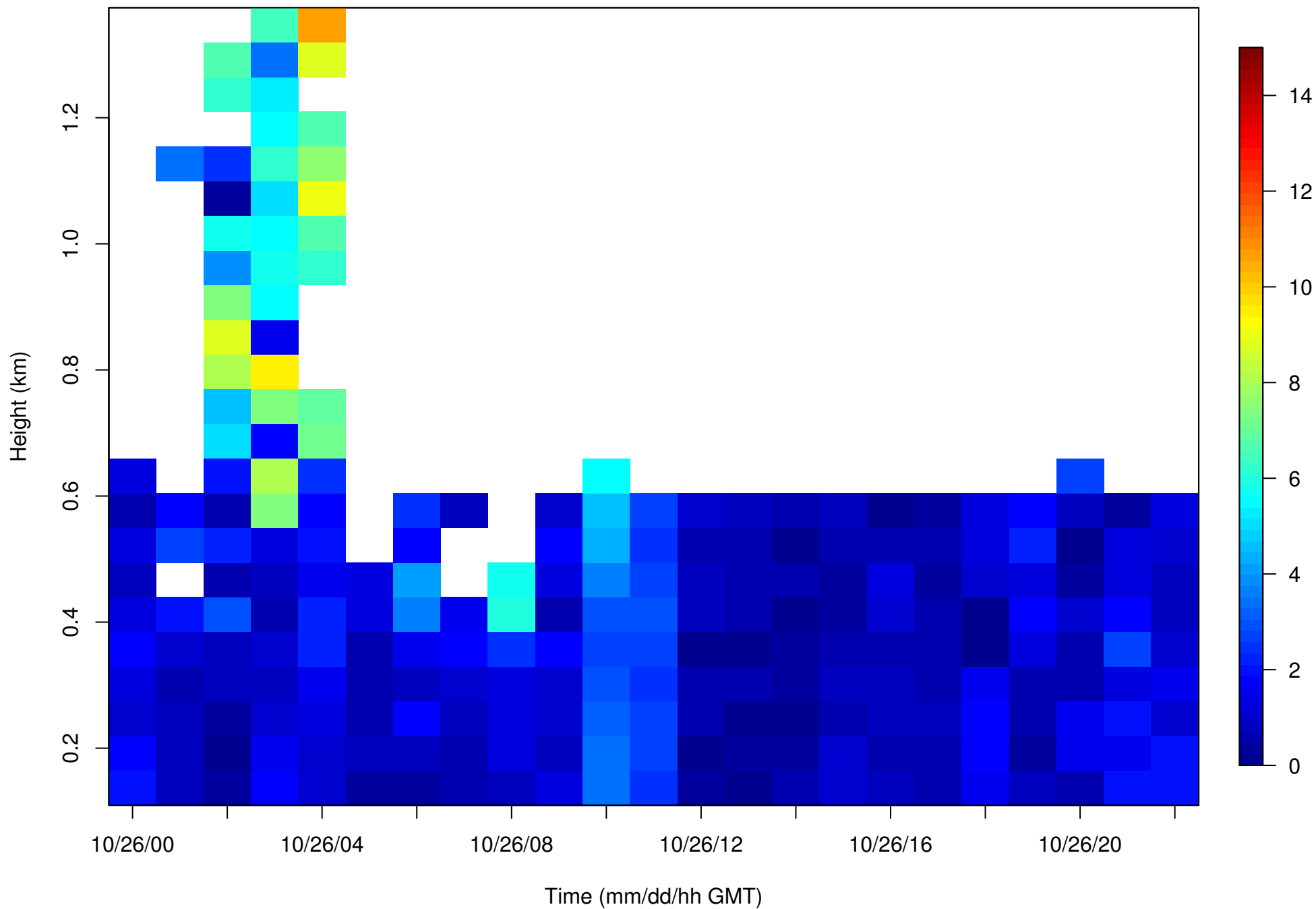
PFL09_low_20001026-SPD-Time_vs_Height
