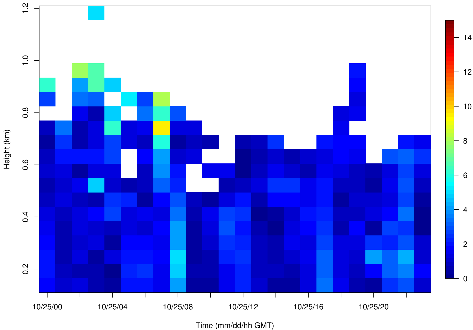
PFL09_low_20001025-SPD-Time_vs_Height
