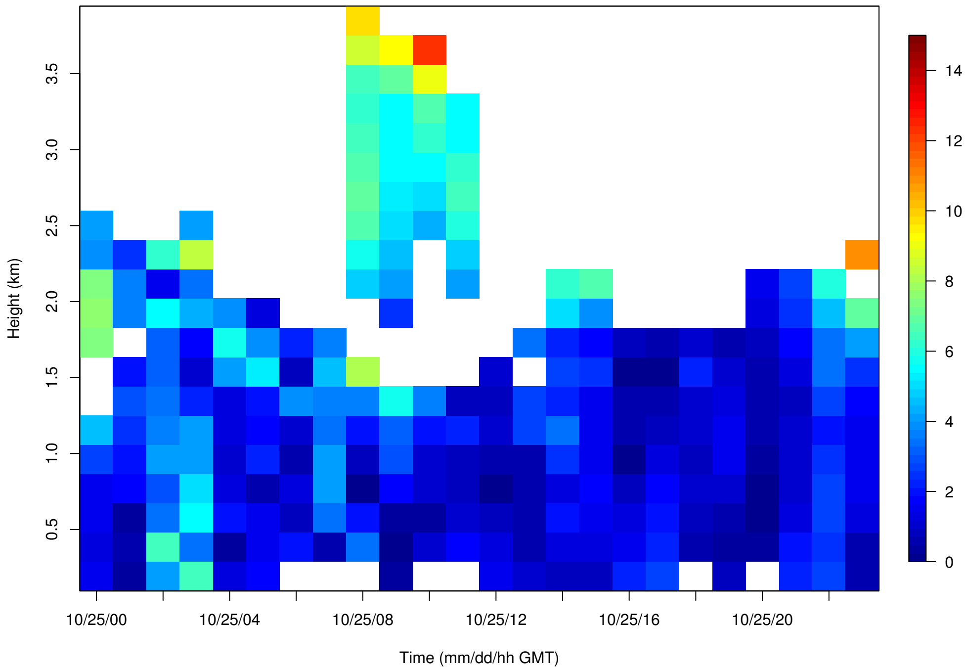
PFL09_high_20001025-SPD-Time_vs_Height
