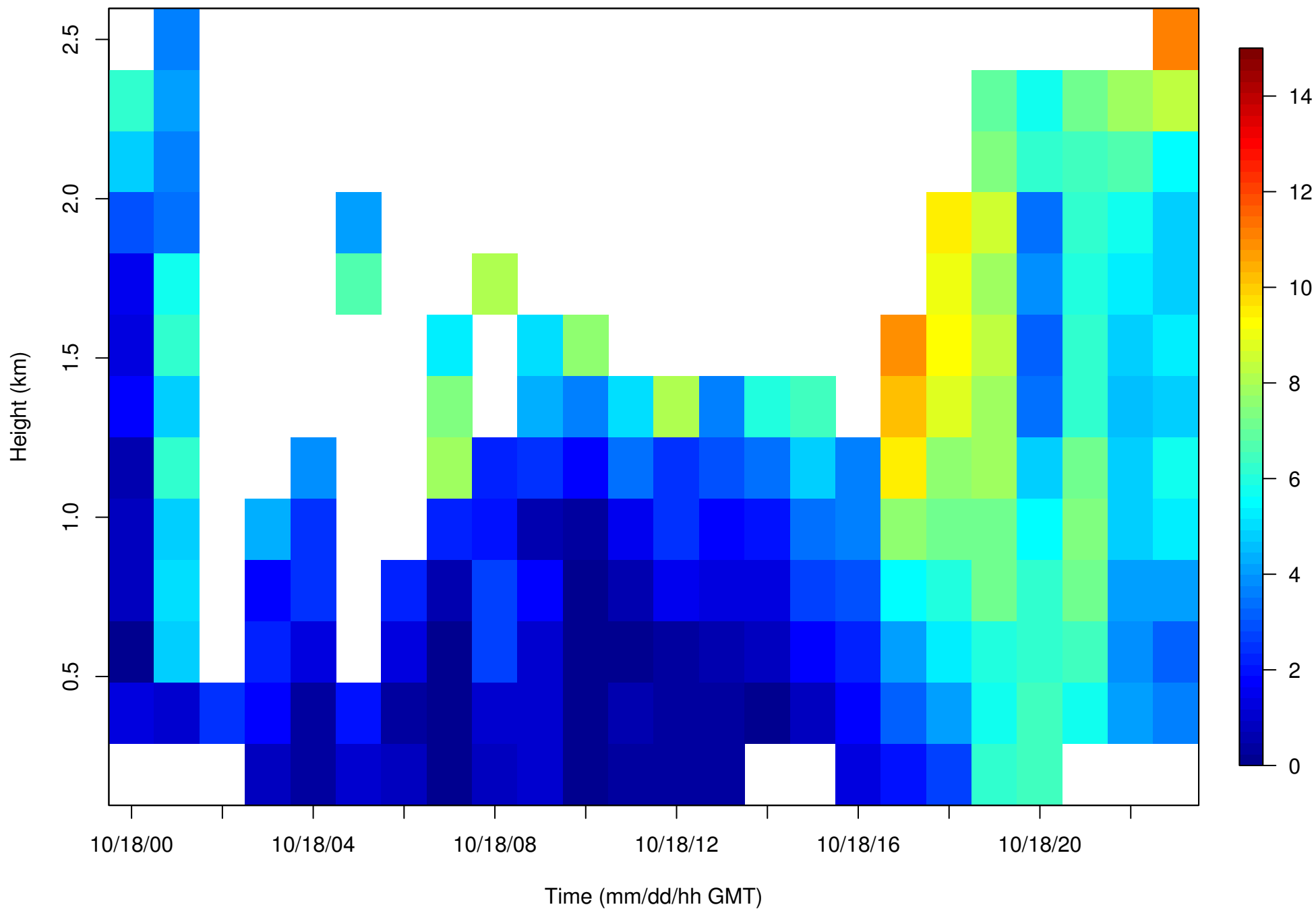
PFL09_high_20001018-SPD-Time_vs_Height
