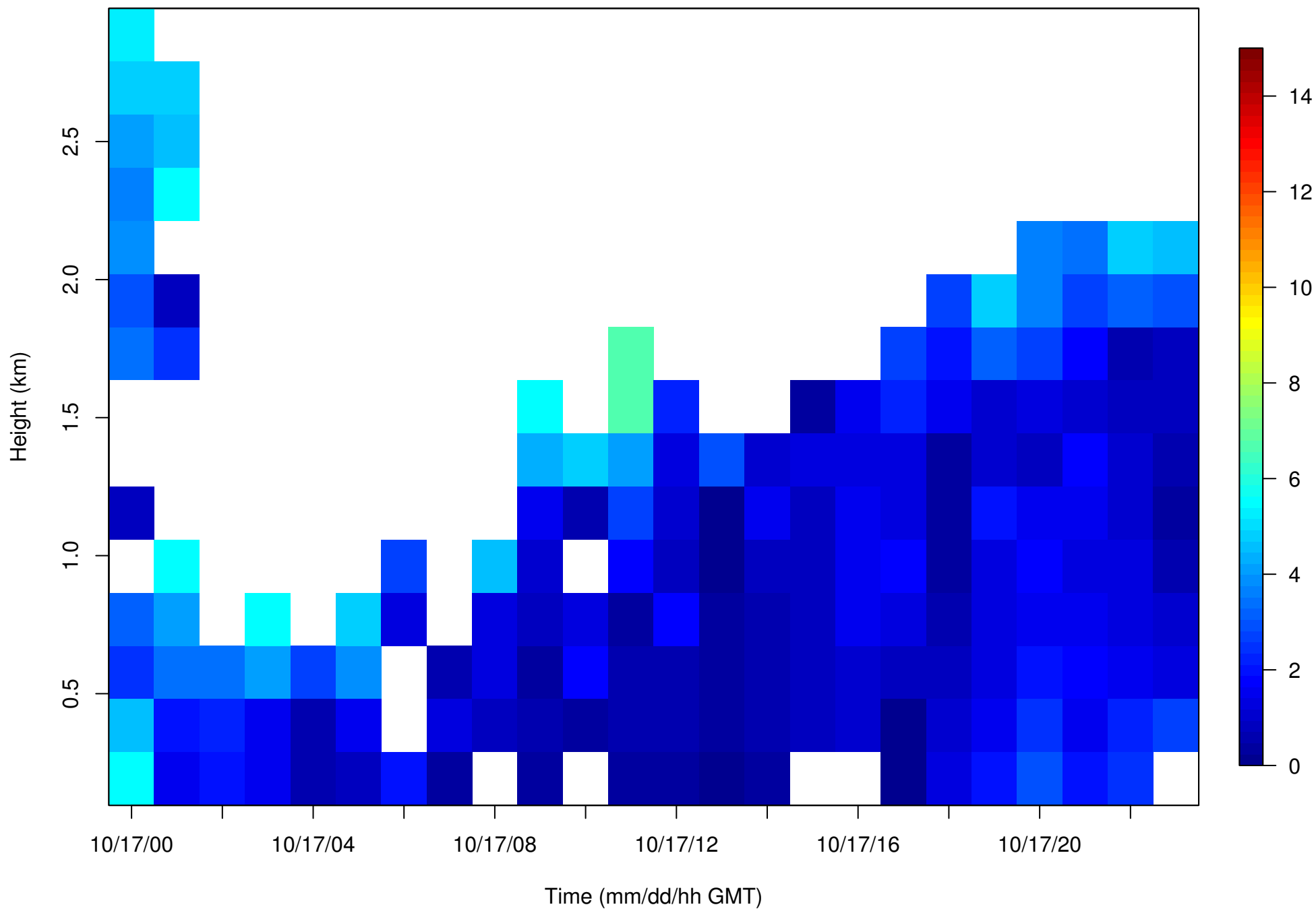
PFL09_high_20001017-SPD-Time_vs_Height
