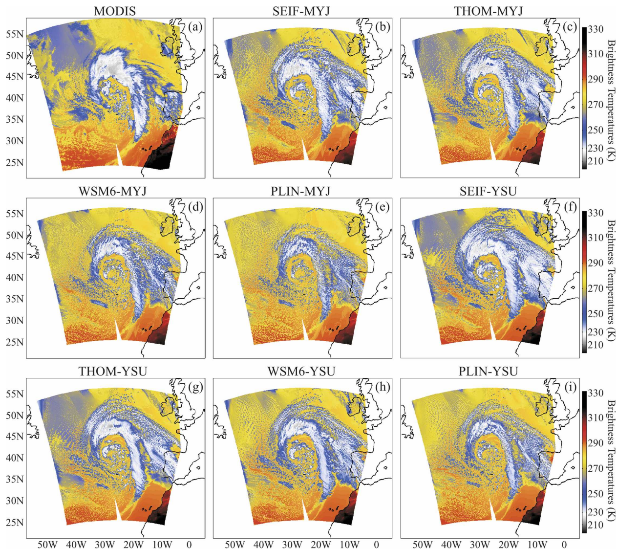
FIG. 5. (a) Composite MODIS 11- \mu m brightness temperatures (K) from the 1405–1415 and 1540–1550 UTC overpasses. Simulated MODIS 11- \mu m brightness temperatures (K) for the (b) SEIF-MYJ, (c) THOM-MYJ, (d) WSM6-MYJ, (e) PLIN-MYJ, (f) SEIF-YSU, (g) THOM-YSU, (h) WSM6-YSU, and (i) PLIN-YSU simulations.
