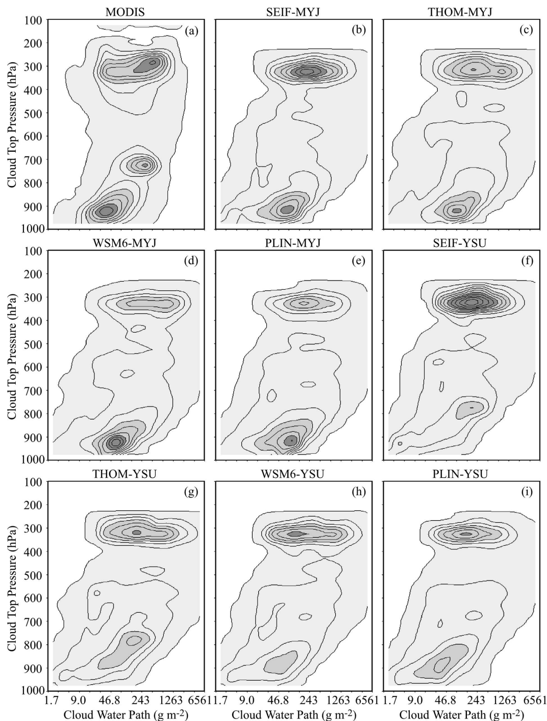
FIG. 7. Cloud water path ( \text{g m}^{-2} )–cloud-top pressure (hPa) probability distributions contoured every 0.3% for the (a) MODIS observations and the (b) SEIF-MYJ, (c) THOM-MYJ, (d) WSM6-MYJ, (e) PLIN-MYJ, (f) SEIF-YSU, (g) THOM-YSU, (h) WSM6-YSU, and (i) PLIN-YSU simulations. Light, medium, and dark shading denote probabilities greater than 0%, 0.9%, and 1.8%, respectively.
