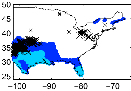
Lifted index 2012040912Z-2012041012Z
