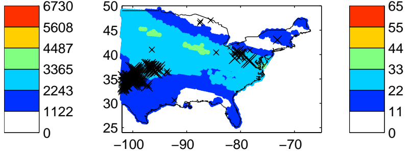
Surf hum (time max CAPE) 2012040912Z-2012041012Z
