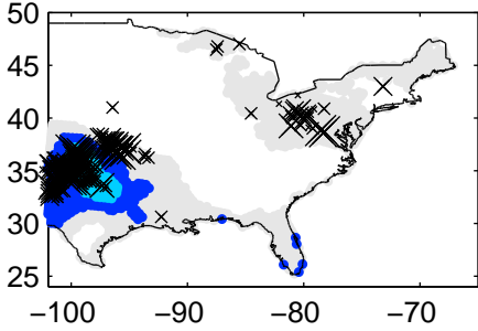
Precip water 2012040912Z-2012041012Z
