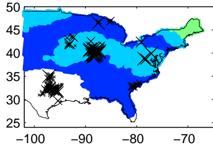
Lifted index 2012040812Z–2012040912Z
