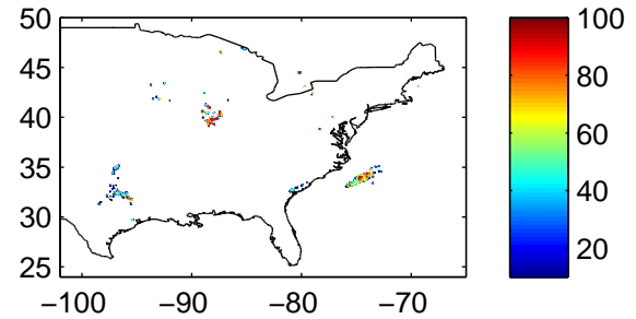
Max POSH 2012040812Z–2012040912Z
