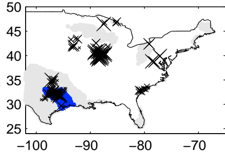
Precip water 2012040812Z–2012040912Z
