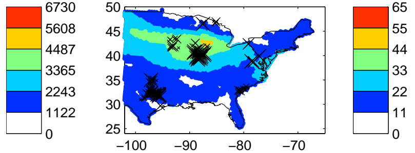
Surf hum (time max CAPE) 2012040812Z–2012040912Z
