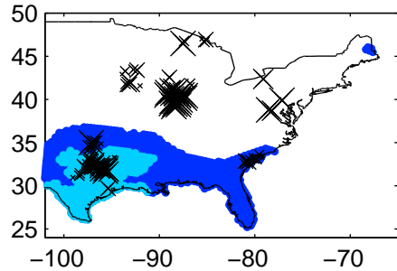
Lifted index 2012040812Z–2012040912Z
