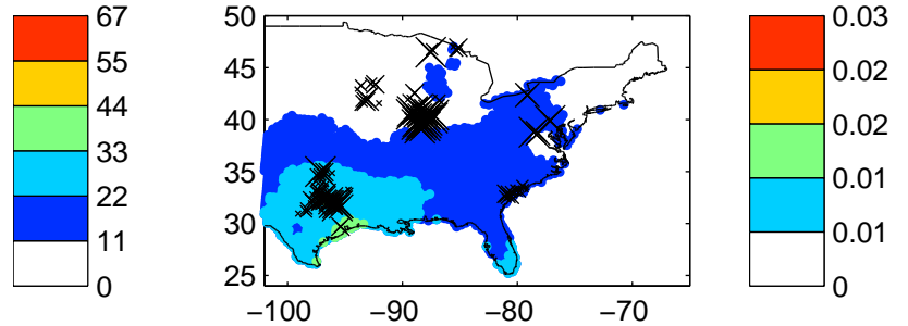
Max POSH 2012040812Z–2012040912Z
