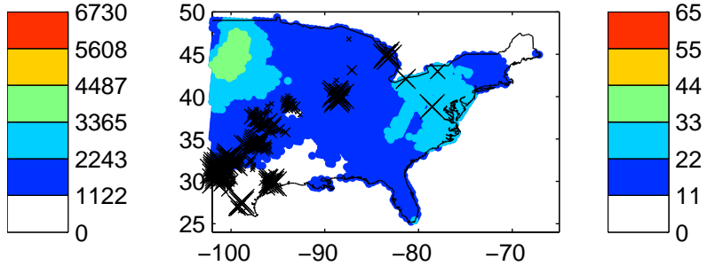
Surf hum (time max CAPE) 2012040712Z–2012040812Z
