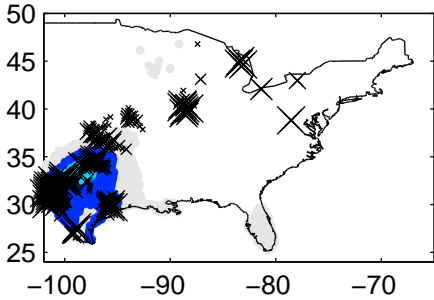
Precip water 2012040712Z–2012040812Z
