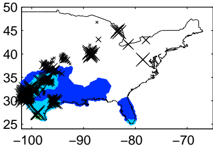
Lifted index 2012040712Z–2012040812Z
