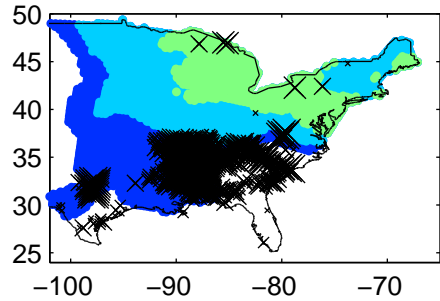
Lifted index 2012040512Z-2012040612Z
