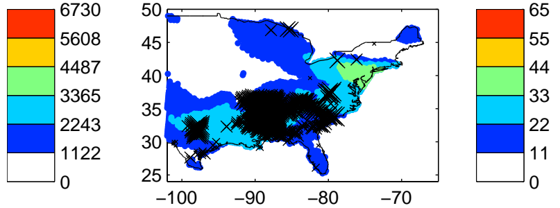
Surf hum (time max CAPE) 2012040512Z-2012040612Z
