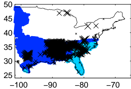
Lifted index 2012040512Z-2012040612Z
