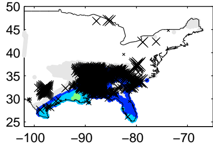
Precip water 2012040512Z-2012040612Z
