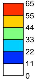
Shear (time max CAPE) 2012040412Z-2012040512Z
