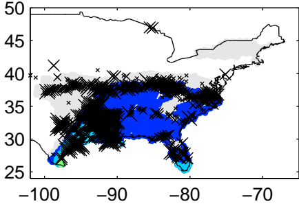
Precip water 2012040412Z-2012040512Z
