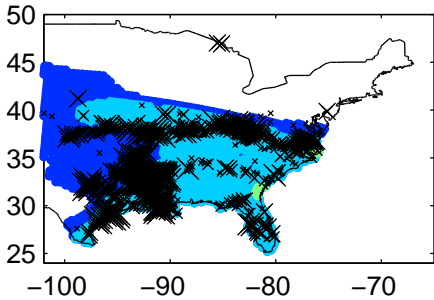
Lifted index 2012040412Z-2012040512Z
