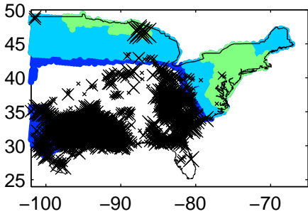
Lifted index 2012040312Z-2012040412Z
