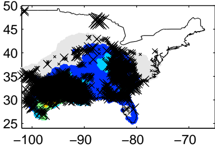
Precip water 2012040312Z-2012040412Z
