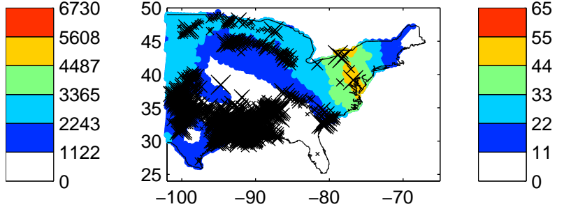
Surf hum (time max CAPE) 2012040212Z-2012040312Z
