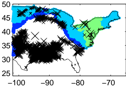
Lifted index 2012040212Z-2012040312Z
