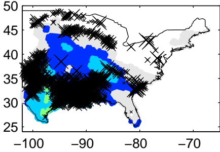
Precip water 2012040212Z-2012040312Z
