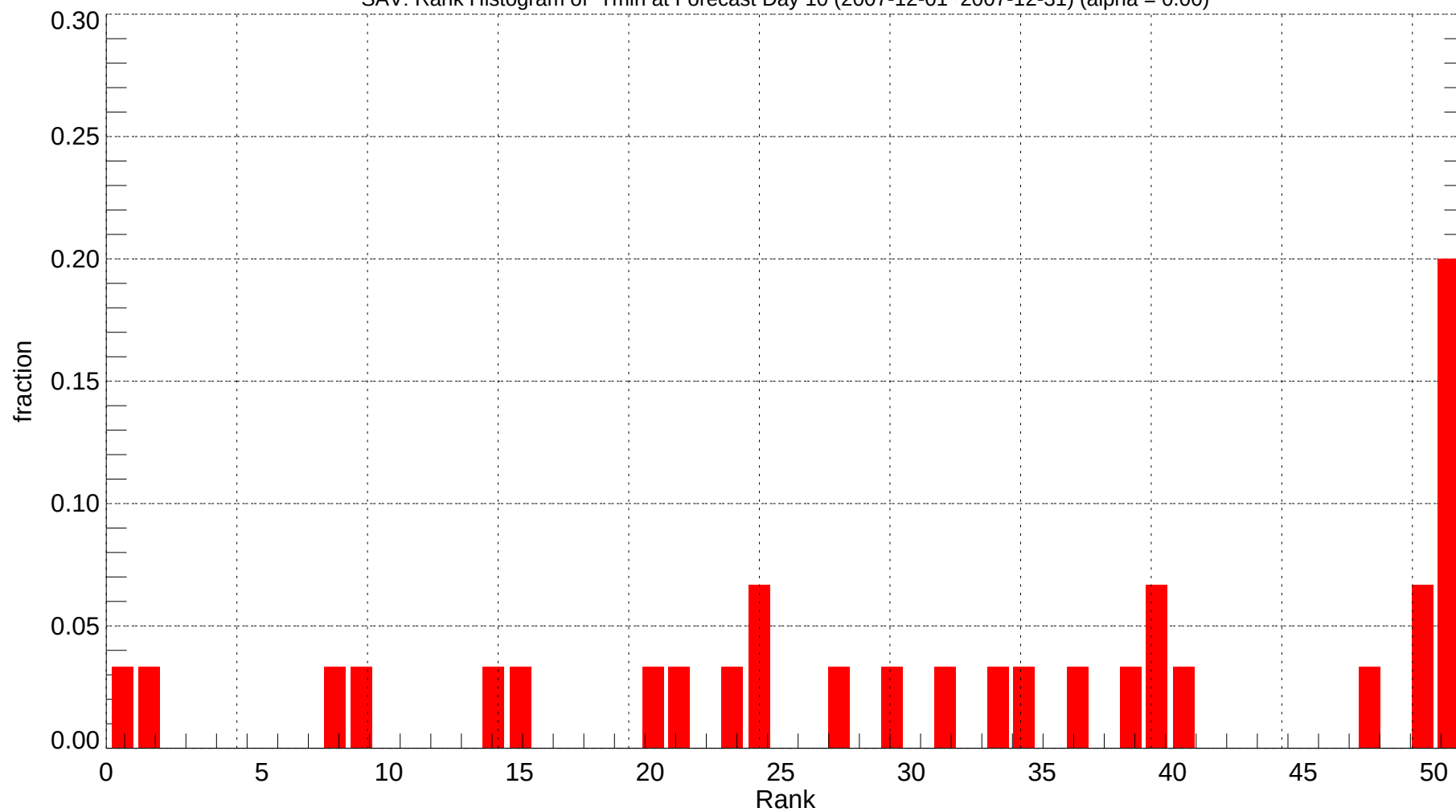
SAV: Rank Histogram of Tmin at Forecast Day 10 (2007-12-01~2007-12-31) (alpha = 0.00)
