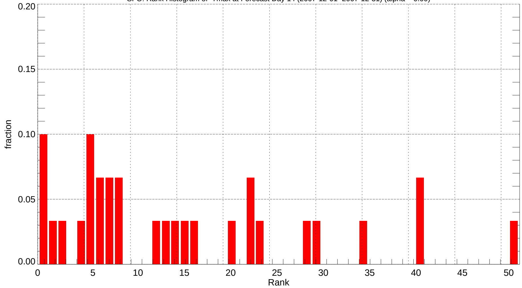
SFO: Rank Histogram of Tmax at Forecast Day 14 (2007-12-01~2007-12-31) (alpha = 0.00)
