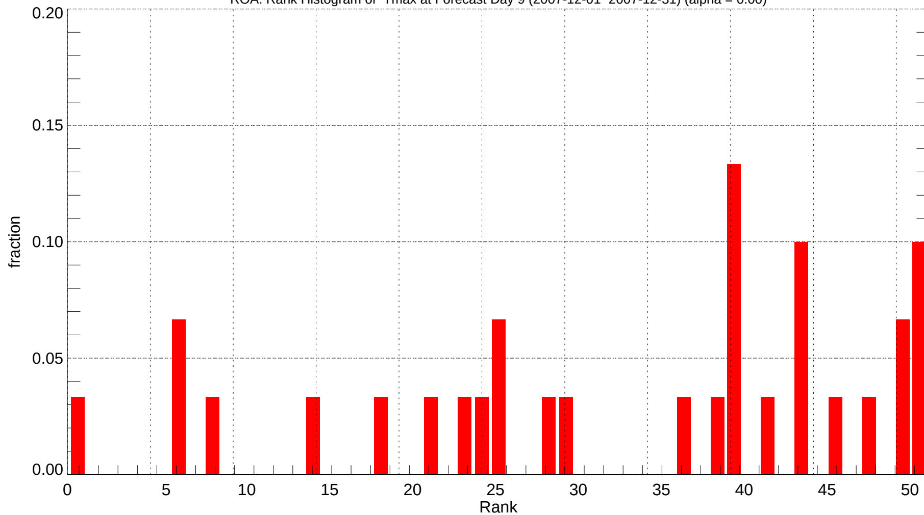
ROA: Rank Histogram of Tmax at Forecast Day 9 (2007-12-01~2007-12-31) (alpha = 0.00)
