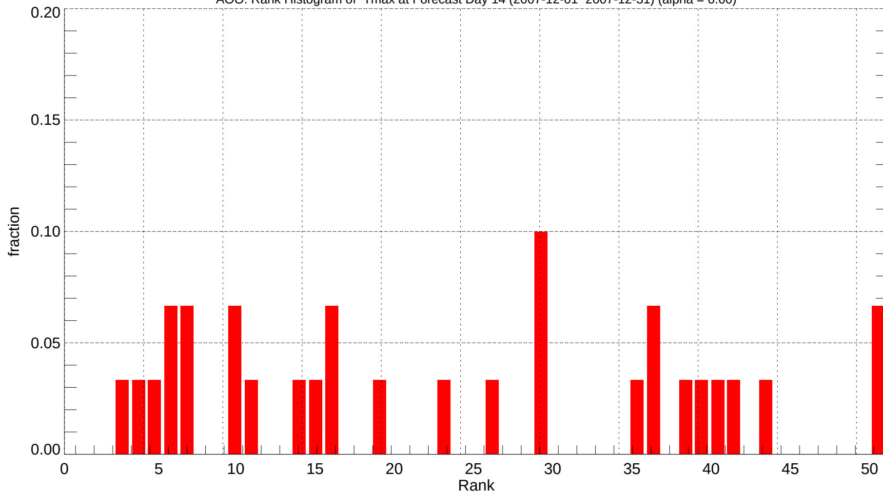
AOO: Rank Histogram of Tmax at Forecast Day 14 (2007-12-01~2007-12-31) (alpha = 0.00)
