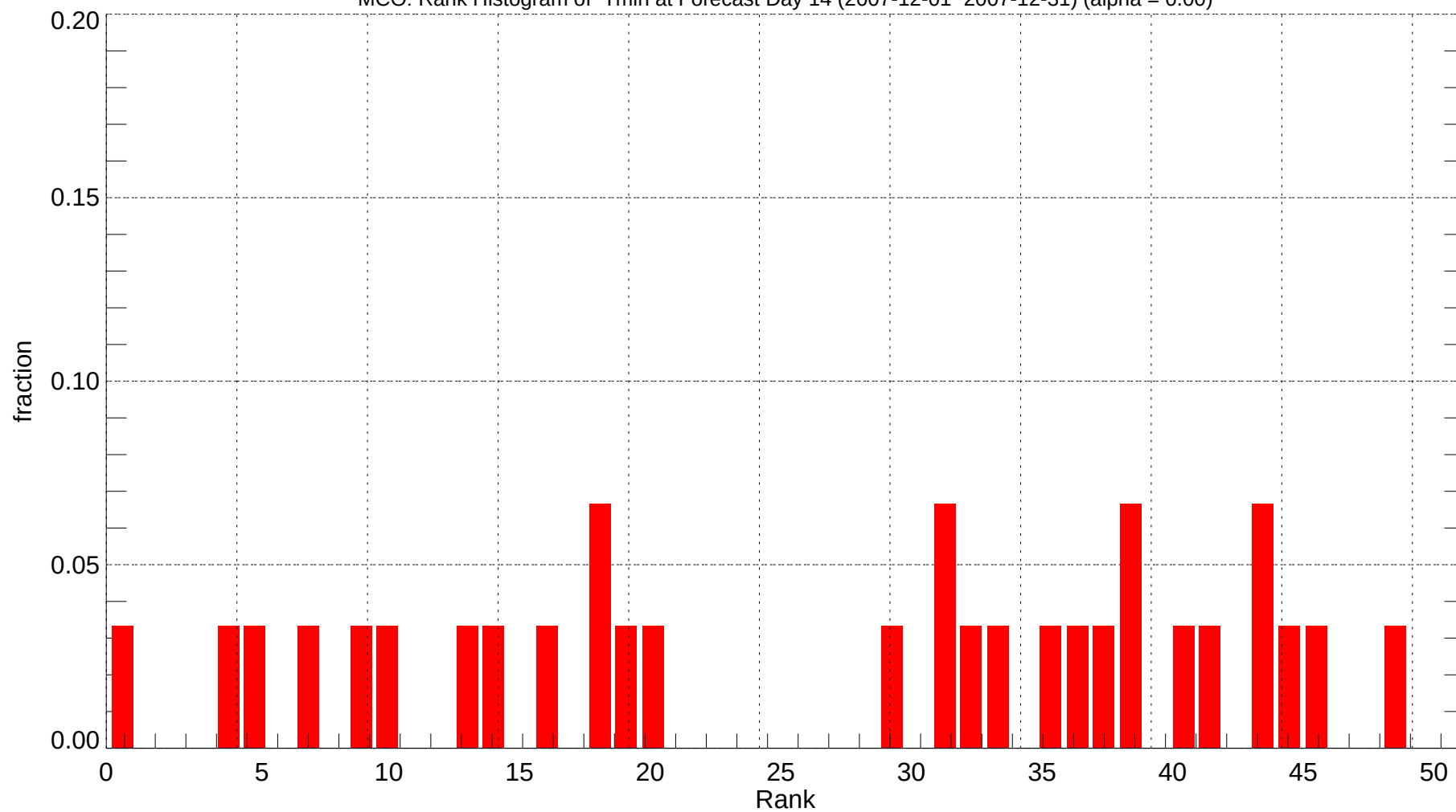
MCO: Rank Histogram of Tmin at Forecast Day 14 (2007-12-01~2007-12-31) (alpha = 0.00)
