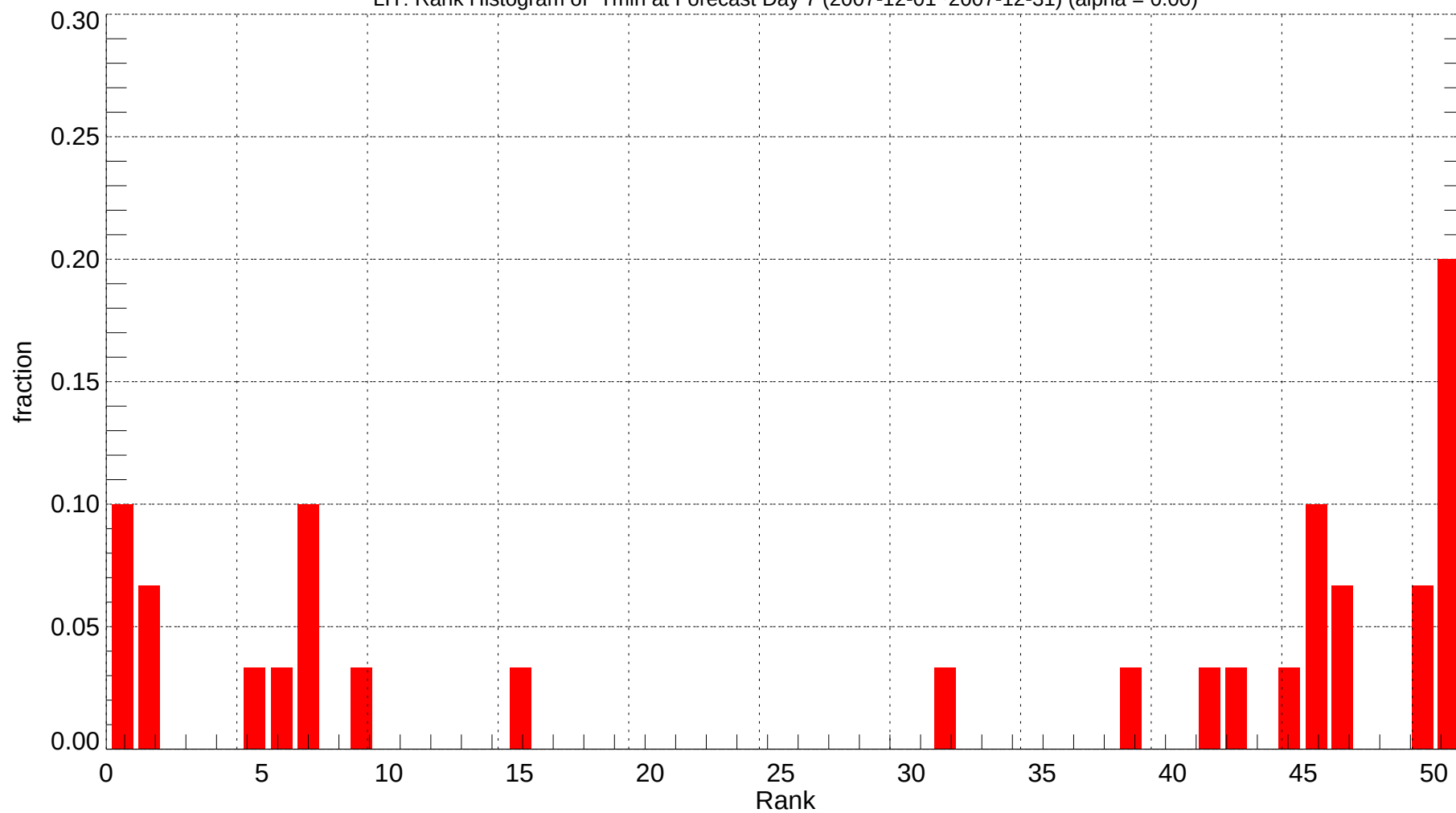
LIT: Rank Histogram of Tmin at Forecast Day 7 (2007-12-01~2007-12-31) (alpha = 0.00)
