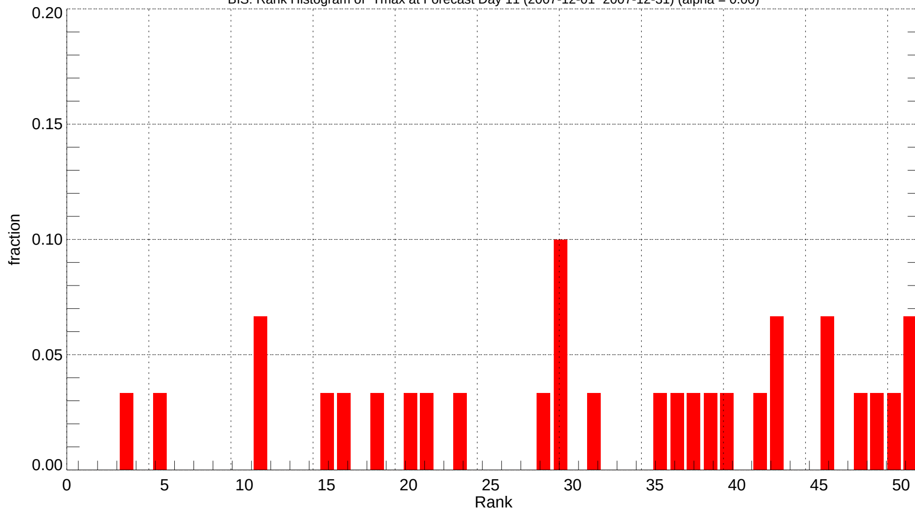
BIS: Rank Histogram of Tmax at Forecast Day 11 (2007-12-01~2007-12-31) (alpha = 0.00)
