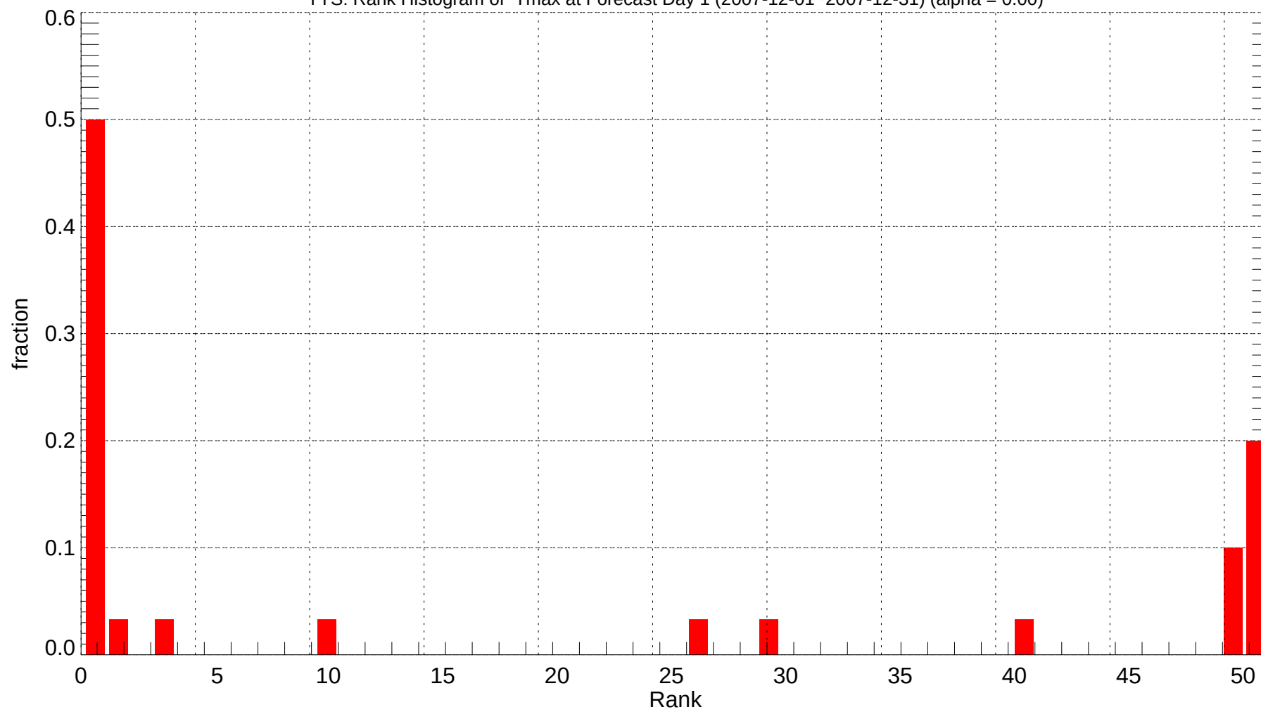
TYS: Rank Histogram of Tmax at Forecast Day 1 (2007-12-01~2007-12-31) (alpha = 0.00)
