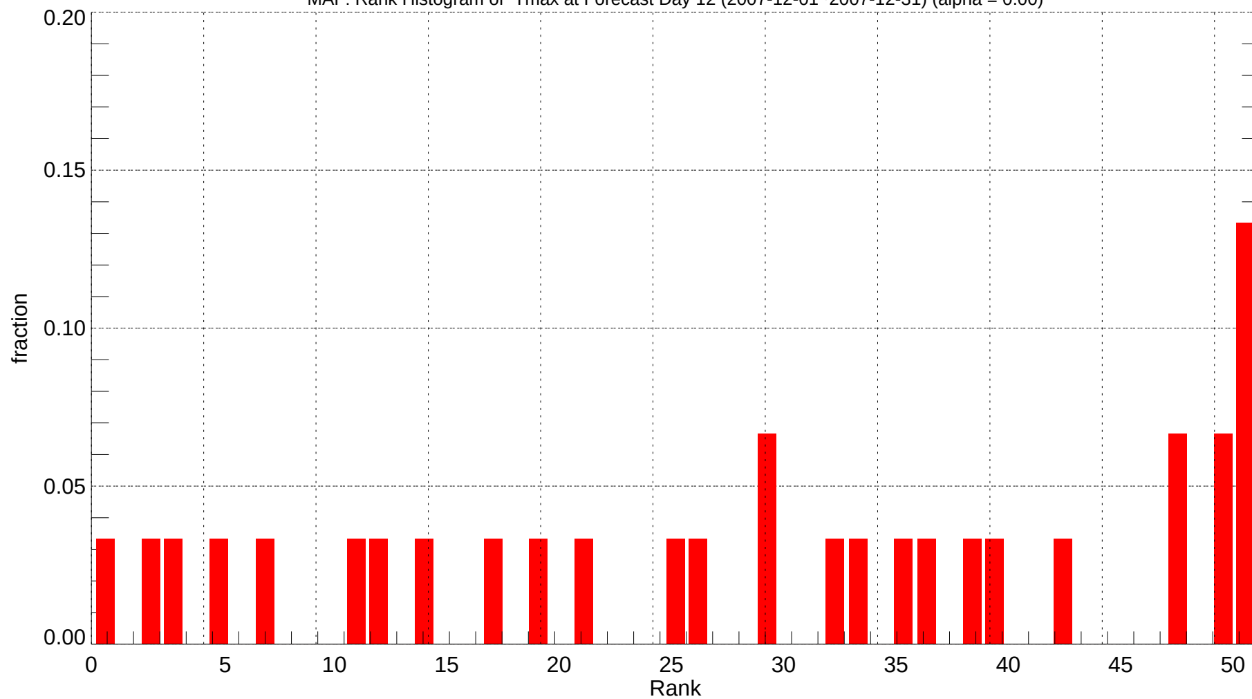
MAF: Rank Histogram of Tmax at Forecast Day 12 (2007-12-01~2007-12-31) (alpha = 0.00)
