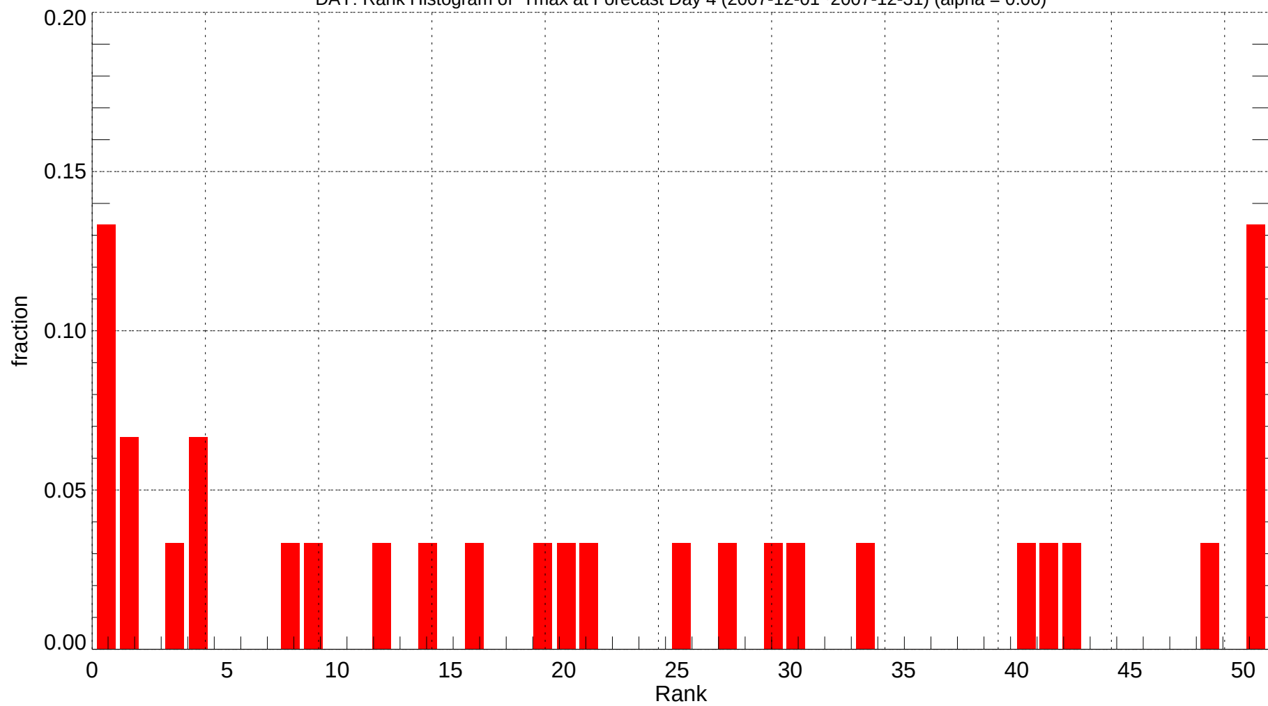
DAY: Rank Histogram of Tmax at Forecast Day 4 (2007-12-01~2007-12-31) (alpha = 0.00)
