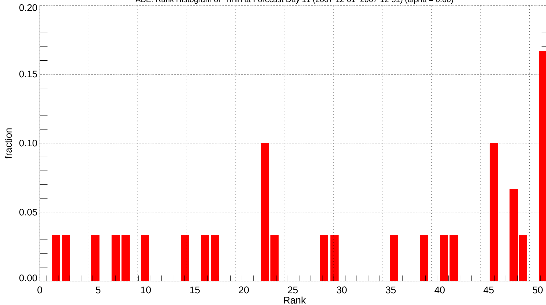
ABE: Rank Histogram of Tmin at Forecast Day 11 (2007-12-01~2007-12-31) (alpha = 0.00)
