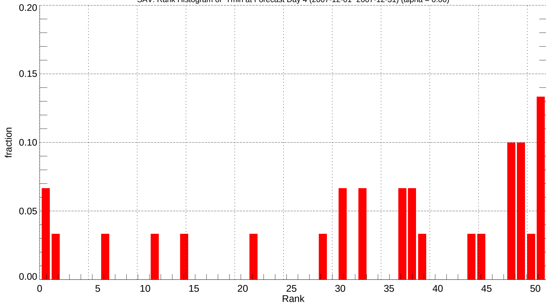
SAV: Rank Histogram of Tmin at Forecast Day 4 (2007-12-01~2007-12-31) (alpha = 0.00)
