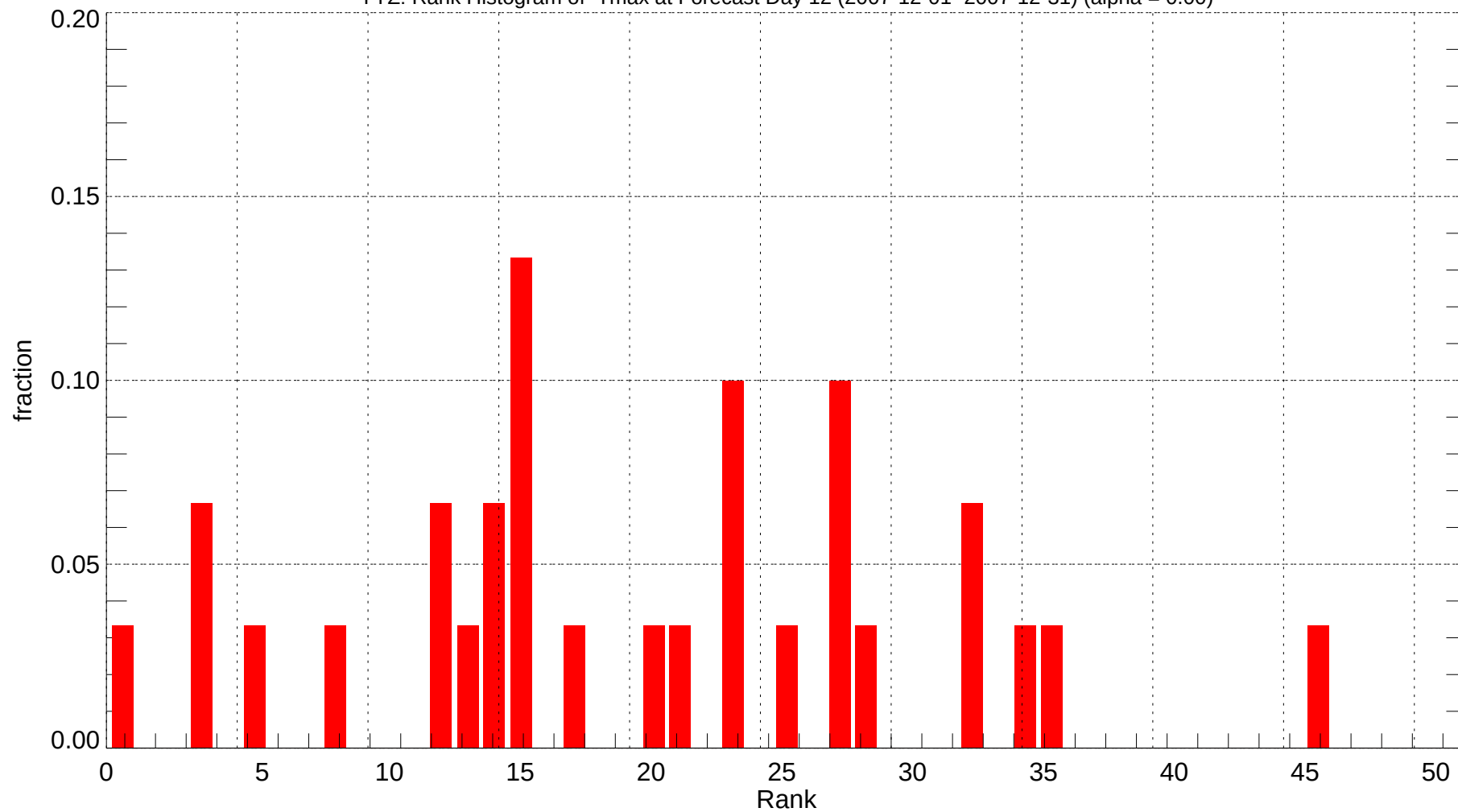
YYZ: Rank Histogram of Tmax at Forecast Day 12 (2007-12-01~2007-12-31) (alpha = 0.00)
