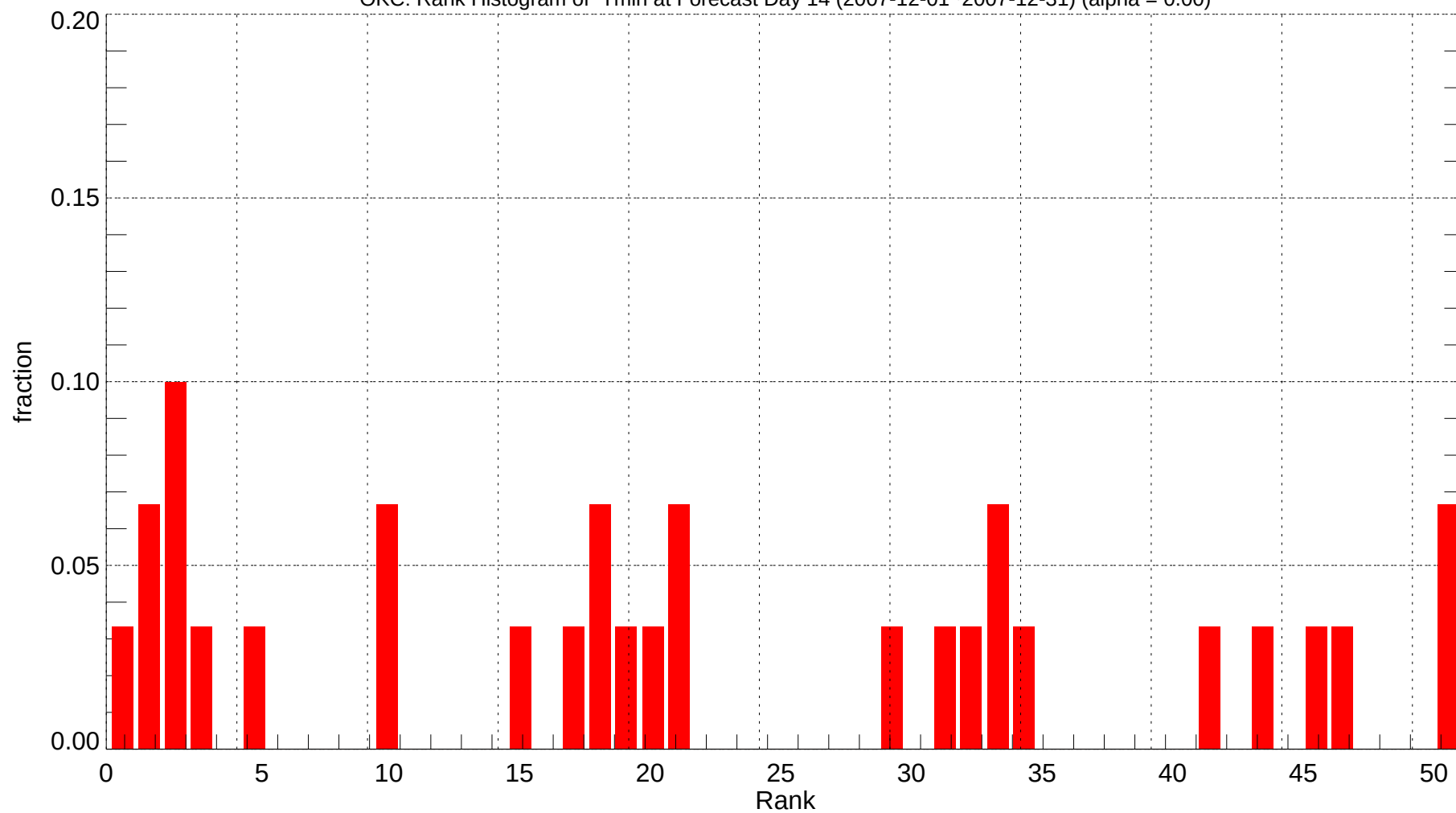
OKC: Rank Histogram of Tmin at Forecast Day 14 (2007-12-01~2007-12-31) (alpha = 0.00)
