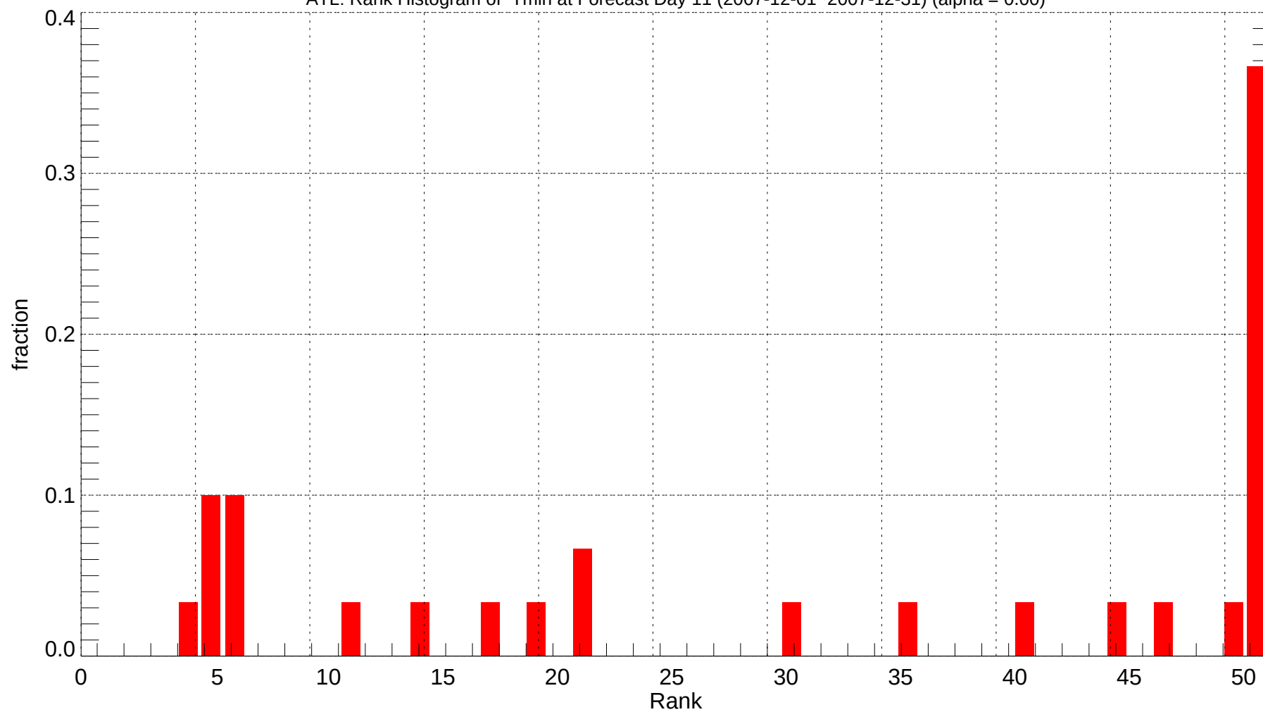
ATL: Rank Histogram of Tmin at Forecast Day 11 (2007-12-01~2007-12-31) (alpha = 0.00)
