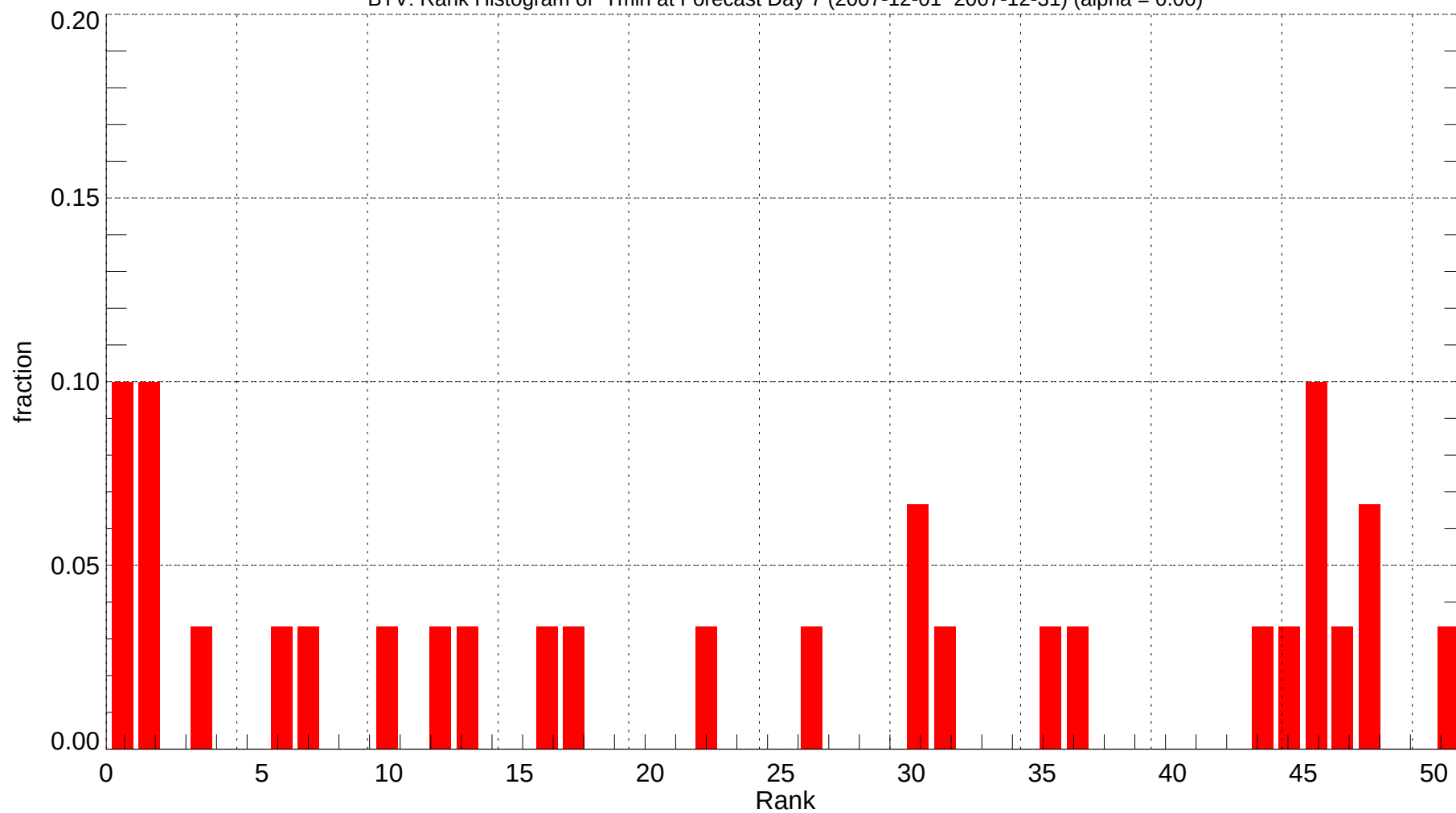
BTV: Rank Histogram of Tmin at Forecast Day 7 (2007-12-01~2007-12-31) (alpha = 0.00)
