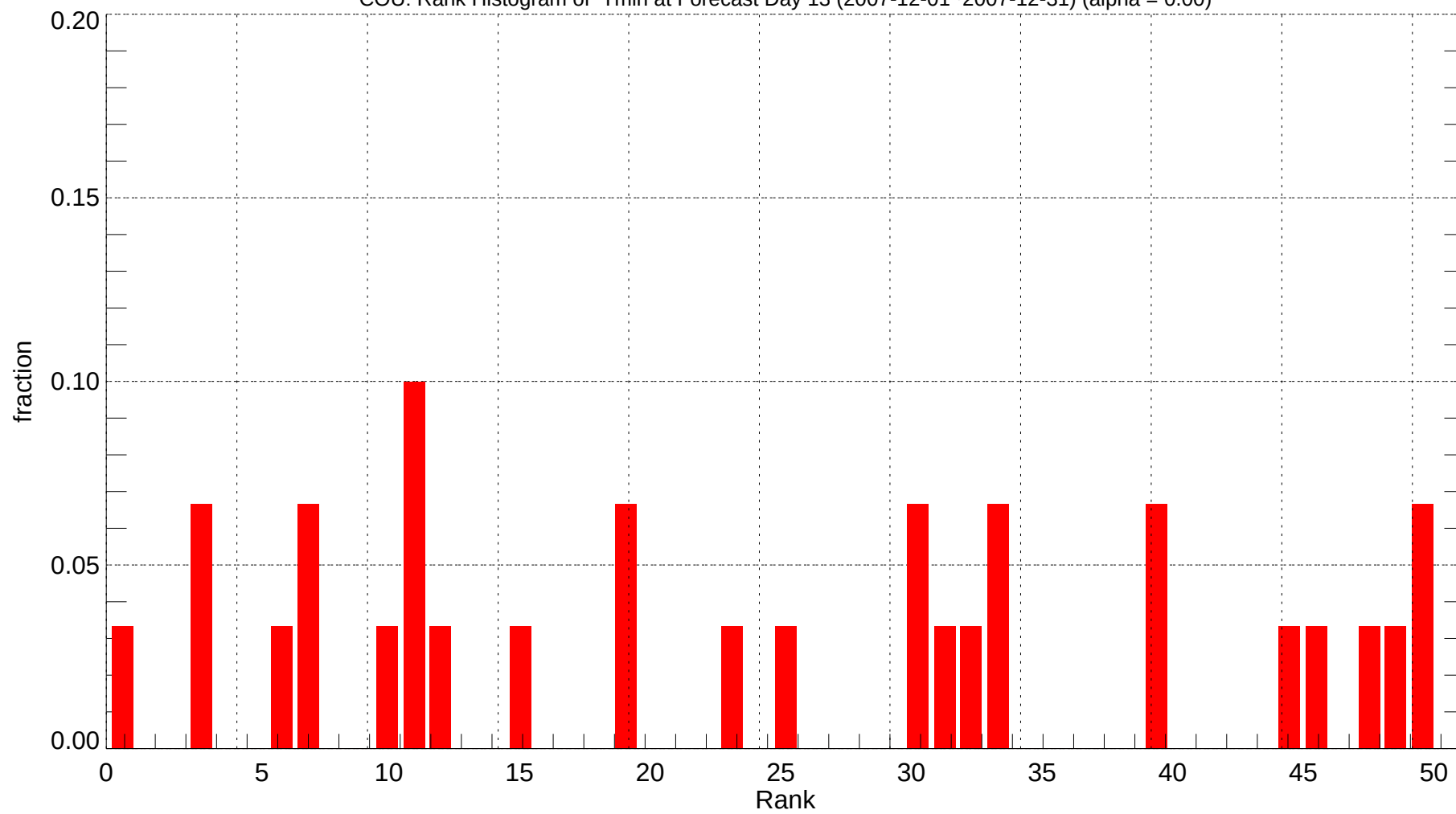
COU: Rank Histogram of Tmin at Forecast Day 13 (2007-12-01~2007-12-31) (alpha = 0.00)
