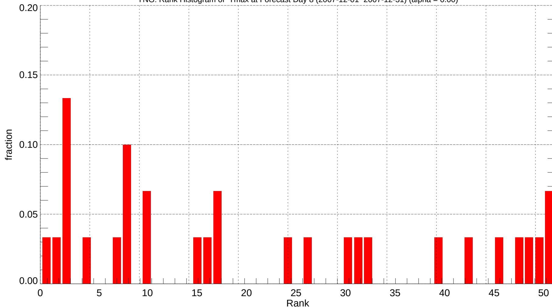
YNG: Rank Histogram of Tmax at Forecast Day 8 (2007-12-01~2007-12-31) (alpha = 0.00)
