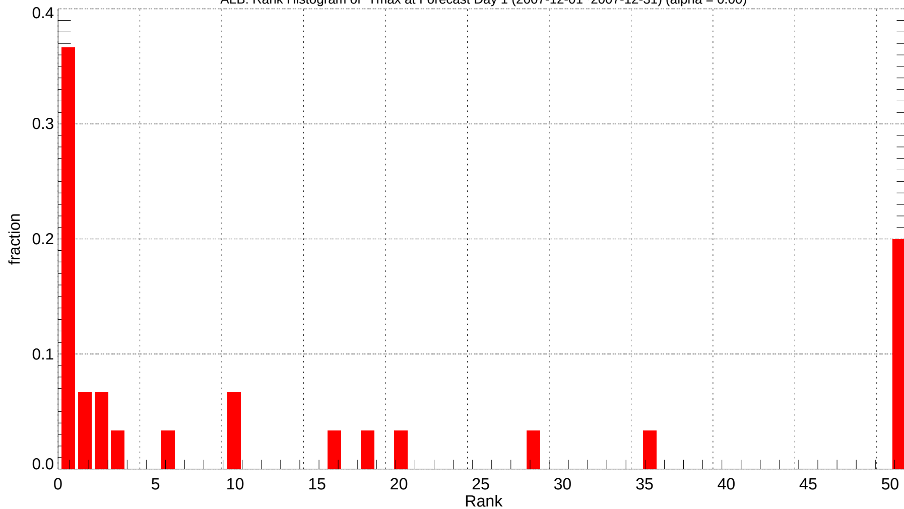
ALB: Rank Histogram of Tmax at Forecast Day 1 (2007-12-01~2007-12-31) (alpha = 0.00)
