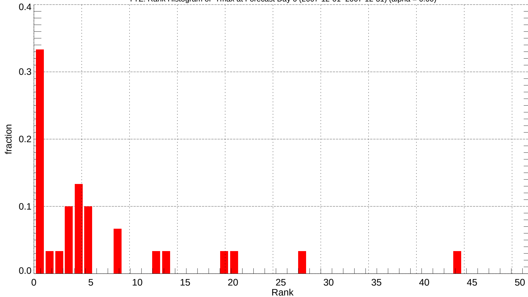
YYZ: Rank Histogram of Tmax at Forecast Day 6 (2007-12-01~2007-12-31) (alpha = 0.00)
