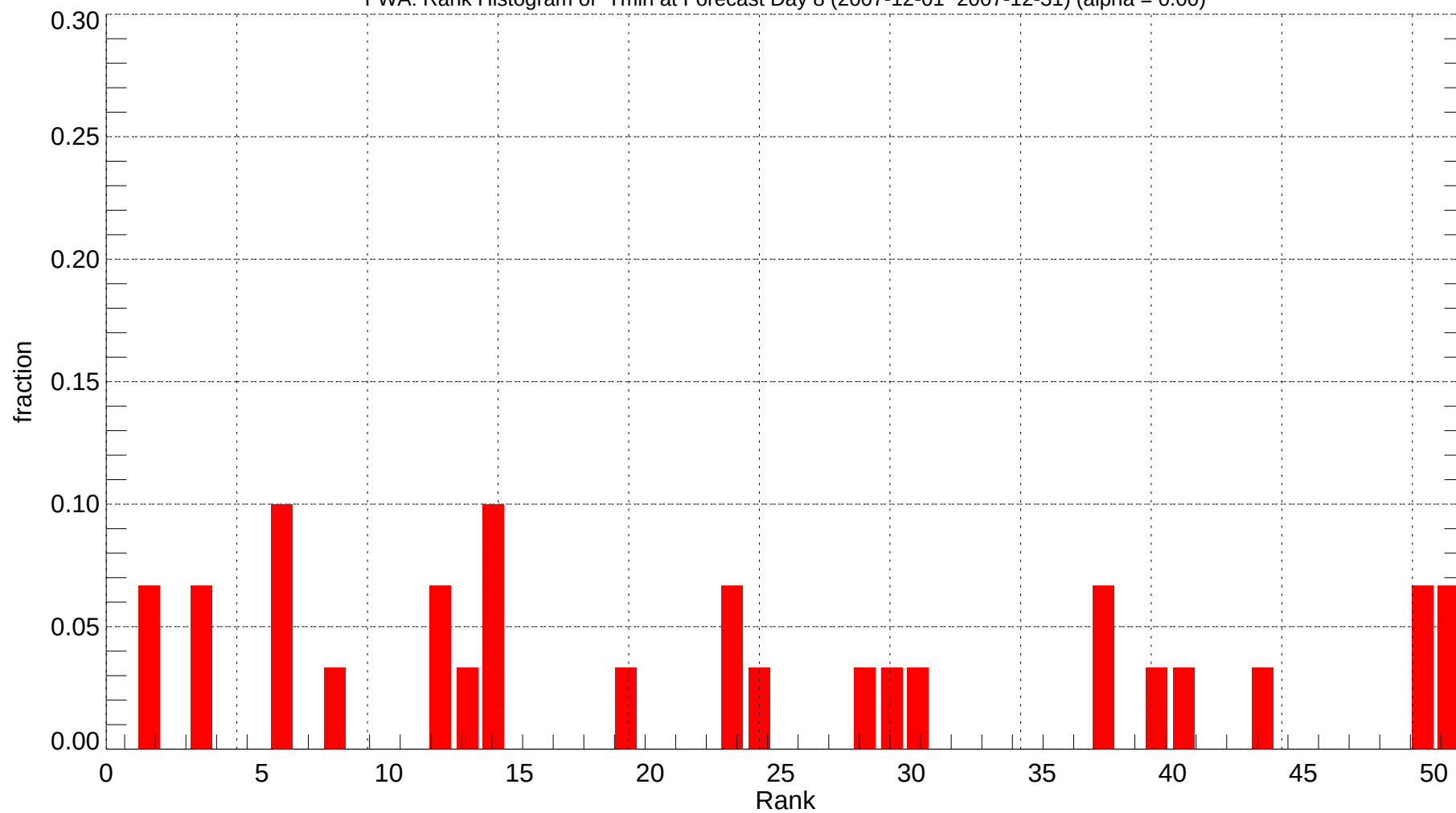
FWA: Rank Histogram of Tmin at Forecast Day 8 (2007-12-01~2007-12-31) (alpha = 0.00)
