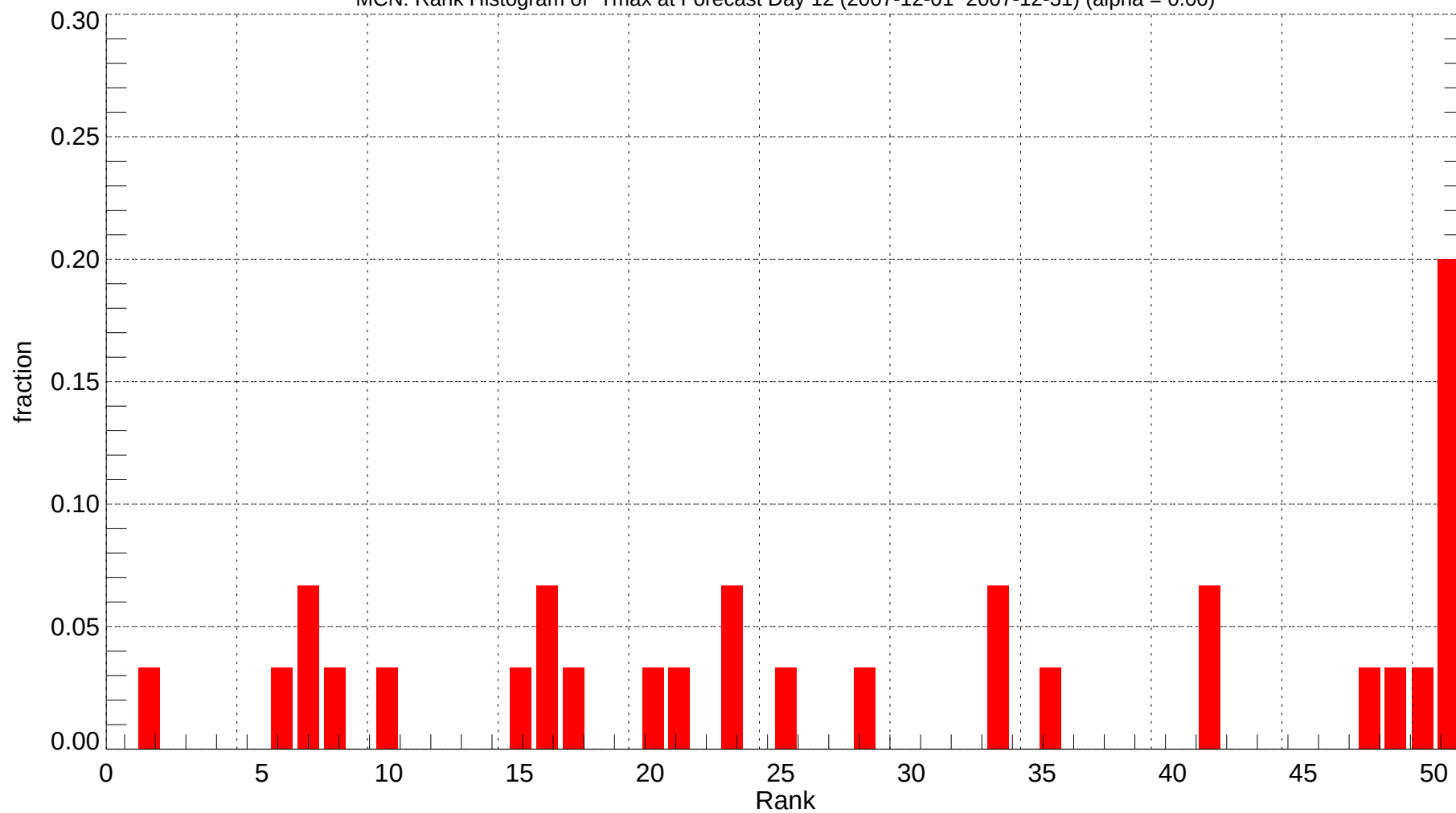
MCN: Rank Histogram of Tmax at Forecast Day 12 (2007-12-01~2007-12-31) (alpha = 0.00)
