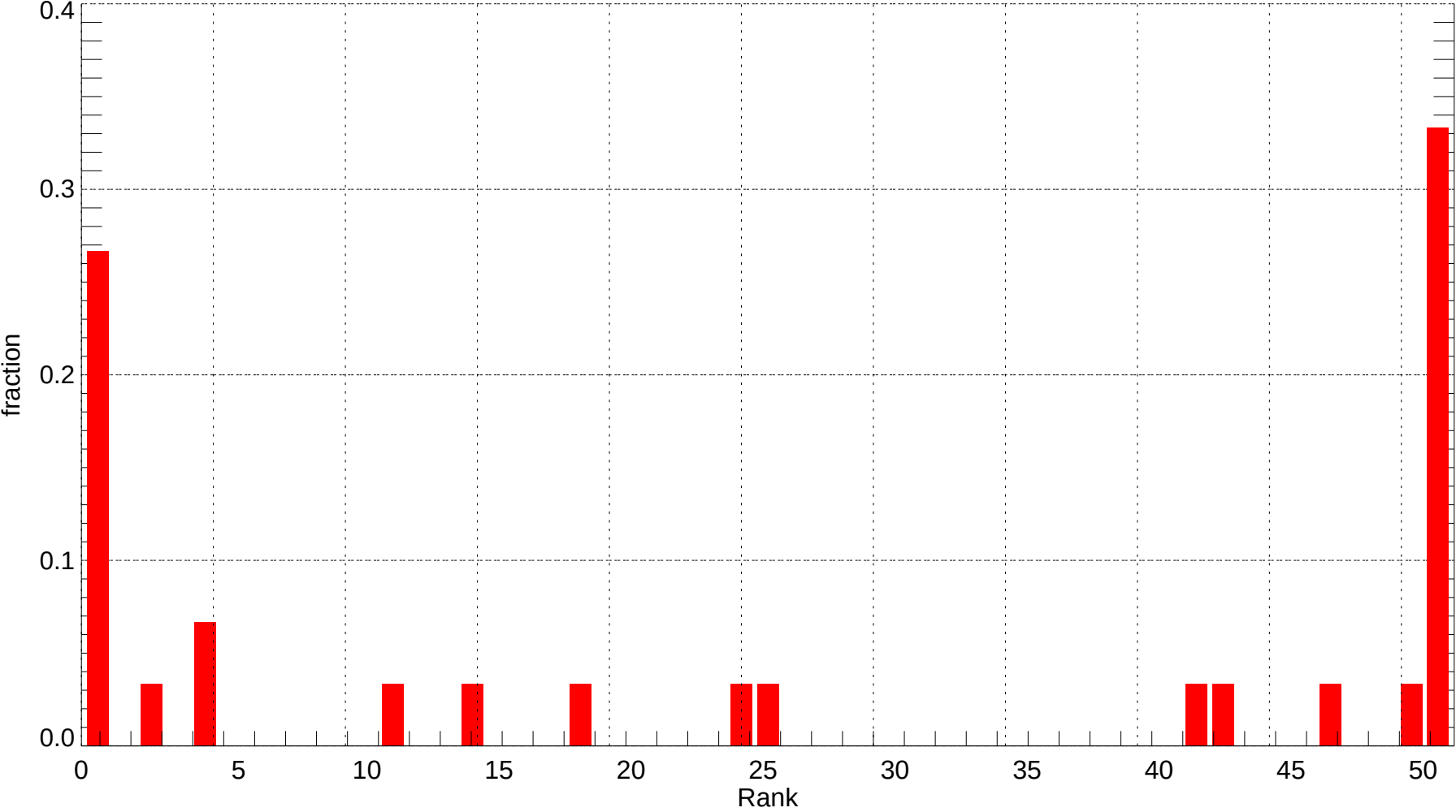
BIS: Rank Histogram of Tmax at Forecast Day 1 (2007-12-01~2007-12-31) (alpha = 0.00)
