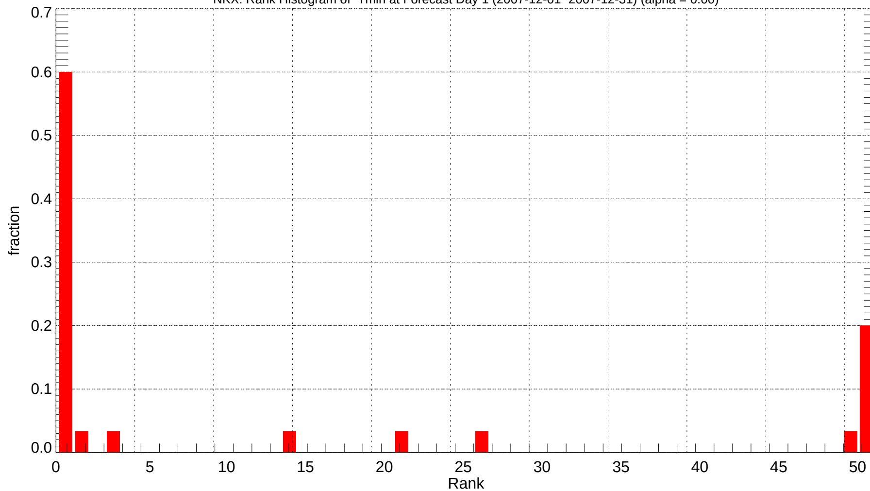
NKX: Rank Histogram of Tmin at Forecast Day 1 (2007-12-01~2007-12-31) (alpha = 0.00)
