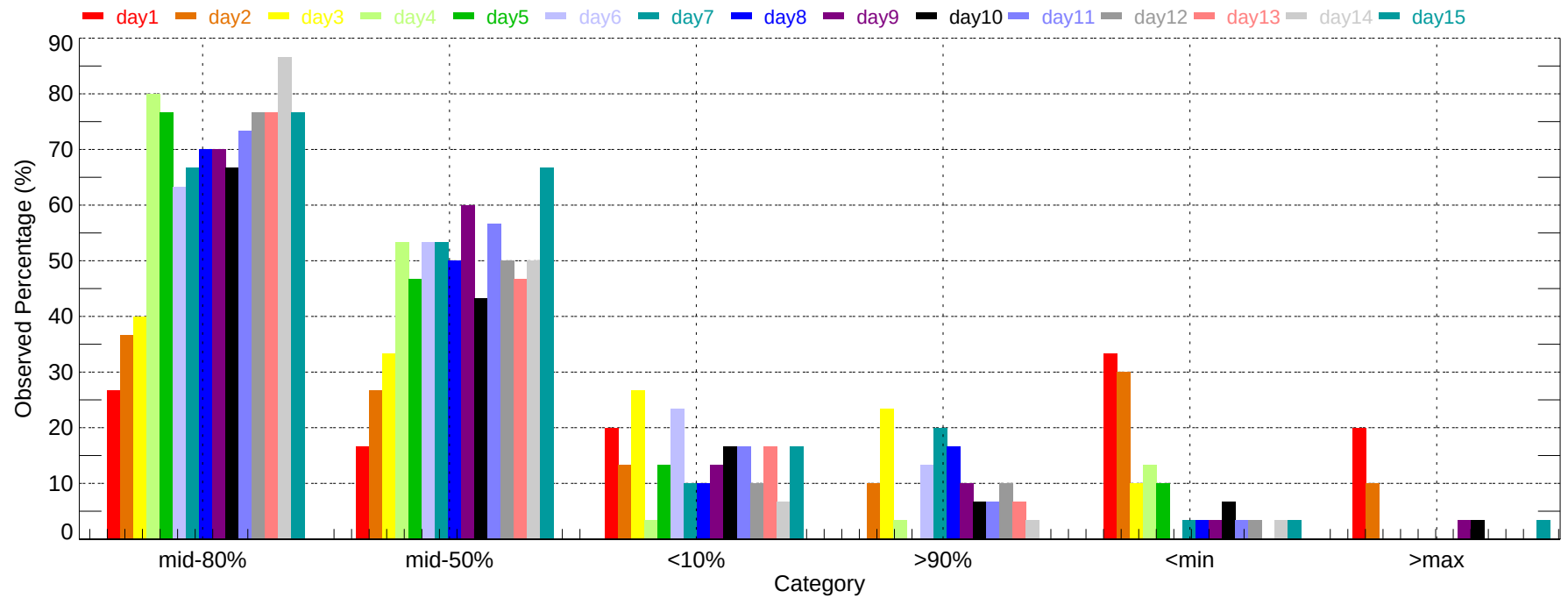
Observed Percentage of Ensembles - ALB: Max Temperature (2007-12-01~2007-12-31)
