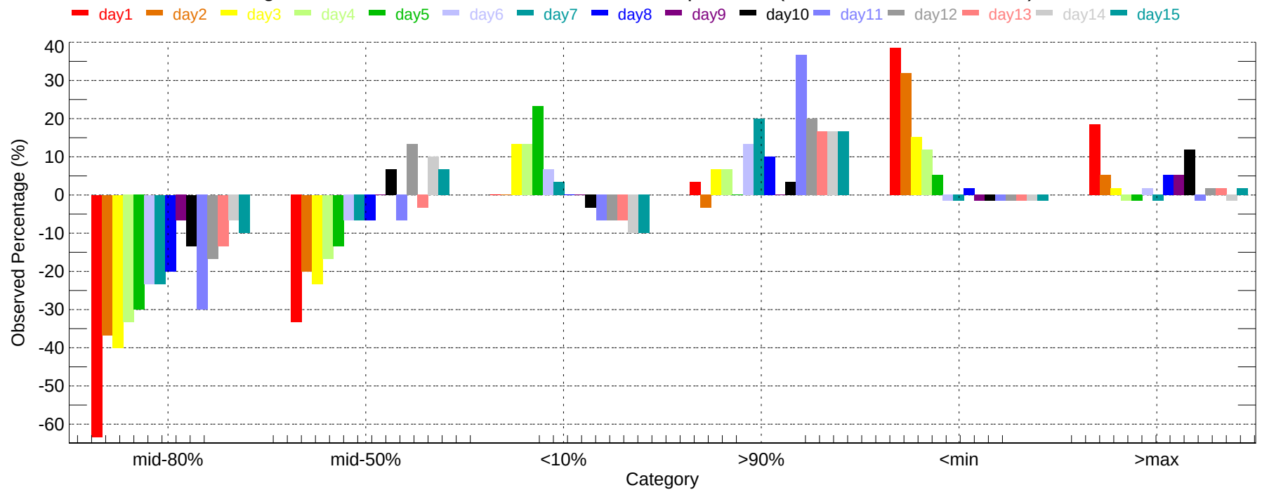
Observed Percentage Deviation of Ensembles - ERI: Min Temperature (2007-12-01~2007-12-31)
