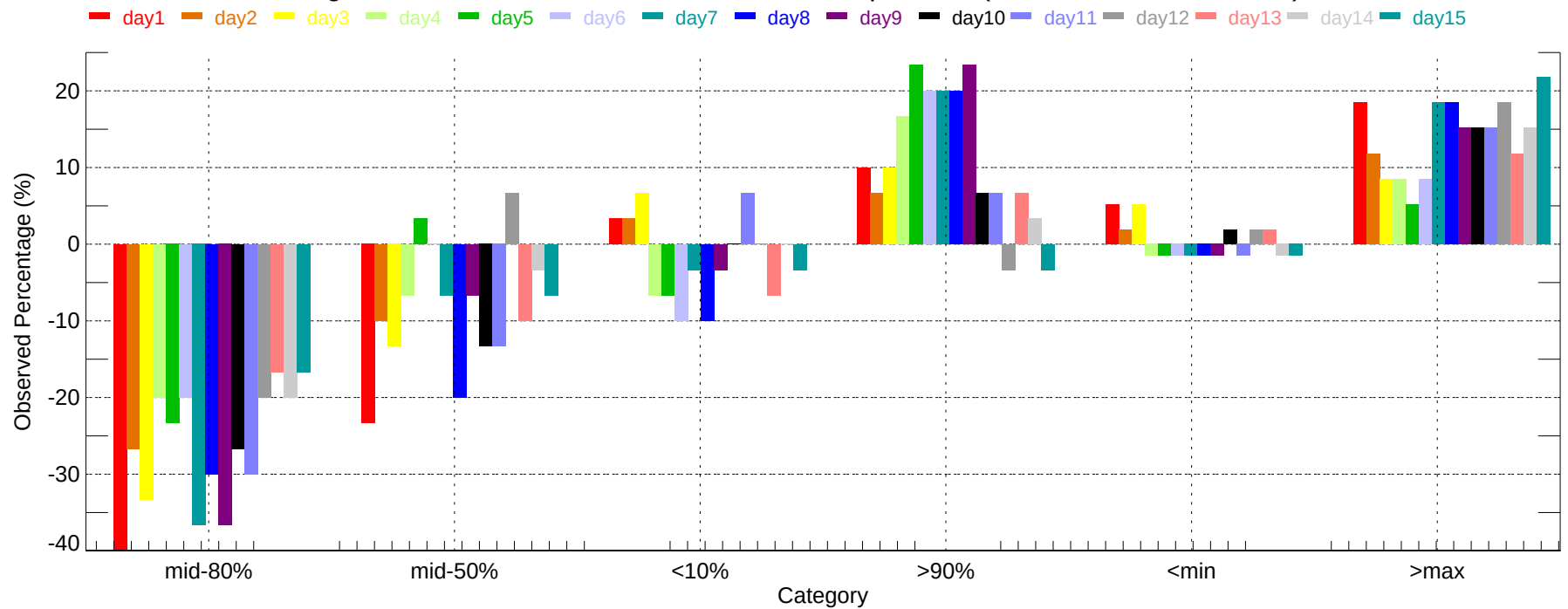
Observed Percentage Deviation of Ensembles - HOU: Min Temperature (2007-12-01~2007-12-31)
