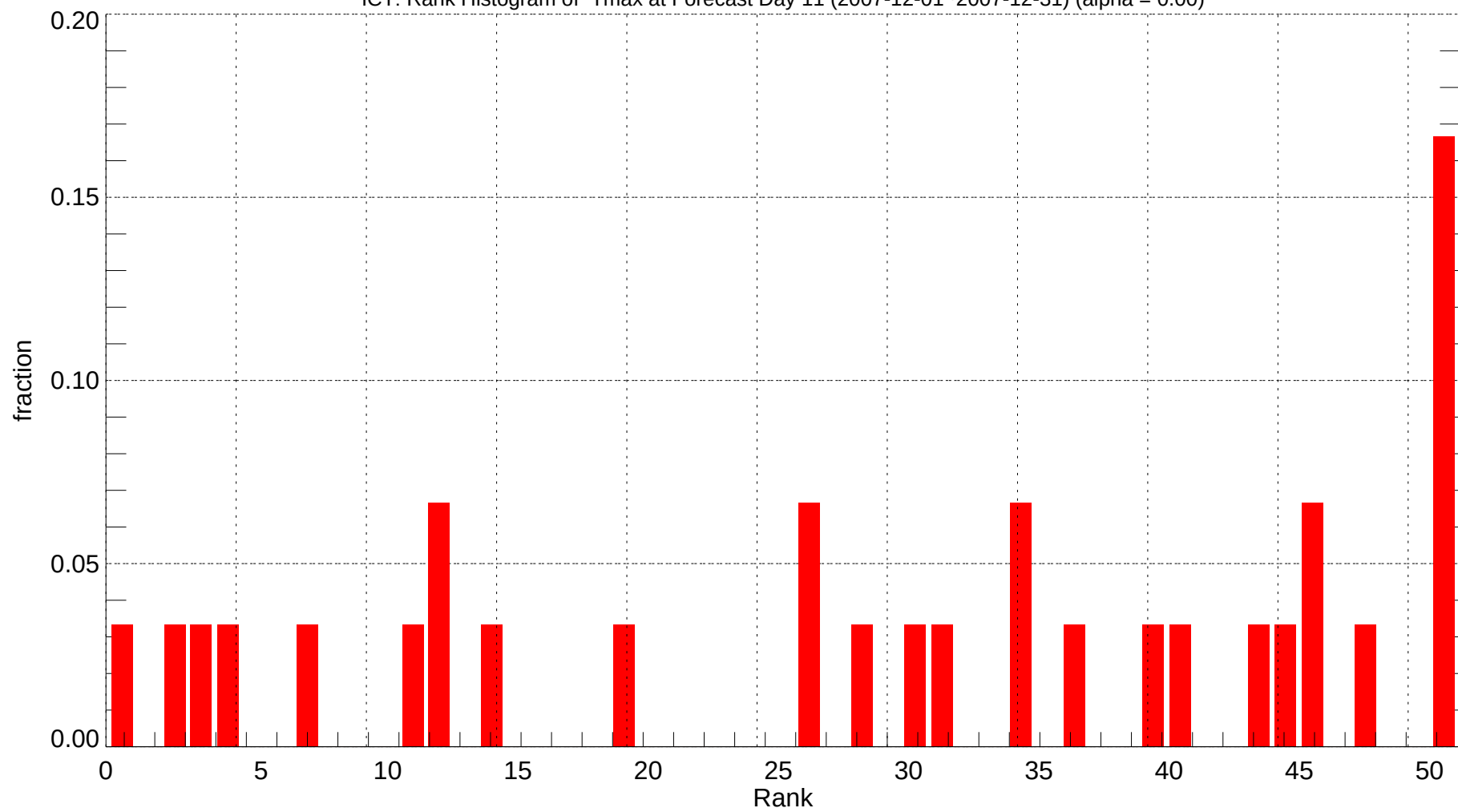
ICT: Rank Histogram of Tmax at Forecast Day 11 (2007-12-01~2007-12-31) (alpha = 0.00)
