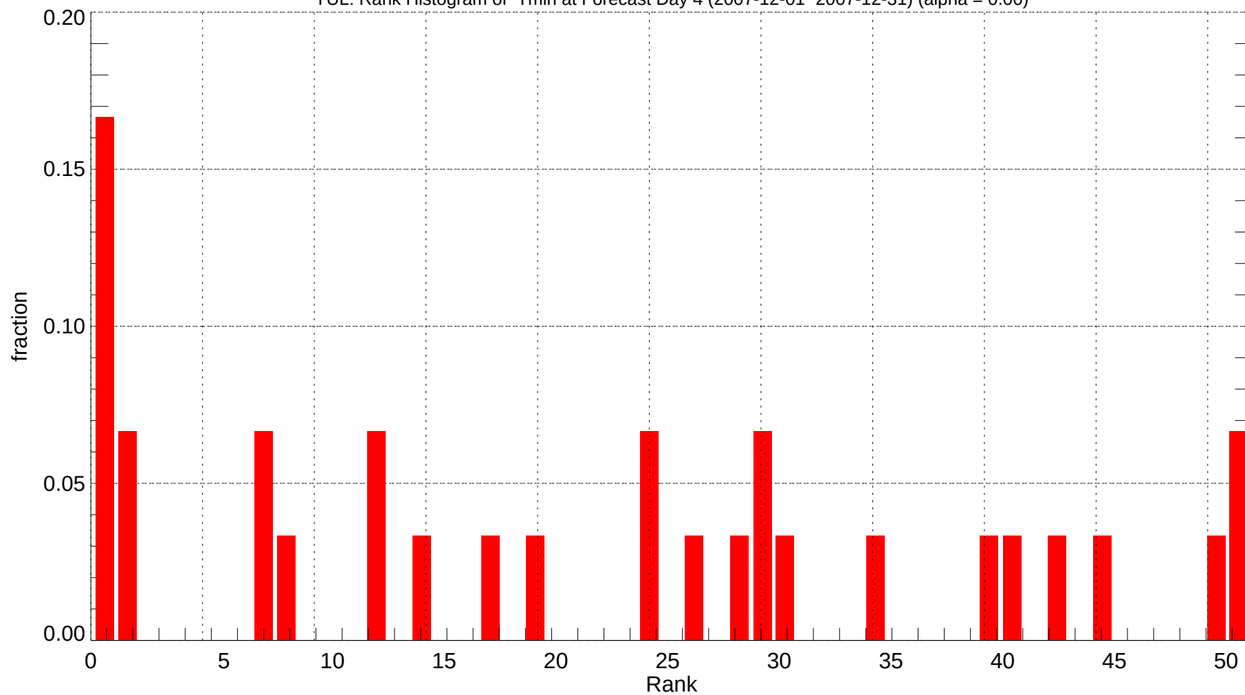
YUL: Rank Histogram of Tmin at Forecast Day 4 (2007-12-01~2007-12-31) (alpha = 0.00)
