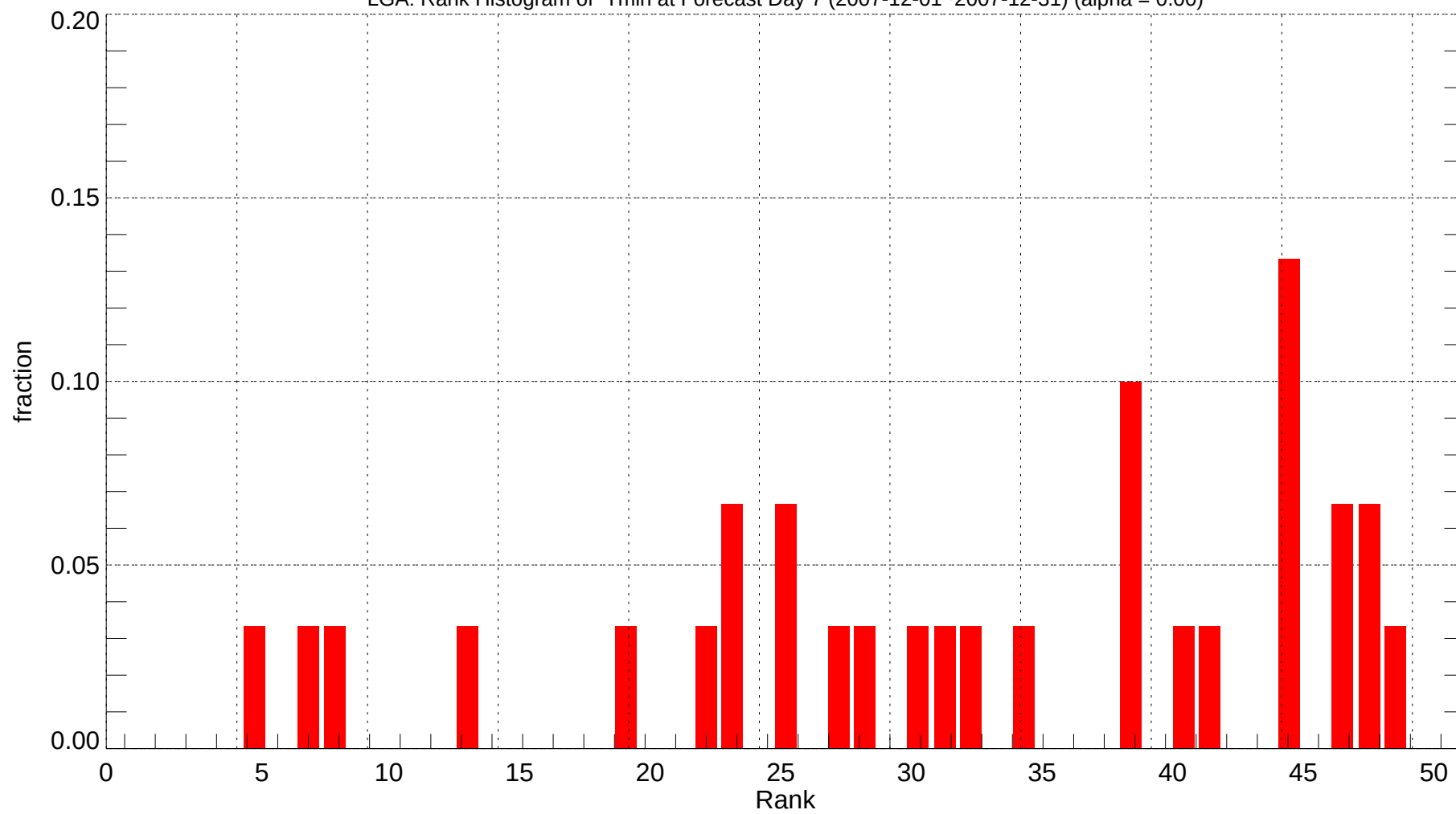
LGA: Rank Histogram of Tmin at Forecast Day 7 (2007-12-01~2007-12-31) (alpha = 0.00)
