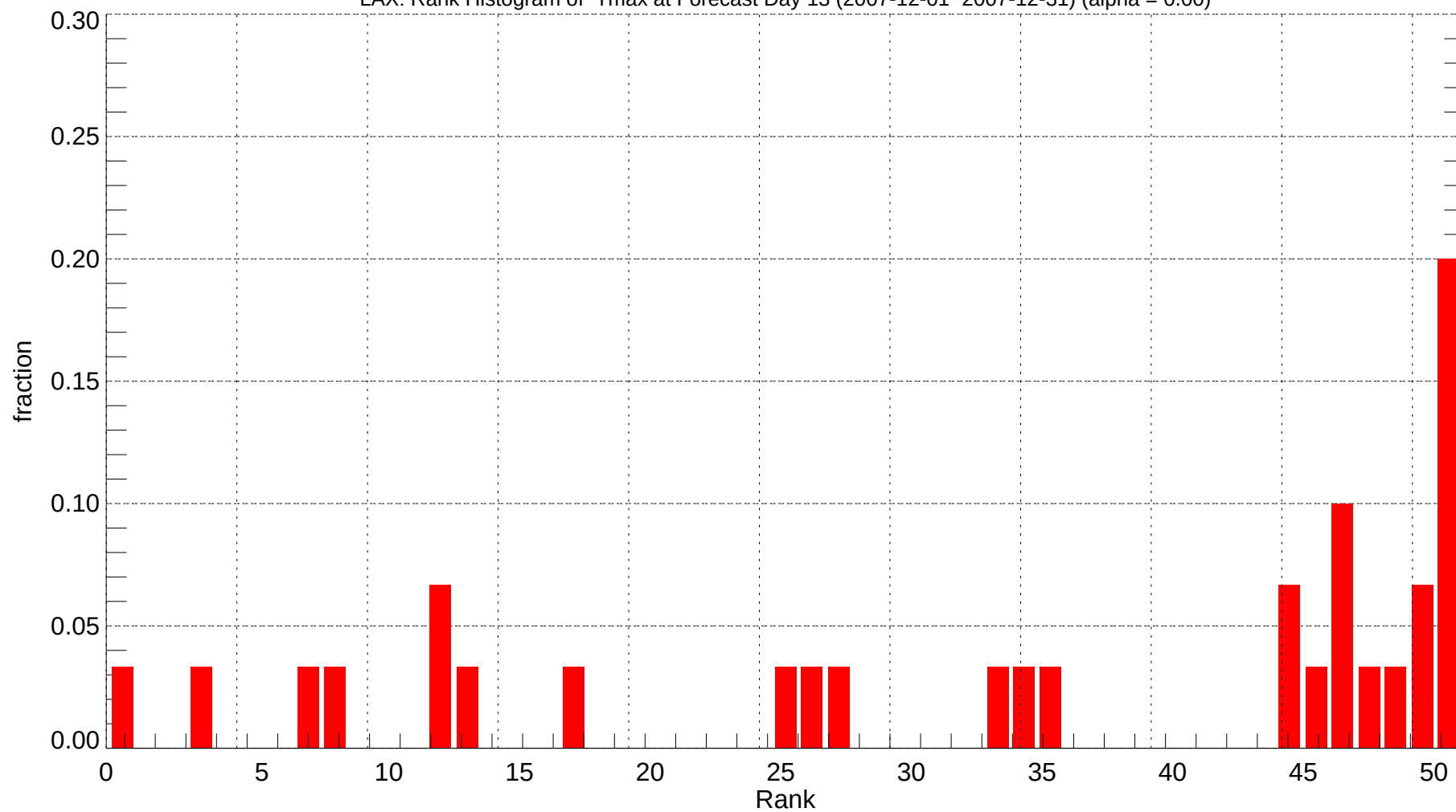
LAX: Rank Histogram of Tmax at Forecast Day 13 (2007-12-01~2007-12-31) (alpha = 0.00)
