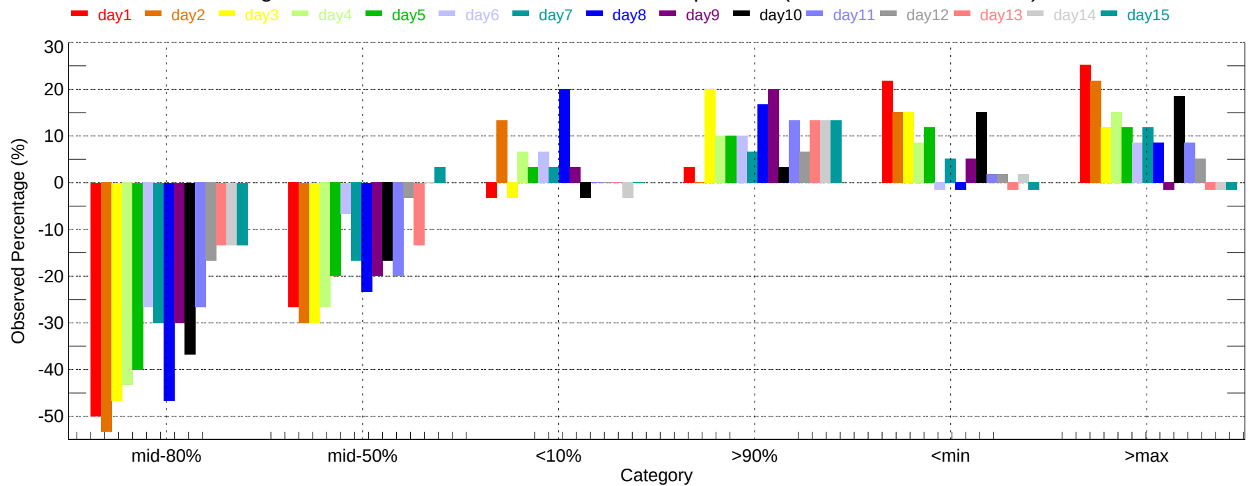
Observed Percentage Deviation of Ensembles - COU: Min Temperature (2007-12-01~2007-12-31)
