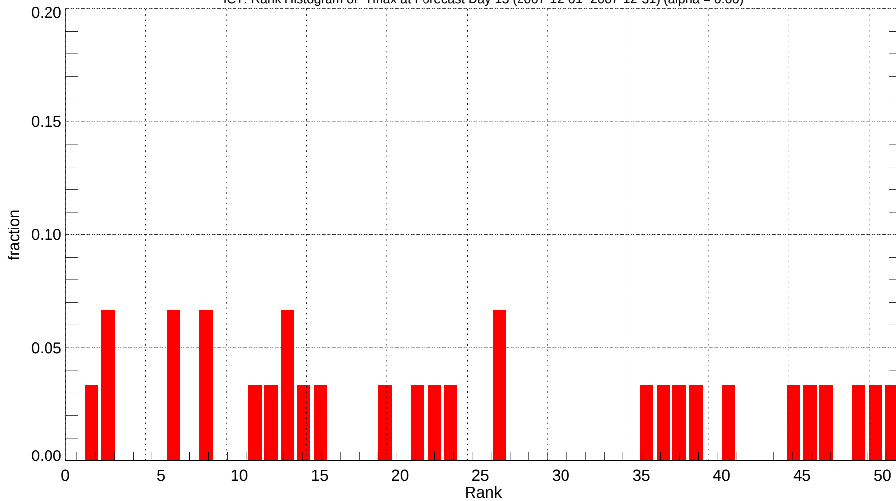
ICT: Rank Histogram of Tmax at Forecast Day 15 (2007-12-01~2007-12-31) (alpha = 0.00)
