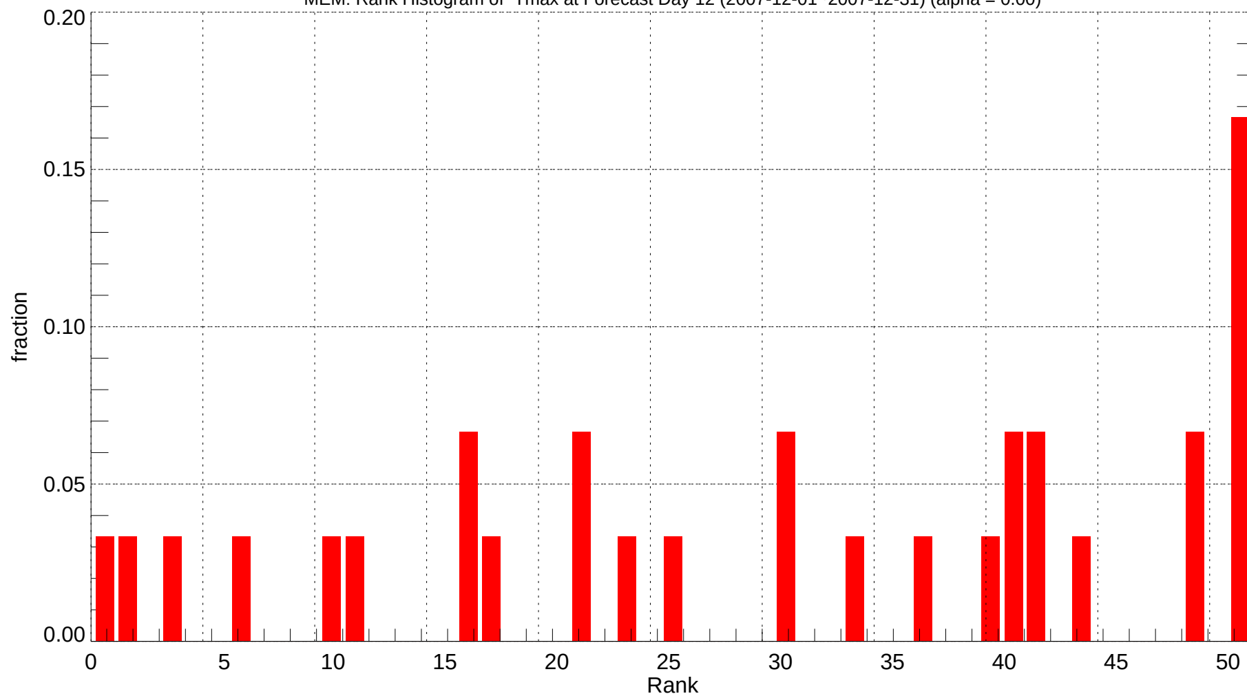
MEM: Rank Histogram of Tmax at Forecast Day 12 (2007-12-01~2007-12-31) (alpha = 0.00)
