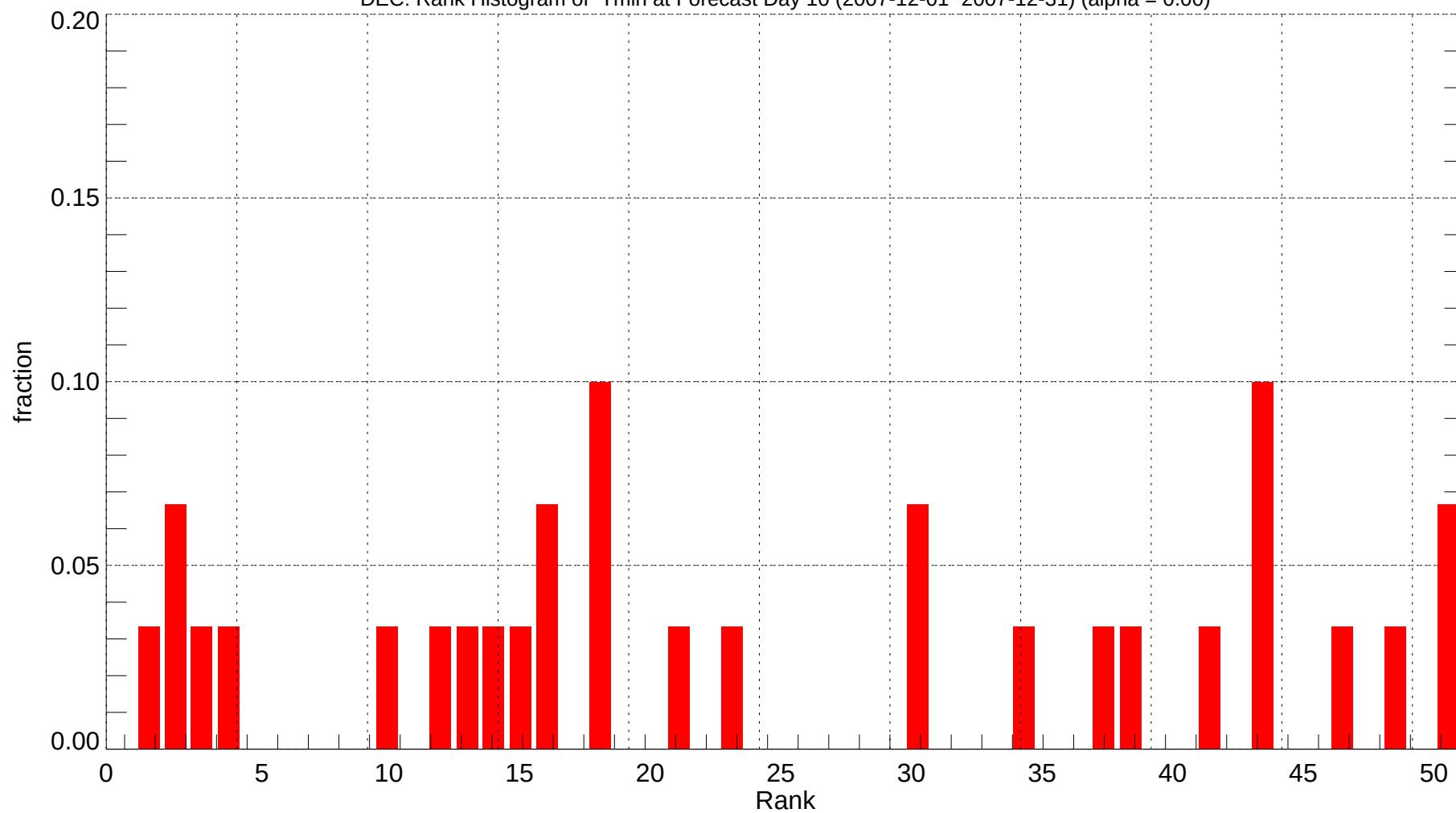
DEC: Rank Histogram of Tmin at Forecast Day 10 (2007-12-01~2007-12-31) (alpha = 0.00)
