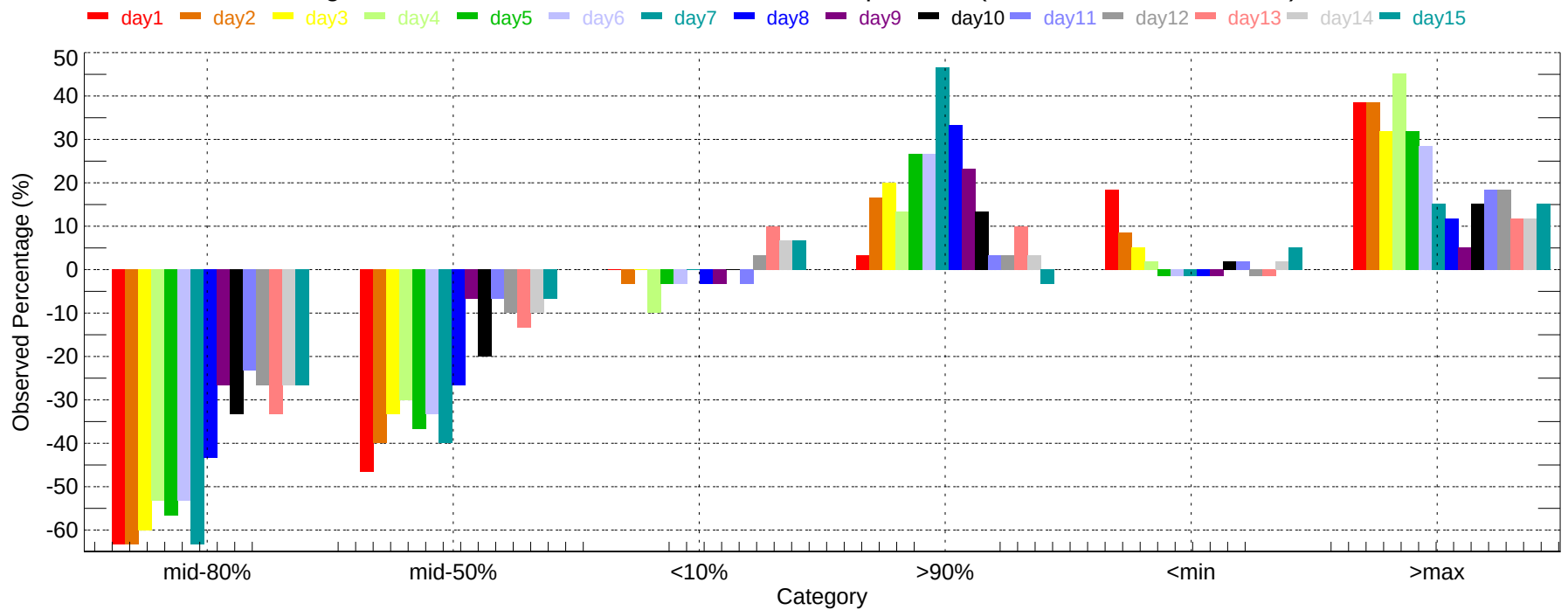
Observed Percentage Deviation of Ensembles - BUR: Min Temperature (2007-12-01~2007-12-31)
