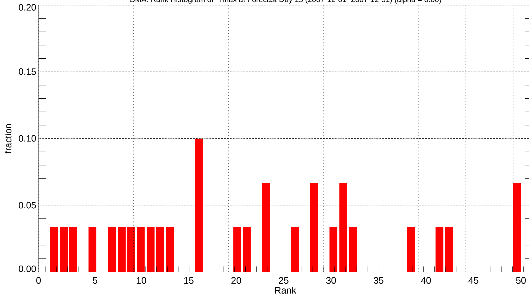
OMA: Rank Histogram of Tmax at Forecast Day 15 (2007-12-01~2007-12-31) (alpha = 0.00)
