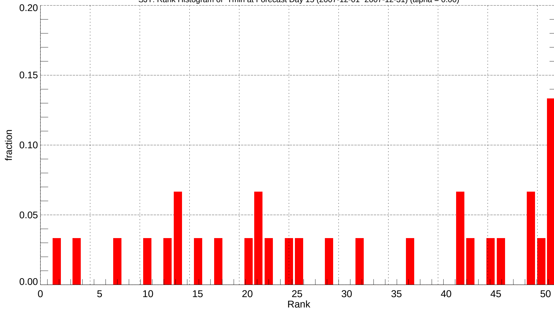
SJT: Rank Histogram of Tmin at Forecast Day 15 (2007-12-01~2007-12-31) (alpha = 0.00)
