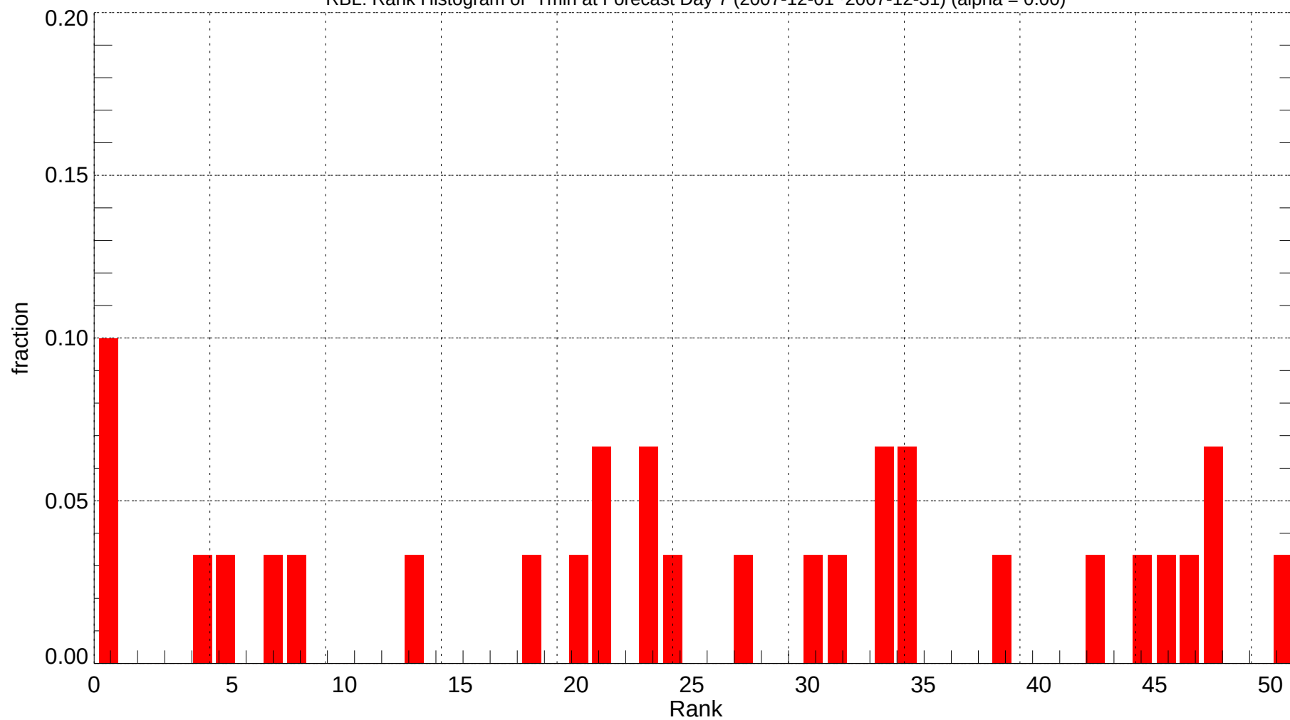
RBL: Rank Histogram of Tmin at Forecast Day 7 (2007-12-01~2007-12-31) (alpha = 0.00)
