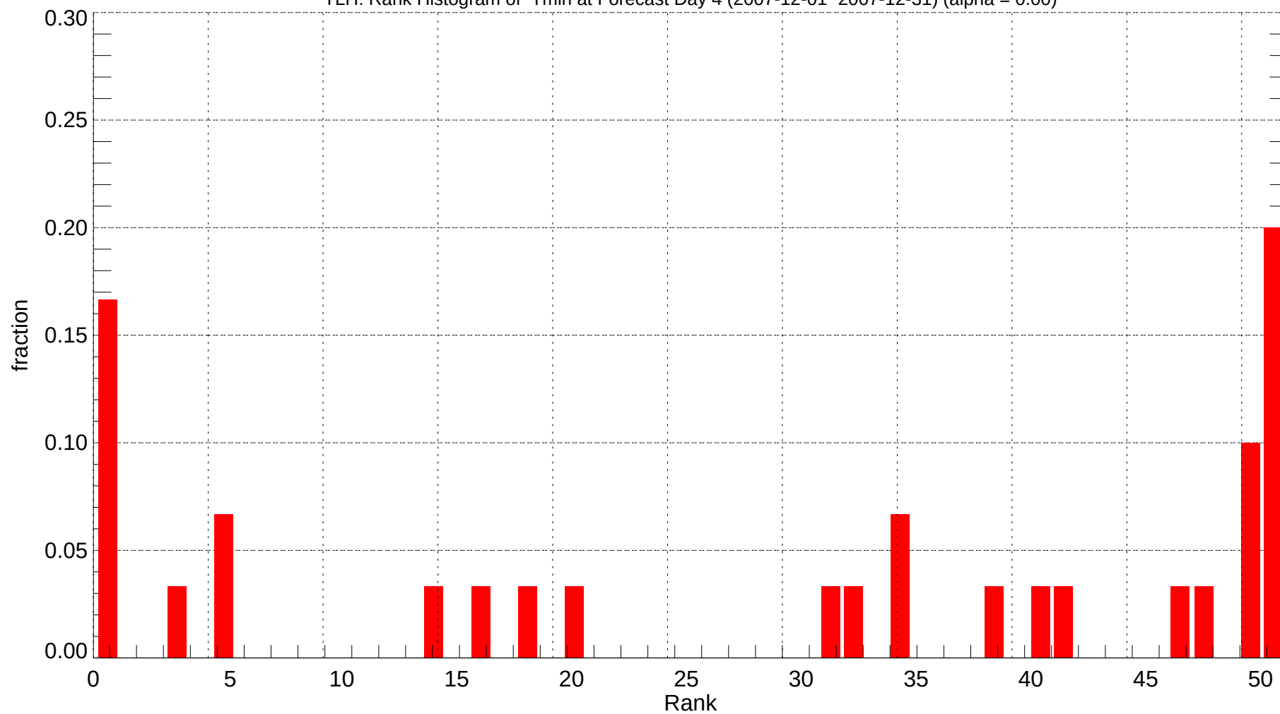
TLH: Rank Histogram of Tmin at Forecast Day 4 (2007-12-01~2007-12-31) (alpha = 0.00)
