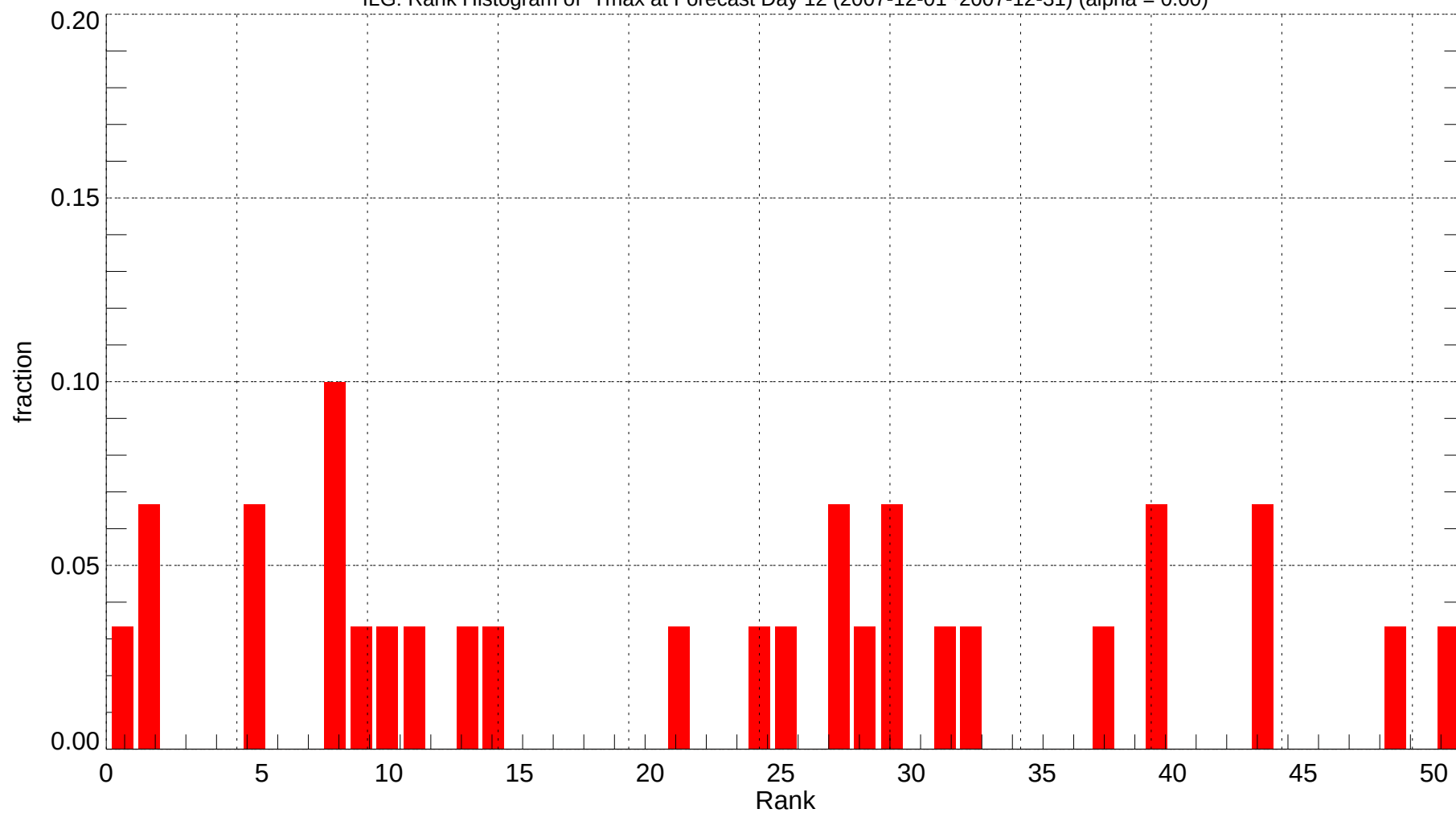
ILG: Rank Histogram of Tmax at Forecast Day 12 (2007-12-01~2007-12-31) (alpha = 0.00)
