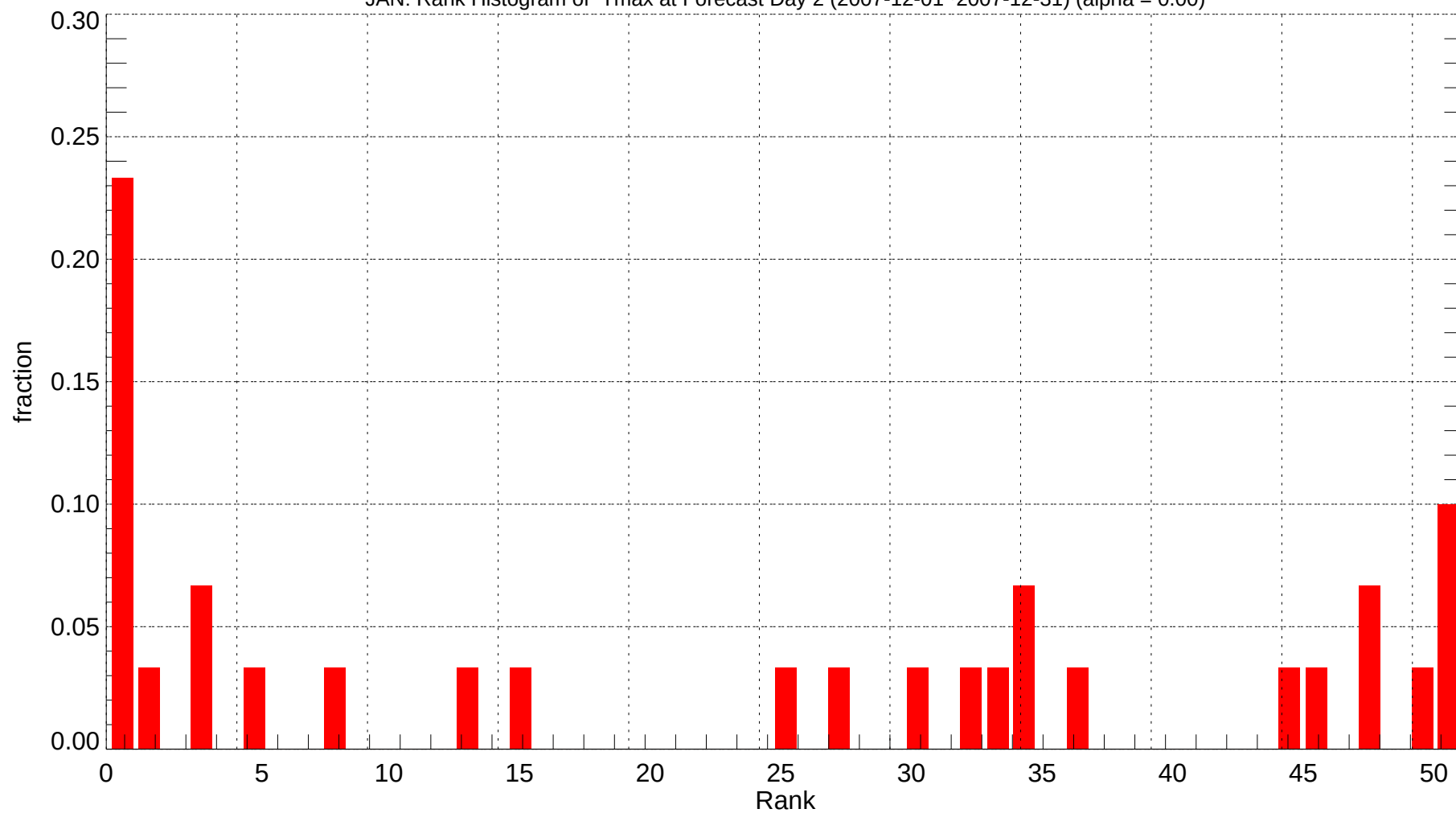
JAN: Rank Histogram of Tmax at Forecast Day 2 (2007-12-01~2007-12-31) (alpha = 0.00)
