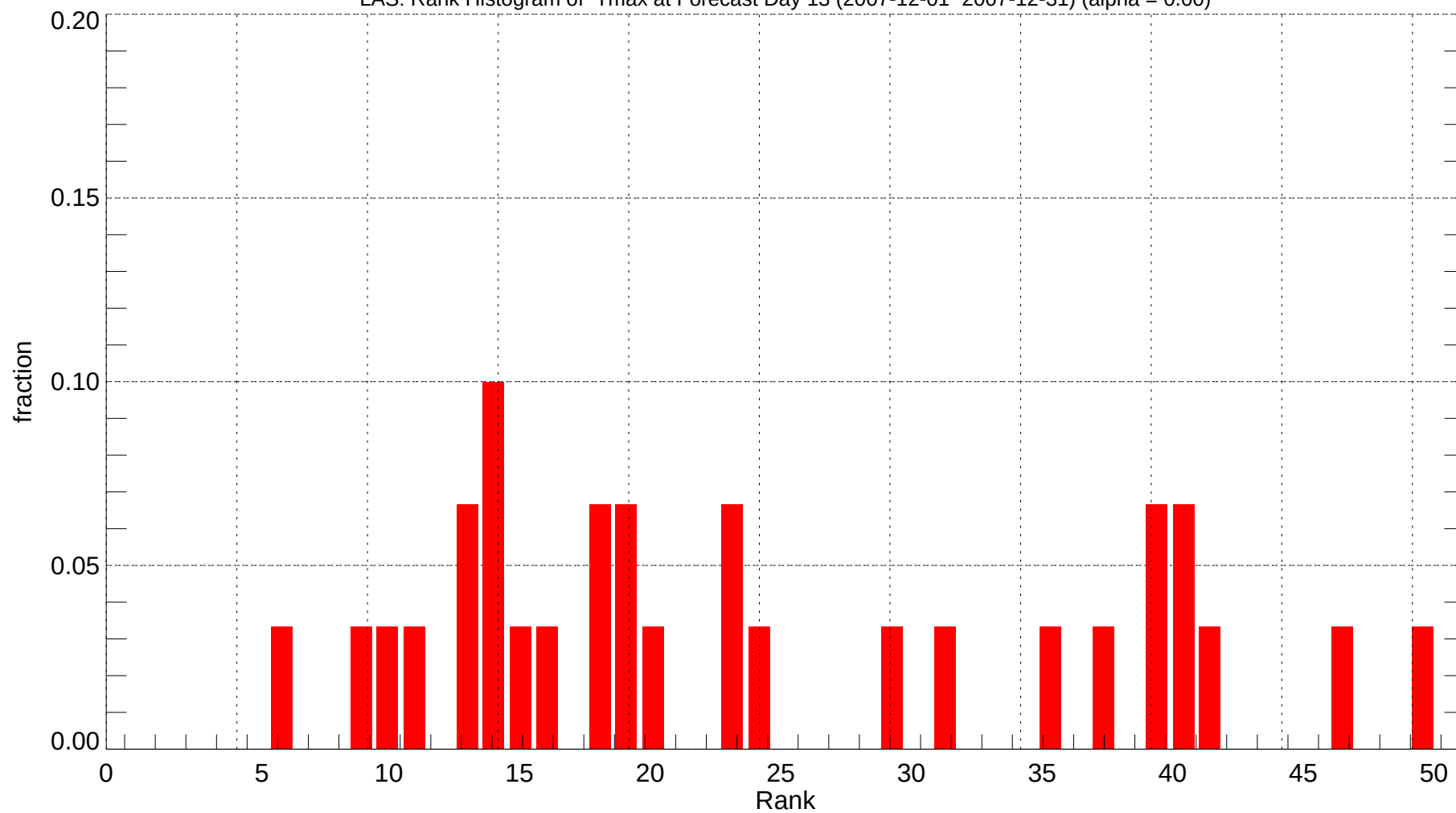
LAS: Rank Histogram of Tmax at Forecast Day 13 (2007-12-01~2007-12-31) (alpha = 0.00)
