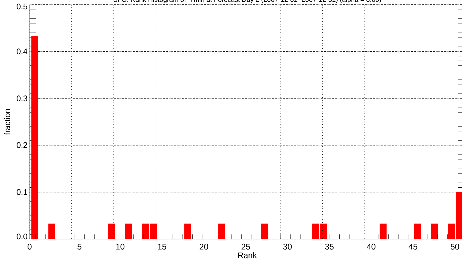
SFO: Rank Histogram of Tmin at Forecast Day 2 (2007-12-01~2007-12-31) (alpha = 0.00)
