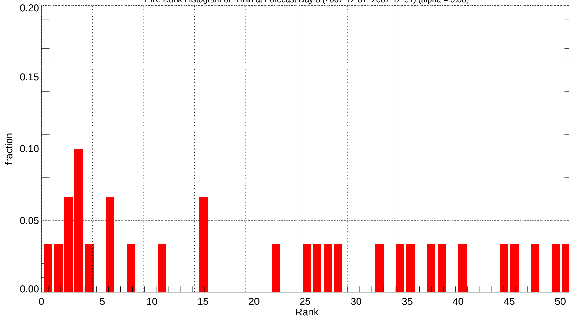
PIR: Rank Histogram of Tmin at Forecast Day 8 (2007-12-01~2007-12-31) (alpha = 0.00)
