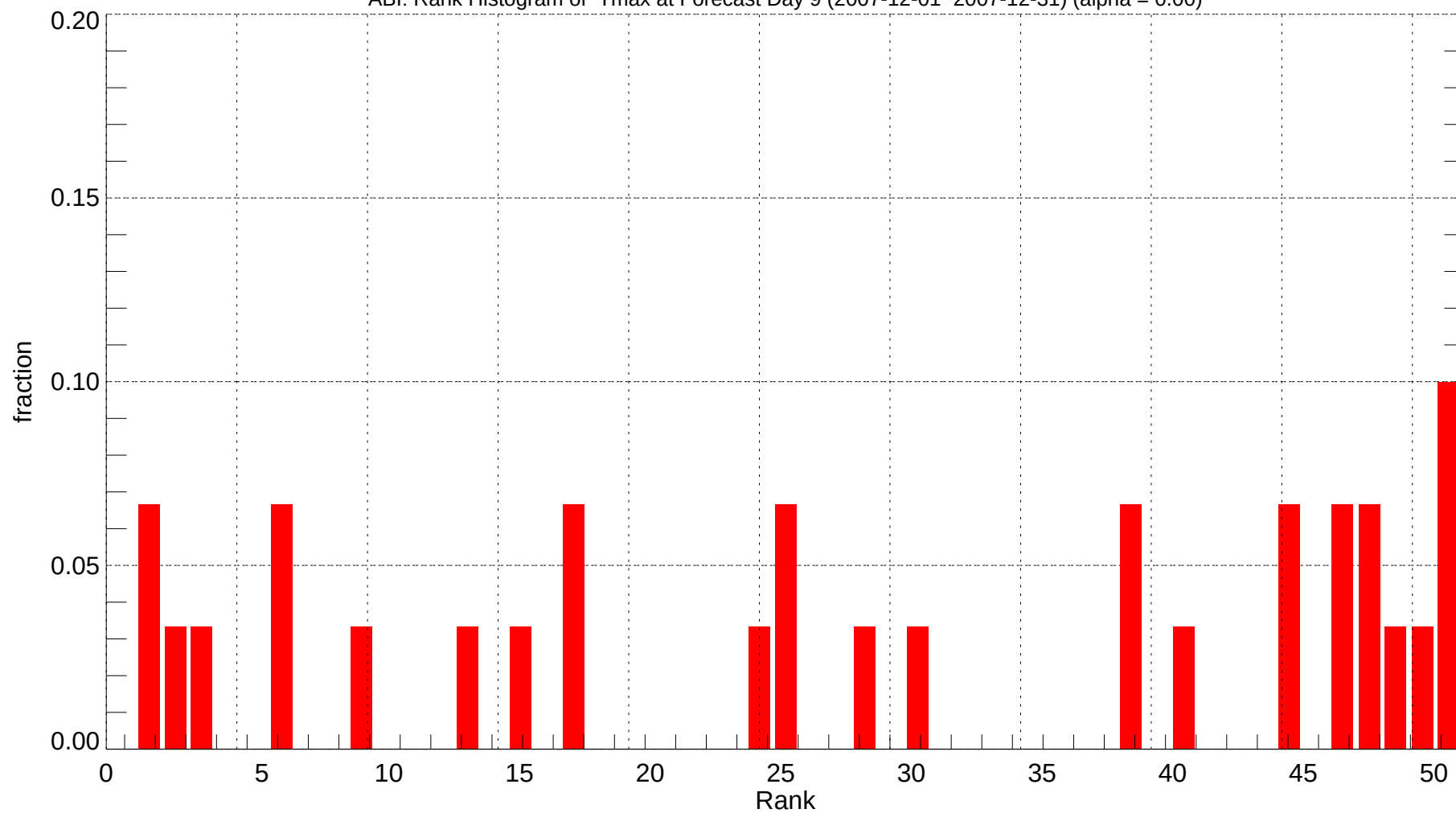
ABI: Rank Histogram of Tmax at Forecast Day 9 (2007-12-01~2007-12-31) (alpha = 0.00)
