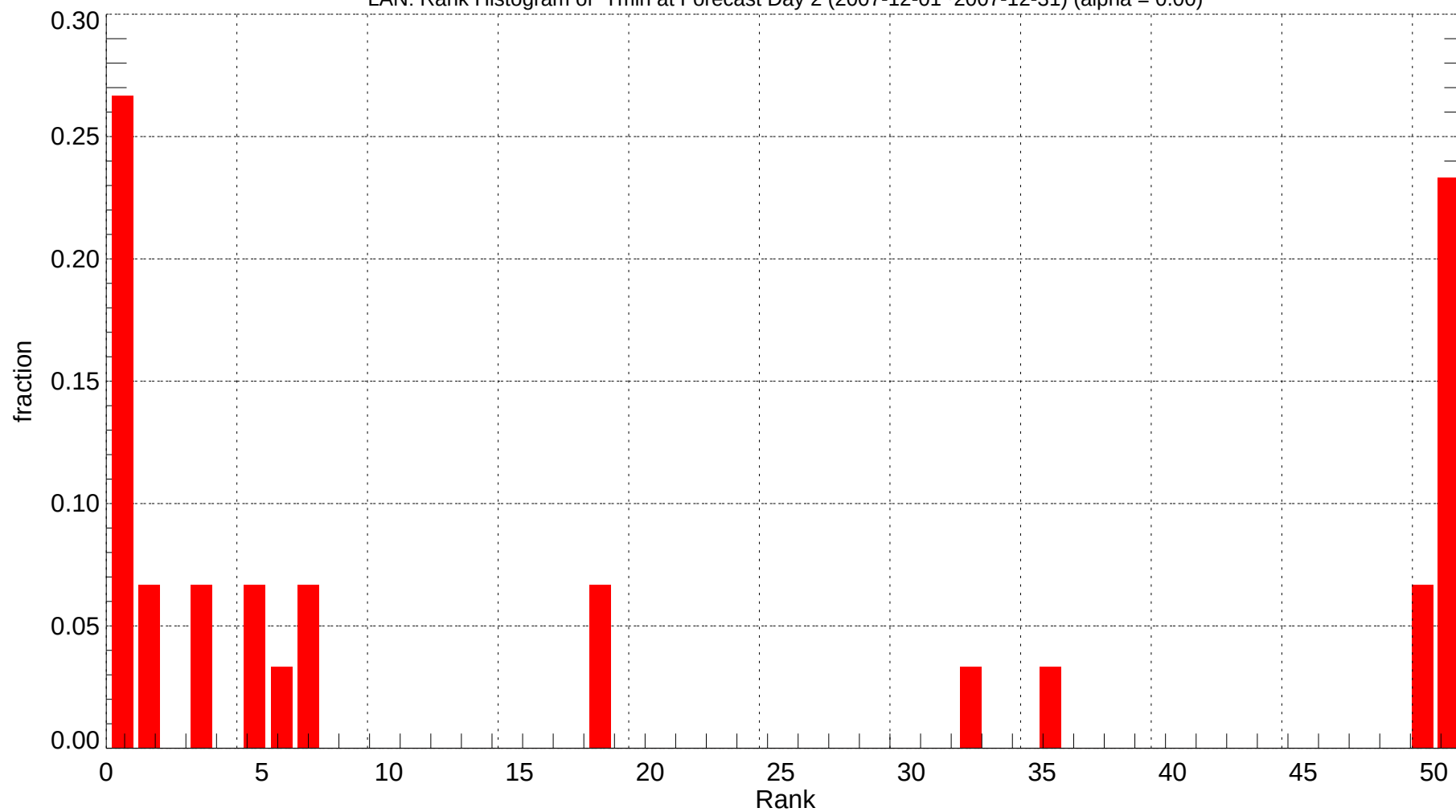
LAN: Rank Histogram of Tmin at Forecast Day 2 (2007-12-01~2007-12-31) (alpha = 0.00)
