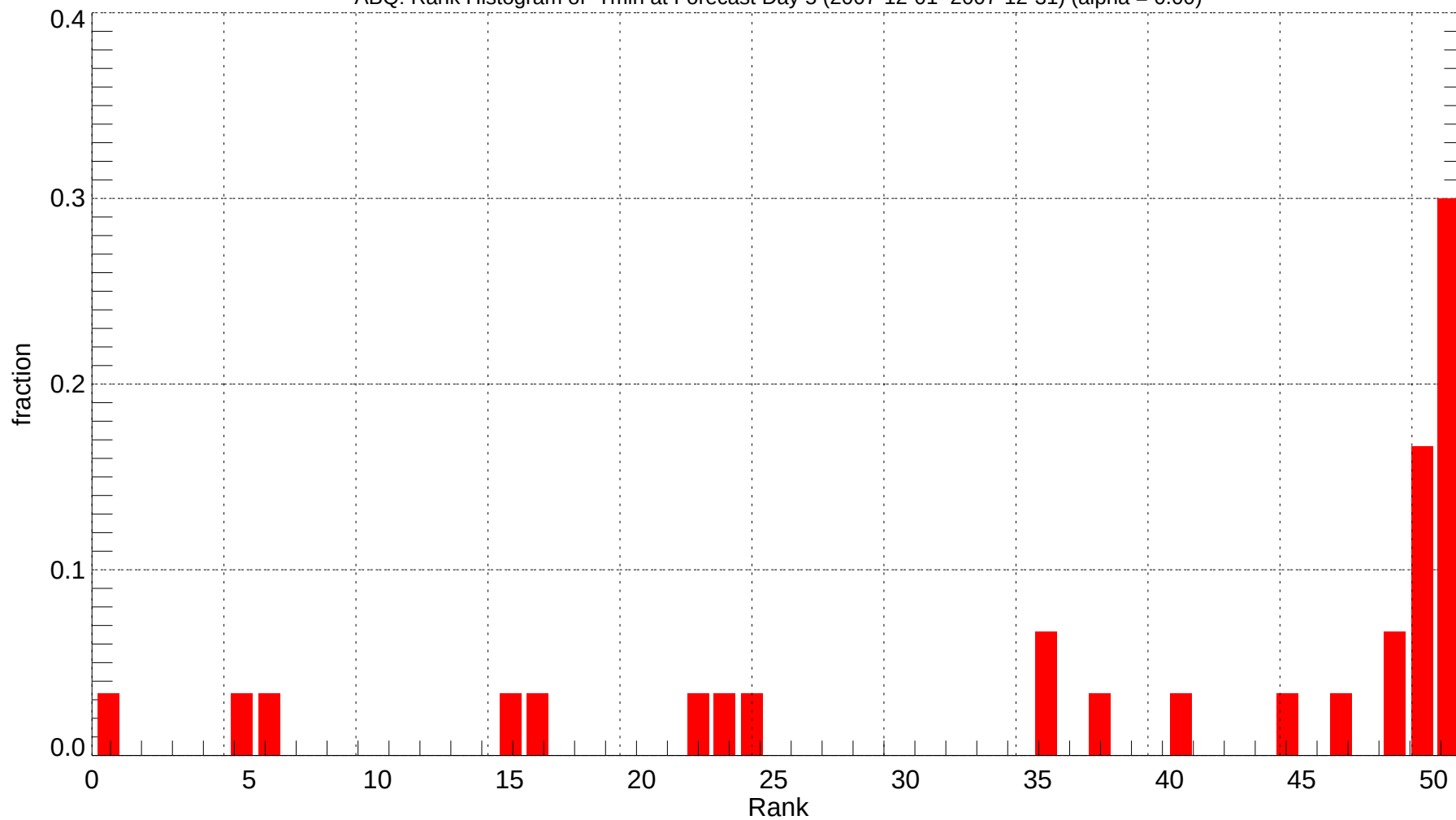
ABQ: Rank Histogram of Tmin at Forecast Day 5 (2007-12-01~2007-12-31) (alpha = 0.00)
