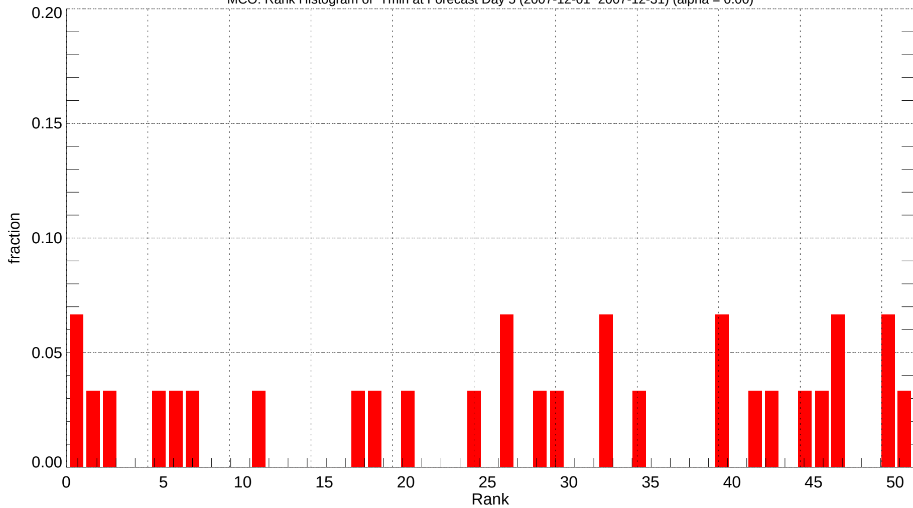
MCO: Rank Histogram of Tmin at Forecast Day 5 (2007-12-01~2007-12-31) (alpha = 0.00)
