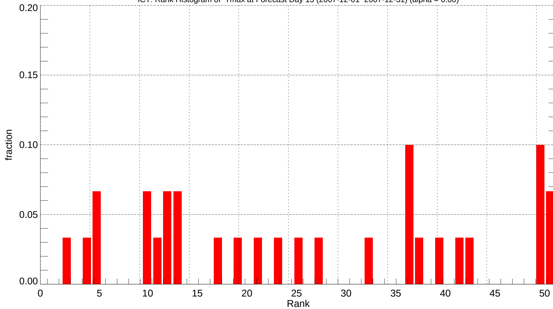
ICT: Rank Histogram of Tmax at Forecast Day 13 (2007-12-01~2007-12-31) (alpha = 0.00)
