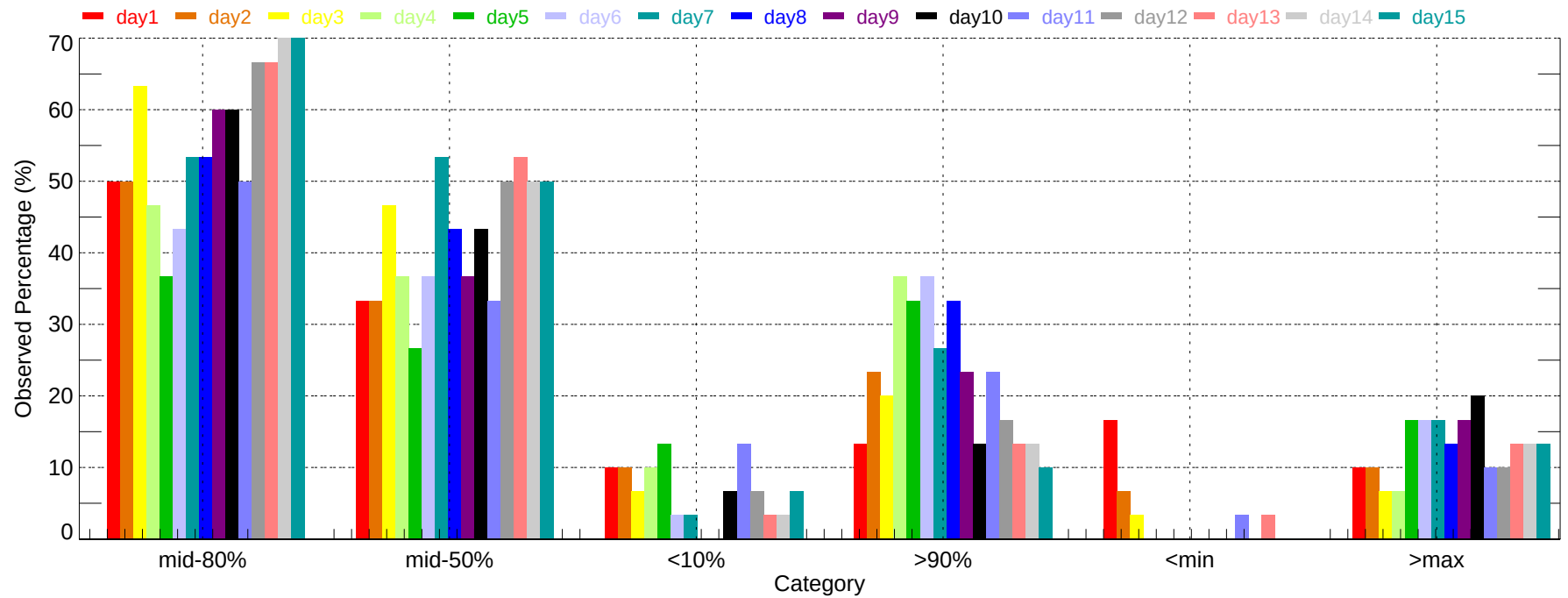
Observed Percentage of Ensembles - CAE: Min Temperature (2007-12-01~2007-12-31)
