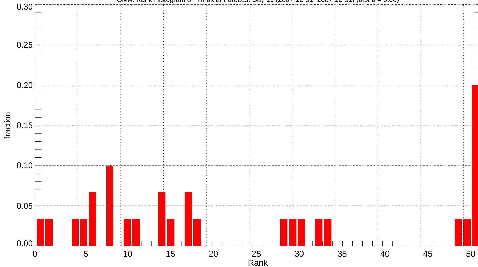
OMA: Rank Histogram of Tmax at Forecast Day 11 (2007-12-01~2007-12-31) (alpha = 0.00)
