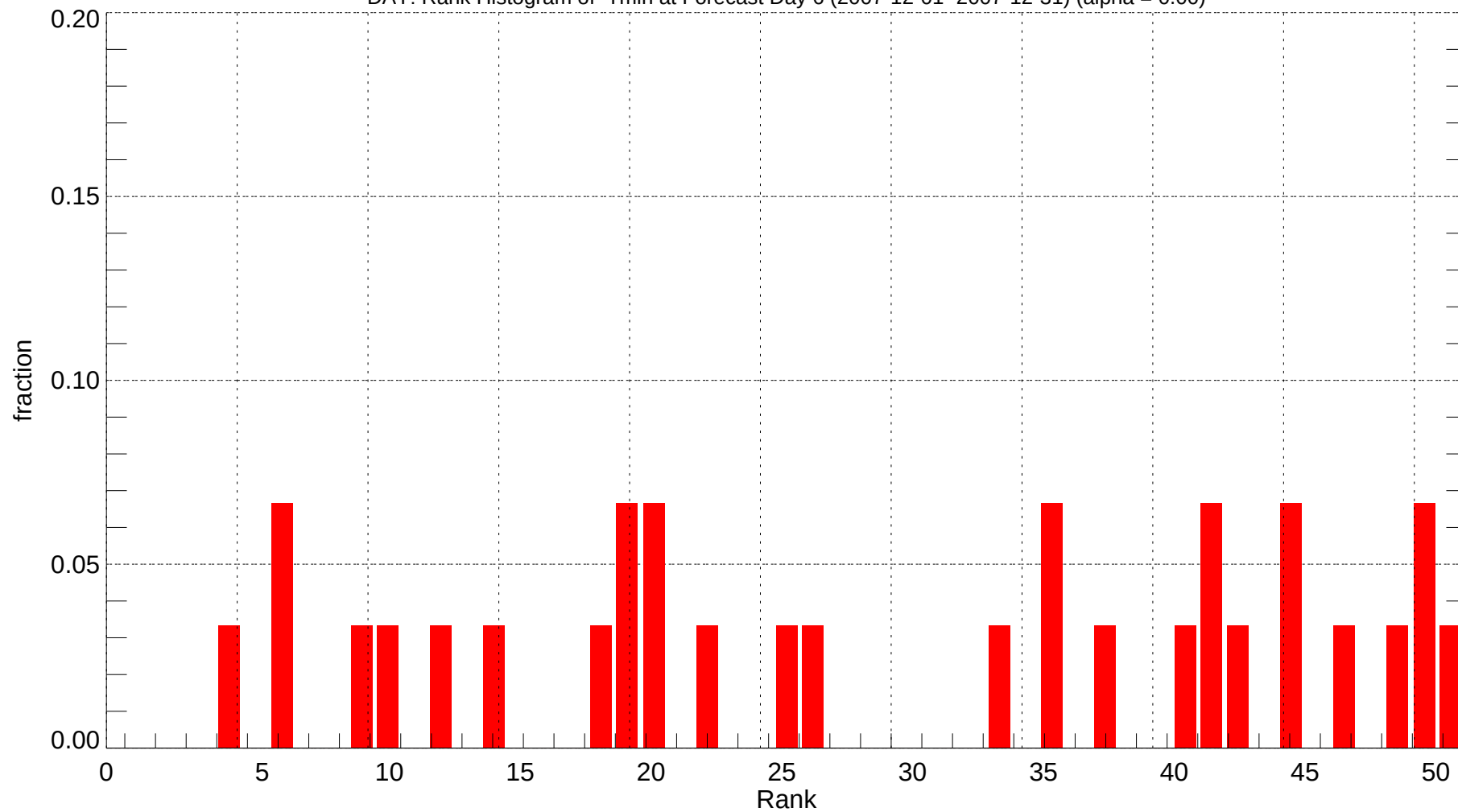
DAY: Rank Histogram of Tmin at Forecast Day 6 (2007-12-01~2007-12-31) (alpha = 0.00)
