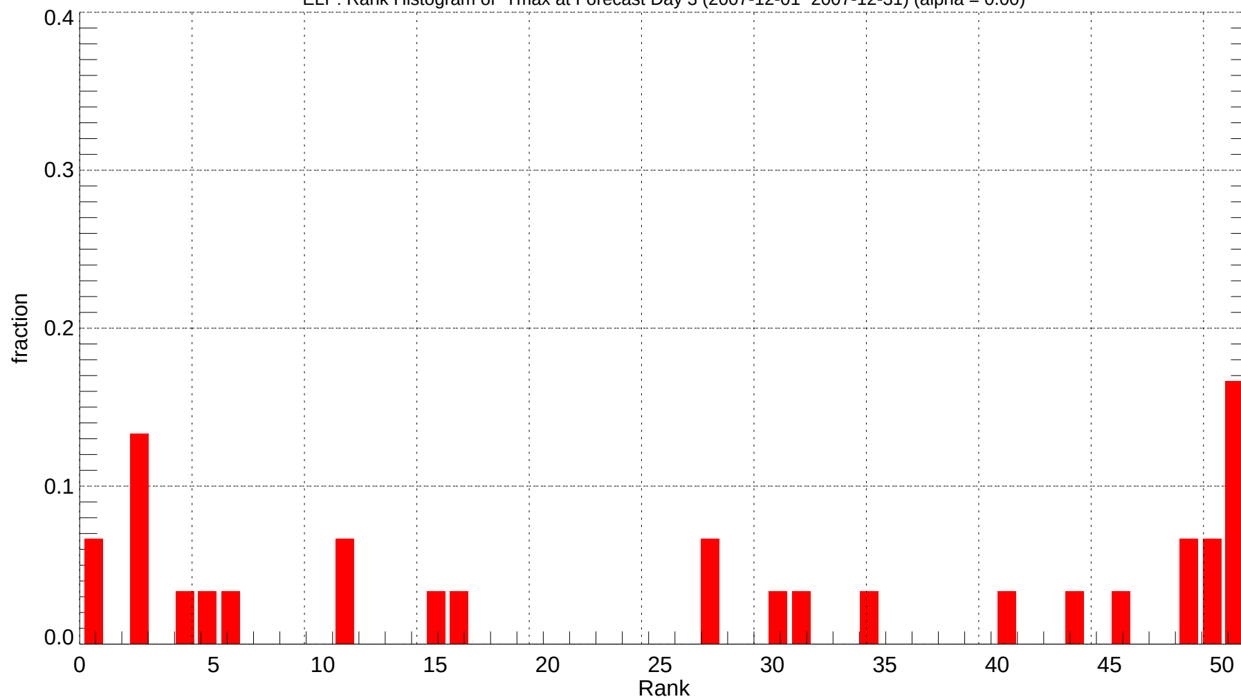
ELP: Rank Histogram of Tmax at Forecast Day 3 (2007-12-01~2007-12-31) (alpha = 0.00)
