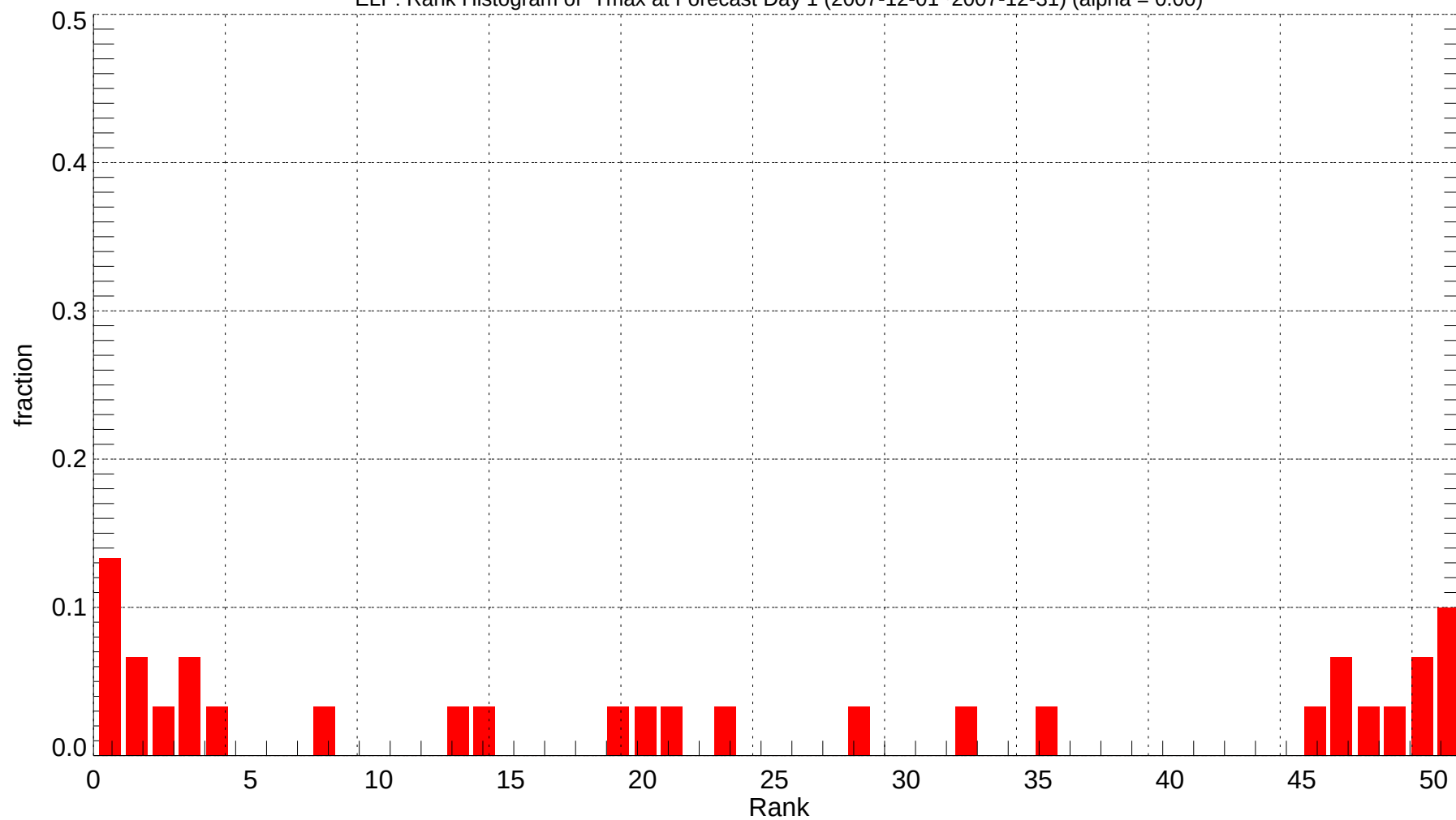
ELP: Rank Histogram of Tmax at Forecast Day 1 (2007-12-01~2007-12-31) (alpha = 0.00)
