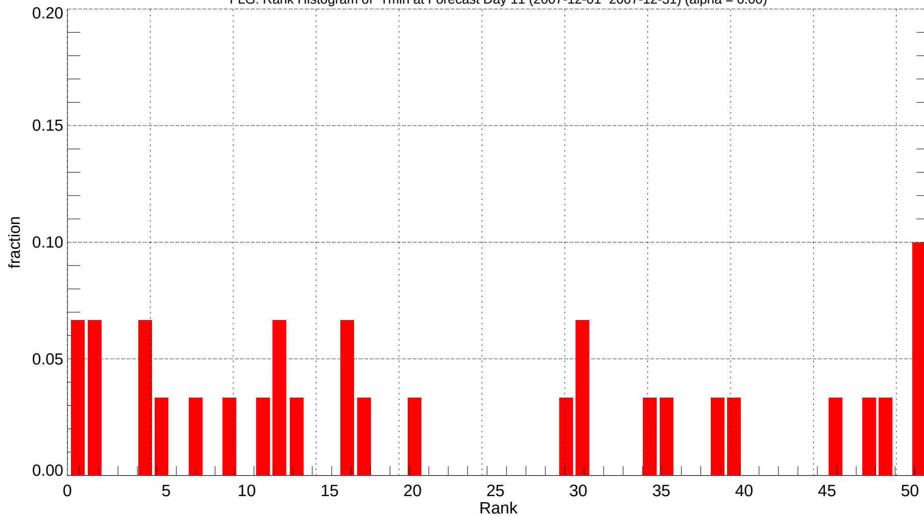
FLG: Rank Histogram of Tmin at Forecast Day 11 (2007-12-01~2007-12-31) (alpha = 0.00)
