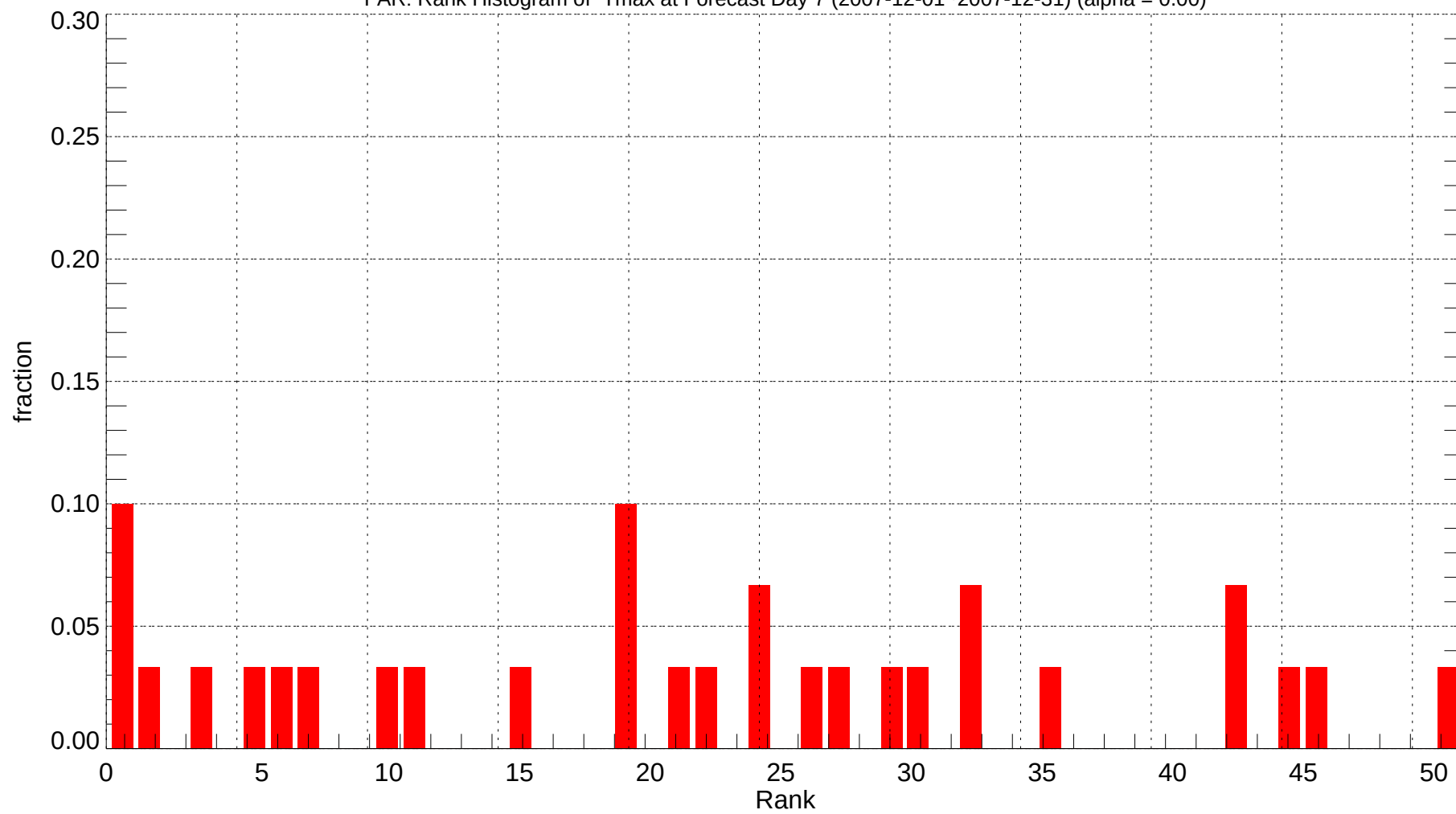
FAR: Rank Histogram of Tmax at Forecast Day 7 (2007-12-01~2007-12-31) (alpha = 0.00)
