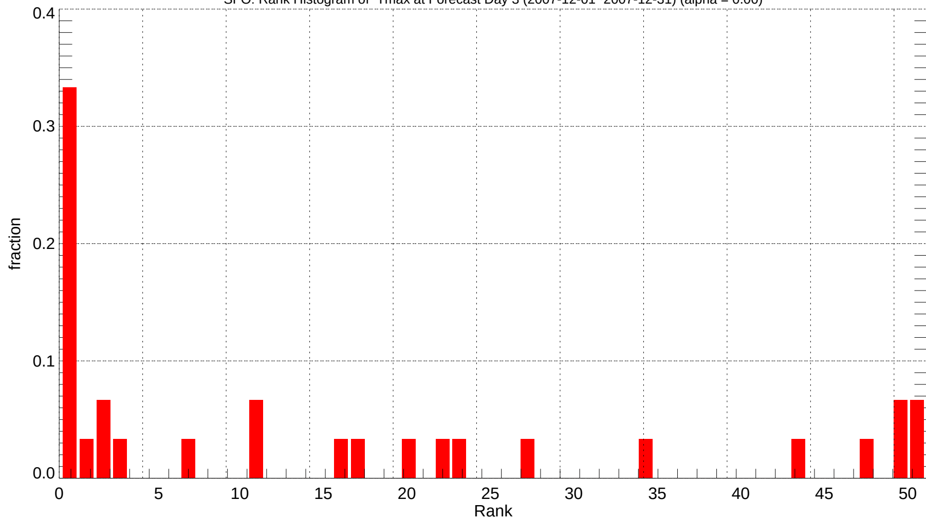
SFO: Rank Histogram of Tmax at Forecast Day 3 (2007-12-01~2007-12-31) (alpha = 0.00)
