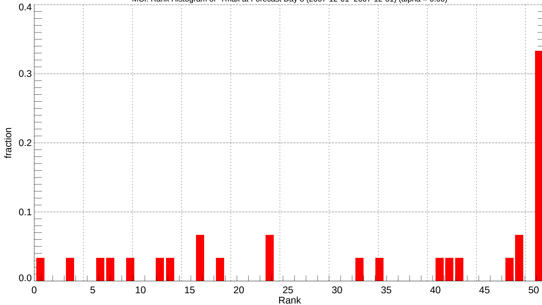
MCI: Rank Histogram of Tmax at Forecast Day 8 (2007-12-01~2007-12-31) (alpha = 0.00)
