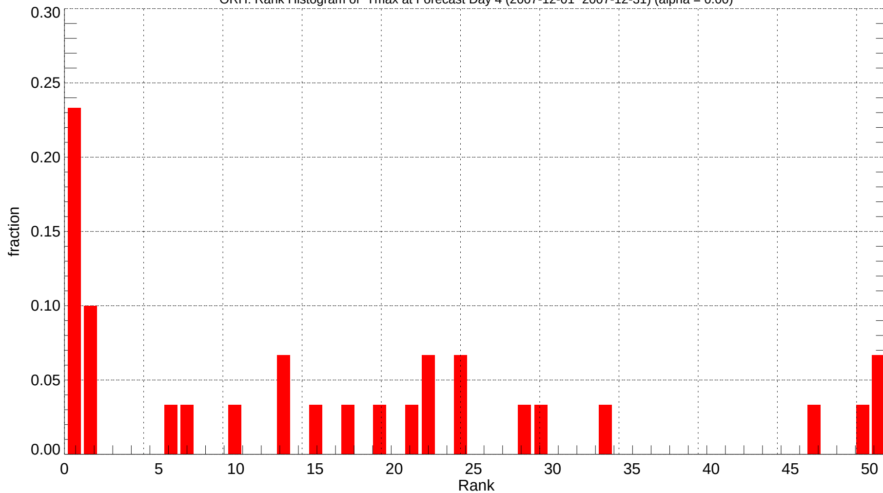
ORH: Rank Histogram of Tmax at Forecast Day 4 (2007-12-01~2007-12-31) (alpha = 0.00)
