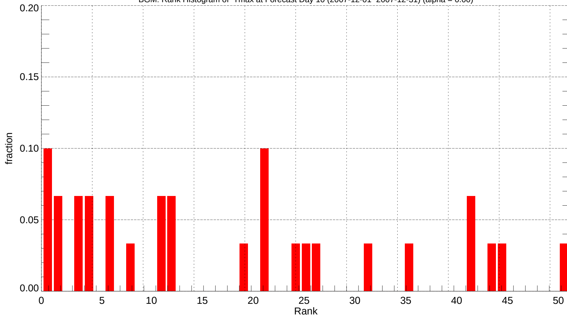
BGM: Rank Histogram of Tmax at Forecast Day 10 (2007-12-01~2007-12-31) (alpha = 0.00)
