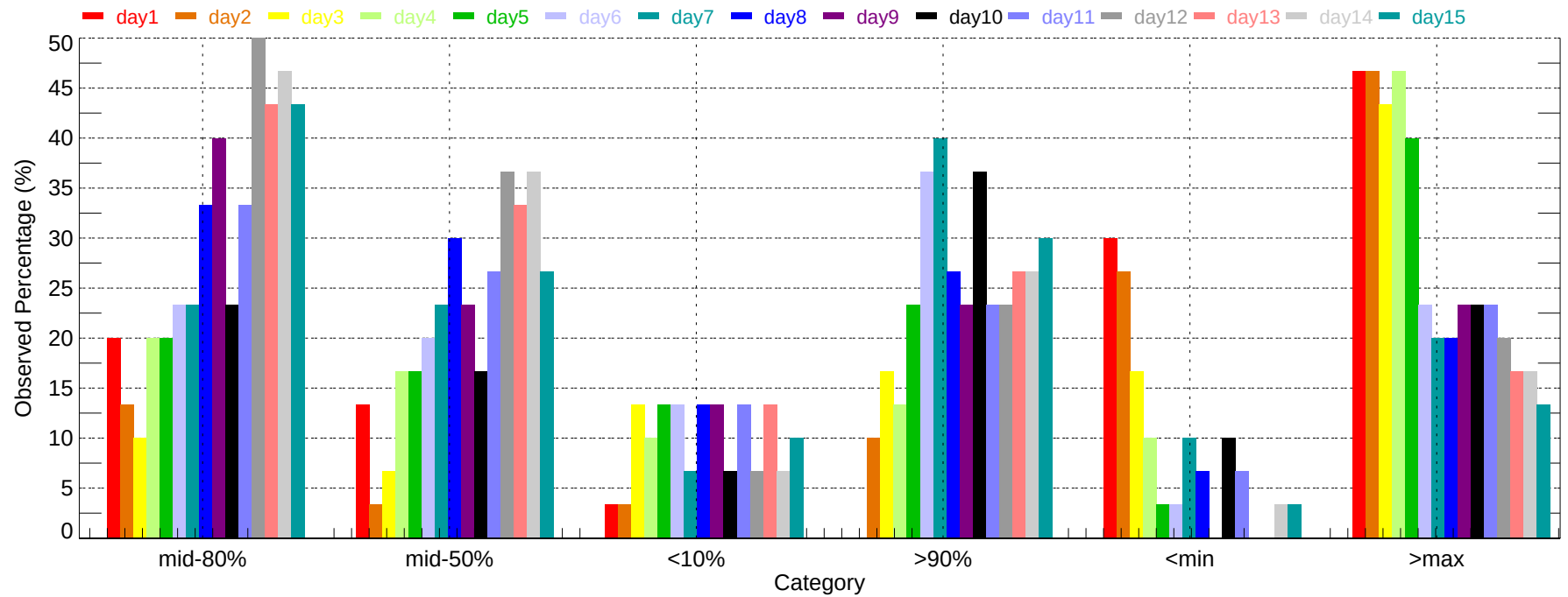
Observed Percentage of Ensembles - PDT: Min Temperature (2007-12-01~2007-12-31)
