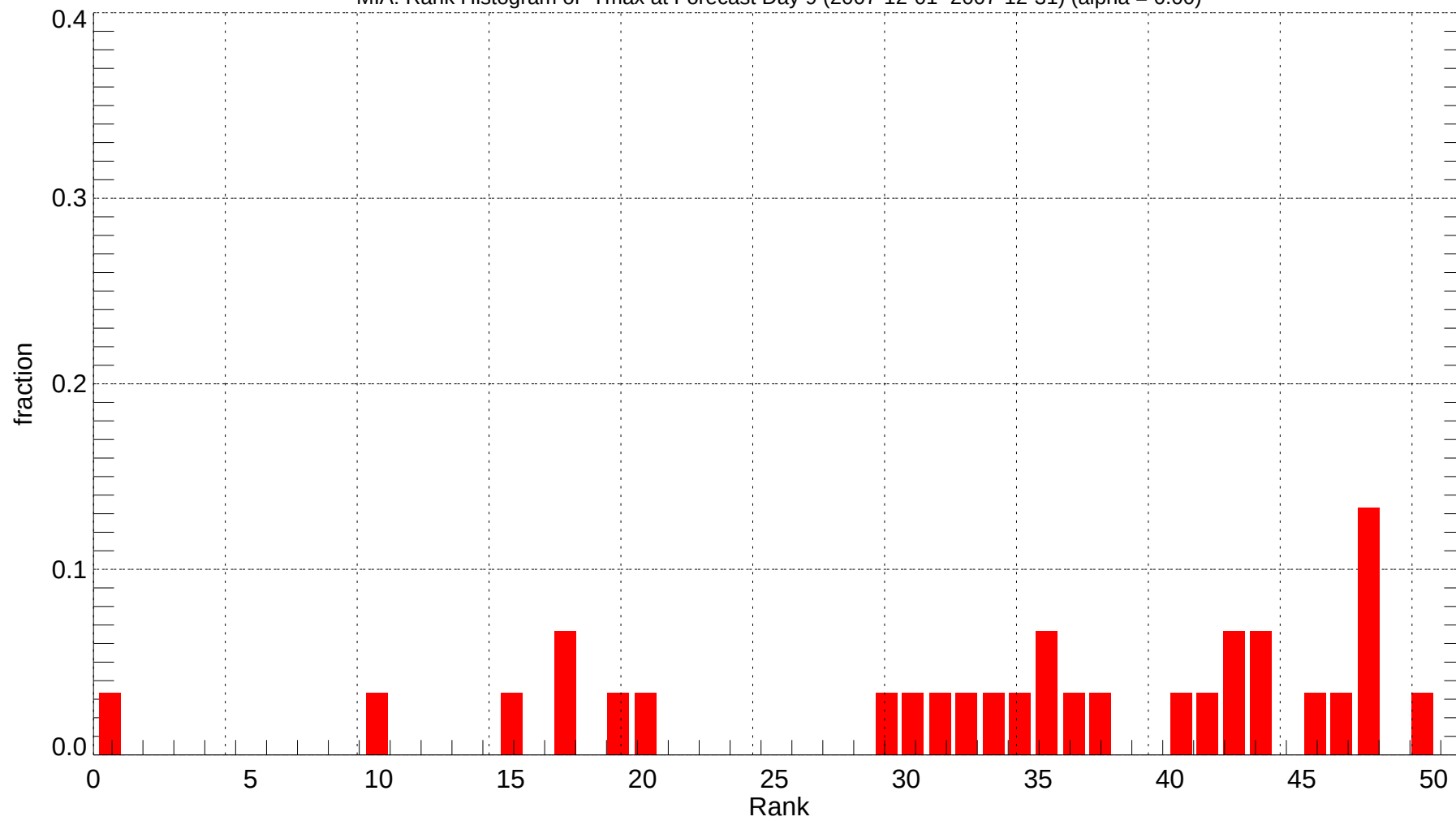
MIA: Rank Histogram of Tmax at Forecast Day 9 (2007-12-01~2007-12-31) (alpha = 0.00)
