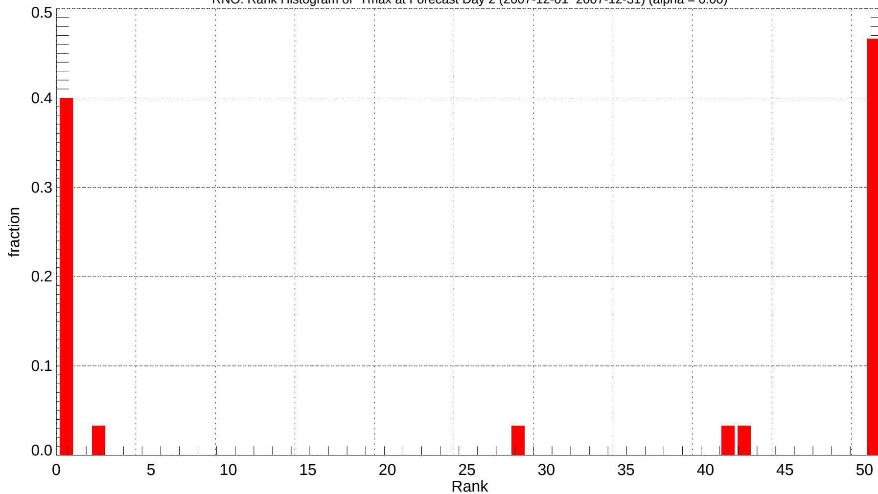
RNO: Rank Histogram of Tmax at Forecast Day 2 (2007-12-01~2007-12-31) (alpha = 0.00)
