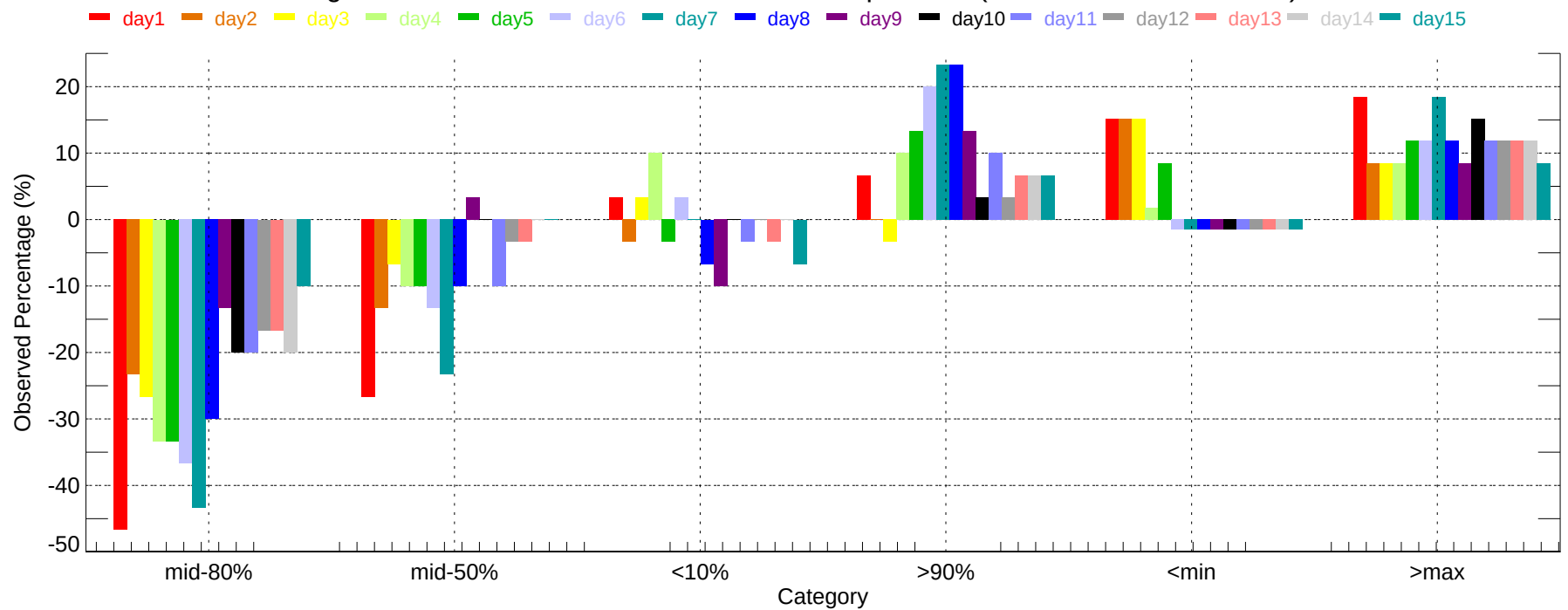
Observed Percentage Deviation of Ensembles - CHA: Min Temperature (2007-12-01~2007-12-31)
