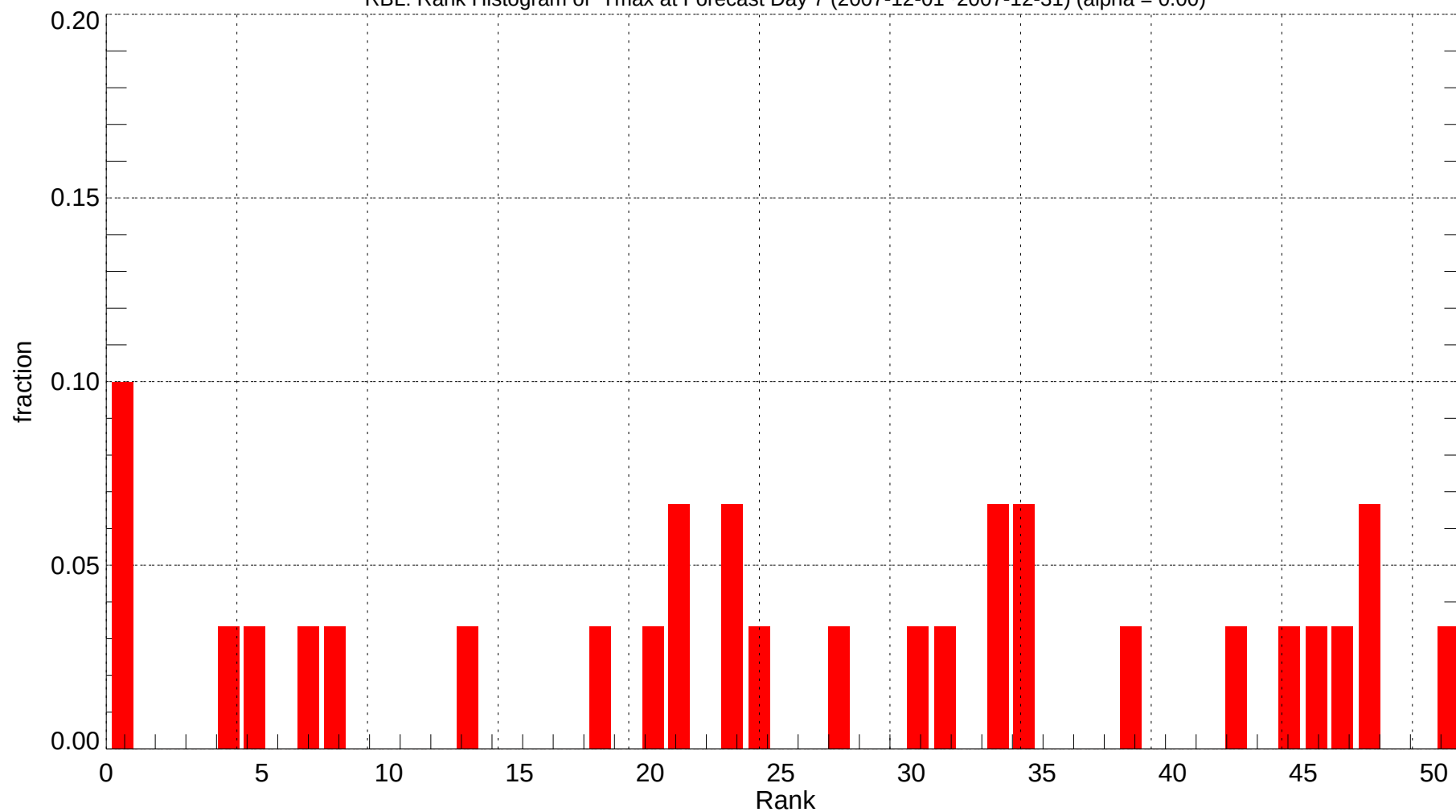
RBL: Rank Histogram of Tmax at Forecast Day 7 (2007-12-01~2007-12-31) (alpha = 0.00)
