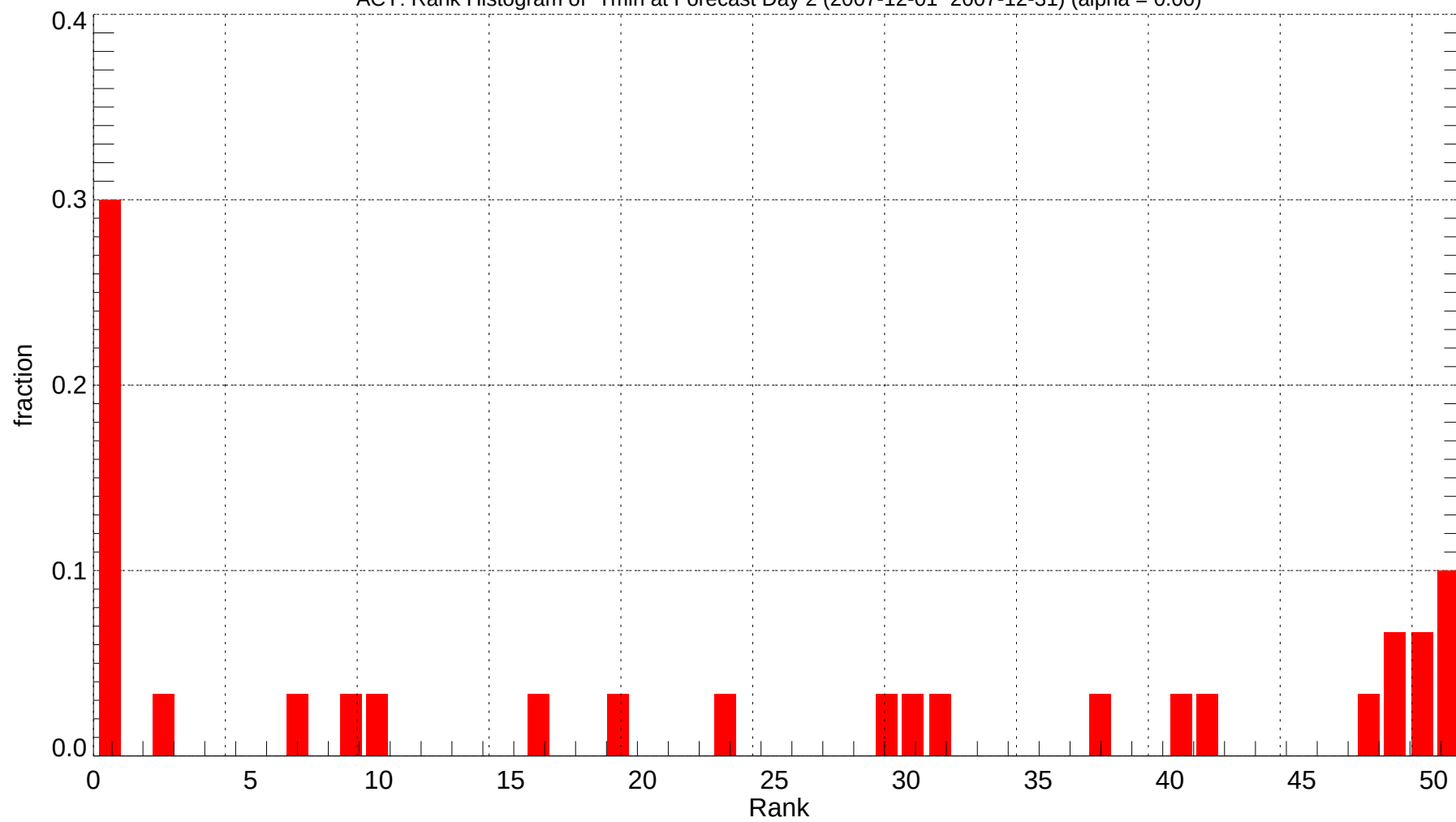
ACY: Rank Histogram of Tmin at Forecast Day 2 (2007-12-01~2007-12-31) (alpha = 0.00)
