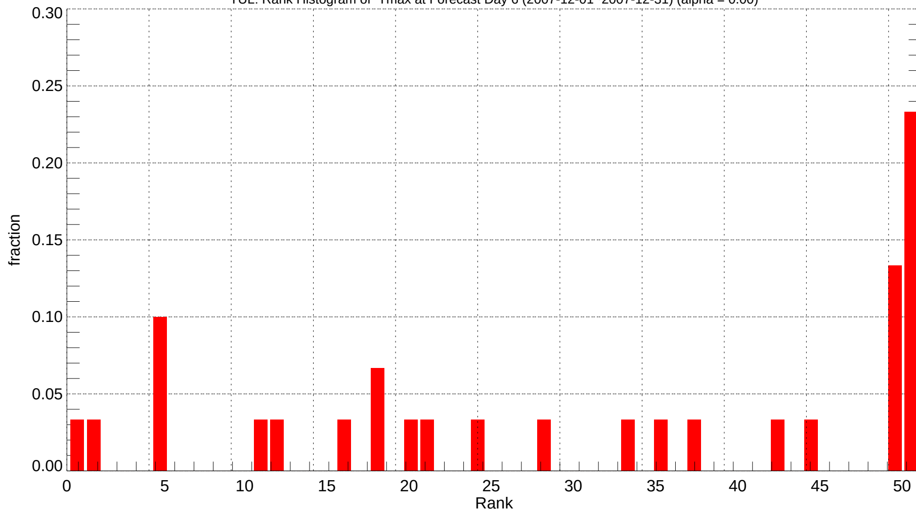
TUL: Rank Histogram of Tmax at Forecast Day 6 (2007-12-01~2007-12-31) (alpha = 0.00)
