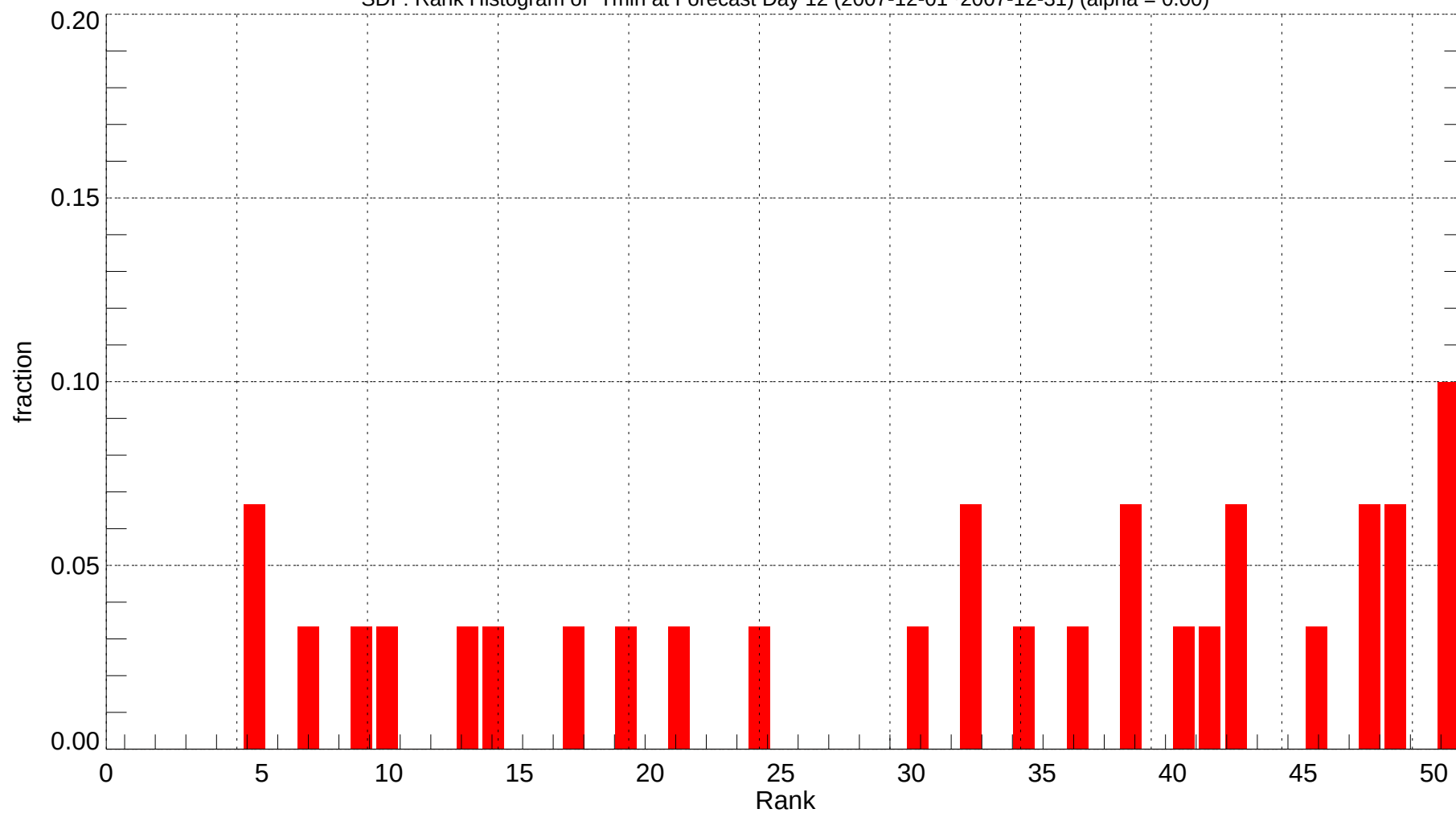
SDF: Rank Histogram of Tmin at Forecast Day 12 (2007-12-01~2007-12-31) (alpha = 0.00)
