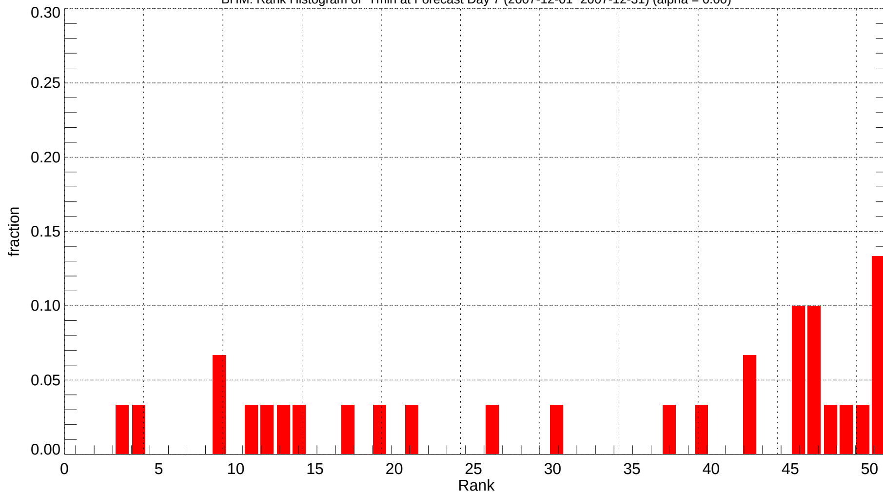
BHM: Rank Histogram of Tmin at Forecast Day 7 (2007-12-01~2007-12-31) (alpha = 0.00)
