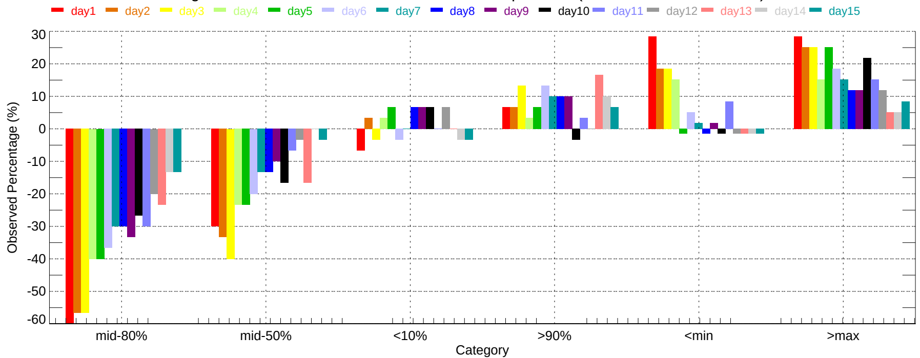
Observed Percentage Deviation of Ensembles - MWL: Min Temperature (2007-12-01~2007-12-31)
