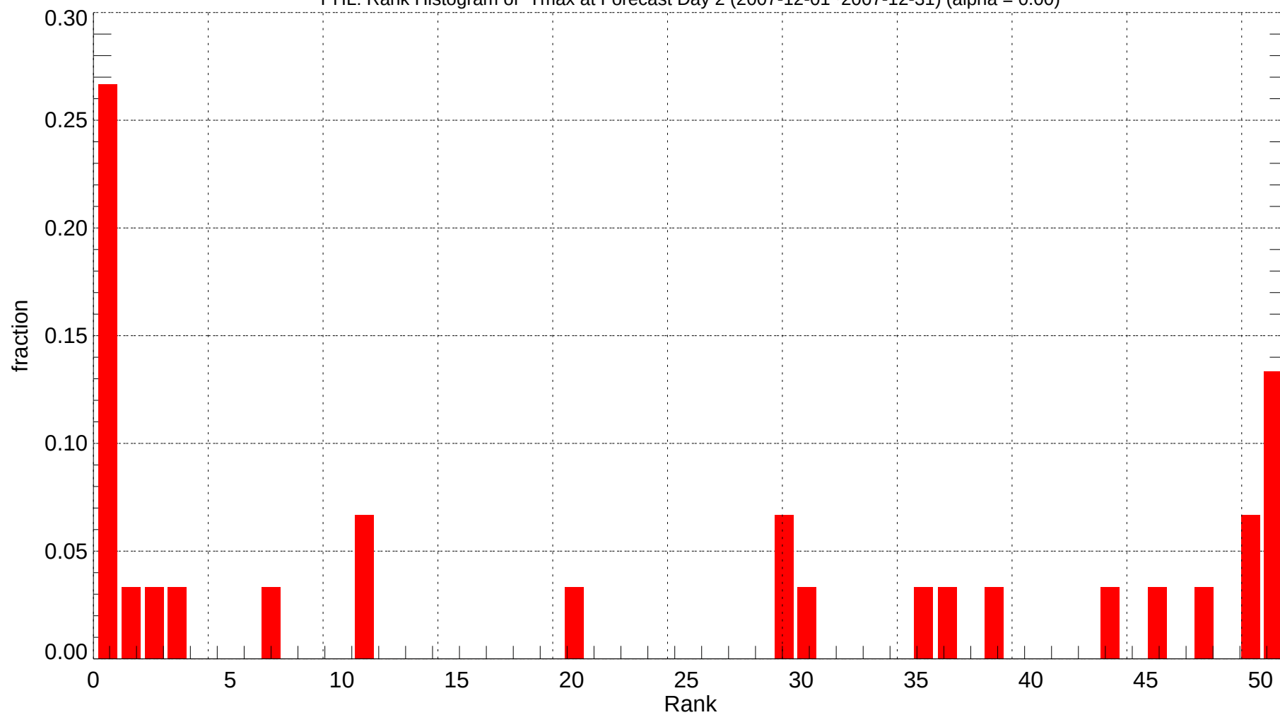
PHL: Rank Histogram of Tmax at Forecast Day 2 (2007-12-01~2007-12-31) (alpha = 0.00)
