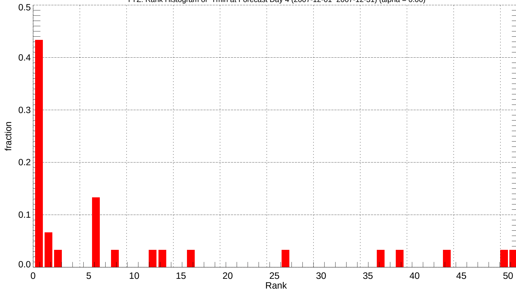
YYZ: Rank Histogram of Tmin at Forecast Day 4 (2007-12-01~2007-12-31) (alpha = 0.00)
