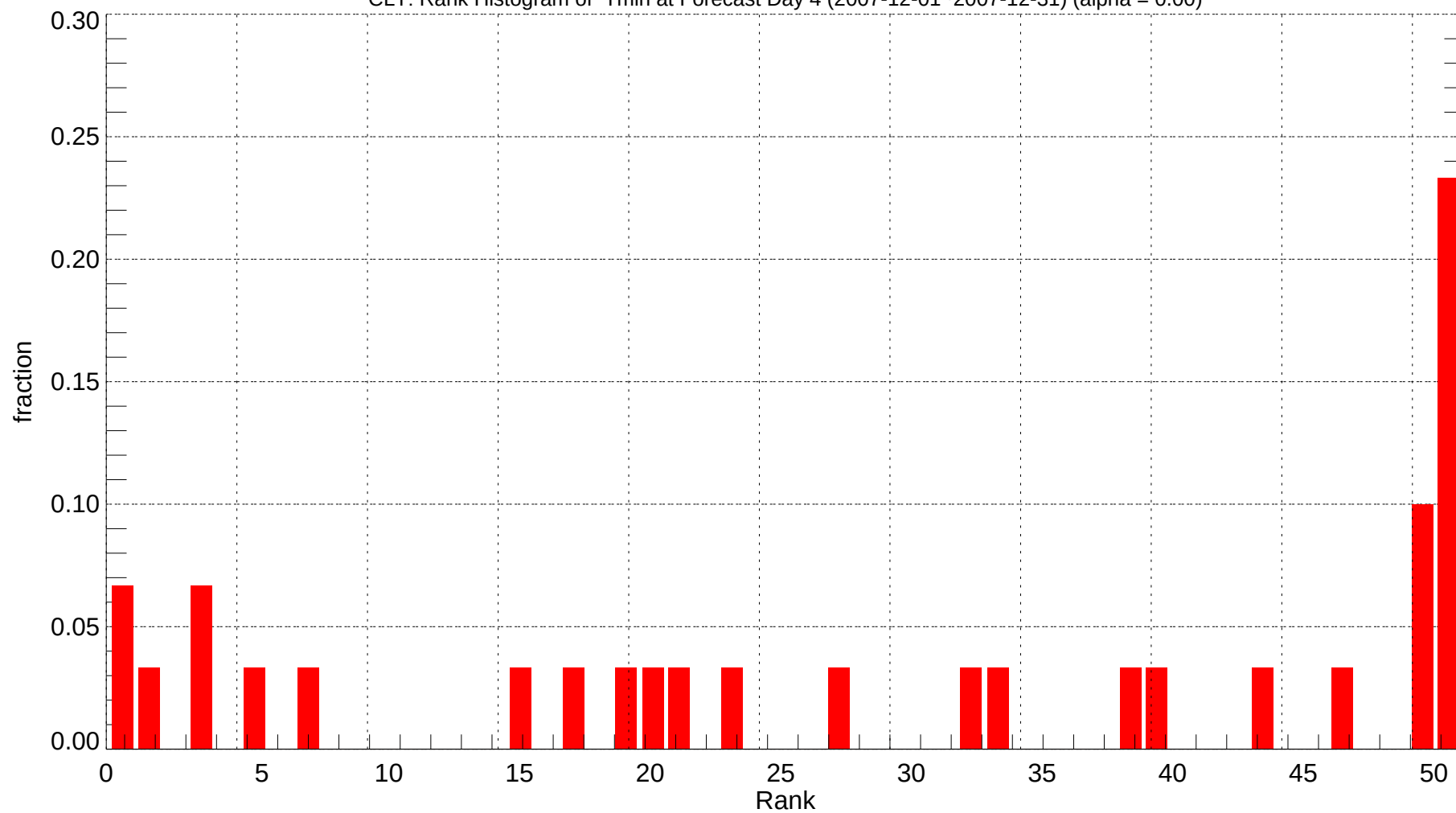
CLT: Rank Histogram of Tmin at Forecast Day 4 (2007-12-01~2007-12-31) (alpha = 0.00)
