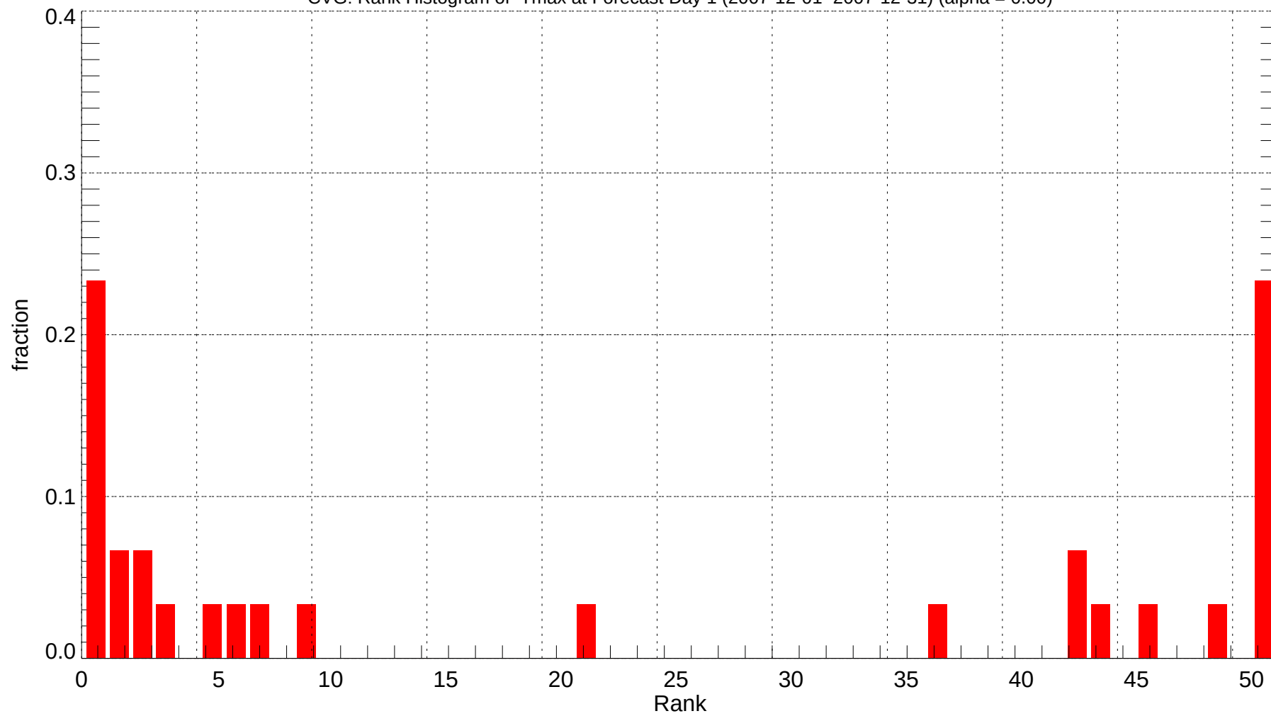
CVG: Rank Histogram of Tmax at Forecast Day 1 (2007-12-01~2007-12-31) (alpha = 0.00)
