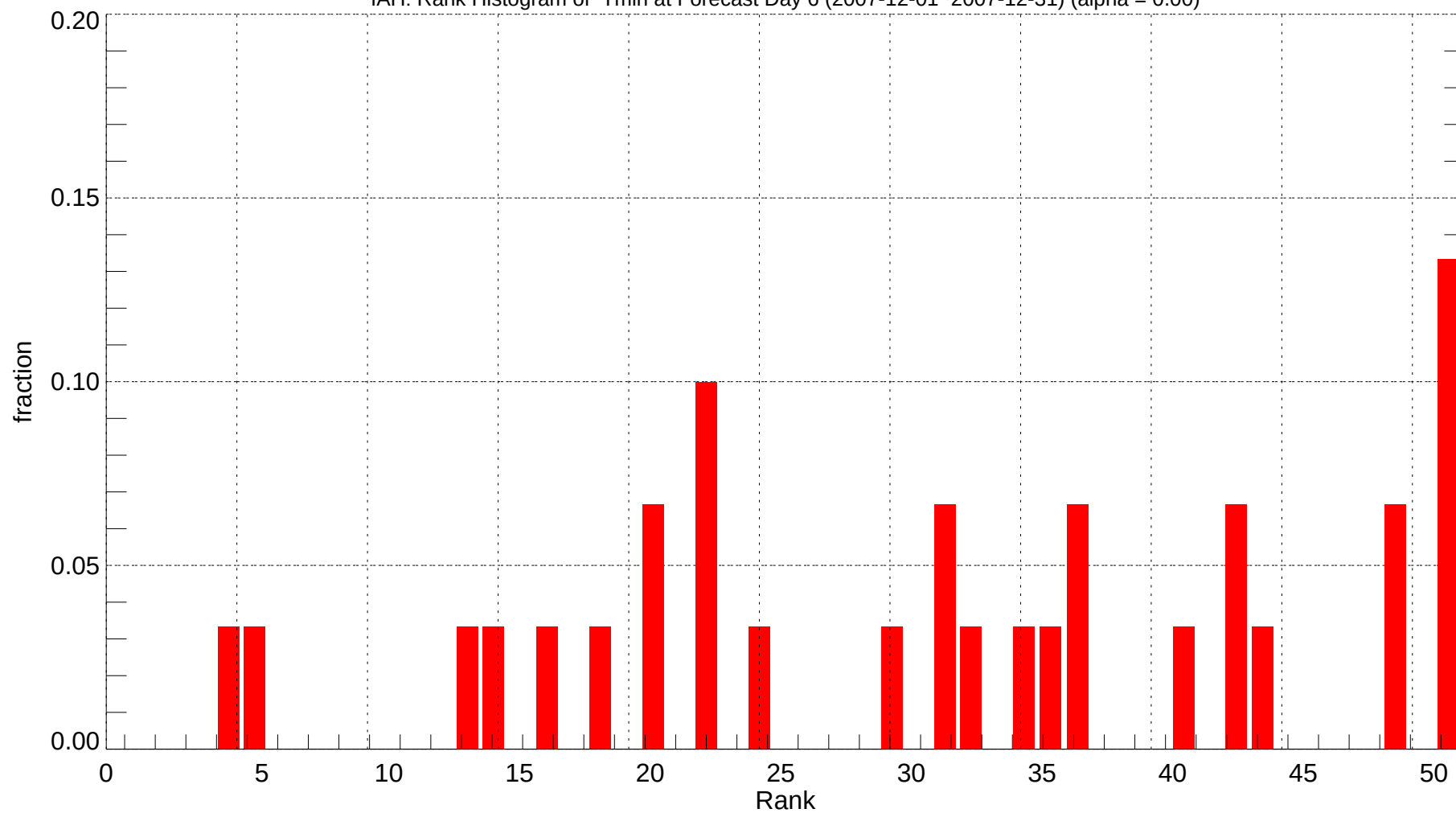
IAH: Rank Histogram of Tmin at Forecast Day 6 (2007-12-01~2007-12-31) (alpha = 0.00)
