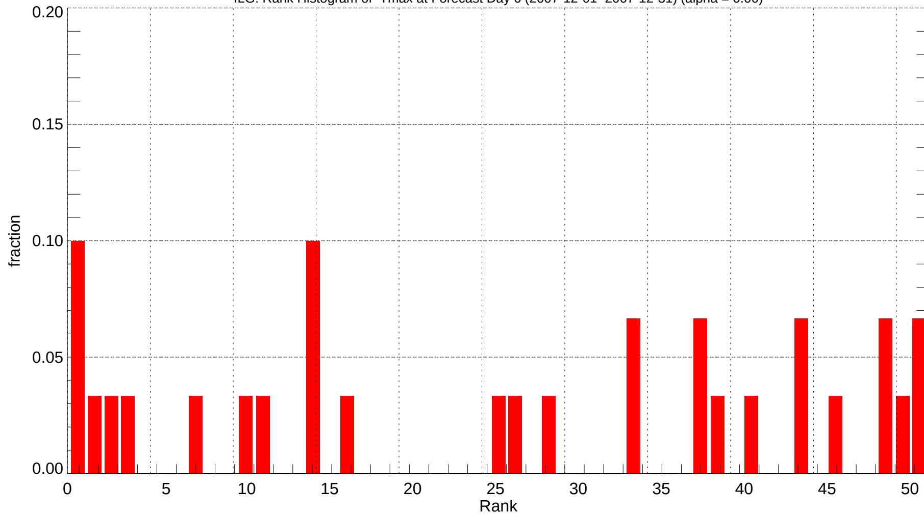
ILG: Rank Histogram of Tmax at Forecast Day 6 (2007-12-01~2007-12-31) (alpha = 0.00)
