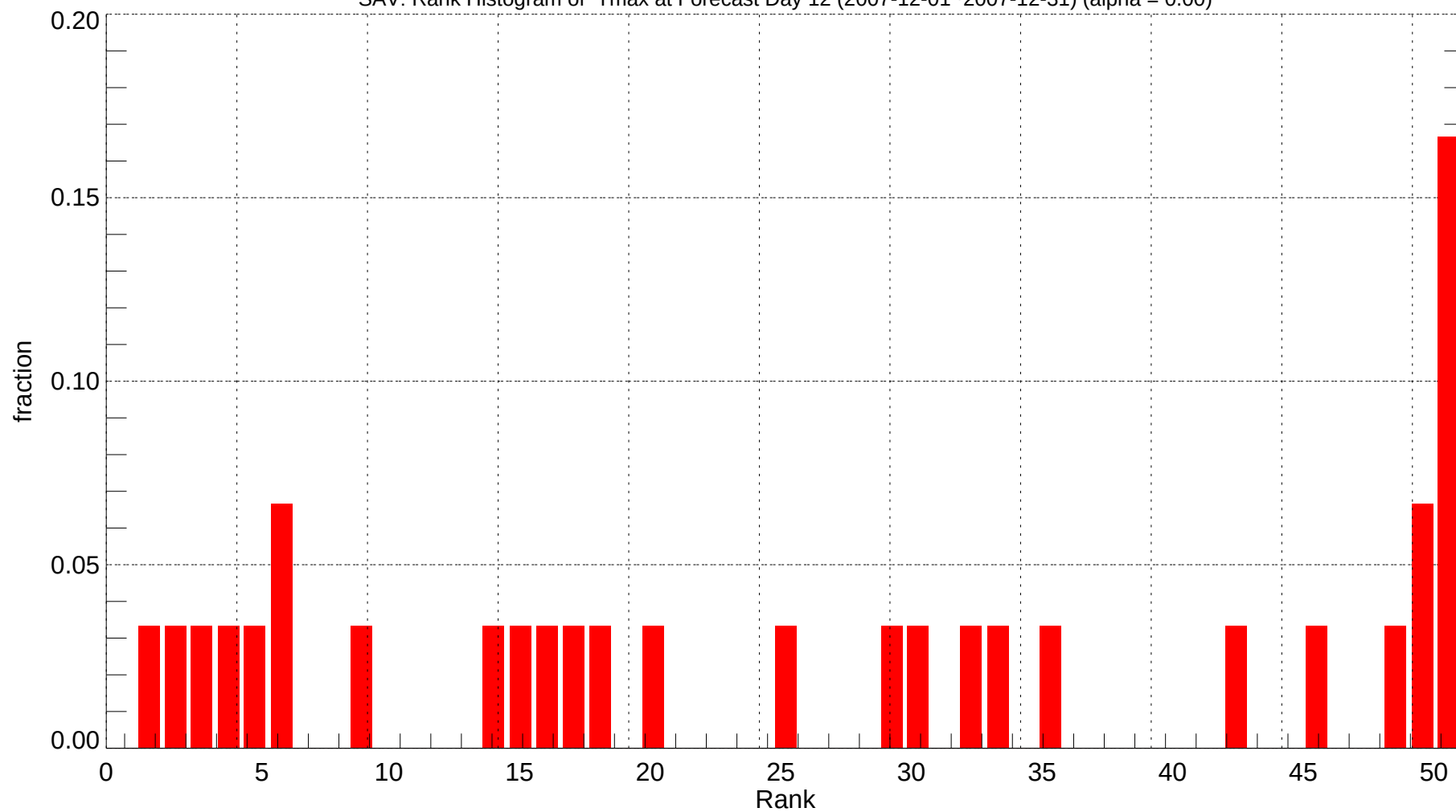
SAV: Rank Histogram of Tmax at Forecast Day 12 (2007-12-01~2007-12-31) (alpha = 0.00)
