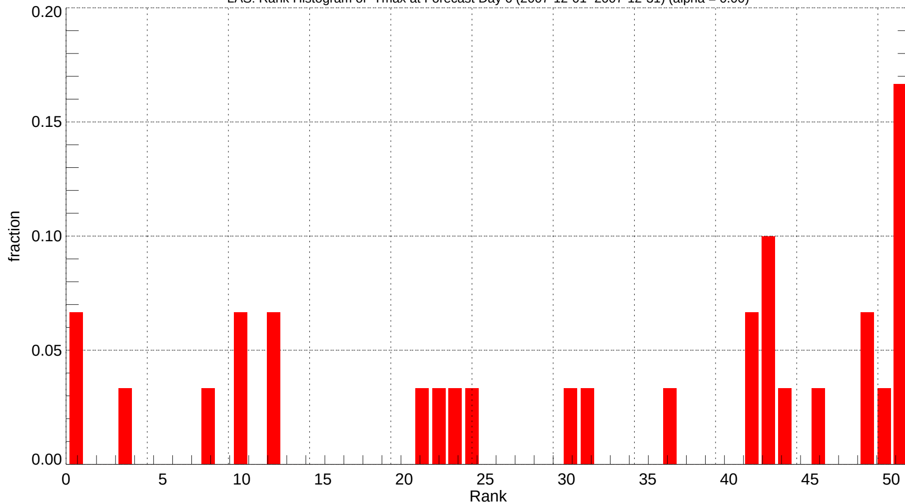
LAS: Rank Histogram of Tmax at Forecast Day 6 (2007-12-01~2007-12-31) (alpha = 0.00)
