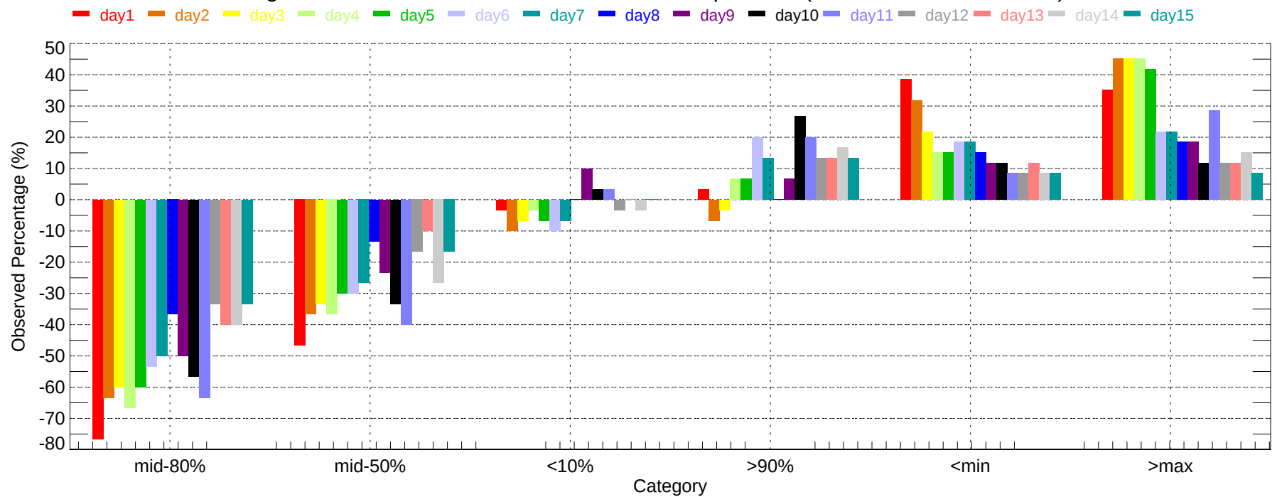
Observed Percentage Deviation of Ensembles - ALW: Max Temperature (2007-12-01~2007-12-31)
