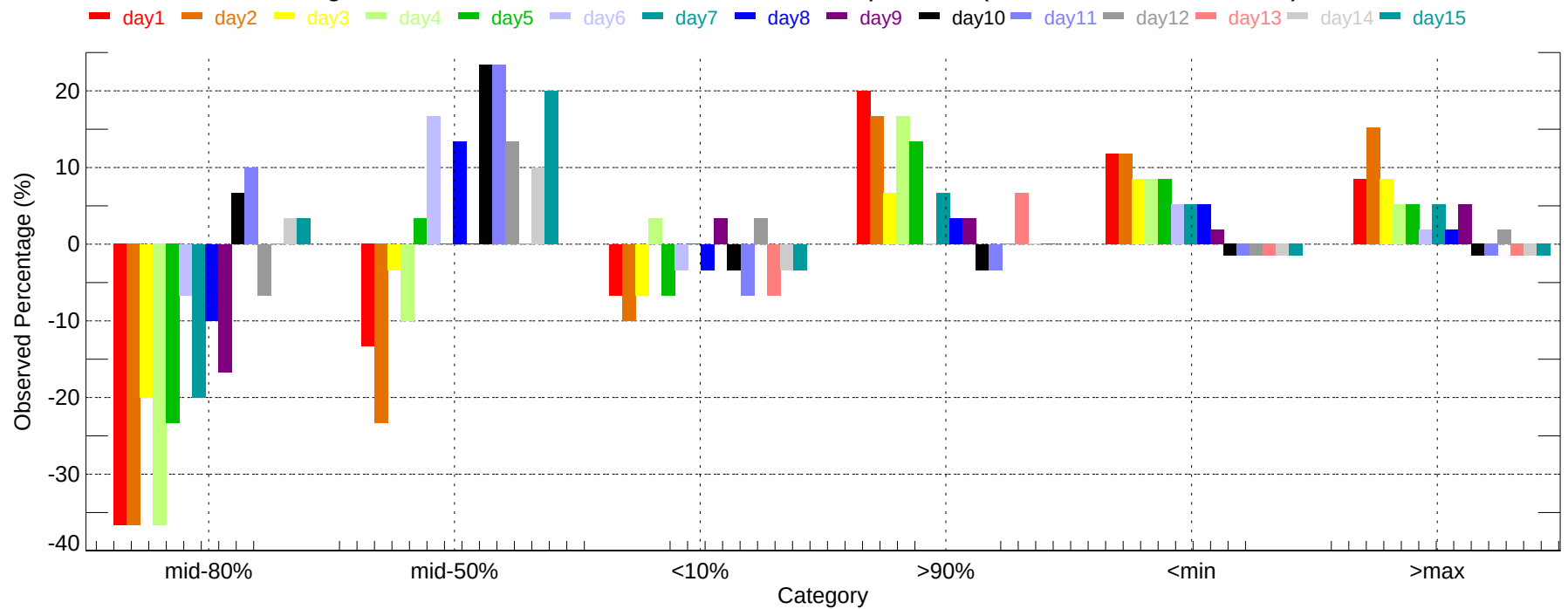
Observed Percentage Deviation of Ensembles - FAT: Max Temperature (2007-12-01~2007-12-31)
