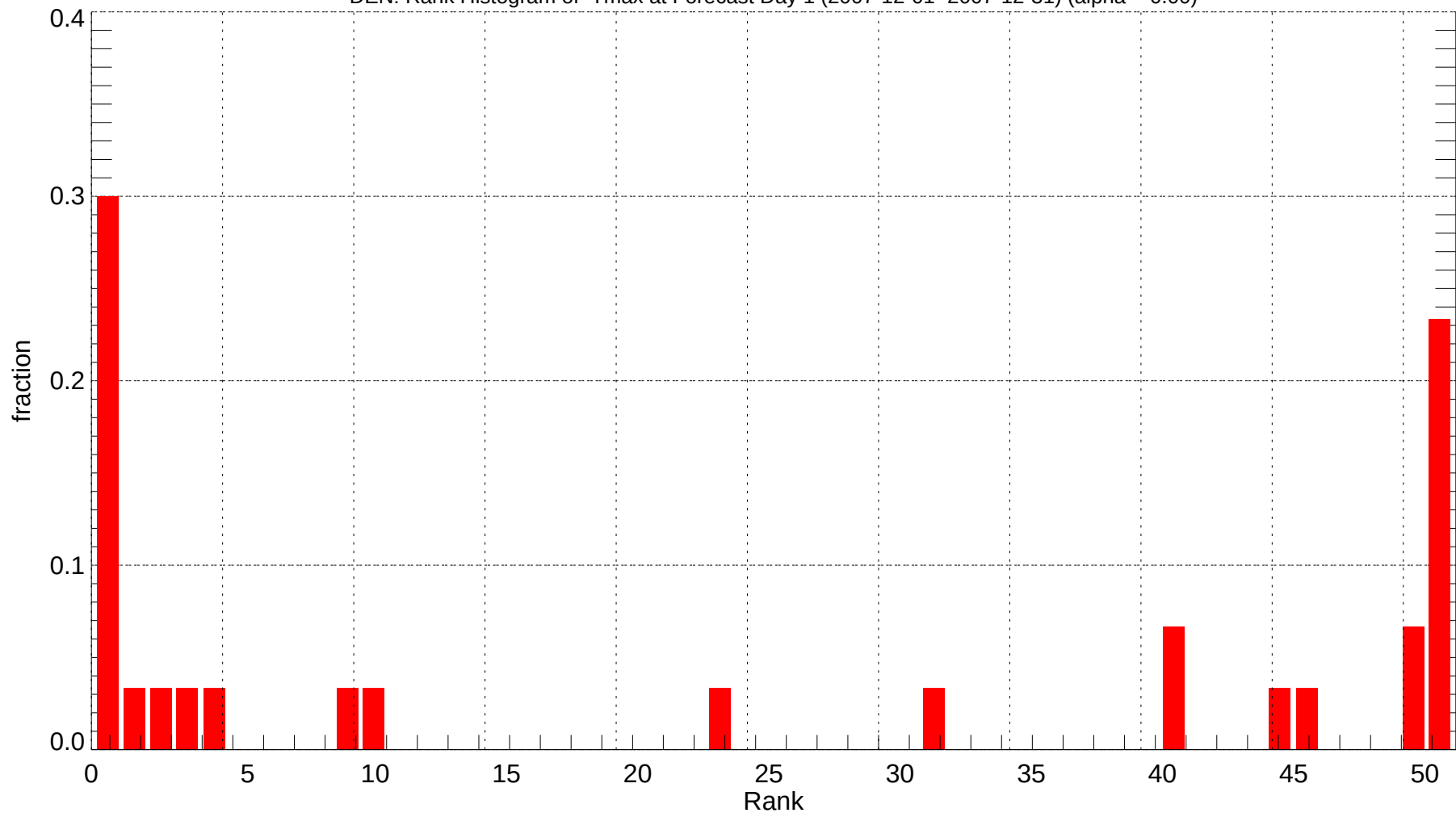
DEN: Rank Histogram of Tmax at Forecast Day 1 (2007-12-01~2007-12-31) (alpha = 0.00)
