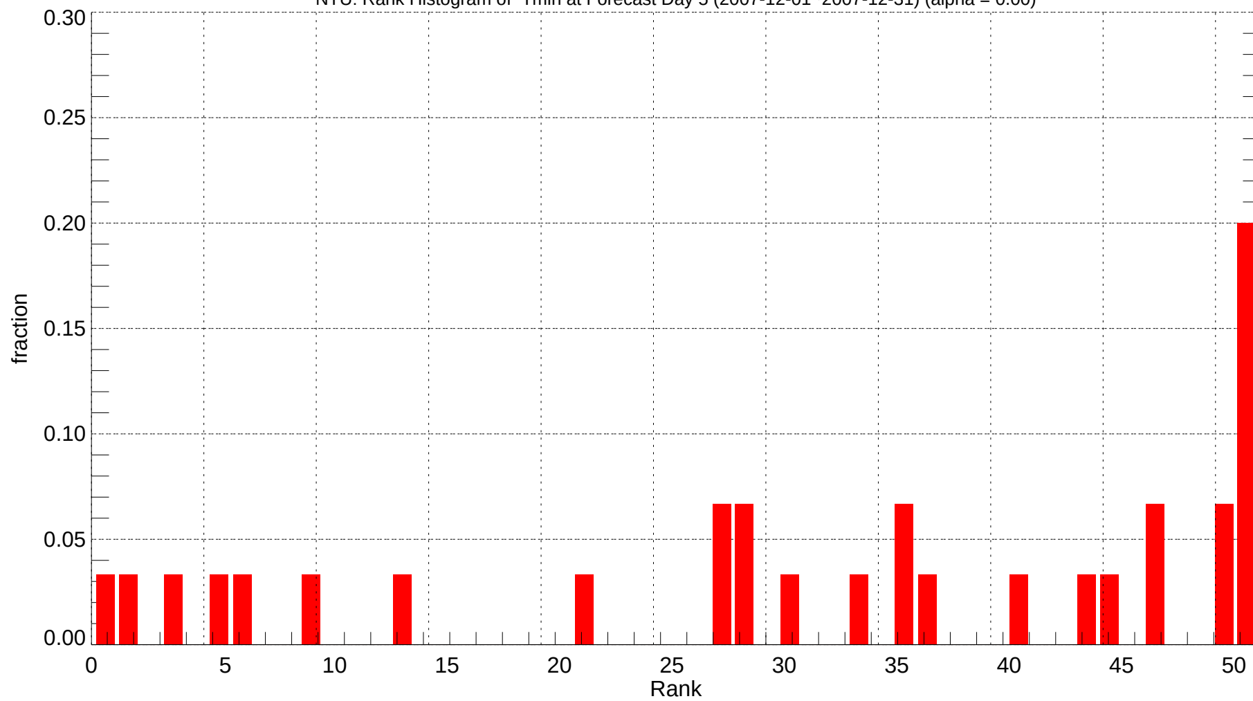
NTU: Rank Histogram of Tmin at Forecast Day 5 (2007-12-01~2007-12-31) (alpha = 0.00)
