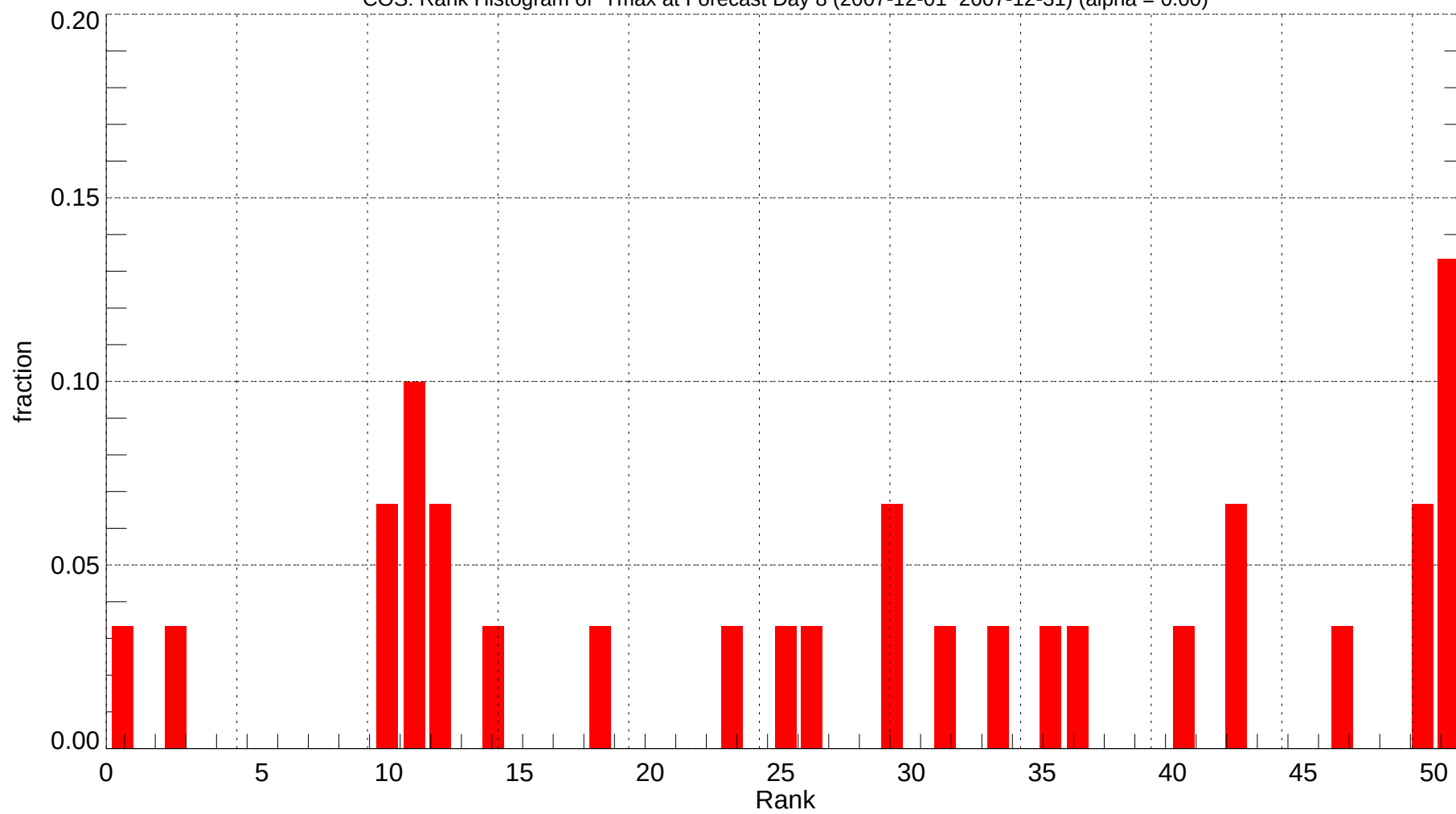
COS: Rank Histogram of Tmax at Forecast Day 8 (2007-12-01~2007-12-31) (alpha = 0.00)
