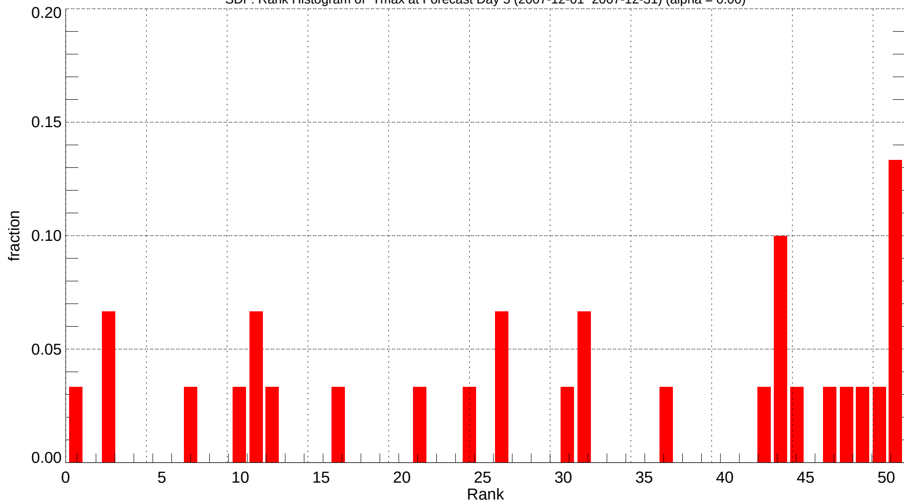
SDF: Rank Histogram of Tmax at Forecast Day 5 (2007-12-01~2007-12-31) (alpha = 0.00)
