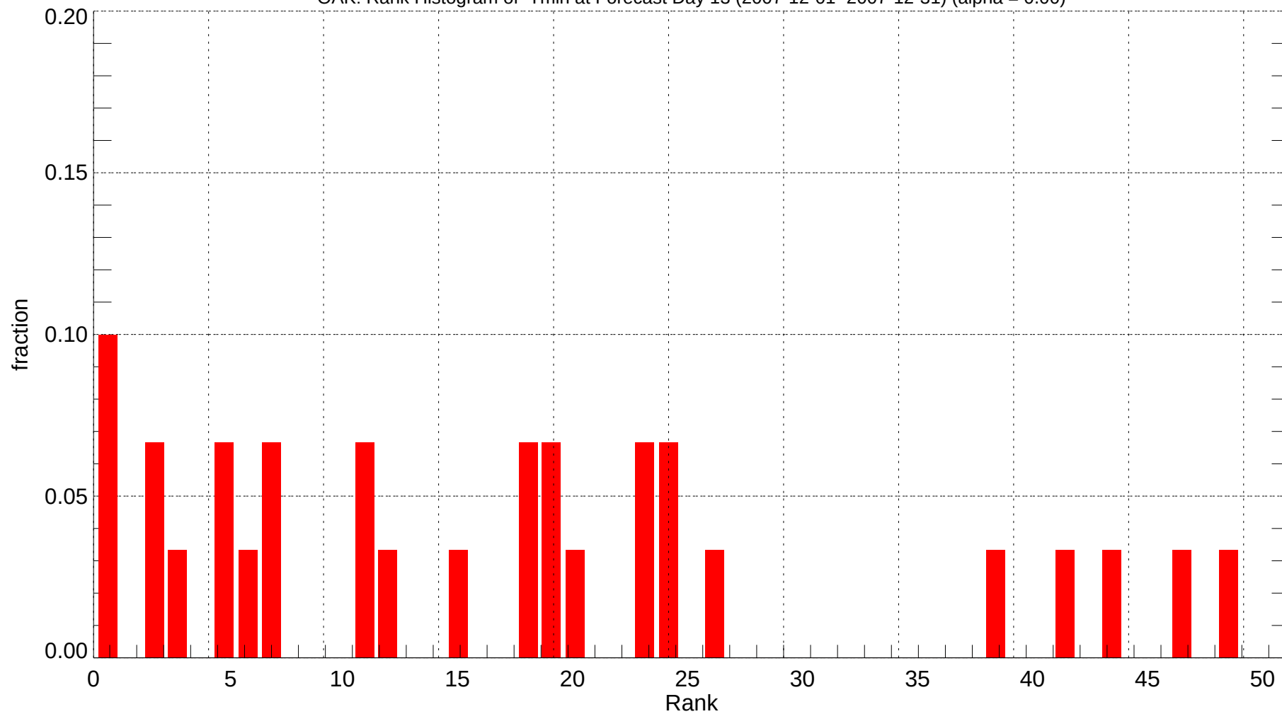
OAK: Rank Histogram of Tmin at Forecast Day 13 (2007-12-01~2007-12-31) (alpha = 0.00)
