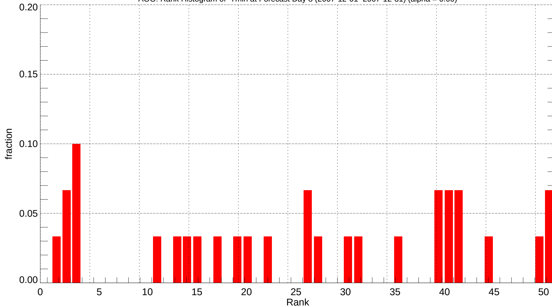
AOO: Rank Histogram of Tmin at Forecast Day 8 (2007-12-01~2007-12-31) (alpha = 0.00)
