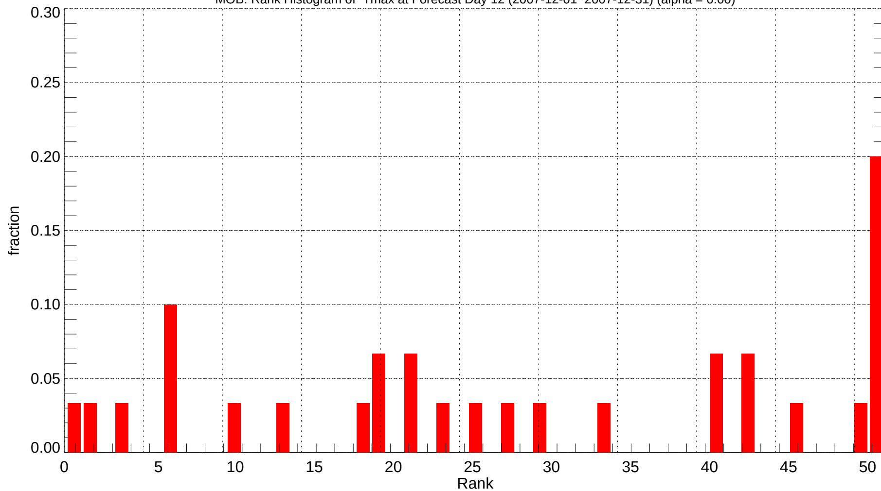
MOB: Rank Histogram of Tmax at Forecast Day 12 (2007-12-01~2007-12-31) (alpha = 0.00)
