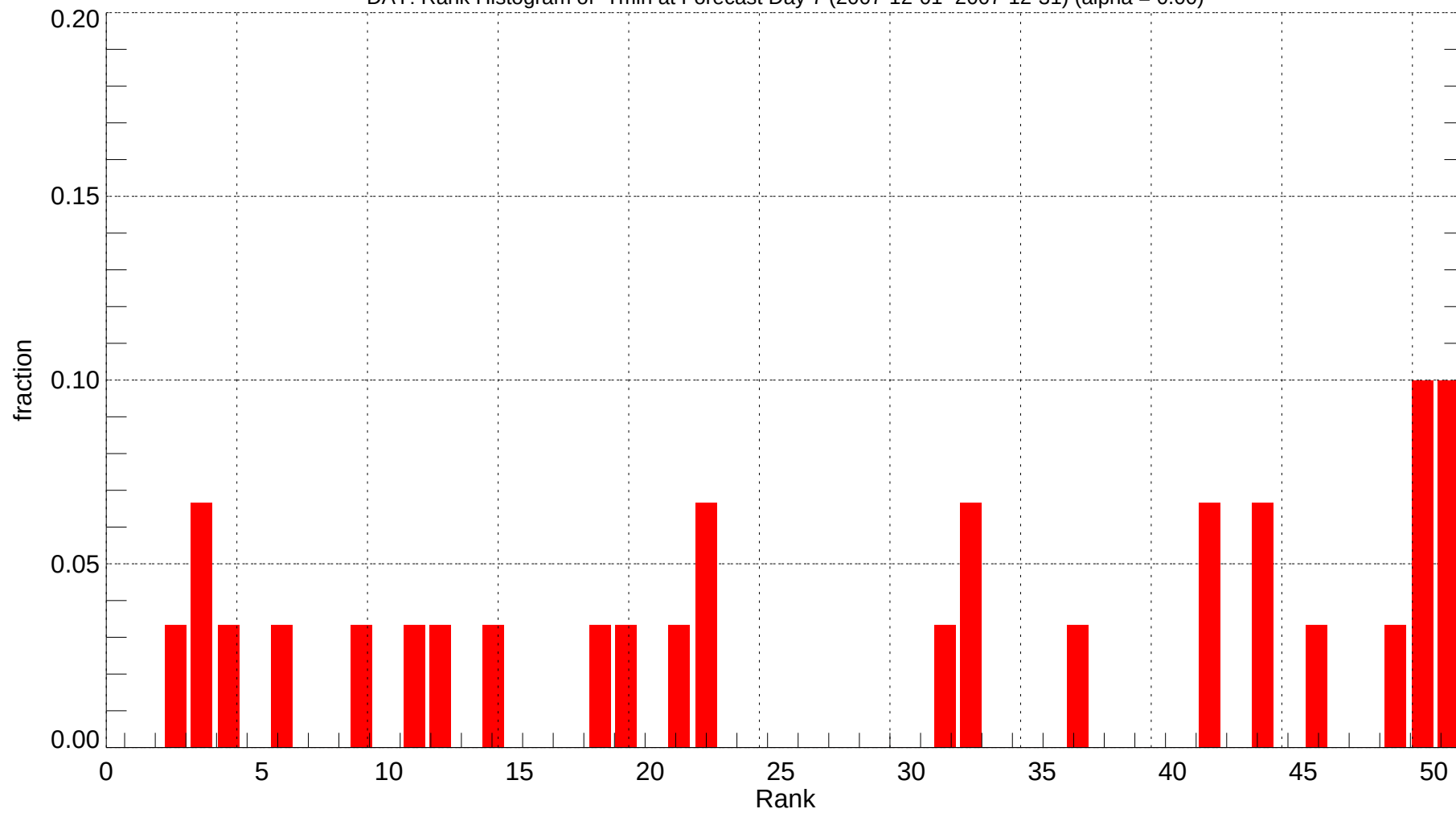
DAY: Rank Histogram of Tmin at Forecast Day 7 (2007-12-01~2007-12-31) (alpha = 0.00)
