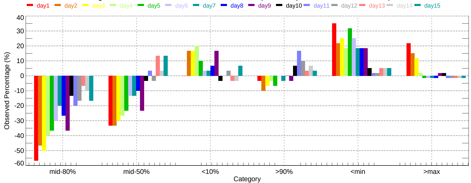
Observed Percentage Deviation of Ensembles - ROC: Min Temperature (2007-12-01~2007-12-31)
