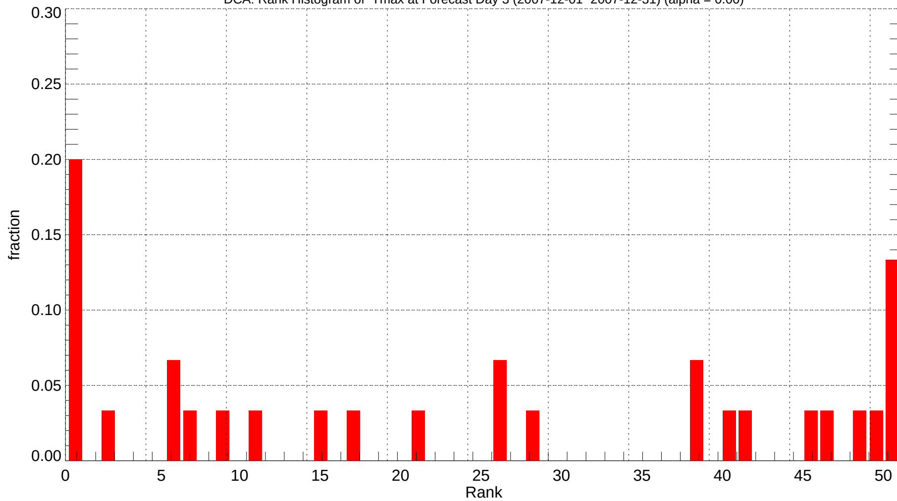
DCA: Rank Histogram of Tmax at Forecast Day 3 (2007-12-01~2007-12-31) (alpha = 0.00)
