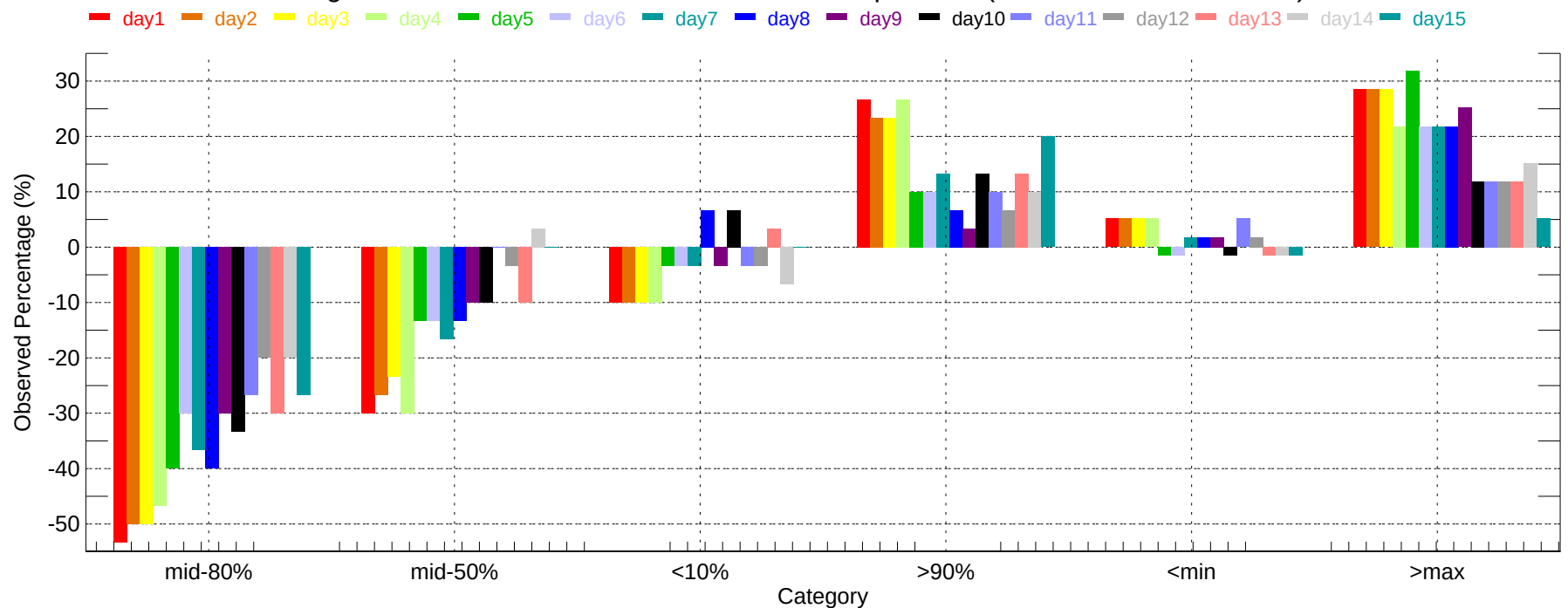
Observed Percentage Deviation of Ensembles - MAF: Max Temperature (2007-12-01~2007-12-31)
