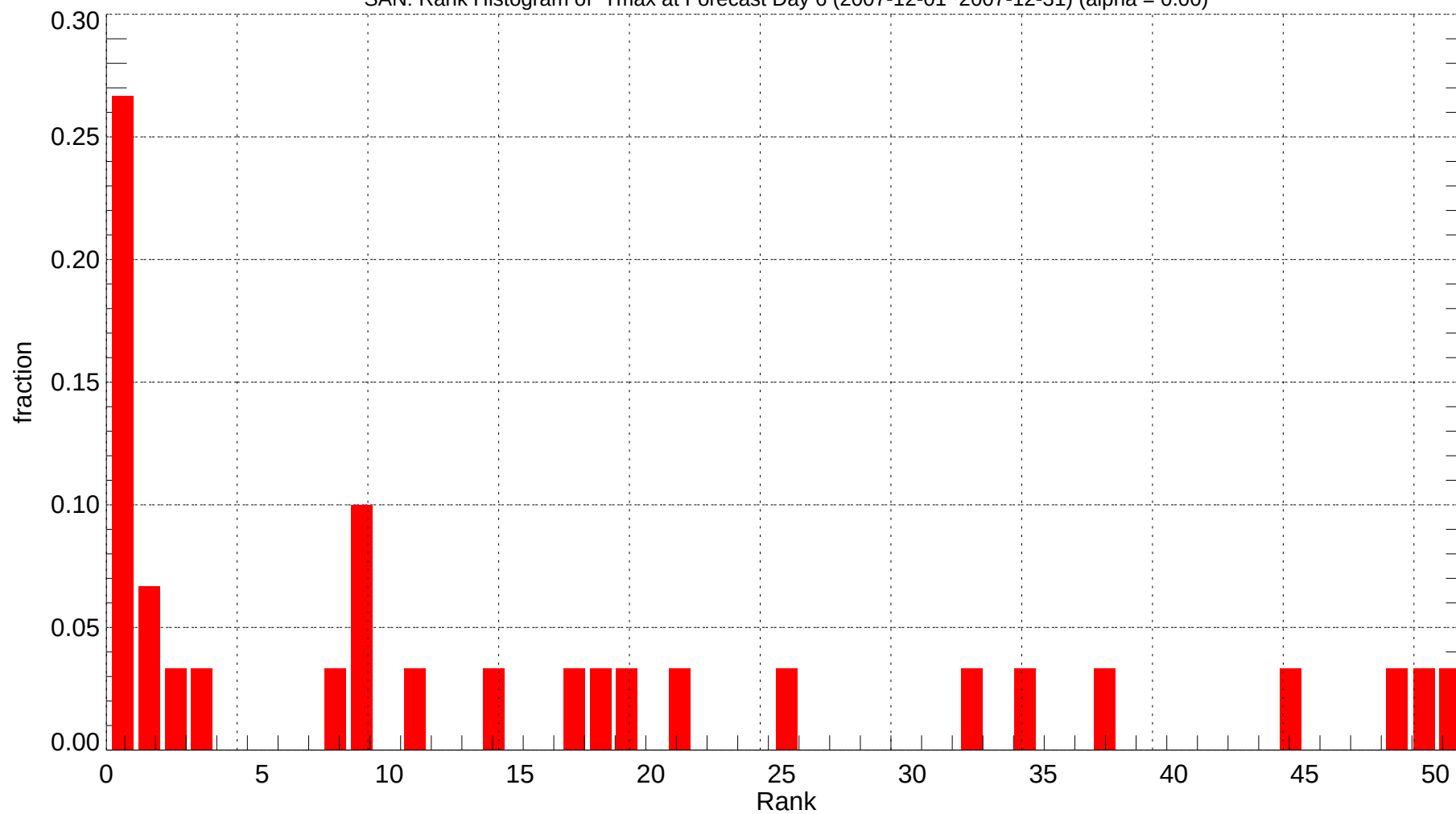
SAN: Rank Histogram of Tmax at Forecast Day 6 (2007-12-01~2007-12-31) (alpha = 0.00)
