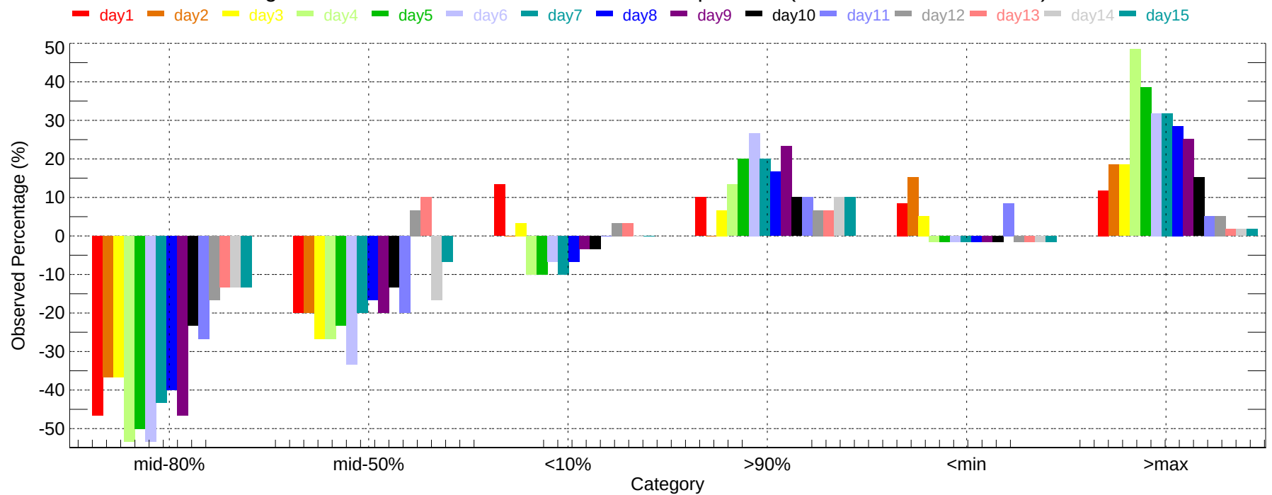
Observed Percentage Deviation of Ensembles - ELP: Min Temperature (2007-12-01~2007-12-31)
