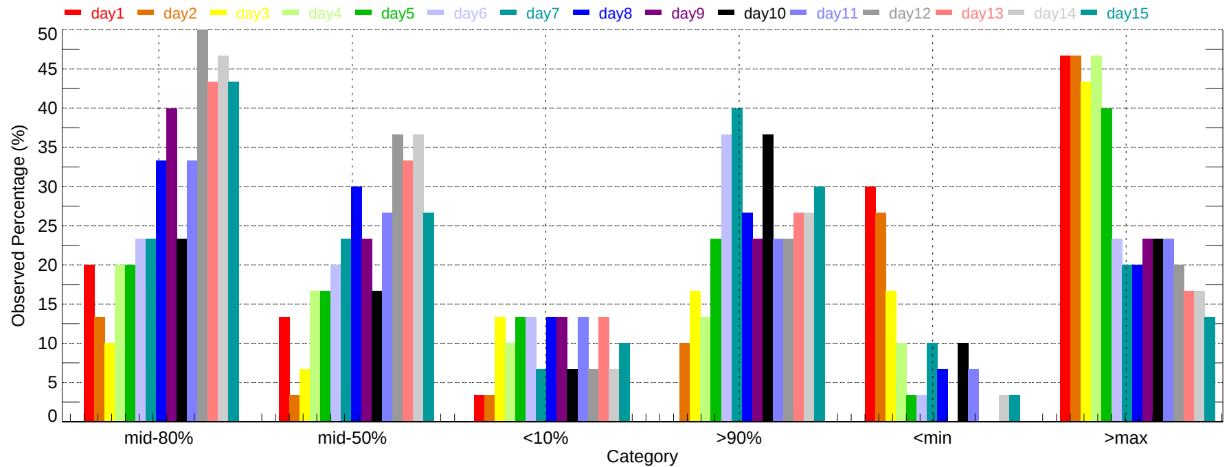
Observed Percentage of Ensembles - PDT: Max Temperature (2007-12-01~2007-12-31)
