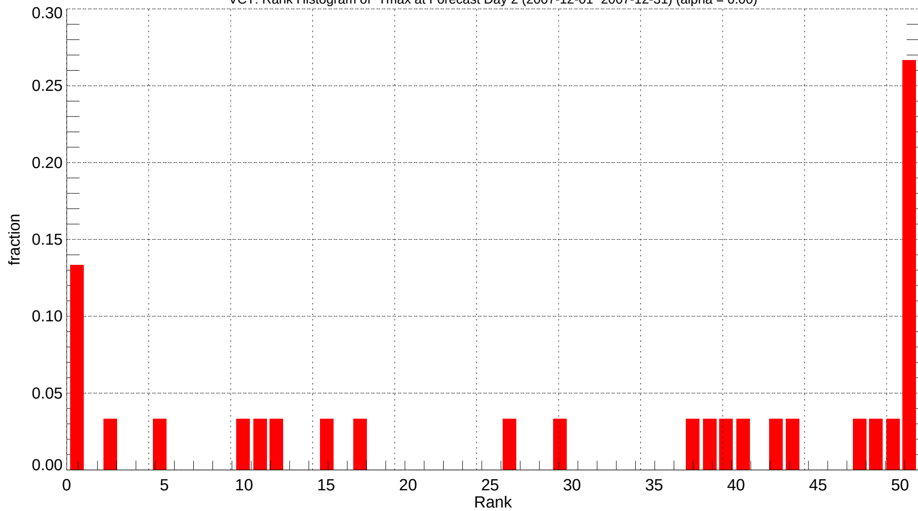
VCT: Rank Histogram of Tmax at Forecast Day 2 (2007-12-01~2007-12-31) (alpha = 0.00)
