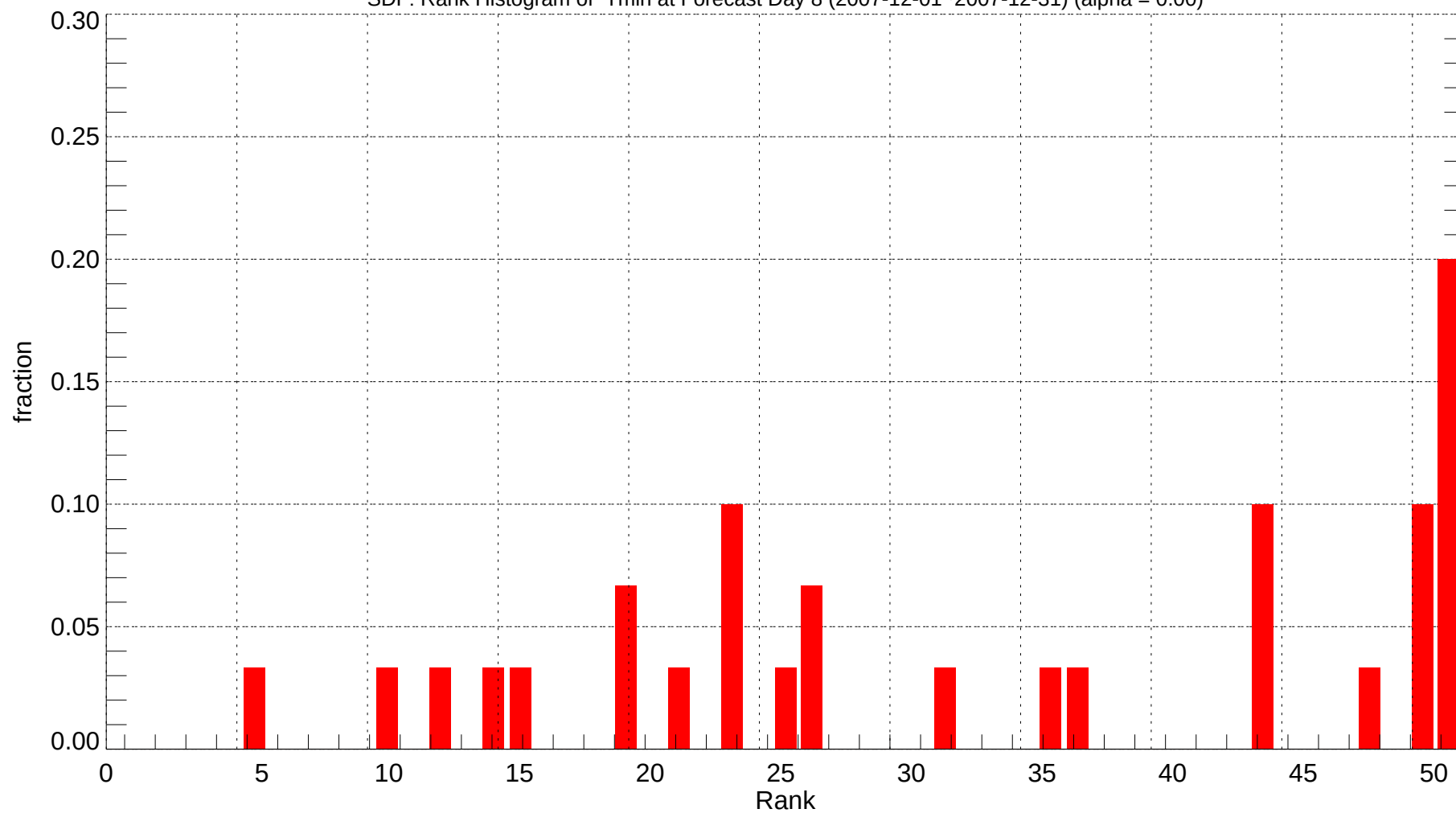
SDF: Rank Histogram of Tmin at Forecast Day 8 (2007-12-01~2007-12-31) (alpha = 0.00)
