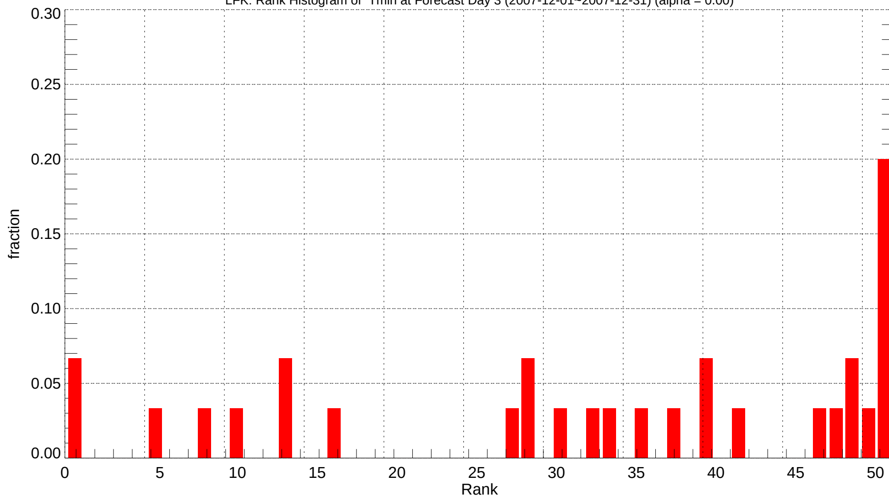
LFK: Rank Histogram of Tmin at Forecast Day 3 (2007-12-01~2007-12-31) (alpha = 0.00)
