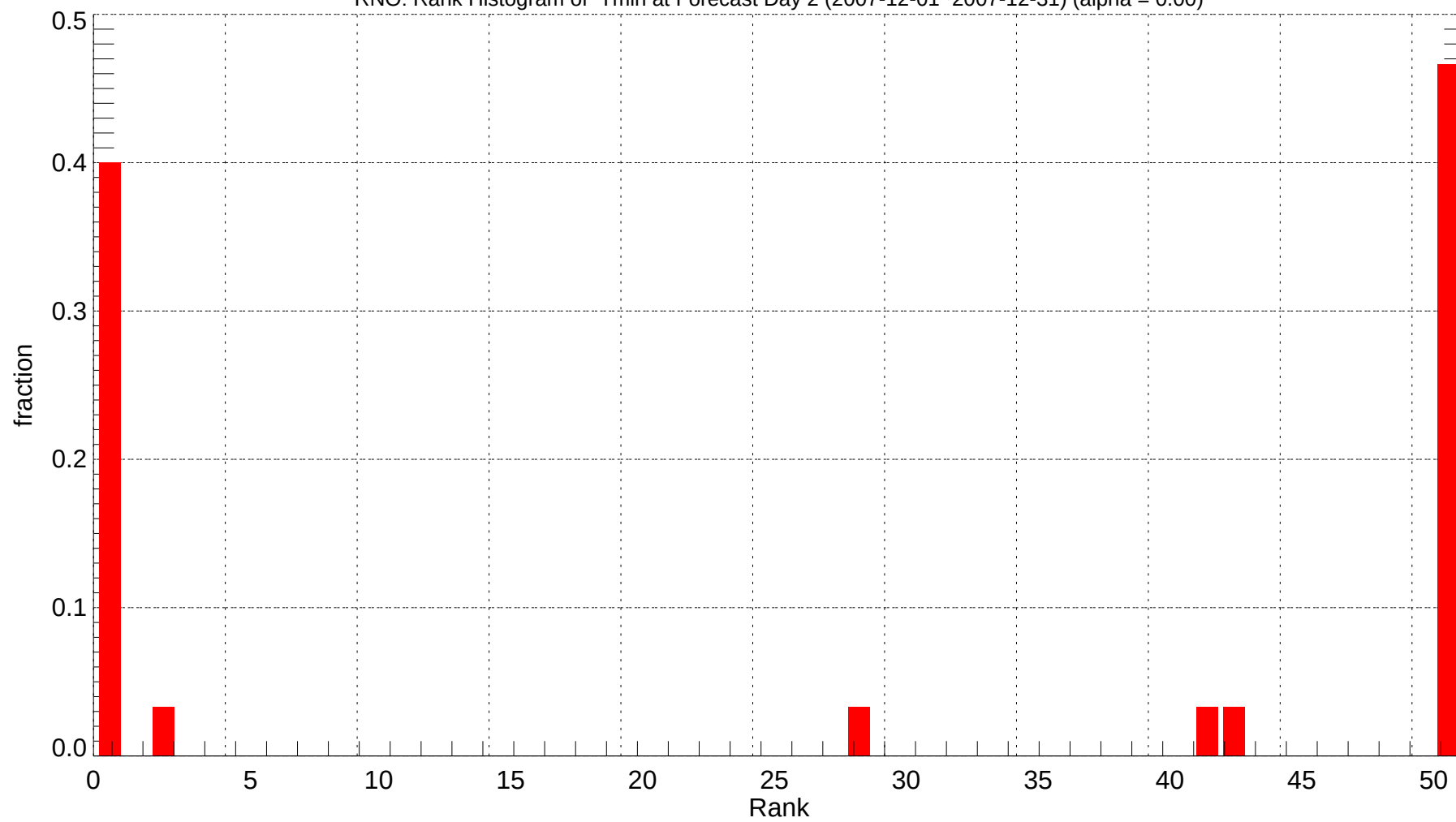
RNO: Rank Histogram of Tmin at Forecast Day 2 (2007-12-01~2007-12-31) (alpha = 0.00)
