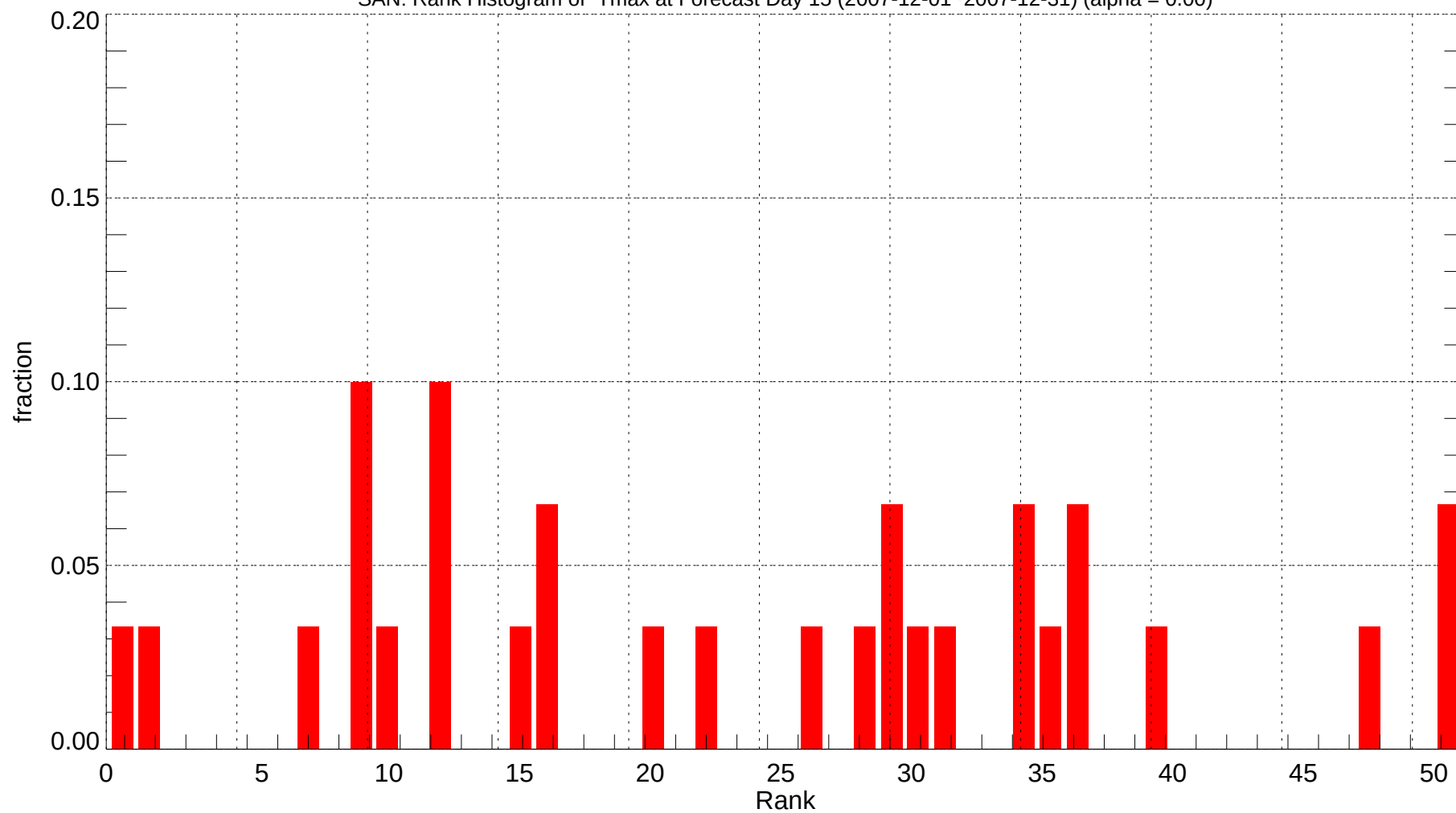
SAN: Rank Histogram of Tmax at Forecast Day 15 (2007-12-01~2007-12-31) (alpha = 0.00)
