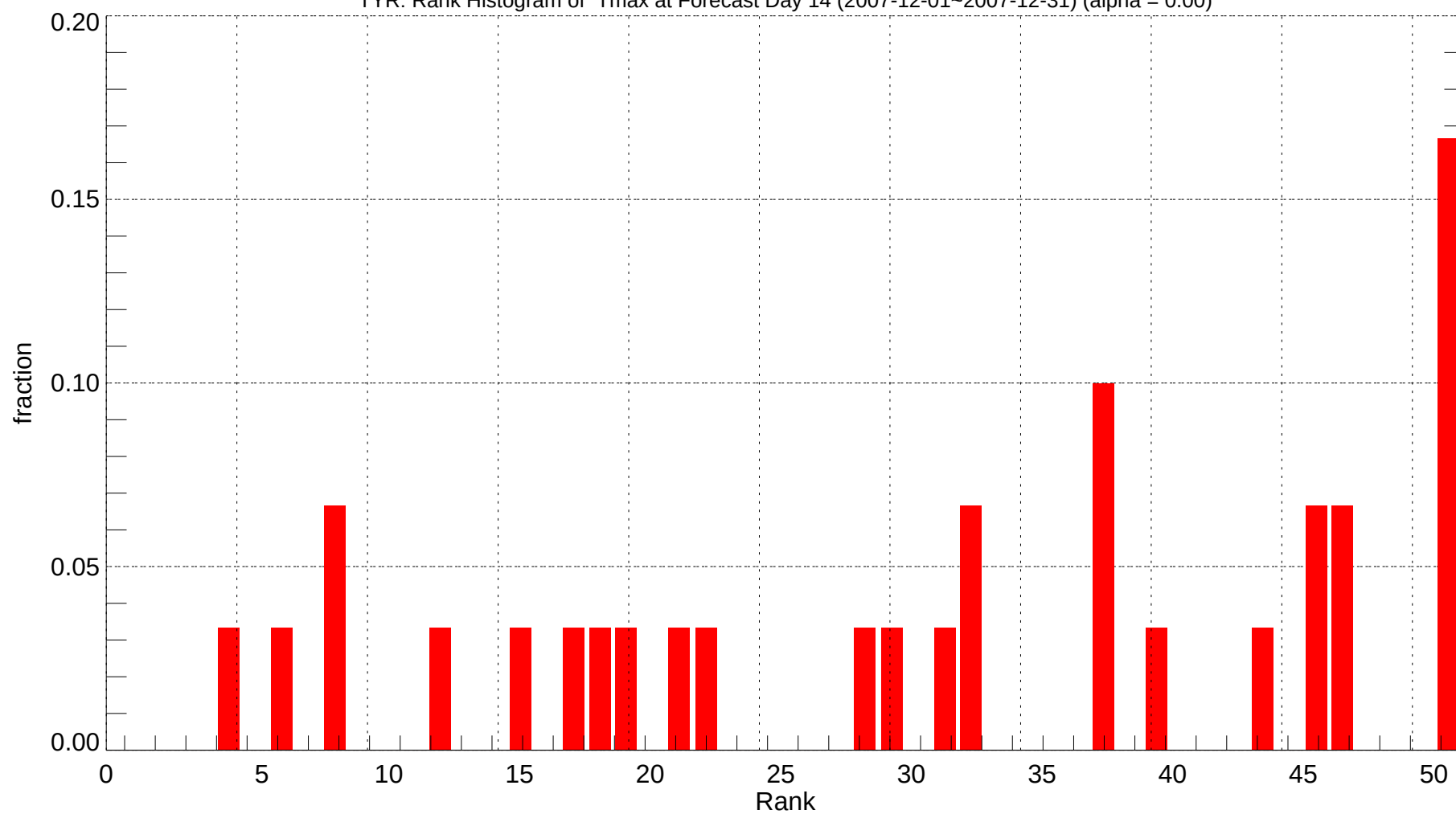
TYR: Rank Histogram of Tmax at Forecast Day 14 (2007-12-01~2007-12-31) (alpha = 0.00)
