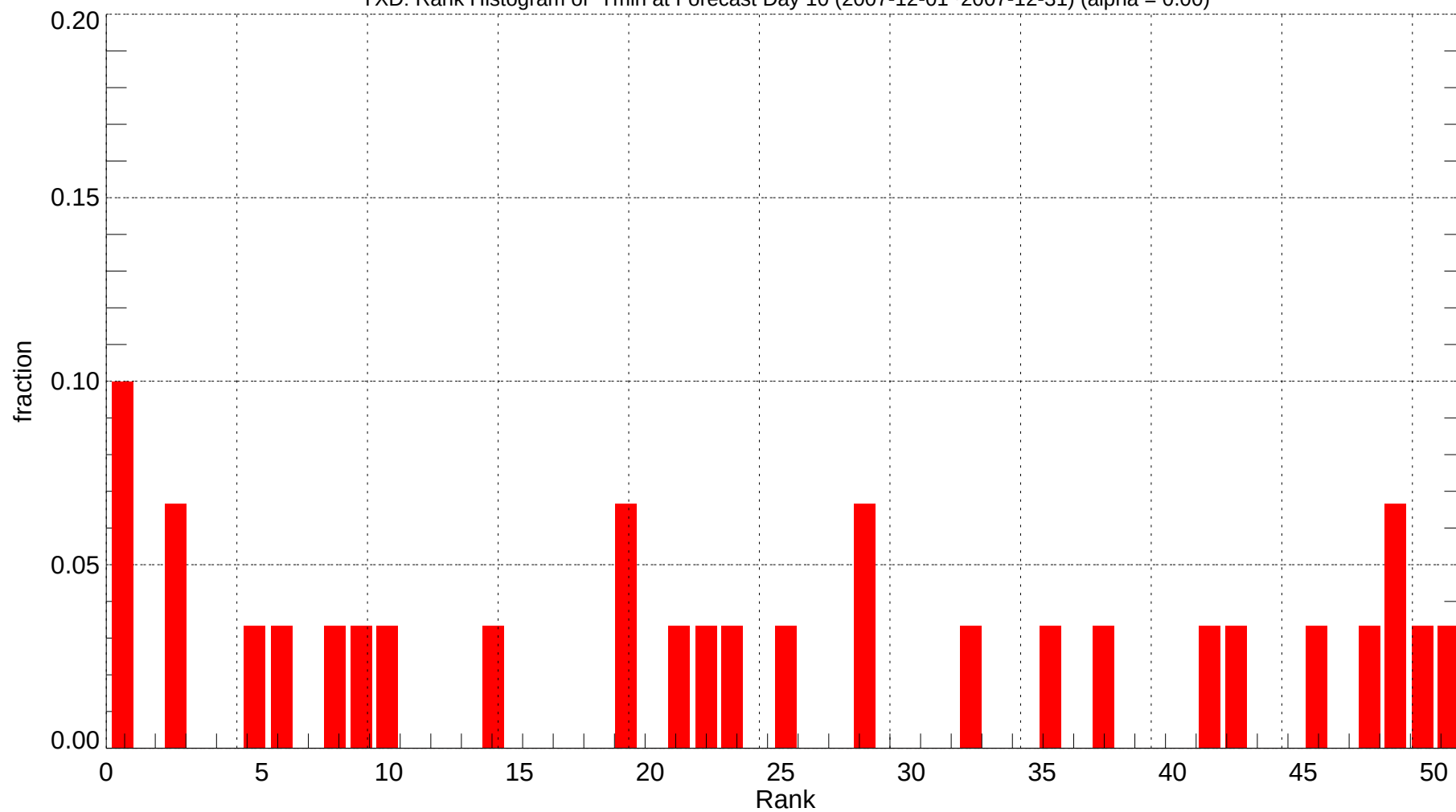
YXD: Rank Histogram of Tmin at Forecast Day 10 (2007-12-01~2007-12-31) (alpha = 0.00)
