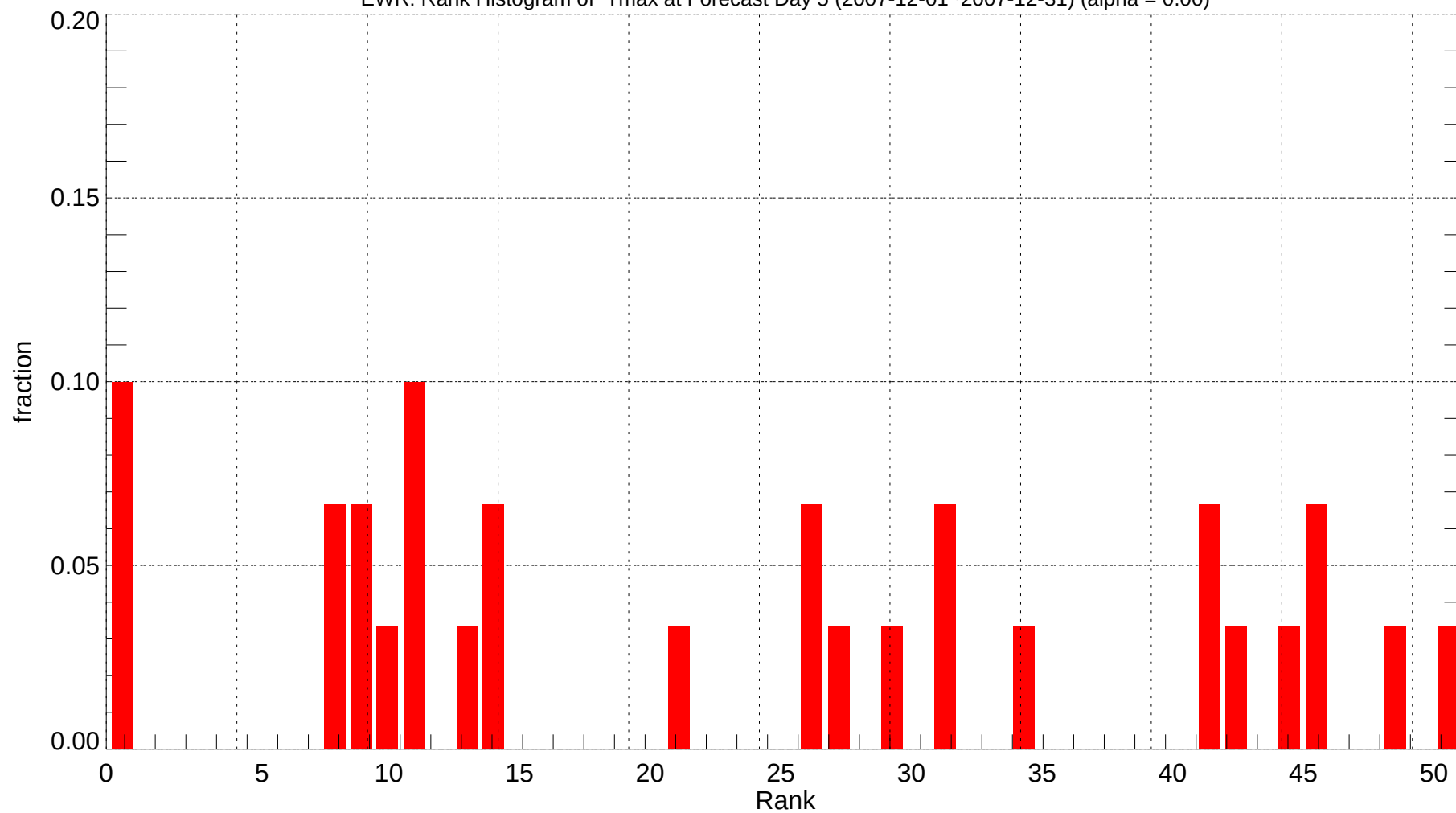
EWR: Rank Histogram of Tmax at Forecast Day 5 (2007-12-01~2007-12-31) (alpha = 0.00)
