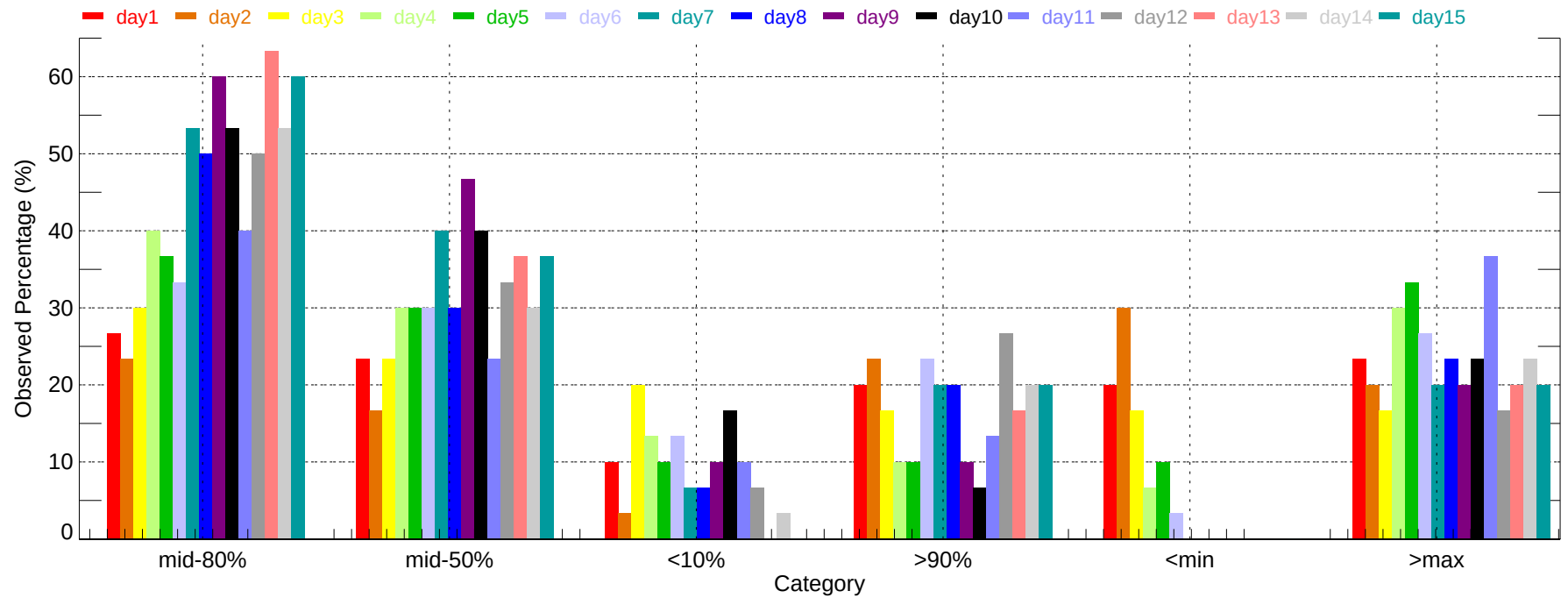
Observed Percentage of Ensembles - ATL: Min Temperature (2007-12-01~2007-12-31)
