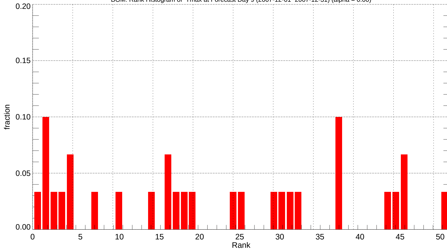
BGM: Rank Histogram of Tmax at Forecast Day 9 (2007-12-01~2007-12-31) (alpha = 0.00)
