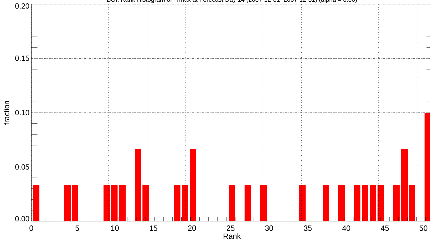
BOI: Rank Histogram of Tmax at Forecast Day 14 (2007-12-01~2007-12-31) (alpha = 0.00)
