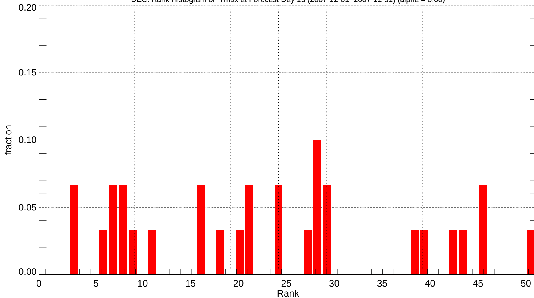
DEC: Rank Histogram of Tmax at Forecast Day 13 (2007-12-01~2007-12-31) (alpha = 0.00)
