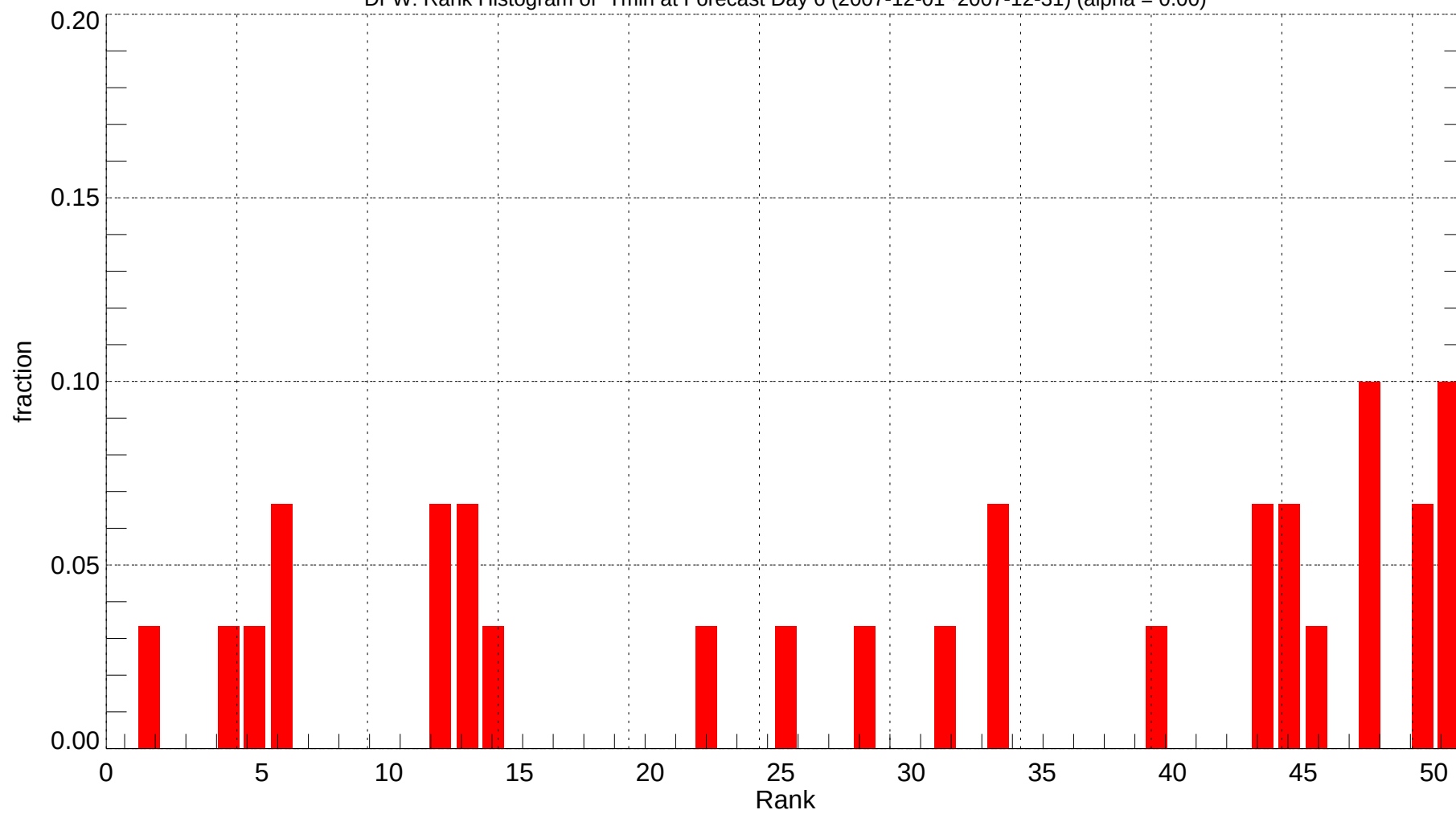
DFW: Rank Histogram of Tmin at Forecast Day 6 (2007-12-01~2007-12-31) (alpha = 0.00)
