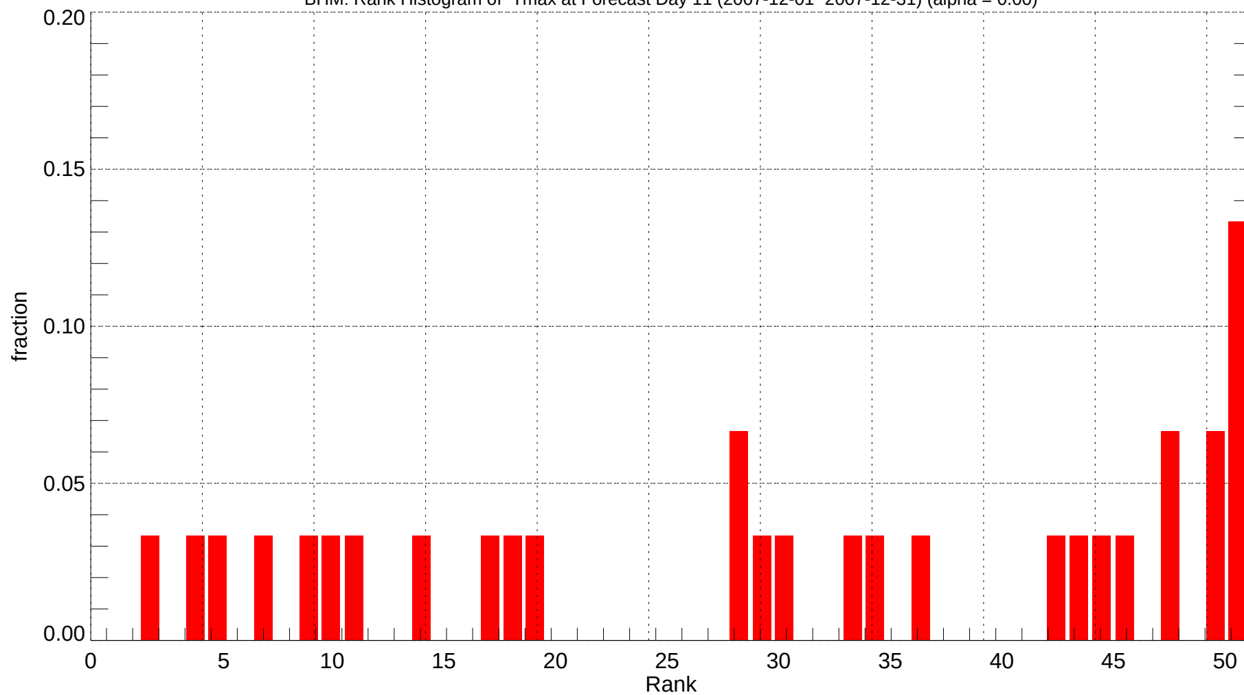
BHM: Rank Histogram of Tmax at Forecast Day 11 (2007-12-01~2007-12-31) (alpha = 0.00)
