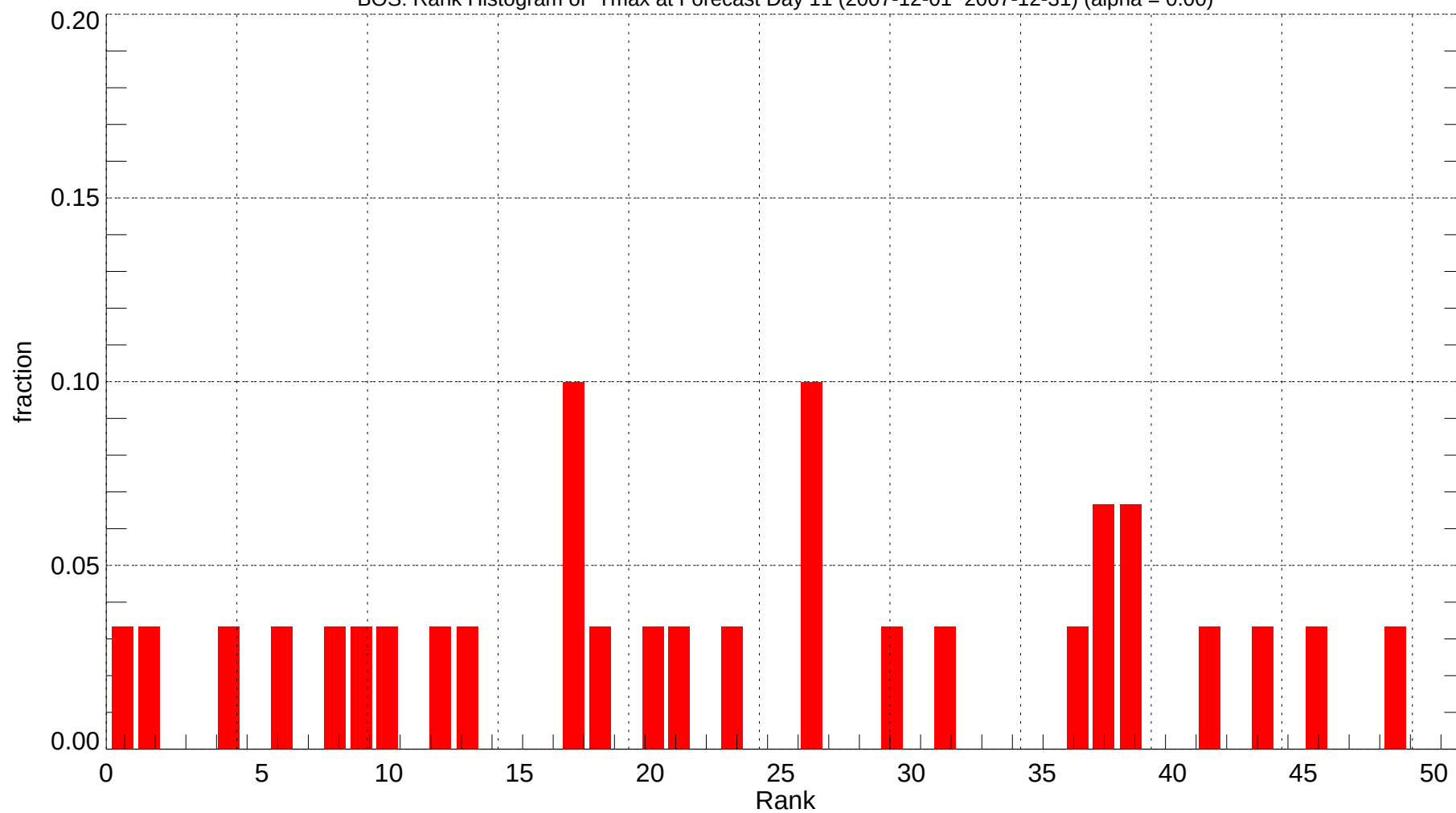
BOS: Rank Histogram of Tmax at Forecast Day 11 (2007-12-01~2007-12-31) (alpha = 0.00)
