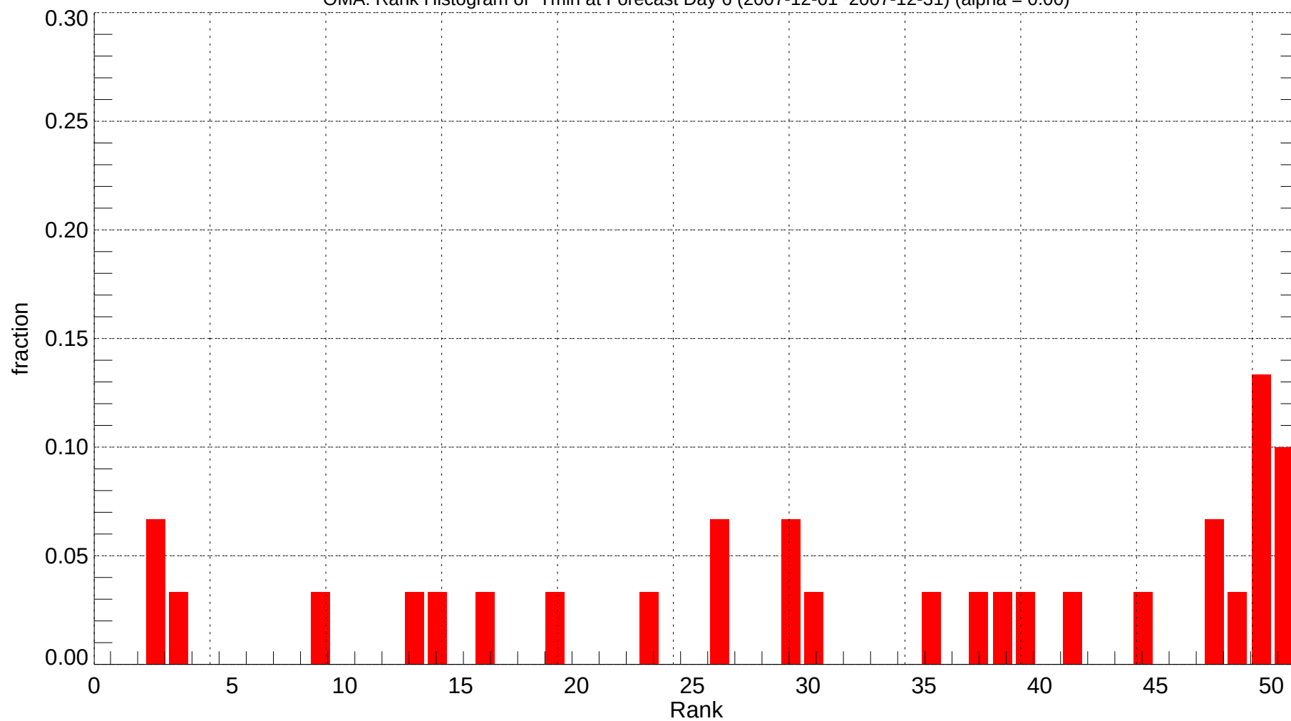
OMA: Rank Histogram of Tmin at Forecast Day 6 (2007-12-01~2007-12-31) (alpha = 0.00)
