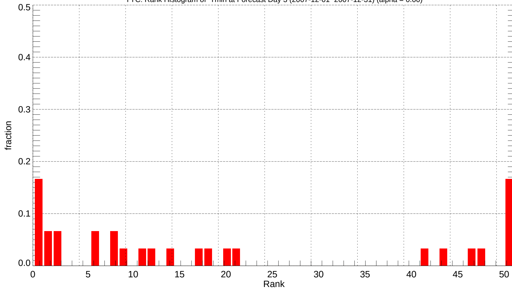
YYC: Rank Histogram of Tmin at Forecast Day 3 (2007-12-01~2007-12-31) (alpha = 0.00)
