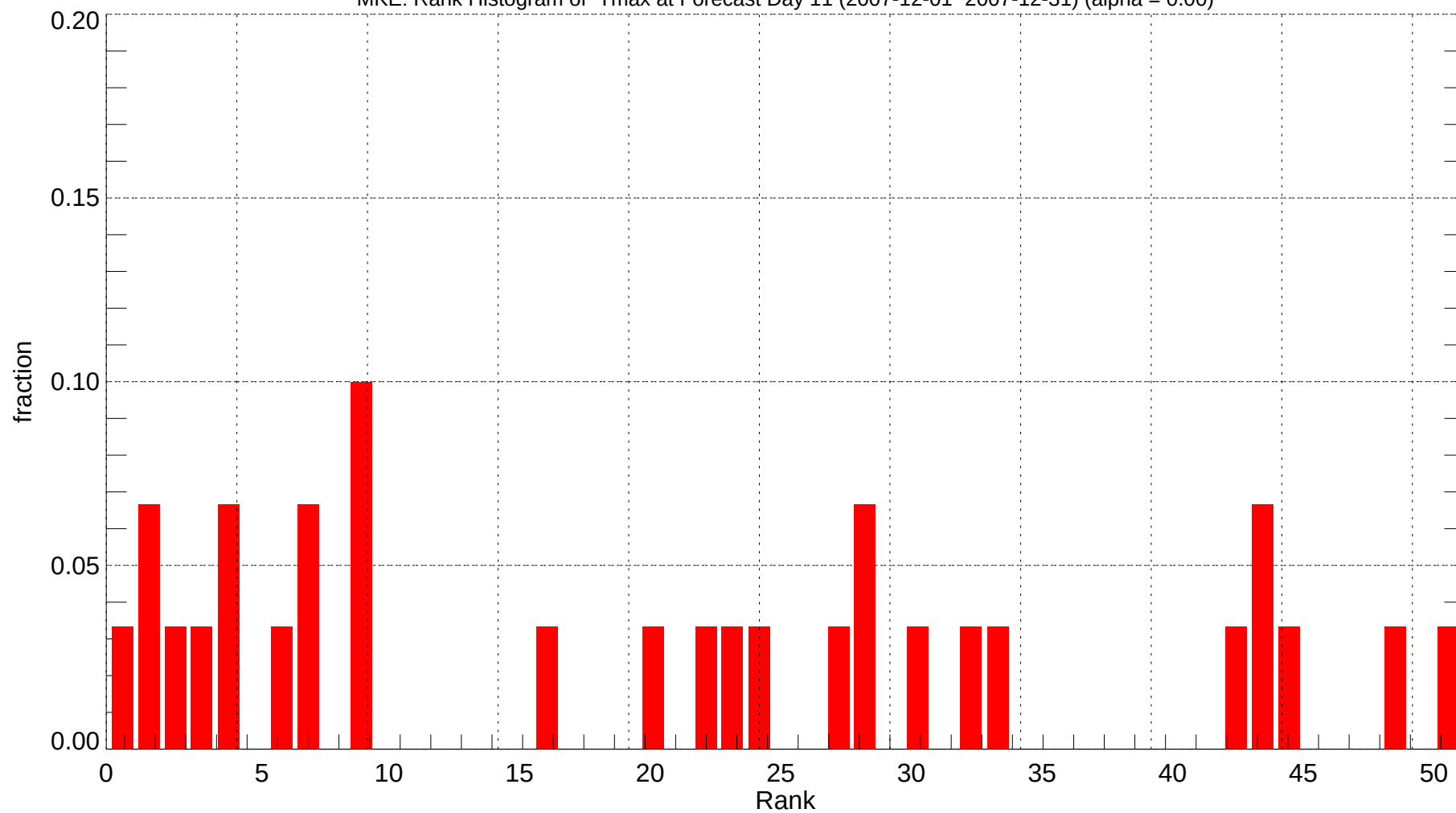
MKE: Rank Histogram of Tmax at Forecast Day 11 (2007-12-01~2007-12-31) (alpha = 0.00)
