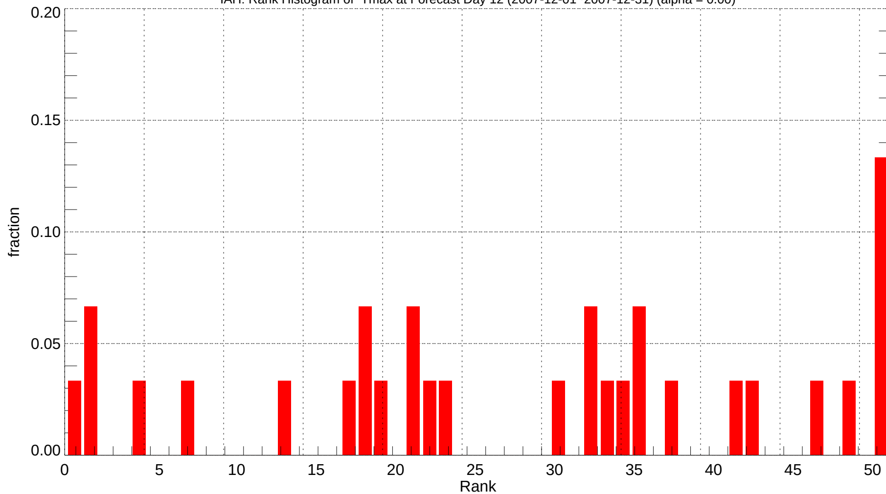
IAH: Rank Histogram of Tmax at Forecast Day 12 (2007-12-01~2007-12-31) (alpha = 0.00)
