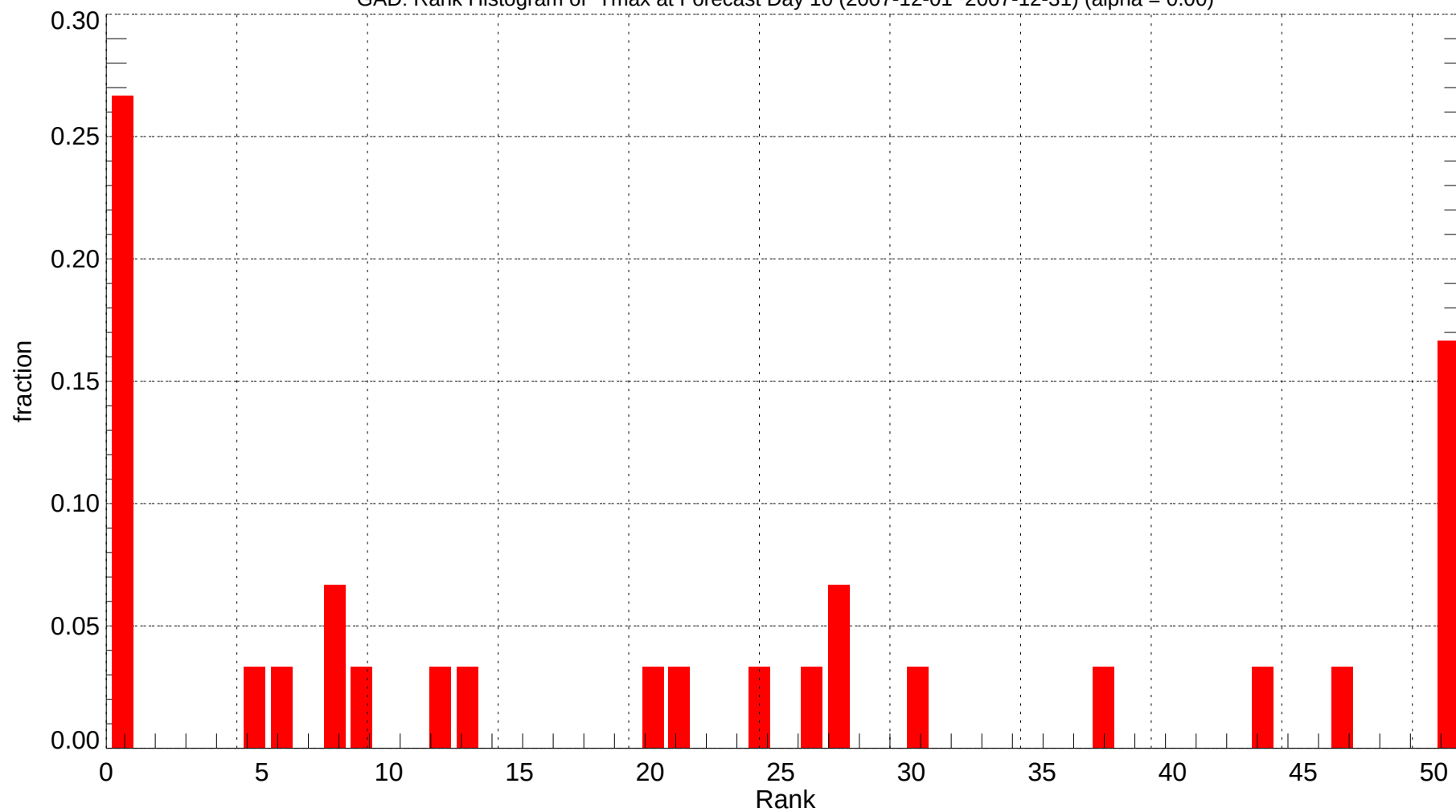
GAD: Rank Histogram of Tmax at Forecast Day 10 (2007-12-01~2007-12-31) (alpha = 0.00)
