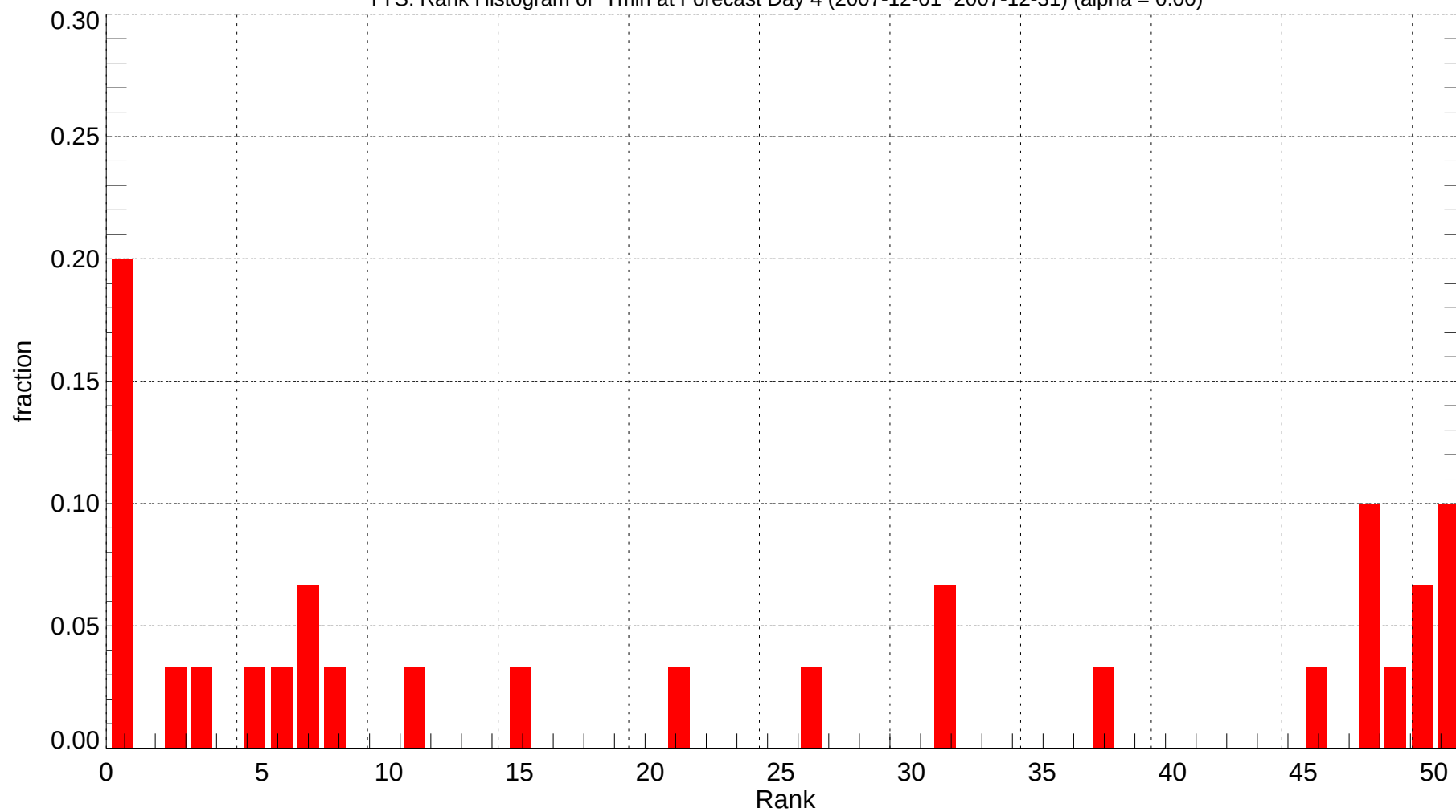
TYS: Rank Histogram of Tmin at Forecast Day 4 (2007-12-01~2007-12-31) (alpha = 0.00)
