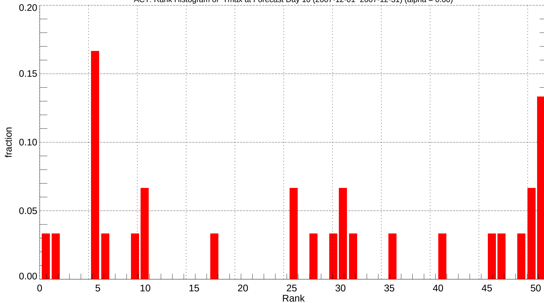
ACT: Rank Histogram of Tmax at Forecast Day 10 (2007-12-01~2007-12-31) (alpha = 0.00)
