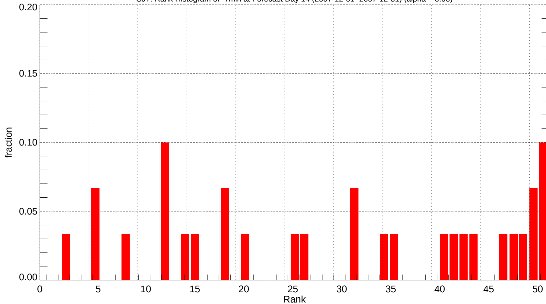
SJT: Rank Histogram of Tmin at Forecast Day 14 (2007-12-01~2007-12-31) (alpha = 0.00)
