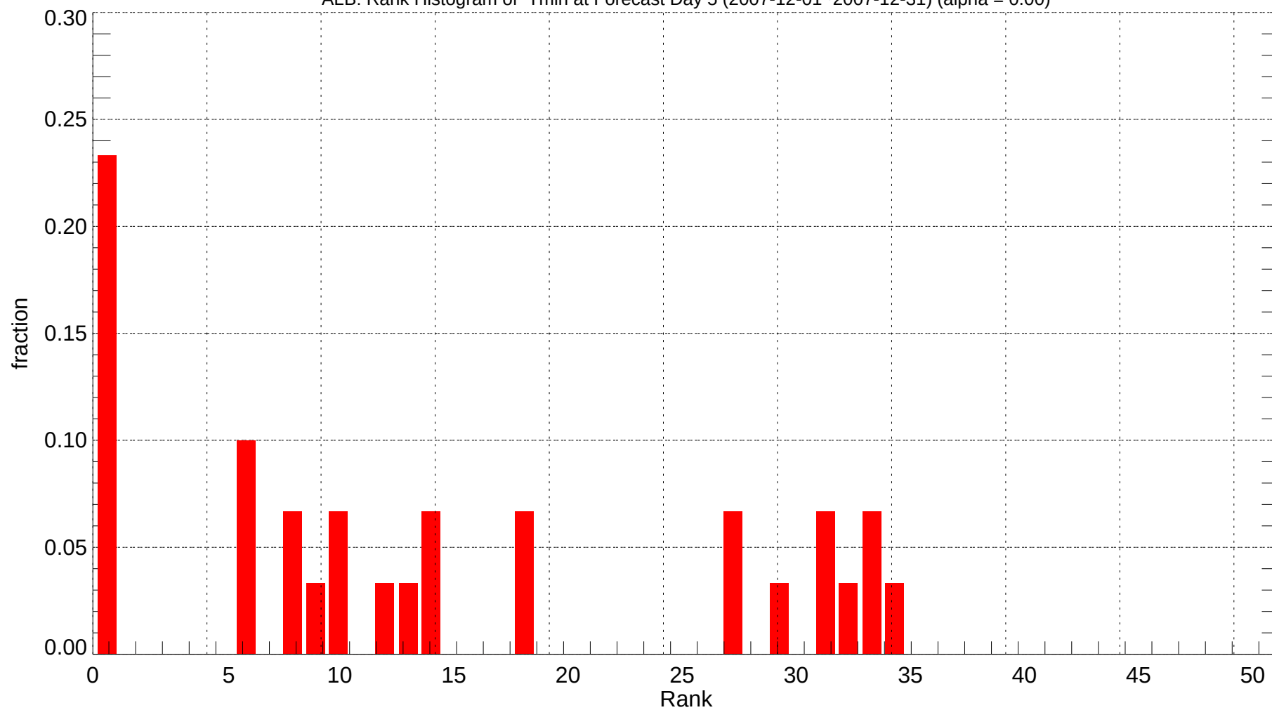
ALB: Rank Histogram of Tmin at Forecast Day 5 (2007-12-01~2007-12-31) (alpha = 0.00)
