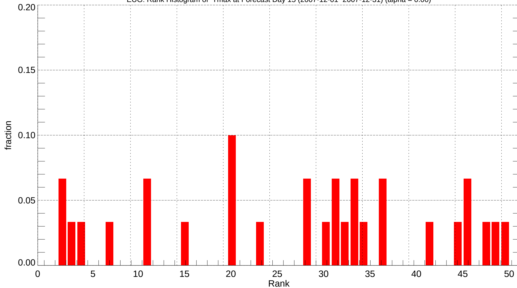
EUG: Rank Histogram of Tmax at Forecast Day 15 (2007-12-01~2007-12-31) (alpha = 0.00)
