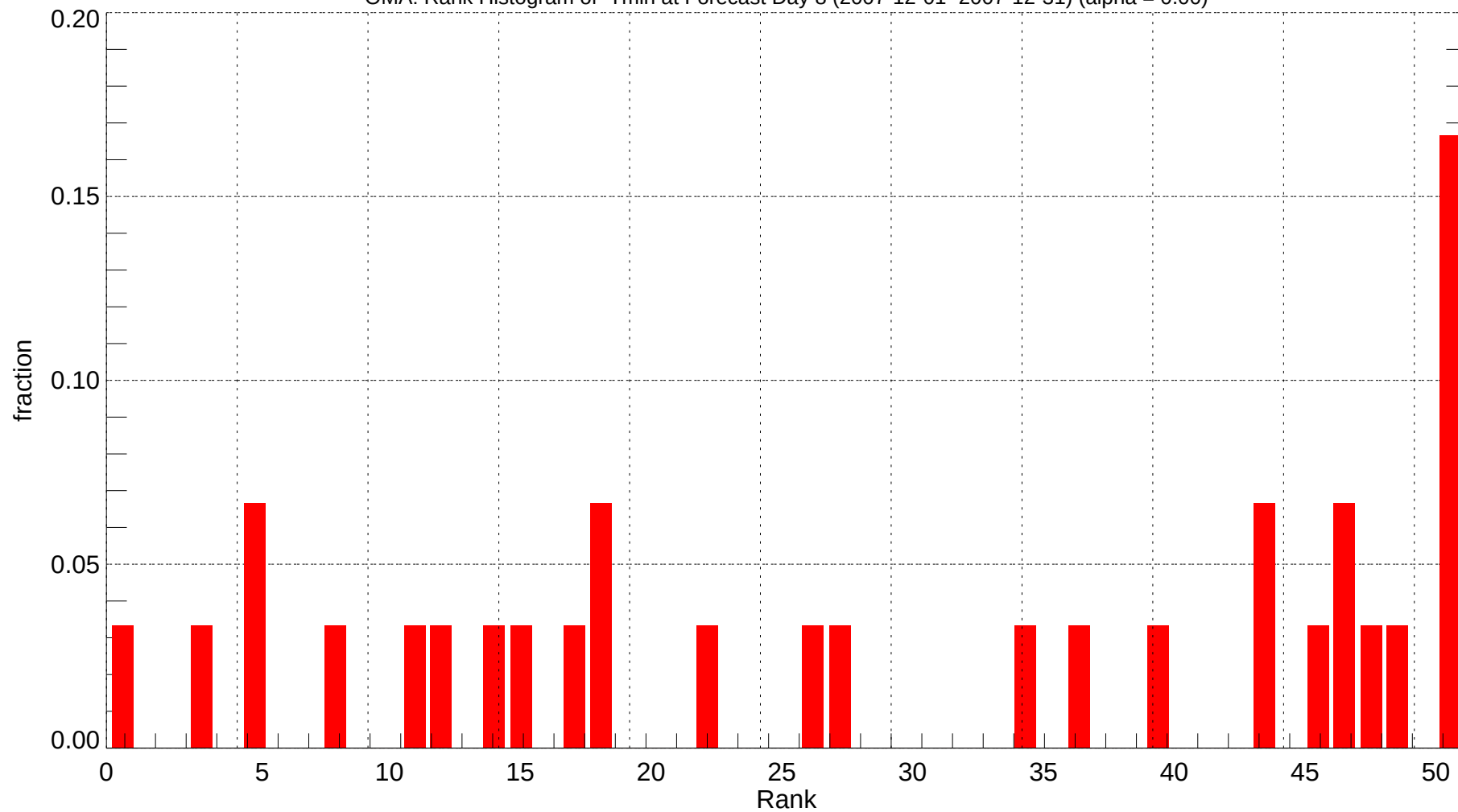
OMA: Rank Histogram of Tmin at Forecast Day 8 (2007-12-01~2007-12-31) (alpha = 0.00)
