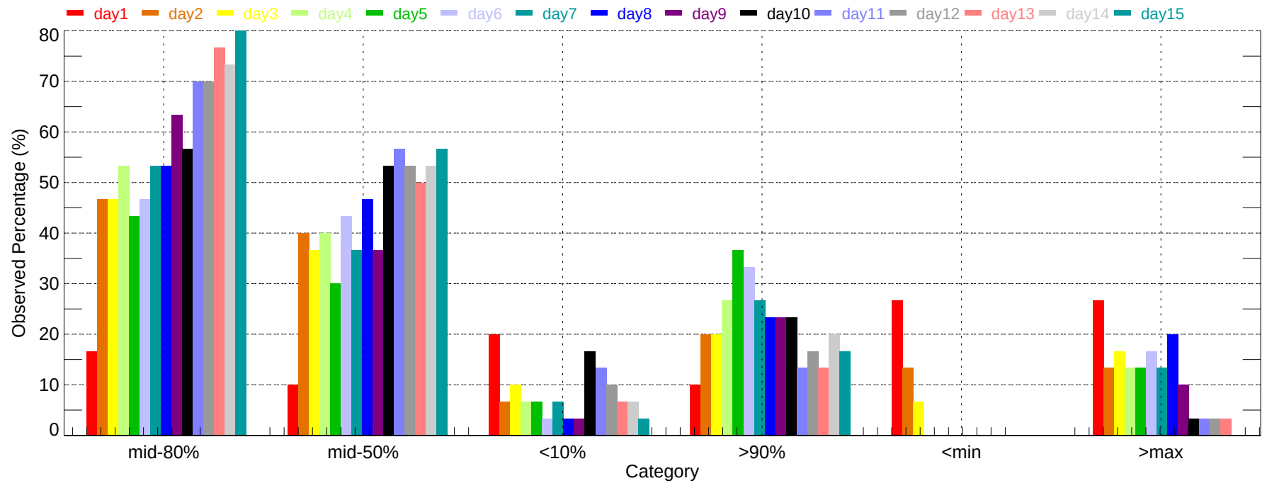
Observed Percentage of Ensembles - DEC: Min Temperature (2007-12-01~2007-12-31)
