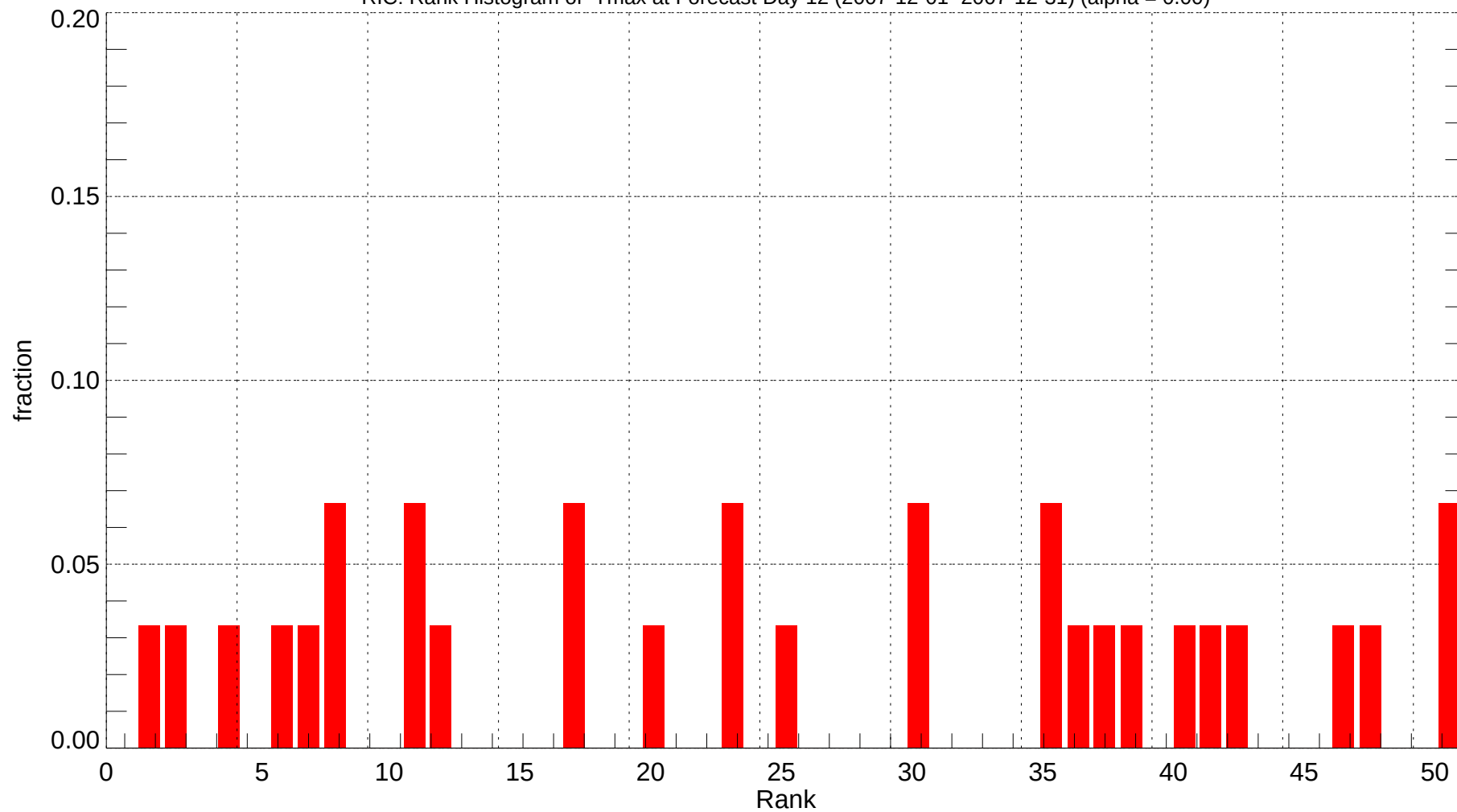
RIC: Rank Histogram of Tmax at Forecast Day 12 (2007-12-01~2007-12-31) (alpha = 0.00)
