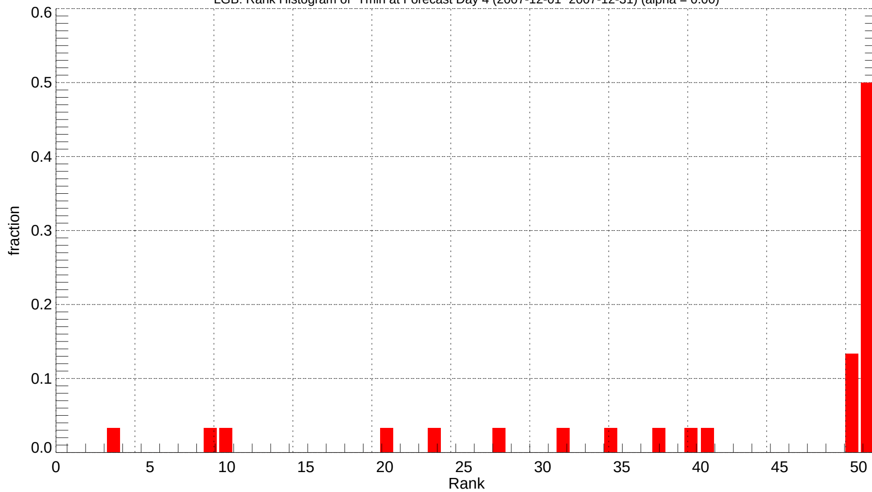
LGB: Rank Histogram of Tmin at Forecast Day 4 (2007-12-01~2007-12-31) (alpha = 0.00)
