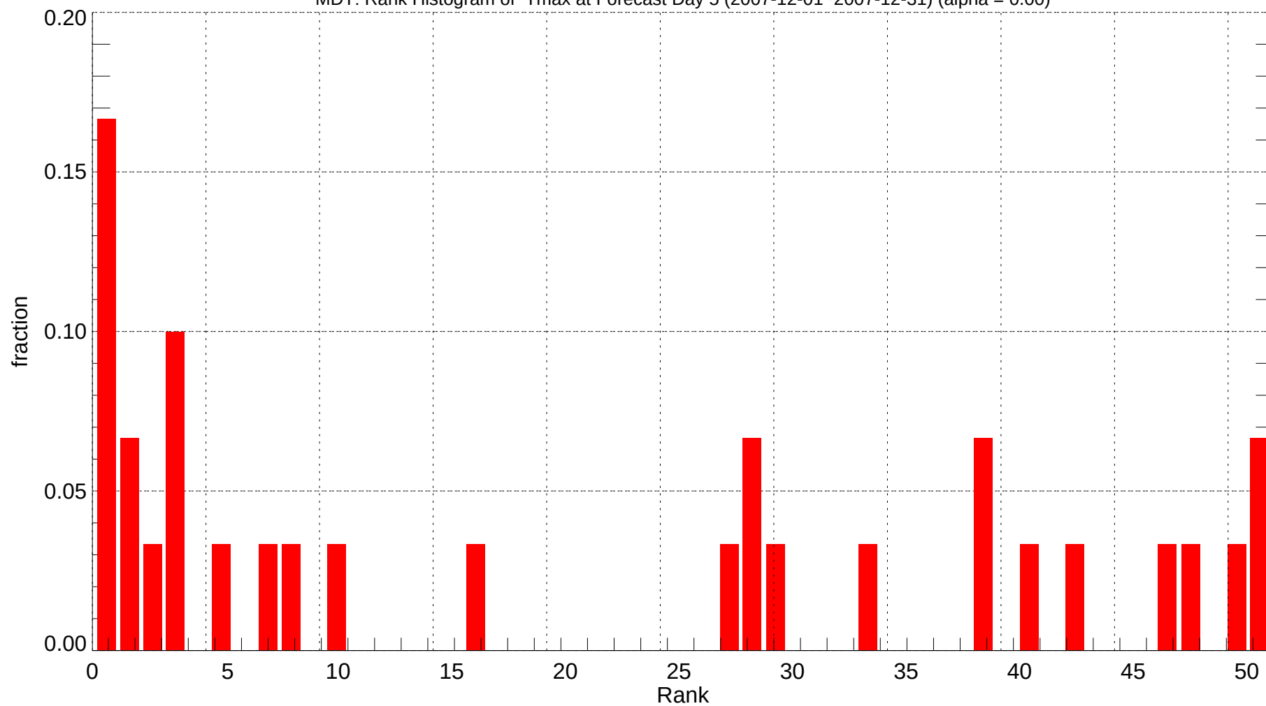
MDT: Rank Histogram of Tmax at Forecast Day 5 (2007-12-01~2007-12-31) (alpha = 0.00)
