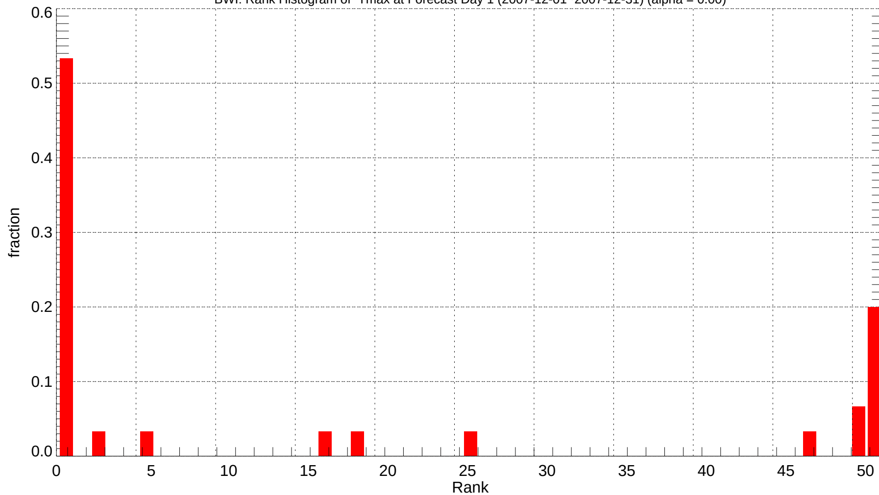
BWI: Rank Histogram of Tmax at Forecast Day 1 (2007-12-01~2007-12-31) (alpha = 0.00)
