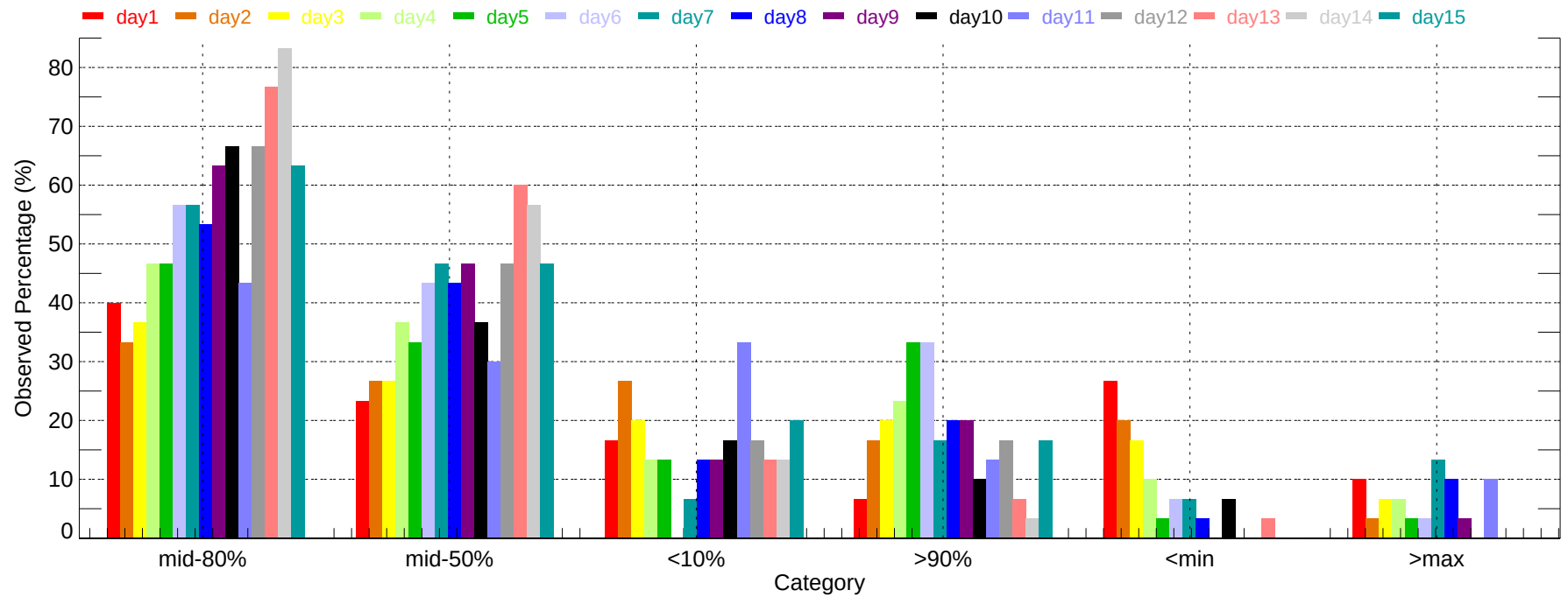
Observed Percentage of Ensembles - DBQ: Max Temperature (2007-12-01~2007-12-31)
