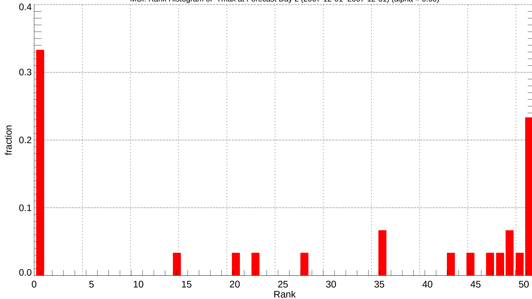
MCI: Rank Histogram of Tmax at Forecast Day 2 (2007-12-01~2007-12-31) (alpha = 0.00)
