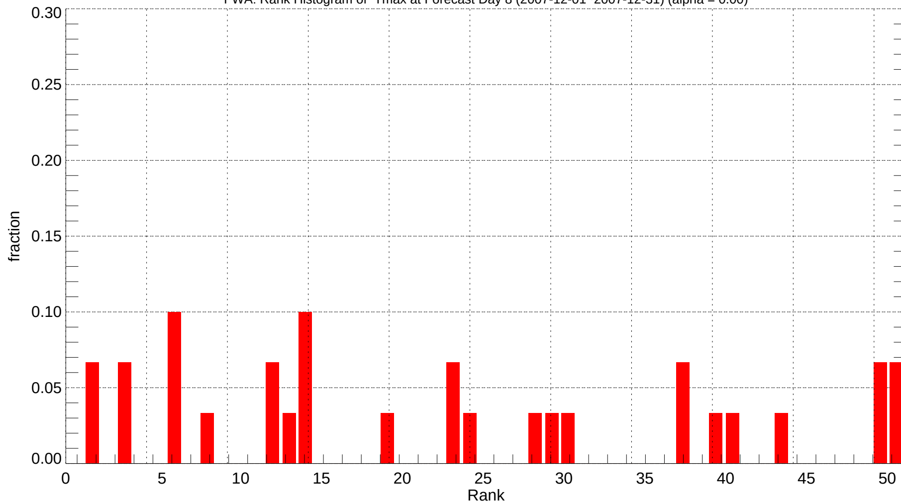
FWA: Rank Histogram of Tmax at Forecast Day 8 (2007-12-01~2007-12-31) (alpha = 0.00)
