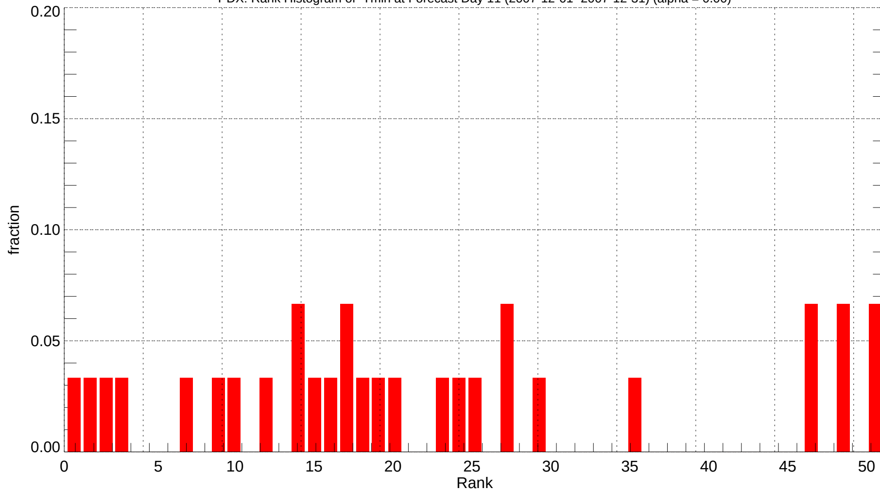
PDX: Rank Histogram of Tmin at Forecast Day 11 (2007-12-01~2007-12-31) (alpha = 0.00)
