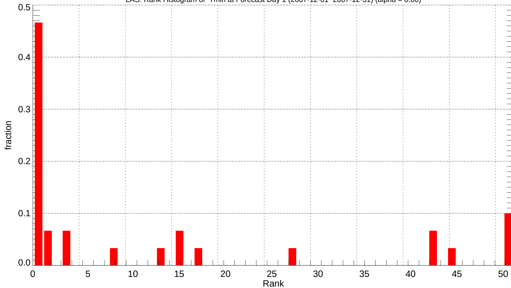
LAS: Rank Histogram of Tmin at Forecast Day 1 (2007-12-01~2007-12-31) (alpha = 0.00)
