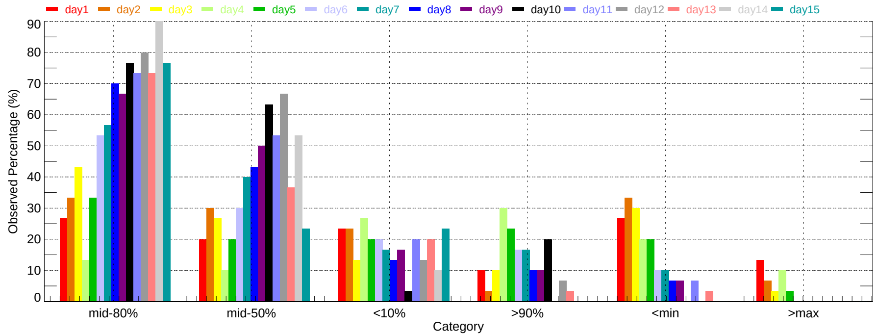
Observed Percentage of Ensembles - TRM: Max Temperature (2007-12-01~2007-12-31)
