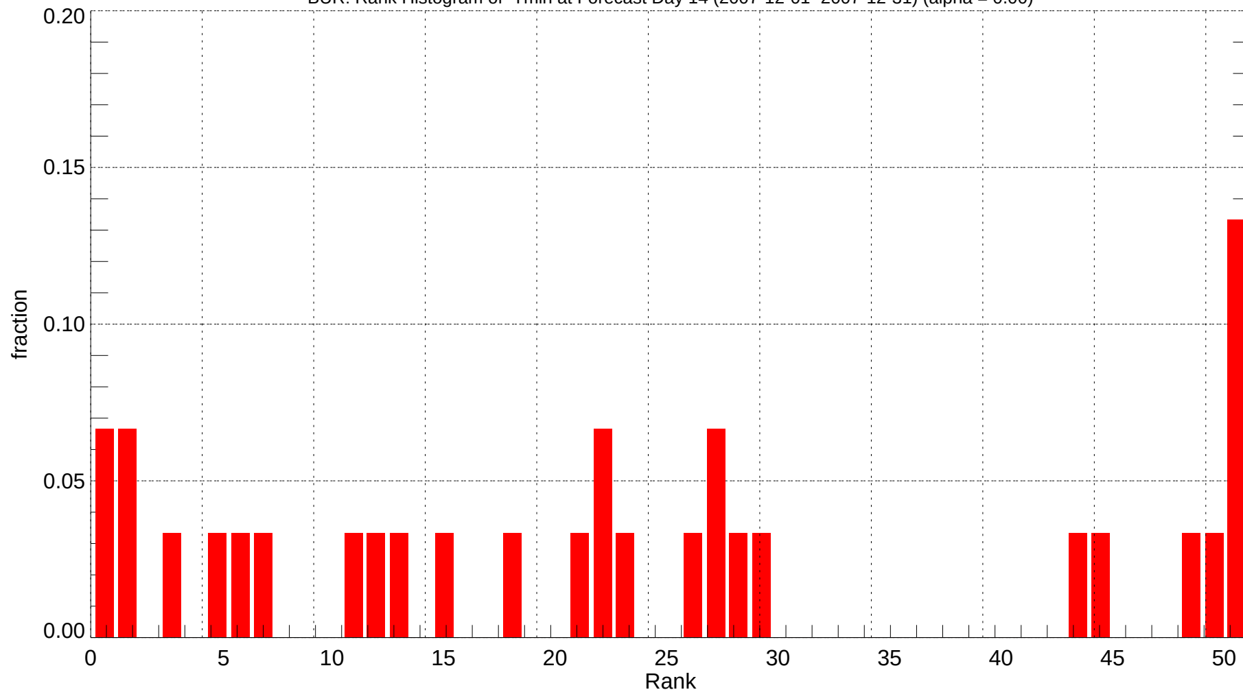
BUR: Rank Histogram of Tmin at Forecast Day 14 (2007-12-01~2007-12-31) (alpha = 0.00)
