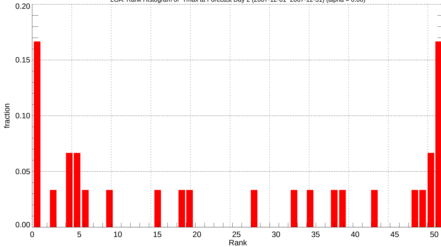
LGA: Rank Histogram of Tmax at Forecast Day 2 (2007-12-01~2007-12-31) (alpha = 0.00)
