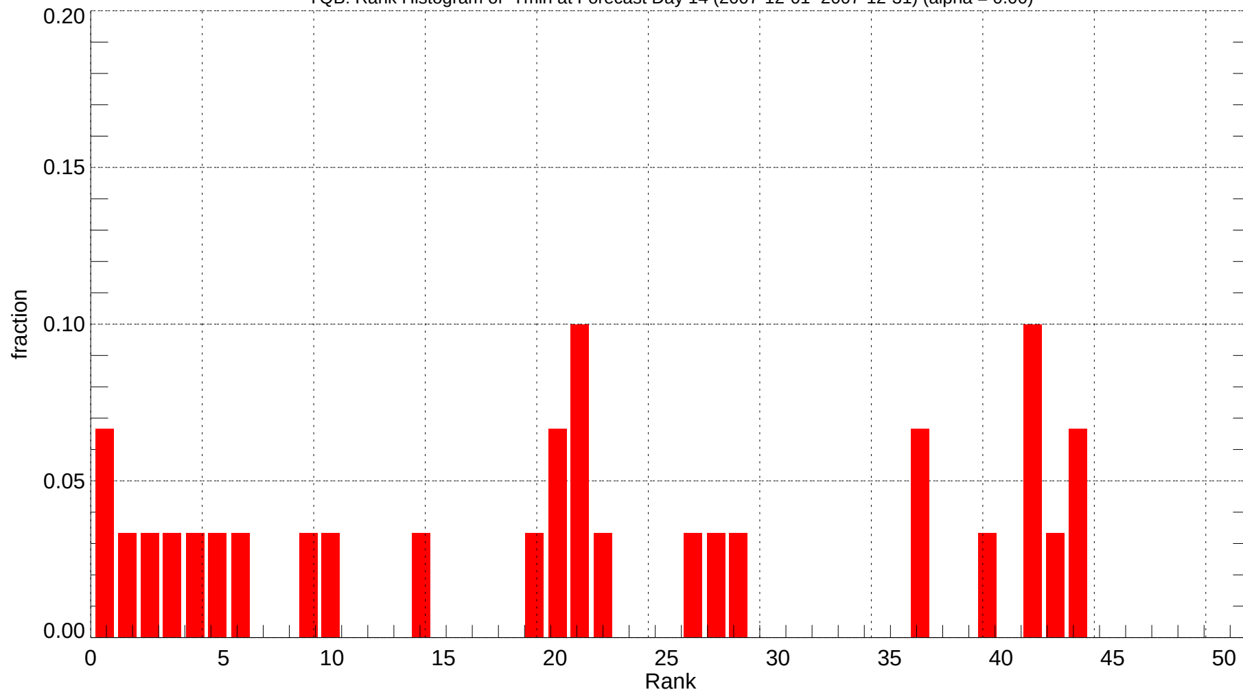
YQB: Rank Histogram of Tmin at Forecast Day 14 (2007-12-01~2007-12-31) (alpha = 0.00)
