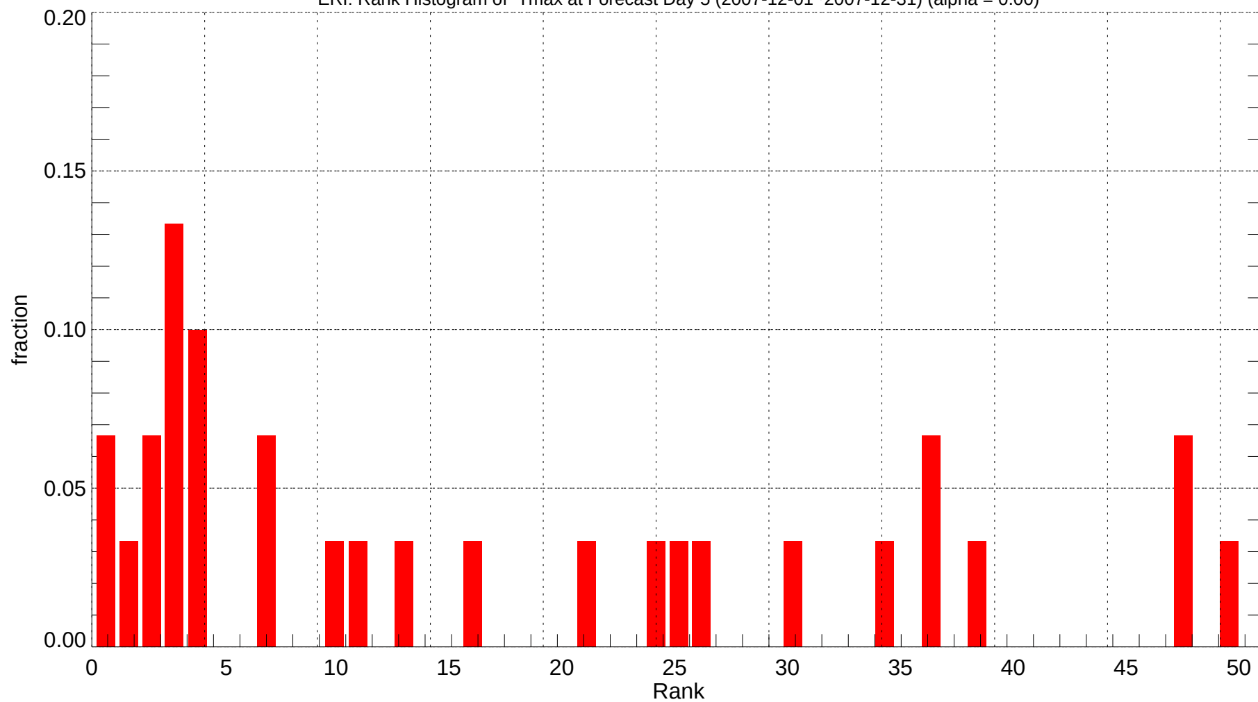
ERI: Rank Histogram of Tmax at Forecast Day 5 (2007-12-01~2007-12-31) (alpha = 0.00)
