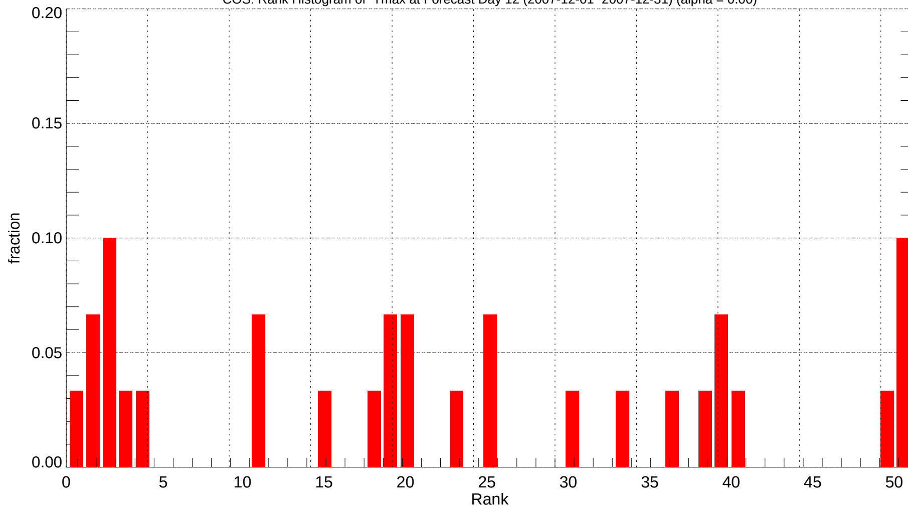
COS: Rank Histogram of Tmax at Forecast Day 12 (2007-12-01~2007-12-31) (alpha = 0.00)
