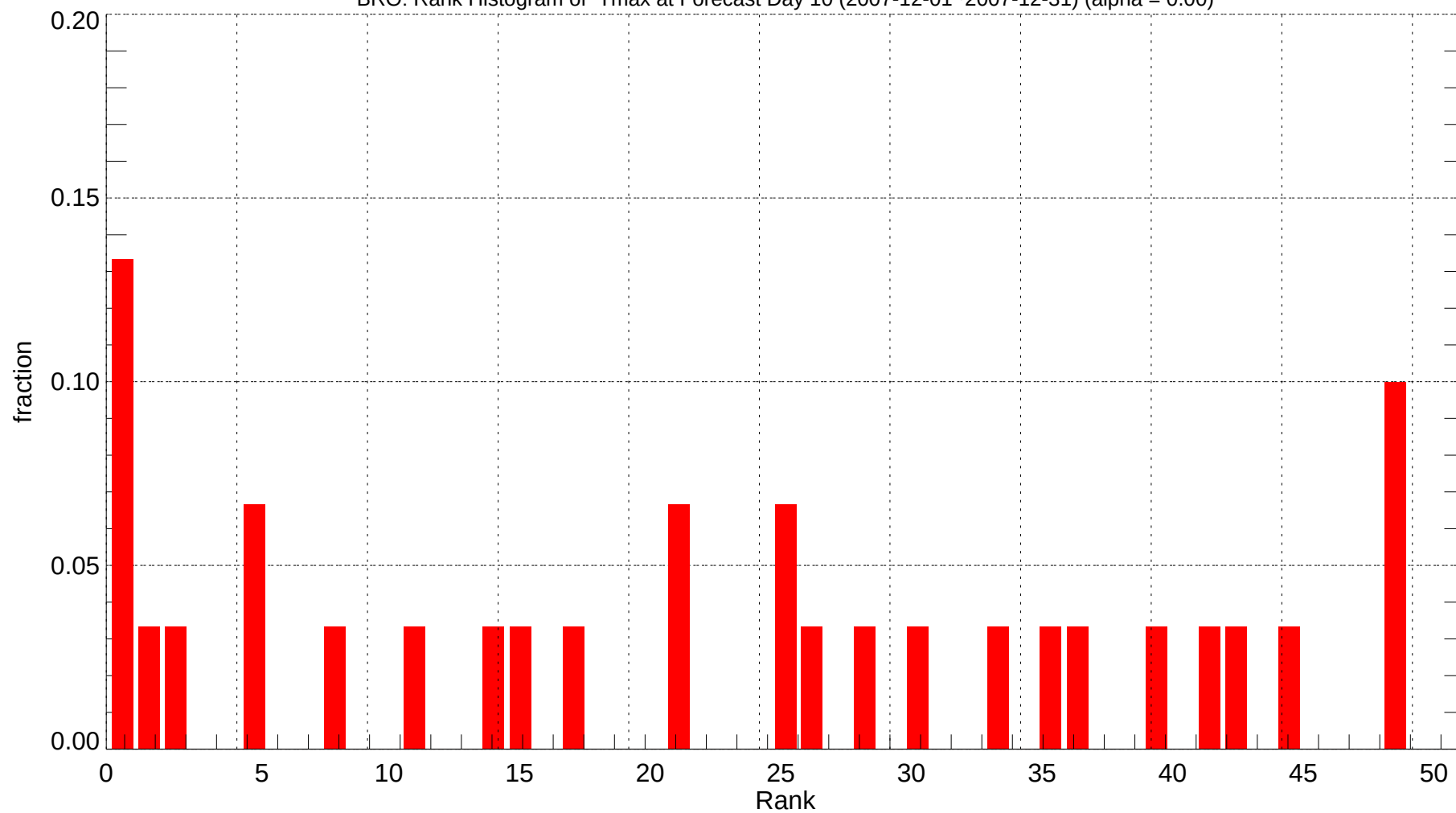
BRO: Rank Histogram of Tmax at Forecast Day 10 (2007-12-01~2007-12-31) (alpha = 0.00)
