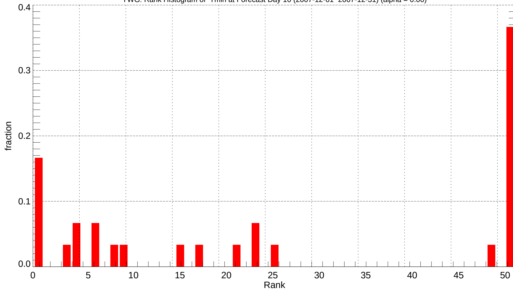
YWG: Rank Histogram of Tmin at Forecast Day 10 (2007-12-01~2007-12-31) (alpha = 0.00)
