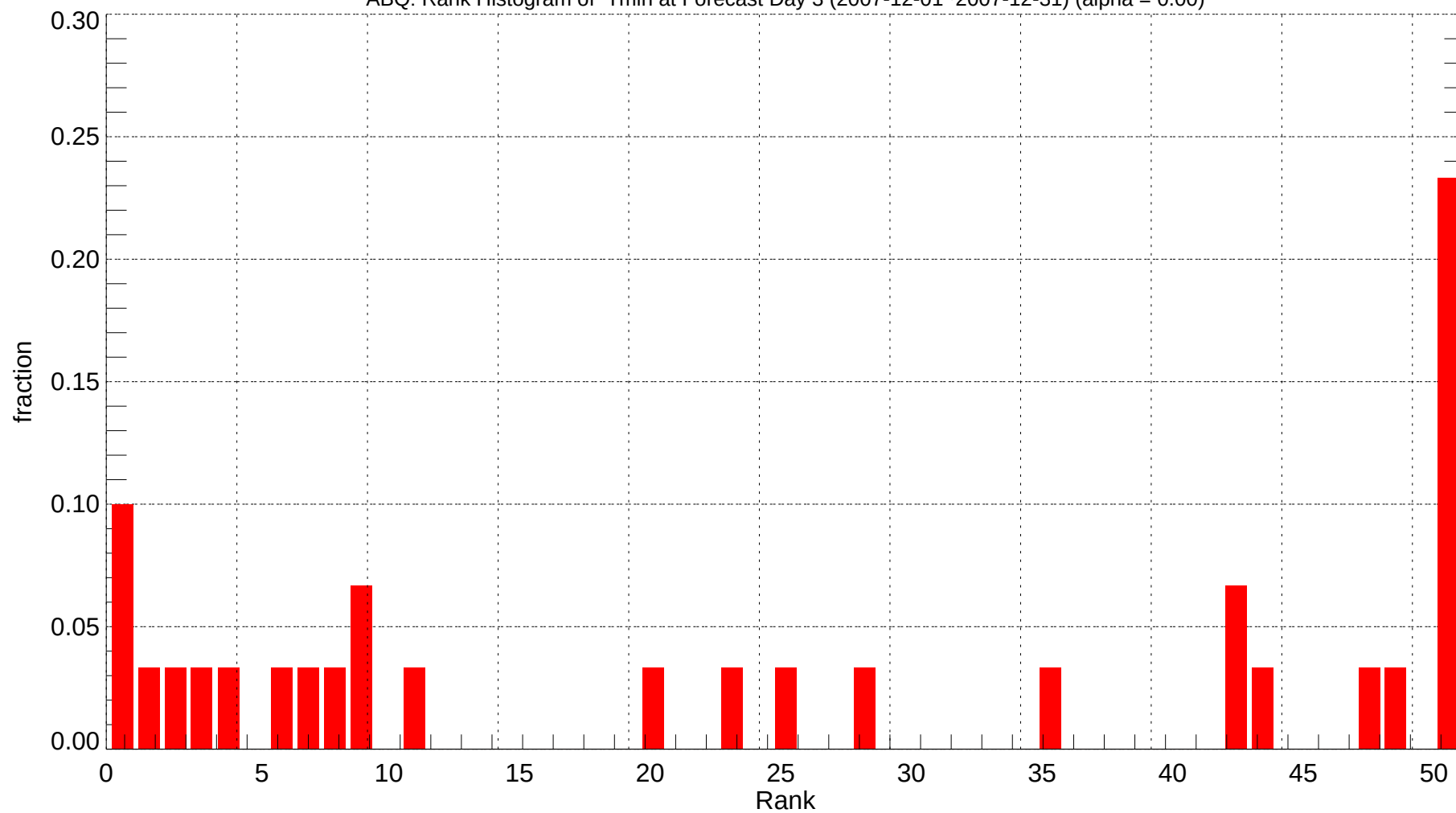
ABQ: Rank Histogram of Tmin at Forecast Day 3 (2007-12-01~2007-12-31) (alpha = 0.00)
