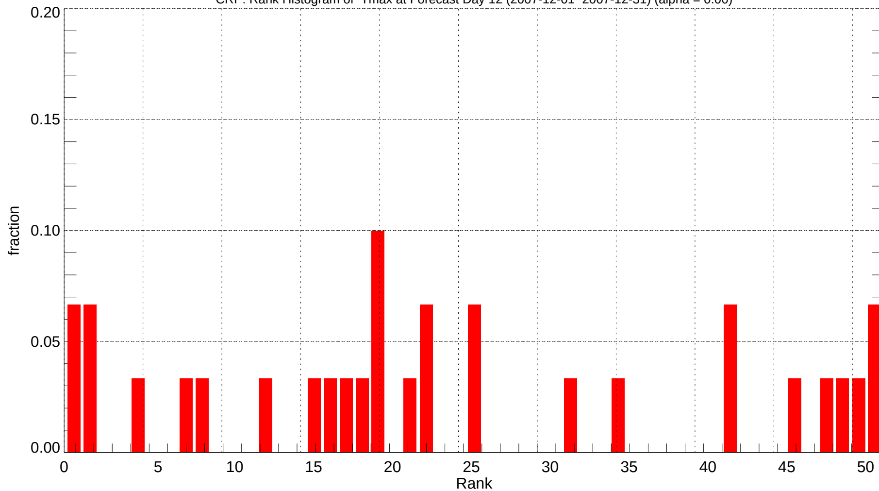
CRP: Rank Histogram of Tmax at Forecast Day 12 (2007-12-01~2007-12-31) (alpha = 0.00)
