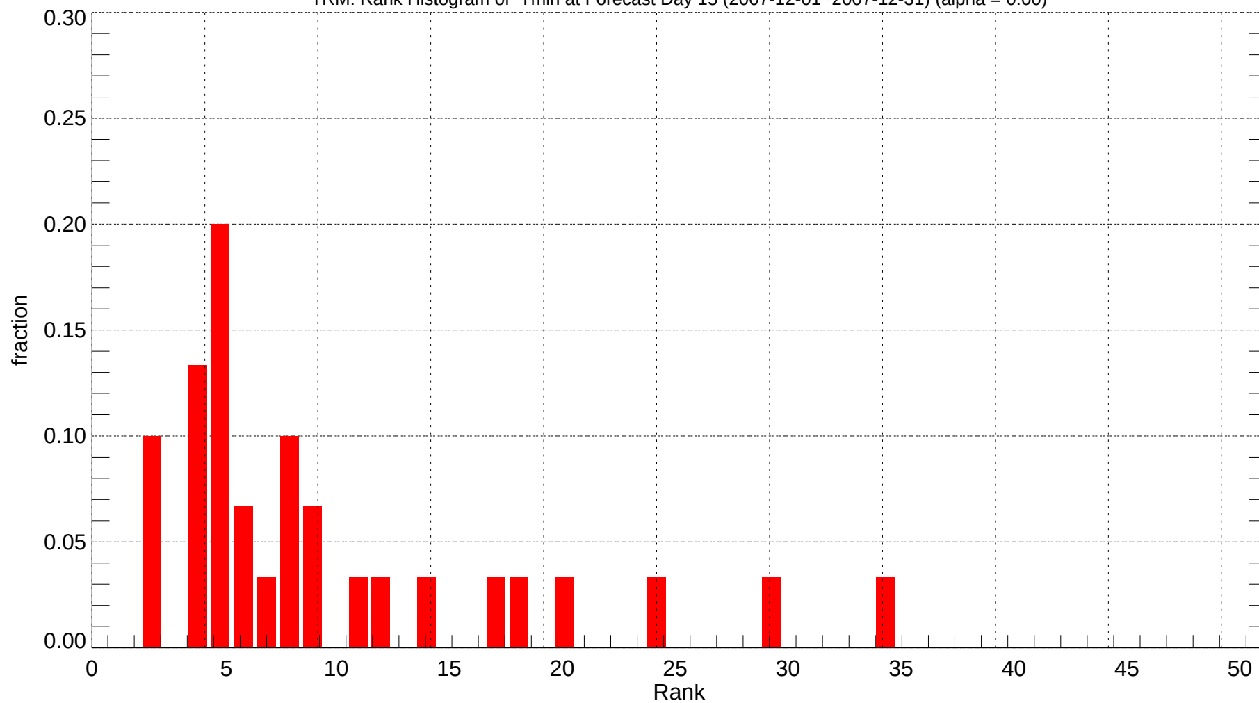
TRM: Rank Histogram of Tmin at Forecast Day 15 (2007-12-01~2007-12-31) (alpha = 0.00)
