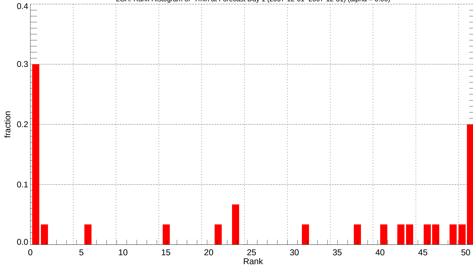
LGA: Rank Histogram of Tmin at Forecast Day 1 (2007-12-01~2007-12-31) (alpha = 0.00)
