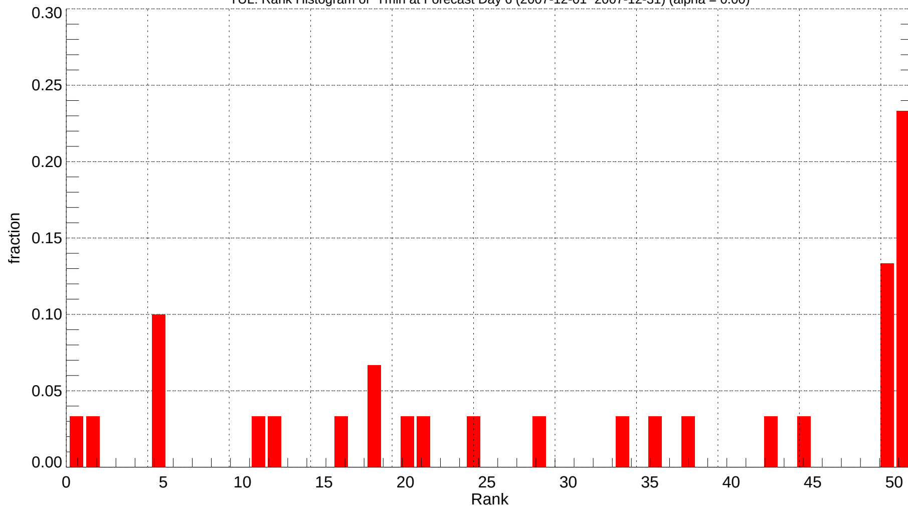
TUL: Rank Histogram of Tmin at Forecast Day 6 (2007-12-01~2007-12-31) (alpha = 0.00)
