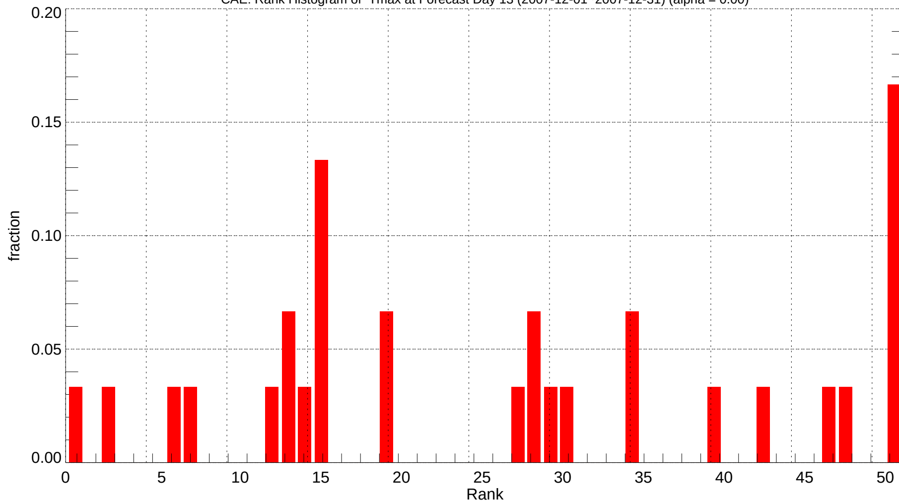
CAE: Rank Histogram of Tmax at Forecast Day 13 (2007-12-01~2007-12-31) (alpha = 0.00)
