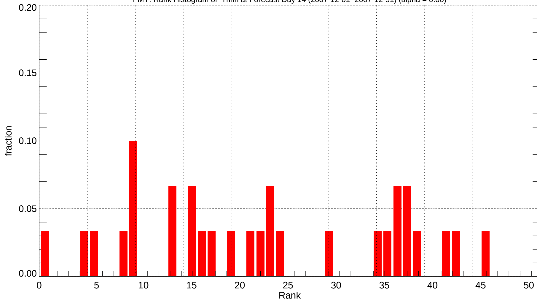
FMY: Rank Histogram of Tmin at Forecast Day 14 (2007-12-01~2007-12-31) (alpha = 0.00)
