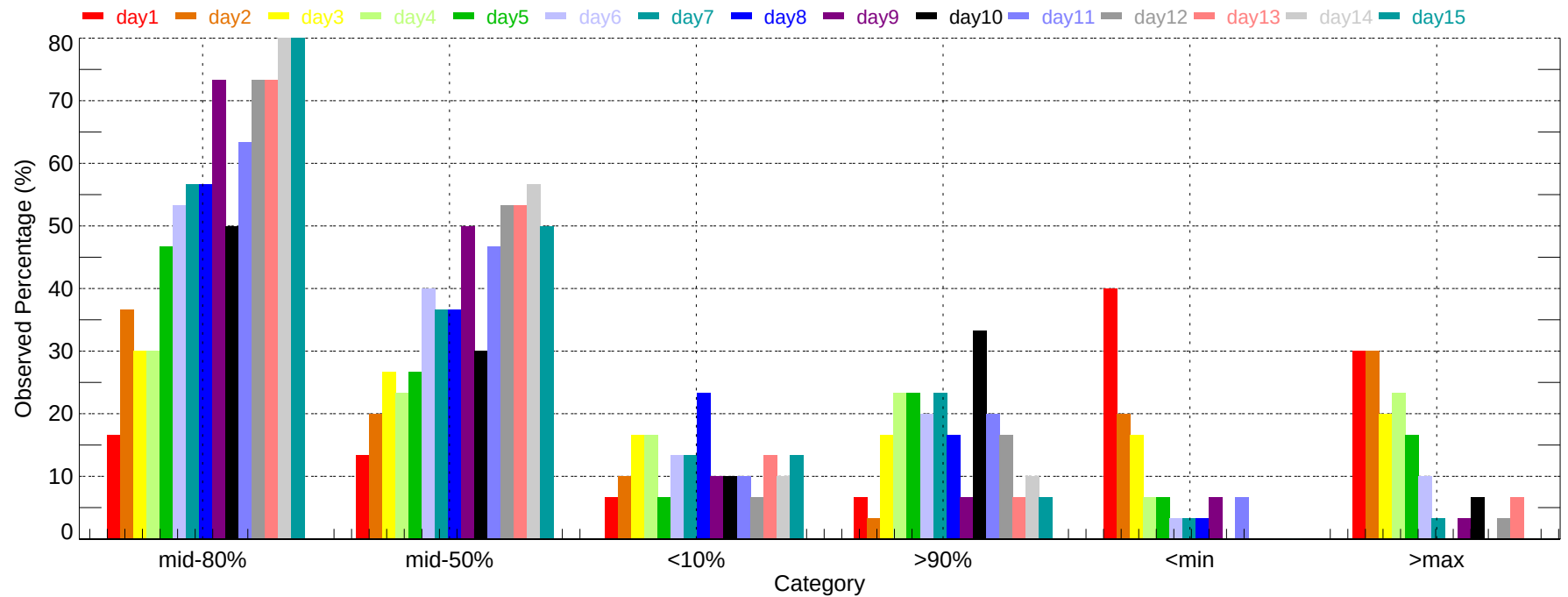
Observed Percentage of Ensembles - PIR: Min Temperature (2007-12-01~2007-12-31)
