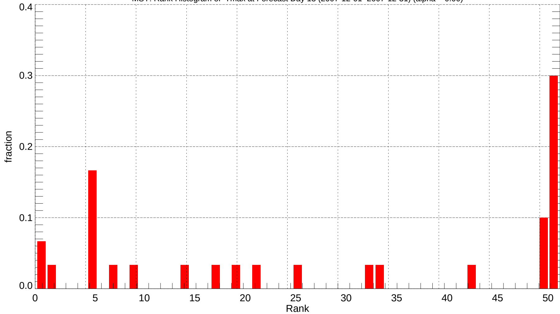
MSY: Rank Histogram of Tmax at Forecast Day 13 (2007-12-01~2007-12-31) (alpha = 0.00)
