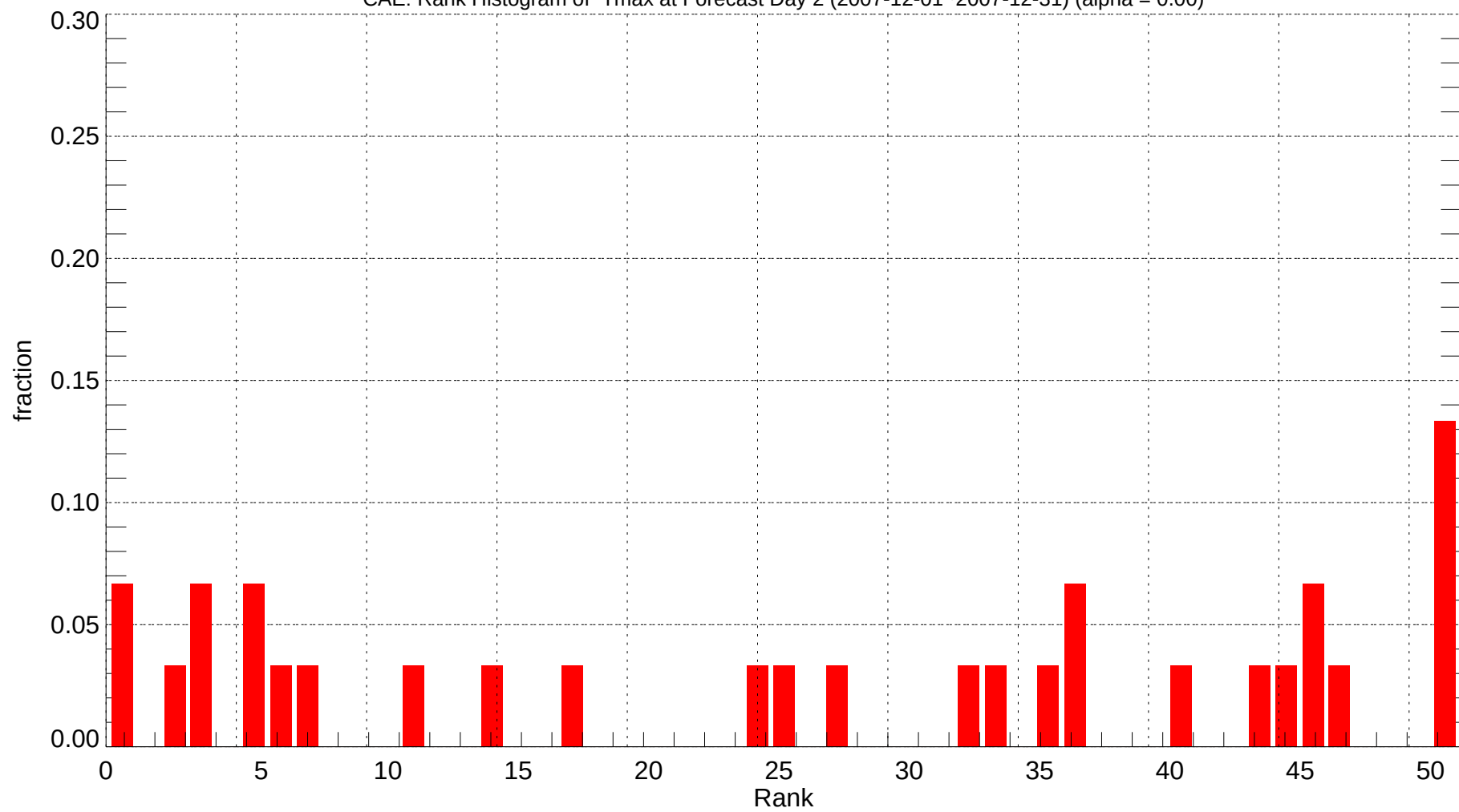
CAE: Rank Histogram of Tmax at Forecast Day 2 (2007-12-01~2007-12-31) (alpha = 0.00)
