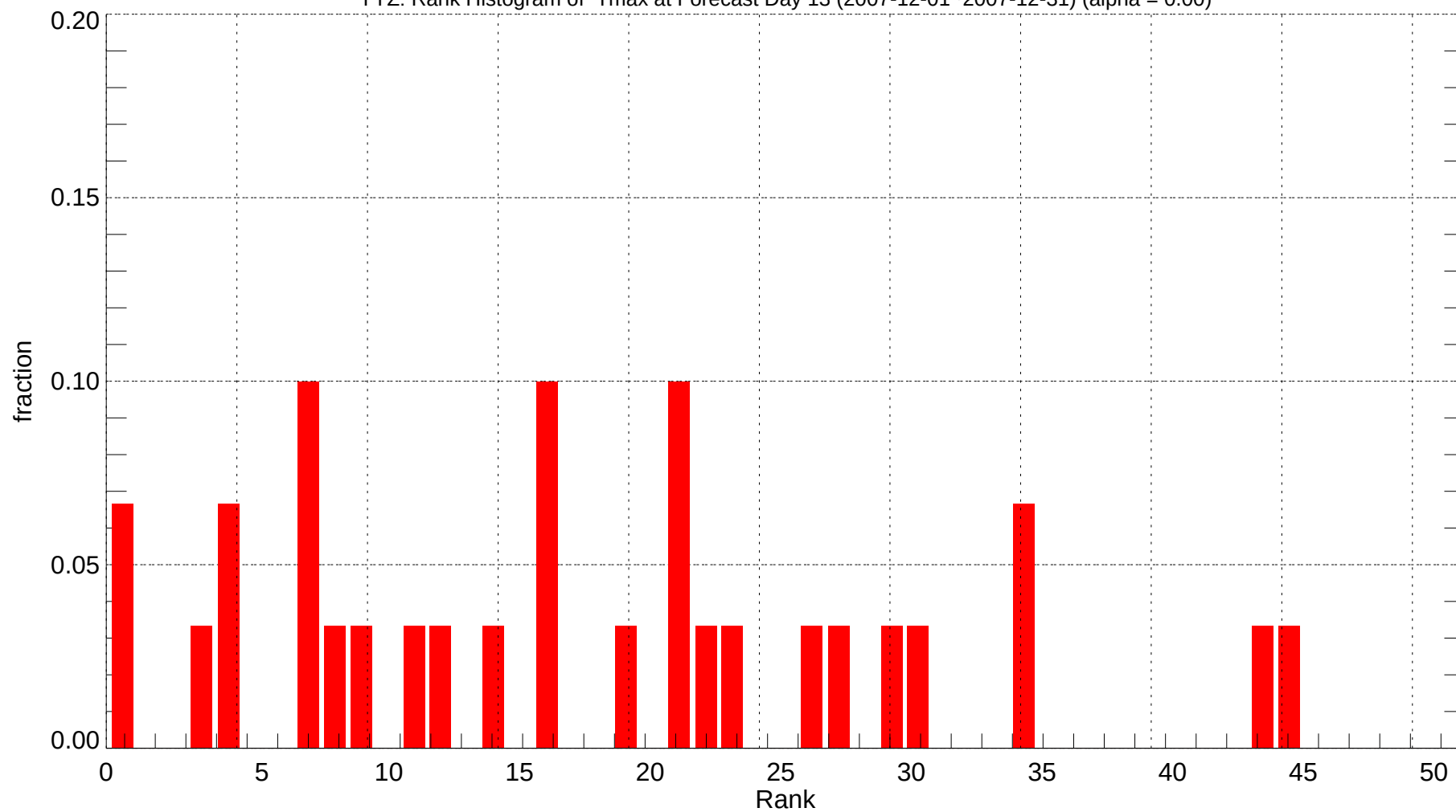
YYZ: Rank Histogram of Tmax at Forecast Day 13 (2007-12-01~2007-12-31) (alpha = 0.00)
