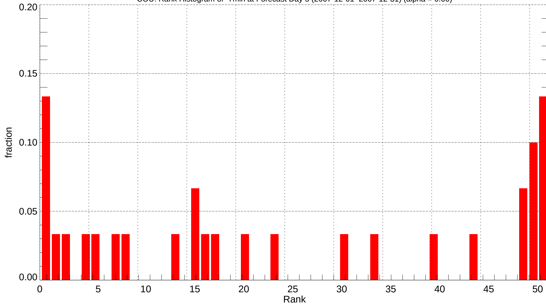
COU: Rank Histogram of Tmin at Forecast Day 5 (2007-12-01~2007-12-31) (alpha = 0.00)
