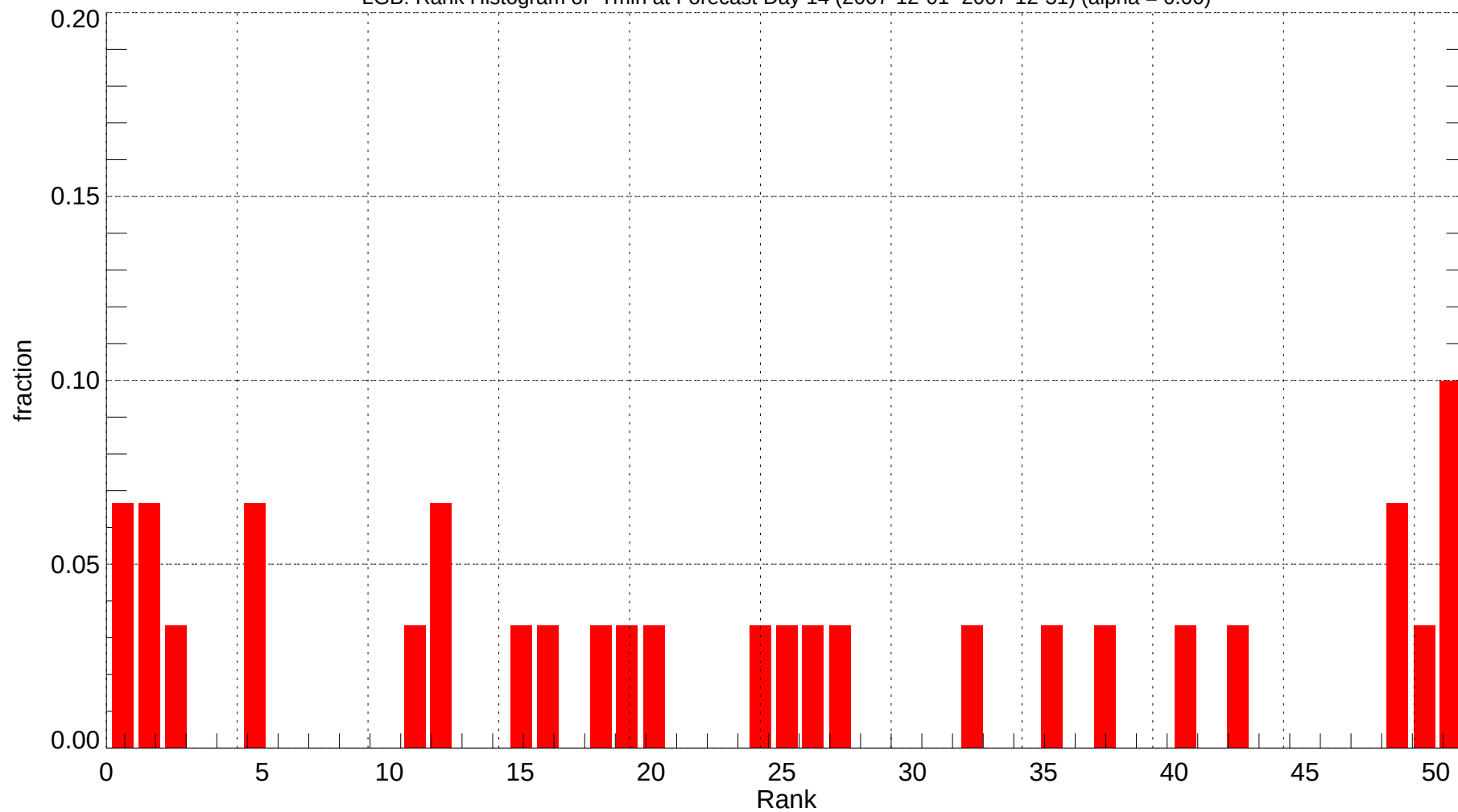
LGB: Rank Histogram of Tmin at Forecast Day 14 (2007-12-01~2007-12-31) (alpha = 0.00)
