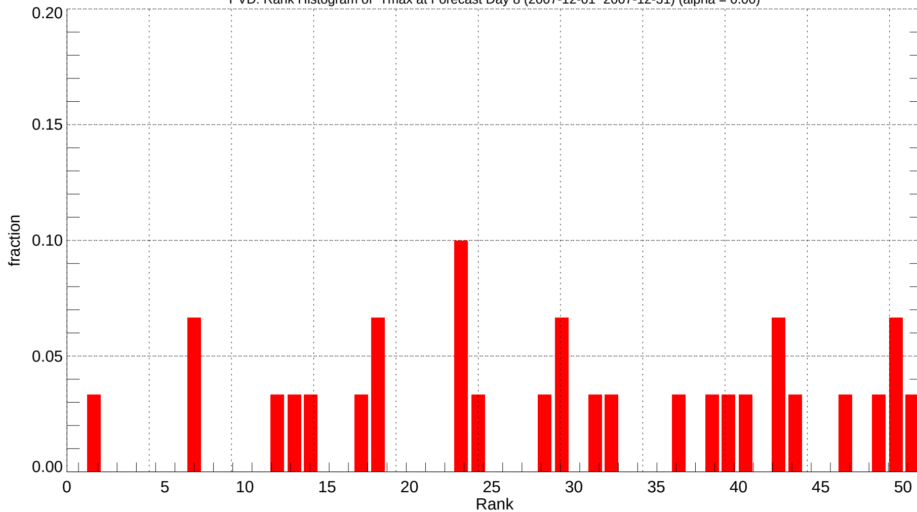
PVD: Rank Histogram of Tmax at Forecast Day 8 (2007-12-01~2007-12-31) (alpha = 0.00)
