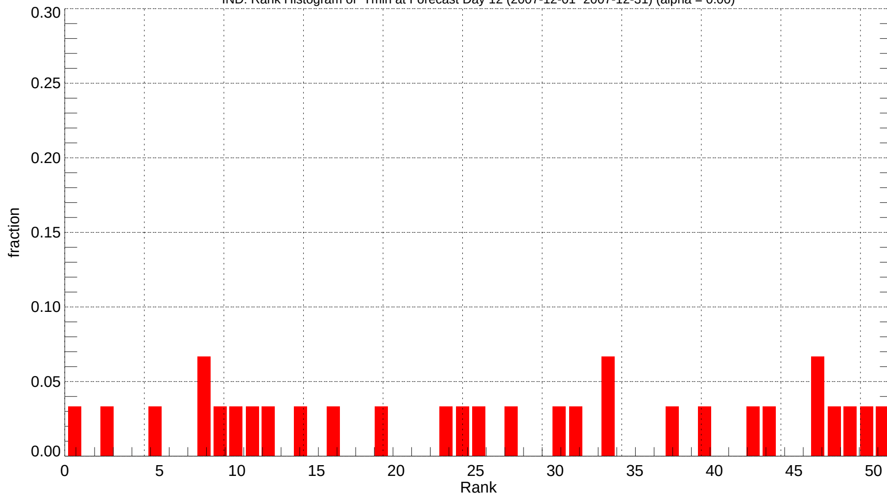
IND: Rank Histogram of Tmin at Forecast Day 12 (2007-12-01~2007-12-31) (alpha = 0.00)
