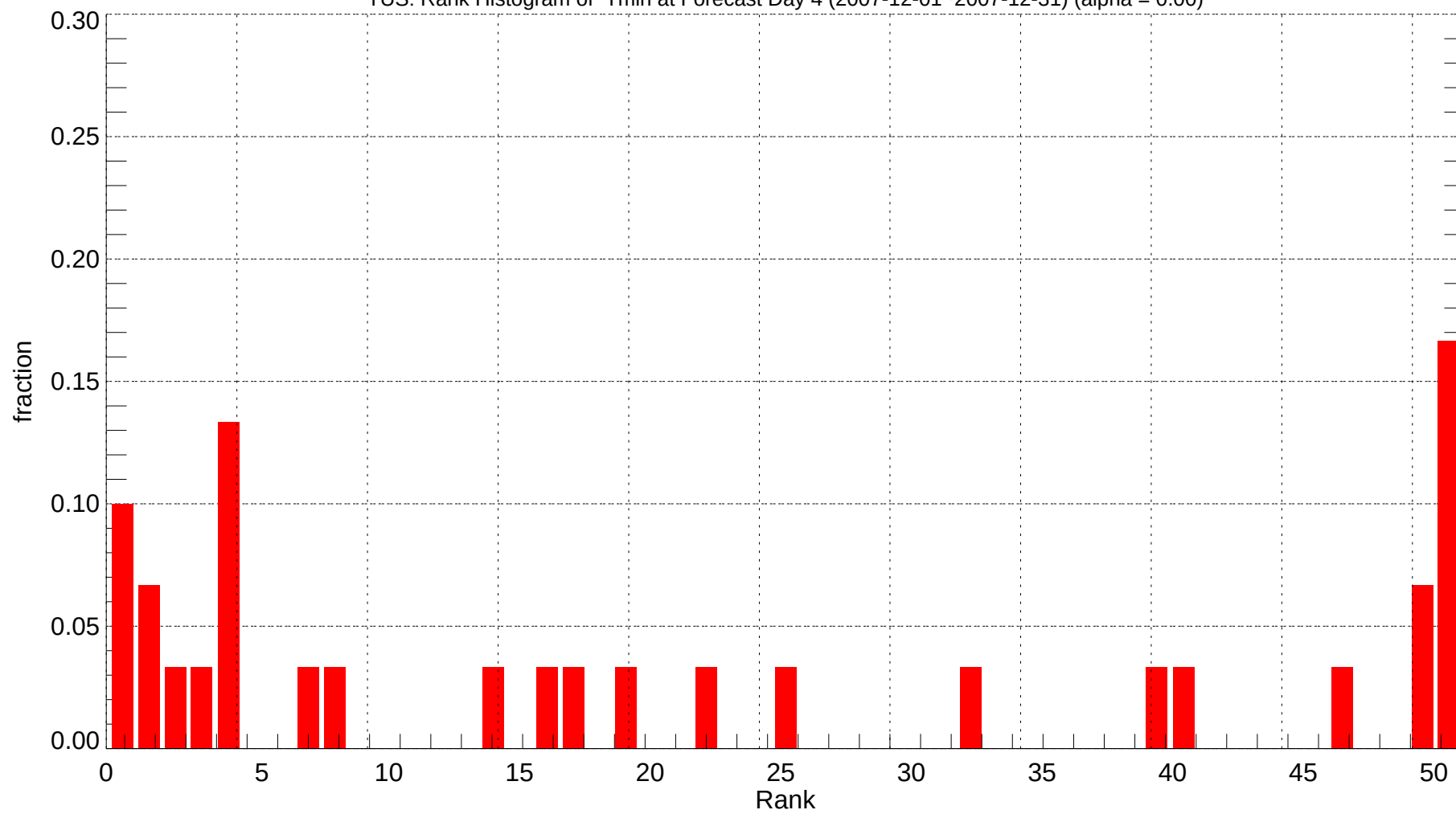
TUS: Rank Histogram of Tmin at Forecast Day 4 (2007-12-01~2007-12-31) (alpha = 0.00)
