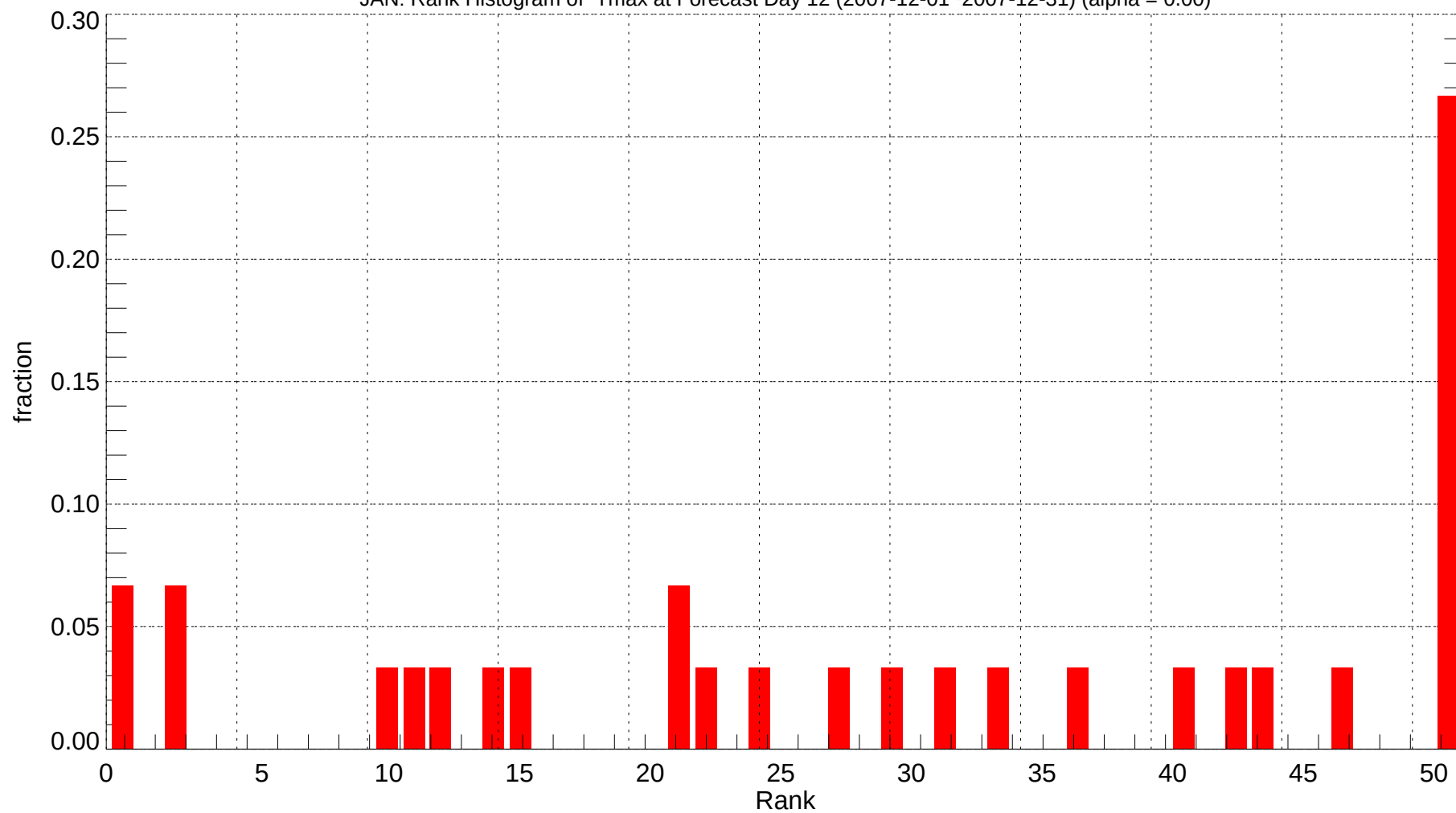
JAN: Rank Histogram of Tmax at Forecast Day 12 (2007-12-01~2007-12-31) (alpha = 0.00)
