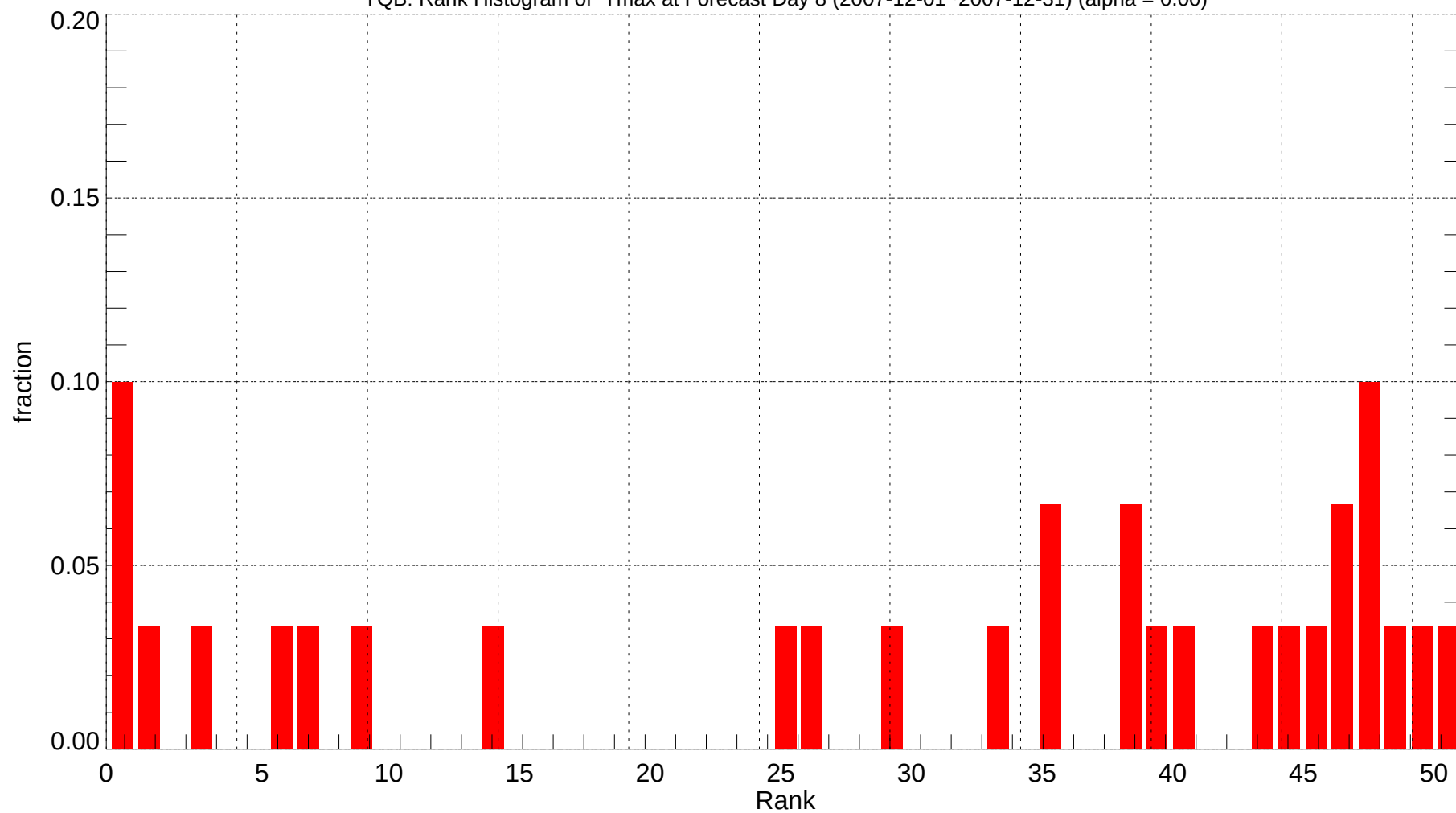
YQB: Rank Histogram of Tmax at Forecast Day 8 (2007-12-01~2007-12-31) (alpha = 0.00)
