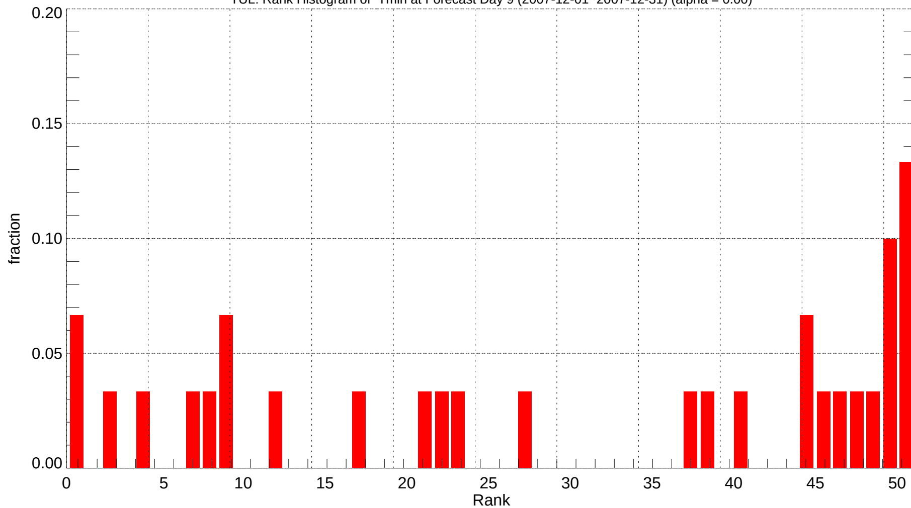
TUL: Rank Histogram of Tmin at Forecast Day 9 (2007-12-01~2007-12-31) (alpha = 0.00)
