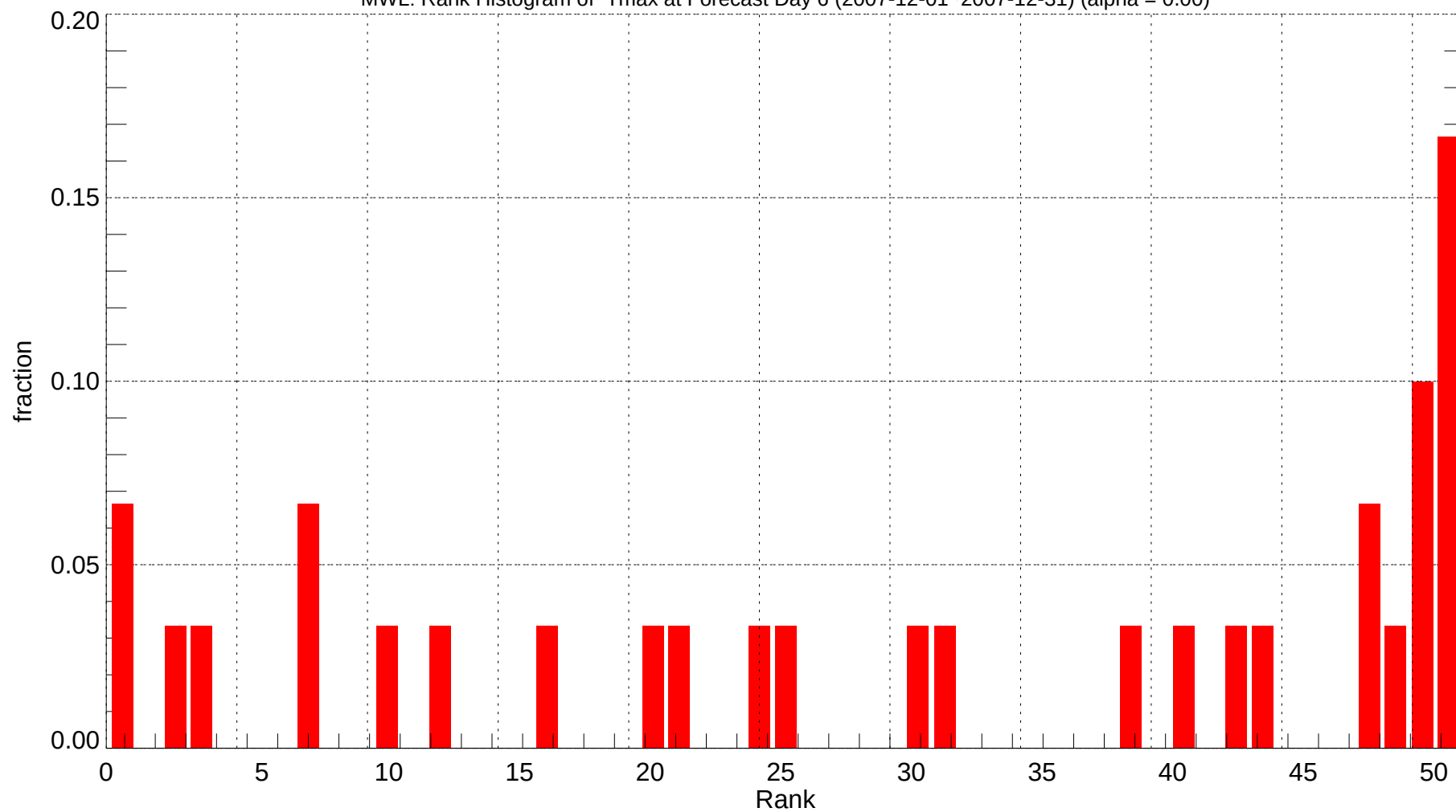
MWL: Rank Histogram of Tmax at Forecast Day 6 (2007-12-01~2007-12-31) (alpha = 0.00)
