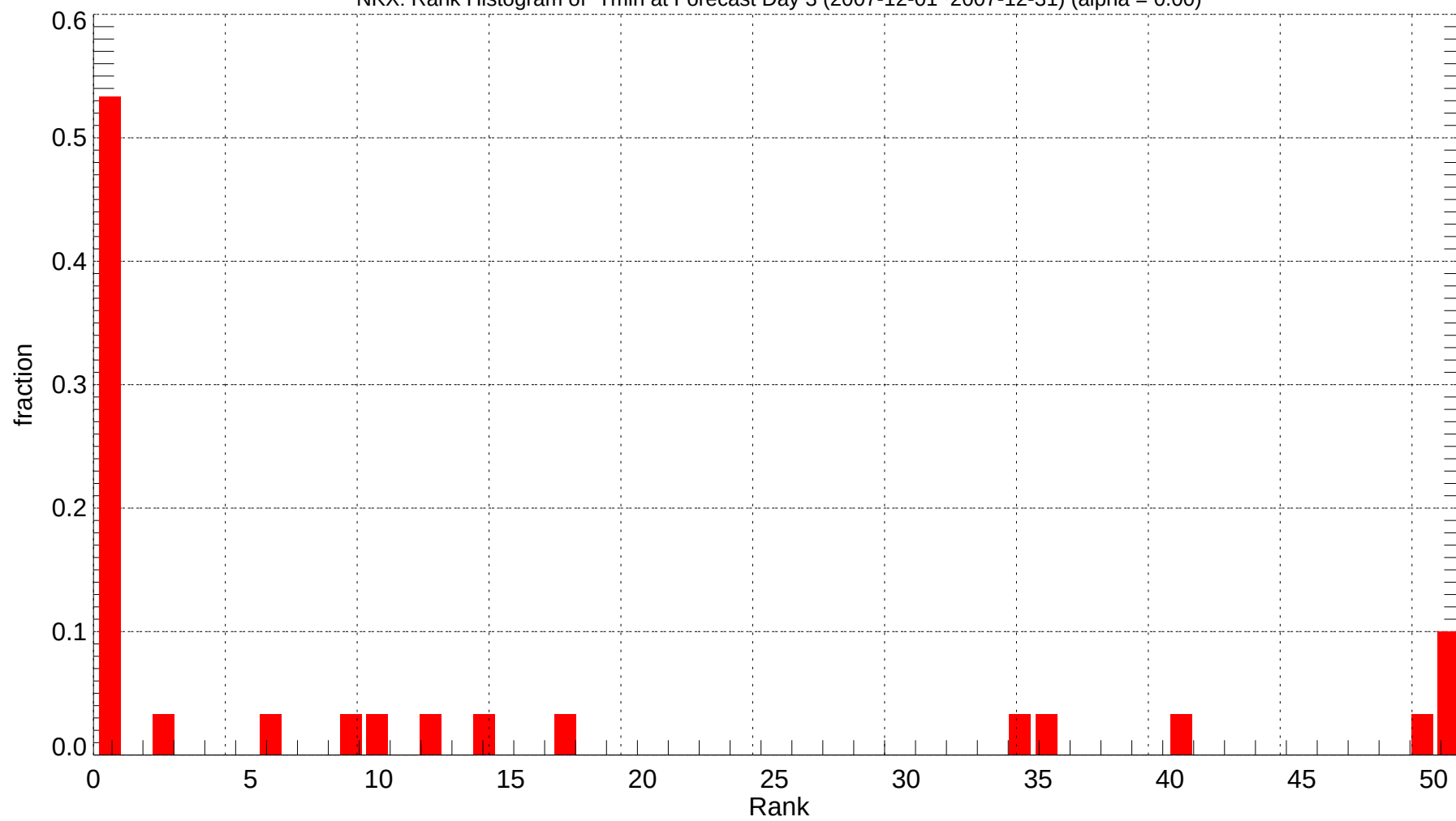
NKX: Rank Histogram of Tmin at Forecast Day 3 (2007-12-01~2007-12-31) (alpha = 0.00)
