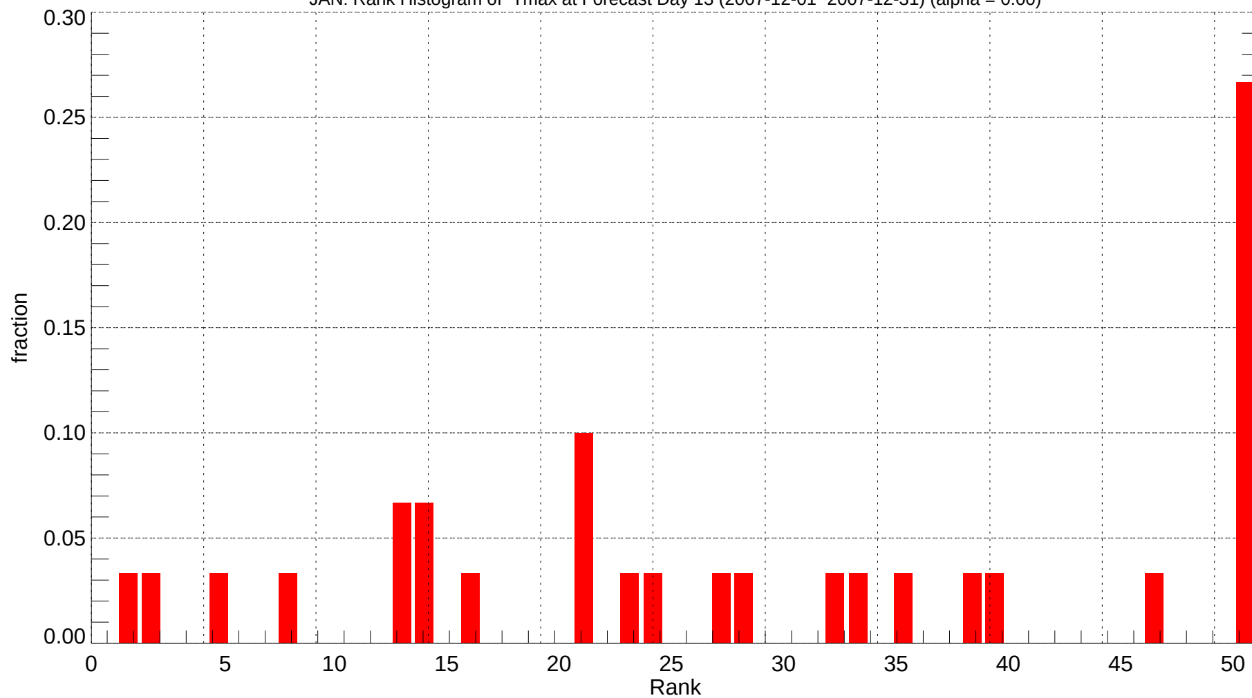
JAN: Rank Histogram of Tmax at Forecast Day 13 (2007-12-01~2007-12-31) (alpha = 0.00)
