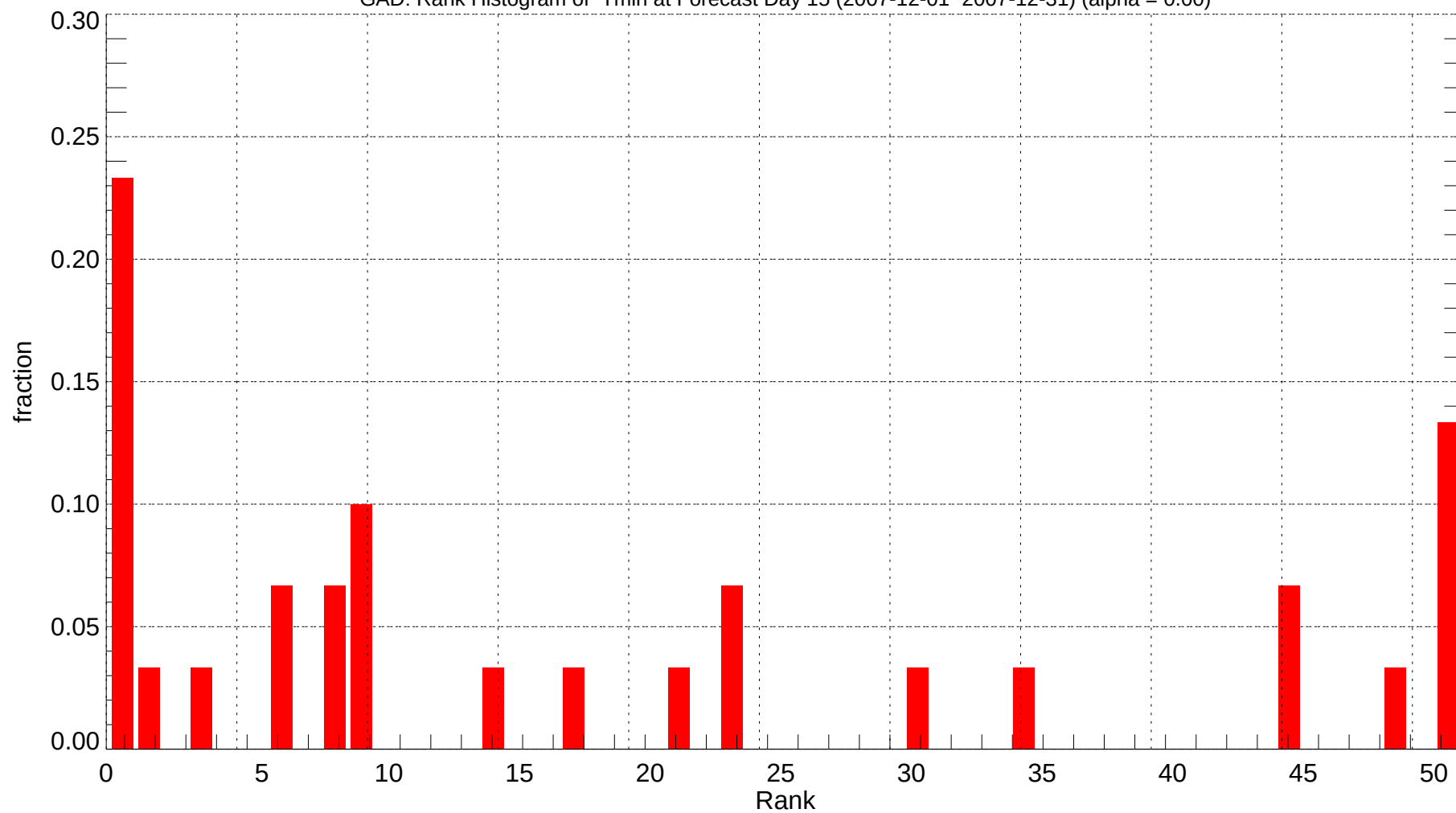
GAD: Rank Histogram of Tmin at Forecast Day 15 (2007-12-01~2007-12-31) (alpha = 0.00)
