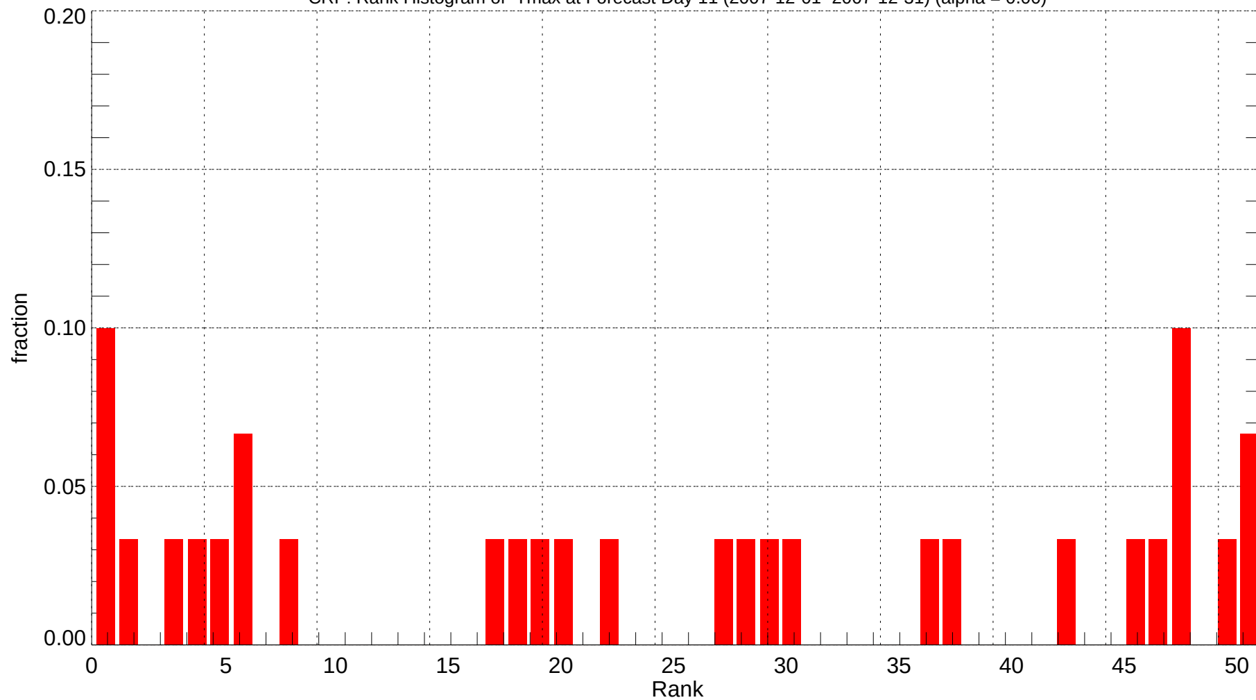
CRP: Rank Histogram of Tmax at Forecast Day 11 (2007-12-01~2007-12-31) (alpha = 0.00)
