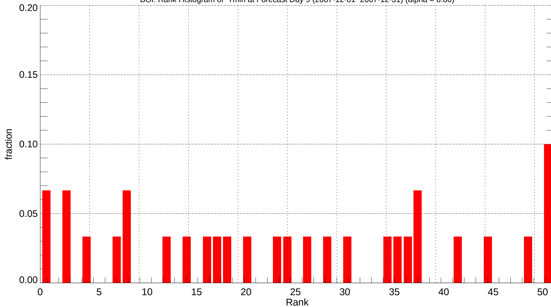
BOI: Rank Histogram of Tmin at Forecast Day 9 (2007-12-01~2007-12-31) (alpha = 0.00)
