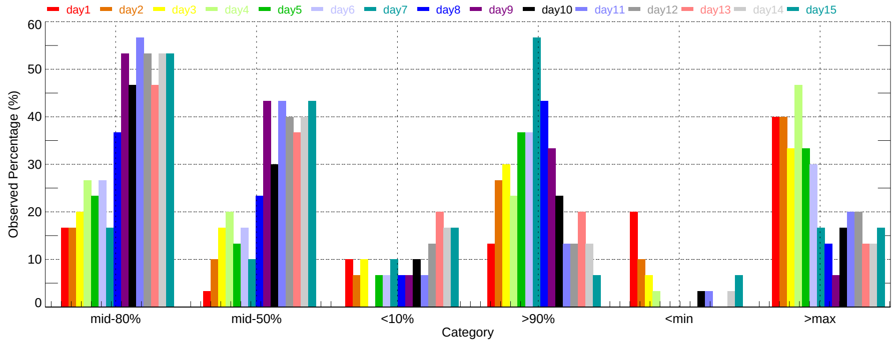
Observed Percentage of Ensembles - BUR: Max Temperature (2007-12-01~2007-12-31)
