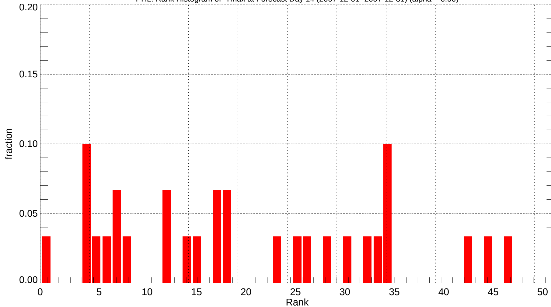
PHL: Rank Histogram of Tmax at Forecast Day 14 (2007-12-01~2007-12-31) (alpha = 0.00)
