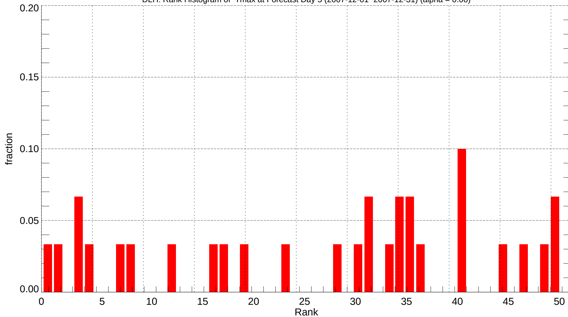
DLH: Rank Histogram of Tmax at Forecast Day 5 (2007-12-01~2007-12-31) (alpha = 0.00)
