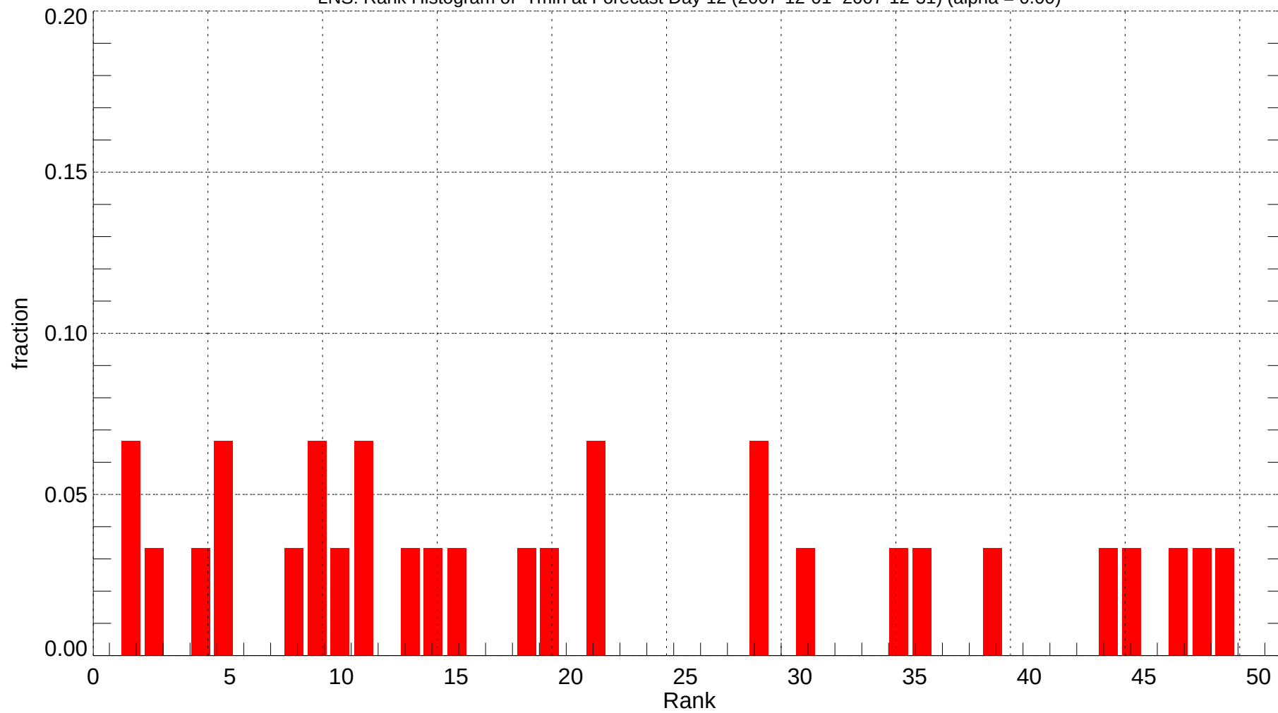
LNS: Rank Histogram of Tmin at Forecast Day 12 (2007-12-01~2007-12-31) (alpha = 0.00)
