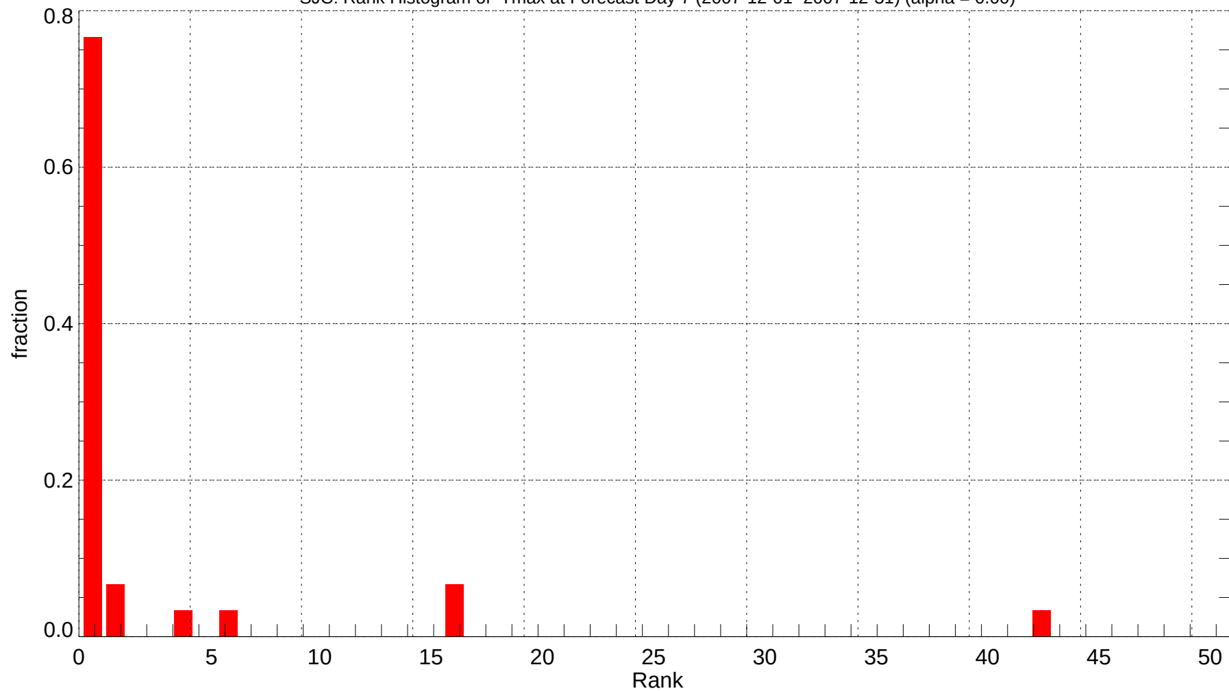
SJC: Rank Histogram of Tmax at Forecast Day 7 (2007-12-01~2007-12-31) (alpha = 0.00)
