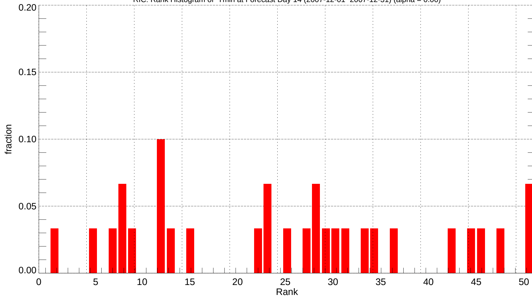
RIC: Rank Histogram of Tmin at Forecast Day 14 (2007-12-01~2007-12-31) (alpha = 0.00)
