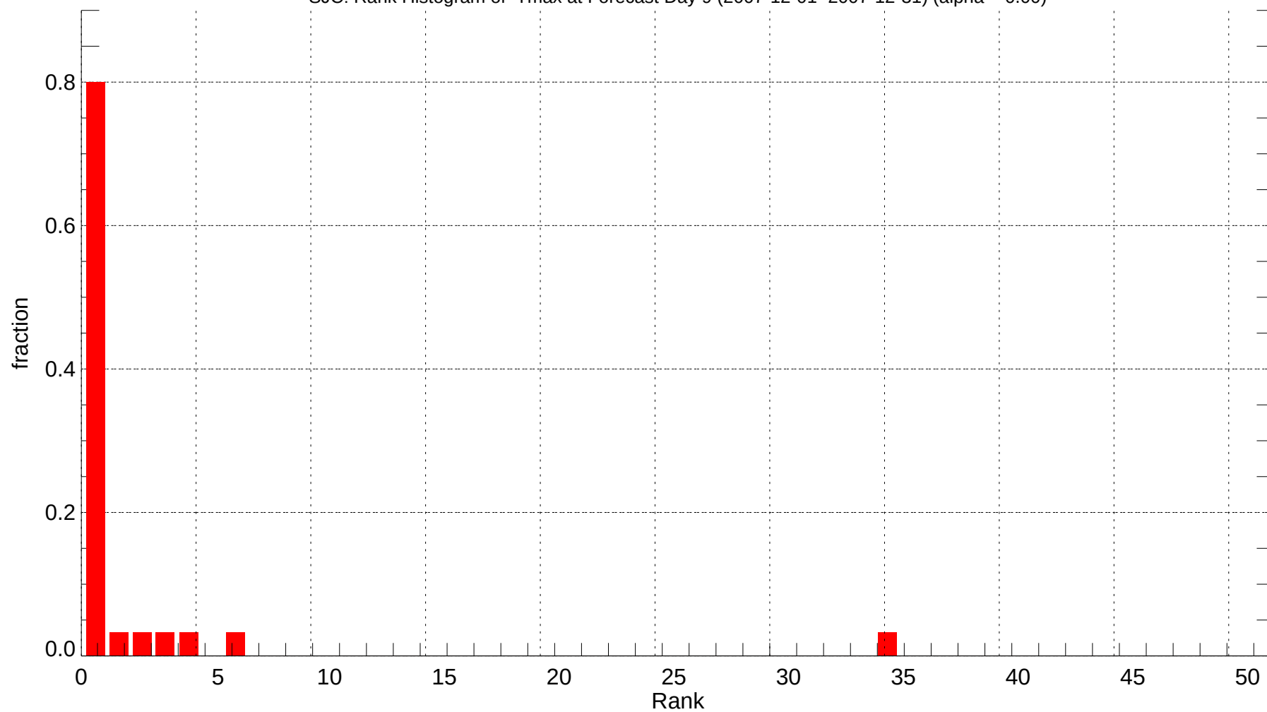
SJC: Rank Histogram of Tmax at Forecast Day 9 (2007-12-01~2007-12-31) (alpha = 0.00)
