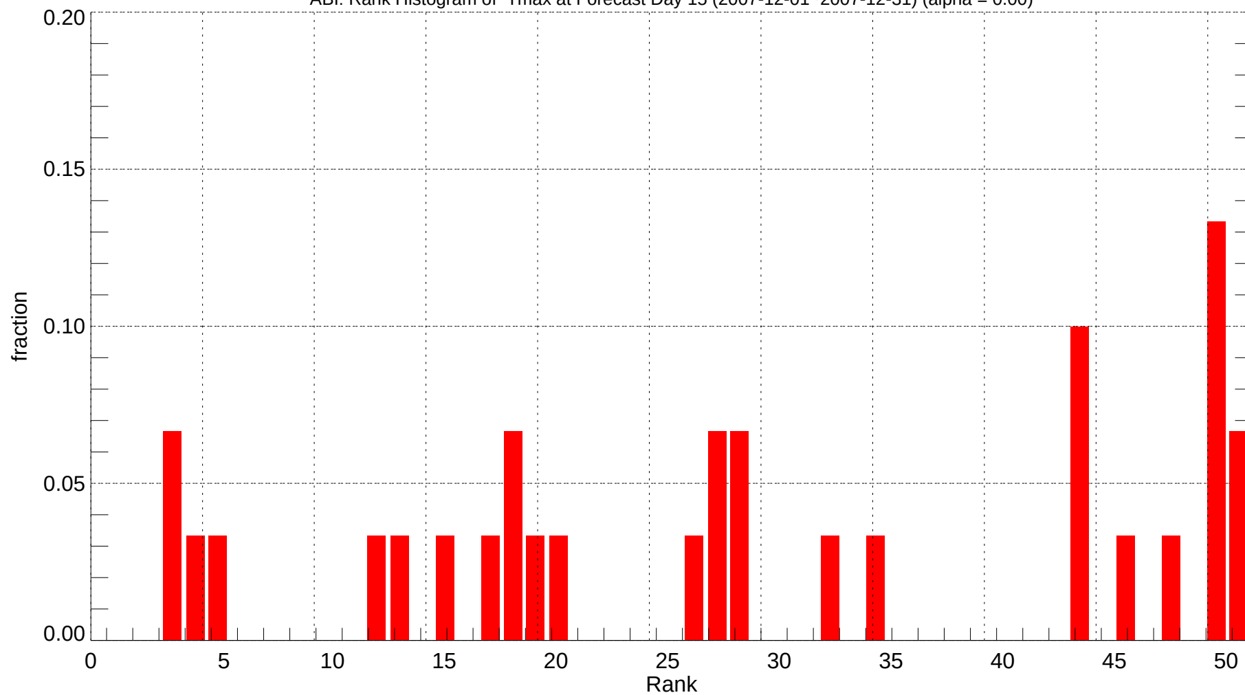
ABI: Rank Histogram of Tmax at Forecast Day 15 (2007-12-01~2007-12-31) (alpha = 0.00)
