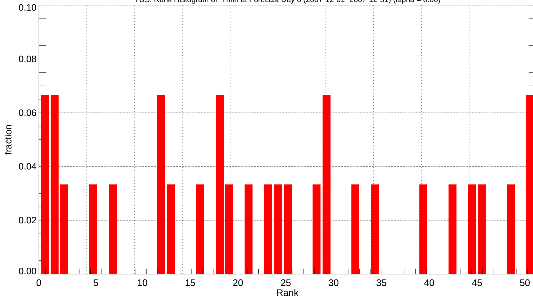
TUS: Rank Histogram of Tmin at Forecast Day 6 (2007-12-01~2007-12-31) (alpha = 0.00)
