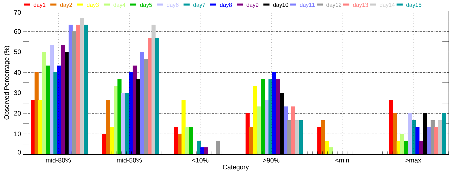
Observed Percentage of Ensembles - HSV: Max Temperature (2007-12-01~2007-12-31)
