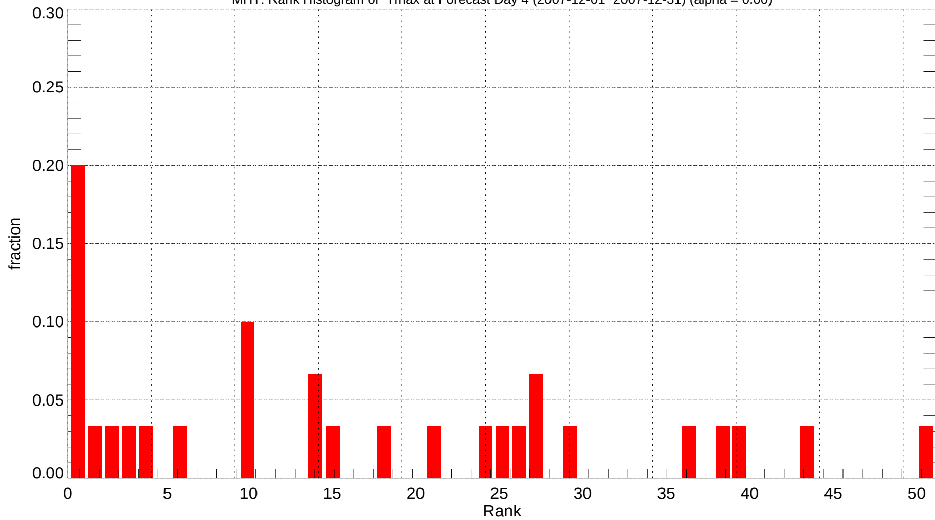
MHT: Rank Histogram of Tmax at Forecast Day 4 (2007-12-01~2007-12-31) (alpha = 0.00)
