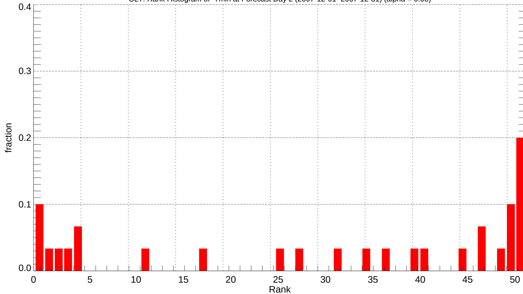
CLT: Rank Histogram of Tmin at Forecast Day 2 (2007-12-01~2007-12-31) (alpha = 0.00)
