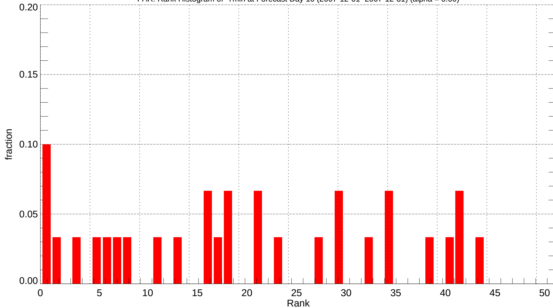
FAR: Rank Histogram of Tmin at Forecast Day 10 (2007-12-01~2007-12-31) (alpha = 0.00)
