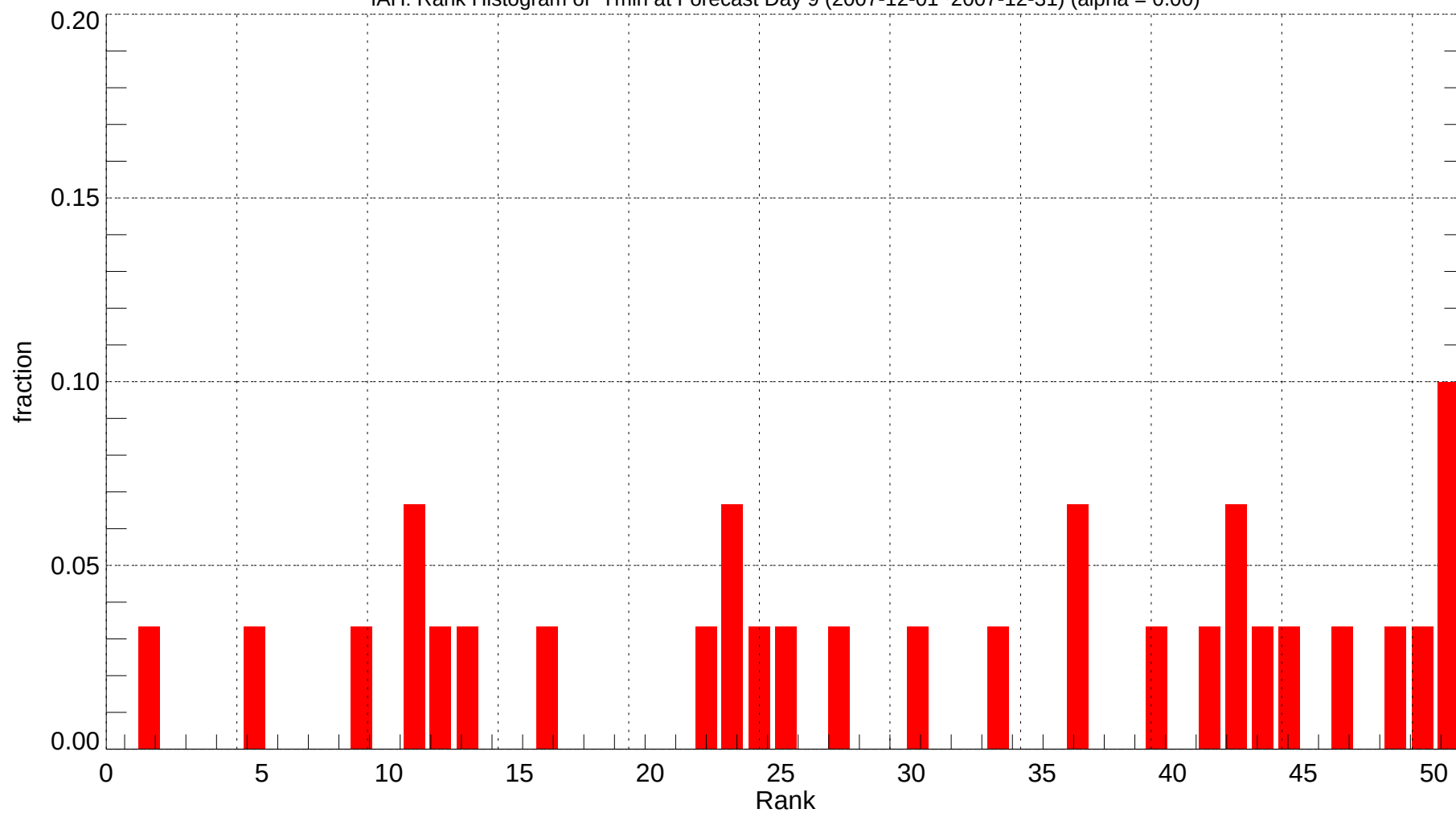
IAH: Rank Histogram of Tmin at Forecast Day 9 (2007-12-01~2007-12-31) (alpha = 0.00)
