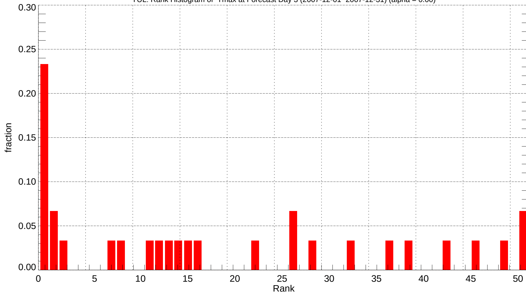
YUL: Rank Histogram of Tmax at Forecast Day 3 (2007-12-01~2007-12-31) (alpha = 0.00)
