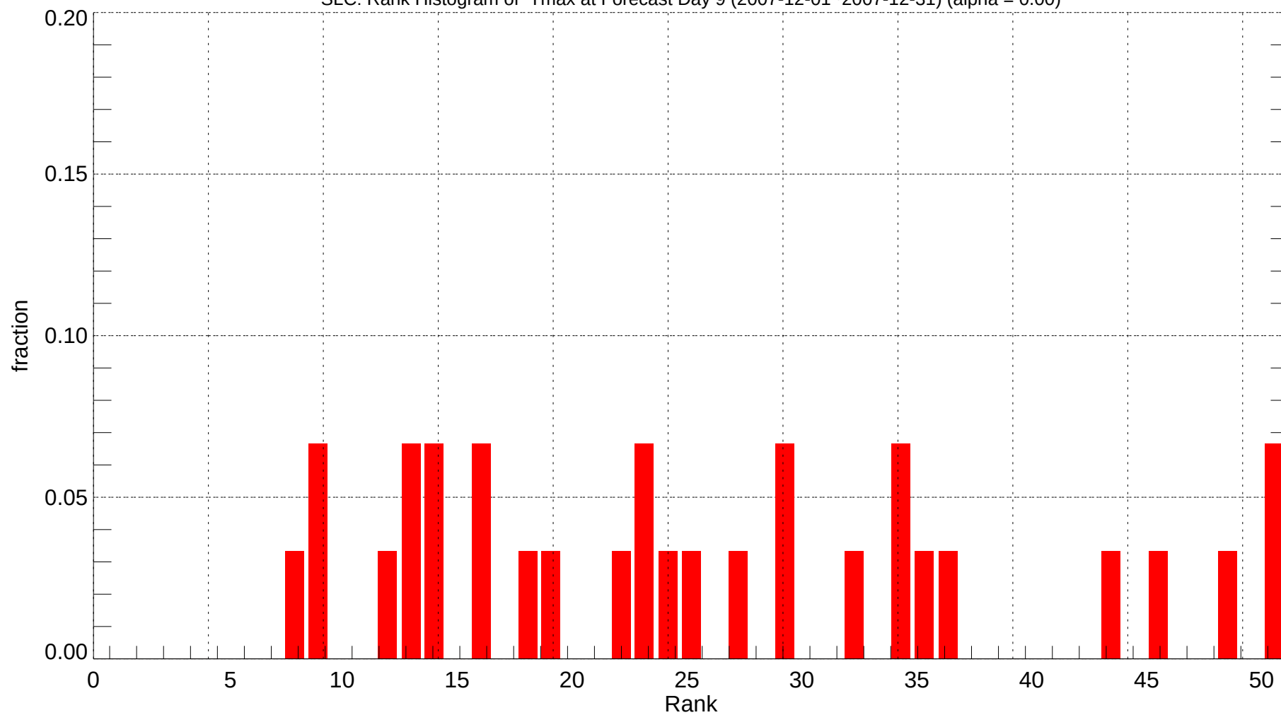
SLC: Rank Histogram of Tmax at Forecast Day 9 (2007-12-01~2007-12-31) (alpha = 0.00)
