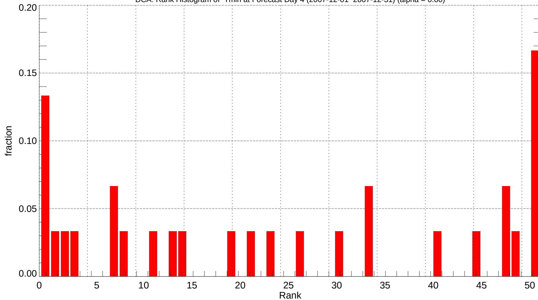
DCA: Rank Histogram of Tmin at Forecast Day 4 (2007-12-01~2007-12-31) (alpha = 0.00)
