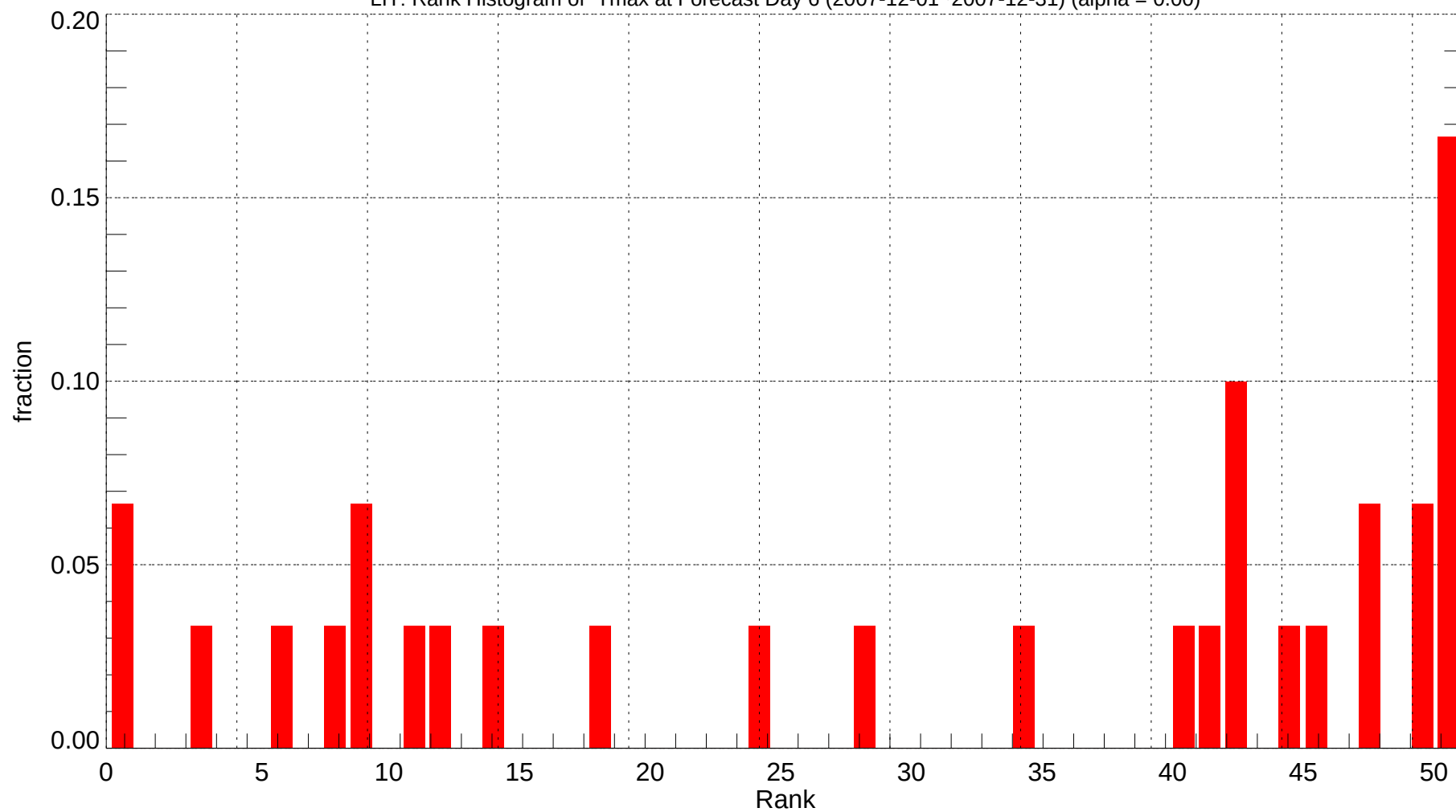
LIT: Rank Histogram of Tmax at Forecast Day 6 (2007-12-01~2007-12-31) (alpha = 0.00)
