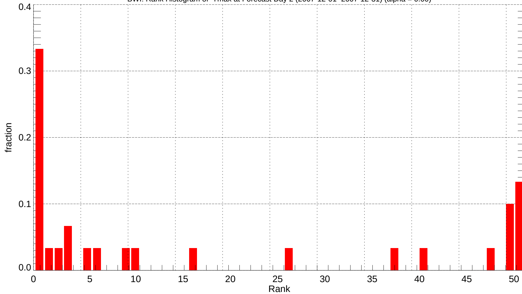
BWI: Rank Histogram of Tmax at Forecast Day 2 (2007-12-01~2007-12-31) (alpha = 0.00)
