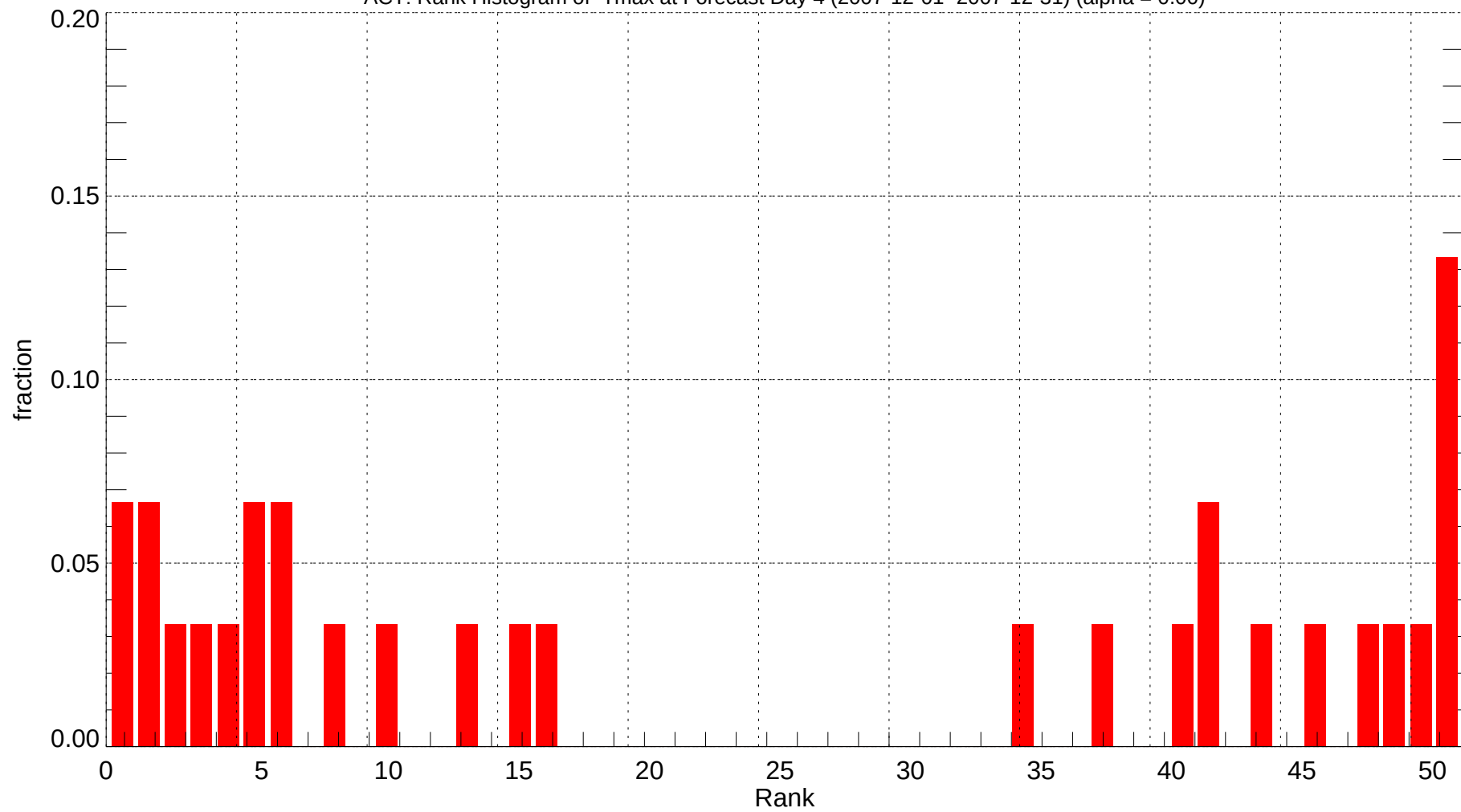
ACT: Rank Histogram of Tmax at Forecast Day 4 (2007-12-01~2007-12-31) (alpha = 0.00)
