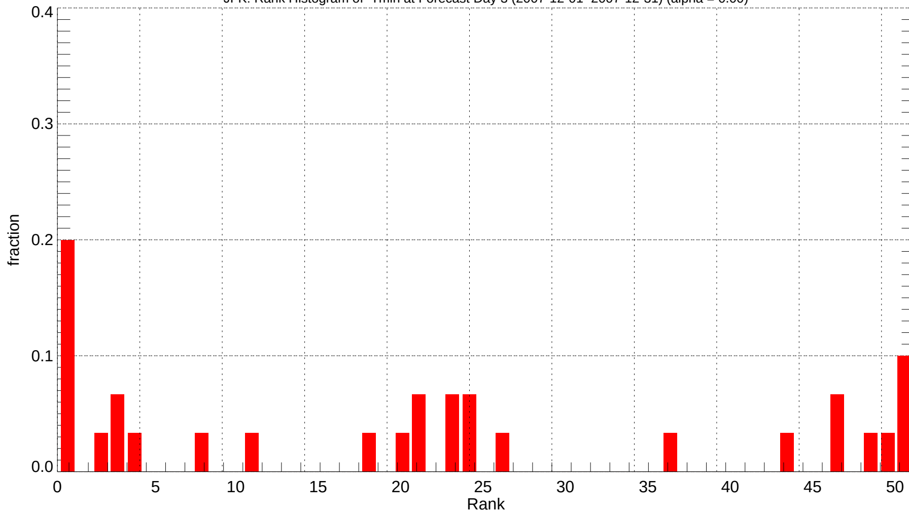
JFK: Rank Histogram of Tmin at Forecast Day 3 (2007-12-01~2007-12-31) (alpha = 0.00)
