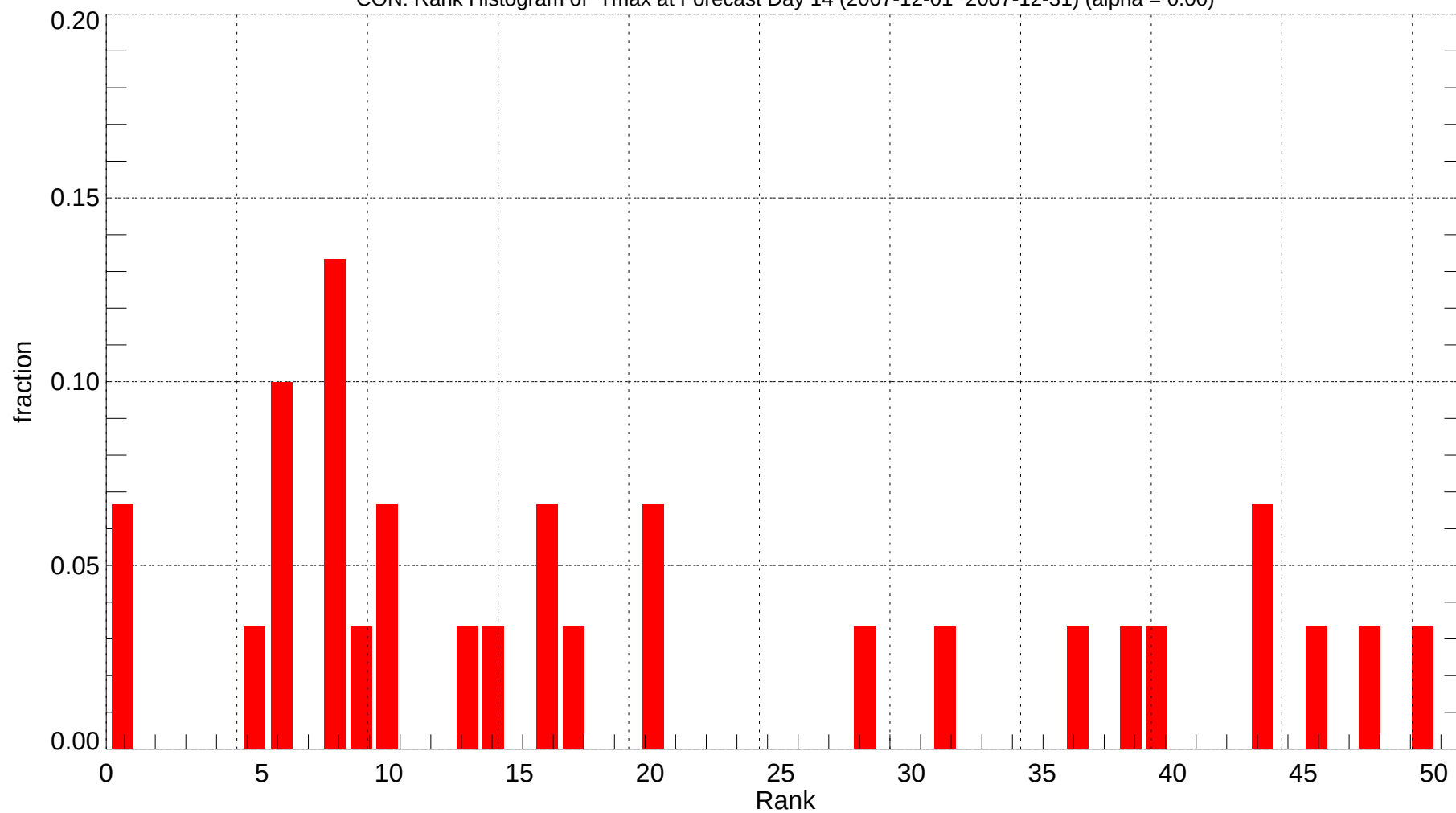
CON: Rank Histogram of Tmax at Forecast Day 14 (2007-12-01~2007-12-31) (alpha = 0.00)
