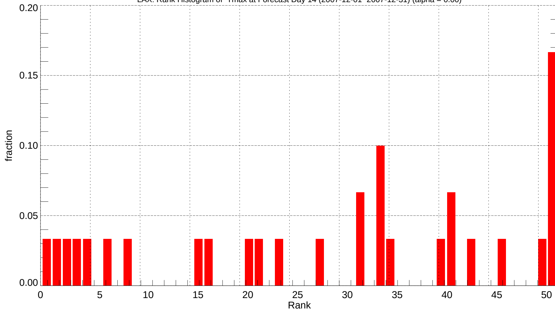
LAX: Rank Histogram of Tmax at Forecast Day 14 (2007-12-01~2007-12-31) (alpha = 0.00)
