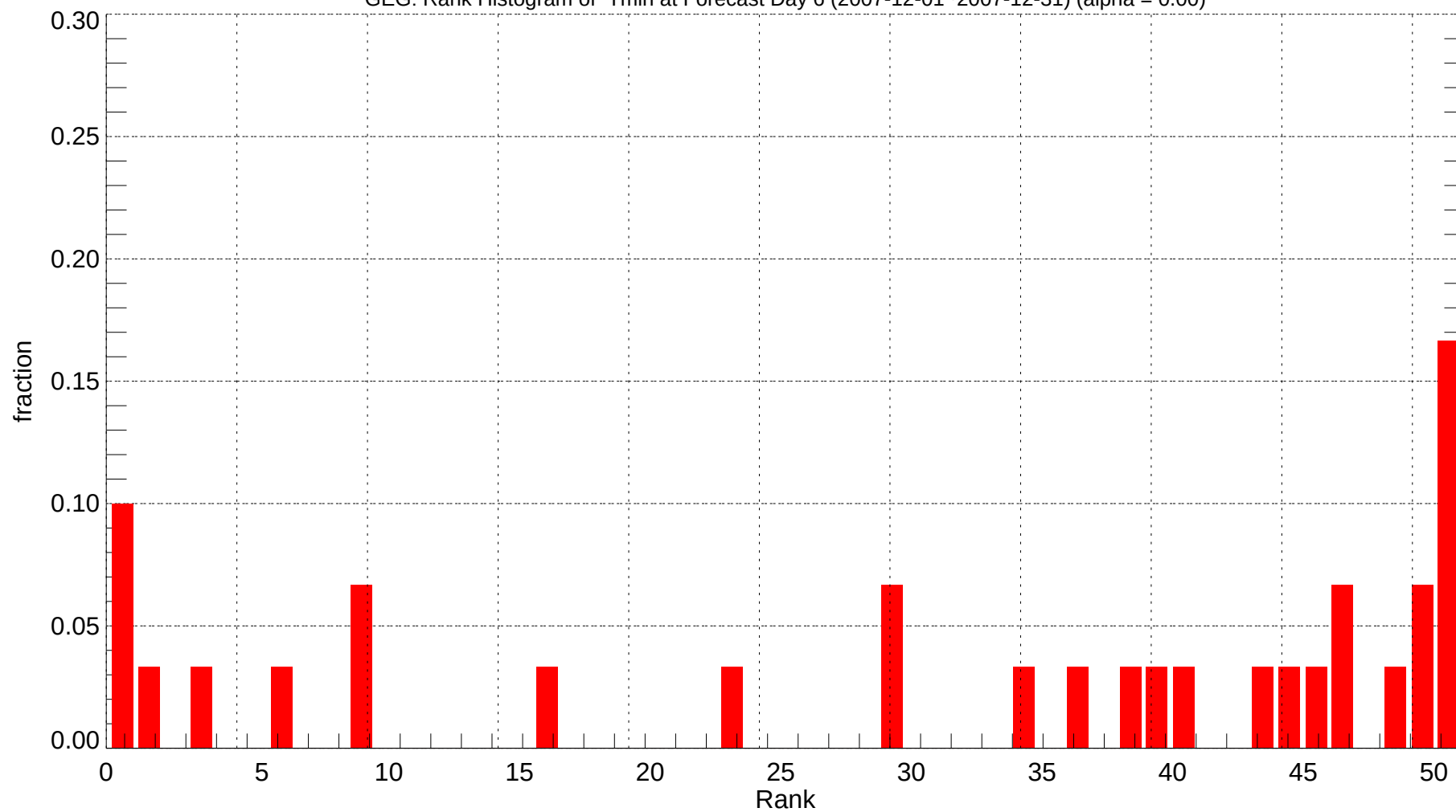
GEG: Rank Histogram of Tmin at Forecast Day 6 (2007-12-01~2007-12-31) (alpha = 0.00)
