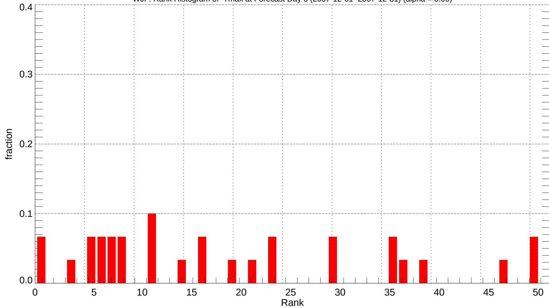
WJF: Rank Histogram of Tmax at Forecast Day 6 (2007-12-01~2007-12-31) (alpha = 0.00)
