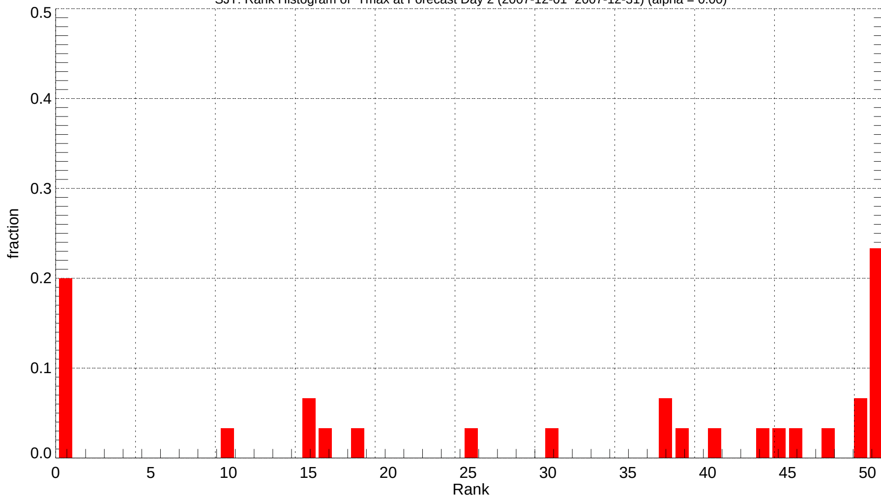
SJT: Rank Histogram of Tmax at Forecast Day 2 (2007-12-01~2007-12-31) (alpha = 0.00)
