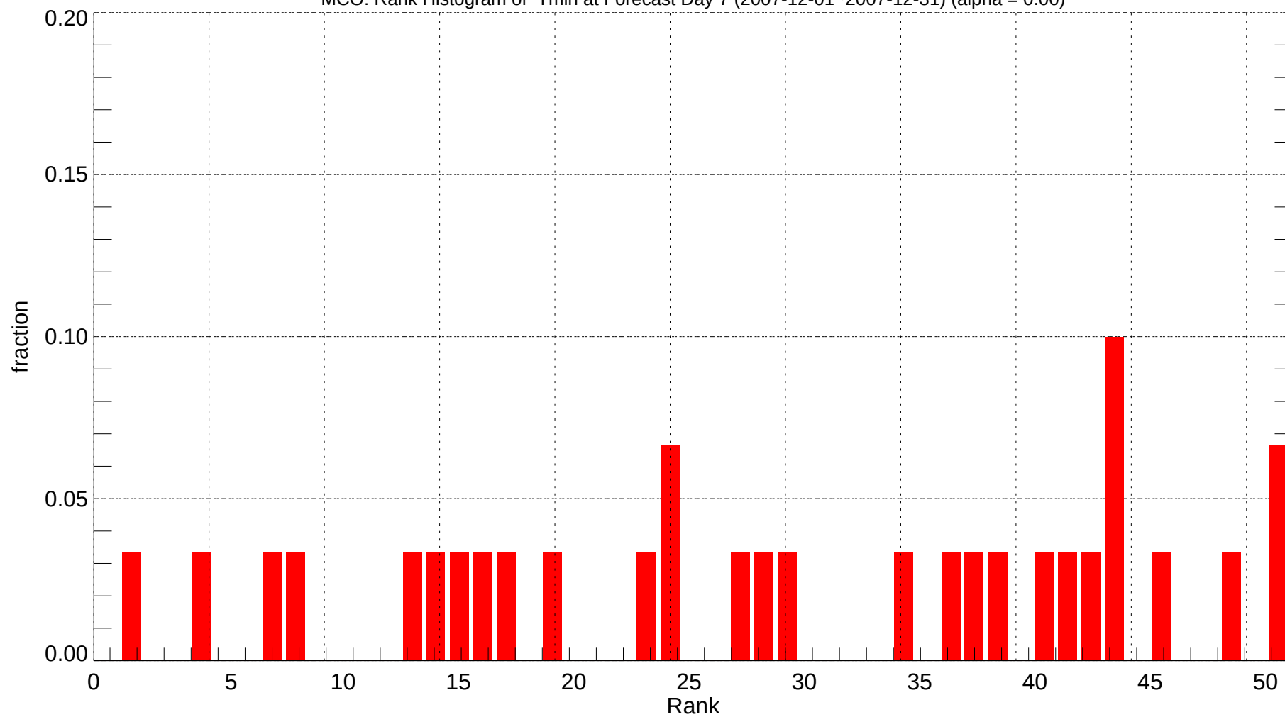
MCO: Rank Histogram of Tmin at Forecast Day 7 (2007-12-01~2007-12-31) (alpha = 0.00)
