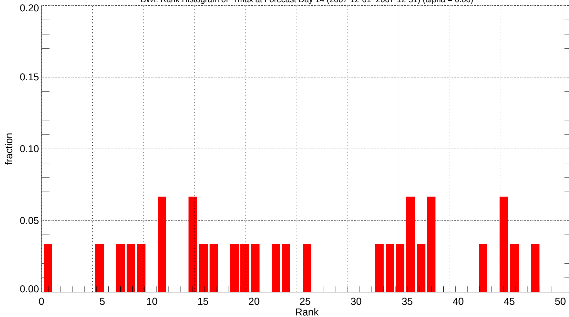
BWI: Rank Histogram of Tmax at Forecast Day 14 (2007-12-01~2007-12-31) (alpha = 0.00)
