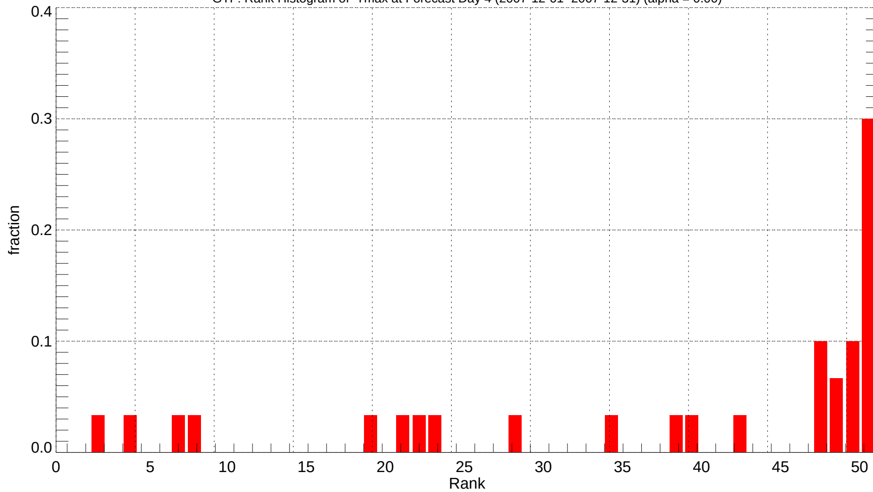
GTF: Rank Histogram of Tmax at Forecast Day 4 (2007-12-01~2007-12-31) (alpha = 0.00)
