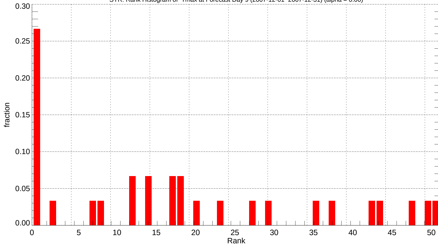
SYR: Rank Histogram of Tmax at Forecast Day 9 (2007-12-01~2007-12-31) (alpha = 0.00)
