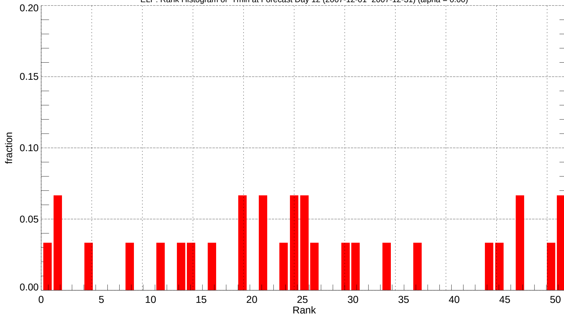
ELP: Rank Histogram of Tmin at Forecast Day 12 (2007-12-01~2007-12-31) (alpha = 0.00)
