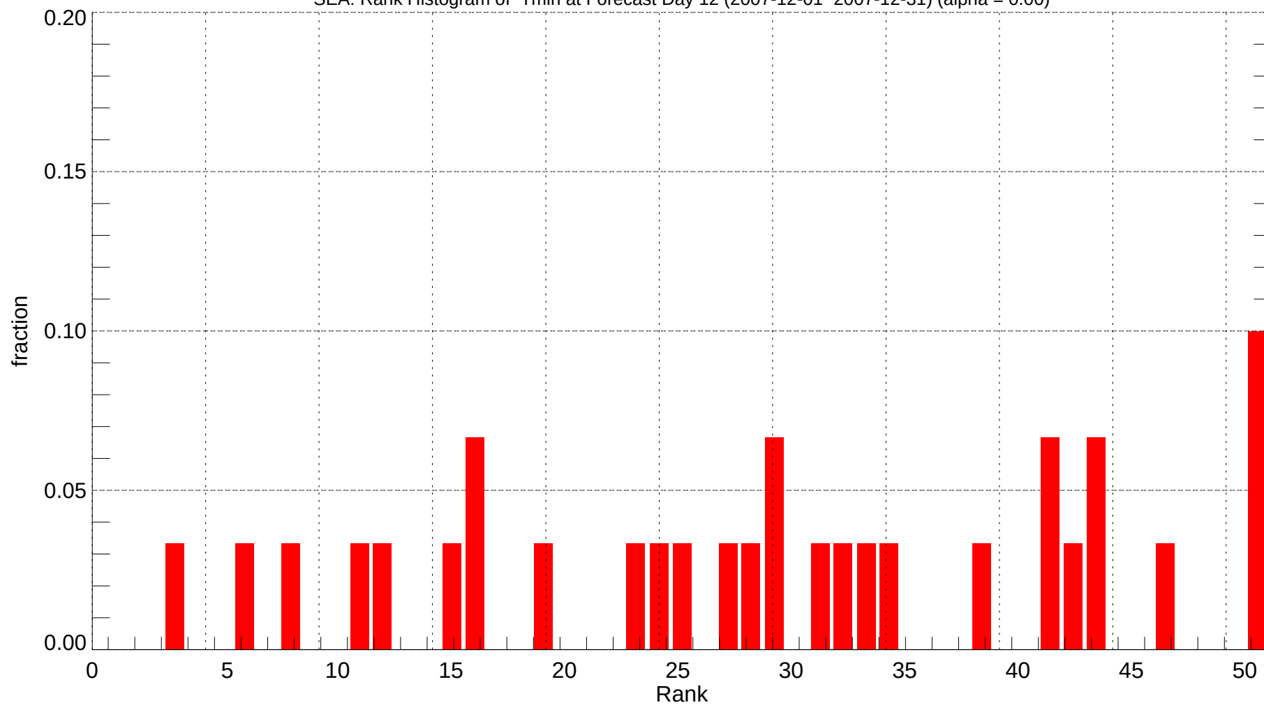
SEA: Rank Histogram of Tmin at Forecast Day 12 (2007-12-01~2007-12-31) (alpha = 0.00)
