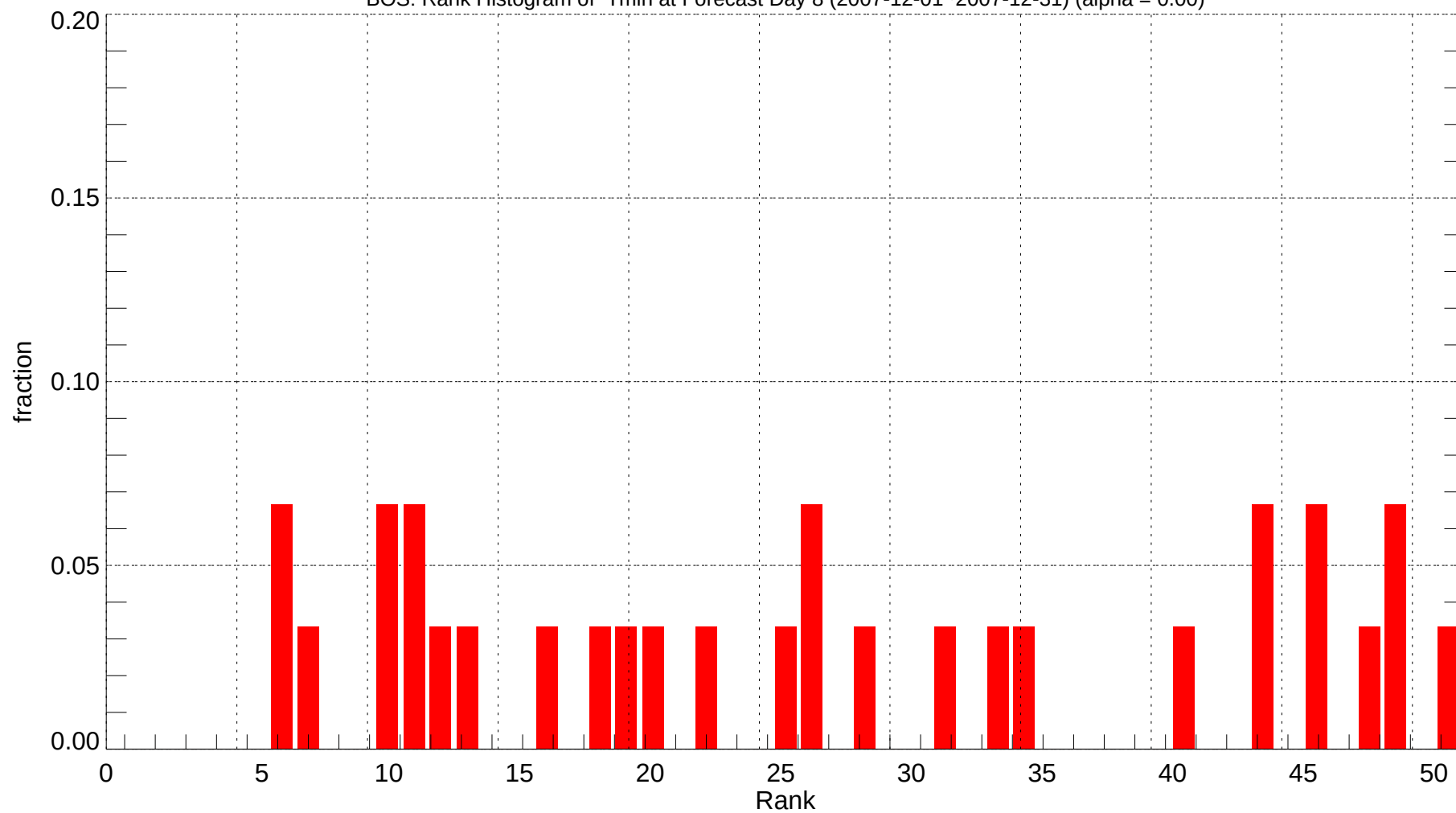
BOS: Rank Histogram of Tmin at Forecast Day 8 (2007-12-01~2007-12-31) (alpha = 0.00)
