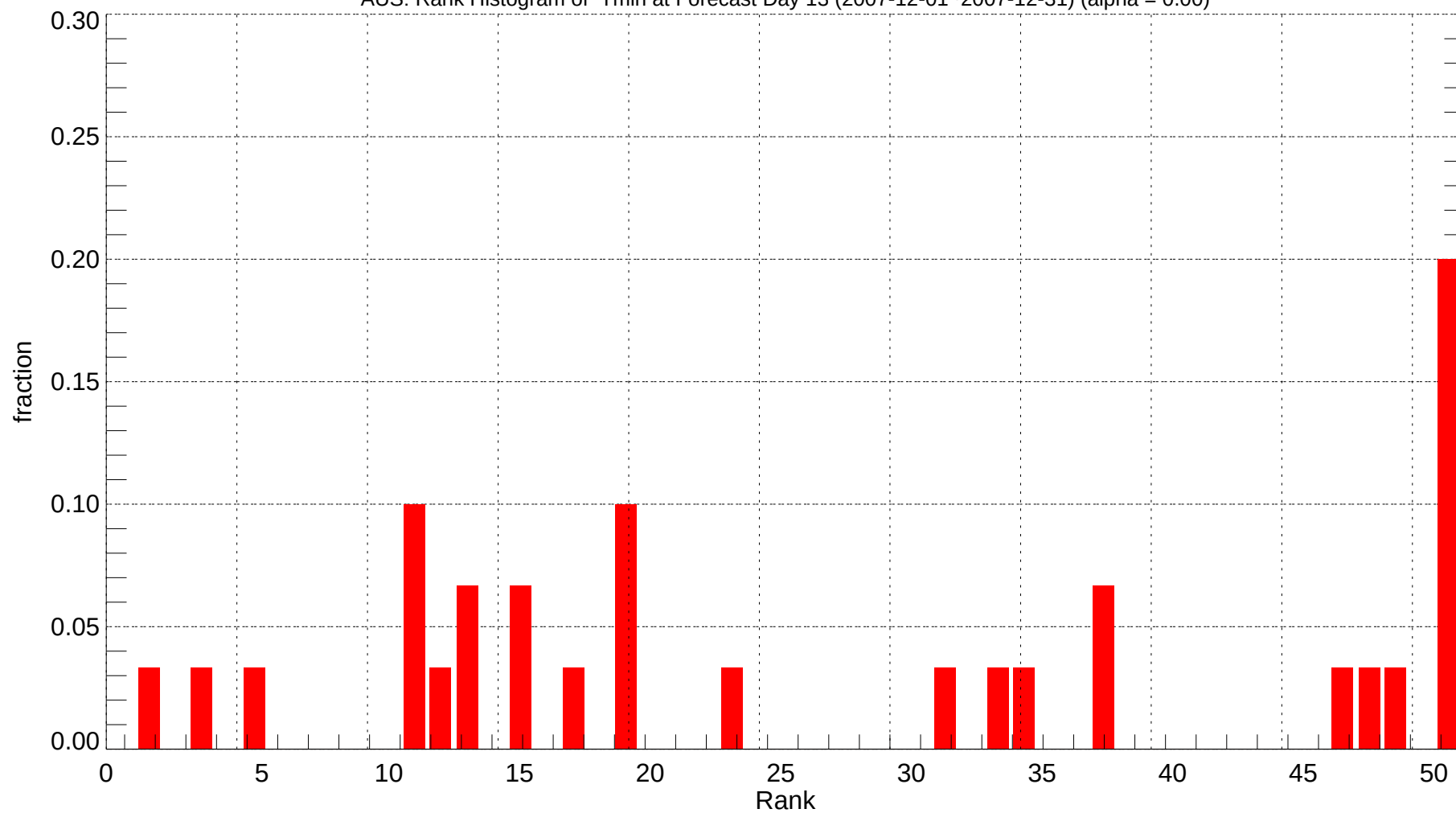
AUS: Rank Histogram of Tmin at Forecast Day 13 (2007-12-01~2007-12-31) (alpha = 0.00)
