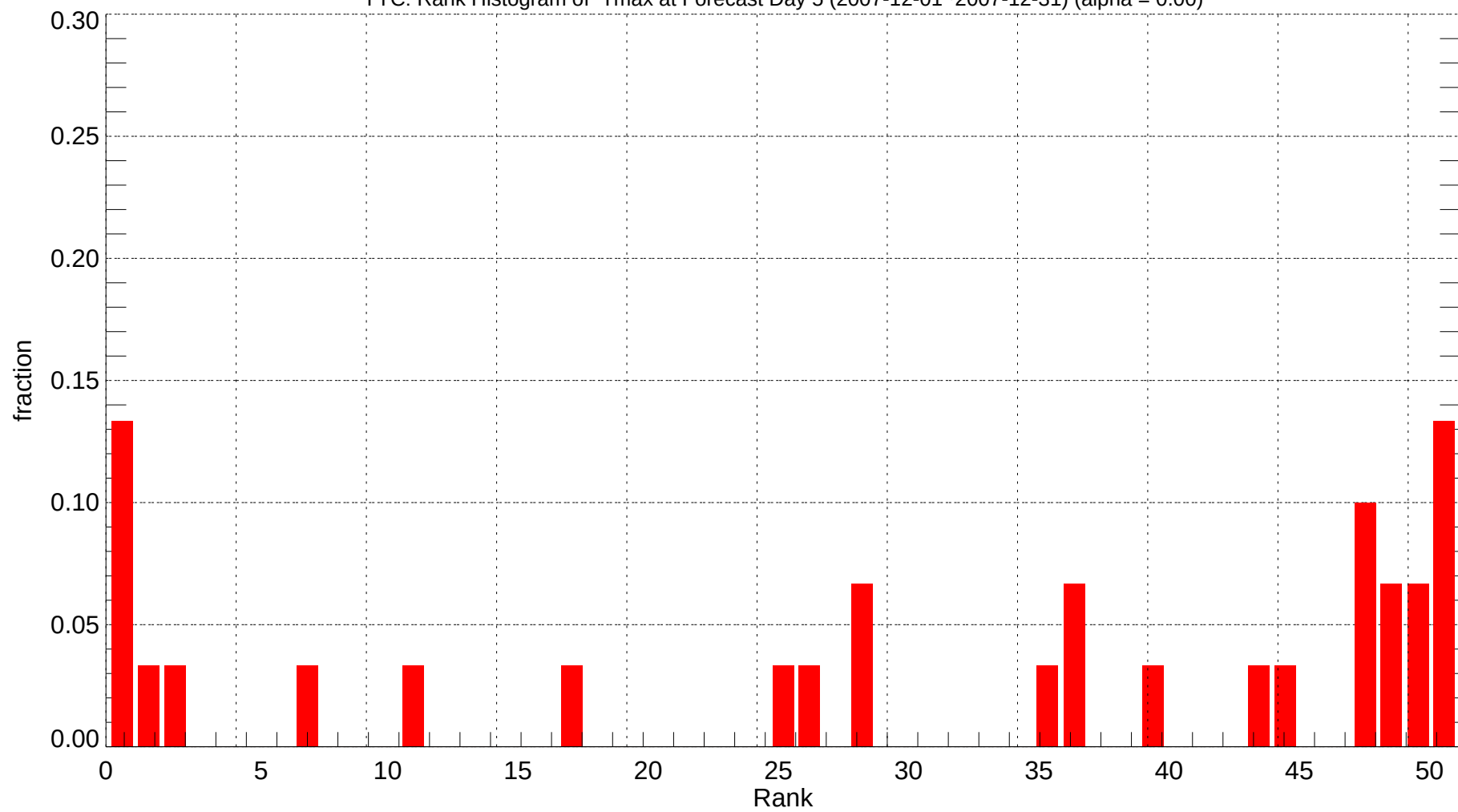
YYC: Rank Histogram of Tmax at Forecast Day 5 (2007-12-01~2007-12-31) (alpha = 0.00)
