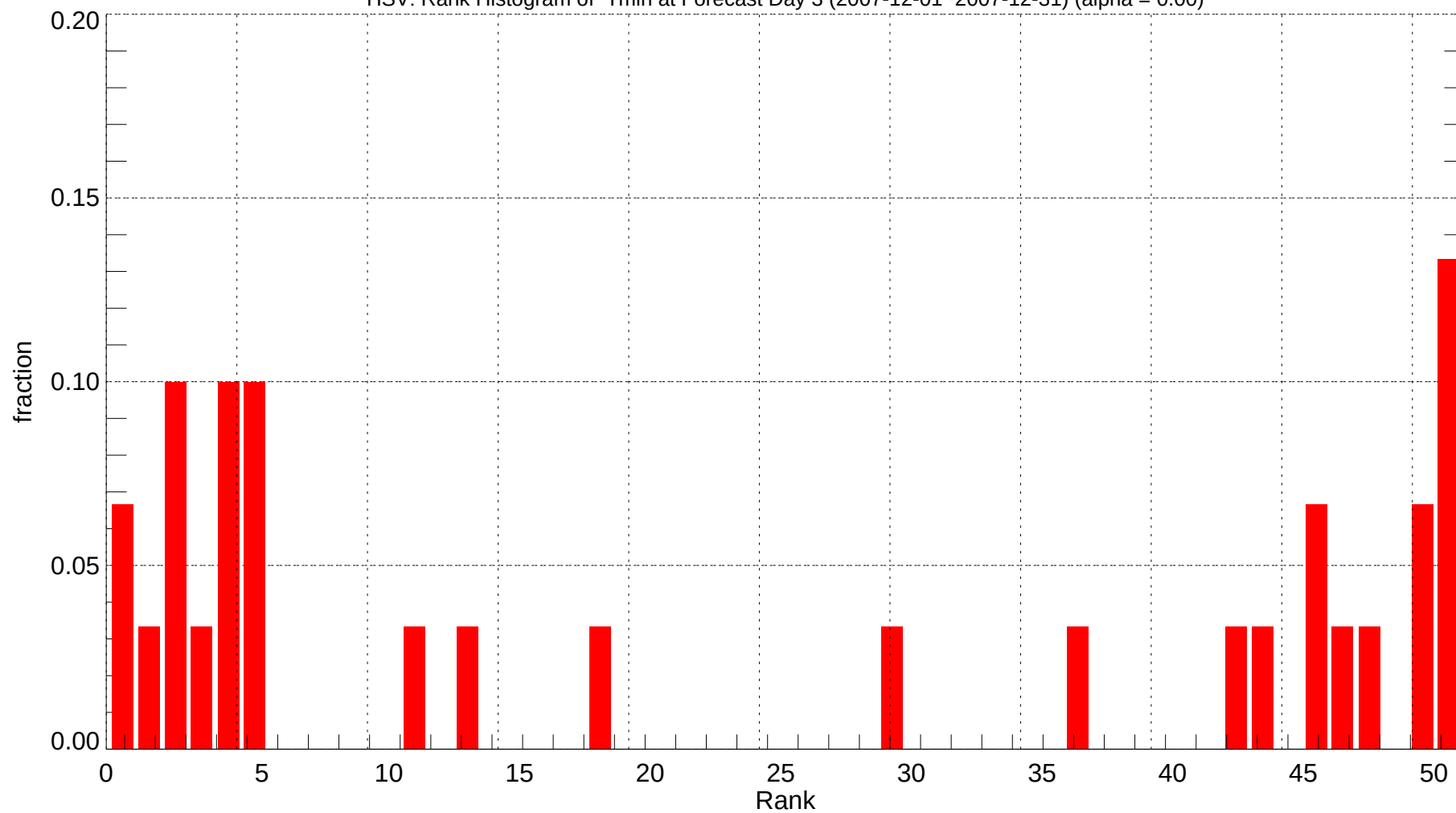
HSV: Rank Histogram of Tmin at Forecast Day 3 (2007-12-01~2007-12-31) (alpha = 0.00)
