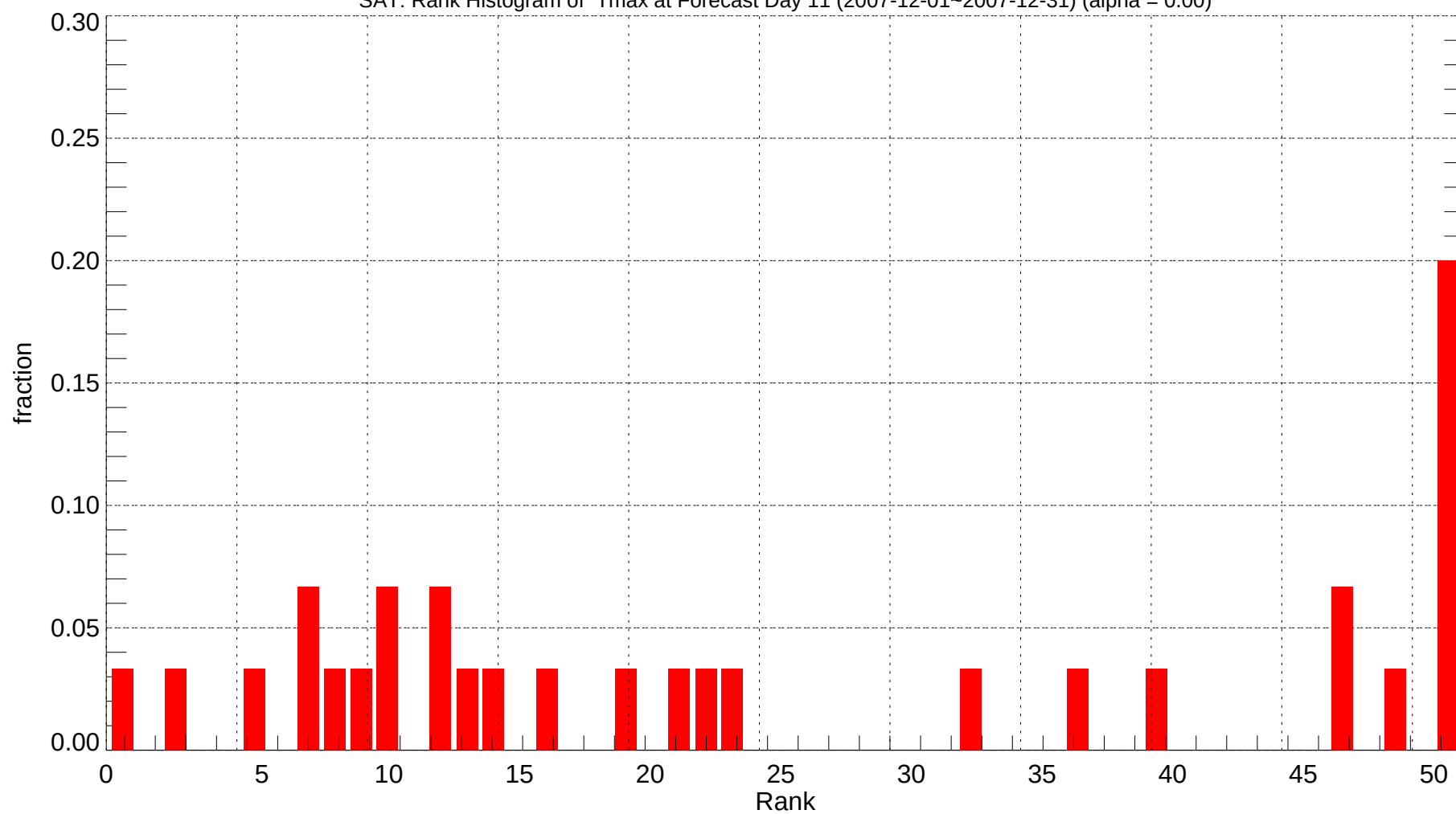
SAT: Rank Histogram of Tmax at Forecast Day 11 (2007-12-01~2007-12-31) (alpha = 0.00)
