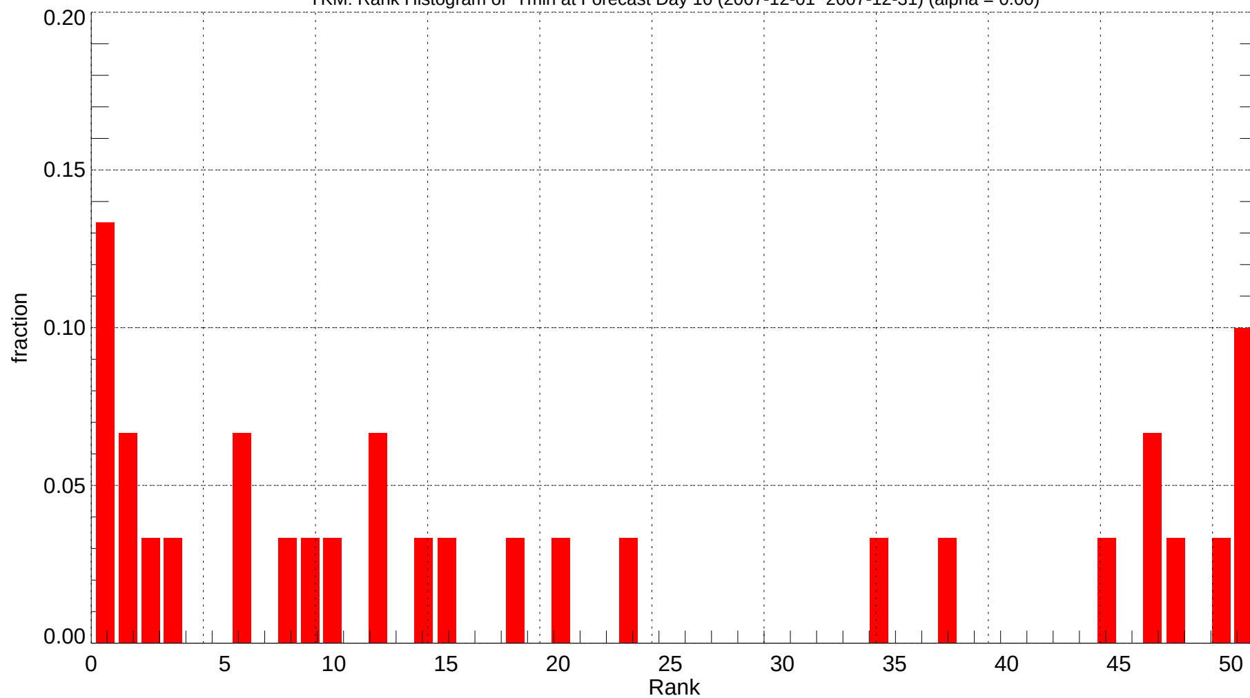
YKM: Rank Histogram of Tmin at Forecast Day 10 (2007-12-01~2007-12-31) (alpha = 0.00)
