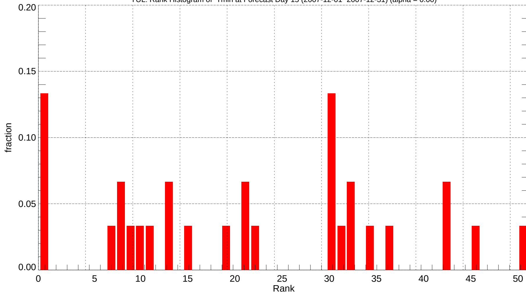
YUL: Rank Histogram of Tmin at Forecast Day 15 (2007-12-01~2007-12-31) (alpha = 0.00)
