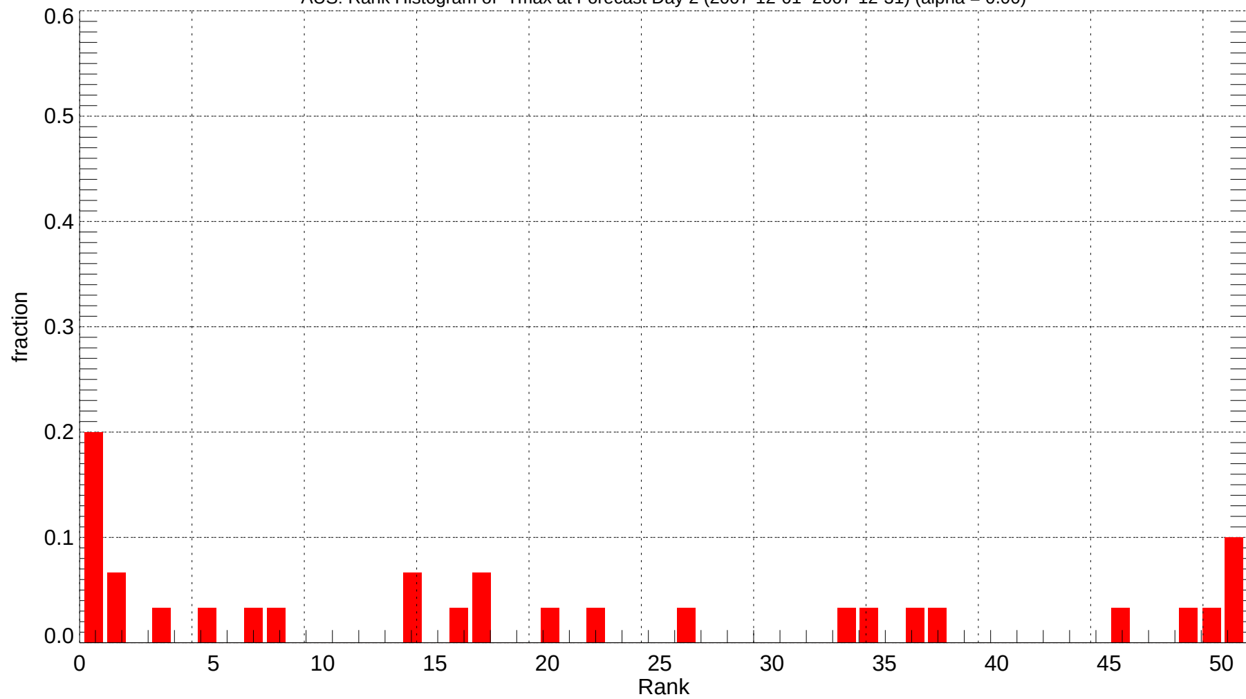
AUS: Rank Histogram of Tmax at Forecast Day 2 (2007-12-01~2007-12-31) (alpha = 0.00)
