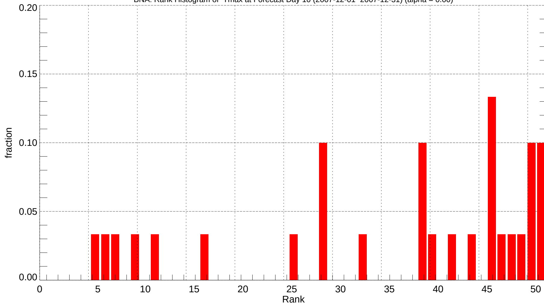
BNA: Rank Histogram of Tmax at Forecast Day 10 (2007-12-01~2007-12-31) (alpha = 0.00)
