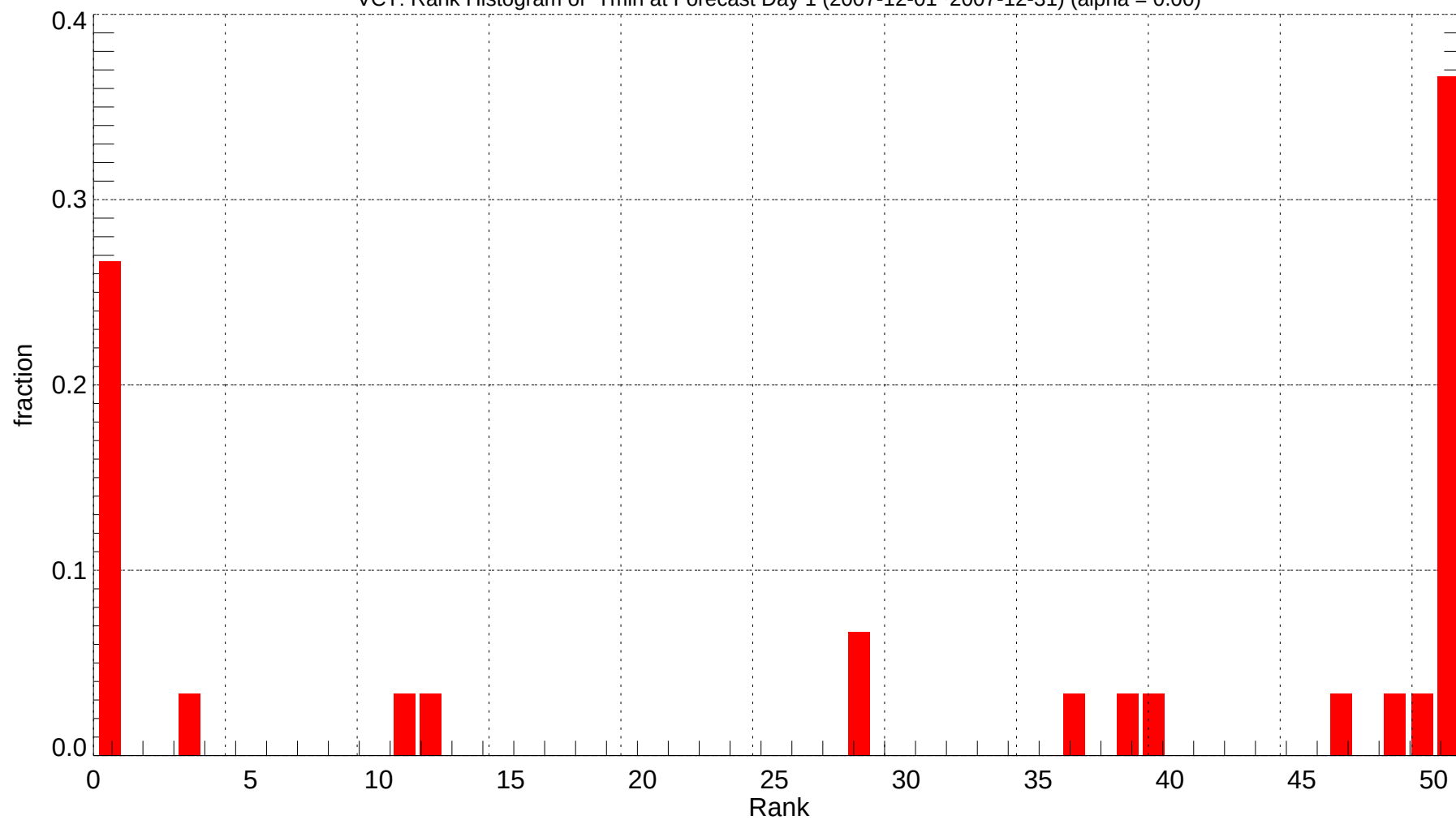
VCT: Rank Histogram of Tmin at Forecast Day 1 (2007-12-01~2007-12-31) (alpha = 0.00)
