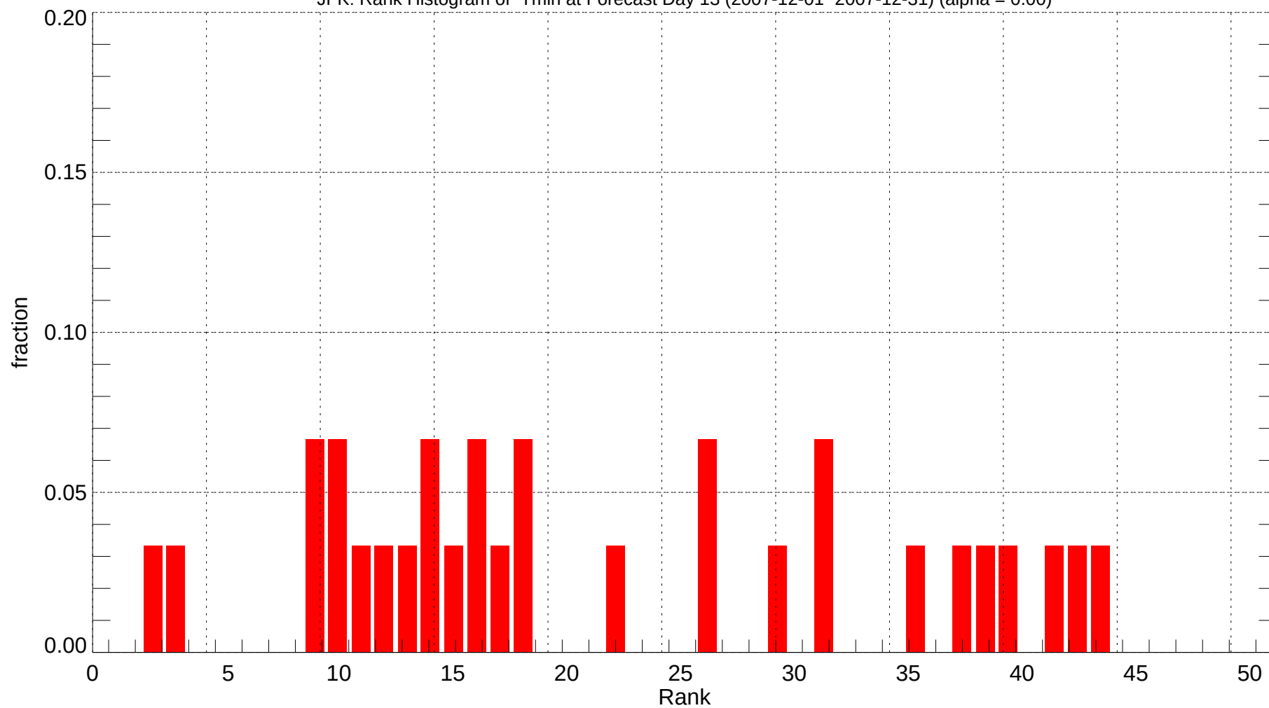
JFK: Rank Histogram of Tmin at Forecast Day 13 (2007-12-01~2007-12-31) (alpha = 0.00)
