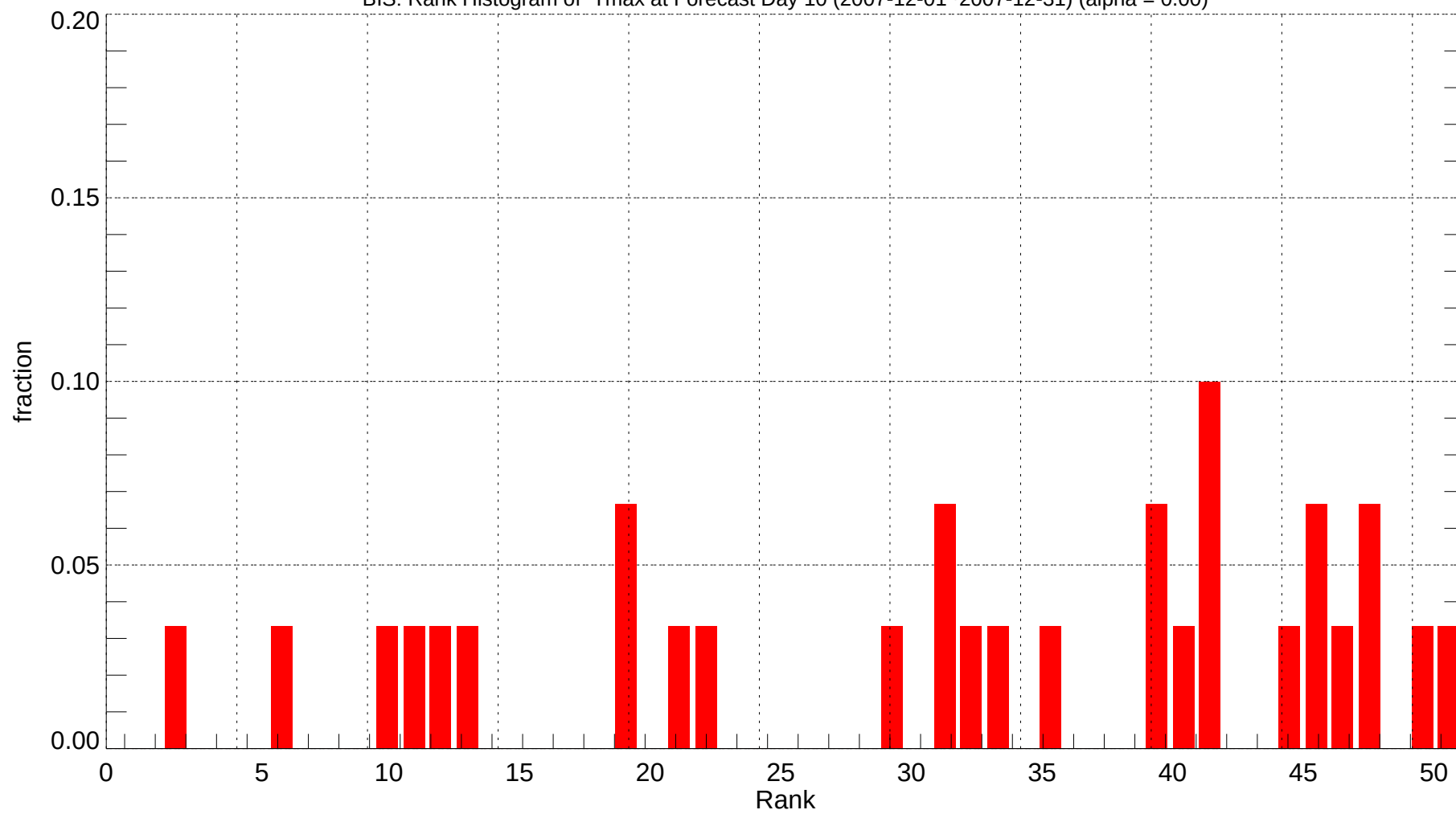
BIS: Rank Histogram of Tmax at Forecast Day 10 (2007-12-01~2007-12-31) (alpha = 0.00)
