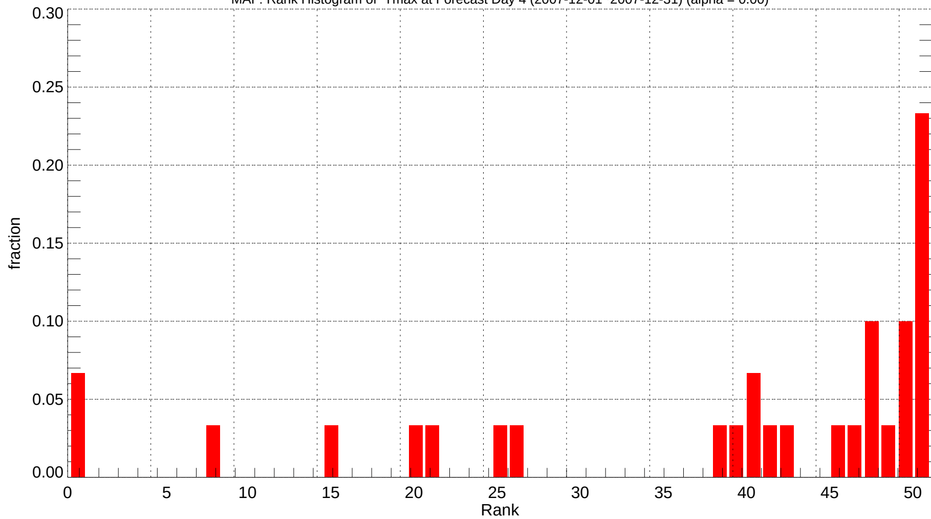
MAF: Rank Histogram of Tmax at Forecast Day 4 (2007-12-01~2007-12-31) (alpha = 0.00)
