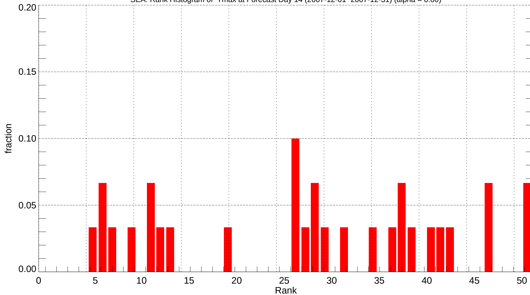
SEA: Rank Histogram of Tmax at Forecast Day 14 (2007-12-01~2007-12-31) (alpha = 0.00)
