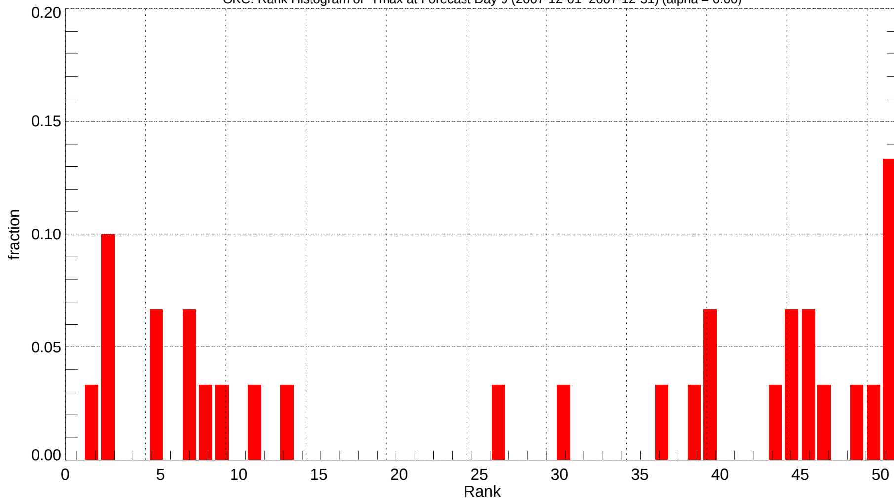
OKC: Rank Histogram of Tmax at Forecast Day 9 (2007-12-01~2007-12-31) (alpha = 0.00)
