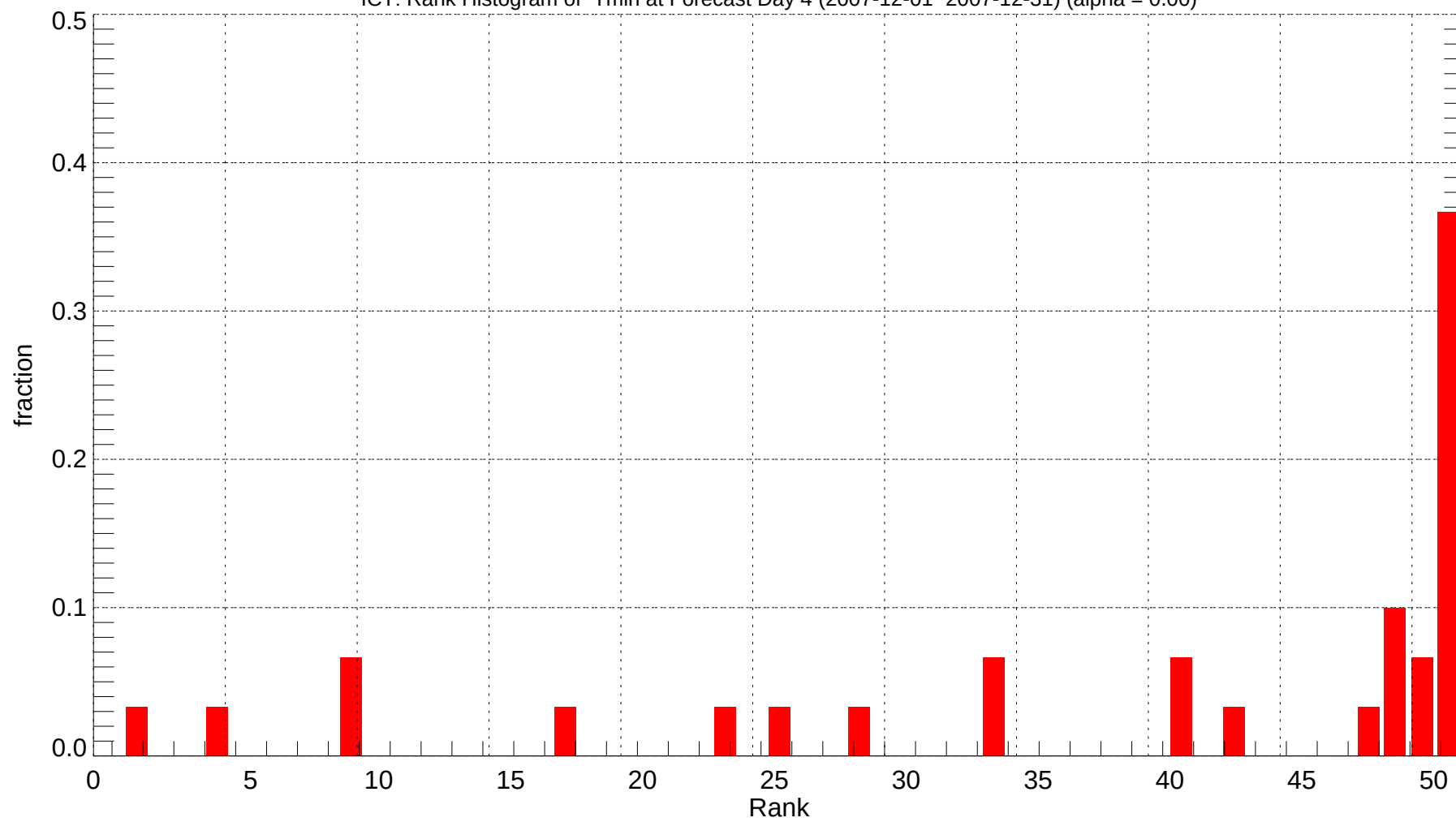
ICT: Rank Histogram of Tmin at Forecast Day 4 (2007-12-01~2007-12-31) (alpha = 0.00)
