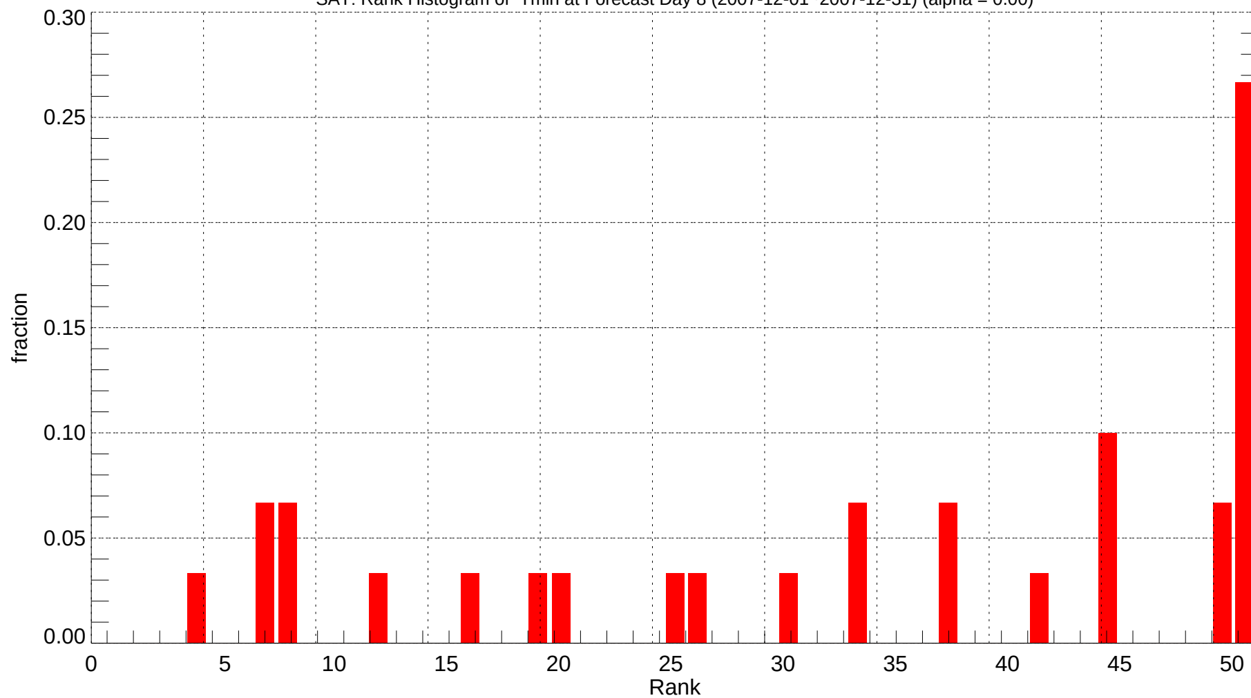
SAT: Rank Histogram of Tmin at Forecast Day 8 (2007-12-01~2007-12-31) (alpha = 0.00)
