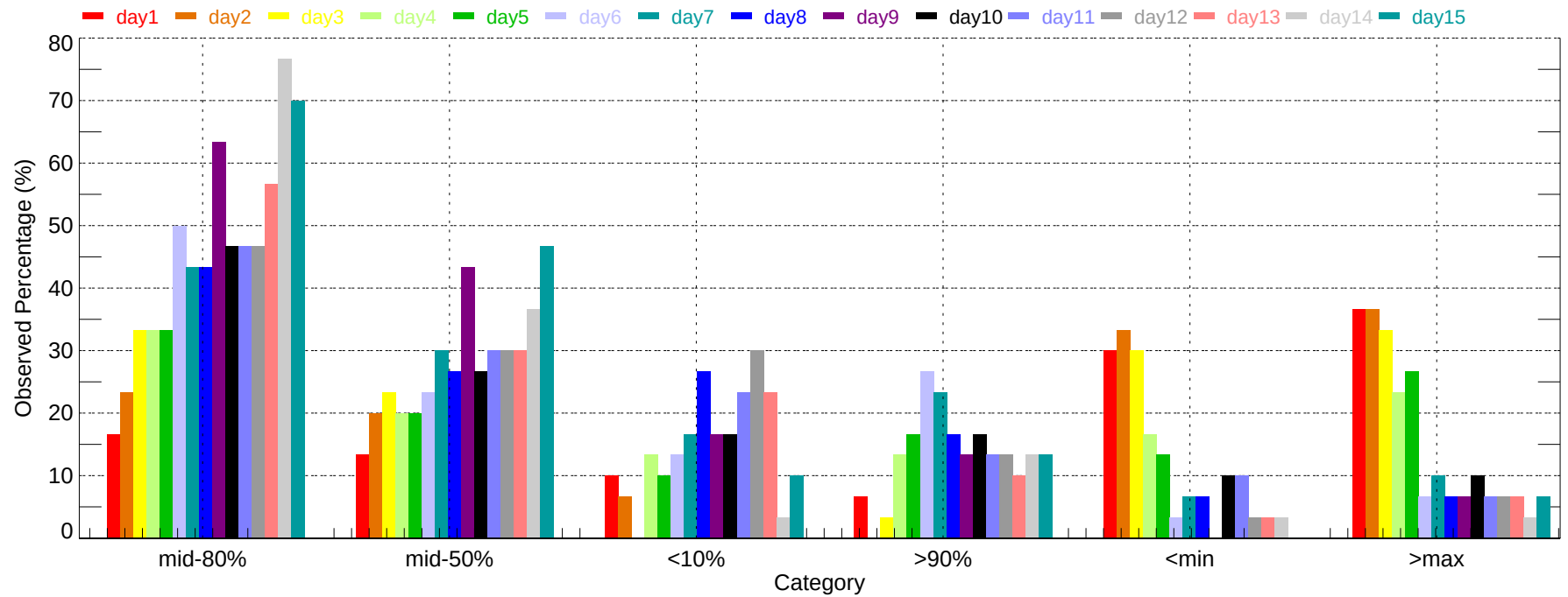
Observed Percentage of Ensembles - YKM: Min Temperature (2007-12-01~2007-12-31)
