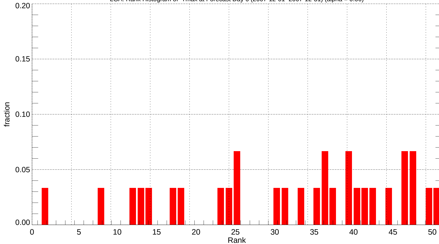
LGA: Rank Histogram of Tmax at Forecast Day 6 (2007-12-01~2007-12-31) (alpha = 0.00)
