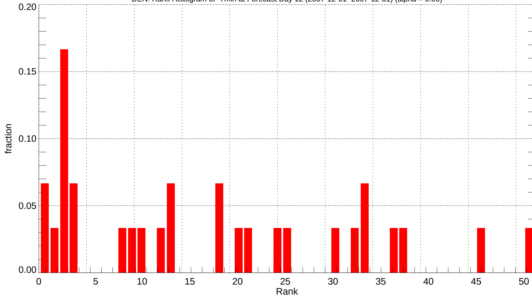
DEN: Rank Histogram of Tmin at Forecast Day 12 (2007-12-01~2007-12-31) (alpha = 0.00)
