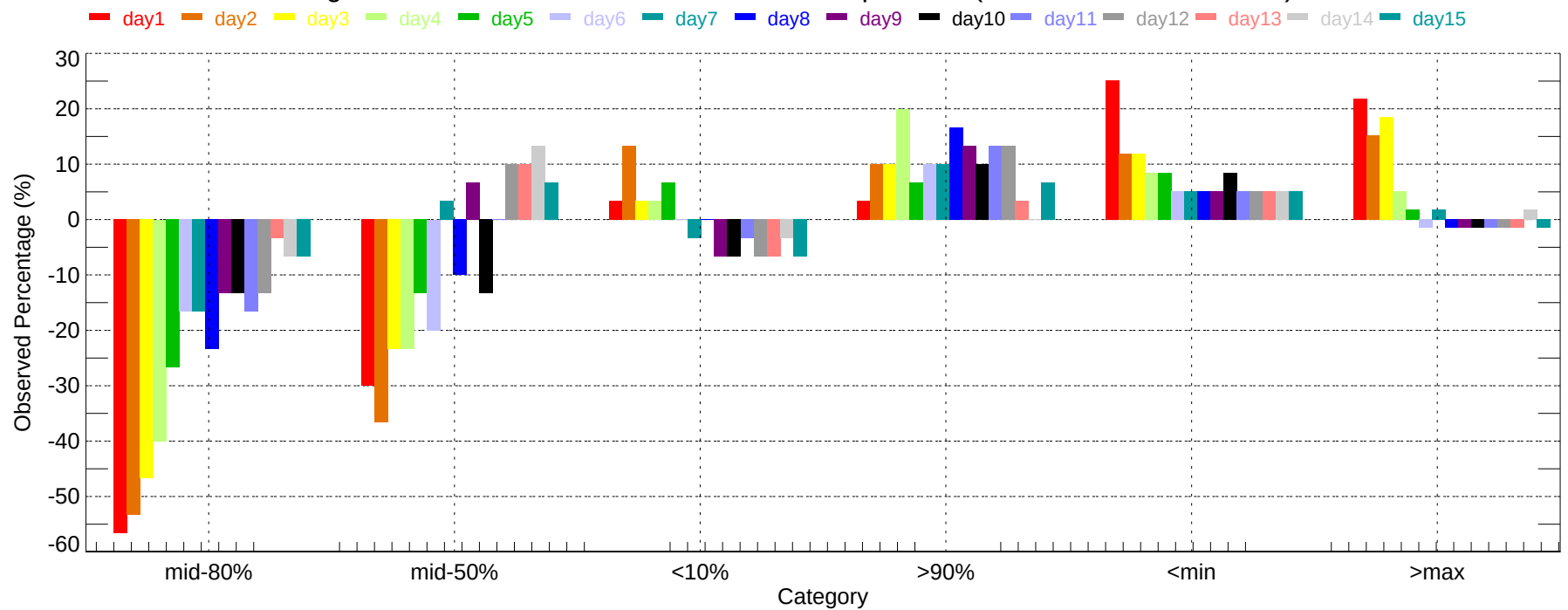
Observed Percentage Deviation of Ensembles - RBL: Min Temperature (2007-12-01~2007-12-31)
