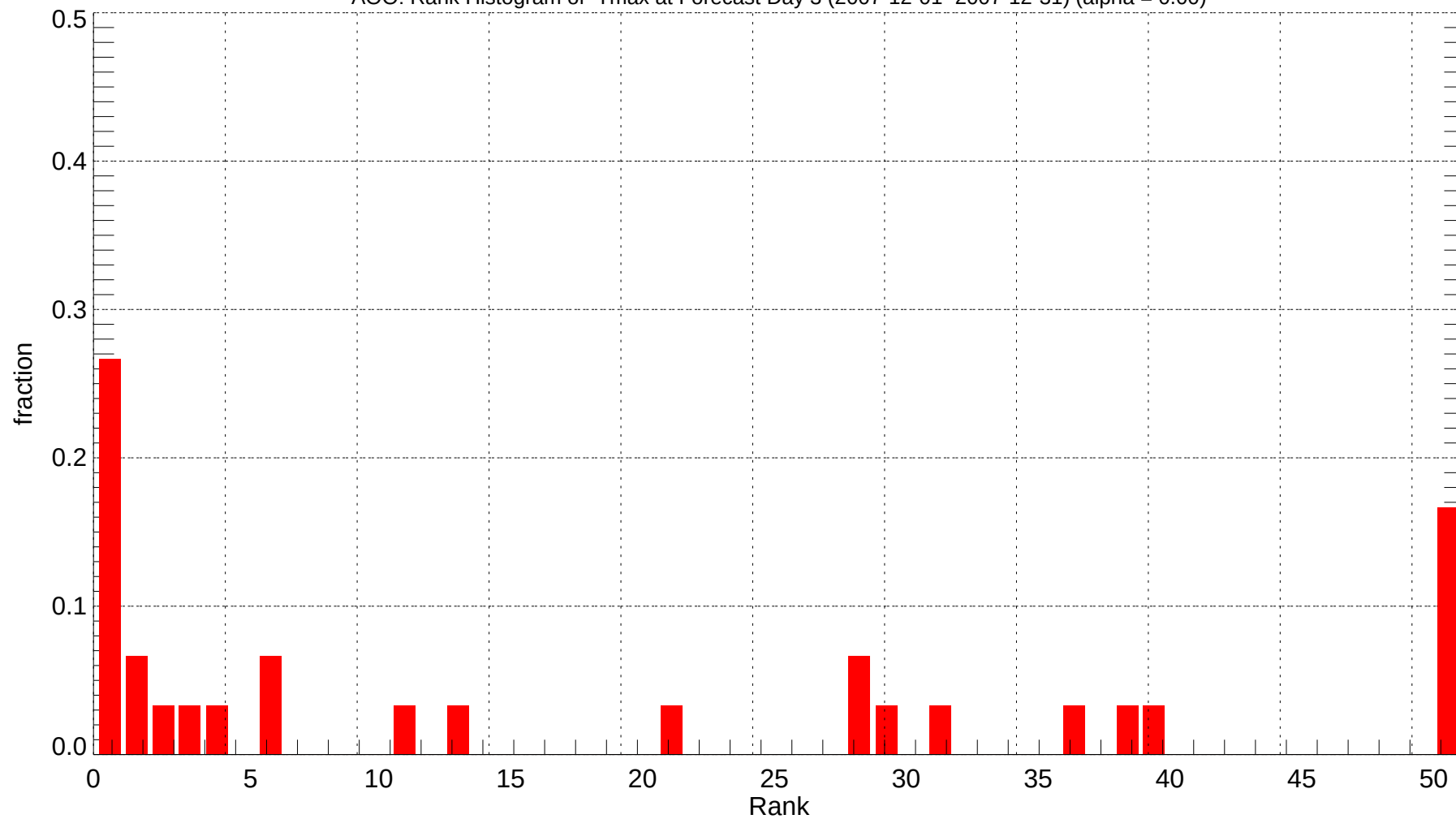
AOO: Rank Histogram of Tmax at Forecast Day 3 (2007-12-01~2007-12-31) (alpha = 0.00)
