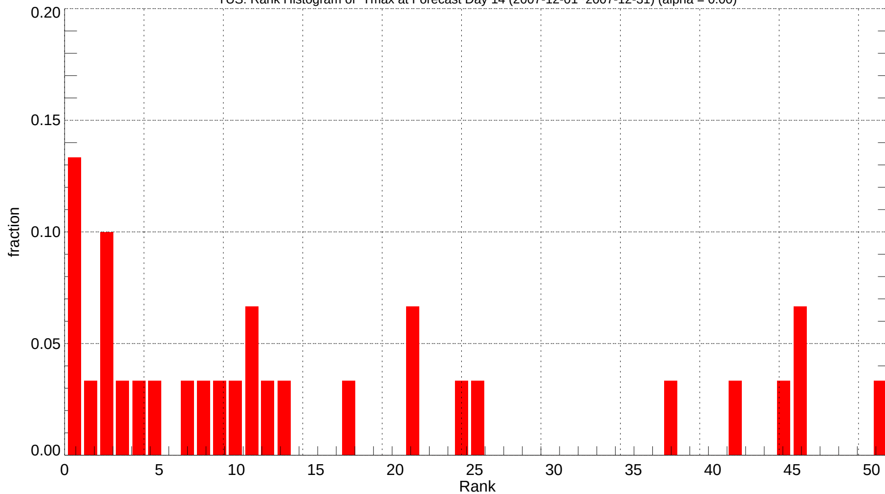
TUS: Rank Histogram of Tmax at Forecast Day 14 (2007-12-01~2007-12-31) (alpha = 0.00)
