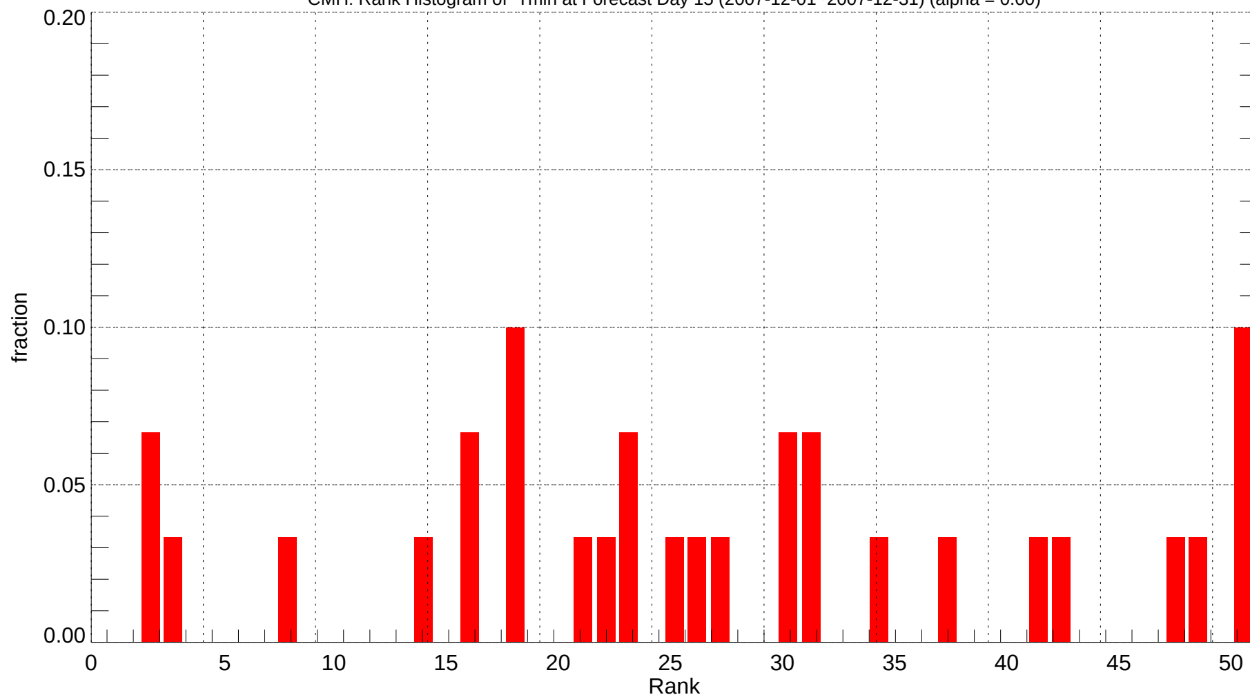
CMH: Rank Histogram of Tmin at Forecast Day 15 (2007-12-01~2007-12-31) (alpha = 0.00)
