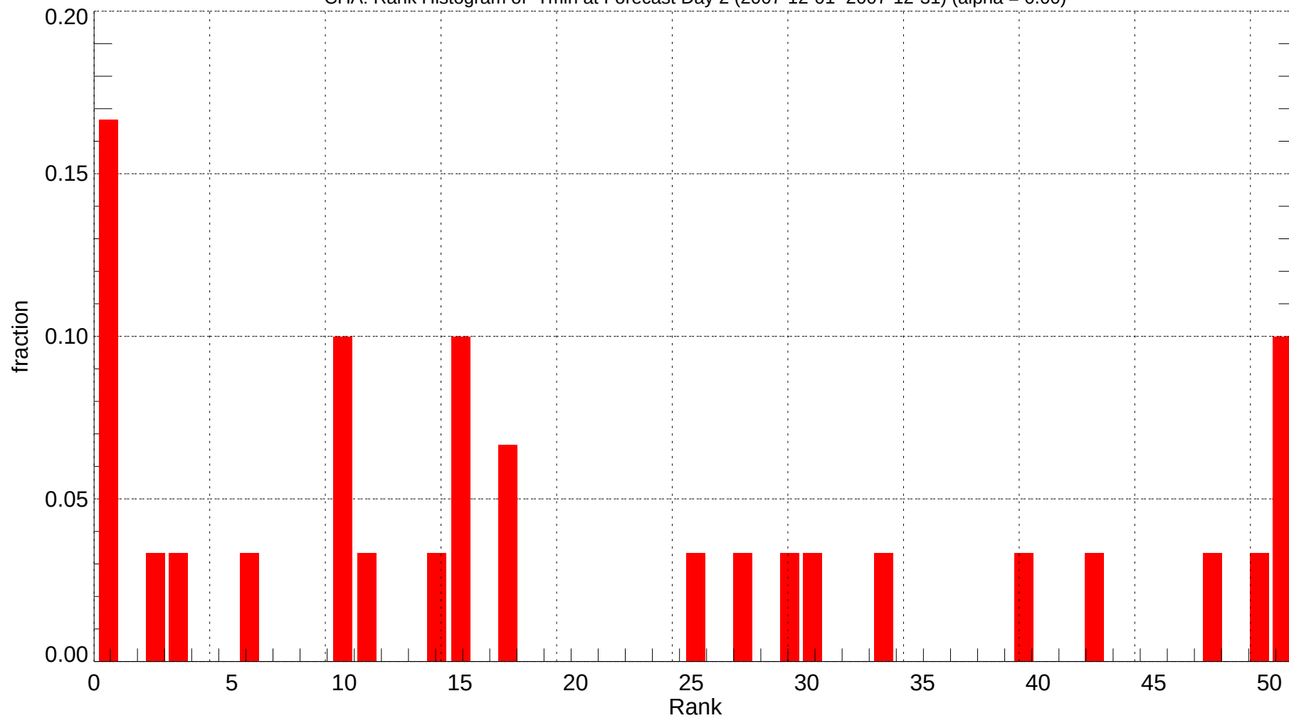
CHA: Rank Histogram of Tmin at Forecast Day 2 (2007-12-01~2007-12-31) (alpha = 0.00)
