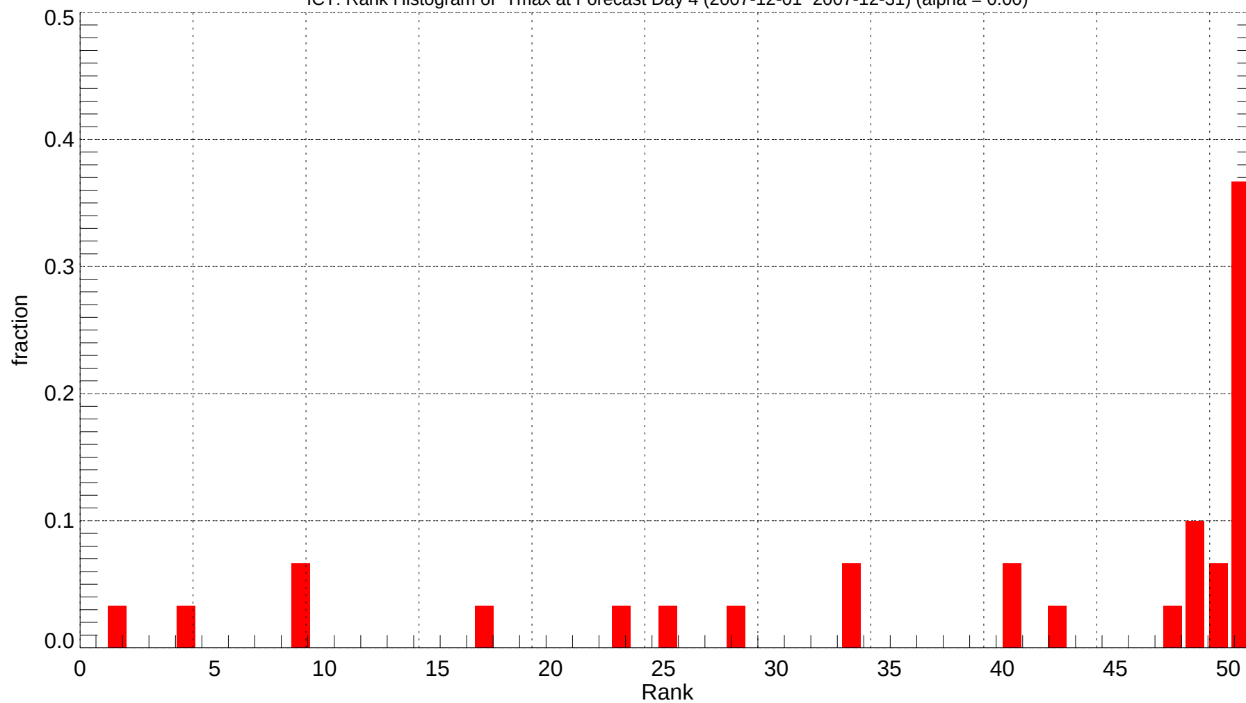
ICT: Rank Histogram of Tmax at Forecast Day 4 (2007-12-01~2007-12-31) (alpha = 0.00)
