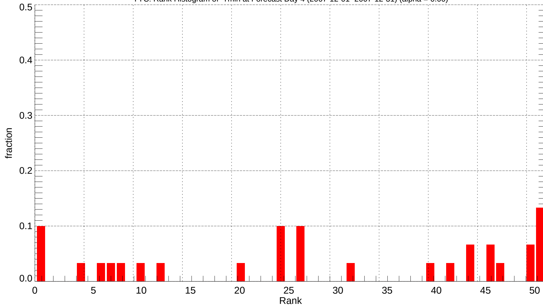
YYC: Rank Histogram of Tmin at Forecast Day 4 (2007-12-01~2007-12-31) (alpha = 0.00)
