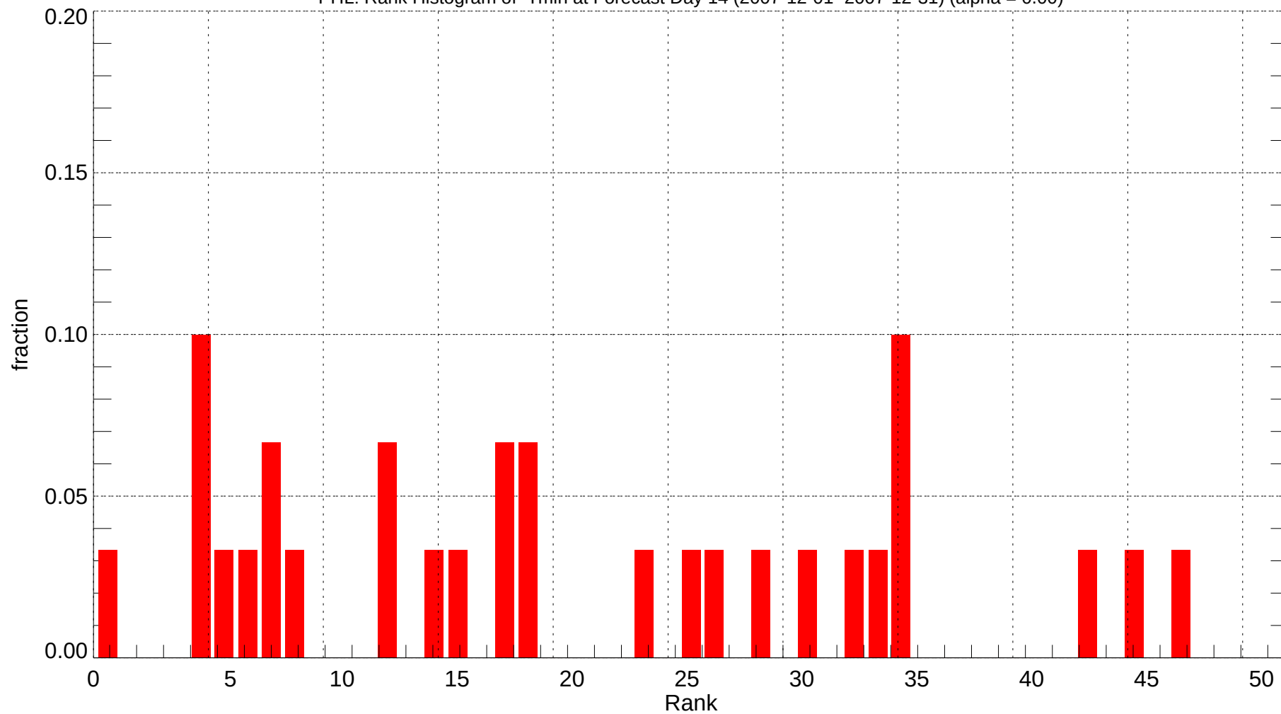
PHL: Rank Histogram of Tmin at Forecast Day 14 (2007-12-01~2007-12-31) (alpha = 0.00)
