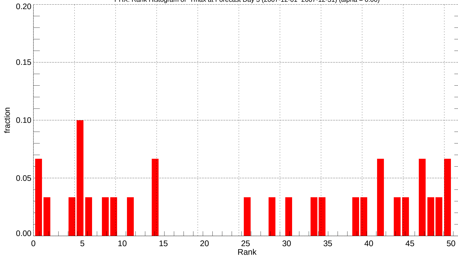
PHX: Rank Histogram of Tmax at Forecast Day 3 (2007-12-01~2007-12-31) (alpha = 0.00)
