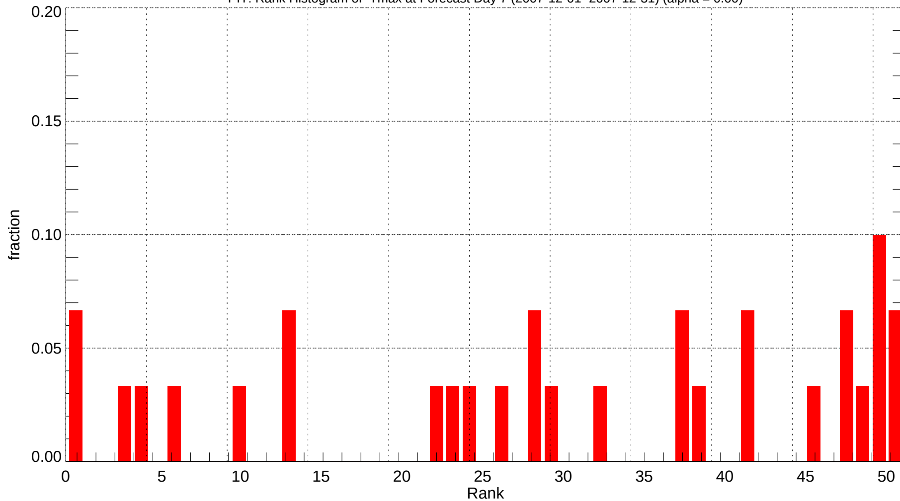
PIT: Rank Histogram of Tmax at Forecast Day 7 (2007-12-01~2007-12-31) (alpha = 0.00)
