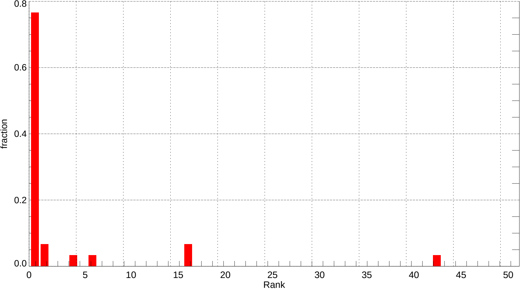
SJC: Rank Histogram of Tmin at Forecast Day 7 (2007-12-01~2007-12-31) (alpha = 0.00)
