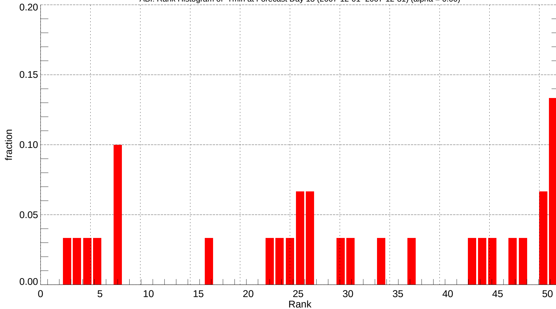
ABI: Rank Histogram of Tmin at Forecast Day 13 (2007-12-01~2007-12-31) (alpha = 0.00)
