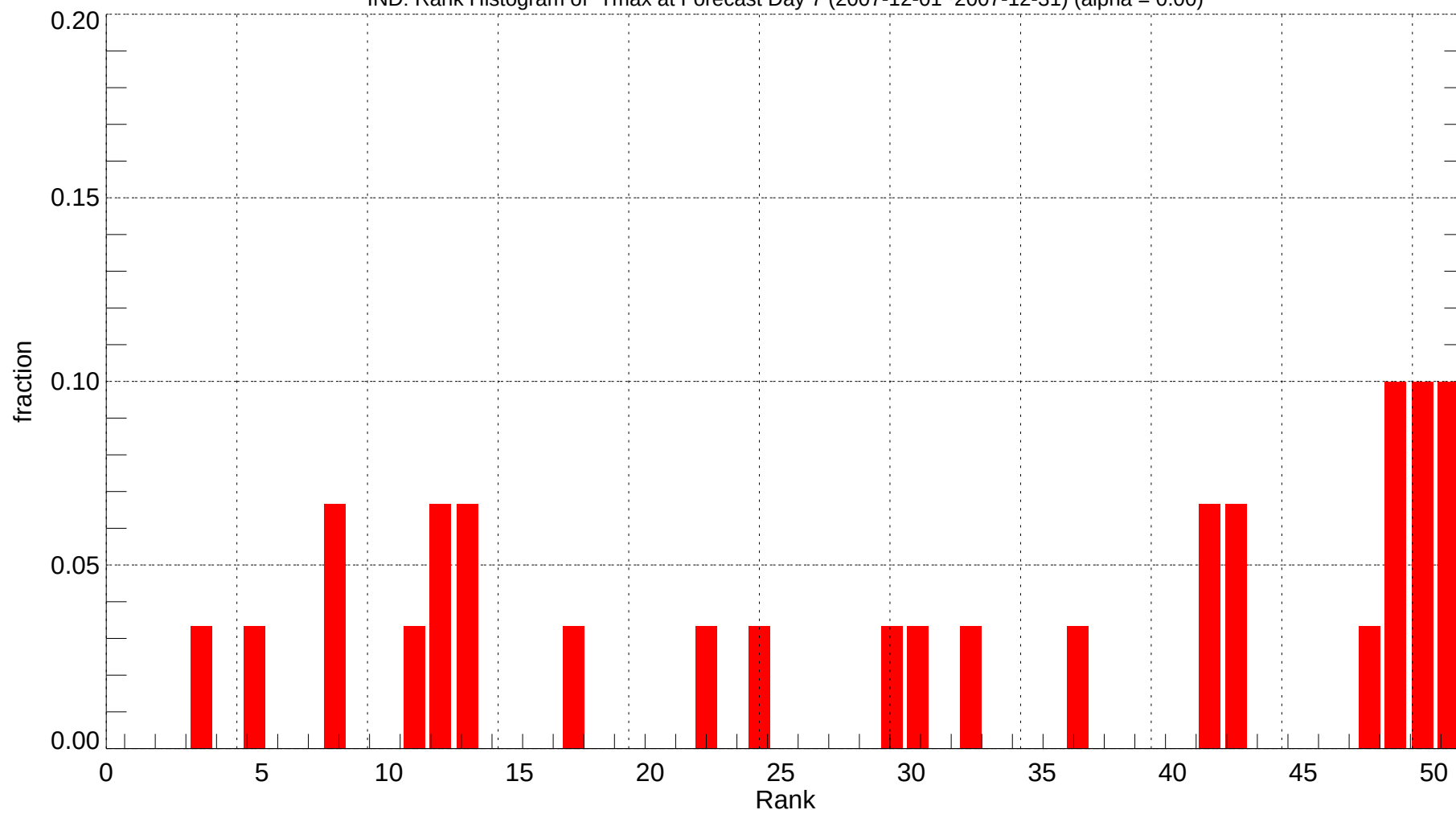
IND: Rank Histogram of Tmax at Forecast Day 7 (2007-12-01~2007-12-31) (alpha = 0.00)
