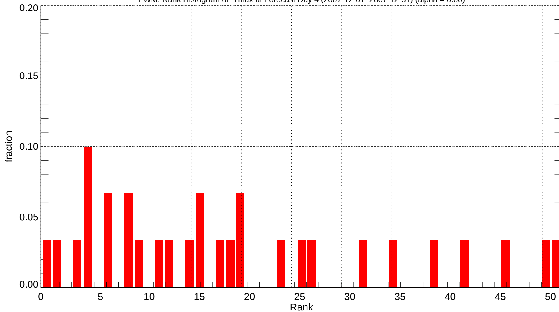
PWM: Rank Histogram of Tmax at Forecast Day 4 (2007-12-01~2007-12-31) (alpha = 0.00)
