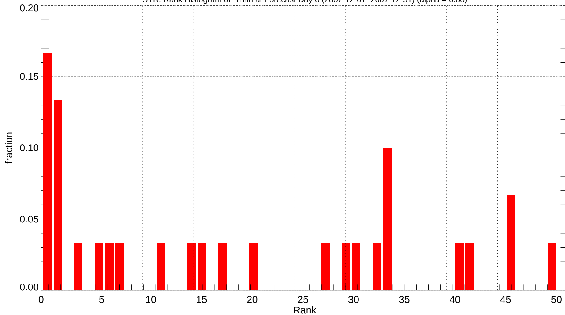
SYR: Rank Histogram of Tmin at Forecast Day 6 (2007-12-01~2007-12-31) (alpha = 0.00)
