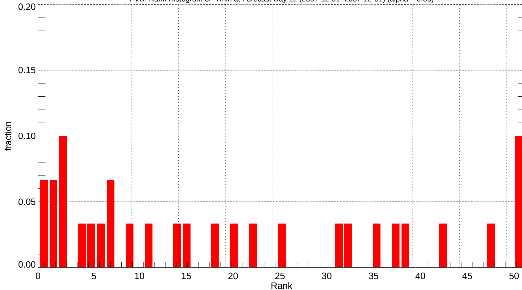
PVD: Rank Histogram of Tmin at Forecast Day 12 (2007-12-01~2007-12-31) (alpha = 0.00)
