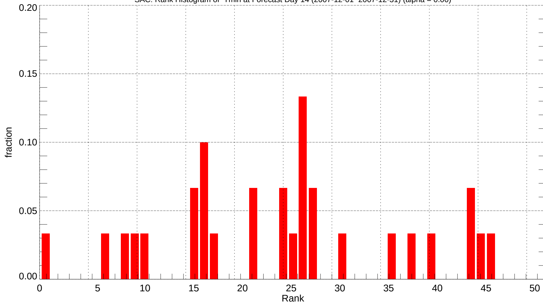
SAC: Rank Histogram of Tmin at Forecast Day 14 (2007-12-01~2007-12-31) (alpha = 0.00)
