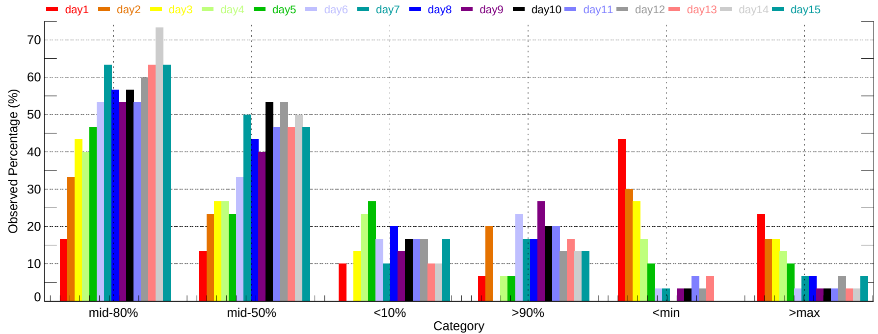
Observed Percentage of Ensembles - AOO: Min Temperature (2007-12-01~2007-12-31)
