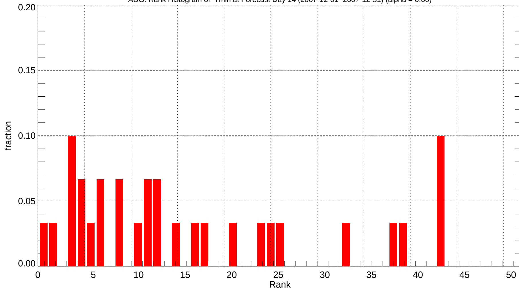
AUG: Rank Histogram of Tmin at Forecast Day 14 (2007-12-01~2007-12-31) (alpha = 0.00)
