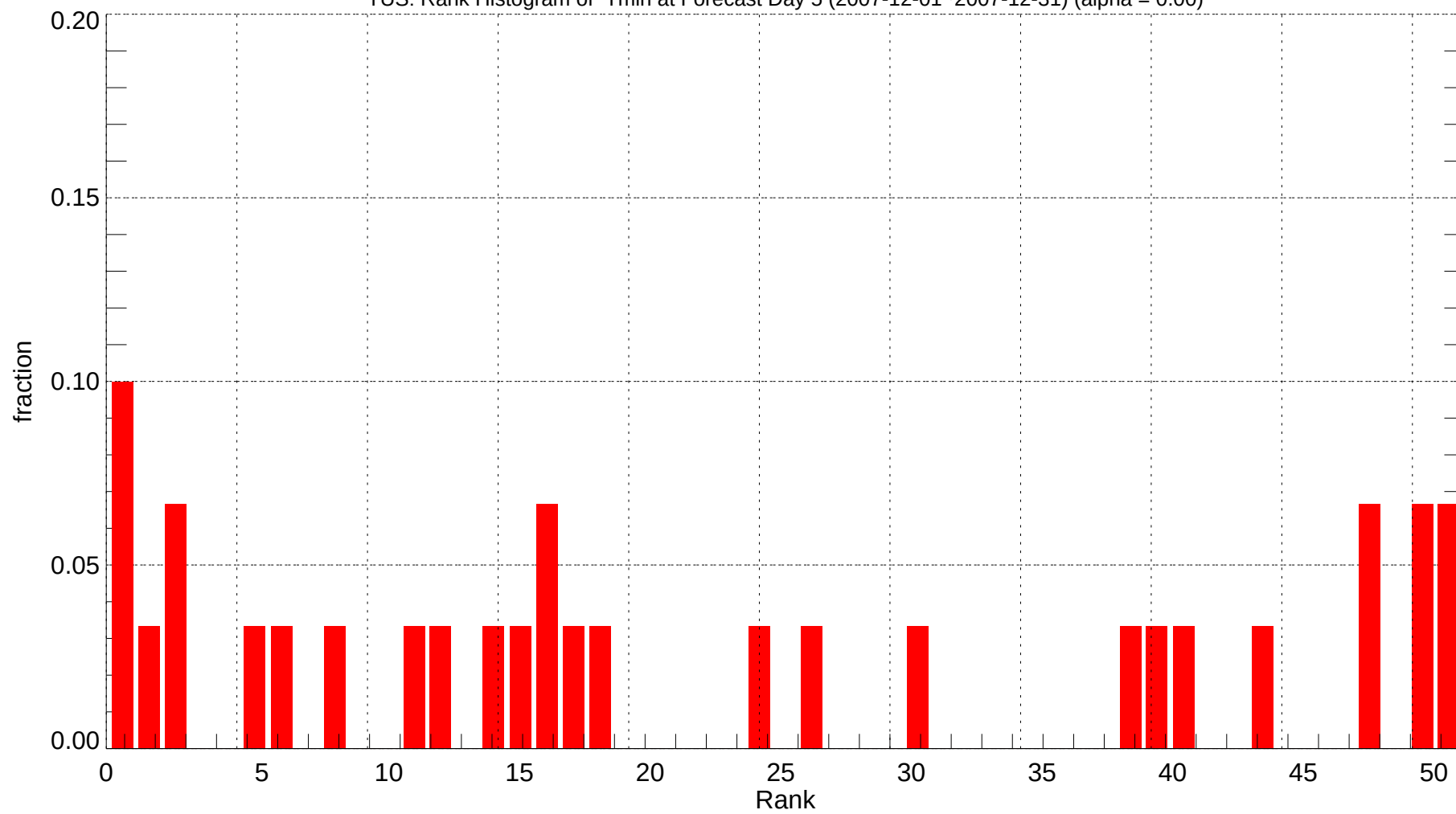
TUS: Rank Histogram of Tmin at Forecast Day 5 (2007-12-01~2007-12-31) (alpha = 0.00)
