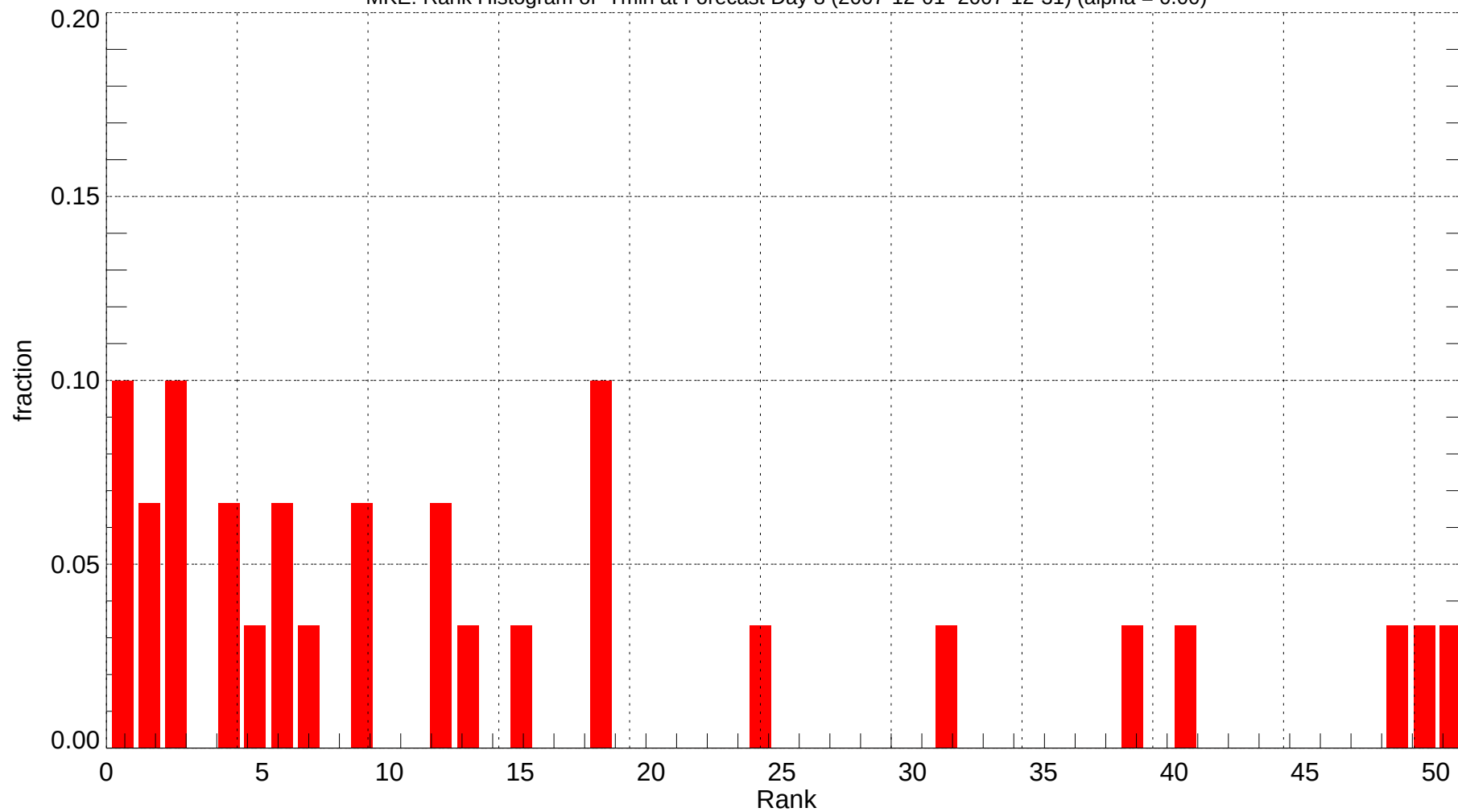
MKE: Rank Histogram of Tmin at Forecast Day 8 (2007-12-01~2007-12-31) (alpha = 0.00)
