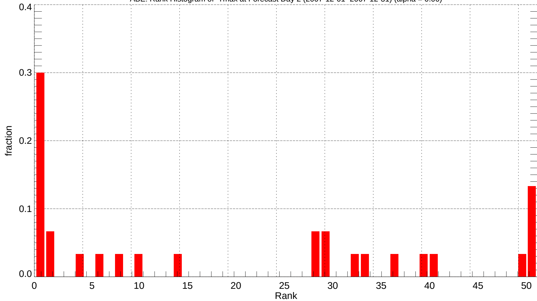
ABE: Rank Histogram of Tmax at Forecast Day 2 (2007-12-01~2007-12-31) (alpha = 0.00)
