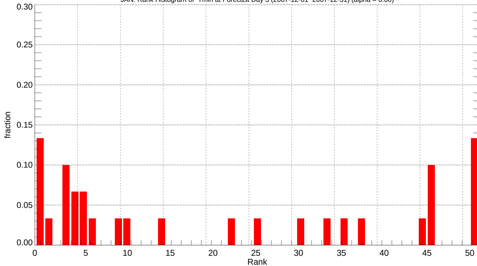
JAN: Rank Histogram of Tmin at Forecast Day 3 (2007-12-01~2007-12-31) (alpha = 0.00)
