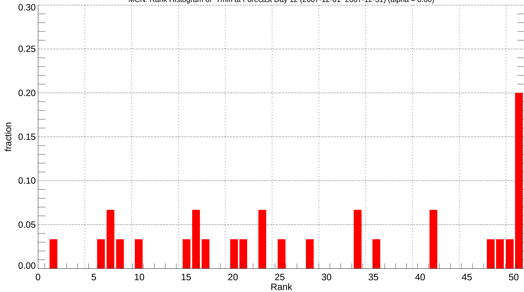
MCN: Rank Histogram of Tmin at Forecast Day 12 (2007-12-01~2007-12-31) (alpha = 0.00)
