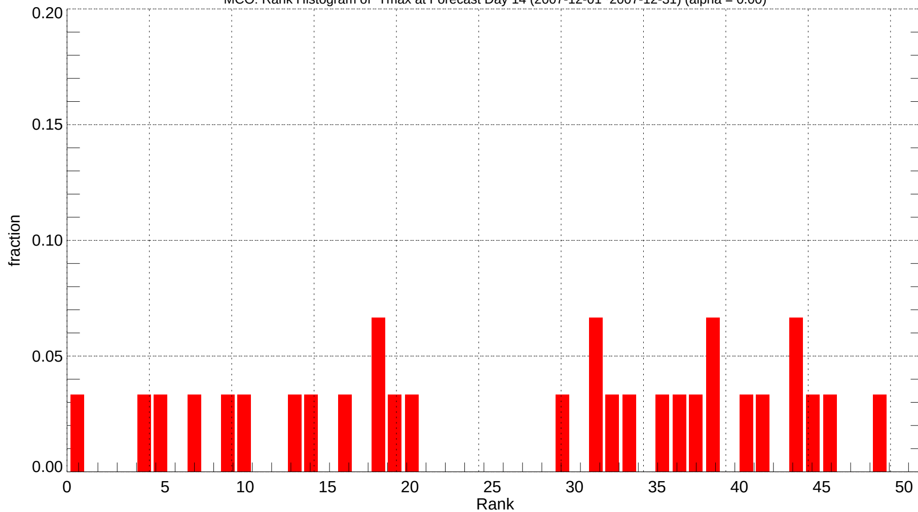
MCO: Rank Histogram of Tmax at Forecast Day 14 (2007-12-01~2007-12-31) (alpha = 0.00)
