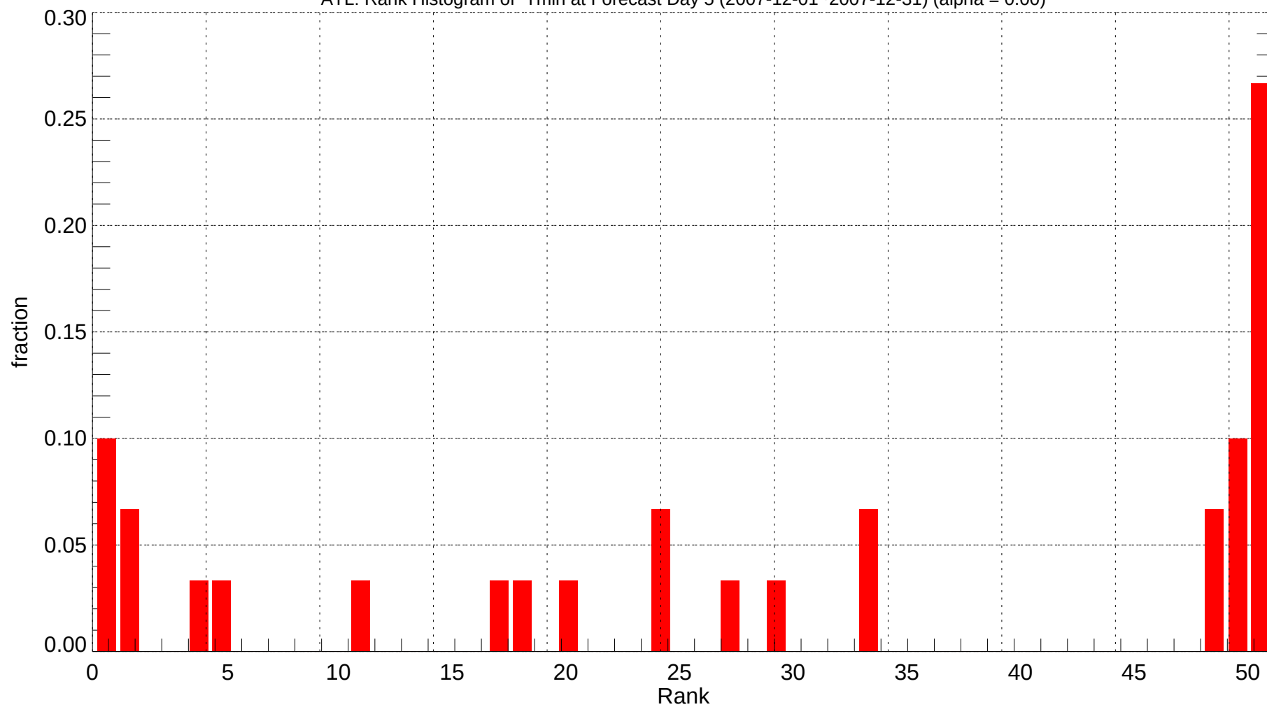
ATL: Rank Histogram of Tmin at Forecast Day 5 (2007-12-01~2007-12-31) (alpha = 0.00)
