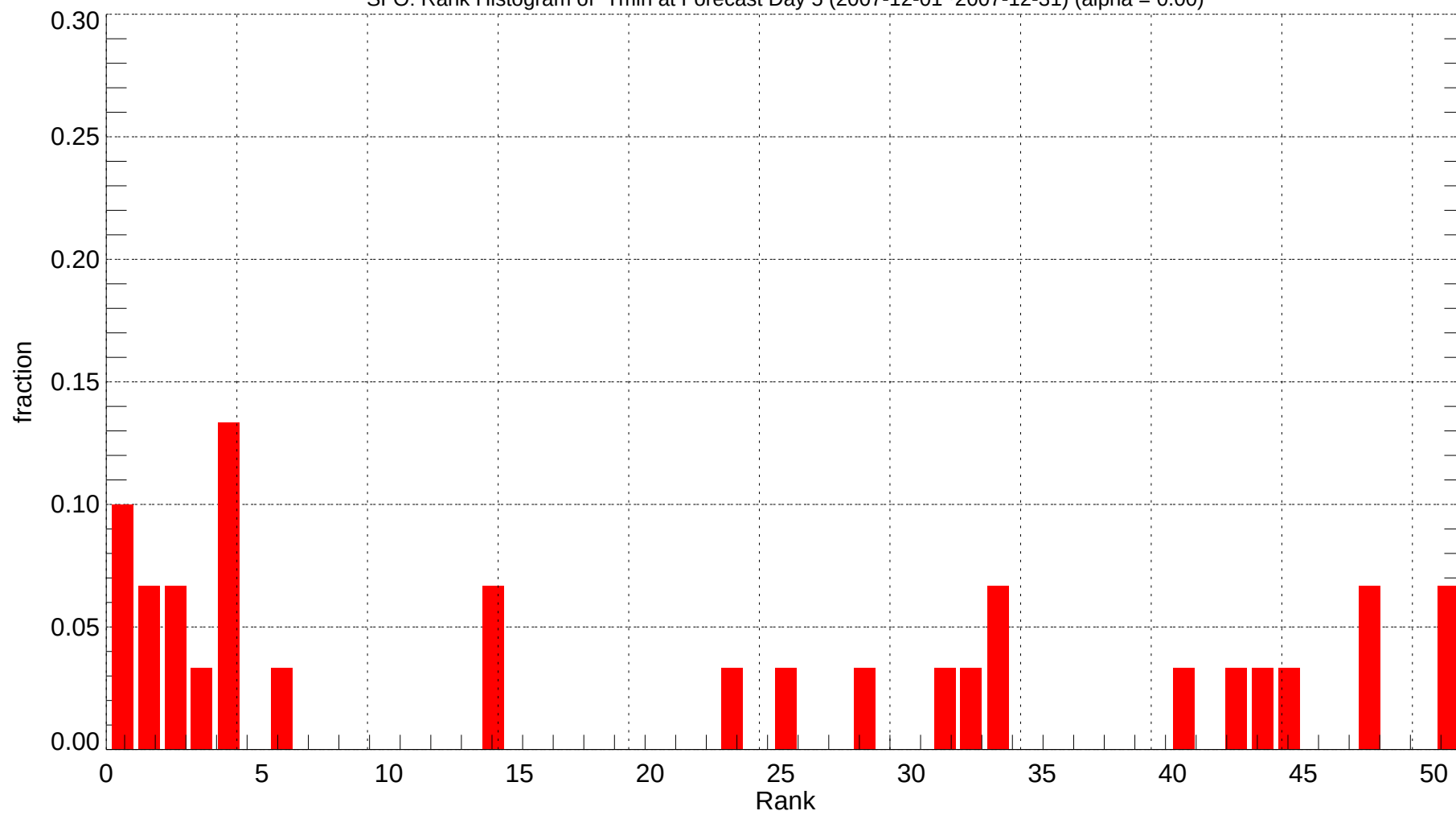
SFO: Rank Histogram of Tmin at Forecast Day 5 (2007-12-01~2007-12-31) (alpha = 0.00)
