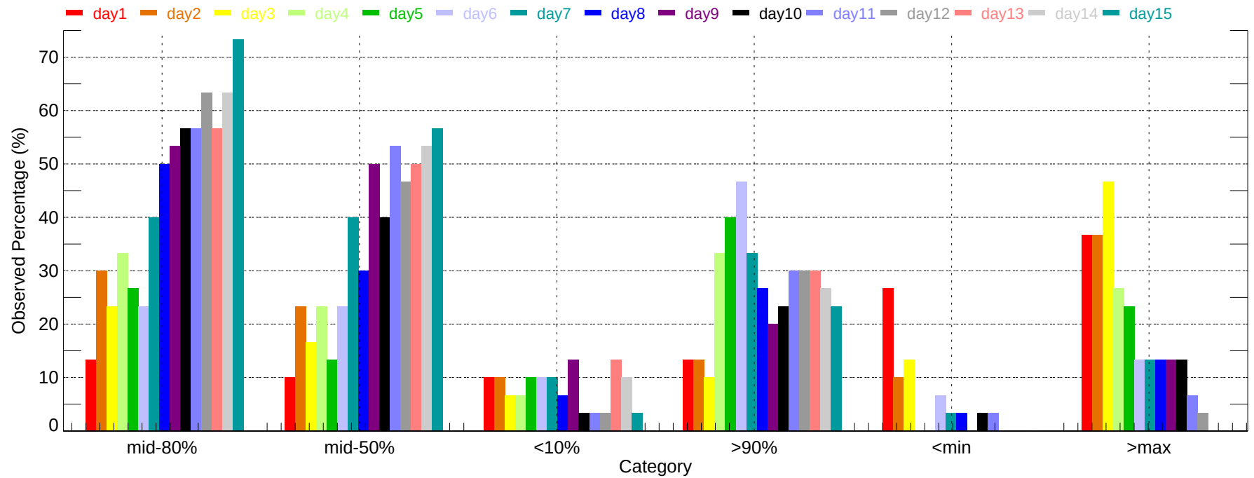
Observed Percentage of Ensembles - GTF: Min Temperature (2007-12-01~2007-12-31)
