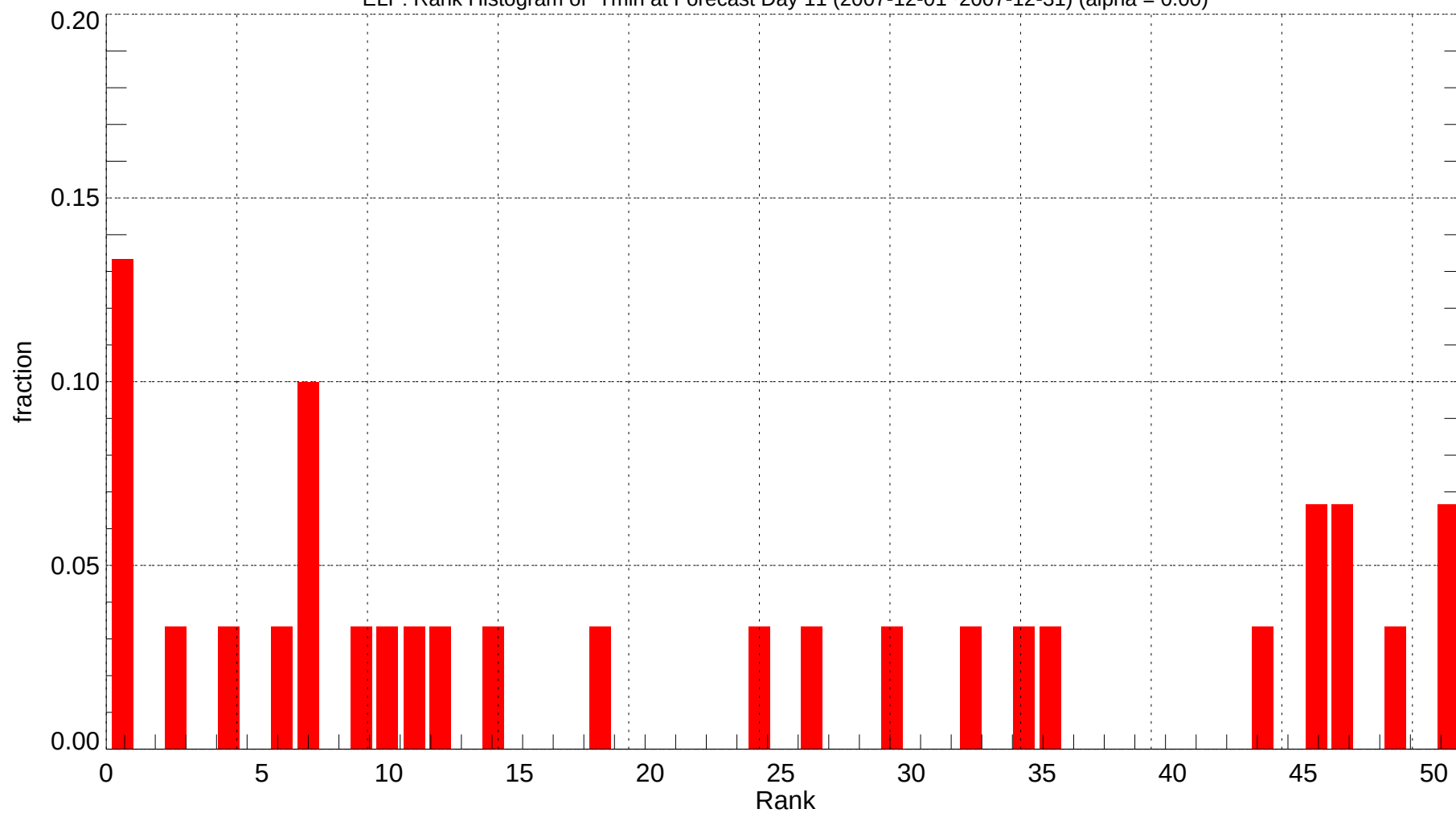
ELP: Rank Histogram of Tmin at Forecast Day 11 (2007-12-01~2007-12-31) (alpha = 0.00)
