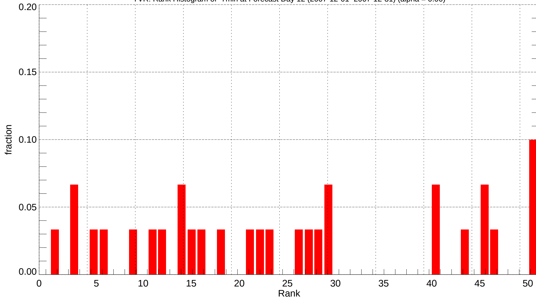
YVR: Rank Histogram of Tmin at Forecast Day 12 (2007-12-01~2007-12-31) (alpha = 0.00)
