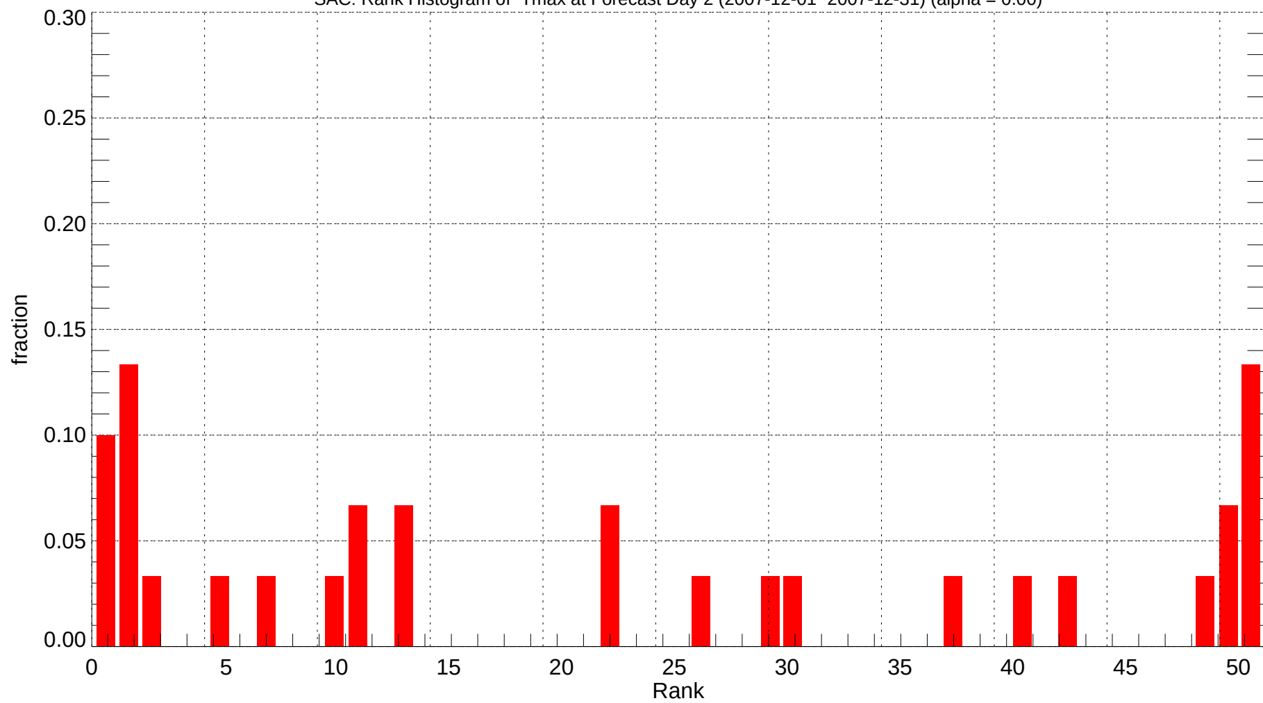
SAC: Rank Histogram of Tmax at Forecast Day 2 (2007-12-01~2007-12-31) (alpha = 0.00)
