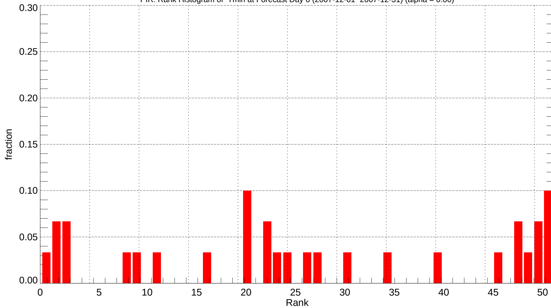
PIR: Rank Histogram of Tmin at Forecast Day 6 (2007-12-01~2007-12-31) (alpha = 0.00)
