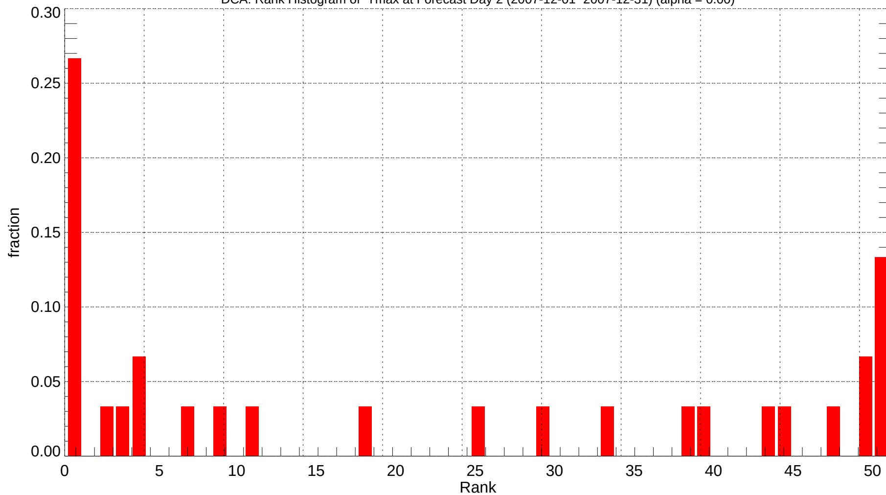
DCA: Rank Histogram of Tmax at Forecast Day 2 (2007-12-01~2007-12-31) (alpha = 0.00)
