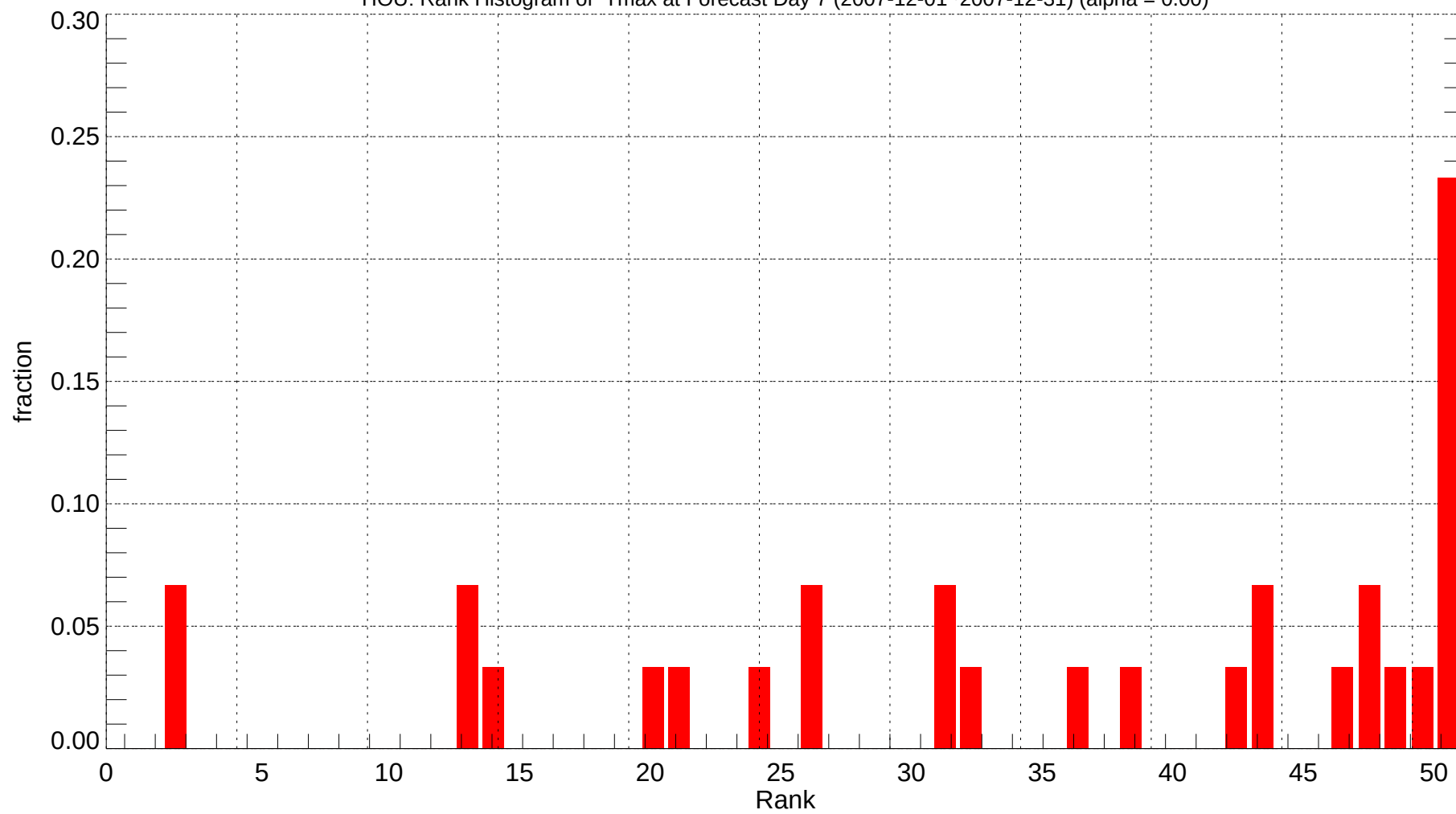
HOU: Rank Histogram of Tmax at Forecast Day 7 (2007-12-01~2007-12-31) (alpha = 0.00)
