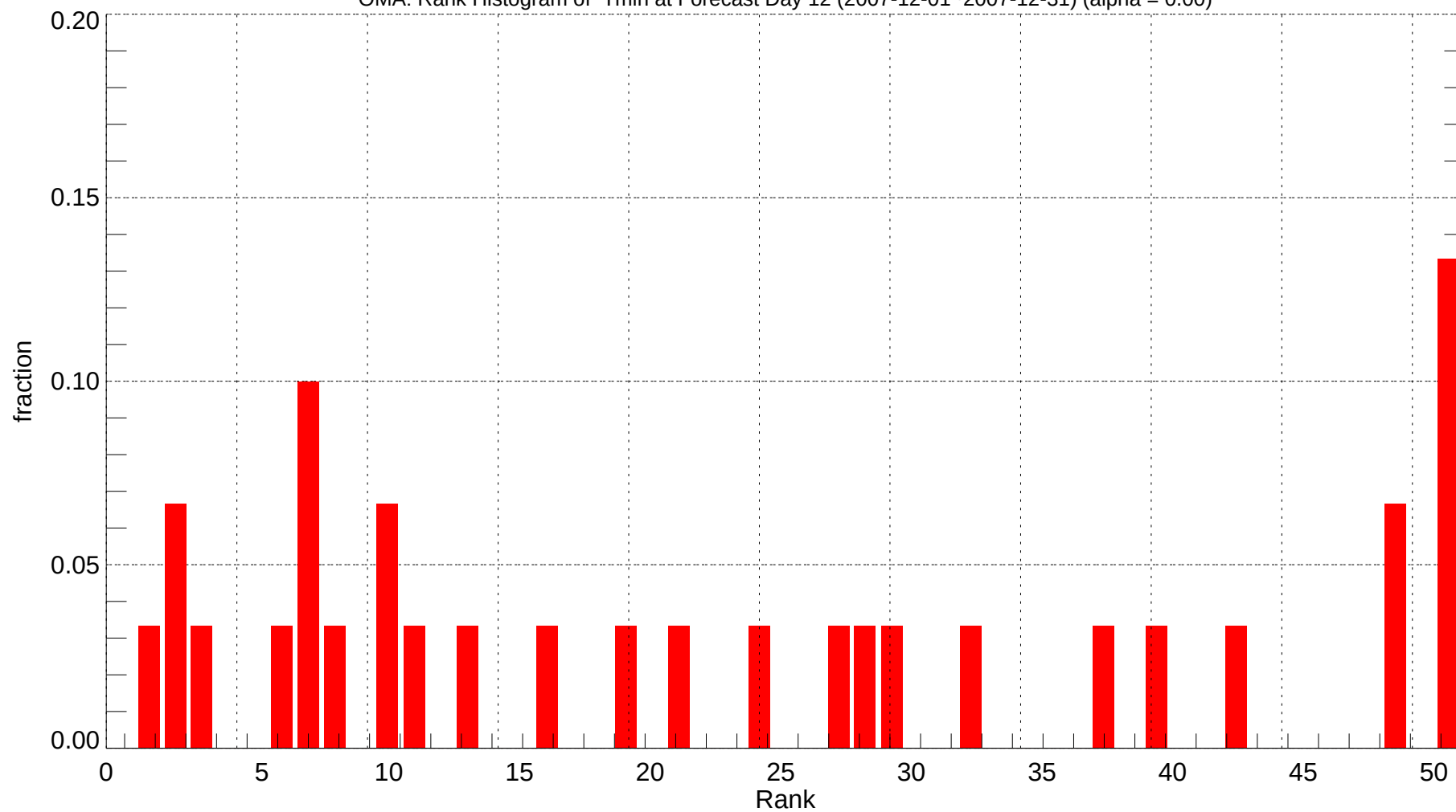
OMA: Rank Histogram of Tmin at Forecast Day 12 (2007-12-01~2007-12-31) (alpha = 0.00)
