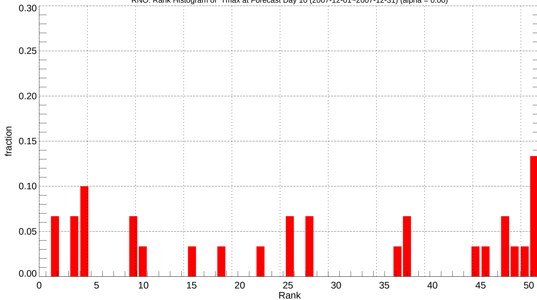
RNO: Rank Histogram of Tmax at Forecast Day 10 (2007-12-01~2007-12-31) (alpha = 0.00)
