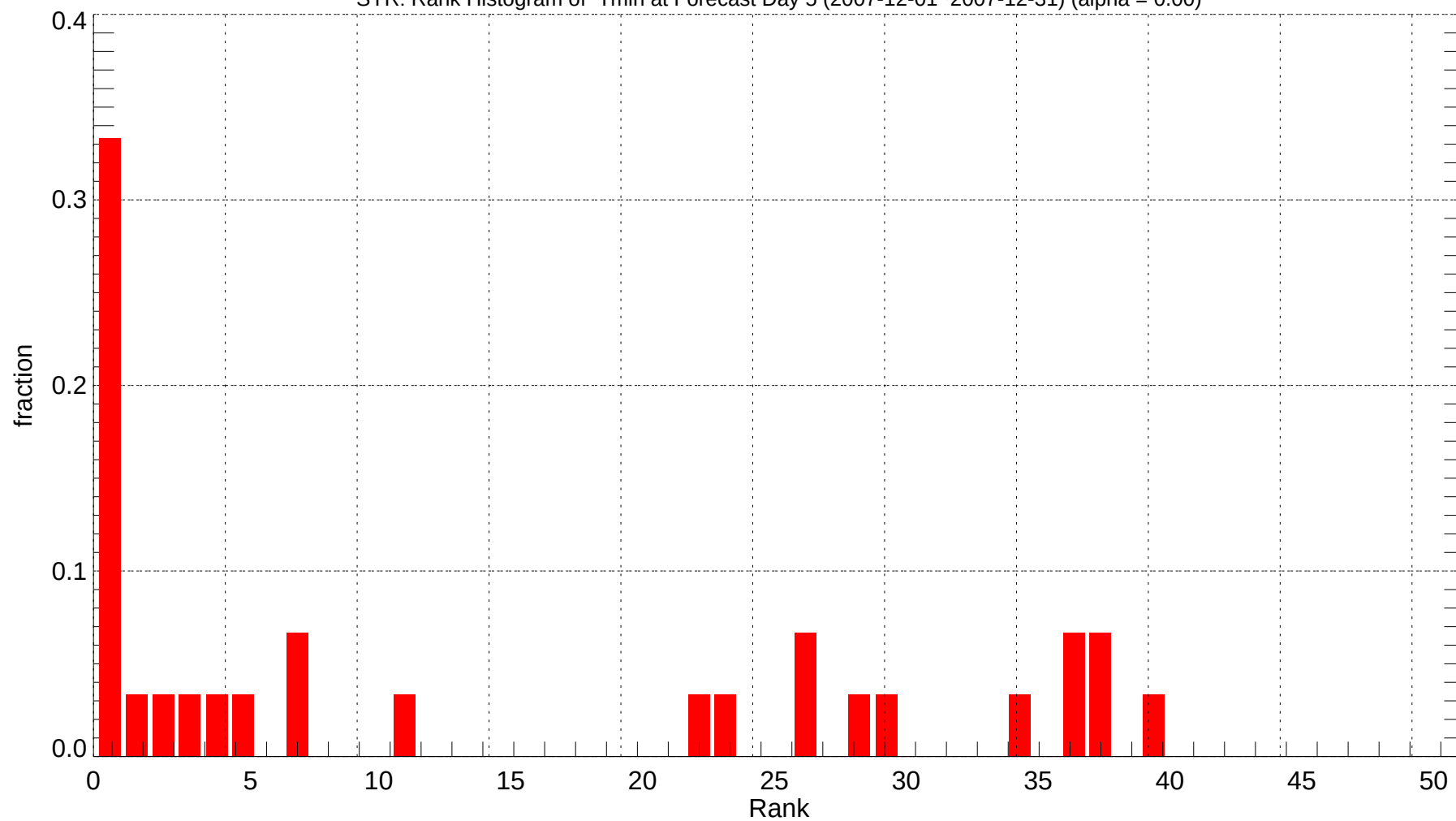
SYR: Rank Histogram of Tmin at Forecast Day 5 (2007-12-01~2007-12-31) (alpha = 0.00)
