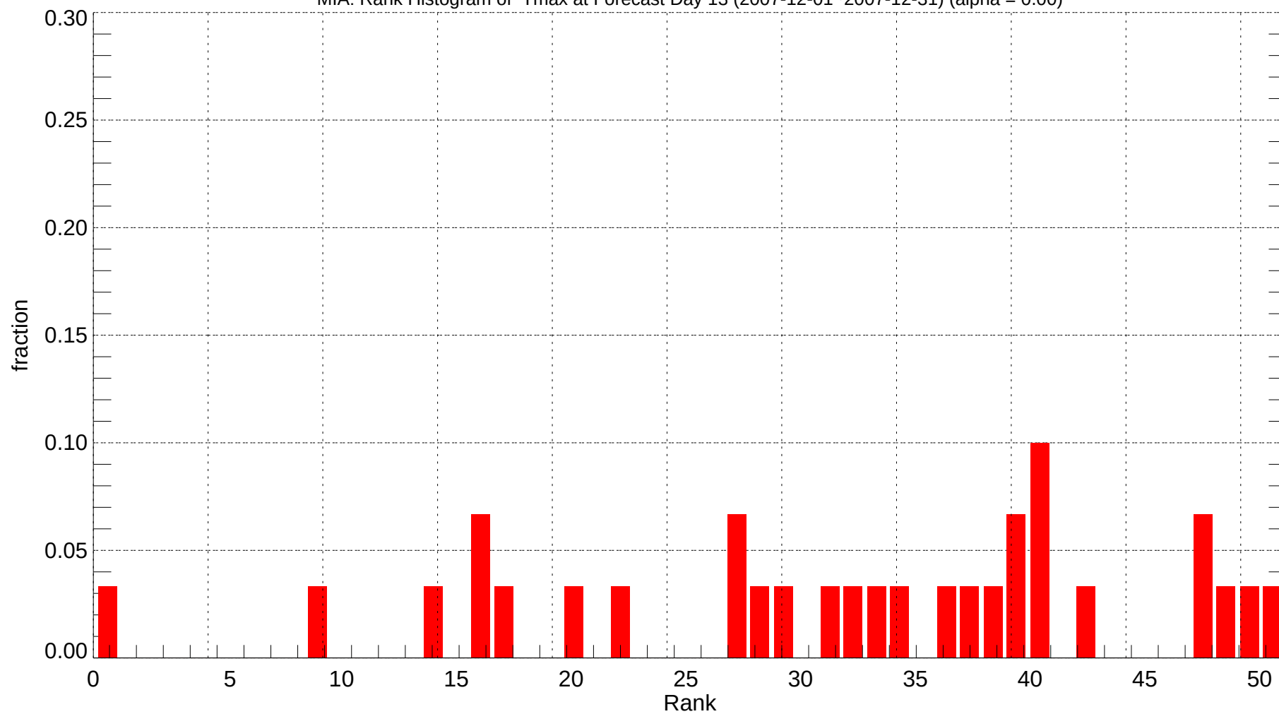
MIA: Rank Histogram of Tmax at Forecast Day 13 (2007-12-01~2007-12-31) (alpha = 0.00)
