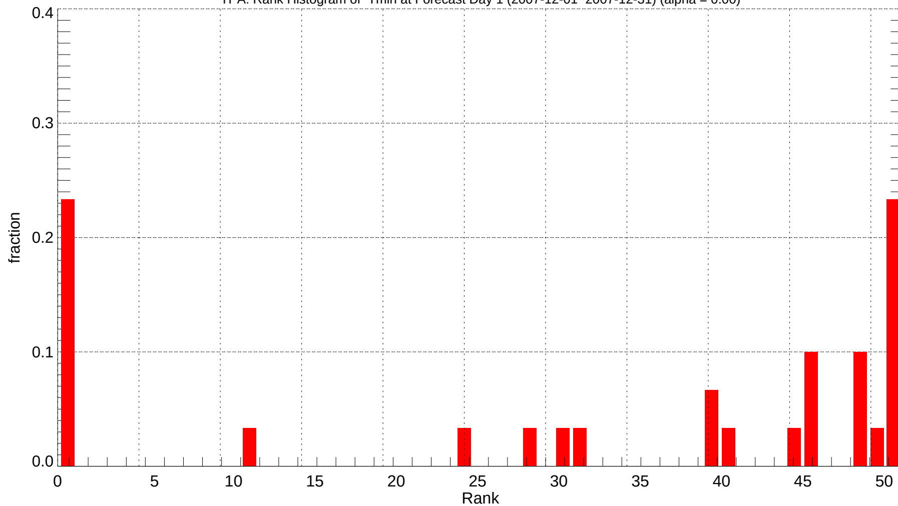
TPA: Rank Histogram of Tmin at Forecast Day 1 (2007-12-01~2007-12-31) (alpha = 0.00)
