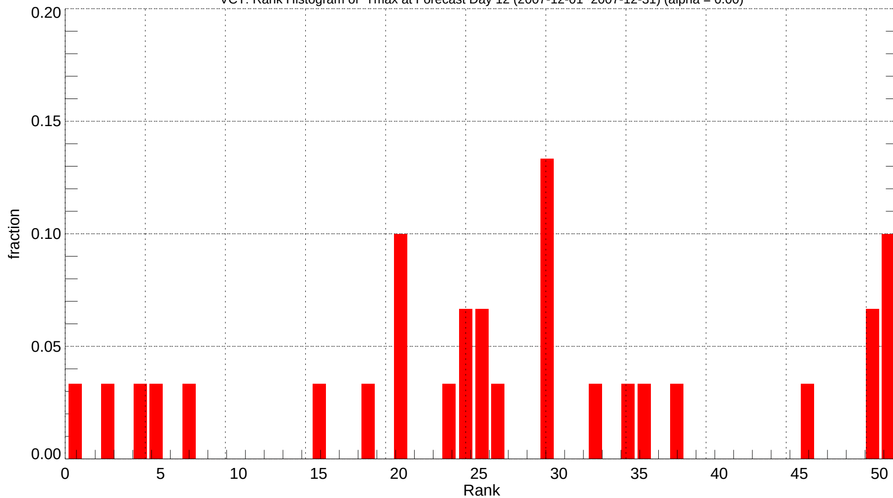
VCT: Rank Histogram of Tmax at Forecast Day 12 (2007-12-01~2007-12-31) (alpha = 0.00)
