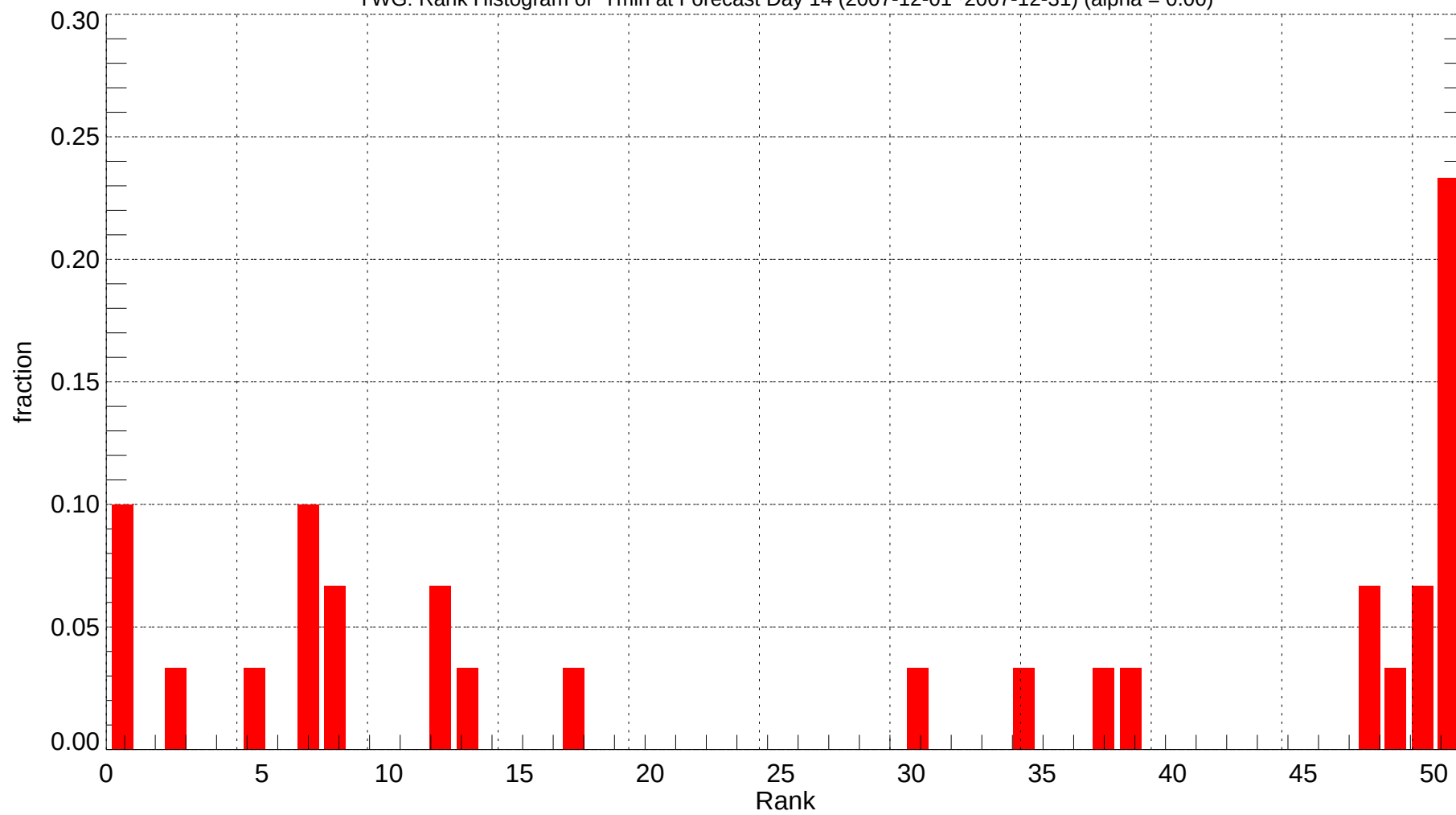
YWG: Rank Histogram of Tmin at Forecast Day 14 (2007-12-01~2007-12-31) (alpha = 0.00)
