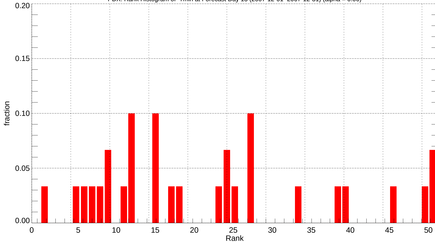
PDX: Rank Histogram of Tmin at Forecast Day 13 (2007-12-01~2007-12-31) (alpha = 0.00)
