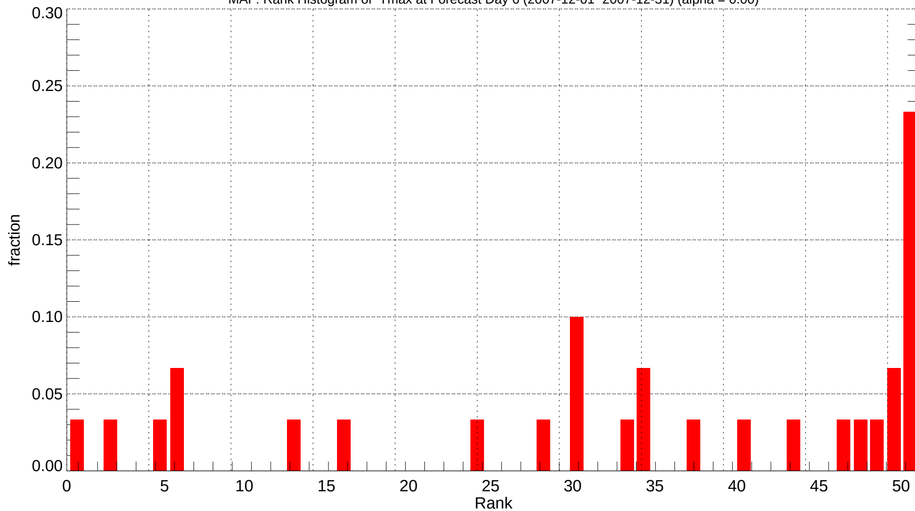
MAF: Rank Histogram of Tmax at Forecast Day 6 (2007-12-01~2007-12-31) (alpha = 0.00)
