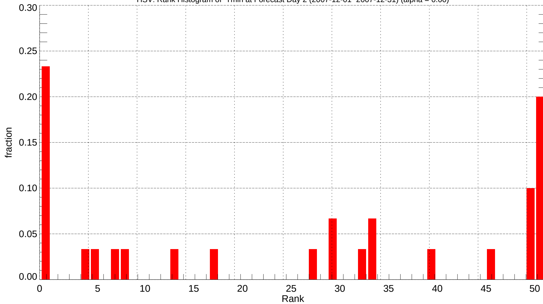
HSV: Rank Histogram of Tmin at Forecast Day 2 (2007-12-01~2007-12-31) (alpha = 0.00)
