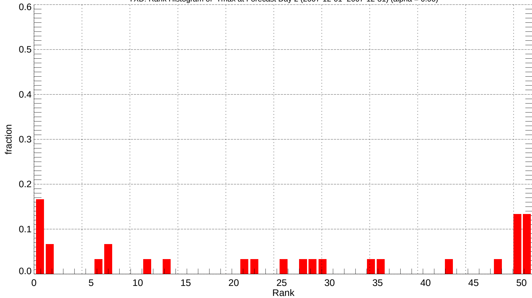
YXD: Rank Histogram of Tmax at Forecast Day 2 (2007-12-01~2007-12-31) (alpha = 0.00)
