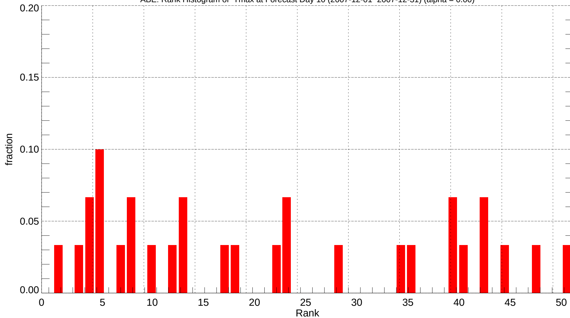
ABE: Rank Histogram of Tmax at Forecast Day 10 (2007-12-01~2007-12-31) (alpha = 0.00)
