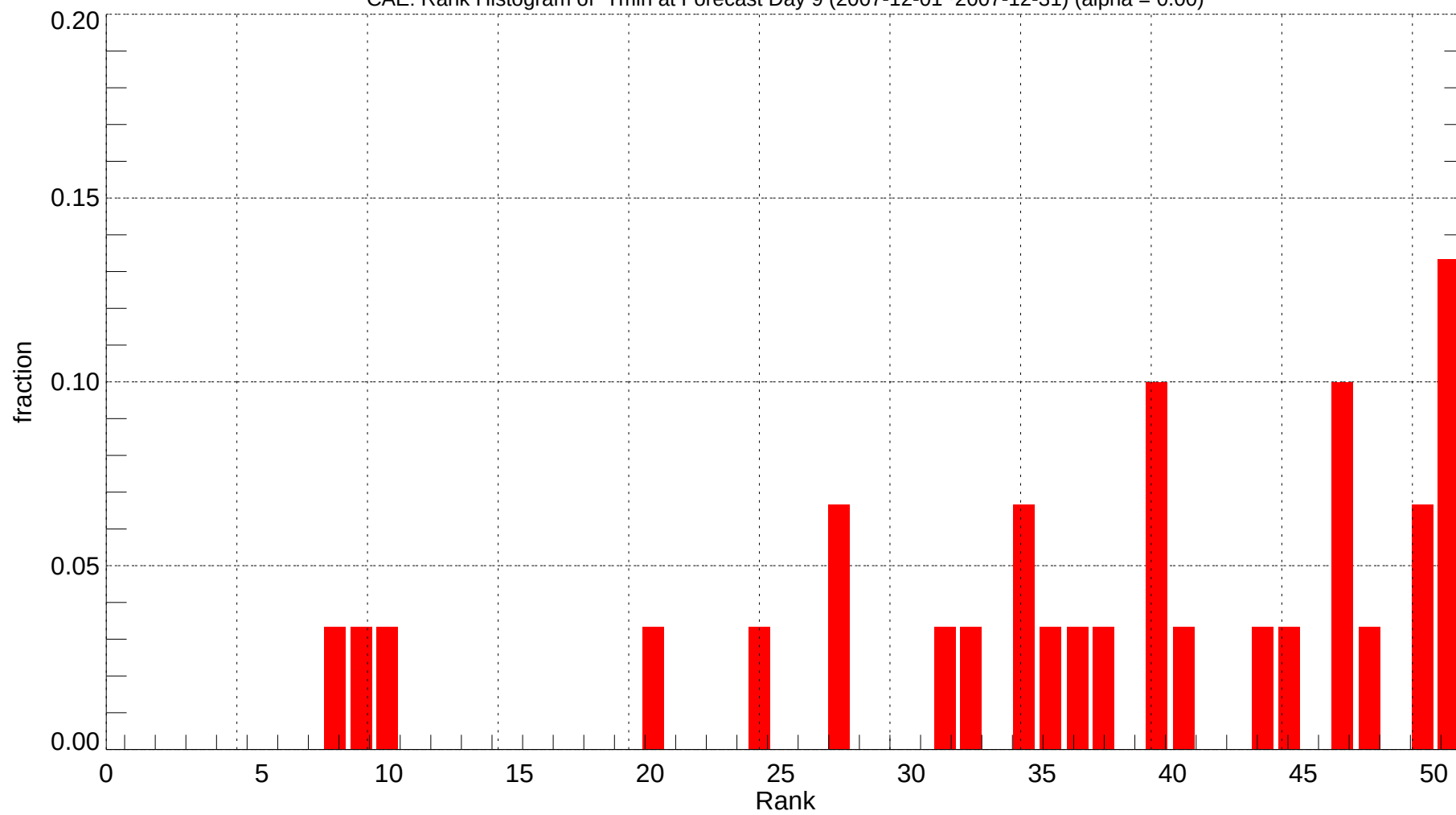
CAE: Rank Histogram of Tmin at Forecast Day 9 (2007-12-01~2007-12-31) (alpha = 0.00)
