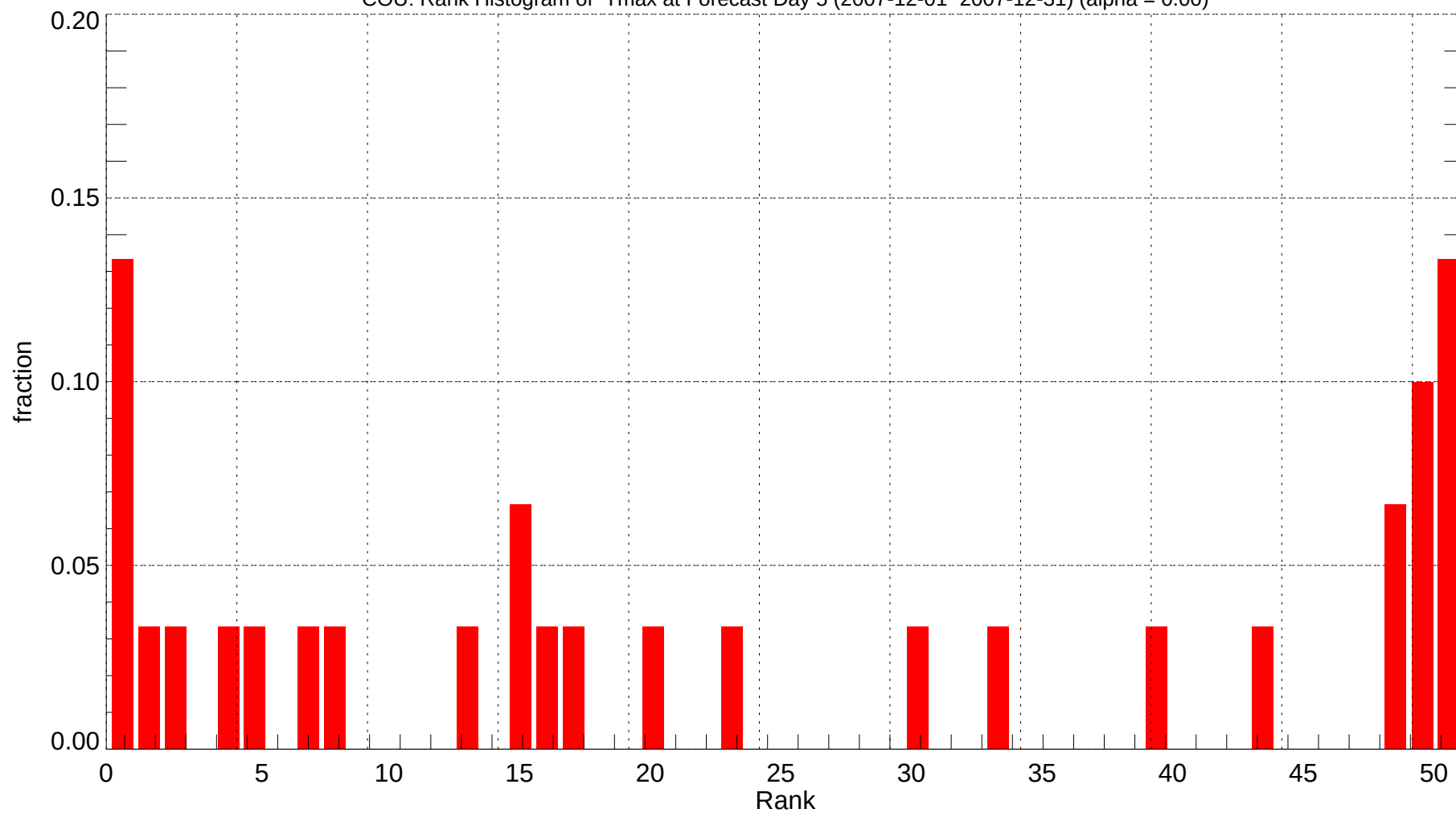
COU: Rank Histogram of Tmax at Forecast Day 5 (2007-12-01~2007-12-31) (alpha = 0.00)
