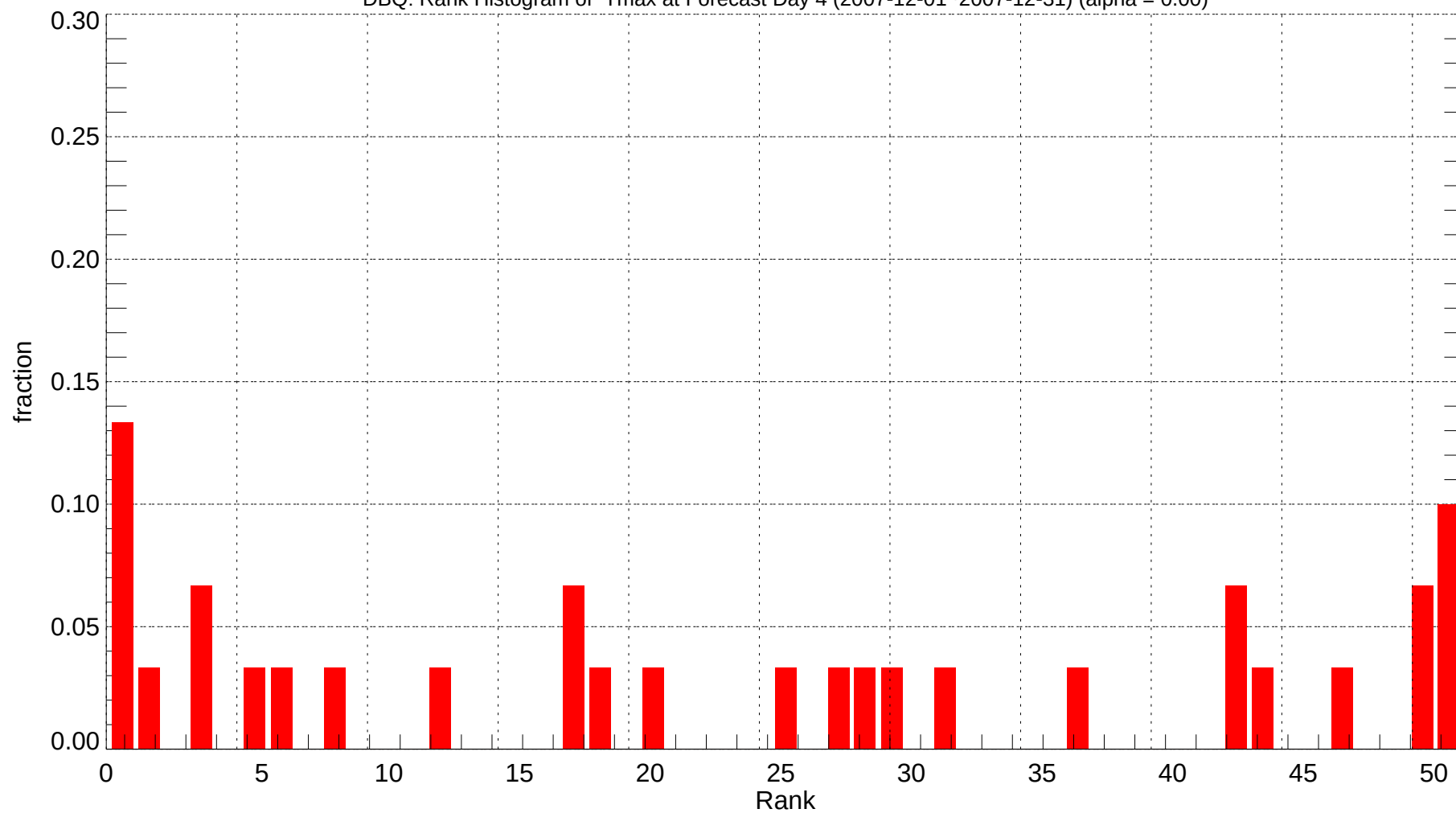
DBQ: Rank Histogram of Tmax at Forecast Day 4 (2007-12-01~2007-12-31) (alpha = 0.00)
