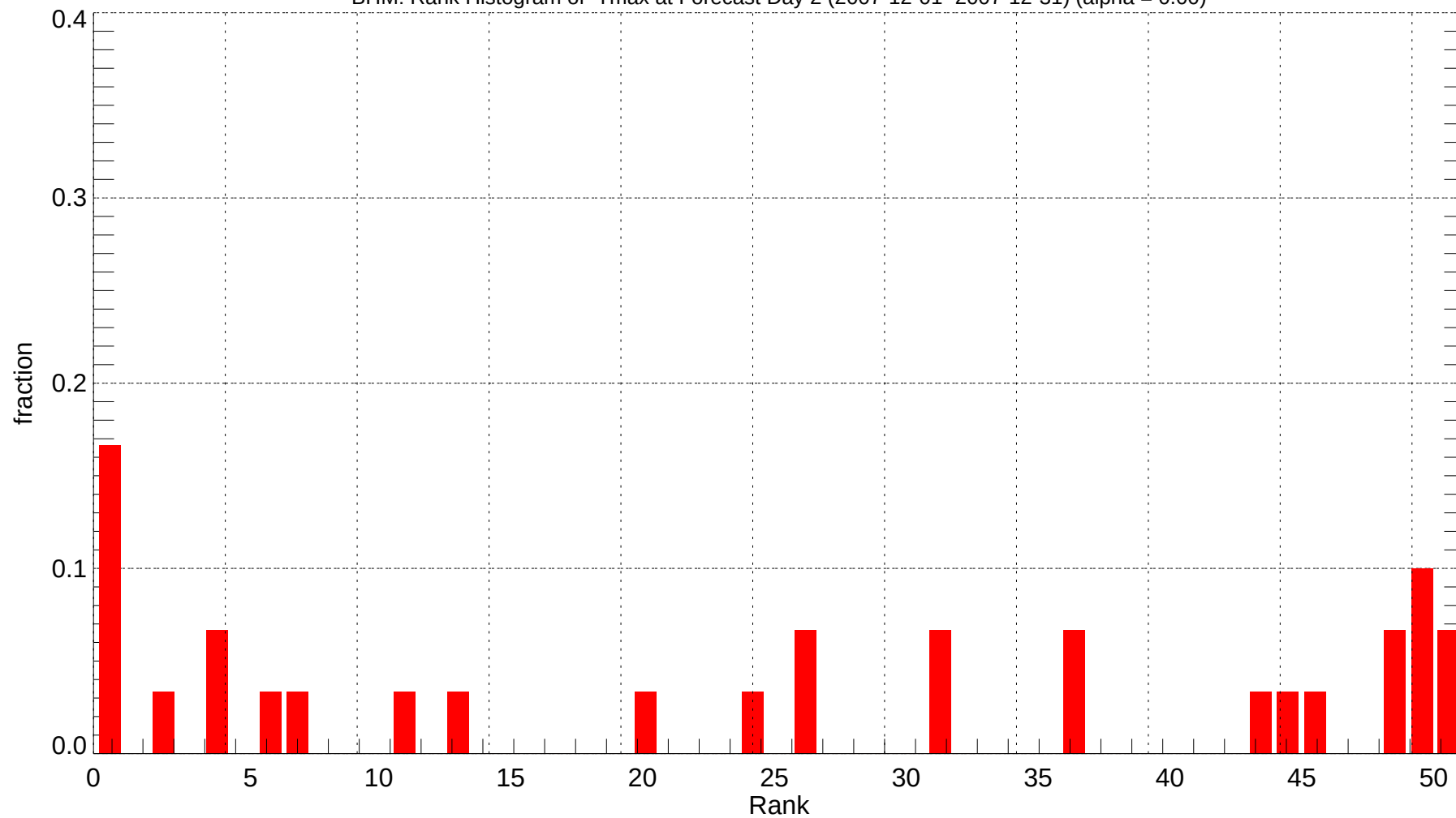
BHM: Rank Histogram of Tmax at Forecast Day 2 (2007-12-01~2007-12-31) (alpha = 0.00)
