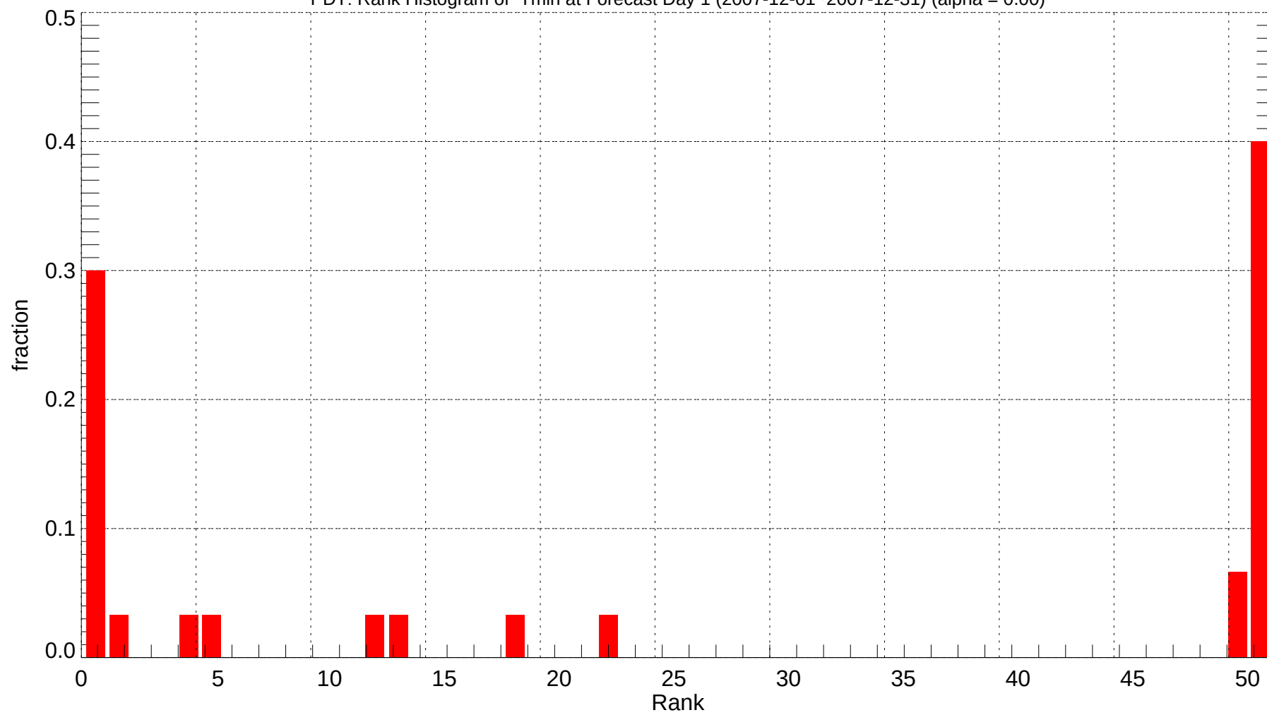
PDT: Rank Histogram of Tmin at Forecast Day 1 (2007-12-01~2007-12-31) (alpha = 0.00)
