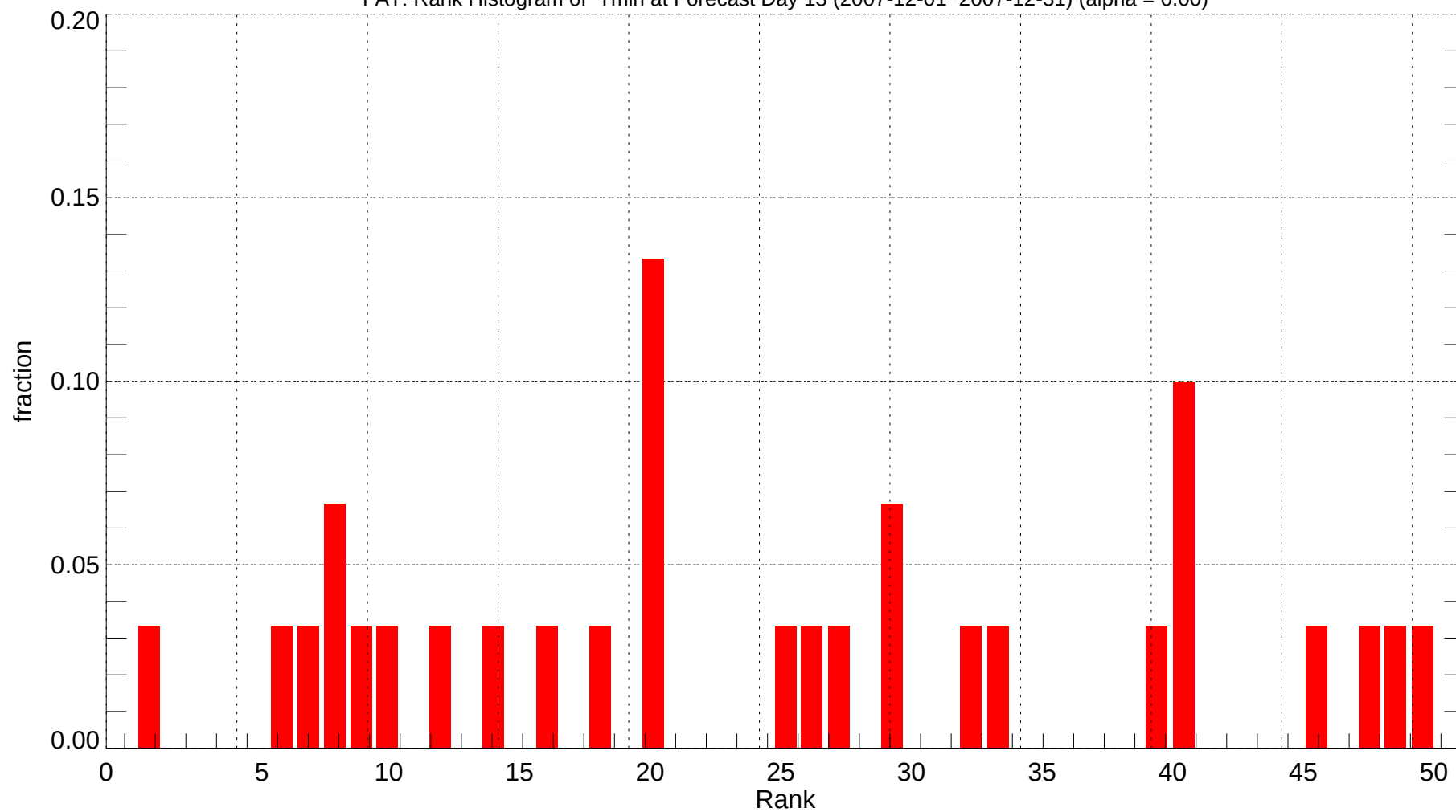
FAT: Rank Histogram of Tmin at Forecast Day 13 (2007-12-01~2007-12-31) (alpha = 0.00)
