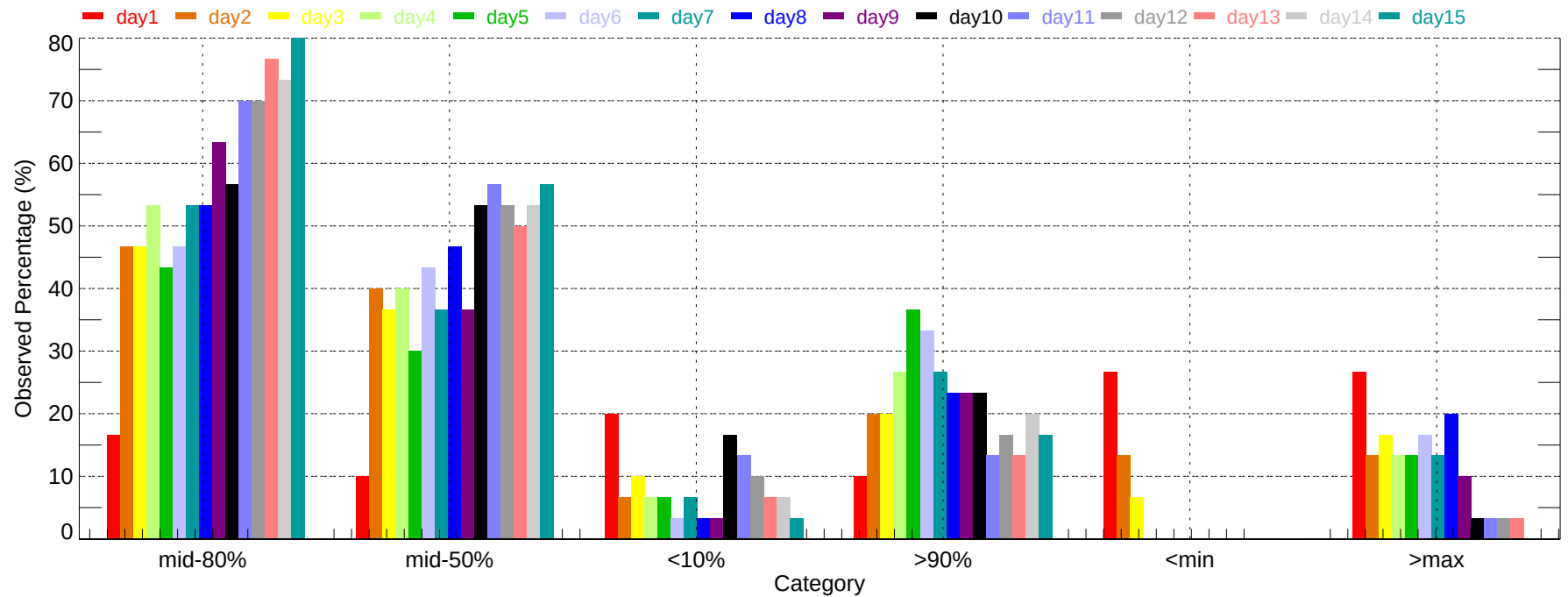
Observed Percentage of Ensembles - DEC: Max Temperature (2007-12-01~2007-12-31)
