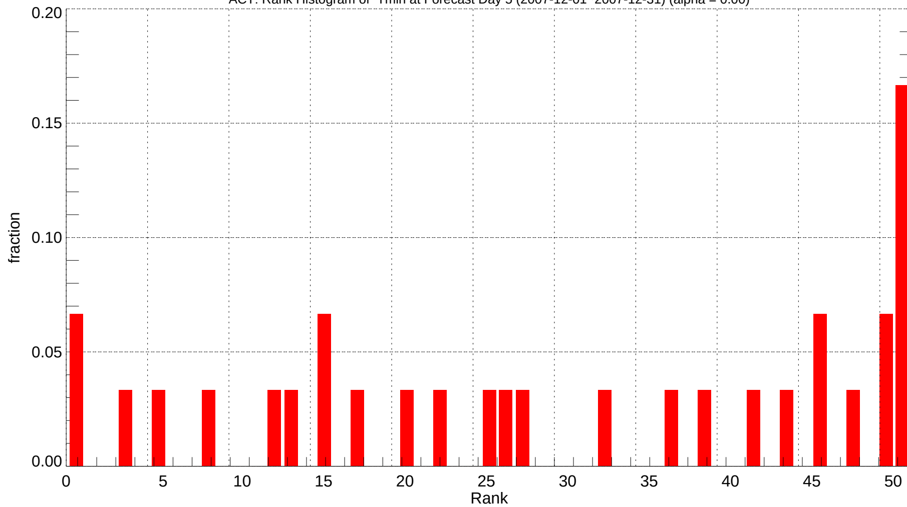
ACT: Rank Histogram of Tmin at Forecast Day 5 (2007-12-01~2007-12-31) (alpha = 0.00)
