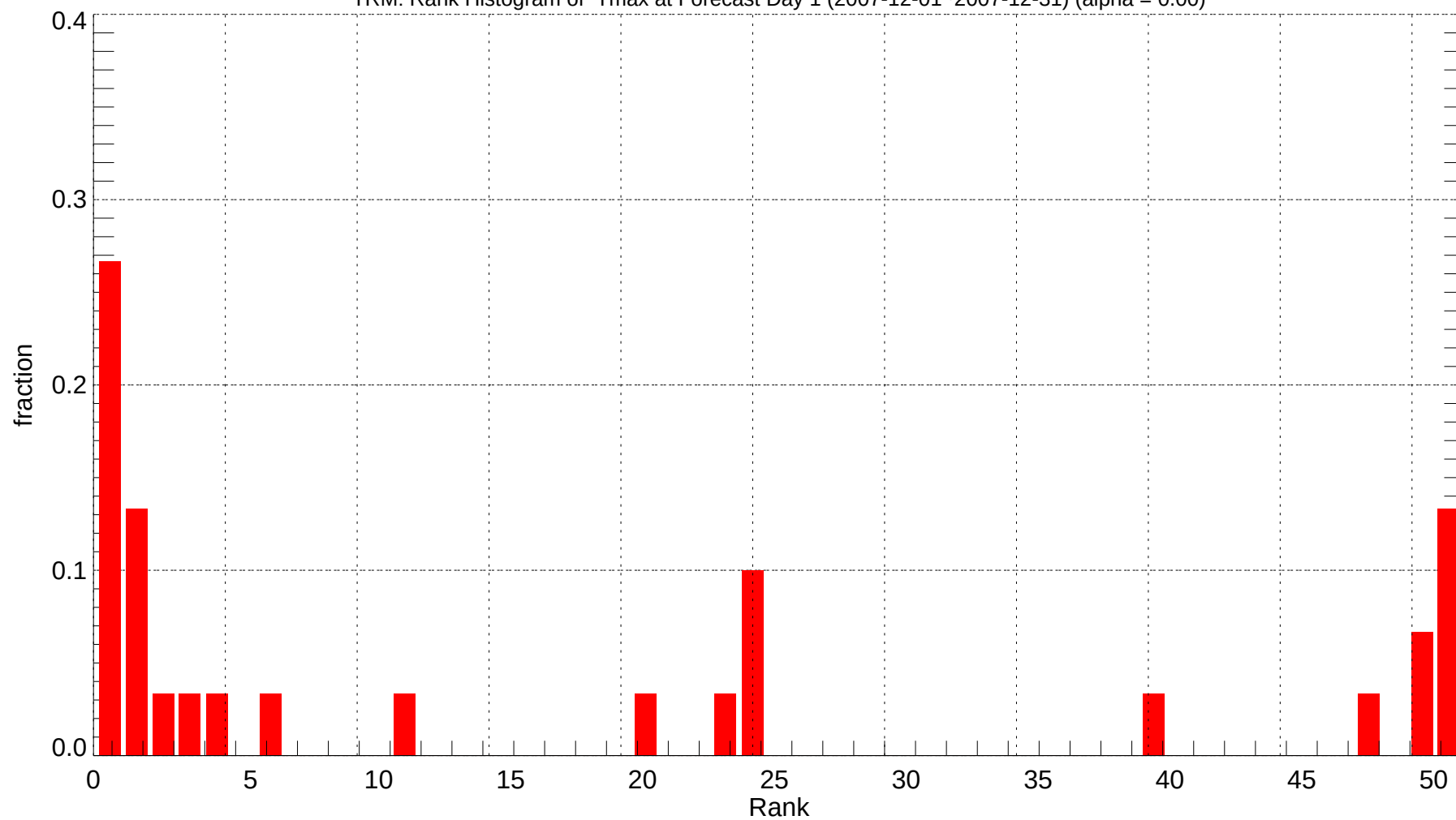
TRM: Rank Histogram of Tmax at Forecast Day 1 (2007-12-01~2007-12-31) (alpha = 0.00)
