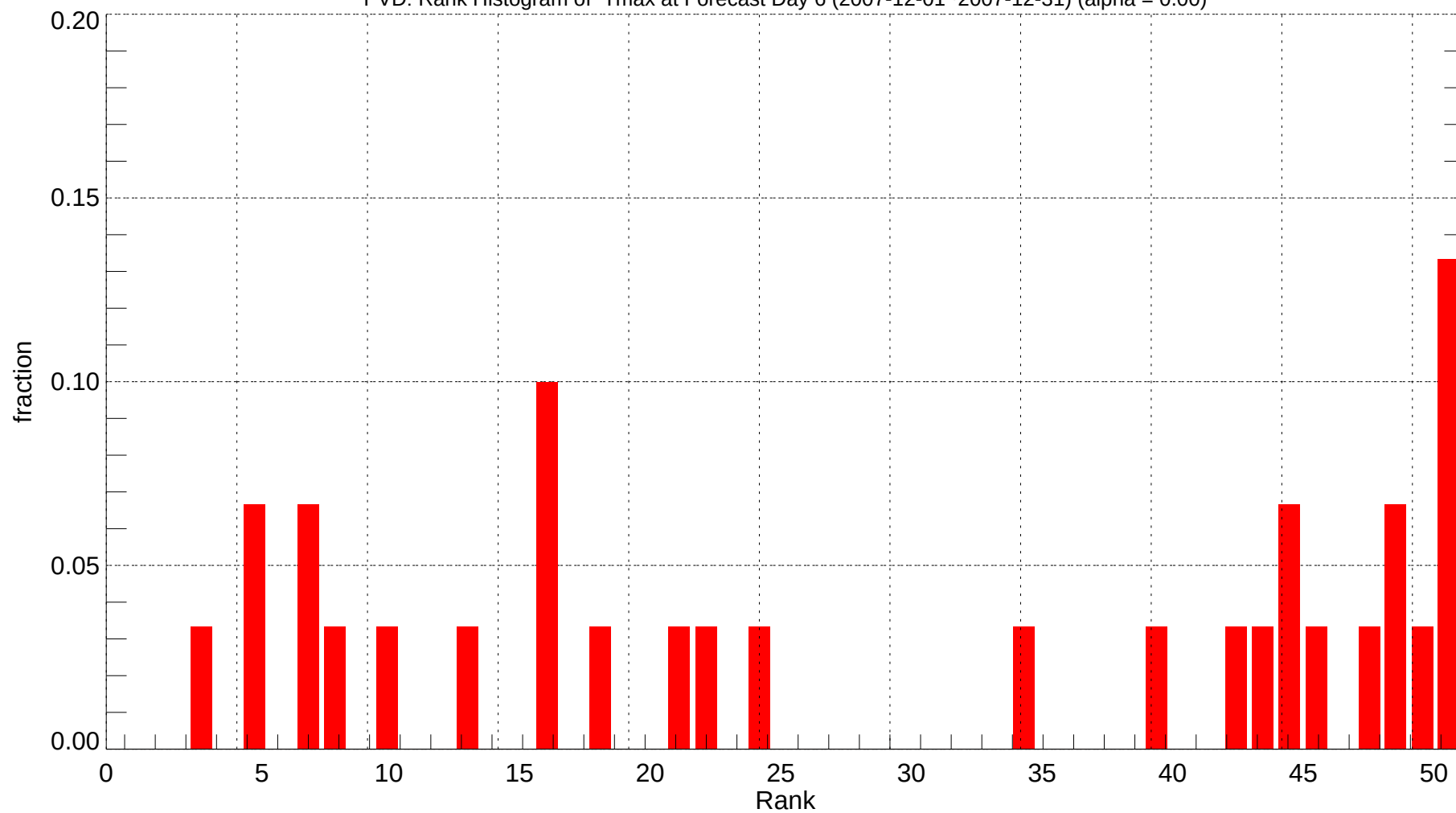
PVD: Rank Histogram of Tmax at Forecast Day 6 (2007-12-01~2007-12-31) (alpha = 0.00)
