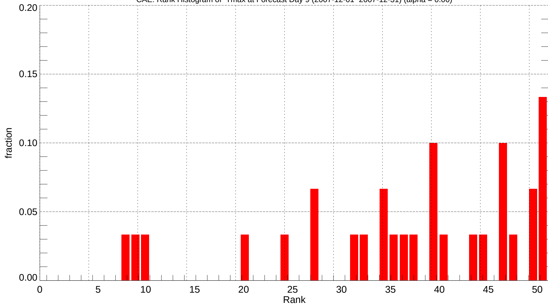
CAE: Rank Histogram of Tmax at Forecast Day 9 (2007-12-01~2007-12-31) (alpha = 0.00)
