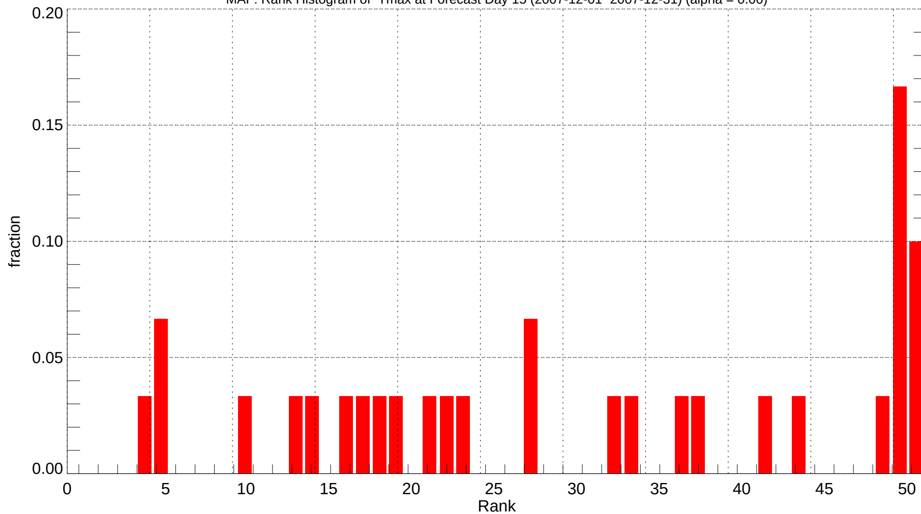
MAF: Rank Histogram of Tmax at Forecast Day 15 (2007-12-01~2007-12-31) (alpha = 0.00)
