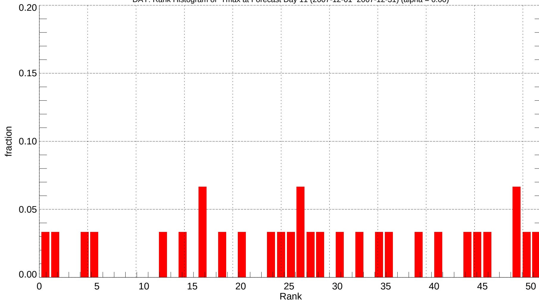
DAY: Rank Histogram of Tmax at Forecast Day 11 (2007-12-01~2007-12-31) (alpha = 0.00)
