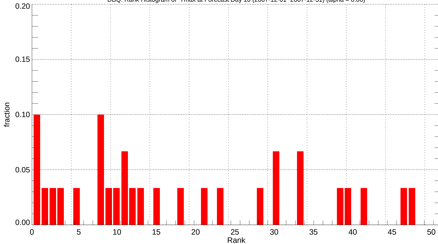
DBQ: Rank Histogram of Tmax at Forecast Day 10 (2007-12-01~2007-12-31) (alpha = 0.00)
