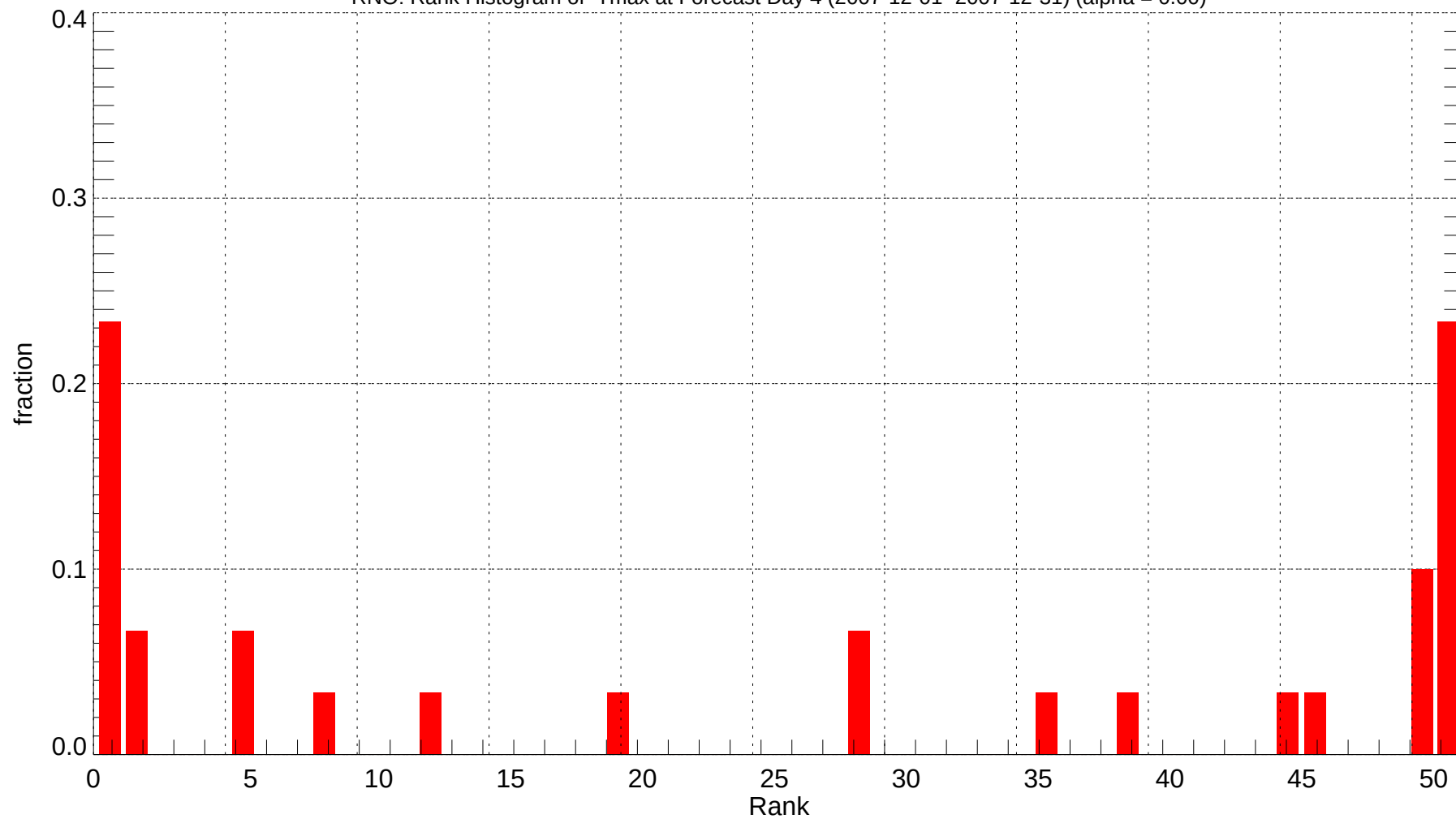
RNO: Rank Histogram of Tmax at Forecast Day 4 (2007-12-01~2007-12-31) (alpha = 0.00)
