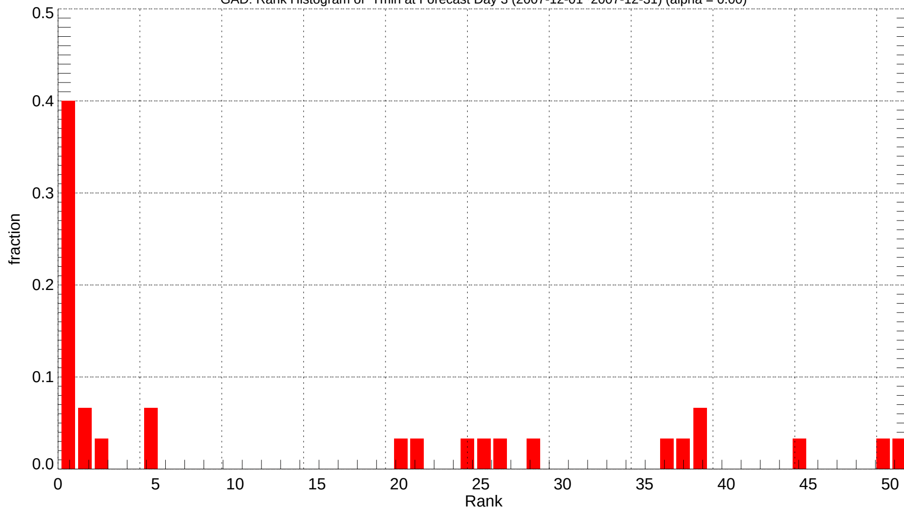
GAD: Rank Histogram of Tmin at Forecast Day 3 (2007-12-01~2007-12-31) (alpha = 0.00)
