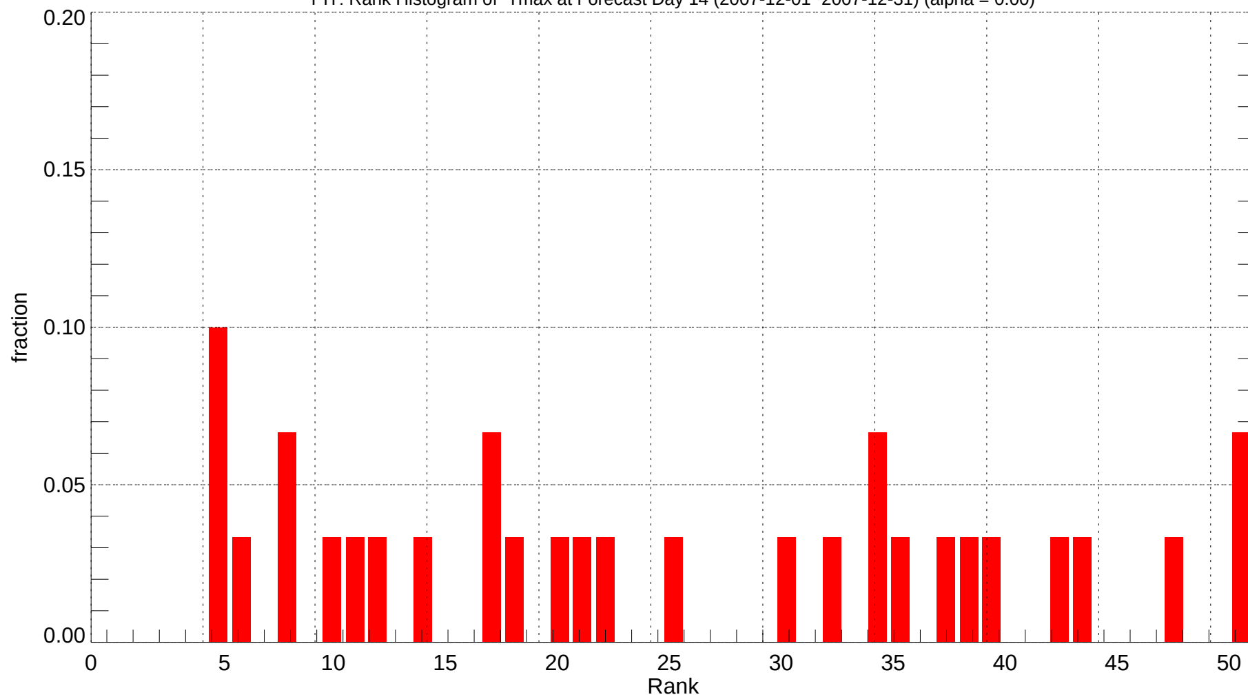
PIT: Rank Histogram of Tmax at Forecast Day 14 (2007-12-01~2007-12-31) (alpha = 0.00)
