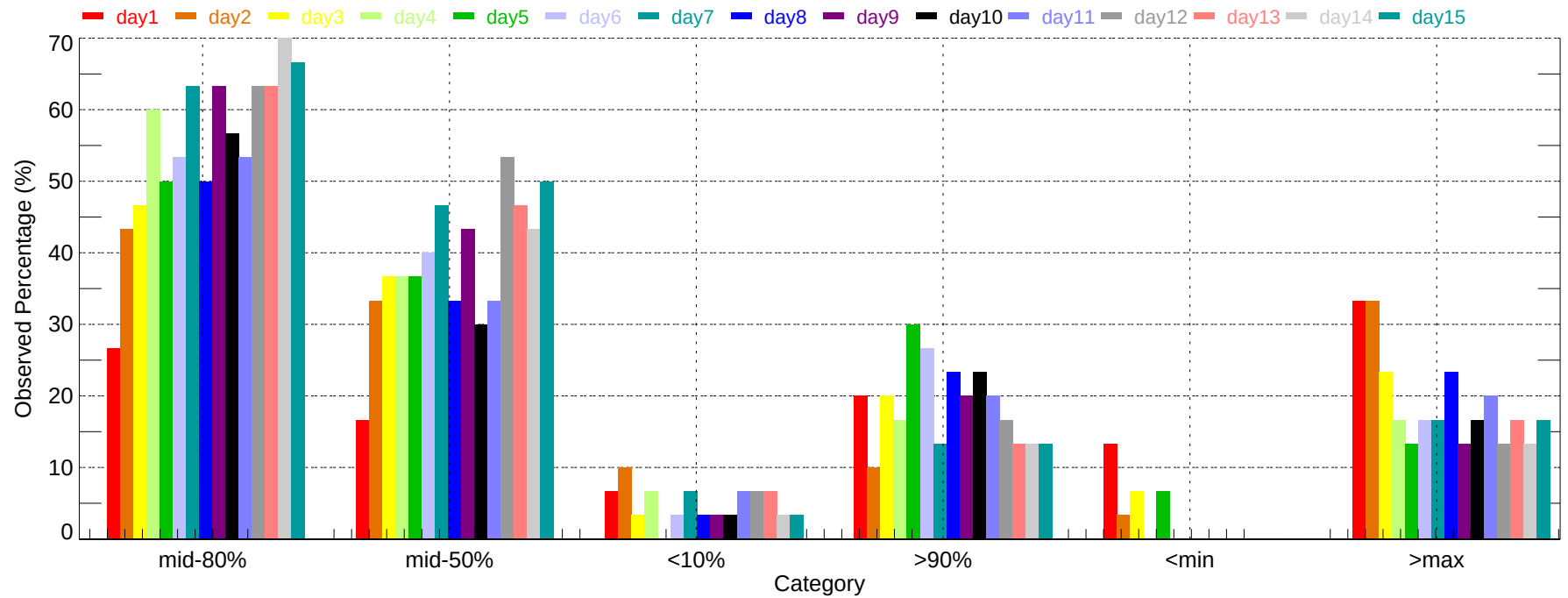
Observed Percentage of Ensembles - LFK: Min Temperature (2007-12-01~2007-12-31)
