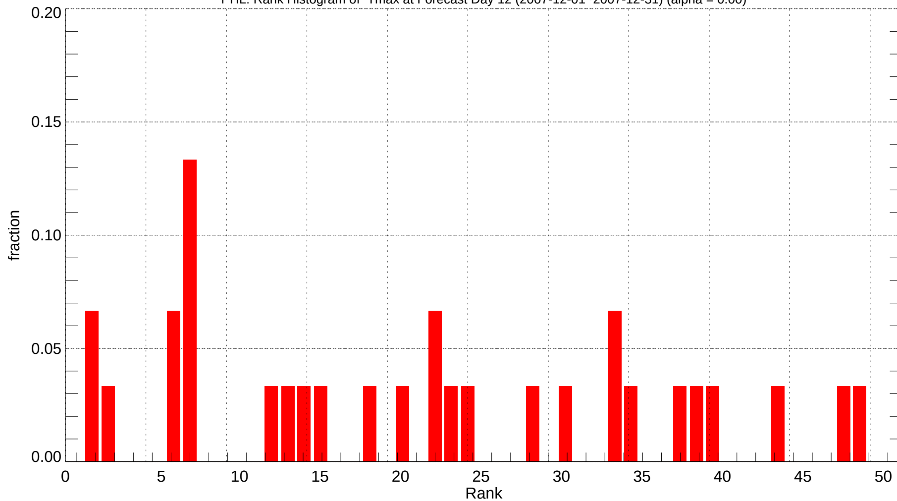
PHL: Rank Histogram of Tmax at Forecast Day 12 (2007-12-01~2007-12-31) (alpha = 0.00)
