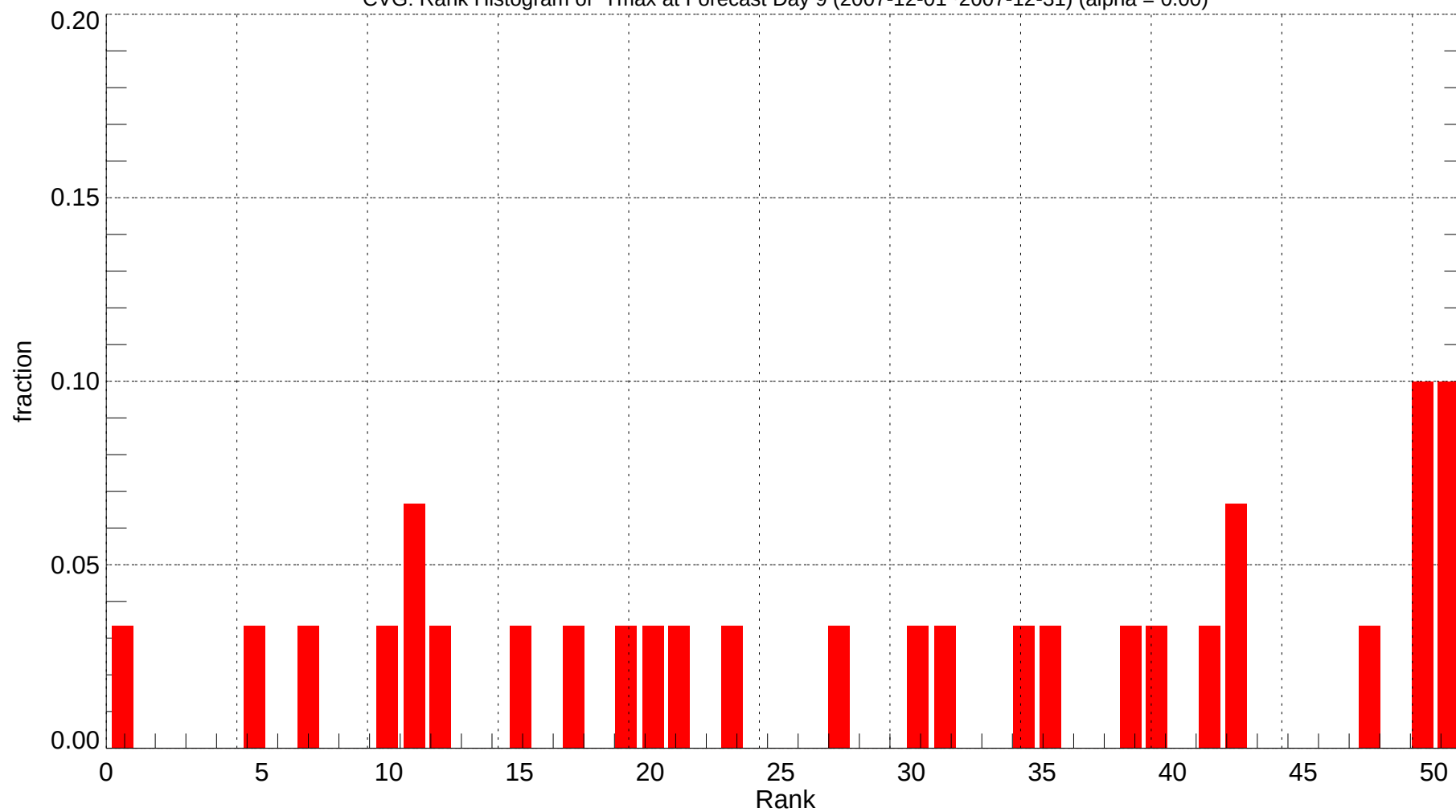
CVG: Rank Histogram of Tmax at Forecast Day 9 (2007-12-01~2007-12-31) (alpha = 0.00)
