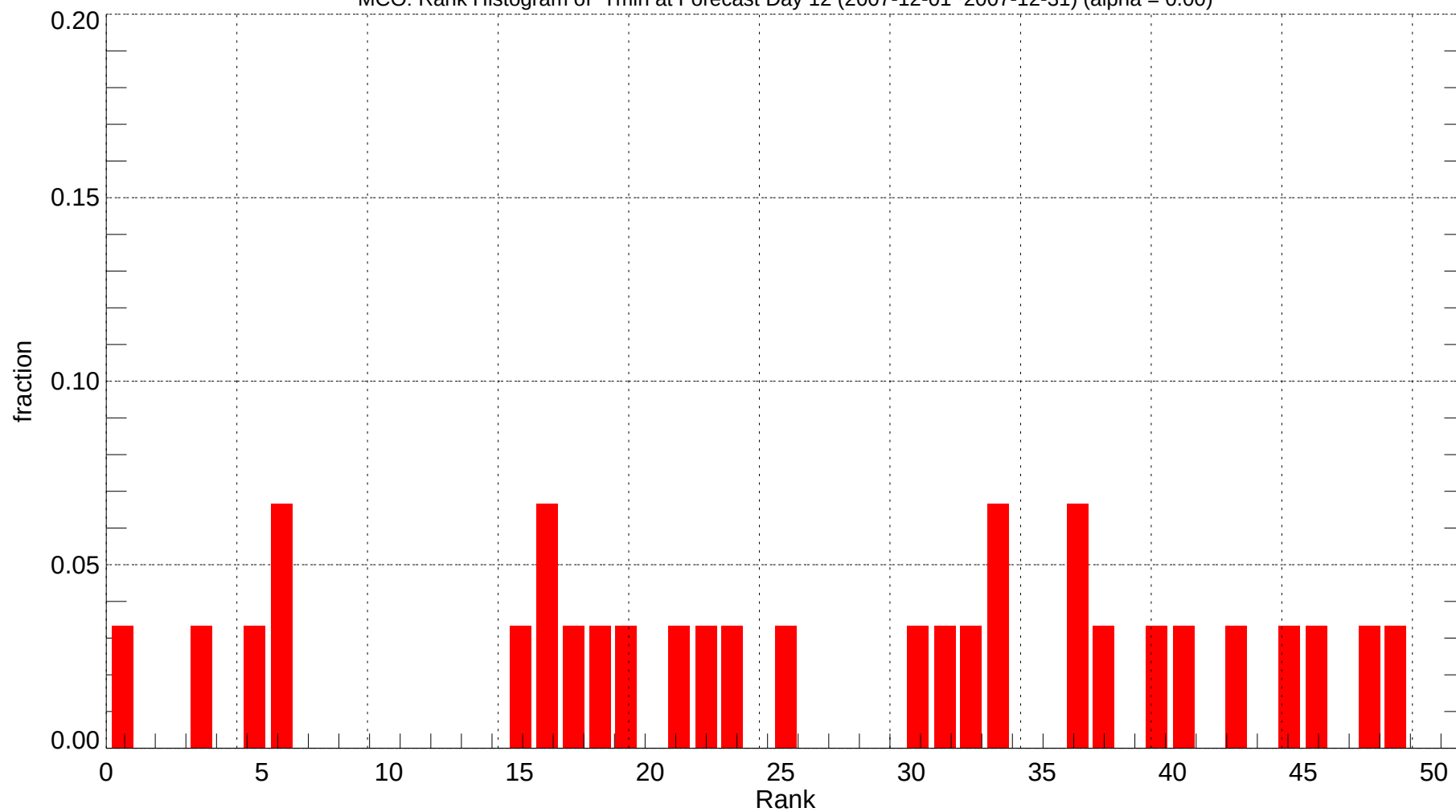
MCO: Rank Histogram of Tmin at Forecast Day 12 (2007-12-01~2007-12-31) (alpha = 0.00)
