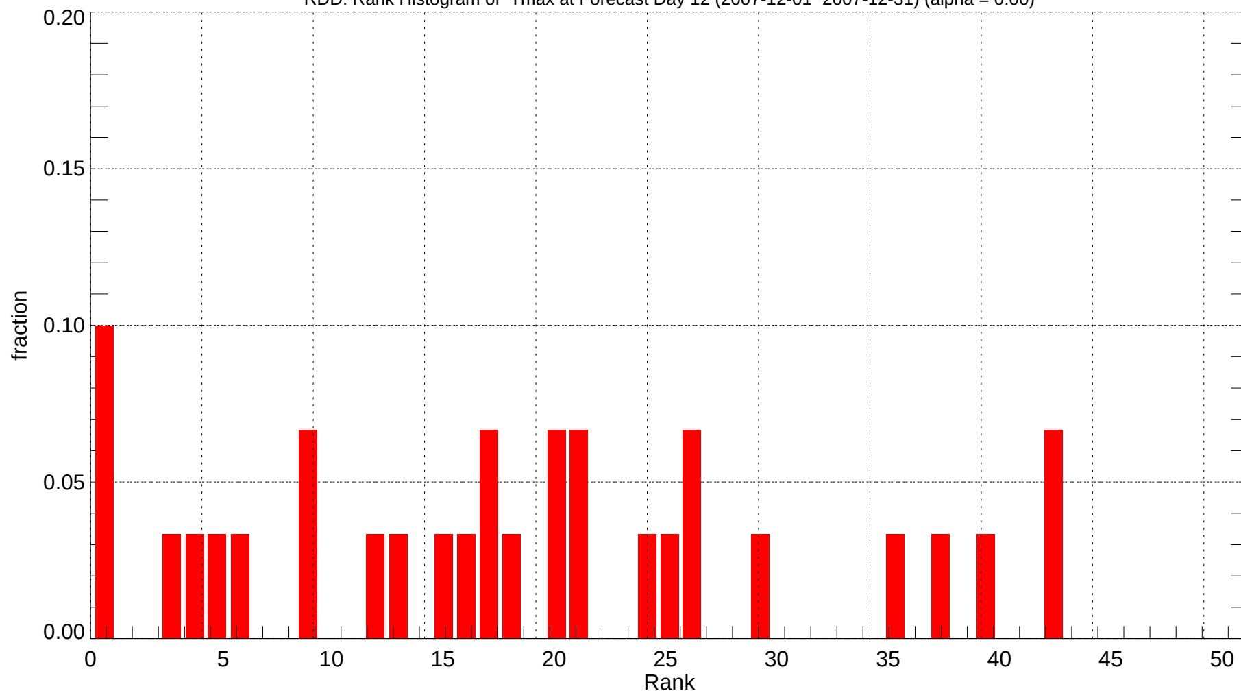
RDD: Rank Histogram of Tmax at Forecast Day 12 (2007-12-01~2007-12-31) (alpha = 0.00)
