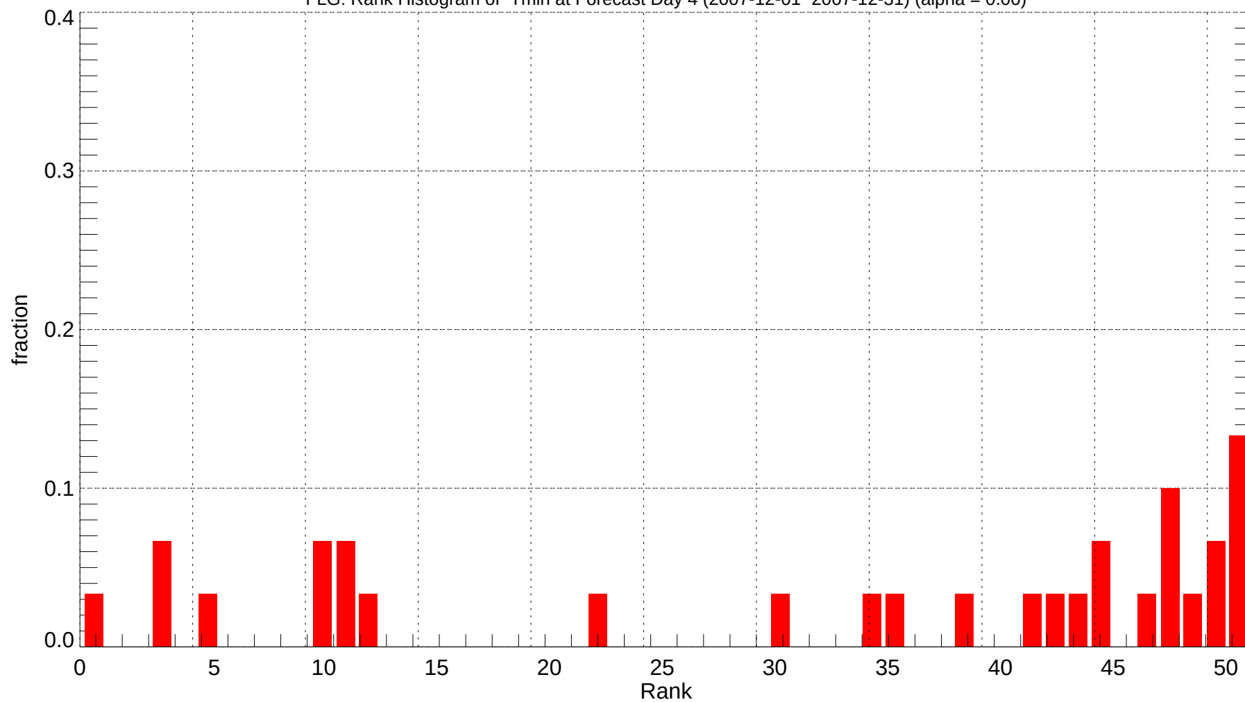
FLG: Rank Histogram of Tmin at Forecast Day 4 (2007-12-01~2007-12-31) (alpha = 0.00)
