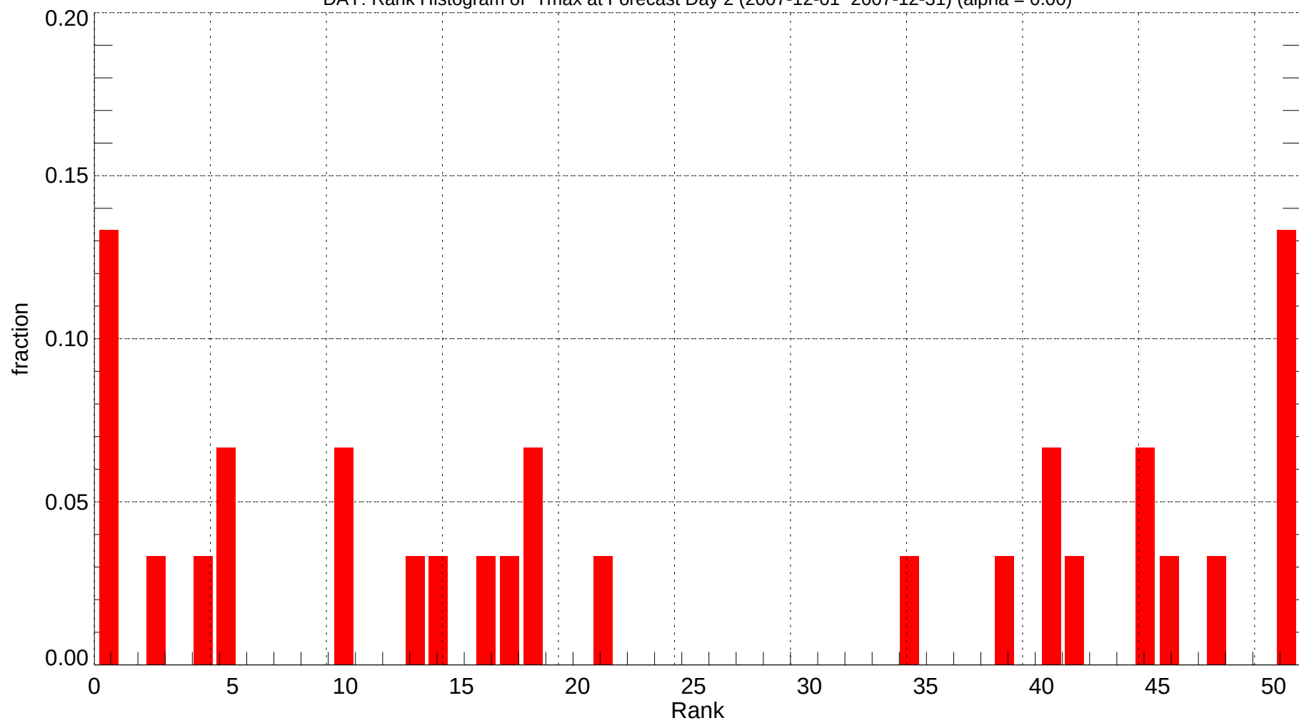
DAY: Rank Histogram of Tmax at Forecast Day 2 (2007-12-01~2007-12-31) (alpha = 0.00)
