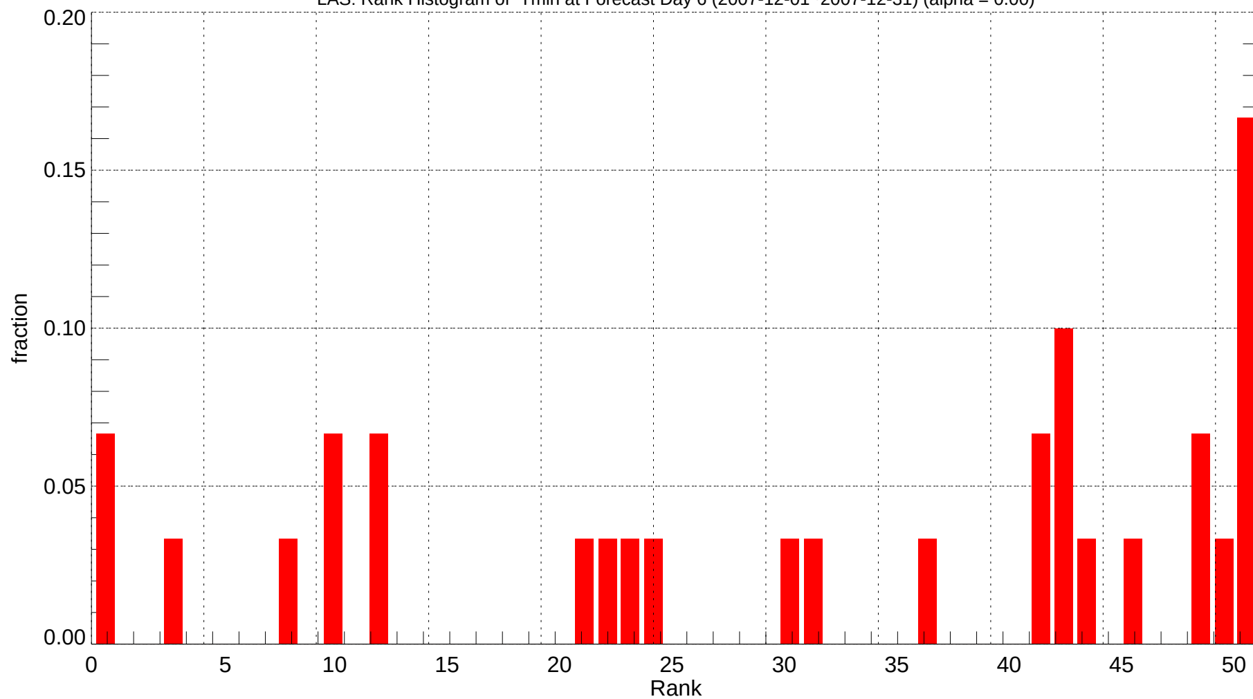
LAS: Rank Histogram of Tmin at Forecast Day 6 (2007-12-01~2007-12-31) (alpha = 0.00)
