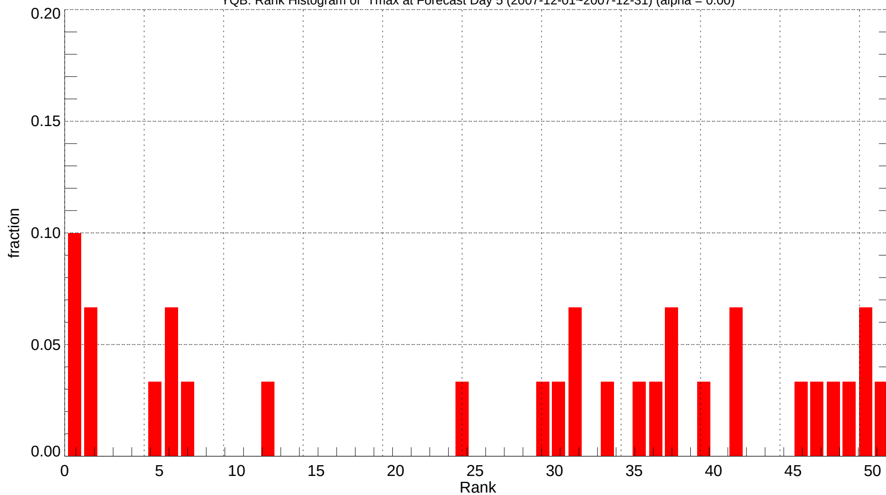
YQB: Rank Histogram of Tmax at Forecast Day 5 (2007-12-01~2007-12-31) (alpha = 0.00)
