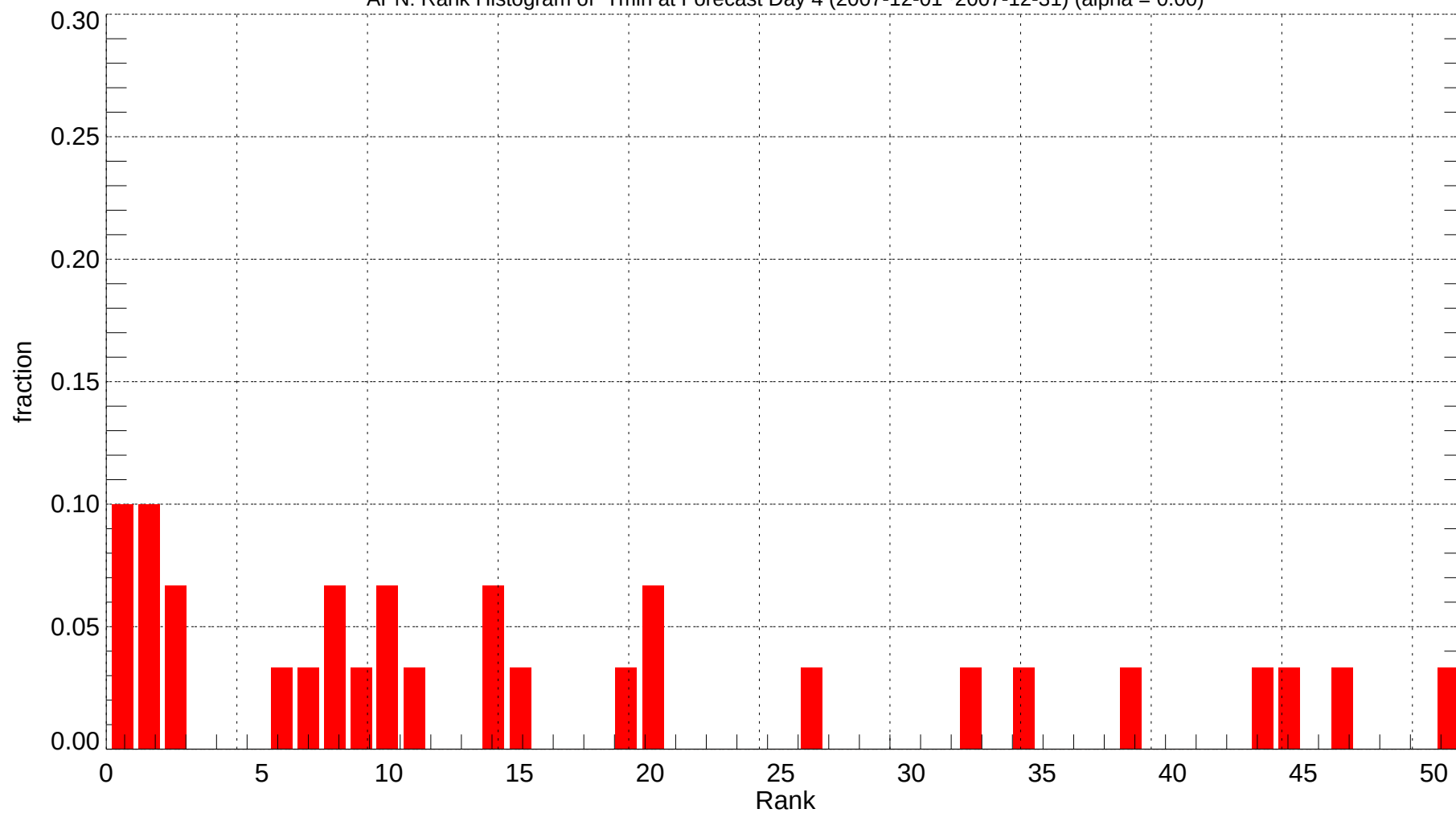
APN: Rank Histogram of Tmin at Forecast Day 4 (2007-12-01~2007-12-31) (alpha = 0.00)
