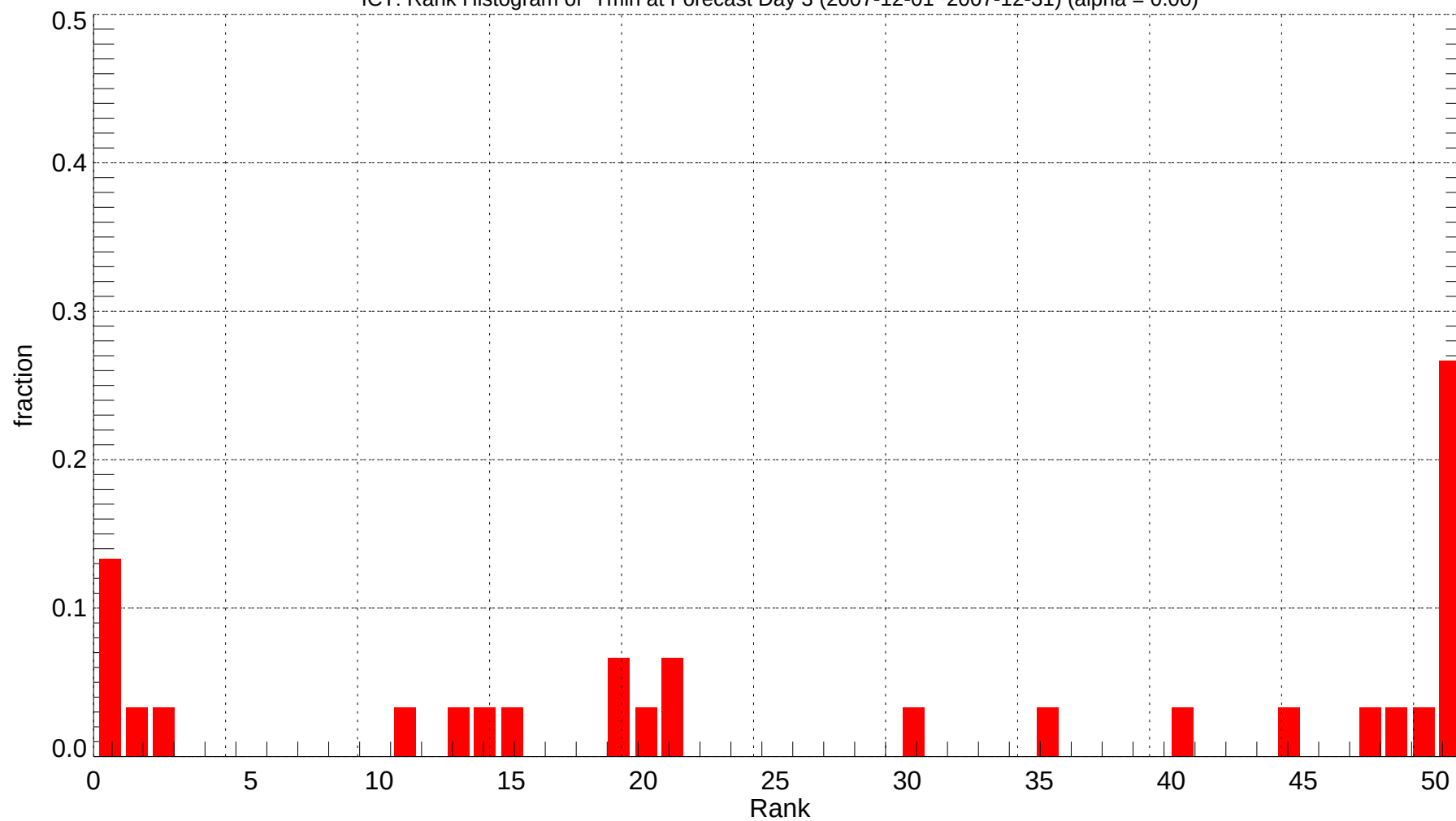
ICT: Rank Histogram of Tmin at Forecast Day 3 (2007-12-01~2007-12-31) (alpha = 0.00)
