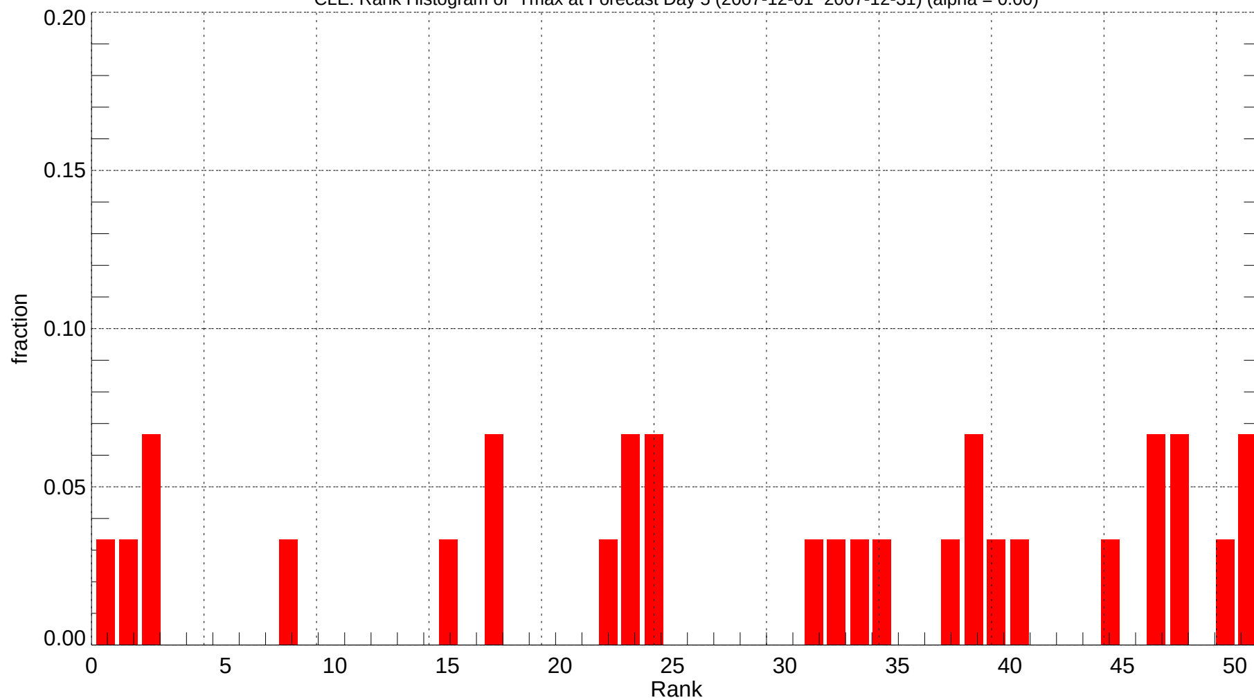
CLE: Rank Histogram of Tmax at Forecast Day 5 (2007-12-01~2007-12-31) (alpha = 0.00)
