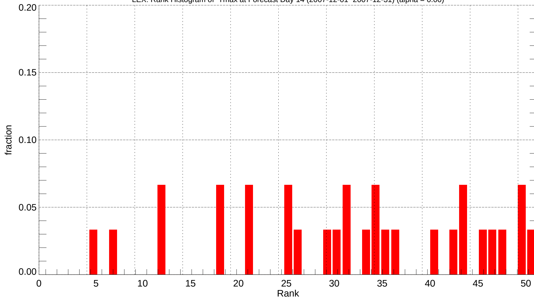
LEX: Rank Histogram of Tmax at Forecast Day 14 (2007-12-01~2007-12-31) (alpha = 0.00)
