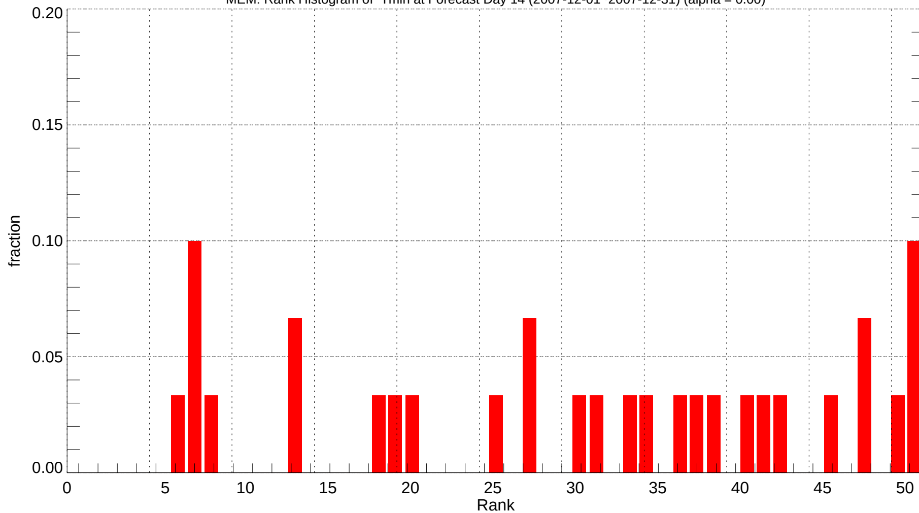
MEM: Rank Histogram of Tmin at Forecast Day 14 (2007-12-01~2007-12-31) (alpha = 0.00)
