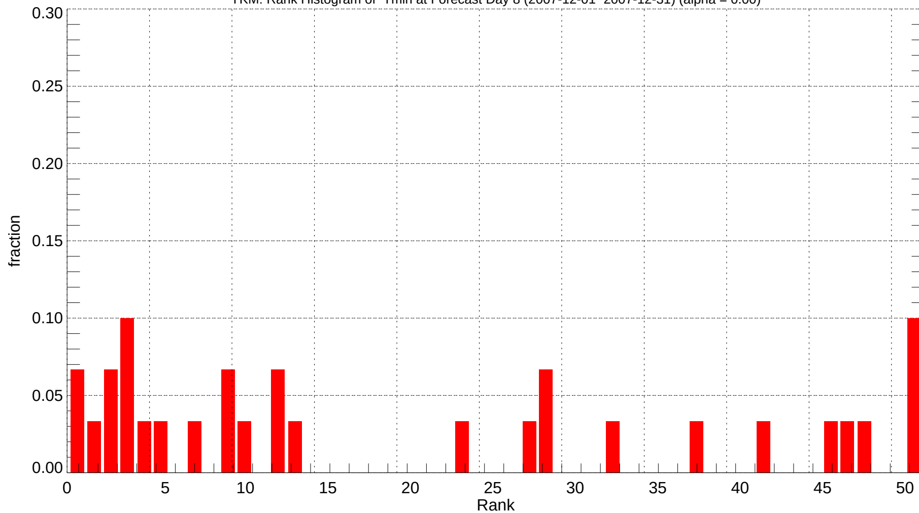
YKM: Rank Histogram of Tmin at Forecast Day 8 (2007-12-01~2007-12-31) (alpha = 0.00)
