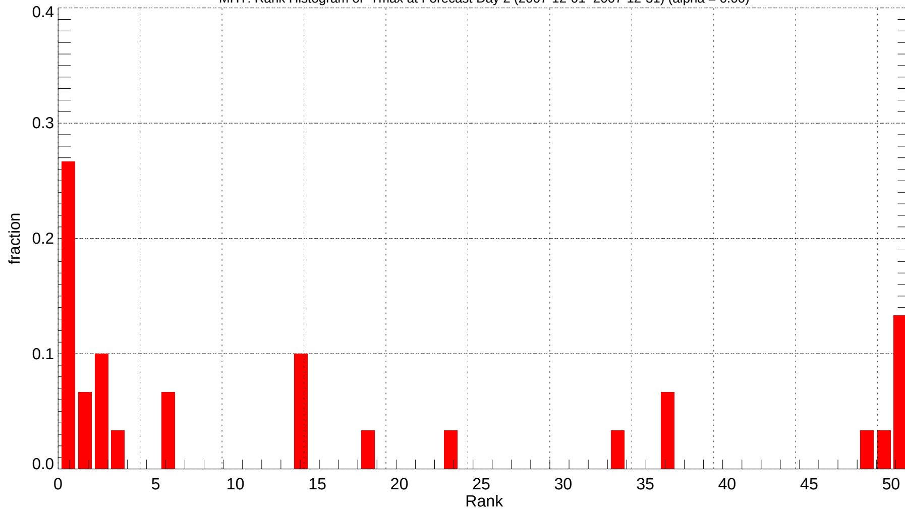
MHT: Rank Histogram of Tmax at Forecast Day 2 (2007-12-01~2007-12-31) (alpha = 0.00)
