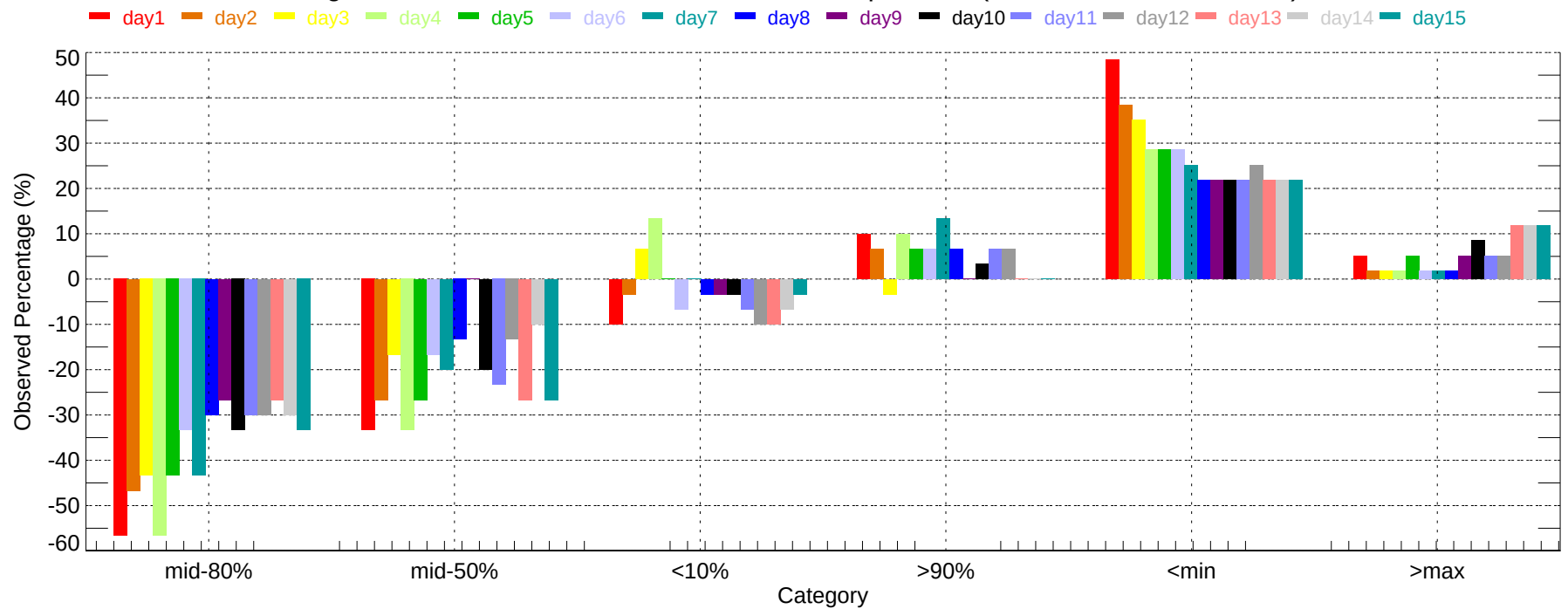
Observed Percentage Deviation of Ensembles - GAD: Min Temperature (2007-12-01~2007-12-31)
