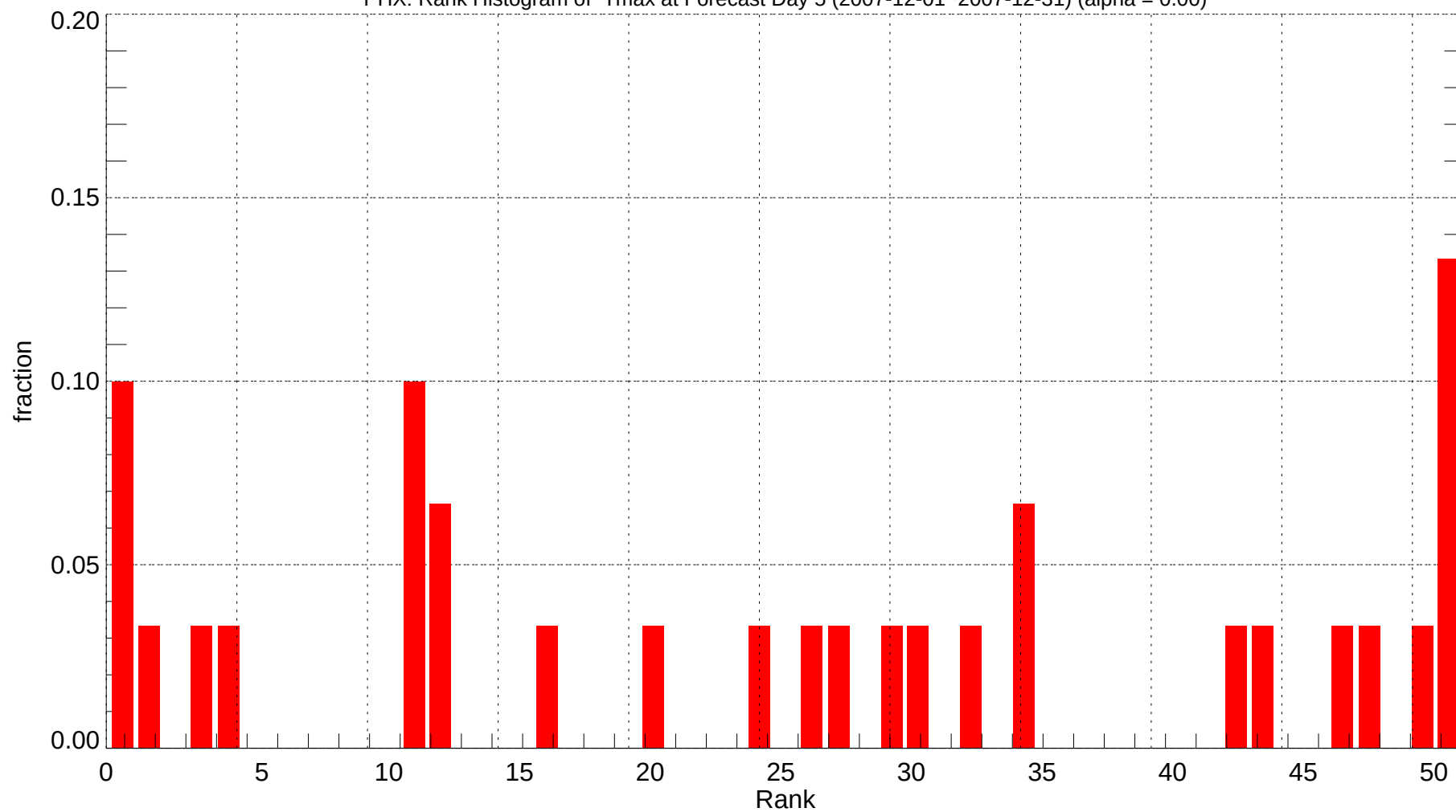
PHX: Rank Histogram of Tmax at Forecast Day 5 (2007-12-01~2007-12-31) (alpha = 0.00)
