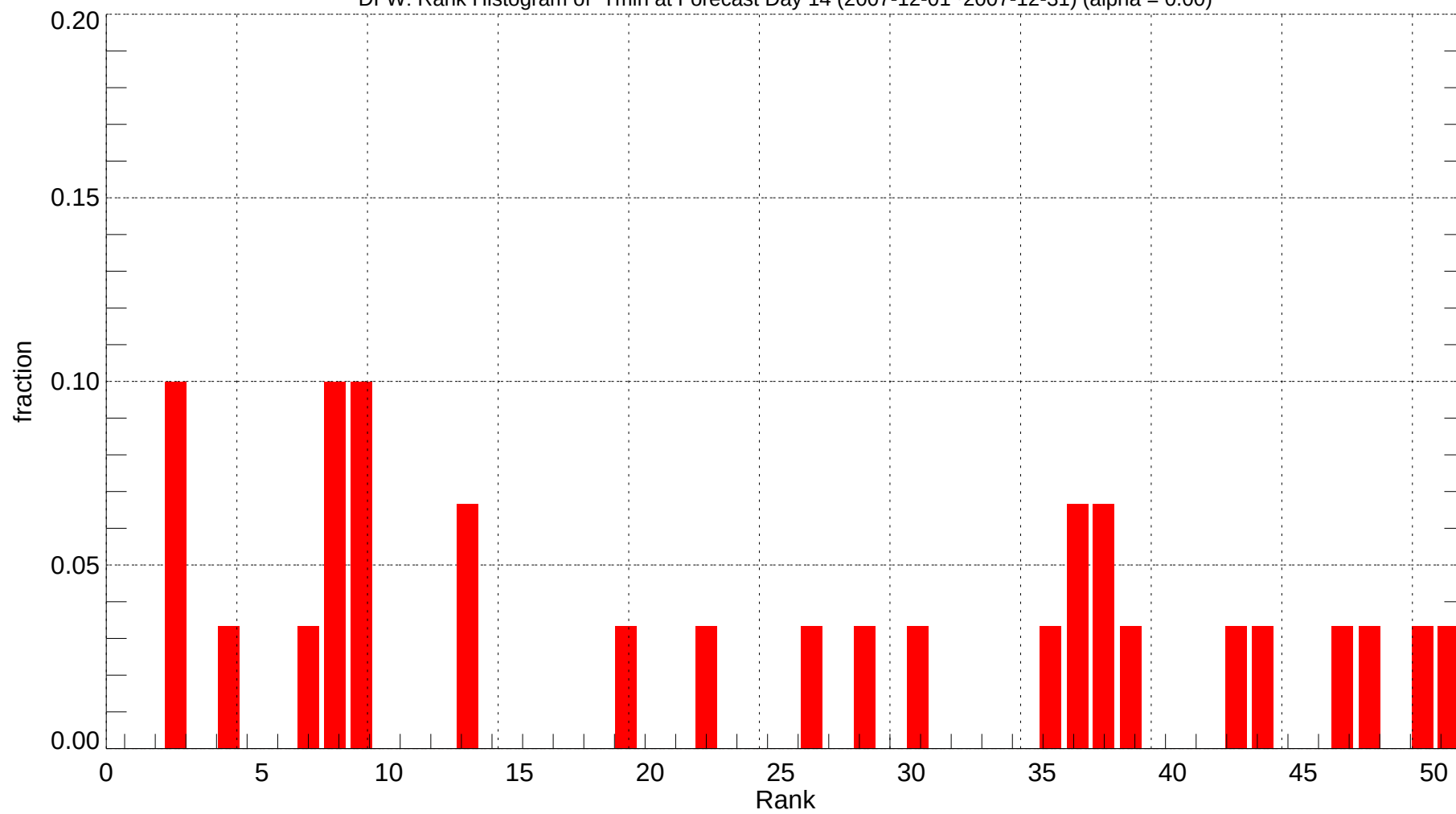
DFW: Rank Histogram of Tmin at Forecast Day 14 (2007-12-01~2007-12-31) (alpha = 0.00)
