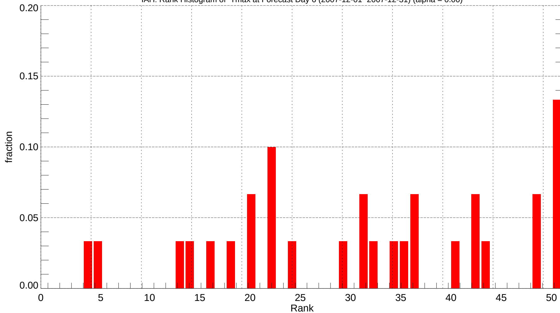
IAH: Rank Histogram of Tmax at Forecast Day 6 (2007-12-01~2007-12-31) (alpha = 0.00)
