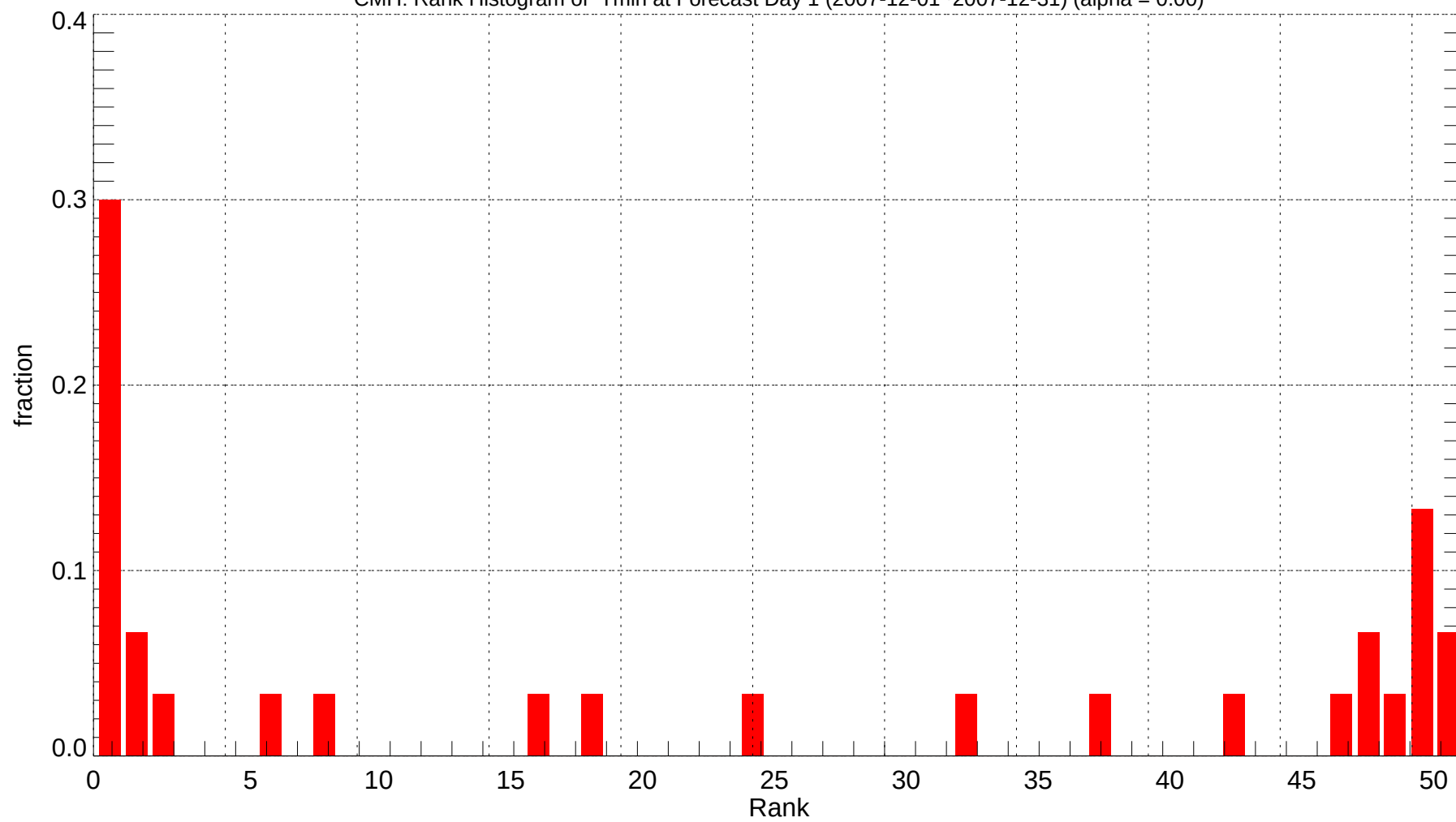
CMH: Rank Histogram of Tmin at Forecast Day 1 (2007-12-01~2007-12-31) (alpha = 0.00)
