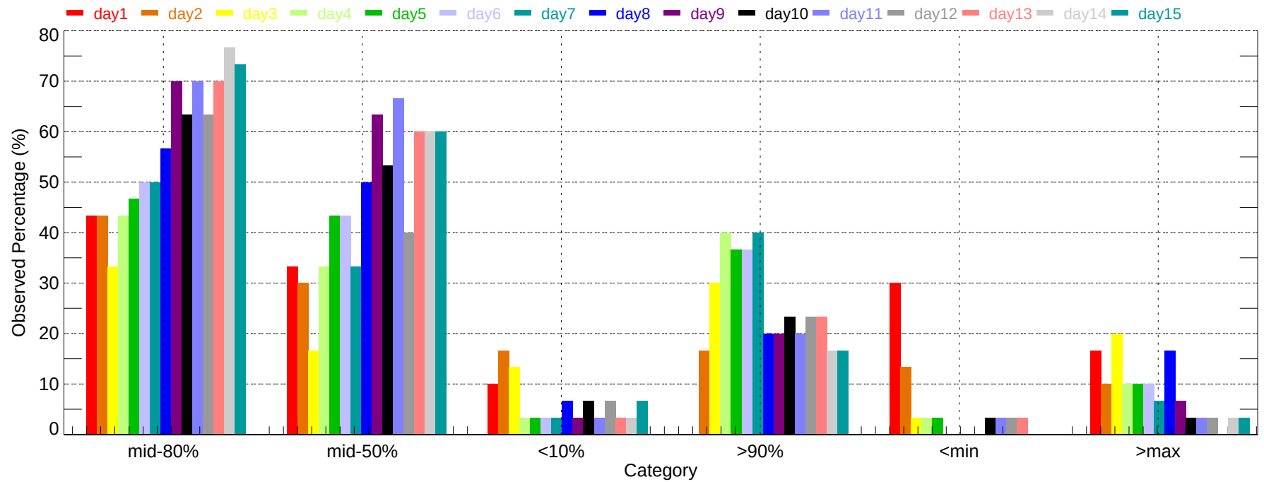
Observed Percentage of Ensembles - IND: Min Temperature (2007-12-01~2007-12-31)
