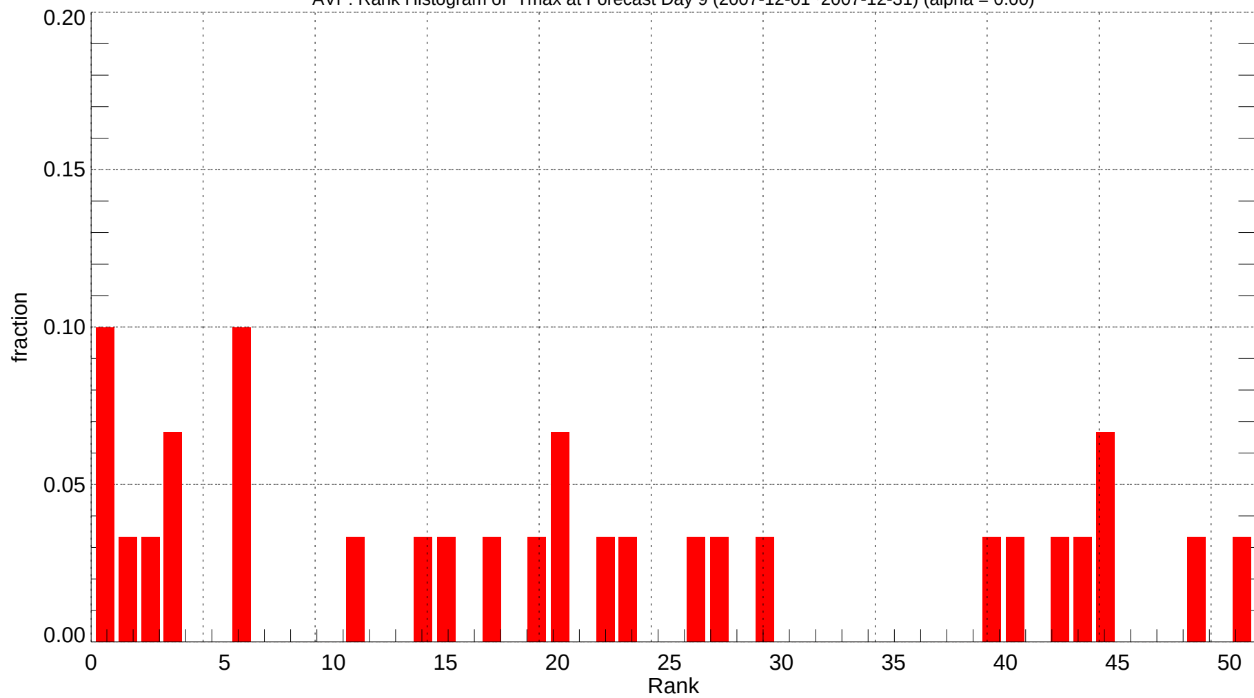
AVP: Rank Histogram of Tmax at Forecast Day 9 (2007-12-01~2007-12-31) (alpha = 0.00)
