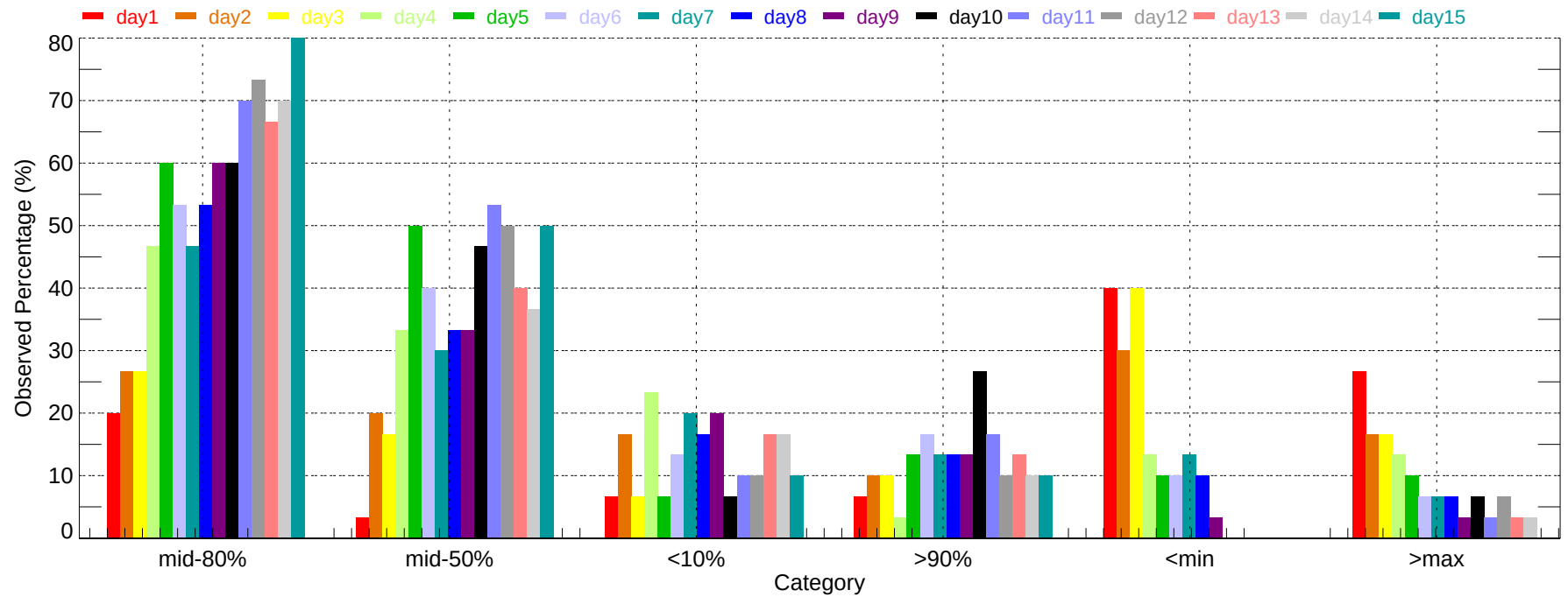
Observed Percentage of Ensembles - RAP: Min Temperature (2007-12-01~2007-12-31)
