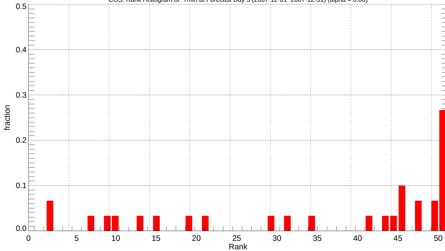
COS: Rank Histogram of Tmin at Forecast Day 5 (2007-12-01~2007-12-31) (alpha = 0.00)
