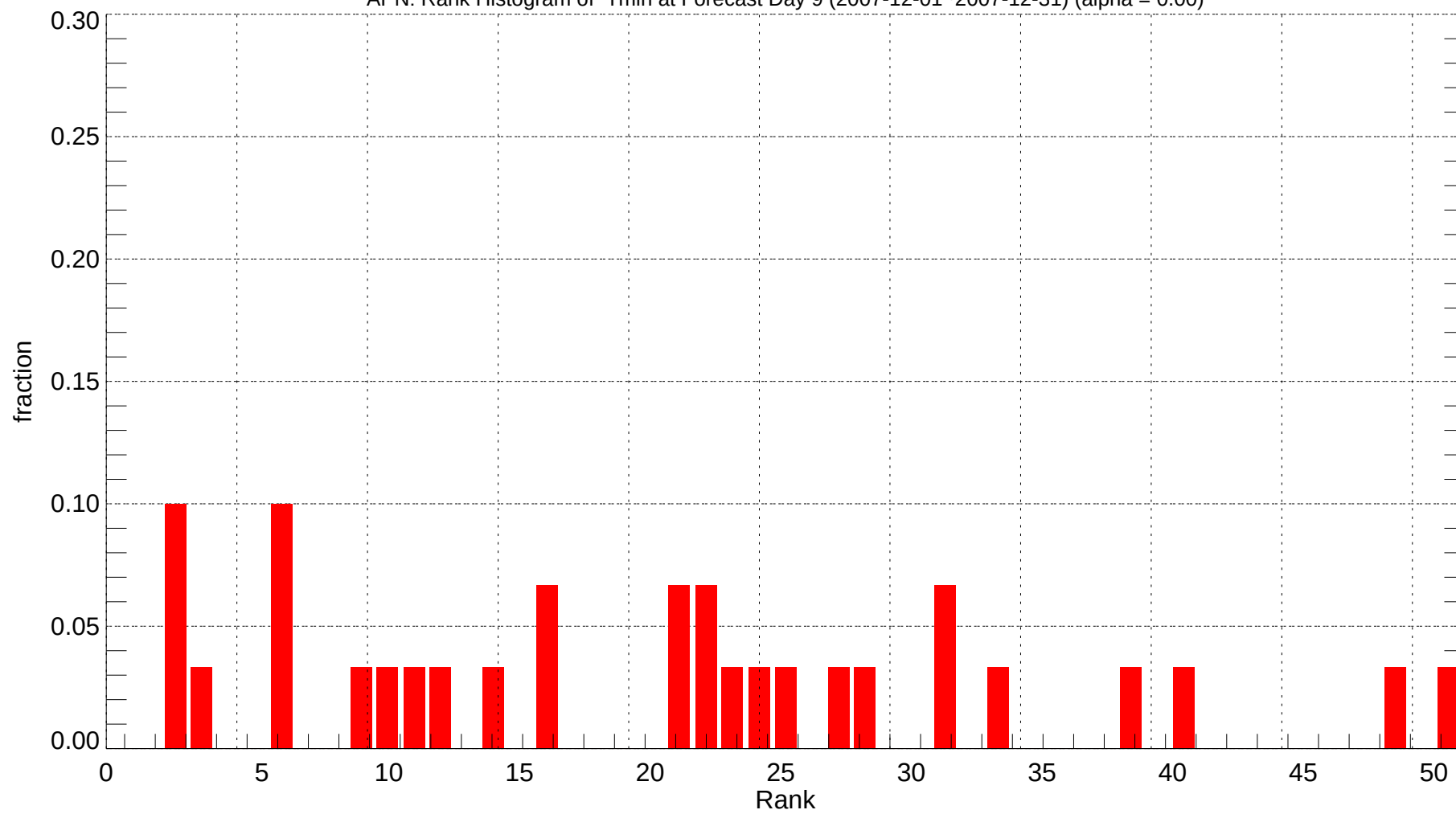
APN: Rank Histogram of Tmin at Forecast Day 9 (2007-12-01~2007-12-31) (alpha = 0.00)
