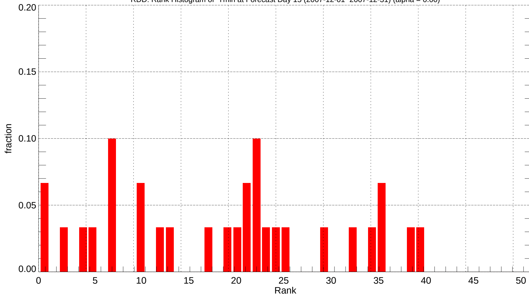
RDD: Rank Histogram of Tmin at Forecast Day 15 (2007-12-01~2007-12-31) (alpha = 0.00)
