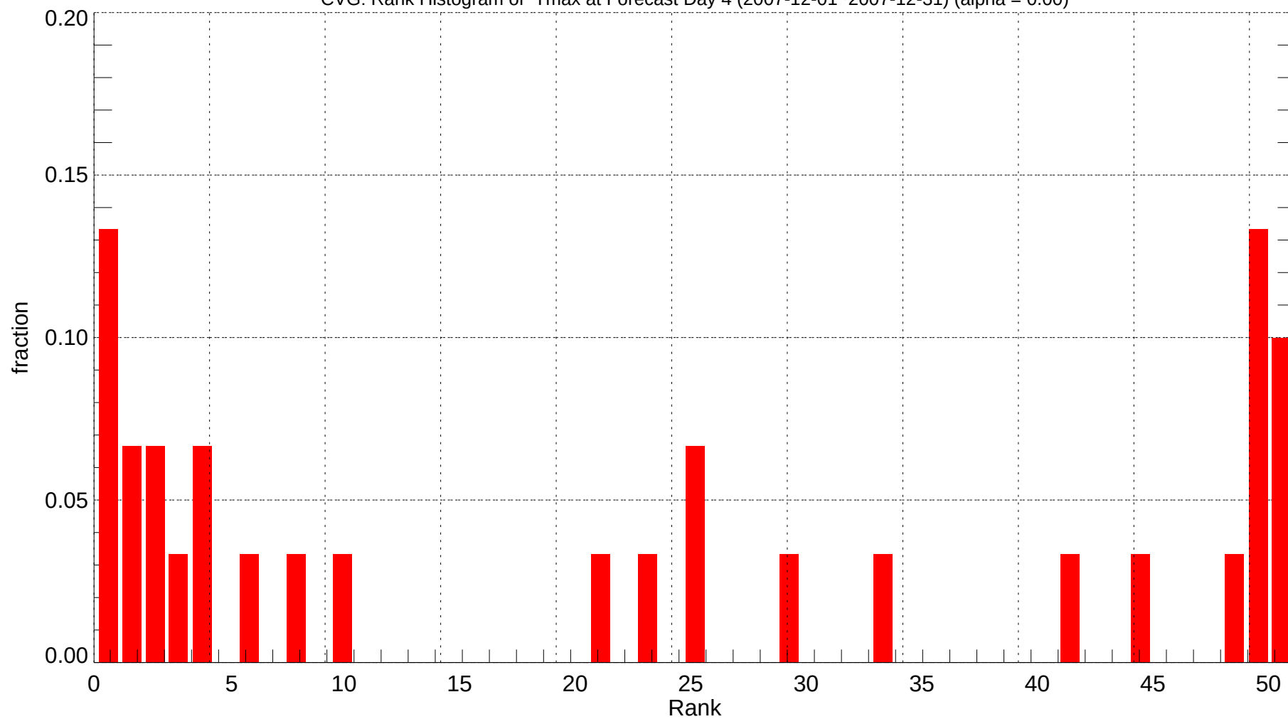
CVG: Rank Histogram of Tmax at Forecast Day 4 (2007-12-01~2007-12-31) (alpha = 0.00)
