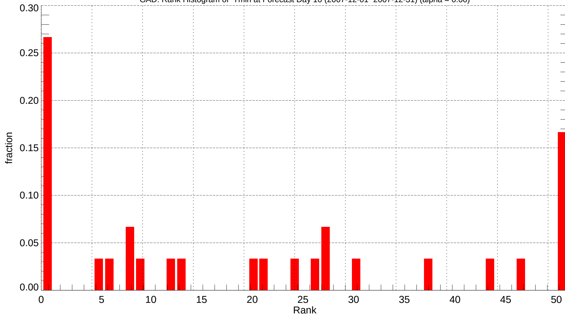
GAD: Rank Histogram of Tmin at Forecast Day 10 (2007-12-01~2007-12-31) (alpha = 0.00)
