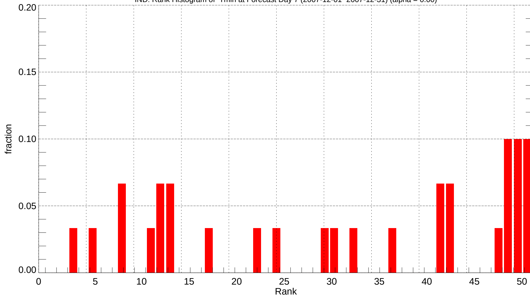
IND: Rank Histogram of Tmin at Forecast Day 7 (2007-12-01~2007-12-31) (alpha = 0.00)
