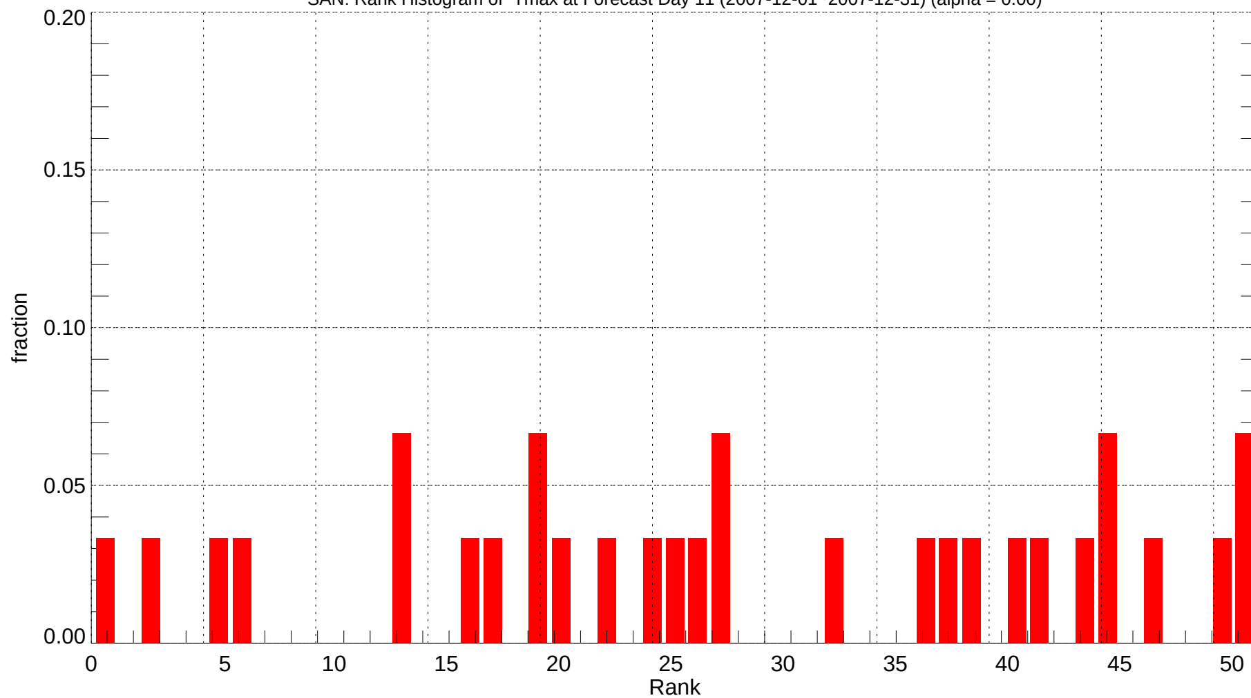
SAN: Rank Histogram of Tmax at Forecast Day 11 (2007-12-01~2007-12-31) (alpha = 0.00)
