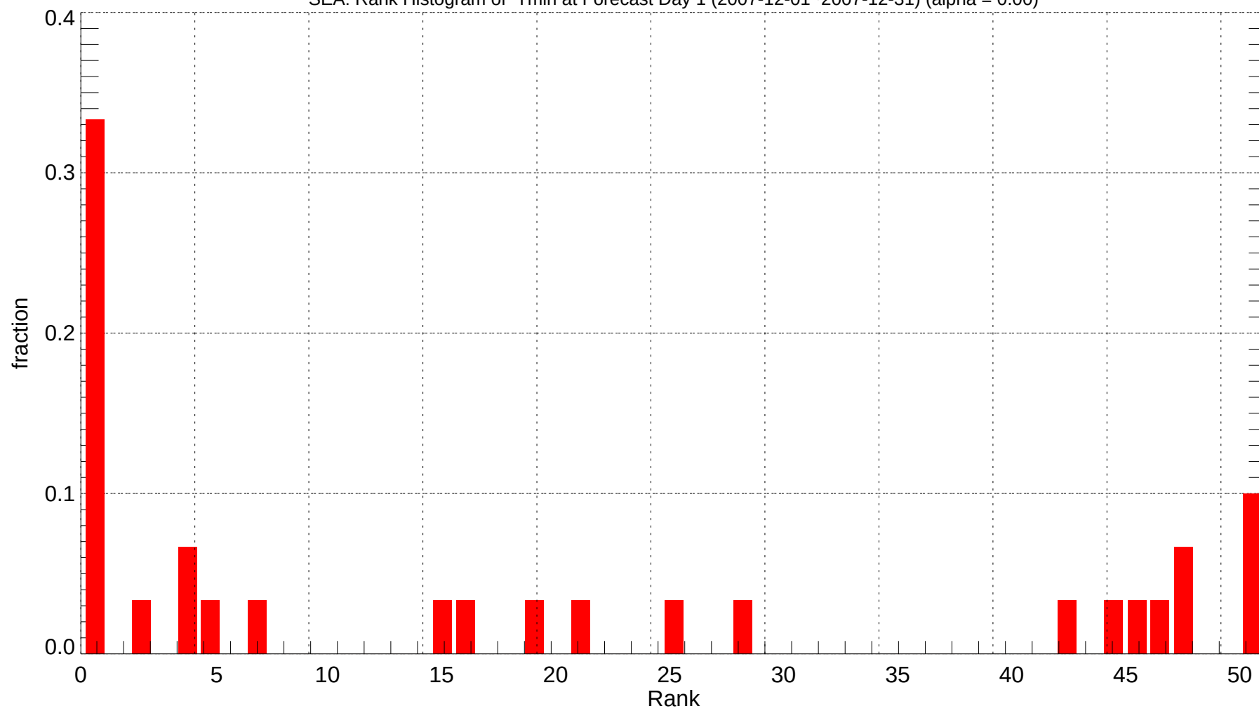
SEA: Rank Histogram of Tmin at Forecast Day 1 (2007-12-01~2007-12-31) (alpha = 0.00)
