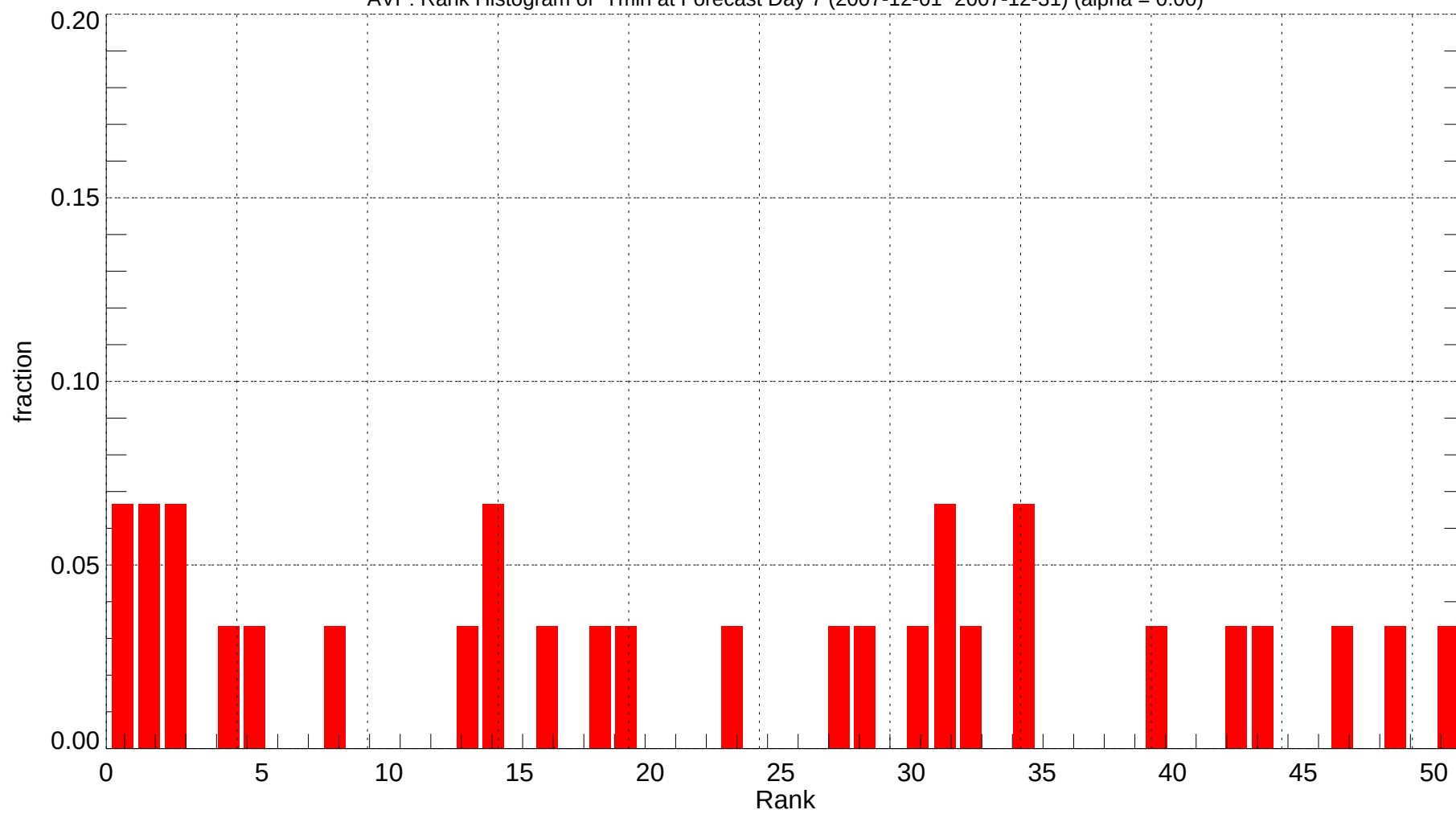
AVP: Rank Histogram of Tmin at Forecast Day 7 (2007-12-01~2007-12-31) (alpha = 0.00)
