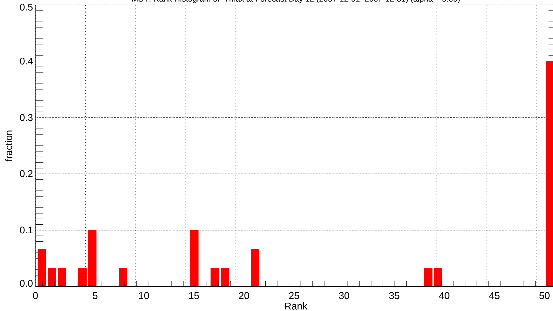
MSY: Rank Histogram of Tmax at Forecast Day 12 (2007-12-01~2007-12-31) (alpha = 0.00)
