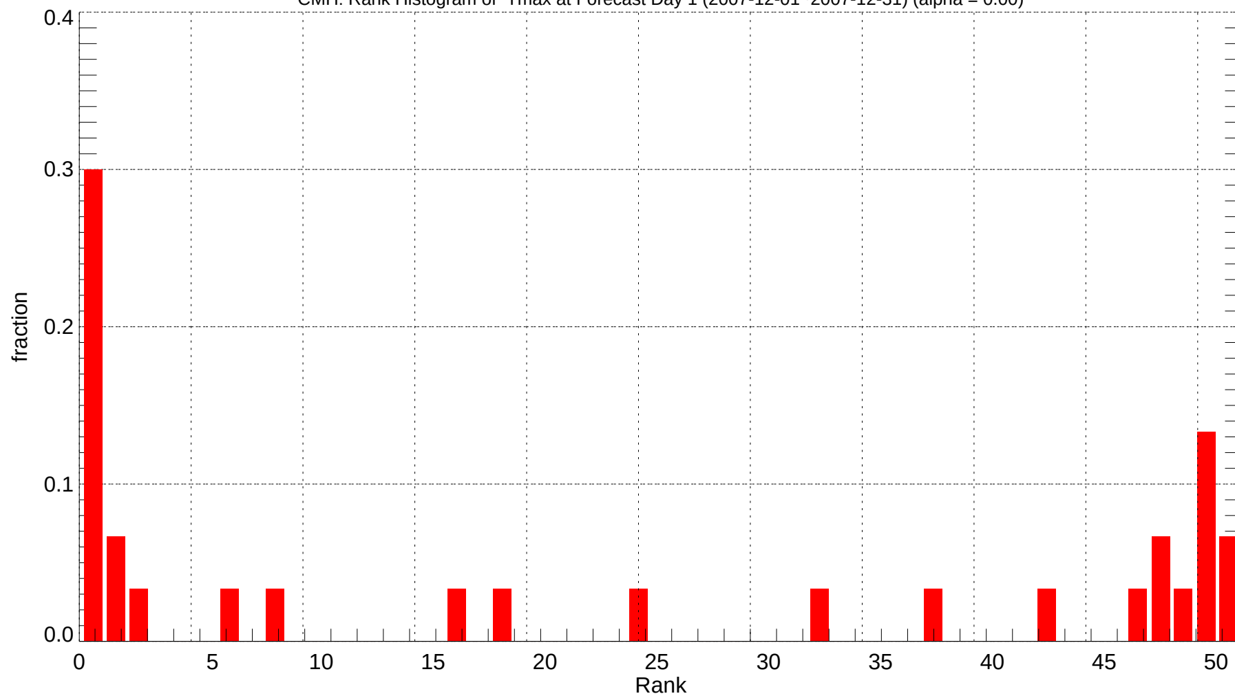
CMH: Rank Histogram of Tmax at Forecast Day 1 (2007-12-01~2007-12-31) (alpha = 0.00)
