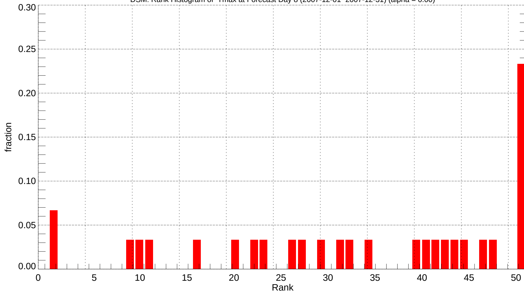
DSM: Rank Histogram of Tmax at Forecast Day 8 (2007-12-01~2007-12-31) (alpha = 0.00)
