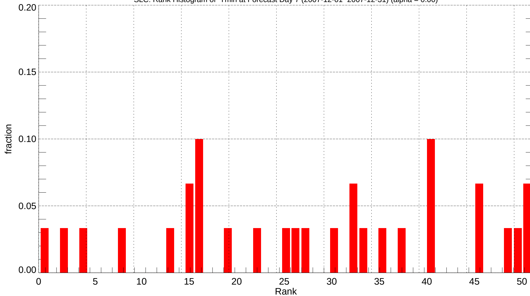
SLC: Rank Histogram of Tmin at Forecast Day 7 (2007-12-01~2007-12-31) (alpha = 0.00)
