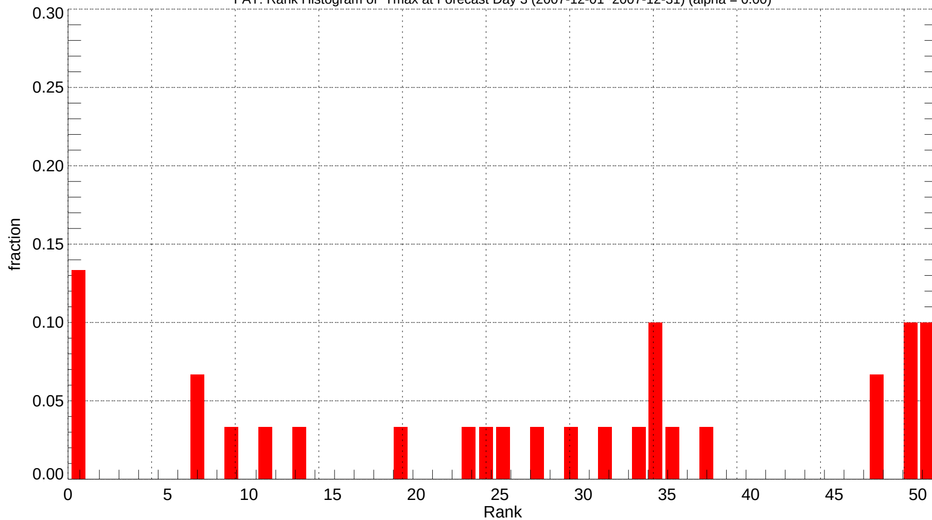
FAT: Rank Histogram of Tmax at Forecast Day 3 (2007-12-01~2007-12-31) (alpha = 0.00)
