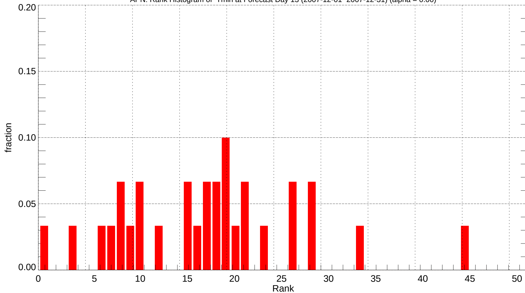
APN: Rank Histogram of Tmin at Forecast Day 13 (2007-12-01~2007-12-31) (alpha = 0.00)
