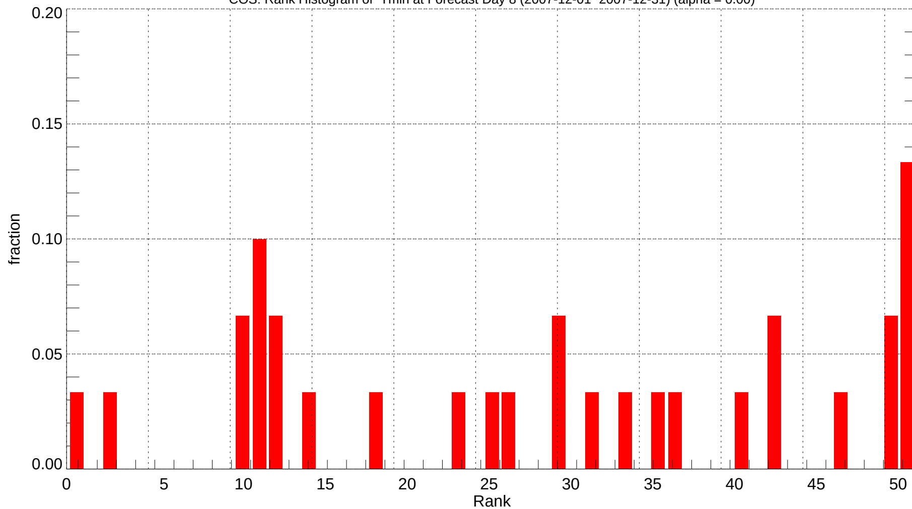
COS: Rank Histogram of Tmin at Forecast Day 8 (2007-12-01~2007-12-31) (alpha = 0.00)
