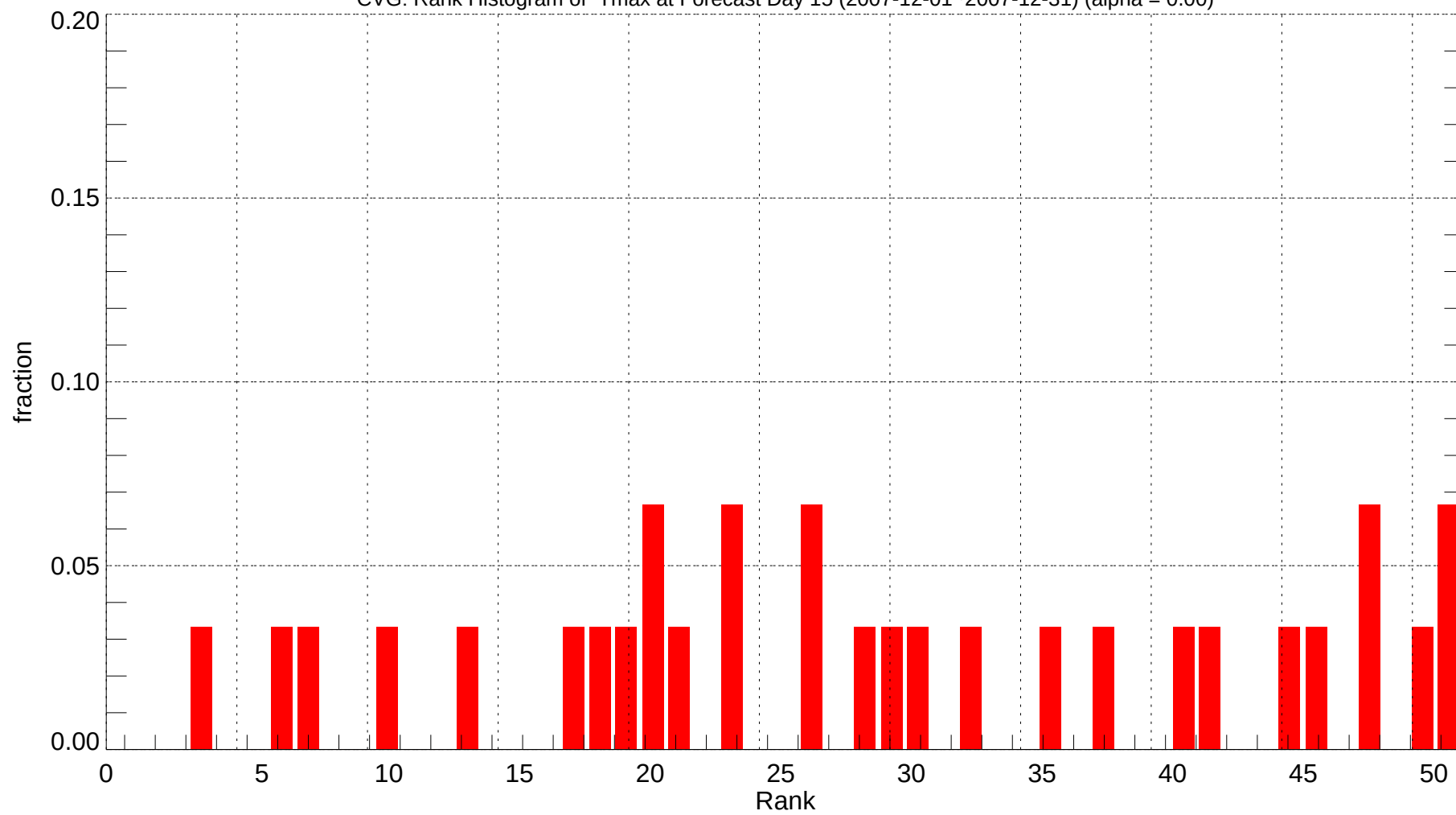
CVG: Rank Histogram of Tmax at Forecast Day 15 (2007-12-01~2007-12-31) (alpha = 0.00)
