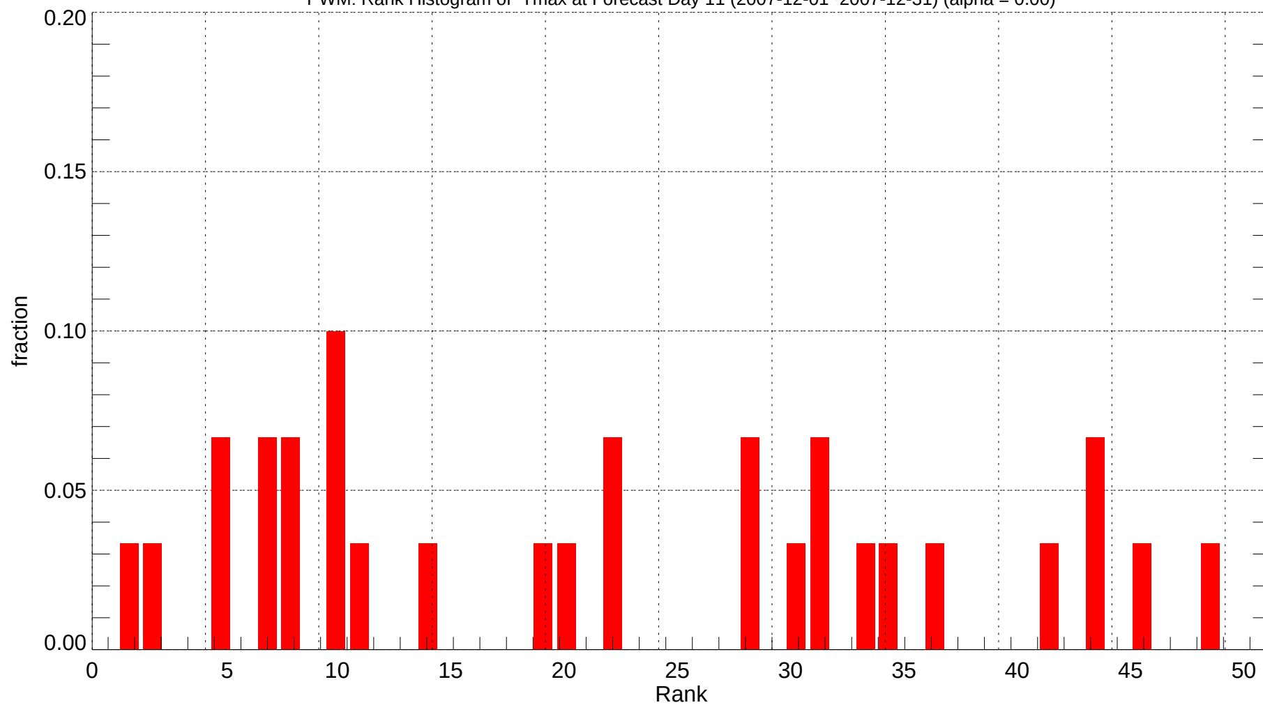
PWM: Rank Histogram of Tmax at Forecast Day 11 (2007-12-01~2007-12-31) (alpha = 0.00)
