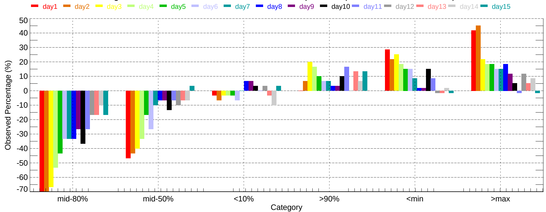
Observed Percentage Deviation of Ensembles - EUG: Max Temperature (2007-12-01~2007-12-31)
