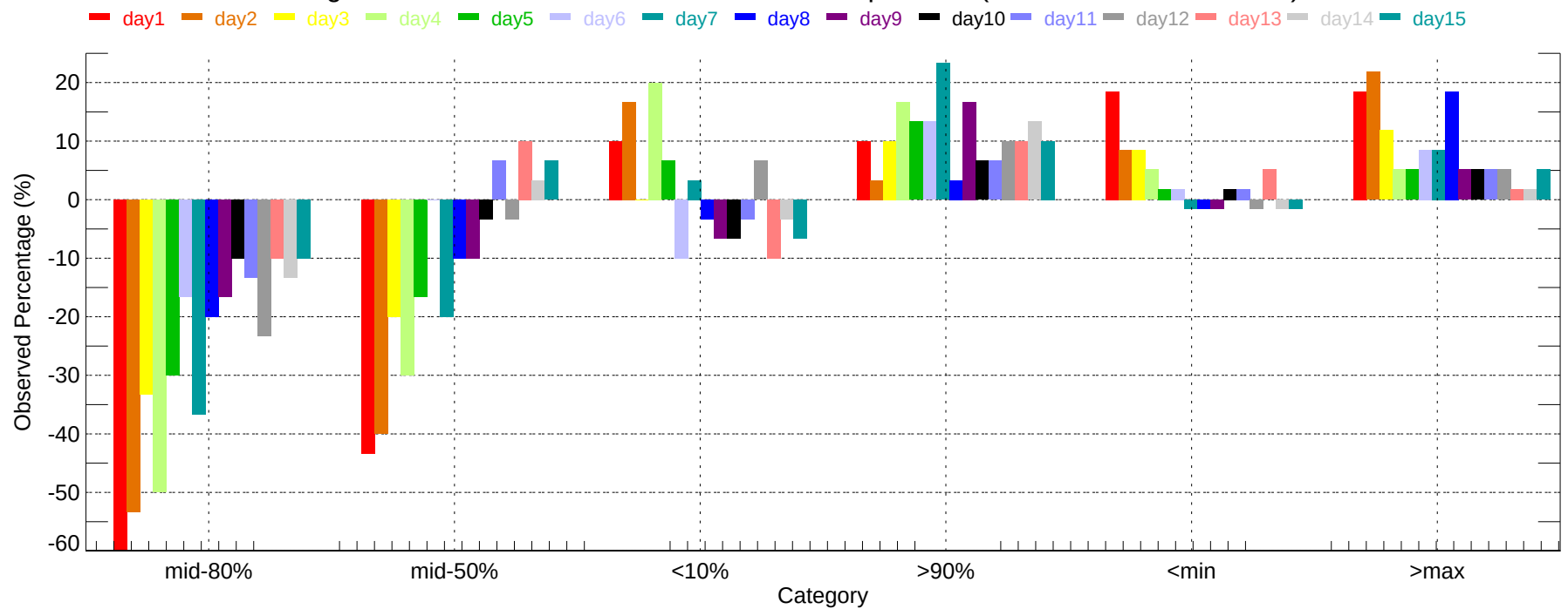
Observed Percentage Deviation of Ensembles - CVG: Min Temperature (2007-12-01~2007-12-31)
