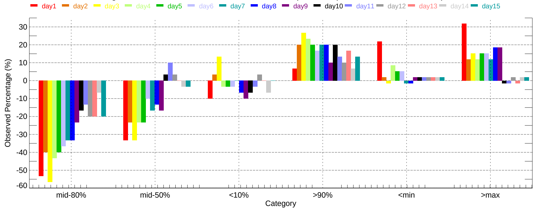
Observed Percentage Deviation of Ensembles - TPA: Max Temperature (2007-12-01~2007-12-31)
