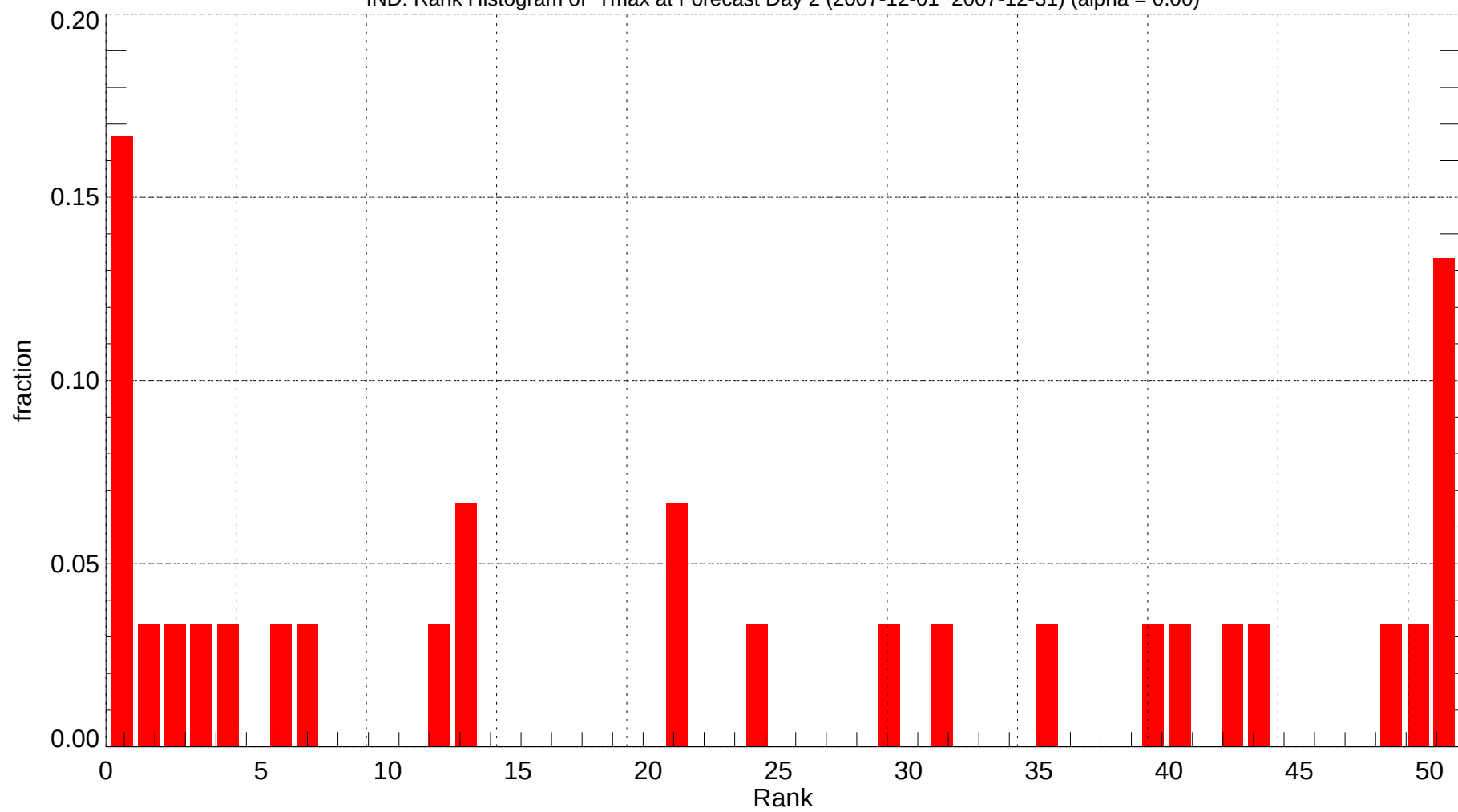
IND: Rank Histogram of Tmax at Forecast Day 2 (2007-12-01~2007-12-31) (alpha = 0.00)
