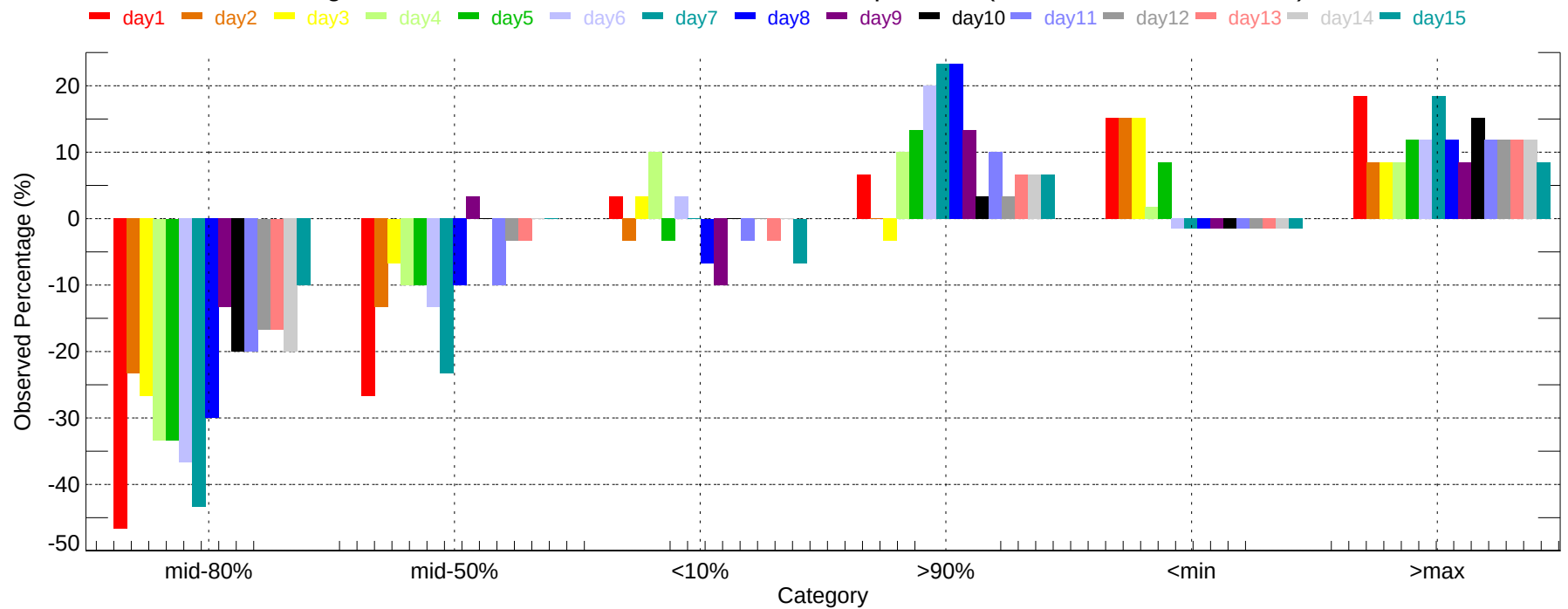
Observed Percentage Deviation of Ensembles - CHA: Max Temperature (2007-12-01~2007-12-31)
