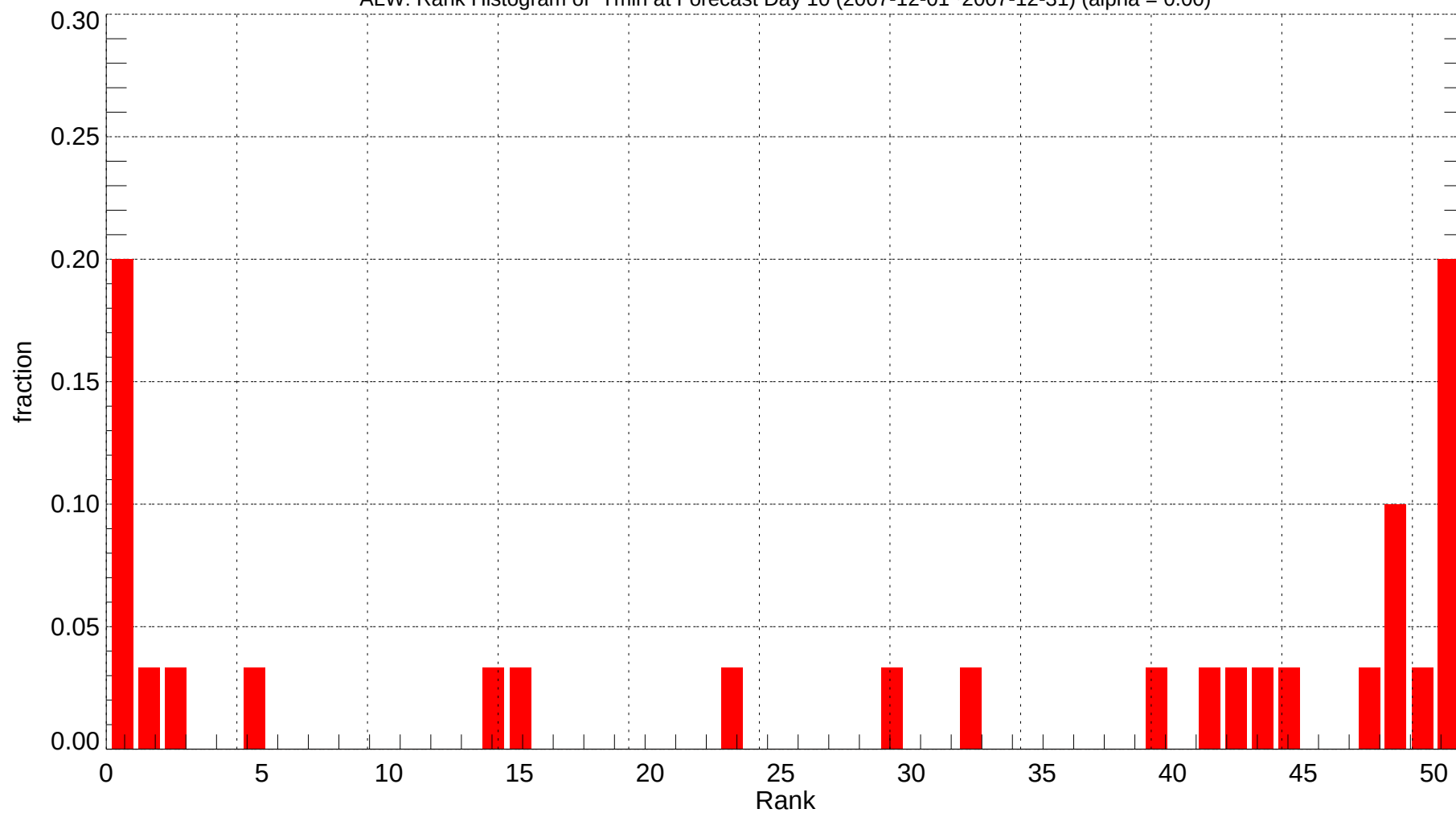
ALW: Rank Histogram of Tmin at Forecast Day 10 (2007-12-01~2007-12-31) (alpha = 0.00)
