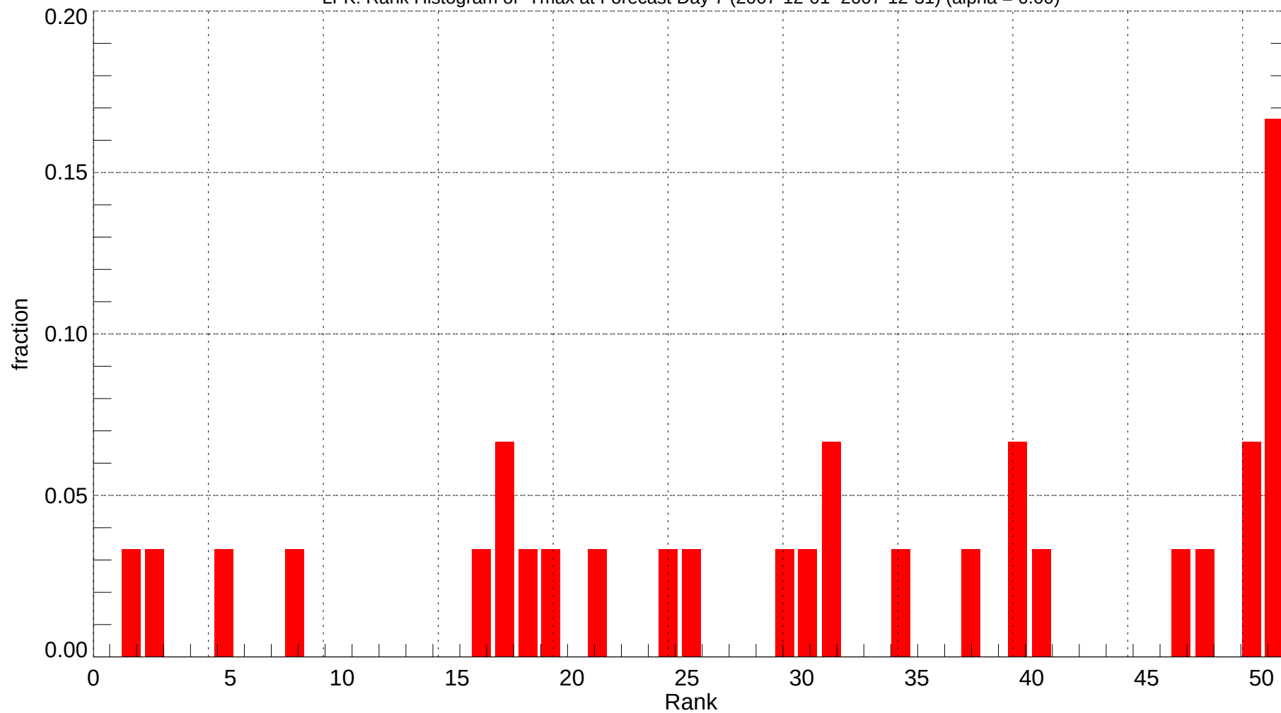
LFK: Rank Histogram of Tmax at Forecast Day 7 (2007-12-01~2007-12-31) (alpha = 0.00)
