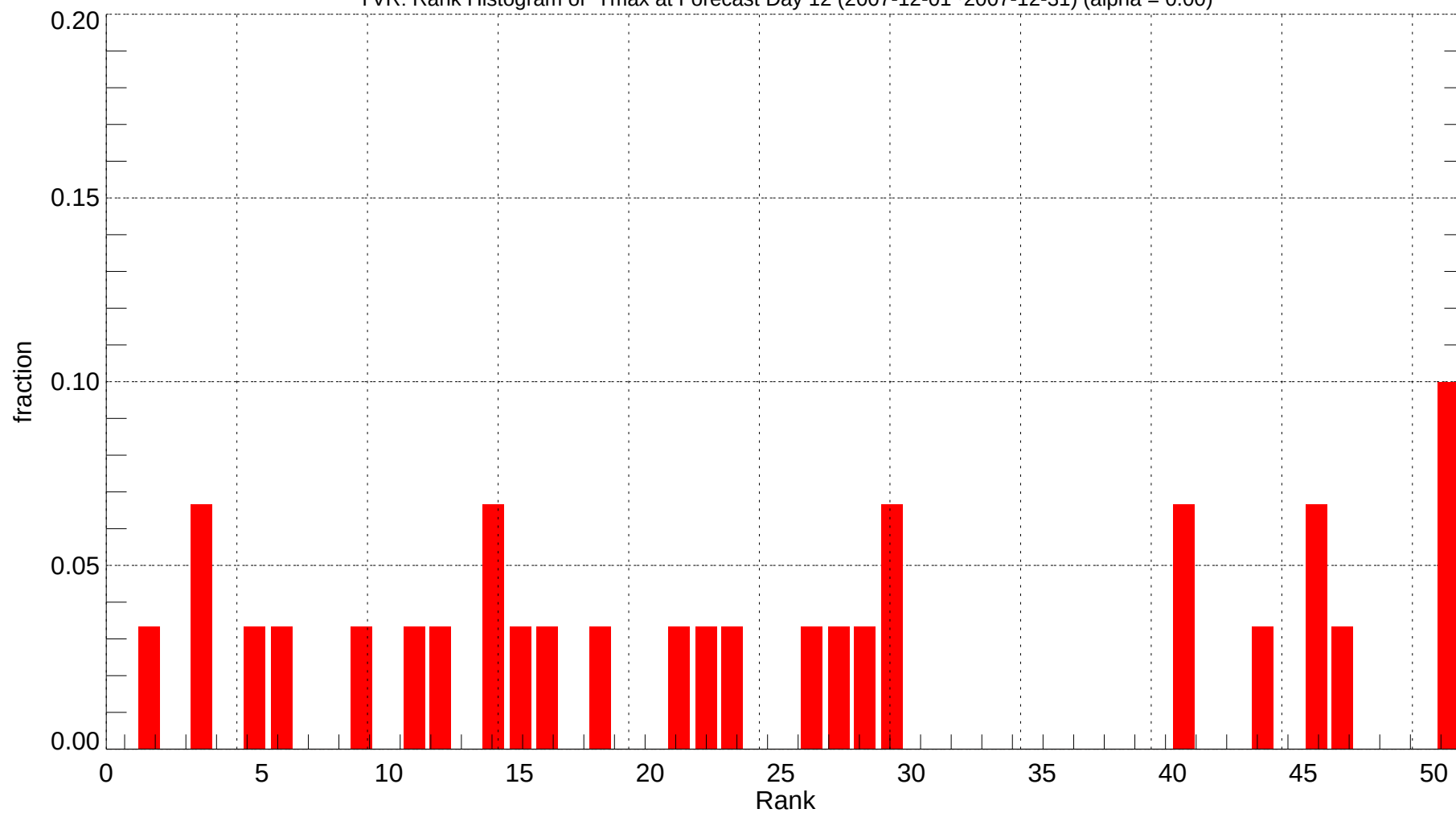
YVR: Rank Histogram of Tmax at Forecast Day 12 (2007-12-01~2007-12-31) (alpha = 0.00)
