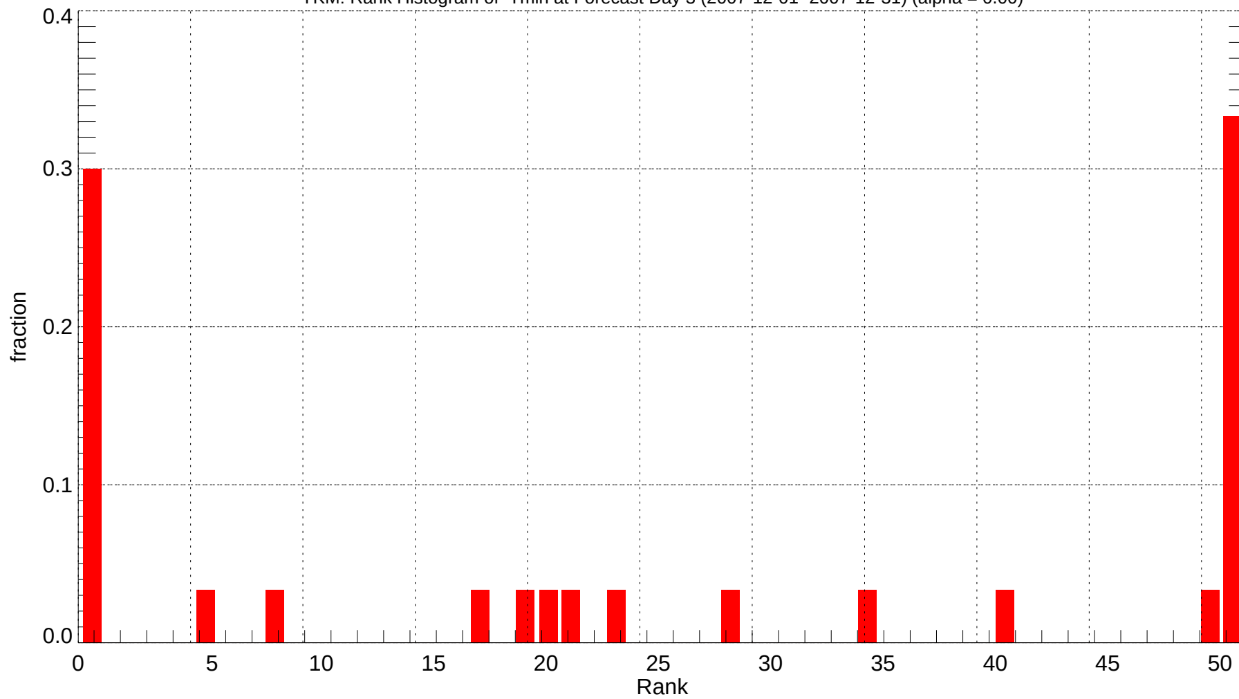
YKM: Rank Histogram of Tmin at Forecast Day 3 (2007-12-01~2007-12-31) (alpha = 0.00)
