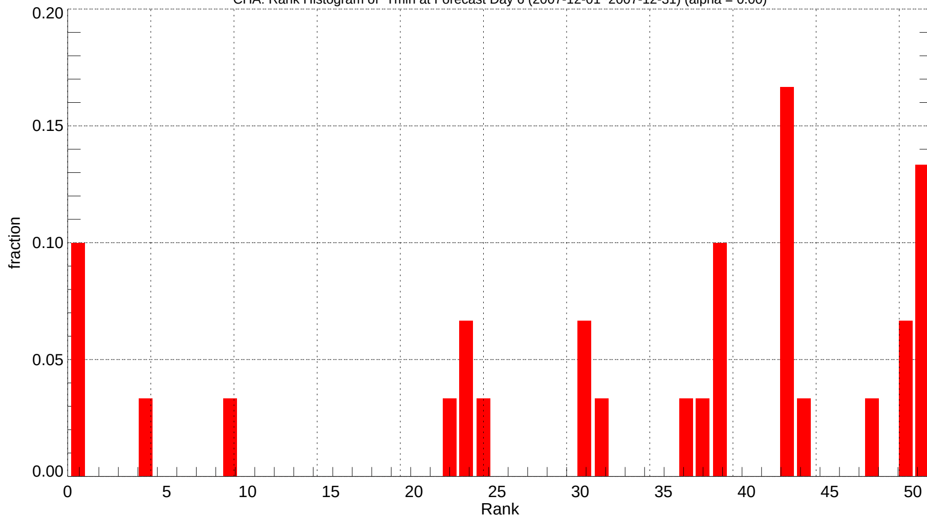
CHA: Rank Histogram of Tmin at Forecast Day 6 (2007-12-01~2007-12-31) (alpha = 0.00)
