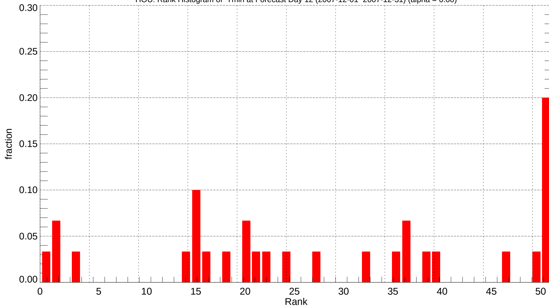
HOU: Rank Histogram of Tmin at Forecast Day 12 (2007-12-01~2007-12-31) (alpha = 0.00)
