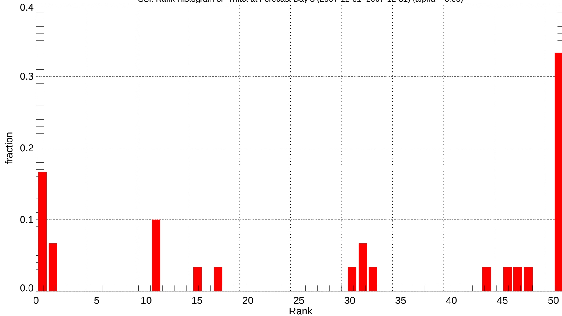
SSI: Rank Histogram of Tmax at Forecast Day 5 (2007-12-01~2007-12-31) (alpha = 0.00)
