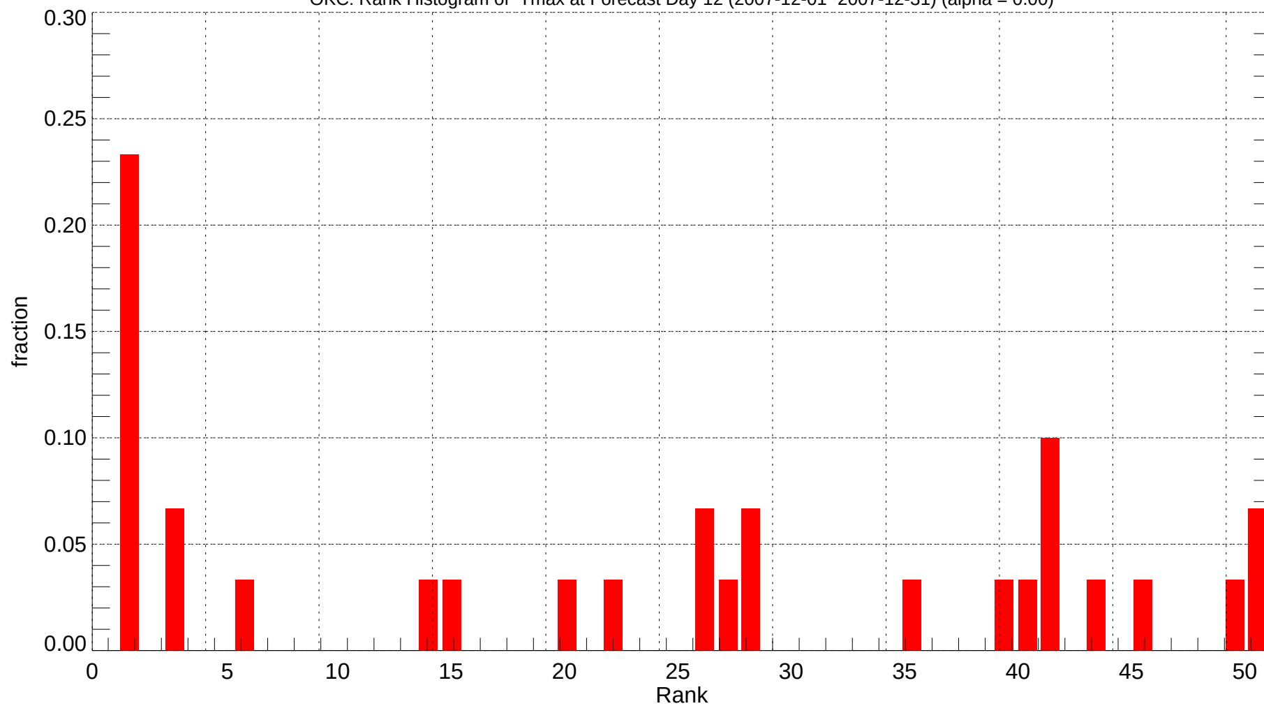
OKC: Rank Histogram of Tmax at Forecast Day 12 (2007-12-01~2007-12-31) (alpha = 0.00)
