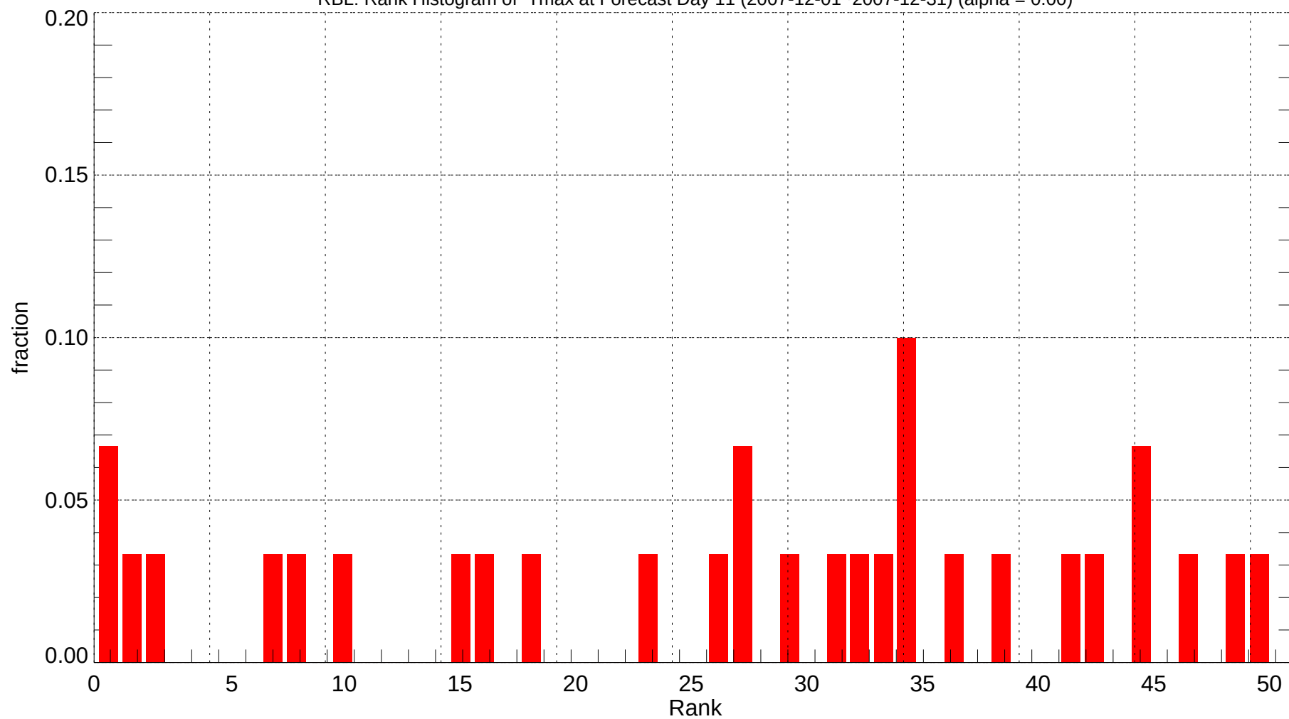
RBL: Rank Histogram of Tmax at Forecast Day 11 (2007-12-01~2007-12-31) (alpha = 0.00)
