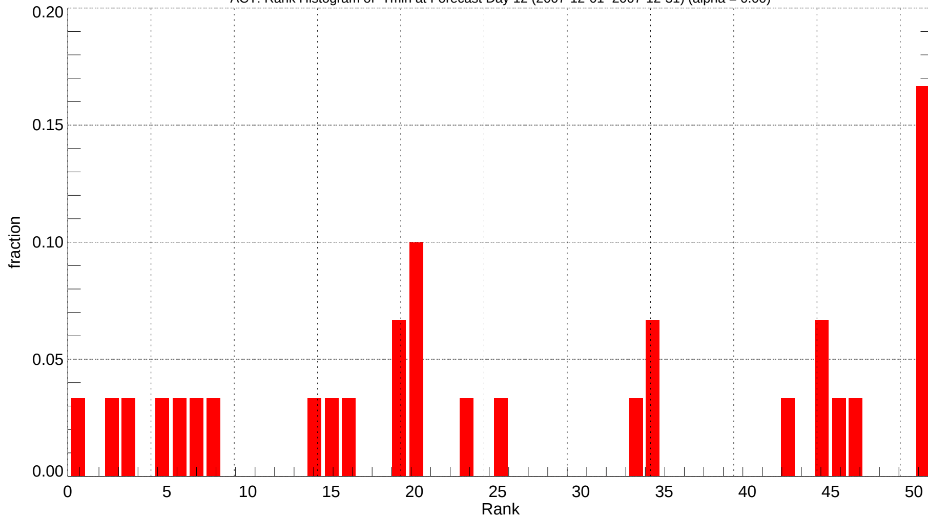
ACT: Rank Histogram of Tmin at Forecast Day 12 (2007-12-01~2007-12-31) (alpha = 0.00)
