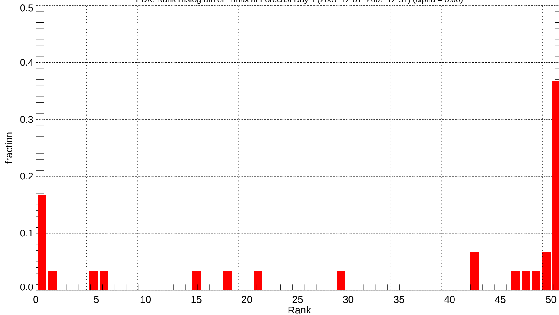
PDX: Rank Histogram of Tmax at Forecast Day 1 (2007-12-01~2007-12-31) (alpha = 0.00)
