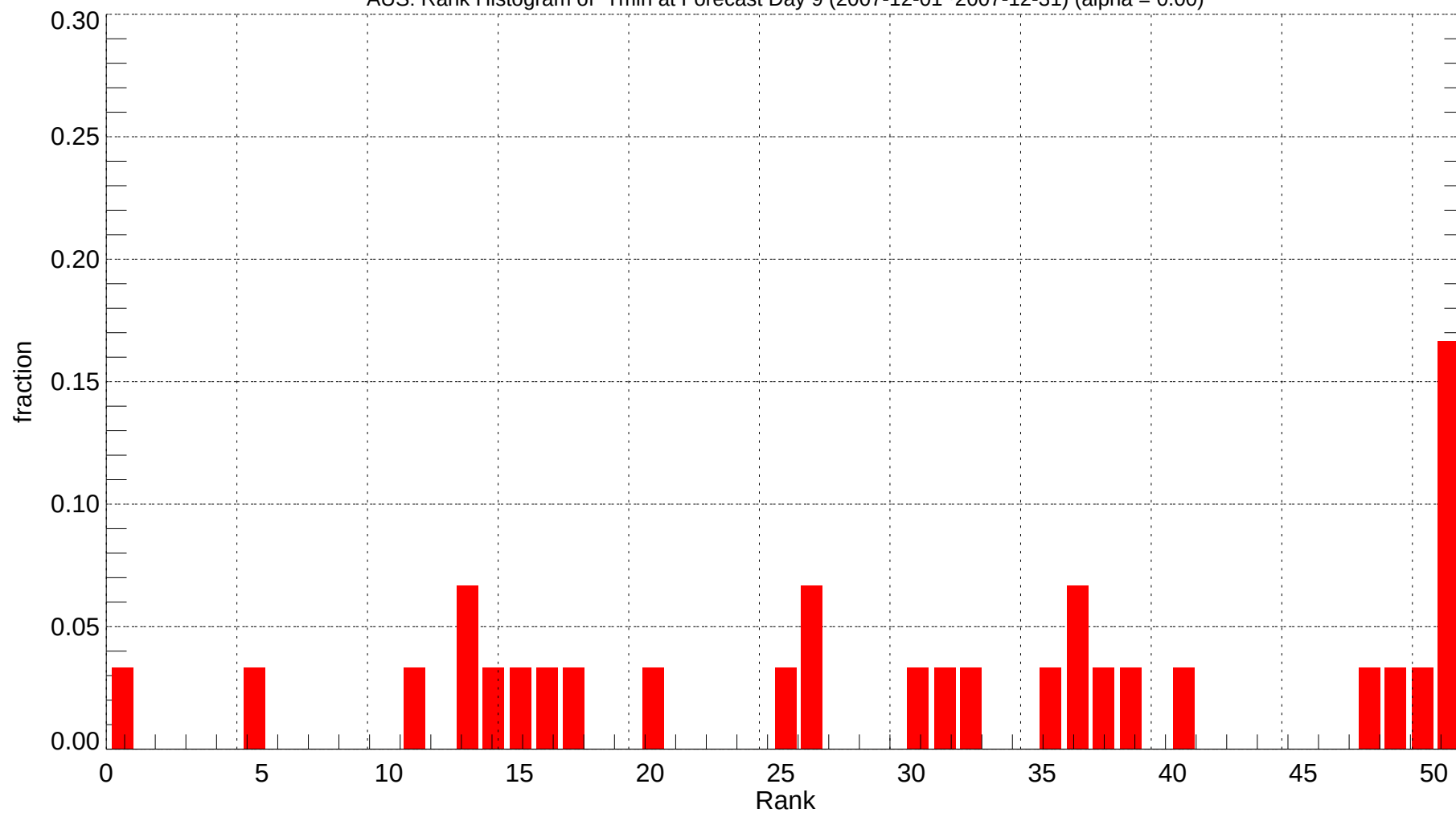
AUS: Rank Histogram of Tmin at Forecast Day 9 (2007-12-01~2007-12-31) (alpha = 0.00)
