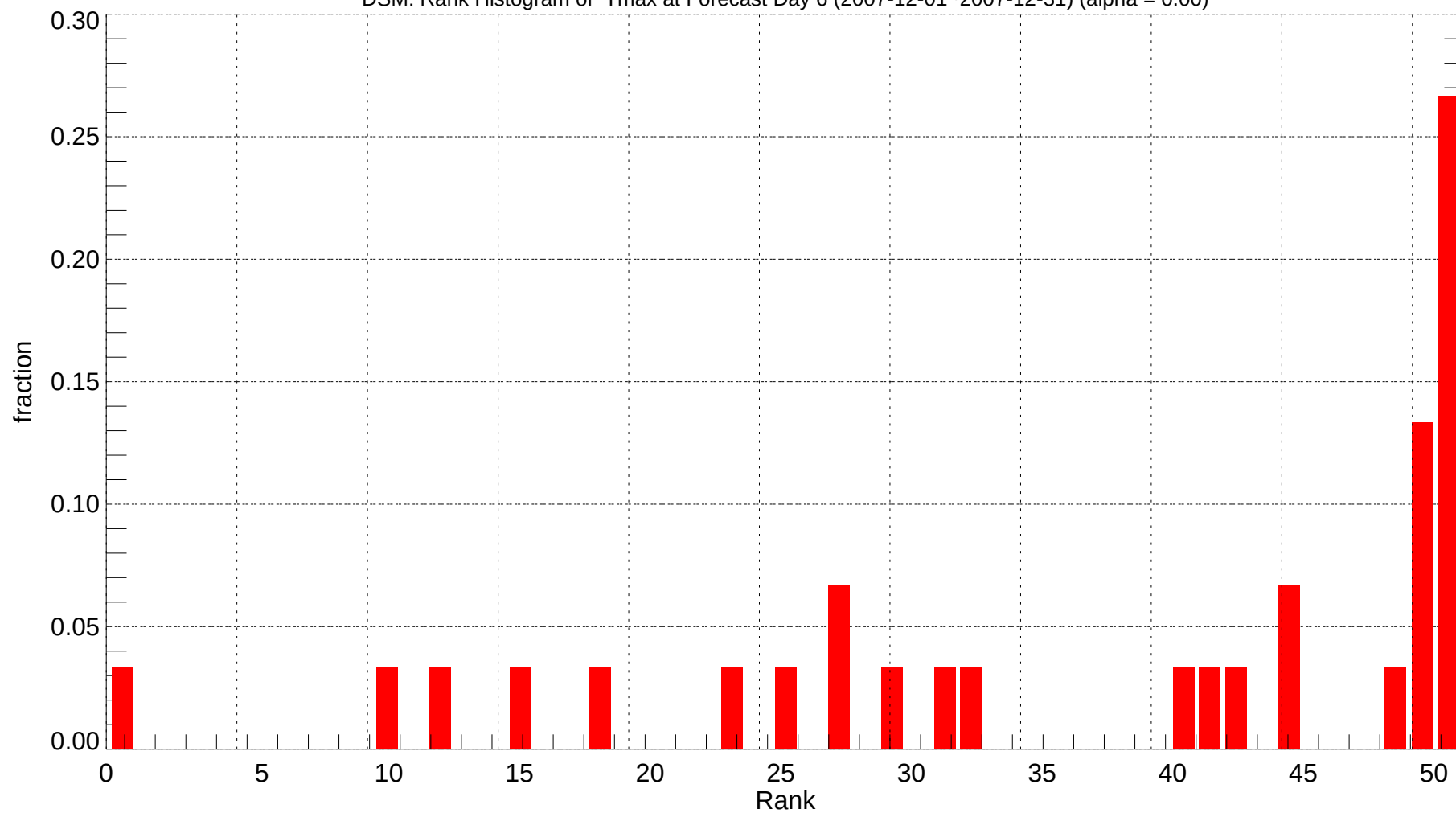
DSM: Rank Histogram of Tmax at Forecast Day 6 (2007-12-01~2007-12-31) (alpha = 0.00)
