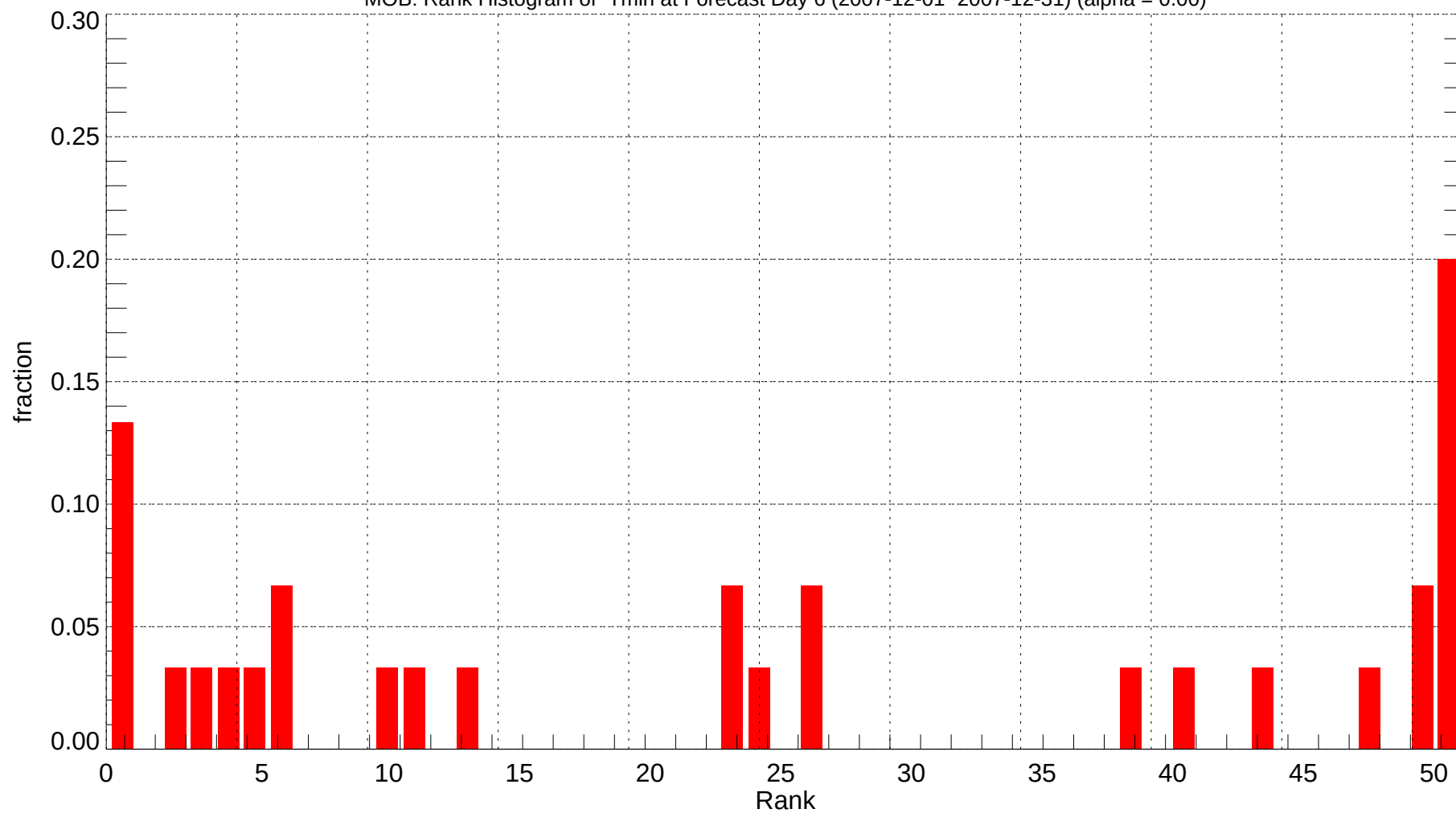
MOB: Rank Histogram of Tmin at Forecast Day 6 (2007-12-01~2007-12-31) (alpha = 0.00)
