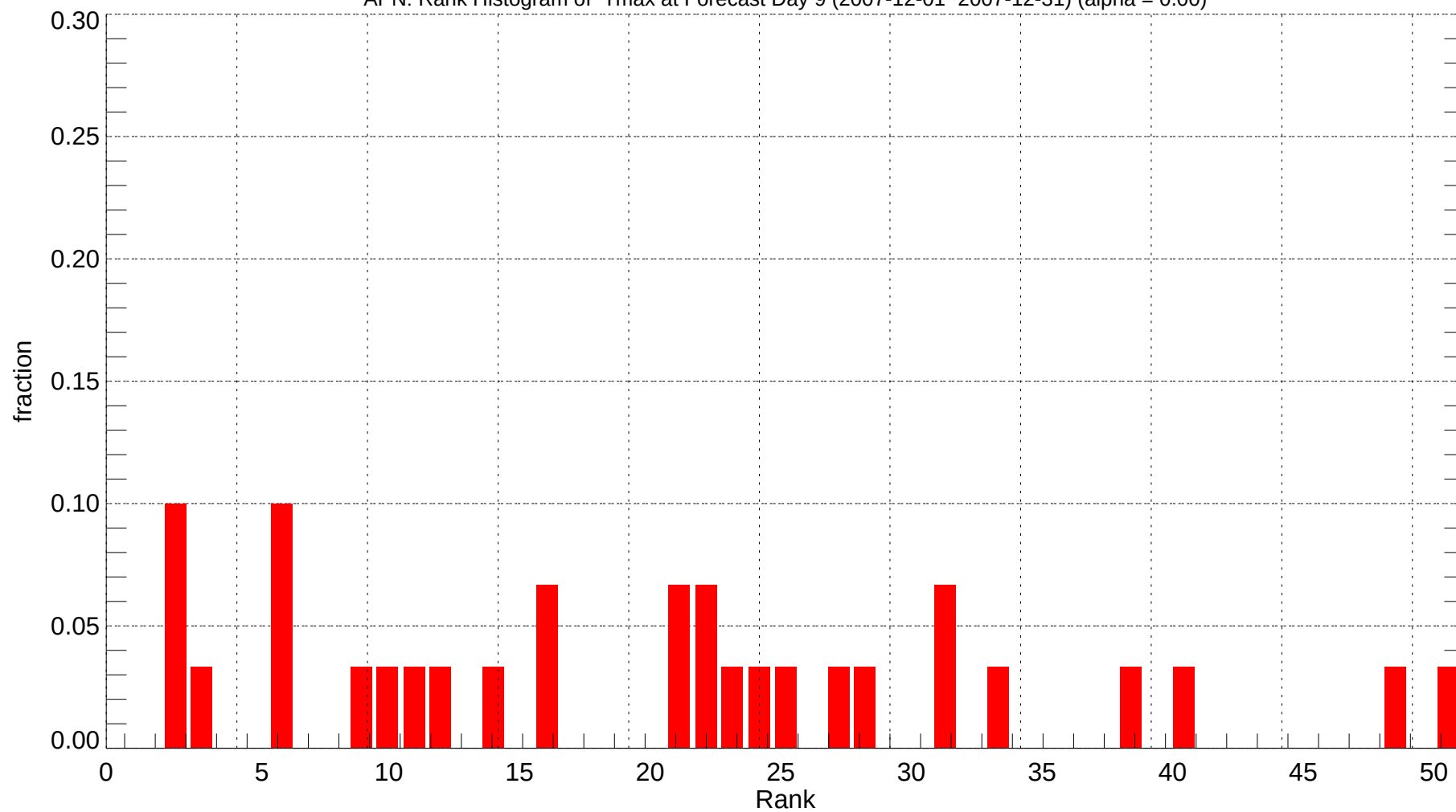
APN: Rank Histogram of Tmax at Forecast Day 9 (2007-12-01~2007-12-31) (alpha = 0.00)
