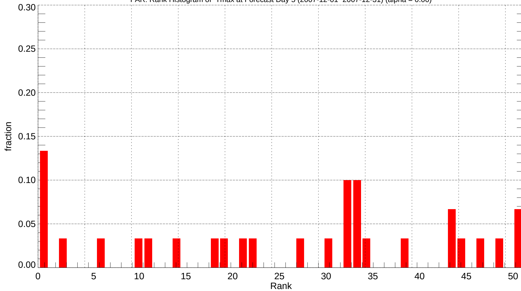
FAR: Rank Histogram of Tmax at Forecast Day 5 (2007-12-01~2007-12-31) (alpha = 0.00)
