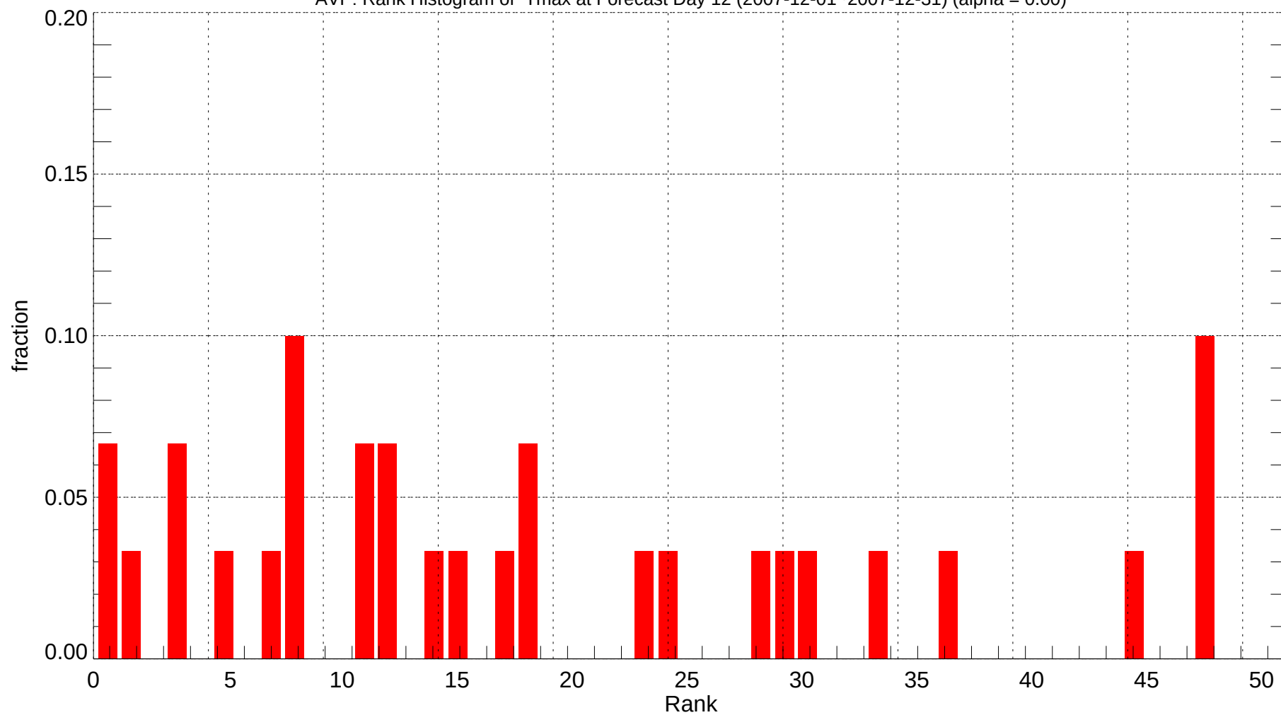
AVP: Rank Histogram of Tmax at Forecast Day 12 (2007-12-01~2007-12-31) (alpha = 0.00)
