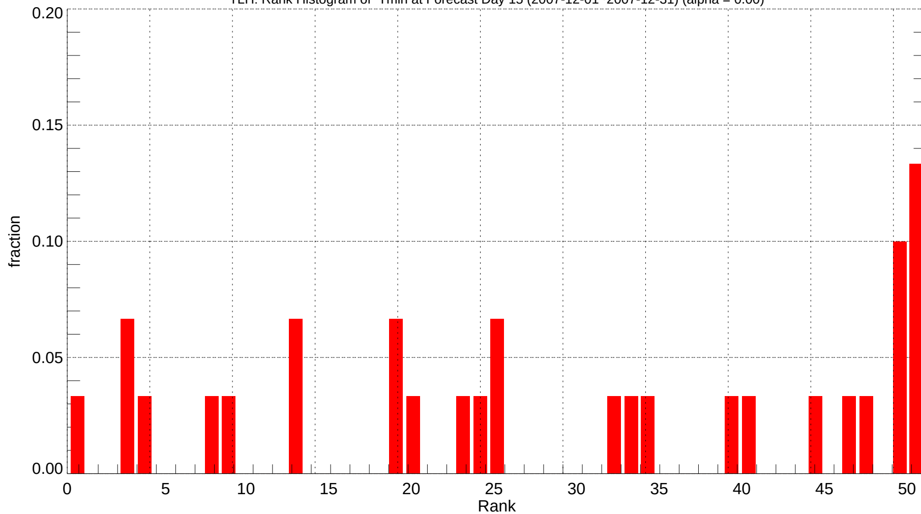
TLH: Rank Histogram of Tmin at Forecast Day 15 (2007-12-01~2007-12-31) (alpha = 0.00)
