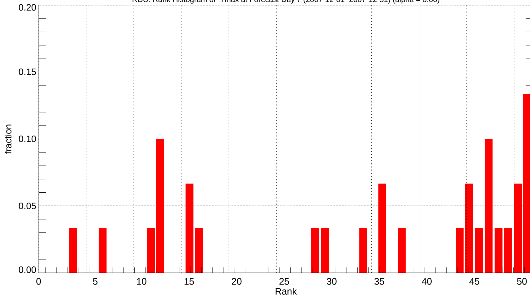
RDU: Rank Histogram of Tmax at Forecast Day 7 (2007-12-01~2007-12-31) (alpha = 0.00)
