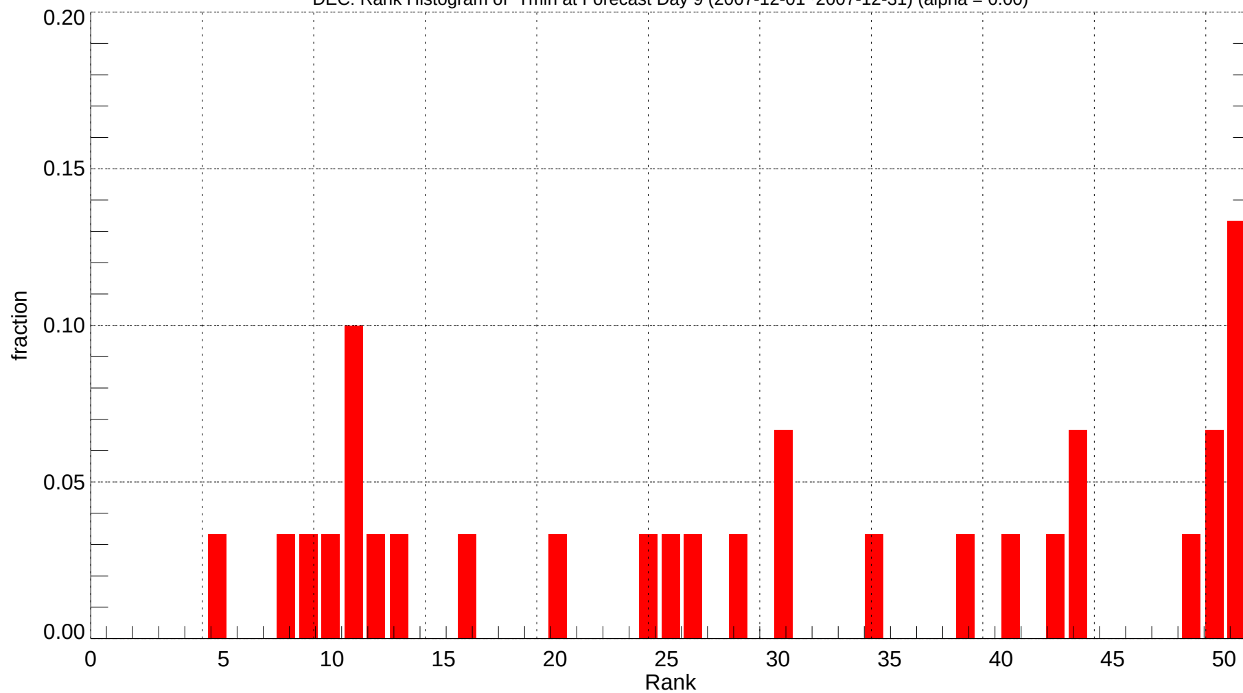
DEC: Rank Histogram of Tmin at Forecast Day 9 (2007-12-01~2007-12-31) (alpha = 0.00)
