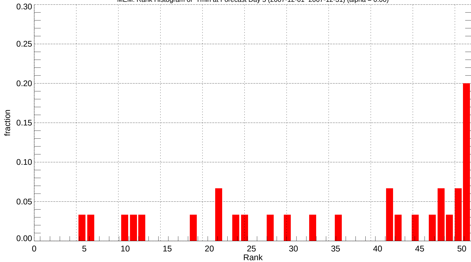
MEM: Rank Histogram of Tmin at Forecast Day 5 (2007-12-01~2007-12-31) (alpha = 0.00)
