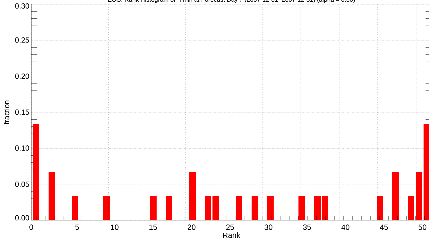
EUG: Rank Histogram of Tmin at Forecast Day 7 (2007-12-01~2007-12-31) (alpha = 0.00)
