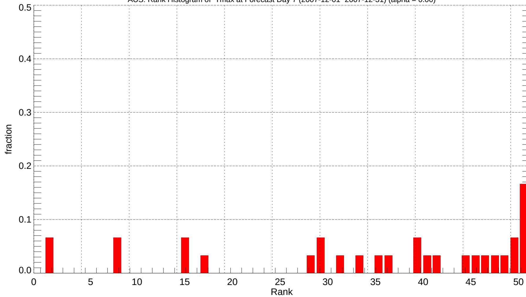
AUS: Rank Histogram of Tmax at Forecast Day 7 (2007-12-01~2007-12-31) (alpha = 0.00)
