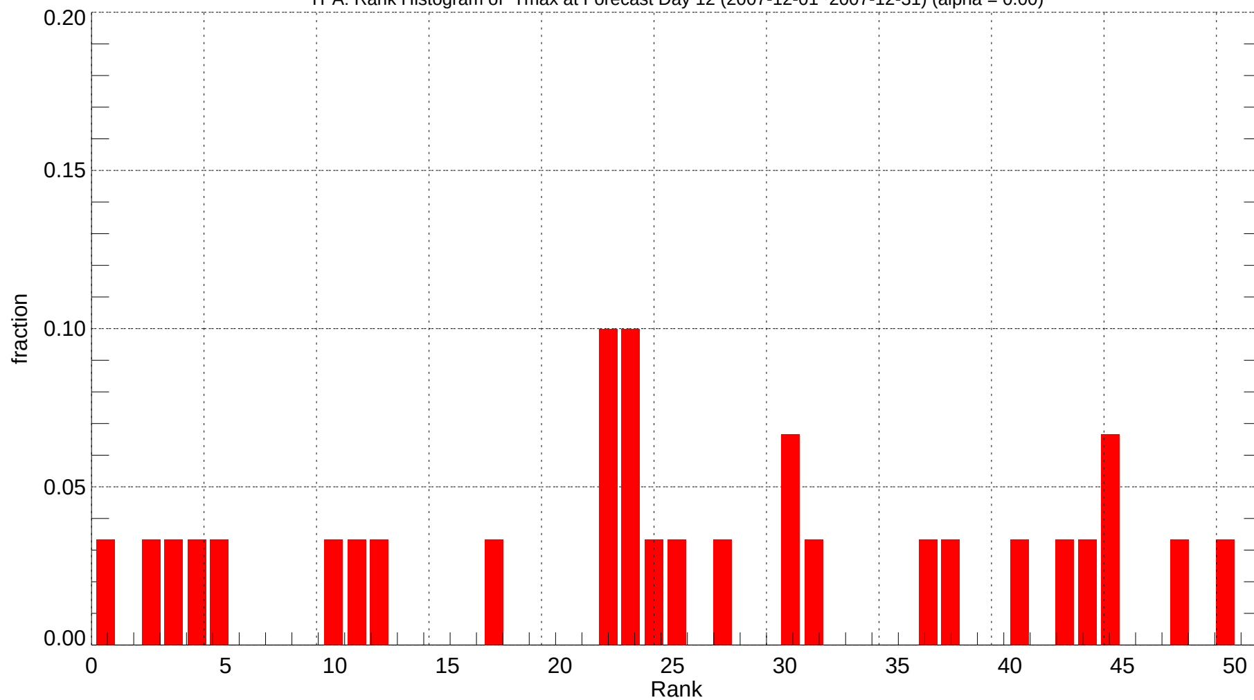
TPA: Rank Histogram of Tmax at Forecast Day 12 (2007-12-01~2007-12-31) (alpha = 0.00)
