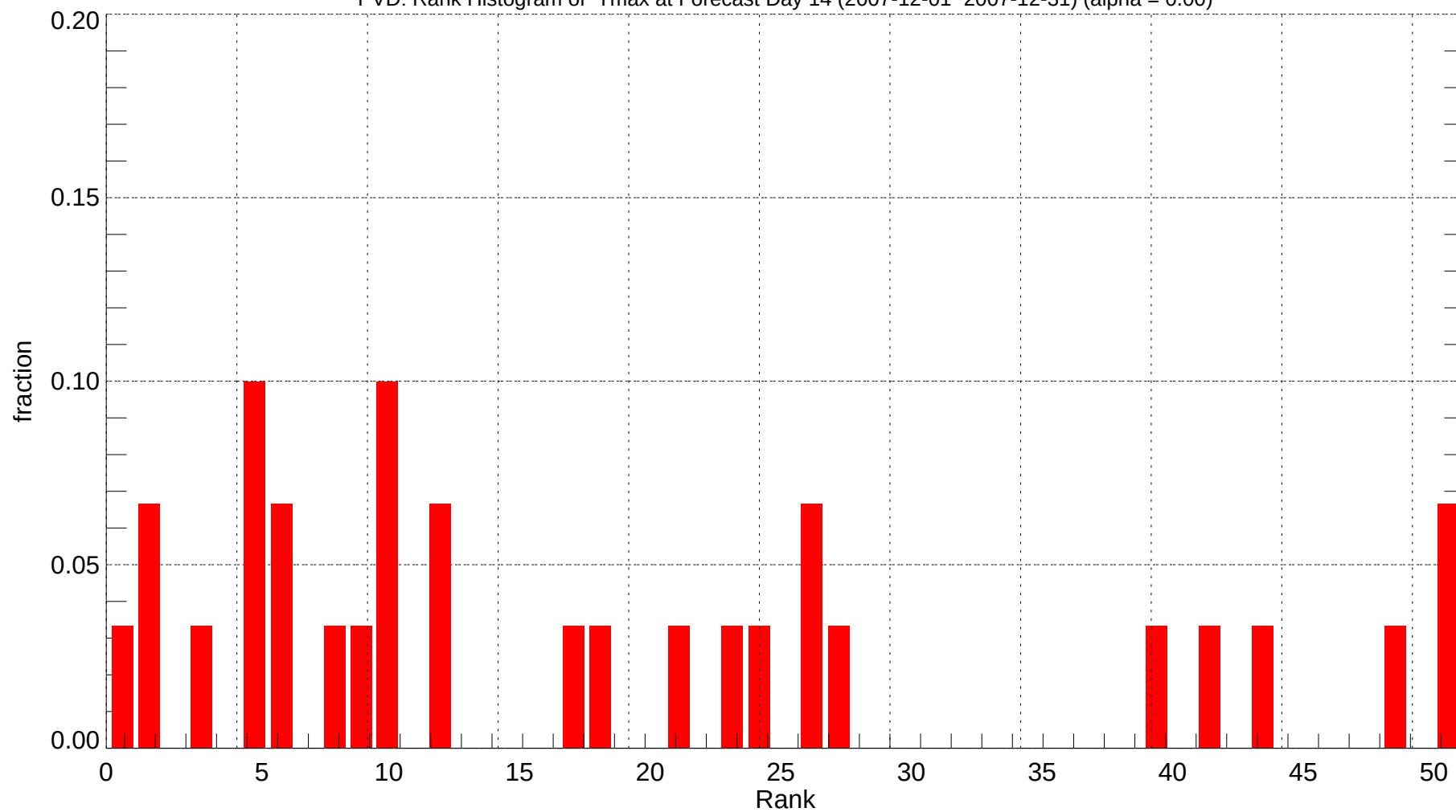
PVD: Rank Histogram of Tmax at Forecast Day 14 (2007-12-01~2007-12-31) (alpha = 0.00)
