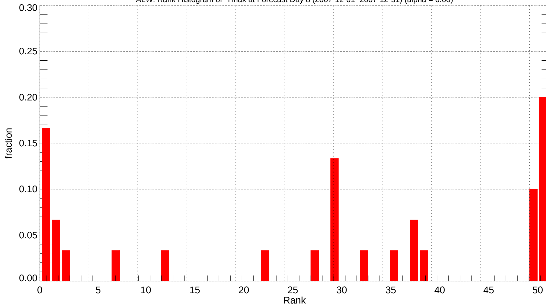
ALW: Rank Histogram of Tmax at Forecast Day 8 (2007-12-01~2007-12-31) (alpha = 0.00)
