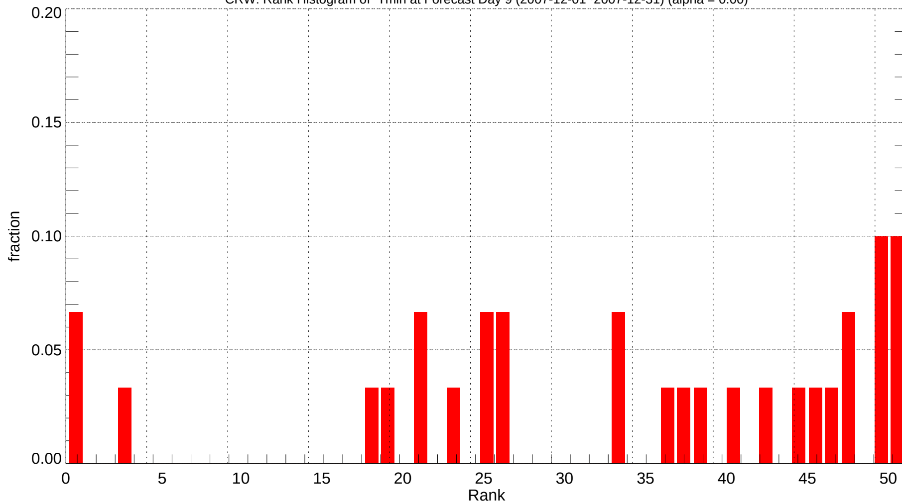
CRW: Rank Histogram of Tmin at Forecast Day 9 (2007-12-01~2007-12-31) (alpha = 0.00)
