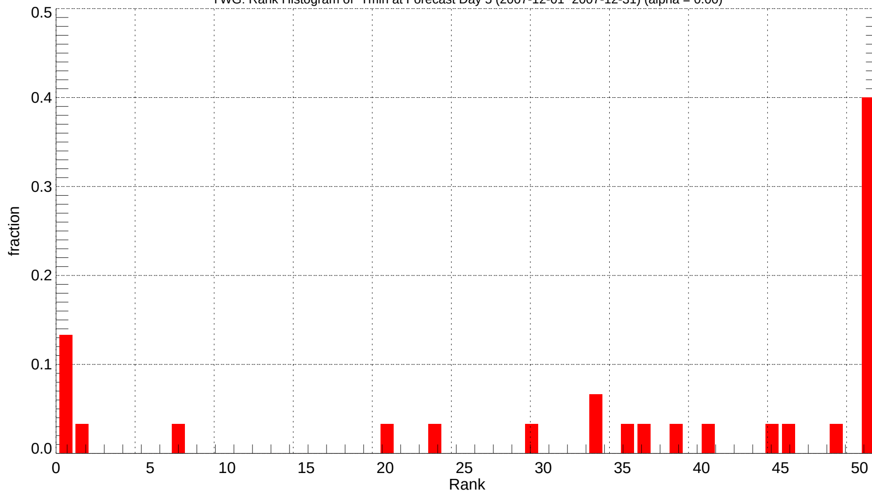
YWG: Rank Histogram of Tmin at Forecast Day 5 (2007-12-01~2007-12-31) (alpha = 0.00)
