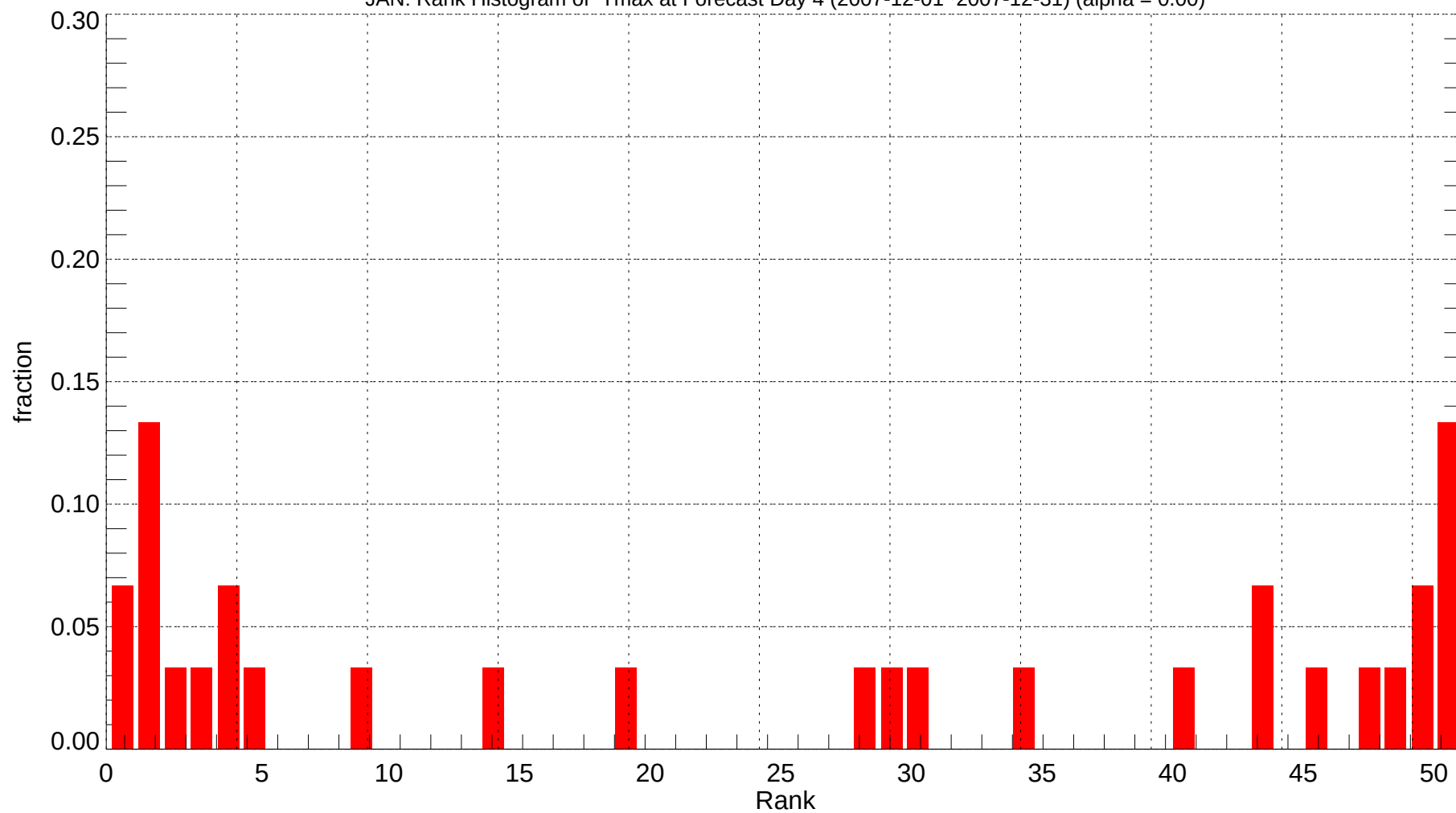
JAN: Rank Histogram of Tmax at Forecast Day 4 (2007-12-01~2007-12-31) (alpha = 0.00)
