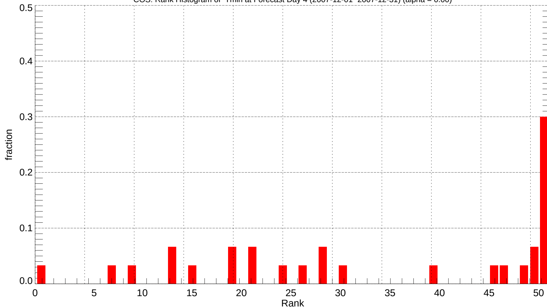
COS: Rank Histogram of Tmin at Forecast Day 4 (2007-12-01~2007-12-31) (alpha = 0.00)
