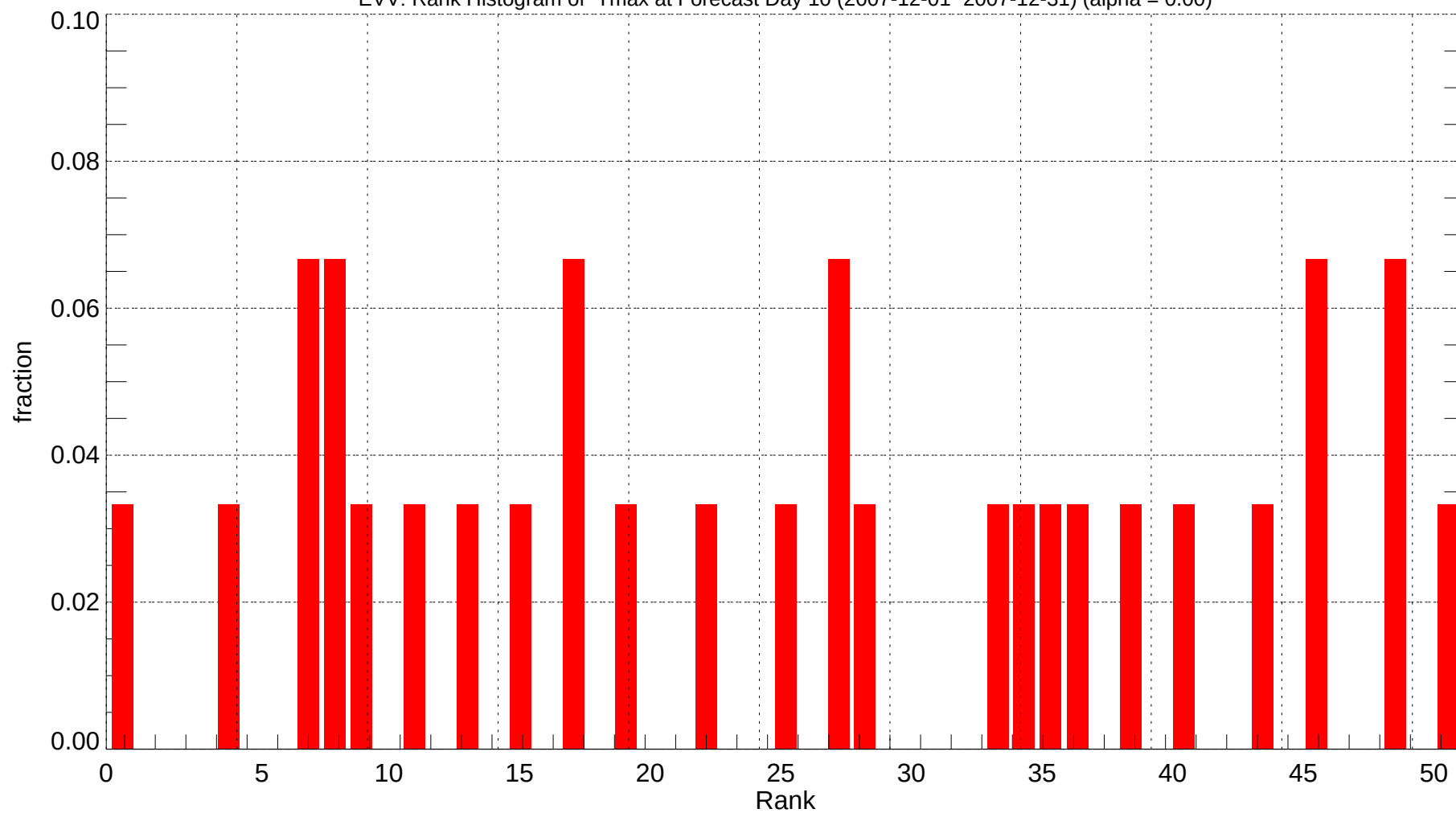
EVV: Rank Histogram of Tmax at Forecast Day 10 (2007-12-01~2007-12-31) (alpha = 0.00)
