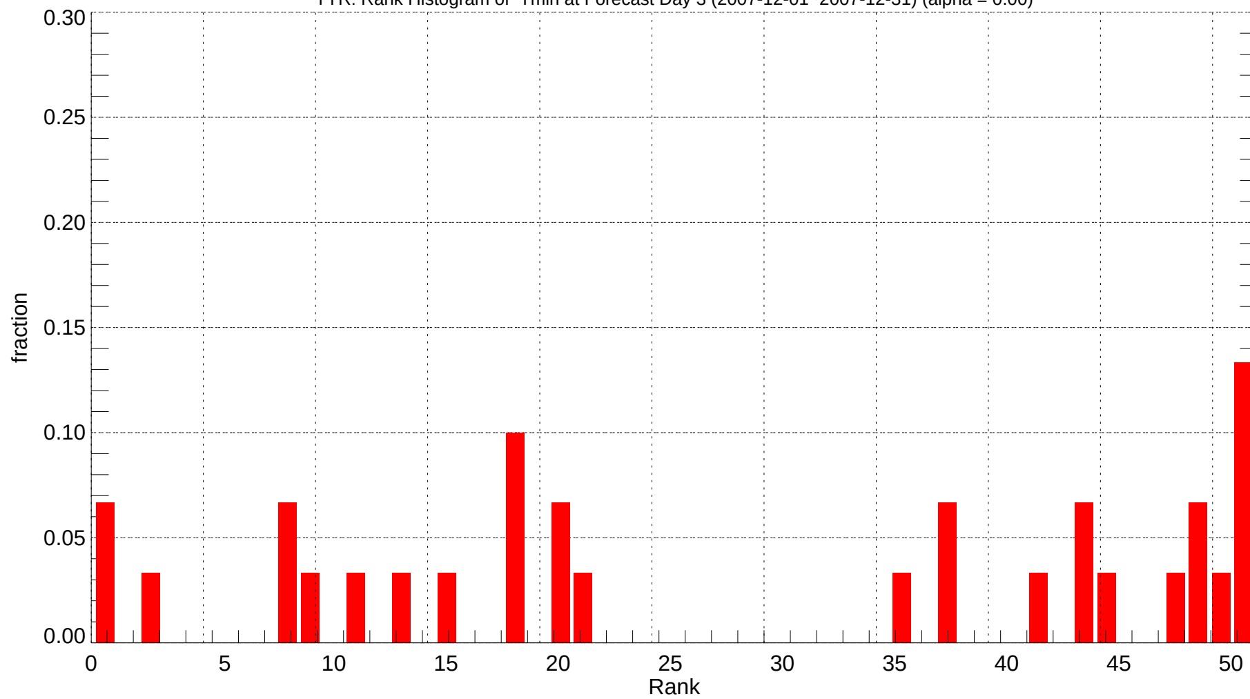
TYR: Rank Histogram of Tmin at Forecast Day 3 (2007-12-01~2007-12-31) (alpha = 0.00)
