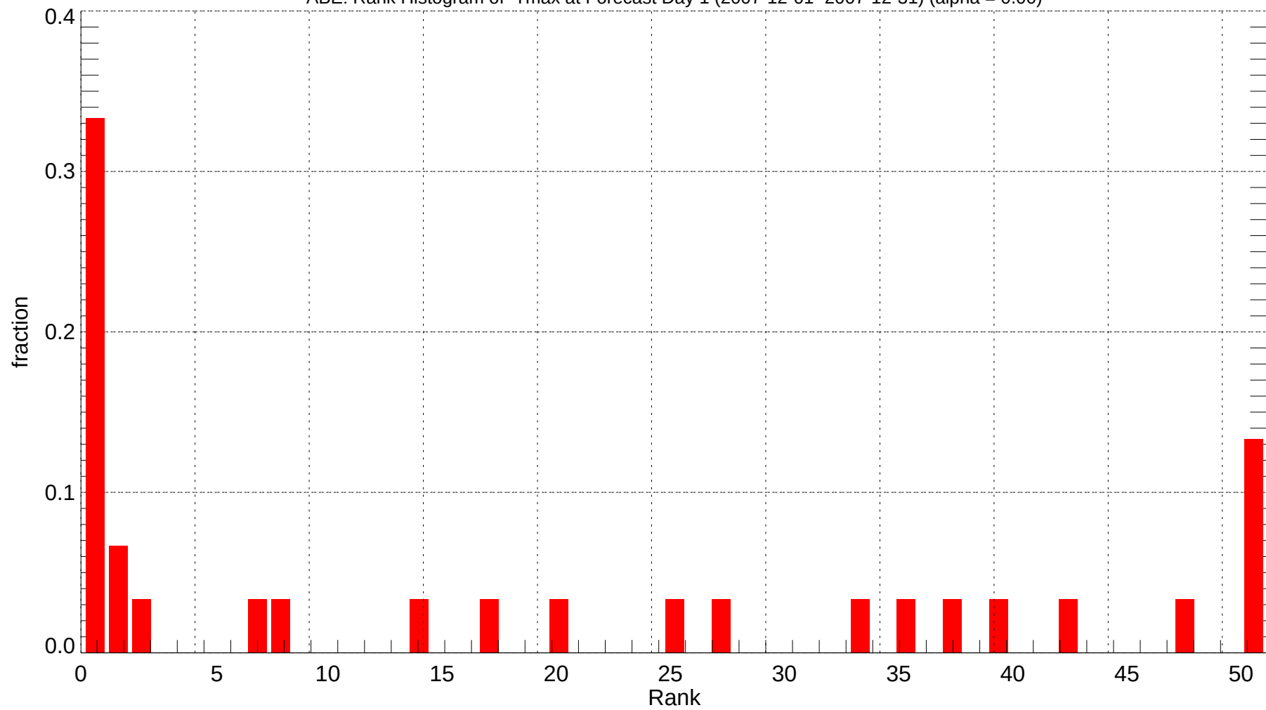
ABE: Rank Histogram of Tmax at Forecast Day 1 (2007-12-01~2007-12-31) (alpha = 0.00)
