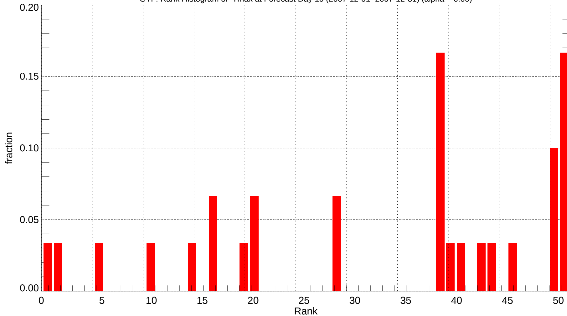
GTF: Rank Histogram of Tmax at Forecast Day 10 (2007-12-01~2007-12-31) (alpha = 0.00)
