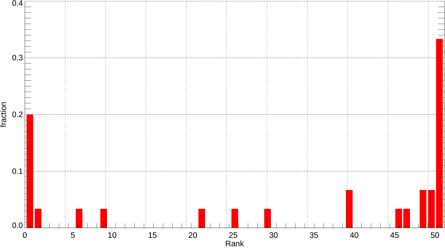
MCI: Rank Histogram of Tmin at Forecast Day 3 (2007-12-01~2007-12-31) (alpha = 0.00)
