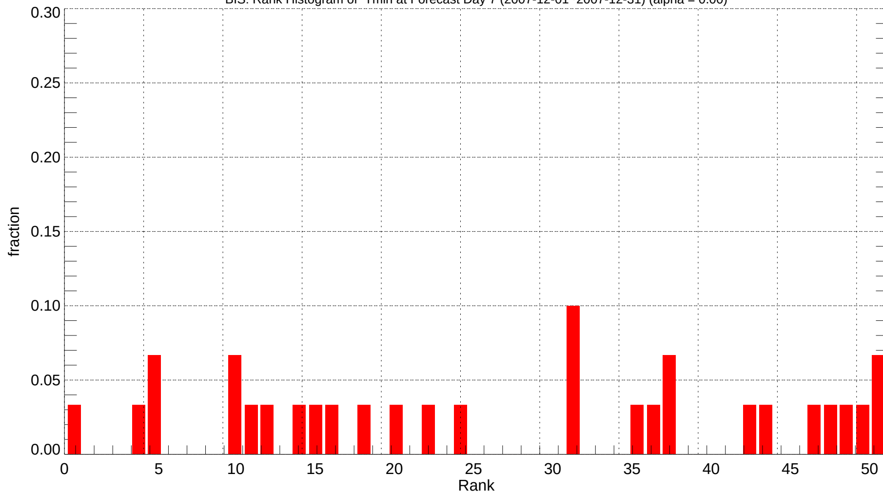
BIS: Rank Histogram of Tmin at Forecast Day 7 (2007-12-01~2007-12-31) (alpha = 0.00)
