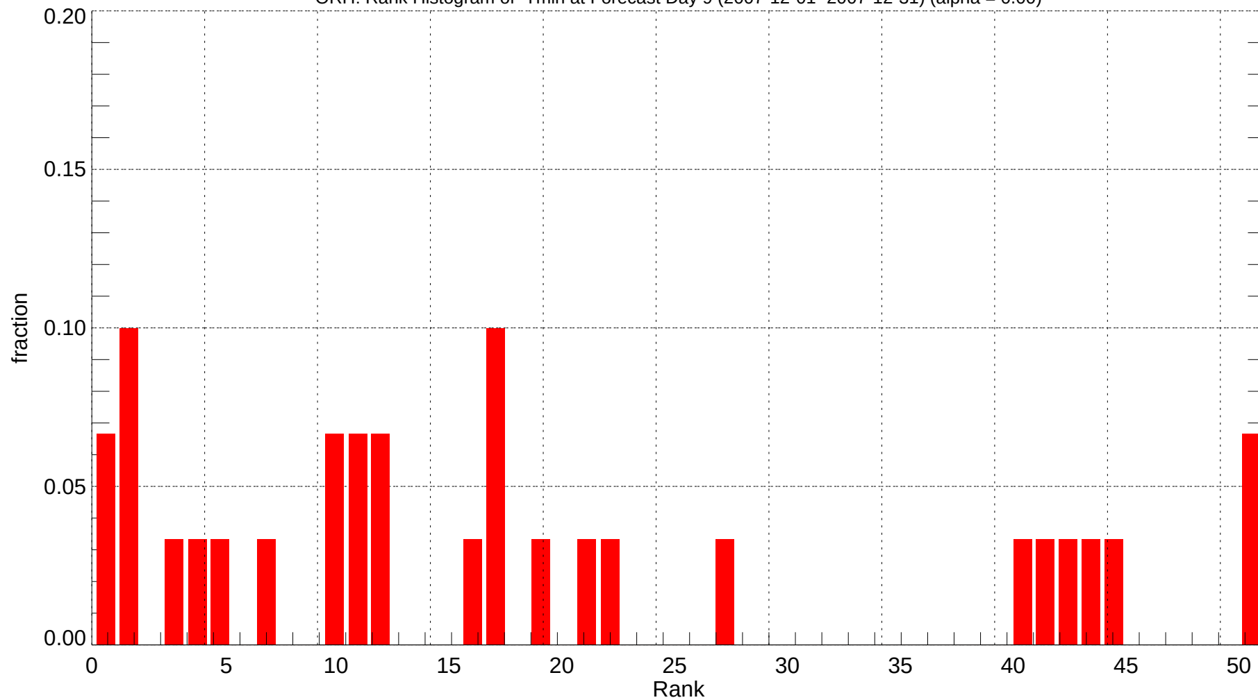
ORH: Rank Histogram of Tmin at Forecast Day 9 (2007-12-01~2007-12-31) (alpha = 0.00)
