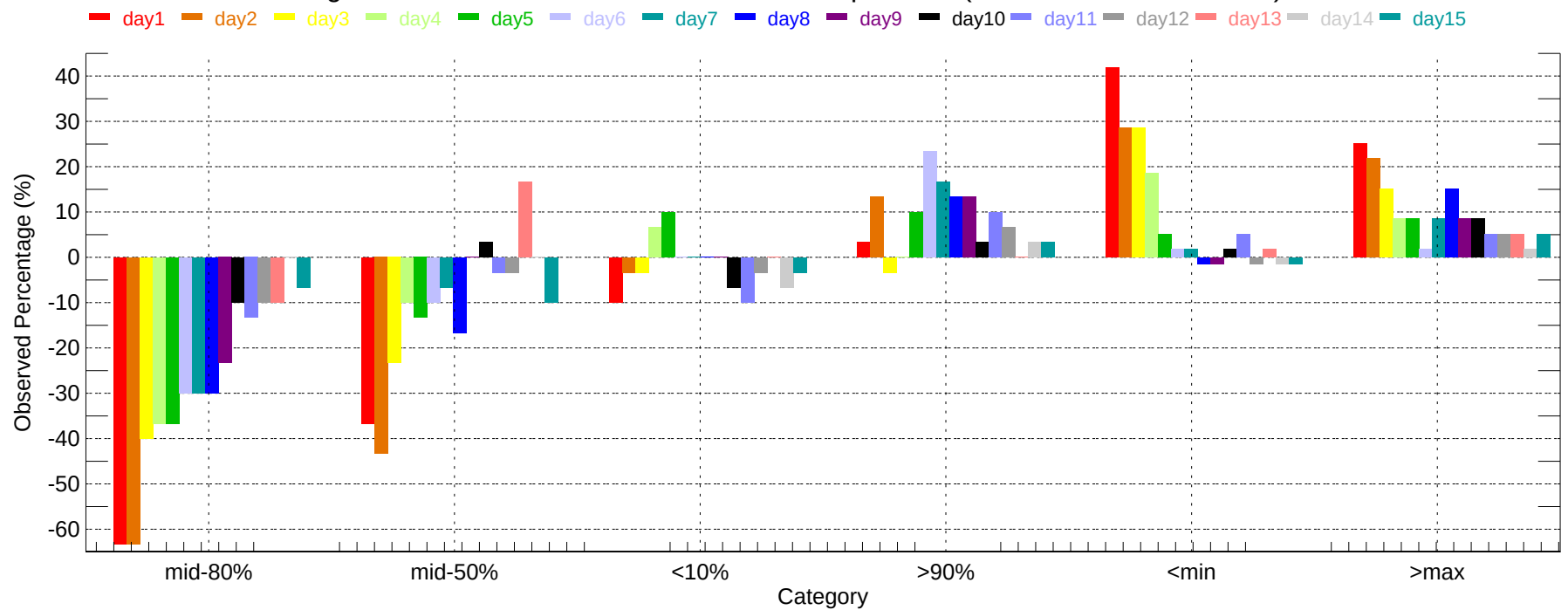
Observed Percentage Deviation of Ensembles - PIT: Min Temperature (2007-12-01~2007-12-31)
