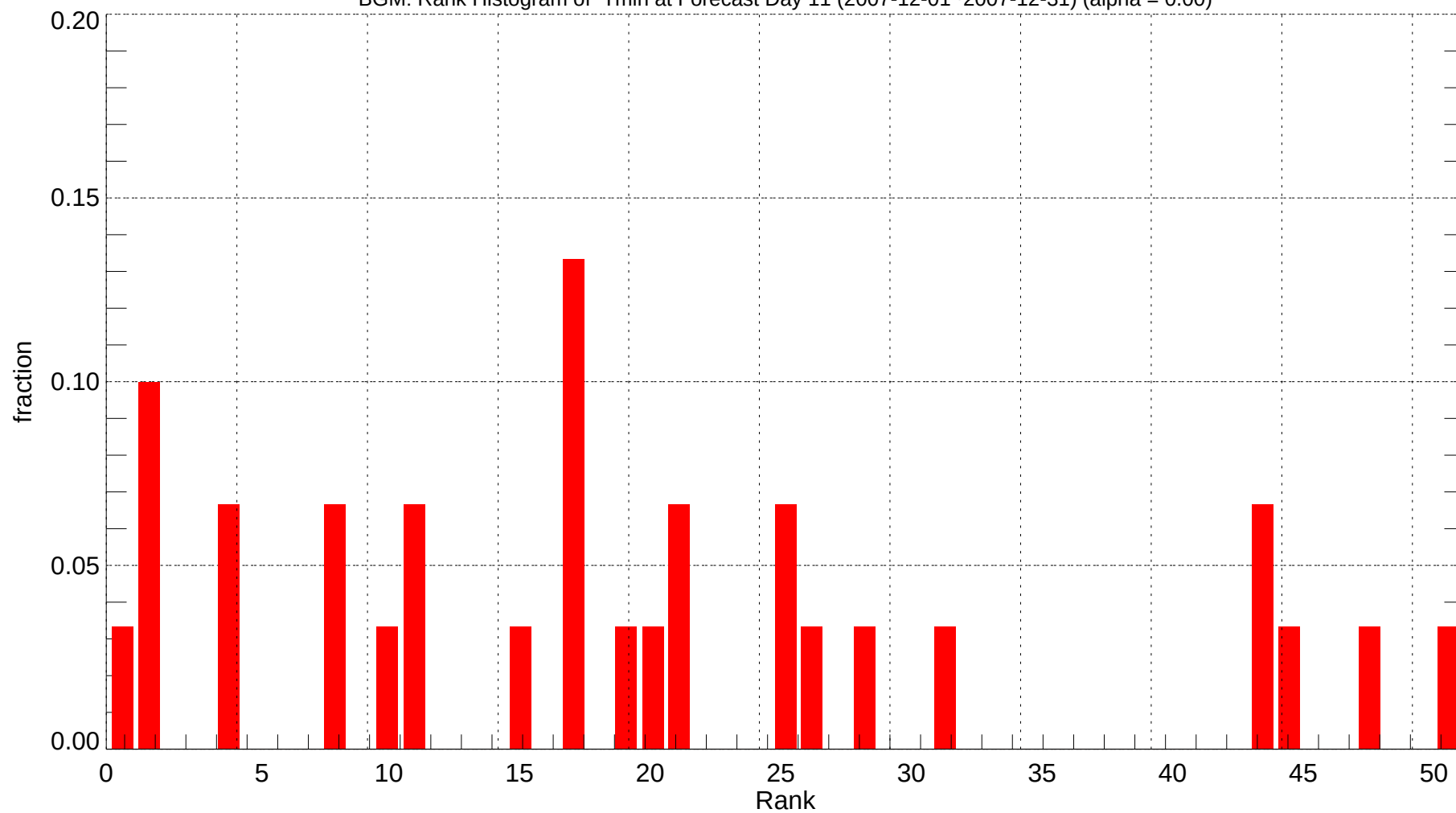
BGM: Rank Histogram of Tmin at Forecast Day 11 (2007-12-01~2007-12-31) (alpha = 0.00)
