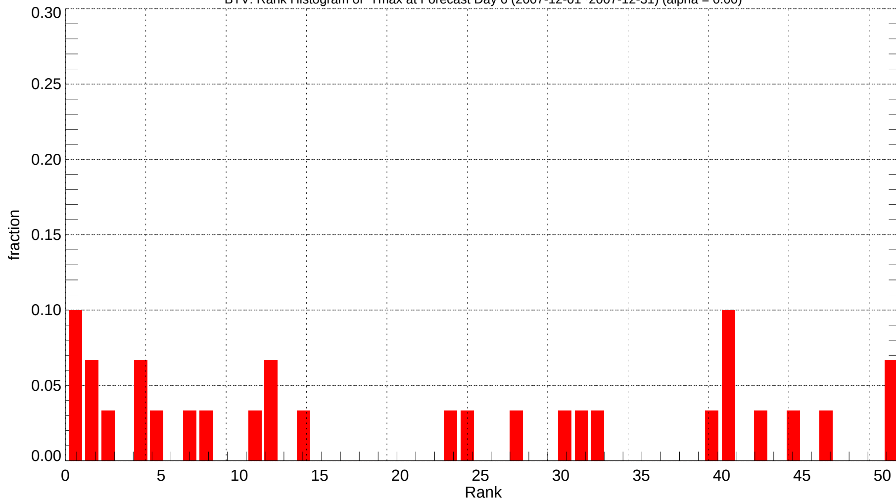
BTV: Rank Histogram of Tmax at Forecast Day 6 (2007-12-01~2007-12-31) (alpha = 0.00)
