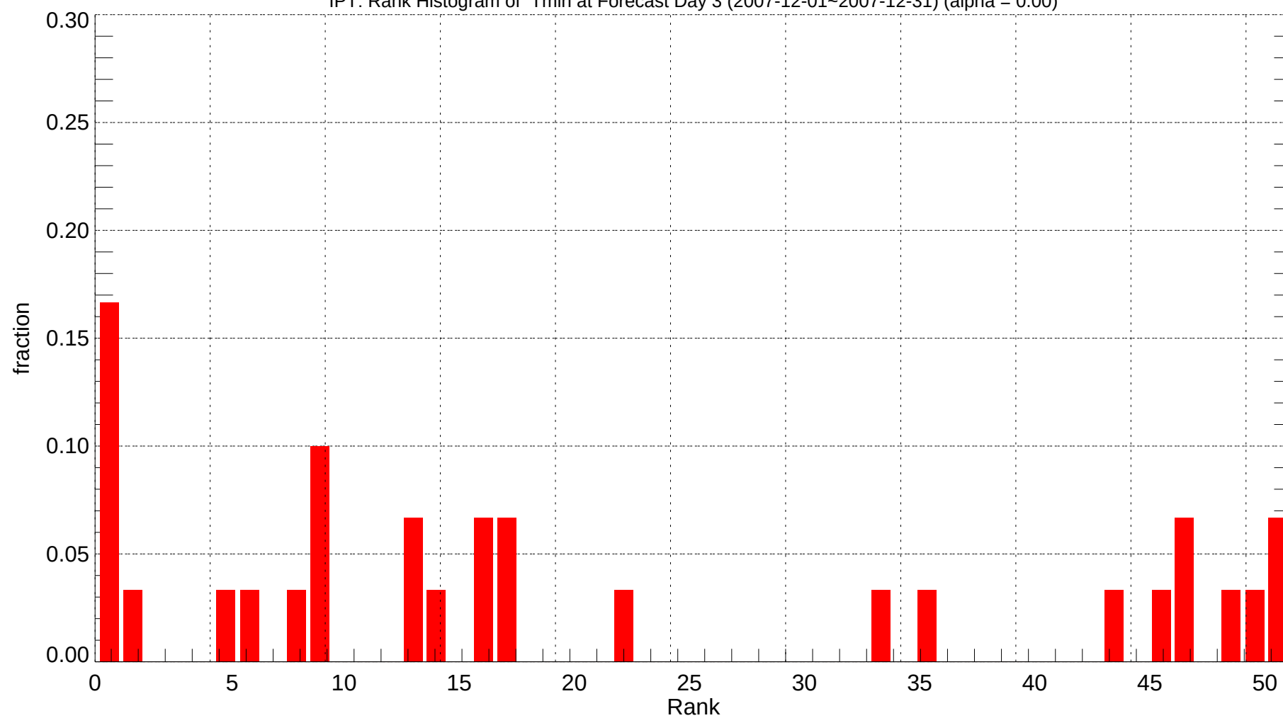
IPT: Rank Histogram of Tmin at Forecast Day 3 (2007-12-01~2007-12-31) (alpha = 0.00)
