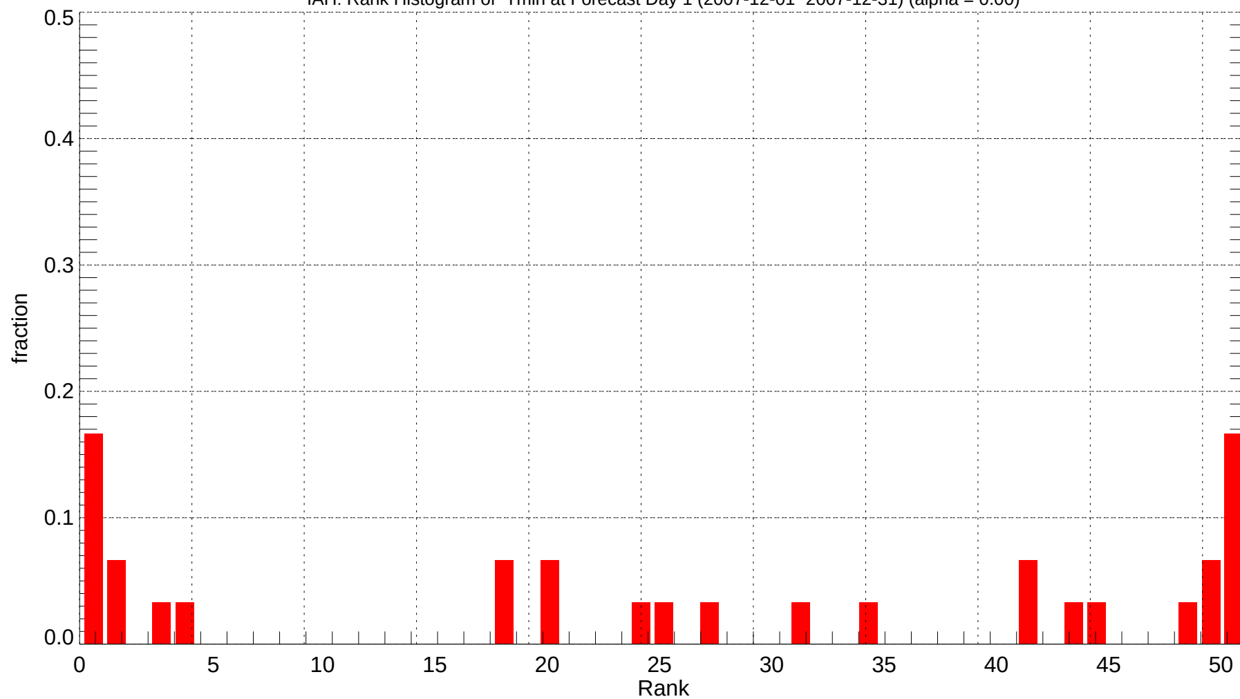
IAH: Rank Histogram of Tmin at Forecast Day 1 (2007-12-01~2007-12-31) (alpha = 0.00)
