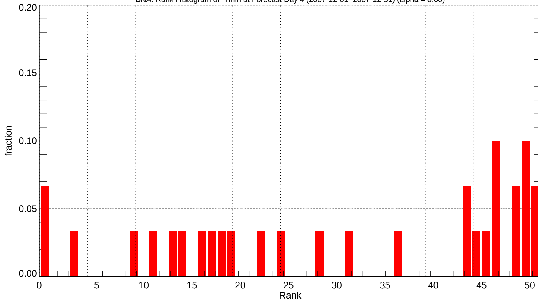
BNA: Rank Histogram of Tmin at Forecast Day 4 (2007-12-01~2007-12-31) (alpha = 0.00)
