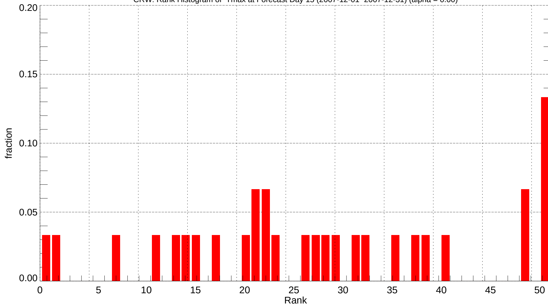
CRW: Rank Histogram of Tmax at Forecast Day 15 (2007-12-01~2007-12-31) (alpha = 0.00)
