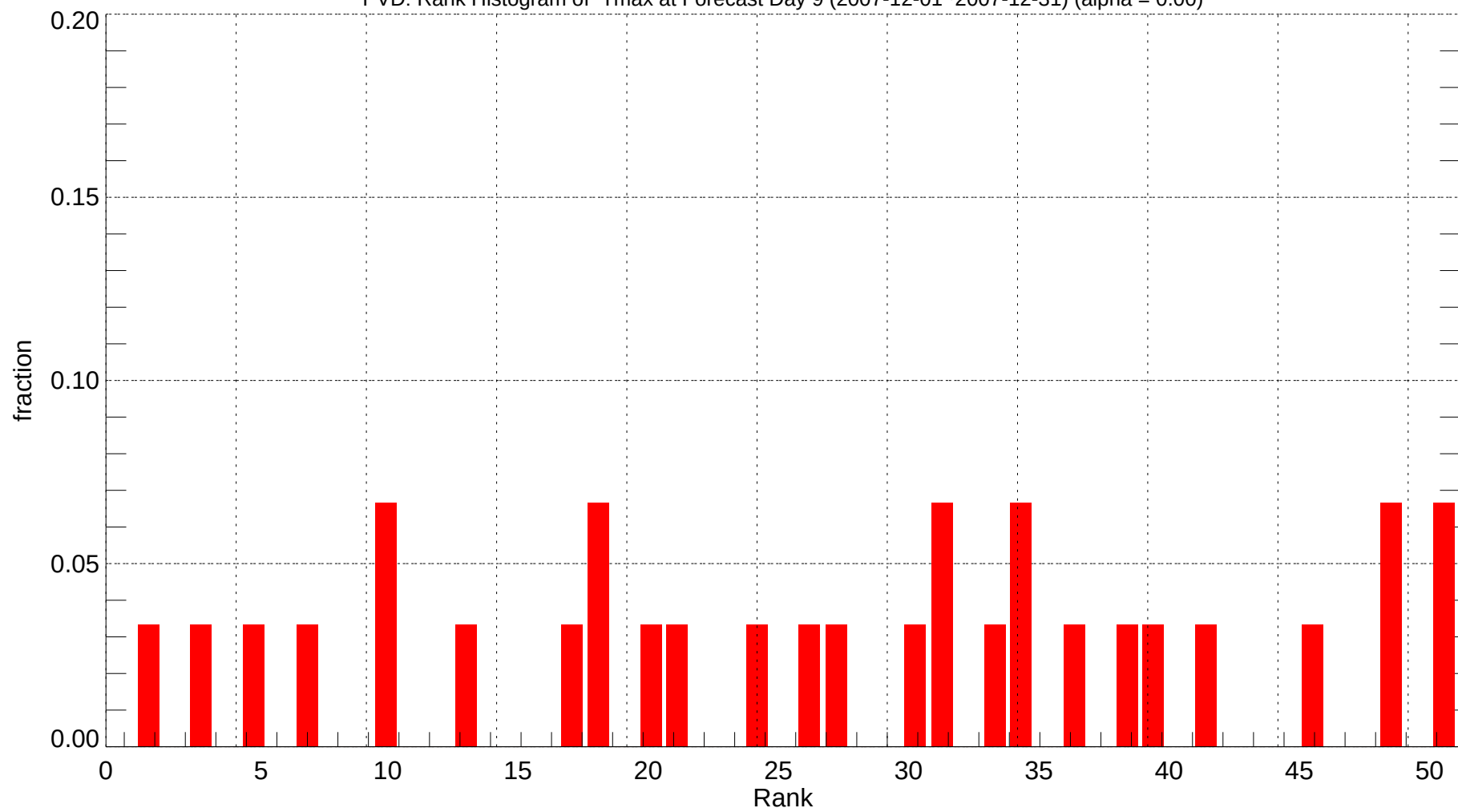
PVD: Rank Histogram of Tmax at Forecast Day 9 (2007-12-01~2007-12-31) (alpha = 0.00)
