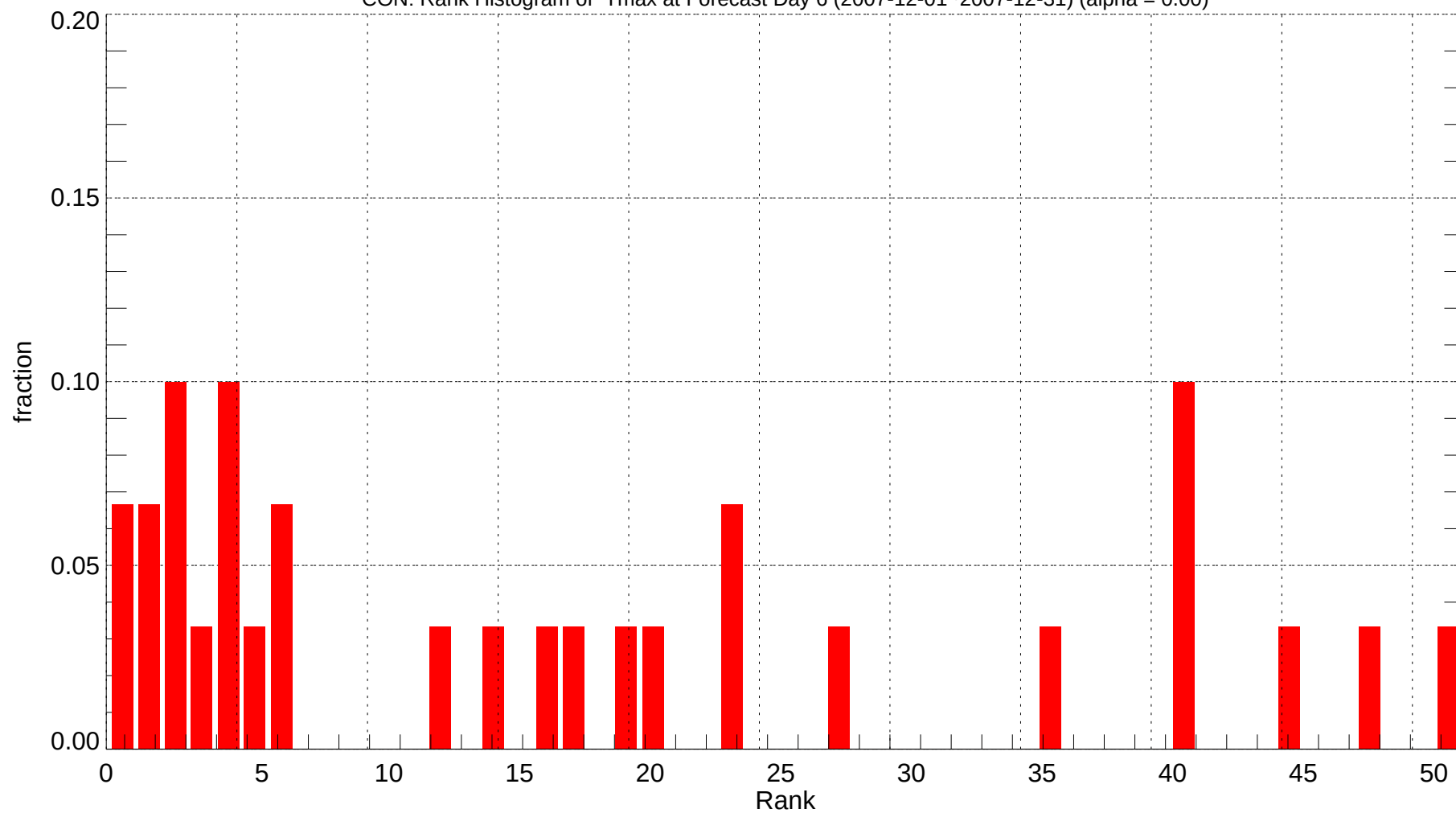
CON: Rank Histogram of Tmax at Forecast Day 6 (2007-12-01~2007-12-31) (alpha = 0.00)
