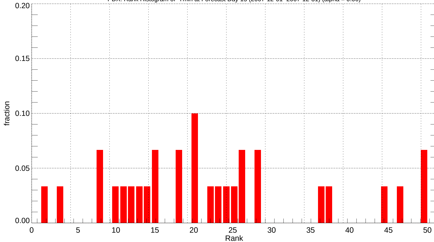
PDX: Rank Histogram of Tmin at Forecast Day 15 (2007-12-01~2007-12-31) (alpha = 0.00)
