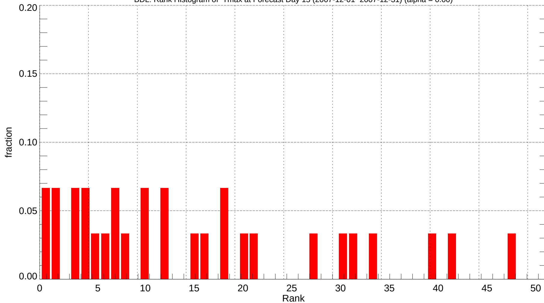
BDL: Rank Histogram of Tmax at Forecast Day 15 (2007-12-01~2007-12-31) (alpha = 0.00)
