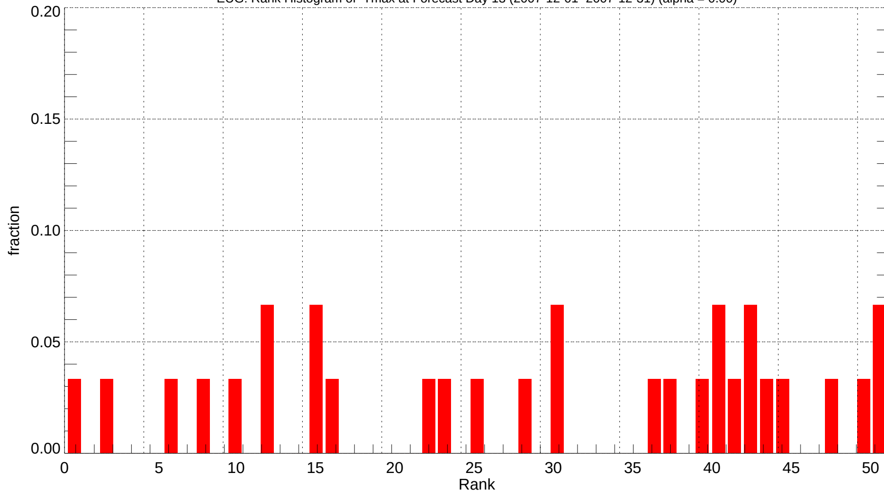
EUG: Rank Histogram of Tmax at Forecast Day 13 (2007-12-01~2007-12-31) (alpha = 0.00)
