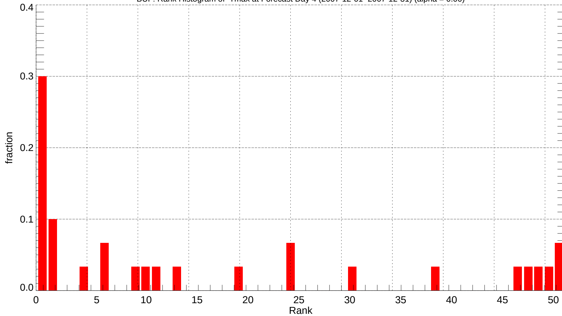
BUF: Rank Histogram of Tmax at Forecast Day 4 (2007-12-01~2007-12-31) (alpha = 0.00)
