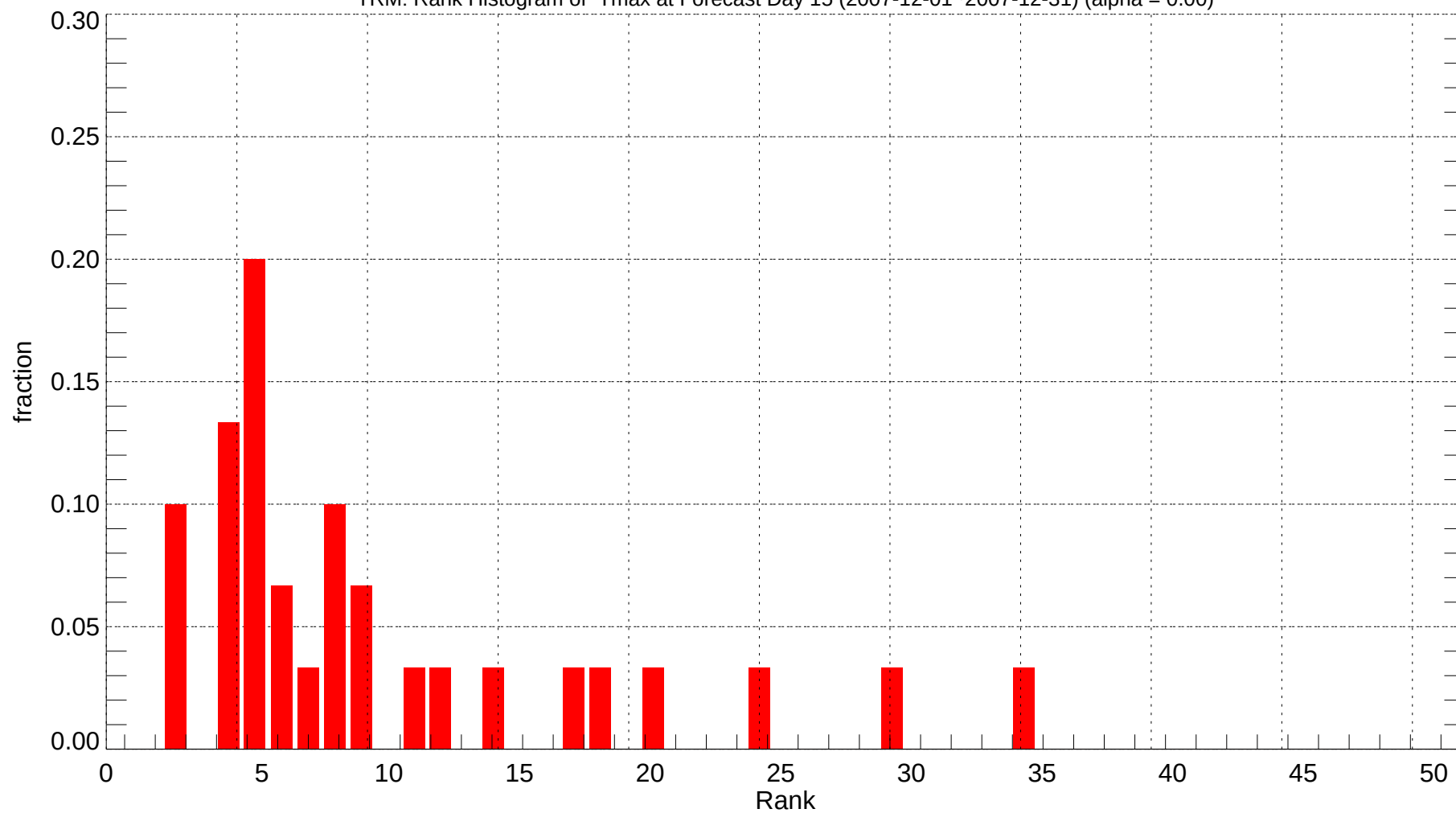
TRM: Rank Histogram of Tmax at Forecast Day 15 (2007-12-01~2007-12-31) (alpha = 0.00)
