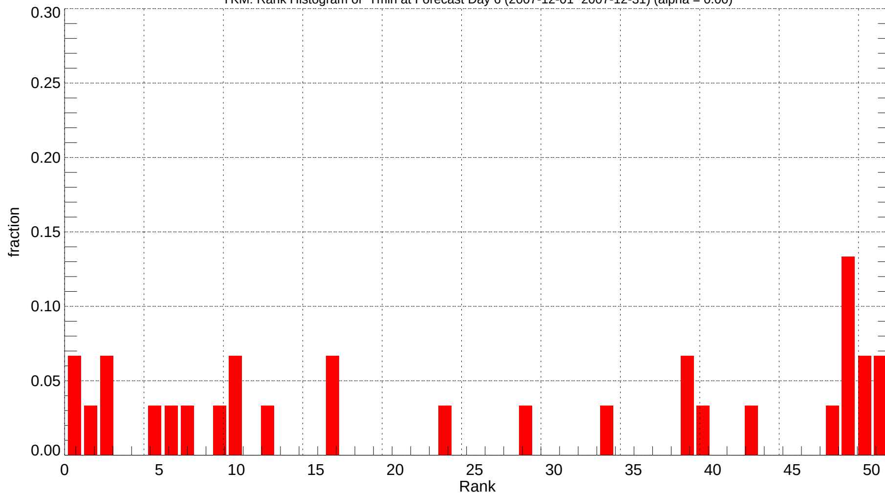
YKM: Rank Histogram of Tmin at Forecast Day 6 (2007-12-01~2007-12-31) (alpha = 0.00)
