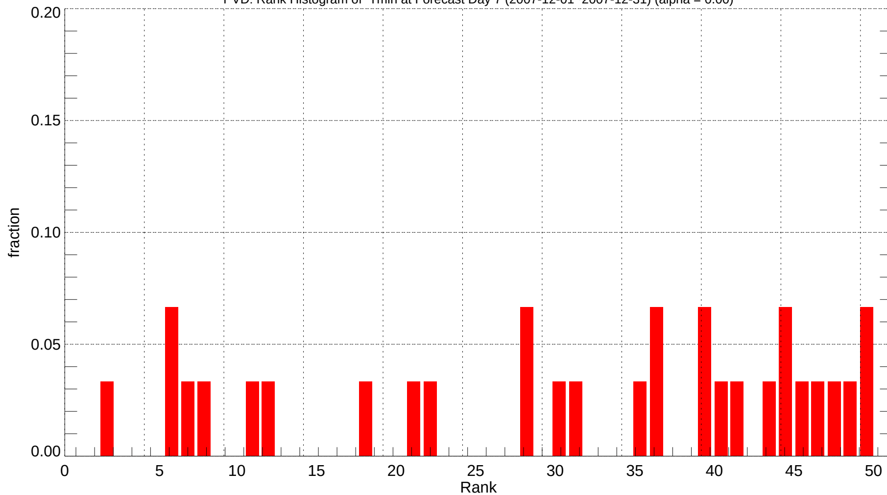
PVD: Rank Histogram of Tmin at Forecast Day 7 (2007-12-01~2007-12-31) (alpha = 0.00)
