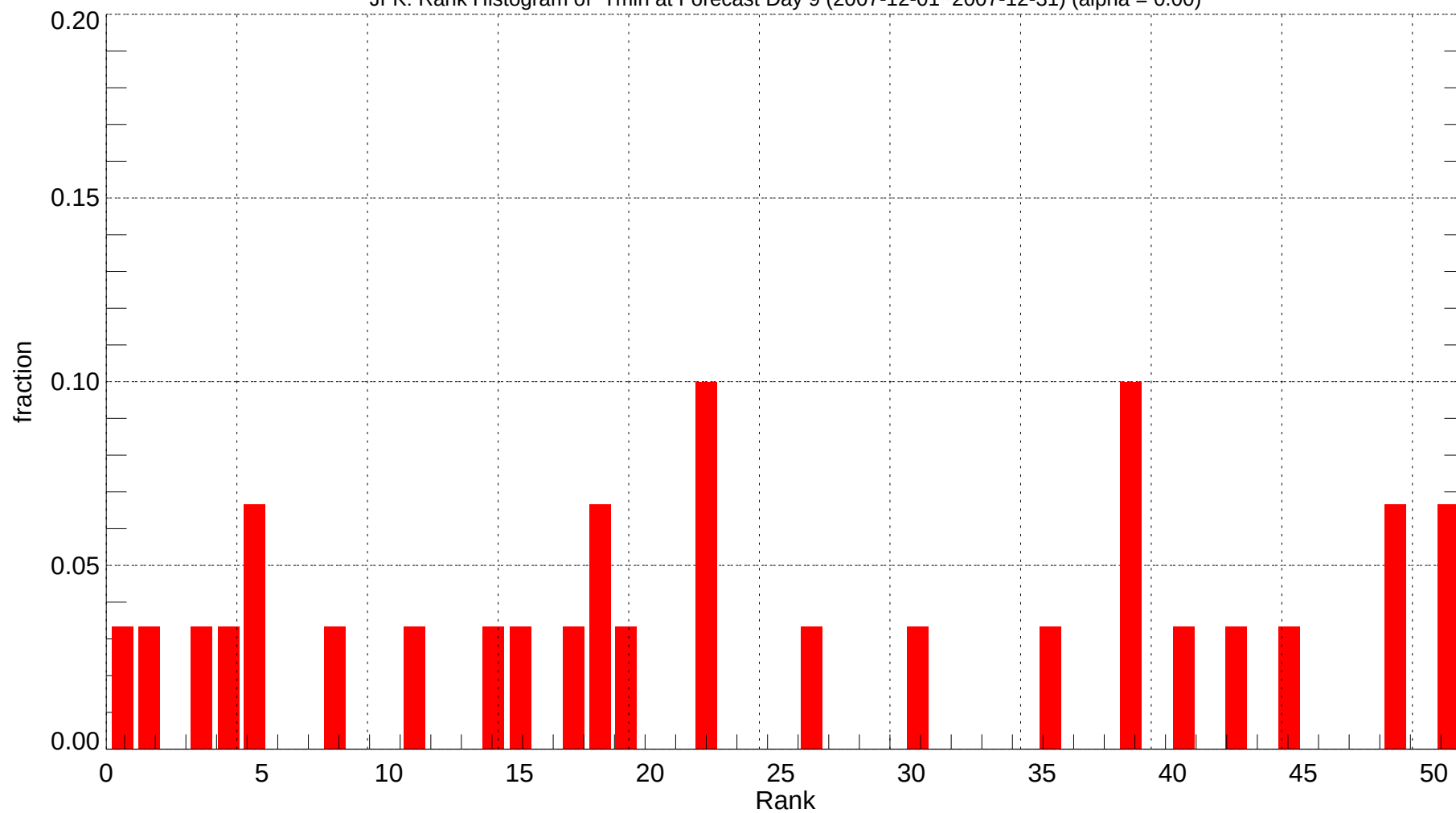
JFK: Rank Histogram of Tmin at Forecast Day 9 (2007-12-01~2007-12-31) (alpha = 0.00)
