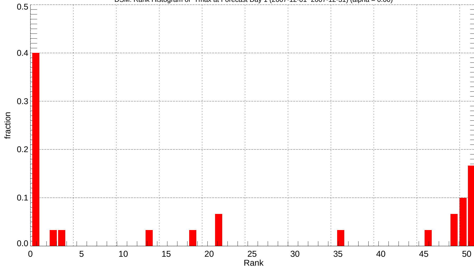
DSM: Rank Histogram of Tmax at Forecast Day 1 (2007-12-01~2007-12-31) (alpha = 0.00)
