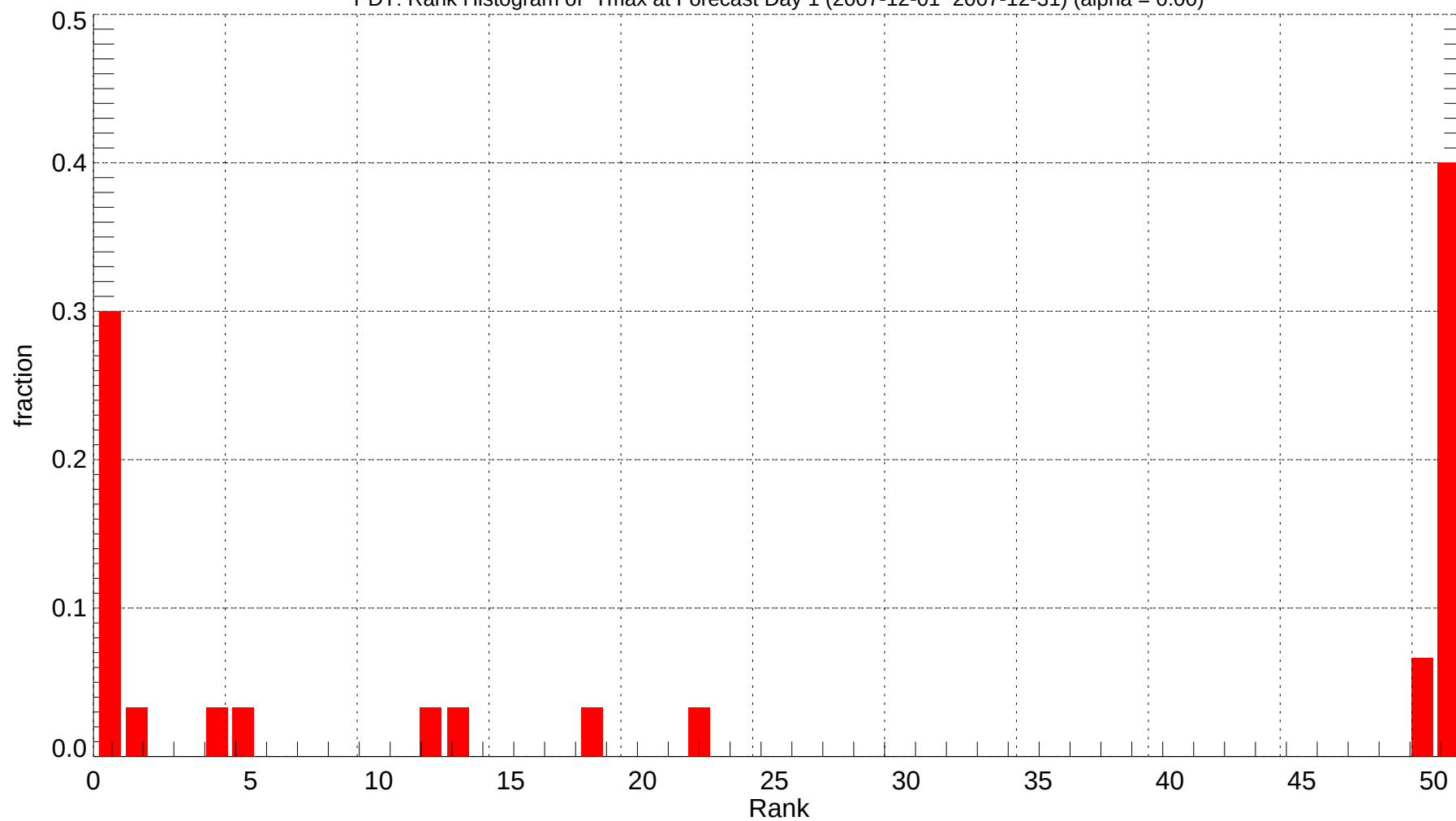
PDT: Rank Histogram of Tmax at Forecast Day 1 (2007-12-01~2007-12-31) (alpha = 0.00)
