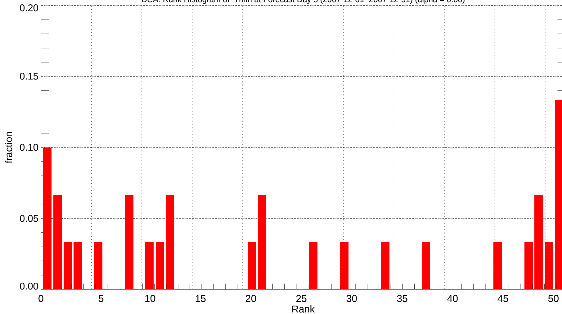
DCA: Rank Histogram of Tmin at Forecast Day 5 (2007-12-01~2007-12-31) (alpha = 0.00)
