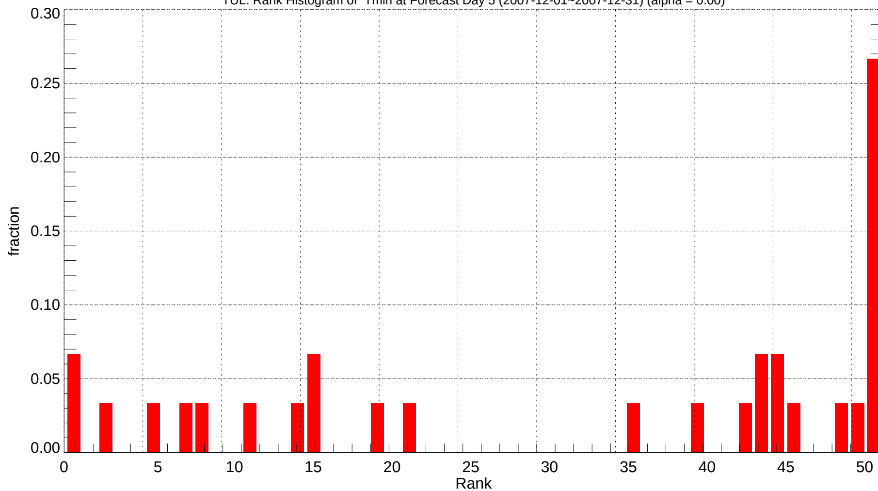
TUL: Rank Histogram of Tmin at Forecast Day 5 (2007-12-01~2007-12-31) (alpha = 0.00)
