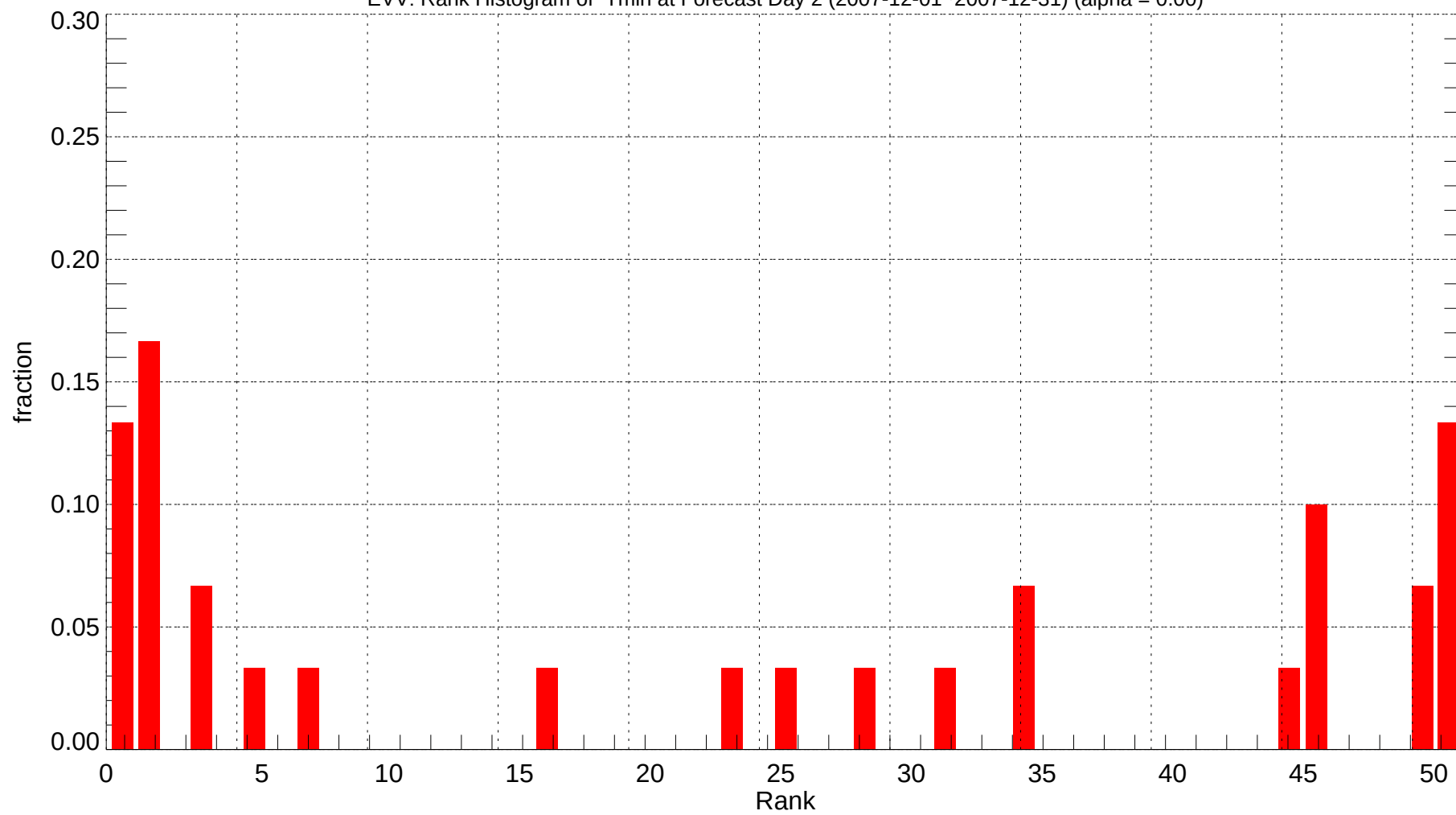
EVV: Rank Histogram of Tmin at Forecast Day 2 (2007-12-01~2007-12-31) (alpha = 0.00)
