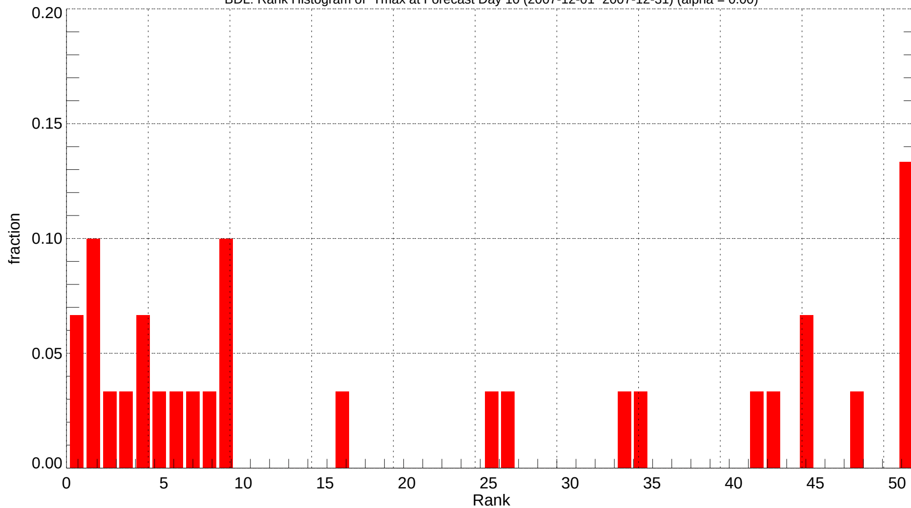
BDL: Rank Histogram of Tmax at Forecast Day 10 (2007-12-01~2007-12-31) (alpha = 0.00)
