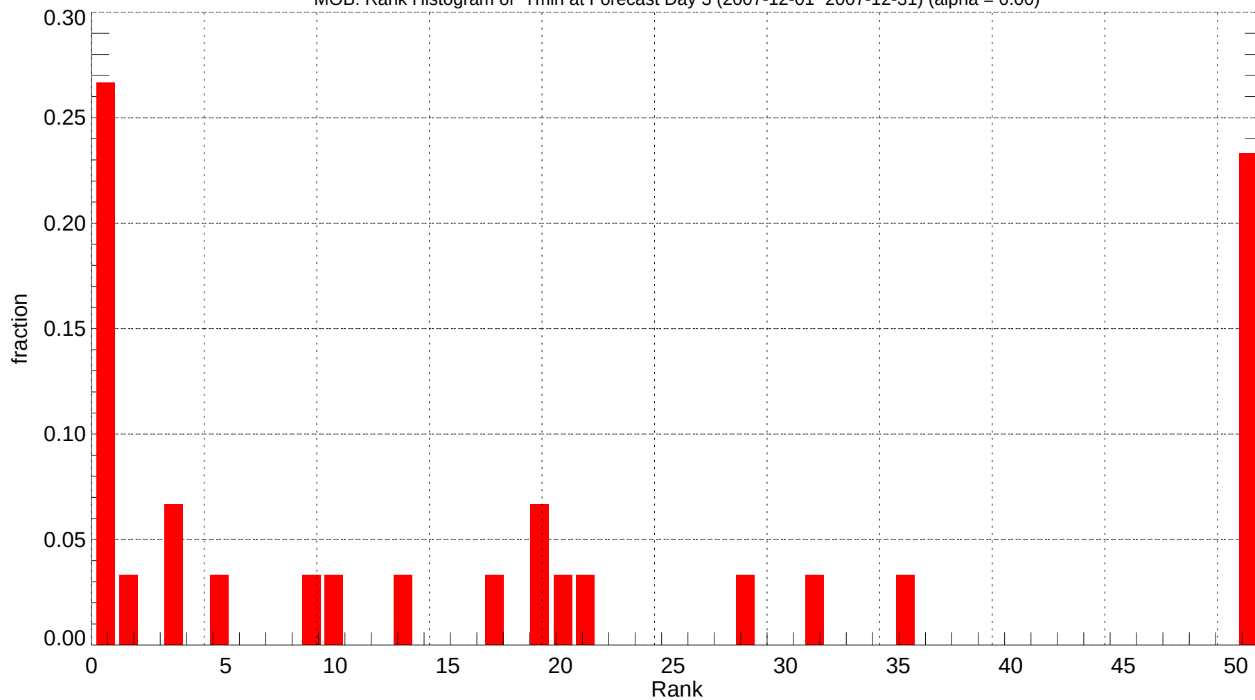
MOB: Rank Histogram of Tmin at Forecast Day 3 (2007-12-01~2007-12-31) (alpha = 0.00)
