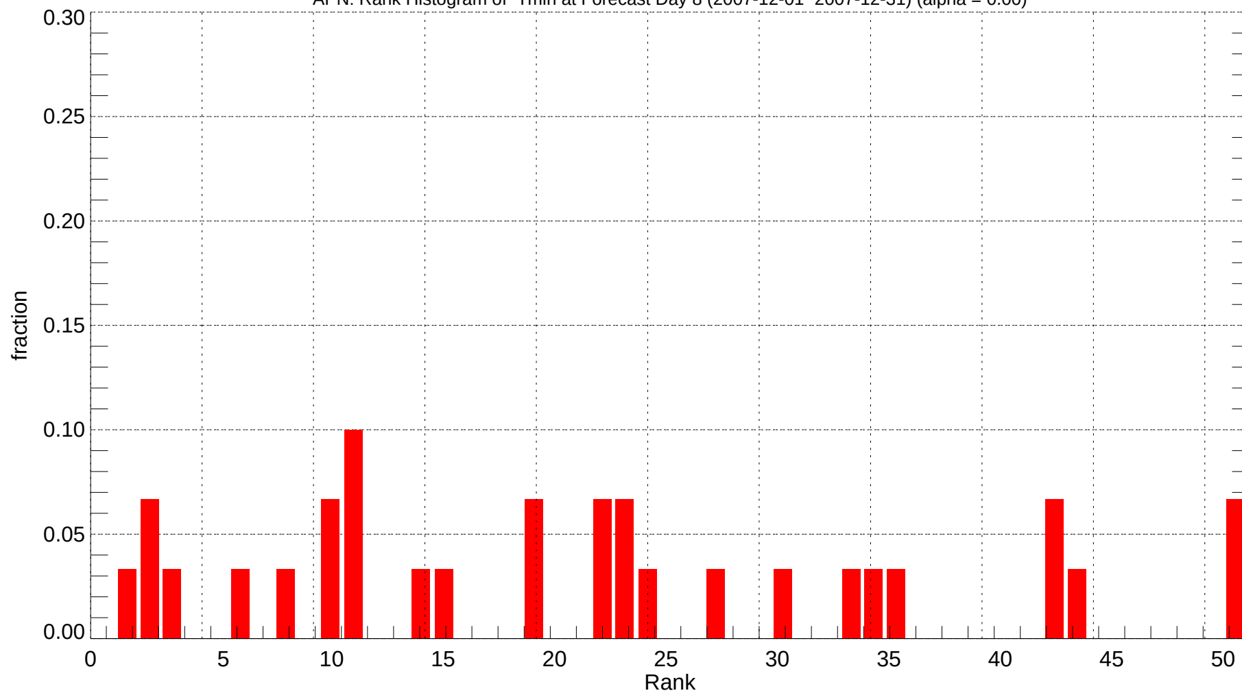
APN: Rank Histogram of Tmin at Forecast Day 8 (2007-12-01~2007-12-31) (alpha = 0.00)
