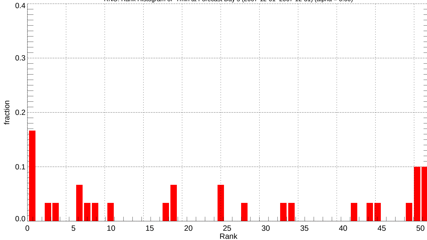
RNO: Rank Histogram of Tmin at Forecast Day 5 (2007-12-01~2007-12-31) (alpha = 0.00)
