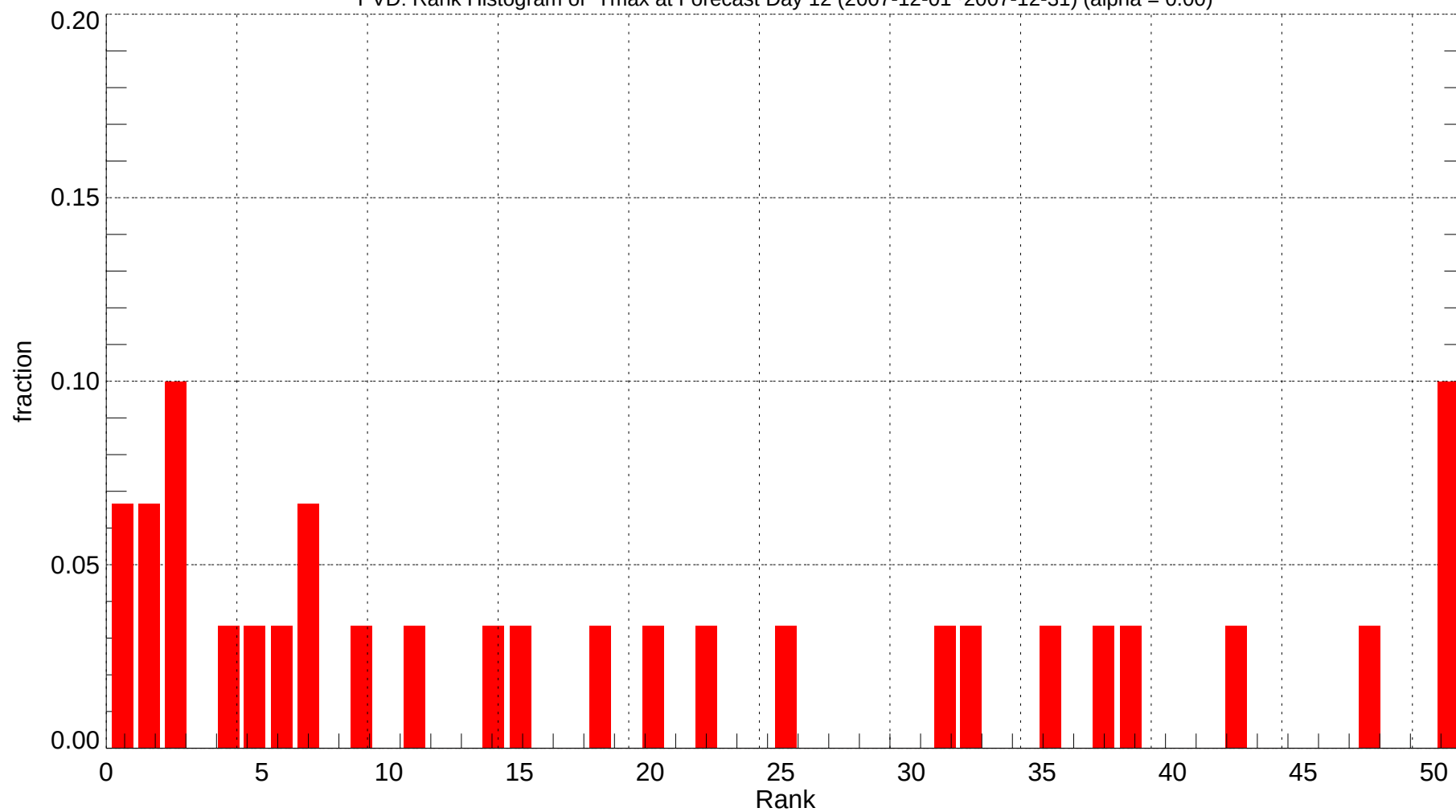
PVD: Rank Histogram of Tmax at Forecast Day 12 (2007-12-01~2007-12-31) (alpha = 0.00)
