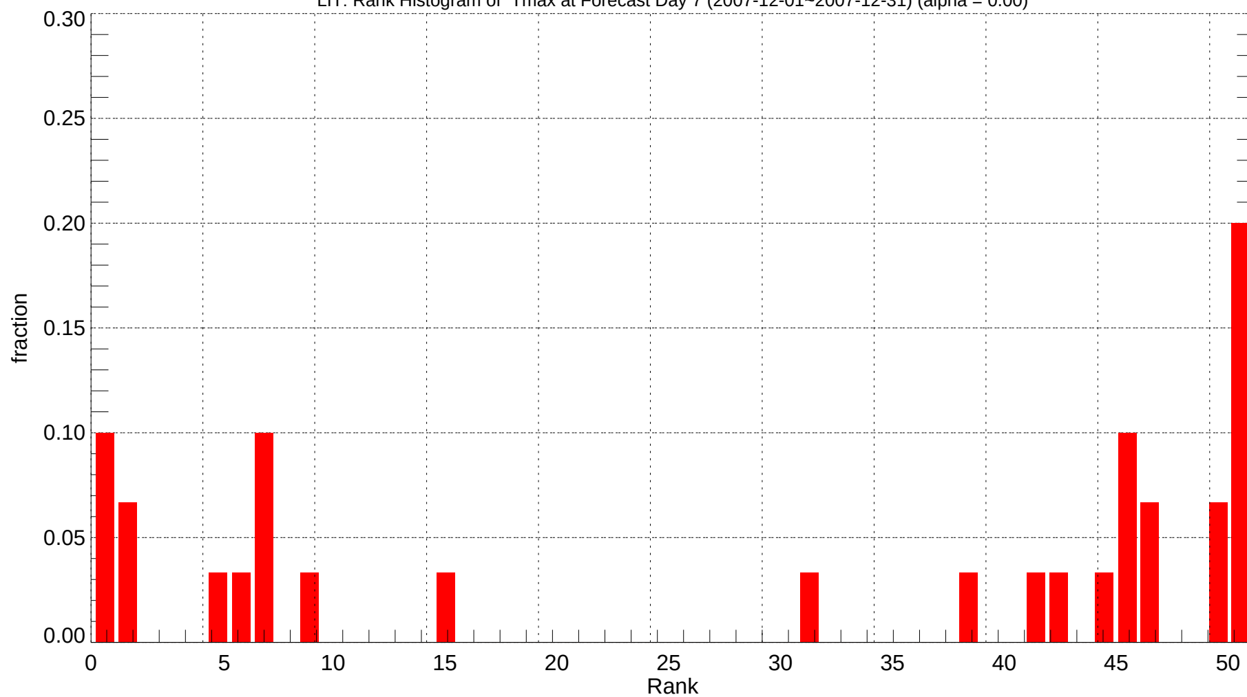
LIT: Rank Histogram of Tmax at Forecast Day 7 (2007-12-01~2007-12-31) (alpha = 0.00)
