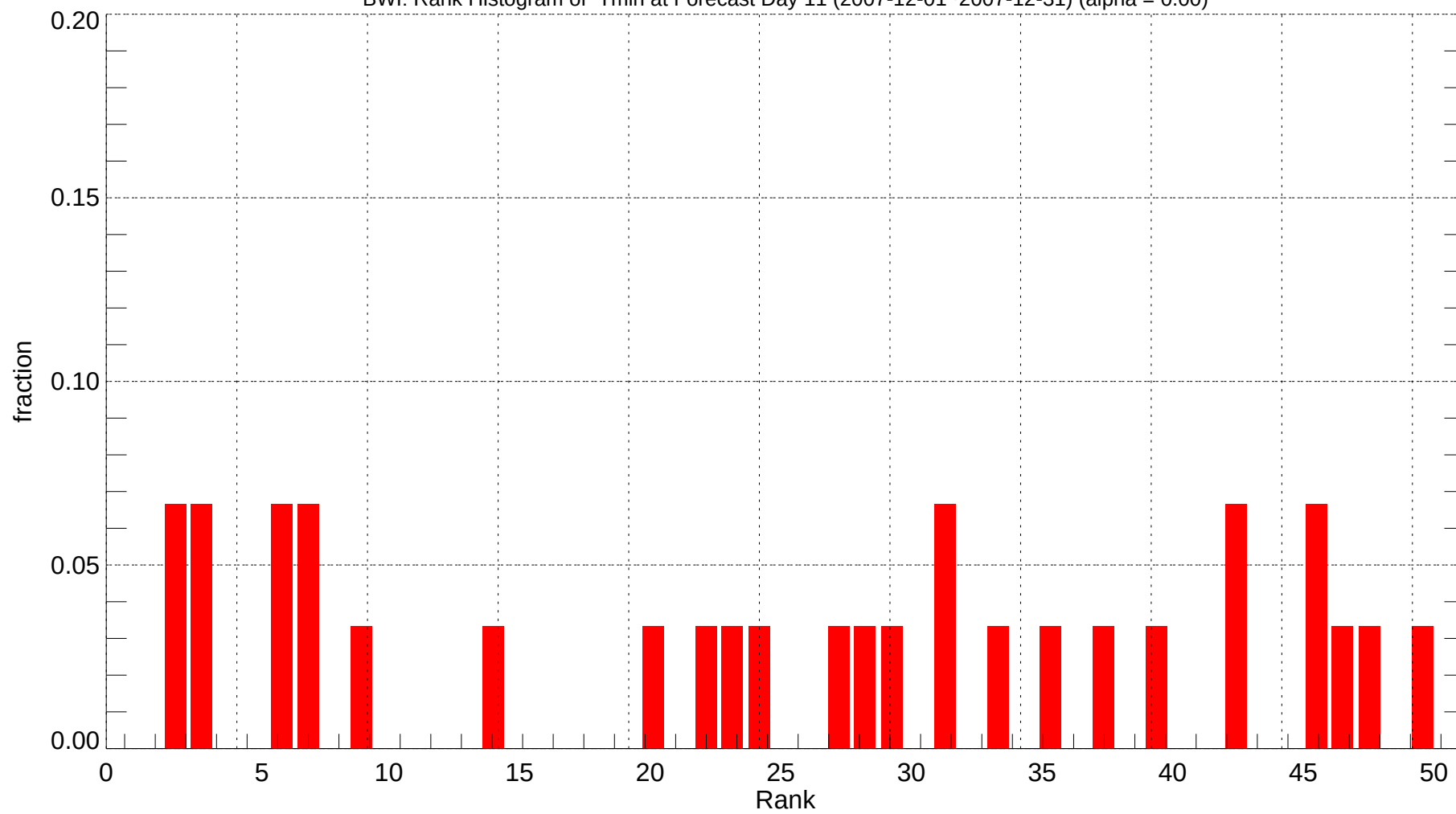
BWl: Rank Histogram of Tmin at Forecast Day 11 (2007-12-01~2007-12-31) (alpha = 0.00)
