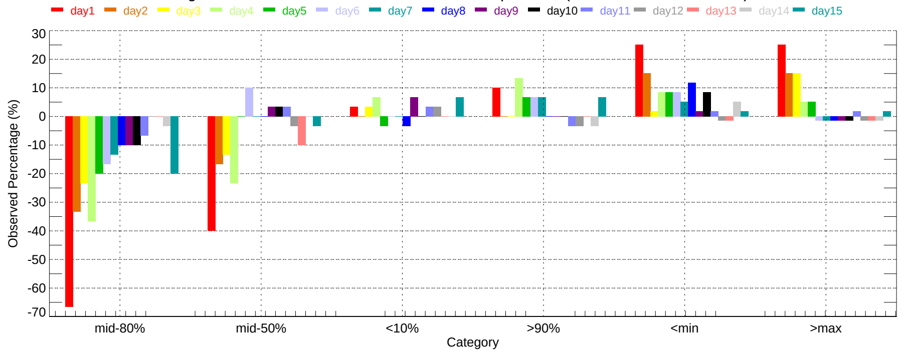
Observed Percentage Deviation of Ensembles - FAR: Max Temperature (2007-12-01~2007-12-31)
