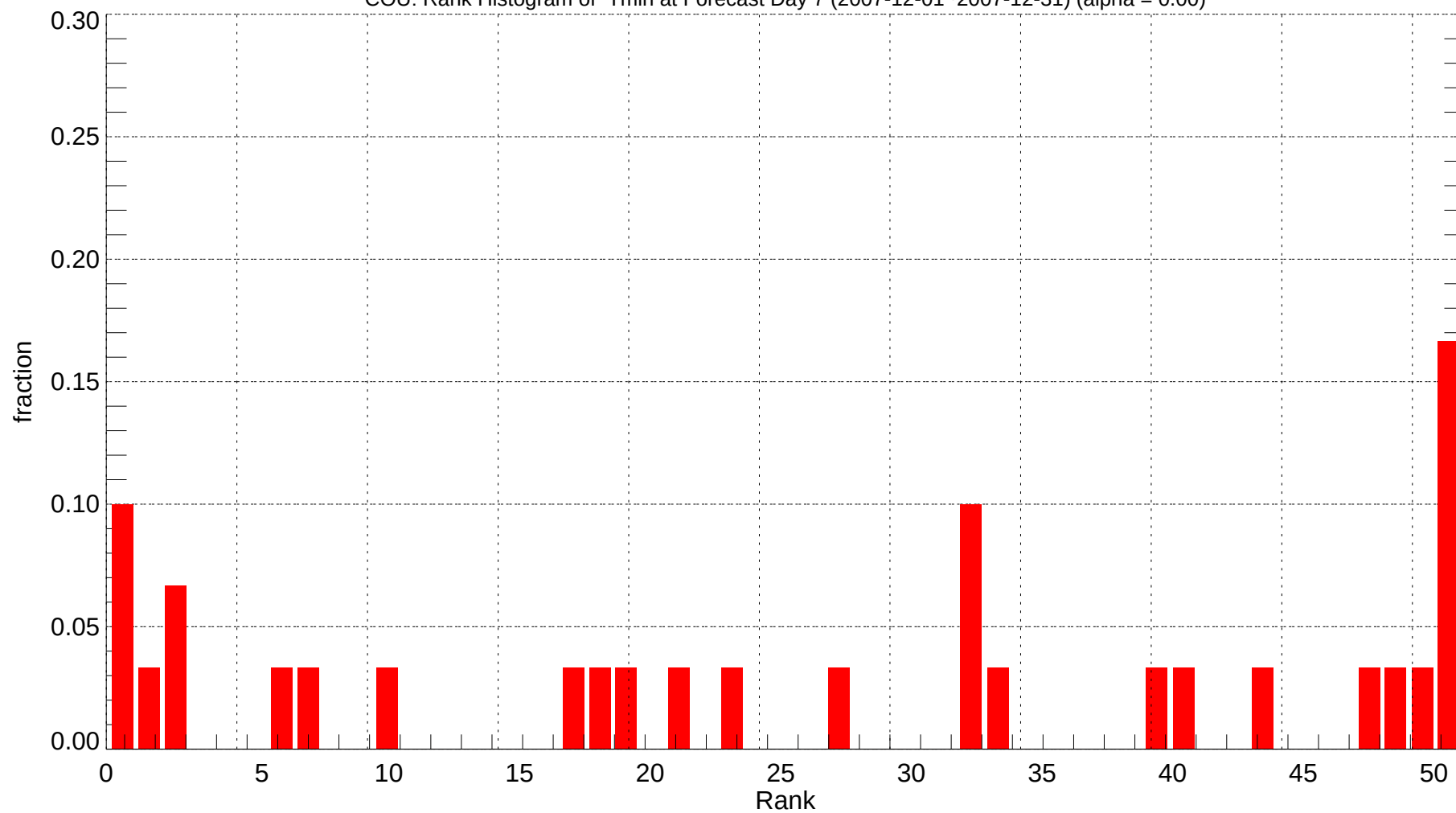
COU: Rank Histogram of Tmin at Forecast Day 7 (2007-12-01~2007-12-31) (alpha = 0.00)
