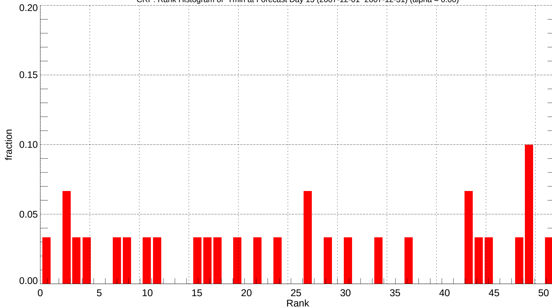
CRP: Rank Histogram of Tmin at Forecast Day 13 (2007-12-01~2007-12-31) (alpha = 0.00)
