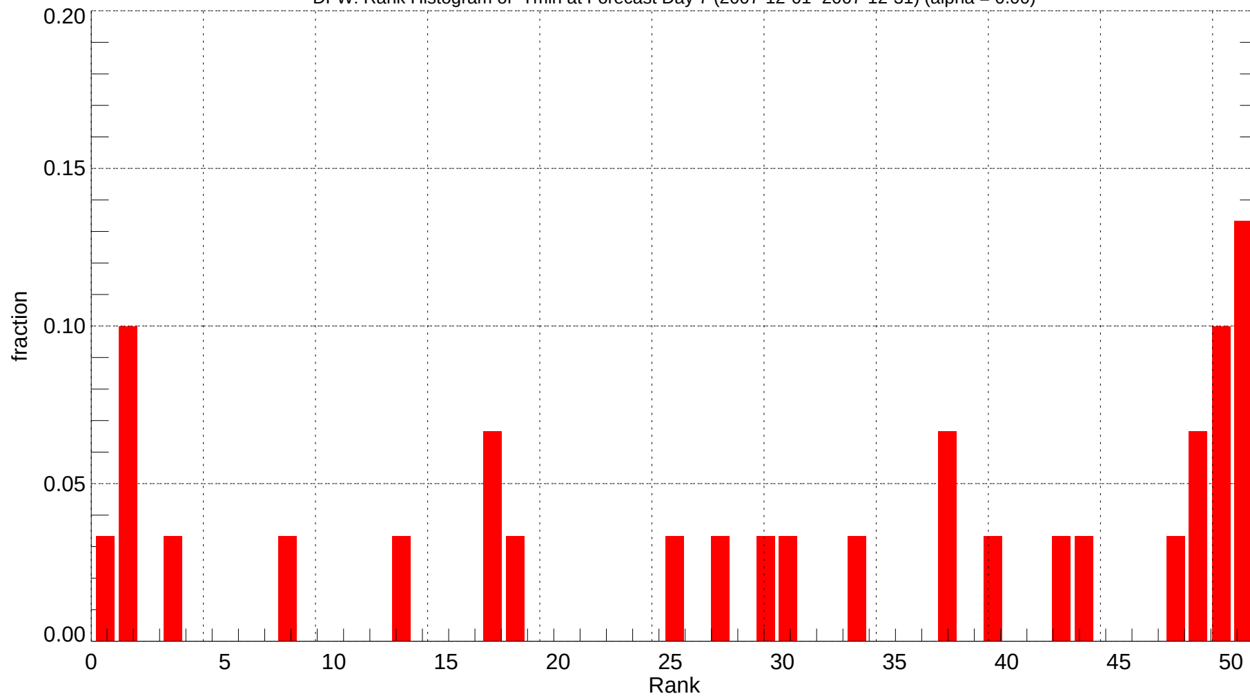
DFW: Rank Histogram of Tmin at Forecast Day 7 (2007-12-01~2007-12-31) (alpha = 0.00)
