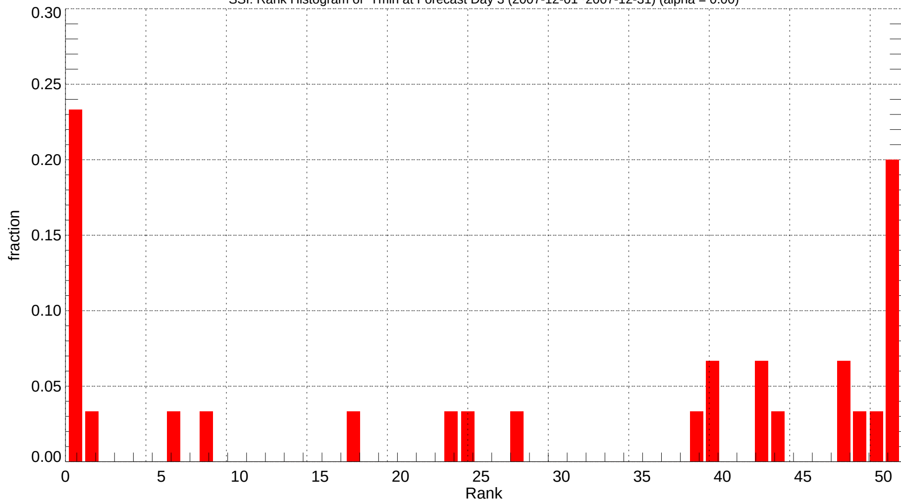
SSI: Rank Histogram of Tmin at Forecast Day 3 (2007-12-01~2007-12-31) (alpha = 0.00)
