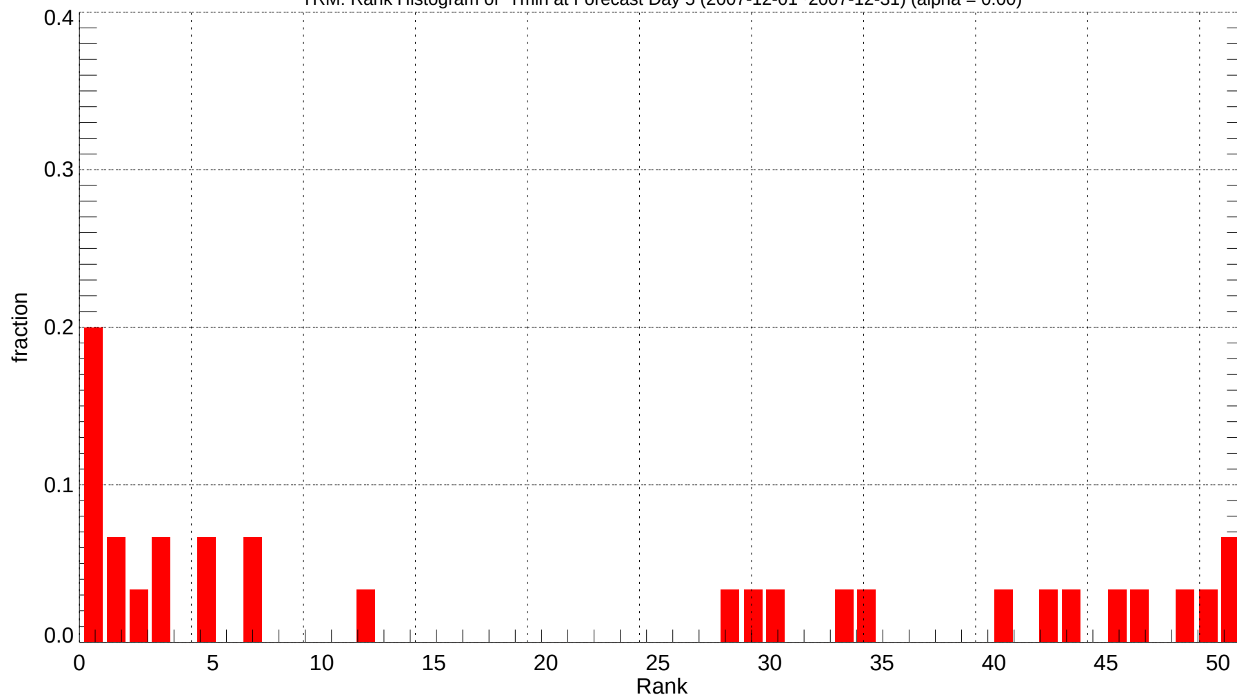
TRM: Rank Histogram of Tmin at Forecast Day 5 (2007-12-01~2007-12-31) (alpha = 0.00)
