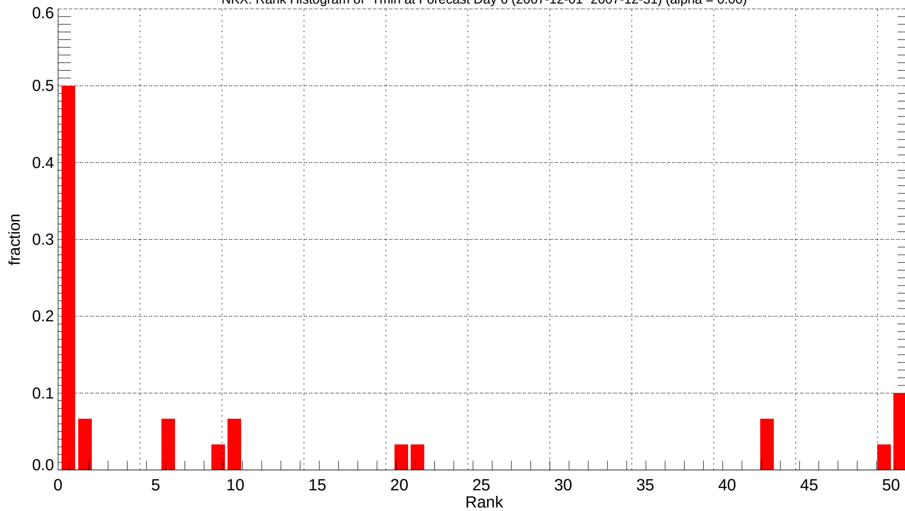
NKX: Rank Histogram of Tmin at Forecast Day 6 (2007-12-01~2007-12-31) (alpha = 0.00)
