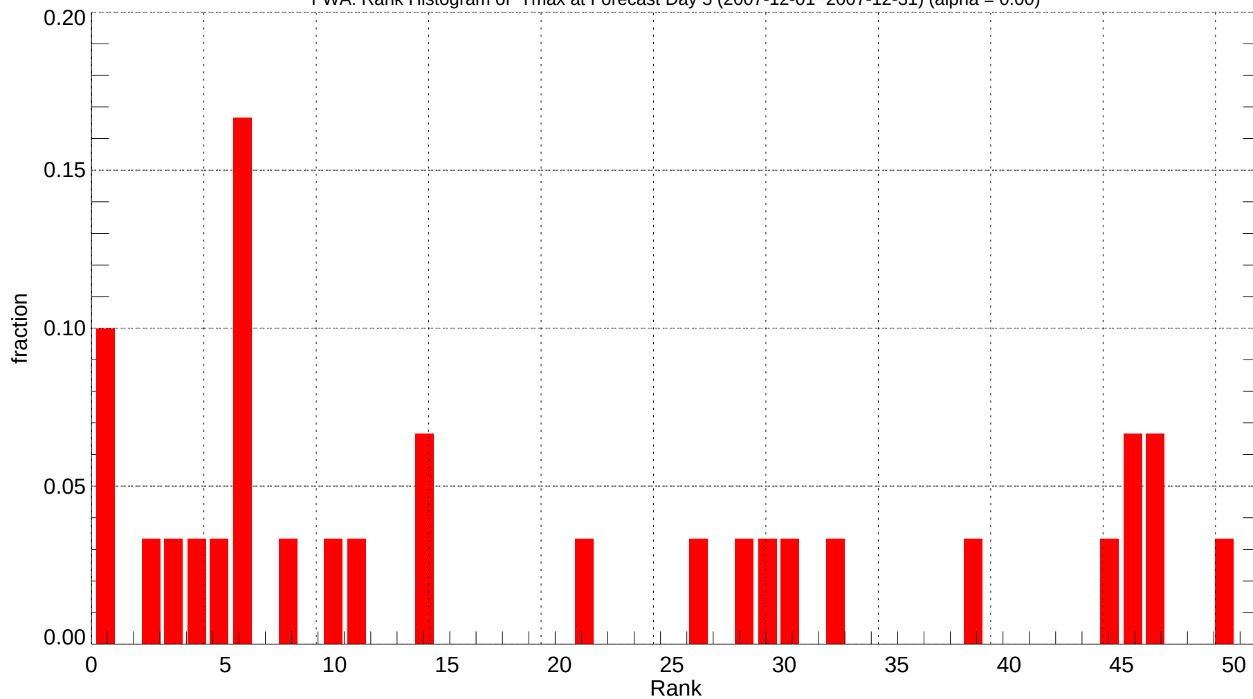
FWA: Rank Histogram of Tmax at Forecast Day 5 (2007-12-01~2007-12-31) (alpha = 0.00)
