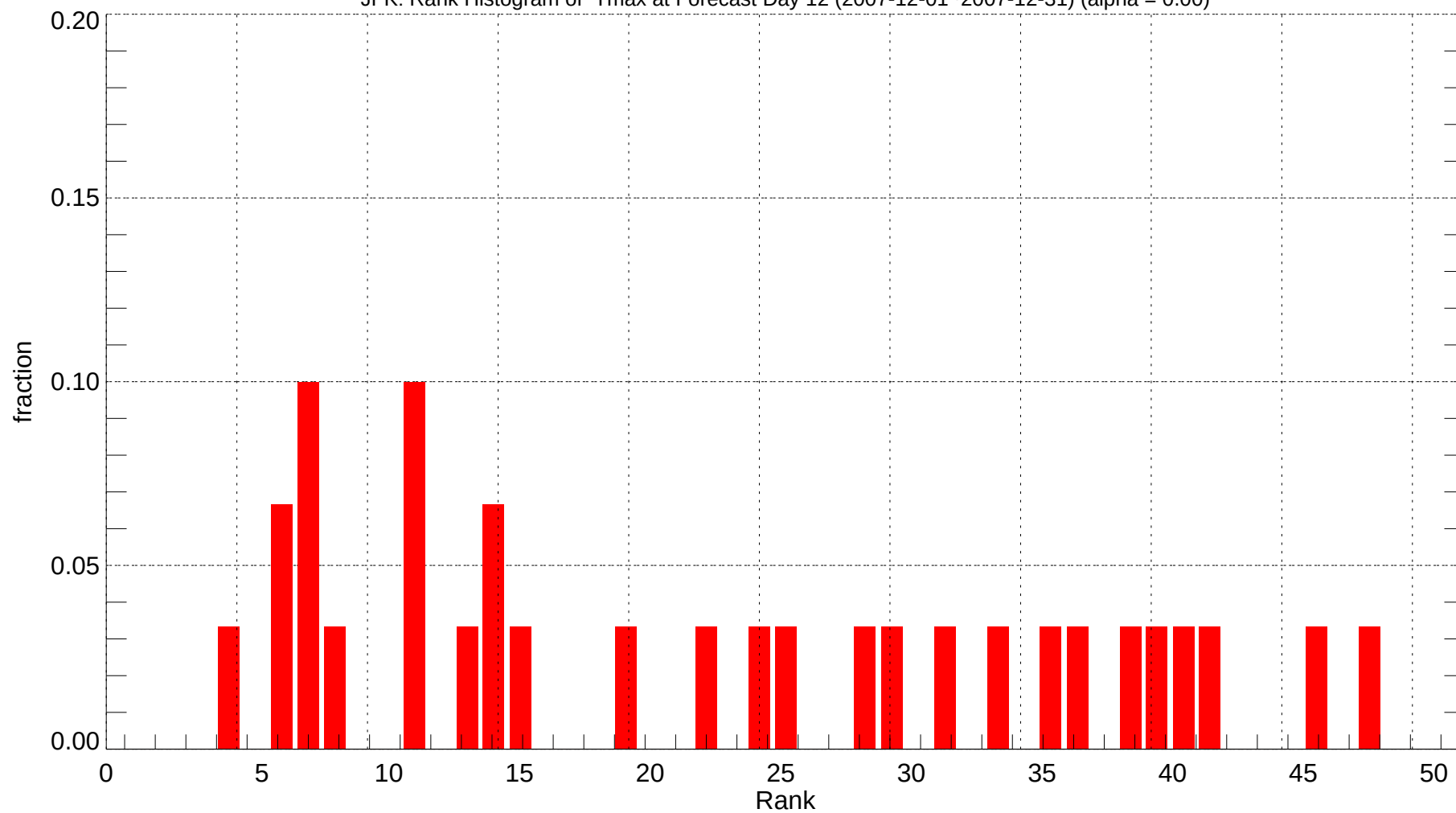
JFK: Rank Histogram of Tmax at Forecast Day 12 (2007-12-01~2007-12-31) (alpha = 0.00)
