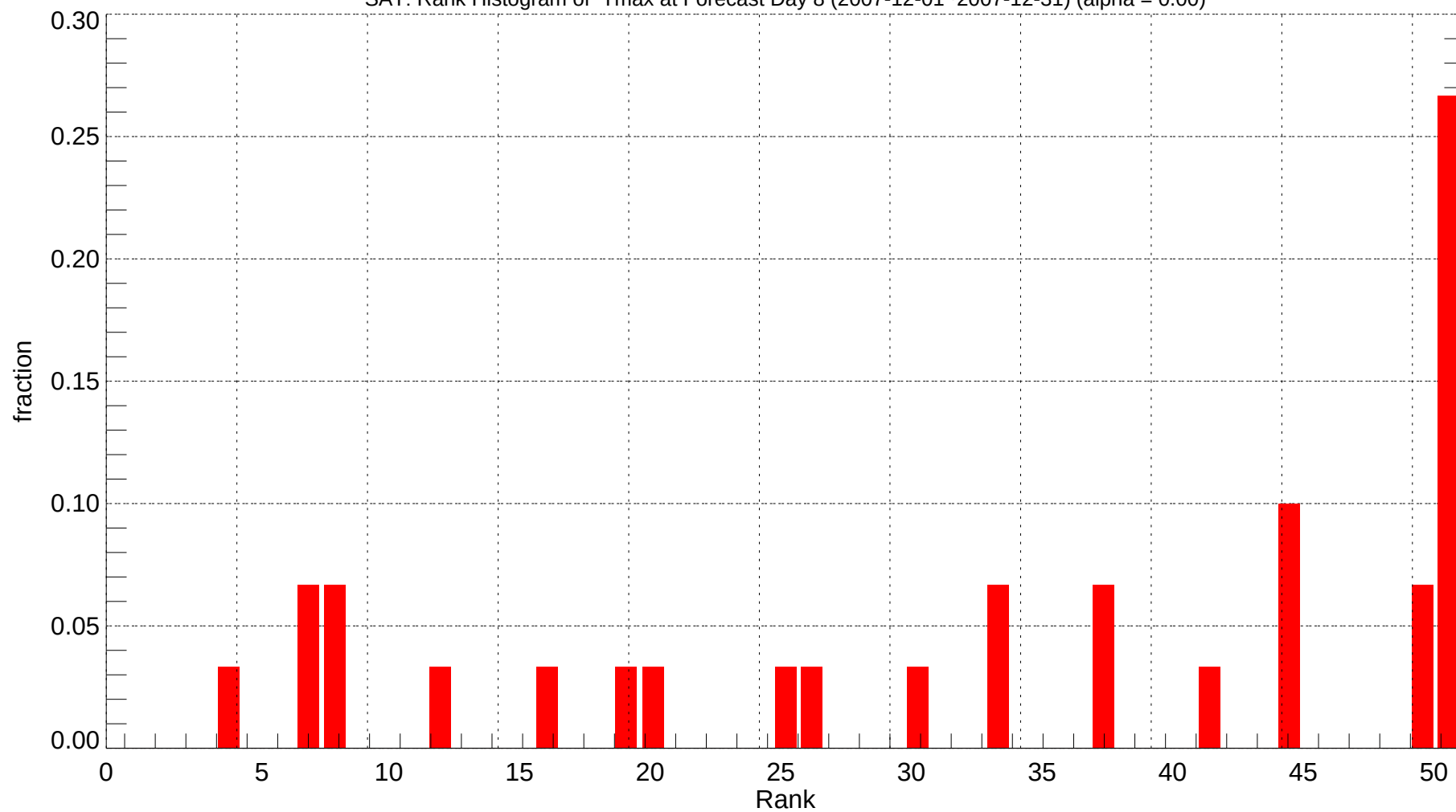
SAT: Rank Histogram of Tmax at Forecast Day 8 (2007-12-01~2007-12-31) (alpha = 0.00)
