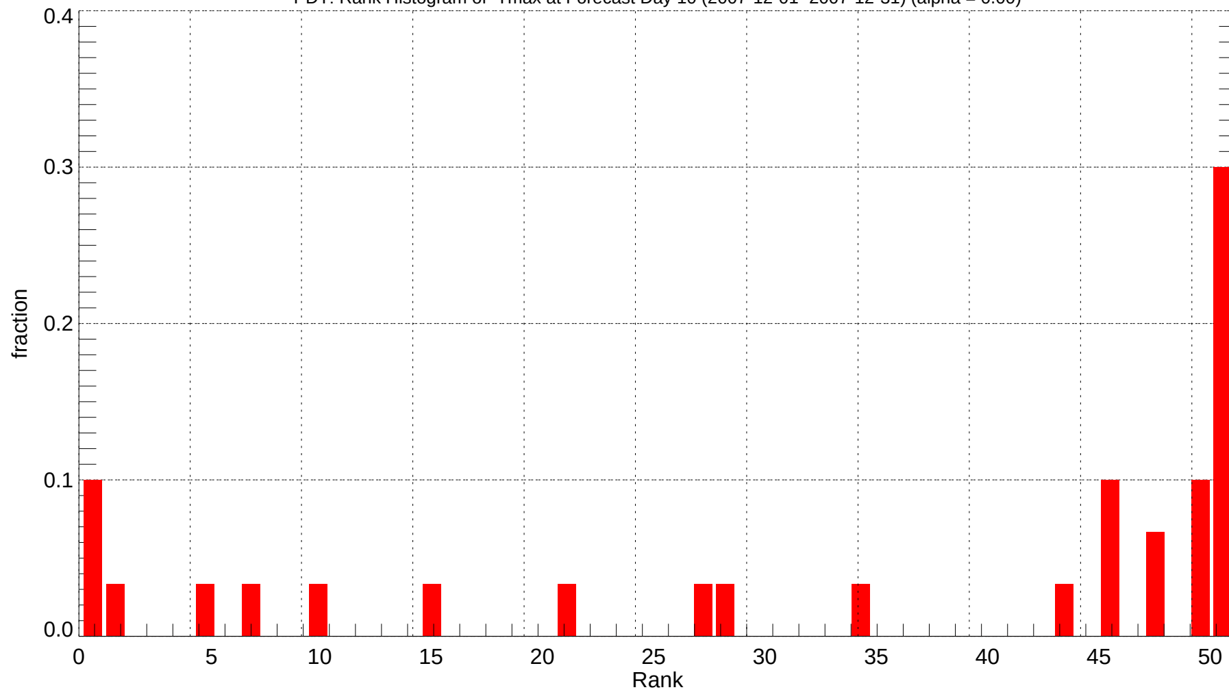
PDT: Rank Histogram of Tmax at Forecast Day 10 (2007-12-01~2007-12-31) (alpha = 0.00)
