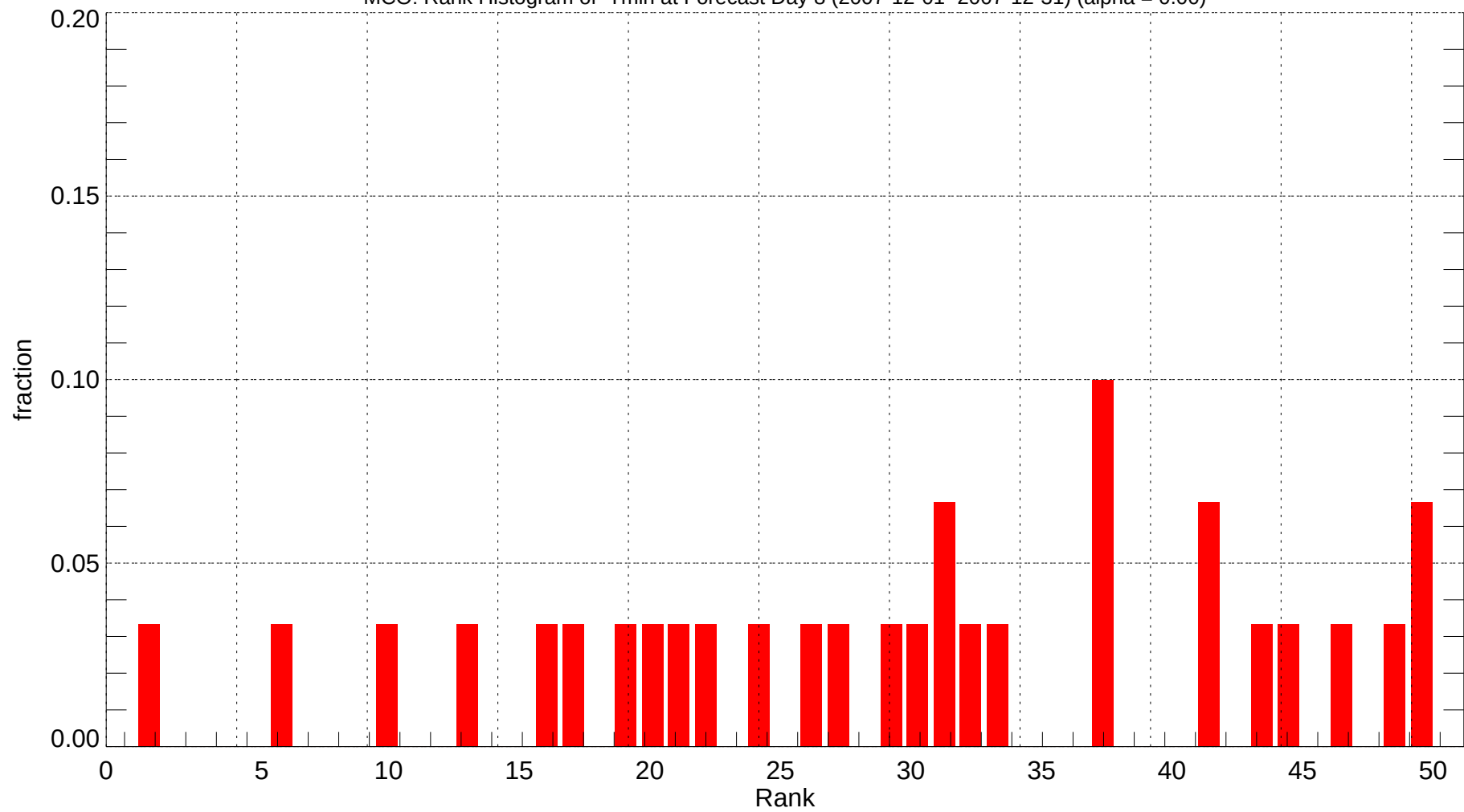
MCO: Rank Histogram of Tmin at Forecast Day 8 (2007-12-01~2007-12-31) (alpha = 0.00)
