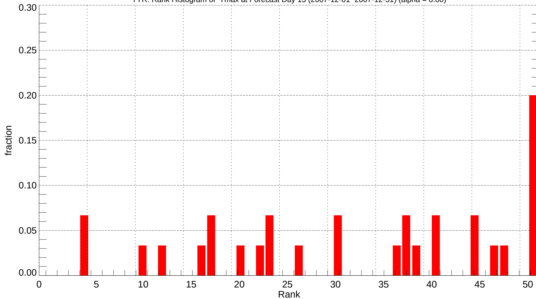
TYR: Rank Histogram of Tmax at Forecast Day 13 (2007-12-01~2007-12-31) (alpha = 0.00)
