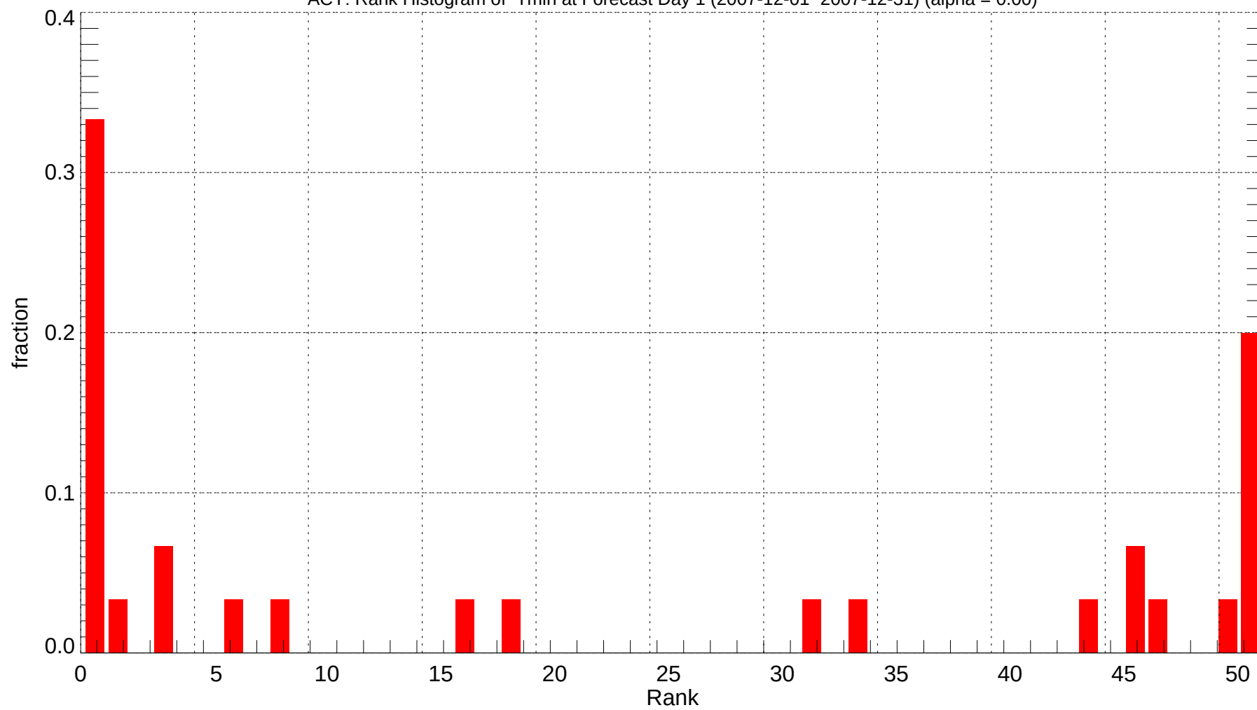
ACY: Rank Histogram of Tmin at Forecast Day 1 (2007-12-01~2007-12-31) (alpha = 0.00)
