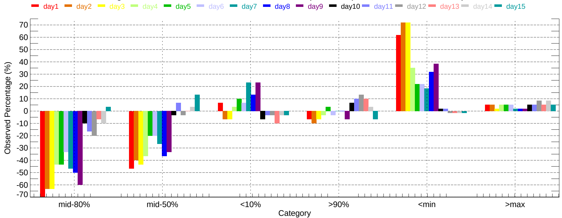
Observed Percentage Deviation of Ensembles - SAN: Min Temperature (2007-12-01~2007-12-31)
