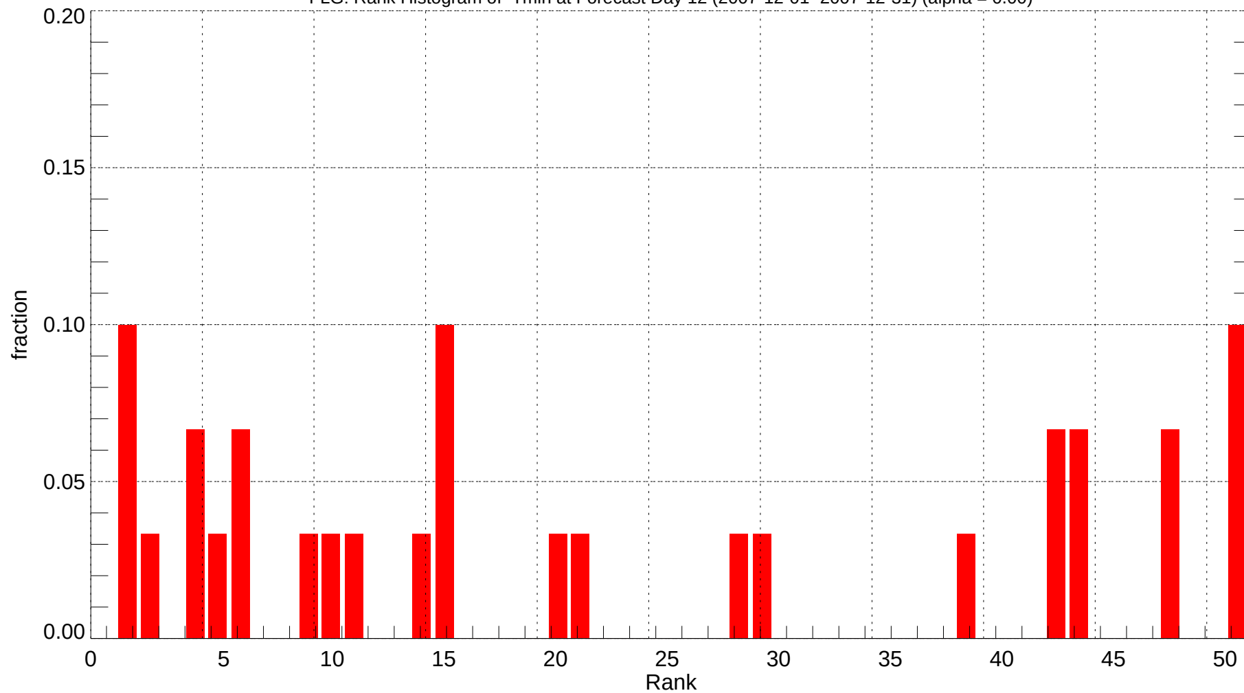
FLG: Rank Histogram of Tmin at Forecast Day 12 (2007-12-01~2007-12-31) (alpha = 0.00)
