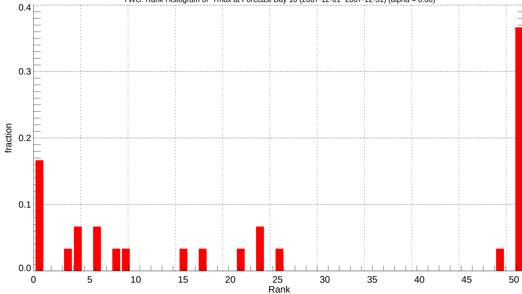
YWG: Rank Histogram of Tmax at Forecast Day 10 (2007-12-01~2007-12-31) (alpha = 0.00)
