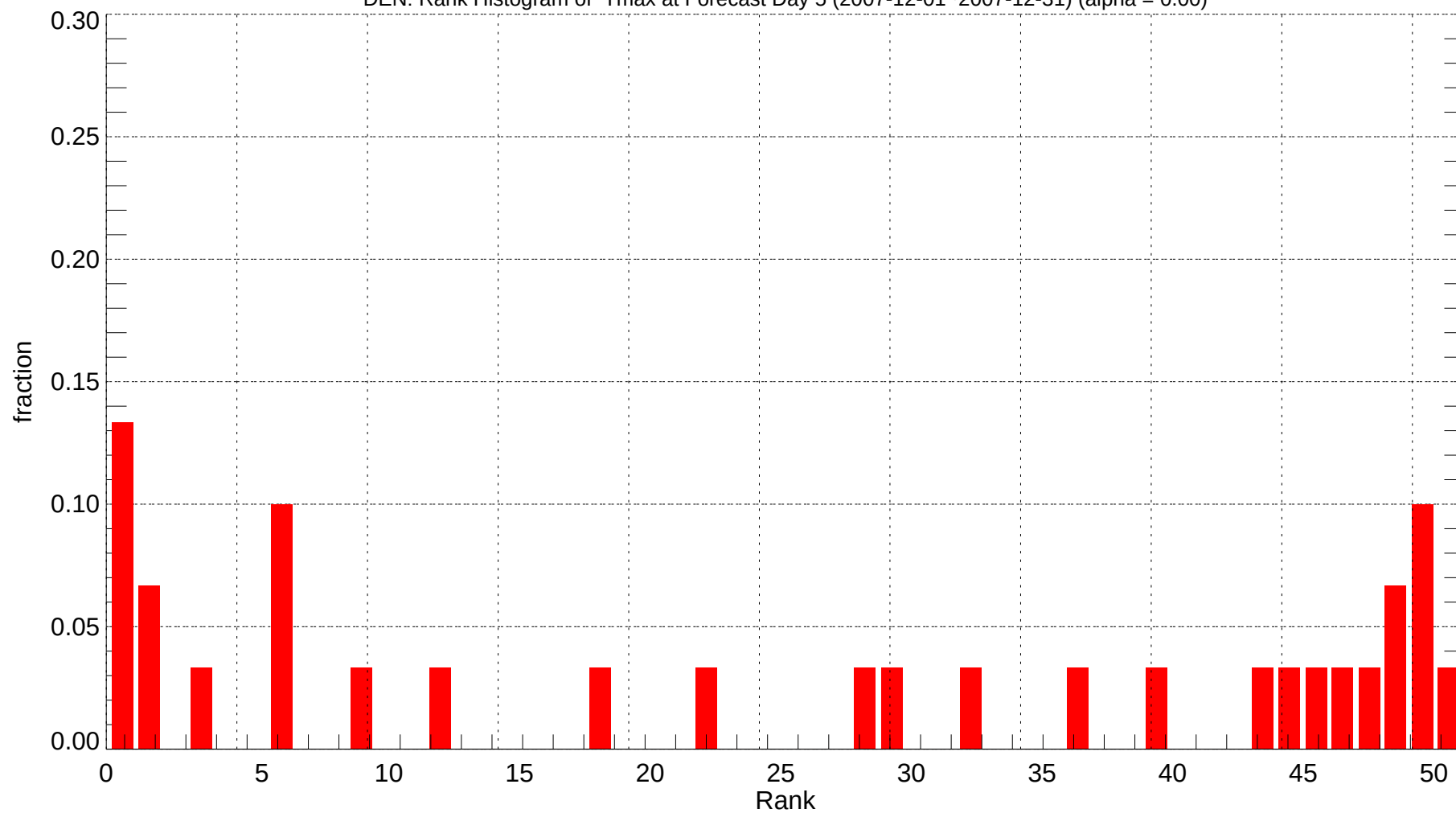
DEN: Rank Histogram of Tmax at Forecast Day 5 (2007-12-01~2007-12-31) (alpha = 0.00)
