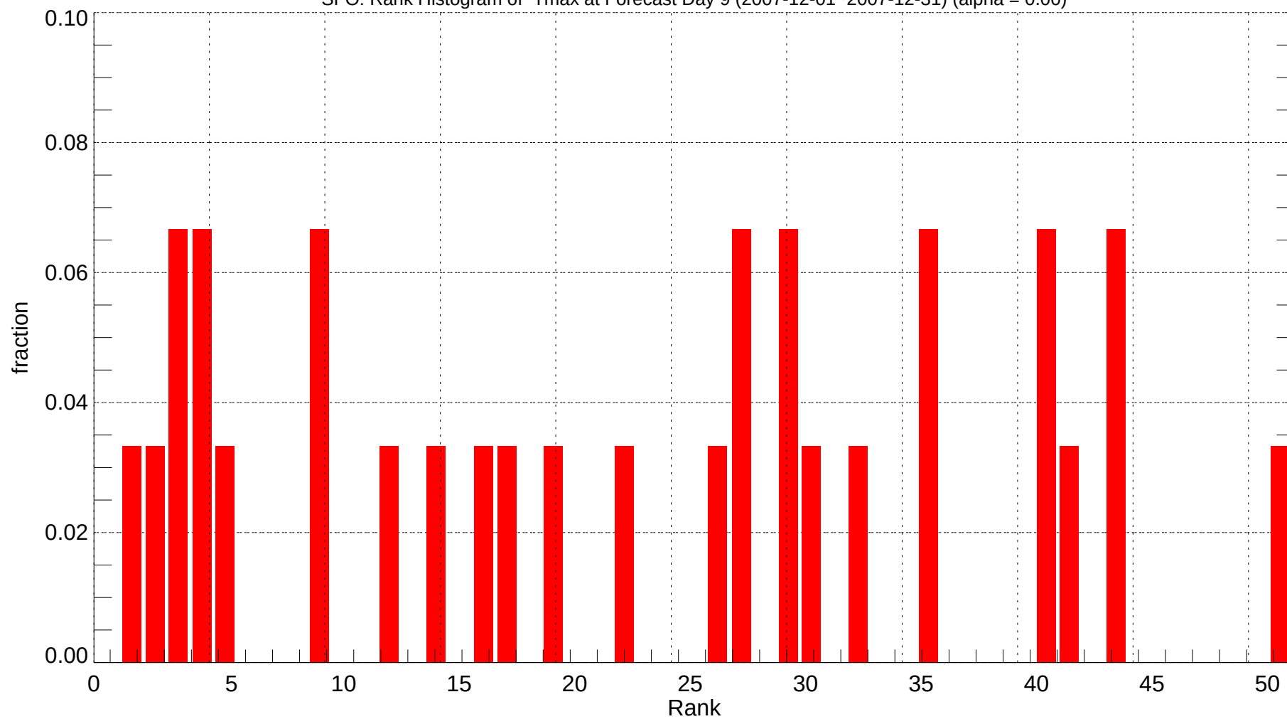
SFO: Rank Histogram of Tmax at Forecast Day 9 (2007-12-01~2007-12-31) (alpha = 0.00)
