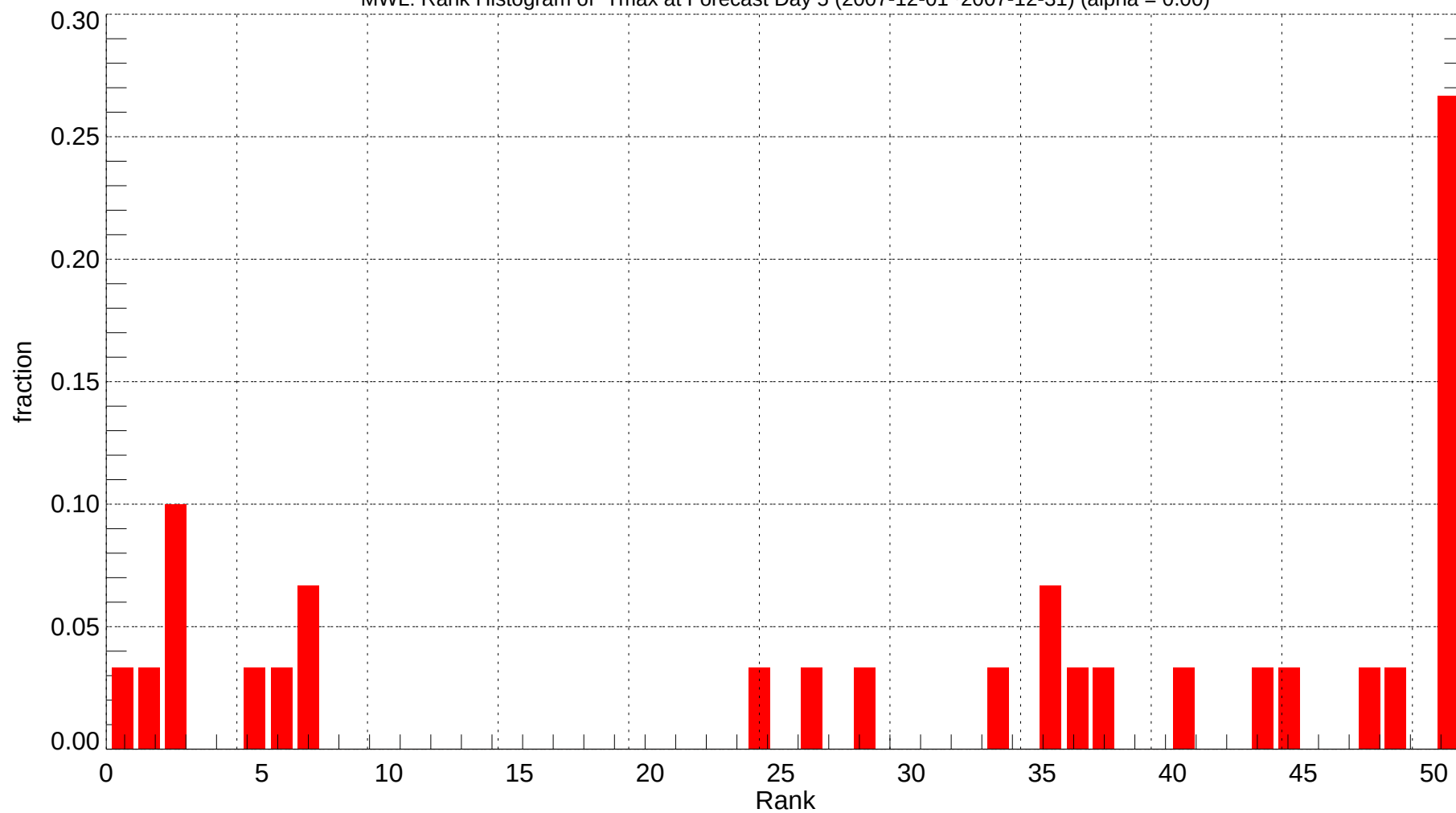
MWL: Rank Histogram of Tmax at Forecast Day 5 (2007-12-01~2007-12-31) (alpha = 0.00)
