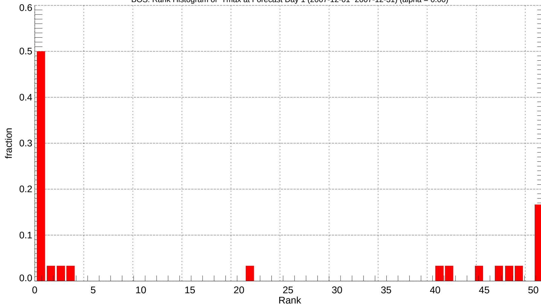
BOS: Rank Histogram of Tmax at Forecast Day 1 (2007-12-01~2007-12-31) (alpha = 0.00)
