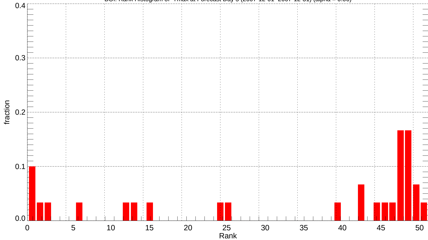
BOI: Rank Histogram of Tmax at Forecast Day 5 (2007-12-01~2007-12-31) (alpha = 0.00)
