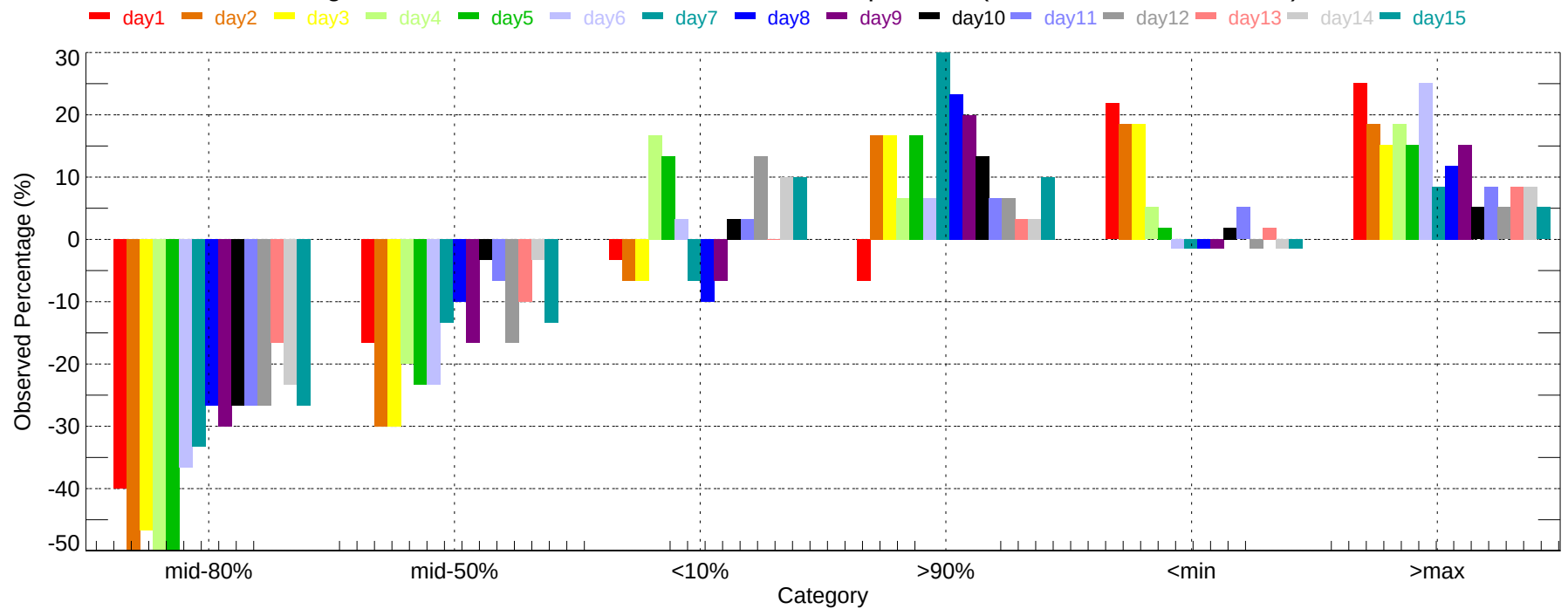
Observed Percentage Deviation of Ensembles - RDU: Min Temperature (2007-12-01~2007-12-31)
