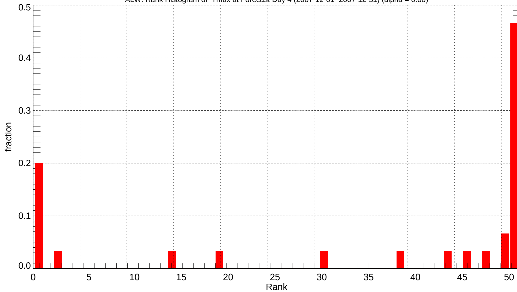
ALW: Rank Histogram of Tmax at Forecast Day 4 (2007-12-01~2007-12-31) (alpha = 0.00)
