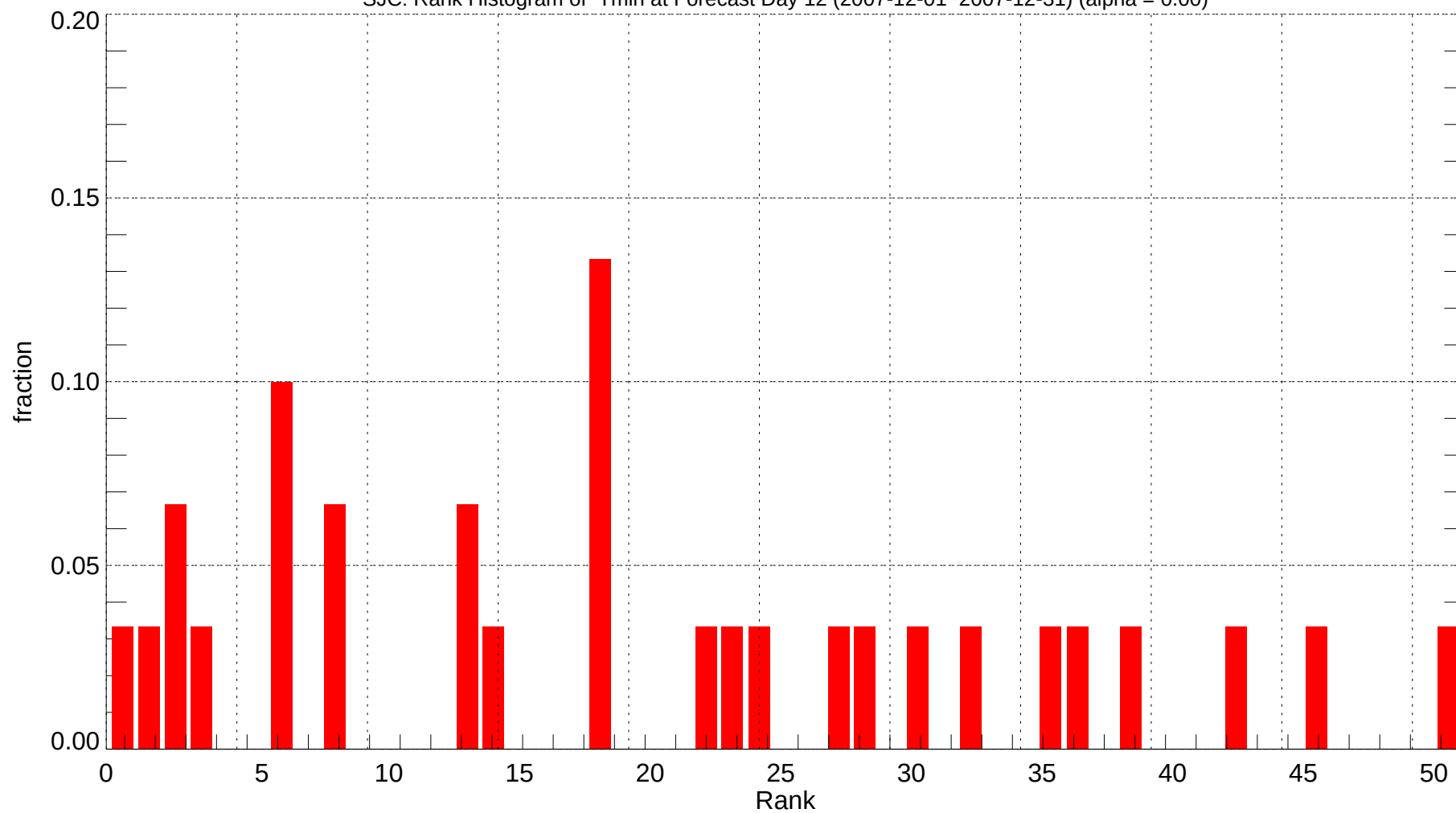
SJC: Rank Histogram of Tmin at Forecast Day 12 (2007-12-01~2007-12-31) (alpha = 0.00)
