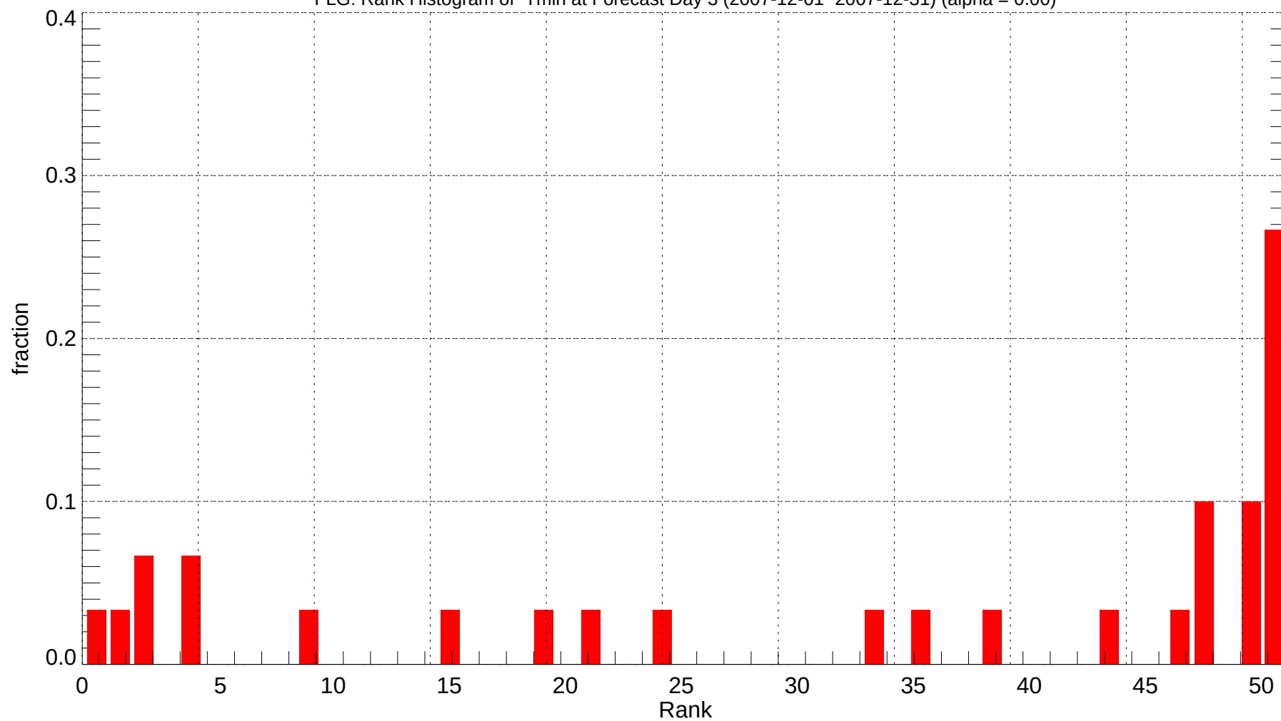
FLG: Rank Histogram of Tmin at Forecast Day 3 (2007-12-01~2007-12-31) (alpha = 0.00)
