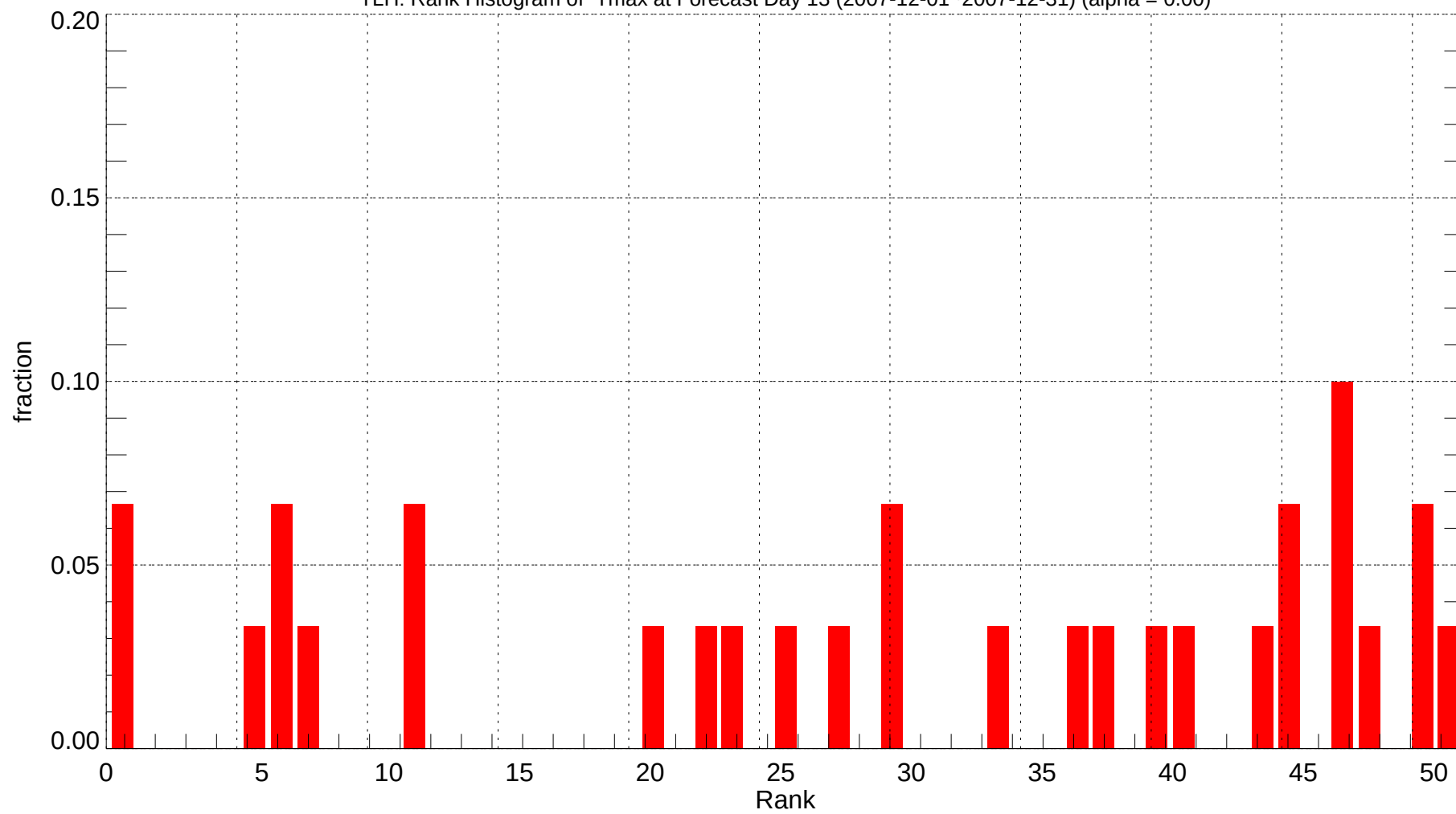
TLH: Rank Histogram of Tmax at Forecast Day 13 (2007-12-01~2007-12-31) (alpha = 0.00)
