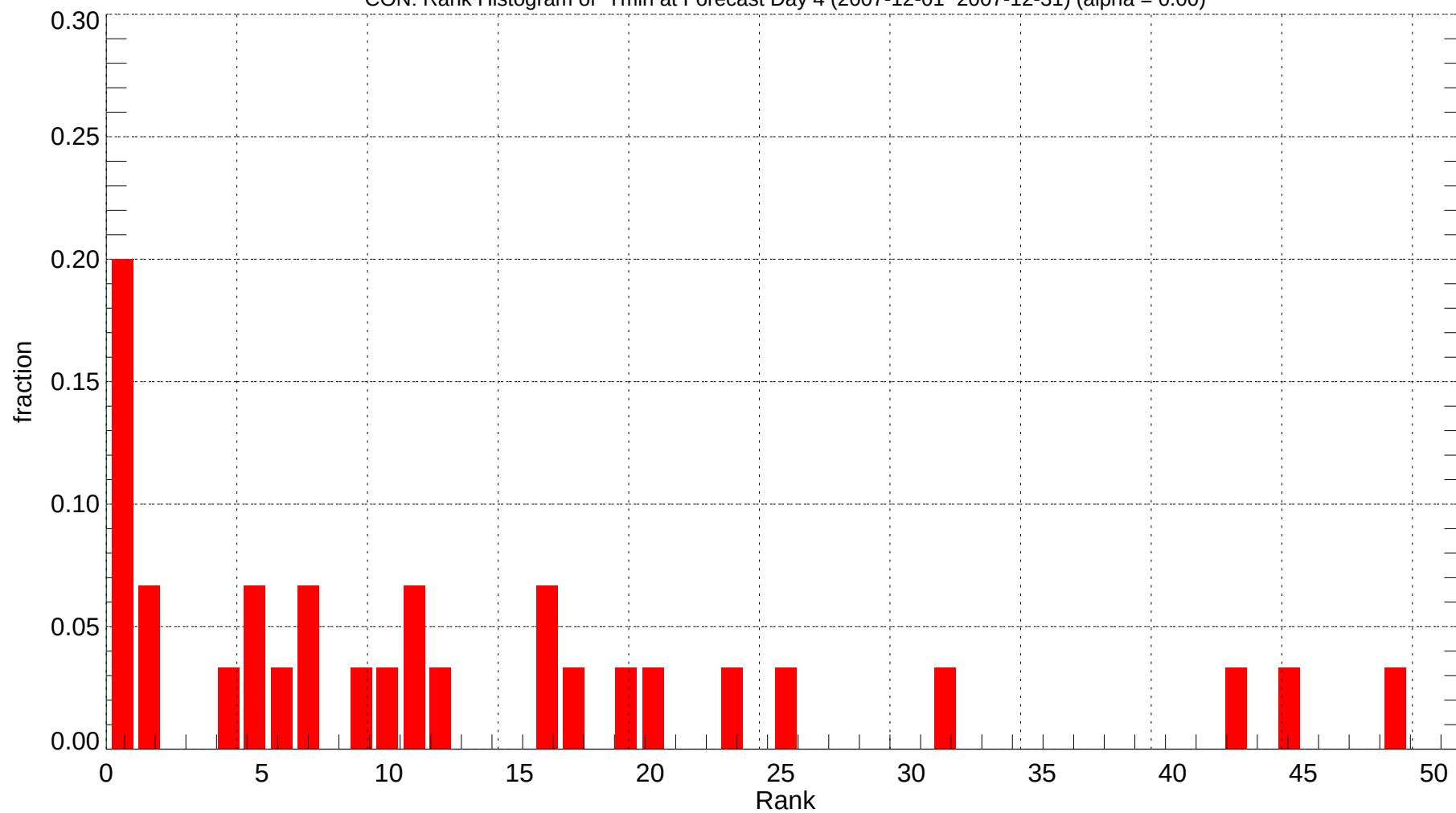
CON: Rank Histogram of Tmin at Forecast Day 4 (2007-12-01~2007-12-31) (alpha = 0.00)
