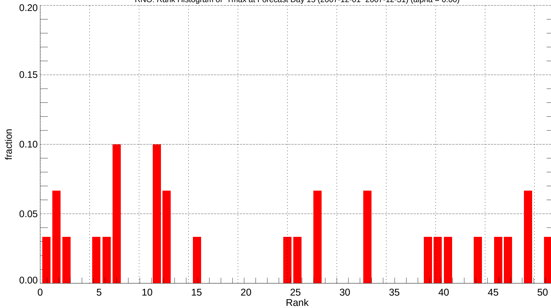
RNO: Rank Histogram of Tmax at Forecast Day 15 (2007-12-01~2007-12-31) (alpha = 0.00)
