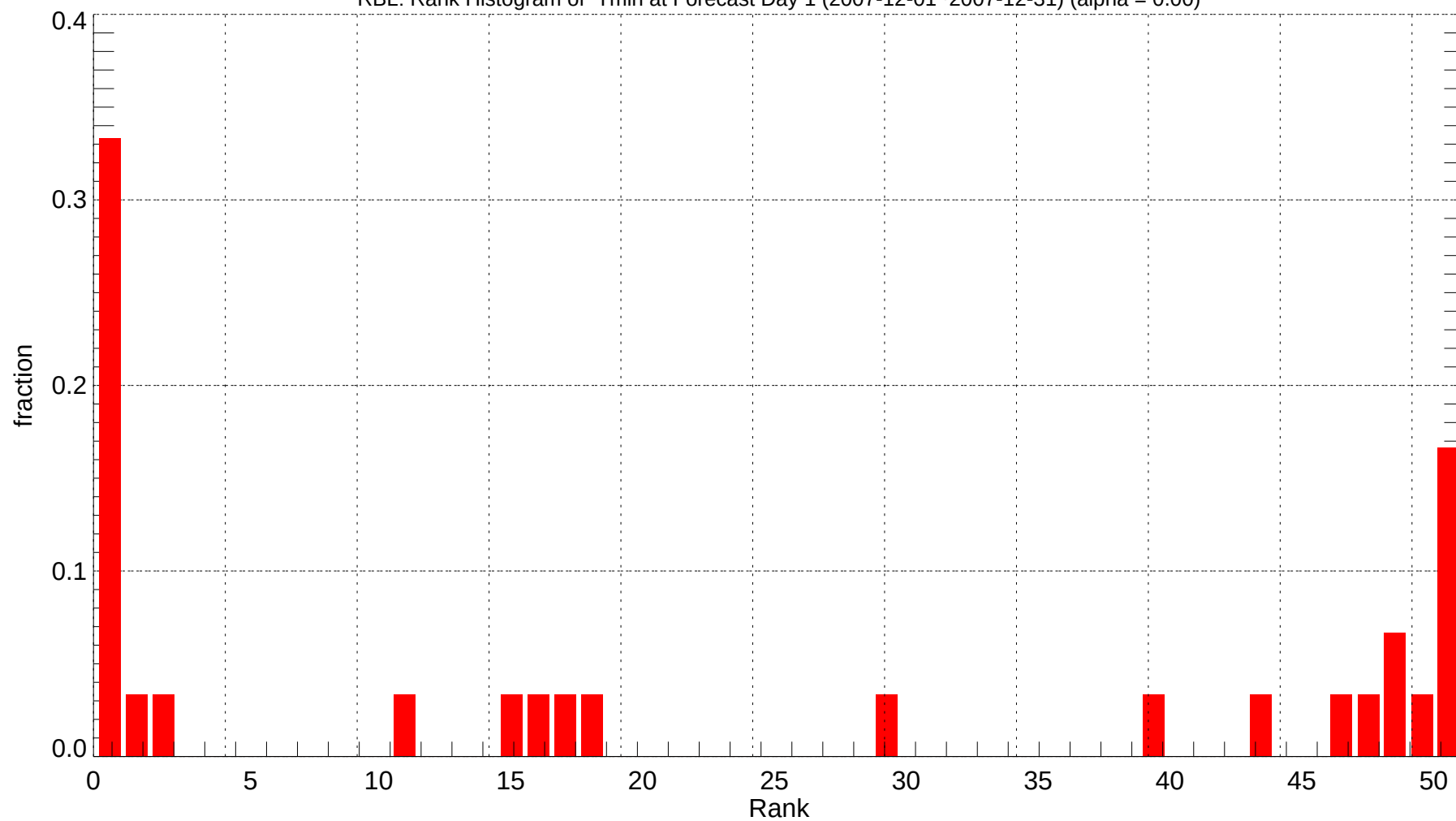
RBL: Rank Histogram of Tmin at Forecast Day 1 (2007-12-01~2007-12-31) (alpha = 0.00)
