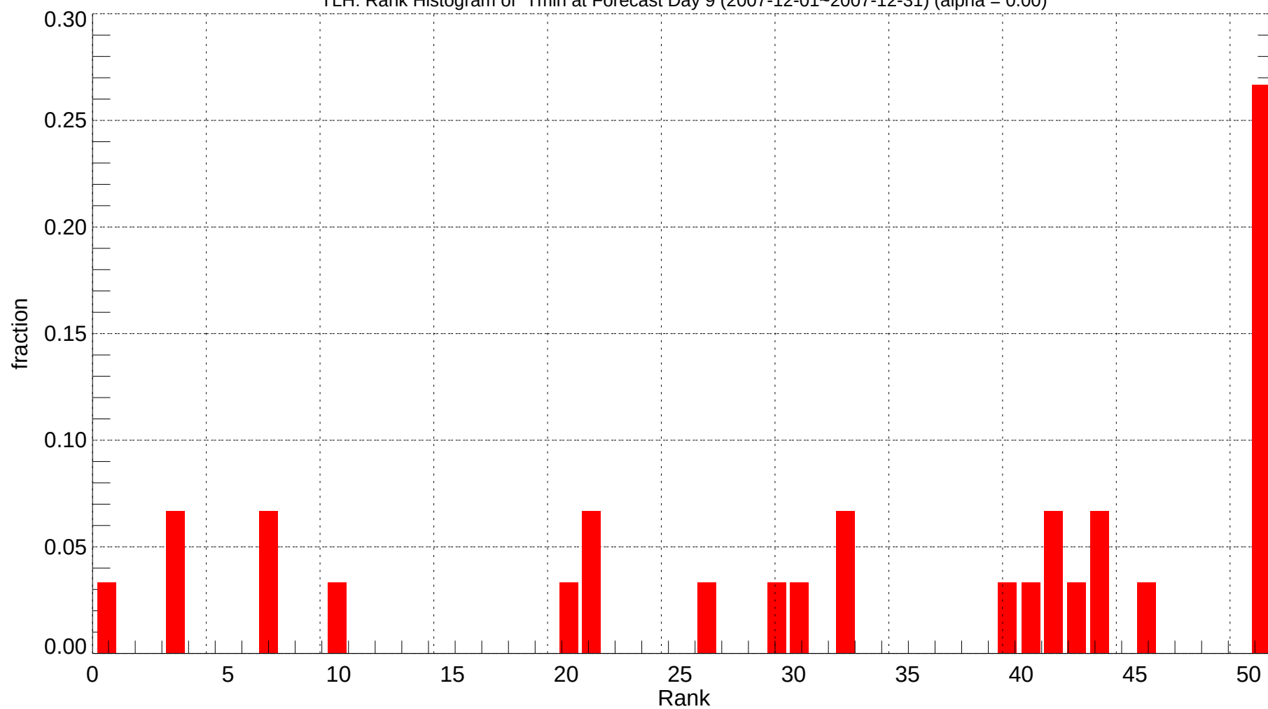
TLH: Rank Histogram of Tmin at Forecast Day 9 (2007-12-01~2007-12-31) (alpha = 0.00)
