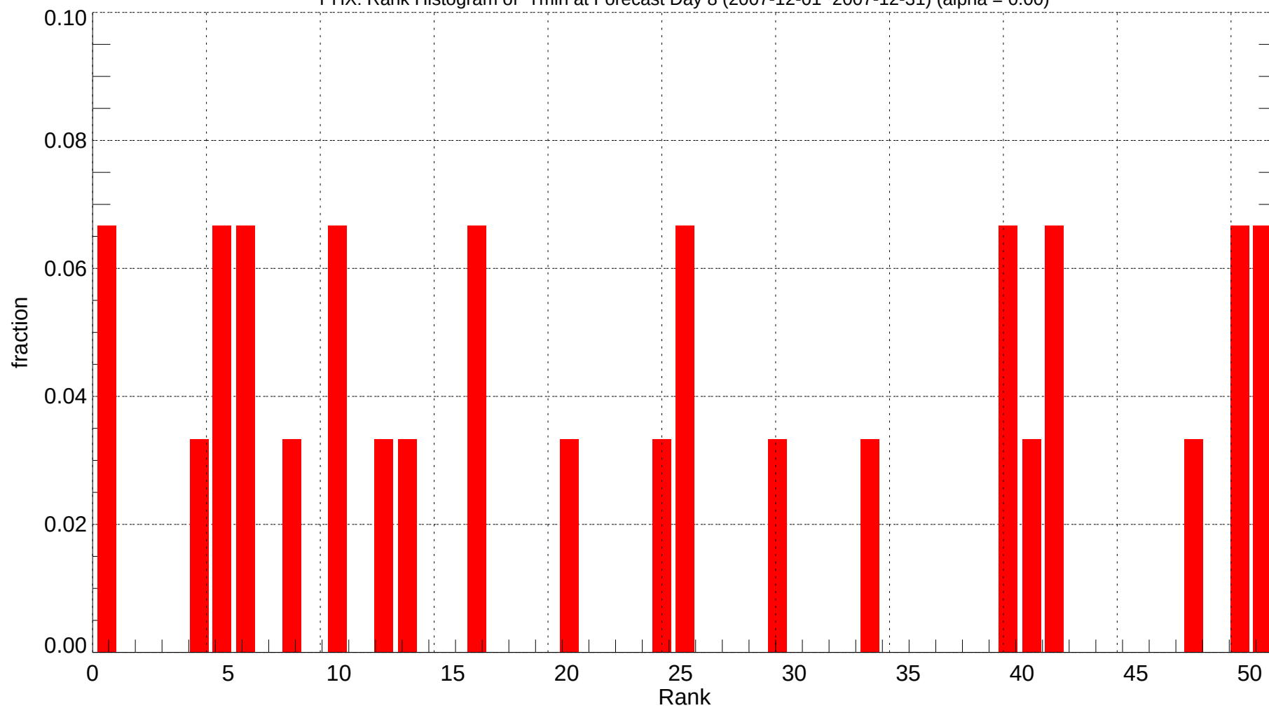
PHX: Rank Histogram of Tmin at Forecast Day 8 (2007-12-01~2007-12-31) (alpha = 0.00)
