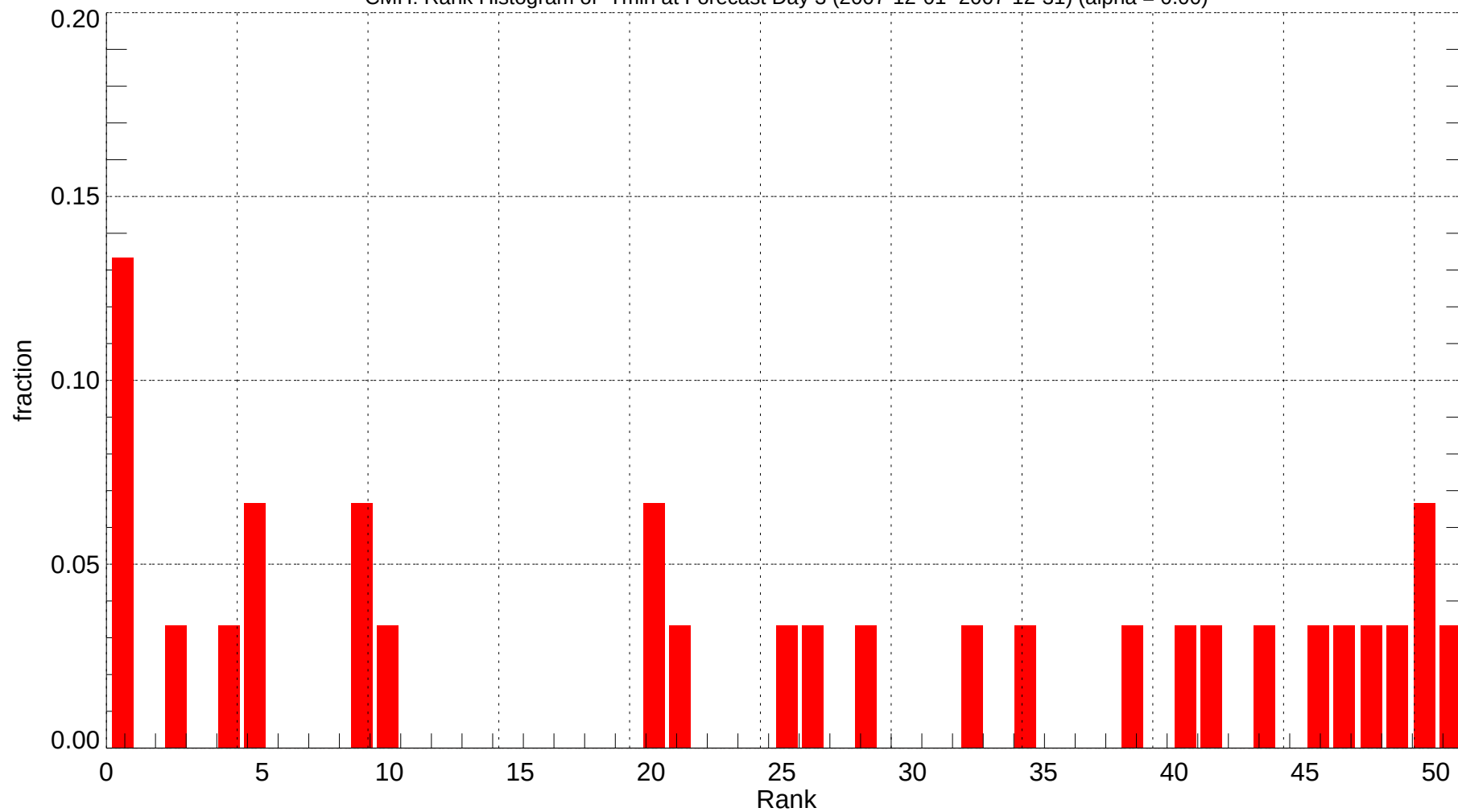
CMH: Rank Histogram of Tmin at Forecast Day 3 (2007-12-01~2007-12-31) (alpha = 0.00)
