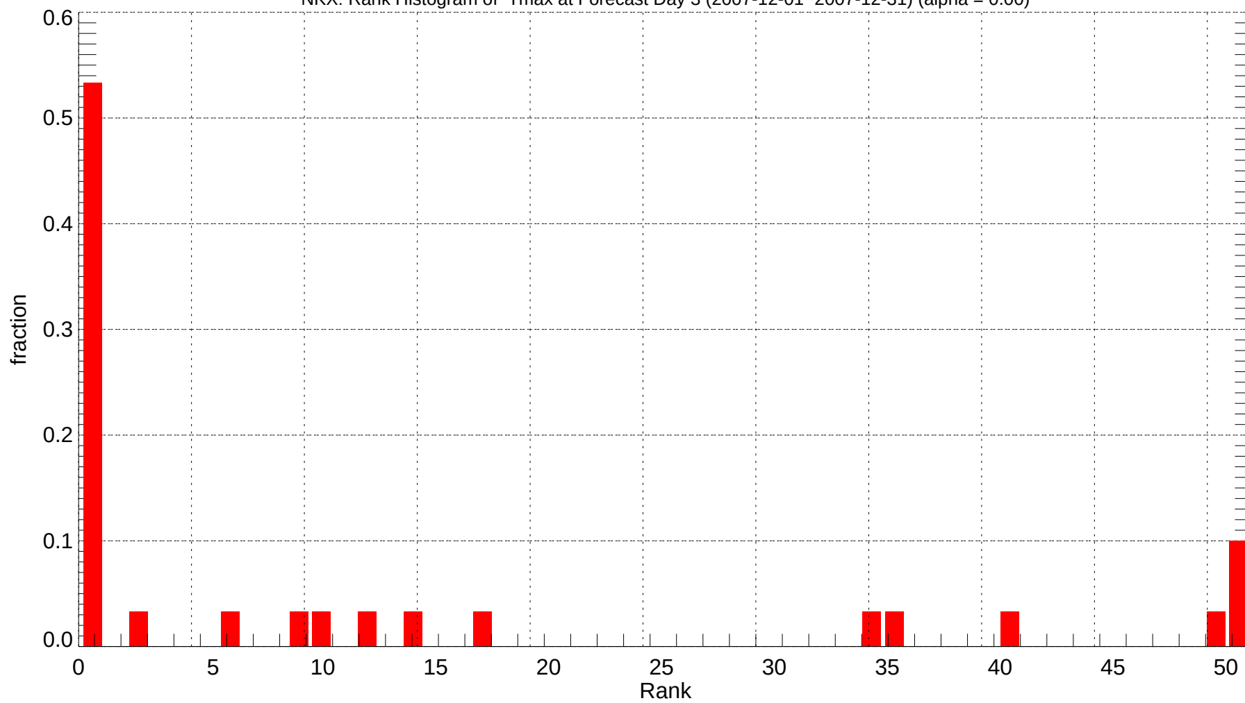
NKX: Rank Histogram of Tmax at Forecast Day 3 (2007-12-01~2007-12-31) (alpha = 0.00)
