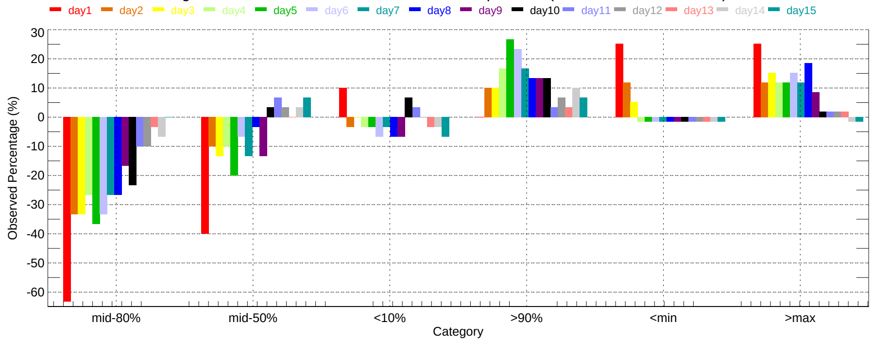
Observed Percentage Deviation of Ensembles - DEC: Max Temperature (2007-12-01~2007-12-31)
