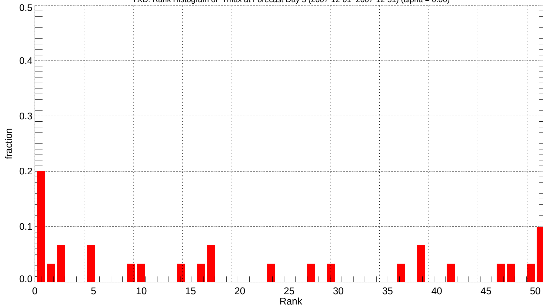
YXD: Rank Histogram of Tmax at Forecast Day 3 (2007-12-01~2007-12-31) (alpha = 0.00)
