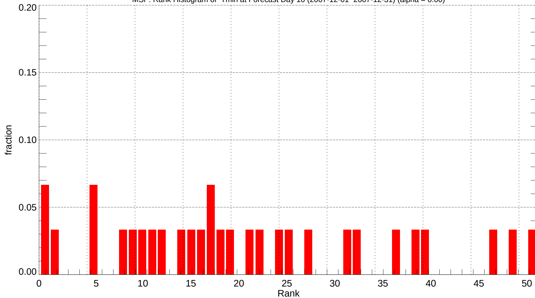
MSP: Rank Histogram of Tmin at Forecast Day 10 (2007-12-01~2007-12-31) (alpha = 0.00)
