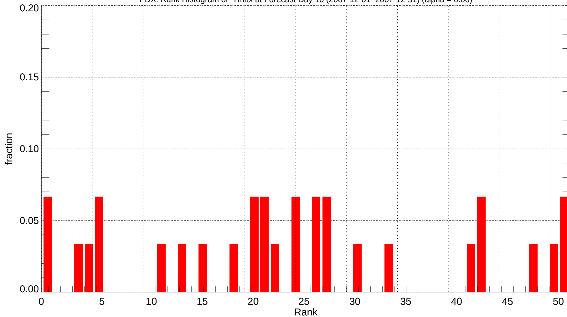
PDX: Rank Histogram of Tmax at Forecast Day 10 (2007-12-01~2007-12-31) (alpha = 0.00)
