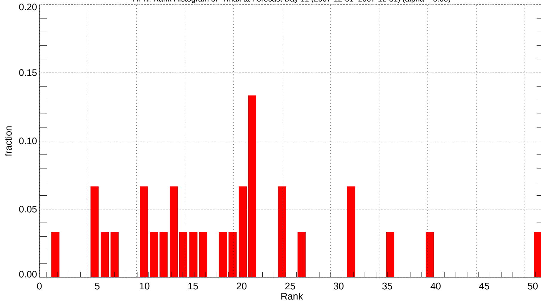
APN: Rank Histogram of Tmax at Forecast Day 11 (2007-12-01~2007-12-31) (alpha = 0.00)
