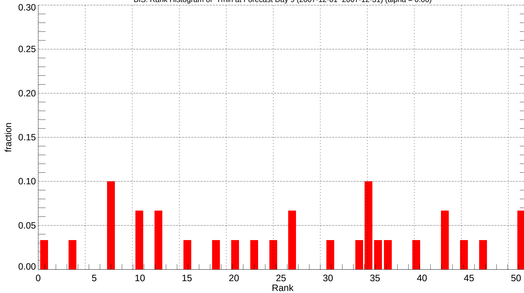
BIS: Rank Histogram of Tmin at Forecast Day 9 (2007-12-01~2007-12-31) (alpha = 0.00)
