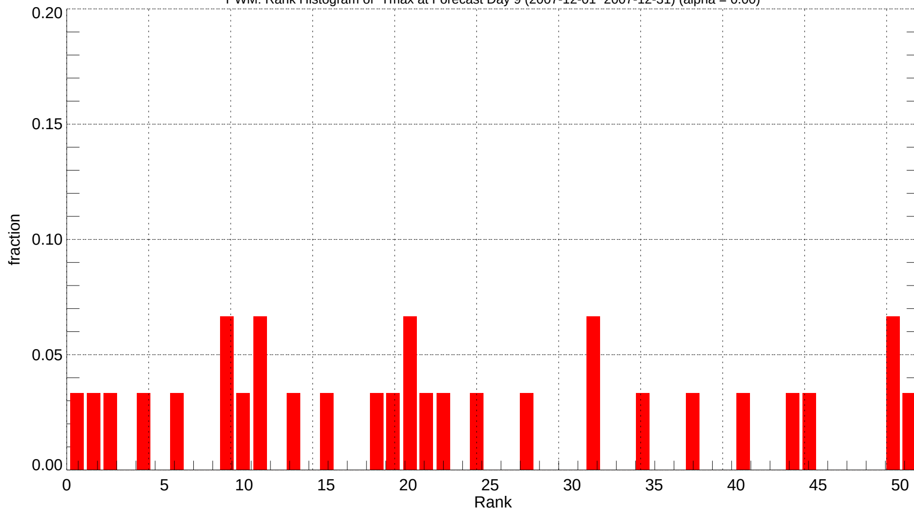
PWM: Rank Histogram of Tmax at Forecast Day 9 (2007-12-01~2007-12-31) (alpha = 0.00)
