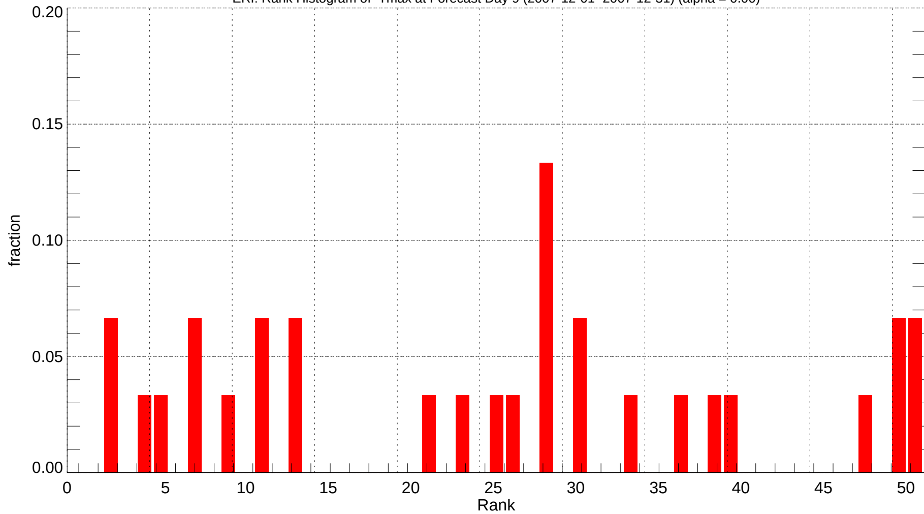
ERI: Rank Histogram of Tmax at Forecast Day 9 (2007-12-01~2007-12-31) (alpha = 0.00)
