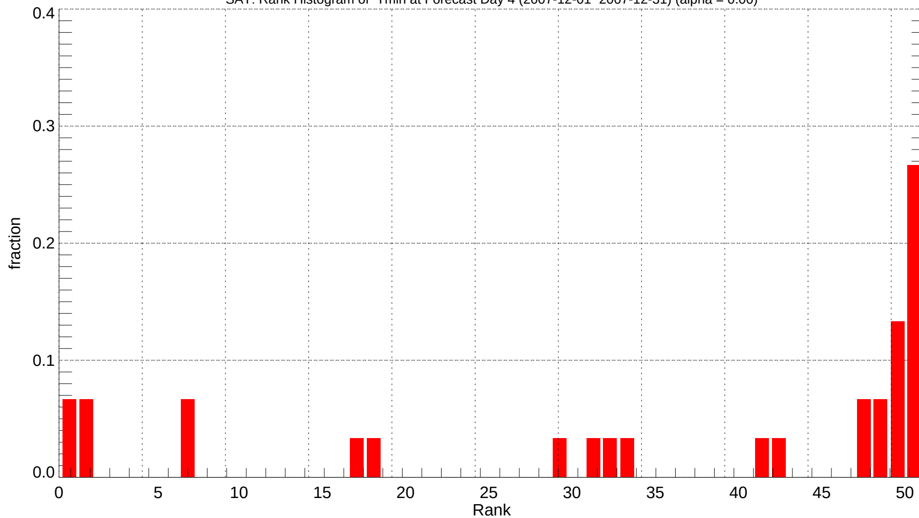
SAT: Rank Histogram of Tmin at Forecast Day 4 (2007-12-01~2007-12-31) (alpha = 0.00)
