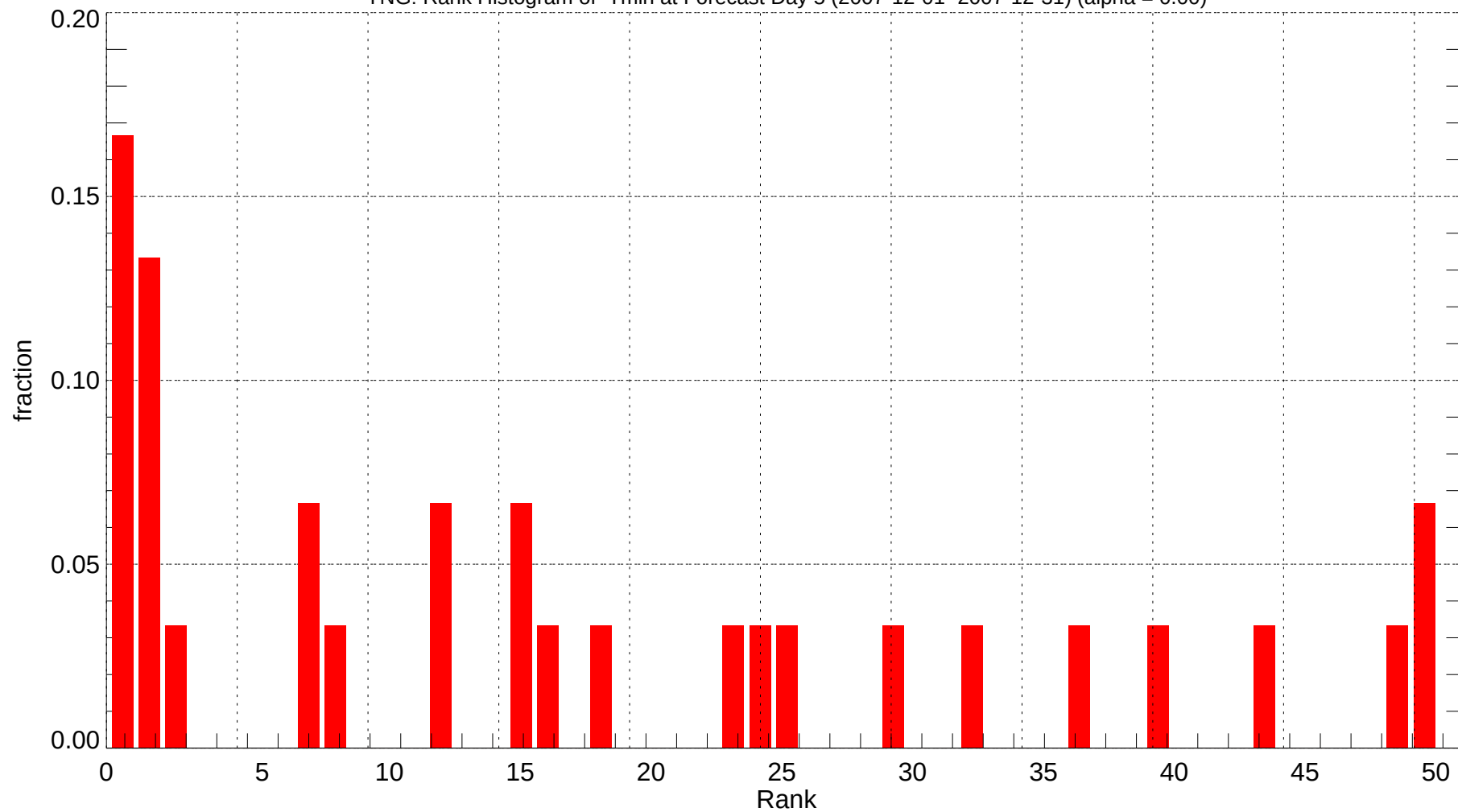
YNG: Rank Histogram of Tmin at Forecast Day 5 (2007-12-01~2007-12-31) (alpha = 0.00)
