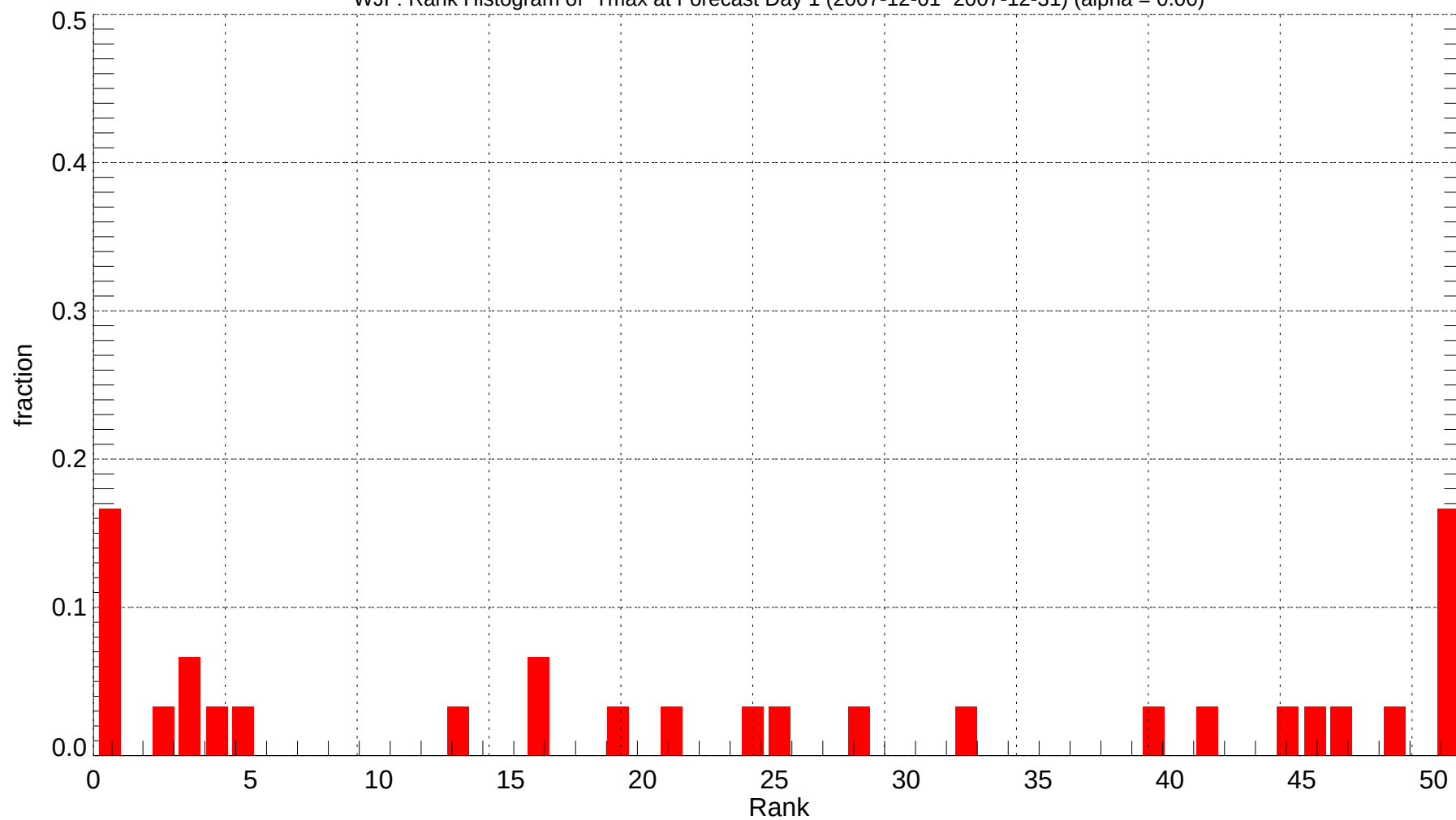
WJF: Rank Histogram of Tmax at Forecast Day 1 (2007-12-01~2007-12-31) (alpha = 0.00)
