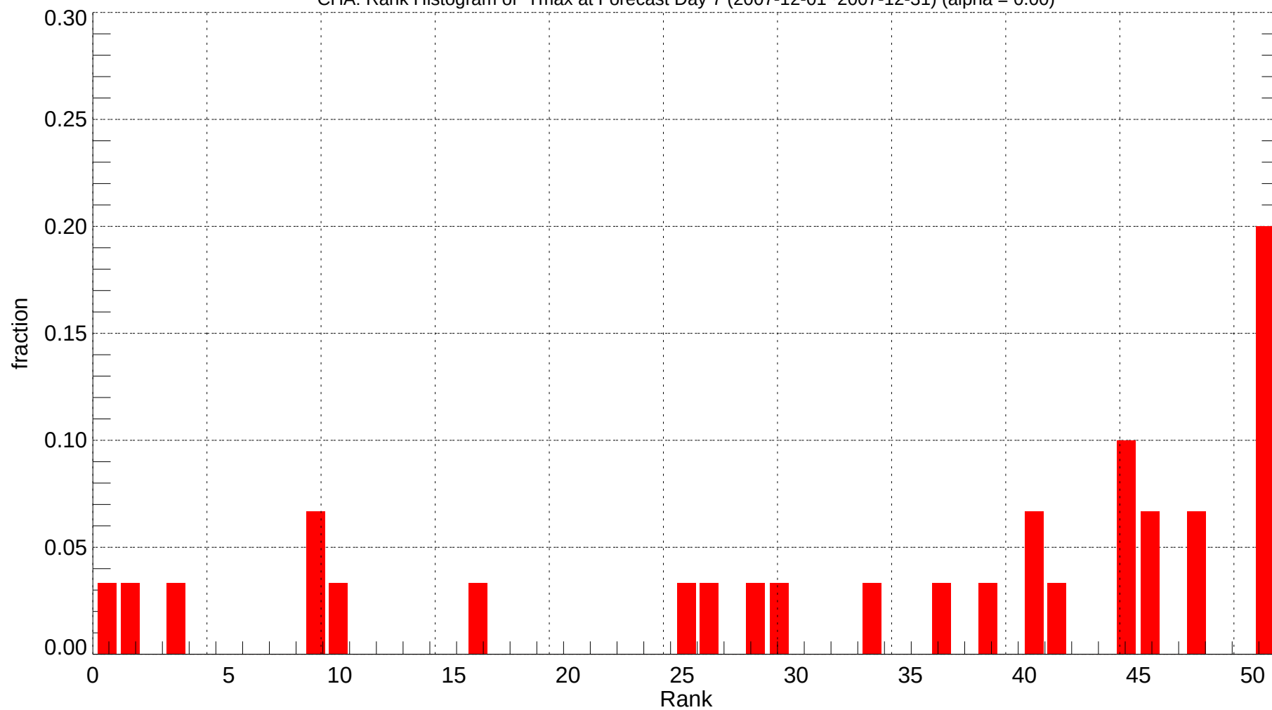
CHA: Rank Histogram of Tmax at Forecast Day 7 (2007-12-01~2007-12-31) (alpha = 0.00)
