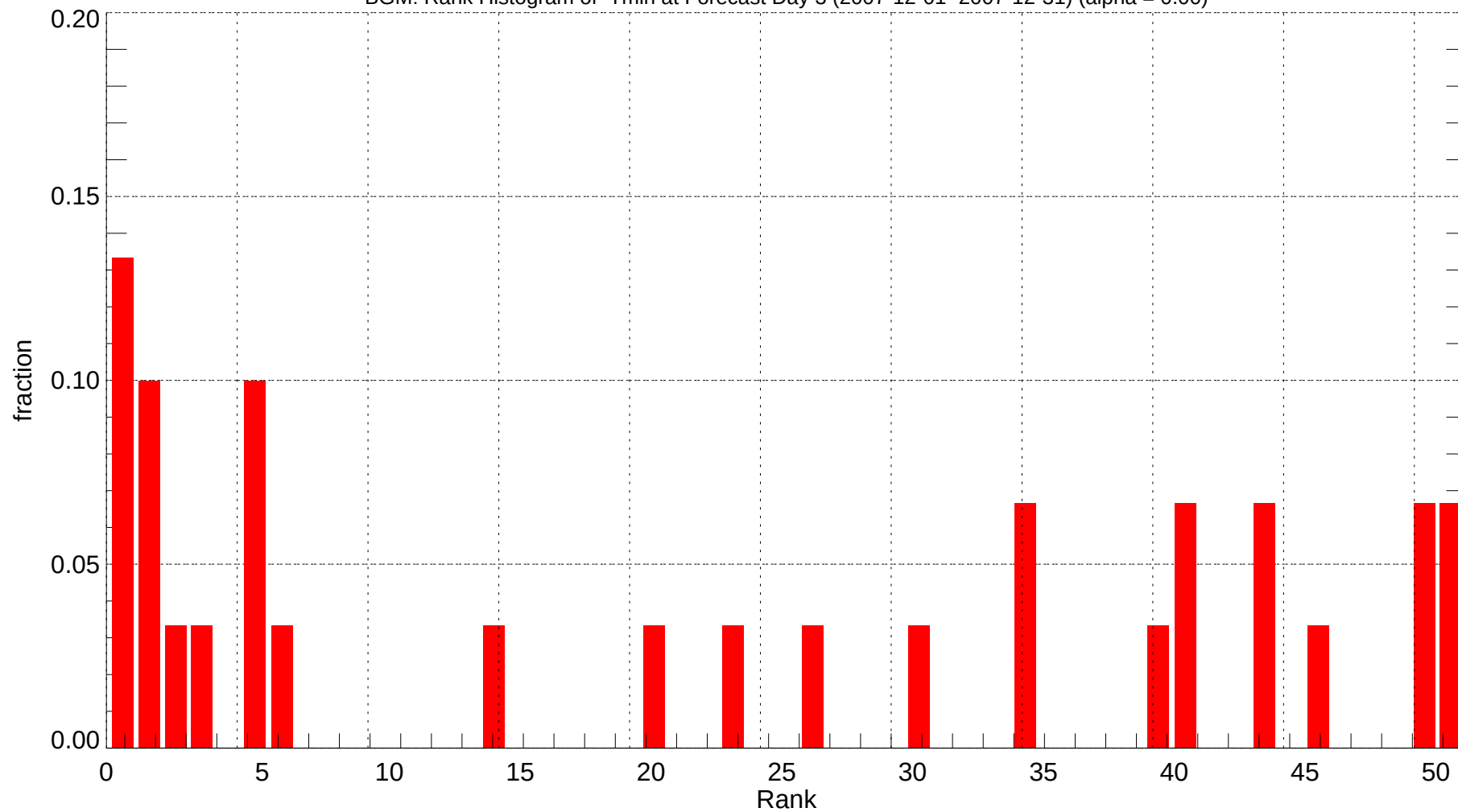
BGM: Rank Histogram of Tmin at Forecast Day 3 (2007-12-01~2007-12-31) (alpha = 0.00)
