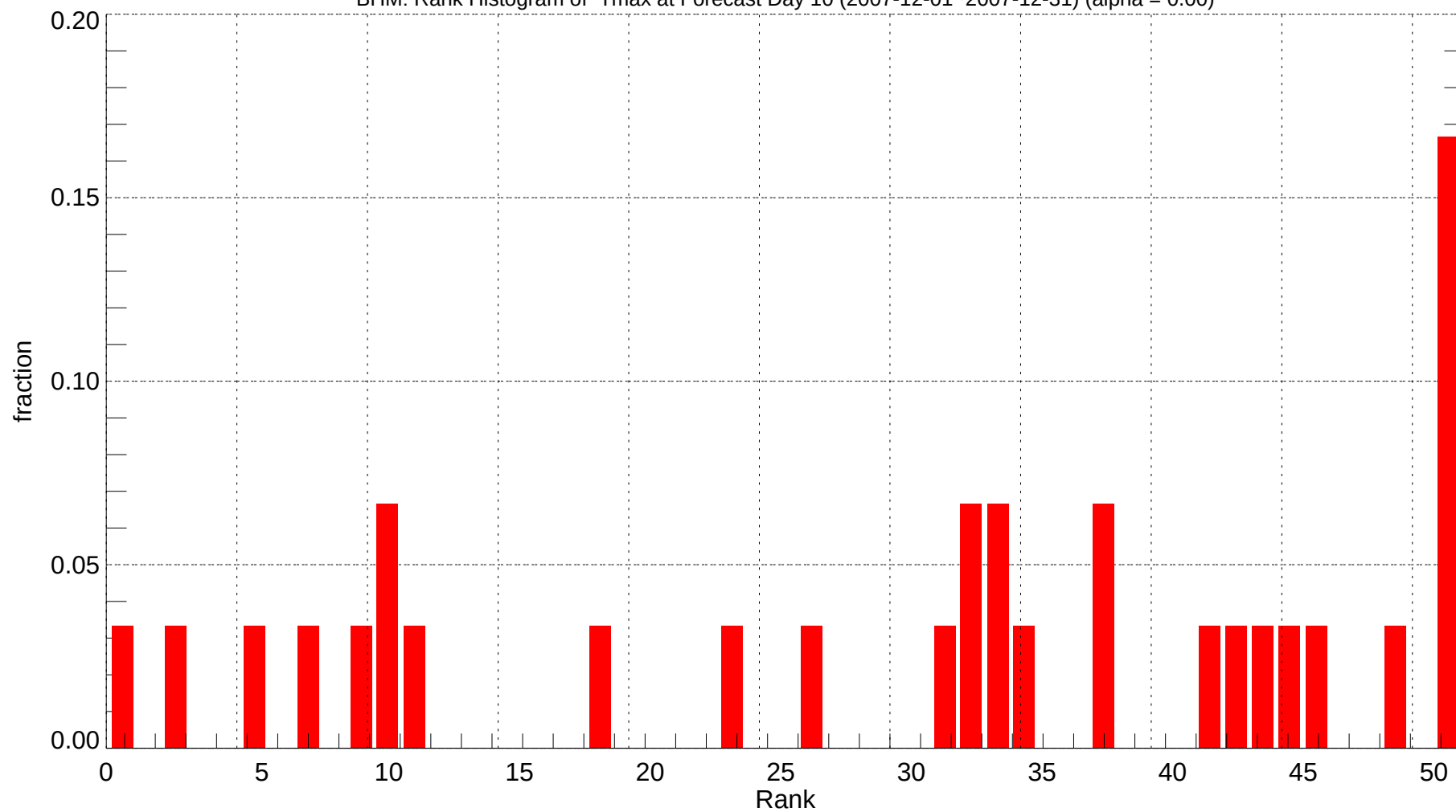
BHM: Rank Histogram of Tmax at Forecast Day 10 (2007-12-01~2007-12-31) (alpha = 0.00)
