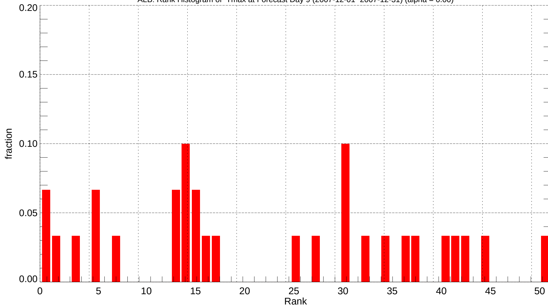
ALB: Rank Histogram of Tmax at Forecast Day 9 (2007-12-01~2007-12-31) (alpha = 0.00)
