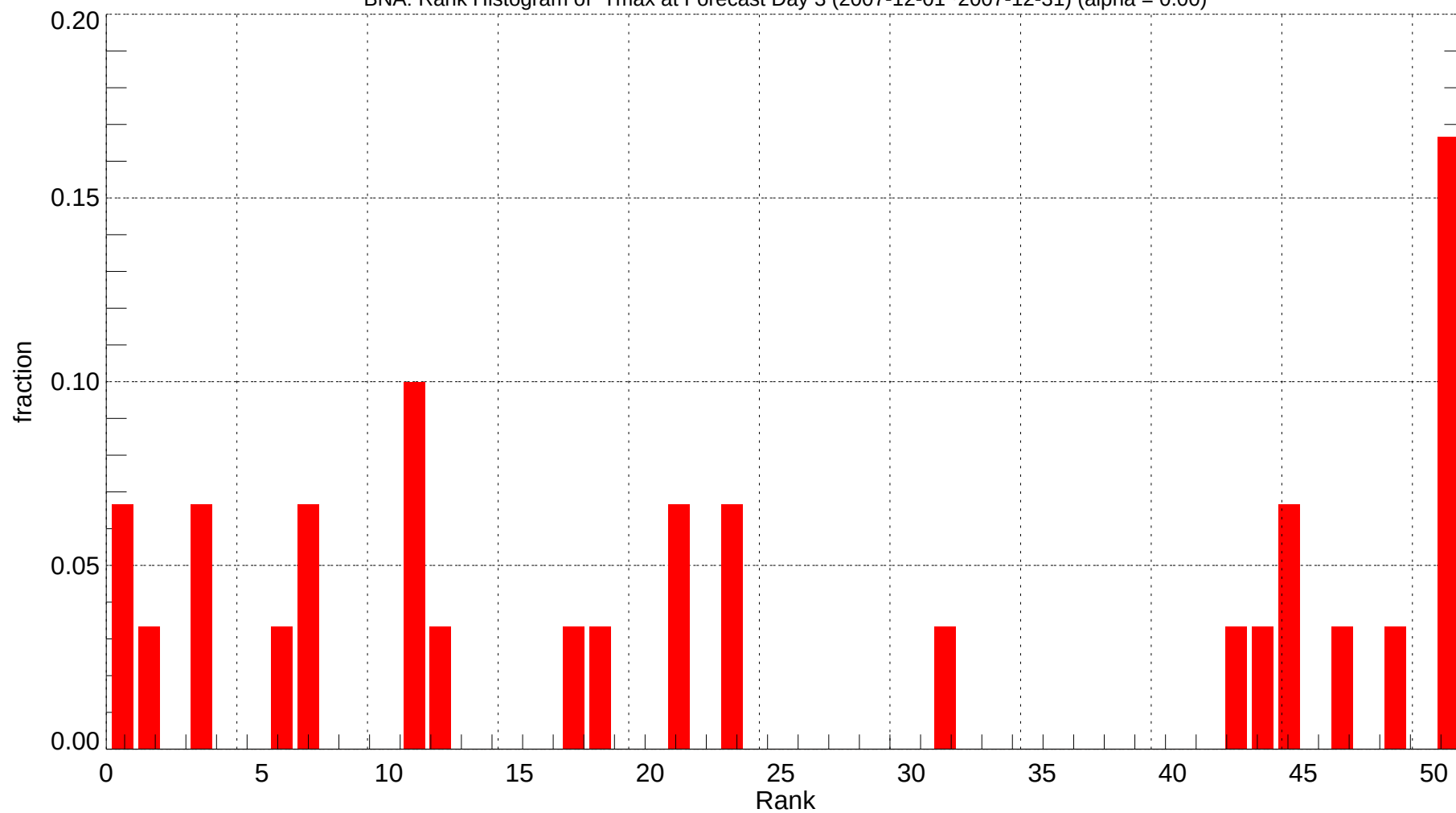
BNA: Rank Histogram of Tmax at Forecast Day 3 (2007-12-01~2007-12-31) (alpha = 0.00)
