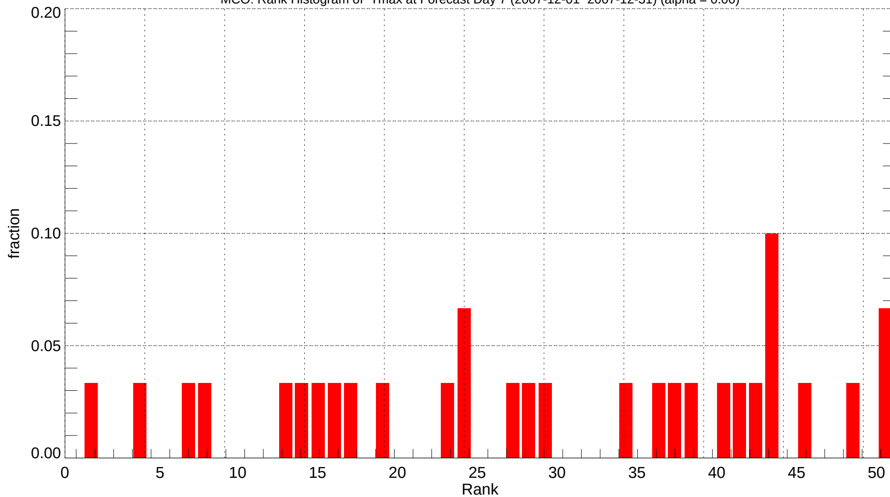
MCO: Rank Histogram of Tmax at Forecast Day 7 (2007-12-01~2007-12-31) (alpha = 0.00)
