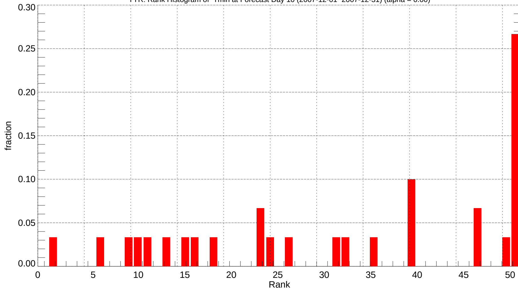
TYR: Rank Histogram of Tmin at Forecast Day 10 (2007-12-01~2007-12-31) (alpha = 0.00)
