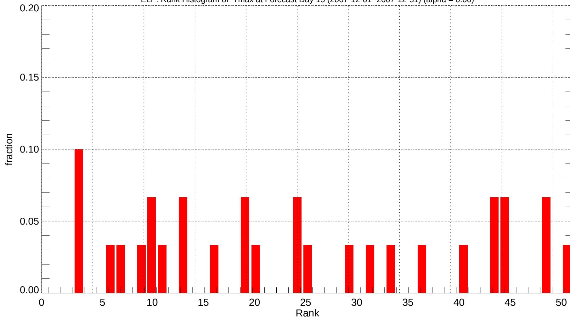
ELP: Rank Histogram of Tmax at Forecast Day 15 (2007-12-01~2007-12-31) (alpha = 0.00)
