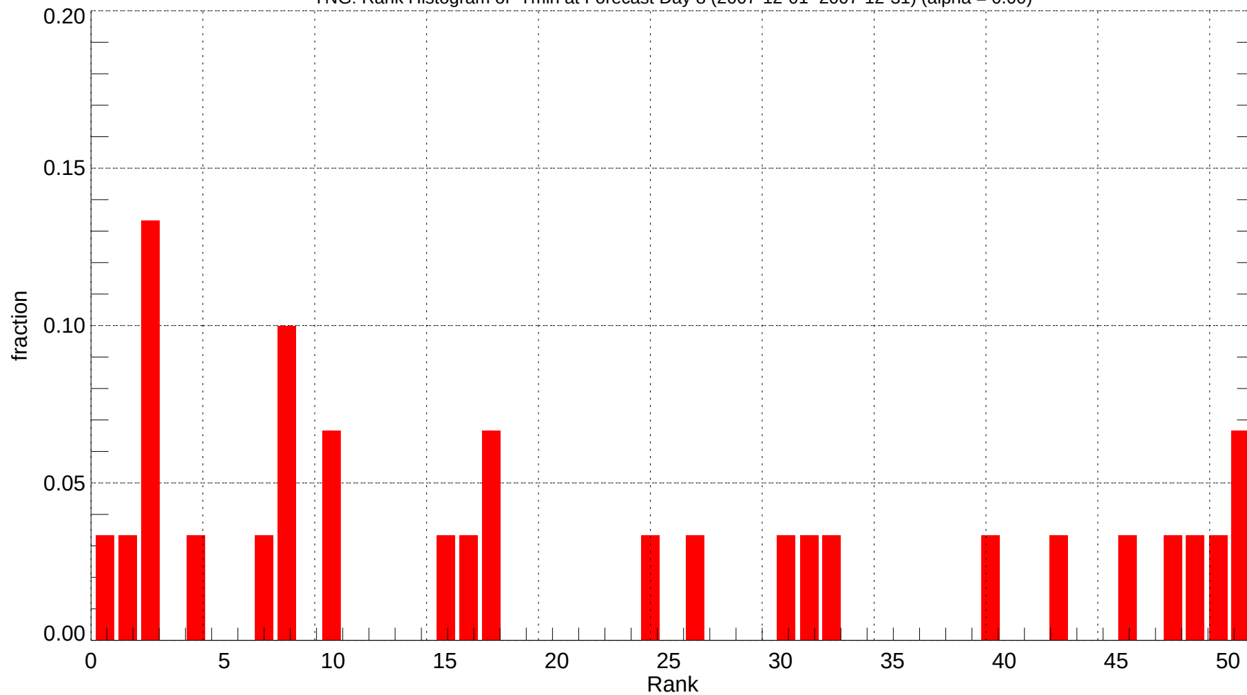
YNG: Rank Histogram of Tmin at Forecast Day 8 (2007-12-01~2007-12-31) (alpha = 0.00)
