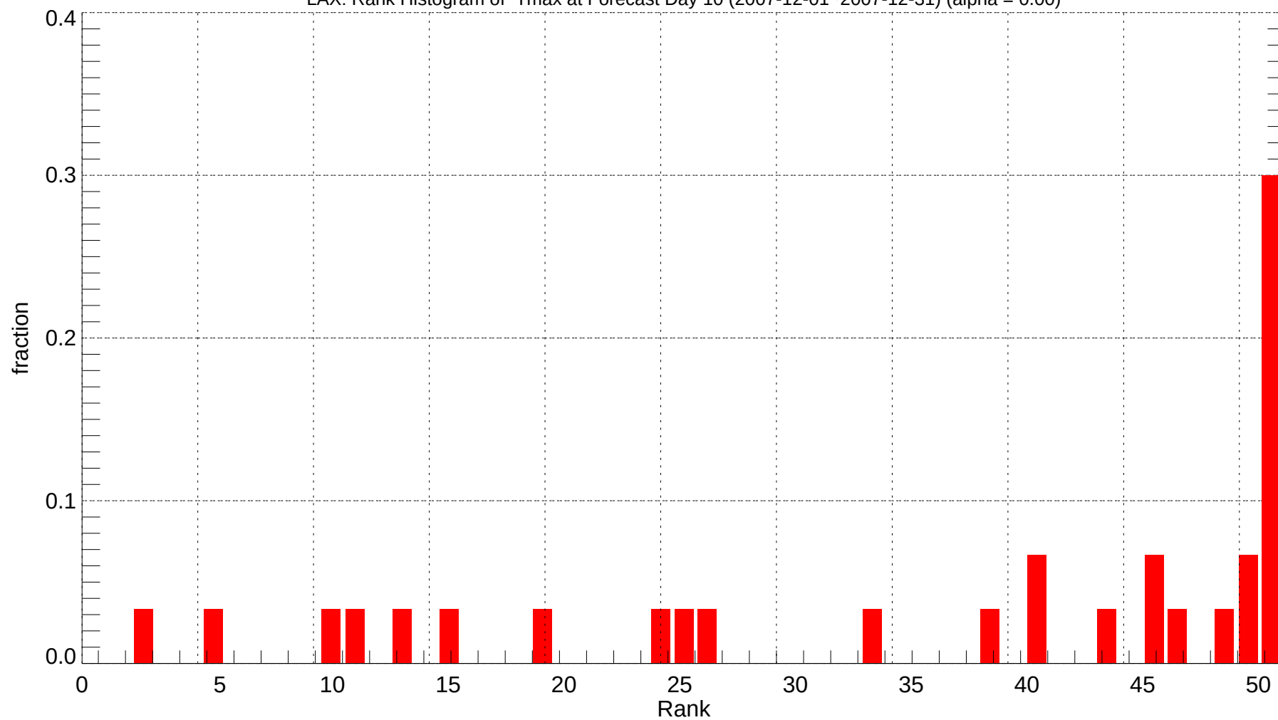
LAX: Rank Histogram of Tmax at Forecast Day 10 (2007-12-01~2007-12-31) (alpha = 0.00)
