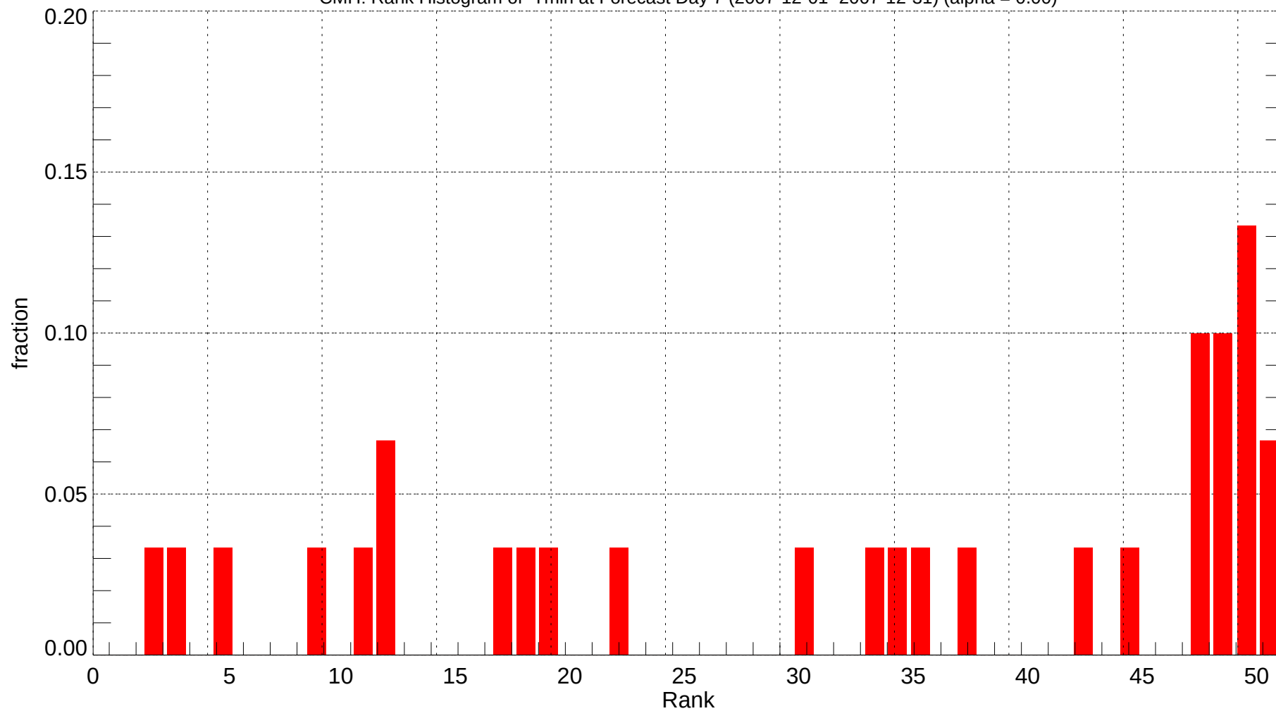
CMH: Rank Histogram of Tmin at Forecast Day 7 (2007-12-01~2007-12-31) (alpha = 0.00)
