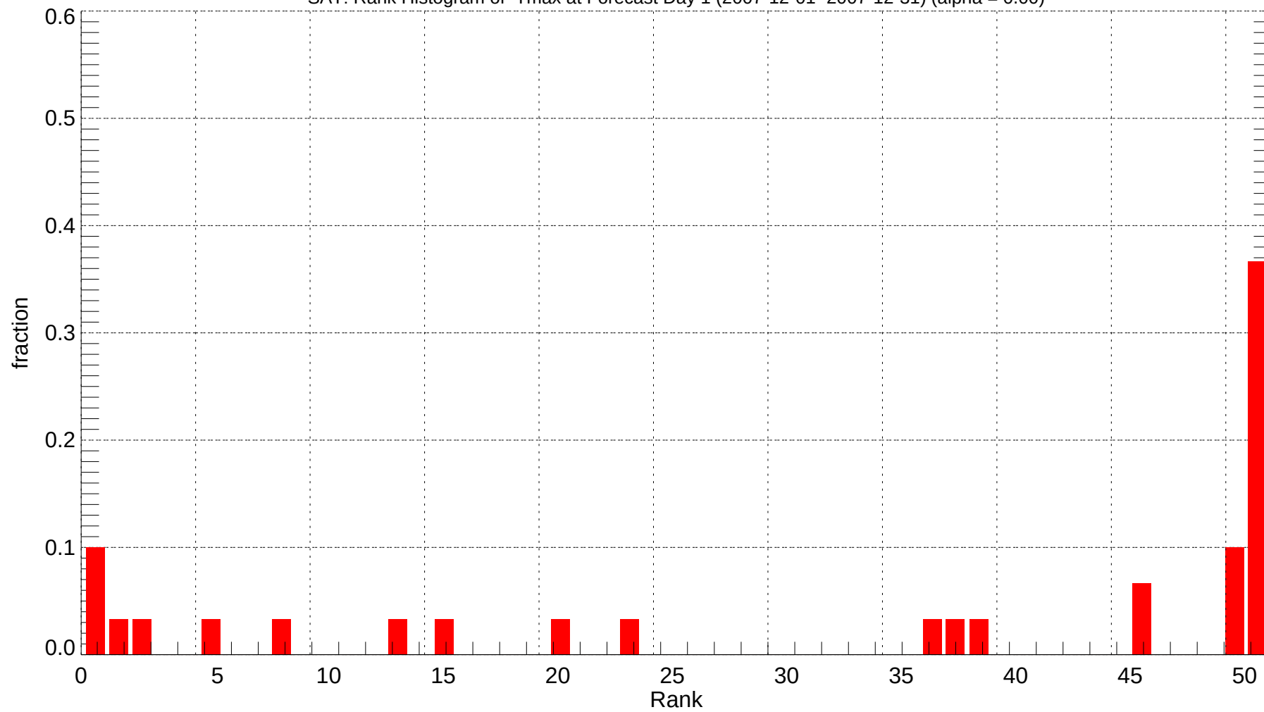
SAT: Rank Histogram of Tmax at Forecast Day 1 (2007-12-01~2007-12-31) (alpha = 0.00)
