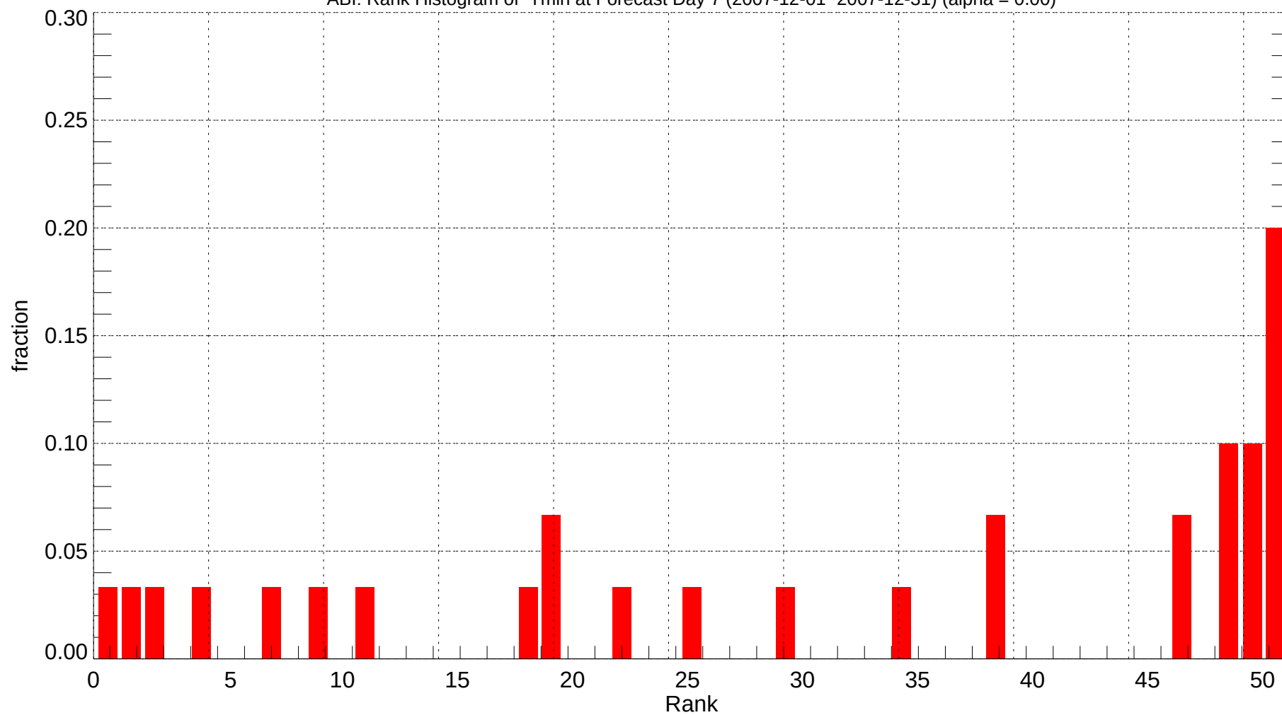
ABI: Rank Histogram of Tmin at Forecast Day 7 (2007-12-01~2007-12-31) (alpha = 0.00)
