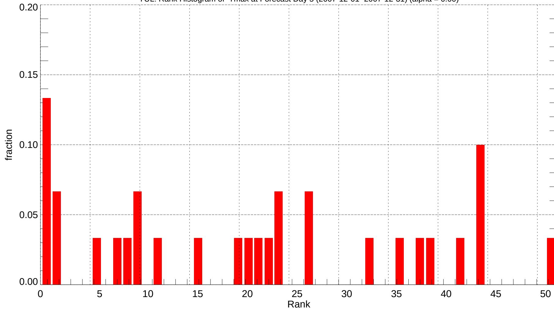
YUL: Rank Histogram of Tmax at Forecast Day 5 (2007-12-01~2007-12-31) (alpha = 0.00)
