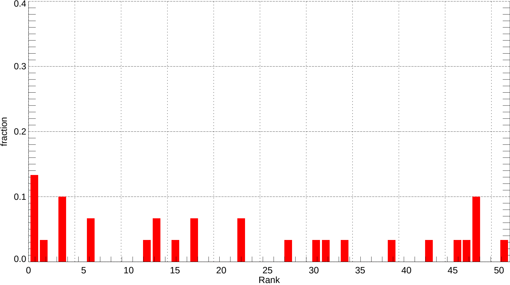
IPT: Rank Histogram of Tmax at Forecast Day 4 (2007-12-01~2007-12-31) (alpha = 0.00)
