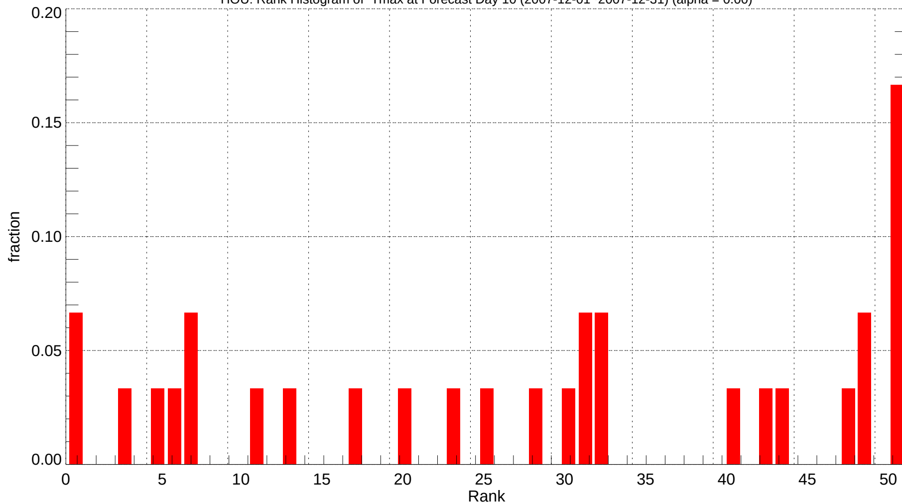
HOU: Rank Histogram of Tmax at Forecast Day 10 (2007-12-01~2007-12-31) (alpha = 0.00)
