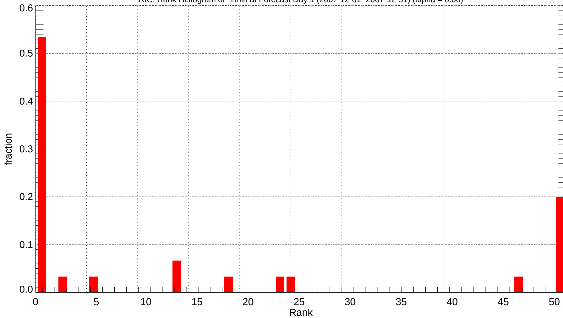
RIC: Rank Histogram of Tmin at Forecast Day 1 (2007-12-01~2007-12-31) (alpha = 0.00)
