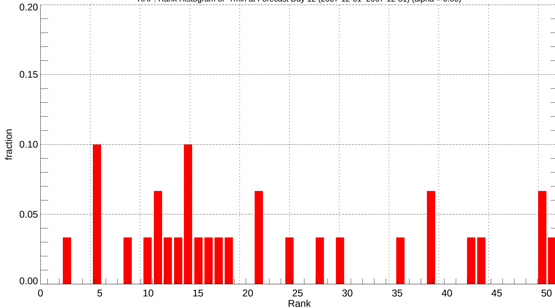
RAP: Rank Histogram of Tmin at Forecast Day 12 (2007-12-01~2007-12-31) (alpha = 0.00)
