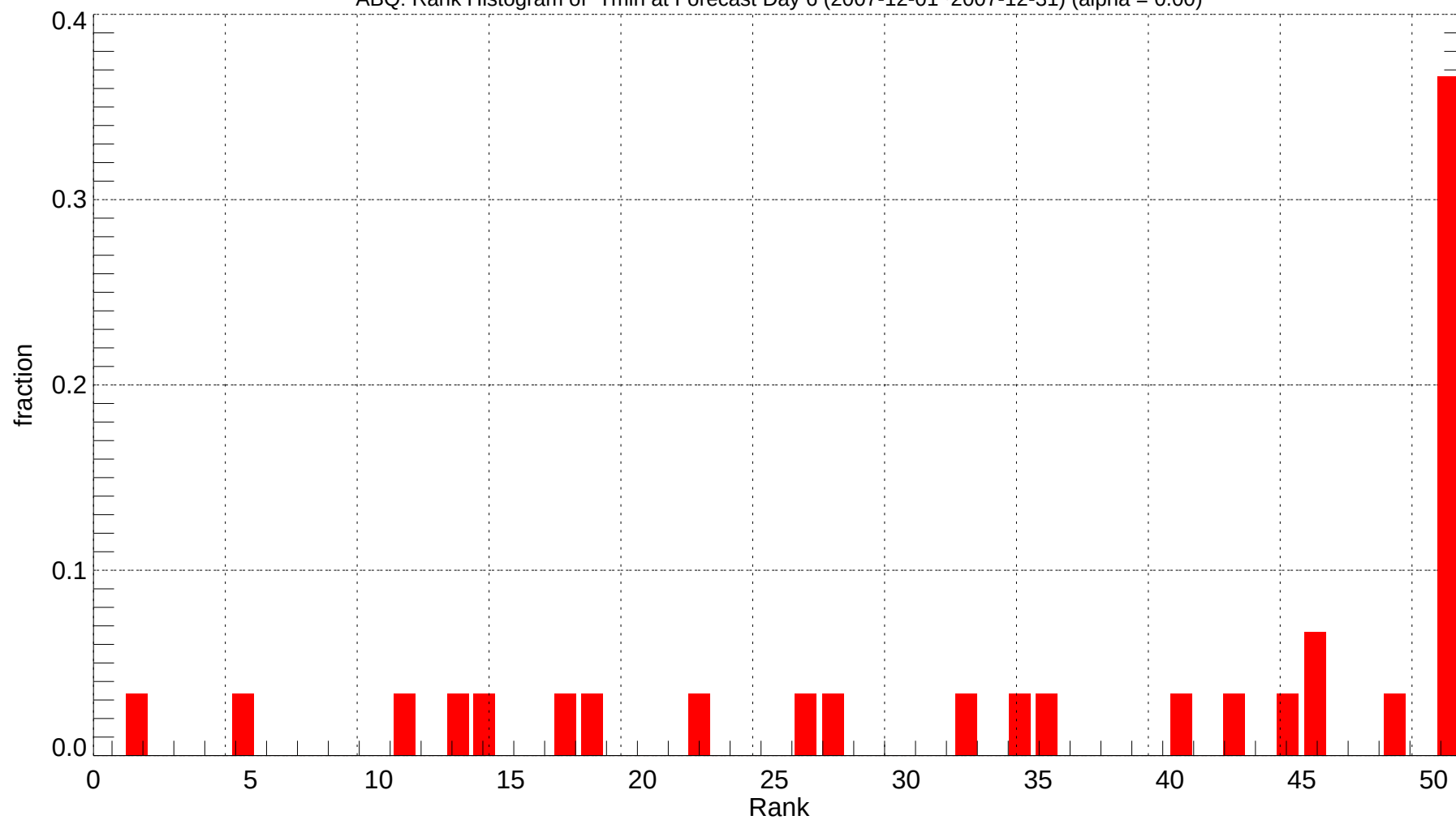
ABQ: Rank Histogram of Tmin at Forecast Day 6 (2007-12-01~2007-12-31) (alpha = 0.00)
