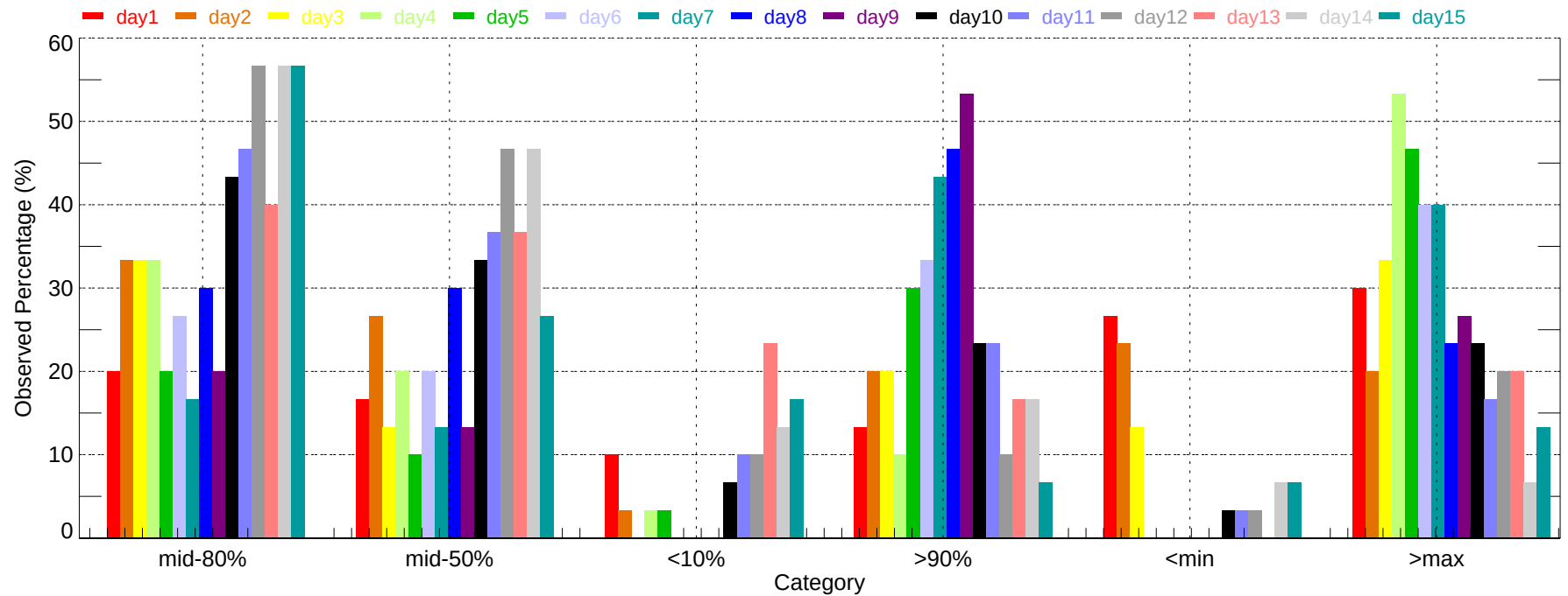
Observed Percentage of Ensembles - LGB: Max Temperature (2007-12-01~2007-12-31)
