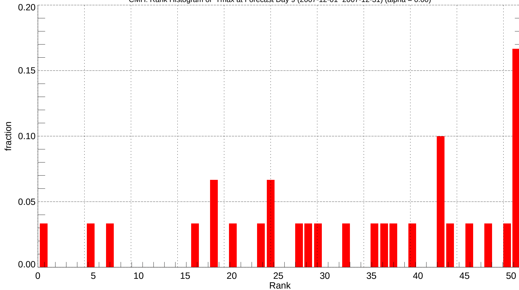
CMH: Rank Histogram of Tmax at Forecast Day 9 (2007-12-01~2007-12-31) (alpha = 0.00)
