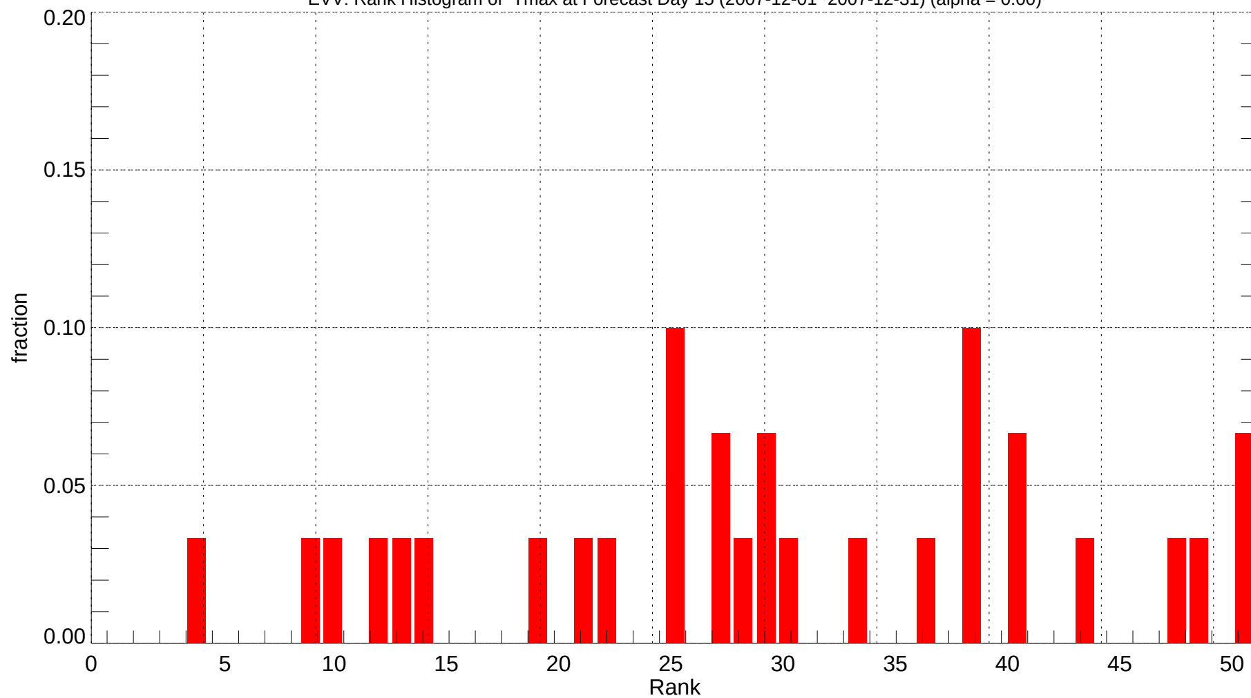
EVV: Rank Histogram of Tmax at Forecast Day 15 (2007-12-01~2007-12-31) (alpha = 0.00)
