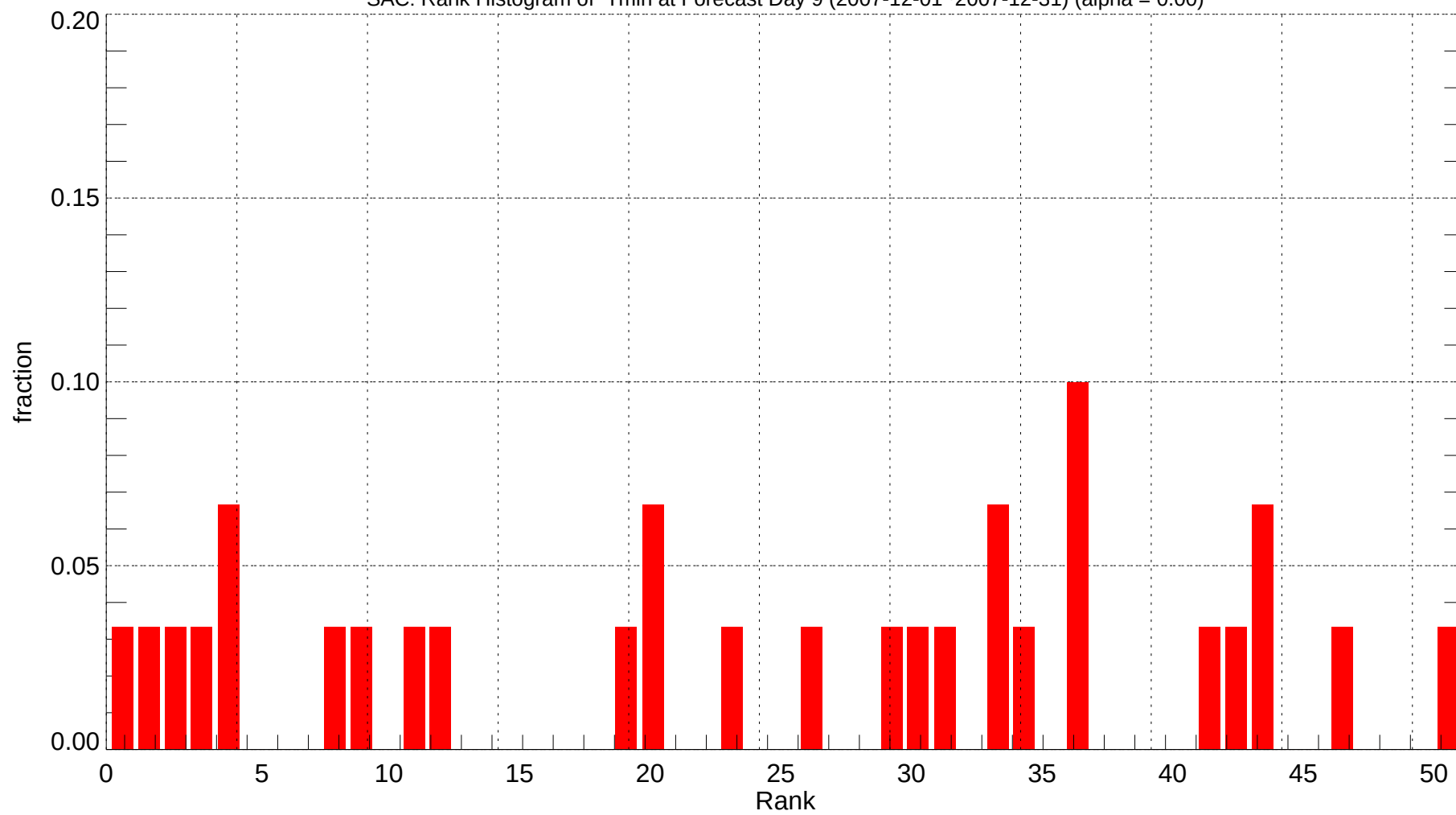
SAC: Rank Histogram of Tmin at Forecast Day 9 (2007-12-01~2007-12-31) (alpha = 0.00)
