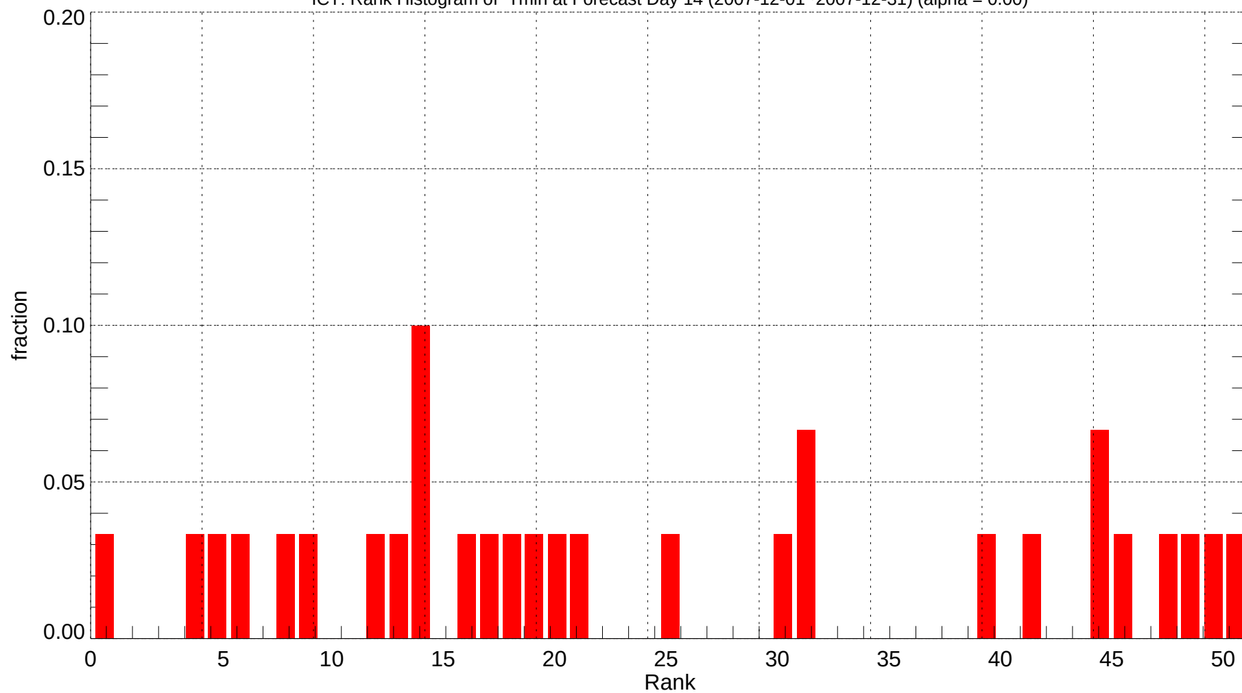
ICT: Rank Histogram of Tmin at Forecast Day 14 (2007-12-01~2007-12-31) (alpha = 0.00)
