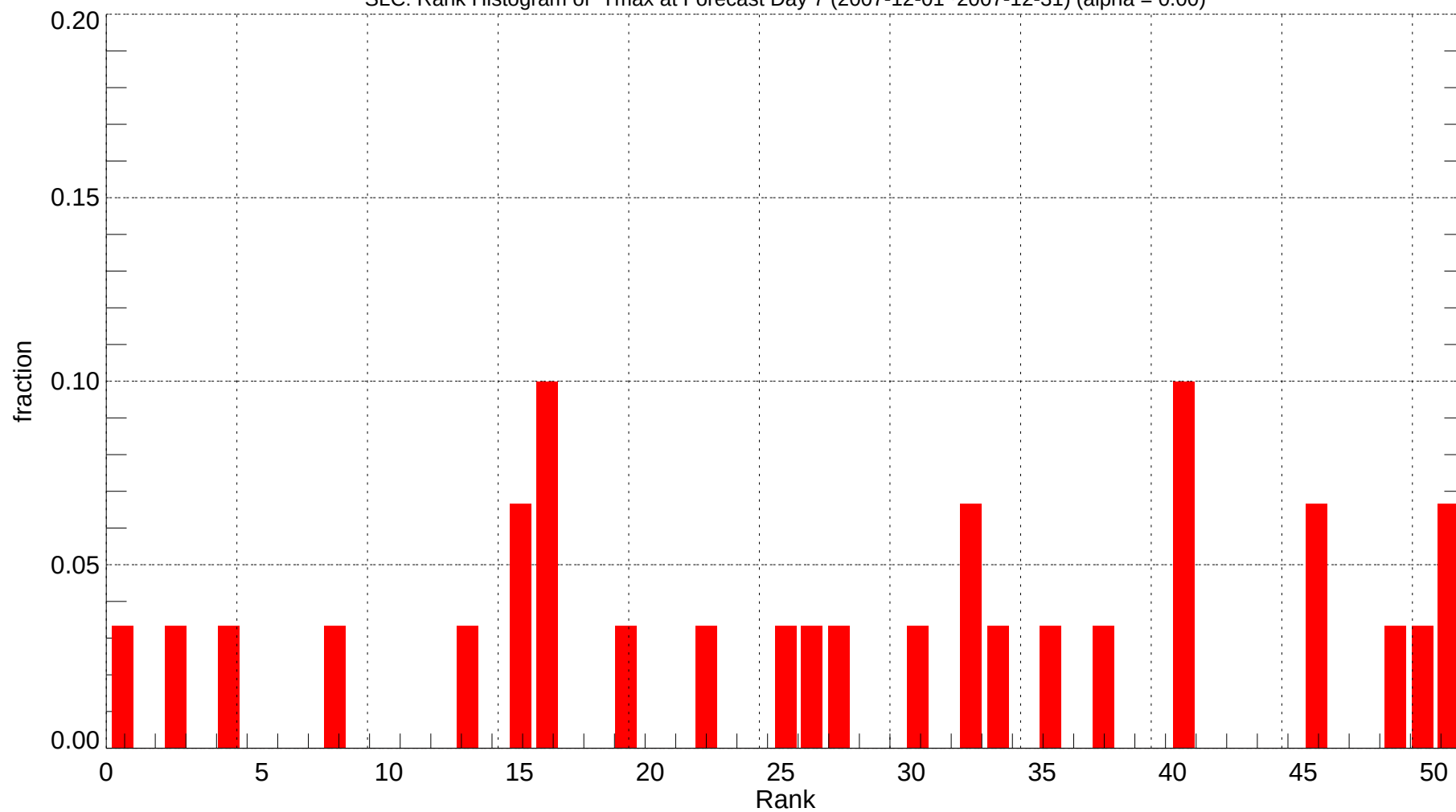
SLC: Rank Histogram of Tmax at Forecast Day 7 (2007-12-01~2007-12-31) (alpha = 0.00)
