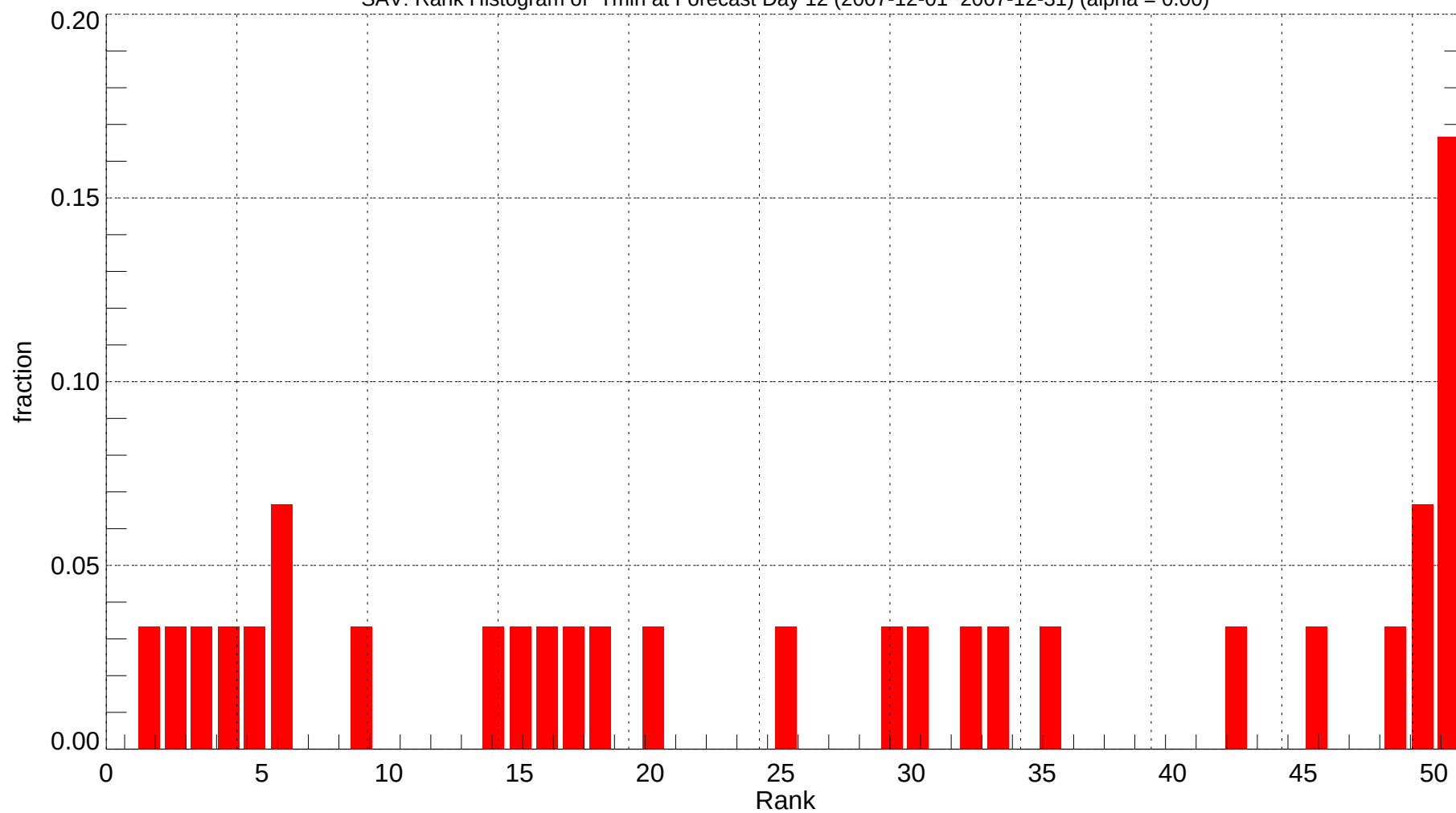
SAV: Rank Histogram of Tmin at Forecast Day 12 (2007-12-01~2007-12-31) (alpha = 0.00)
