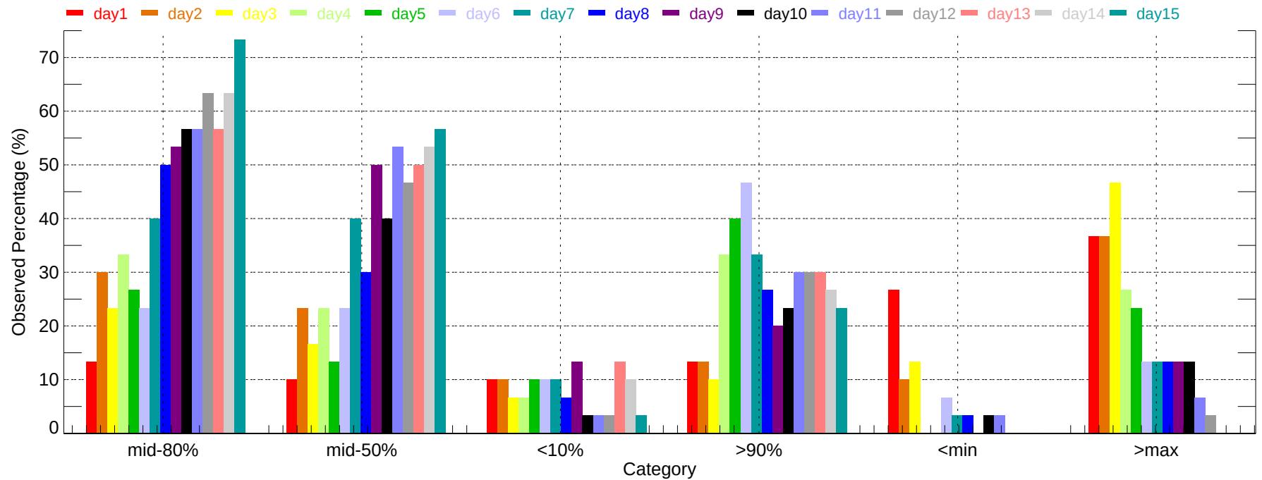
Observed Percentage of Ensembles - GTF: Max Temperature (2007-12-01~2007-12-31)
