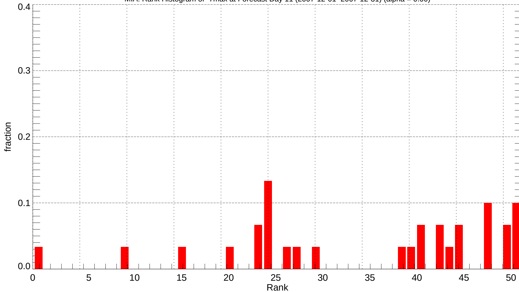
MIA: Rank Histogram of Tmax at Forecast Day 11 (2007-12-01~2007-12-31) (alpha = 0.00)
