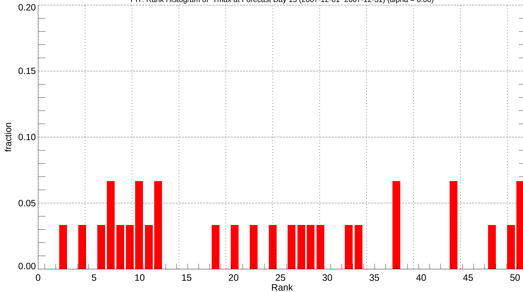
PIT: Rank Histogram of Tmax at Forecast Day 15 (2007-12-01~2007-12-31) (alpha = 0.00)
