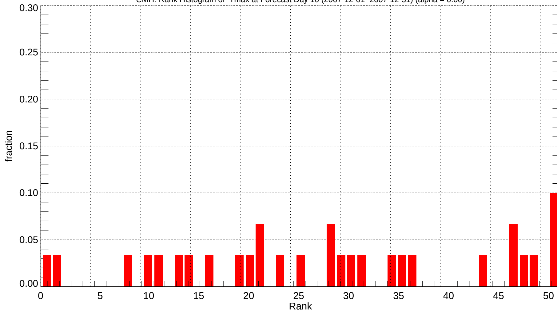
CMH: Rank Histogram of Tmax at Forecast Day 10 (2007-12-01~2007-12-31) (alpha = 0.00)
