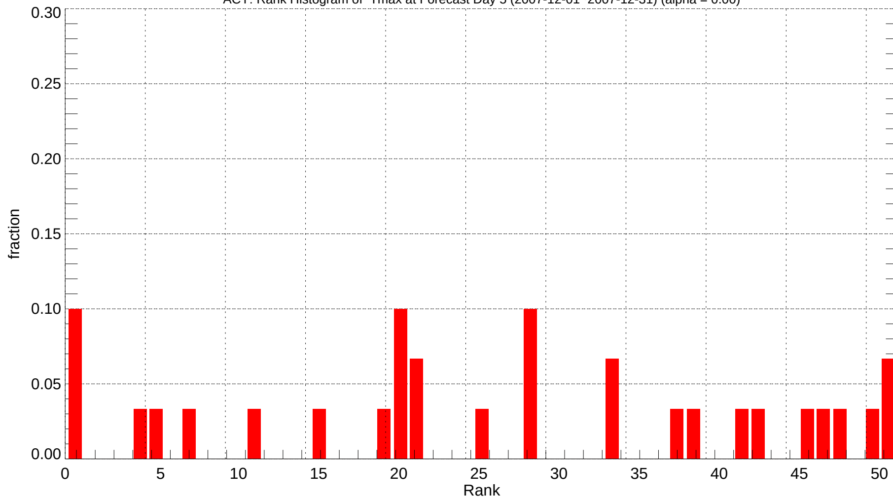
ACY: Rank Histogram of Tmax at Forecast Day 5 (2007-12-01~2007-12-31) (alpha = 0.00)
