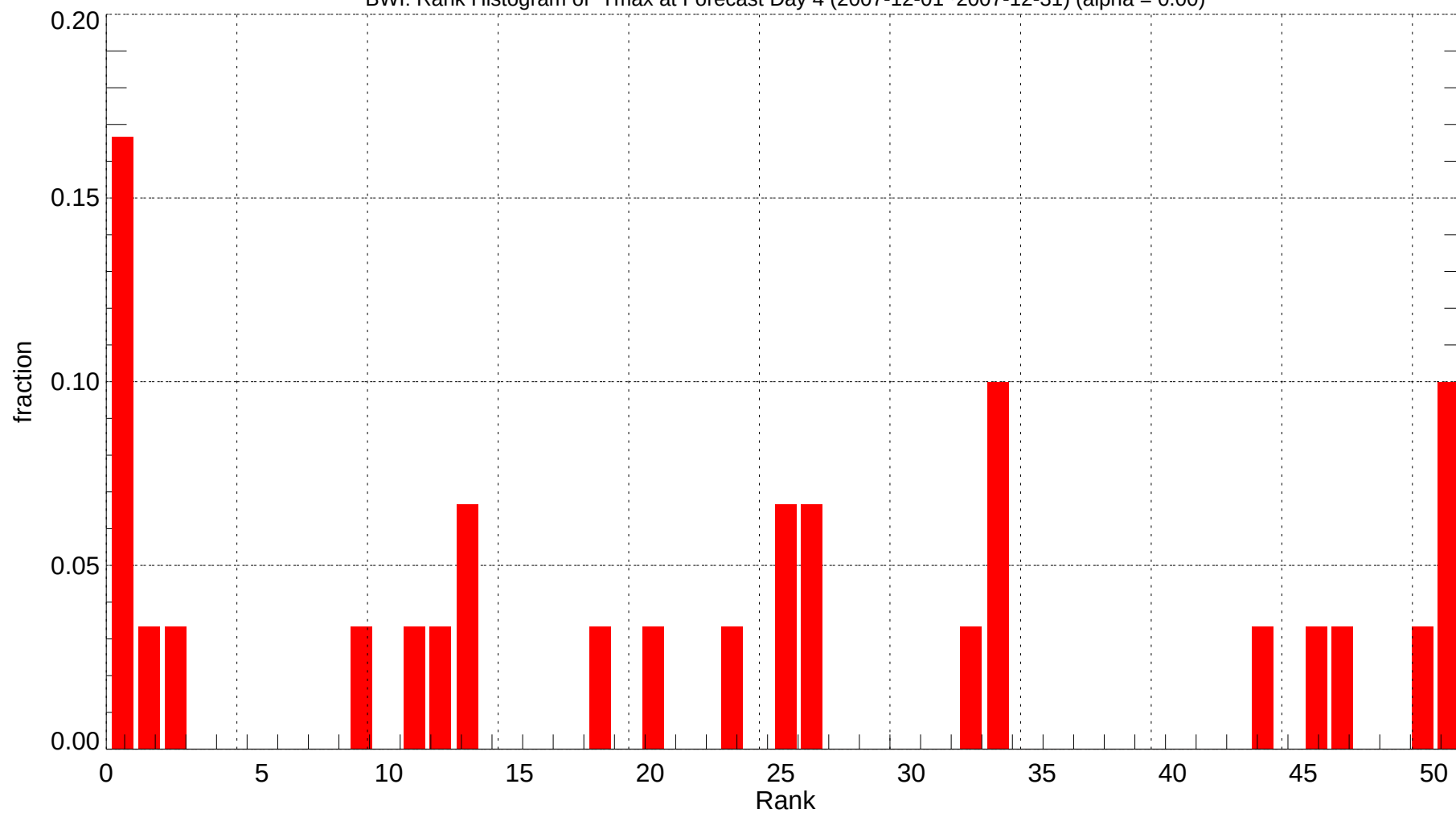
BWI: Rank Histogram of Tmax at Forecast Day 4 (2007-12-01~2007-12-31) (alpha = 0.00)
