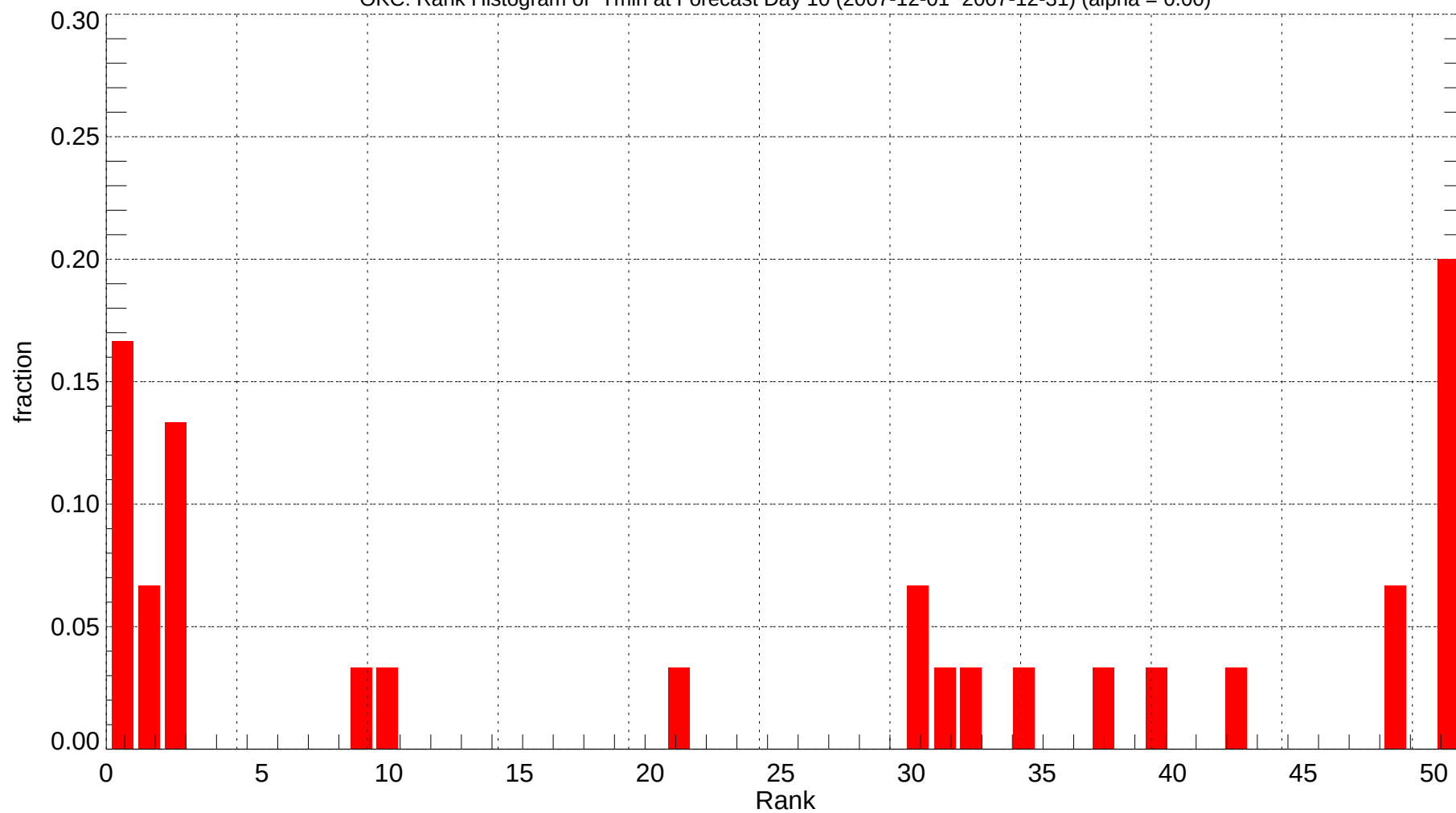
OKC: Rank Histogram of Tmin at Forecast Day 10 (2007-12-01~2007-12-31) (alpha = 0.00)
