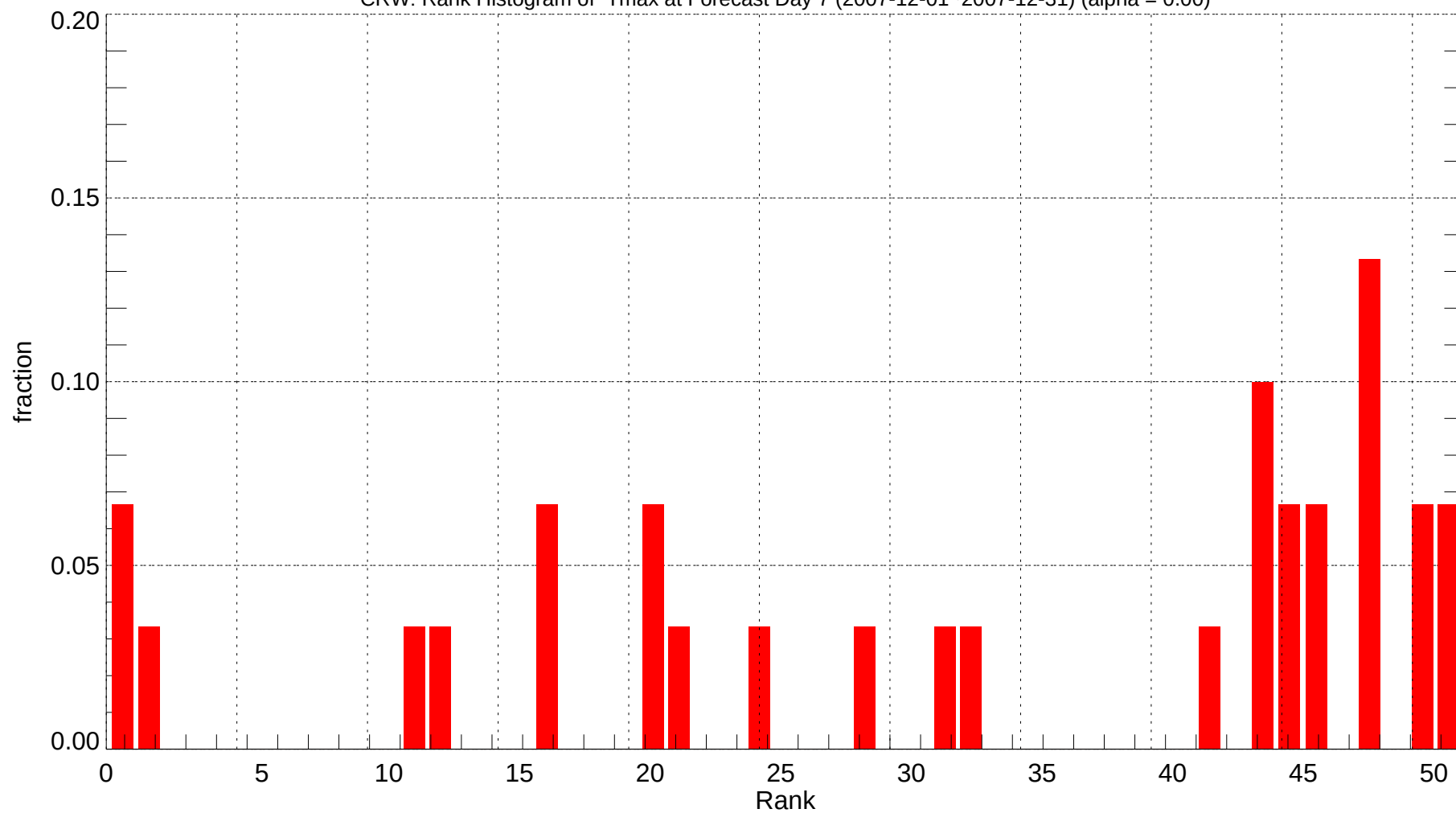
CRW: Rank Histogram of Tmax at Forecast Day 7 (2007-12-01~2007-12-31) (alpha = 0.00)
