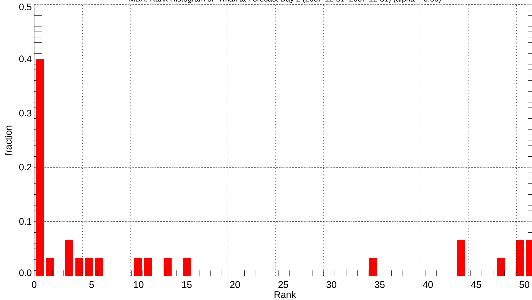
MBA: Rank Histogram of Tmax at Forecast Day 2 (2007-12-01~2007-12-31) (alpha = 0.00)
