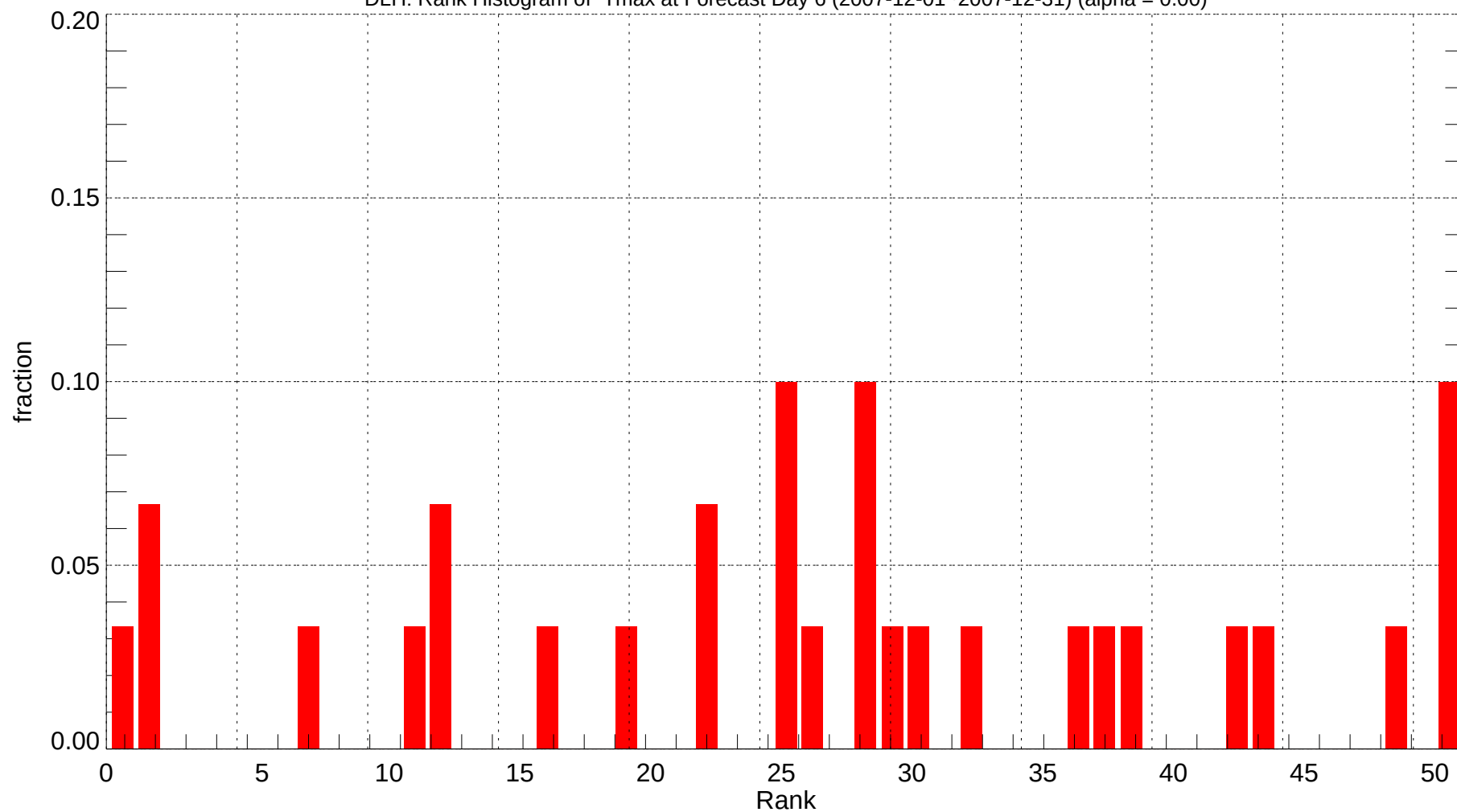
DLH: Rank Histogram of Tmax at Forecast Day 6 (2007-12-01~2007-12-31) (alpha = 0.00)
