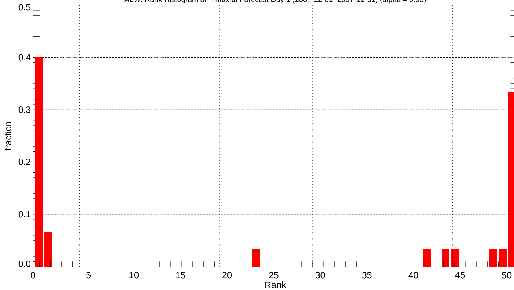
ALW: Rank Histogram of Tmax at Forecast Day 1 (2007-12-01~2007-12-31) (alpha = 0.00)
