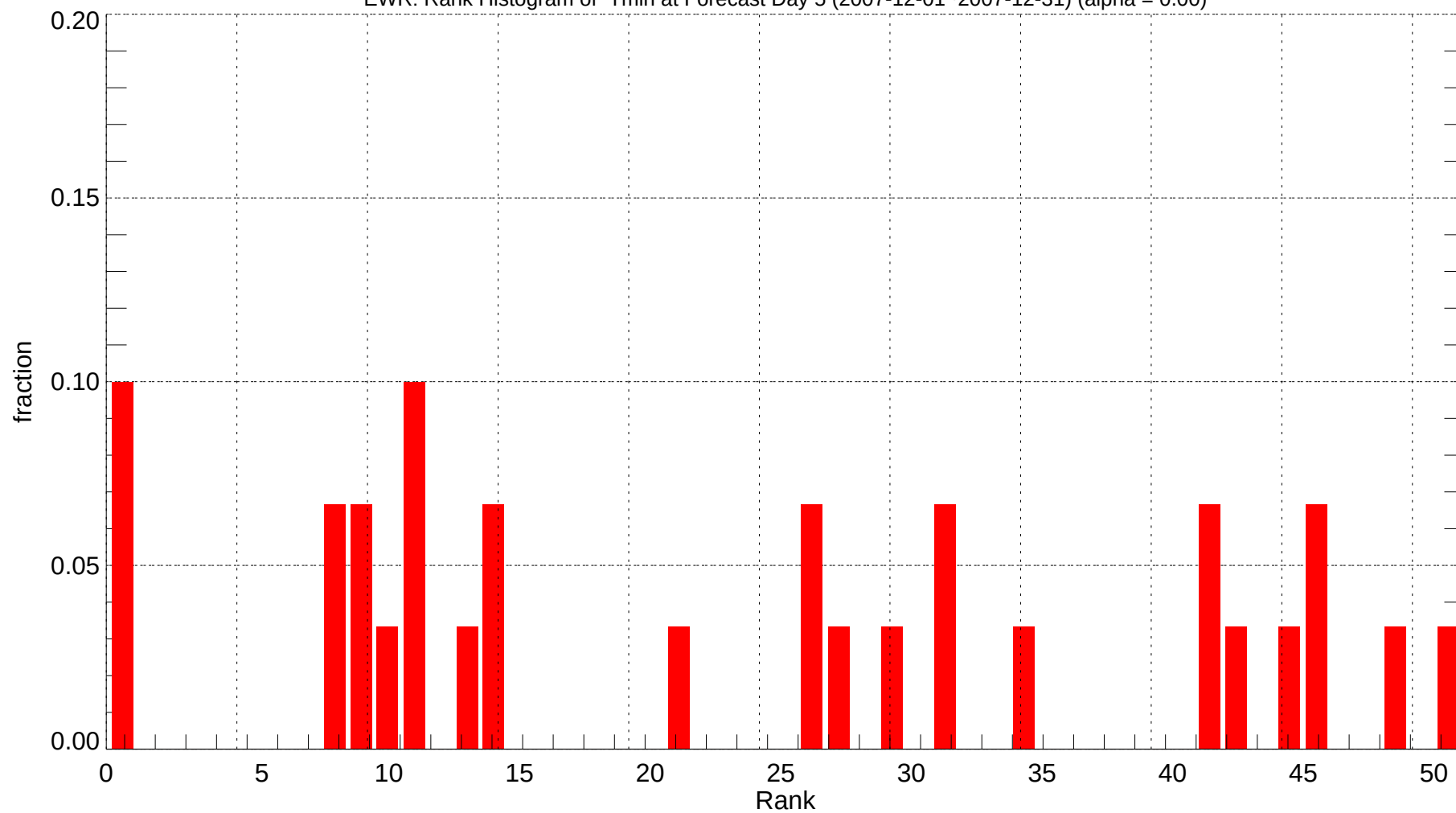
EWR: Rank Histogram of Tmin at Forecast Day 5 (2007-12-01~2007-12-31) (alpha = 0.00)
