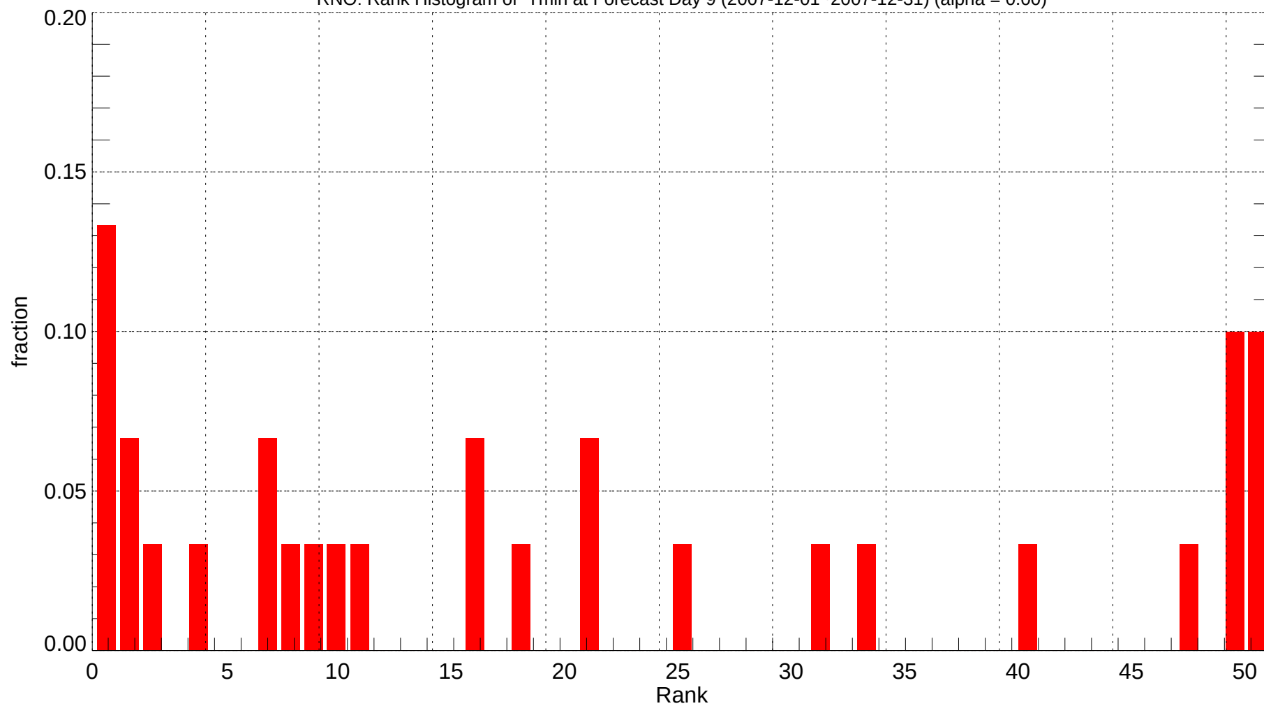
RNO: Rank Histogram of Tmin at Forecast Day 9 (2007-12-01~2007-12-31) (alpha = 0.00)
