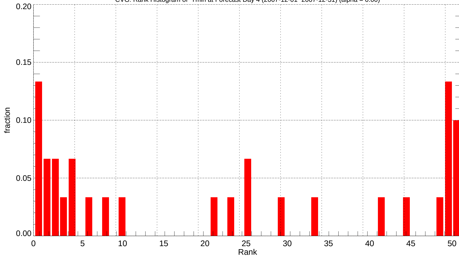
CVG: Rank Histogram of Tmin at Forecast Day 4 (2007-12-01~2007-12-31) (alpha = 0.00)
