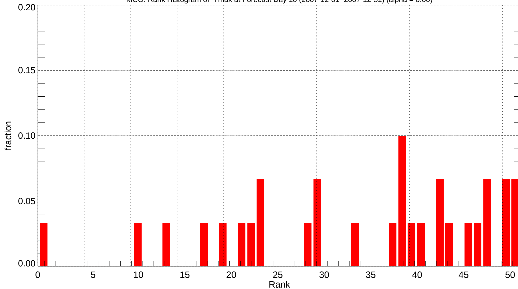
MCO: Rank Histogram of Tmax at Forecast Day 10 (2007-12-01~2007-12-31) (alpha = 0.00)
