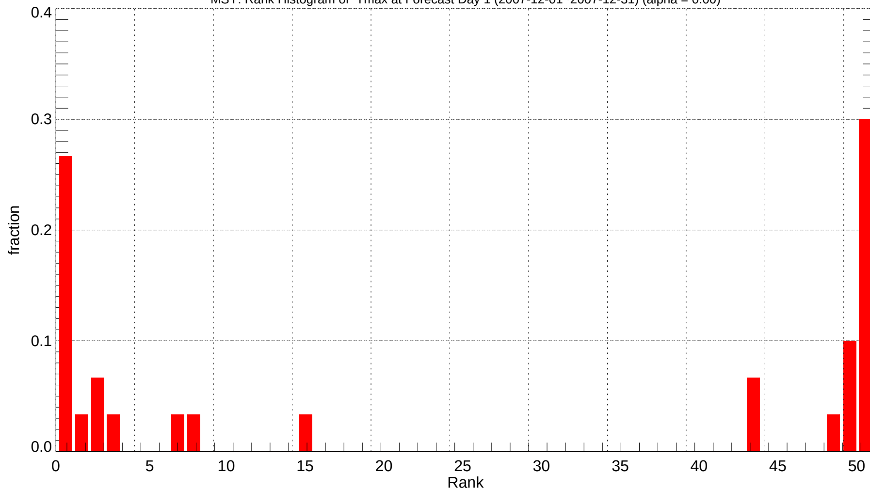
MSY: Rank Histogram of Tmax at Forecast Day 1 (2007-12-01~2007-12-31) (alpha = 0.00)
