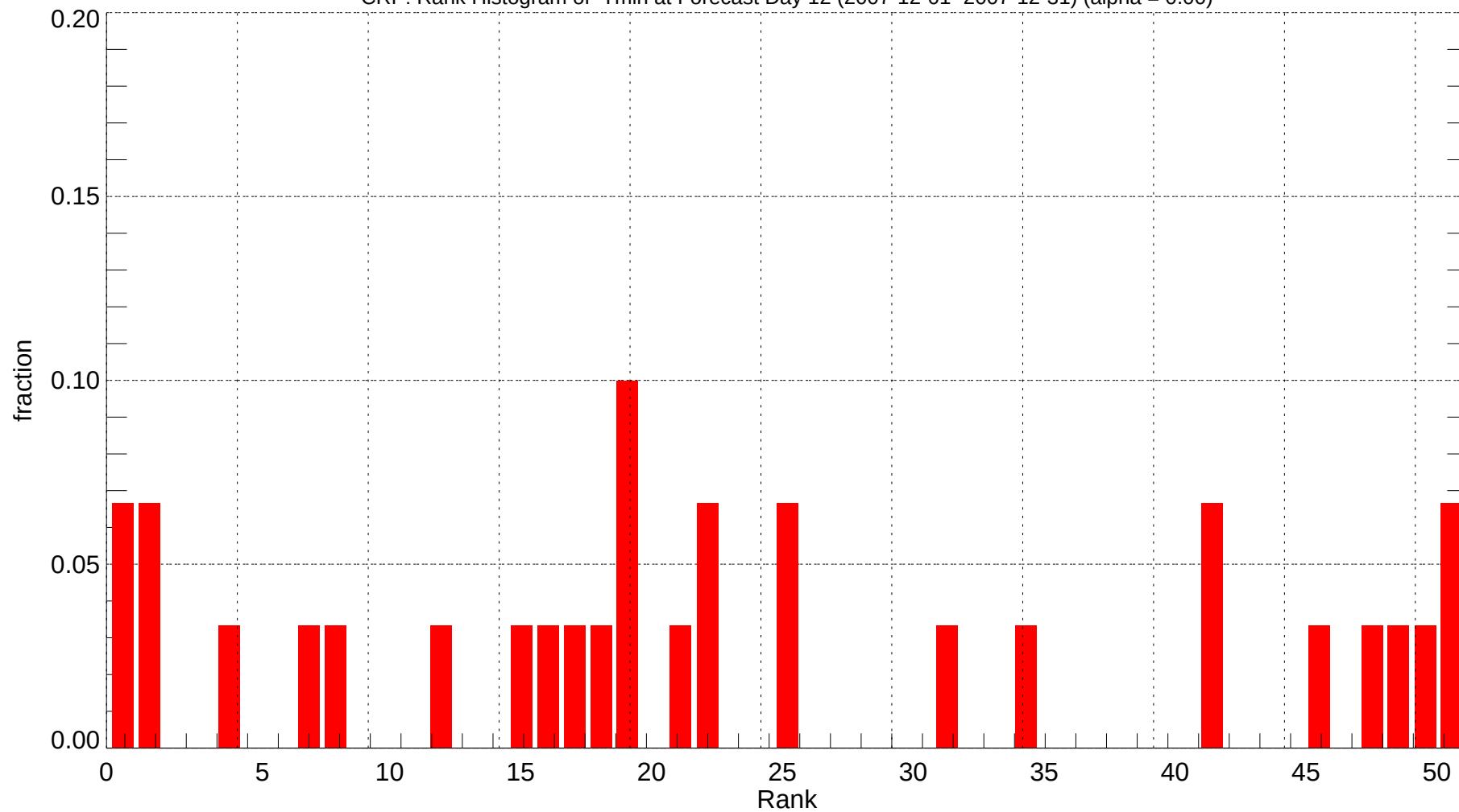
CRP: Rank Histogram of Tmin at Forecast Day 12 (2007-12-01~2007-12-31) (alpha = 0.00)
