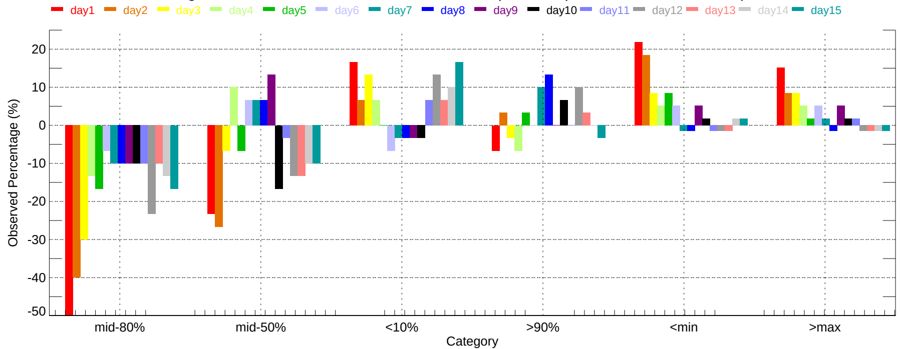
Observed Percentage Deviation of Ensembles - AUG: Min Temperature (2007-12-01~2007-12-31)
