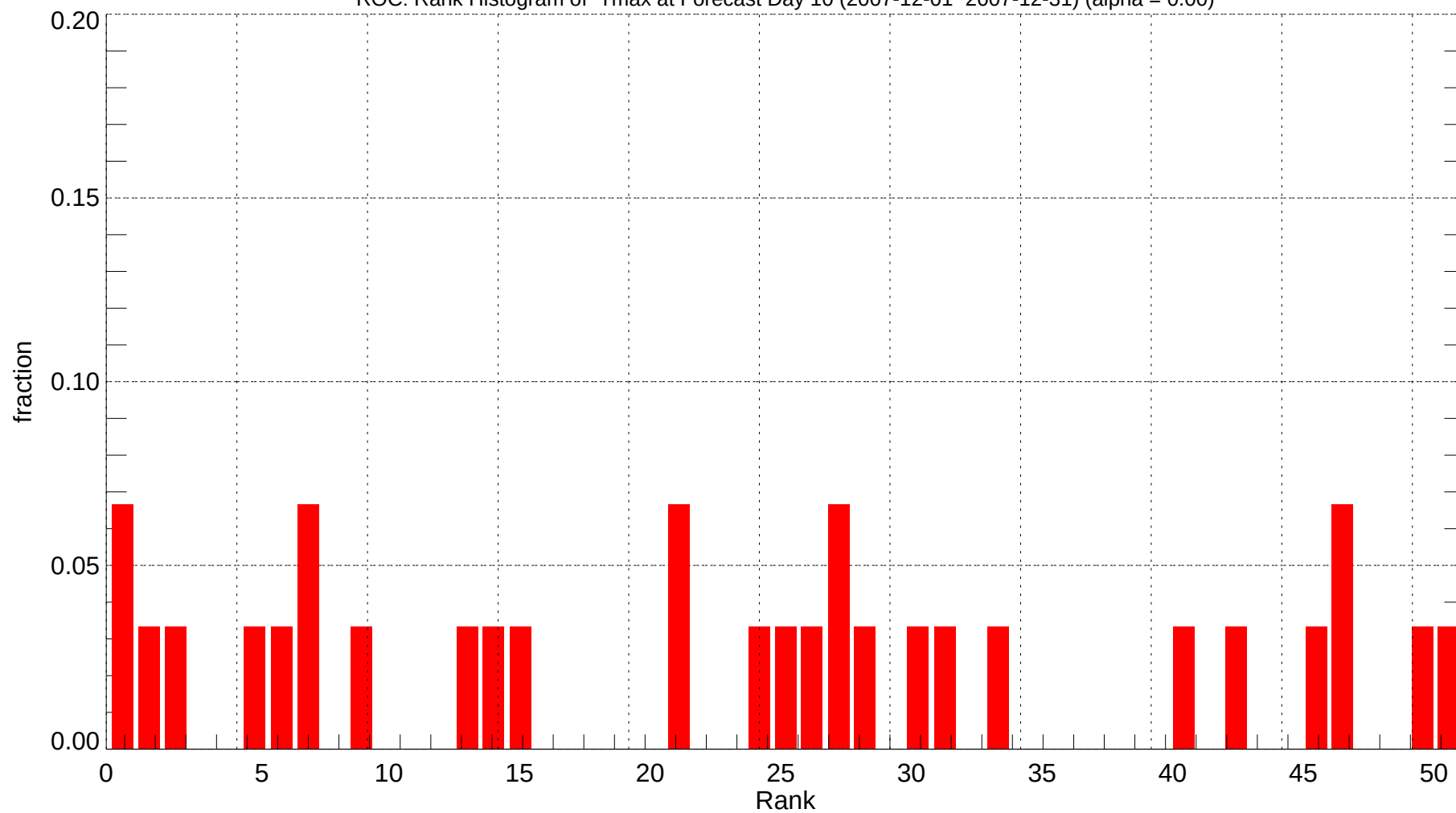
ROC: Rank Histogram of Tmax at Forecast Day 10 (2007-12-01~2007-12-31) (alpha = 0.00)
