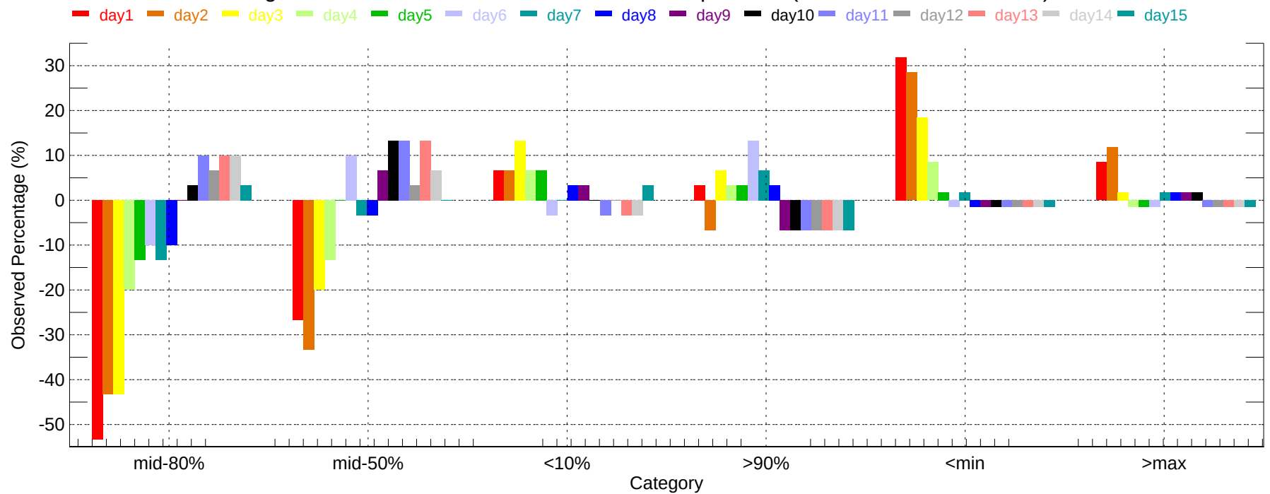
Observed Percentage Deviation of Ensembles - APN: Min Temperature (2007-12-01~2007-12-31)
