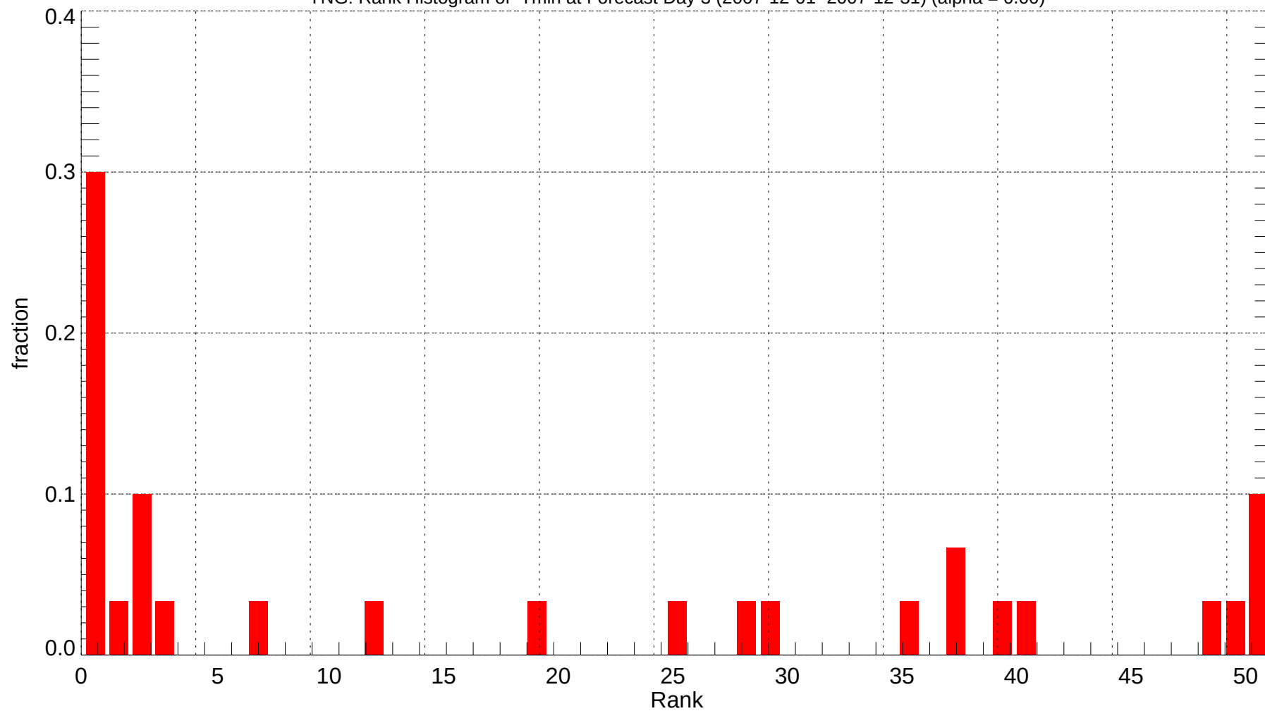
YNG: Rank Histogram of Tmin at Forecast Day 3 (2007-12-01~2007-12-31) (alpha = 0.00)
