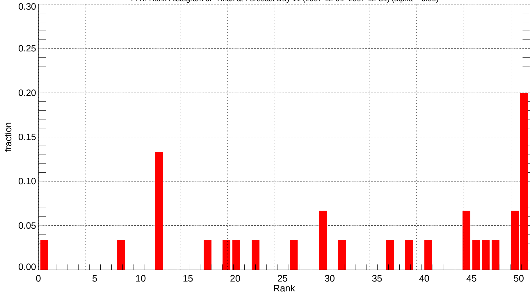
TYR: Rank Histogram of Tmax at Forecast Day 11 (2007-12-01~2007-12-31) (alpha = 0.00)
