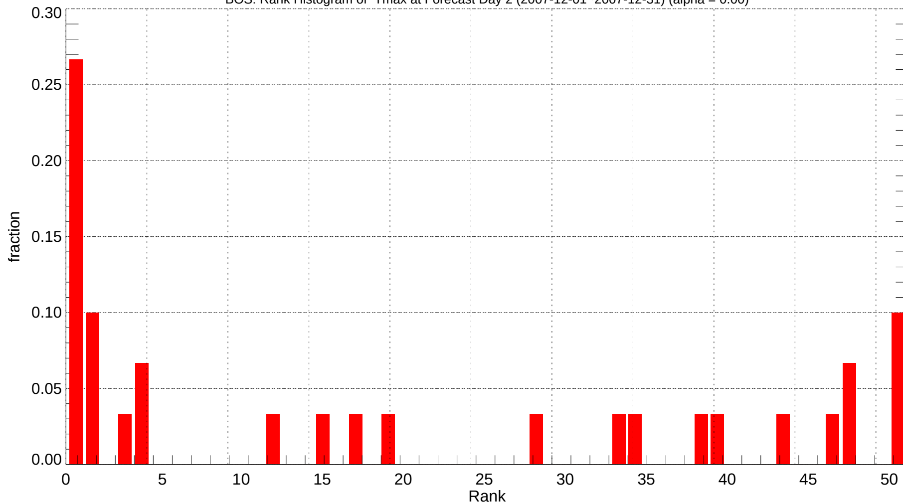
BOS: Rank Histogram of Tmax at Forecast Day 2 (2007-12-01~2007-12-31) (alpha = 0.00)
