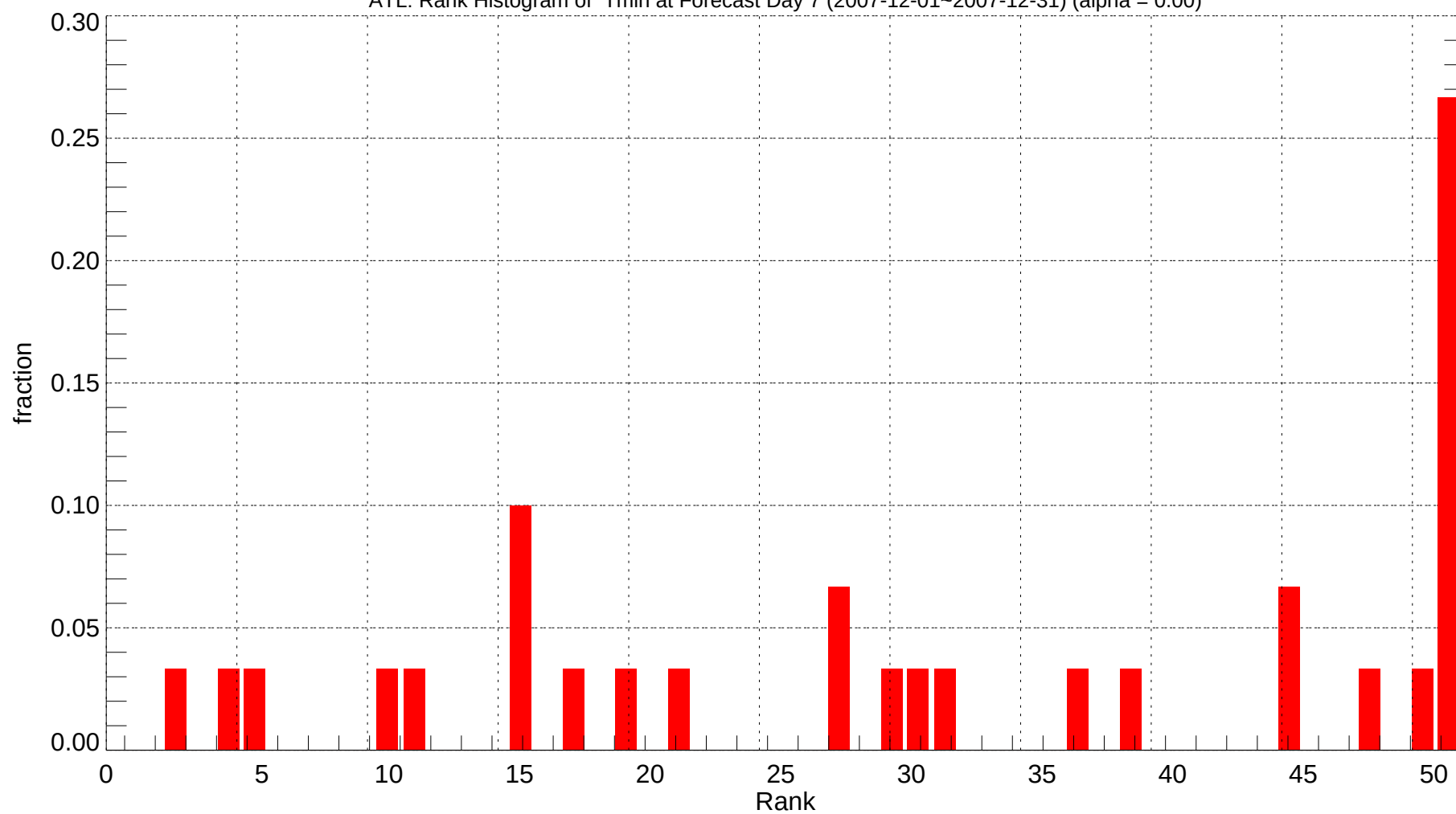
ATL: Rank Histogram of Tmin at Forecast Day 7 (2007-12-01~2007-12-31) (alpha = 0.00)
