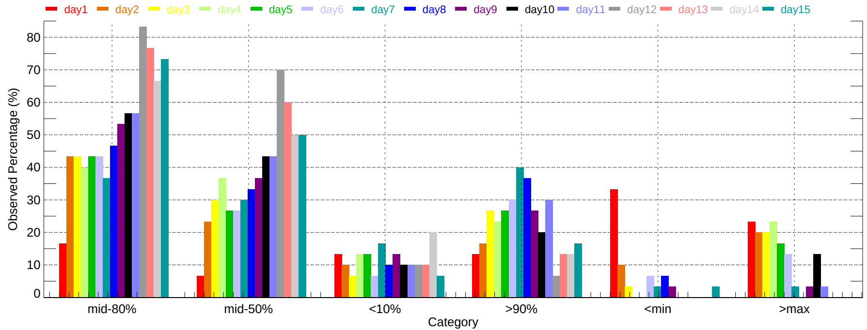
Observed Percentage of Ensembles - FSD: Max Temperature (2007-12-01~2007-12-31)
