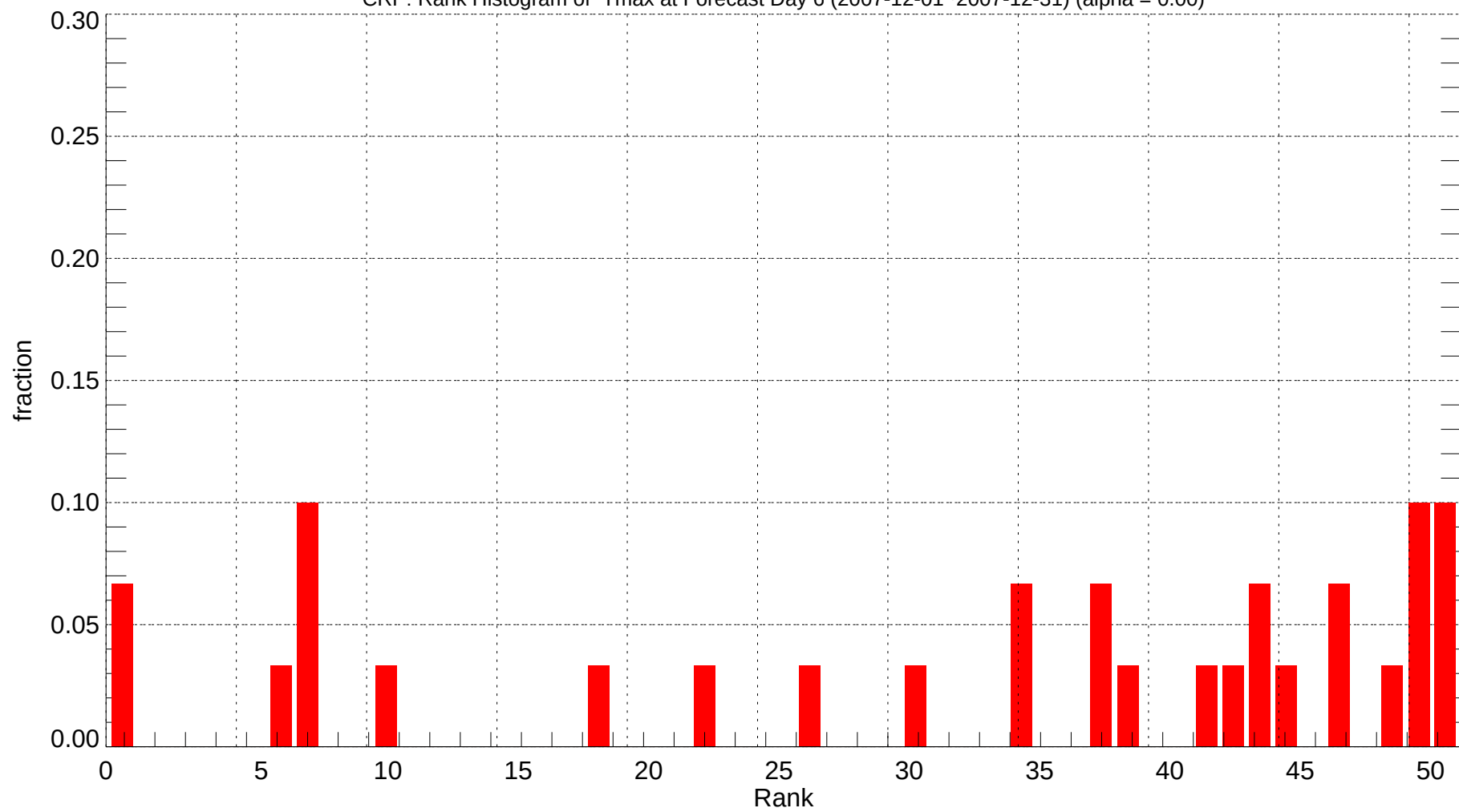
CRP: Rank Histogram of Tmax at Forecast Day 6 (2007-12-01~2007-12-31) (alpha = 0.00)
