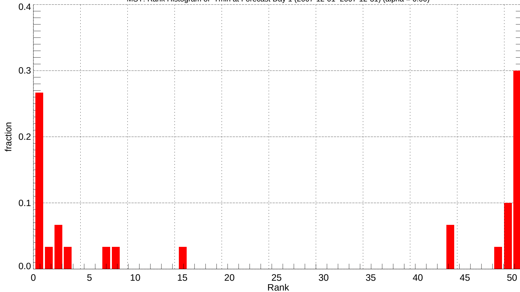
MSY: Rank Histogram of Tmin at Forecast Day 1 (2007-12-01~2007-12-31) (alpha = 0.00)
