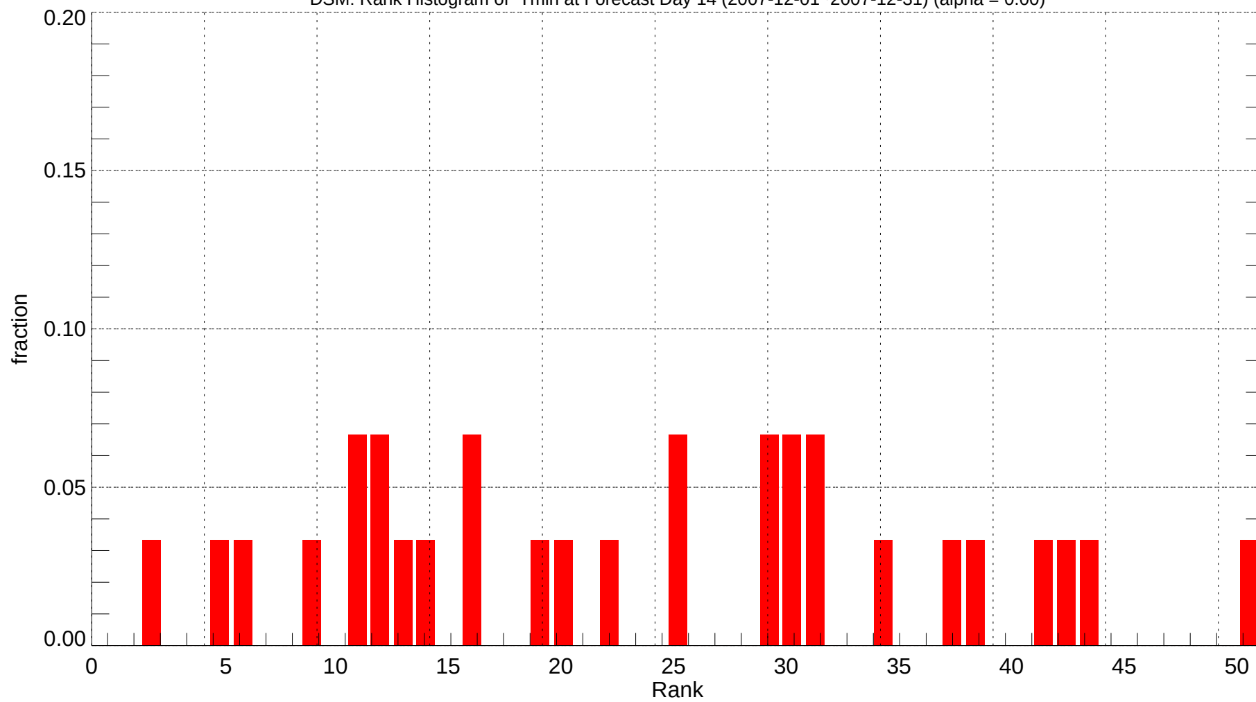
DSM: Rank Histogram of Tmin at Forecast Day 14 (2007-12-01~2007-12-31) (alpha = 0.00)
