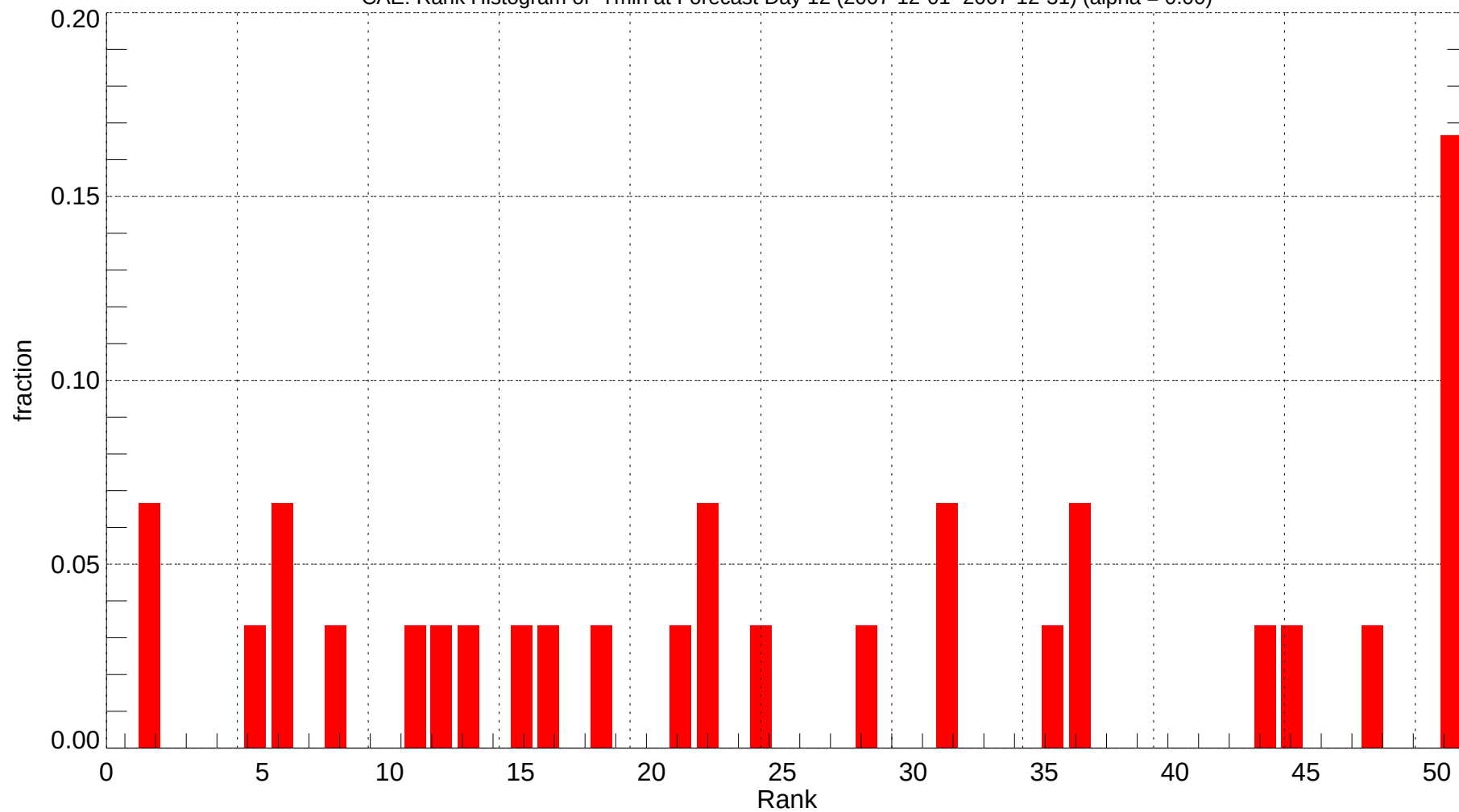
CAE: Rank Histogram of Tmin at Forecast Day 12 (2007-12-01~2007-12-31) (alpha = 0.00)
