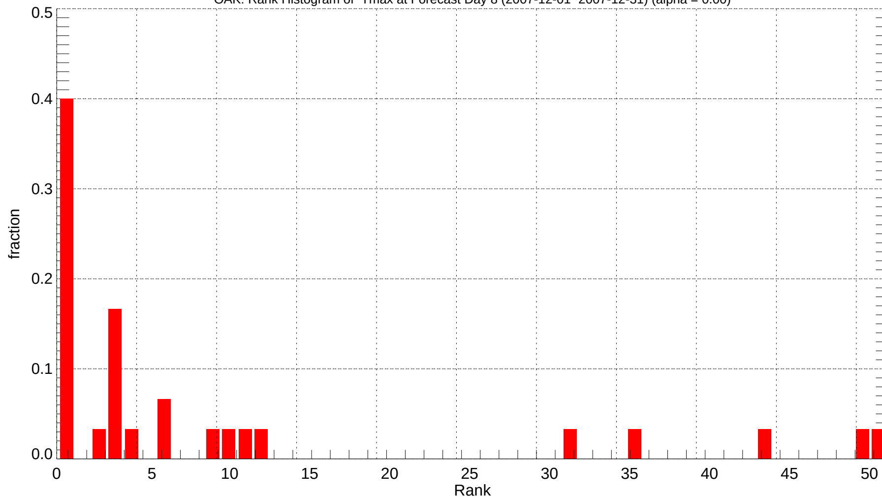
OAK: Rank Histogram of Tmax at Forecast Day 8 (2007-12-01~2007-12-31) (alpha = 0.00)
