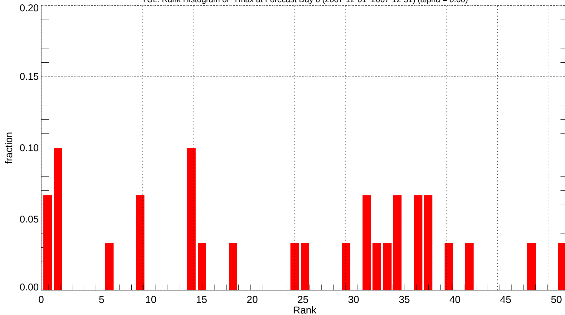
YUL: Rank Histogram of Tmax at Forecast Day 6 (2007-12-01~2007-12-31) (alpha = 0.00)
