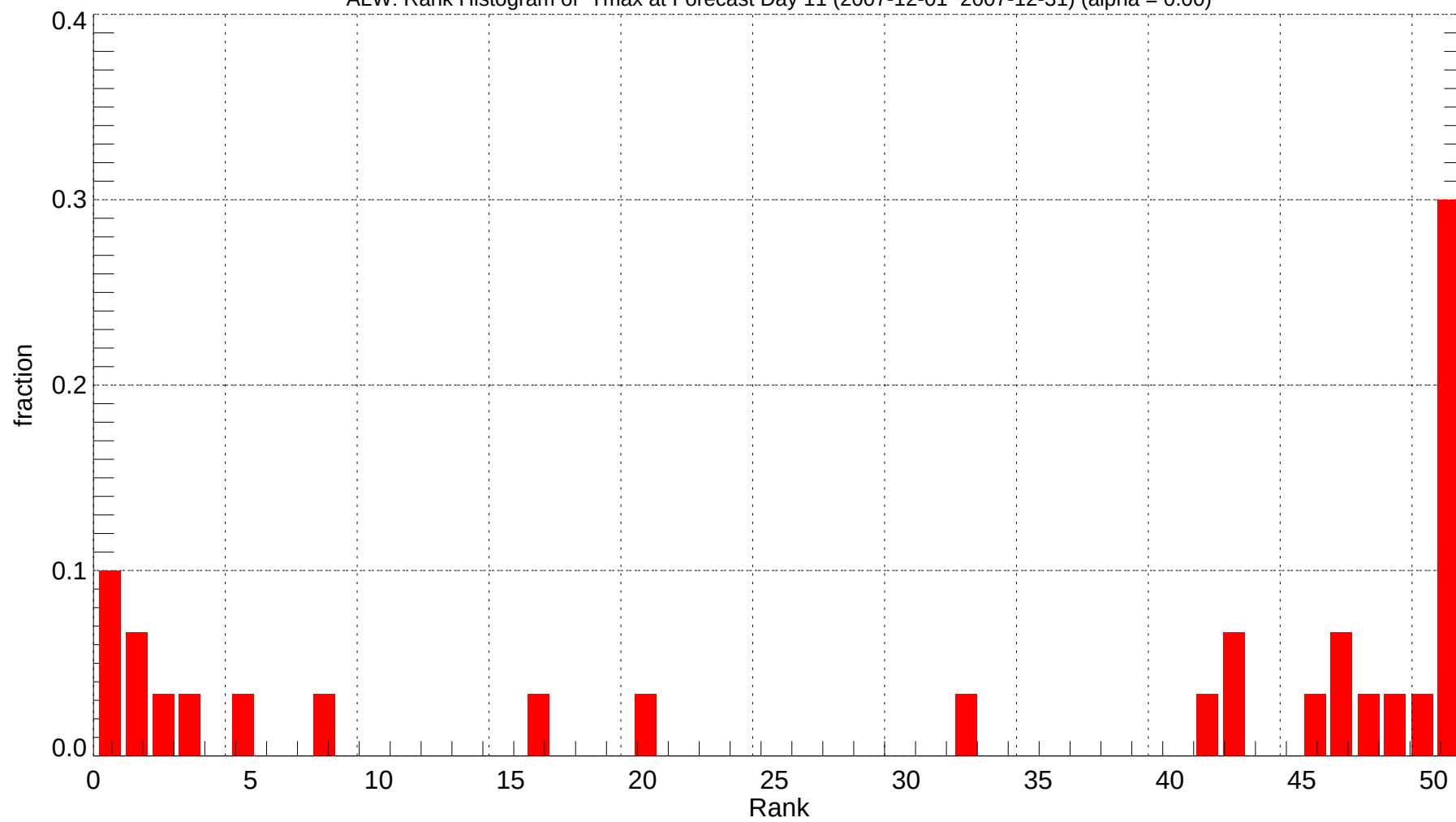
ALW: Rank Histogram of Tmax at Forecast Day 11 (2007-12-01~2007-12-31) (alpha = 0.00)
