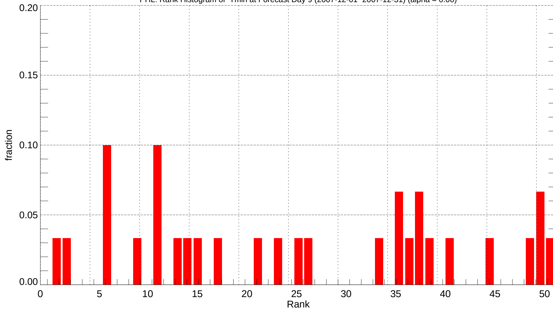
PHL: Rank Histogram of Tmin at Forecast Day 9 (2007-12-01~2007-12-31) (alpha = 0.00)
