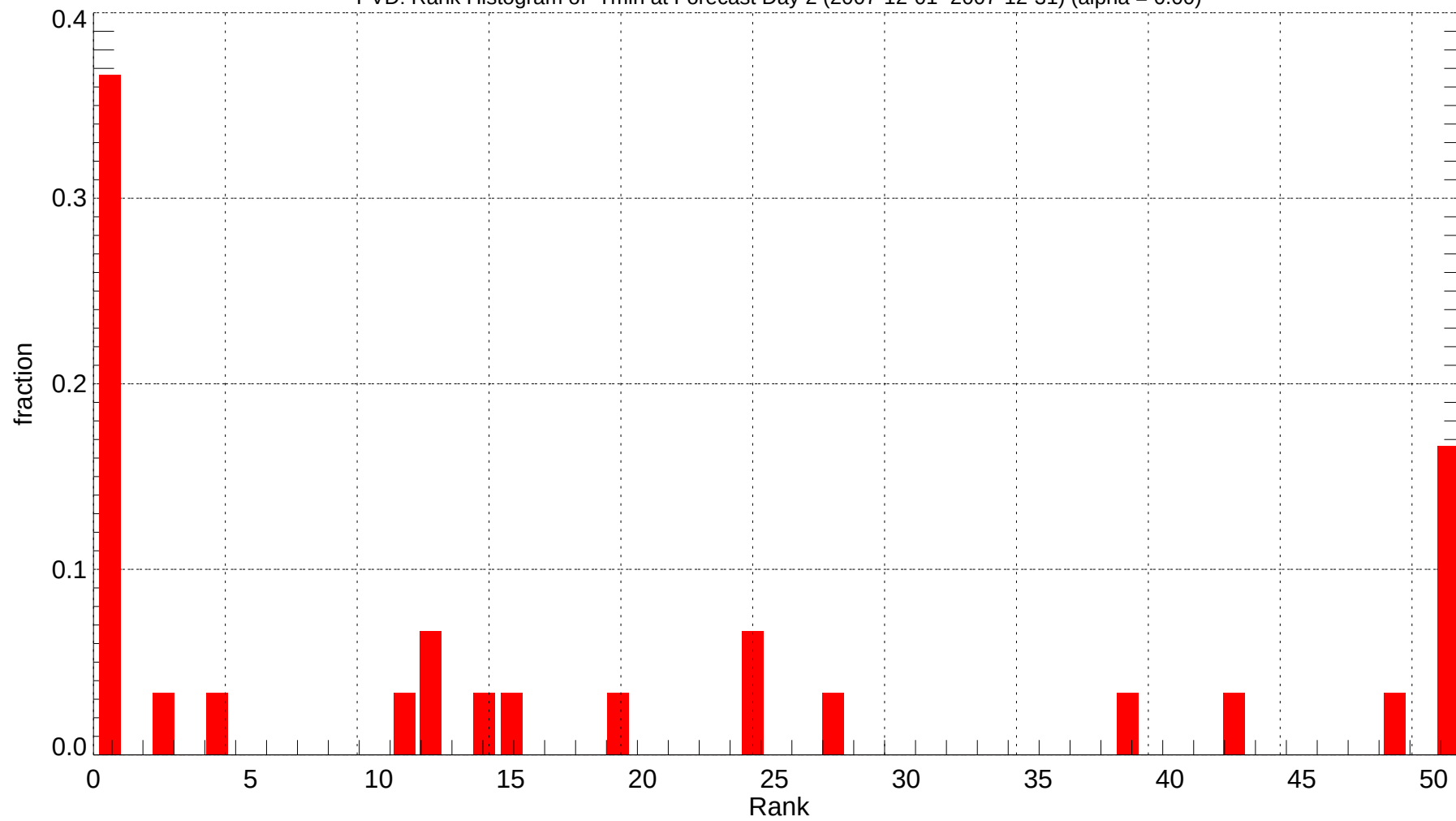
PVD: Rank Histogram of Tmin at Forecast Day 2 (2007-12-01~2007-12-31) (alpha = 0.00)
