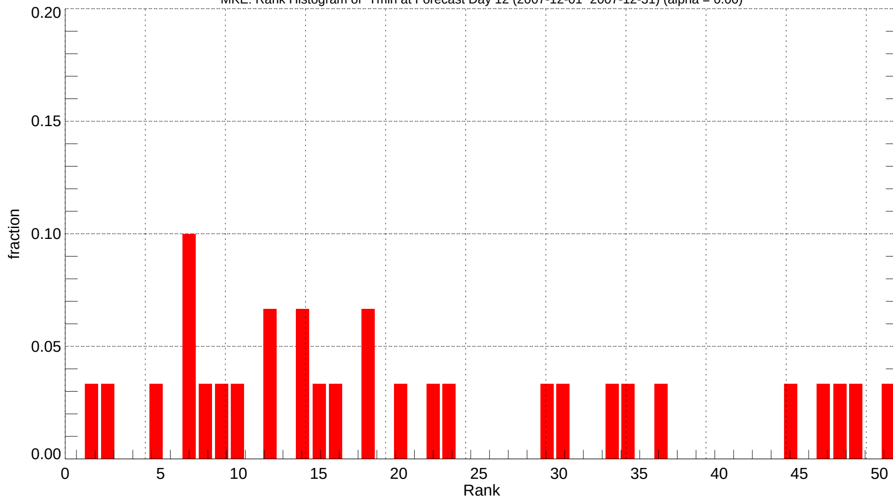
MKE: Rank Histogram of Tmin at Forecast Day 12 (2007-12-01~2007-12-31) (alpha = 0.00)
