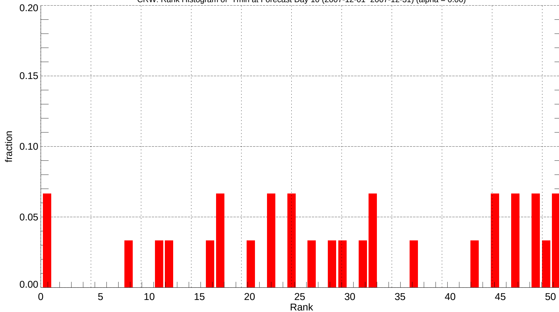
CRW: Rank Histogram of Tmin at Forecast Day 10 (2007-12-01~2007-12-31) (alpha = 0.00)
