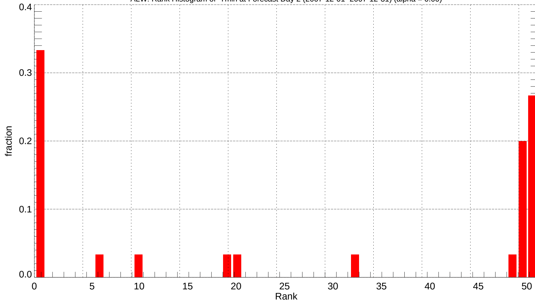
ALW: Rank Histogram of Tmin at Forecast Day 2 (2007-12-01~2007-12-31) (alpha = 0.00)
