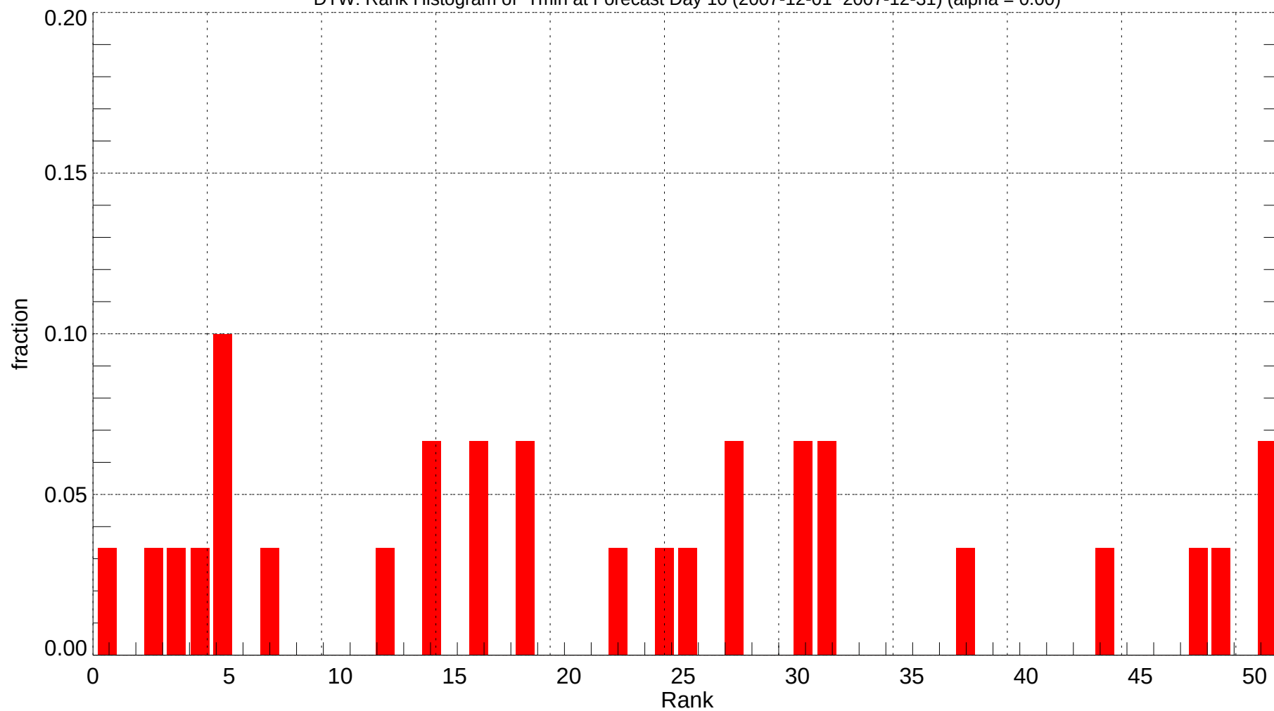
DTW: Rank Histogram of Tmin at Forecast Day 10 (2007-12-01~2007-12-31) (alpha = 0.00)
