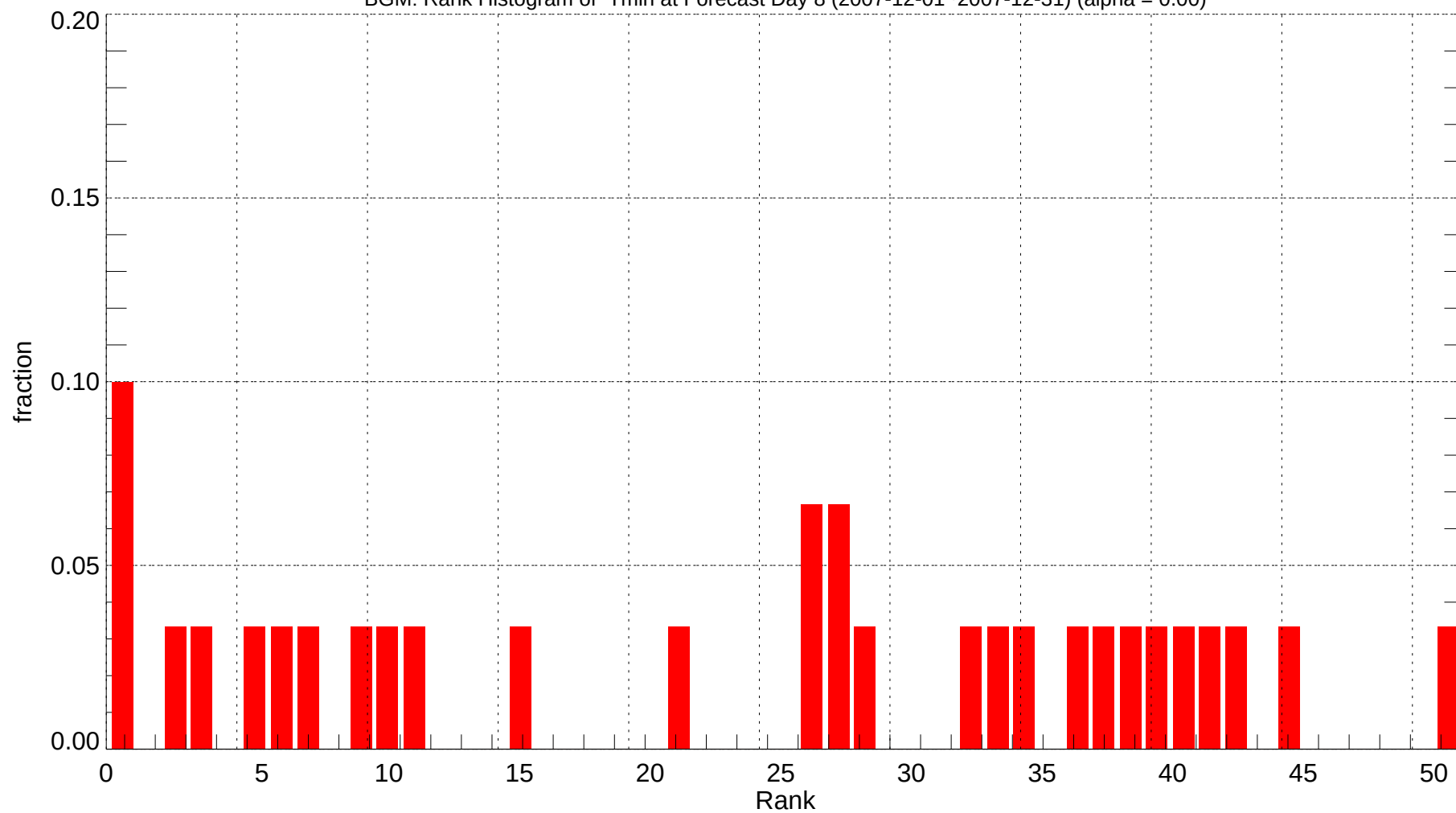
BGM: Rank Histogram of Tmin at Forecast Day 8 (2007-12-01~2007-12-31) (alpha = 0.00)
