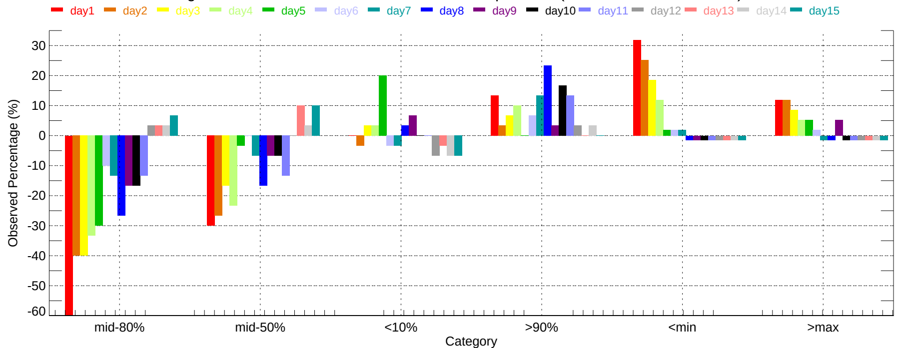
Observed Percentage Deviation of Ensembles - JFK: Max Temperature (2007-12-01~2007-12-31)
