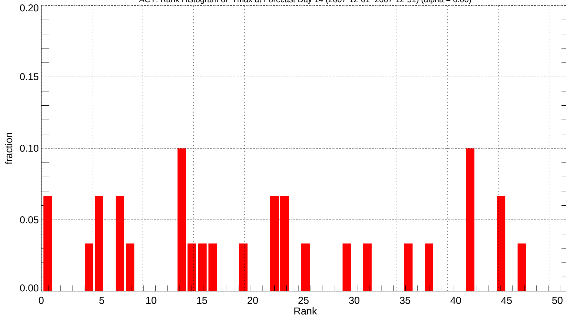
ACY: Rank Histogram of Tmax at Forecast Day 14 (2007-12-01~2007-12-31) (alpha = 0.00)
