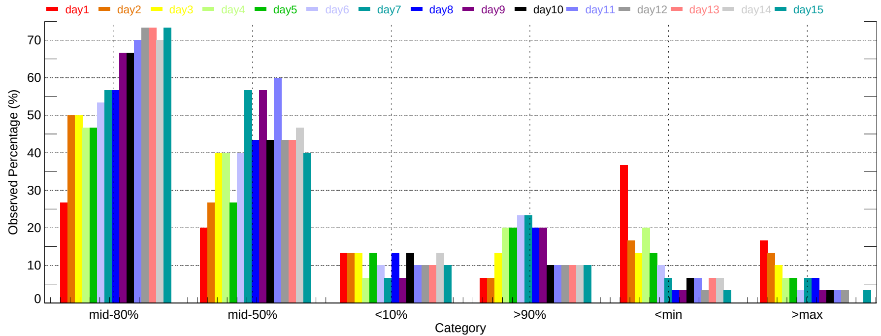
Observed Percentage of Ensembles - ILG: Max Temperature (2007-12-01~2007-12-31)
