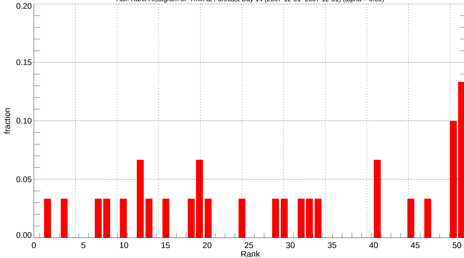
ABI: Rank Histogram of Tmin at Forecast Day 14 (2007-12-01~2007-12-31) (alpha = 0.00)
