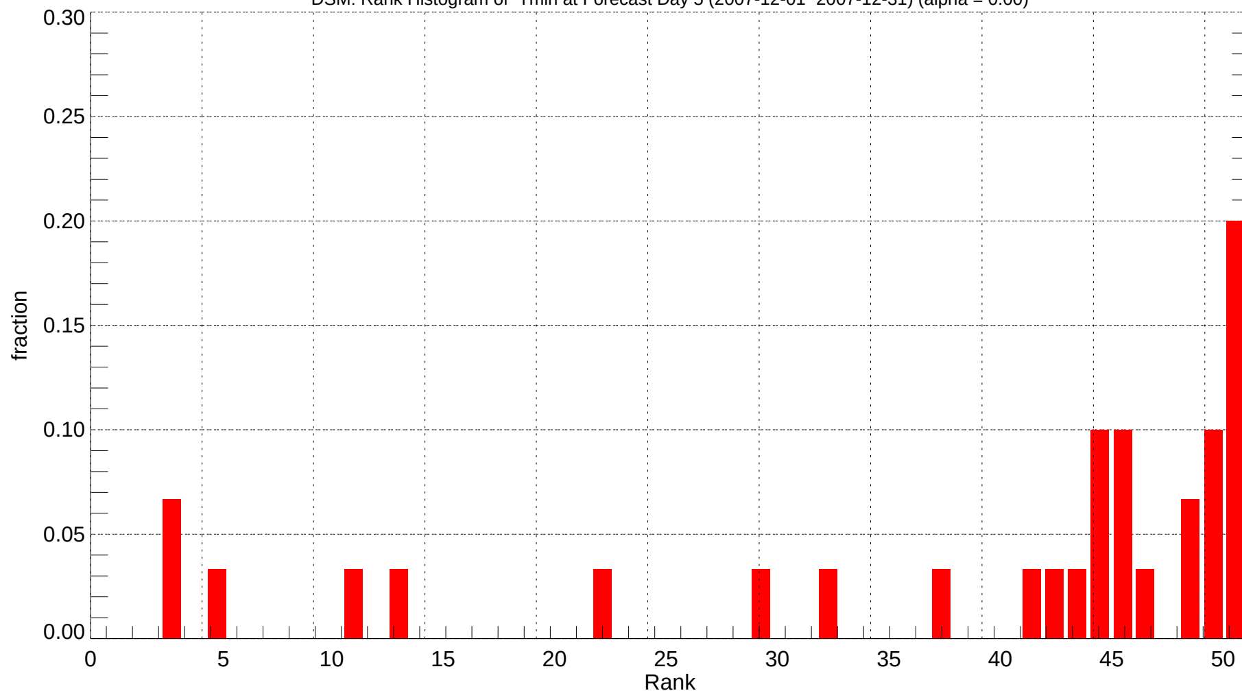
DSM: Rank Histogram of Tmin at Forecast Day 5 (2007-12-01~2007-12-31) (alpha = 0.00)
