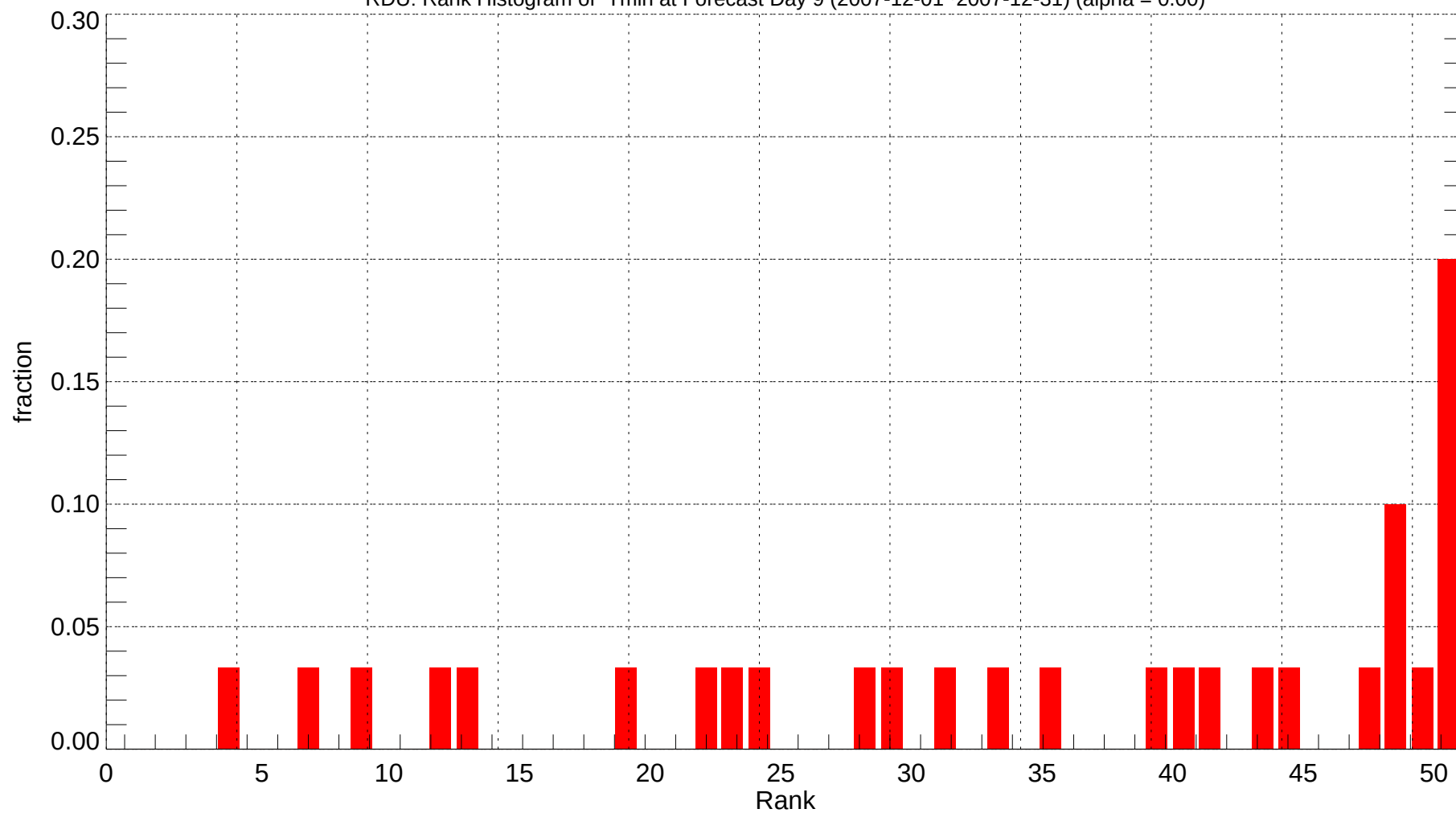
RDU: Rank Histogram of Tmin at Forecast Day 9 (2007-12-01~2007-12-31) (alpha = 0.00)
