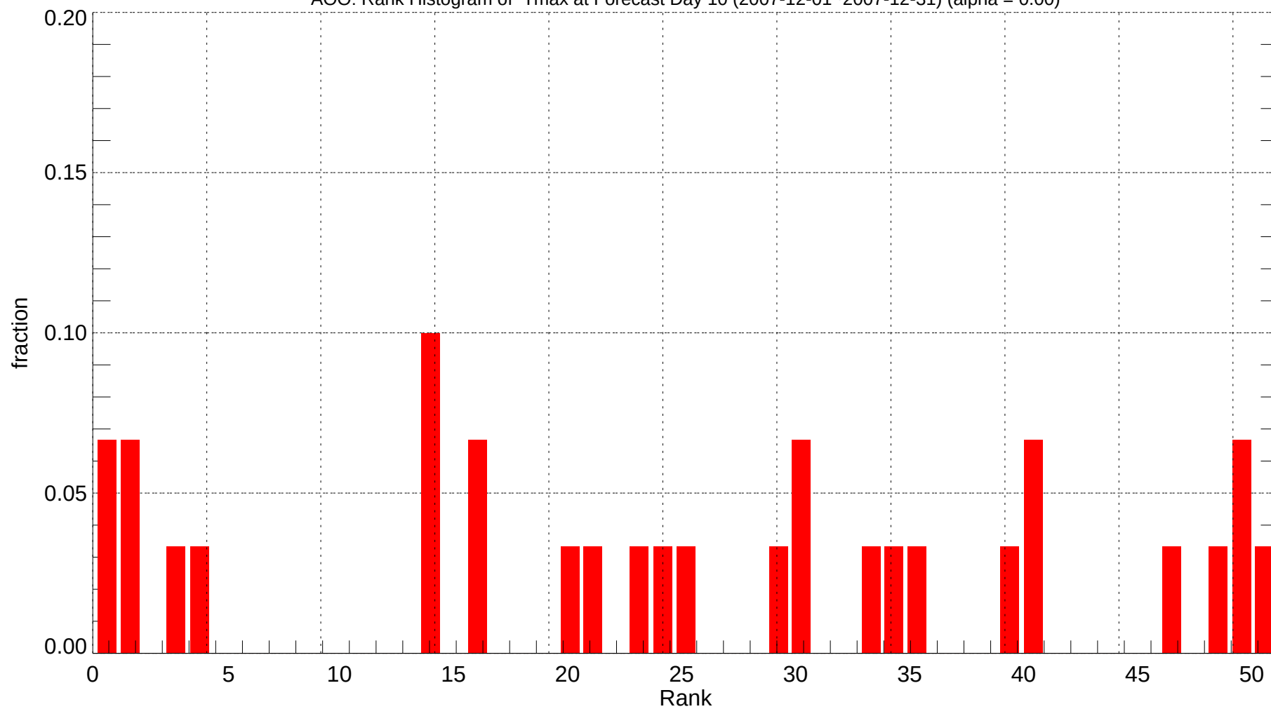
AOO: Rank Histogram of Tmax at Forecast Day 10 (2007-12-01~2007-12-31) (alpha = 0.00)
