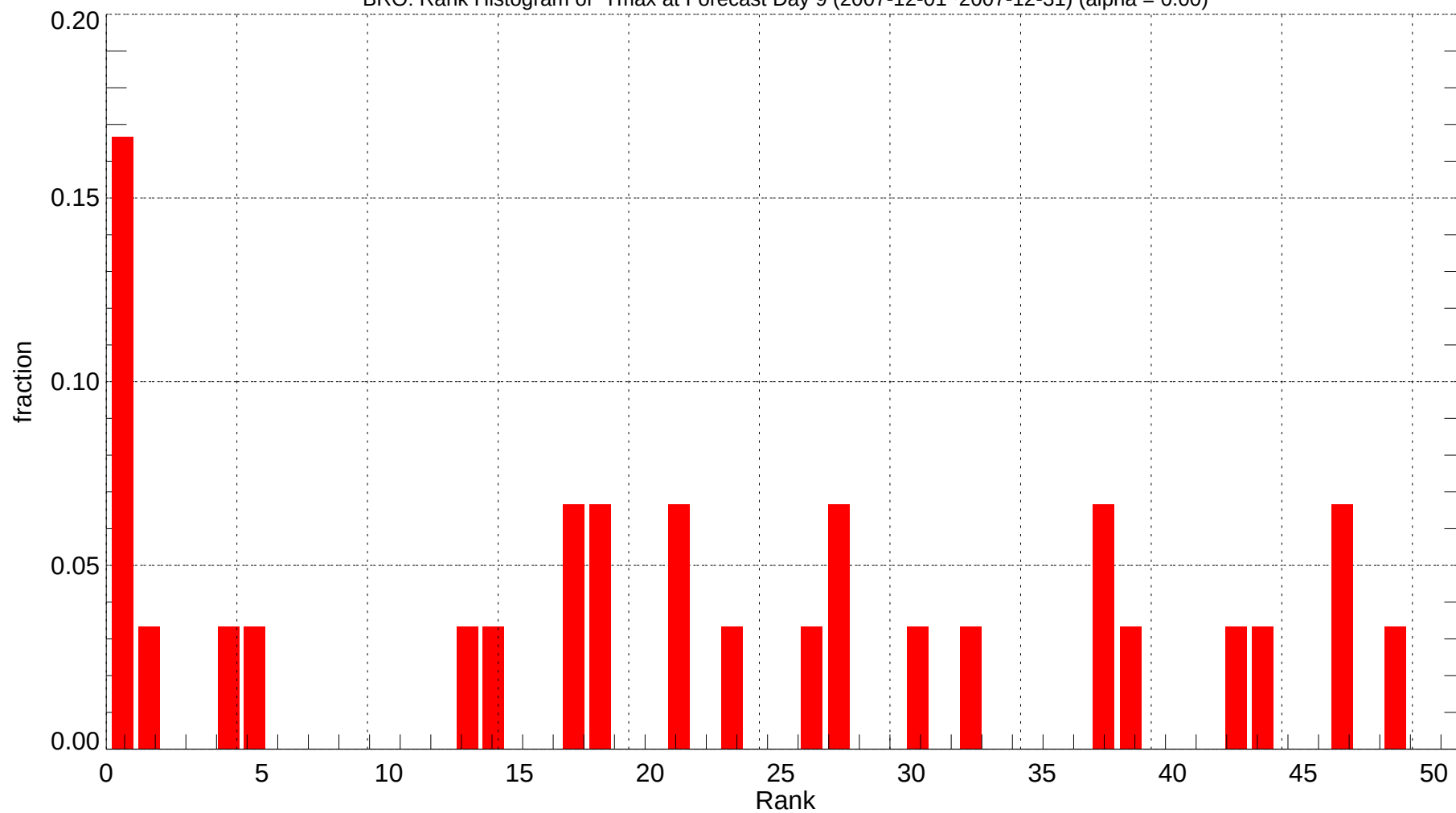
BRO: Rank Histogram of Tmax at Forecast Day 9 (2007-12-01~2007-12-31) (alpha = 0.00)
