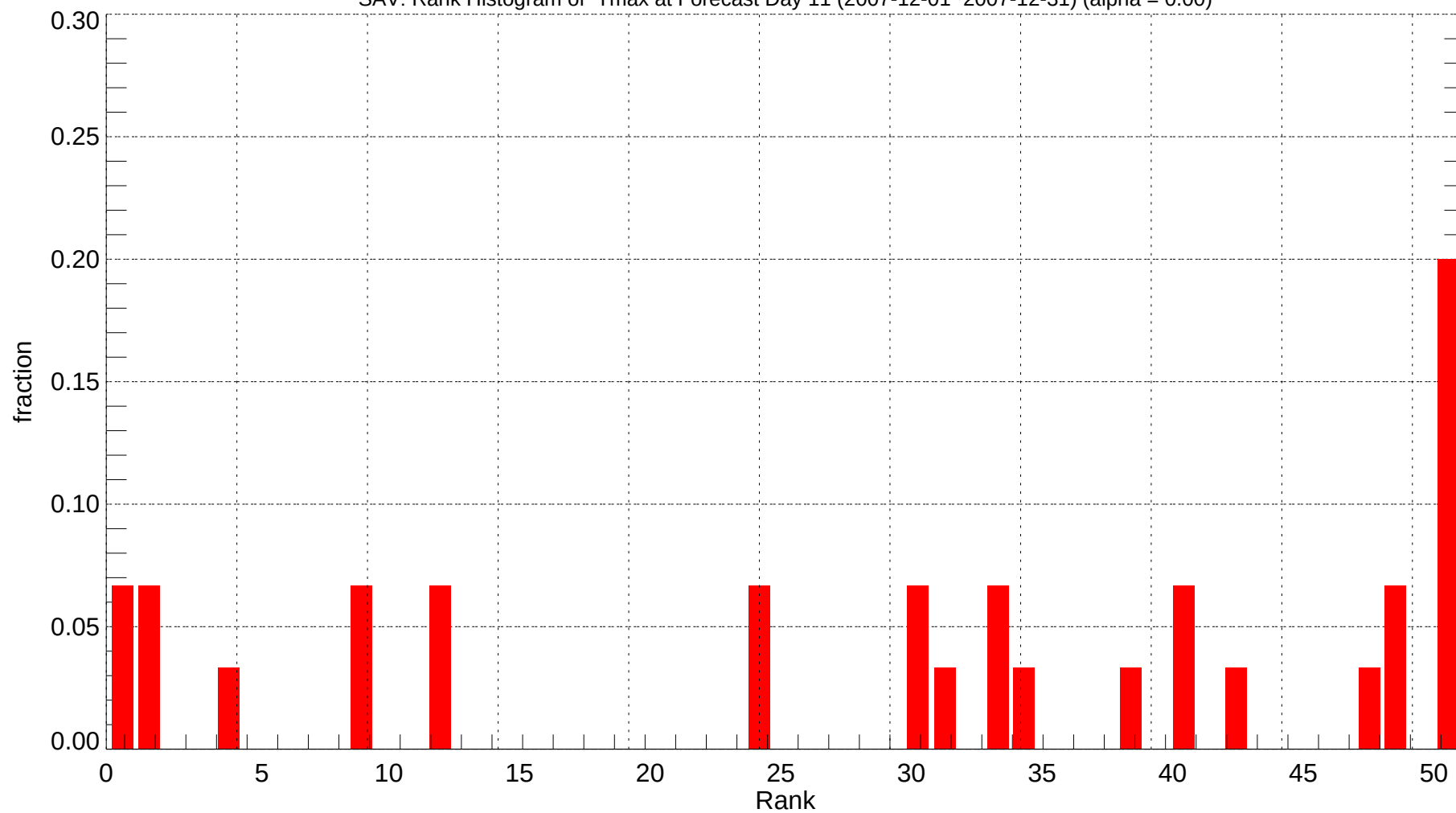
SAV: Rank Histogram of Tmax at Forecast Day 11 (2007-12-01~2007-12-31) (alpha = 0.00)
