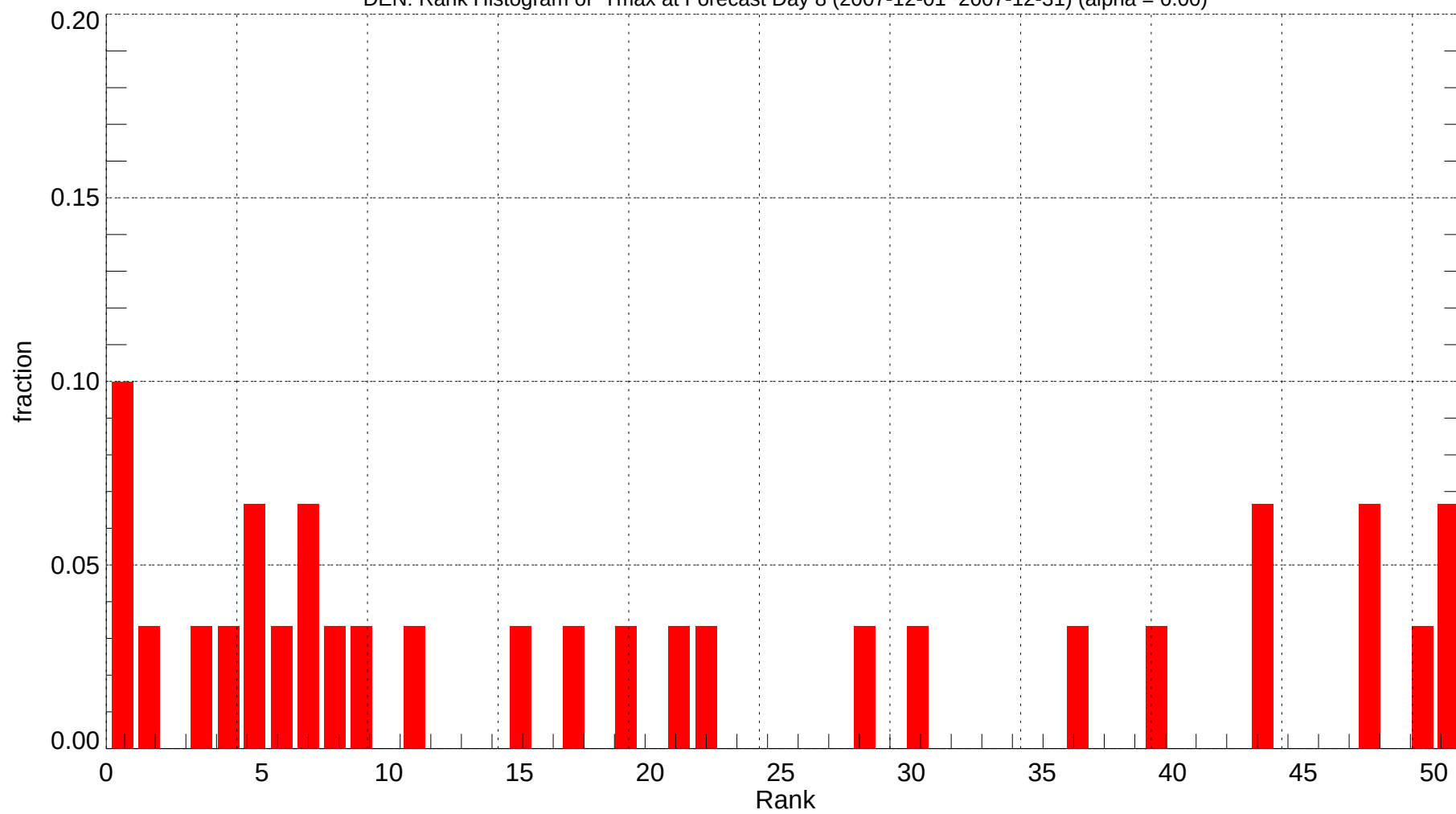
DEN: Rank Histogram of Tmax at Forecast Day 8 (2007-12-01~2007-12-31) (alpha = 0.00)
