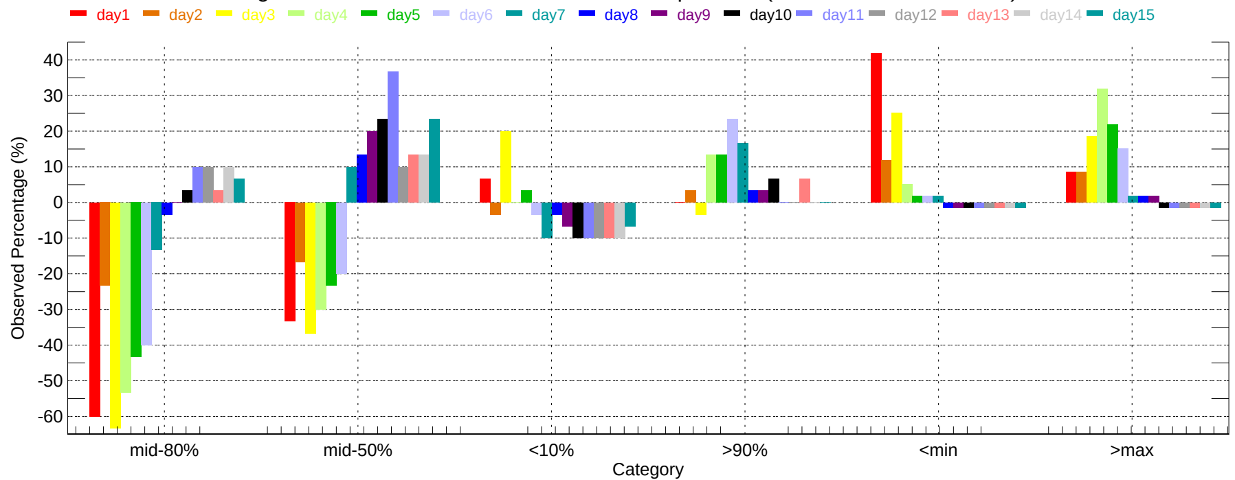
Observed Percentage Deviation of Ensembles - LAS: Min Temperature (2007-12-01~2007-12-31)
