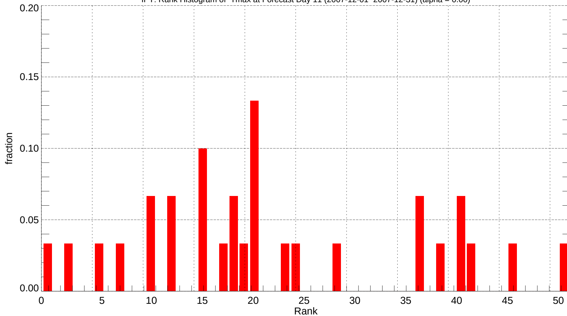
IPT: Rank Histogram of Tmax at Forecast Day 11 (2007-12-01~2007-12-31) (alpha = 0.00)
