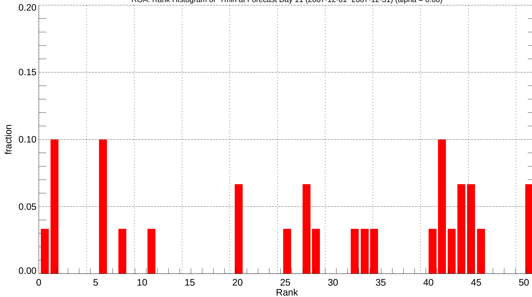
ROA: Rank Histogram of Tmin at Forecast Day 11 (2007-12-01~2007-12-31) (alpha = 0.00)
