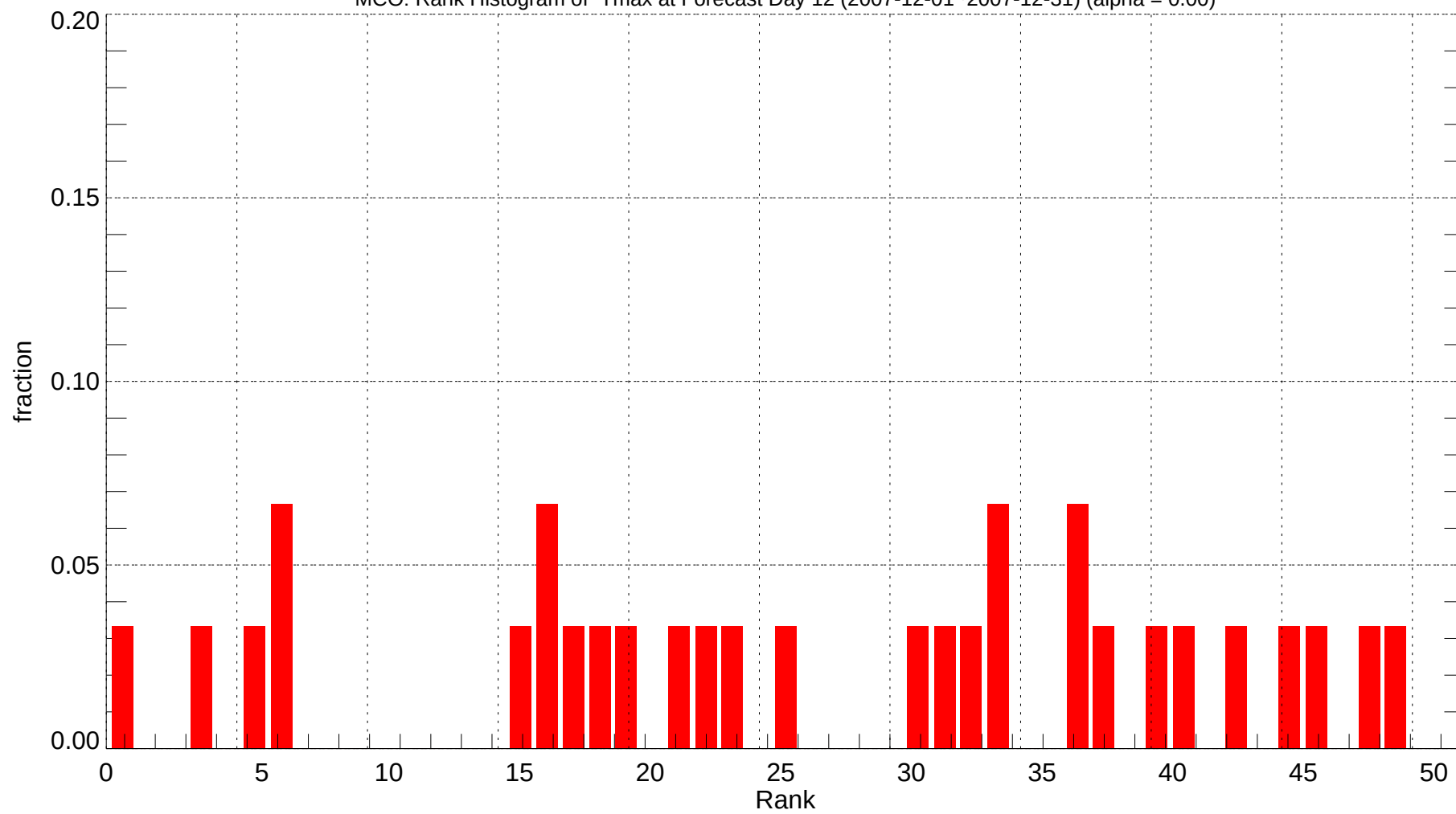
MCO: Rank Histogram of Tmax at Forecast Day 12 (2007-12-01~2007-12-31) (alpha = 0.00)
