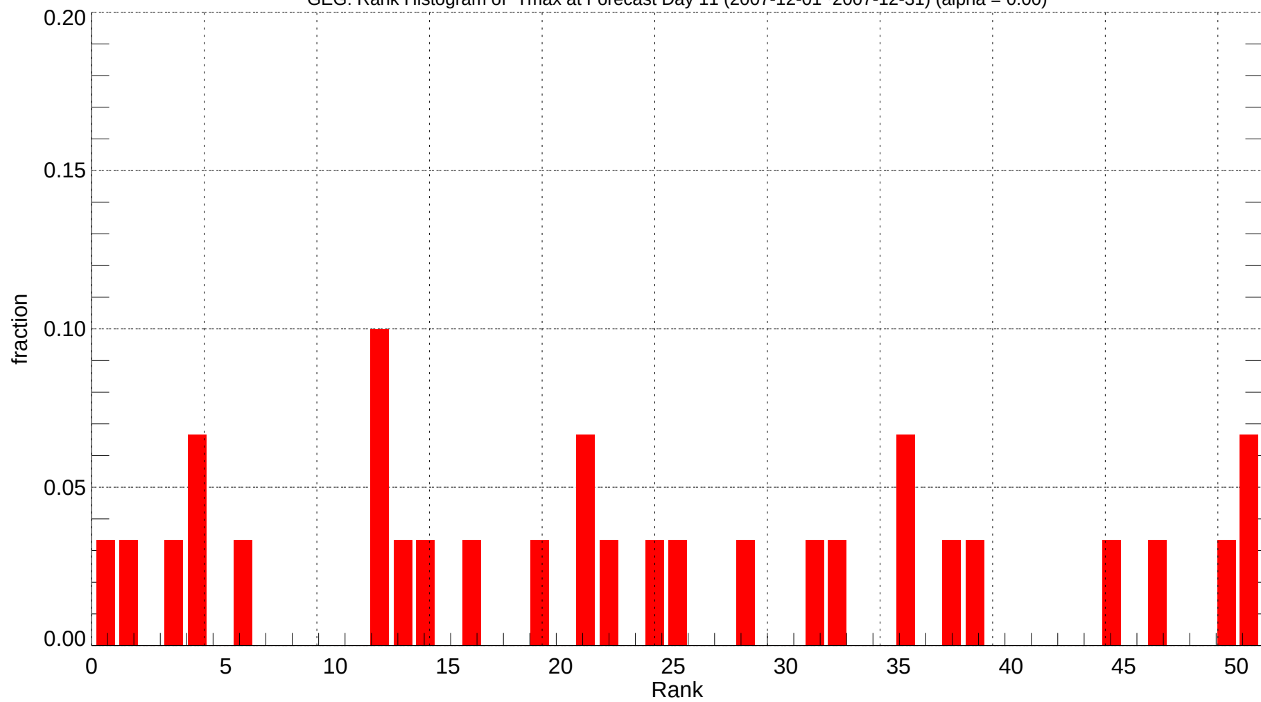
GEG: Rank Histogram of Tmax at Forecast Day 11 (2007-12-01~2007-12-31) (alpha = 0.00)
