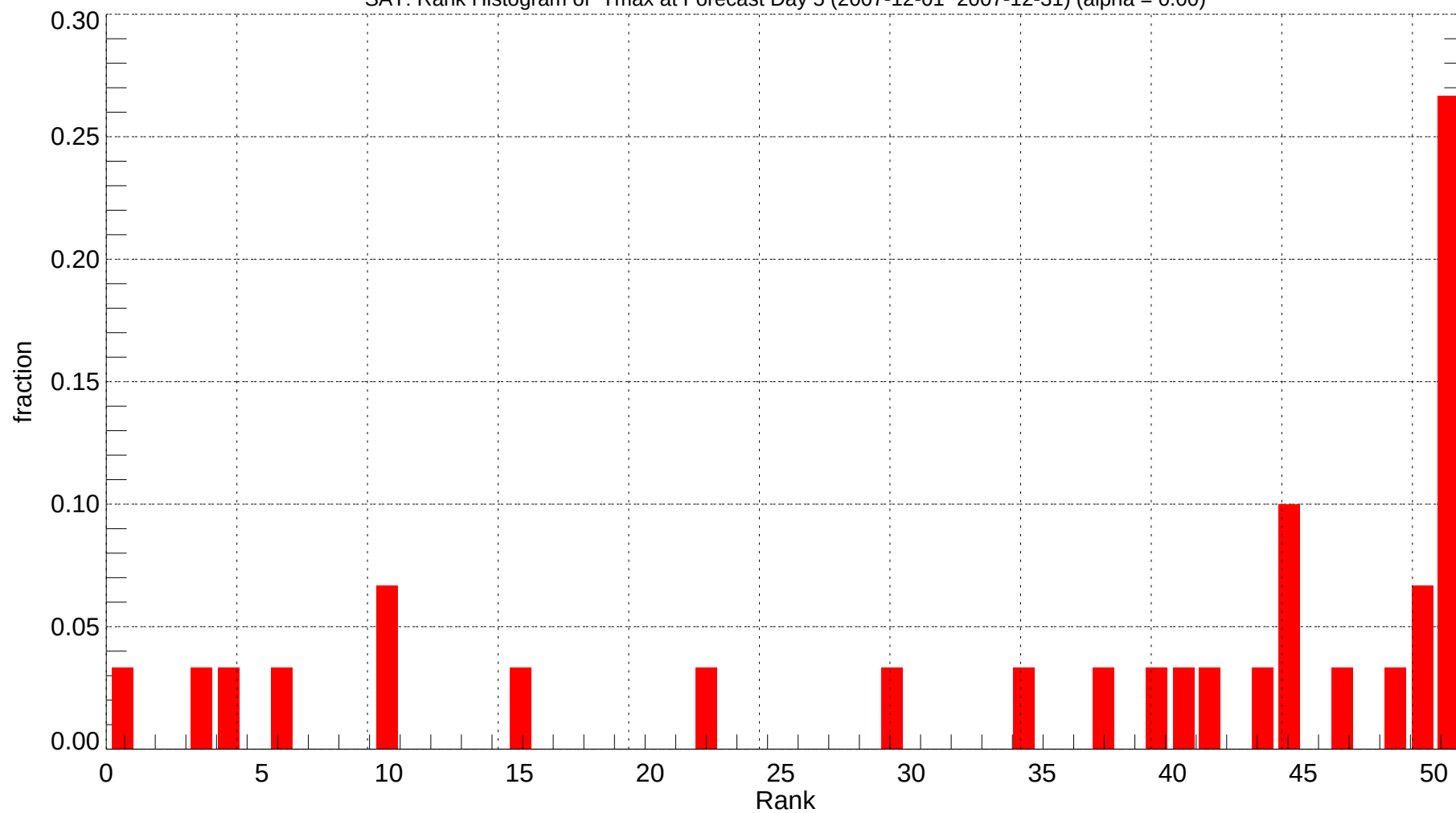
SAT: Rank Histogram of Tmax at Forecast Day 5 (2007-12-01~2007-12-31) (alpha = 0.00)
