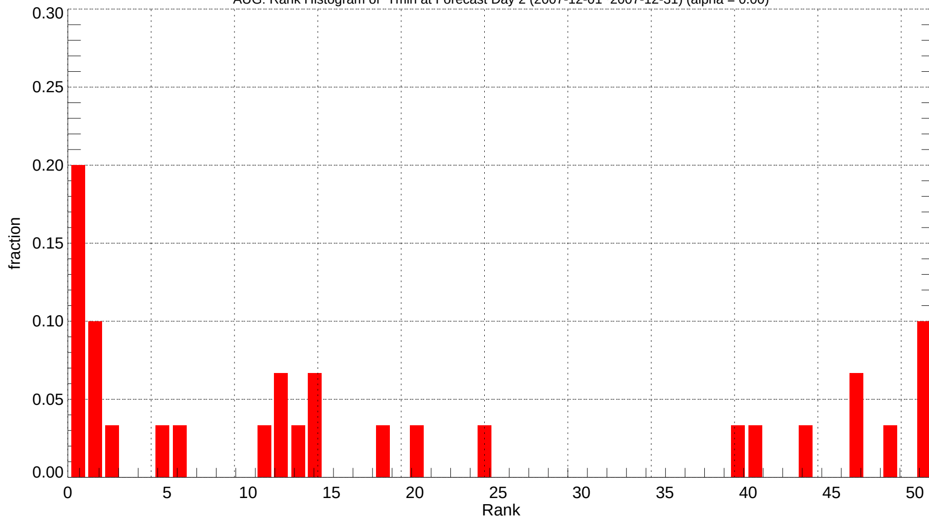
AUG: Rank Histogram of Tmin at Forecast Day 2 (2007-12-01~2007-12-31) (alpha = 0.00)
