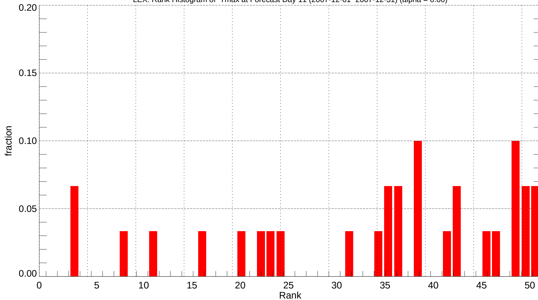
LEX: Rank Histogram of Tmax at Forecast Day 11 (2007-12-01~2007-12-31) (alpha = 0.00)
