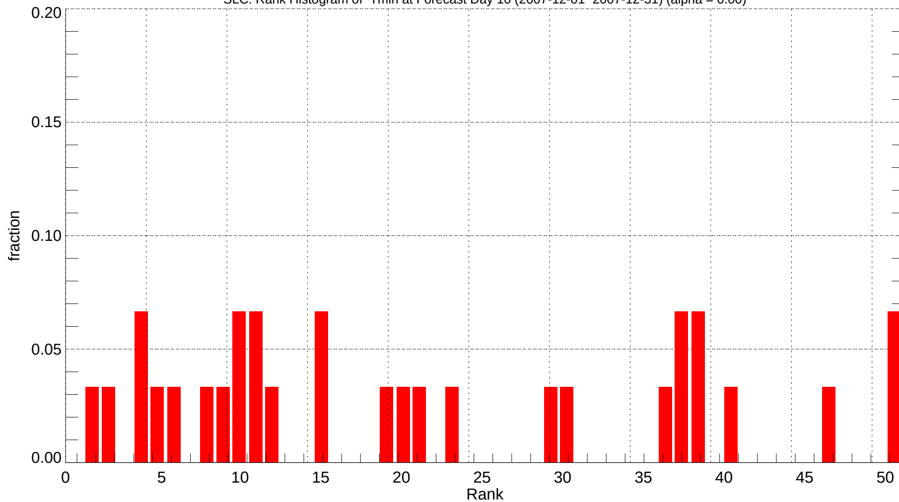
SLC: Rank Histogram of Tmin at Forecast Day 10 (2007-12-01~2007-12-31) (alpha = 0.00)
