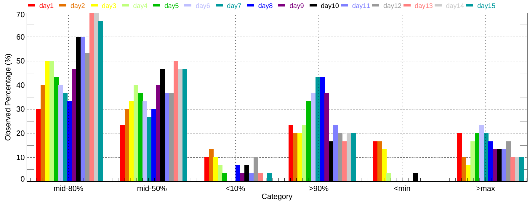
Observed Percentage of Ensembles - MEM: Min Temperature (2007-12-01~2007-12-31)
