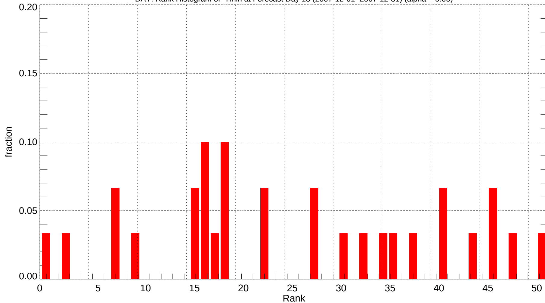
DAY: Rank Histogram of Tmin at Forecast Day 13 (2007-12-01~2007-12-31) (alpha = 0.00)
