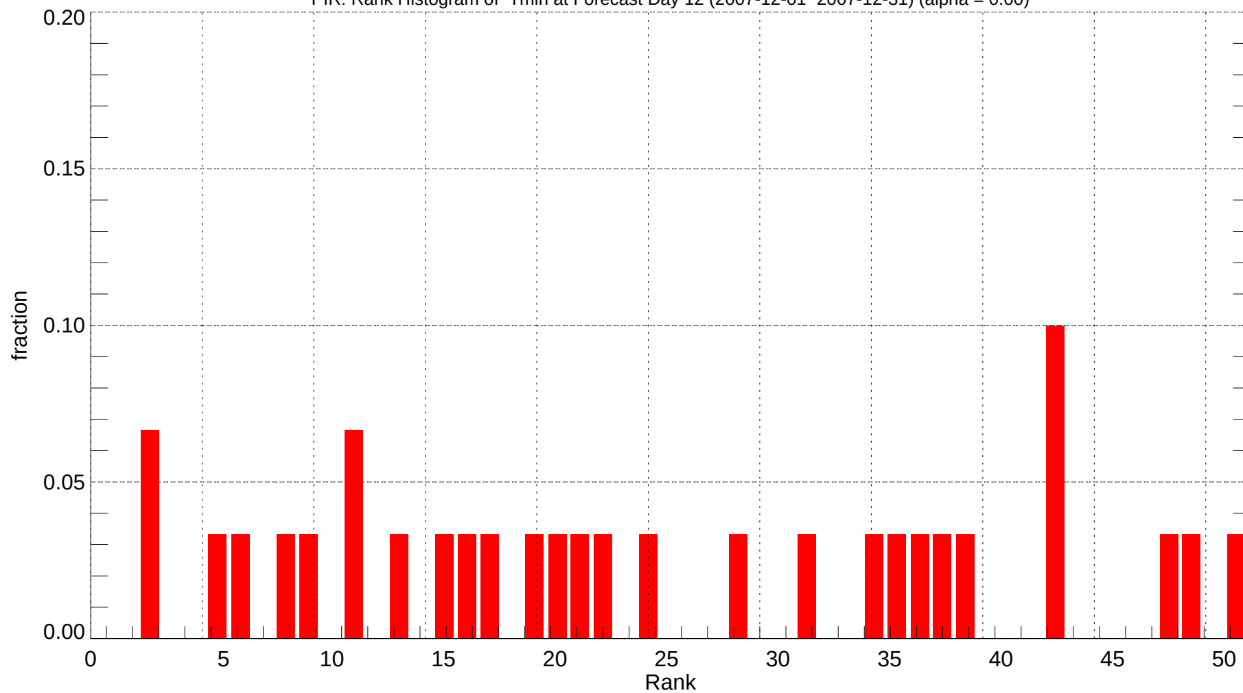
PIR: Rank Histogram of Tmin at Forecast Day 12 (2007-12-01~2007-12-31) (alpha = 0.00)
