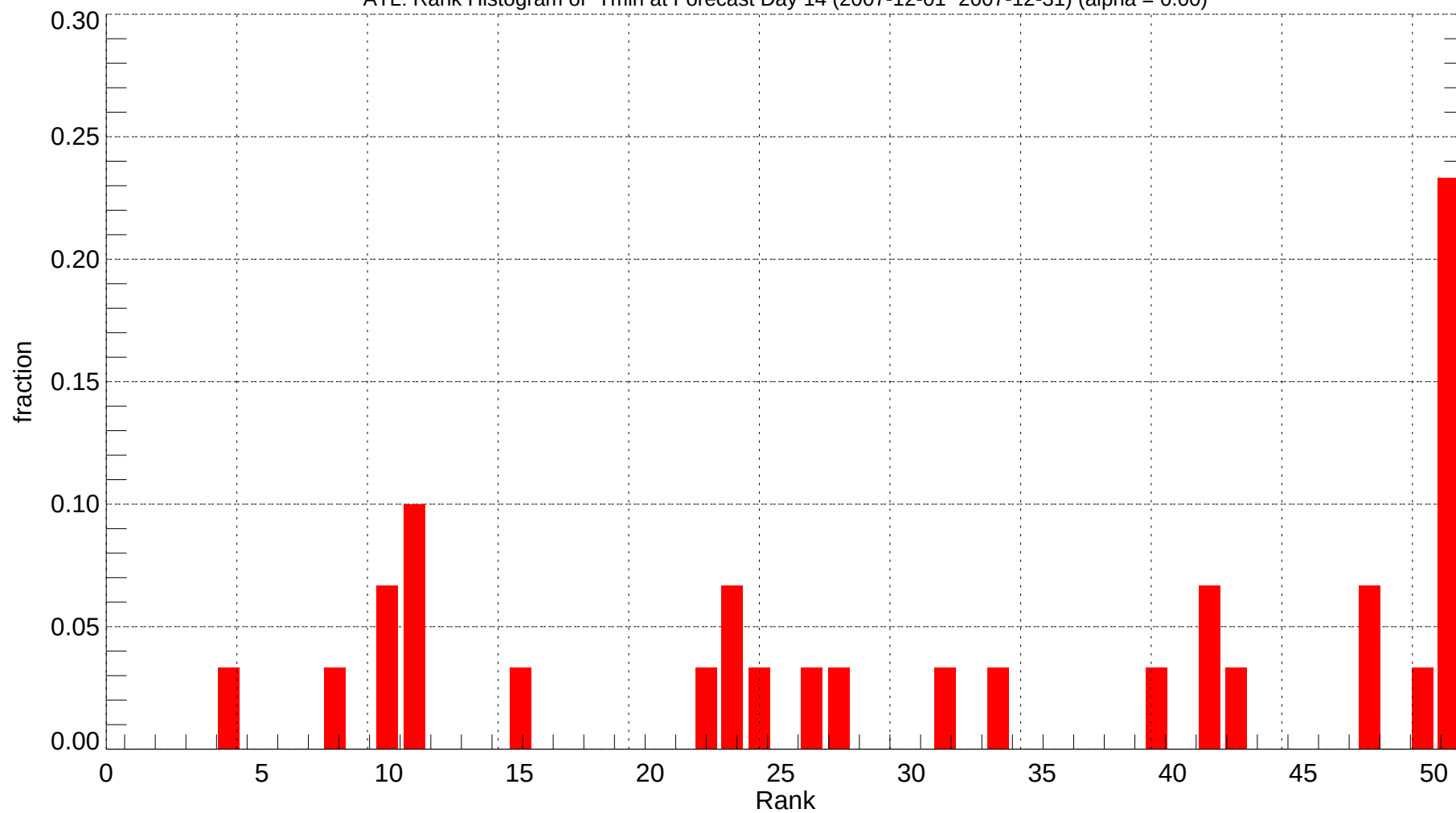
ATL: Rank Histogram of Tmin at Forecast Day 14 (2007-12-01~2007-12-31) (alpha = 0.00)
