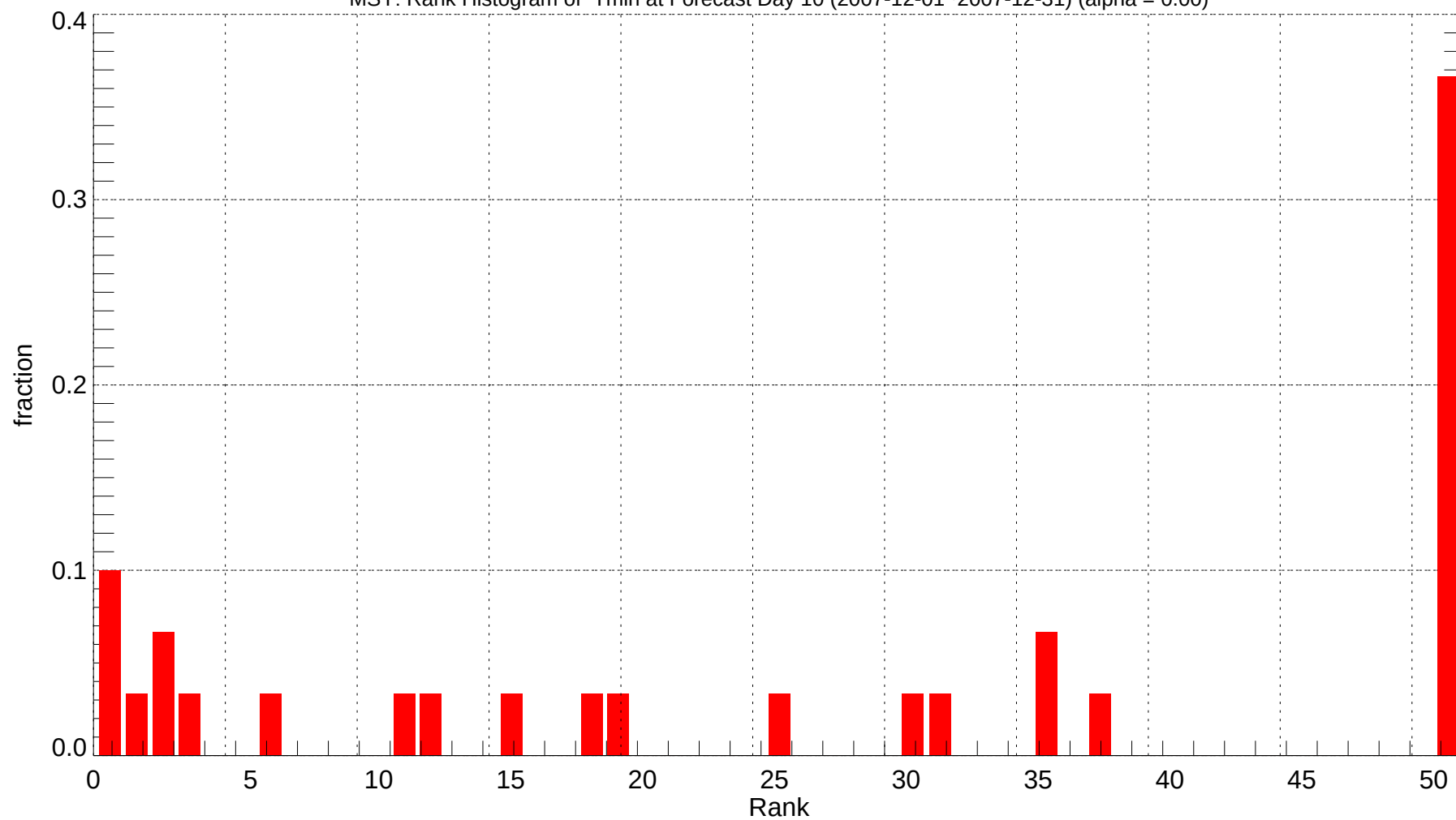
MSY: Rank Histogram of Tmin at Forecast Day 10 (2007-12-01~2007-12-31) (alpha = 0.00)
