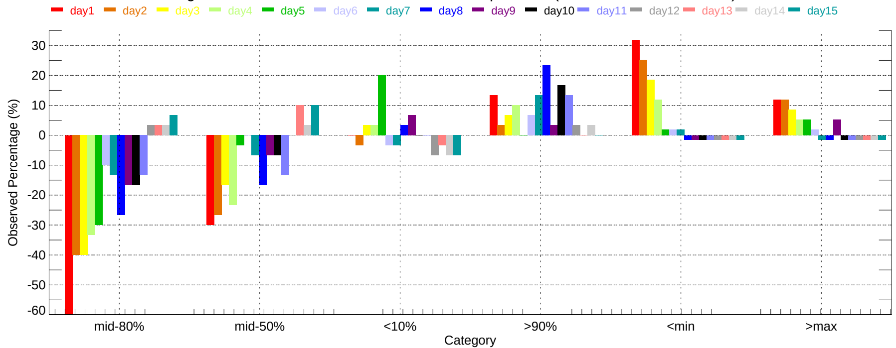
Observed Percentage Deviation of Ensembles - JFK: Min Temperature (2007-12-01~2007-12-31)
