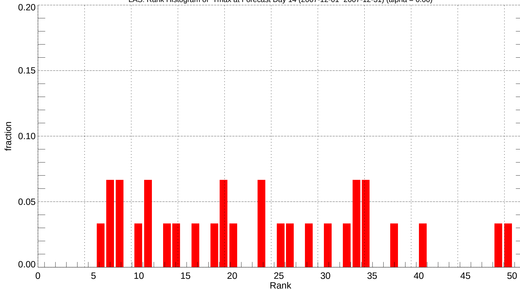
LAS: Rank Histogram of Tmax at Forecast Day 14 (2007-12-01~2007-12-31) (alpha = 0.00)
