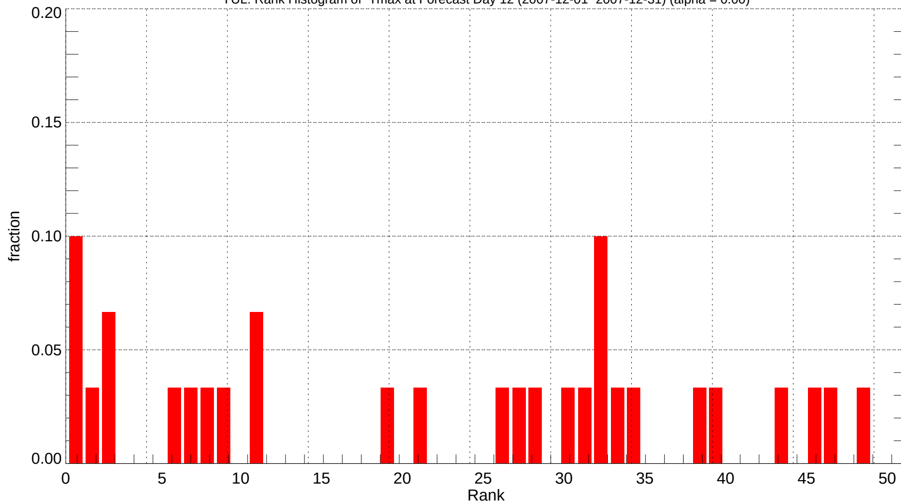
YUL: Rank Histogram of Tmax at Forecast Day 12 (2007-12-01~2007-12-31) (alpha = 0.00)
