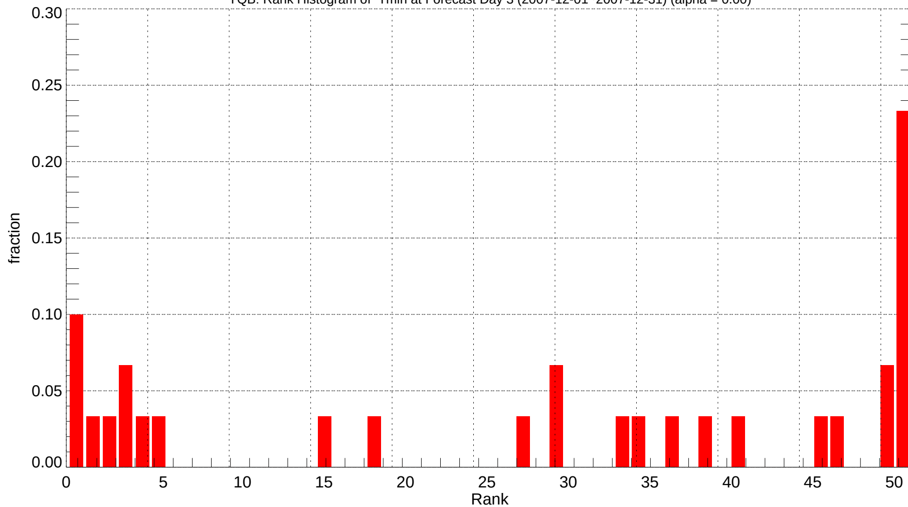
YQB: Rank Histogram of Tmin at Forecast Day 3 (2007-12-01~2007-12-31) (alpha = 0.00)
