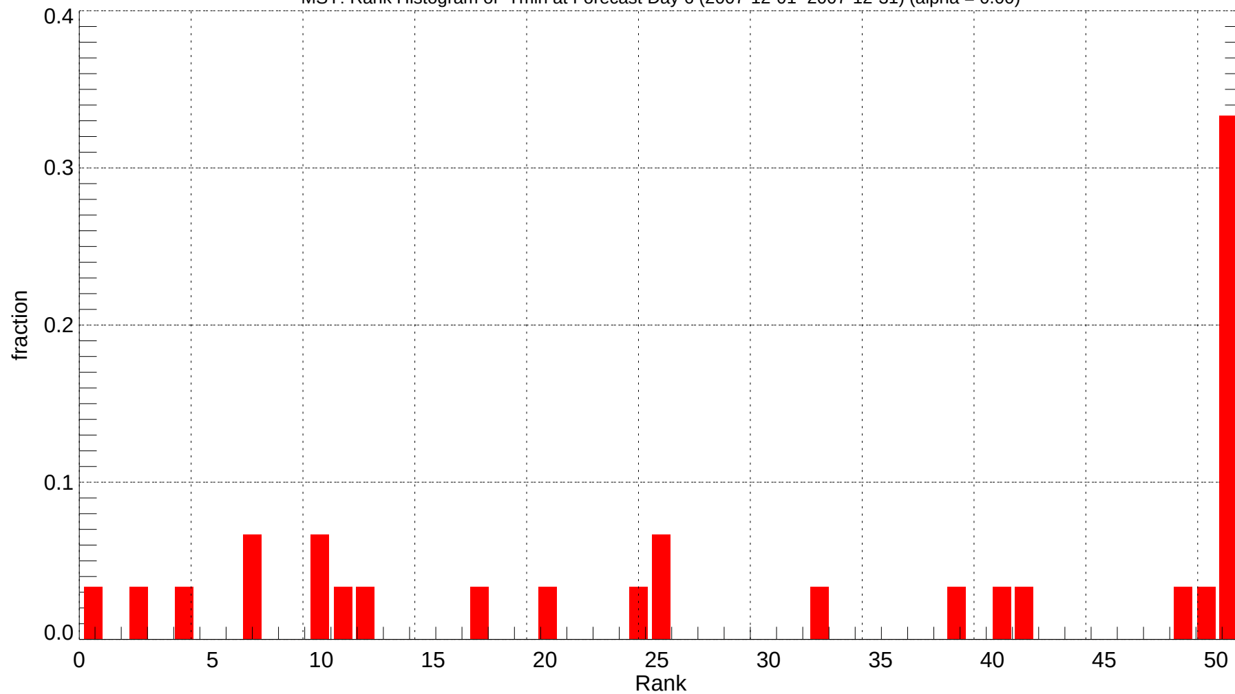
MSY: Rank Histogram of Tmin at Forecast Day 6 (2007-12-01~2007-12-31) (alpha = 0.00)
