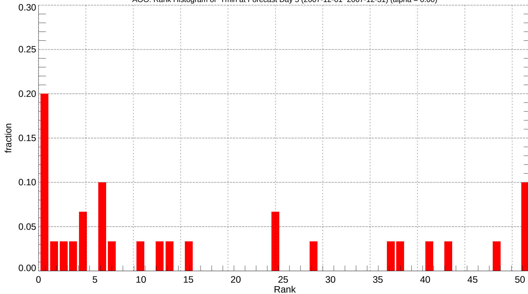
AOO: Rank Histogram of Tmin at Forecast Day 5 (2007-12-01~2007-12-31) (alpha = 0.00)
