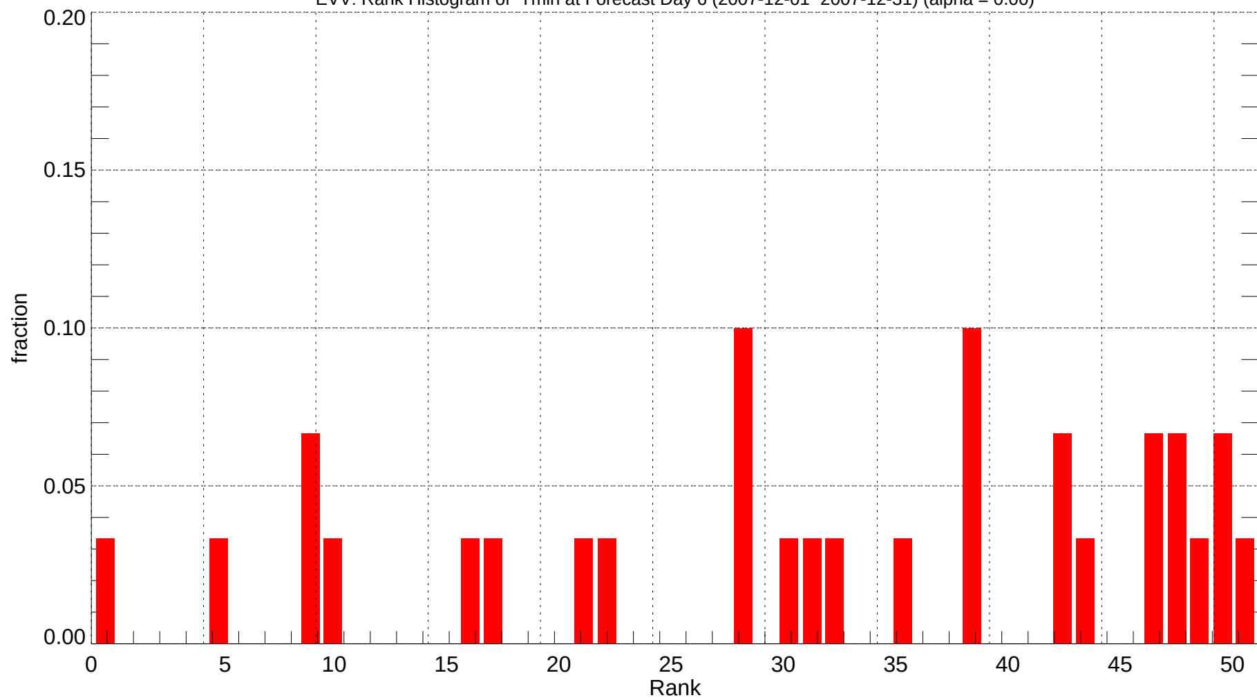
EVV: Rank Histogram of Tmin at Forecast Day 6 (2007-12-01~2007-12-31) (alpha = 0.00)
