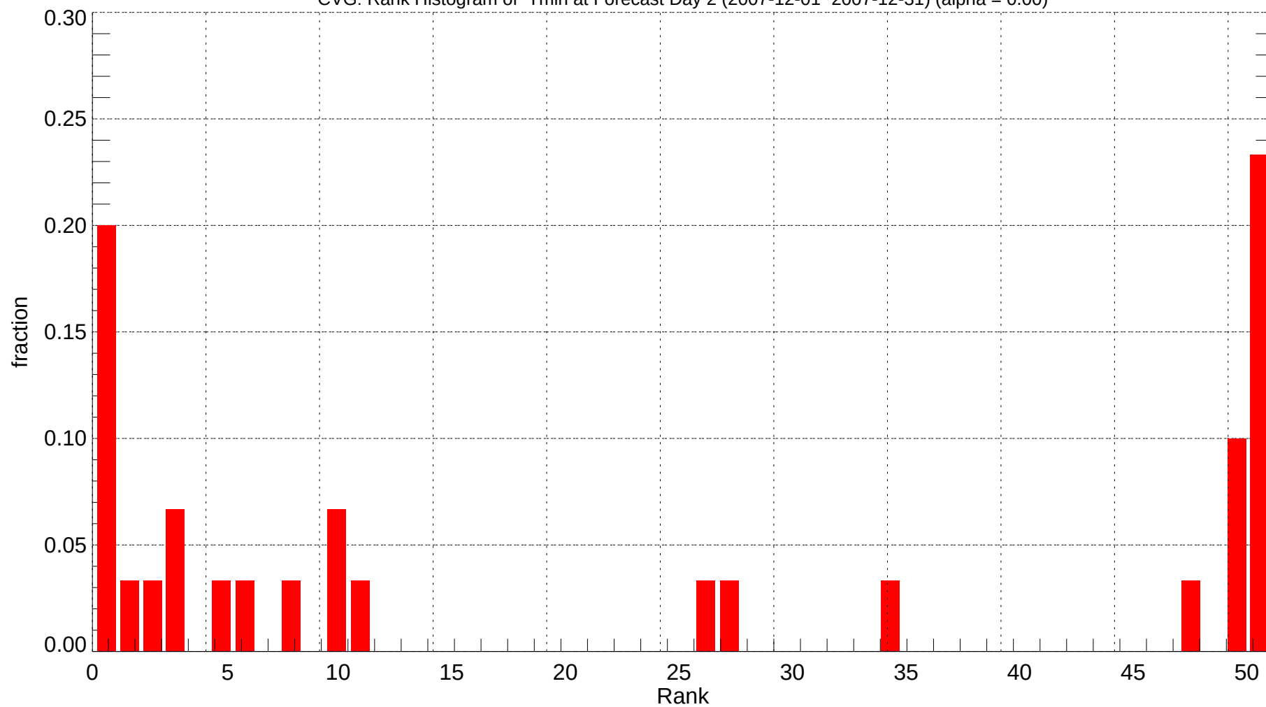
CVG: Rank Histogram of Tmin at Forecast Day 2 (2007-12-01~2007-12-31) (alpha = 0.00)
