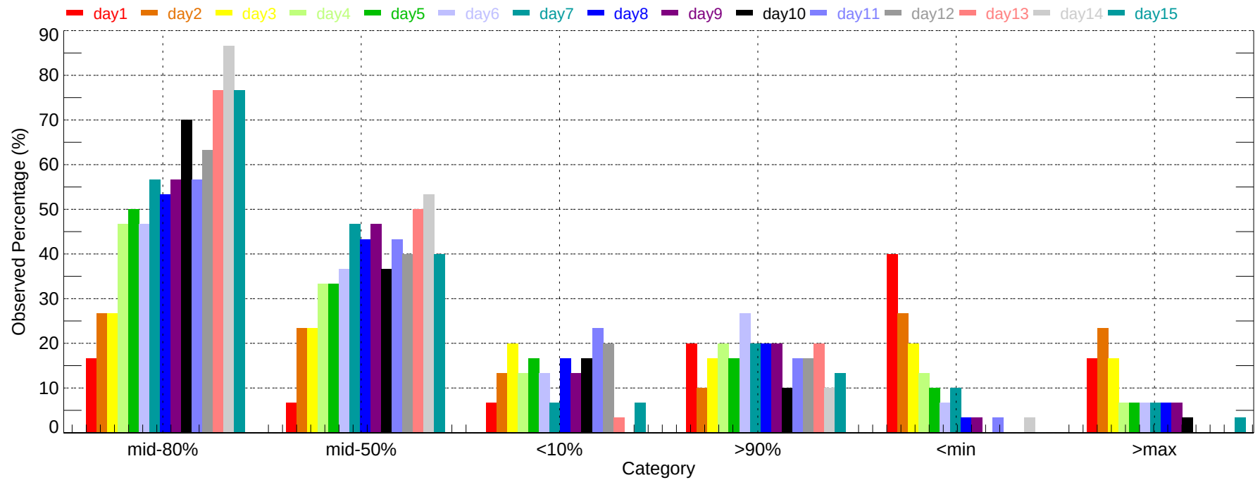
Observed Percentage of Ensembles - LNS: Min Temperature (2007-12-01~2007-12-31)
