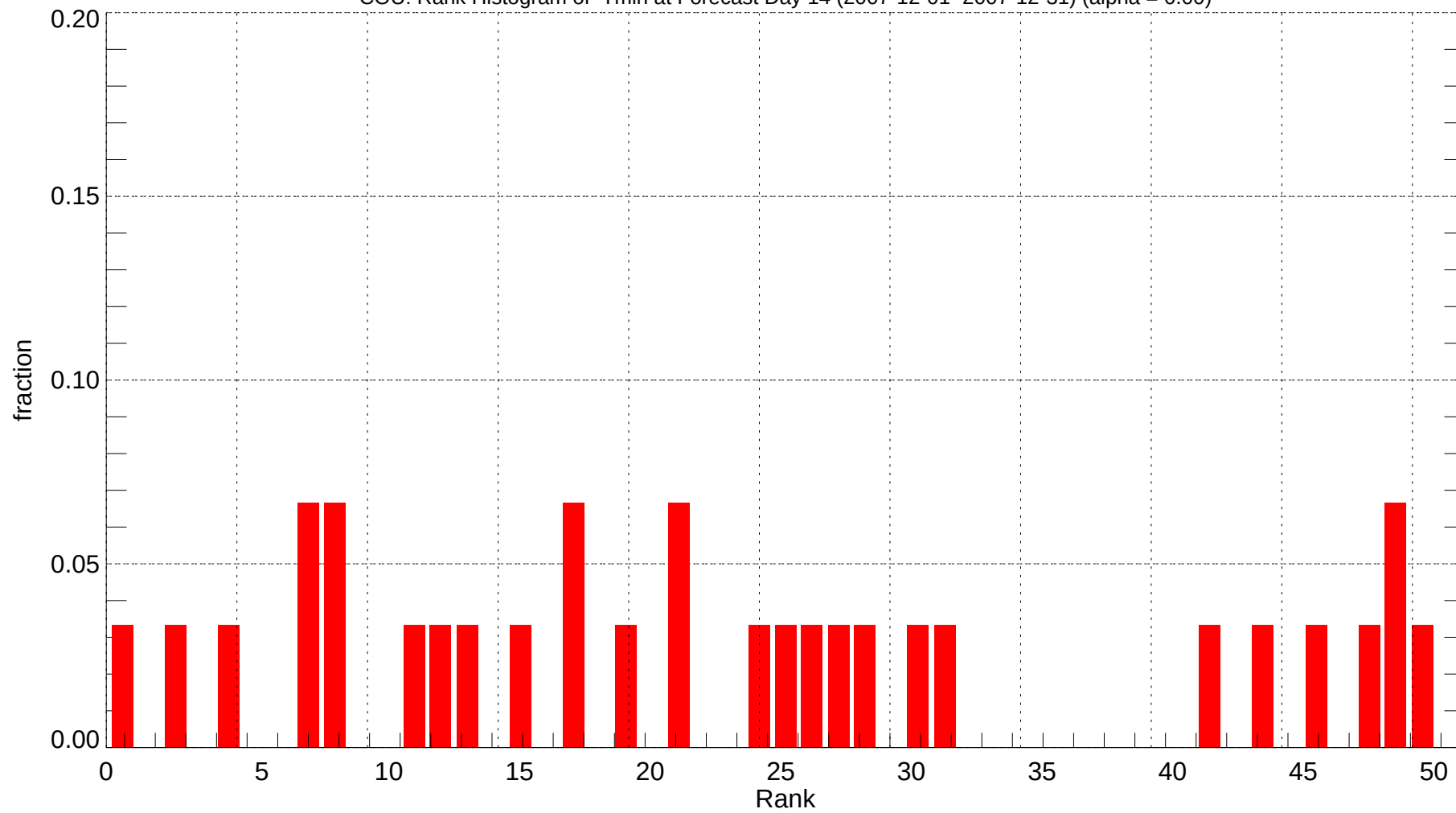
COU: Rank Histogram of Tmin at Forecast Day 14 (2007-12-01~2007-12-31) (alpha = 0.00)
