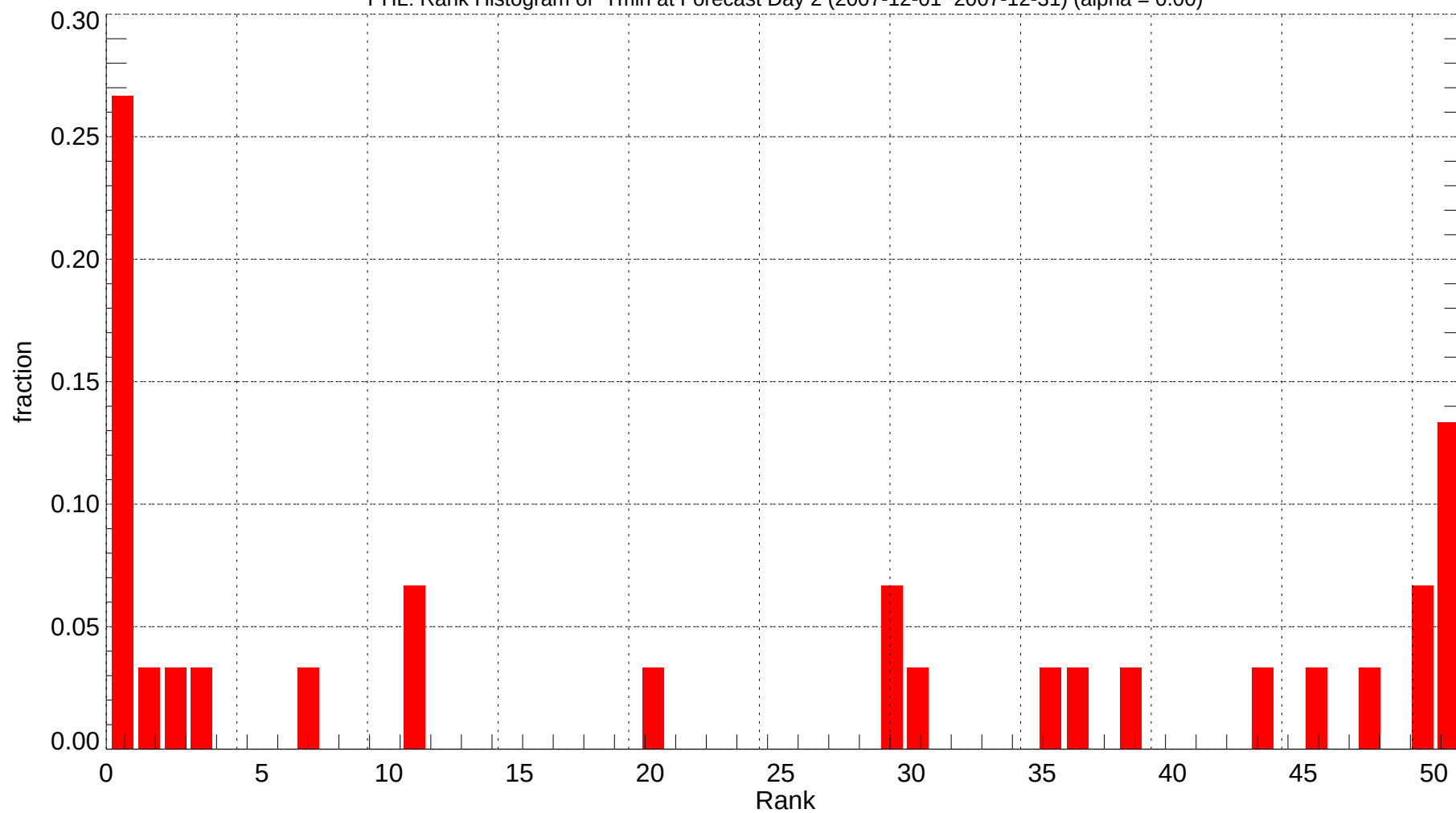
PHL: Rank Histogram of Tmin at Forecast Day 2 (2007-12-01~2007-12-31) (alpha = 0.00)
