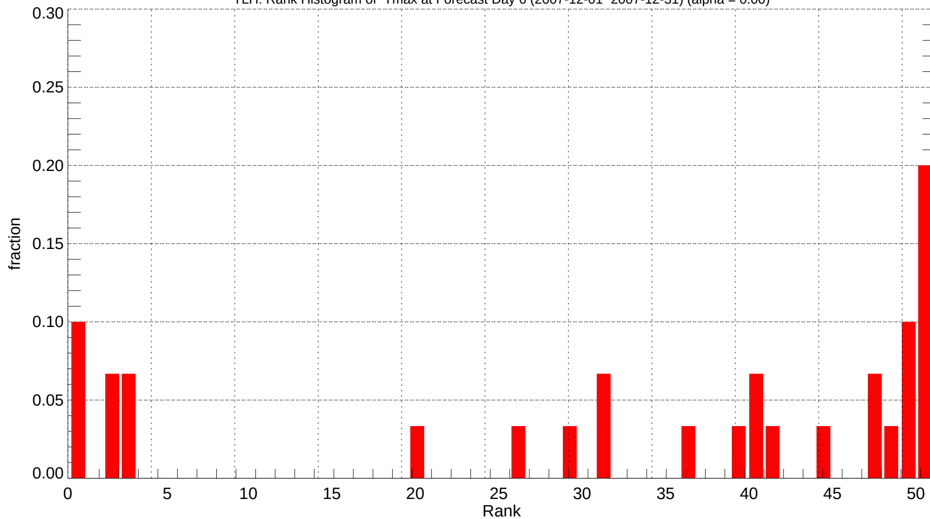
TLH: Rank Histogram of Tmax at Forecast Day 6 (2007-12-01~2007-12-31) (alpha = 0.00)
