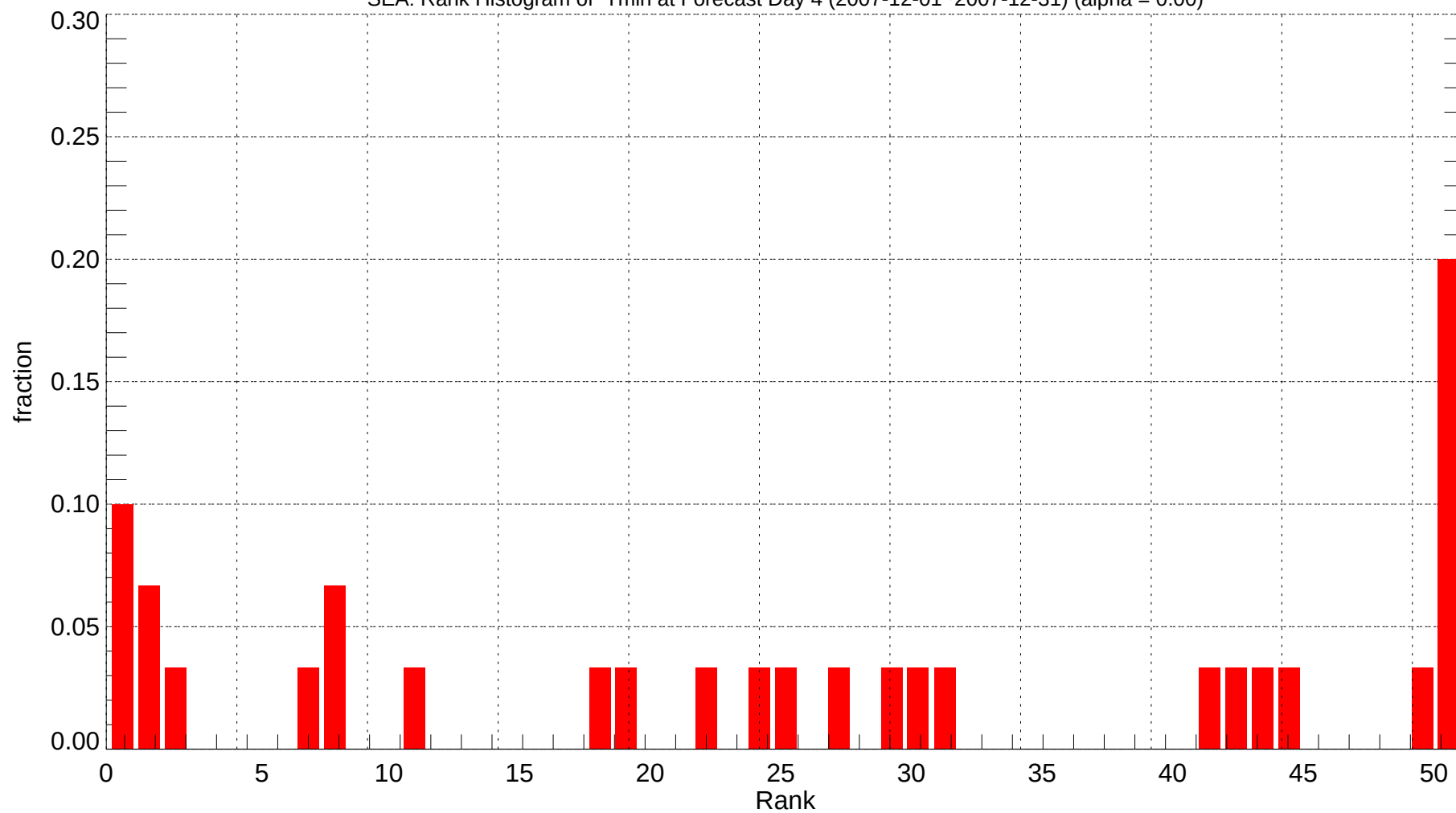
SEA: Rank Histogram of Tmin at Forecast Day 4 (2007-12-01~2007-12-31) (alpha = 0.00)
