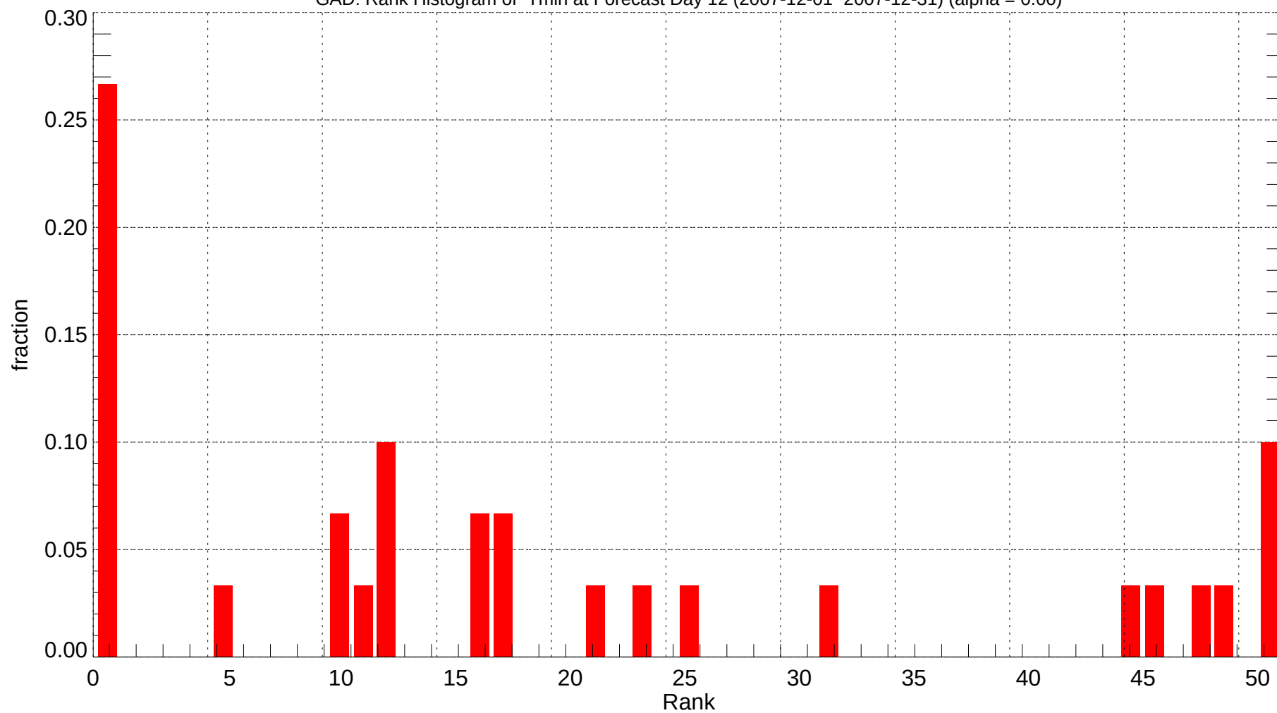
GAD: Rank Histogram of Tmin at Forecast Day 12 (2007-12-01~2007-12-31) (alpha = 0.00)
