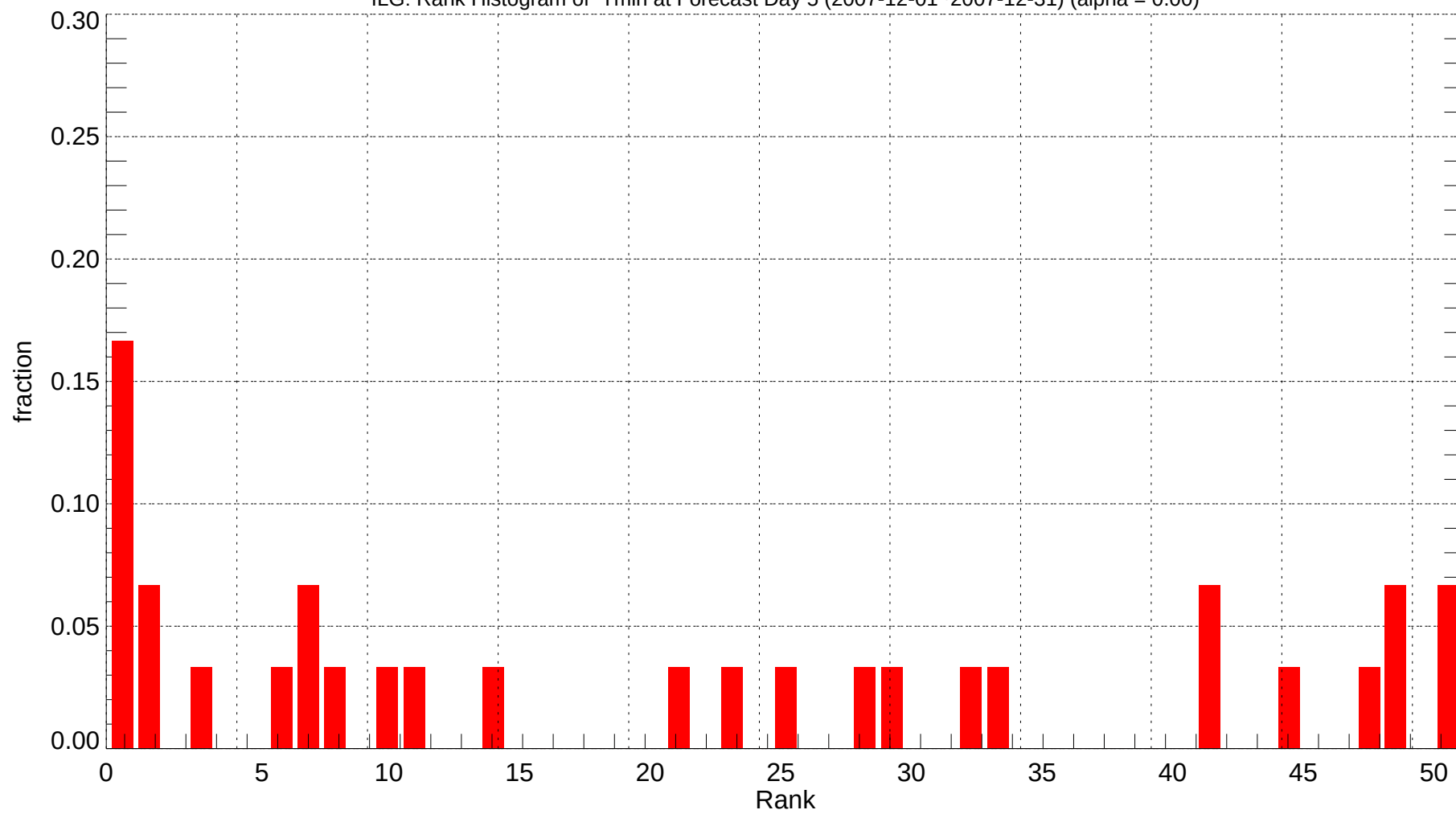
ILG: Rank Histogram of Tmin at Forecast Day 5 (2007-12-01~2007-12-31) (alpha = 0.00)
