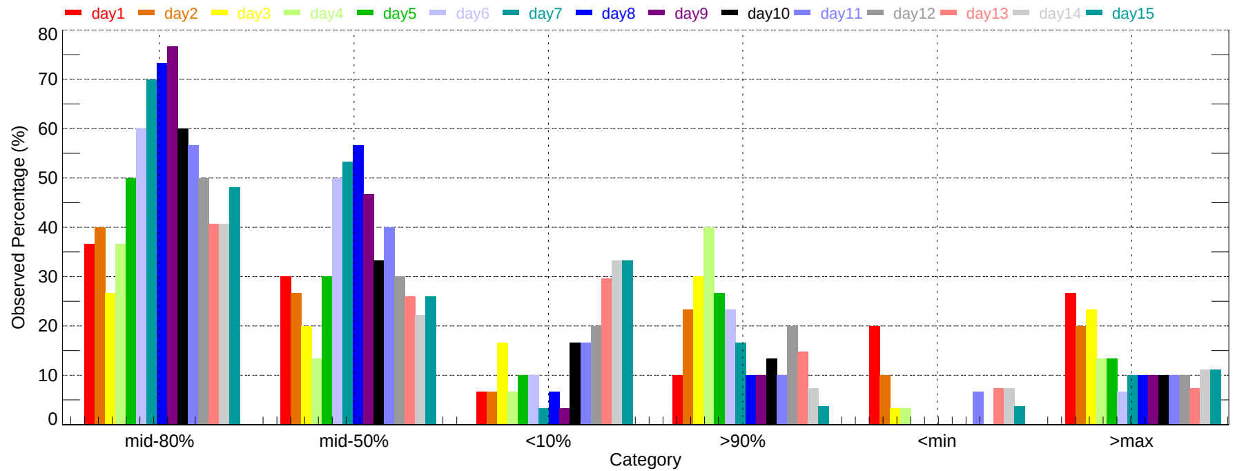
Observed Percentage of Ensembles - FLG: Max Temperature (2007-12-01~2007-12-31)
