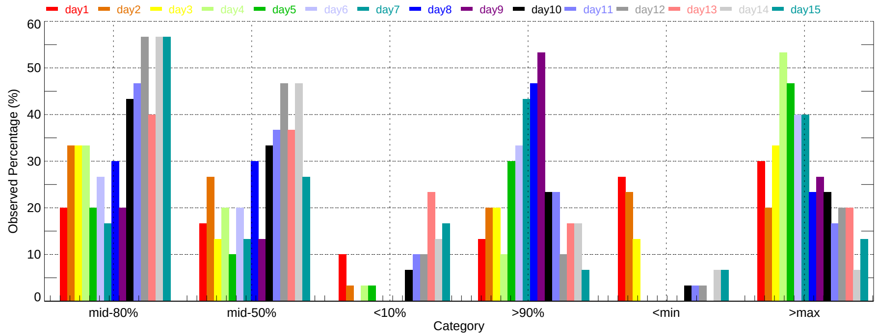
Observed Percentage of Ensembles - LGB: Min Temperature (2007-12-01~2007-12-31)
