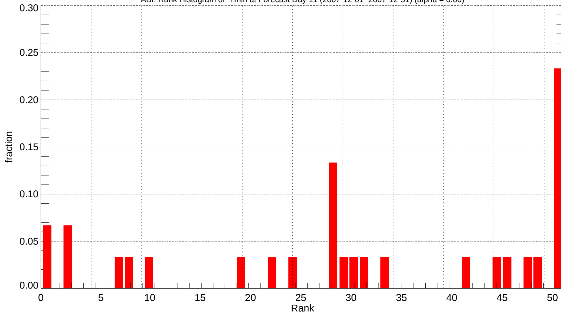
ABI: Rank Histogram of Tmin at Forecast Day 11 (2007-12-01~2007-12-31) (alpha = 0.00)
