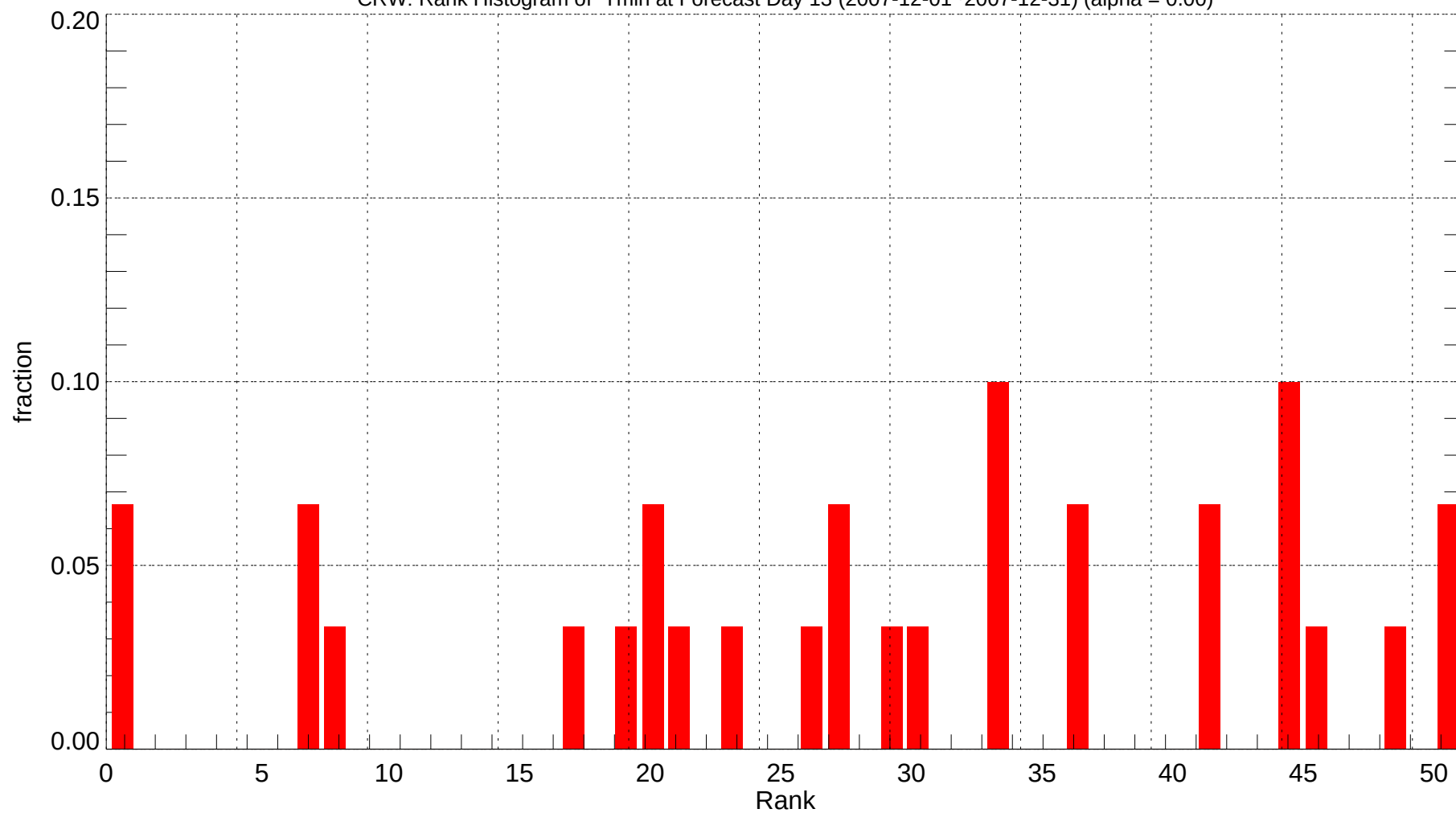
CRW: Rank Histogram of Tmin at Forecast Day 13 (2007-12-01~2007-12-31) (alpha = 0.00)
