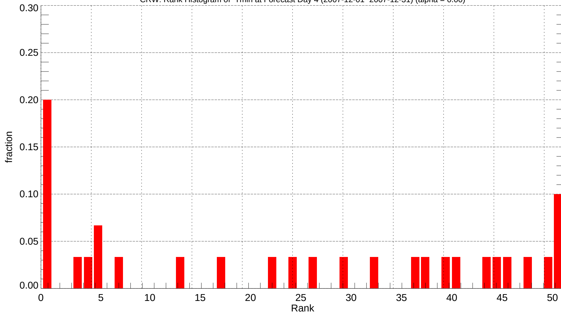
CRW: Rank Histogram of Tmin at Forecast Day 4 (2007-12-01~2007-12-31) (alpha = 0.00)
