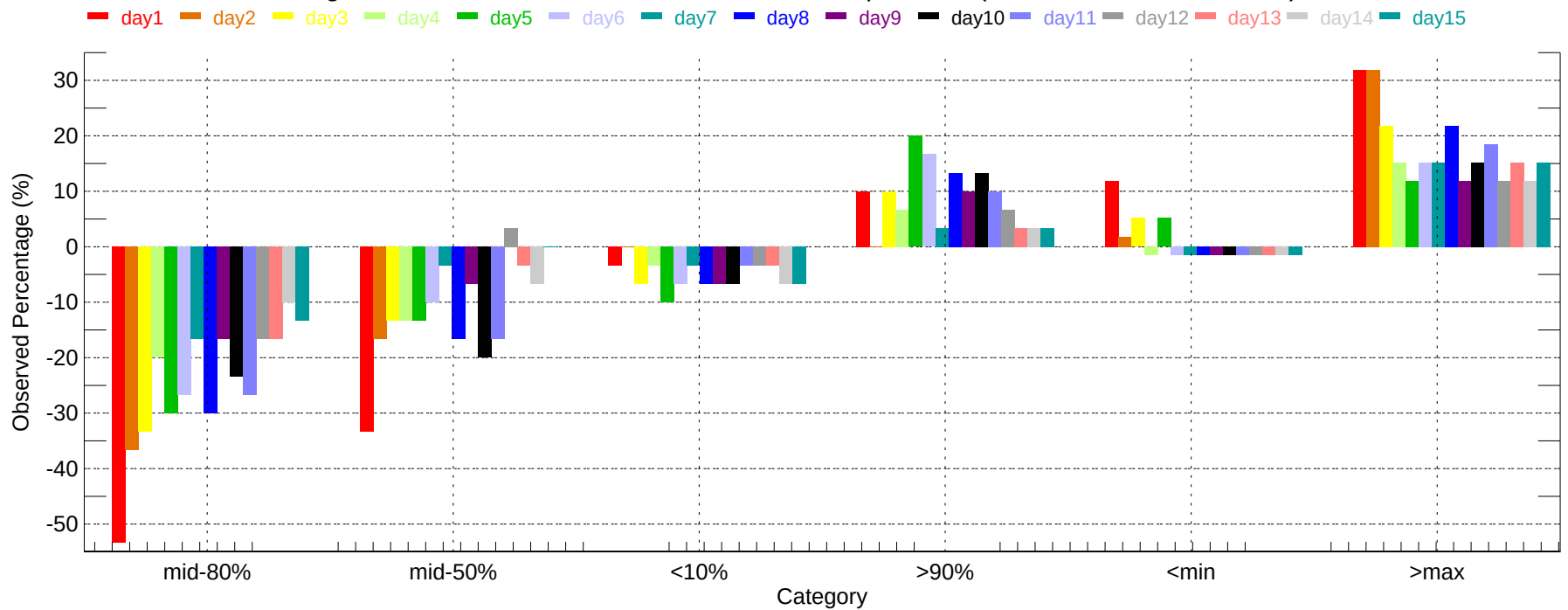
Observed Percentage Deviation of Ensembles - LFK: Max Temperature (2007-12-01~2007-12-31)
