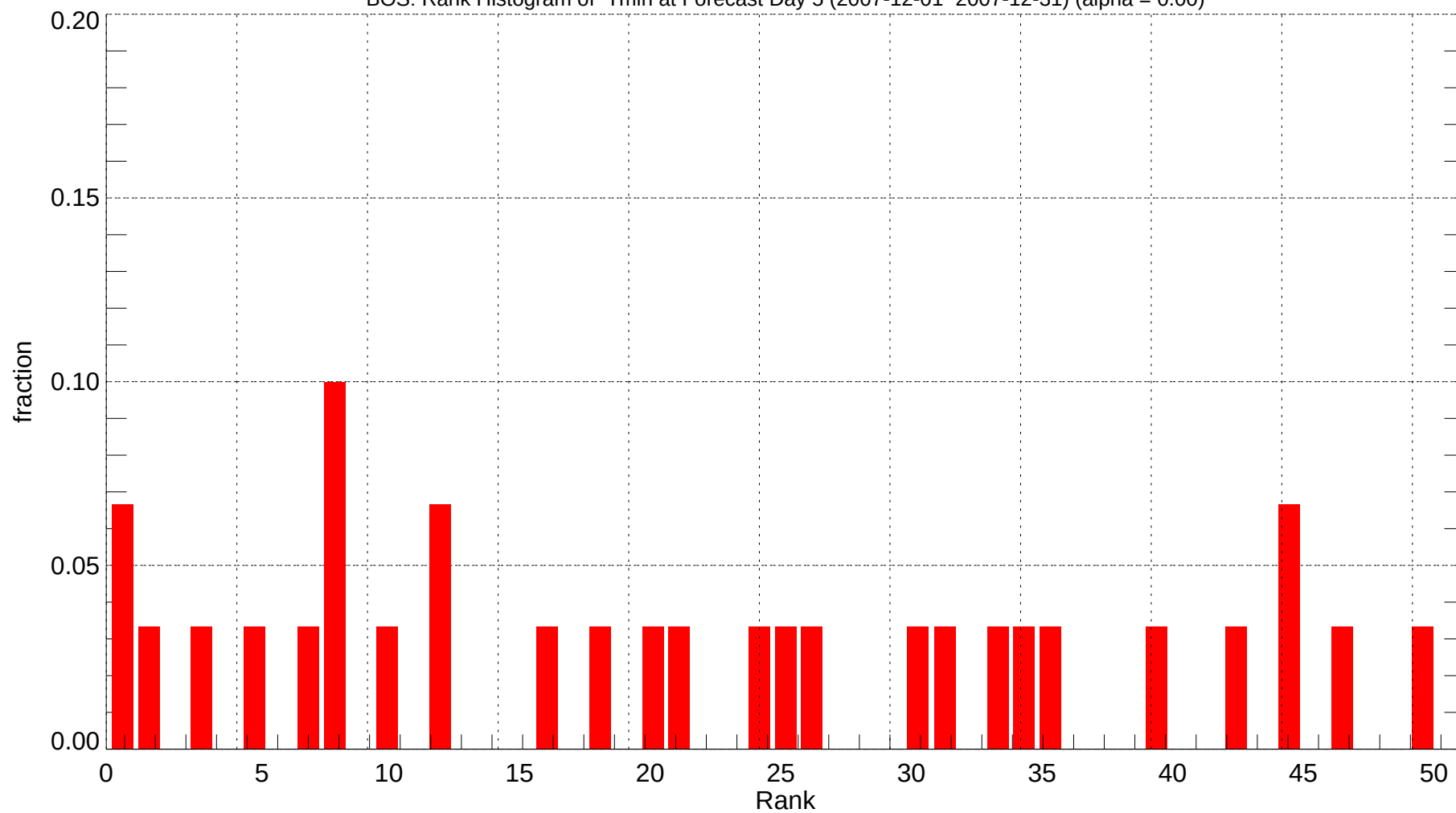
BOS: Rank Histogram of Tmin at Forecast Day 5 (2007-12-01~2007-12-31) (alpha = 0.00)
