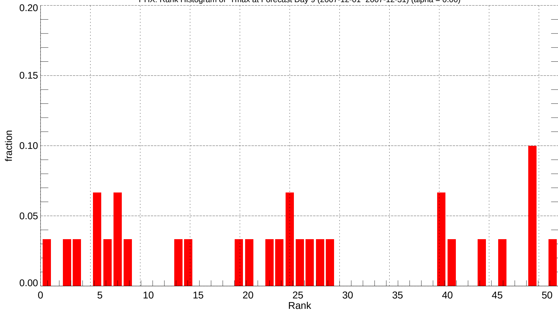
PHX: Rank Histogram of Tmax at Forecast Day 9 (2007-12-01~2007-12-31) (alpha = 0.00)
