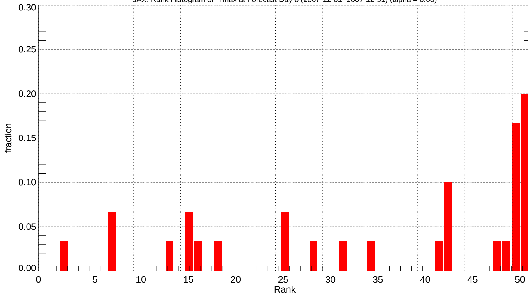
JAX: Rank Histogram of Tmax at Forecast Day 8 (2007-12-01~2007-12-31) (alpha = 0.00)
