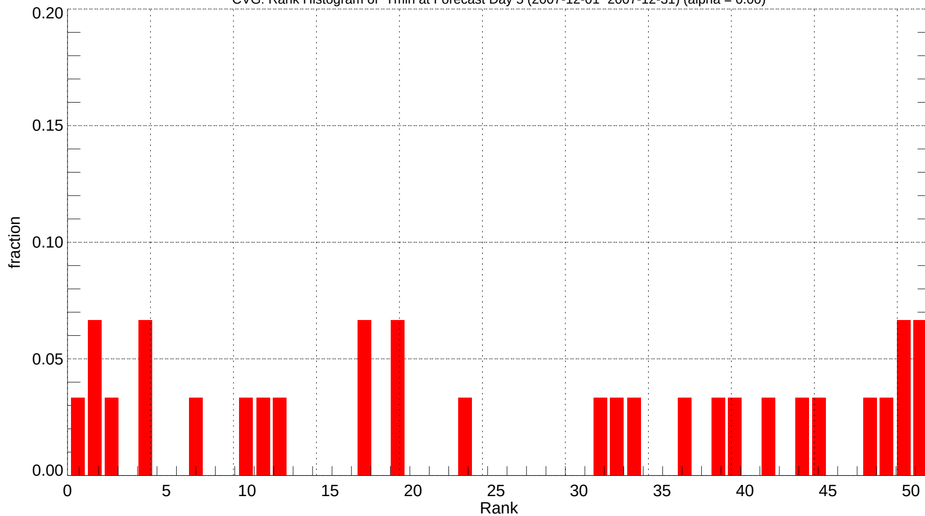
CVG: Rank Histogram of Tmin at Forecast Day 5 (2007-12-01~2007-12-31) (alpha = 0.00)
