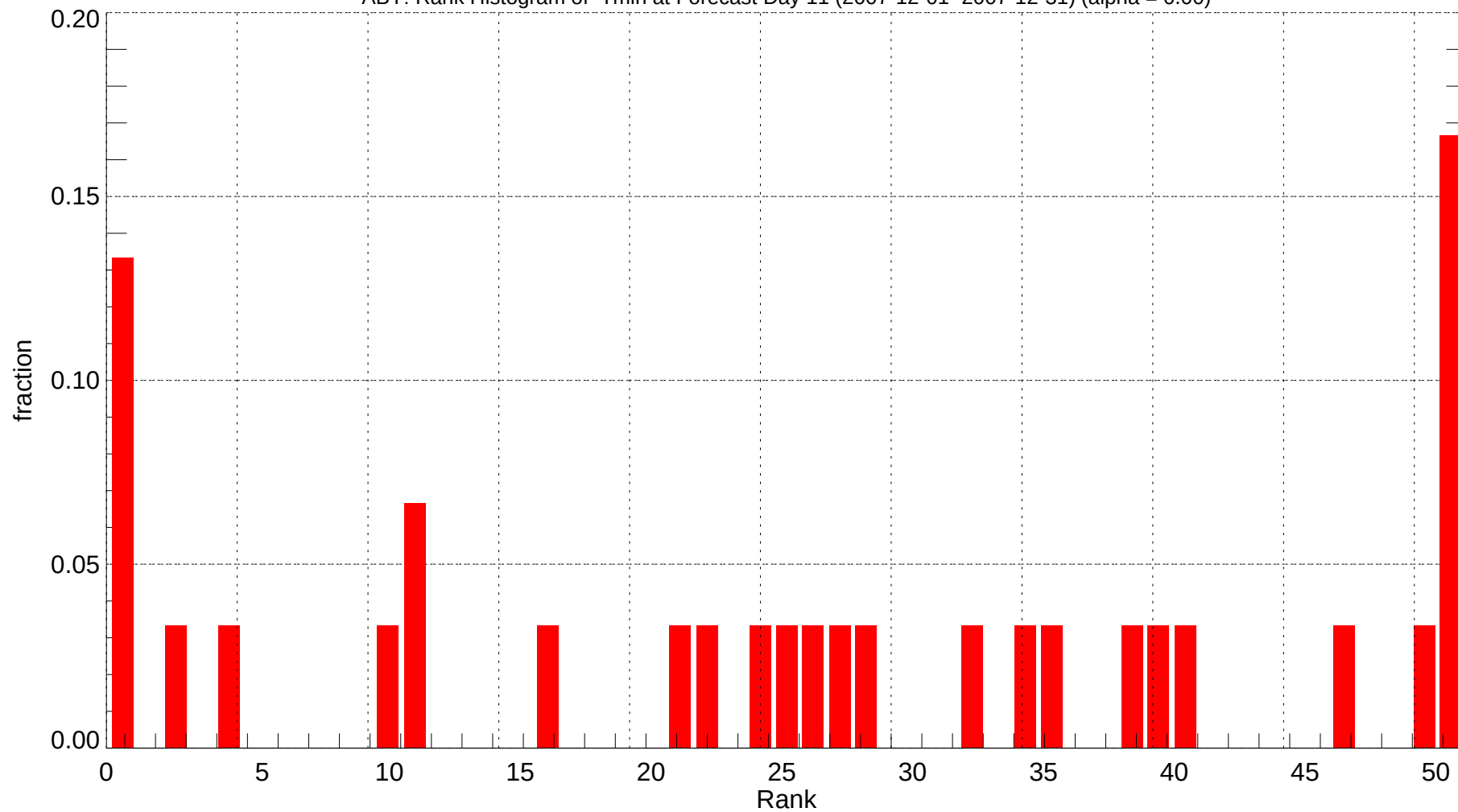
ABY: Rank Histogram of Tmin at Forecast Day 11 (2007-12-01~2007-12-31) (alpha = 0.00)
