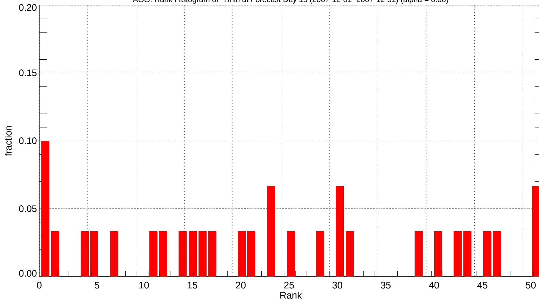
AOO: Rank Histogram of Tmin at Forecast Day 13 (2007-12-01~2007-12-31) (alpha = 0.00)
