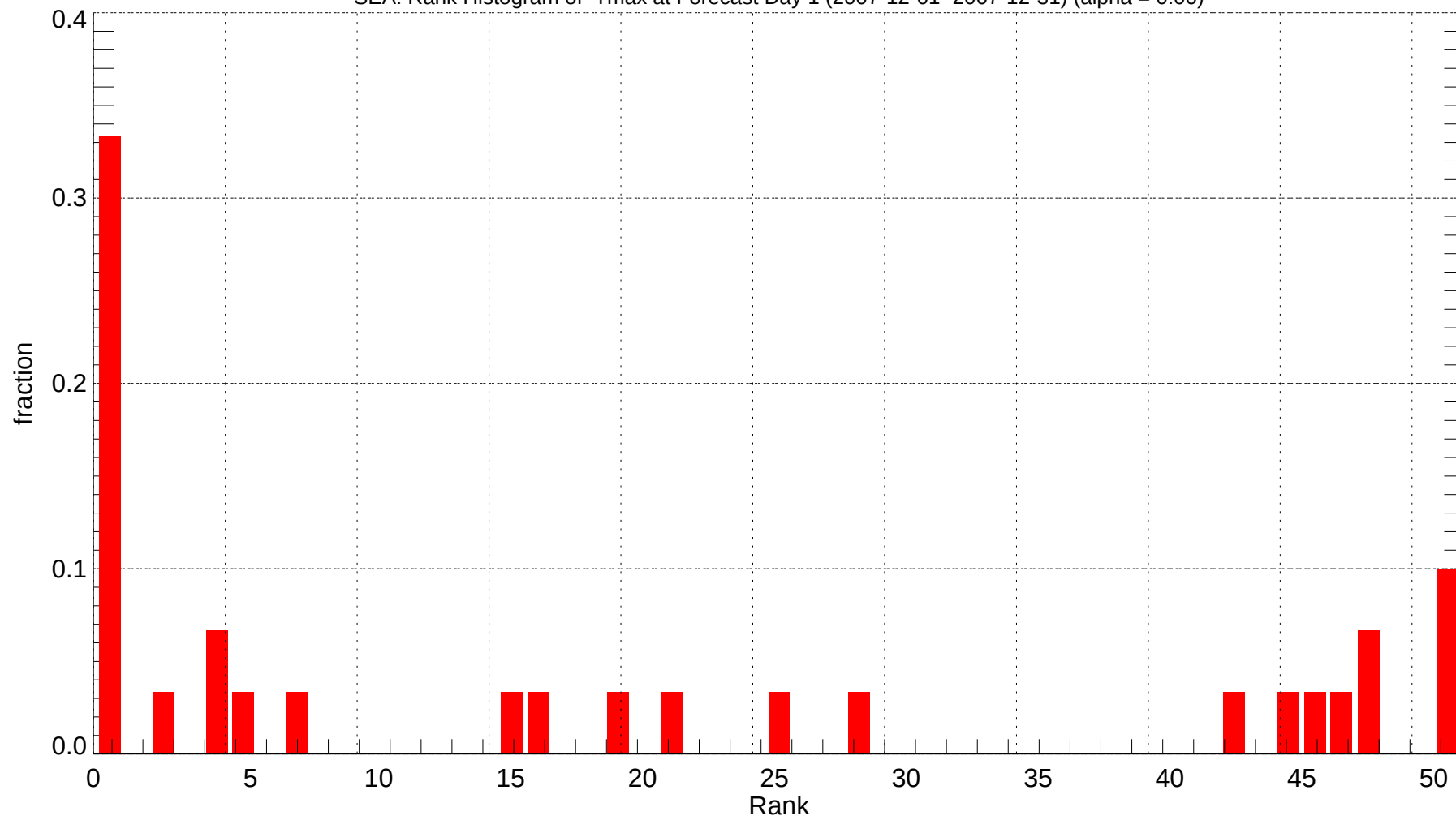
SEA: Rank Histogram of Tmax at Forecast Day 1 (2007-12-01~2007-12-31) (alpha = 0.00)
