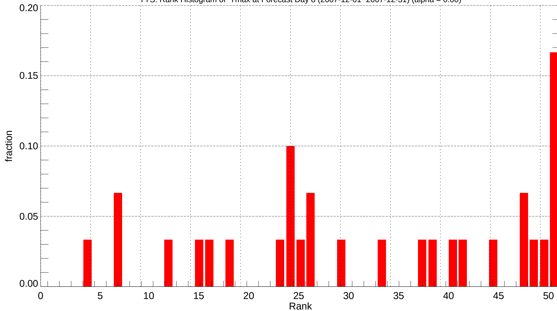
TYS: Rank Histogram of Tmax at Forecast Day 8 (2007-12-01~2007-12-31) (alpha = 0.00)
