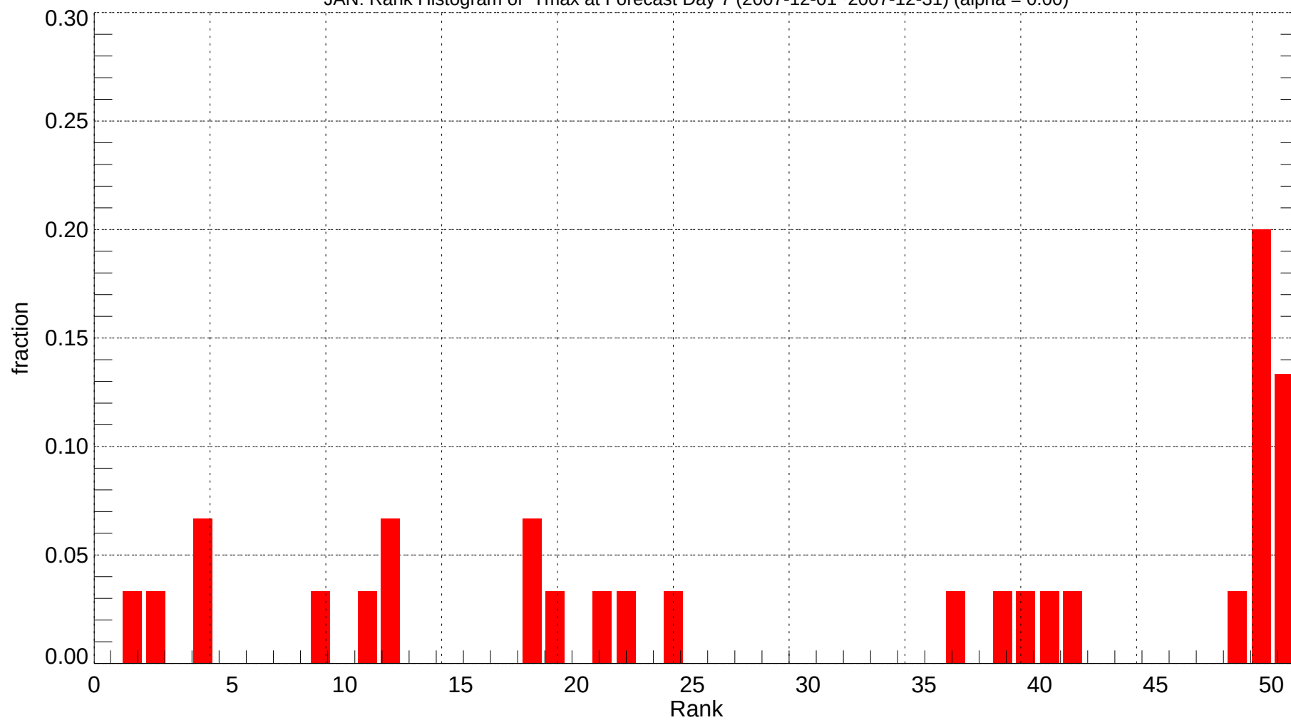
JAN: Rank Histogram of Tmax at Forecast Day 7 (2007-12-01~2007-12-31) (alpha = 0.00)
