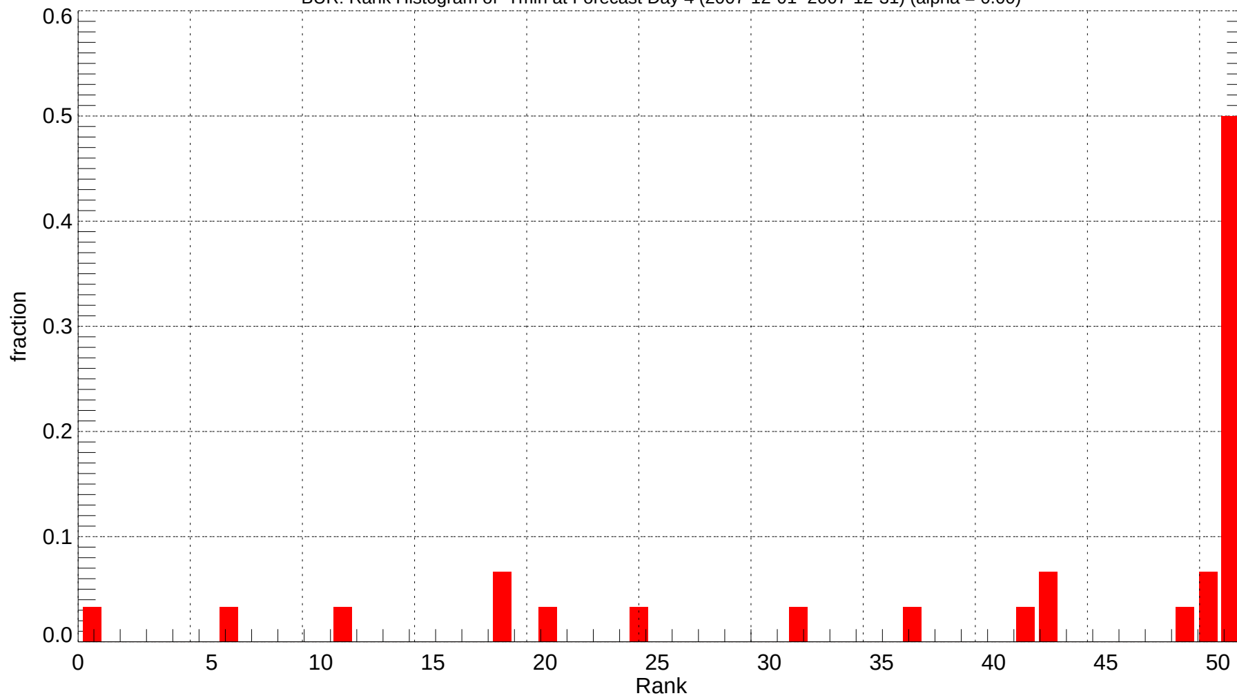
BUR: Rank Histogram of Tmin at Forecast Day 4 (2007-12-01~2007-12-31) (alpha = 0.00)
