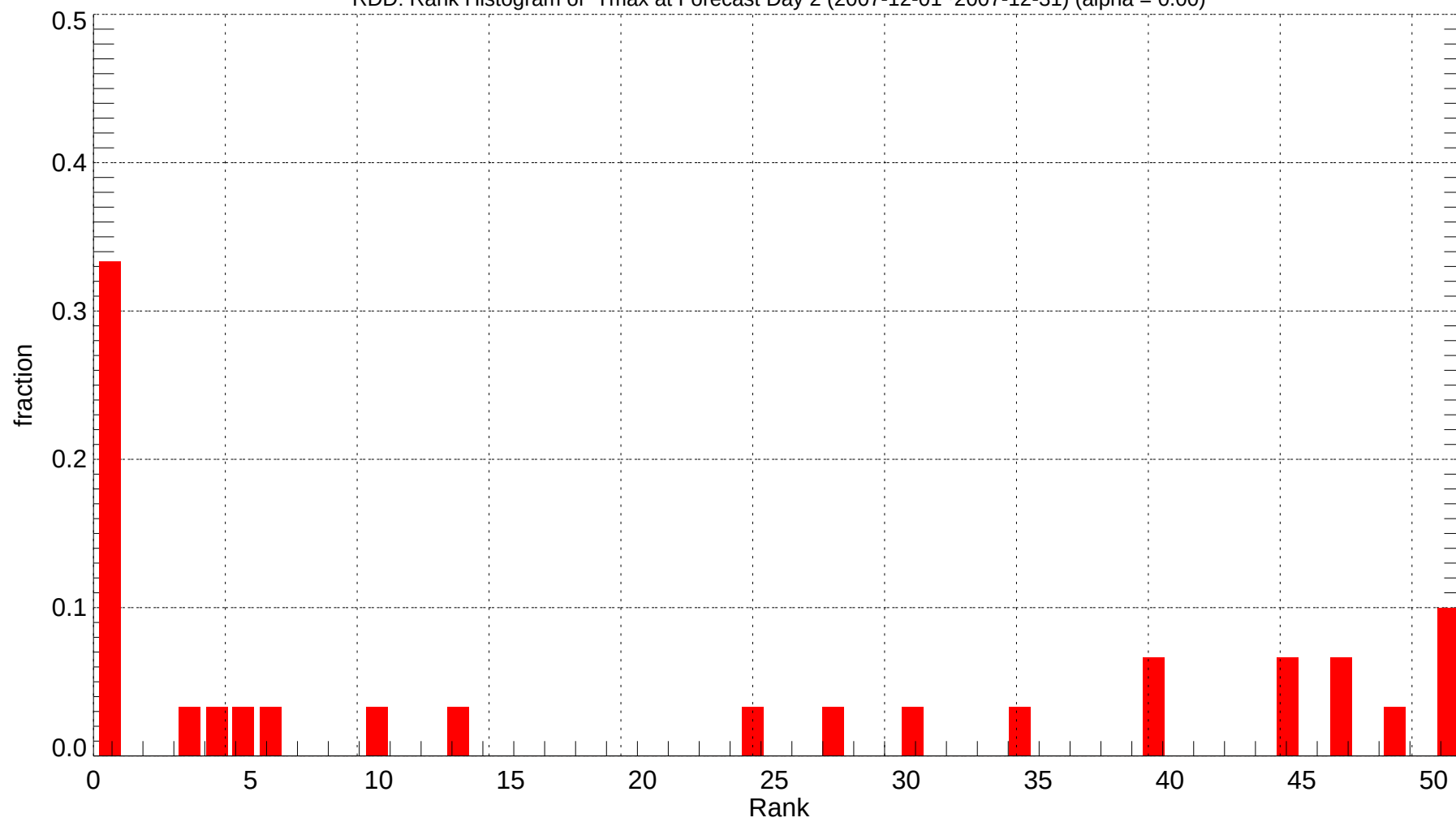
RDD: Rank Histogram of Tmax at Forecast Day 2 (2007-12-01~2007-12-31) (alpha = 0.00)
