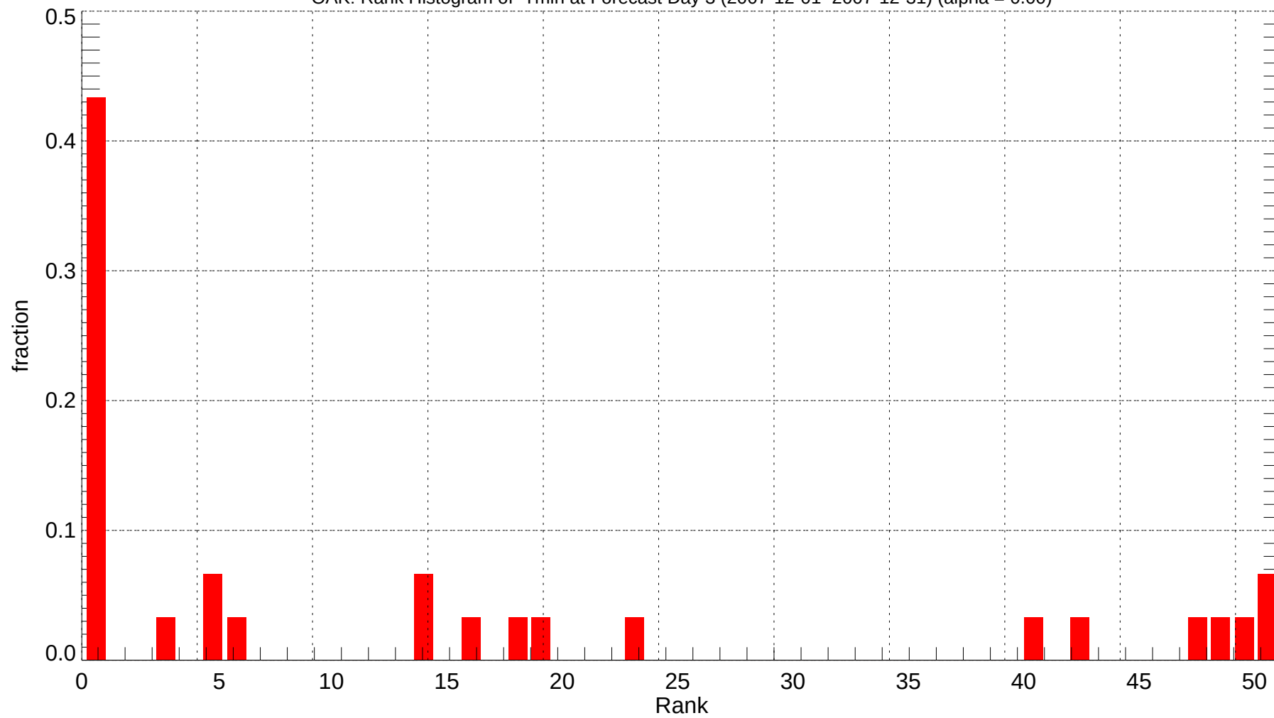
OAK: Rank Histogram of Tmin at Forecast Day 3 (2007-12-01~2007-12-31) (alpha = 0.00)
