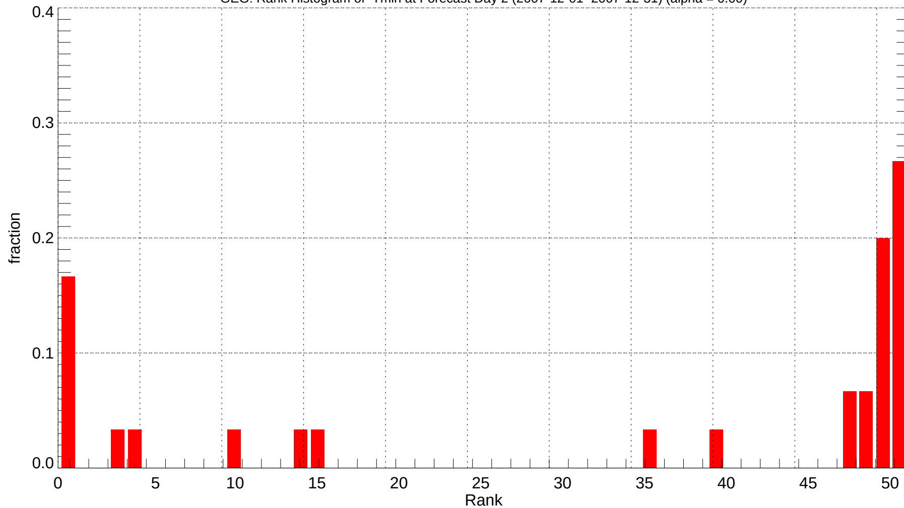
GEG: Rank Histogram of Tmin at Forecast Day 2 (2007-12-01~2007-12-31) (alpha = 0.00)
