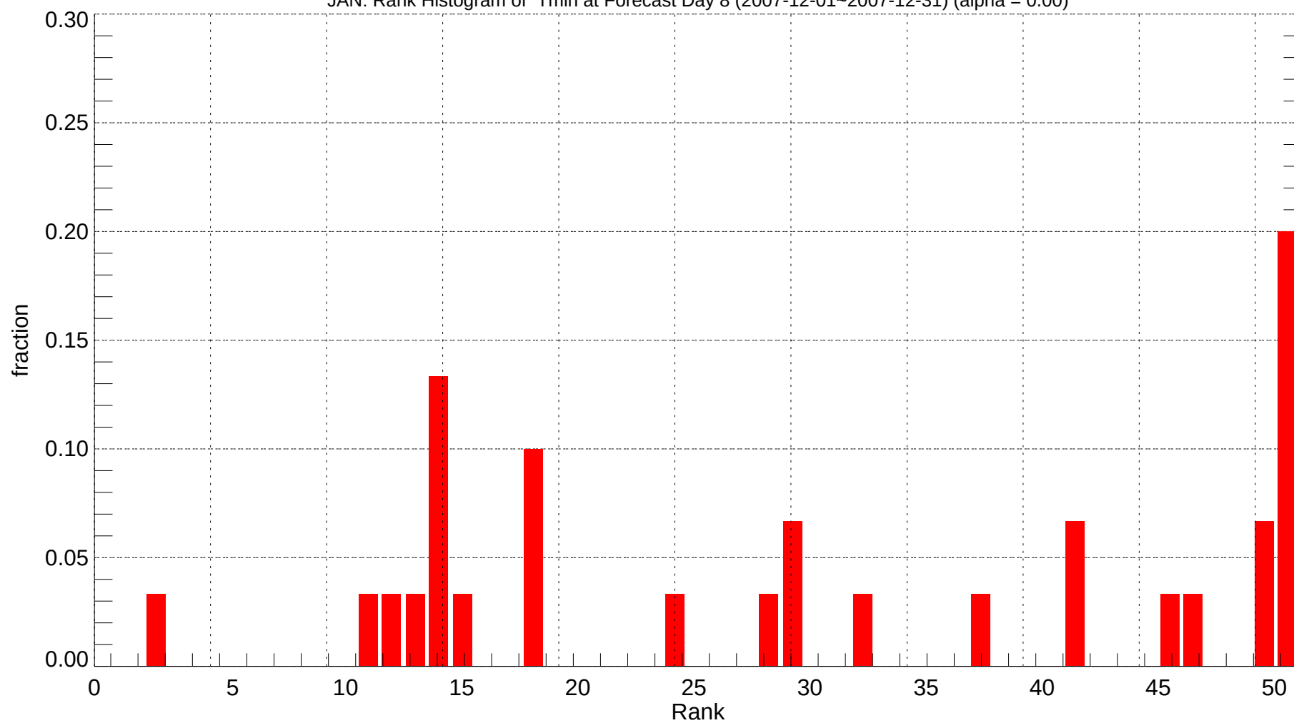
JAN: Rank Histogram of Tmin at Forecast Day 8 (2007-12-01~2007-12-31) (alpha = 0.00)
