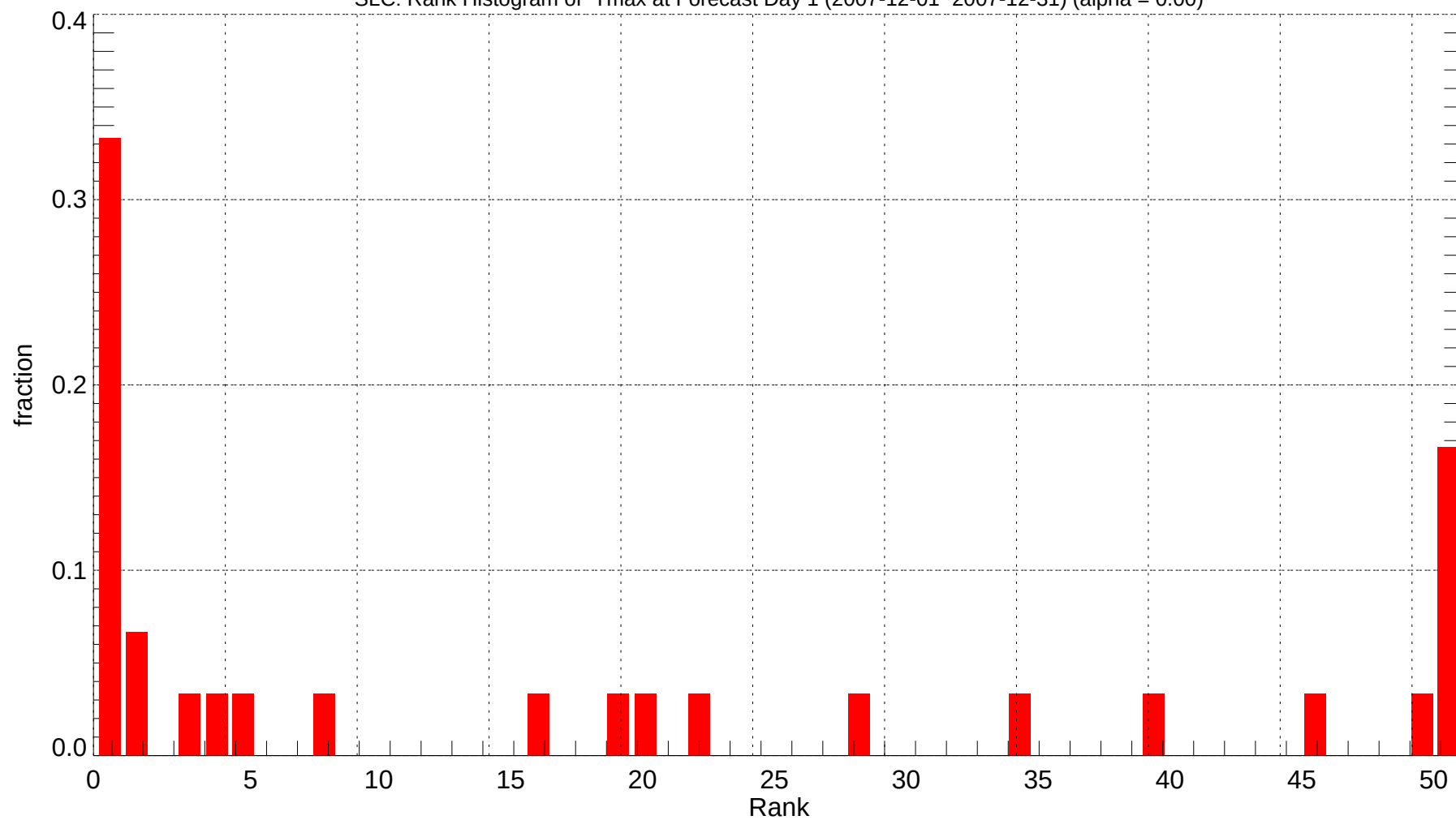
SLC: Rank Histogram of Tmax at Forecast Day 1 (2007-12-01~2007-12-31) (alpha = 0.00)
