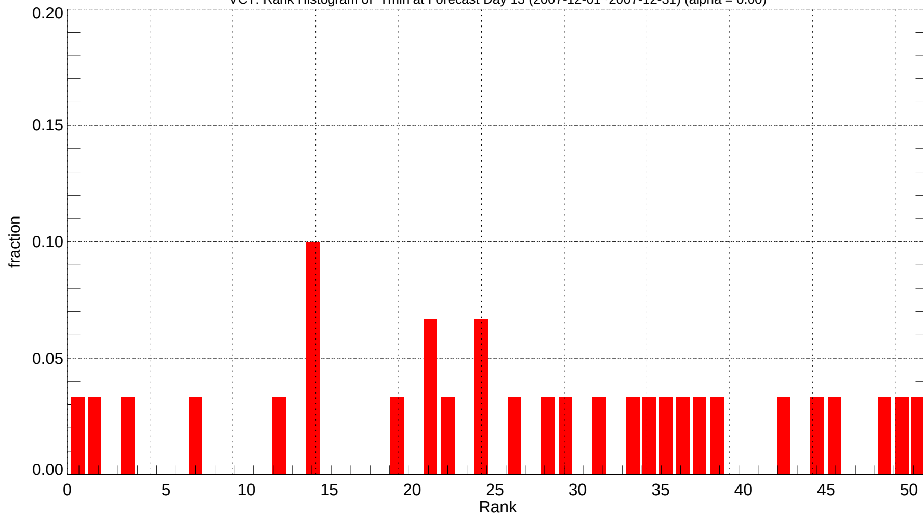
VCT: Rank Histogram of Tmin at Forecast Day 13 (2007-12-01~2007-12-31) (alpha = 0.00)
