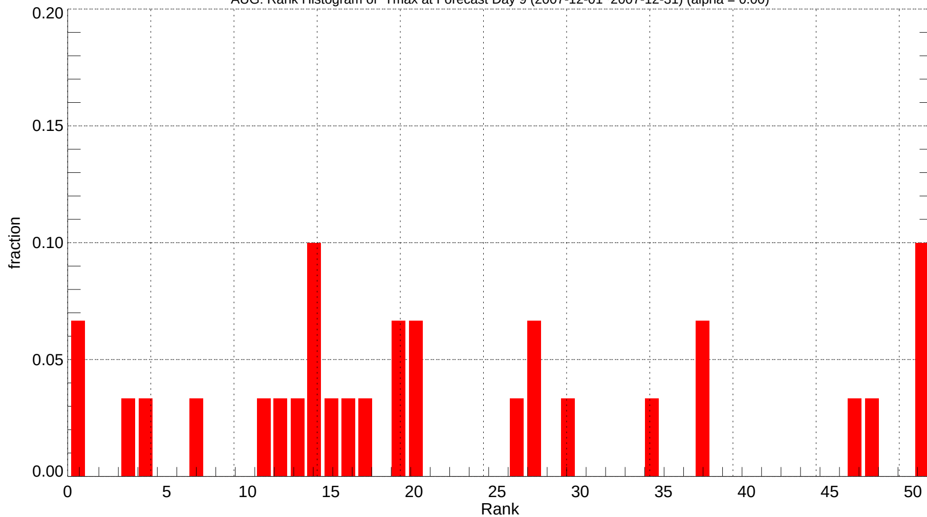
AUG: Rank Histogram of Tmax at Forecast Day 9 (2007-12-01~2007-12-31) (alpha = 0.00)
