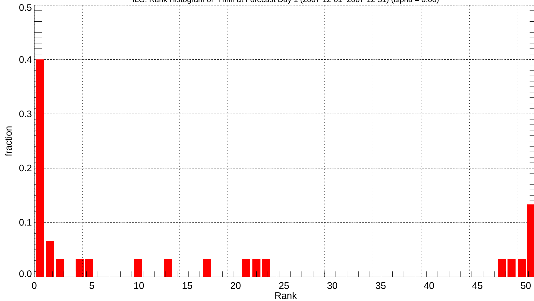
ILG: Rank Histogram of Tmin at Forecast Day 1 (2007-12-01~2007-12-31) (alpha = 0.00)
