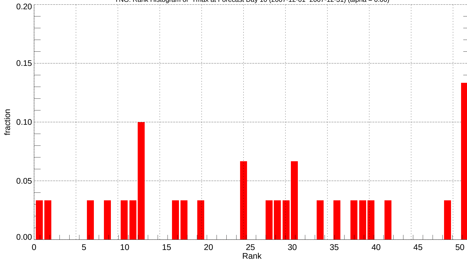
YNG: Rank Histogram of Tmax at Forecast Day 10 (2007-12-01~2007-12-31) (alpha = 0.00)
