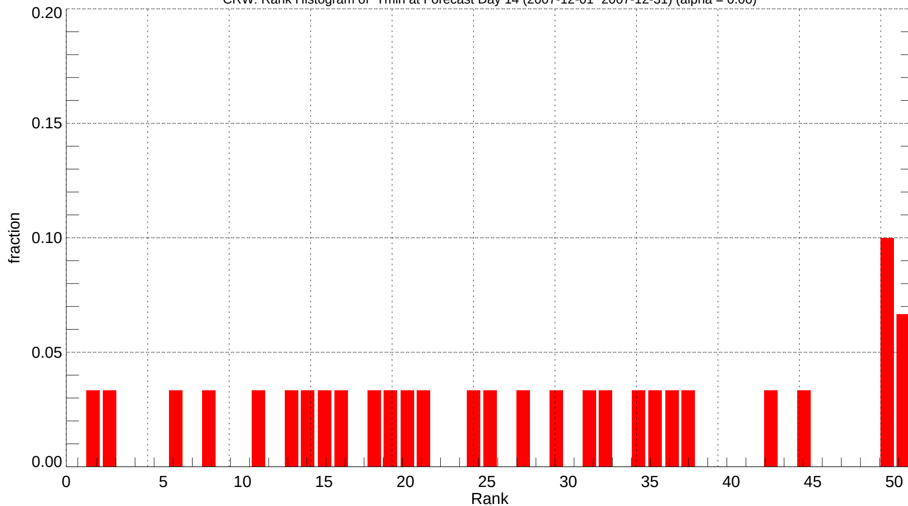
CRW: Rank Histogram of Tmin at Forecast Day 14 (2007-12-01~2007-12-31) (alpha = 0.00)
