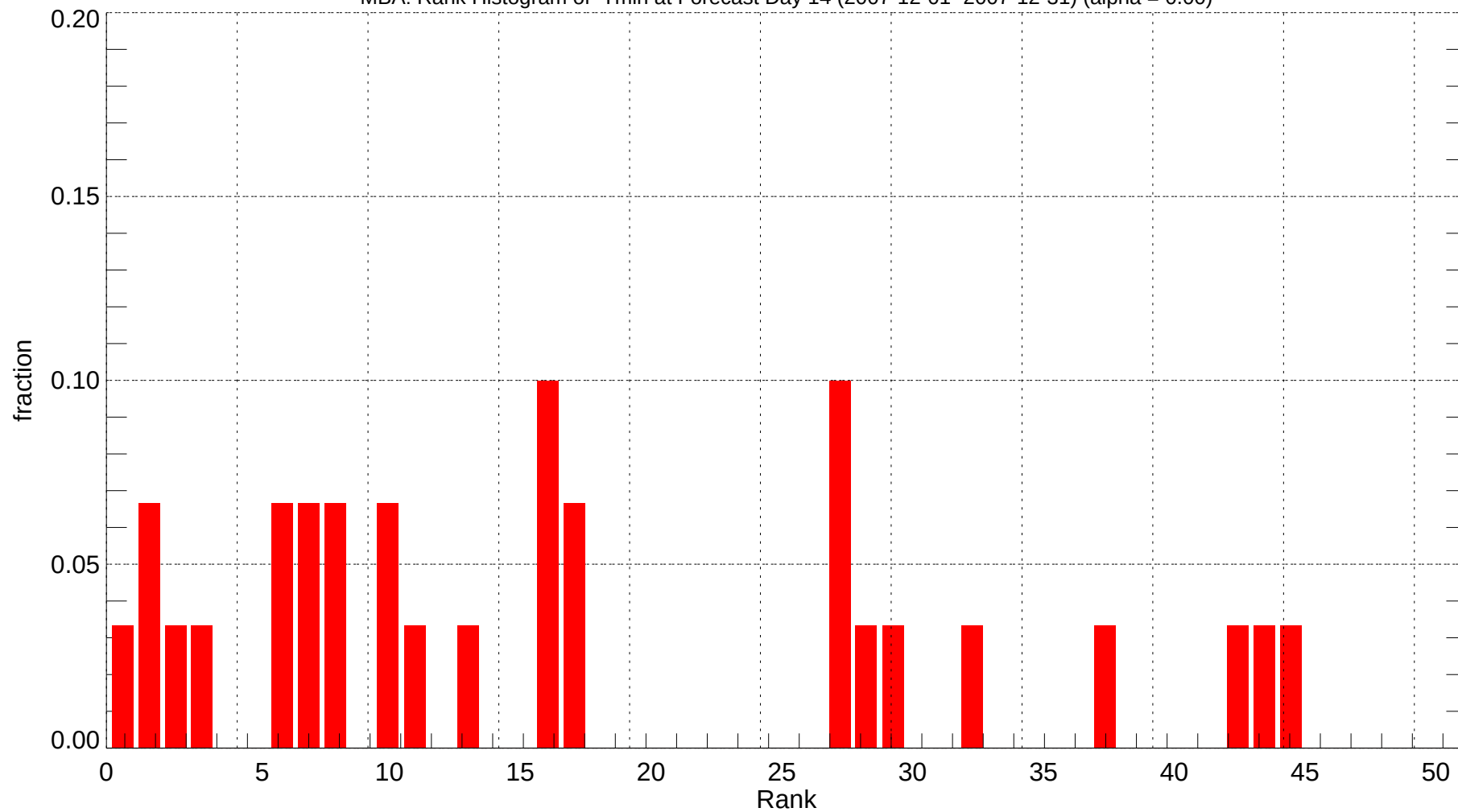
MBA: Rank Histogram of Tmin at Forecast Day 14 (2007-12-01~2007-12-31) (alpha = 0.00)
