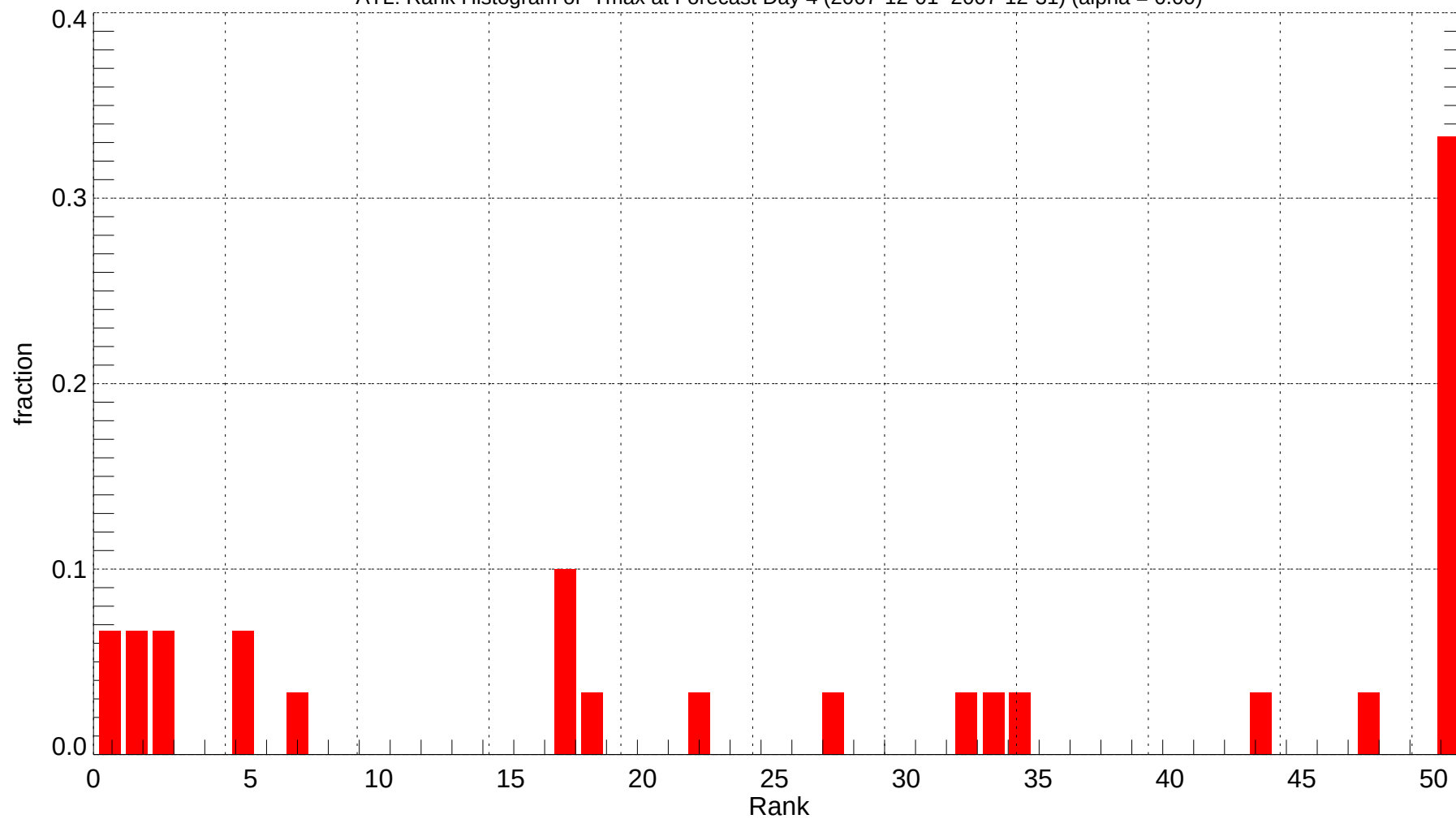
ATL: Rank Histogram of Tmax at Forecast Day 4 (2007-12-01~2007-12-31) (alpha = 0.00)
