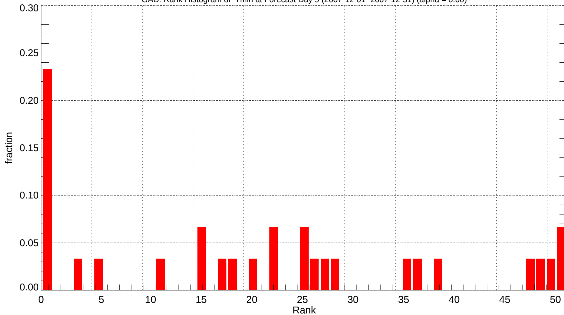
GAD: Rank Histogram of Tmin at Forecast Day 9 (2007-12-01~2007-12-31) (alpha = 0.00)
