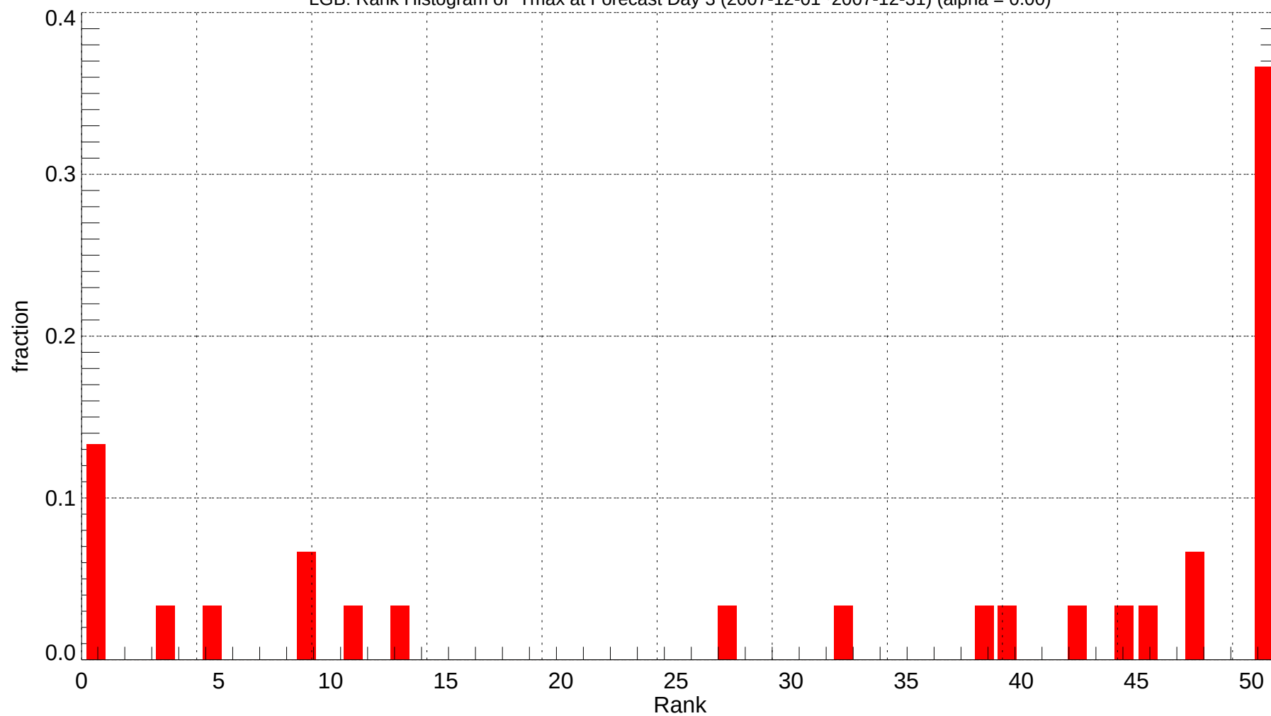
LGB: Rank Histogram of Tmax at Forecast Day 3 (2007-12-01~2007-12-31) (alpha = 0.00)
