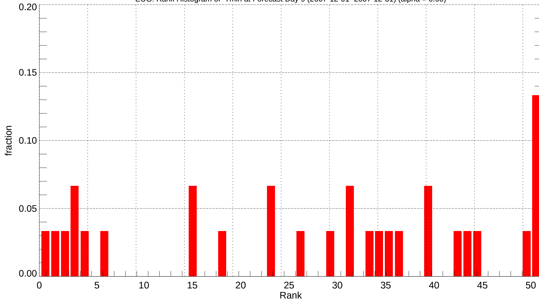
EUG: Rank Histogram of Tmin at Forecast Day 9 (2007-12-01~2007-12-31) (alpha = 0.00)
