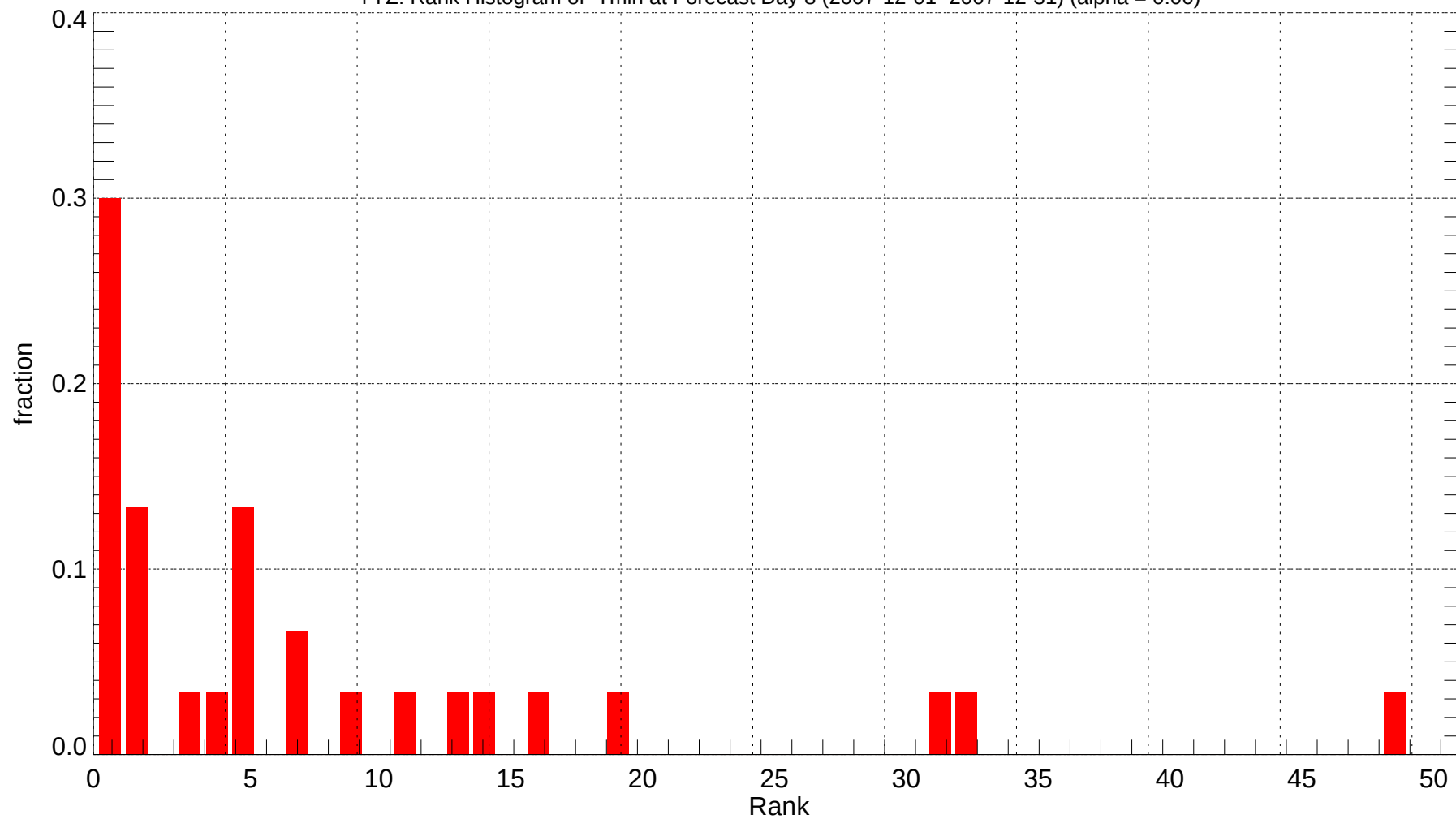
YYZ: Rank Histogram of Tmin at Forecast Day 8 (2007-12-01~2007-12-31) (alpha = 0.00)
