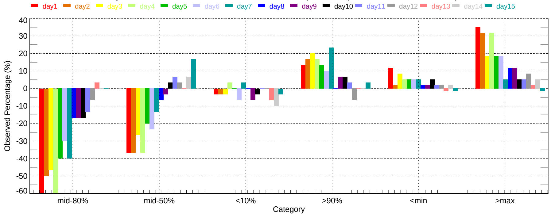
Observed Percentage Deviation of Ensembles - PDX: Max Temperature (2007-12-01~2007-12-31)
