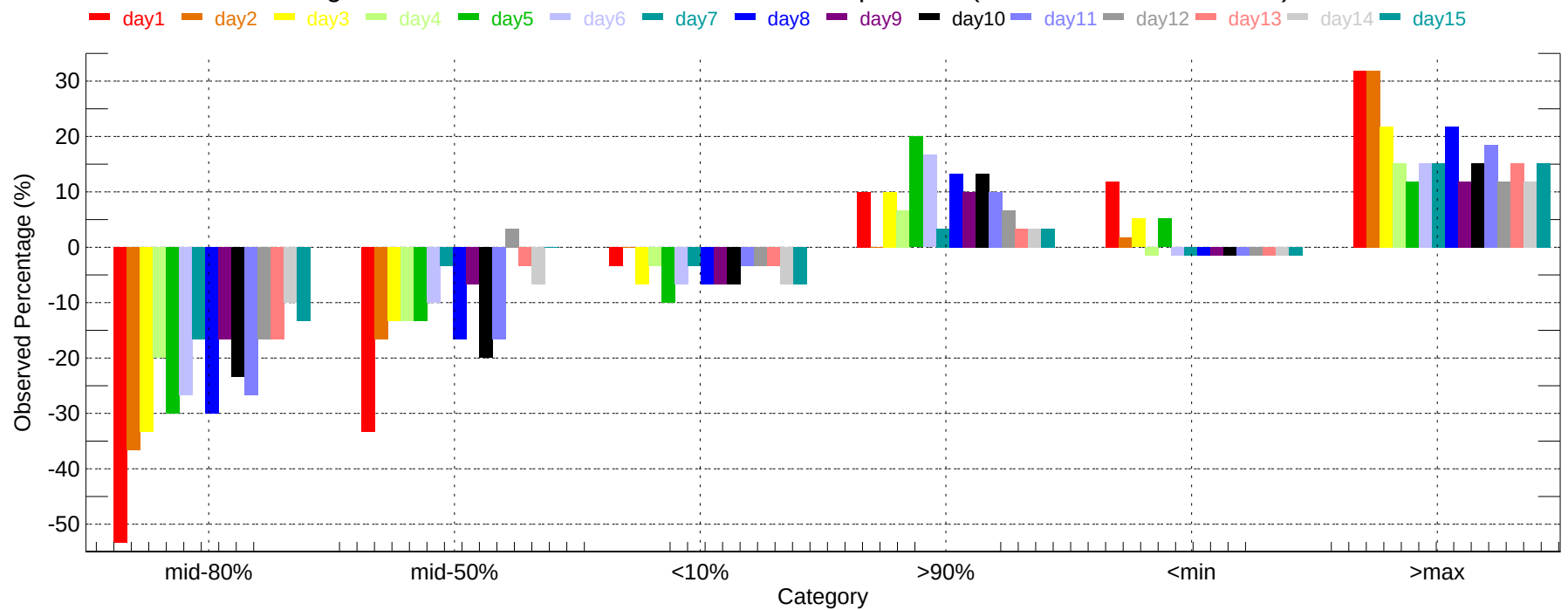
Observed Percentage Deviation of Ensembles - LFK: Min Temperature (2007-12-01~2007-12-31)
