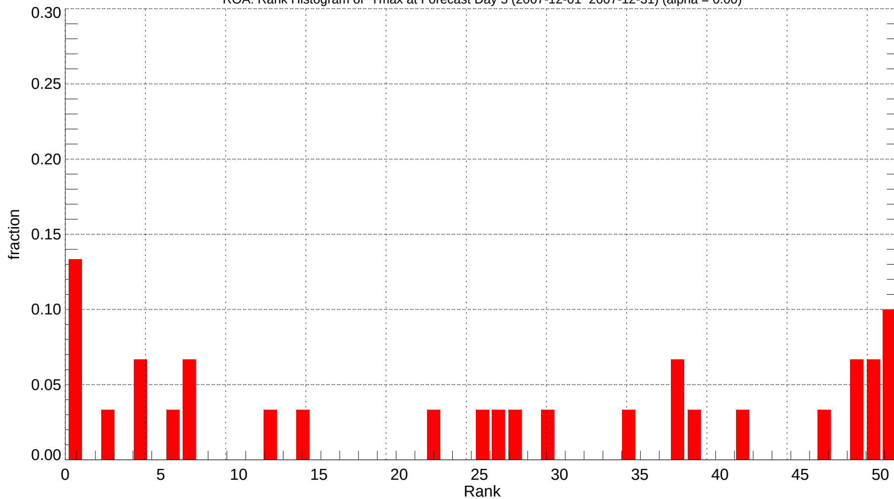
ROA: Rank Histogram of Tmax at Forecast Day 5 (2007-12-01~2007-12-31) (alpha = 0.00)
