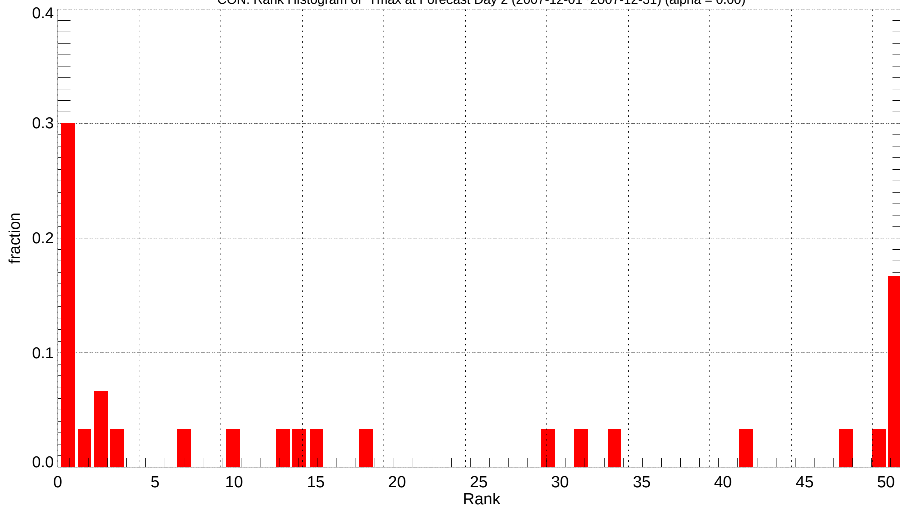
CON: Rank Histogram of Tmax at Forecast Day 2 (2007-12-01~2007-12-31) (alpha = 0.00)
