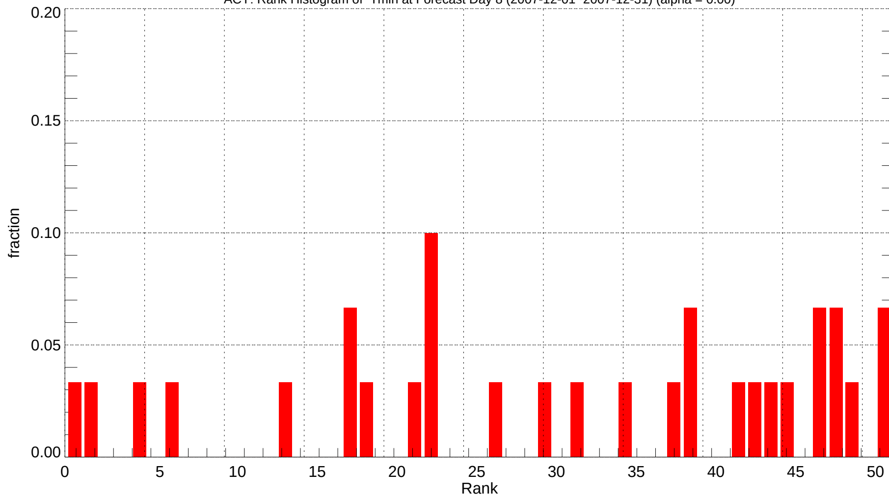
ACY: Rank Histogram of Tmin at Forecast Day 8 (2007-12-01~2007-12-31) (alpha = 0.00)
