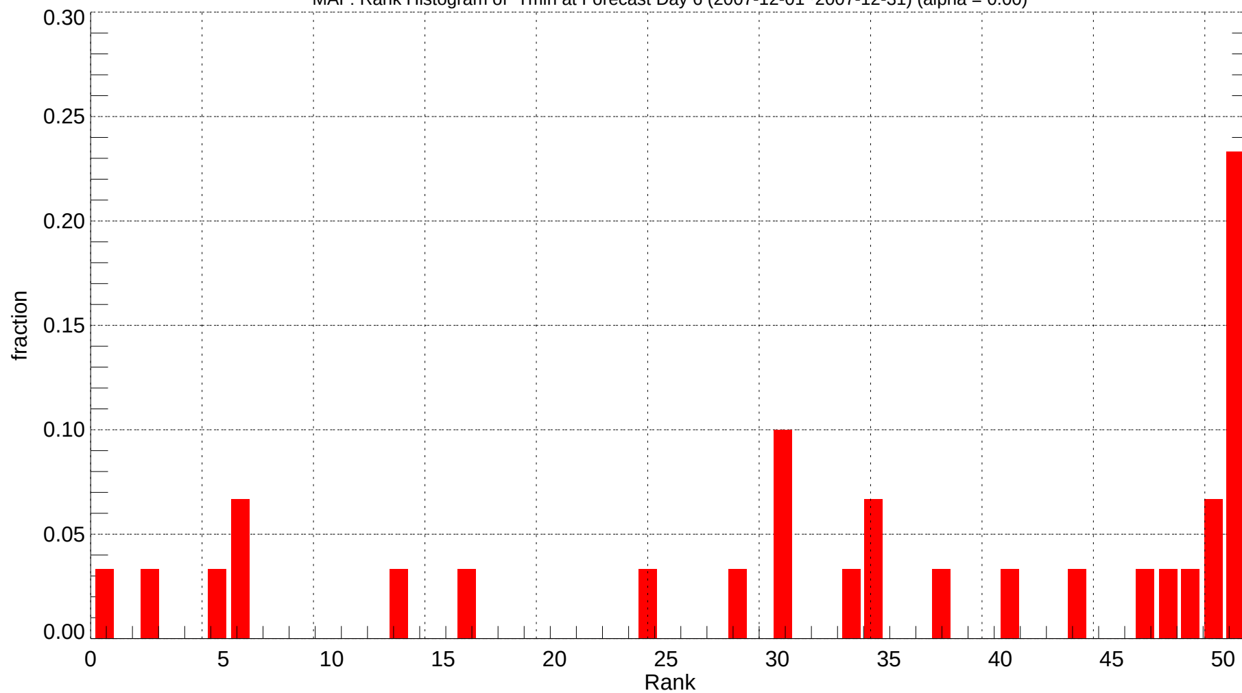
MAF: Rank Histogram of Tmin at Forecast Day 6 (2007-12-01~2007-12-31) (alpha = 0.00)
