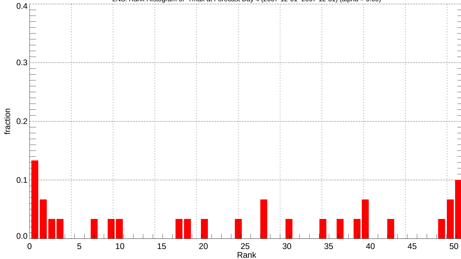
LNS: Rank Histogram of Tmax at Forecast Day 4 (2007-12-01~2007-12-31) (alpha = 0.00)
