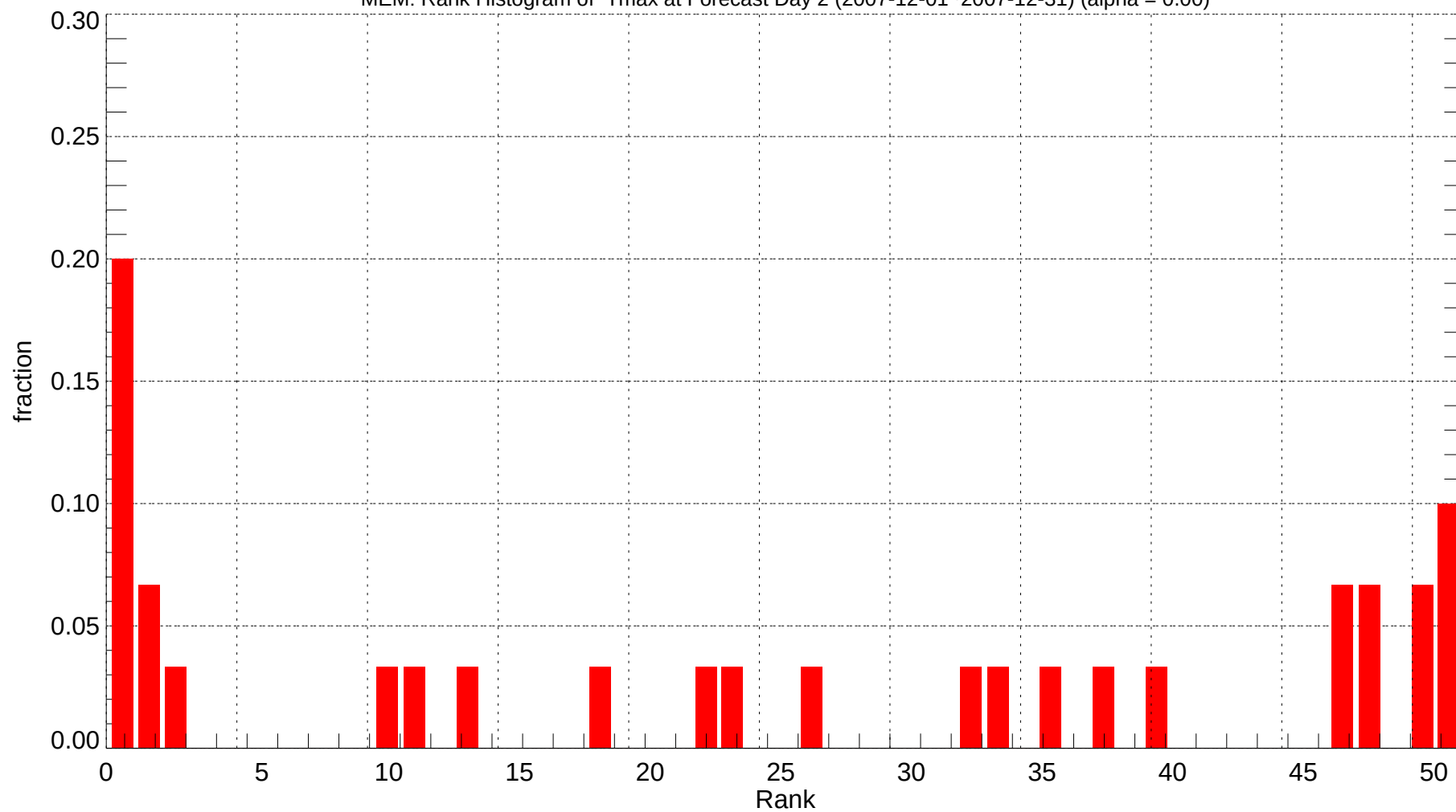
MEM: Rank Histogram of Tmax at Forecast Day 2 (2007-12-01~2007-12-31) (alpha = 0.00)
