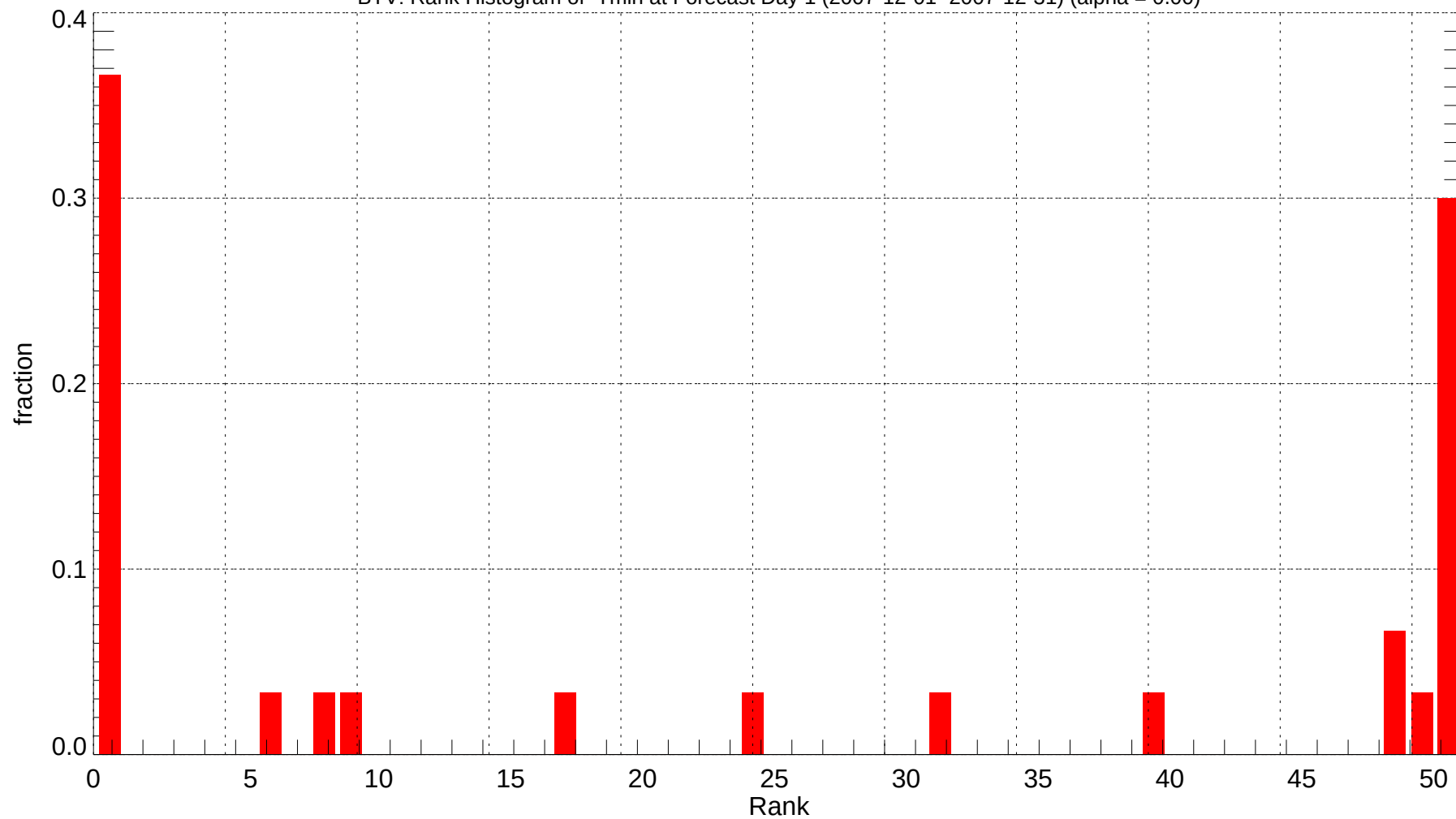
BTV: Rank Histogram of Tmin at Forecast Day 1 (2007-12-01~2007-12-31) (alpha = 0.00)
