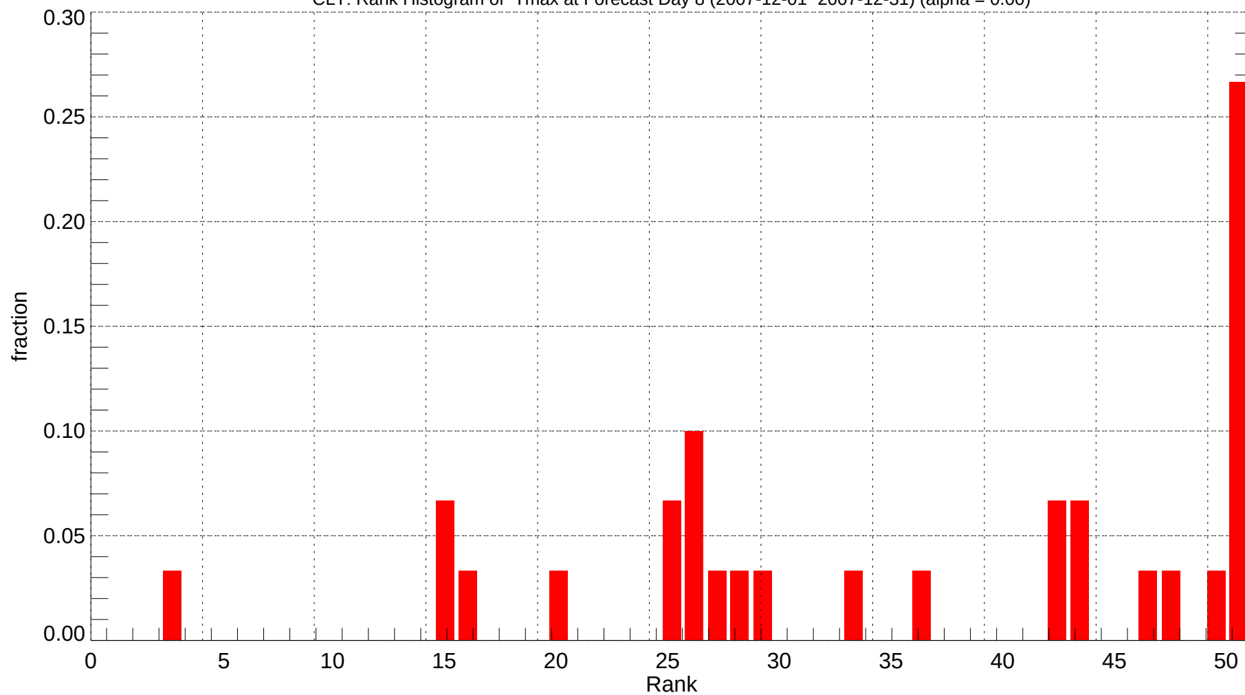
CLT: Rank Histogram of Tmax at Forecast Day 8 (2007-12-01~2007-12-31) (alpha = 0.00)
