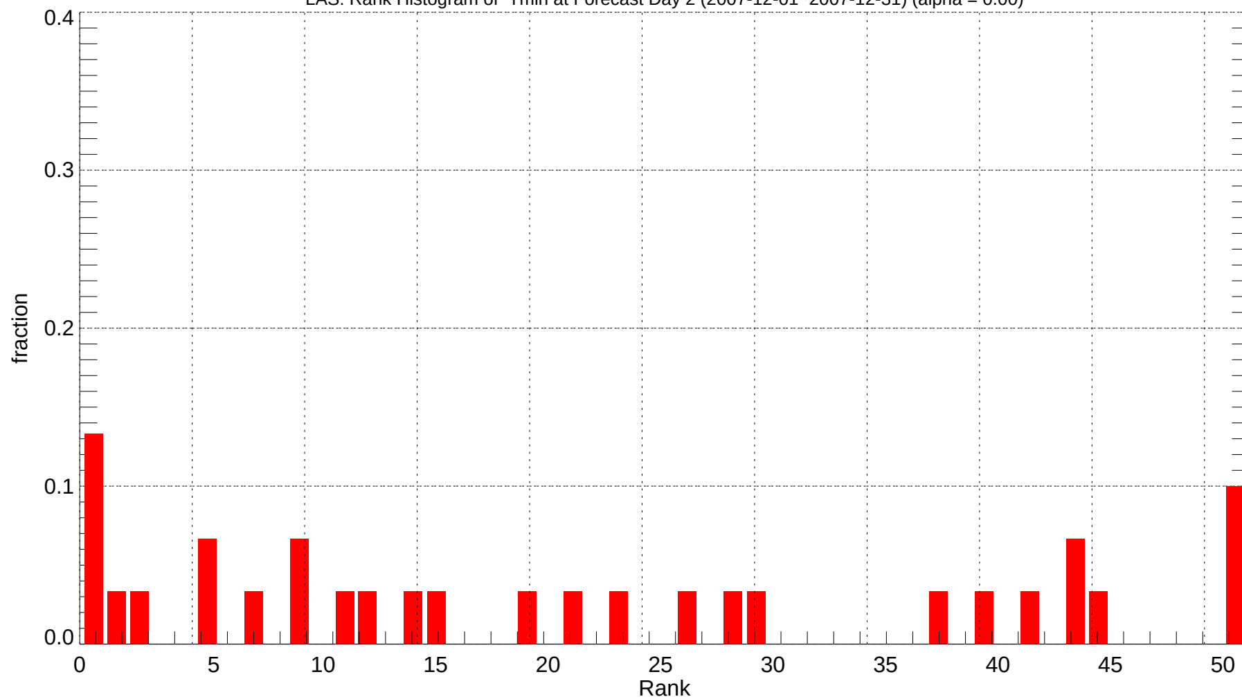
LAS: Rank Histogram of Tmin at Forecast Day 2 (2007-12-01~2007-12-31) (alpha = 0.00)
