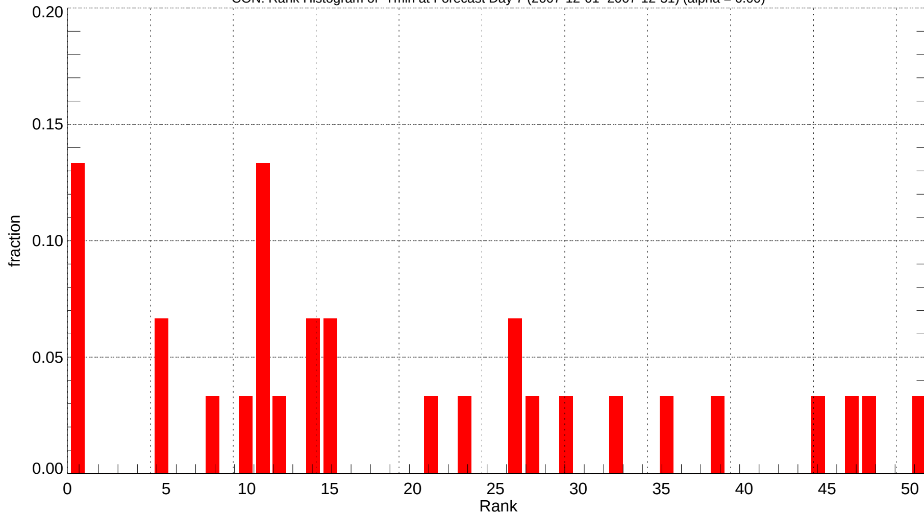
CON: Rank Histogram of Tmin at Forecast Day 7 (2007-12-01~2007-12-31) (alpha = 0.00)
