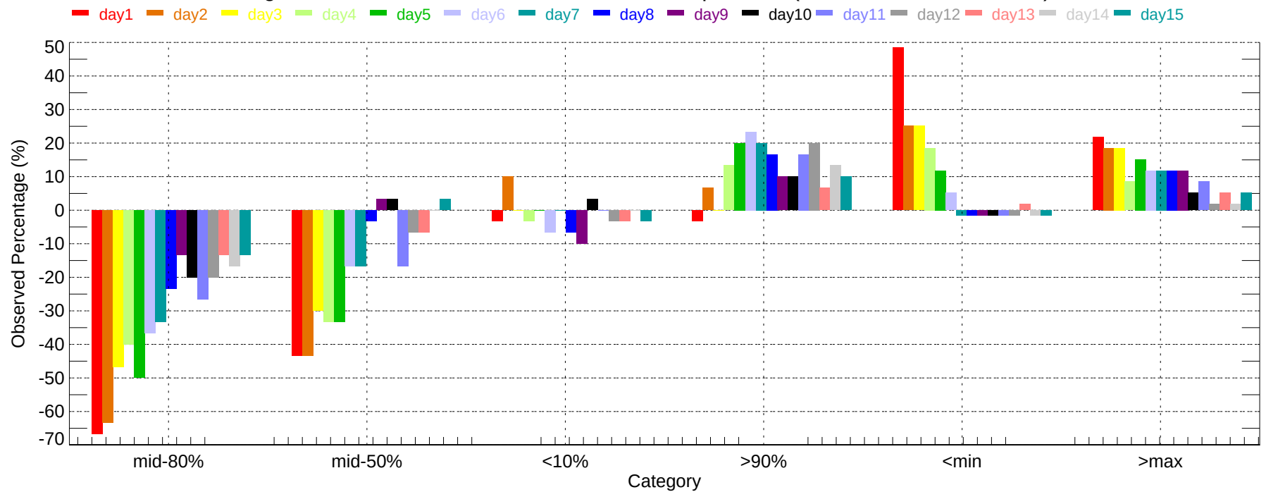
Observed Percentage Deviation of Ensembles - TYS: Max Temperature (2007-12-01~2007-12-31)
