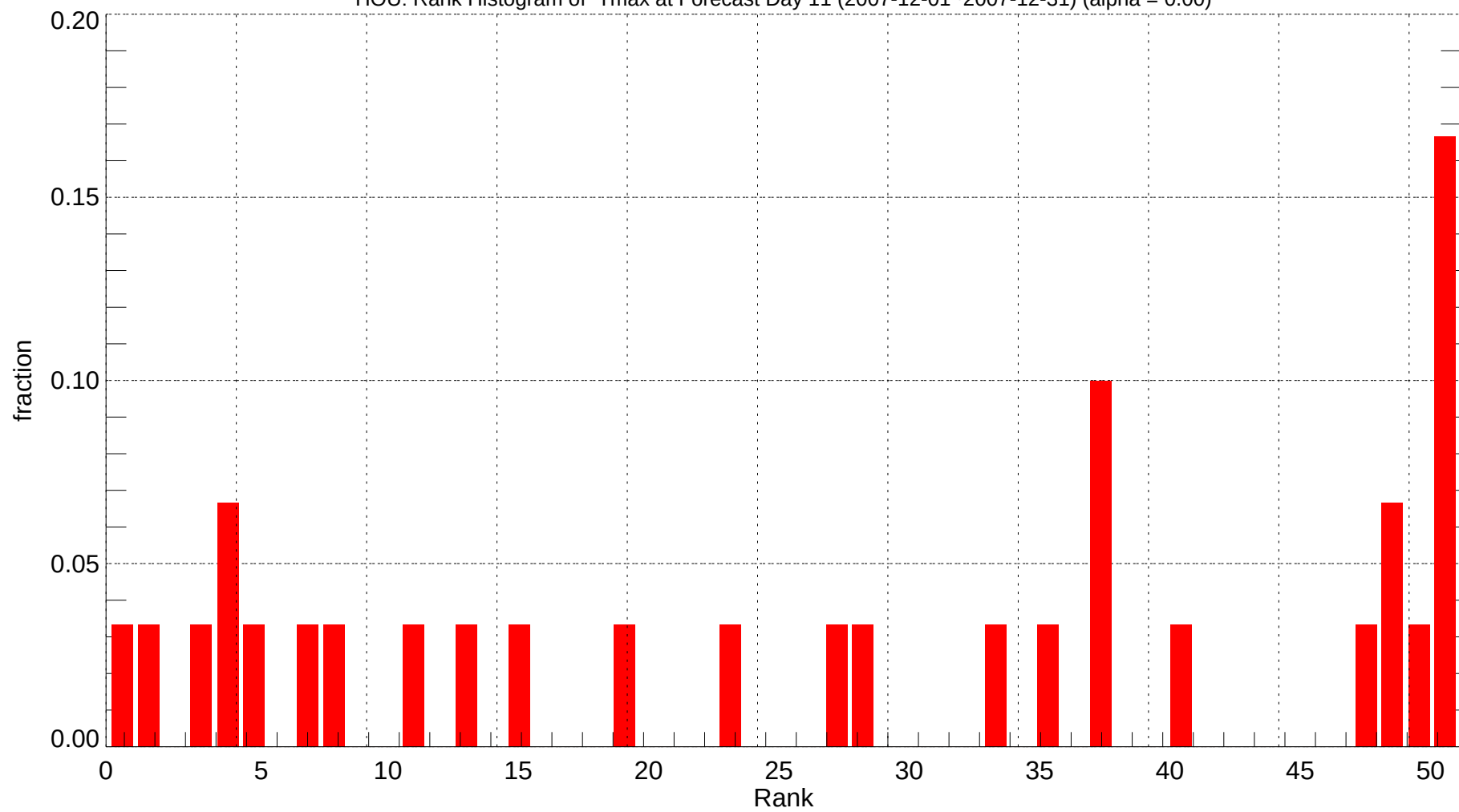
HOU: Rank Histogram of Tmax at Forecast Day 11 (2007-12-01~2007-12-31) (alpha = 0.00)
