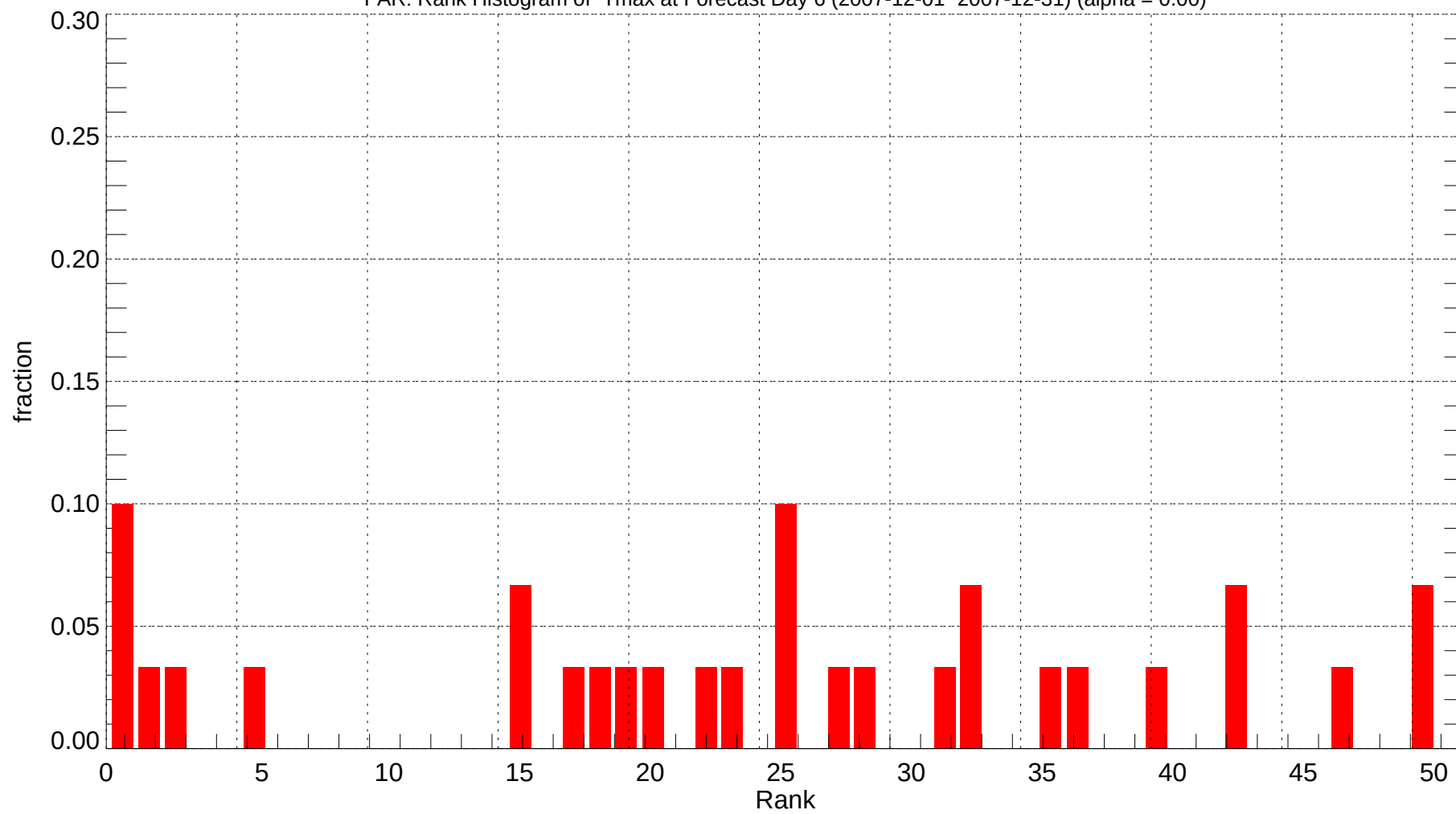
FAR: Rank Histogram of Tmax at Forecast Day 6 (2007-12-01~2007-12-31) (alpha = 0.00)
