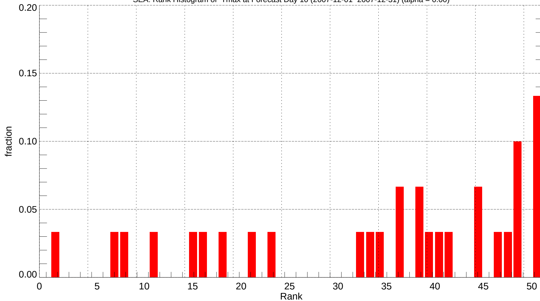
SEA: Rank Histogram of Tmax at Forecast Day 10 (2007-12-01~2007-12-31) (alpha = 0.00)
