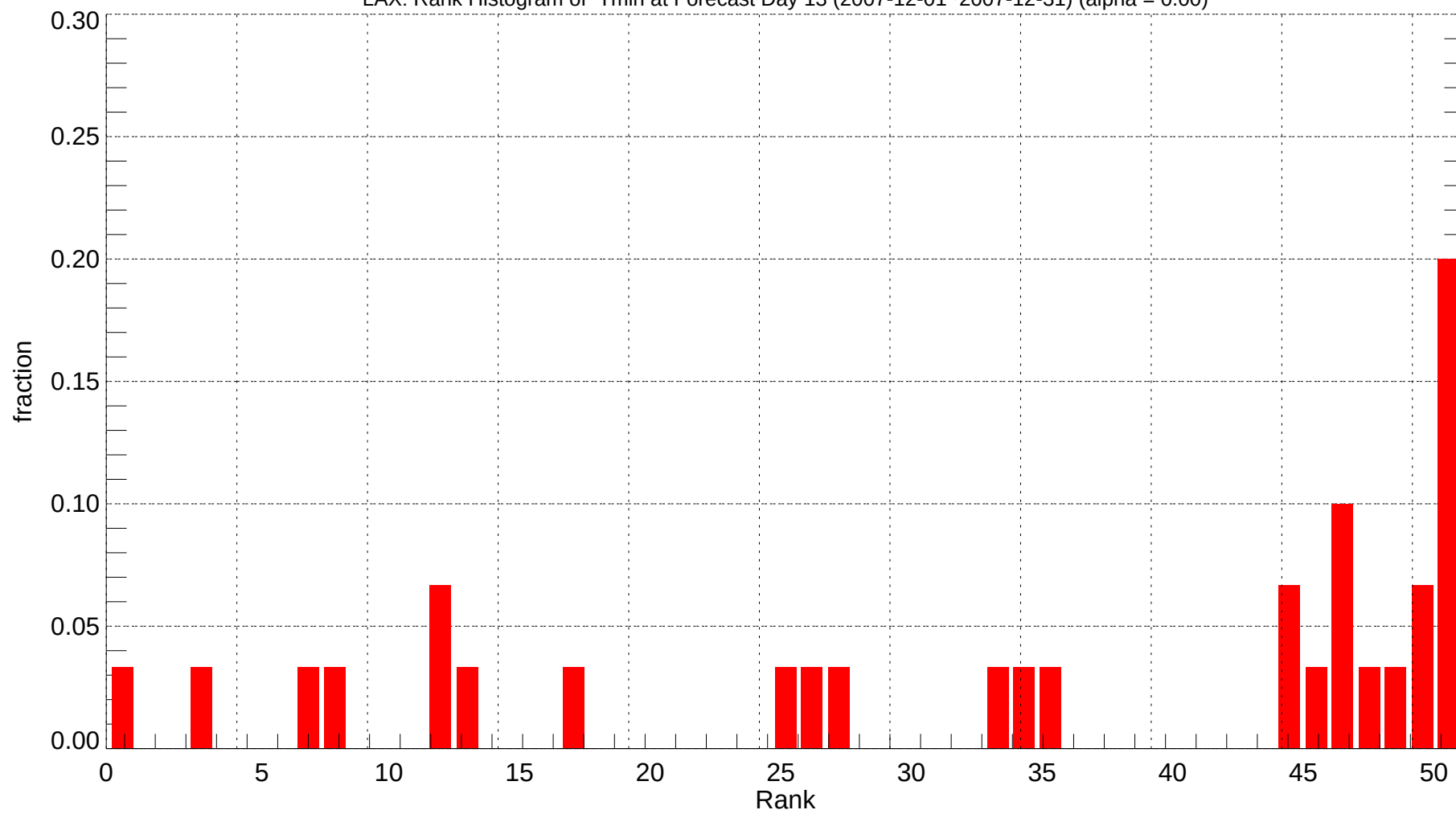
LAX: Rank Histogram of Tmin at Forecast Day 13 (2007-12-01~2007-12-31) (alpha = 0.00)
