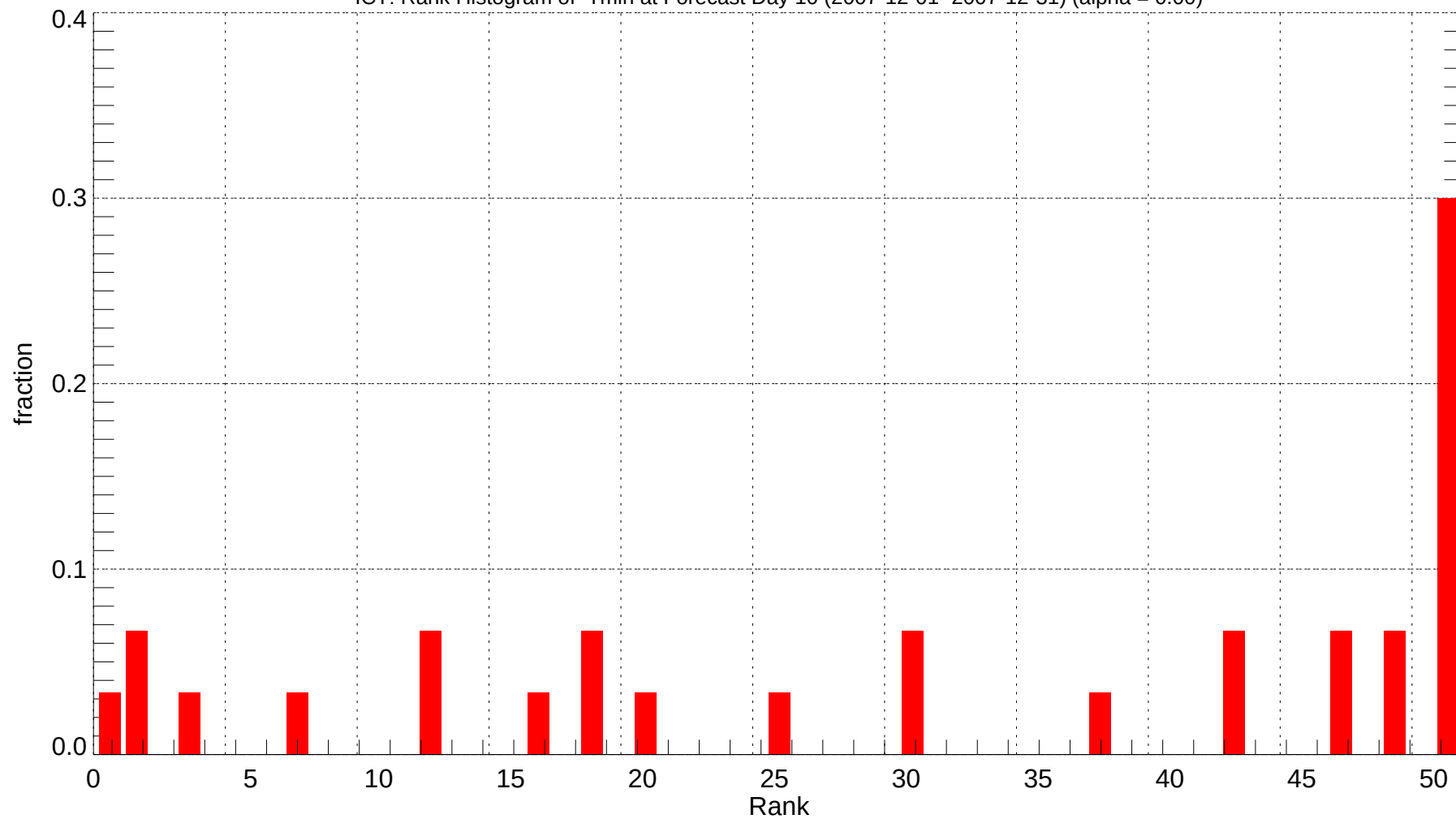
ICT: Rank Histogram of Tmin at Forecast Day 10 (2007-12-01~2007-12-31) (alpha = 0.00)
