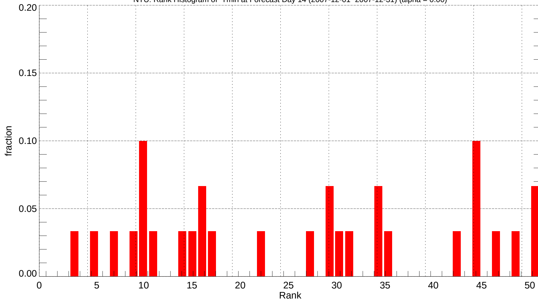
NTU: Rank Histogram of Tmin at Forecast Day 14 (2007-12-01~2007-12-31) (alpha = 0.00)
