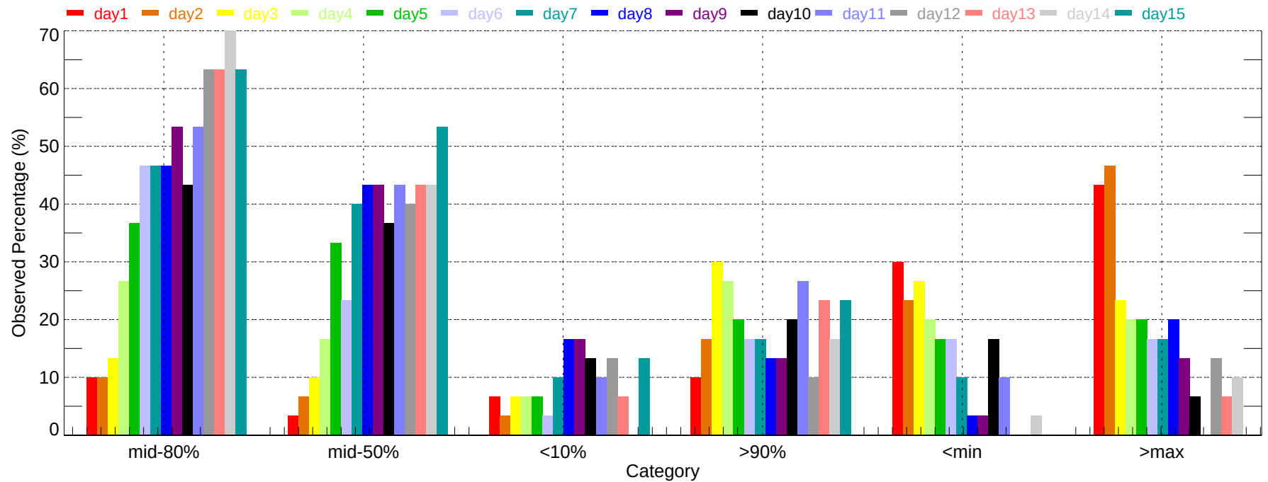
Observed Percentage of Ensembles - EUG: Min Temperature (2007-12-01~2007-12-31)
