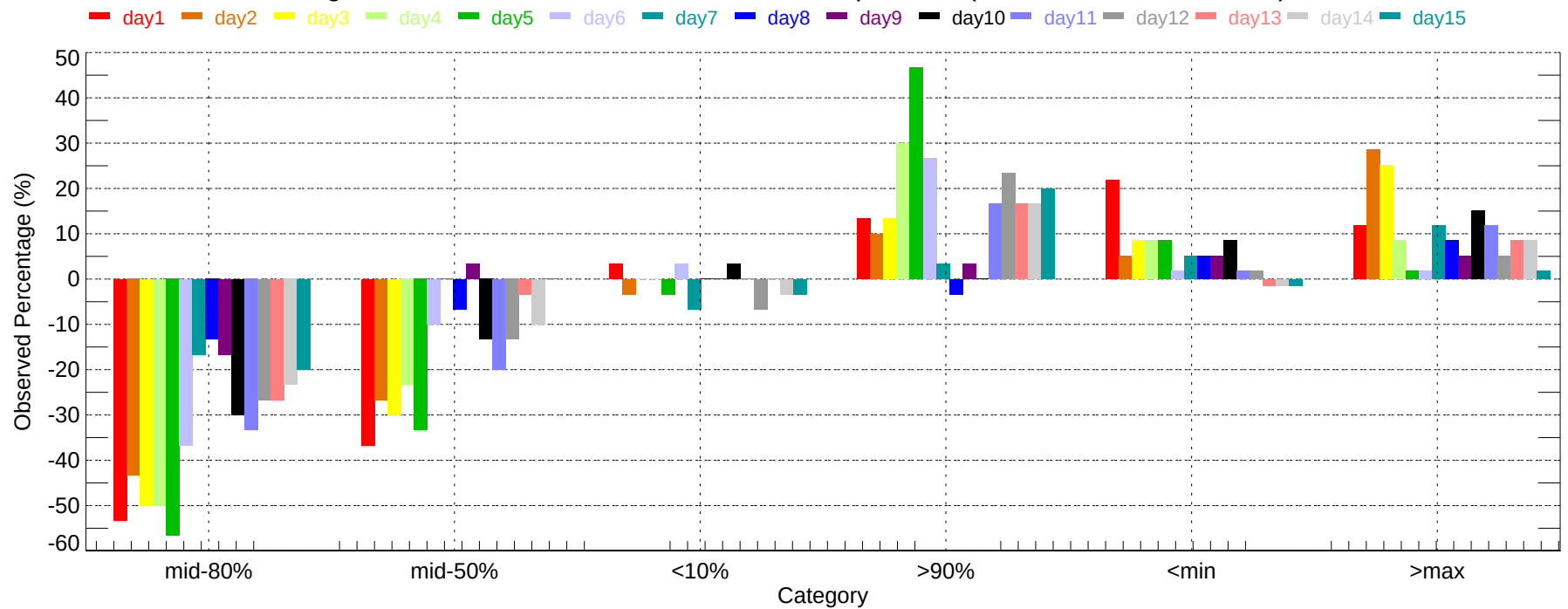
Observed Percentage Deviation of Ensembles - BOI: Min Temperature (2007-12-01~2007-12-31)
