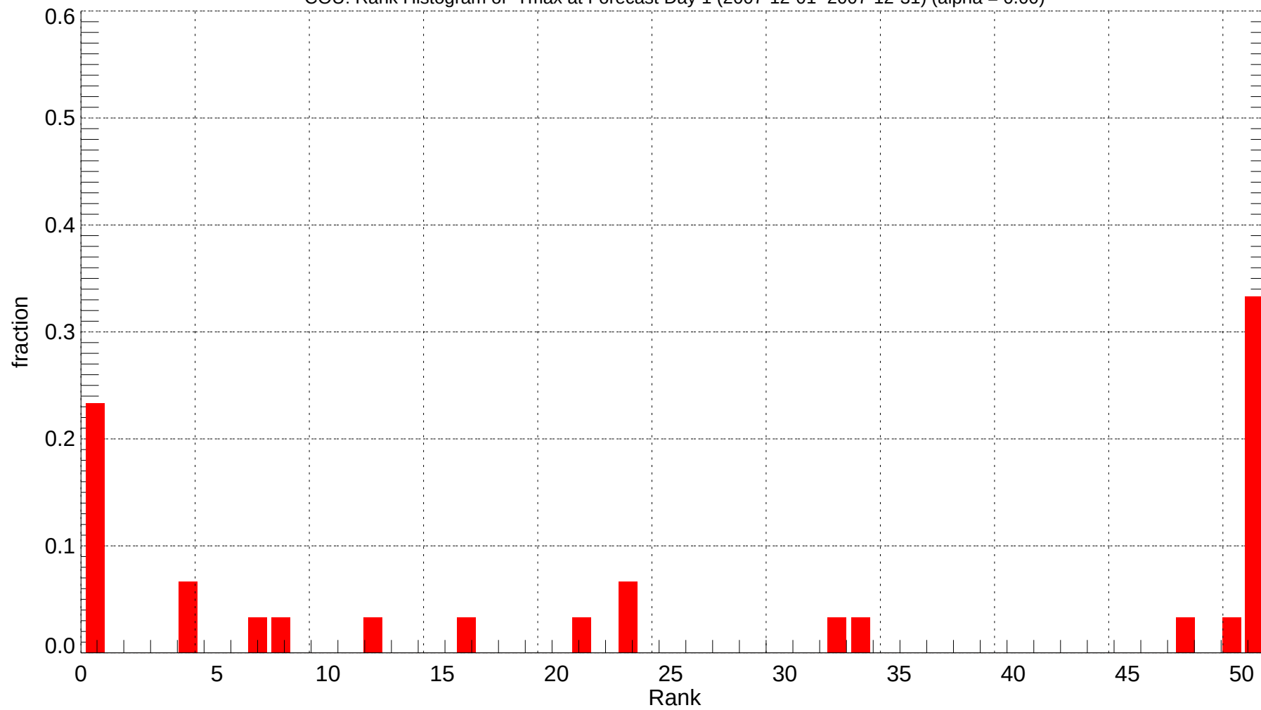
COU: Rank Histogram of Tmax at Forecast Day 1 (2007-12-01~2007-12-31) (alpha = 0.00)
