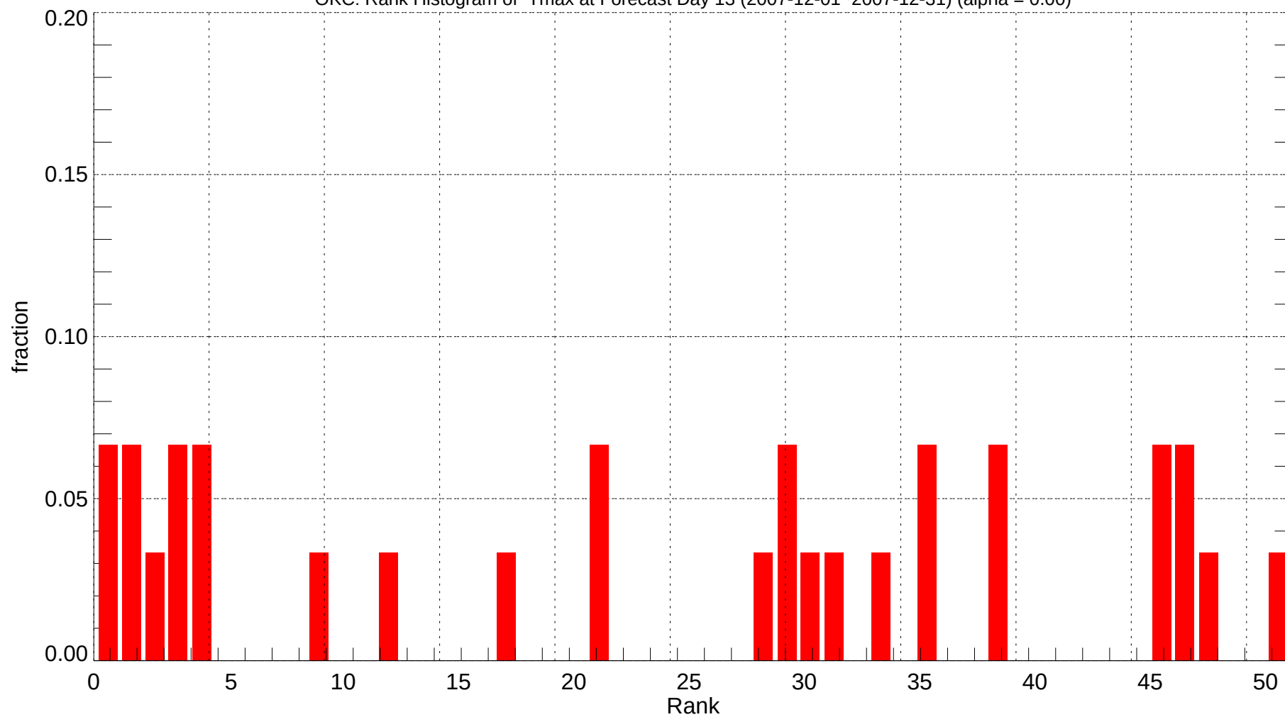
OKC: Rank Histogram of Tmax at Forecast Day 13 (2007-12-01~2007-12-31) (alpha = 0.00)
