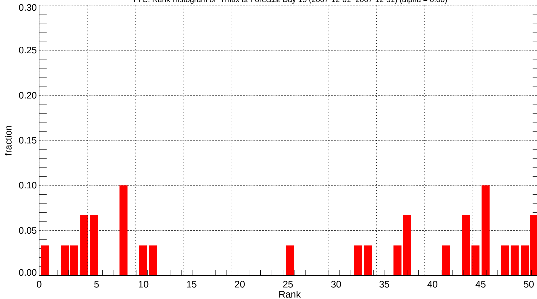
YYC: Rank Histogram of Tmax at Forecast Day 13 (2007-12-01~2007-12-31) (alpha = 0.00)
