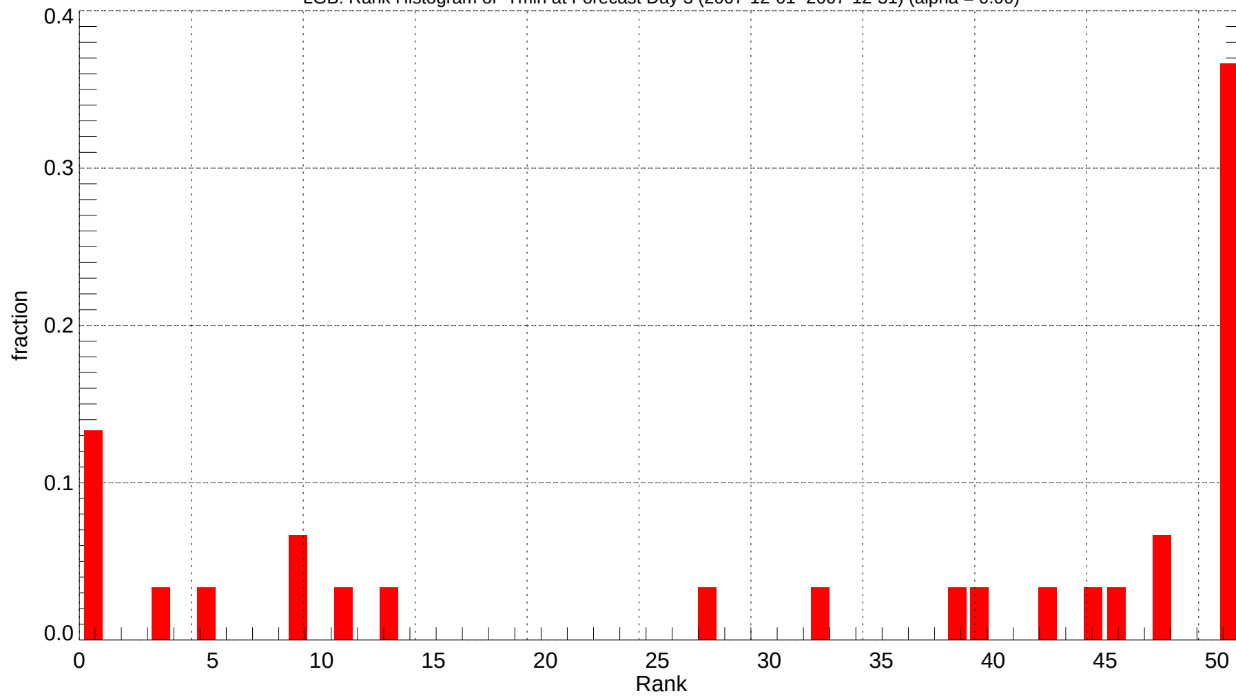
LGB: Rank Histogram of Tmin at Forecast Day 3 (2007-12-01~2007-12-31) (alpha = 0.00)
