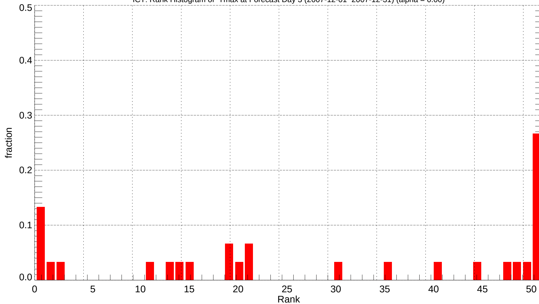
ICT: Rank Histogram of Tmax at Forecast Day 3 (2007-12-01~2007-12-31) (alpha = 0.00)
