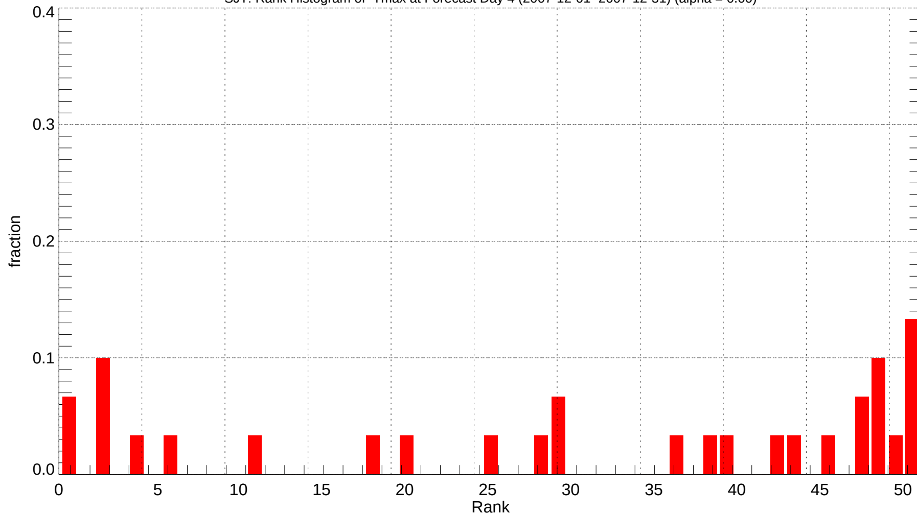
SJT: Rank Histogram of Tmax at Forecast Day 4 (2007-12-01~2007-12-31) (alpha = 0.00)
