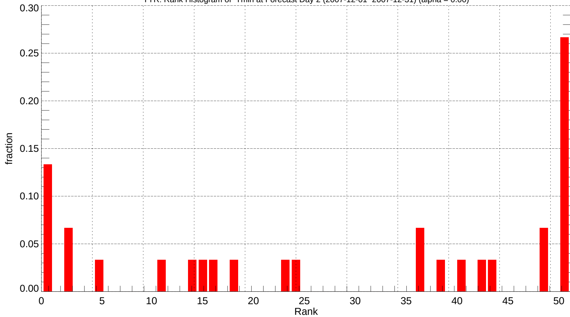
TYR: Rank Histogram of Tmin at Forecast Day 2 (2007-12-01~2007-12-31) (alpha = 0.00)
