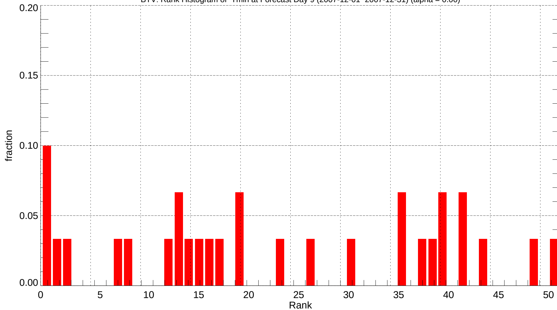
BTV: Rank Histogram of Tmin at Forecast Day 9 (2007-12-01~2007-12-31) (alpha = 0.00)
