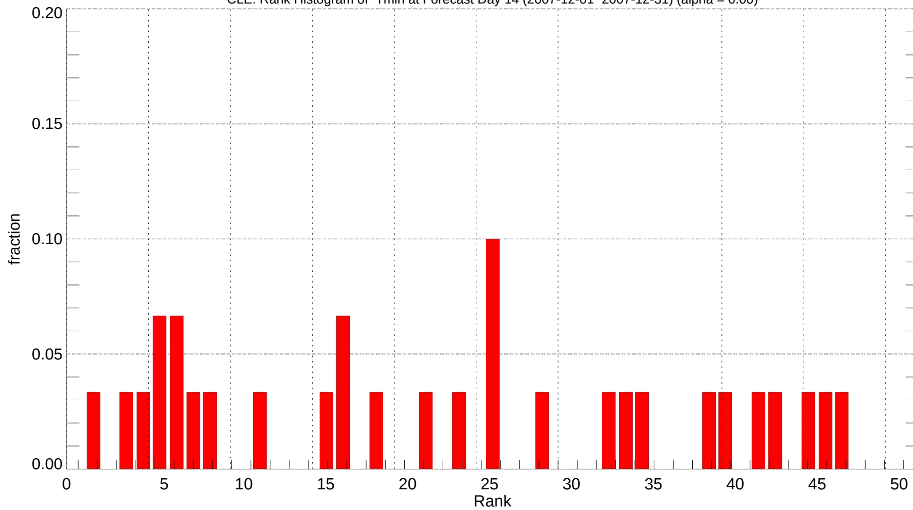
CLE: Rank Histogram of Tmin at Forecast Day 14 (2007-12-01~2007-12-31) (alpha = 0.00)
