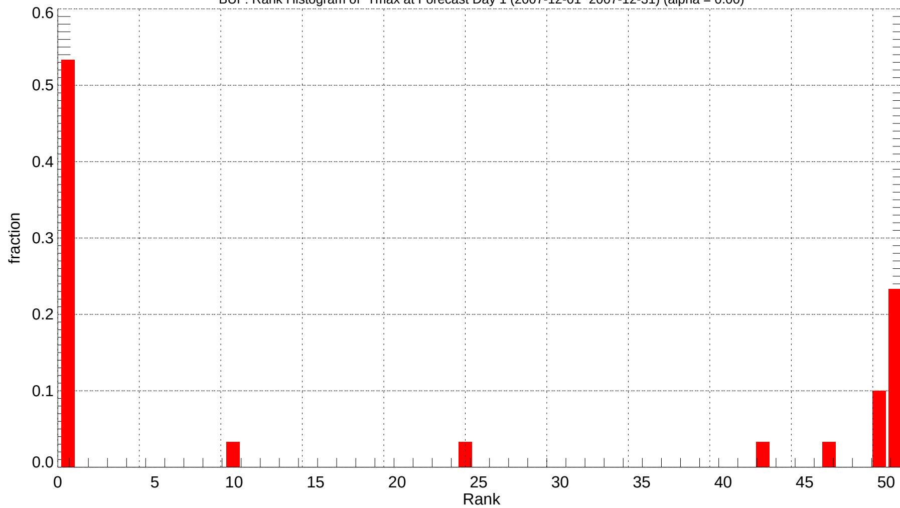
BUF: Rank Histogram of Tmax at Forecast Day 1 (2007-12-01~2007-12-31) (alpha = 0.00)
