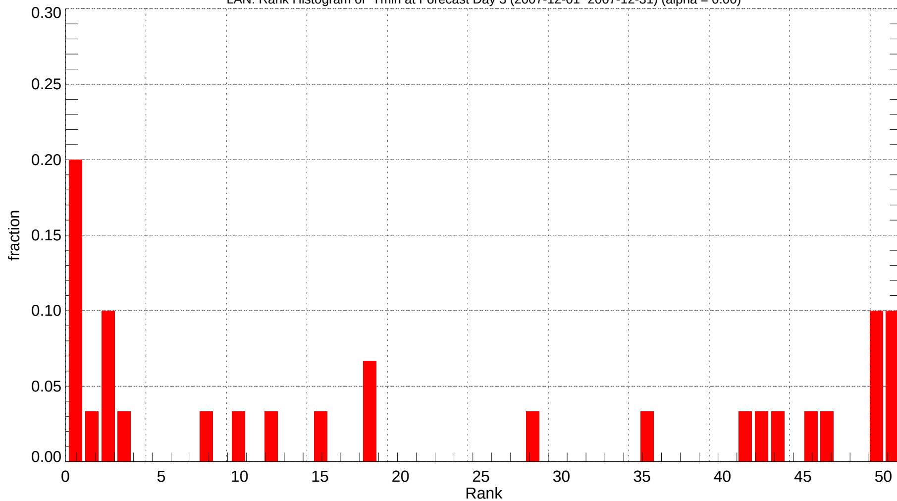
LAN: Rank Histogram of Tmin at Forecast Day 3 (2007-12-01~2007-12-31) (alpha = 0.00)
