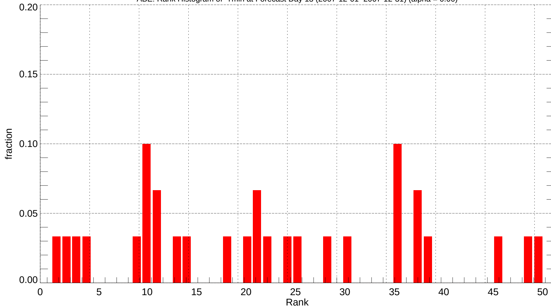
ABE: Rank Histogram of Tmin at Forecast Day 13 (2007-12-01~2007-12-31) (alpha = 0.00)
