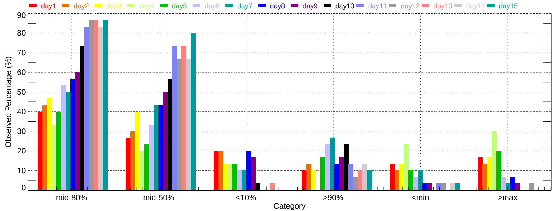
Observed Percentage of Ensembles - SAC: Min Temperature (2007-12-01~2007-12-31)
