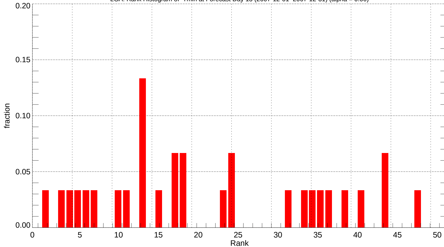
LGA: Rank Histogram of Tmin at Forecast Day 13 (2007-12-01~2007-12-31) (alpha = 0.00)
