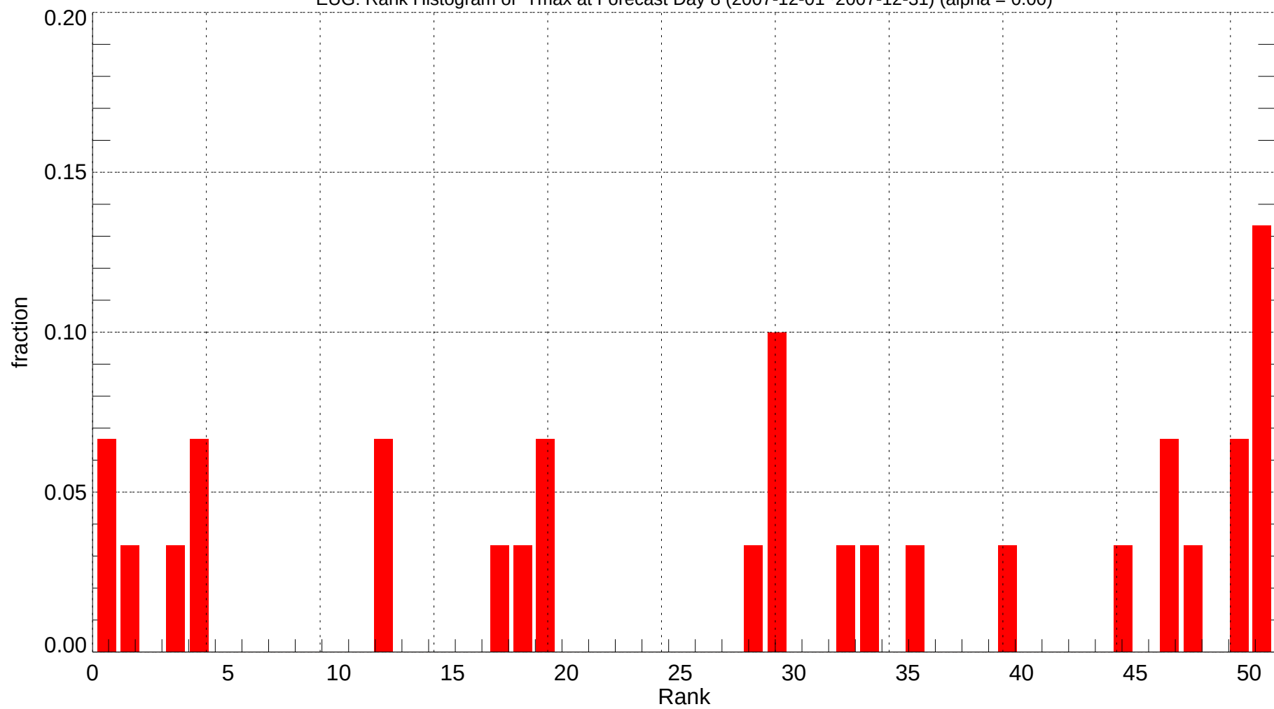
EUG: Rank Histogram of Tmax at Forecast Day 8 (2007-12-01~2007-12-31) (alpha = 0.00)
