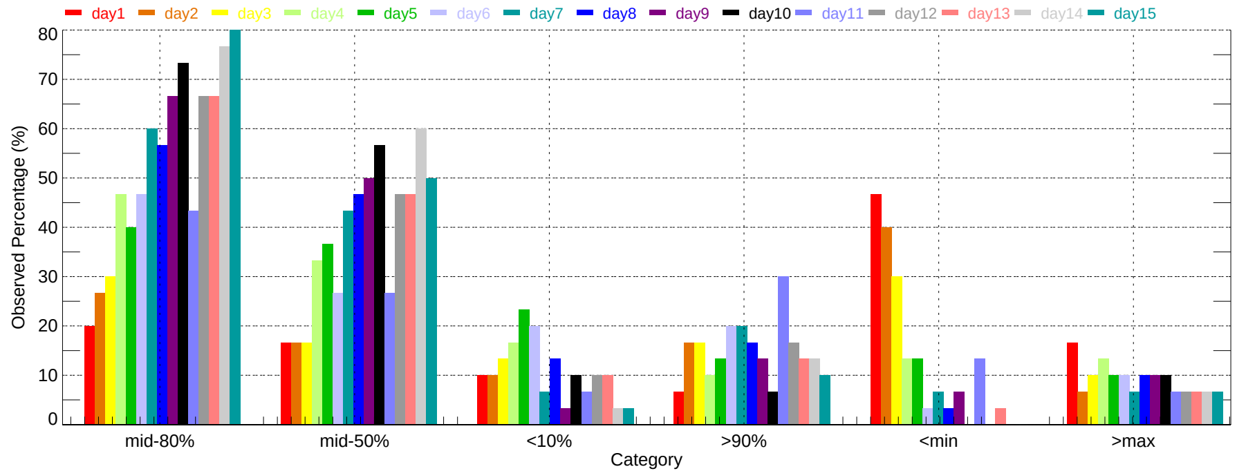
Observed Percentage of Ensembles - RIC: Min Temperature (2007-12-01~2007-12-31)
