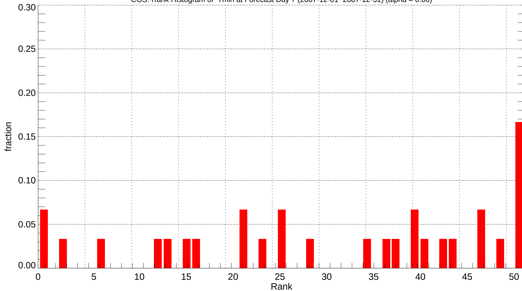
COS: Rank Histogram of Tmin at Forecast Day 7 (2007-12-01~2007-12-31) (alpha = 0.00)
