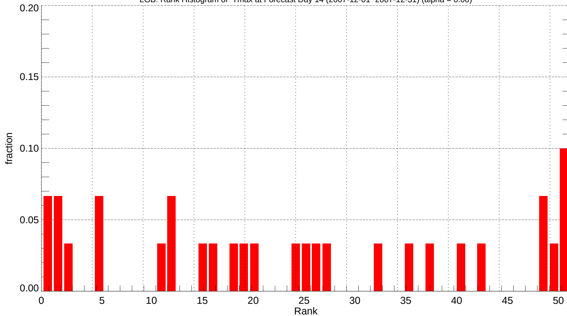
LGB: Rank Histogram of Tmax at Forecast Day 14 (2007-12-01~2007-12-31) (alpha = 0.00)
