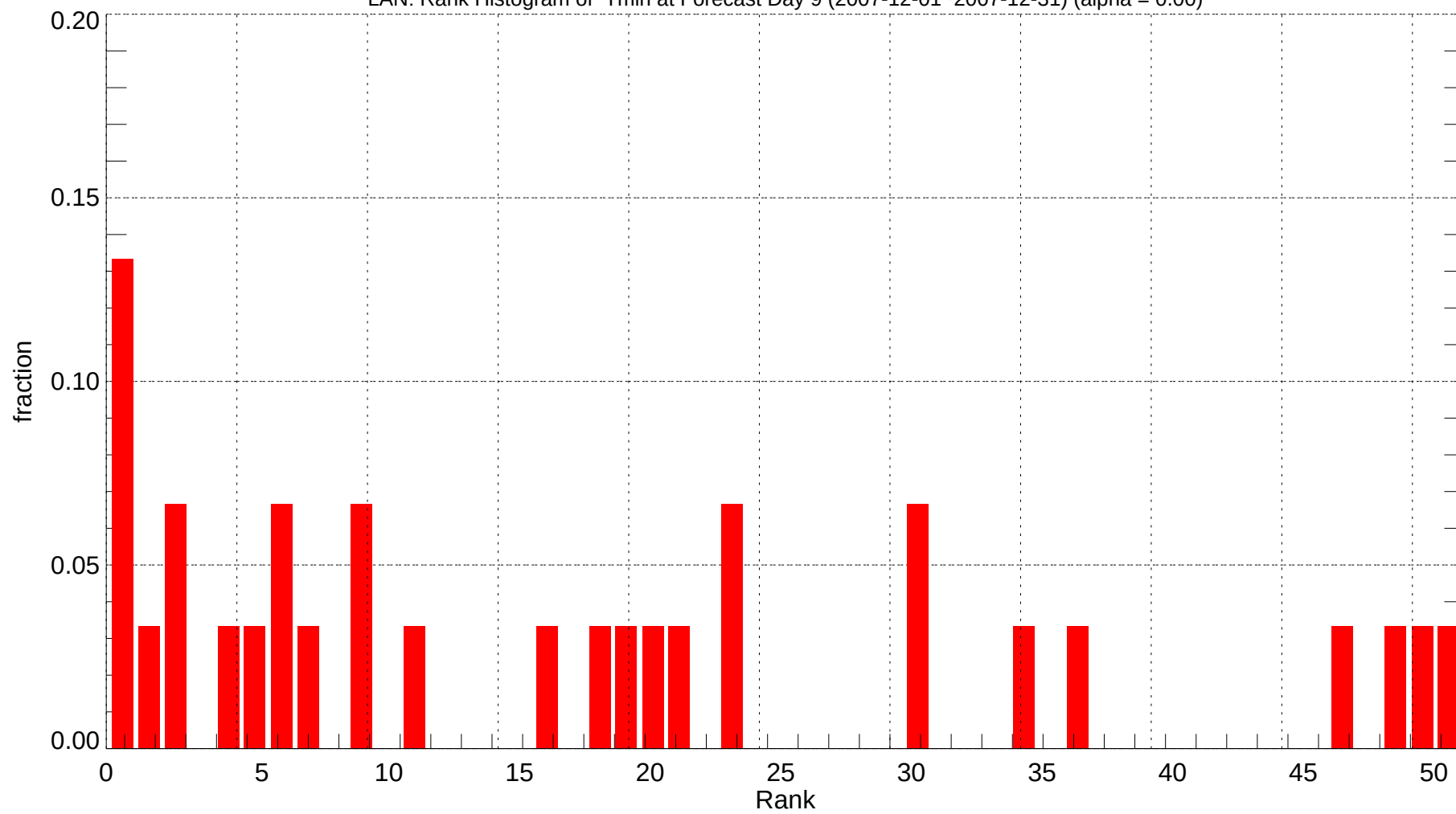
LAN: Rank Histogram of Tmin at Forecast Day 9 (2007-12-01~2007-12-31) (alpha = 0.00)
