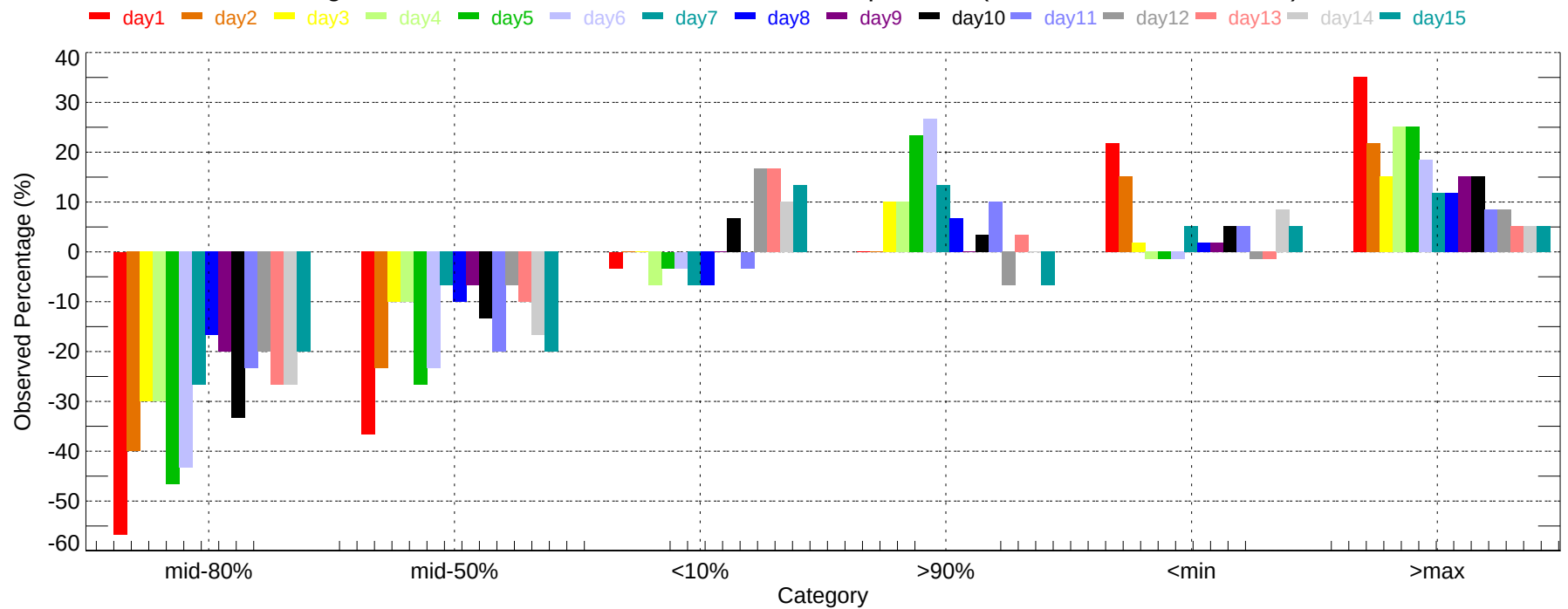
Observed Percentage Deviation of Ensembles - COS: Min Temperature (2007-12-01~2007-12-31)
