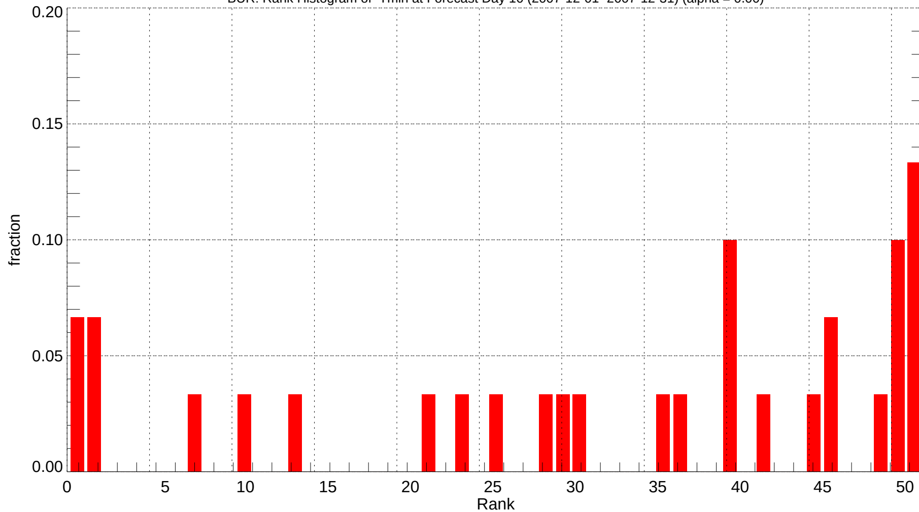
BUR: Rank Histogram of Tmin at Forecast Day 10 (2007-12-01~2007-12-31) (alpha = 0.00)
