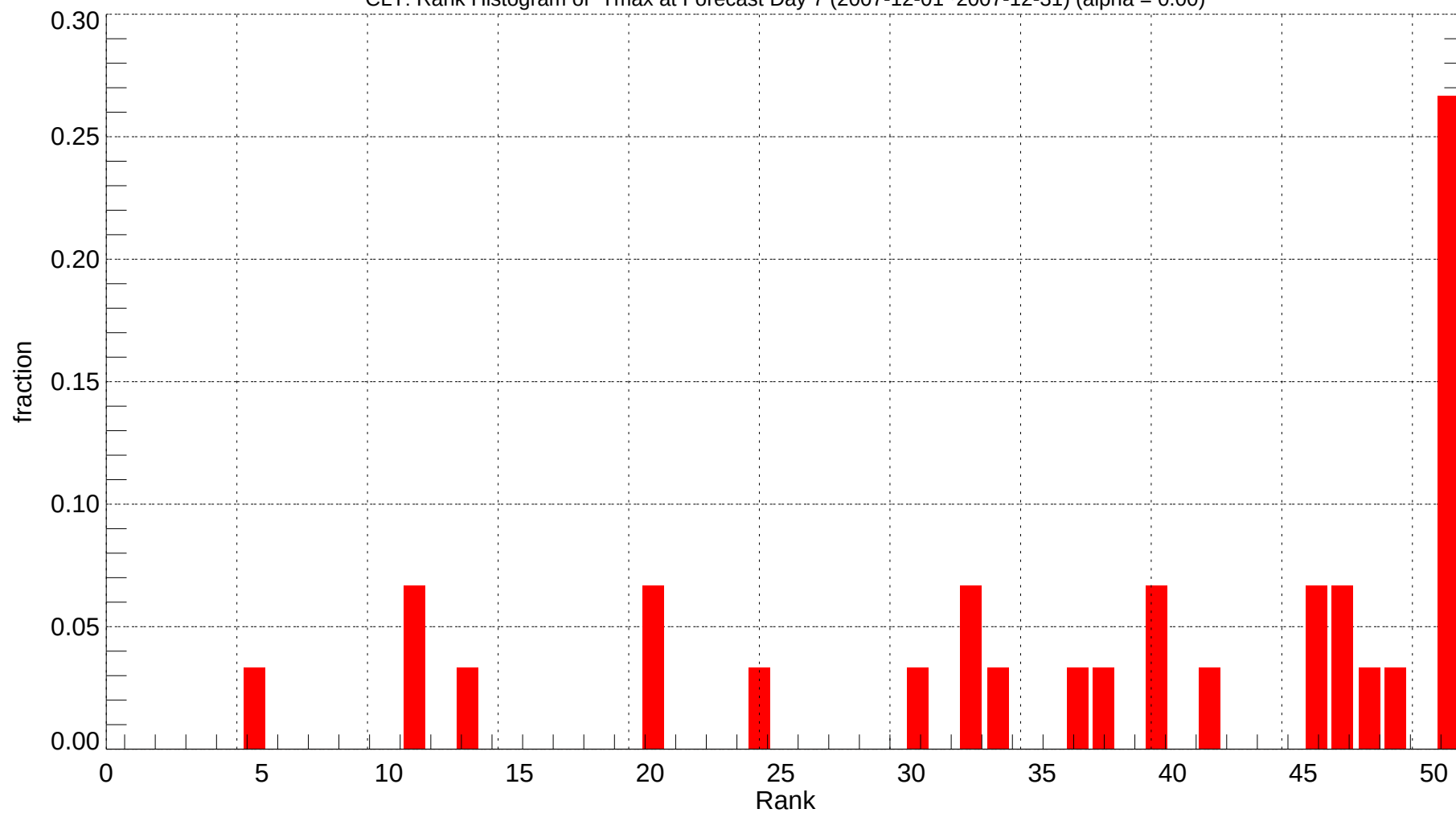
CLT: Rank Histogram of Tmax at Forecast Day 7 (2007-12-01~2007-12-31) (alpha = 0.00)
