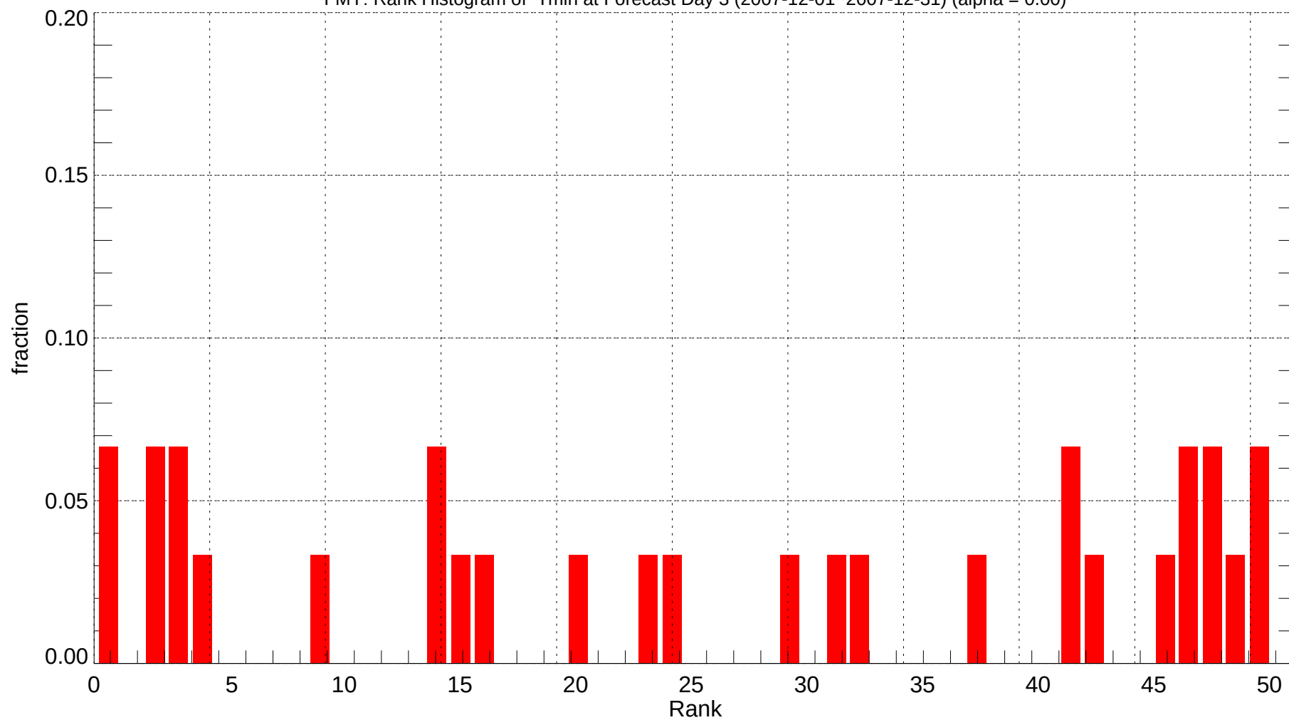
FMY: Rank Histogram of Tmin at Forecast Day 3 (2007-12-01~2007-12-31) (alpha = 0.00)
