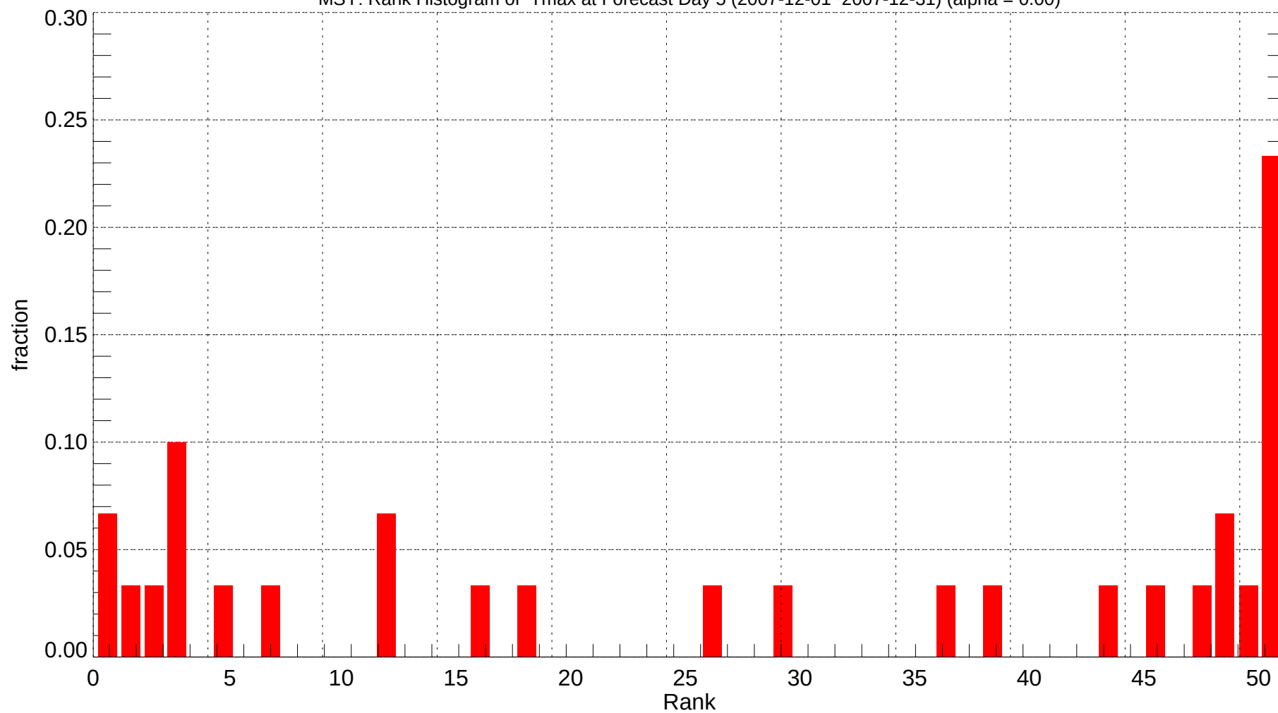
MSY: Rank Histogram of Tmax at Forecast Day 5 (2007-12-01~2007-12-31) (alpha = 0.00)
