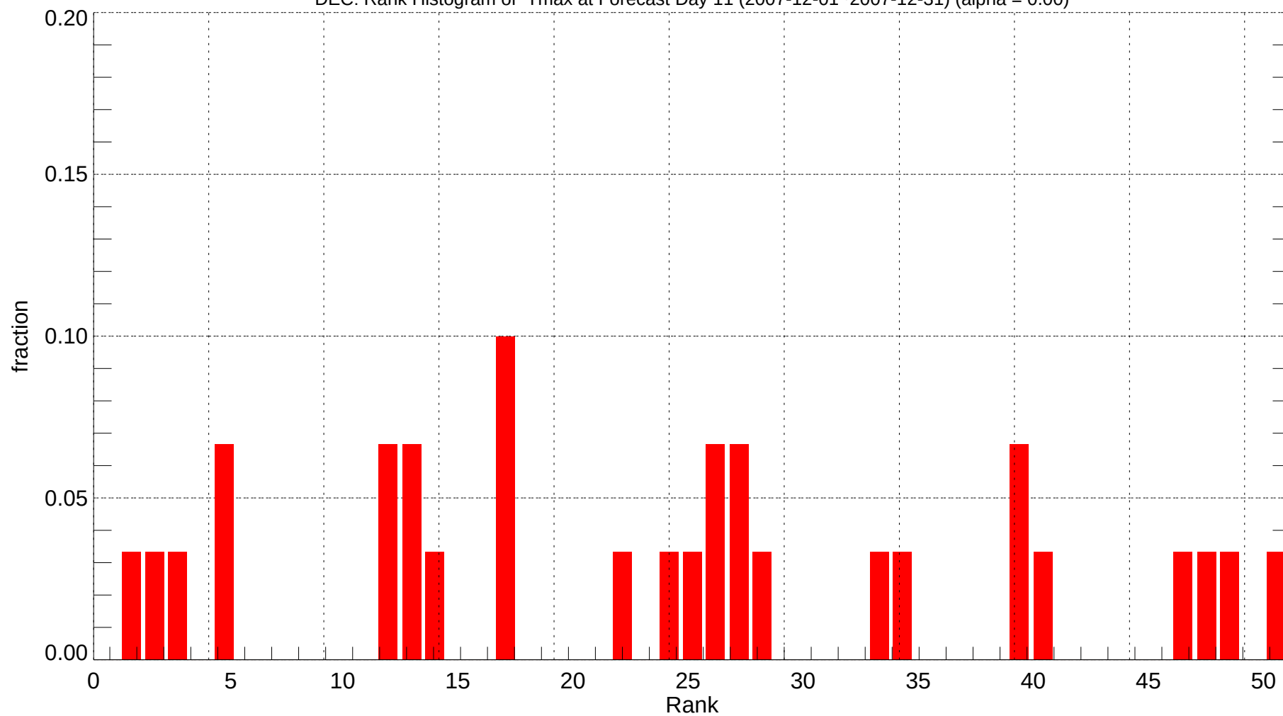
DEC: Rank Histogram of Tmax at Forecast Day 11 (2007-12-01~2007-12-31) (alpha = 0.00)
