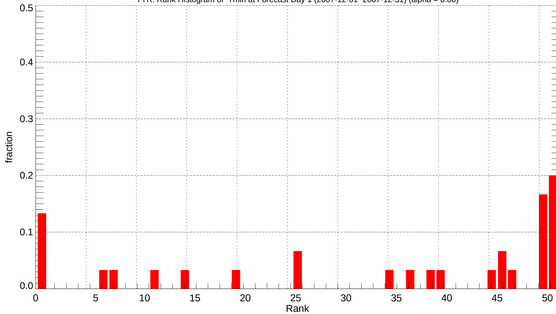
TYR: Rank Histogram of Tmin at Forecast Day 1 (2007-12-01~2007-12-31) (alpha = 0.00)
