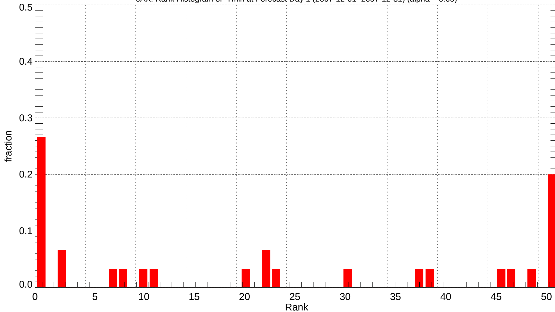
JAX: Rank Histogram of Tmin at Forecast Day 1 (2007-12-01~2007-12-31) (alpha = 0.00)
