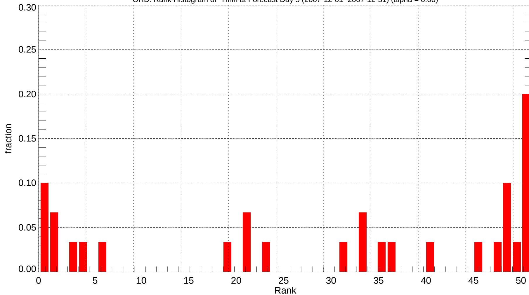
ORD: Rank Histogram of Tmin at Forecast Day 5 (2007-12-01~2007-12-31) (alpha = 0.00)
