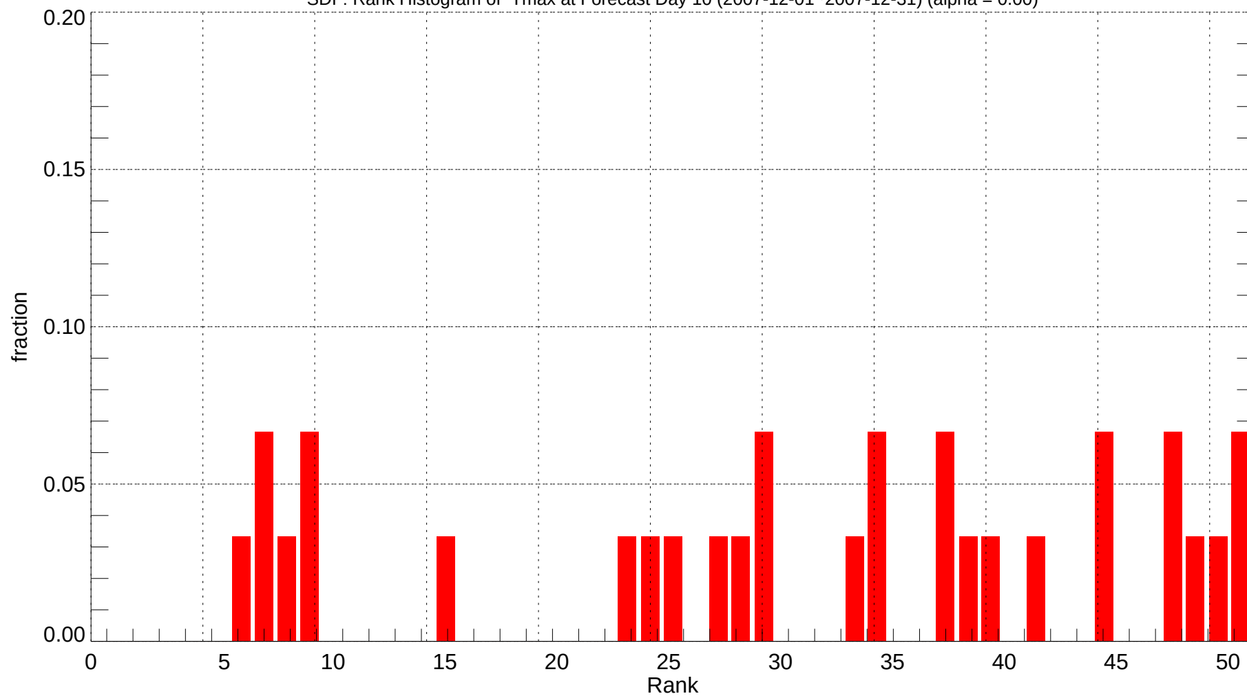
SDF: Rank Histogram of Tmax at Forecast Day 10 (2007-12-01~2007-12-31) (alpha = 0.00)
