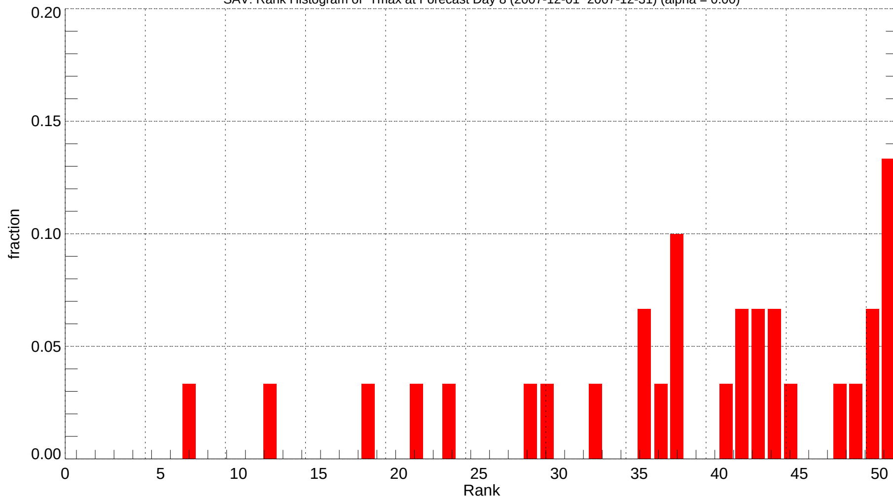
SAV: Rank Histogram of Tmax at Forecast Day 8 (2007-12-01~2007-12-31) (alpha = 0.00)
