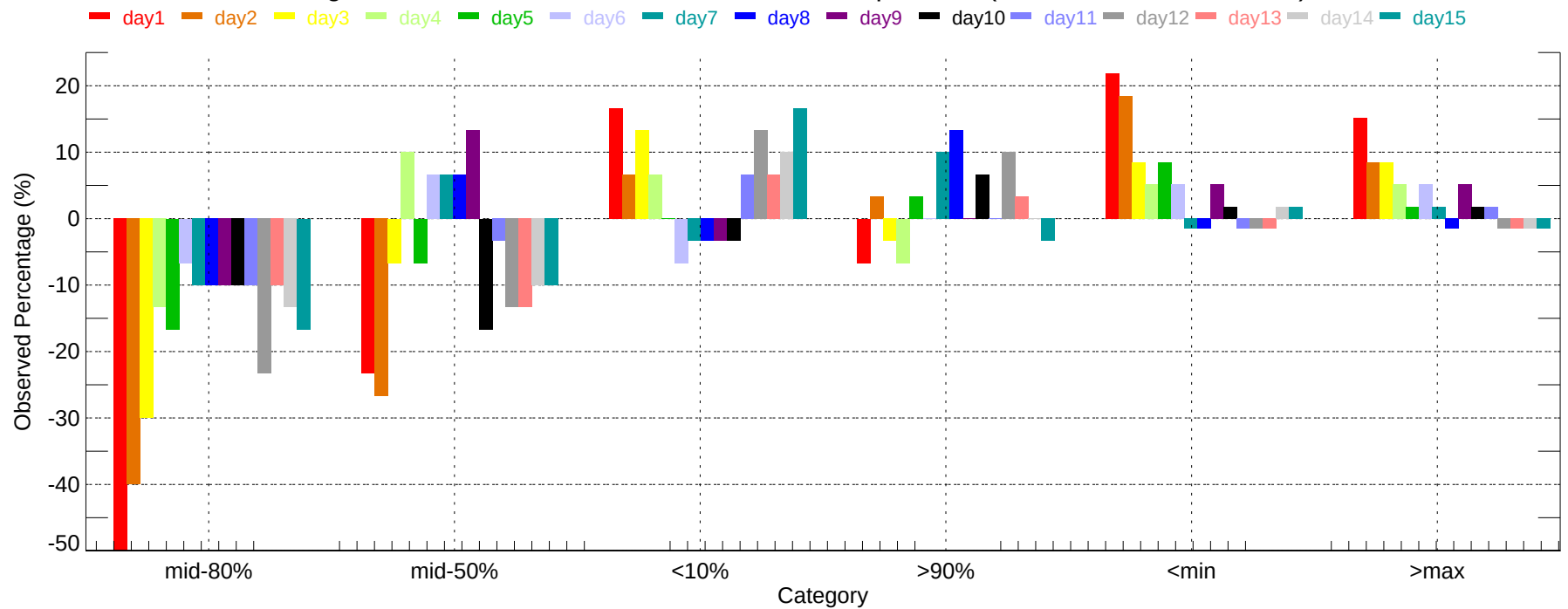
Observed Percentage Deviation of Ensembles - AUG: Max Temperature (2007-12-01~2007-12-31)
