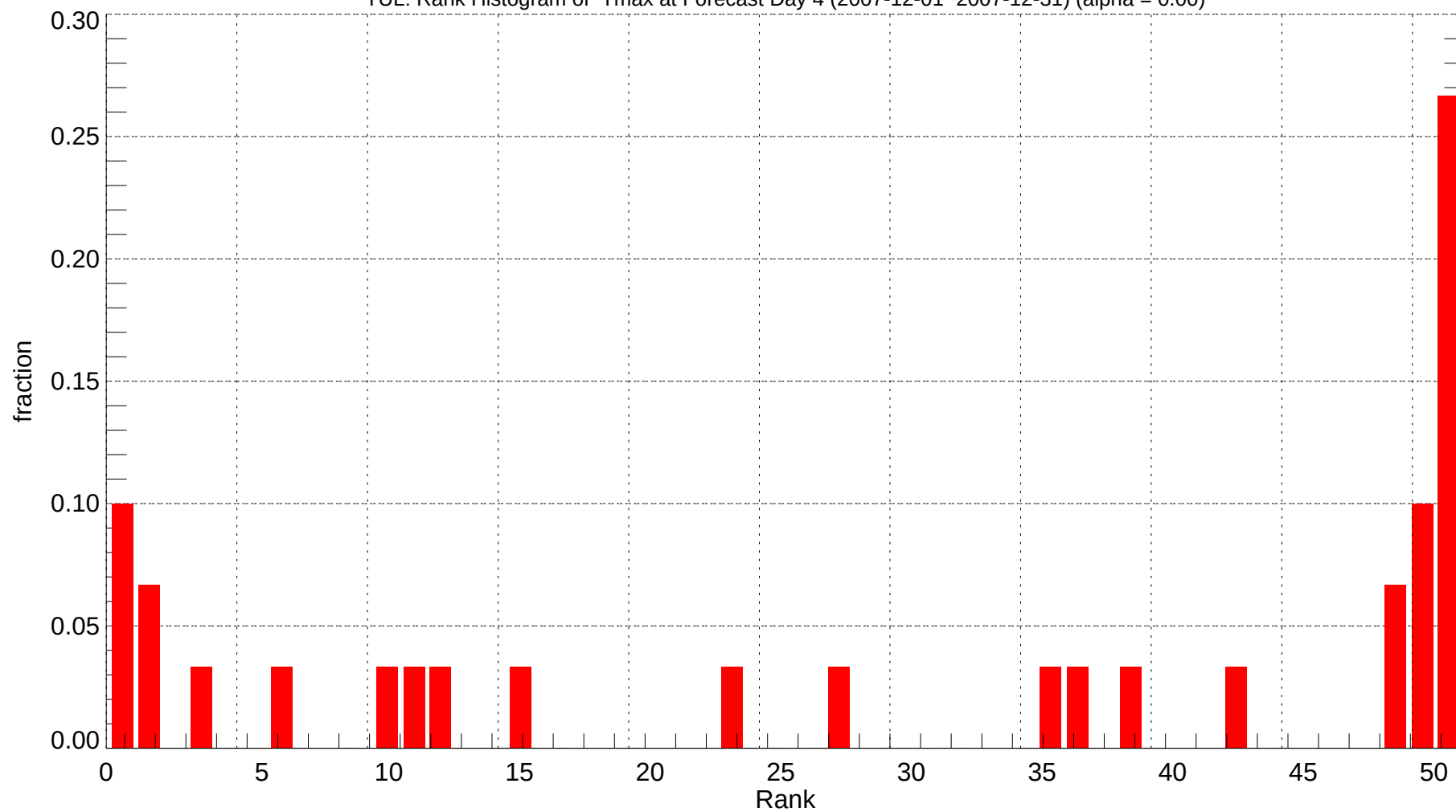
TUL: Rank Histogram of Tmax at Forecast Day 4 (2007-12-01~2007-12-31) (alpha = 0.00)
