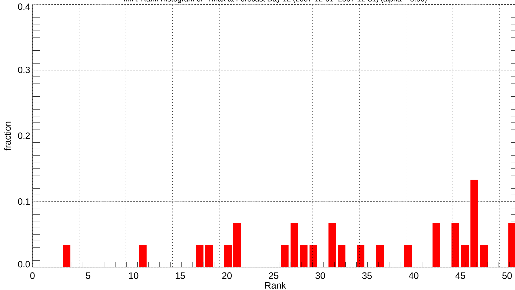
MIA: Rank Histogram of Tmax at Forecast Day 12 (2007-12-01~2007-12-31) (alpha = 0.00)
