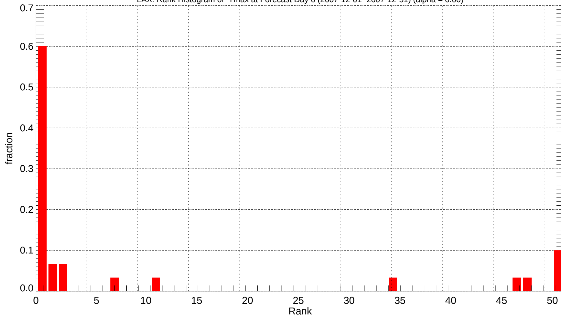
LAX: Rank Histogram of Tmax at Forecast Day 6 (2007-12-01~2007-12-31) (alpha = 0.00)
