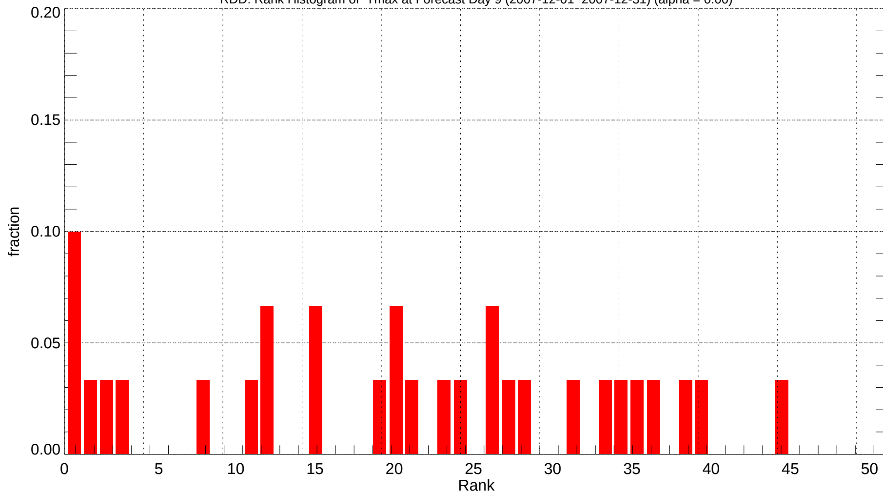
RDD: Rank Histogram of Tmax at Forecast Day 9 (2007-12-01~2007-12-31) (alpha = 0.00)
