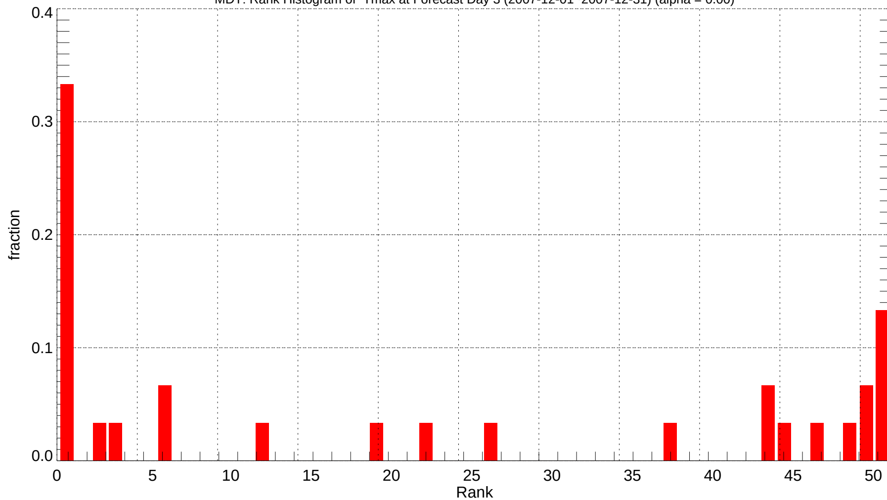
MDT: Rank Histogram of Tmax at Forecast Day 3 (2007-12-01~2007-12-31) (alpha = 0.00)
