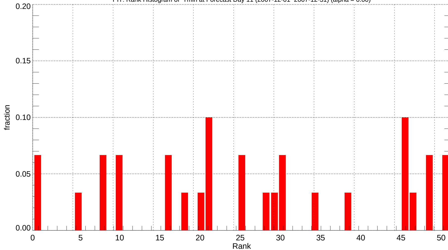
PIT: Rank Histogram of Tmin at Forecast Day 11 (2007-12-01~2007-12-31) (alpha = 0.00)
