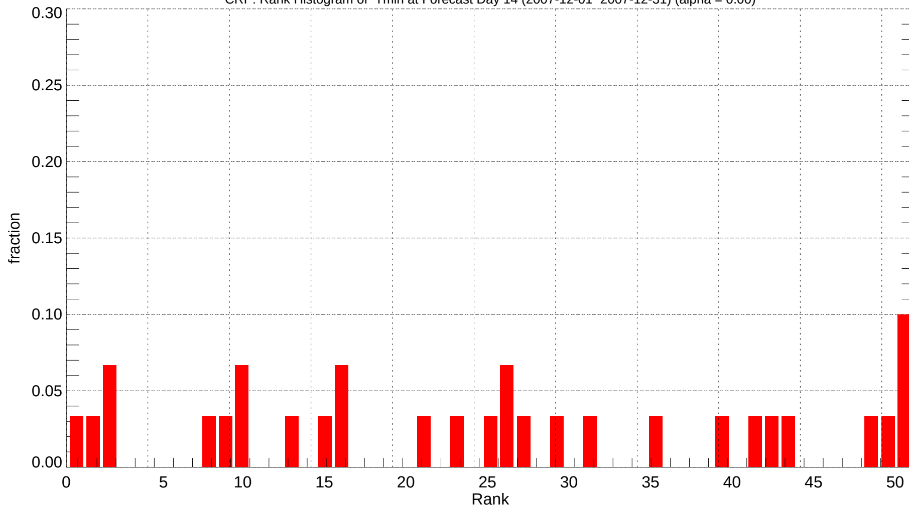
CRP: Rank Histogram of Tmin at Forecast Day 14 (2007-12-01~2007-12-31) (alpha = 0.00)
