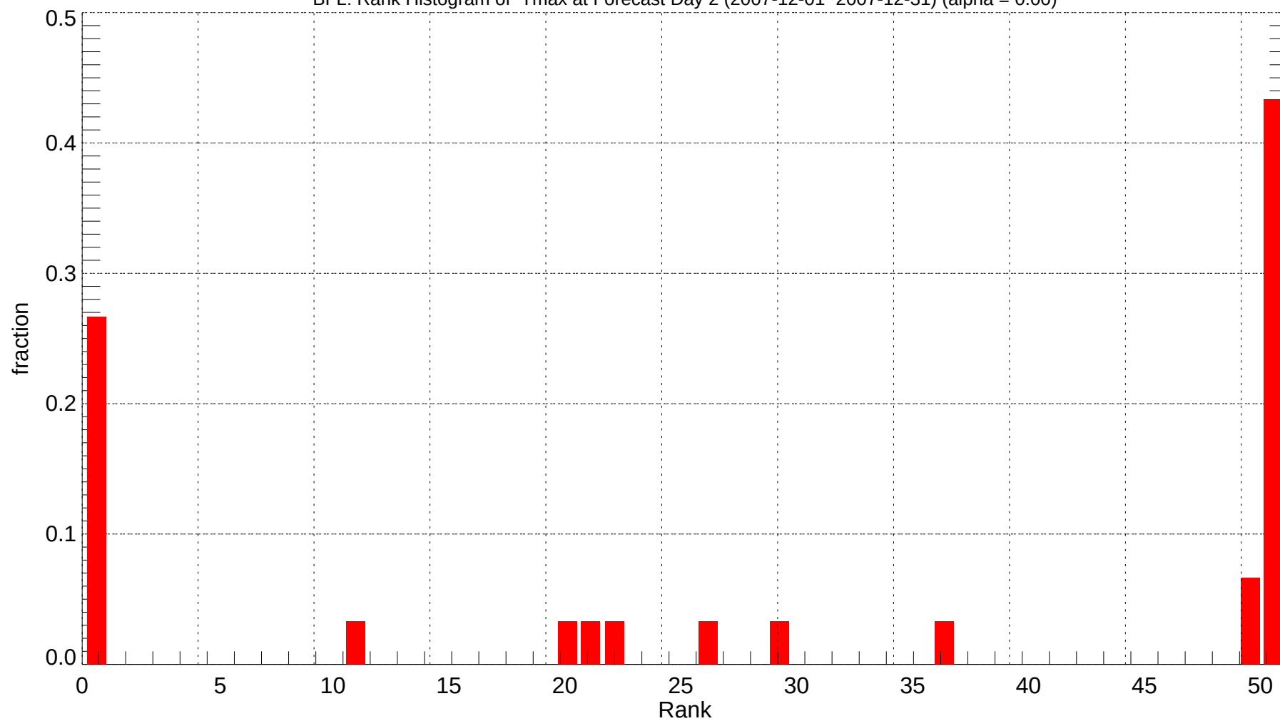
BFL: Rank Histogram of Tmax at Forecast Day 2 (2007-12-01~2007-12-31) (alpha = 0.00)
