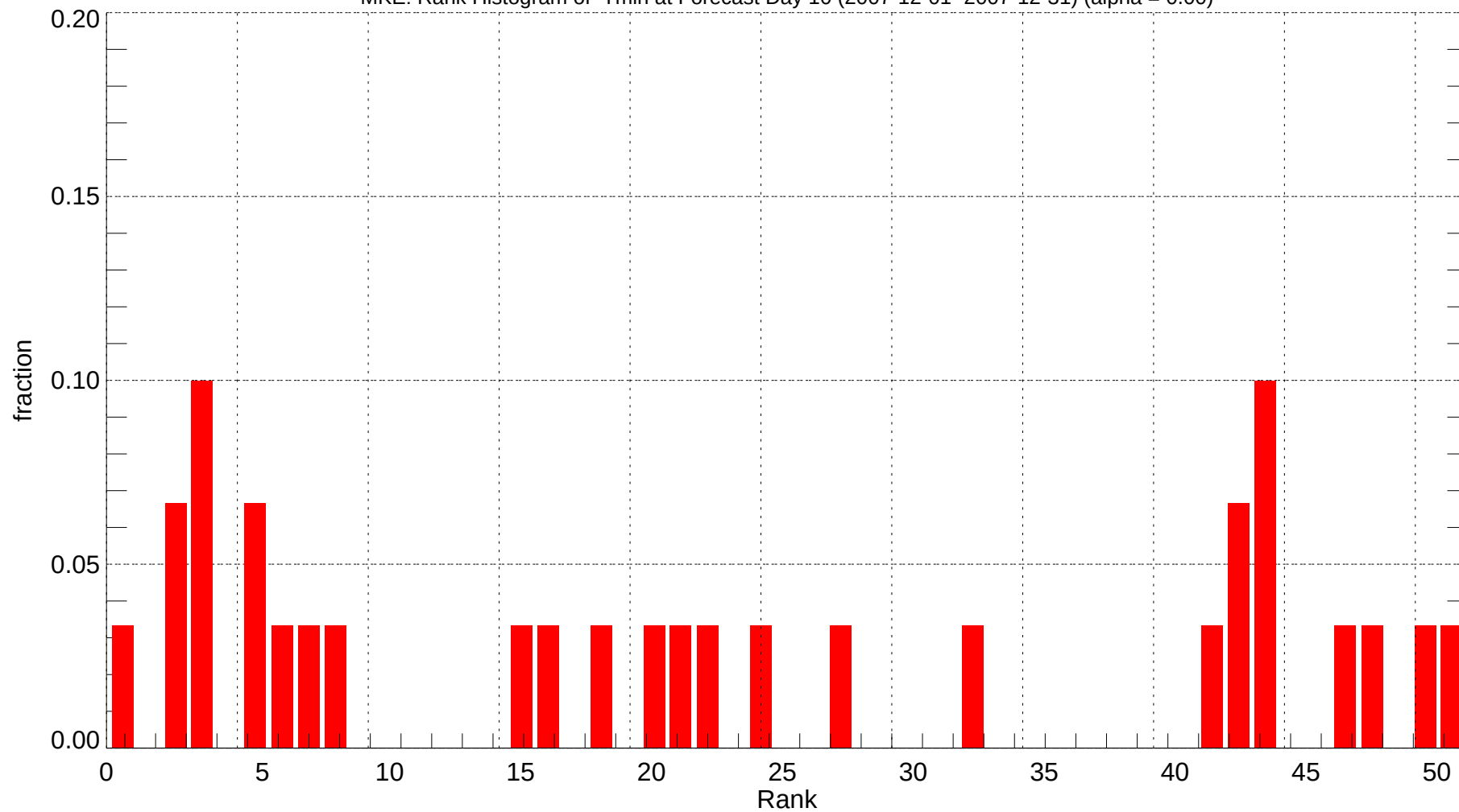
MKE: Rank Histogram of Tmin at Forecast Day 10 (2007-12-01~2007-12-31) (alpha = 0.00)
