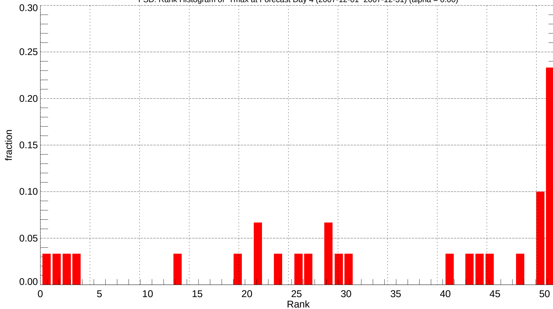
FSD: Rank Histogram of Tmax at Forecast Day 4 (2007-12-01~2007-12-31) (alpha = 0.00)
