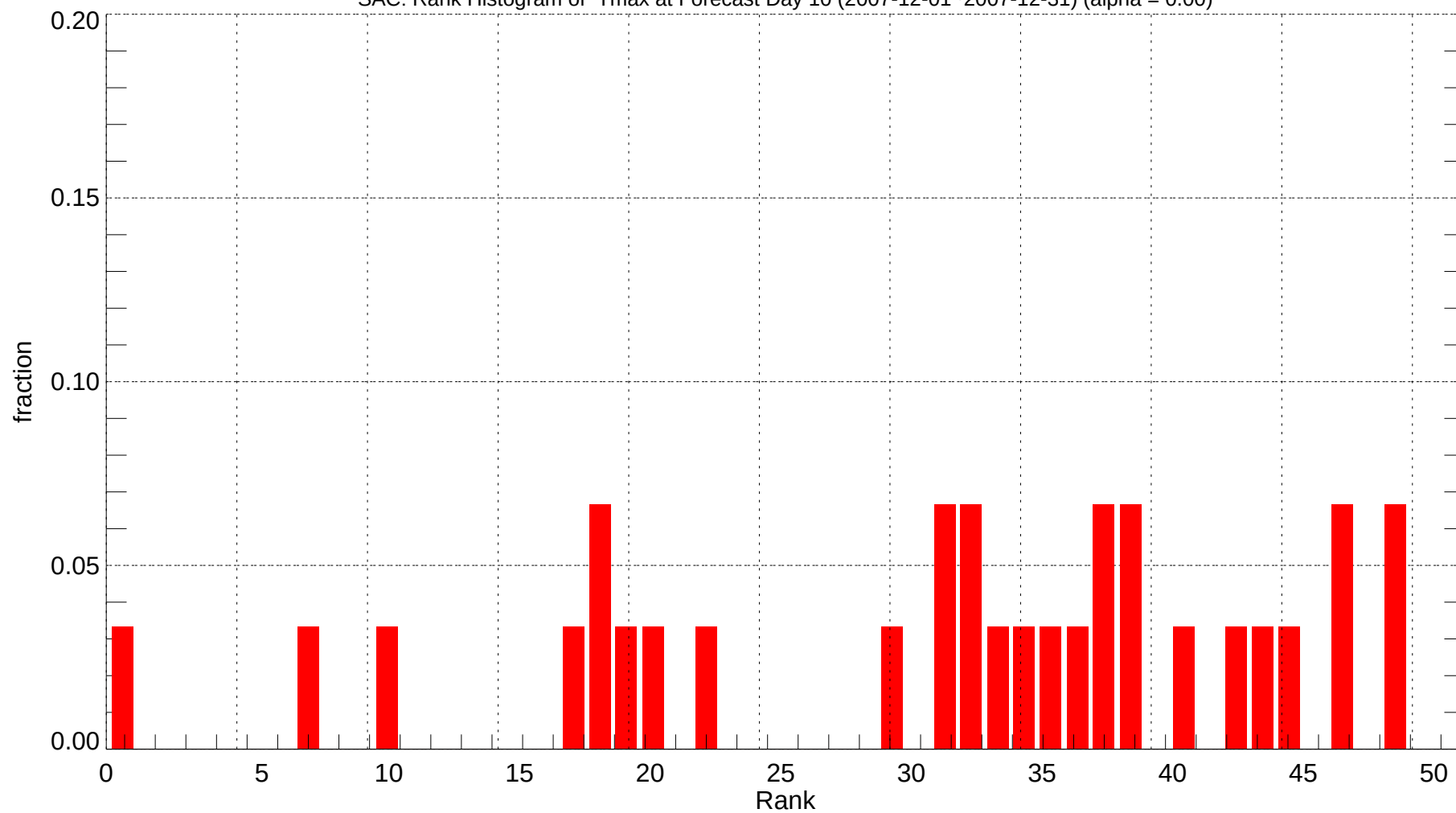
SAC: Rank Histogram of Tmax at Forecast Day 10 (2007-12-01~2007-12-31) (alpha = 0.00)
