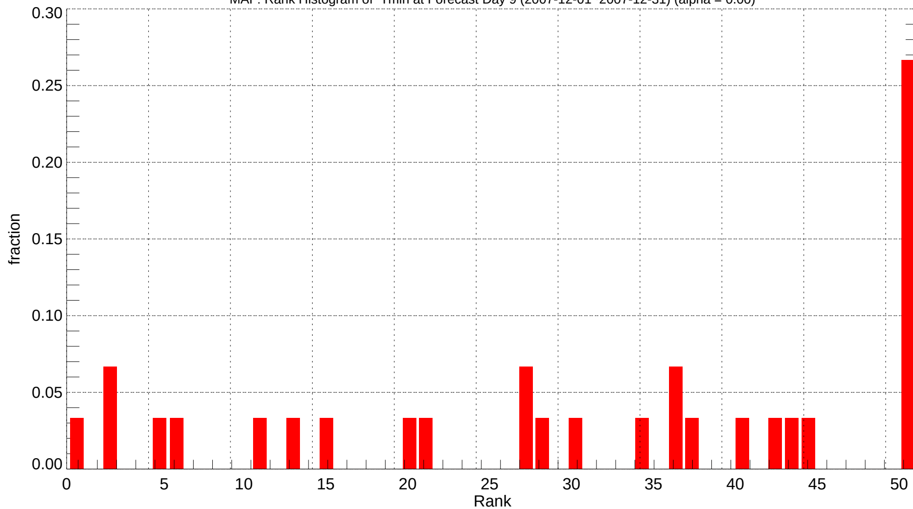
MAF: Rank Histogram of Tmin at Forecast Day 9 (2007-12-01~2007-12-31) (alpha = 0.00)
