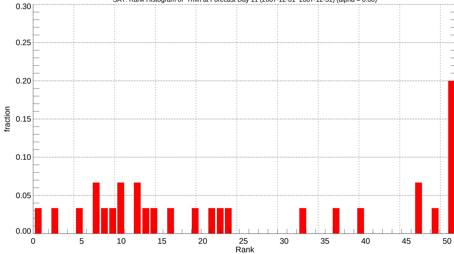
SAT: Rank Histogram of Tmin at Forecast Day 11 (2007-12-01~2007-12-31) (alpha = 0.00)
