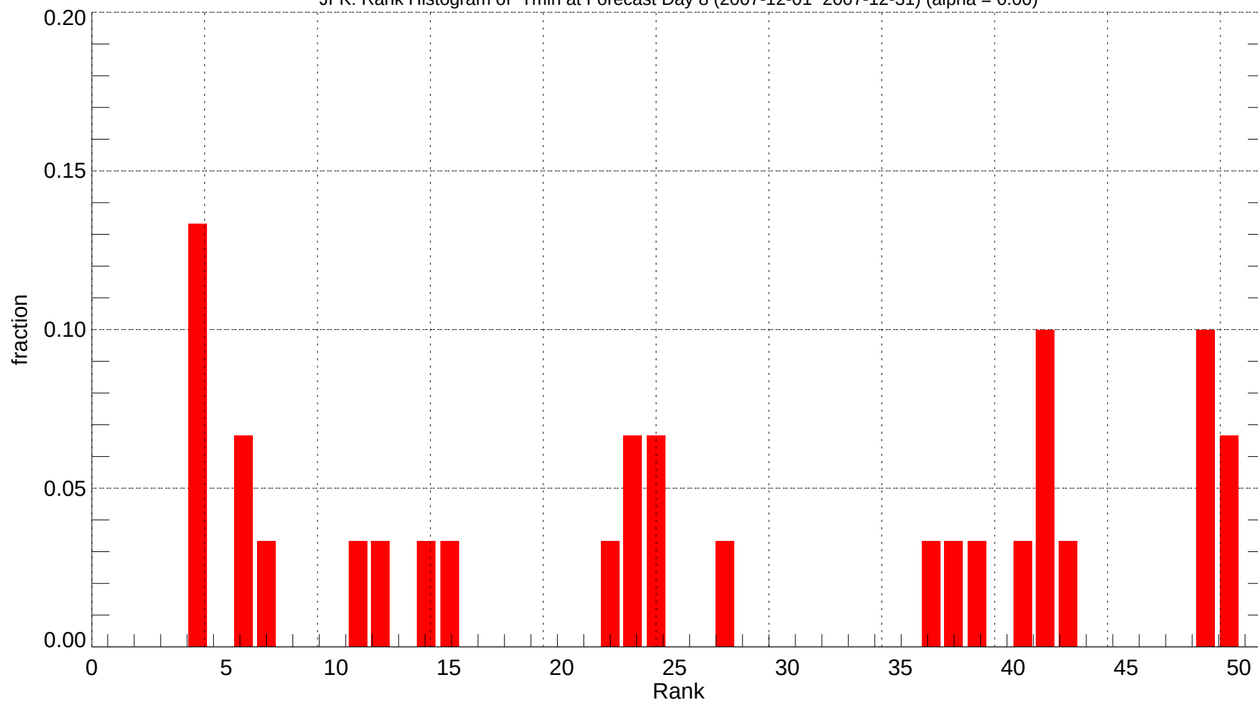
JFK: Rank Histogram of Tmin at Forecast Day 8 (2007-12-01~2007-12-31) (alpha = 0.00)
