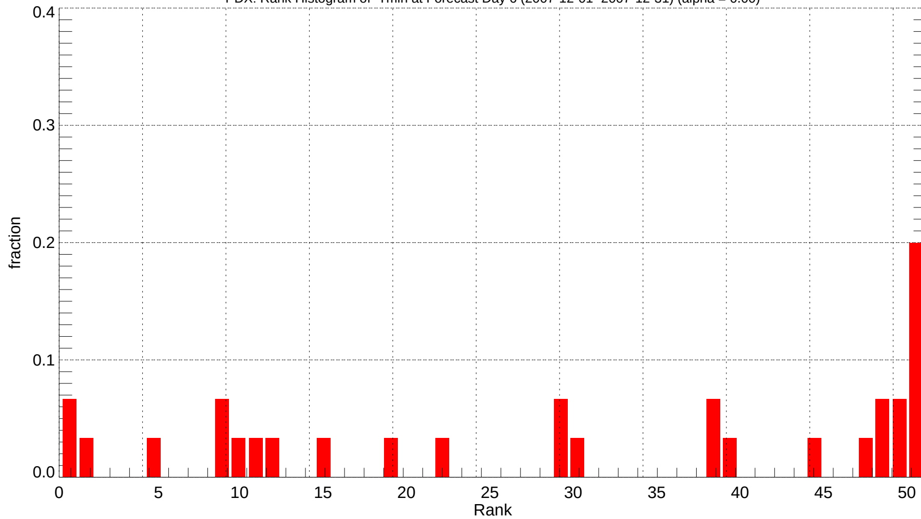
PDX: Rank Histogram of Tmin at Forecast Day 6 (2007-12-01~2007-12-31) (alpha = 0.00)
