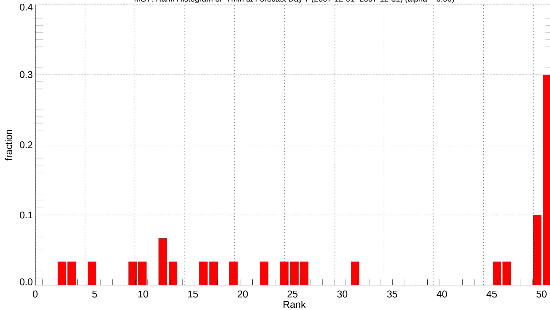
MSY: Rank Histogram of Tmin at Forecast Day 7 (2007-12-01~2007-12-31) (alpha = 0.00)
