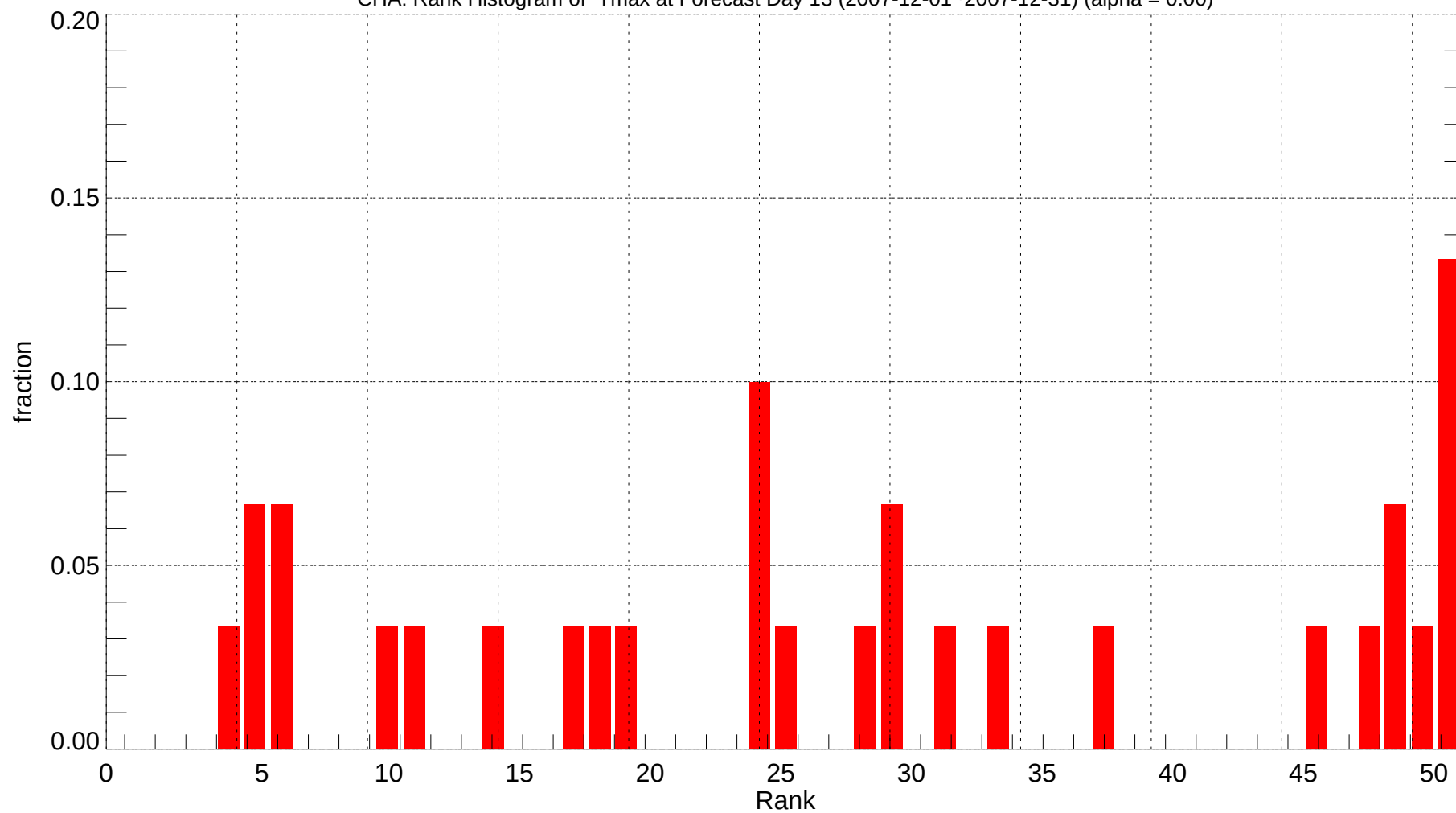
CHA: Rank Histogram of Tmax at Forecast Day 13 (2007-12-01~2007-12-31) (alpha = 0.00)
