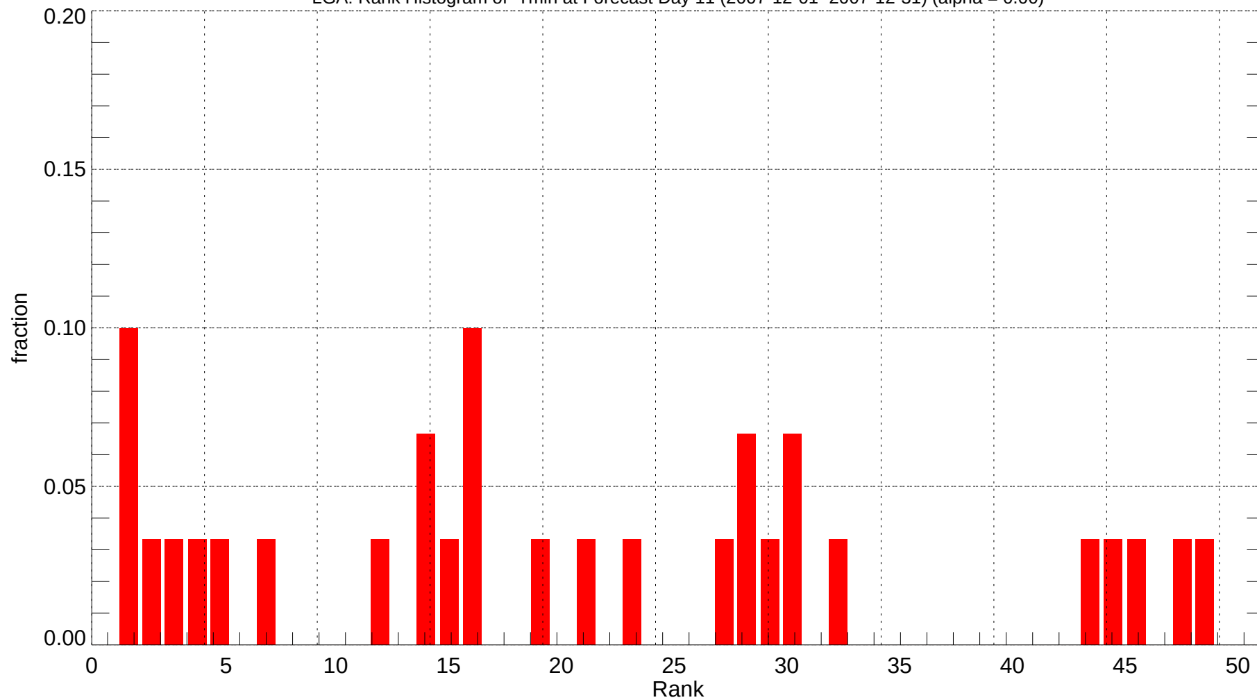
LGA: Rank Histogram of Tmin at Forecast Day 11 (2007-12-01~2007-12-31) (alpha = 0.00)
