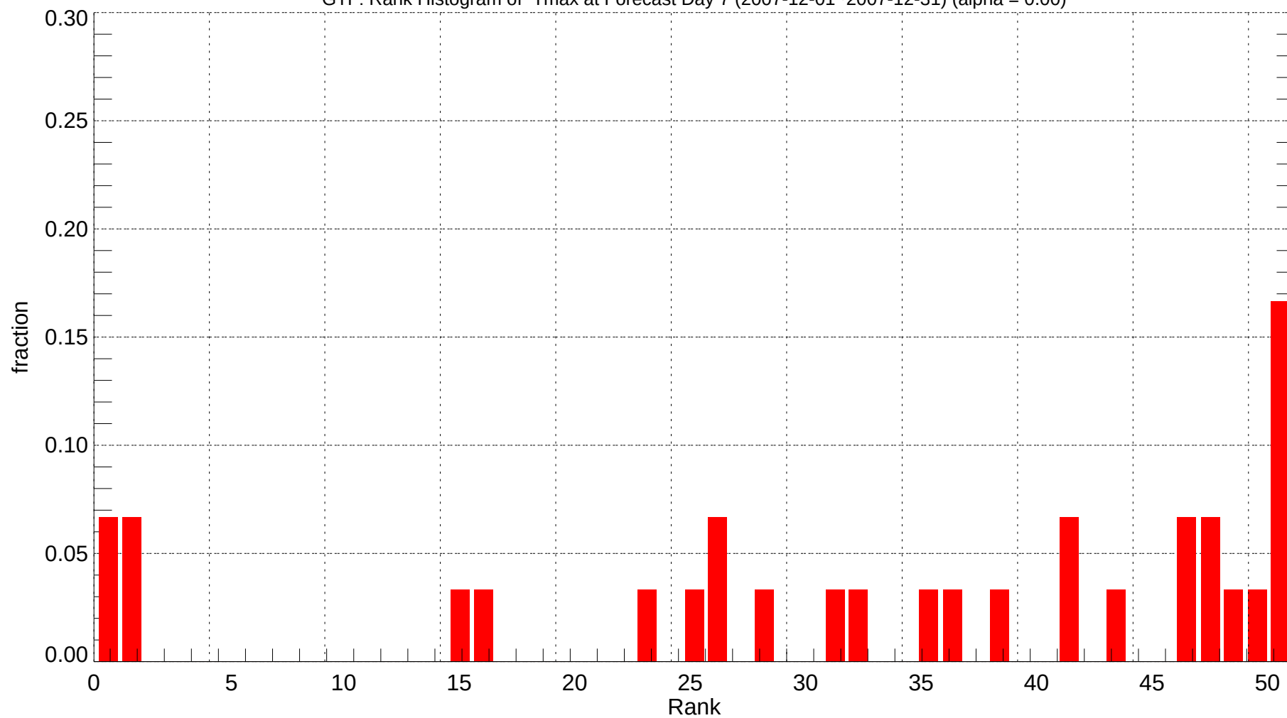
GTF: Rank Histogram of Tmax at Forecast Day 7 (2007-12-01~2007-12-31) (alpha = 0.00)
