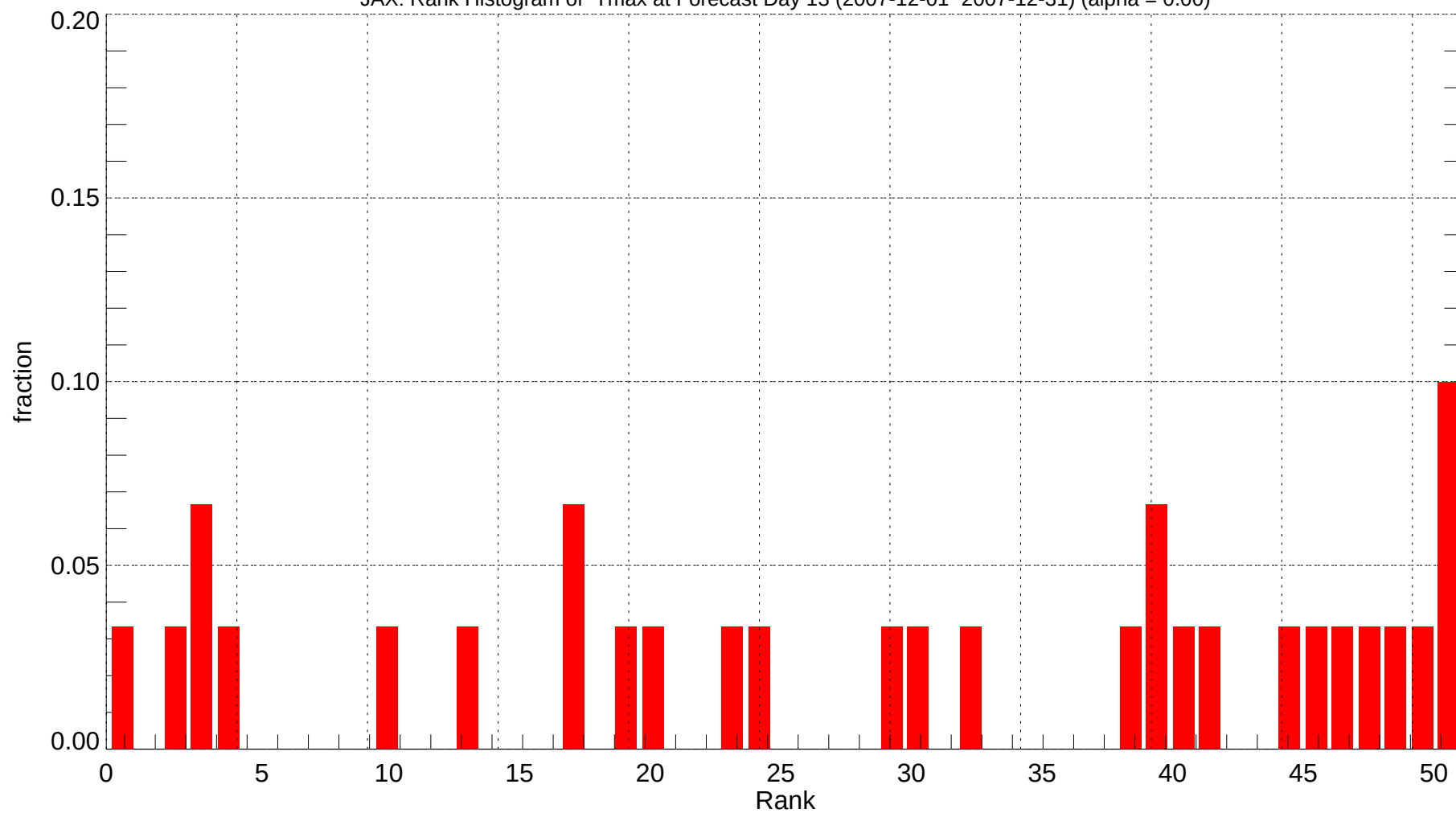
JAX: Rank Histogram of Tmax at Forecast Day 13 (2007-12-01~2007-12-31) (alpha = 0.00)
