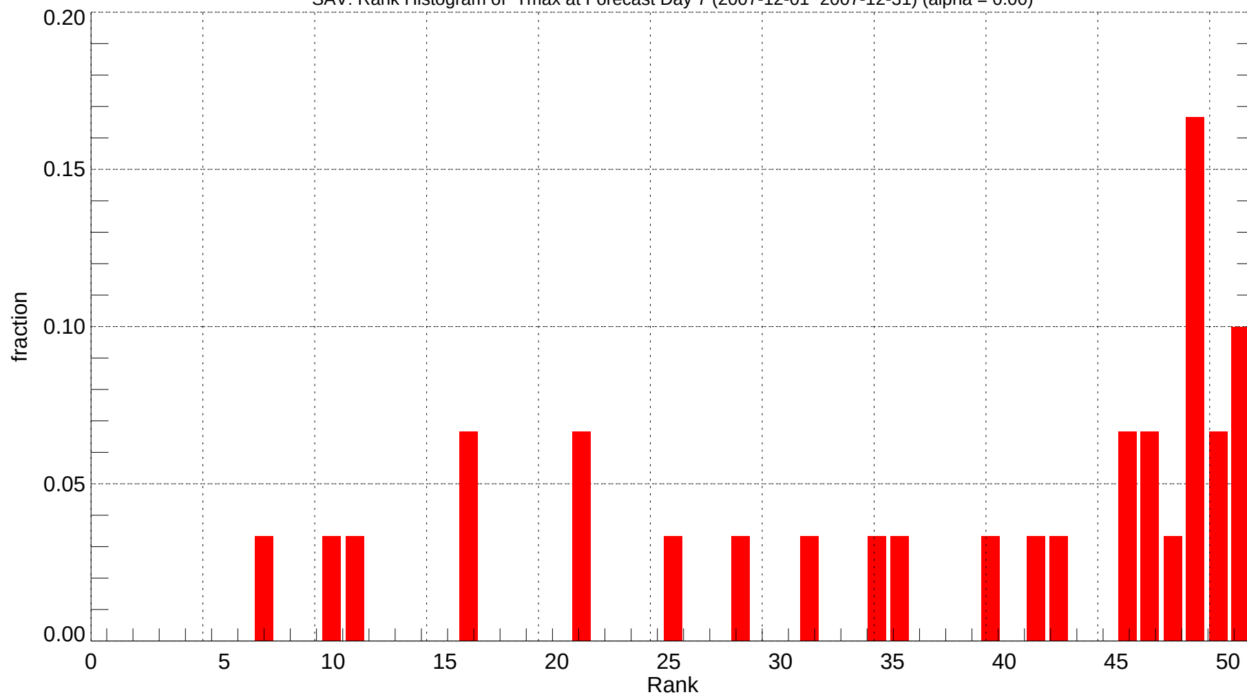
SAV: Rank Histogram of Tmax at Forecast Day 7 (2007-12-01~2007-12-31) (alpha = 0.00)
