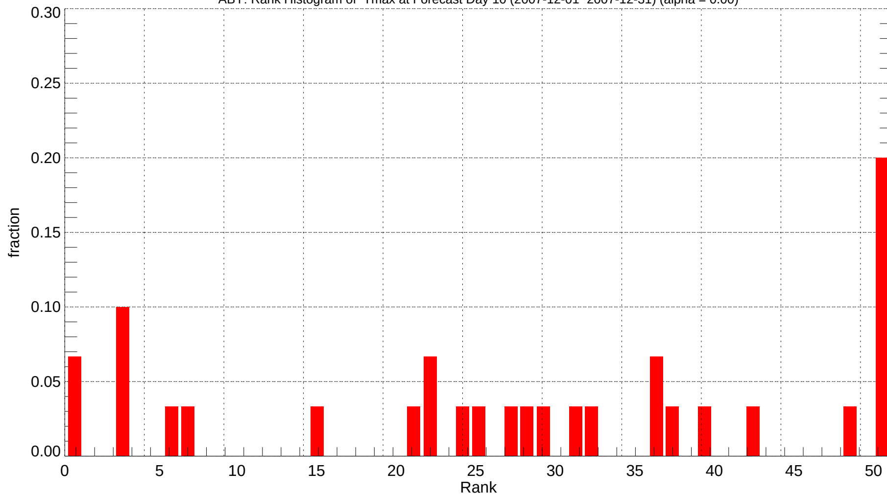
ABY: Rank Histogram of Tmax at Forecast Day 10 (2007-12-01~2007-12-31) (alpha = 0.00)
