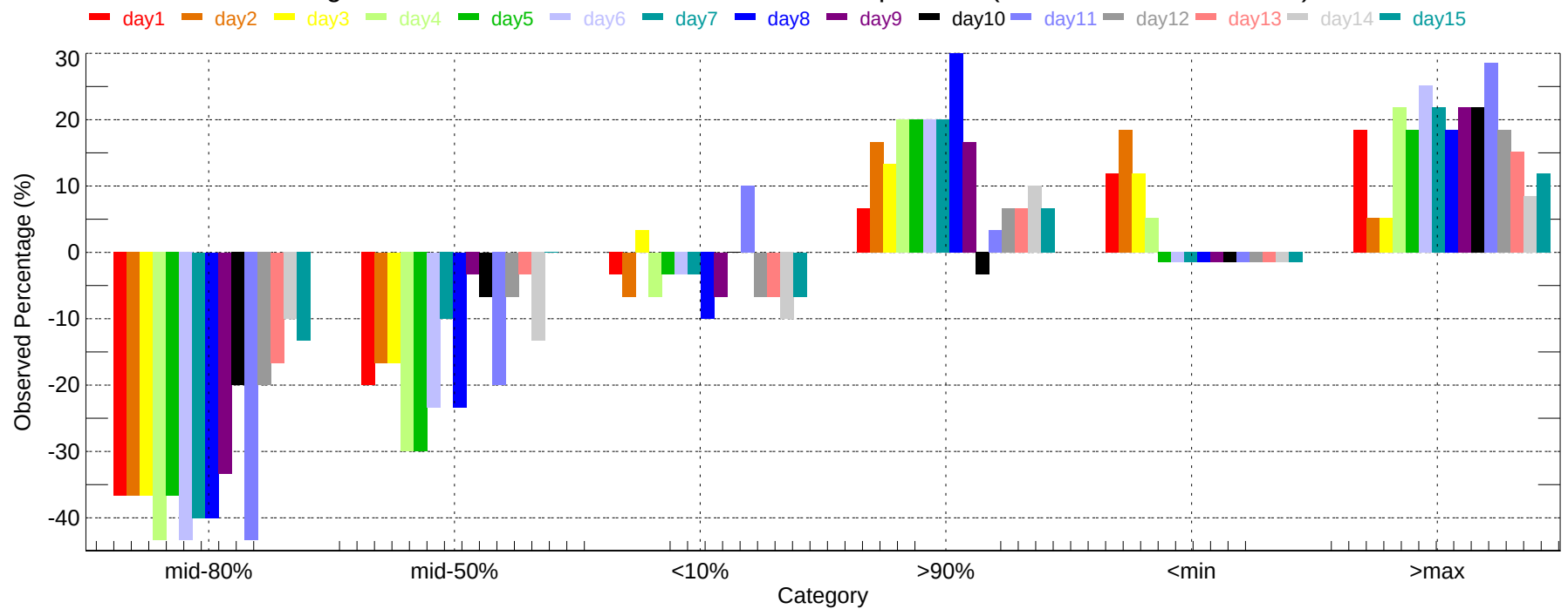
Observed Percentage Deviation of Ensembles - MCN: Max Temperature (2007-12-01~2007-12-31)
