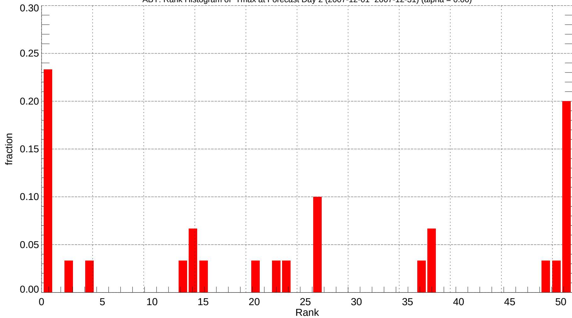
ABY: Rank Histogram of Tmax at Forecast Day 2 (2007-12-01~2007-12-31) (alpha = 0.00)
