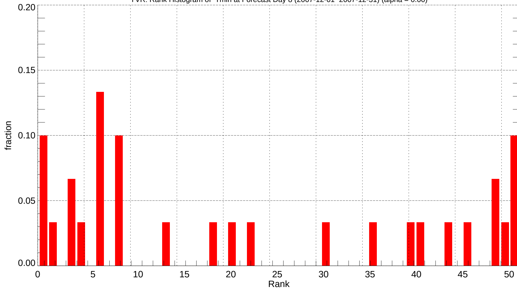
YVR: Rank Histogram of Tmin at Forecast Day 8 (2007-12-01~2007-12-31) (alpha = 0.00)
