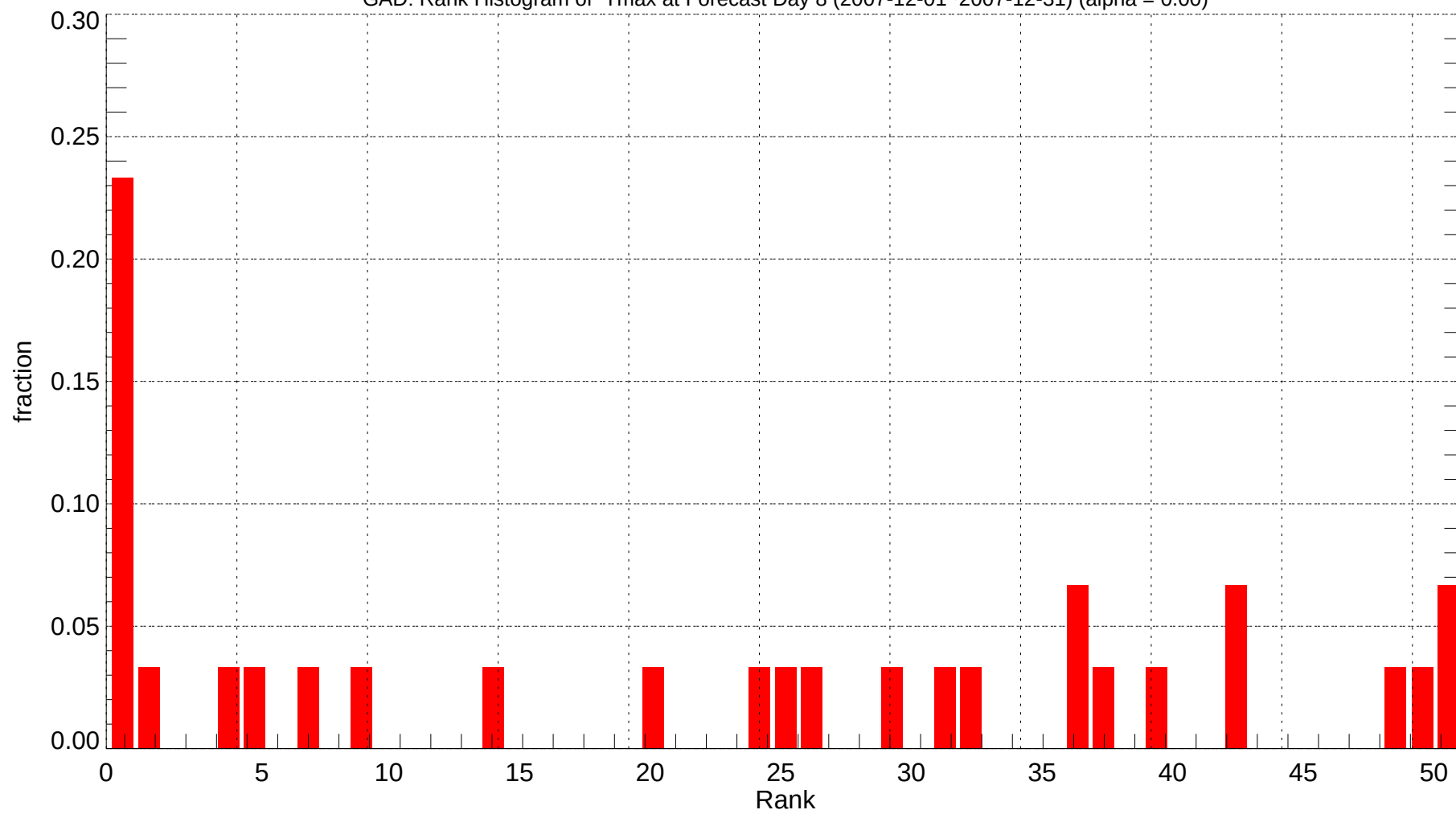
GAD: Rank Histogram of Tmax at Forecast Day 8 (2007-12-01~2007-12-31) (alpha = 0.00)
