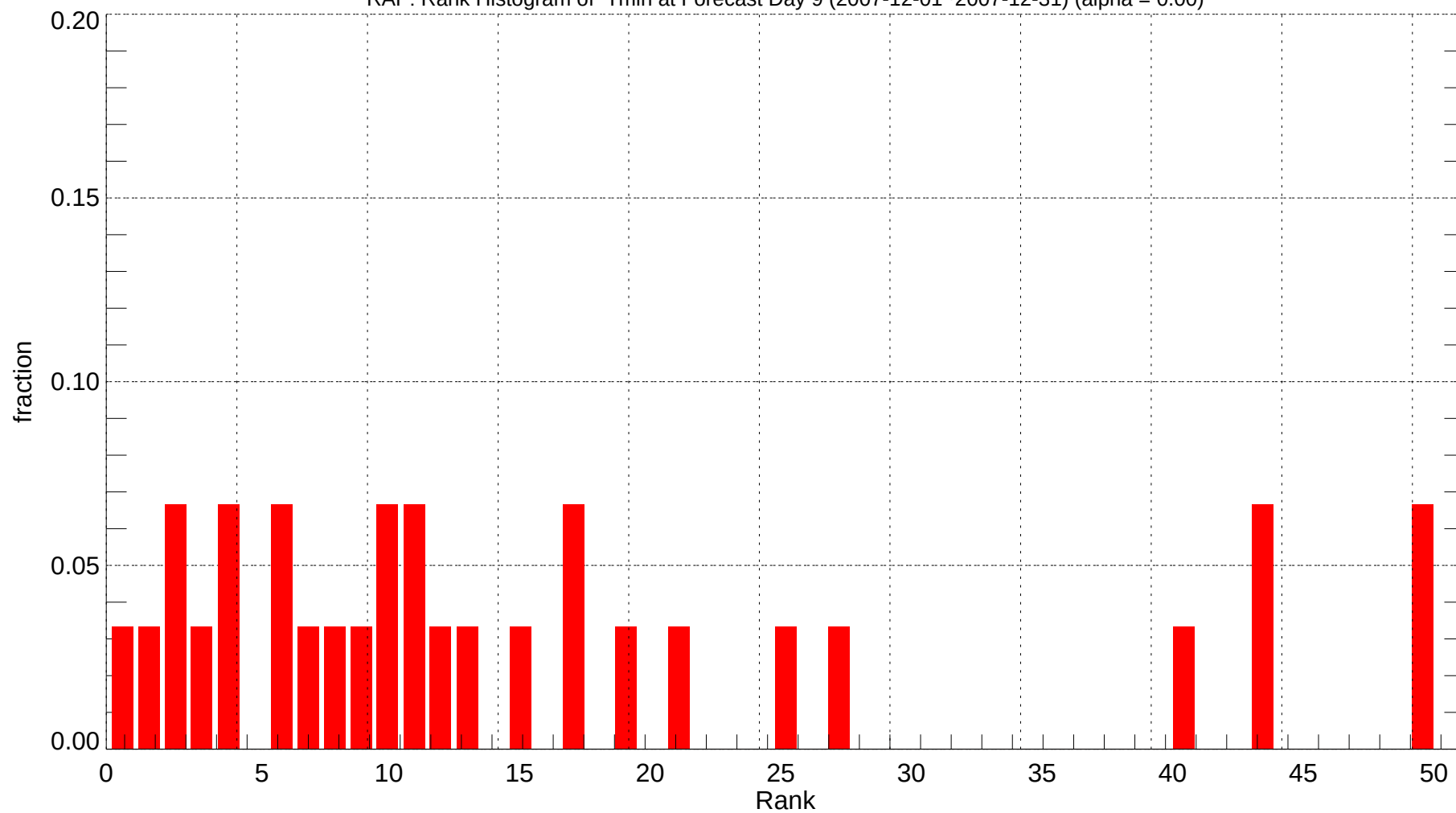
RAP: Rank Histogram of Tmin at Forecast Day 9 (2007-12-01~2007-12-31) (alpha = 0.00)
