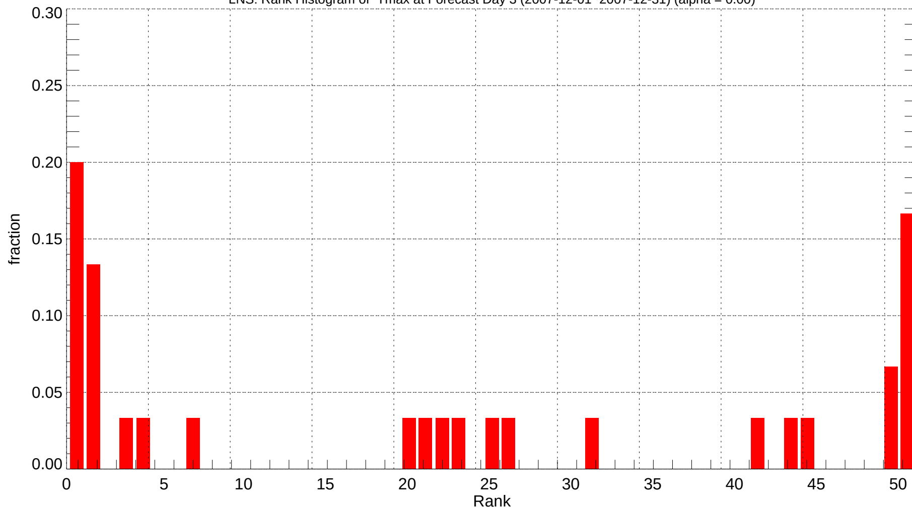
LNS: Rank Histogram of Tmax at Forecast Day 3 (2007-12-01~2007-12-31) (alpha = 0.00)
