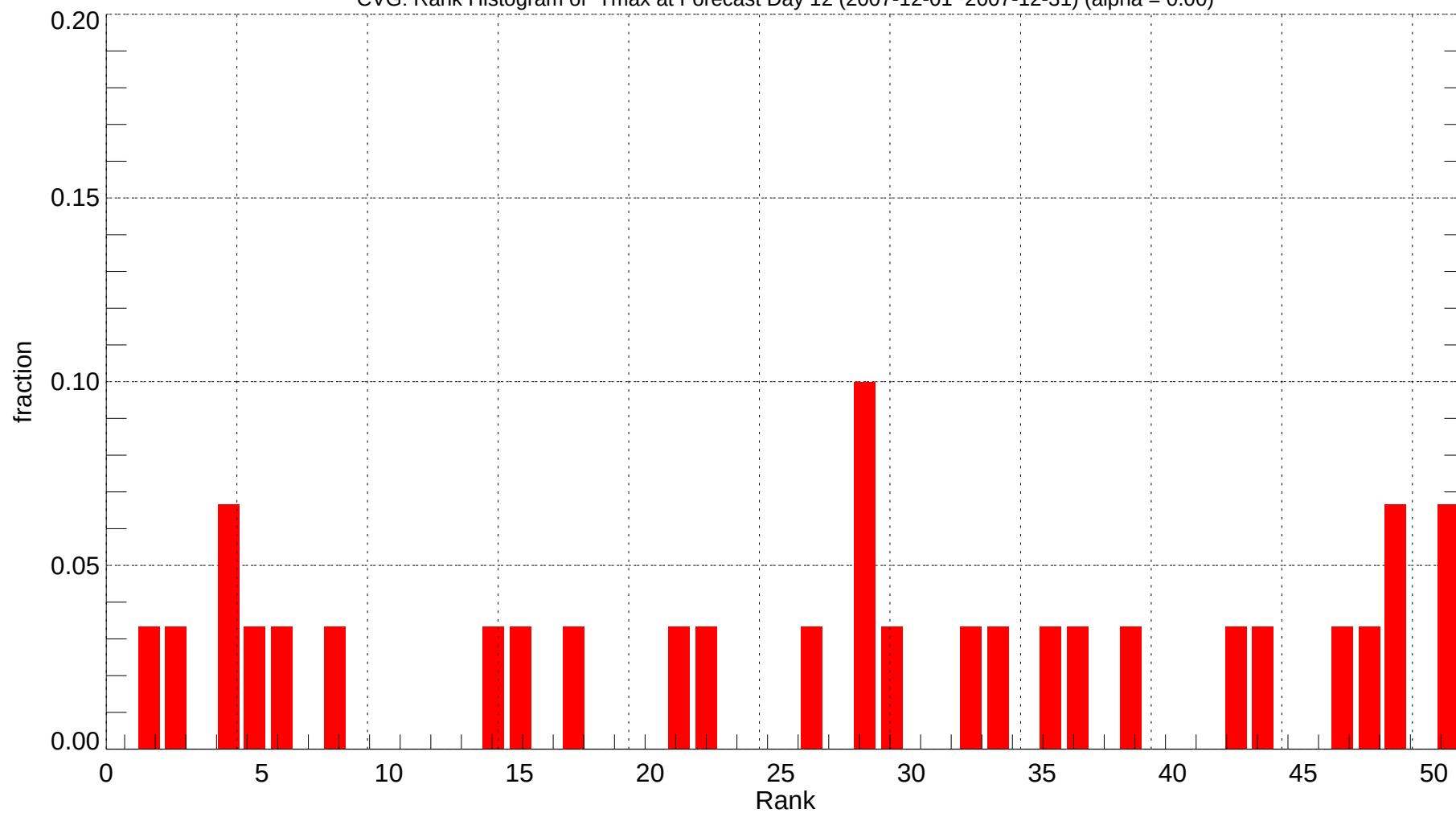
CVG: Rank Histogram of Tmax at Forecast Day 12 (2007-12-01~2007-12-31) (alpha = 0.00)
