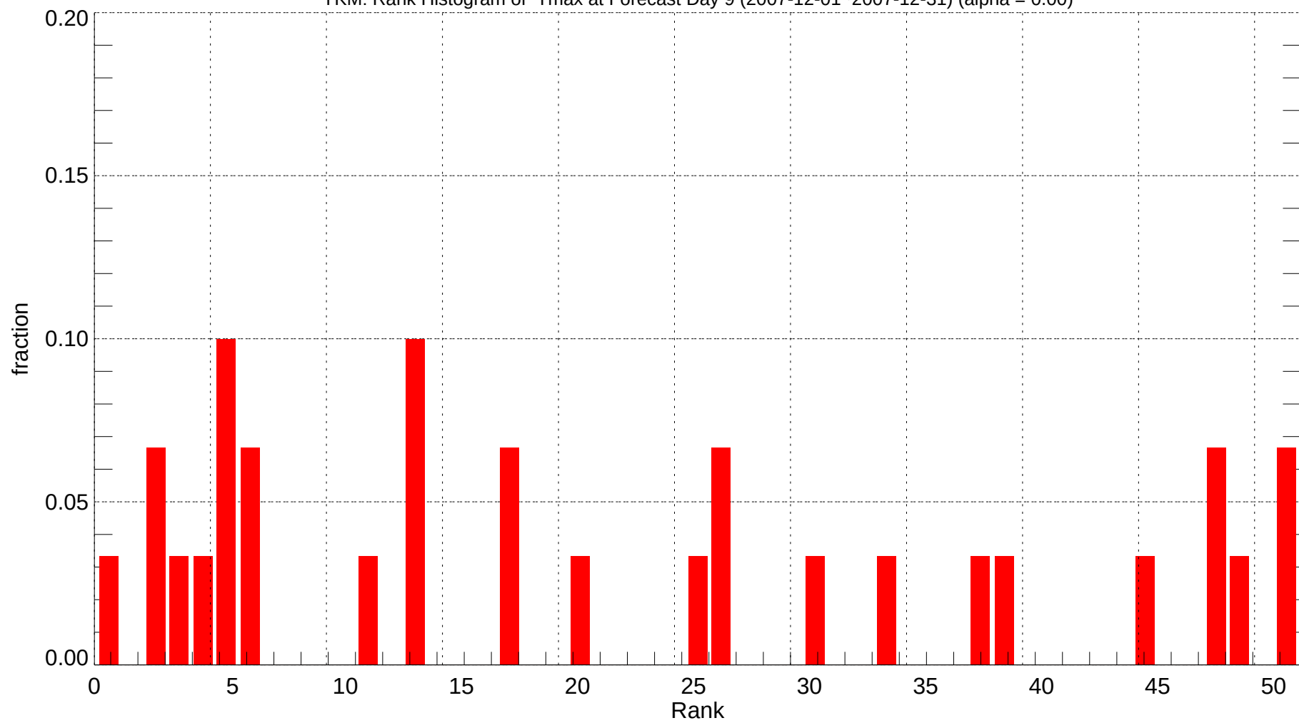
YKM: Rank Histogram of Tmax at Forecast Day 9 (2007-12-01~2007-12-31) (alpha = 0.00)
