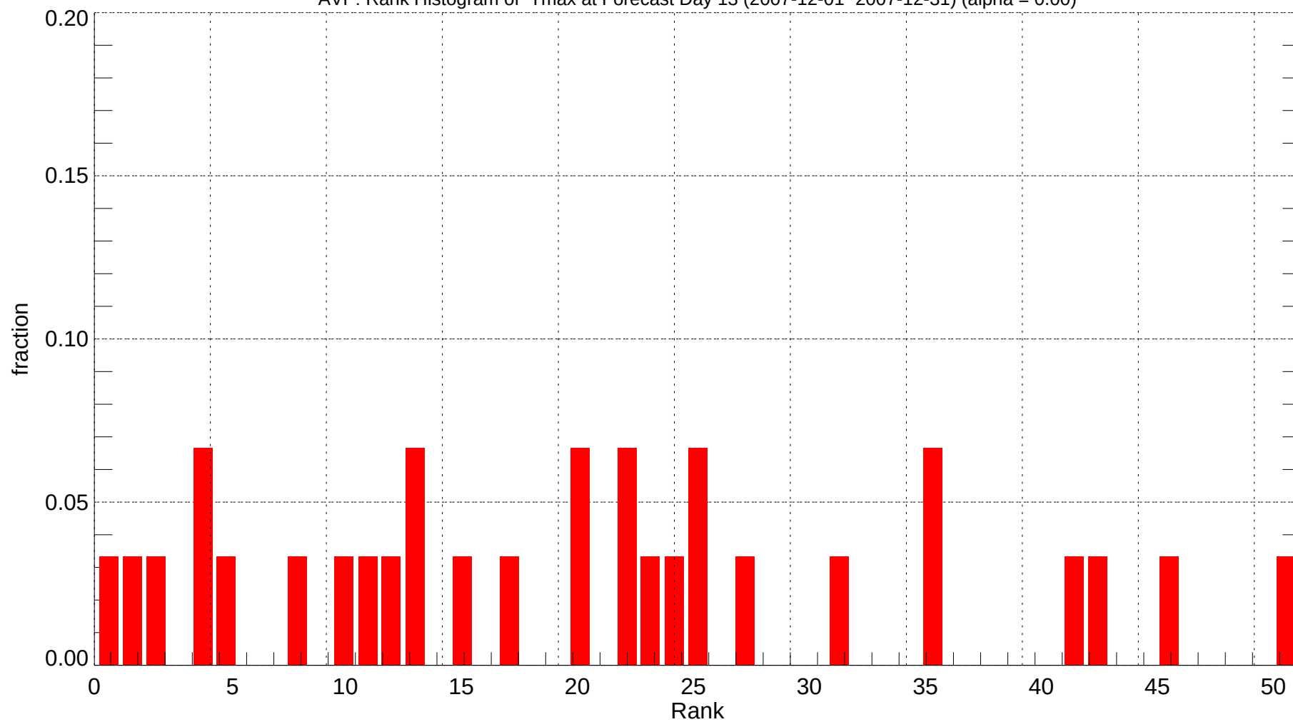
AVP: Rank Histogram of Tmax at Forecast Day 13 (2007-12-01~2007-12-31) (alpha = 0.00)
