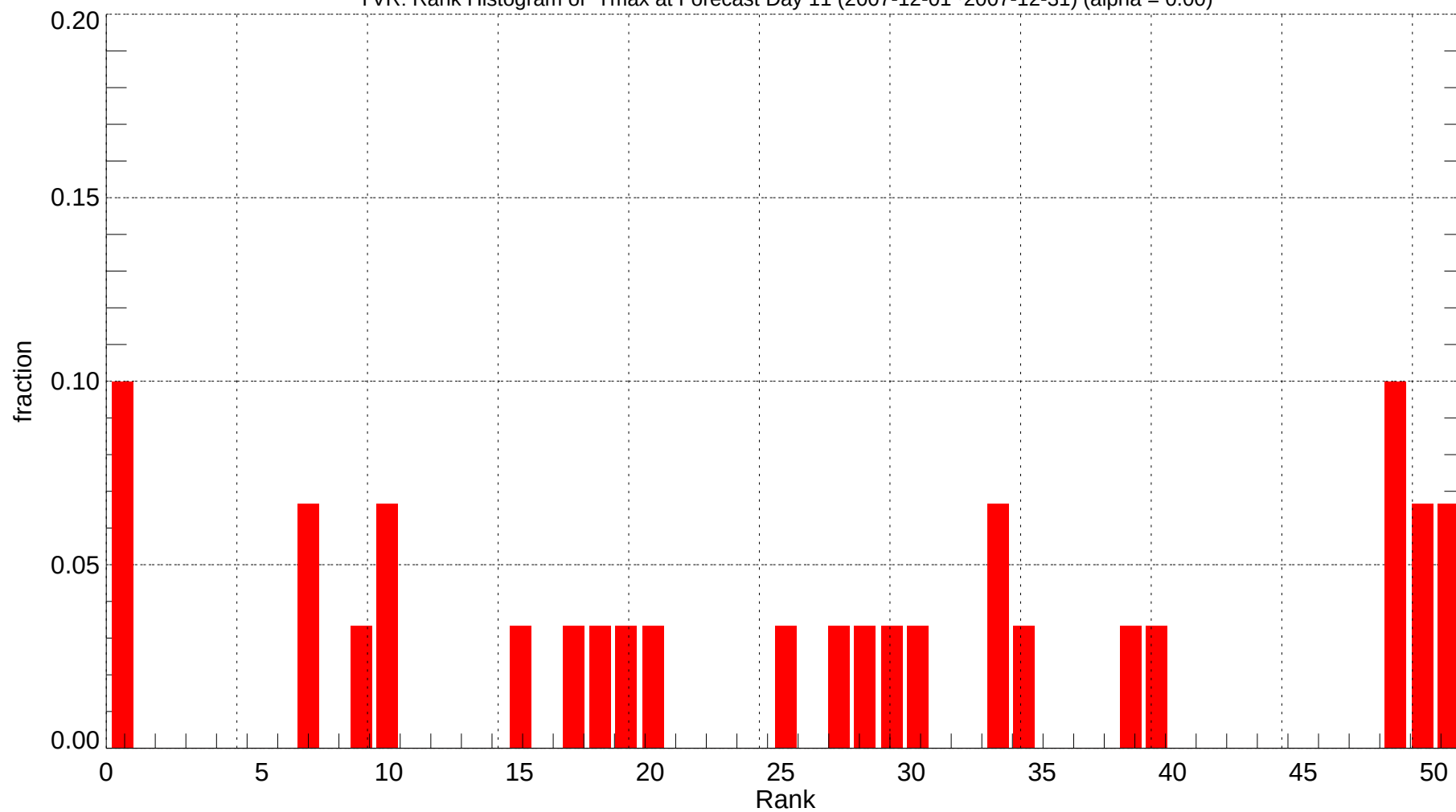
YVR: Rank Histogram of Tmax at Forecast Day 11 (2007-12-01~2007-12-31) (alpha = 0.00)
