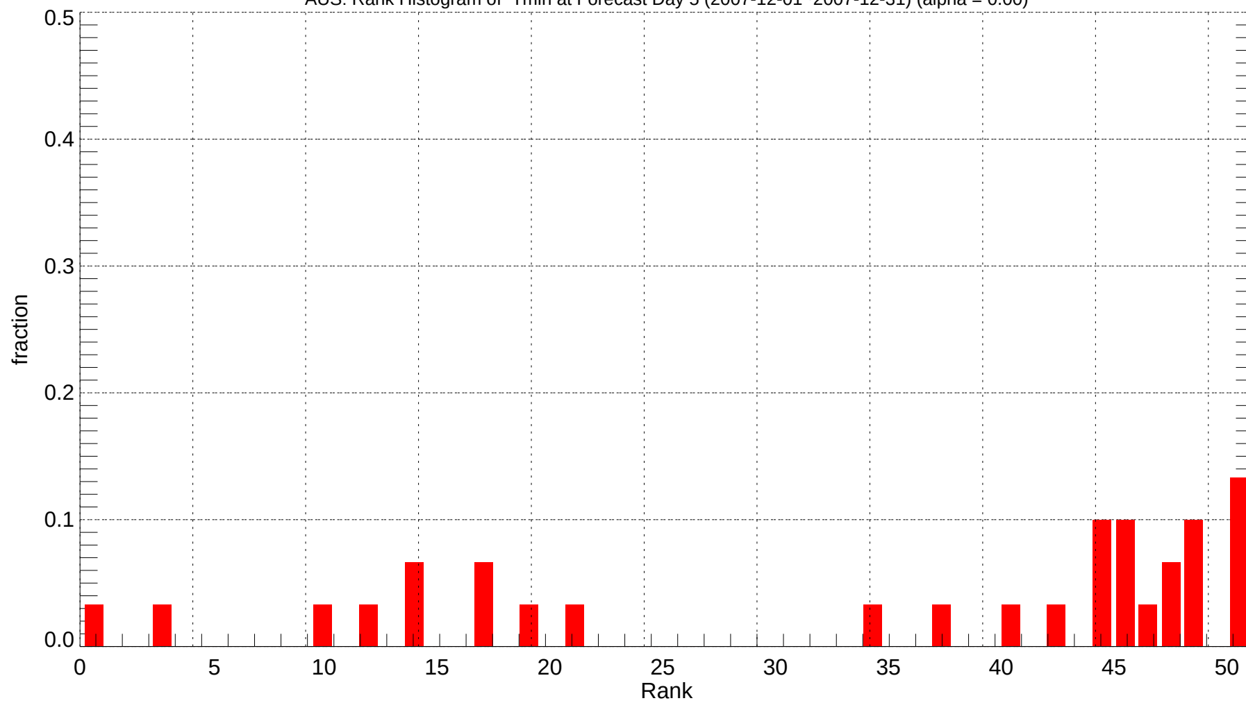
AUS: Rank Histogram of Tmin at Forecast Day 5 (2007-12-01~2007-12-31) (alpha = 0.00)
