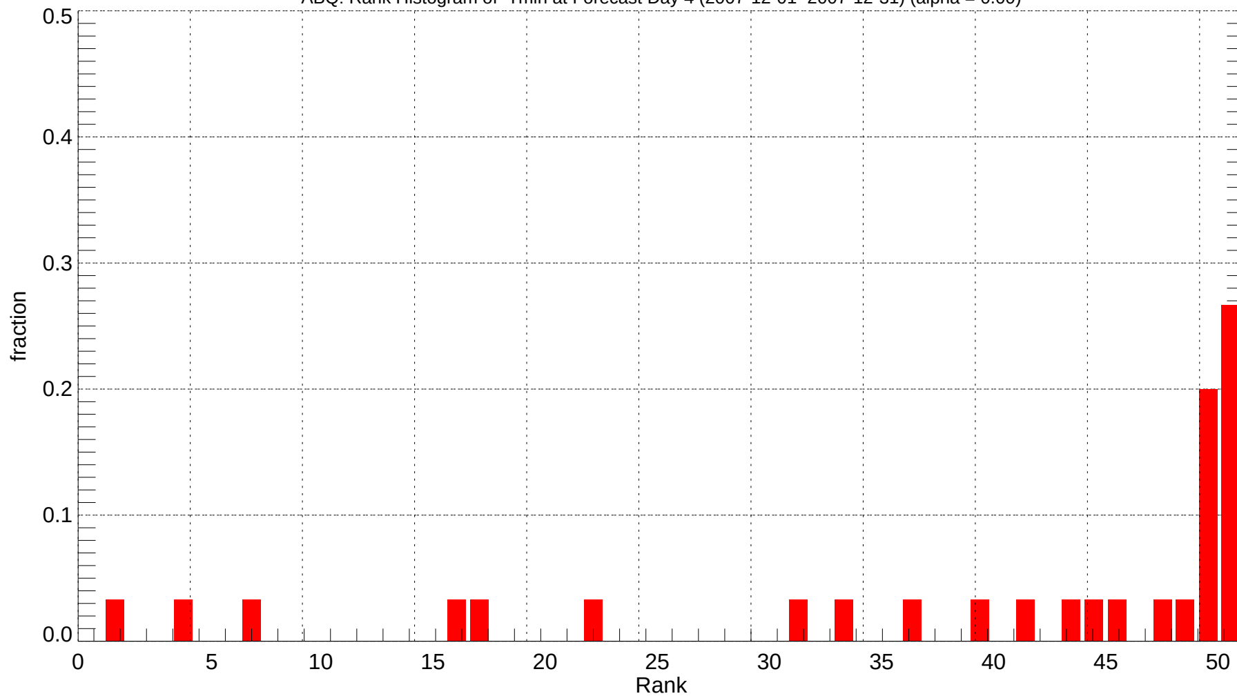
ABQ: Rank Histogram of Tmin at Forecast Day 4 (2007-12-01~2007-12-31) (alpha = 0.00)
