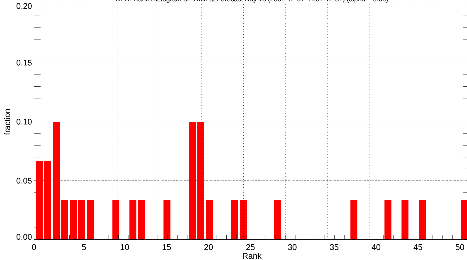
DEN: Rank Histogram of Tmin at Forecast Day 13 (2007-12-01~2007-12-31) (alpha = 0.00)
