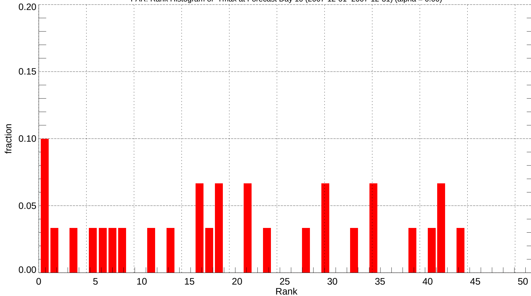
FAR: Rank Histogram of Tmax at Forecast Day 10 (2007-12-01~2007-12-31) (alpha = 0.00)
