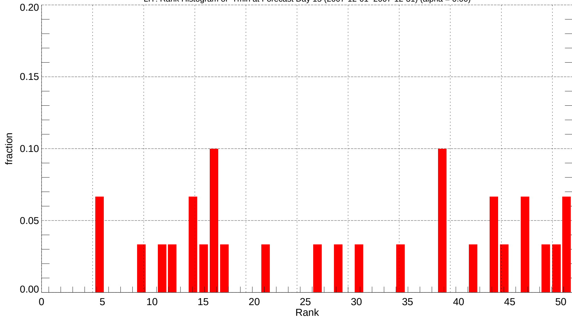
LIT: Rank Histogram of Tmin at Forecast Day 15 (2007-12-01~2007-12-31) (alpha = 0.00)
