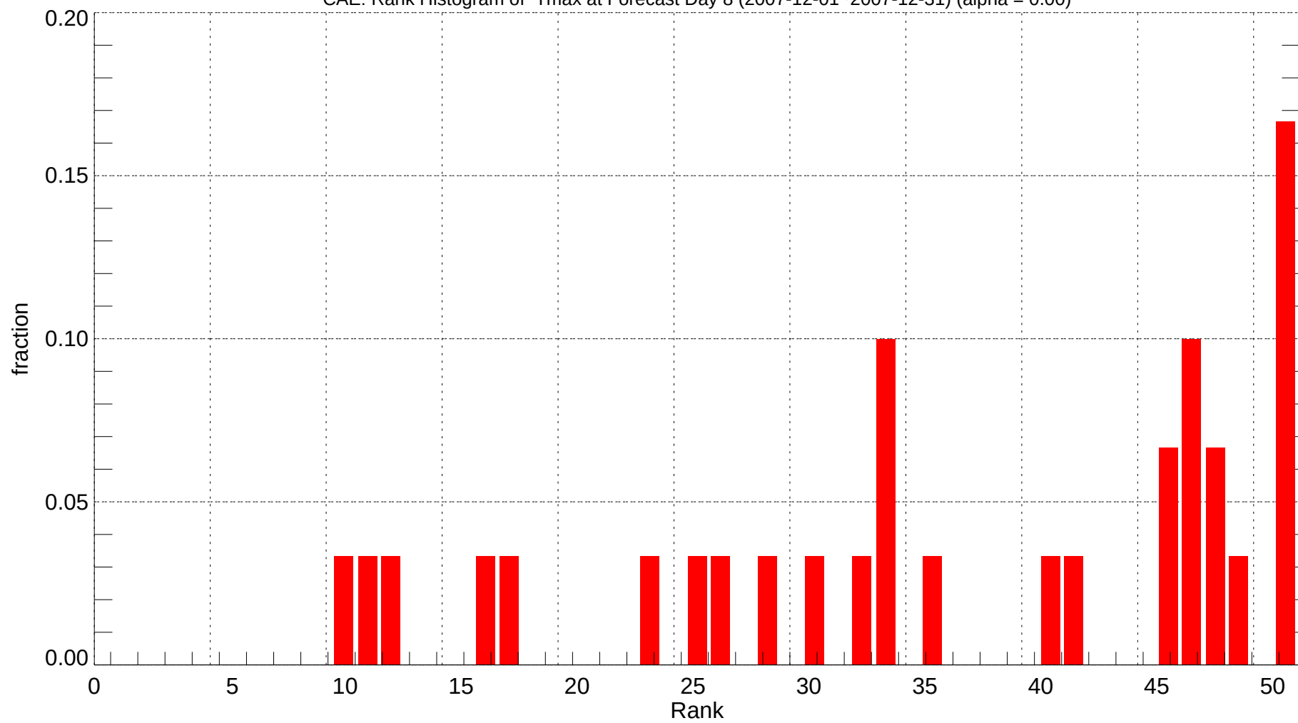
CAE: Rank Histogram of Tmax at Forecast Day 8 (2007-12-01~2007-12-31) (alpha = 0.00)
