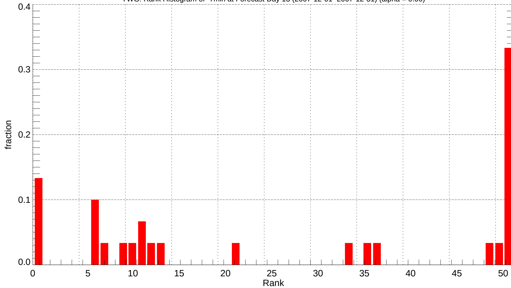
YWG: Rank Histogram of Tmin at Forecast Day 13 (2007-12-01~2007-12-31) (alpha = 0.00)
