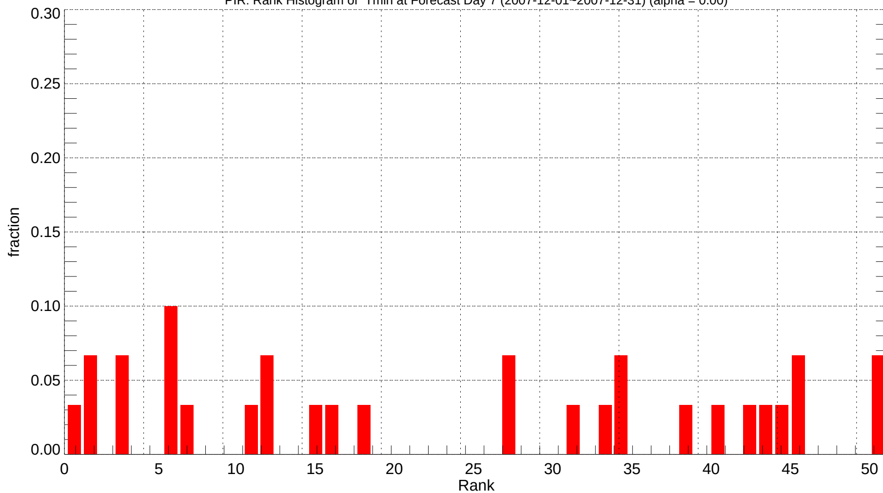
PIR: Rank Histogram of Tmin at Forecast Day 7 (2007-12-01~2007-12-31) (alpha = 0.00)
