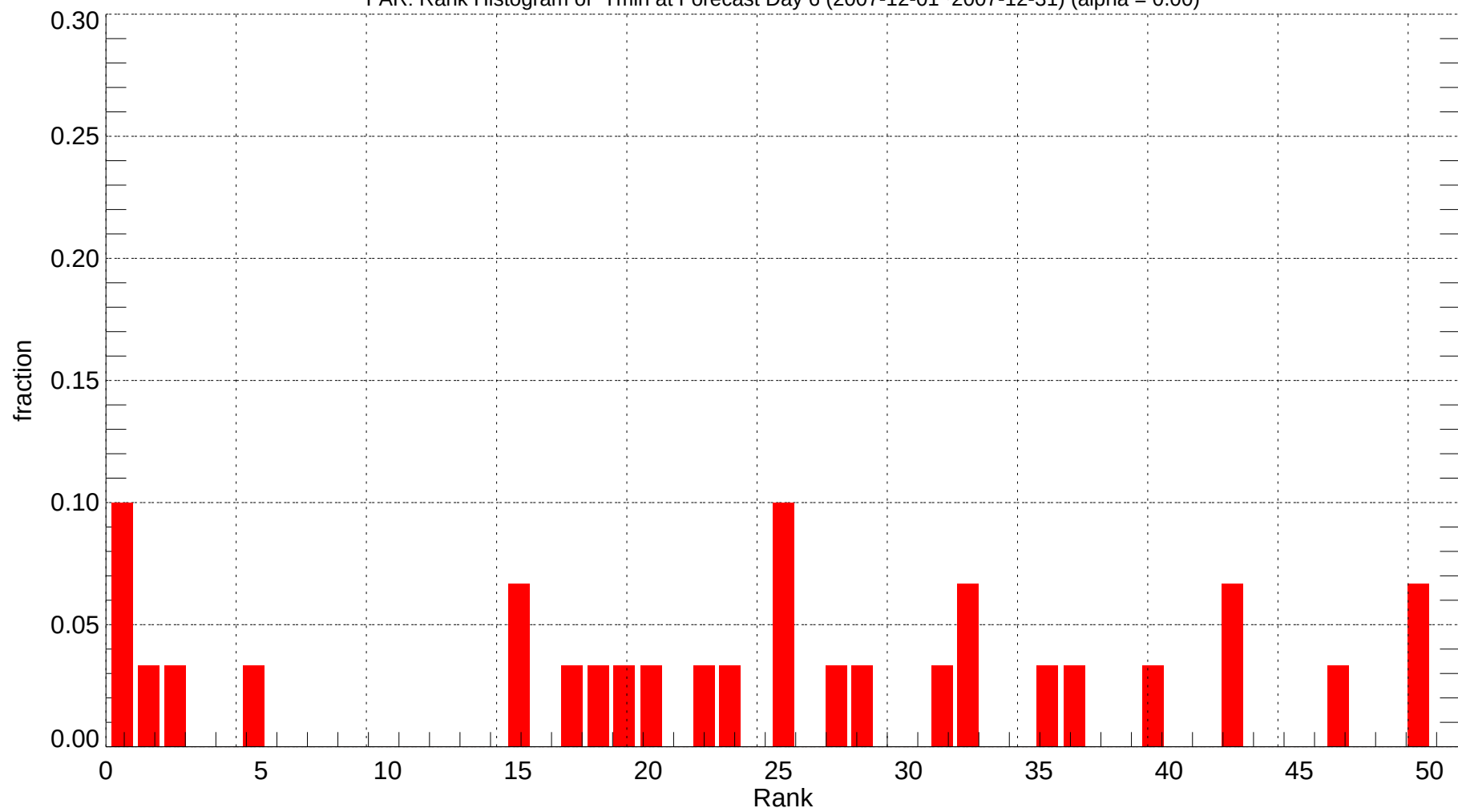
FAR: Rank Histogram of Tmin at Forecast Day 6 (2007-12-01~2007-12-31) (alpha = 0.00)
