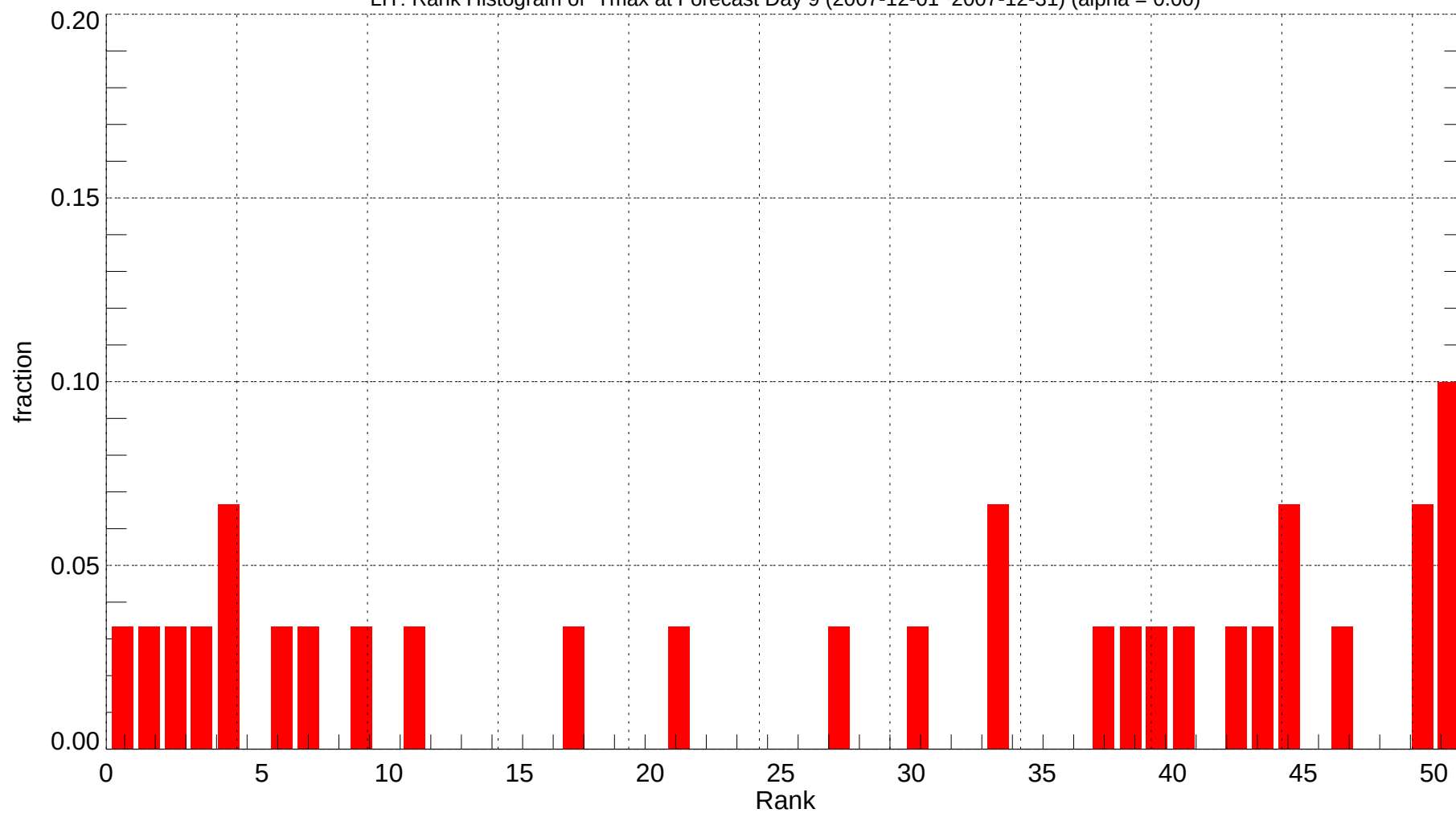
LIT: Rank Histogram of Tmax at Forecast Day 9 (2007-12-01~2007-12-31) (alpha = 0.00)
