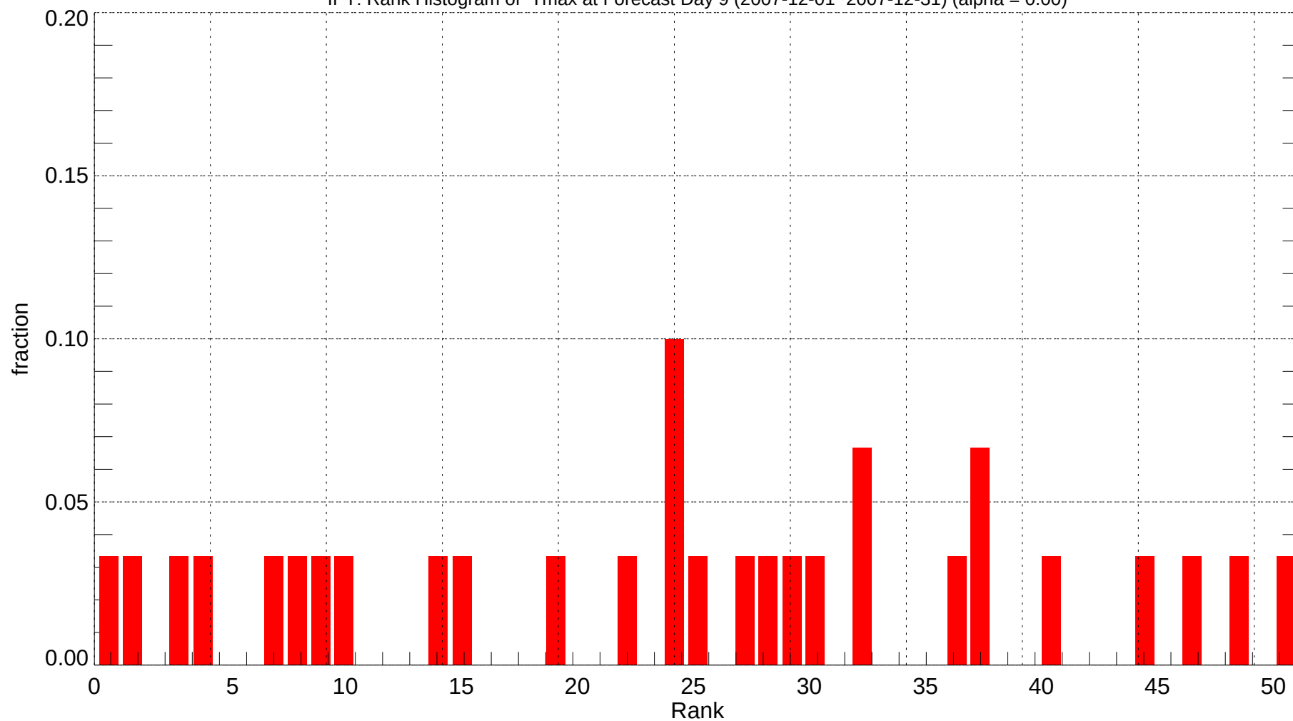
IPT: Rank Histogram of Tmax at Forecast Day 9 (2007-12-01~2007-12-31) (alpha = 0.00)
