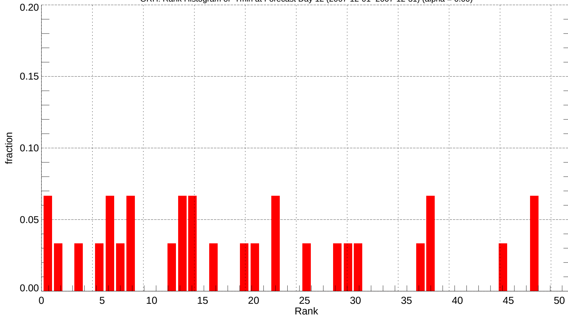
ORH: Rank Histogram of Tmin at Forecast Day 12 (2007-12-01~2007-12-31) (alpha = 0.00)
