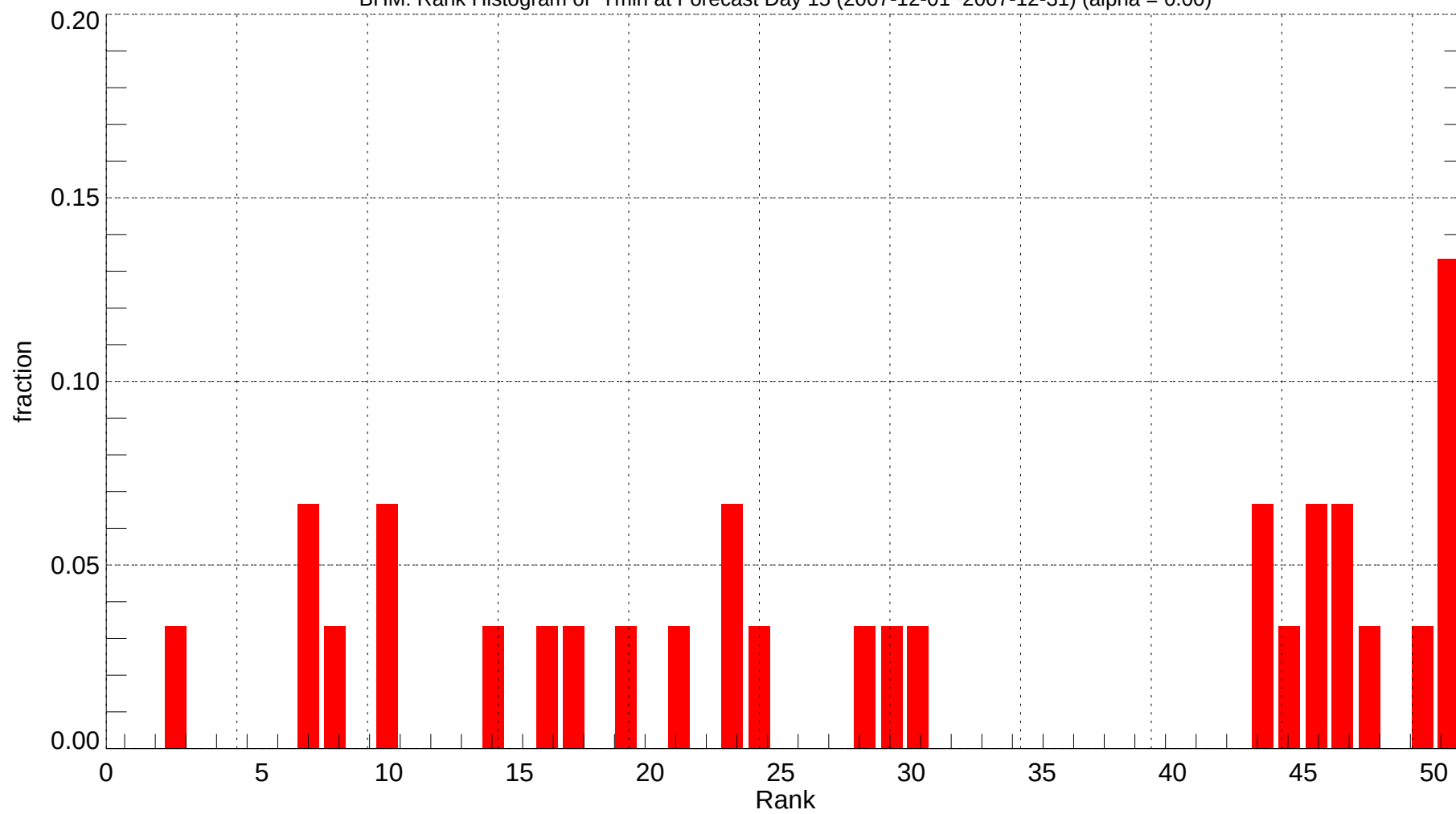
BHM: Rank Histogram of Tmin at Forecast Day 15 (2007-12-01~2007-12-31) (alpha = 0.00)
