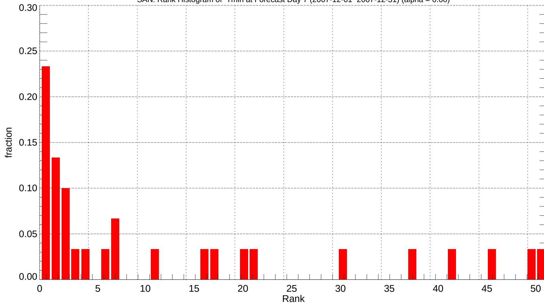
SAN: Rank Histogram of Tmin at Forecast Day 7 (2007-12-01~2007-12-31) (alpha = 0.00)
