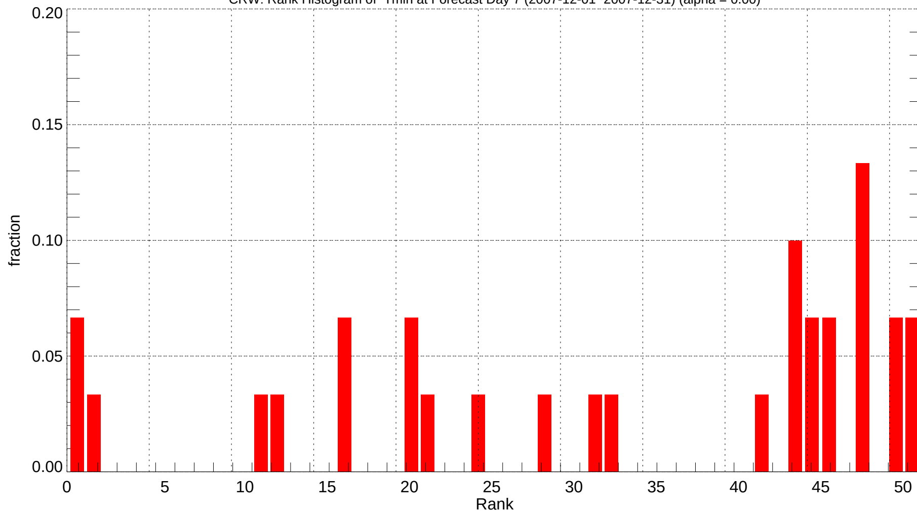
CRW: Rank Histogram of Tmin at Forecast Day 7 (2007-12-01~2007-12-31) (alpha = 0.00)
