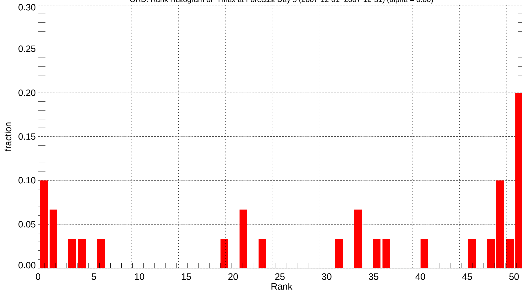
ORD: Rank Histogram of Tmax at Forecast Day 5 (2007-12-01~2007-12-31) (alpha = 0.00)
