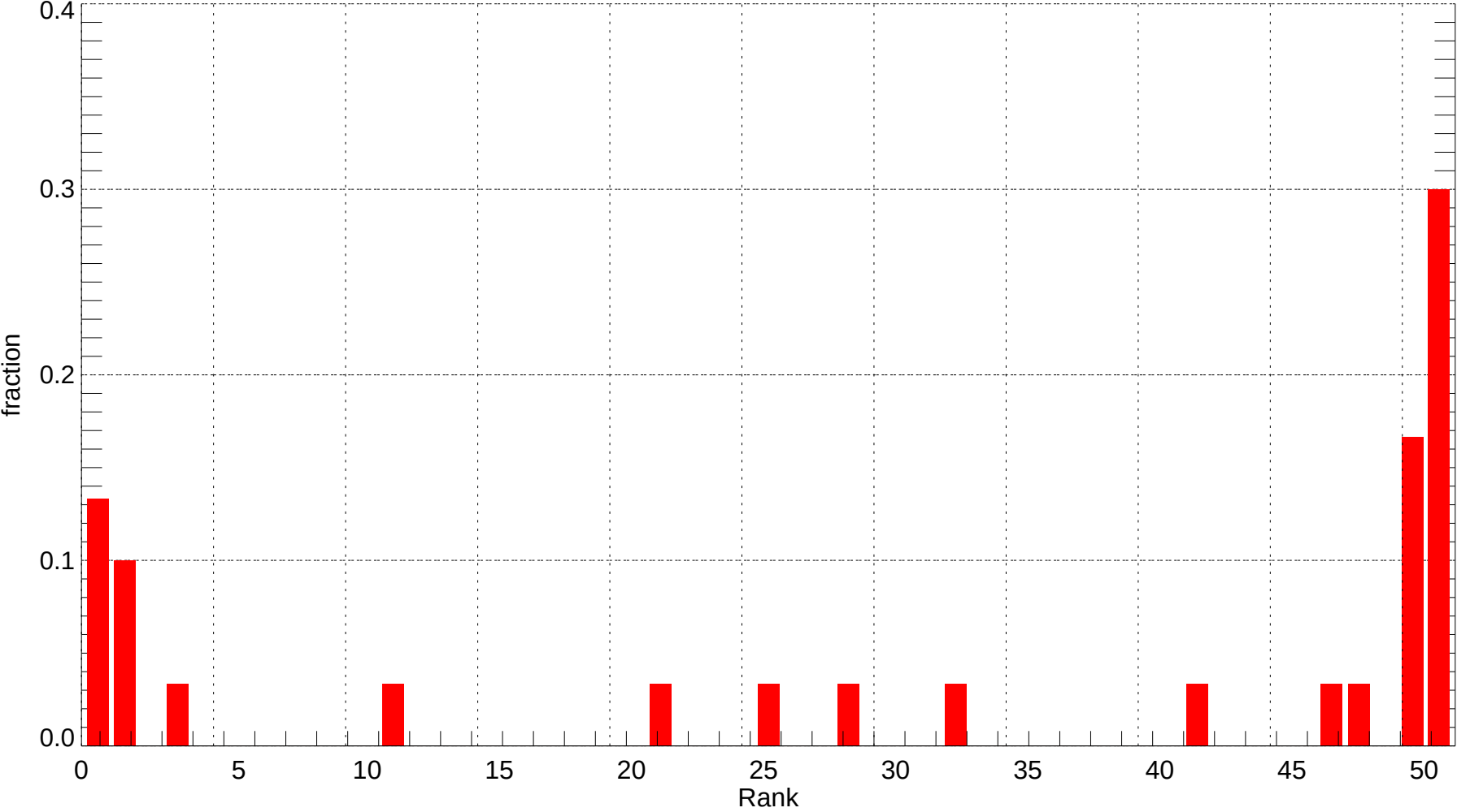
BFL: Rank Histogram of Tmin at Forecast Day 3 (2007-12-01~2007-12-31) (alpha = 0.00)
