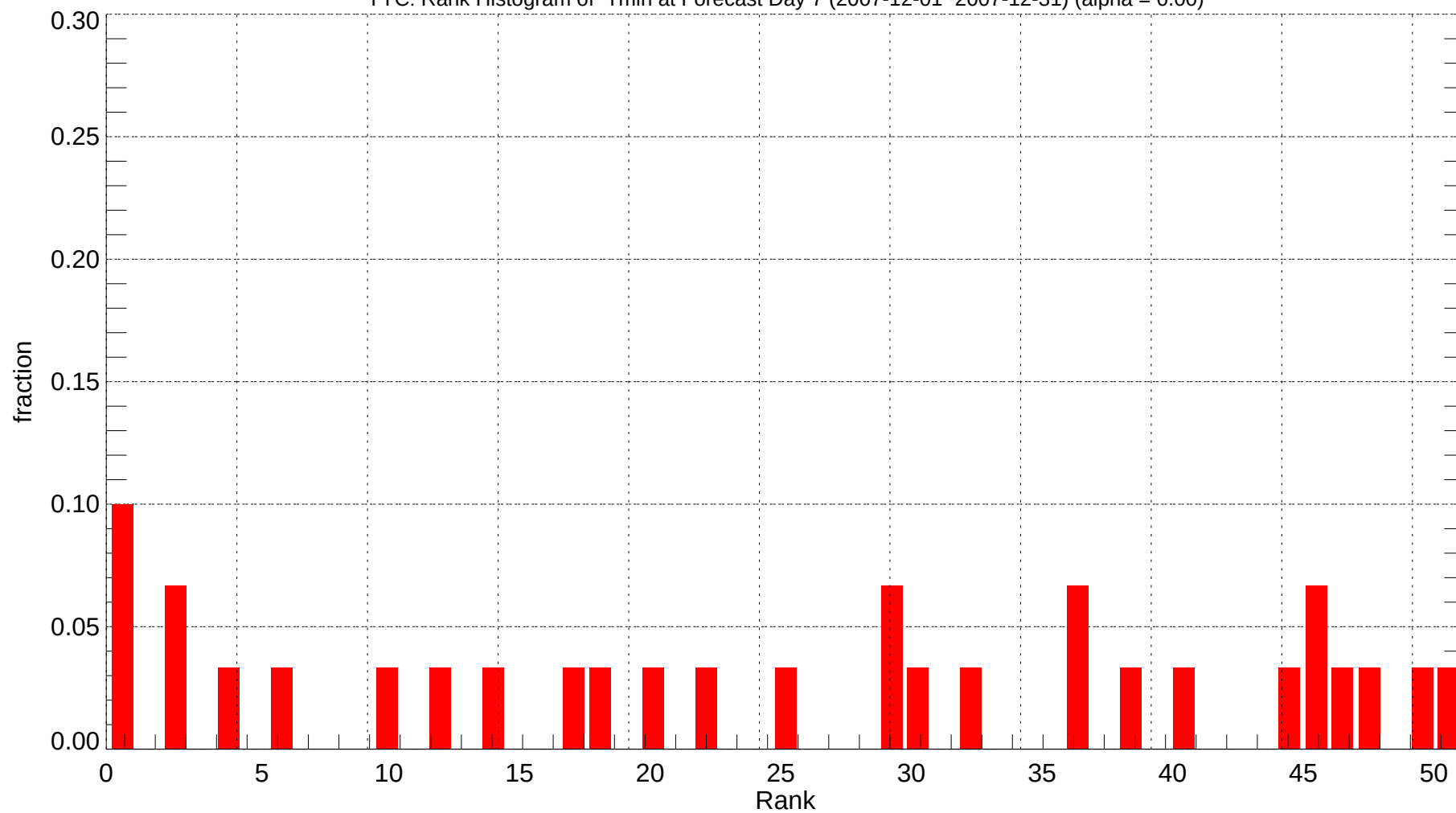
YYC: Rank Histogram of Tmin at Forecast Day 7 (2007-12-01~2007-12-31) (alpha = 0.00)
