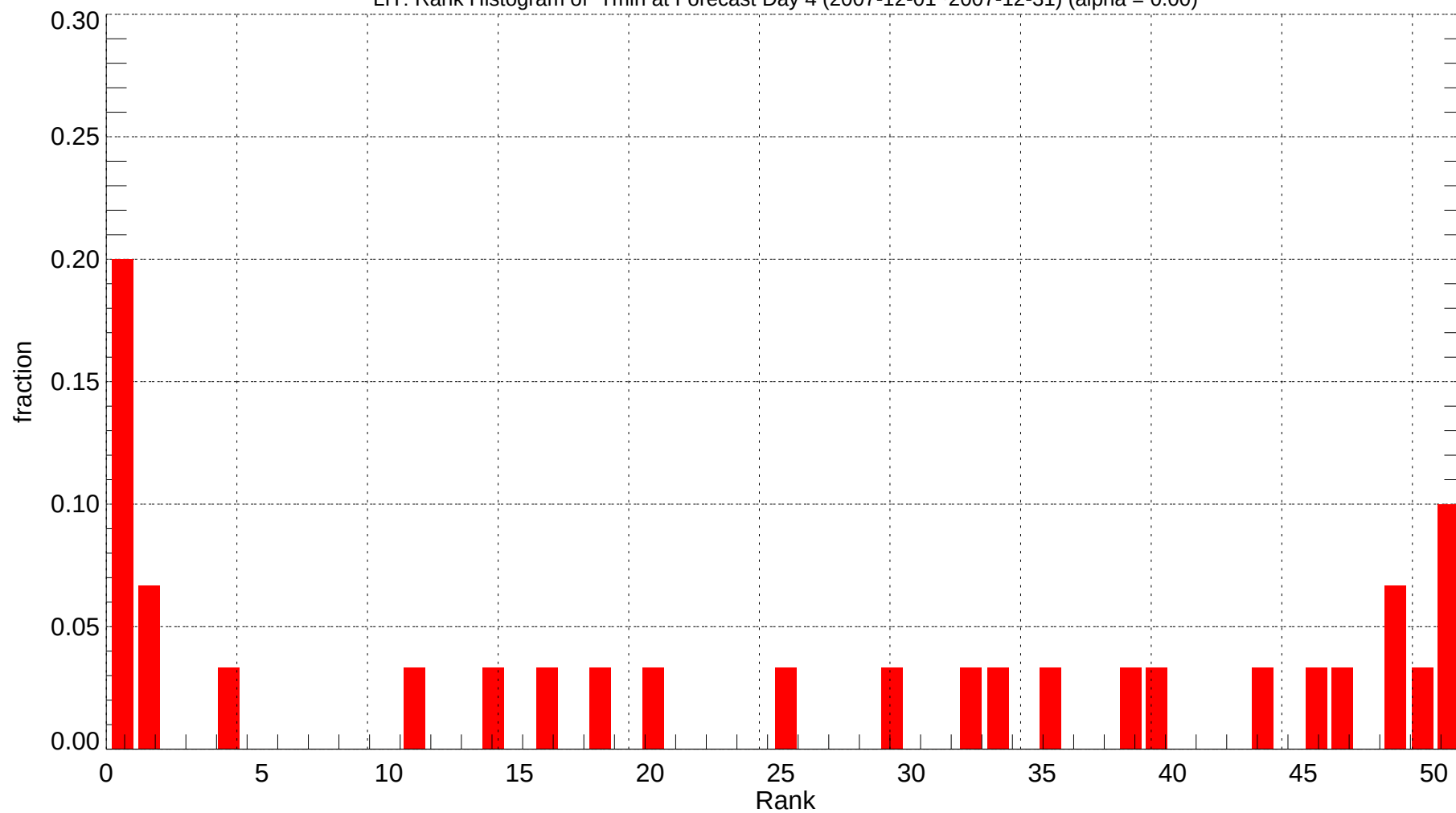
LIT: Rank Histogram of Tmin at Forecast Day 4 (2007-12-01~2007-12-31) (alpha = 0.00)
