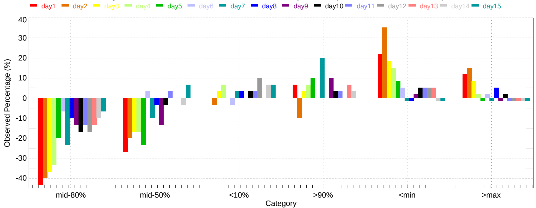
Observed Percentage Deviation of Ensembles - FWA: Min Temperature (2007-12-01~2007-12-31)
