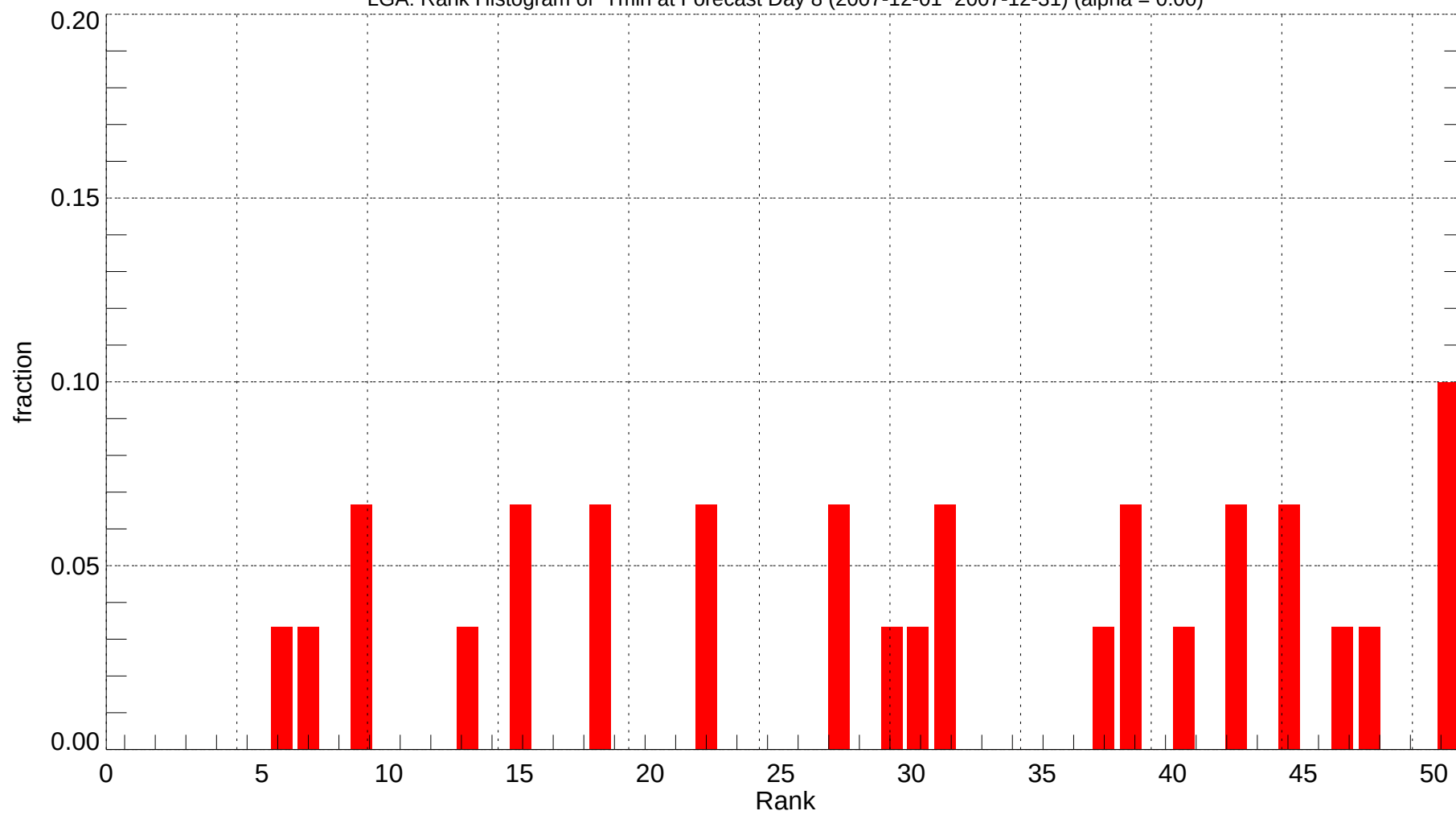
LGA: Rank Histogram of Tmin at Forecast Day 8 (2007-12-01~2007-12-31) (alpha = 0.00)
