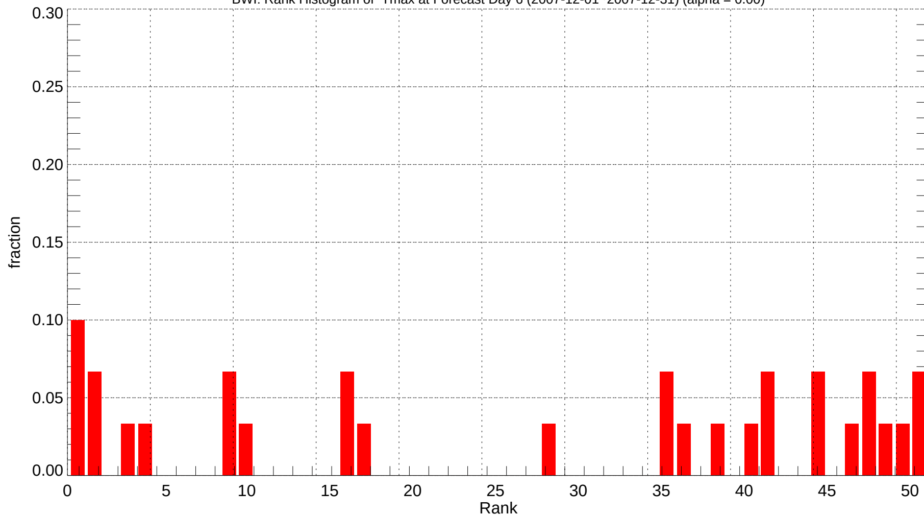
BWI: Rank Histogram of Tmax at Forecast Day 6 (2007-12-01~2007-12-31) (alpha = 0.00)
