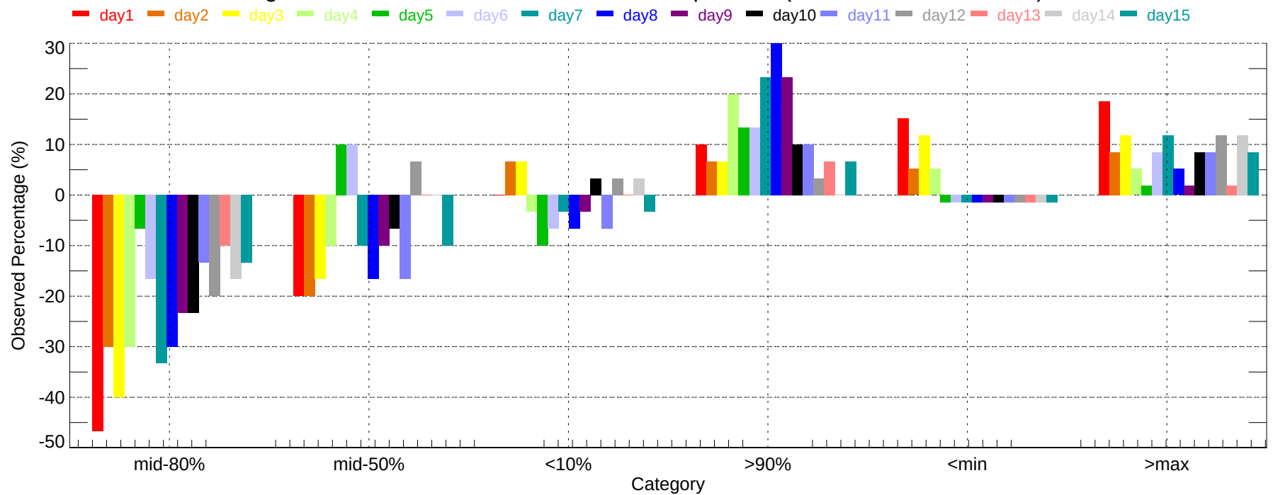
Observed Percentage Deviation of Ensembles - IAH: Min Temperature (2007-12-01~2007-12-31)
