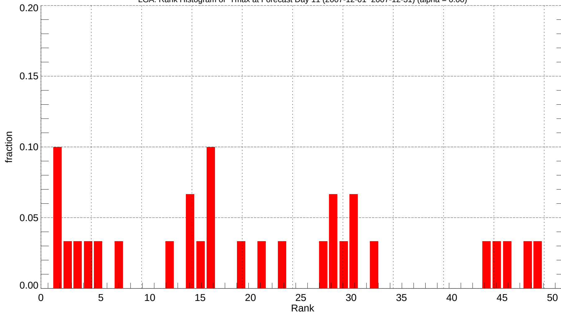
LGA: Rank Histogram of Tmax at Forecast Day 11 (2007-12-01~2007-12-31) (alpha = 0.00)
