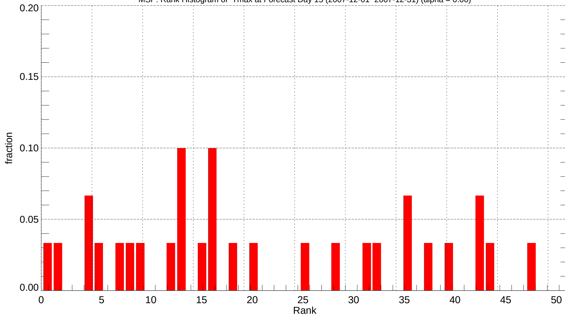
MSP: Rank Histogram of Tmax at Forecast Day 15 (2007-12-01~2007-12-31) (alpha = 0.00)
