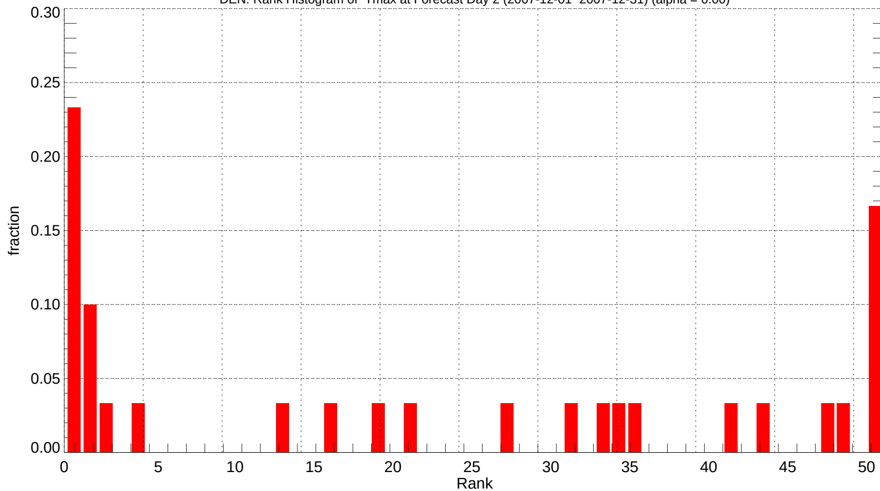
DEN: Rank Histogram of Tmax at Forecast Day 2 (2007-12-01~2007-12-31) (alpha = 0.00)
