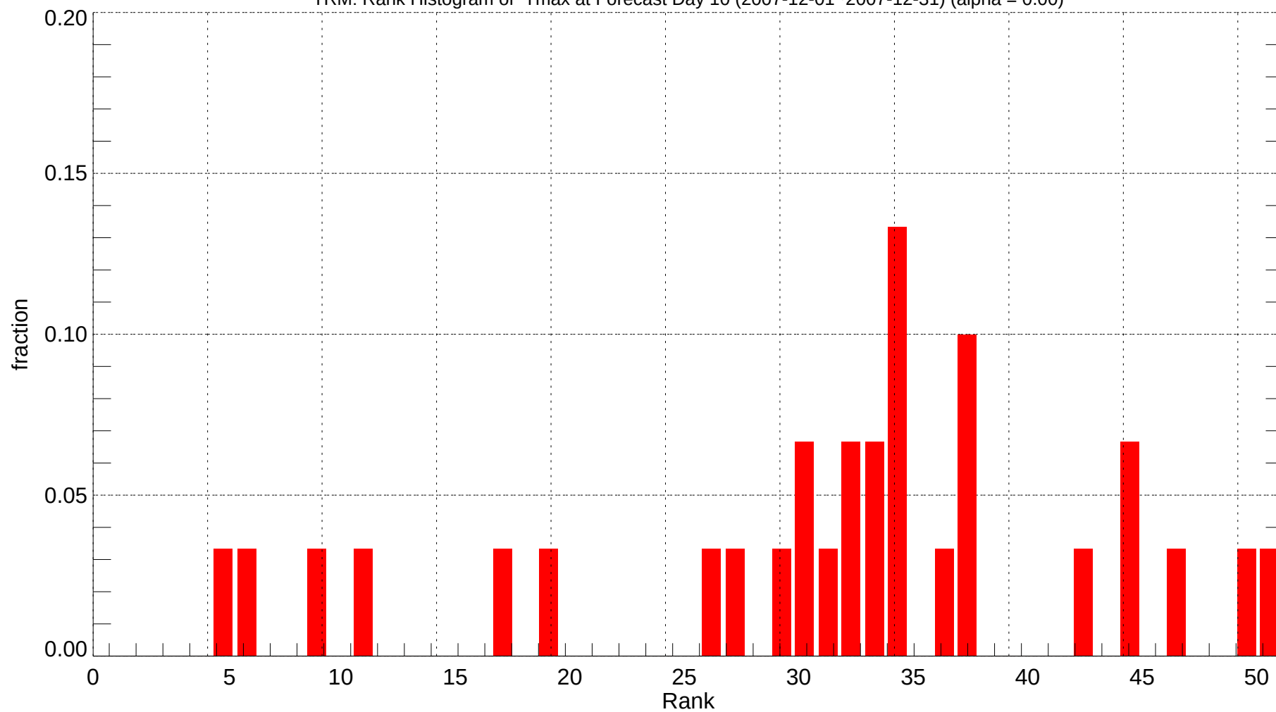
TRM: Rank Histogram of Tmax at Forecast Day 10 (2007-12-01~2007-12-31) (alpha = 0.00)
