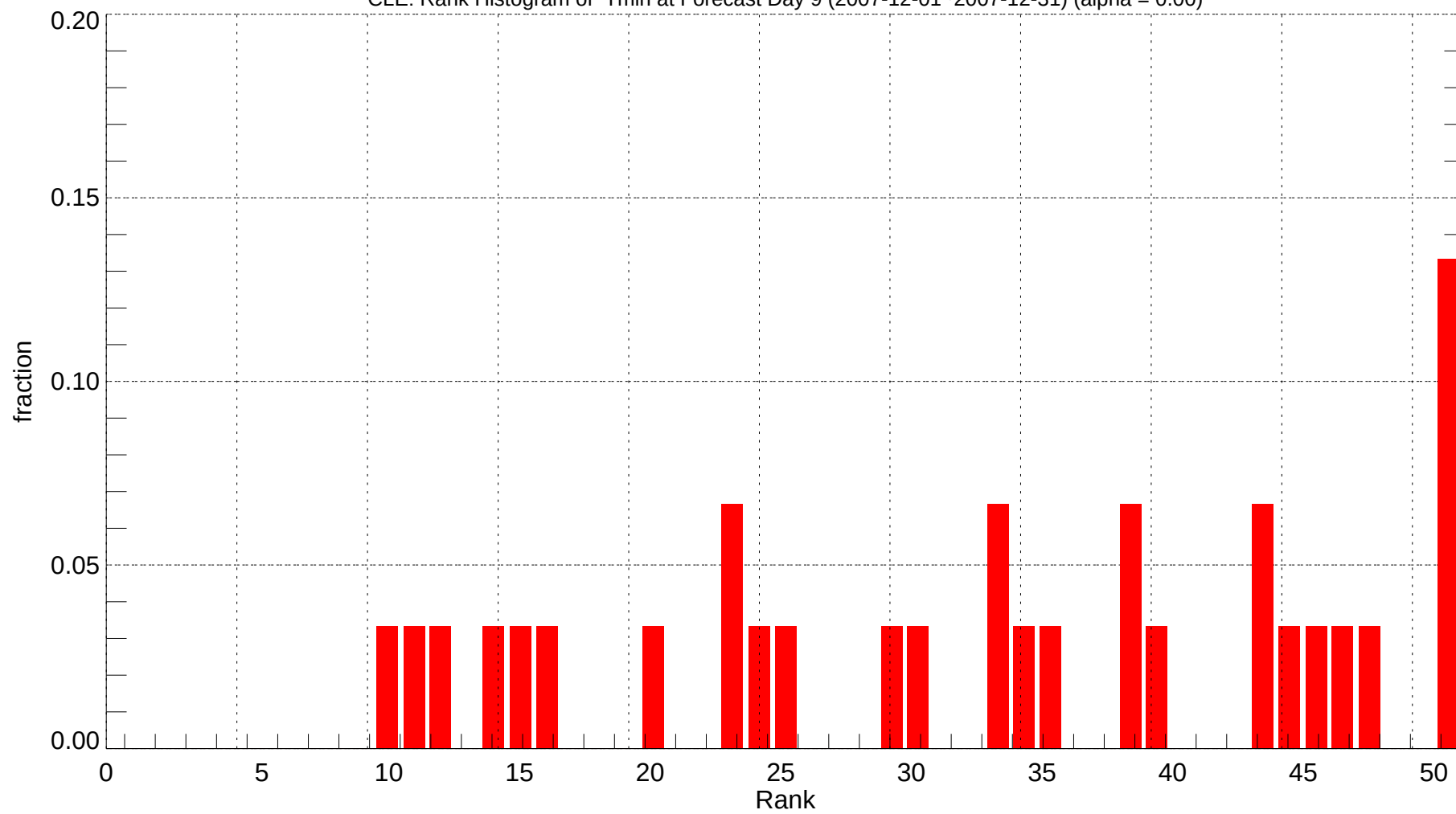
CLE: Rank Histogram of Tmin at Forecast Day 9 (2007-12-01~2007-12-31) (alpha = 0.00)
