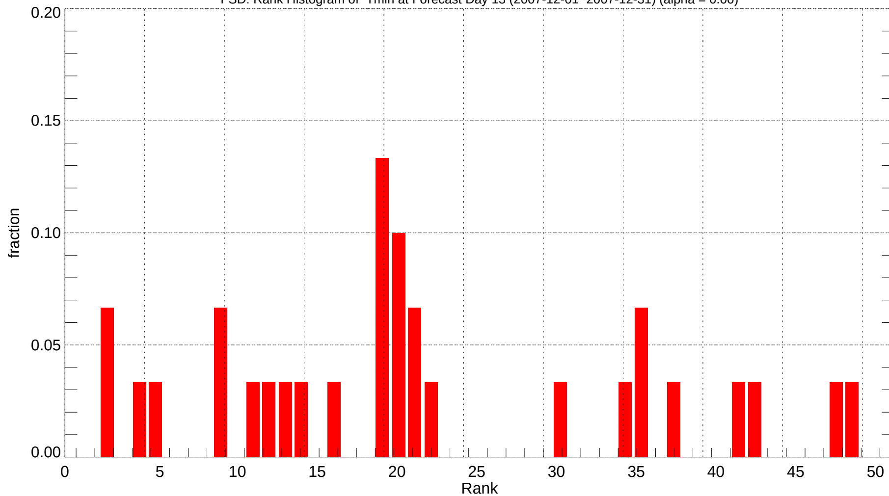
FSD: Rank Histogram of Tmin at Forecast Day 13 (2007-12-01~2007-12-31) (alpha = 0.00)
