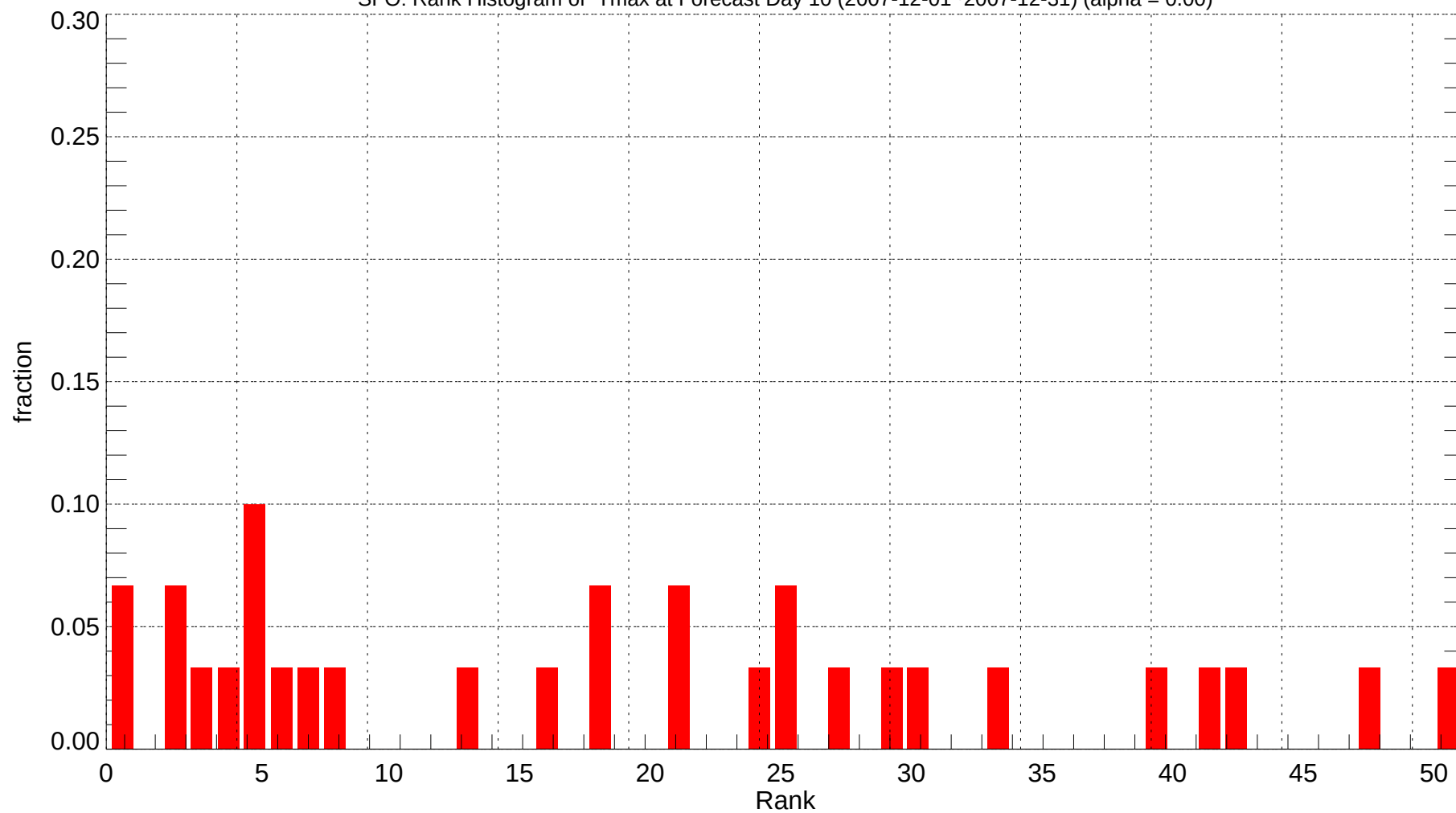
SFO: Rank Histogram of Tmax at Forecast Day 10 (2007-12-01~2007-12-31) (alpha = 0.00)
