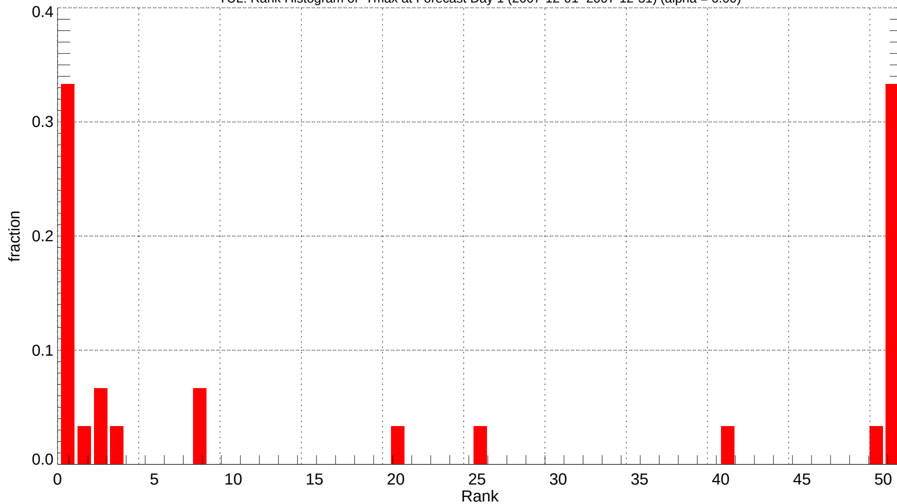
TUL: Rank Histogram of Tmax at Forecast Day 1 (2007-12-01~2007-12-31) (alpha = 0.00)
