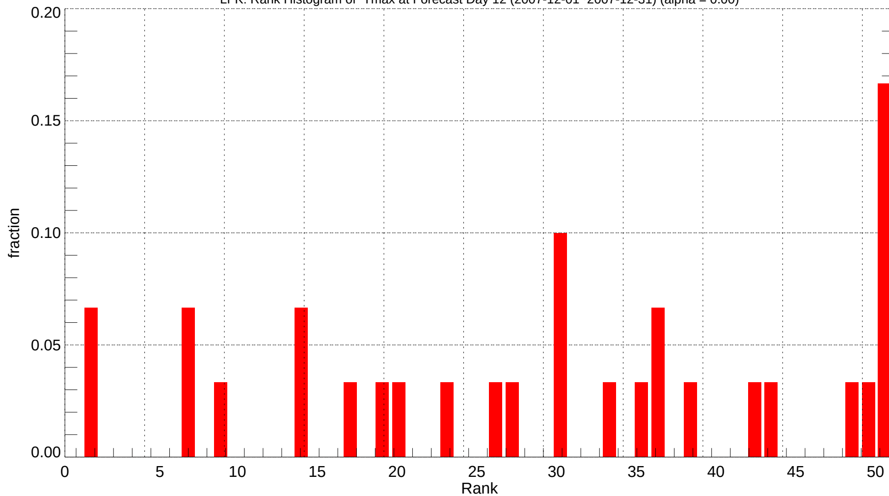
LFK: Rank Histogram of Tmax at Forecast Day 12 (2007-12-01~2007-12-31) (alpha = 0.00)
