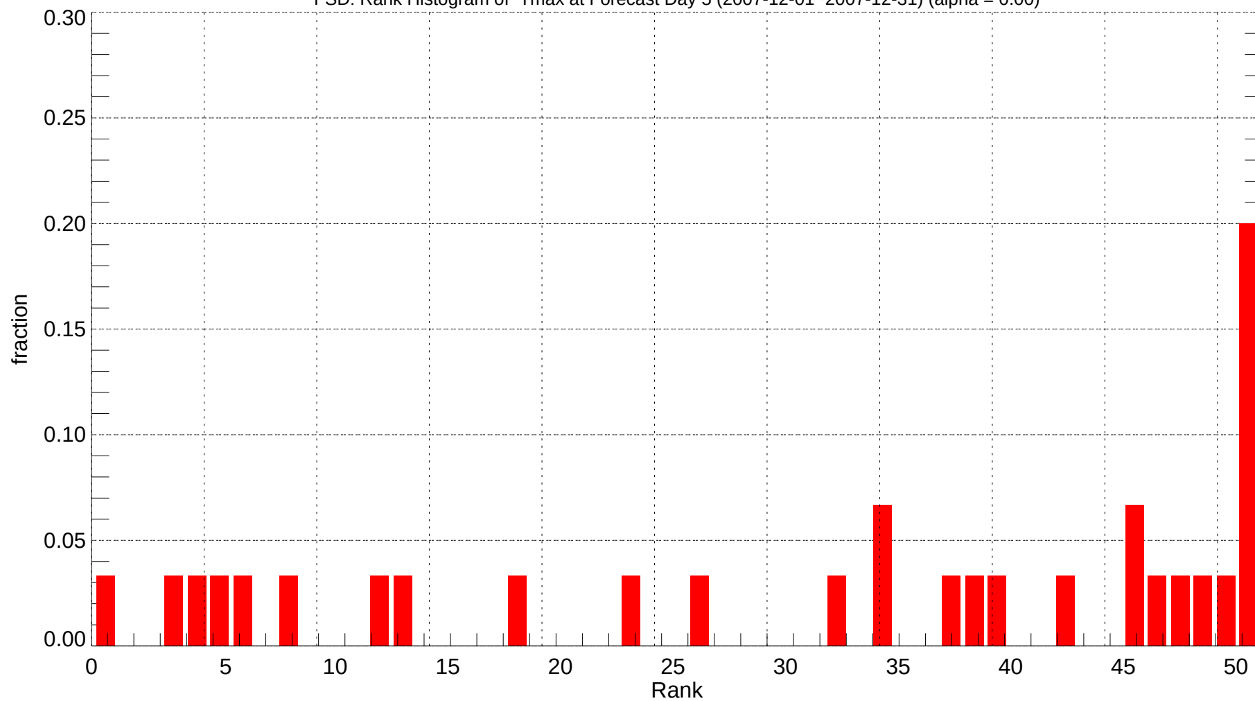
FSD: Rank Histogram of Tmax at Forecast Day 5 (2007-12-01~2007-12-31) (alpha = 0.00)
