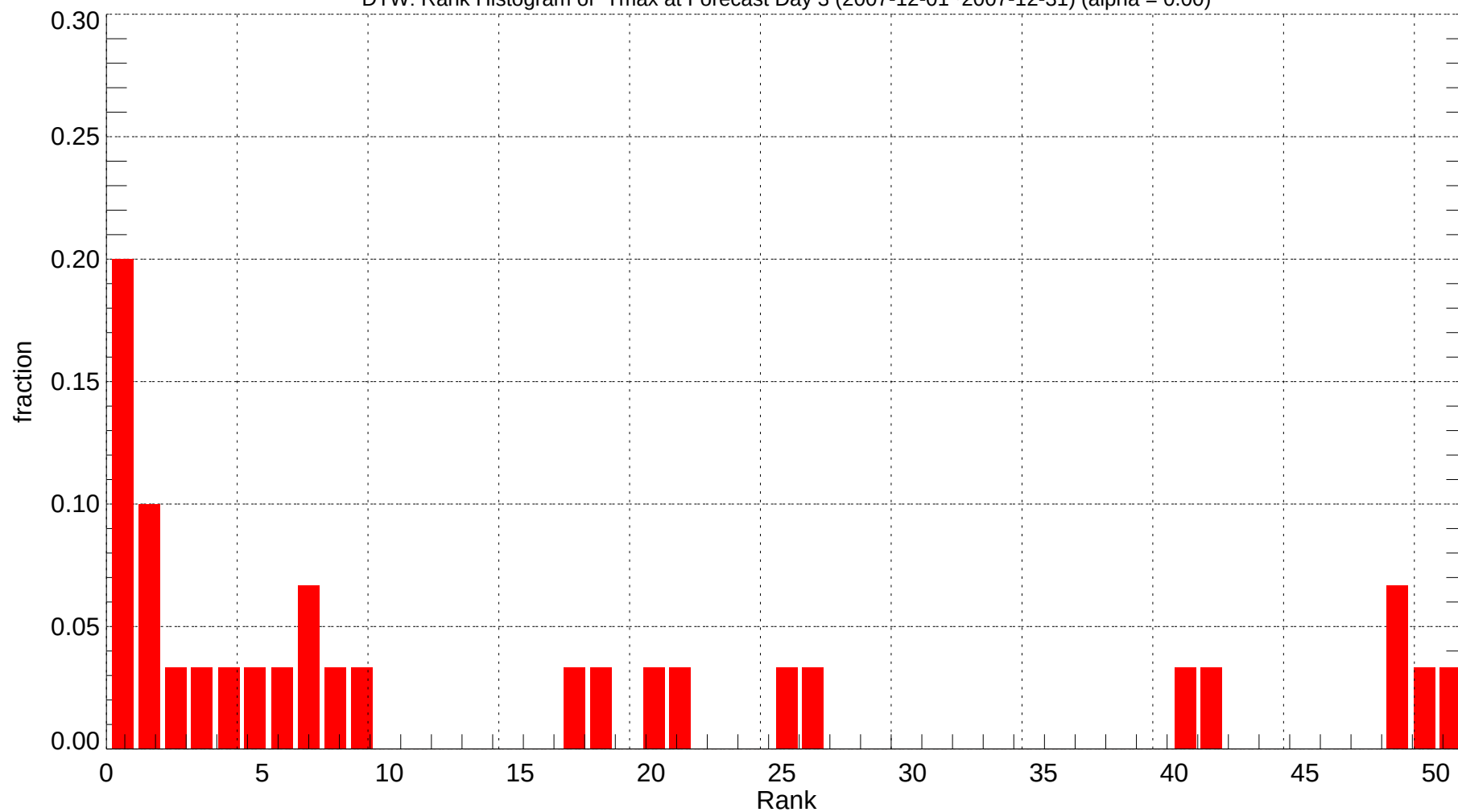
DTW: Rank Histogram of Tmax at Forecast Day 3 (2007-12-01~2007-12-31) (alpha = 0.00)
