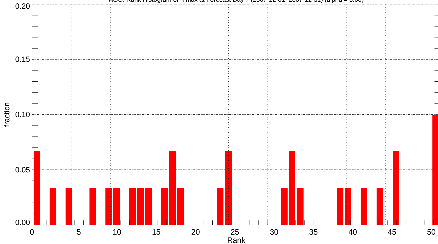
AOO: Rank Histogram of Tmax at Forecast Day 7 (2007-12-01~2007-12-31) (alpha = 0.00)
