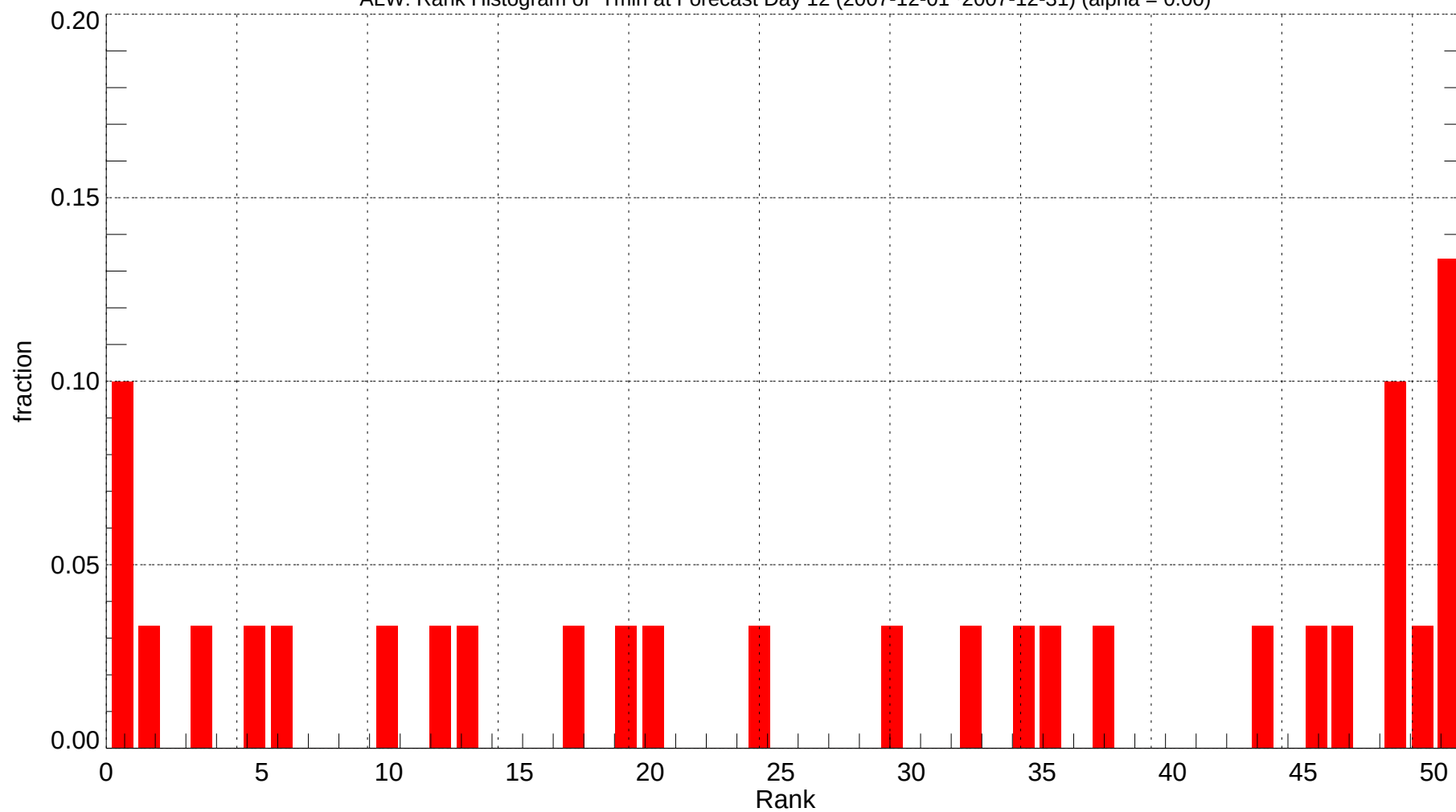
ALW: Rank Histogram of Tmin at Forecast Day 12 (2007-12-01~2007-12-31) (alpha = 0.00)
