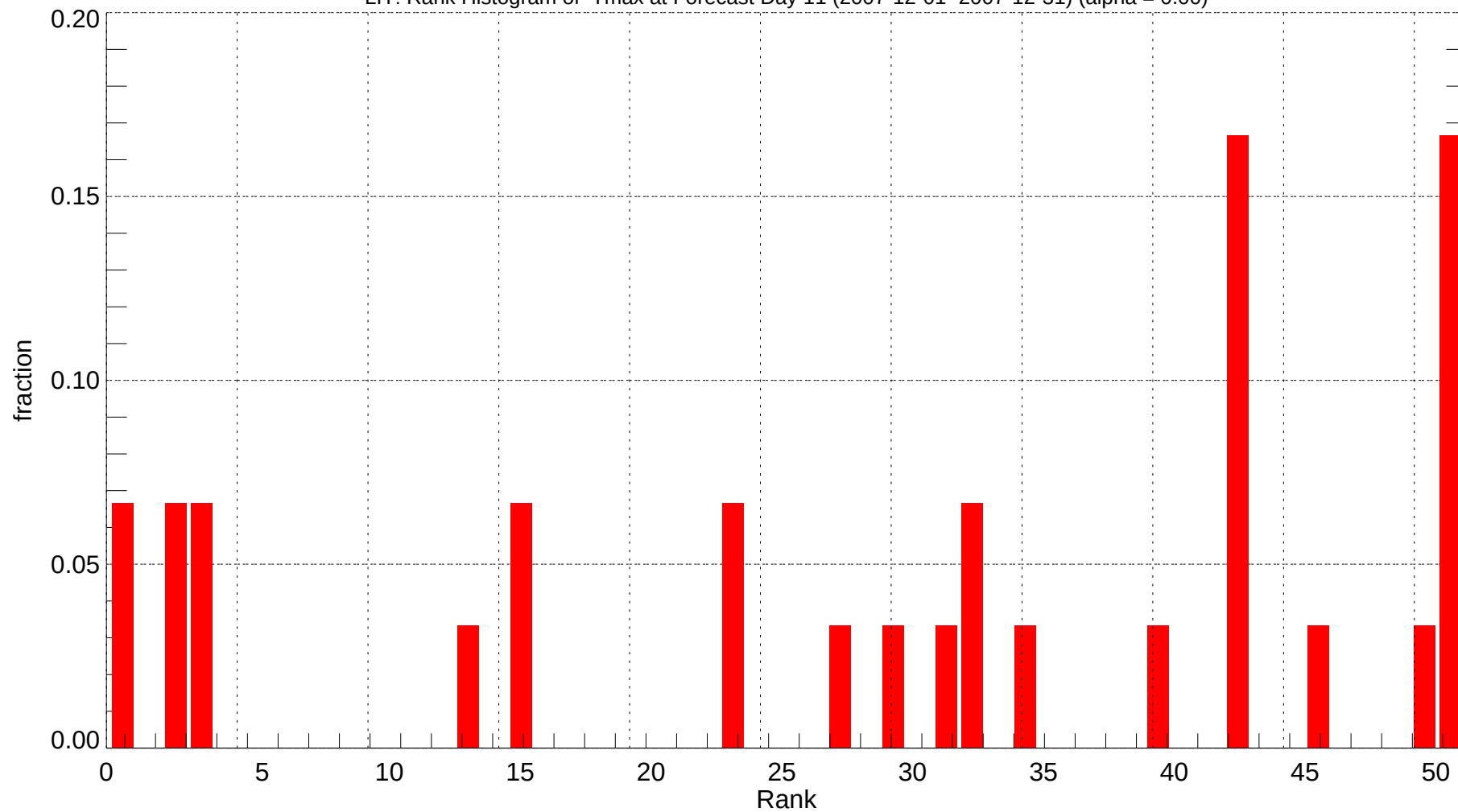
LIT: Rank Histogram of Tmax at Forecast Day 11 (2007-12-01~2007-12-31) (alpha = 0.00)
