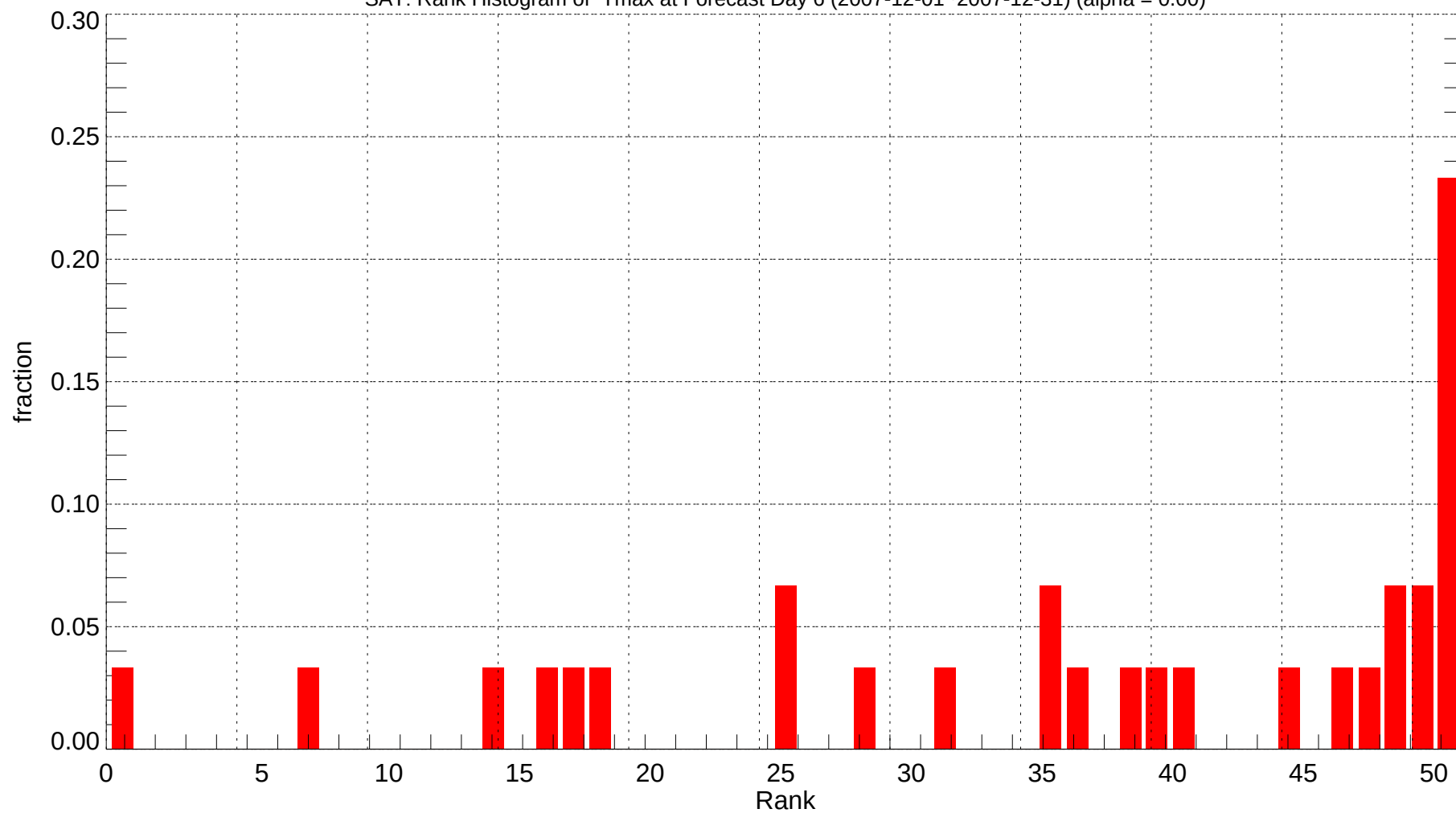
SAT: Rank Histogram of Tmax at Forecast Day 6 (2007-12-01~2007-12-31) (alpha = 0.00)
