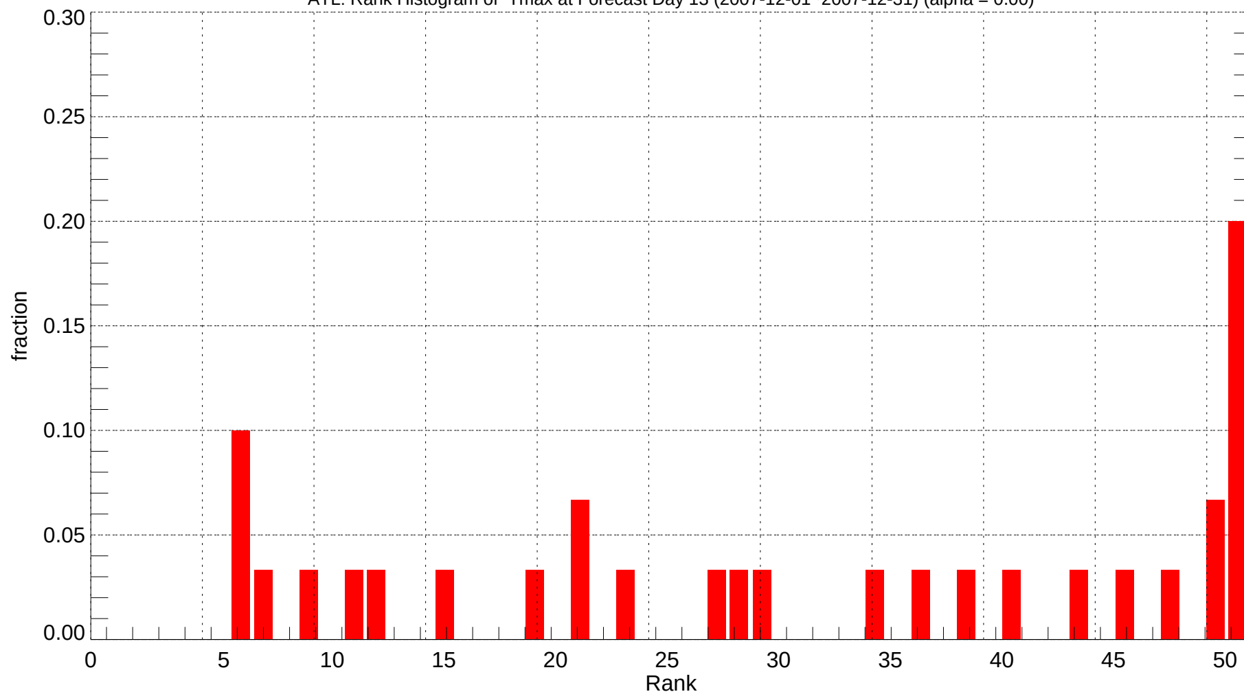
ATL: Rank Histogram of Tmax at Forecast Day 13 (2007-12-01~2007-12-31) (alpha = 0.00)
