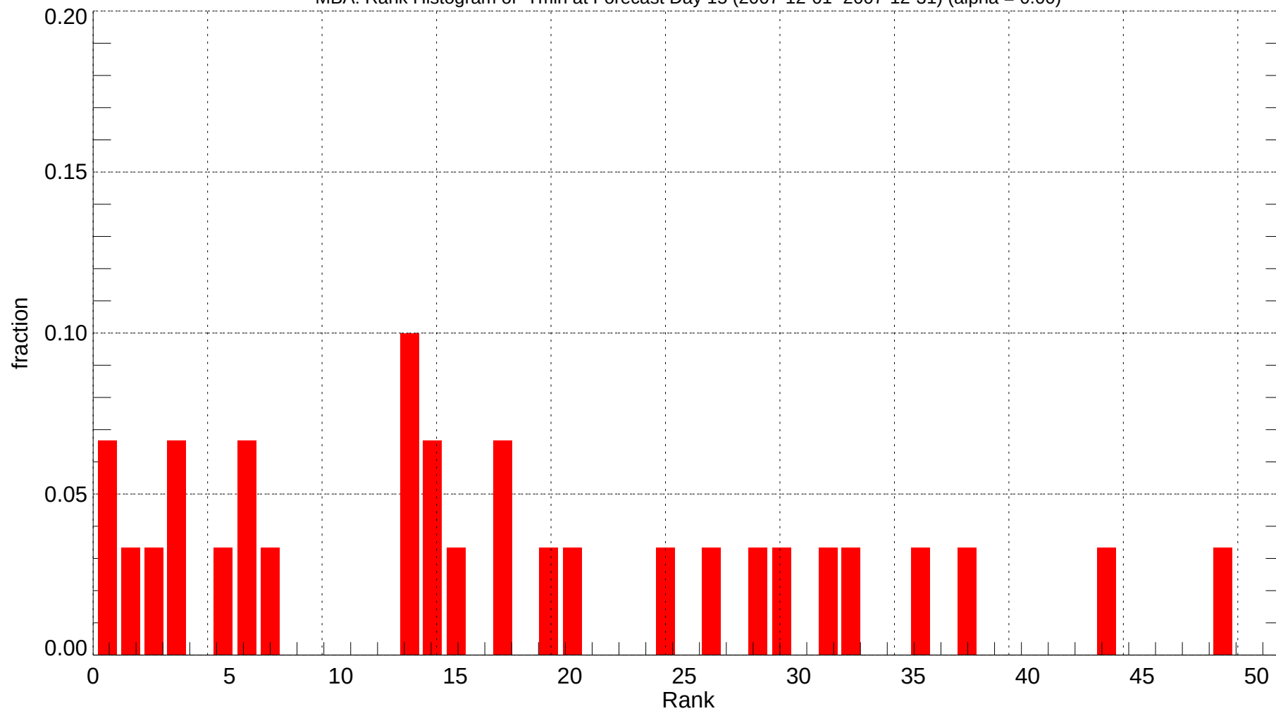
MBA: Rank Histogram of Tmin at Forecast Day 15 (2007-12-01~2007-12-31) (alpha = 0.00)
