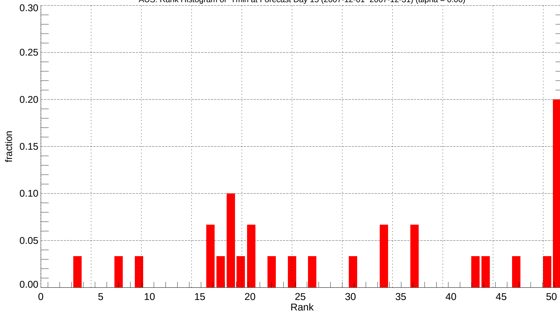
AUS: Rank Histogram of Tmin at Forecast Day 15 (2007-12-01~2007-12-31) (alpha = 0.00)
