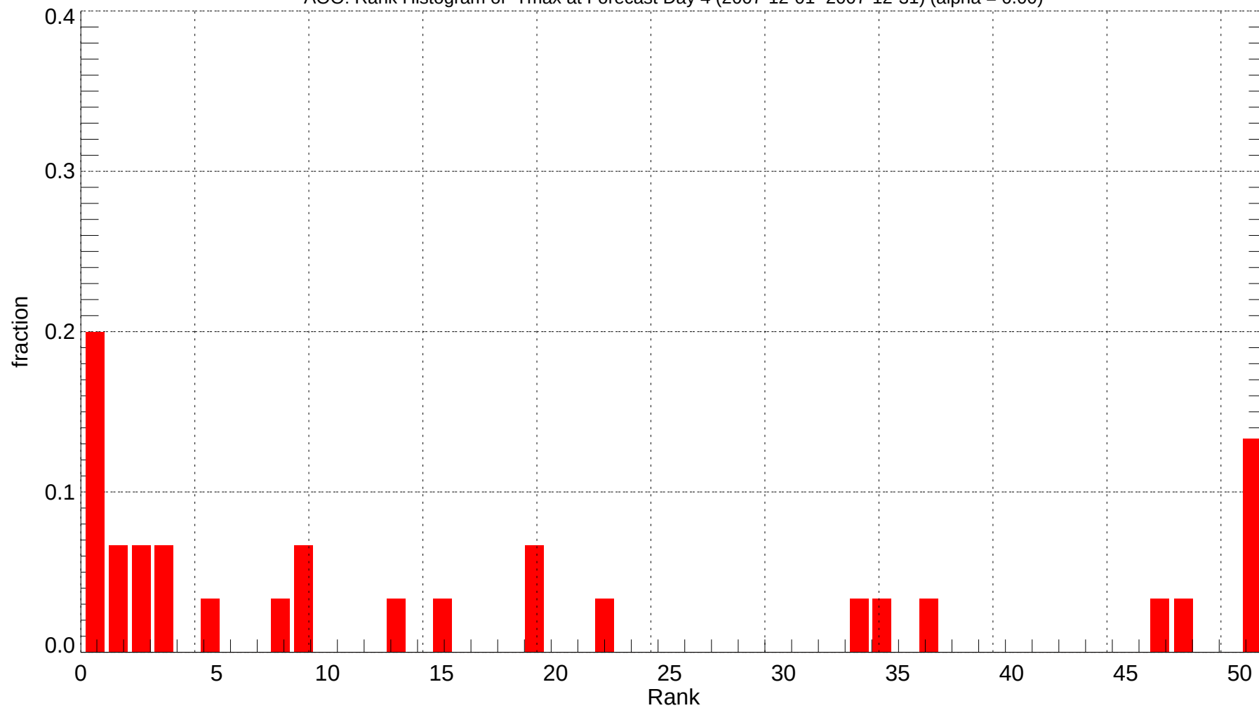
AOO: Rank Histogram of Tmax at Forecast Day 4 (2007-12-01~2007-12-31) (alpha = 0.00)
