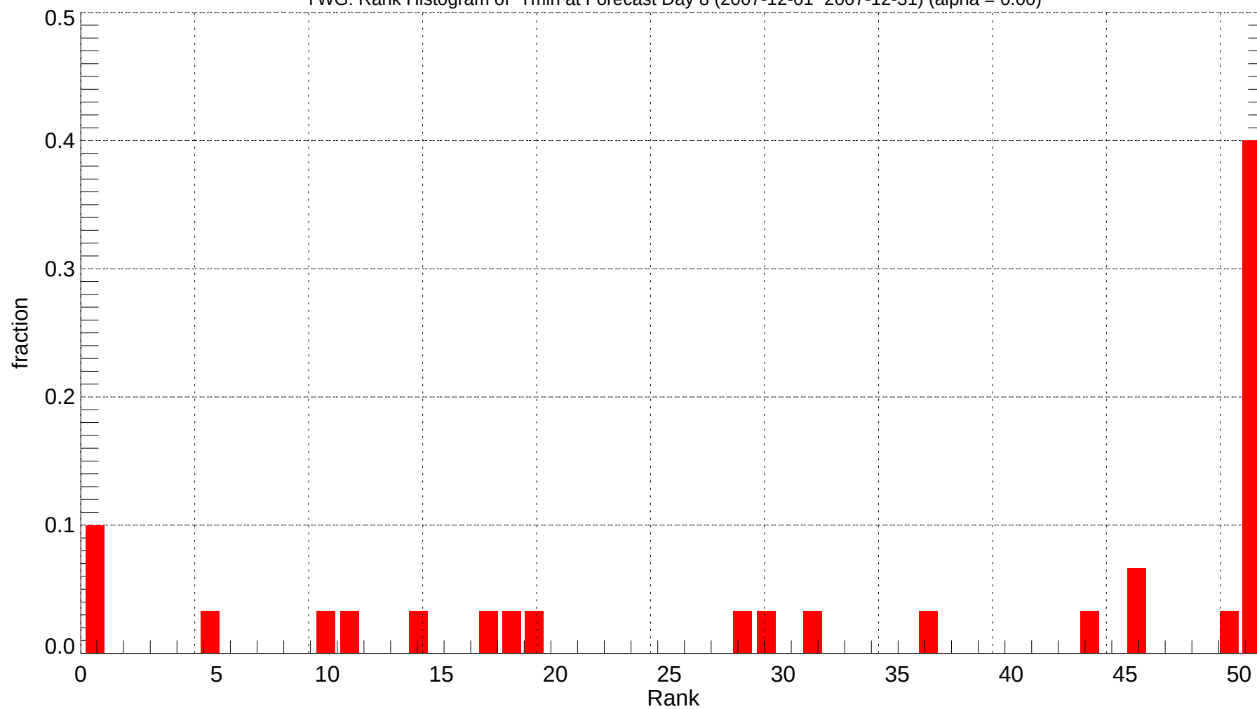
YWG: Rank Histogram of Tmin at Forecast Day 8 (2007-12-01~2007-12-31) (alpha = 0.00)
