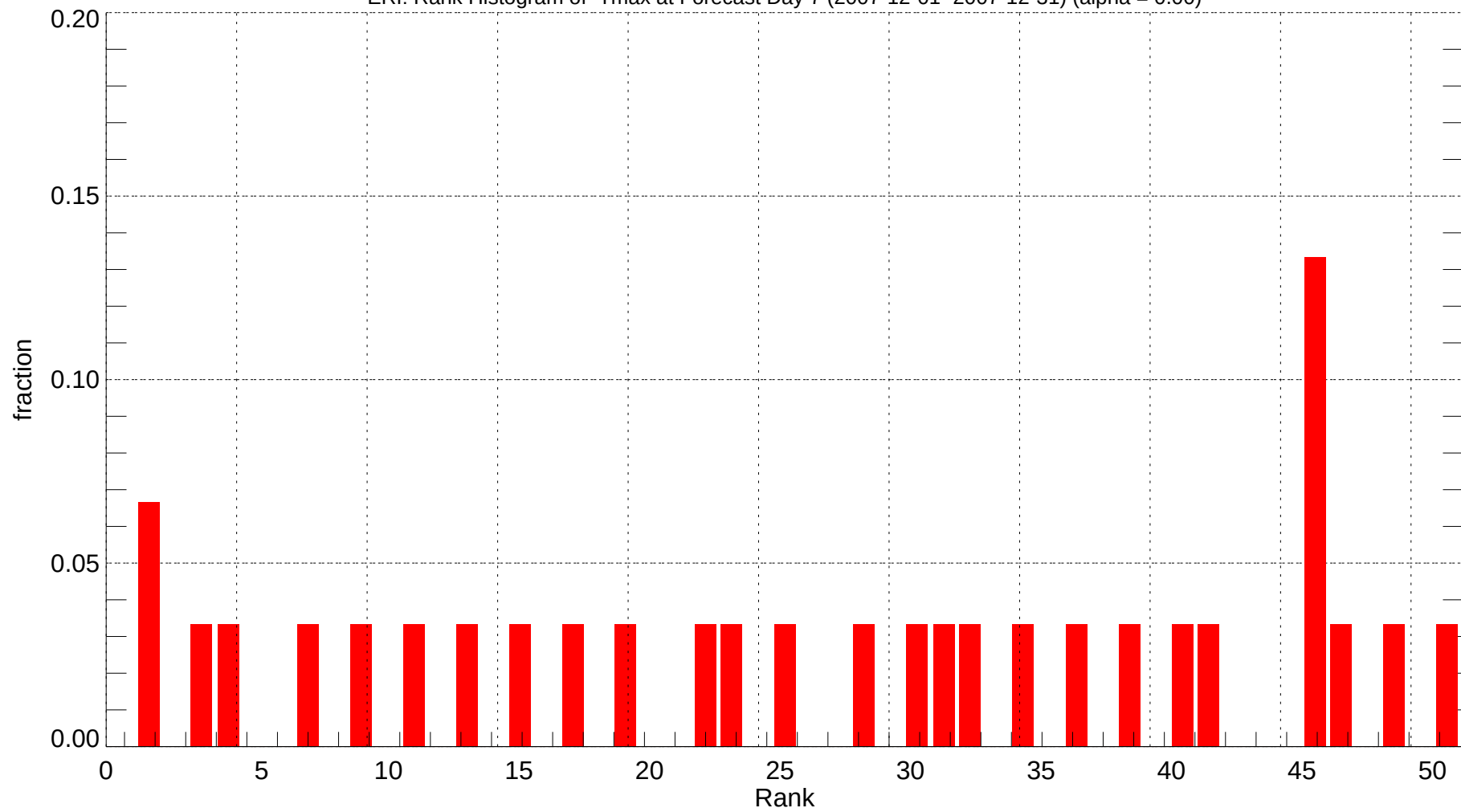
ERI: Rank Histogram of Tmax at Forecast Day 7 (2007-12-01~2007-12-31) (alpha = 0.00)
