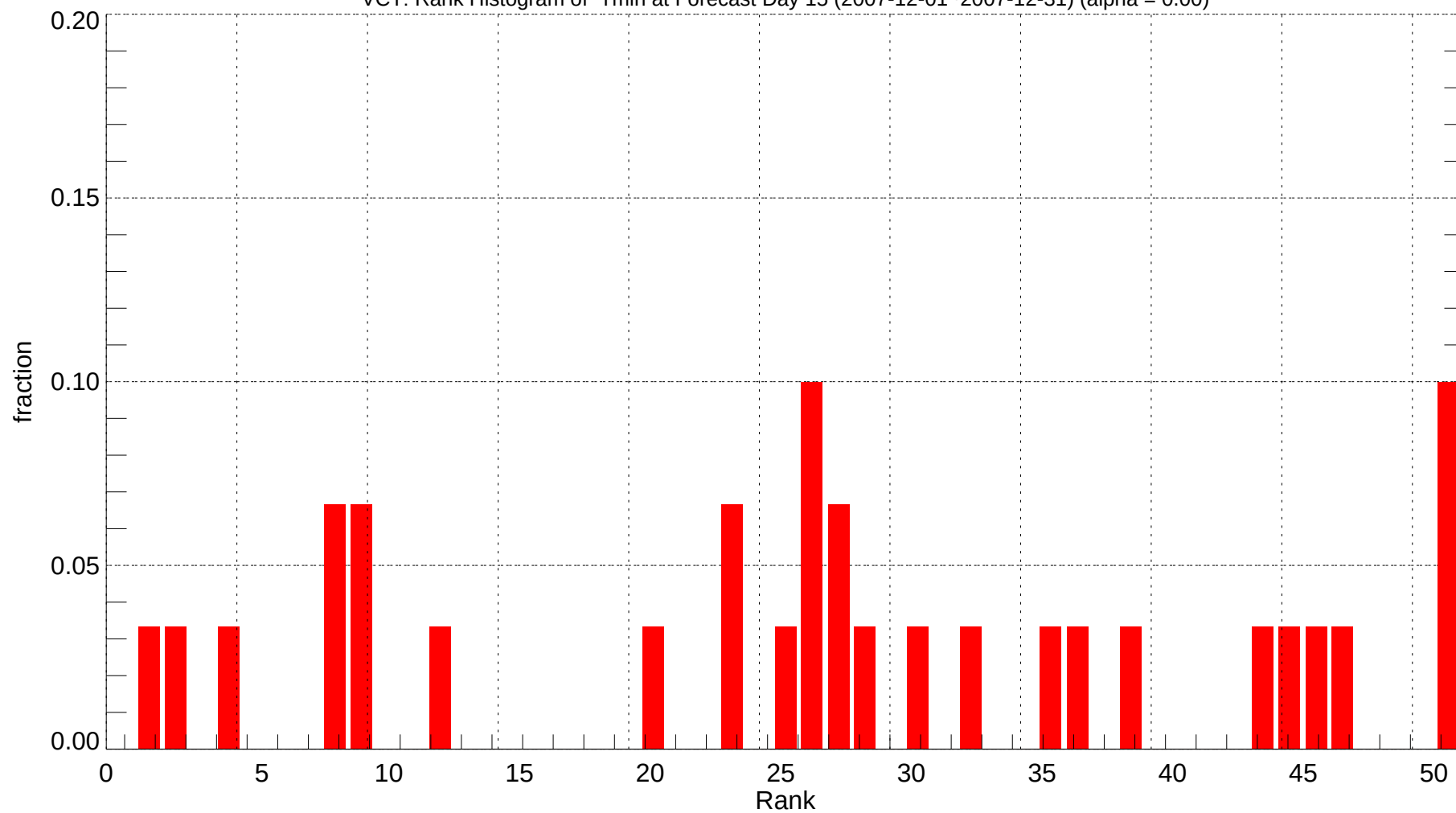
VCT: Rank Histogram of Tmin at Forecast Day 15 (2007-12-01~2007-12-31) (alpha = 0.00)
