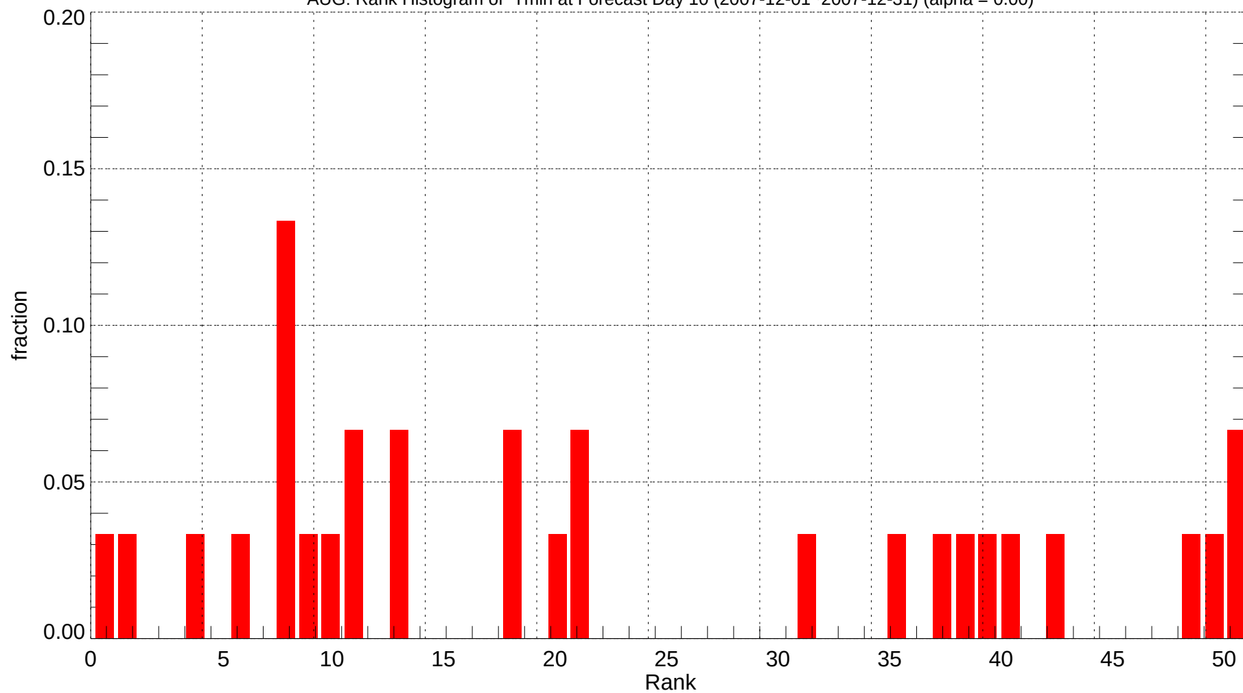
AUG: Rank Histogram of Tmin at Forecast Day 10 (2007-12-01~2007-12-31) (alpha = 0.00)
