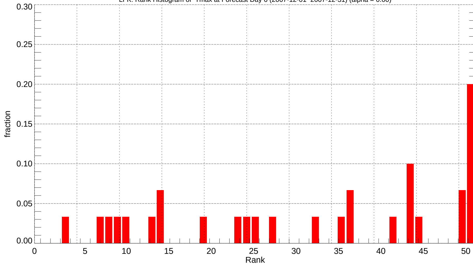
LFK: Rank Histogram of Tmax at Forecast Day 6 (2007-12-01~2007-12-31) (alpha = 0.00)
