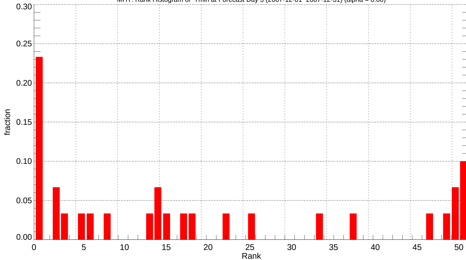
MHT: Rank Histogram of Tmin at Forecast Day 3 (2007-12-01~2007-12-31) (alpha = 0.00)
