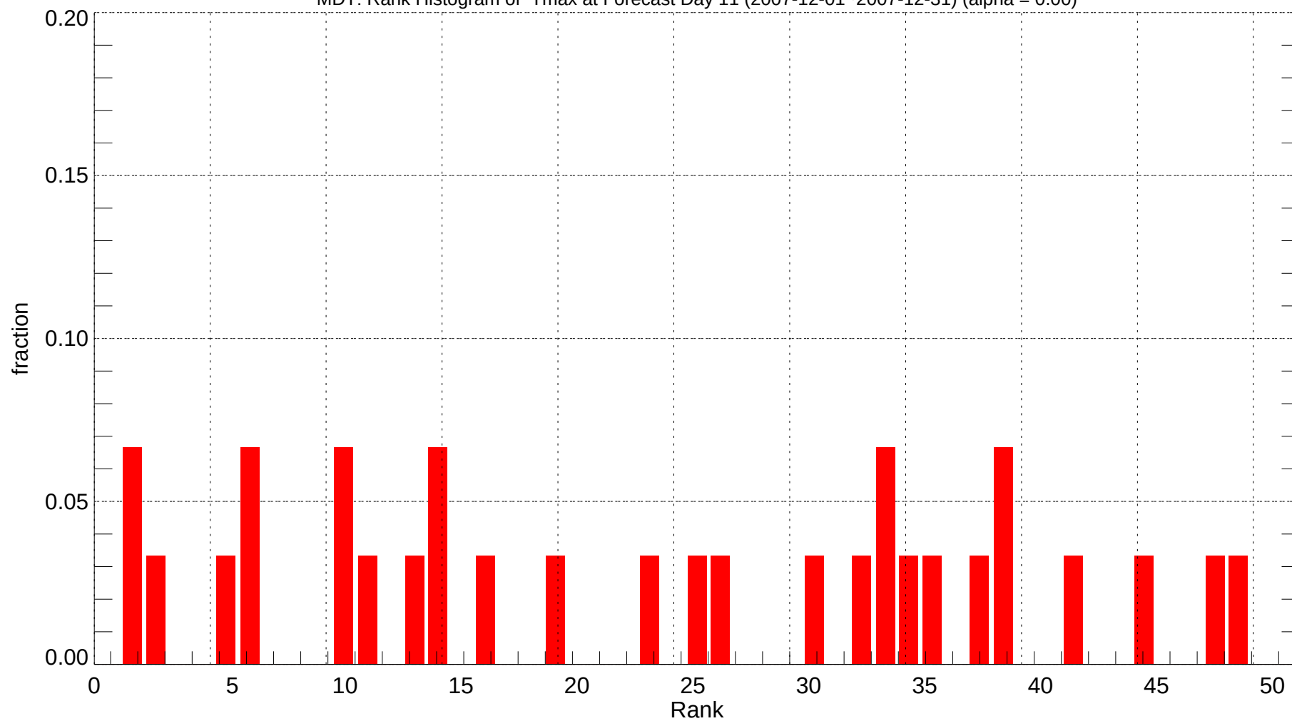
MDT: Rank Histogram of Tmax at Forecast Day 11 (2007-12-01~2007-12-31) (alpha = 0.00)
