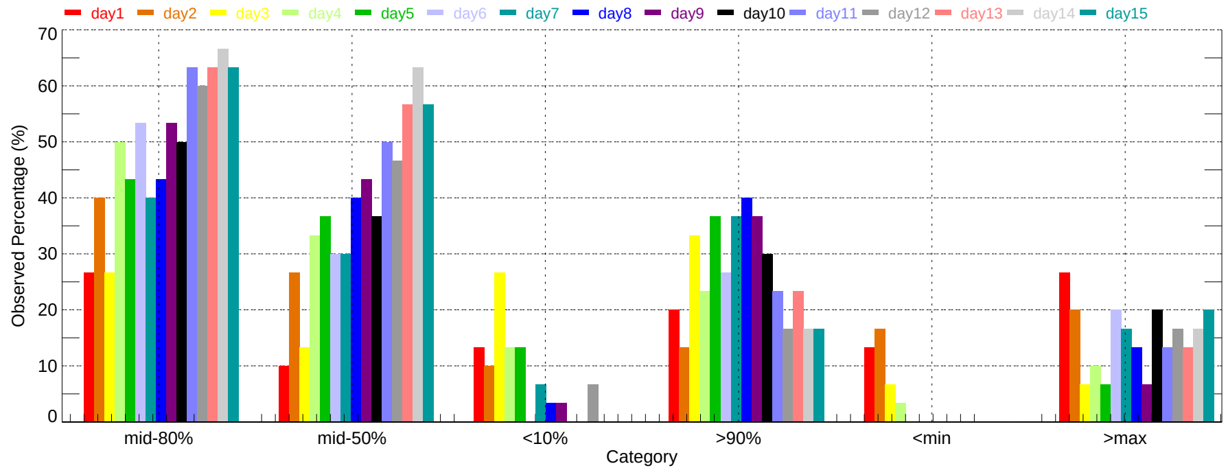
Observed Percentage of Ensembles - HSV: Min Temperature (2007-12-01~2007-12-31)
