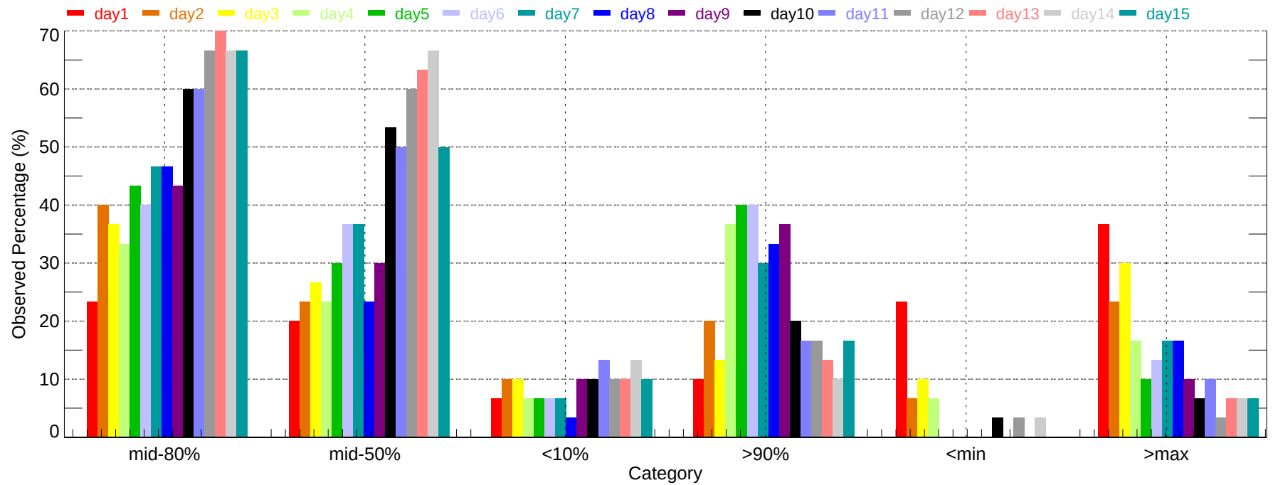
Observed Percentage of Ensembles - VCT: Max Temperature (2007-12-01~2007-12-31)
