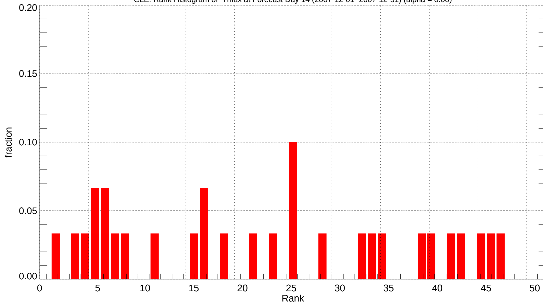
CLE: Rank Histogram of Tmax at Forecast Day 14 (2007-12-01~2007-12-31) (alpha = 0.00)
