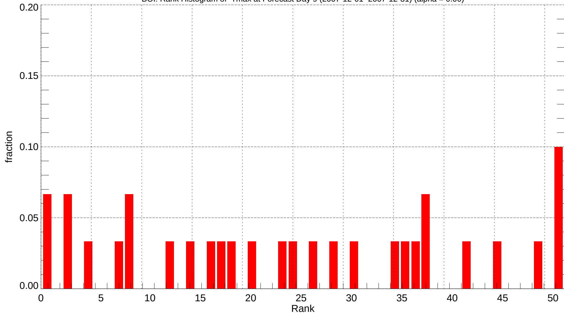
BOI: Rank Histogram of Tmax at Forecast Day 9 (2007-12-01~2007-12-31) (alpha = 0.00)
