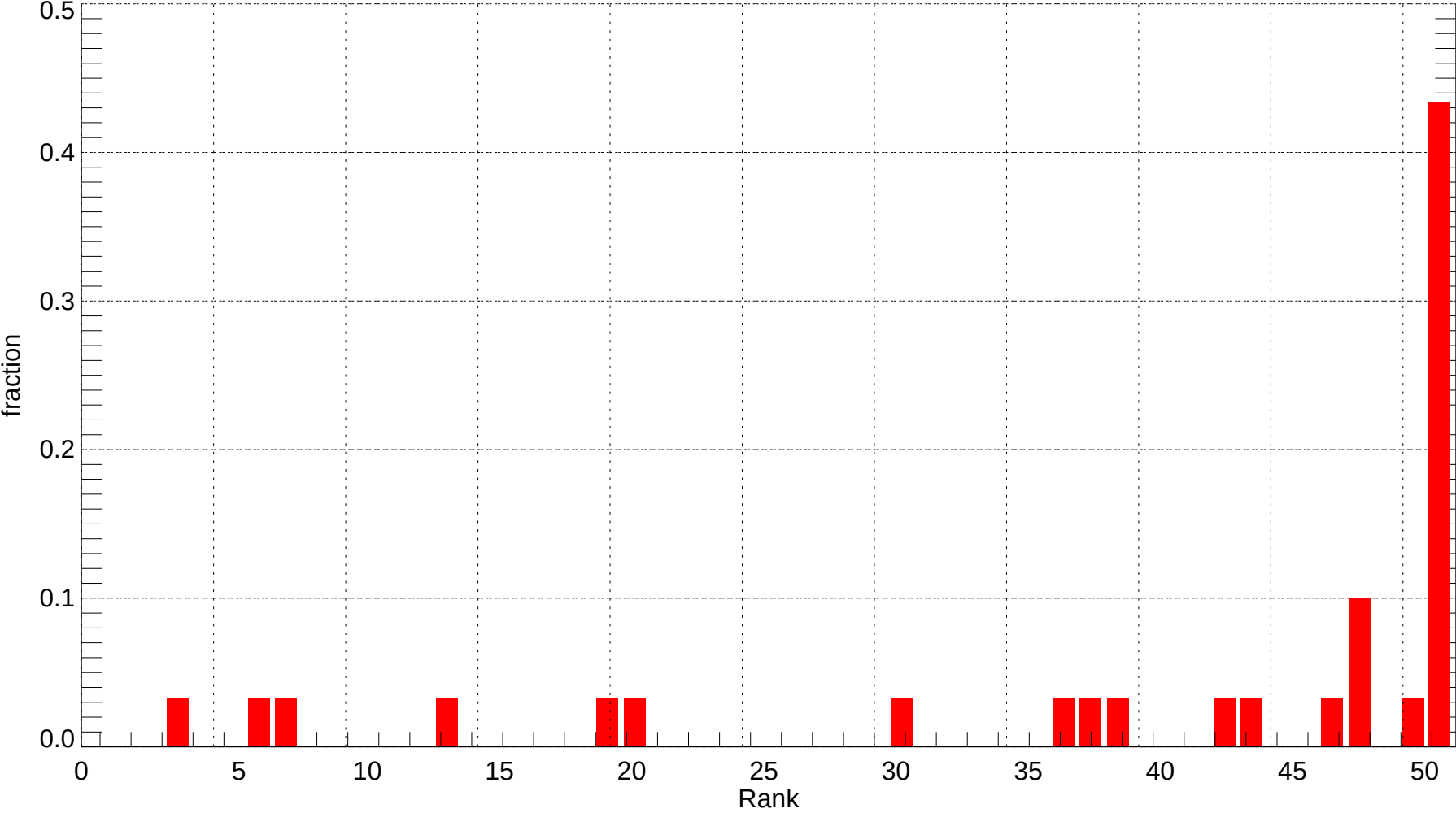
BFL: Rank Histogram of Tmin at Forecast Day 6 (2007-12-01~2007-12-31) (alpha = 0.00)
