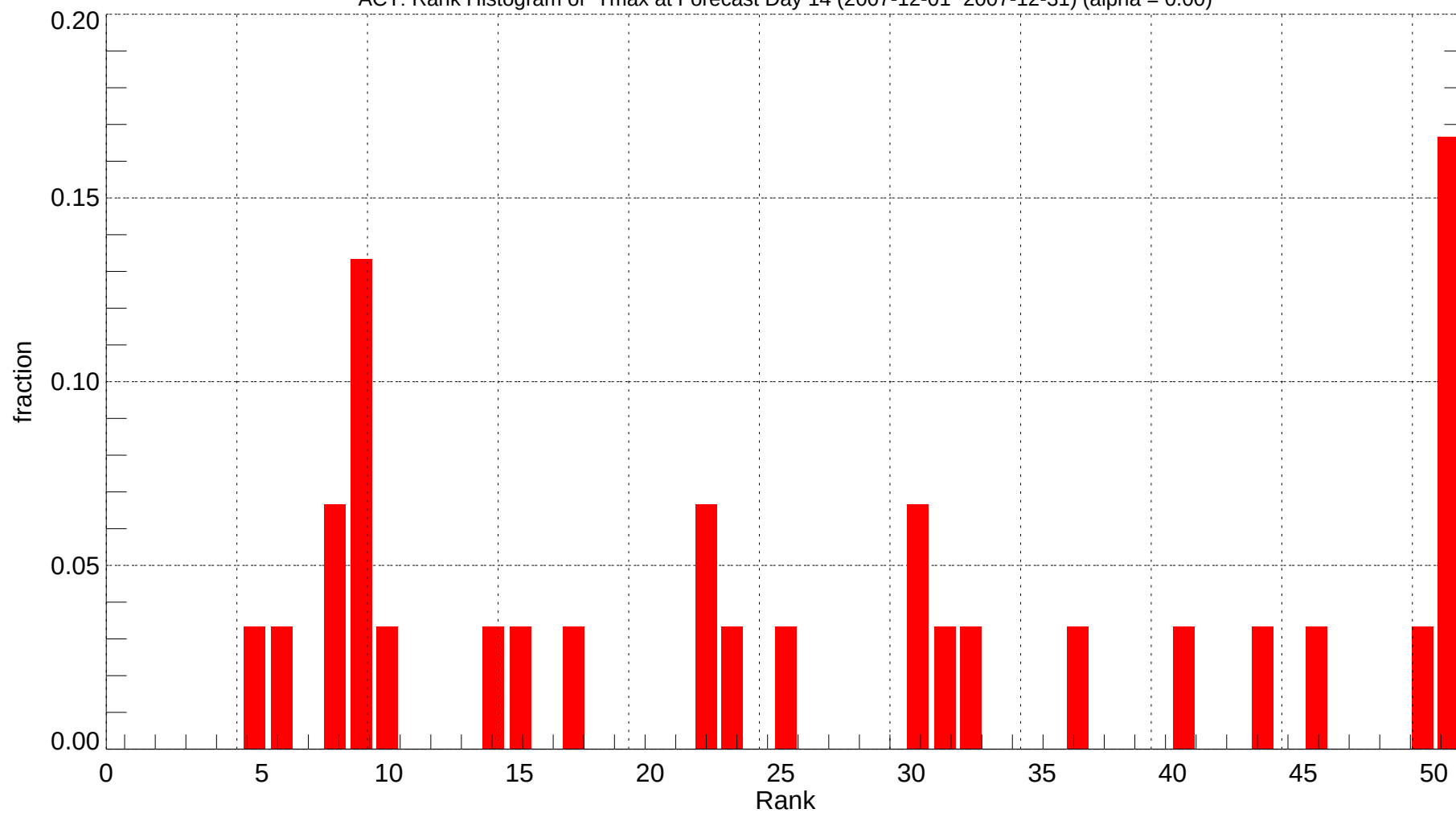
ACT: Rank Histogram of Tmax at Forecast Day 14 (2007-12-01~2007-12-31) (alpha = 0.00)
