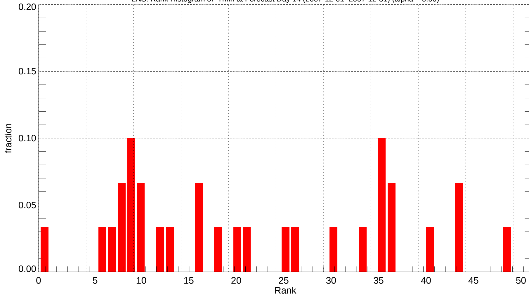
LNS: Rank Histogram of Tmin at Forecast Day 14 (2007-12-01~2007-12-31) (alpha = 0.00)
