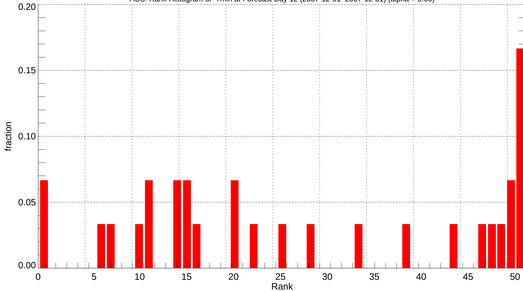
AUS: Rank Histogram of Tmin at Forecast Day 12 (2007-12-01~2007-12-31) (alpha = 0.00)
