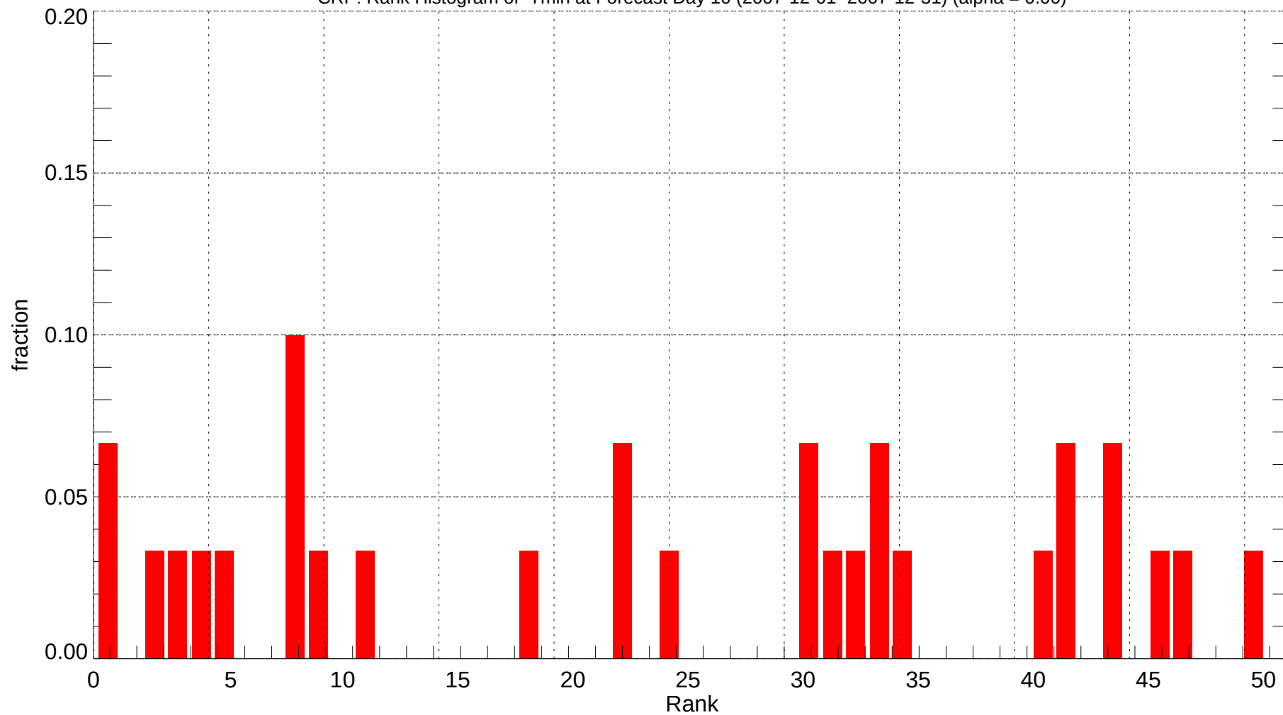
CRP: Rank Histogram of Tmin at Forecast Day 10 (2007-12-01~2007-12-31) (alpha = 0.00)
