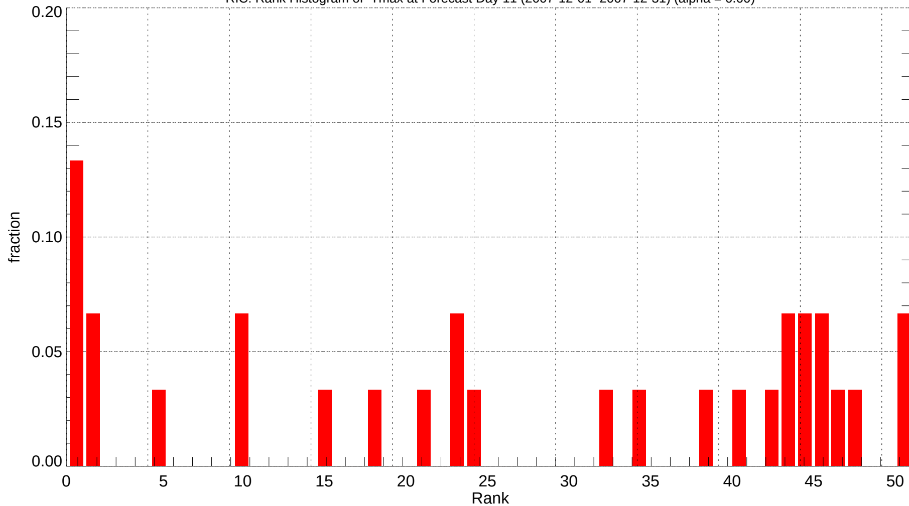
RIC: Rank Histogram of Tmax at Forecast Day 11 (2007-12-01~2007-12-31) (alpha = 0.00)
