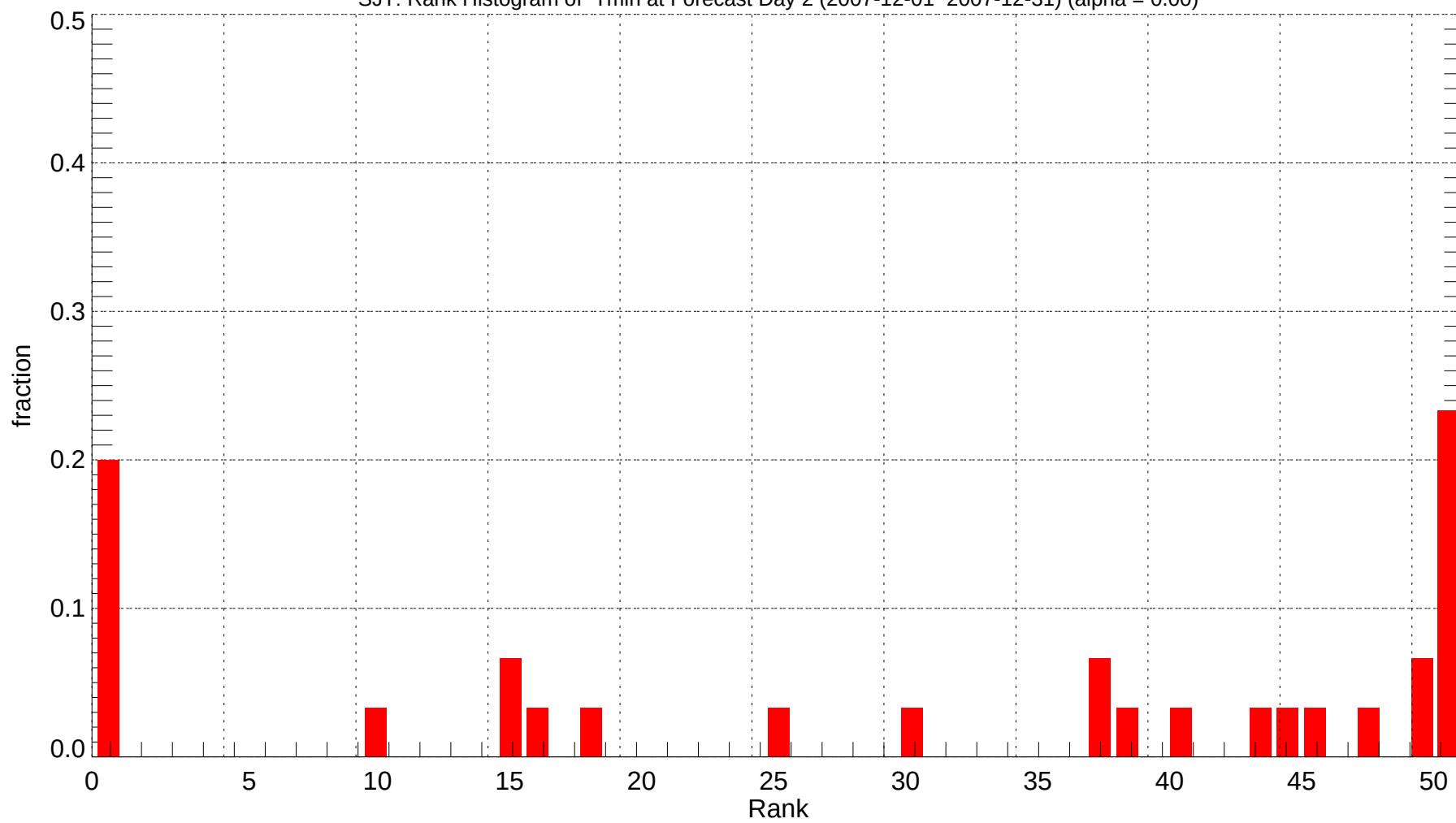
SJT: Rank Histogram of Tmin at Forecast Day 2 (2007-12-01~2007-12-31) (alpha = 0.00)
