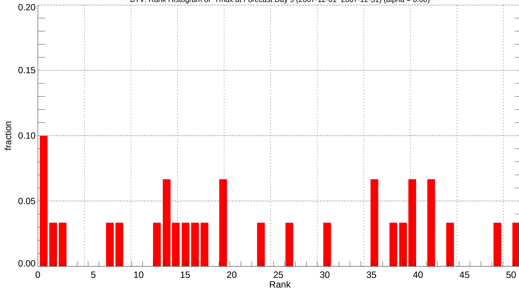
BTV: Rank Histogram of Tmax at Forecast Day 9 (2007-12-01~2007-12-31) (alpha = 0.00)
