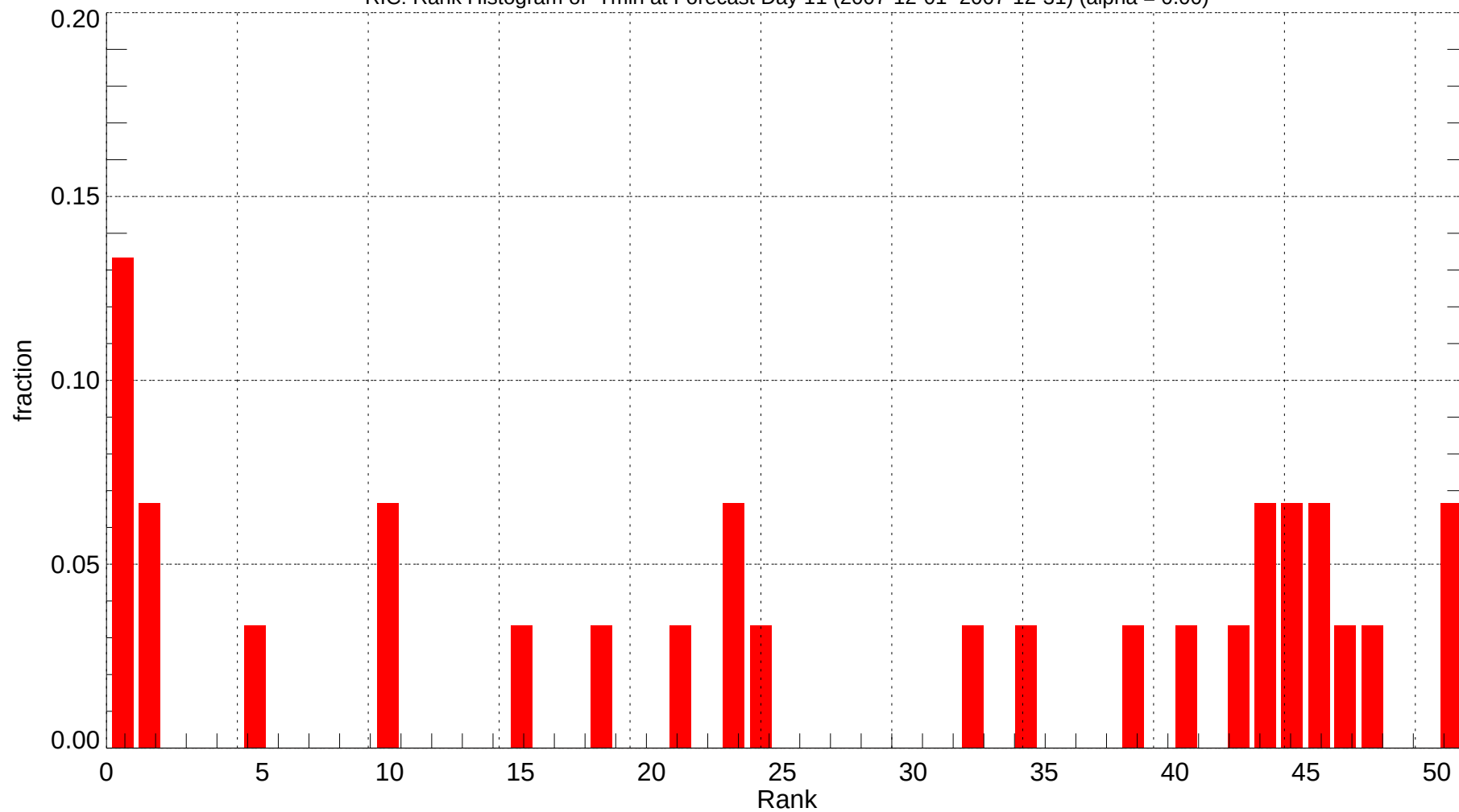
RIC: Rank Histogram of Tmin at Forecast Day 11 (2007-12-01~2007-12-31) (alpha = 0.00)
