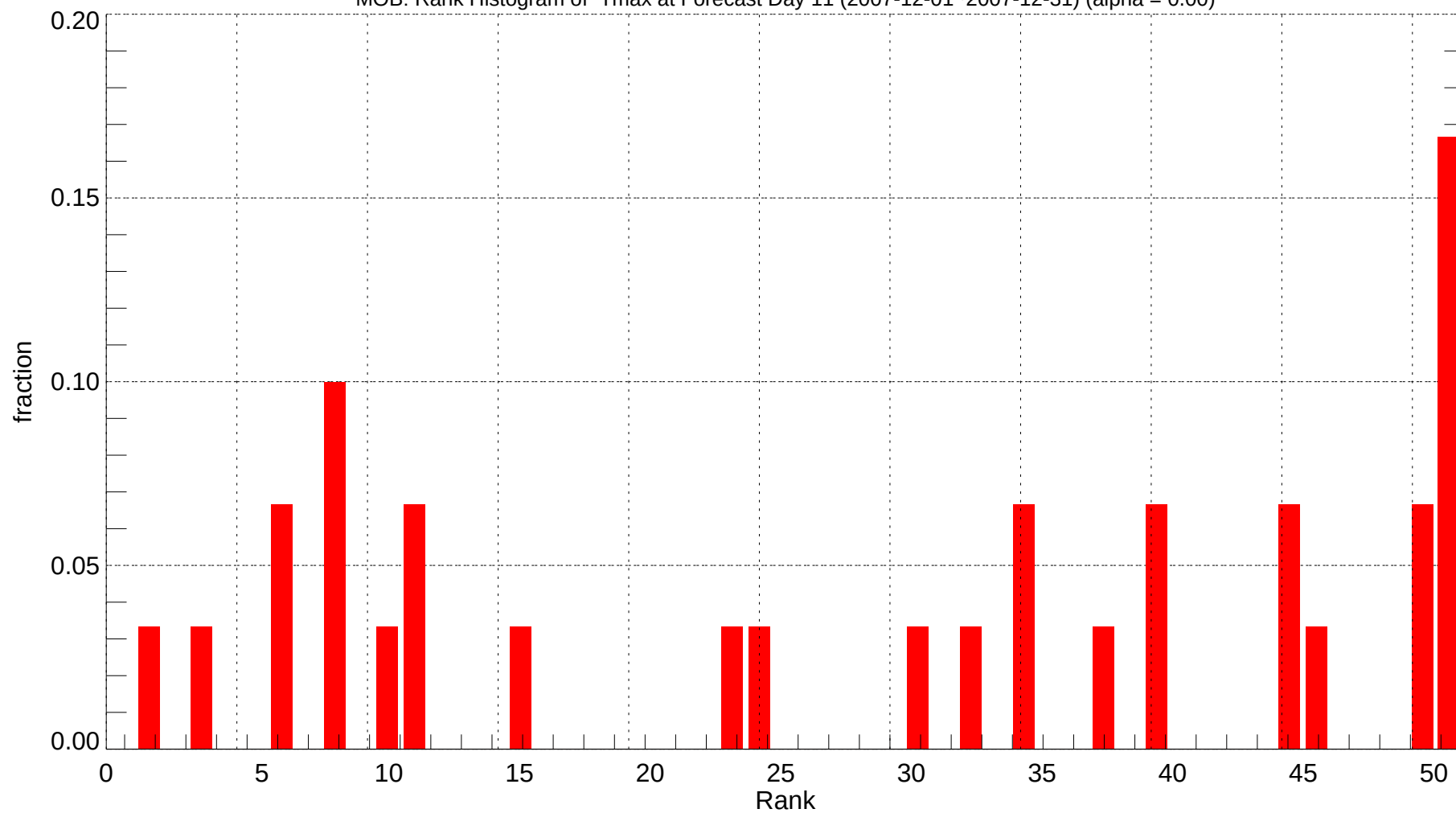
MOB: Rank Histogram of Tmax at Forecast Day 11 (2007-12-01~2007-12-31) (alpha = 0.00)
