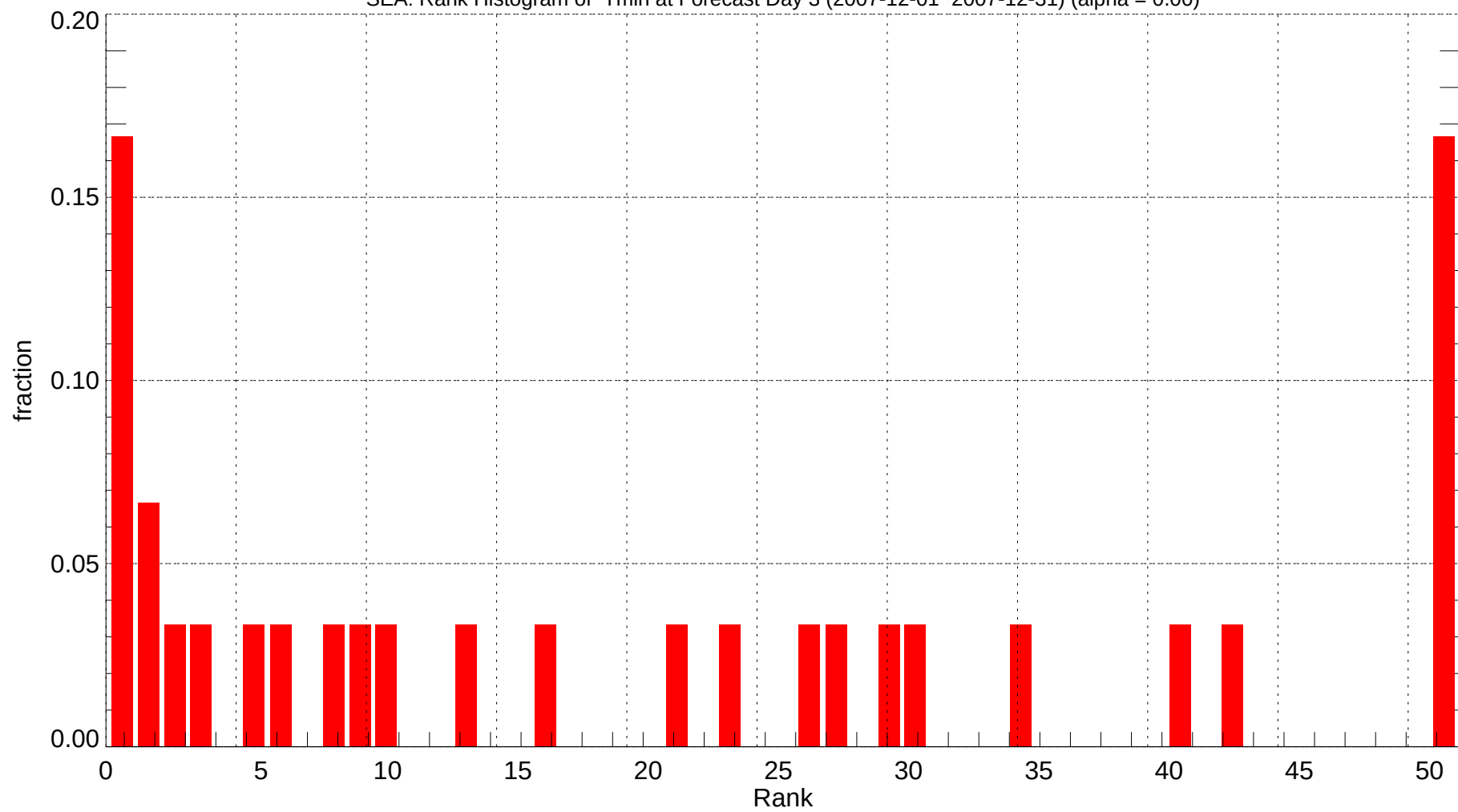
SEA: Rank Histogram of Tmin at Forecast Day 3 (2007-12-01~2007-12-31) (alpha = 0.00)
