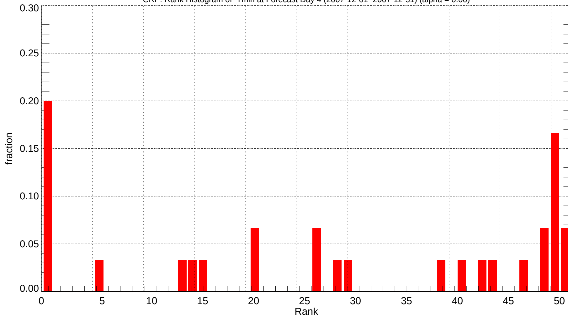
CRP: Rank Histogram of Tmin at Forecast Day 4 (2007-12-01~2007-12-31) (alpha = 0.00)
