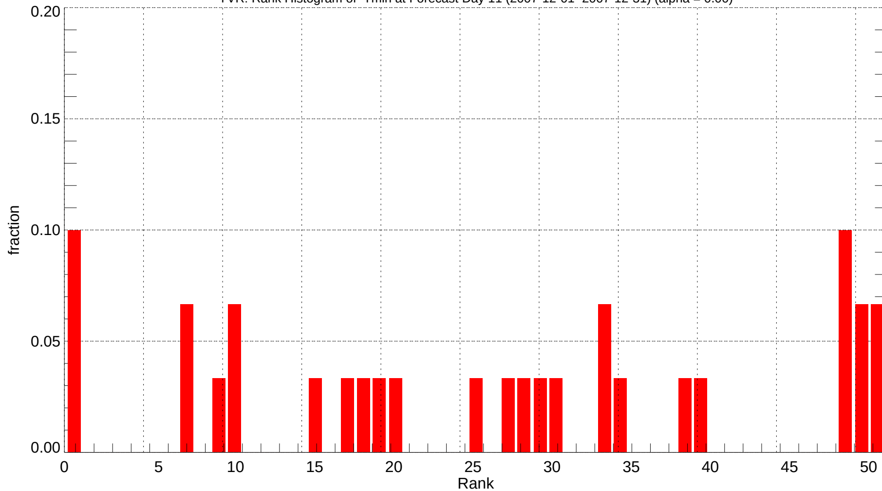
YVR: Rank Histogram of Tmin at Forecast Day 11 (2007-12-01~2007-12-31) (alpha = 0.00)
