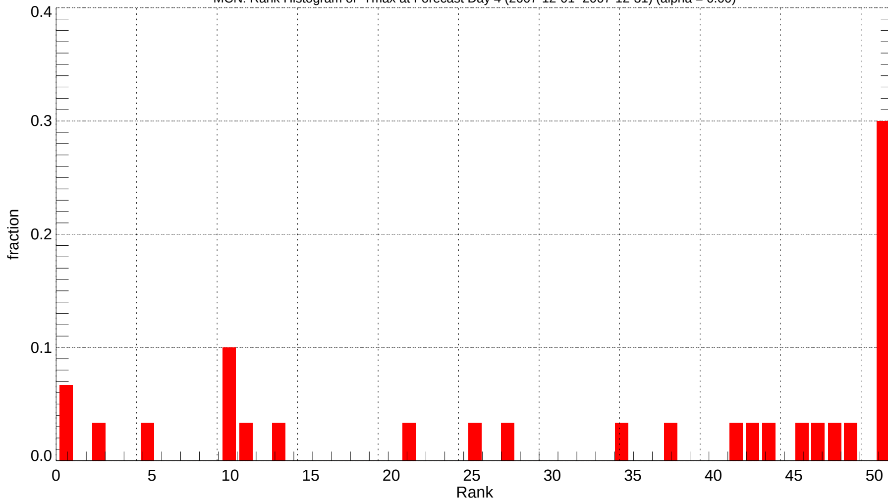
MCN: Rank Histogram of Tmax at Forecast Day 4 (2007-12-01~2007-12-31) (alpha = 0.00)
