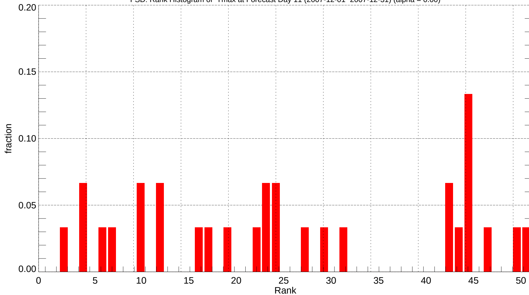
FSD: Rank Histogram of Tmax at Forecast Day 11 (2007-12-01~2007-12-31) (alpha = 0.00)
