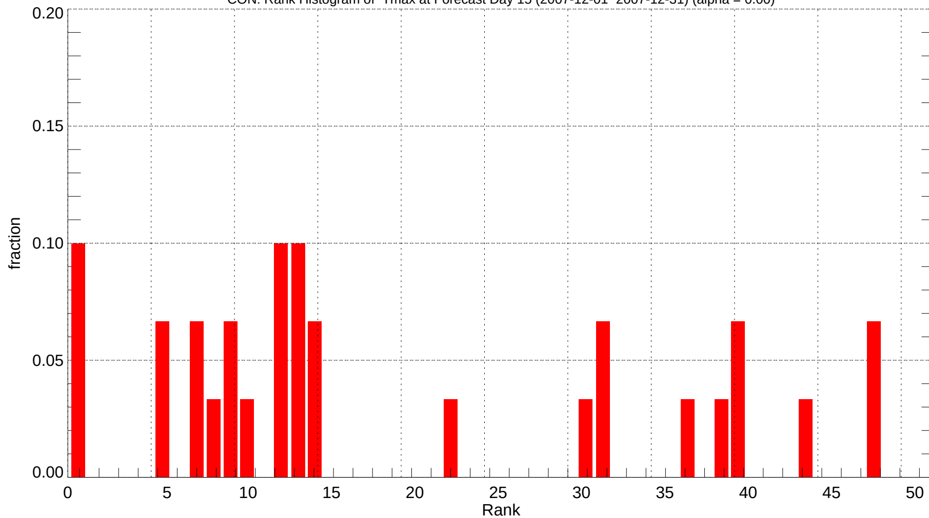
CON: Rank Histogram of Tmax at Forecast Day 15 (2007-12-01~2007-12-31) (alpha = 0.00)
