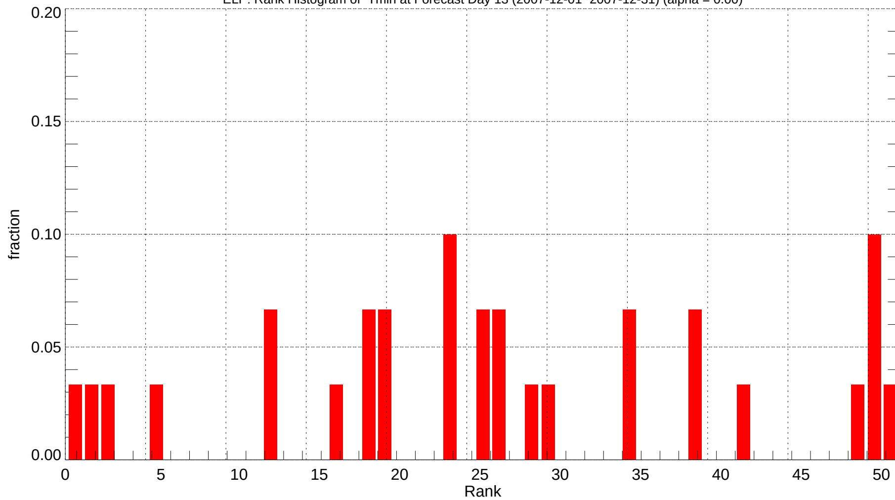
ELP: Rank Histogram of Tmin at Forecast Day 13 (2007-12-01~2007-12-31) (alpha = 0.00)
