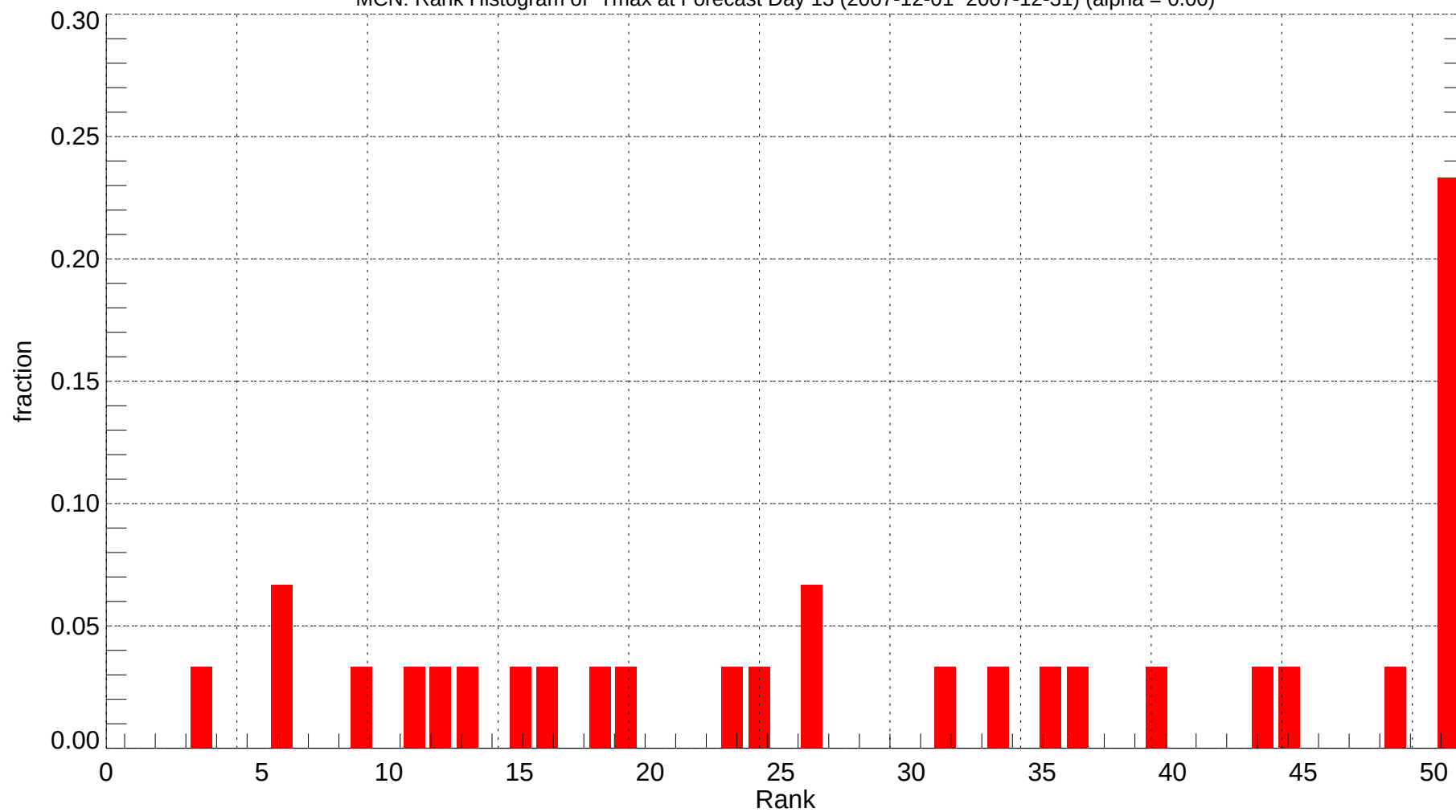
MCN: Rank Histogram of Tmax at Forecast Day 13 (2007-12-01~2007-12-31) (alpha = 0.00)
