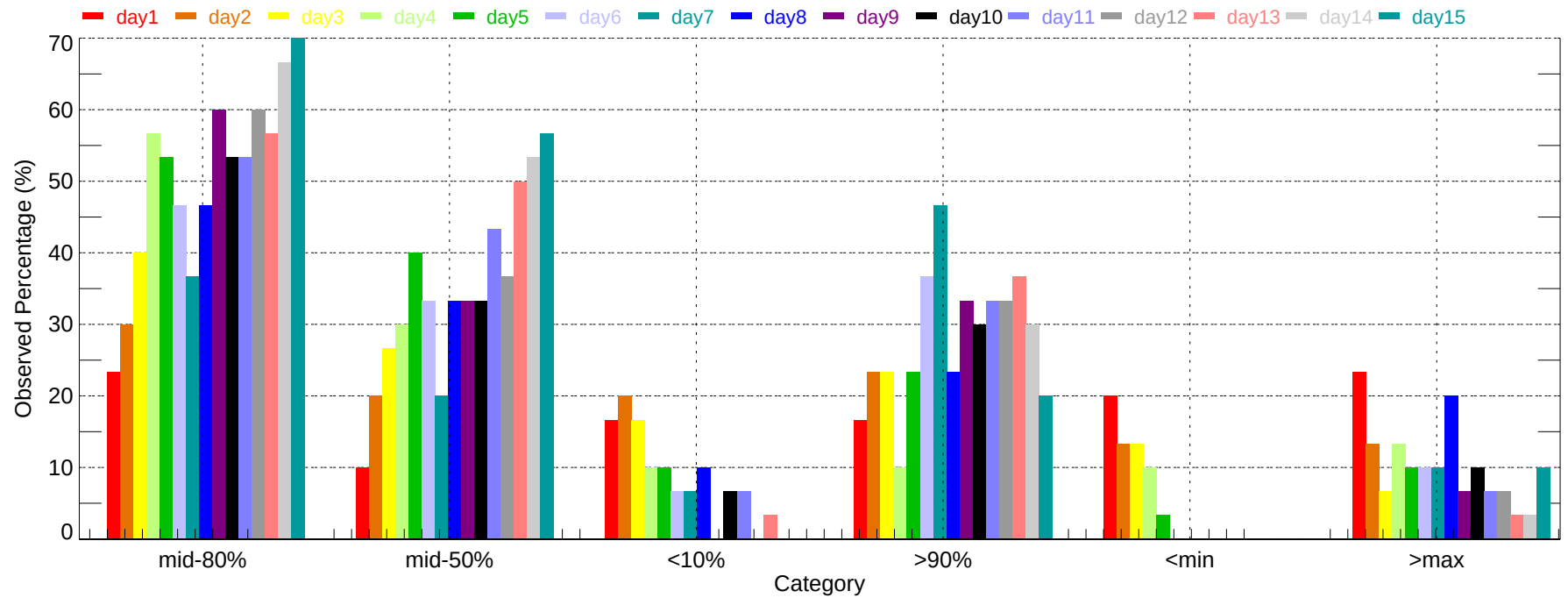
Observed Percentage of Ensembles - LEX: Min Temperature (2007-12-01~2007-12-31)
