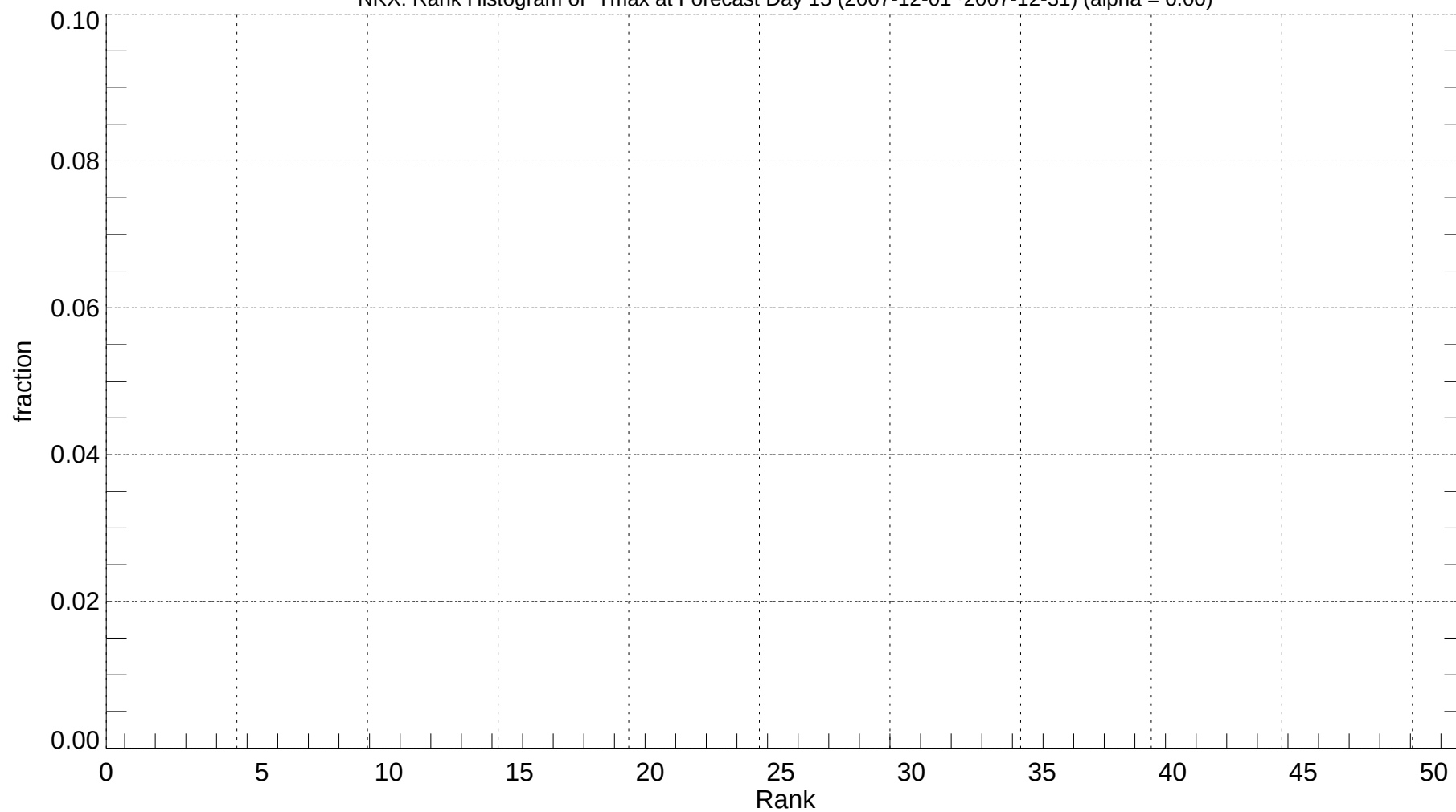
NKX: Rank Histogram of Tmax at Forecast Day 15 (2007-12-01~2007-12-31) (alpha = 0.00)
