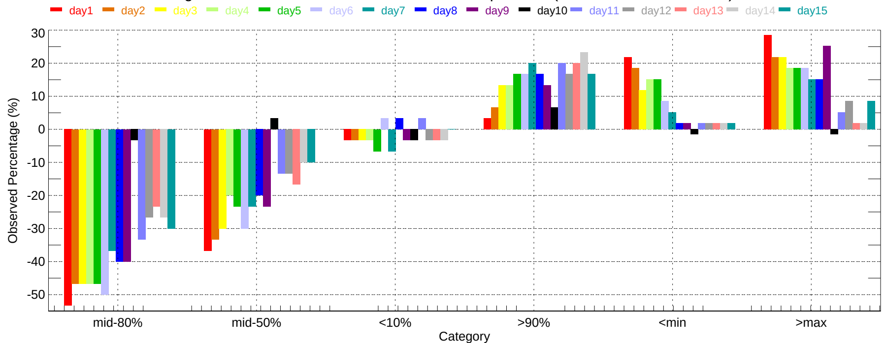
Observed Percentage Deviation of Ensembles - TLH: Max Temperature (2007-12-01~2007-12-31)
