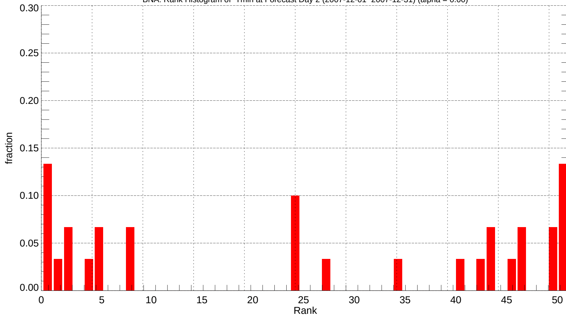
BNA: Rank Histogram of Tmin at Forecast Day 2 (2007-12-01~2007-12-31) (alpha = 0.00)
