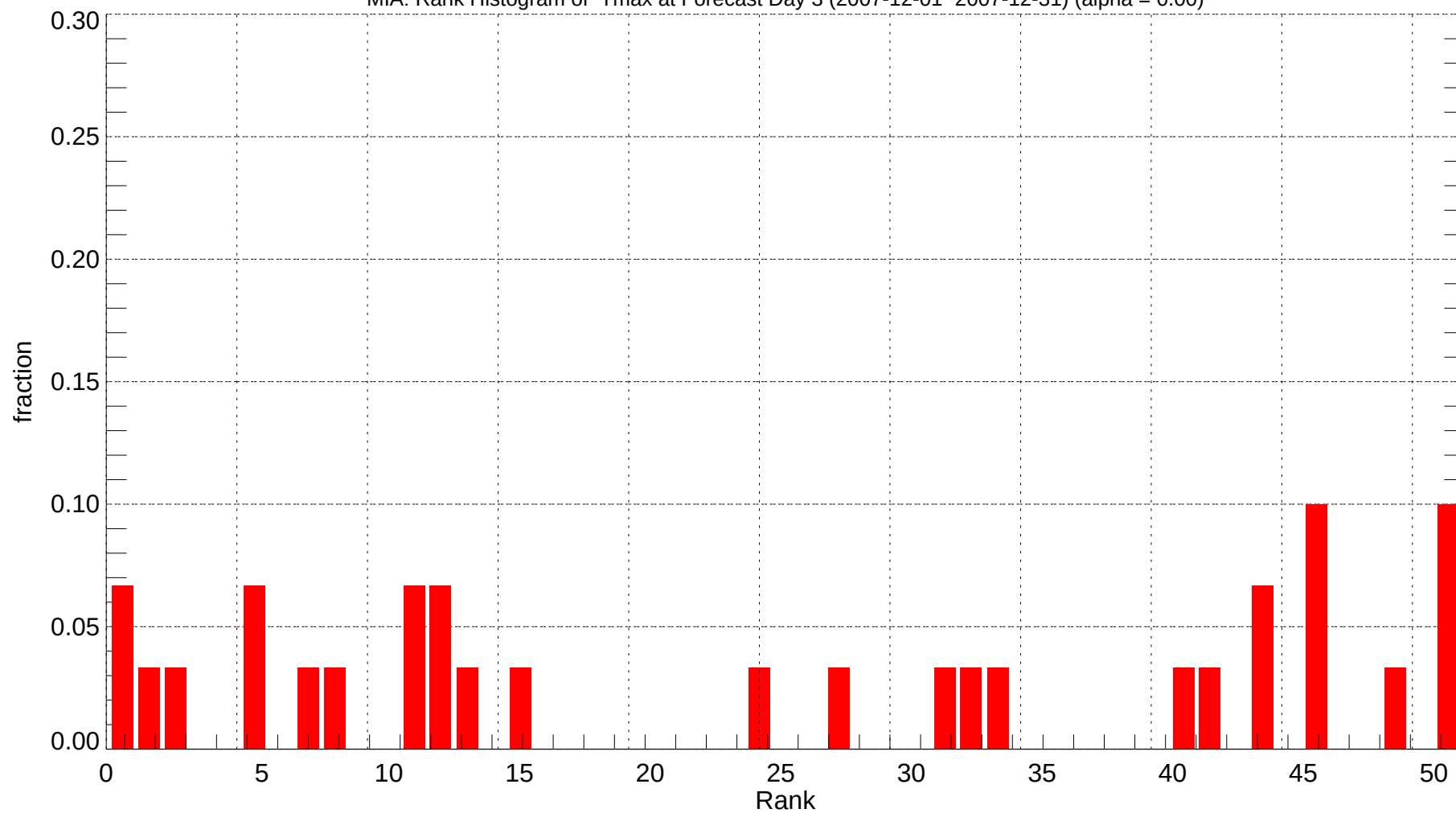
MIA: Rank Histogram of Tmax at Forecast Day 3 (2007-12-01~2007-12-31) (alpha = 0.00)
