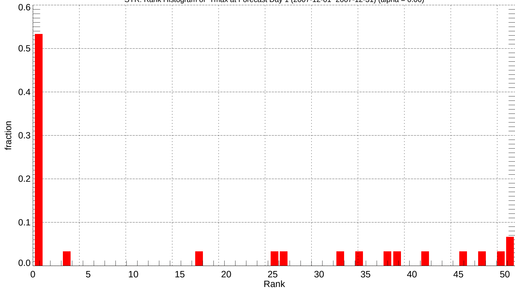
SYR: Rank Histogram of Tmax at Forecast Day 1 (2007-12-01~2007-12-31) (alpha = 0.00)
