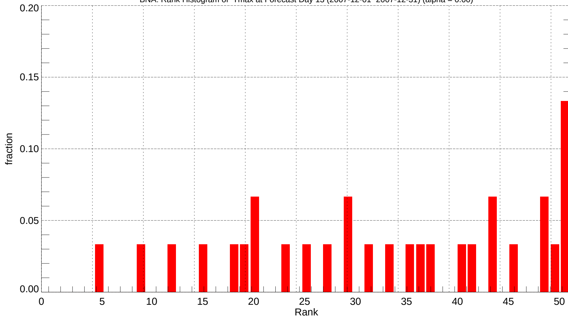
BNA: Rank Histogram of Tmax at Forecast Day 13 (2007-12-01~2007-12-31) (alpha = 0.00)
