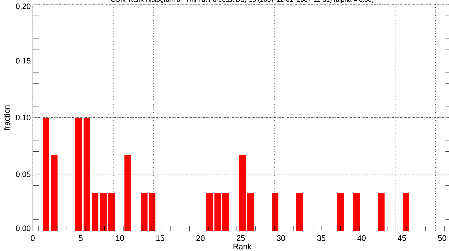
CON: Rank Histogram of Tmin at Forecast Day 13 (2007-12-01~2007-12-31) (alpha = 0.00)
