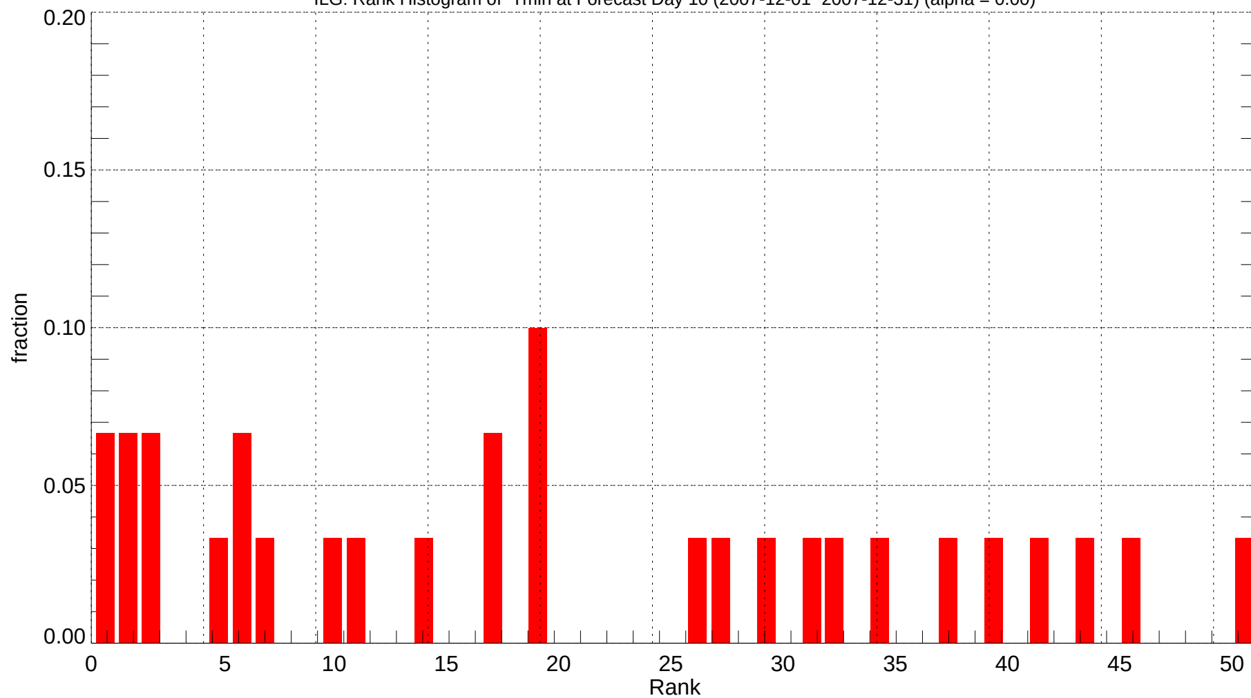
ILG: Rank Histogram of Tmin at Forecast Day 10 (2007-12-01~2007-12-31) (alpha = 0.00)
