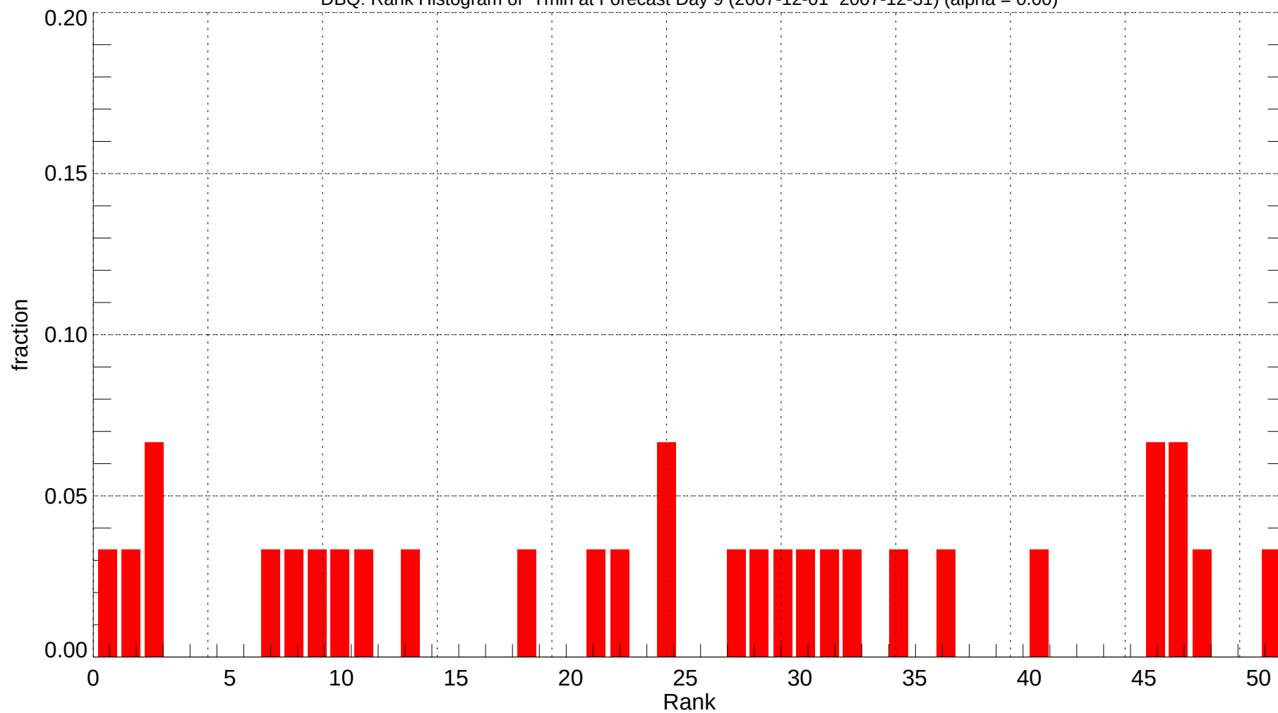
DBQ: Rank Histogram of Tmin at Forecast Day 9 (2007-12-01~2007-12-31) (alpha = 0.00)
