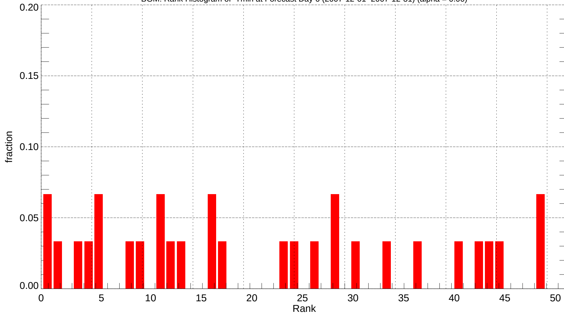
BGM: Rank Histogram of Tmin at Forecast Day 6 (2007-12-01~2007-12-31) (alpha = 0.00)
