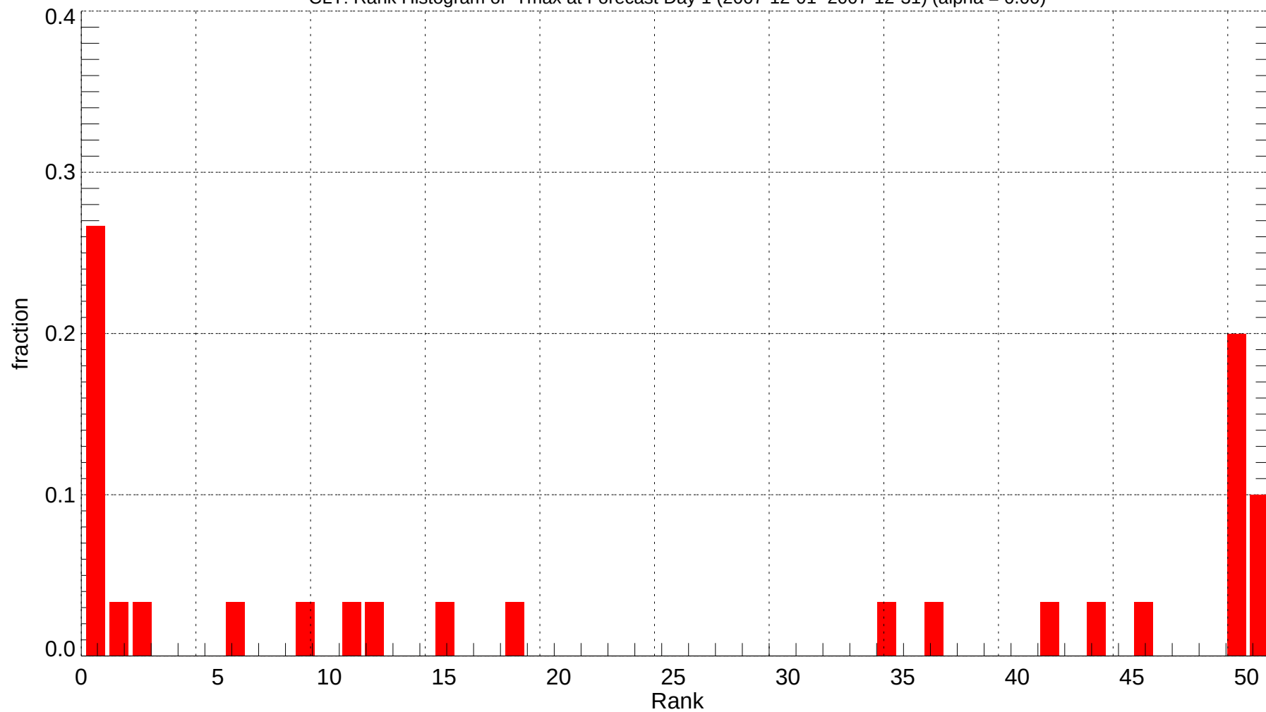
CLT: Rank Histogram of Tmax at Forecast Day 1 (2007-12-01~2007-12-31) (alpha = 0.00)
