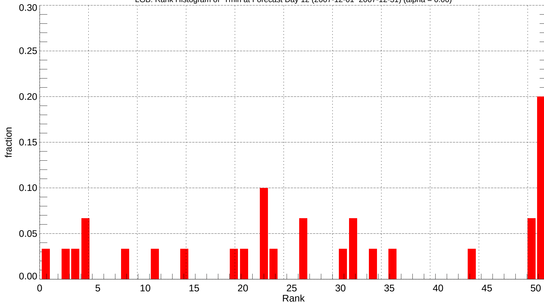
LGB: Rank Histogram of Tmin at Forecast Day 12 (2007-12-01~2007-12-31) (alpha = 0.00)
