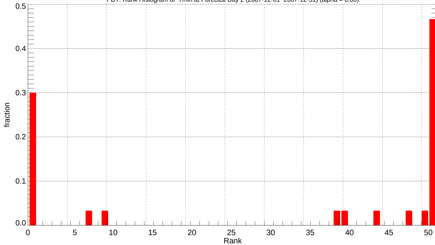
PDT: Rank Histogram of Tmin at Forecast Day 2 (2007-12-01~2007-12-31) (alpha = 0.00)
