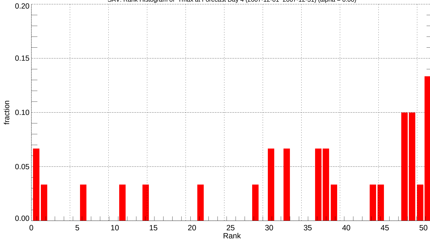
SAV: Rank Histogram of Tmax at Forecast Day 4 (2007-12-01~2007-12-31) (alpha = 0.00)
