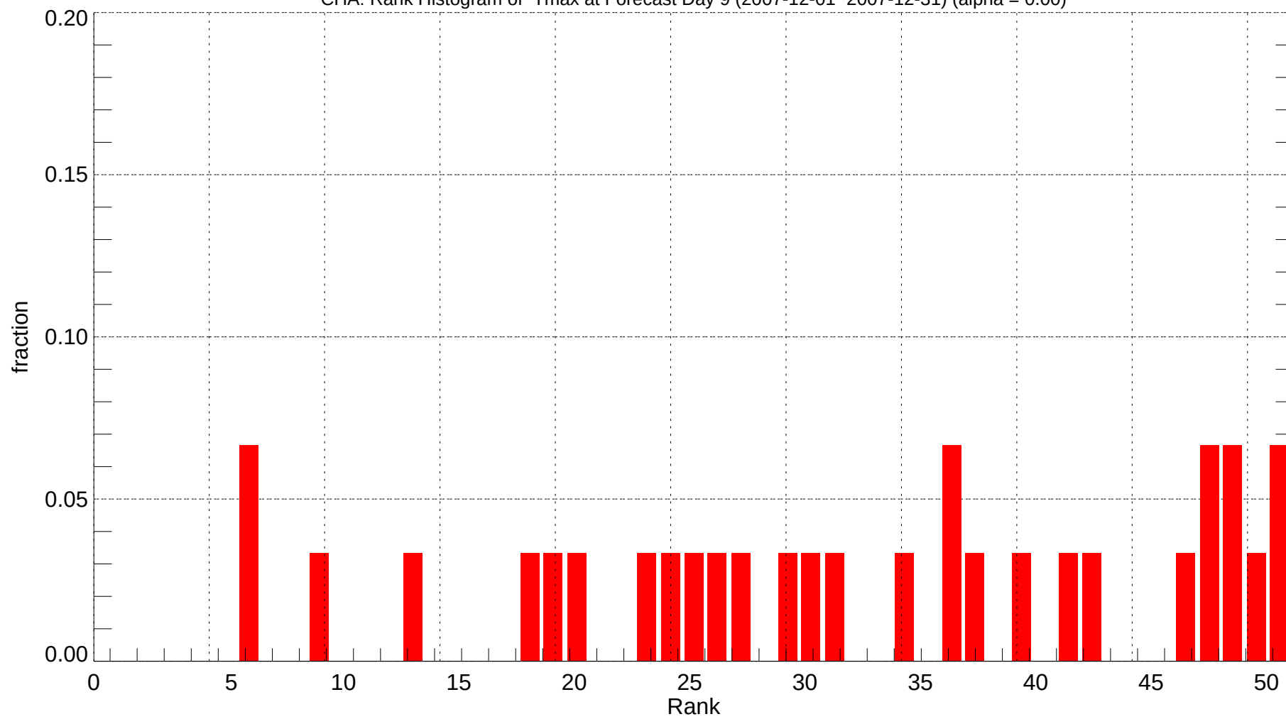
CHA: Rank Histogram of Tmax at Forecast Day 9 (2007-12-01~2007-12-31) (alpha = 0.00)
