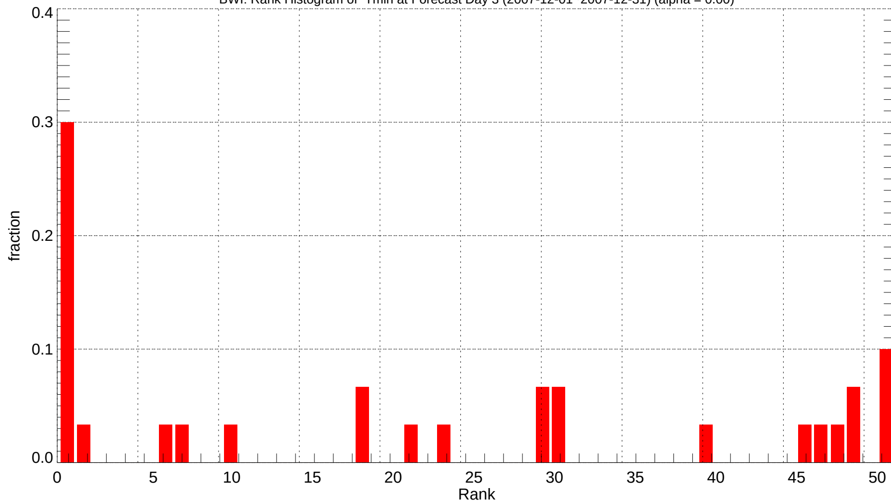
BWI: Rank Histogram of Tmin at Forecast Day 3 (2007-12-01~2007-12-31) (alpha = 0.00)
