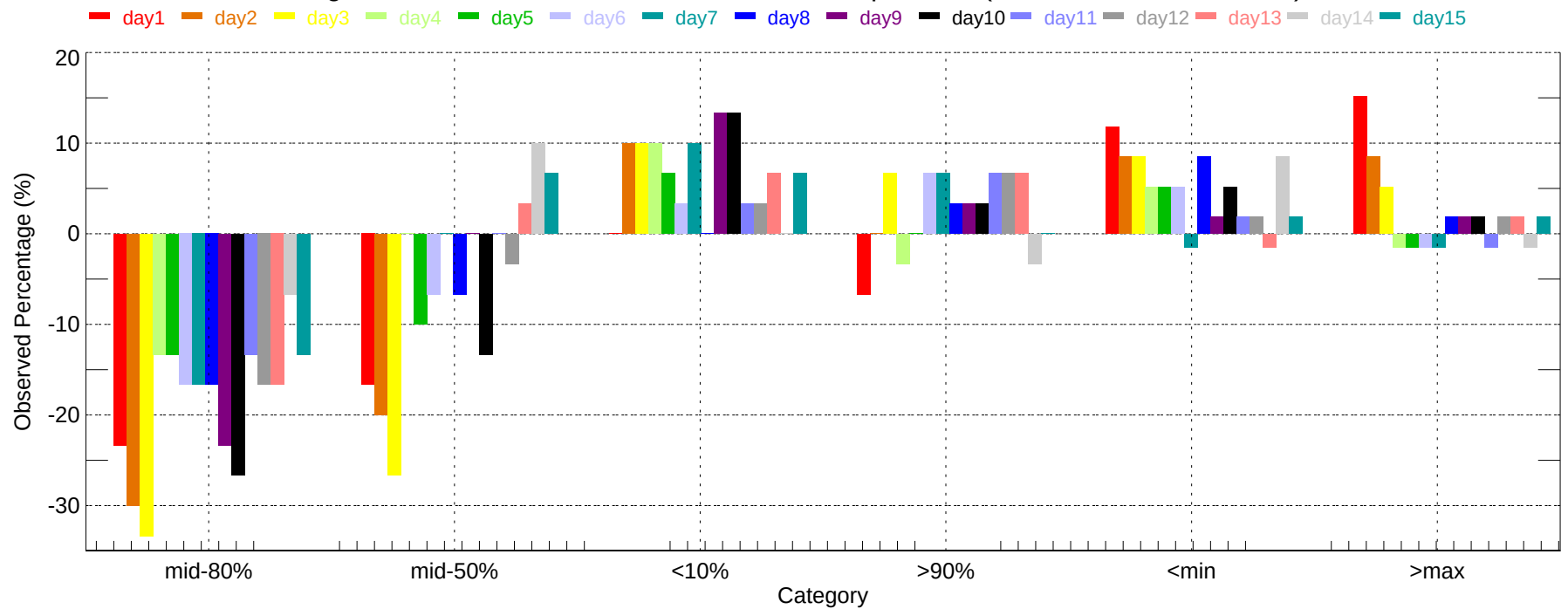
Observed Percentage Deviation of Ensembles - BGM: Min Temperature (2007-12-01~2007-12-31)
