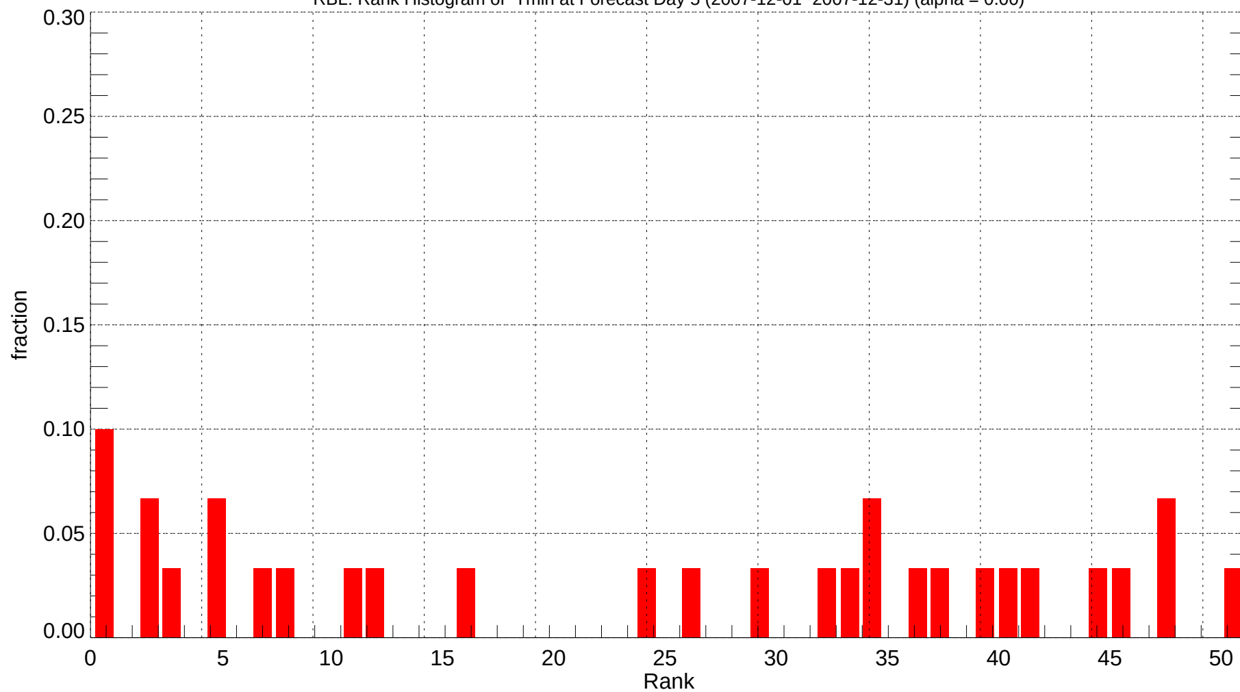
RBL: Rank Histogram of Tmin at Forecast Day 5 (2007-12-01~2007-12-31) (alpha = 0.00)
