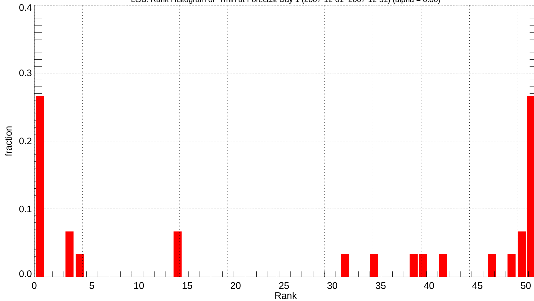
LGB: Rank Histogram of Tmin at Forecast Day 1 (2007-12-01~2007-12-31) (alpha = 0.00)
