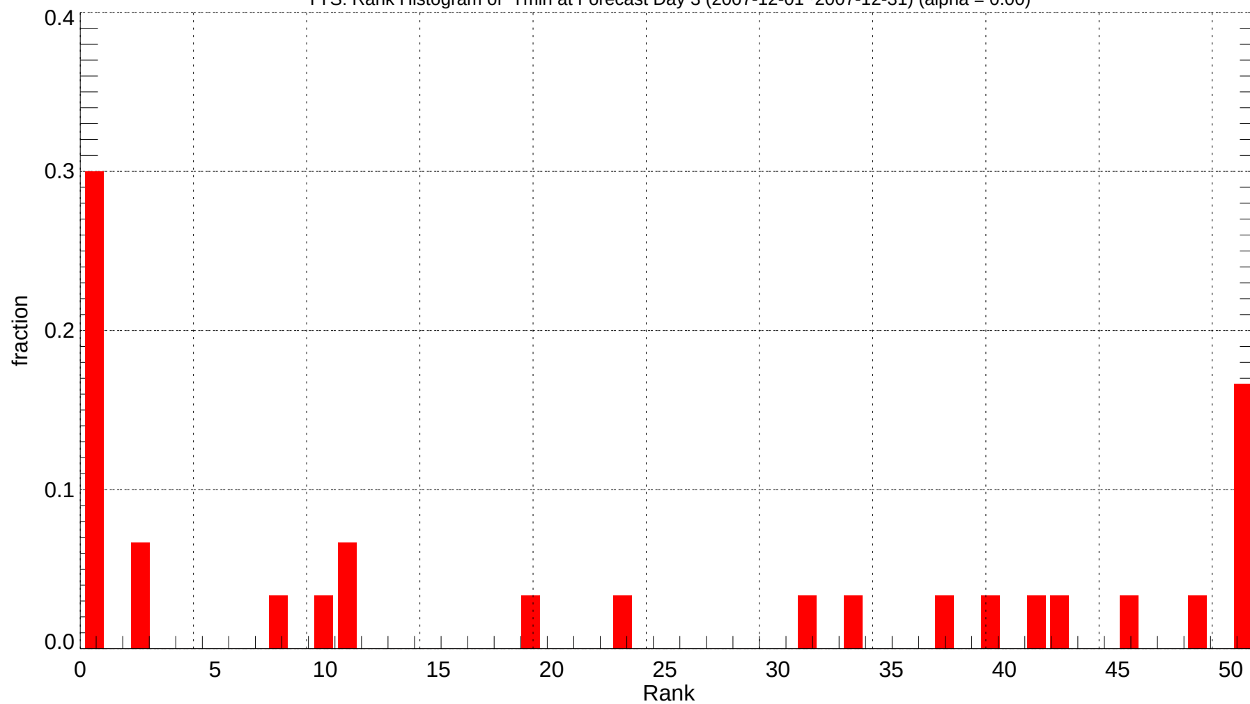
TYS: Rank Histogram of Tmin at Forecast Day 3 (2007-12-01~2007-12-31) (alpha = 0.00)
