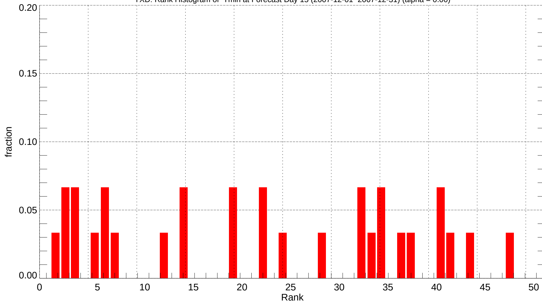
YXD: Rank Histogram of Tmin at Forecast Day 15 (2007-12-01~2007-12-31) (alpha = 0.00)
