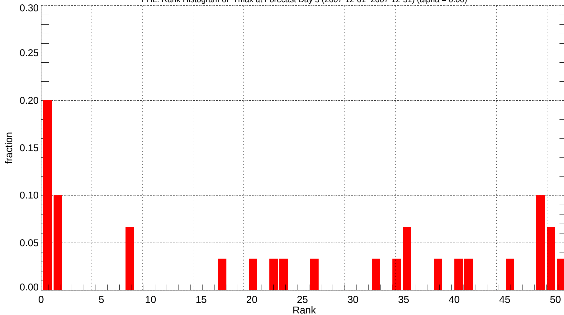
PHL: Rank Histogram of Tmax at Forecast Day 3 (2007-12-01~2007-12-31) (alpha = 0.00)
