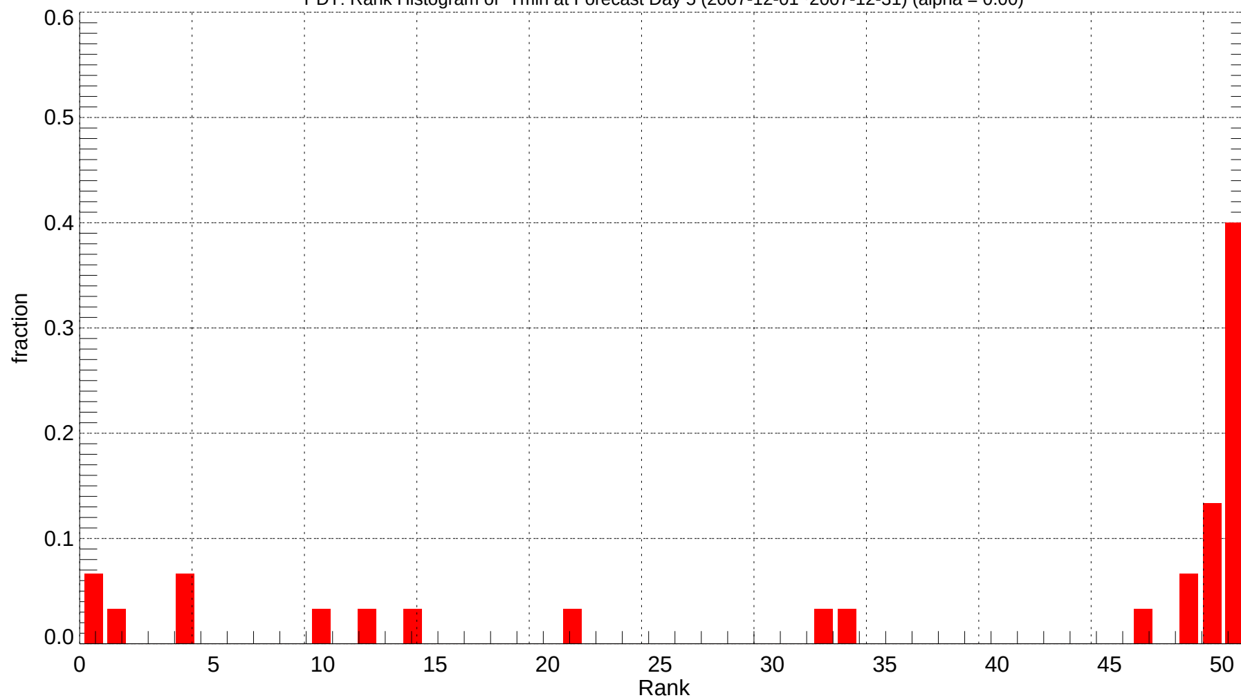
PDT: Rank Histogram of Tmin at Forecast Day 5 (2007-12-01~2007-12-31) (alpha = 0.00)
