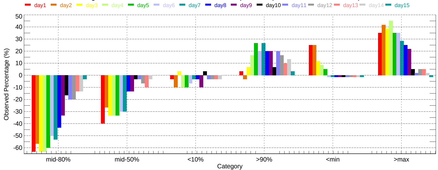
Observed Percentage Deviation of Ensembles - BFL: Min Temperature (2007-12-01~2007-12-31)
