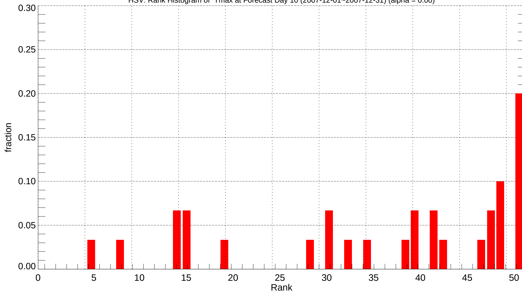
HSV: Rank Histogram of Tmax at Forecast Day 10 (2007-12-01~2007-12-31) (alpha = 0.00)
