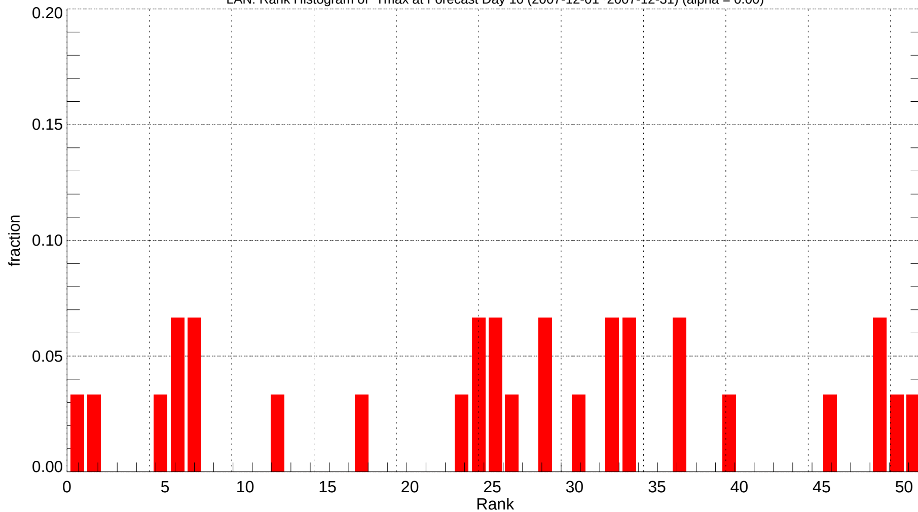
LAN: Rank Histogram of Tmax at Forecast Day 10 (2007-12-01~2007-12-31) (alpha = 0.00)
