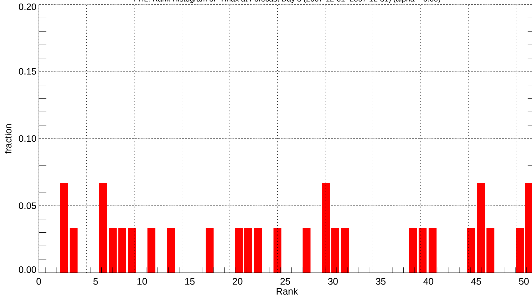
PHL: Rank Histogram of Tmax at Forecast Day 8 (2007-12-01~2007-12-31) (alpha = 0.00)
