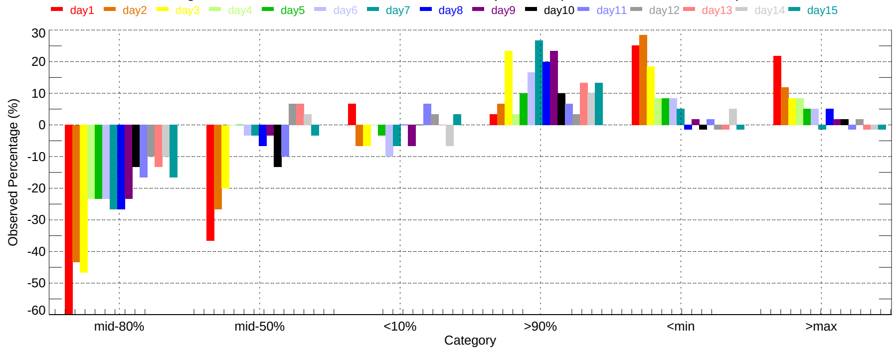
Observed Percentage Deviation of Ensembles - ACY: Min Temperature (2007-12-01~2007-12-31)
