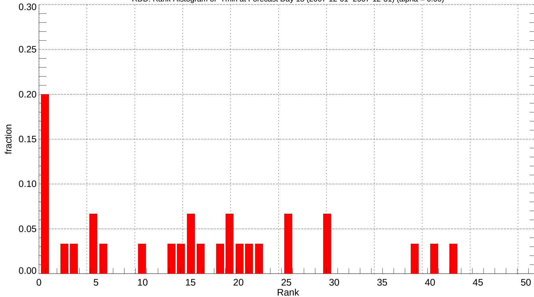
RDD: Rank Histogram of Tmin at Forecast Day 13 (2007-12-01~2007-12-31) (alpha = 0.00)
