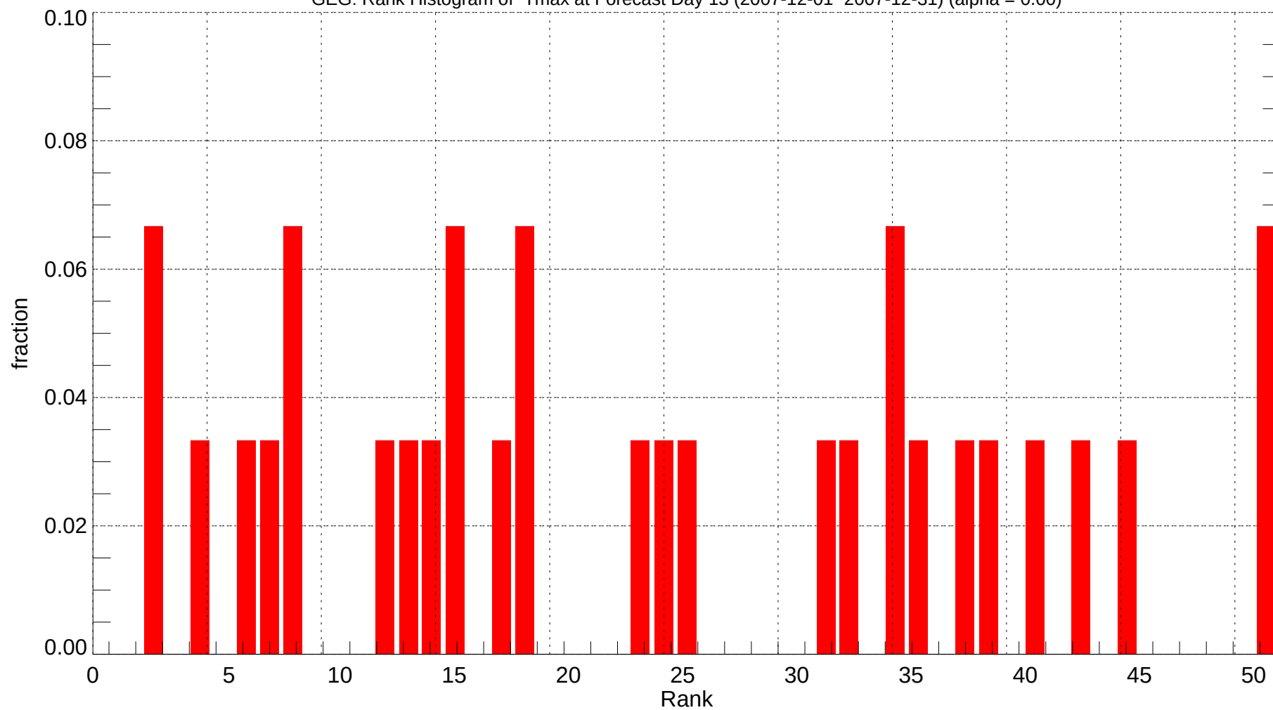
GEG: Rank Histogram of Tmax at Forecast Day 13 (2007-12-01~2007-12-31) (alpha = 0.00)
