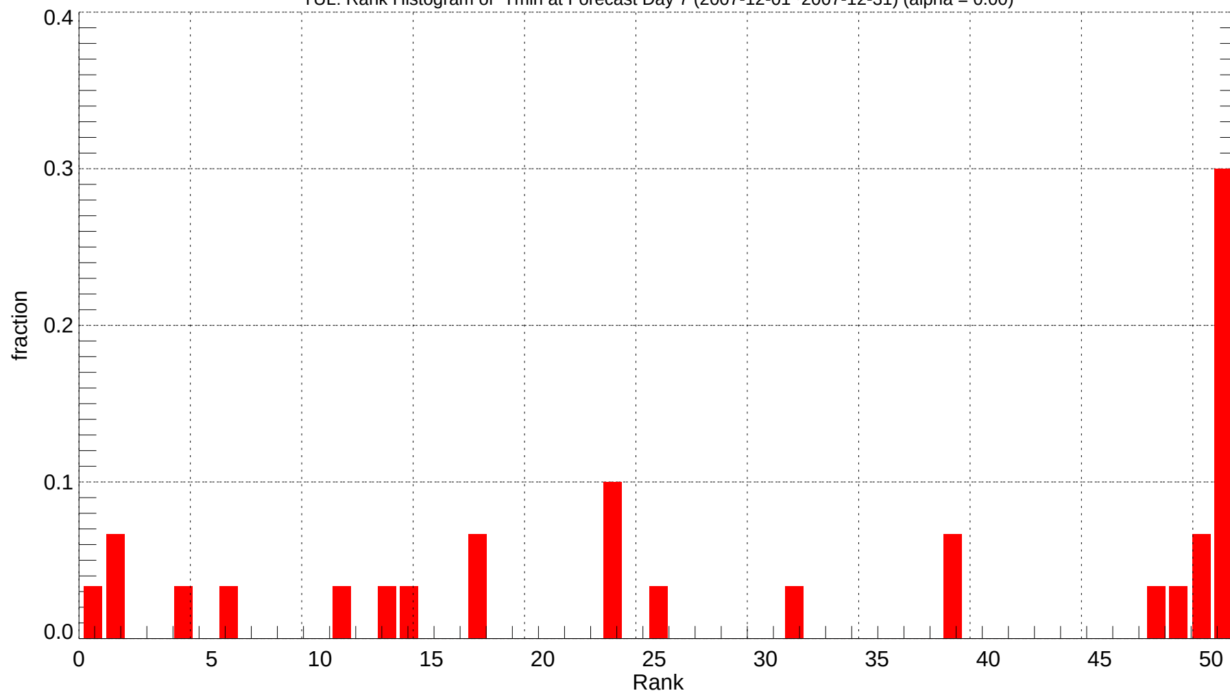
TUL: Rank Histogram of Tmin at Forecast Day 7 (2007-12-01~2007-12-31) (alpha = 0.00)
