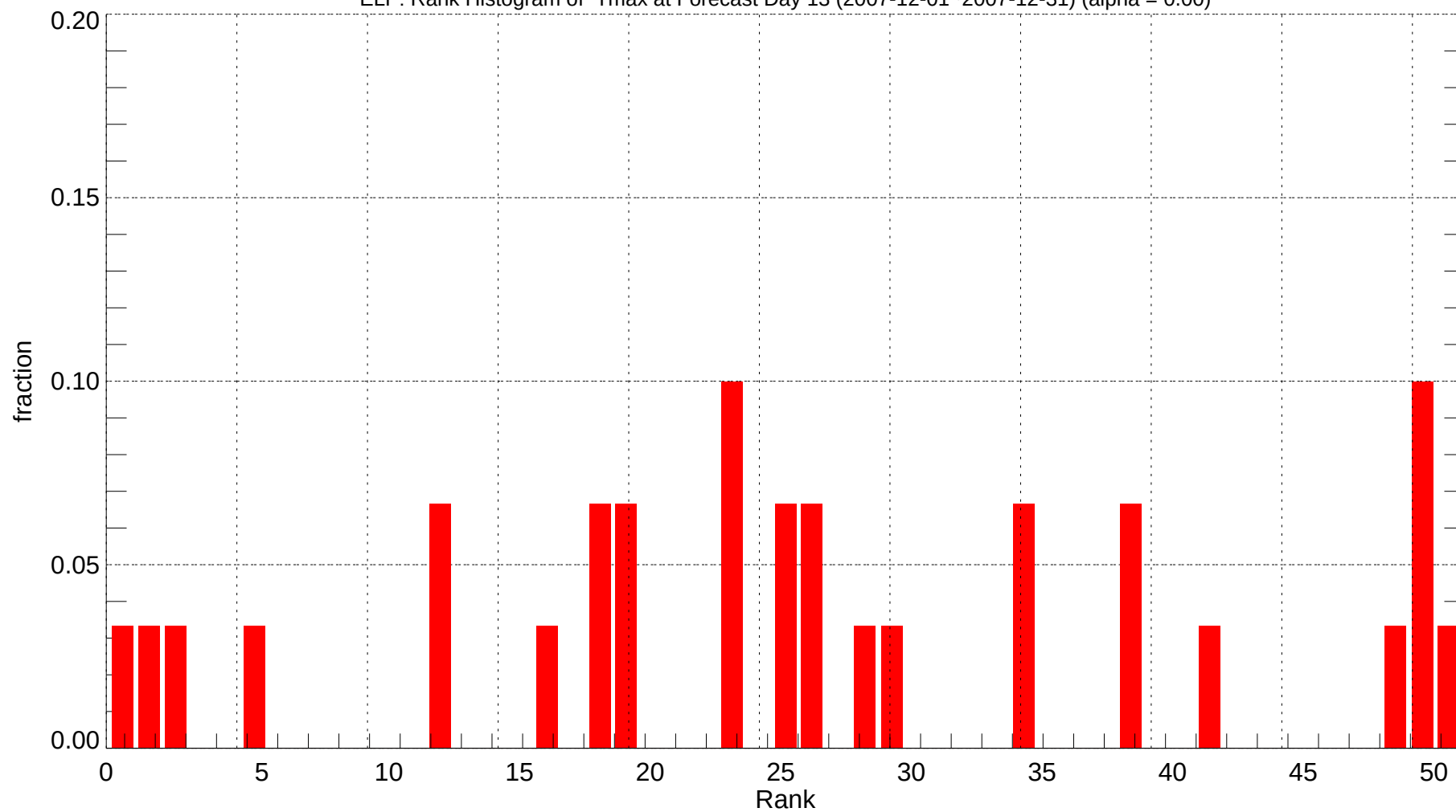
ELP: Rank Histogram of Tmax at Forecast Day 13 (2007-12-01~2007-12-31) (alpha = 0.00)
