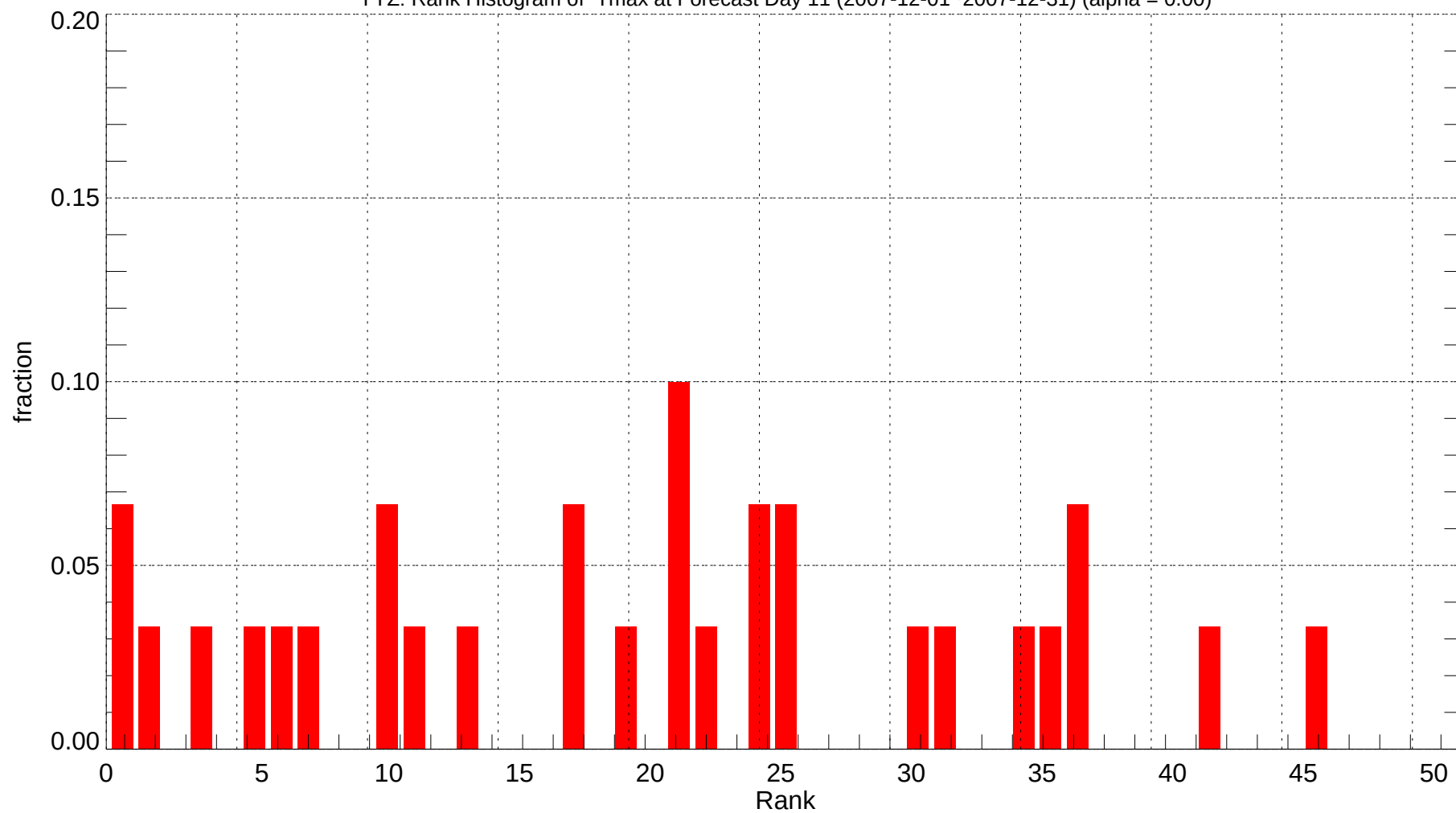
YYZ: Rank Histogram of Tmax at Forecast Day 11 (2007-12-01~2007-12-31) (alpha = 0.00)
