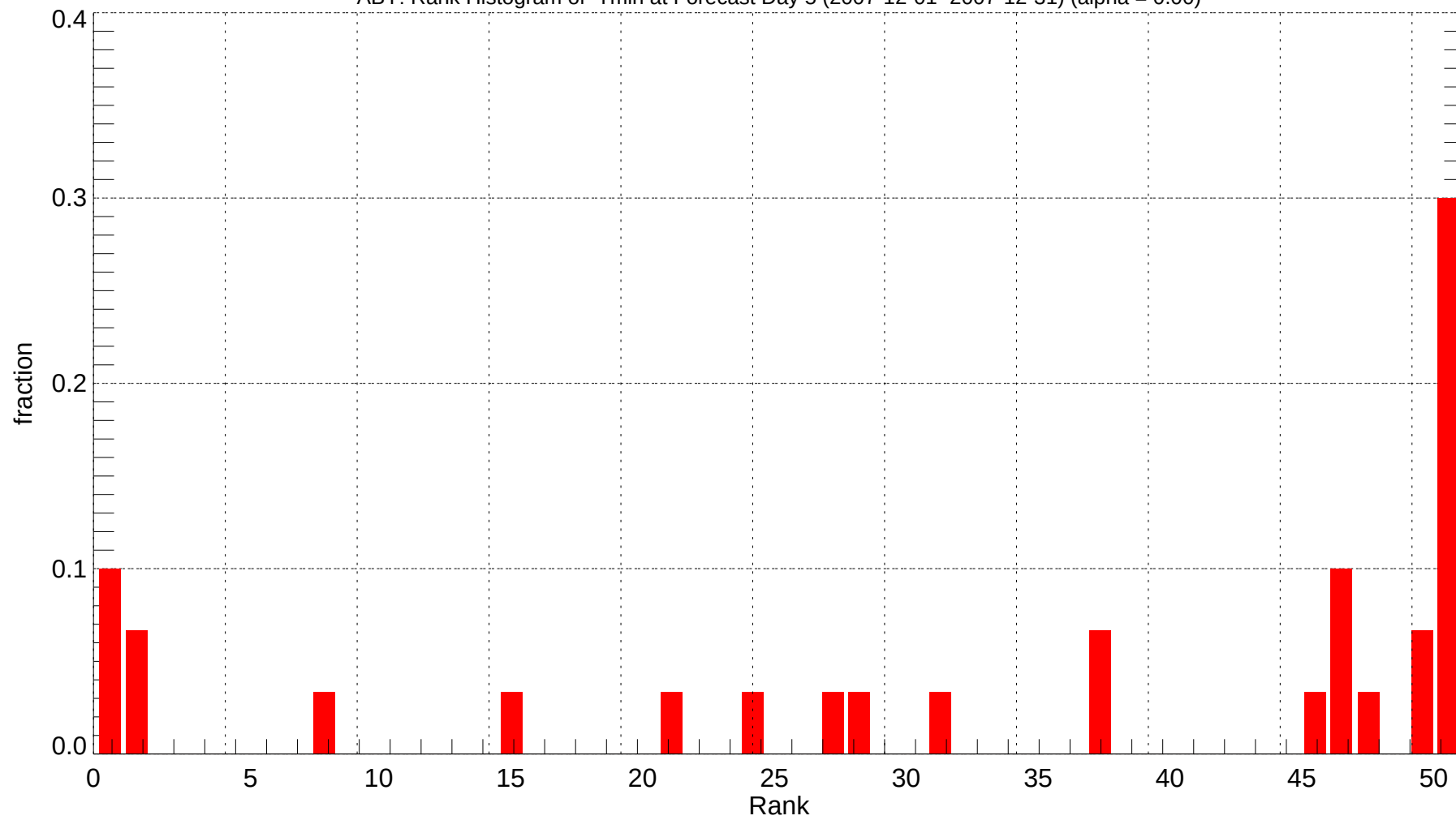
ABY: Rank Histogram of Tmin at Forecast Day 5 (2007-12-01~2007-12-31) (alpha = 0.00)
