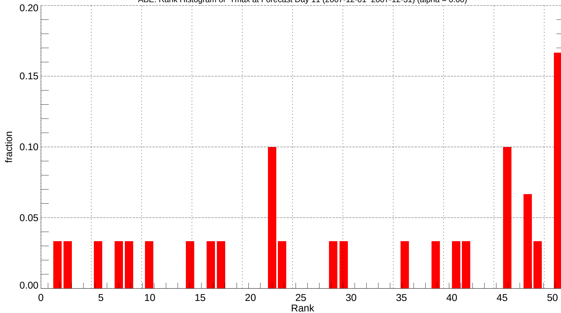
ABE: Rank Histogram of Tmax at Forecast Day 11 (2007-12-01~2007-12-31) (alpha = 0.00)
