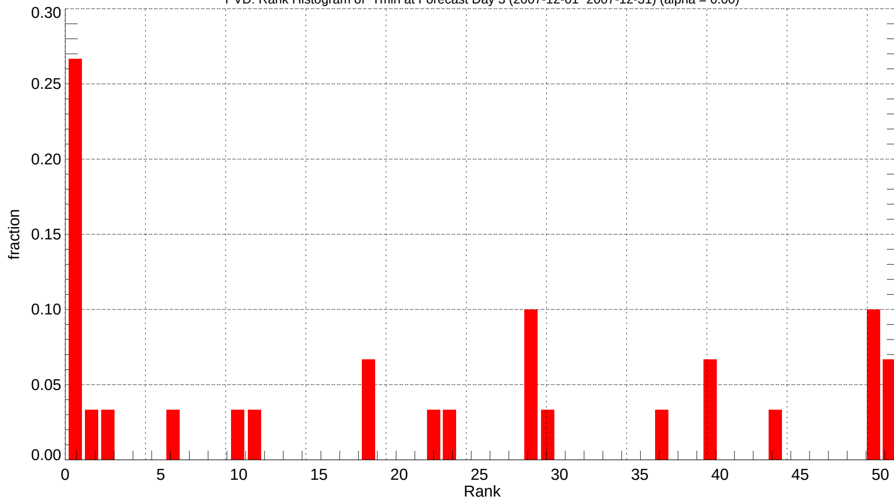
PVD: Rank Histogram of Tmin at Forecast Day 3 (2007-12-01~2007-12-31) (alpha = 0.00)
