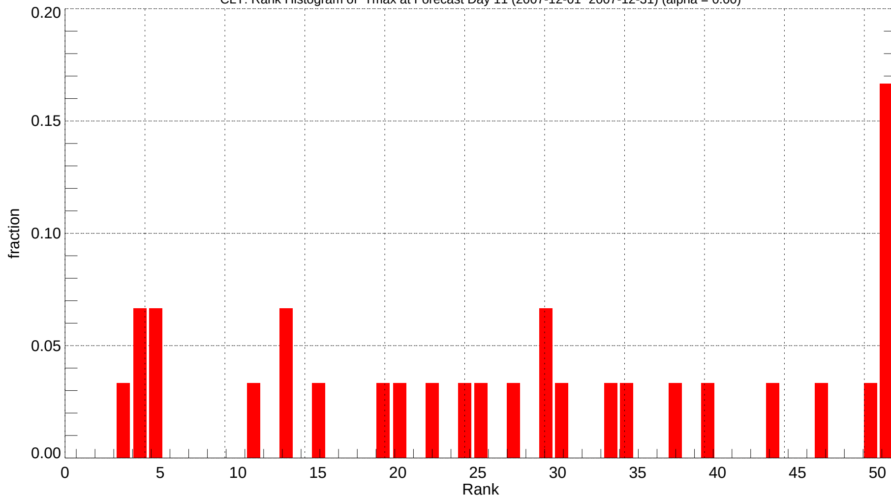
CLT: Rank Histogram of Tmax at Forecast Day 11 (2007-12-01~2007-12-31) (alpha = 0.00)
