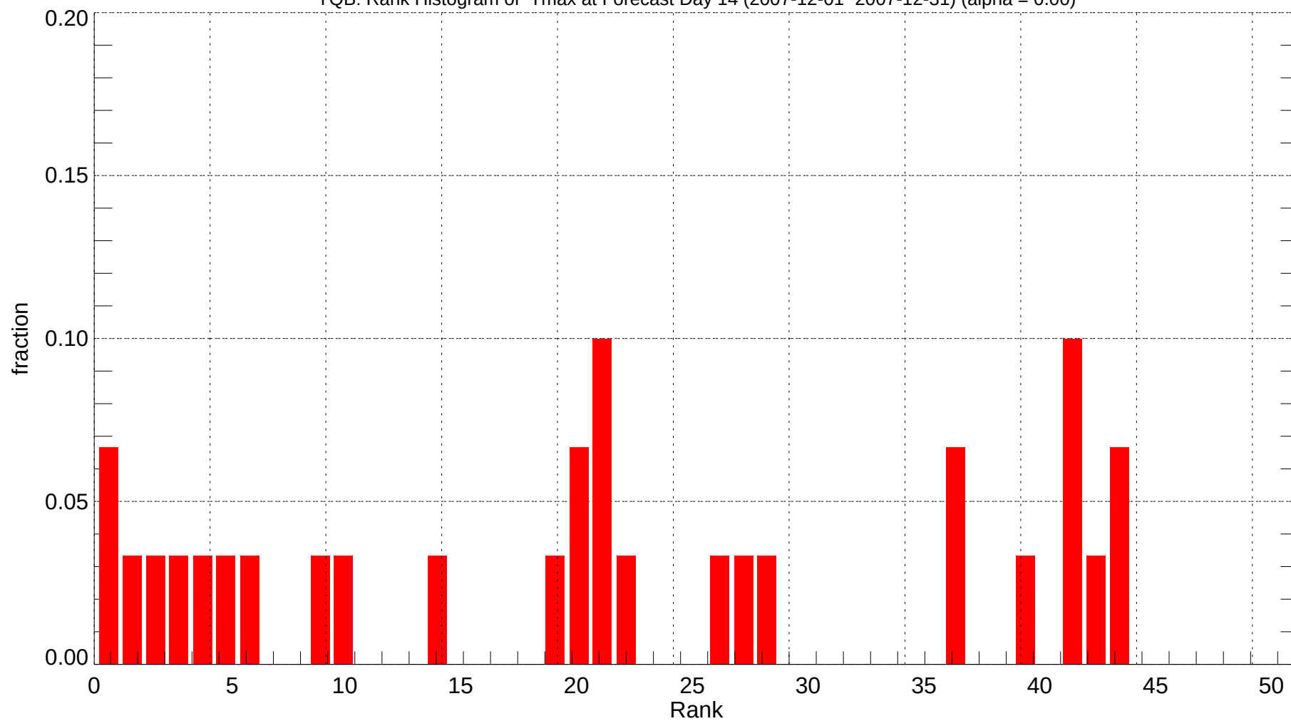
YQB: Rank Histogram of Tmax at Forecast Day 14 (2007-12-01~2007-12-31) (alpha = 0.00)
