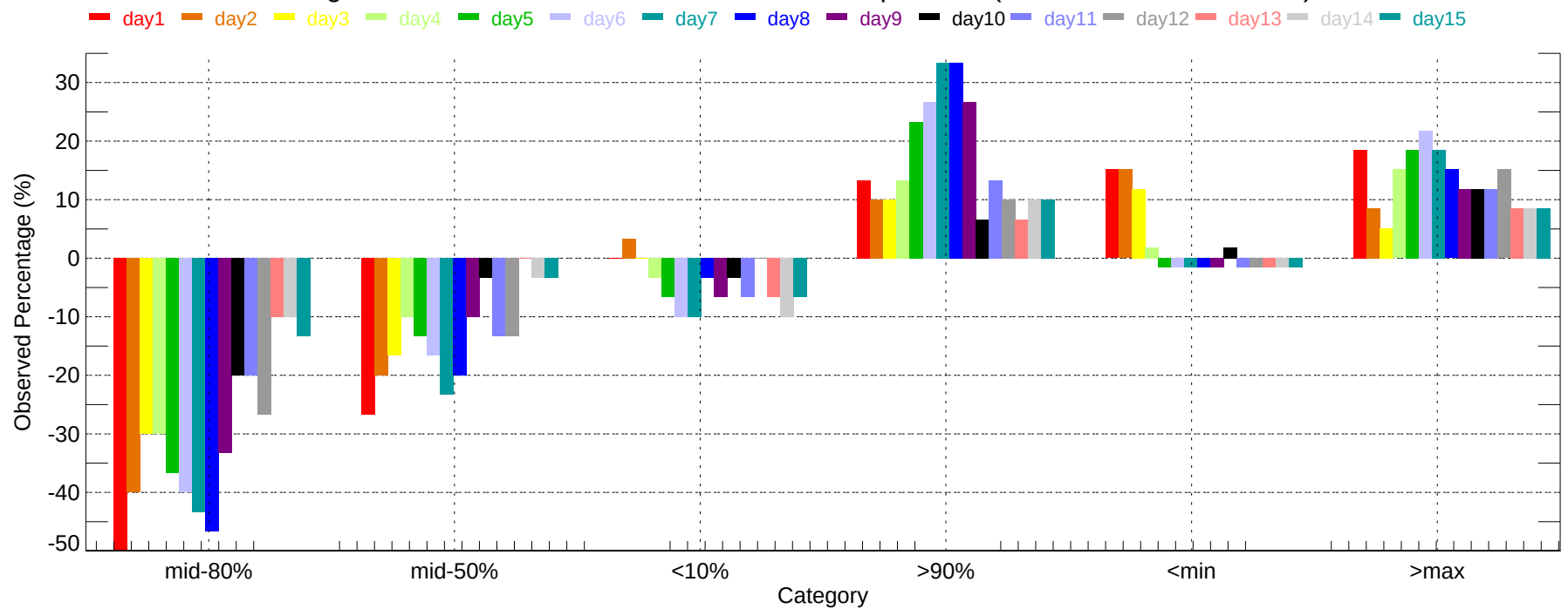
Observed Percentage Deviation of Ensembles - MEM: Max Temperature (2007-12-01~2007-12-31)
