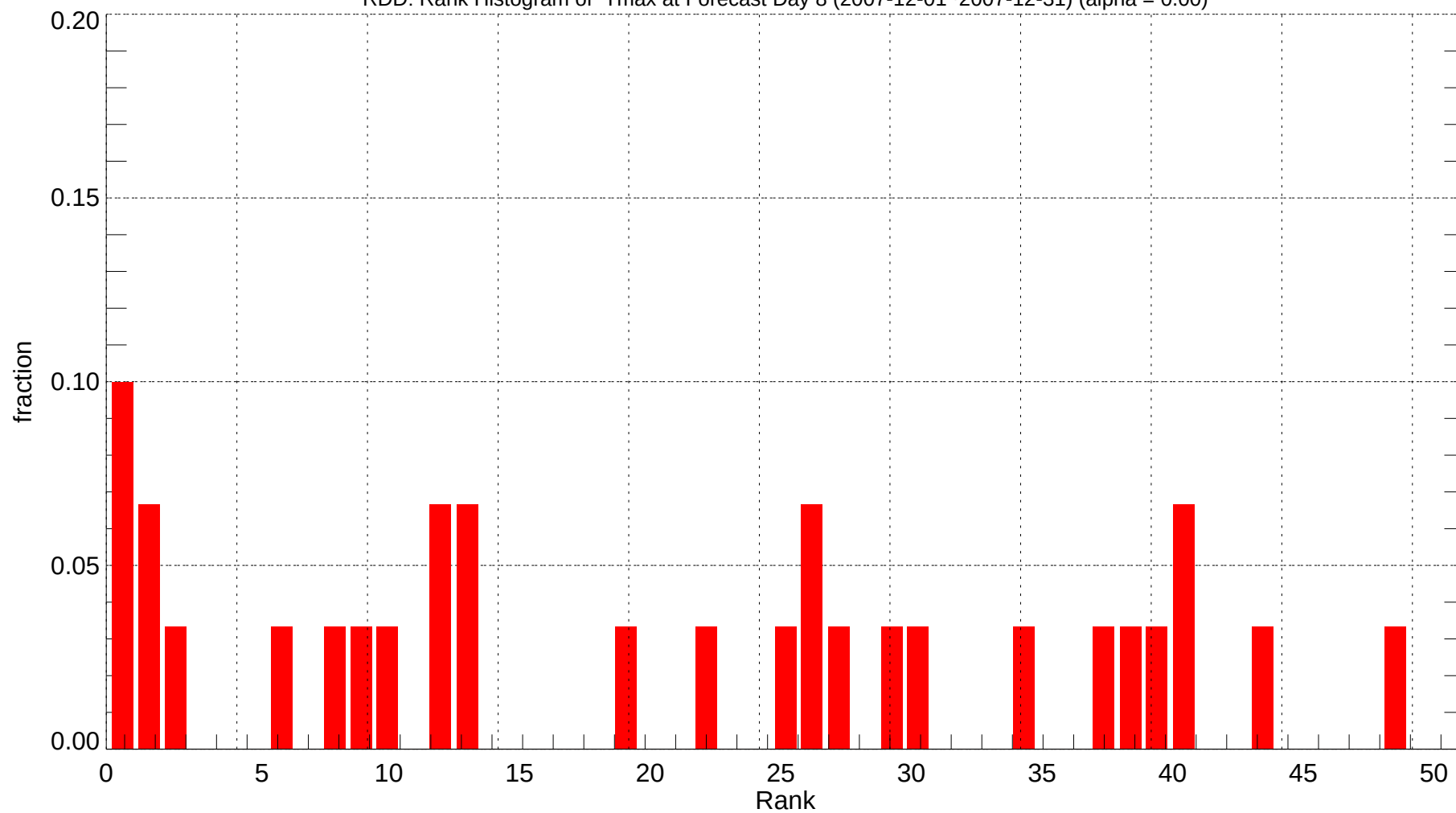
RDD: Rank Histogram of Tmax at Forecast Day 8 (2007-12-01~2007-12-31) (alpha = 0.00)
