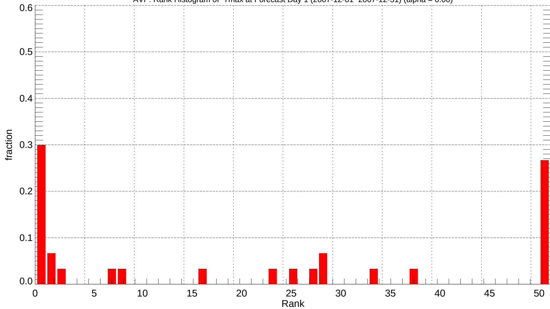
AVP: Rank Histogram of Tmax at Forecast Day 1 (2007-12-01~2007-12-31) (alpha = 0.00)
