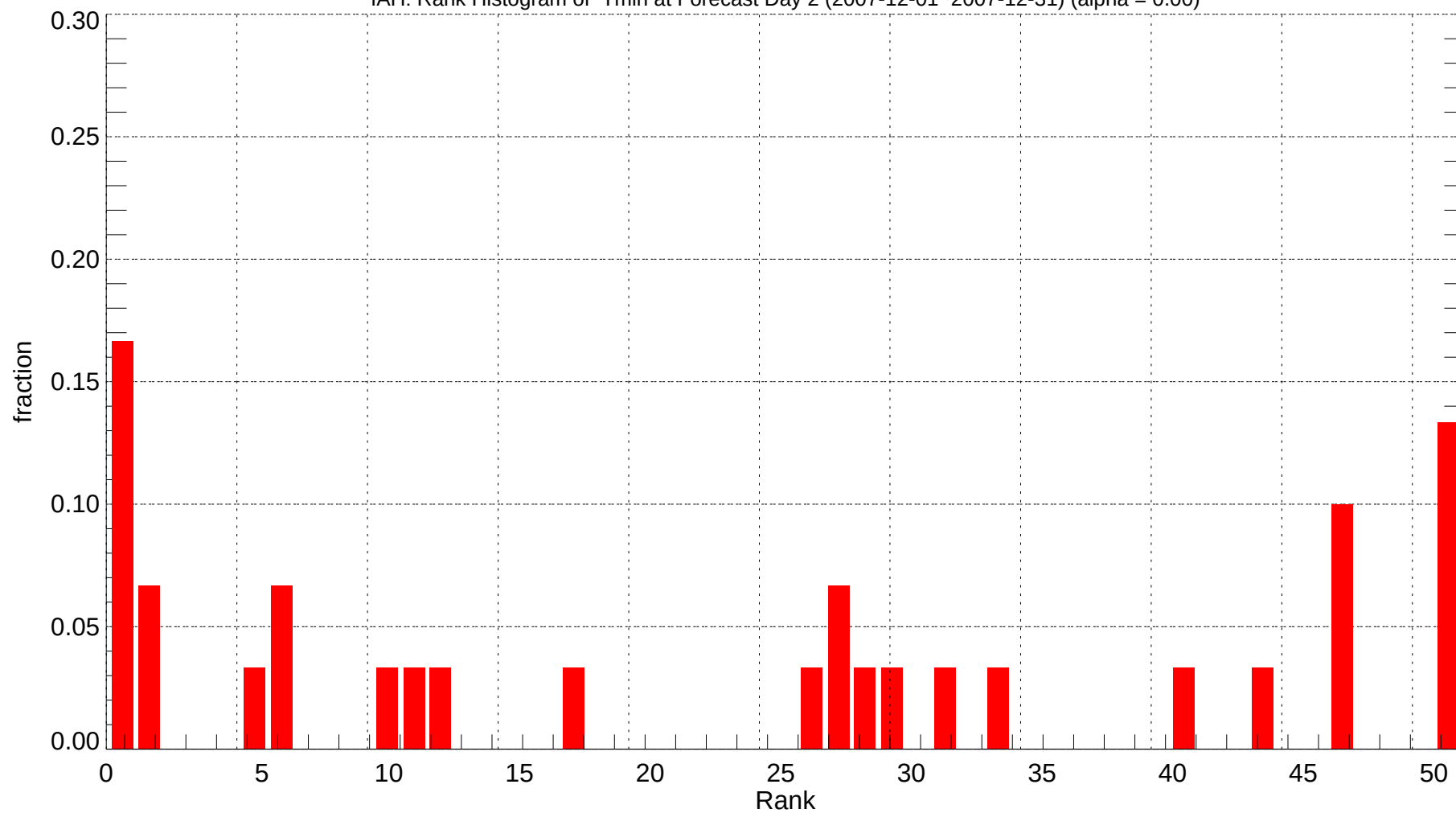
IAH: Rank Histogram of Tmin at Forecast Day 2 (2007-12-01~2007-12-31) (alpha = 0.00)
