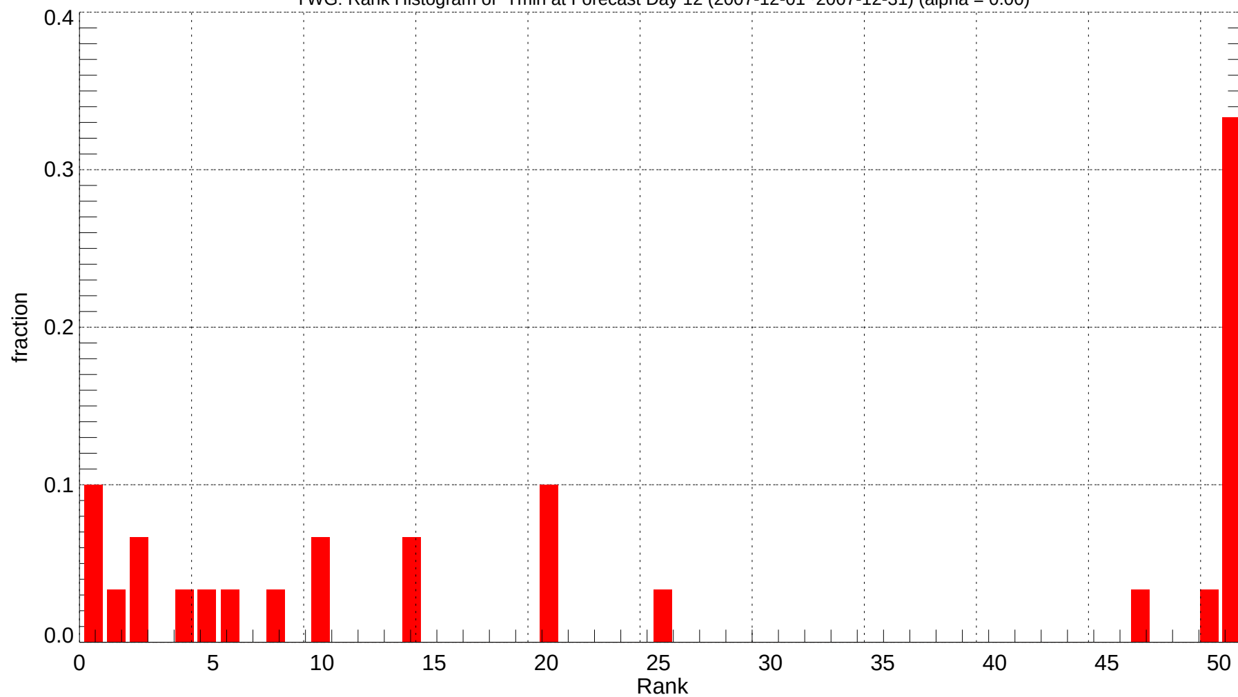
YWG: Rank Histogram of Tmin at Forecast Day 12 (2007-12-01~2007-12-31) (alpha = 0.00)
