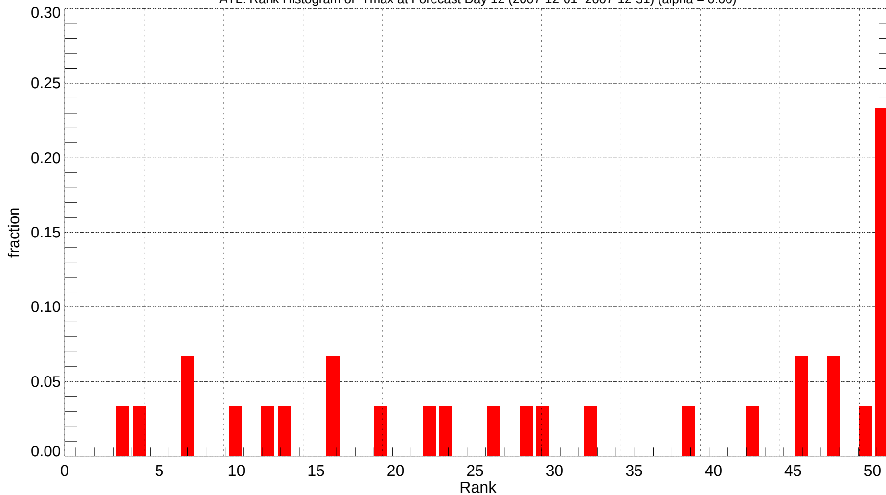
ATL: Rank Histogram of Tmax at Forecast Day 12 (2007-12-01~2007-12-31) (alpha = 0.00)
