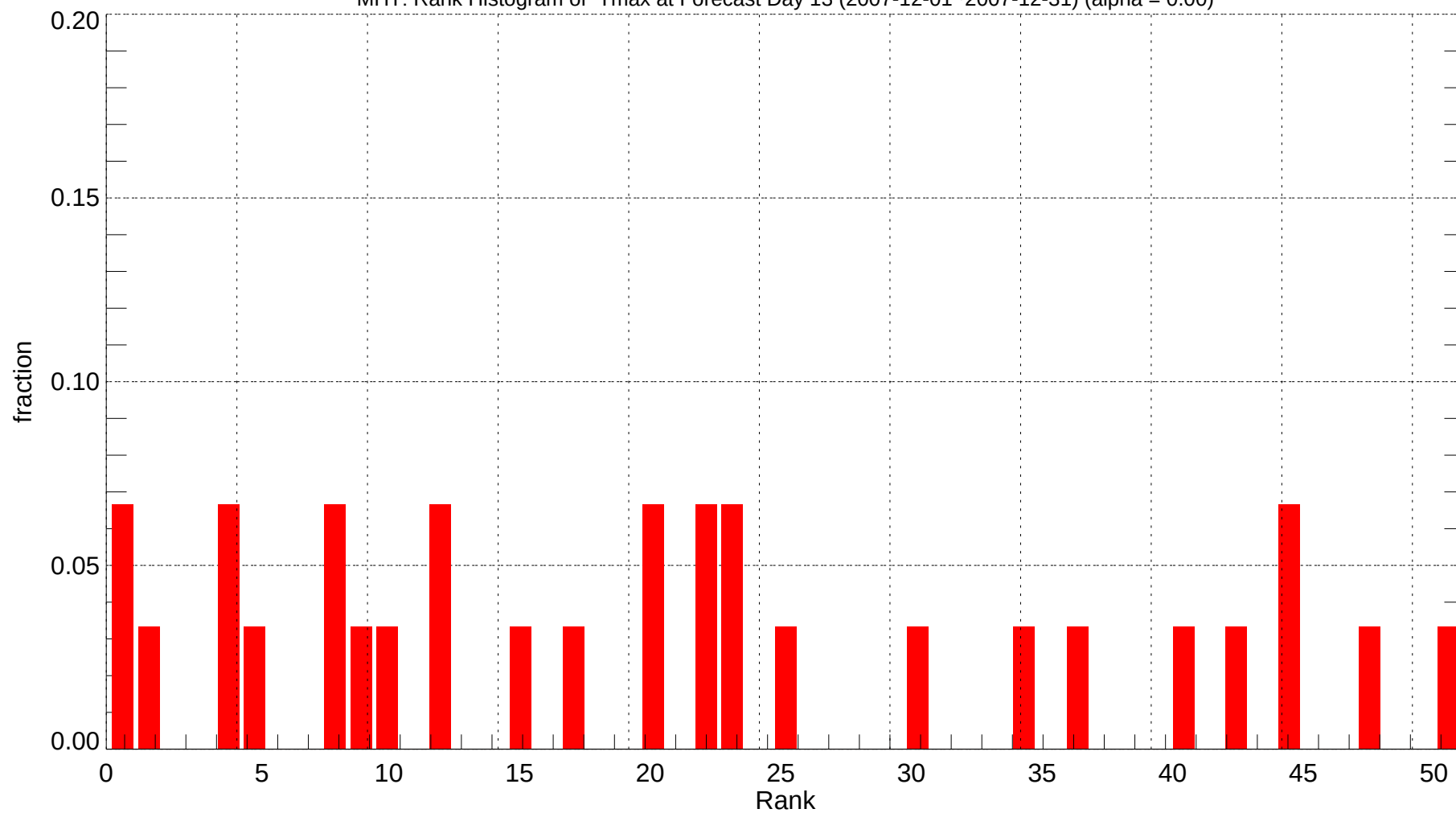
MHT: Rank Histogram of Tmax at Forecast Day 13 (2007-12-01~2007-12-31) (alpha = 0.00)
