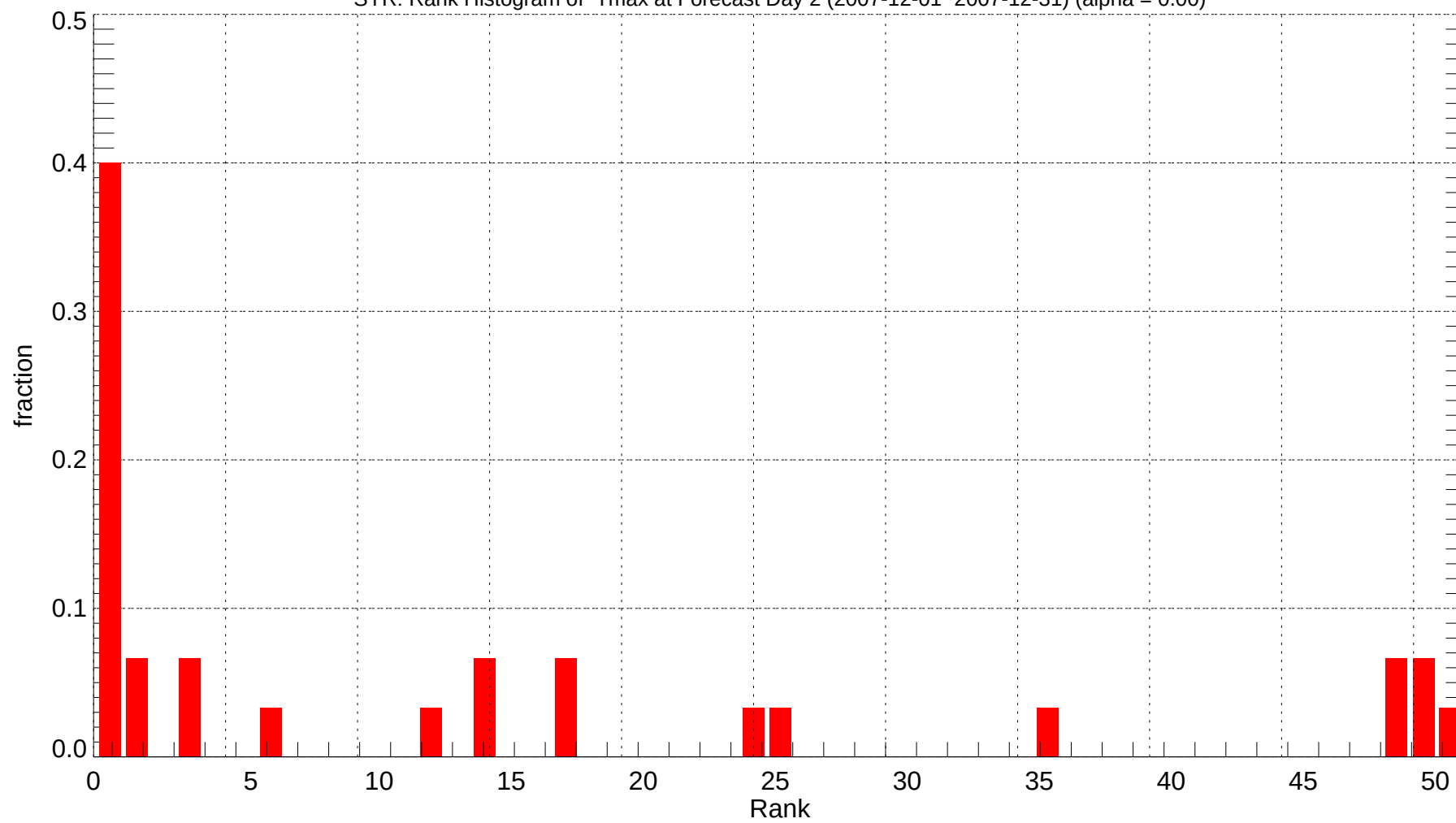
SYR: Rank Histogram of Tmax at Forecast Day 2 (2007-12-01~2007-12-31) (alpha = 0.00)
