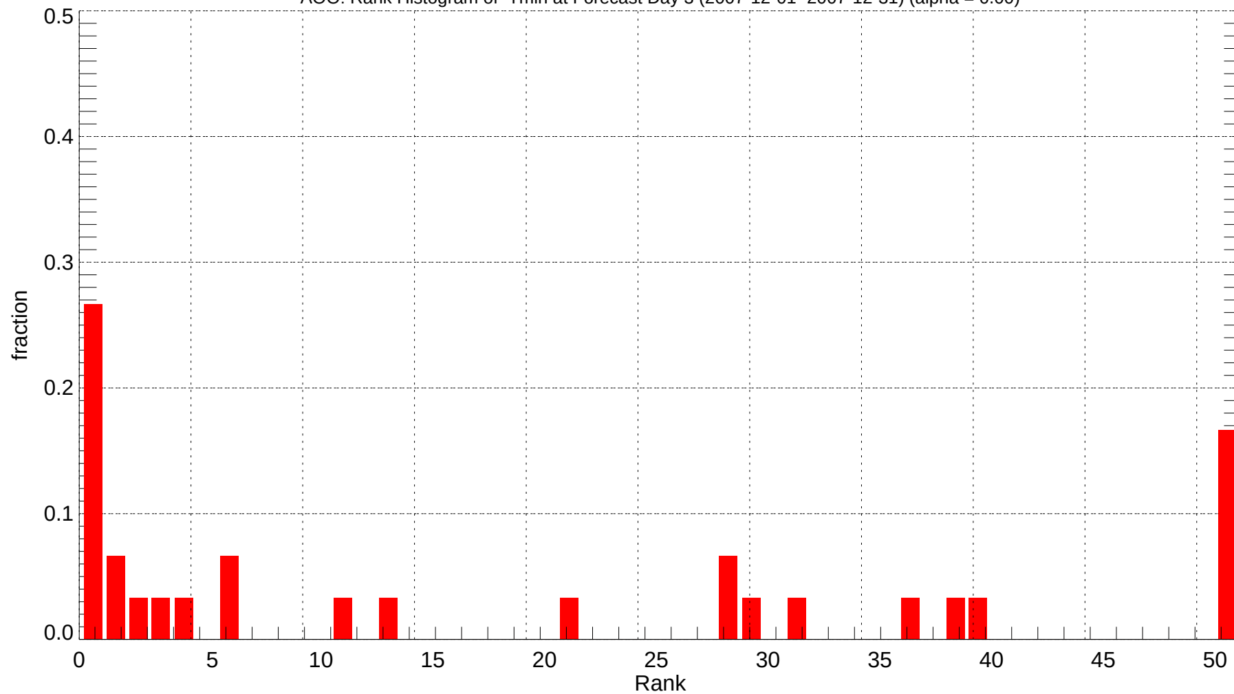
AOO: Rank Histogram of Tmin at Forecast Day 3 (2007-12-01~2007-12-31) (alpha = 0.00)
