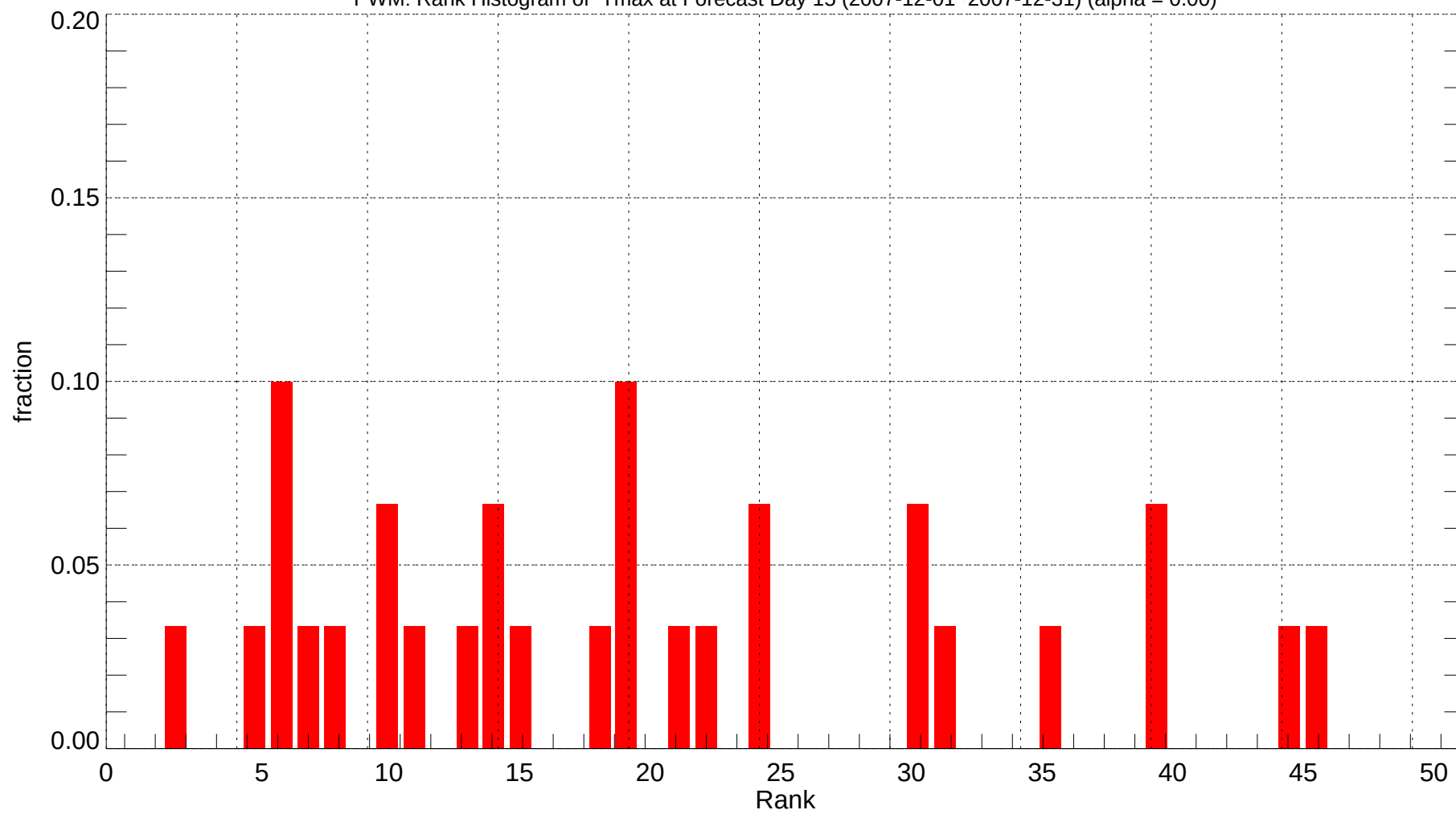
PWM: Rank Histogram of Tmax at Forecast Day 15 (2007-12-01~2007-12-31) (alpha = 0.00)
