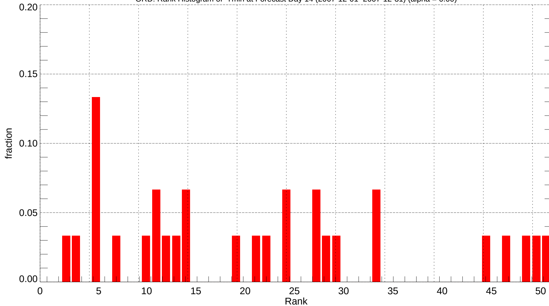
ORD: Rank Histogram of Tmin at Forecast Day 14 (2007-12-01~2007-12-31) (alpha = 0.00)
