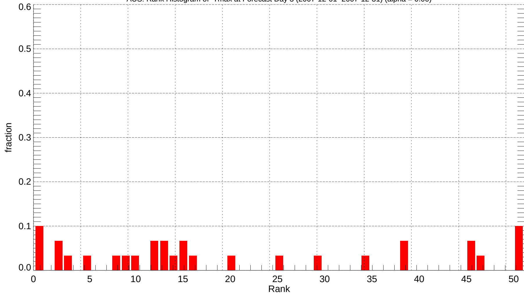
AUS: Rank Histogram of Tmax at Forecast Day 3 (2007-12-01~2007-12-31) (alpha = 0.00)
