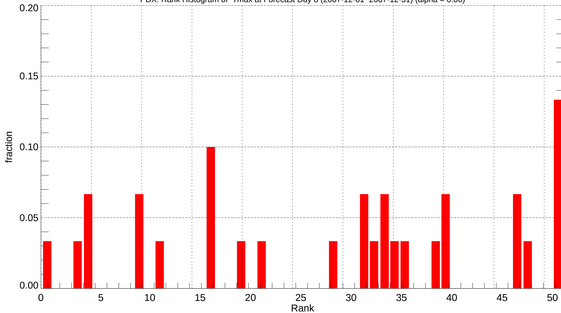
PDX: Rank Histogram of Tmax at Forecast Day 8 (2007-12-01~2007-12-31) (alpha = 0.00)
