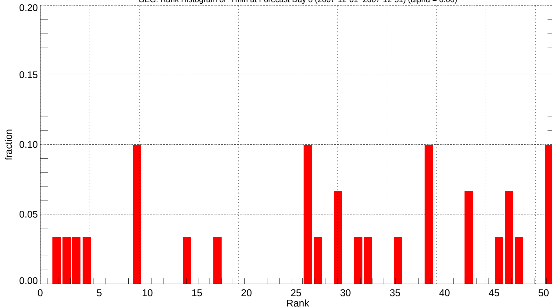
GEG: Rank Histogram of Tmin at Forecast Day 8 (2007-12-01~2007-12-31) (alpha = 0.00)
