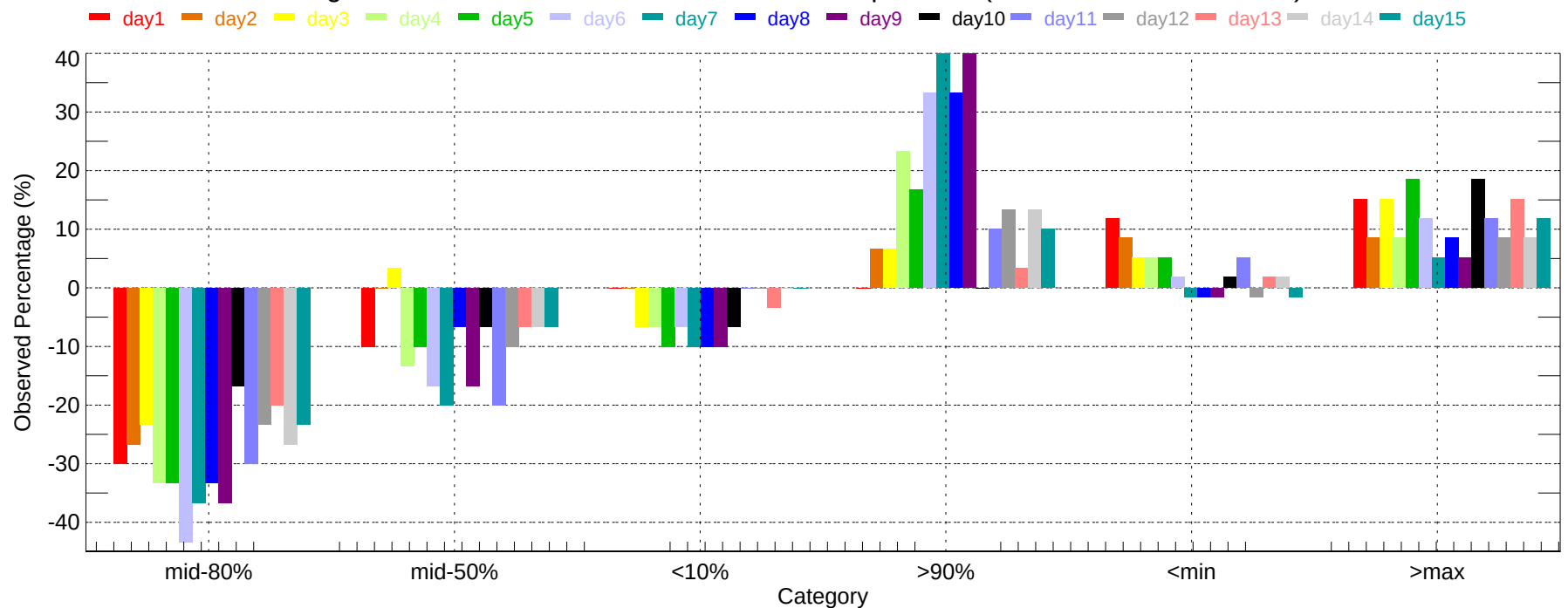
Observed Percentage Deviation of Ensembles - SAV: Max Temperature (2007-12-01~2007-12-31)
