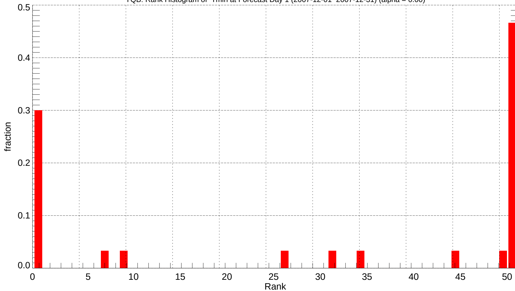
YQB: Rank Histogram of Tmin at Forecast Day 1 (2007-12-01~2007-12-31) (alpha = 0.00)
