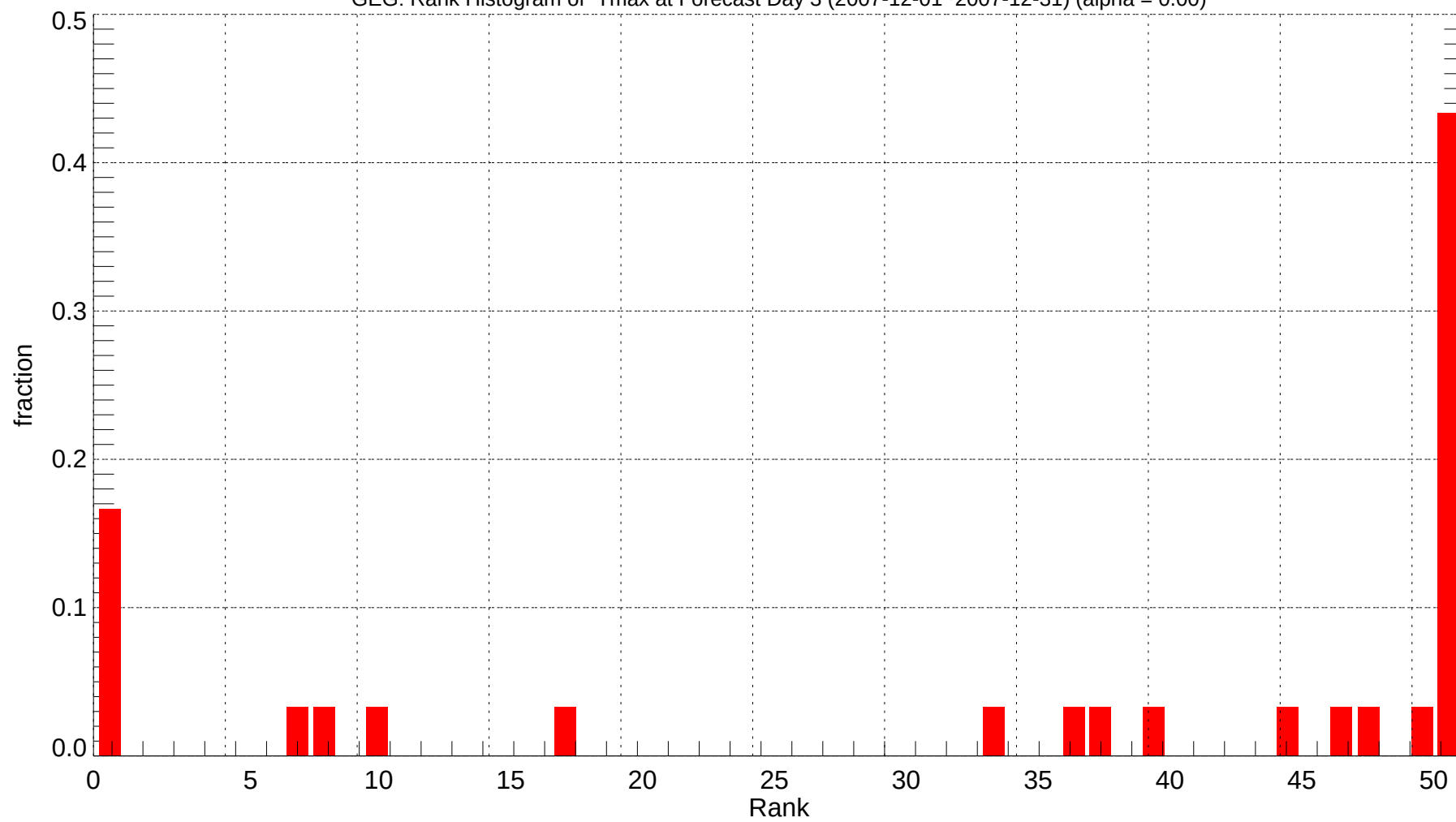
GEG: Rank Histogram of Tmax at Forecast Day 3 (2007-12-01~2007-12-31) (alpha = 0.00)
