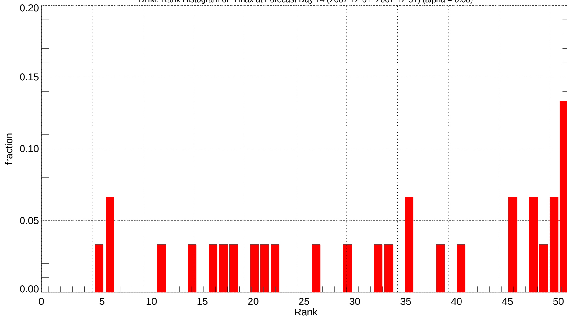
BHM: Rank Histogram of Tmax at Forecast Day 14 (2007-12-01~2007-12-31) (alpha = 0.00)
