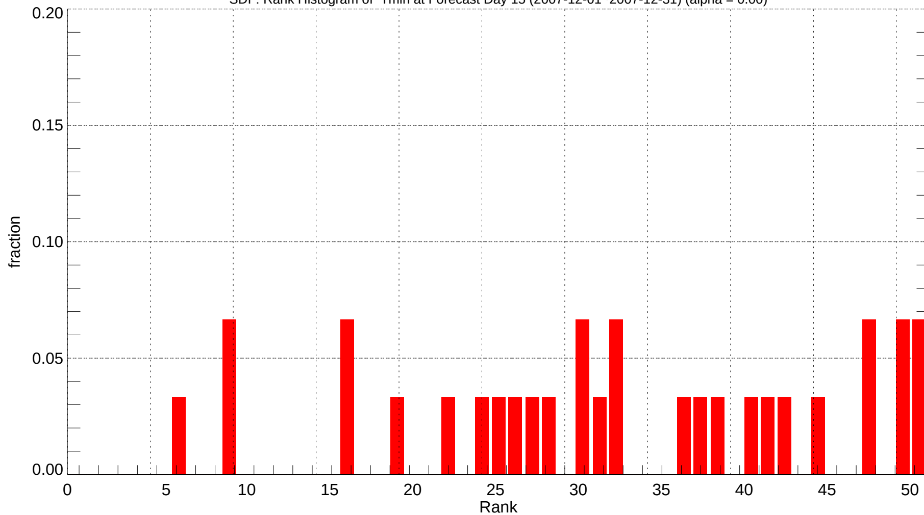
SDF: Rank Histogram of Tmin at Forecast Day 15 (2007-12-01~2007-12-31) (alpha = 0.00)
