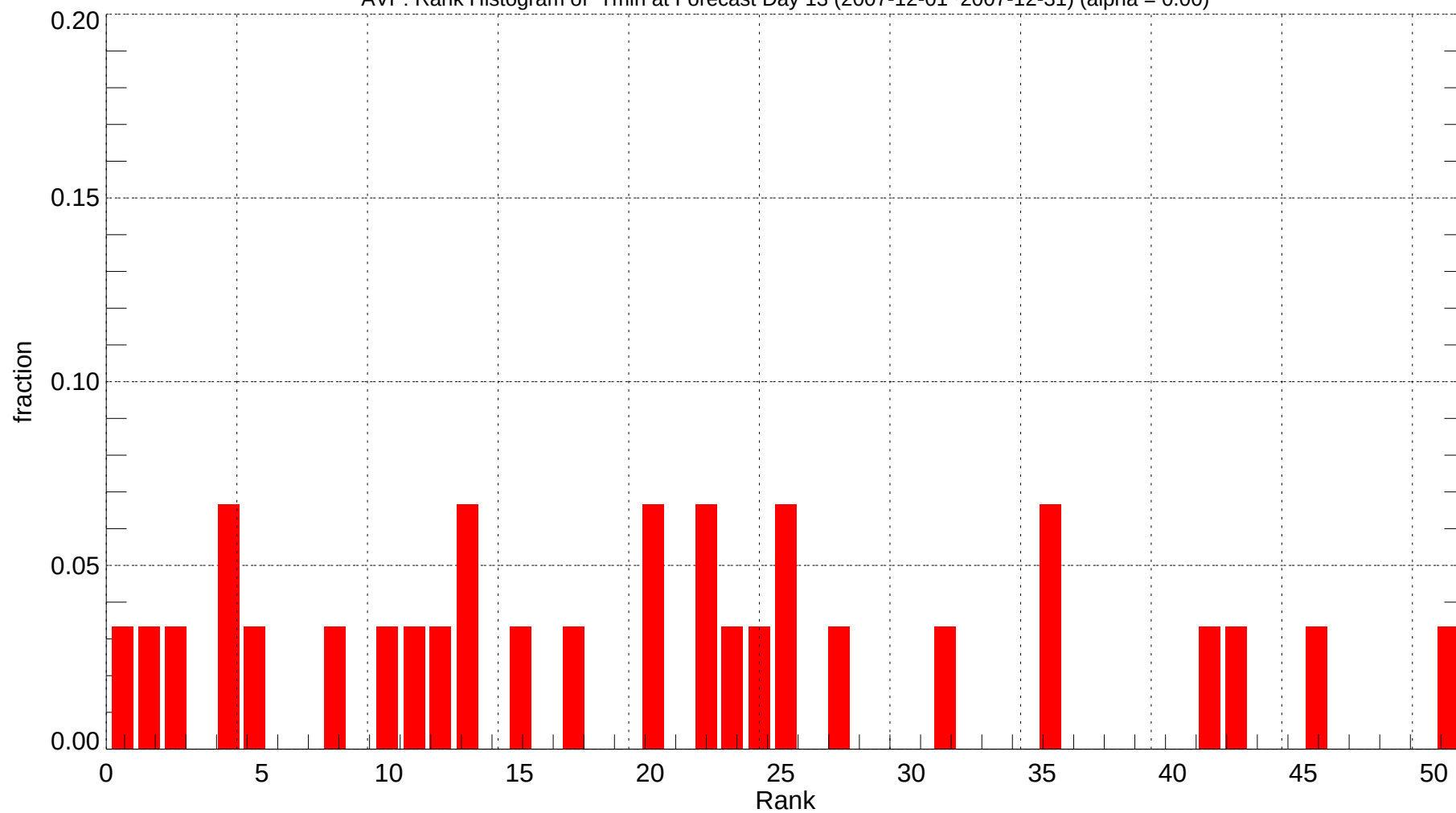
AVP: Rank Histogram of Tmin at Forecast Day 13 (2007-12-01~2007-12-31) (alpha = 0.00)
