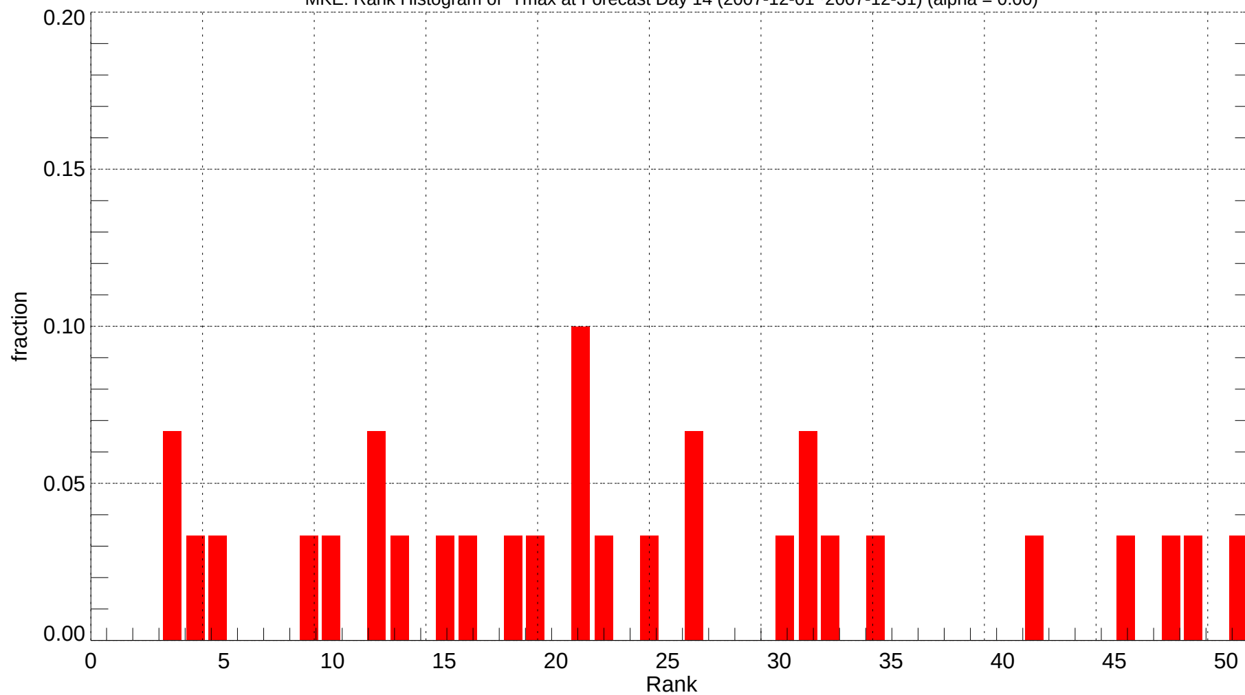
MKE: Rank Histogram of Tmax at Forecast Day 14 (2007-12-01~2007-12-31) (alpha = 0.00)
