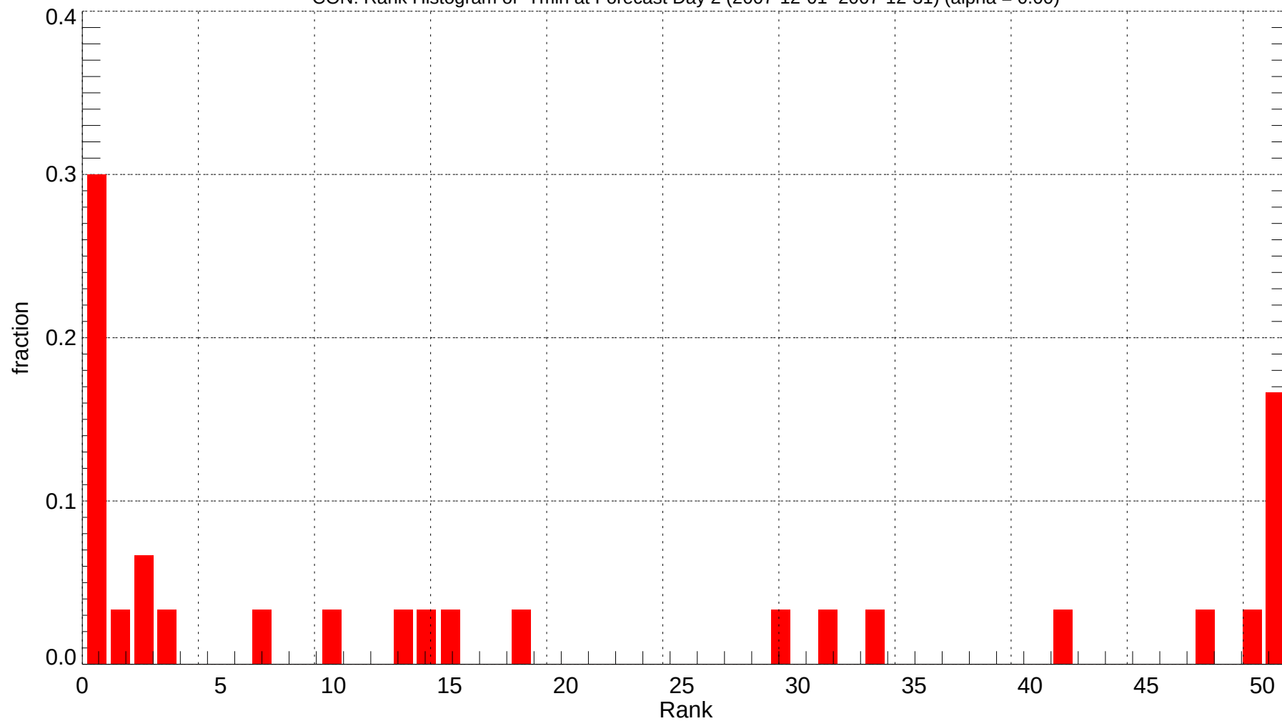
CON: Rank Histogram of Tmin at Forecast Day 2 (2007-12-01~2007-12-31) (alpha = 0.00)
