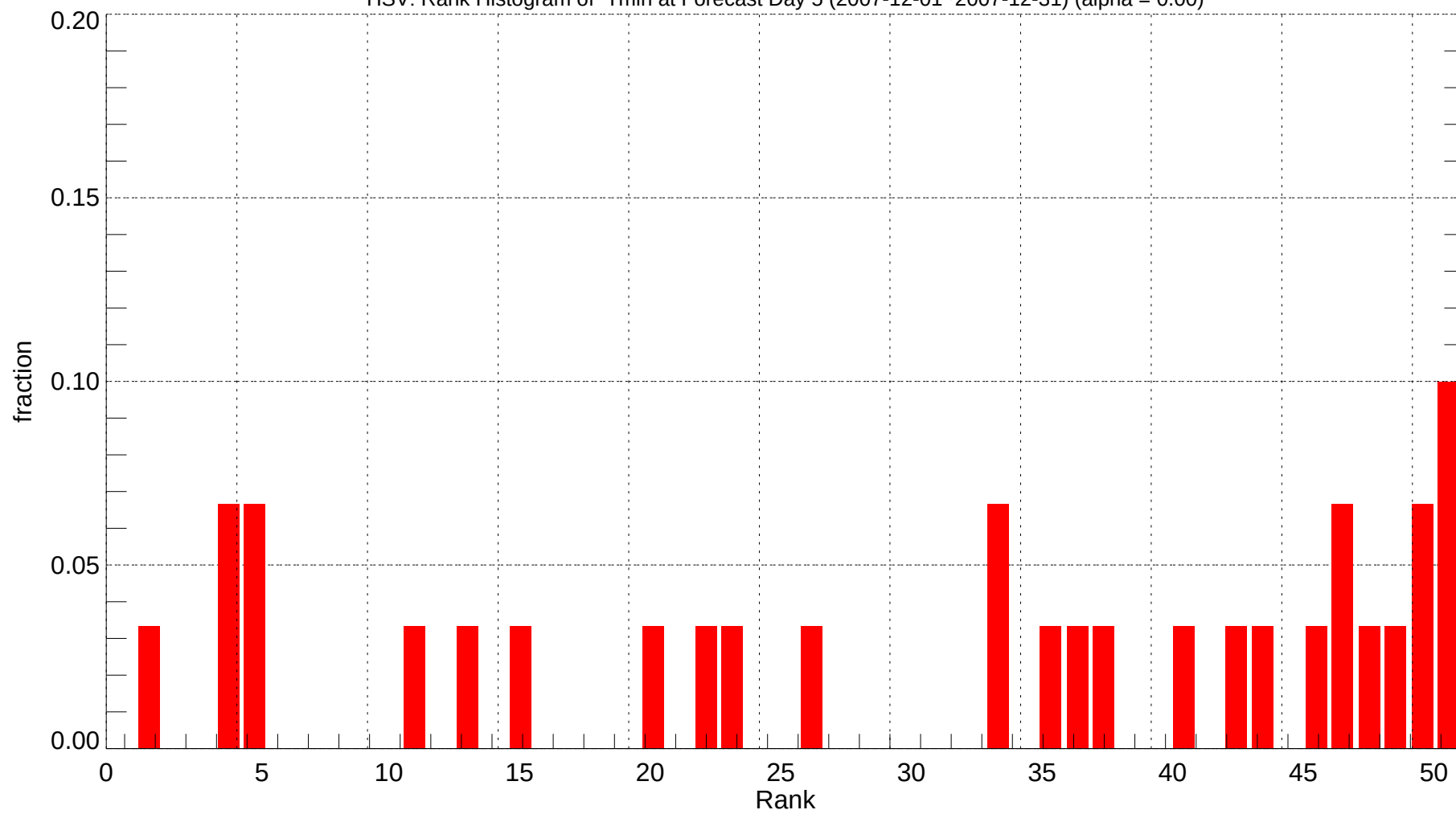
HSV: Rank Histogram of Tmin at Forecast Day 5 (2007-12-01~2007-12-31) (alpha = 0.00)
