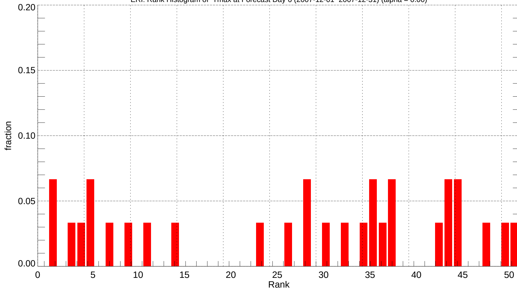
ERI: Rank Histogram of Tmax at Forecast Day 6 (2007-12-01~2007-12-31) (alpha = 0.00)
