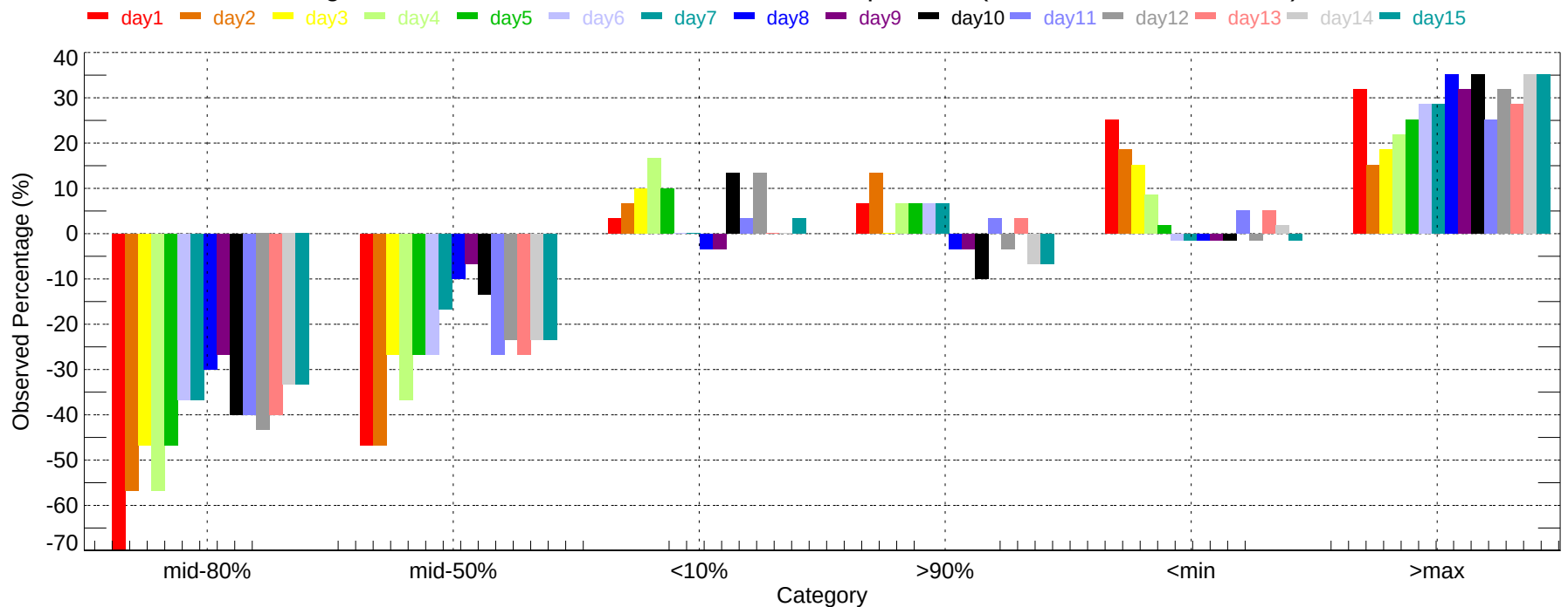
Observed Percentage Deviation of Ensembles - MSY: Min Temperature (2007-12-01~2007-12-31)
