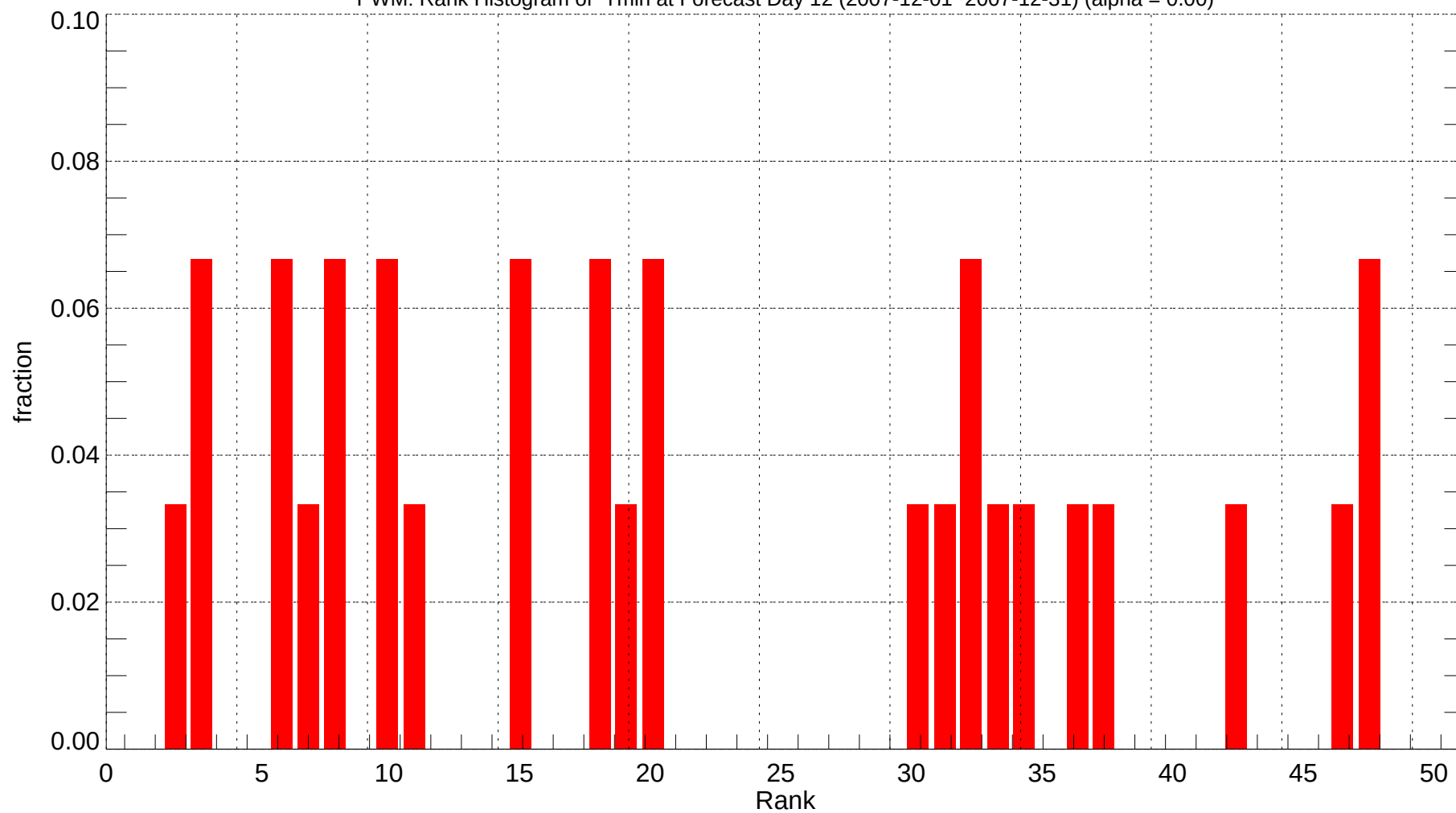
PWM: Rank Histogram of Tmin at Forecast Day 12 (2007-12-01~2007-12-31) (alpha = 0.00)
