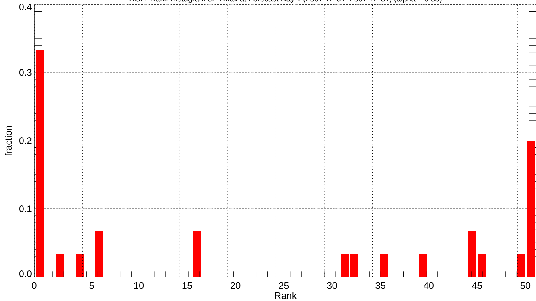
ROA: Rank Histogram of Tmax at Forecast Day 1 (2007-12-01~2007-12-31) (alpha = 0.00)
