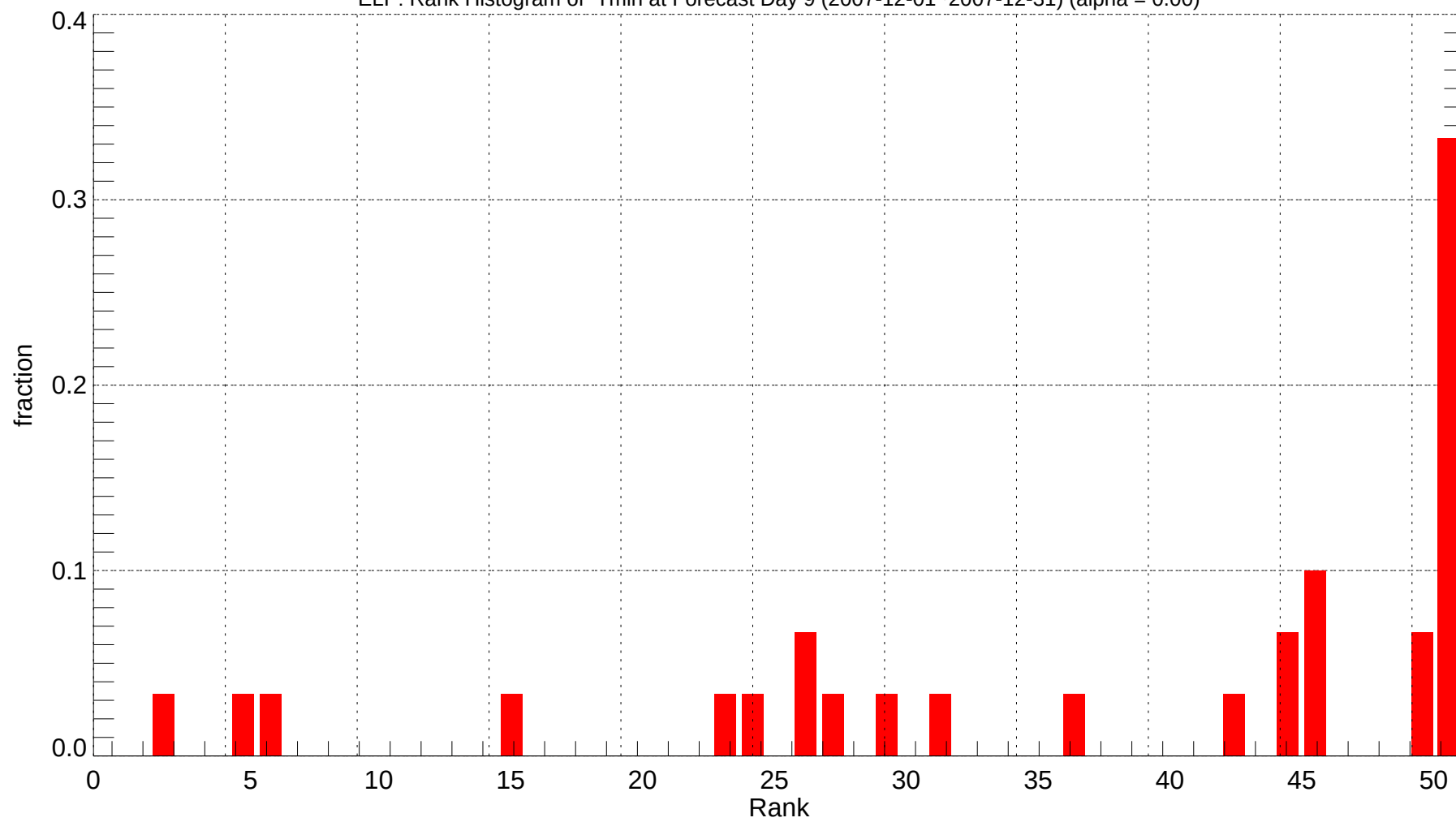
ELP: Rank Histogram of Tmin at Forecast Day 9 (2007-12-01~2007-12-31) (alpha = 0.00)
