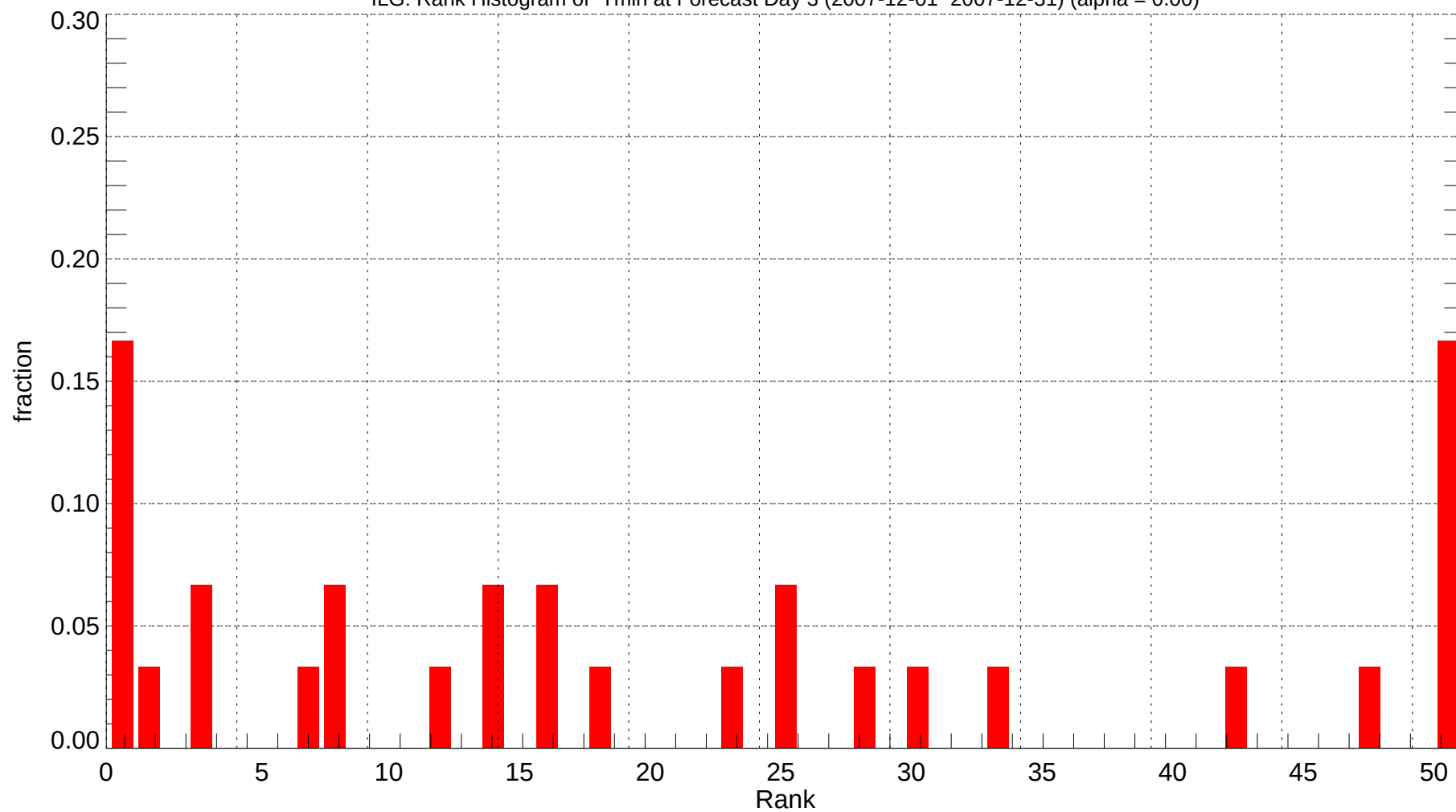
ILG: Rank Histogram of Tmin at Forecast Day 3 (2007-12-01~2007-12-31) (alpha = 0.00)
