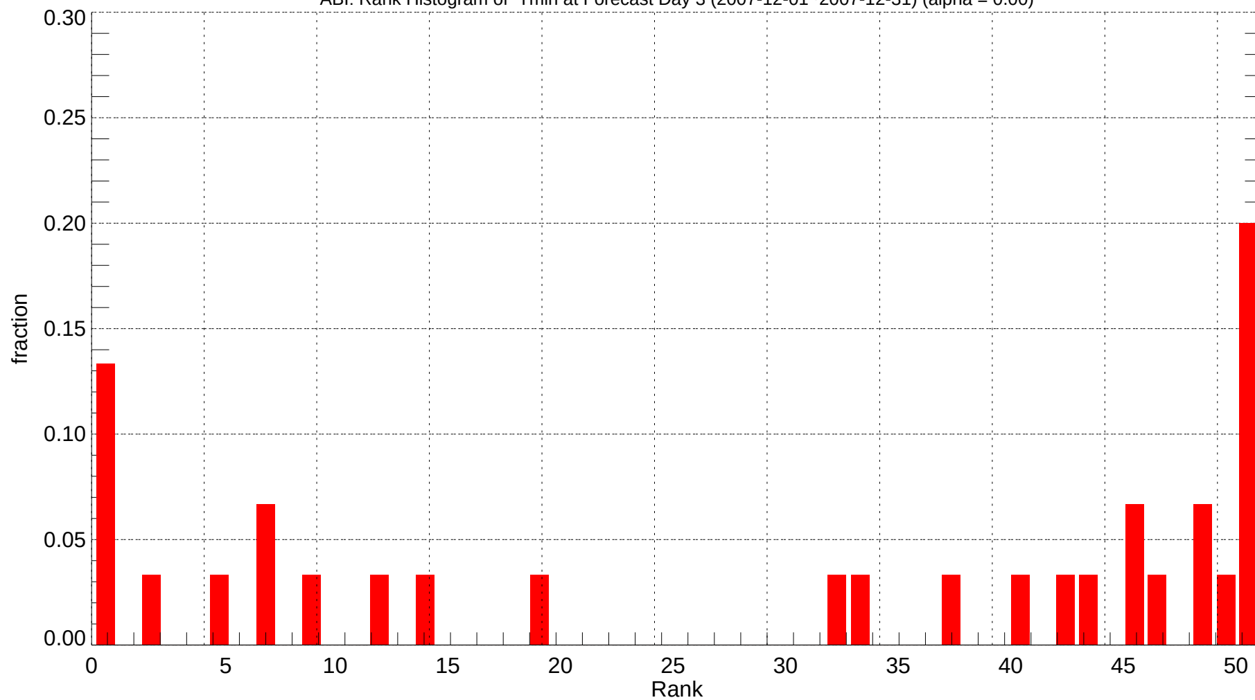
ABI: Rank Histogram of Tmin at Forecast Day 3 (2007-12-01~2007-12-31) (alpha = 0.00)
