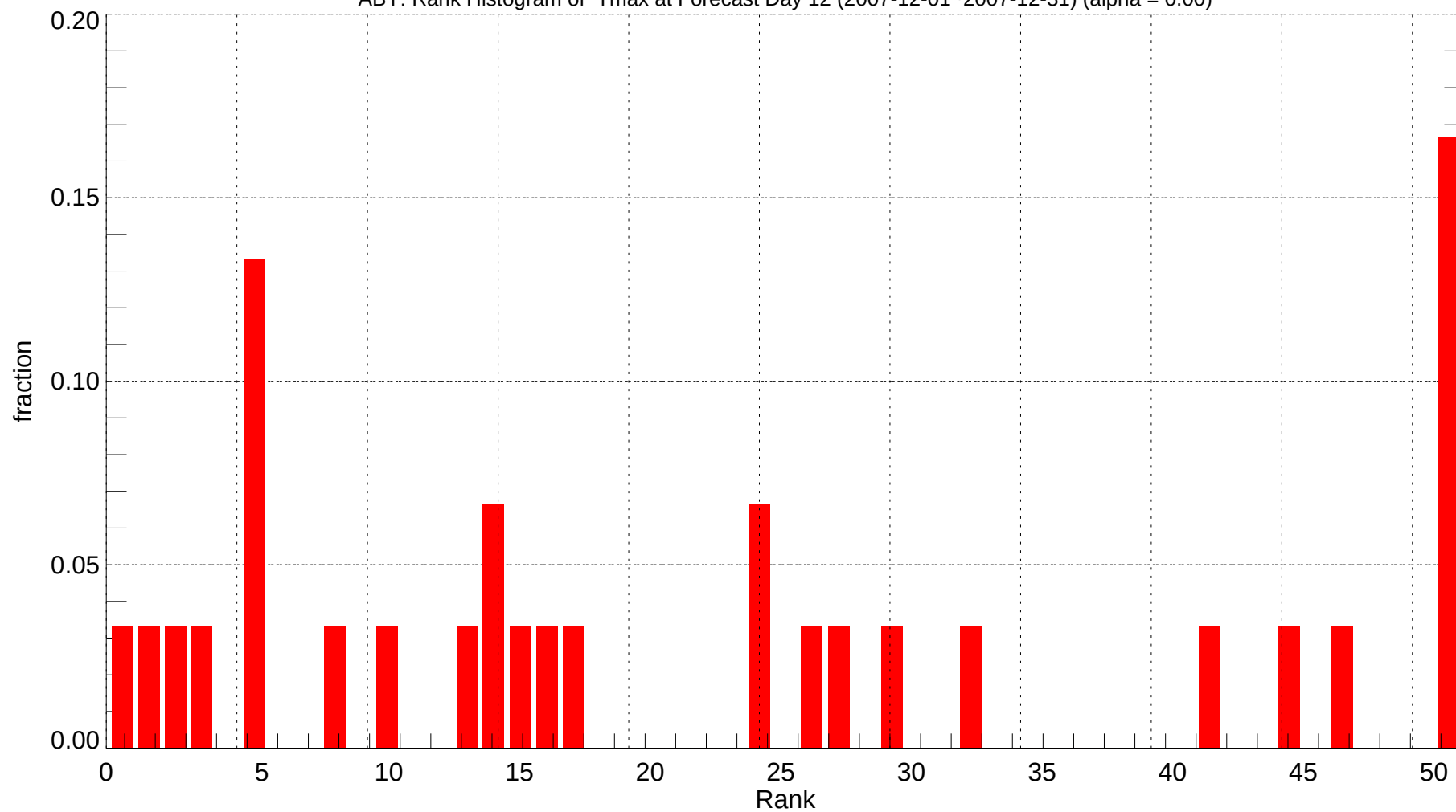
ABY: Rank Histogram of Tmax at Forecast Day 12 (2007-12-01~2007-12-31) (alpha = 0.00)
