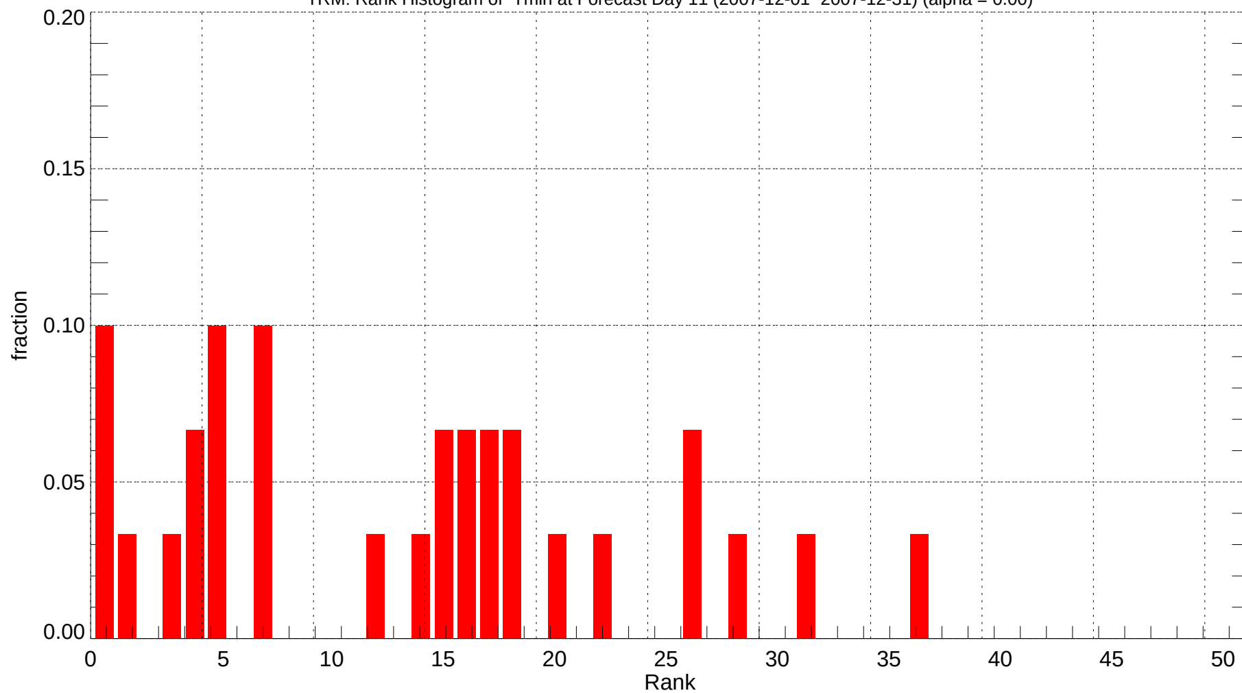
TRM: Rank Histogram of Tmin at Forecast Day 11 (2007-12-01~2007-12-31) (alpha = 0.00)
