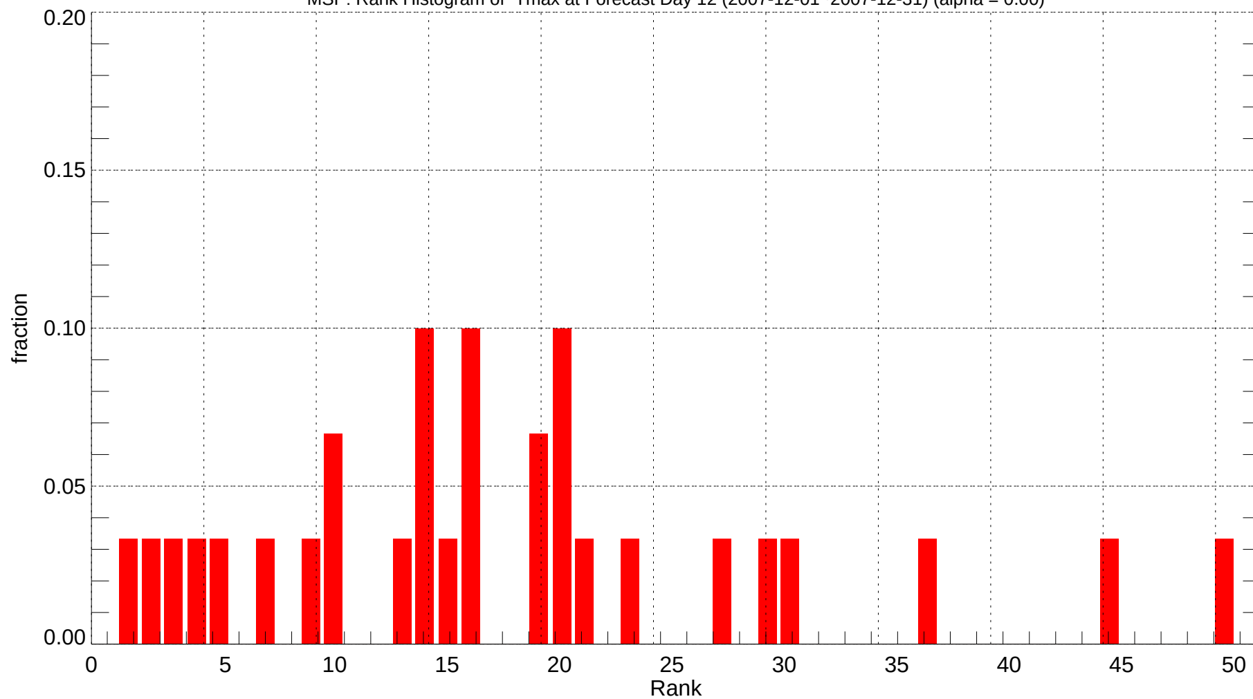
MSP: Rank Histogram of Tmax at Forecast Day 12 (2007-12-01~2007-12-31) (alpha = 0.00)
