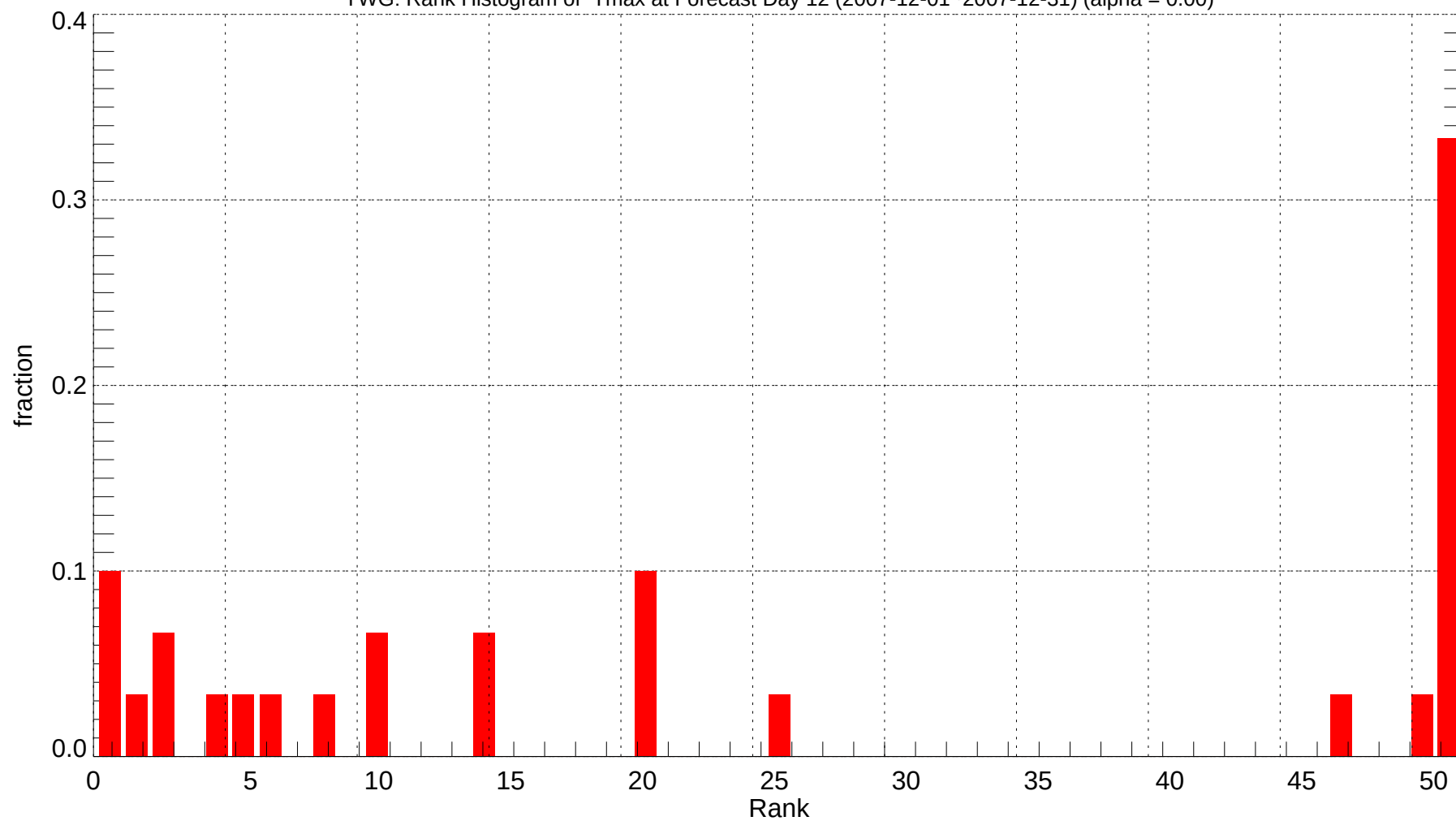
YWG: Rank Histogram of Tmax at Forecast Day 12 (2007-12-01~2007-12-31) (alpha = 0.00)
