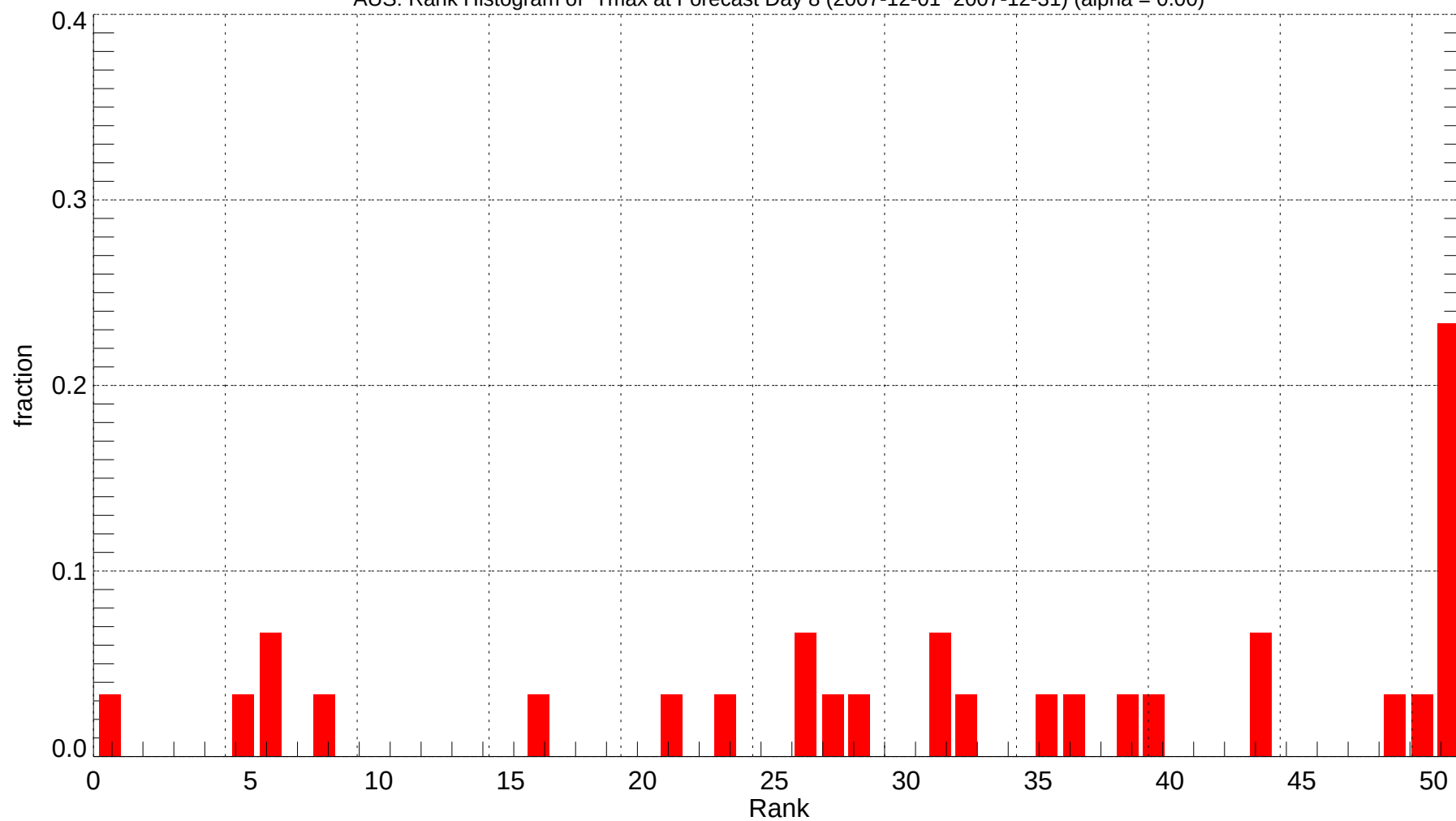
AUS: Rank Histogram of Tmax at Forecast Day 8 (2007-12-01~2007-12-31) (alpha = 0.00)
