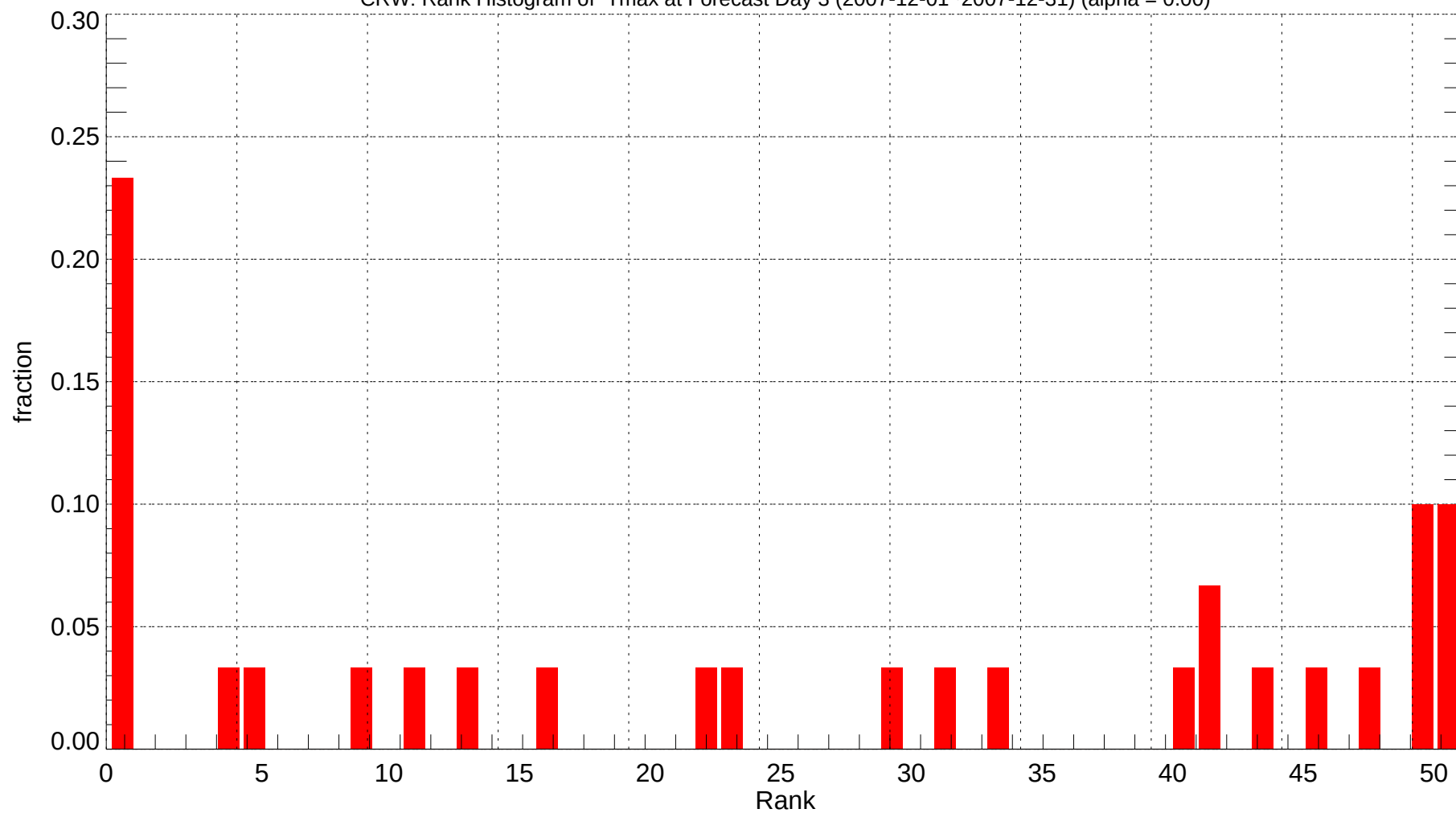
CRW: Rank Histogram of Tmax at Forecast Day 3 (2007-12-01~2007-12-31) (alpha = 0.00)
