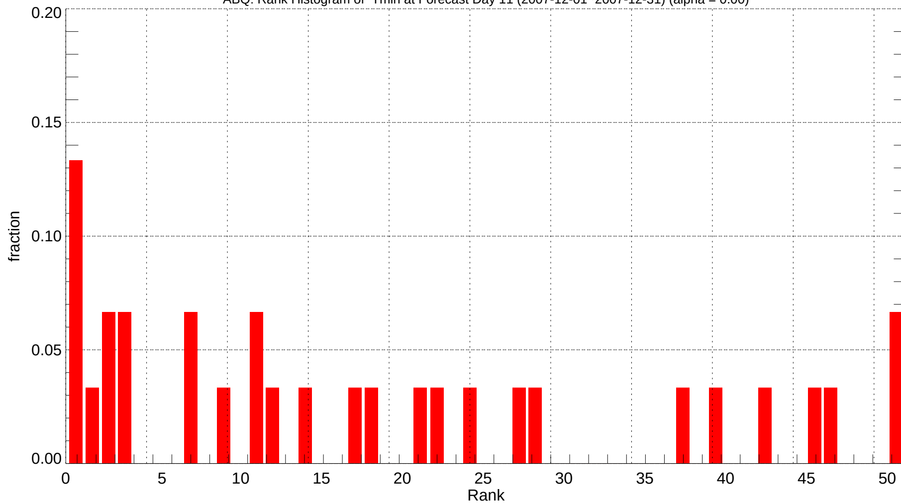
ABQ: Rank Histogram of Tmin at Forecast Day 11 (2007-12-01~2007-12-31) (alpha = 0.00)
