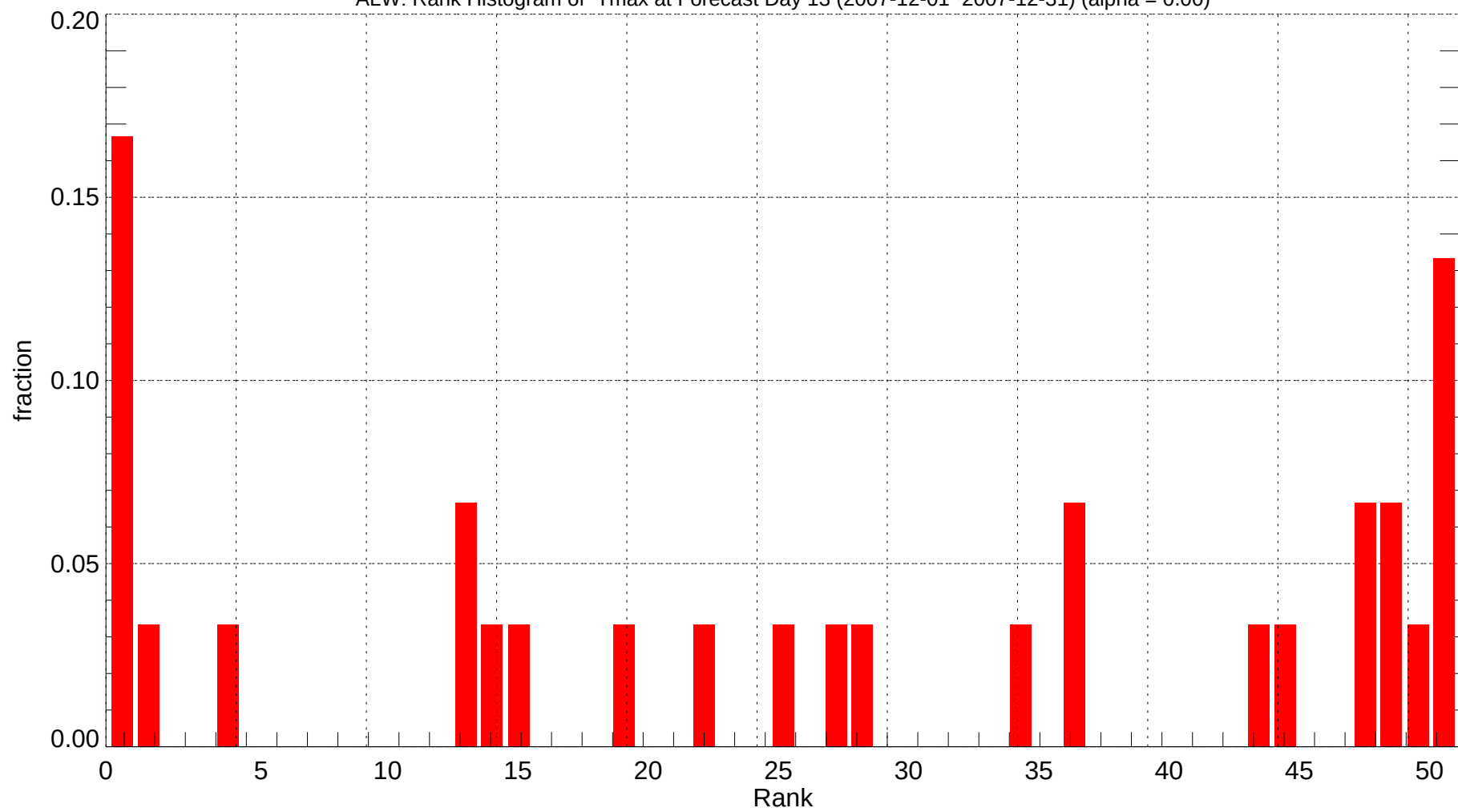
ALW: Rank Histogram of Tmax at Forecast Day 13 (2007-12-01~2007-12-31) (alpha = 0.00)
