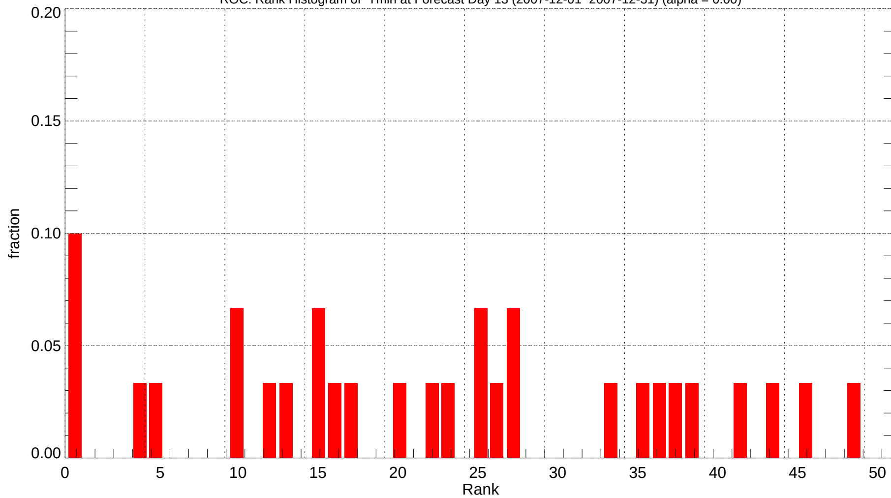
ROC: Rank Histogram of Tmin at Forecast Day 13 (2007-12-01~2007-12-31) (alpha = 0.00)
