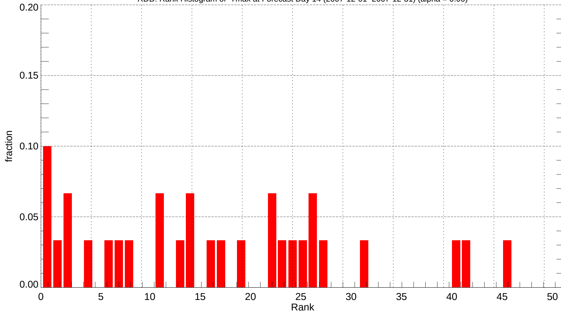
RDD: Rank Histogram of Tmax at Forecast Day 14 (2007-12-01~2007-12-31) (alpha = 0.00)
