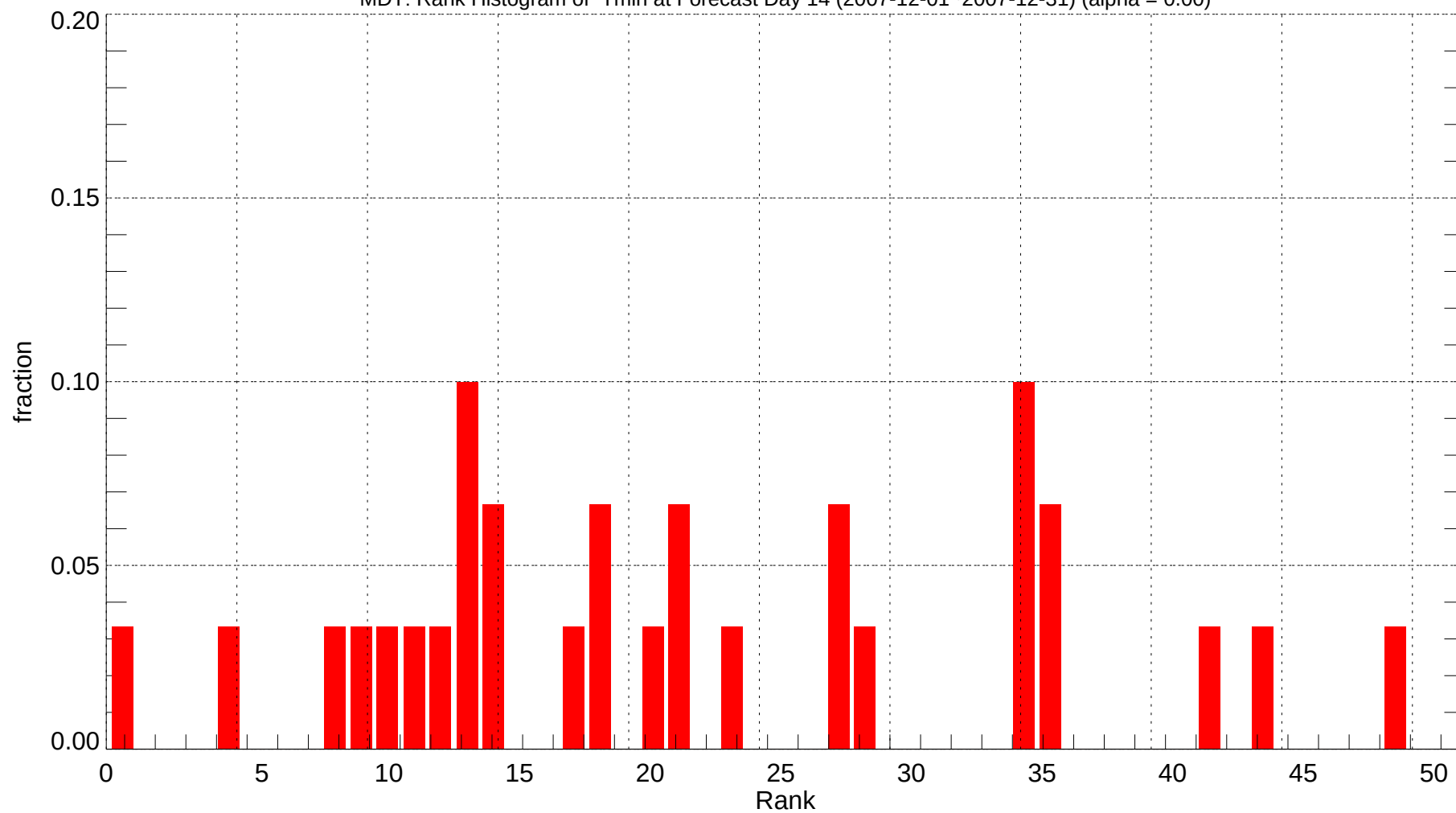
MDT: Rank Histogram of Tmin at Forecast Day 14 (2007-12-01~2007-12-31) (alpha = 0.00)
