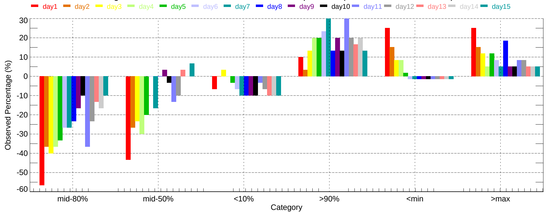
Observed Percentage Deviation of Ensembles - SDF: Max Temperature (2007-12-01~2007-12-31)
