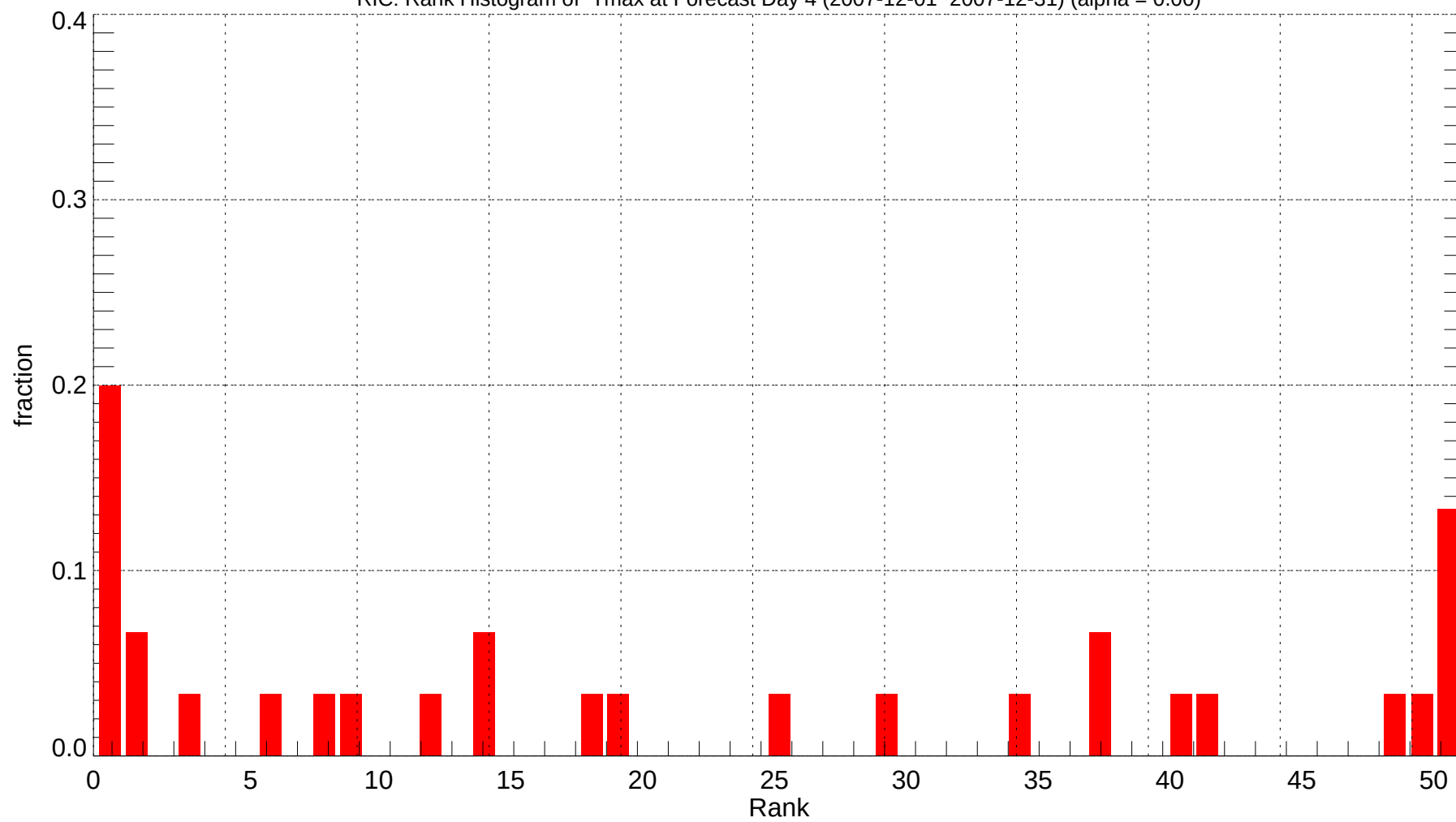
RIC: Rank Histogram of Tmax at Forecast Day 4 (2007-12-01~2007-12-31) (alpha = 0.00)
