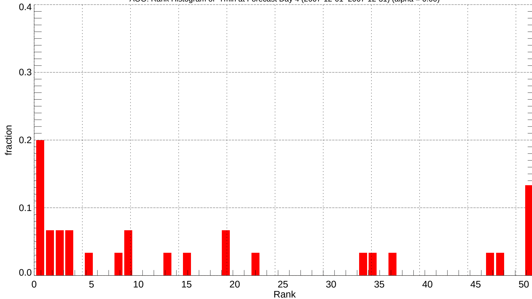
AOO: Rank Histogram of Tmin at Forecast Day 4 (2007-12-01~2007-12-31) (alpha = 0.00)
