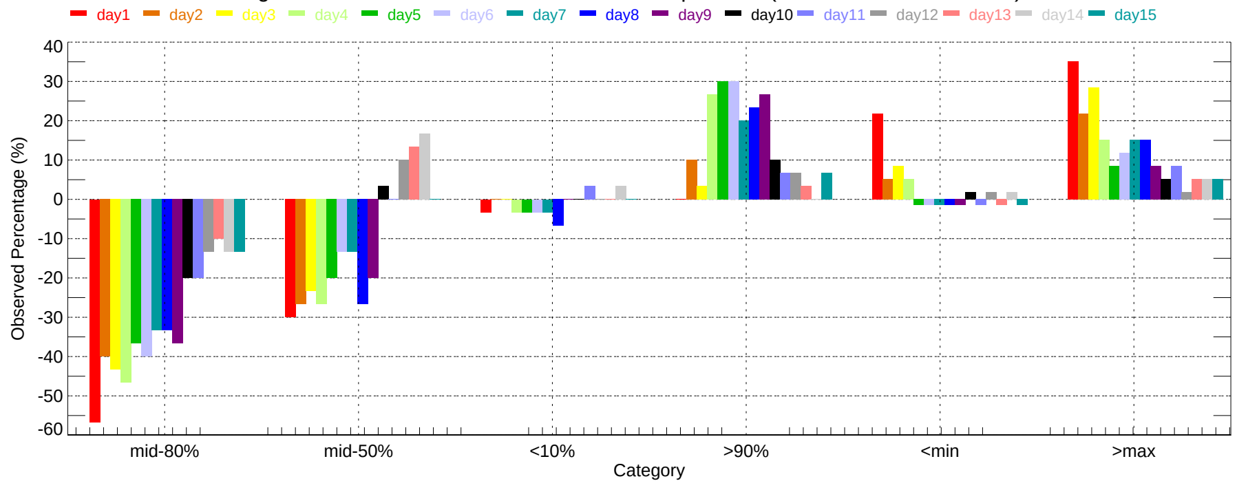
Observed Percentage Deviation of Ensembles - VCT: Min Temperature (2007-12-01~2007-12-31)
