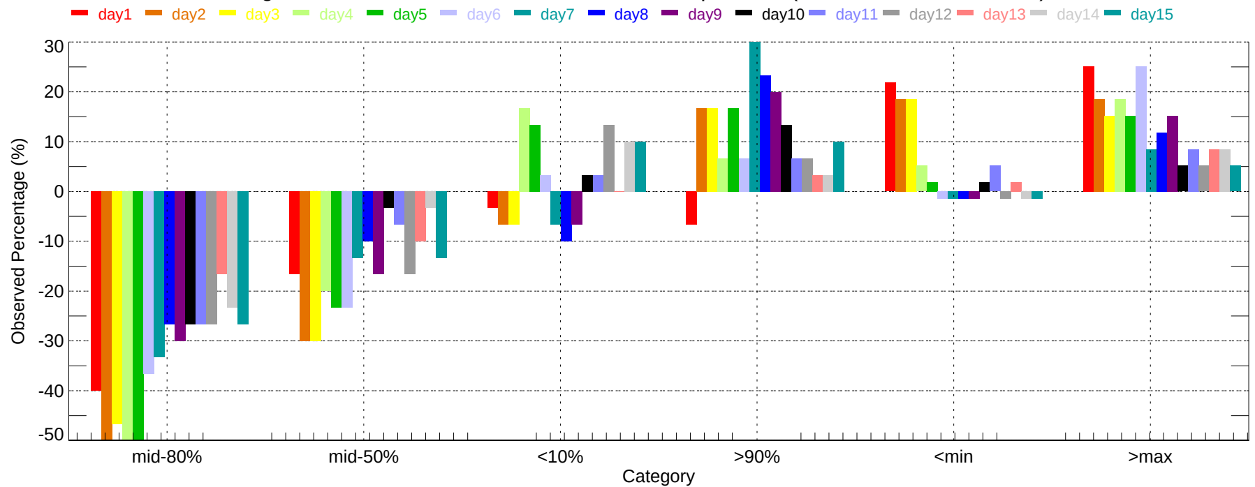
Observed Percentage Deviation of Ensembles - RDU: Max Temperature (2007-12-01~2007-12-31)
