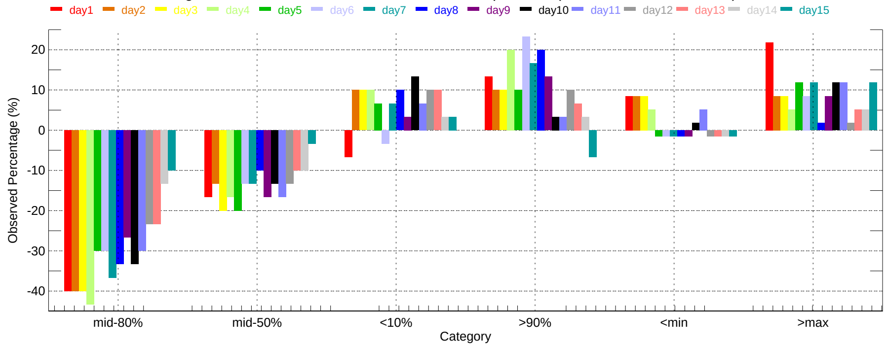
Observed Percentage Deviation of Ensembles - DFW: Min Temperature (2007-12-01~2007-12-31)
