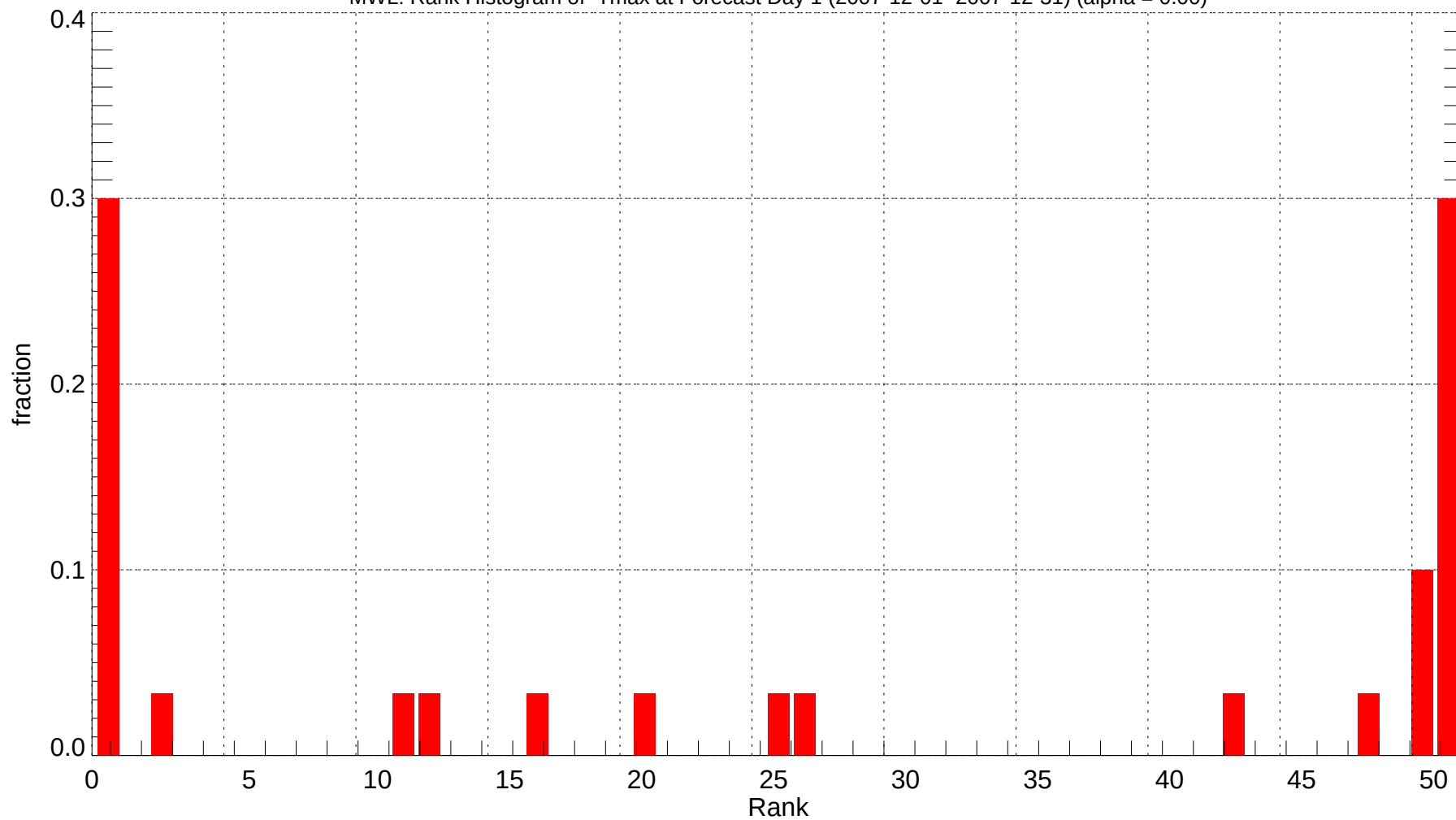
MWL: Rank Histogram of Tmax at Forecast Day 1 (2007-12-01~2007-12-31) (alpha = 0.00)
