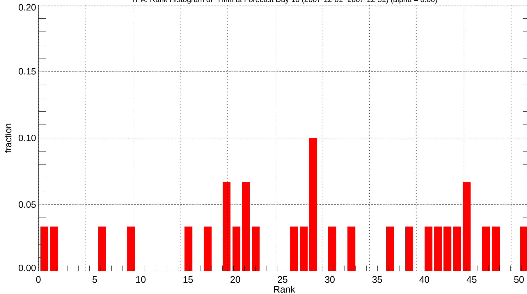
TPA: Rank Histogram of Tmin at Forecast Day 10 (2007-12-01~2007-12-31) (alpha = 0.00)
