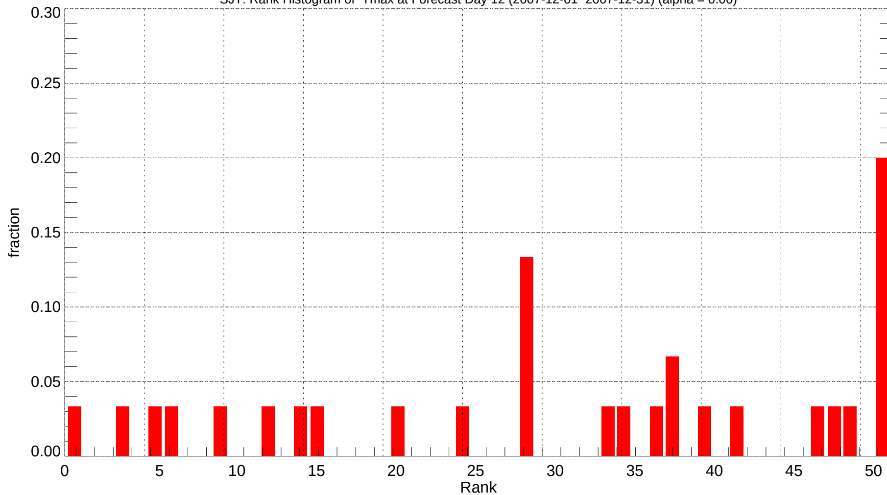
SJT: Rank Histogram of Tmax at Forecast Day 12 (2007-12-01~2007-12-31) (alpha = 0.00)
