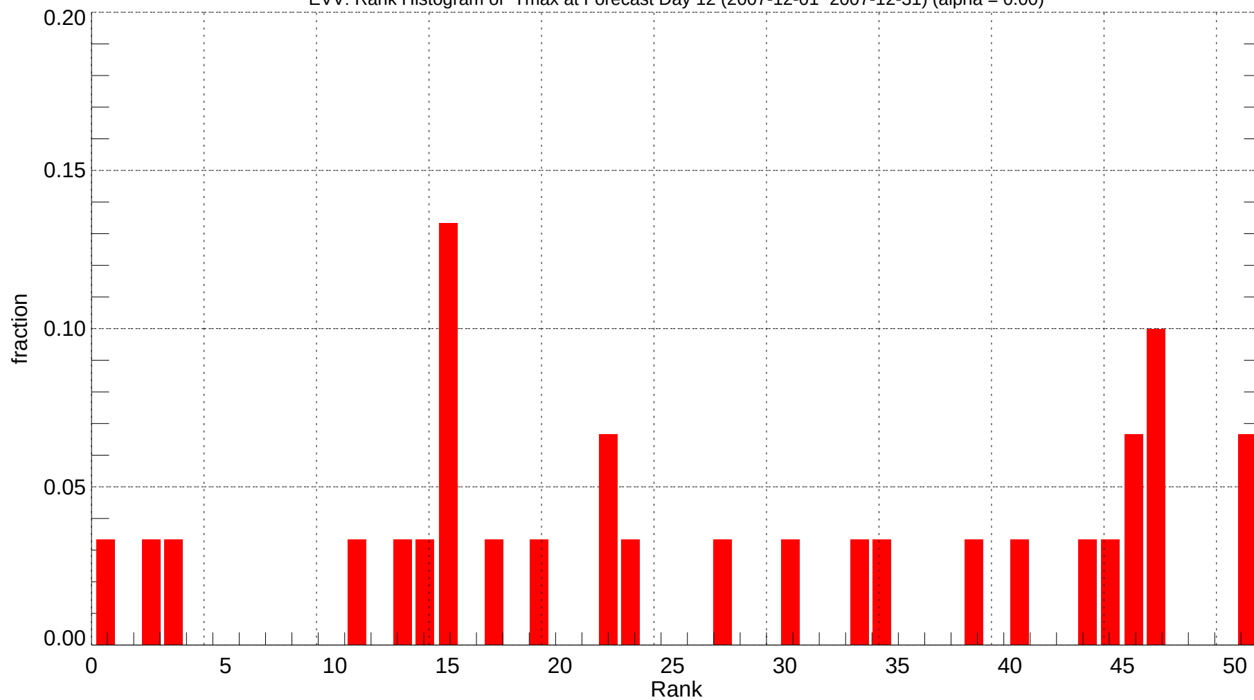
EVV: Rank Histogram of Tmax at Forecast Day 12 (2007-12-01~2007-12-31) (alpha = 0.00)
