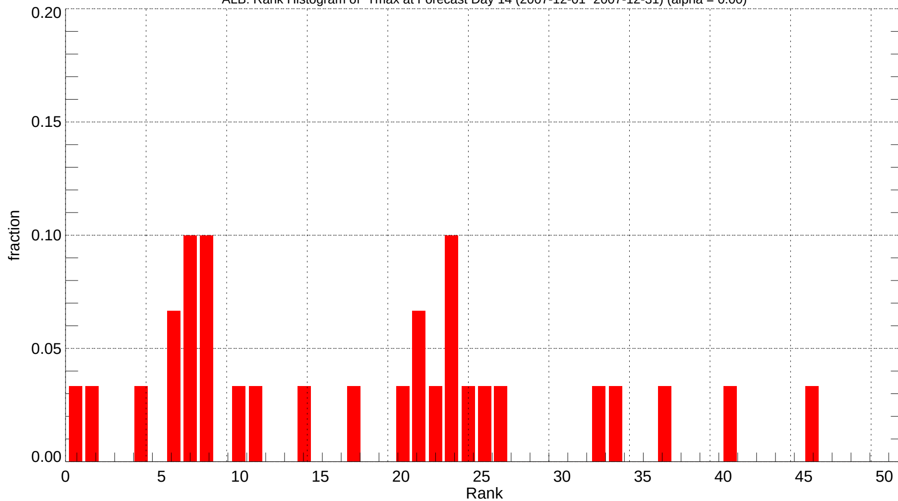
ALB: Rank Histogram of Tmax at Forecast Day 14 (2007-12-01~2007-12-31) (alpha = 0.00)
