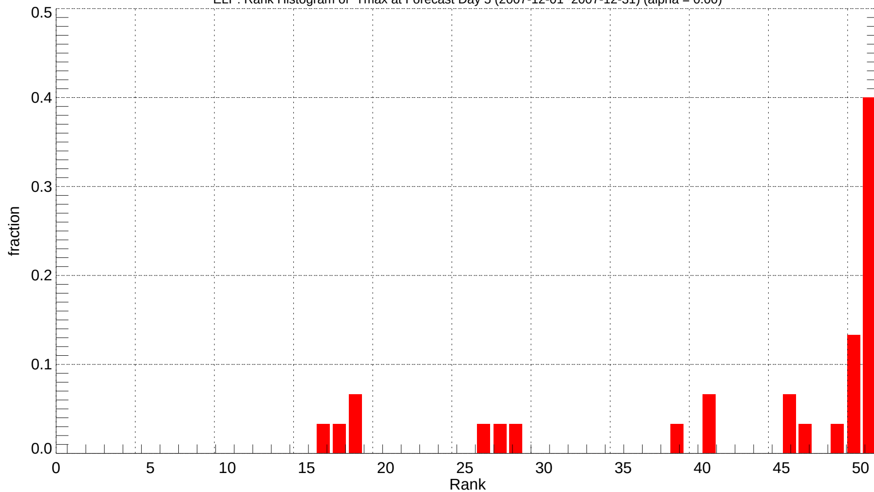
ELP: Rank Histogram of Tmax at Forecast Day 5 (2007-12-01~2007-12-31) (alpha = 0.00)
