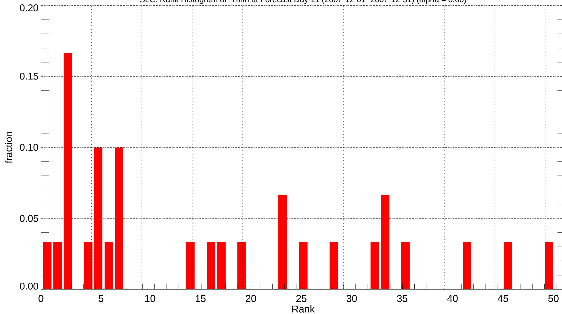
SLC: Rank Histogram of Tmin at Forecast Day 11 (2007-12-01~2007-12-31) (alpha = 0.00)
