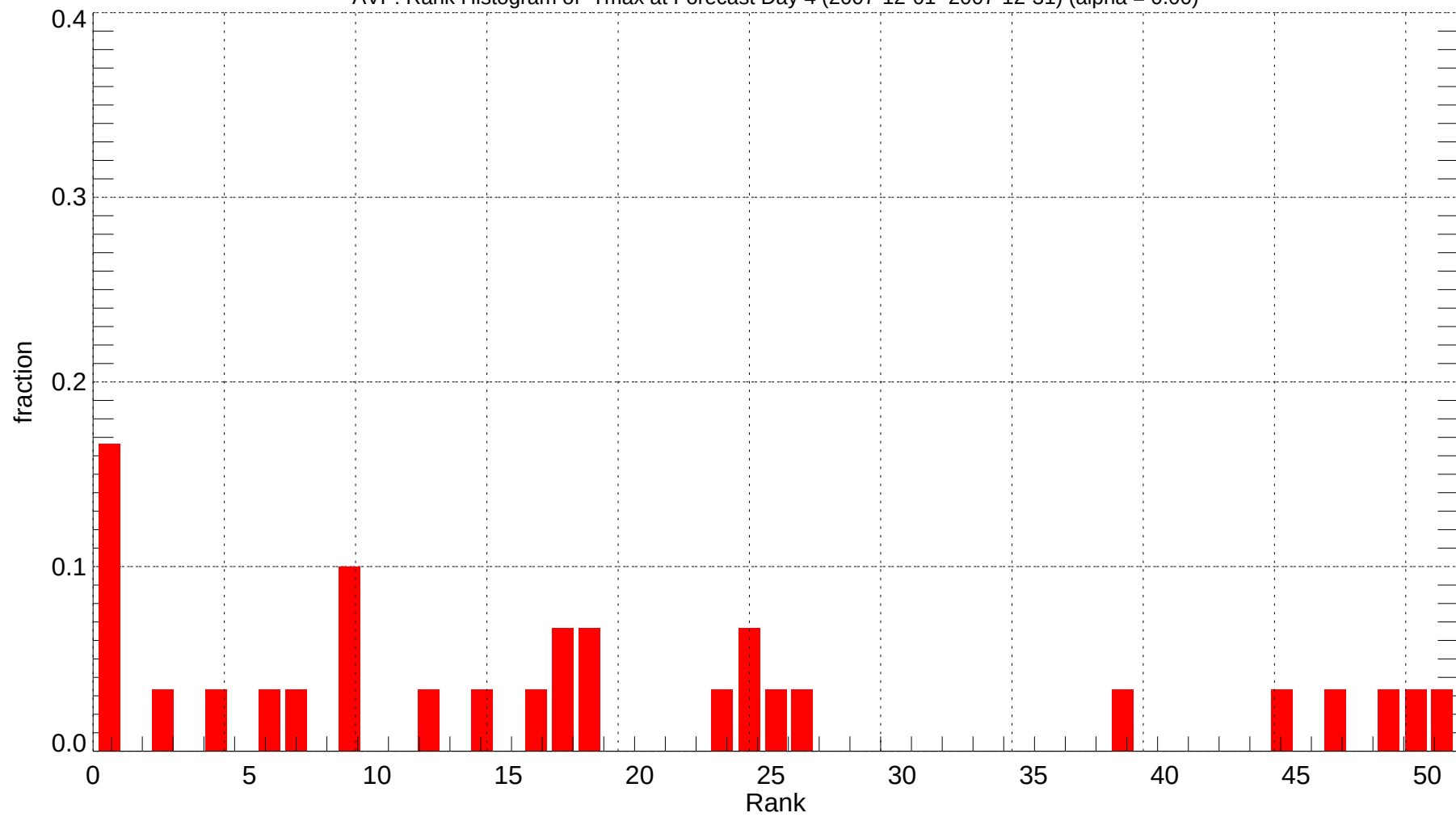
AVP: Rank Histogram of Tmax at Forecast Day 4 (2007-12-01~2007-12-31) (alpha = 0.00)
