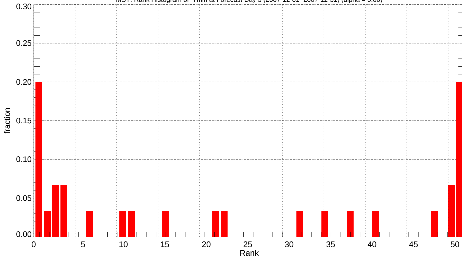
MSY: Rank Histogram of Tmin at Forecast Day 3 (2007-12-01~2007-12-31) (alpha = 0.00)
