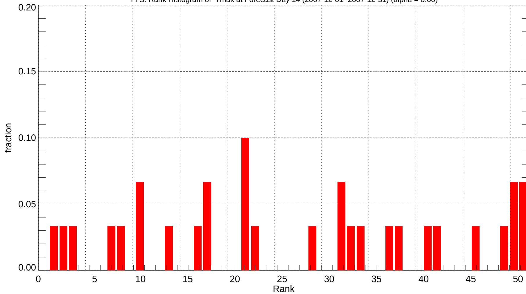
TYS: Rank Histogram of Tmax at Forecast Day 14 (2007-12-01~2007-12-31) (alpha = 0.00)
