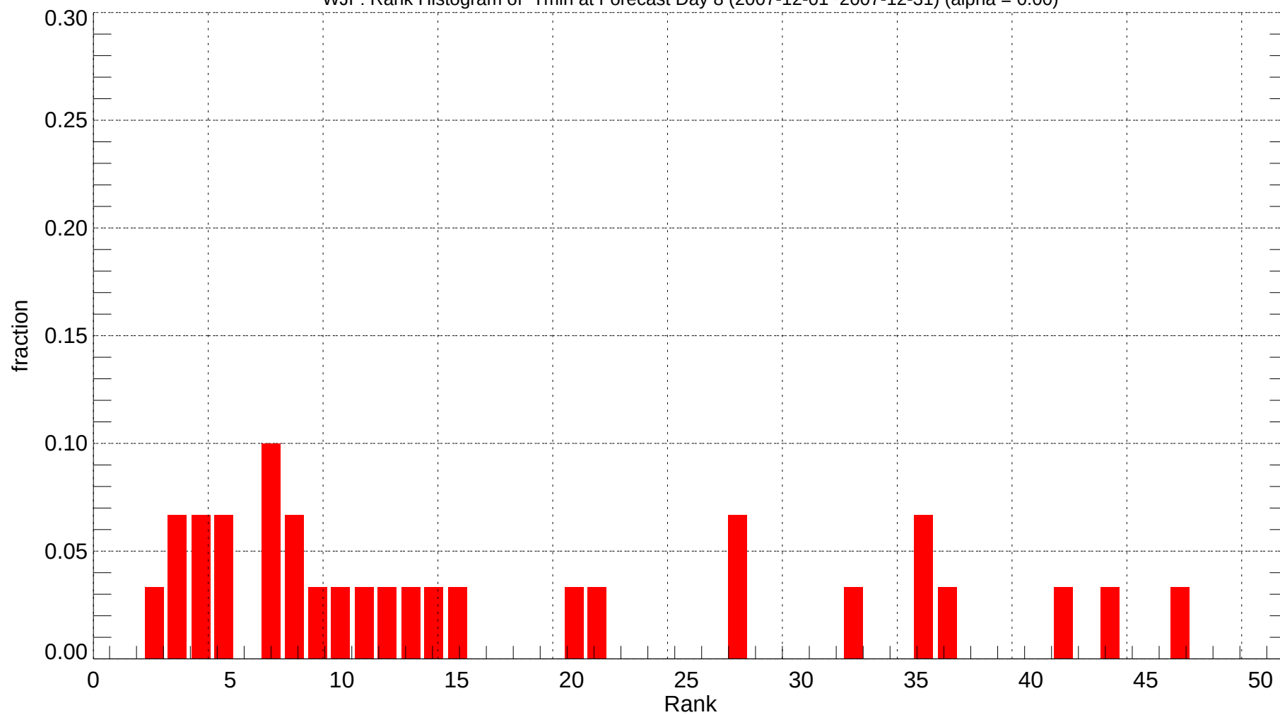
WJF: Rank Histogram of Tmin at Forecast Day 8 (2007-12-01~2007-12-31) (alpha = 0.00)
