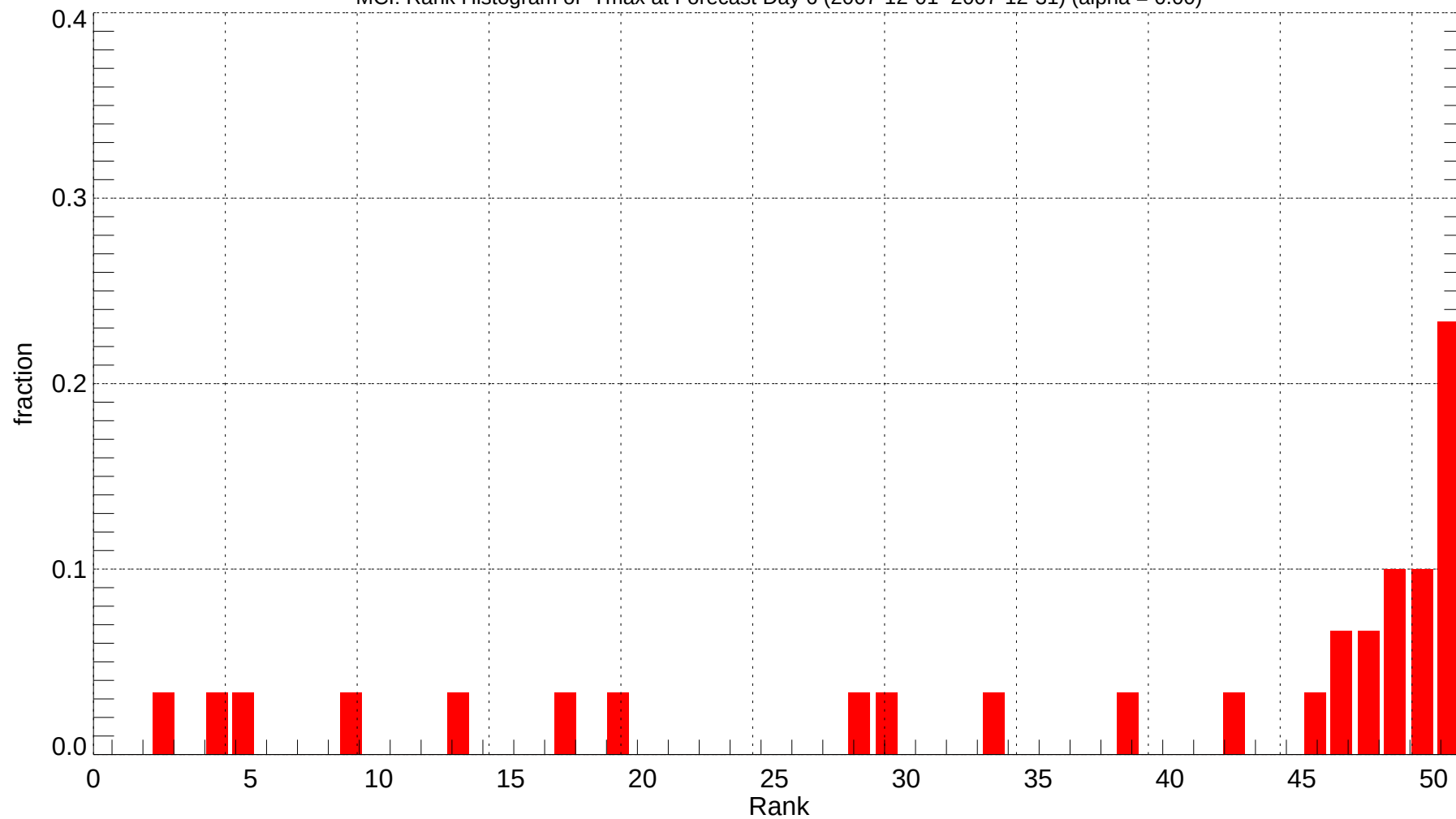
MCI: Rank Histogram of Tmax at Forecast Day 6 (2007-12-01~2007-12-31) (alpha = 0.00)
