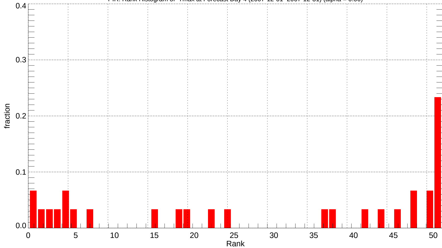
PIR: Rank Histogram of Tmax at Forecast Day 4 (2007-12-01~2007-12-31) (alpha = 0.00)
