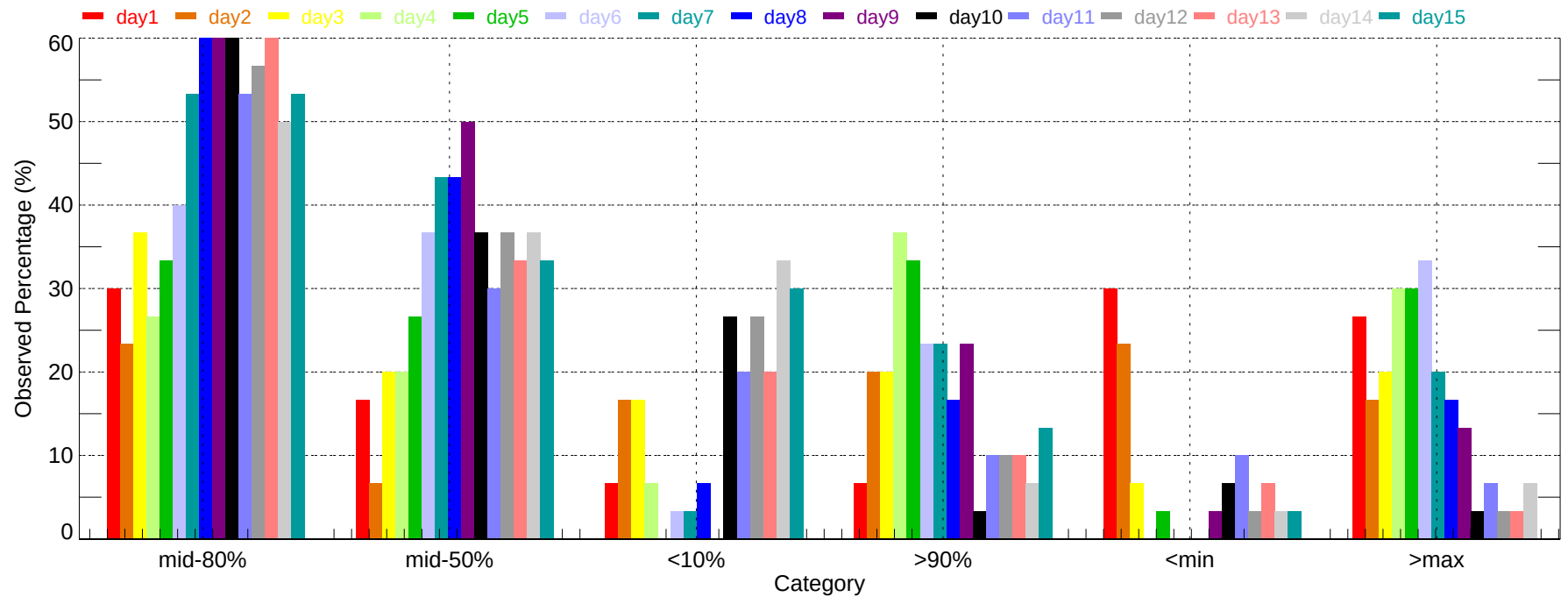
Observed Percentage of Ensembles - ABQ: Min Temperature (2007-12-01~2007-12-31)
