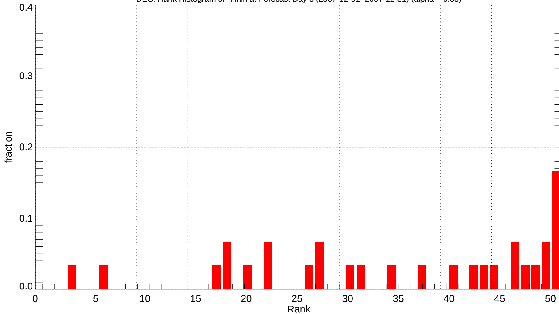
DEC: Rank Histogram of Tmin at Forecast Day 6 (2007-12-01~2007-12-31) (alpha = 0.00)
