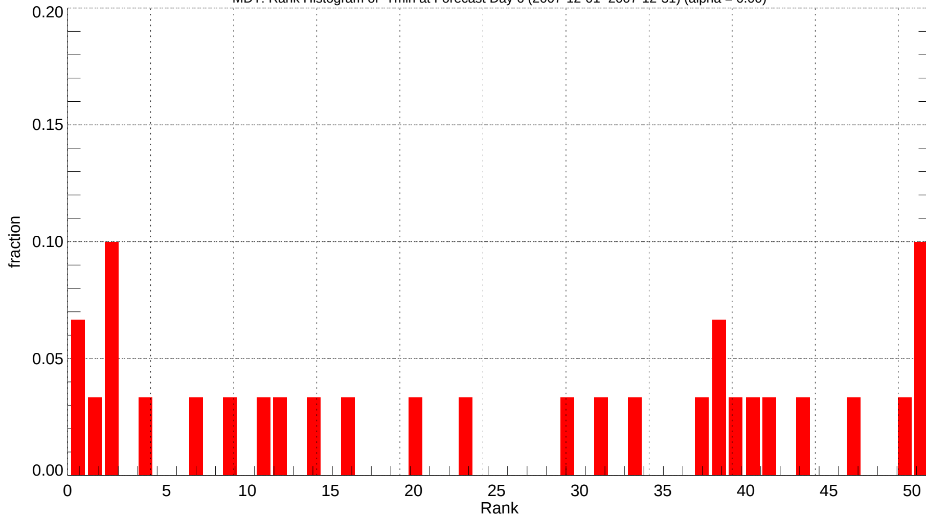
MDT: Rank Histogram of Tmin at Forecast Day 6 (2007-12-01~2007-12-31) (alpha = 0.00)
