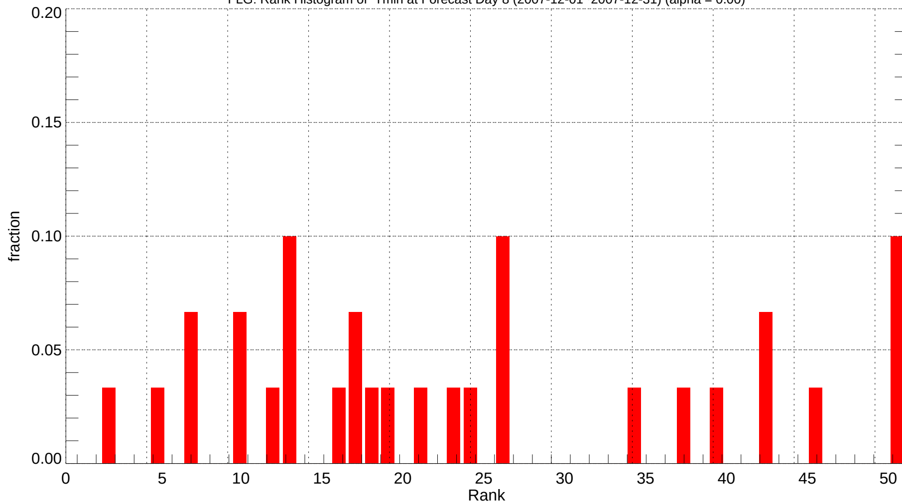
FLG: Rank Histogram of Tmin at Forecast Day 8 (2007-12-01~2007-12-31) (alpha = 0.00)
