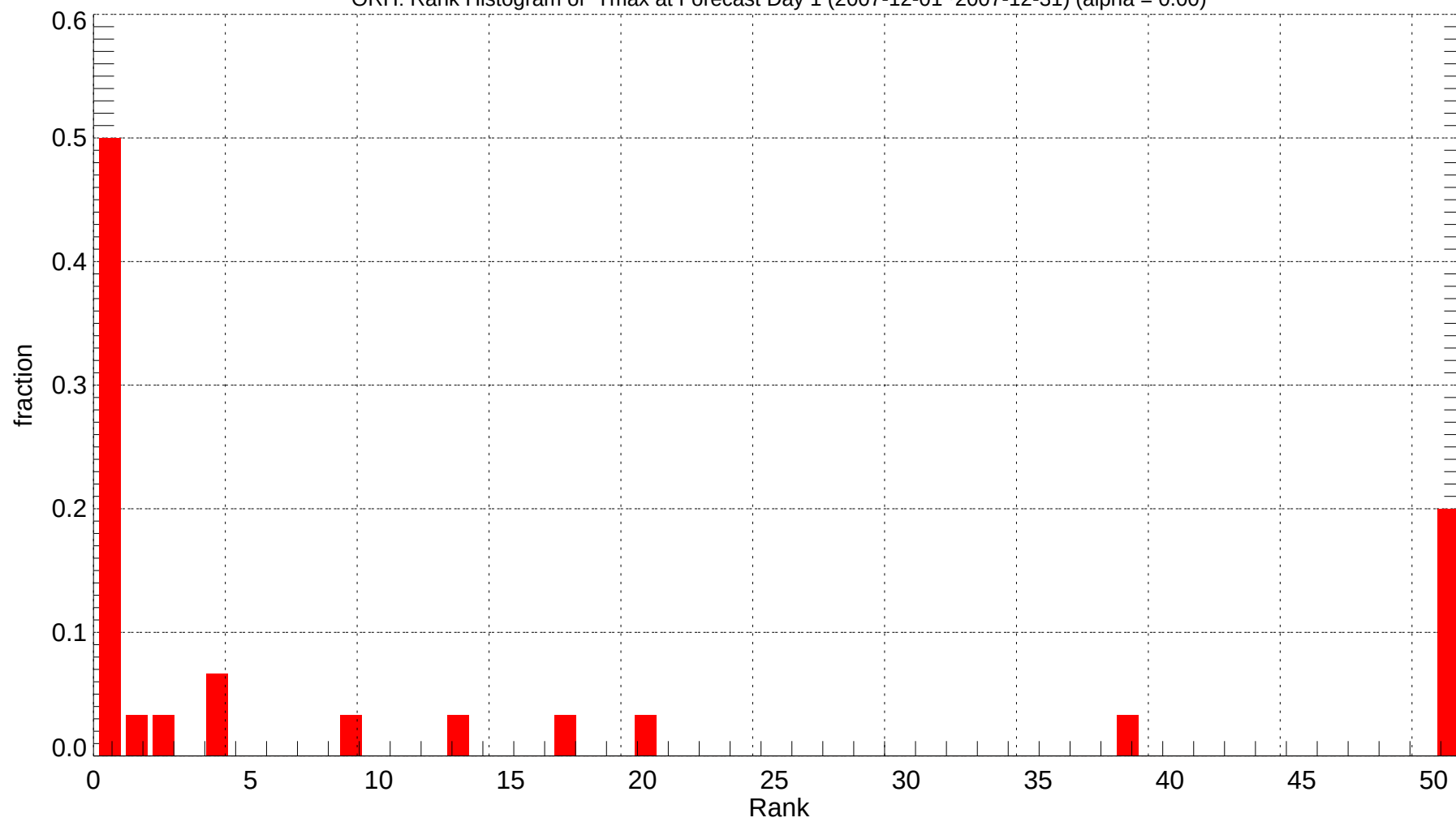
ORH: Rank Histogram of Tmax at Forecast Day 1 (2007-12-01~2007-12-31) (alpha = 0.00)
