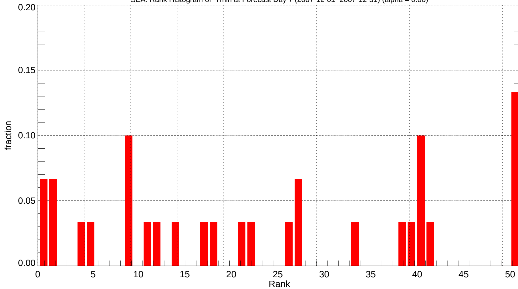
SEA: Rank Histogram of Tmin at Forecast Day 7 (2007-12-01~2007-12-31) (alpha = 0.00)
