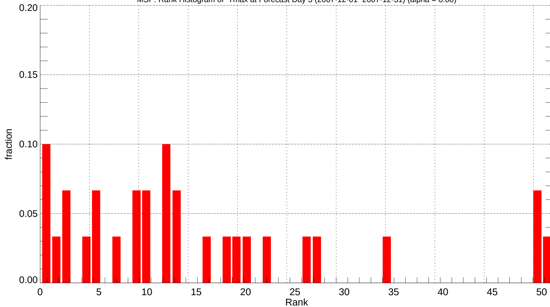
MSP: Rank Histogram of Tmax at Forecast Day 3 (2007-12-01~2007-12-31) (alpha = 0.00)
