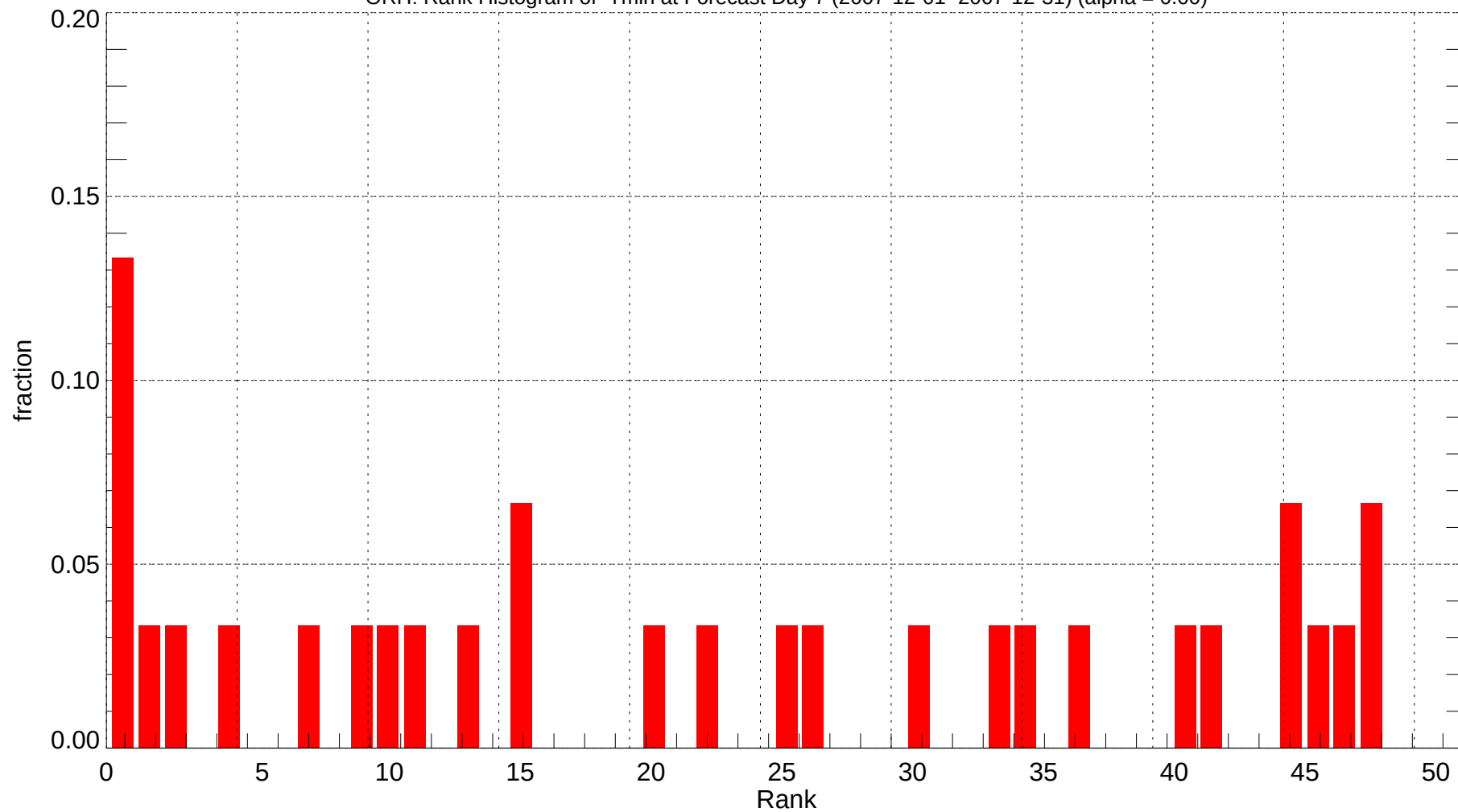
ORH: Rank Histogram of Tmin at Forecast Day 7 (2007-12-01~2007-12-31) (alpha = 0.00)
