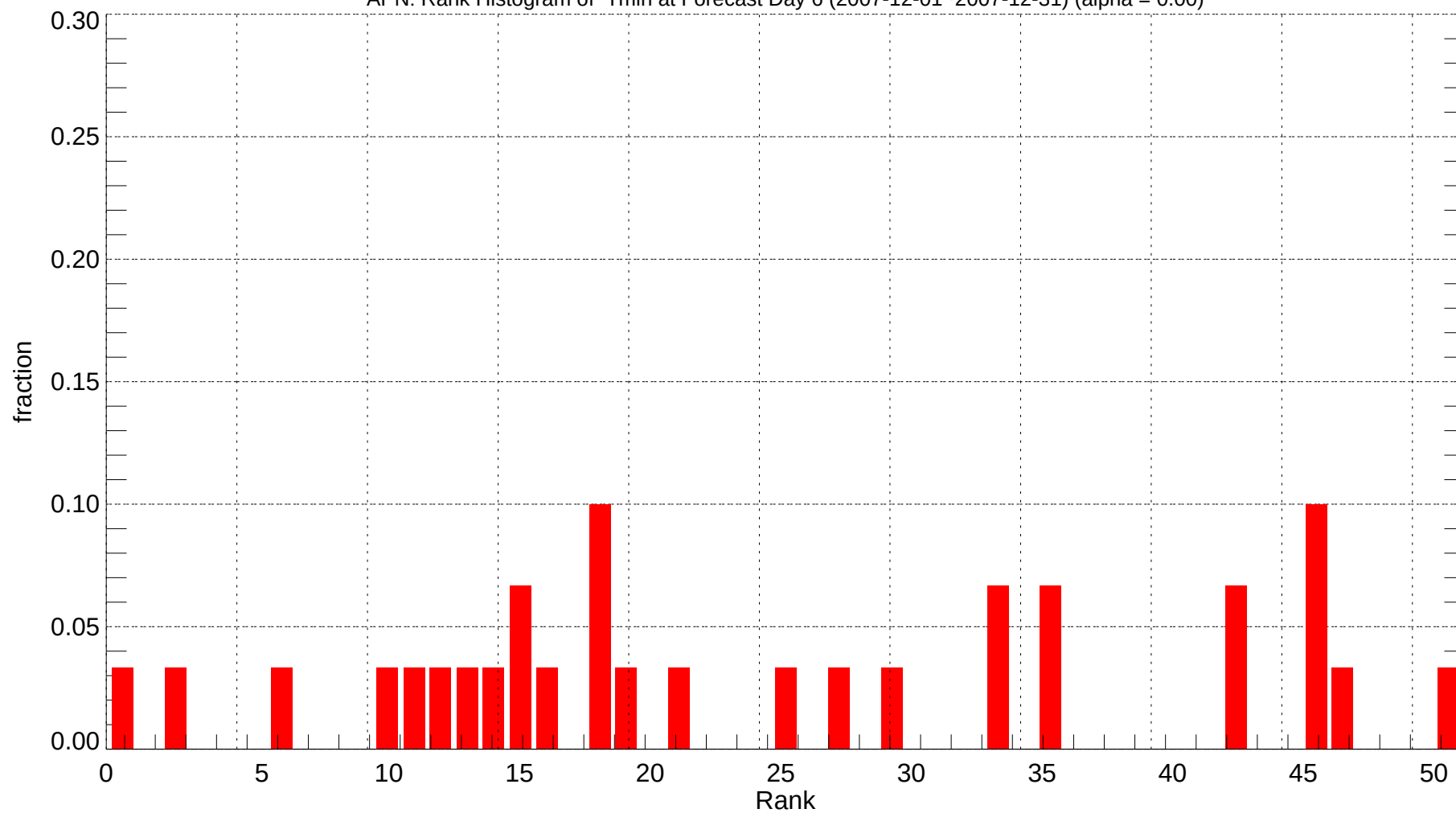
APN: Rank Histogram of Tmin at Forecast Day 6 (2007-12-01~2007-12-31) (alpha = 0.00)
