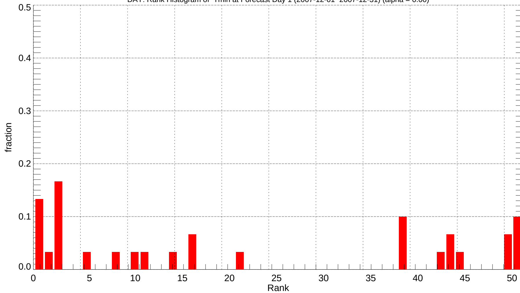
DAY: Rank Histogram of Tmin at Forecast Day 1 (2007-12-01~2007-12-31) (alpha = 0.00)
