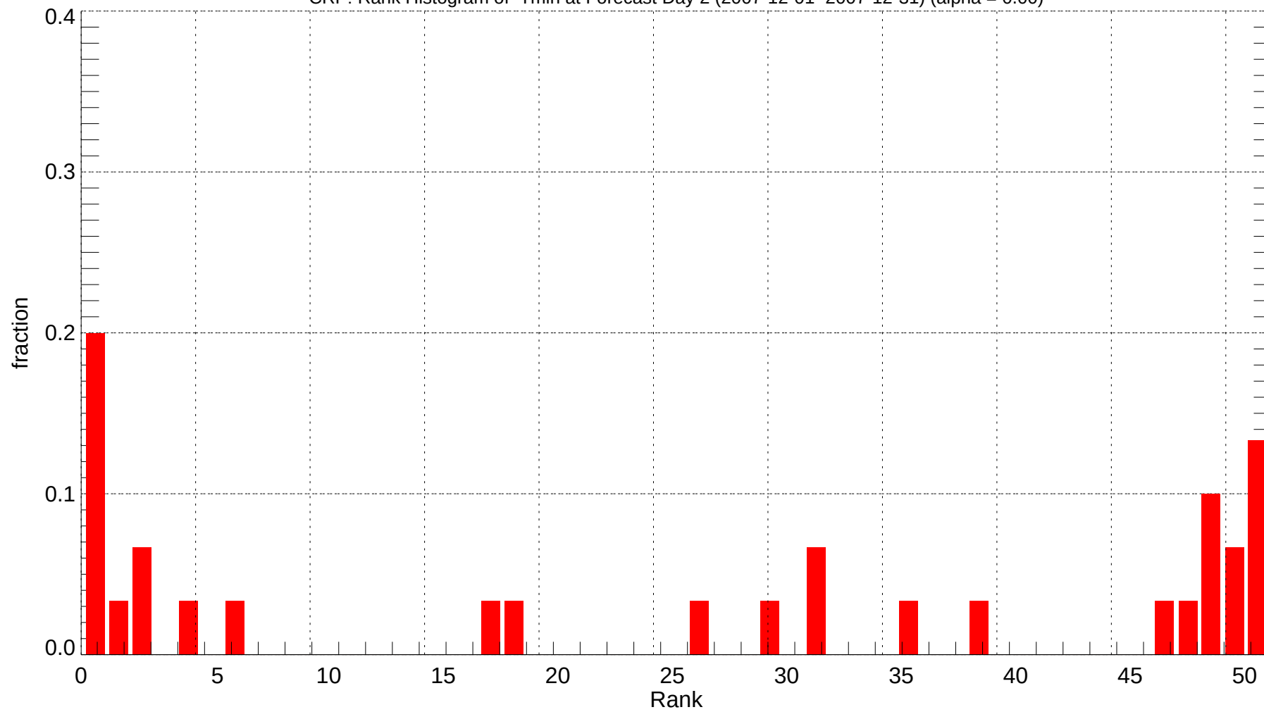
CRP: Rank Histogram of Tmin at Forecast Day 2 (2007-12-01~2007-12-31) (alpha = 0.00)
