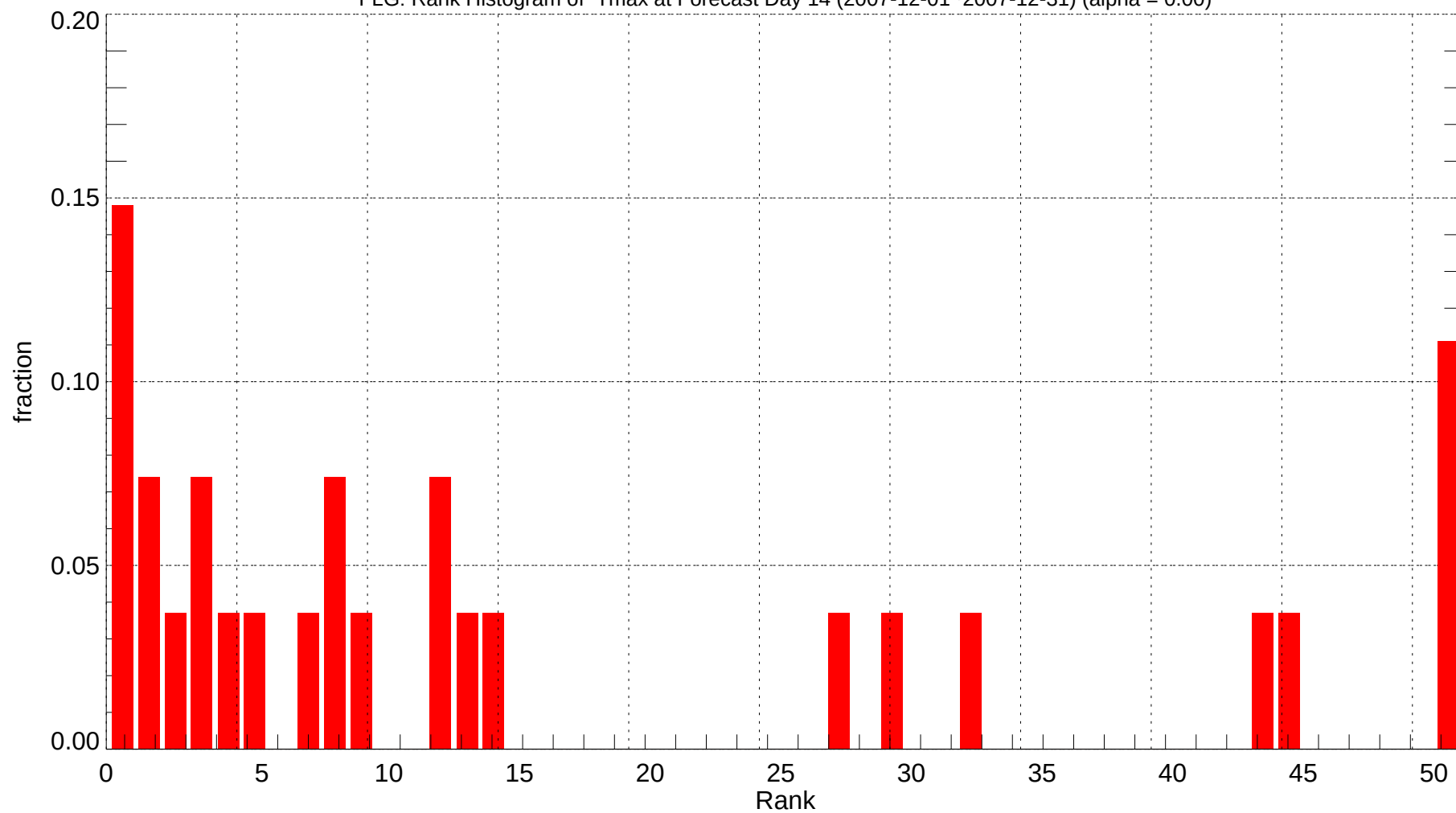
FLG: Rank Histogram of Tmax at Forecast Day 14 (2007-12-01~2007-12-31) (alpha = 0.00)
