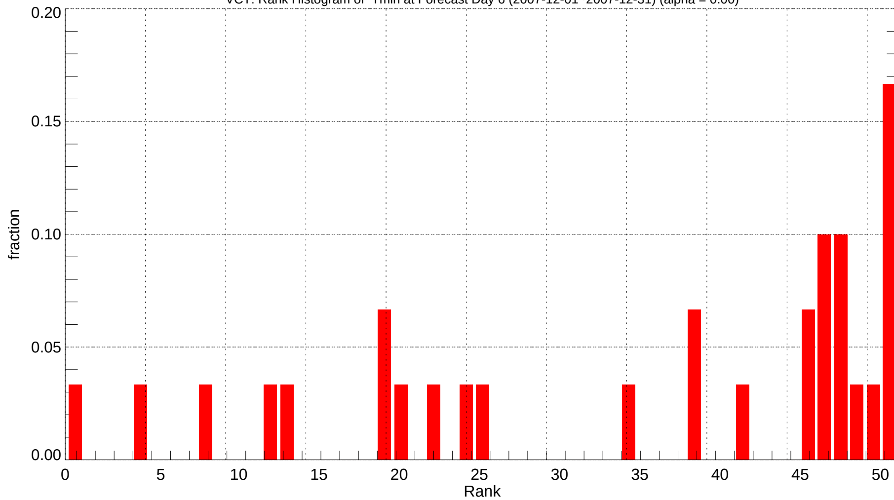
VCT: Rank Histogram of Tmin at Forecast Day 6 (2007-12-01~2007-12-31) (alpha = 0.00)
