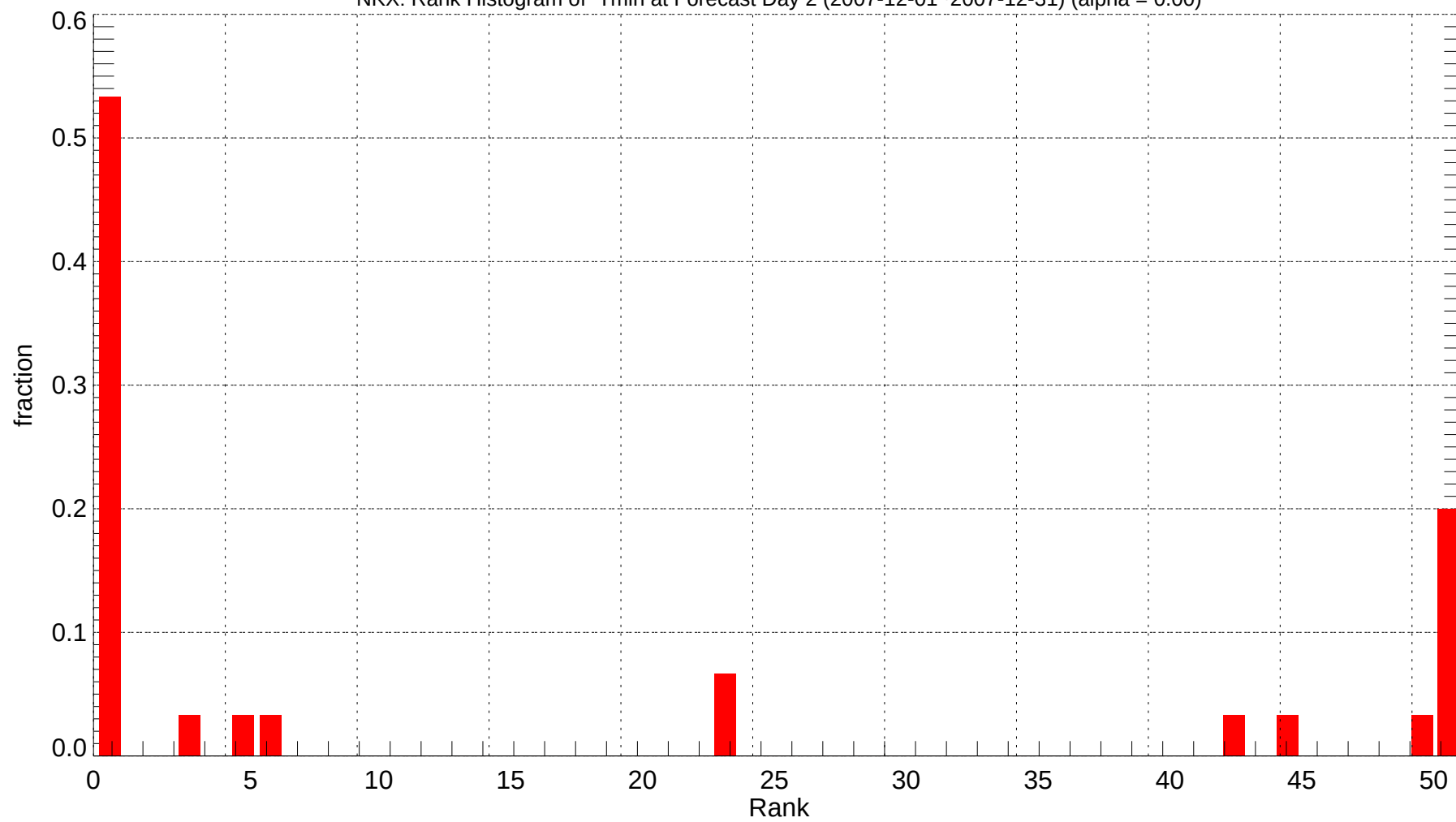
NKX: Rank Histogram of Tmin at Forecast Day 2 (2007-12-01~2007-12-31) (alpha = 0.00)
