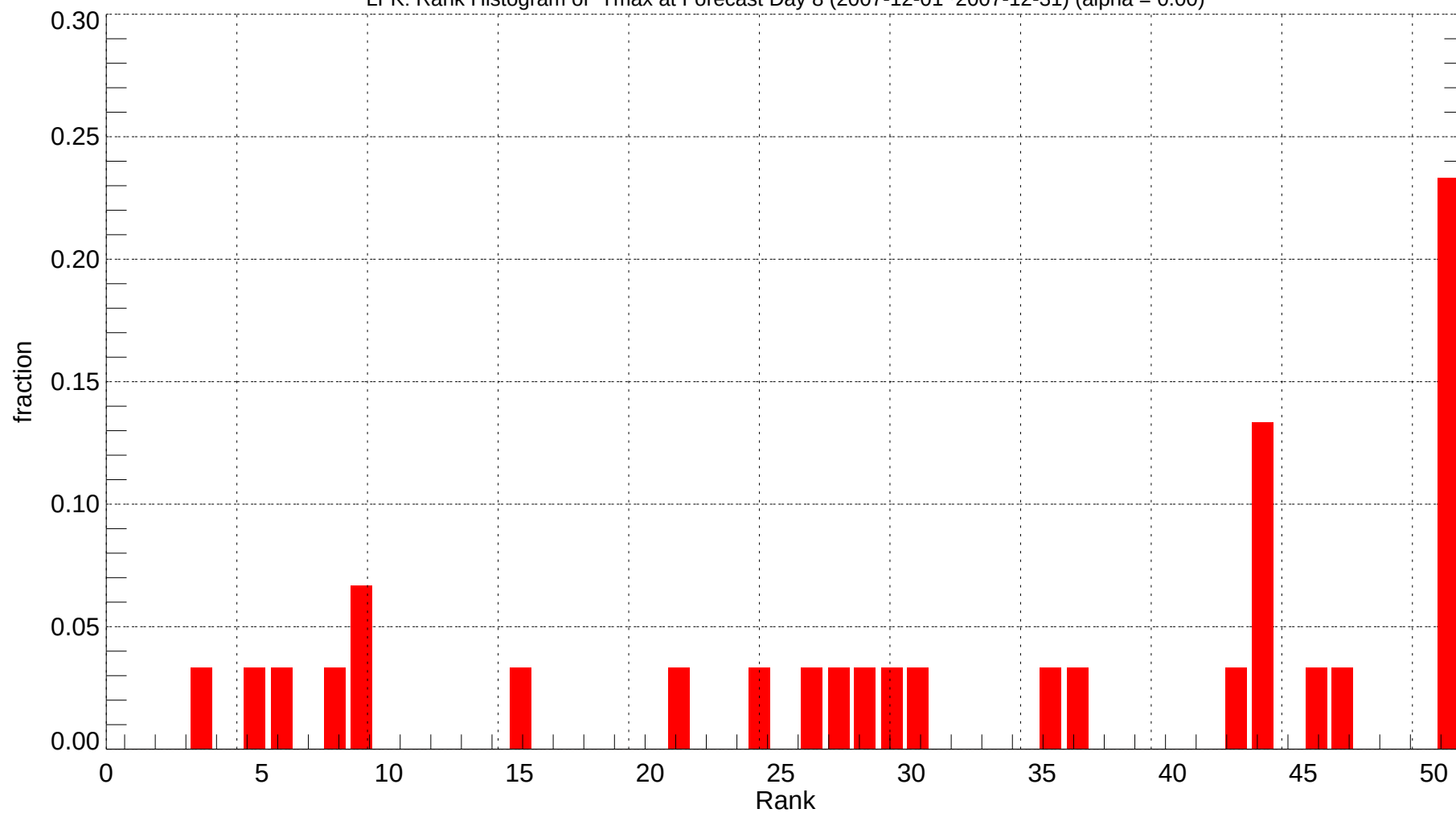
LFK: Rank Histogram of Tmax at Forecast Day 8 (2007-12-01~2007-12-31) (alpha = 0.00)
