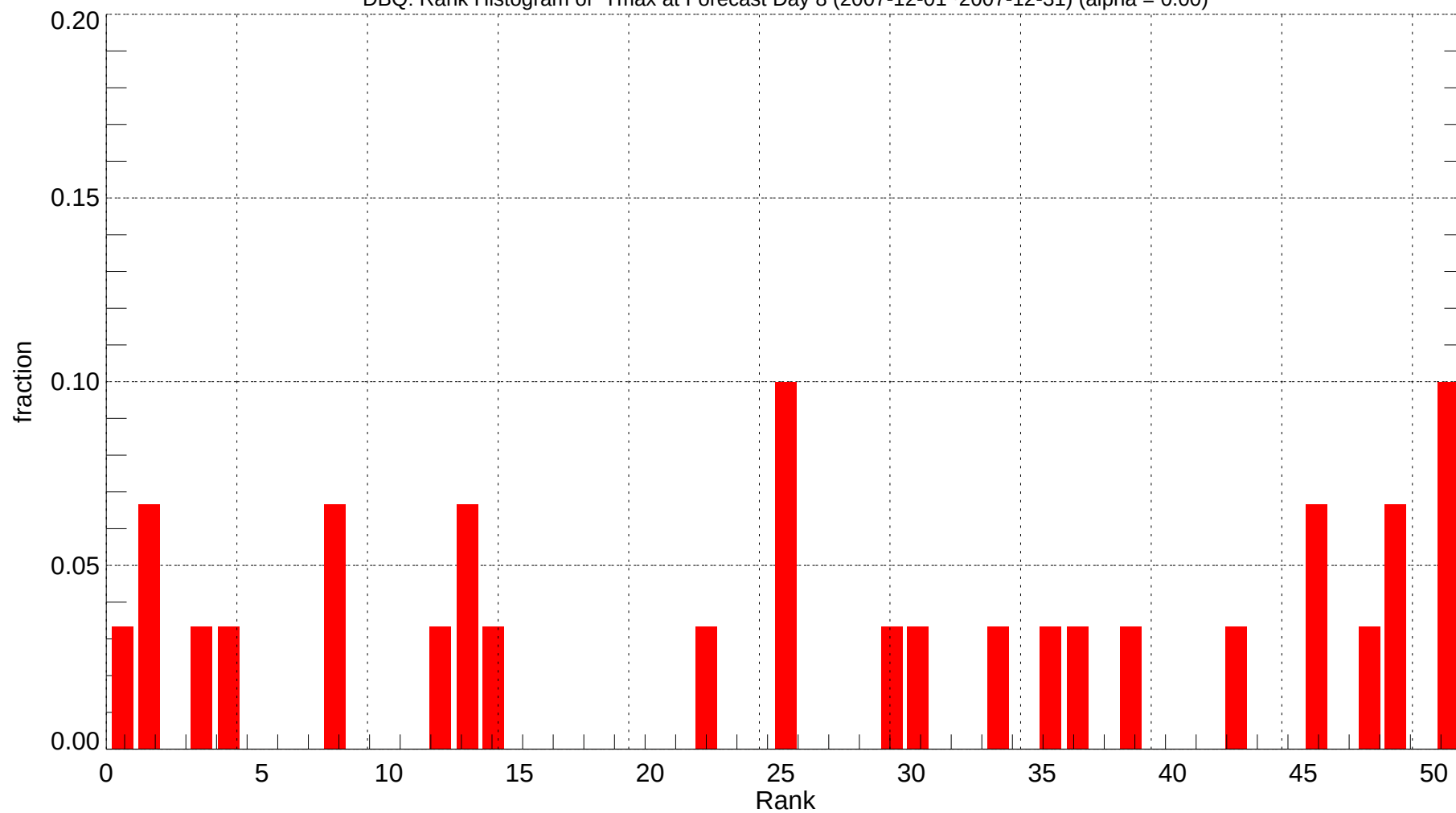
DBQ: Rank Histogram of Tmax at Forecast Day 8 (2007-12-01~2007-12-31) (alpha = 0.00)
