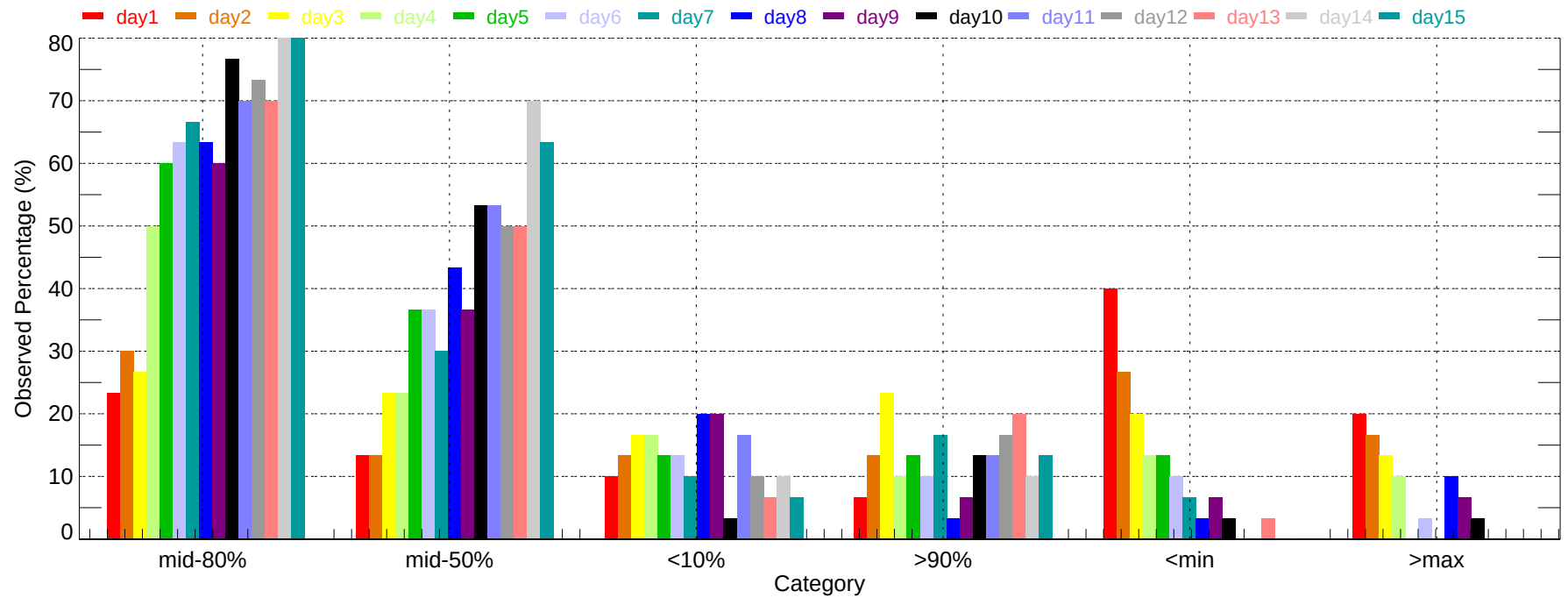
Observed Percentage of Ensembles - LAN: Min Temperature (2007-12-01~2007-12-31)
