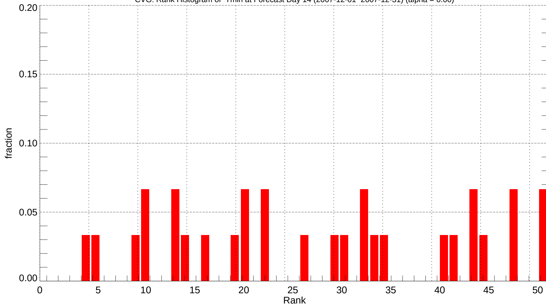
CVG: Rank Histogram of Tmin at Forecast Day 14 (2007-12-01~2007-12-31) (alpha = 0.00)
