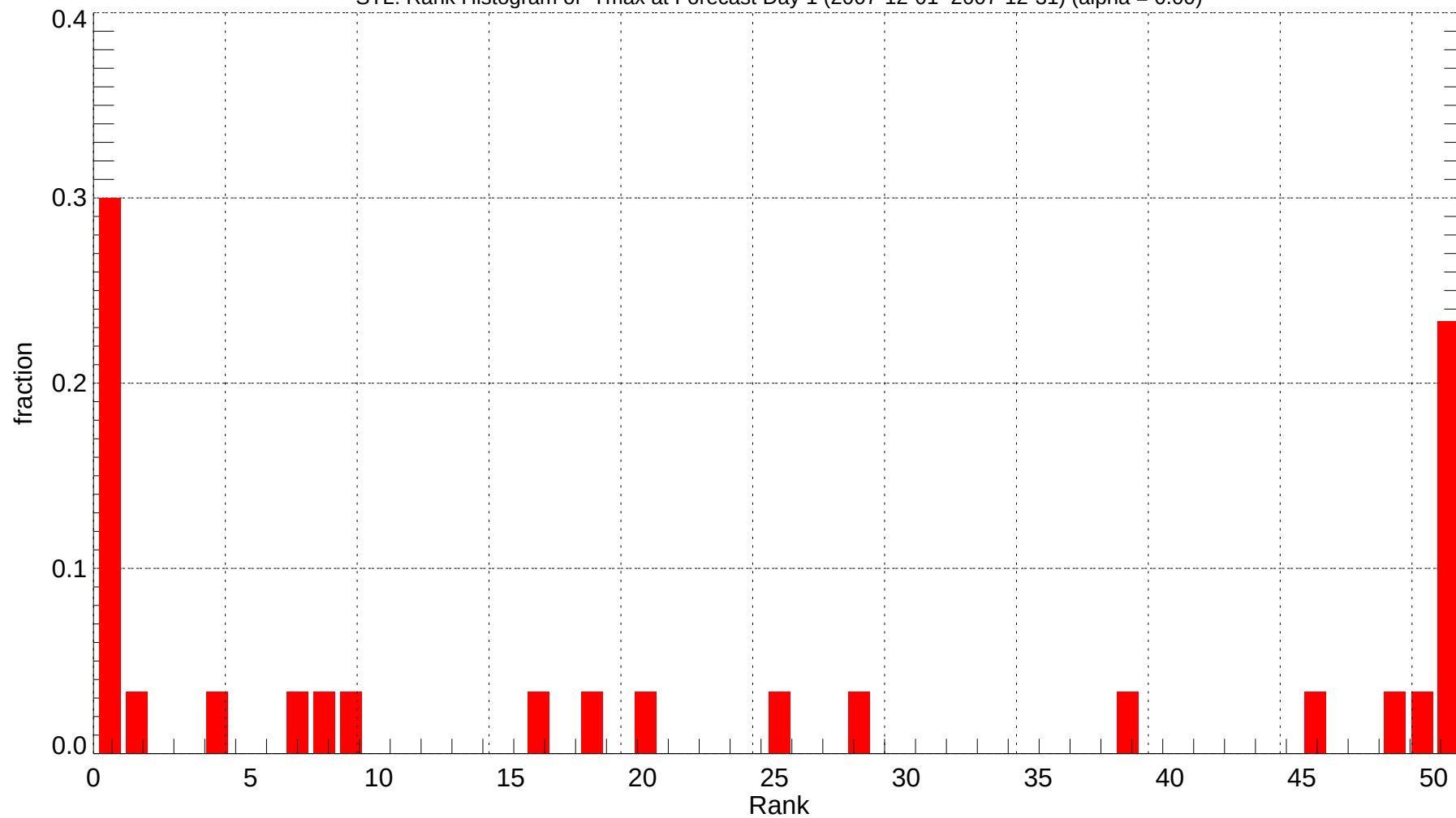
STL: Rank Histogram of Tmax at Forecast Day 1 (2007-12-01~2007-12-31) (alpha = 0.00)
