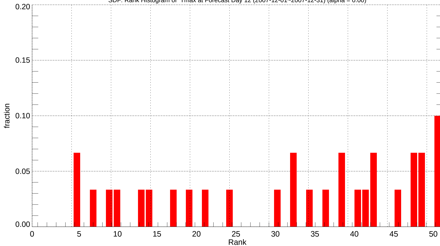
SDF: Rank Histogram of Tmax at Forecast Day 12 (2007-12-01~2007-12-31) (alpha = 0.00)
