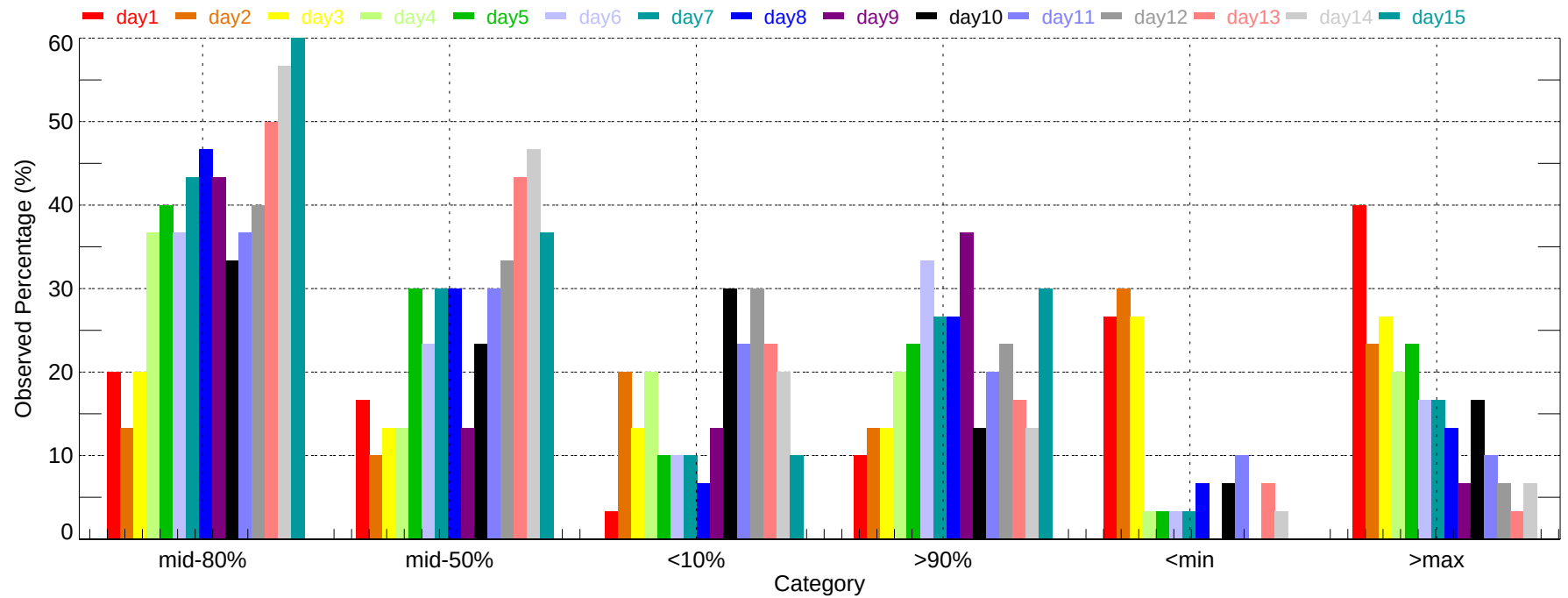
Observed Percentage of Ensembles - OKC: Min Temperature (2007-12-01~2007-12-31)
