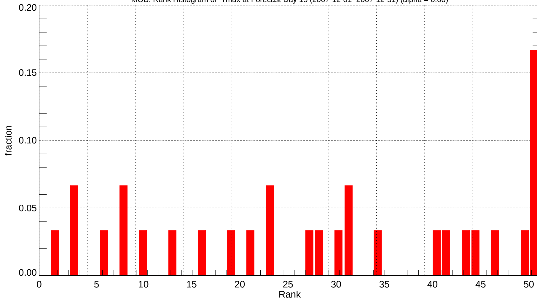
MOB: Rank Histogram of Tmax at Forecast Day 13 (2007-12-01~2007-12-31) (alpha = 0.00)
