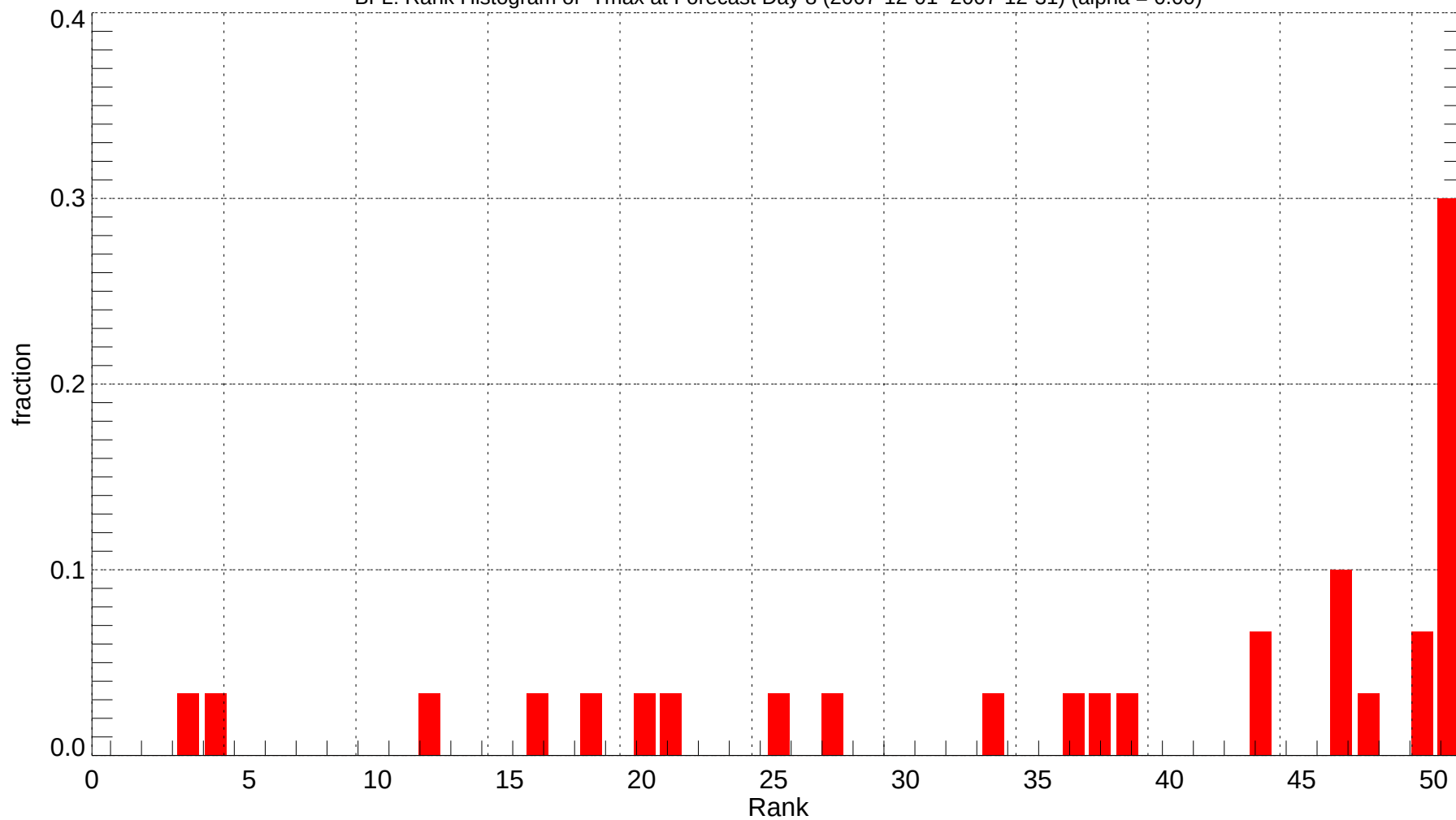
BFL: Rank Histogram of Tmax at Forecast Day 8 (2007-12-01~2007-12-31) (alpha = 0.00)
