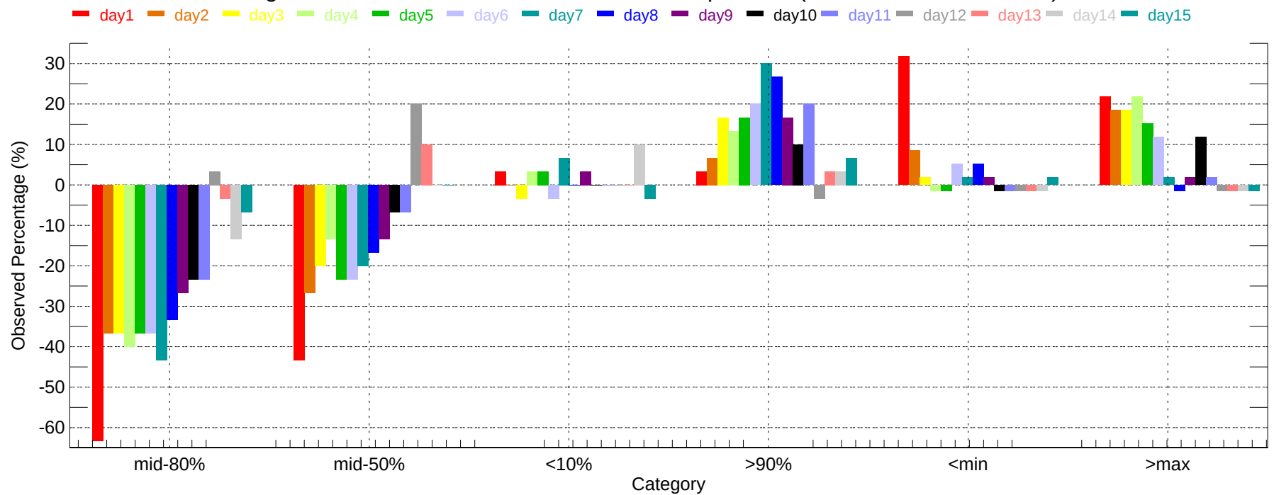
Observed Percentage Deviation of Ensembles - FSD: Max Temperature (2007-12-01~2007-12-31)
