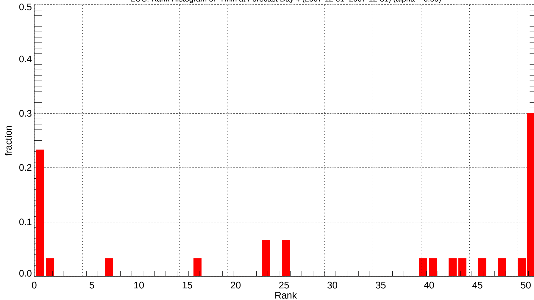
EUG: Rank Histogram of Tmin at Forecast Day 4 (2007-12-01~2007-12-31) (alpha = 0.00)
