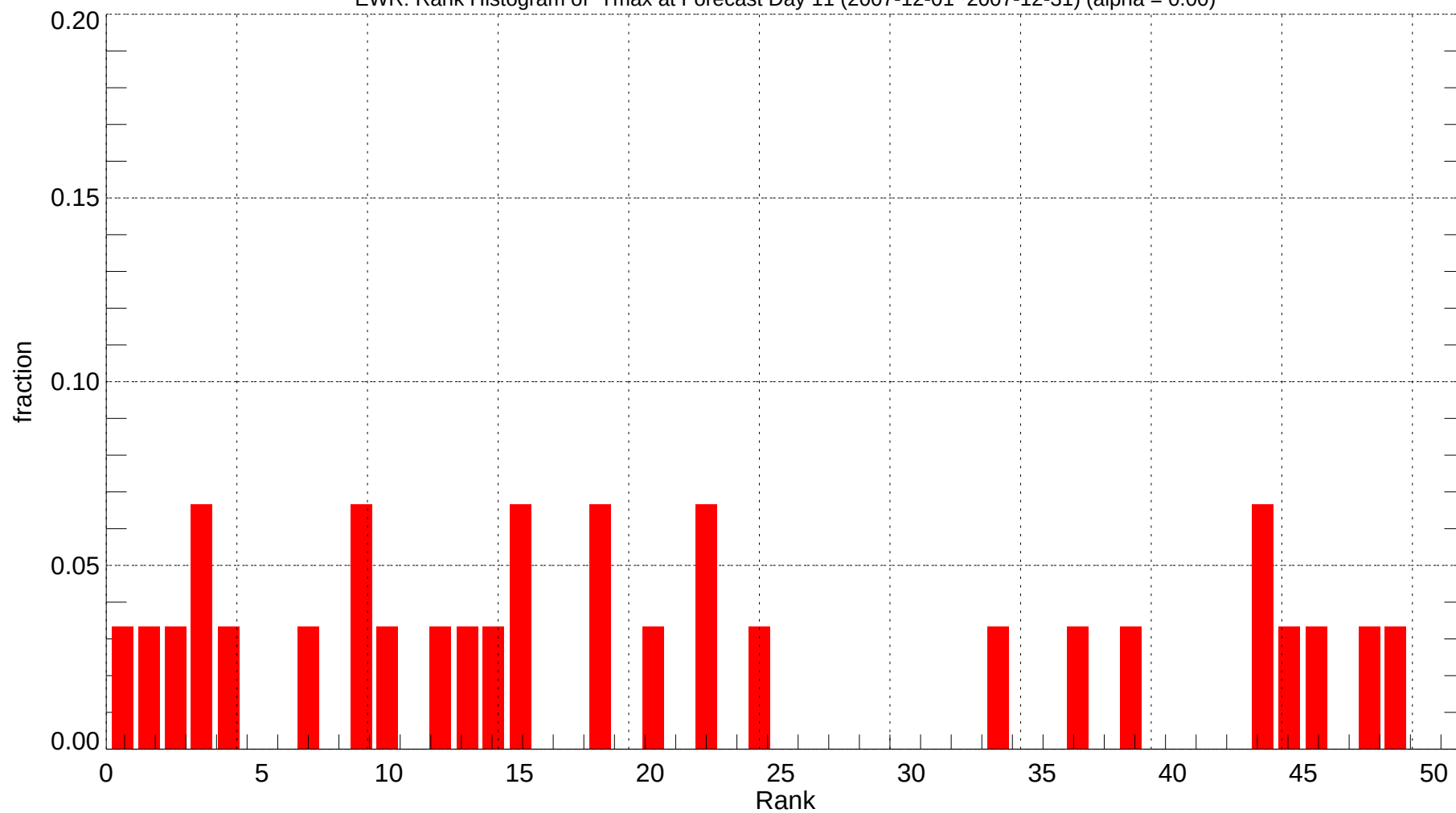
EW: Rank Histogram of Tmax at Forecast Day 11 (2007-12-01~2007-12-31) (alpha = 0.00)
