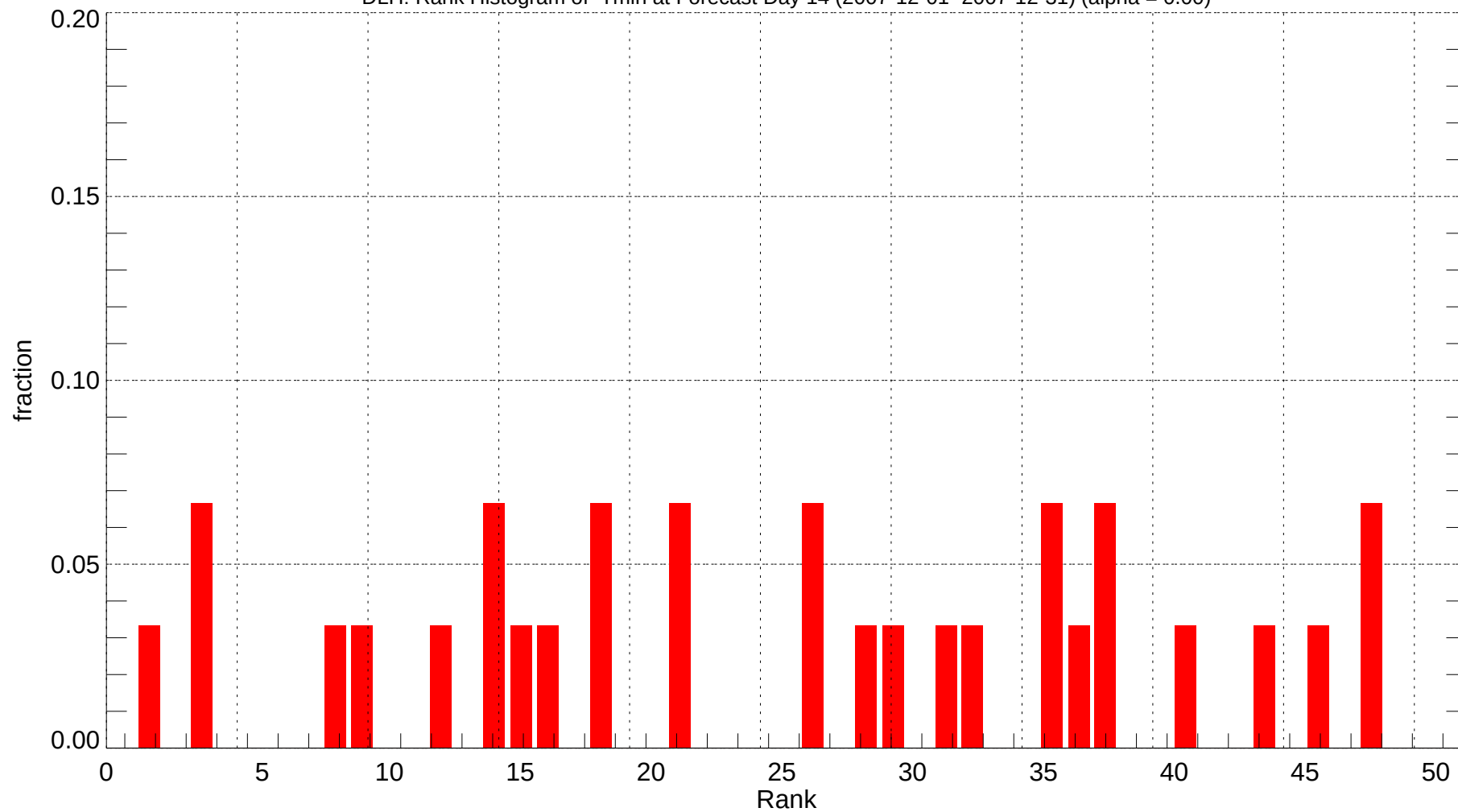
DLH: Rank Histogram of Tmin at Forecast Day 14 (2007-12-01~2007-12-31) (alpha = 0.00)
