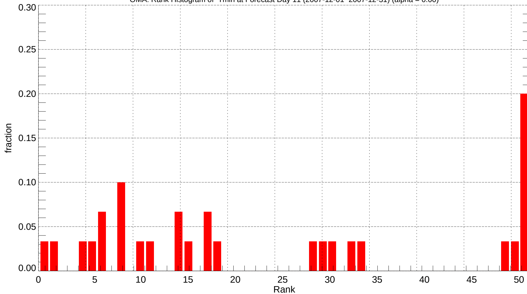
OMA: Rank Histogram of Tmin at Forecast Day 11 (2007-12-01~2007-12-31) (alpha = 0.00)
