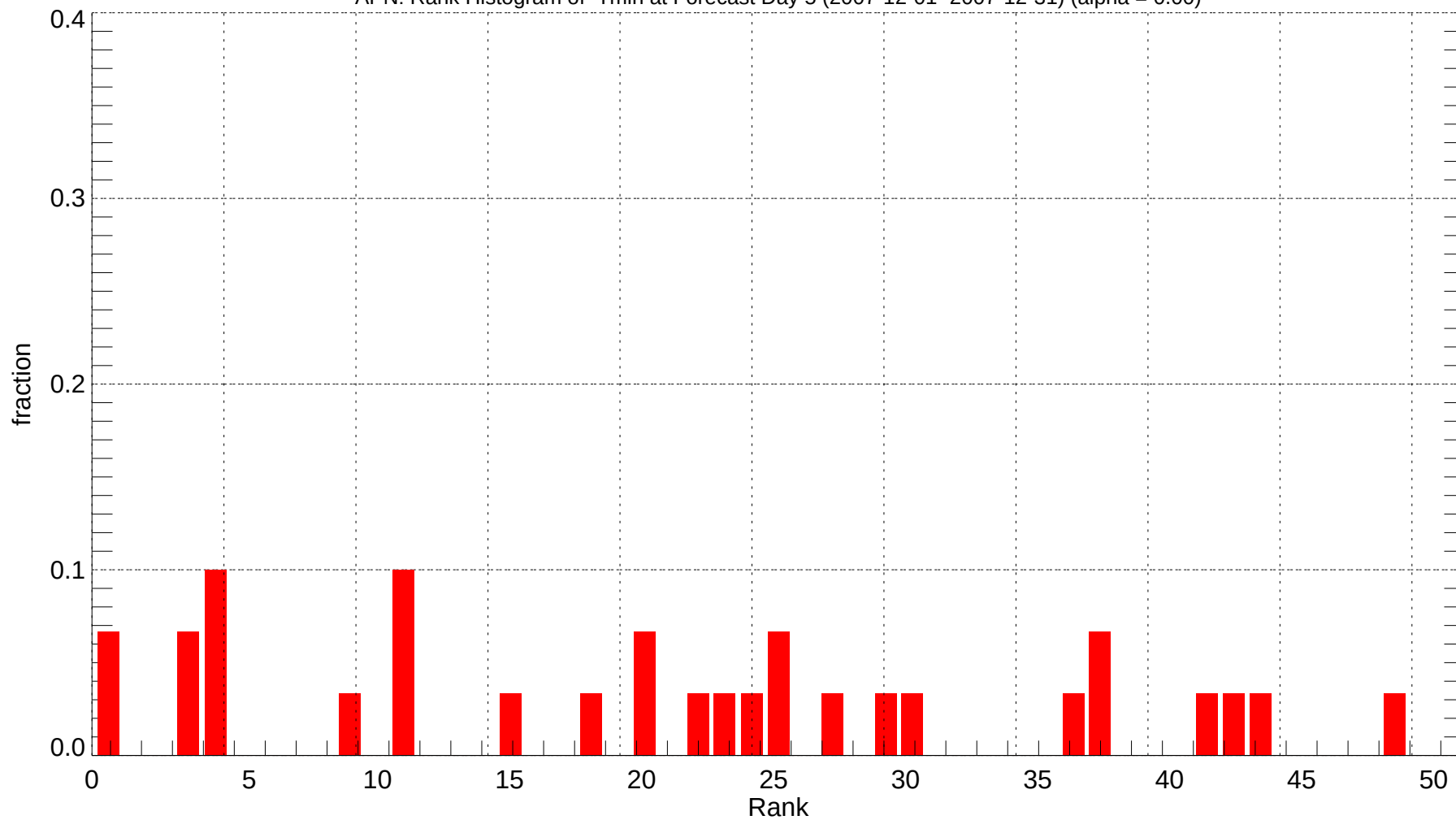
APN: Rank Histogram of Tmin at Forecast Day 5 (2007-12-01~2007-12-31) (alpha = 0.00)
