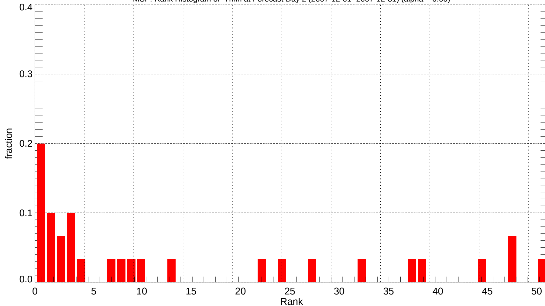
MSP: Rank Histogram of Tmin at Forecast Day 2 (2007-12-01~2007-12-31) (alpha = 0.00)
