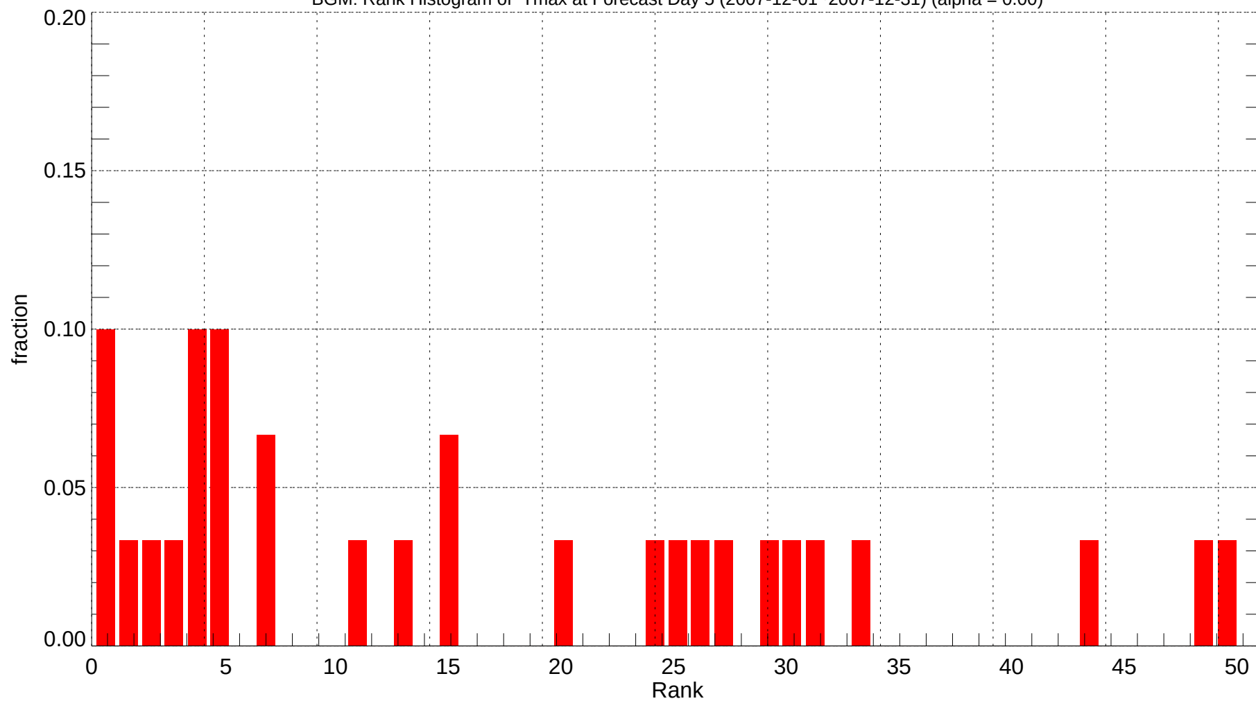
BGM: Rank Histogram of Tmax at Forecast Day 5 (2007-12-01~2007-12-31) (alpha = 0.00)
