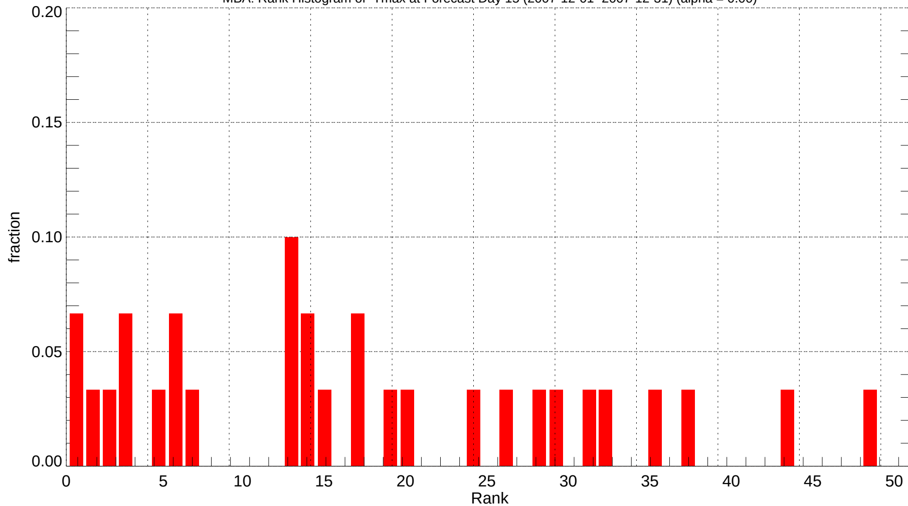
MBA: Rank Histogram of Tmax at Forecast Day 15 (2007-12-01~2007-12-31) (alpha = 0.00)
