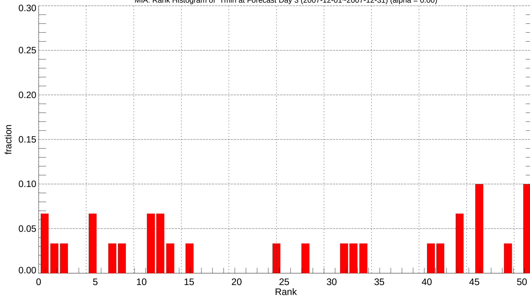
MIA: Rank Histogram of Tmin at Forecast Day 3 (2007-12-01~2007-12-31) (alpha = 0.00)
