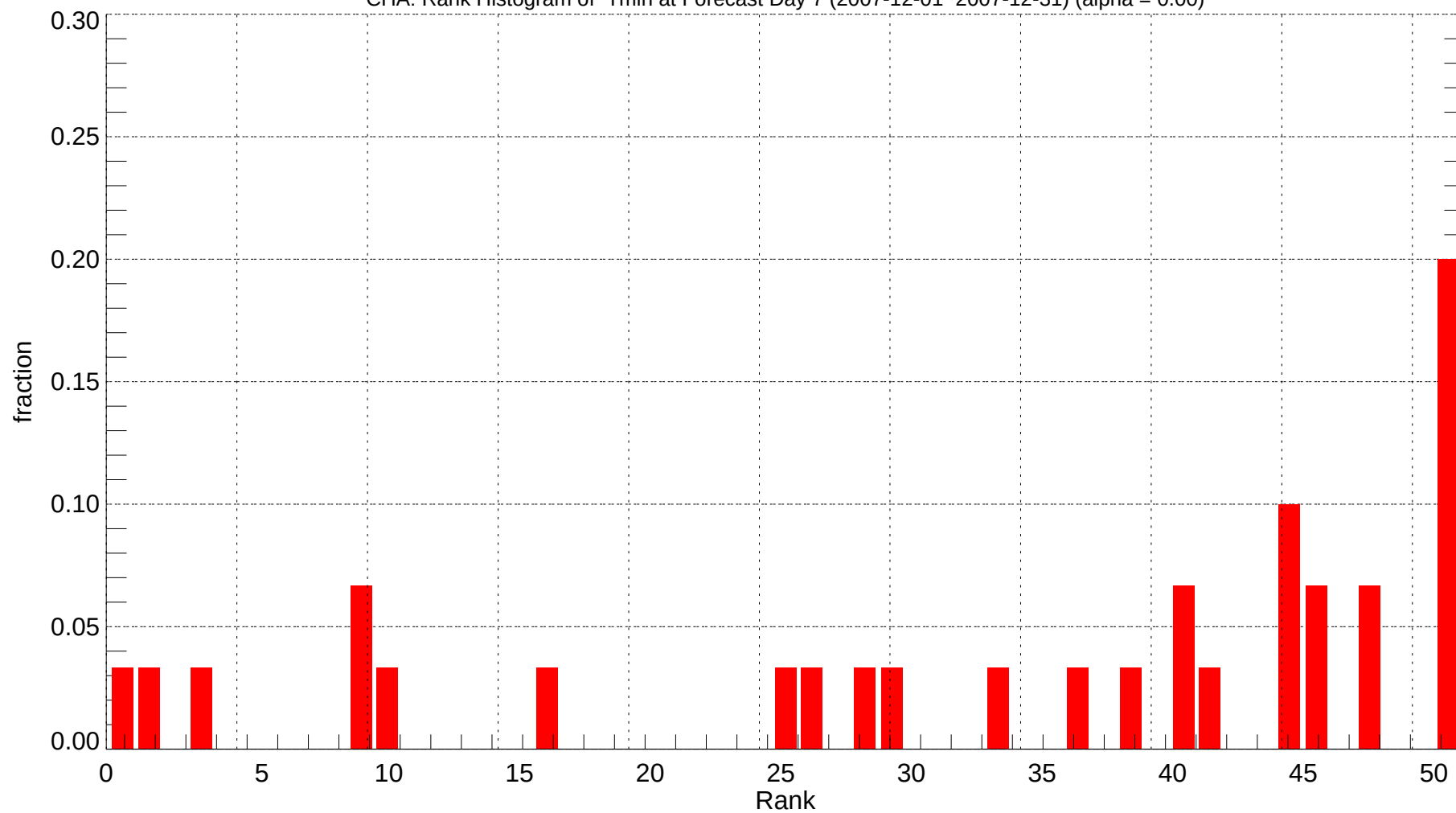
CHA: Rank Histogram of Tmin at Forecast Day 7 (2007-12-01~2007-12-31) (alpha = 0.00)
