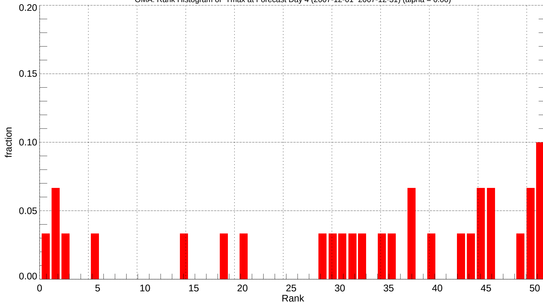
OMA: Rank Histogram of Tmax at Forecast Day 4 (2007-12-01~2007-12-31) (alpha = 0.00)
