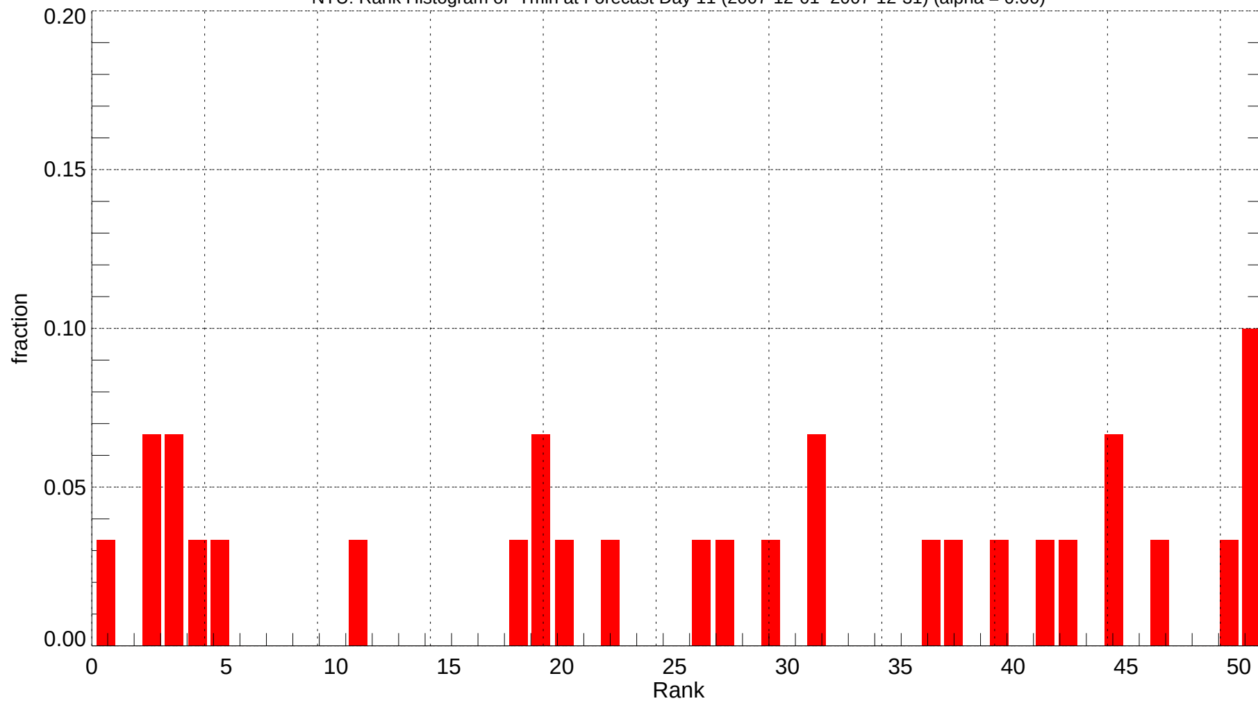
NTU: Rank Histogram of Tmin at Forecast Day 11 (2007-12-01~2007-12-31) (alpha = 0.00)
