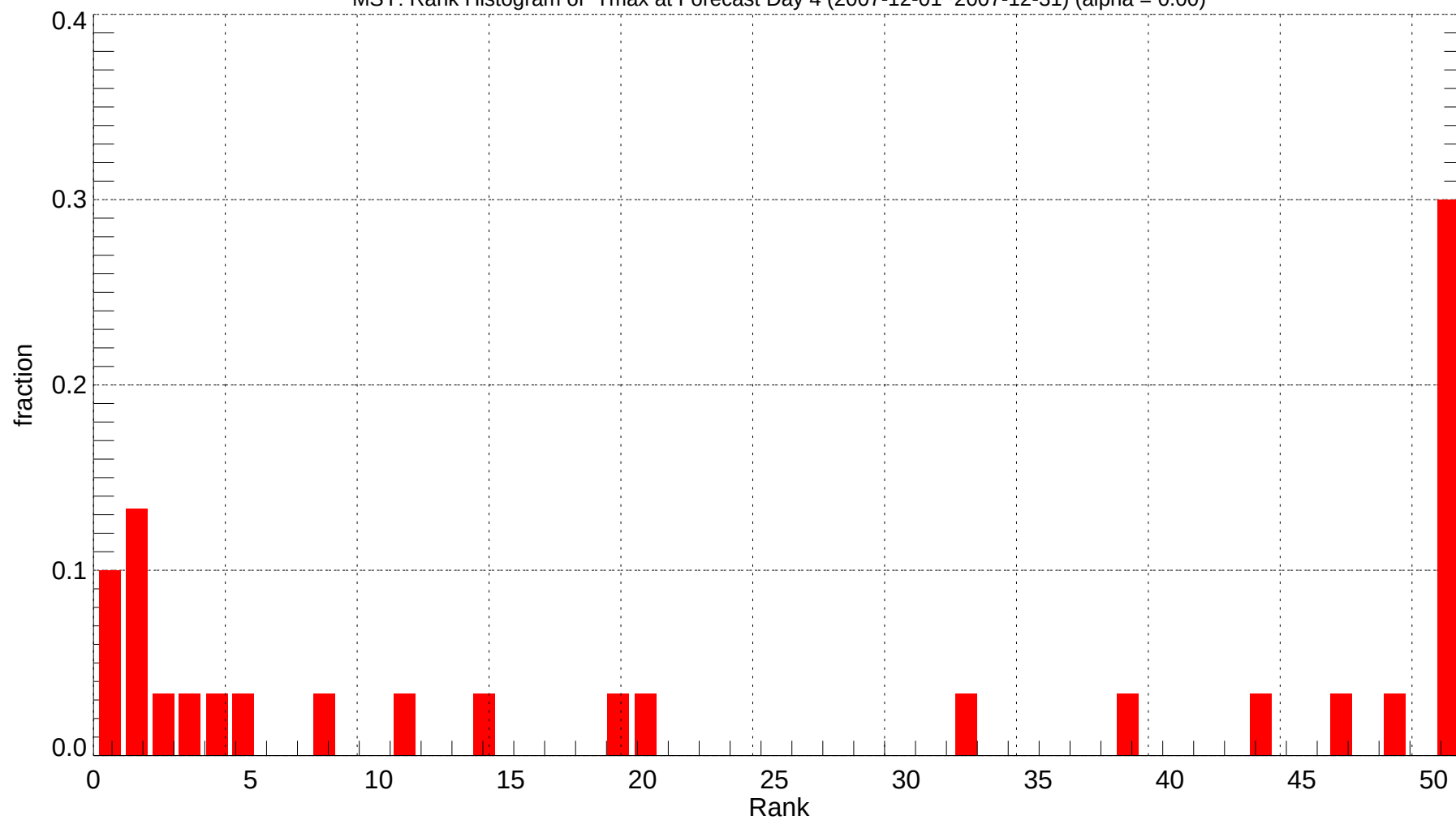
MSY: Rank Histogram of Tmax at Forecast Day 4 (2007-12-01~2007-12-31) (alpha = 0.00)
