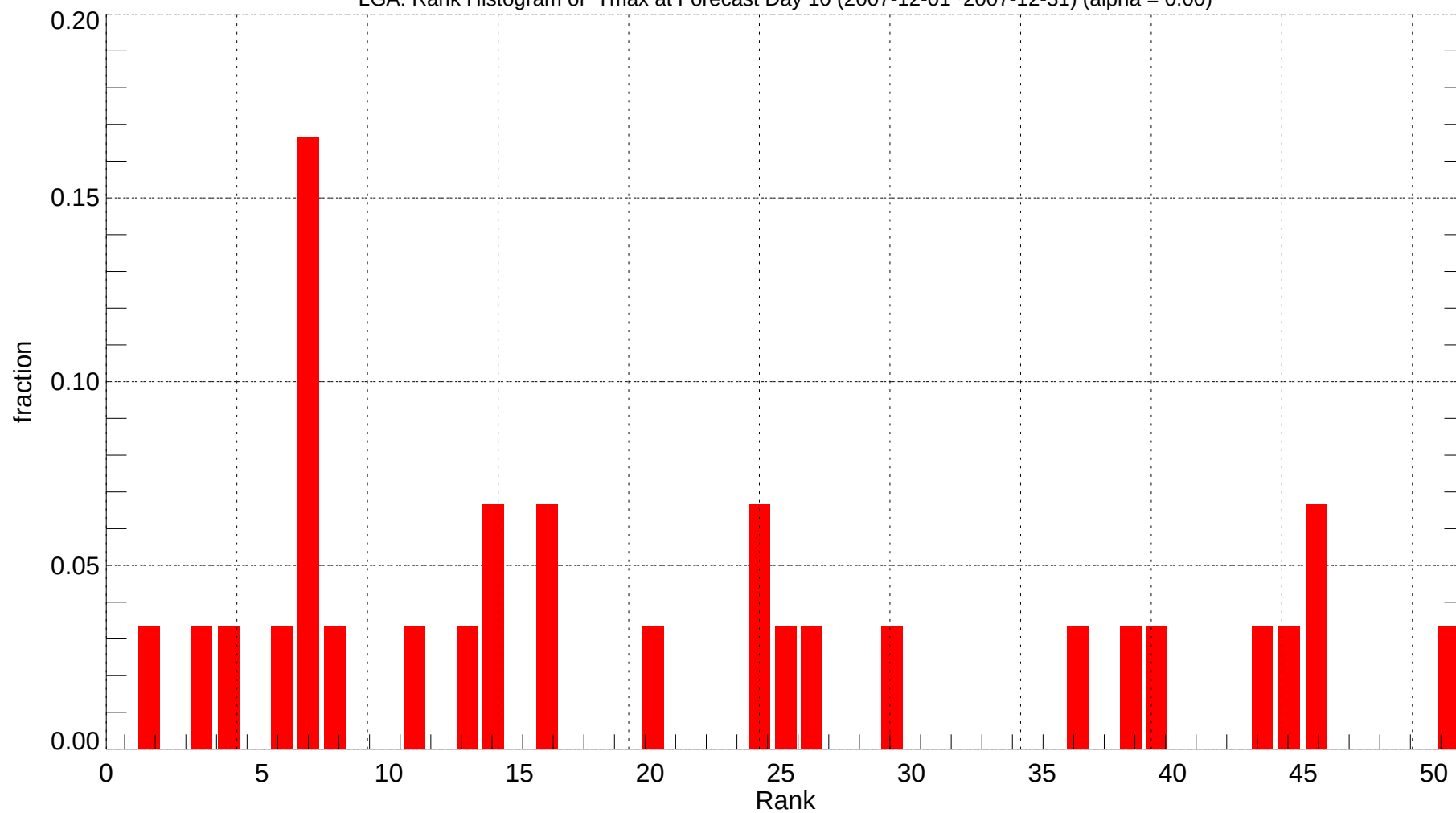
LGA: Rank Histogram of Tmax at Forecast Day 10 (2007-12-01~2007-12-31) (alpha = 0.00)
