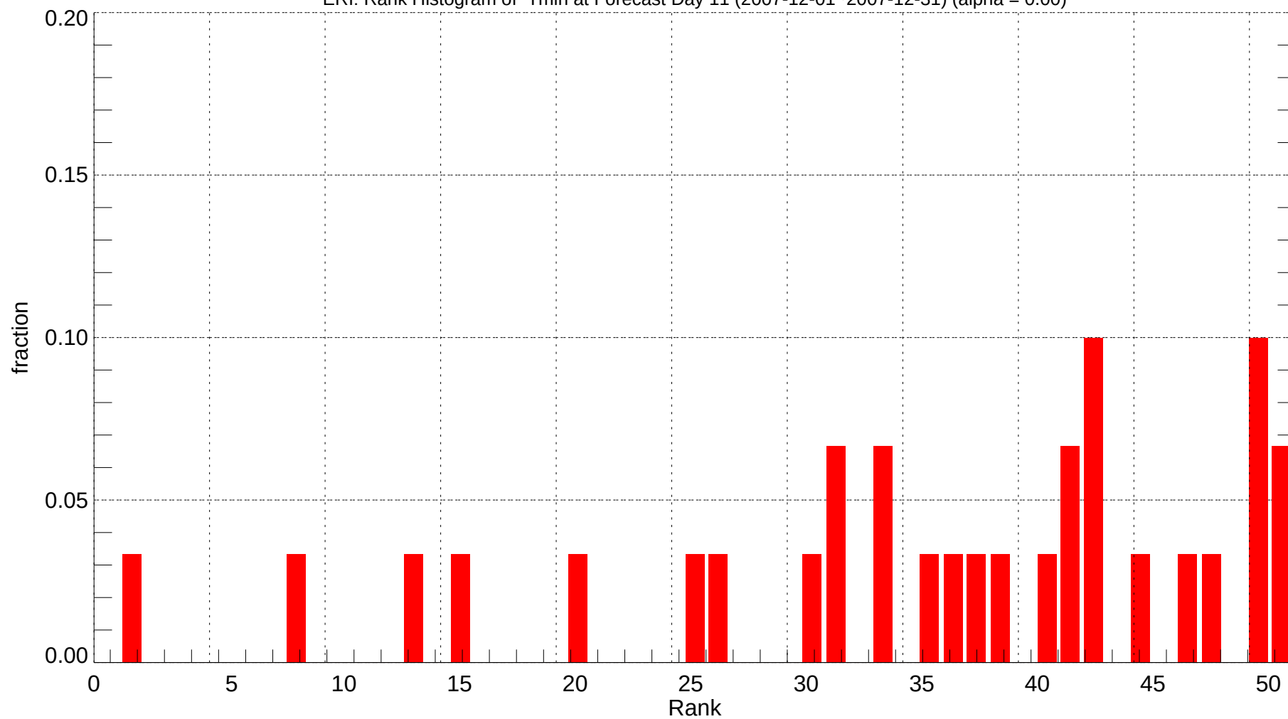
ERI: Rank Histogram of Tmin at Forecast Day 11 (2007-12-01~2007-12-31) (alpha = 0.00)
