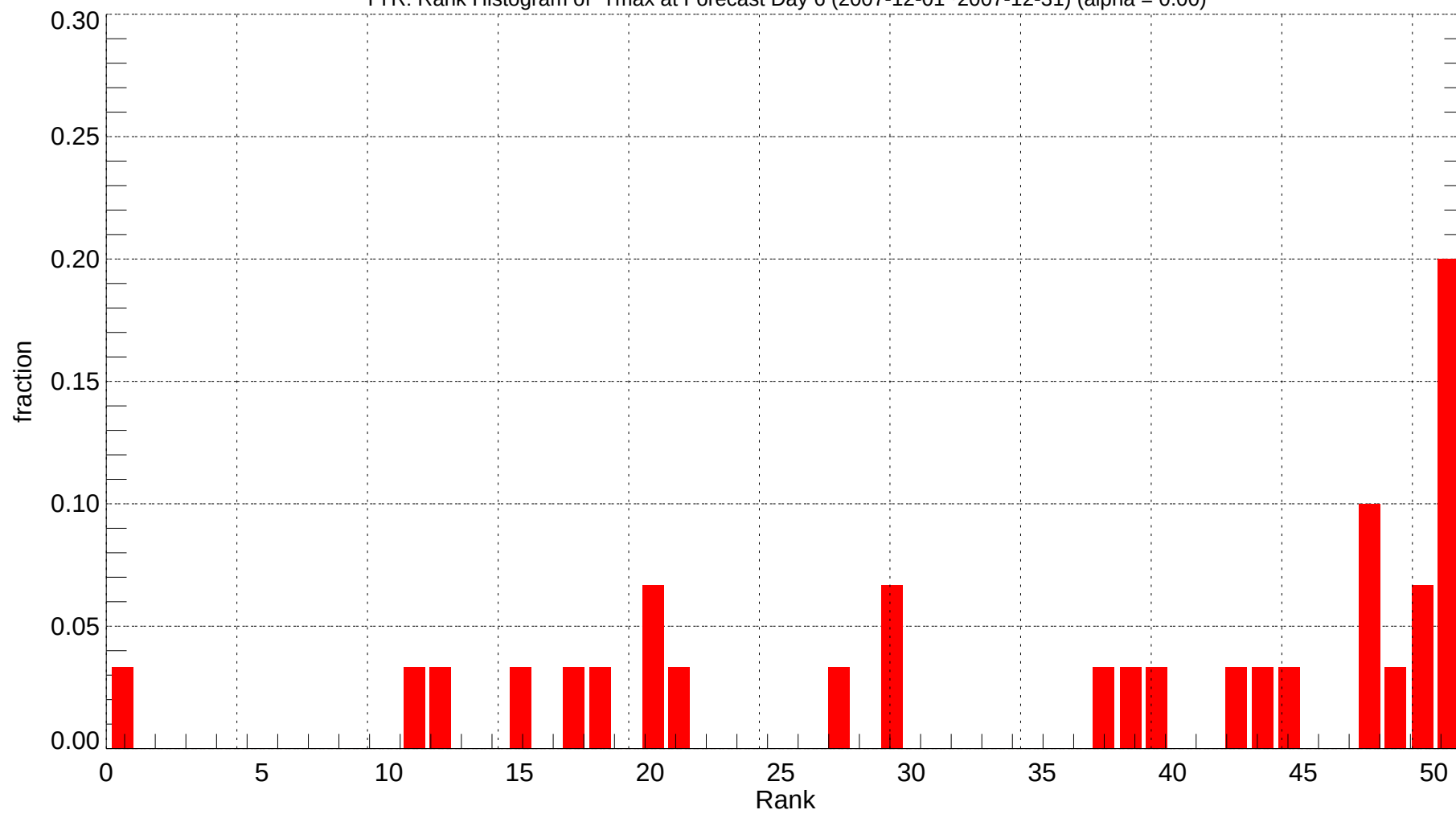
TYR: Rank Histogram of Tmax at Forecast Day 6 (2007-12-01~2007-12-31) (alpha = 0.00)
