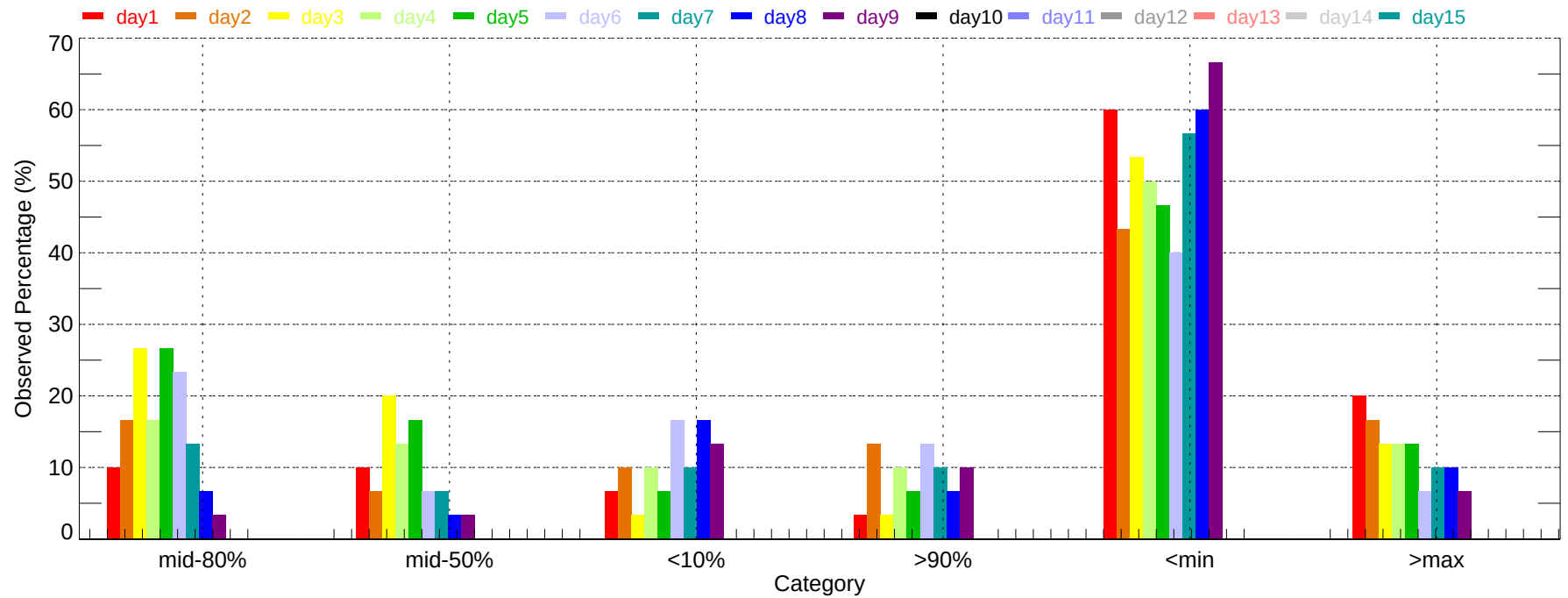
Observed Percentage of Ensembles - NKX: Max Temperature (2007-12-01~2007-12-31)
