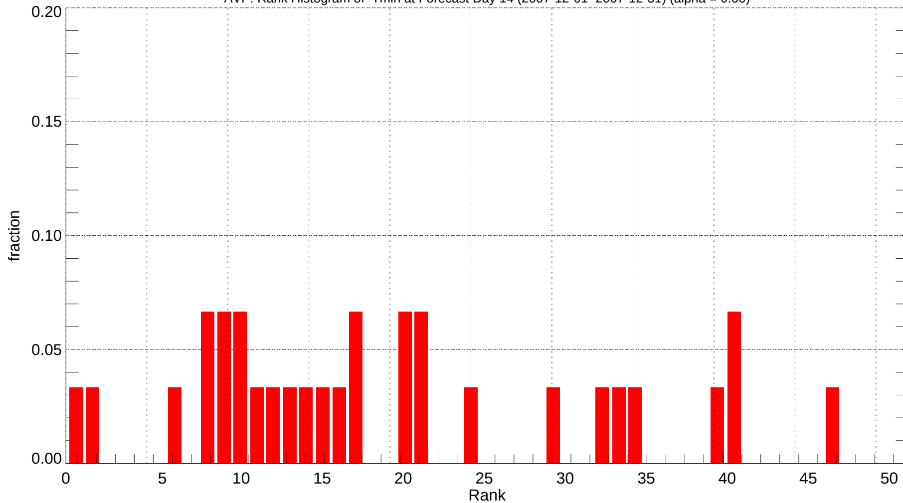
AVP: Rank Histogram of Tmin at Forecast Day 14 (2007-12-01~2007-12-31) (alpha = 0.00)
