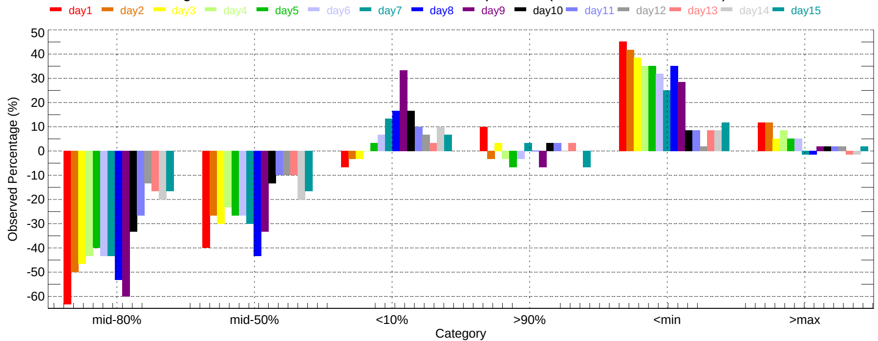
Observed Percentage Deviation of Ensembles - OAK: Min Temperature (2007-12-01~2007-12-31)
