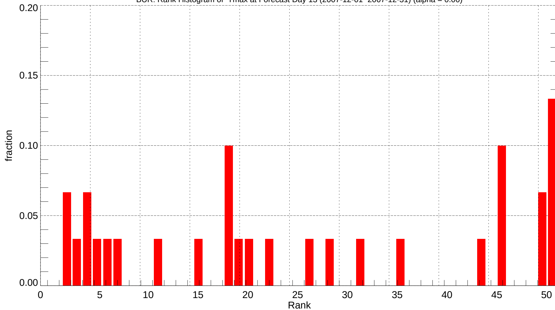
BUR: Rank Histogram of Tmax at Forecast Day 13 (2007-12-01~2007-12-31) (alpha = 0.00)
