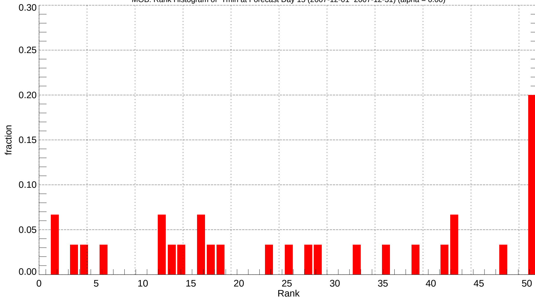
MOB: Rank Histogram of Tmin at Forecast Day 15 (2007-12-01~2007-12-31) (alpha = 0.00)
