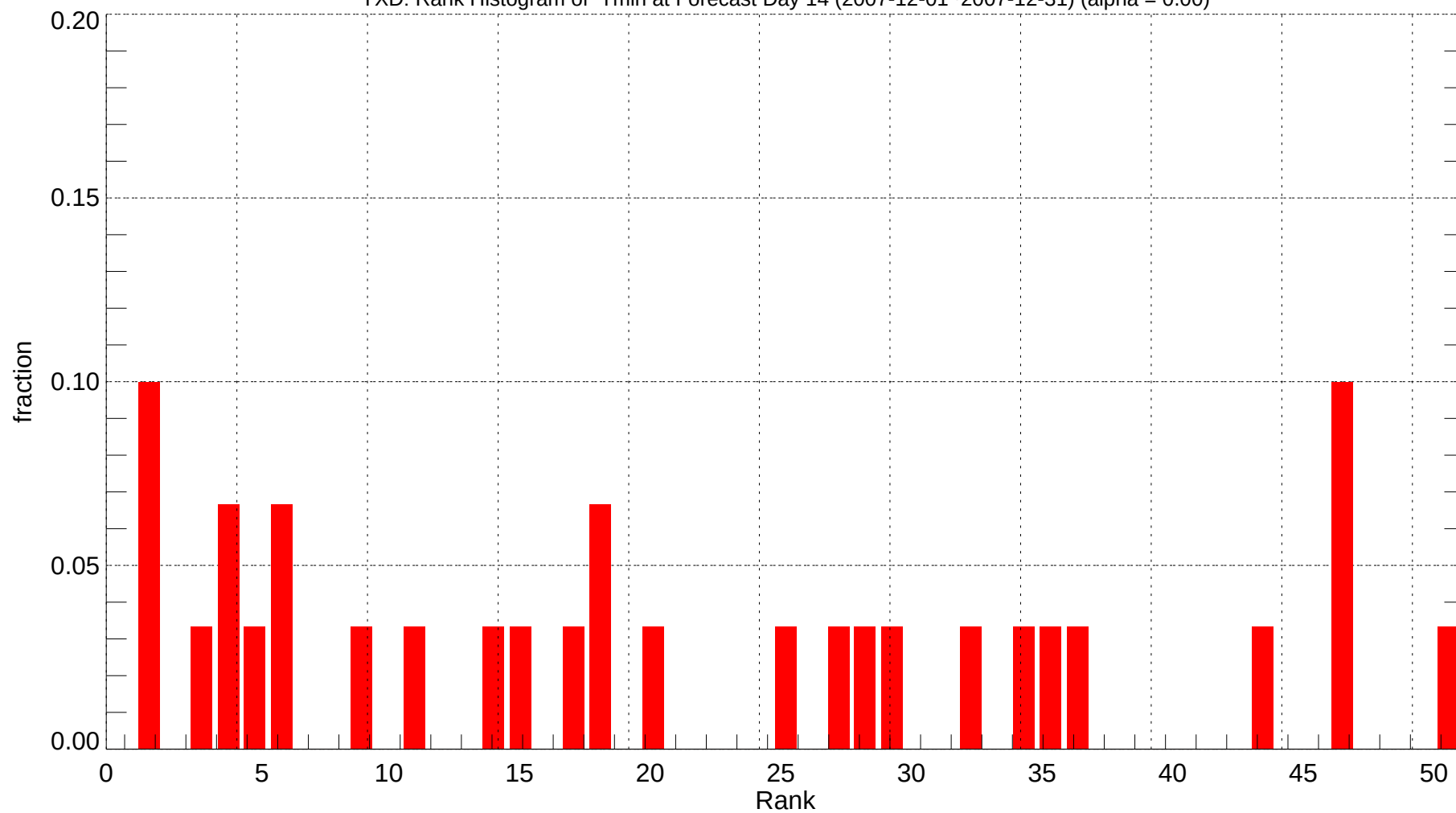
YXD: Rank Histogram of Tmin at Forecast Day 14 (2007-12-01~2007-12-31) (alpha = 0.00)
