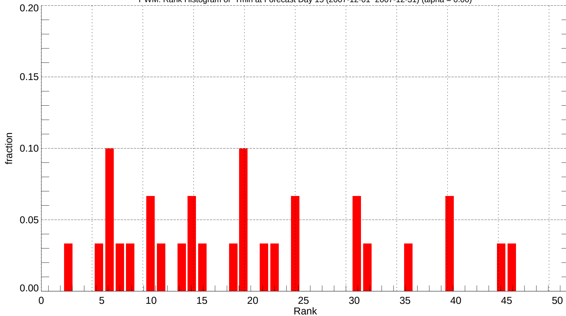
PWM: Rank Histogram of Tmin at Forecast Day 15 (2007-12-01~2007-12-31) (alpha = 0.00)
