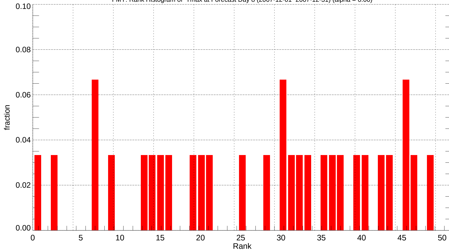
FMY: Rank Histogram of Tmax at Forecast Day 8 (2007-12-01~2007-12-31) (alpha = 0.00)
