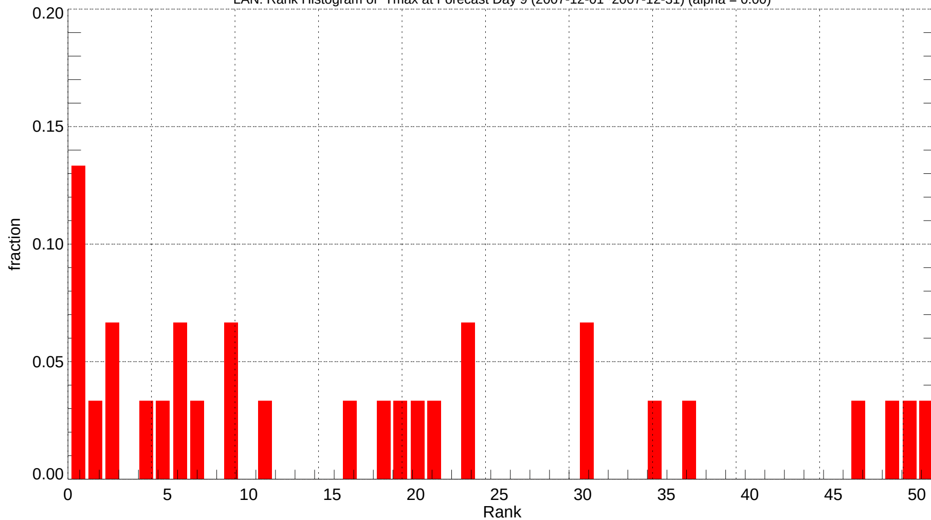
LAN: Rank Histogram of Tmax at Forecast Day 9 (2007-12-01~2007-12-31) (alpha = 0.00)
