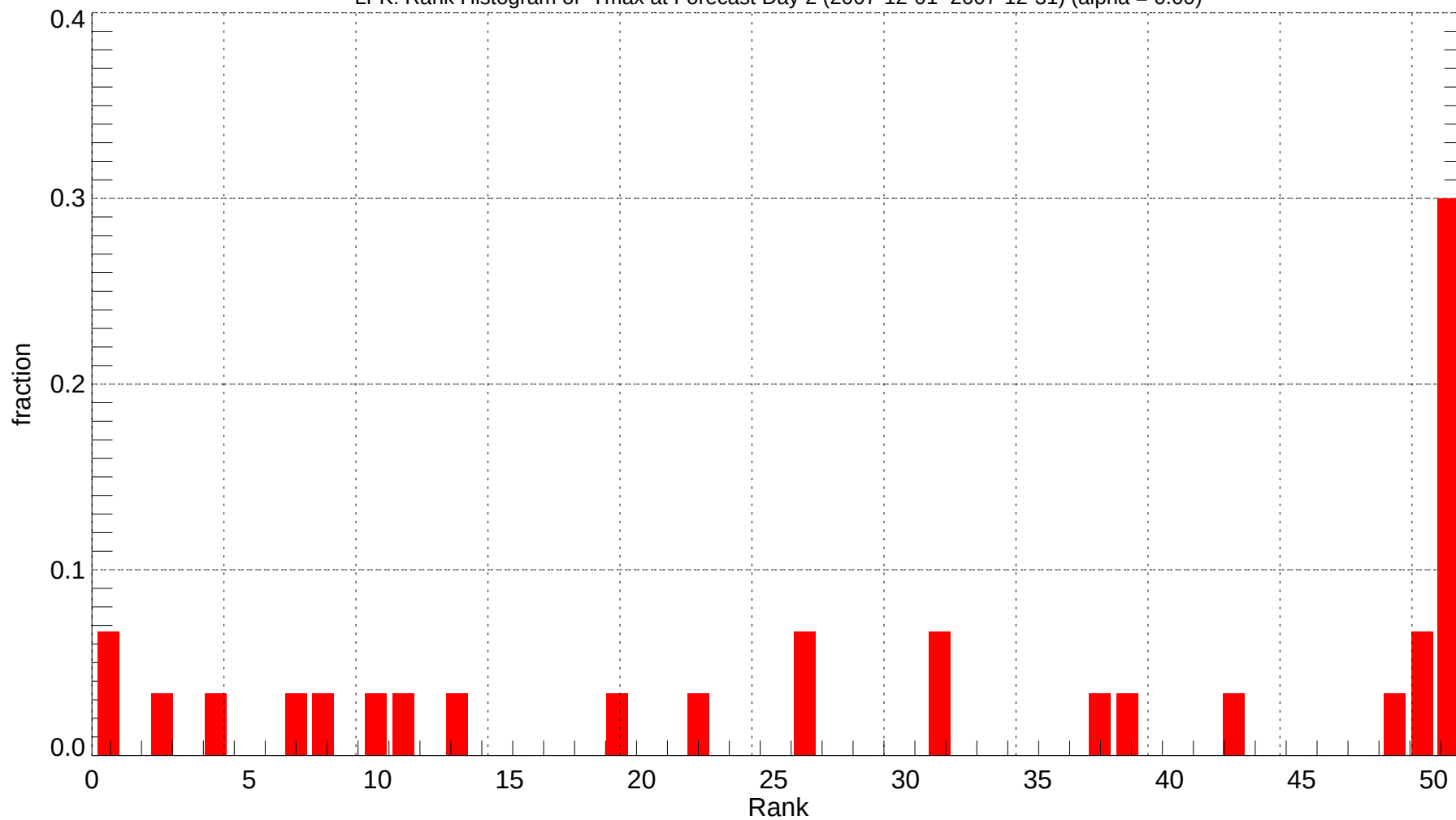
LFK: Rank Histogram of Tmax at Forecast Day 2 (2007-12-01~2007-12-31) (alpha = 0.00)
