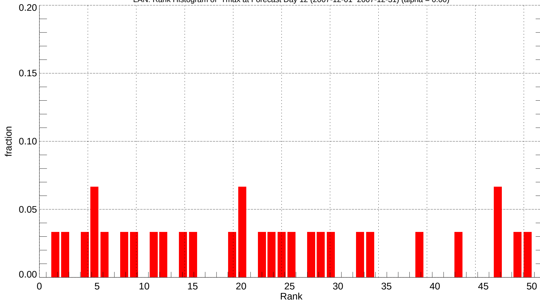
LAN: Rank Histogram of Tmax at Forecast Day 12 (2007-12-01~2007-12-31) (alpha = 0.00)
