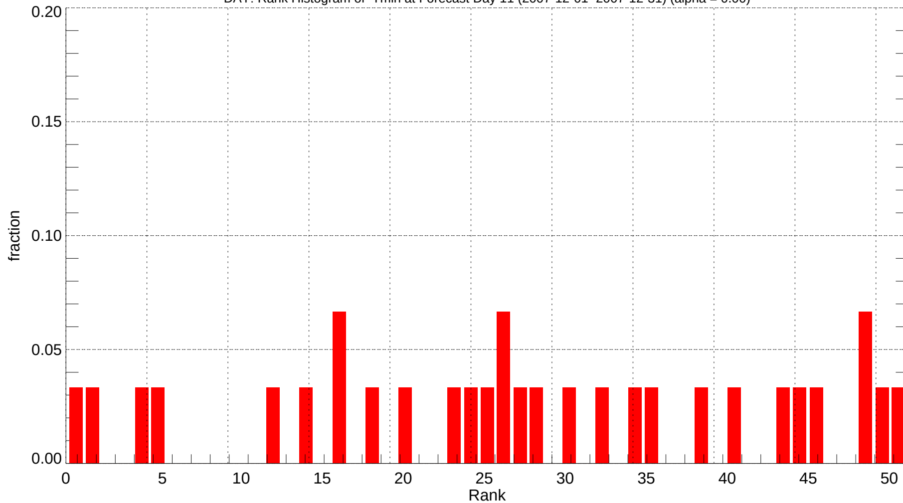
DAY: Rank Histogram of Tmin at Forecast Day 11 (2007-12-01~2007-12-31) (alpha = 0.00)
