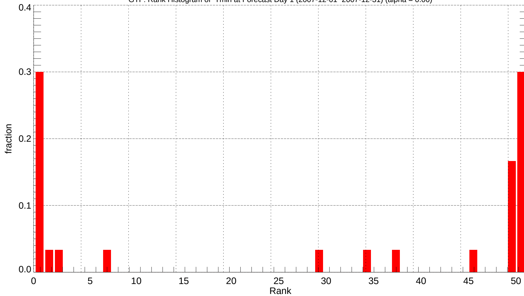
GTF: Rank Histogram of Tmin at Forecast Day 1 (2007-12-01~2007-12-31) (alpha = 0.00)
