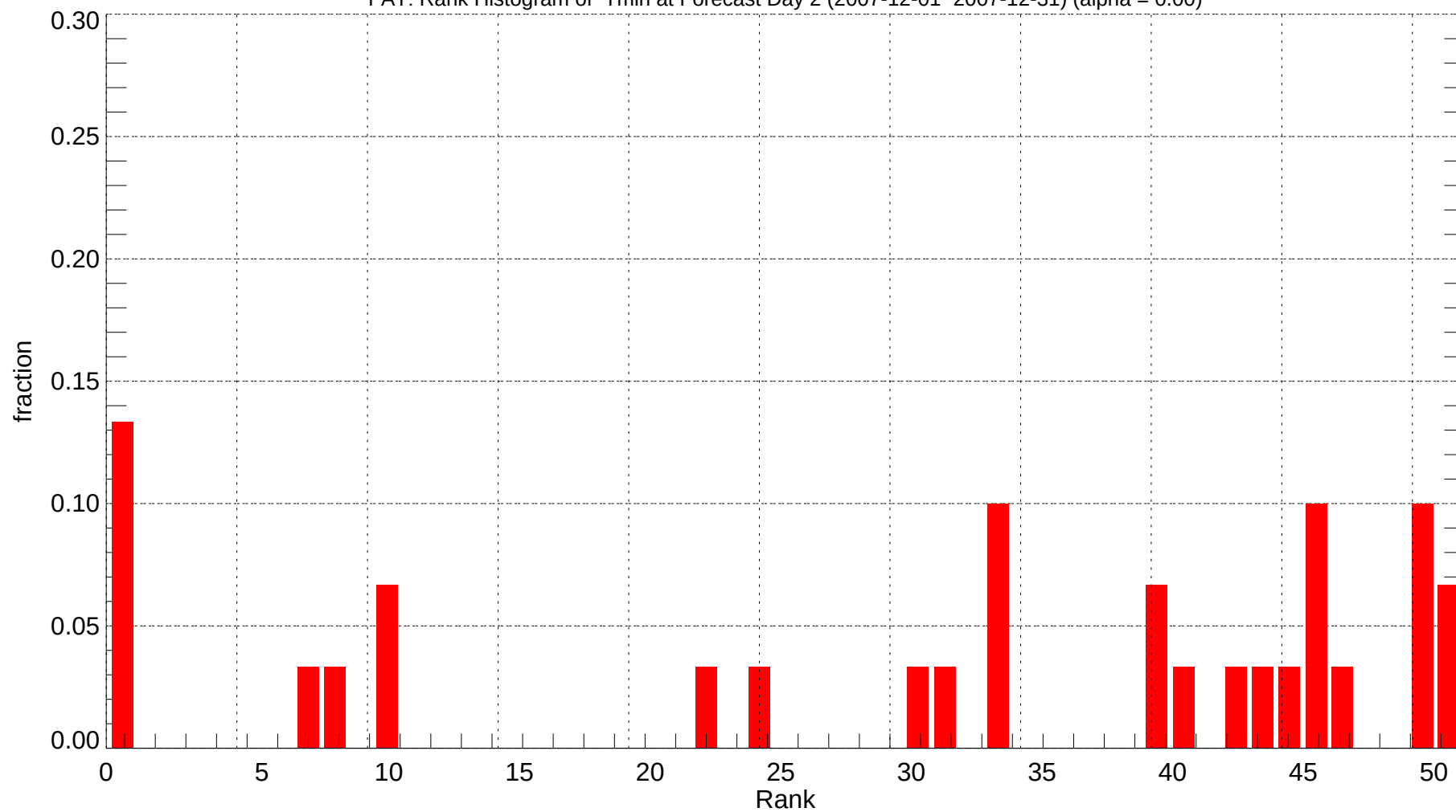
FAT: Rank Histogram of Tmin at Forecast Day 2 (2007-12-01~2007-12-31) (alpha = 0.00)
