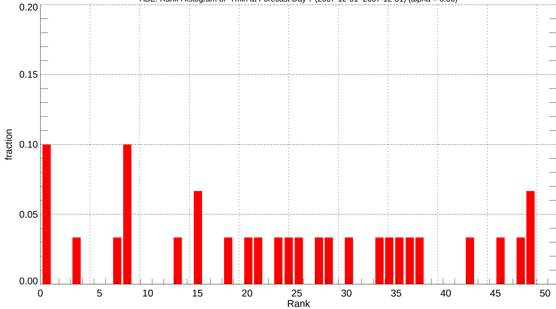
ABE: Rank Histogram of Tmin at Forecast Day 7 (2007-12-01~2007-12-31) (alpha = 0.00)
