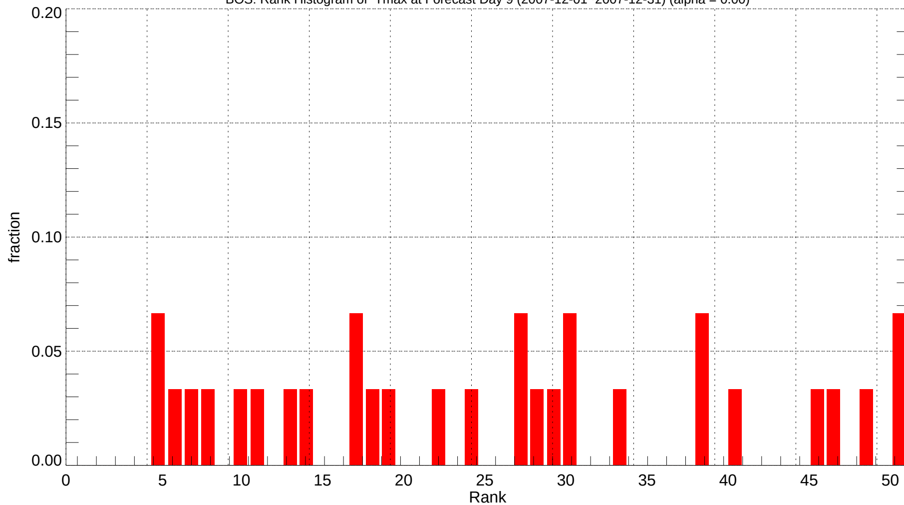
BOS: Rank Histogram of Tmax at Forecast Day 9 (2007-12-01~2007-12-31) (alpha = 0.00)
