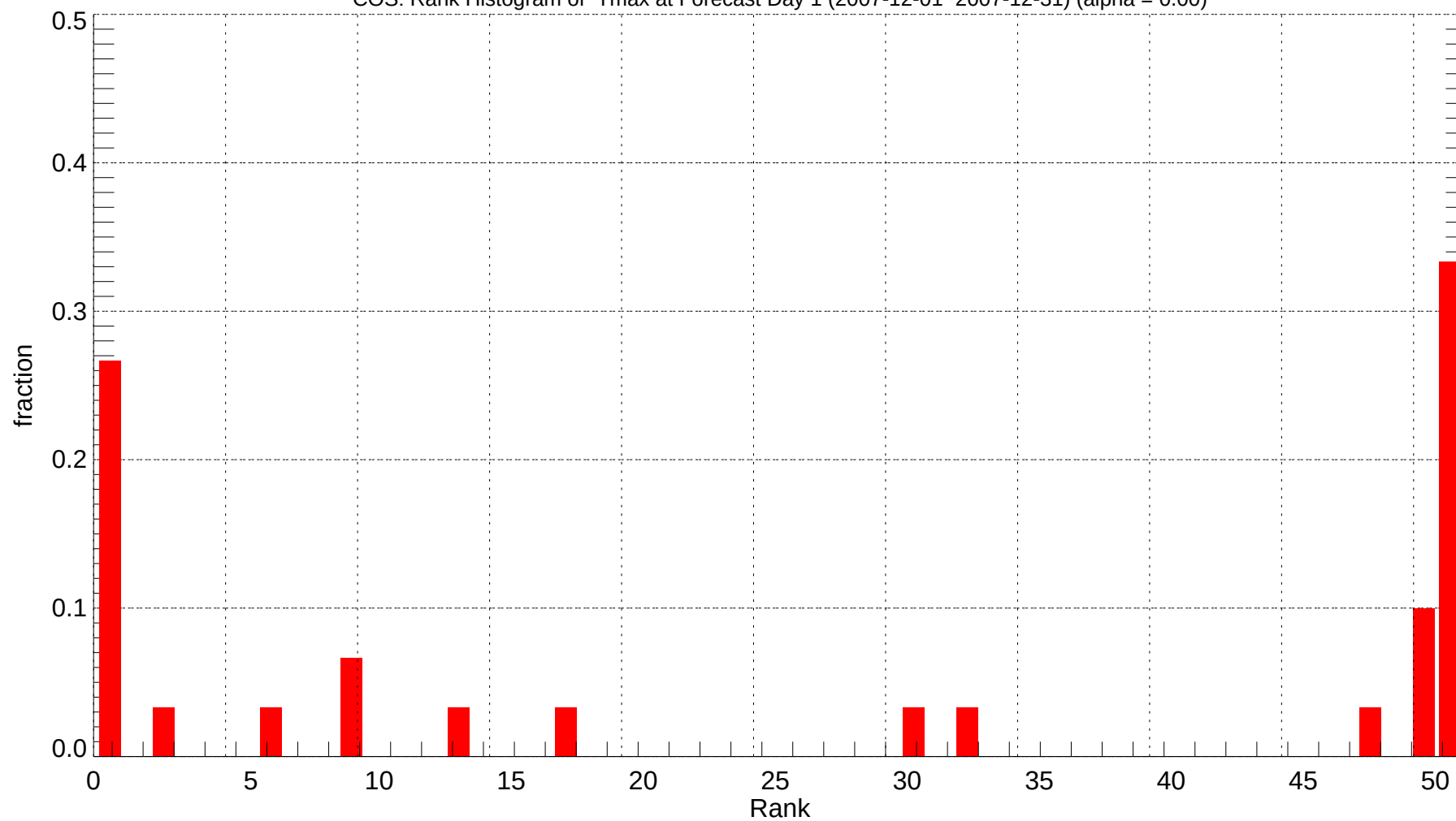
COS: Rank Histogram of Tmax at Forecast Day 1 (2007-12-01~2007-12-31) (alpha = 0.00)
