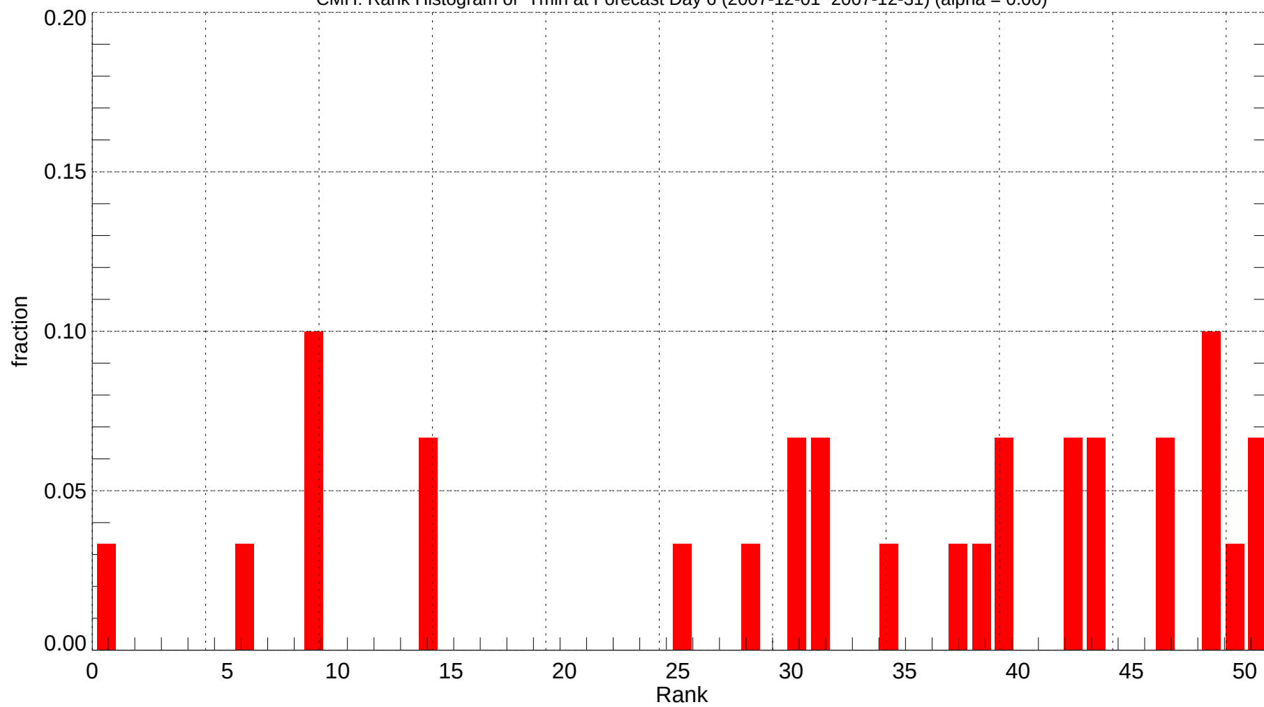
CMH: Rank Histogram of Tmin at Forecast Day 6 (2007-12-01~2007-12-31) (alpha = 0.00)
