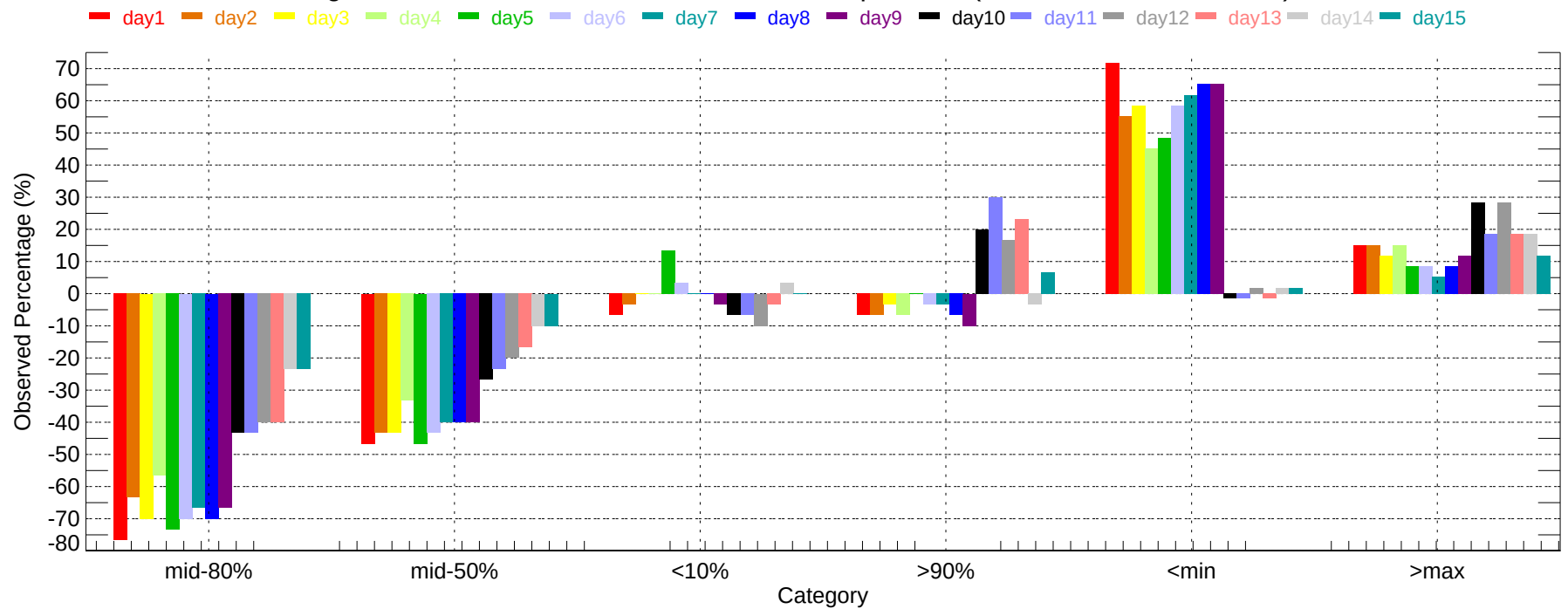
Observed Percentage Deviation of Ensembles - LAX: Min Temperature (2007-12-01~2007-12-31)
