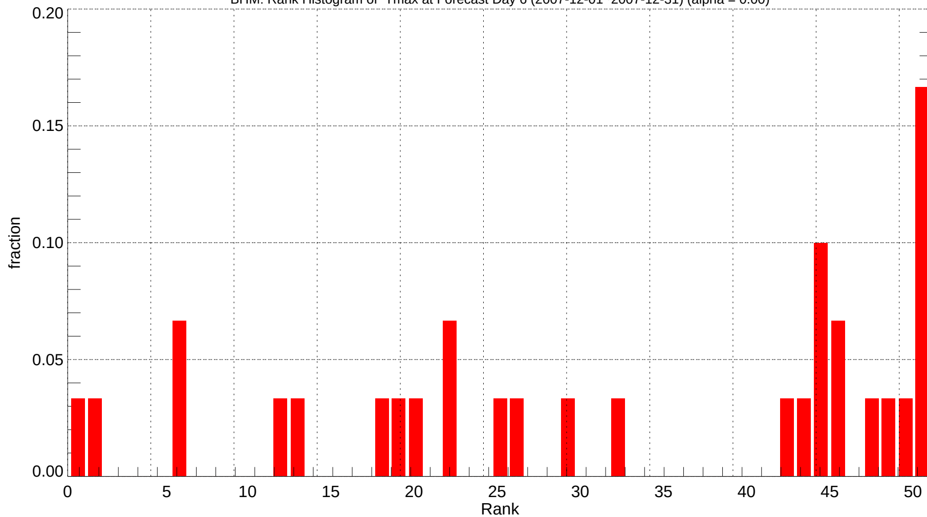
BHM: Rank Histogram of Tmax at Forecast Day 6 (2007-12-01~2007-12-31) (alpha = 0.00)
