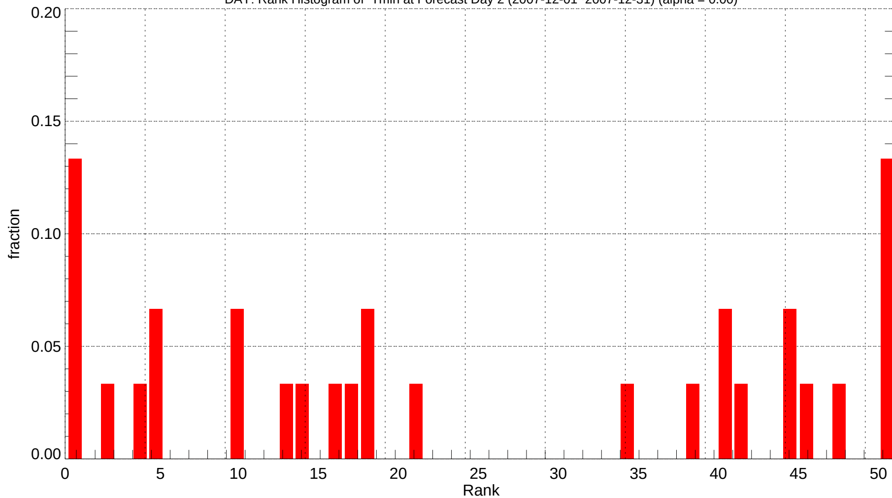
DAY: Rank Histogram of Tmin at Forecast Day 2 (2007-12-01~2007-12-31) (alpha = 0.00)
