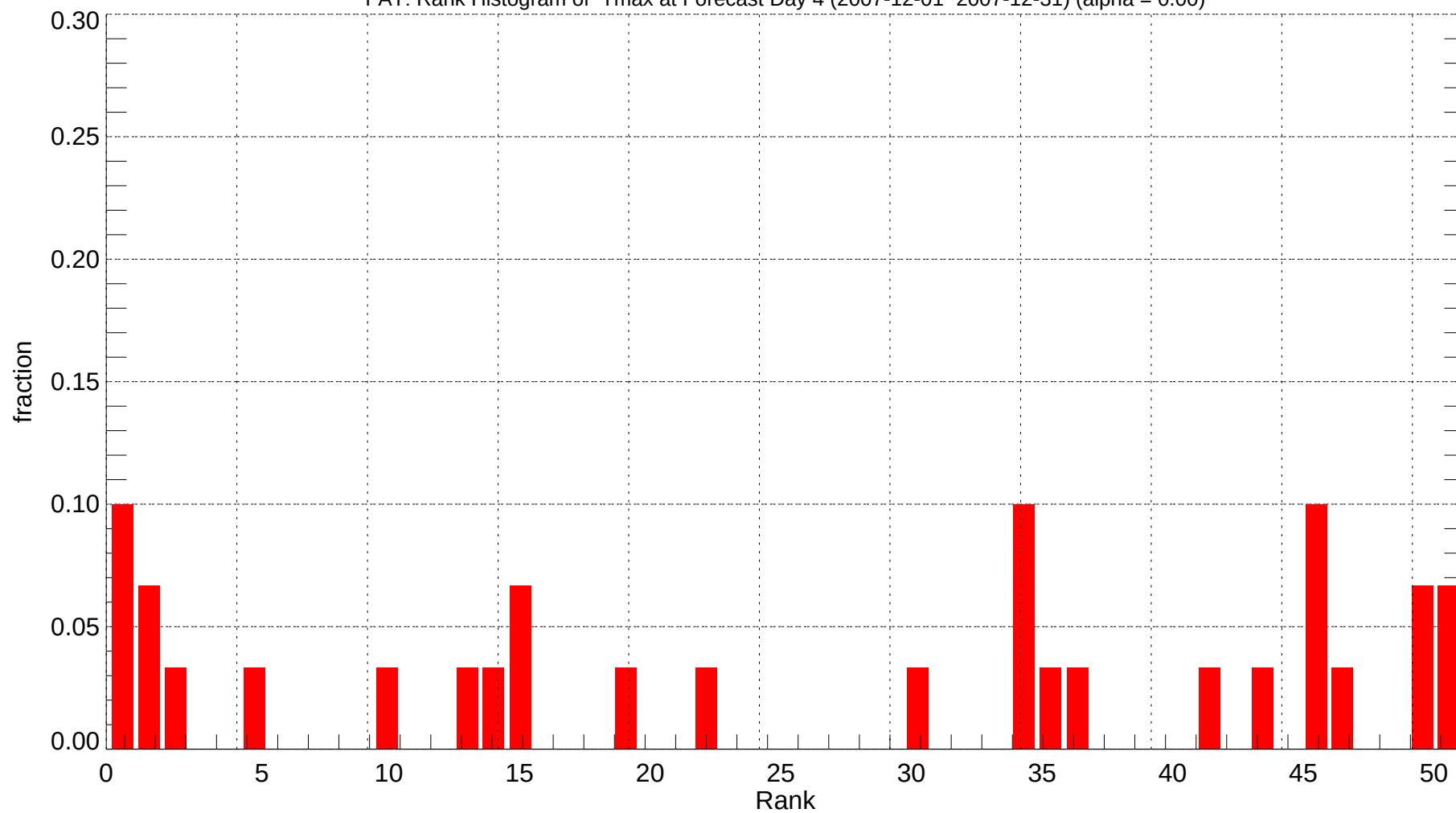
FAT: Rank Histogram of Tmax at Forecast Day 4 (2007-12-01~2007-12-31) (alpha = 0.00)
