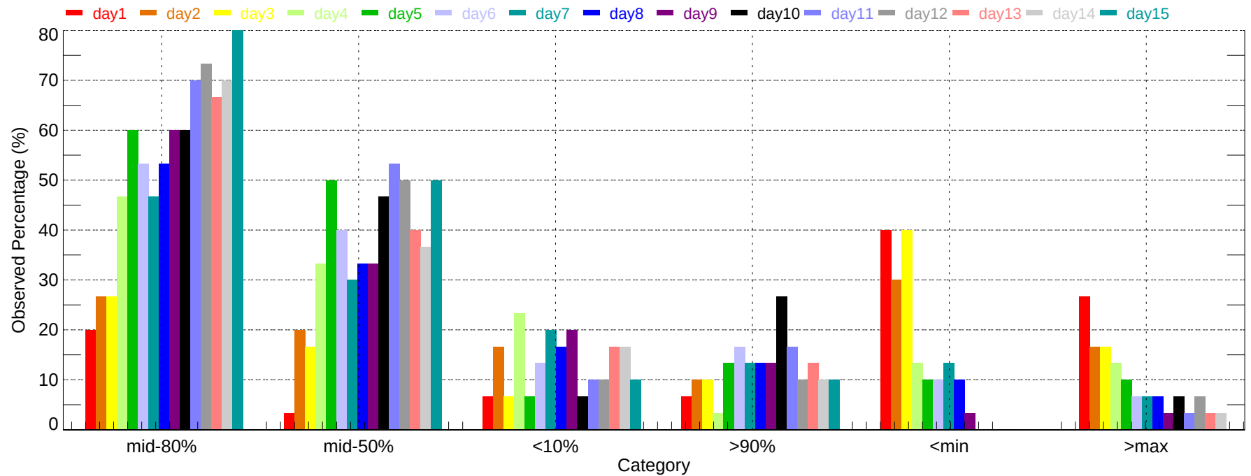
Observed Percentage of Ensembles - RAP: Max Temperature (2007-12-01~2007-12-31)
