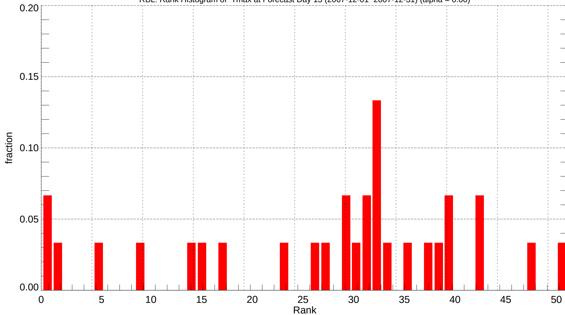
RBL: Rank Histogram of Tmax at Forecast Day 13 (2007-12-01~2007-12-31) (alpha = 0.00)
