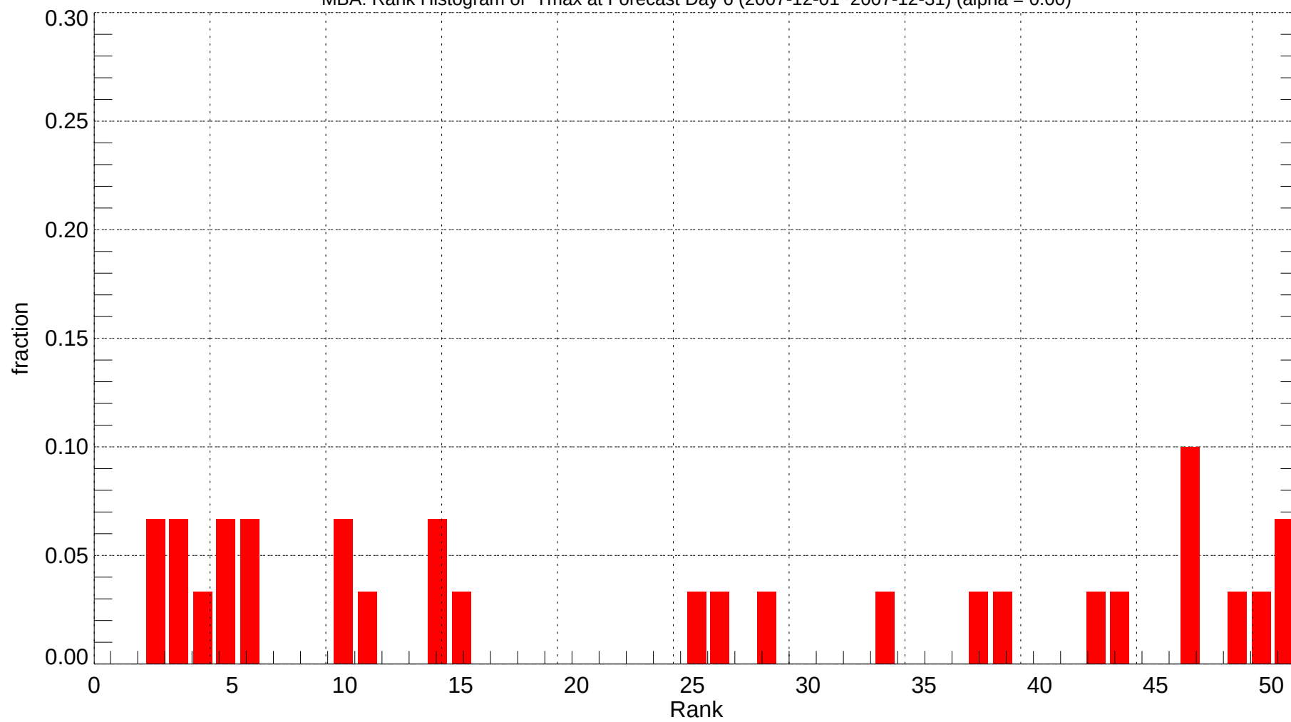
MBA: Rank Histogram of Tmax at Forecast Day 6 (2007-12-01~2007-12-31) (alpha = 0.00)
