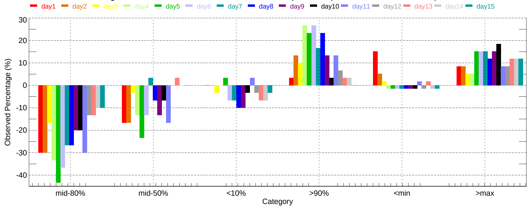
Observed Percentage Deviation of Ensembles - CAE: Min Temperature (2007-12-01~2007-12-31)
