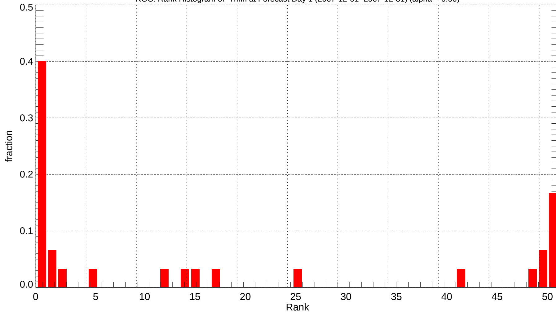
ROC: Rank Histogram of Tmin at Forecast Day 1 (2007-12-01~2007-12-31) (alpha = 0.00)
