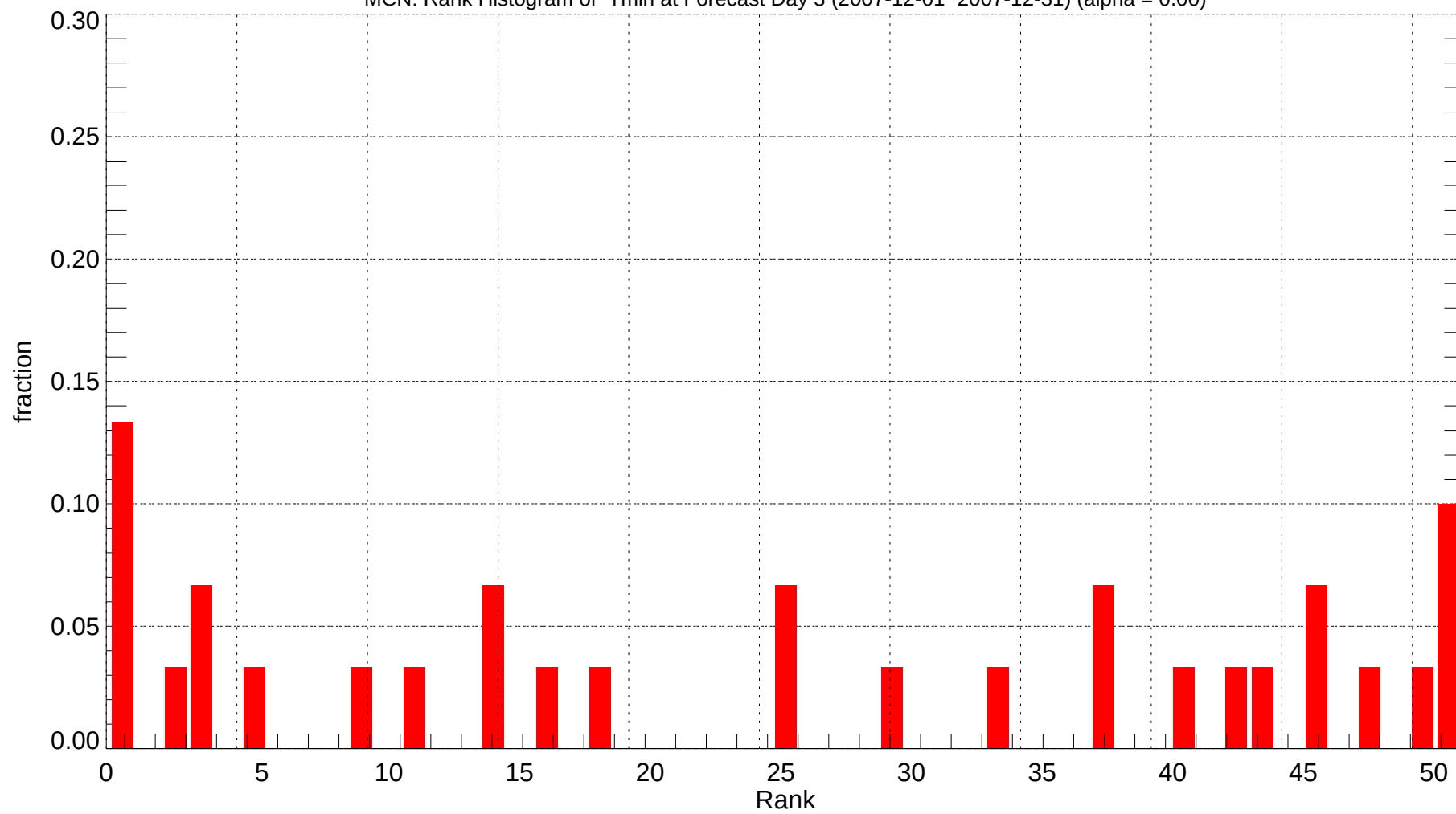
MCN: Rank Histogram of Tmin at Forecast Day 3 (2007-12-01~2007-12-31) (alpha = 0.00)
