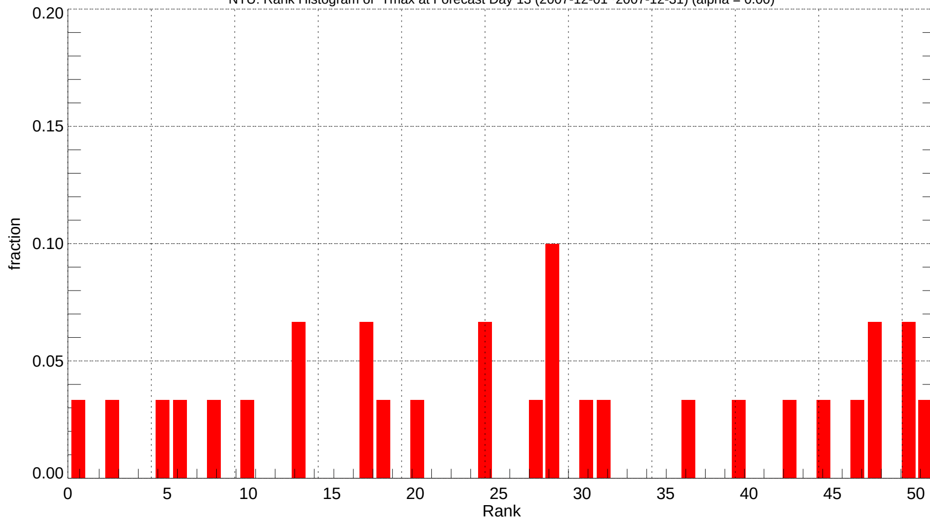
NTU: Rank Histogram of Tmax at Forecast Day 13 (2007-12-01~2007-12-31) (alpha = 0.00)
