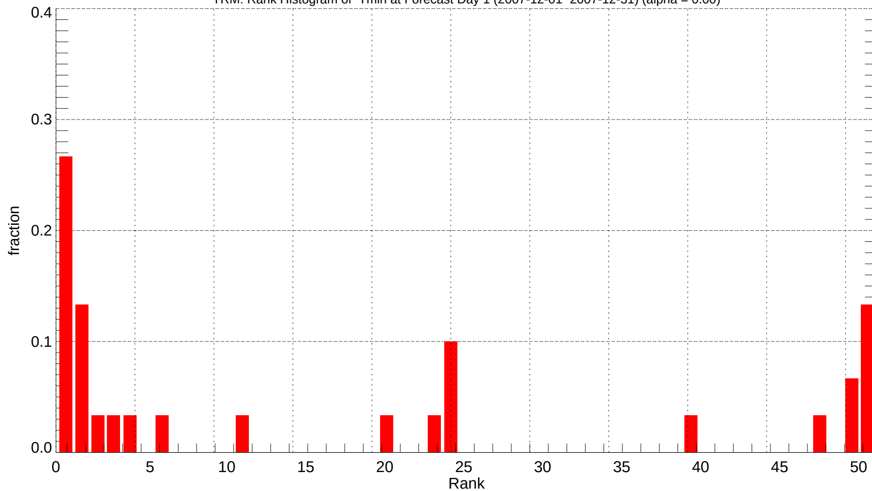
TRM: Rank Histogram of Tmin at Forecast Day 1 (2007-12-01~2007-12-31) (alpha = 0.00)
