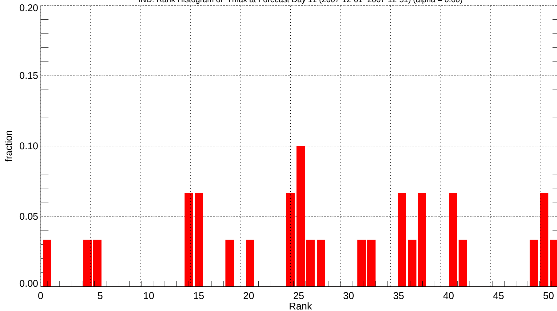
IND: Rank Histogram of Tmax at Forecast Day 11 (2007-12-01~2007-12-31) (alpha = 0.00)
