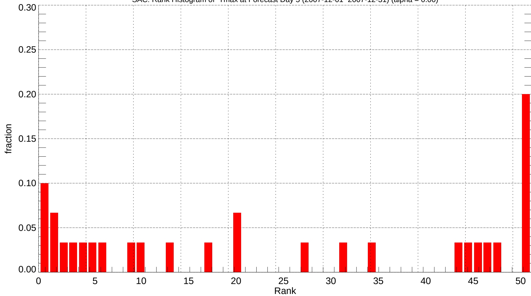
SAC: Rank Histogram of Tmax at Forecast Day 5 (2007-12-01~2007-12-31) (alpha = 0.00)
