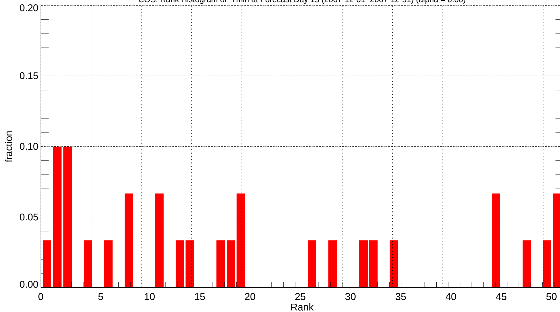
COS: Rank Histogram of Tmin at Forecast Day 13 (2007-12-01~2007-12-31) (alpha = 0.00)
