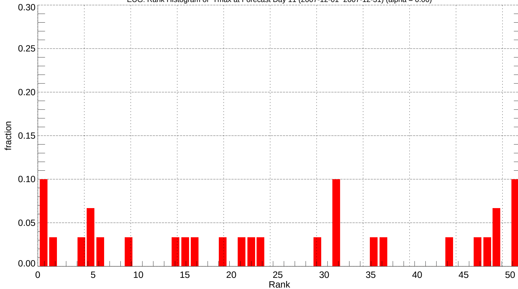
EUG: Rank Histogram of Tmax at Forecast Day 11 (2007-12-01~2007-12-31) (alpha = 0.00)
