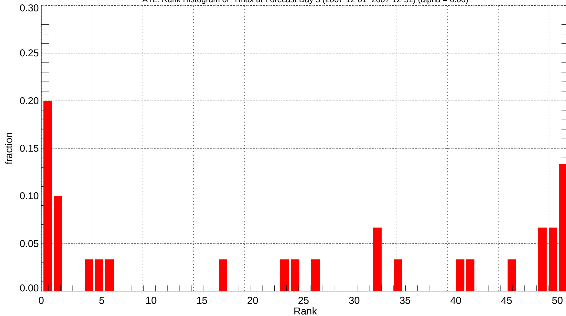
ATL: Rank Histogram of Tmax at Forecast Day 3 (2007-12-01~2007-12-31) (alpha = 0.00)
