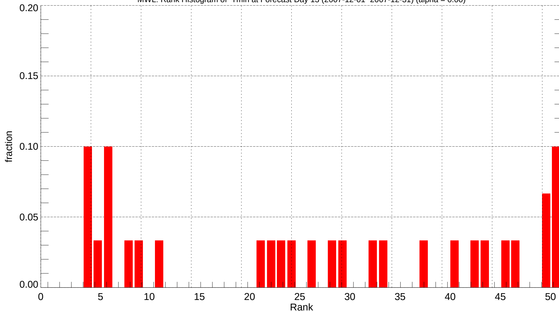
MWL: Rank Histogram of Tmin at Forecast Day 13 (2007-12-01~2007-12-31) (alpha = 0.00)
