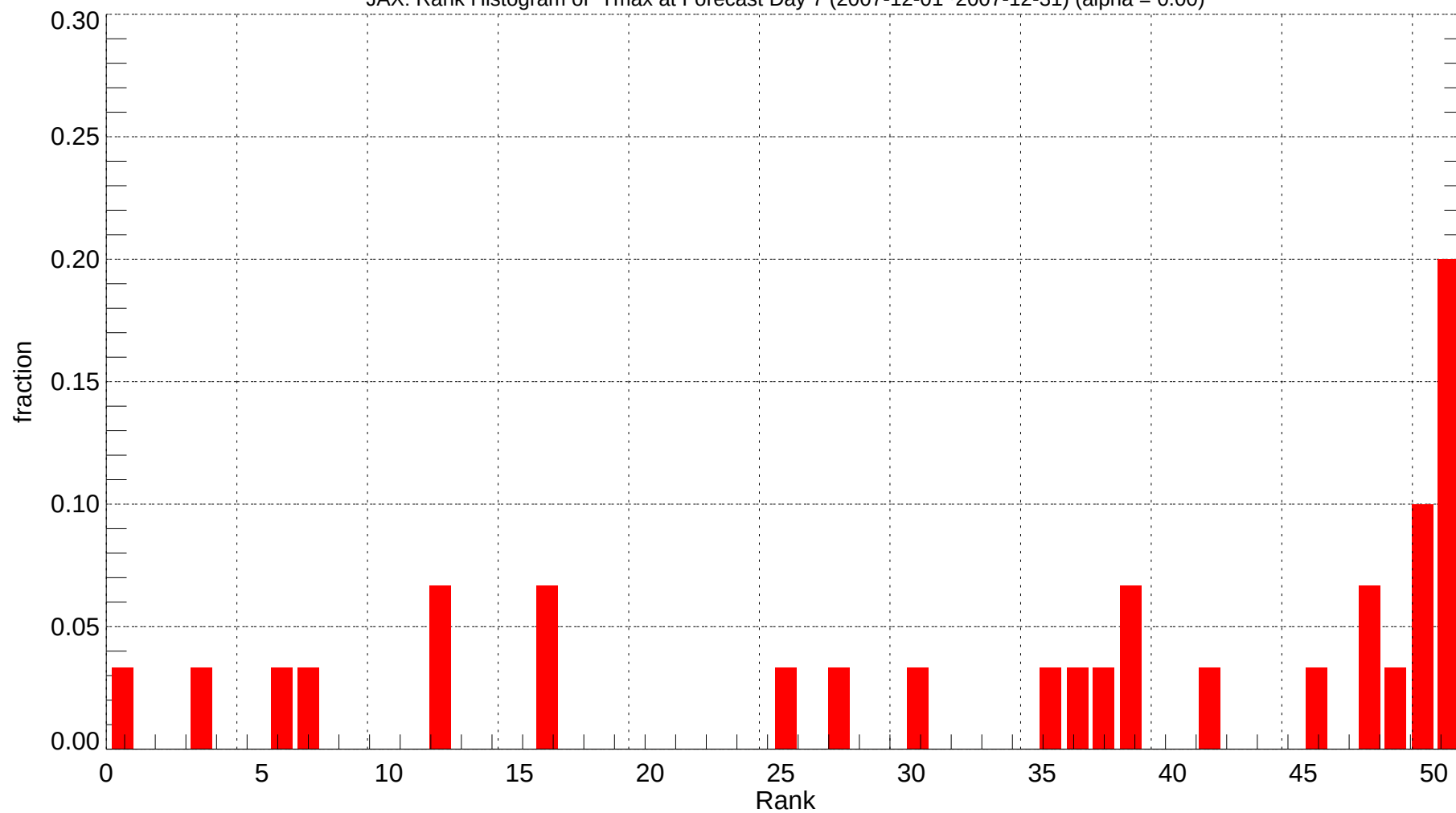
JAX: Rank Histogram of Tmax at Forecast Day 7 (2007-12-01~2007-12-31) (alpha = 0.00)
