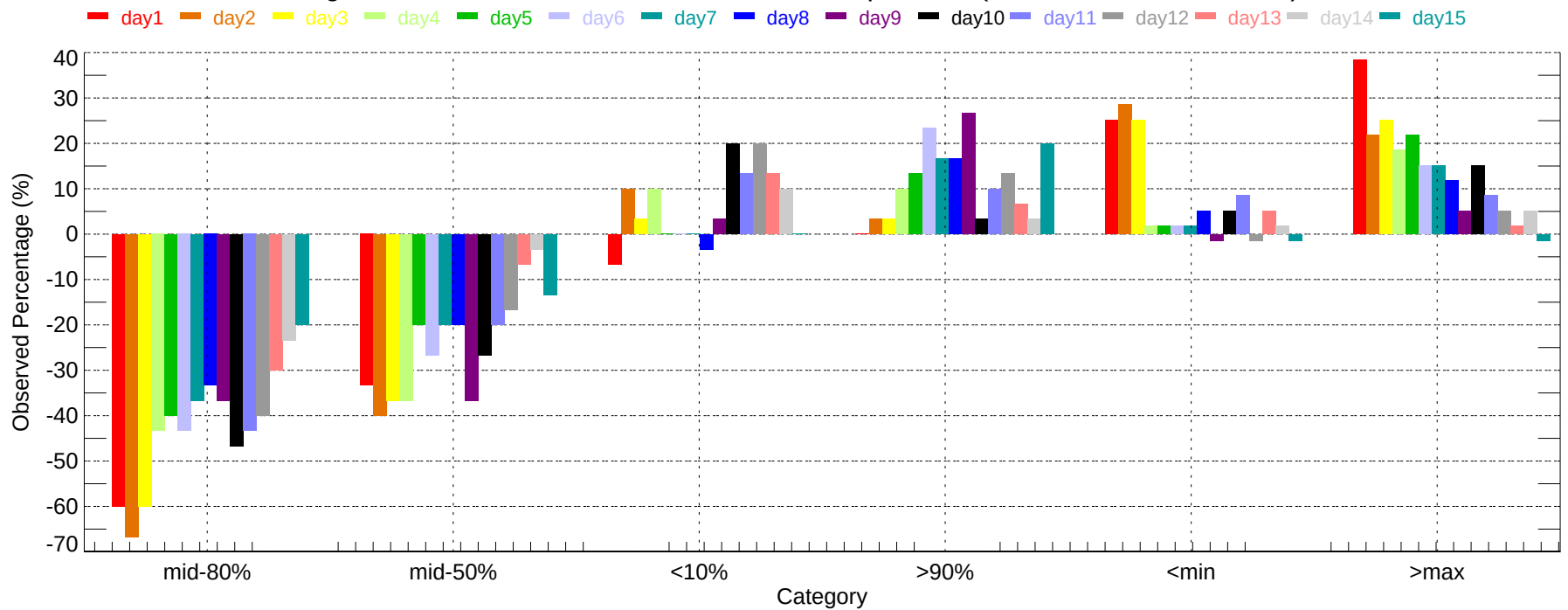
Observed Percentage Deviation of Ensembles - OKC: Min Temperature (2007-12-01~2007-12-31)
