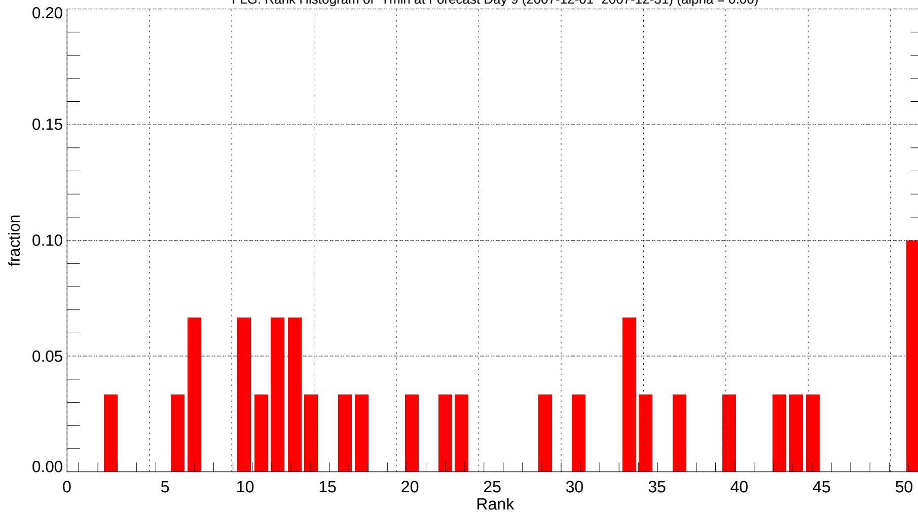
FLG: Rank Histogram of Tmin at Forecast Day 9 (2007-12-01~2007-12-31) (alpha = 0.00)
