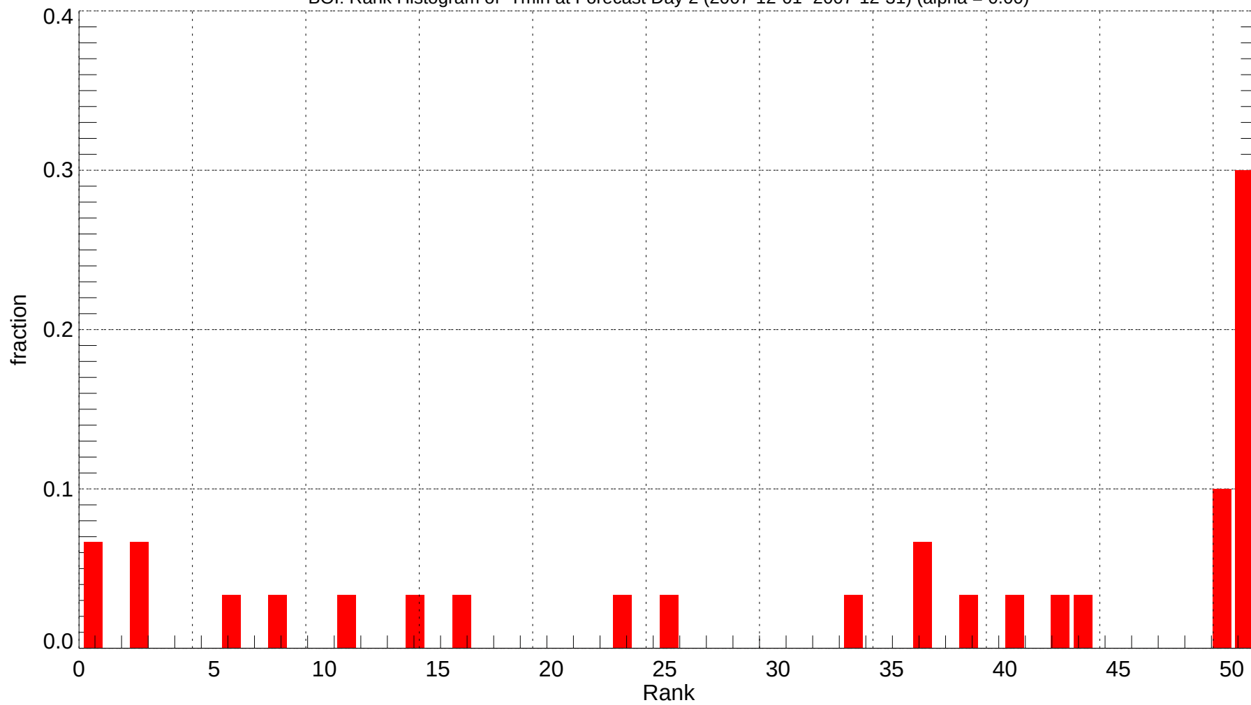
BOI: Rank Histogram of Tmin at Forecast Day 2 (2007-12-01~2007-12-31) (alpha = 0.00)
