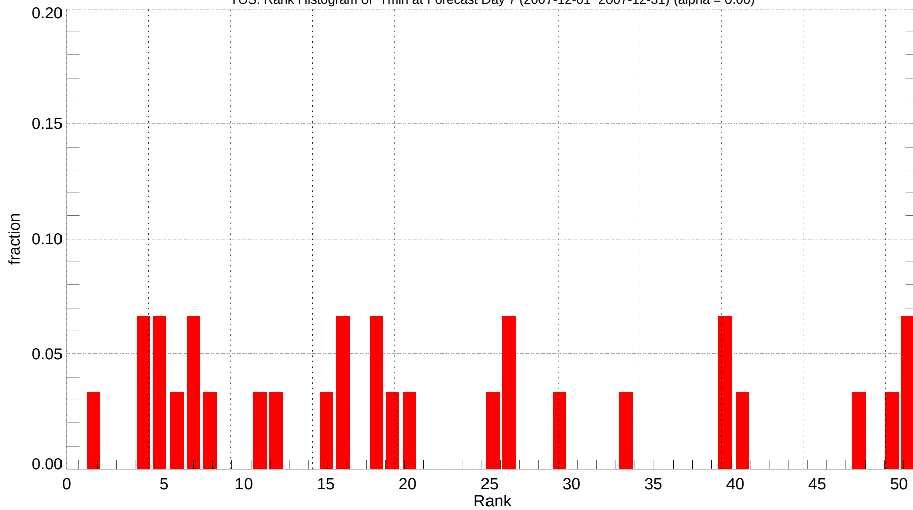
TUS: Rank Histogram of Tmin at Forecast Day 7 (2007-12-01~2007-12-31) (alpha = 0.00)
