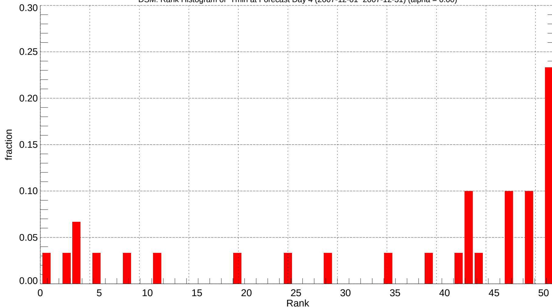
DSM: Rank Histogram of Tmin at Forecast Day 4 (2007-12-01~2007-12-31) (alpha = 0.00)
