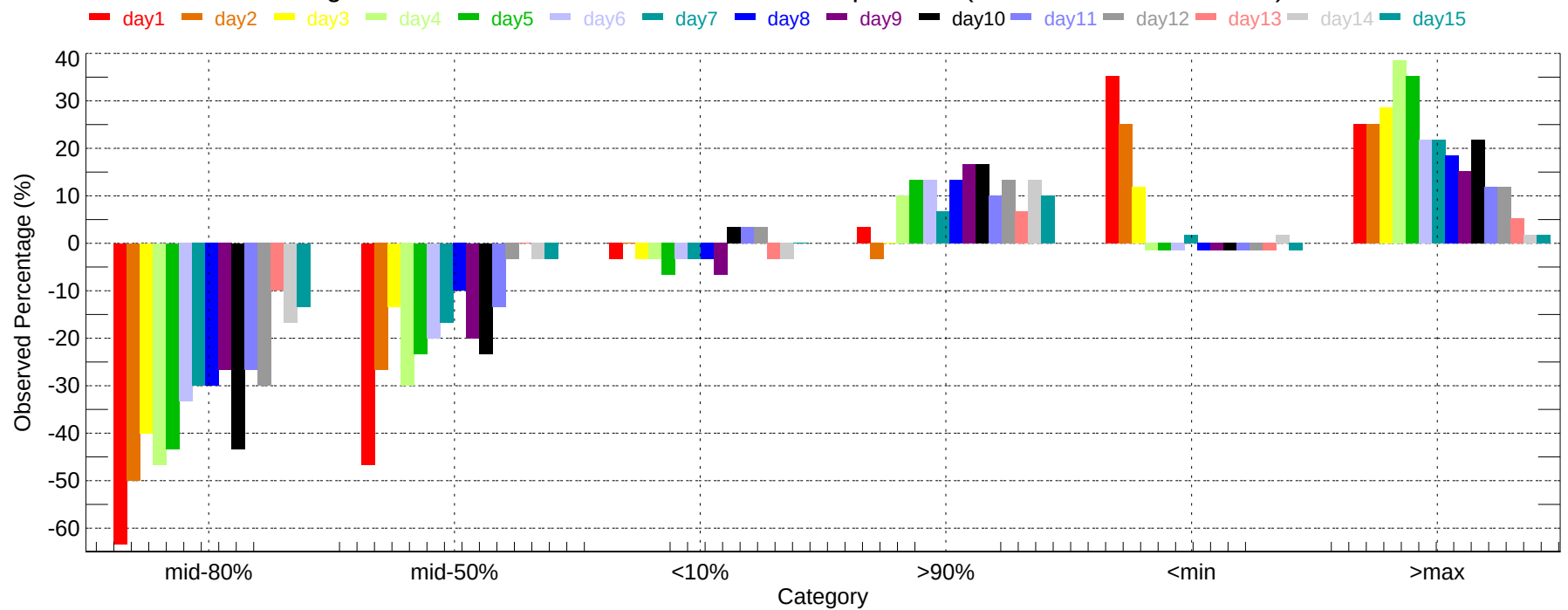
Observed Percentage Deviation of Ensembles - ICT: Min Temperature (2007-12-01~2007-12-31)
