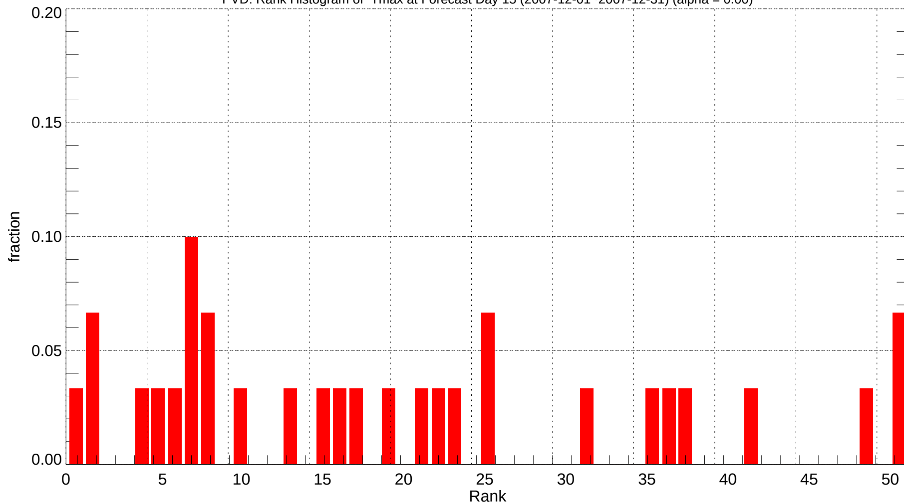
PVD: Rank Histogram of Tmax at Forecast Day 15 (2007-12-01~2007-12-31) (alpha = 0.00)
