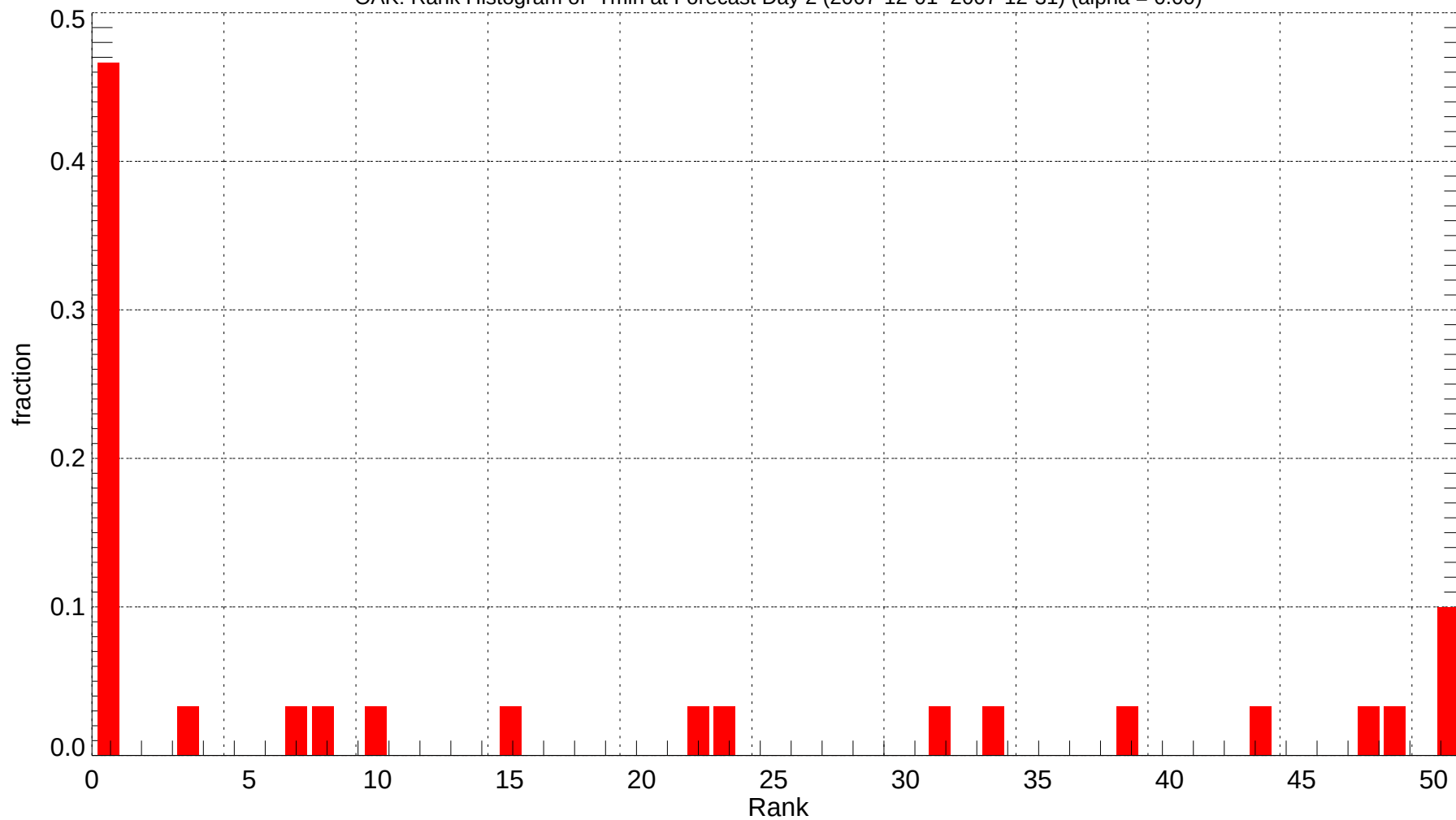
OAK: Rank Histogram of Tmin at Forecast Day 2 (2007-12-01~2007-12-31) (alpha = 0.00)
