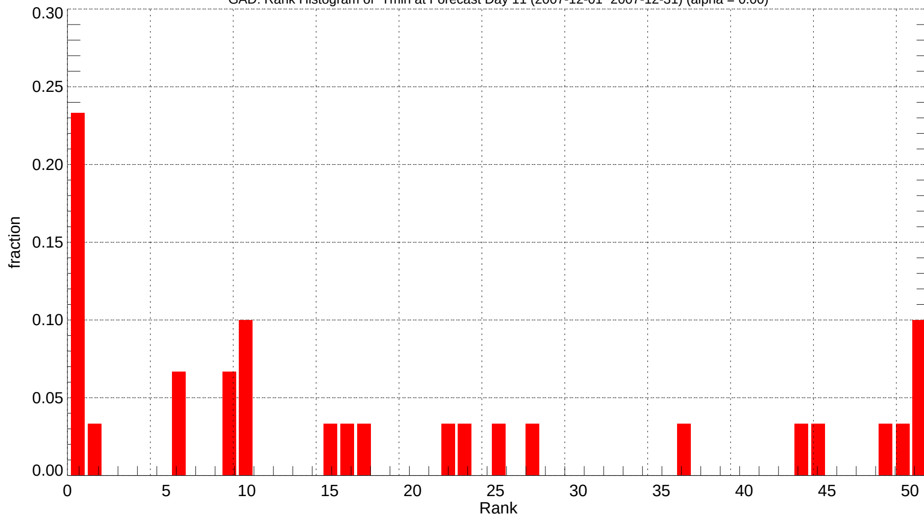
GAD: Rank Histogram of Tmin at Forecast Day 11 (2007-12-01~2007-12-31) (alpha = 0.00)
