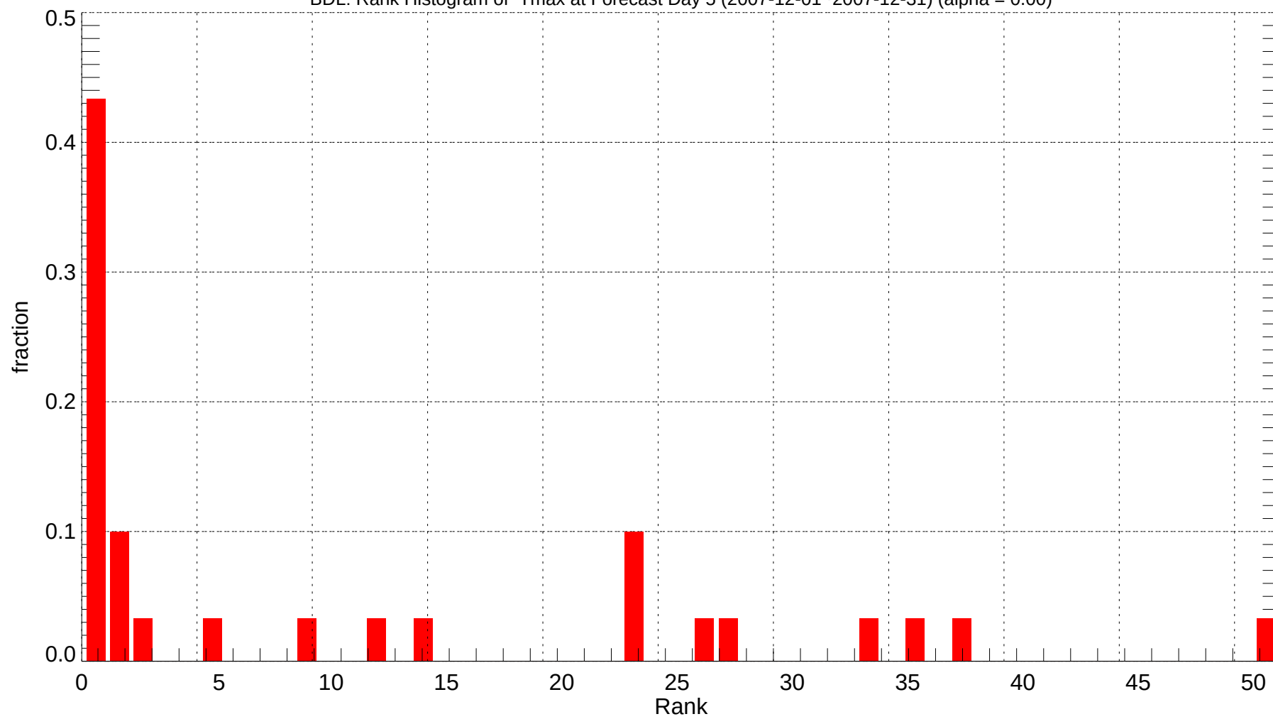
BDL: Rank Histogram of Tmax at Forecast Day 5 (2007-12-01~2007-12-31) (alpha = 0.00)
