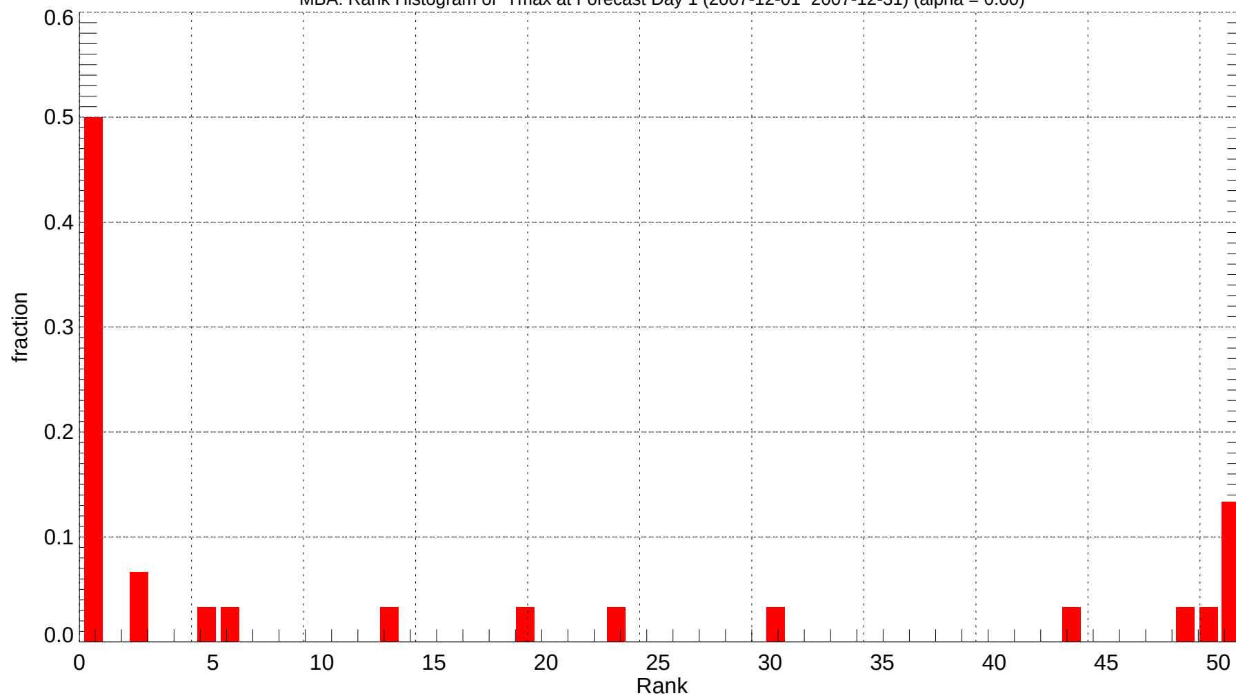
MBA: Rank Histogram of Tmax at Forecast Day 1 (2007-12-01~2007-12-31) (alpha = 0.00)
