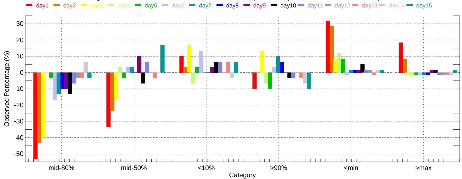
Observed Percentage Deviation of Ensembles - ALB: Min Temperature (2007-12-01~2007-12-31)
