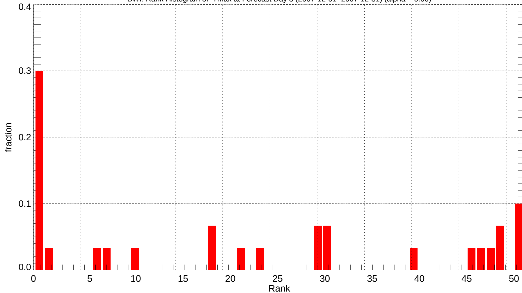
BWI: Rank Histogram of Tmax at Forecast Day 3 (2007-12-01~2007-12-31) (alpha = 0.00)
