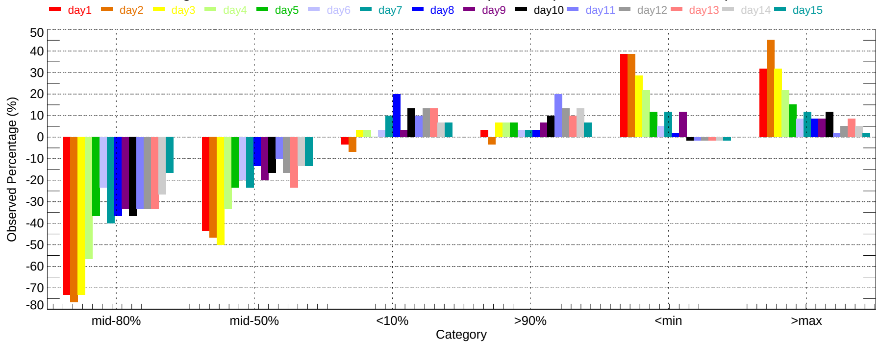
Observed Percentage Deviation of Ensembles - RNO: Min Temperature (2007-12-01~2007-12-31)
