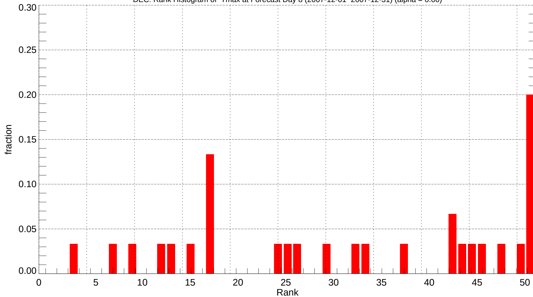
DEC: Rank Histogram of Tmax at Forecast Day 8 (2007-12-01~2007-12-31) (alpha = 0.00)
