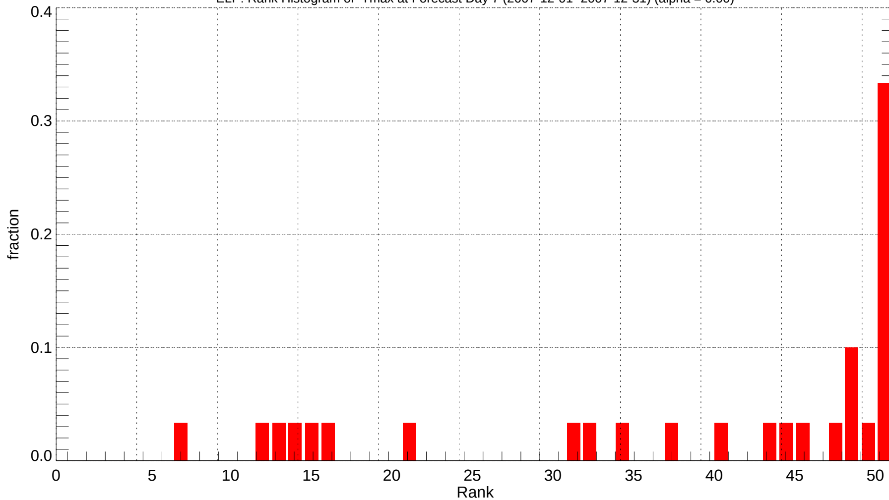
ELP: Rank Histogram of Tmax at Forecast Day 7 (2007-12-01~2007-12-31) (alpha = 0.00)
