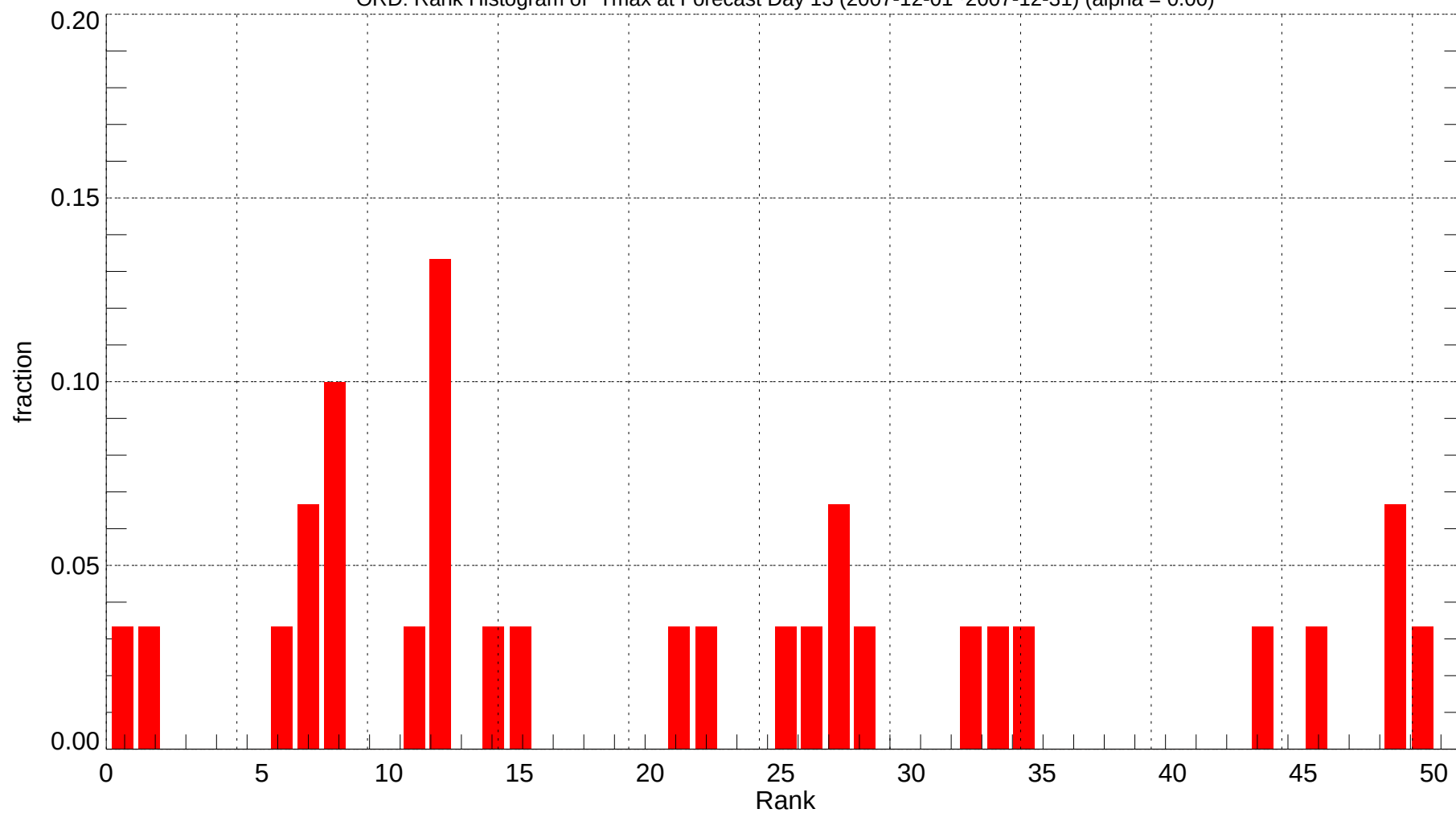
ORD: Rank Histogram of Tmax at Forecast Day 13 (2007-12-01~2007-12-31) (alpha = 0.00)
