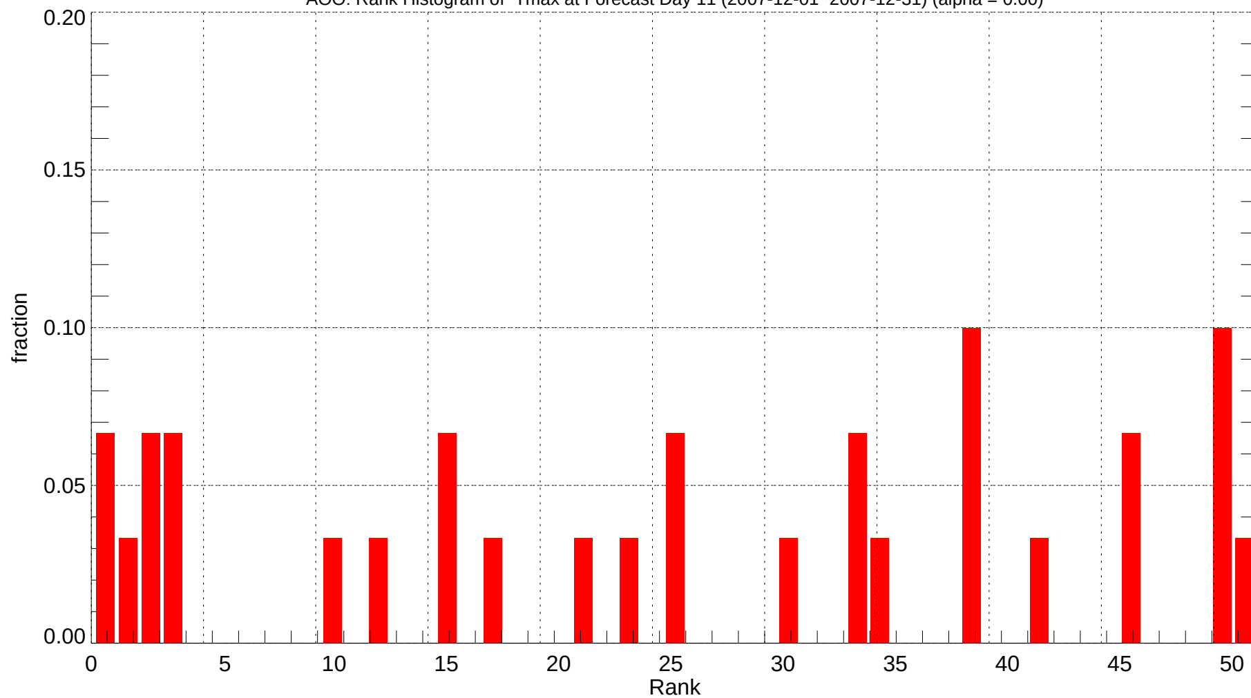
AOO: Rank Histogram of Tmax at Forecast Day 11 (2007-12-01~2007-12-31) (alpha = 0.00)
