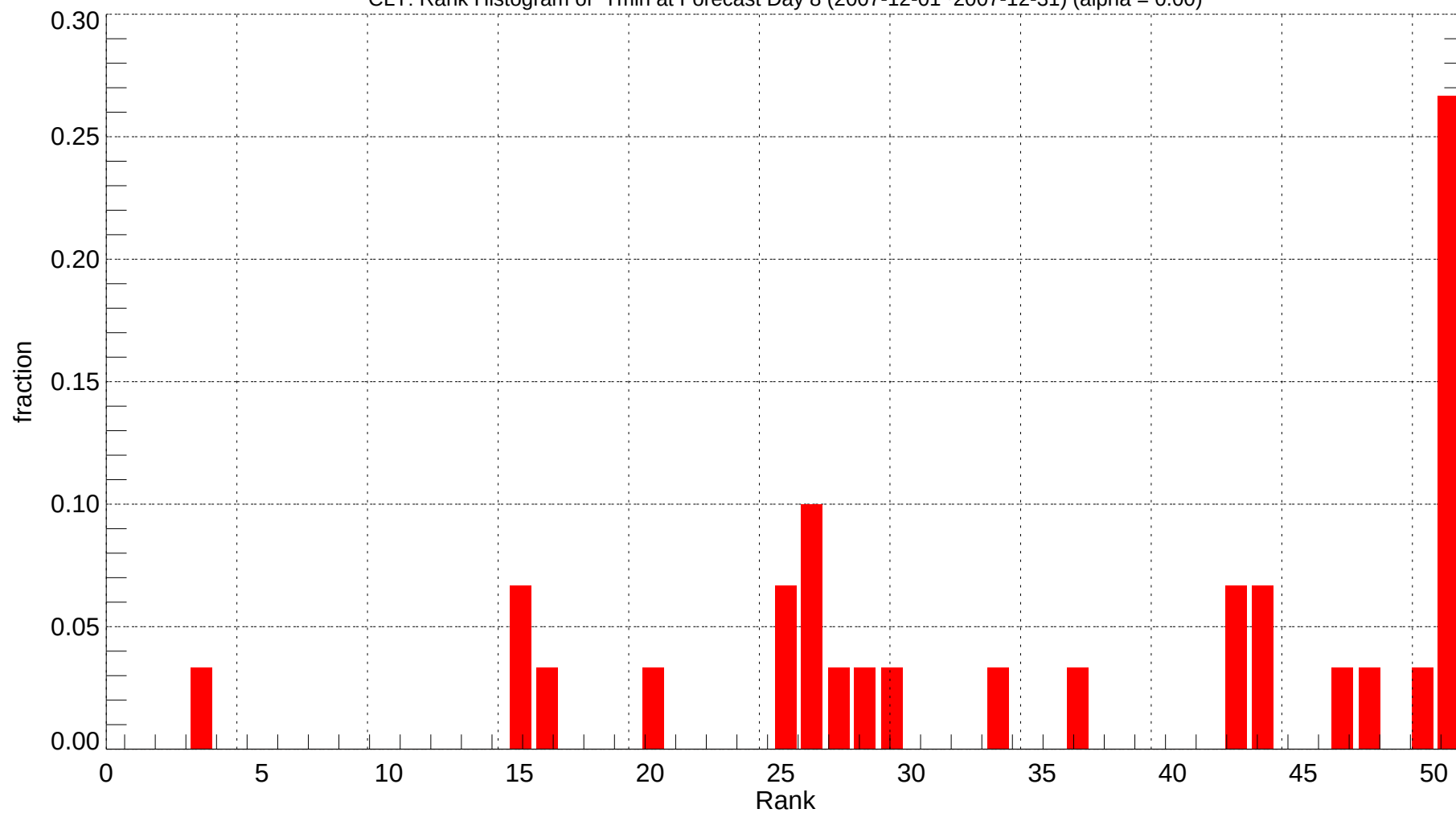
CLT: Rank Histogram of Tmin at Forecast Day 8 (2007-12-01~2007-12-31) (alpha = 0.00)
