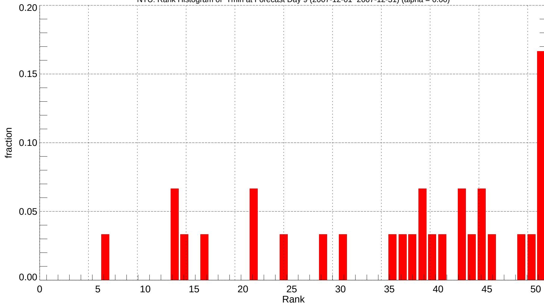
NTU: Rank Histogram of Tmin at Forecast Day 9 (2007-12-01~2007-12-31) (alpha = 0.00)
