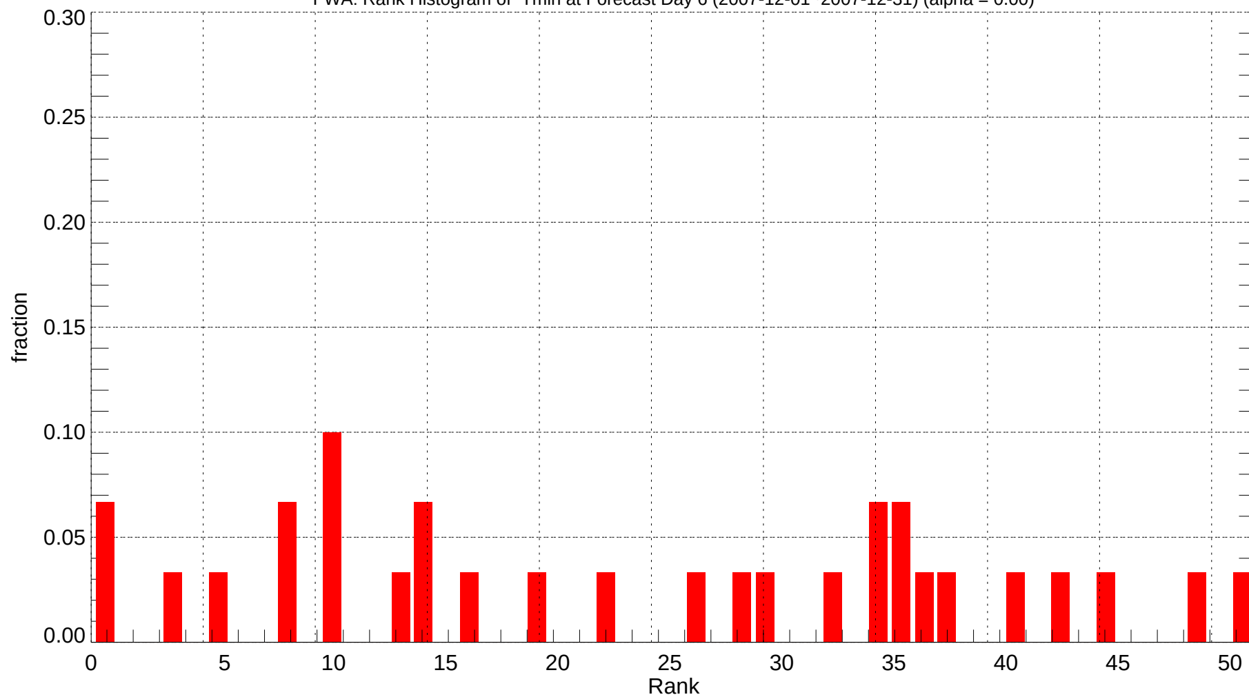
FWA: Rank Histogram of Tmin at Forecast Day 6 (2007-12-01~2007-12-31) (alpha = 0.00)
