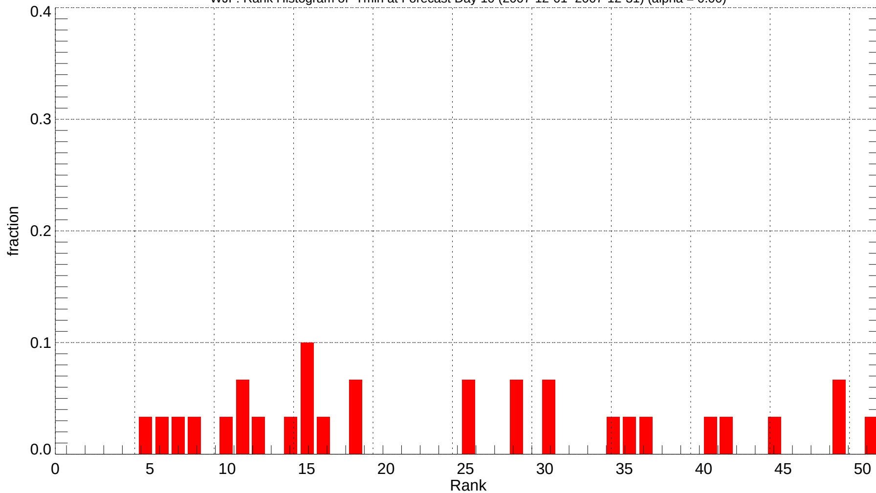
WJF: Rank Histogram of Tmin at Forecast Day 10 (2007-12-01~2007-12-31) (alpha = 0.00)
