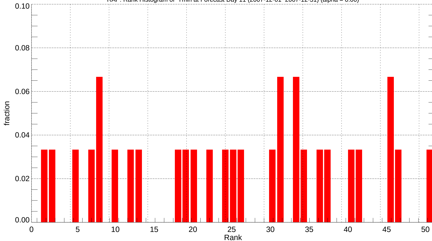
RAP: Rank Histogram of Tmin at Forecast Day 11 (2007-12-01~2007-12-31) (alpha = 0.00)
