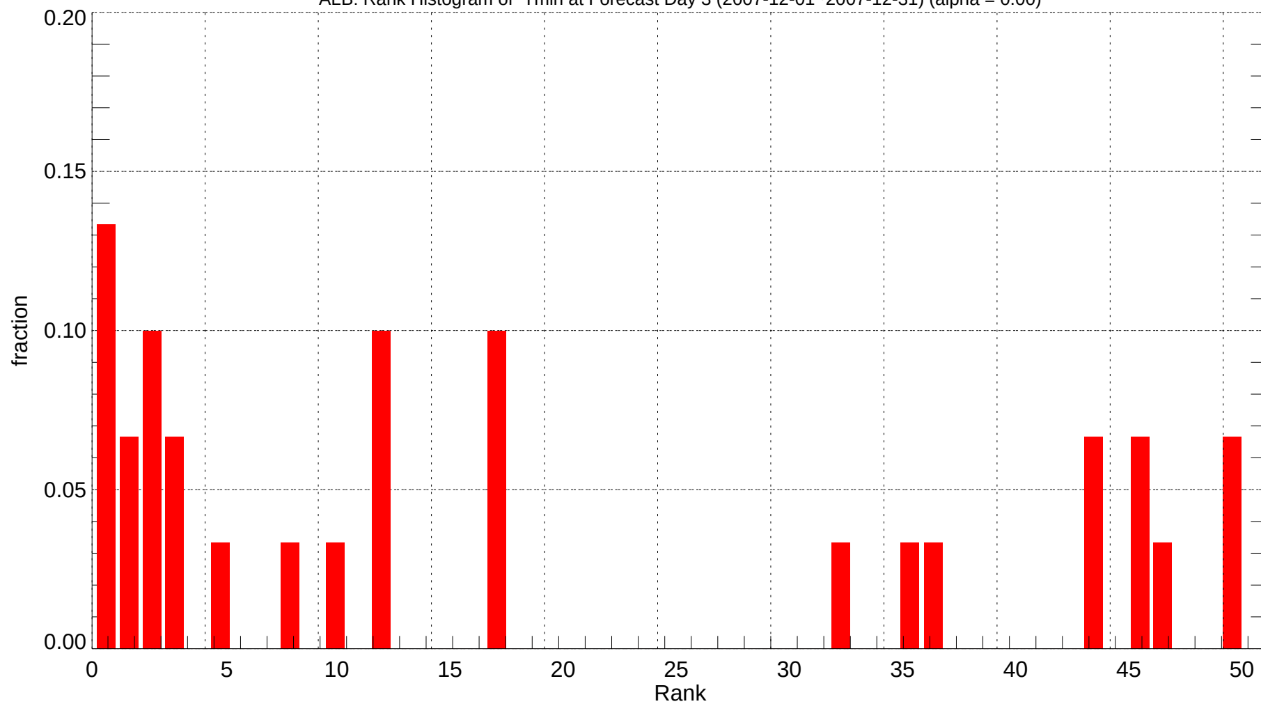
ALB: Rank Histogram of Tmin at Forecast Day 3 (2007-12-01~2007-12-31) (alpha = 0.00)
