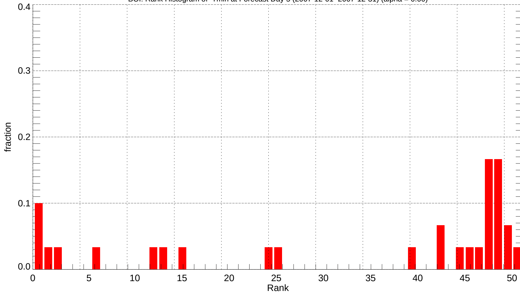
BOI: Rank Histogram of Tmin at Forecast Day 5 (2007-12-01~2007-12-31) (alpha = 0.00)
