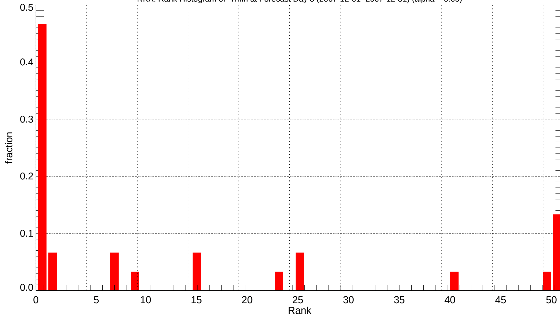
NKX: Rank Histogram of Tmin at Forecast Day 5 (2007-12-01~2007-12-31) (alpha = 0.00)
