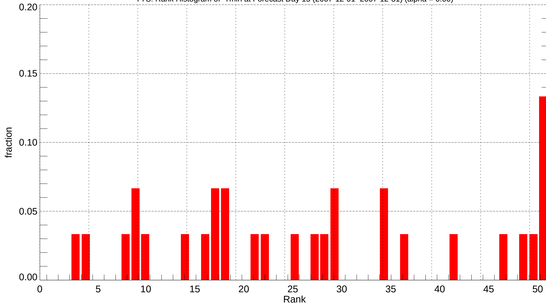
TYS: Rank Histogram of Tmin at Forecast Day 15 (2007-12-01~2007-12-31) (alpha = 0.00)
