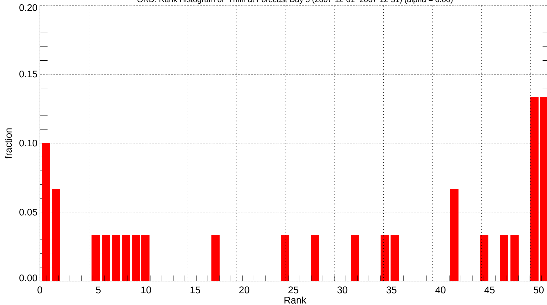
ORD: Rank Histogram of Tmin at Forecast Day 3 (2007-12-01~2007-12-31) (alpha = 0.00)
