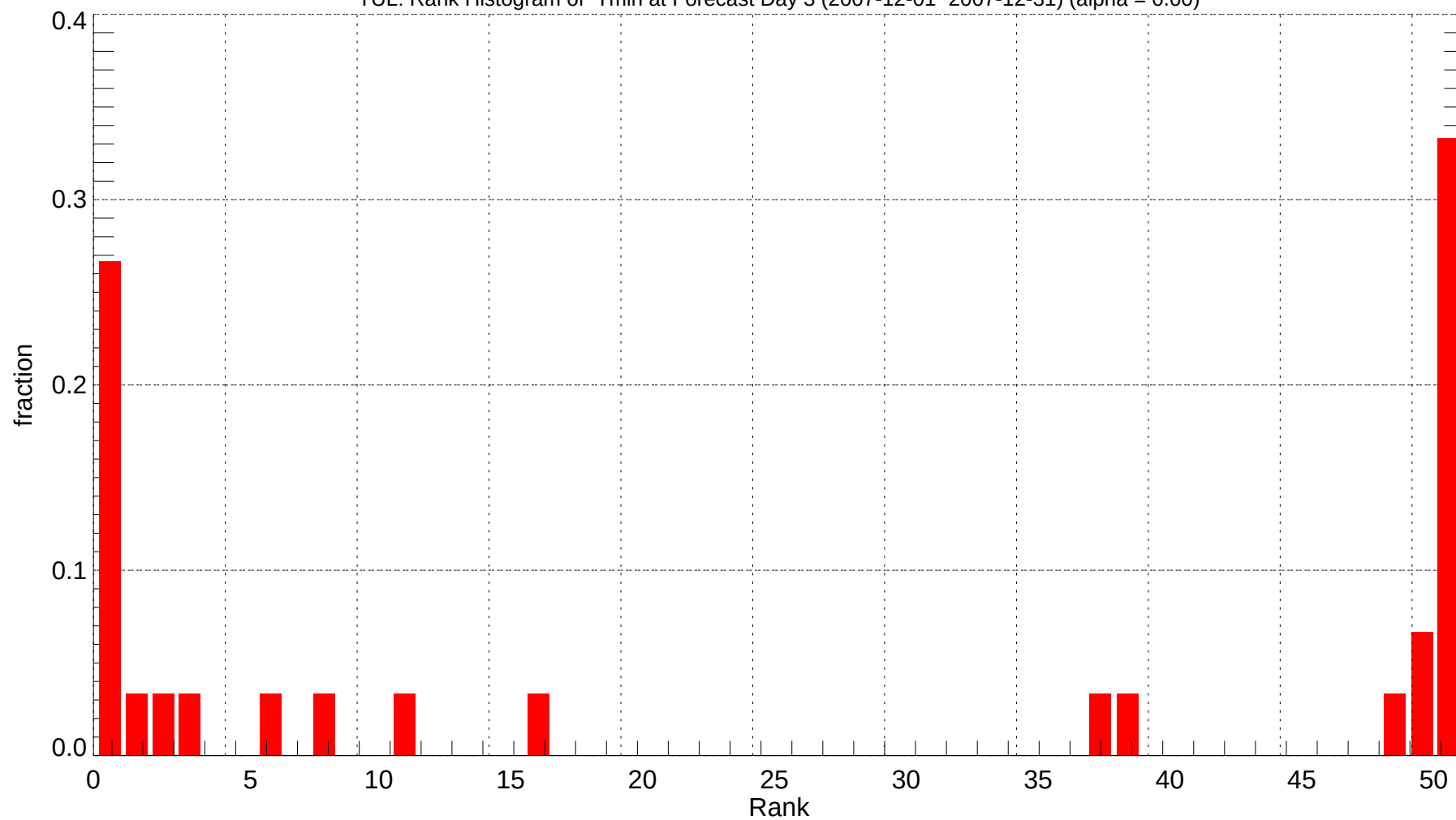
TUL: Rank Histogram of Tmin at Forecast Day 3 (2007-12-01~2007-12-31) (alpha = 0.00)
