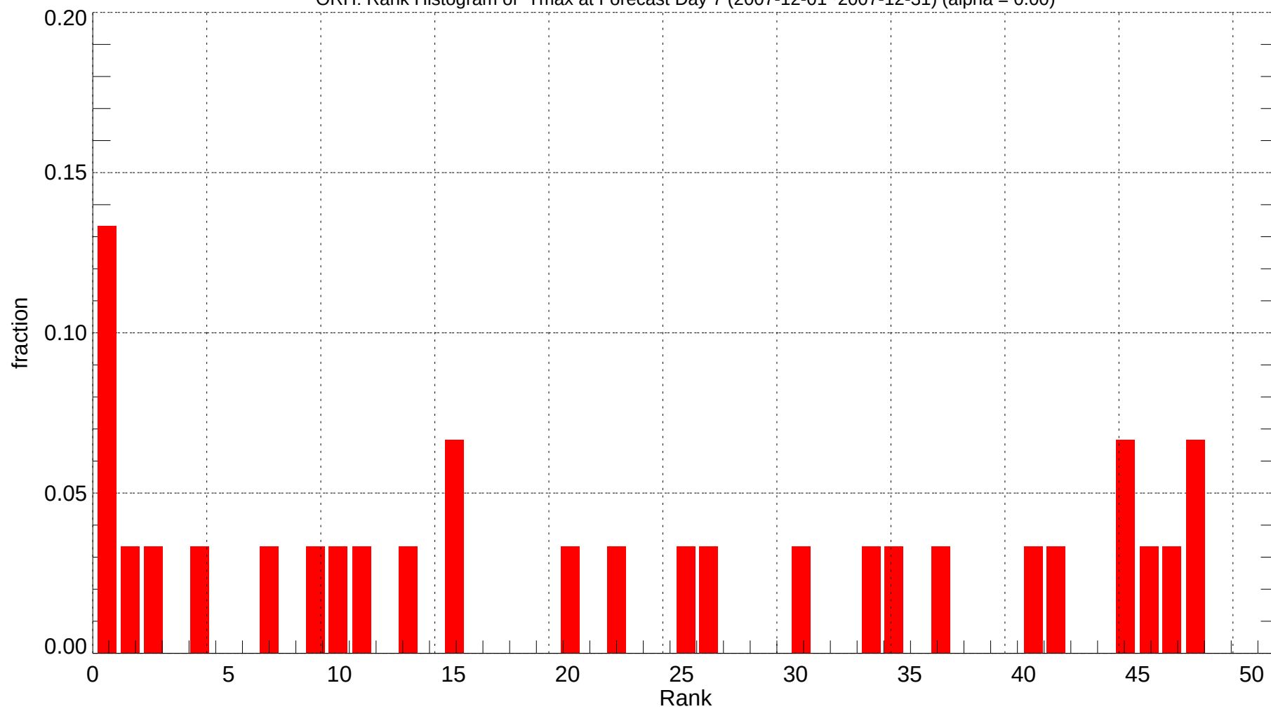
ORH: Rank Histogram of Tmax at Forecast Day 7 (2007-12-01~2007-12-31) (alpha = 0.00)
