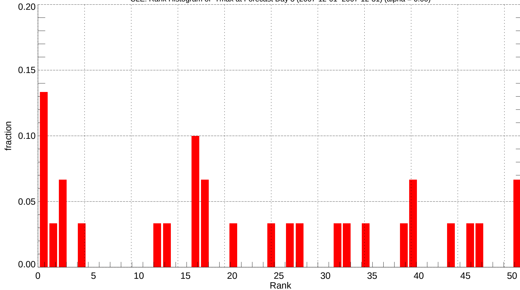
CLE: Rank Histogram of Tmax at Forecast Day 3 (2007-12-01~2007-12-31) (alpha = 0.00)
