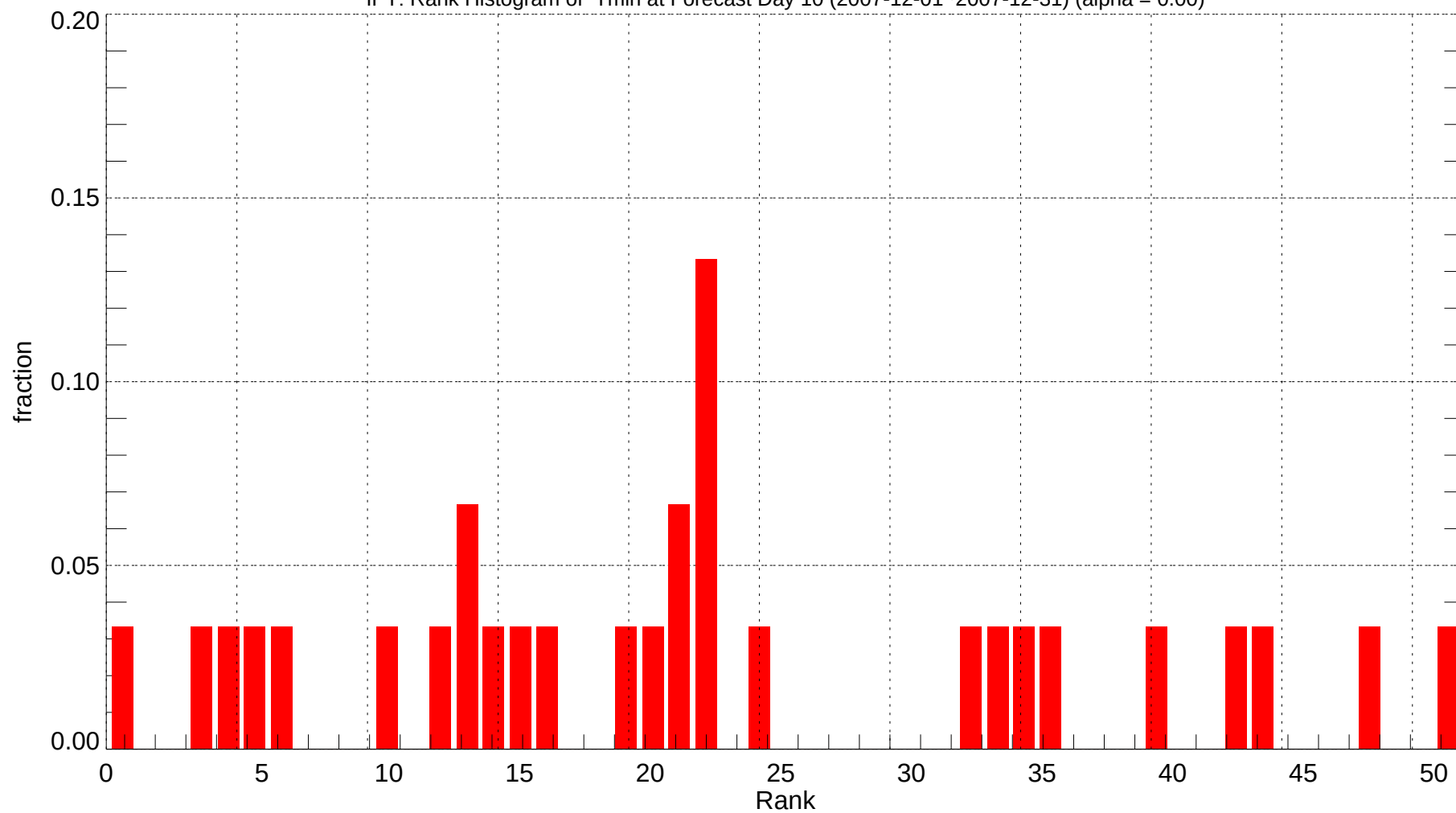
IPT: Rank Histogram of Tmin at Forecast Day 10 (2007-12-01~2007-12-31) (alpha = 0.00)
