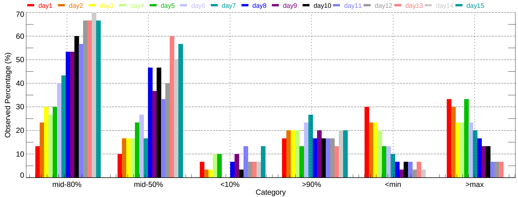
Observed Percentage of Ensembles - SSI: Min Temperature (2007-12-01~2007-12-31)
