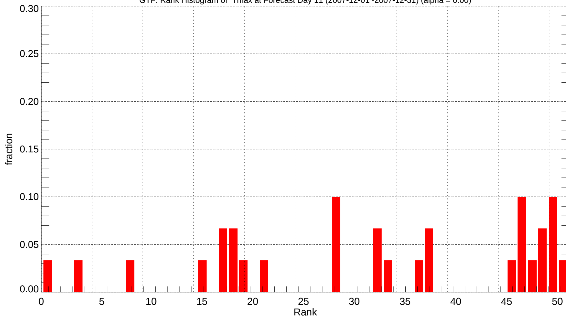
GTF: Rank Histogram of Tmax at Forecast Day 11 (2007-12-01~2007-12-31) (alpha = 0.00)
