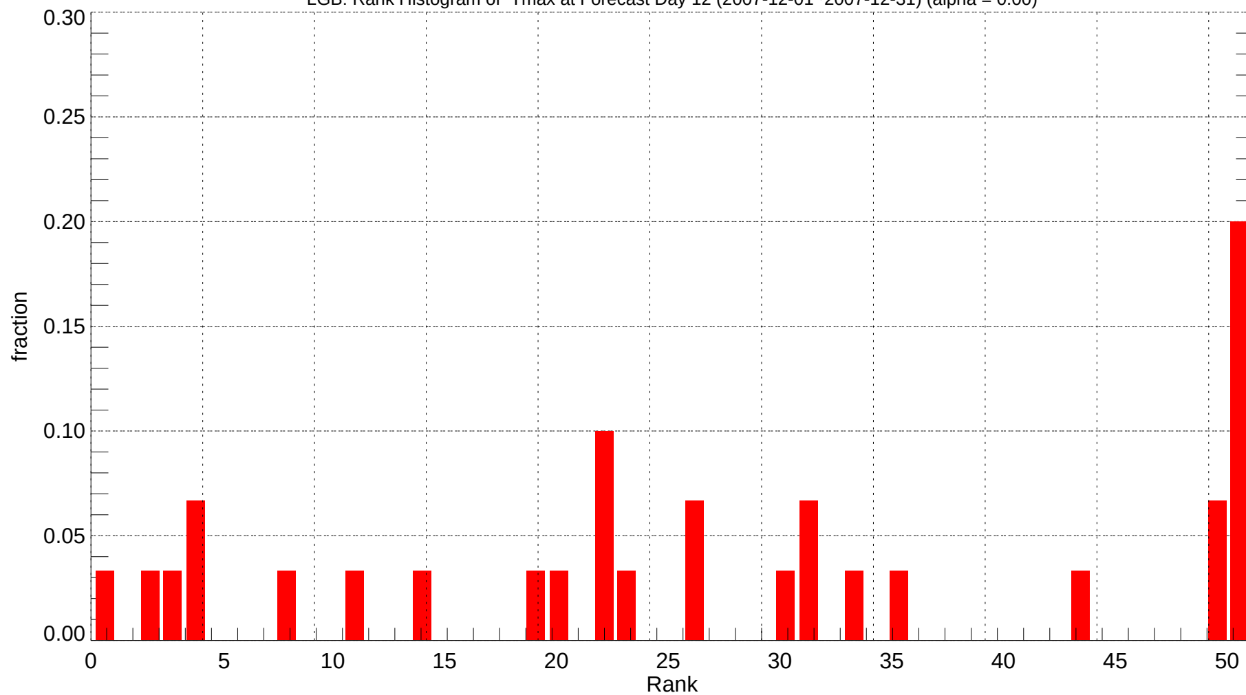
LGB: Rank Histogram of Tmax at Forecast Day 12 (2007-12-01~2007-12-31) (alpha = 0.00)
