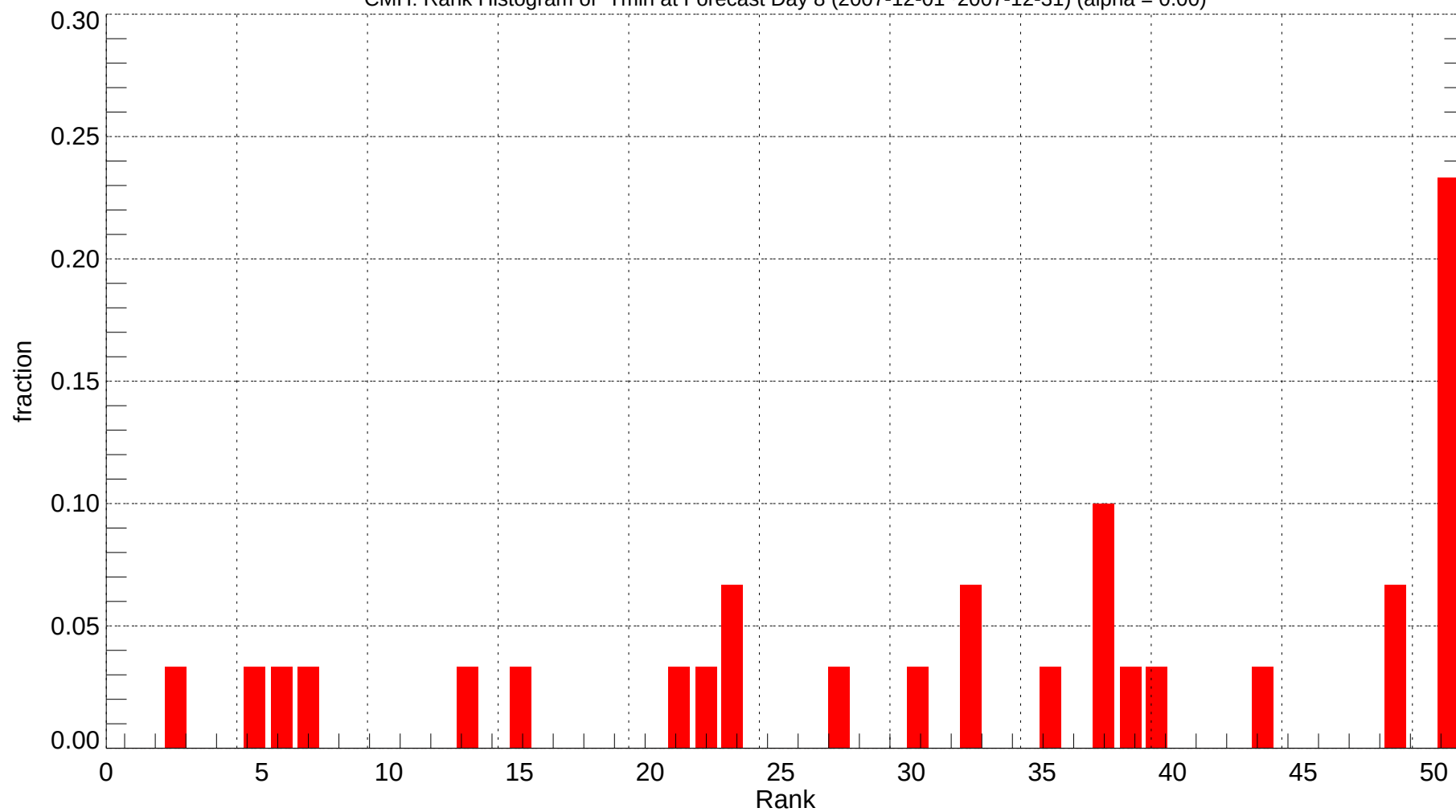
CMH: Rank Histogram of Tmin at Forecast Day 8 (2007-12-01~2007-12-31) (alpha = 0.00)
