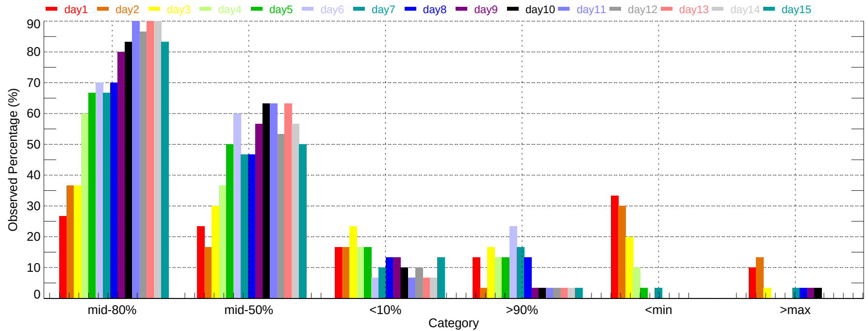
Observed Percentage of Ensembles - APN: Min Temperature (2007-12-01~2007-12-31)
