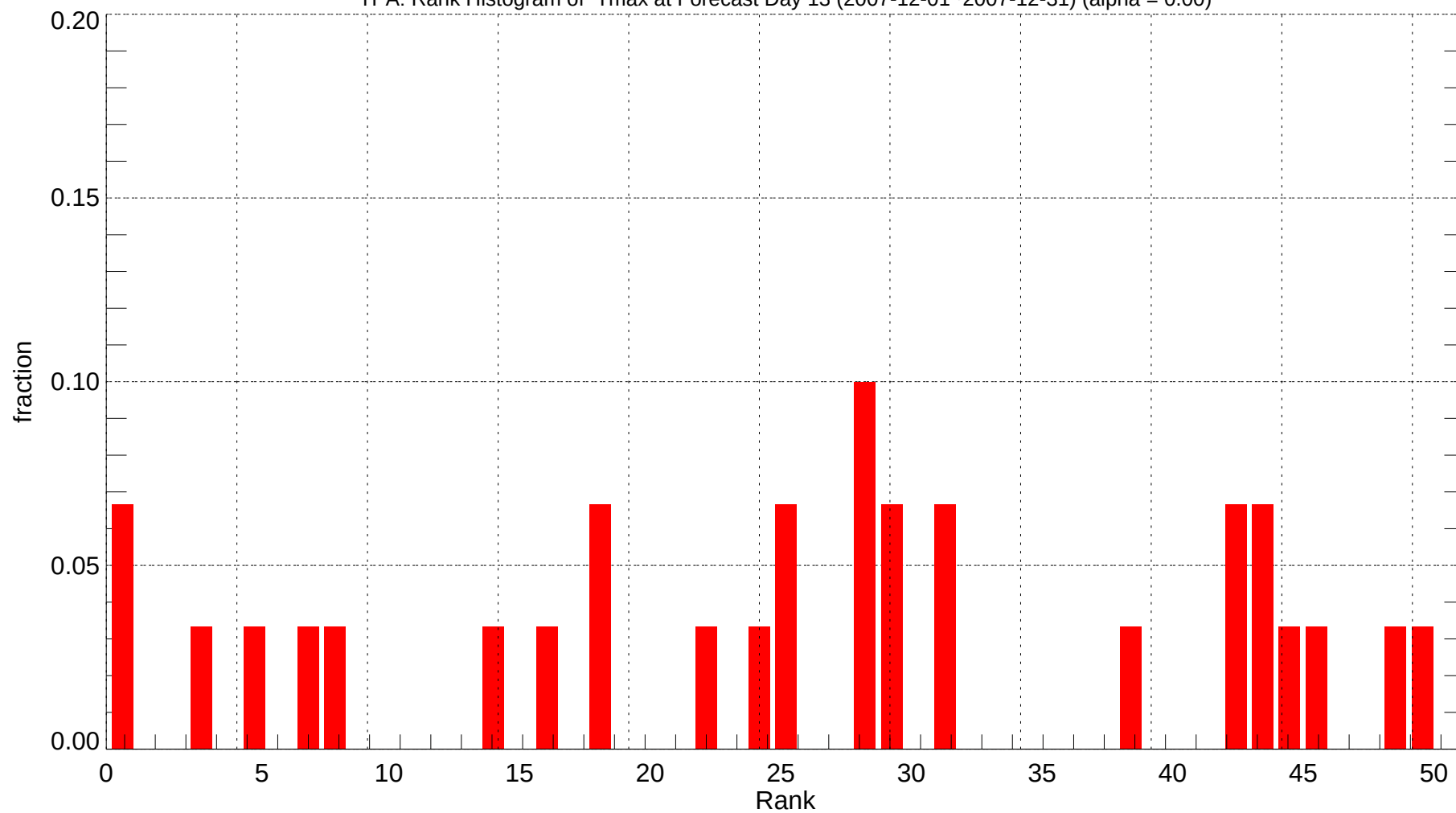
TPA: Rank Histogram of Tmax at Forecast Day 13 (2007-12-01~2007-12-31) (alpha = 0.00)
