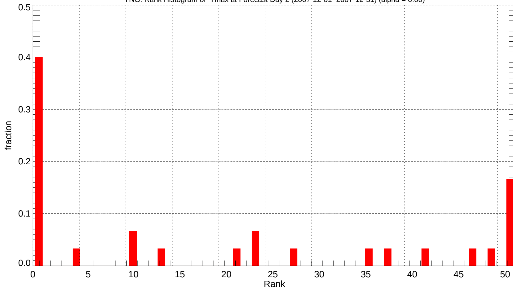
YNG: Rank Histogram of Tmax at Forecast Day 2 (2007-12-01~2007-12-31) (alpha = 0.00)
