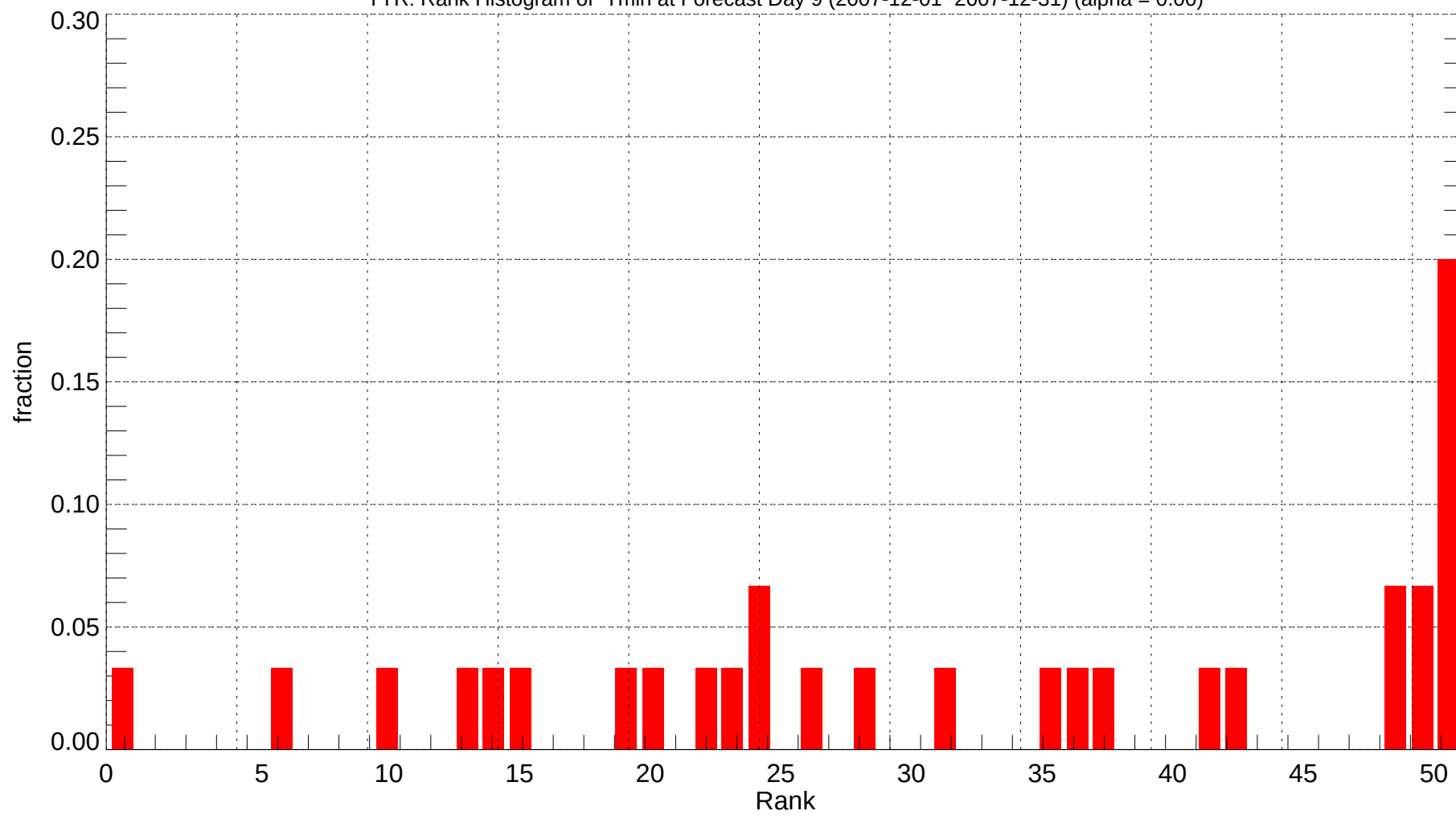
TYR: Rank Histogram of Tmin at Forecast Day 9 (2007-12-01~2007-12-31) (alpha = 0.00)
