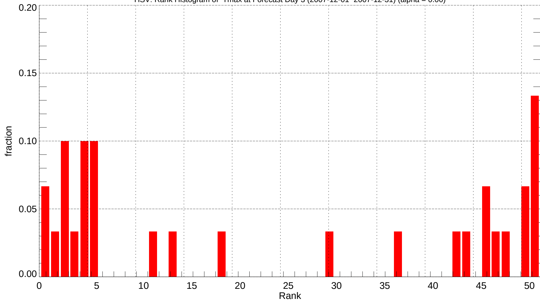
HSV: Rank Histogram of Tmax at Forecast Day 3 (2007-12-01~2007-12-31) (alpha = 0.00)
