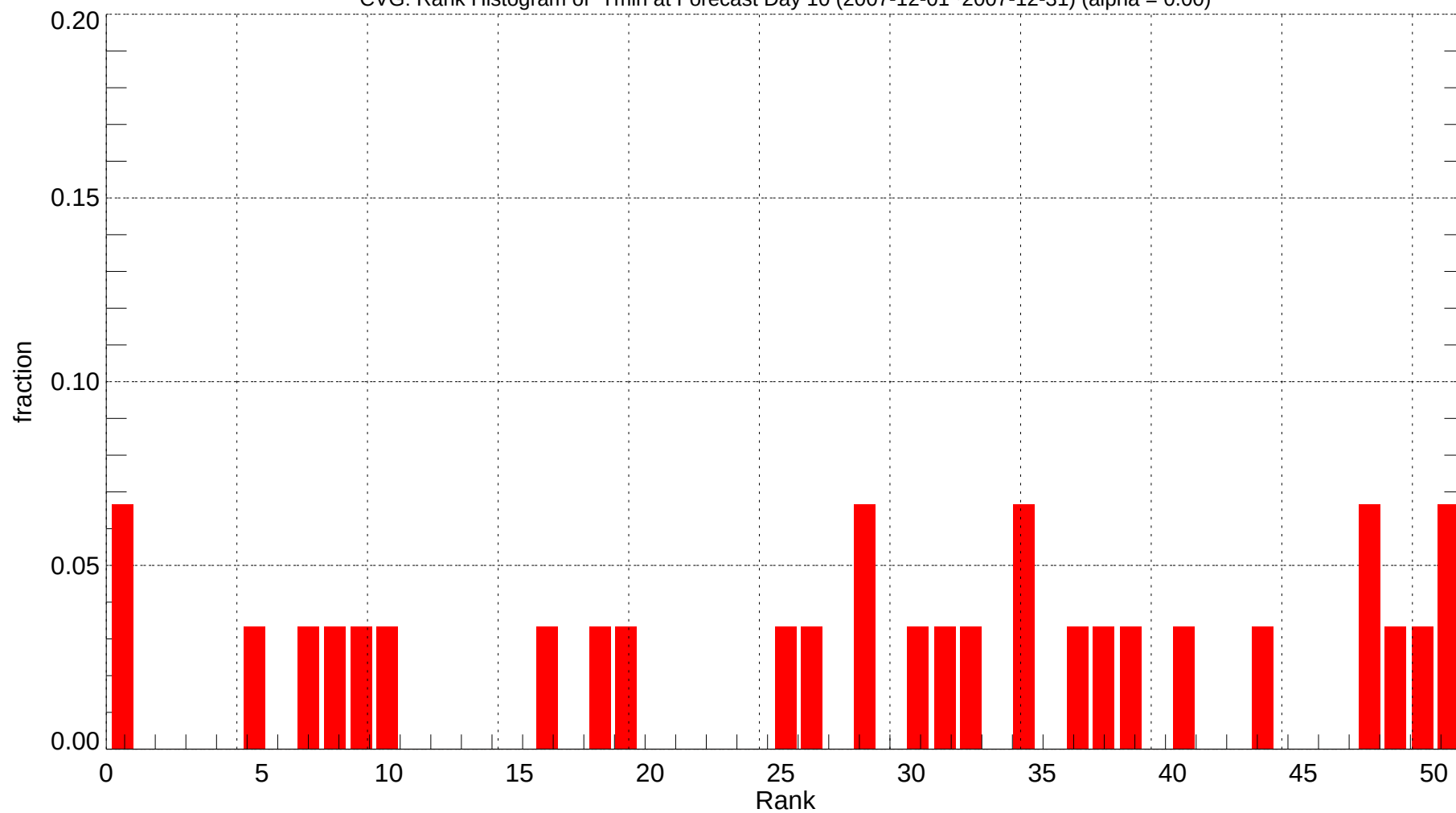
CVG: Rank Histogram of Tmin at Forecast Day 10 (2007-12-01~2007-12-31) (alpha = 0.00)
