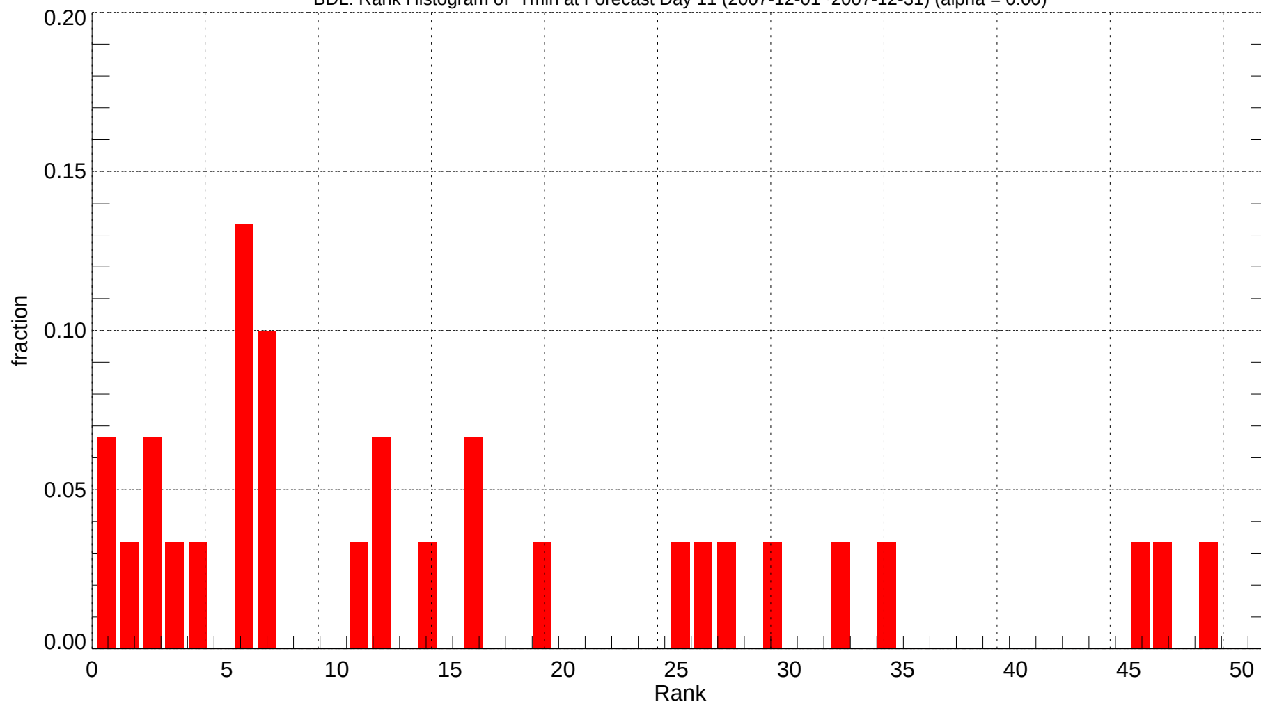
BDL: Rank Histogram of Tmin at Forecast Day 11 (2007-12-01~2007-12-31) (alpha = 0.00)
