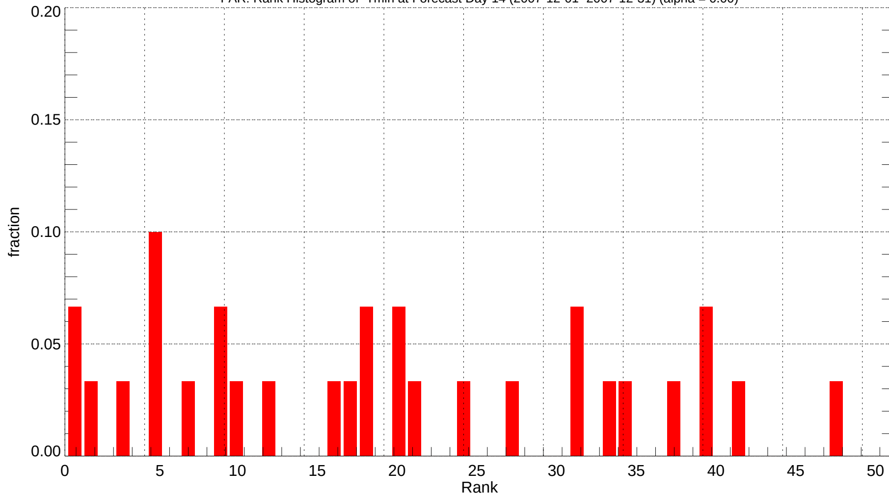
FAR: Rank Histogram of Tmin at Forecast Day 14 (2007-12-01~2007-12-31) (alpha = 0.00)
