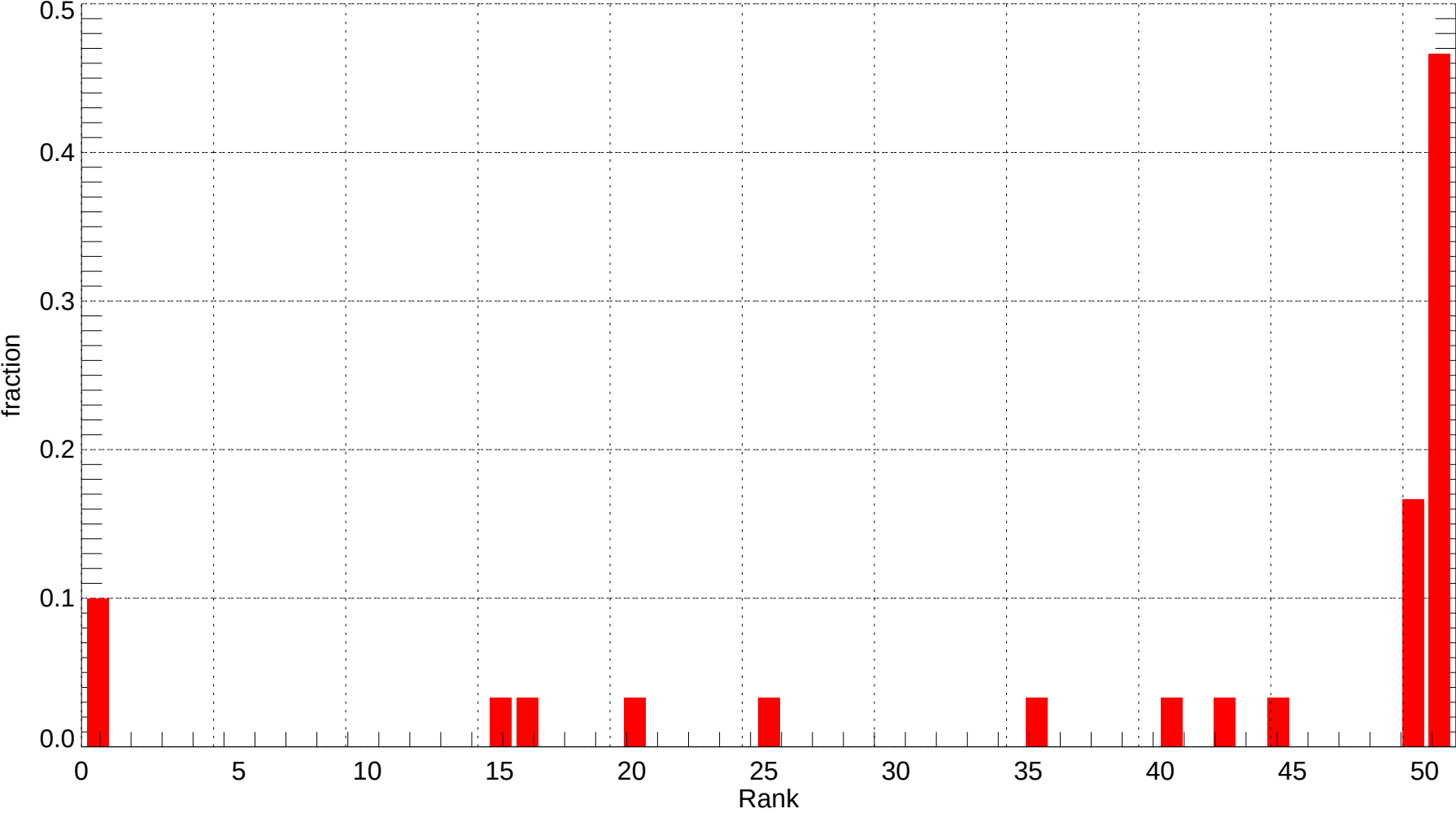
BFL: Rank Histogram of Tmin at Forecast Day 4 (2007-12-01~2007-12-31) (alpha = 0.00)
