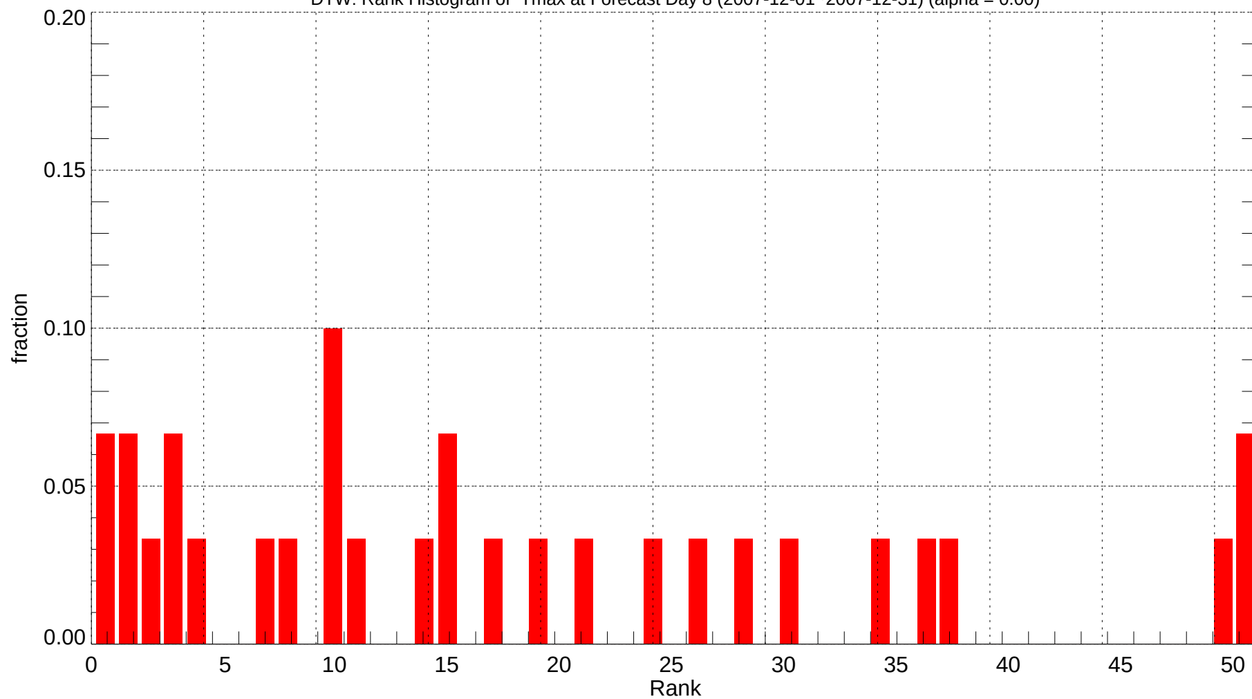
DTW: Rank Histogram of Tmax at Forecast Day 8 (2007-12-01~2007-12-31) (alpha = 0.00)
