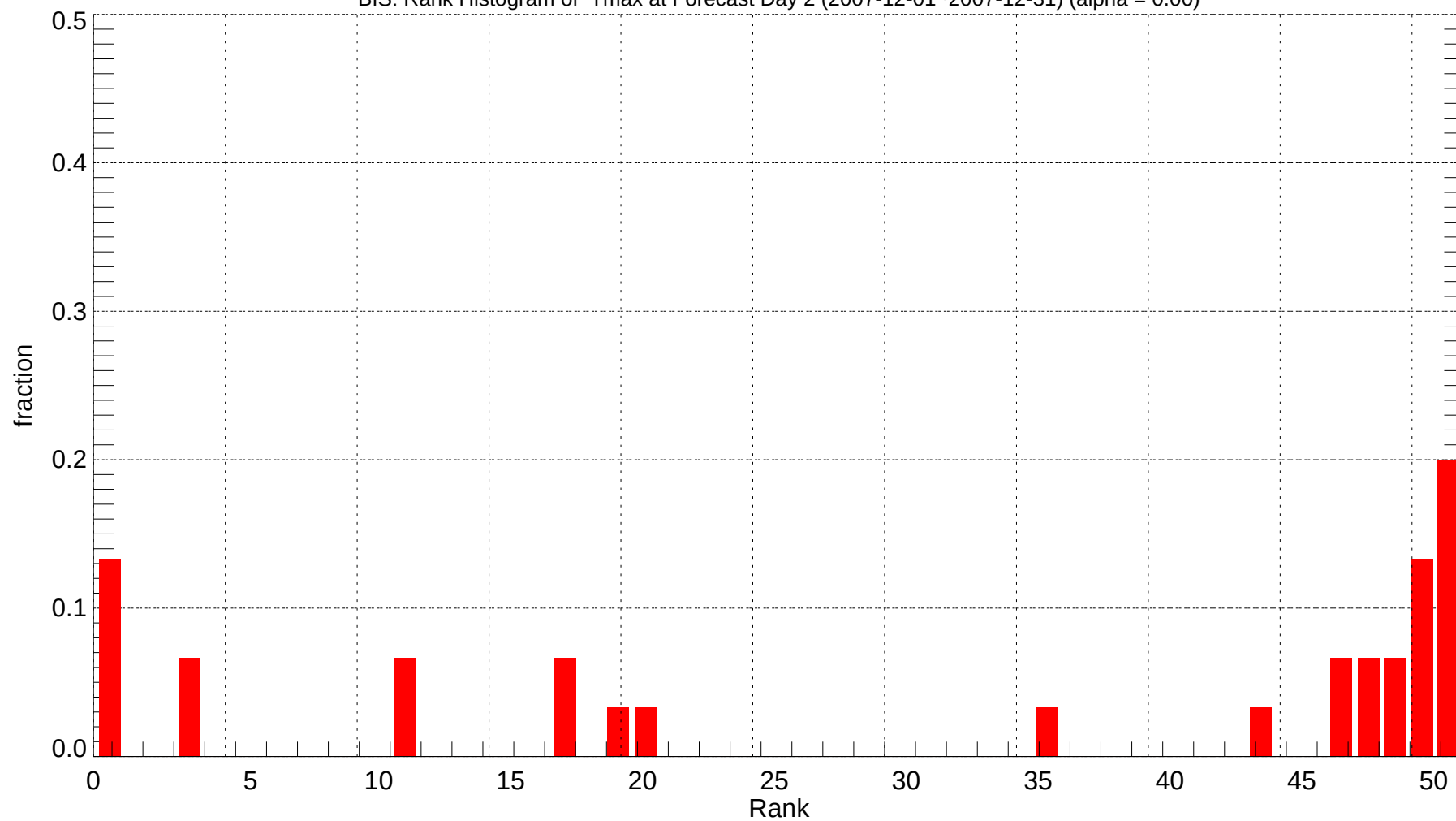
BIS: Rank Histogram of Tmax at Forecast Day 2 (2007-12-01~2007-12-31) (alpha = 0.00)
