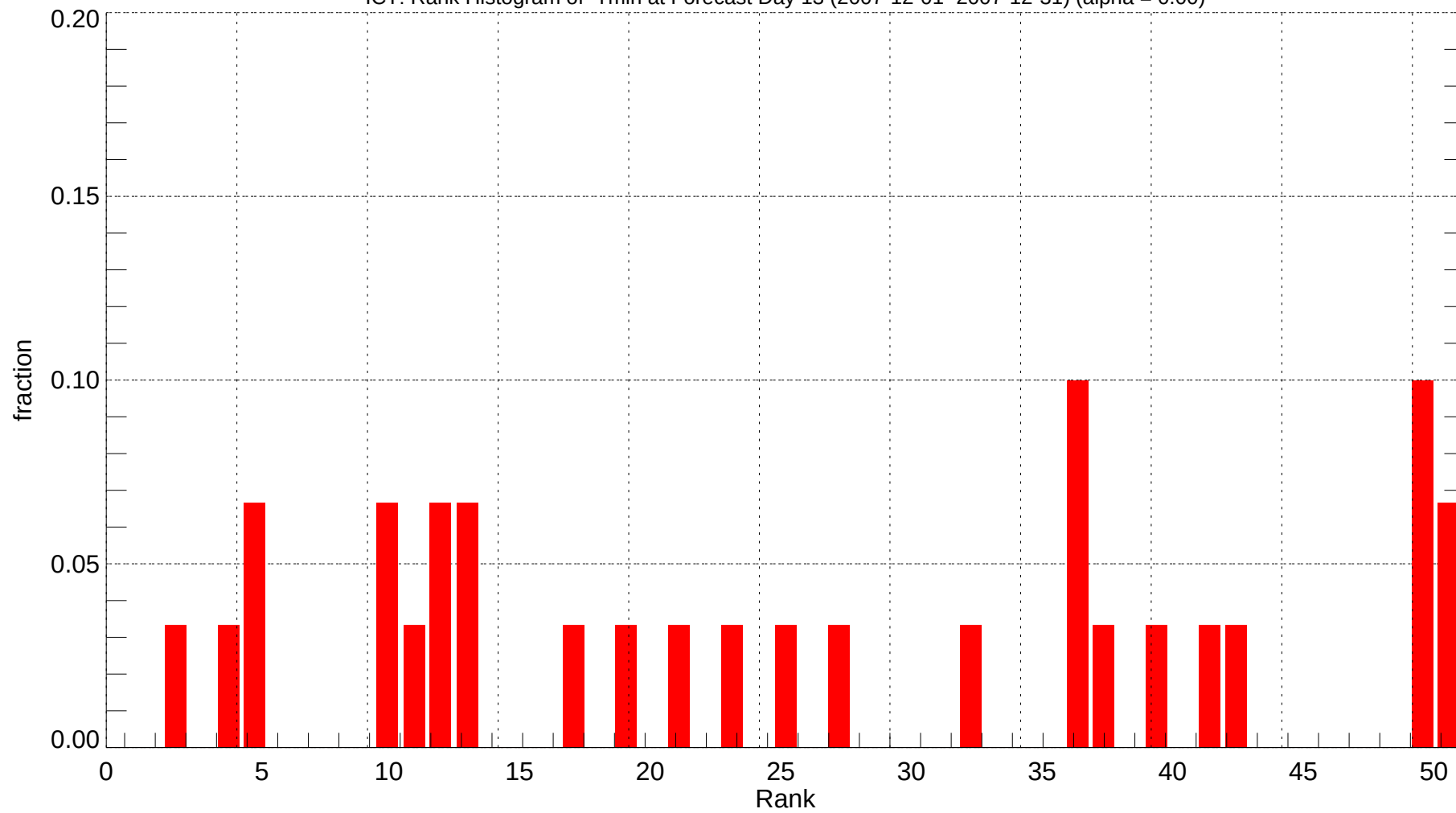
ICT: Rank Histogram of Tmin at Forecast Day 13 (2007-12-01~2007-12-31) (alpha = 0.00)
