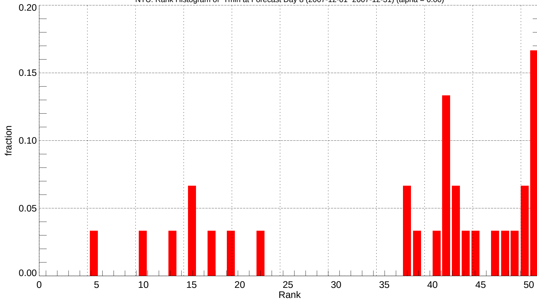
NTU: Rank Histogram of Tmin at Forecast Day 8 (2007-12-01~2007-12-31) (alpha = 0.00)
