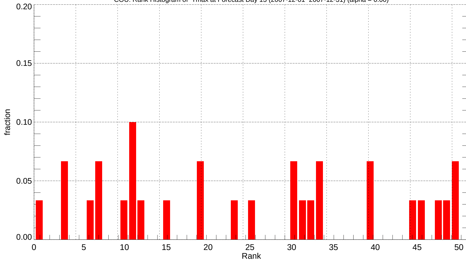
COU: Rank Histogram of Tmax at Forecast Day 13 (2007-12-01~2007-12-31) (alpha = 0.00)
