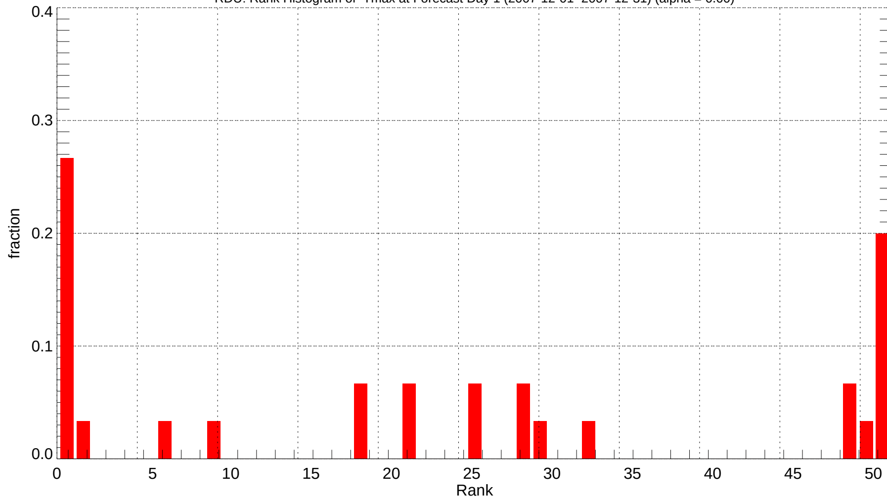
RDU: Rank Histogram of Tmax at Forecast Day 1 (2007-12-01~2007-12-31) (alpha = 0.00)
