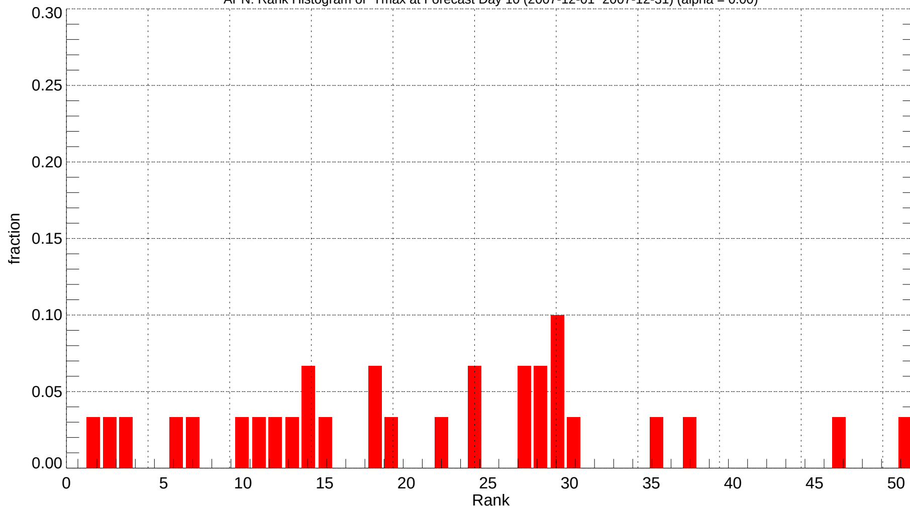
APN: Rank Histogram of Tmax at Forecast Day 10 (2007-12-01~2007-12-31) (alpha = 0.00)
