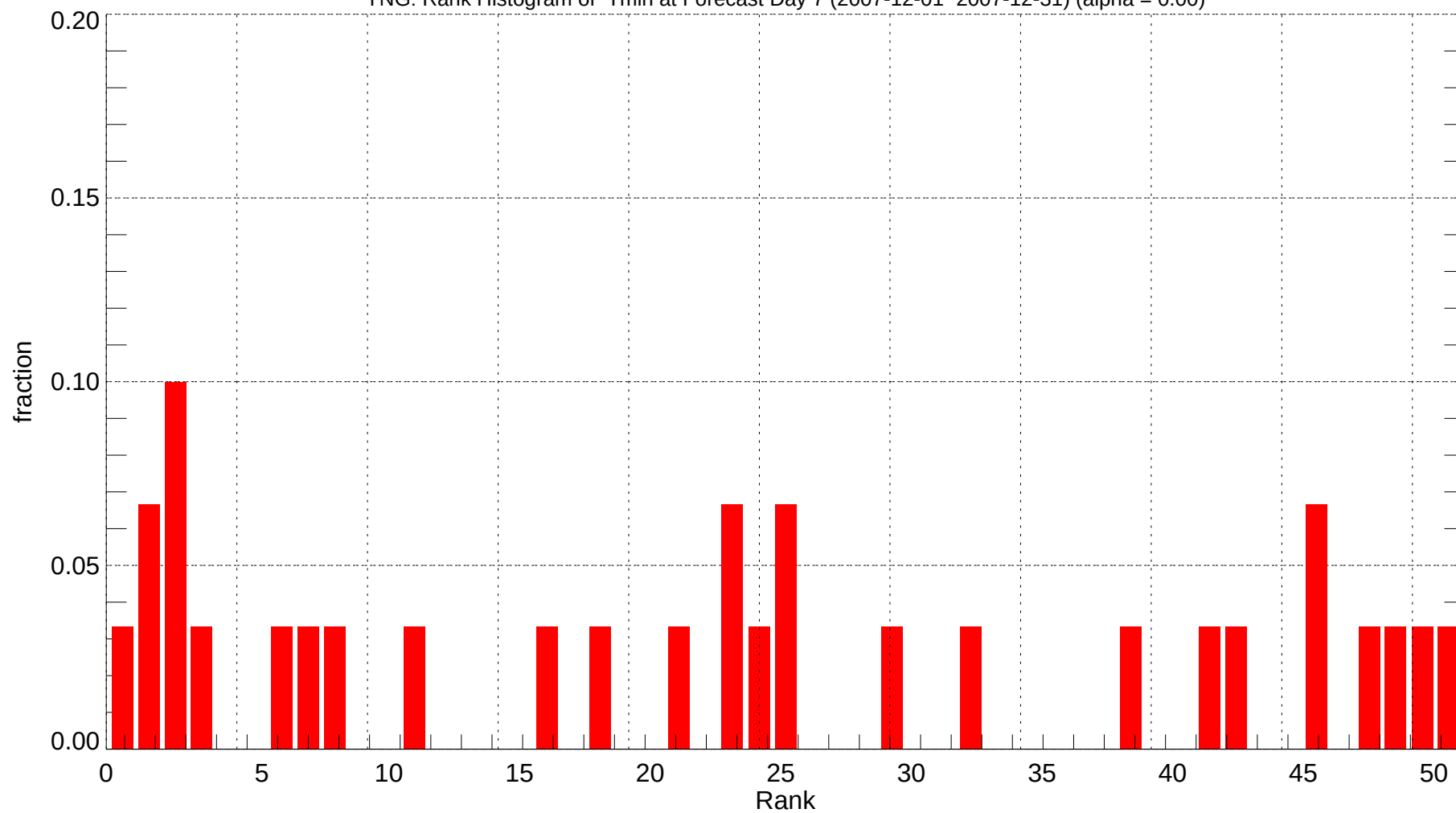
YNG: Rank Histogram of Tmin at Forecast Day 7 (2007-12-01~2007-12-31) (alpha = 0.00)
