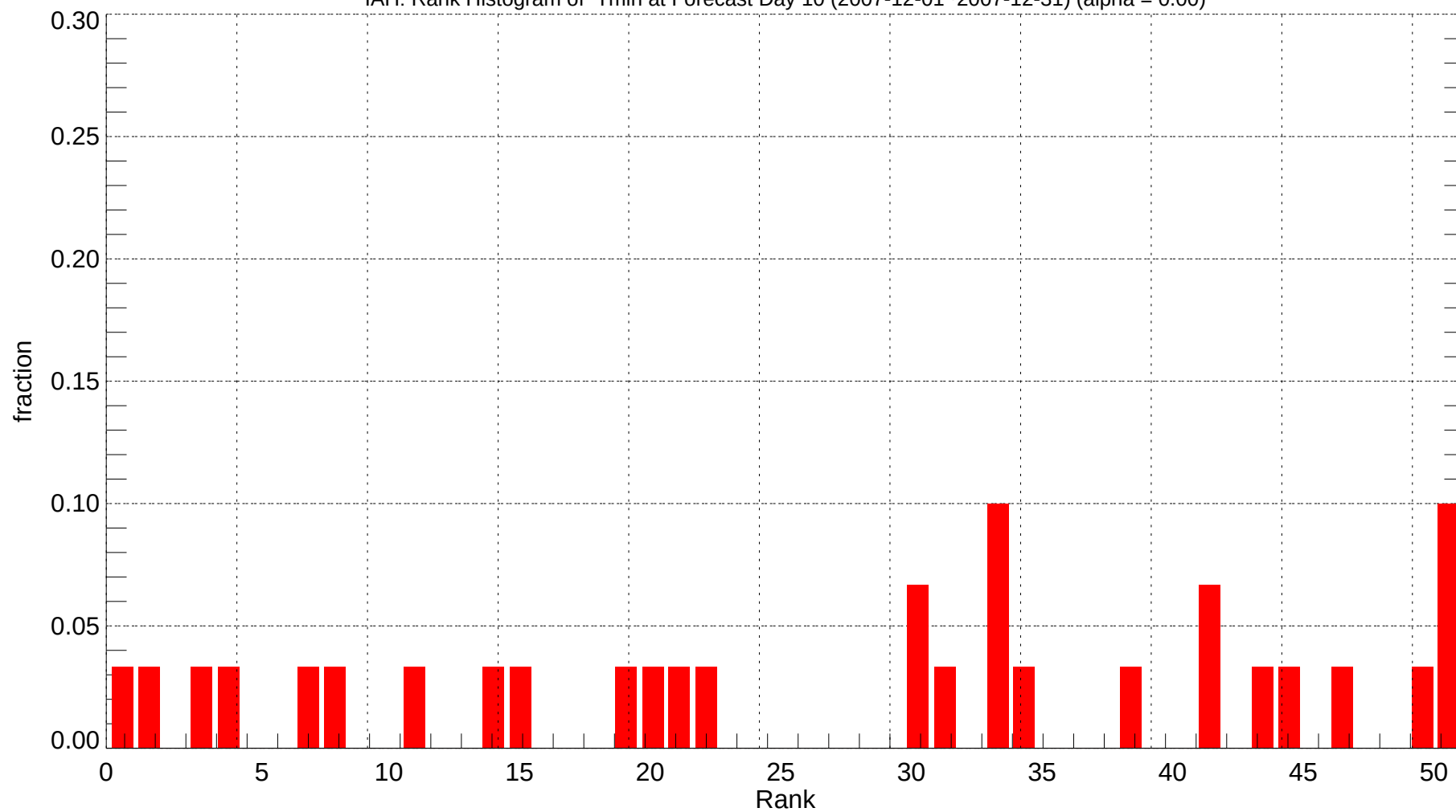
IAH: Rank Histogram of Tmin at Forecast Day 10 (2007-12-01~2007-12-31) (alpha = 0.00)
