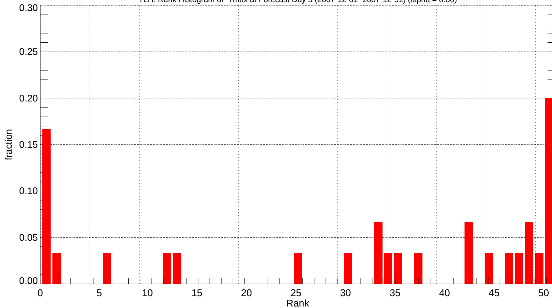
TLH: Rank Histogram of Tmax at Forecast Day 5 (2007-12-01~2007-12-31) (alpha = 0.00)
