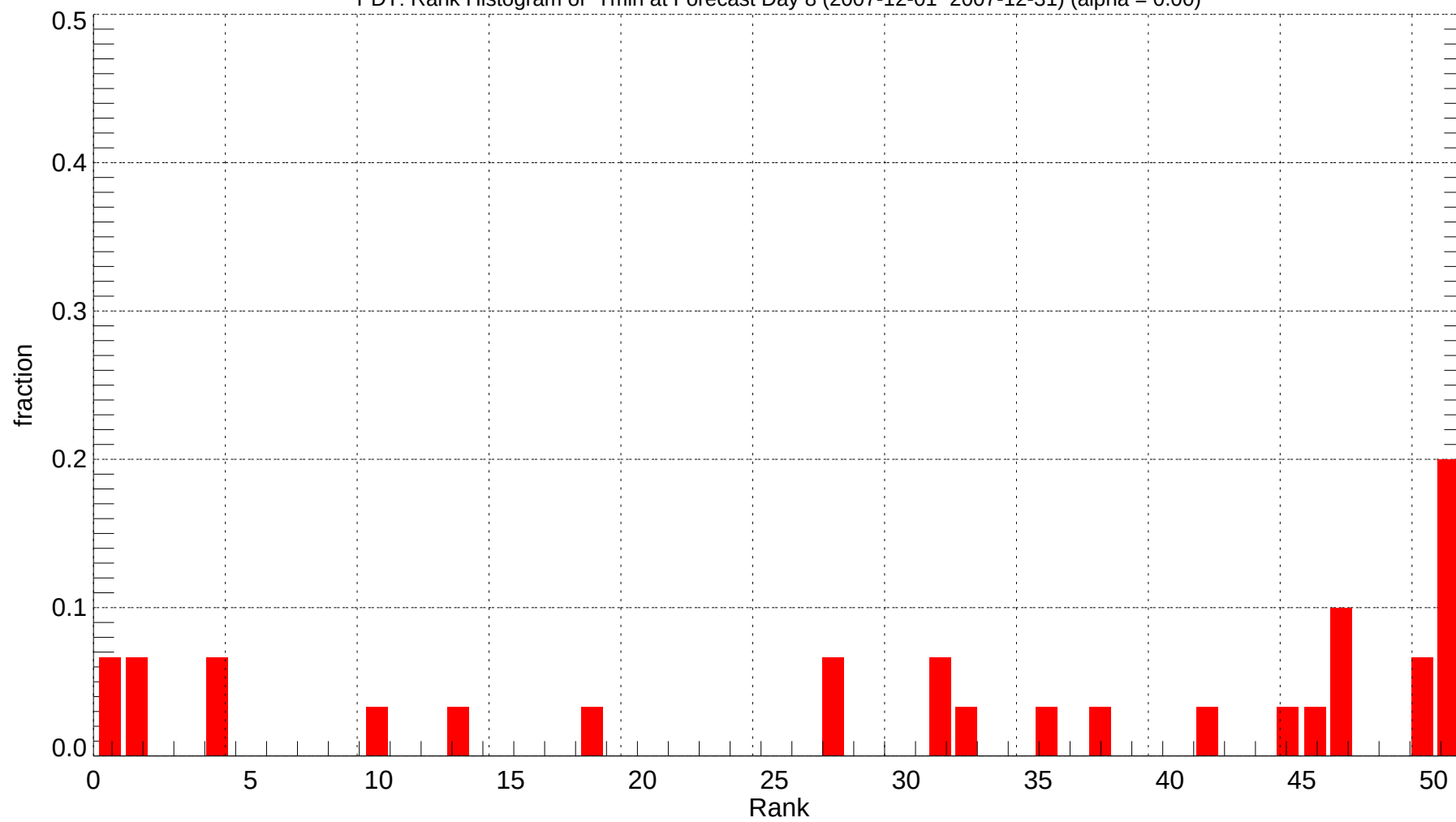
PDT: Rank Histogram of Tmin at Forecast Day 8 (2007-12-01~2007-12-31) (alpha = 0.00)
