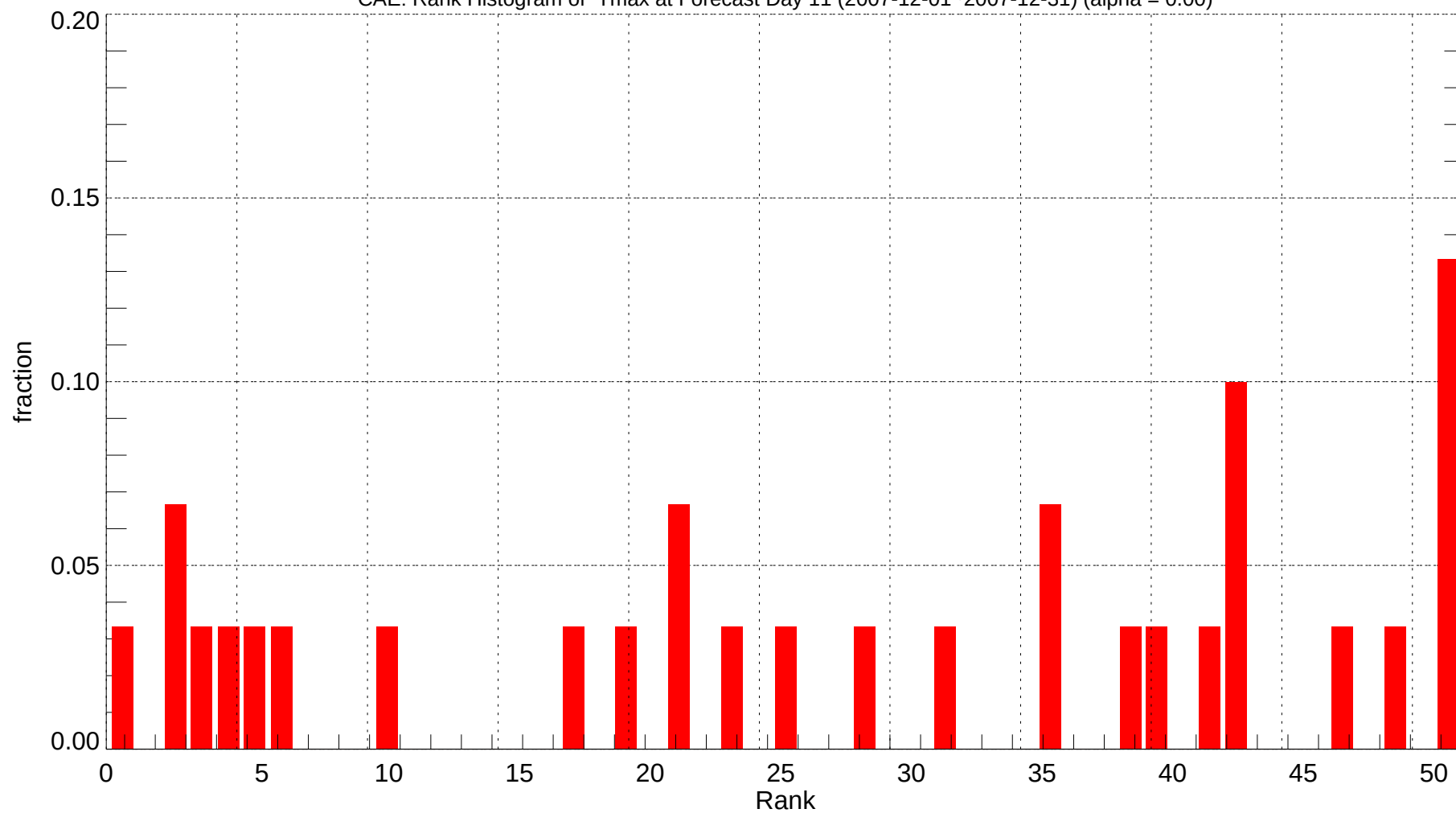
CAE: Rank Histogram of Tmax at Forecast Day 11 (2007-12-01~2007-12-31) (alpha = 0.00)
