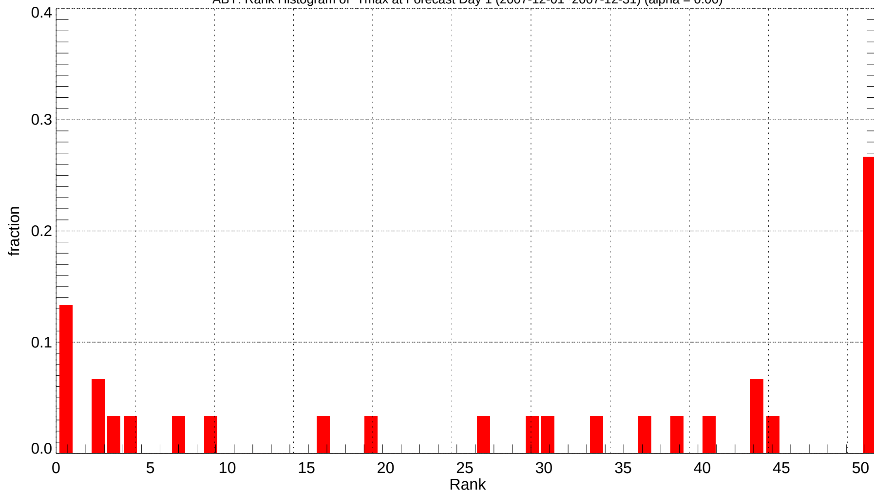
ABY: Rank Histogram of Tmax at Forecast Day 1 (2007-12-01~2007-12-31) (alpha = 0.00)
