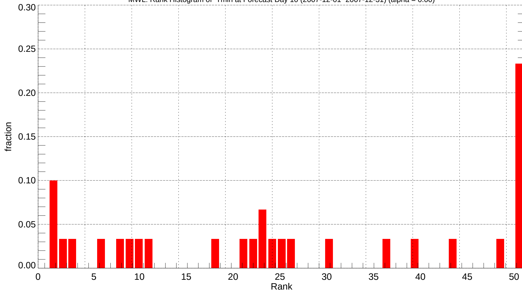
MWL: Rank Histogram of Tmin at Forecast Day 10 (2007-12-01~2007-12-31) (alpha = 0.00)
