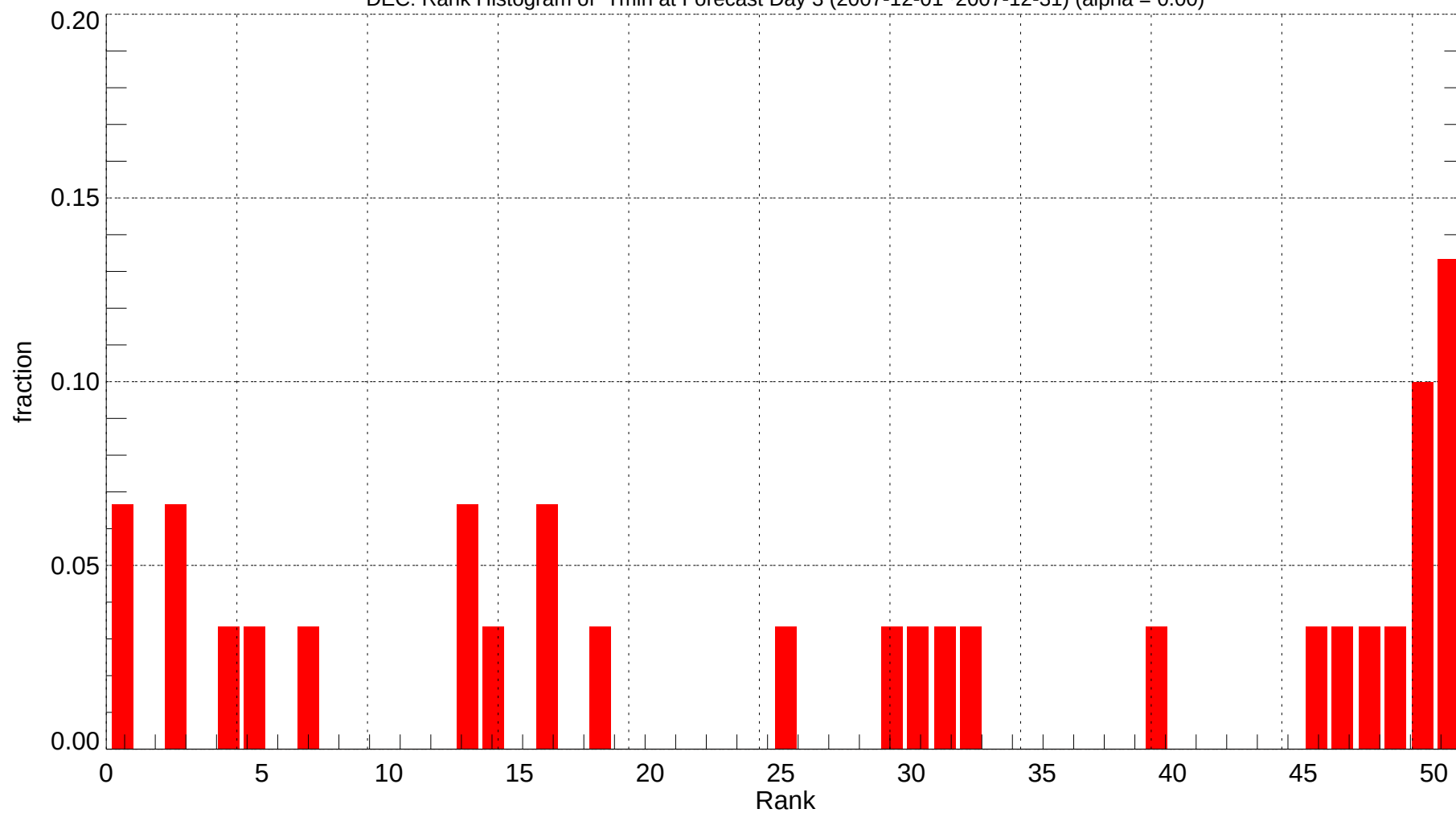
DEC: Rank Histogram of Tmin at Forecast Day 3 (2007-12-01~2007-12-31) (alpha = 0.00)
