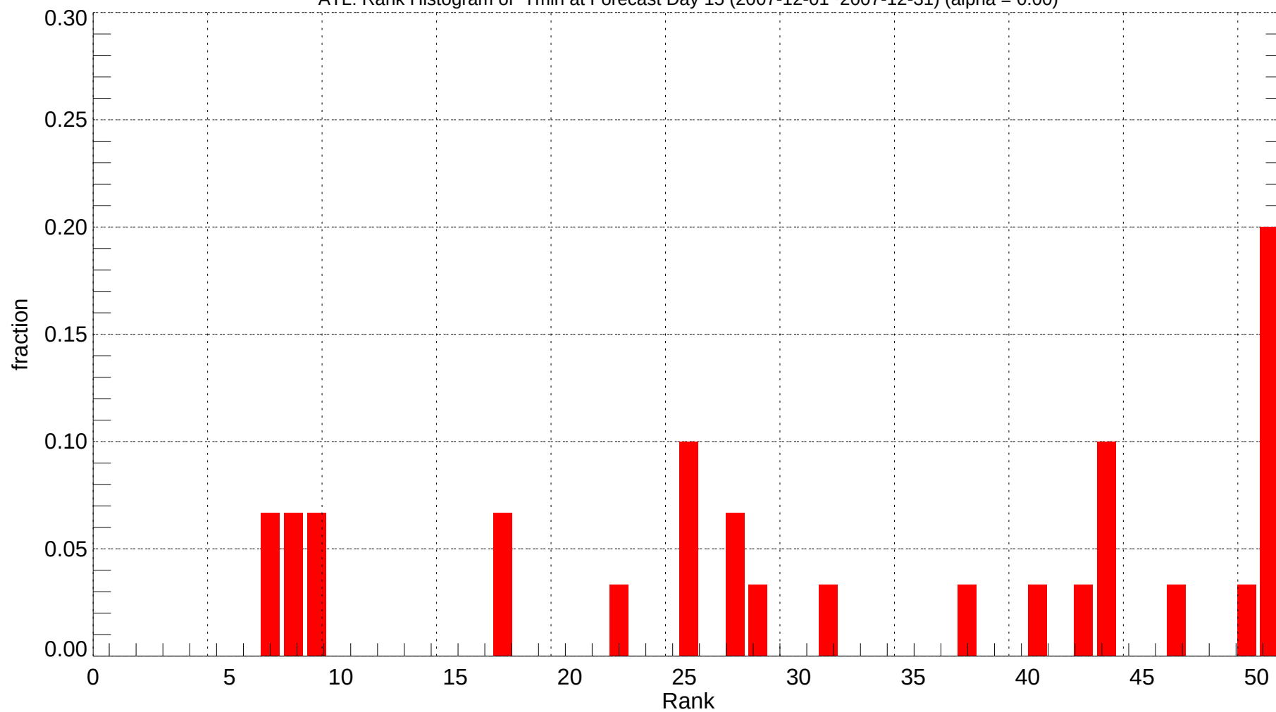
ATL: Rank Histogram of Tmin at Forecast Day 15 (2007-12-01~2007-12-31) (alpha = 0.00)
