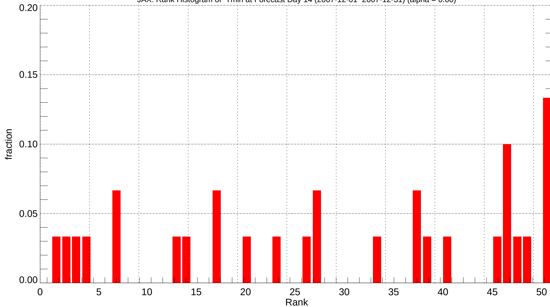
JAX: Rank Histogram of Tmin at Forecast Day 14 (2007-12-01~2007-12-31) (alpha = 0.00)
