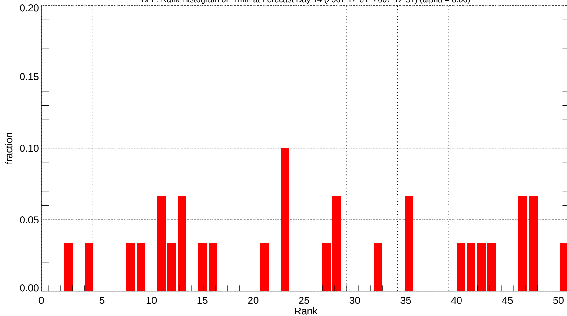
BFL: Rank Histogram of Tmin at Forecast Day 14 (2007-12-01~2007-12-31) (alpha = 0.00)
