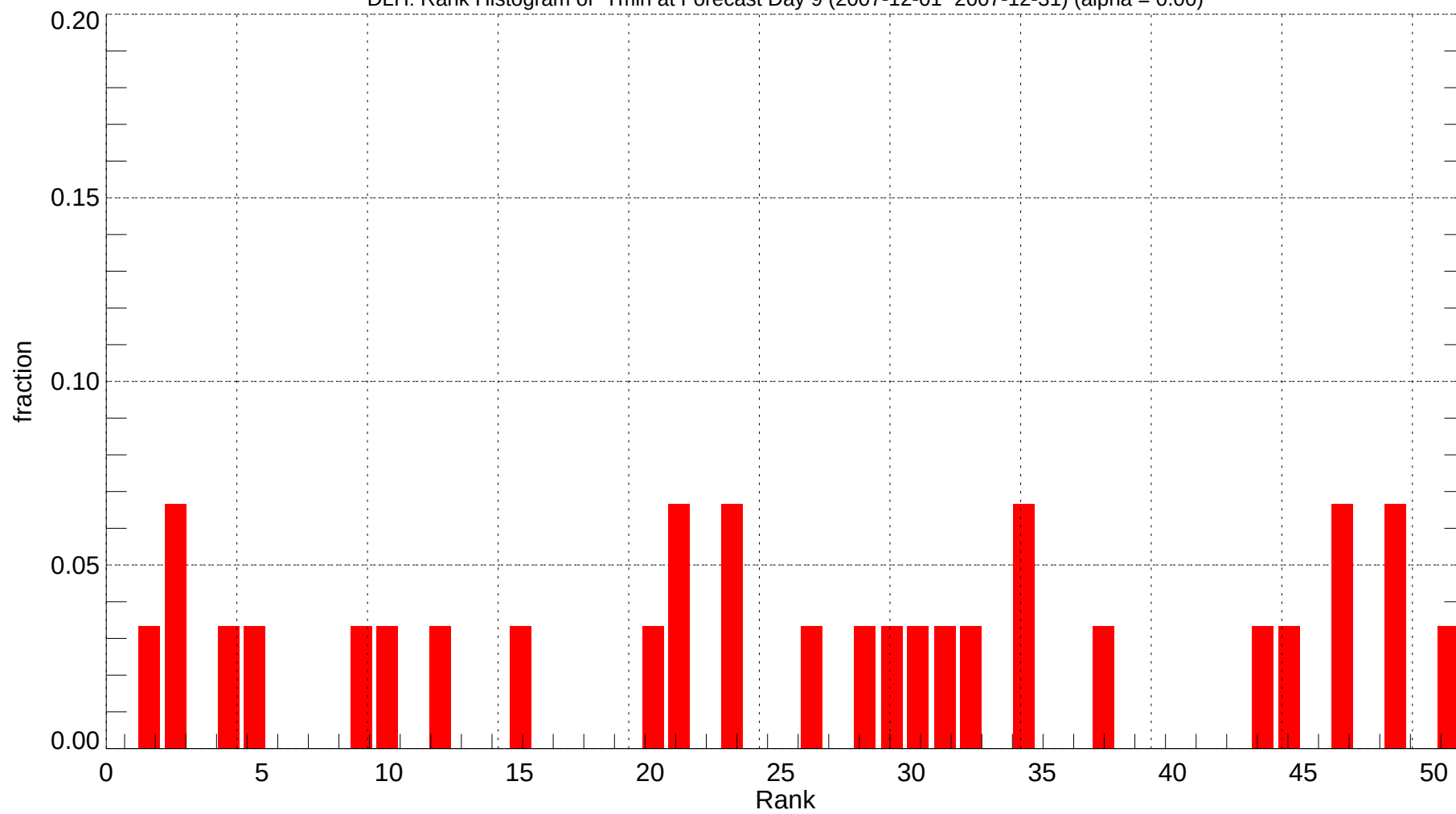
DLH: Rank Histogram of Tmin at Forecast Day 9 (2007-12-01~2007-12-31) (alpha = 0.00)
