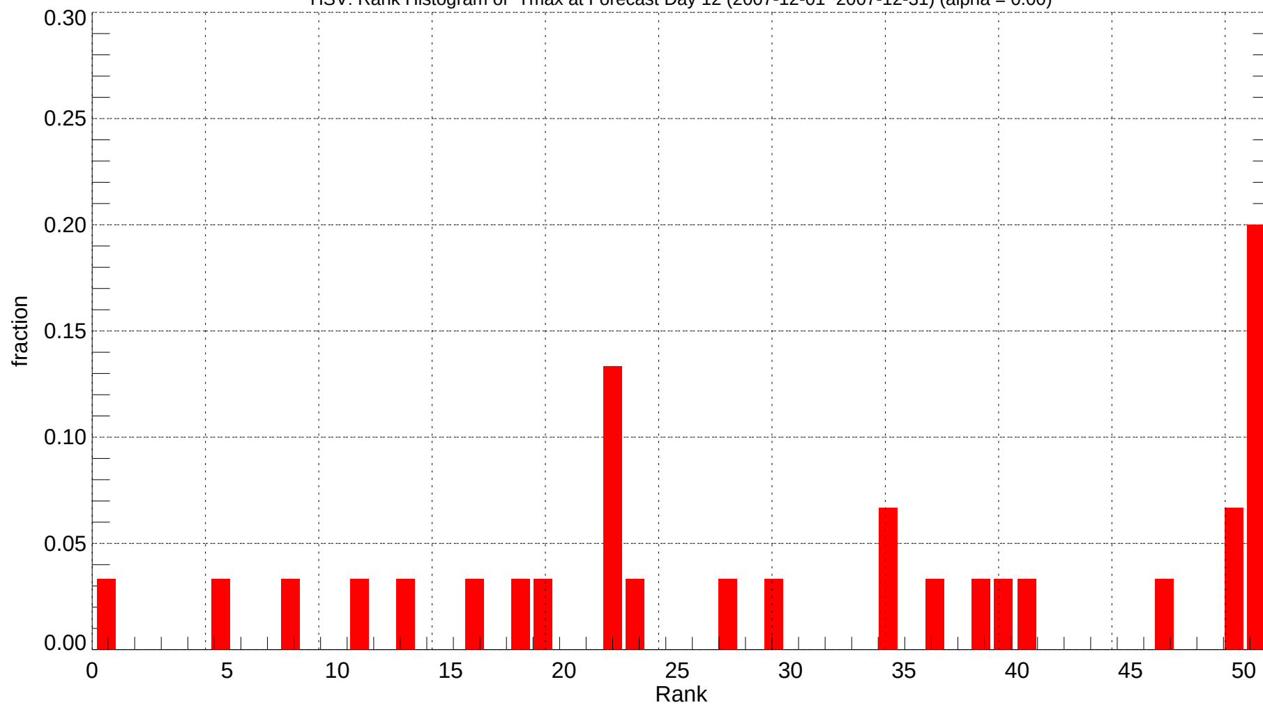
HSV: Rank Histogram of Tmax at Forecast Day 12 (2007-12-01~2007-12-31) (alpha = 0.00)
