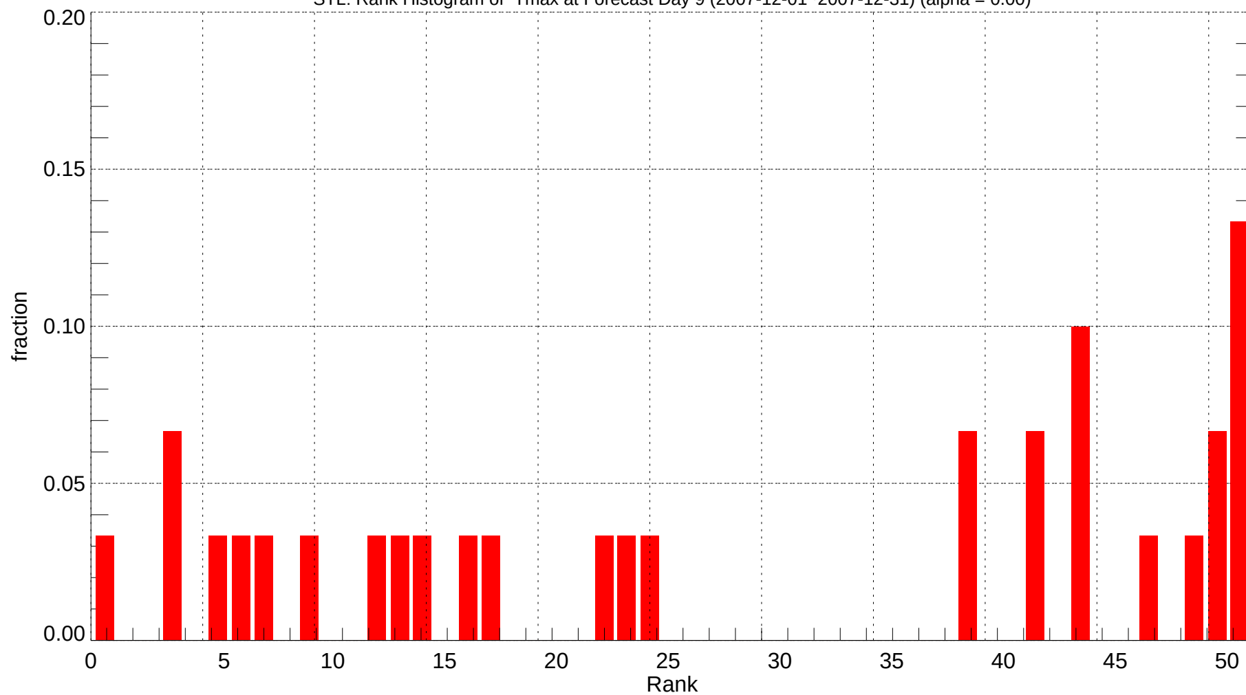
STL: Rank Histogram of Tmax at Forecast Day 9 (2007-12-01~2007-12-31) (alpha = 0.00)
