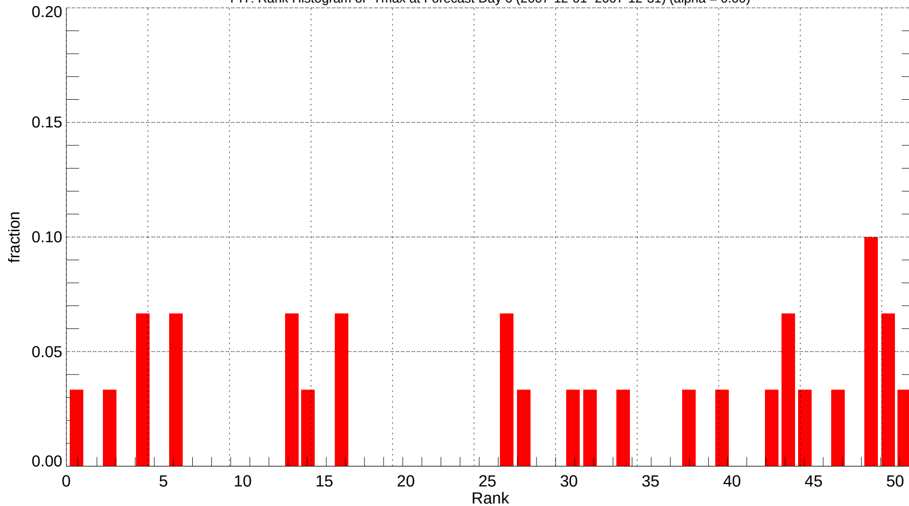
PIT: Rank Histogram of Tmax at Forecast Day 6 (2007-12-01~2007-12-31) (alpha = 0.00)
