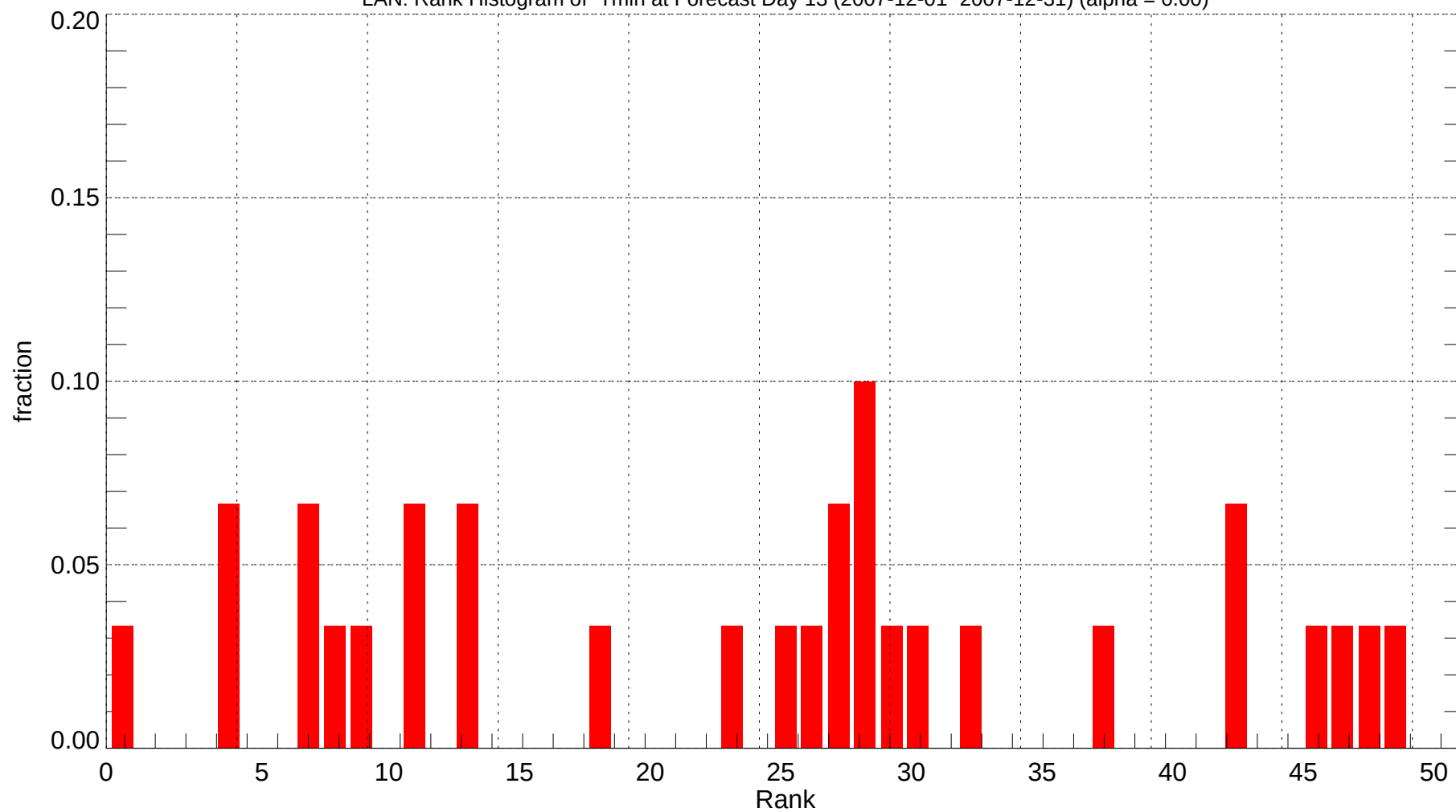
LAN: Rank Histogram of Tmin at Forecast Day 13 (2007-12-01~2007-12-31) (alpha = 0.00)
