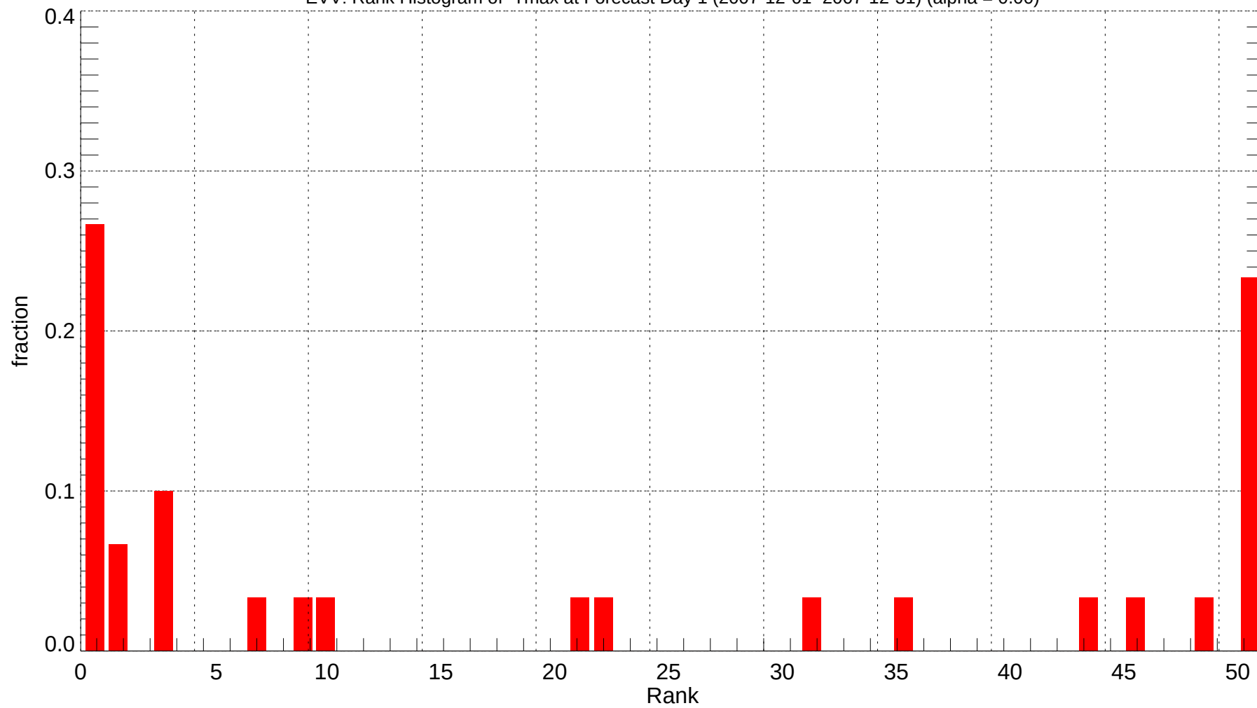
EVV: Rank Histogram of Tmax at Forecast Day 1 (2007-12-01~2007-12-31) (alpha = 0.00)
