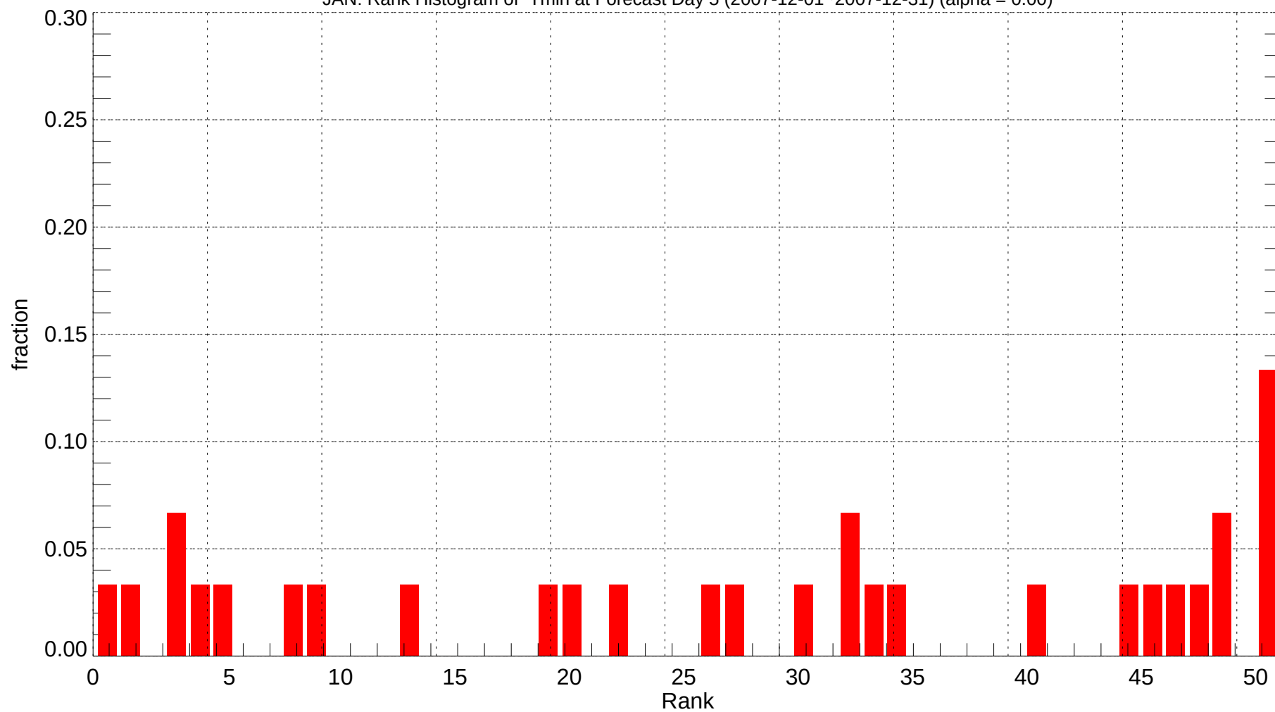
JAN: Rank Histogram of Tmin at Forecast Day 5 (2007-12-01~2007-12-31) (alpha = 0.00)
