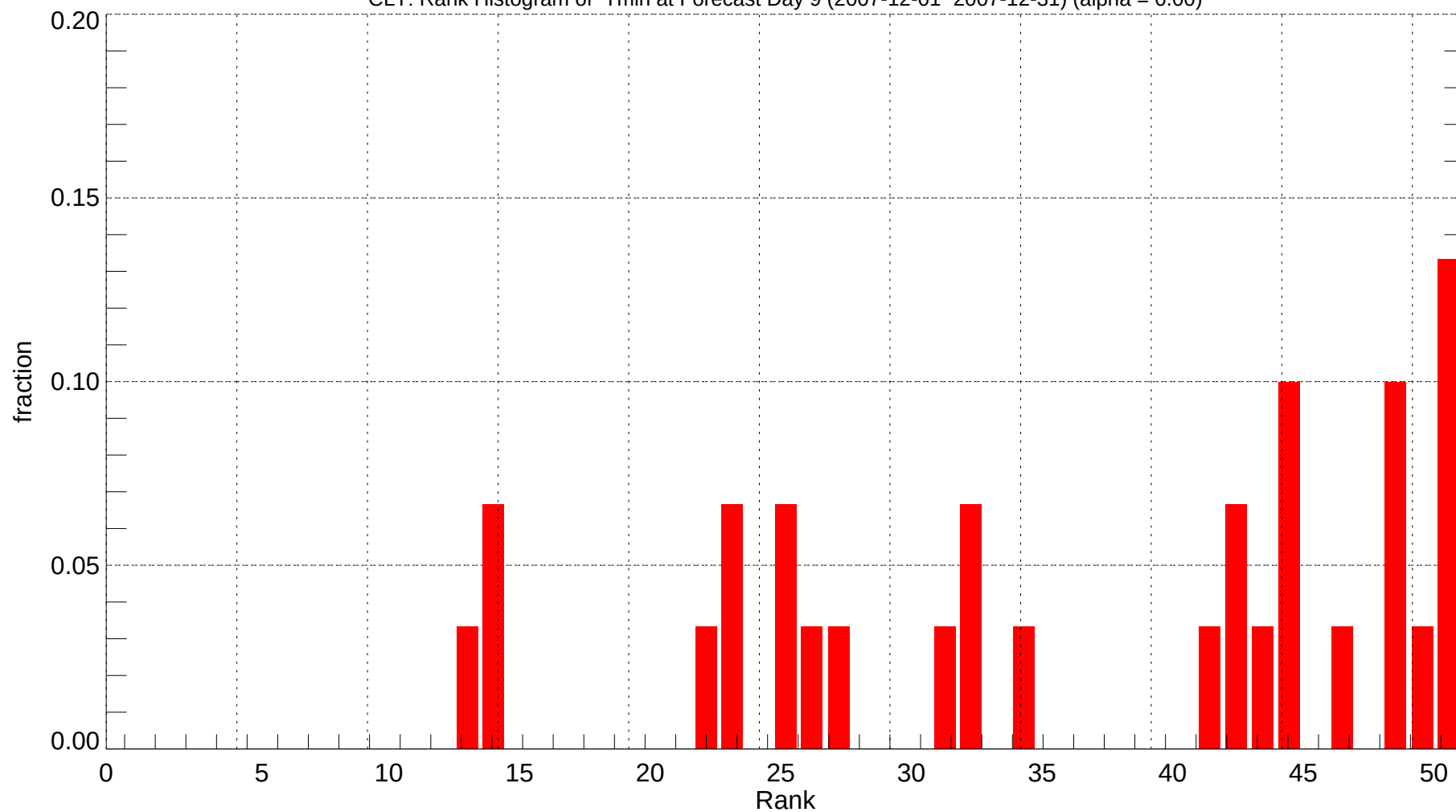
CLT: Rank Histogram of Tmin at Forecast Day 9 (2007-12-01~2007-12-31) (alpha = 0.00)
