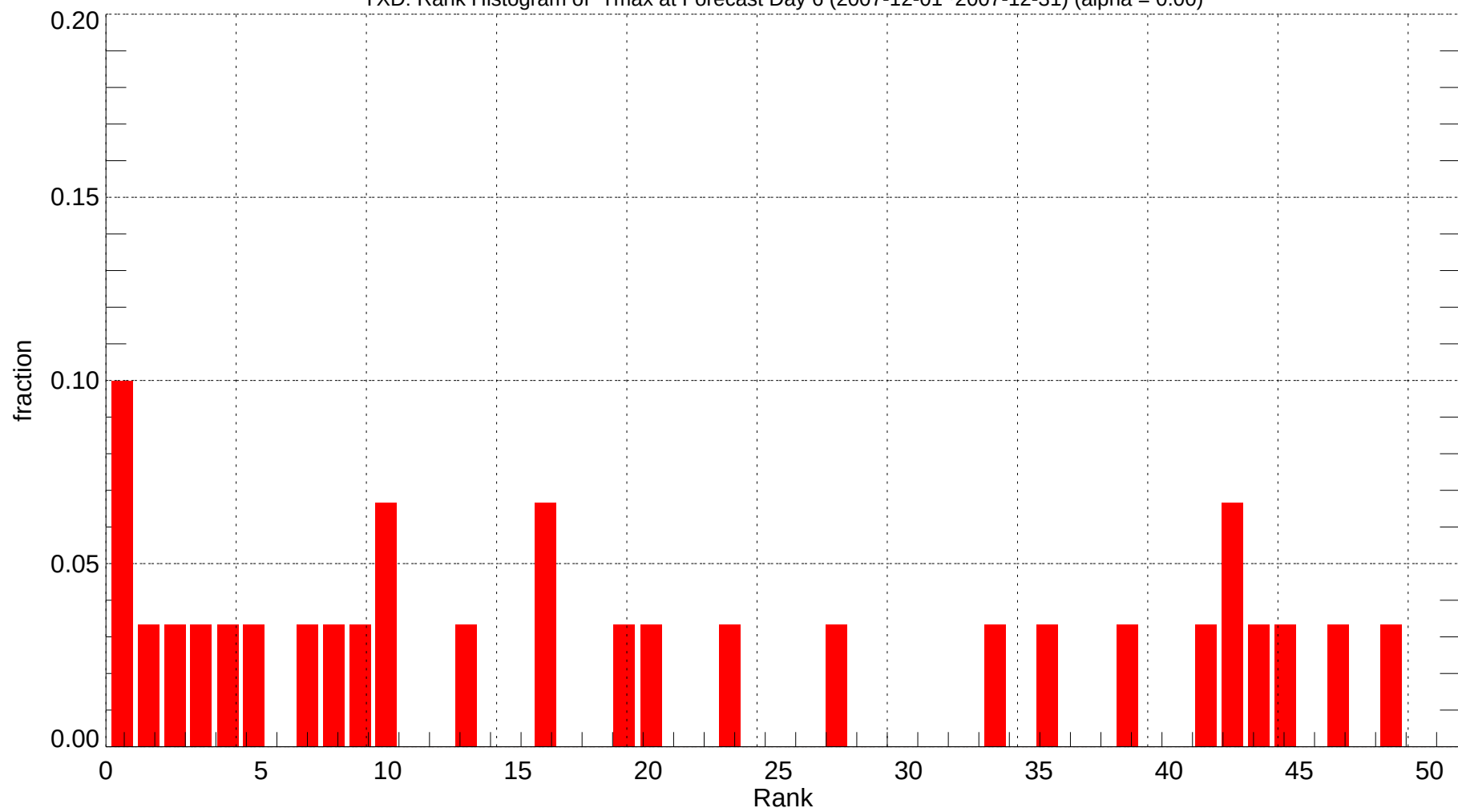
YXD: Rank Histogram of Tmax at Forecast Day 6 (2007-12-01~2007-12-31) (alpha = 0.00)
