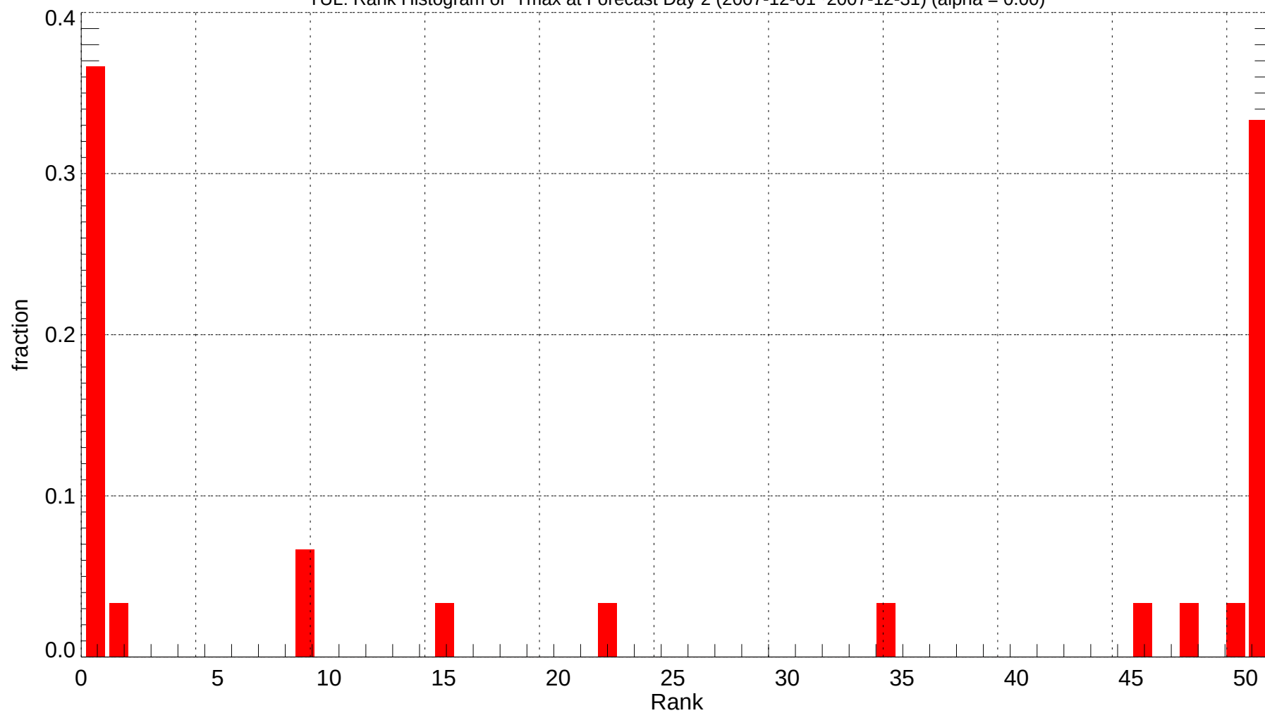
TUL: Rank Histogram of Tmax at Forecast Day 2 (2007-12-01~2007-12-31) (alpha = 0.00)
