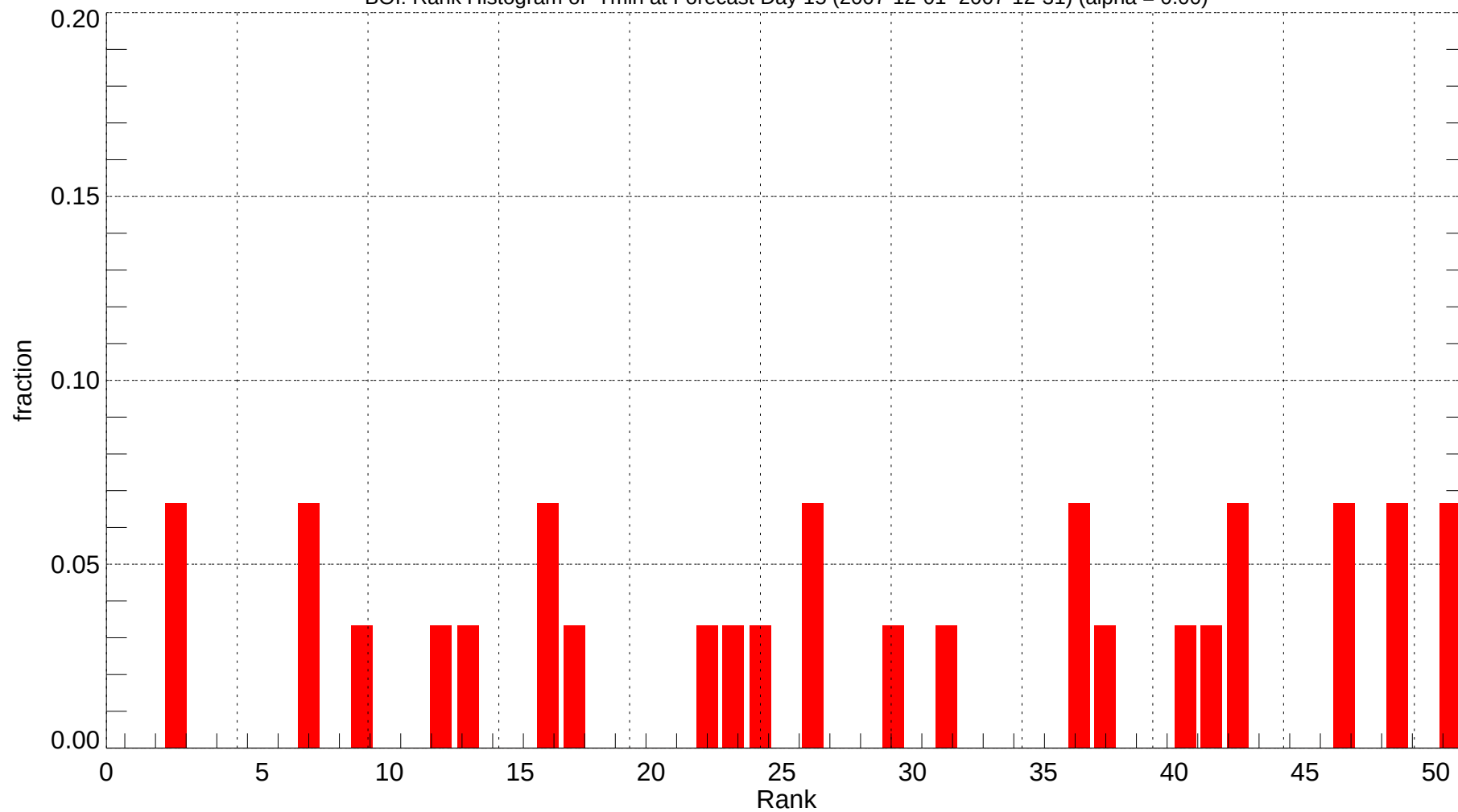
BOI: Rank Histogram of Tmin at Forecast Day 15 (2007-12-01~2007-12-31) (alpha = 0.00)
