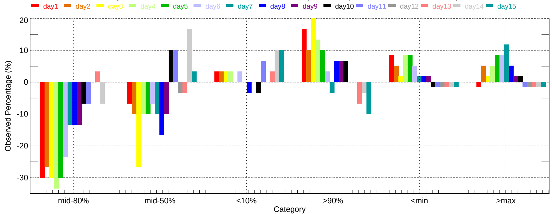
Observed Percentage Deviation of Ensembles - PHX: Max Temperature (2007-12-01~2007-12-31)
