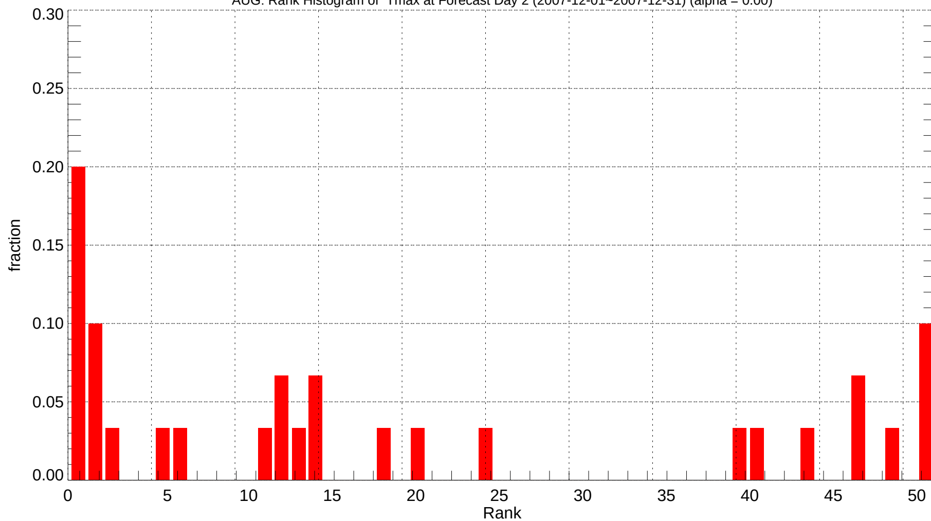
AUG: Rank Histogram of Tmax at Forecast Day 2 (2007-12-01~2007-12-31) (alpha = 0.00)
