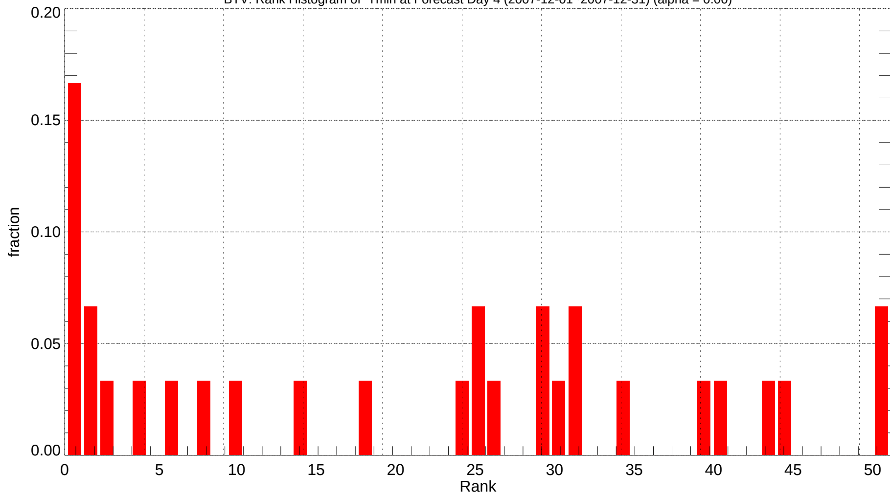
BTV: Rank Histogram of Tmin at Forecast Day 4 (2007-12-01~2007-12-31) (alpha = 0.00)
