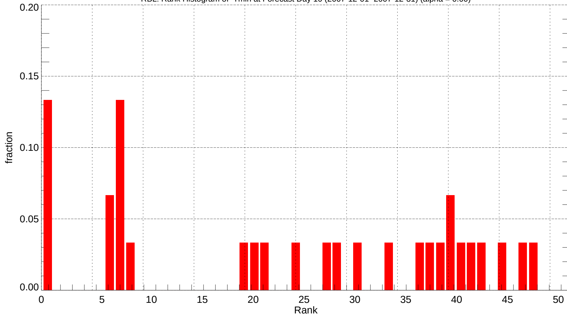
RBL: Rank Histogram of Tmin at Forecast Day 10 (2007-12-01~2007-12-31) (alpha = 0.00)
