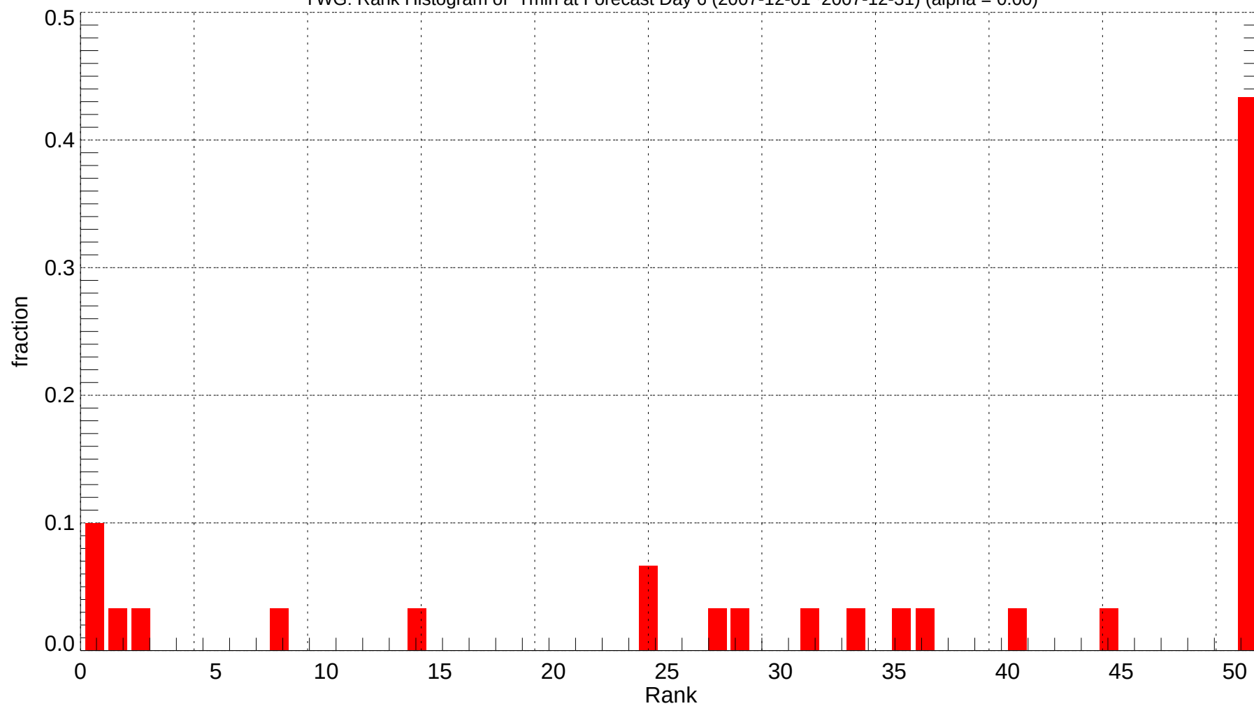
YWG: Rank Histogram of Tmin at Forecast Day 6 (2007-12-01~2007-12-31) (alpha = 0.00)
