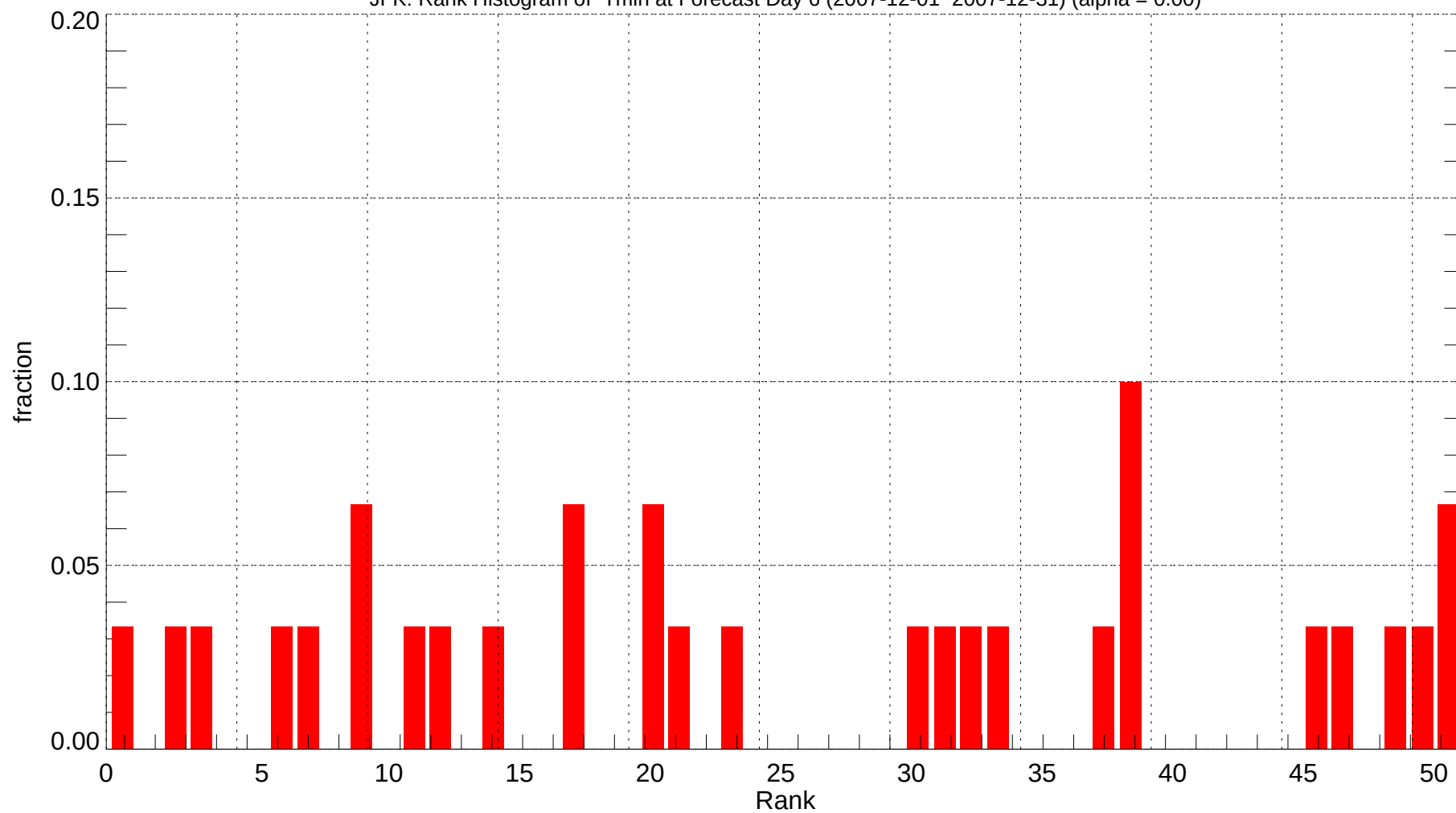
JFK: Rank Histogram of Tmin at Forecast Day 6 (2007-12-01~2007-12-31) (alpha = 0.00)
