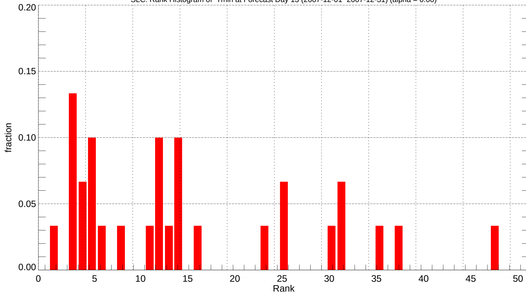
SLC: Rank Histogram of Tmin at Forecast Day 13 (2007-12-01~2007-12-31) (alpha = 0.00)
