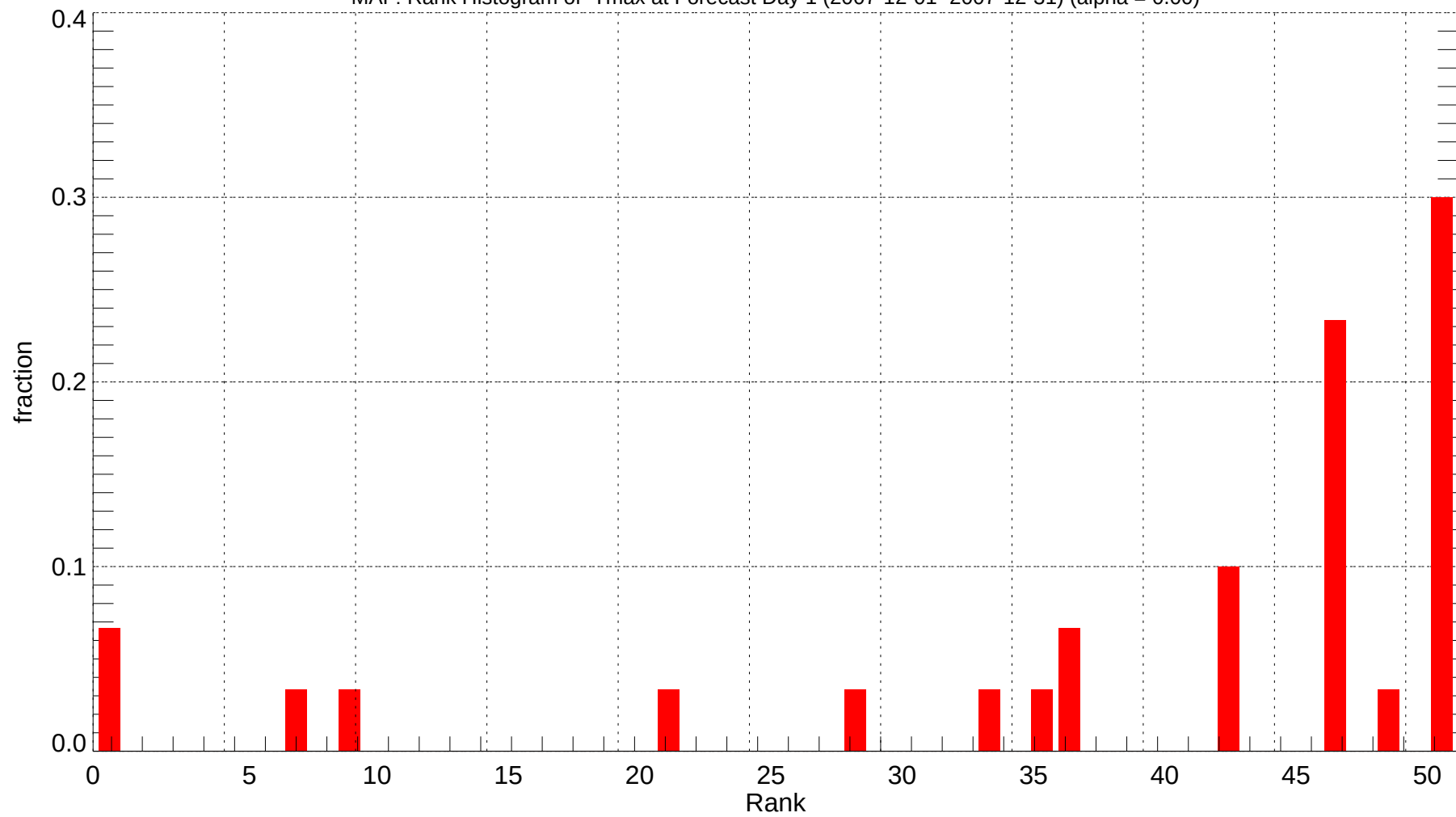
MAF: Rank Histogram of Tmax at Forecast Day 1 (2007-12-01~2007-12-31) (alpha = 0.00)
