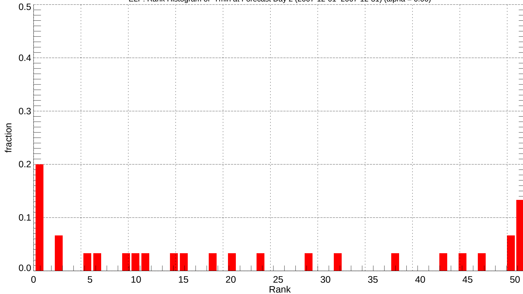
ELP: Rank Histogram of Tmin at Forecast Day 2 (2007-12-01~2007-12-31) (alpha = 0.00)
