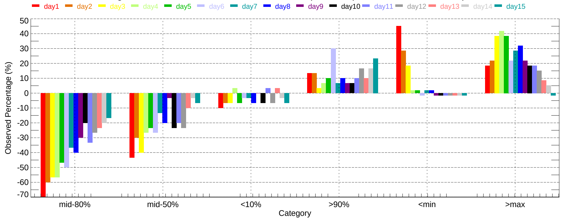
Observed Percentage Deviation of Ensembles - MCI: Max Temperature (2007-12-01~2007-12-31)
