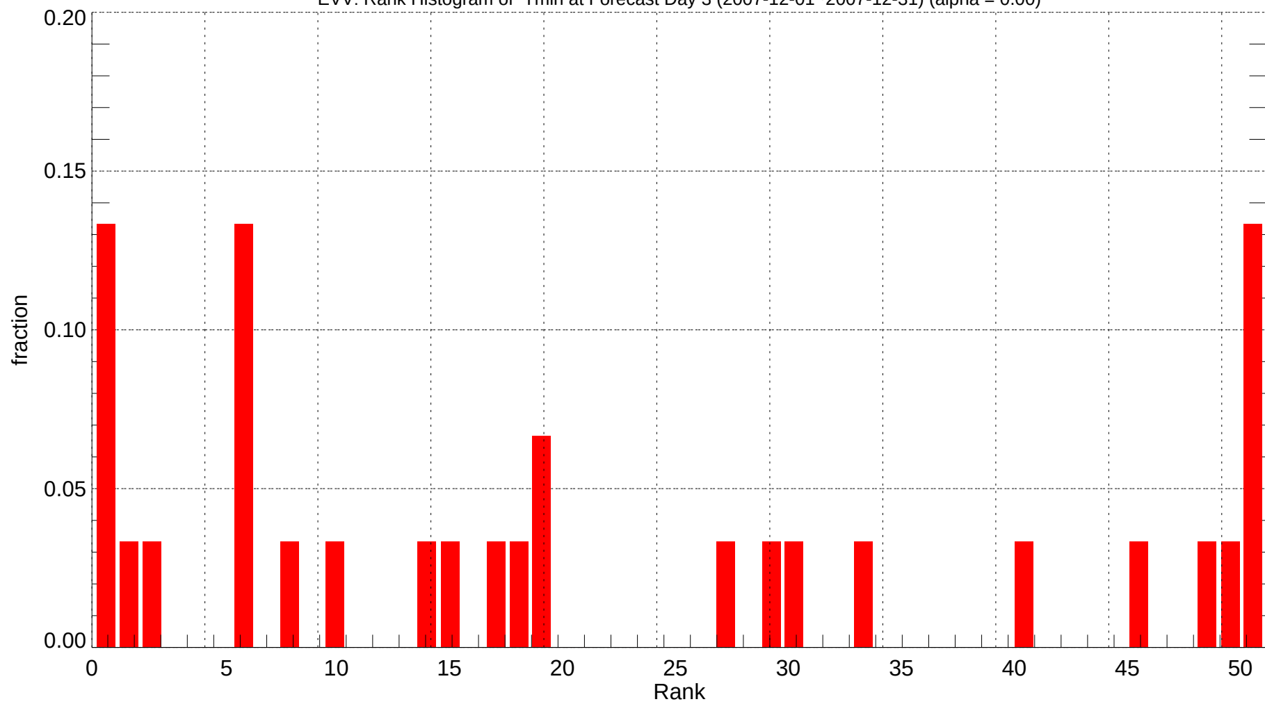
EVV: Rank Histogram of Tmin at Forecast Day 3 (2007-12-01~2007-12-31) (alpha = 0.00)
