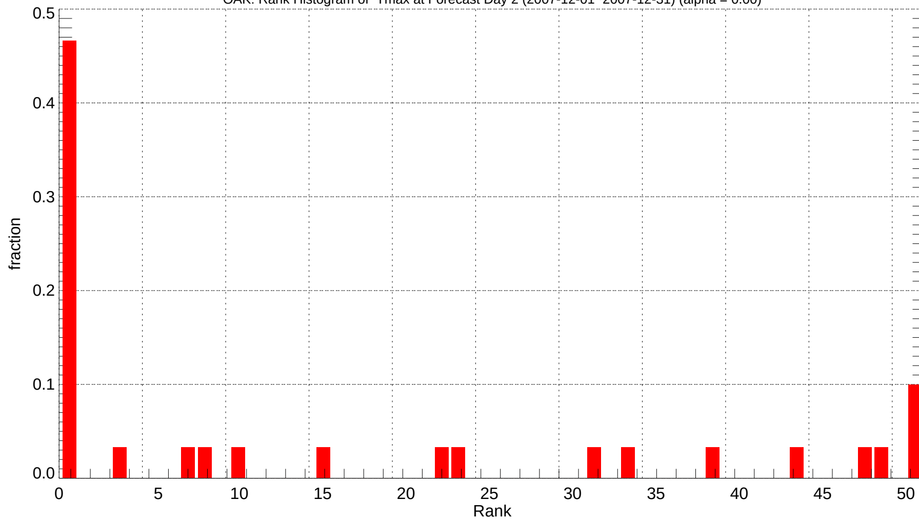
OAK: Rank Histogram of Tmax at Forecast Day 2 (2007-12-01~2007-12-31) (alpha = 0.00)
