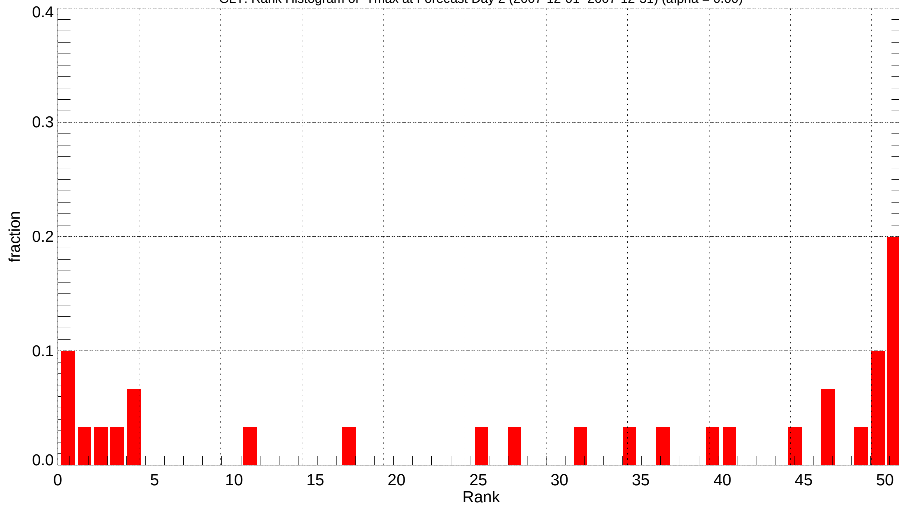
CLT: Rank Histogram of Tmax at Forecast Day 2 (2007-12-01~2007-12-31) (alpha = 0.00)
