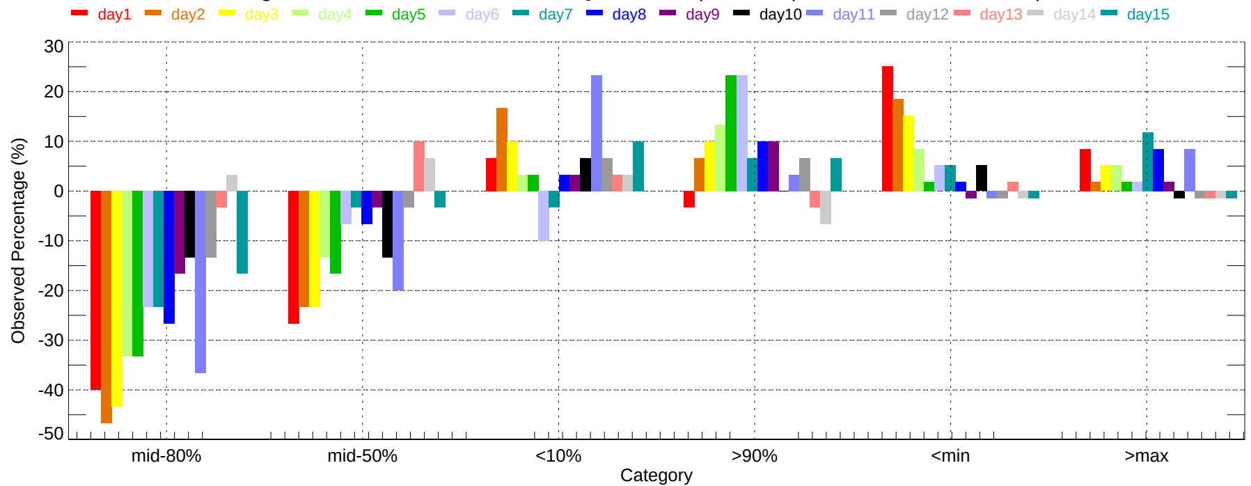
Observed Percentage Deviation of Ensembles - DBQ: Max Temperature (2007-12-01~2007-12-31)
