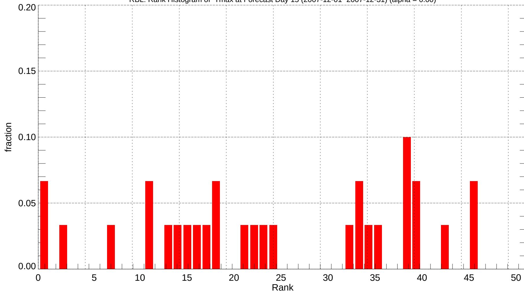
RBL: Rank Histogram of Tmax at Forecast Day 15 (2007-12-01~2007-12-31) (alpha = 0.00)
