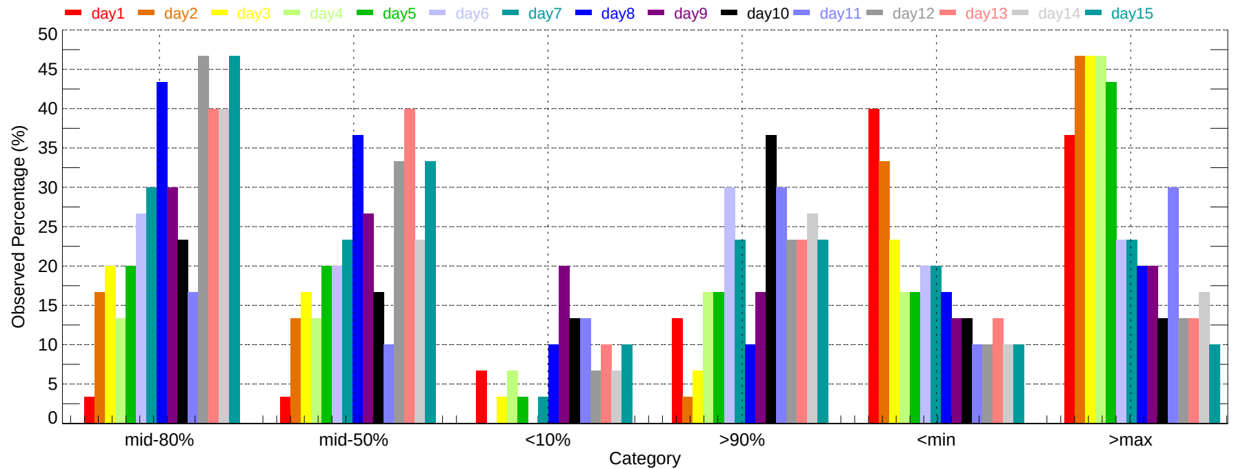
Observed Percentage of Ensembles - ALW: Max Temperature (2007-12-01~2007-12-31)
