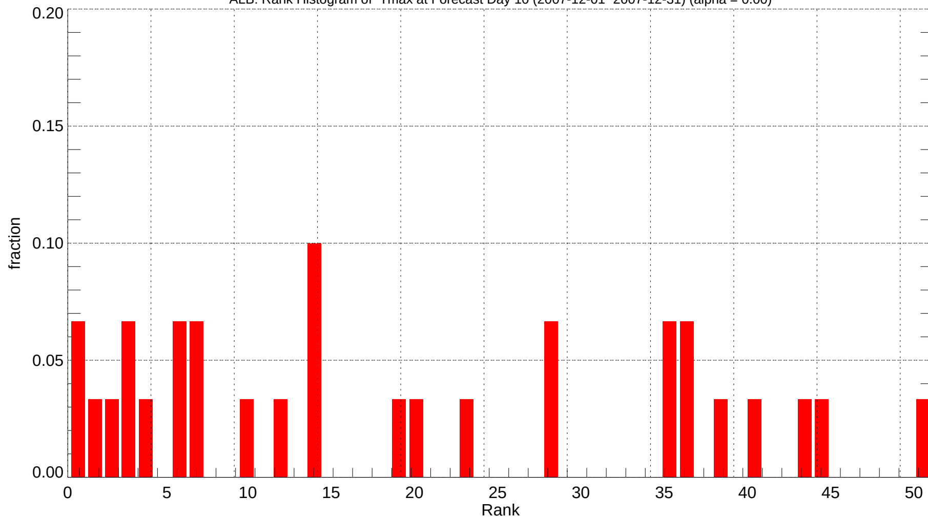
ALB: Rank Histogram of Tmax at Forecast Day 10 (2007-12-01~2007-12-31) (alpha = 0.00)
