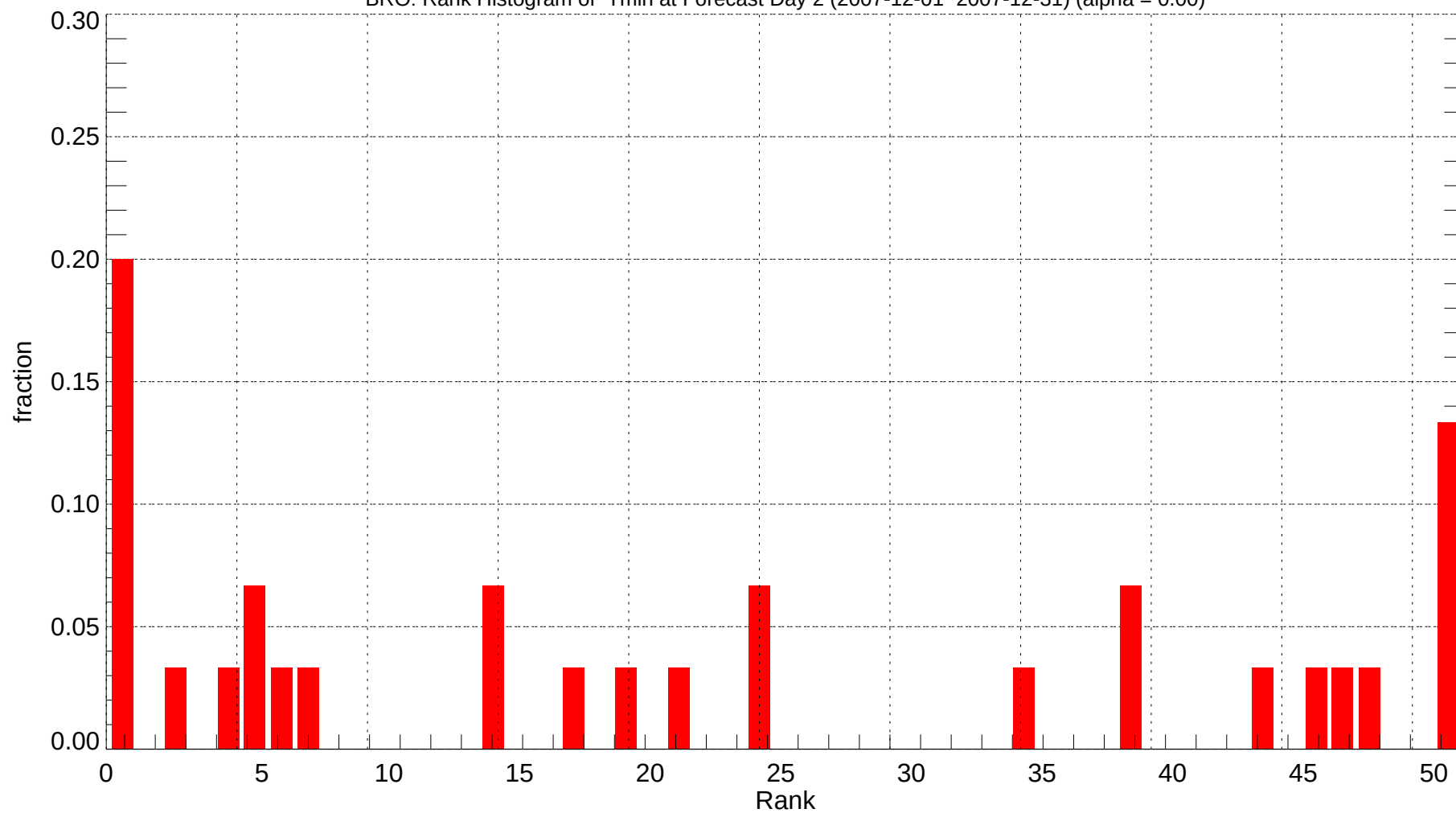
BRO: Rank Histogram of Tmin at Forecast Day 2 (2007-12-01~2007-12-31) (alpha = 0.00)
