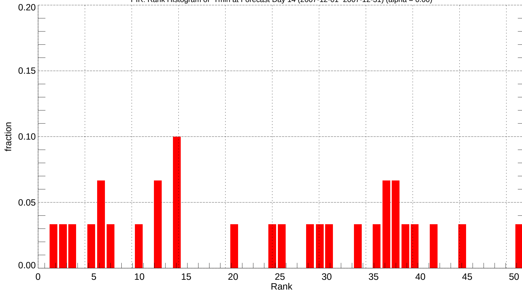
PIR: Rank Histogram of Tmin at Forecast Day 14 (2007-12-01~2007-12-31) (alpha = 0.00)
