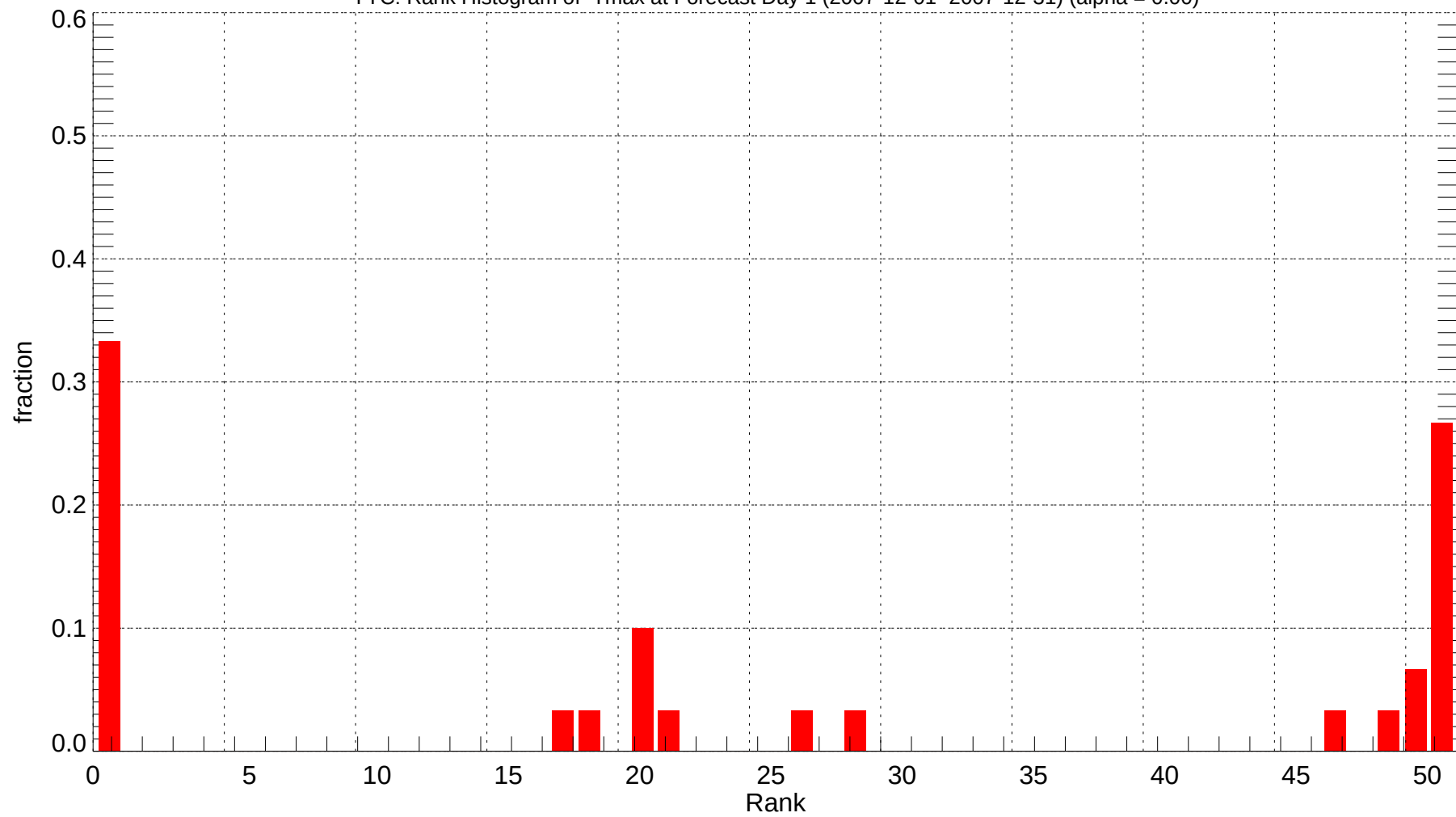
YYC: Rank Histogram of Tmax at Forecast Day 1 (2007-12-01~2007-12-31) (alpha = 0.00)
