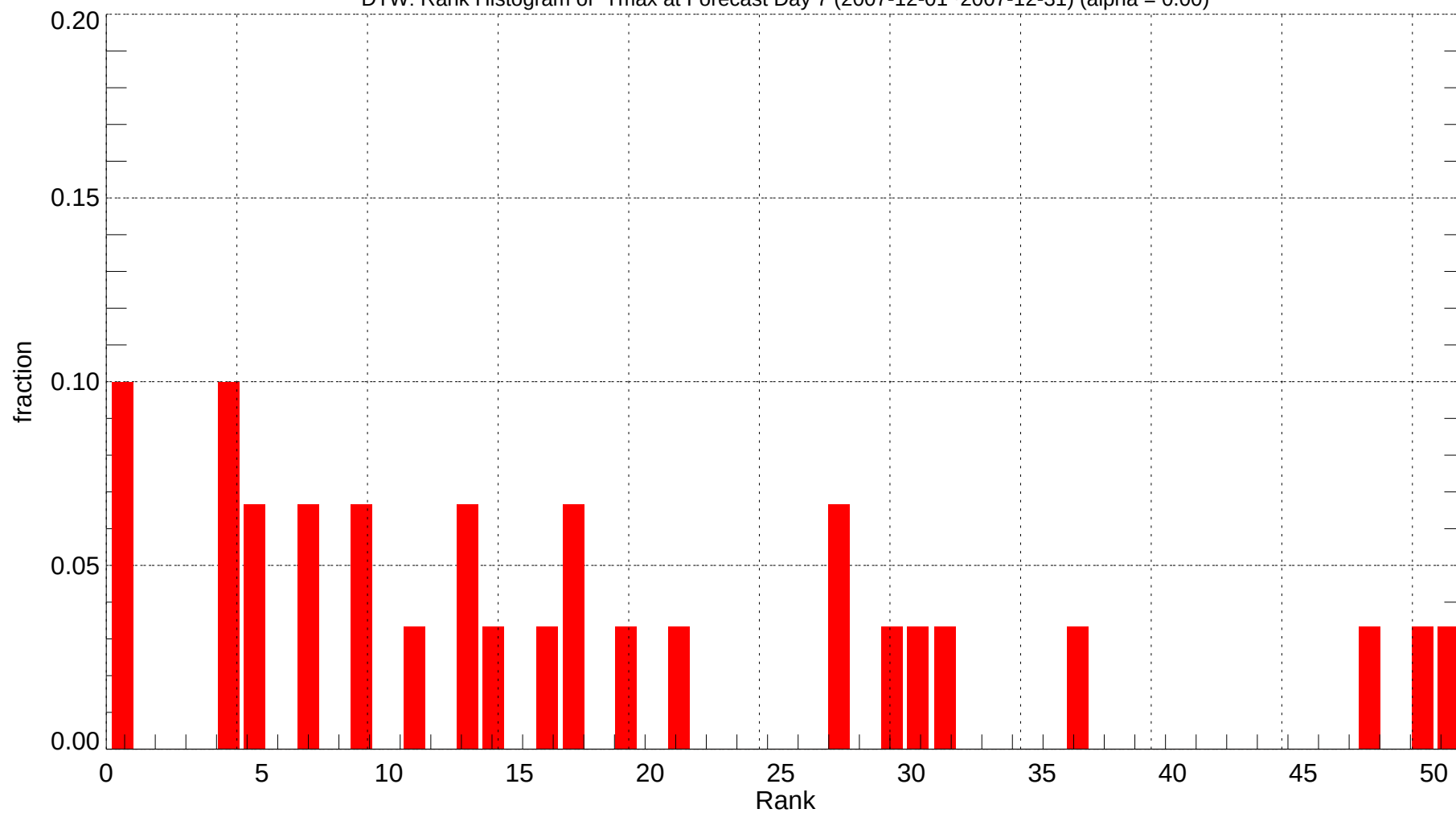
DTW: Rank Histogram of Tmax at Forecast Day 7 (2007-12-01~2007-12-31) (alpha = 0.00)
