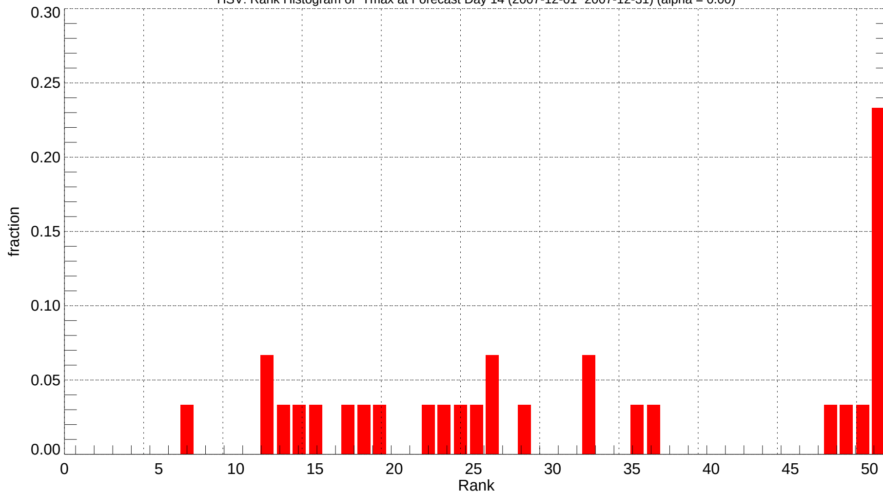
HSV: Rank Histogram of Tmax at Forecast Day 14 (2007-12-01~2007-12-31) (alpha = 0.00)
