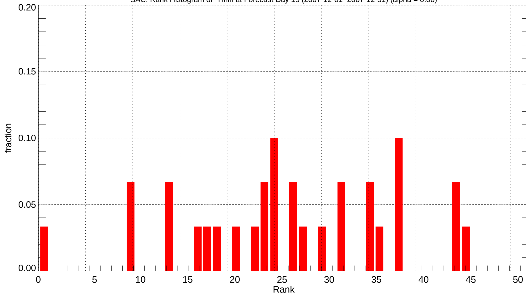
SAC: Rank Histogram of Tmin at Forecast Day 15 (2007-12-01~2007-12-31) (alpha = 0.00)
