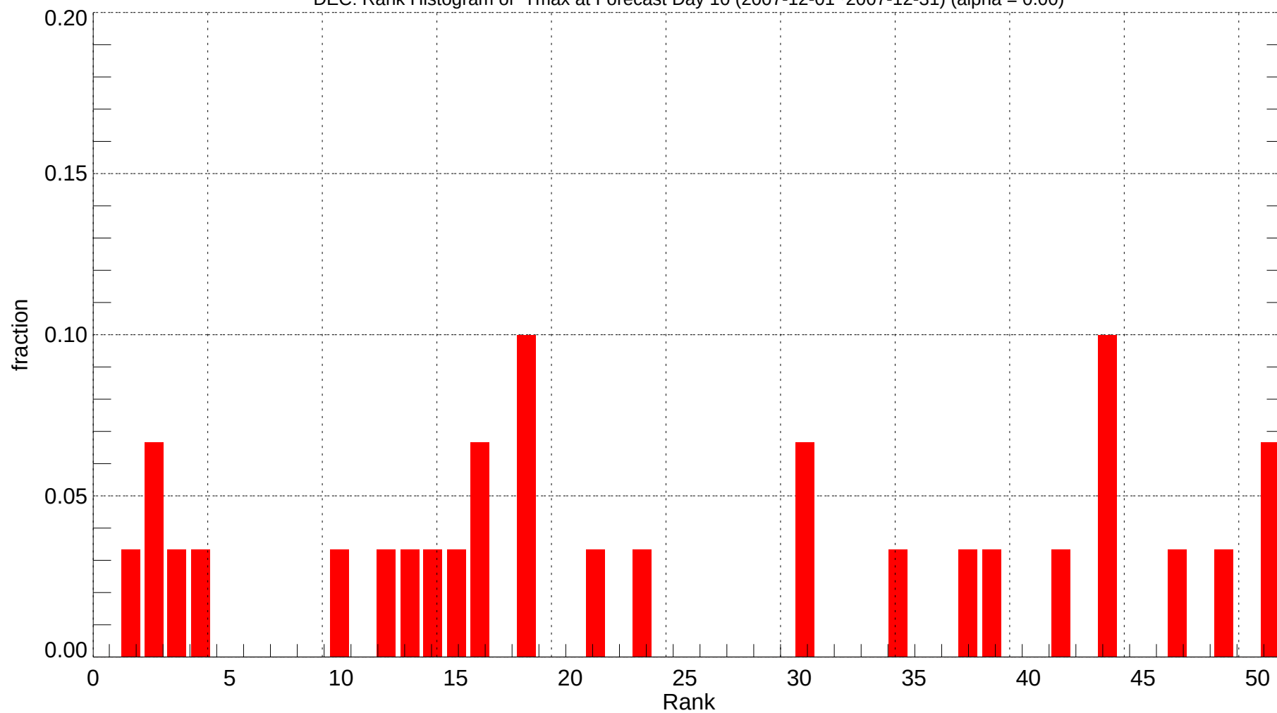
DEC: Rank Histogram of Tmax at Forecast Day 10 (2007-12-01~2007-12-31) (alpha = 0.00)
