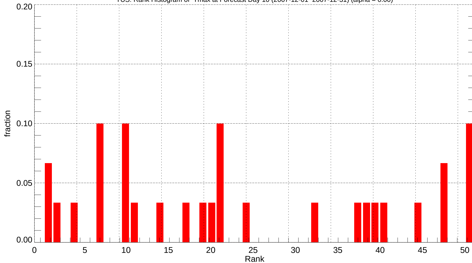
TUS: Rank Histogram of Tmax at Forecast Day 10 (2007-12-01~2007-12-31) (alpha = 0.00)
