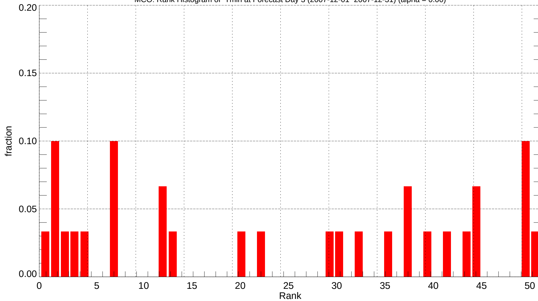
MCO: Rank Histogram of Tmin at Forecast Day 3 (2007-12-01~2007-12-31) (alpha = 0.00)
