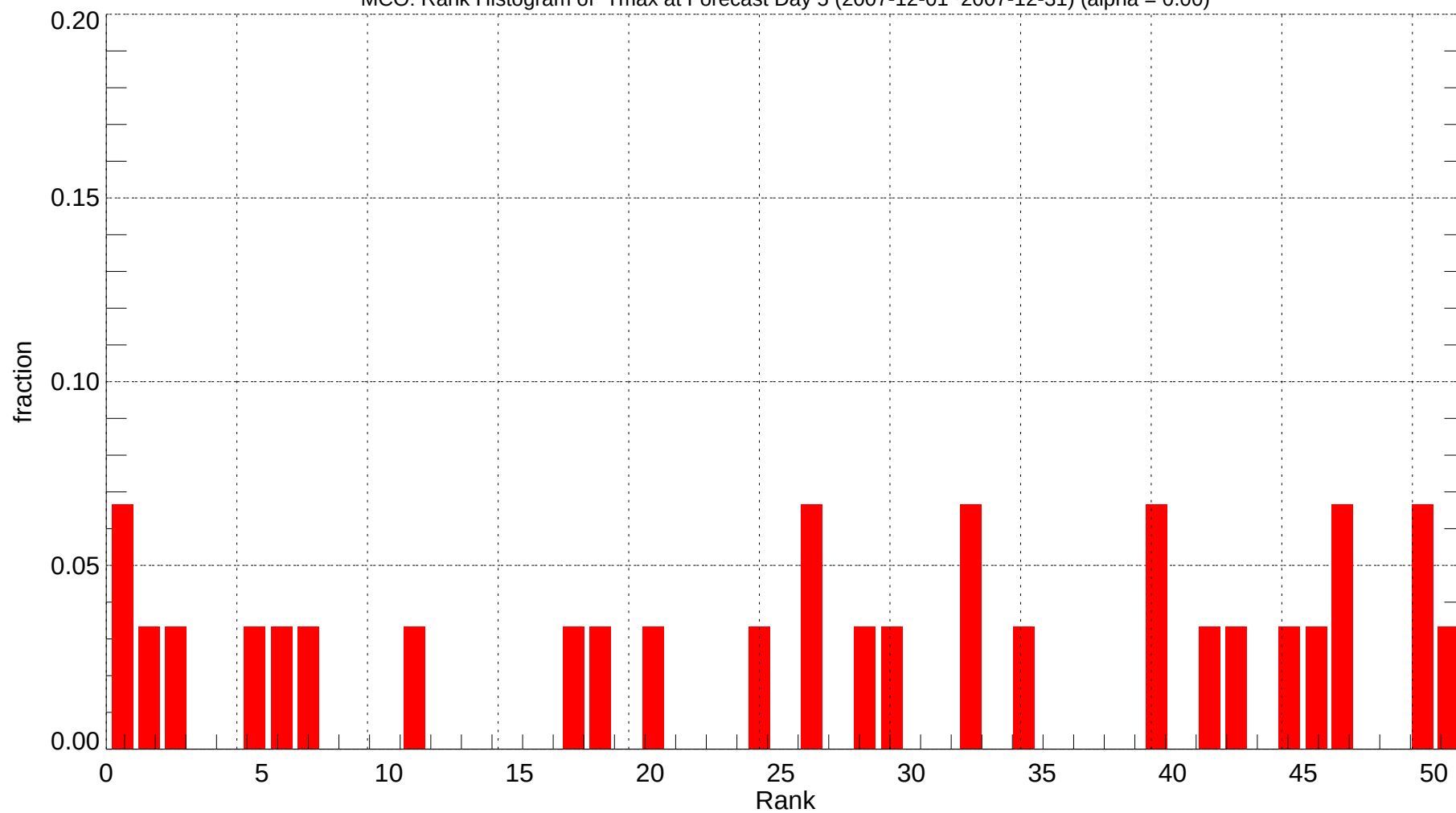
MCO: Rank Histogram of Tmax at Forecast Day 5 (2007-12-01~2007-12-31) (alpha = 0.00)
