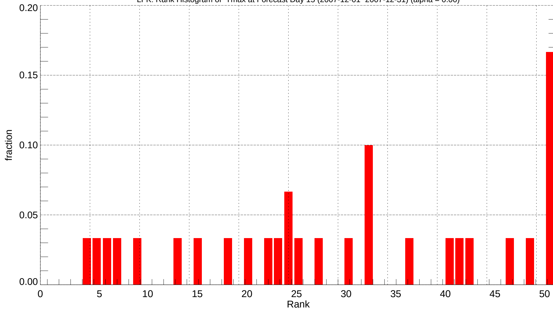
LFK: Rank Histogram of Tmax at Forecast Day 15 (2007-12-01~2007-12-31) (alpha = 0.00)
