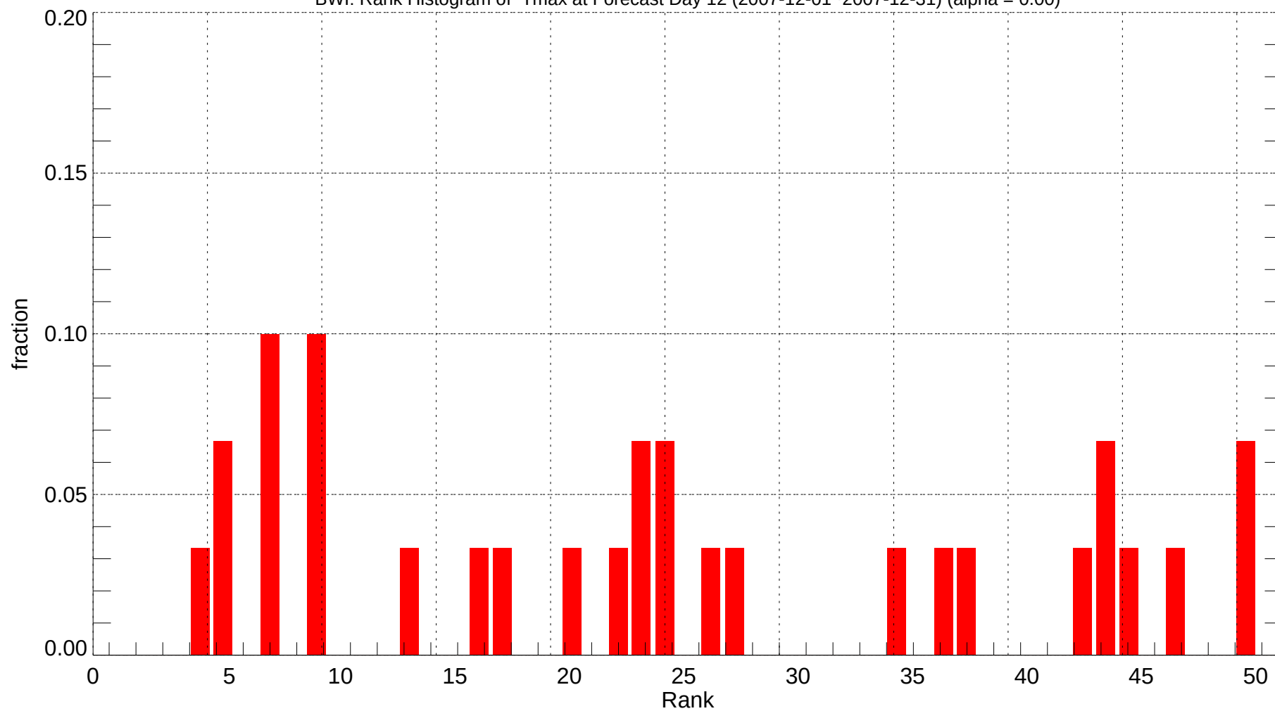
BWI: Rank Histogram of Tmax at Forecast Day 12 (2007-12-01~2007-12-31) (alpha = 0.00)
