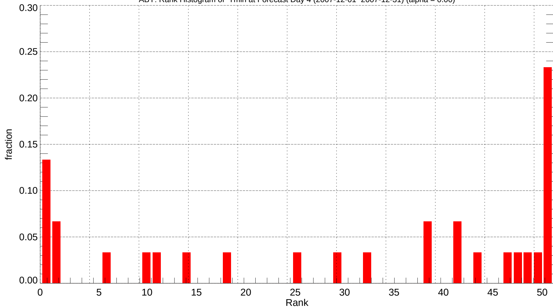
ABY: Rank Histogram of Tmin at Forecast Day 4 (2007-12-01~2007-12-31) (alpha = 0.00)
