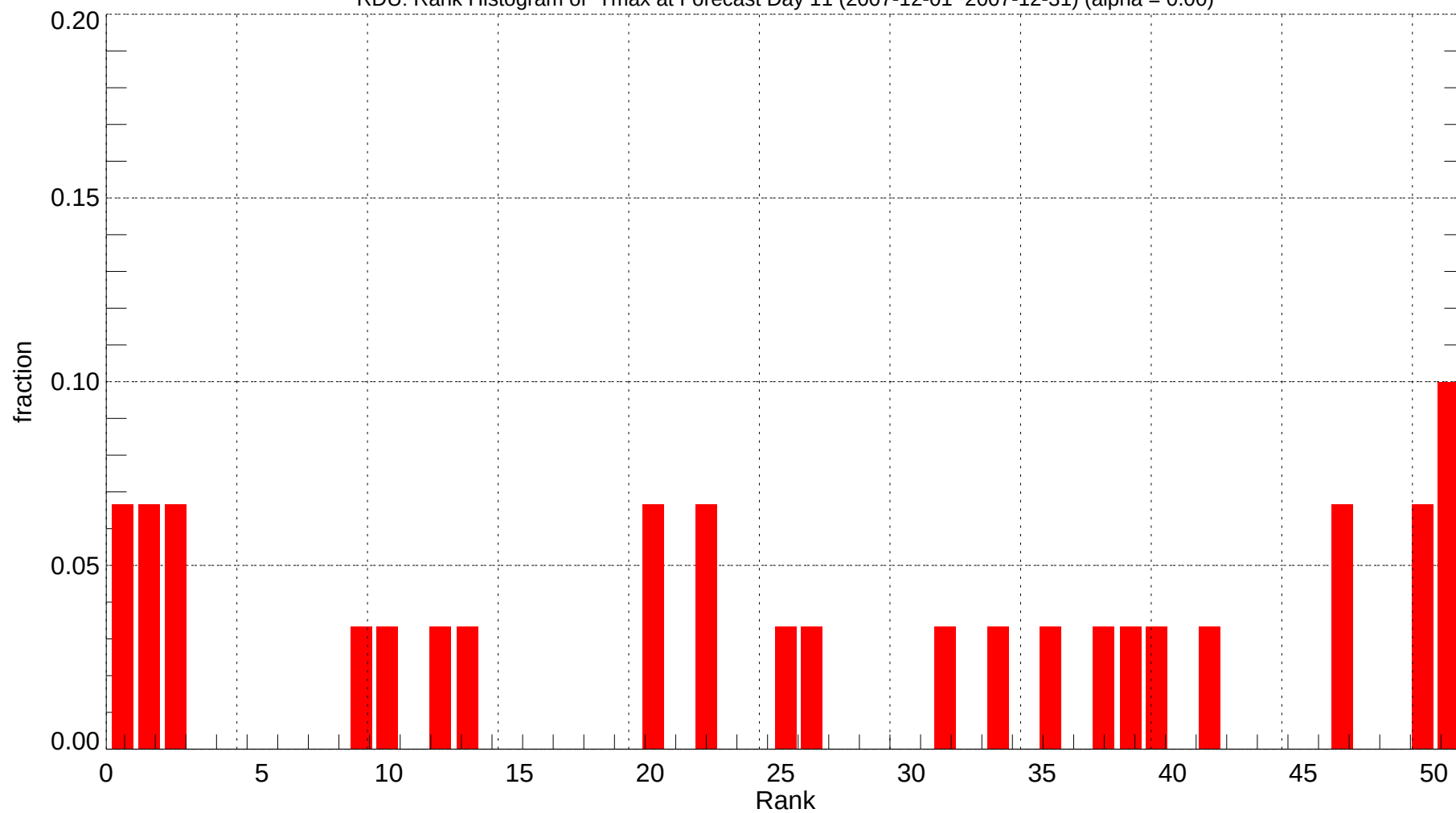
RDU: Rank Histogram of Tmax at Forecast Day 11 (2007-12-01~2007-12-31) (alpha = 0.00)
