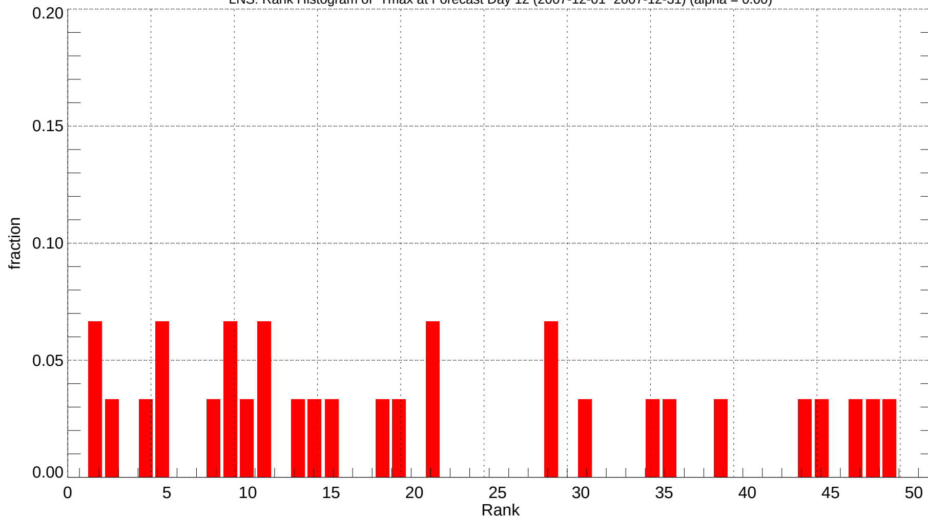
LNS: Rank Histogram of Tmax at Forecast Day 12 (2007-12-01~2007-12-31) (alpha = 0.00)
