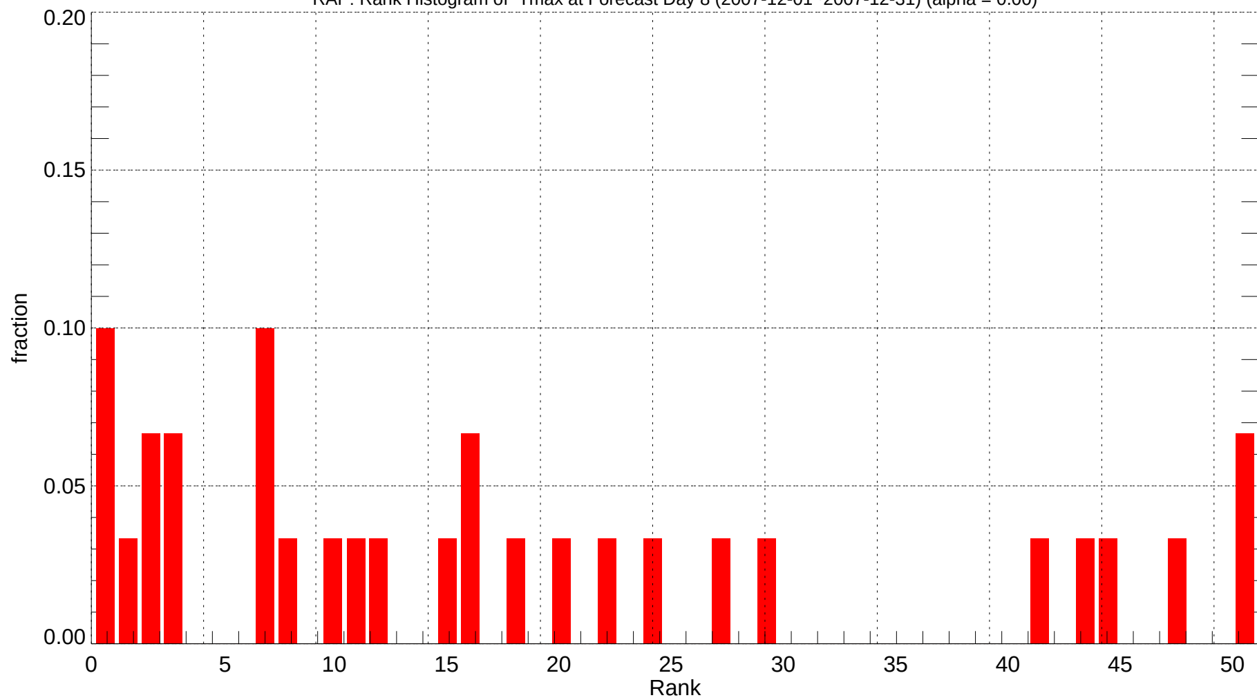
RAP: Rank Histogram of Tmax at Forecast Day 8 (2007-12-01~2007-12-31) (alpha = 0.00)
