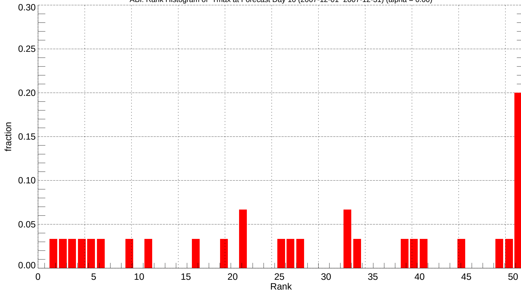
ABI: Rank Histogram of Tmax at Forecast Day 10 (2007-12-01~2007-12-31) (alpha = 0.00)
