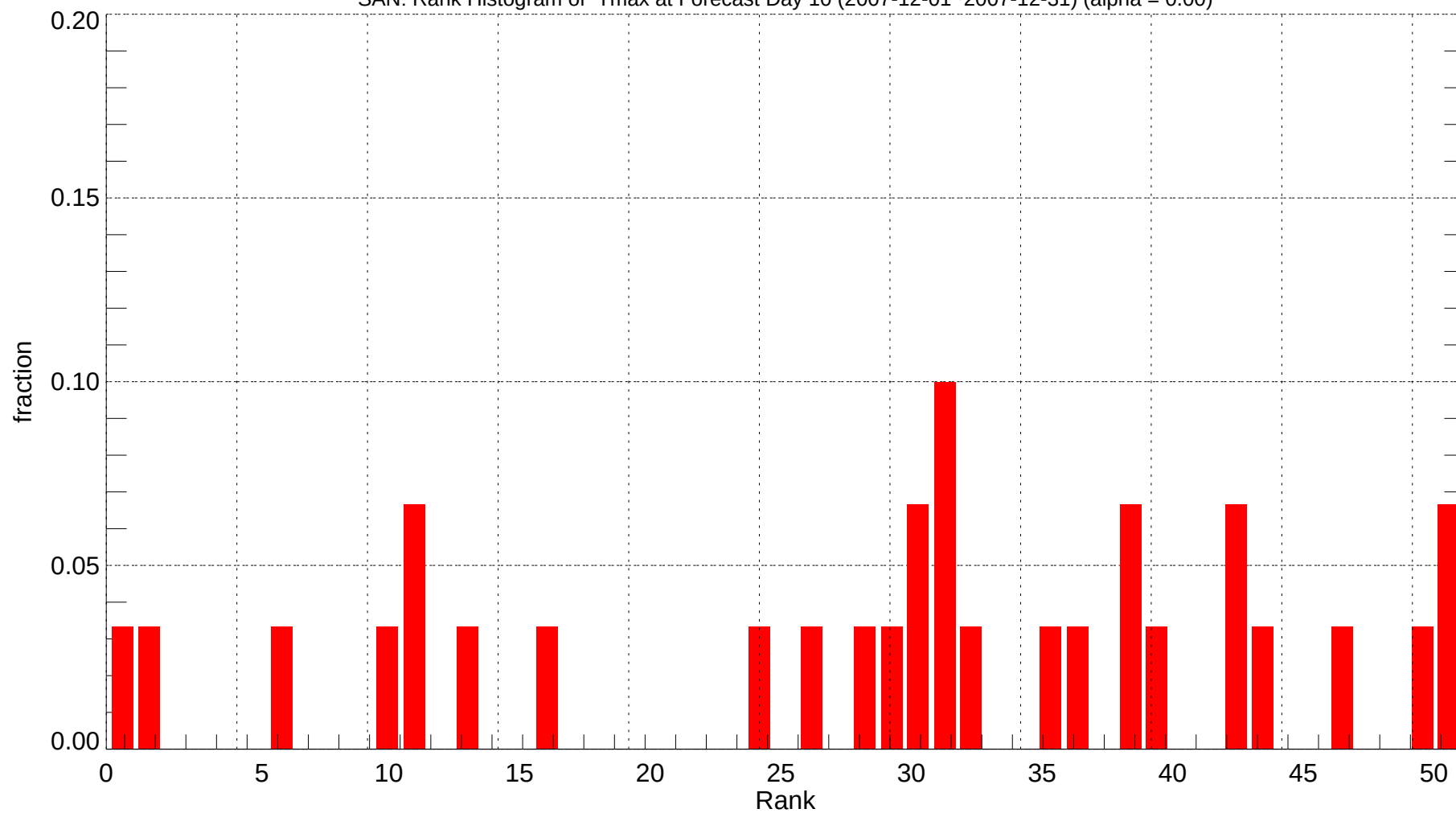
SAN: Rank Histogram of Tmax at Forecast Day 10 (2007-12-01~2007-12-31) (alpha = 0.00)
