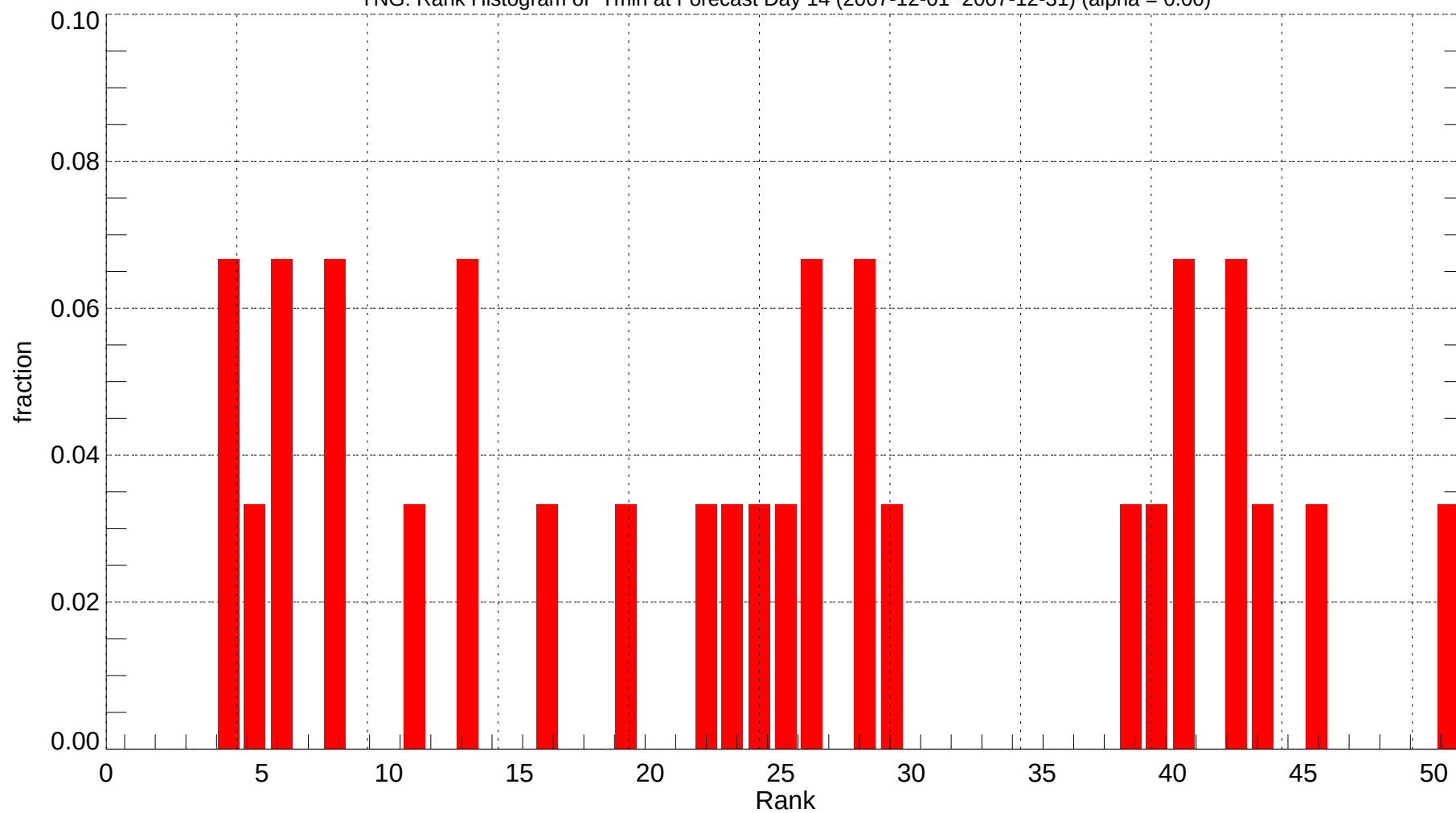
YNG: Rank Histogram of Tmin at Forecast Day 14 (2007-12-01~2007-12-31) (alpha = 0.00)
