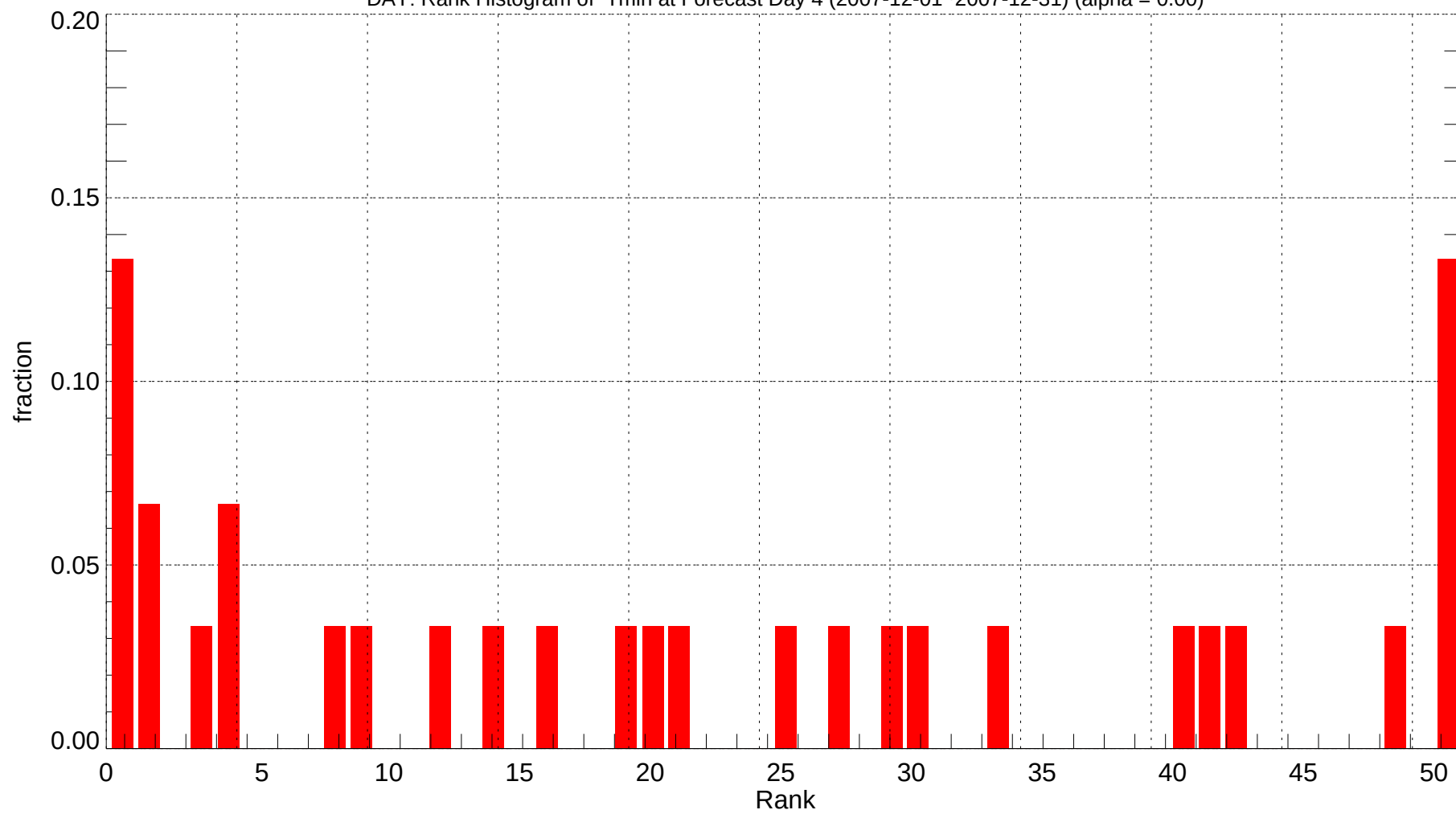
DAY: Rank Histogram of Tmin at Forecast Day 4 (2007-12-01~2007-12-31) (alpha = 0.00)
