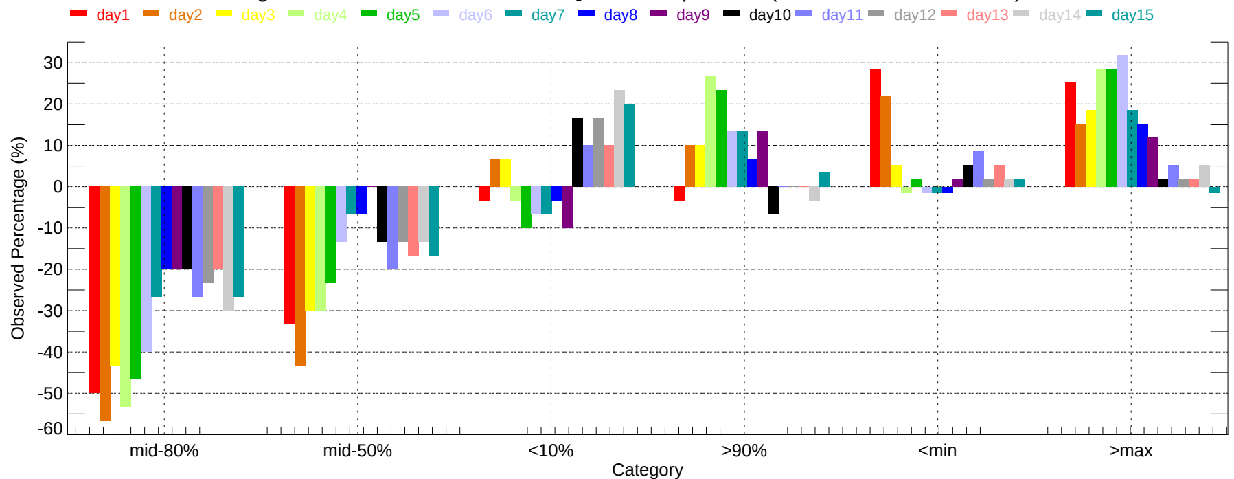
Observed Percentage Deviation of Ensembles - ABQ: Min Temperature (2007-12-01~2007-12-31)
