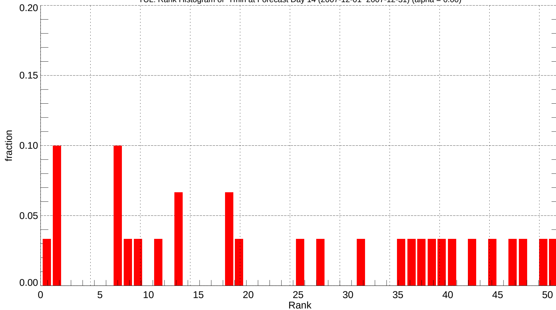
TUL: Rank Histogram of Tmin at Forecast Day 14 (2007-12-01~2007-12-31) (alpha = 0.00)
