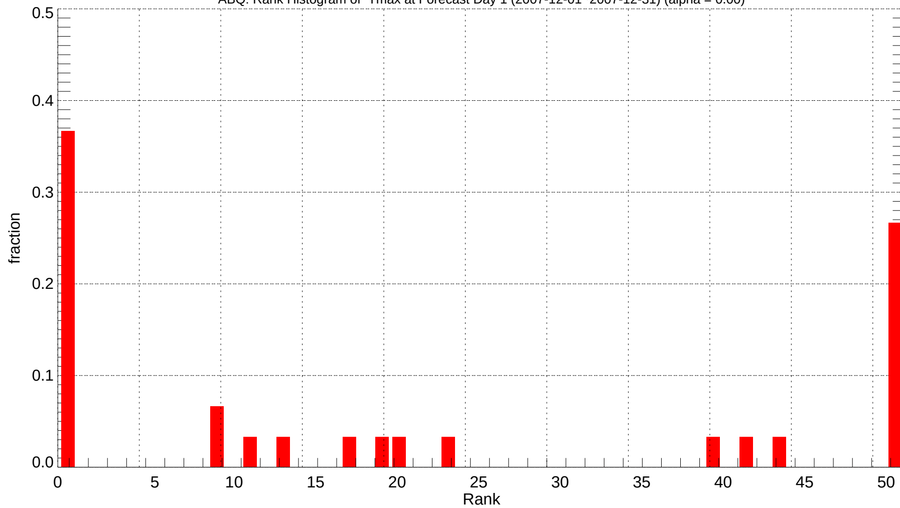
ABQ: Rank Histogram of Tmax at Forecast Day 1 (2007-12-01~2007-12-31) (alpha = 0.00)
