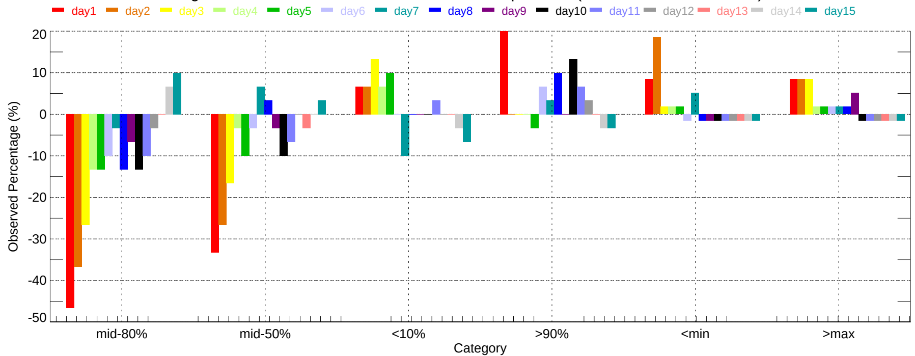
Observed Percentage Deviation of Ensembles - PWM: Min Temperature (2007-12-01~2007-12-31)
