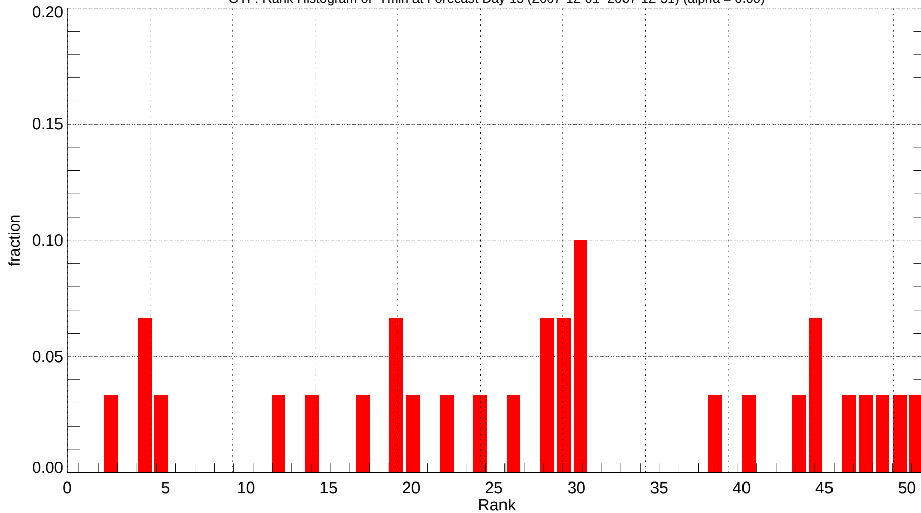
GTF: Rank Histogram of Tmin at Forecast Day 13 (2007-12-01~2007-12-31) (alpha = 0.00)
