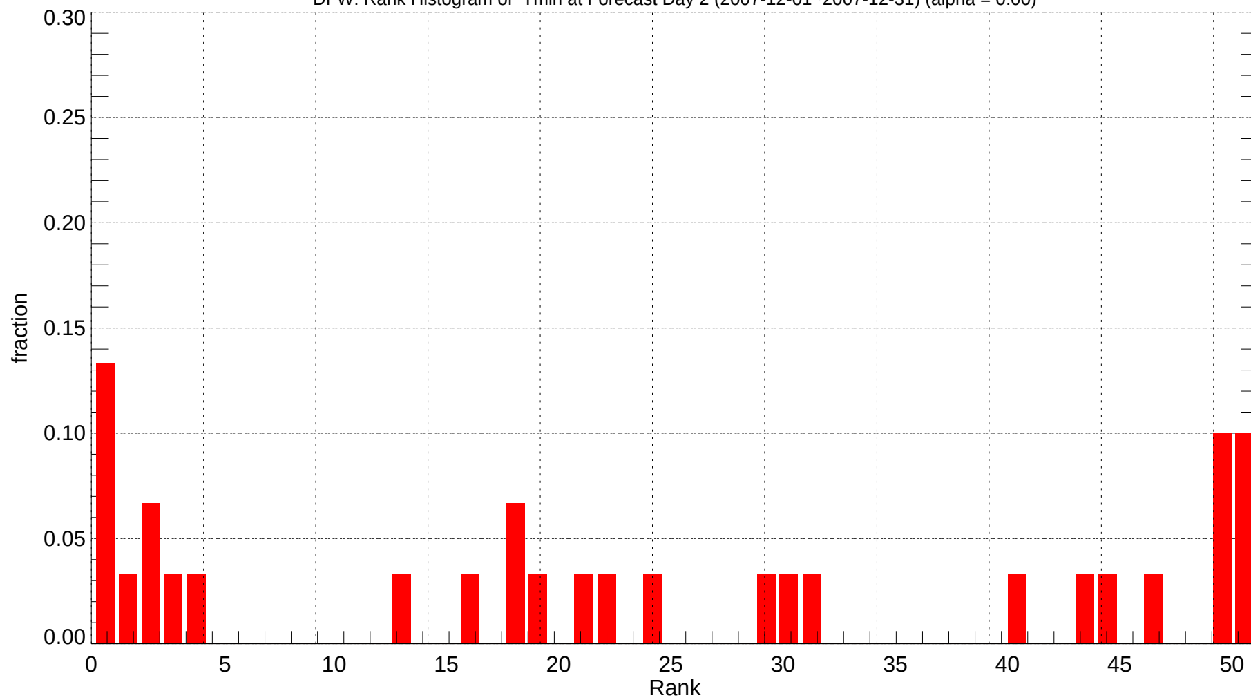
DFW: Rank Histogram of Tmin at Forecast Day 2 (2007-12-01~2007-12-31) (alpha = 0.00)
