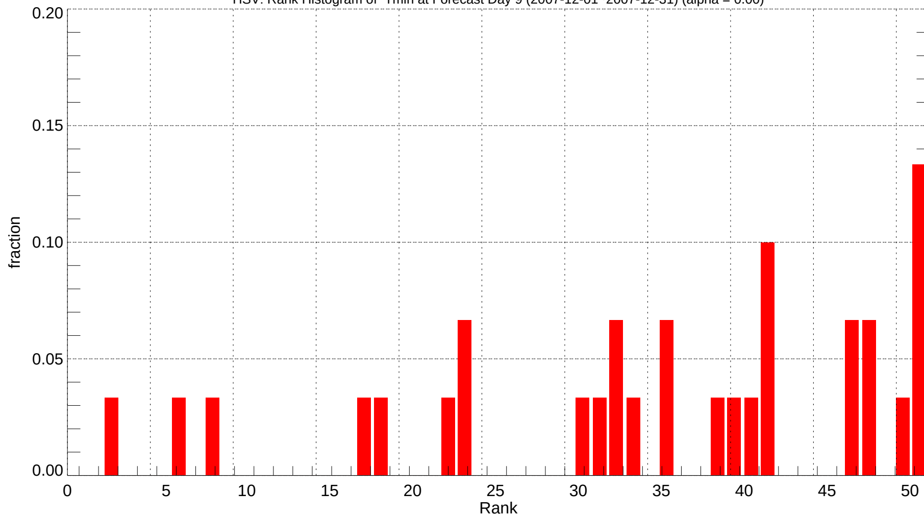
HSV: Rank Histogram of Tmin at Forecast Day 9 (2007-12-01~2007-12-31) (alpha = 0.00)
