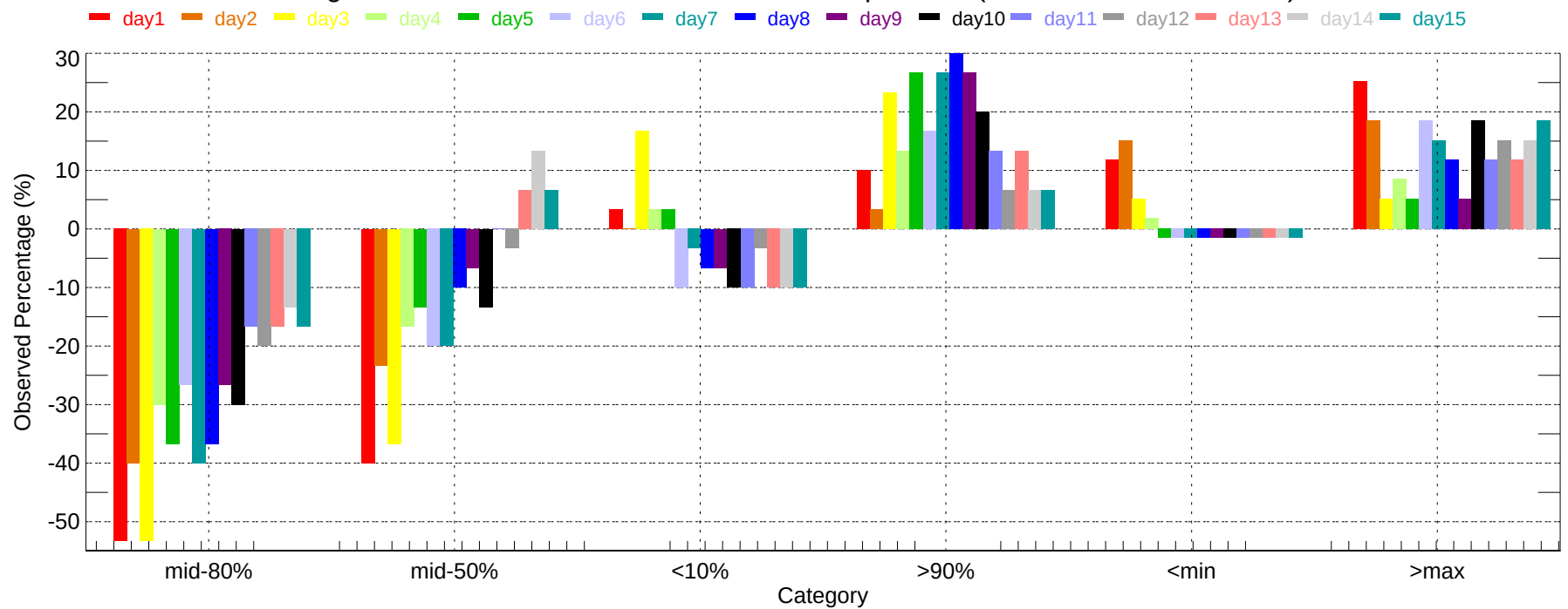
Observed Percentage Deviation of Ensembles - HSV: Min Temperature (2007-12-01~2007-12-31)
