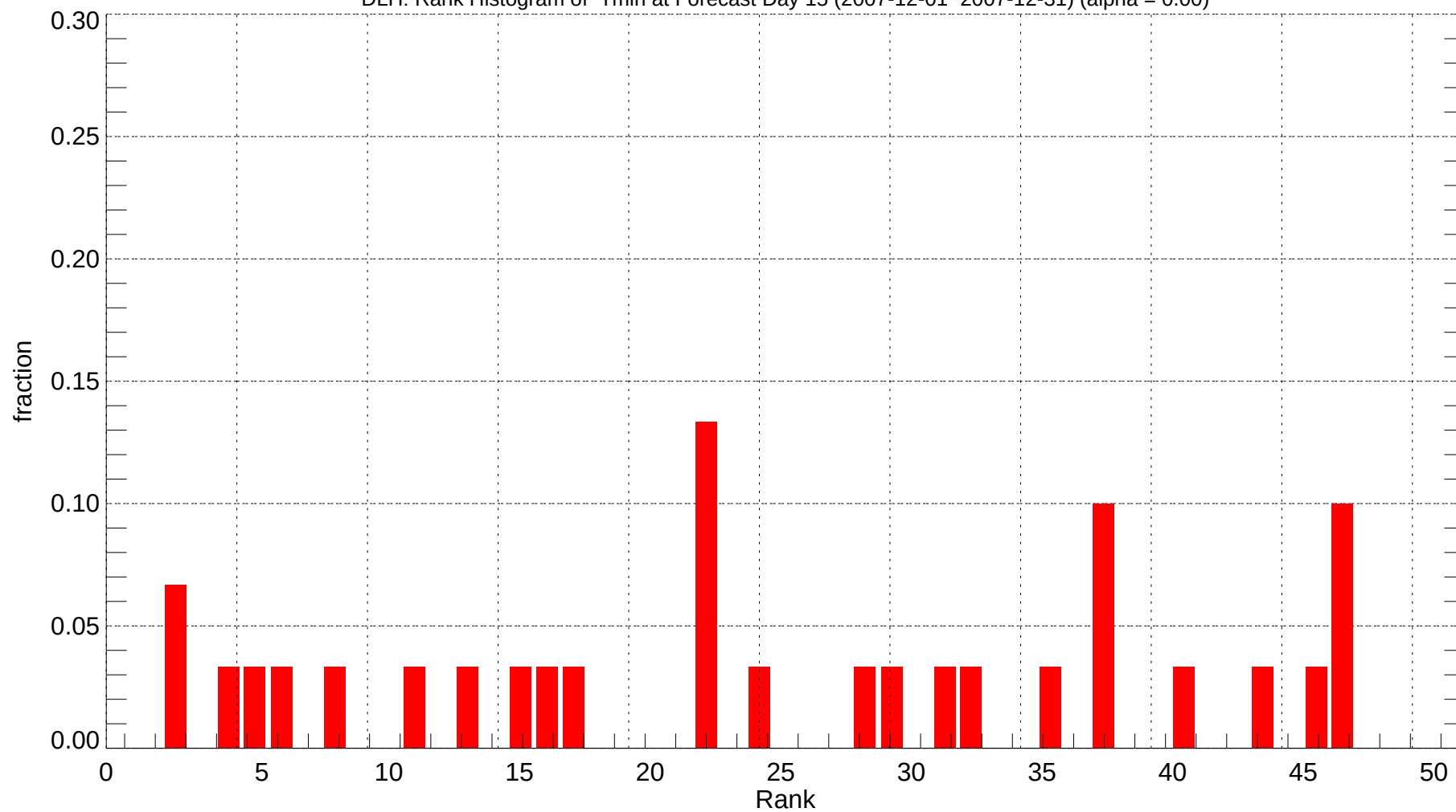
DLH: Rank Histogram of Tmin at Forecast Day 15 (2007-12-01~2007-12-31) (alpha = 0.00)
