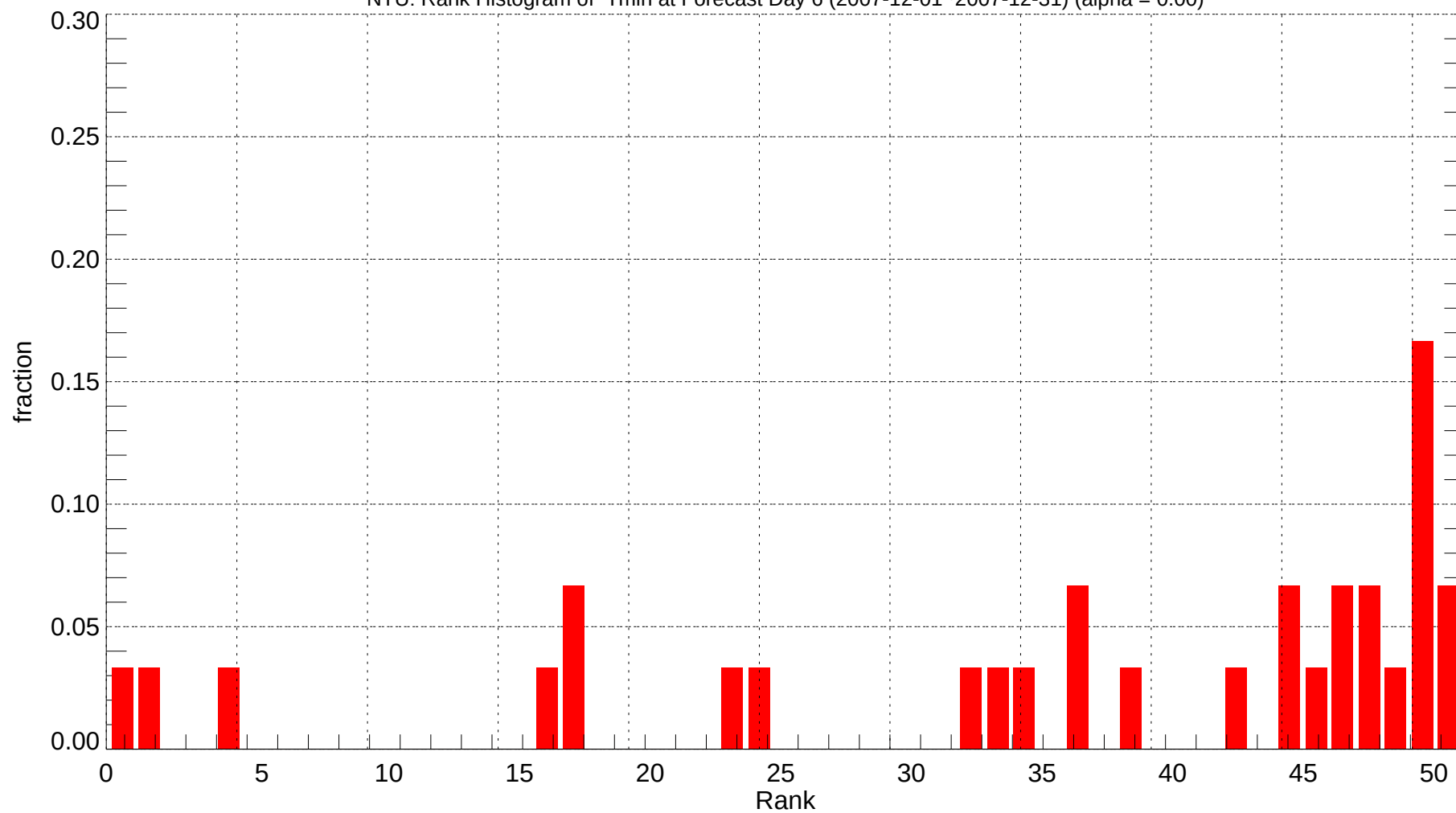
NTU: Rank Histogram of Tmin at Forecast Day 6 (2007-12-01~2007-12-31) (alpha = 0.00)
