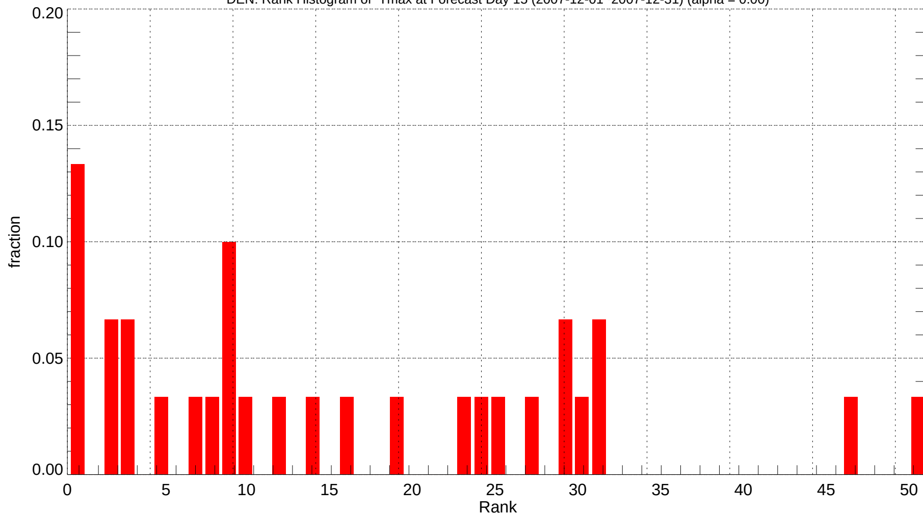
DEN: Rank Histogram of Tmax at Forecast Day 15 (2007-12-01~2007-12-31) (alpha = 0.00)
