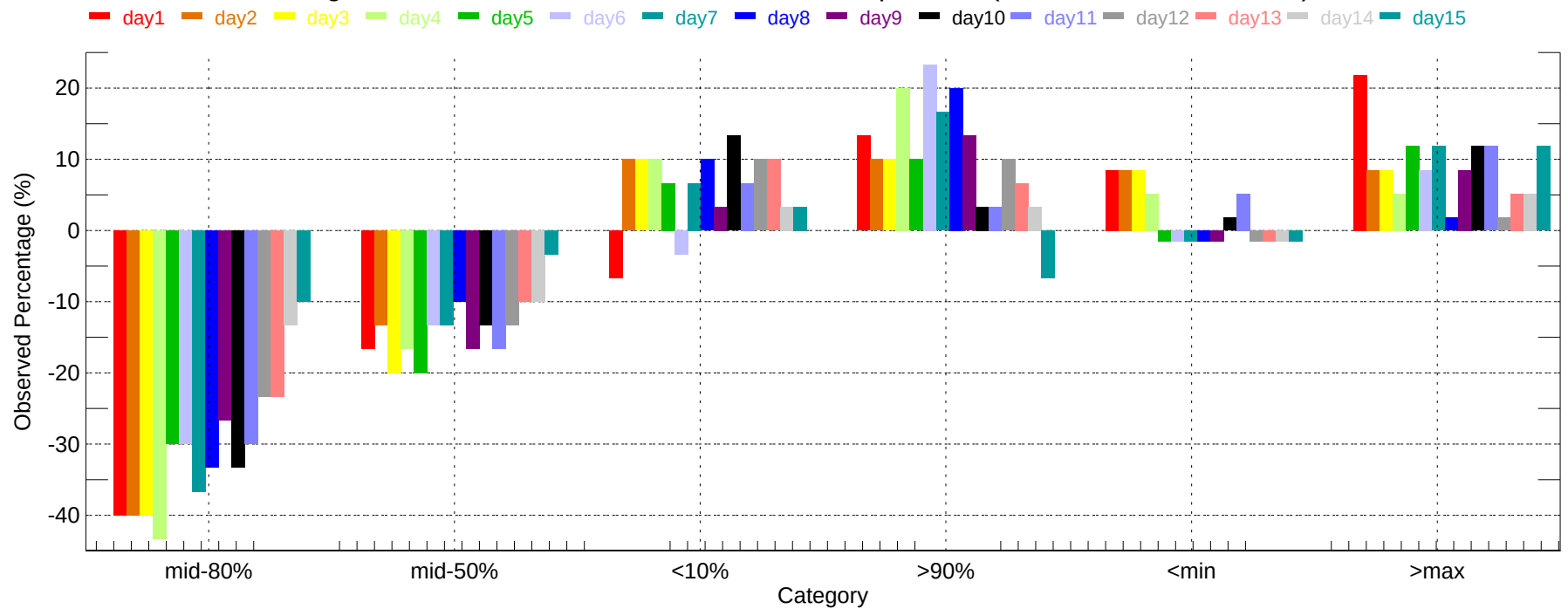
Observed Percentage Deviation of Ensembles - DFW: Max Temperature (2007-12-01~2007-12-31)
