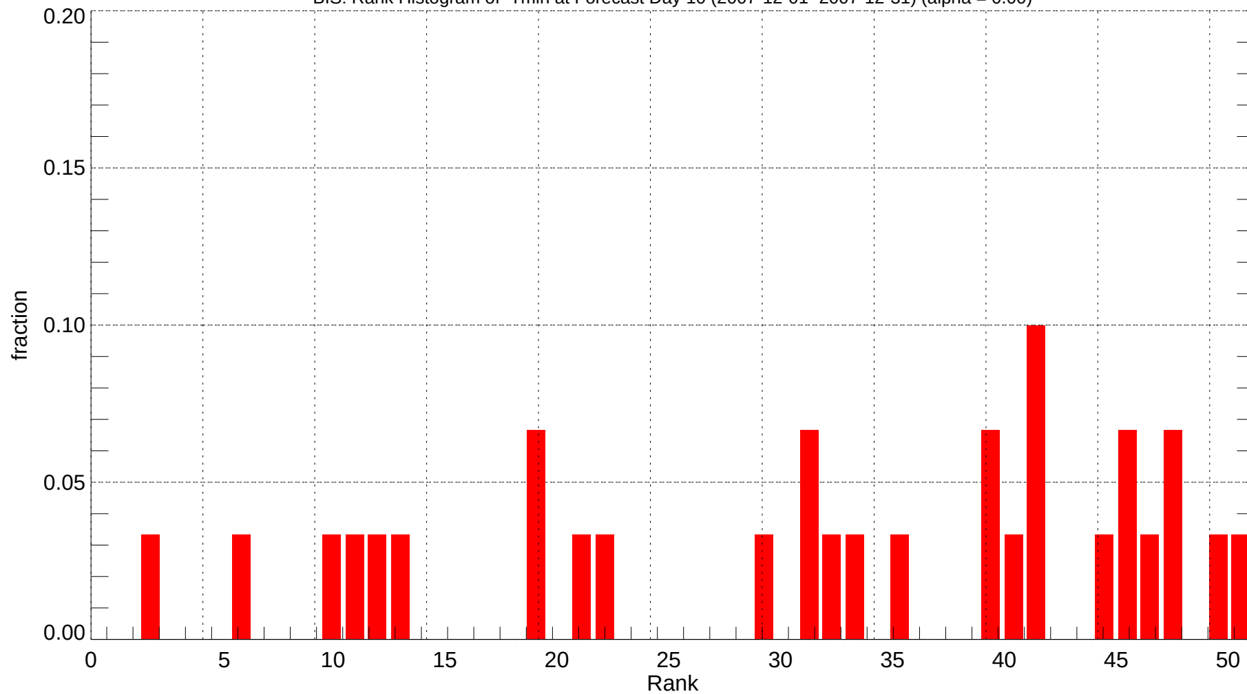
BIS: Rank Histogram of Tmin at Forecast Day 10 (2007-12-01~2007-12-31) (alpha = 0.00)
