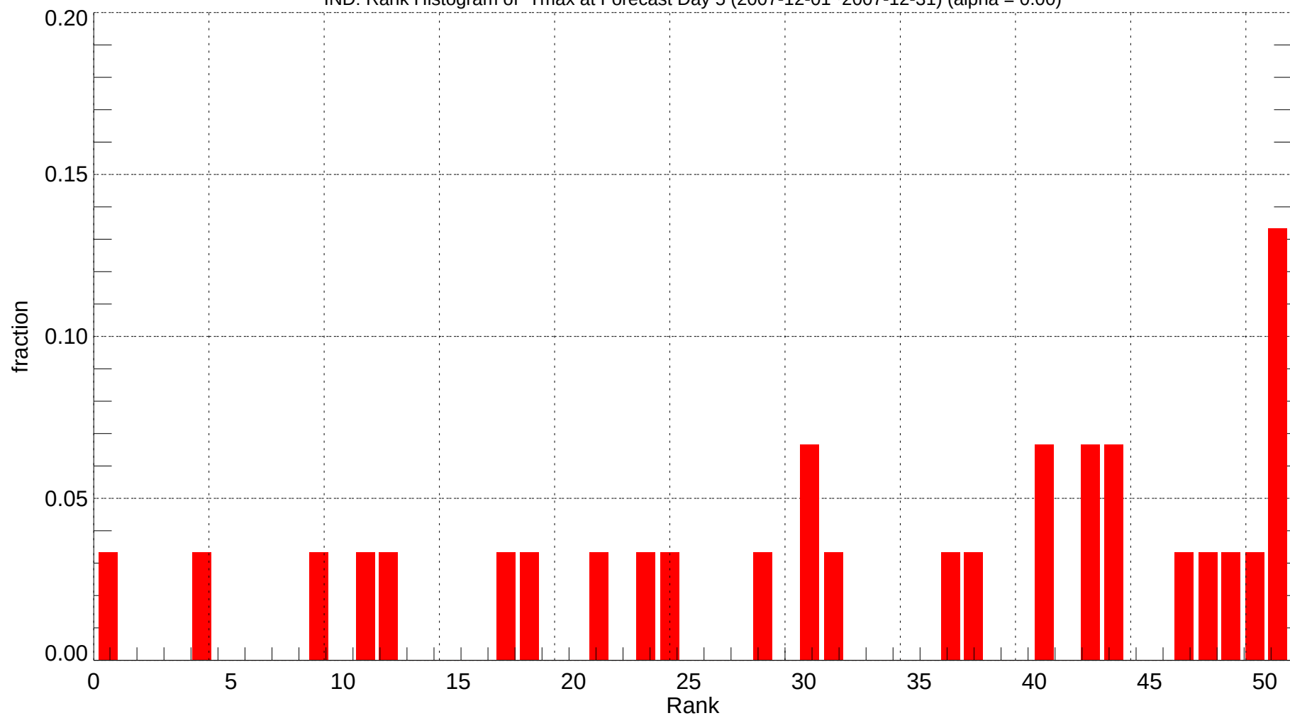
IND: Rank Histogram of Tmax at Forecast Day 5 (2007-12-01~2007-12-31) (alpha = 0.00)
