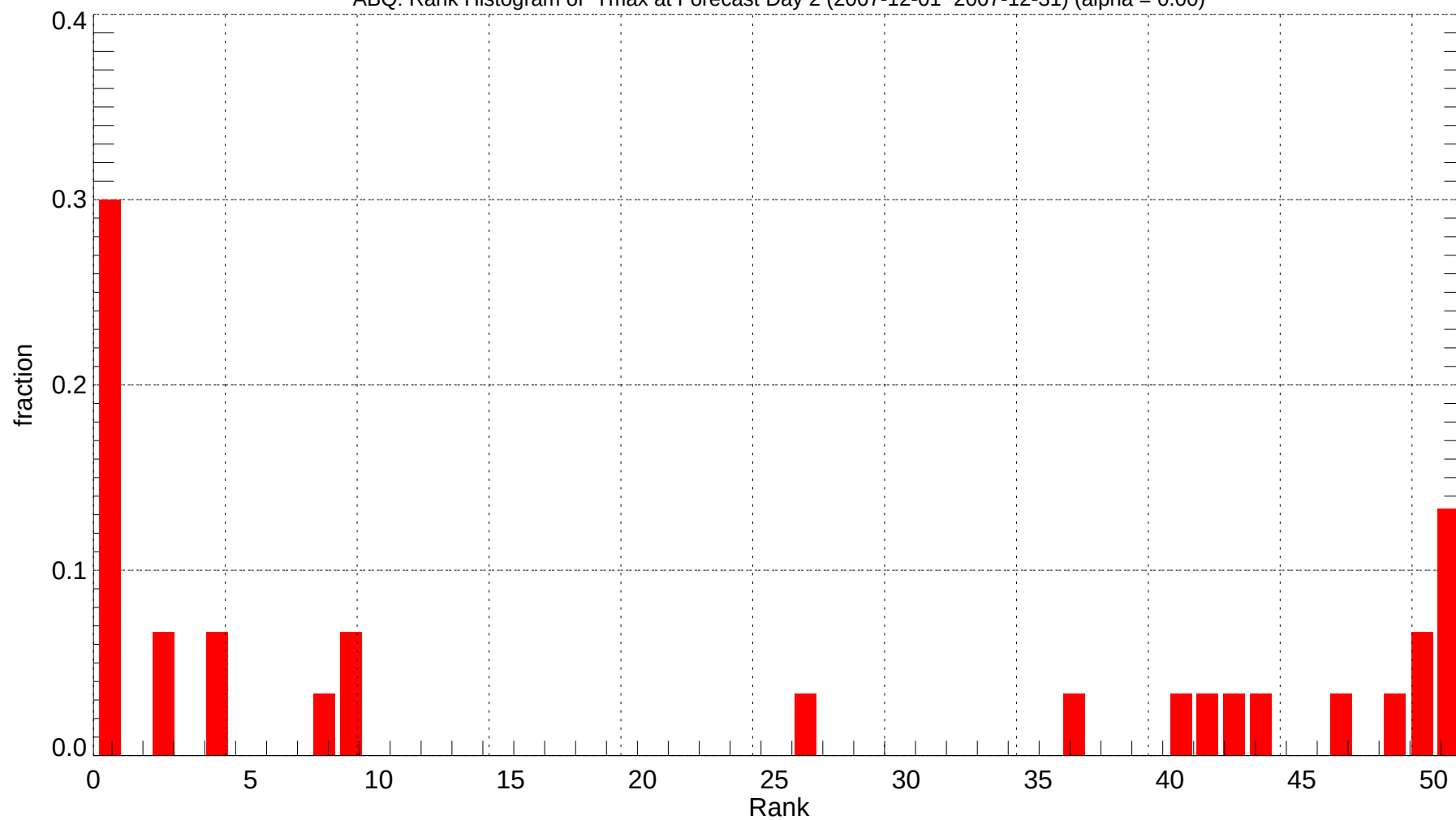
ABQ: Rank Histogram of Tmax at Forecast Day 2 (2007-12-01~2007-12-31) (alpha = 0.00)
