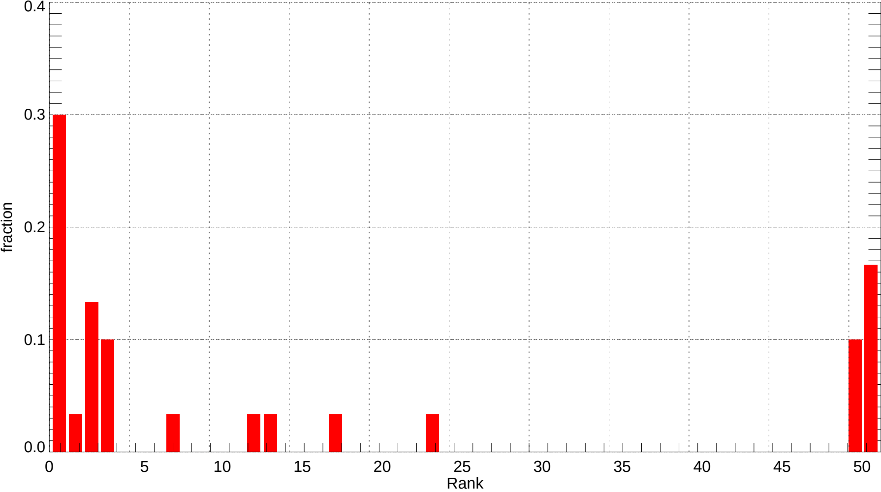
LAS: Rank Histogram of Tmin at Forecast Day 3 (2007-12-01~2007-12-31) (alpha = 0.00)
