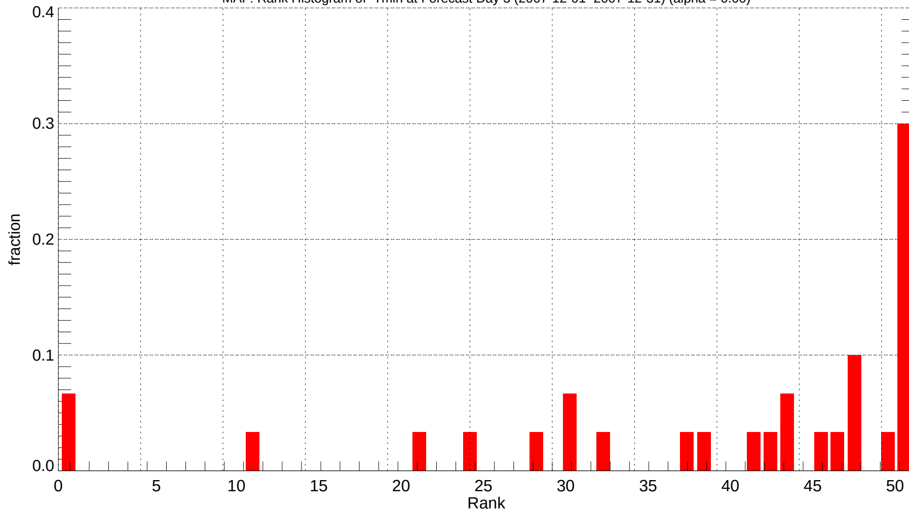
MAF: Rank Histogram of Tmin at Forecast Day 3 (2007-12-01~2007-12-31) (alpha = 0.00)
