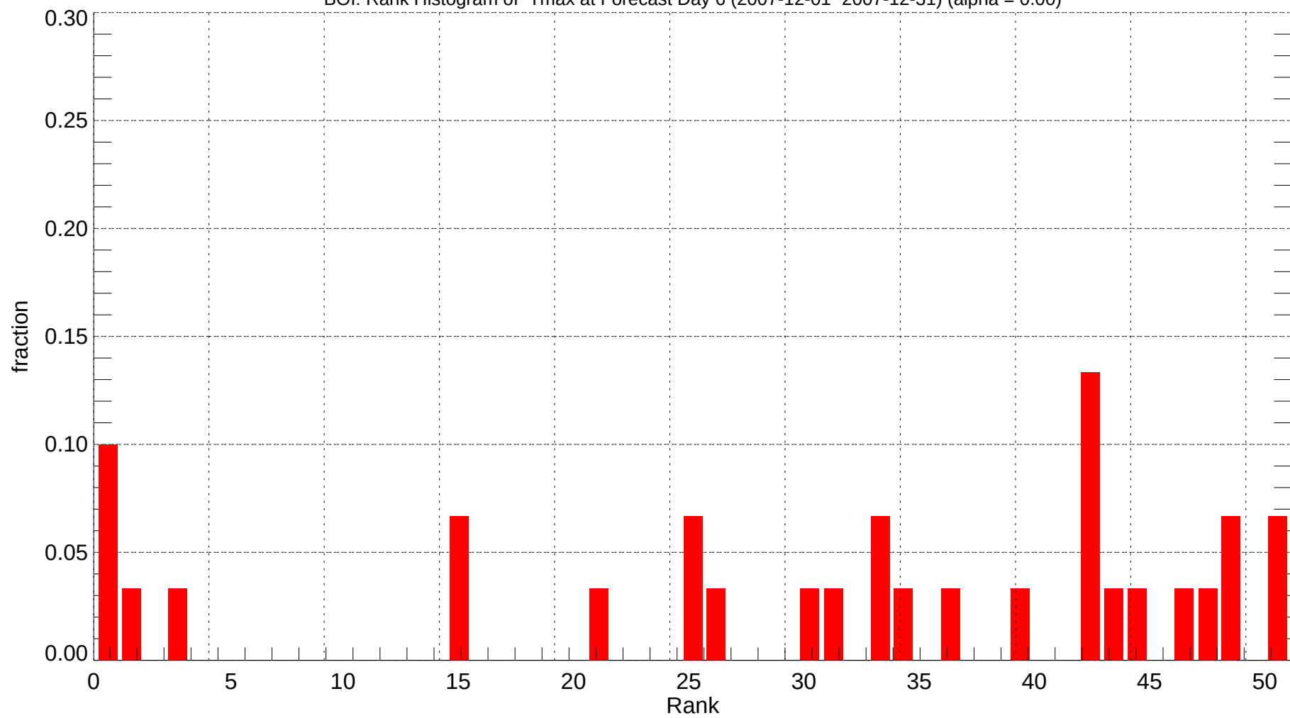
BOI: Rank Histogram of Tmax at Forecast Day 6 (2007-12-01~2007-12-31) (alpha = 0.00)
