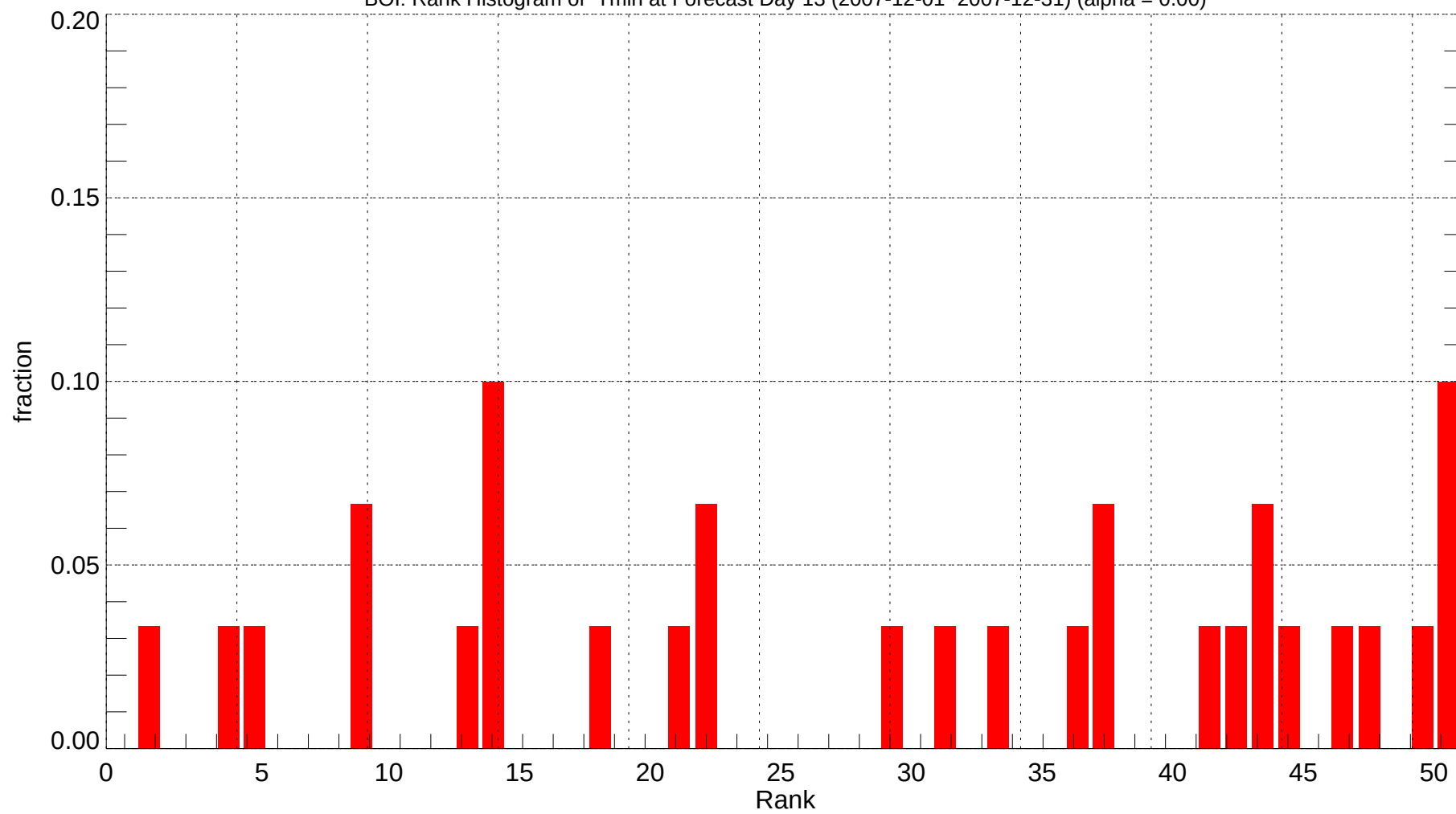
BOI: Rank Histogram of Tmin at Forecast Day 13 (2007-12-01~2007-12-31) (alpha = 0.00)
