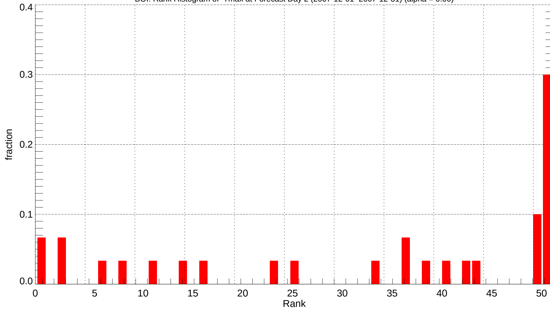
BOI: Rank Histogram of Tmax at Forecast Day 2 (2007-12-01~2007-12-31) (alpha = 0.00)
