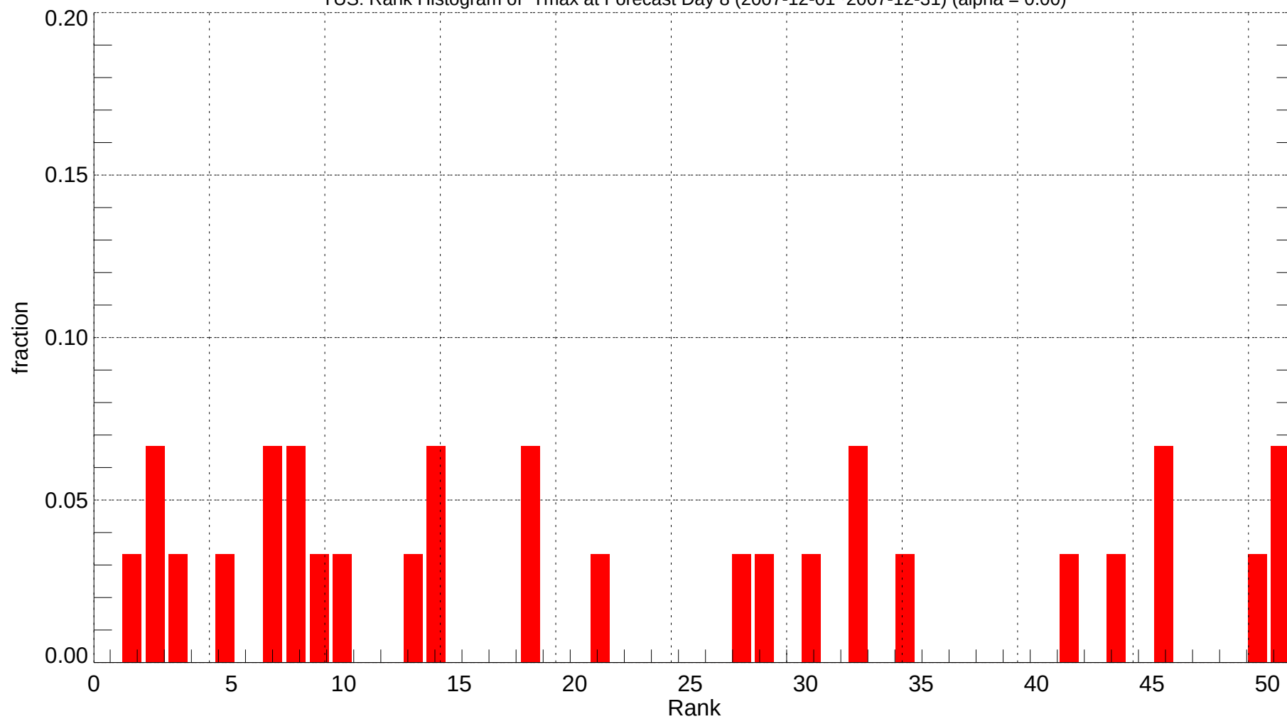
TUS: Rank Histogram of Tmax at Forecast Day 8 (2007-12-01~2007-12-31) (alpha = 0.00)
