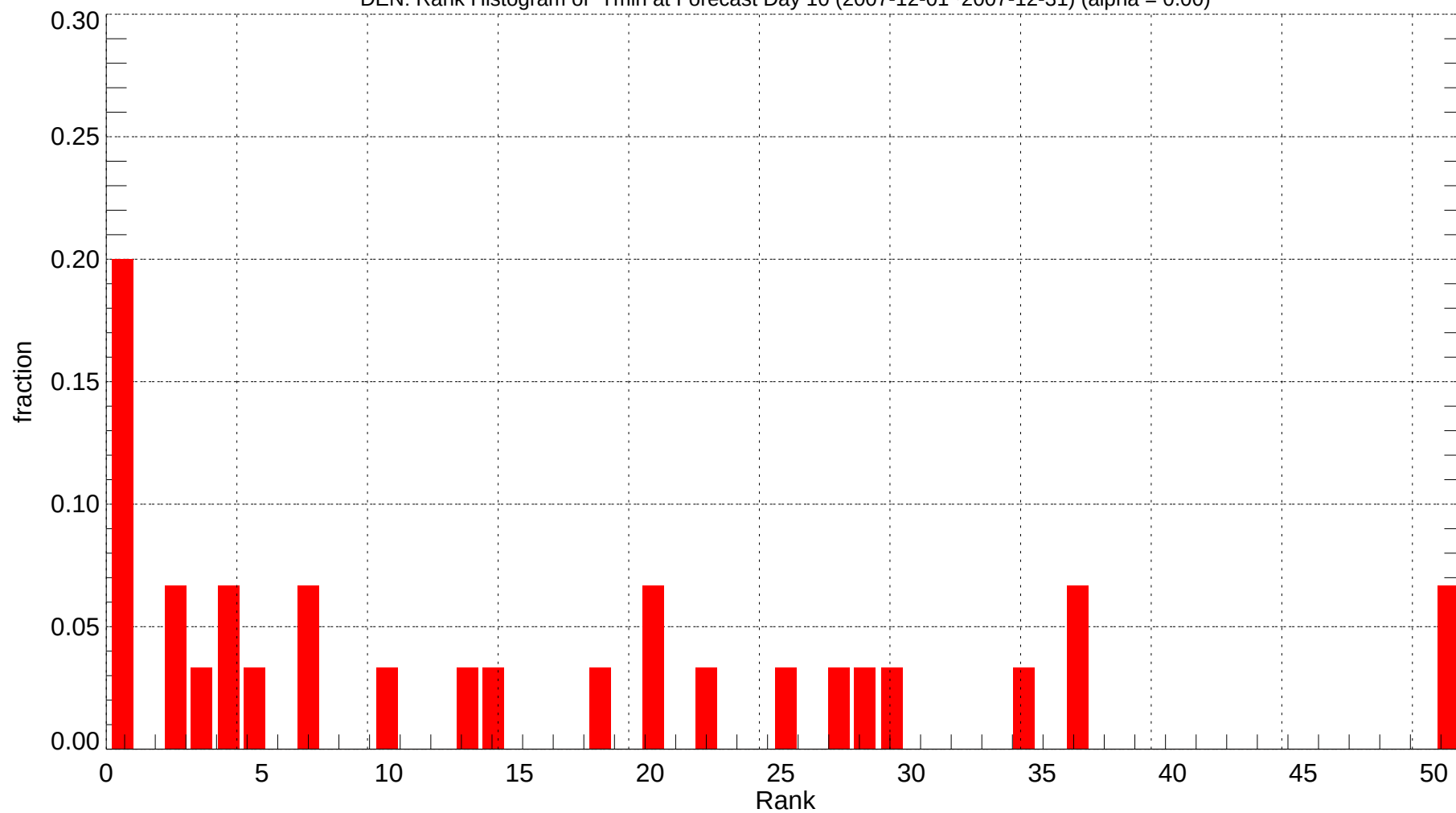
DEN: Rank Histogram of Tmin at Forecast Day 10 (2007-12-01~2007-12-31) (alpha = 0.00)
