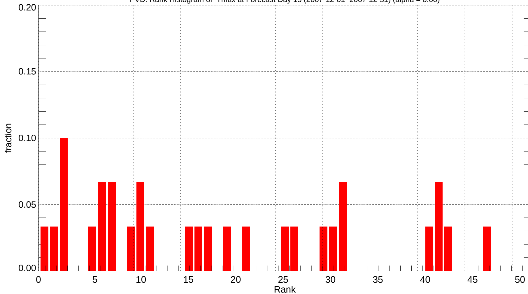
PVD: Rank Histogram of Tmax at Forecast Day 13 (2007-12-01~2007-12-31) (alpha = 0.00)
