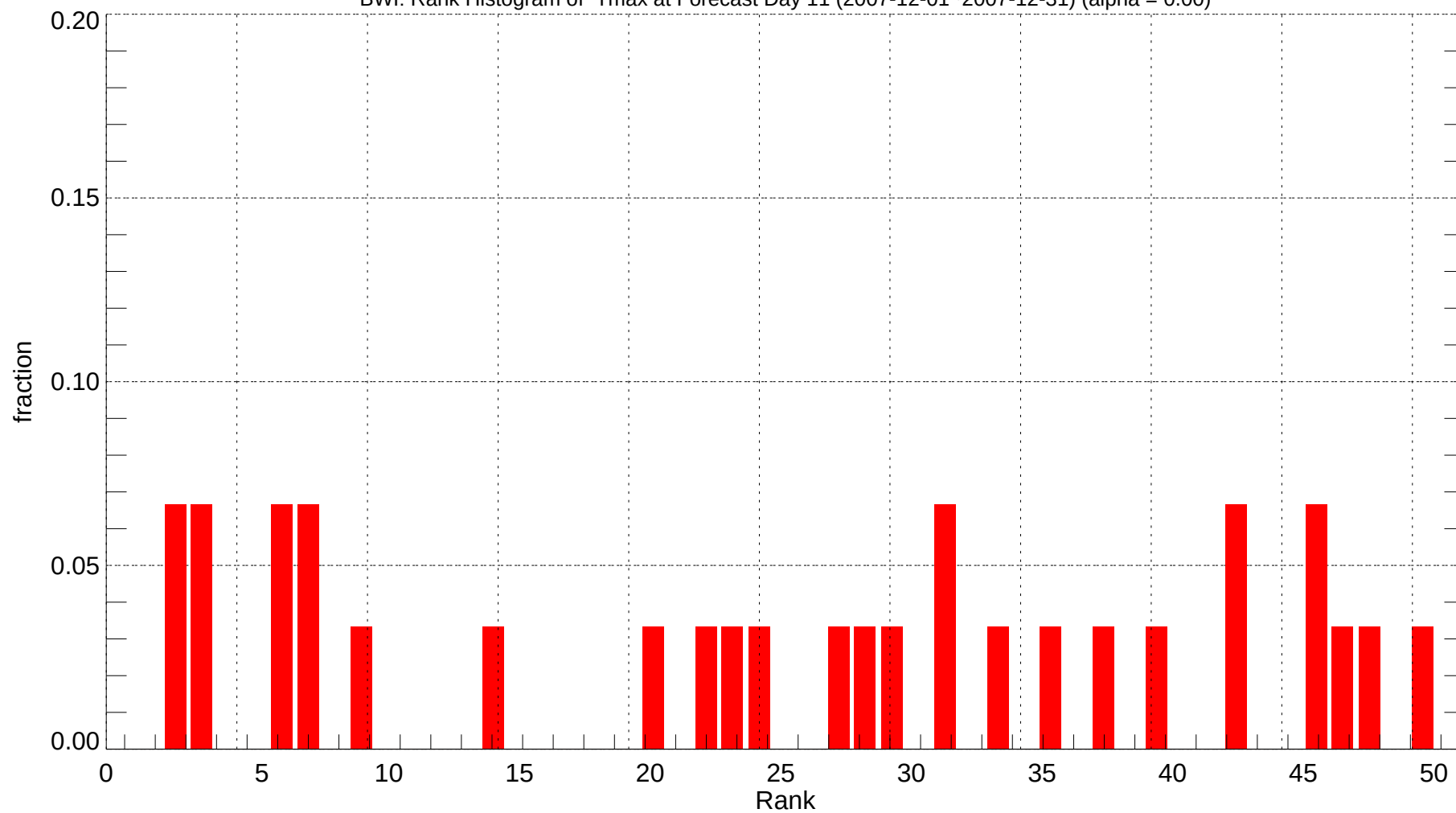
BWI: Rank Histogram of Tmax at Forecast Day 11 (2007-12-01~2007-12-31) (alpha = 0.00)
