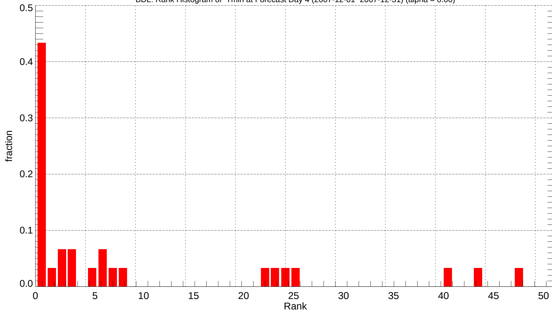
BDL: Rank Histogram of Tmin at Forecast Day 4 (2007-12-01~2007-12-31) (alpha = 0.00)
