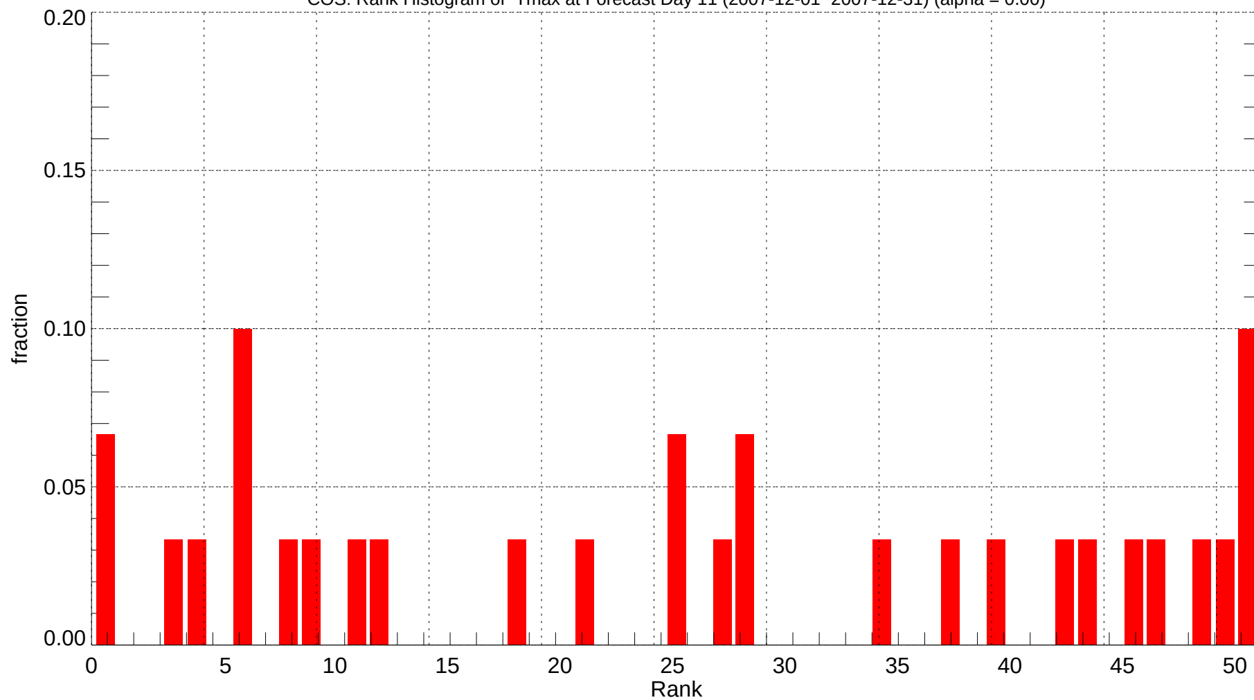
COS: Rank Histogram of Tmax at Forecast Day 11 (2007-12-01~2007-12-31) (alpha = 0.00)
