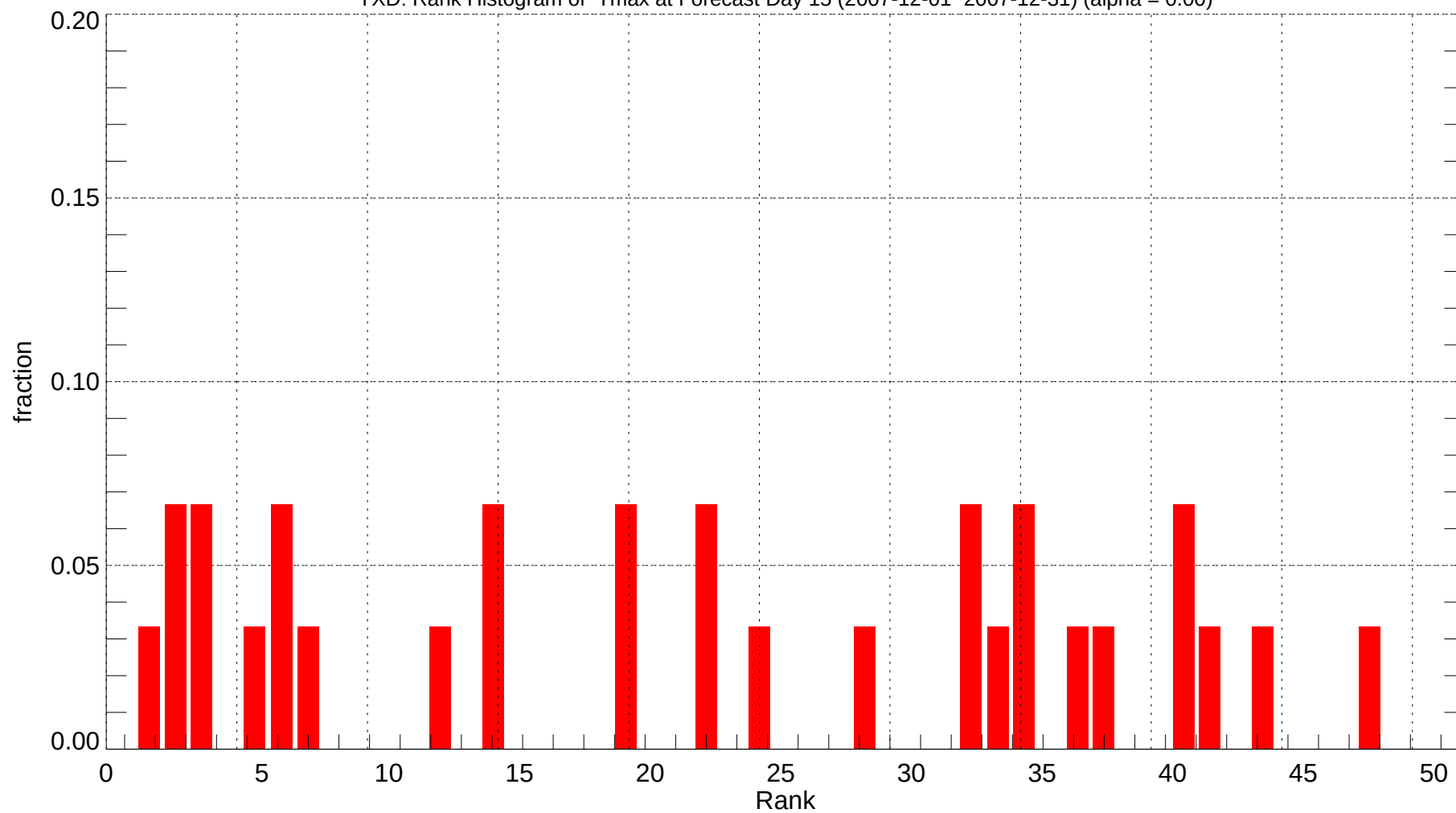
YXD: Rank Histogram of Tmax at Forecast Day 15 (2007-12-01~2007-12-31) (alpha = 0.00)
