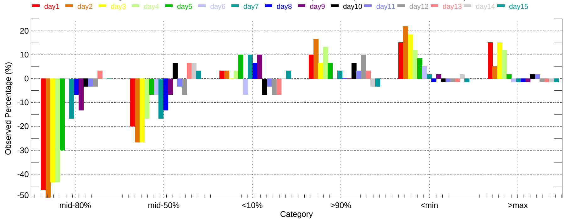
Observed Percentage Deviation of Ensembles - WJF: Min Temperature (2007-12-01~2007-12-31)
