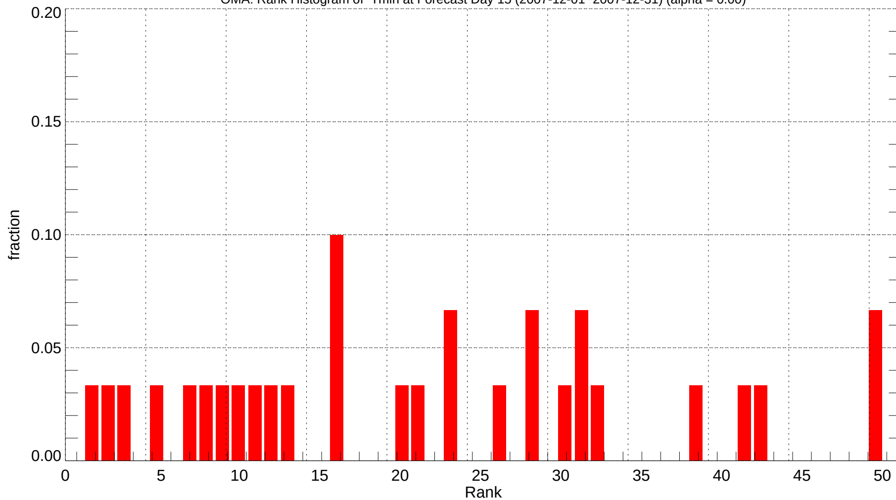
OMA: Rank Histogram of Tmin at Forecast Day 15 (2007-12-01~2007-12-31) (alpha = 0.00)
