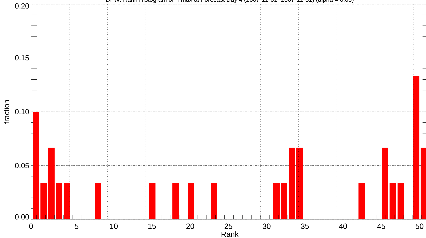
DFW: Rank Histogram of Tmax at Forecast Day 4 (2007-12-01~2007-12-31) (alpha = 0.00)
