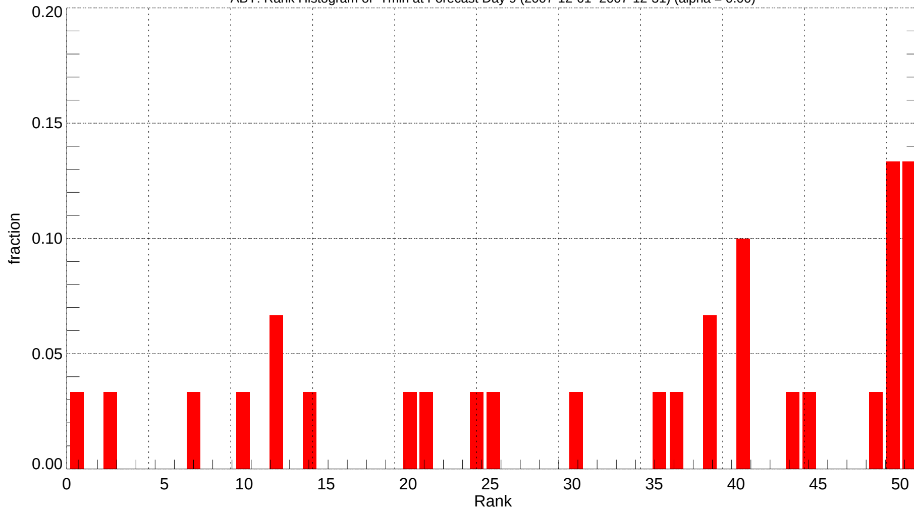
ABY: Rank Histogram of Tmin at Forecast Day 9 (2007-12-01~2007-12-31) (alpha = 0.00)
