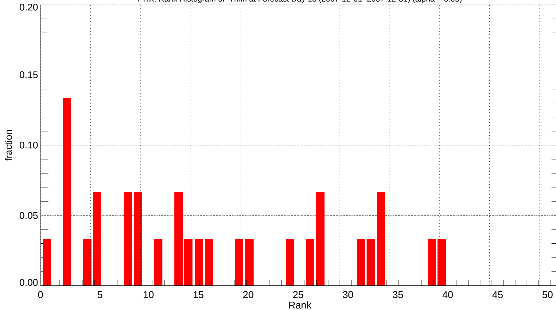
PHX: Rank Histogram of Tmin at Forecast Day 15 (2007-12-01~2007-12-31) (alpha = 0.00)
