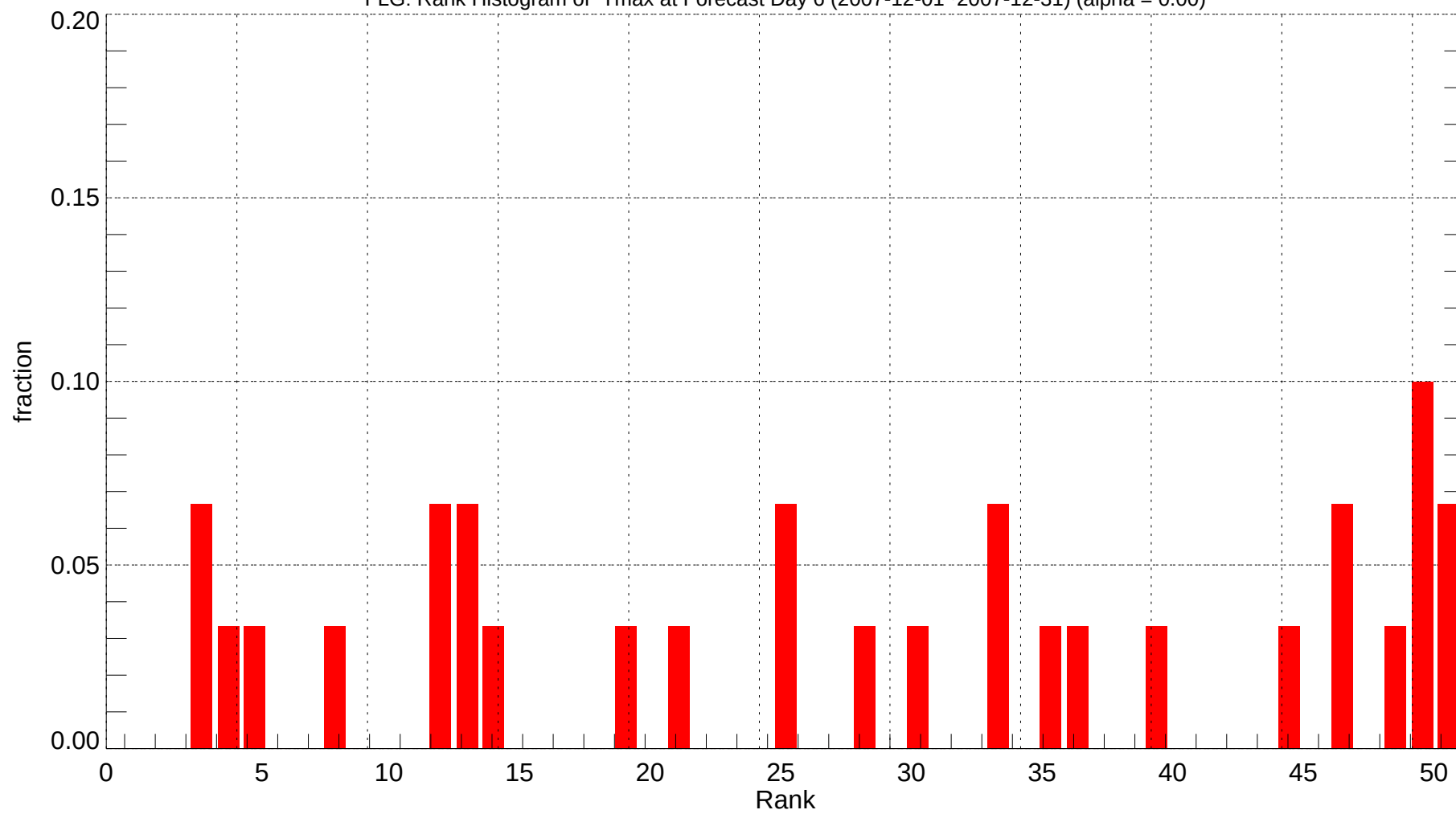
FLG: Rank Histogram of Tmax at Forecast Day 6 (2007-12-01~2007-12-31) (alpha = 0.00)
