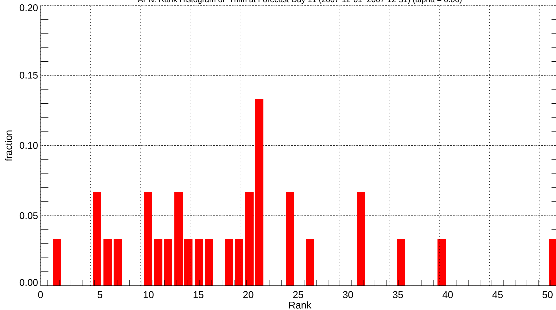
APN: Rank Histogram of Tmin at Forecast Day 11 (2007-12-01~2007-12-31) (alpha = 0.00)
