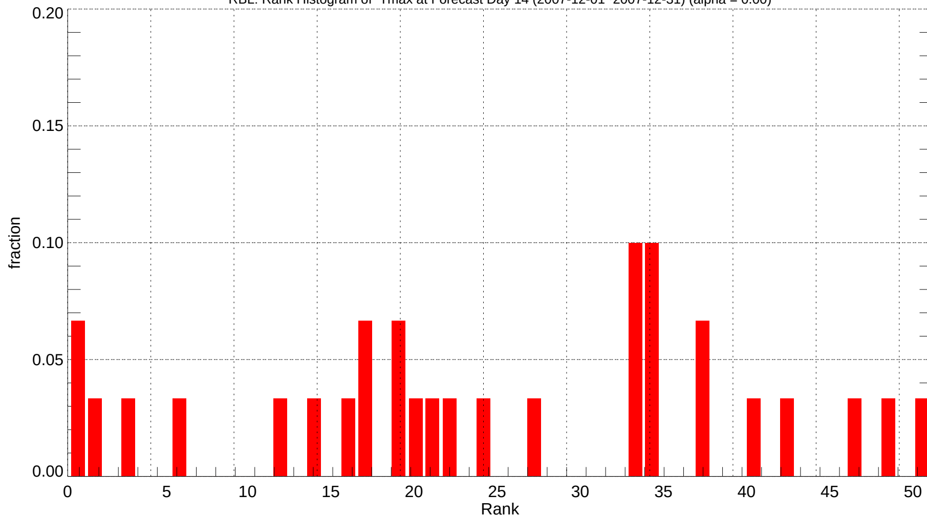
RBL: Rank Histogram of Tmax at Forecast Day 14 (2007-12-01~2007-12-31) (alpha = 0.00)
