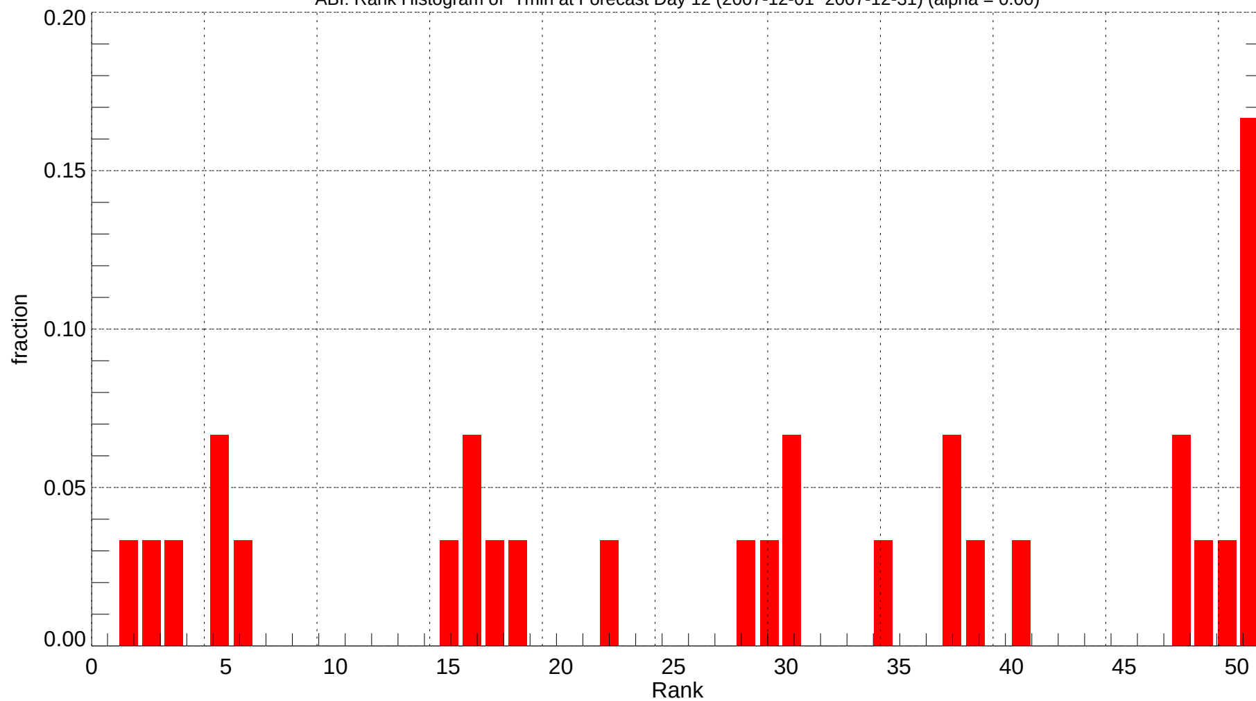
ABI: Rank Histogram of Tmin at Forecast Day 12 (2007-12-01~2007-12-31) (alpha = 0.00)
