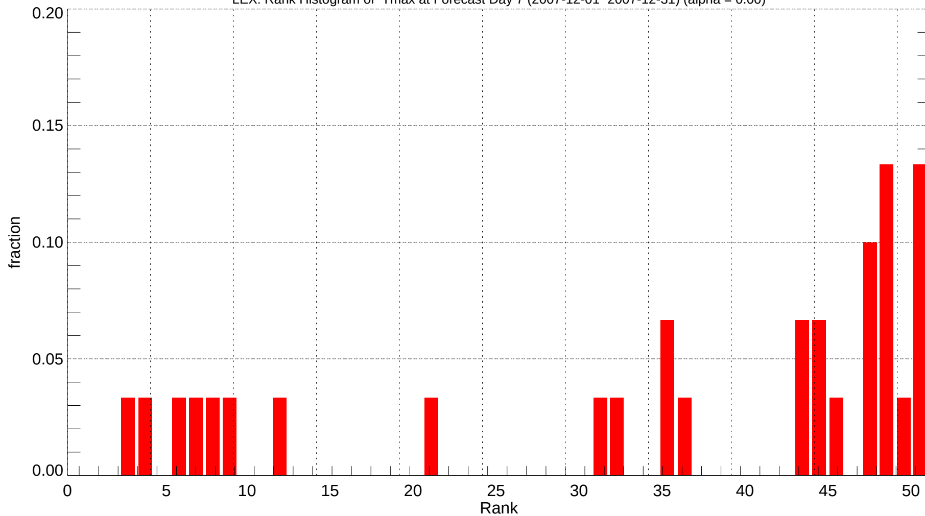
LEX: Rank Histogram of Tmax at Forecast Day 7 (2007-12-01~2007-12-31) (alpha = 0.00)
