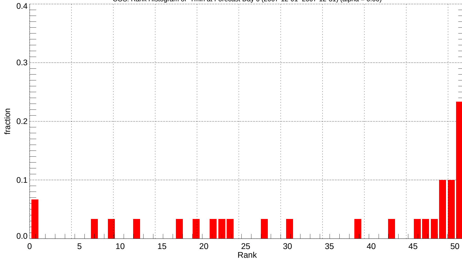
COS: Rank Histogram of Tmin at Forecast Day 6 (2007-12-01~2007-12-31) (alpha = 0.00)
