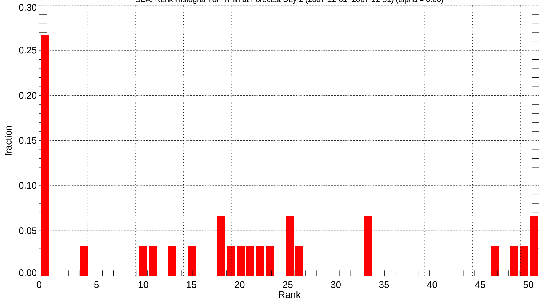
SEA: Rank Histogram of Tmin at Forecast Day 2 (2007-12-01~2007-12-31) (alpha = 0.00)
