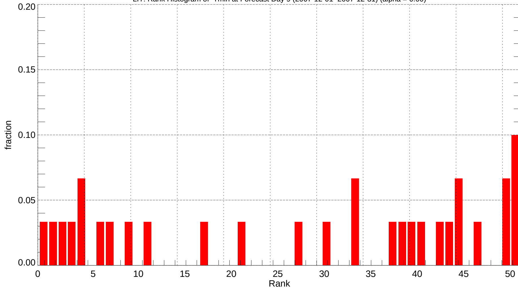
LIT: Rank Histogram of Tmin at Forecast Day 9 (2007-12-01~2007-12-31) (alpha = 0.00)
