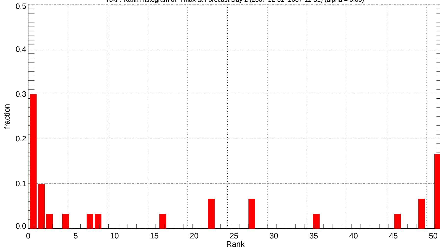
RAP: Rank Histogram of Tmax at Forecast Day 2 (2007-12-01~2007-12-31) (alpha = 0.00)
