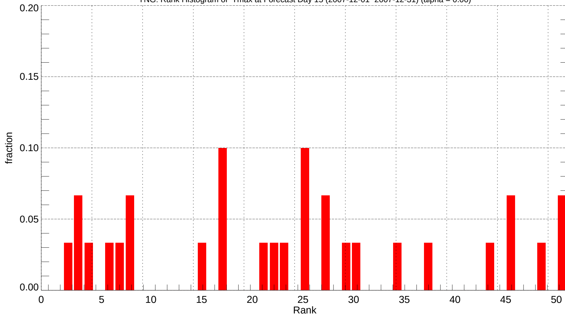
YNG: Rank Histogram of Tmax at Forecast Day 15 (2007-12-01~2007-12-31) (alpha = 0.00)
