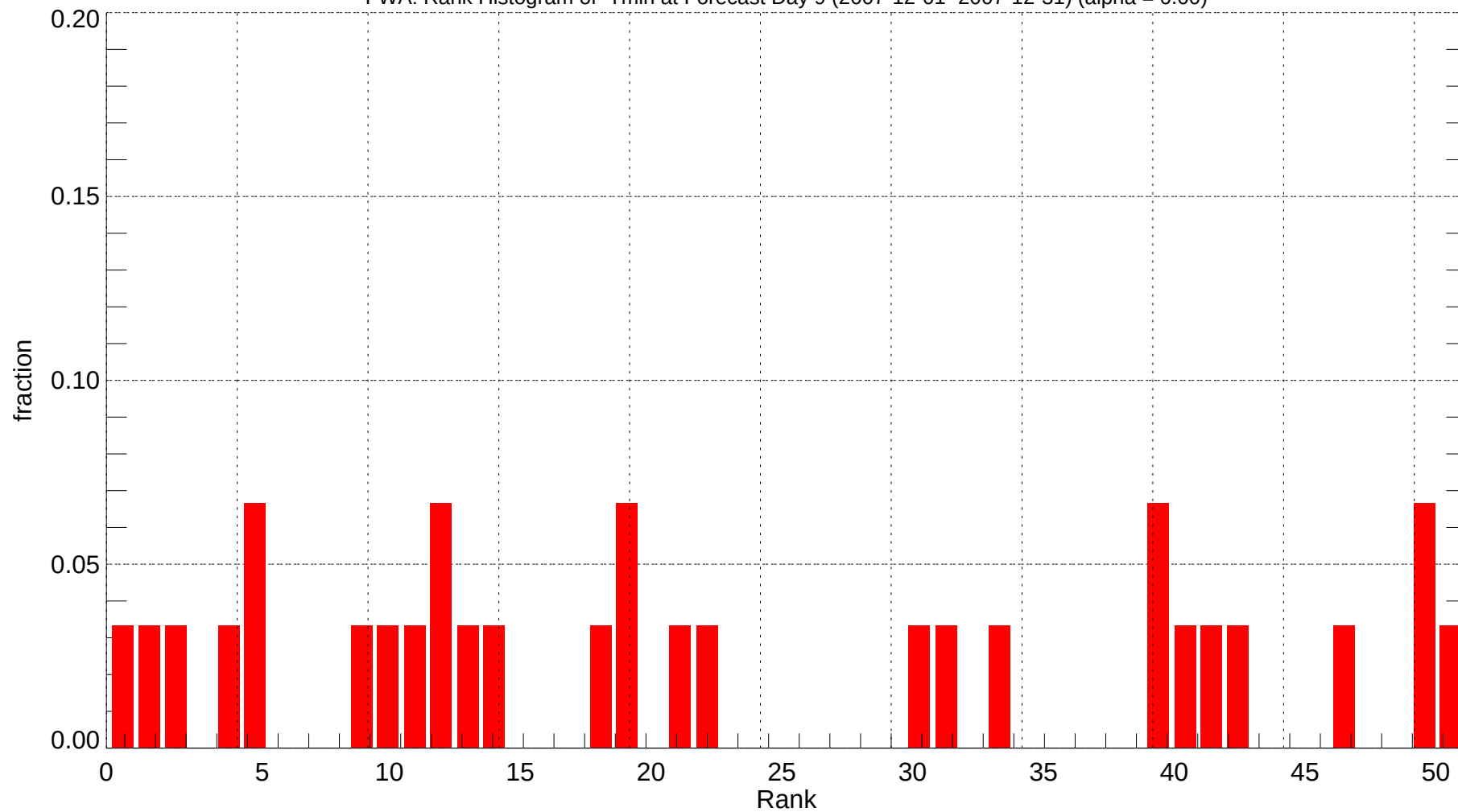
FWA: Rank Histogram of Tmin at Forecast Day 9 (2007-12-01~2007-12-31) (alpha = 0.00)
