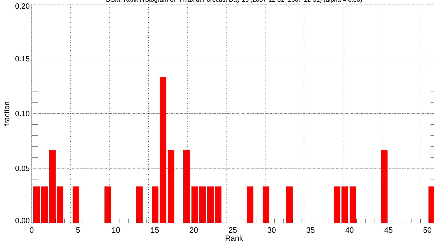
BGM: Rank Histogram of Tmax at Forecast Day 15 (2007-12-01~2007-12-31) (alpha = 0.00)
