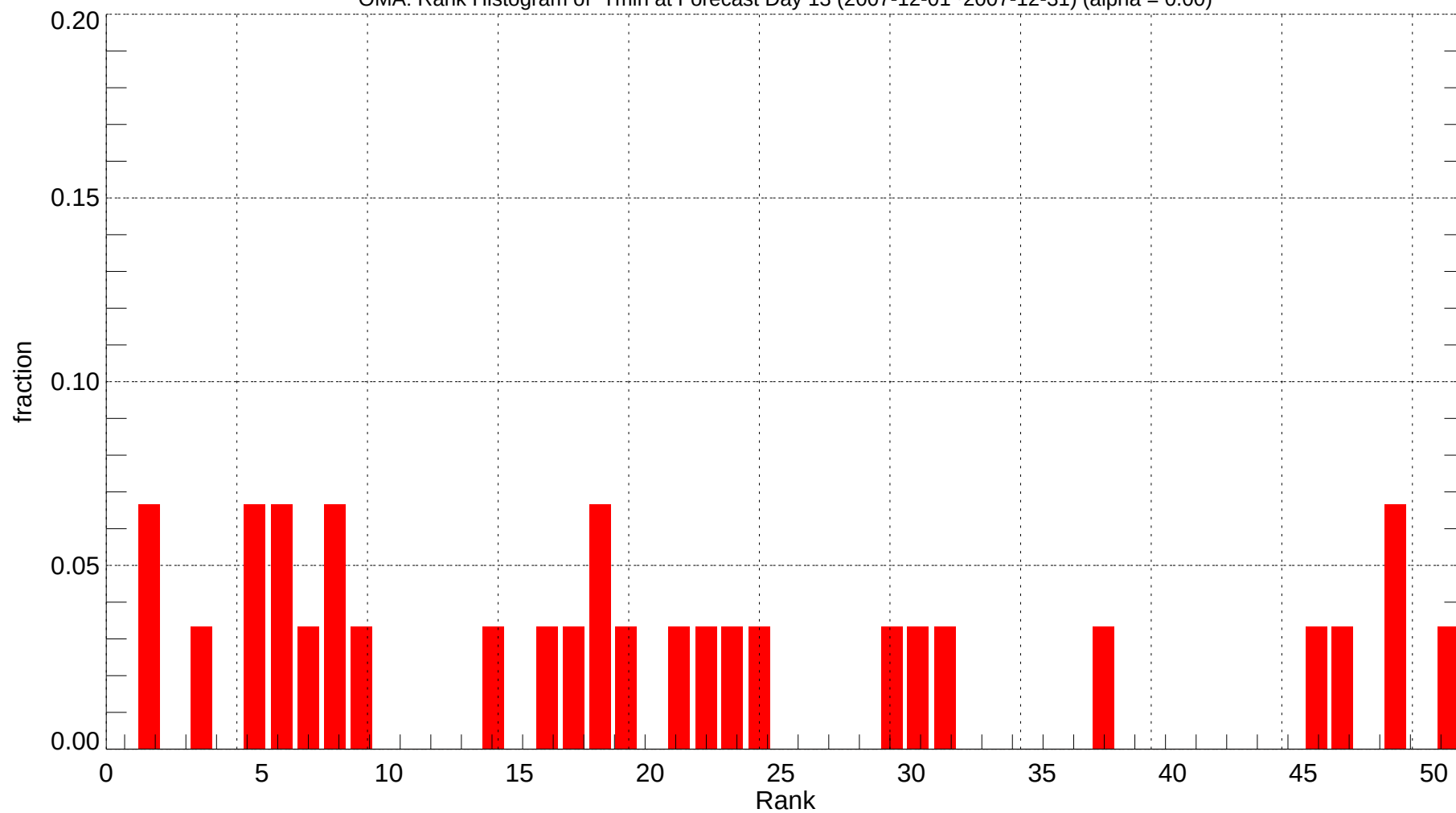
OMA: Rank Histogram of Tmin at Forecast Day 13 (2007-12-01~2007-12-31) (alpha = 0.00)
