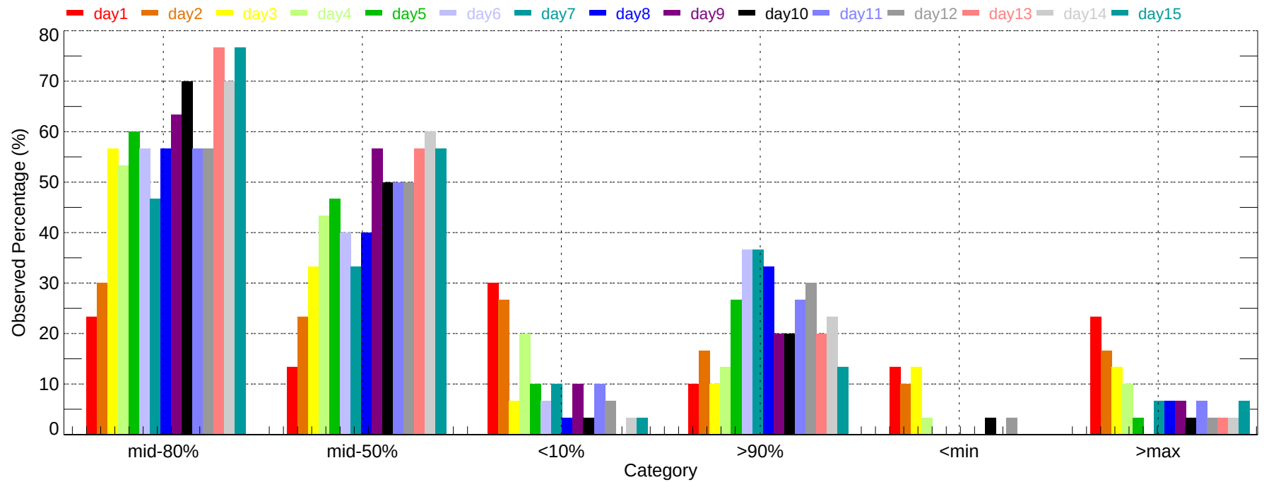
Observed Percentage of Ensembles - EVV: Min Temperature (2007-12-01~2007-12-31)
