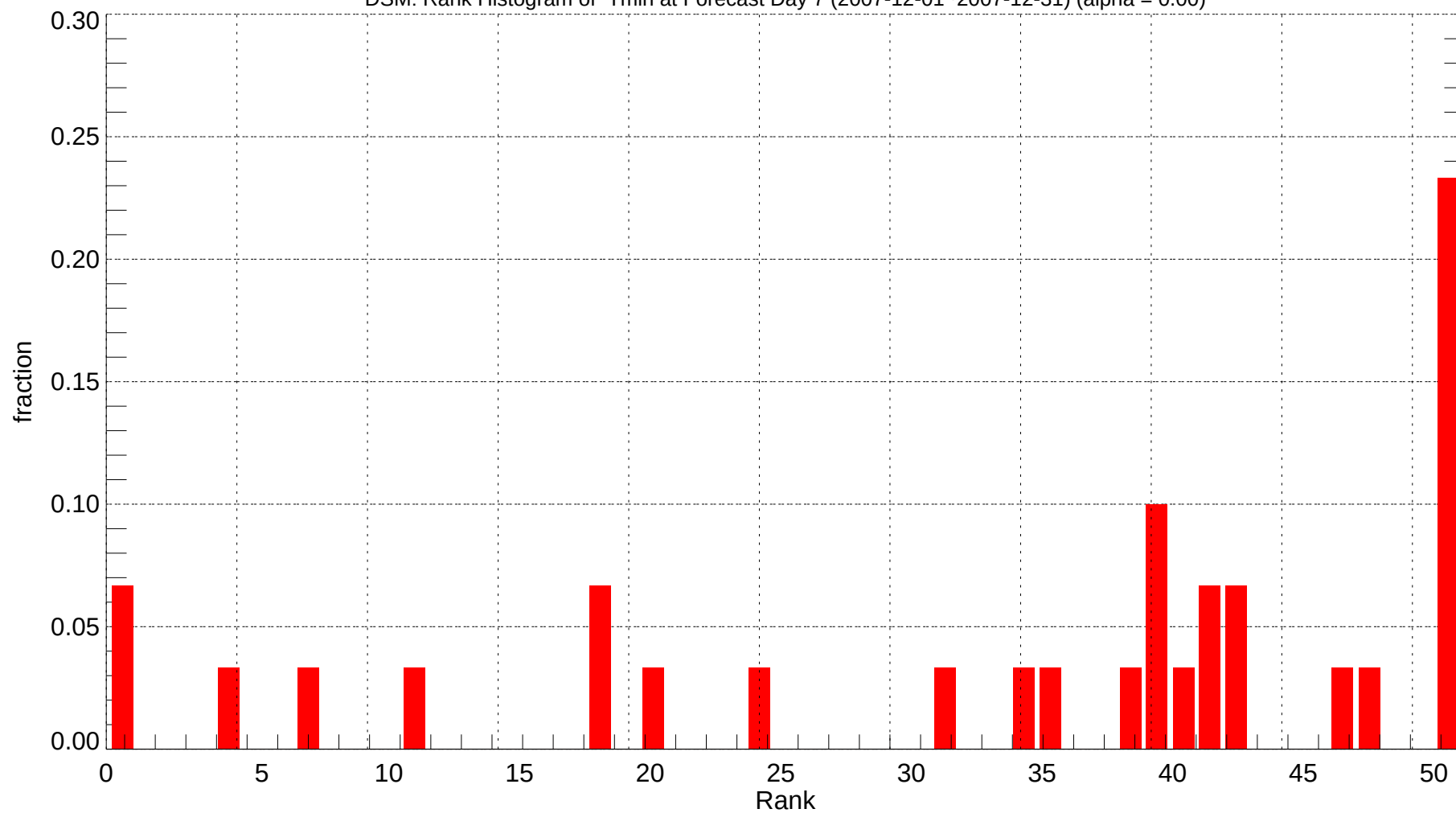
DSM: Rank Histogram of Tmin at Forecast Day 7 (2007-12-01~2007-12-31) (alpha = 0.00)
