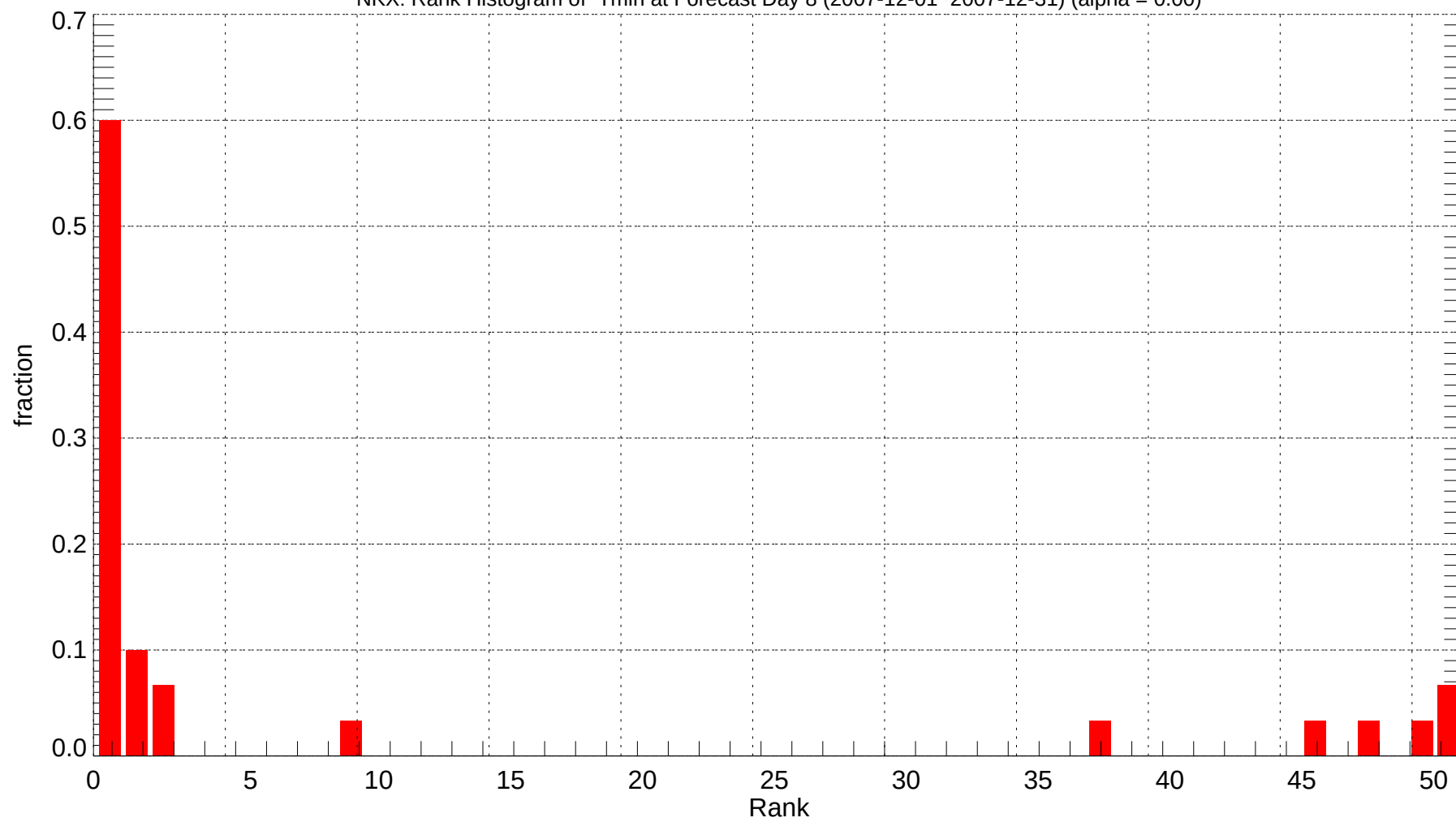
NKX: Rank Histogram of Tmin at Forecast Day 8 (2007-12-01~2007-12-31) (alpha = 0.00)
