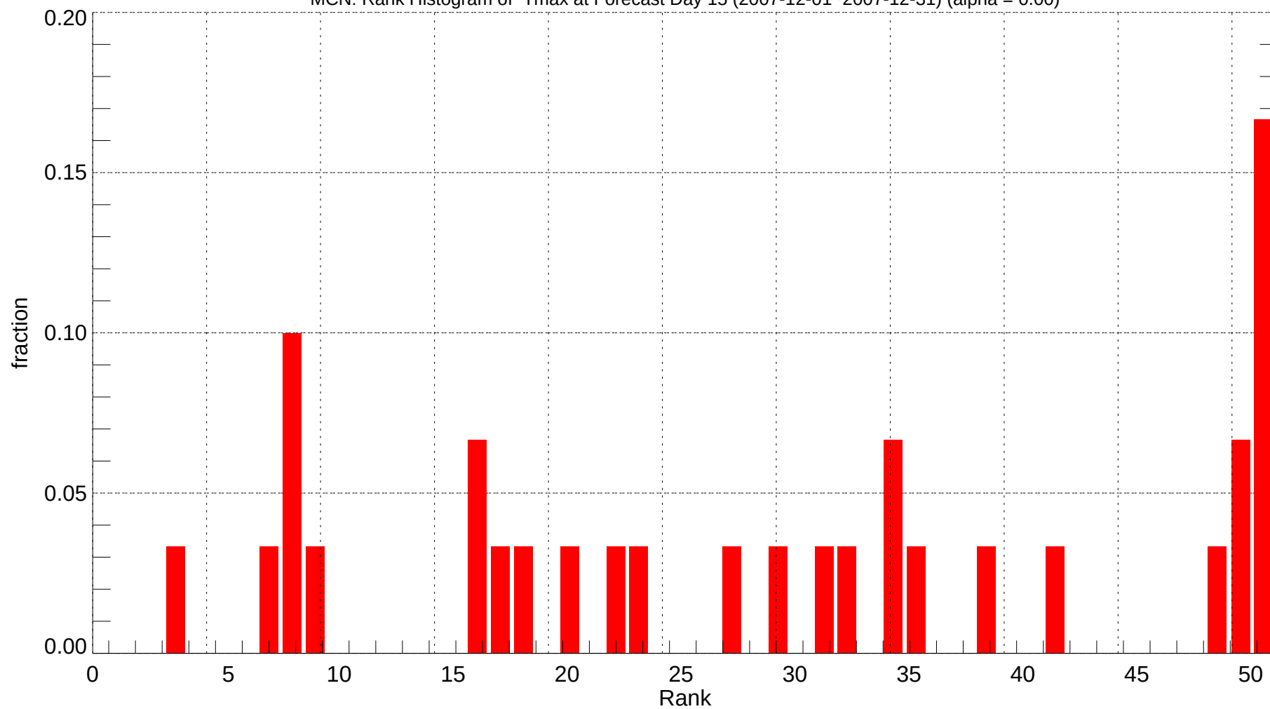
MCN: Rank Histogram of Tmax at Forecast Day 15 (2007-12-01~2007-12-31) (alpha = 0.00)
