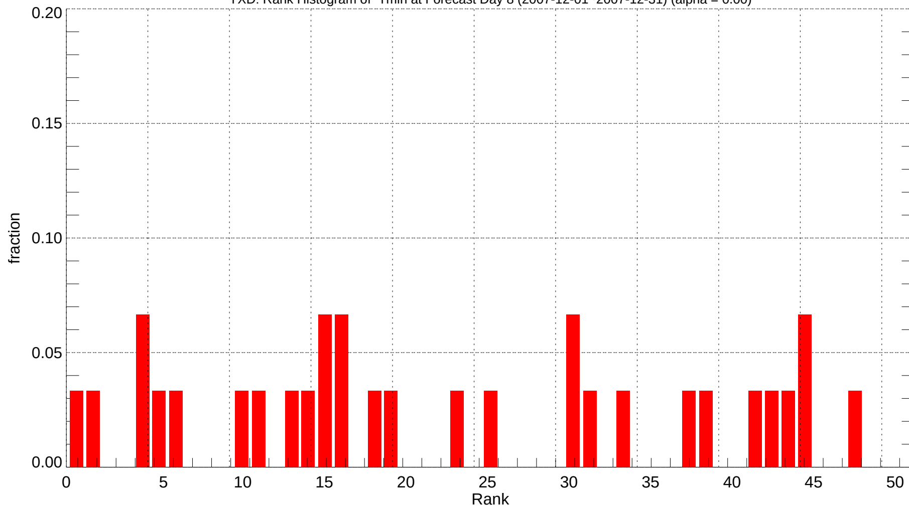
YXD: Rank Histogram of Tmin at Forecast Day 8 (2007-12-01~2007-12-31) (alpha = 0.00)
