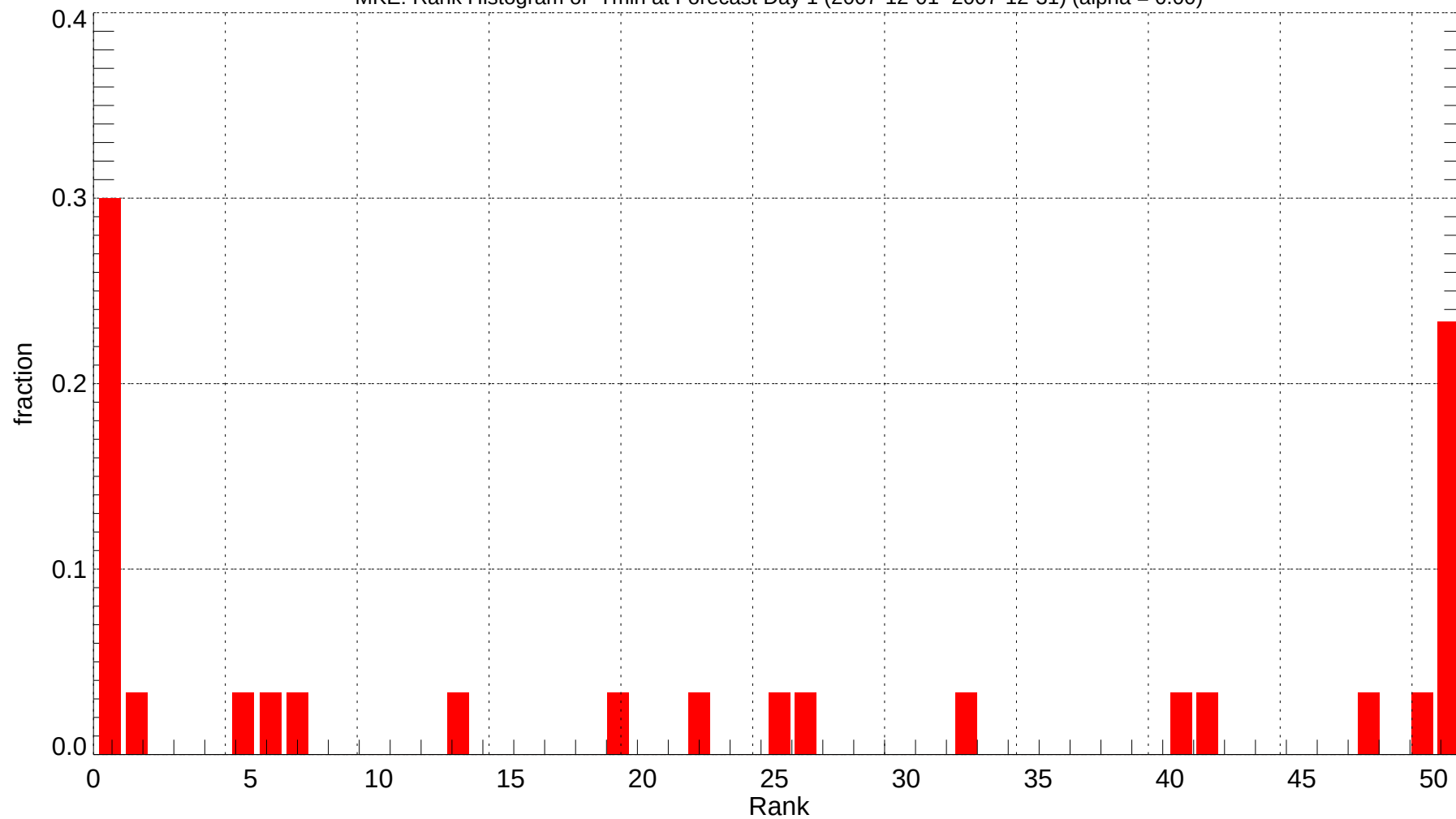
MKE: Rank Histogram of Tmin at Forecast Day 1 (2007-12-01~2007-12-31) (alpha = 0.00)
