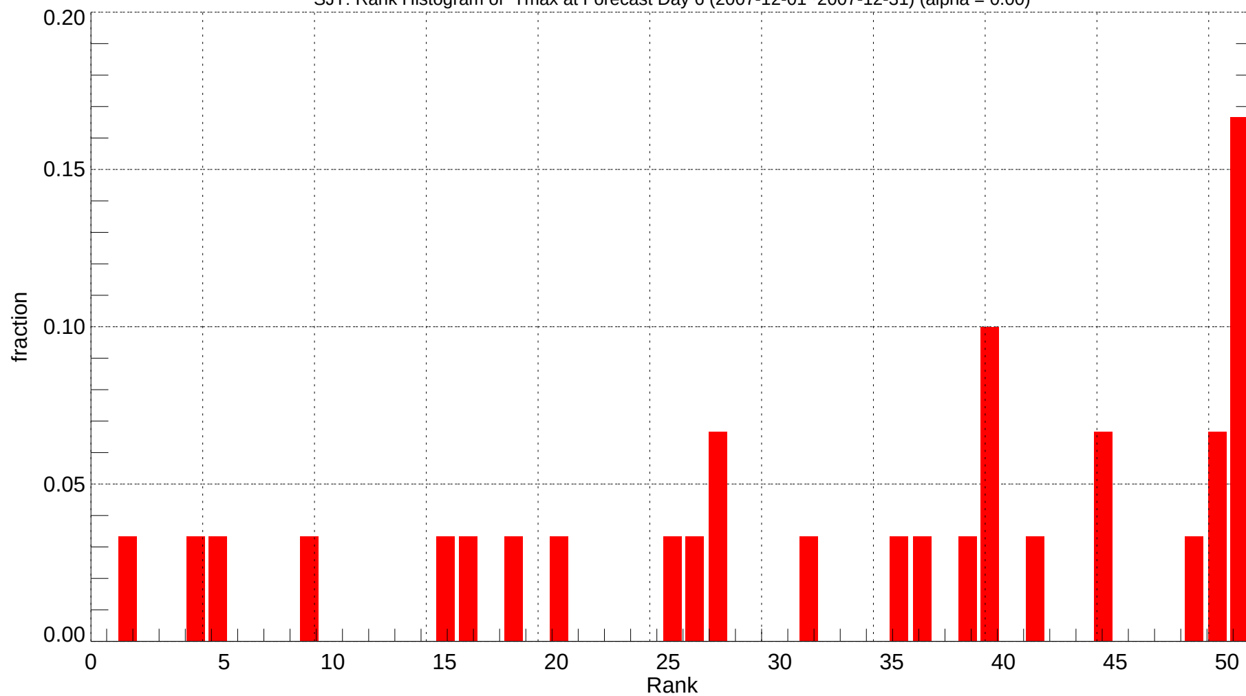
SJT: Rank Histogram of Tmax at Forecast Day 6 (2007-12-01~2007-12-31) (alpha = 0.00)
