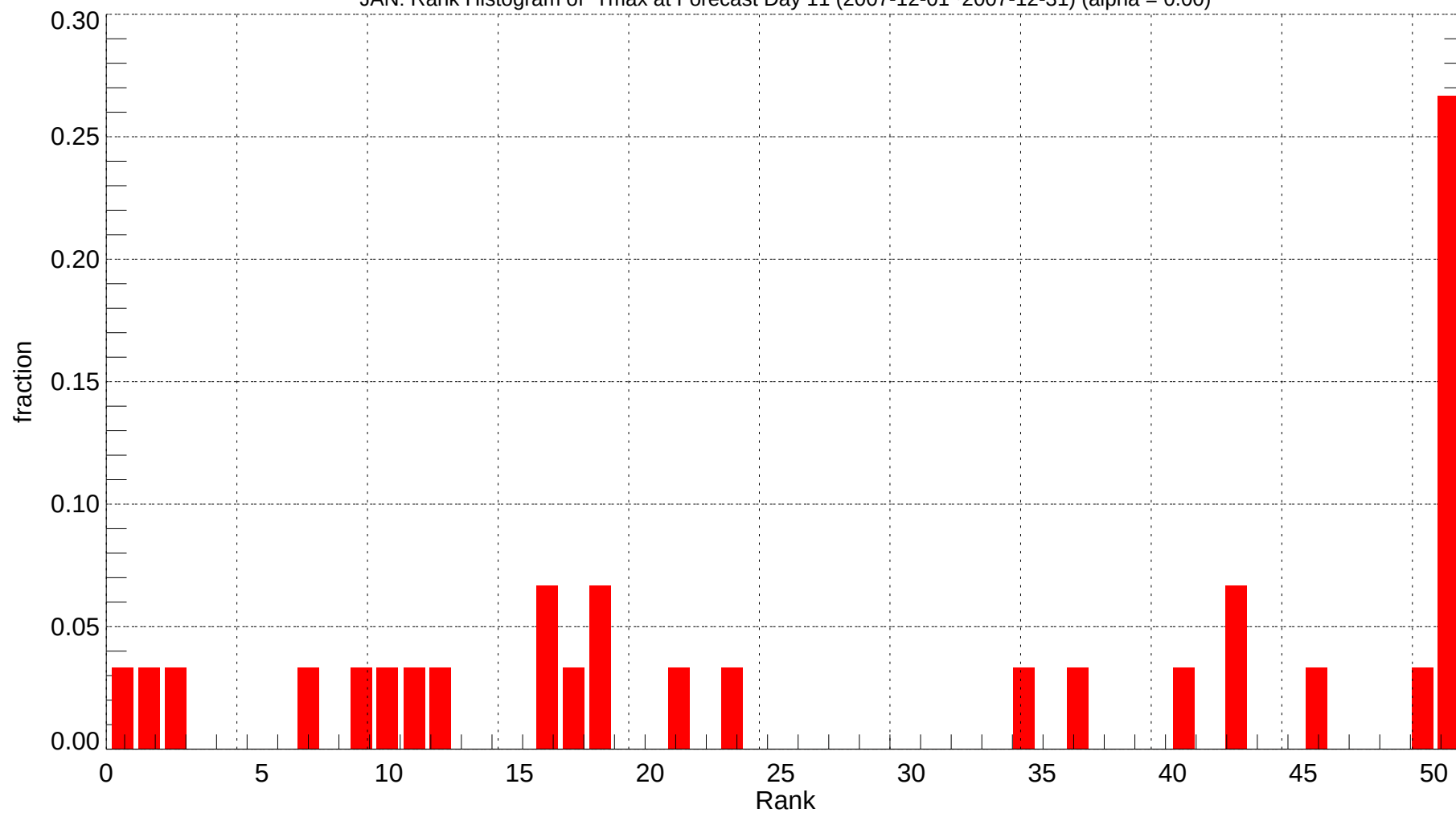
JAN: Rank Histogram of Tmax at Forecast Day 11 (2007-12-01~2007-12-31) (alpha = 0.00)
