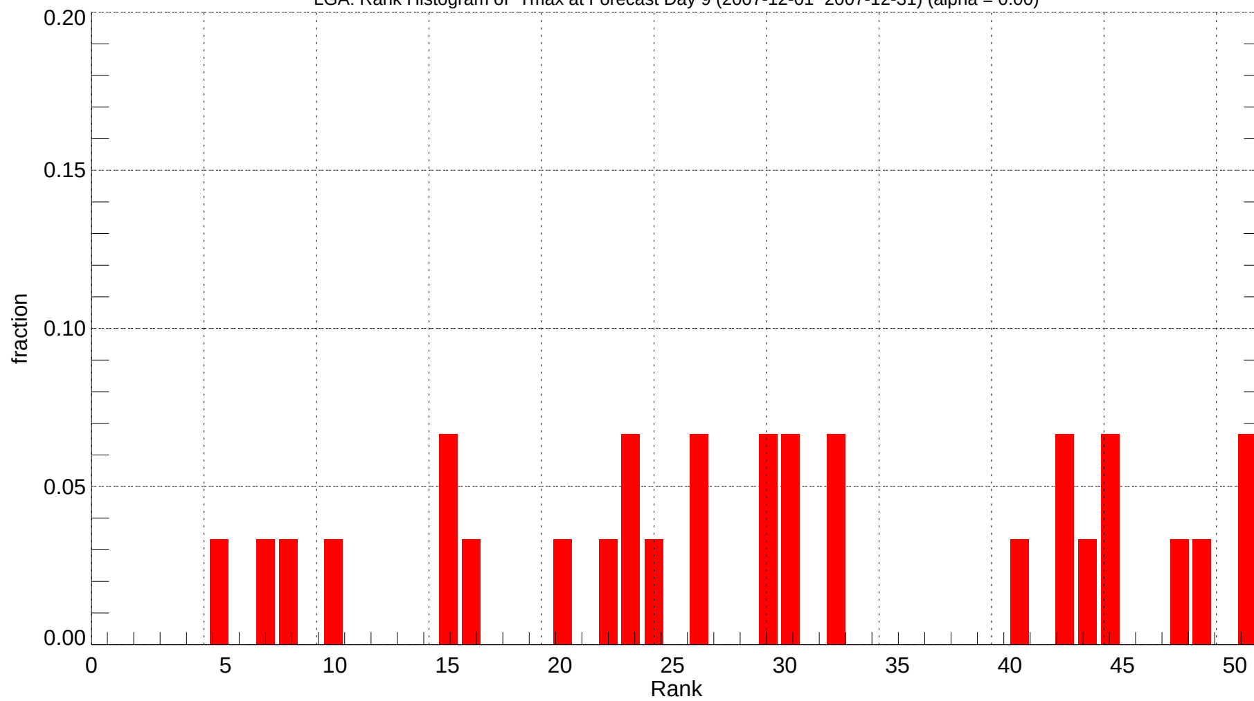
LGA: Rank Histogram of Tmax at Forecast Day 9 (2007-12-01~2007-12-31) (alpha = 0.00)
