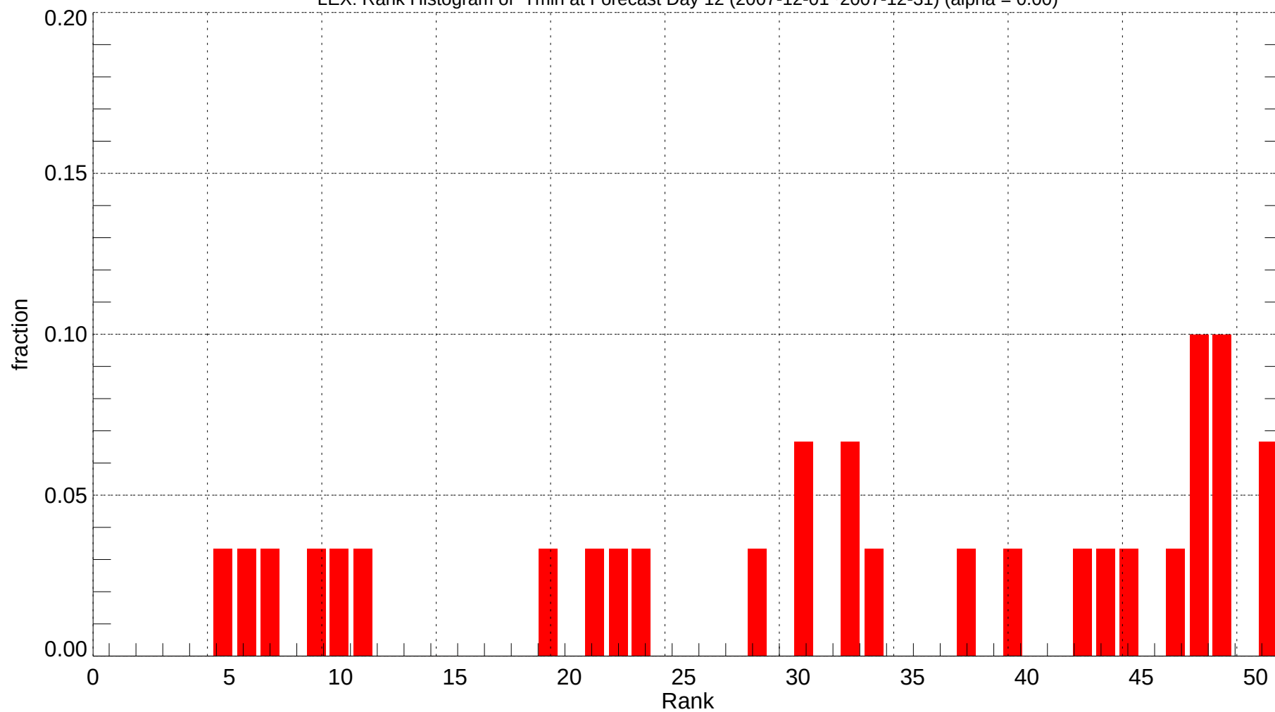
LEX: Rank Histogram of Tmin at Forecast Day 12 (2007-12-01~2007-12-31) (alpha = 0.00)
