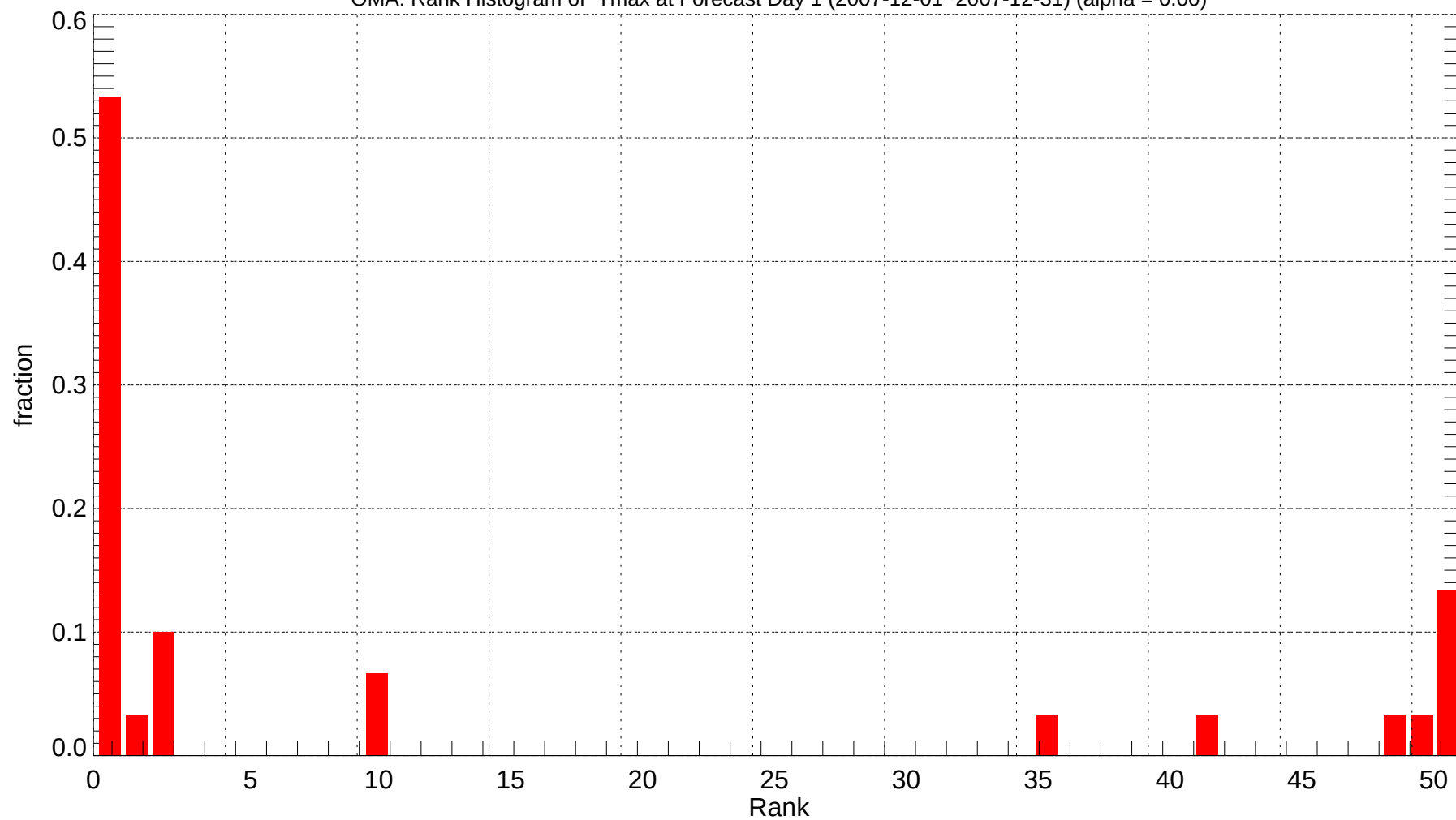
OMA: Rank Histogram of Tmax at Forecast Day 1 (2007-12-01~2007-12-31) (alpha = 0.00)
