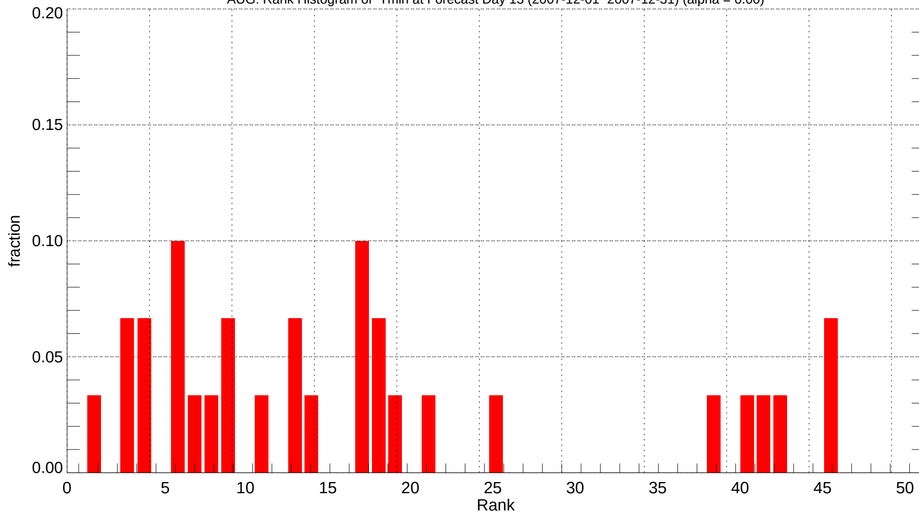
AUG: Rank Histogram of Tmin at Forecast Day 13 (2007-12-01~2007-12-31) (alpha = 0.00)
