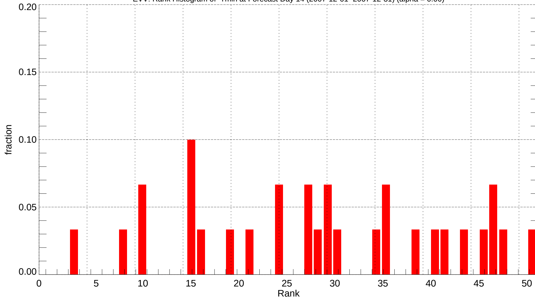
EVV: Rank Histogram of Tmin at Forecast Day 14 (2007-12-01~2007-12-31) (alpha = 0.00)
