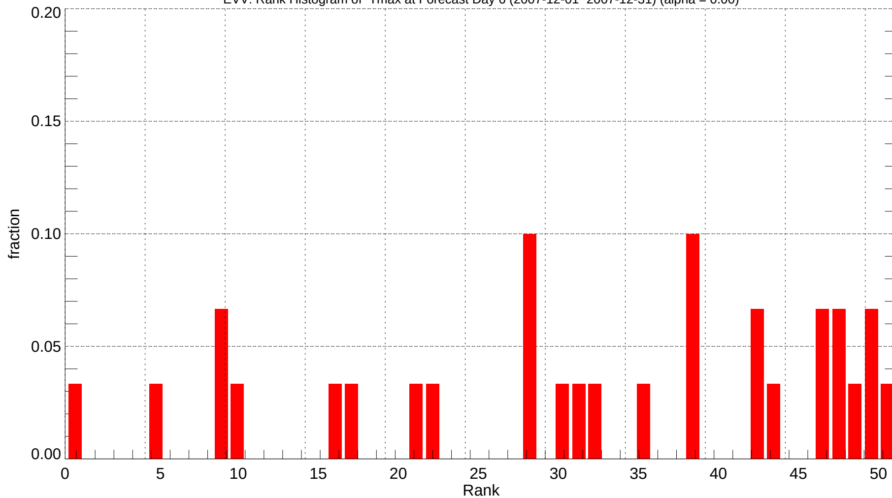
EVV: Rank Histogram of Tmax at Forecast Day 6 (2007-12-01~2007-12-31) (alpha = 0.00)
