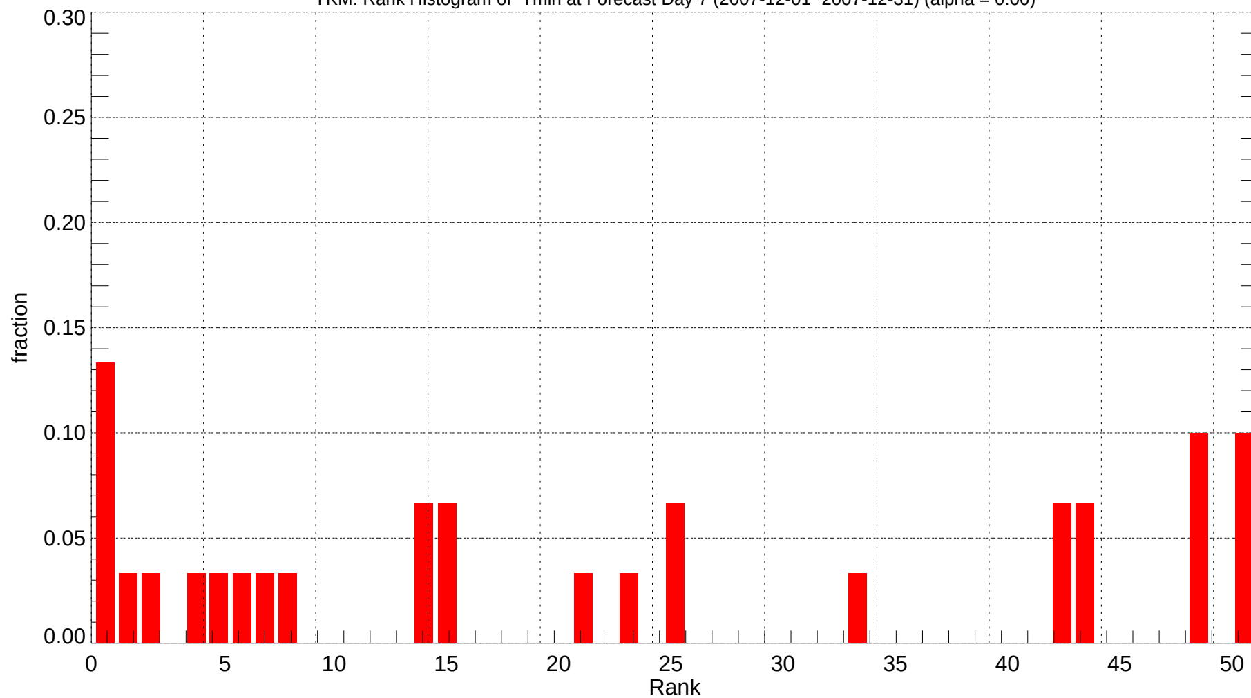
YKM: Rank Histogram of Tmin at Forecast Day 7 (2007-12-01~2007-12-31) (alpha = 0.00)
