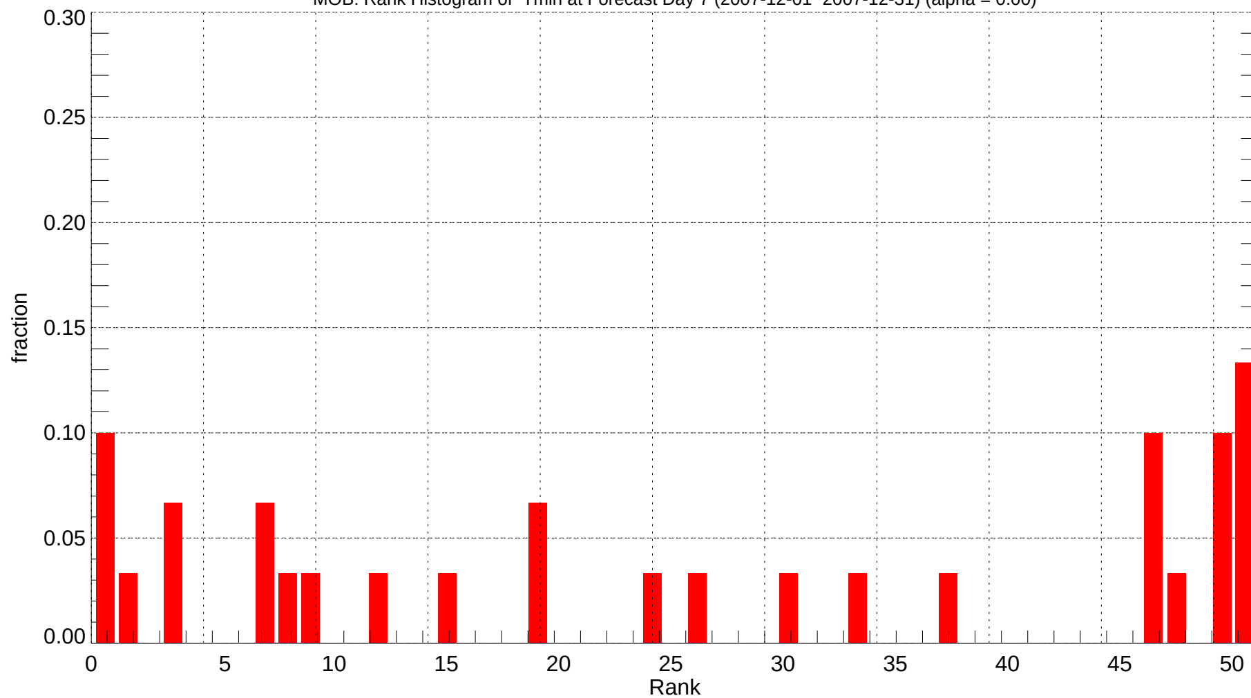
MOB: Rank Histogram of Tmin at Forecast Day 7 (2007-12-01~2007-12-31) (alpha = 0.00)
