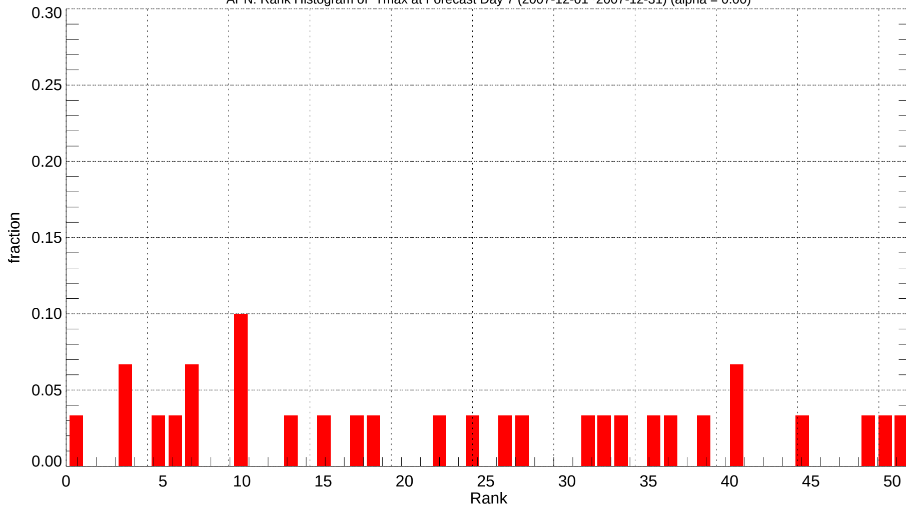
APN: Rank Histogram of Tmax at Forecast Day 7 (2007-12-01~2007-12-31) (alpha = 0.00)
