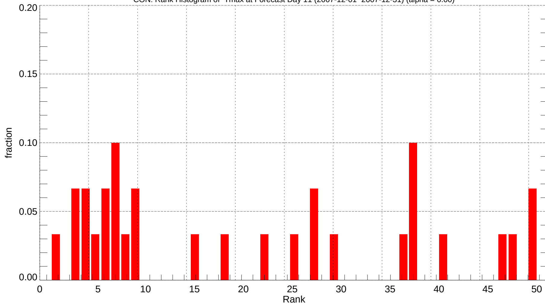
CON: Rank Histogram of Tmax at Forecast Day 11 (2007-12-01~2007-12-31) (alpha = 0.00)
