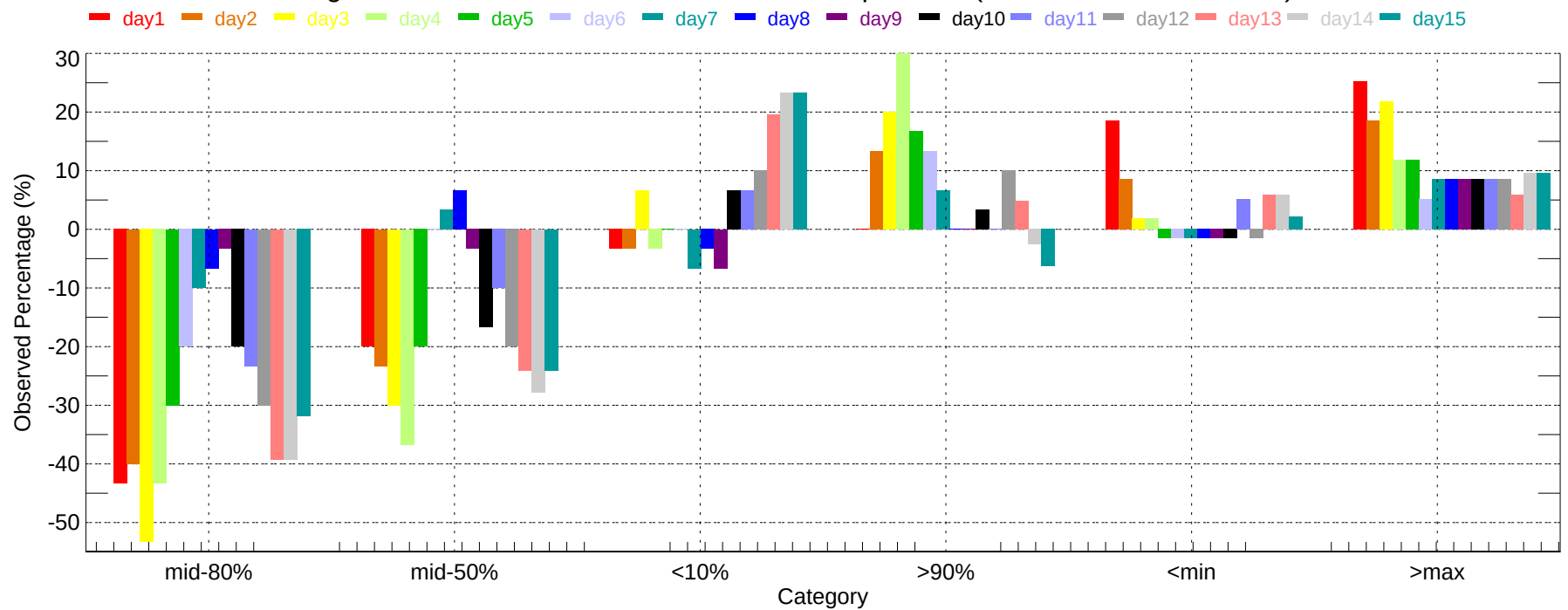
Observed Percentage Deviation of Ensembles - FLG: Min Temperature (2007-12-01~2007-12-31)
