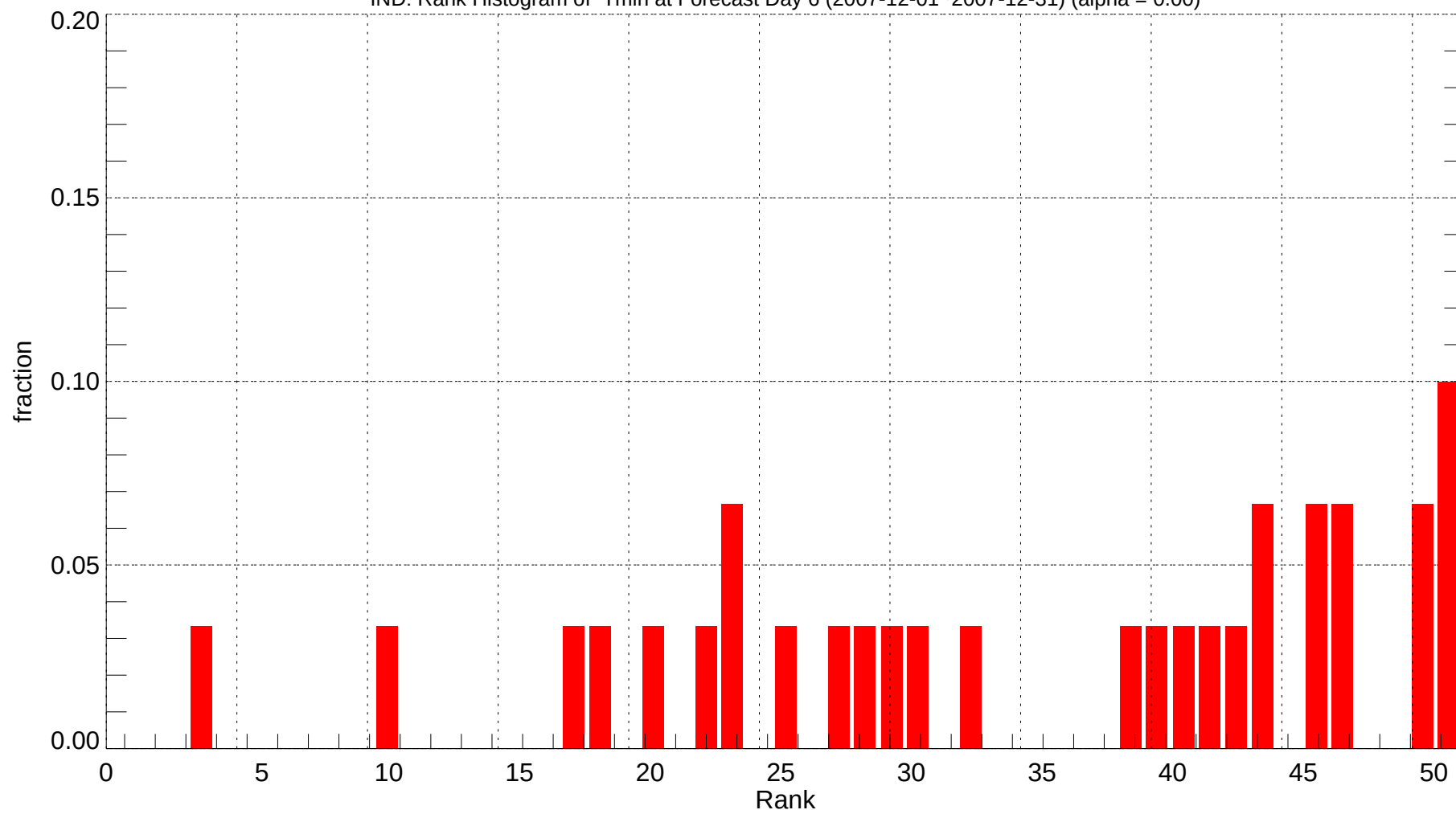
IND: Rank Histogram of Tmin at Forecast Day 6 (2007-12-01~2007-12-31) (alpha = 0.00)
