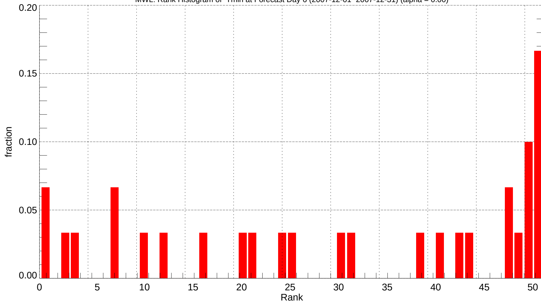
MWL: Rank Histogram of Tmin at Forecast Day 6 (2007-12-01~2007-12-31) (alpha = 0.00)
