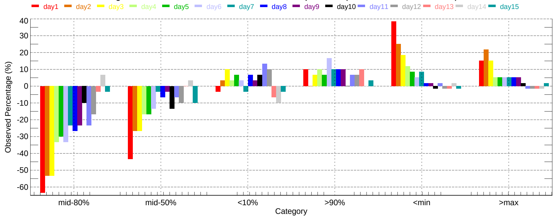
Observed Percentage Deviation of Ensembles - LNS: Min Temperature (2007-12-01~2007-12-31)
