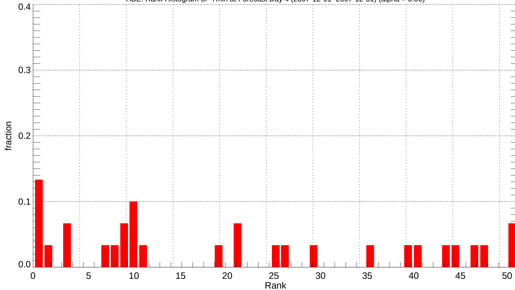
ABE: Rank Histogram of Tmin at Forecast Day 4 (2007-12-01~2007-12-31) (alpha = 0.00)
