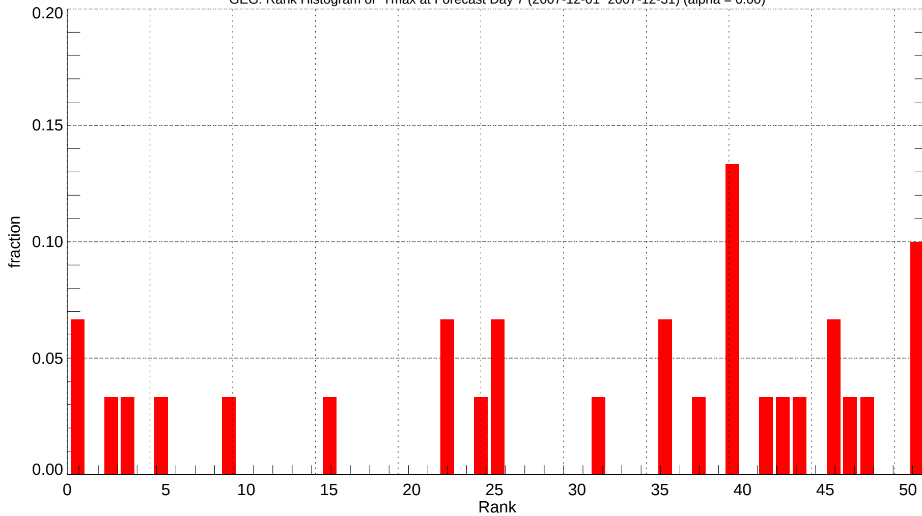
GEG: Rank Histogram of Tmax at Forecast Day 7 (2007-12-01~2007-12-31) (alpha = 0.00)
