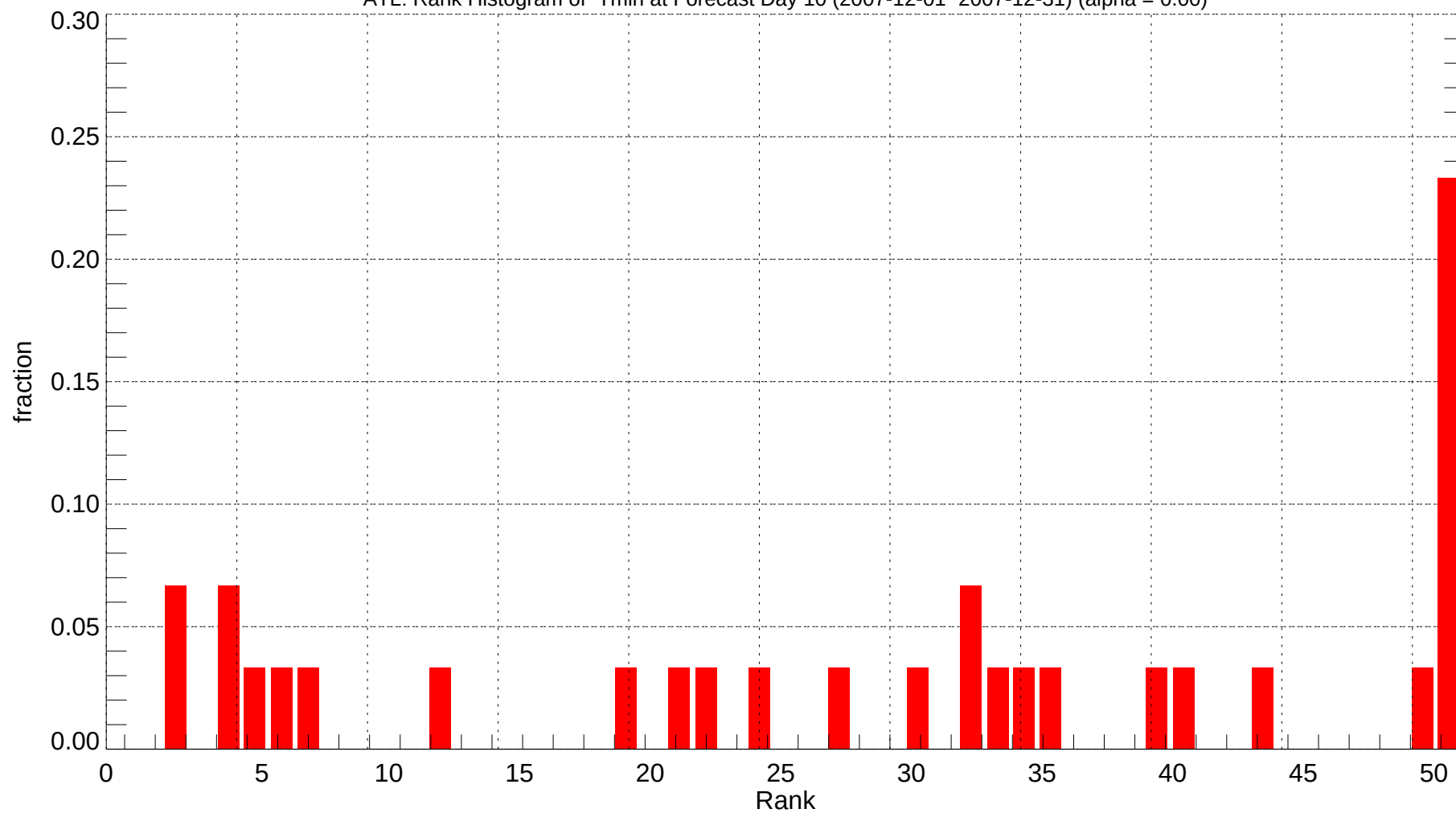
ATL: Rank Histogram of Tmin at Forecast Day 10 (2007-12-01~2007-12-31) (alpha = 0.00)
