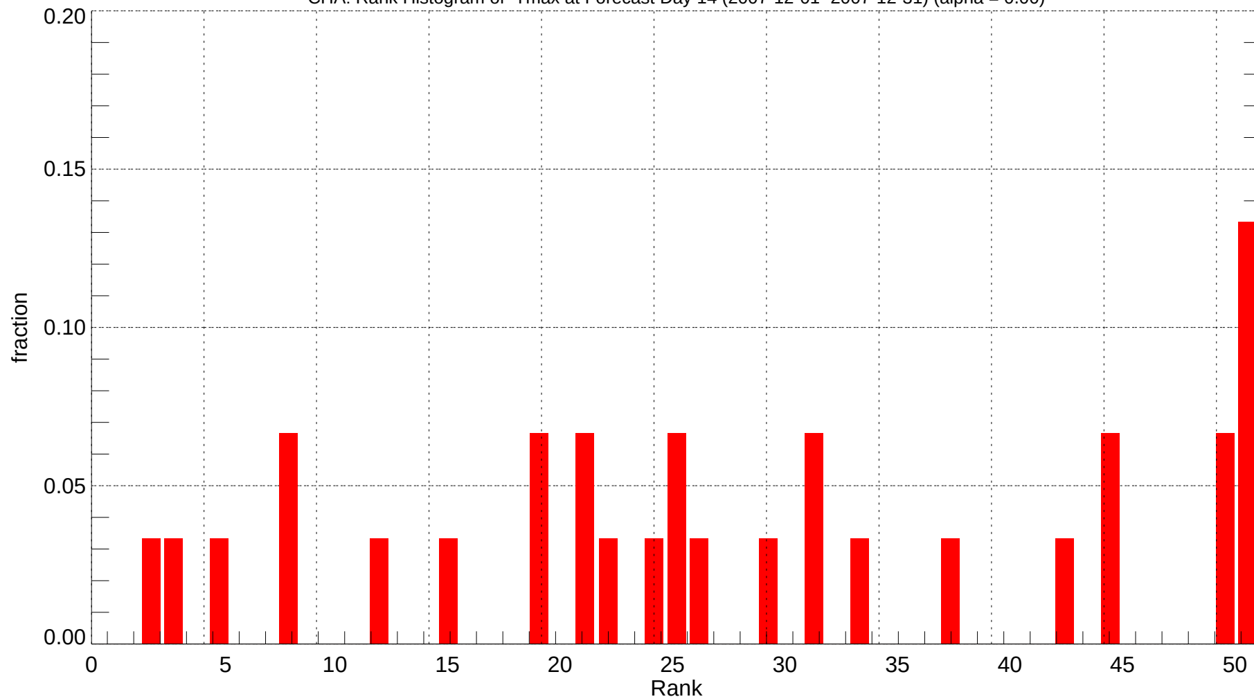
CHA: Rank Histogram of Tmax at Forecast Day 14 (2007-12-01~2007-12-31) (alpha = 0.00)
