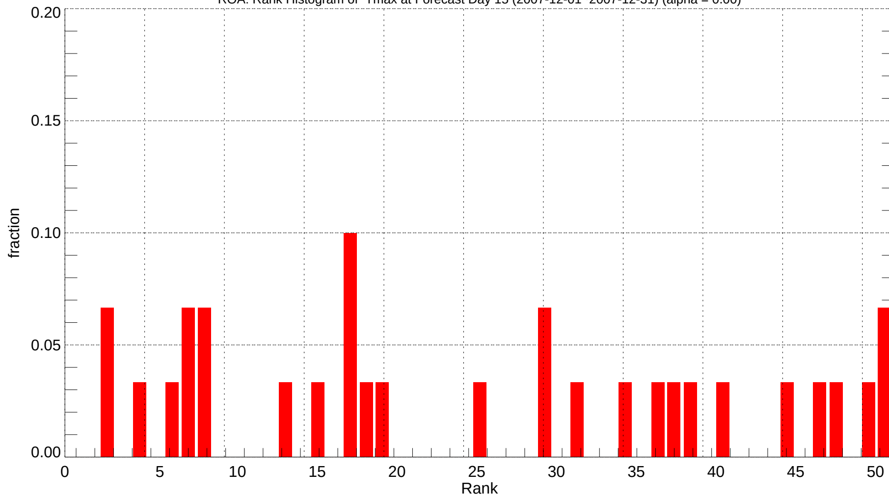
ROA: Rank Histogram of Tmax at Forecast Day 15 (2007-12-01~2007-12-31) (alpha = 0.00)
