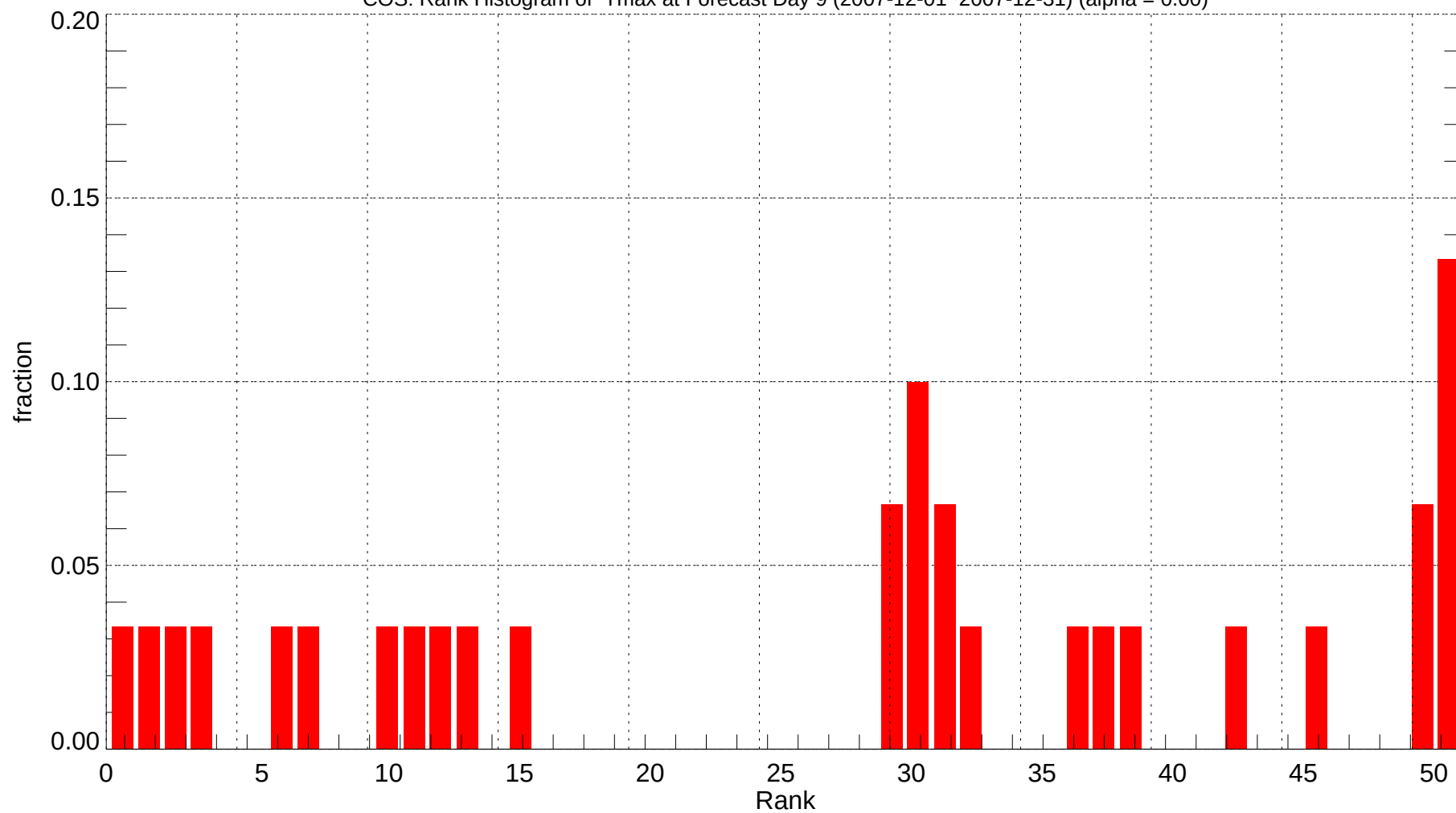
COS: Rank Histogram of Tmax at Forecast Day 9 (2007-12-01~2007-12-31) (alpha = 0.00)
