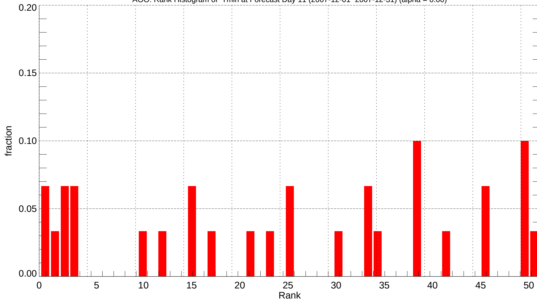
AOO: Rank Histogram of Tmin at Forecast Day 11 (2007-12-01~2007-12-31) (alpha = 0.00)
