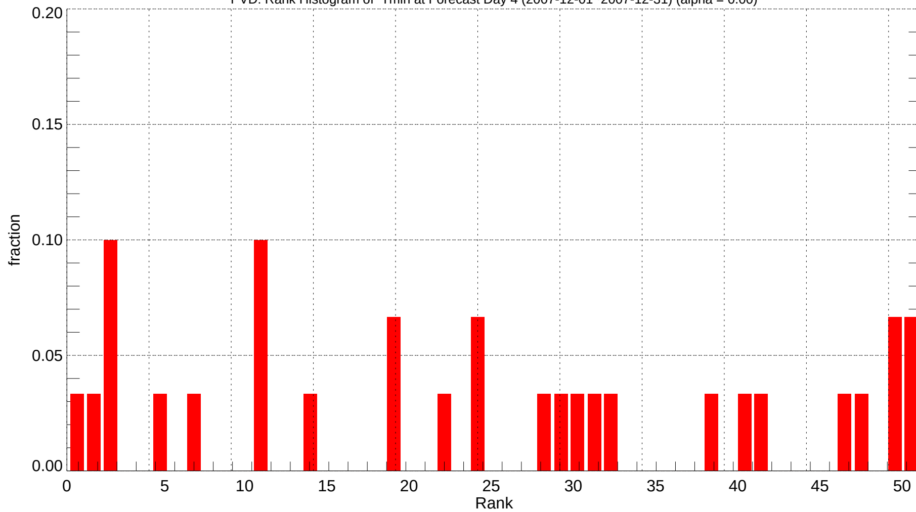
PVD: Rank Histogram of Tmin at Forecast Day 4 (2007-12-01~2007-12-31) (alpha = 0.00)
