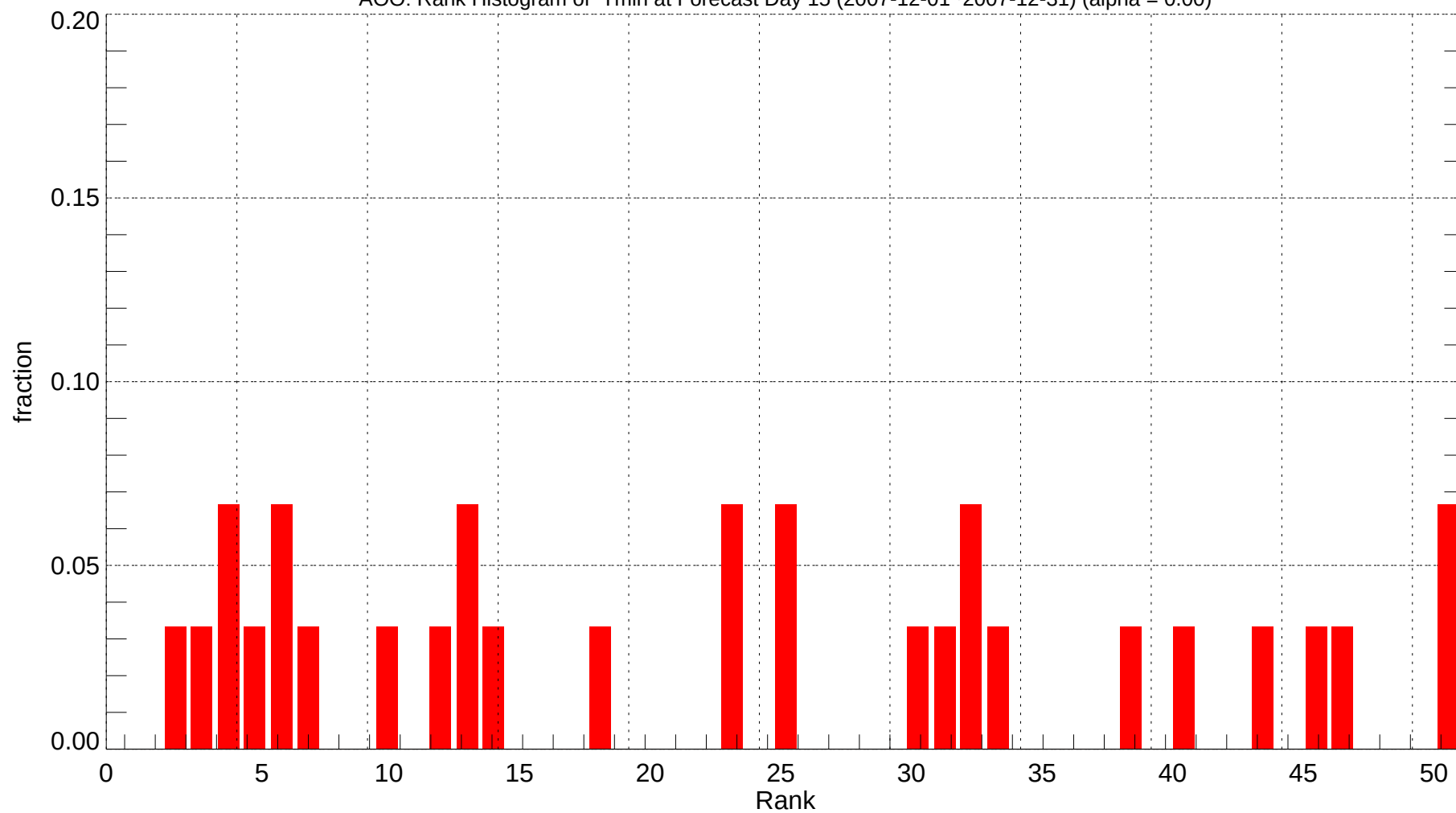
AOO: Rank Histogram of Tmin at Forecast Day 15 (2007-12-01~2007-12-31) (alpha = 0.00)
