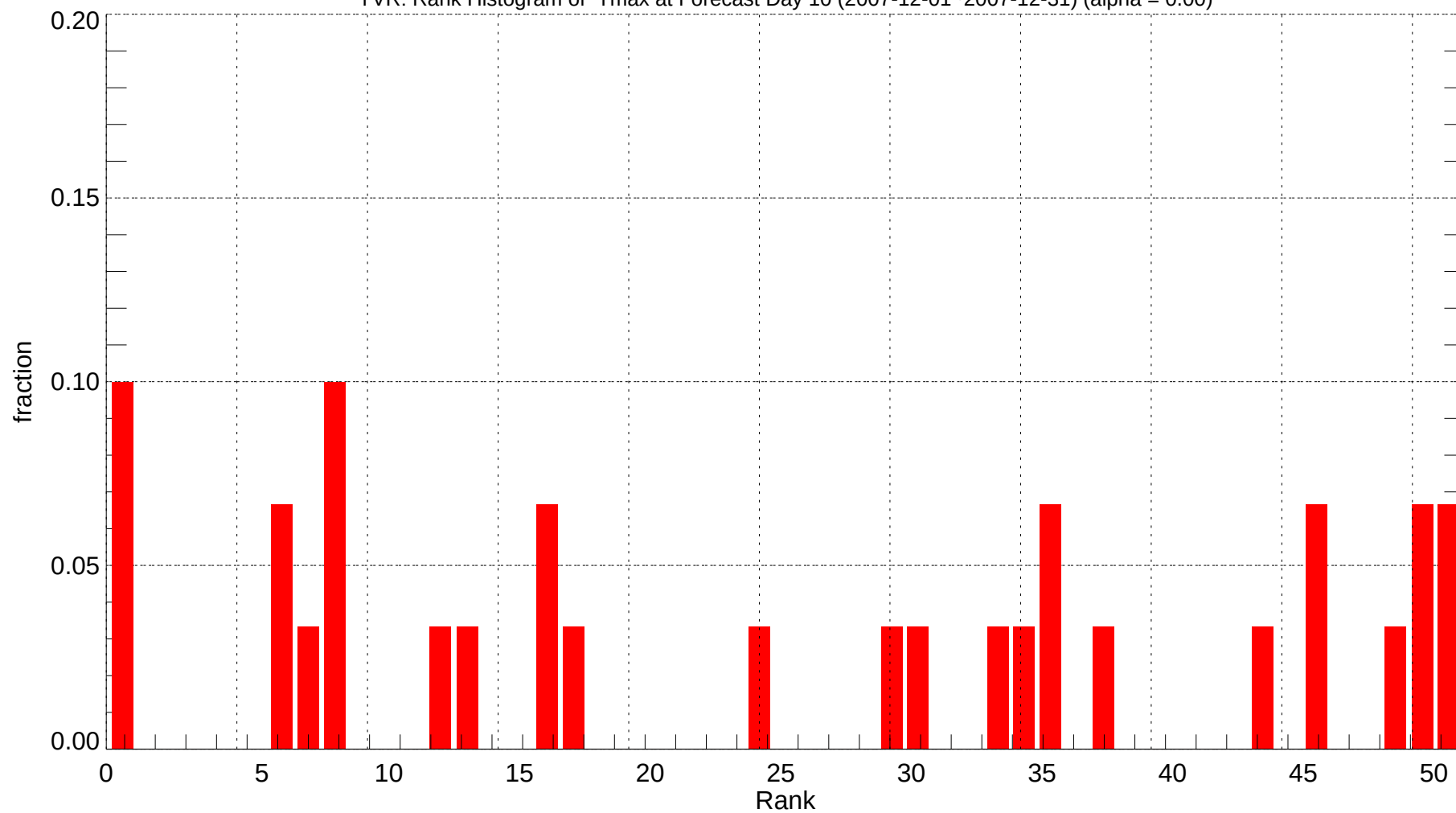
YVR: Rank Histogram of Tmax at Forecast Day 10 (2007-12-01~2007-12-31) (alpha = 0.00)
