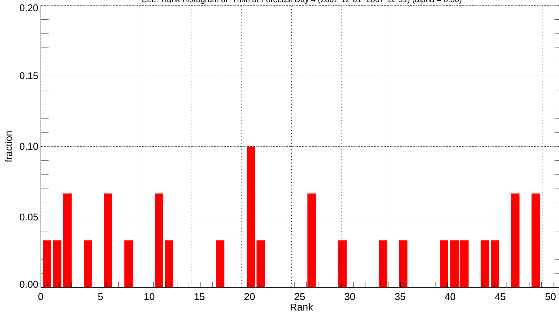
CLE: Rank Histogram of Tmin at Forecast Day 4 (2007-12-01~2007-12-31) (alpha = 0.00)
