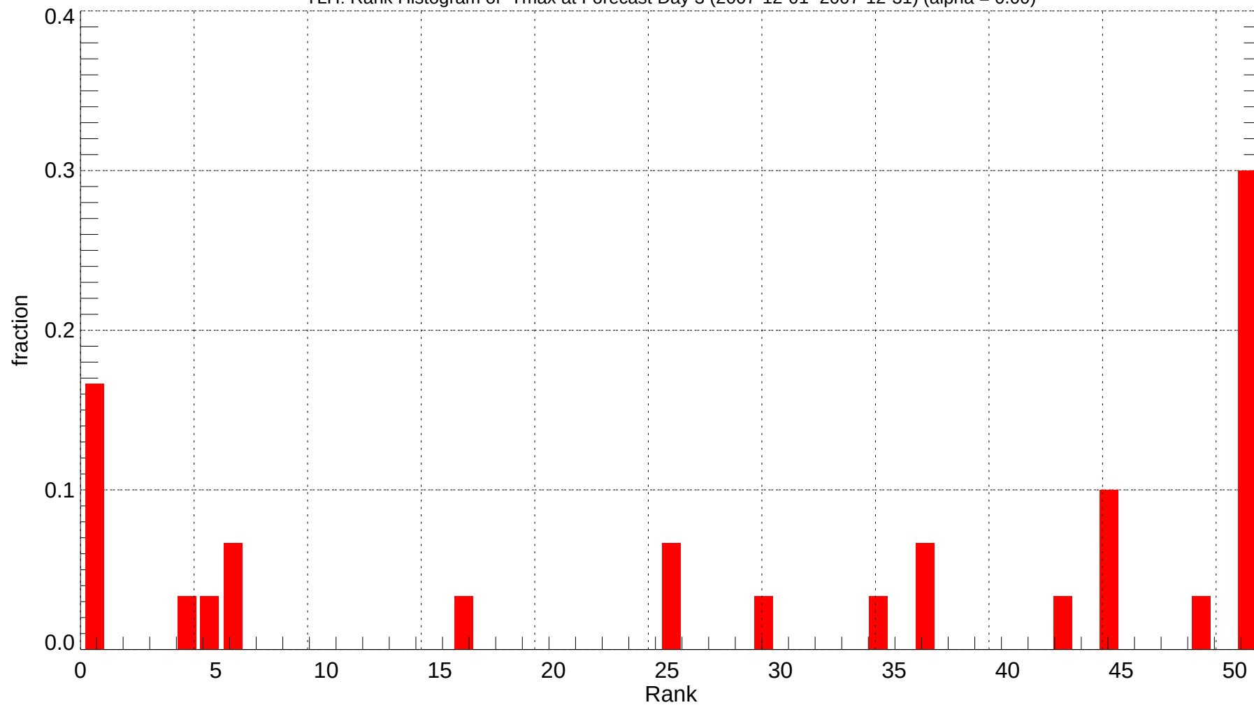
TLH: Rank Histogram of Tmax at Forecast Day 3 (2007-12-01~2007-12-31) (alpha = 0.00)
