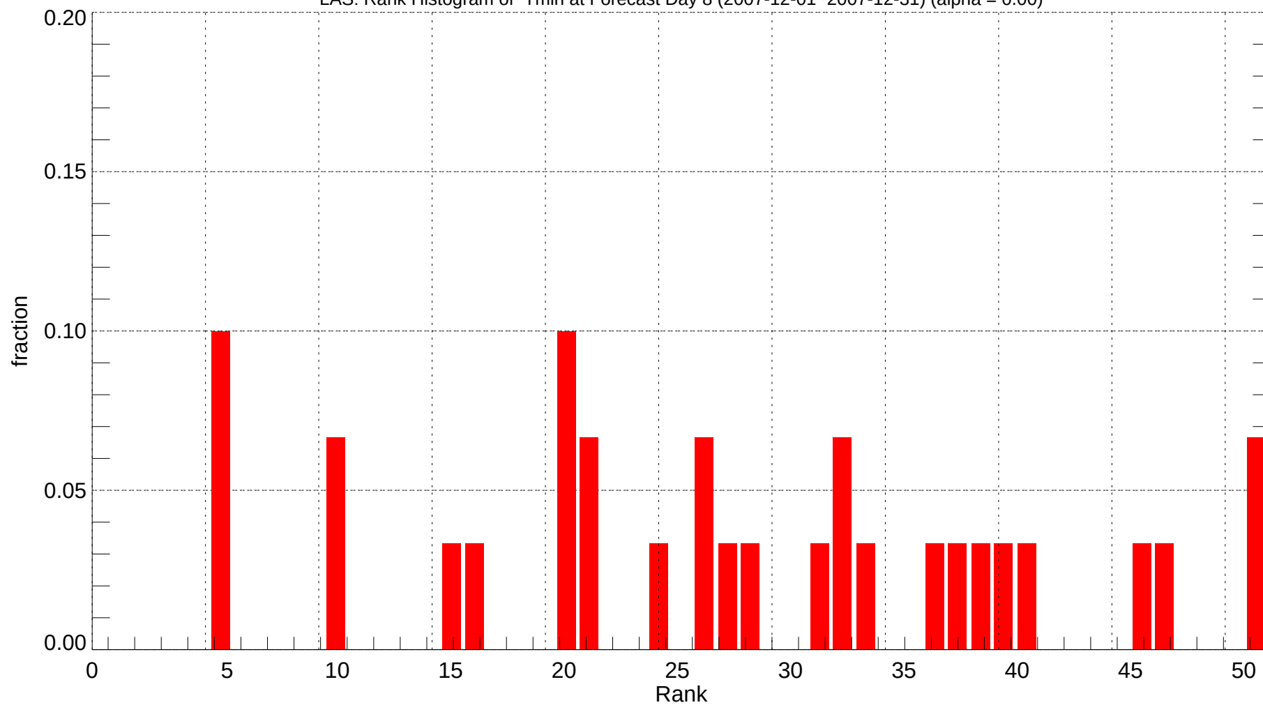
LAS: Rank Histogram of Tmin at Forecast Day 8 (2007-12-01~2007-12-31) (alpha = 0.00)
