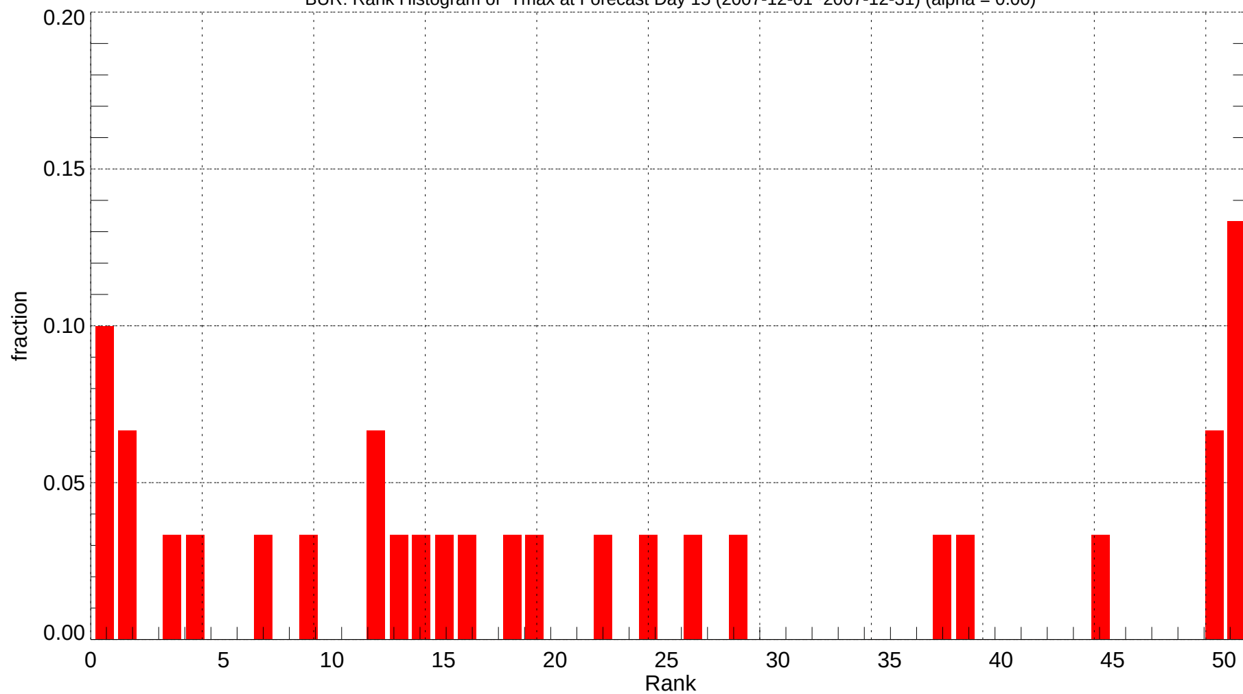
BUR: Rank Histogram of Tmax at Forecast Day 15 (2007-12-01~2007-12-31) (alpha = 0.00)
