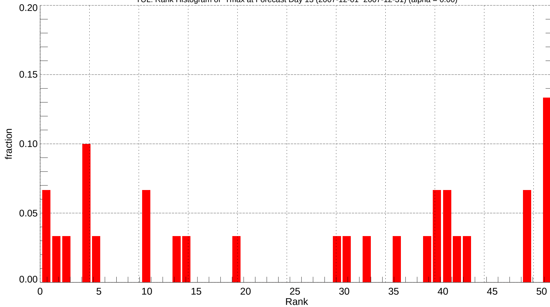
TUL: Rank Histogram of Tmax at Forecast Day 13 (2007-12-01~2007-12-31) (alpha = 0.00)
