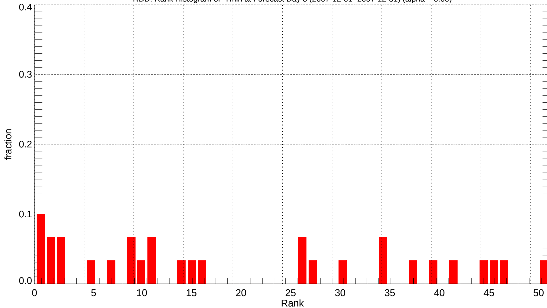
RDD: Rank Histogram of Tmin at Forecast Day 5 (2007-12-01~2007-12-31) (alpha = 0.00)
