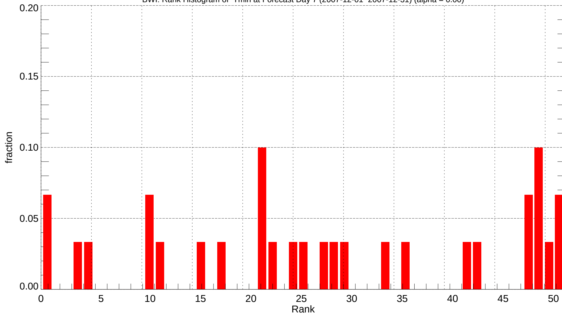
BWI: Rank Histogram of Tmin at Forecast Day 7 (2007-12-01~2007-12-31) (alpha = 0.00)
