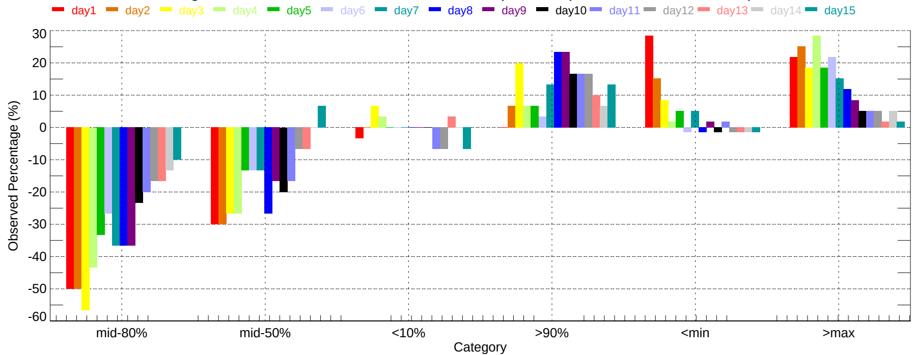
Observed Percentage Deviation of Ensembles - STL: Min Temperature (2007-12-01~2007-12-31)
