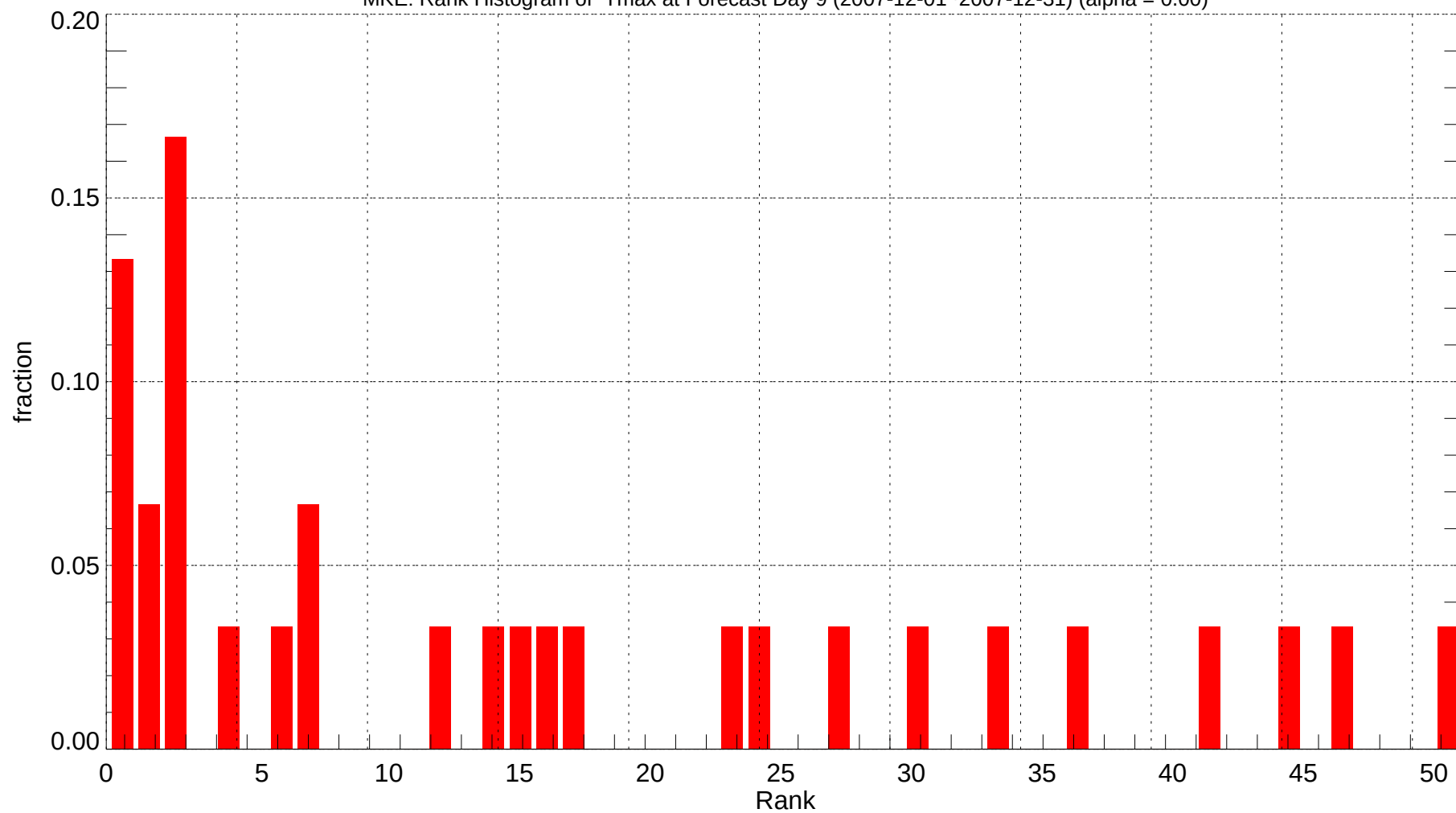
MKE: Rank Histogram of Tmax at Forecast Day 9 (2007-12-01~2007-12-31) (alpha = 0.00)
