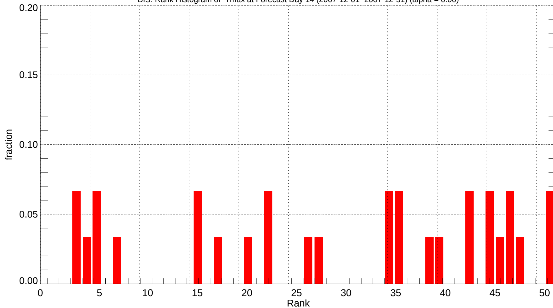
BIS: Rank Histogram of Tmax at Forecast Day 14 (2007-12-01~2007-12-31) (alpha = 0.00)
