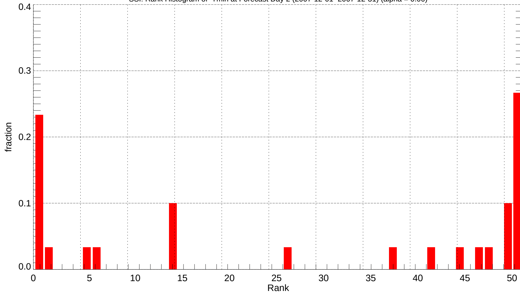
SSI: Rank Histogram of Tmin at Forecast Day 2 (2007-12-01~2007-12-31) (alpha = 0.00)
