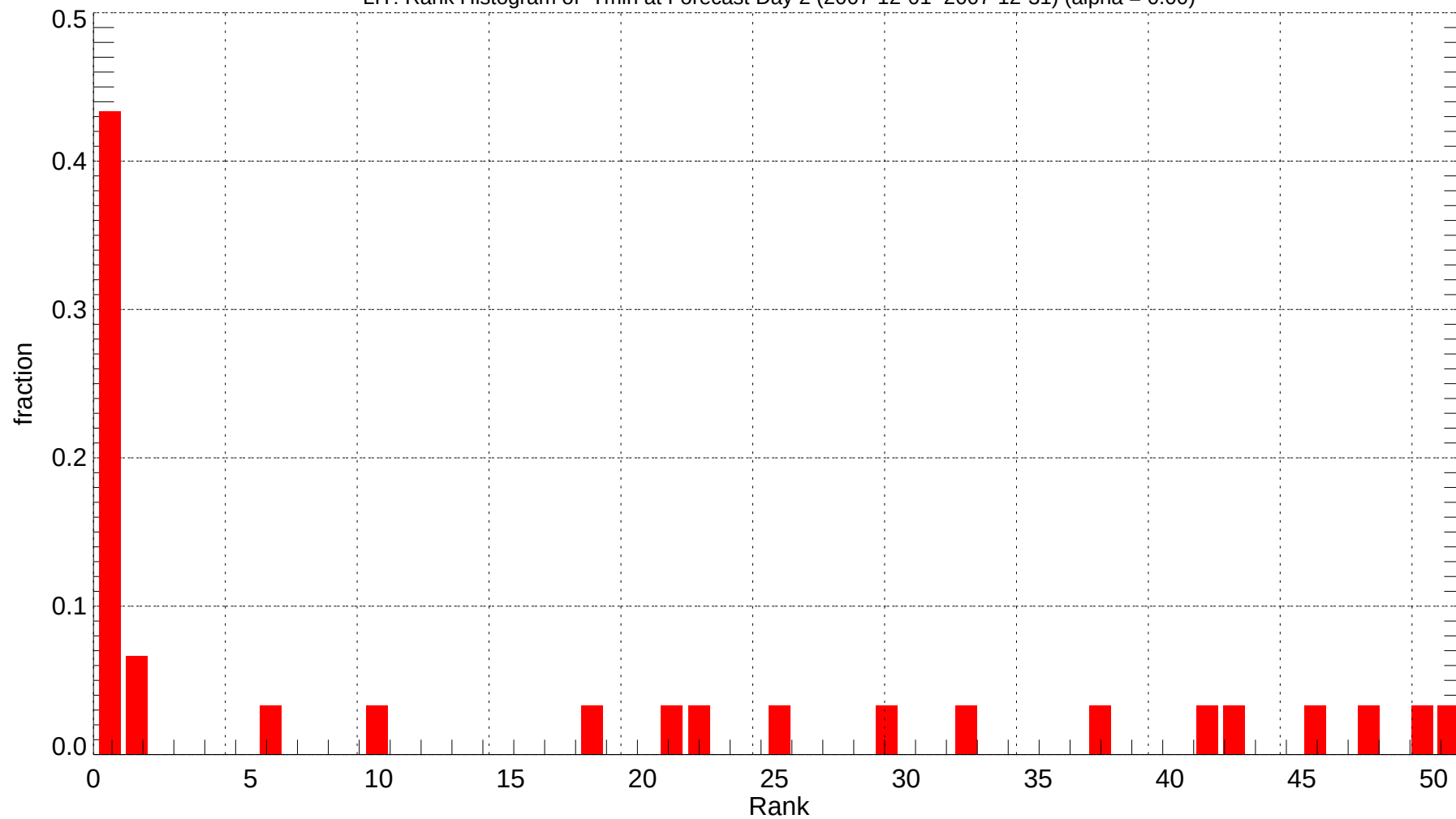
LIT: Rank Histogram of Tmin at Forecast Day 2 (2007-12-01~2007-12-31) (alpha = 0.00)
