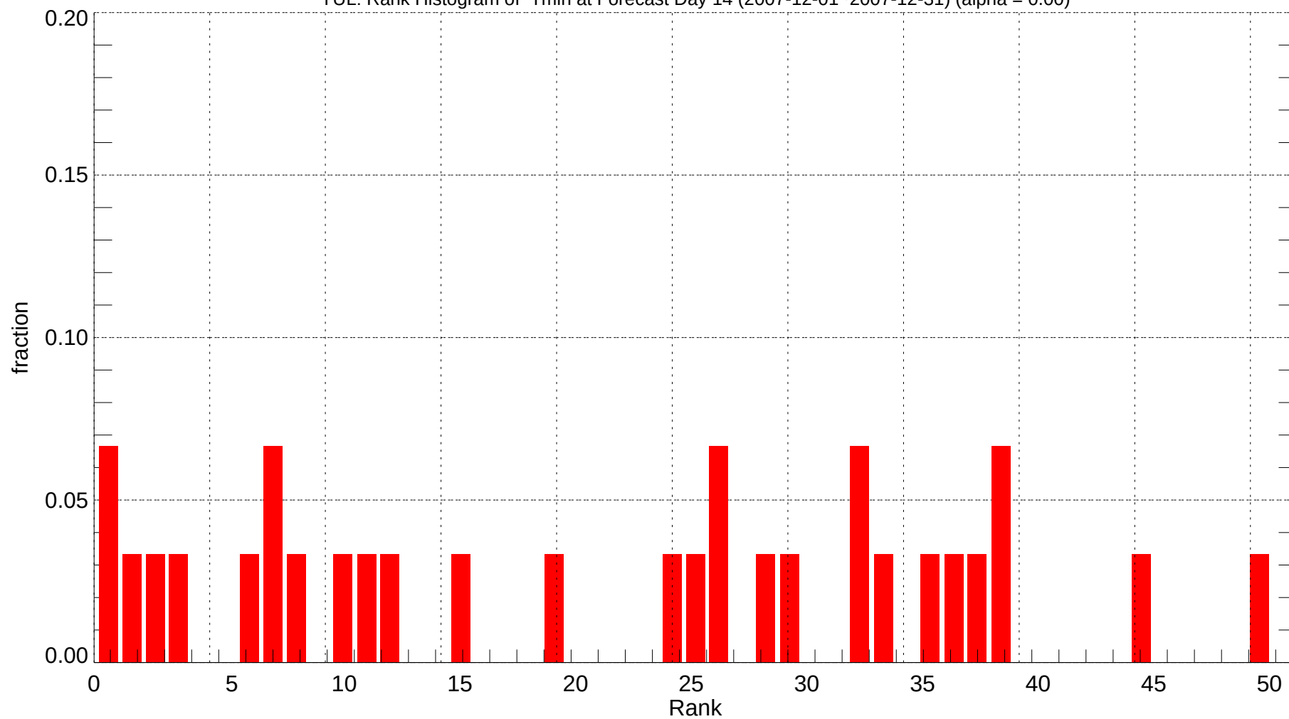
YUL: Rank Histogram of Tmin at Forecast Day 14 (2007-12-01~2007-12-31) (alpha = 0.00)
