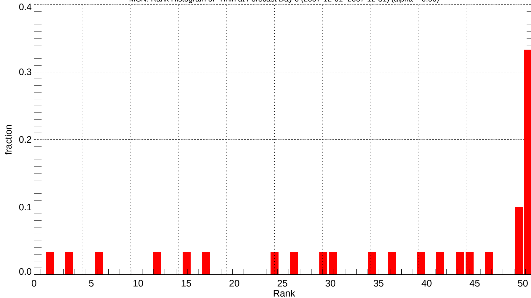
MCN: Rank Histogram of Tmin at Forecast Day 6 (2007-12-01~2007-12-31) (alpha = 0.00)
