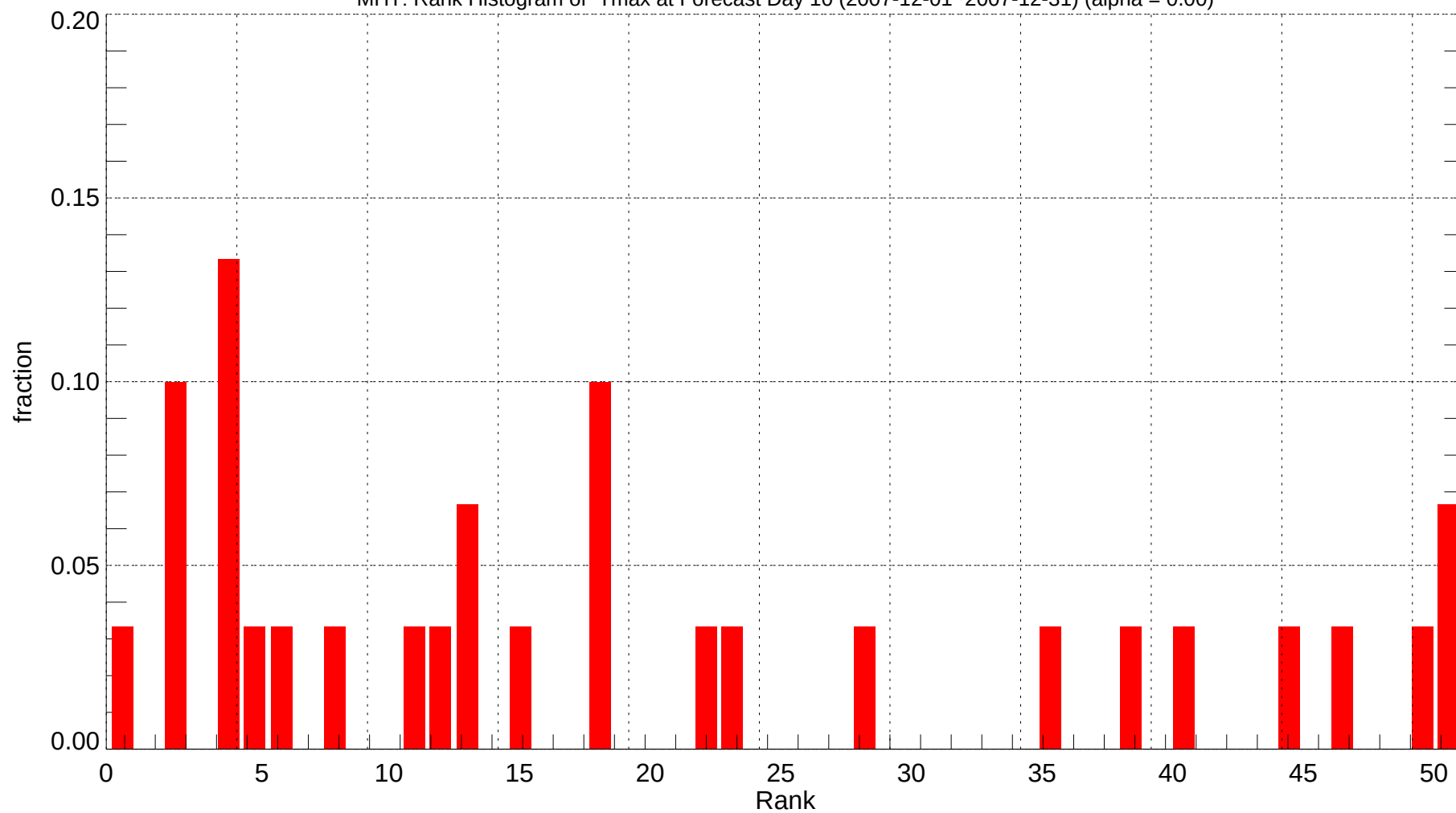
MHT: Rank Histogram of Tmax at Forecast Day 10 (2007-12-01~2007-12-31) (alpha = 0.00)
