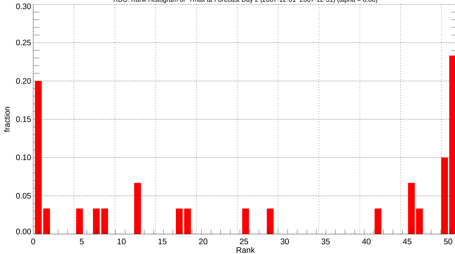
RDU: Rank Histogram of Tmax at Forecast Day 2 (2007-12-01~2007-12-31) (alpha = 0.00)
