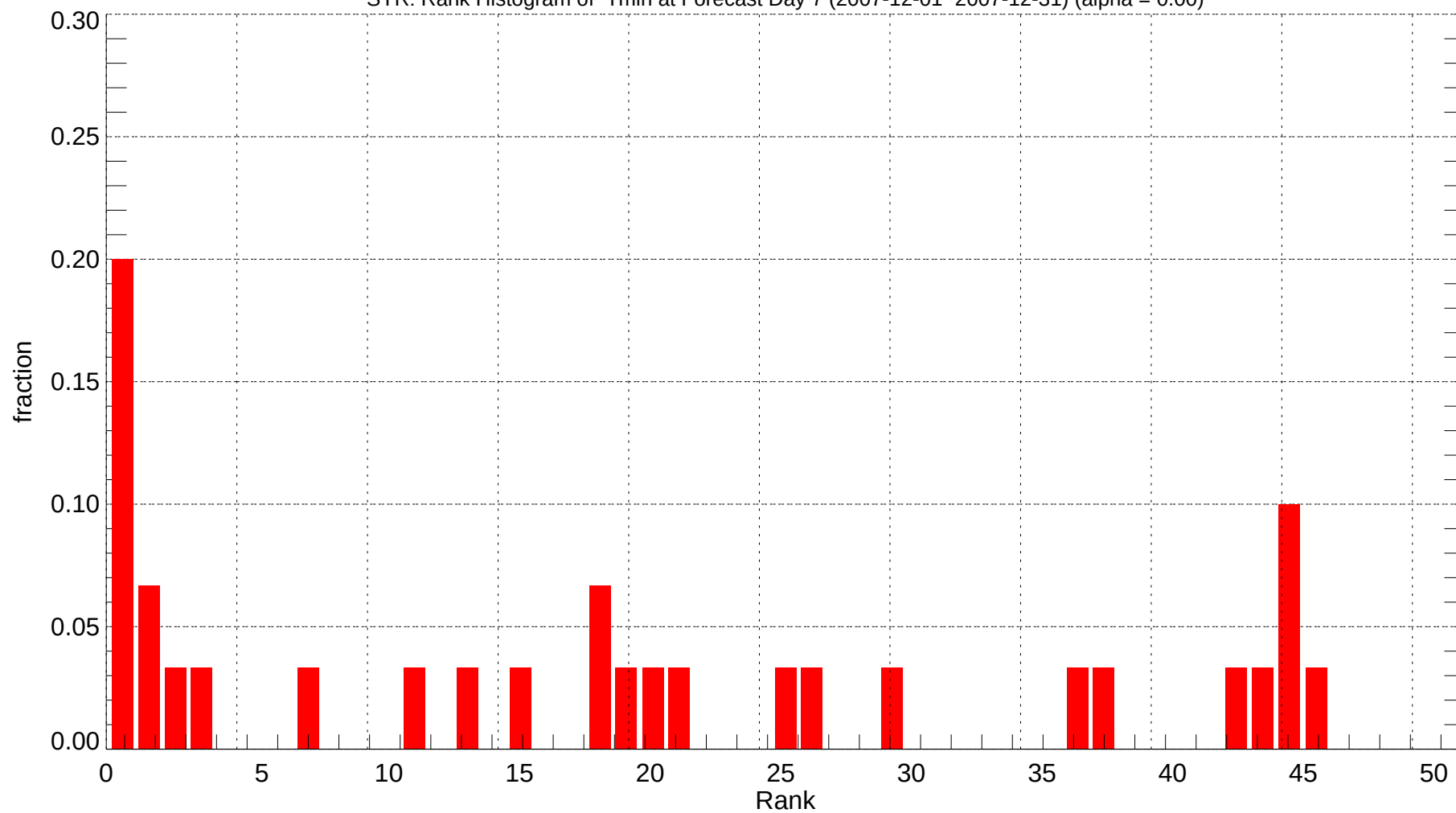
SYR: Rank Histogram of Tmin at Forecast Day 7 (2007-12-01~2007-12-31) (alpha = 0.00)
