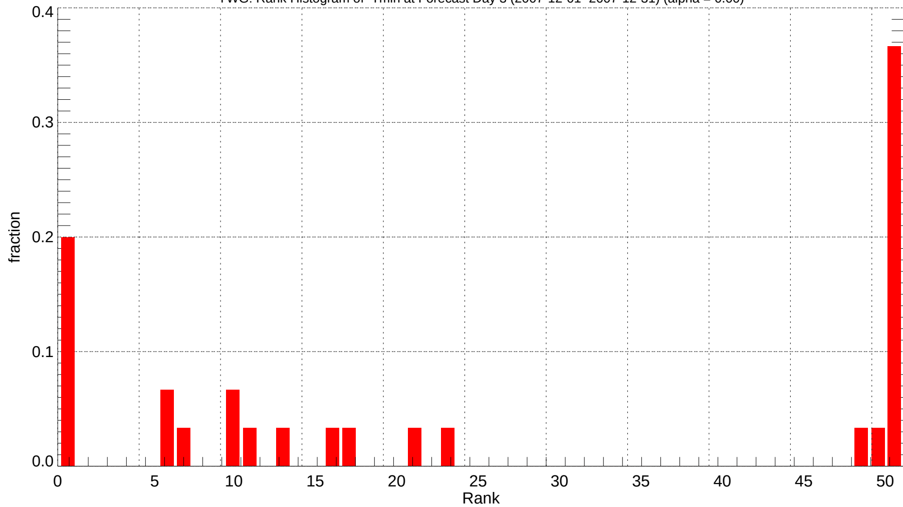
YWG: Rank Histogram of Tmin at Forecast Day 3 (2007-12-01~2007-12-31) (alpha = 0.00)
