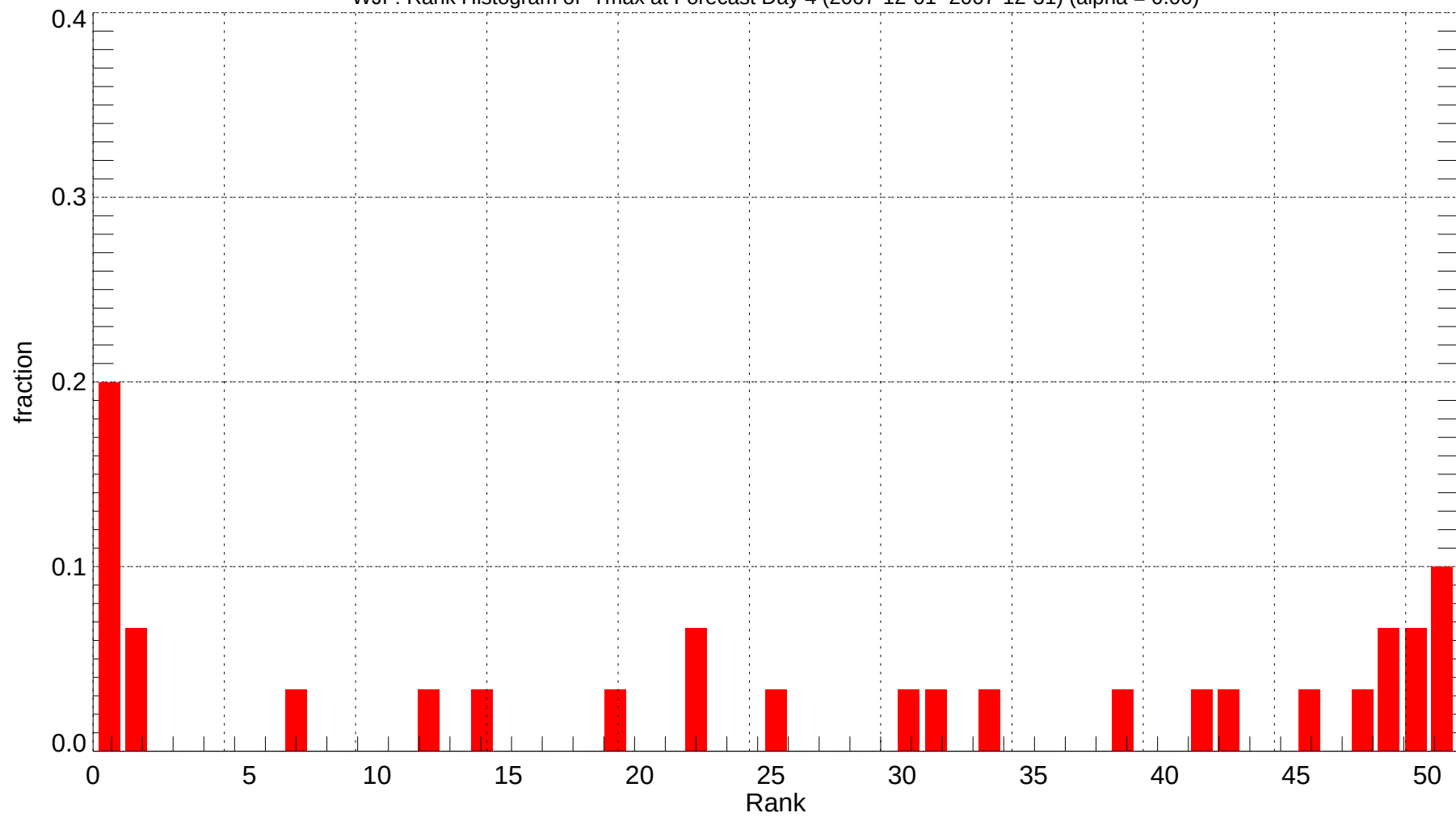
WJF: Rank Histogram of Tmax at Forecast Day 4 (2007-12-01~2007-12-31) (alpha = 0.00)
