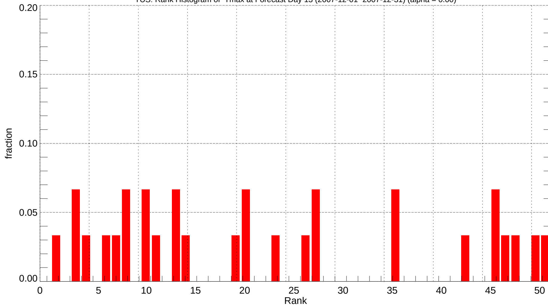
TUS: Rank Histogram of Tmax at Forecast Day 13 (2007-12-01~2007-12-31) (alpha = 0.00)
