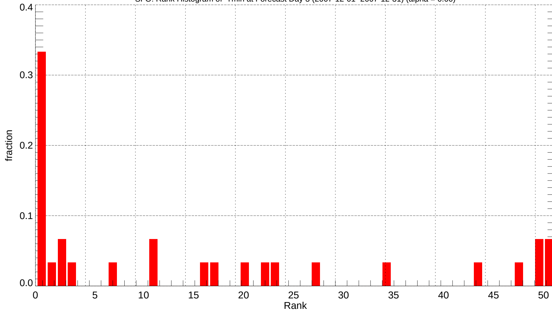
SFO: Rank Histogram of Tmin at Forecast Day 3 (2007-12-01~2007-12-31) (alpha = 0.00)
