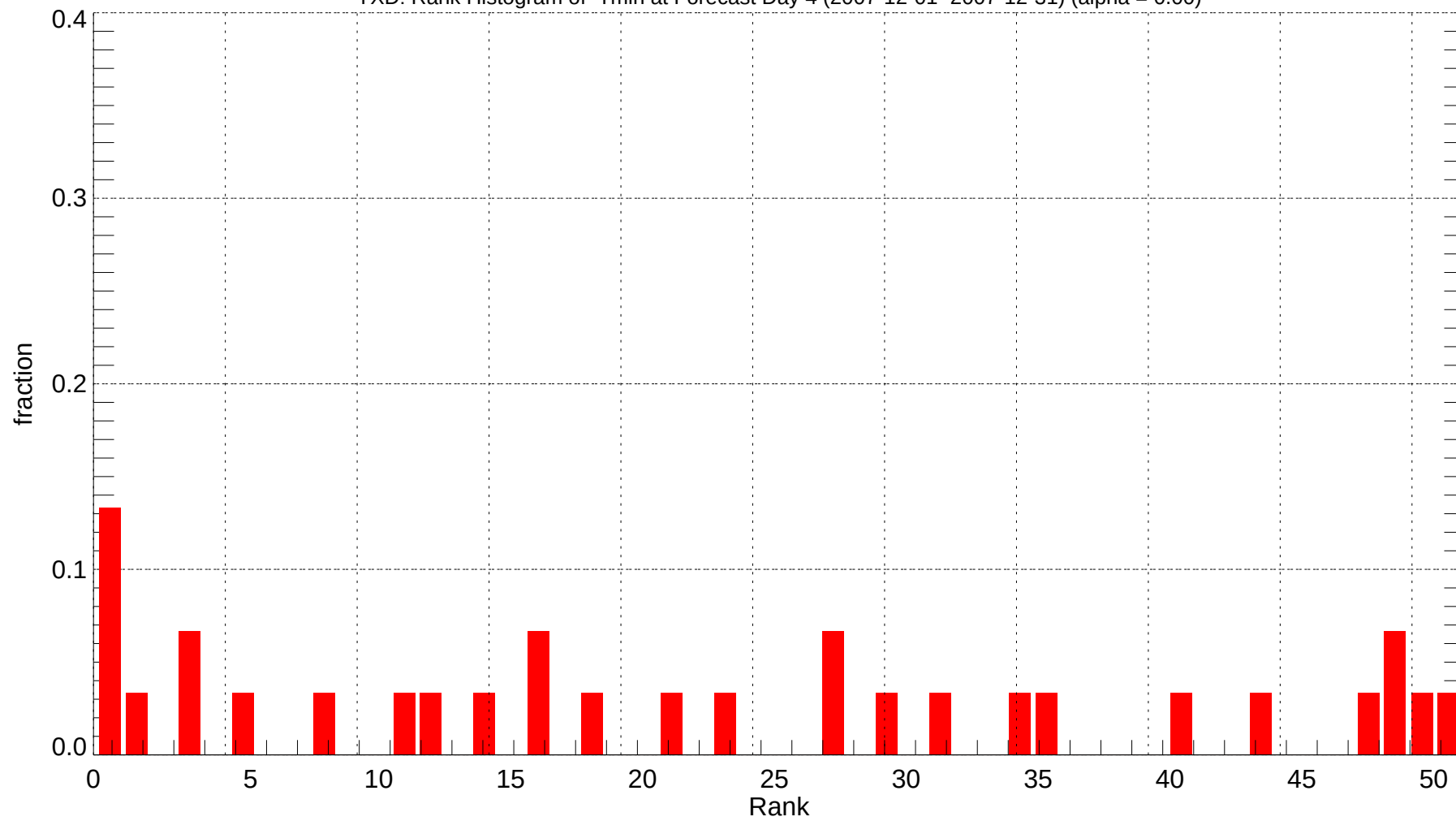
YXD: Rank Histogram of Tmin at Forecast Day 4 (2007-12-01~2007-12-31) (alpha = 0.00)
