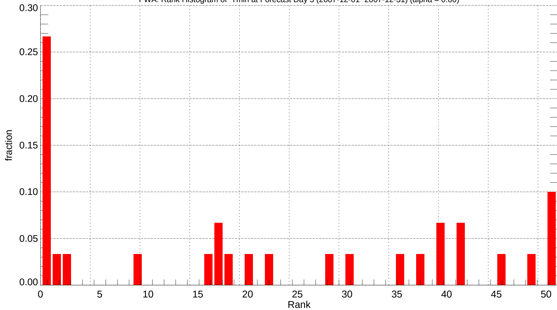
FWA: Rank Histogram of Tmin at Forecast Day 3 (2007-12-01~2007-12-31) (alpha = 0.00)
