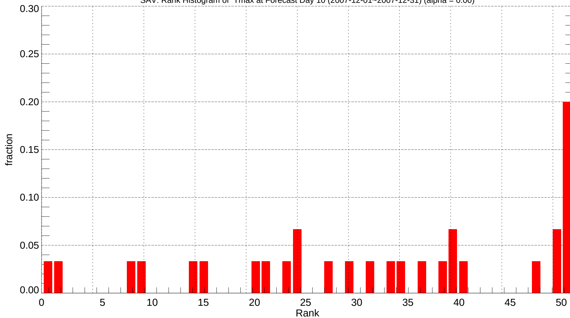
SAV: Rank Histogram of Tmax at Forecast Day 10 (2007-12-01~2007-12-31) (alpha = 0.00)
