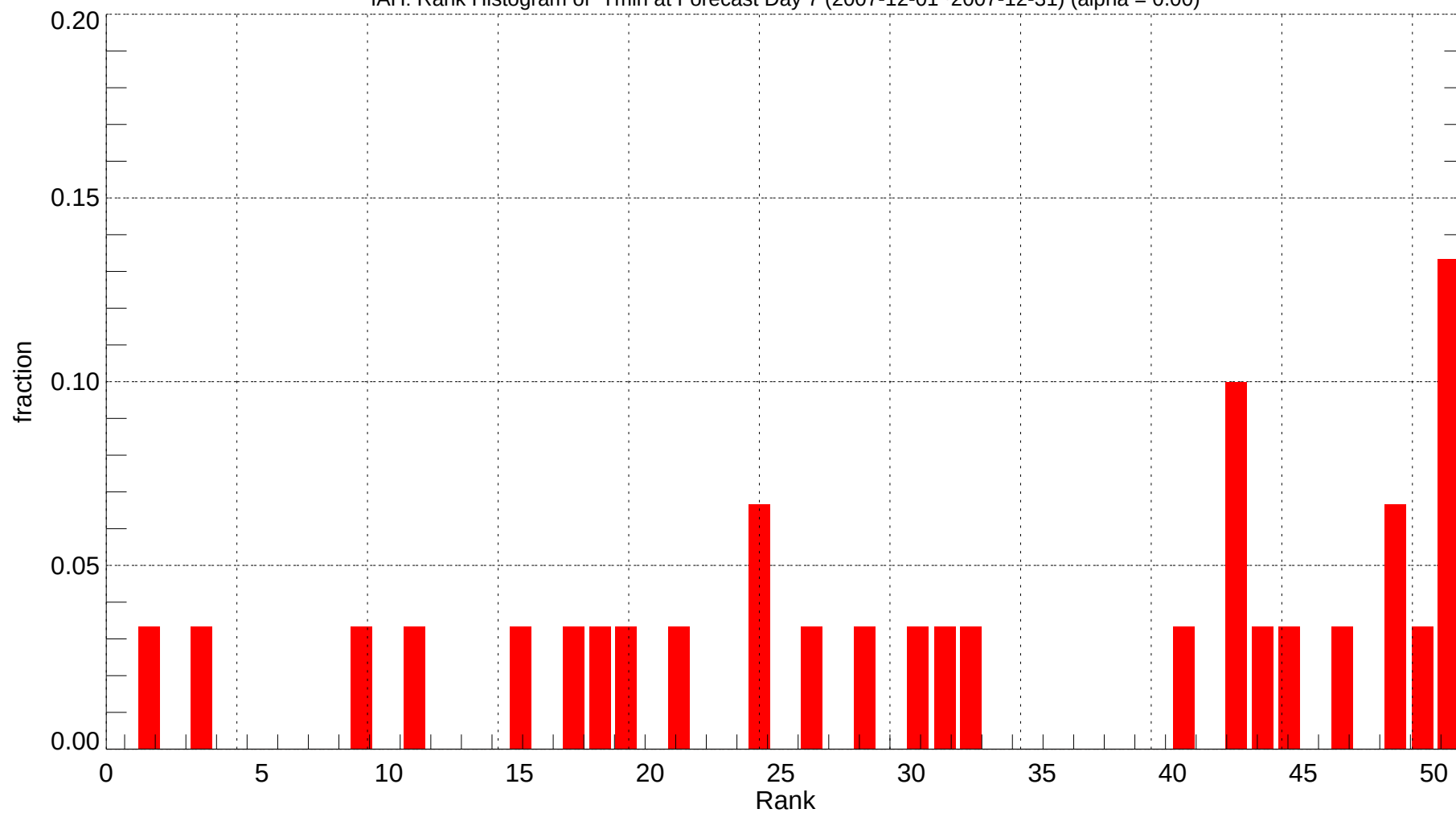
IAH: Rank Histogram of Tmin at Forecast Day 7 (2007-12-01~2007-12-31) (alpha = 0.00)
