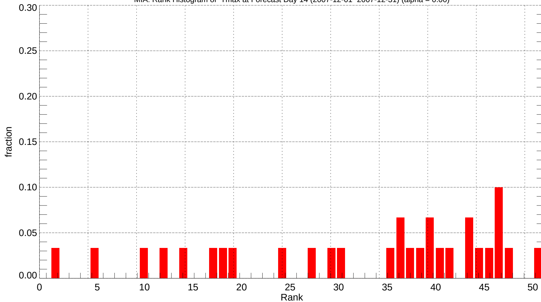
MIA: Rank Histogram of Tmax at Forecast Day 14 (2007-12-01~2007-12-31) (alpha = 0.00)
