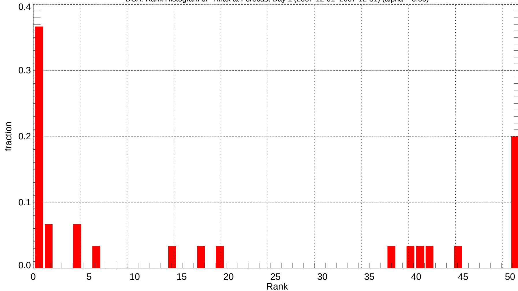
DCA: Rank Histogram of Tmax at Forecast Day 1 (2007-12-01~2007-12-31) (alpha = 0.00)
