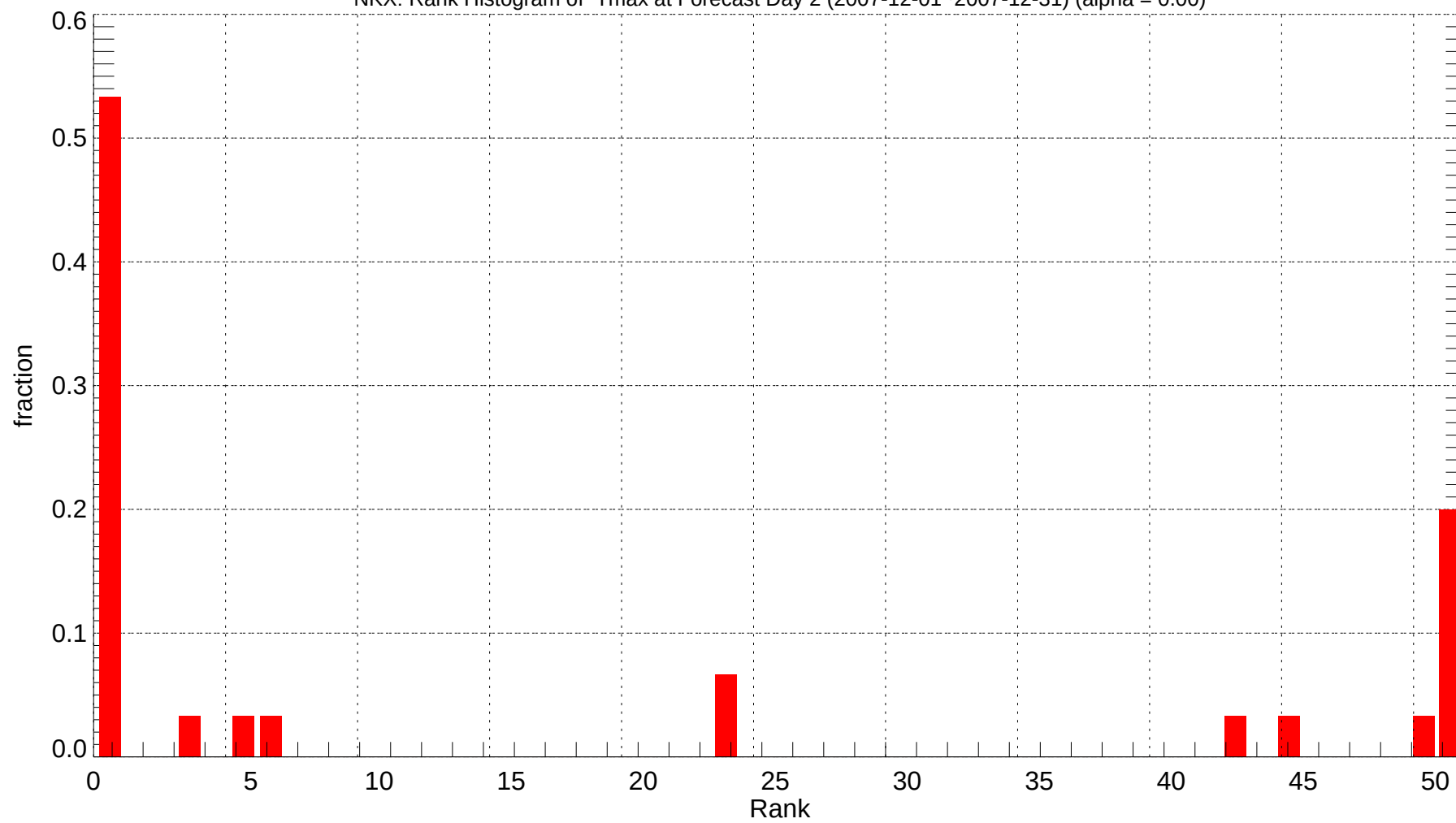
NKX: Rank Histogram of Tmax at Forecast Day 2 (2007-12-01~2007-12-31) (alpha = 0.00)
