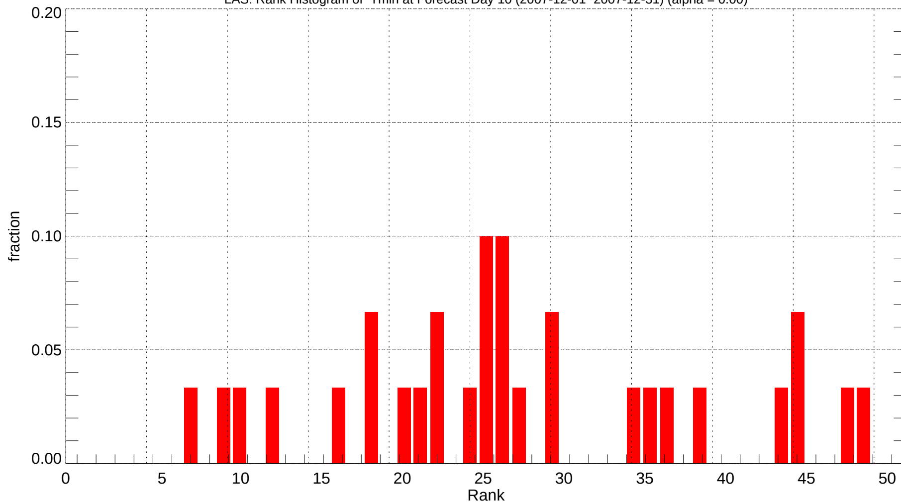
LAS: Rank Histogram of Tmin at Forecast Day 10 (2007-12-01~2007-12-31) (alpha = 0.00)
