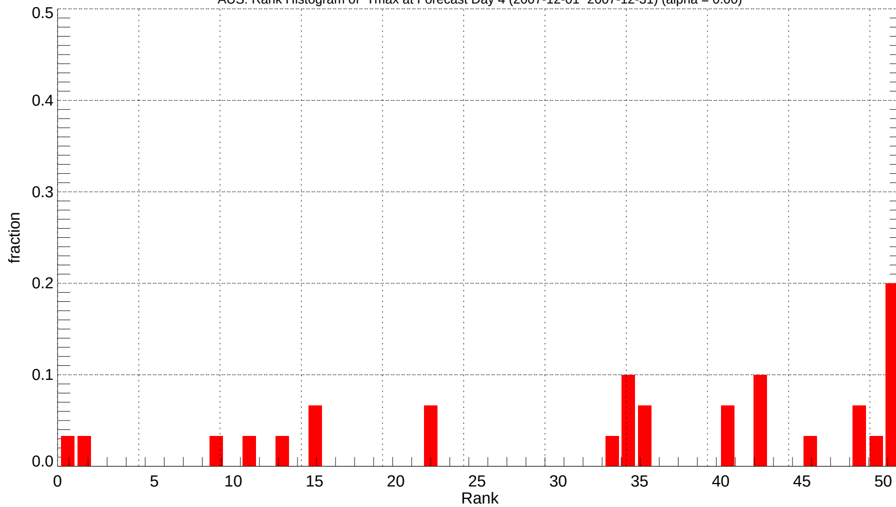
AUS: Rank Histogram of Tmax at Forecast Day 4 (2007-12-01~2007-12-31) (alpha = 0.00)
