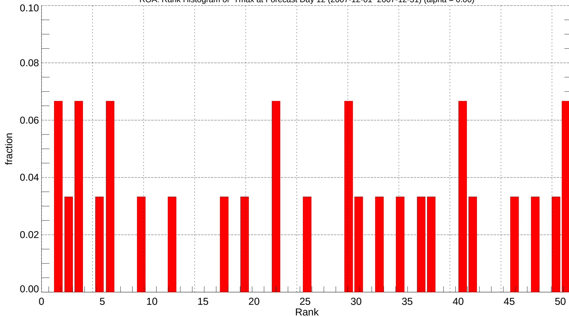
ROA: Rank Histogram of Tmax at Forecast Day 12 (2007-12-01~2007-12-31) (alpha = 0.00)
