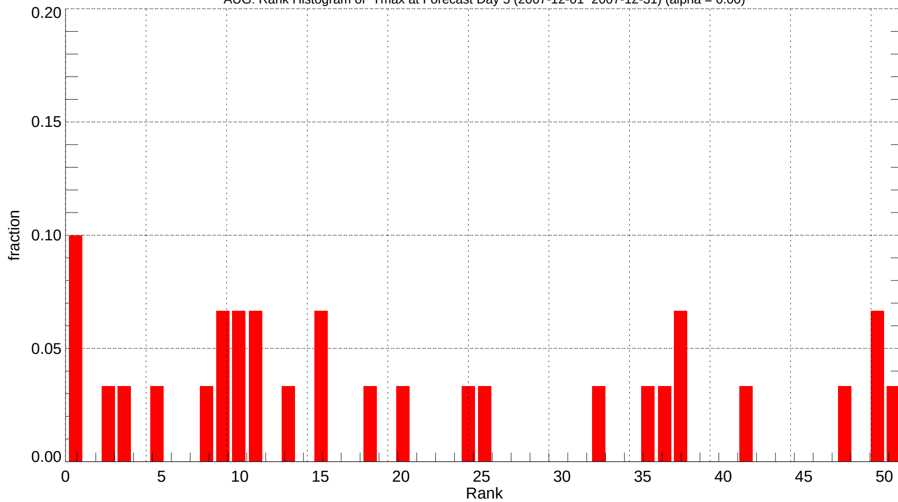
AUG: Rank Histogram of Tmax at Forecast Day 5 (2007-12-01~2007-12-31) (alpha = 0.00)
