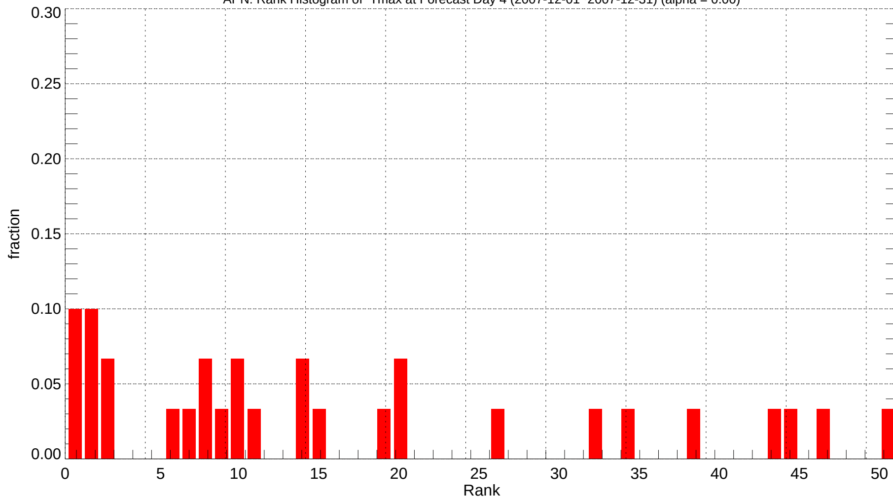
APN: Rank Histogram of Tmax at Forecast Day 4 (2007-12-01~2007-12-31) (alpha = 0.00)
