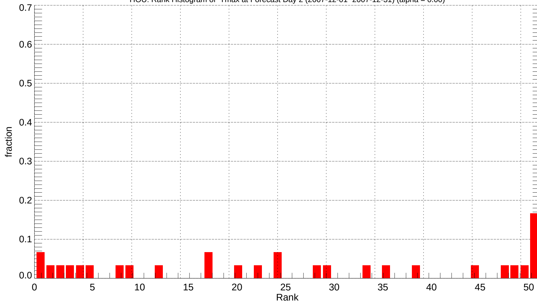
HOU: Rank Histogram of Tmax at Forecast Day 2 (2007-12-01~2007-12-31) (alpha = 0.00)
