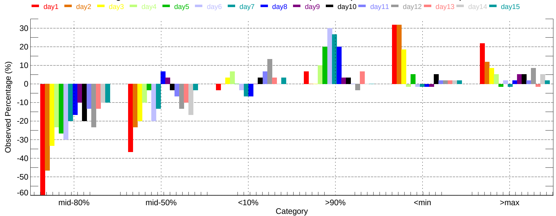
Observed Percentage Deviation of Ensembles - PVD: Max Temperature (2007-12-01~2007-12-31)
