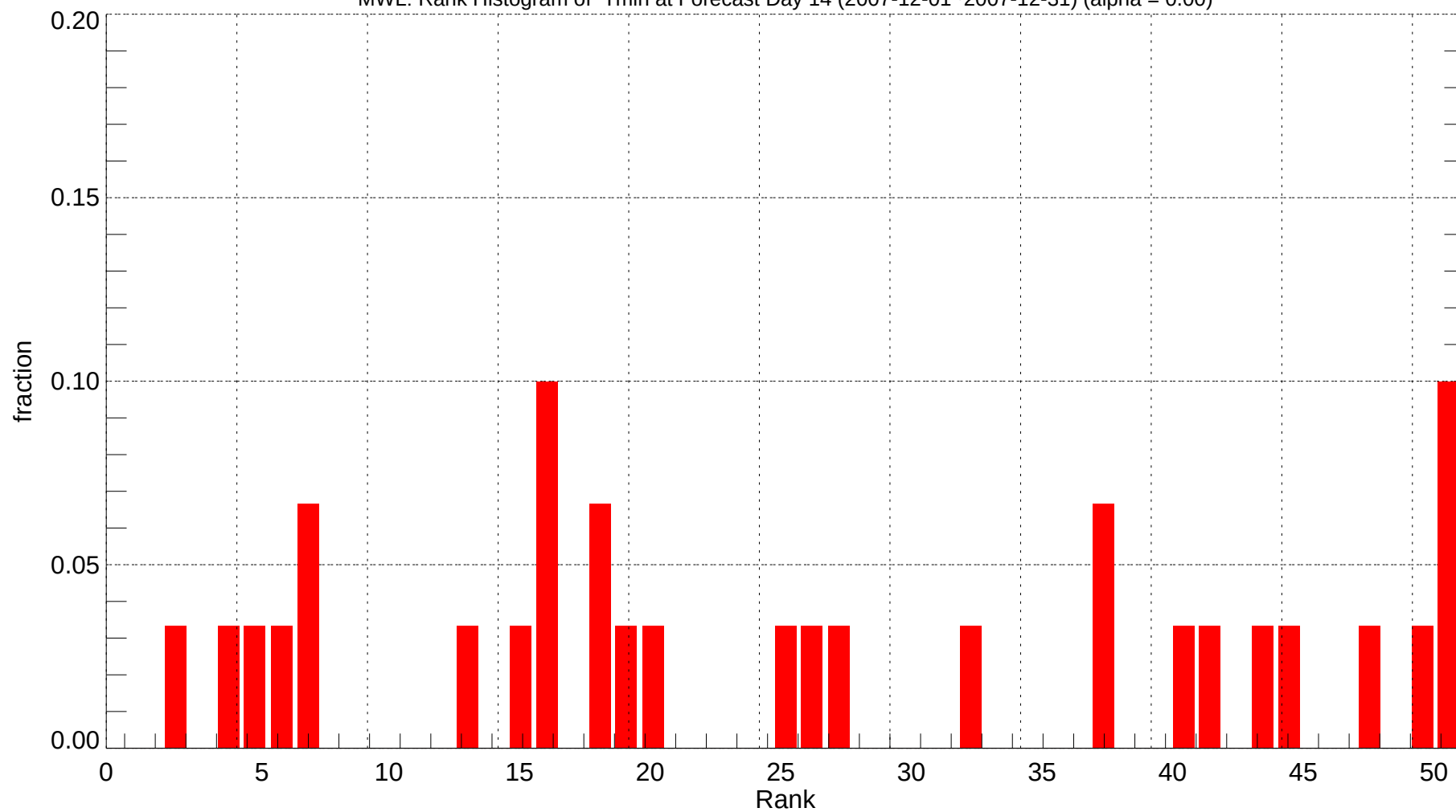
MWL: Rank Histogram of Tmin at Forecast Day 14 (2007-12-01~2007-12-31) (alpha = 0.00)
