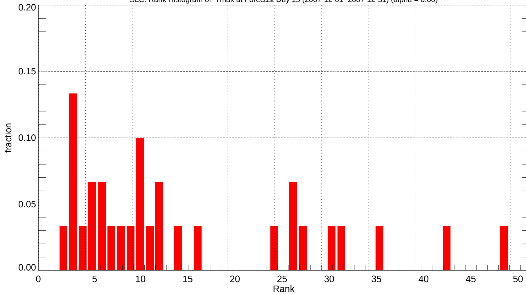
SLC: Rank Histogram of Tmax at Forecast Day 15 (2007-12-01~2007-12-31) (alpha = 0.00)
