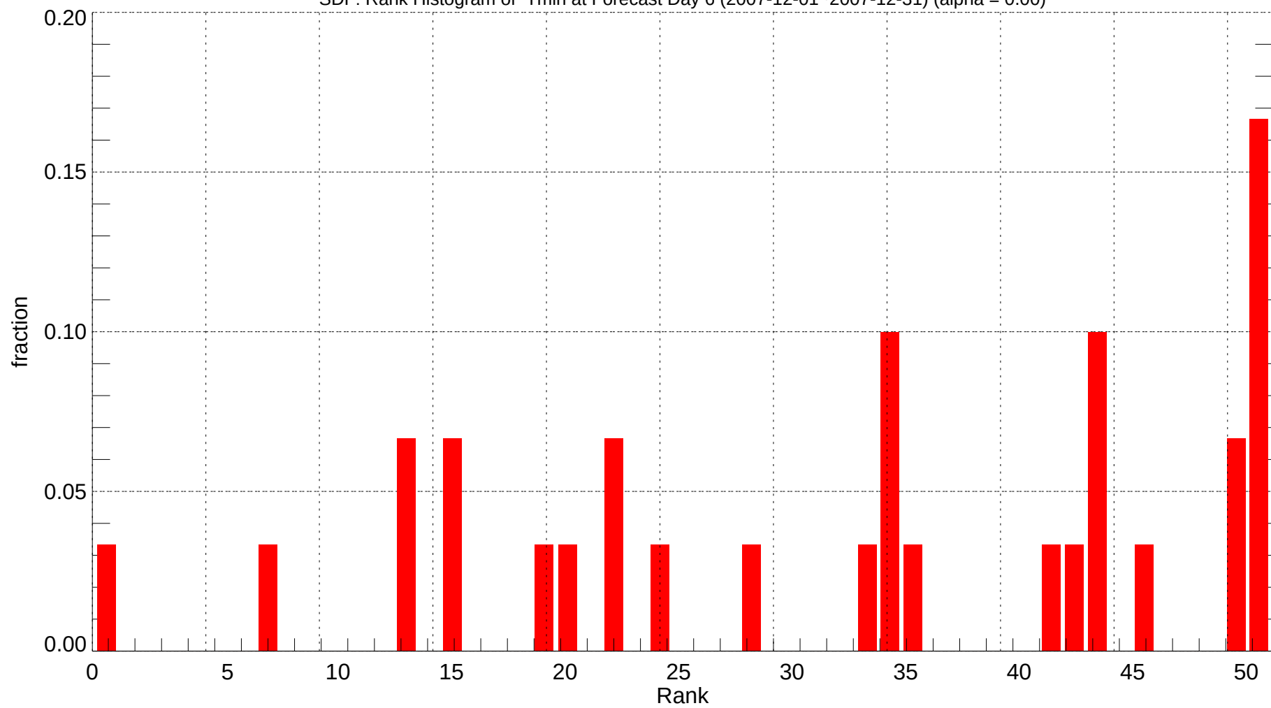
SDF: Rank Histogram of Tmin at Forecast Day 6 (2007-12-01~2007-12-31) (alpha = 0.00)
