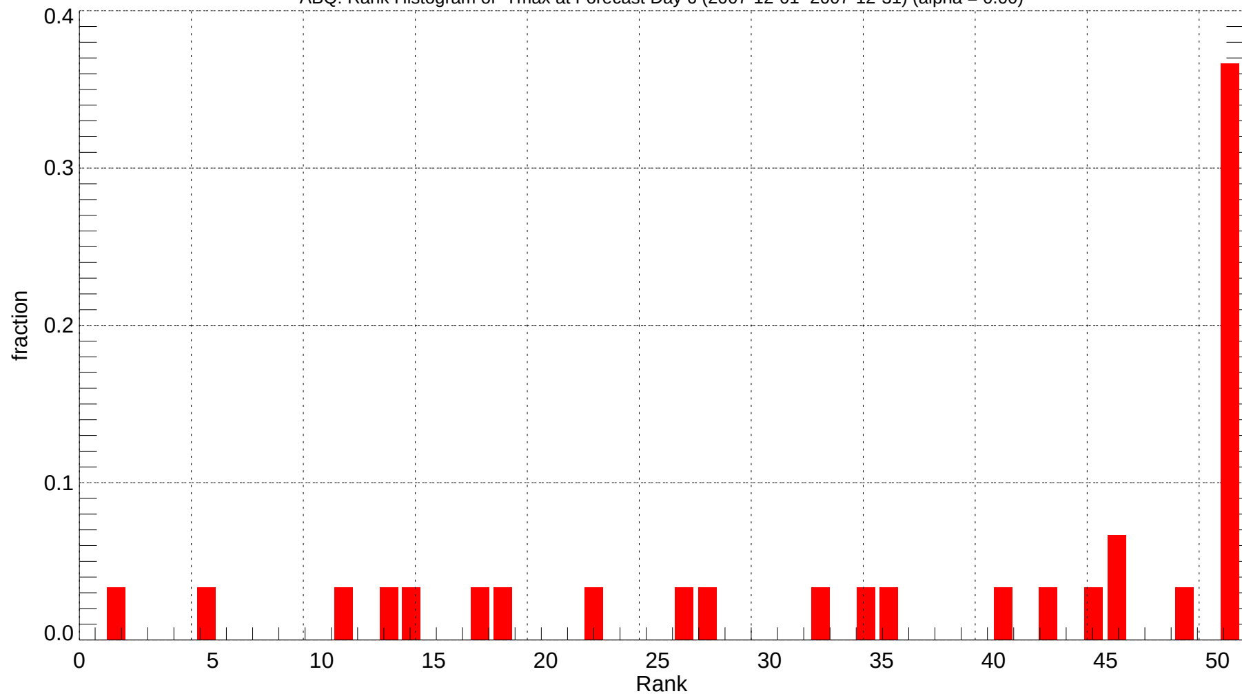
ABQ: Rank Histogram of Tmax at Forecast Day 6 (2007-12-01~2007-12-31) (alpha = 0.00)
