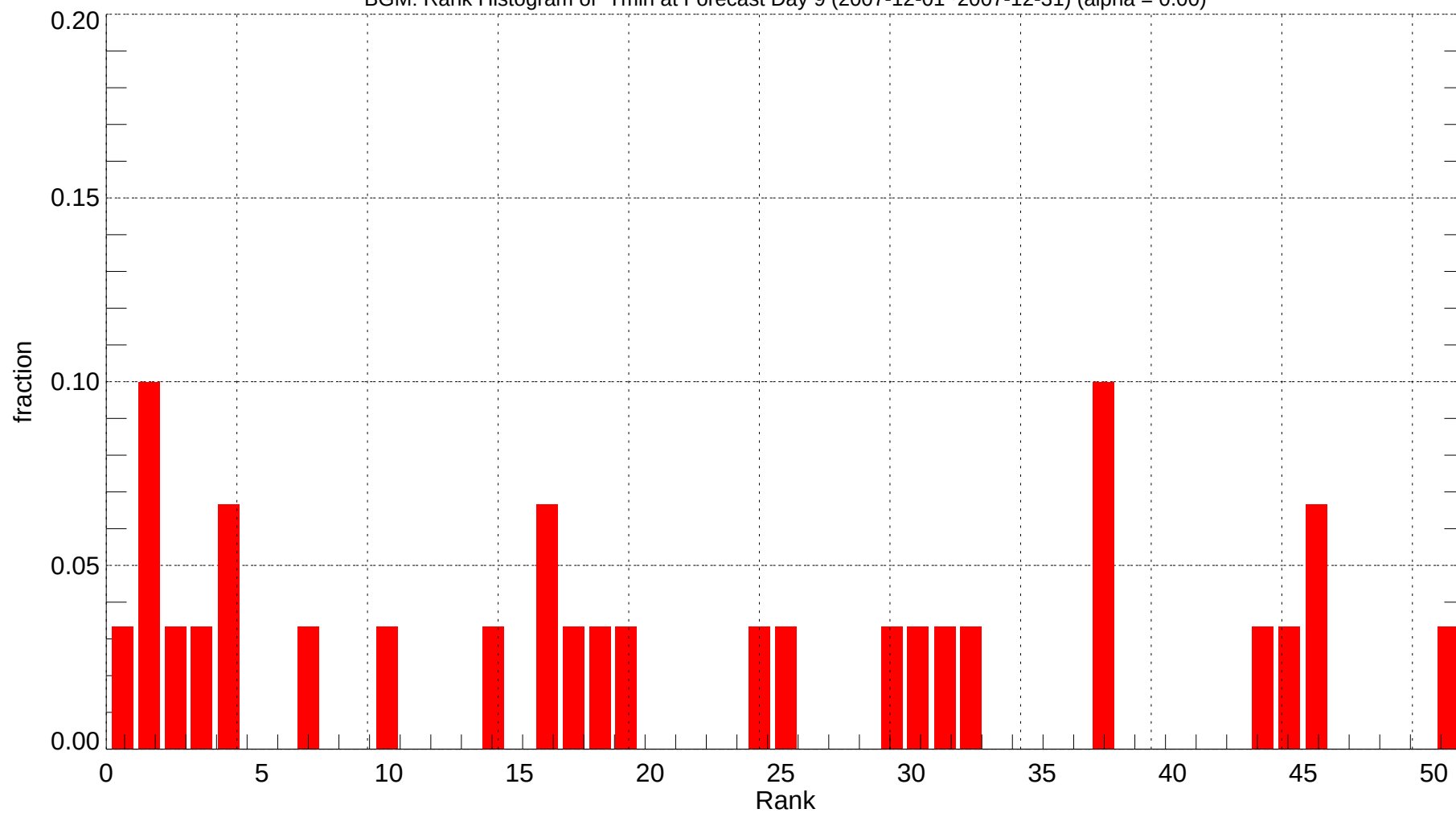
BGM: Rank Histogram of Tmin at Forecast Day 9 (2007-12-01~2007-12-31) (alpha = 0.00)
