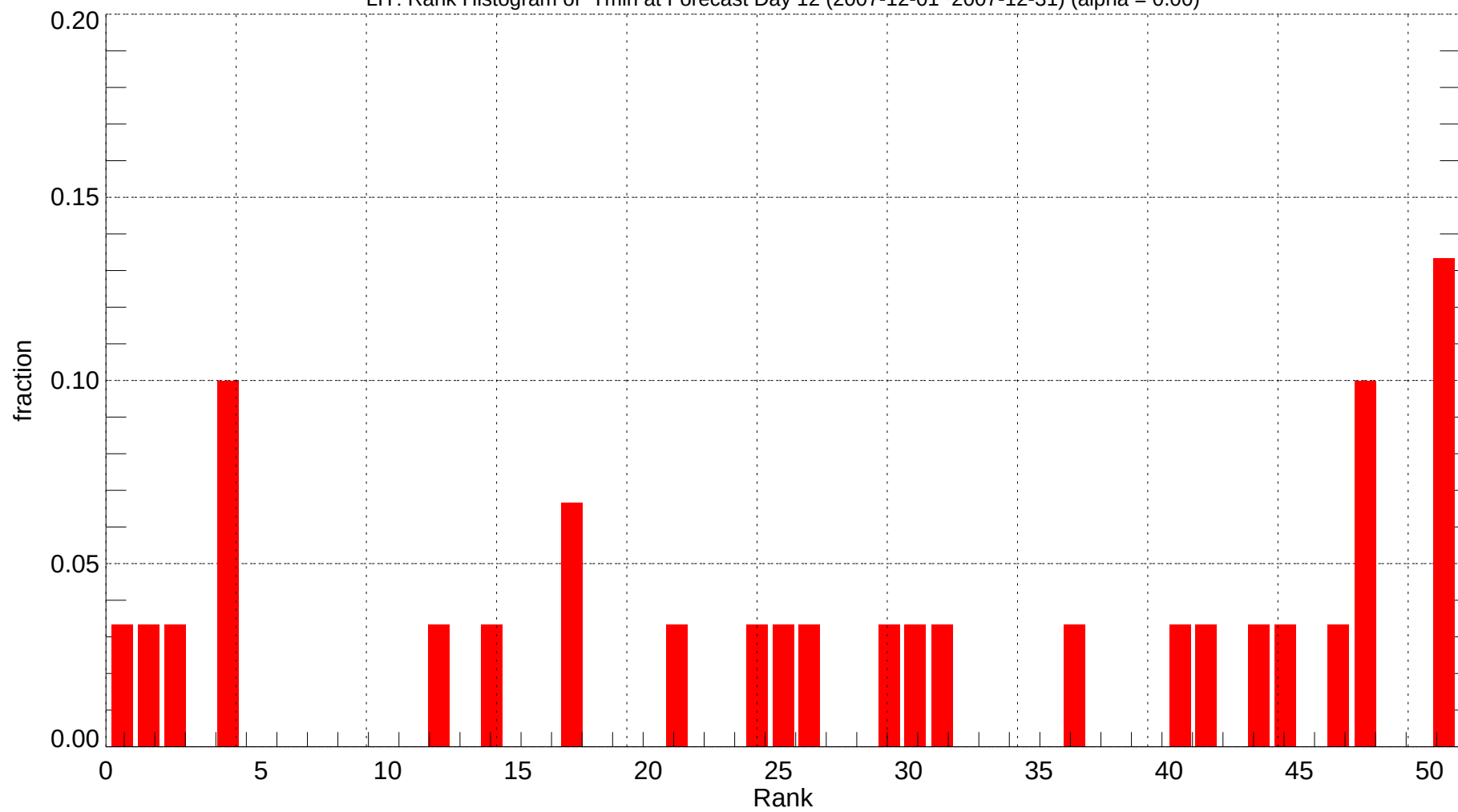
LIT: Rank Histogram of Tmin at Forecast Day 12 (2007-12-01~2007-12-31) (alpha = 0.00)
