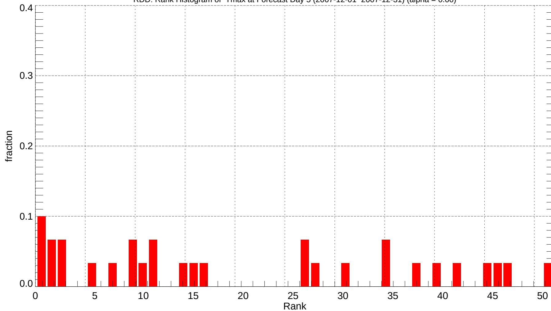
RDD: Rank Histogram of Tmax at Forecast Day 5 (2007-12-01~2007-12-31) (alpha = 0.00)
