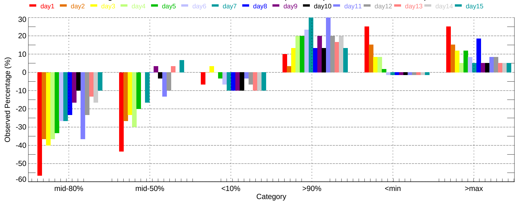
Observed Percentage Deviation of Ensembles - SDF: Min Temperature (2007-12-01~2007-12-31)
