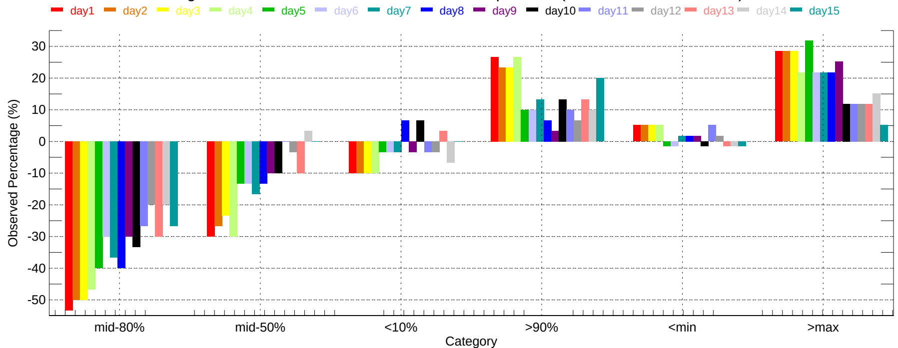
Observed Percentage Deviation of Ensembles - MAF: Min Temperature (2007-12-01~2007-12-31)
