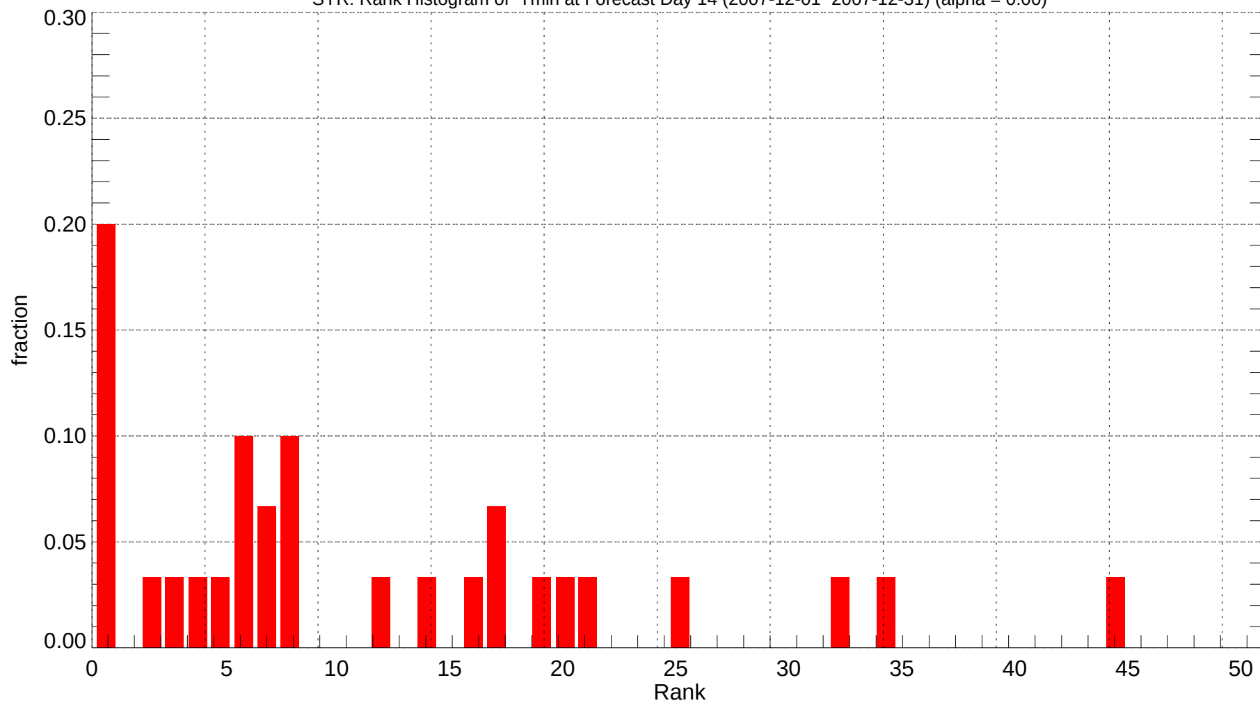
SYR: Rank Histogram of Tmin at Forecast Day 14 (2007-12-01~2007-12-31) (alpha = 0.00)
