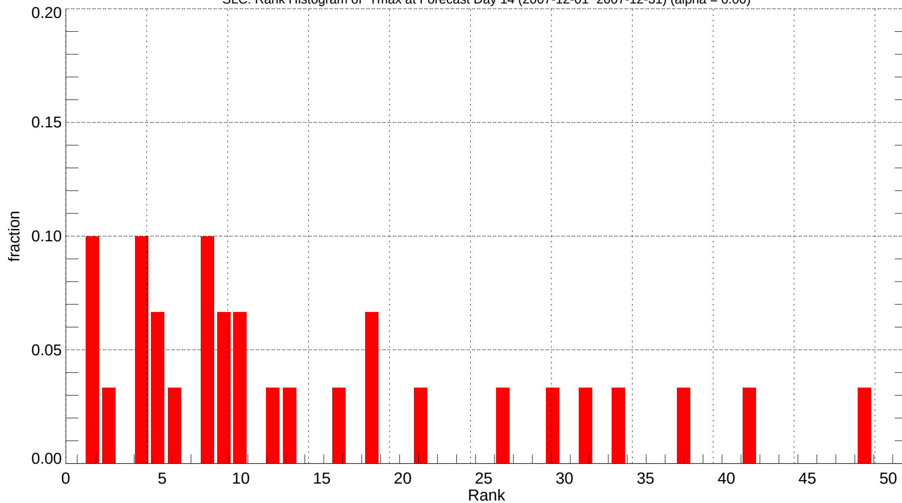
SLC: Rank Histogram of Tmax at Forecast Day 14 (2007-12-01~2007-12-31) (alpha = 0.00)
