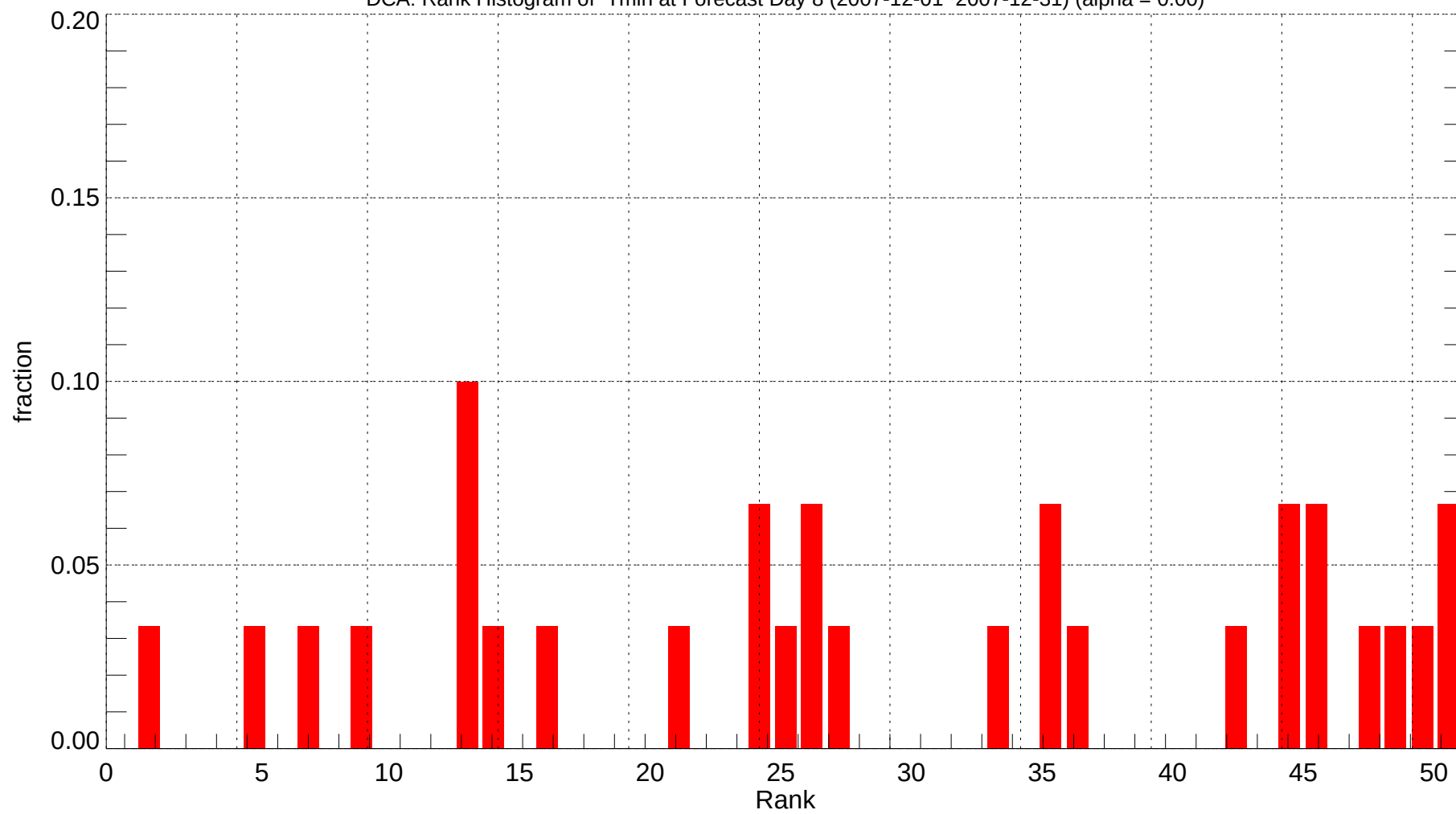
DCA: Rank Histogram of Tmin at Forecast Day 8 (2007-12-01~2007-12-31) (alpha = 0.00)
