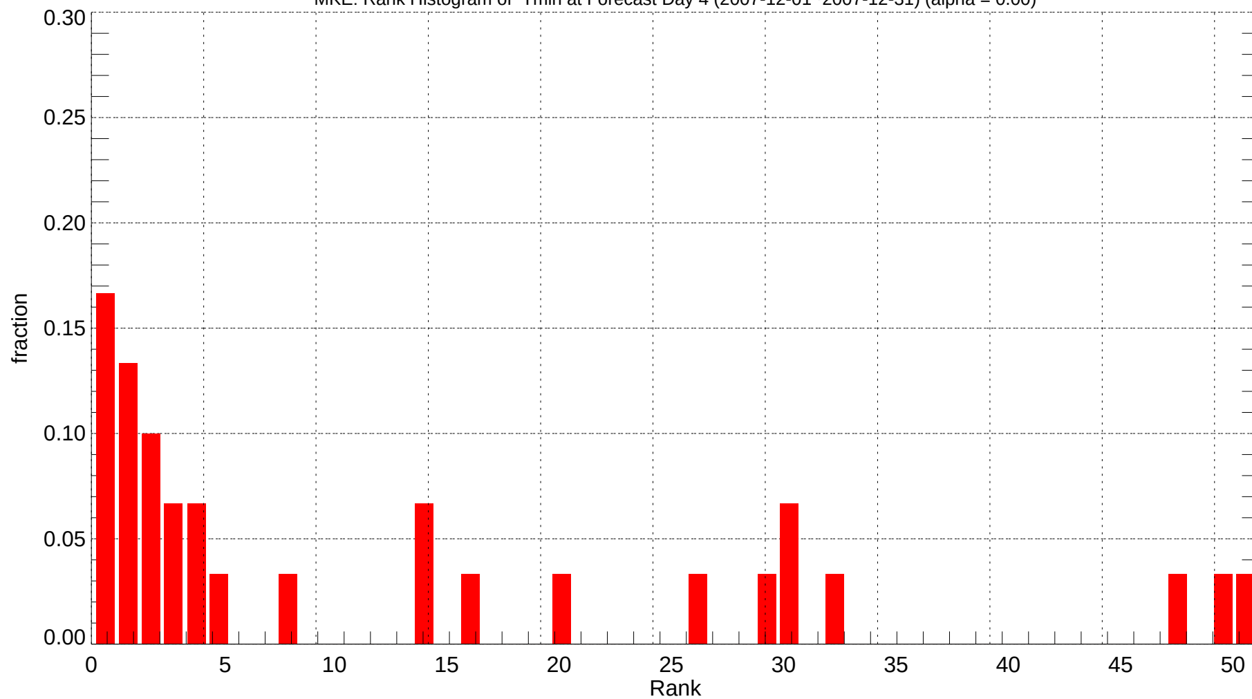
MKE: Rank Histogram of Tmin at Forecast Day 4 (2007-12-01~2007-12-31) (alpha = 0.00)
