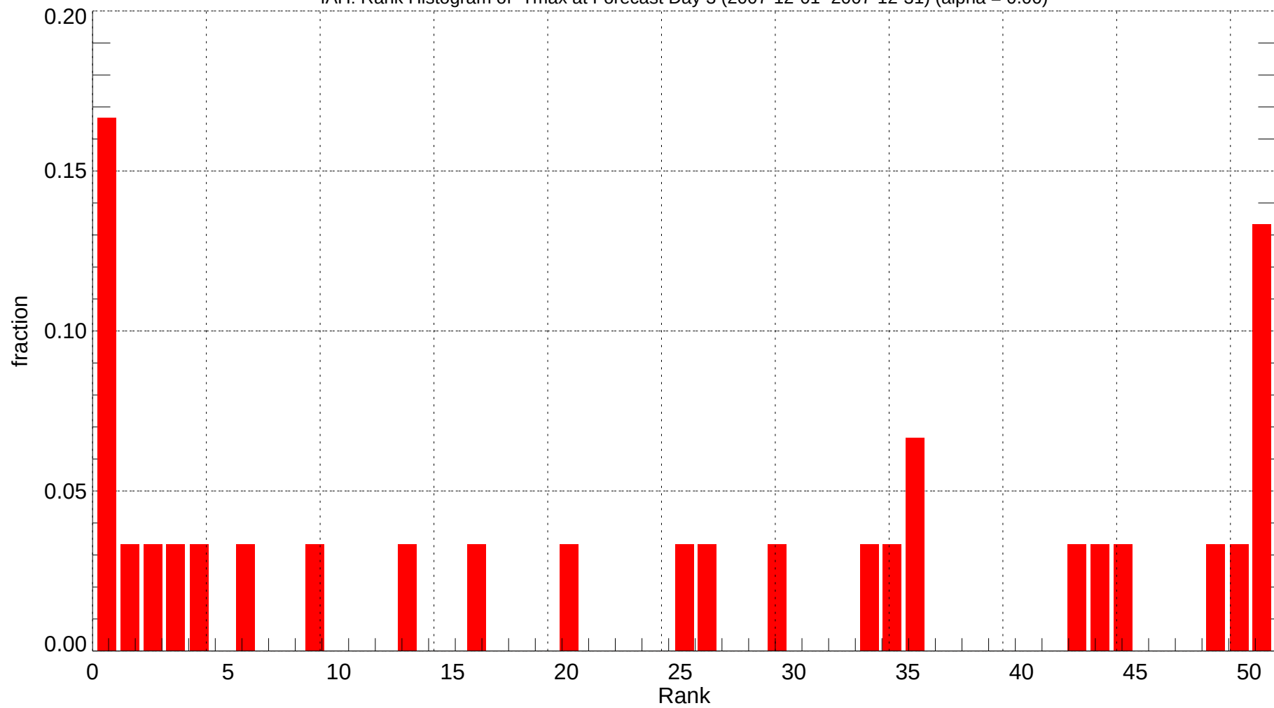
IAH: Rank Histogram of Tmax at Forecast Day 3 (2007-12-01~2007-12-31) (alpha = 0.00)
