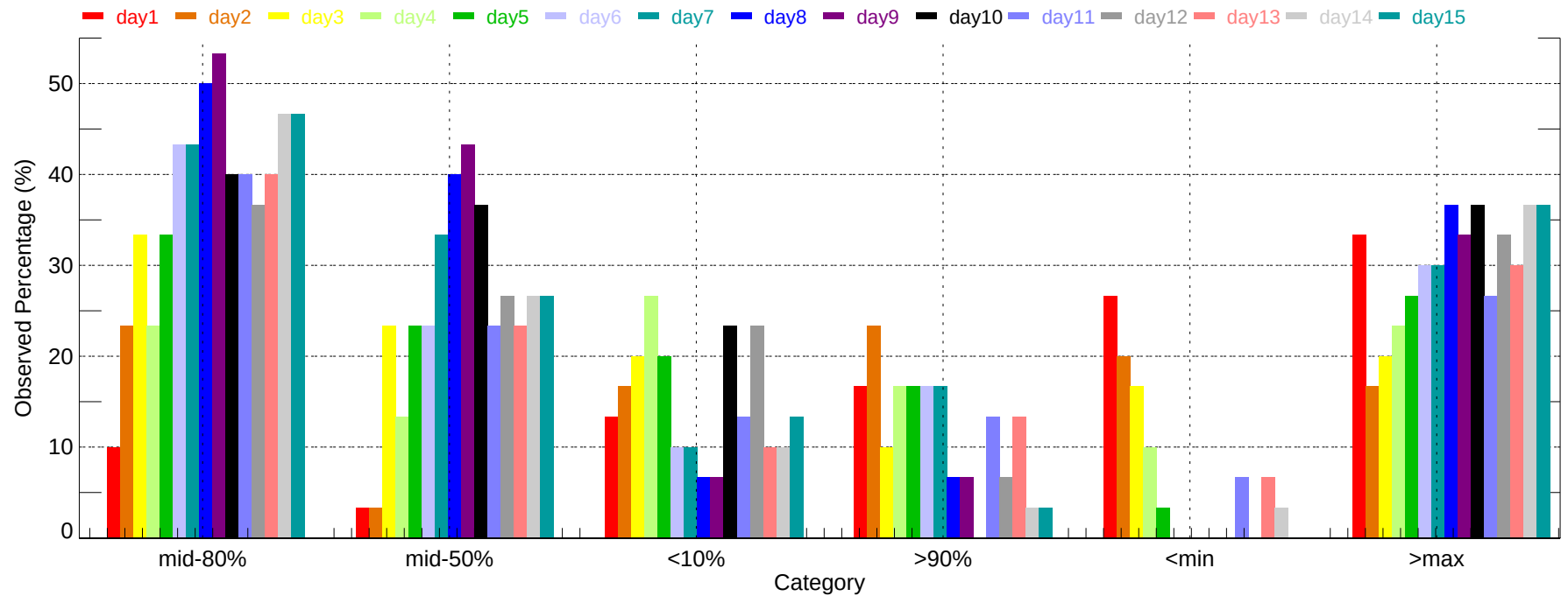
Observed Percentage of Ensembles - MSY: Min Temperature (2007-12-01~2007-12-31)
