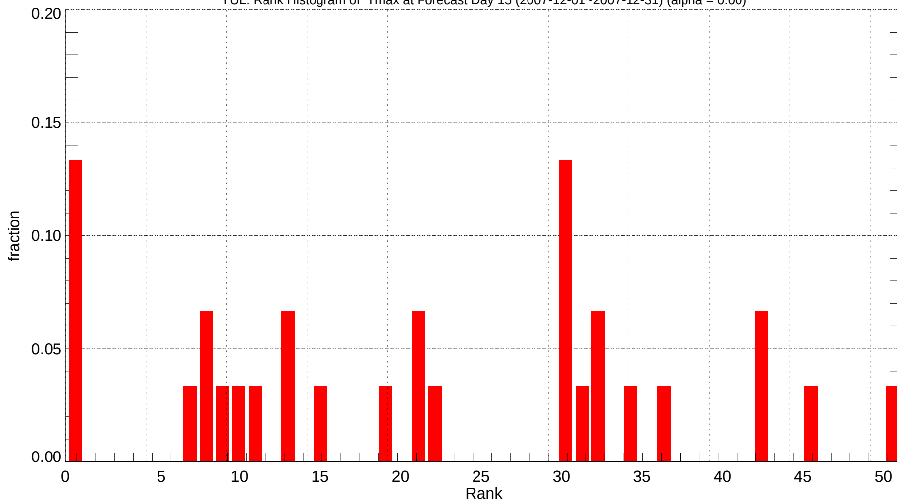
YUL: Rank Histogram of Tmax at Forecast Day 15 (2007-12-01~2007-12-31) (alpha = 0.00)
