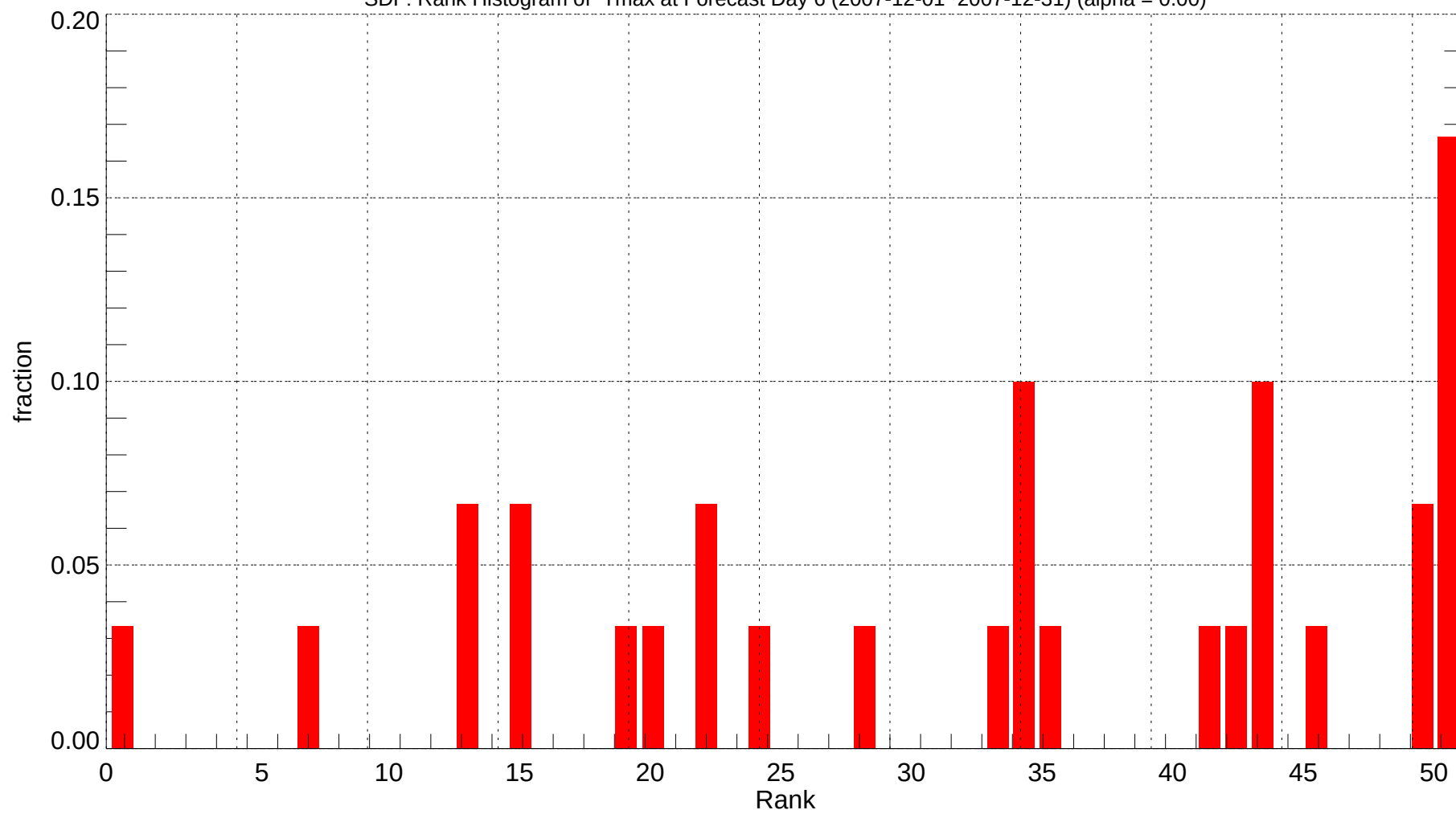
SDF: Rank Histogram of Tmax at Forecast Day 6 (2007-12-01~2007-12-31) (alpha = 0.00)
