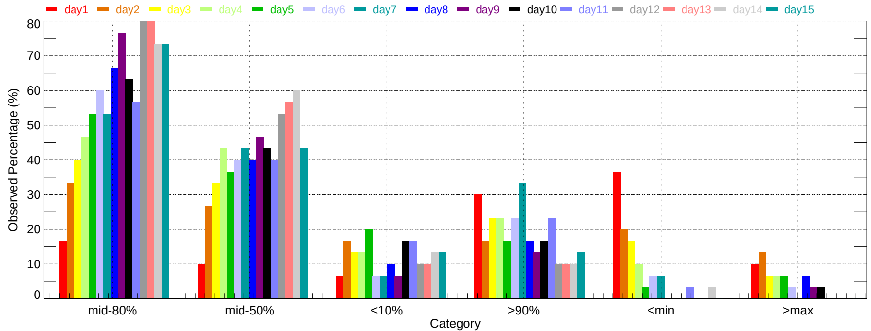
Observed Percentage of Ensembles - PHL: Min Temperature (2007-12-01~2007-12-31)
