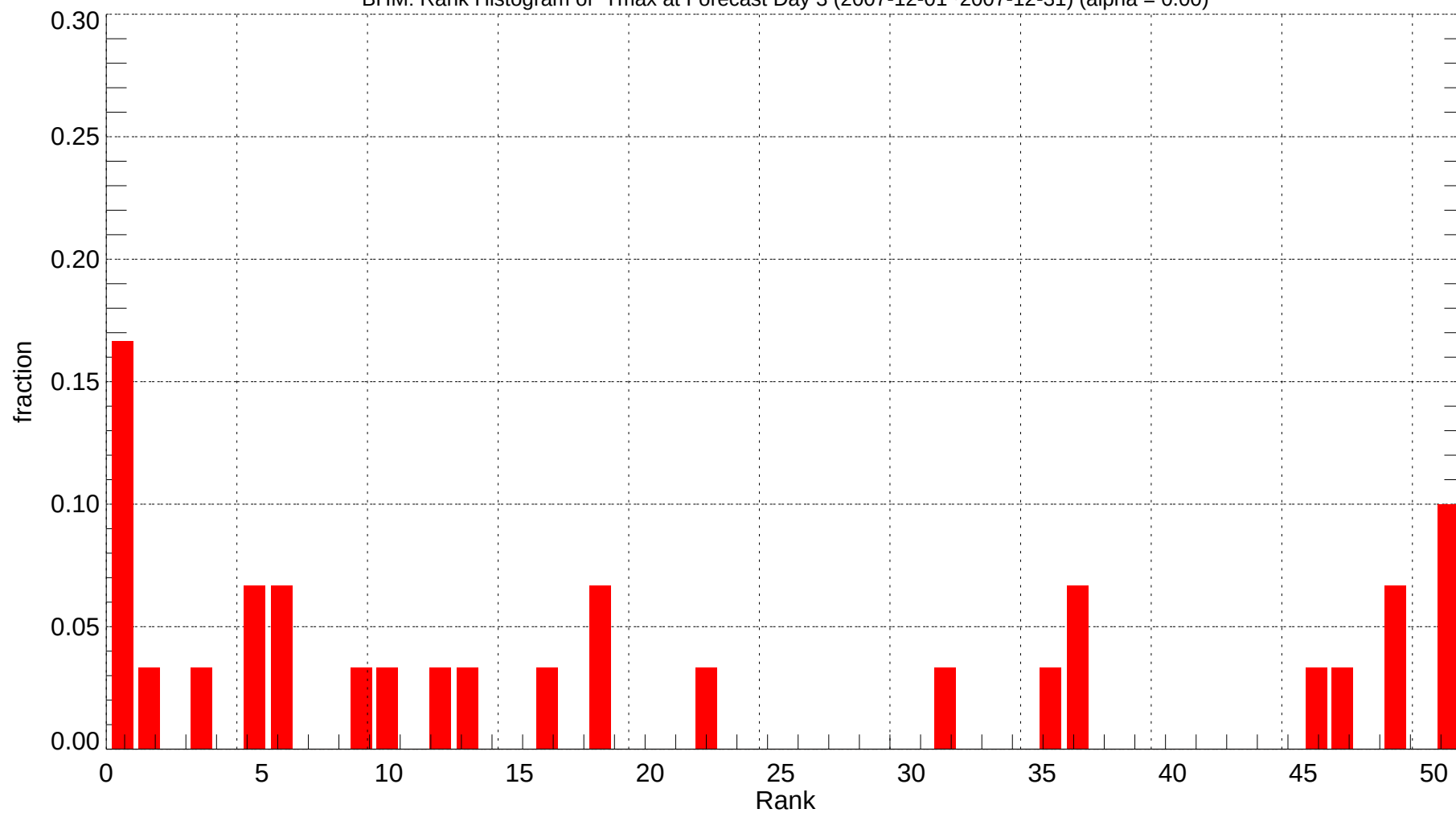
BHM: Rank Histogram of Tmax at Forecast Day 3 (2007-12-01~2007-12-31) (alpha = 0.00)
