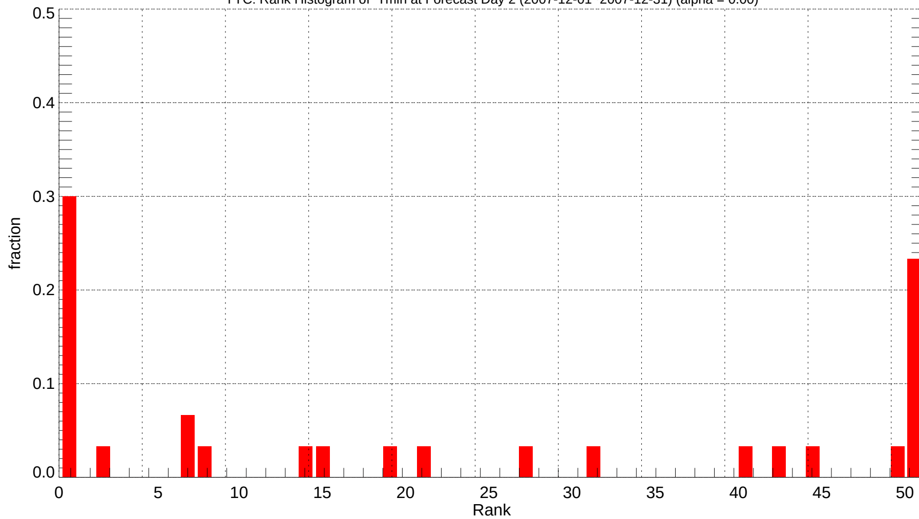
YYC: Rank Histogram of Tmin at Forecast Day 2 (2007-12-01~2007-12-31) (alpha = 0.00)
