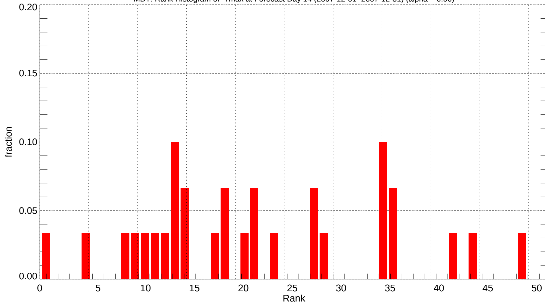
MDT: Rank Histogram of Tmax at Forecast Day 14 (2007-12-01~2007-12-31) (alpha = 0.00)
