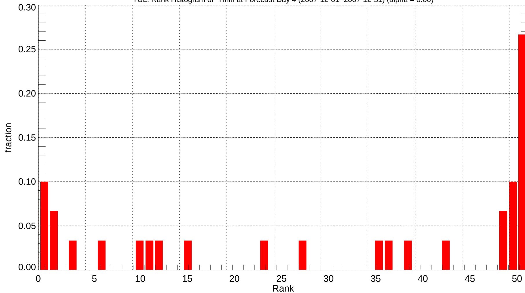
TUL: Rank Histogram of Tmin at Forecast Day 4 (2007-12-01~2007-12-31) (alpha = 0.00)
