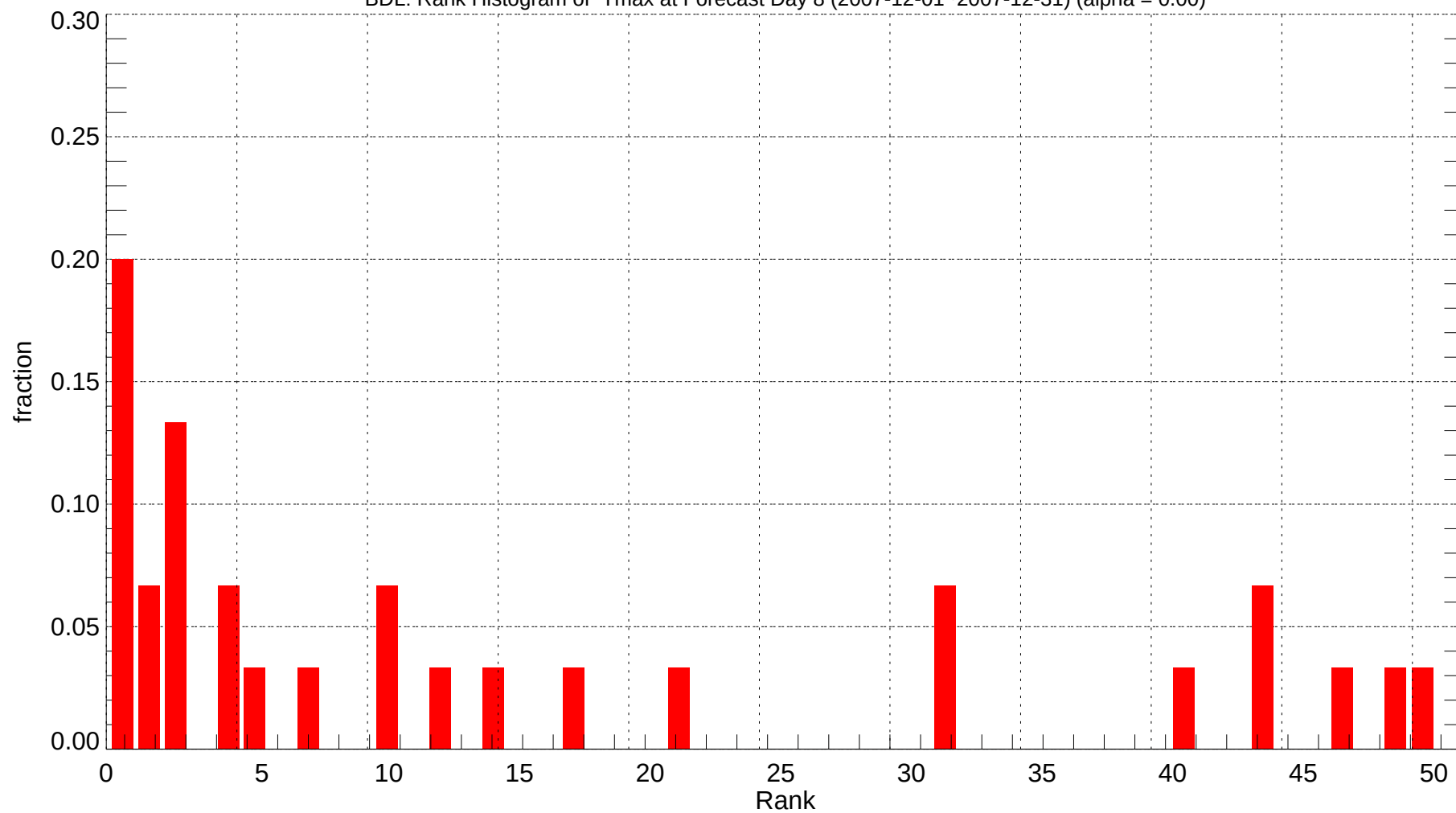
BDL: Rank Histogram of Tmax at Forecast Day 8 (2007-12-01~2007-12-31) (alpha = 0.00)
