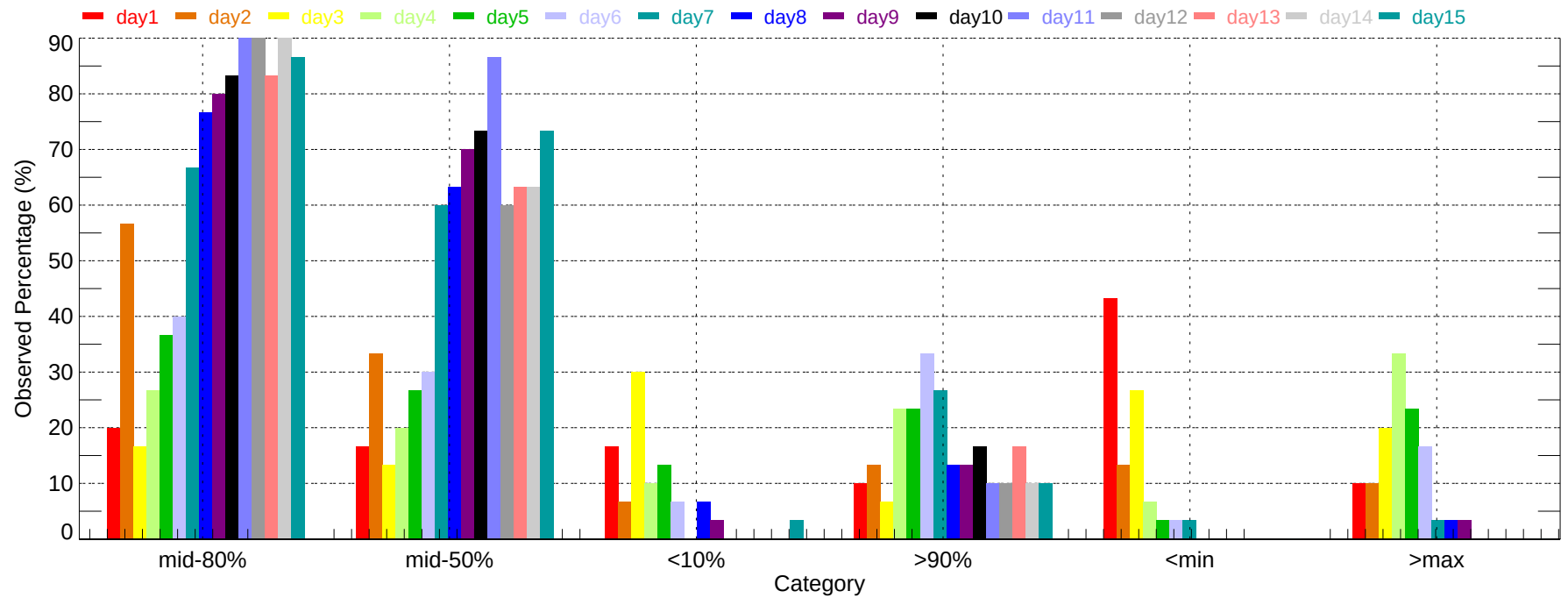
Observed Percentage of Ensembles - LAS: Min Temperature (2007-12-01~2007-12-31)
