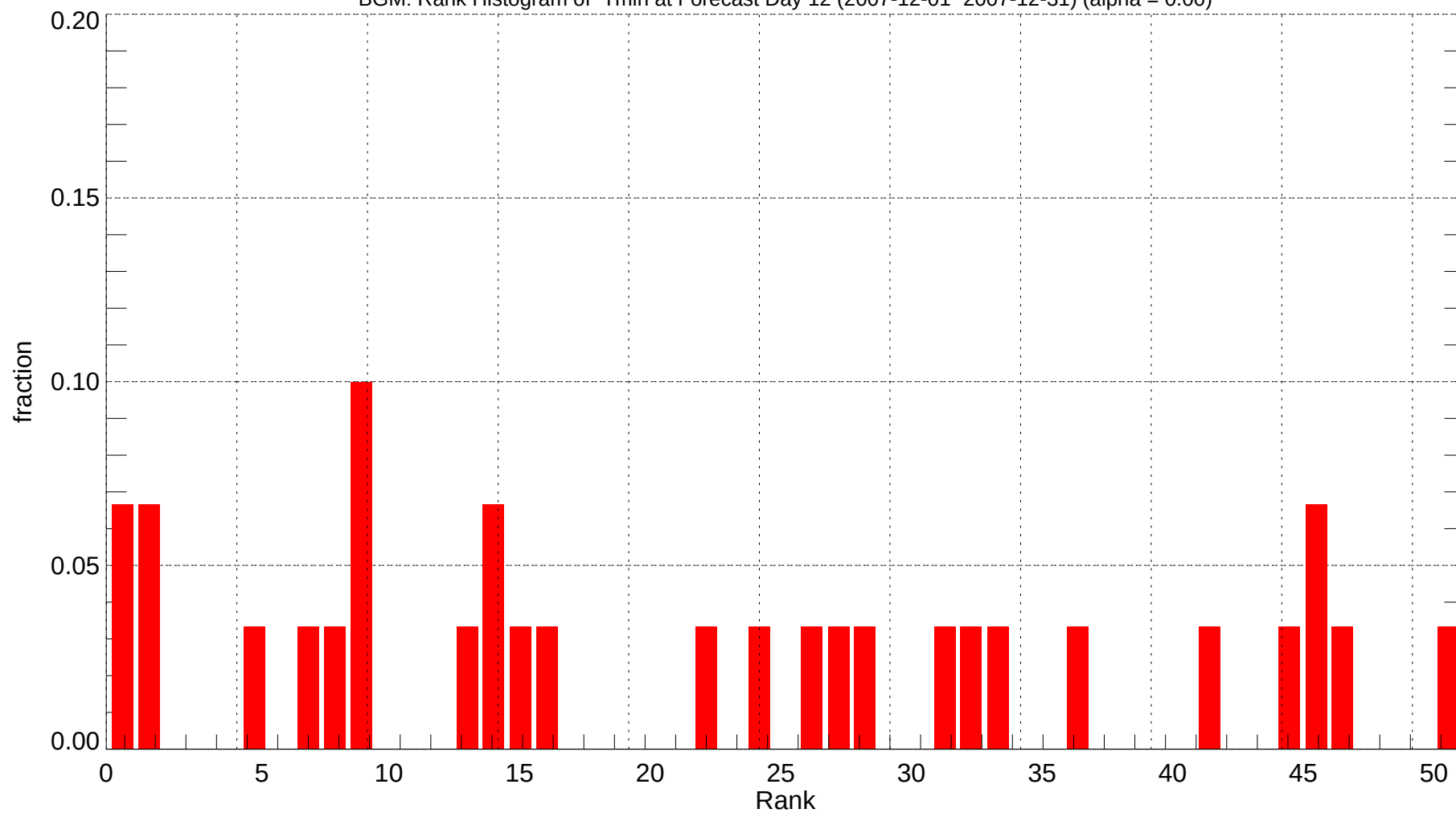
BGM: Rank Histogram of Tmin at Forecast Day 12 (2007-12-01~2007-12-31) (alpha = 0.00)
