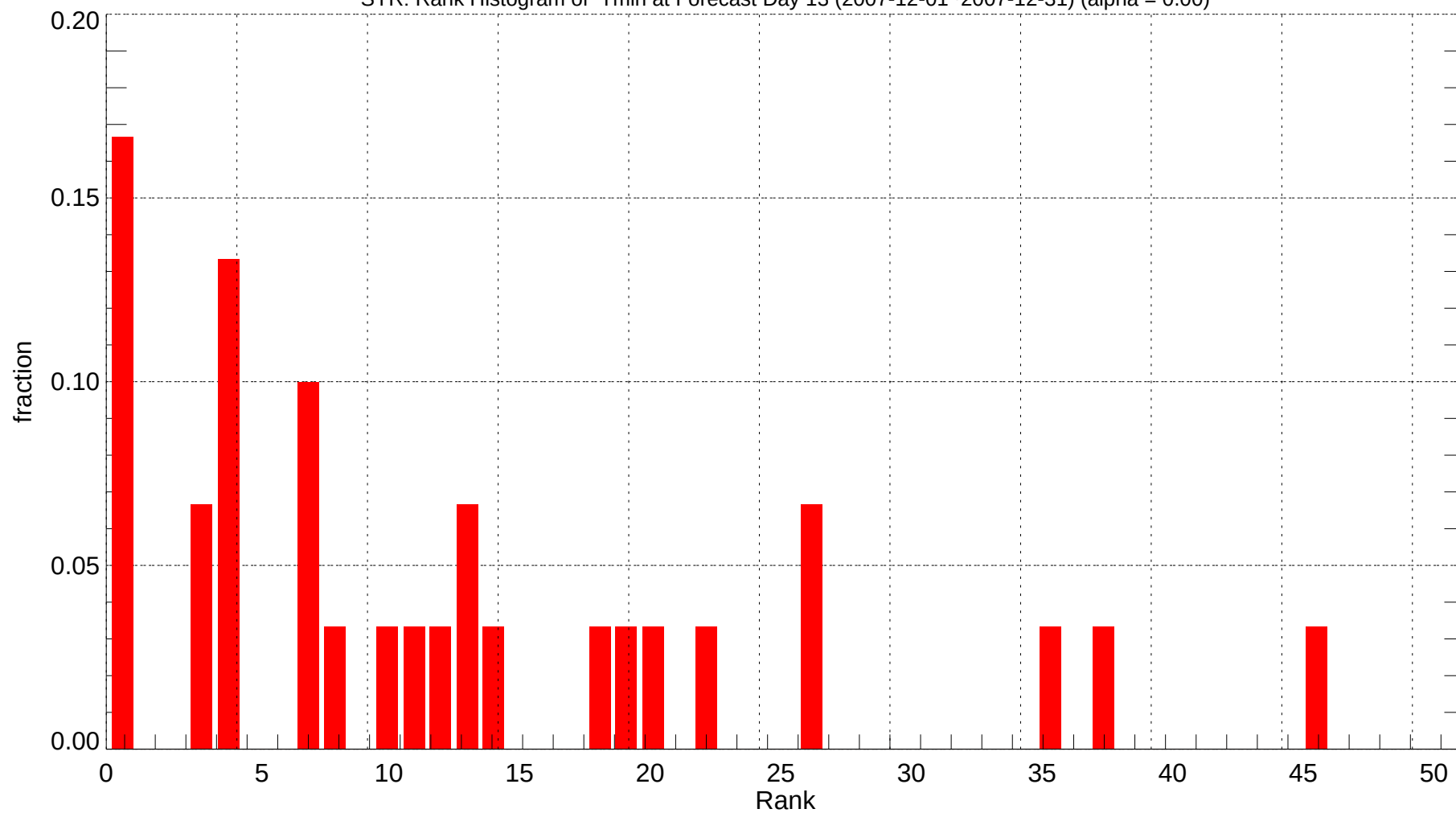
SYR: Rank Histogram of Tmin at Forecast Day 13 (2007-12-01~2007-12-31) (alpha = 0.00)
