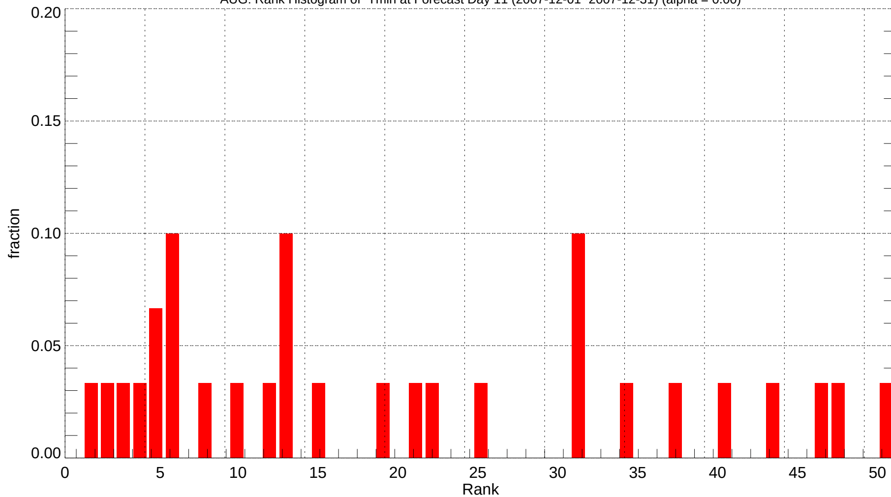
AUG: Rank Histogram of Tmin at Forecast Day 11 (2007-12-01~2007-12-31) (alpha = 0.00)
