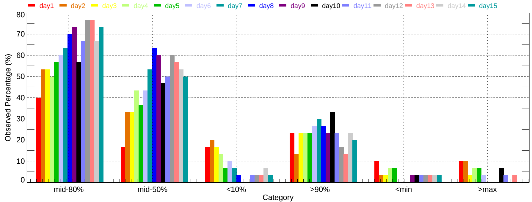
Observed Percentage of Ensembles - MCO: Min Temperature (2007-12-01~2007-12-31)
