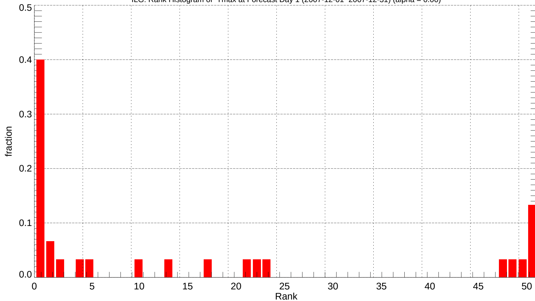
ILG: Rank Histogram of Tmax at Forecast Day 1 (2007-12-01~2007-12-31) (alpha = 0.00)
