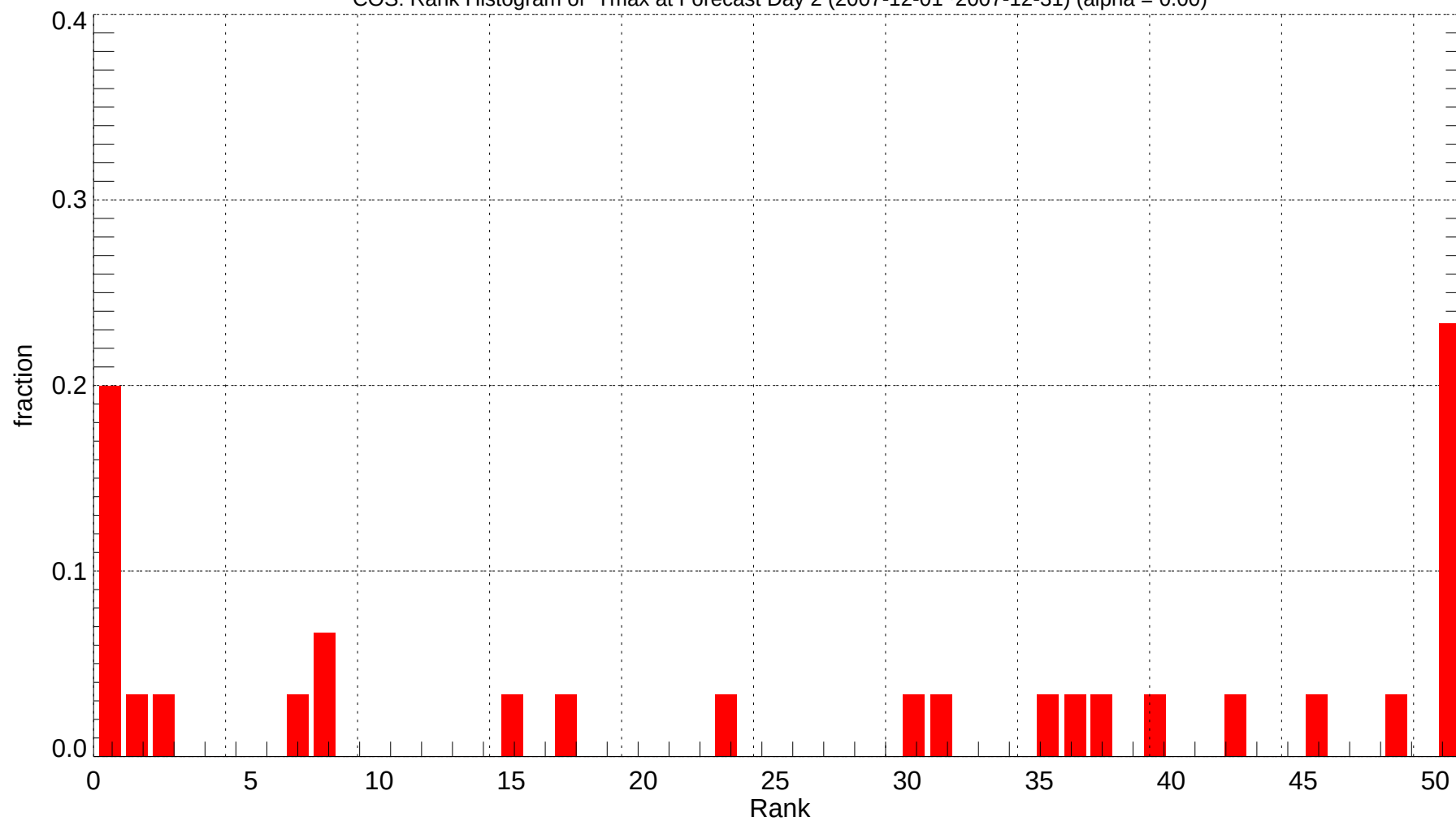
COS: Rank Histogram of Tmax at Forecast Day 2 (2007-12-01~2007-12-31) (alpha = 0.00)
