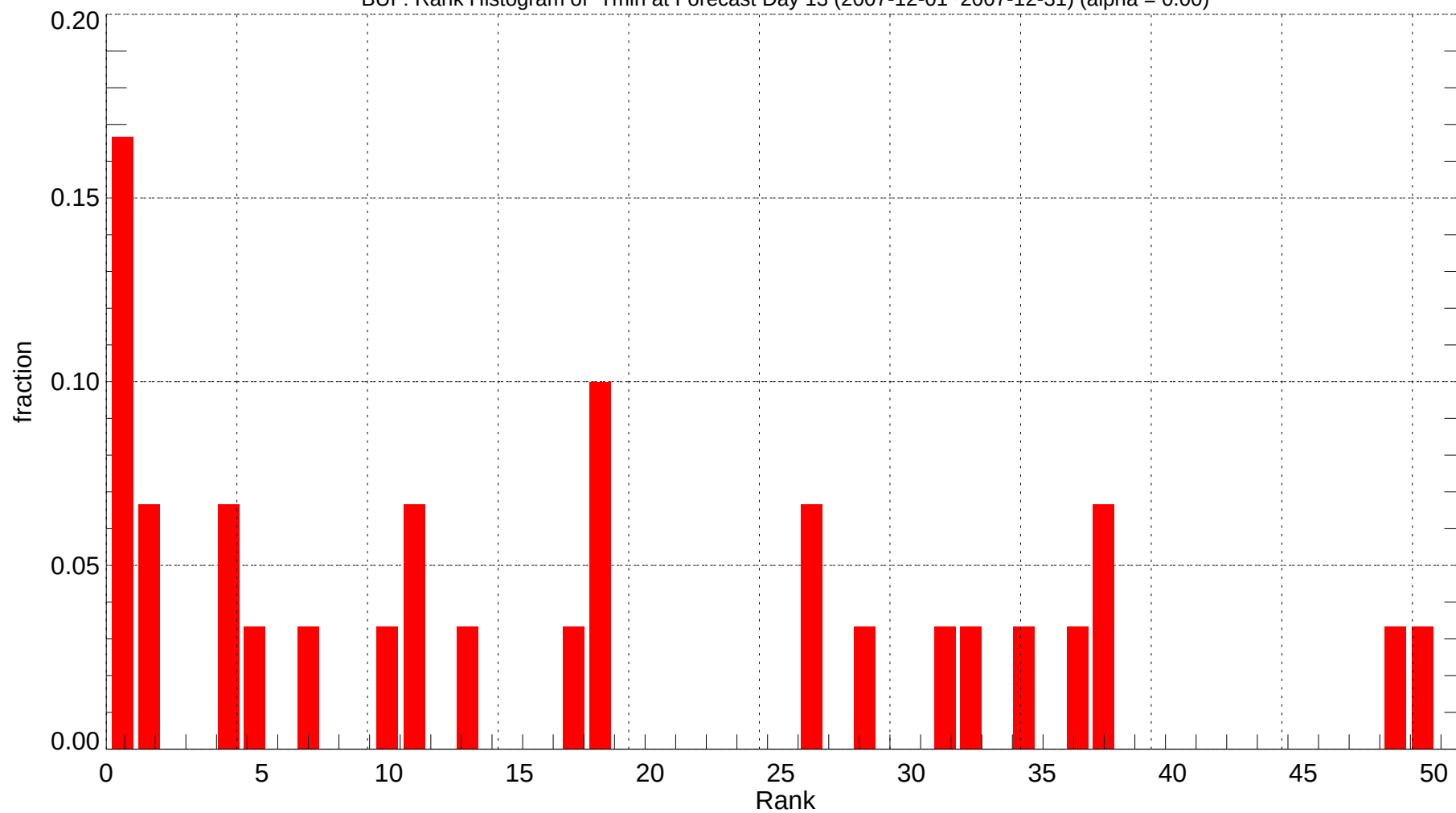
BUF: Rank Histogram of Tmin at Forecast Day 13 (2007-12-01~2007-12-31) (alpha = 0.00)
