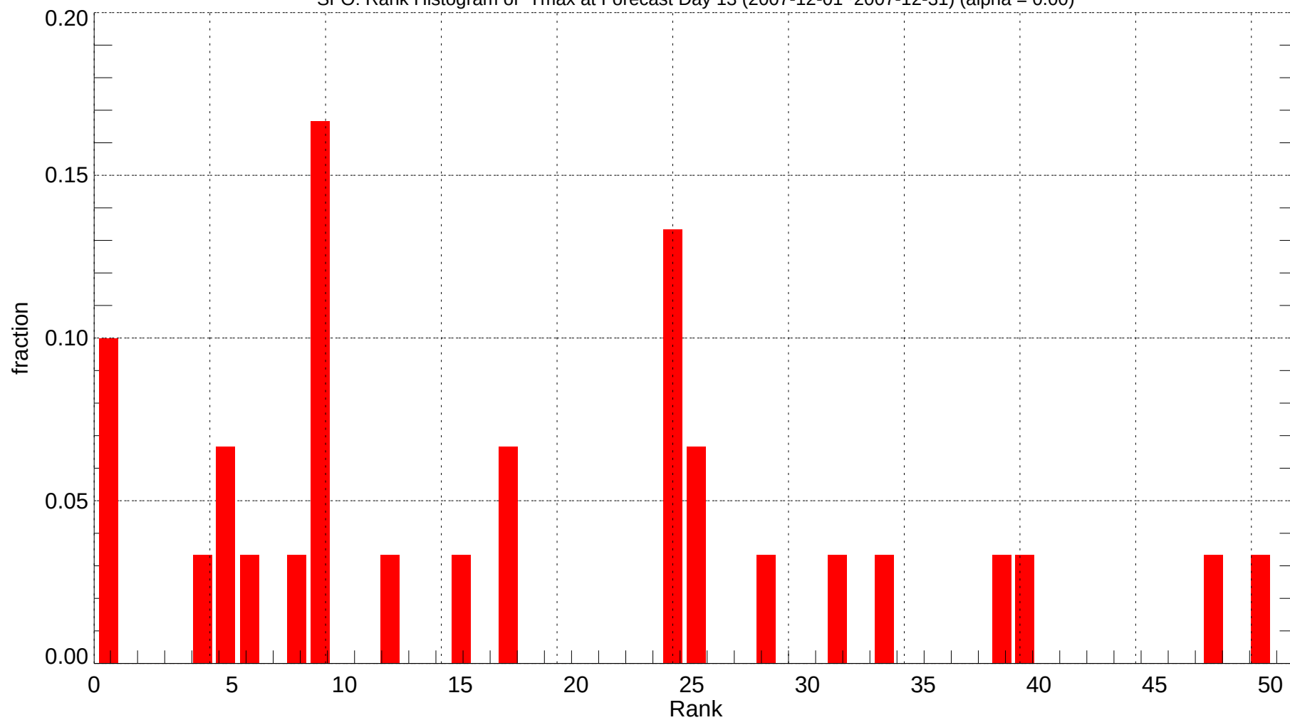
SFO: Rank Histogram of Tmax at Forecast Day 13 (2007-12-01~2007-12-31) (alpha = 0.00)
