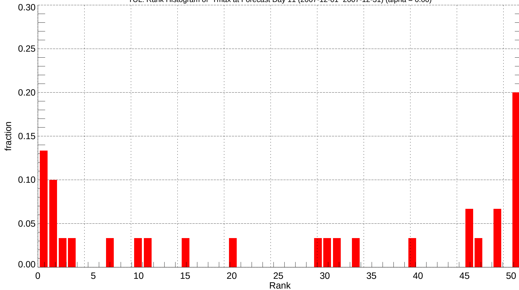
TUL: Rank Histogram of Tmax at Forecast Day 11 (2007-12-01~2007-12-31) (alpha = 0.00)
