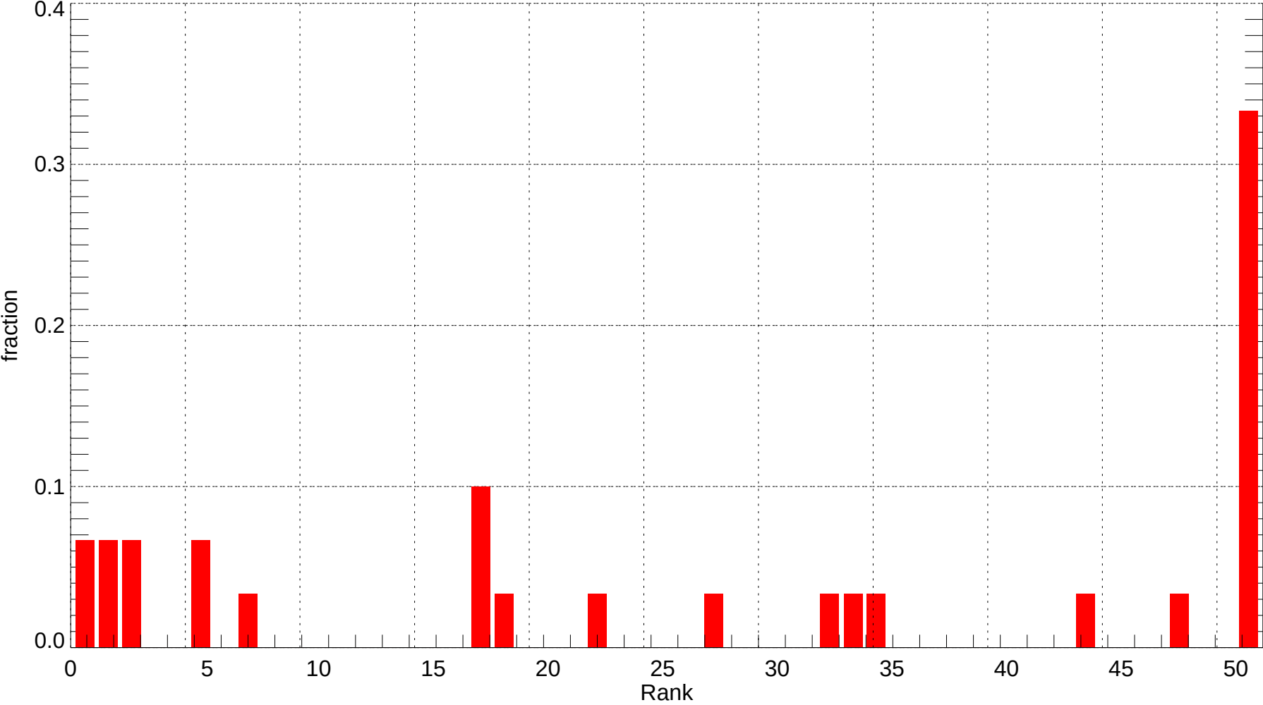
ATL: Rank Histogram of Tmin at Forecast Day 4 (2007-12-01~2007-12-31) (alpha = 0.00)
