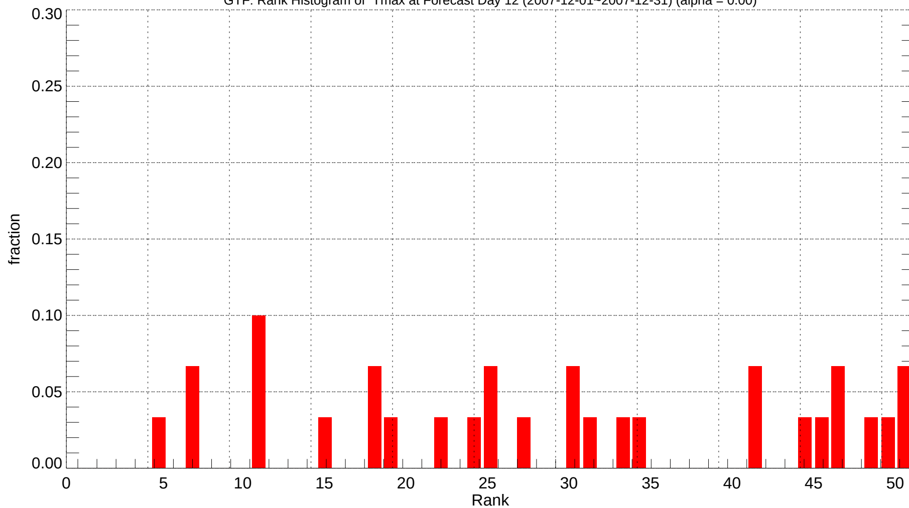
GTF: Rank Histogram of Tmax at Forecast Day 12 (2007-12-01~2007-12-31) (alpha = 0.00)
