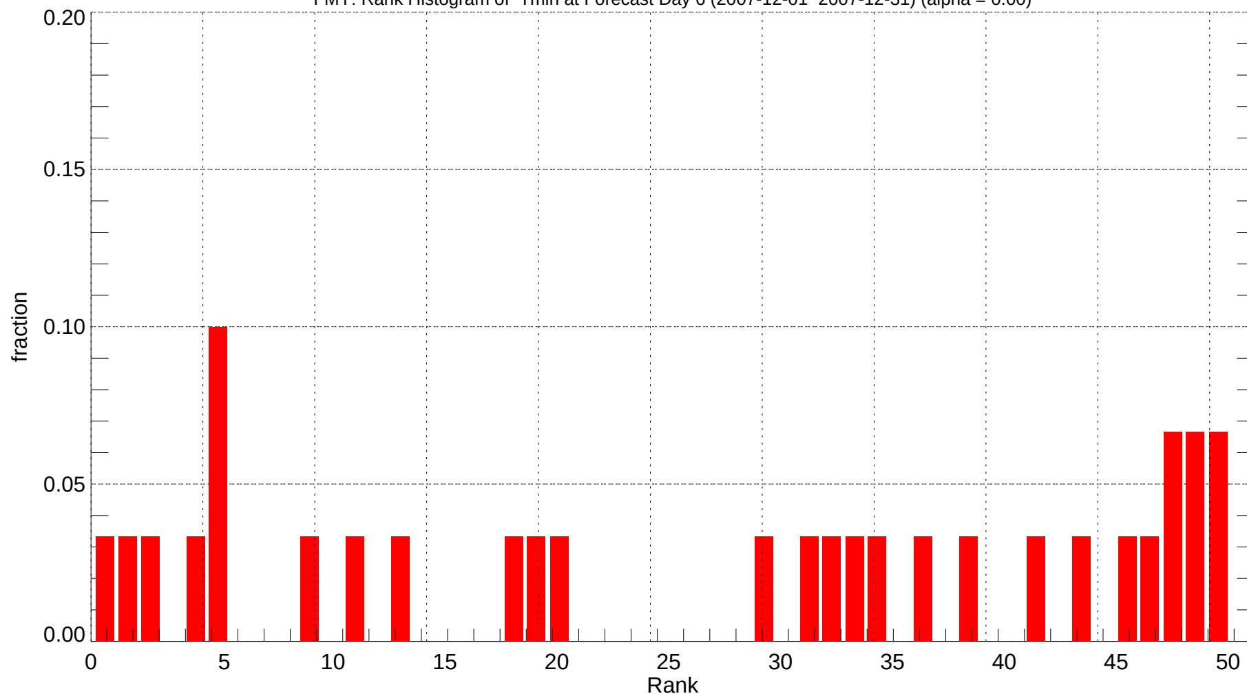
FMY: Rank Histogram of Tmin at Forecast Day 6 (2007-12-01~2007-12-31) (alpha = 0.00)
