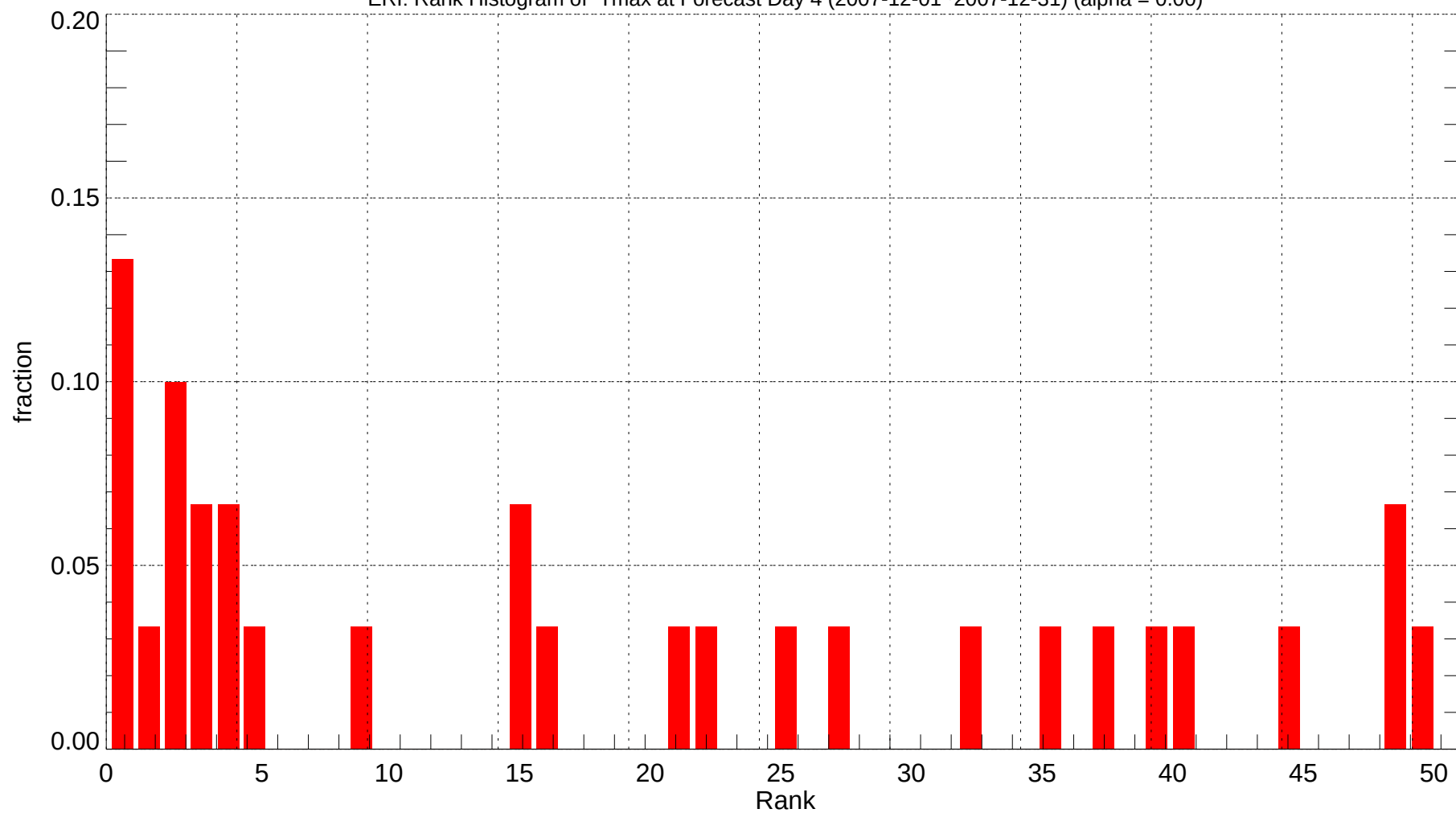
ERI: Rank Histogram of Tmax at Forecast Day 4 (2007-12-01~2007-12-31) (alpha = 0.00)
