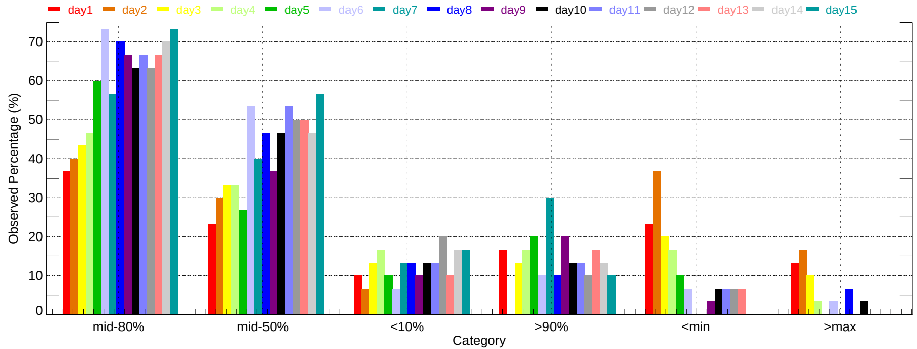
Observed Percentage of Ensembles - FWA: Max Temperature (2007-12-01~2007-12-31)
