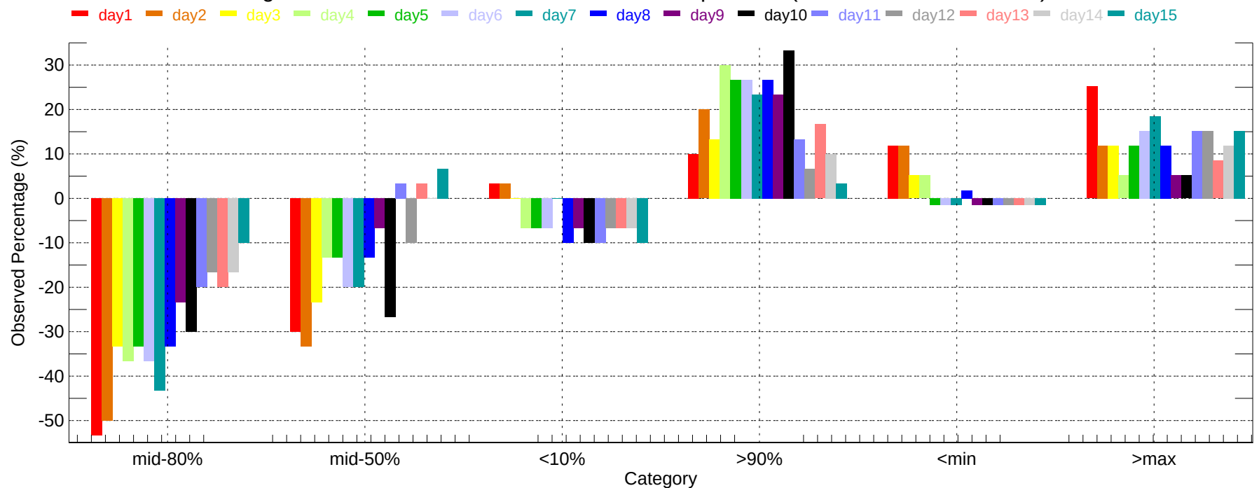
Observed Percentage Deviation of Ensembles - BNA: Max Temperature (2007-12-01~2007-12-31)
