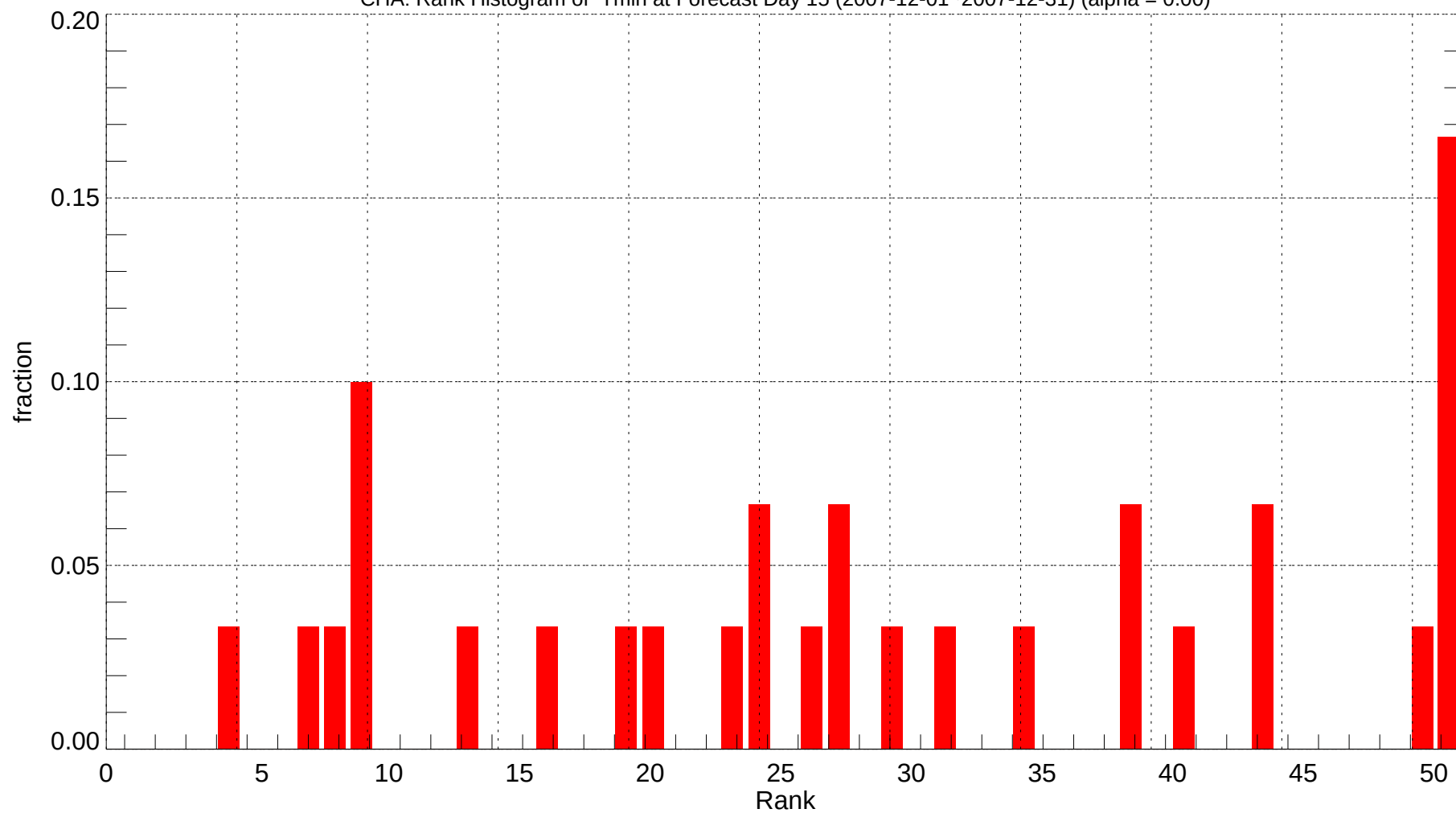
CHA: Rank Histogram of Tmin at Forecast Day 15 (2007-12-01~2007-12-31) (alpha = 0.00)
