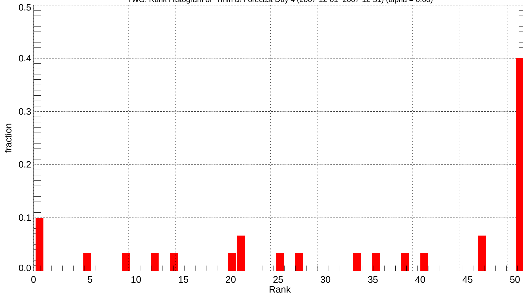
YWG: Rank Histogram of Tmin at Forecast Day 4 (2007-12-01~2007-12-31) (alpha = 0.00)
