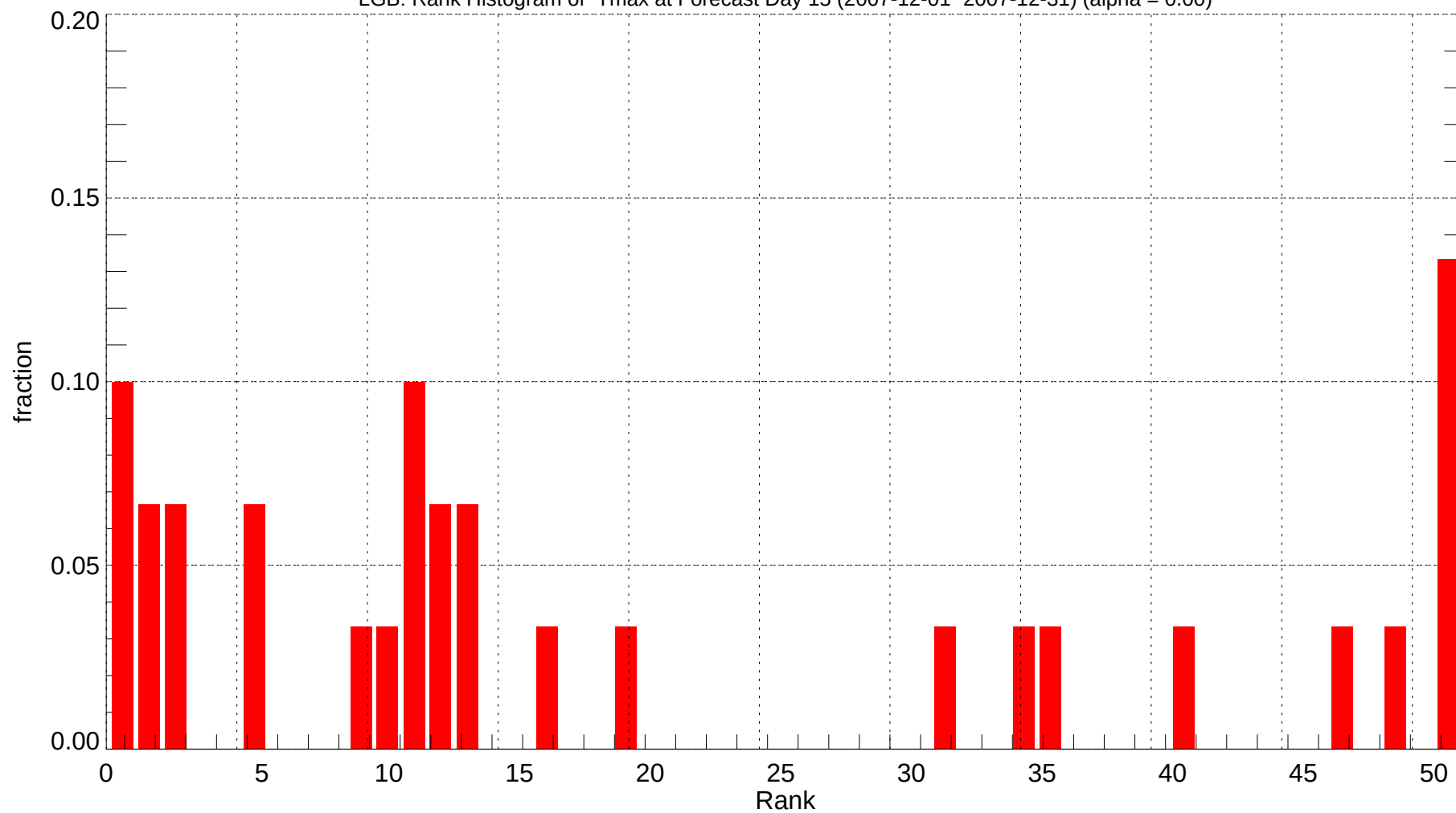
LGB: Rank Histogram of Tmax at Forecast Day 15 (2007-12-01~2007-12-31) (alpha = 0.00)
