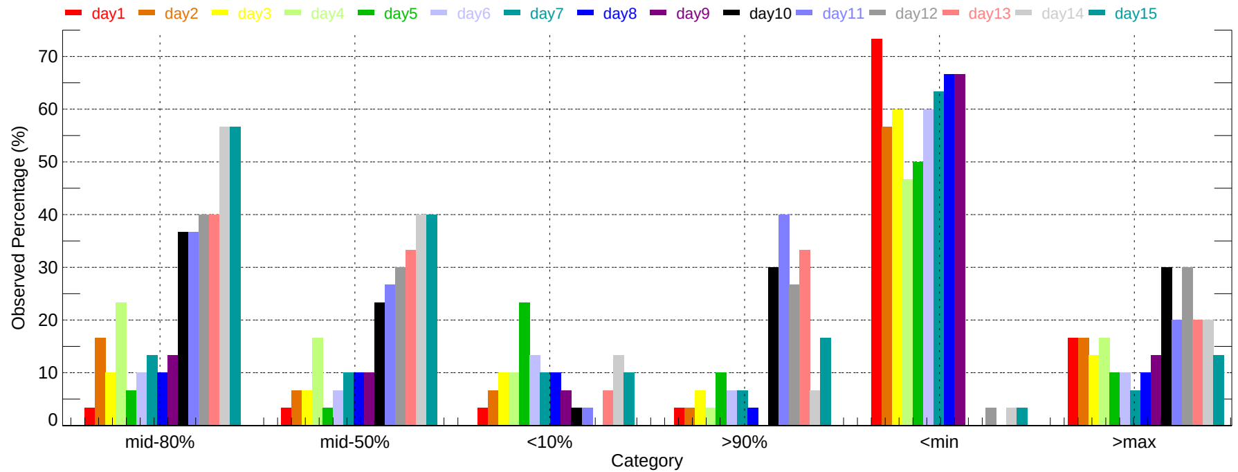
Observed Percentage of Ensembles - LAX: Min Temperature (2007-12-01~2007-12-31)
