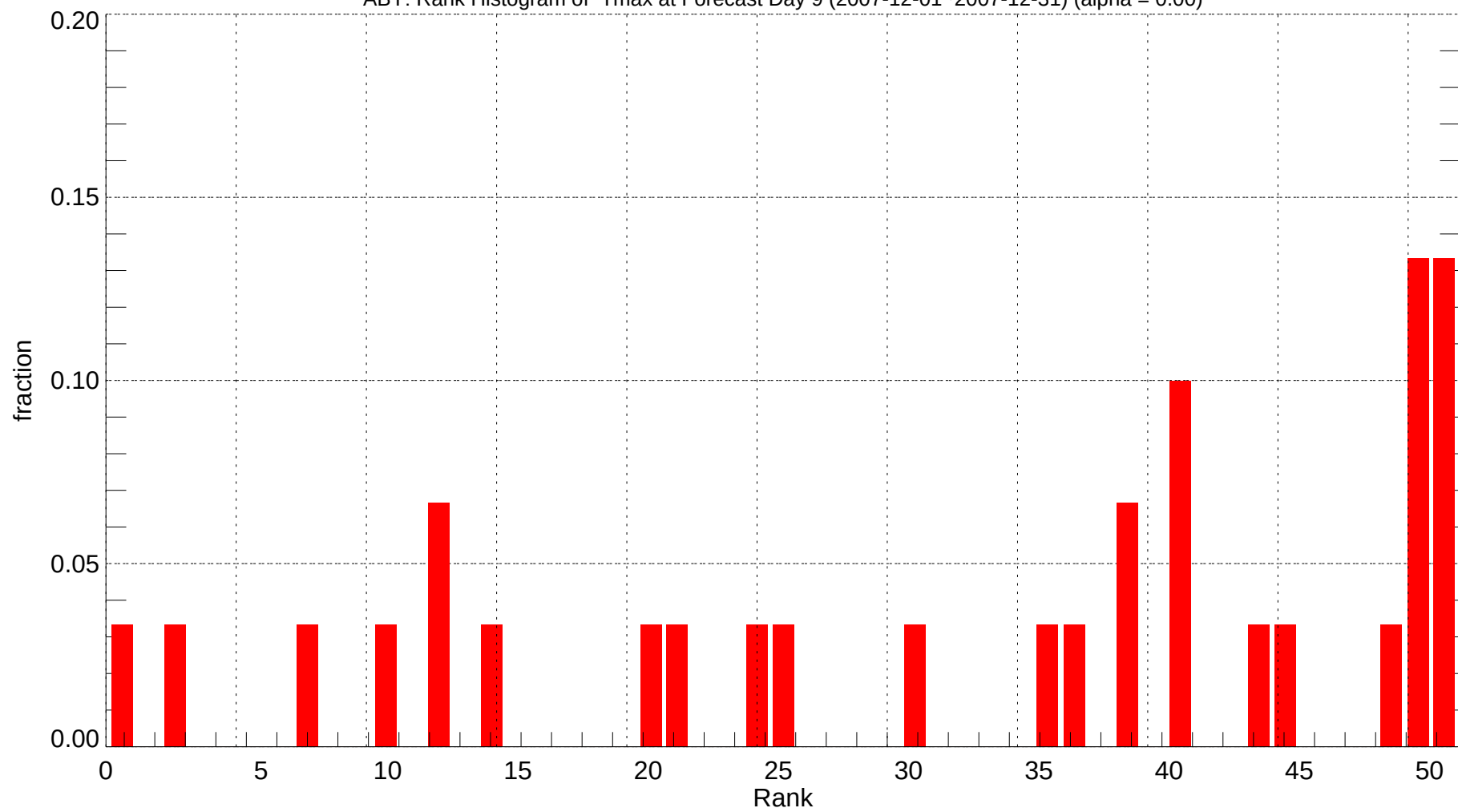
ABY: Rank Histogram of Tmax at Forecast Day 9 (2007-12-01~2007-12-31) (alpha = 0.00)
