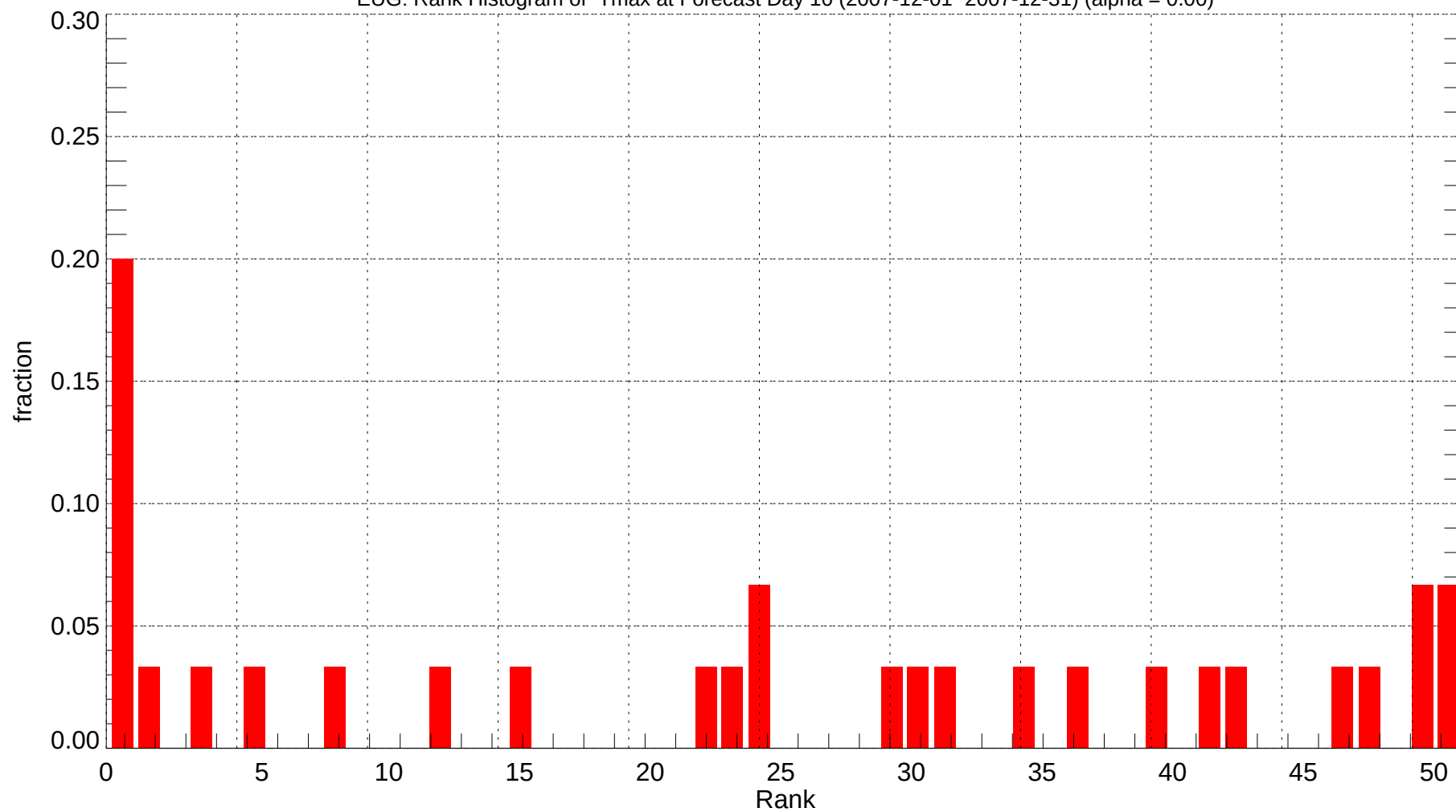
EUG: Rank Histogram of Tmax at Forecast Day 10 (2007-12-01~2007-12-31) (alpha = 0.00)
