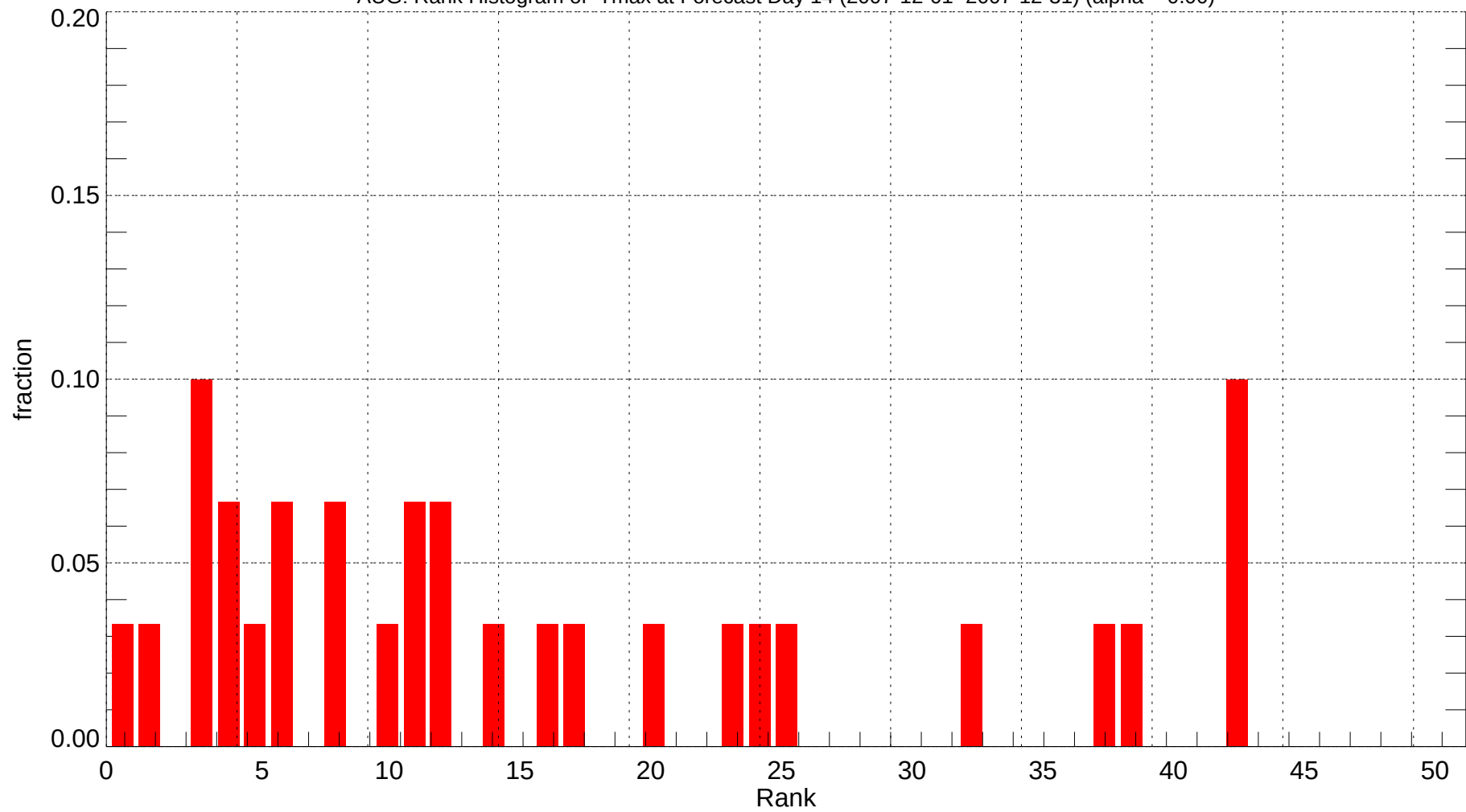
AUG: Rank Histogram of Tmax at Forecast Day 14 (2007-12-01~2007-12-31) (alpha = 0.00)
