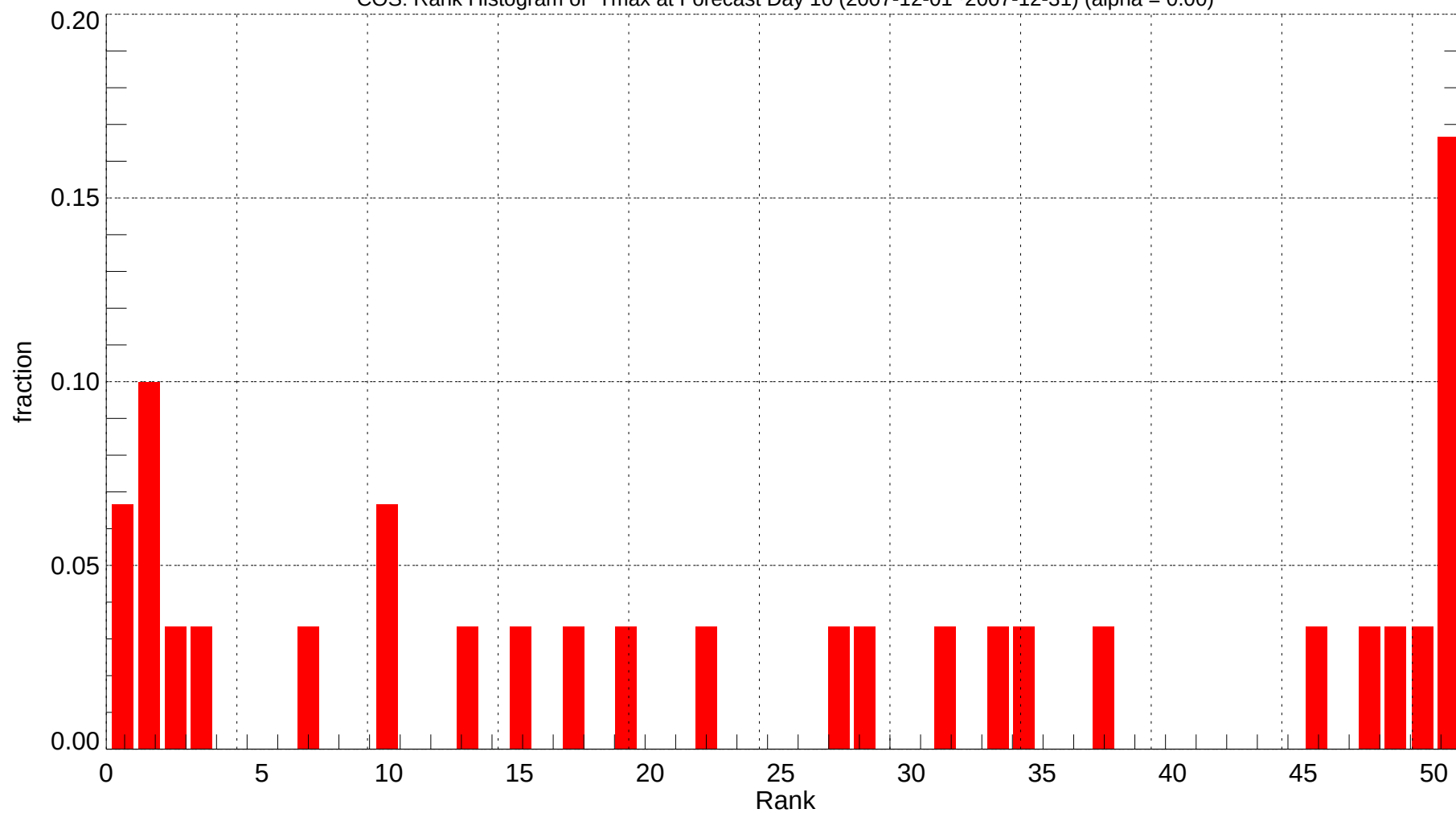
COS: Rank Histogram of Tmax at Forecast Day 10 (2007-12-01~2007-12-31) (alpha = 0.00)
