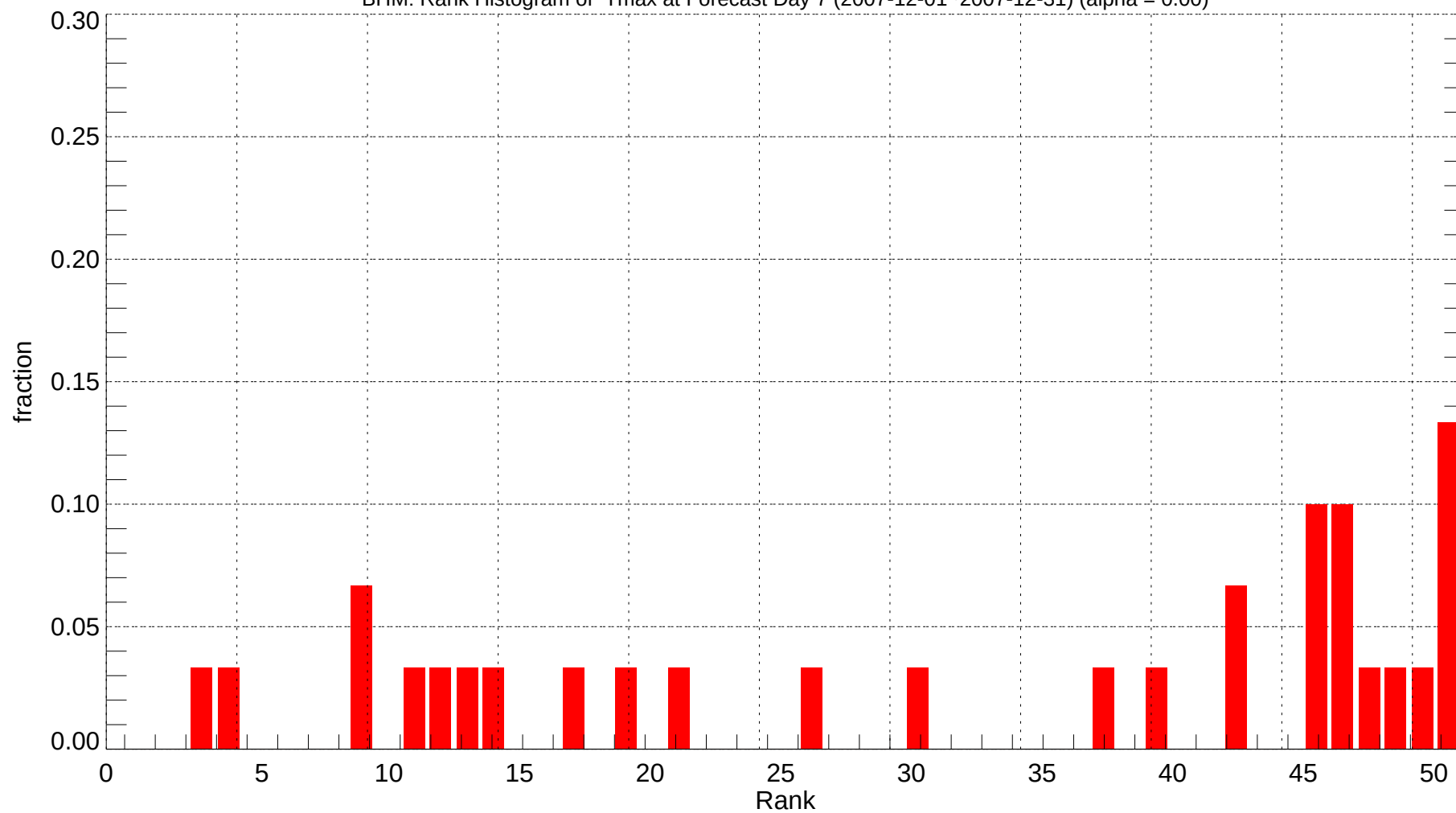
BHM: Rank Histogram of Tmax at Forecast Day 7 (2007-12-01~2007-12-31) (alpha = 0.00)
