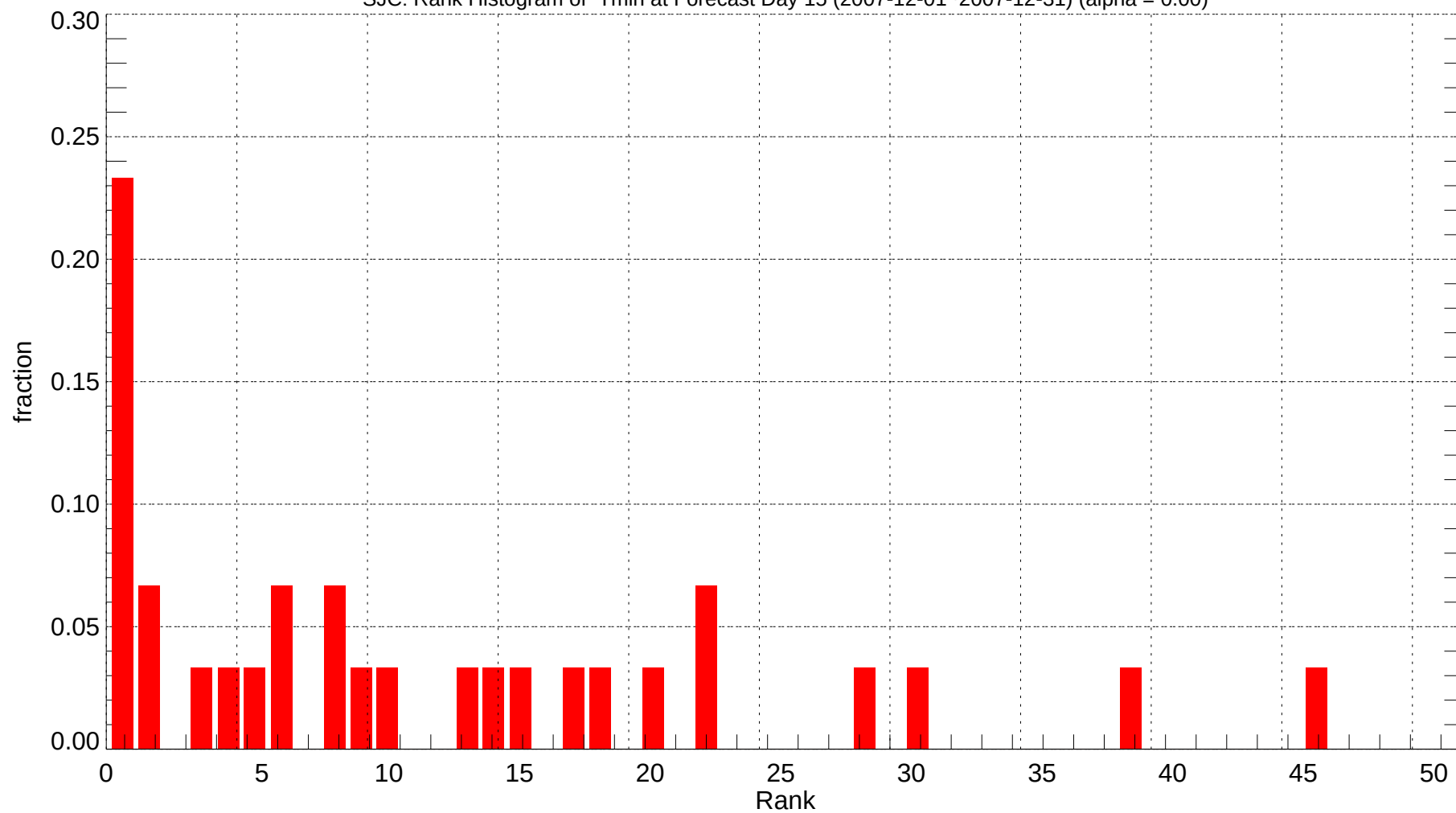
SJC: Rank Histogram of Tmin at Forecast Day 15 (2007-12-01~2007-12-31) (alpha = 0.00)
