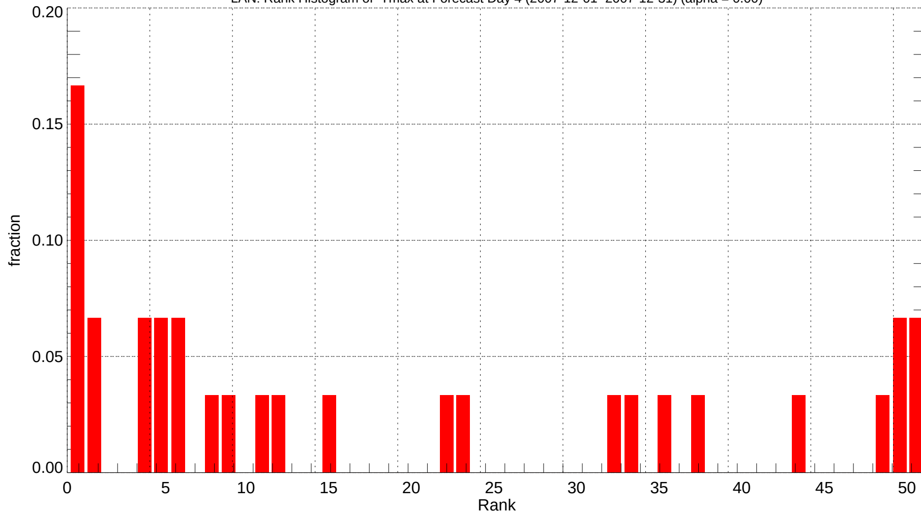
LAN: Rank Histogram of Tmax at Forecast Day 4 (2007-12-01~2007-12-31) (alpha = 0.00)
