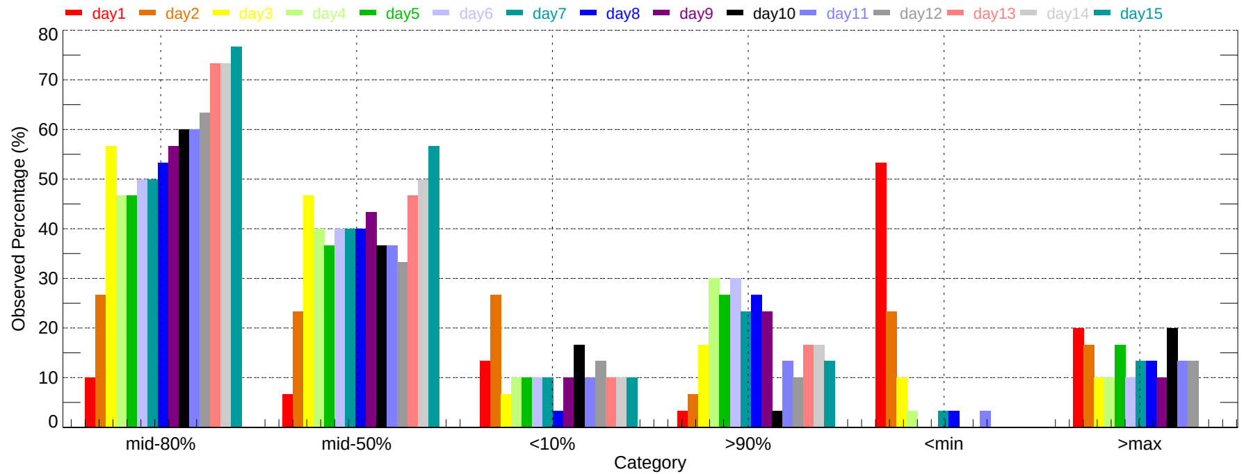
Observed Percentage of Ensembles - OMA: Min Temperature (2007-12-01~2007-12-31)
