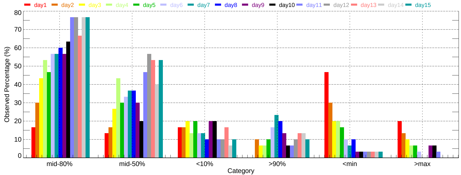
Observed Percentage of Ensembles - ORH: Max Temperature (2007-12-01~2007-12-31)
