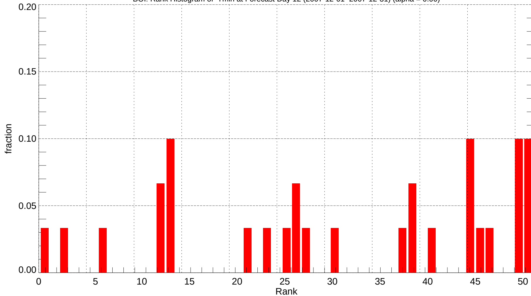
BOI: Rank Histogram of Tmin at Forecast Day 12 (2007-12-01~2007-12-31) (alpha = 0.00)
