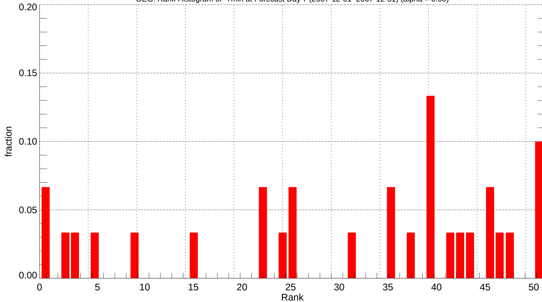
GEG: Rank Histogram of Tmin at Forecast Day 7 (2007-12-01~2007-12-31) (alpha = 0.00)
