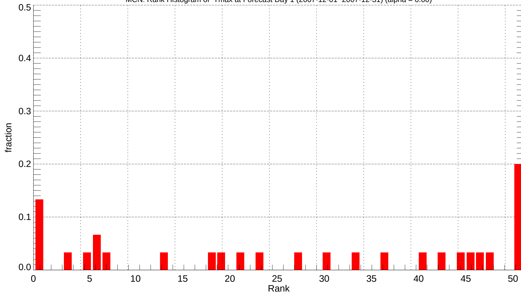
MCN: Rank Histogram of Tmax at Forecast Day 1 (2007-12-01~2007-12-31) (alpha = 0.00)
