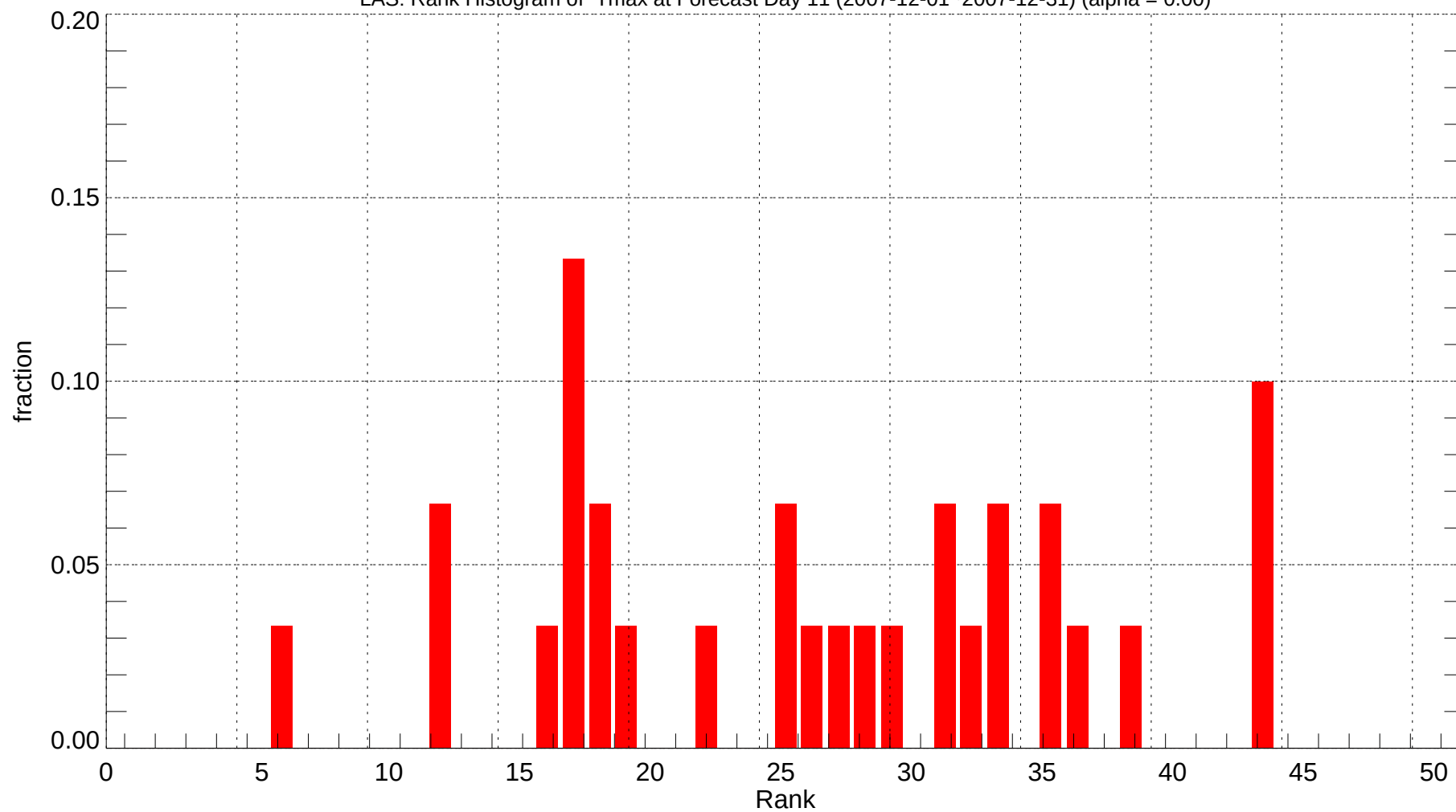
LAS: Rank Histogram of Tmax at Forecast Day 11 (2007-12-01~2007-12-31) (alpha = 0.00)
