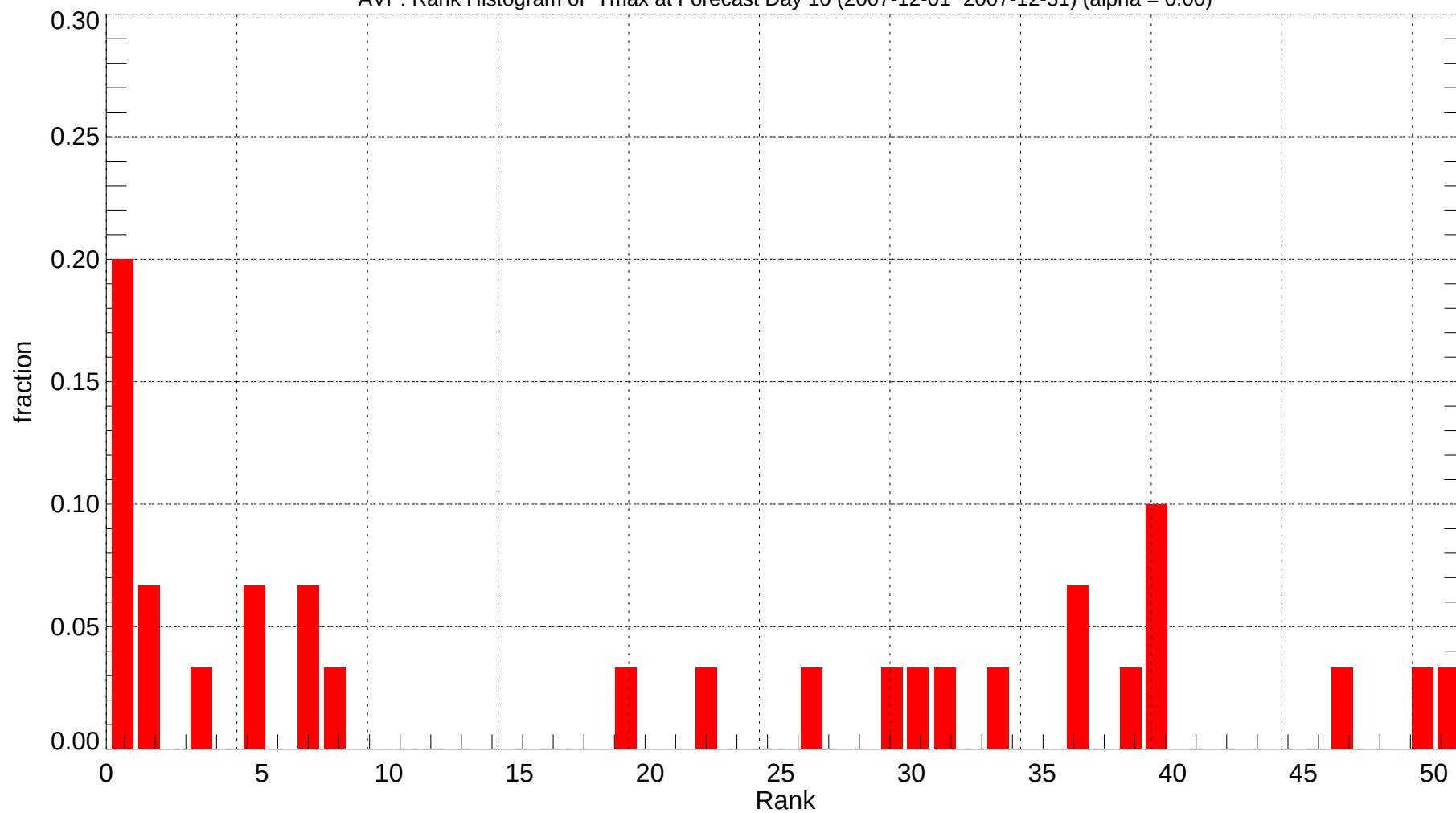
AVP: Rank Histogram of Tmax at Forecast Day 10 (2007-12-01~2007-12-31) (alpha = 0.00)
