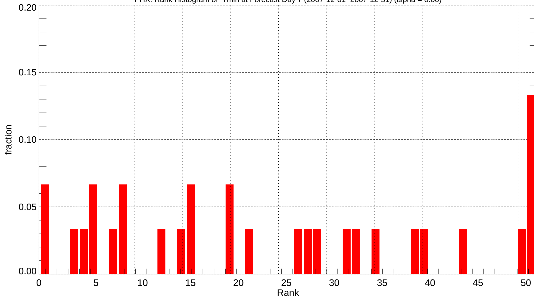
PHX: Rank Histogram of Tmin at Forecast Day 7 (2007-12-01~2007-12-31) (alpha = 0.00)
