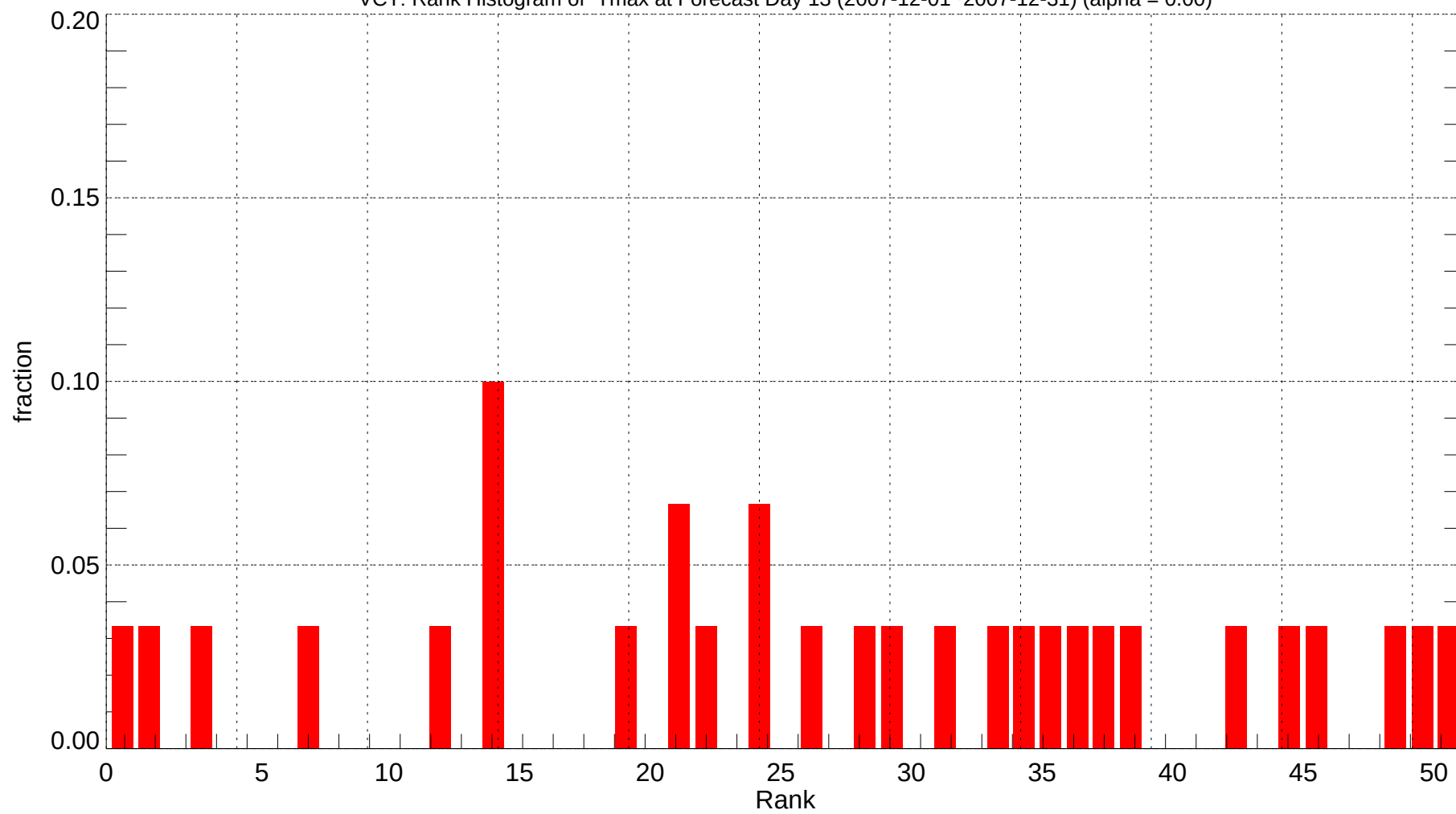
VCT: Rank Histogram of Tmax at Forecast Day 13 (2007-12-01~2007-12-31) (alpha = 0.00)
