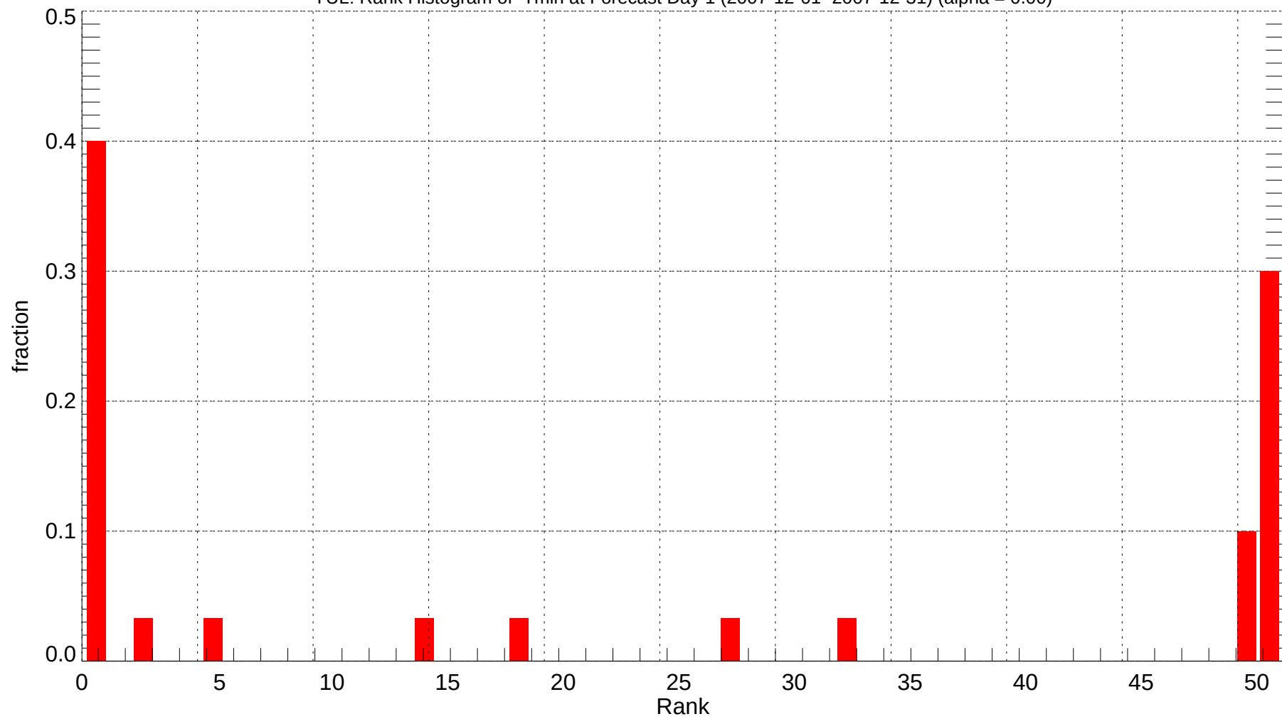
YUL: Rank Histogram of Tmin at Forecast Day 1 (2007-12-01~2007-12-31) (alpha = 0.00)
