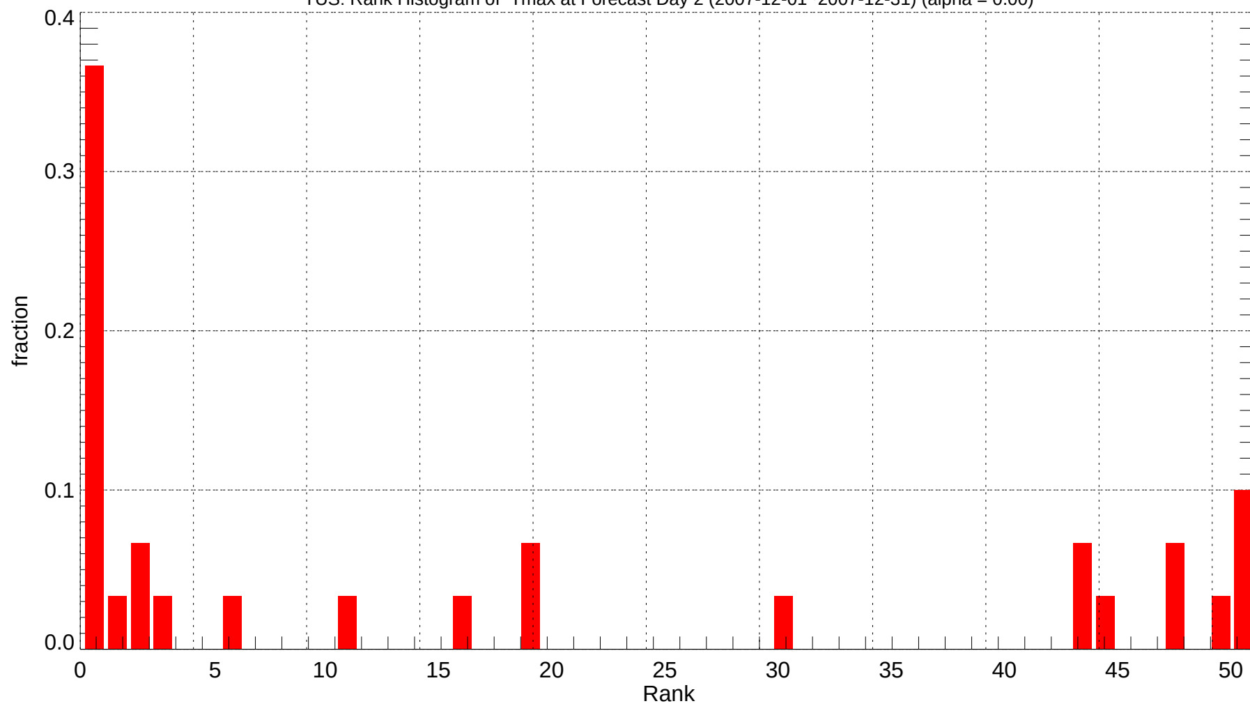
TUS: Rank Histogram of Tmax at Forecast Day 2 (2007-12-01~2007-12-31) (alpha = 0.00)
