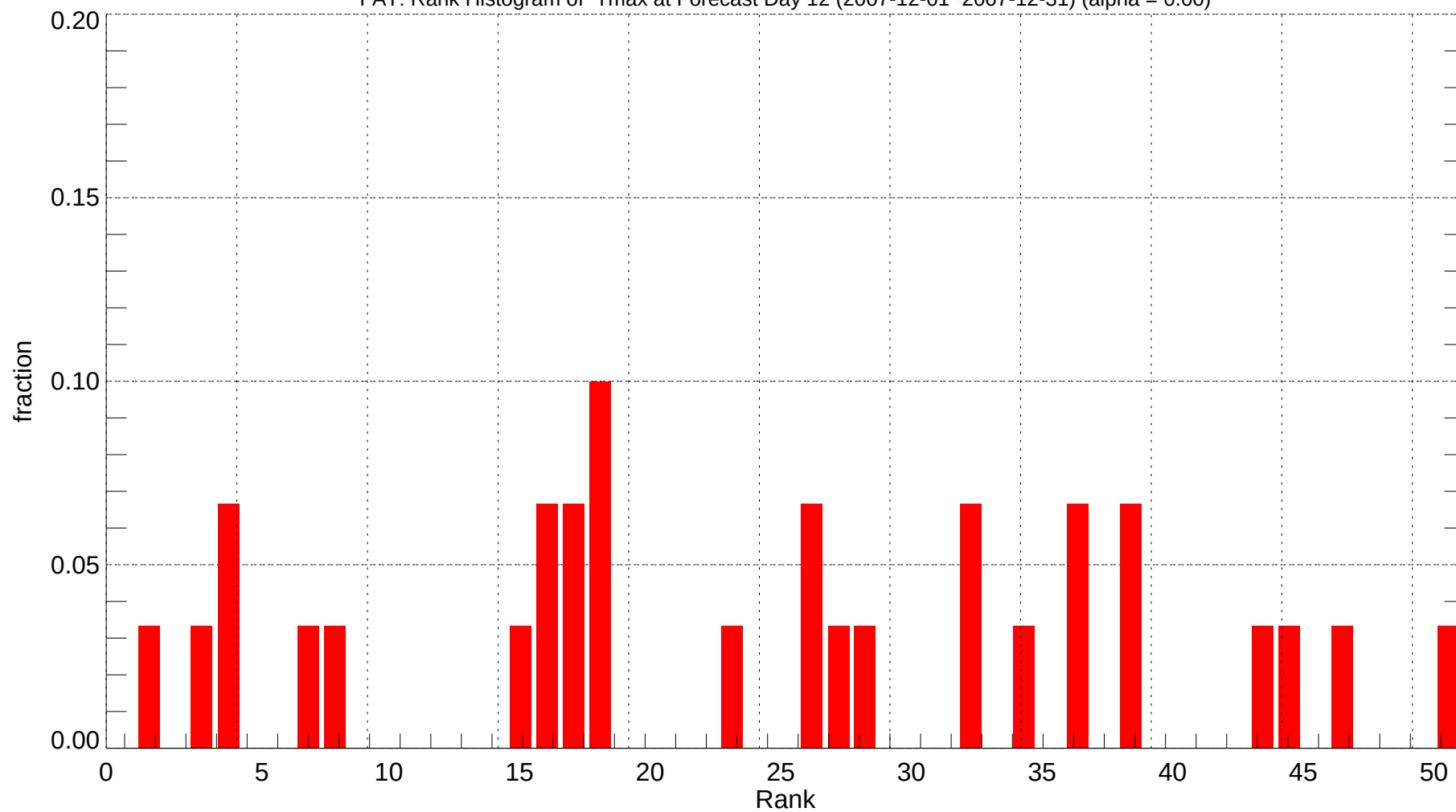
FAT: Rank Histogram of Tmax at Forecast Day 12 (2007-12-01~2007-12-31) (alpha = 0.00)
