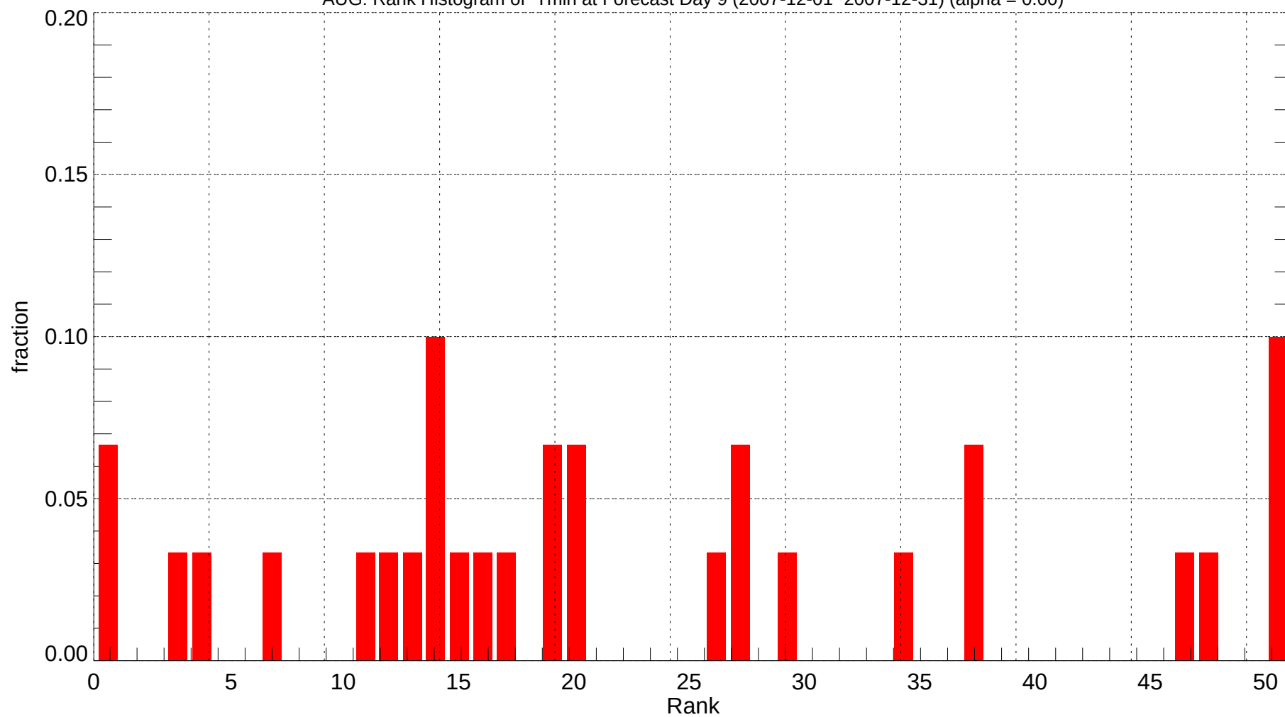
AUG: Rank Histogram of Tmin at Forecast Day 9 (2007-12-01~2007-12-31) (alpha = 0.00)
