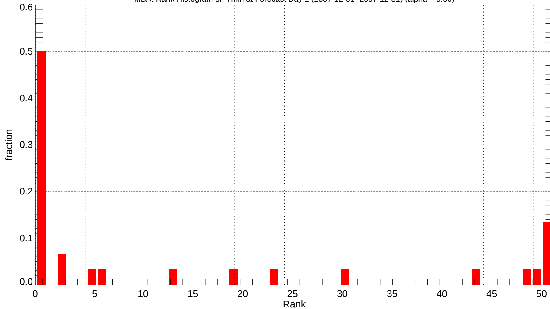
MBA: Rank Histogram of Tmin at Forecast Day 1 (2007-12-01~2007-12-31) (alpha = 0.00)
