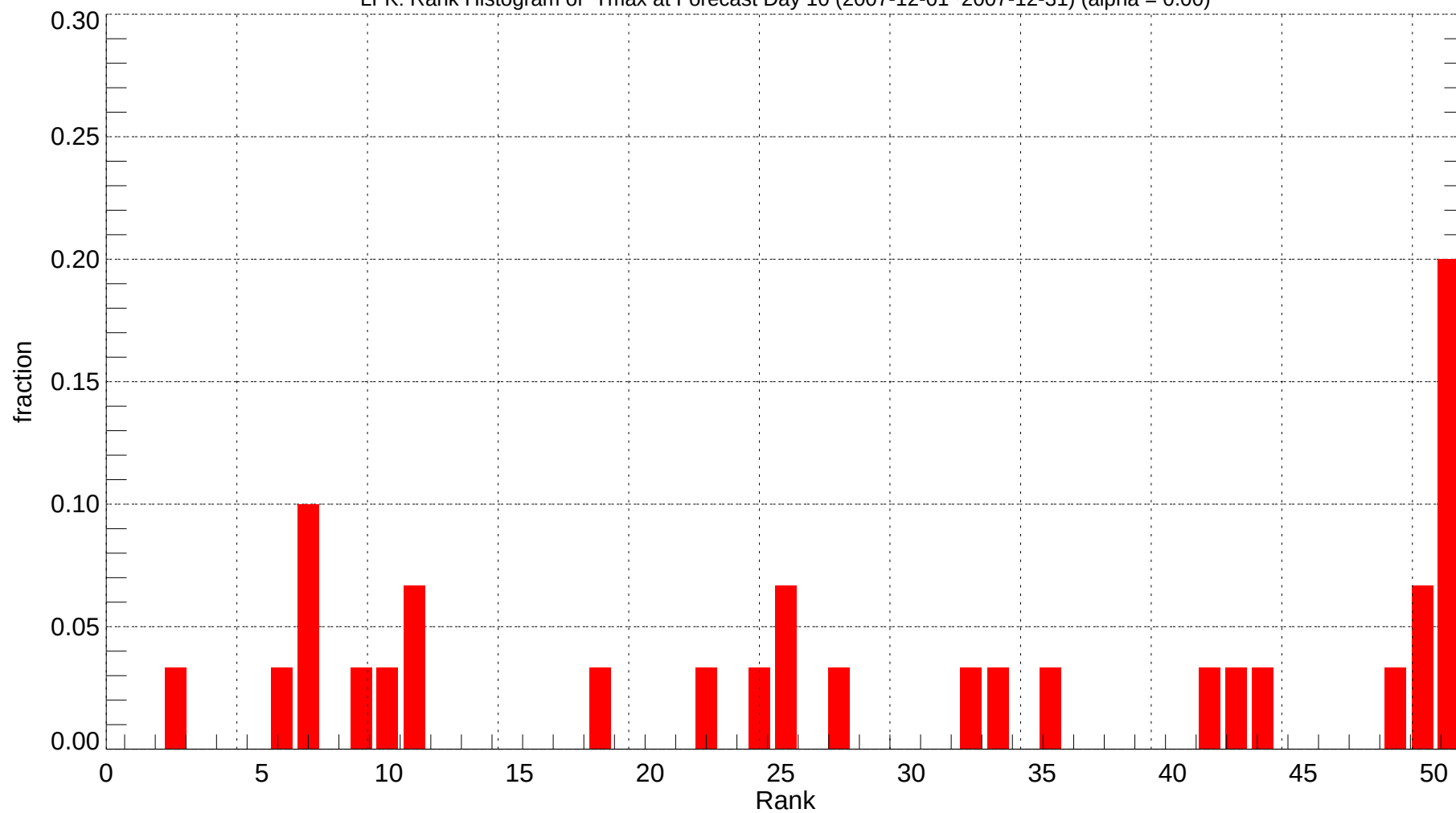
LFK: Rank Histogram of Tmax at Forecast Day 10 (2007-12-01~2007-12-31) (alpha = 0.00)
