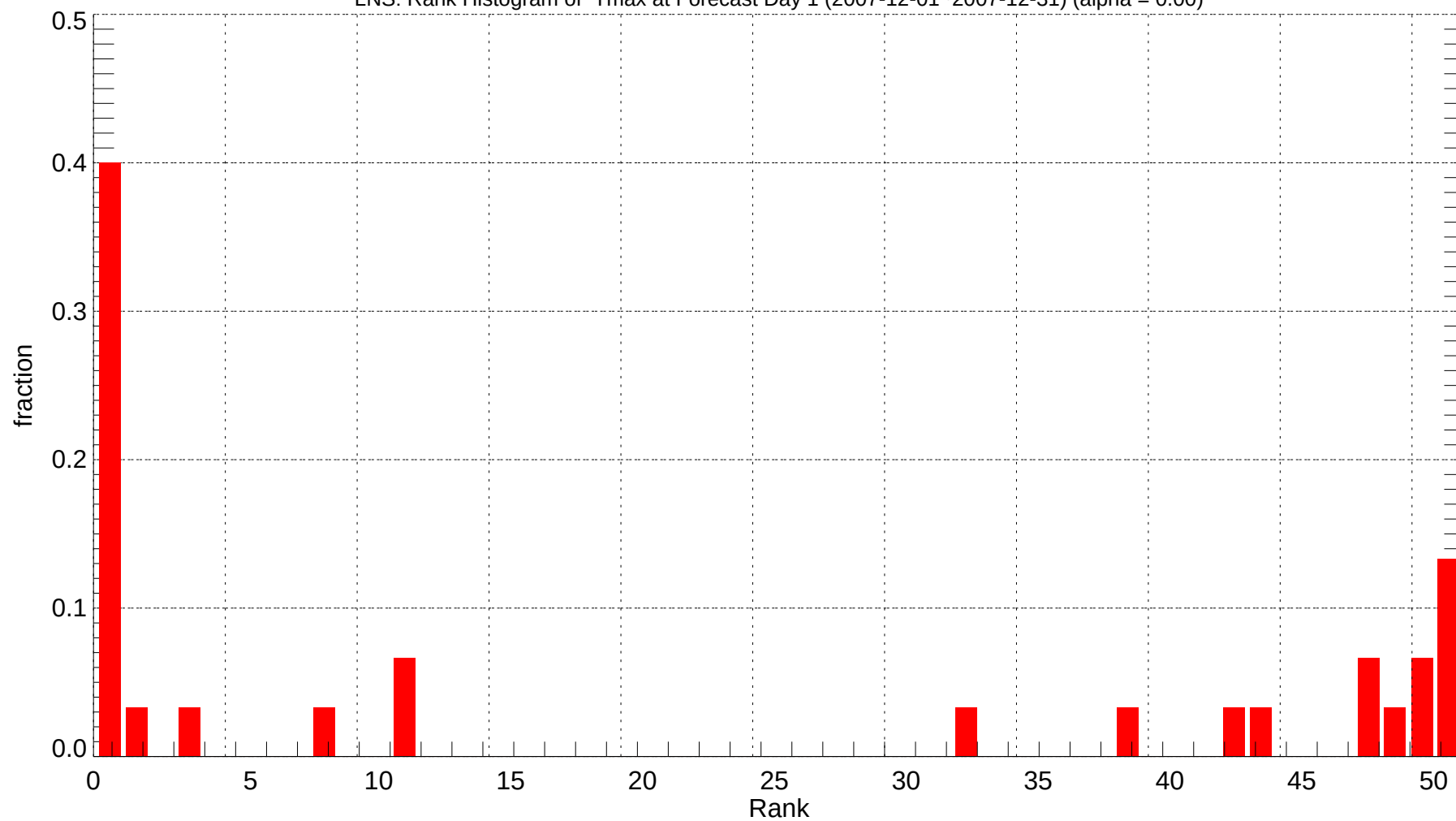
LNS: Rank Histogram of Tmax at Forecast Day 1 (2007-12-01~2007-12-31) (alpha = 0.00)
