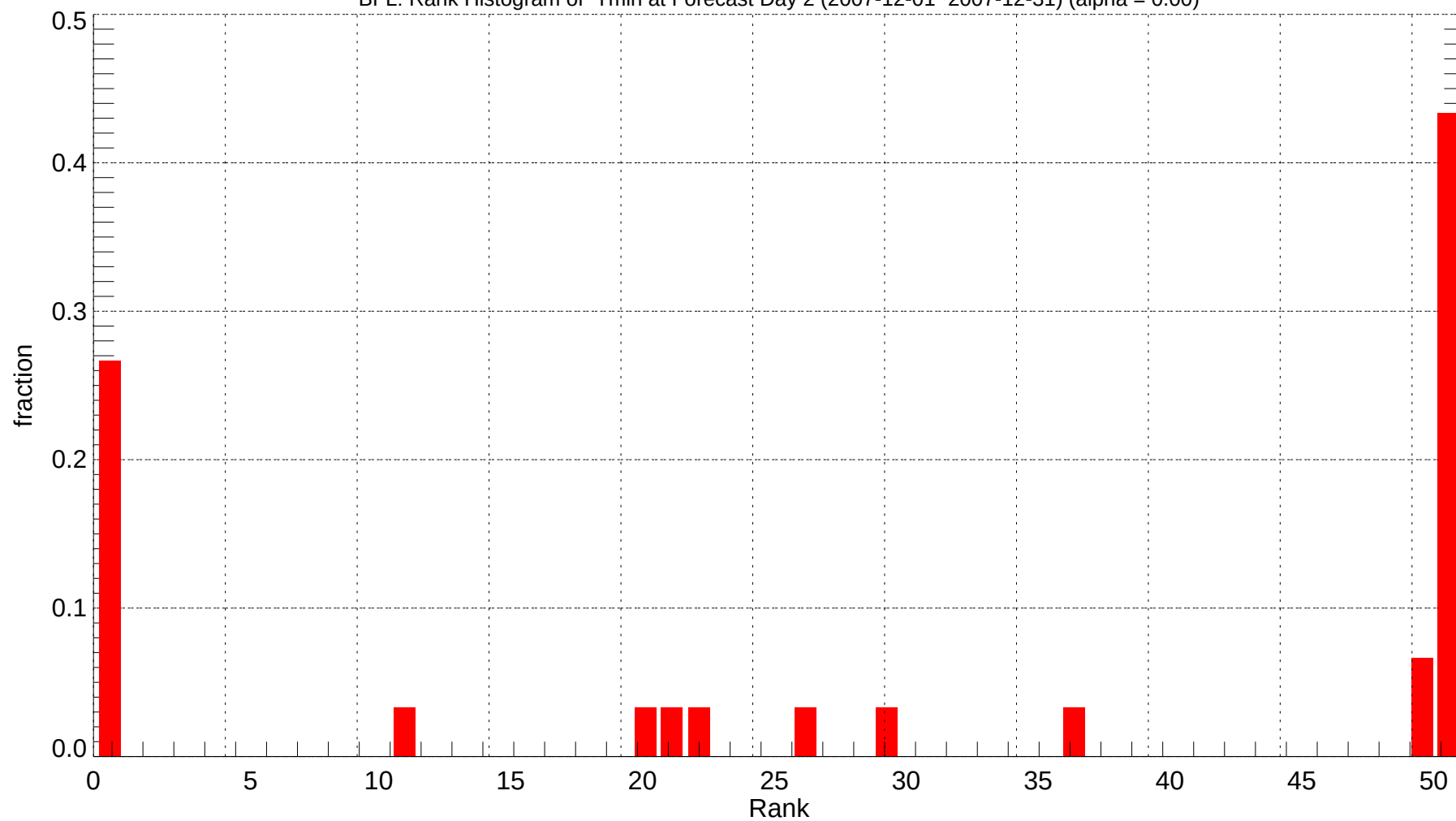
BFL: Rank Histogram of Tmin at Forecast Day 2 (2007-12-01~2007-12-31) (alpha = 0.00)
