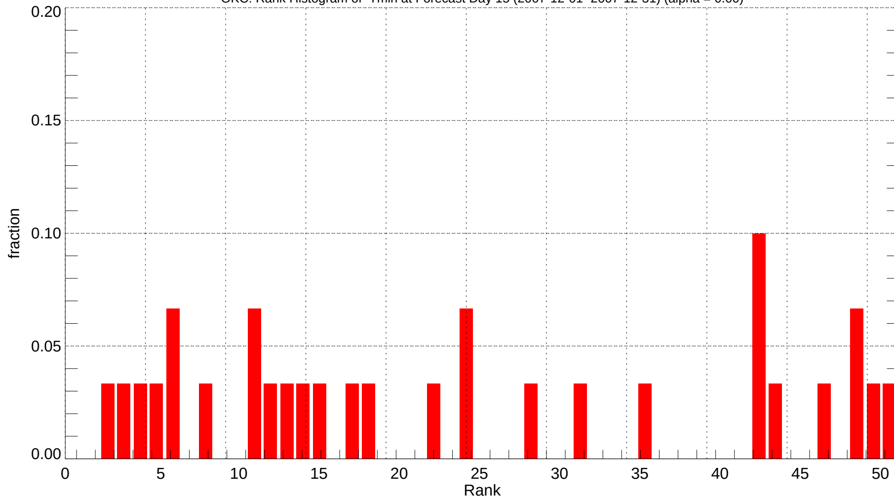
OKC: Rank Histogram of Tmin at Forecast Day 15 (2007-12-01~2007-12-31) (alpha = 0.00)
