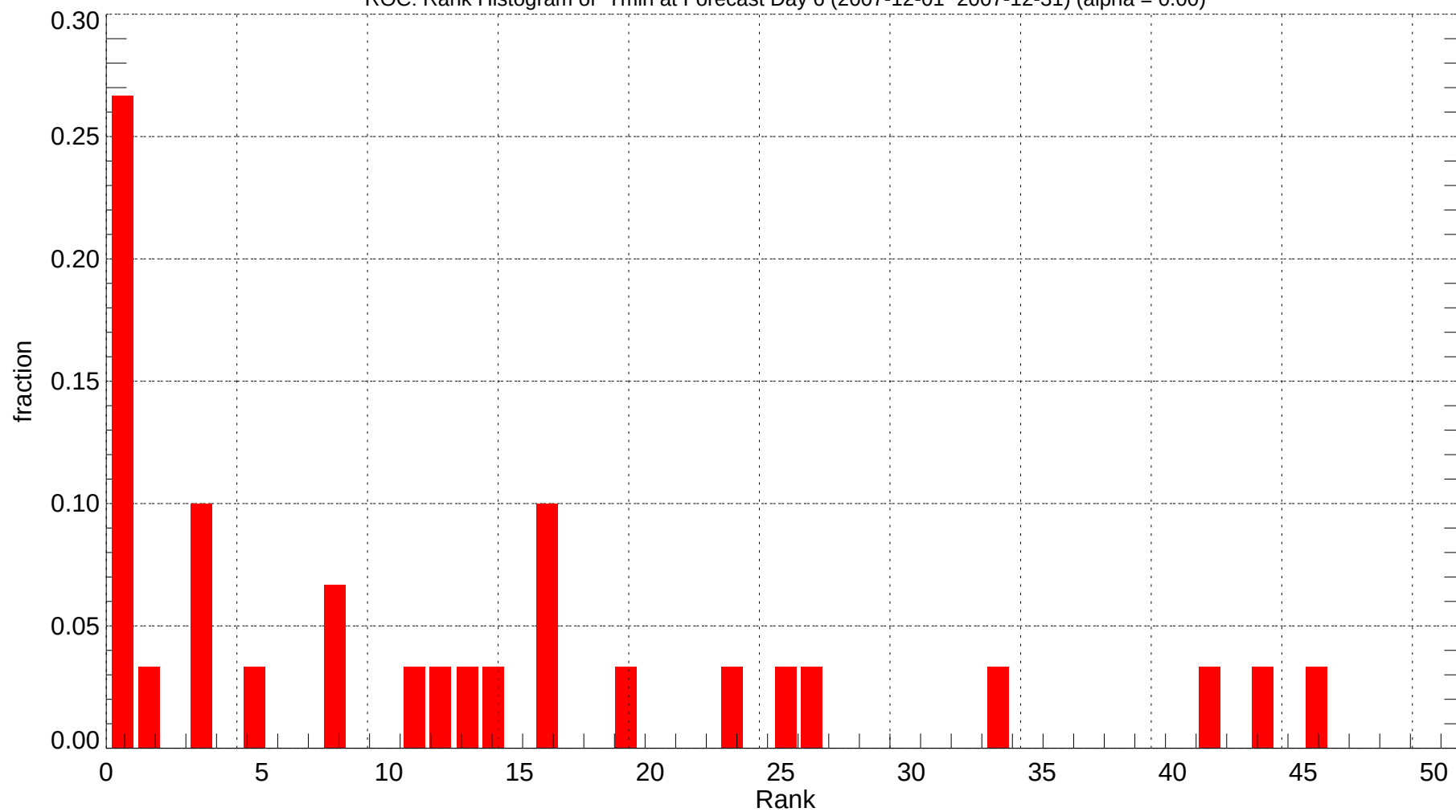
ROC: Rank Histogram of Tmin at Forecast Day 6 (2007-12-01~2007-12-31) (alpha = 0.00)
