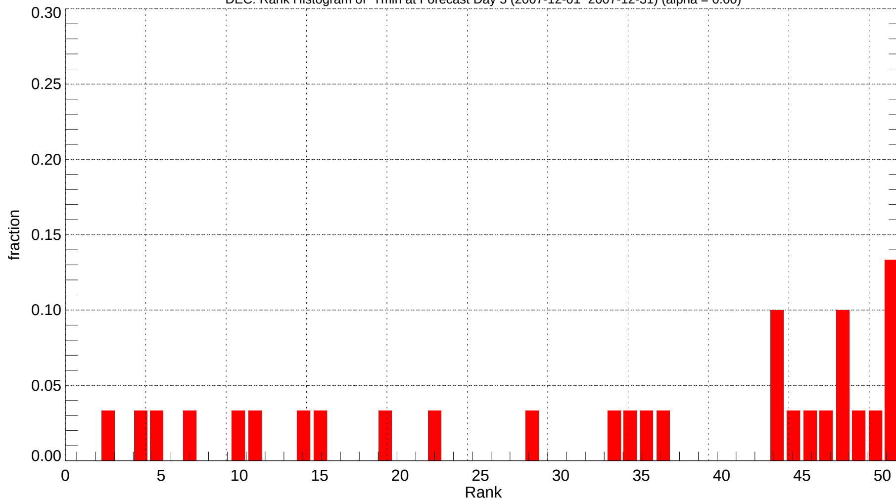
DEC: Rank Histogram of Tmin at Forecast Day 5 (2007-12-01~2007-12-31) (alpha = 0.00)
