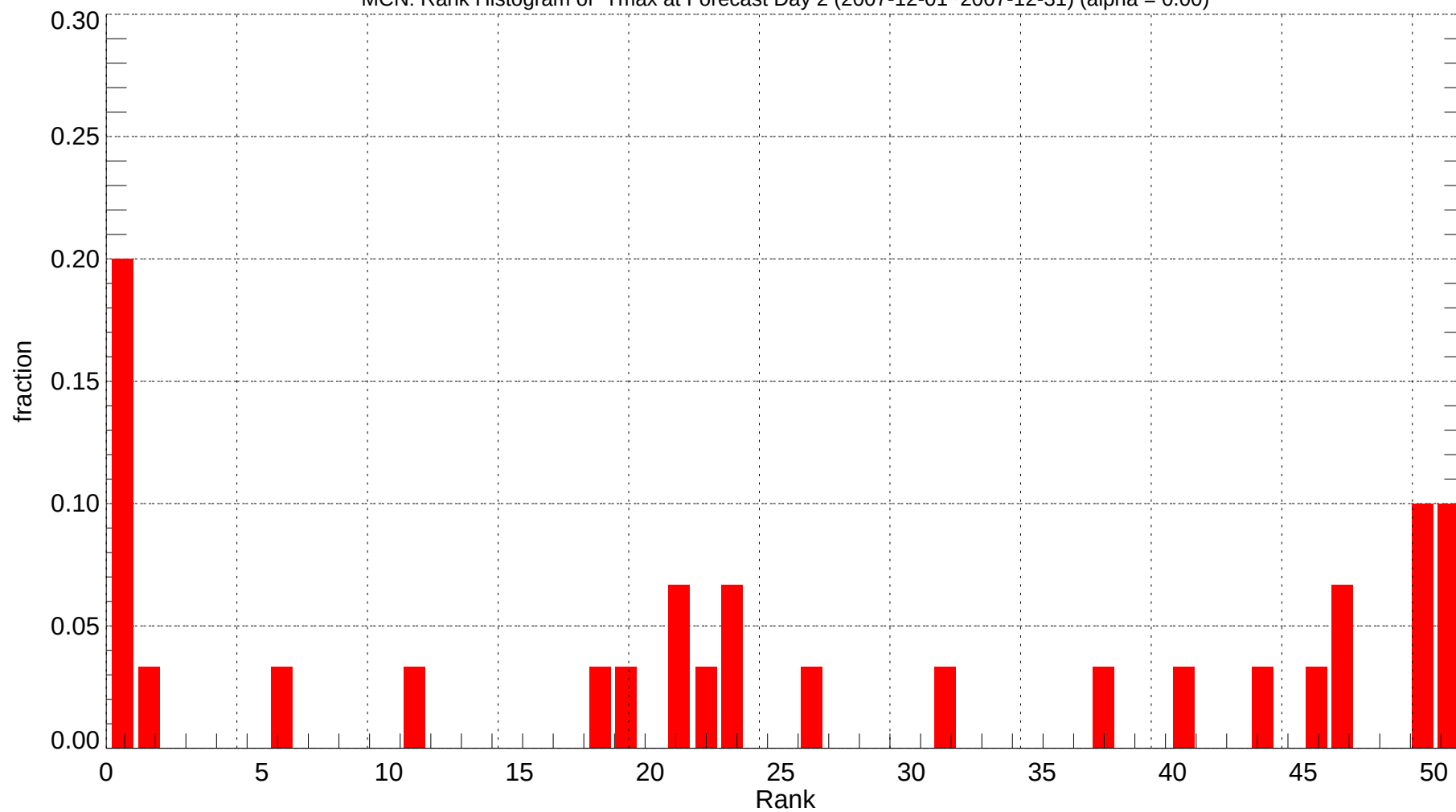
MCN: Rank Histogram of Tmax at Forecast Day 2 (2007-12-01~2007-12-31) (alpha = 0.00)
