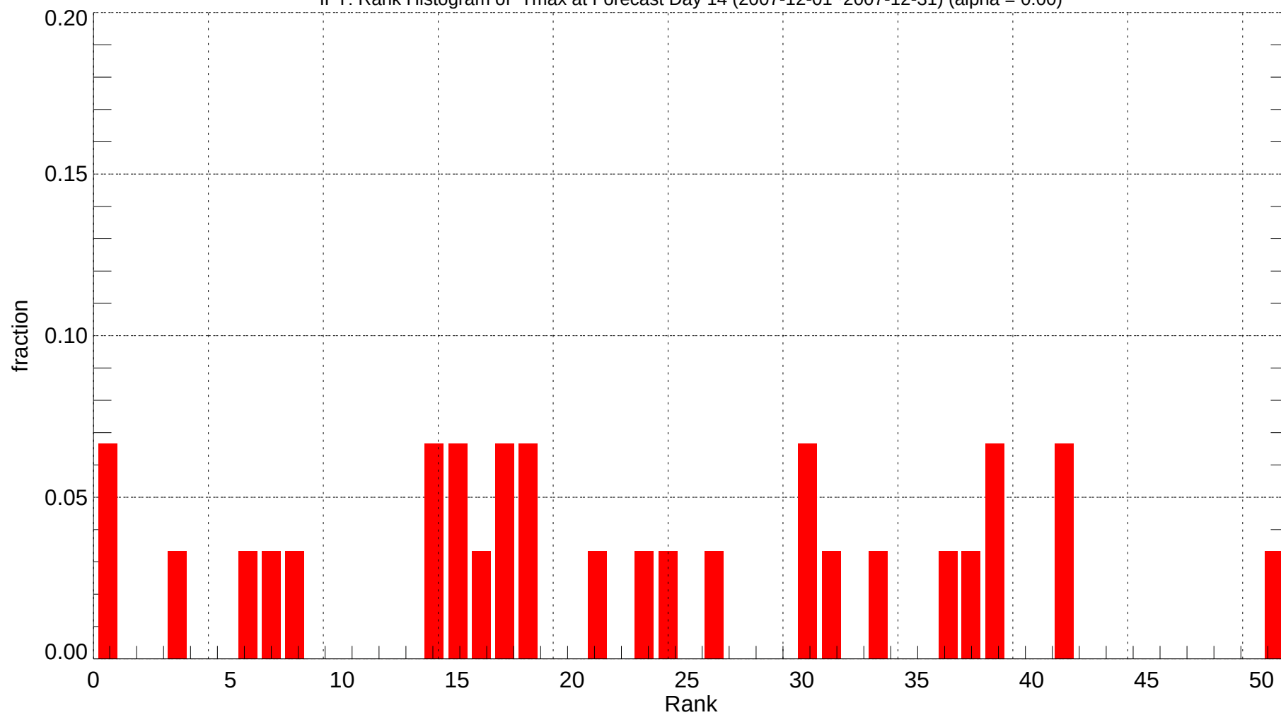
IPT: Rank Histogram of Tmax at Forecast Day 14 (2007-12-01~2007-12-31) (alpha = 0.00)
