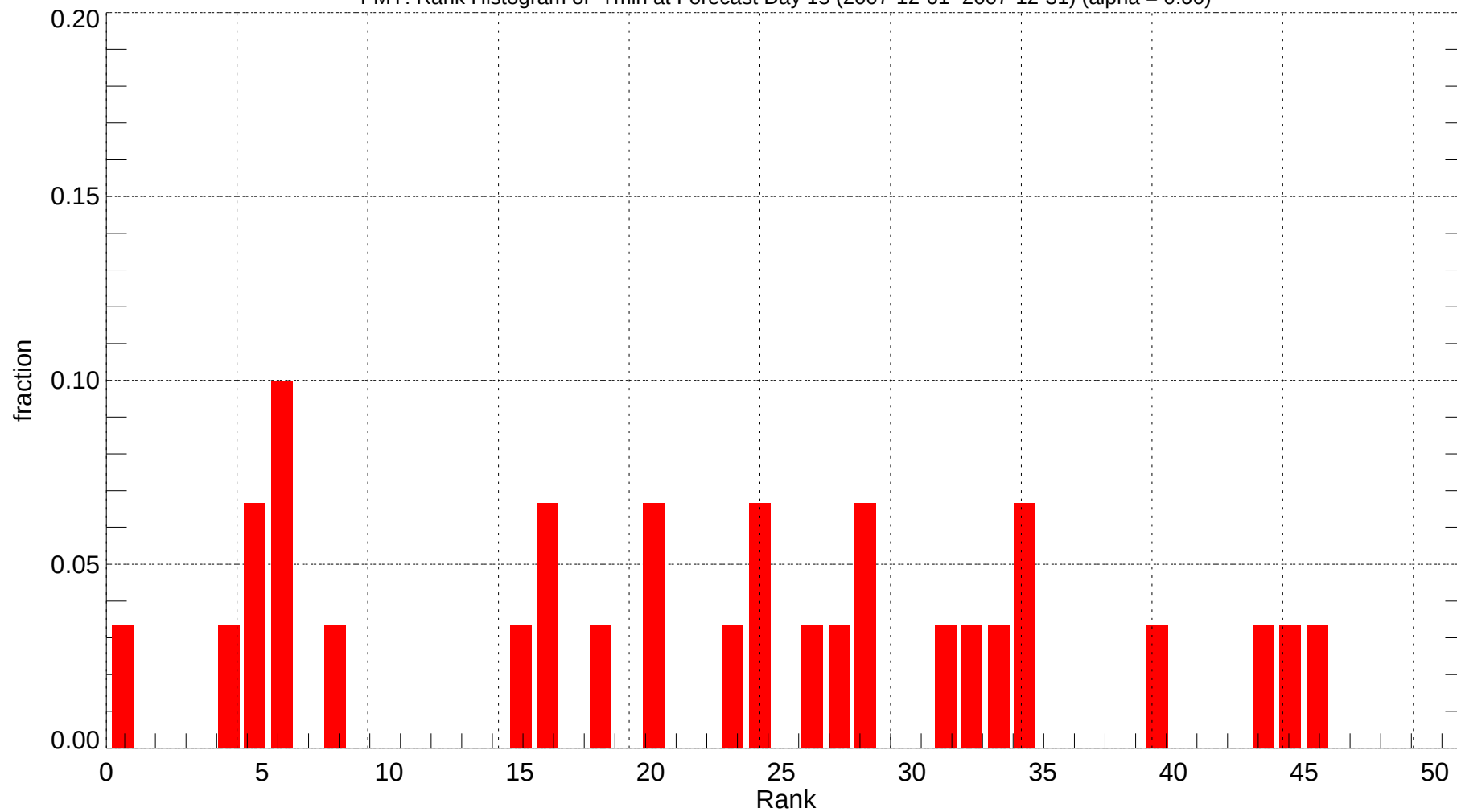
FMY: Rank Histogram of Tmin at Forecast Day 15 (2007-12-01~2007-12-31) (alpha = 0.00)
