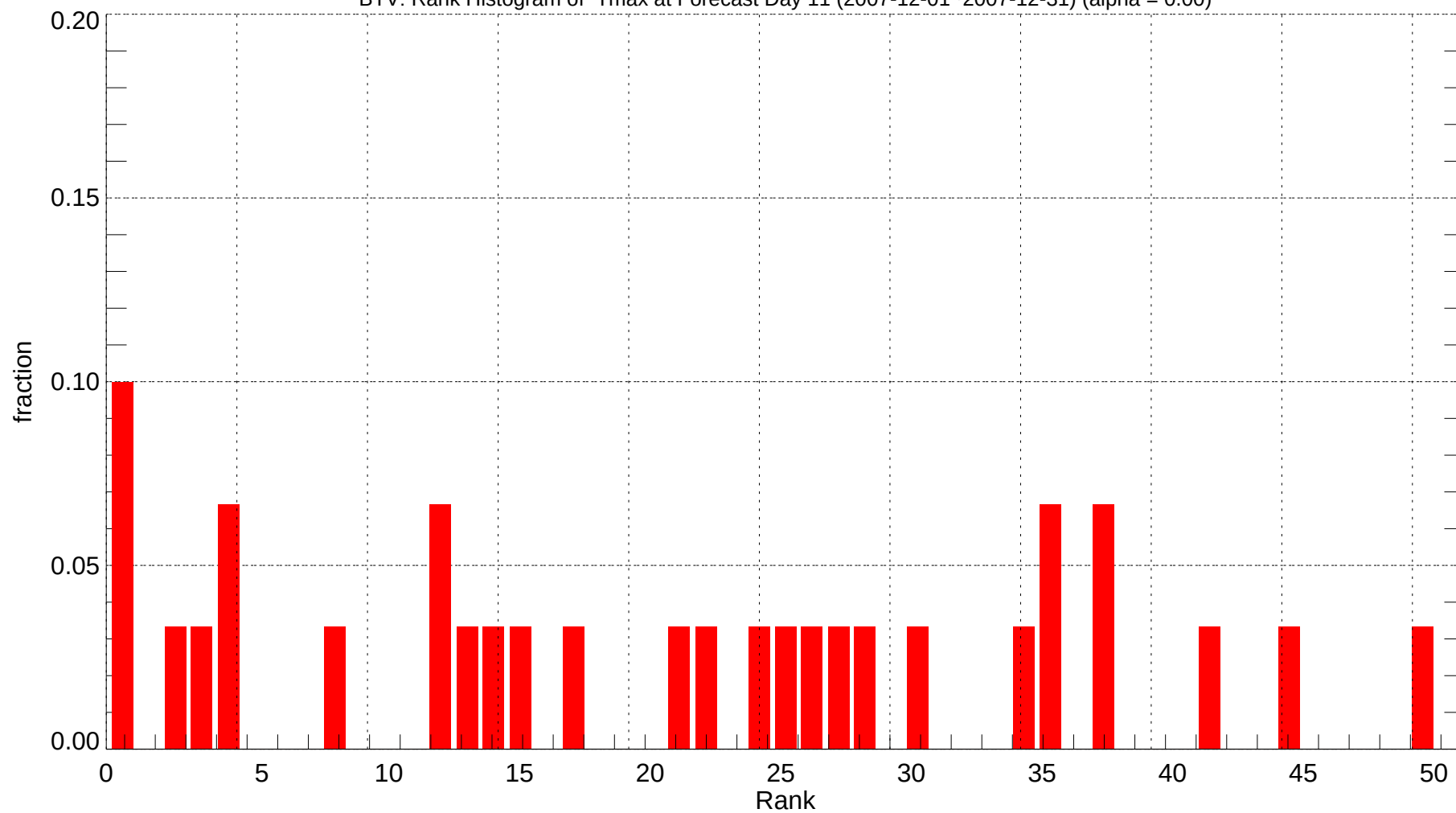
BTV: Rank Histogram of Tmax at Forecast Day 11 (2007-12-01~2007-12-31) (alpha = 0.00)
