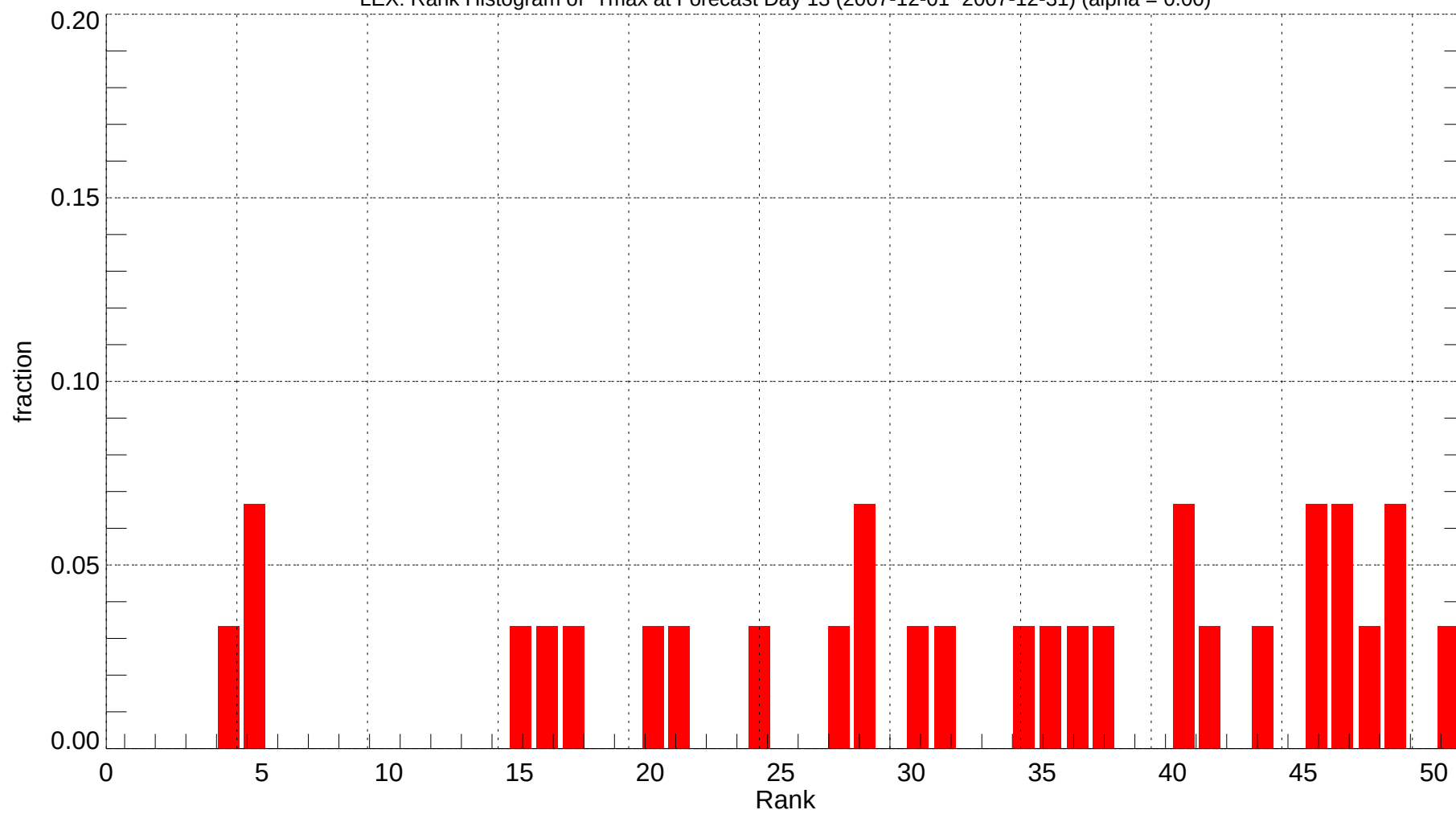
LEX: Rank Histogram of Tmax at Forecast Day 13 (2007-12-01~2007-12-31) (alpha = 0.00)
