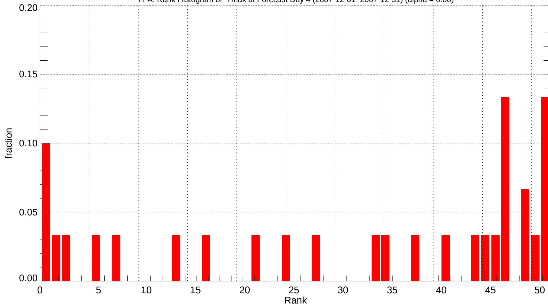
TPA: Rank Histogram of Tmax at Forecast Day 4 (2007-12-01~2007-12-31) (alpha = 0.00)
