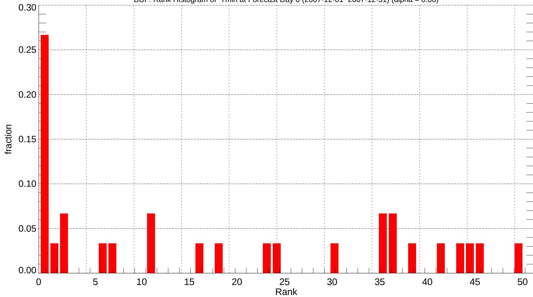
BUF: Rank Histogram of Tmin at Forecast Day 6 (2007-12-01~2007-12-31) (alpha = 0.00)
