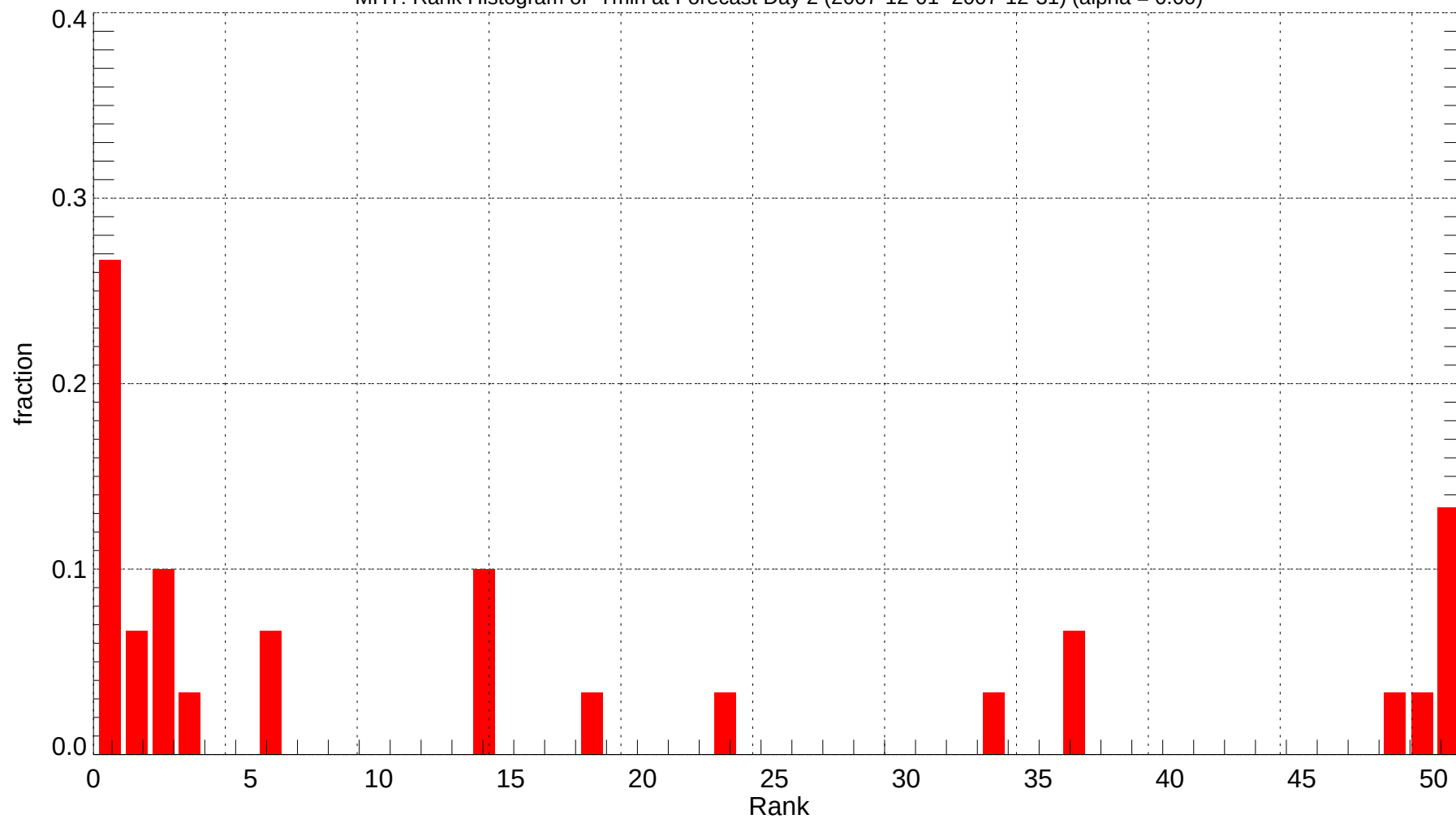
MHT: Rank Histogram of Tmin at Forecast Day 2 (2007-12-01~2007-12-31) (alpha = 0.00)
