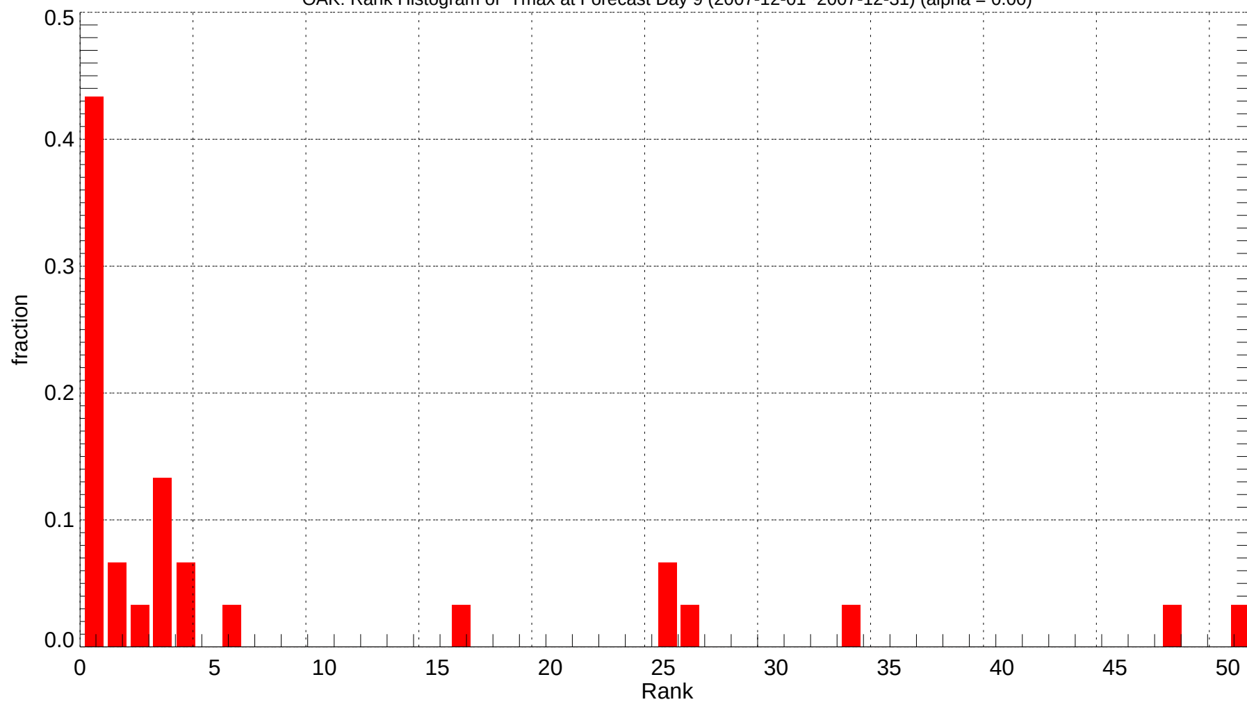
OAK: Rank Histogram of Tmax at Forecast Day 9 (2007-12-01~2007-12-31) (alpha = 0.00)
