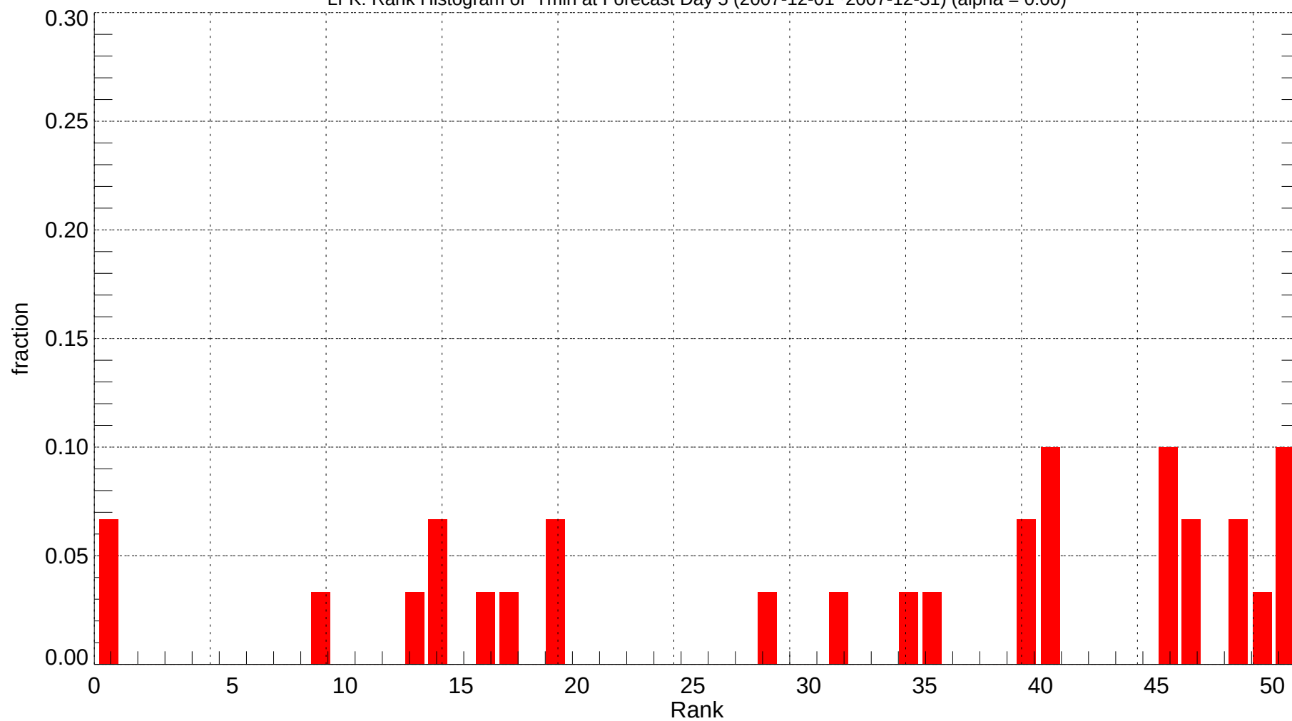
LFK: Rank Histogram of Tmin at Forecast Day 5 (2007-12-01~2007-12-31) (alpha = 0.00)
