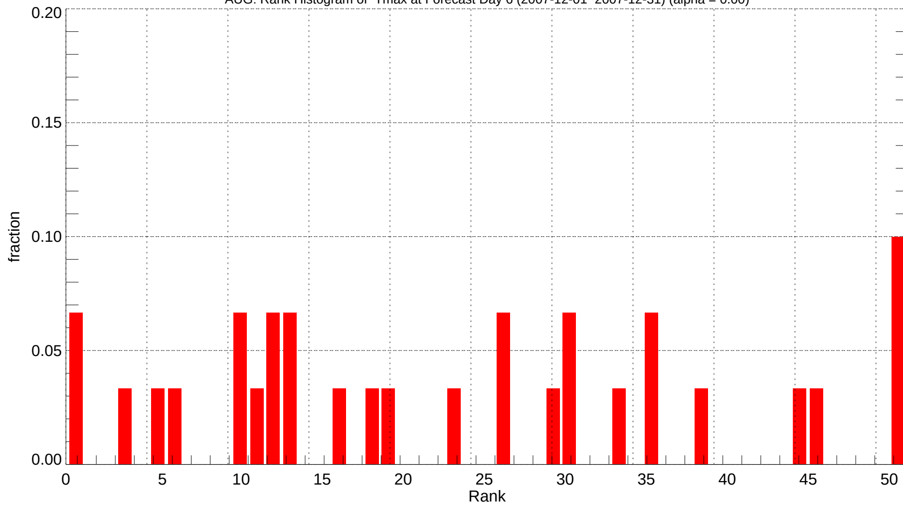
AUG: Rank Histogram of Tmax at Forecast Day 6 (2007-12-01~2007-12-31) (alpha = 0.00)
