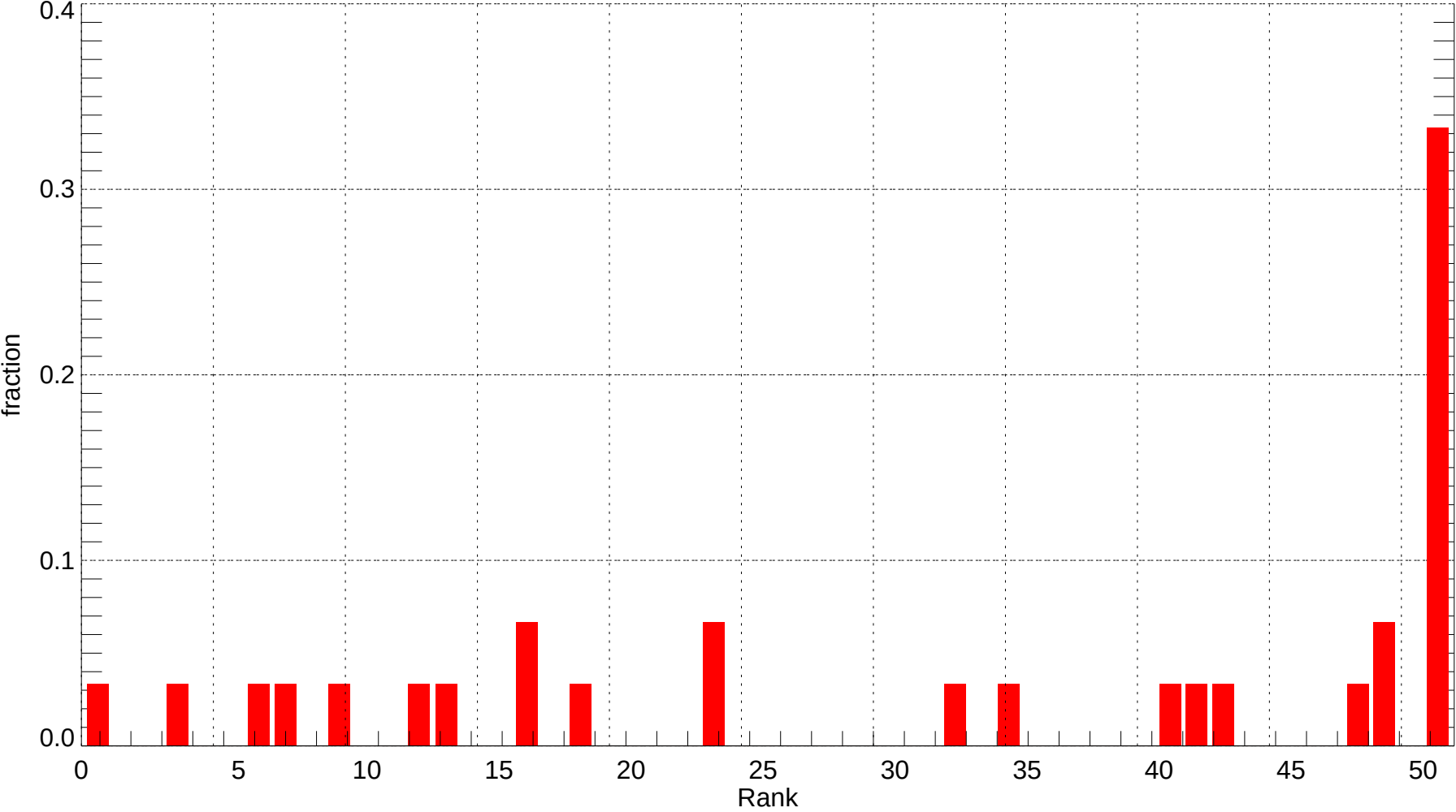
MCI: Rank Histogram of Tmin at Forecast Day 8 (2007-12-01~2007-12-31) (alpha = 0.00)
