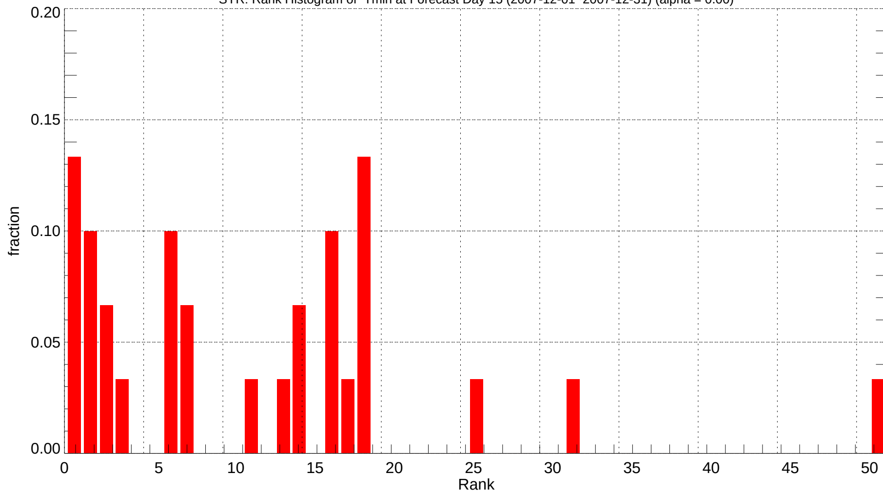
SYR: Rank Histogram of Tmin at Forecast Day 15 (2007-12-01~2007-12-31) (alpha = 0.00)
