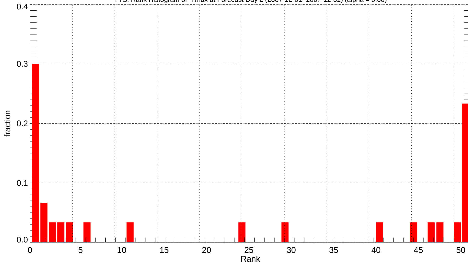
TYS: Rank Histogram of Tmax at Forecast Day 2 (2007-12-01~2007-12-31) (alpha = 0.00)
