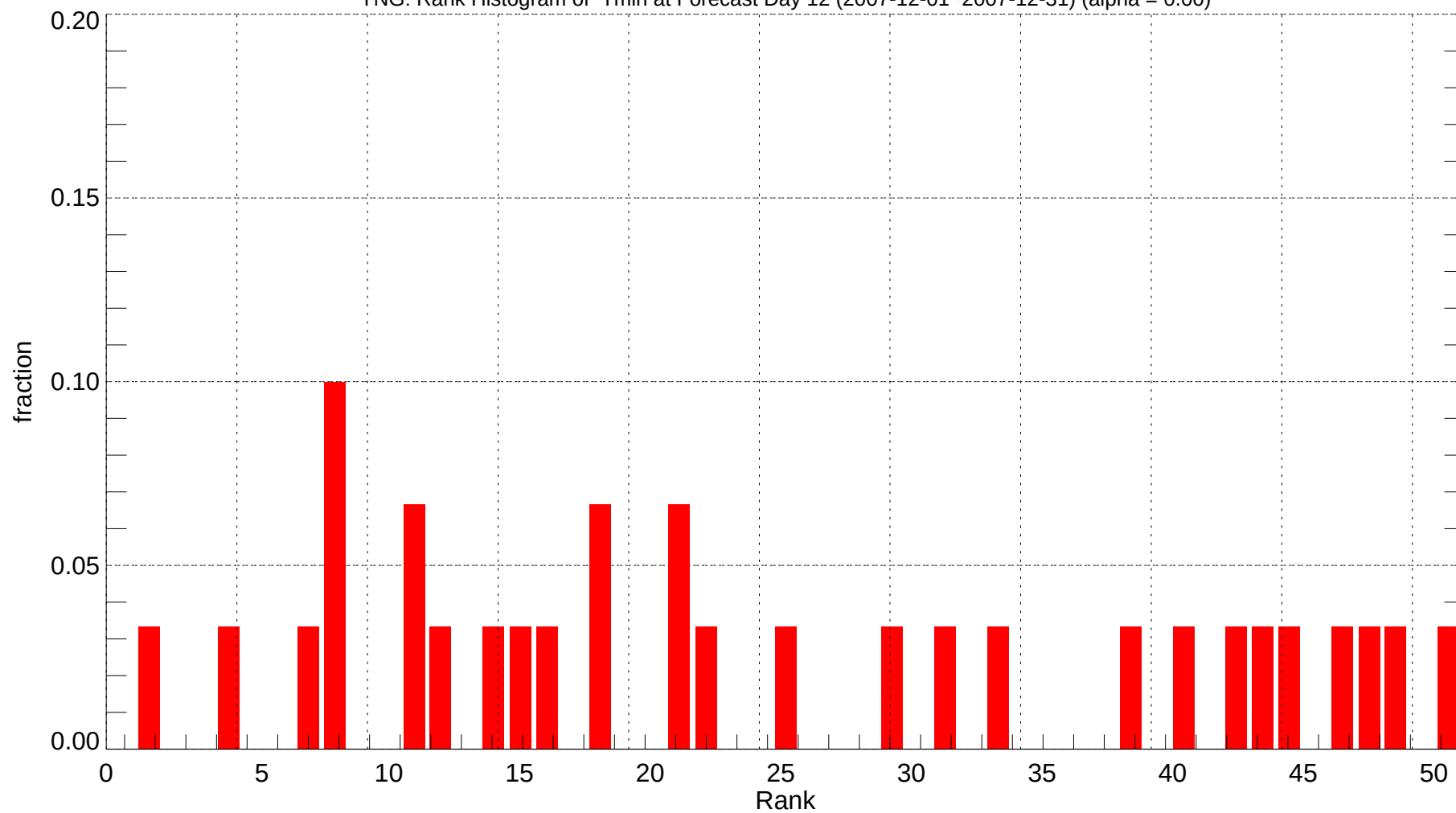
YNG: Rank Histogram of Tmin at Forecast Day 12 (2007-12-01~2007-12-31) (alpha = 0.00)
