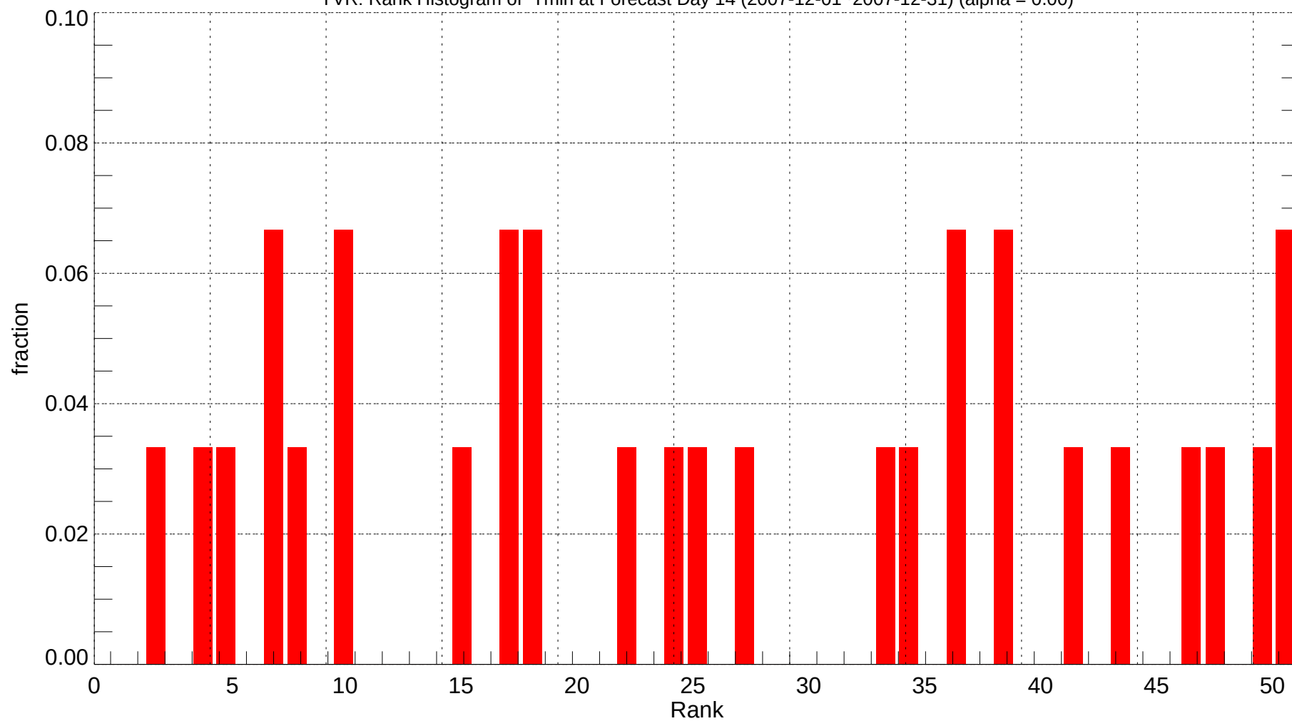
YVR: Rank Histogram of Tmin at Forecast Day 14 (2007-12-01~2007-12-31) (alpha = 0.00)
