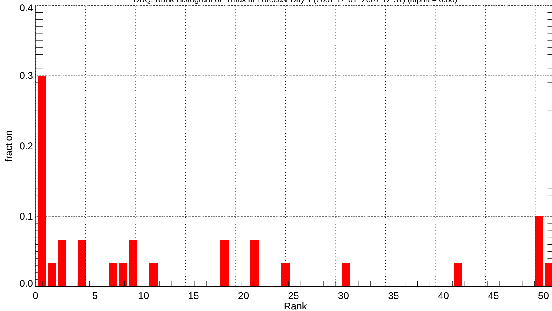
DBQ: Rank Histogram of Tmax at Forecast Day 1 (2007-12-01~2007-12-31) (alpha = 0.00)
