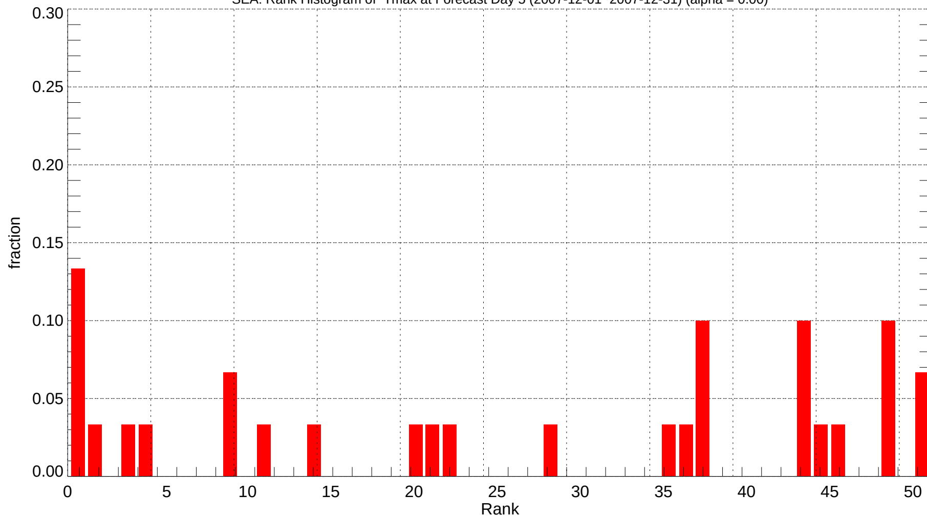
SEA: Rank Histogram of Tmax at Forecast Day 5 (2007-12-01~2007-12-31) (alpha = 0.00)
