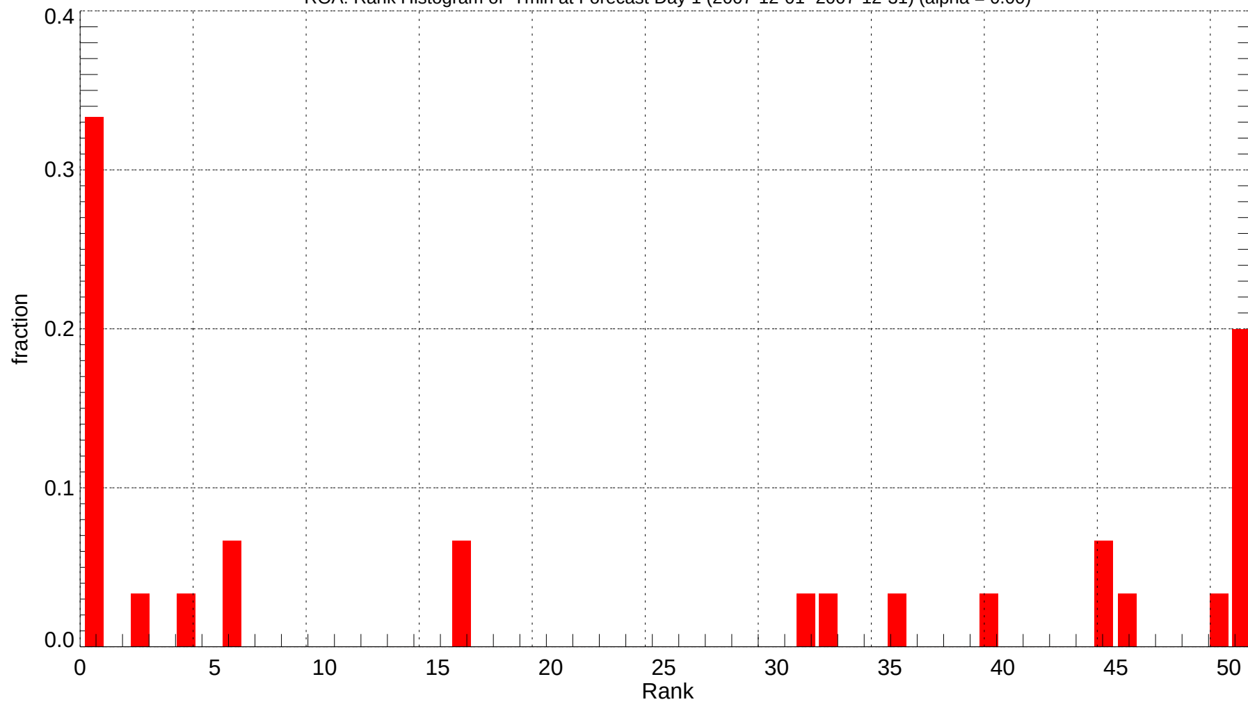
ROA: Rank Histogram of Tmin at Forecast Day 1 (2007-12-01~2007-12-31) (alpha = 0.00)
