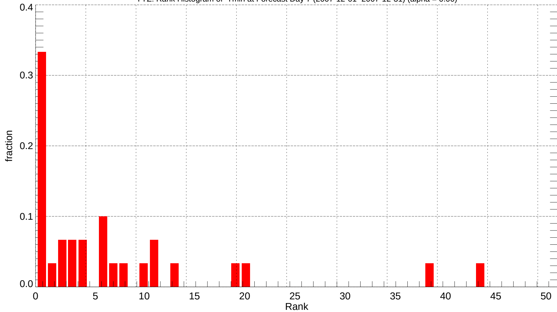
YYZ: Rank Histogram of Tmin at Forecast Day 7 (2007-12-01~2007-12-31) (alpha = 0.00)
