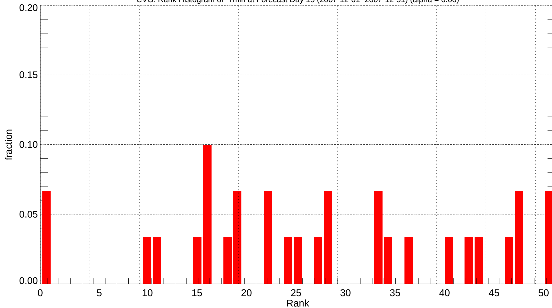
CVG: Rank Histogram of Tmin at Forecast Day 13 (2007-12-01~2007-12-31) (alpha = 0.00)
