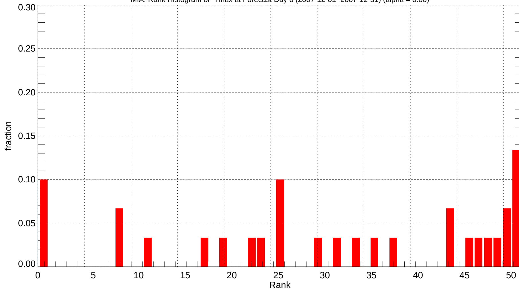
MIA: Rank Histogram of Tmax at Forecast Day 6 (2007-12-01~2007-12-31) (alpha = 0.00)
