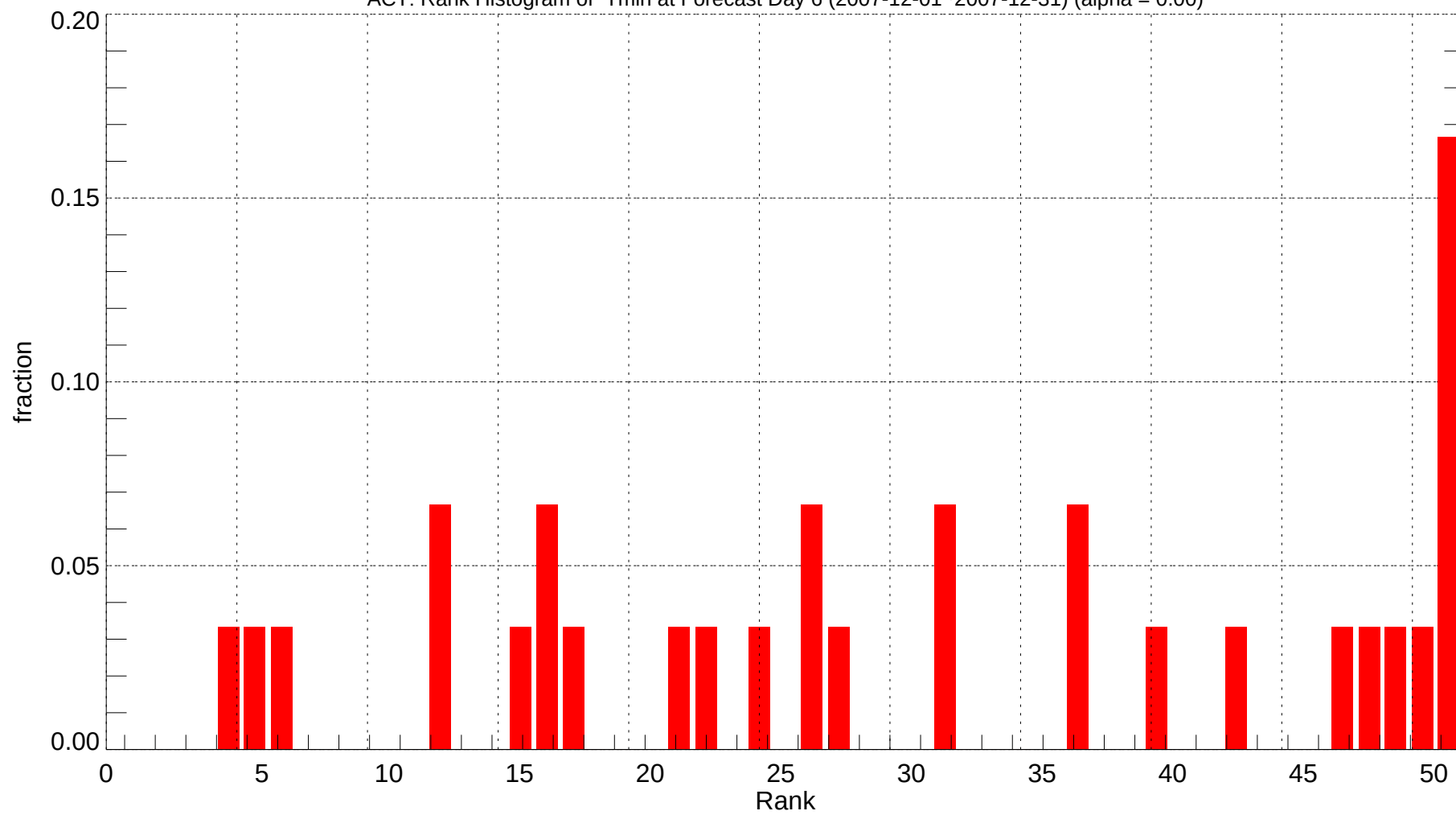
ACT: Rank Histogram of Tmin at Forecast Day 6 (2007-12-01~2007-12-31) (alpha = 0.00)
