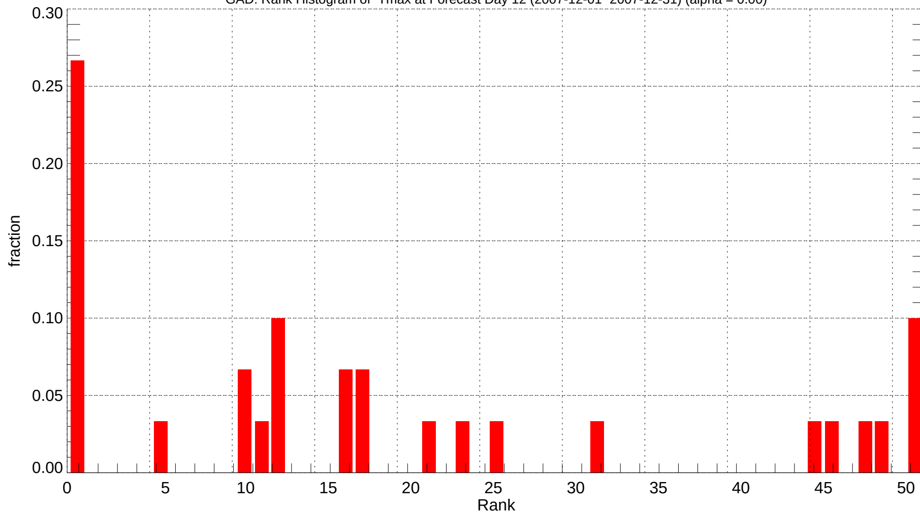
GAD: Rank Histogram of Tmax at Forecast Day 12 (2007-12-01~2007-12-31) (alpha = 0.00)
