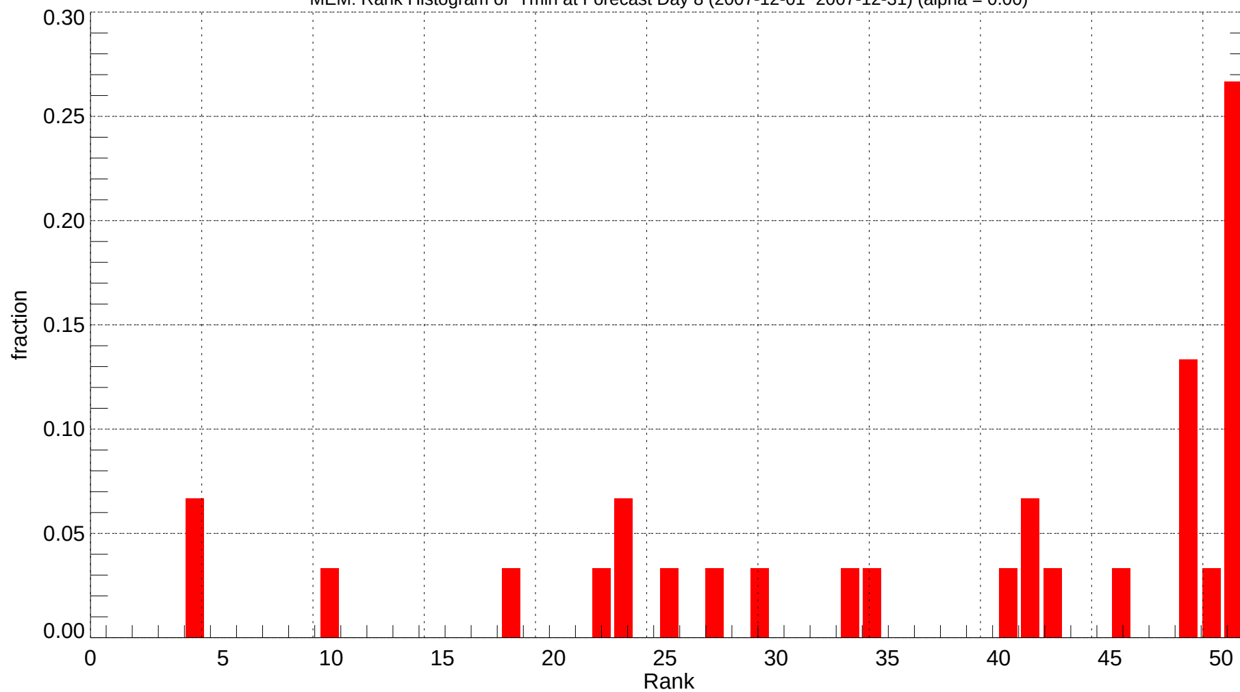
MEM: Rank Histogram of Tmin at Forecast Day 8 (2007-12-01~2007-12-31) (alpha = 0.00)
