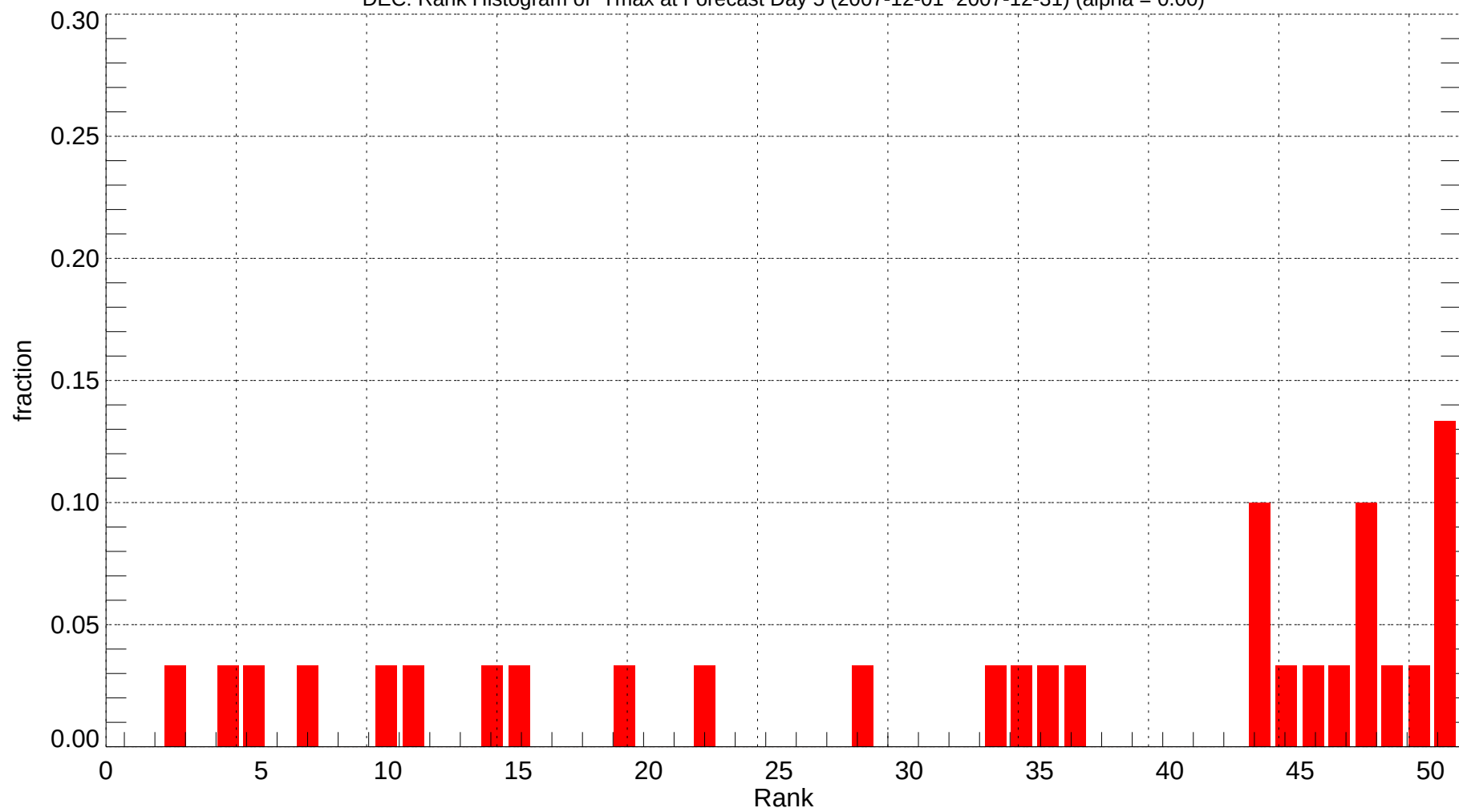
DEC: Rank Histogram of Tmax at Forecast Day 5 (2007-12-01~2007-12-31) (alpha = 0.00)
