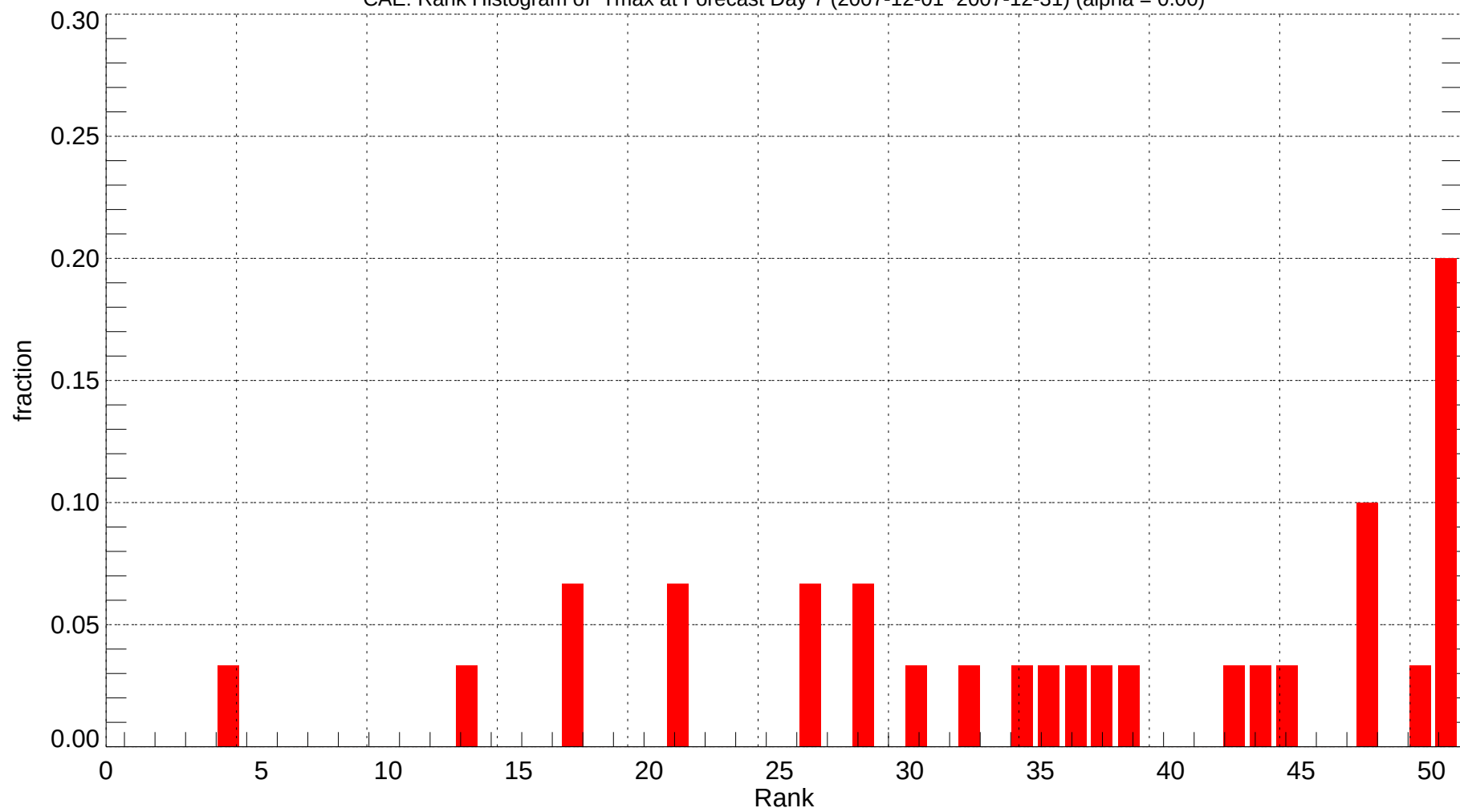
CAE: Rank Histogram of Tmax at Forecast Day 7 (2007-12-01~2007-12-31) (alpha = 0.00)
