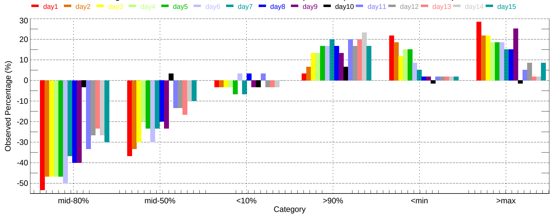
Observed Percentage Deviation of Ensembles - TLH: Min Temperature (2007-12-01~2007-12-31)
