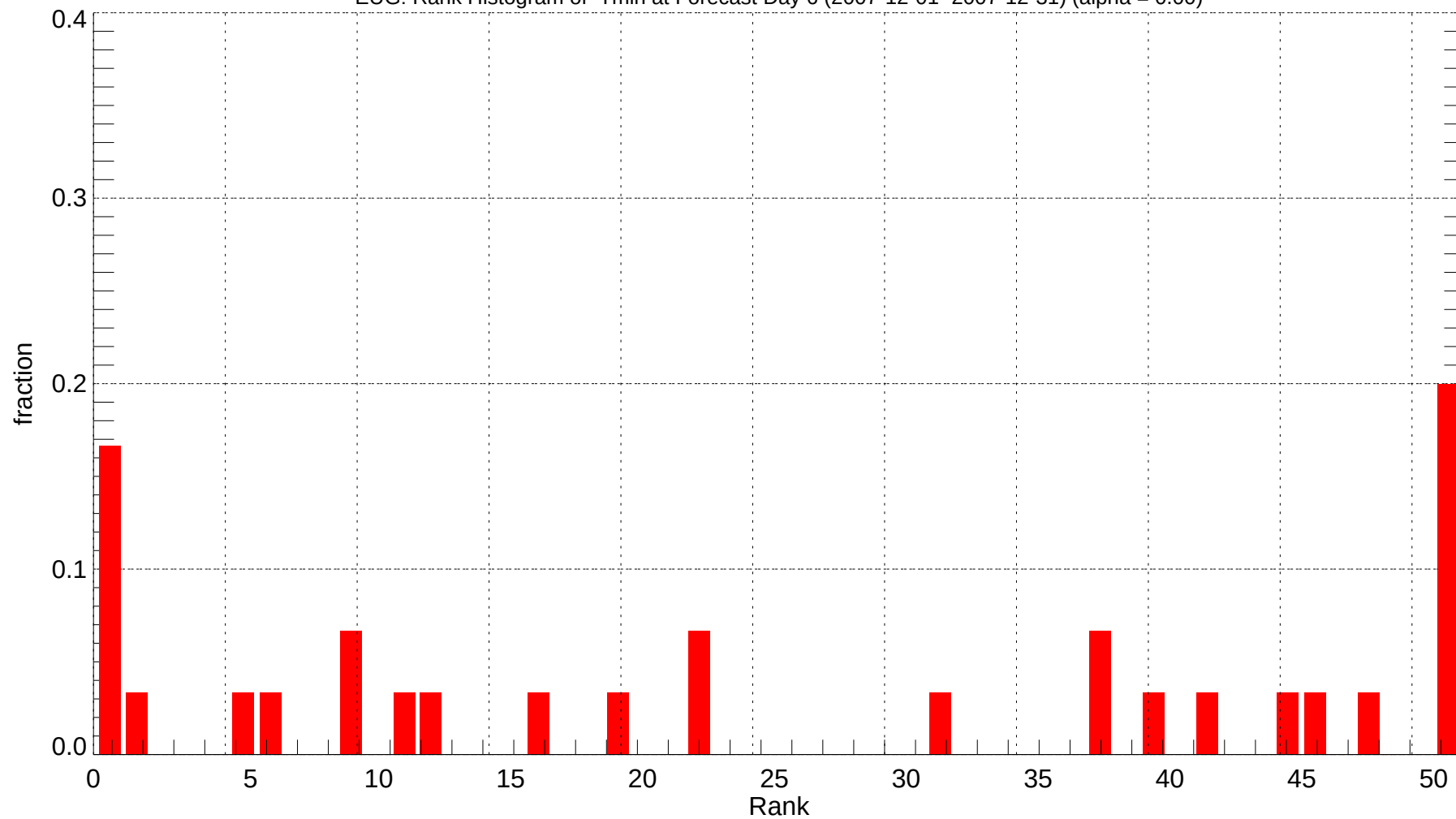
EUG: Rank Histogram of Tmin at Forecast Day 6 (2007-12-01~2007-12-31) (alpha = 0.00)
