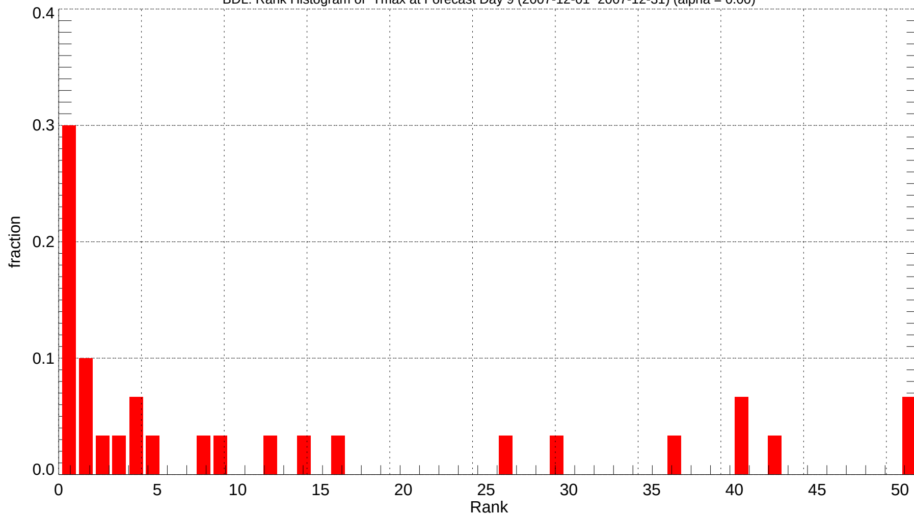
BDL: Rank Histogram of Tmax at Forecast Day 9 (2007-12-01~2007-12-31) (alpha = 0.00)
