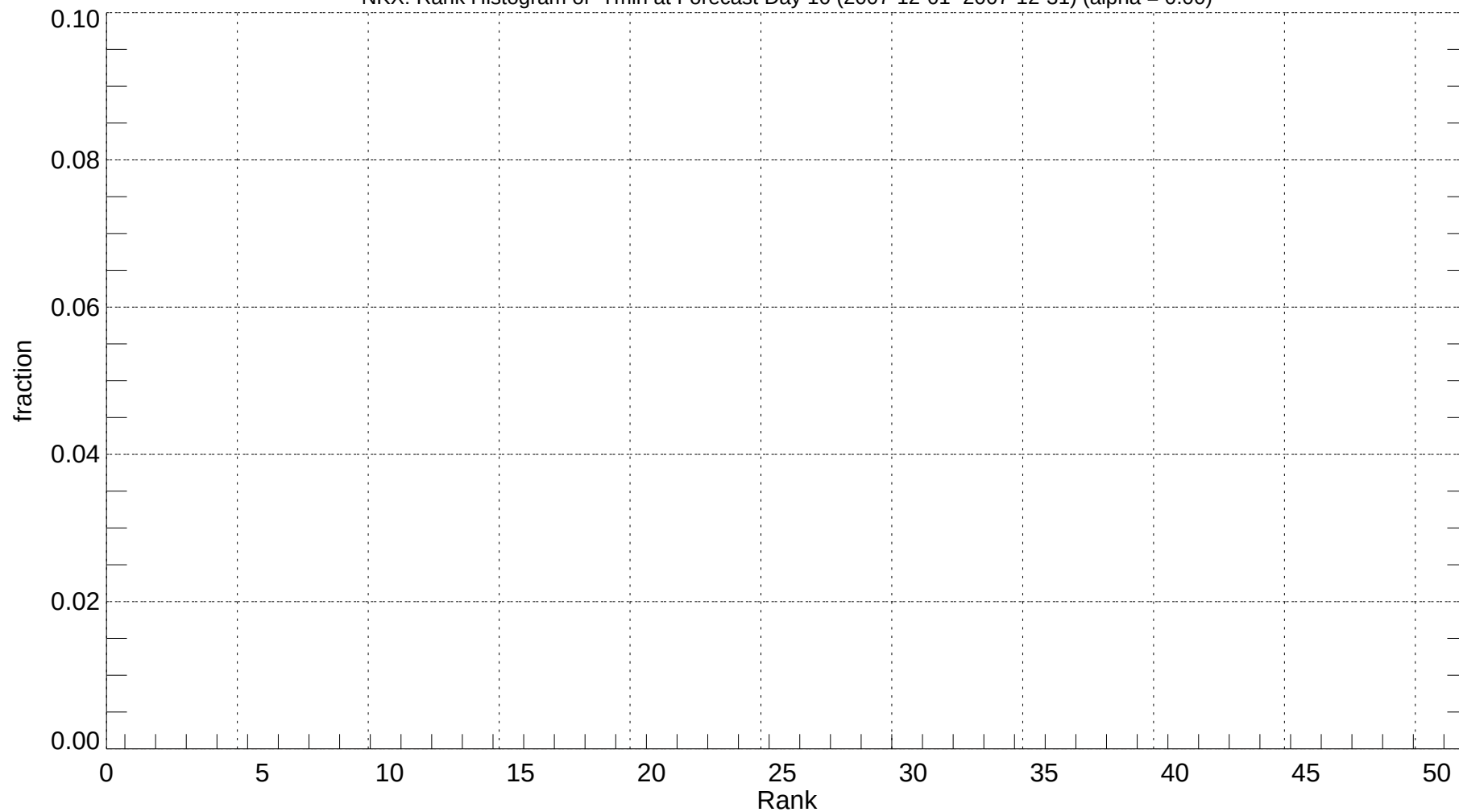
NKX: Rank Histogram of Tmin at Forecast Day 10 (2007-12-01~2007-12-31) (alpha = 0.00)
