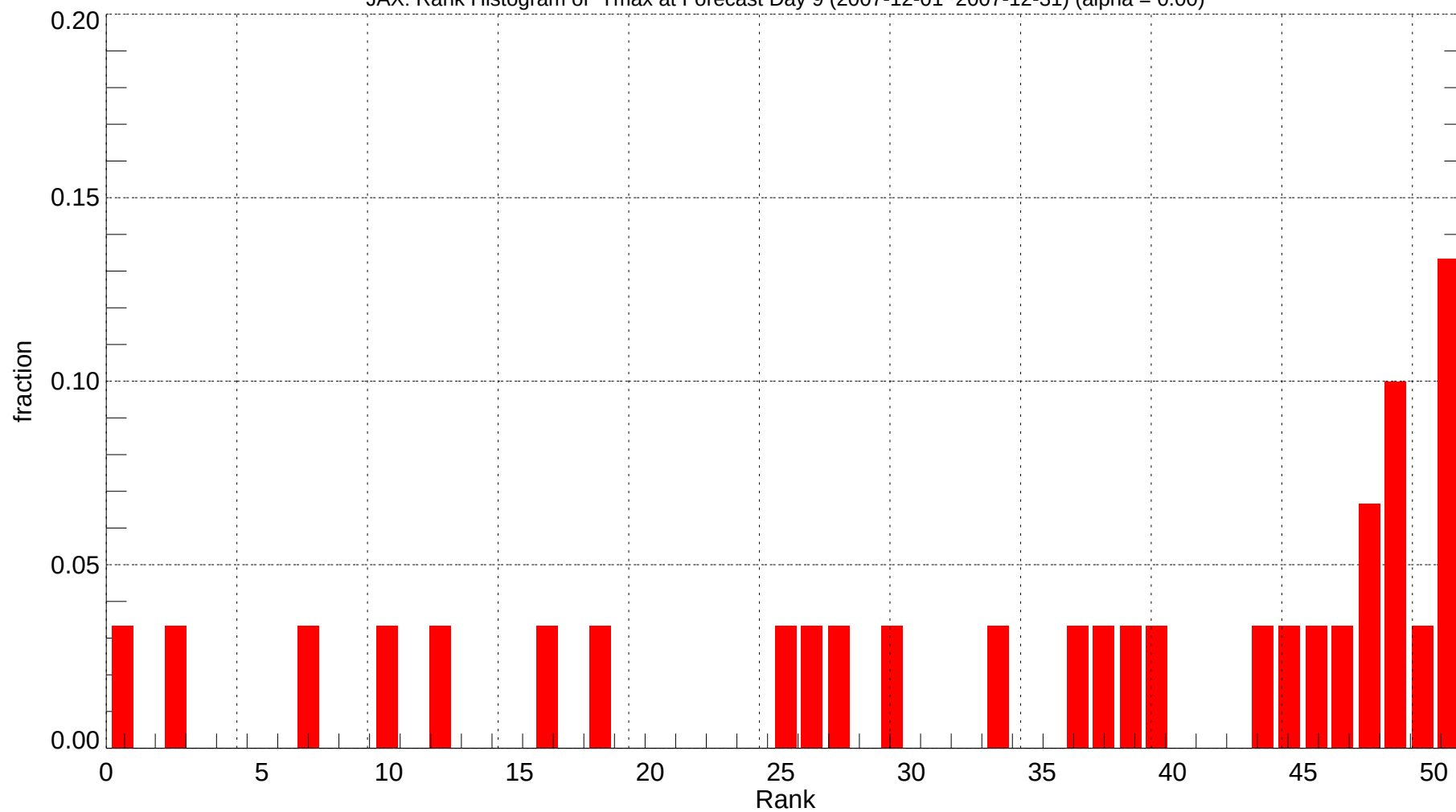
JAX: Rank Histogram of Tmax at Forecast Day 9 (2007-12-01~2007-12-31) (alpha = 0.00)
