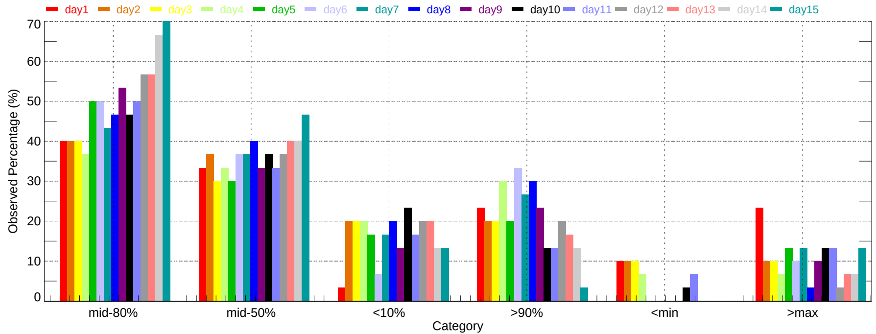
Observed Percentage of Ensembles - DFW: Min Temperature (2007-12-01~2007-12-31)
