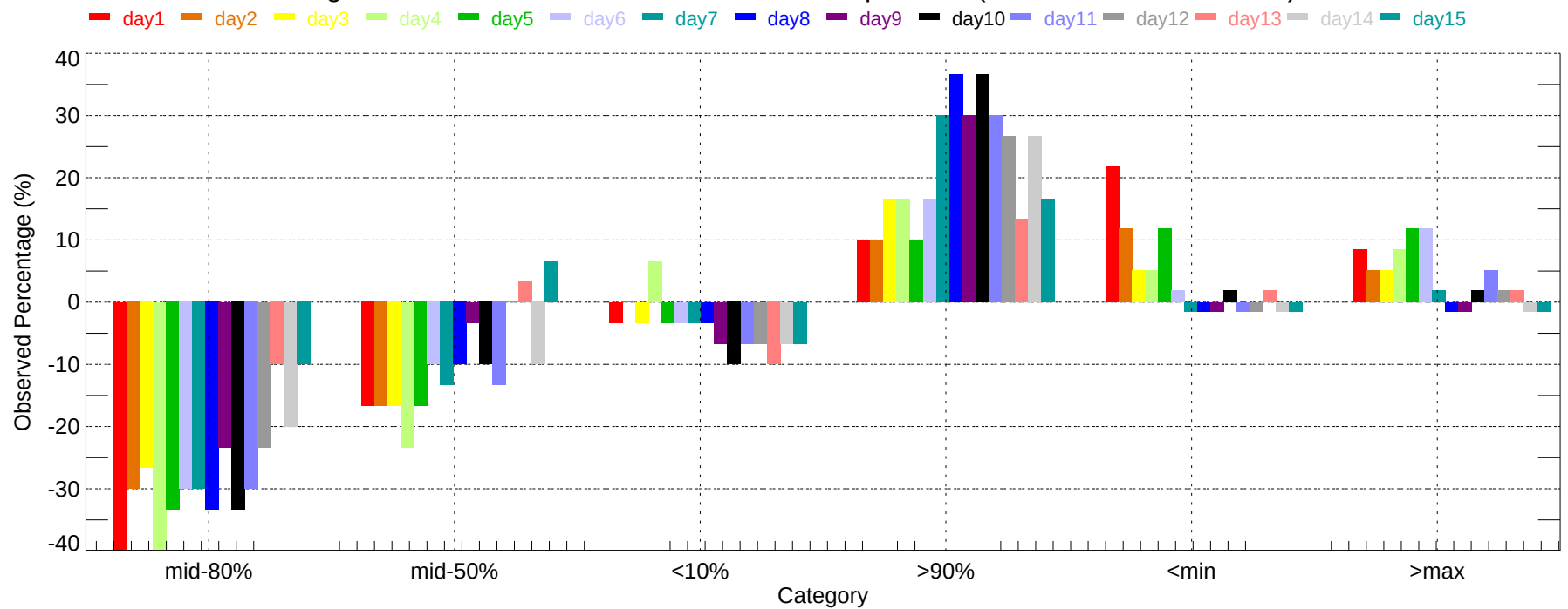
Observed Percentage Deviation of Ensembles - MIA: Max Temperature (2007-12-01~2007-12-31)
