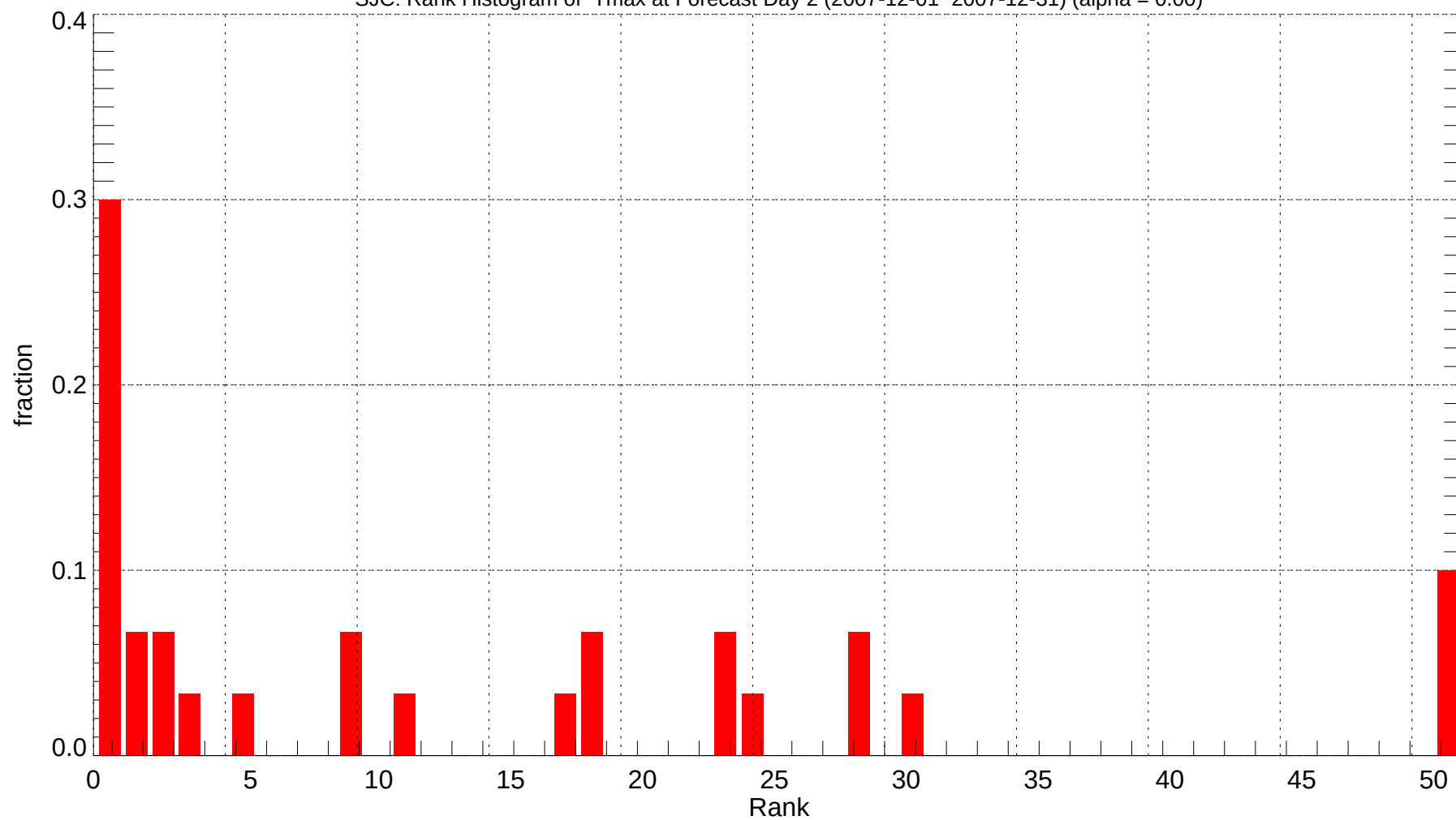
SJC: Rank Histogram of Tmax at Forecast Day 2 (2007-12-01~2007-12-31) (alpha = 0.00)
