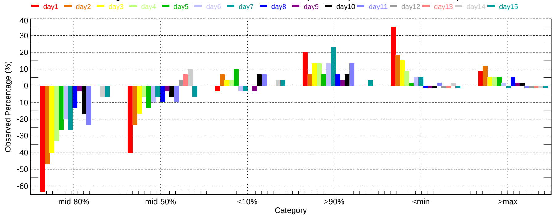
Observed Percentage Deviation of Ensembles - PHL: Max Temperature (2007-12-01~2007-12-31)
