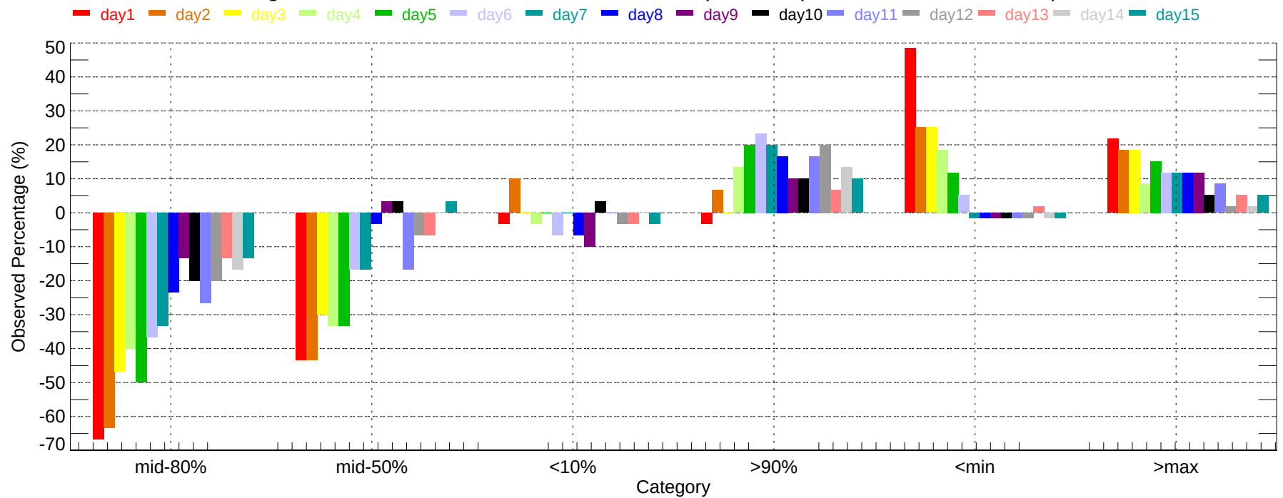
Observed Percentage Deviation of Ensembles - TYS: Min Temperature (2007-12-01~2007-12-31)
