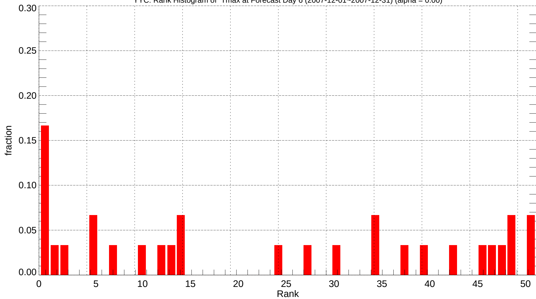
YYC: Rank Histogram of Tmax at Forecast Day 6 (2007-12-01~2007-12-31) (alpha = 0.00)
