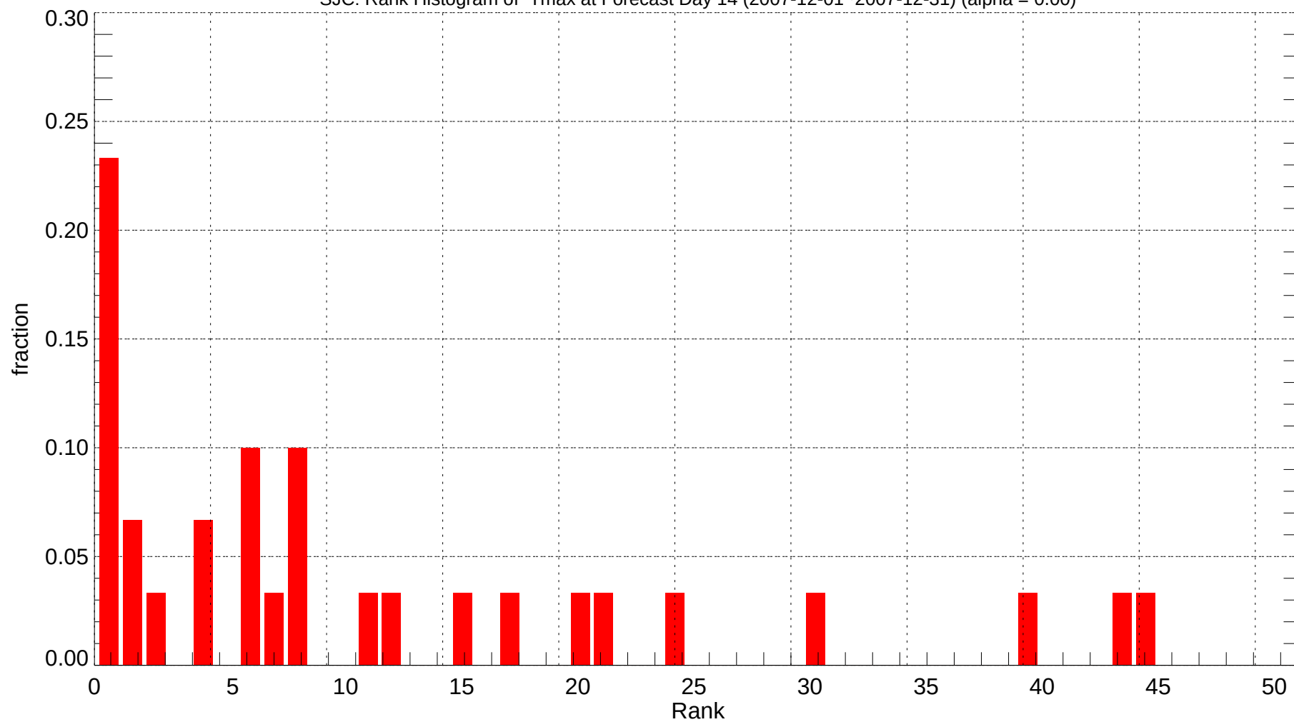
SJC: Rank Histogram of Tmax at Forecast Day 14 (2007-12-01~2007-12-31) (alpha = 0.00)
