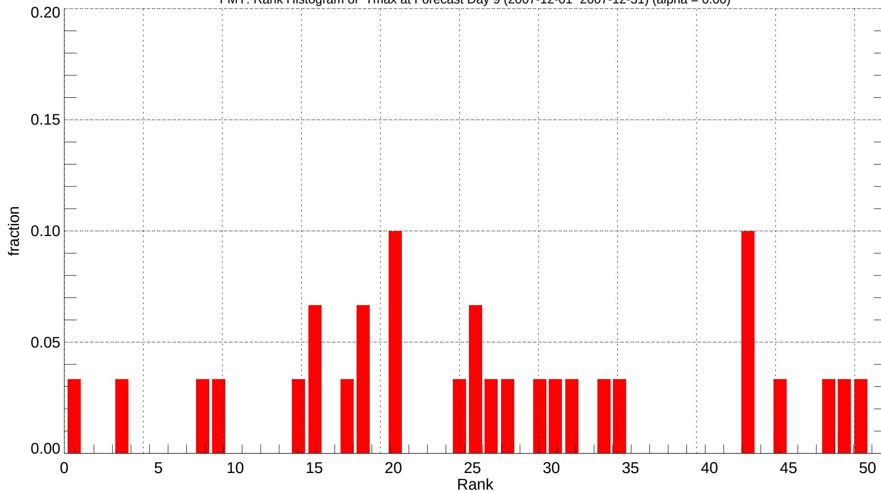
FMY: Rank Histogram of Tmax at Forecast Day 9 (2007-12-01~2007-12-31) (alpha = 0.00)
