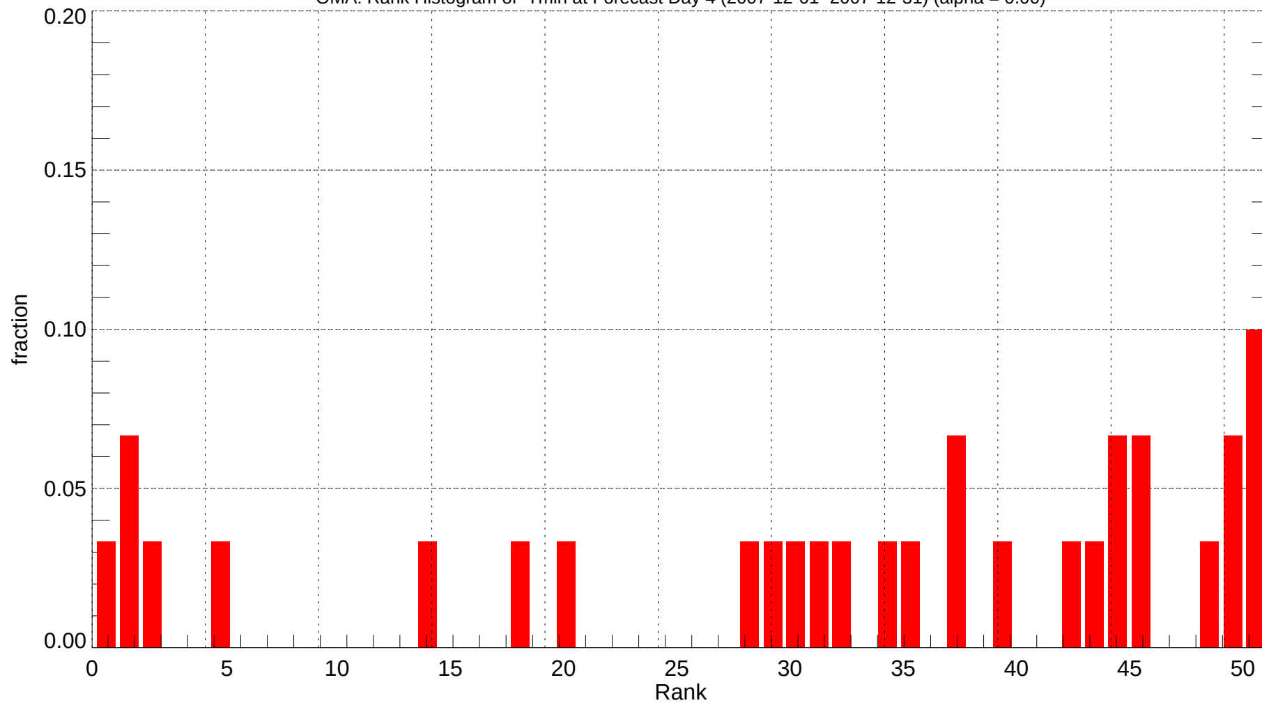
OMA: Rank Histogram of Tmin at Forecast Day 4 (2007-12-01~2007-12-31) (alpha = 0.00)
