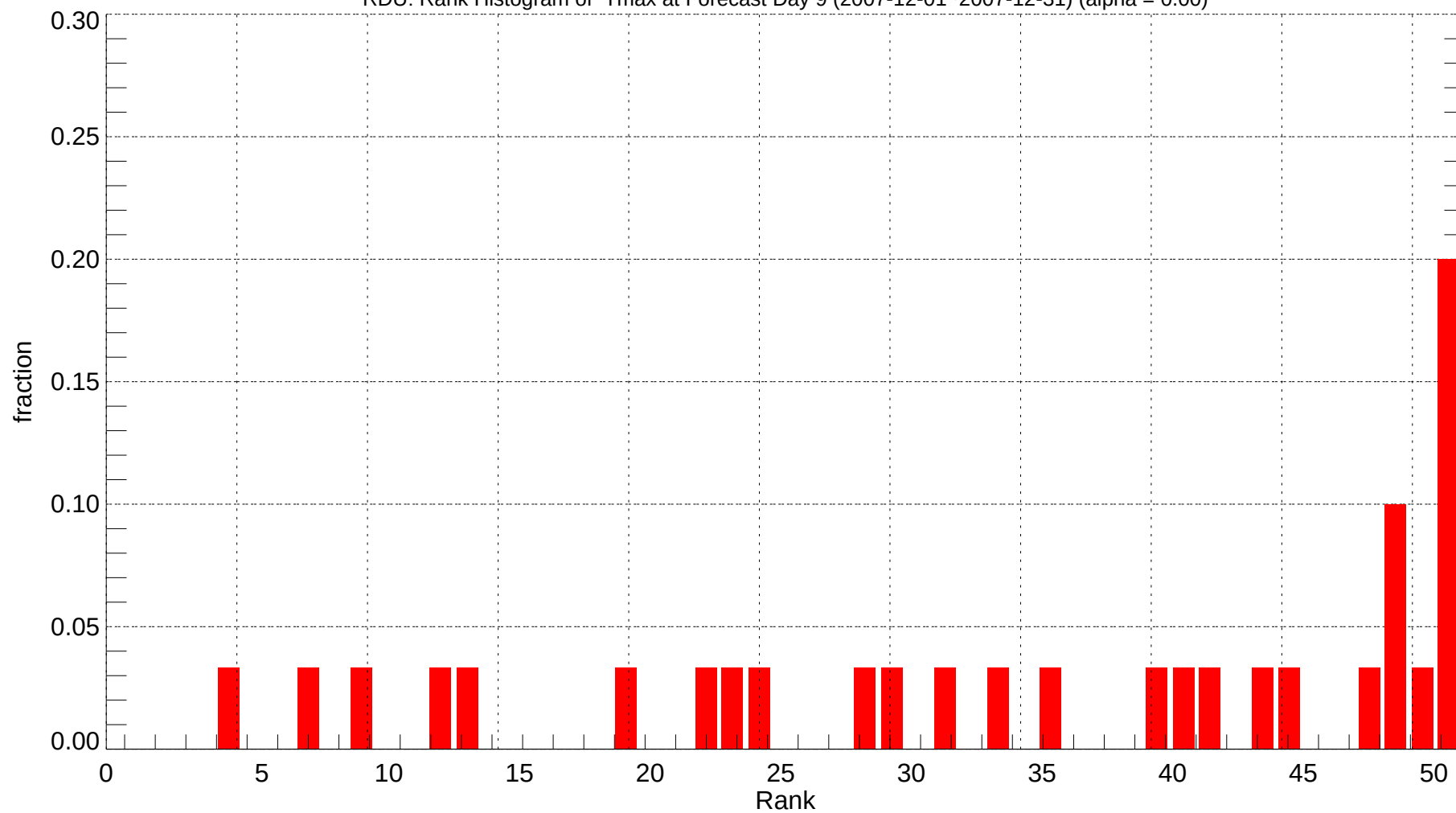
RDU: Rank Histogram of Tmax at Forecast Day 9 (2007-12-01~2007-12-31) (alpha = 0.00)
