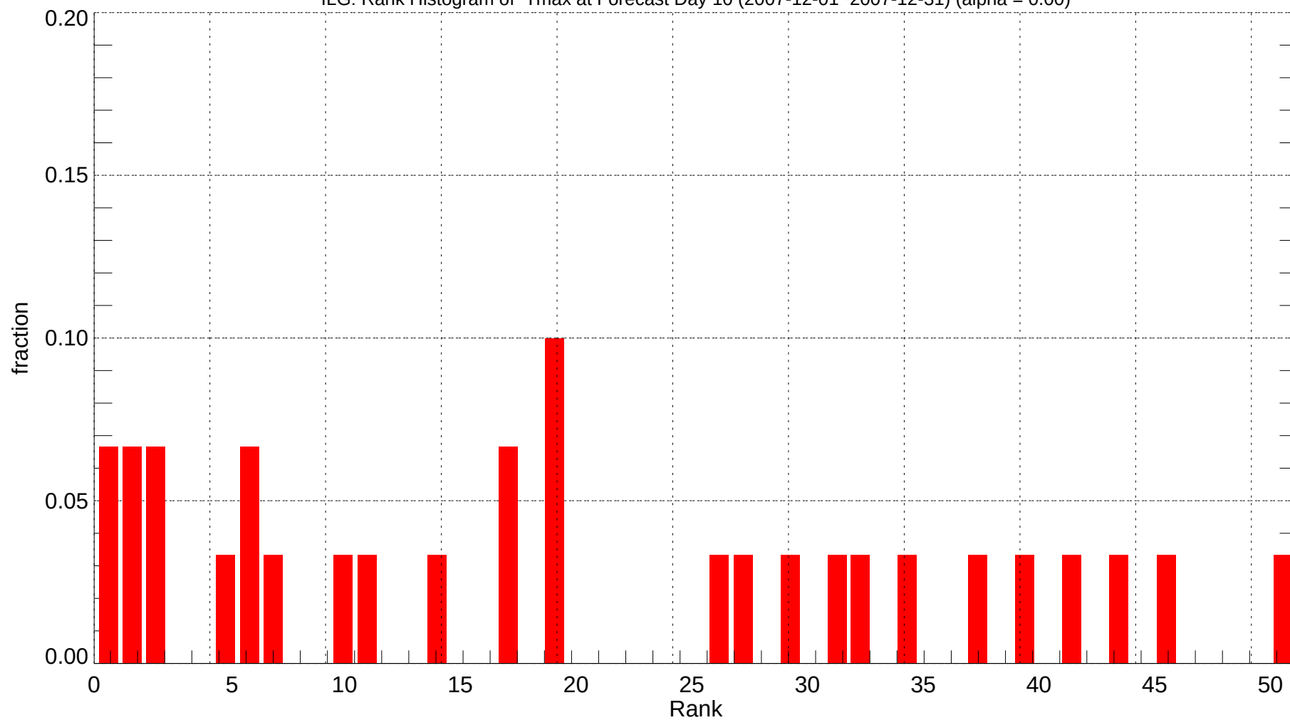
ILG: Rank Histogram of Tmax at Forecast Day 10 (2007-12-01~2007-12-31) (alpha = 0.00)
