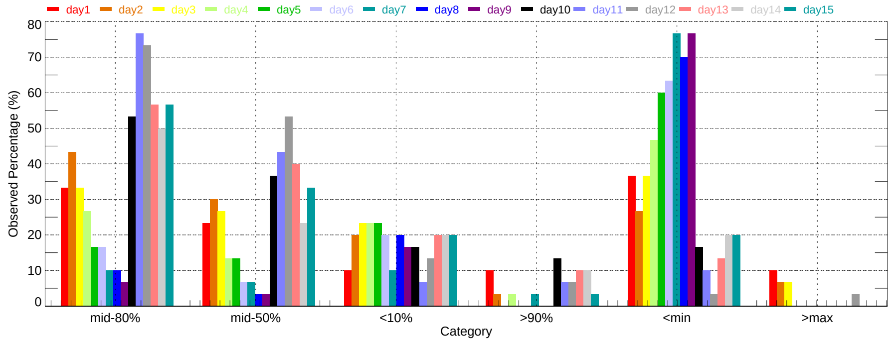
Observed Percentage of Ensembles - SJC: Min Temperature (2007-12-01~2007-12-31)
