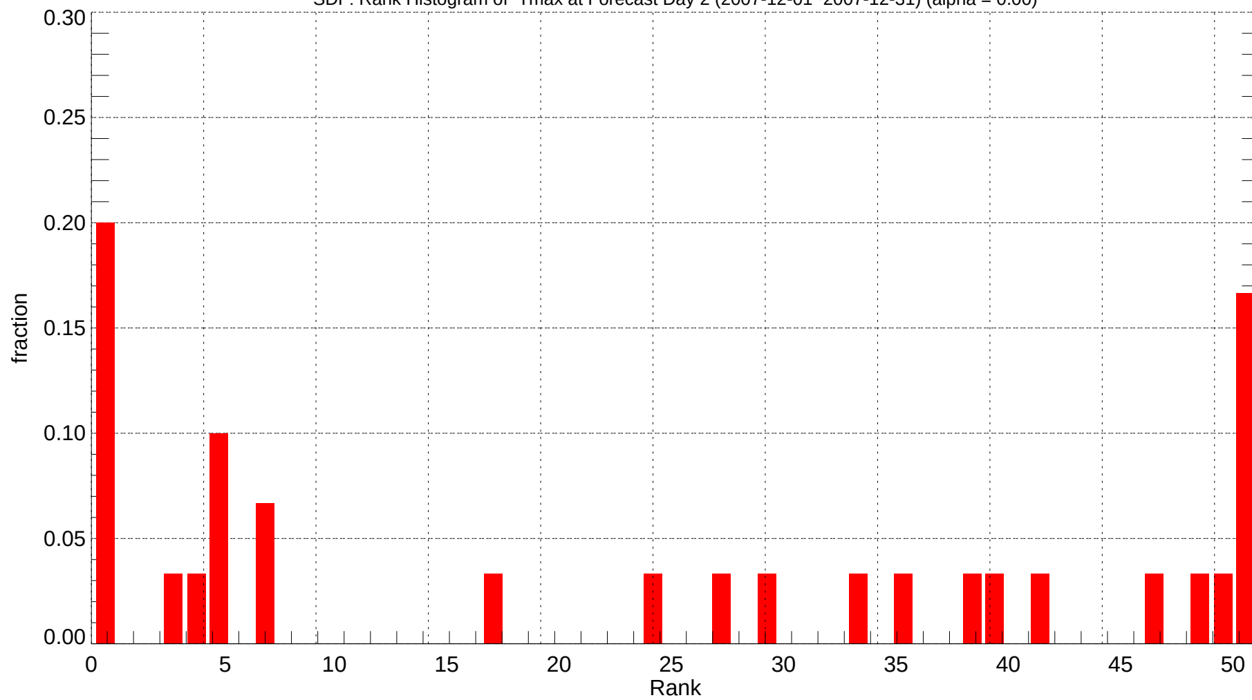
SDF: Rank Histogram of Tmax at Forecast Day 2 (2007-12-01~2007-12-31) (alpha = 0.00)
