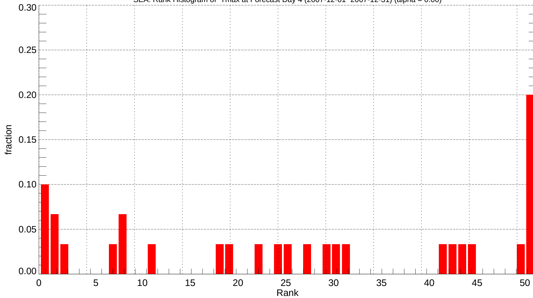
SEA: Rank Histogram of Tmax at Forecast Day 4 (2007-12-01~2007-12-31) (alpha = 0.00)
