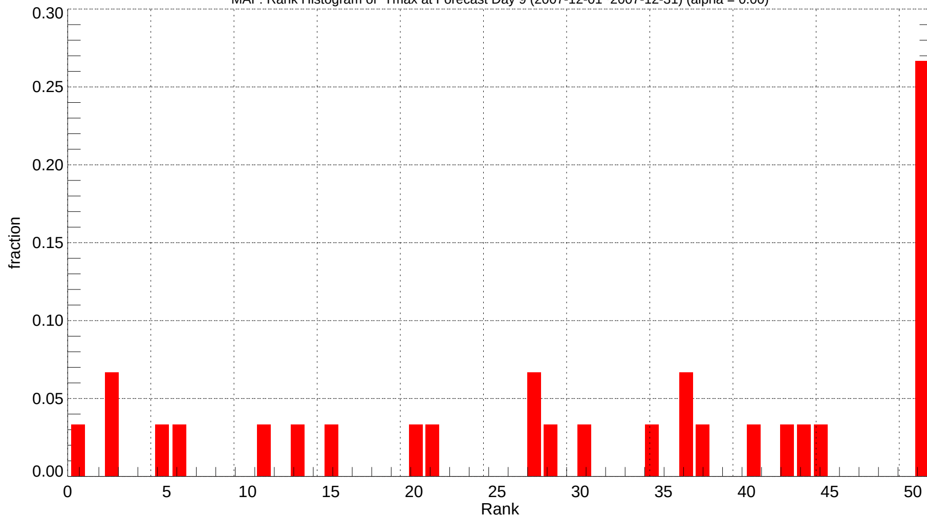
MAF: Rank Histogram of Tmax at Forecast Day 9 (2007-12-01~2007-12-31) (alpha = 0.00)
