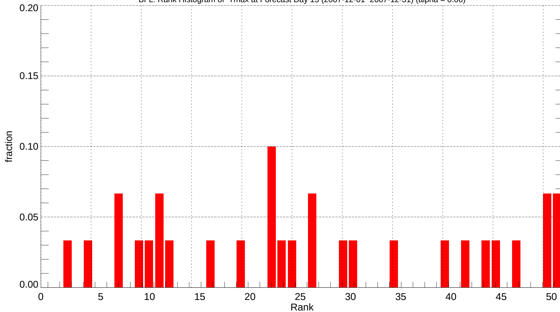
BFL: Rank Histogram of Tmax at Forecast Day 13 (2007-12-01~2007-12-31) (alpha = 0.00)
