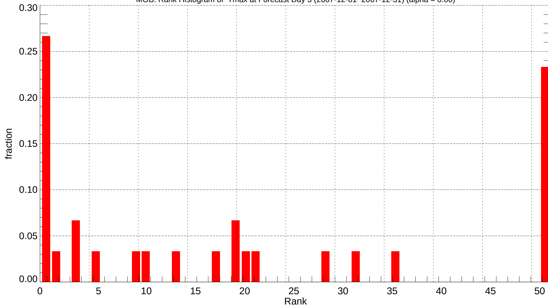
MOB: Rank Histogram of Tmax at Forecast Day 3 (2007-12-01~2007-12-31) (alpha = 0.00)
