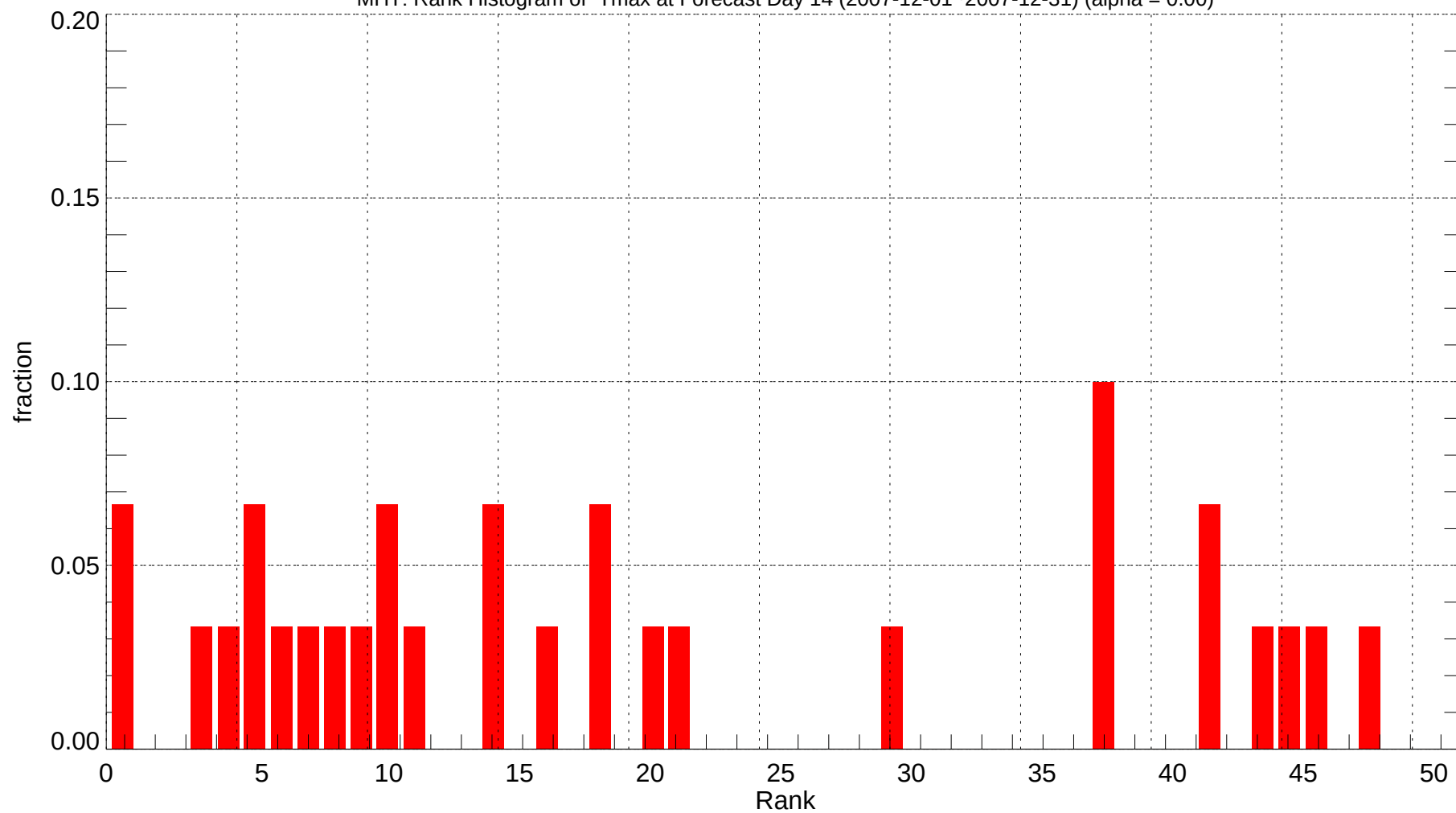
MHT: Rank Histogram of Tmax at Forecast Day 14 (2007-12-01~2007-12-31) (alpha = 0.00)
