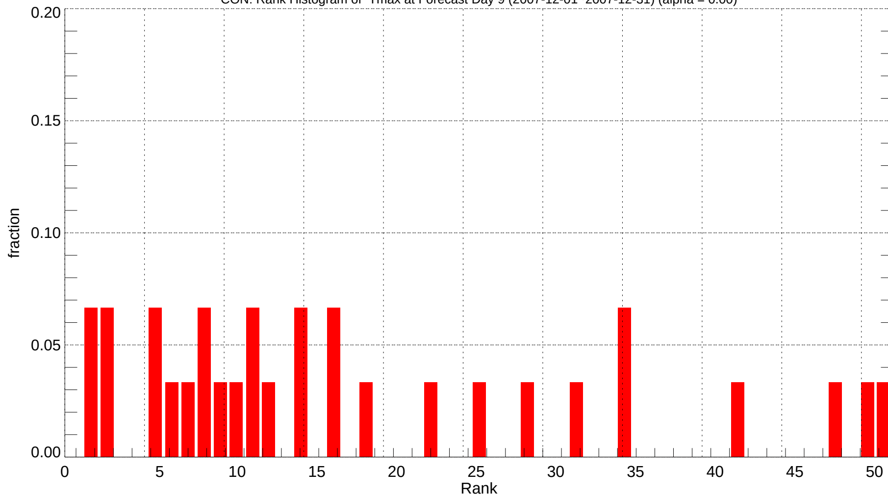
CON: Rank Histogram of Tmax at Forecast Day 9 (2007-12-01~2007-12-31) (alpha = 0.00)
