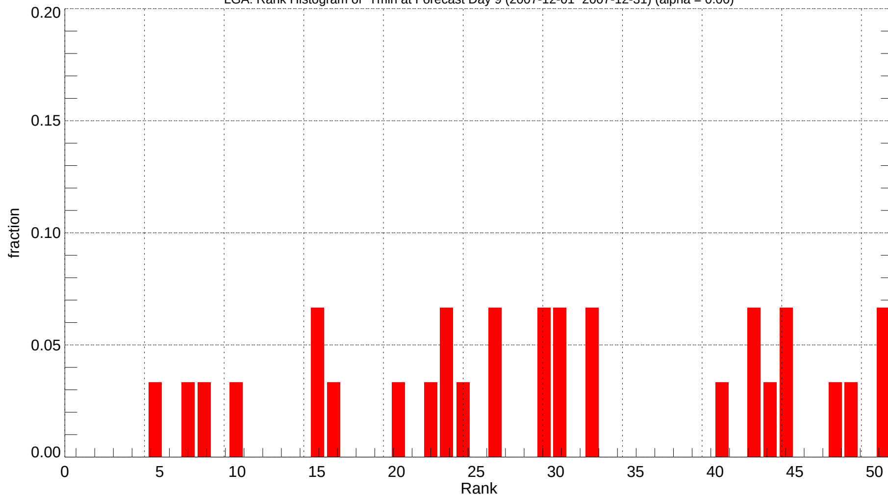
LGA: Rank Histogram of Tmin at Forecast Day 9 (2007-12-01~2007-12-31) (alpha = 0.00)
