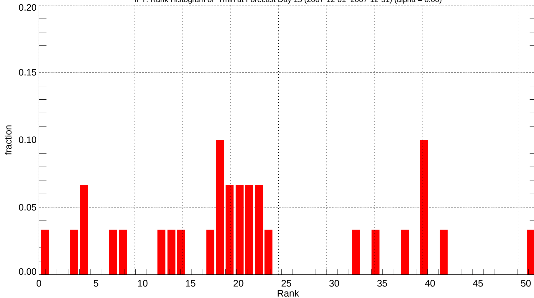
IPT: Rank Histogram of Tmin at Forecast Day 15 (2007-12-01~2007-12-31) (alpha = 0.00)
