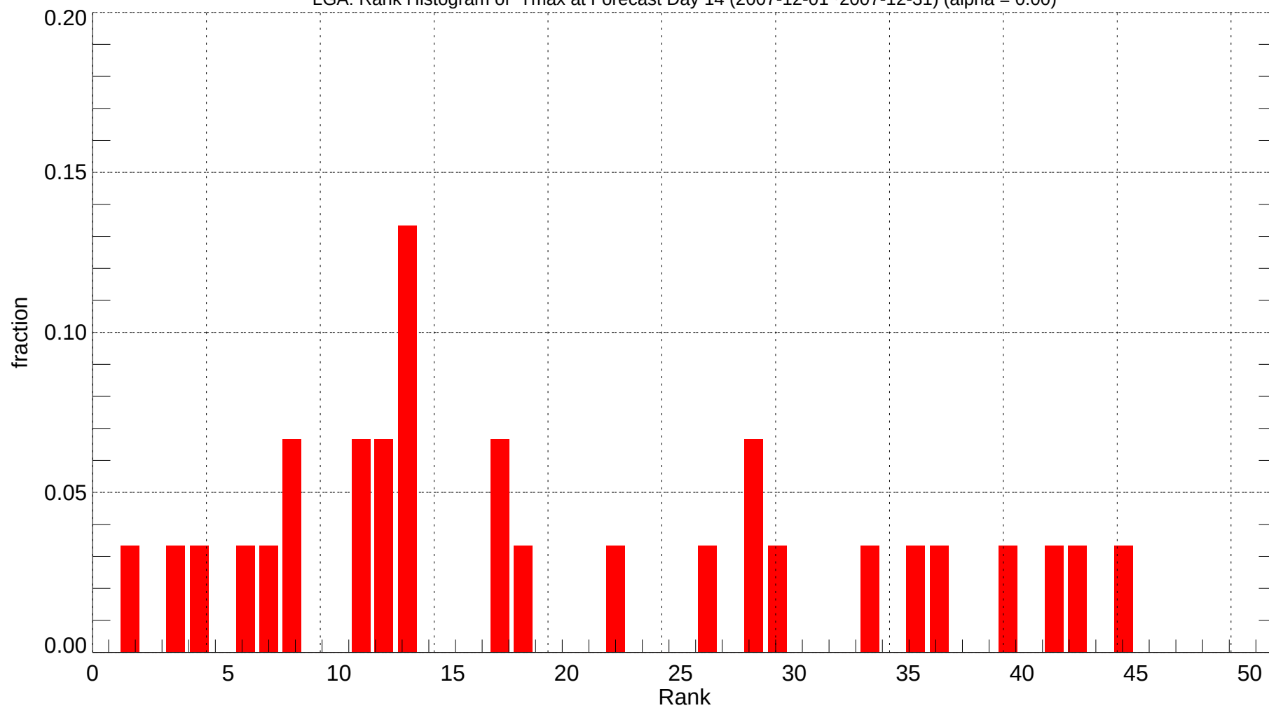
LGA: Rank Histogram of Tmax at Forecast Day 14 (2007-12-01~2007-12-31) (alpha = 0.00)
