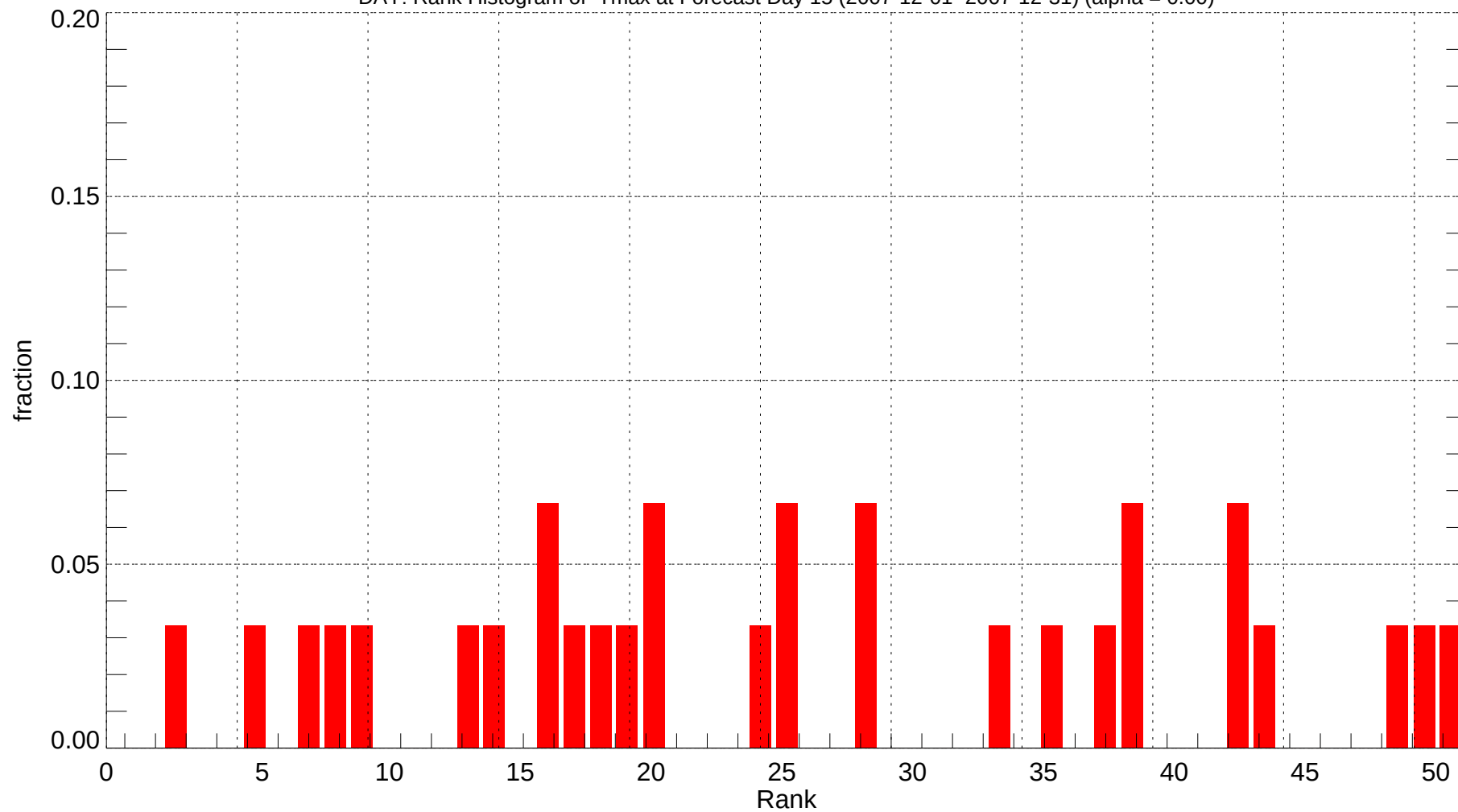
DAY: Rank Histogram of Tmax at Forecast Day 15 (2007-12-01~2007-12-31) (alpha = 0.00)
