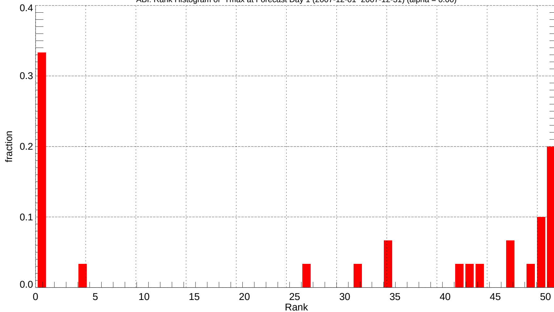
ABI: Rank Histogram of Tmax at Forecast Day 1 (2007-12-01~2007-12-31) (alpha = 0.00)
