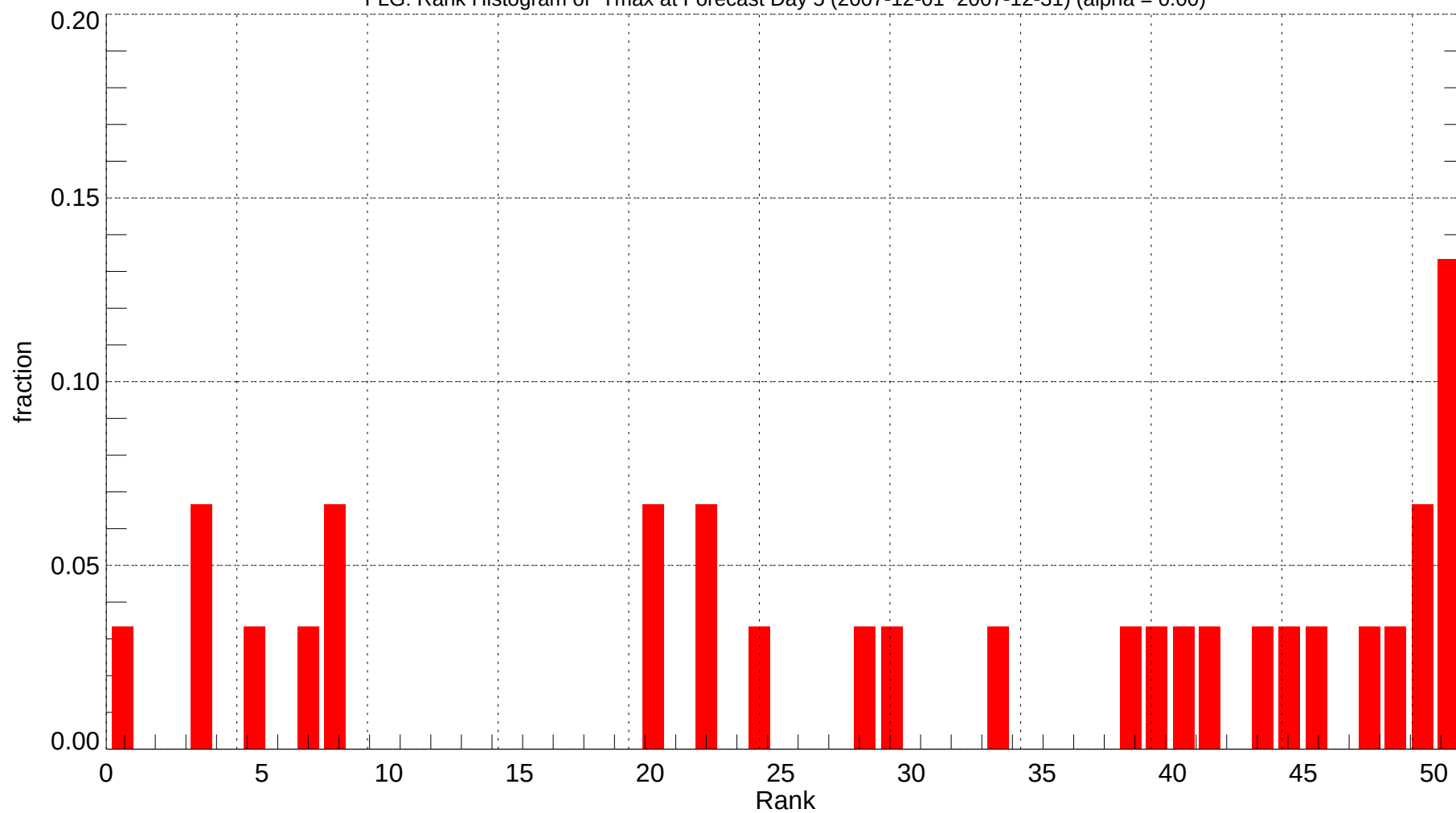
FLG: Rank Histogram of Tmax at Forecast Day 5 (2007-12-01~2007-12-31) (alpha = 0.00)
