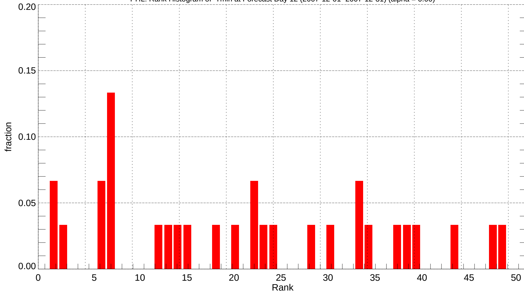
PHL: Rank Histogram of Tmin at Forecast Day 12 (2007-12-01~2007-12-31) (alpha = 0.00)
