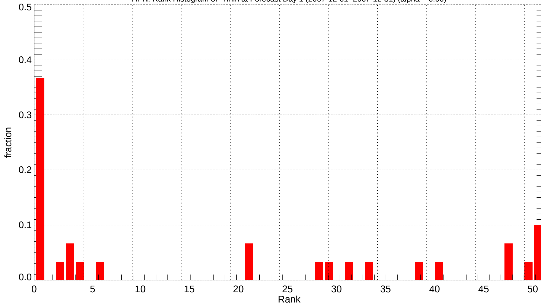
APN: Rank Histogram of Tmin at Forecast Day 1 (2007-12-01~2007-12-31) (alpha = 0.00)
