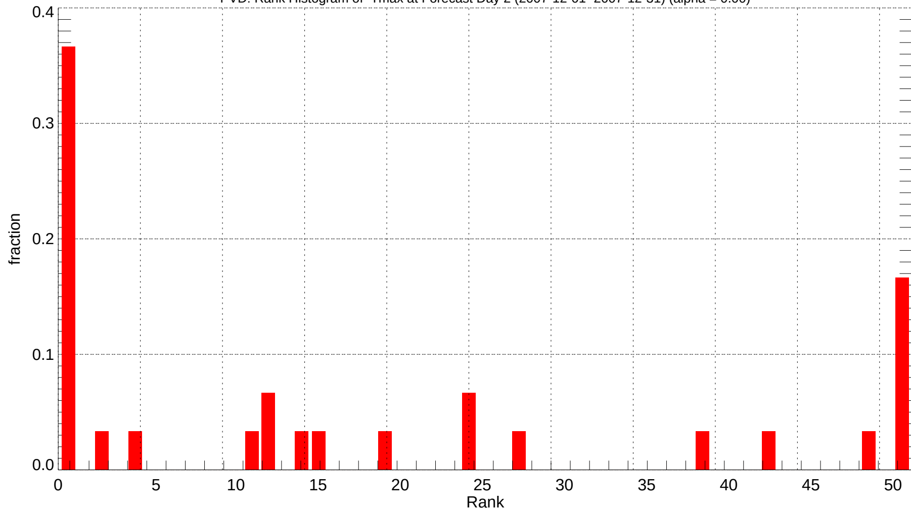
PVD: Rank Histogram of Tmax at Forecast Day 2 (2007-12-01~2007-12-31) (alpha = 0.00)
