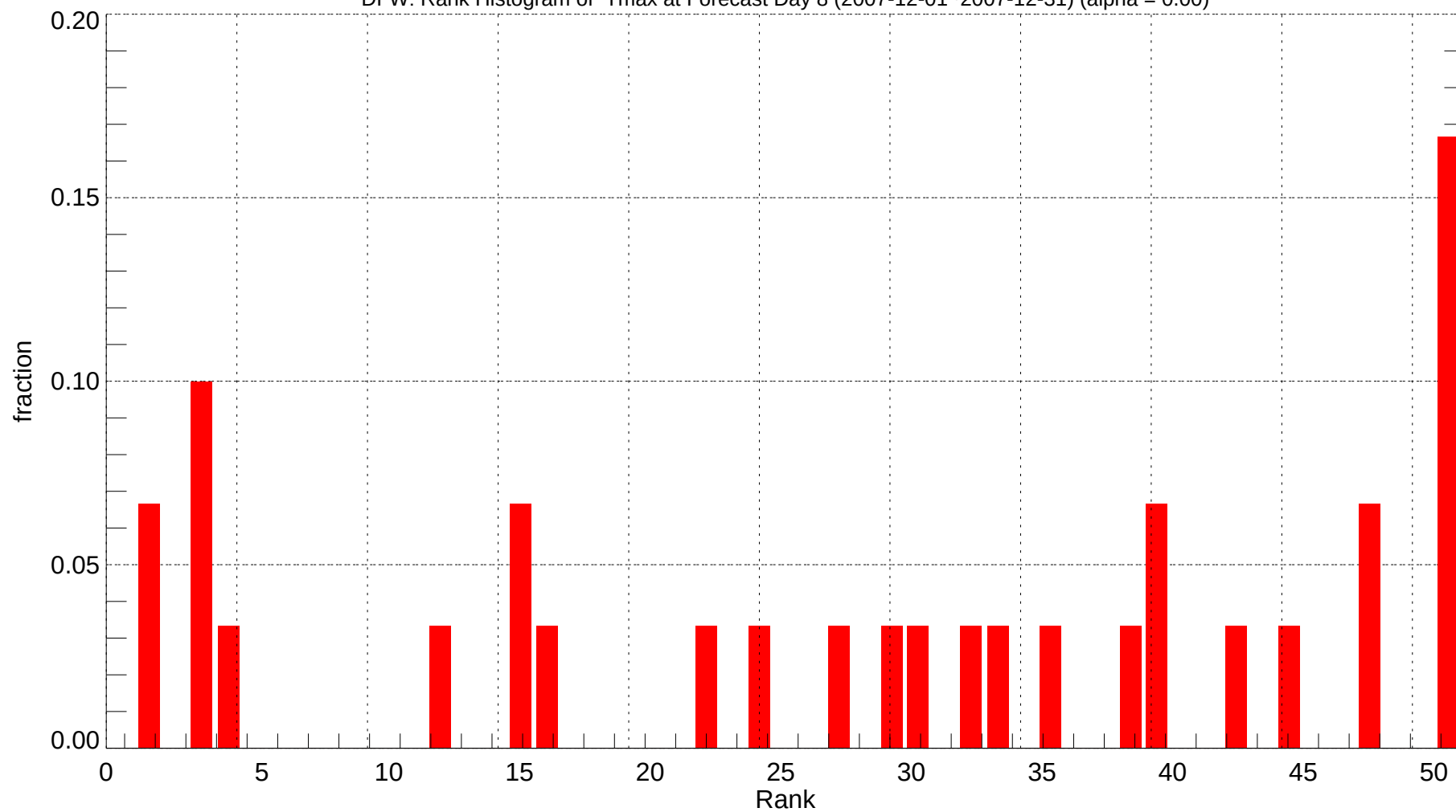
DFW: Rank Histogram of Tmax at Forecast Day 8 (2007-12-01~2007-12-31) (alpha = 0.00)
