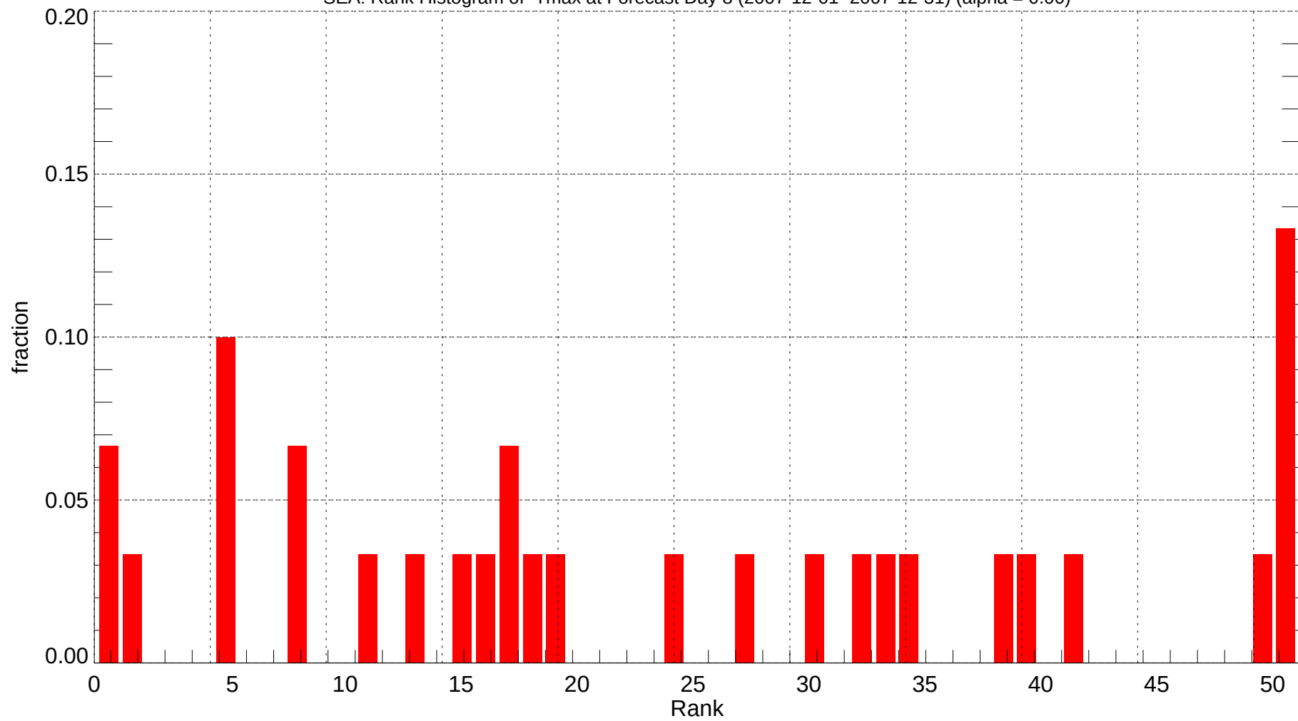
SEA: Rank Histogram of Tmax at Forecast Day 8 (2007-12-01~2007-12-31) (alpha = 0.00)
