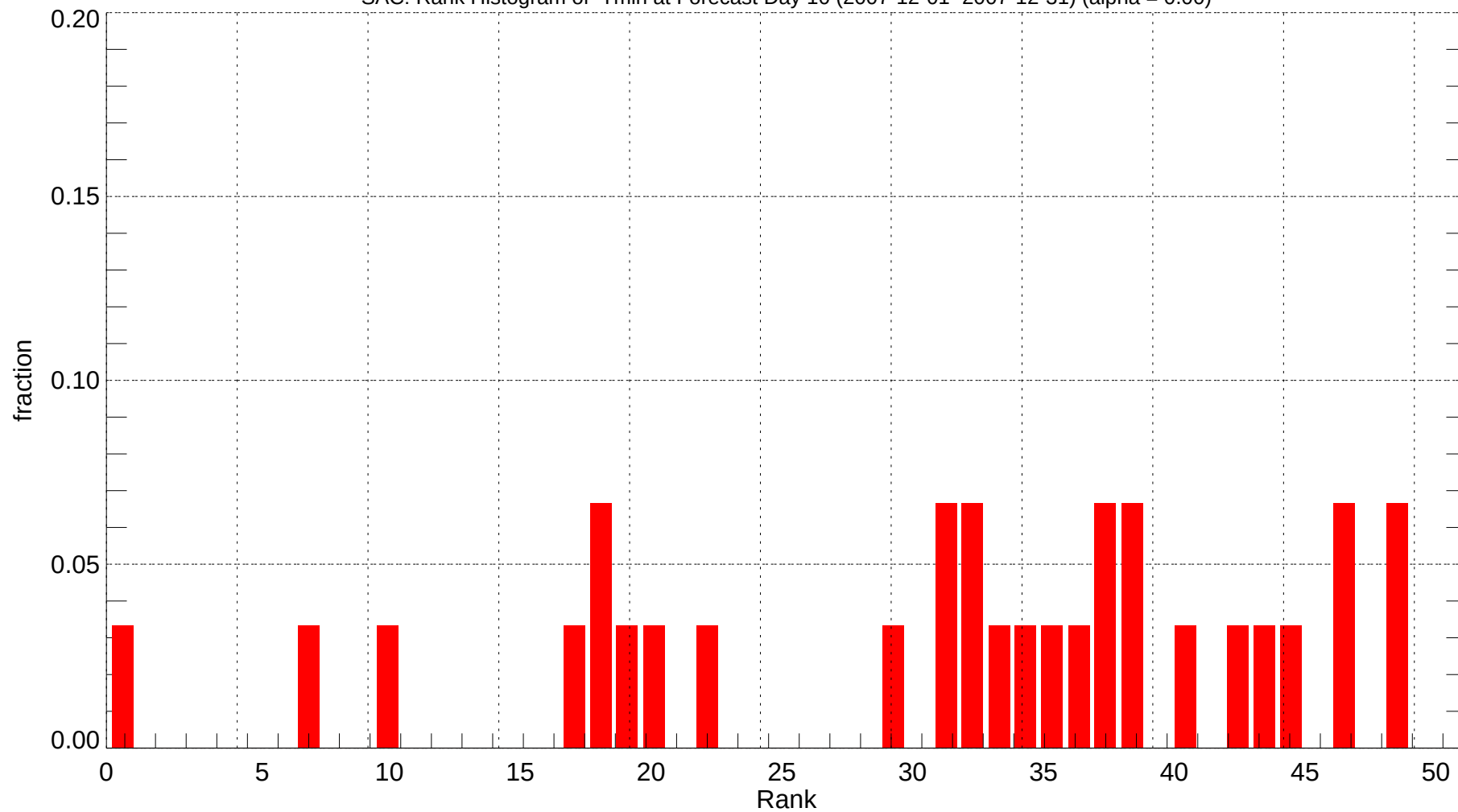
SAC: Rank Histogram of Tmin at Forecast Day 10 (2007-12-01~2007-12-31) (alpha = 0.00)
