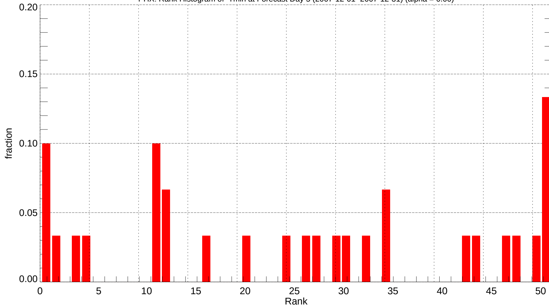
PHX: Rank Histogram of Tmin at Forecast Day 5 (2007-12-01~2007-12-31) (alpha = 0.00)
