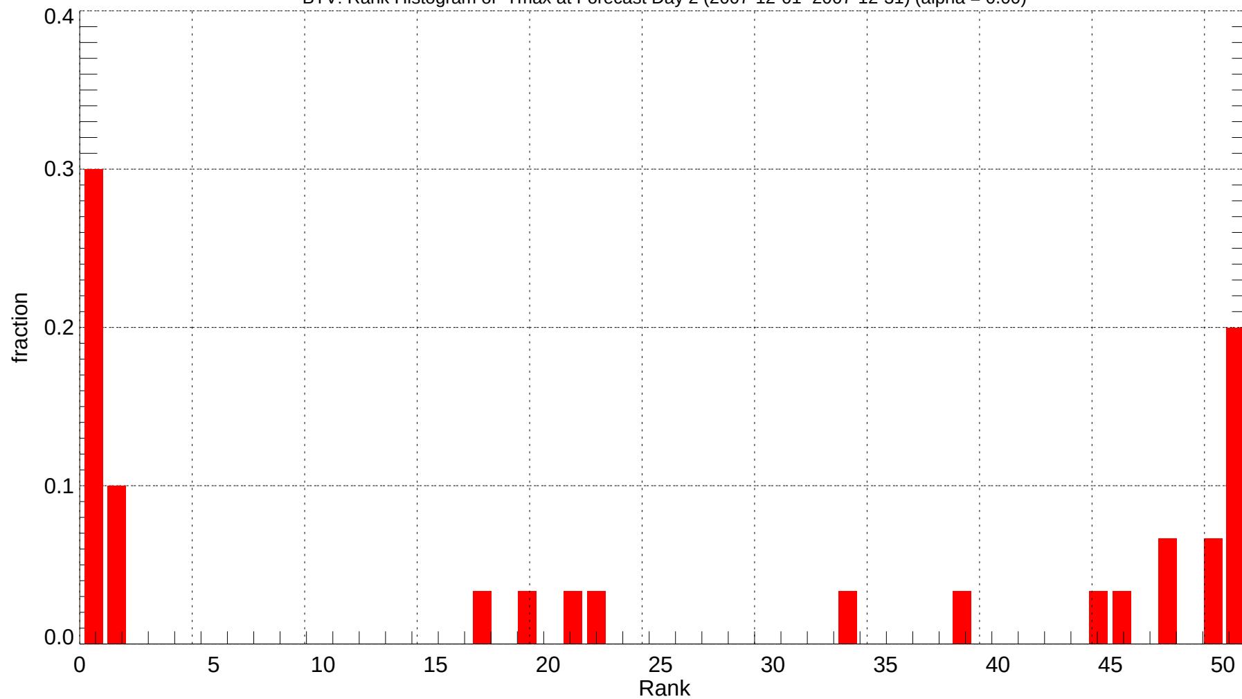
BTV: Rank Histogram of Tmax at Forecast Day 2 (2007-12-01~2007-12-31) (alpha = 0.00)
