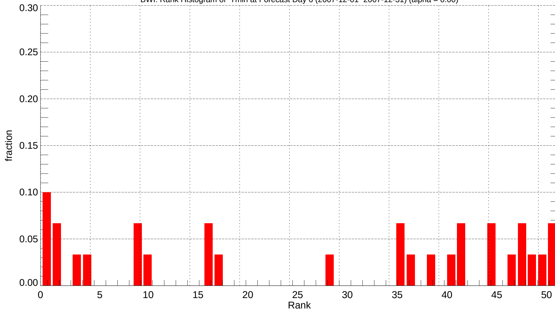
BWI: Rank Histogram of Tmin at Forecast Day 6 (2007-12-01~2007-12-31) (alpha = 0.00)
