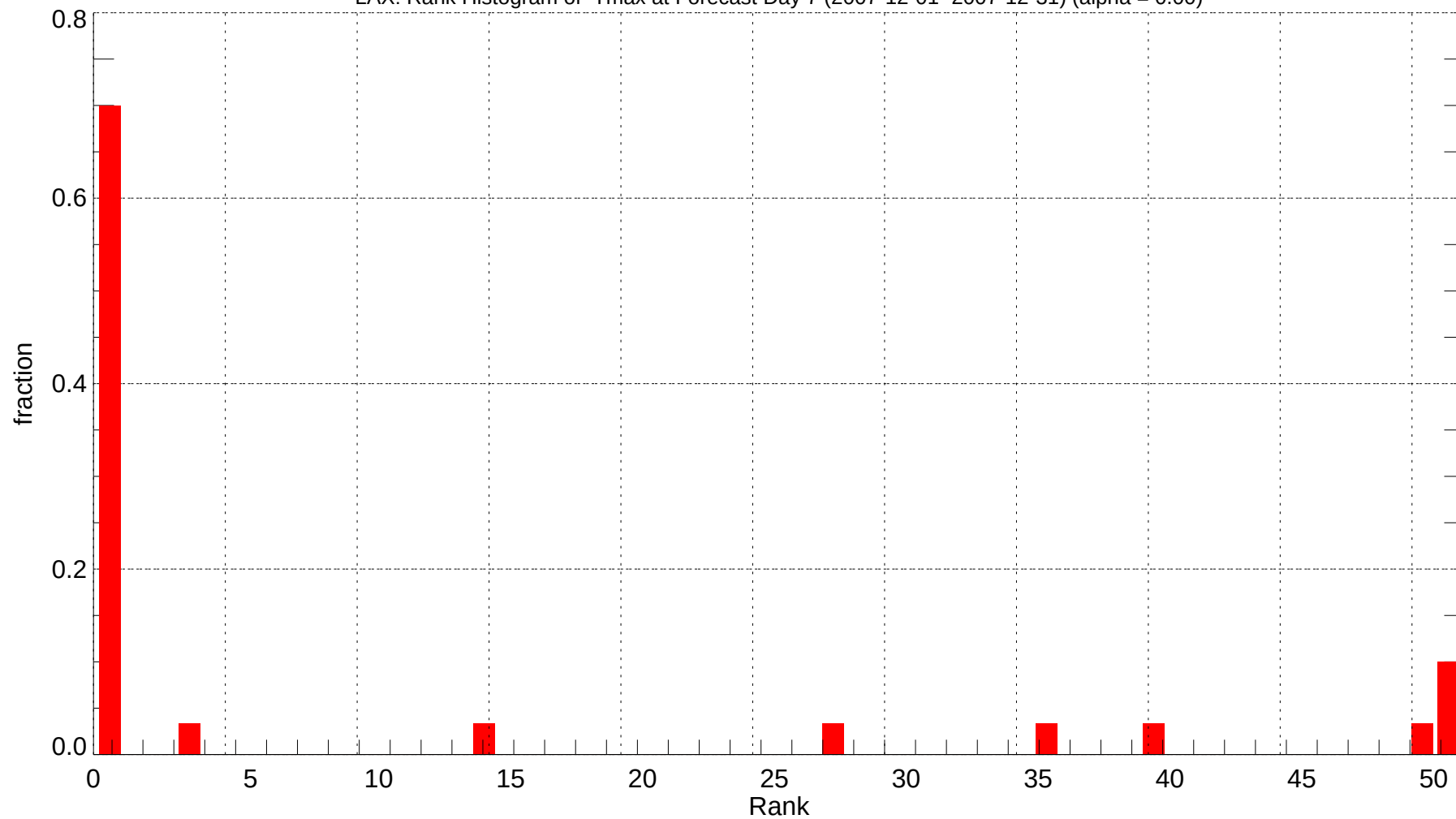
LAX: Rank Histogram of Tmax at Forecast Day 7 (2007-12-01~2007-12-31) (alpha = 0.00)
