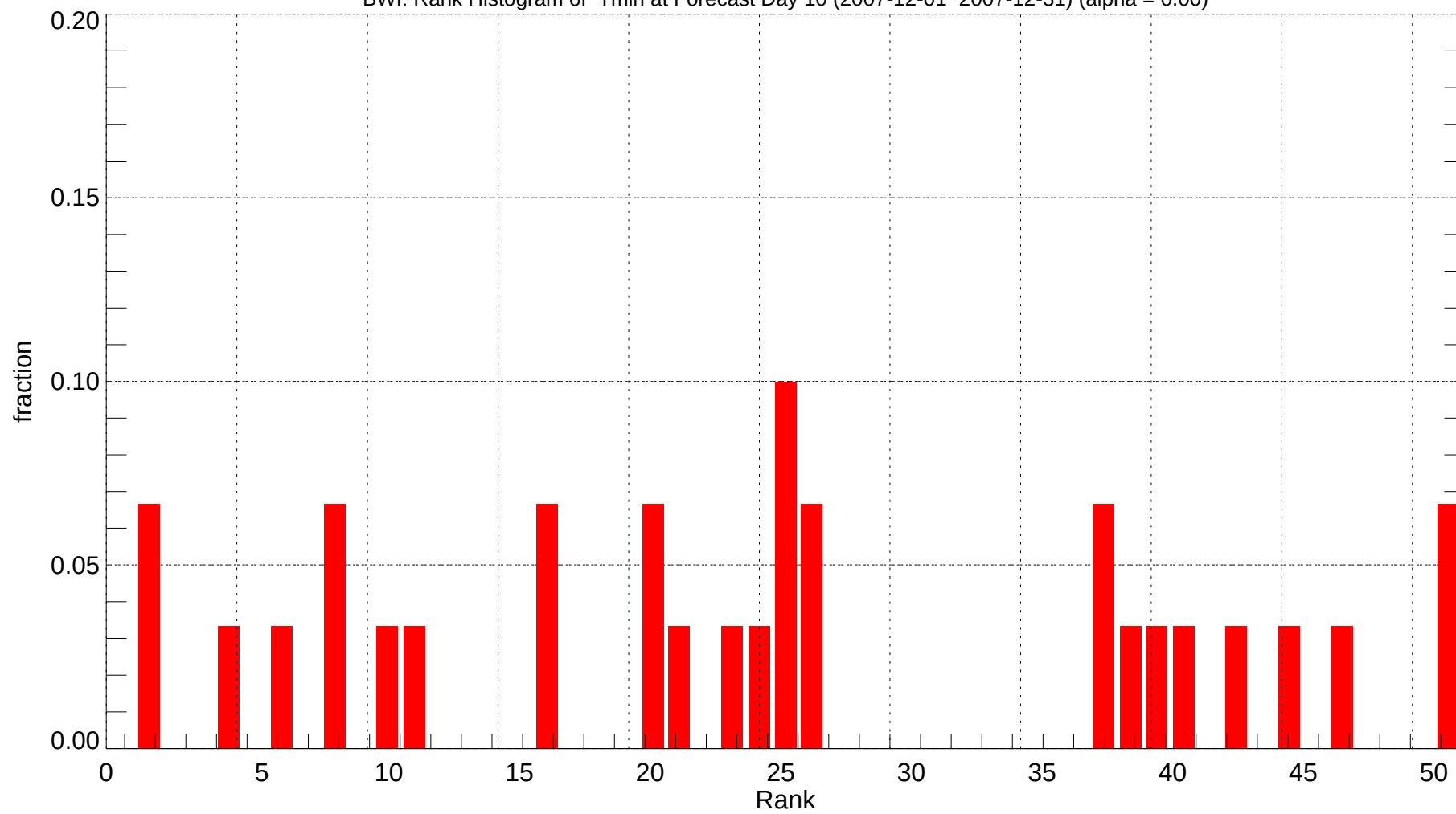
BWl: Rank Histogram of Tmin at Forecast Day 10 (2007-12-01~2007-12-31) (alpha = 0.00)
