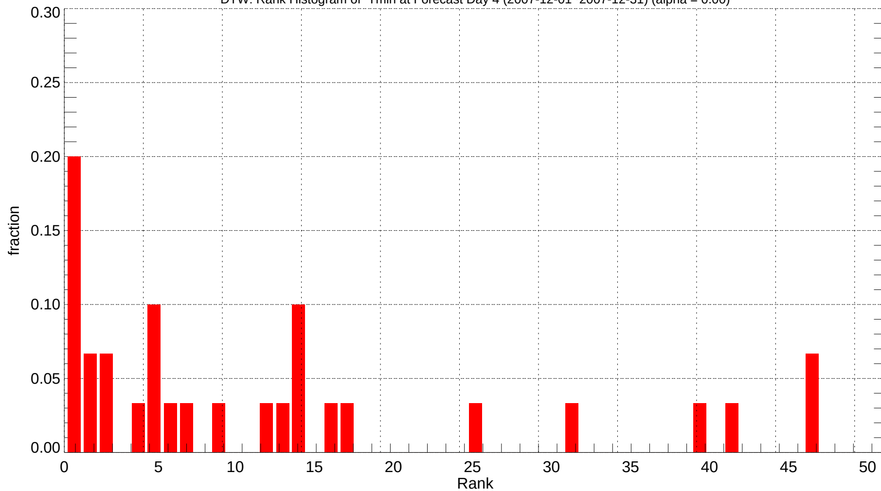
DTW: Rank Histogram of Tmin at Forecast Day 4 (2007-12-01~2007-12-31) (alpha = 0.00)
