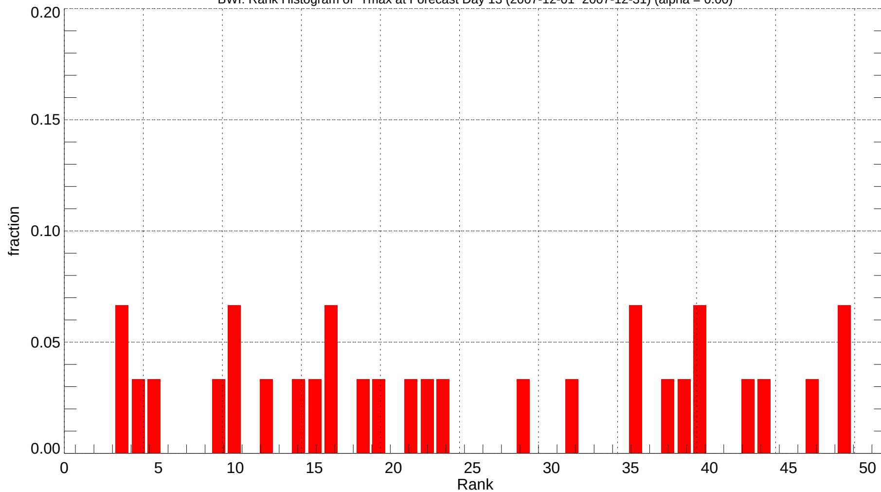
BWI: Rank Histogram of Tmax at Forecast Day 13 (2007-12-01~2007-12-31) (alpha = 0.00)
