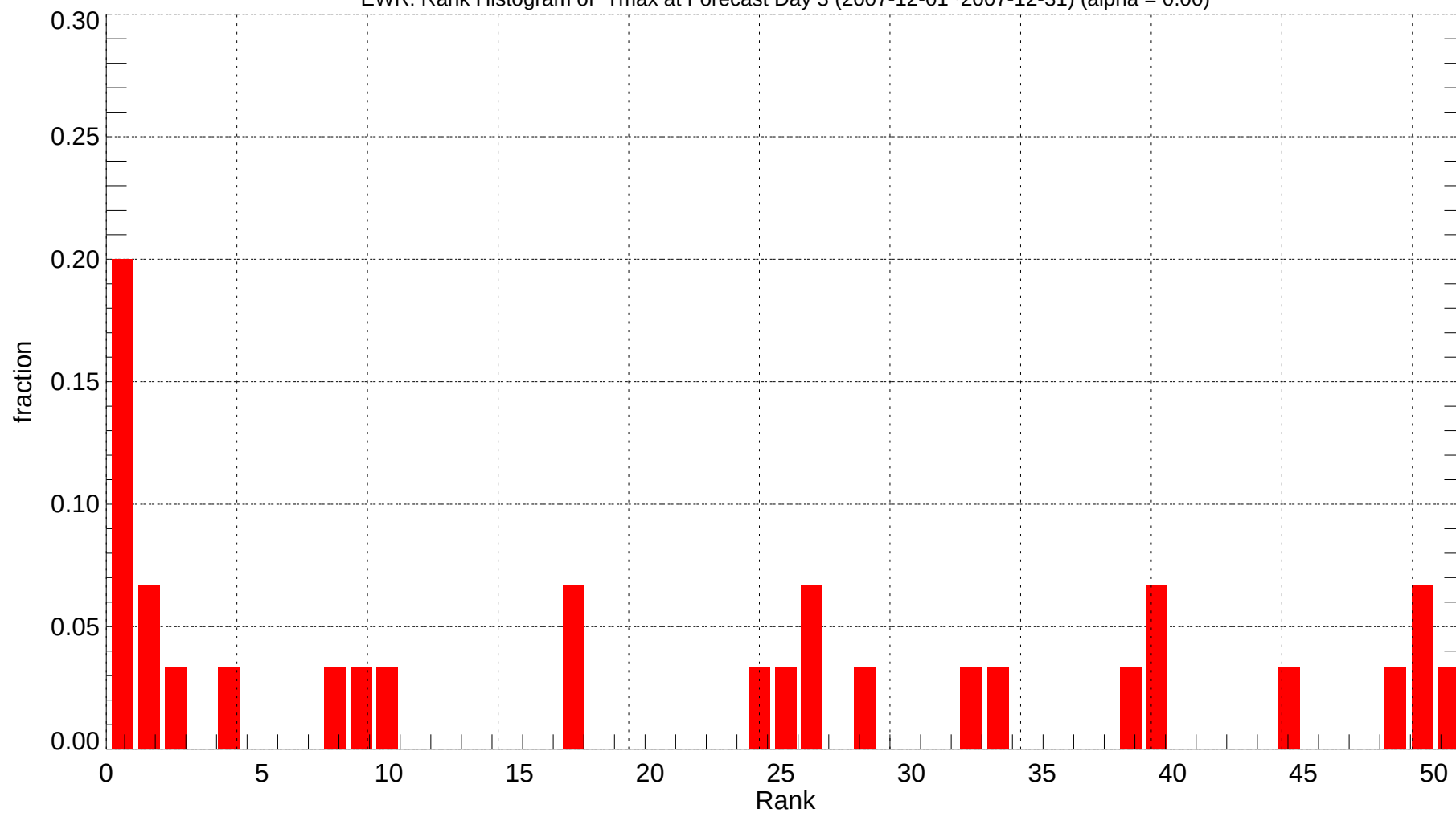
EWR: Rank Histogram of Tmax at Forecast Day 3 (2007-12-01~2007-12-31) (alpha = 0.00)
