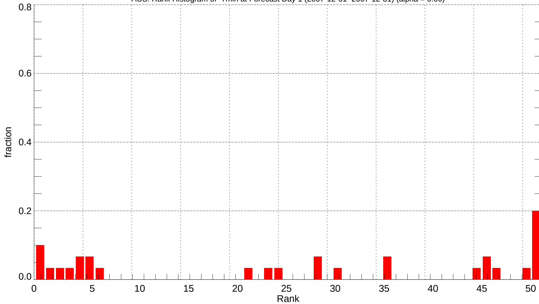
AUS: Rank Histogram of Tmin at Forecast Day 1 (2007-12-01~2007-12-31) (alpha = 0.00)
