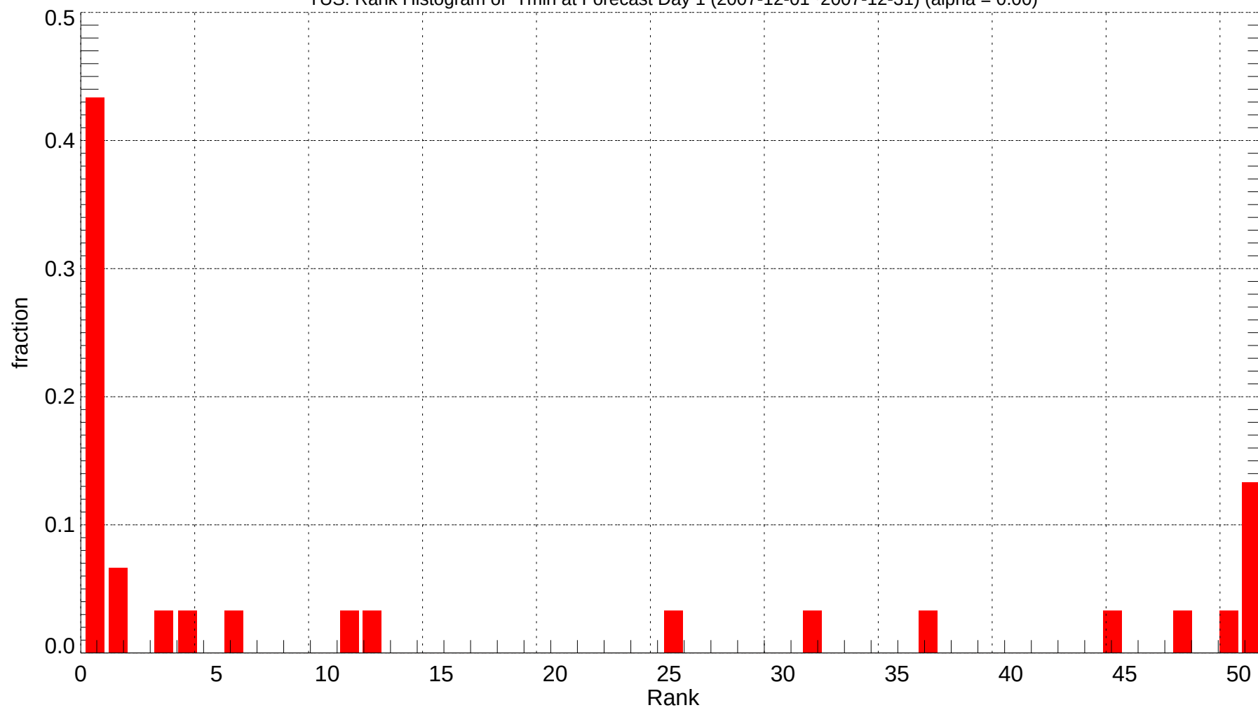
TUS: Rank Histogram of Tmin at Forecast Day 1 (2007-12-01~2007-12-31) (alpha = 0.00)
