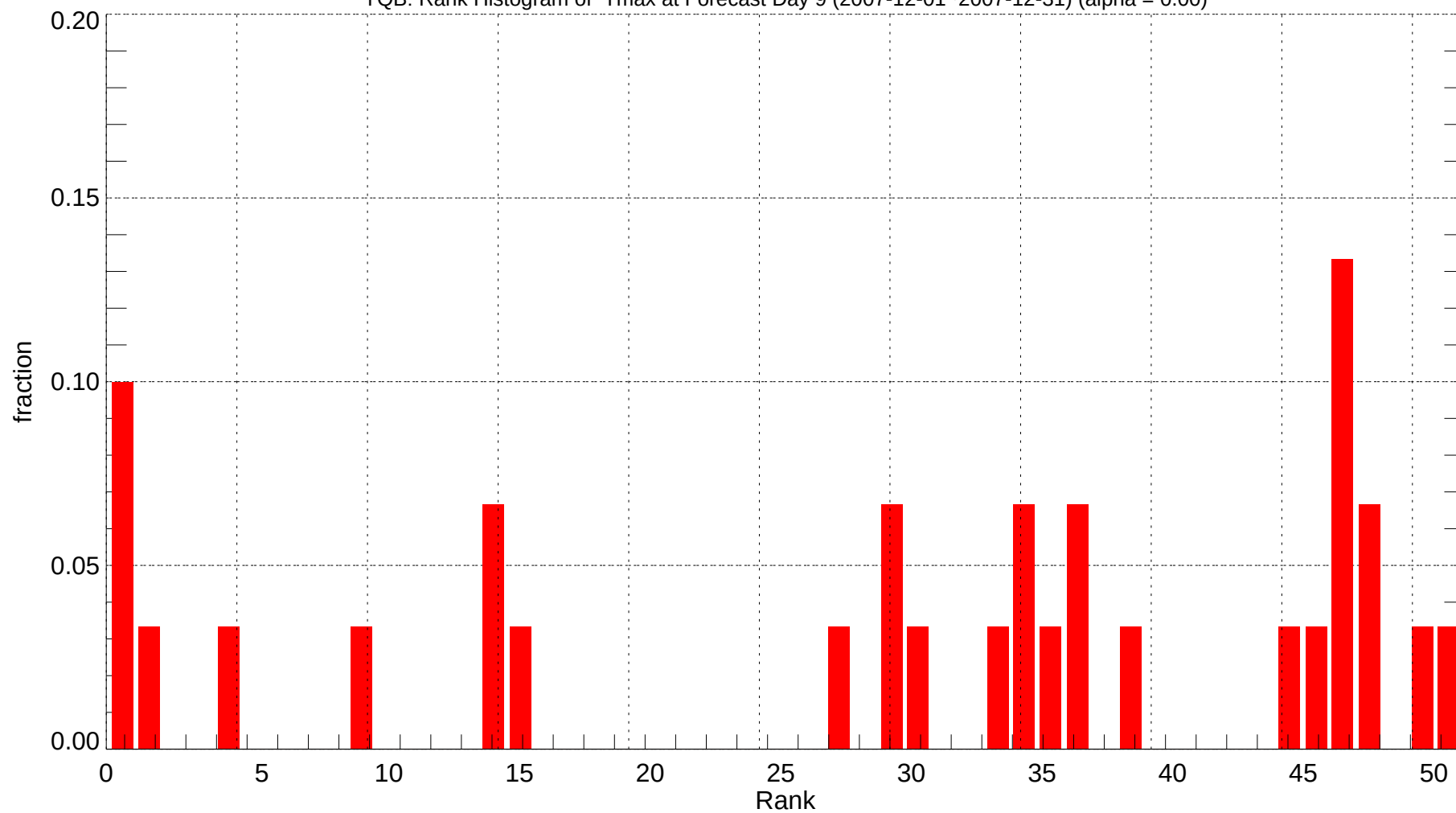
YQB: Rank Histogram of Tmax at Forecast Day 9 (2007-12-01~2007-12-31) (alpha = 0.00)
