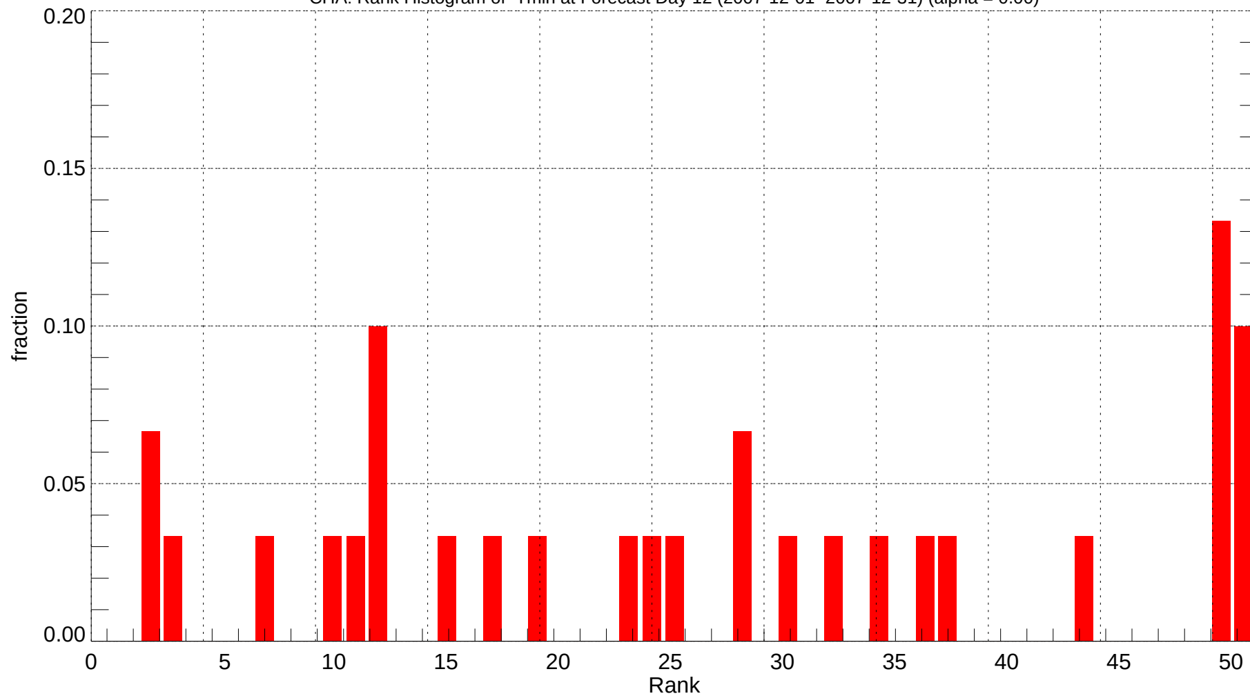
CHA: Rank Histogram of Tmin at Forecast Day 12 (2007-12-01~2007-12-31) (alpha = 0.00)
