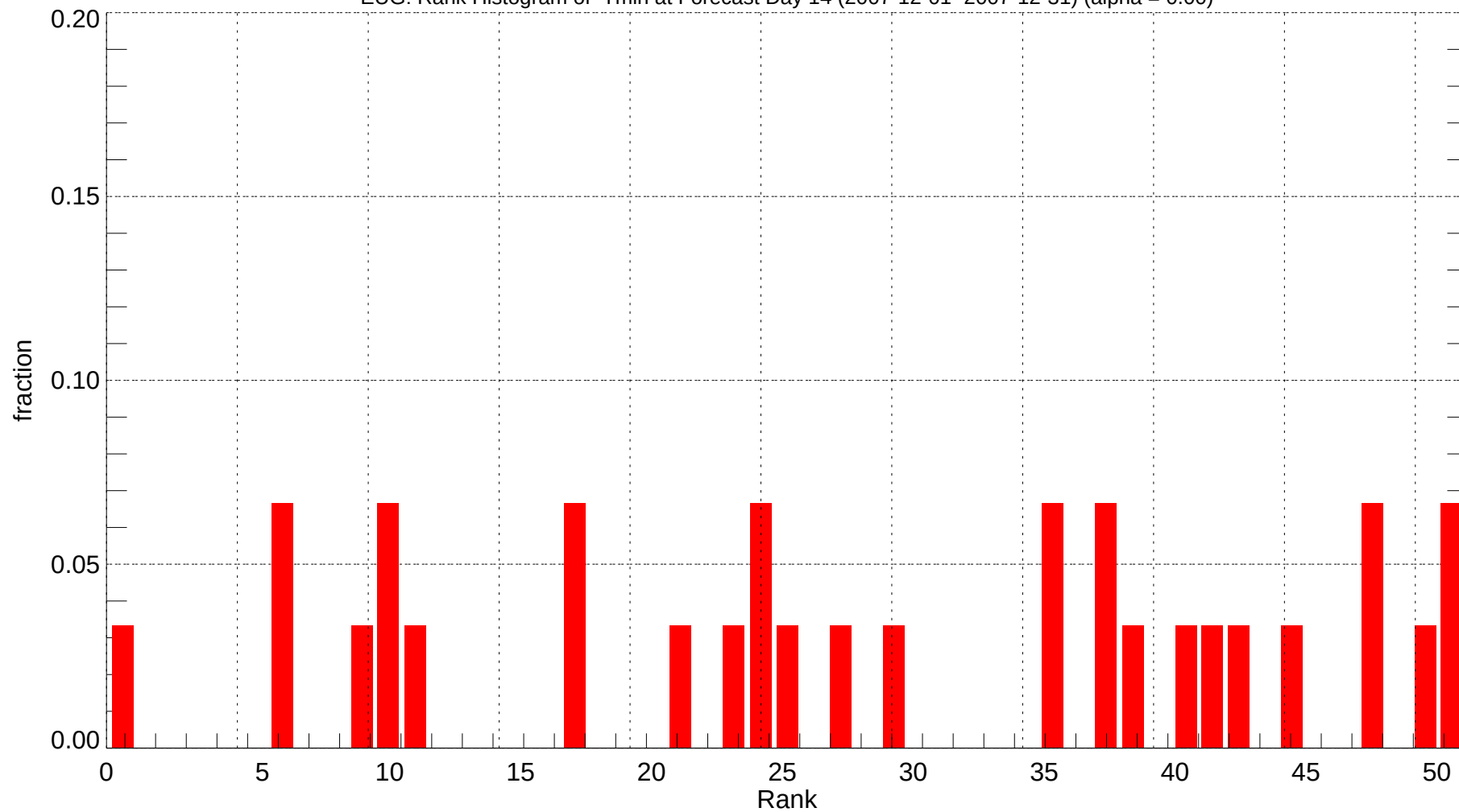
EUG: Rank Histogram of Tmin at Forecast Day 14 (2007-12-01~2007-12-31) (alpha = 0.00)
