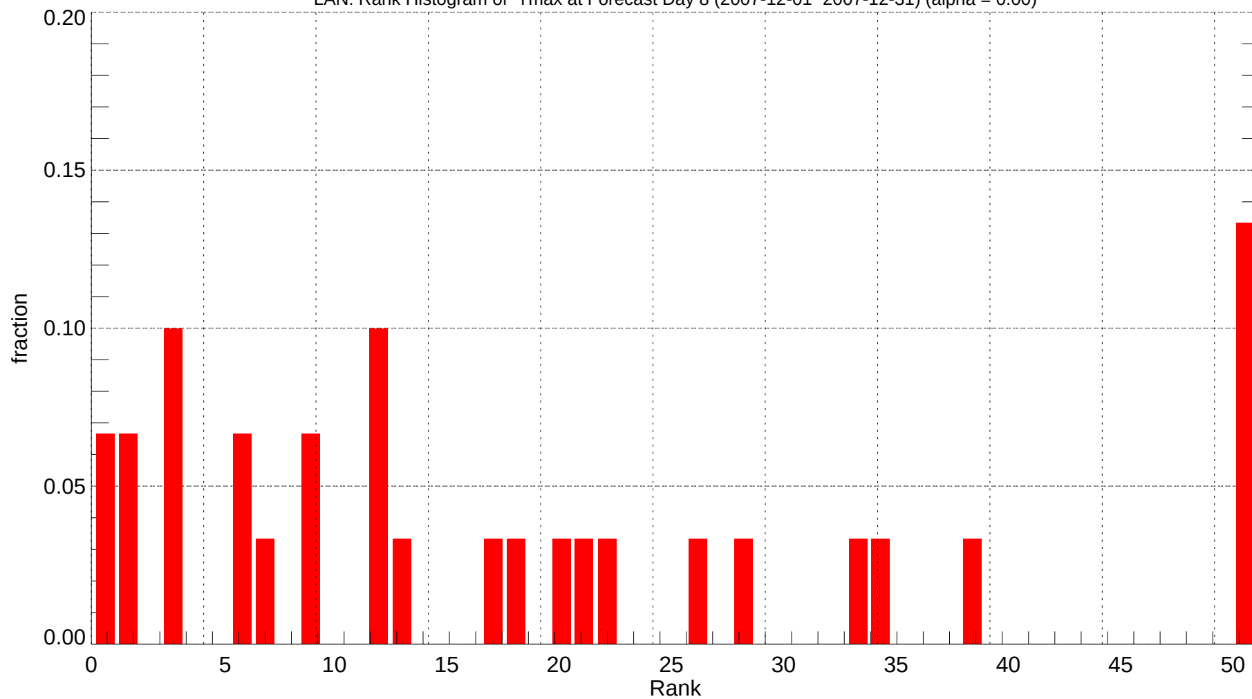
LAN: Rank Histogram of Tmax at Forecast Day 8 (2007-12-01~2007-12-31) (alpha = 0.00)
