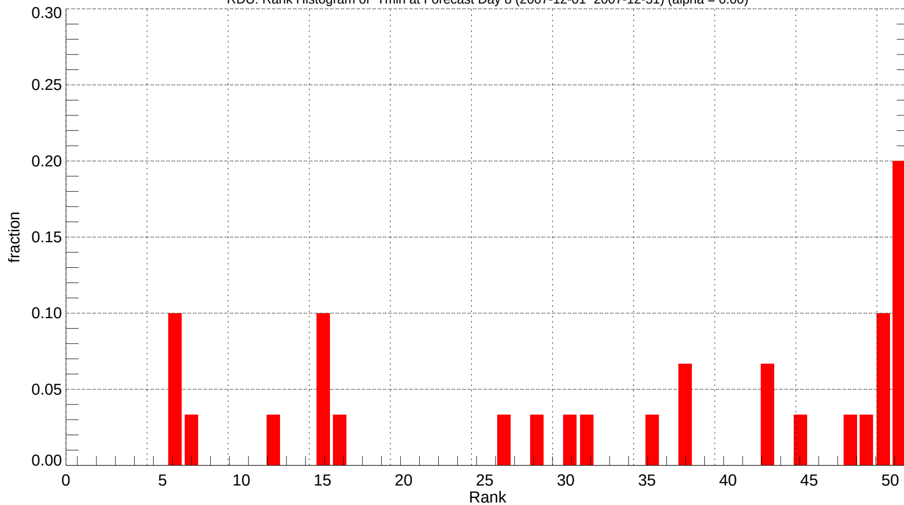
RDU: Rank Histogram of Tmin at Forecast Day 8 (2007-12-01~2007-12-31) (alpha = 0.00)
