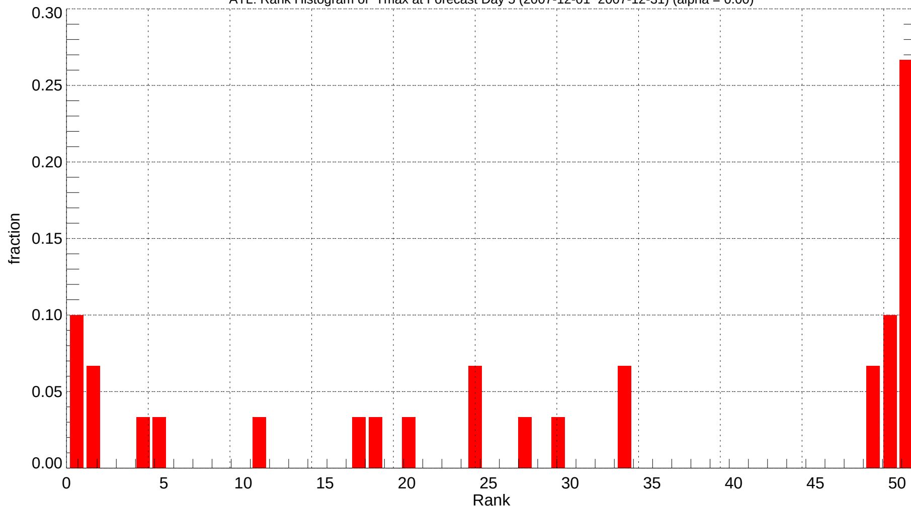
ATL: Rank Histogram of Tmax at Forecast Day 5 (2007-12-01~2007-12-31) (alpha = 0.00)
