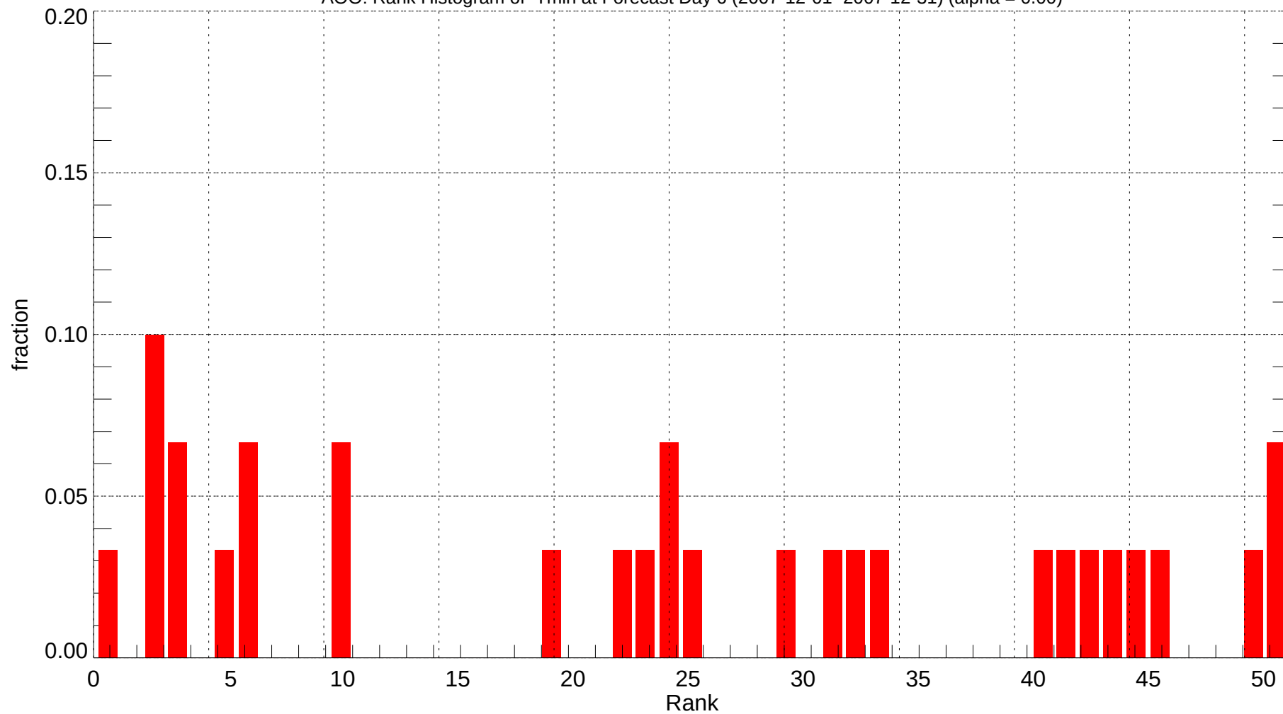
AOO: Rank Histogram of Tmin at Forecast Day 6 (2007-12-01~2007-12-31) (alpha = 0.00)
