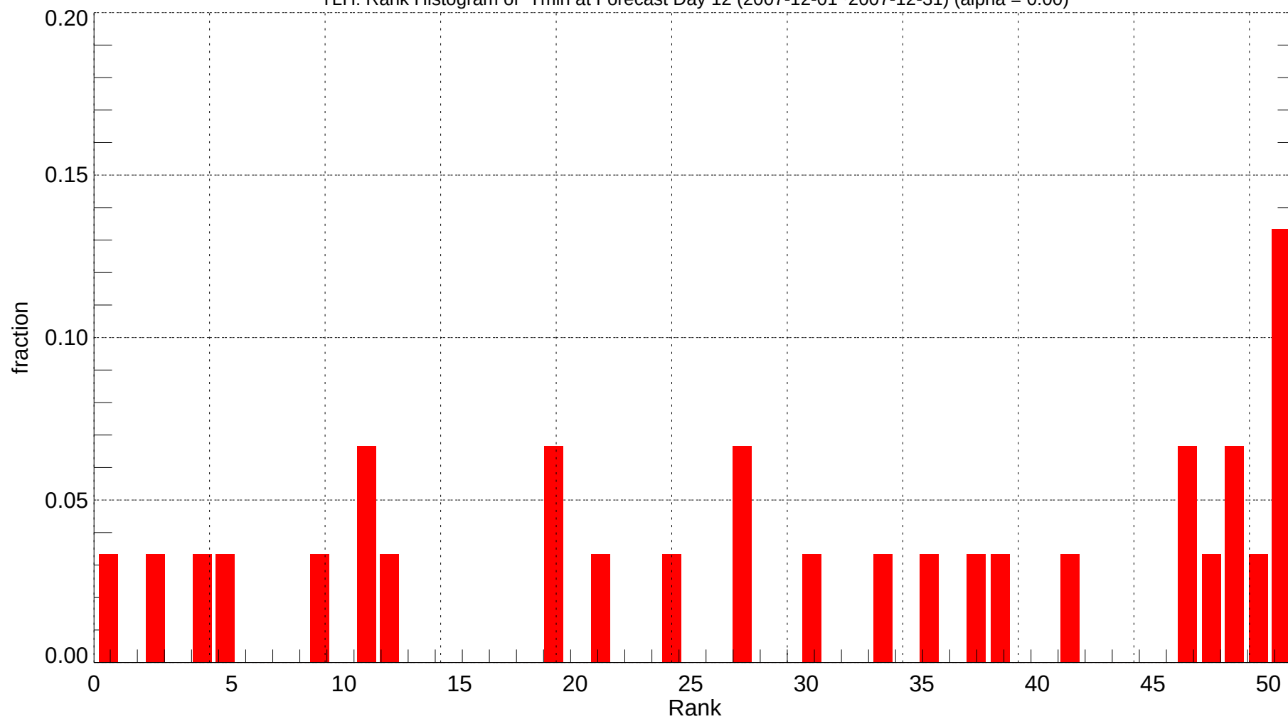
TLH: Rank Histogram of Tmin at Forecast Day 12 (2007-12-01~2007-12-31) (alpha = 0.00)
