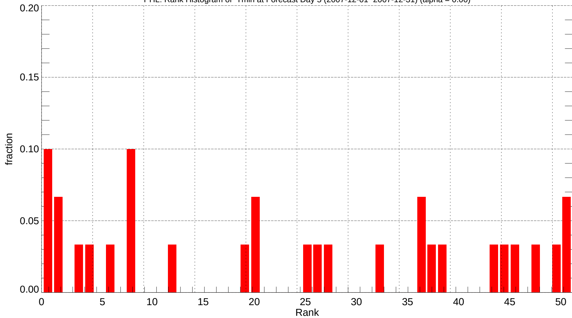
PHL: Rank Histogram of Tmin at Forecast Day 5 (2007-12-01~2007-12-31) (alpha = 0.00)
