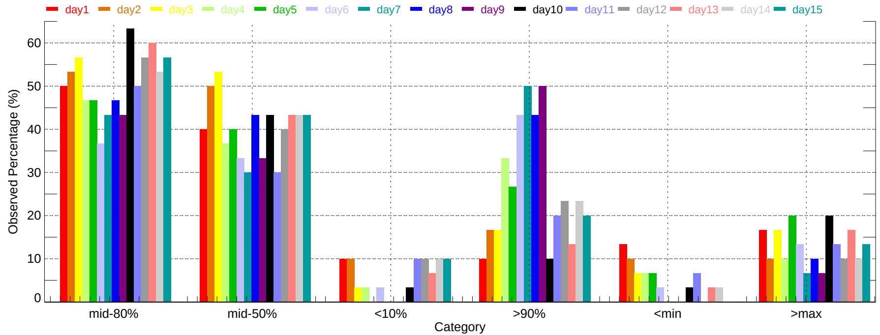
Observed Percentage of Ensembles - SAV: Min Temperature (2007-12-01~2007-12-31)
