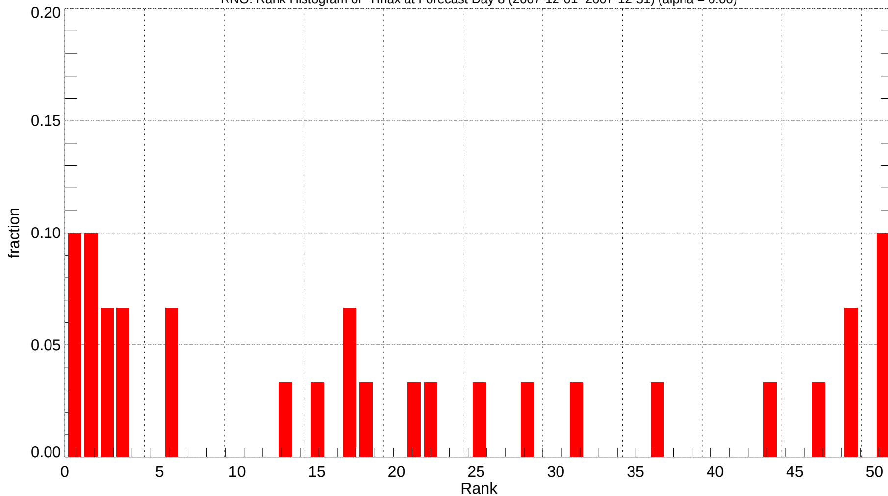
RNO: Rank Histogram of Tmax at Forecast Day 8 (2007-12-01~2007-12-31) (alpha = 0.00)
