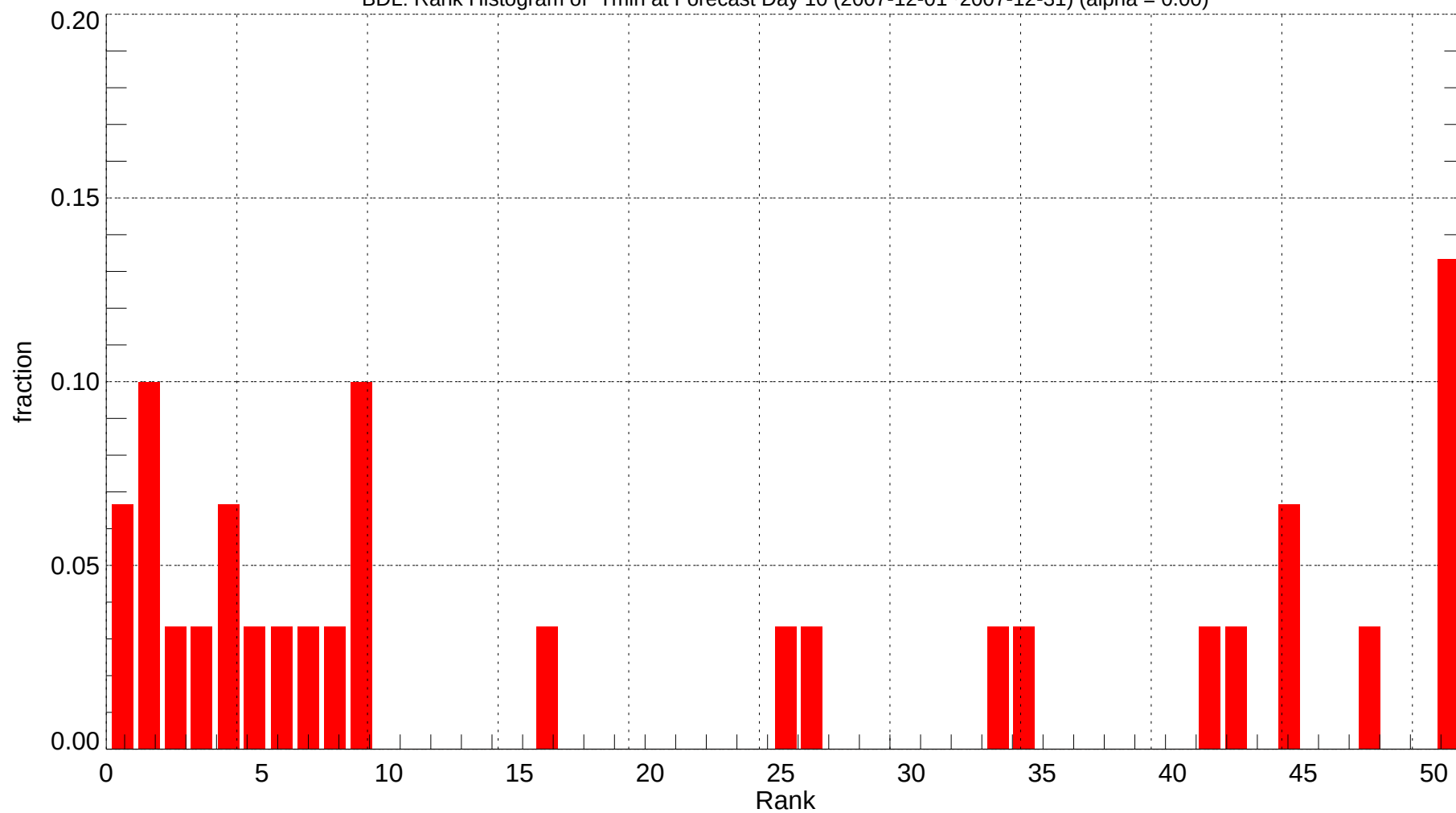
BDL: Rank Histogram of Tmin at Forecast Day 10 (2007-12-01~2007-12-31) (alpha = 0.00)
