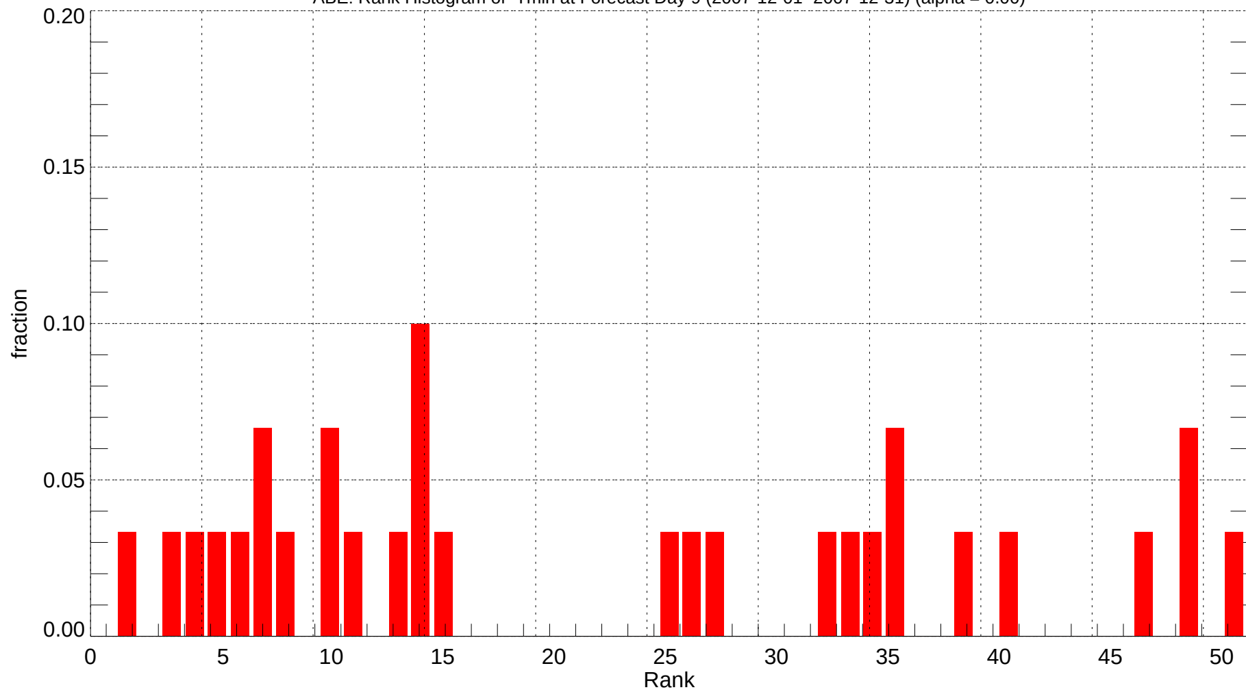
ABE: Rank Histogram of Tmin at Forecast Day 9 (2007-12-01~2007-12-31) (alpha = 0.00)
