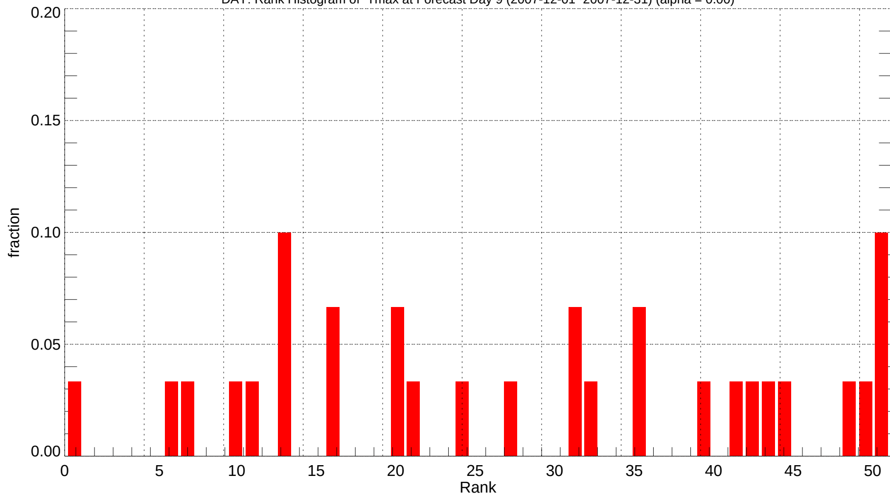
DAY: Rank Histogram of Tmax at Forecast Day 9 (2007-12-01~2007-12-31) (alpha = 0.00)
