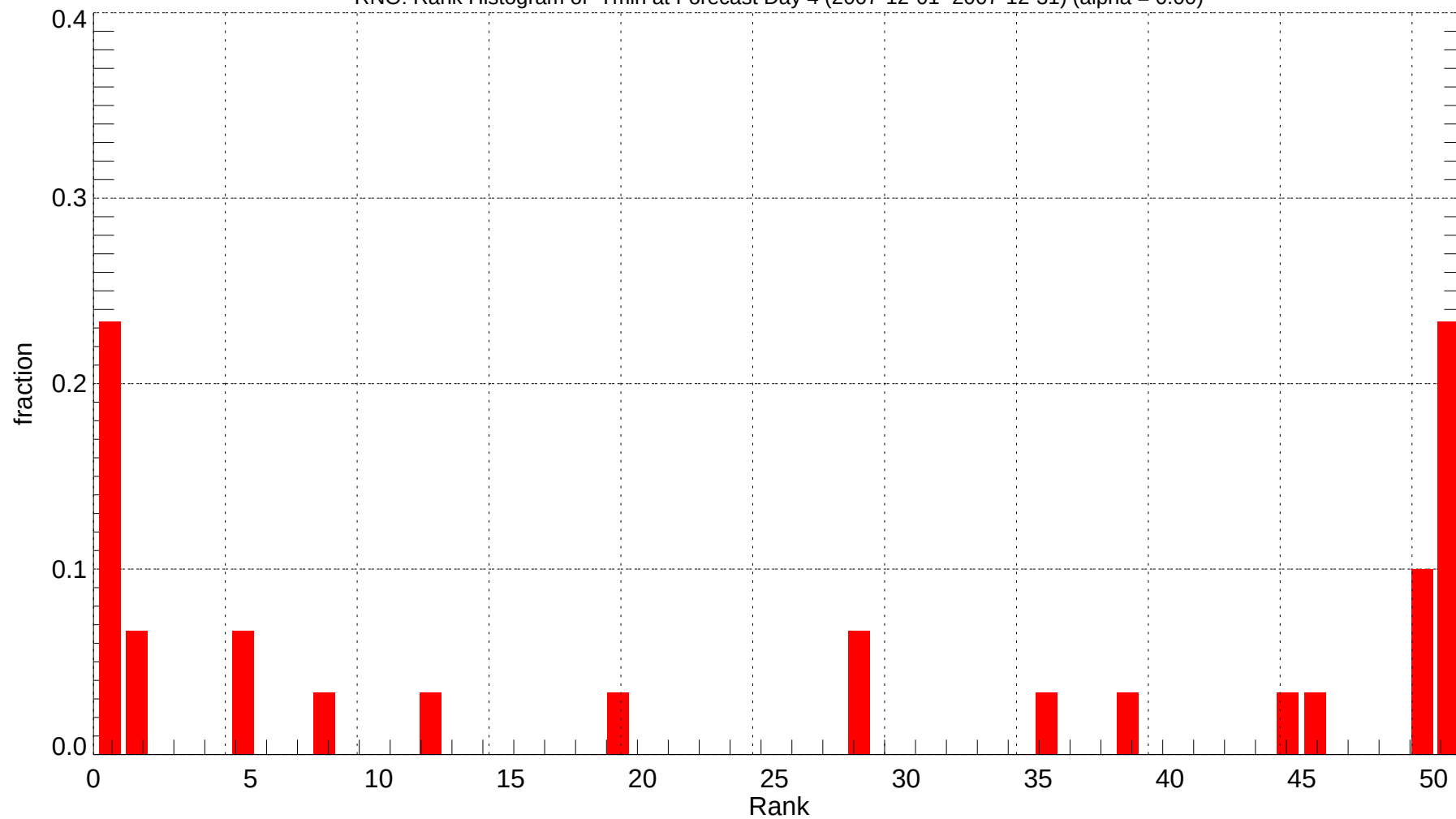
RNO: Rank Histogram of Tmin at Forecast Day 4 (2007-12-01~2007-12-31) (alpha = 0.00)
