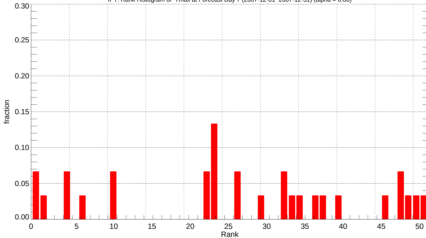
IPT: Rank Histogram of Tmax at Forecast Day 7 (2007-12-01~2007-12-31) (alpha = 0.00)
