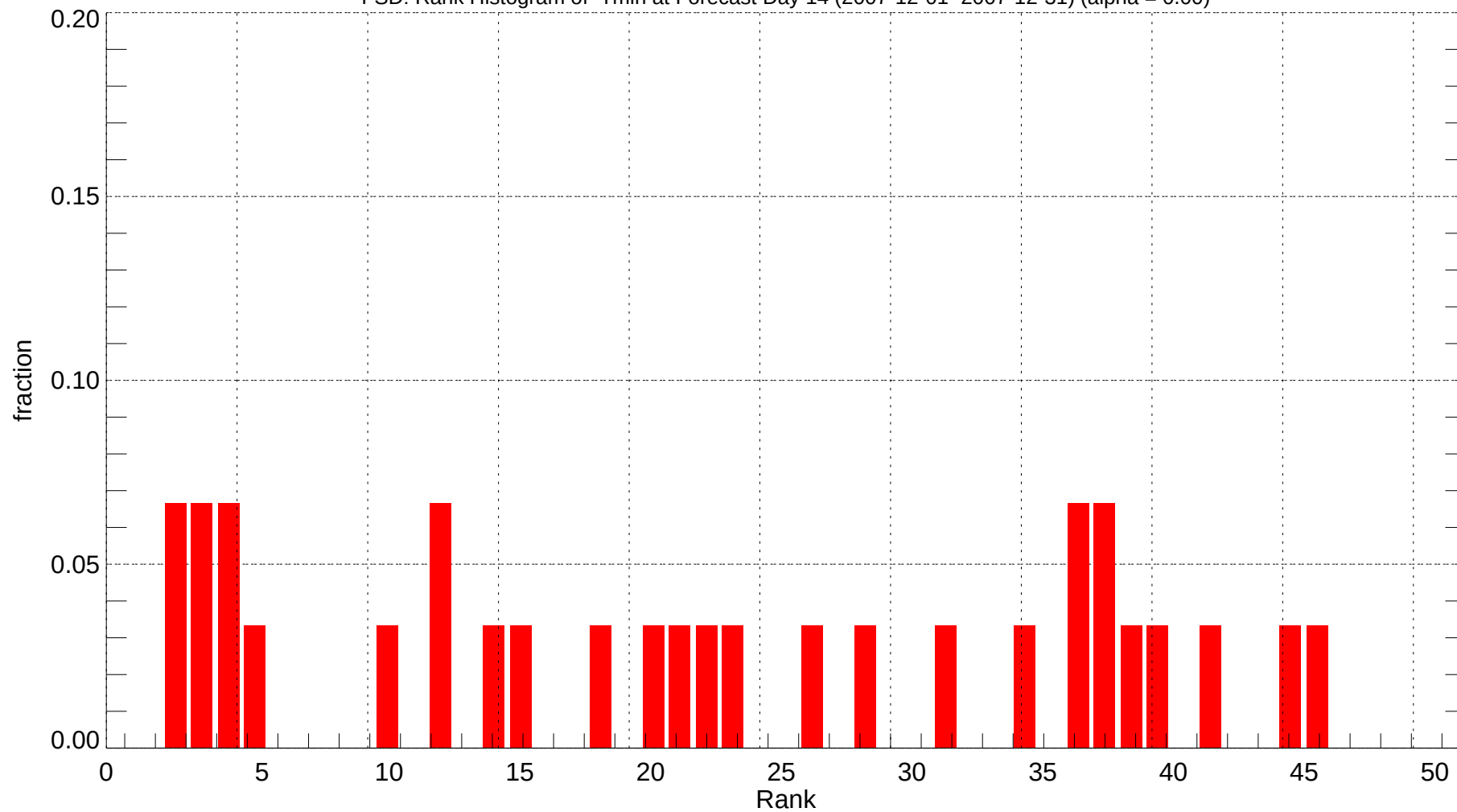
FSD: Rank Histogram of Tmin at Forecast Day 14 (2007-12-01~2007-12-31) (alpha = 0.00)
