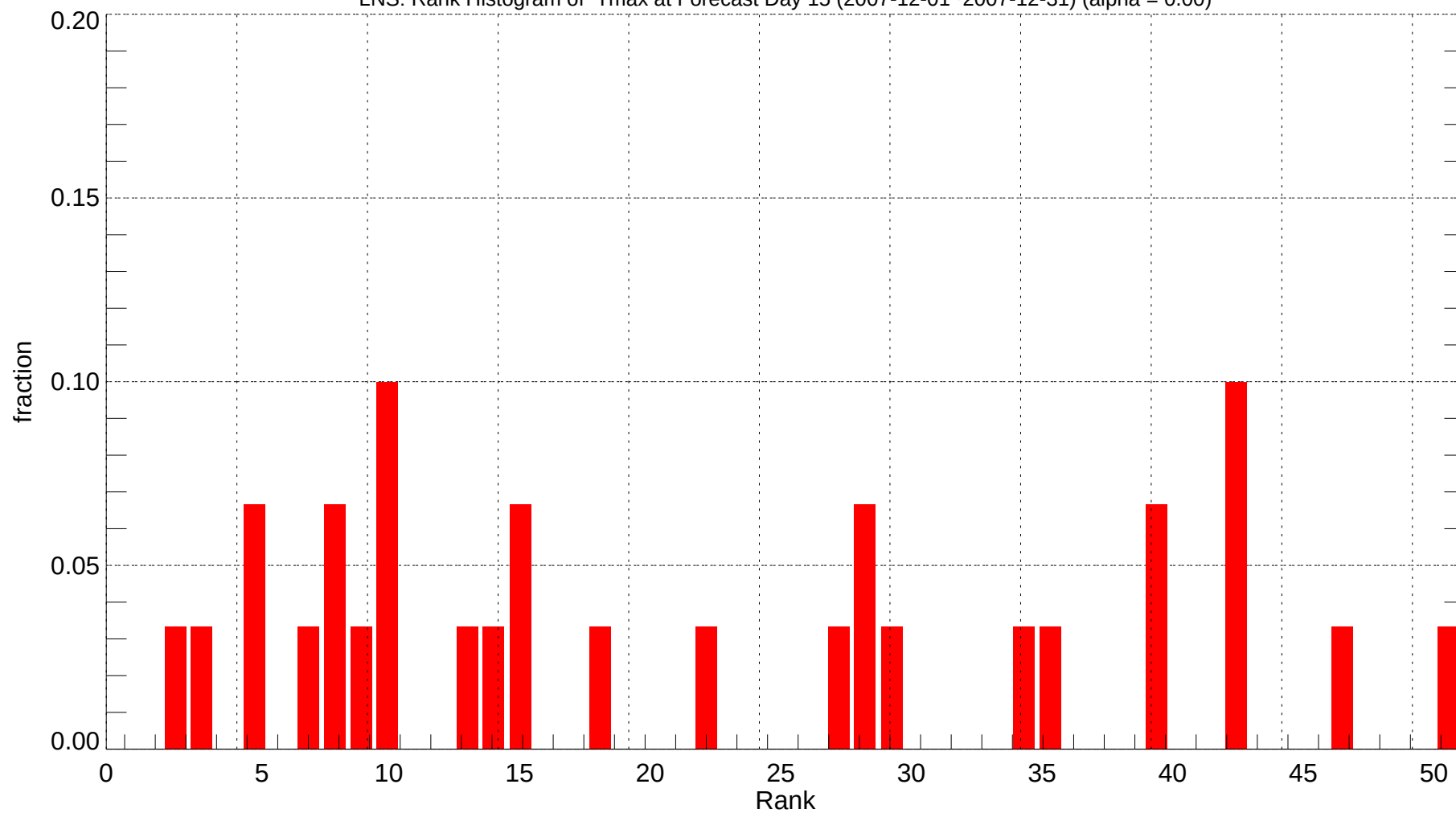
LNS: Rank Histogram of Tmax at Forecast Day 15 (2007-12-01~2007-12-31) (alpha = 0.00)
