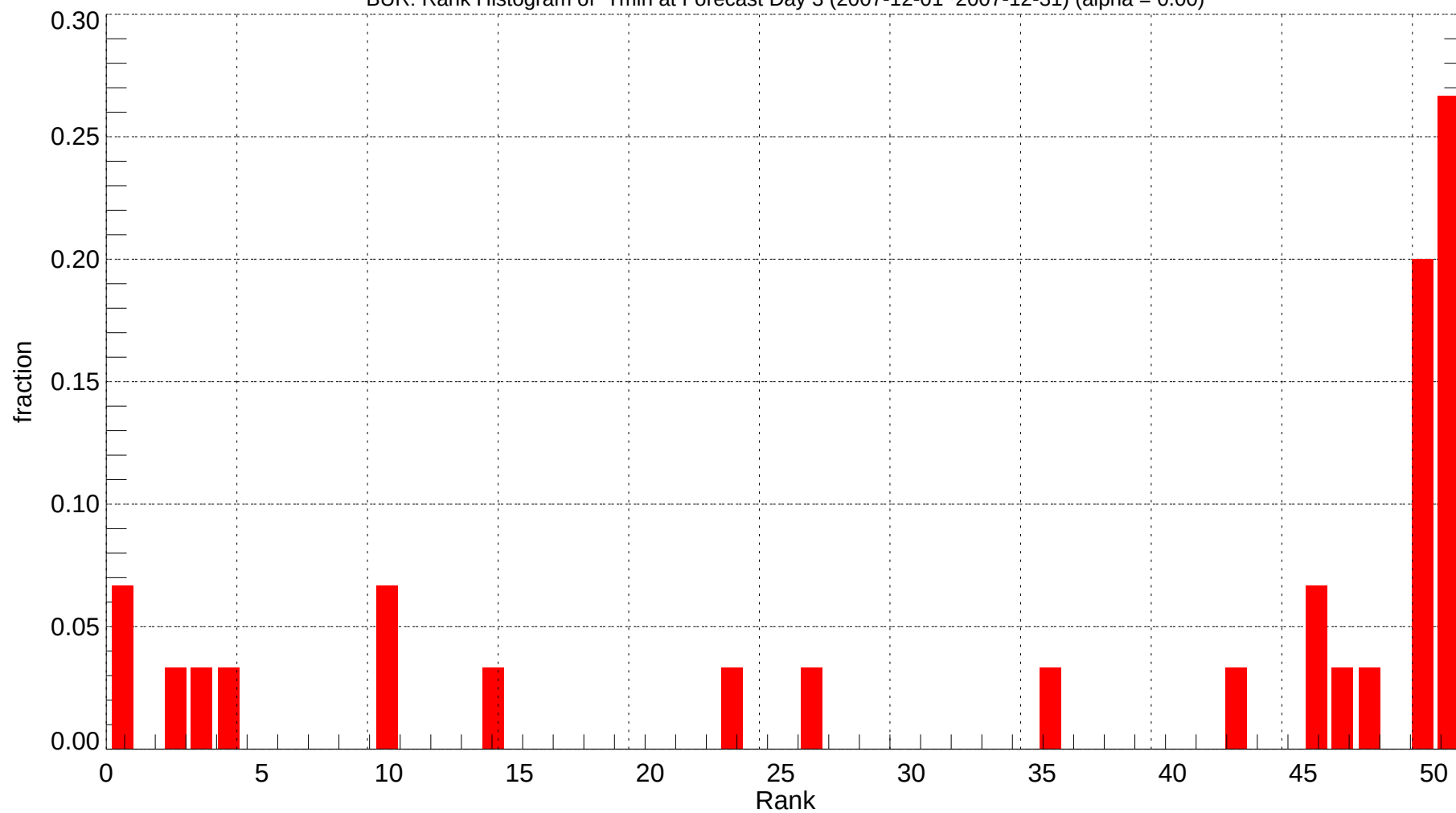
BUR: Rank Histogram of Tmin at Forecast Day 3 (2007-12-01~2007-12-31) (alpha = 0.00)
