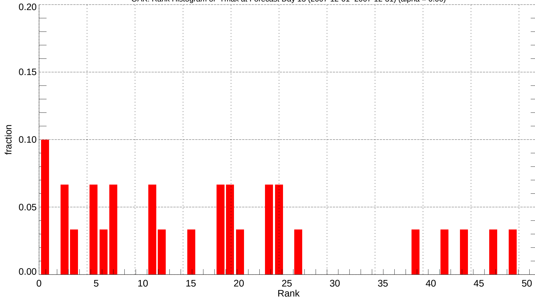
OAK: Rank Histogram of Tmax at Forecast Day 13 (2007-12-01~2007-12-31) (alpha = 0.00)
