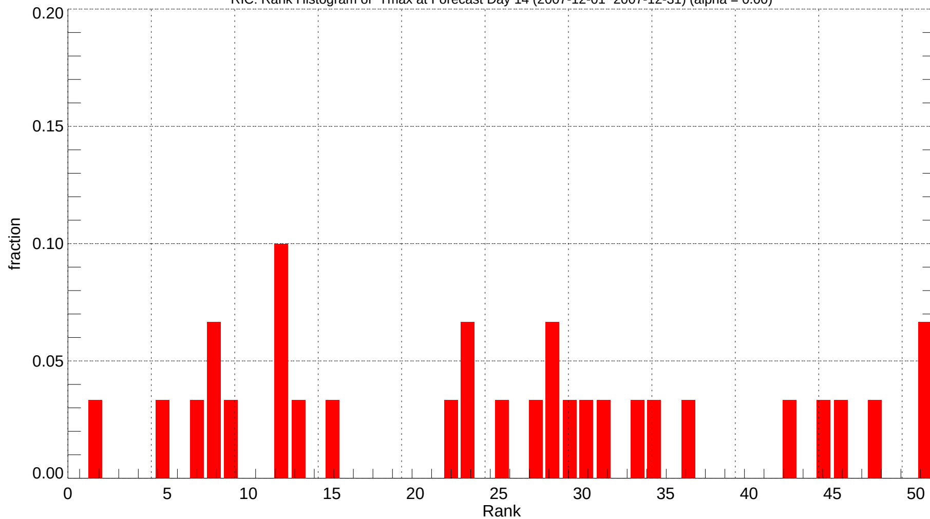
RIC: Rank Histogram of Tmax at Forecast Day 14 (2007-12-01~2007-12-31) (alpha = 0.00)
