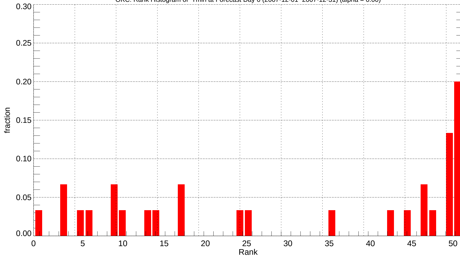
OKC: Rank Histogram of Tmin at Forecast Day 6 (2007-12-01~2007-12-31) (alpha = 0.00)
