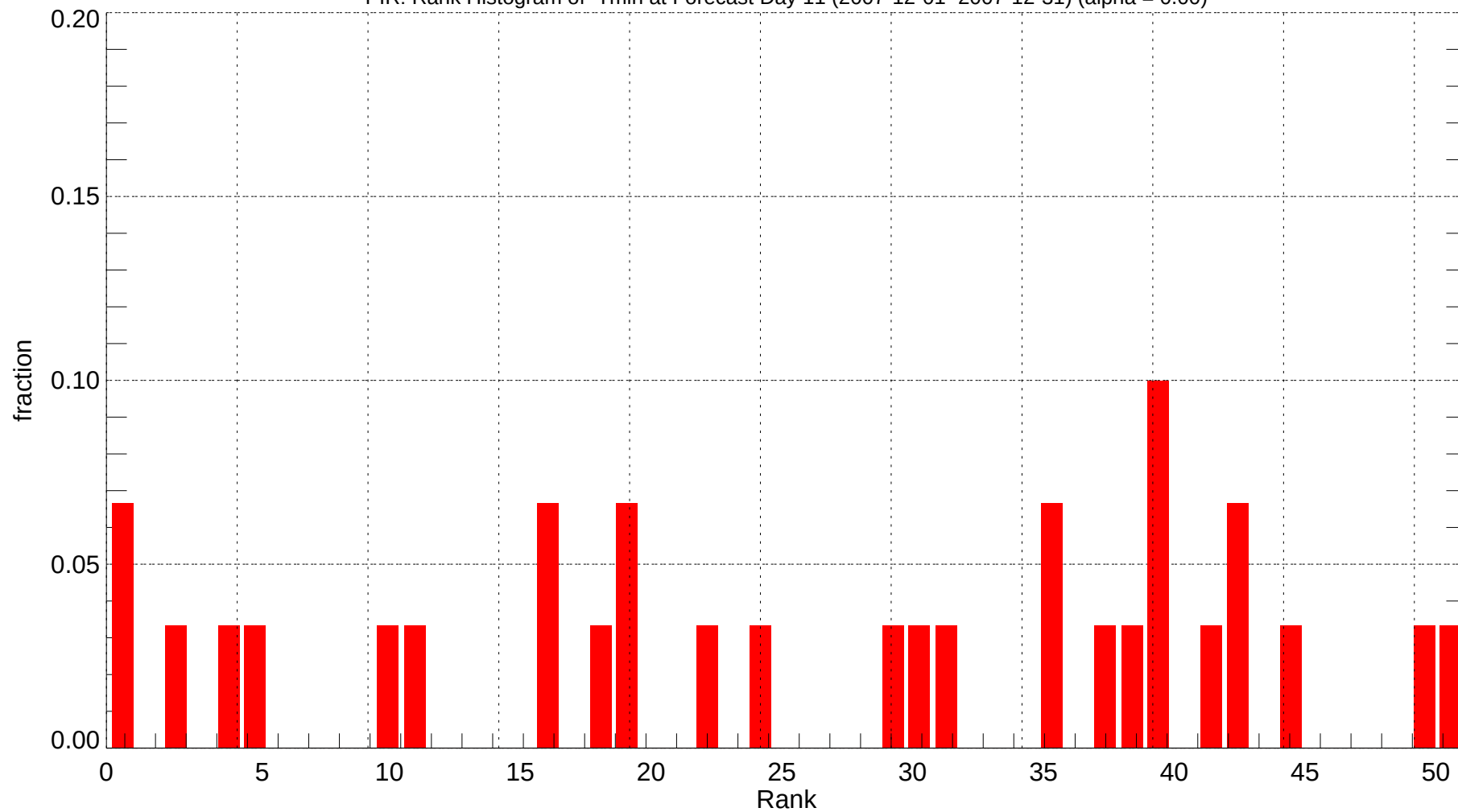
PIR: Rank Histogram of Tmin at Forecast Day 11 (2007-12-01~2007-12-31) (alpha = 0.00)
