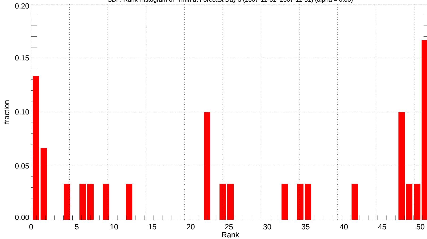
SDF: Rank Histogram of Tmin at Forecast Day 3 (2007-12-01~2007-12-31) (alpha = 0.00)
