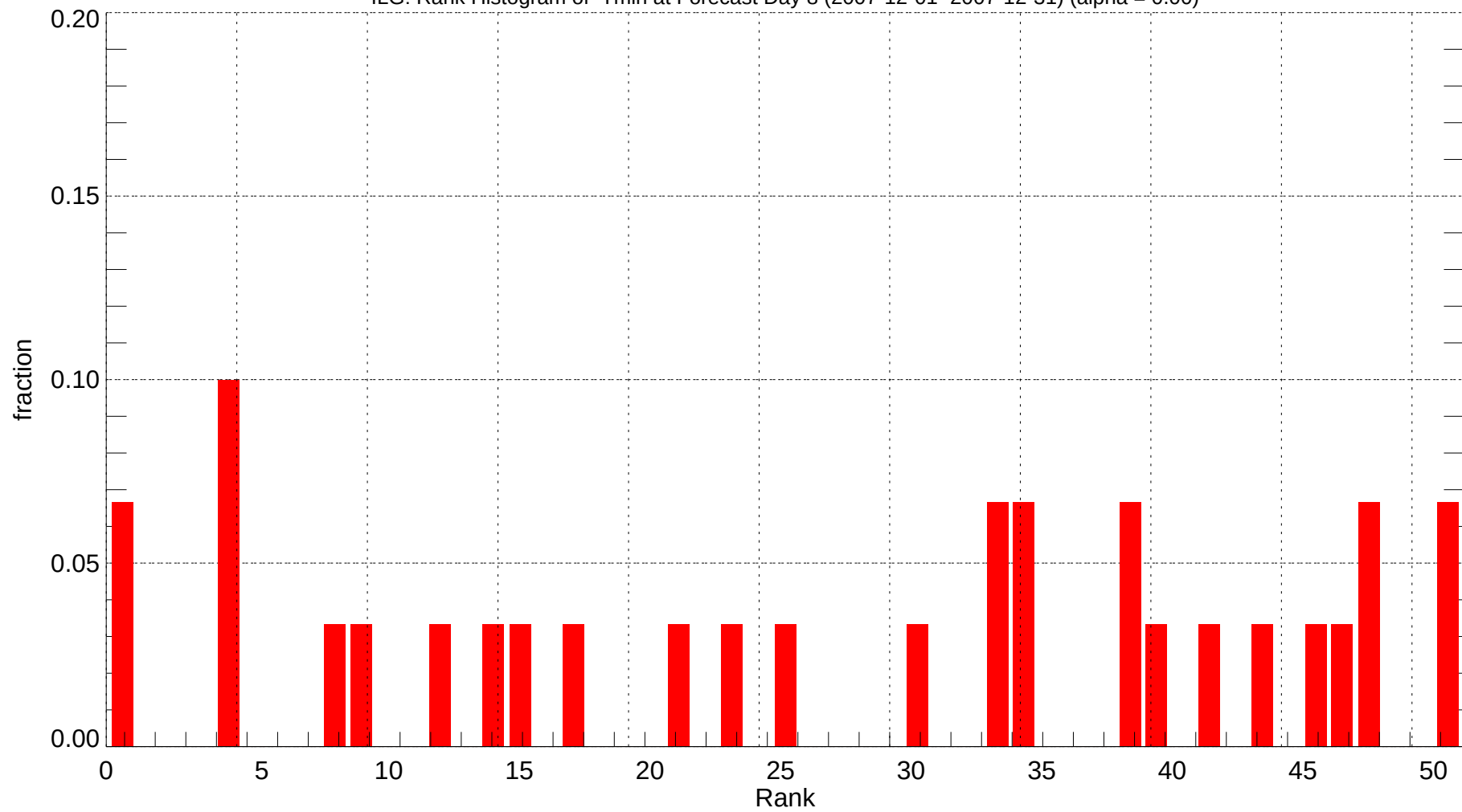
ILG: Rank Histogram of Tmin at Forecast Day 8 (2007-12-01~2007-12-31) (alpha = 0.00)
