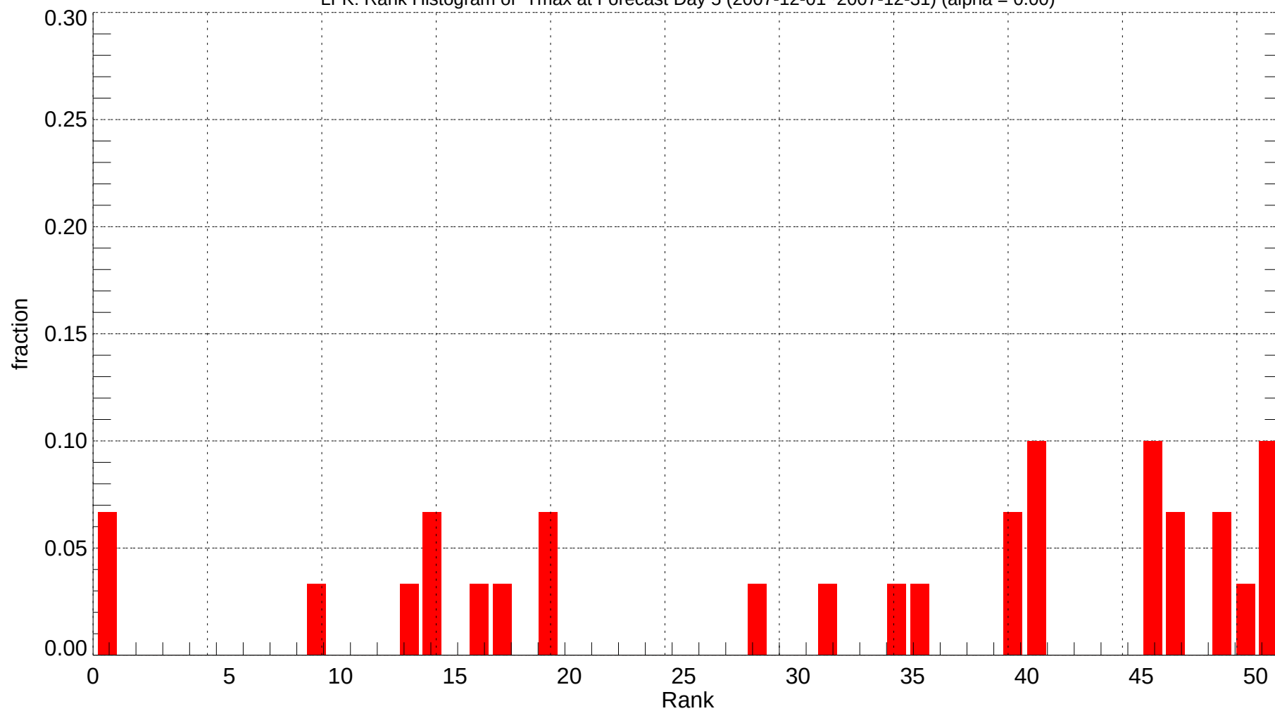
LFK: Rank Histogram of Tmax at Forecast Day 5 (2007-12-01~2007-12-31) (alpha = 0.00)
