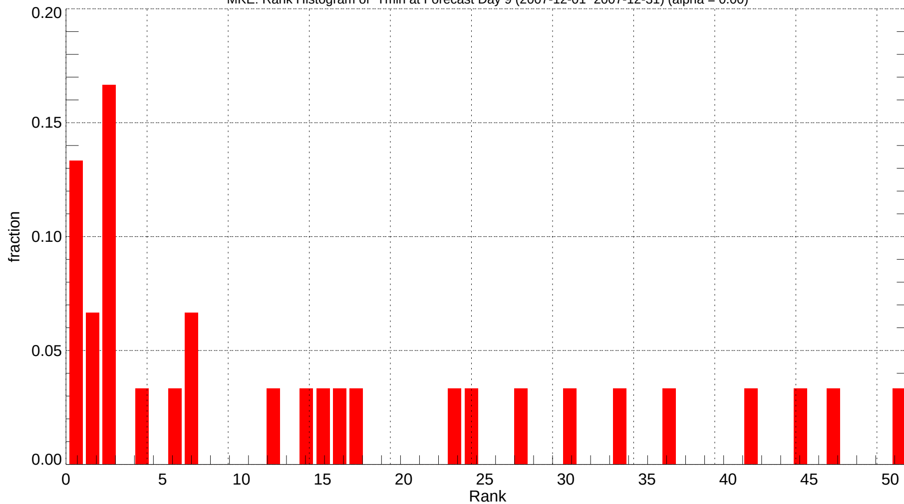
MKE: Rank Histogram of Tmin at Forecast Day 9 (2007-12-01~2007-12-31) (alpha = 0.00)
