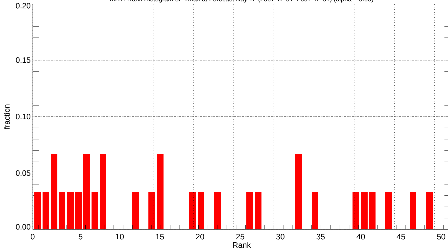
MHT: Rank Histogram of Tmax at Forecast Day 12 (2007-12-01~2007-12-31) (alpha = 0.00)
