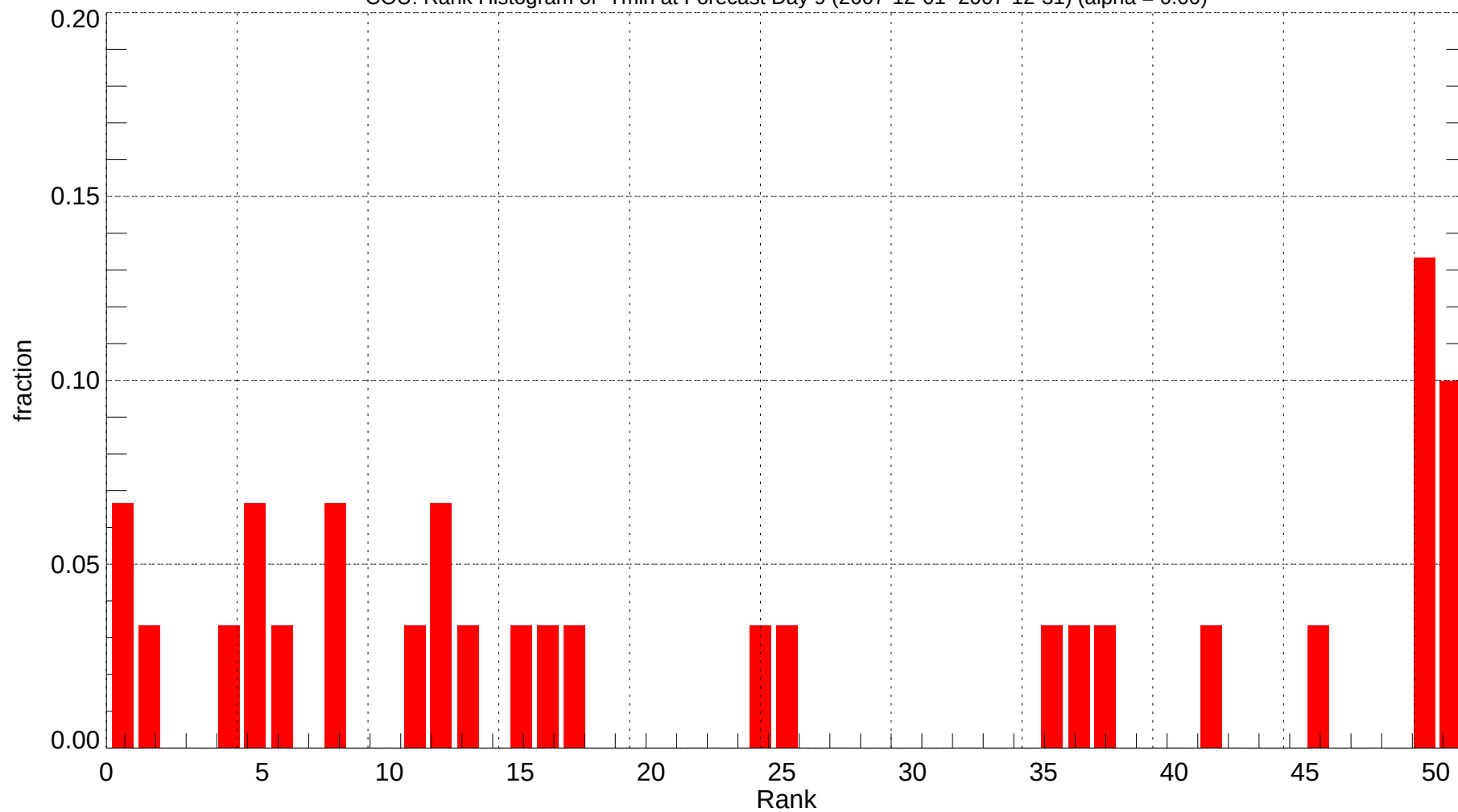
COU: Rank Histogram of Tmin at Forecast Day 9 (2007-12-01~2007-12-31) (alpha = 0.00)
