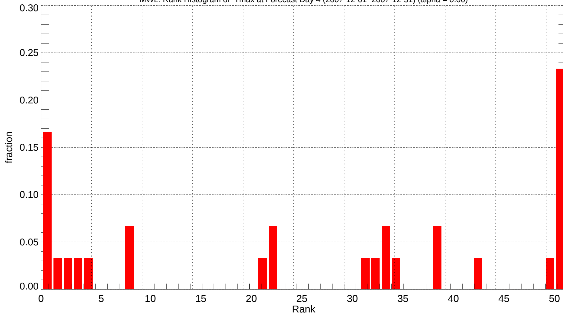
MWL: Rank Histogram of Tmax at Forecast Day 4 (2007-12-01~2007-12-31) (alpha = 0.00)
