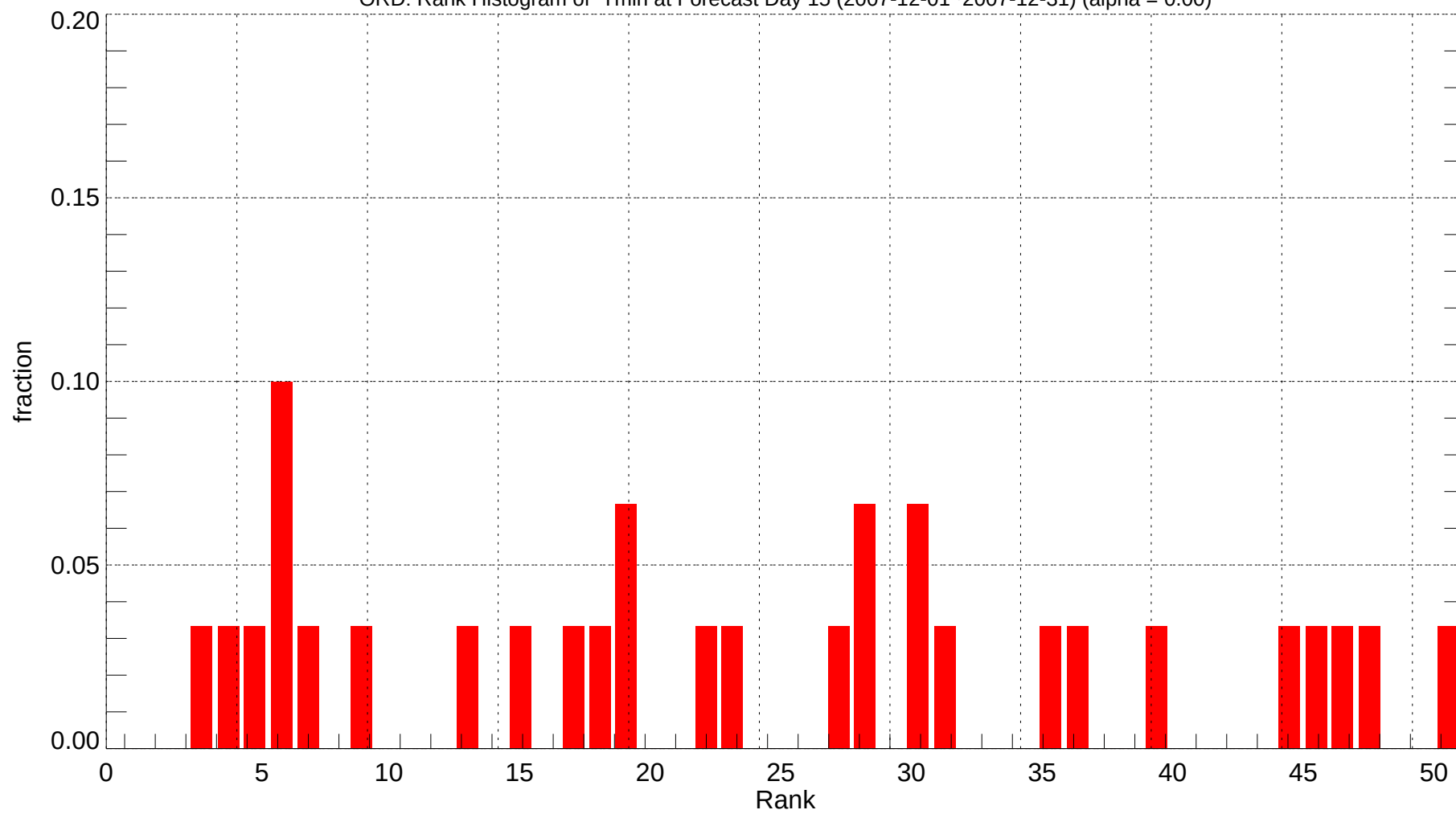
ORD: Rank Histogram of Tmin at Forecast Day 15 (2007-12-01~2007-12-31) (alpha = 0.00)
