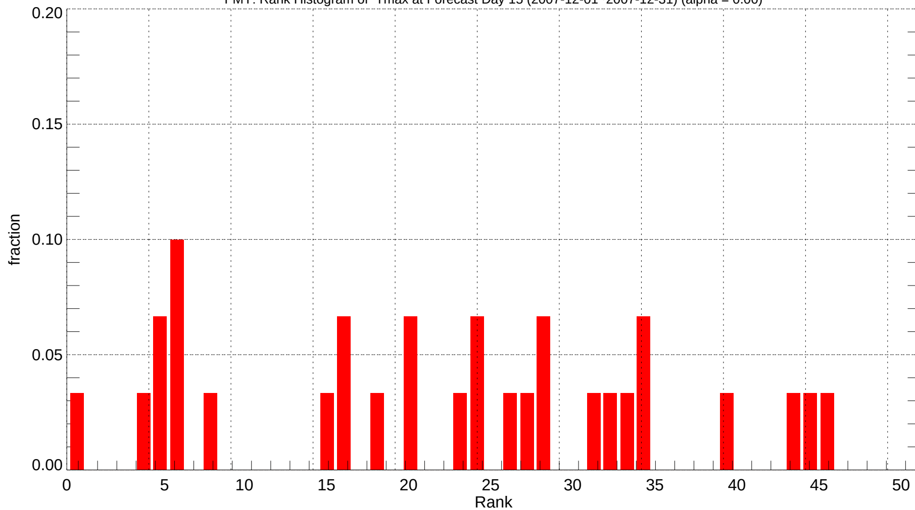
FMY: Rank Histogram of Tmax at Forecast Day 15 (2007-12-01~2007-12-31) (alpha = 0.00)
