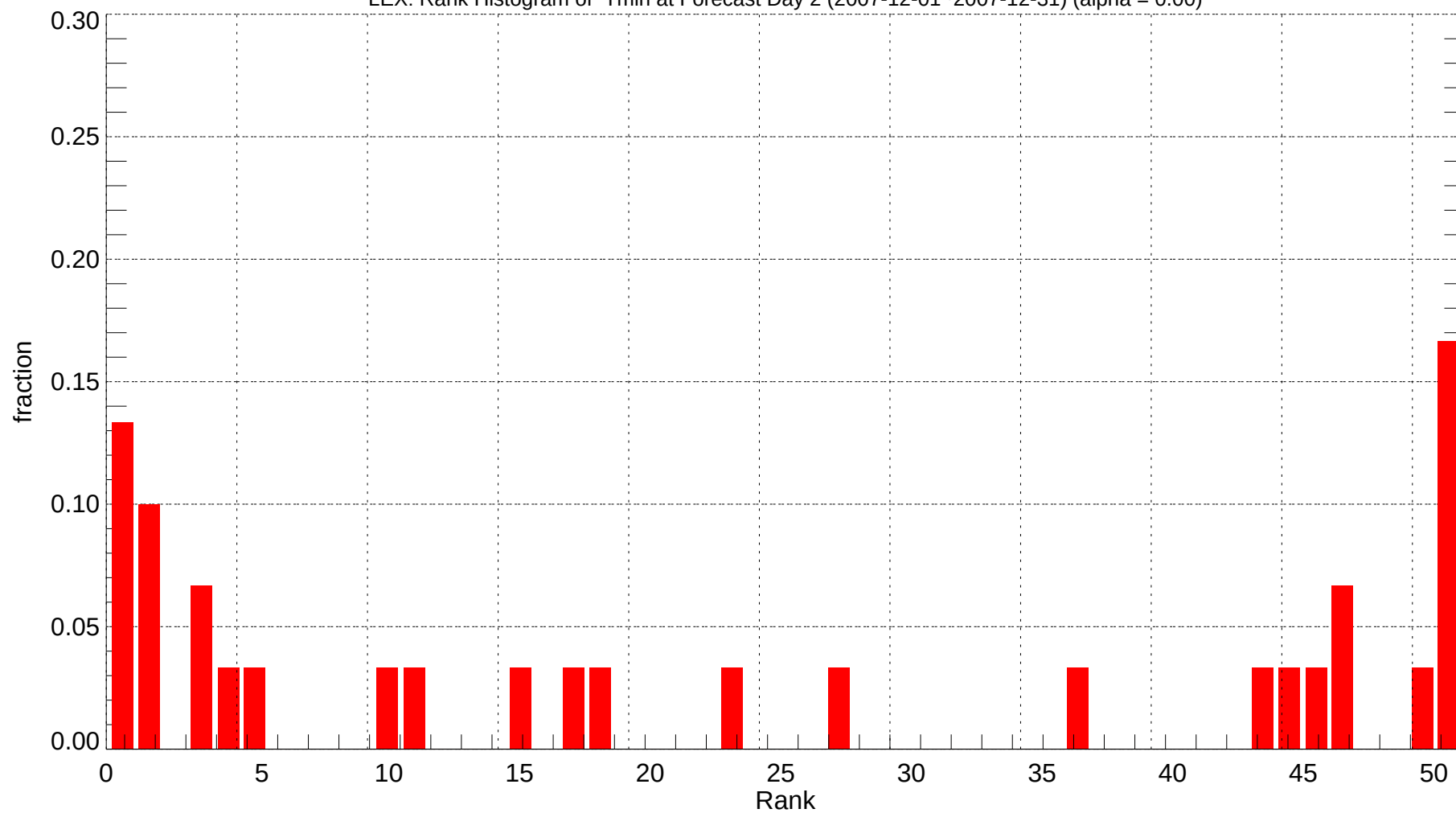
LEX: Rank Histogram of Tmin at Forecast Day 2 (2007-12-01~2007-12-31) (alpha = 0.00)
