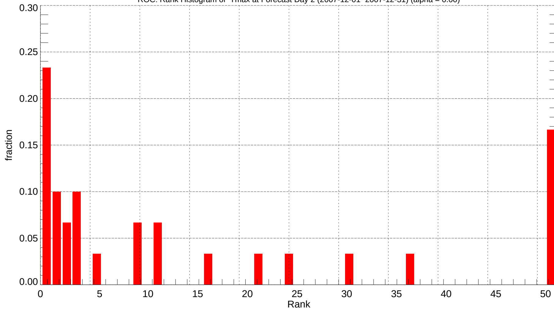
ROC: Rank Histogram of Tmax at Forecast Day 2 (2007-12-01~2007-12-31) (alpha = 0.00)
