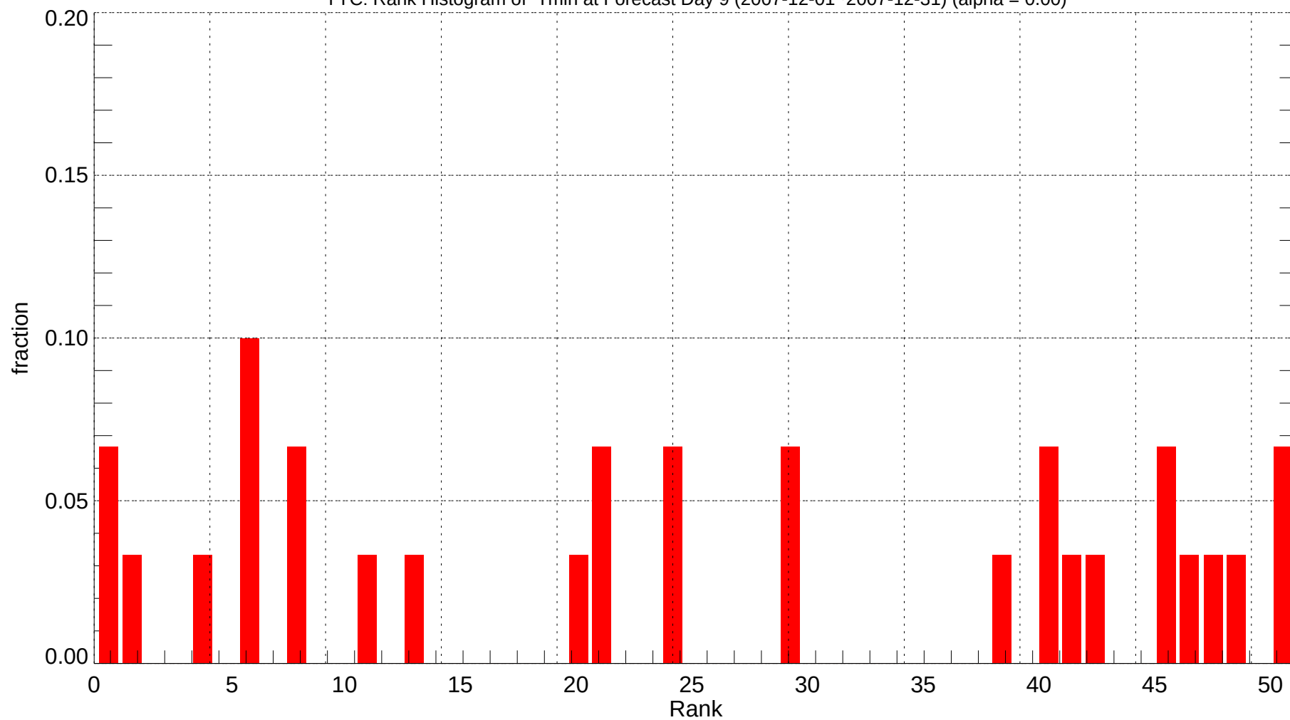
YYC: Rank Histogram of Tmin at Forecast Day 9 (2007-12-01~2007-12-31) (alpha = 0.00)
