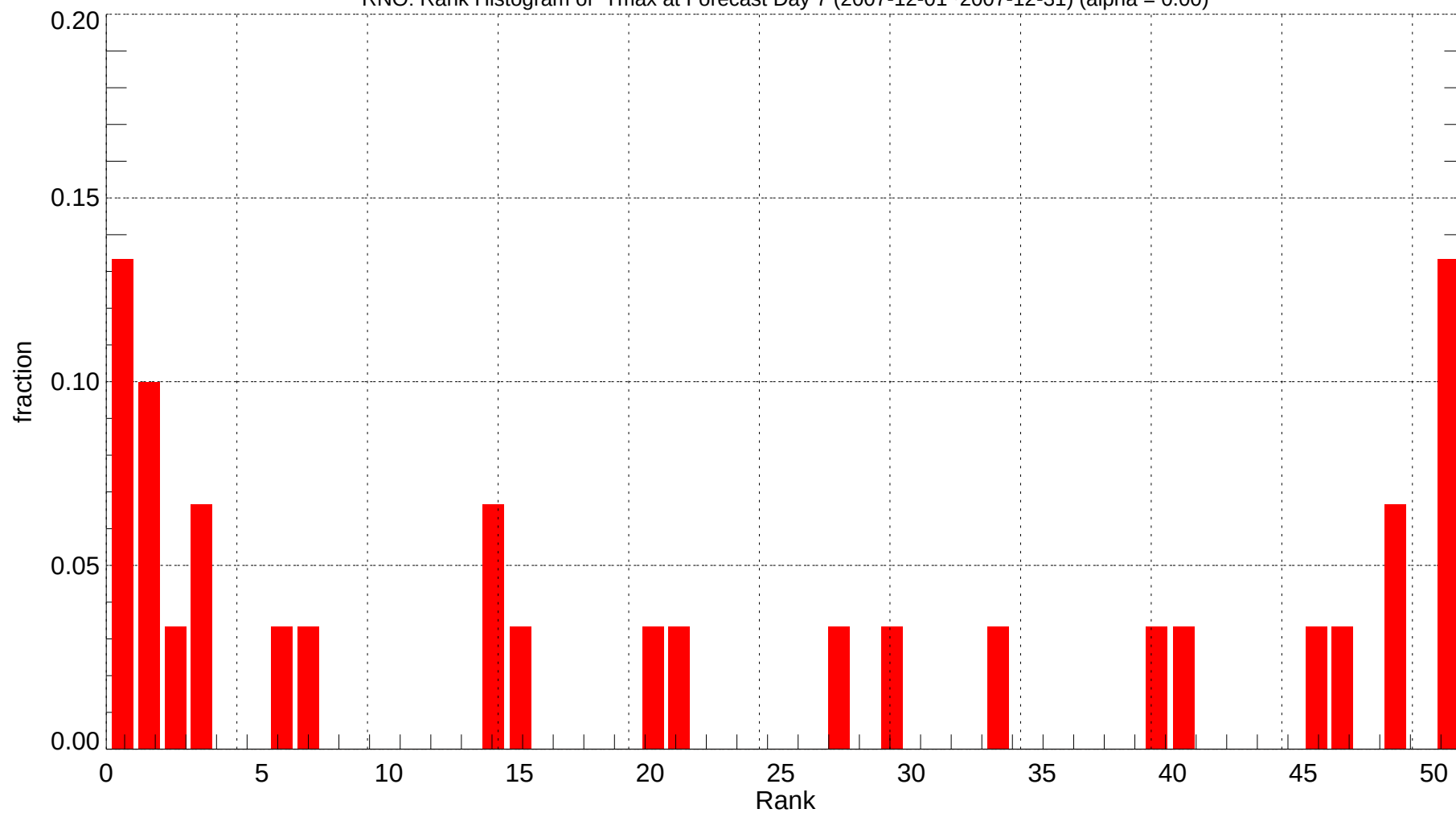
RNO: Rank Histogram of Tmax at Forecast Day 7 (2007-12-01~2007-12-31) (alpha = 0.00)
