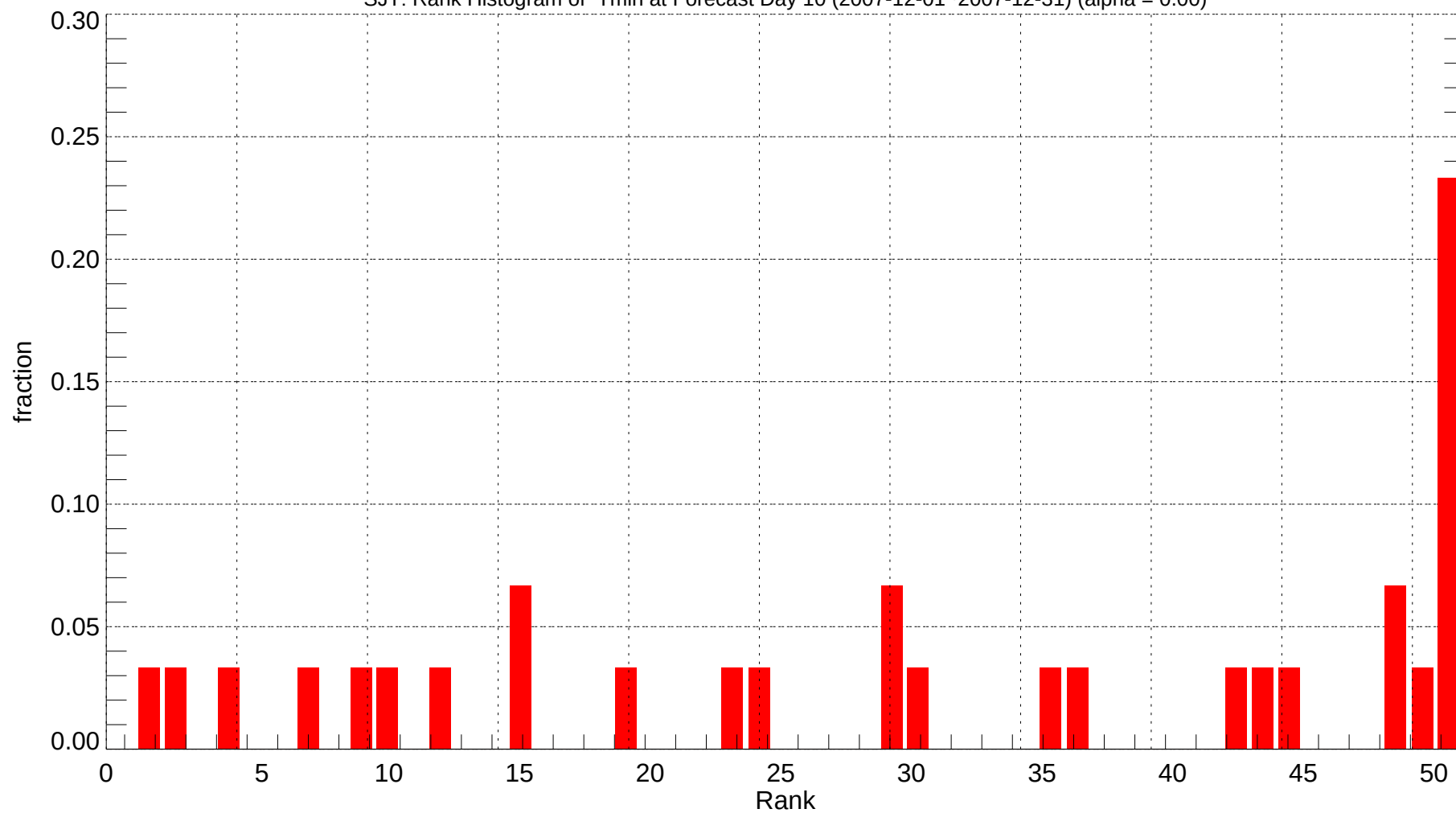
SJT: Rank Histogram of Tmin at Forecast Day 10 (2007-12-01~2007-12-31) (alpha = 0.00)
