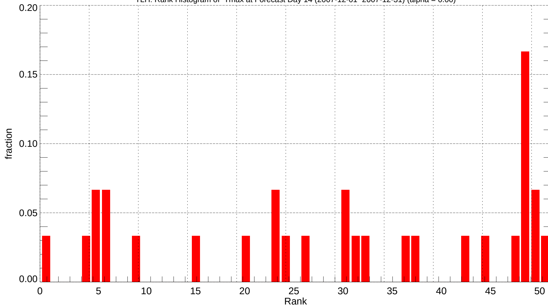
TLH: Rank Histogram of Tmax at Forecast Day 14 (2007-12-01~2007-12-31) (alpha = 0.00)
