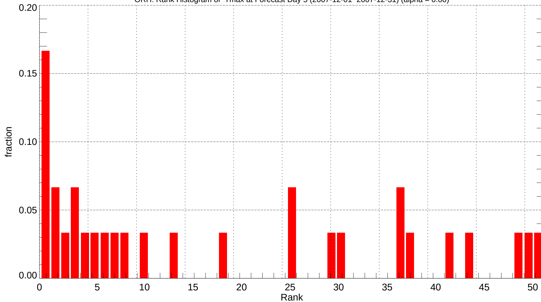
ORH: Rank Histogram of Tmax at Forecast Day 5 (2007-12-01~2007-12-31) (alpha = 0.00)
