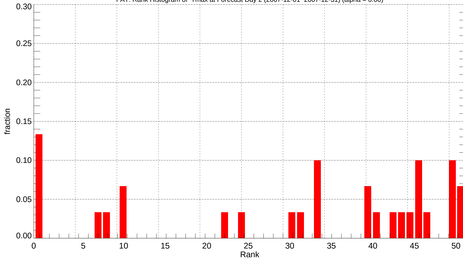
FAT: Rank Histogram of Tmax at Forecast Day 2 (2007-12-01~2007-12-31) (alpha = 0.00)
