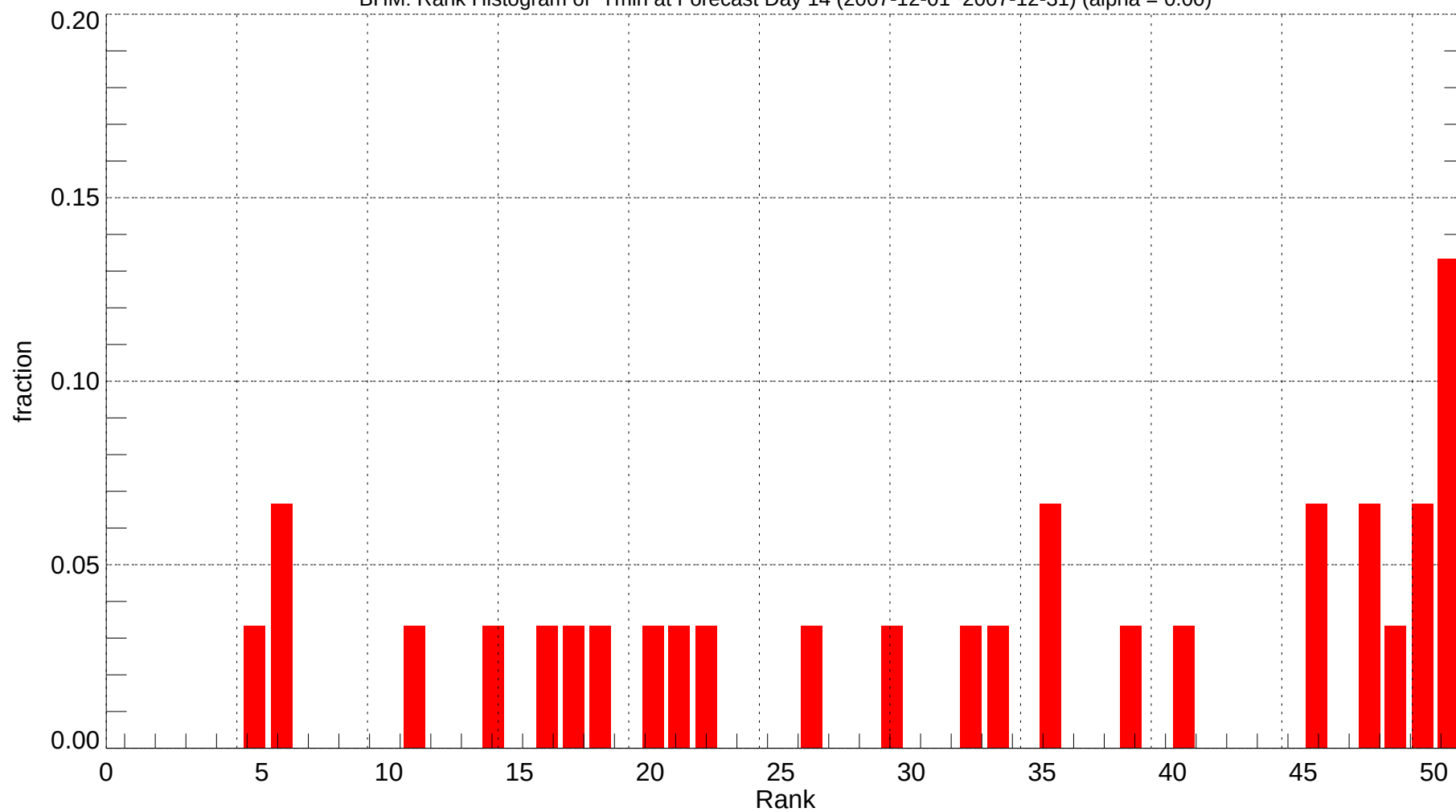
BHM: Rank Histogram of Tmin at Forecast Day 14 (2007-12-01~2007-12-31) (alpha = 0.00)
