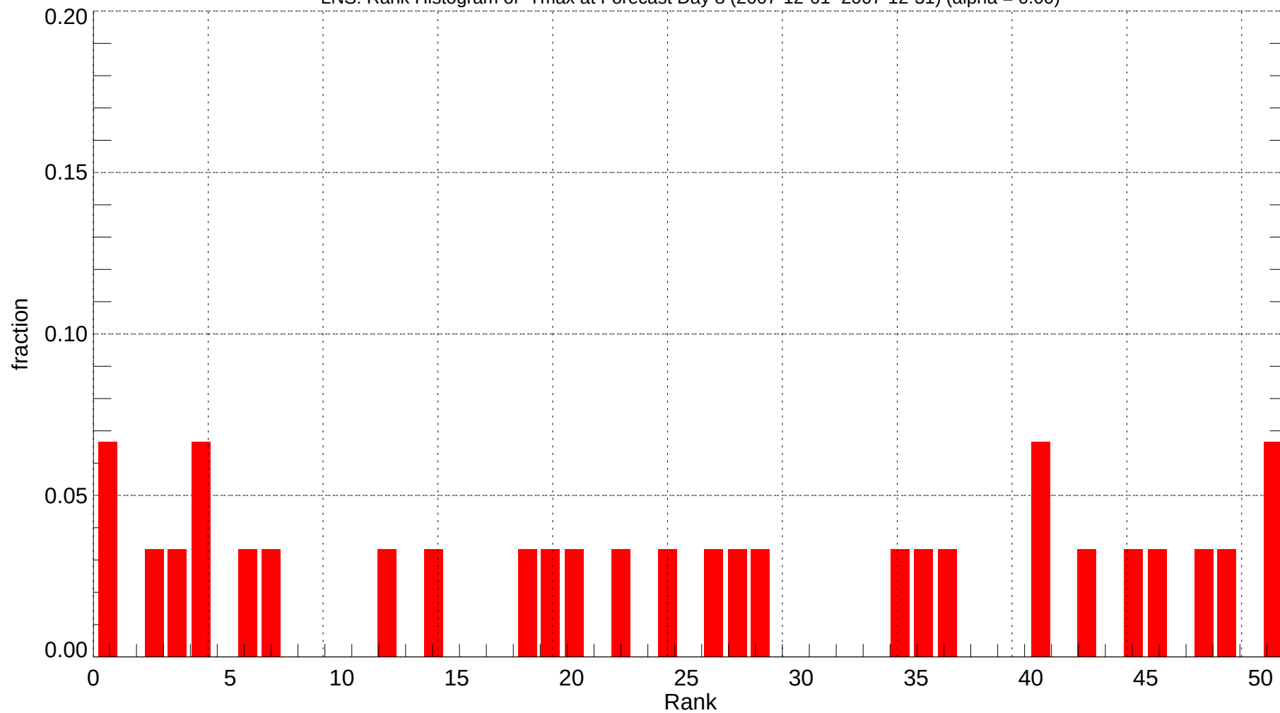
LNS: Rank Histogram of Tmax at Forecast Day 8 (2007-12-01~2007-12-31) (alpha = 0.00)
