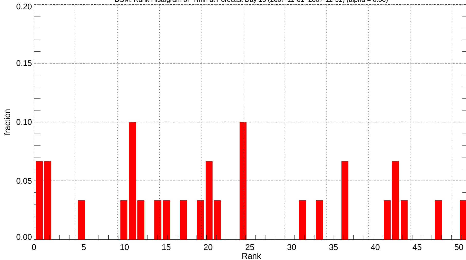
BGM: Rank Histogram of Tmin at Forecast Day 13 (2007-12-01~2007-12-31) (alpha = 0.00)
