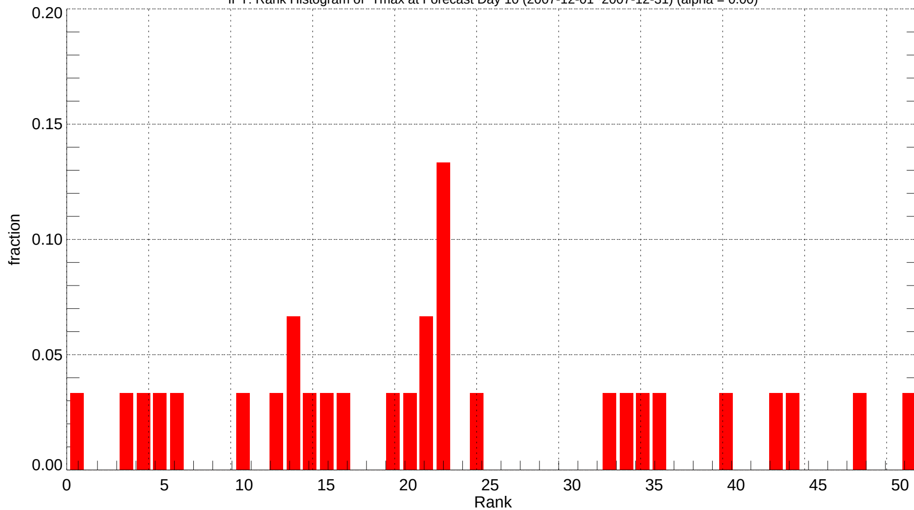
IPT: Rank Histogram of Tmax at Forecast Day 10 (2007-12-01~2007-12-31) (alpha = 0.00)
