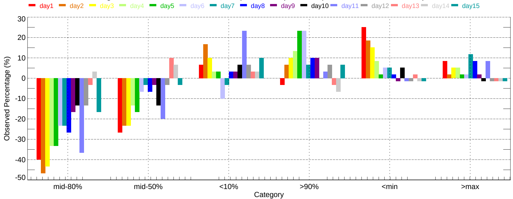
Observed Percentage Deviation of Ensembles - DBQ: Min Temperature (2007-12-01~2007-12-31)
