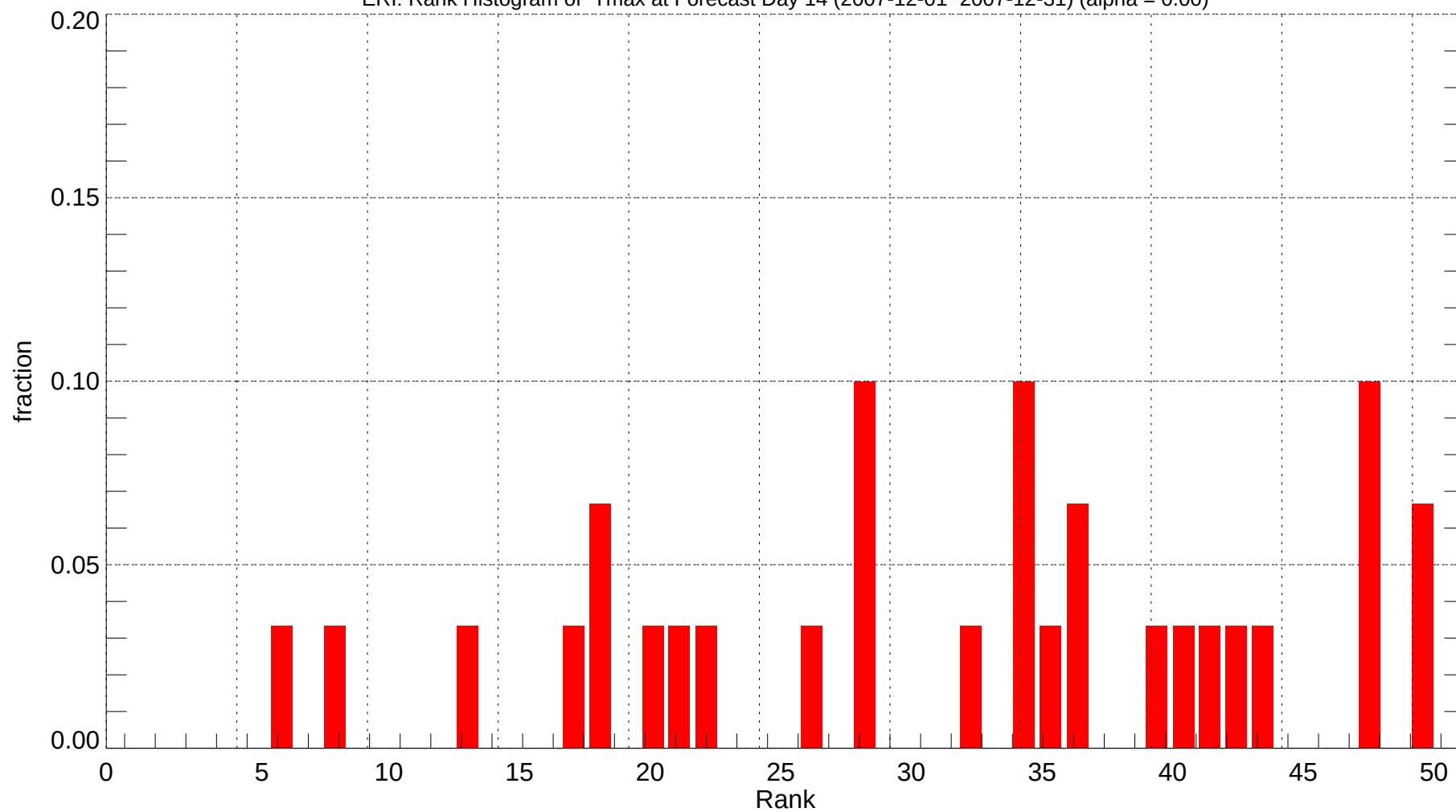
ERI: Rank Histogram of Tmax at Forecast Day 14 (2007-12-01~2007-12-31) (alpha = 0.00)
