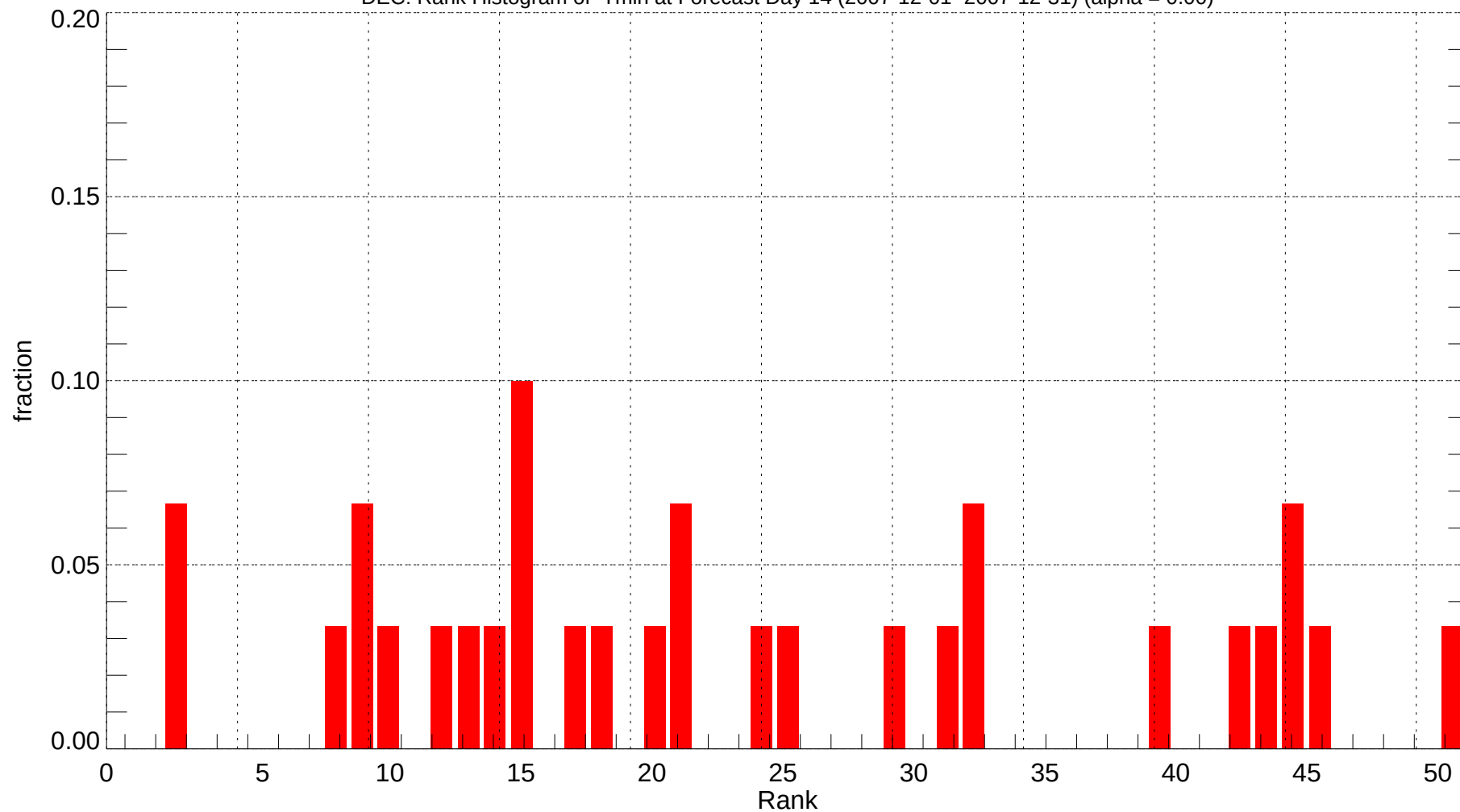
DEC: Rank Histogram of Tmin at Forecast Day 14 (2007-12-01~2007-12-31) (alpha = 0.00)
