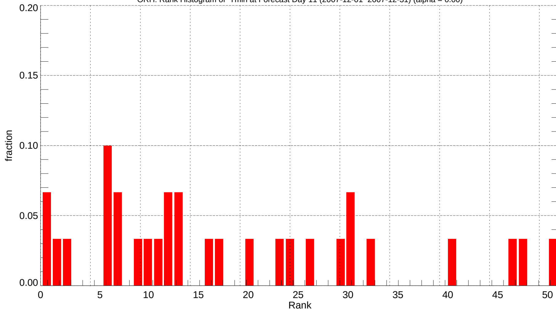
ORH: Rank Histogram of Tmin at Forecast Day 11 (2007-12-01~2007-12-31) (alpha = 0.00)
