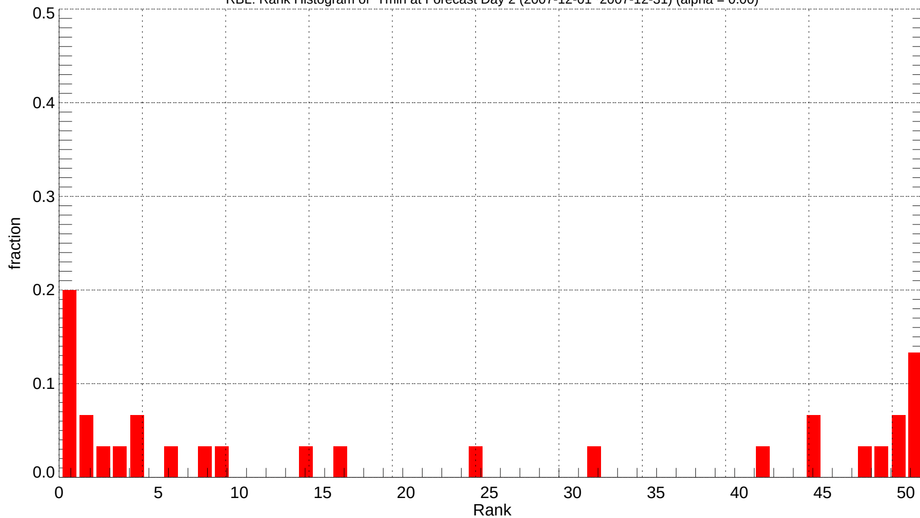
RBL: Rank Histogram of Tmin at Forecast Day 2 (2007-12-01~2007-12-31) (alpha = 0.00)
