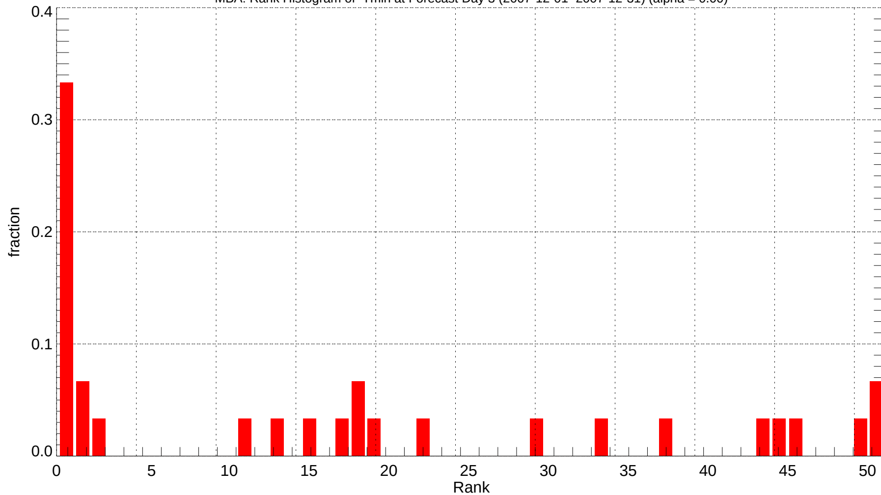
MBA: Rank Histogram of Tmin at Forecast Day 3 (2007-12-01~2007-12-31) (alpha = 0.00)
