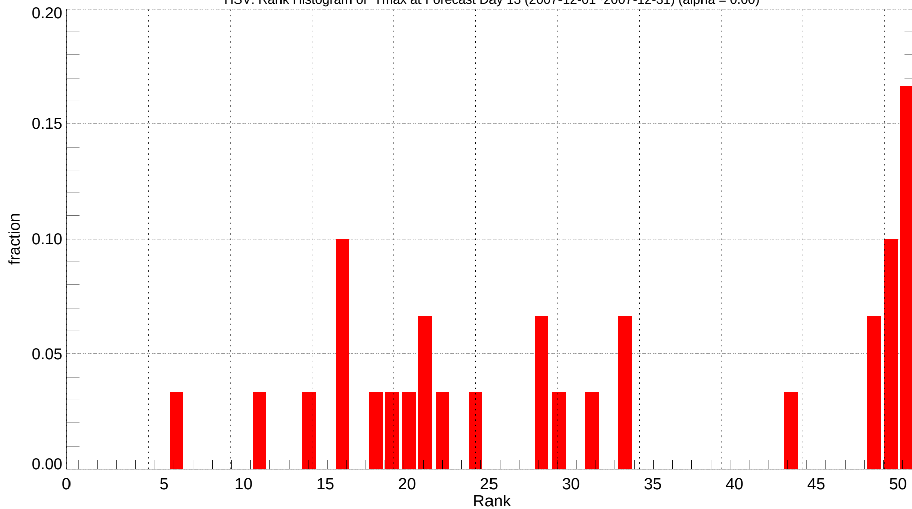
HSV: Rank Histogram of Tmax at Forecast Day 13 (2007-12-01~2007-12-31) (alpha = 0.00)
