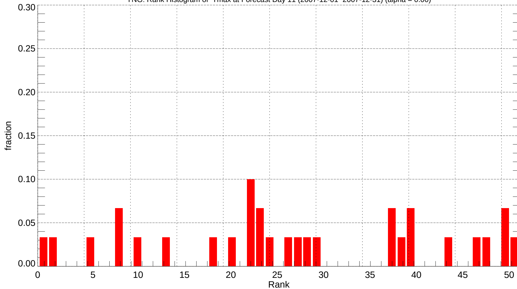
YNG: Rank Histogram of Tmax at Forecast Day 11 (2007-12-01~2007-12-31) (alpha = 0.00)
