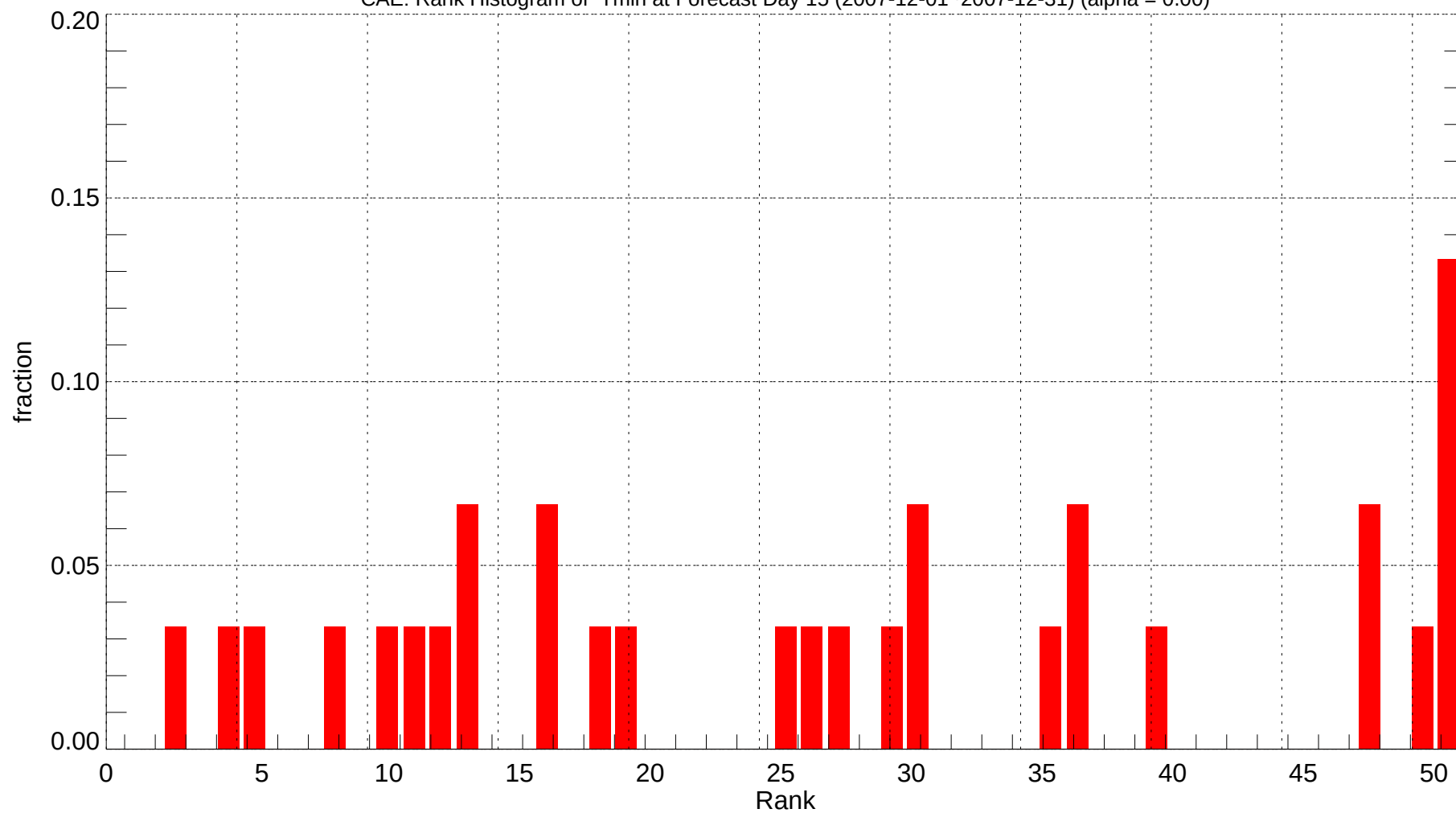
CAE: Rank Histogram of Tmin at Forecast Day 15 (2007-12-01~2007-12-31) (alpha = 0.00)
