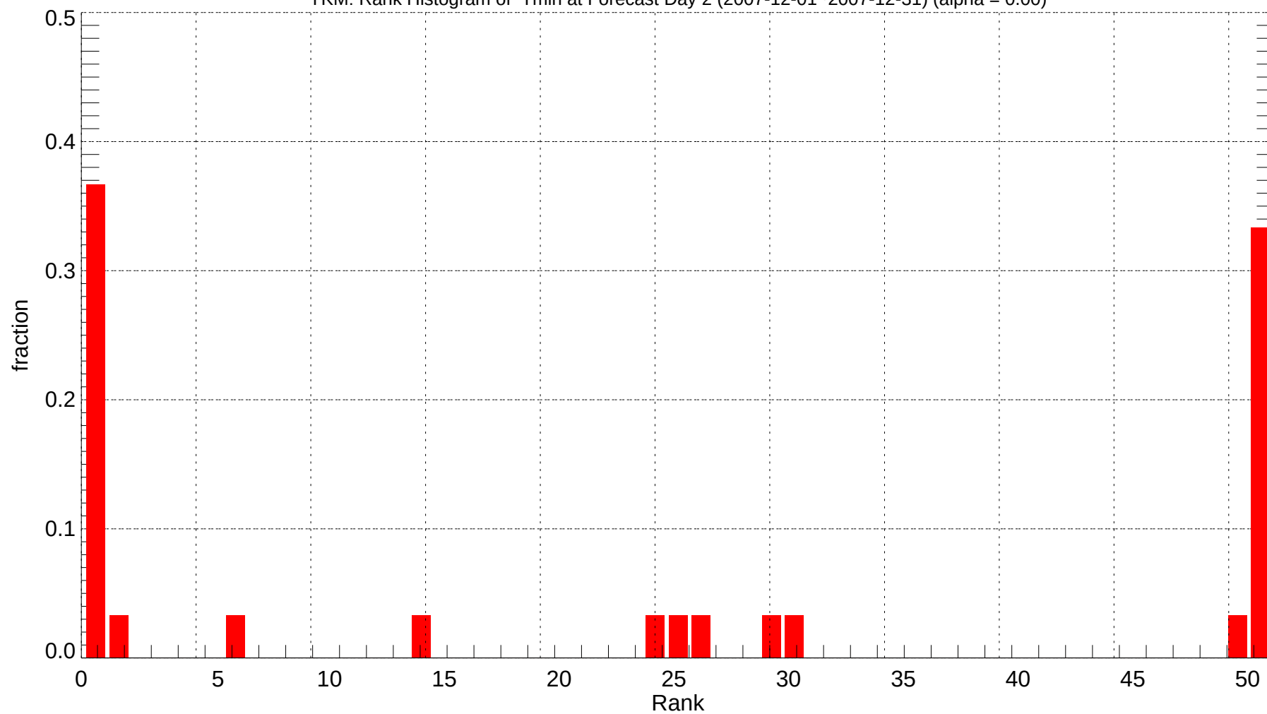
YKM: Rank Histogram of Tmin at Forecast Day 2 (2007-12-01~2007-12-31) (alpha = 0.00)
