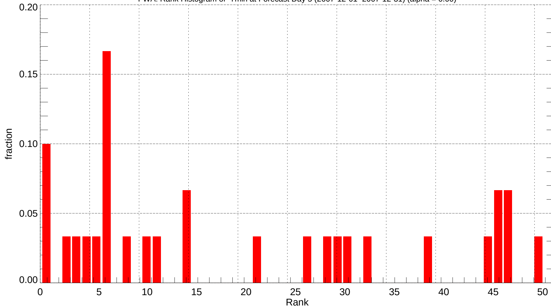
FWA: Rank Histogram of Tmin at Forecast Day 5 (2007-12-01~2007-12-31) (alpha = 0.00)
