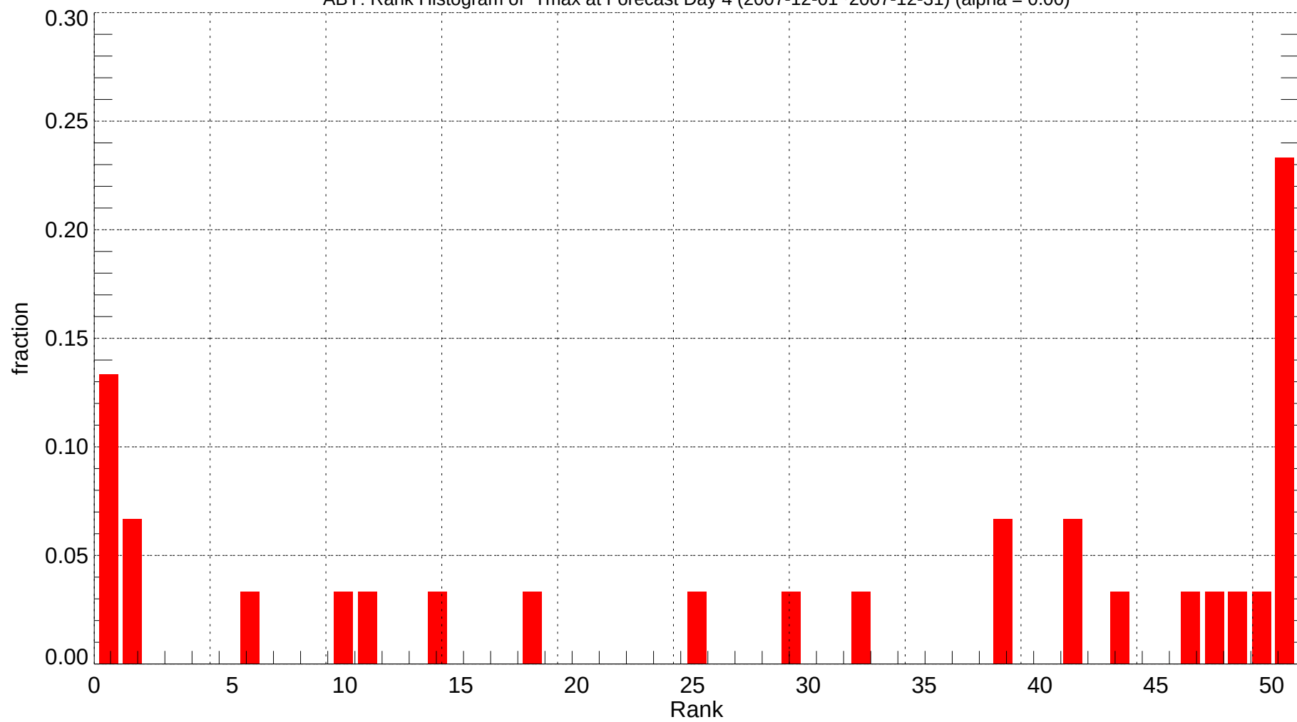
ABY: Rank Histogram of Tmax at Forecast Day 4 (2007-12-01~2007-12-31) (alpha = 0.00)
