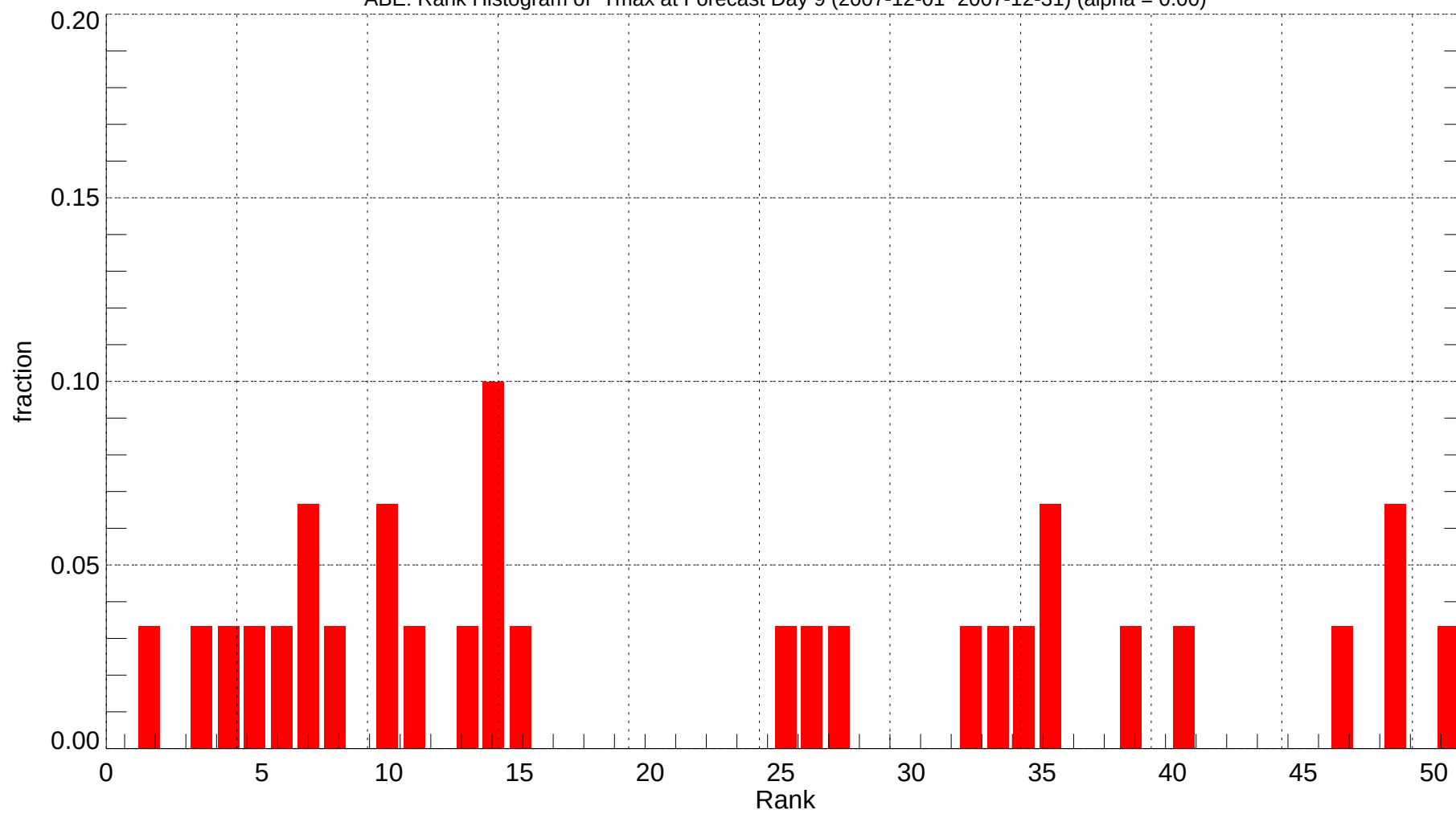
ABE: Rank Histogram of Tmax at Forecast Day 9 (2007-12-01~2007-12-31) (alpha = 0.00)
