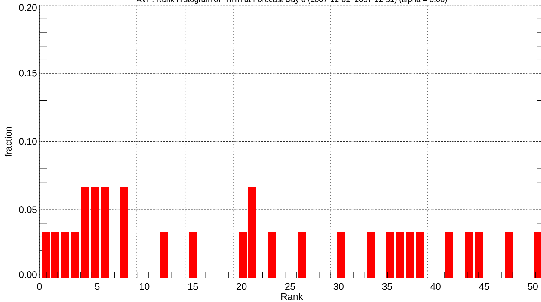
AVP: Rank Histogram of Tmin at Forecast Day 8 (2007-12-01~2007-12-31) (alpha = 0.00)
