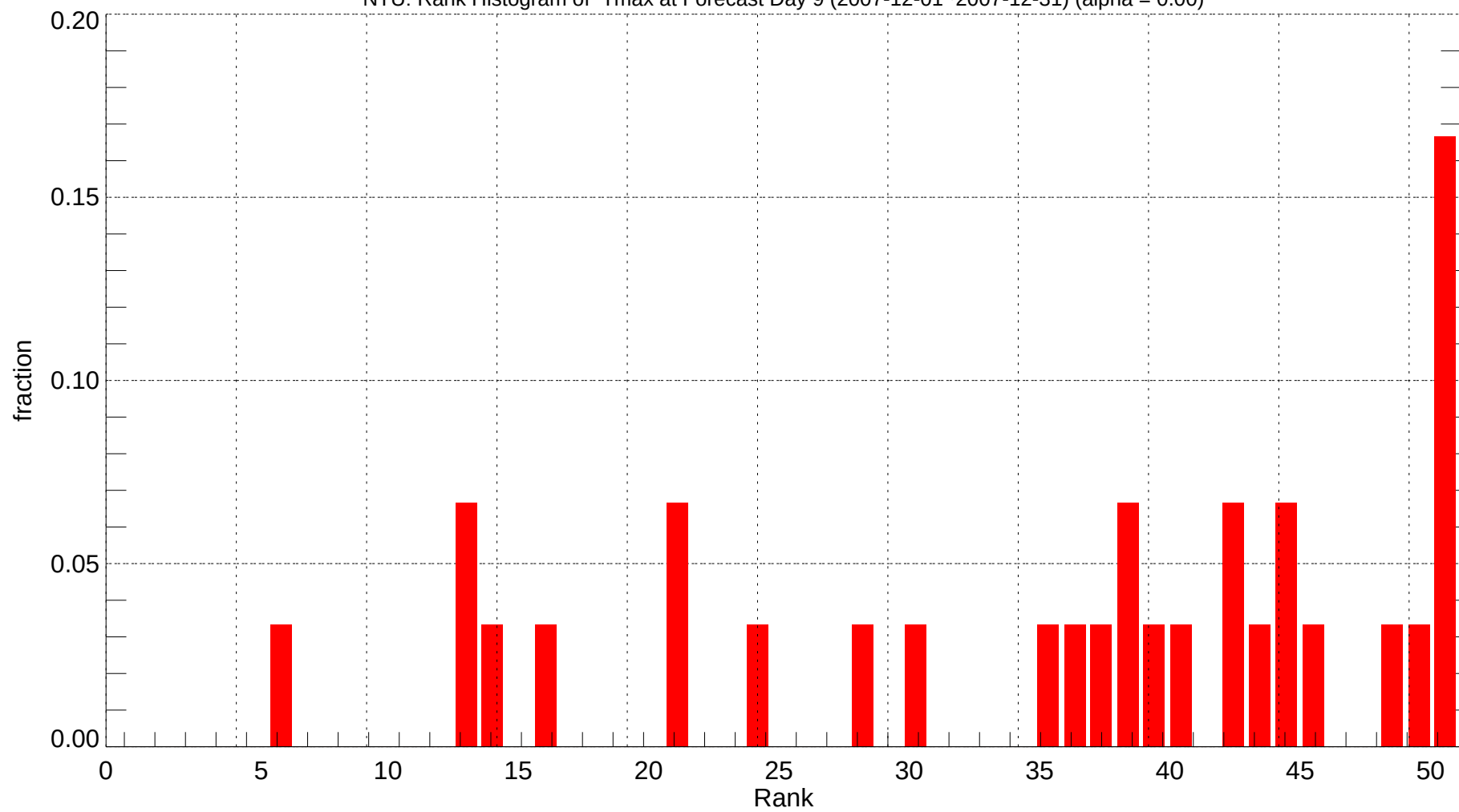
NTU: Rank Histogram of Tmax at Forecast Day 9 (2007-12-01~2007-12-31) (alpha = 0.00)
