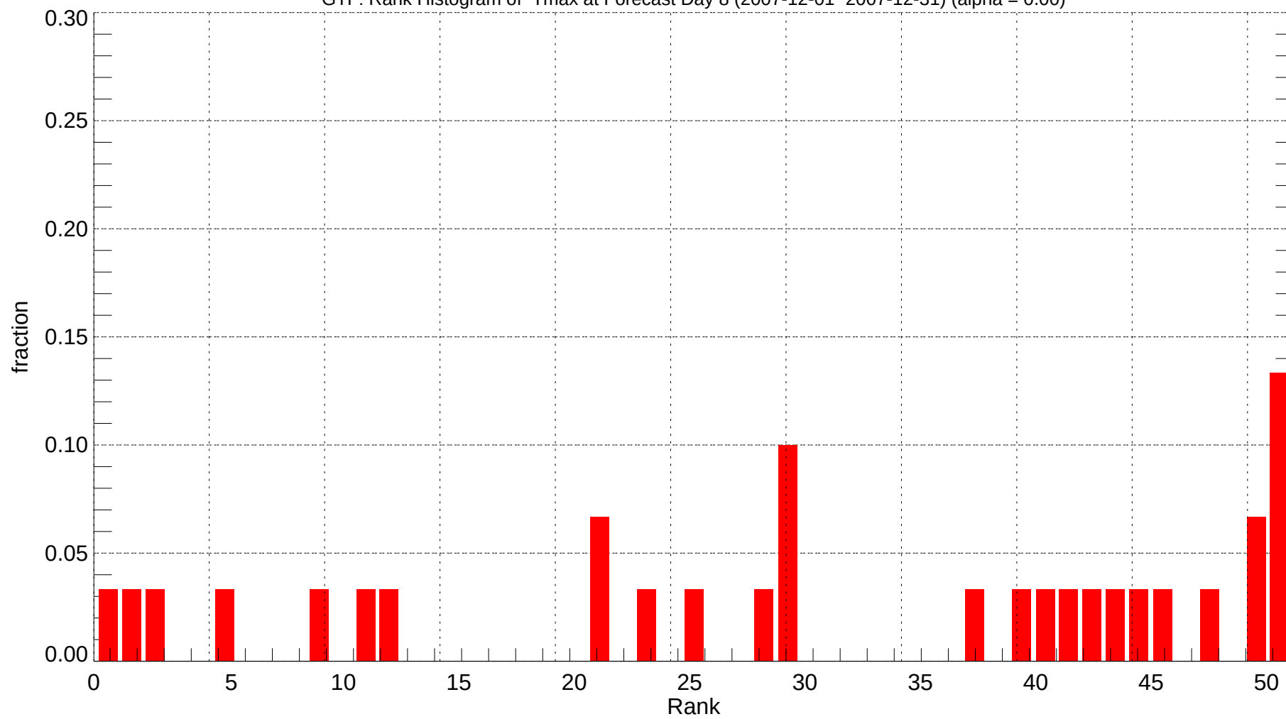
GTF: Rank Histogram of Tmax at Forecast Day 8 (2007-12-01~2007-12-31) (alpha = 0.00)
