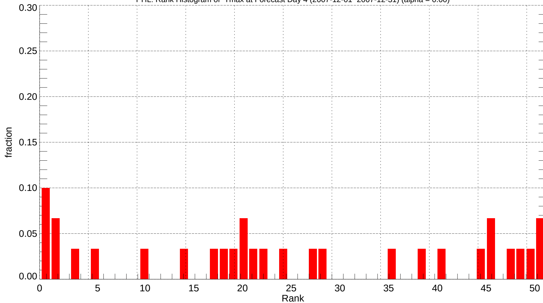
PHL: Rank Histogram of Tmax at Forecast Day 4 (2007-12-01~2007-12-31) (alpha = 0.00)
