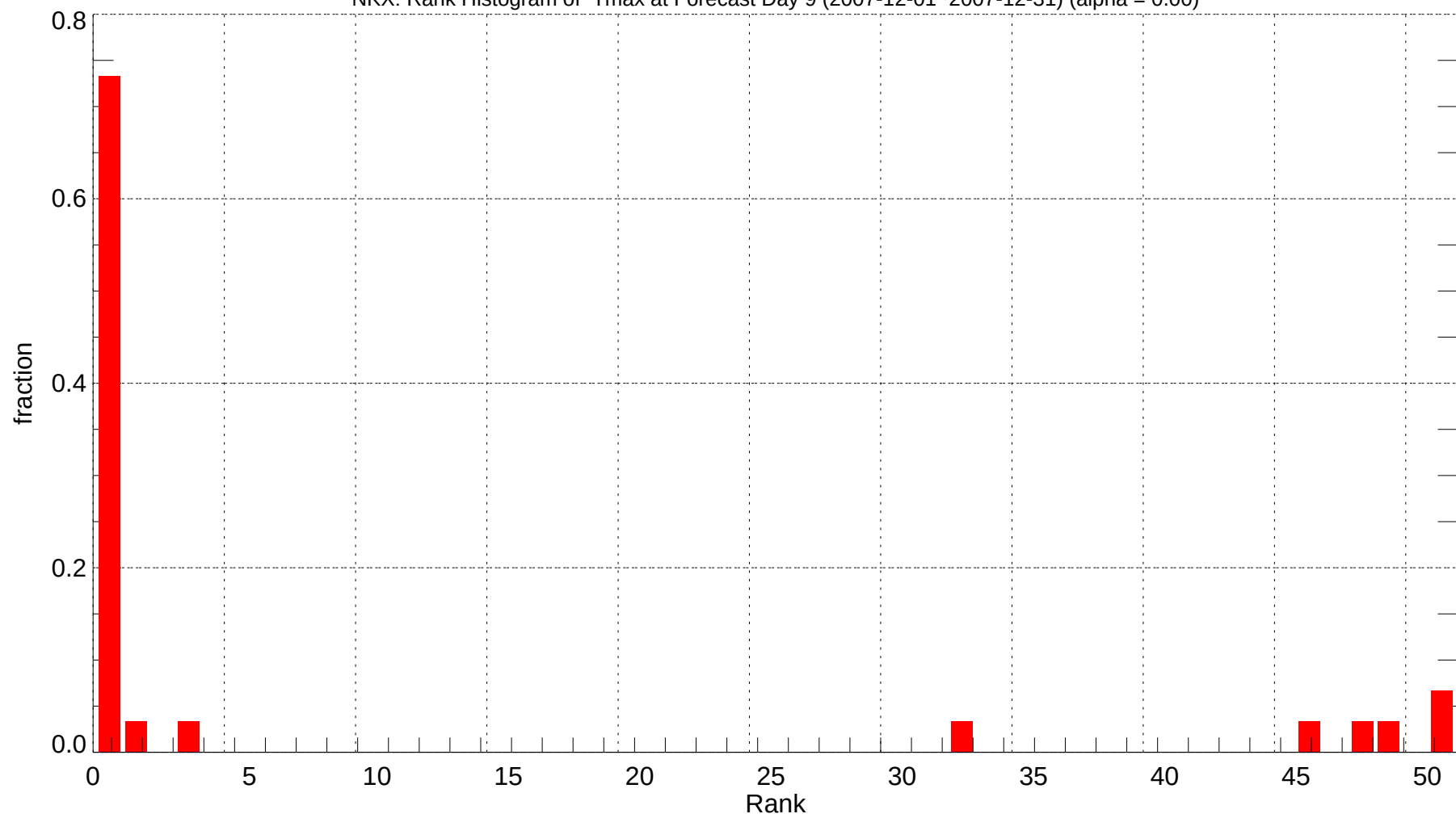
NKX: Rank Histogram of Tmax at Forecast Day 9 (2007-12-01~2007-12-31) (alpha = 0.00)
