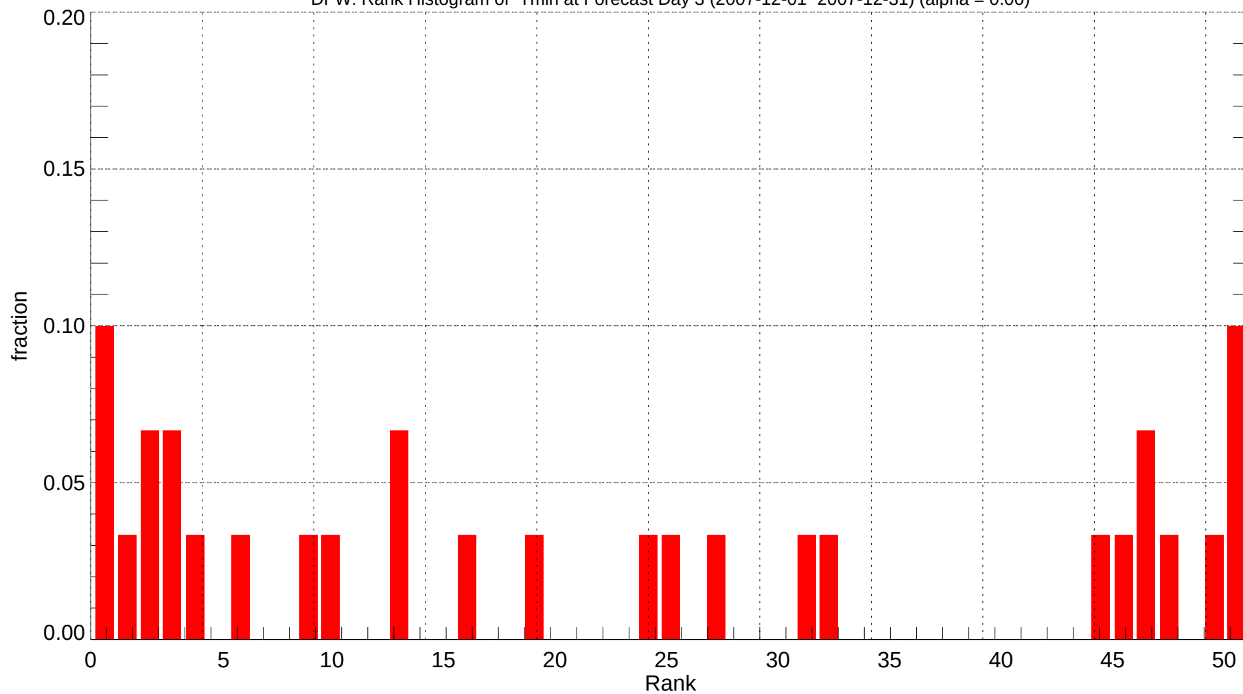
DFW: Rank Histogram of Tmin at Forecast Day 3 (2007-12-01~2007-12-31) (alpha = 0.00)
