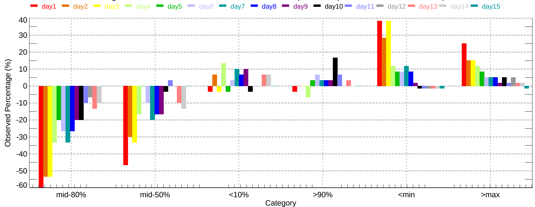
Observed Percentage Deviation of Ensembles - RAP: Max Temperature (2007-12-01~2007-12-31)
