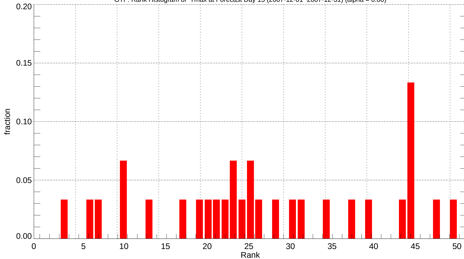
GTF: Rank Histogram of Tmax at Forecast Day 15 (2007-12-01~2007-12-31) (alpha = 0.00)
