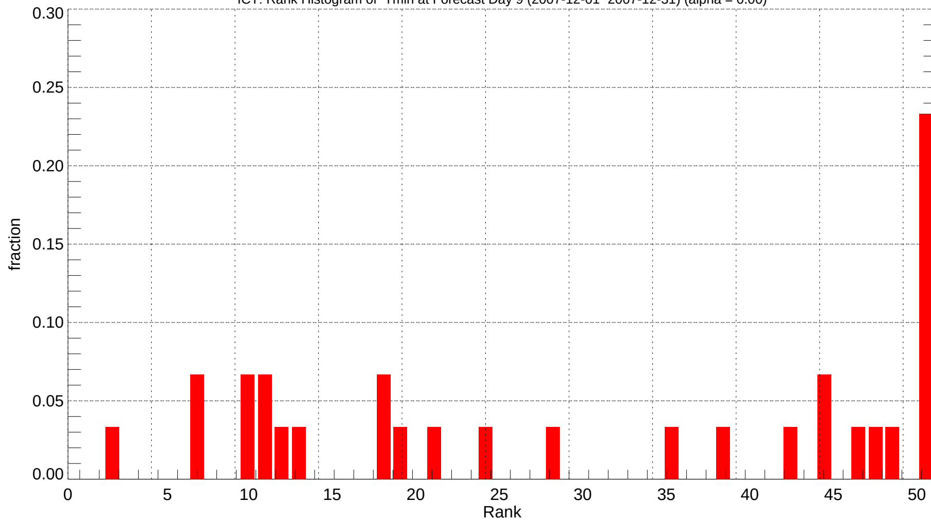
ICT: Rank Histogram of Tmin at Forecast Day 9 (2007-12-01~2007-12-31) (alpha = 0.00)
