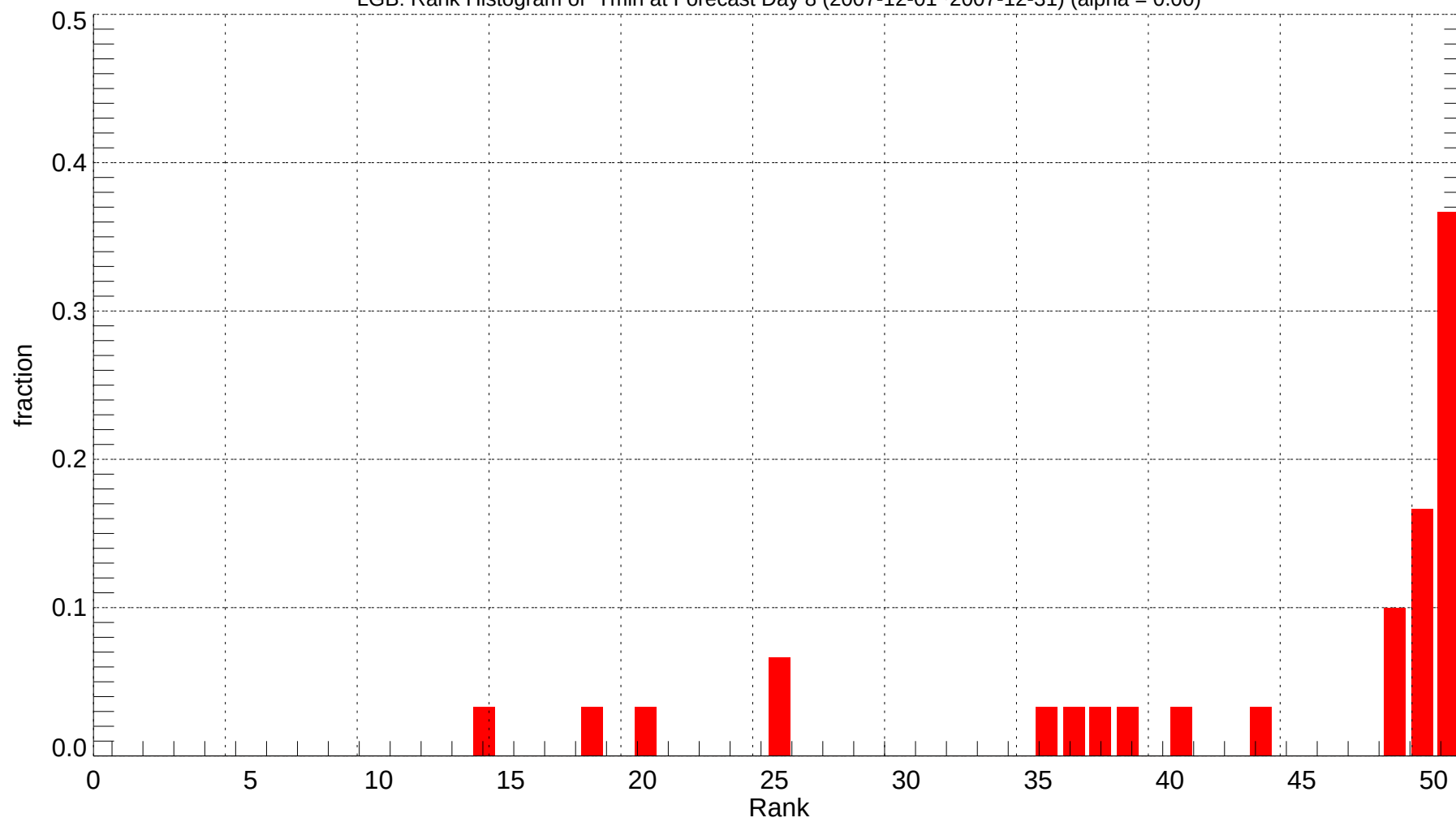
LGB: Rank Histogram of Tmin at Forecast Day 8 (2007-12-01~2007-12-31) (alpha = 0.00)
