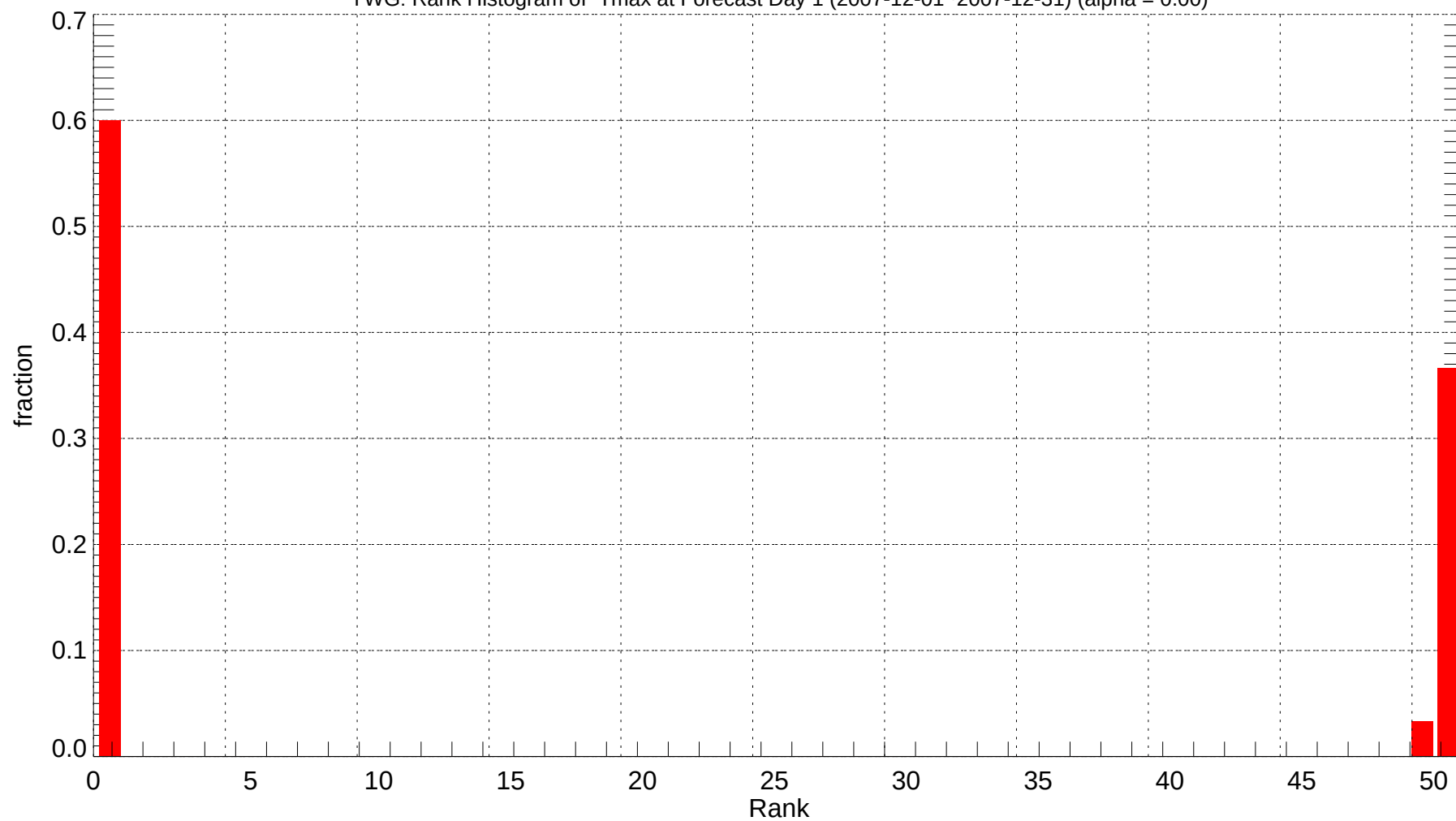
YWG: Rank Histogram of Tmax at Forecast Day 1 (2007-12-01~2007-12-31) (alpha = 0.00)
