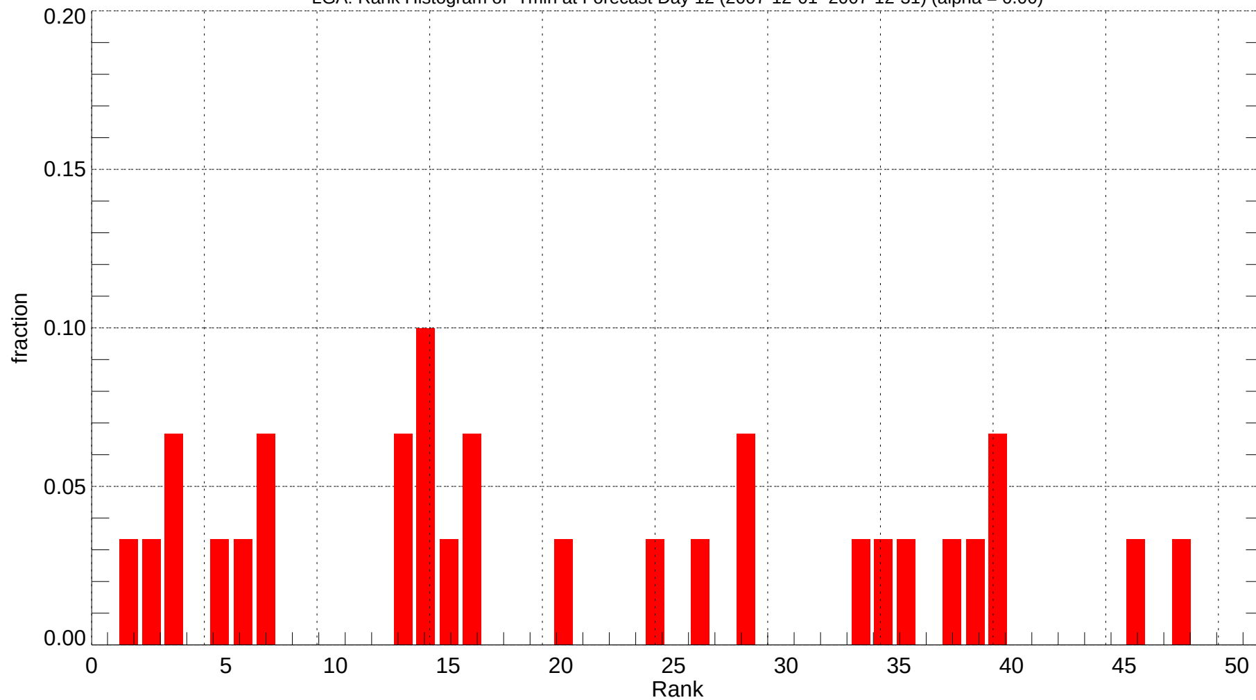
LGA: Rank Histogram of Tmin at Forecast Day 12 (2007-12-01~2007-12-31) (alpha = 0.00)
