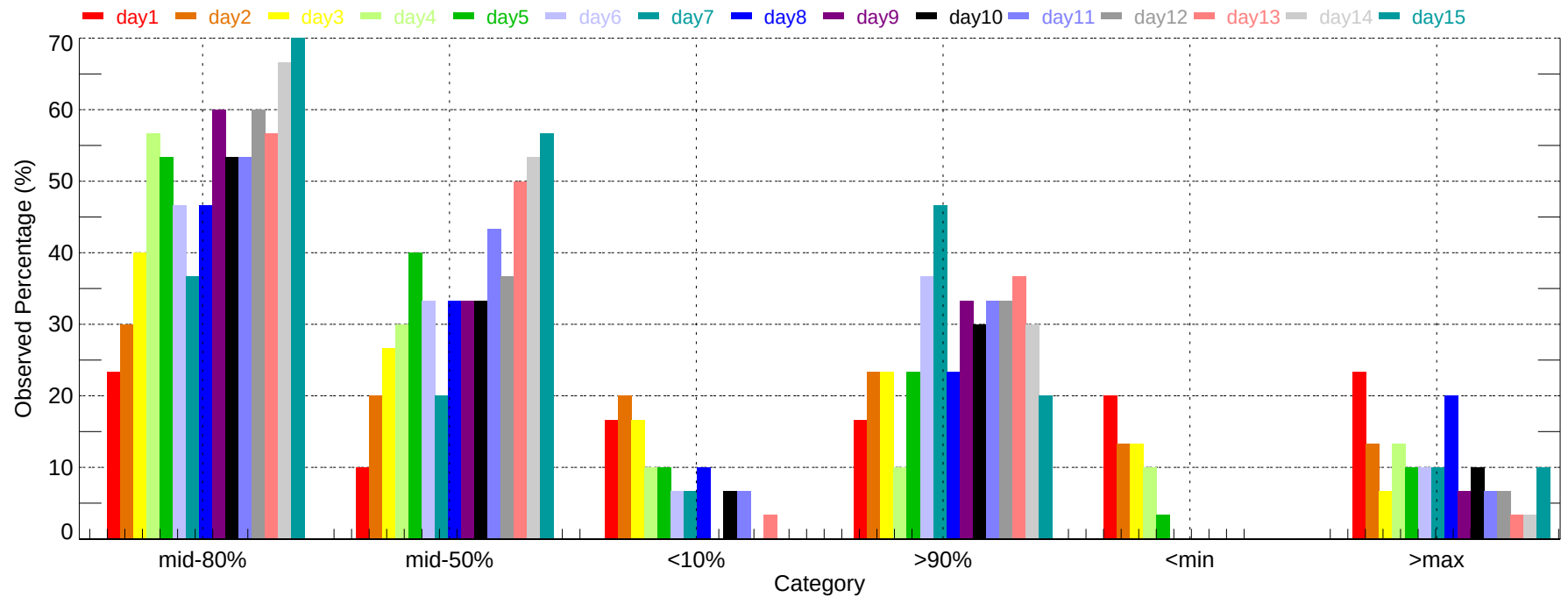
Observed Percentage of Ensembles - LEX: Max Temperature (2007-12-01~2007-12-31)
