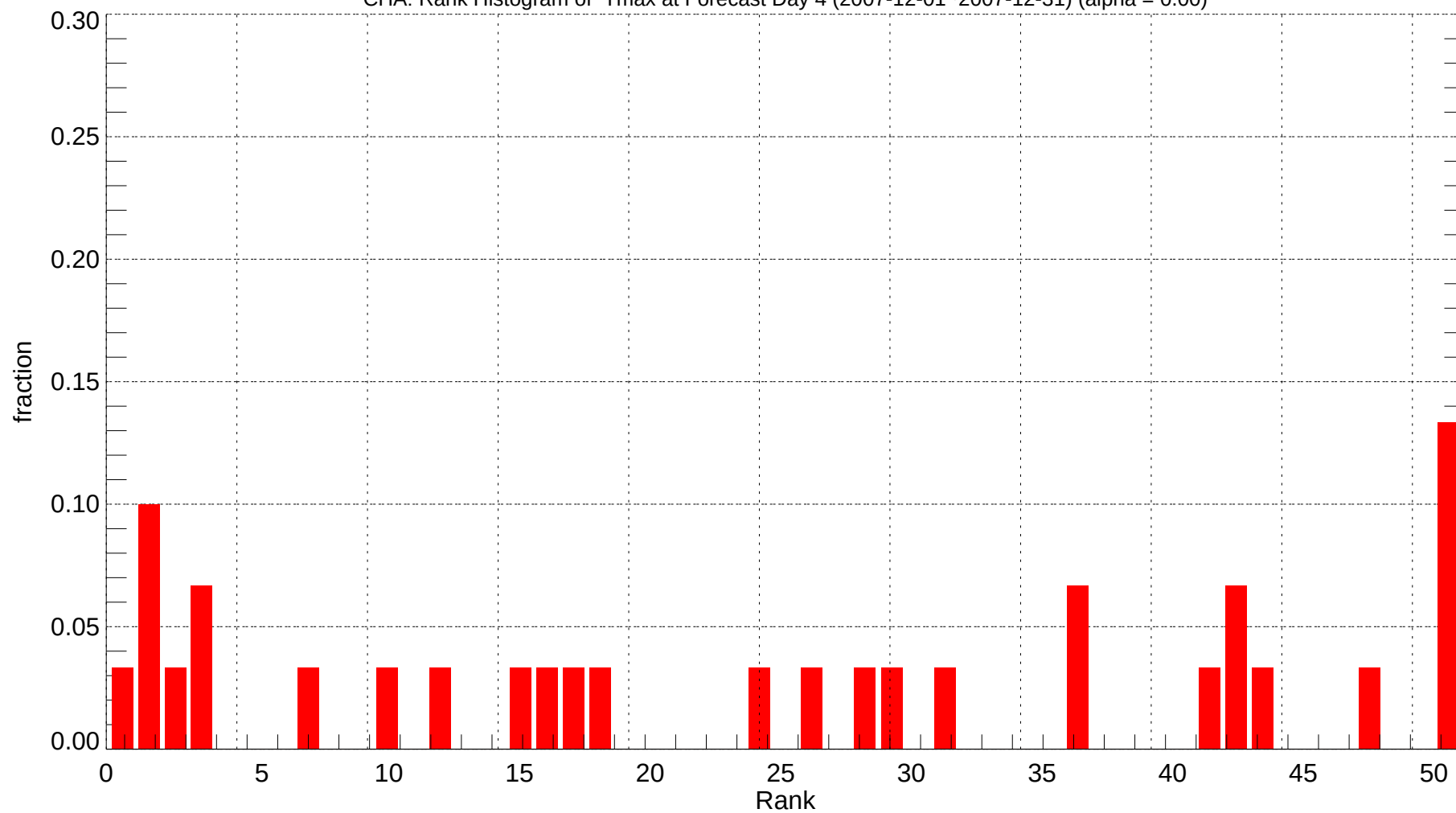
CHA: Rank Histogram of Tmax at Forecast Day 4 (2007-12-01~2007-12-31) (alpha = 0.00)
