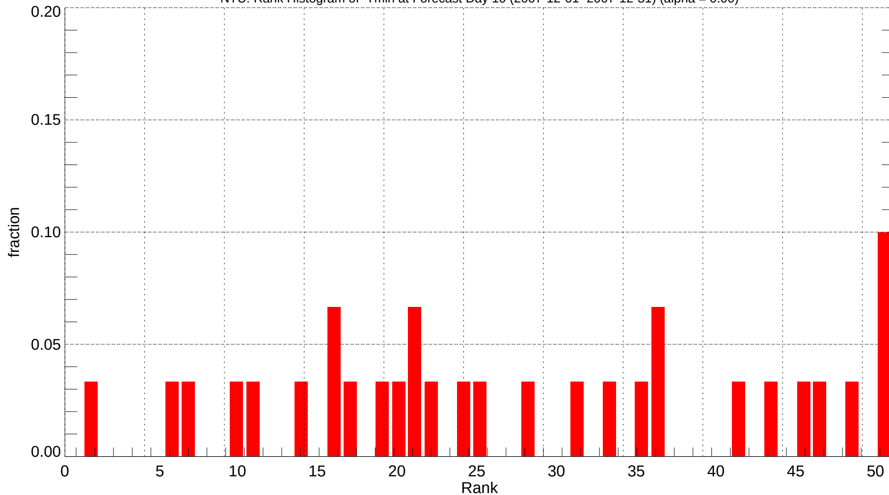
NTU: Rank Histogram of Tmin at Forecast Day 10 (2007-12-01~2007-12-31) (alpha = 0.00)
