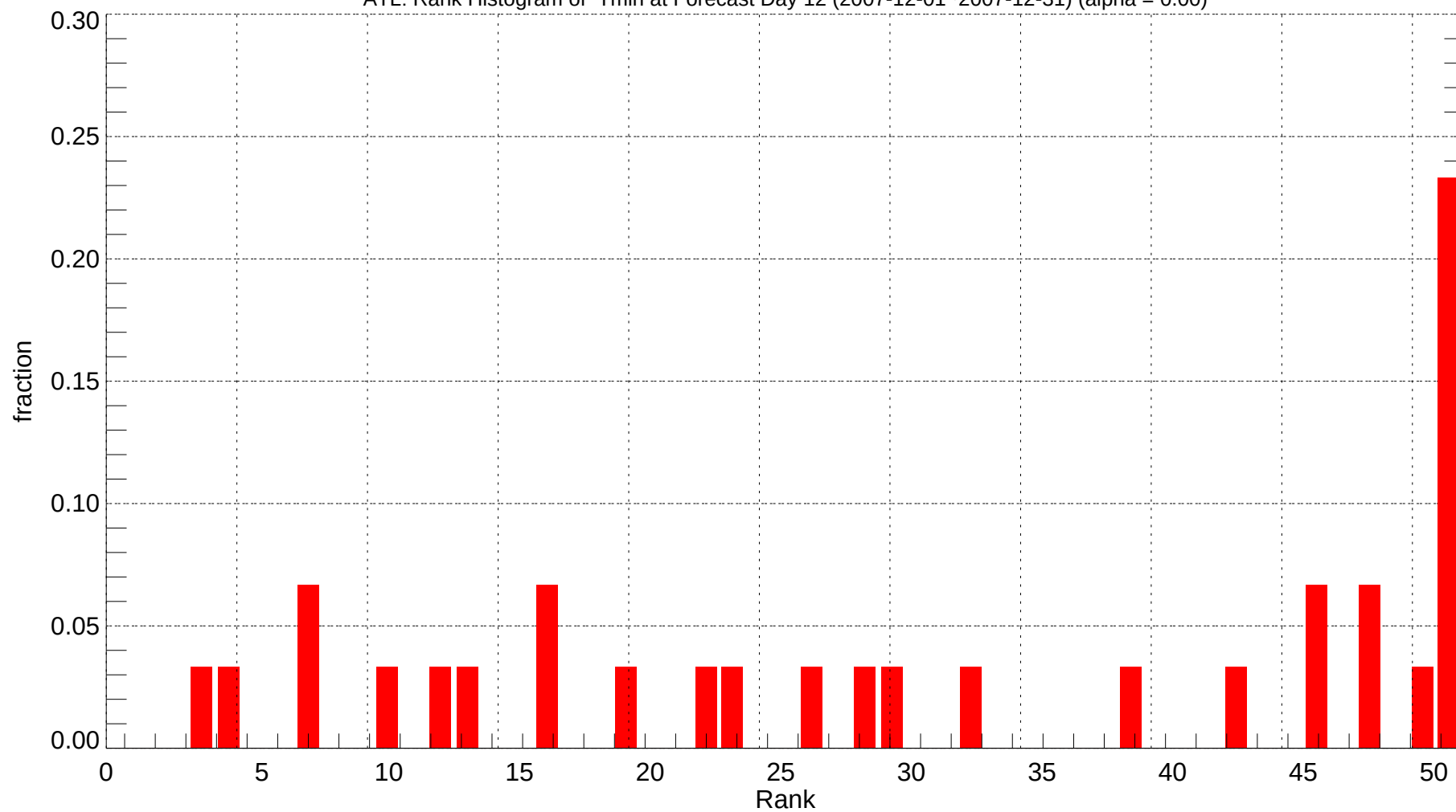
ATL: Rank Histogram of Tmin at Forecast Day 12 (2007-12-01~2007-12-31) (alpha = 0.00)
