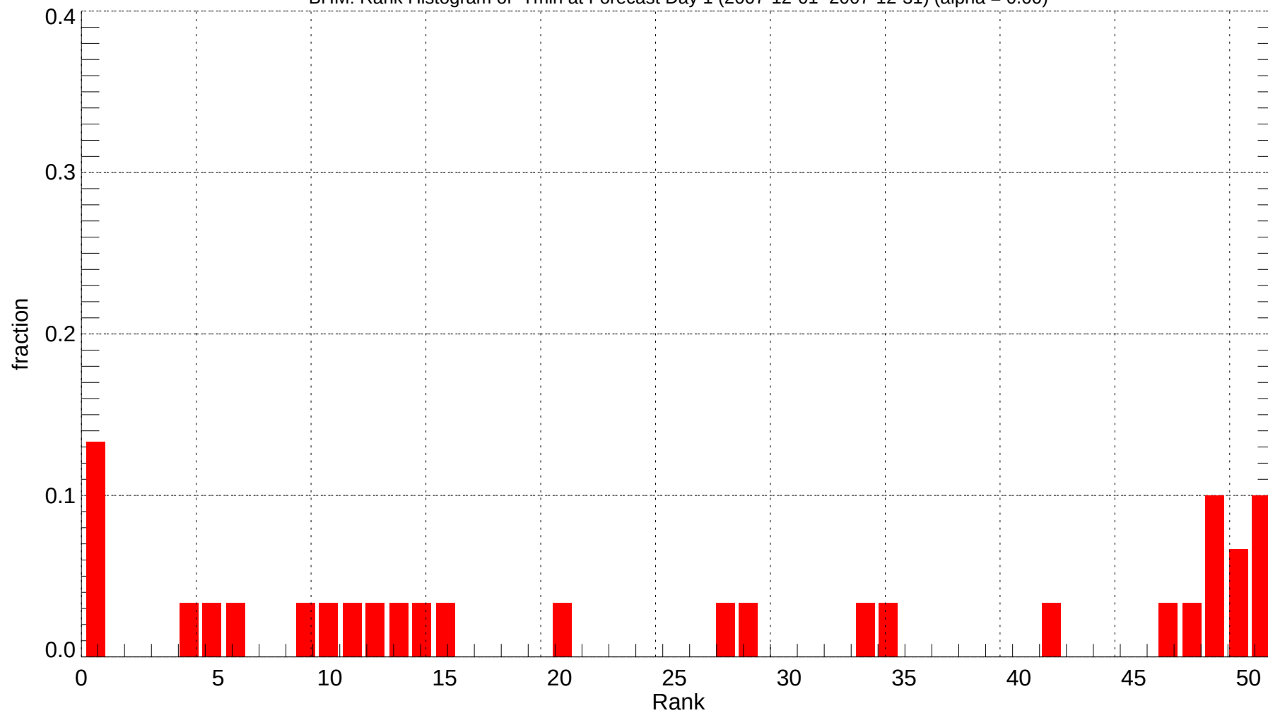
BHM: Rank Histogram of Tmin at Forecast Day 1 (2007-12-01~2007-12-31) (alpha = 0.00)
