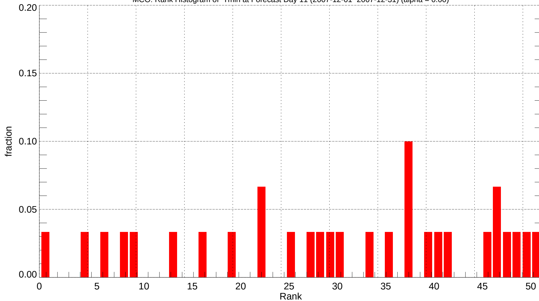
MCO: Rank Histogram of Tmin at Forecast Day 11 (2007-12-01~2007-12-31) (alpha = 0.00)
