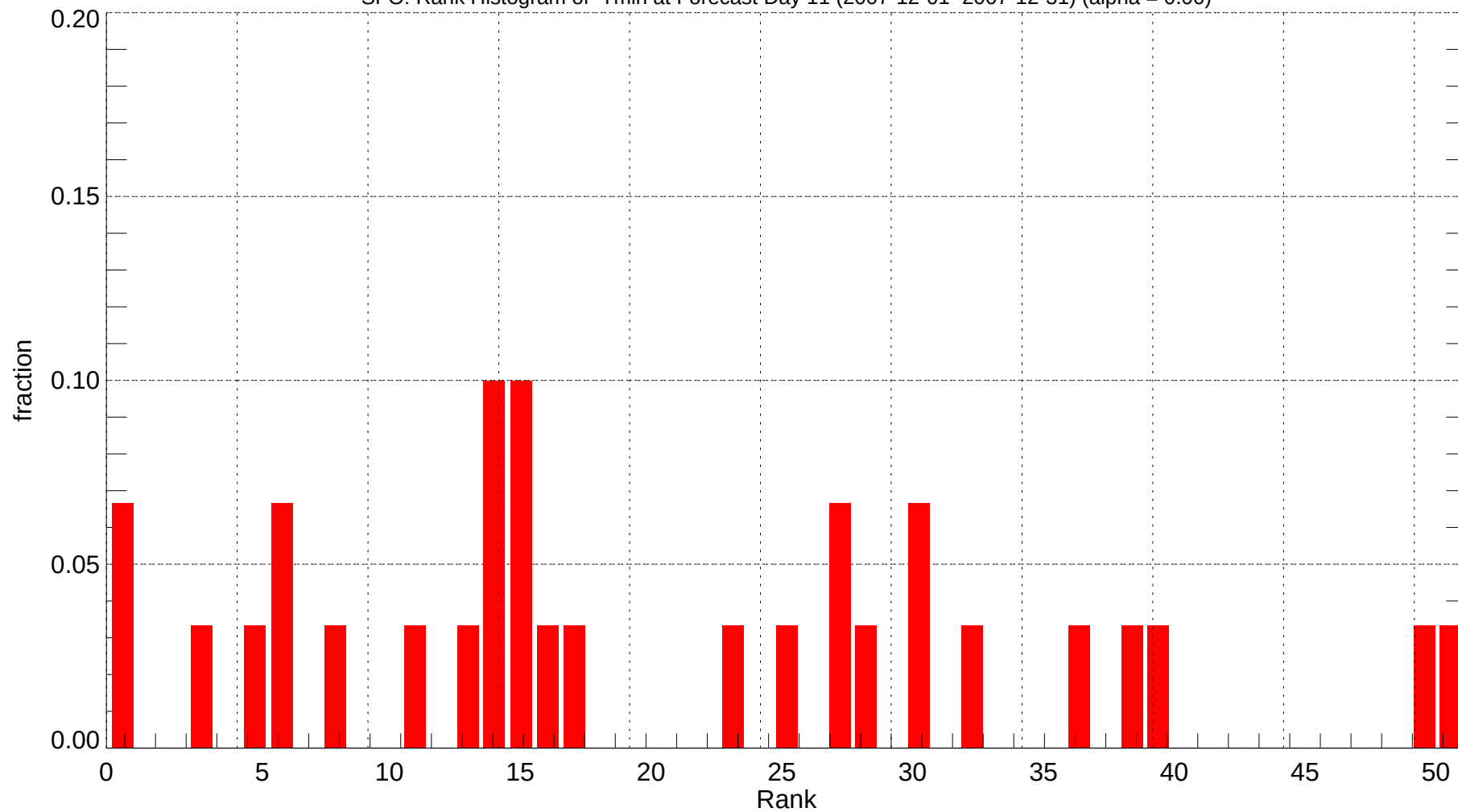
SFO: Rank Histogram of Tmin at Forecast Day 11 (2007-12-01~2007-12-31) (alpha = 0.00)
