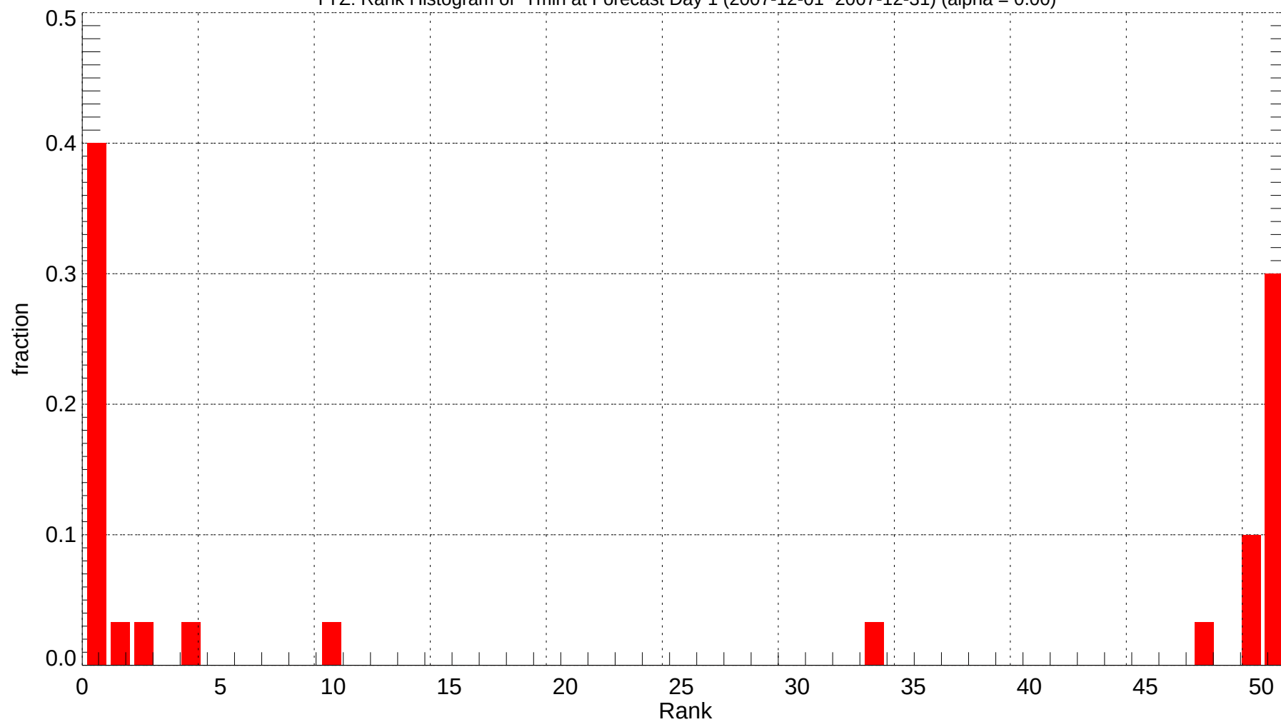
YYZ: Rank Histogram of Tmin at Forecast Day 1 (2007-12-01~2007-12-31) (alpha = 0.00)
