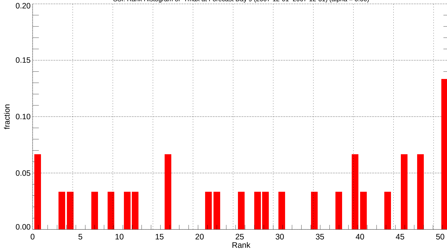
SSI: Rank Histogram of Tmax at Forecast Day 9 (2007-12-01~2007-12-31) (alpha = 0.00)
