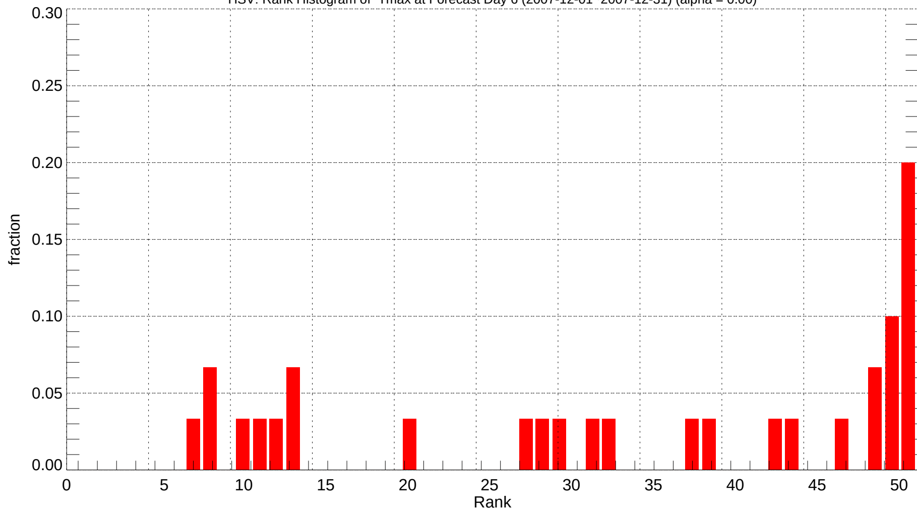
HSV: Rank Histogram of Tmax at Forecast Day 6 (2007-12-01~2007-12-31) (alpha = 0.00)
