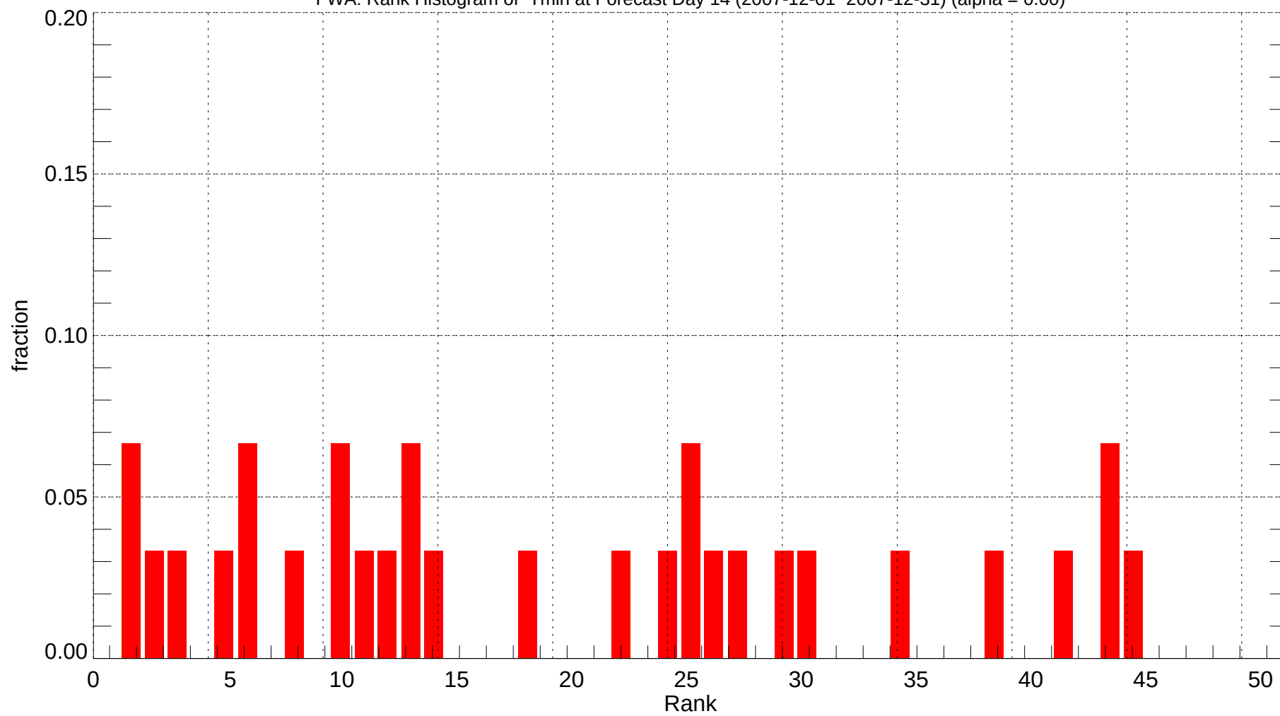
FWA: Rank Histogram of Tmin at Forecast Day 14 (2007-12-01~2007-12-31) (alpha = 0.00)
