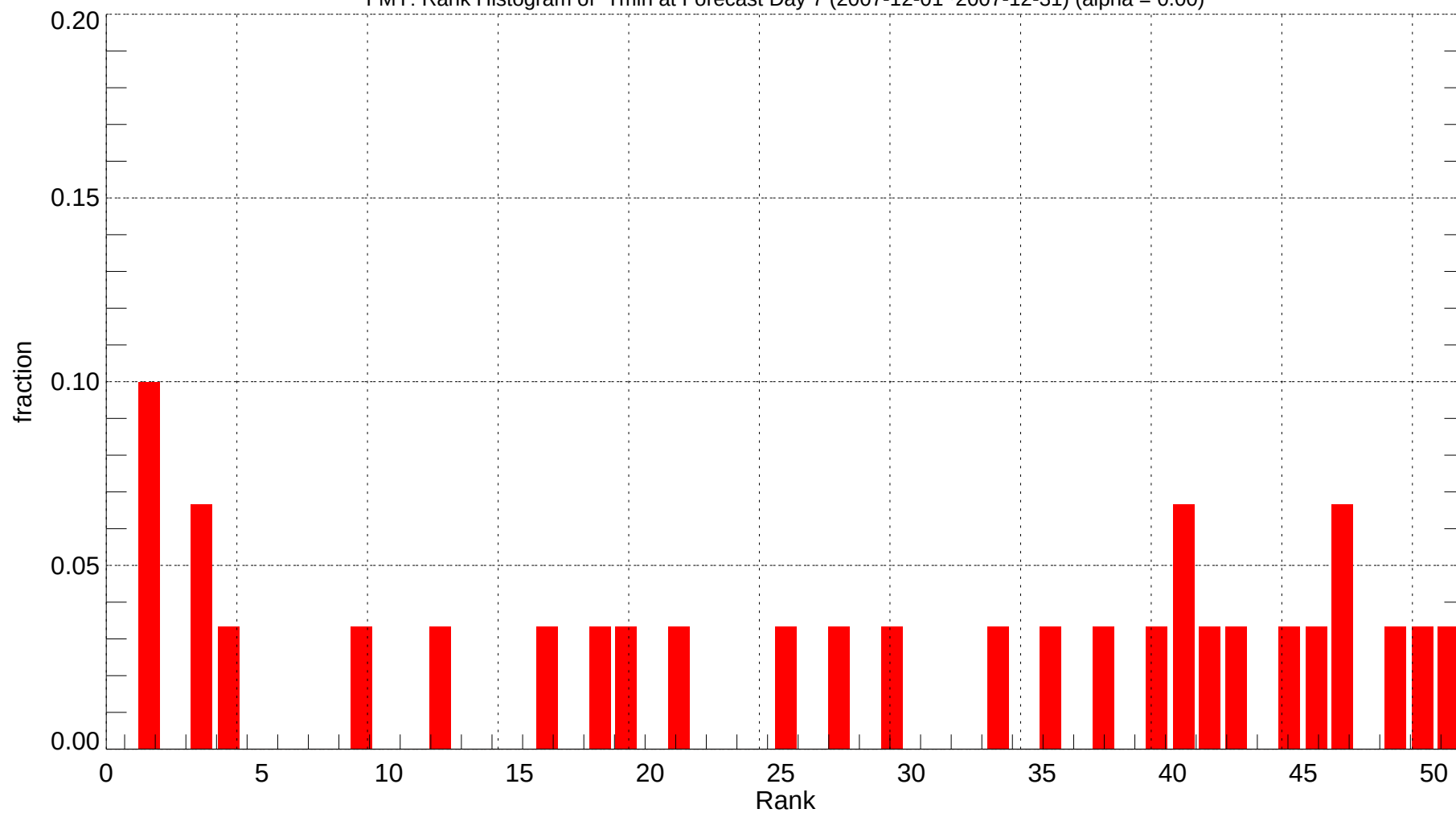
FMY: Rank Histogram of Tmin at Forecast Day 7 (2007-12-01~2007-12-31) (alpha = 0.00)
