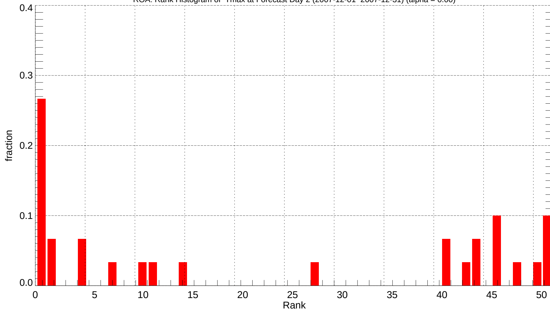
ROA: Rank Histogram of Tmax at Forecast Day 2 (2007-12-01~2007-12-31) (alpha = 0.00)
