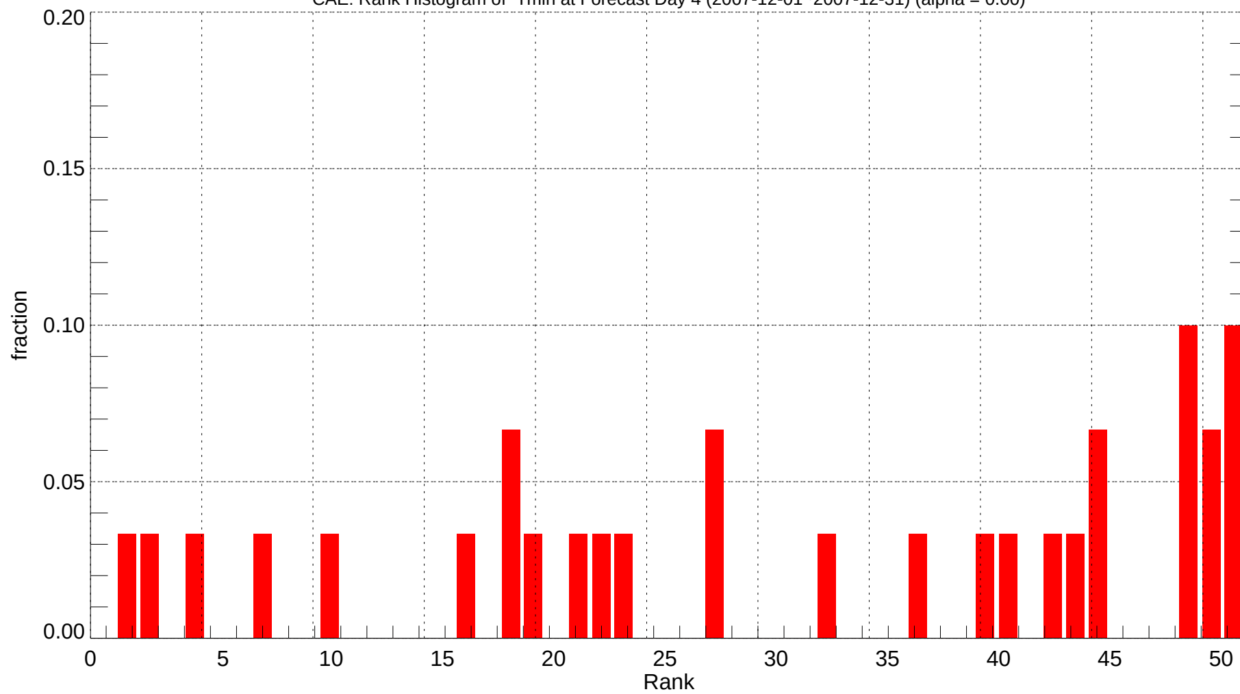
CAE: Rank Histogram of Tmin at Forecast Day 4 (2007-12-01~2007-12-31) (alpha = 0.00)
