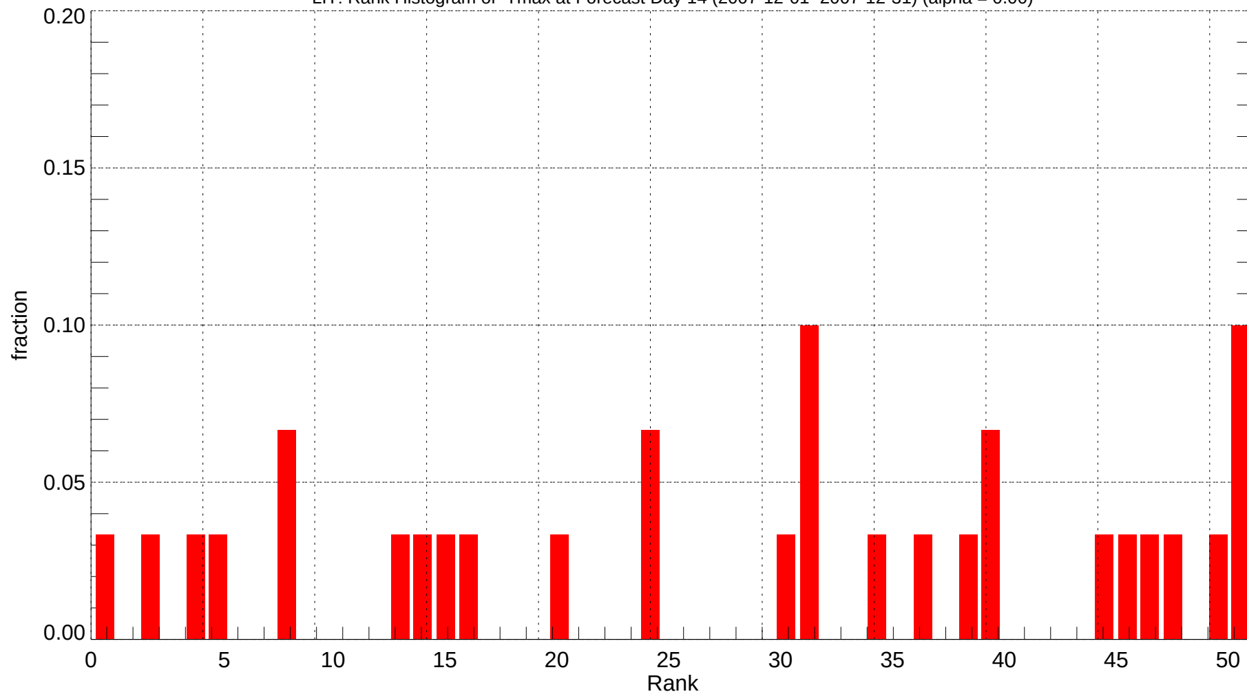
LIT: Rank Histogram of Tmax at Forecast Day 14 (2007-12-01~2007-12-31) (alpha = 0.00)
