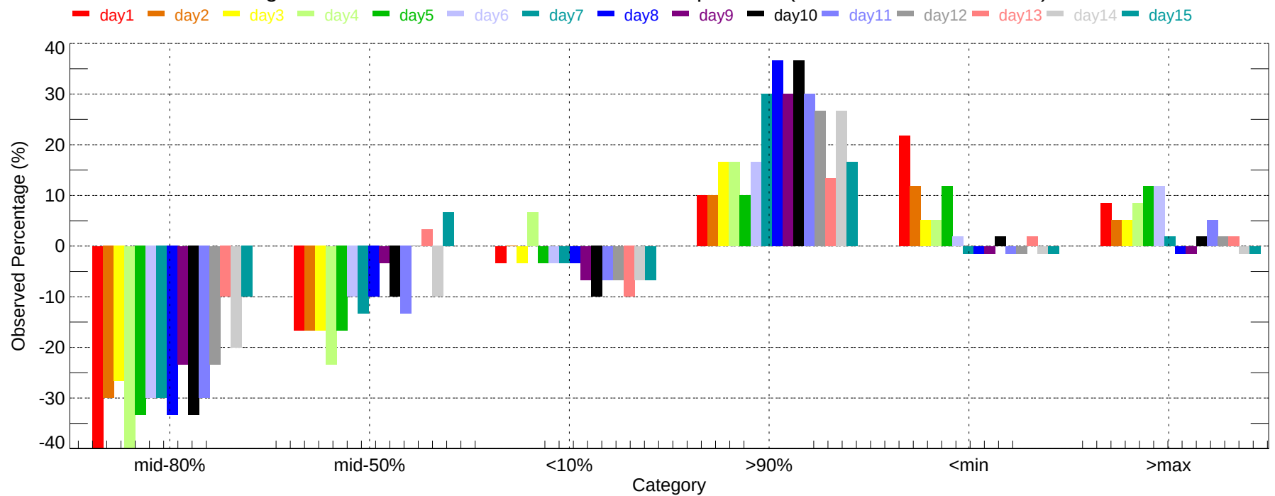
Observed Percentage Deviation of Ensembles - MIA: Min Temperature (2007-12-01~2007-12-31)
