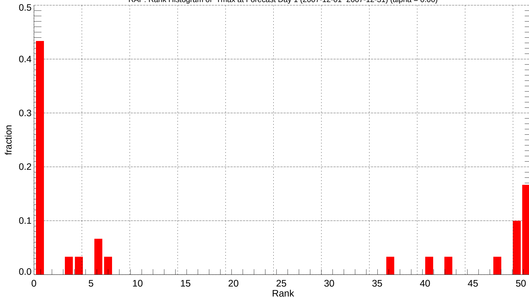
RAP: Rank Histogram of Tmax at Forecast Day 1 (2007-12-01~2007-12-31) (alpha = 0.00)
