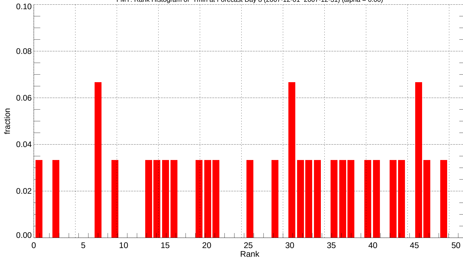
FMY: Rank Histogram of Tmin at Forecast Day 8 (2007-12-01~2007-12-31) (alpha = 0.00)
