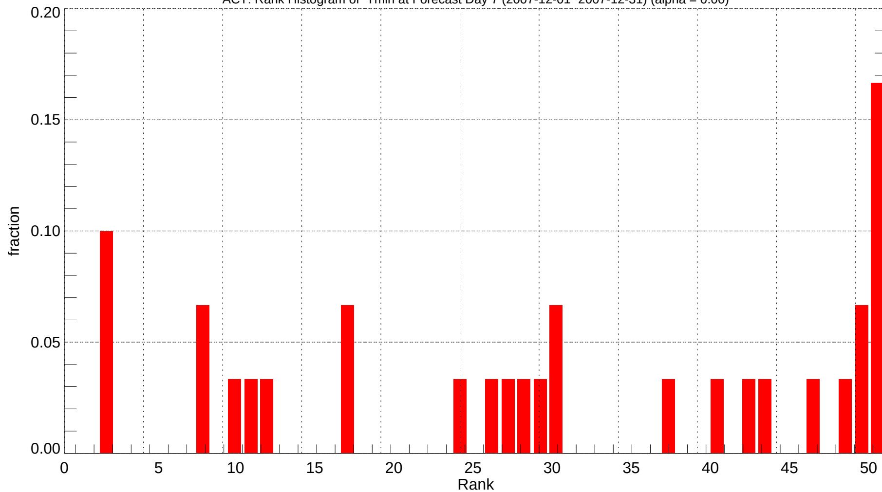
ACT: Rank Histogram of Tmin at Forecast Day 7 (2007-12-01~2007-12-31) (alpha = 0.00)
