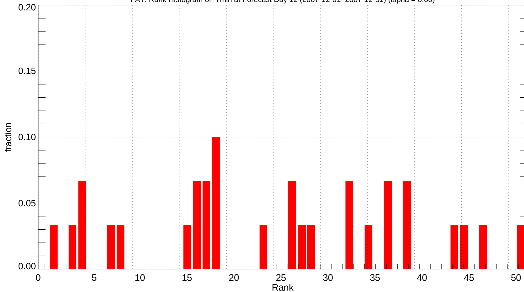
FAT: Rank Histogram of Tmin at Forecast Day 12 (2007-12-01~2007-12-31) (alpha = 0.00)
