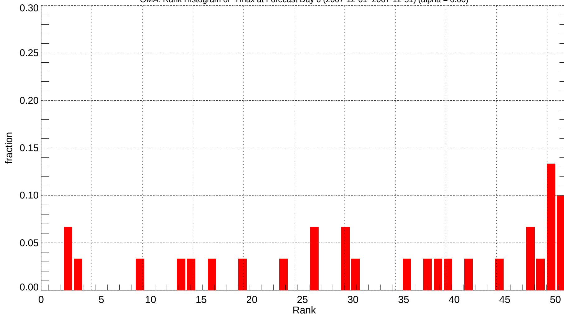
OMA: Rank Histogram of Tmax at Forecast Day 6 (2007-12-01~2007-12-31) (alpha = 0.00)
