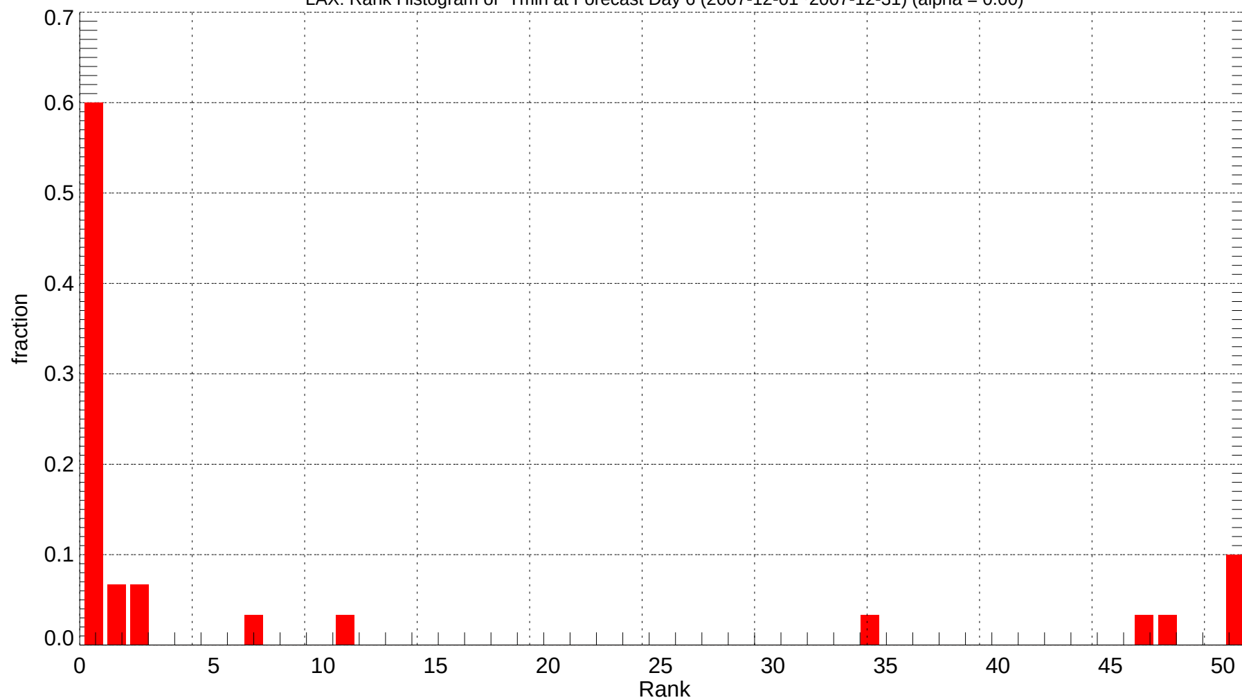
LAX: Rank Histogram of Tmin at Forecast Day 6 (2007-12-01~2007-12-31) (alpha = 0.00)
