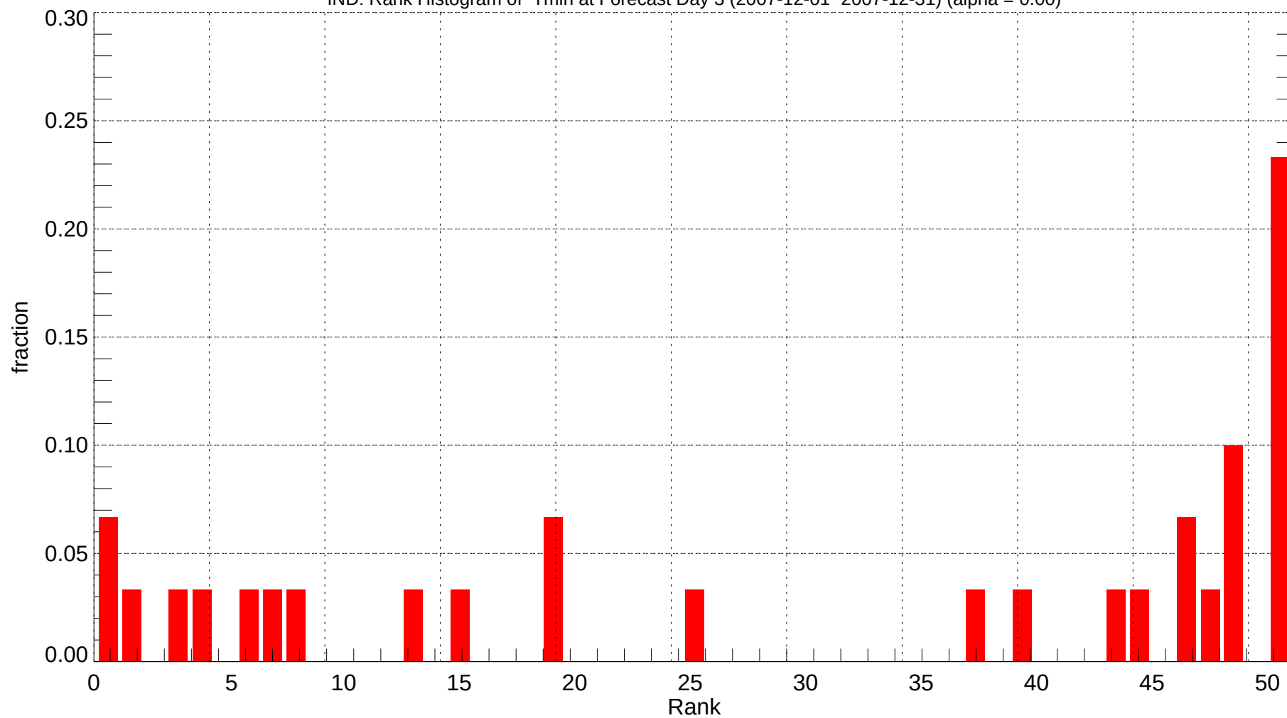
IND: Rank Histogram of Tmin at Forecast Day 3 (2007-12-01~2007-12-31) (alpha = 0.00)
