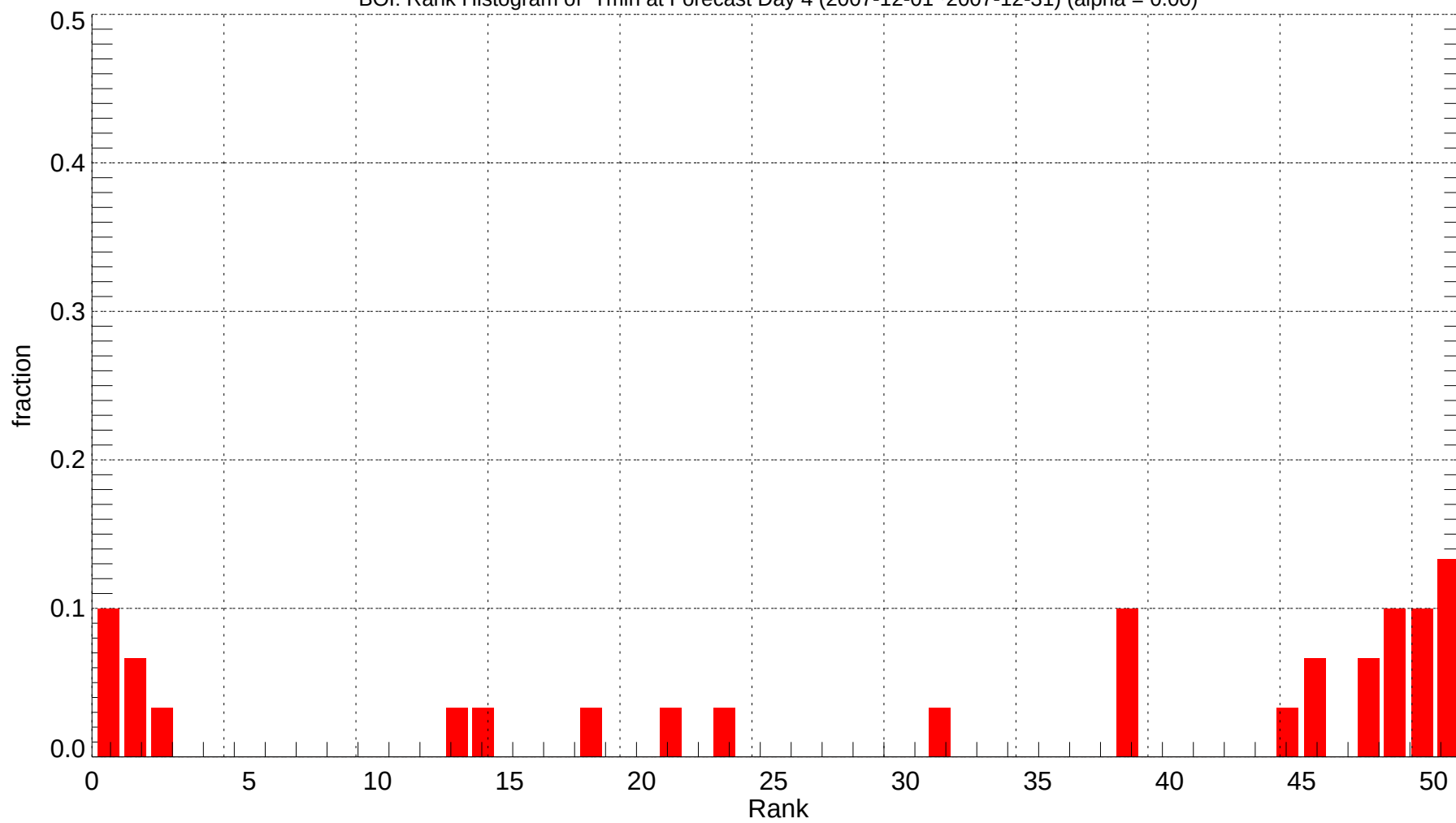
BOI: Rank Histogram of Tmin at Forecast Day 4 (2007-12-01~2007-12-31) (alpha = 0.00)
