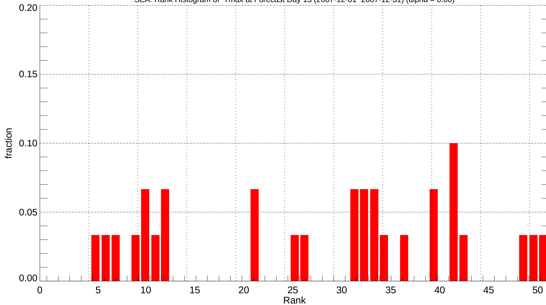
SEA: Rank Histogram of Tmax at Forecast Day 13 (2007-12-01~2007-12-31) (alpha = 0.00)
