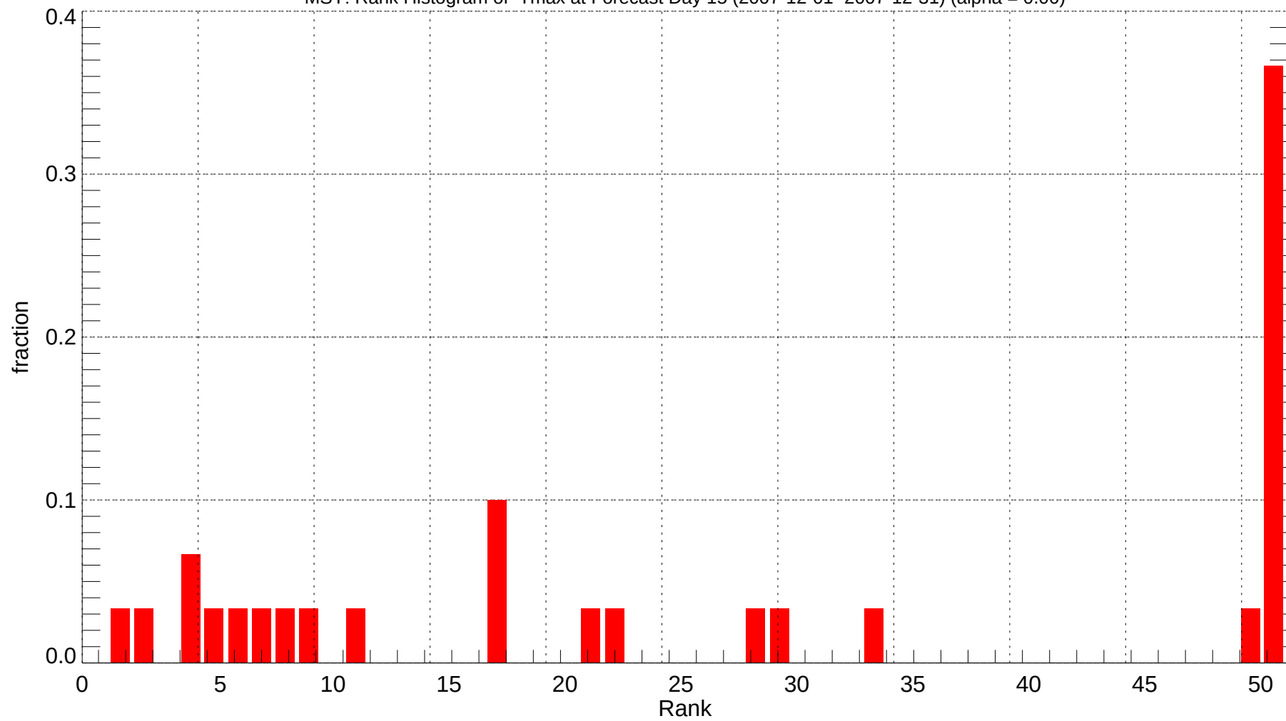
MSY: Rank Histogram of Tmax at Forecast Day 15 (2007-12-01~2007-12-31) (alpha = 0.00)
