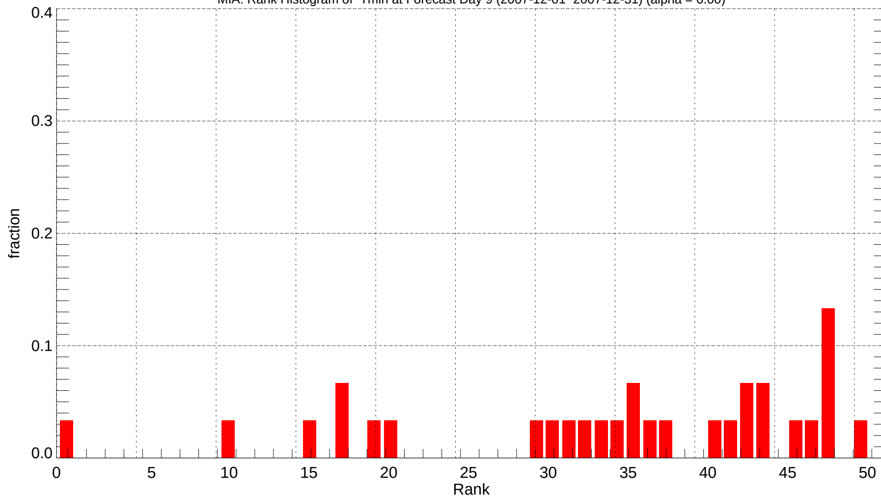
MIA: Rank Histogram of Tmin at Forecast Day 9 (2007-12-01~2007-12-31) (alpha = 0.00)
