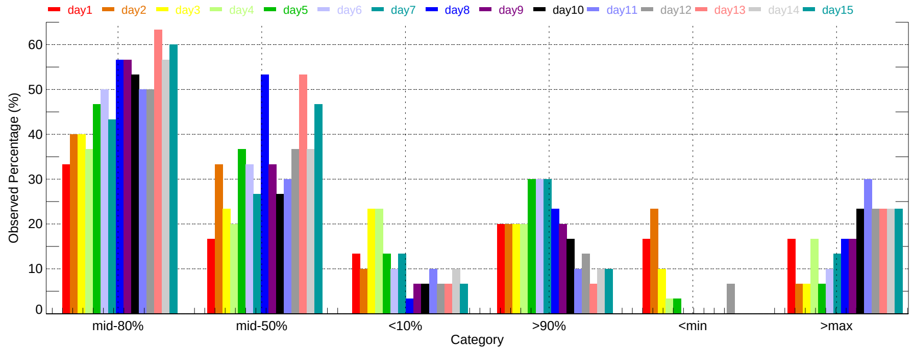
Observed Percentage of Ensembles - JAN: Min Temperature (2007-12-01~2007-12-31)
