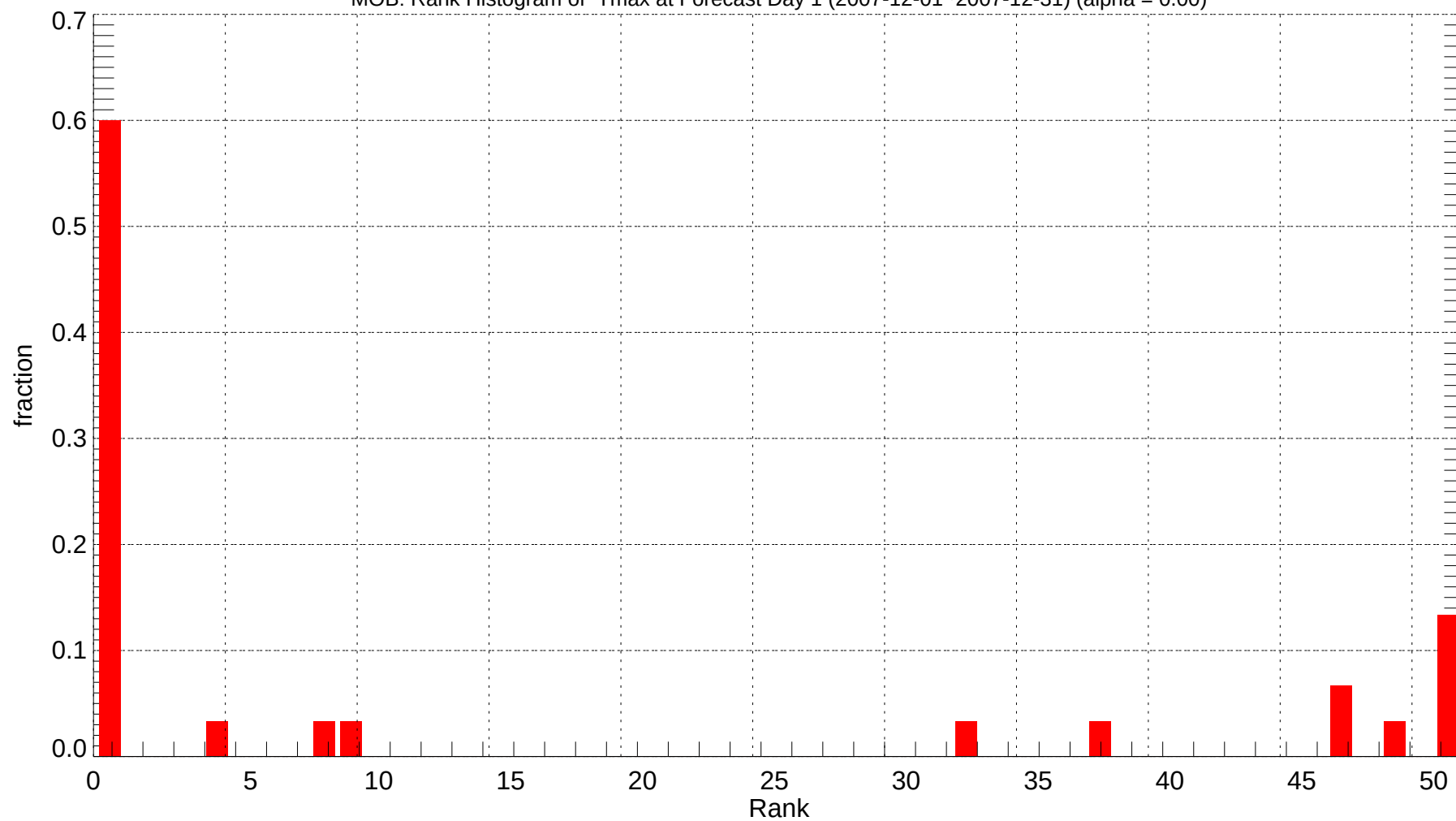
MOB: Rank Histogram of Tmax at Forecast Day 1 (2007-12-01~2007-12-31) (alpha = 0.00)
