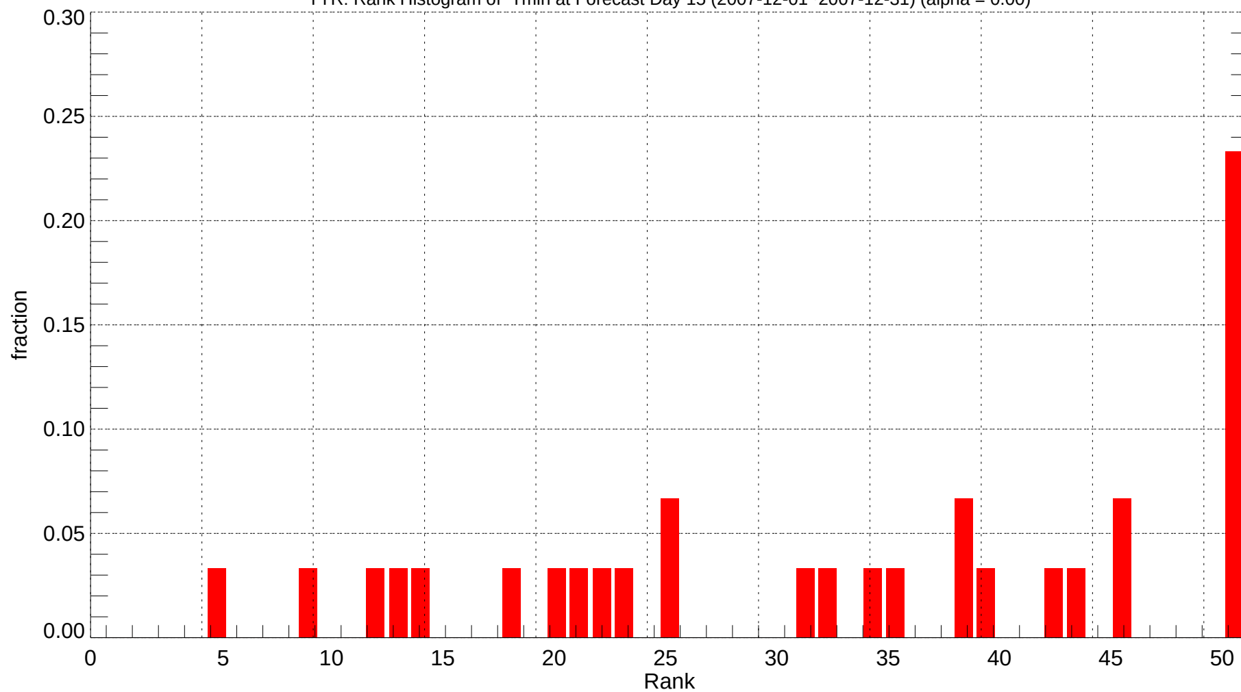
TYR: Rank Histogram of Tmin at Forecast Day 15 (2007-12-01~2007-12-31) (alpha = 0.00)
