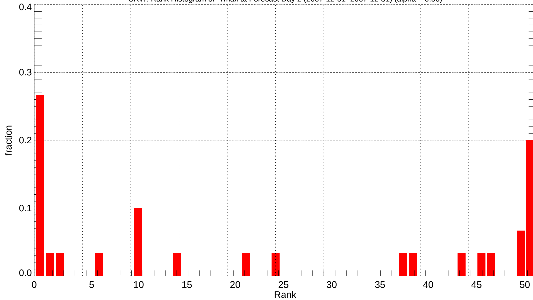
CRW: Rank Histogram of Tmax at Forecast Day 2 (2007-12-01~2007-12-31) (alpha = 0.00)
