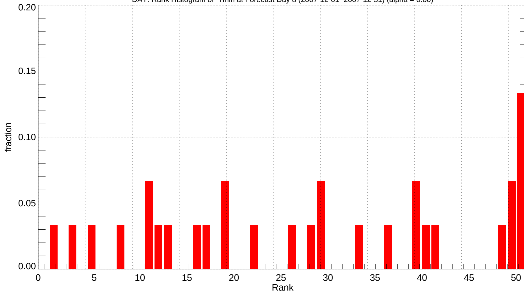
DAY: Rank Histogram of Tmin at Forecast Day 8 (2007-12-01~2007-12-31) (alpha = 0.00)
