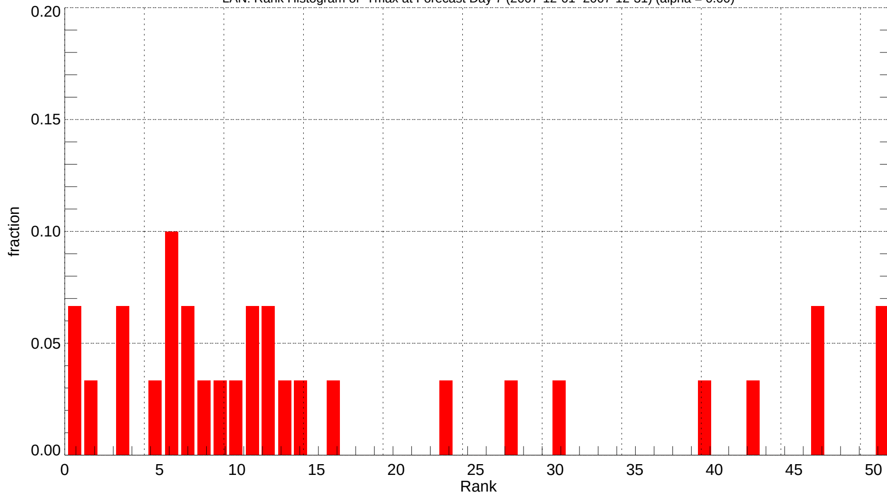
LAN: Rank Histogram of Tmax at Forecast Day 7 (2007-12-01~2007-12-31) (alpha = 0.00)
