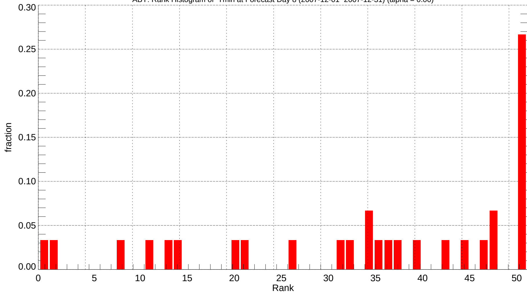
ABY: Rank Histogram of Tmin at Forecast Day 8 (2007-12-01~2007-12-31) (alpha = 0.00)
