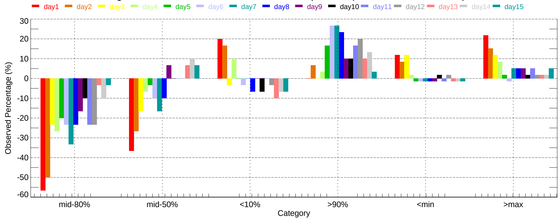
Observed Percentage Deviation of Ensembles - EVV: Max Temperature (2007-12-01~2007-12-31)
