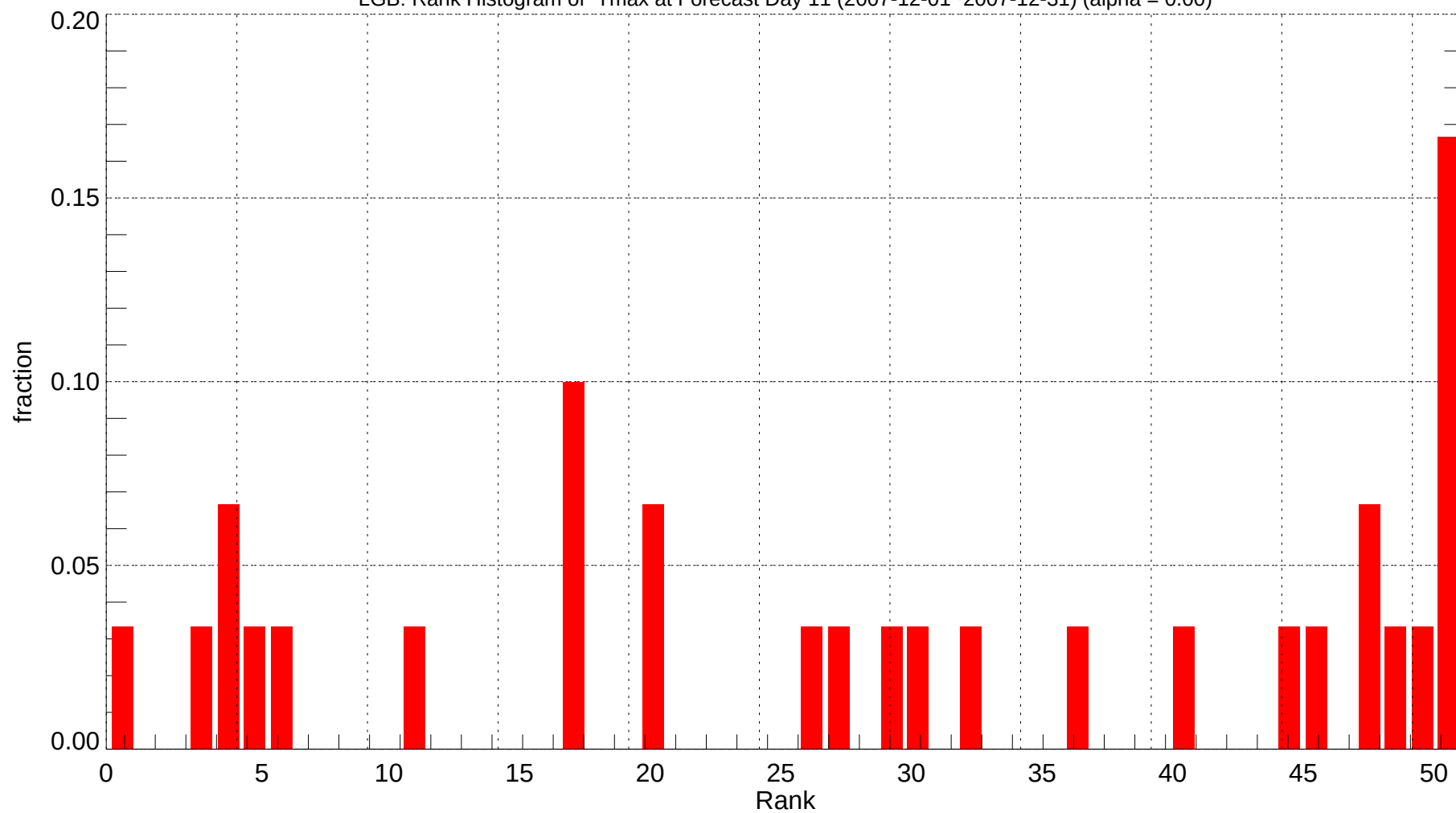
LGB: Rank Histogram of Tmax at Forecast Day 11 (2007-12-01~2007-12-31) (alpha = 0.00)
