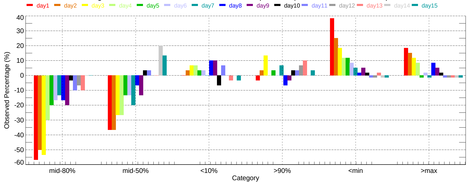
Observed Percentage Deviation of Ensembles - LAN: Max Temperature (2007-12-01~2007-12-31)
