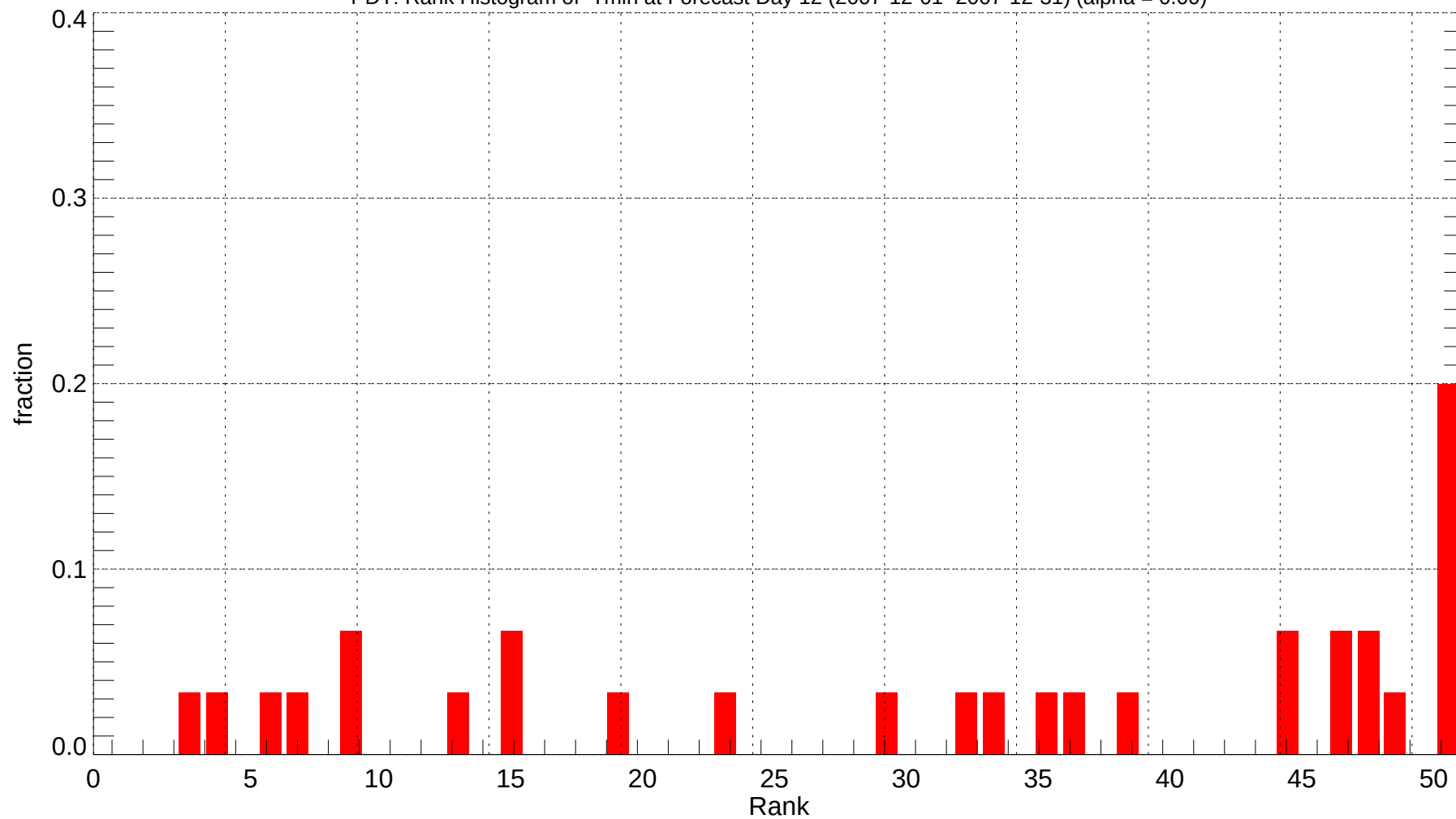
PDT: Rank Histogram of Tmin at Forecast Day 12 (2007-12-01~2007-12-31) (alpha = 0.00)
