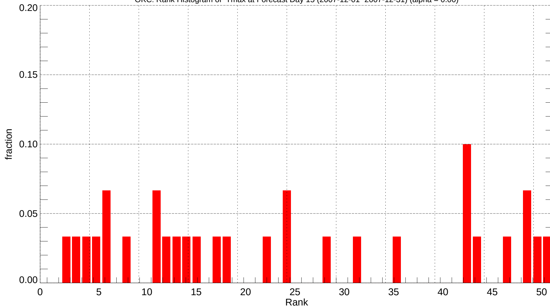
OKC: Rank Histogram of Tmax at Forecast Day 15 (2007-12-01~2007-12-31) (alpha = 0.00)
