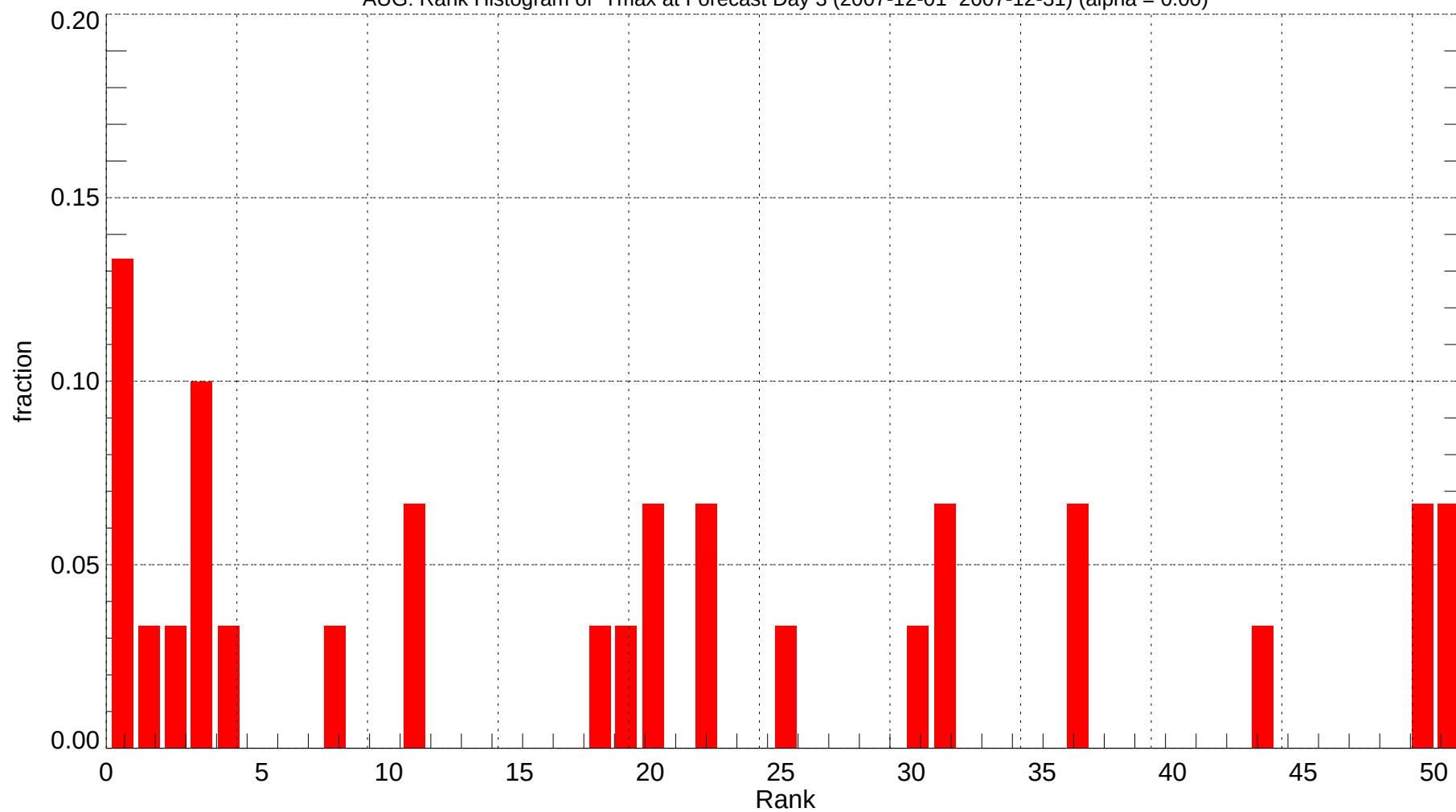
AUG: Rank Histogram of Tmax at Forecast Day 3 (2007-12-01~2007-12-31) (alpha = 0.00)
