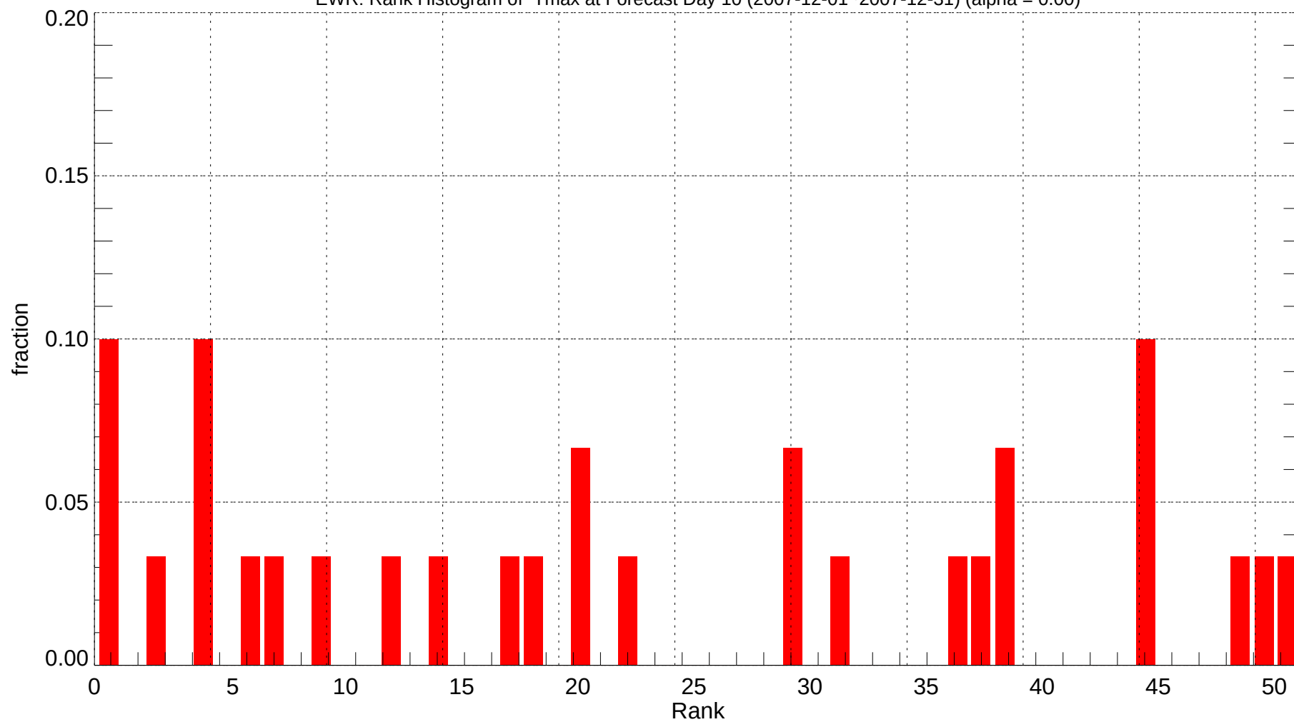
EWR: Rank Histogram of Tmax at Forecast Day 10 (2007-12-01~2007-12-31) (alpha = 0.00)
