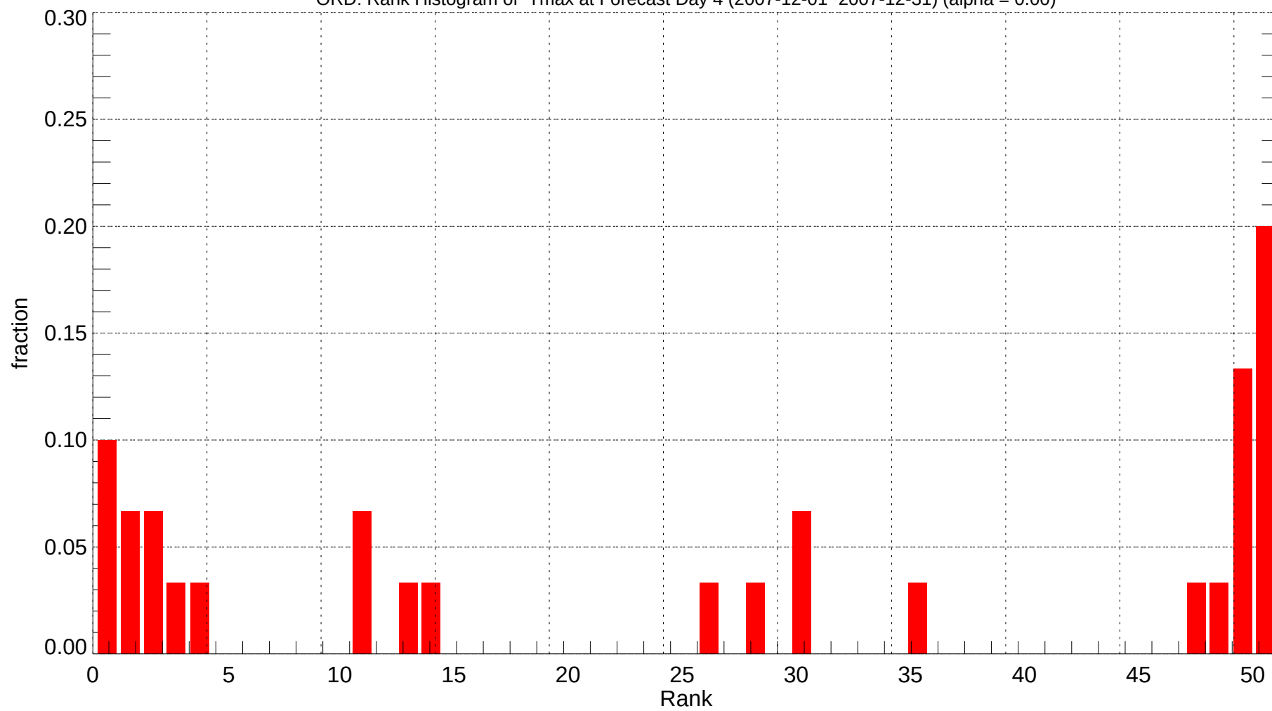
ORD: Rank Histogram of Tmax at Forecast Day 4 (2007-12-01~2007-12-31) (alpha = 0.00)
