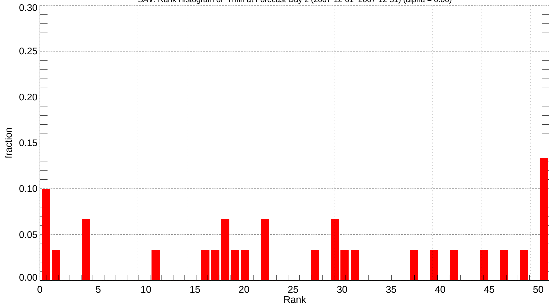
SAV: Rank Histogram of Tmin at Forecast Day 2 (2007-12-01~2007-12-31) (alpha = 0.00)
