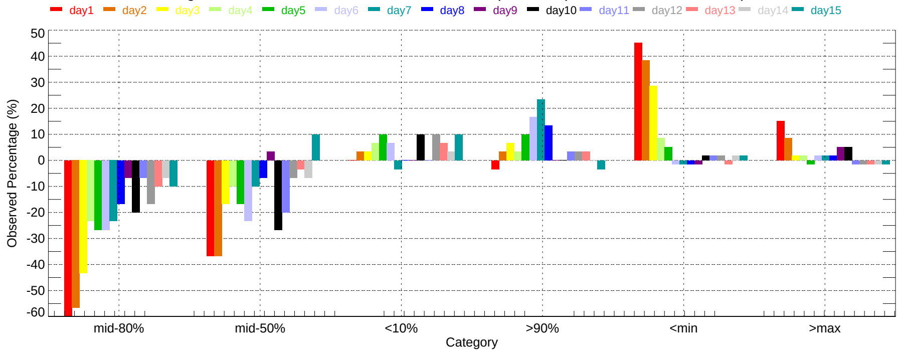
Observed Percentage Deviation of Ensembles - MBA: Min Temperature (2007-12-01~2007-12-31)
