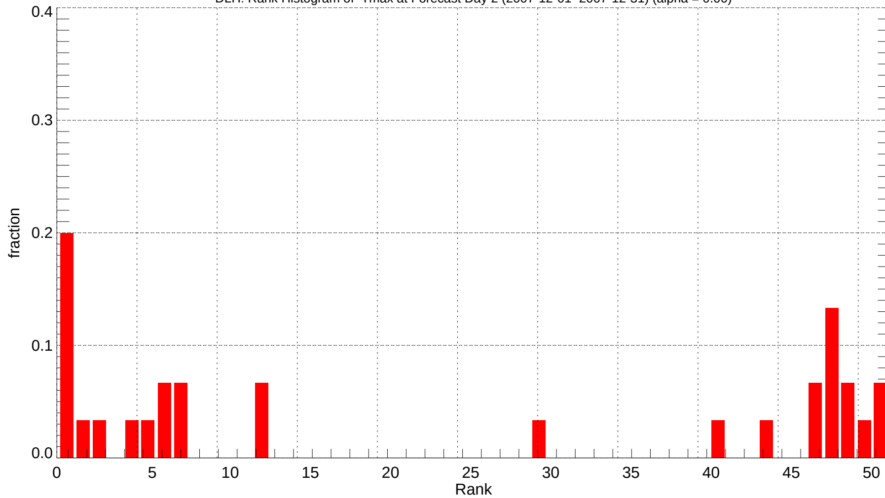
DLH: Rank Histogram of Tmax at Forecast Day 2 (2007-12-01~2007-12-31) (alpha = 0.00)
