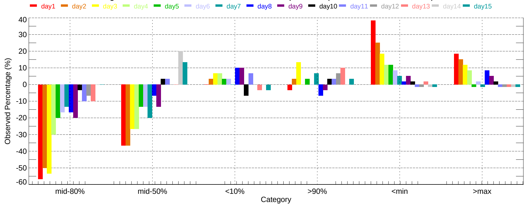
Observed Percentage Deviation of Ensembles - LAN: Min Temperature (2007-12-01~2007-12-31)
