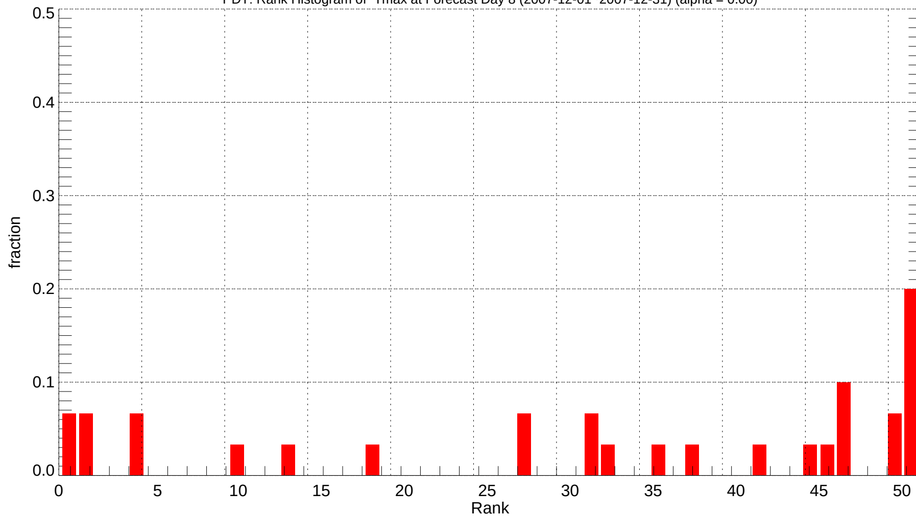
PDT: Rank Histogram of Tmax at Forecast Day 8 (2007-12-01~2007-12-31) (alpha = 0.00)
