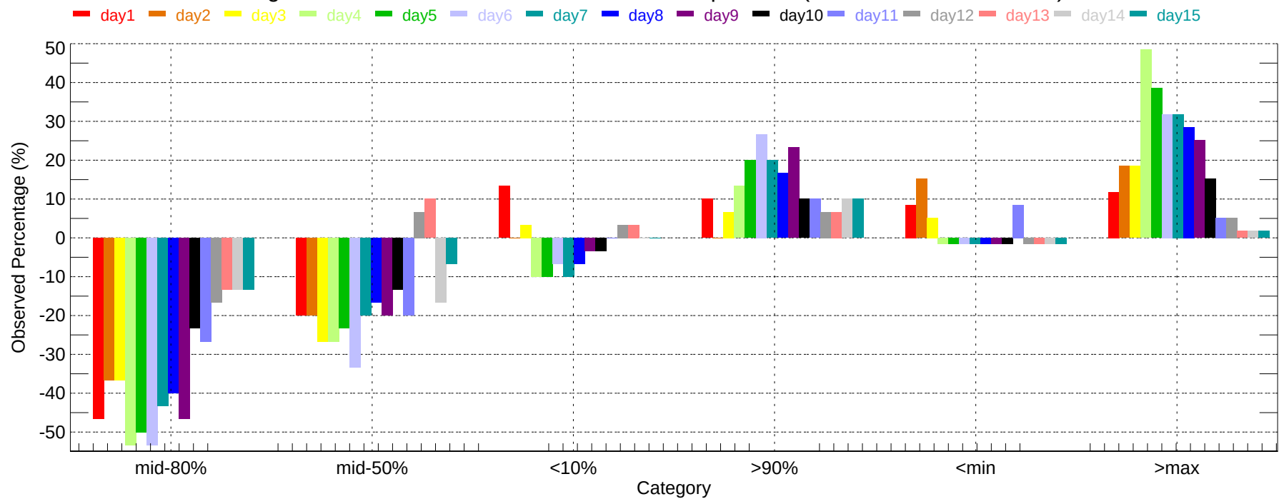
Observed Percentage Deviation of Ensembles - ELP: Max Temperature (2007-12-01~2007-12-31)
