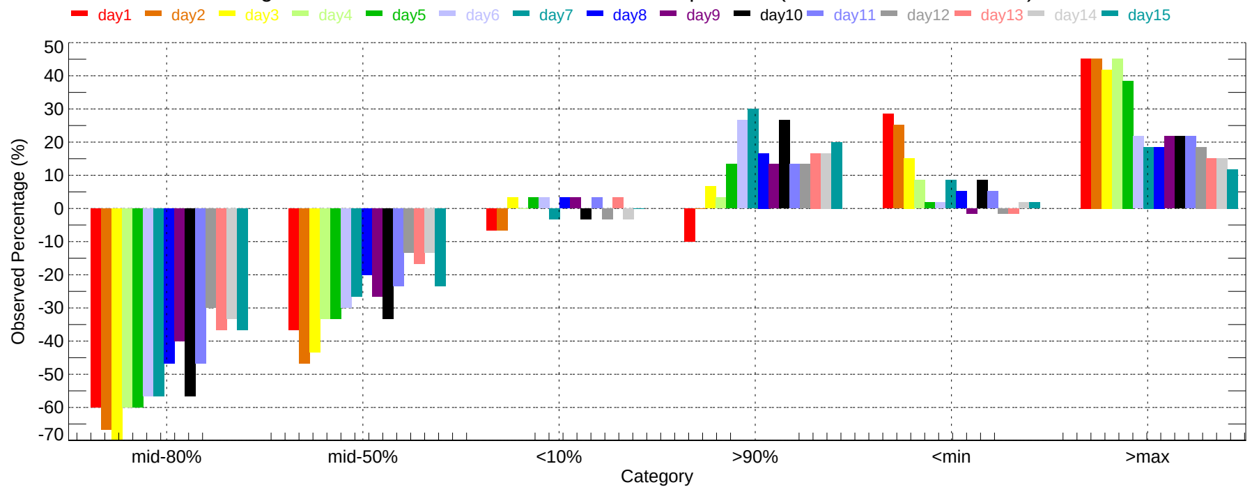
Observed Percentage Deviation of Ensembles - PDT: Min Temperature (2007-12-01~2007-12-31)
