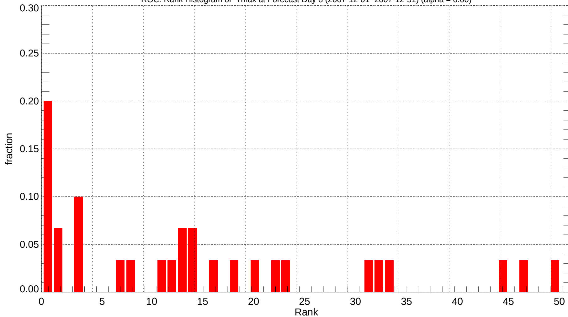
ROC: Rank Histogram of Tmax at Forecast Day 8 (2007-12-01~2007-12-31) (alpha = 0.00)
