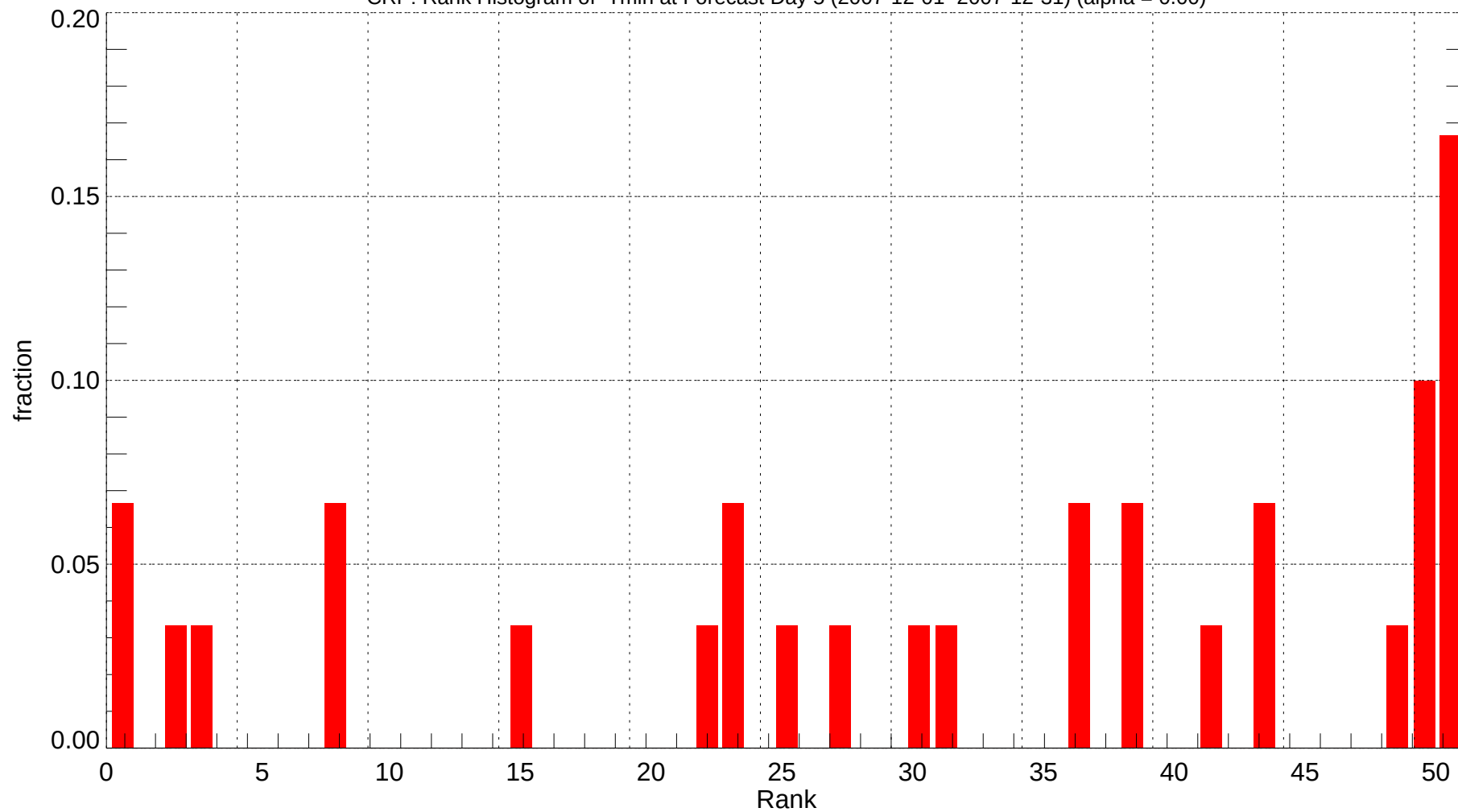
CRP: Rank Histogram of Tmin at Forecast Day 5 (2007-12-01~2007-12-31) (alpha = 0.00)
