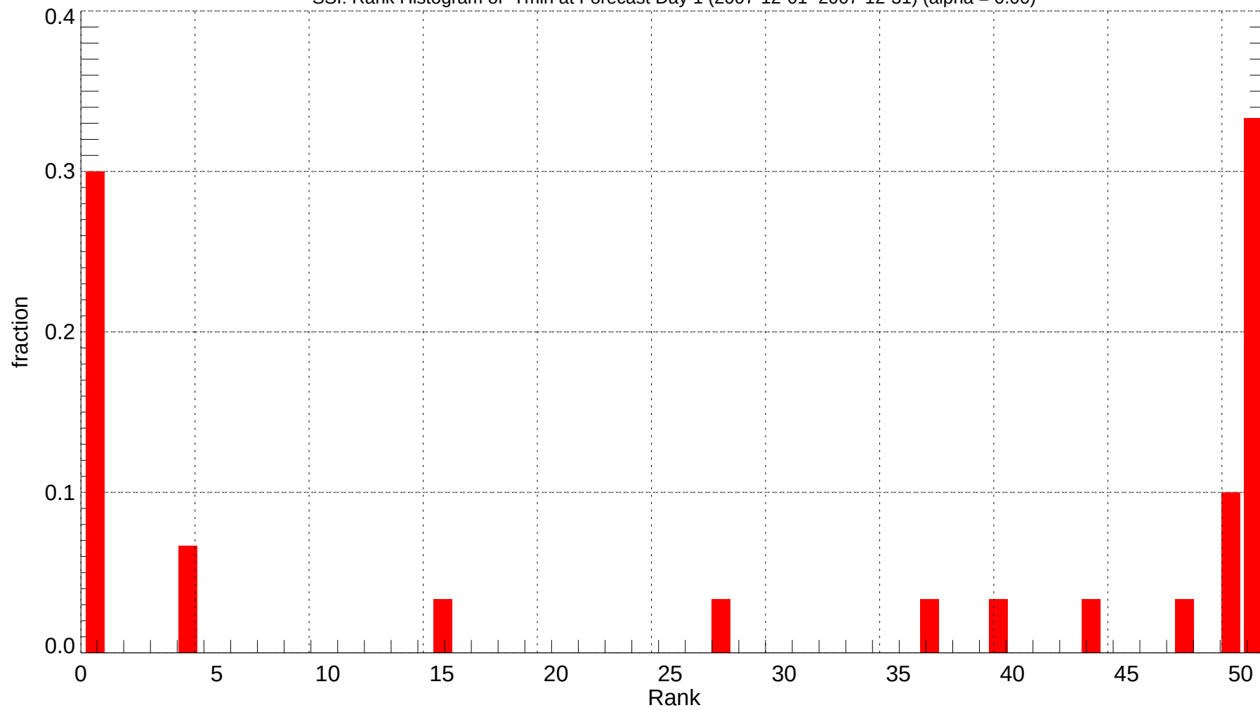
SSI: Rank Histogram of Tmin at Forecast Day 1 (2007-12-01~2007-12-31) (alpha = 0.00)
