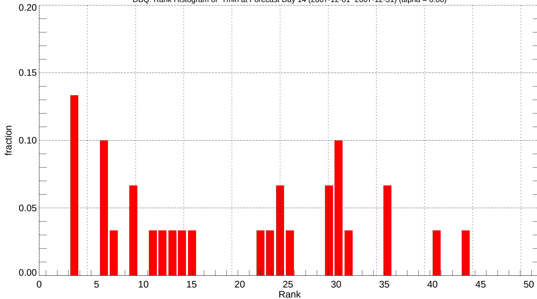
DBQ: Rank Histogram of Tmin at Forecast Day 14 (2007-12-01~2007-12-31) (alpha = 0.00)
