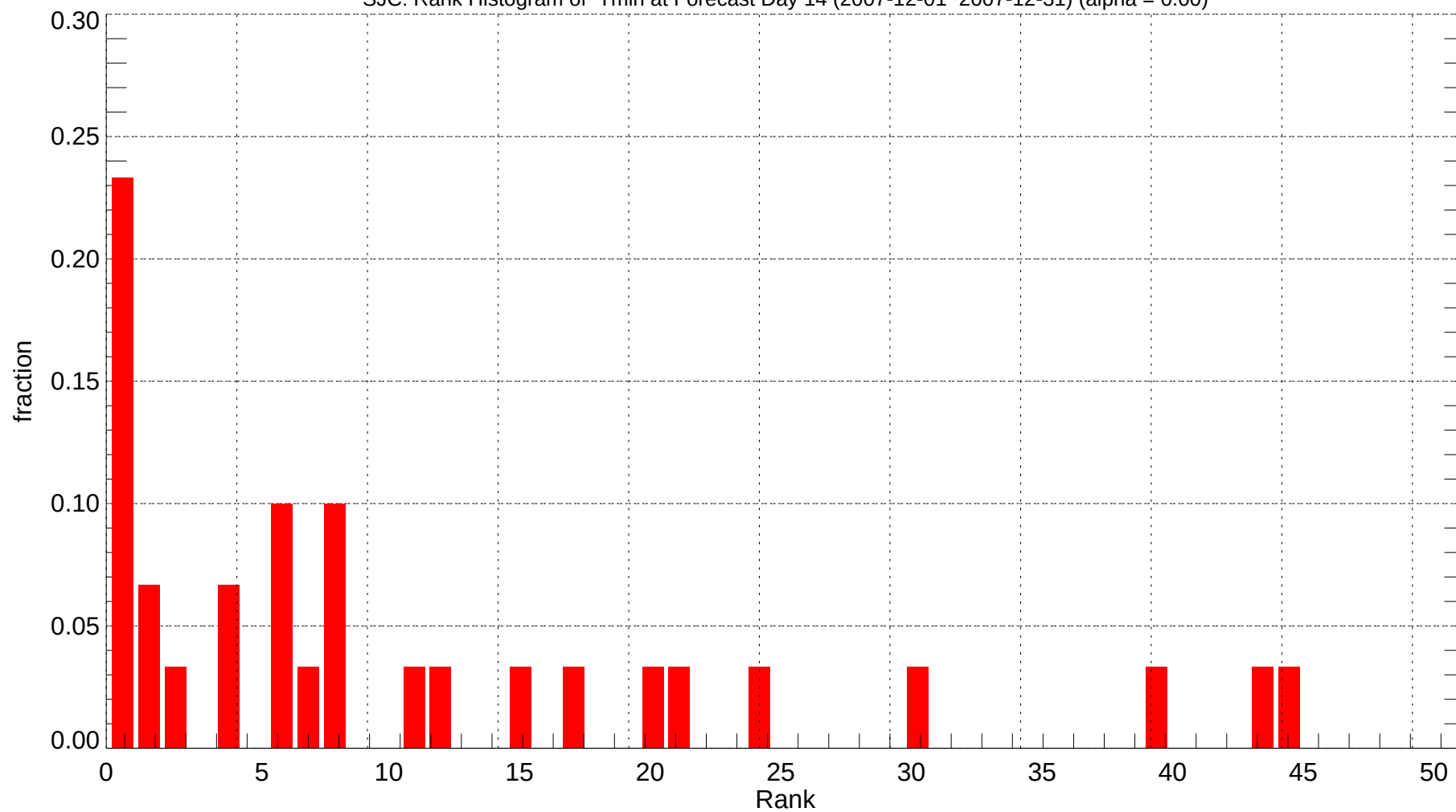
SJC: Rank Histogram of Tmin at Forecast Day 14 (2007-12-01~2007-12-31) (alpha = 0.00)
