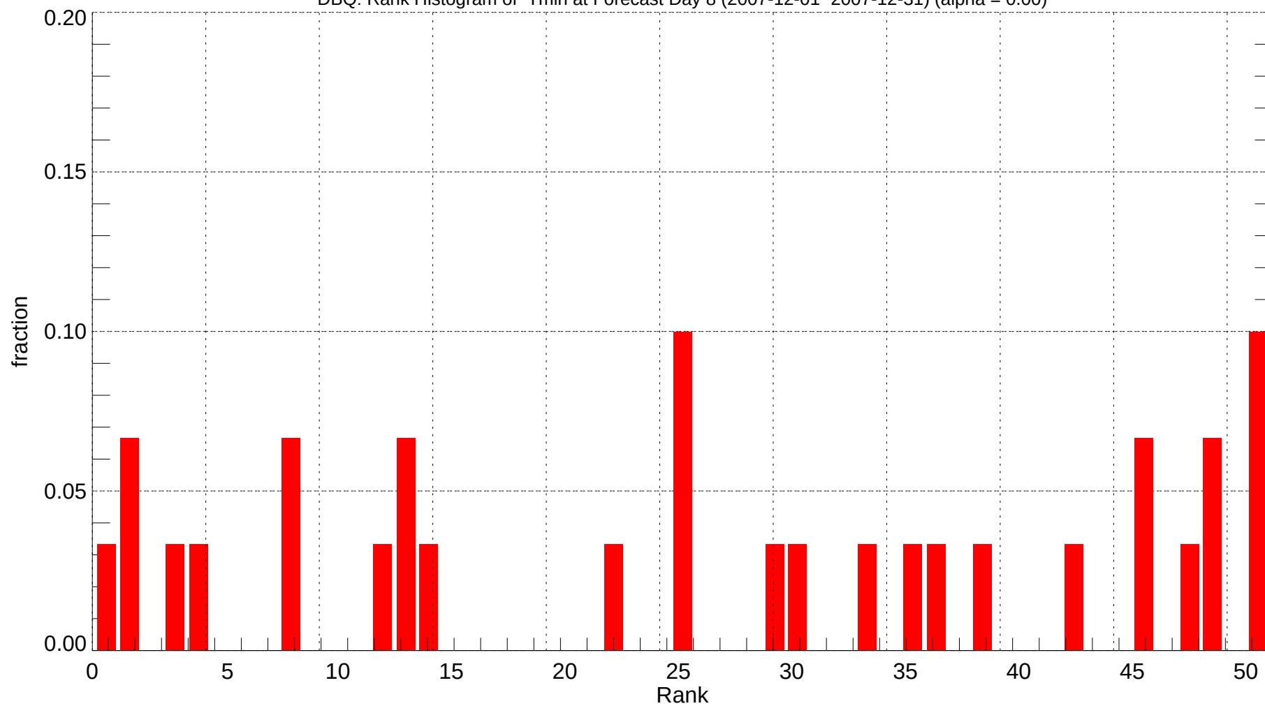
DBQ: Rank Histogram of Tmin at Forecast Day 8 (2007-12-01~2007-12-31) (alpha = 0.00)
