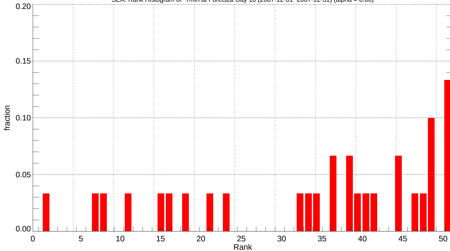
SEA: Rank Histogram of Tmin at Forecast Day 10 (2007-12-01~2007-12-31) (alpha = 0.00)
