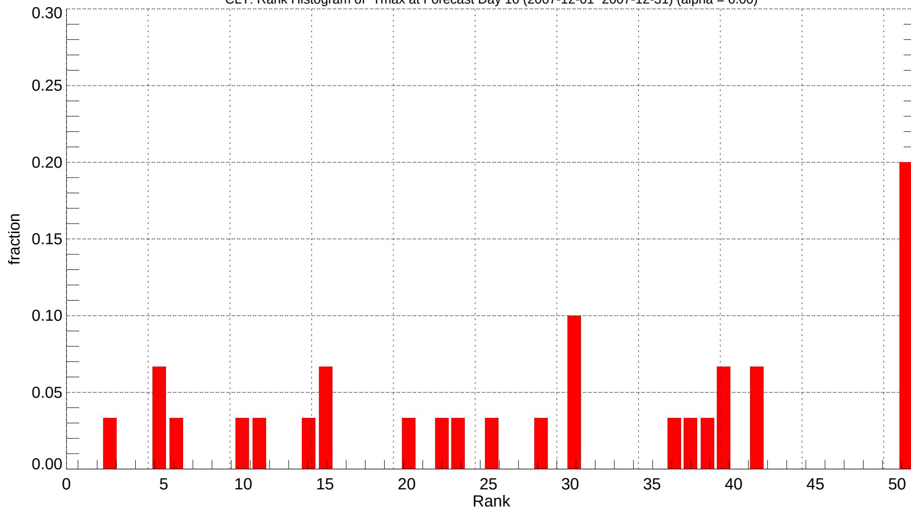
CLT: Rank Histogram of Tmax at Forecast Day 10 (2007-12-01~2007-12-31) (alpha = 0.00)
