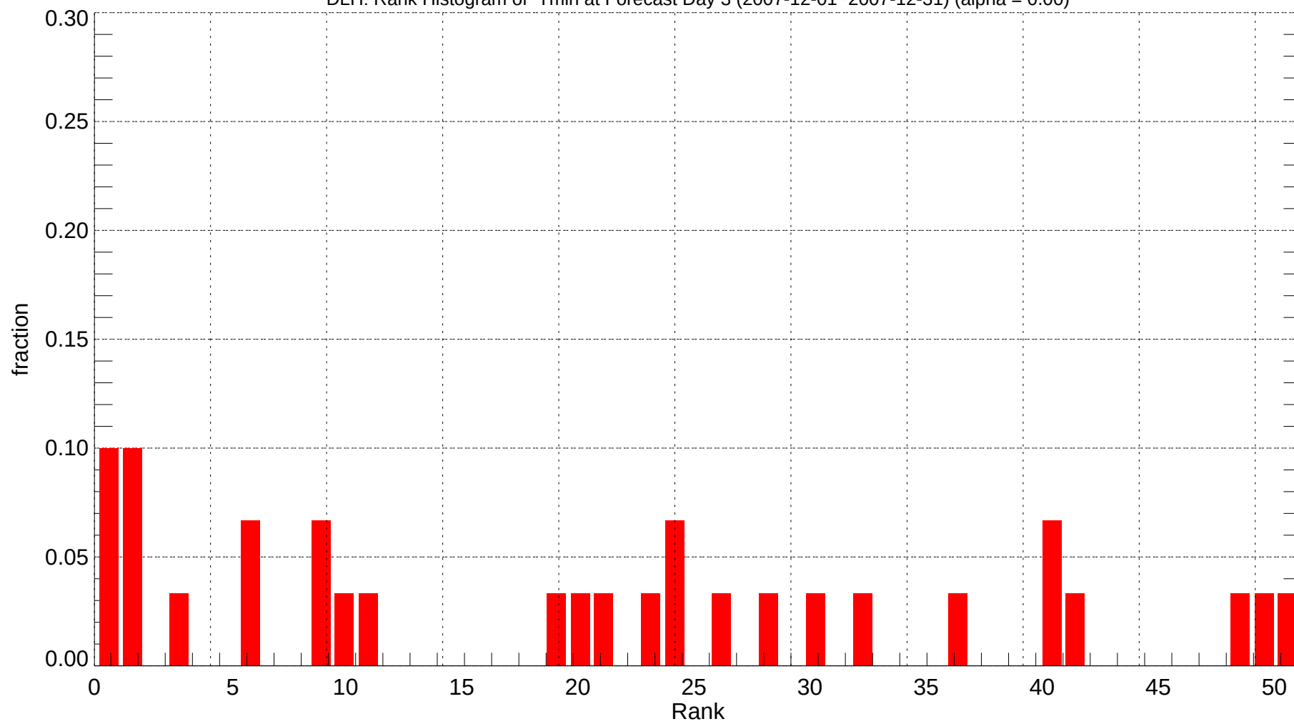
DLH: Rank Histogram of Tmin at Forecast Day 3 (2007-12-01~2007-12-31) (alpha = 0.00)
