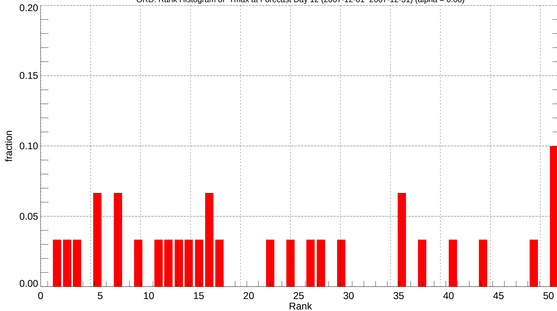
ORD: Rank Histogram of Tmax at Forecast Day 12 (2007-12-01~2007-12-31) (alpha = 0.00)
