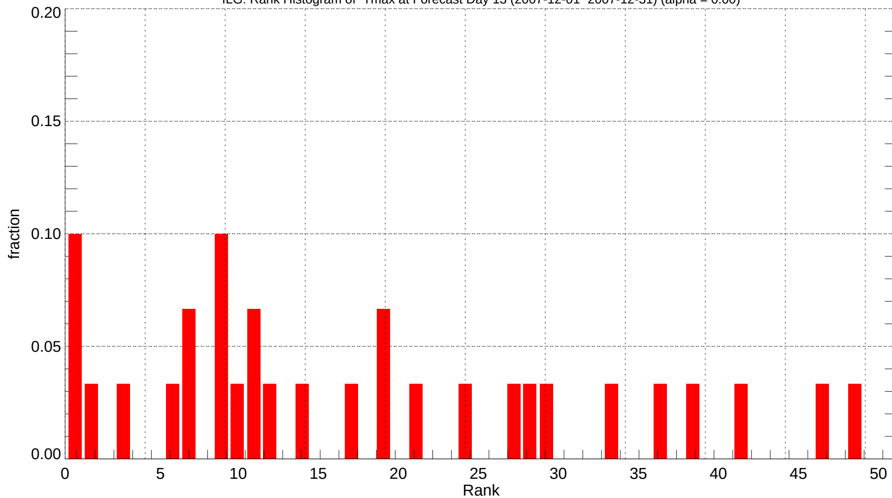
ILG: Rank Histogram of Tmax at Forecast Day 13 (2007-12-01~2007-12-31) (alpha = 0.00)
