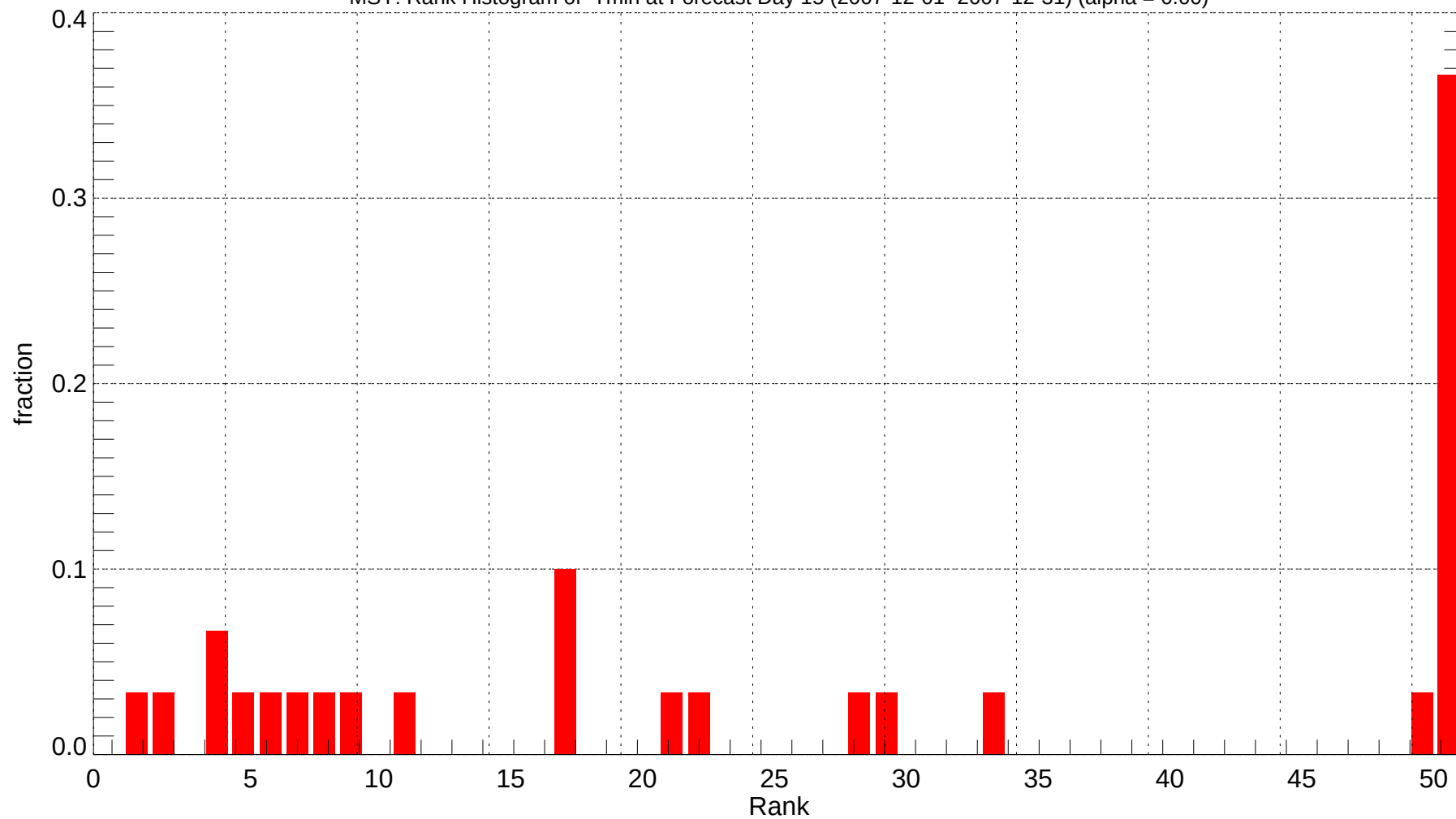
MSY: Rank Histogram of Tmin at Forecast Day 15 (2007-12-01~2007-12-31) (alpha = 0.00)
