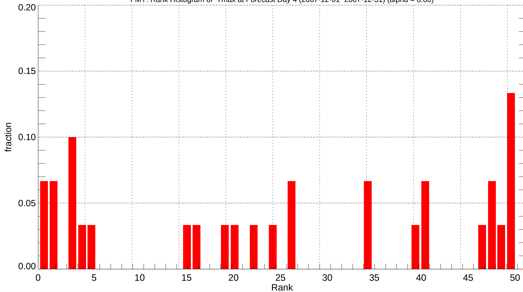
FMY: Rank Histogram of Tmax at Forecast Day 4 (2007-12-01~2007-12-31) (alpha = 0.00)
