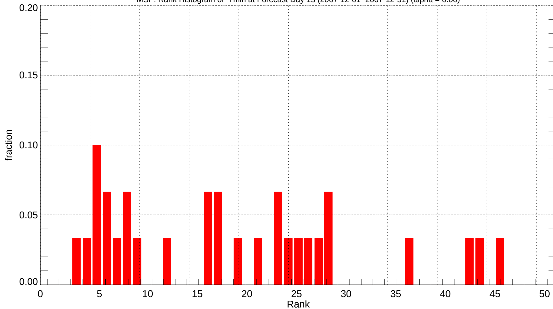
MSP: Rank Histogram of Tmin at Forecast Day 13 (2007-12-01~2007-12-31) (alpha = 0.00)
