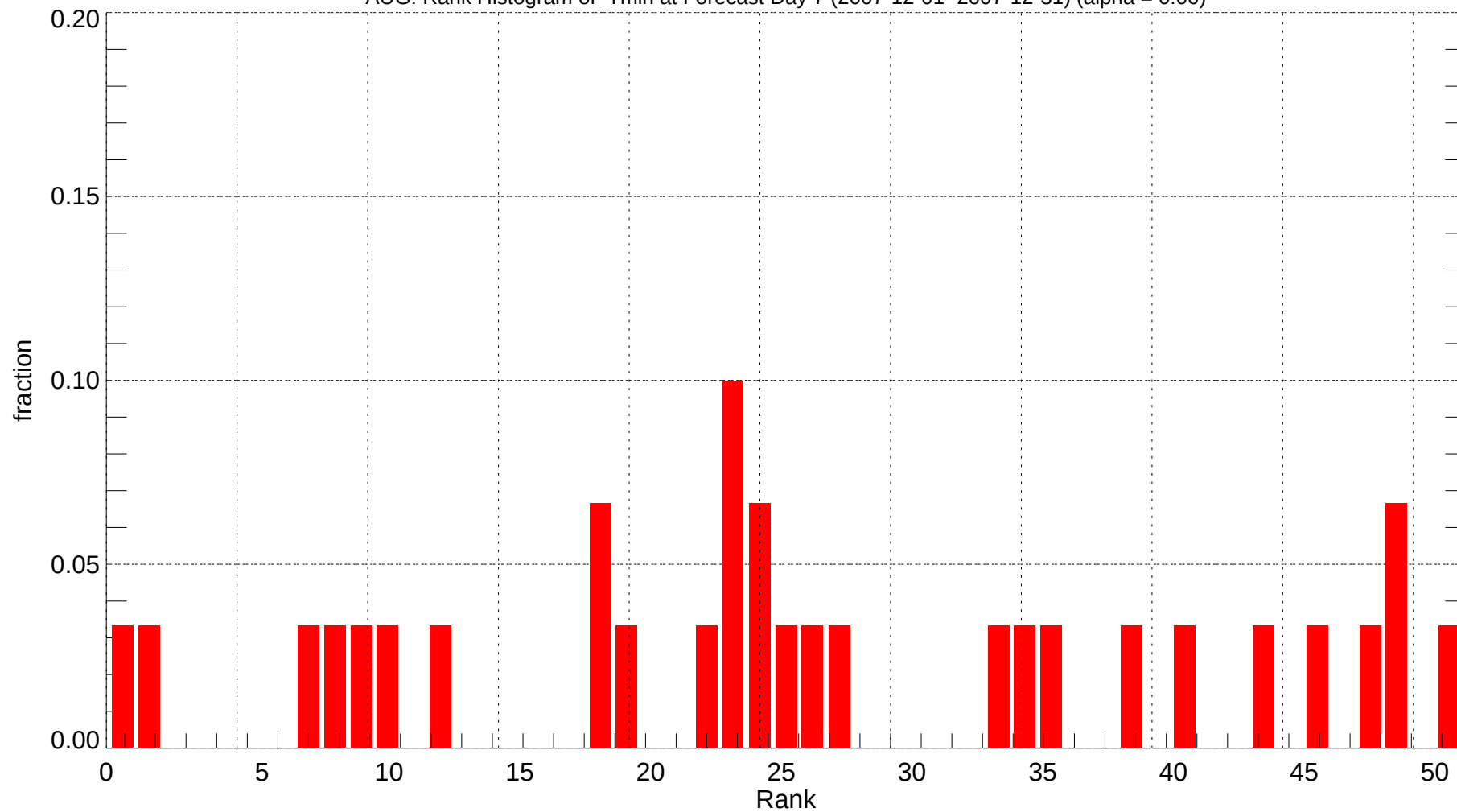
AUG: Rank Histogram of Tmin at Forecast Day 7 (2007-12-01~2007-12-31) (alpha = 0.00)
