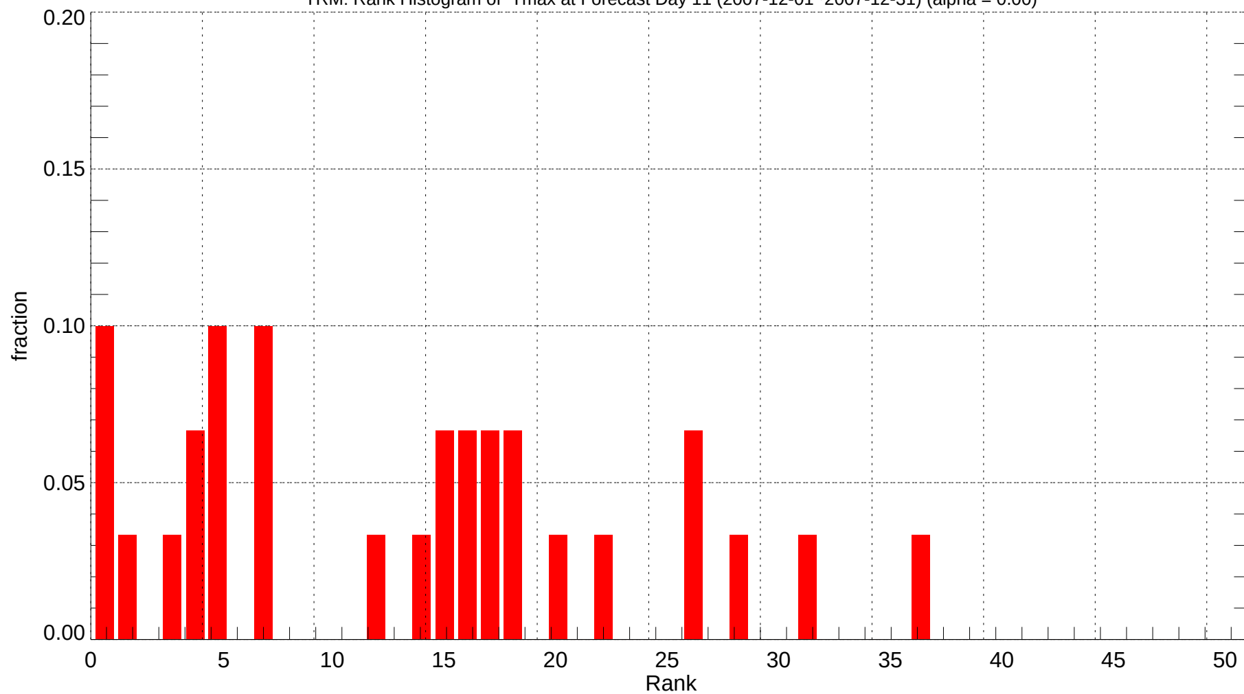
TRM: Rank Histogram of Tmax at Forecast Day 11 (2007-12-01~2007-12-31) (alpha = 0.00)
