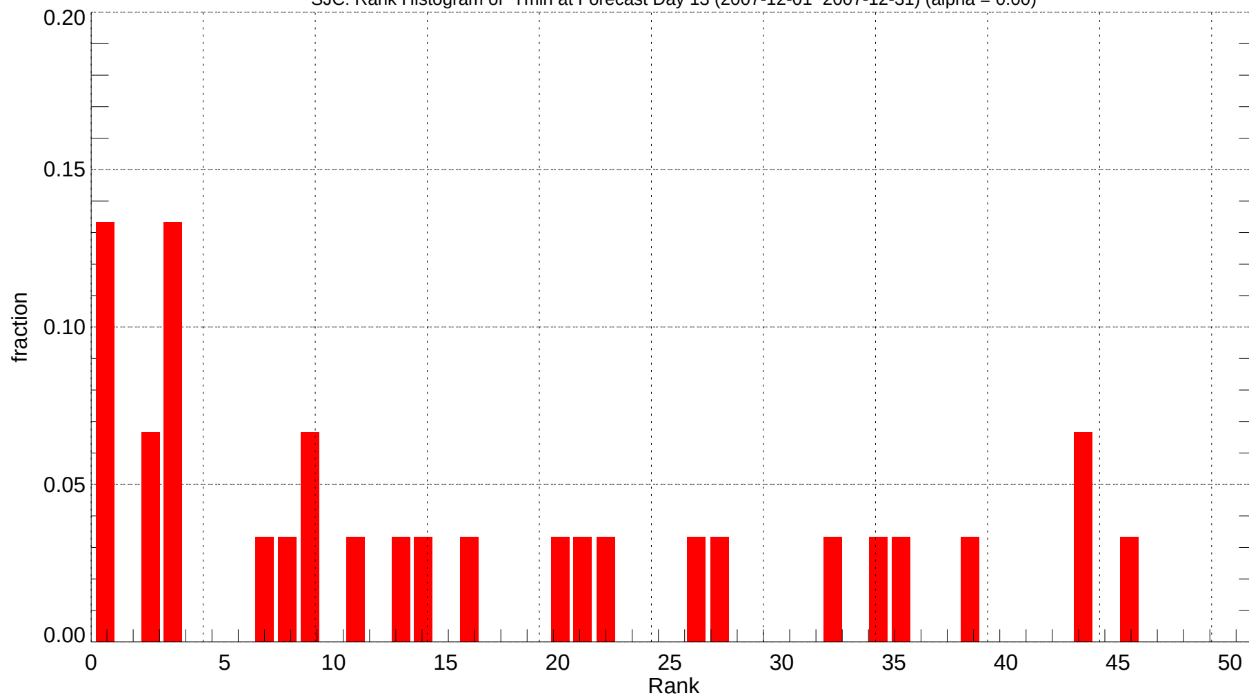
SJC: Rank Histogram of Tmin at Forecast Day 13 (2007-12-01~2007-12-31) (alpha = 0.00)
