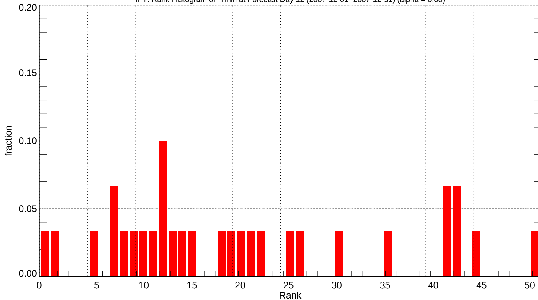
IPT: Rank Histogram of Tmin at Forecast Day 12 (2007-12-01~2007-12-31) (alpha = 0.00)
