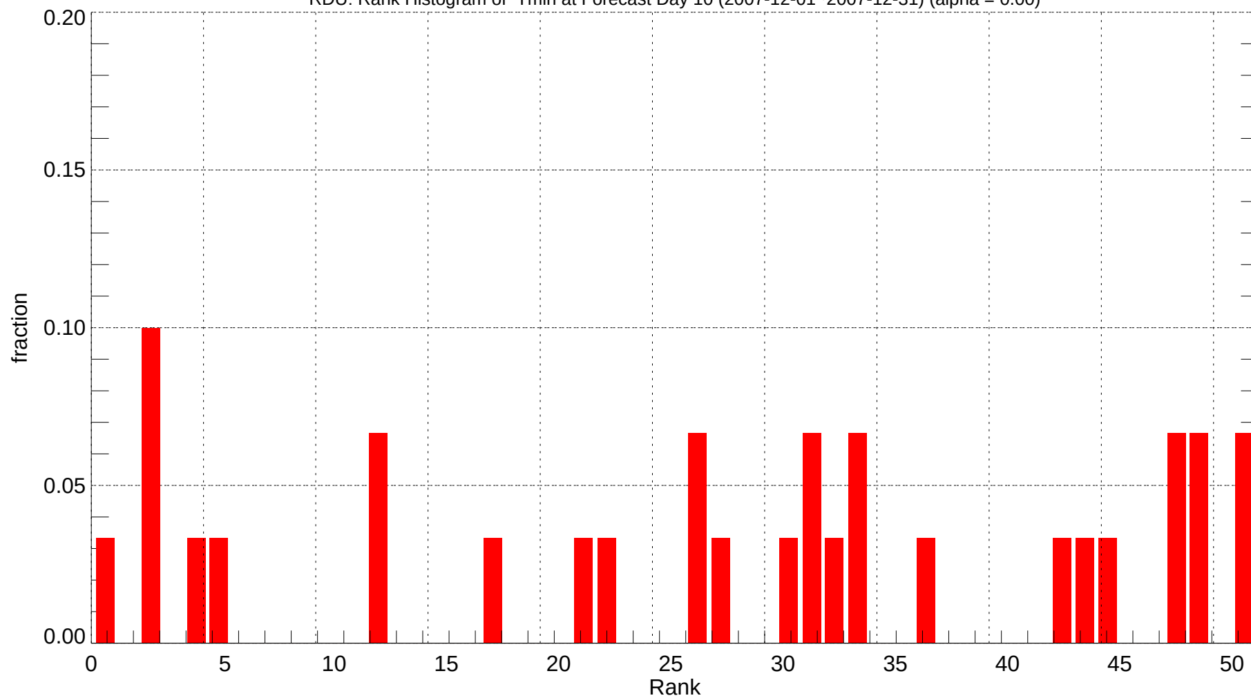
RDU: Rank Histogram of Tmin at Forecast Day 10 (2007-12-01~2007-12-31) (alpha = 0.00)
