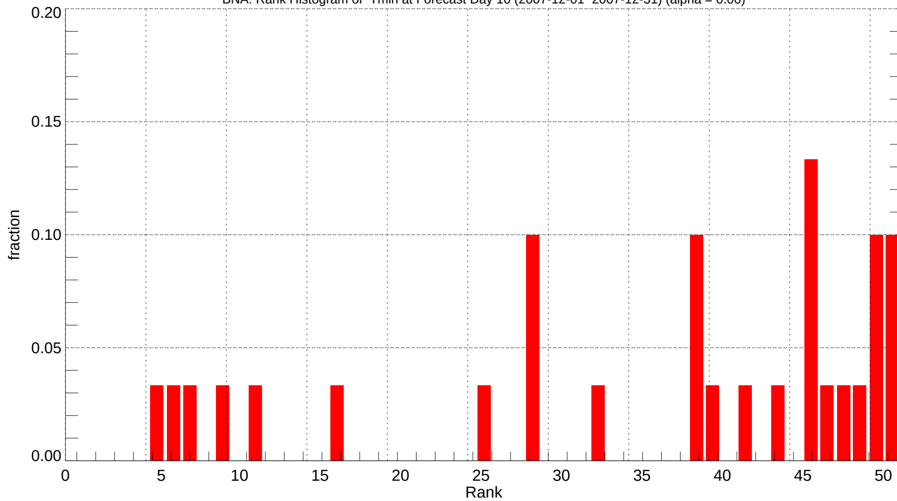
BNA: Rank Histogram of Tmin at Forecast Day 10 (2007-12-01~2007-12-31) (alpha = 0.00)
