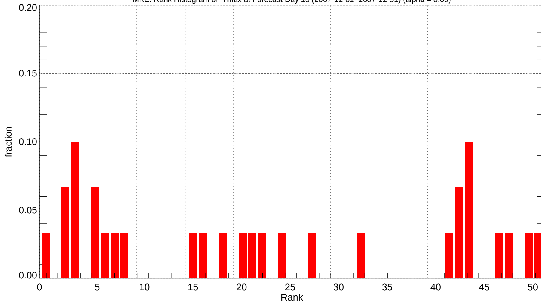
MKE: Rank Histogram of Tmax at Forecast Day 10 (2007-12-01~2007-12-31) (alpha = 0.00)
