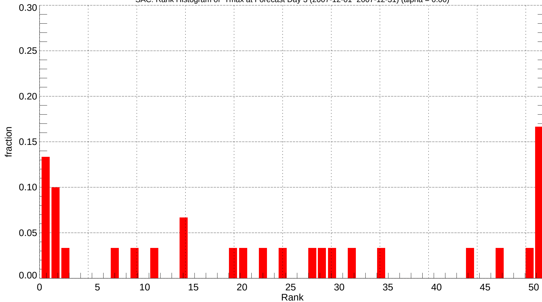
SAC: Rank Histogram of Tmax at Forecast Day 3 (2007-12-01~2007-12-31) (alpha = 0.00)
