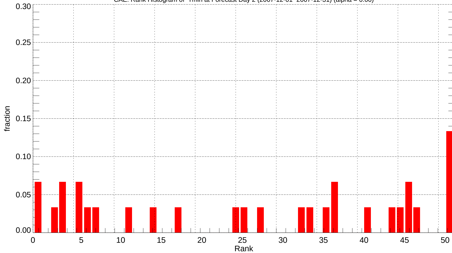
CAE: Rank Histogram of Tmin at Forecast Day 2 (2007-12-01~2007-12-31) (alpha = 0.00)
