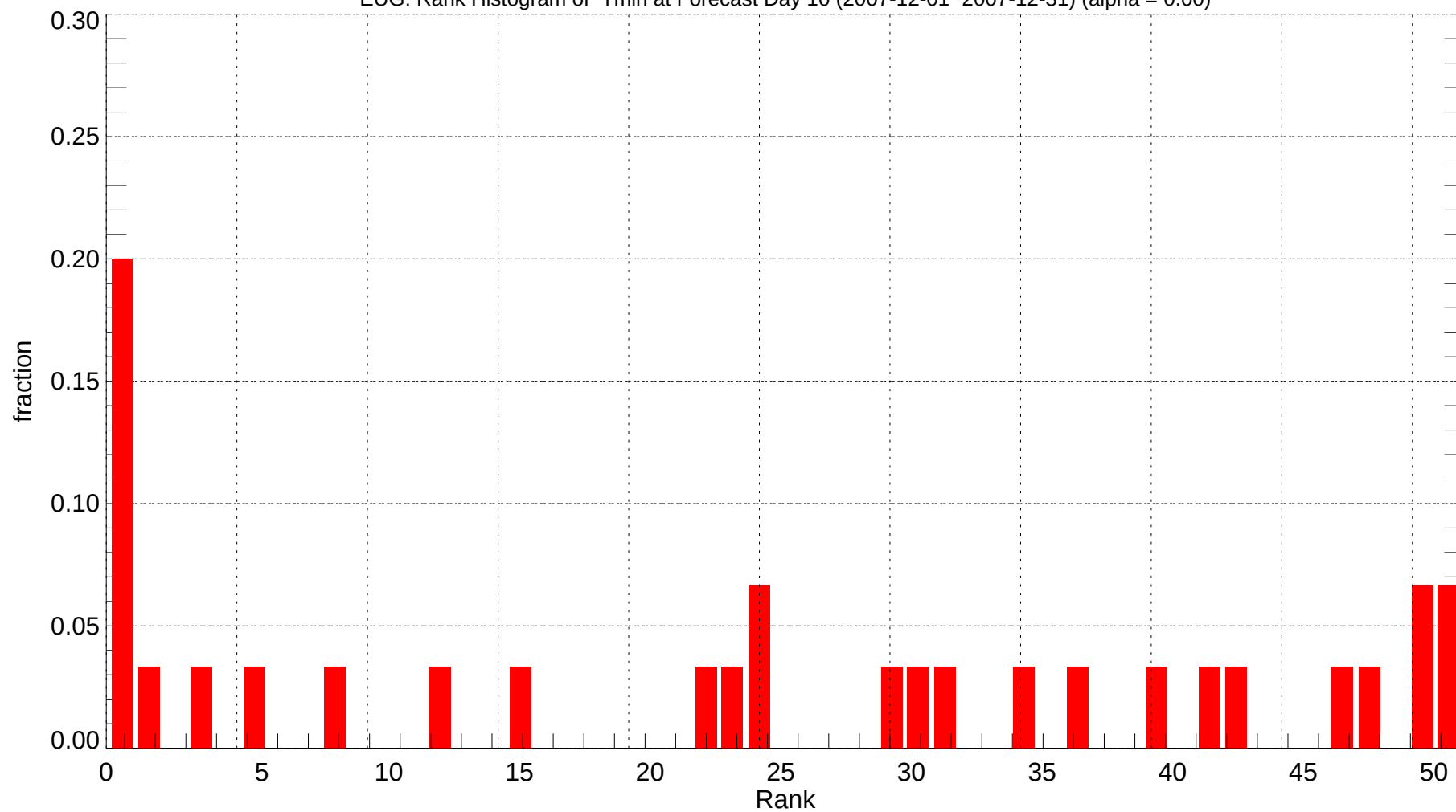
EUG: Rank Histogram of Tmin at Forecast Day 10 (2007-12-01~2007-12-31) (alpha = 0.00)
