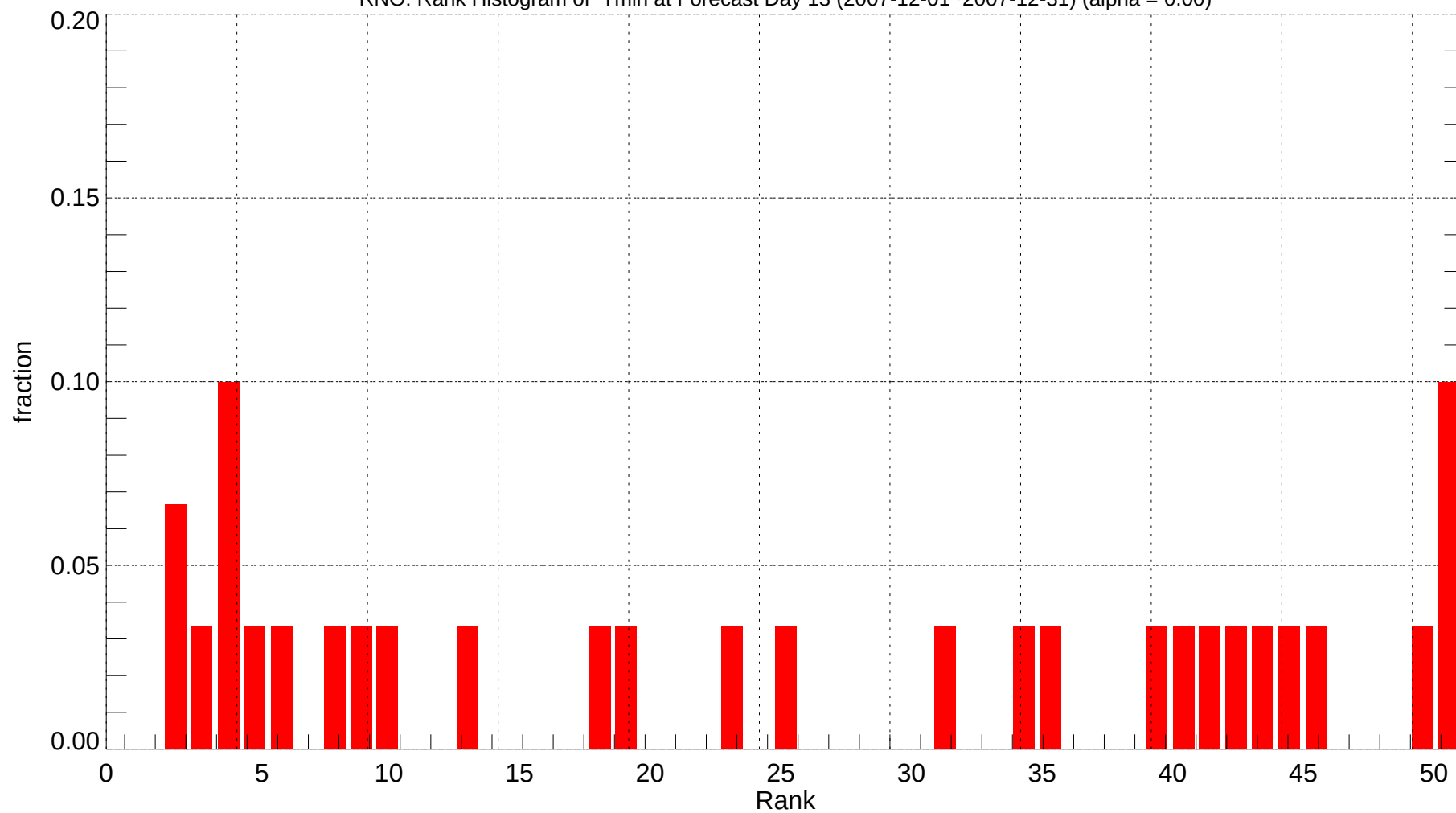
RNO: Rank Histogram of Tmin at Forecast Day 13 (2007-12-01~2007-12-31) (alpha = 0.00)
