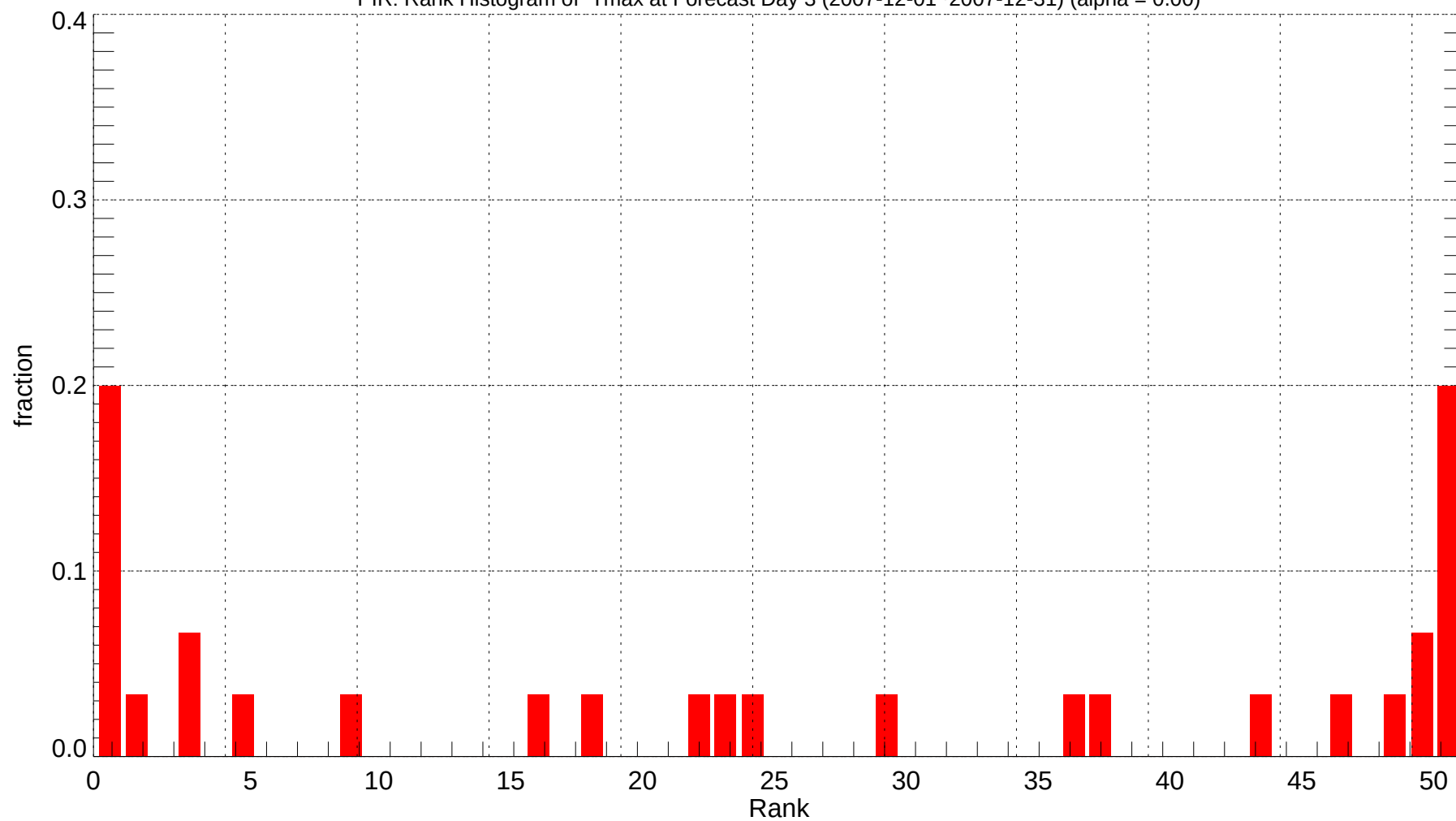
PIR: Rank Histogram of Tmax at Forecast Day 3 (2007-12-01~2007-12-31) (alpha = 0.00)
