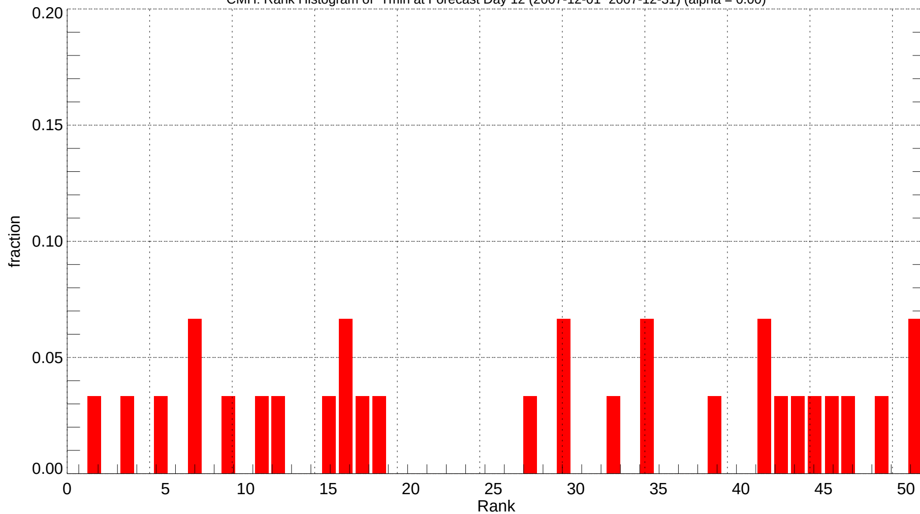
CMH: Rank Histogram of Tmin at Forecast Day 12 (2007-12-01~2007-12-31) (alpha = 0.00)
