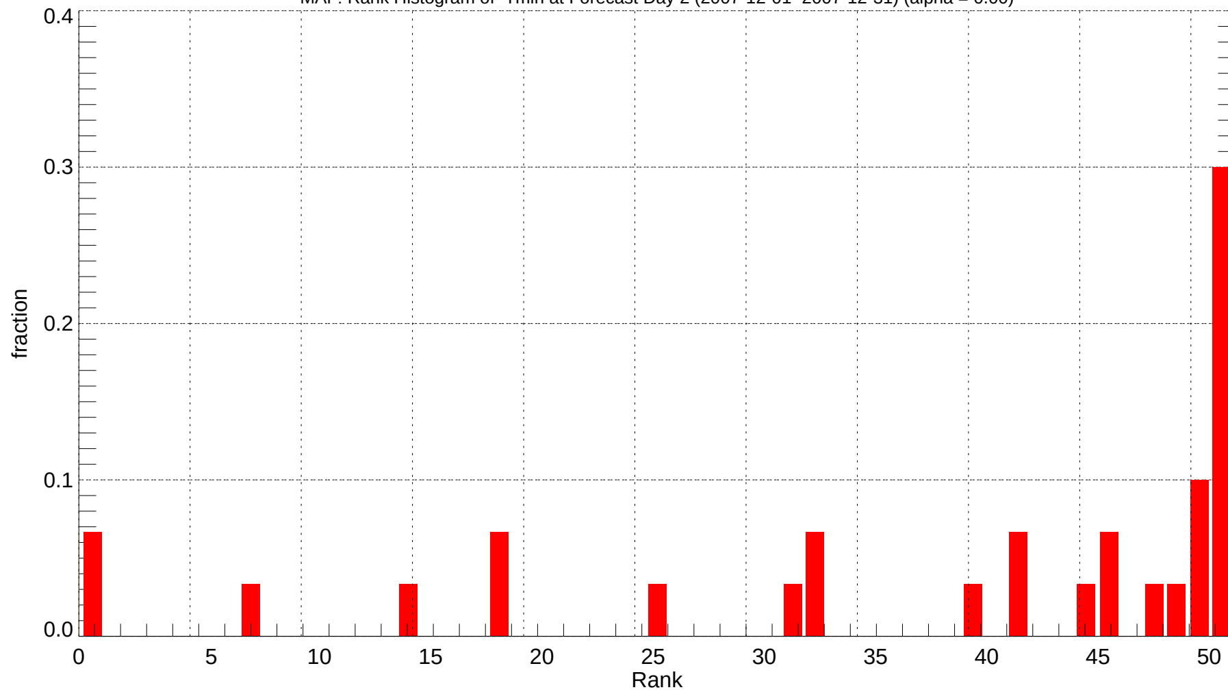
MAF: Rank Histogram of Tmin at Forecast Day 2 (2007-12-01~2007-12-31) (alpha = 0.00)
