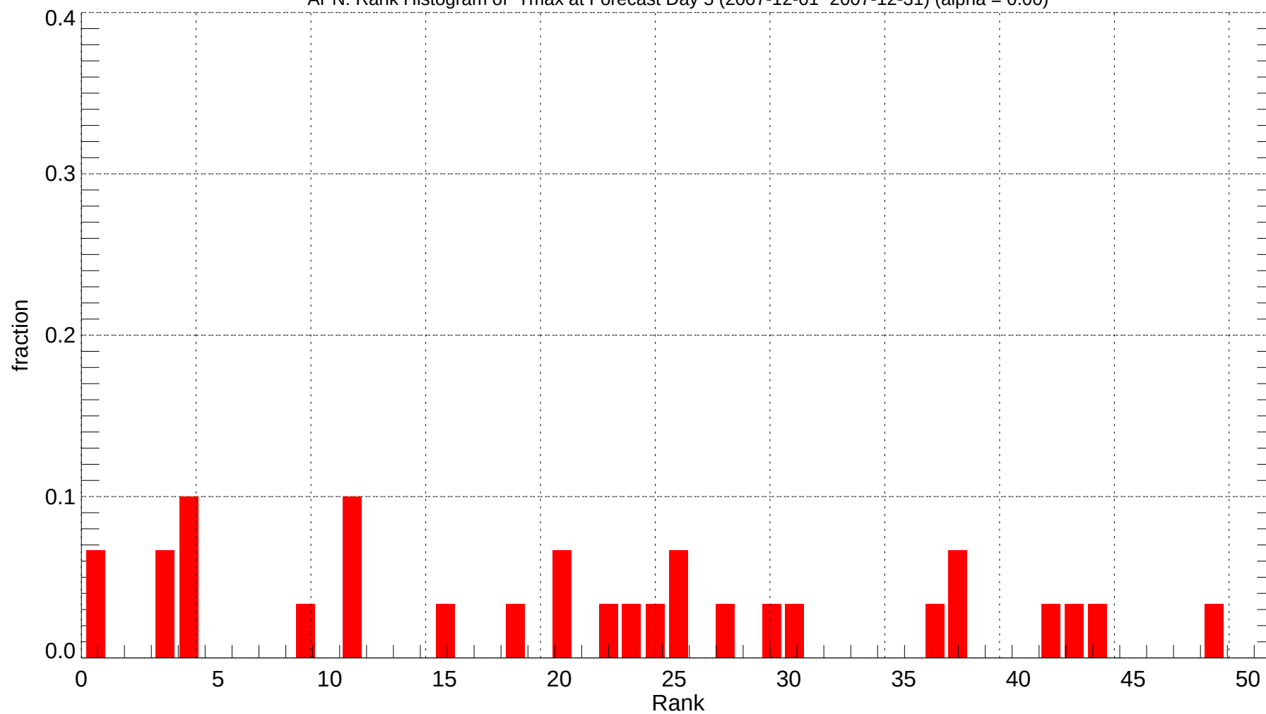
APN: Rank Histogram of Tmax at Forecast Day 5 (2007-12-01~2007-12-31) (alpha = 0.00)
