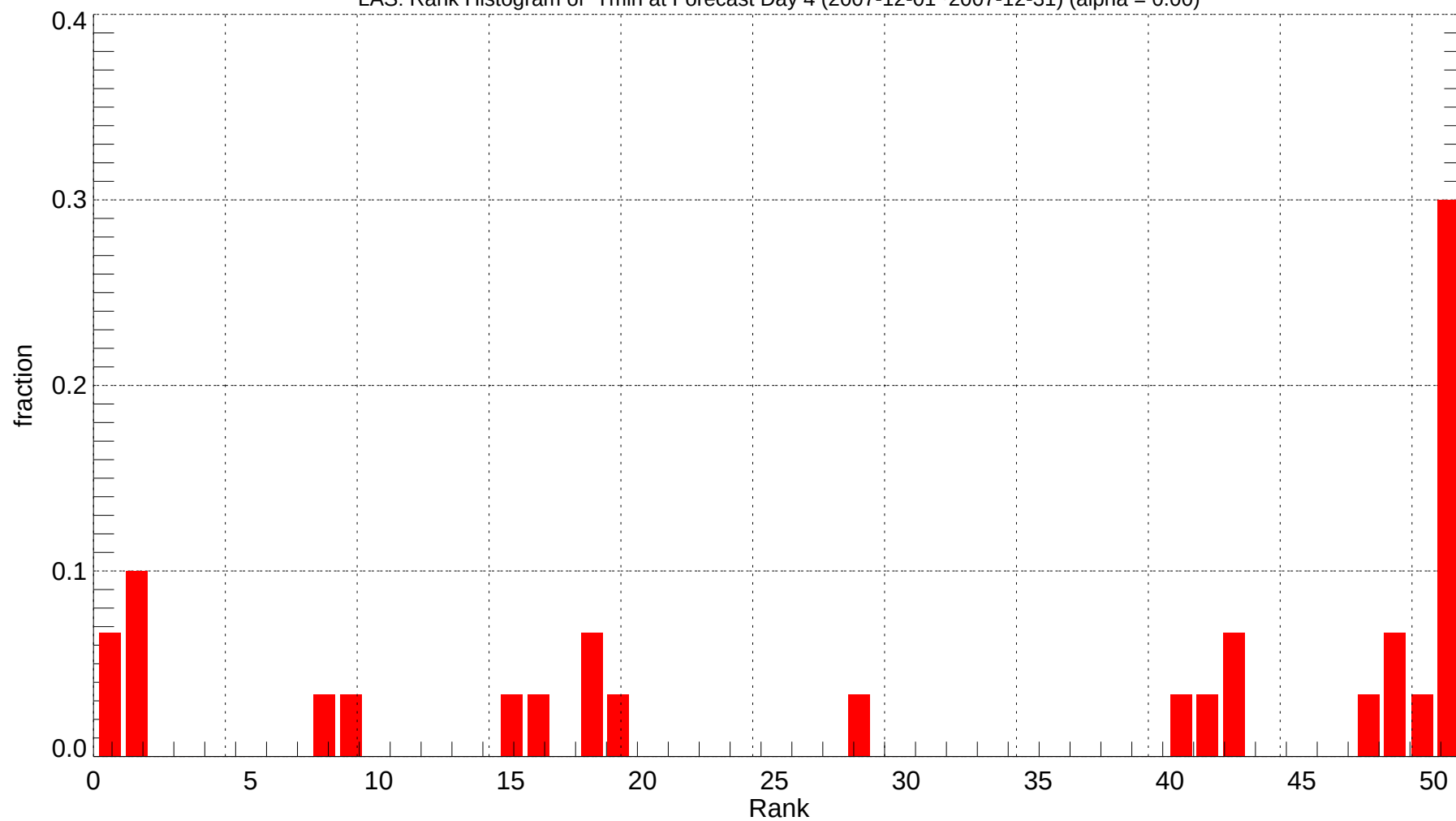
LAS: Rank Histogram of Tmin at Forecast Day 4 (2007-12-01~2007-12-31) (alpha = 0.00)
