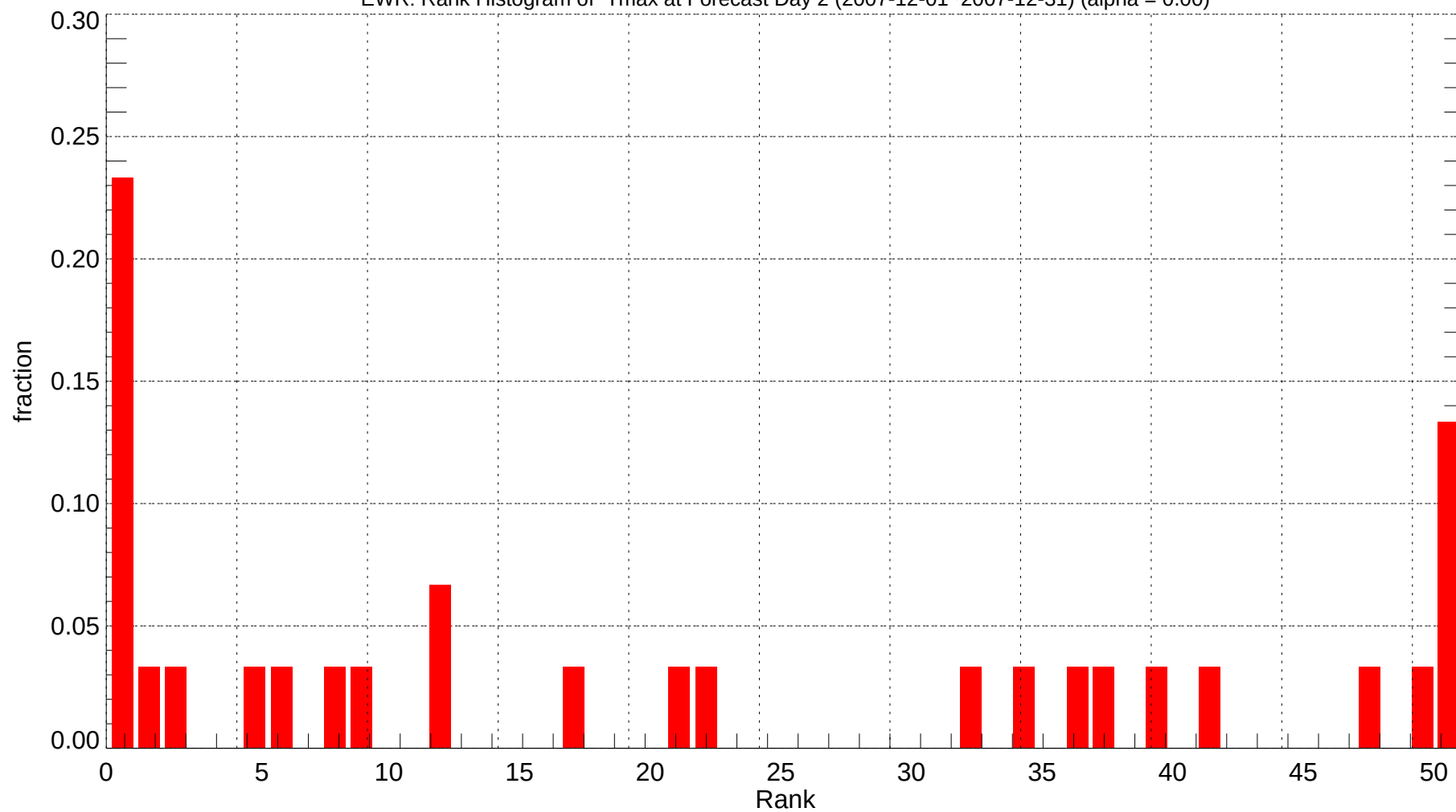
EWR: Rank Histogram of Tmax at Forecast Day 2 (2007-12-01~2007-12-31) (alpha = 0.00)
