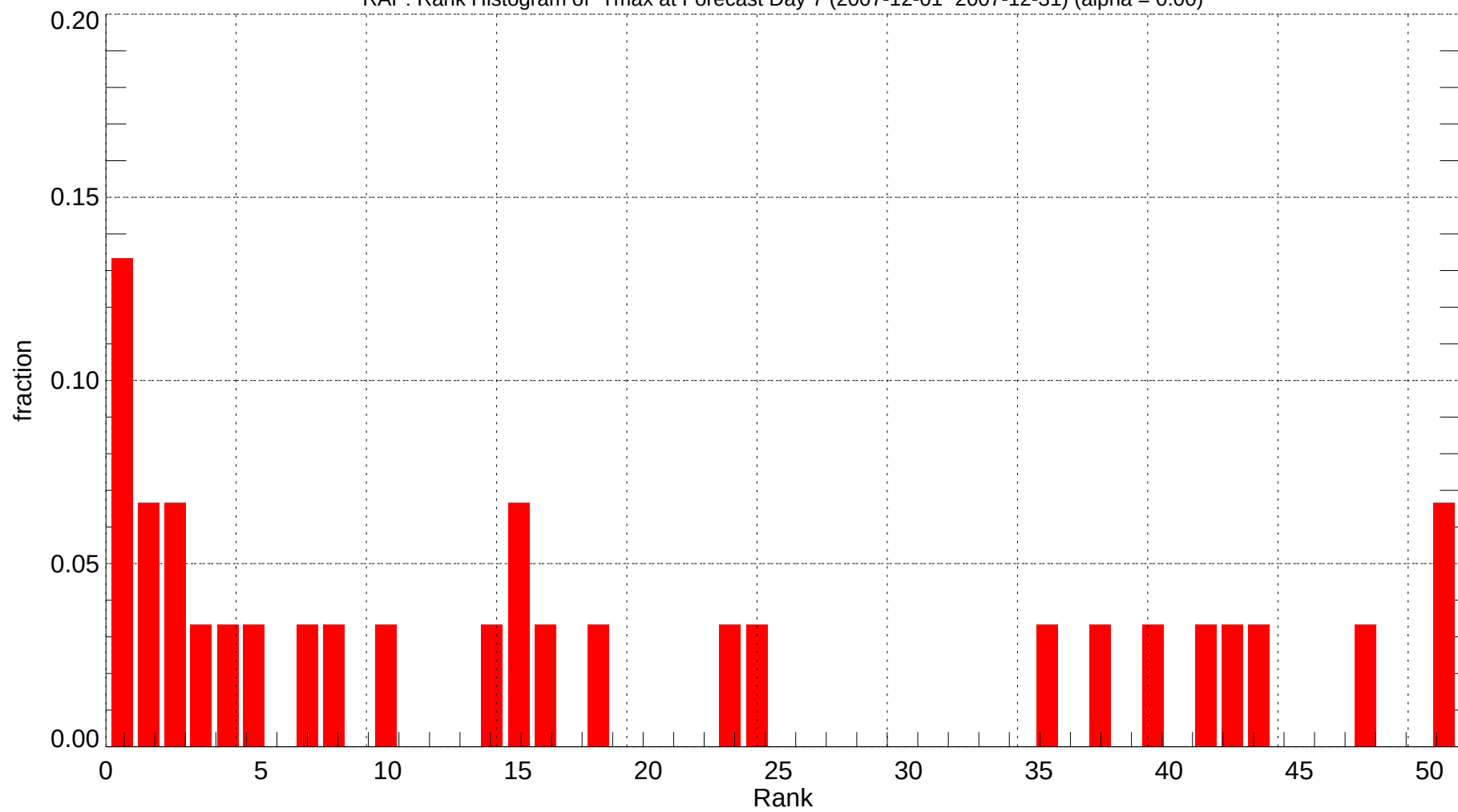
RAP: Rank Histogram of Tmax at Forecast Day 7 (2007-12-01~2007-12-31) (alpha = 0.00)
