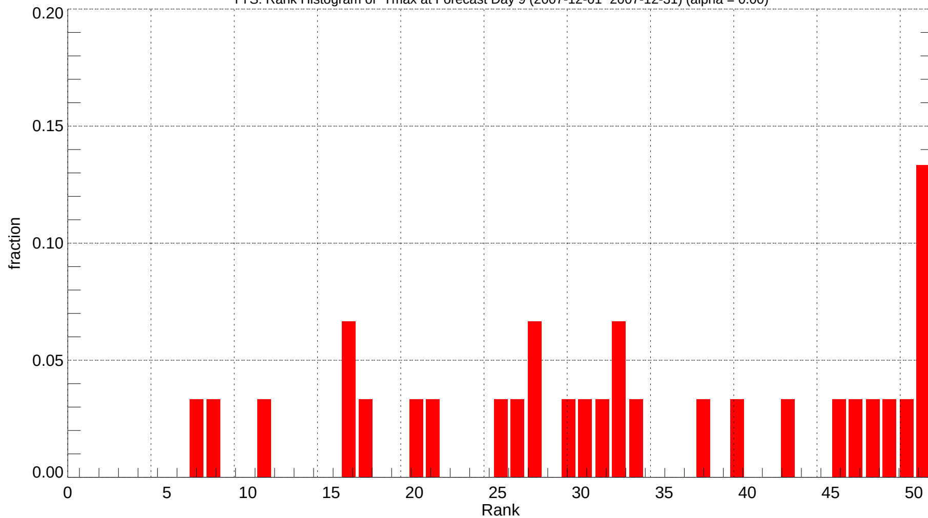
TYS: Rank Histogram of Tmax at Forecast Day 9 (2007-12-01~2007-12-31) (alpha = 0.00)
