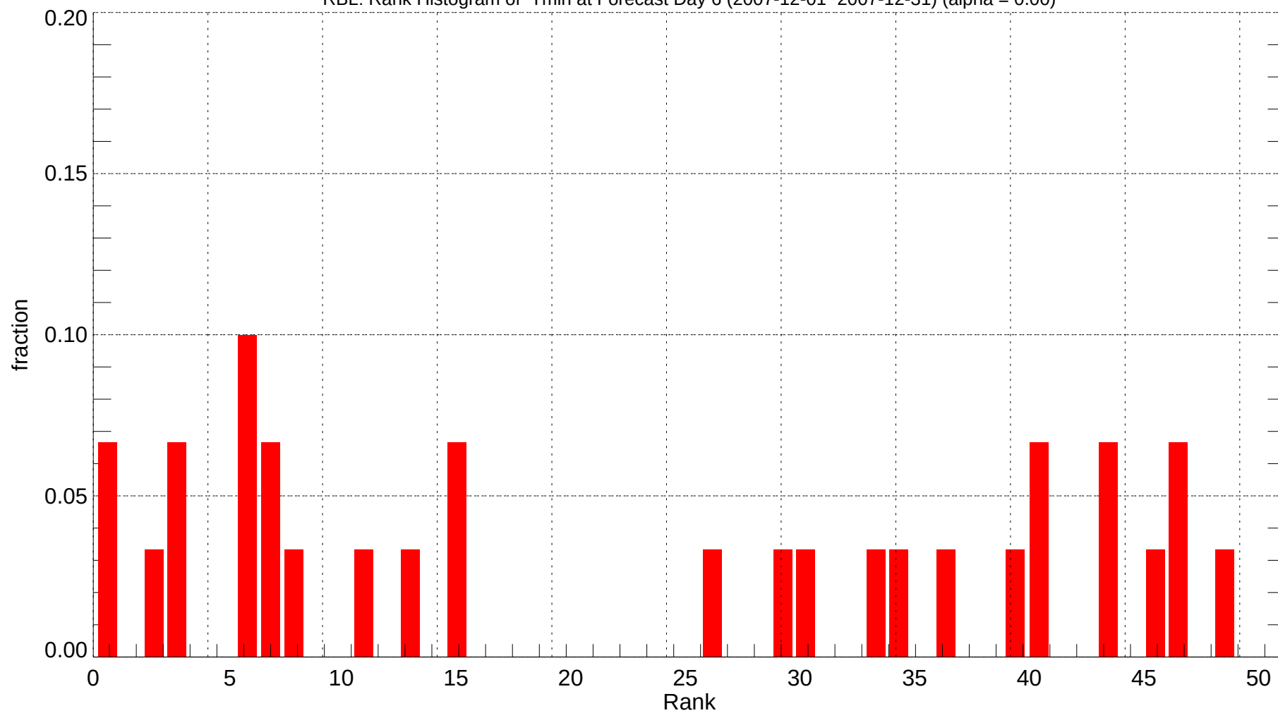
RBL: Rank Histogram of Tmin at Forecast Day 6 (2007-12-01~2007-12-31) (alpha = 0.00)
