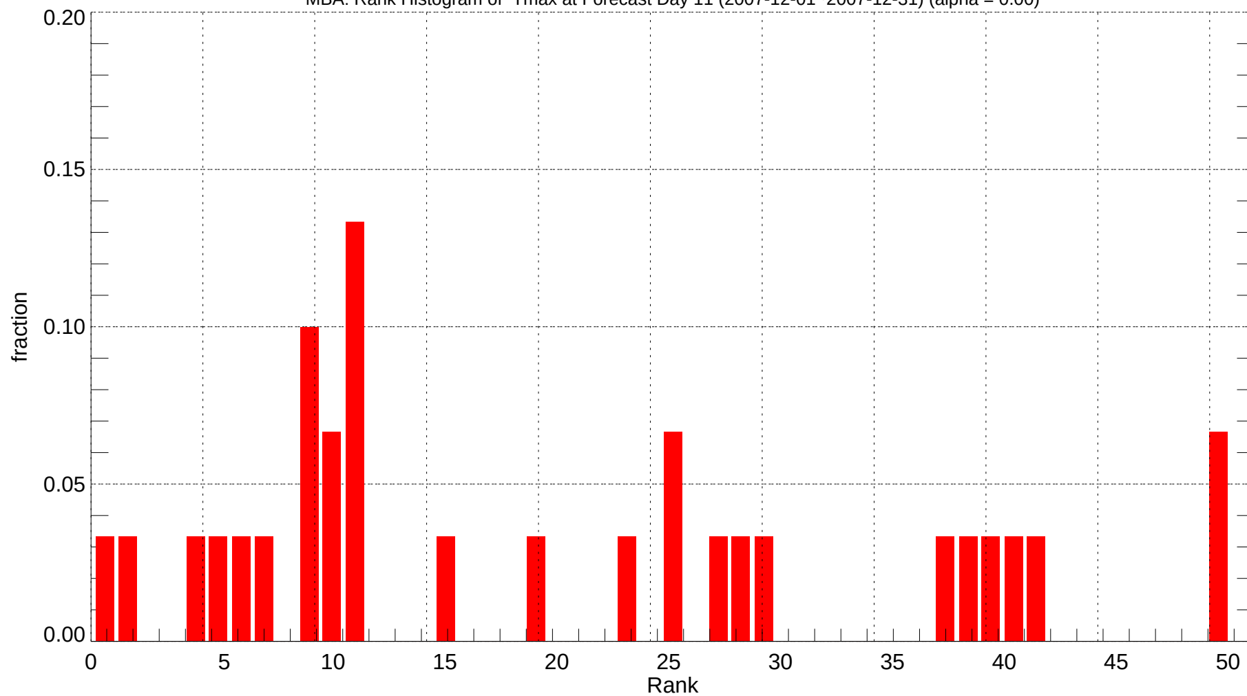
MBA: Rank Histogram of Tmax at Forecast Day 11 (2007-12-01~2007-12-31) (alpha = 0.00)
