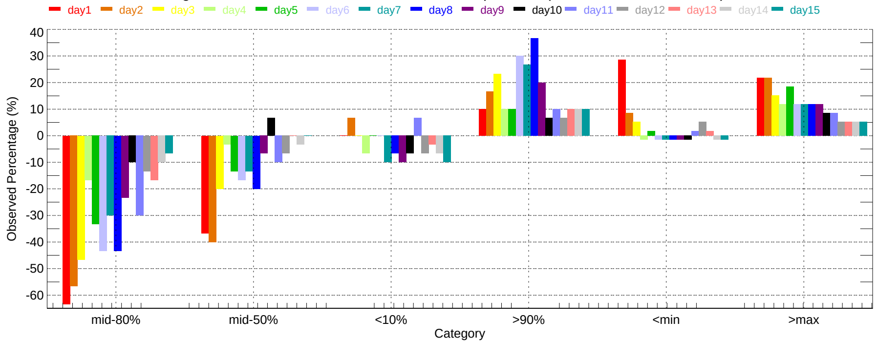
Observed Percentage Deviation of Ensembles - NTU: Min Temperature (2007-12-01~2007-12-31)
