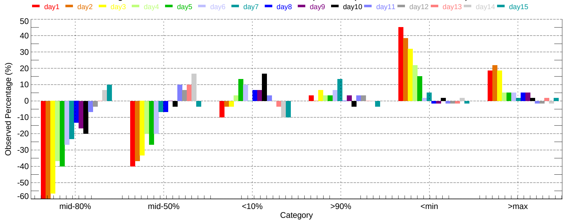
Observed Percentage Deviation of Ensembles - MDT: Min Temperature (2007-12-01~2007-12-31)
