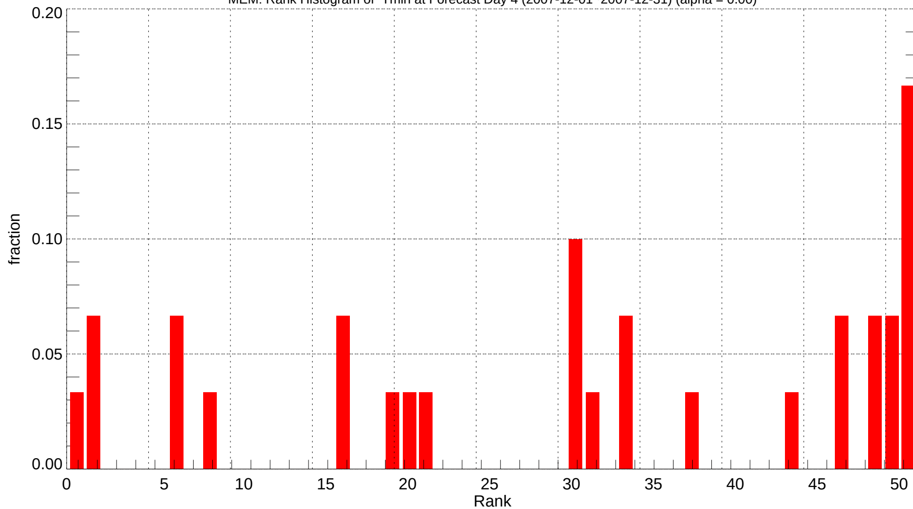
MEM: Rank Histogram of Tmin at Forecast Day 4 (2007-12-01~2007-12-31) (alpha = 0.00)
