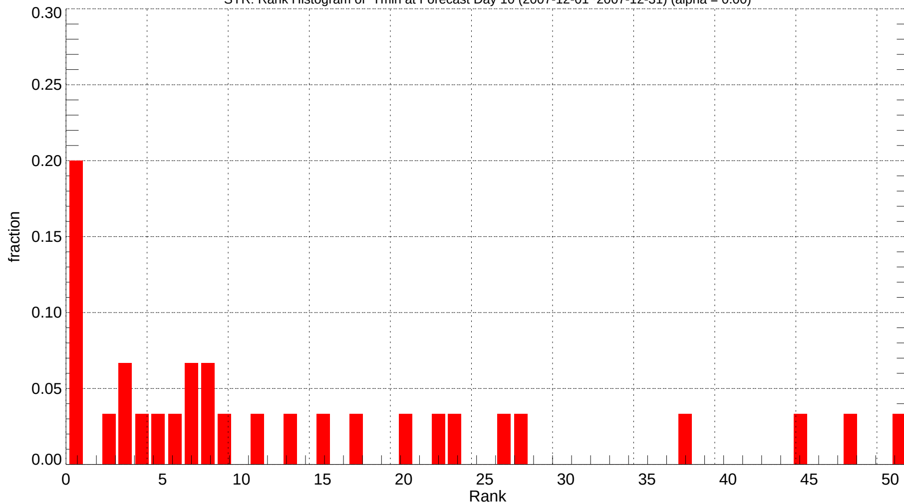
SYR: Rank Histogram of Tmin at Forecast Day 10 (2007-12-01~2007-12-31) (alpha = 0.00)
