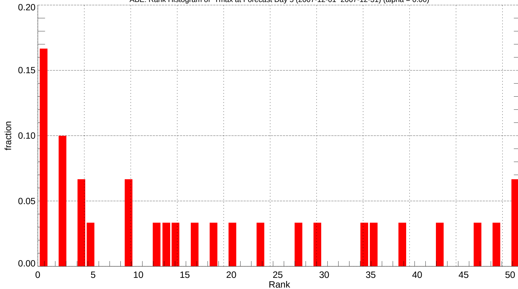
ABE: Rank Histogram of Tmax at Forecast Day 5 (2007-12-01~2007-12-31) (alpha = 0.00)
