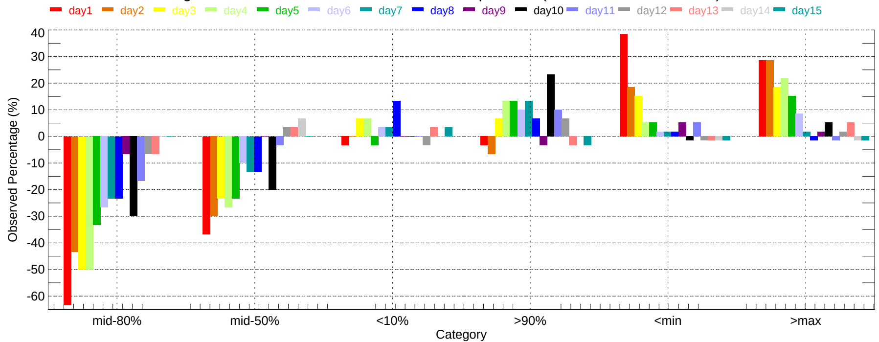
Observed Percentage Deviation of Ensembles - PIR: Min Temperature (2007-12-01~2007-12-31)
