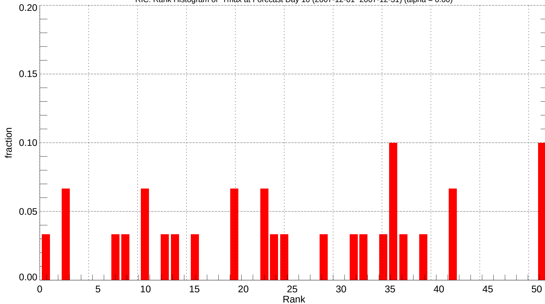
RIC: Rank Histogram of Tmax at Forecast Day 10 (2007-12-01~2007-12-31) (alpha = 0.00)
