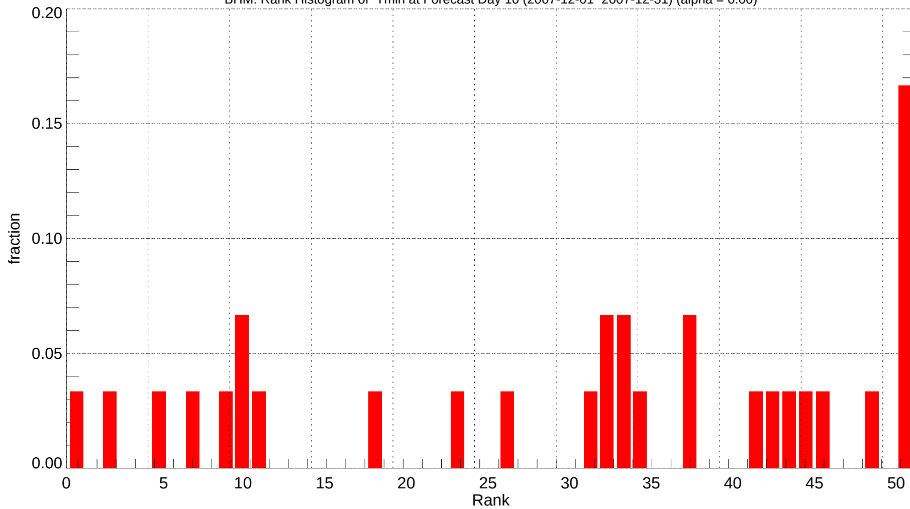
BHM: Rank Histogram of Tmin at Forecast Day 10 (2007-12-01~2007-12-31) (alpha = 0.00)
