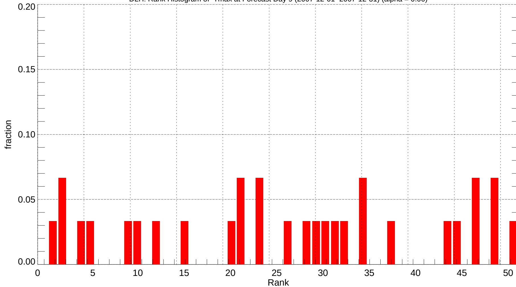
DLH: Rank Histogram of Tmax at Forecast Day 9 (2007-12-01~2007-12-31) (alpha = 0.00)
