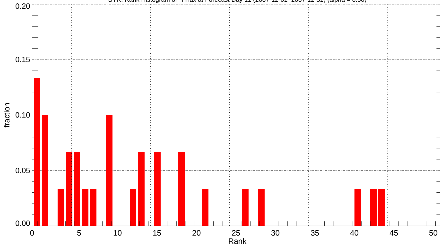
SYR: Rank Histogram of Tmax at Forecast Day 11 (2007-12-01~2007-12-31) (alpha = 0.00)
