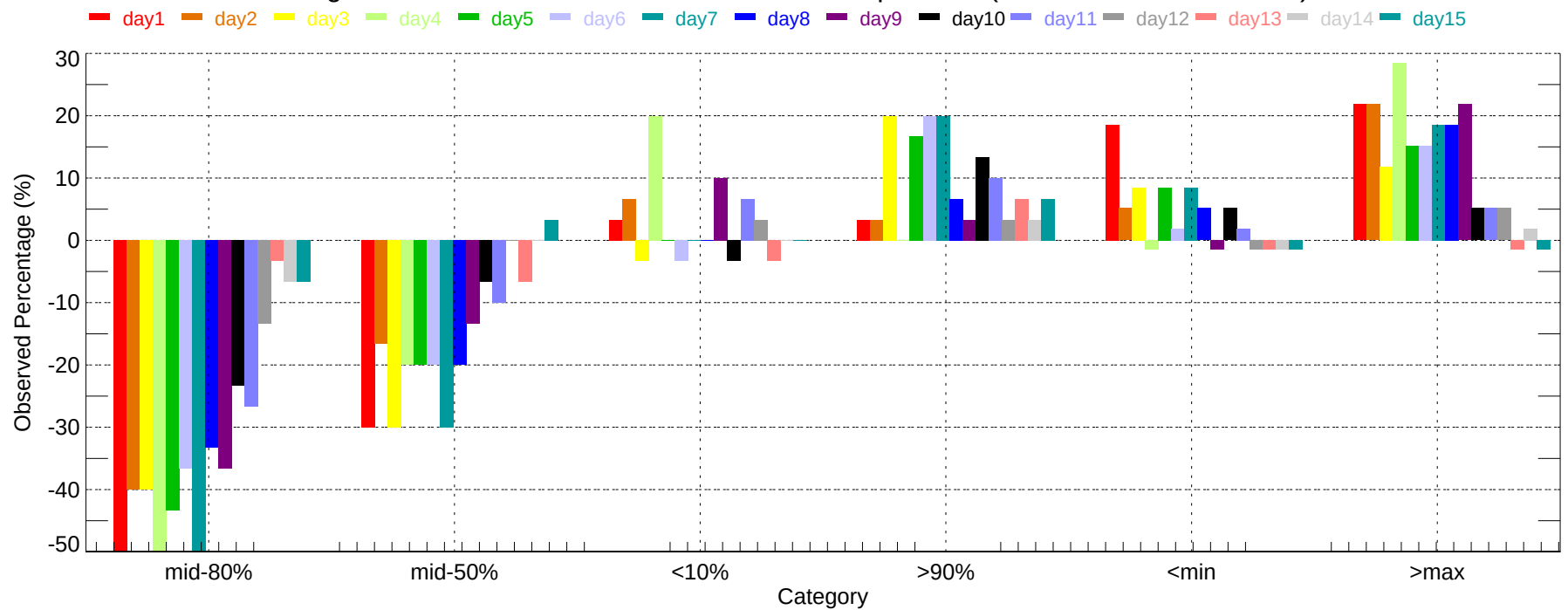
Observed Percentage Deviation of Ensembles - ORD: Max Temperature (2007-12-01~2007-12-31)
