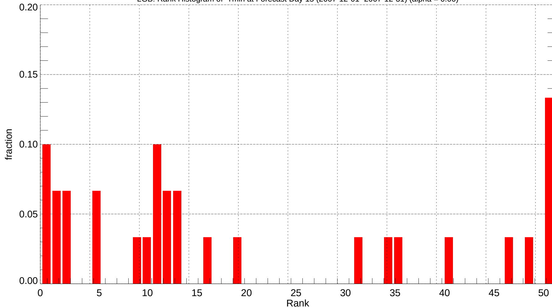
LGB: Rank Histogram of Tmin at Forecast Day 15 (2007-12-01~2007-12-31) (alpha = 0.00)
