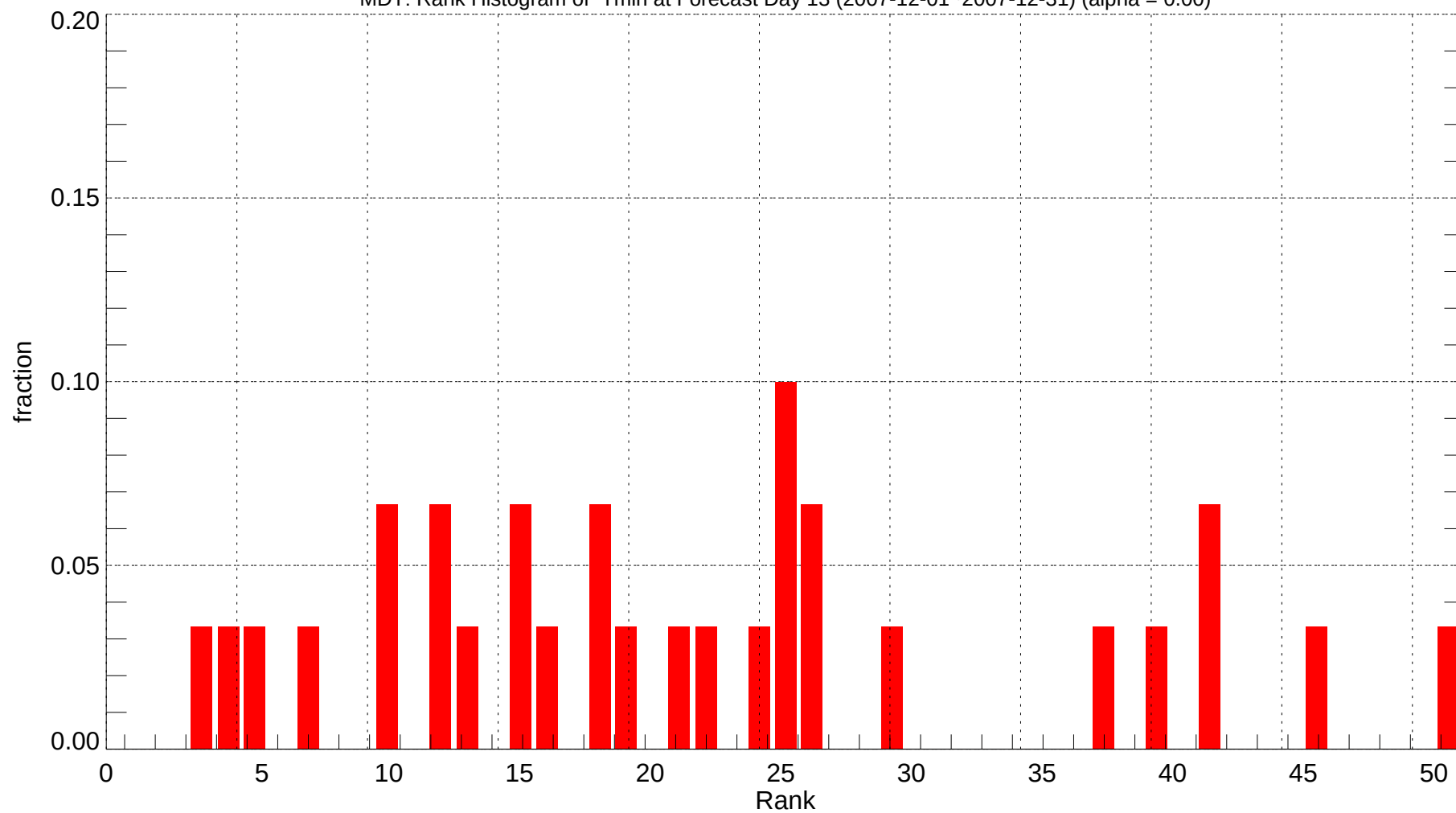
MDT: Rank Histogram of Tmin at Forecast Day 13 (2007-12-01~2007-12-31) (alpha = 0.00)
