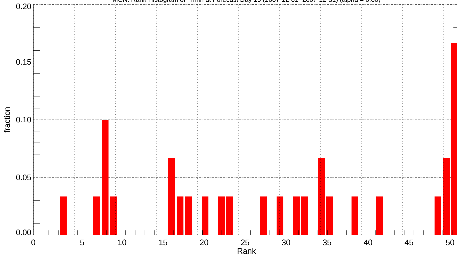
MCN: Rank Histogram of Tmin at Forecast Day 15 (2007-12-01~2007-12-31) (alpha = 0.00)
