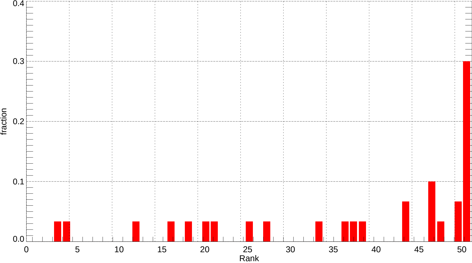
BFL: Rank Histogram of Tmin at Forecast Day 8 (2007-12-01~2007-12-31) (alpha = 0.00)
