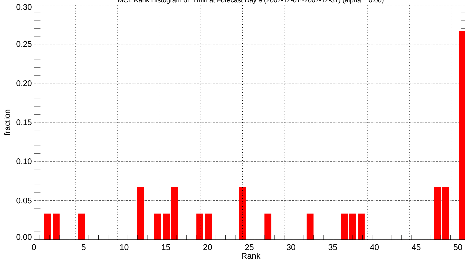
MCI: Rank Histogram of Tmin at Forecast Day 9 (2007-12-01~2007-12-31) (alpha = 0.00)
