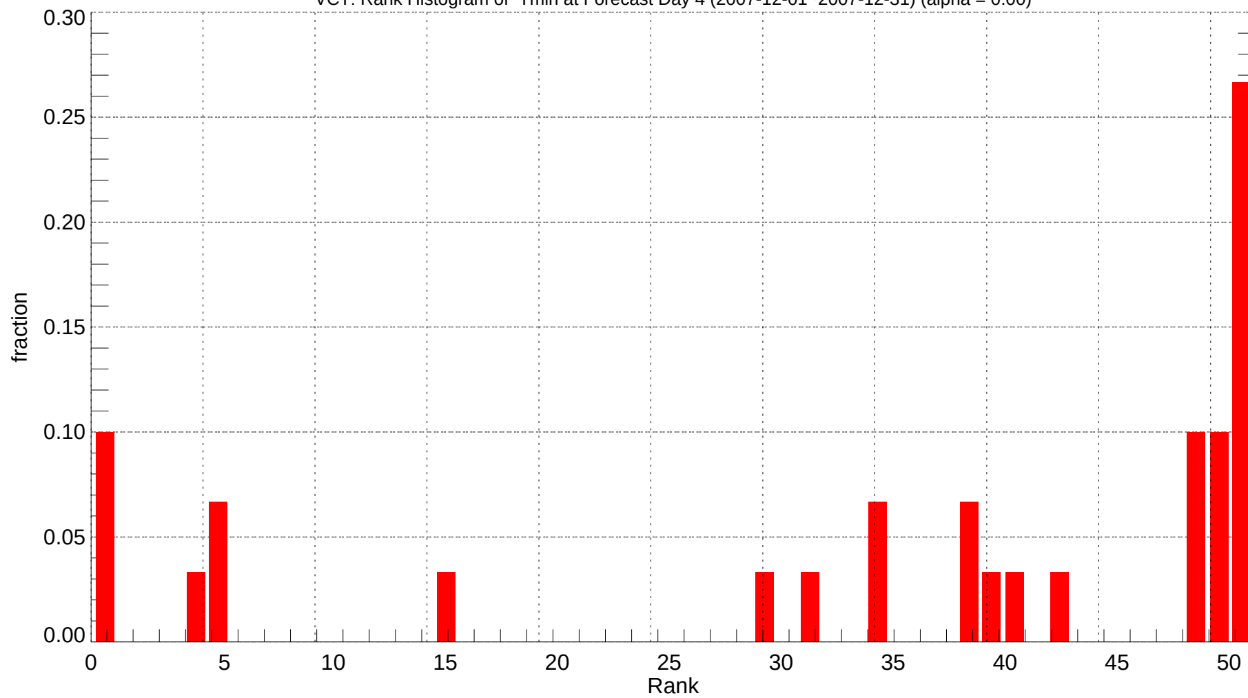
VCT: Rank Histogram of Tmin at Forecast Day 4 (2007-12-01~2007-12-31) (alpha = 0.00)
