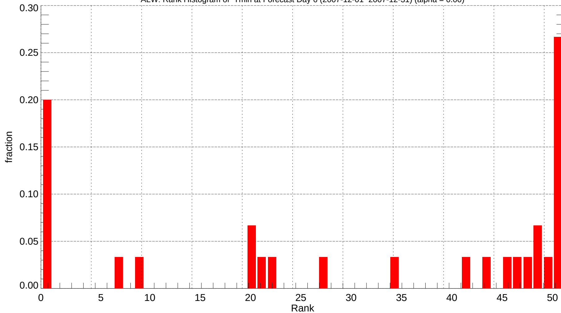
ALW: Rank Histogram of Tmin at Forecast Day 6 (2007-12-01~2007-12-31) (alpha = 0.00)
