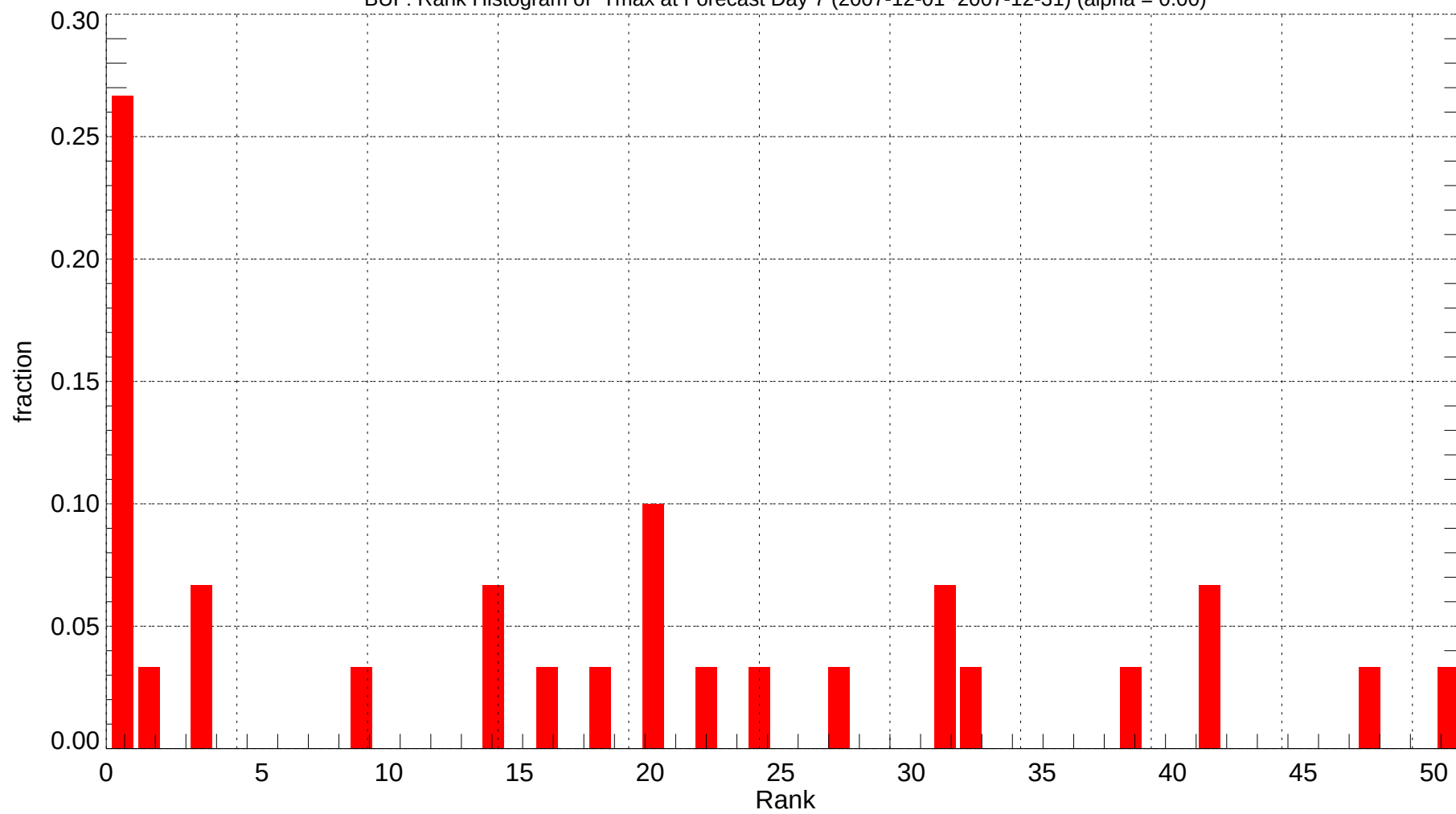
BUF: Rank Histogram of Tmax at Forecast Day 7 (2007-12-01~2007-12-31) (alpha = 0.00)
