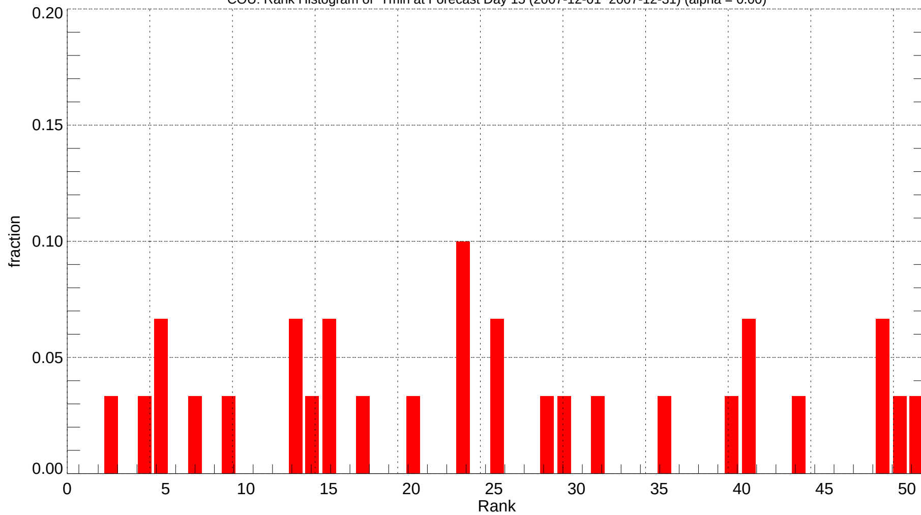
COU: Rank Histogram of Tmin at Forecast Day 15 (2007-12-01~2007-12-31) (alpha = 0.00)
