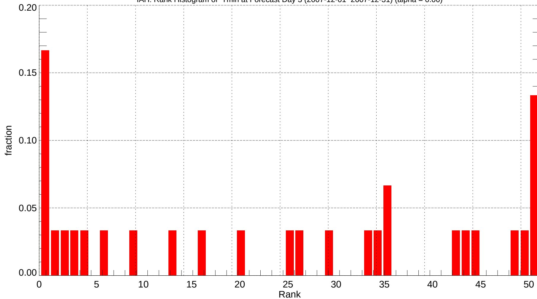
IAH: Rank Histogram of Tmin at Forecast Day 3 (2007-12-01~2007-12-31) (alpha = 0.00)
