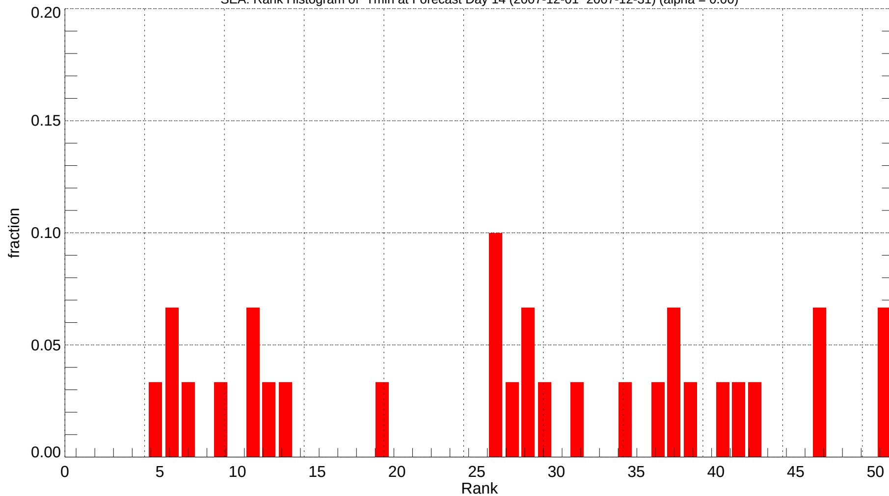
SEA: Rank Histogram of Tmin at Forecast Day 14 (2007-12-01~2007-12-31) (alpha = 0.00)
