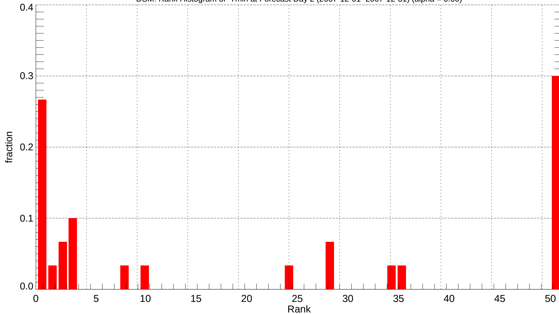
DSM: Rank Histogram of Tmin at Forecast Day 2 (2007-12-01~2007-12-31) (alpha = 0.00)
