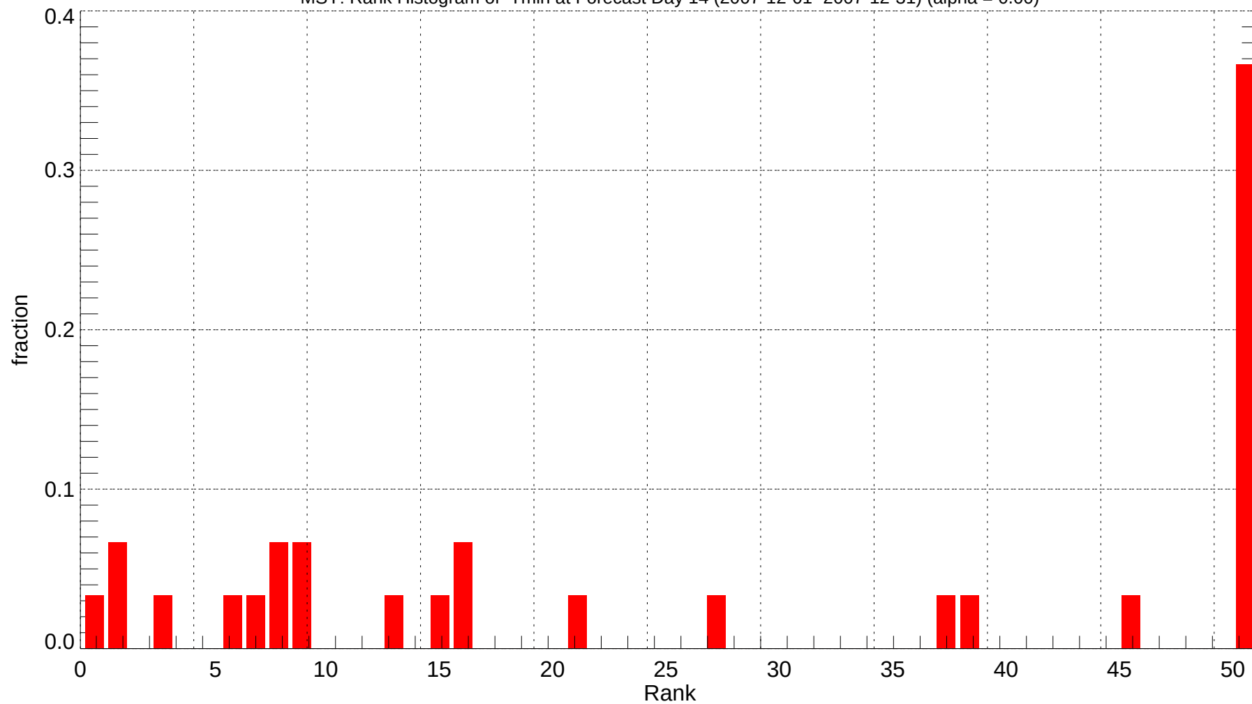
MSY: Rank Histogram of Tmin at Forecast Day 14 (2007-12-01~2007-12-31) (alpha = 0.00)
