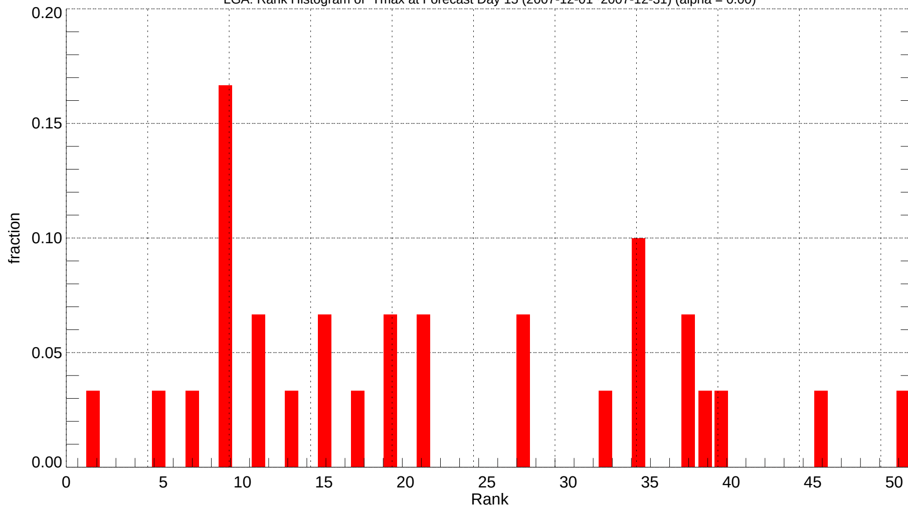
LGA: Rank Histogram of Tmax at Forecast Day 15 (2007-12-01~2007-12-31) (alpha = 0.00)
