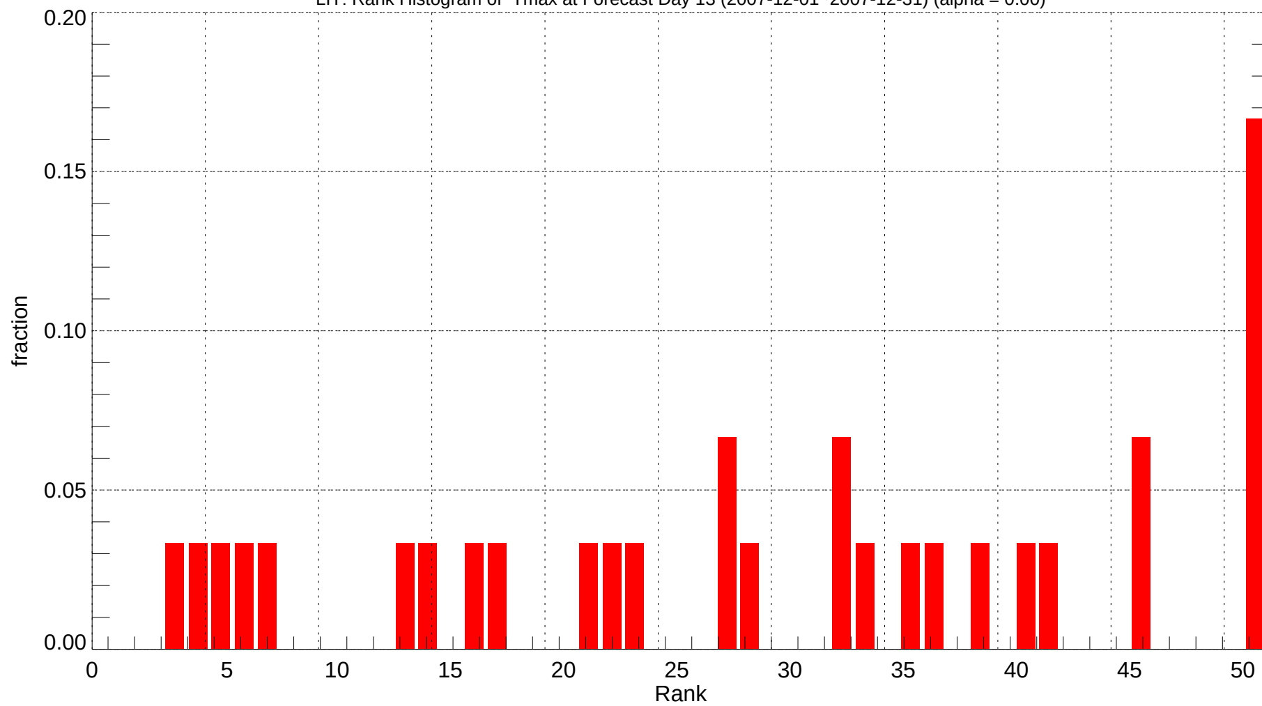
LIT: Rank Histogram of Tmax at Forecast Day 13 (2007-12-01~2007-12-31) (alpha = 0.00)
