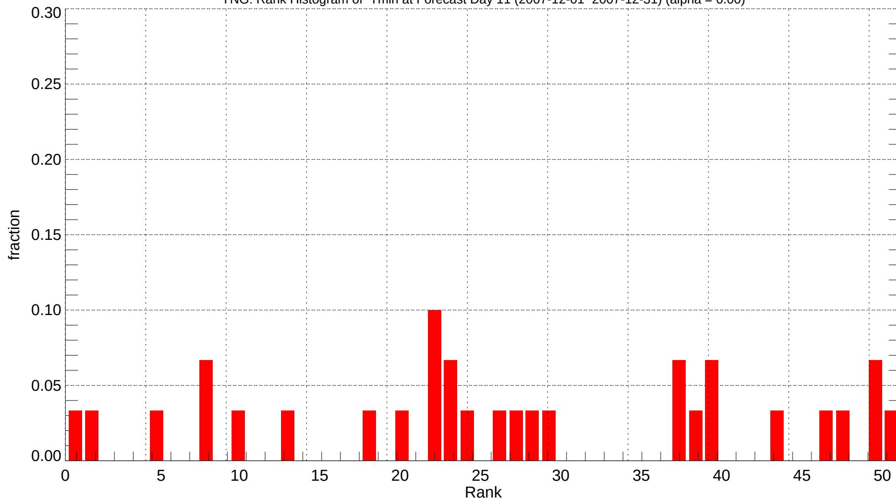
YNG: Rank Histogram of Tmin at Forecast Day 11 (2007-12-01~2007-12-31) (alpha = 0.00)
