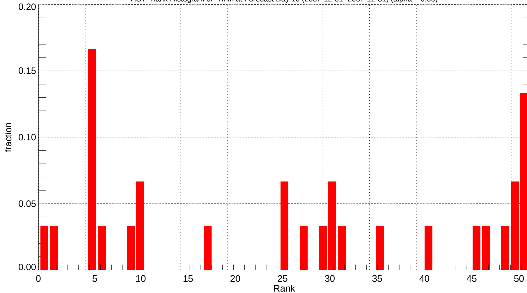
ACT: Rank Histogram of Tmin at Forecast Day 10 (2007-12-01~2007-12-31) (alpha = 0.00)
