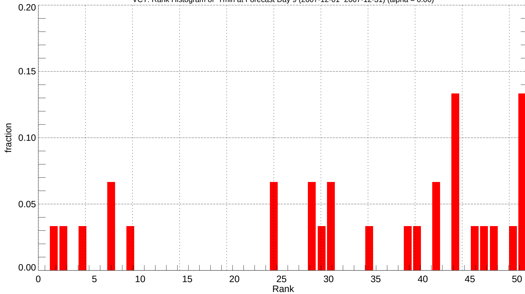
VCT: Rank Histogram of Tmin at Forecast Day 9 (2007-12-01~2007-12-31) (alpha = 0.00)
