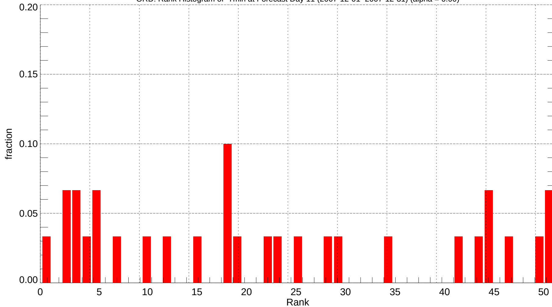
ORD: Rank Histogram of Tmin at Forecast Day 11 (2007-12-01~2007-12-31) (alpha = 0.00)
