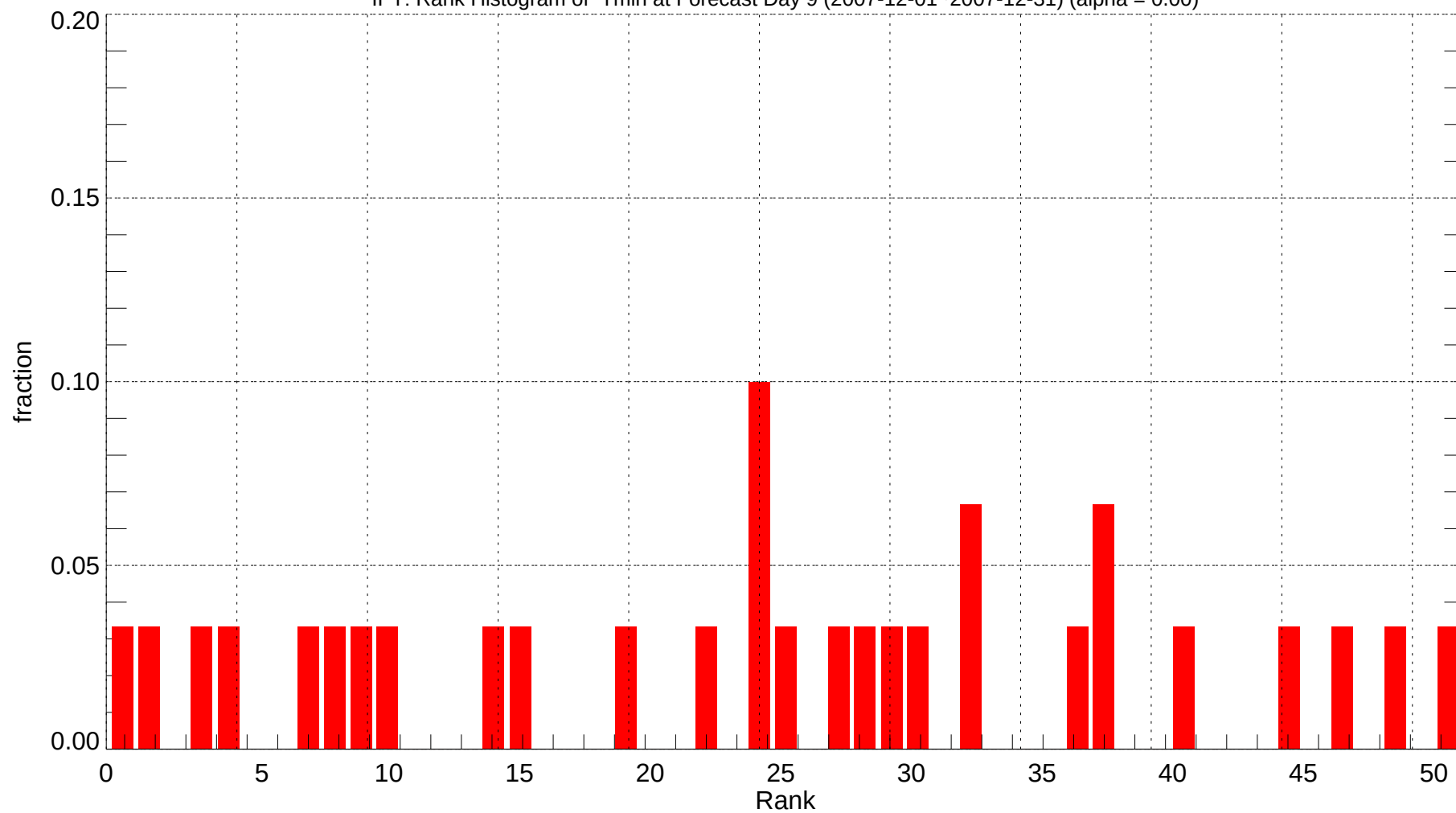
IPT: Rank Histogram of Tmin at Forecast Day 9 (2007-12-01~2007-12-31) (alpha = 0.00)
