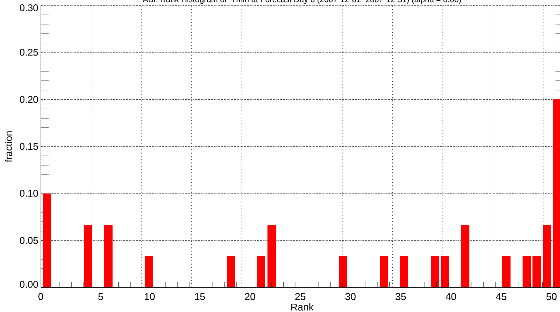
ABI: Rank Histogram of Tmin at Forecast Day 6 (2007-12-01~2007-12-31) (alpha = 0.00)
