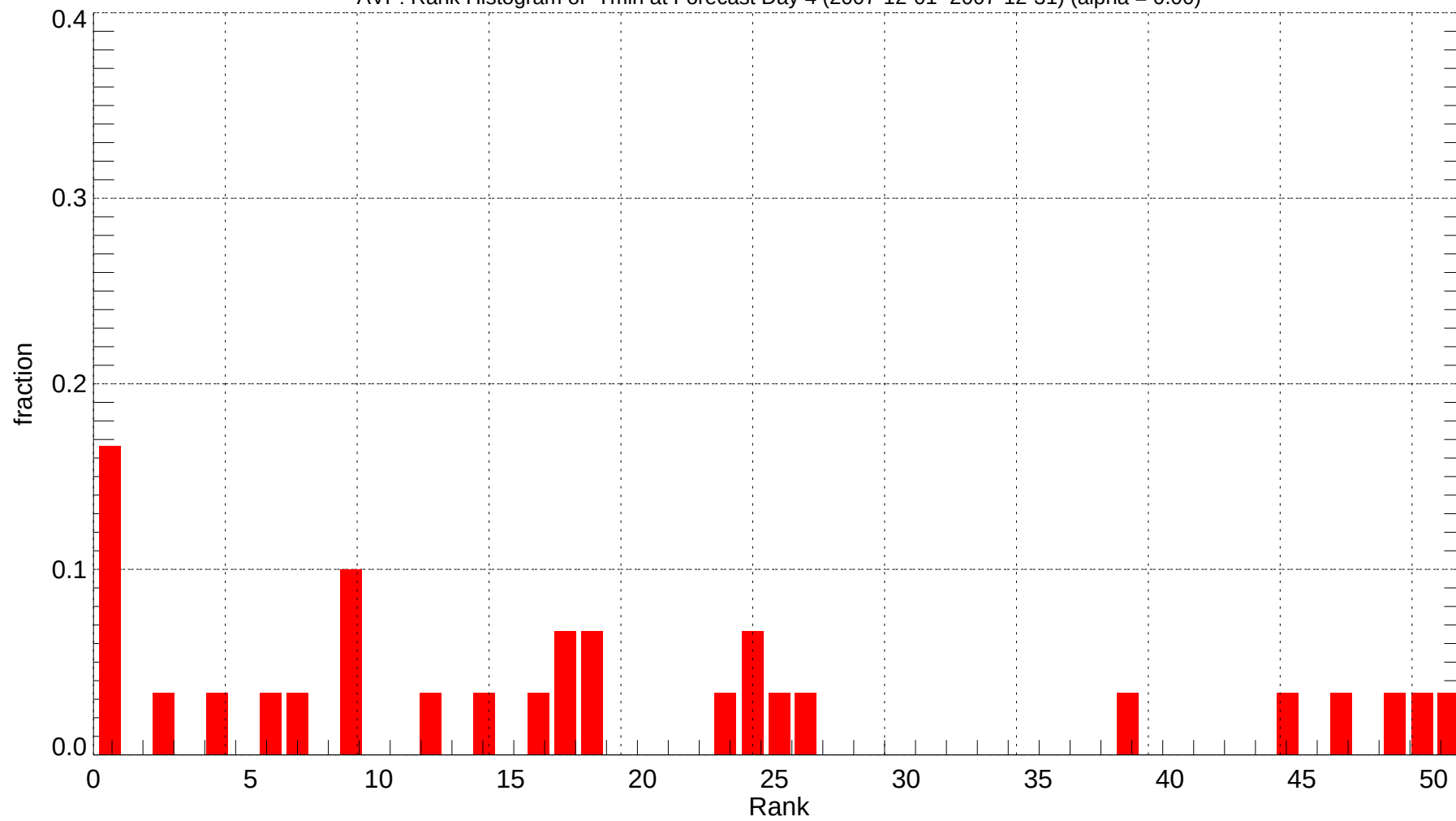
AVP: Rank Histogram of Tmin at Forecast Day 4 (2007-12-01~2007-12-31) (alpha = 0.00)
