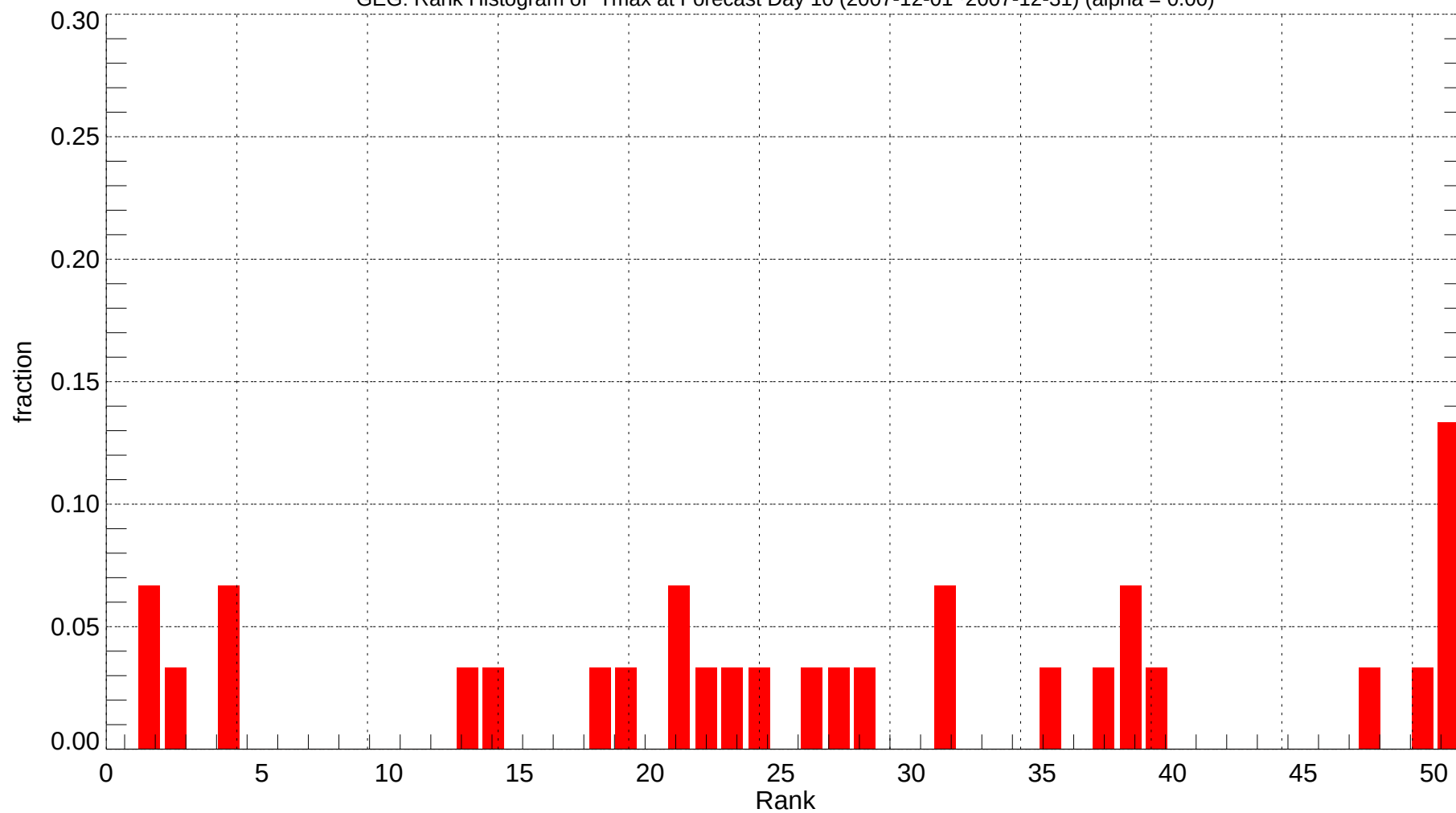
GEG: Rank Histogram of Tmax at Forecast Day 10 (2007-12-01~2007-12-31) (alpha = 0.00)
