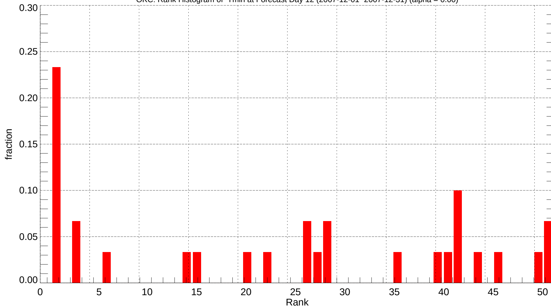
OKC: Rank Histogram of Tmin at Forecast Day 12 (2007-12-01~2007-12-31) (alpha = 0.00)
