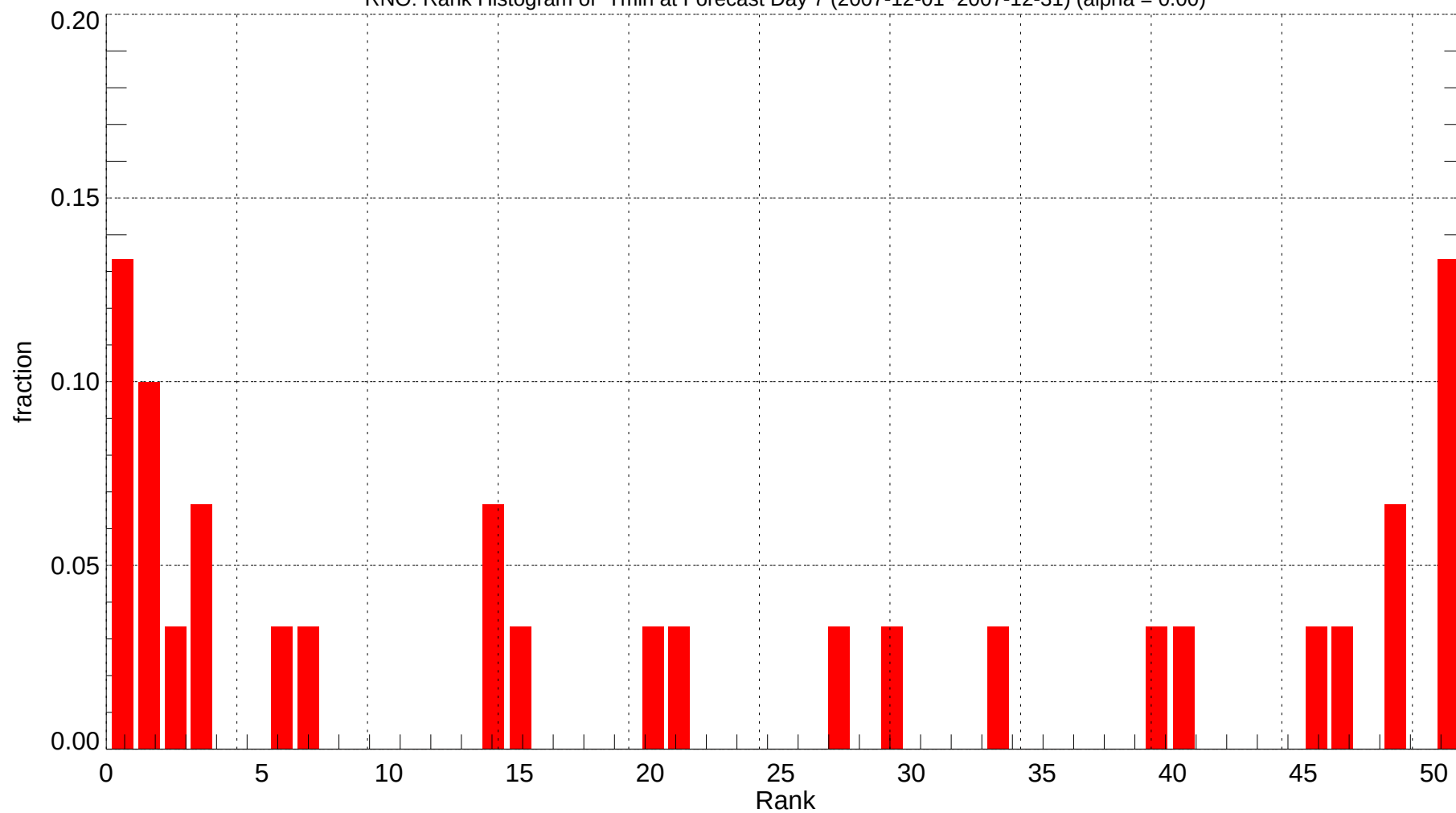
RNO: Rank Histogram of Tmin at Forecast Day 7 (2007-12-01~2007-12-31) (alpha = 0.00)
