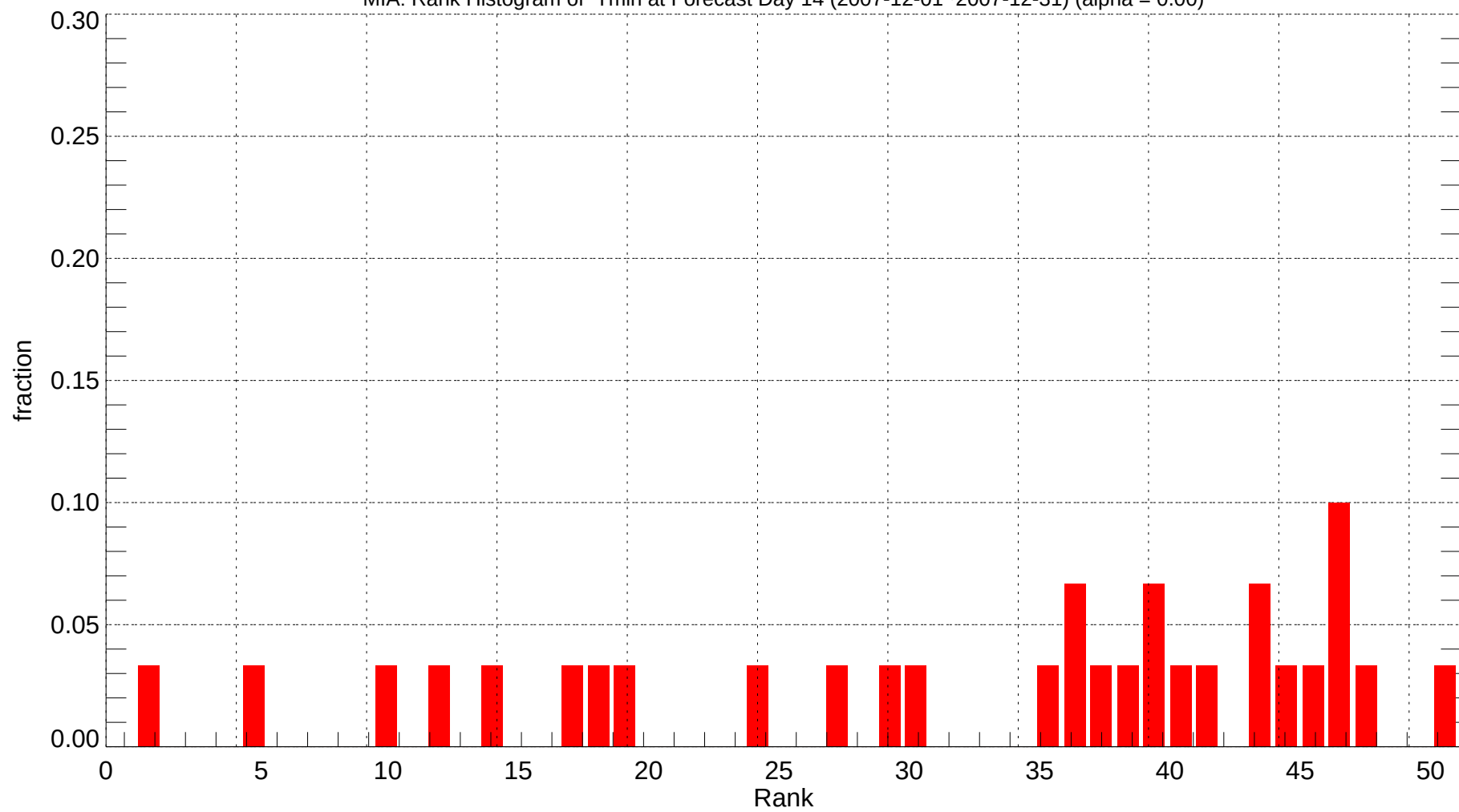
MIA: Rank Histogram of Tmin at Forecast Day 14 (2007-12-01~2007-12-31) (alpha = 0.00)
