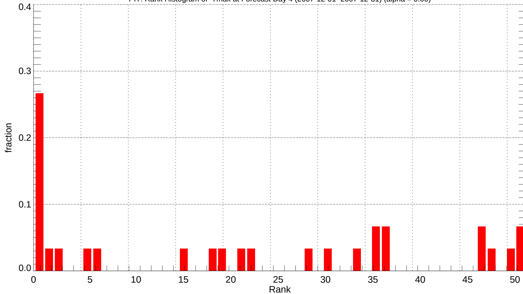
PIT: Rank Histogram of Tmax at Forecast Day 4 (2007-12-01~2007-12-31) (alpha = 0.00)
