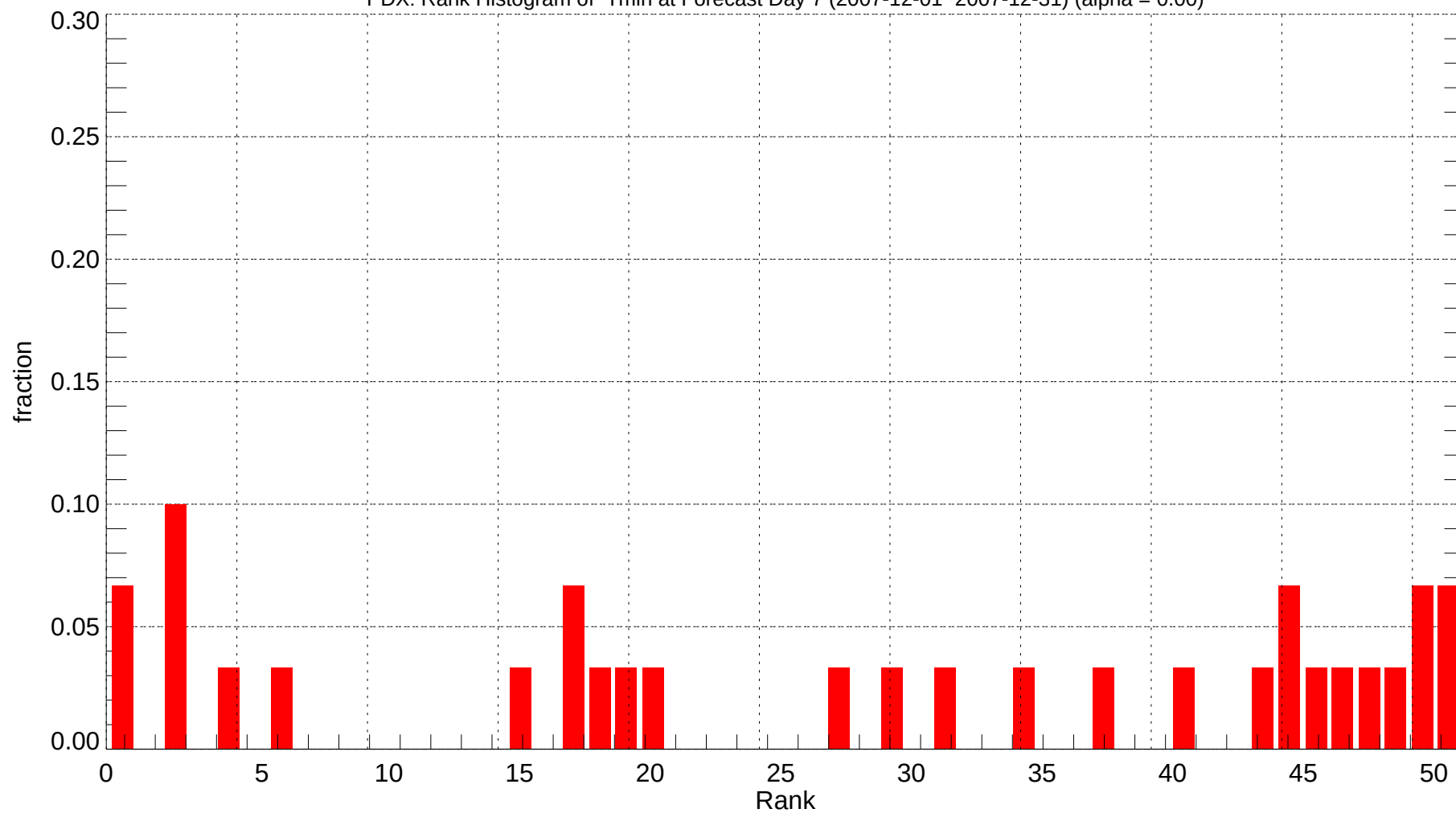
PDX: Rank Histogram of Tmin at Forecast Day 7 (2007-12-01~2007-12-31) (alpha = 0.00)
