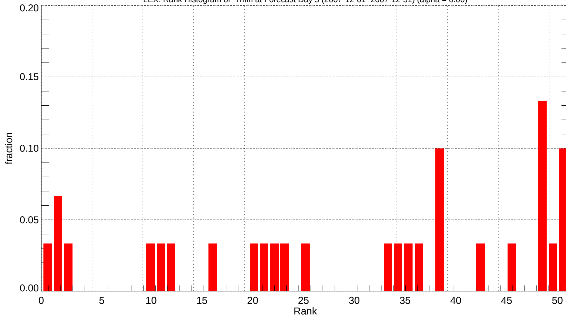
LEX: Rank Histogram of Tmin at Forecast Day 5 (2007-12-01~2007-12-31) (alpha = 0.00)
