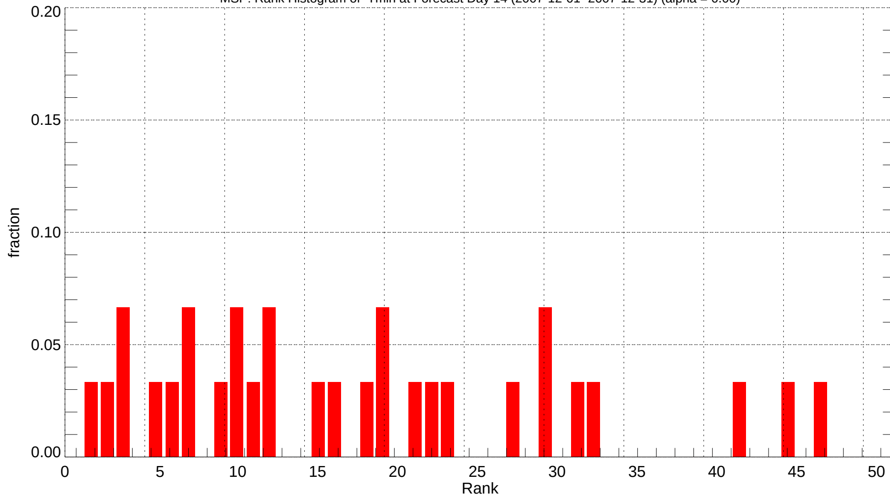
MSP: Rank Histogram of Tmin at Forecast Day 14 (2007-12-01~2007-12-31) (alpha = 0.00)
