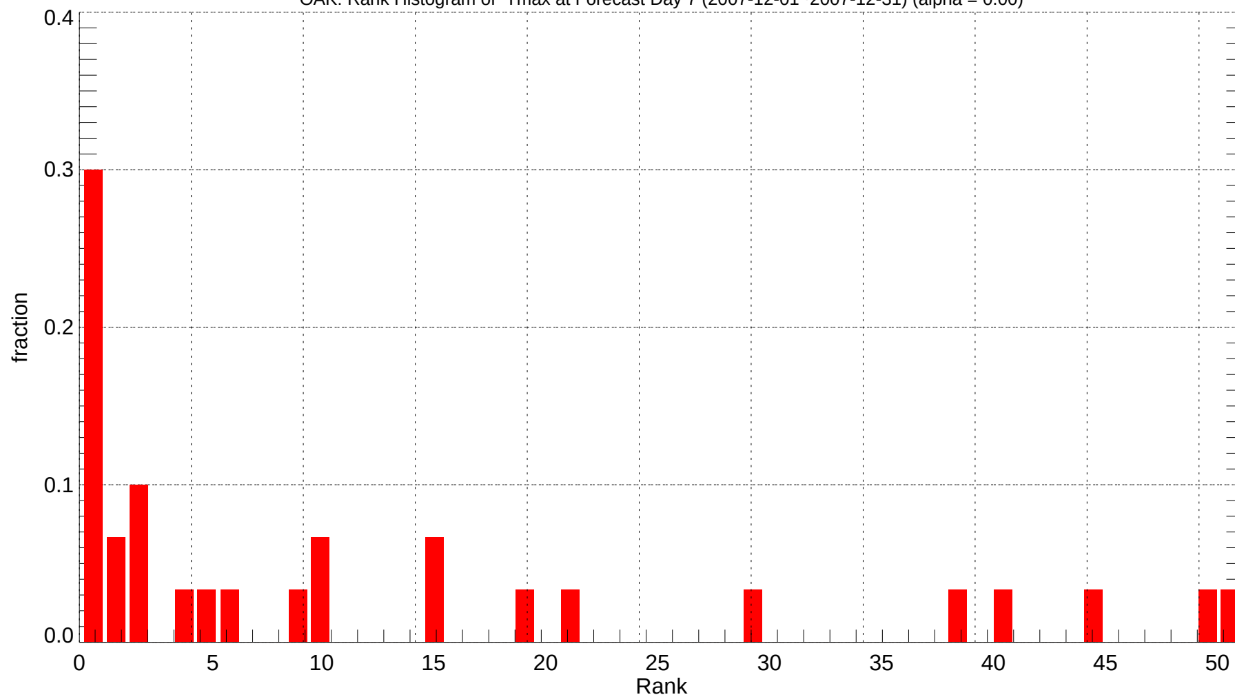
OAK: Rank Histogram of Tmax at Forecast Day 7 (2007-12-01~2007-12-31) (alpha = 0.00)
