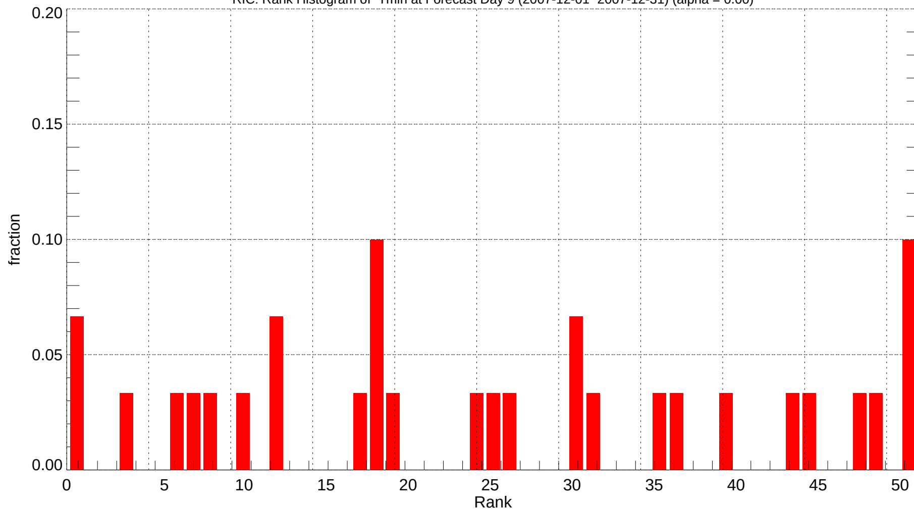
RIC: Rank Histogram of Tmin at Forecast Day 9 (2007-12-01~2007-12-31) (alpha = 0.00)
