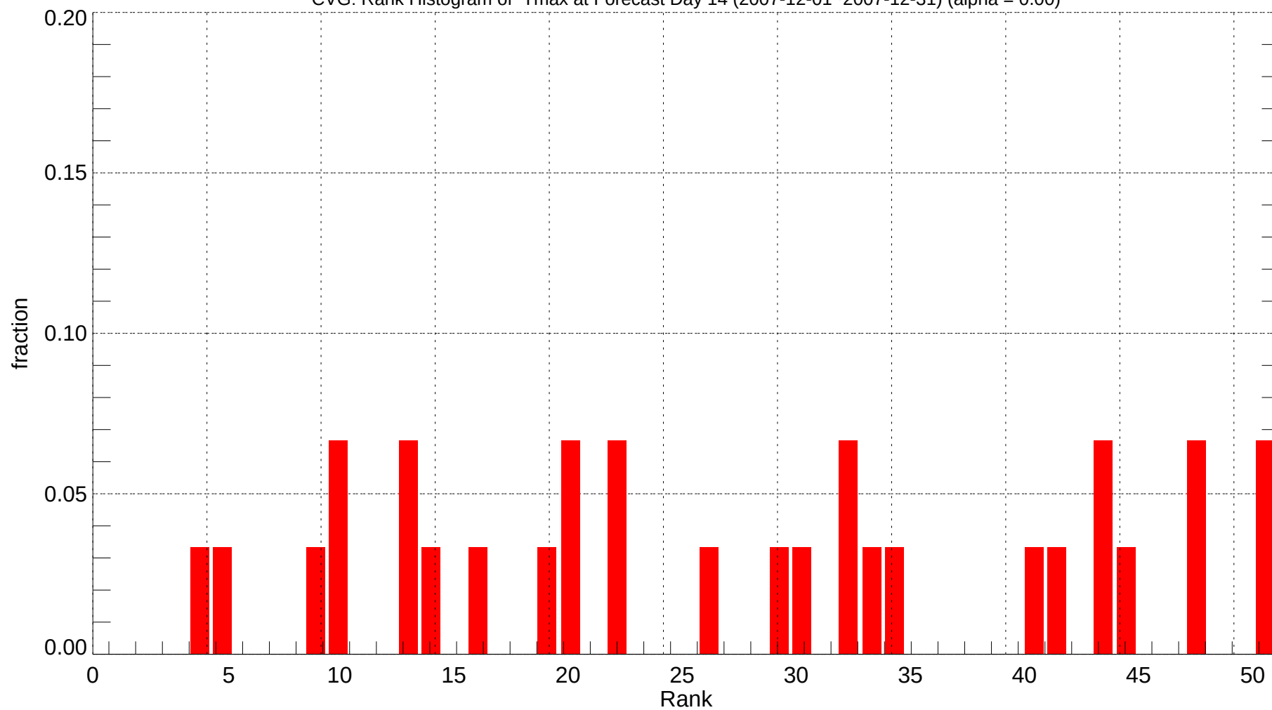
CVG: Rank Histogram of Tmax at Forecast Day 14 (2007-12-01~2007-12-31) (alpha = 0.00)
