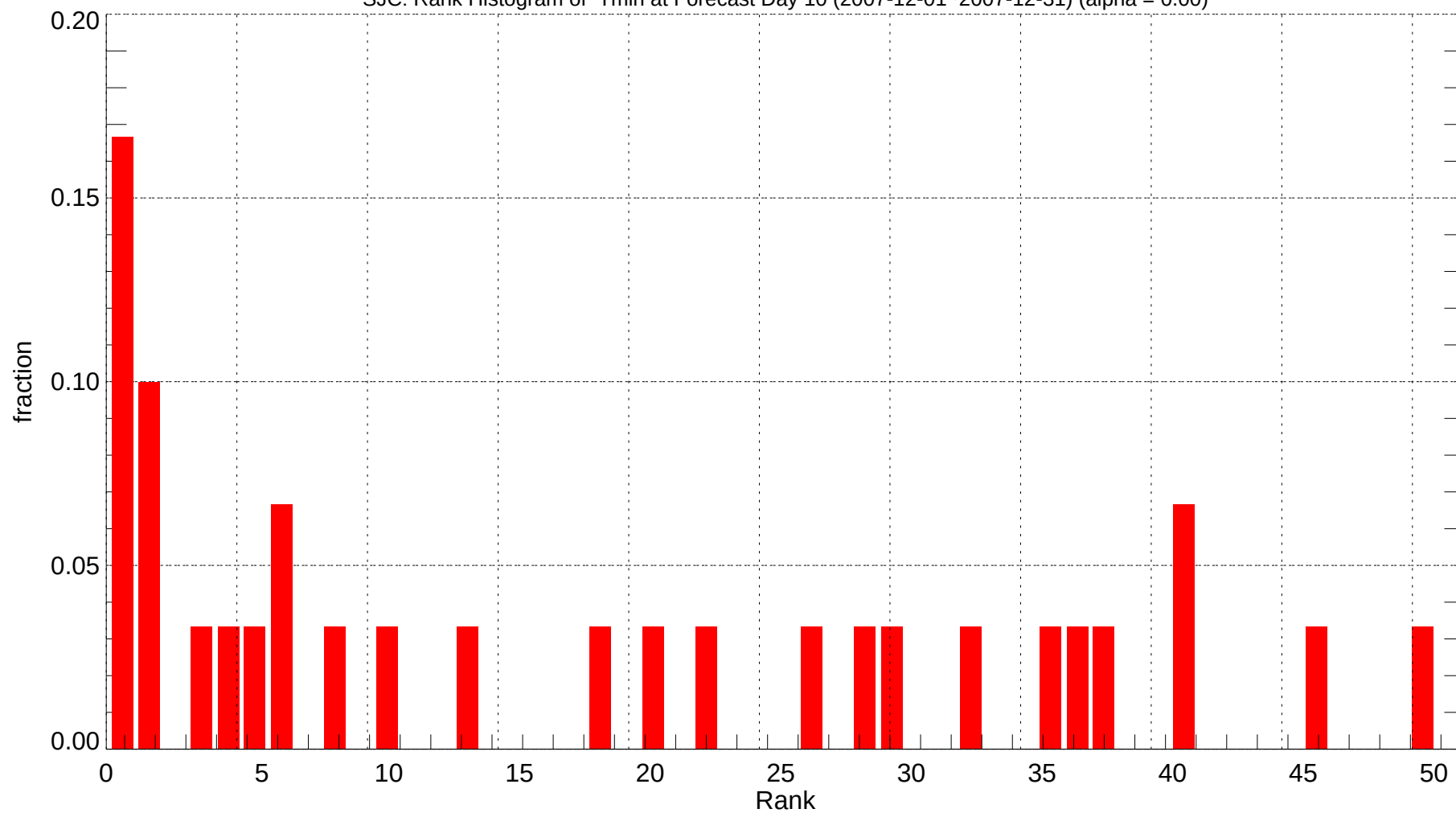
SJC: Rank Histogram of Tmin at Forecast Day 10 (2007-12-01~2007-12-31) (alpha = 0.00)
