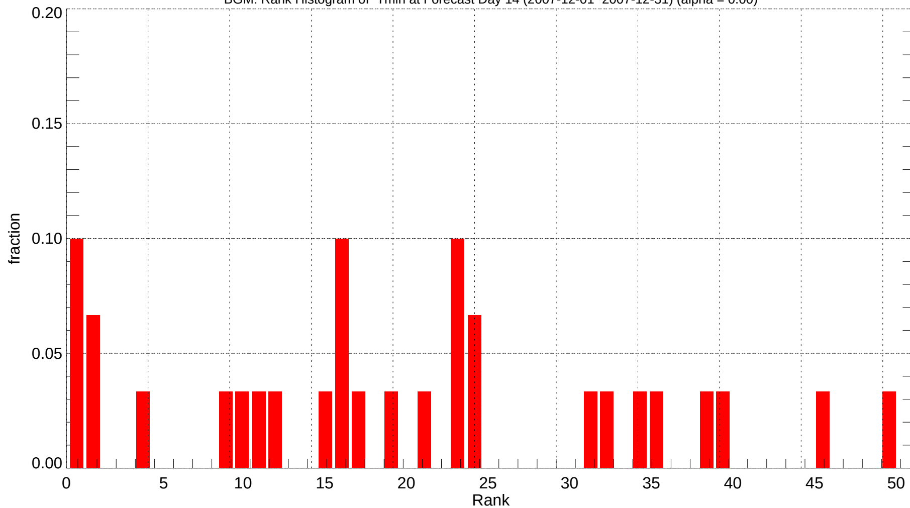
BGM: Rank Histogram of Tmin at Forecast Day 14 (2007-12-01~2007-12-31) (alpha = 0.00)
