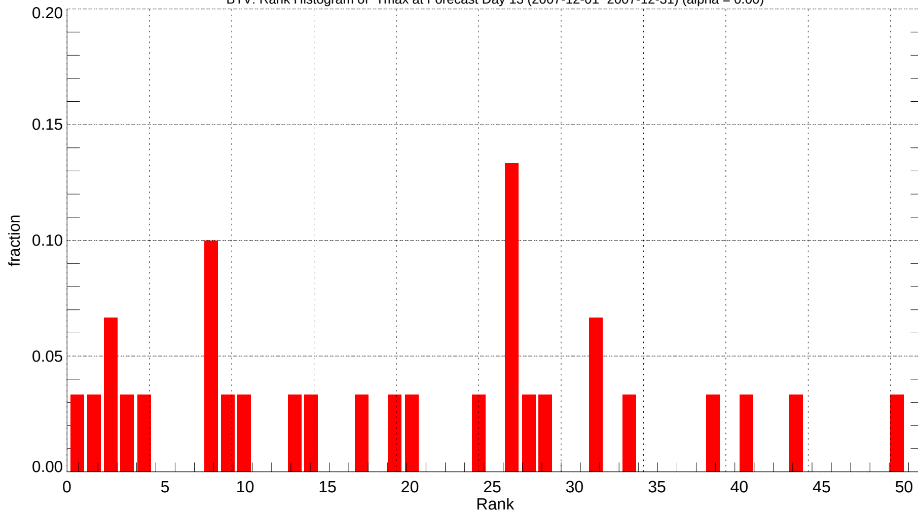
BTV: Rank Histogram of Tmax at Forecast Day 13 (2007-12-01~2007-12-31) (alpha = 0.00)
