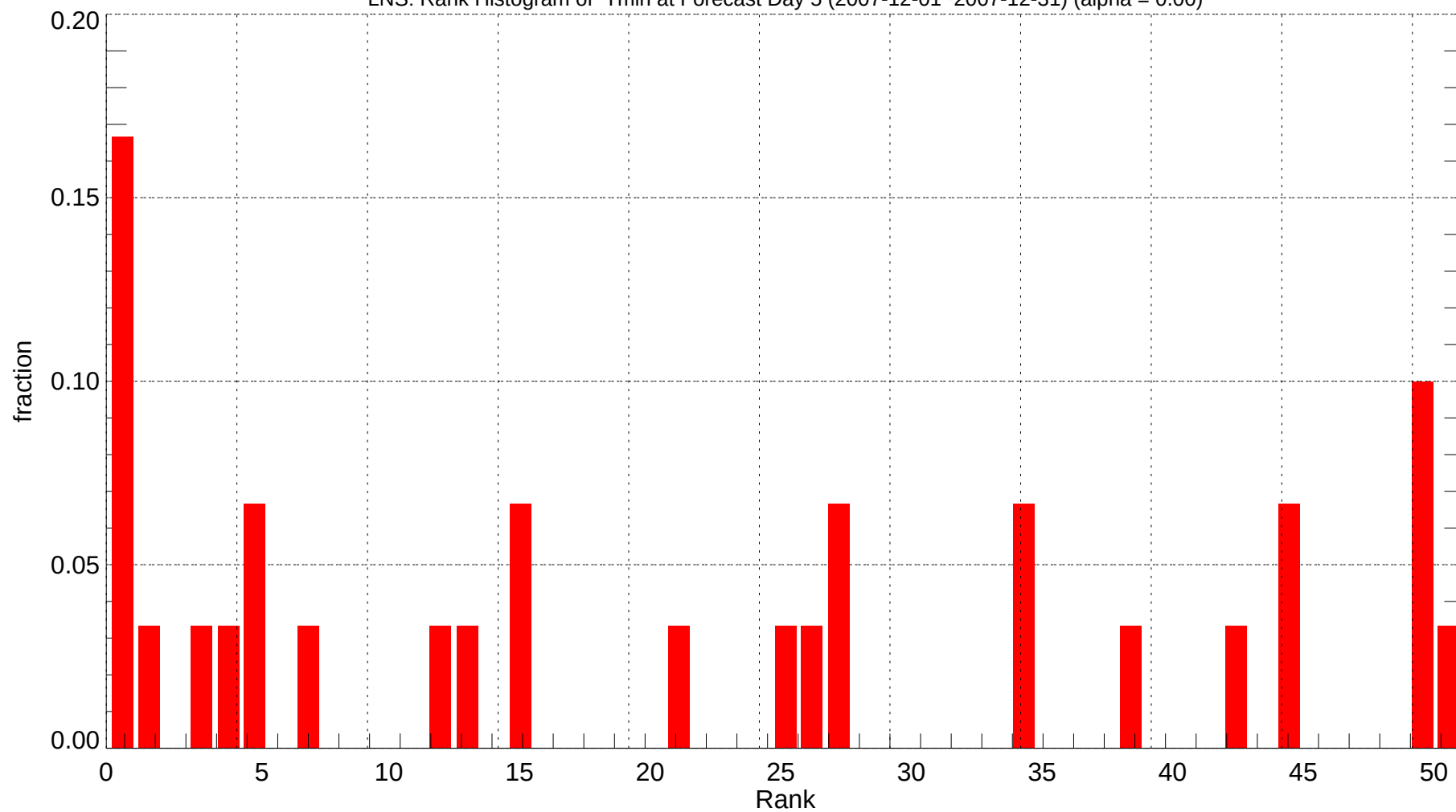
LNS: Rank Histogram of Tmin at Forecast Day 5 (2007-12-01~2007-12-31) (alpha = 0.00)
