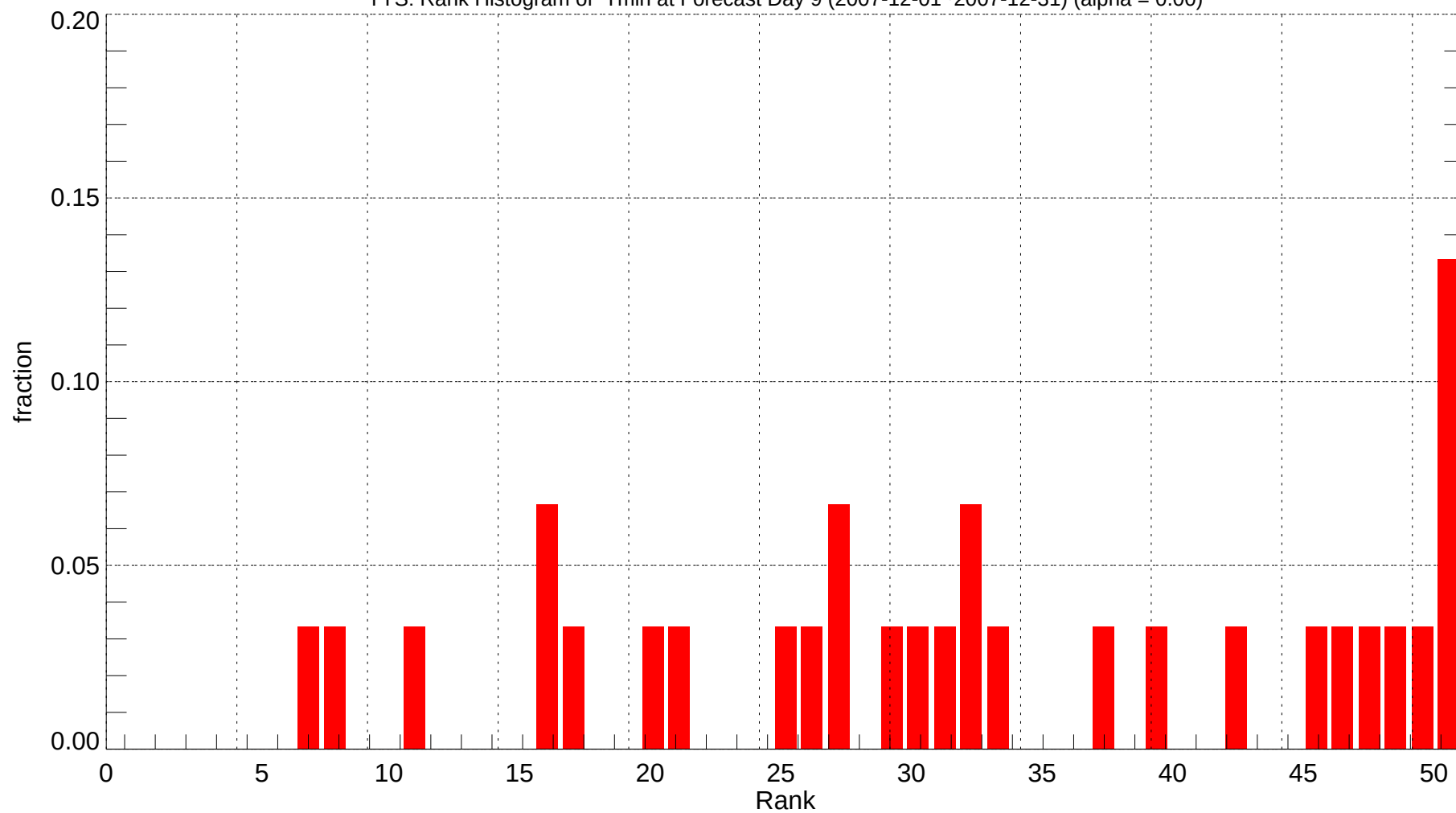
TYS: Rank Histogram of Tmin at Forecast Day 9 (2007-12-01~2007-12-31) (alpha = 0.00)
