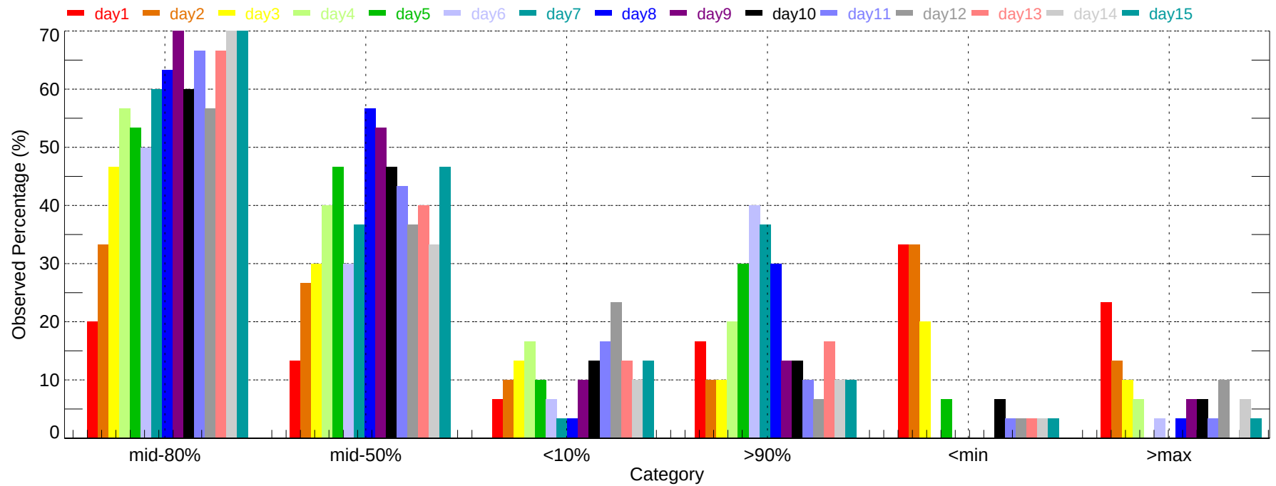
Observed Percentage of Ensembles - PVD: Max Temperature (2007-12-01~2007-12-31)
