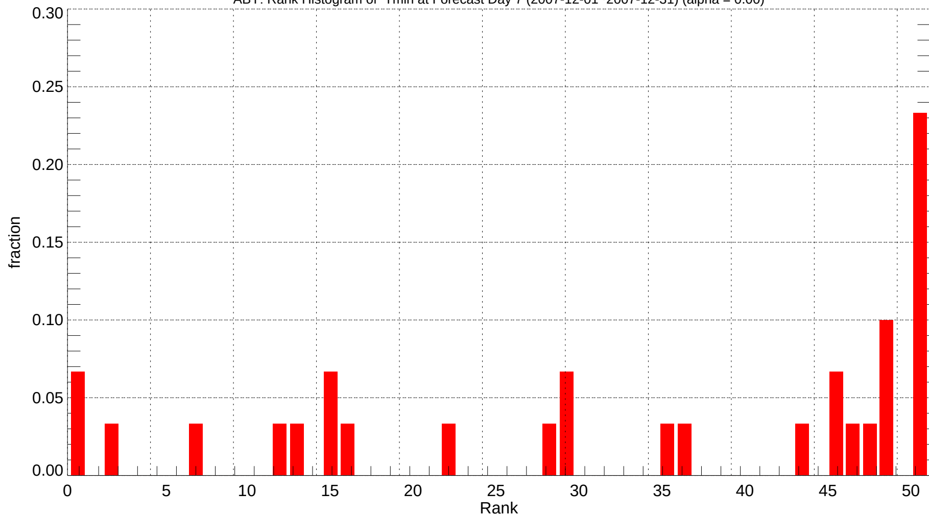
ABY: Rank Histogram of Tmin at Forecast Day 7 (2007-12-01~2007-12-31) (alpha = 0.00)
