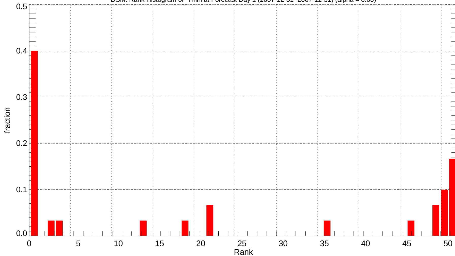
DSM: Rank Histogram of Tmin at Forecast Day 1 (2007-12-01~2007-12-31) (alpha = 0.00)
