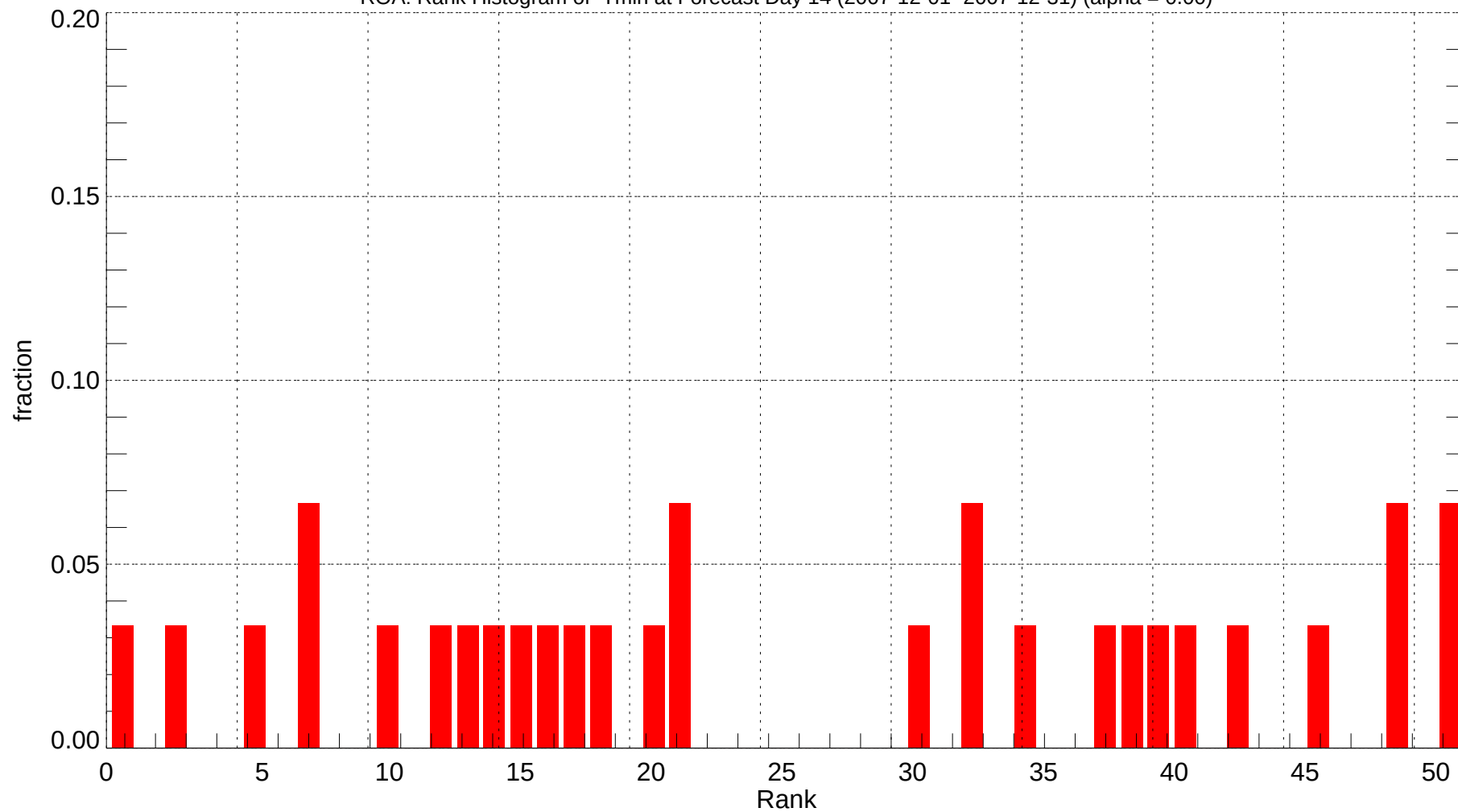
ROA: Rank Histogram of Tmin at Forecast Day 14 (2007-12-01~2007-12-31) (alpha = 0.00)
