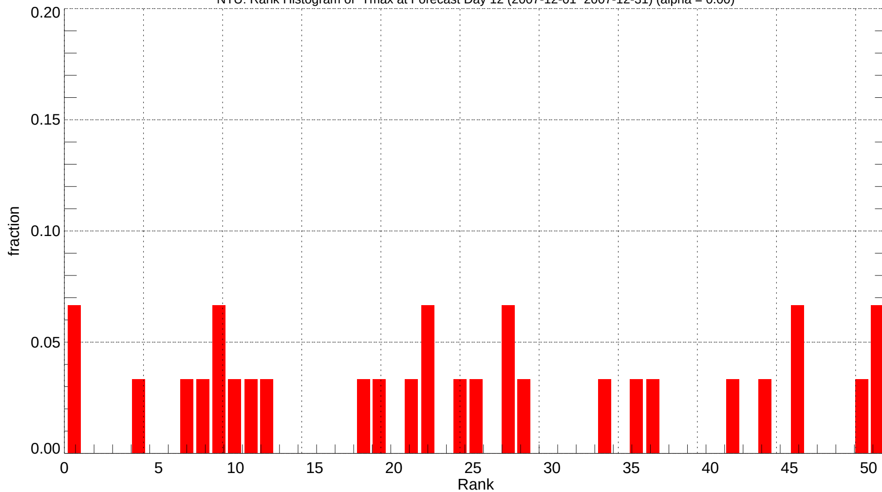
NTU: Rank Histogram of Tmax at Forecast Day 12 (2007-12-01~2007-12-31) (alpha = 0.00)
