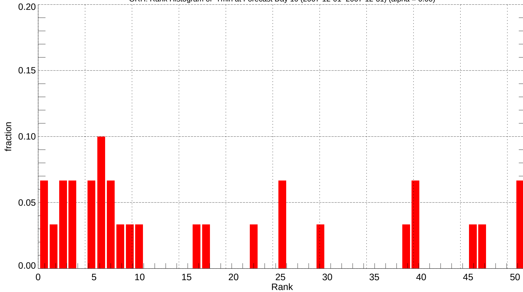
ORH: Rank Histogram of Tmin at Forecast Day 10 (2007-12-01~2007-12-31) (alpha = 0.00)
