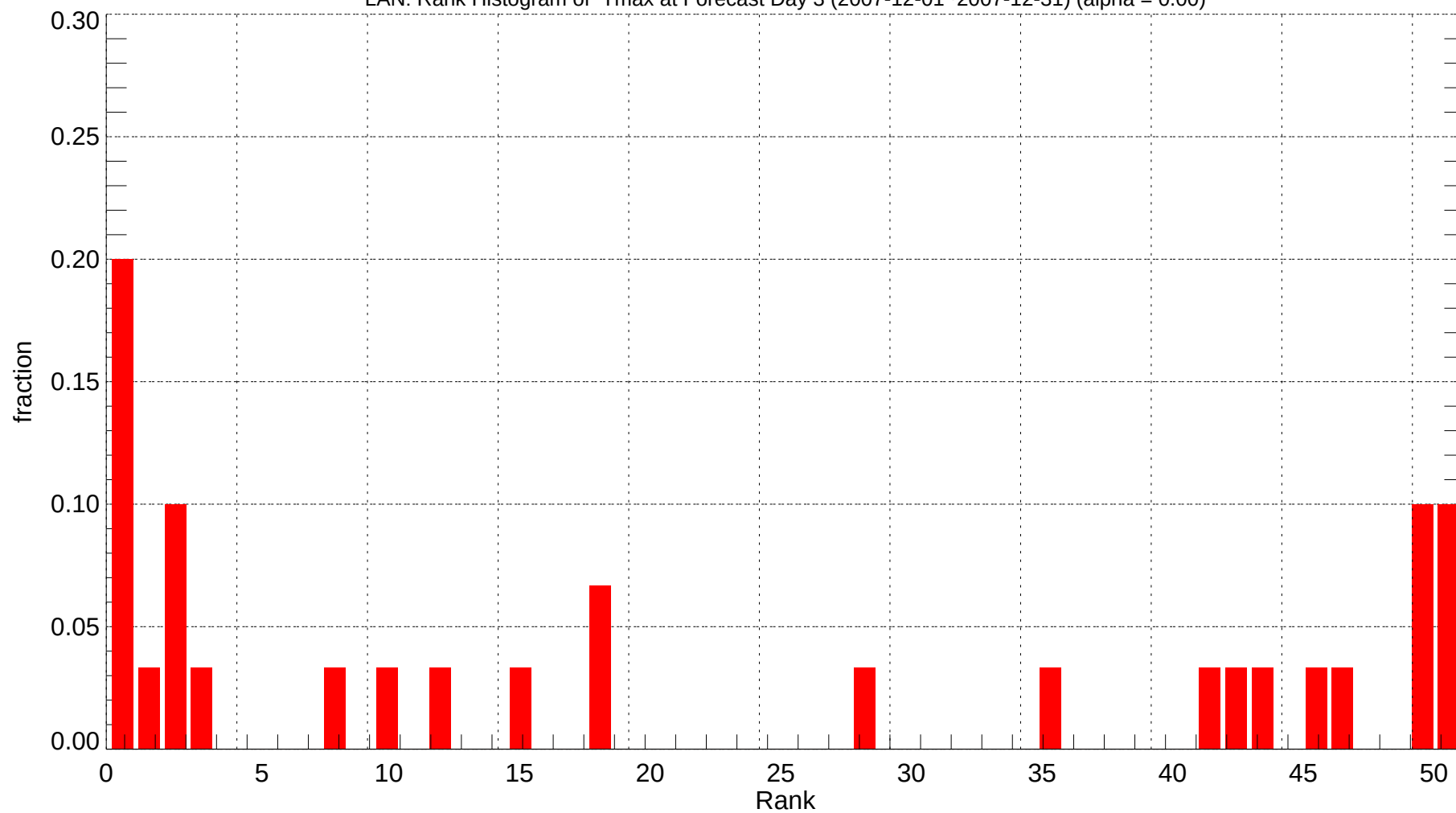
LAN: Rank Histogram of Tmax at Forecast Day 3 (2007-12-01~2007-12-31) (alpha = 0.00)
