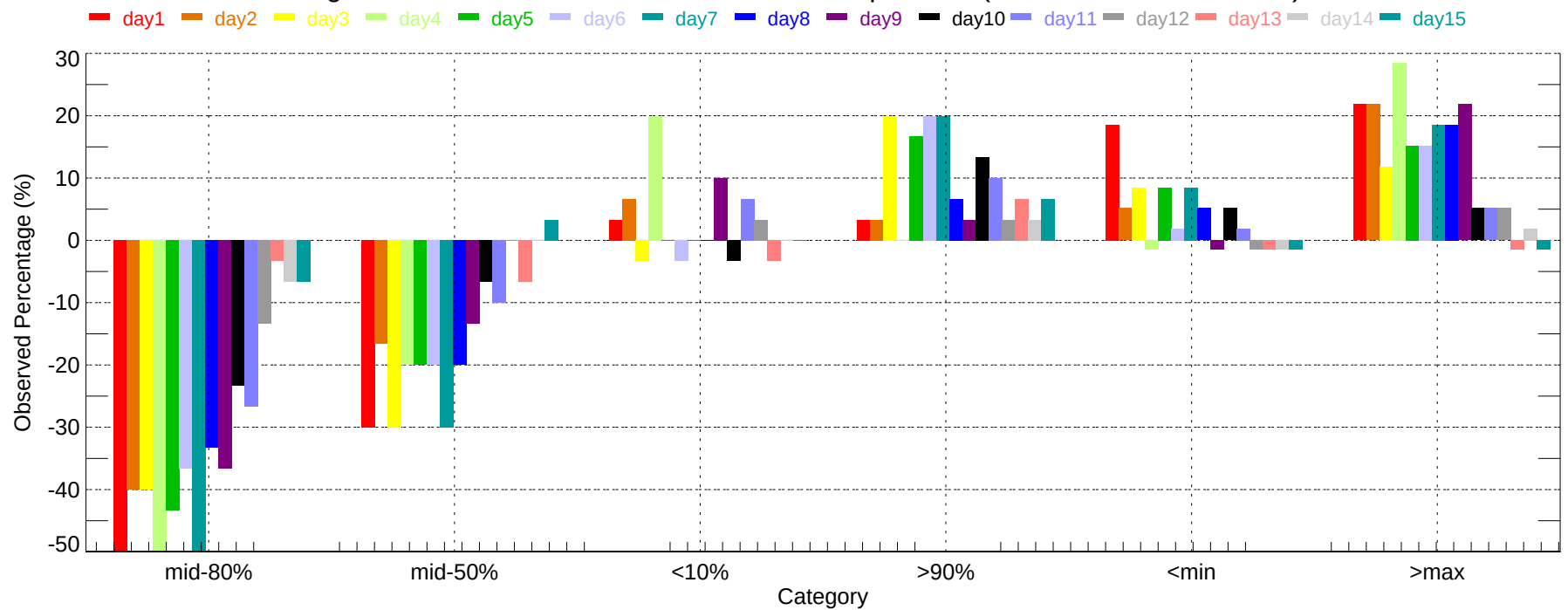
Observed Percentage Deviation of Ensembles - ORD: Min Temperature (2007-12-01~2007-12-31)
