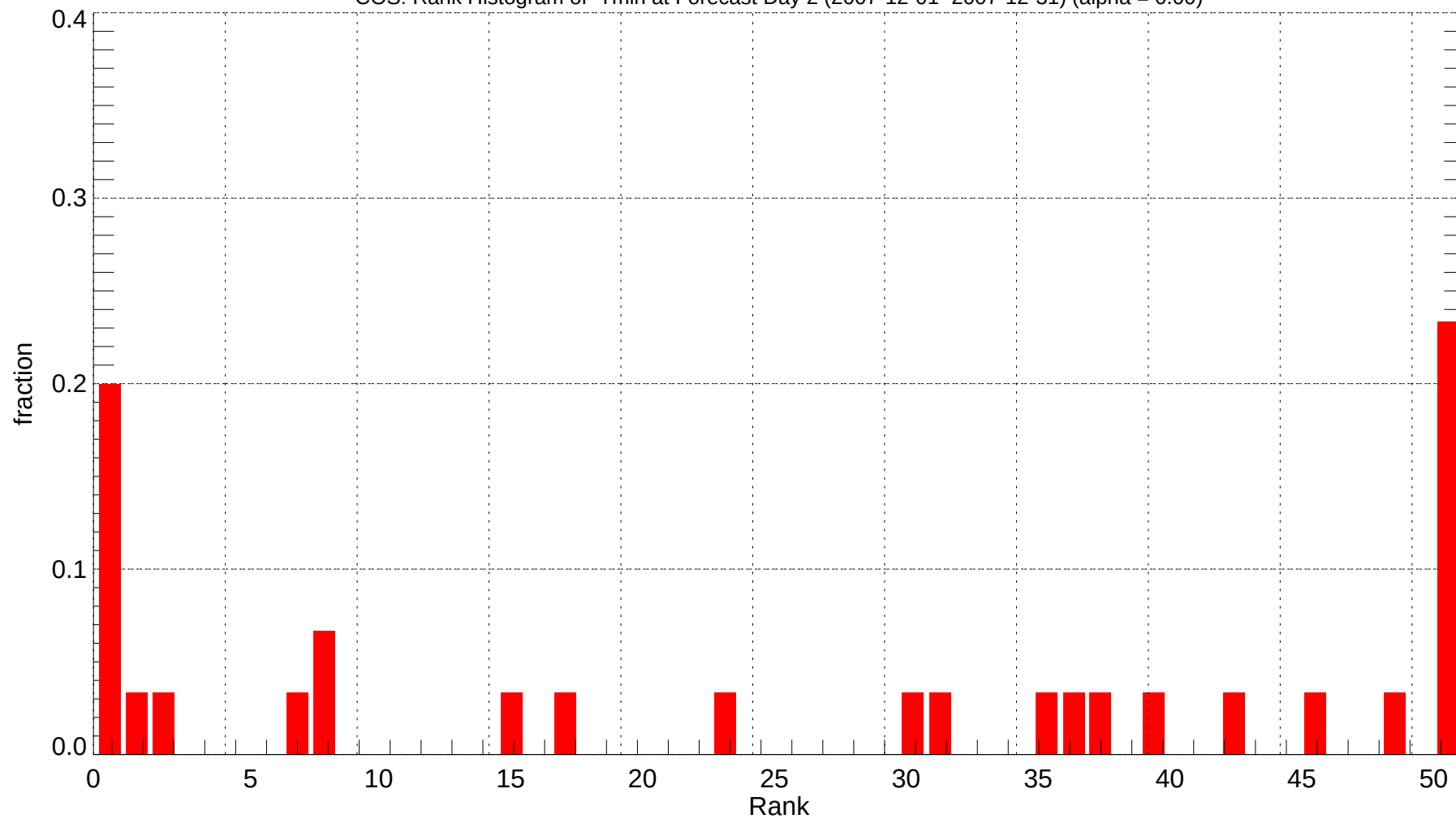
COS: Rank Histogram of Tmin at Forecast Day 2 (2007-12-01~2007-12-31) (alpha = 0.00)
