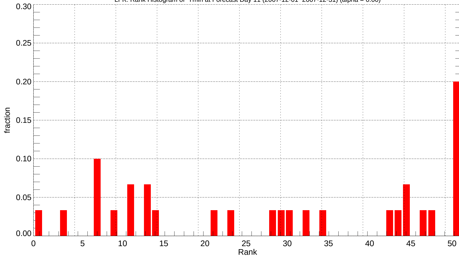
LFK: Rank Histogram of Tmin at Forecast Day 11 (2007-12-01~2007-12-31) (alpha = 0.00)
