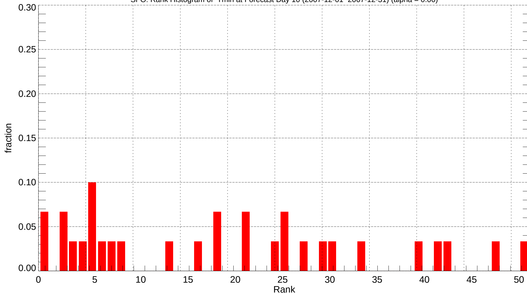
SFO: Rank Histogram of Tmin at Forecast Day 10 (2007-12-01~2007-12-31) (alpha = 0.00)
