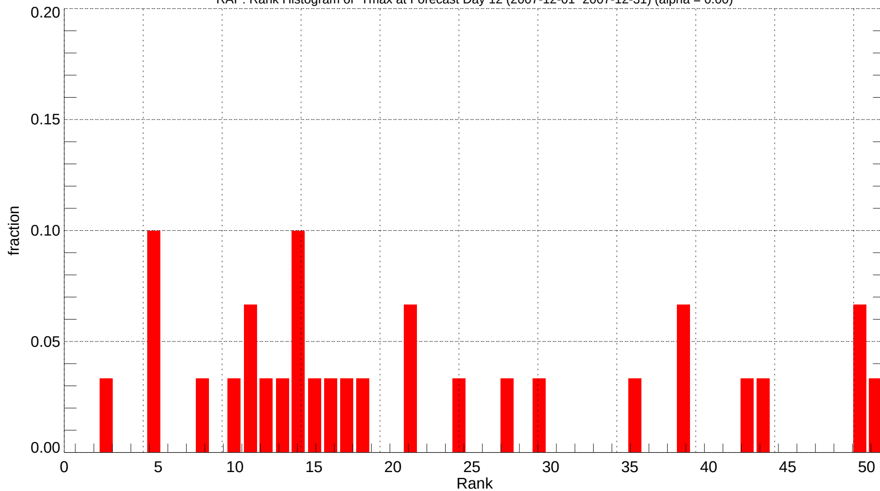
RAP: Rank Histogram of Tmax at Forecast Day 12 (2007-12-01~2007-12-31) (alpha = 0.00)
