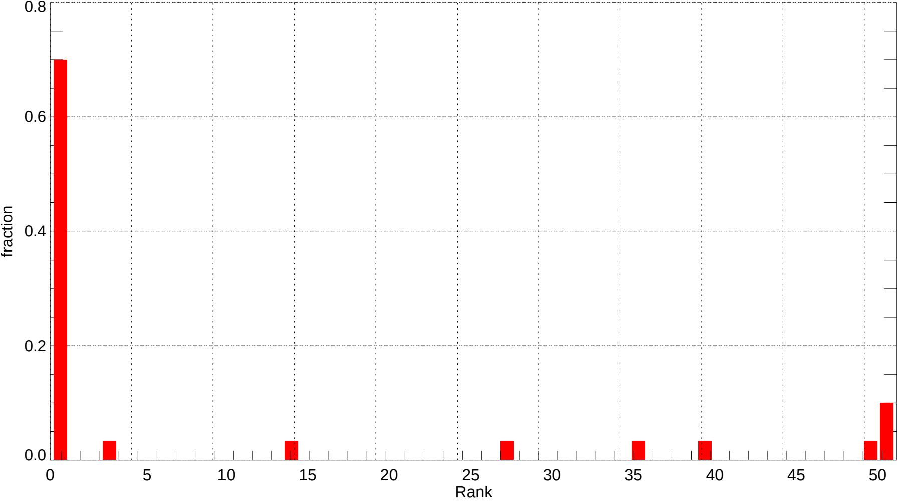
LAX: Rank Histogram of Tmin at Forecast Day 7 (2007-12-01~2007-12-31) (alpha = 0.00)
