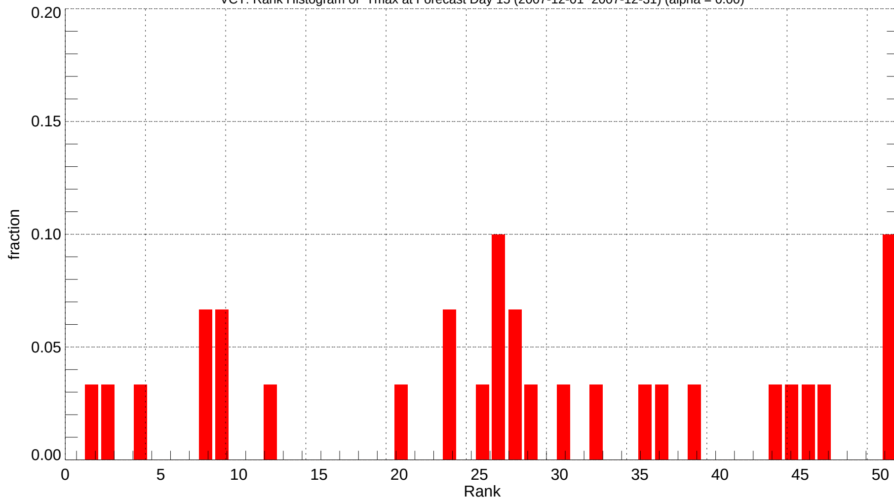
VCT: Rank Histogram of Tmax at Forecast Day 15 (2007-12-01~2007-12-31) (alpha = 0.00)
