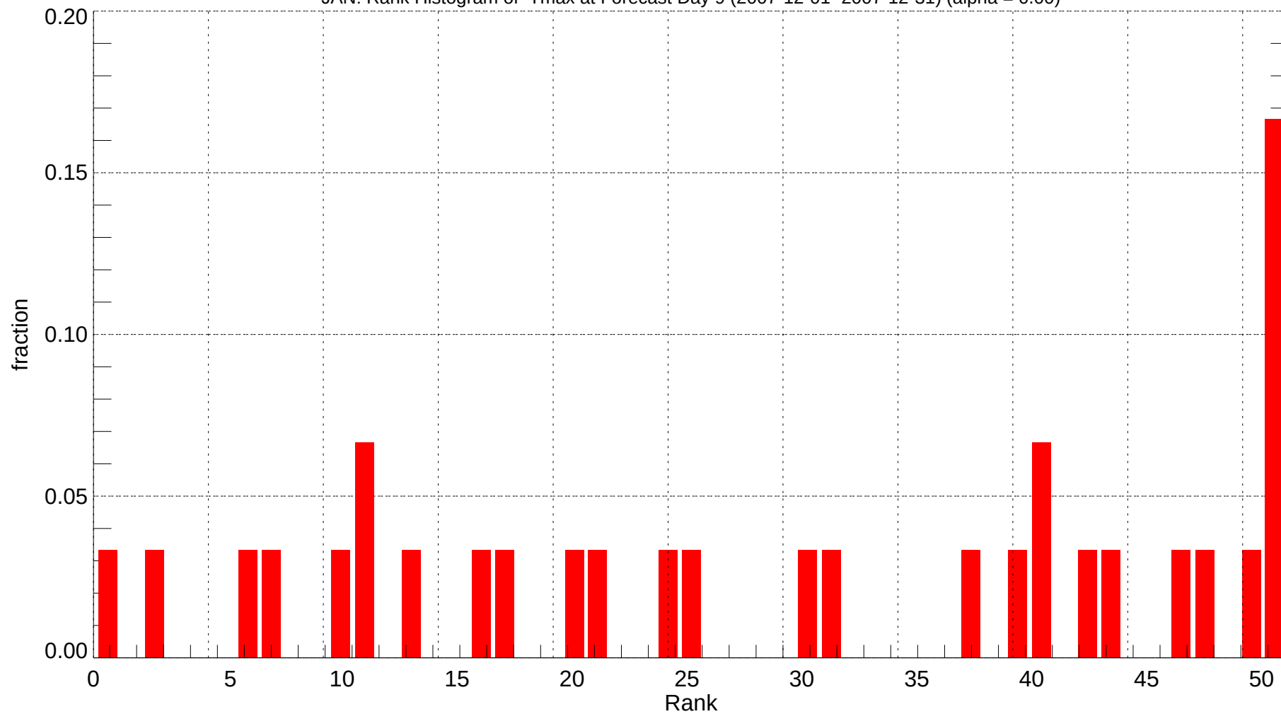
JAN: Rank Histogram of Tmax at Forecast Day 9 (2007-12-01~2007-12-31) (alpha = 0.00)
