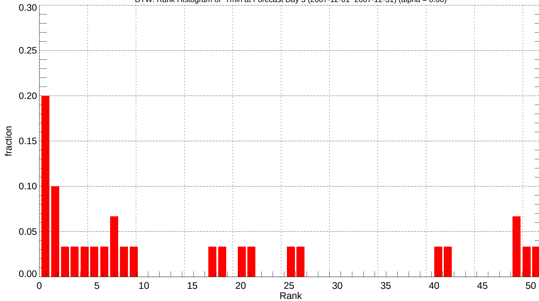
DTW: Rank Histogram of Tmin at Forecast Day 3 (2007-12-01~2007-12-31) (alpha = 0.00)
