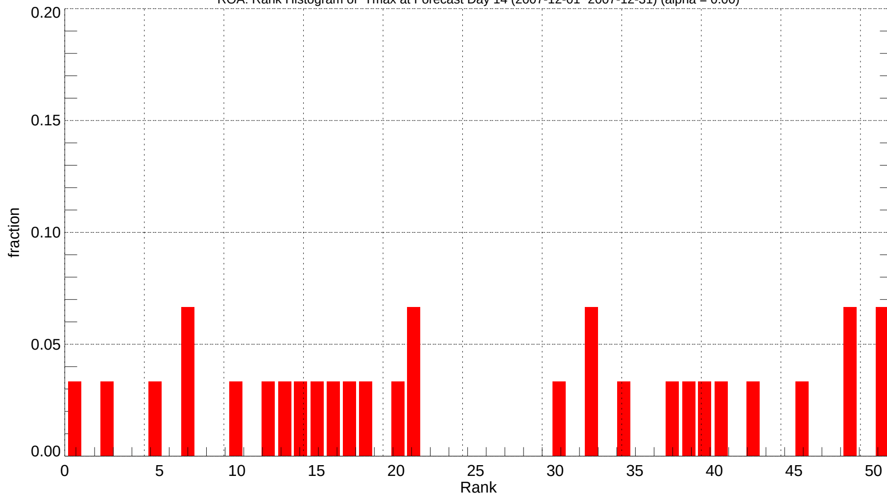
ROA: Rank Histogram of Tmax at Forecast Day 14 (2007-12-01~2007-12-31) (alpha = 0.00)
