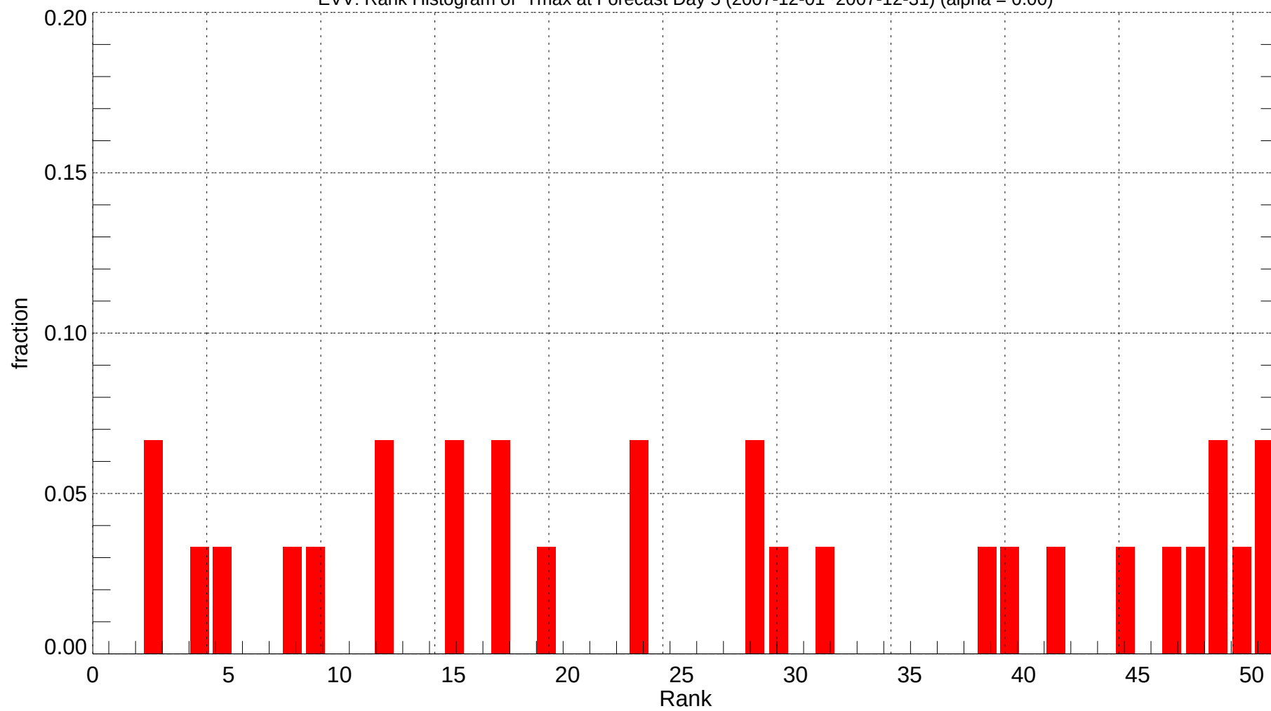
EVV: Rank Histogram of Tmax at Forecast Day 5 (2007-12-01~2007-12-31) (alpha = 0.00)
