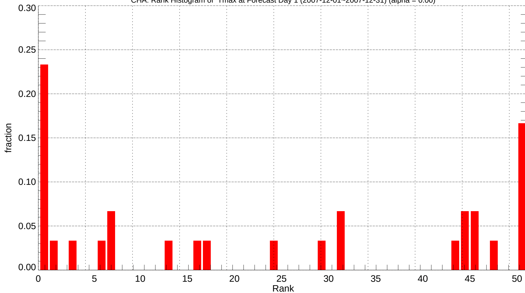
CHA: Rank Histogram of Tmax at Forecast Day 1 (2007-12-01~2007-12-31) (alpha = 0.00)
