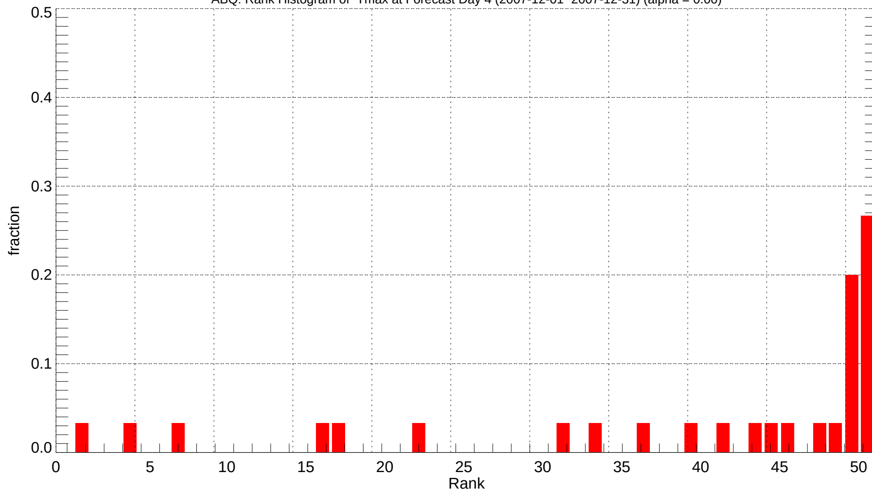
ABQ: Rank Histogram of Tmax at Forecast Day 4 (2007-12-01~2007-12-31) (alpha = 0.00)
