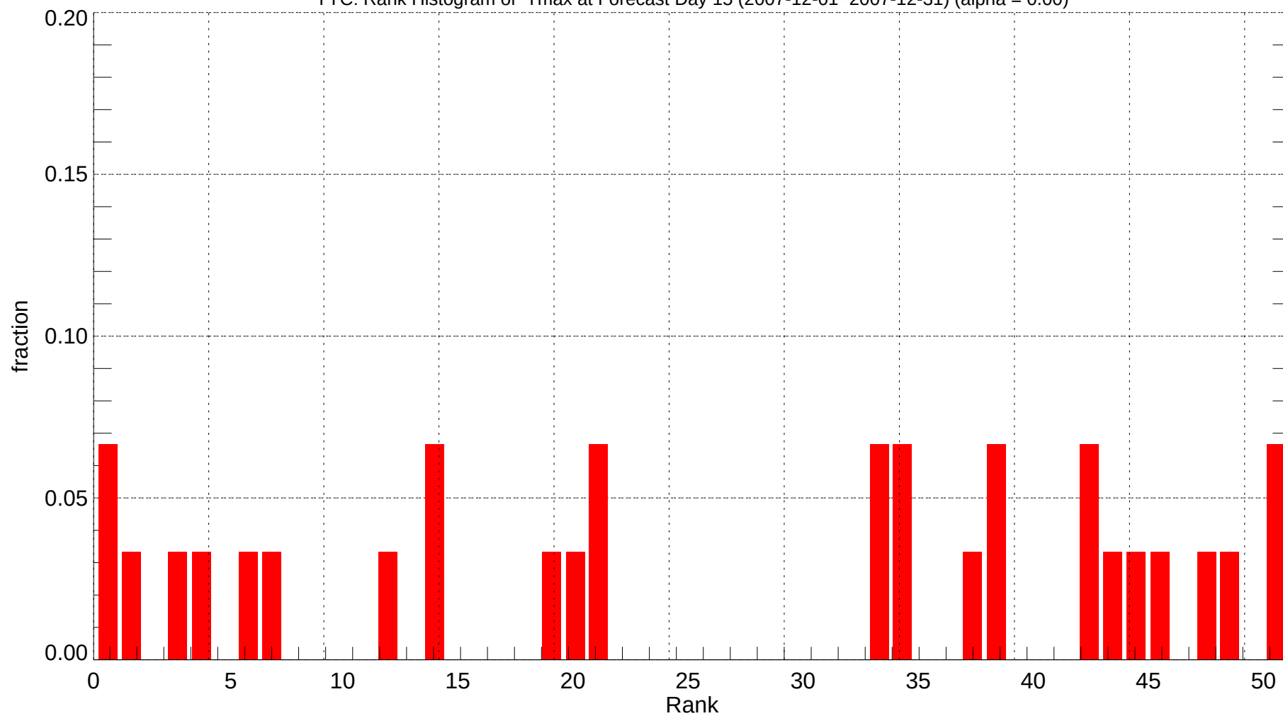
YYC: Rank Histogram of Tmax at Forecast Day 15 (2007-12-01~2007-12-31) (alpha = 0.00)
