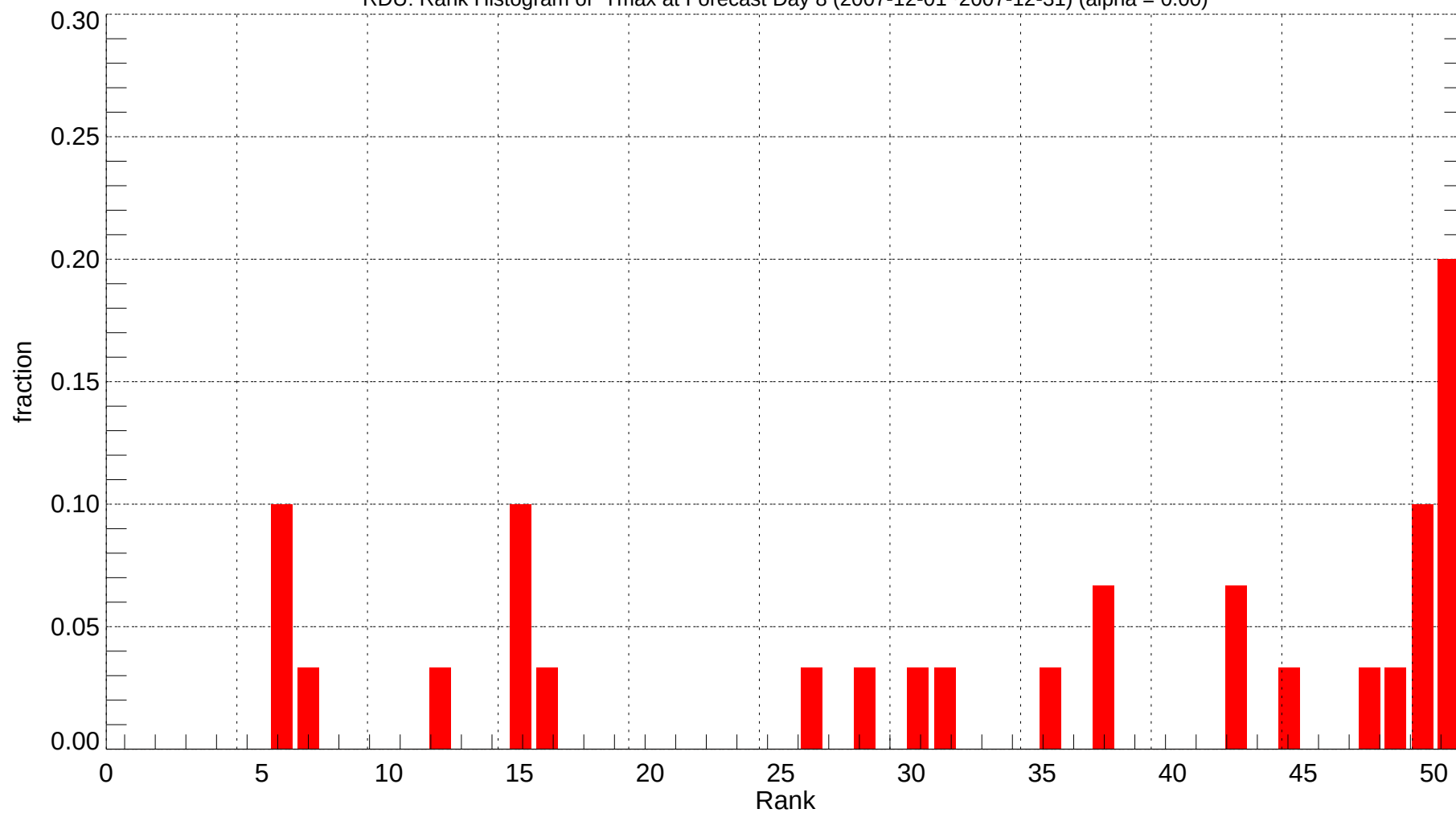
RDU: Rank Histogram of Tmax at Forecast Day 8 (2007-12-01~2007-12-31) (alpha = 0.00)
