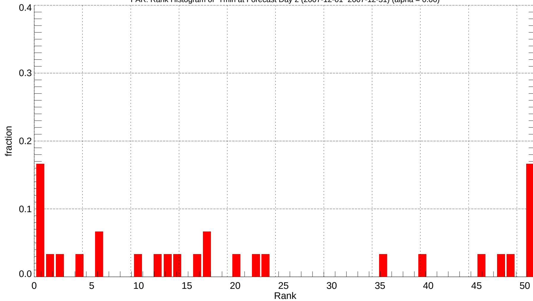
FAR: Rank Histogram of Tmin at Forecast Day 2 (2007-12-01~2007-12-31) (alpha = 0.00)
