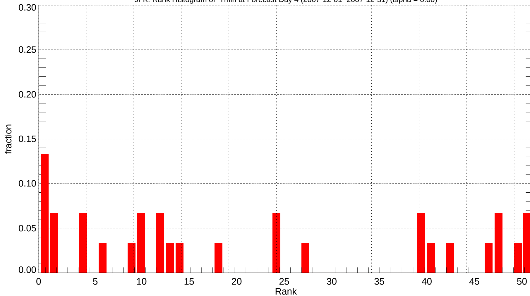
JFK: Rank Histogram of Tmin at Forecast Day 4 (2007-12-01~2007-12-31) (alpha = 0.00)
