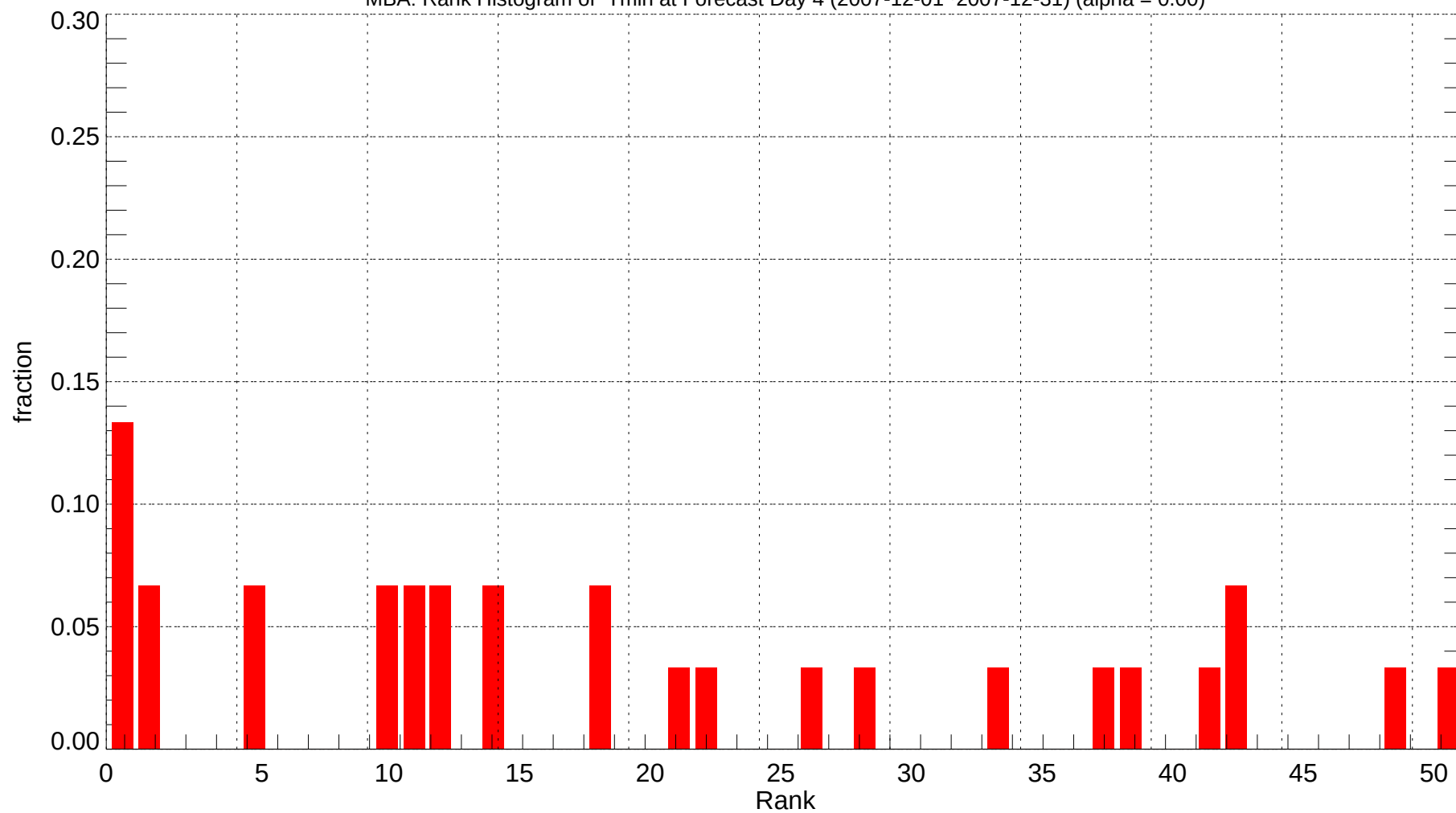
MBA: Rank Histogram of Tmin at Forecast Day 4 (2007-12-01~2007-12-31) (alpha = 0.00)
