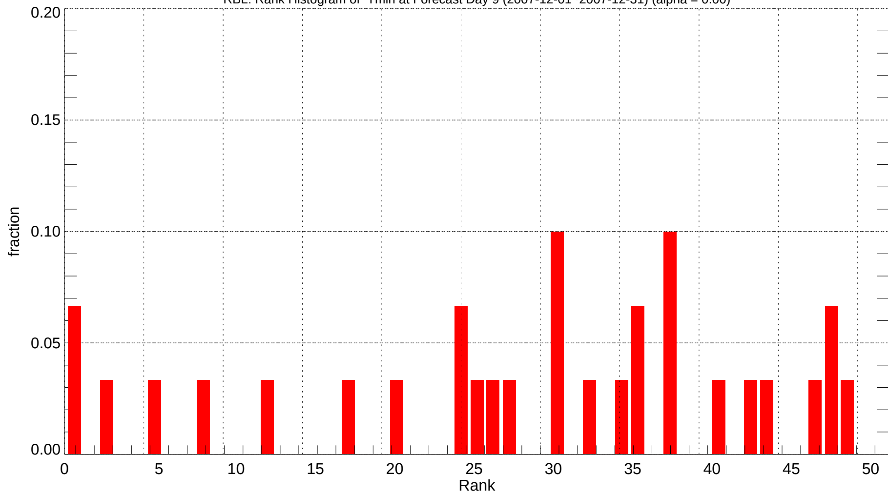
RBL: Rank Histogram of Tmin at Forecast Day 9 (2007-12-01~2007-12-31) (alpha = 0.00)
