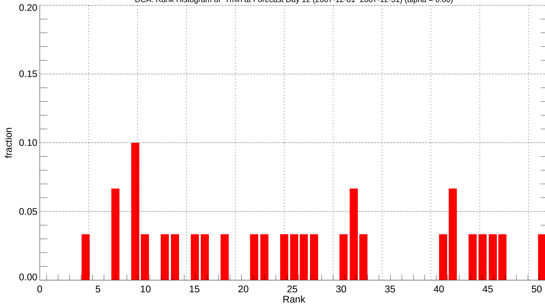
DCA: Rank Histogram of Tmin at Forecast Day 12 (2007-12-01~2007-12-31) (alpha = 0.00)
