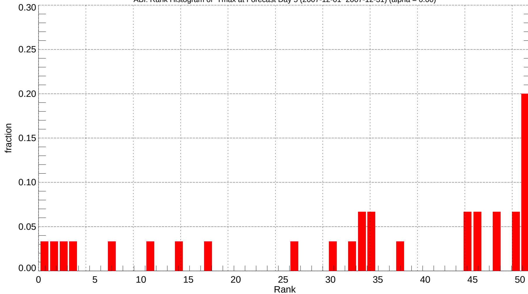
ABI: Rank Histogram of Tmax at Forecast Day 5 (2007-12-01~2007-12-31) (alpha = 0.00)
