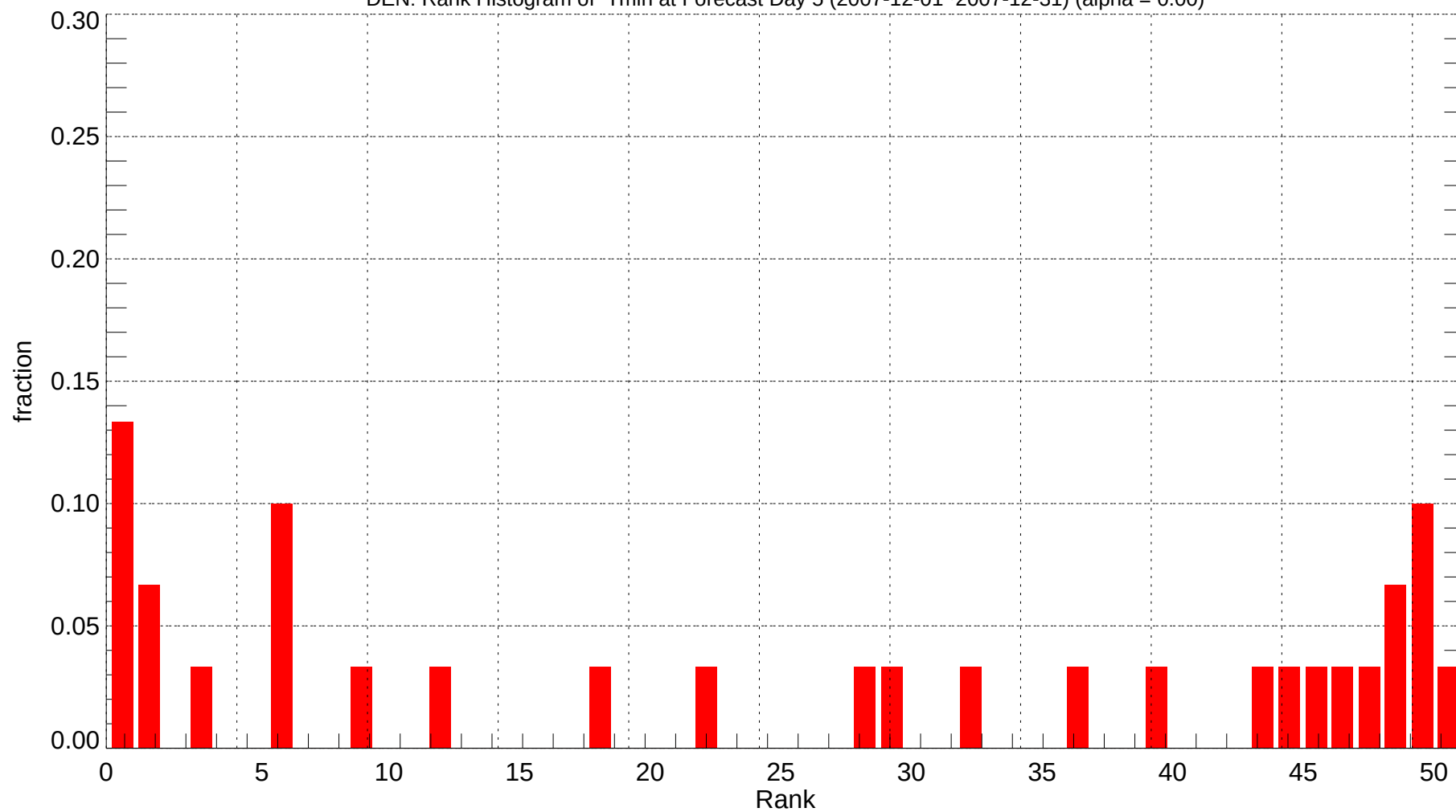
DEN: Rank Histogram of Tmin at Forecast Day 5 (2007-12-01~2007-12-31) (alpha = 0.00)
