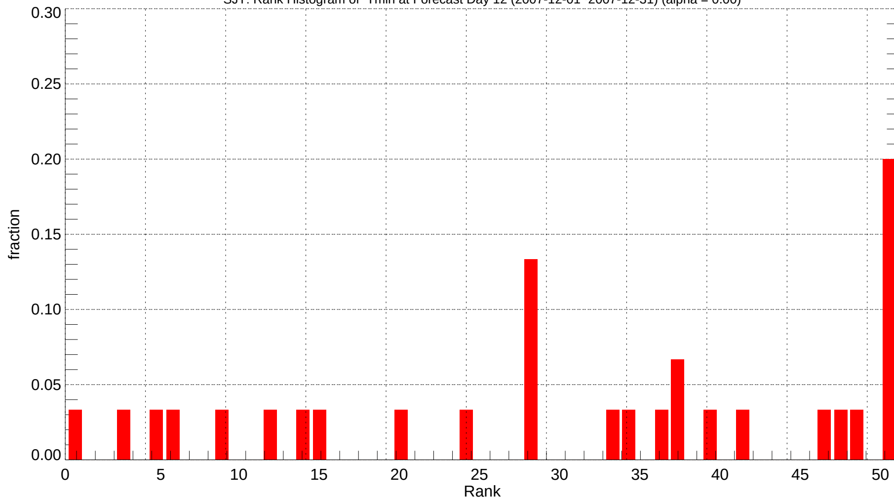
SJT: Rank Histogram of Tmin at Forecast Day 12 (2007-12-01~2007-12-31) (alpha = 0.00)
