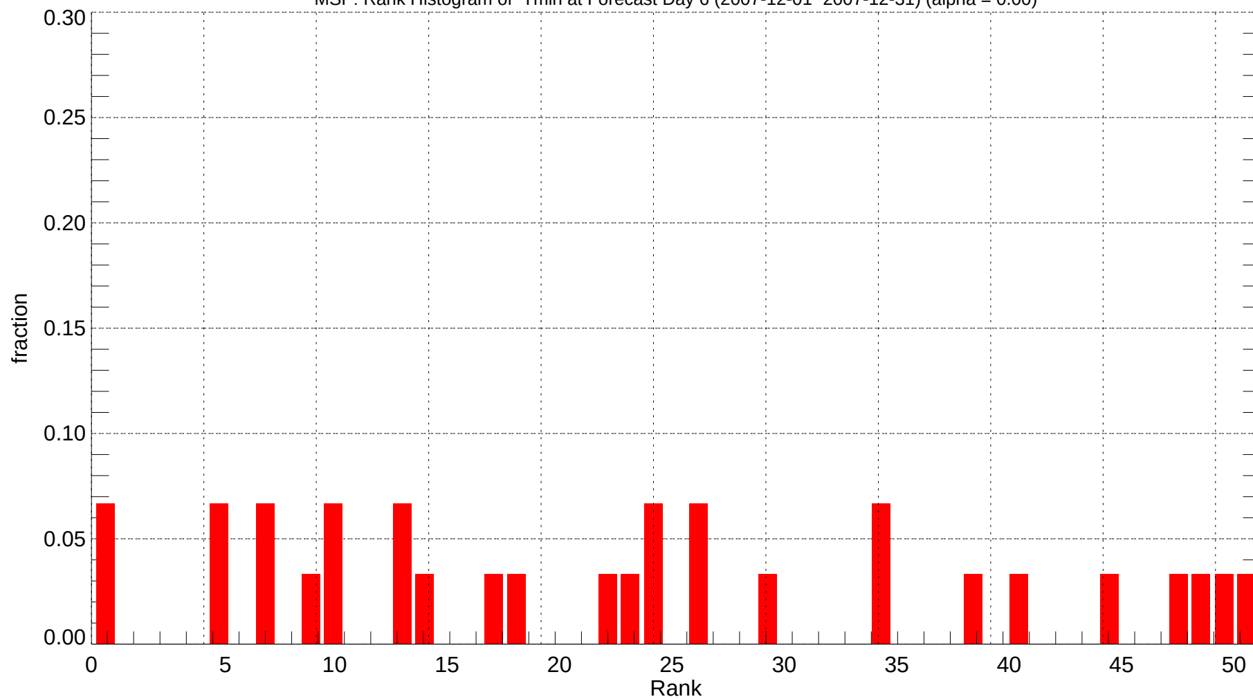
MSP: Rank Histogram of Tmin at Forecast Day 6 (2007-12-01~2007-12-31) (alpha = 0.00)
