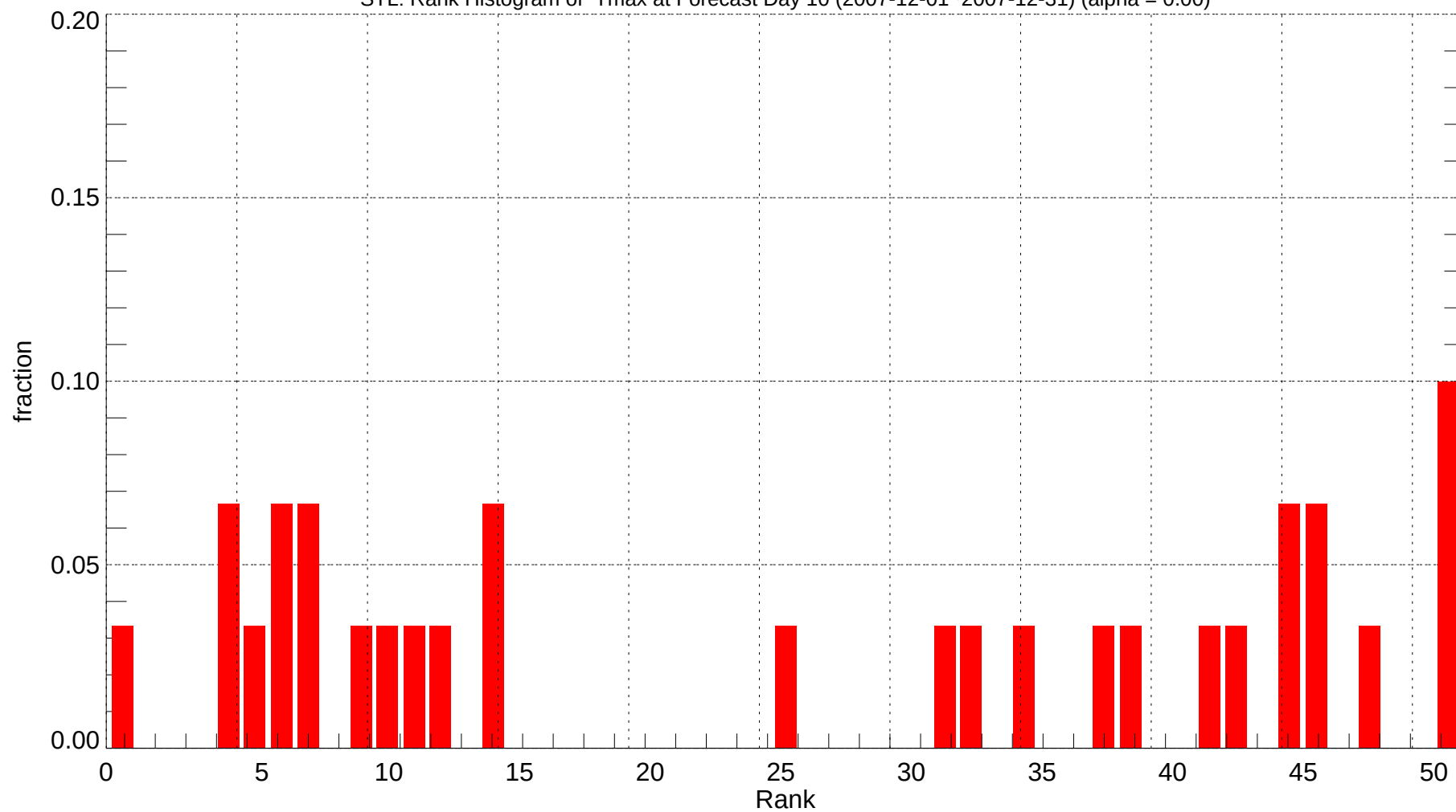
STL: Rank Histogram of Tmax at Forecast Day 10 (2007-12-01~2007-12-31) (alpha = 0.00)
