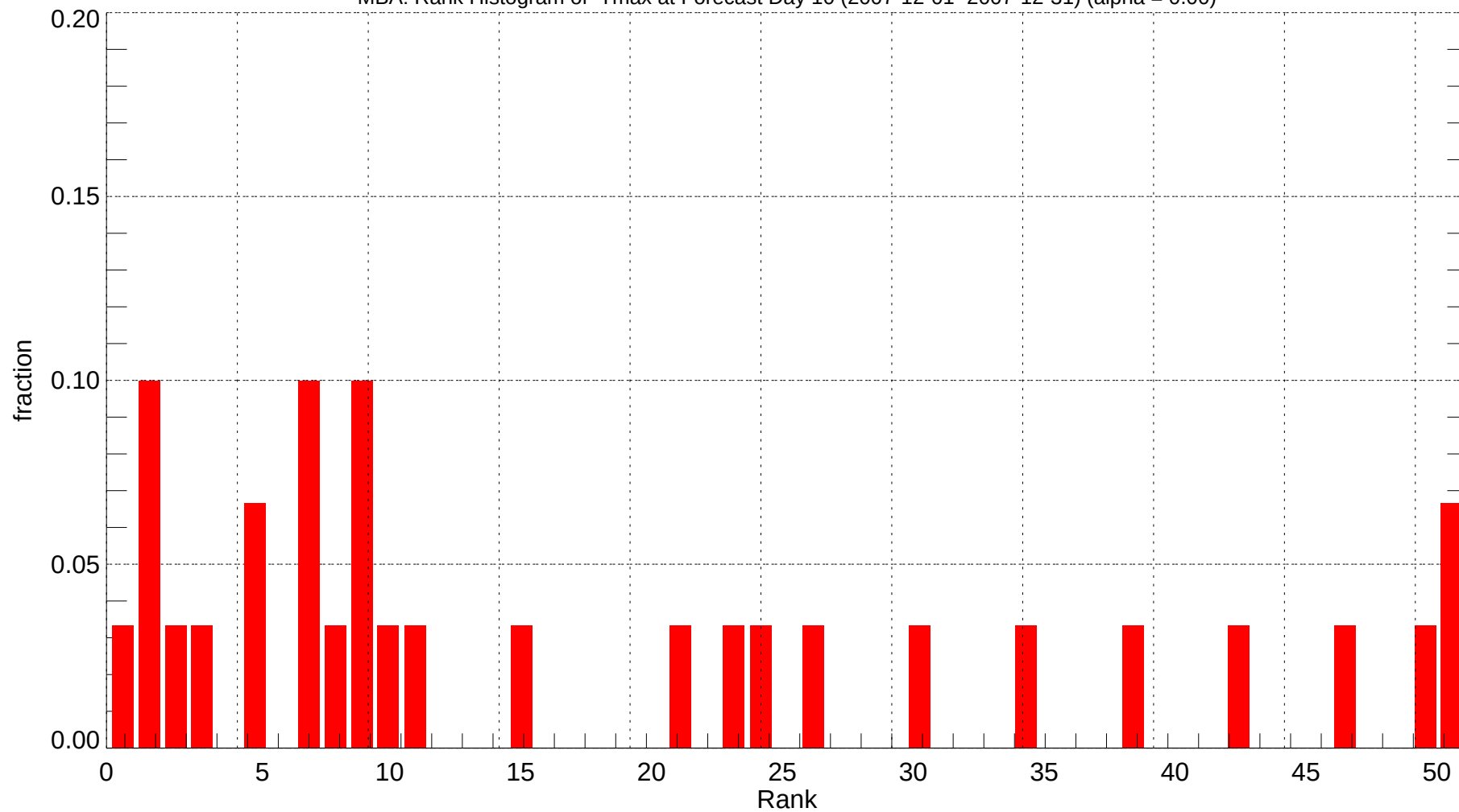
MBA: Rank Histogram of Tmax at Forecast Day 10 (2007-12-01~2007-12-31) (alpha = 0.00)
