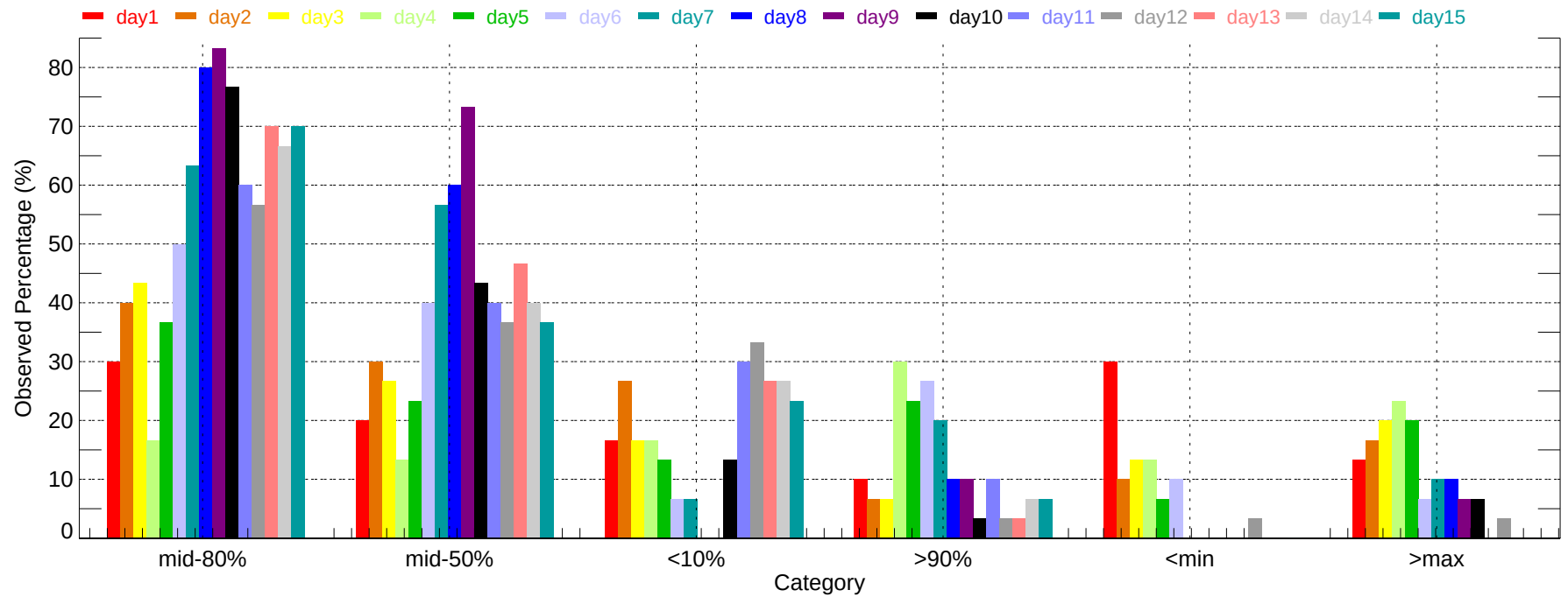
Observed Percentage of Ensembles - SLC: Max Temperature (2007-12-01~2007-12-31)
