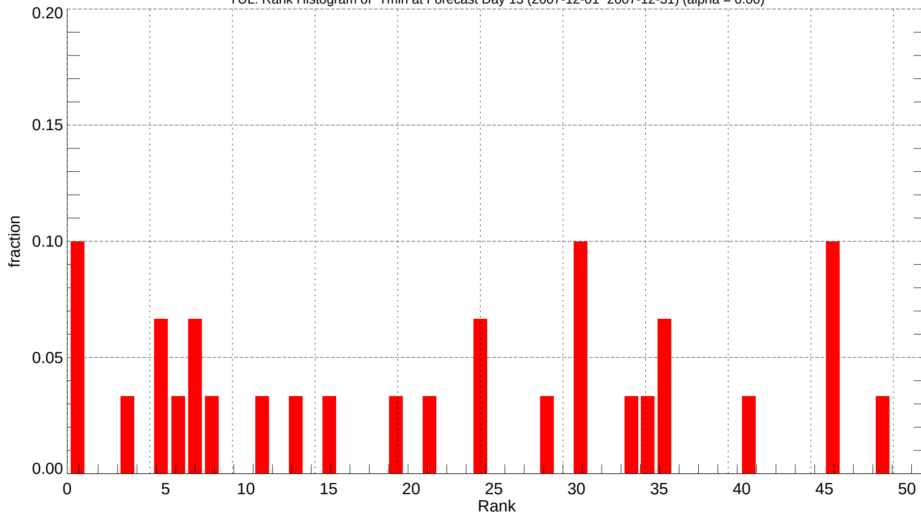
YUL: Rank Histogram of Tmin at Forecast Day 13 (2007-12-01~2007-12-31) (alpha = 0.00)
