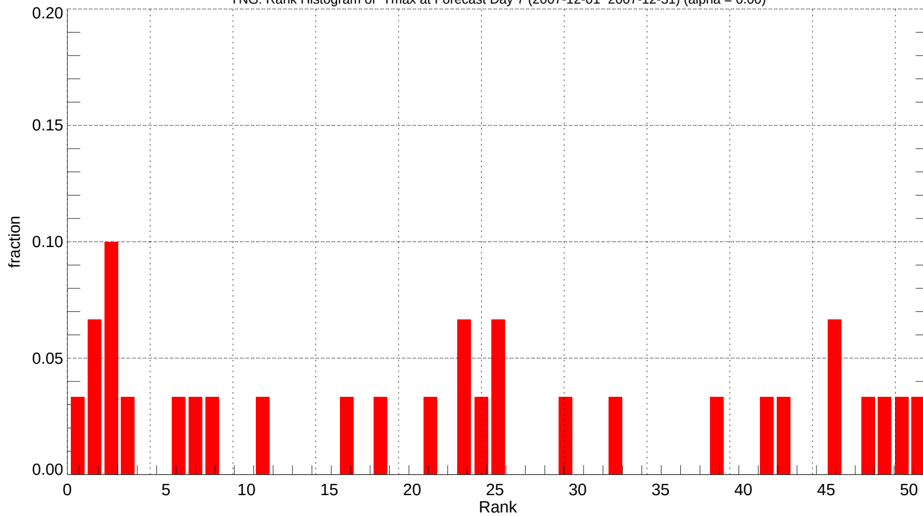
YNG: Rank Histogram of Tmax at Forecast Day 7 (2007-12-01~2007-12-31) (alpha = 0.00)
