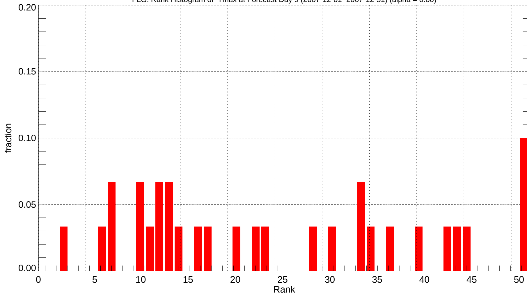
FLG: Rank Histogram of Tmax at Forecast Day 9 (2007-12-01~2007-12-31) (alpha = 0.00)
