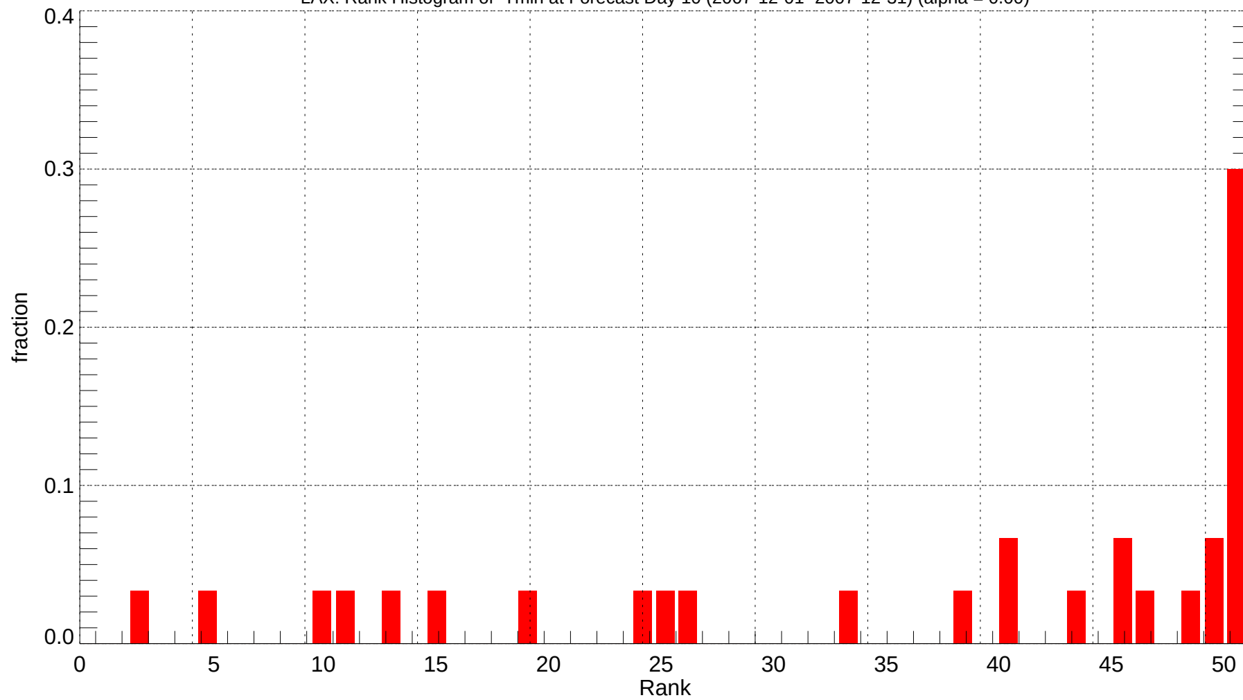
LAX: Rank Histogram of Tmin at Forecast Day 10 (2007-12-01~2007-12-31) (alpha = 0.00)
