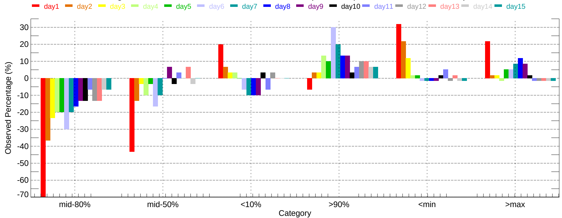
Observed Percentage Deviation of Ensembles - CLE: Max Temperature (2007-12-01~2007-12-31)
