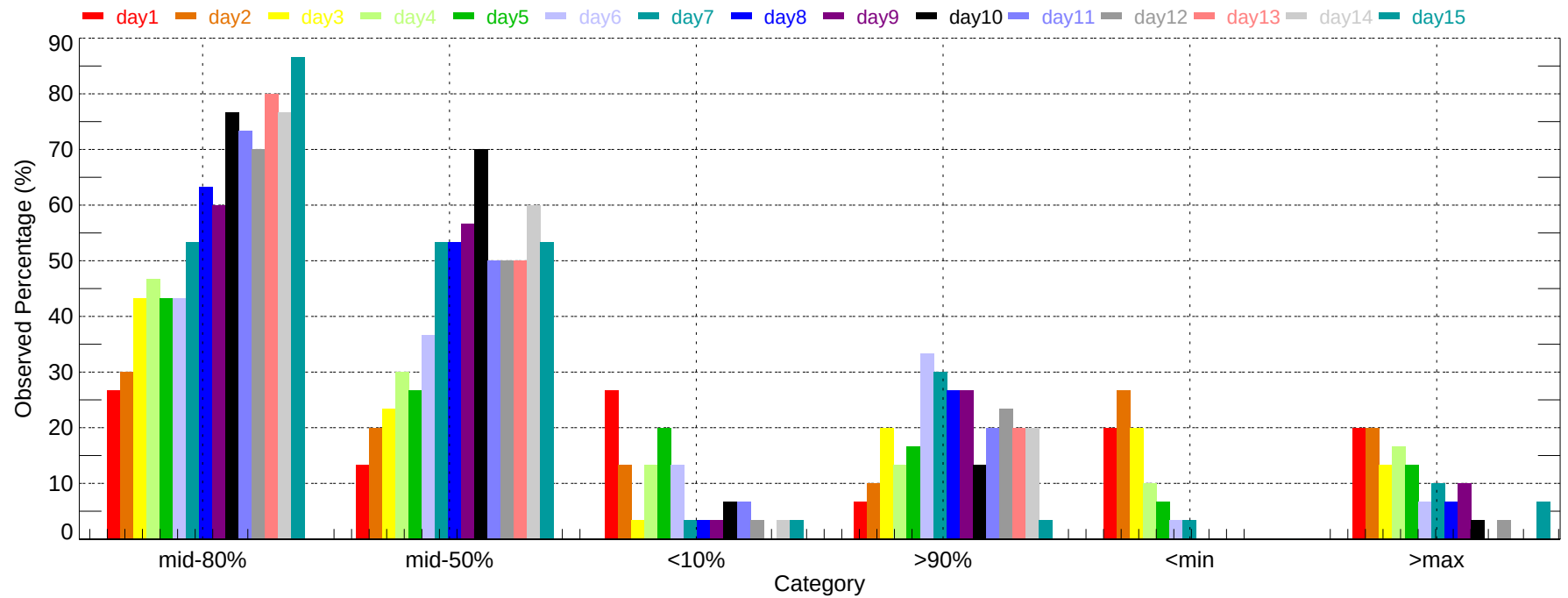
Observed Percentage of Ensembles - DCA: Max Temperature (2007-12-01~2007-12-31)
