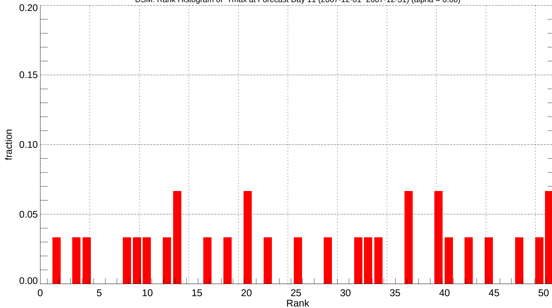
DSM: Rank Histogram of Tmax at Forecast Day 11 (2007-12-01~2007-12-31) (alpha = 0.00)
