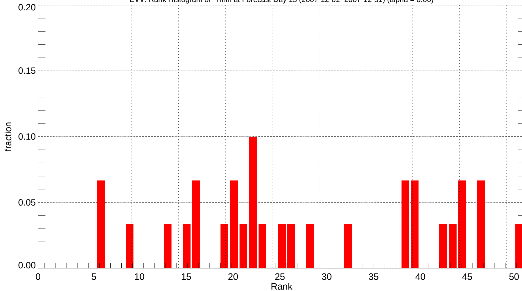
EVV: Rank Histogram of Tmin at Forecast Day 13 (2007-12-01~2007-12-31) (alpha = 0.00)
