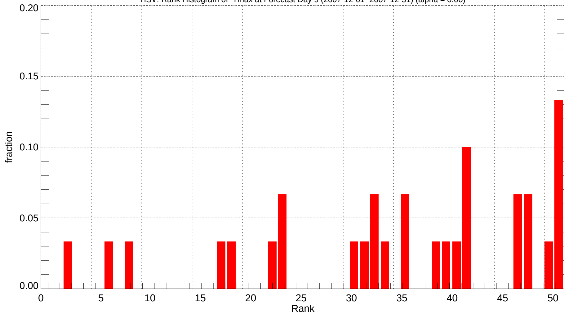
HSV: Rank Histogram of Tmax at Forecast Day 9 (2007-12-01~2007-12-31) (alpha = 0.00)
