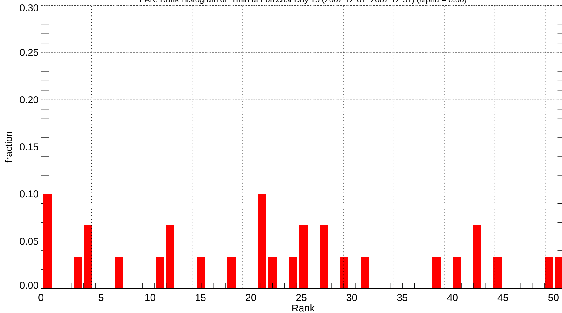
FAR: Rank Histogram of Tmin at Forecast Day 15 (2007-12-01~2007-12-31) (alpha = 0.00)
