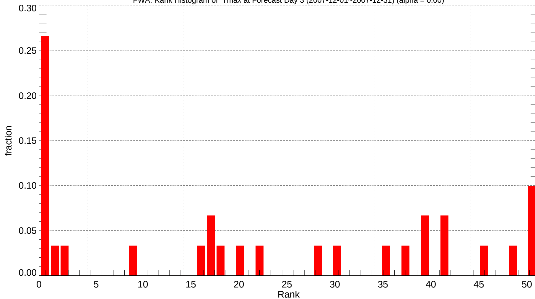
FWA: Rank Histogram of Tmax at Forecast Day 3 (2007-12-01~2007-12-31) (alpha = 0.00)
