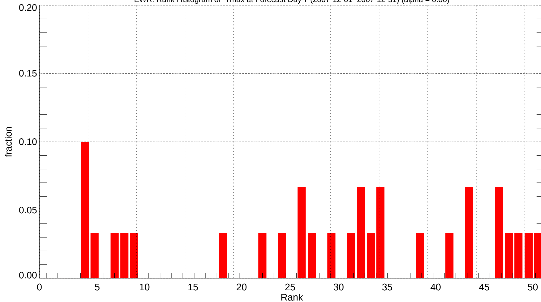
EWR: Rank Histogram of Tmax at Forecast Day 7 (2007-12-01~2007-12-31) (alpha = 0.00)
