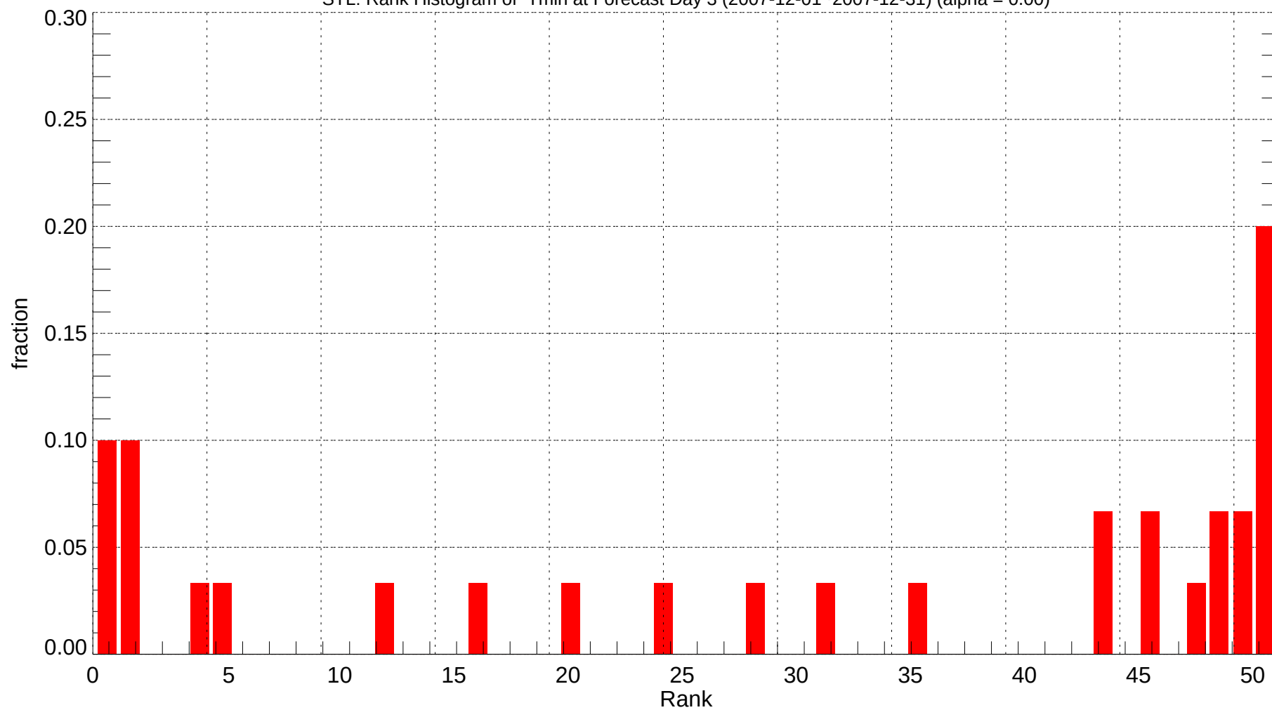
STL: Rank Histogram of Tmin at Forecast Day 3 (2007-12-01~2007-12-31) (alpha = 0.00)
