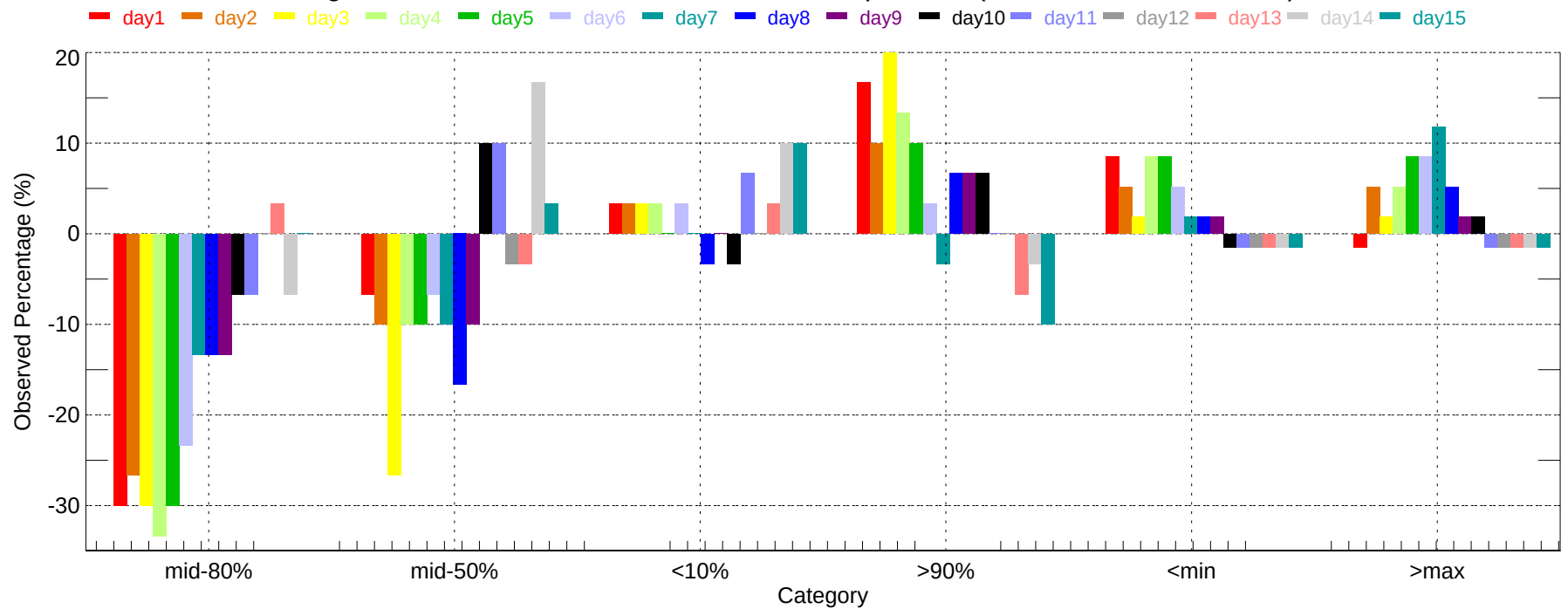
Observed Percentage Deviation of Ensembles - PHX: Min Temperature (2007-12-01~2007-12-31)
