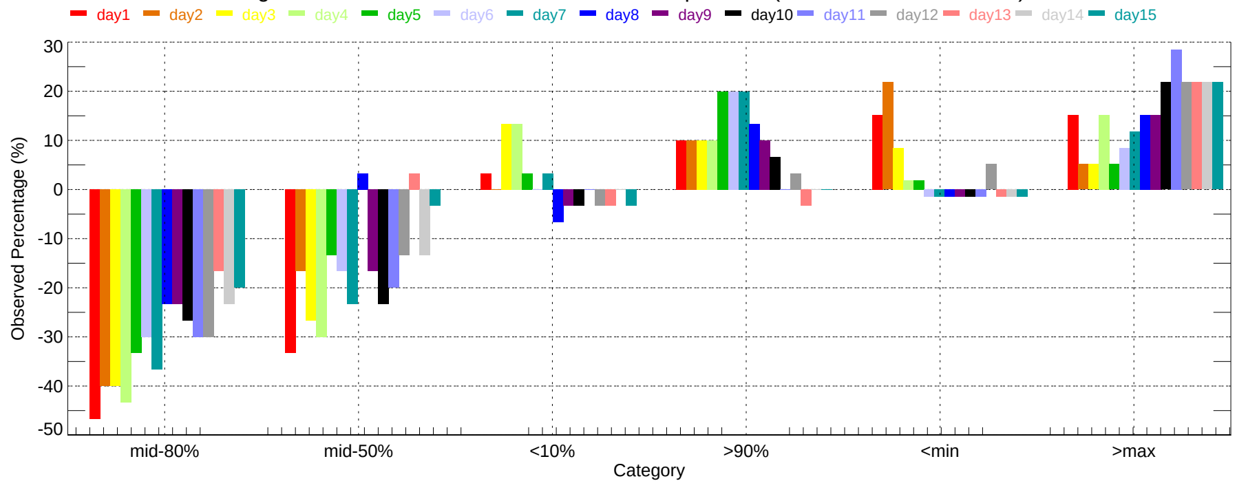
Observed Percentage Deviation of Ensembles - JAN: Max Temperature (2007-12-01~2007-12-31)
