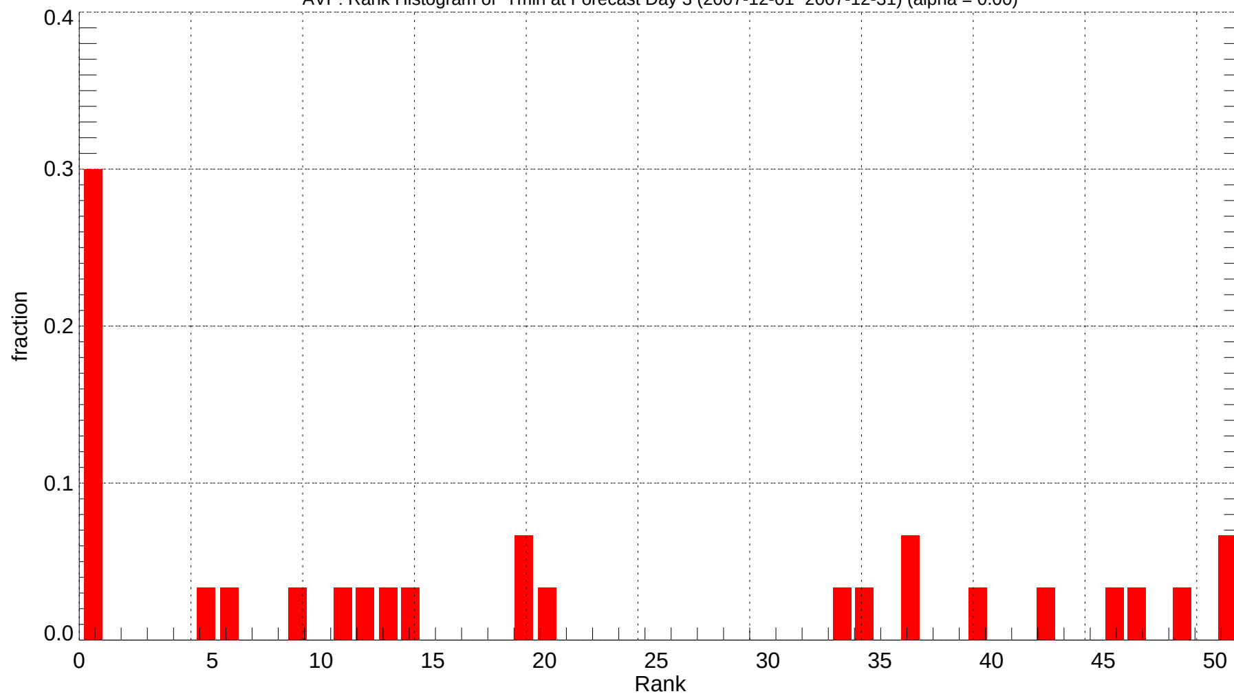
AVP: Rank Histogram of Tmin at Forecast Day 3 (2007-12-01~2007-12-31) (alpha = 0.00)
