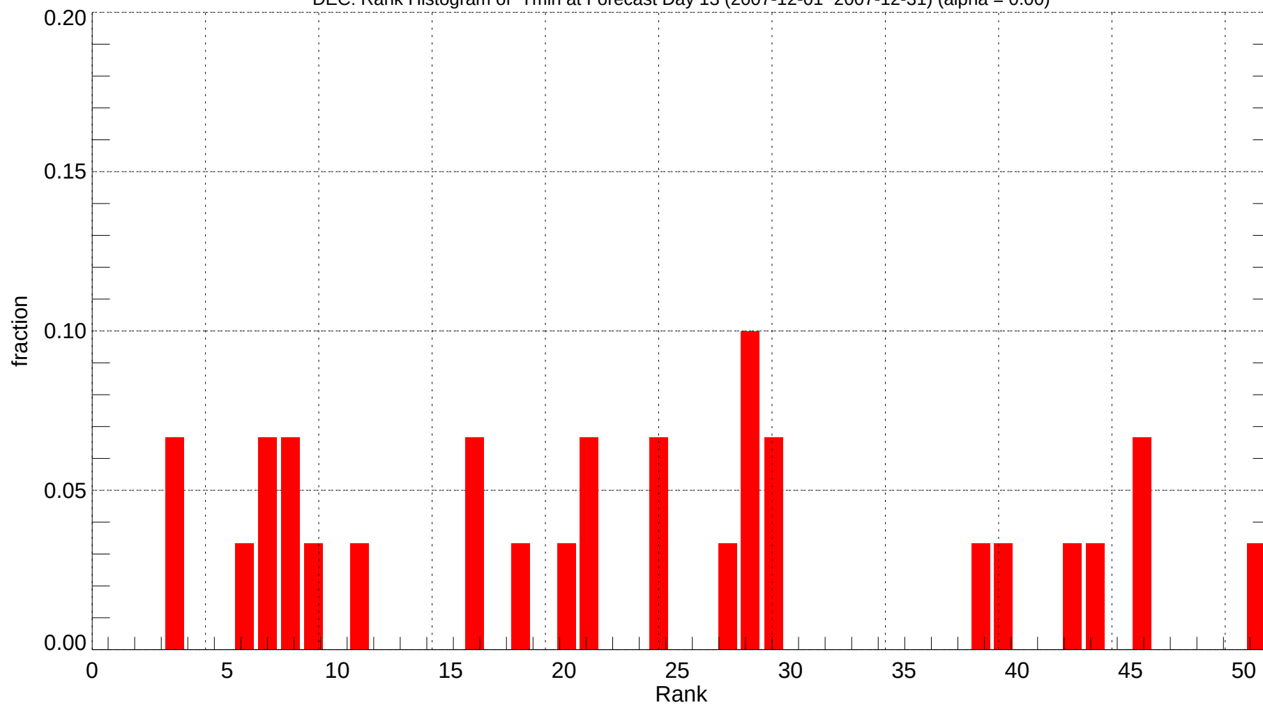
DEC: Rank Histogram of Tmin at Forecast Day 13 (2007-12-01~2007-12-31) (alpha = 0.00)
