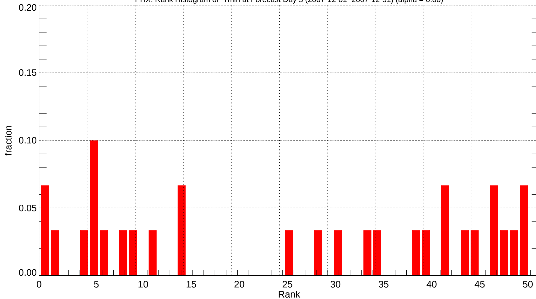
PHX: Rank Histogram of Tmin at Forecast Day 3 (2007-12-01~2007-12-31) (alpha = 0.00)
