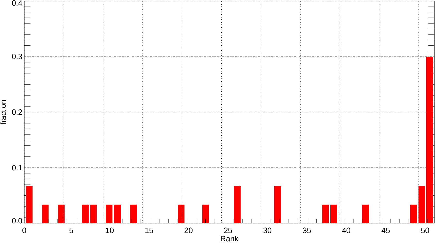
LFK: Rank Histogram of Tmin at Forecast Day 2 (2007-12-01~2007-12-31) (alpha = 0.00)
