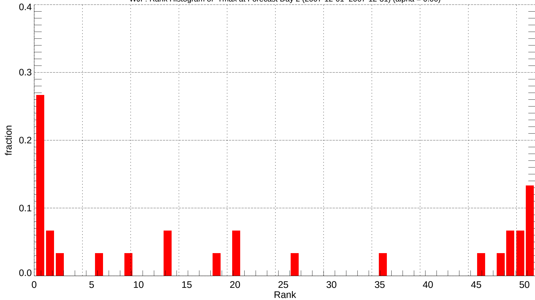
WJF: Rank Histogram of Tmax at Forecast Day 2 (2007-12-01~2007-12-31) (alpha = 0.00)
