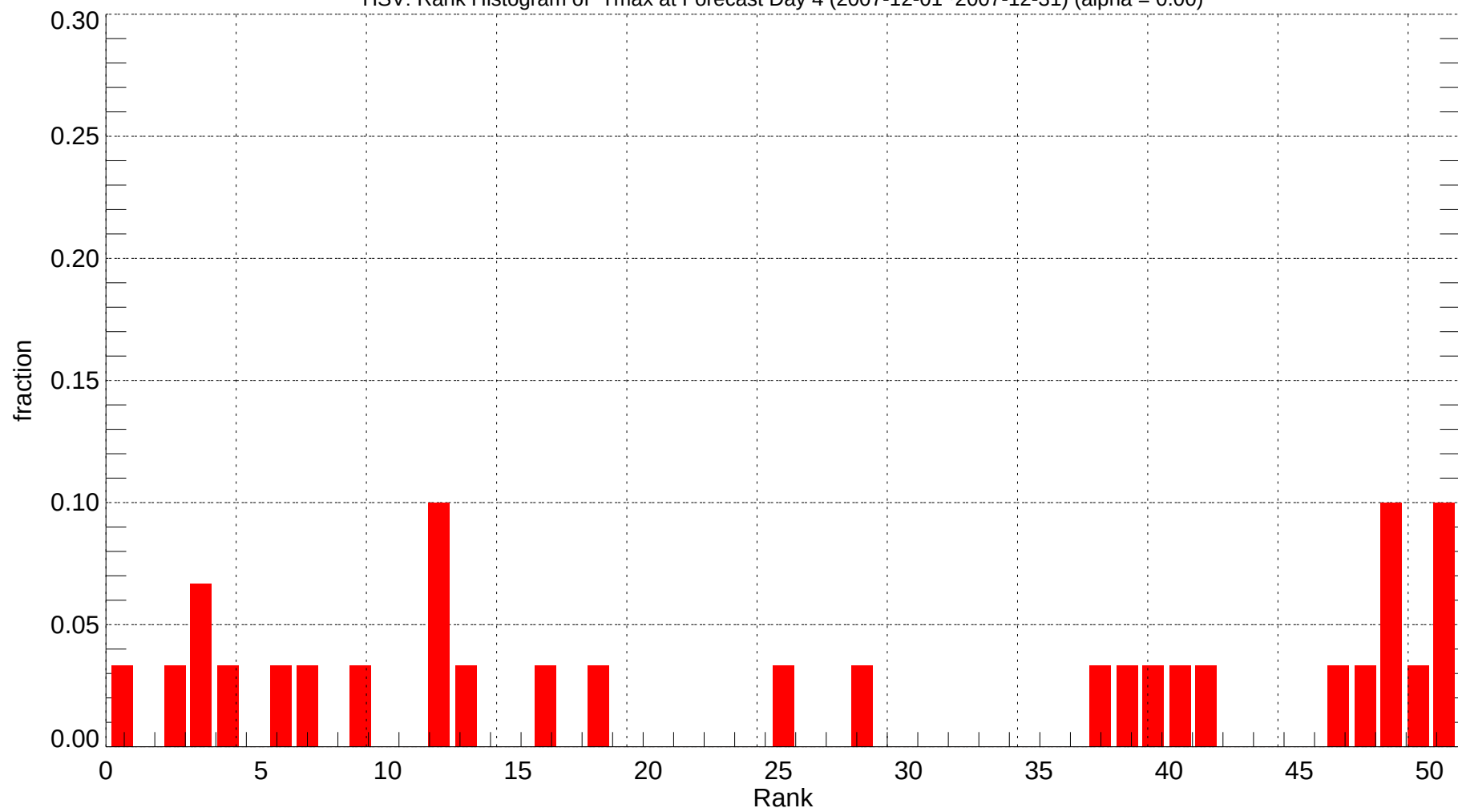
HSV: Rank Histogram of Tmax at Forecast Day 4 (2007-12-01~2007-12-31) (alpha = 0.00)
