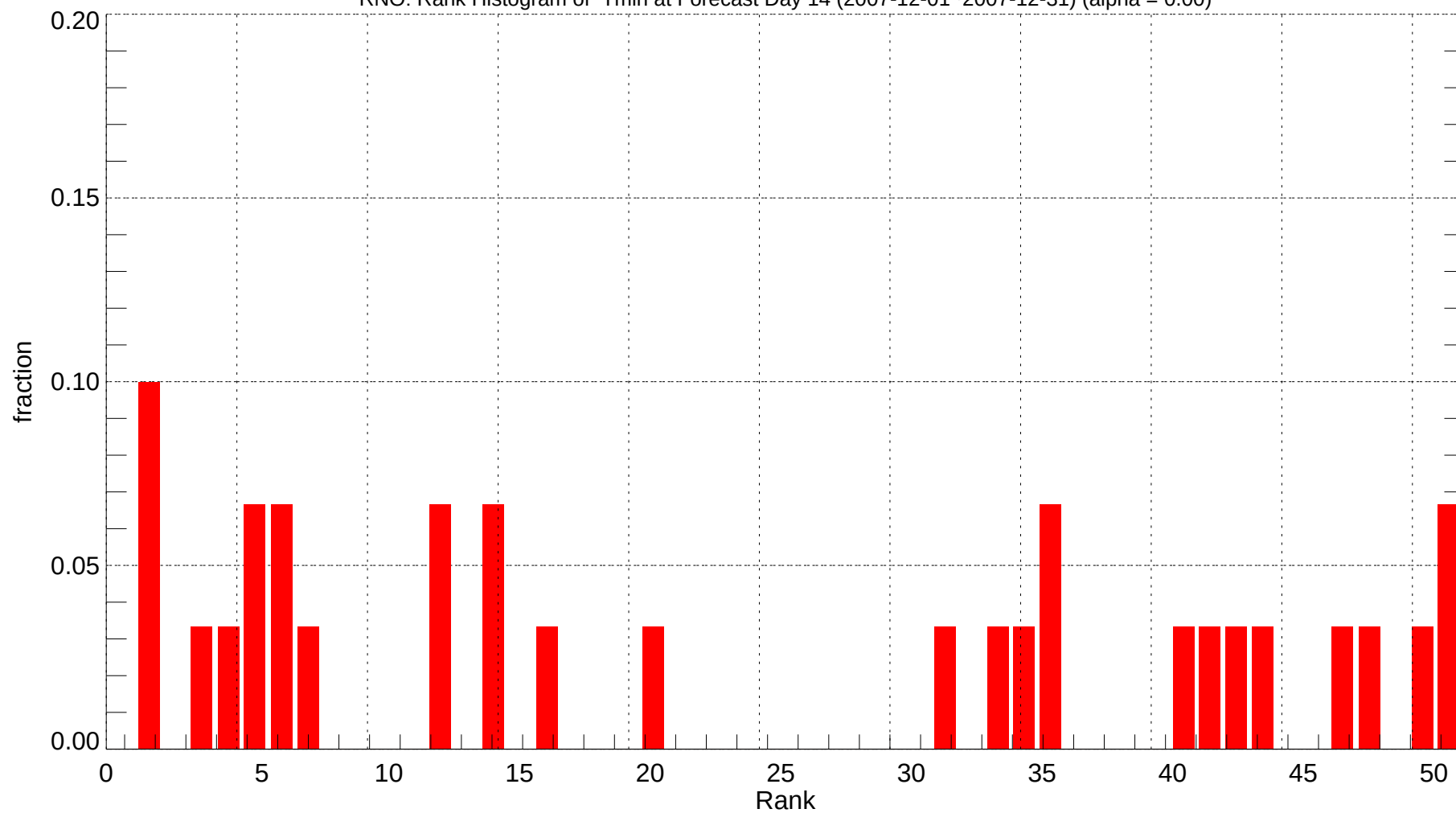
RNO: Rank Histogram of Tmin at Forecast Day 14 (2007-12-01~2007-12-31) (alpha = 0.00)
