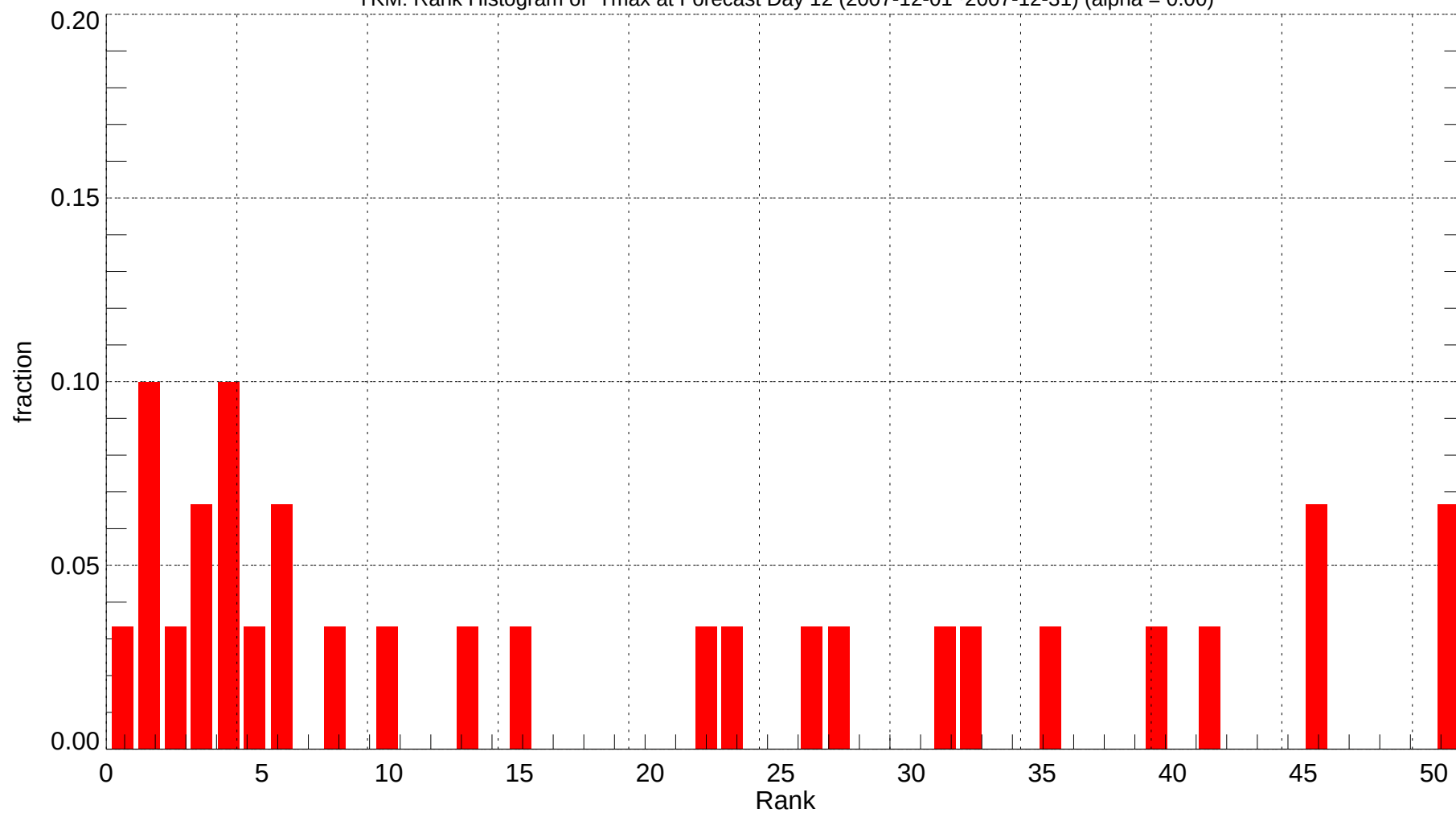
YKM: Rank Histogram of Tmax at Forecast Day 12 (2007-12-01~2007-12-31) (alpha = 0.00)
