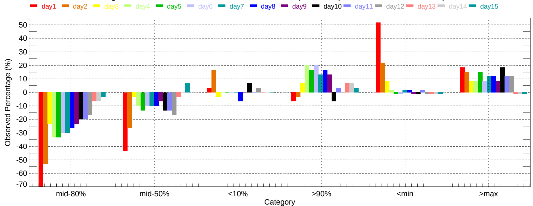
Observed Percentage Deviation of Ensembles - OMA: Max Temperature (2007-12-01~2007-12-31)
