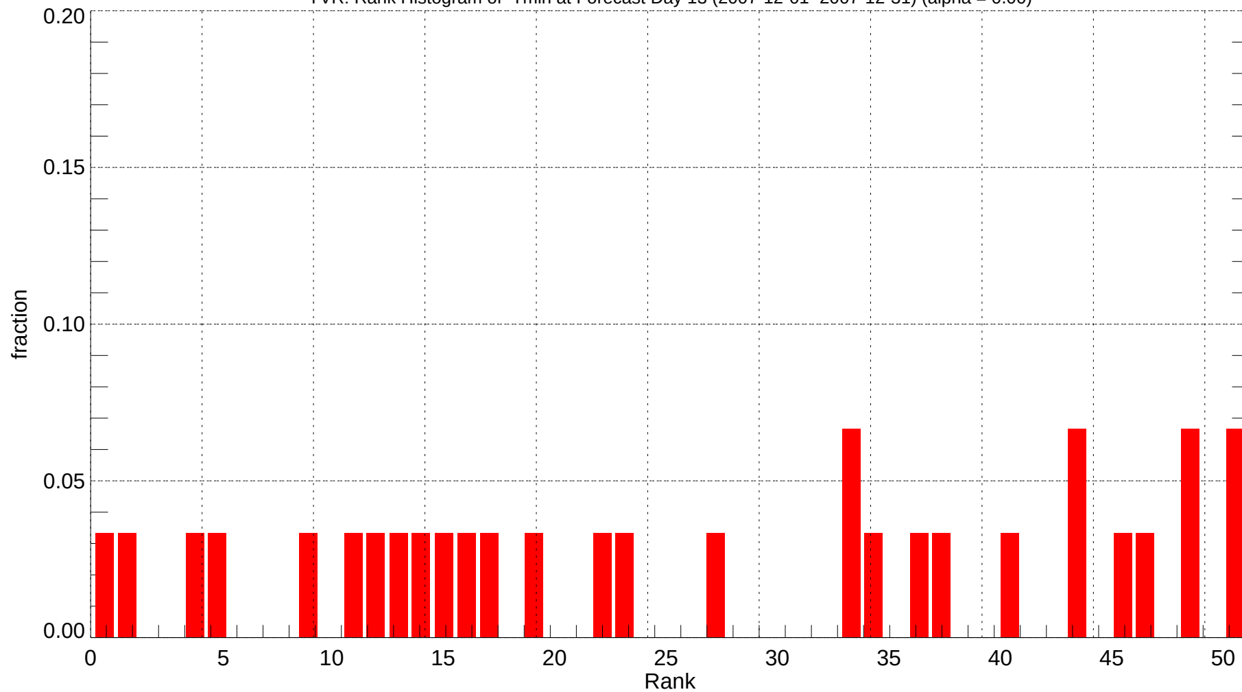
YVR: Rank Histogram of Tmin at Forecast Day 13 (2007-12-01~2007-12-31) (alpha = 0.00)
