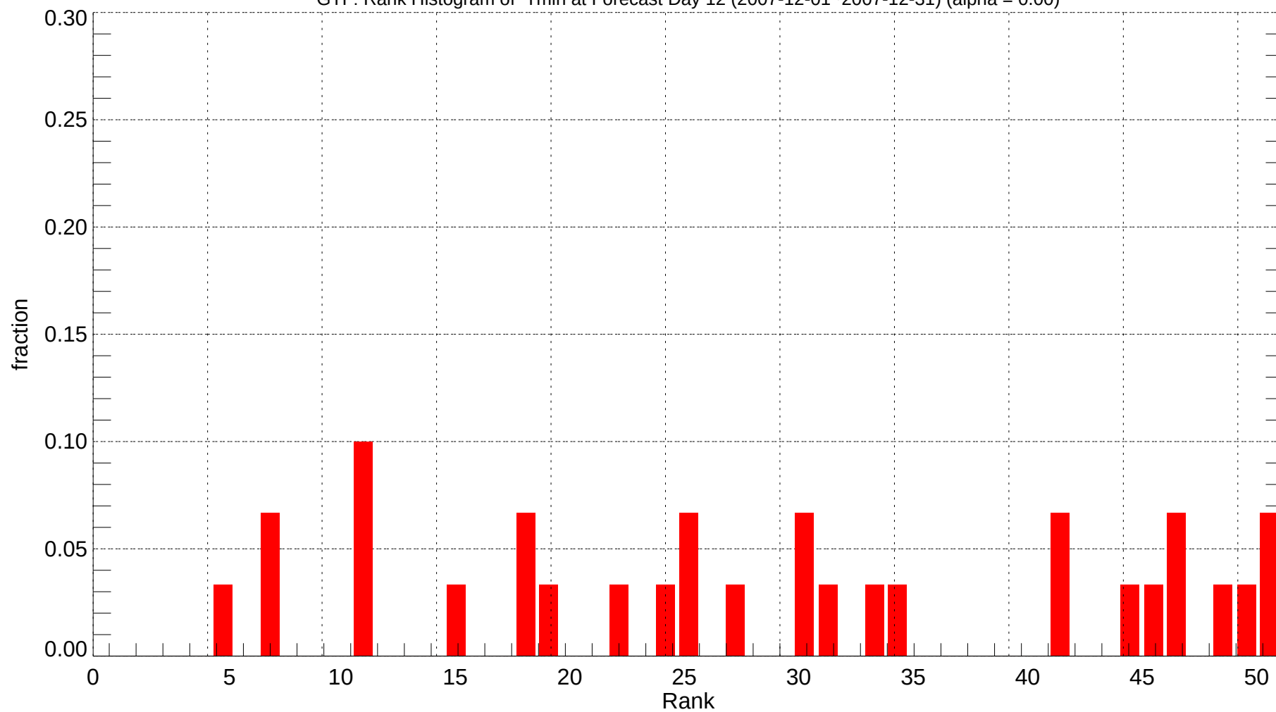
GTF: Rank Histogram of Tmin at Forecast Day 12 (2007-12-01~2007-12-31) (alpha = 0.00)
