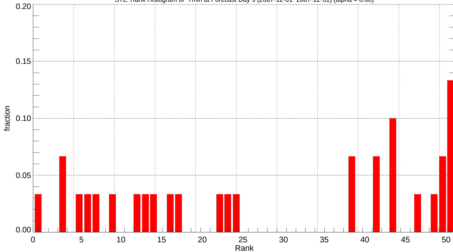
STL: Rank Histogram of Tmin at Forecast Day 9 (2007-12-01~2007-12-31) (alpha = 0.00)
