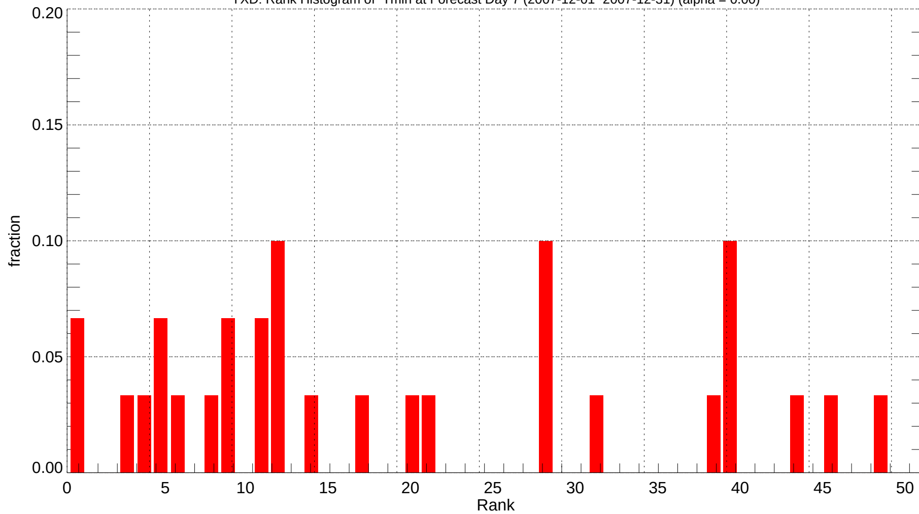
YXD: Rank Histogram of Tmin at Forecast Day 7 (2007-12-01~2007-12-31) (alpha = 0.00)
