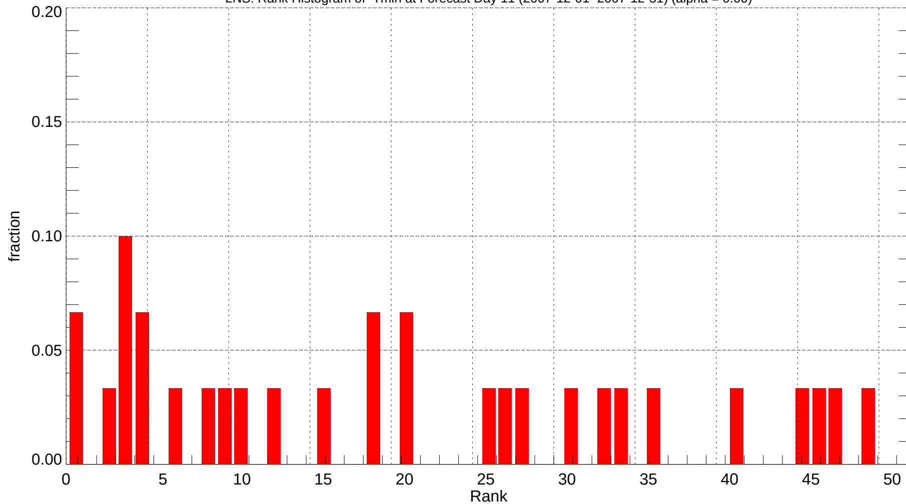
LNS: Rank Histogram of Tmin at Forecast Day 11 (2007-12-01~2007-12-31) (alpha = 0.00)
