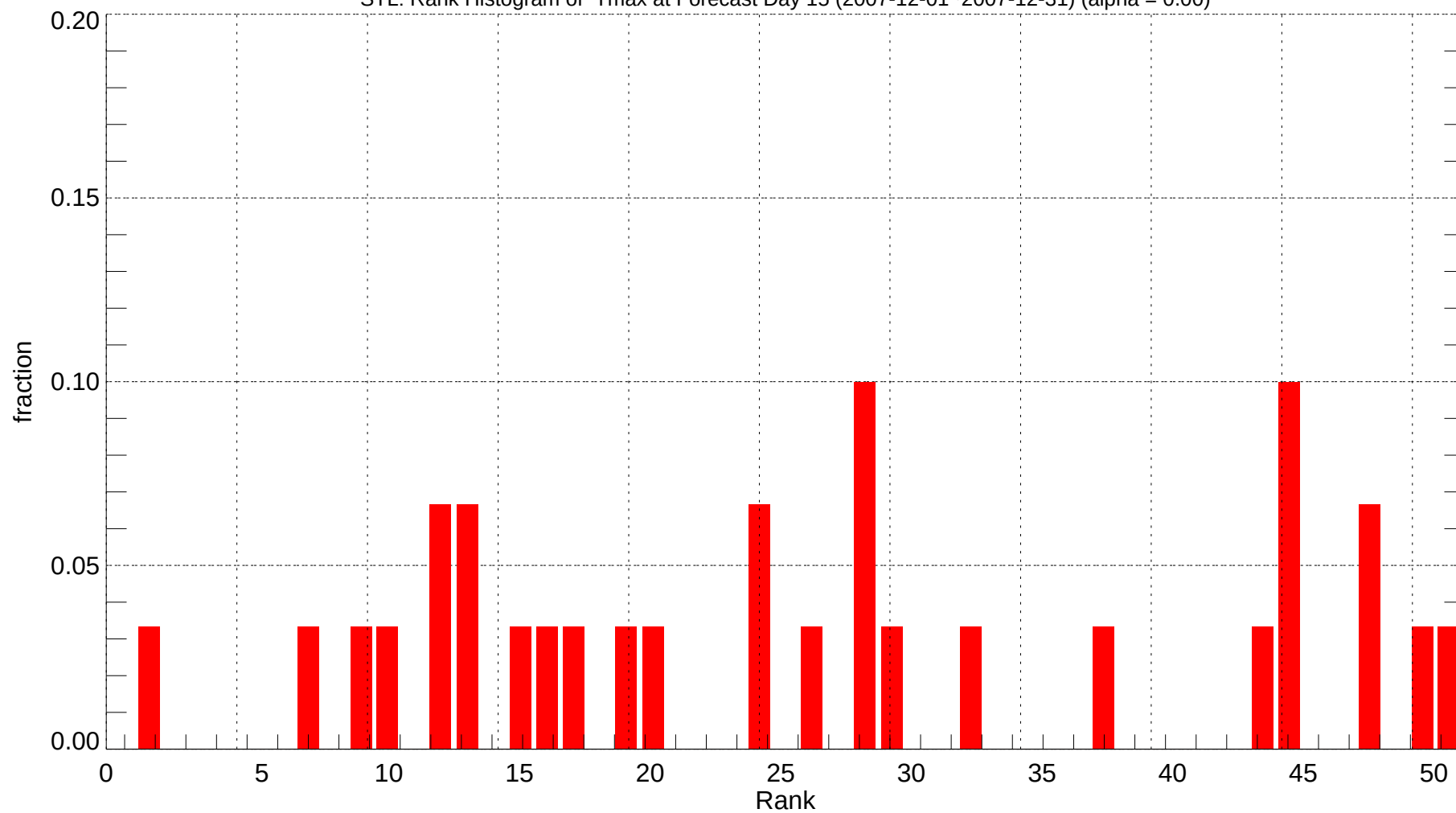
STL: Rank Histogram of Tmax at Forecast Day 15 (2007-12-01~2007-12-31) (alpha = 0.00)
