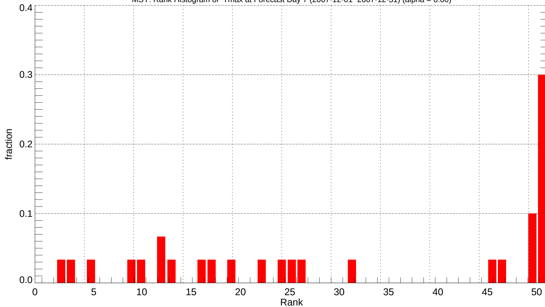
MSY: Rank Histogram of Tmax at Forecast Day 7 (2007-12-01~2007-12-31) (alpha = 0.00)
