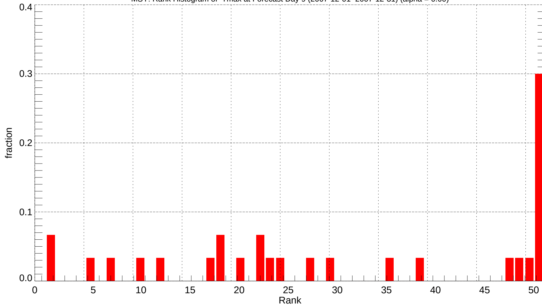
MSY: Rank Histogram of Tmax at Forecast Day 9 (2007-12-01~2007-12-31) (alpha = 0.00)
