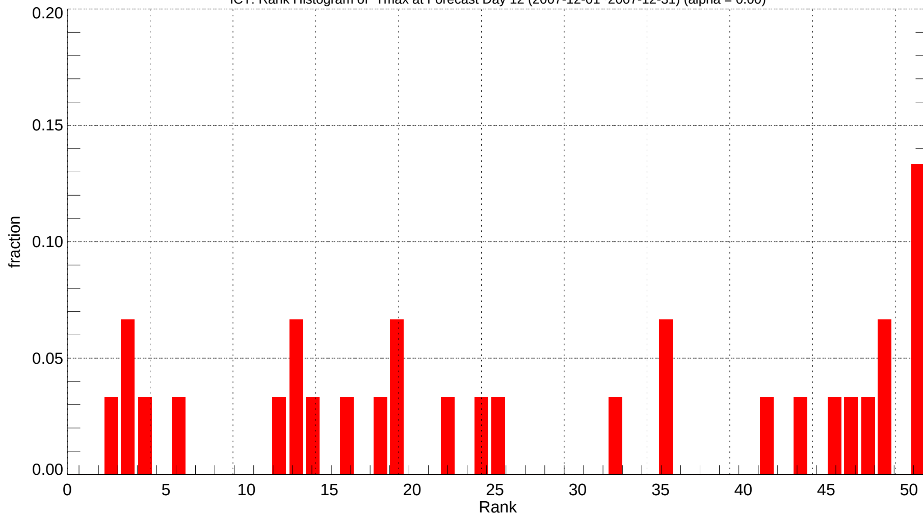
ICT: Rank Histogram of Tmax at Forecast Day 12 (2007-12-01~2007-12-31) (alpha = 0.00)
