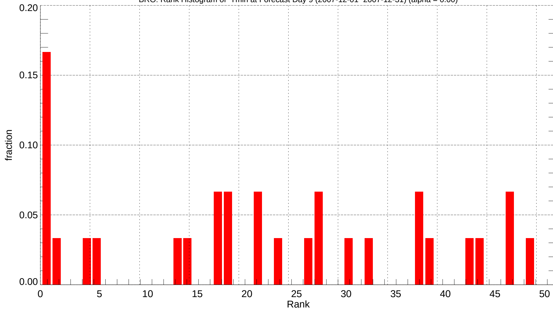
BRO: Rank Histogram of Tmin at Forecast Day 9 (2007-12-01~2007-12-31) (alpha = 0.00)
