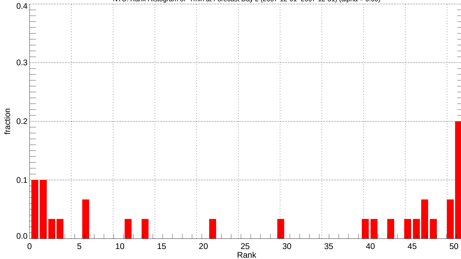
NTU: Rank Histogram of Tmin at Forecast Day 2 (2007-12-01~2007-12-31) (alpha = 0.00)
