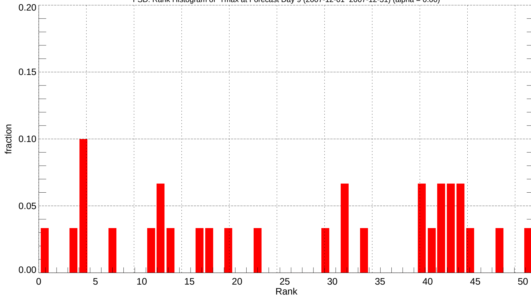
FSD: Rank Histogram of Tmax at Forecast Day 9 (2007-12-01~2007-12-31) (alpha = 0.00)
