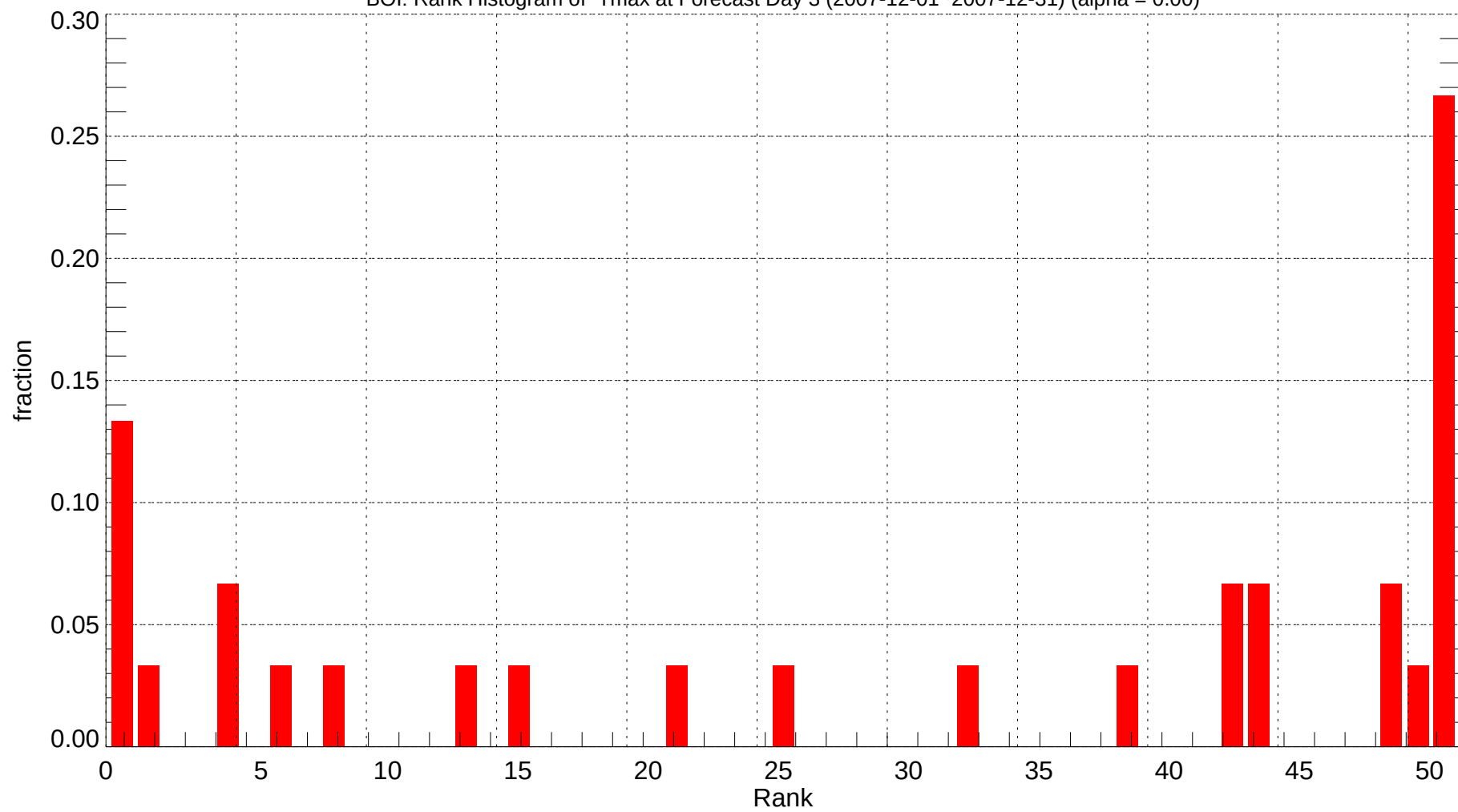
BOI: Rank Histogram of Tmax at Forecast Day 3 (2007-12-01~2007-12-31) (alpha = 0.00)
