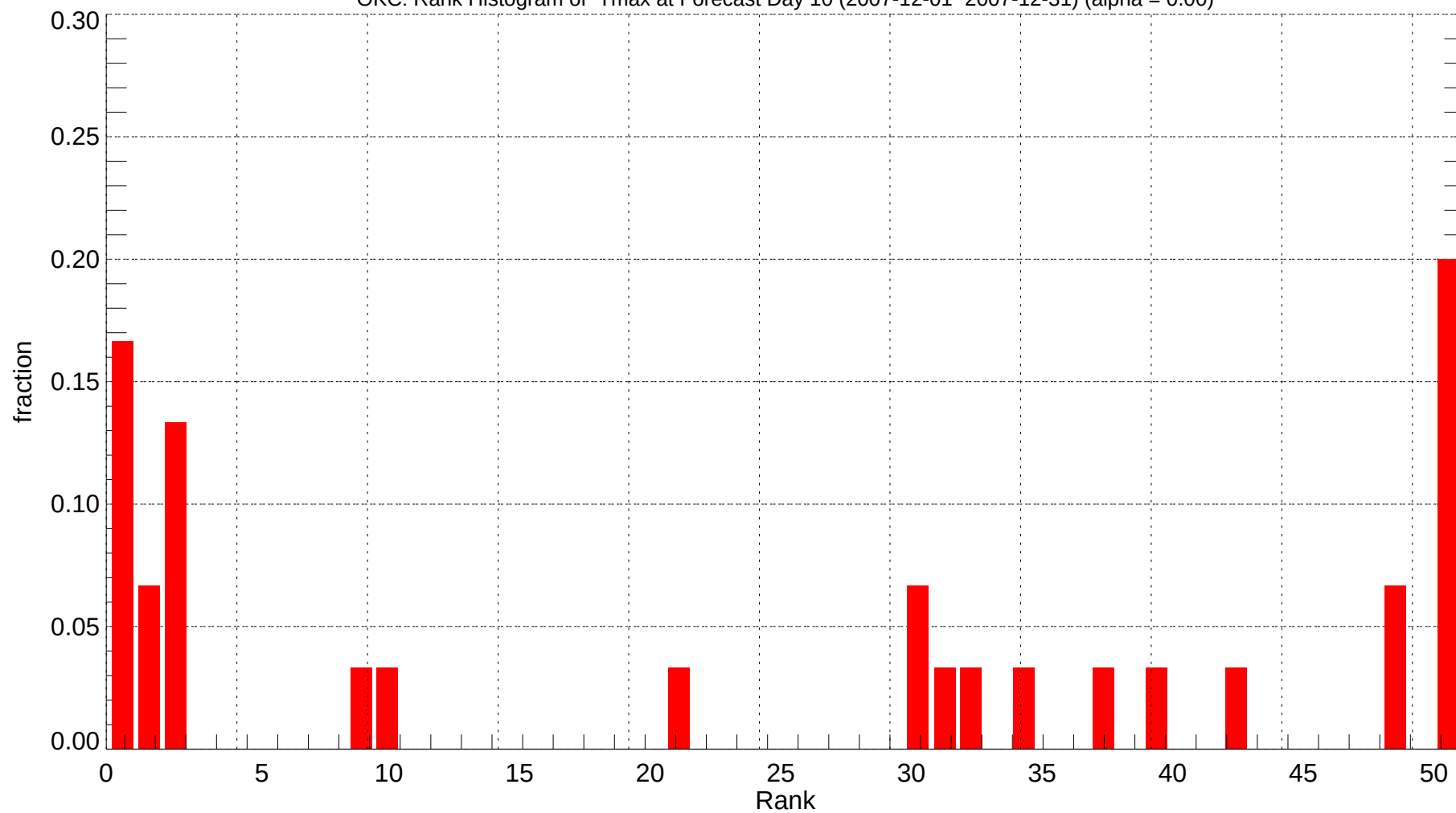
OKC: Rank Histogram of Tmax at Forecast Day 10 (2007-12-01~2007-12-31) (alpha = 0.00)
