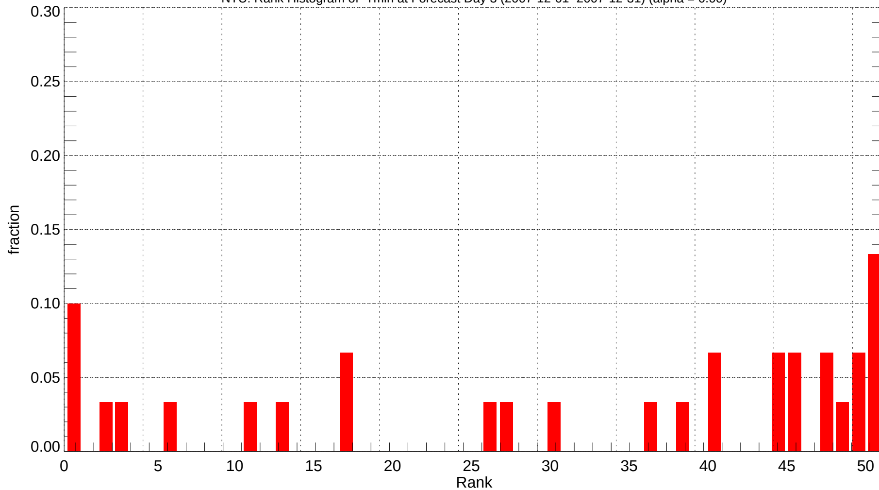
NTU: Rank Histogram of Tmin at Forecast Day 3 (2007-12-01~2007-12-31) (alpha = 0.00)
