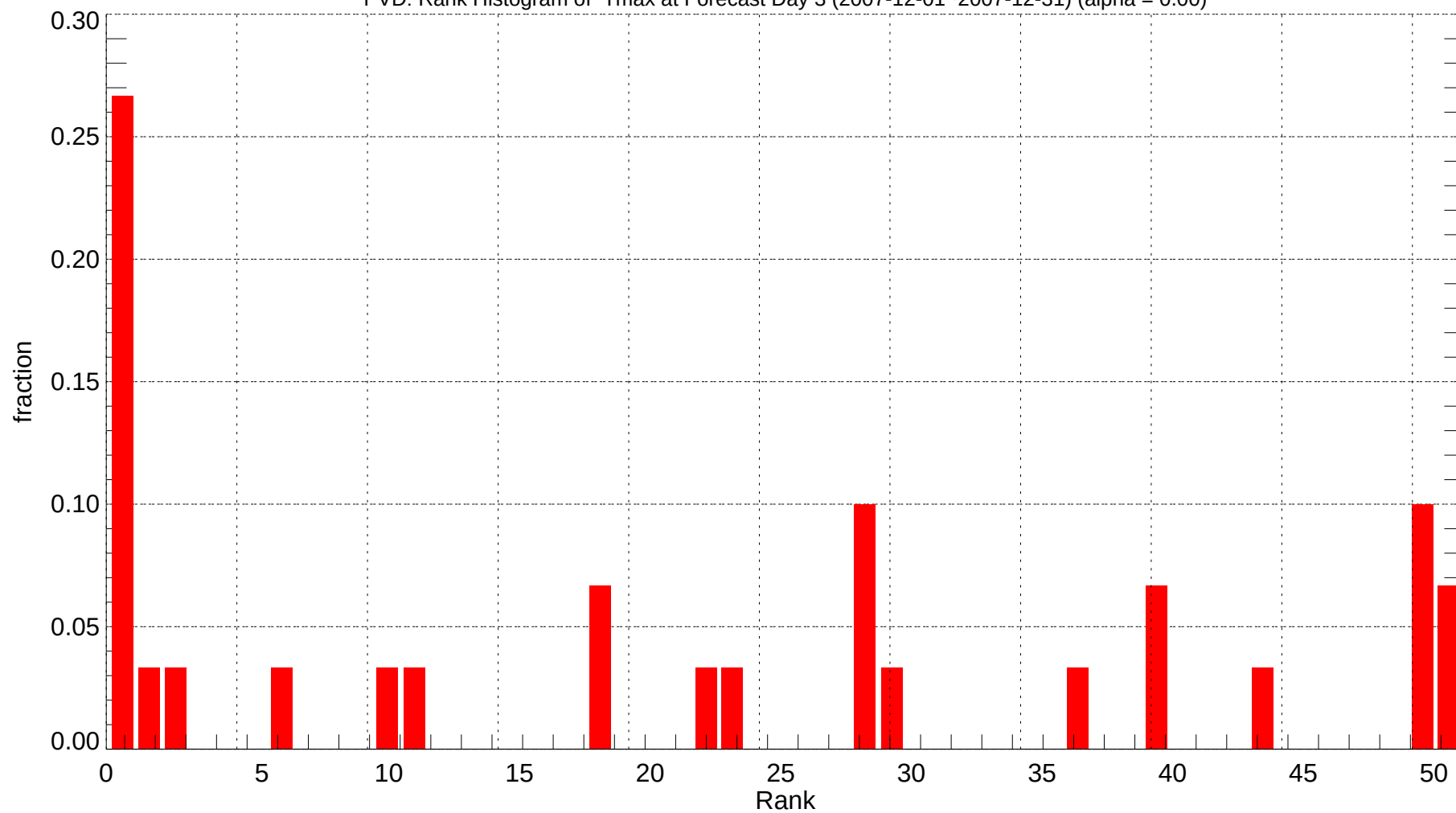
PVD: Rank Histogram of Tmax at Forecast Day 3 (2007-12-01~2007-12-31) (alpha = 0.00)
