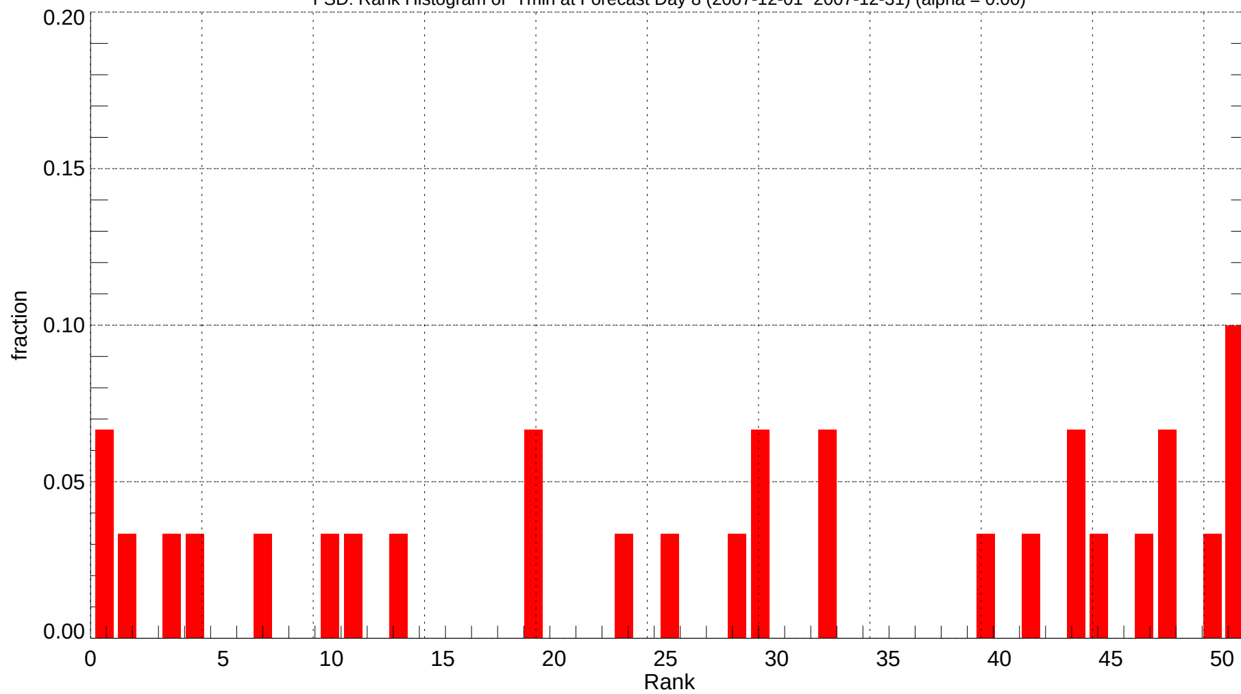
FSD: Rank Histogram of Tmin at Forecast Day 8 (2007-12-01~2007-12-31) (alpha = 0.00)
