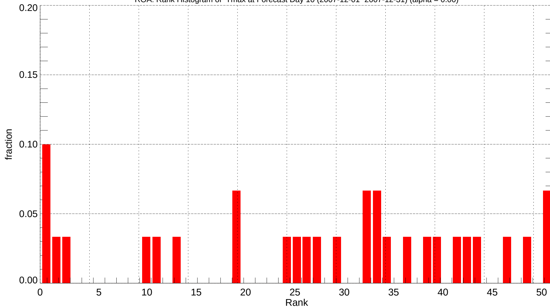
ROA: Rank Histogram of Tmax at Forecast Day 10 (2007-12-01~2007-12-31) (alpha = 0.00)
