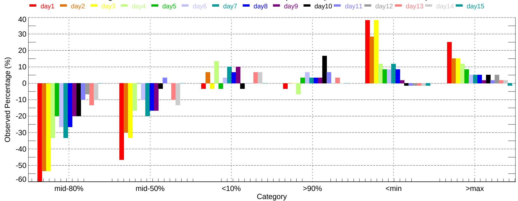
Observed Percentage Deviation of Ensembles - RAP: Min Temperature (2007-12-01~2007-12-31)
