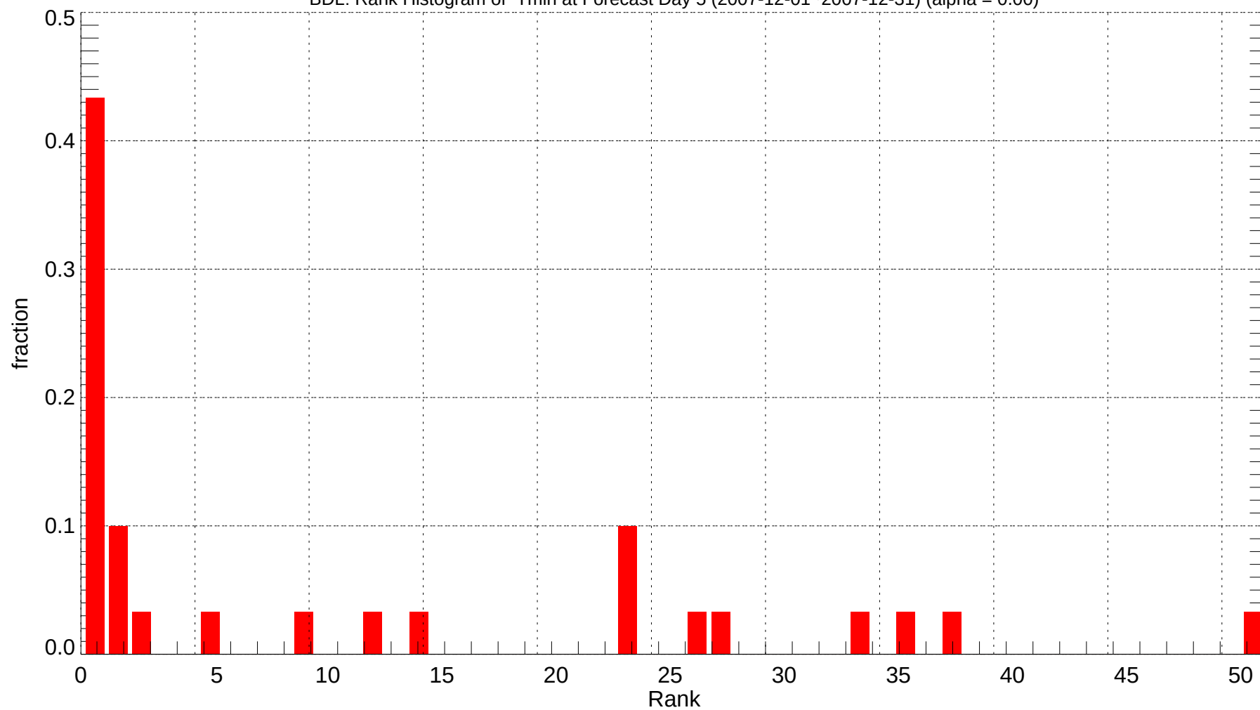
BDL: Rank Histogram of Tmin at Forecast Day 5 (2007-12-01~2007-12-31) (alpha = 0.00)
