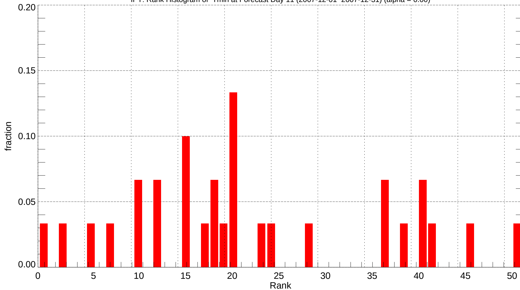
IPT: Rank Histogram of Tmin at Forecast Day 11 (2007-12-01~2007-12-31) (alpha = 0.00)
