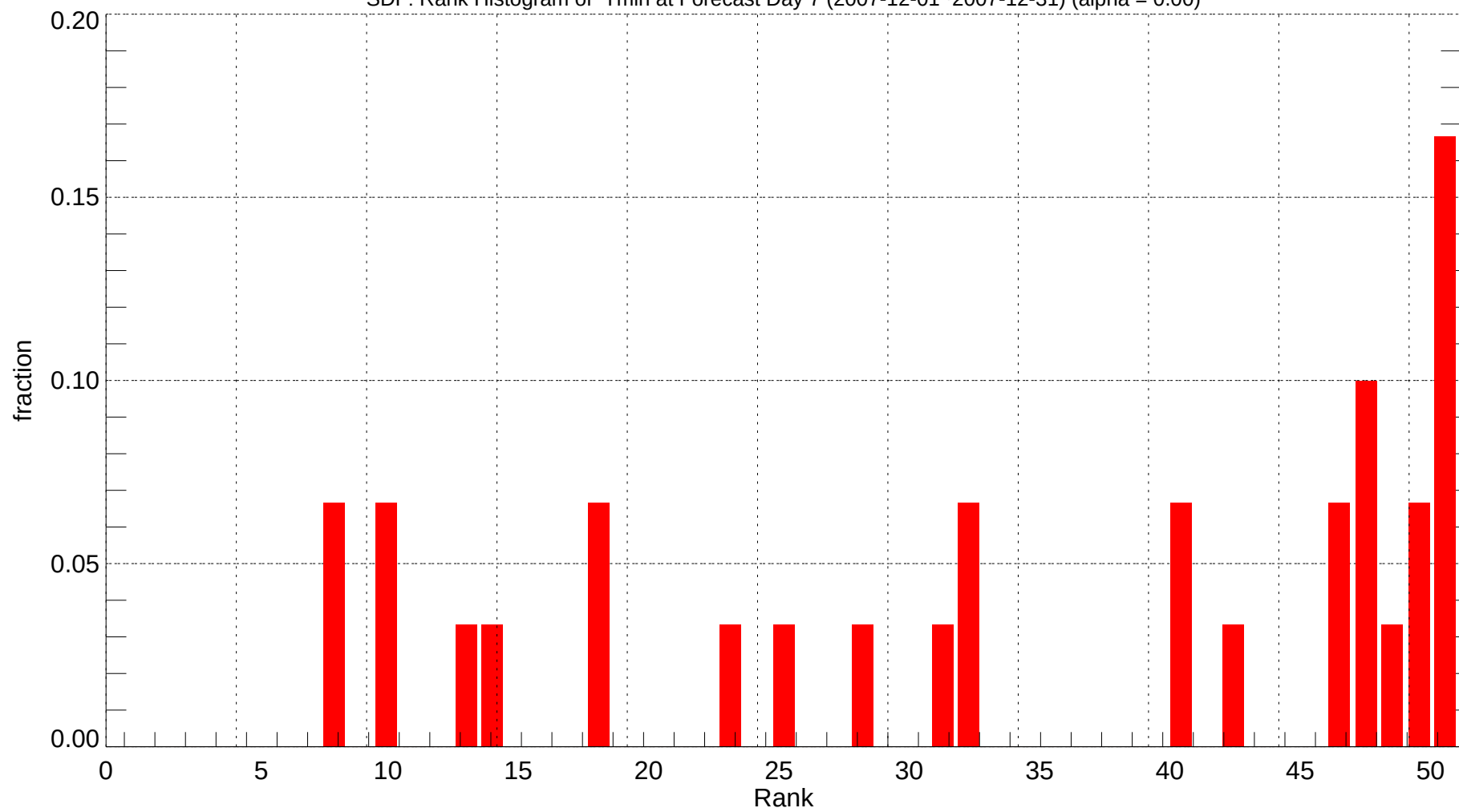
SDF: Rank Histogram of Tmin at Forecast Day 7 (2007-12-01~2007-12-31) (alpha = 0.00)
