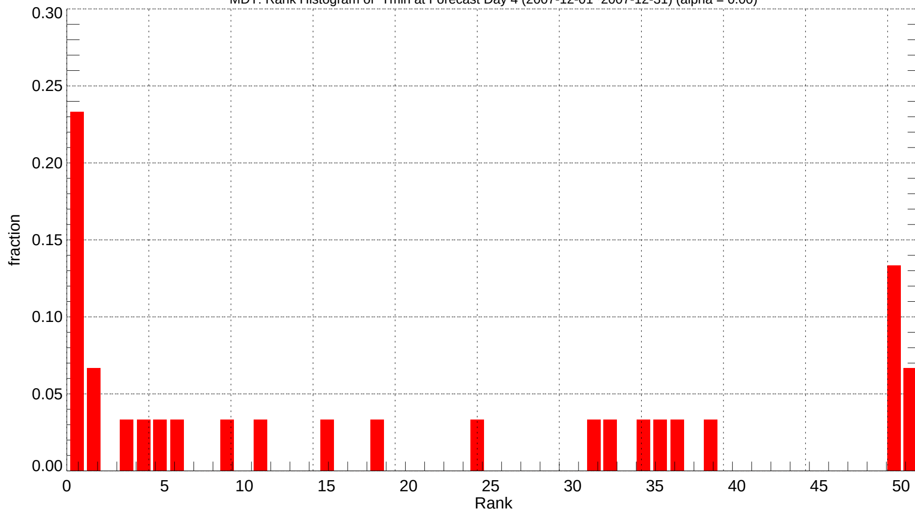
MDT: Rank Histogram of Tmin at Forecast Day 4 (2007-12-01~2007-12-31) (alpha = 0.00)
