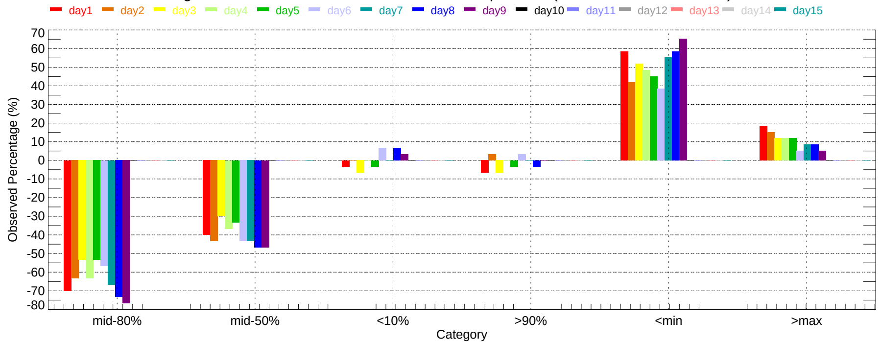
Observed Percentage Deviation of Ensembles - NKX: Max Temperature (2007-12-01~2007-12-31)
