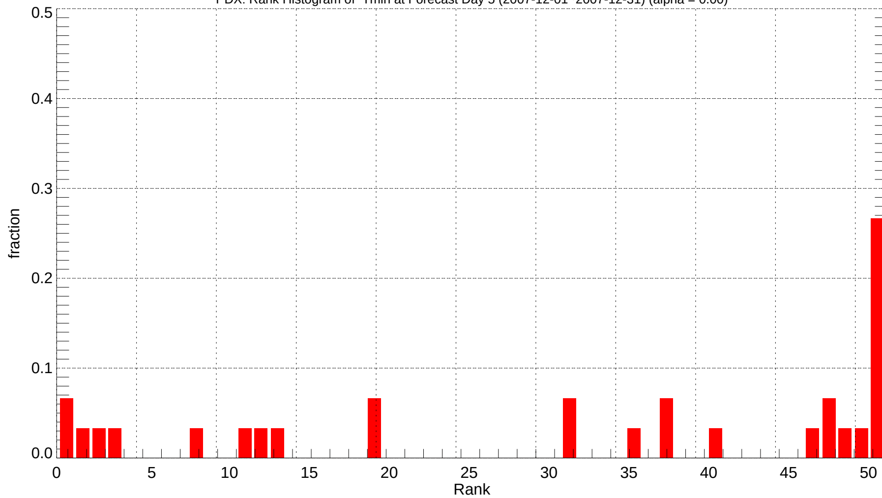
PDX: Rank Histogram of Tmin at Forecast Day 5 (2007-12-01~2007-12-31) (alpha = 0.00)
