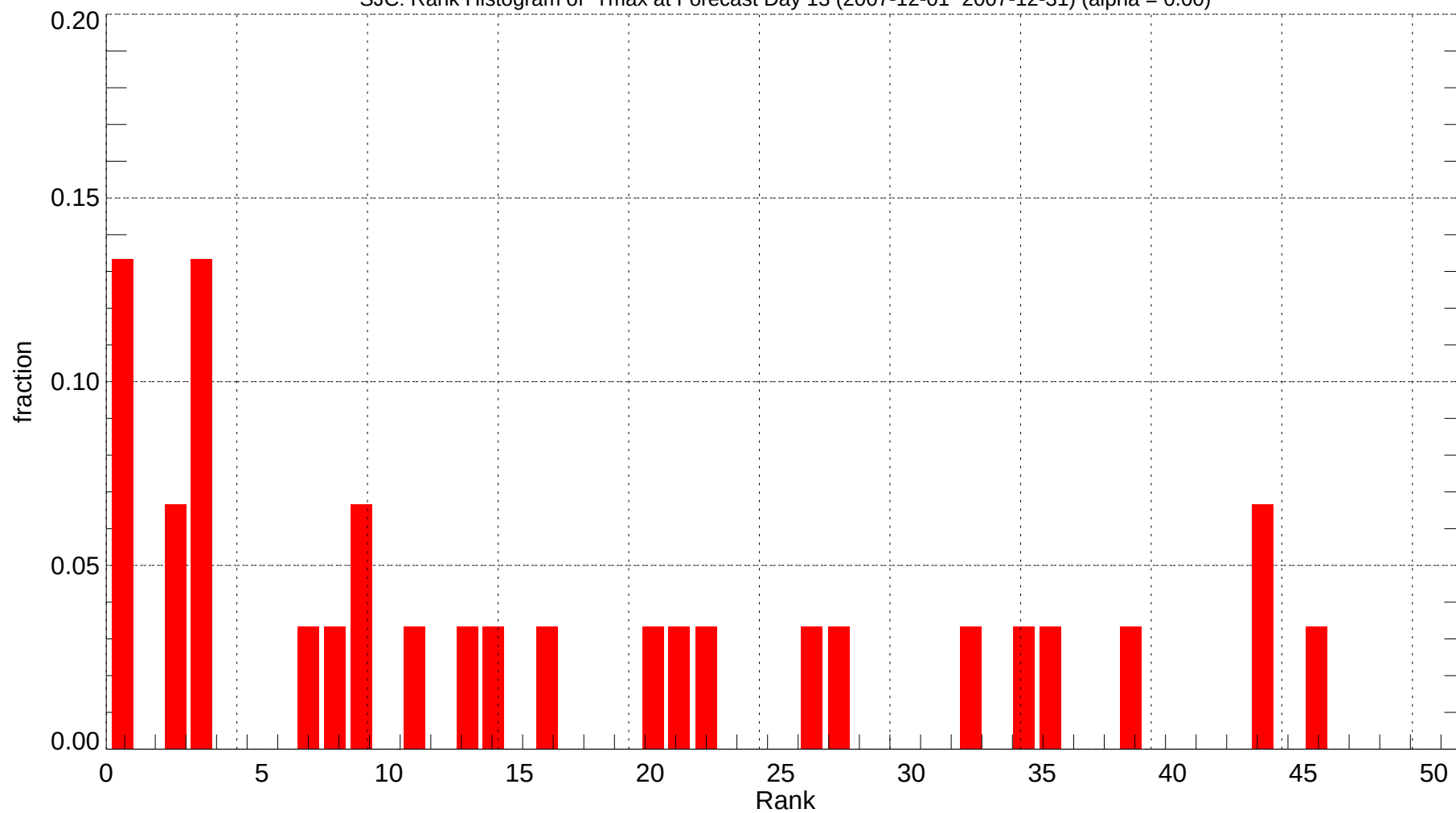
SJC: Rank Histogram of Tmax at Forecast Day 13 (2007-12-01~2007-12-31) (alpha = 0.00)
