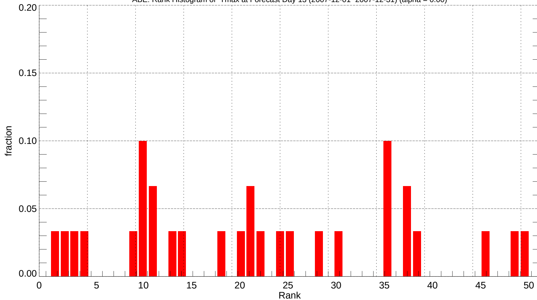
ABE: Rank Histogram of Tmax at Forecast Day 13 (2007-12-01~2007-12-31) (alpha = 0.00)
