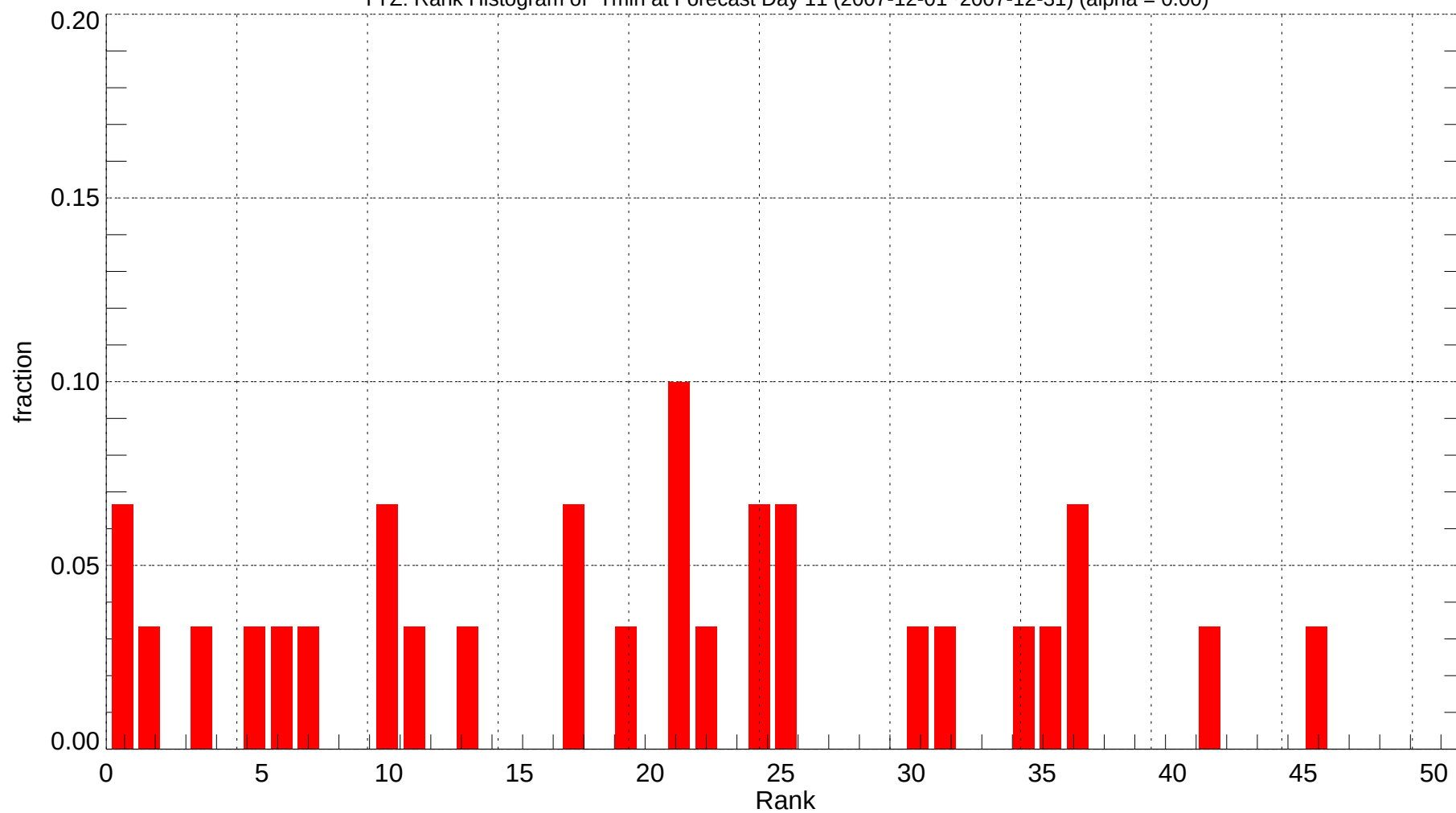
YYZ: Rank Histogram of Tmin at Forecast Day 11 (2007-12-01~2007-12-31) (alpha = 0.00)
