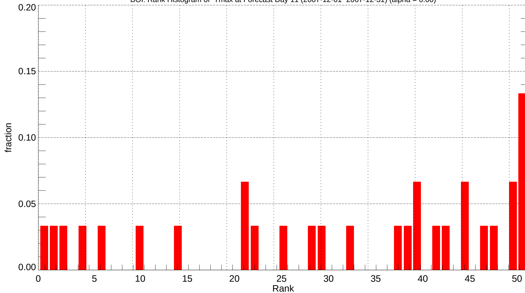
BOI: Rank Histogram of Tmax at Forecast Day 11 (2007-12-01~2007-12-31) (alpha = 0.00)
