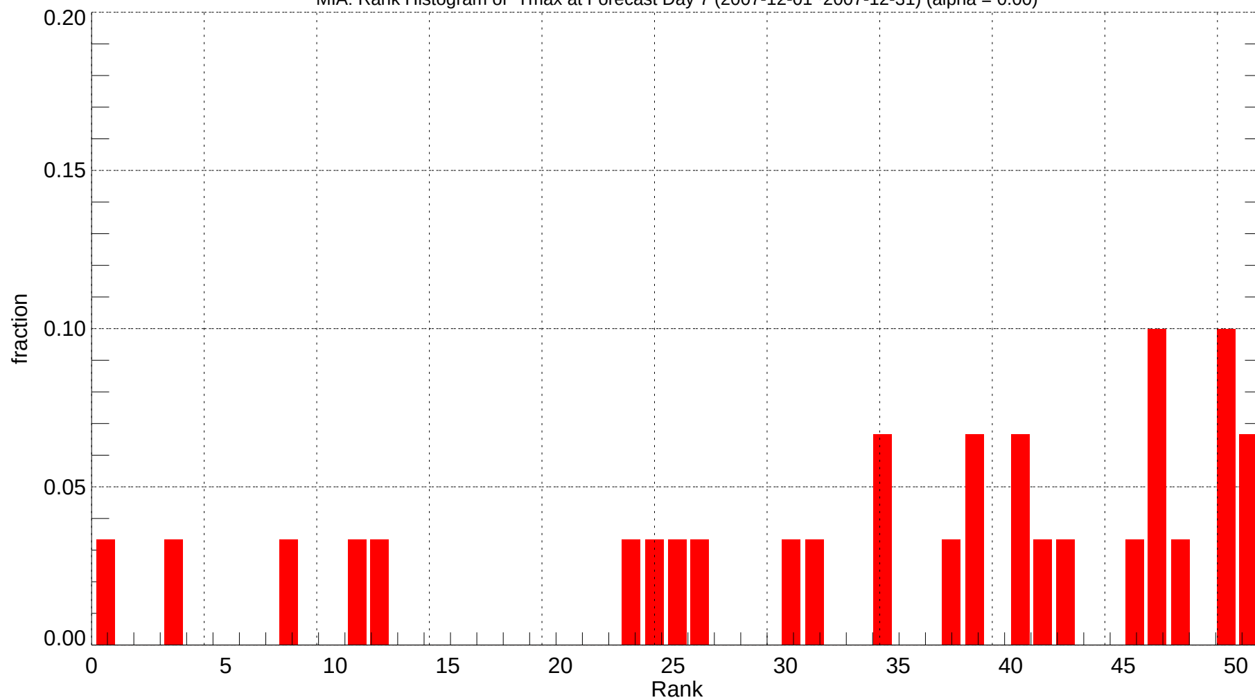
MIA: Rank Histogram of Tmax at Forecast Day 7 (2007-12-01~2007-12-31) (alpha = 0.00)
