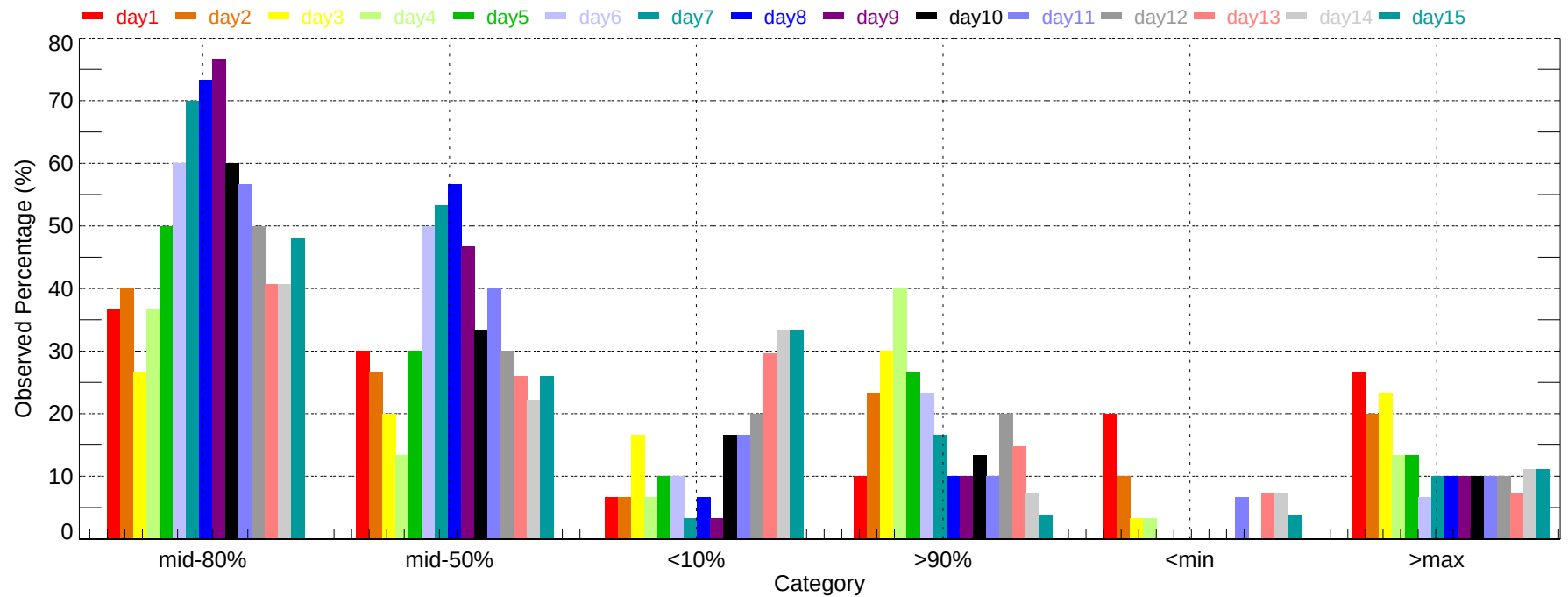
Observed Percentage of Ensembles - FLG: Min Temperature (2007-12-01~2007-12-31)
