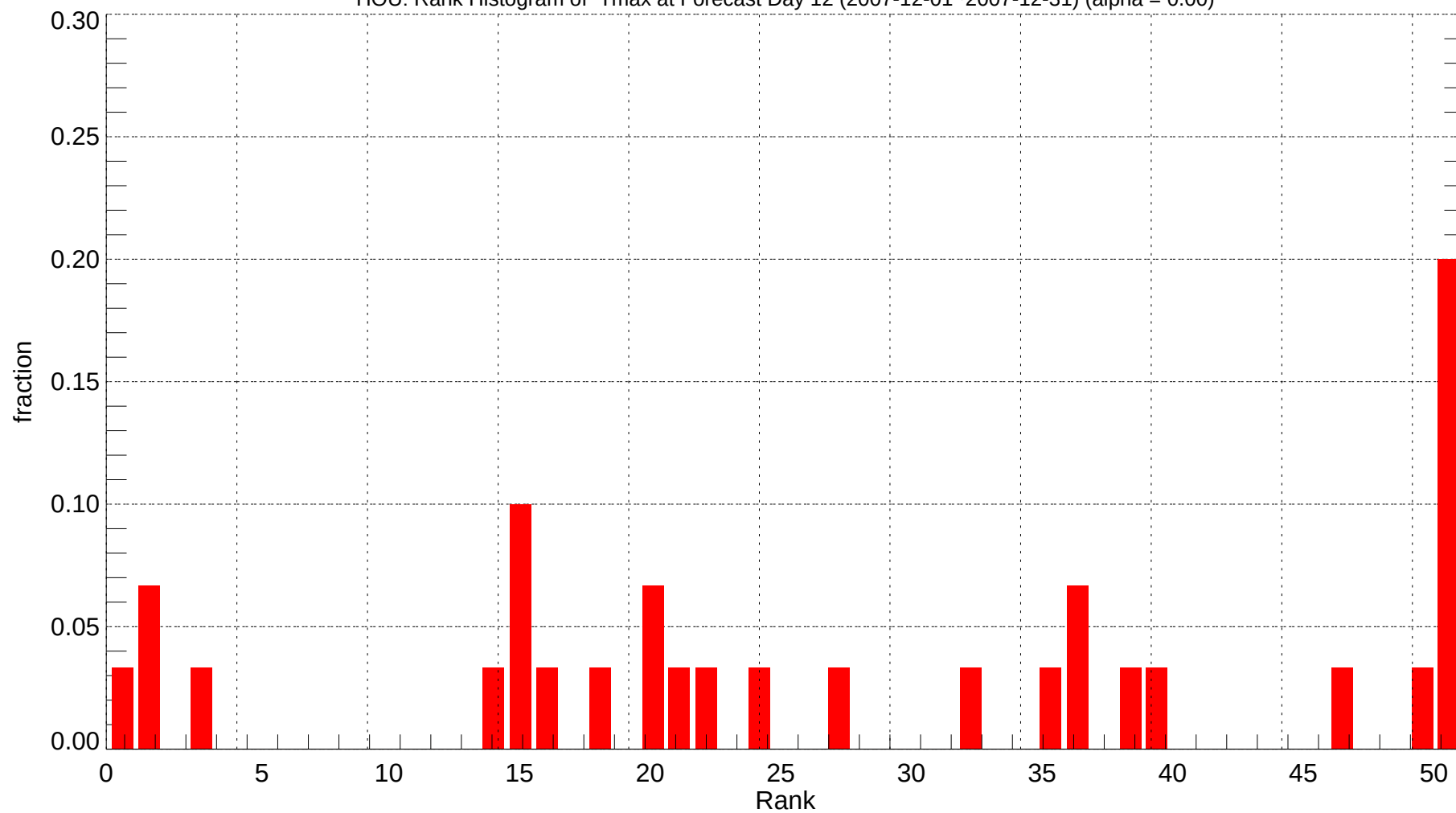
HOU: Rank Histogram of Tmax at Forecast Day 12 (2007-12-01~2007-12-31) (alpha = 0.00)
