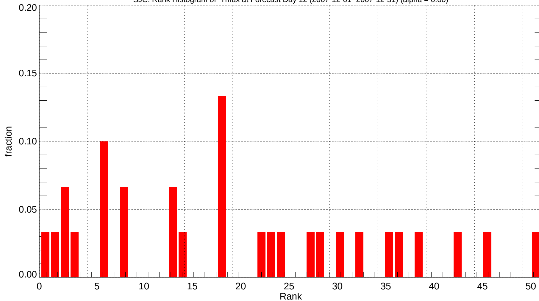
SJC: Rank Histogram of Tmax at Forecast Day 12 (2007-12-01~2007-12-31) (alpha = 0.00)
