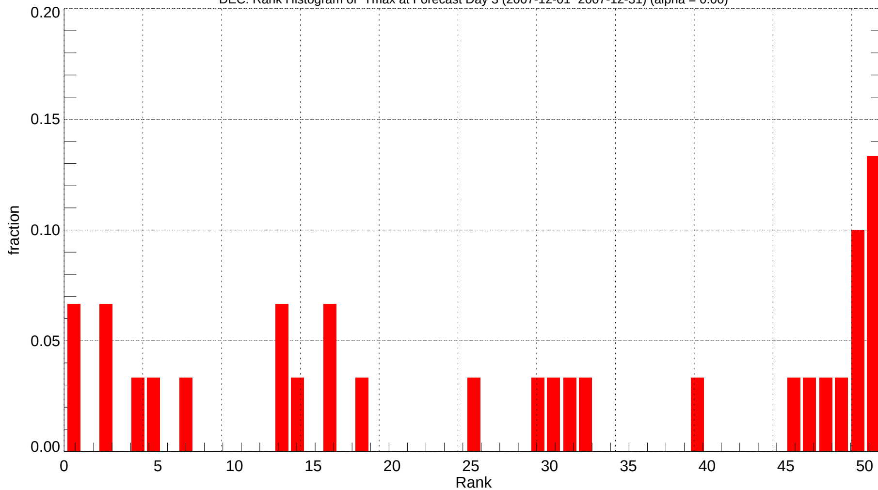
DEC: Rank Histogram of Tmax at Forecast Day 3 (2007-12-01~2007-12-31) (alpha = 0.00)
