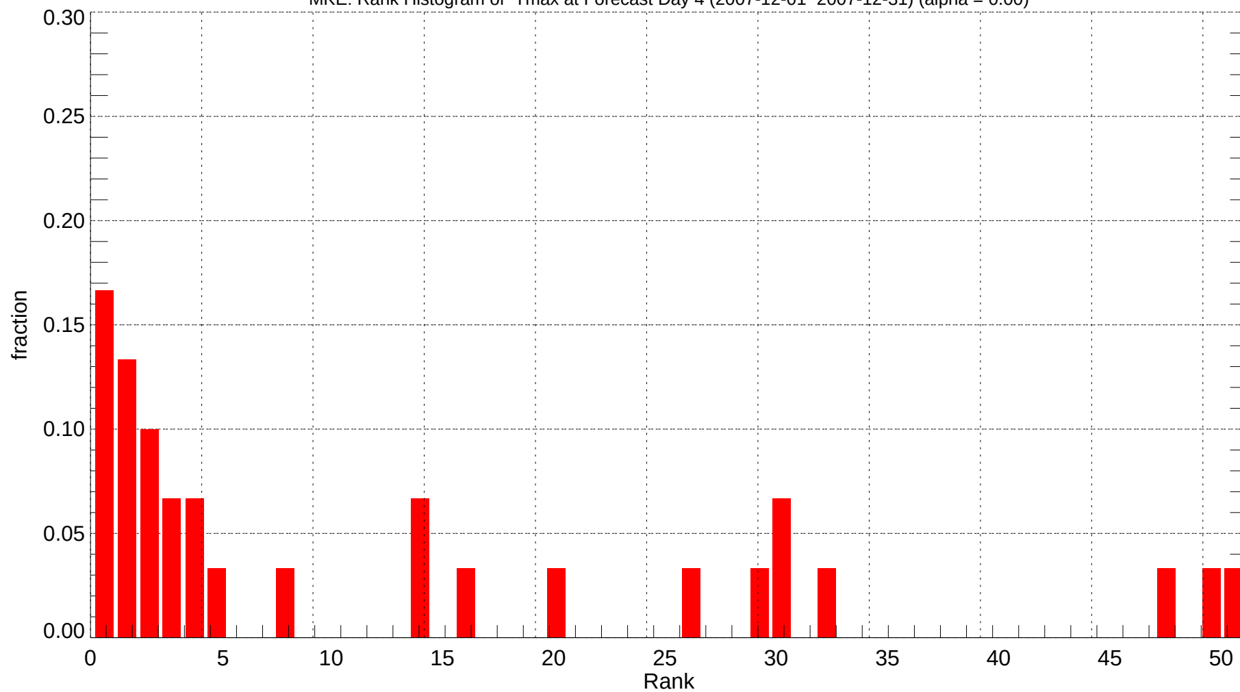
MKE: Rank Histogram of Tmax at Forecast Day 4 (2007-12-01~2007-12-31) (alpha = 0.00)
