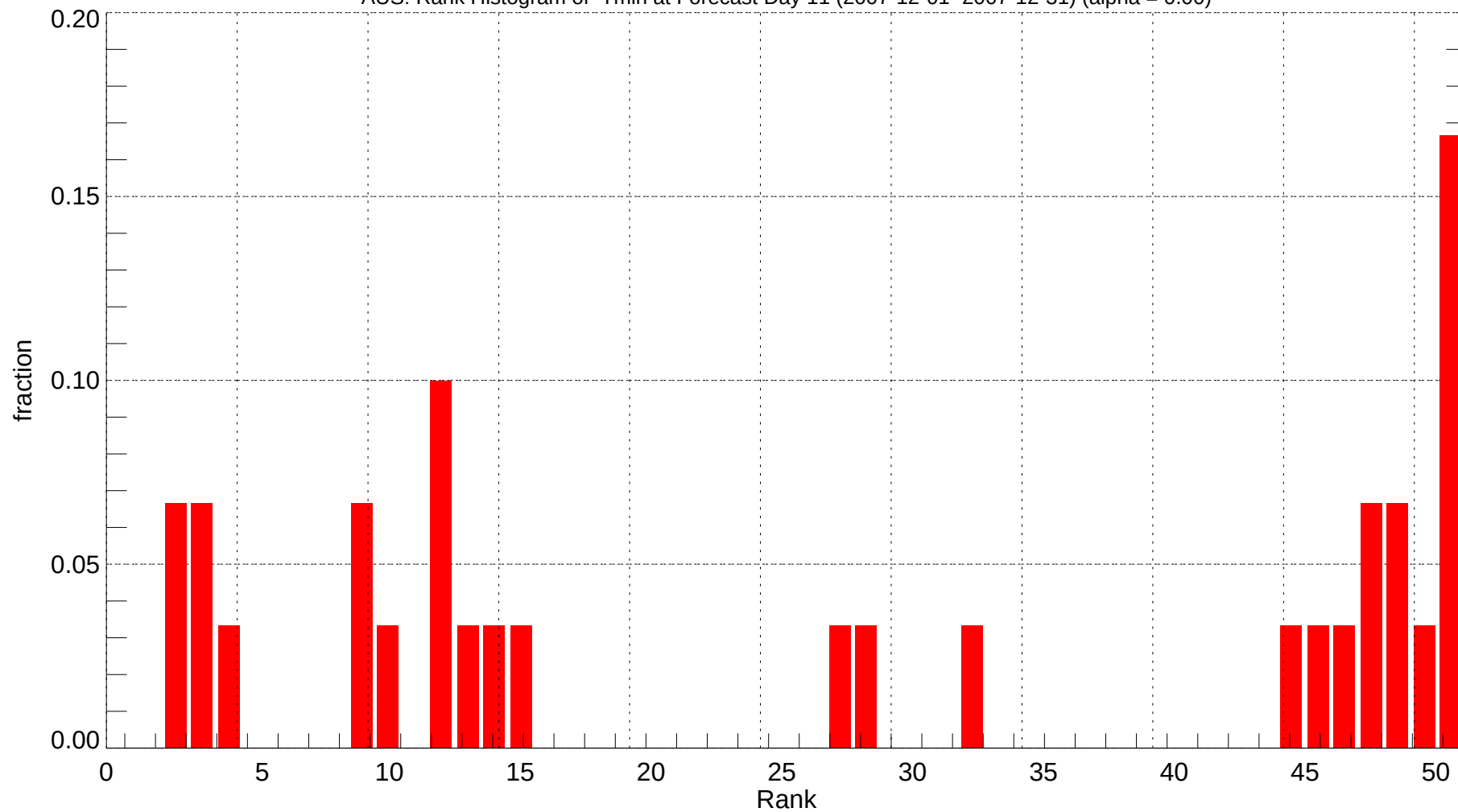
AUS: Rank Histogram of Tmin at Forecast Day 11 (2007-12-01~2007-12-31) (alpha = 0.00)
