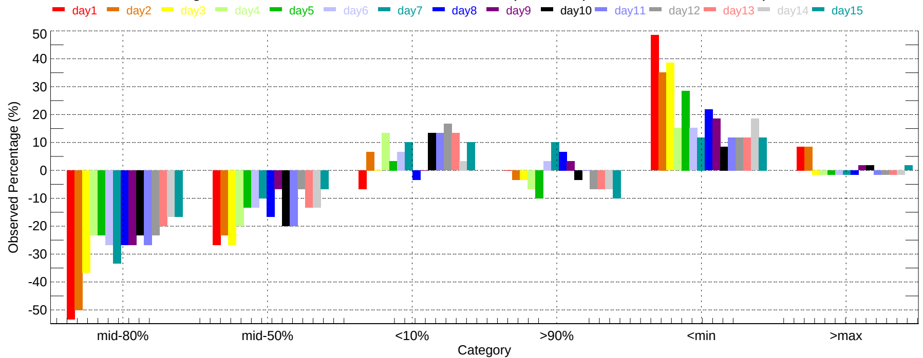
Observed Percentage Deviation of Ensembles - SYR: Max Temperature (2007-12-01~2007-12-31)
