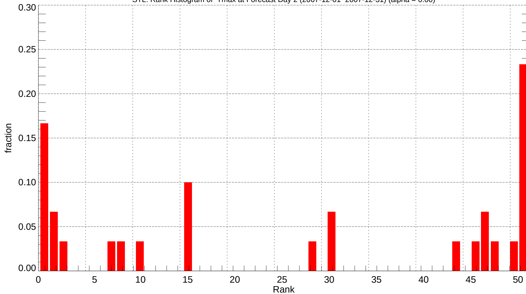
STL: Rank Histogram of Tmax at Forecast Day 2 (2007-12-01~2007-12-31) (alpha = 0.00)
