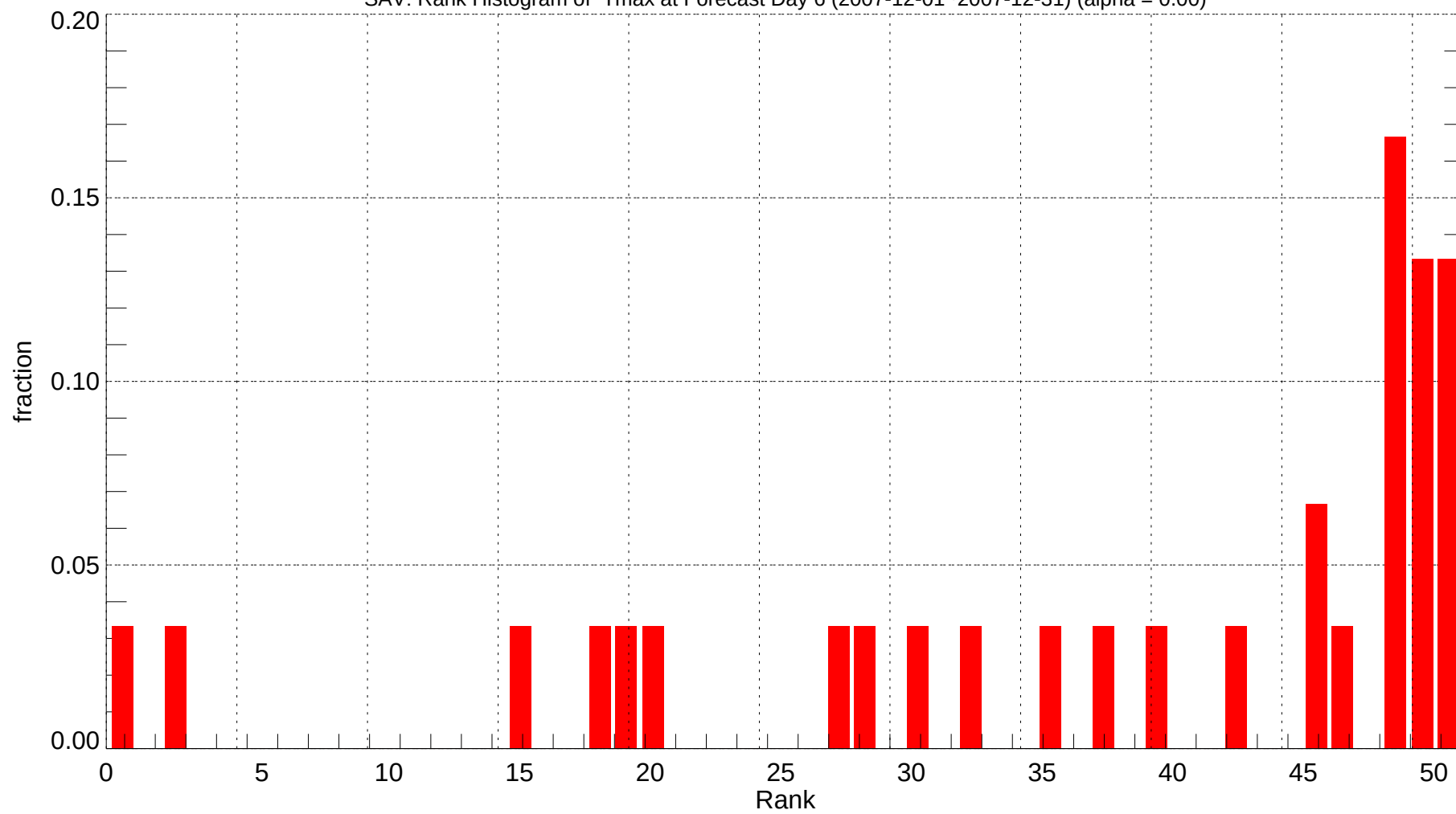
SAV: Rank Histogram of Tmax at Forecast Day 6 (2007-12-01~2007-12-31) (alpha = 0.00)
