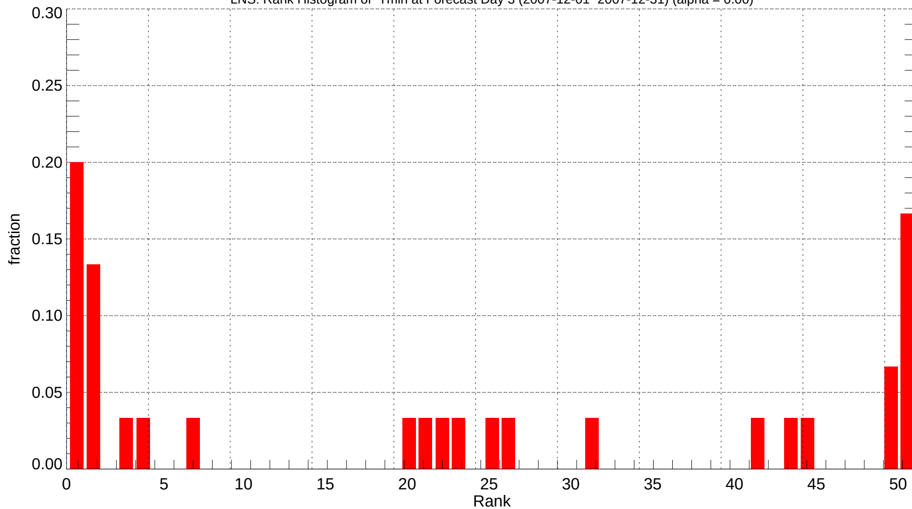
LNS: Rank Histogram of Tmin at Forecast Day 3 (2007-12-01~2007-12-31) (alpha = 0.00)
