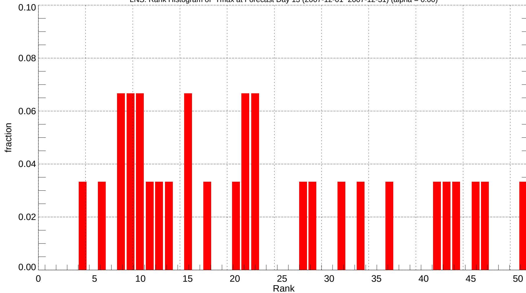
LNS: Rank Histogram of Tmax at Forecast Day 13 (2007-12-01~2007-12-31) (alpha = 0.00)
