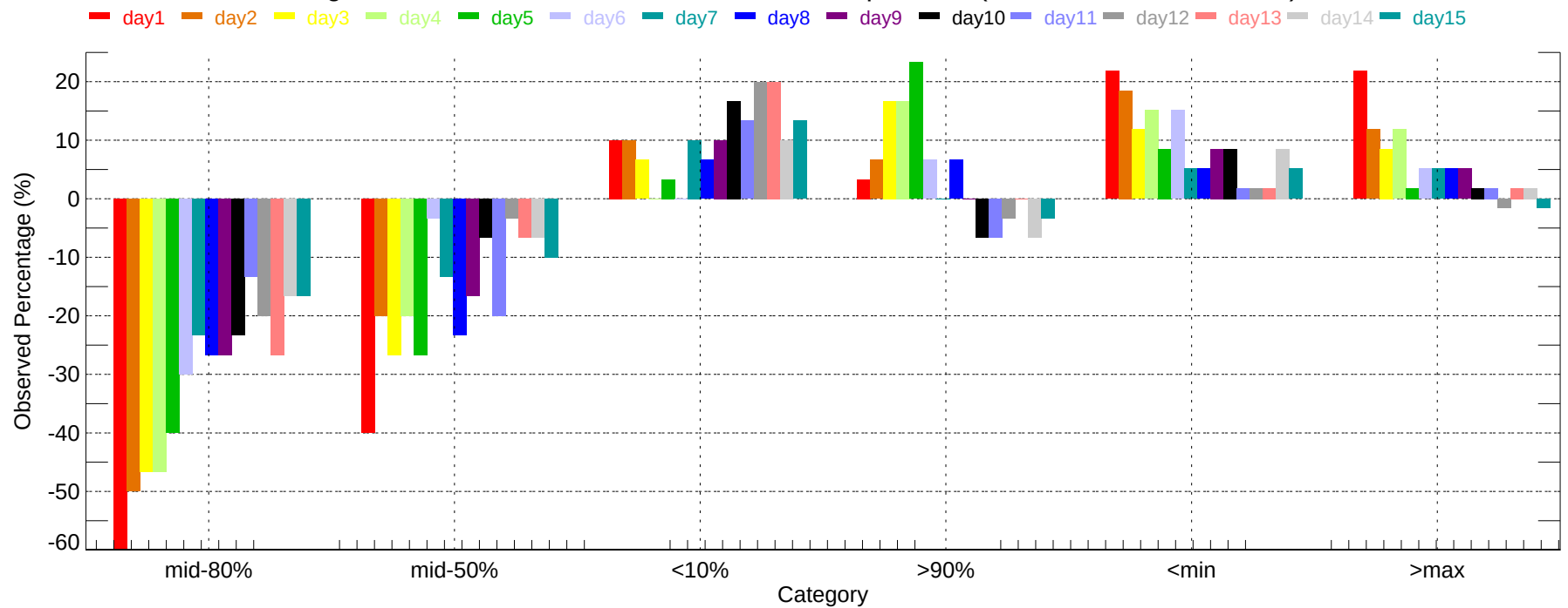
Observed Percentage Deviation of Ensembles - DEN: Min Temperature (2007-12-01~2007-12-31)
