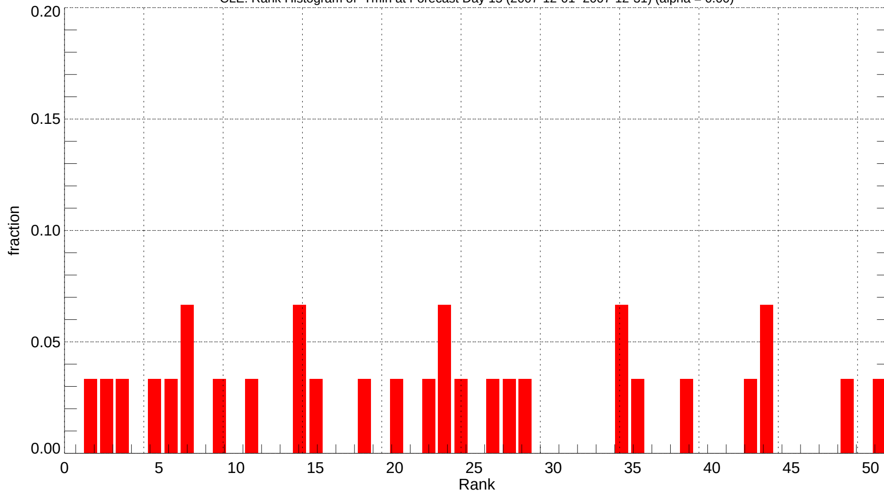
CLE: Rank Histogram of Tmin at Forecast Day 15 (2007-12-01~2007-12-31) (alpha = 0.00)
