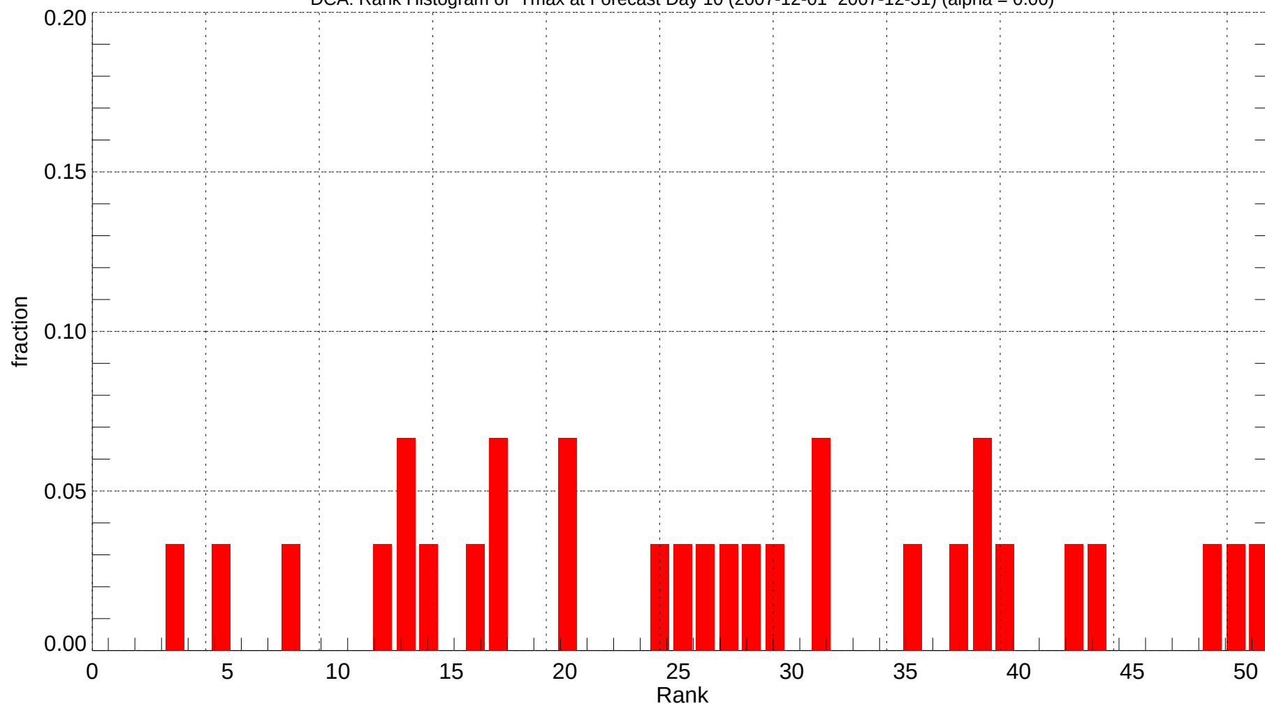
DCA: Rank Histogram of Tmax at Forecast Day 10 (2007-12-01~2007-12-31) (alpha = 0.00)
