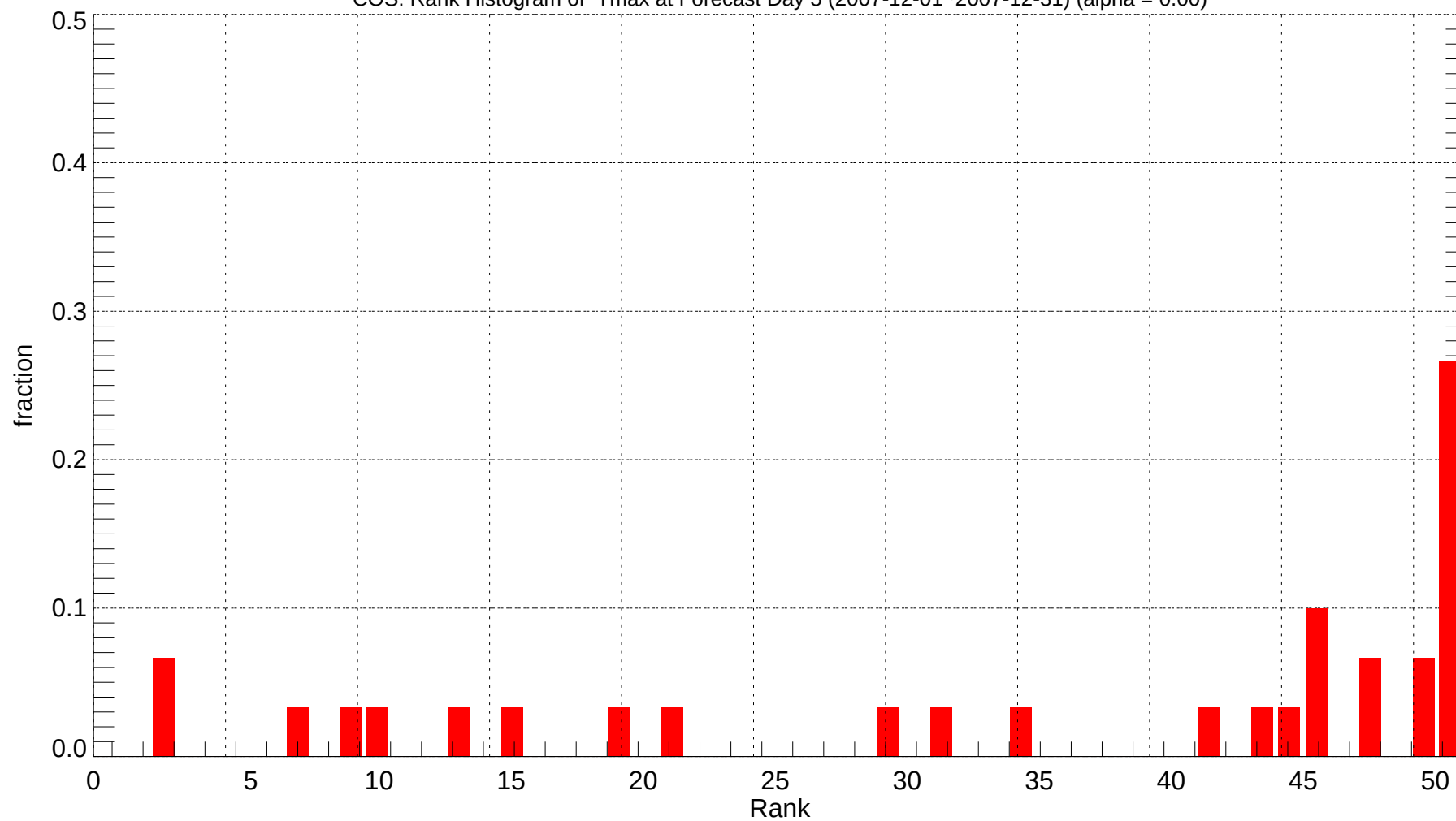
COS: Rank Histogram of Tmax at Forecast Day 5 (2007-12-01~2007-12-31) (alpha = 0.00)
