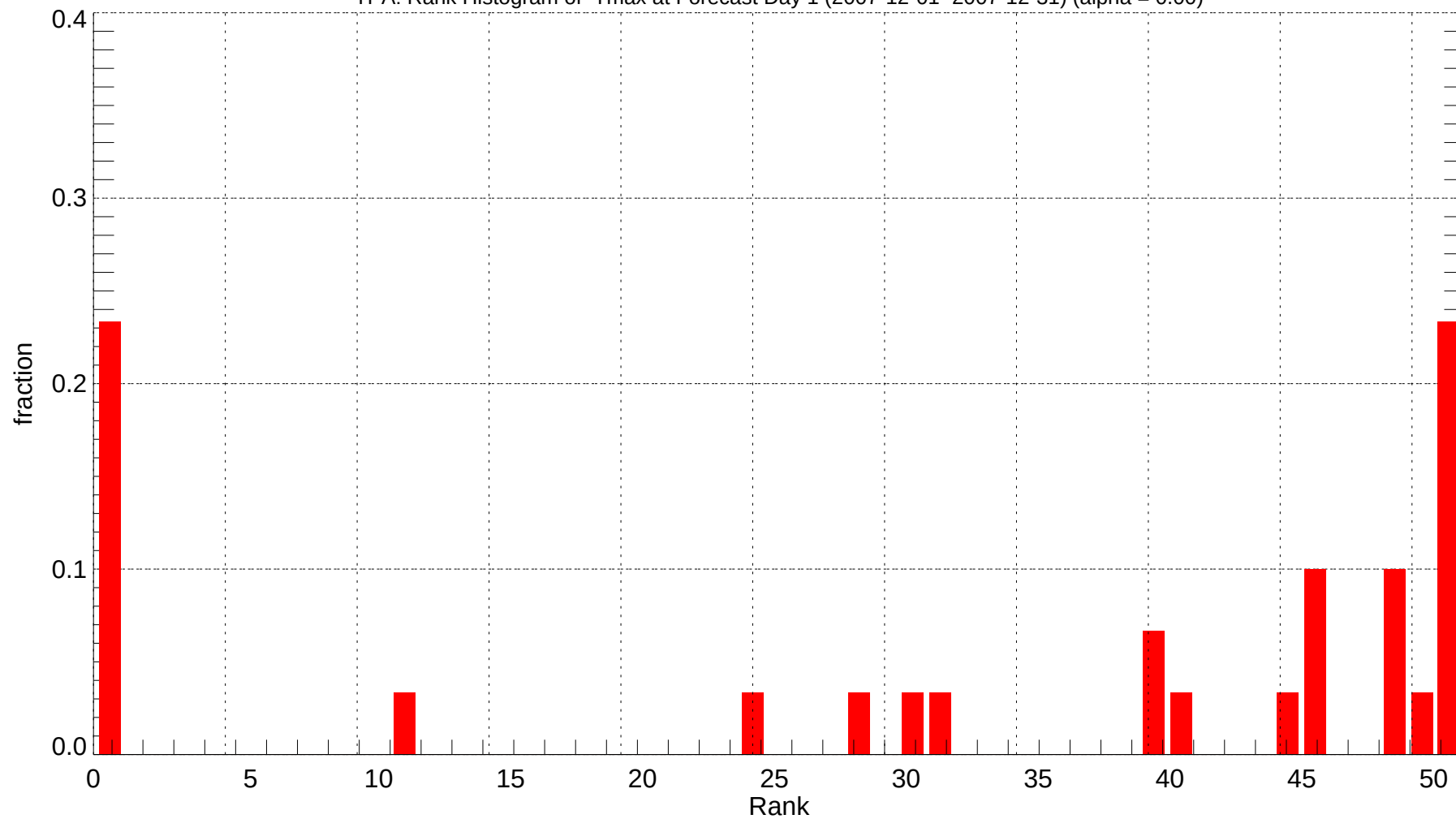
TPA: Rank Histogram of Tmax at Forecast Day 1 (2007-12-01~2007-12-31) (alpha = 0.00)
