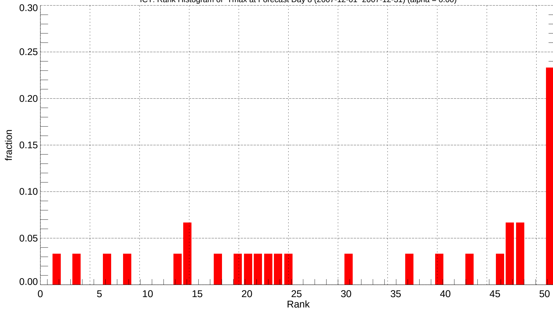
ICT: Rank Histogram of Tmax at Forecast Day 8 (2007-12-01~2007-12-31) (alpha = 0.00)
