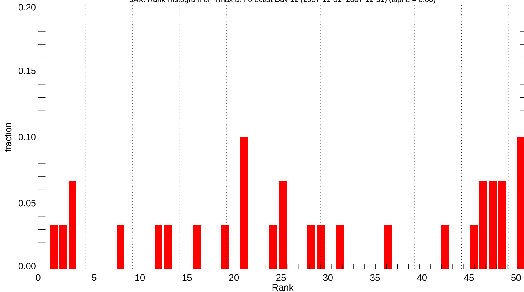
JAX: Rank Histogram of Tmax at Forecast Day 12 (2007-12-01~2007-12-31) (alpha = 0.00)
