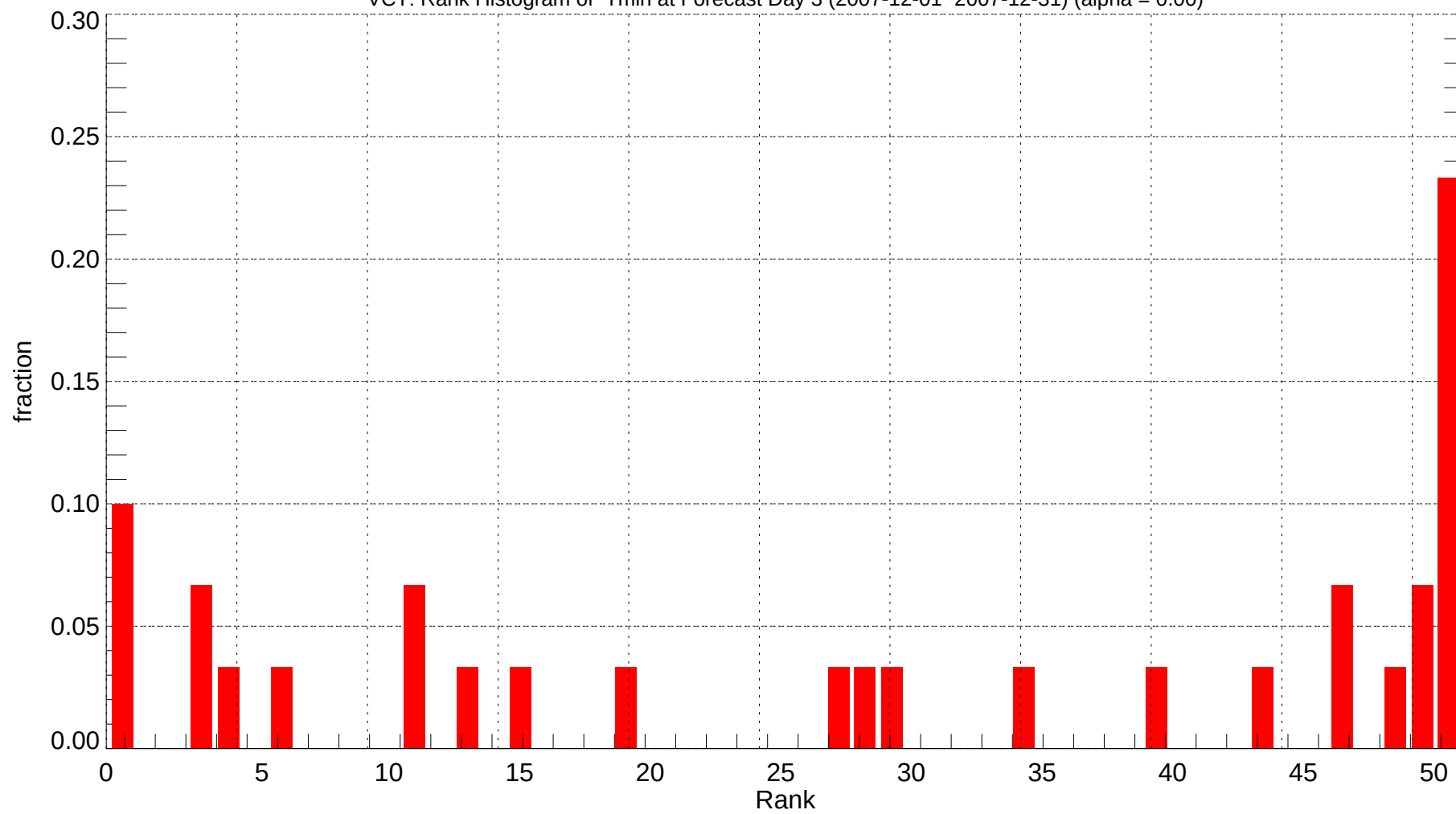
VCT: Rank Histogram of Tmin at Forecast Day 3 (2007-12-01~2007-12-31) (alpha = 0.00)
