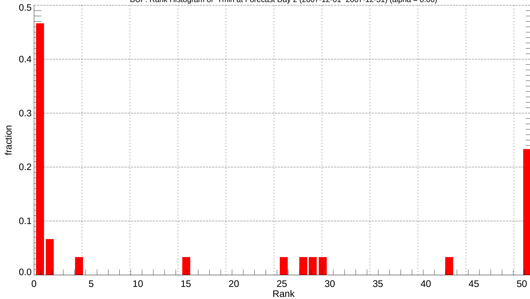
BUF: Rank Histogram of Tmin at Forecast Day 2 (2007-12-01~2007-12-31) (alpha = 0.00)
