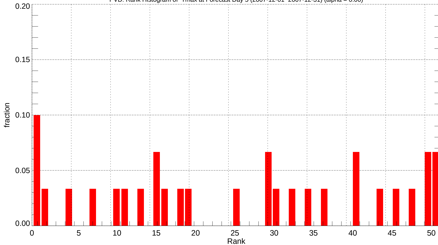
PVD: Rank Histogram of Tmax at Forecast Day 5 (2007-12-01~2007-12-31) (alpha = 0.00)
