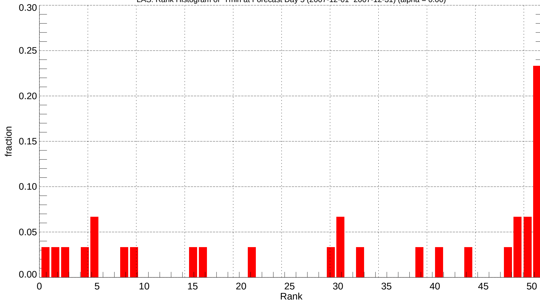
LAS: Rank Histogram of Tmin at Forecast Day 5 (2007-12-01~2007-12-31) (alpha = 0.00)
