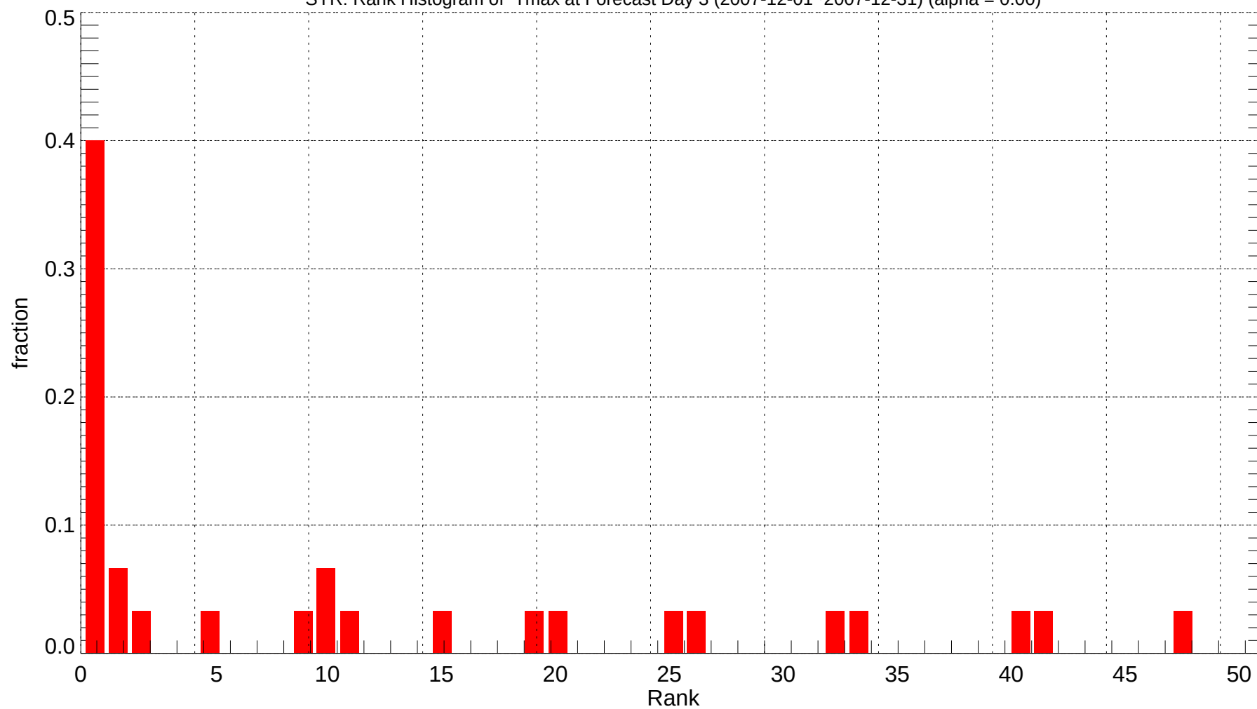
SYR: Rank Histogram of Tmax at Forecast Day 3 (2007-12-01~2007-12-31) (alpha = 0.00)
