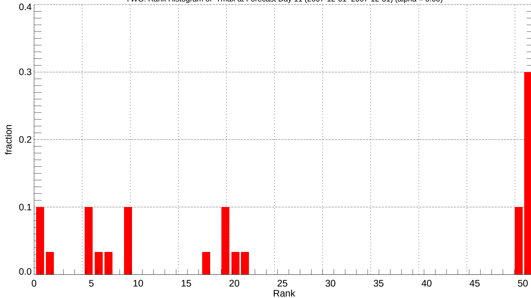
YWG: Rank Histogram of Tmax at Forecast Day 11 (2007-12-01~2007-12-31) (alpha = 0.00)
