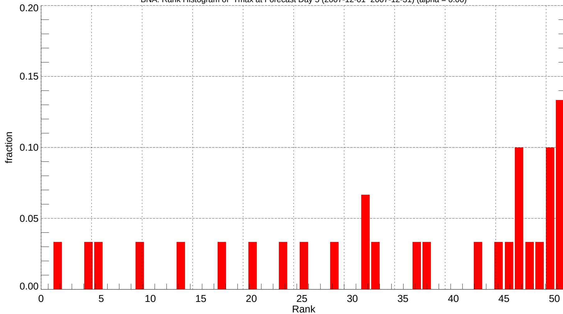
BNA: Rank Histogram of Tmax at Forecast Day 5 (2007-12-01~2007-12-31) (alpha = 0.00)
