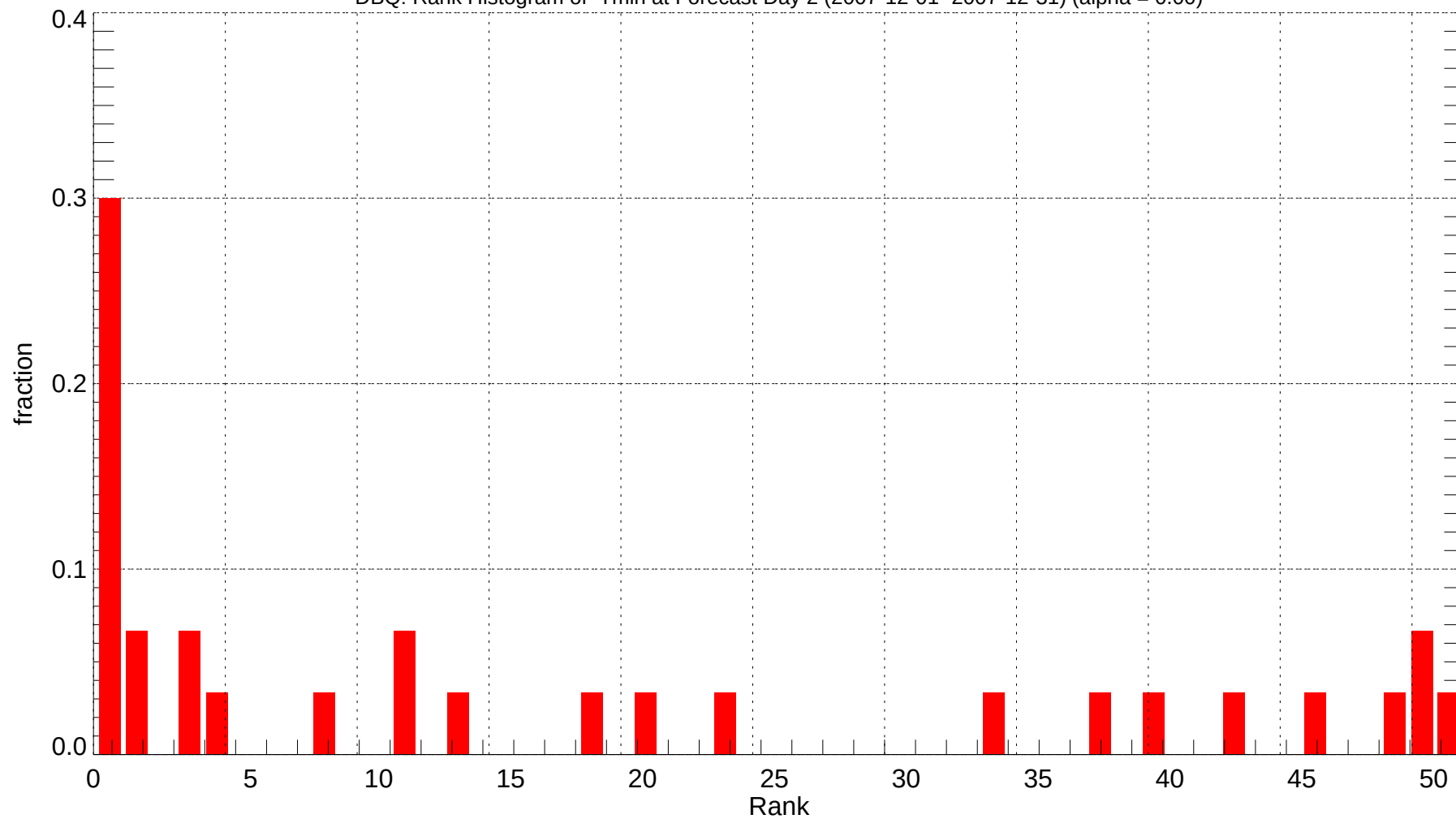
DBQ: Rank Histogram of Tmin at Forecast Day 2 (2007-12-01~2007-12-31) (alpha = 0.00)
