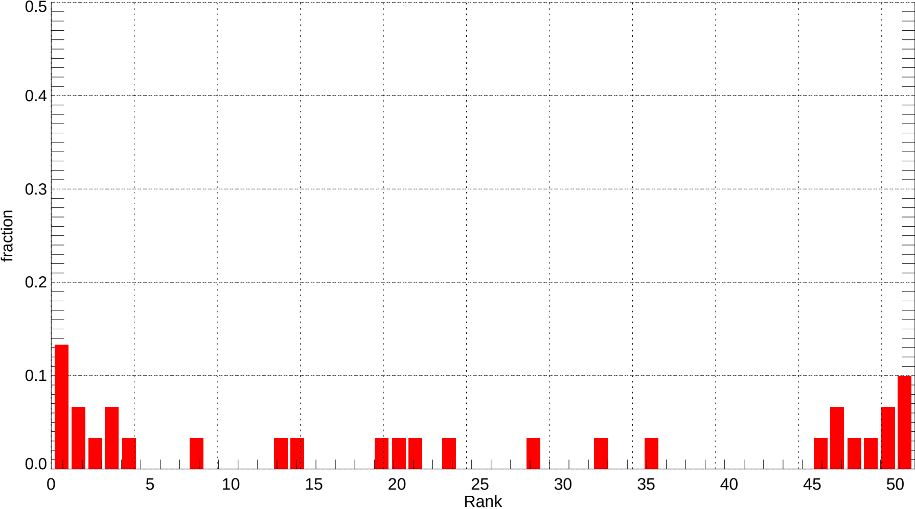
ELP: Rank Histogram of Tmin at Forecast Day 1 (2007-12-01~2007-12-31) (alpha = 0.00)
