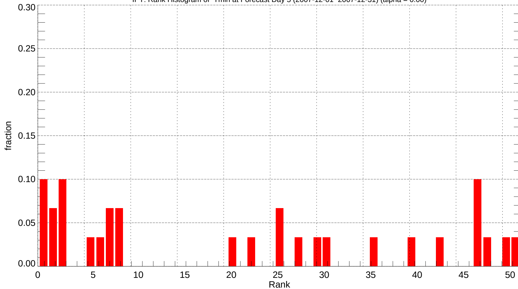
IPT: Rank Histogram of Tmin at Forecast Day 5 (2007-12-01~2007-12-31) (alpha = 0.00)
