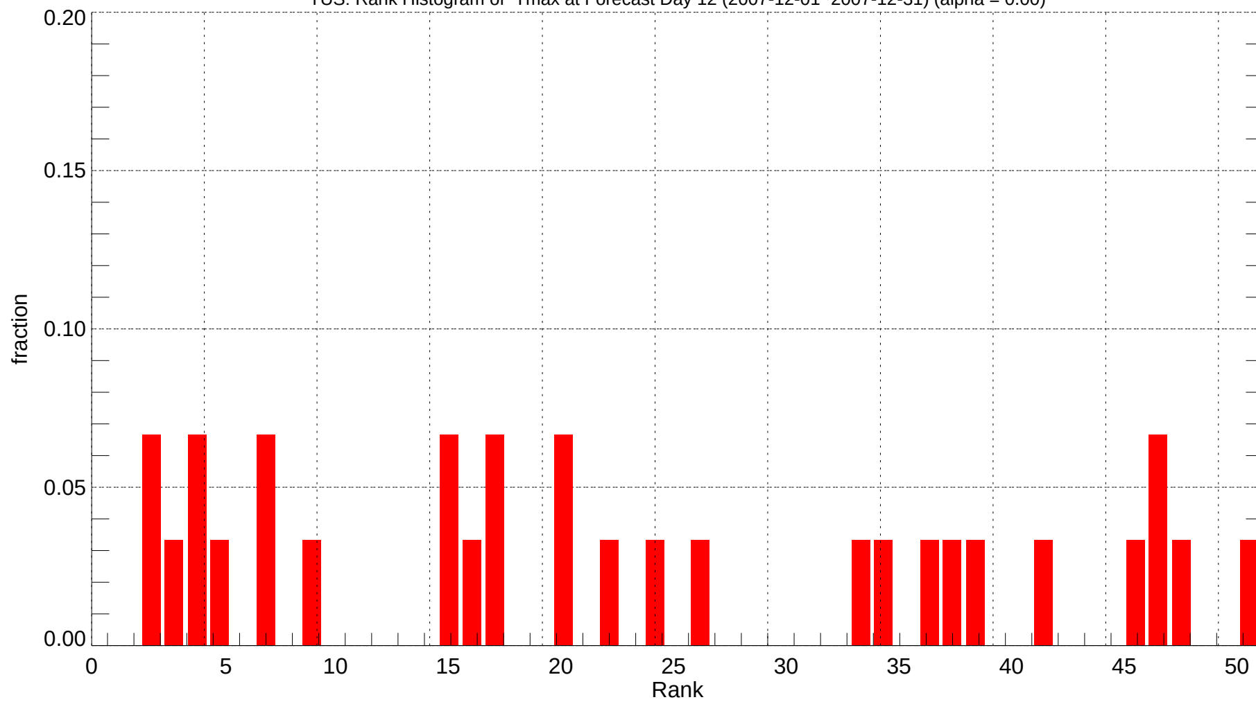
TUS: Rank Histogram of Tmax at Forecast Day 12 (2007-12-01~2007-12-31) (alpha = 0.00)
