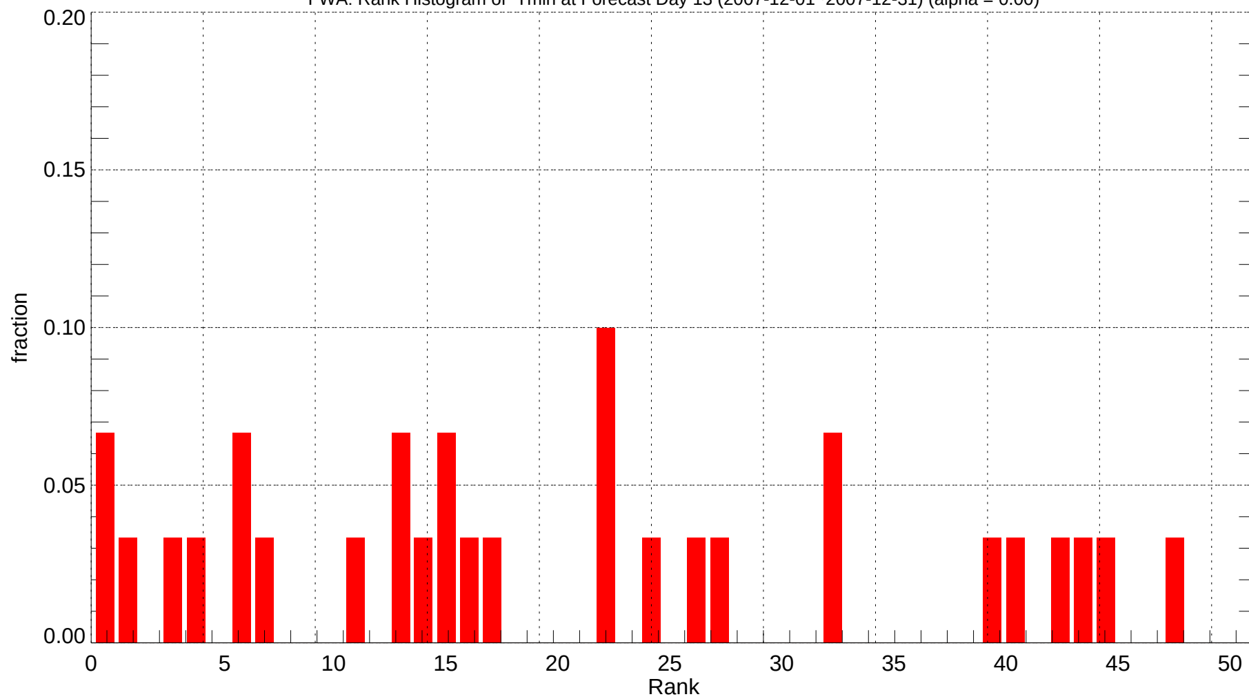
FWA: Rank Histogram of Tmin at Forecast Day 13 (2007-12-01~2007-12-31) (alpha = 0.00)
