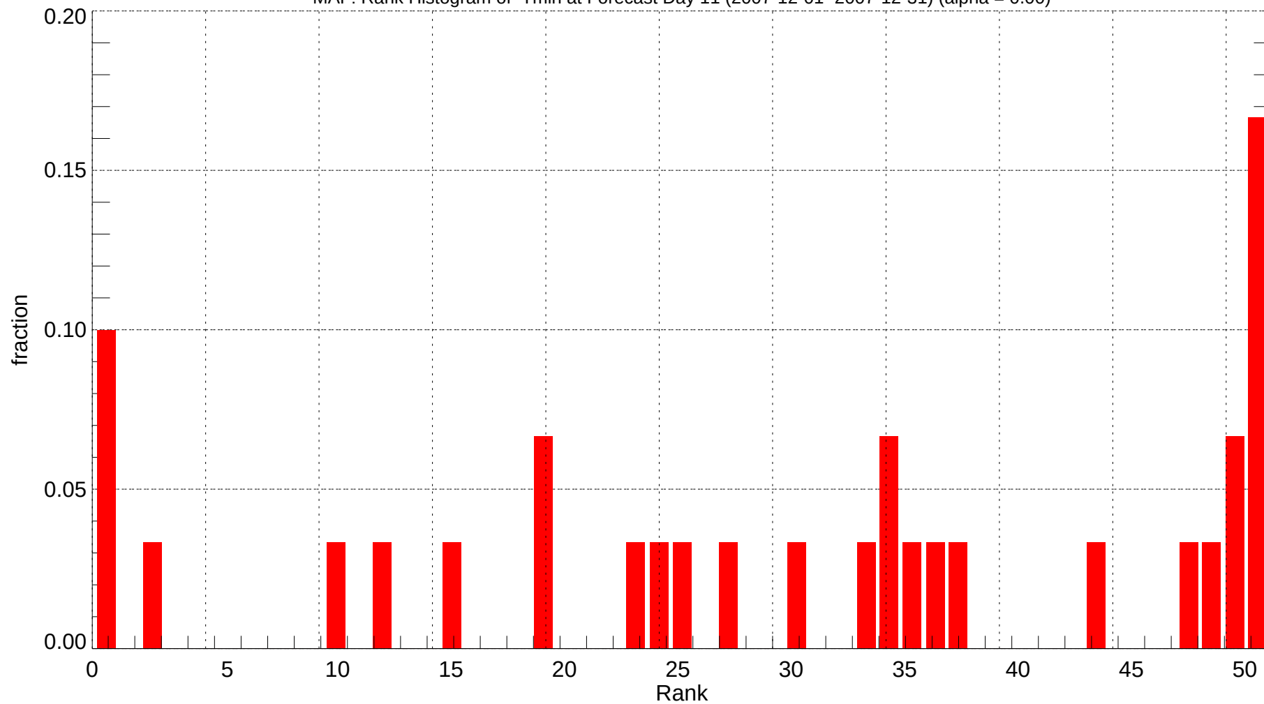
MAF: Rank Histogram of Tmin at Forecast Day 11 (2007-12-01~2007-12-31) (alpha = 0.00)
