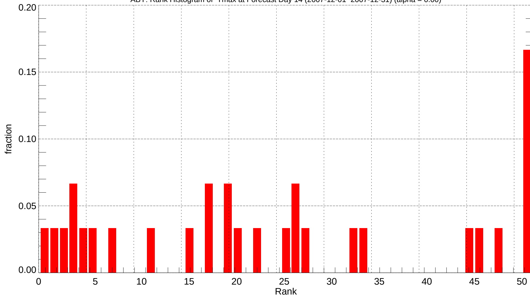
ABY: Rank Histogram of Tmax at Forecast Day 14 (2007-12-01~2007-12-31) (alpha = 0.00)
