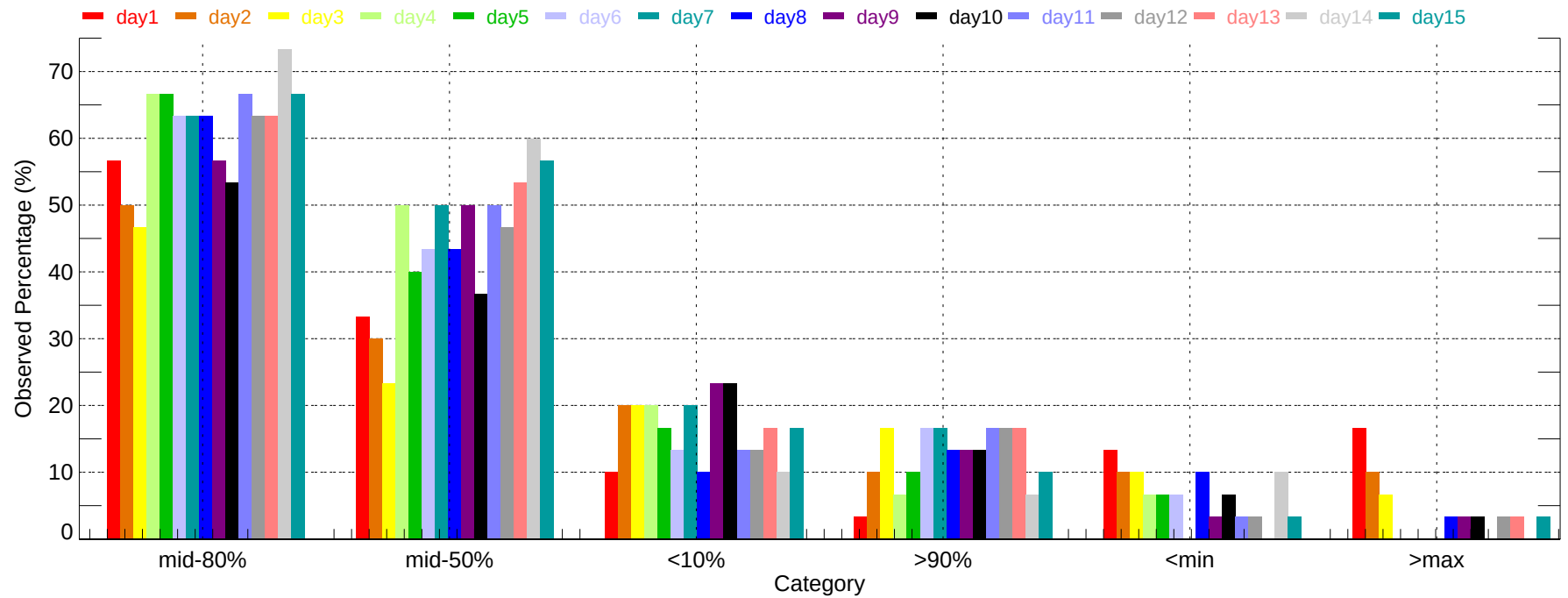
Observed Percentage of Ensembles - BGM: Max Temperature (2007-12-01~2007-12-31)
