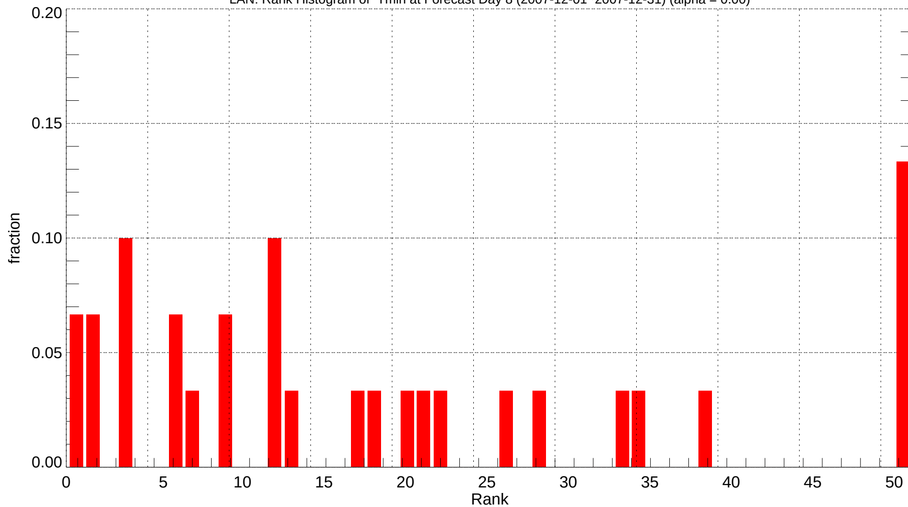
LAN: Rank Histogram of Tmin at Forecast Day 8 (2007-12-01~2007-12-31) (alpha = 0.00)
