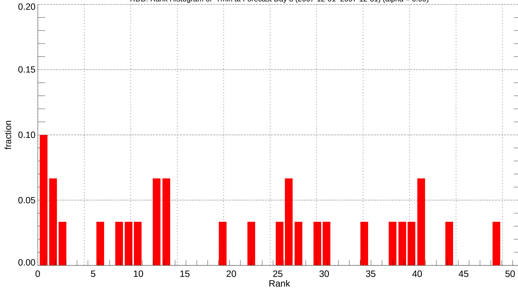
RDD: Rank Histogram of Tmin at Forecast Day 8 (2007-12-01~2007-12-31) (alpha = 0.00)
