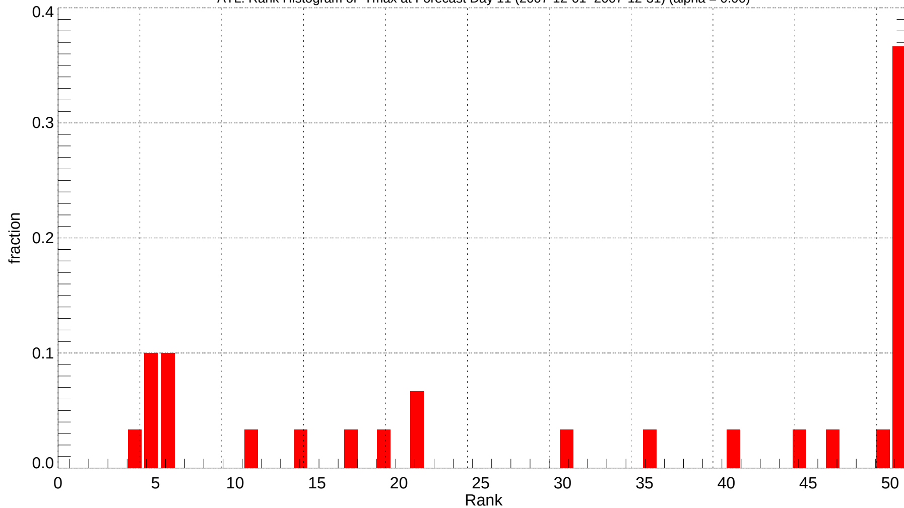
ATL: Rank Histogram of Tmax at Forecast Day 11 (2007-12-01~2007-12-31) (alpha = 0.00)
