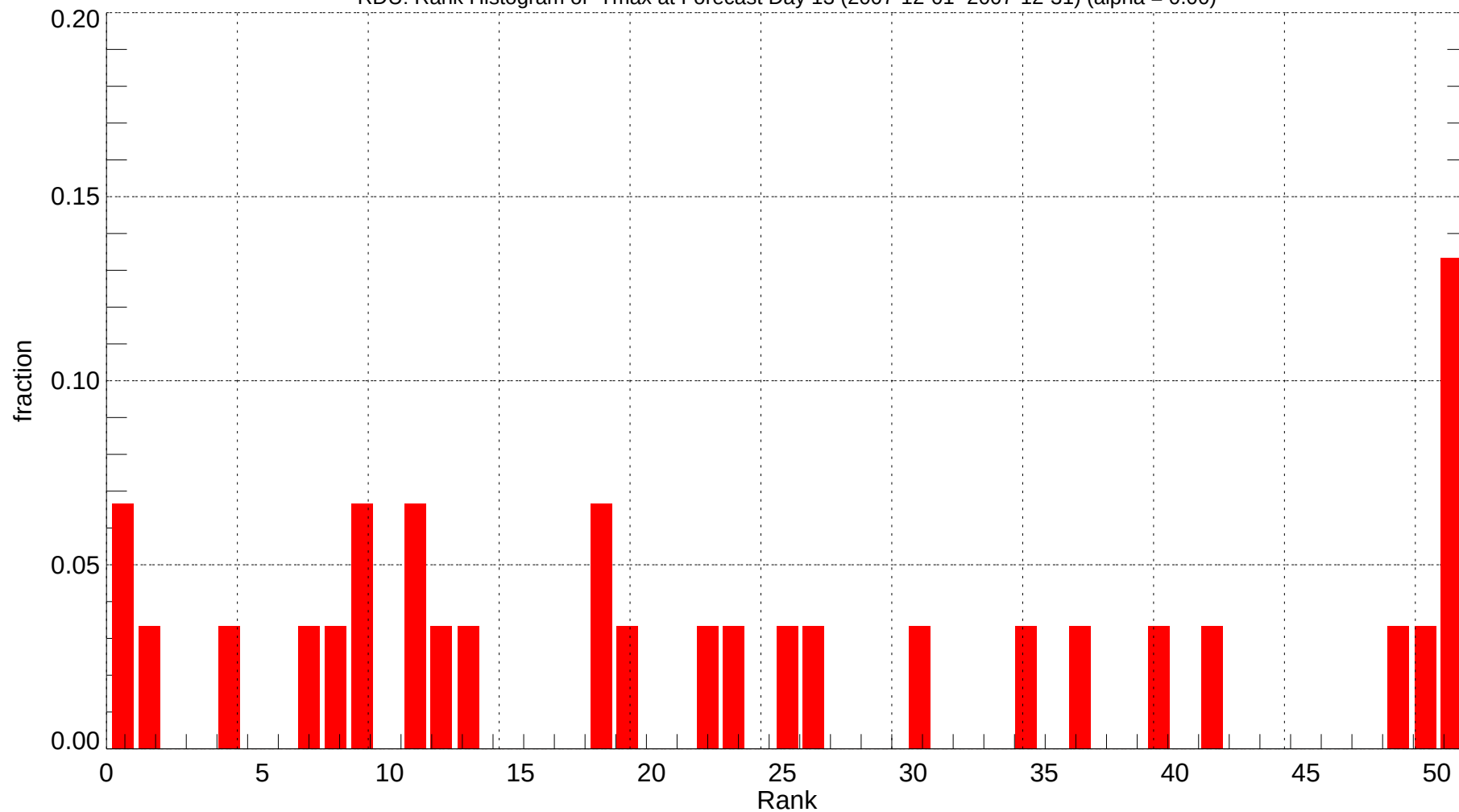
RDU: Rank Histogram of Tmax at Forecast Day 13 (2007-12-01~2007-12-31) (alpha = 0.00)
