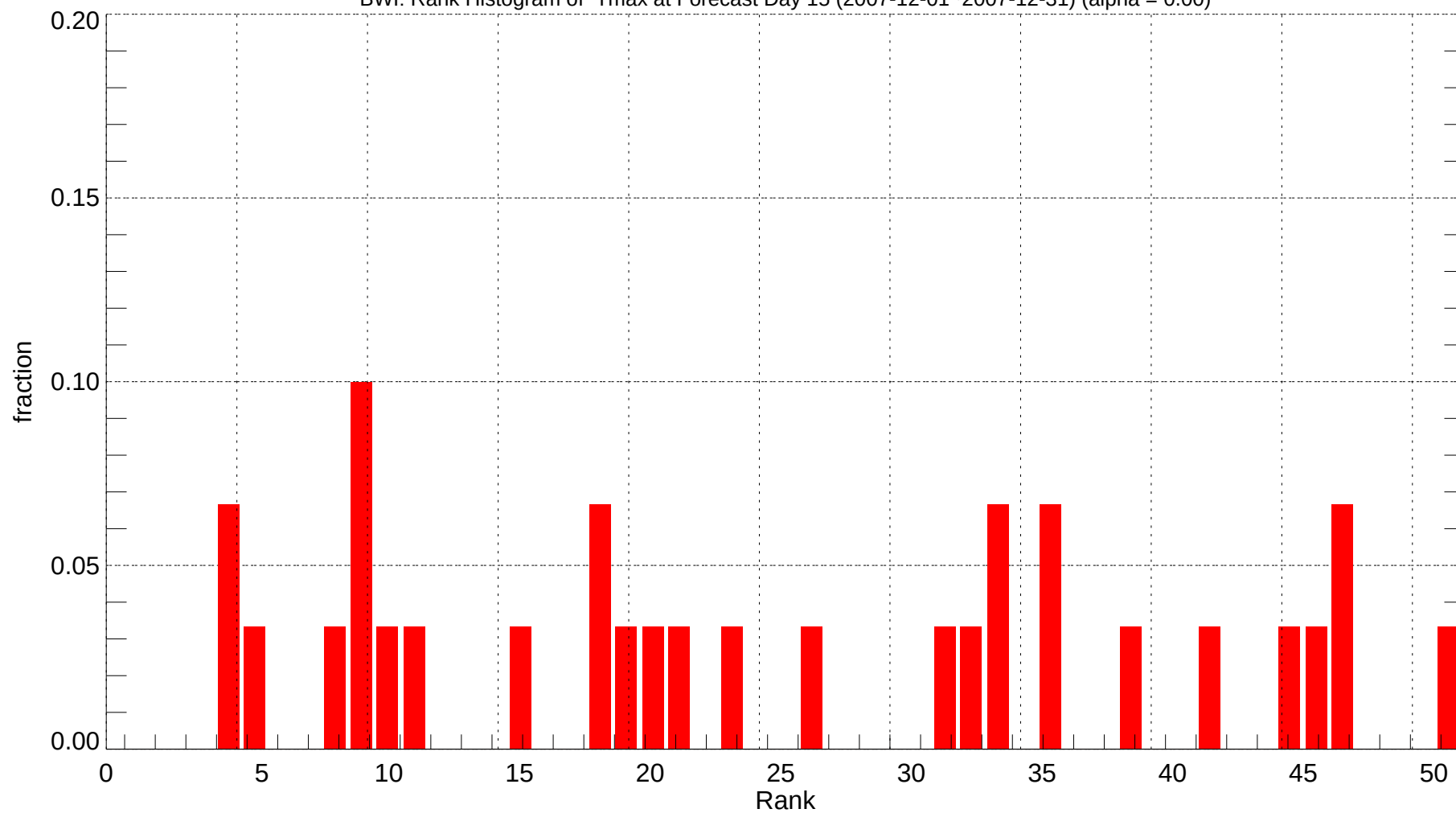
BWI: Rank Histogram of Tmax at Forecast Day 15 (2007-12-01~2007-12-31) (alpha = 0.00)
