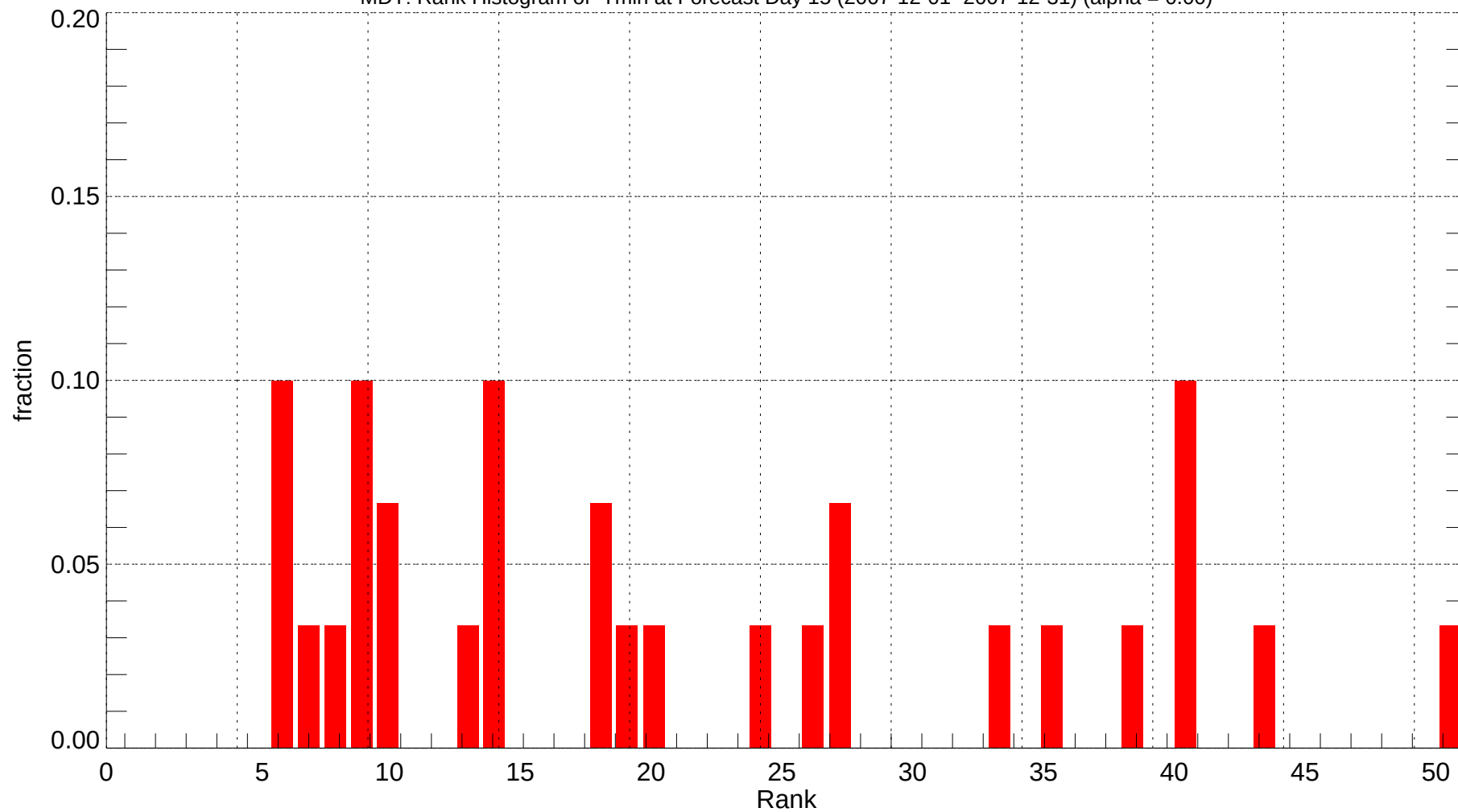
MDT: Rank Histogram of Tmin at Forecast Day 15 (2007-12-01~2007-12-31) (alpha = 0.00)
