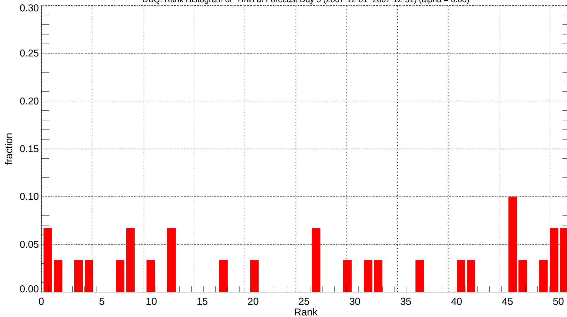
DBQ: Rank Histogram of Tmin at Forecast Day 5 (2007-12-01~2007-12-31) (alpha = 0.00)
