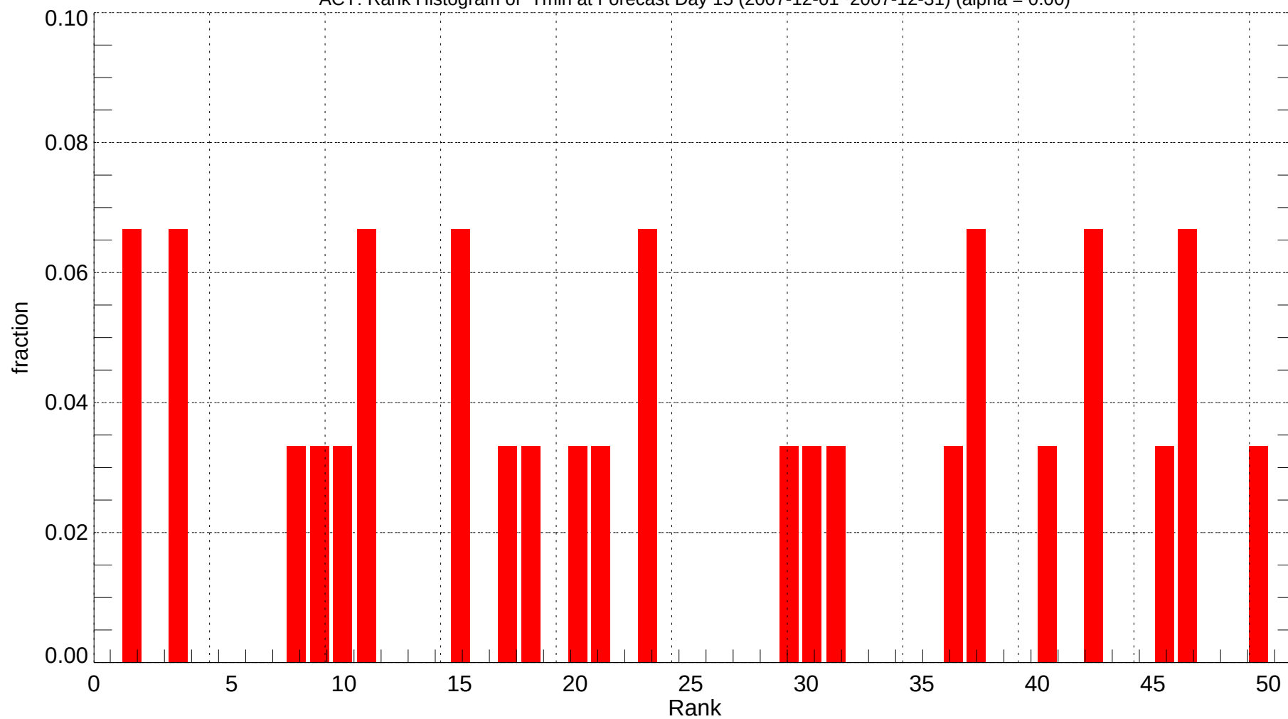
ACY: Rank Histogram of Tmin at Forecast Day 15 (2007-12-01~2007-12-31) (alpha = 0.00)
