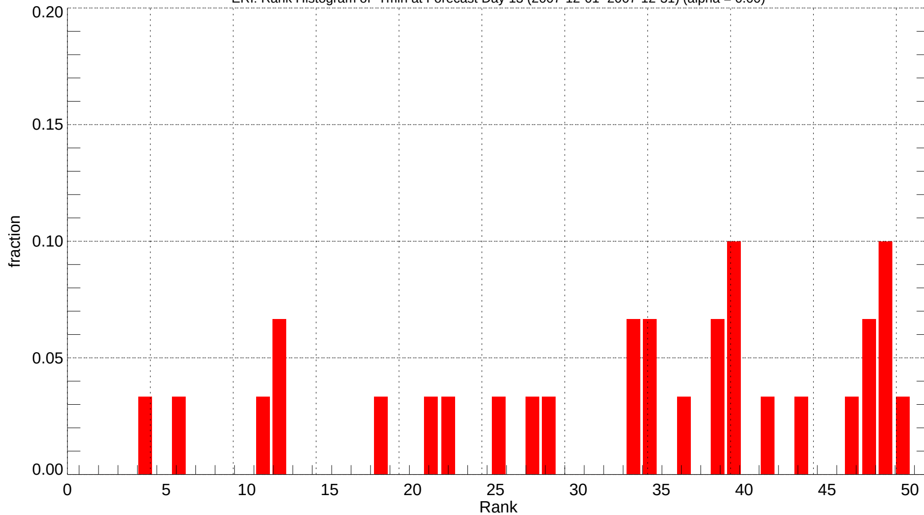
ERI: Rank Histogram of Tmin at Forecast Day 13 (2007-12-01~2007-12-31) (alpha = 0.00)
