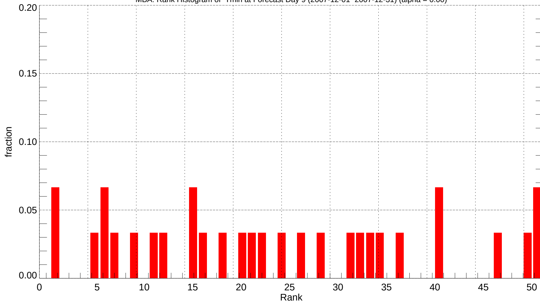
MBA: Rank Histogram of Tmin at Forecast Day 9 (2007-12-01~2007-12-31) (alpha = 0.00)
