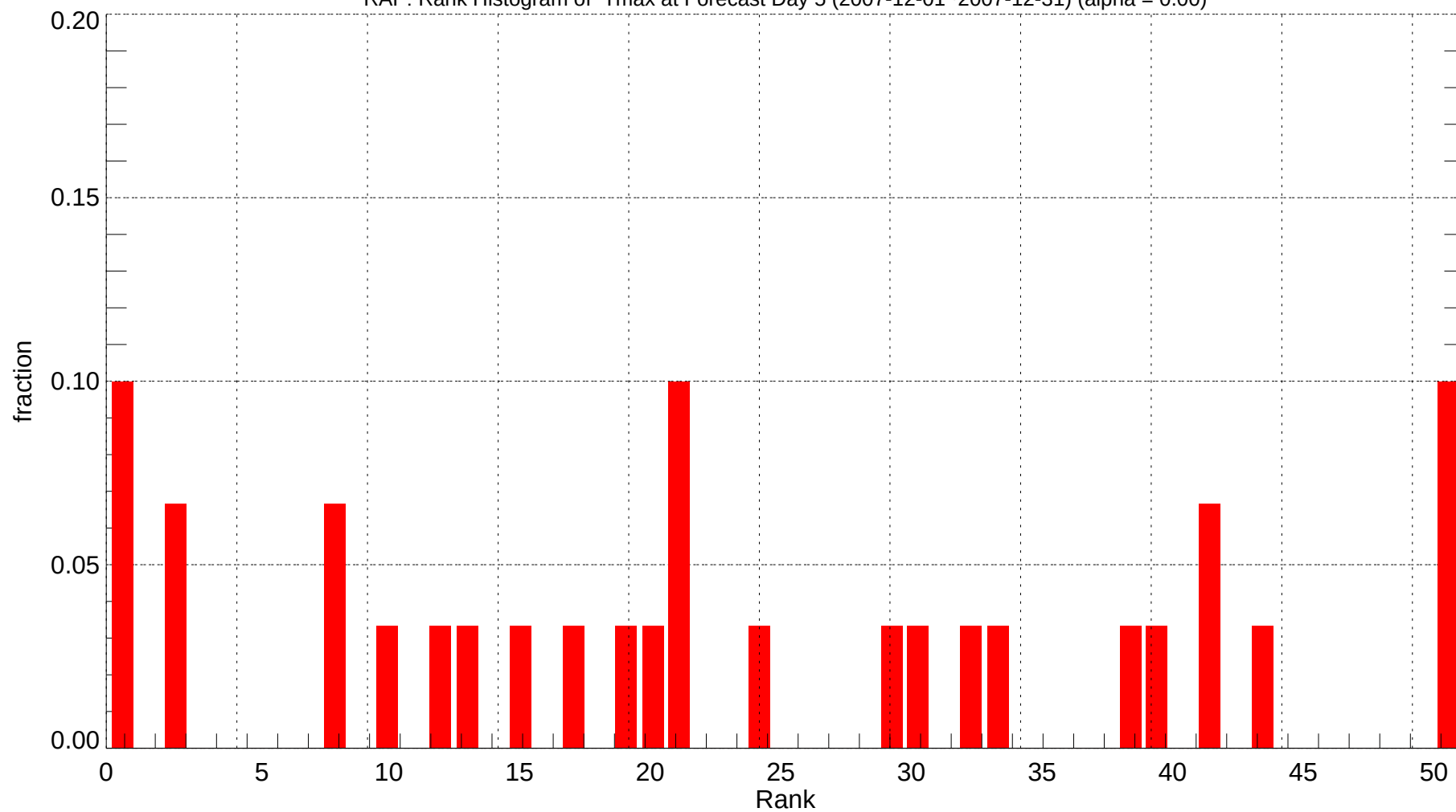
RAP: Rank Histogram of Tmax at Forecast Day 5 (2007-12-01~2007-12-31) (alpha = 0.00)
