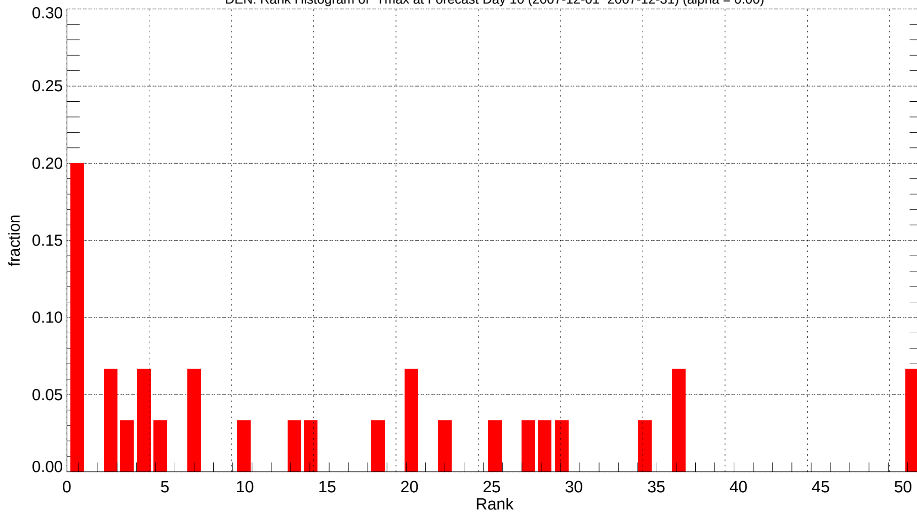
DEN: Rank Histogram of Tmax at Forecast Day 10 (2007-12-01~2007-12-31) (alpha = 0.00)
