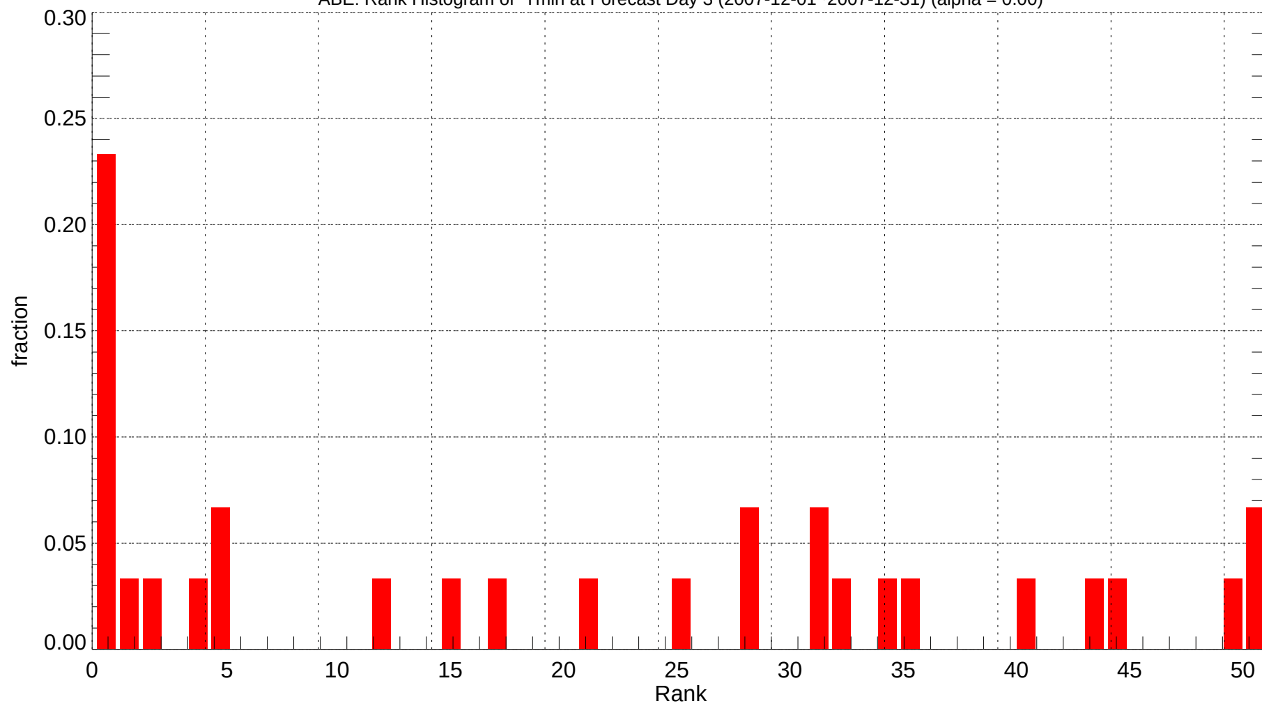
ABE: Rank Histogram of Tmin at Forecast Day 3 (2007-12-01~2007-12-31) (alpha = 0.00)
