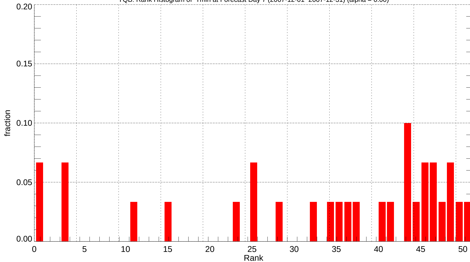
YQB: Rank Histogram of Tmin at Forecast Day 7 (2007-12-01~2007-12-31) (alpha = 0.00)
