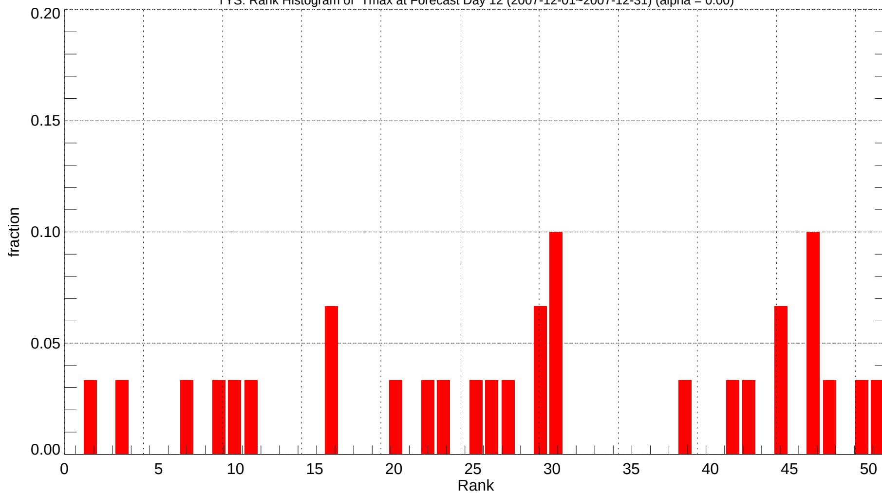
TYS: Rank Histogram of Tmax at Forecast Day 12 (2007-12-01~2007-12-31) (alpha = 0.00)
