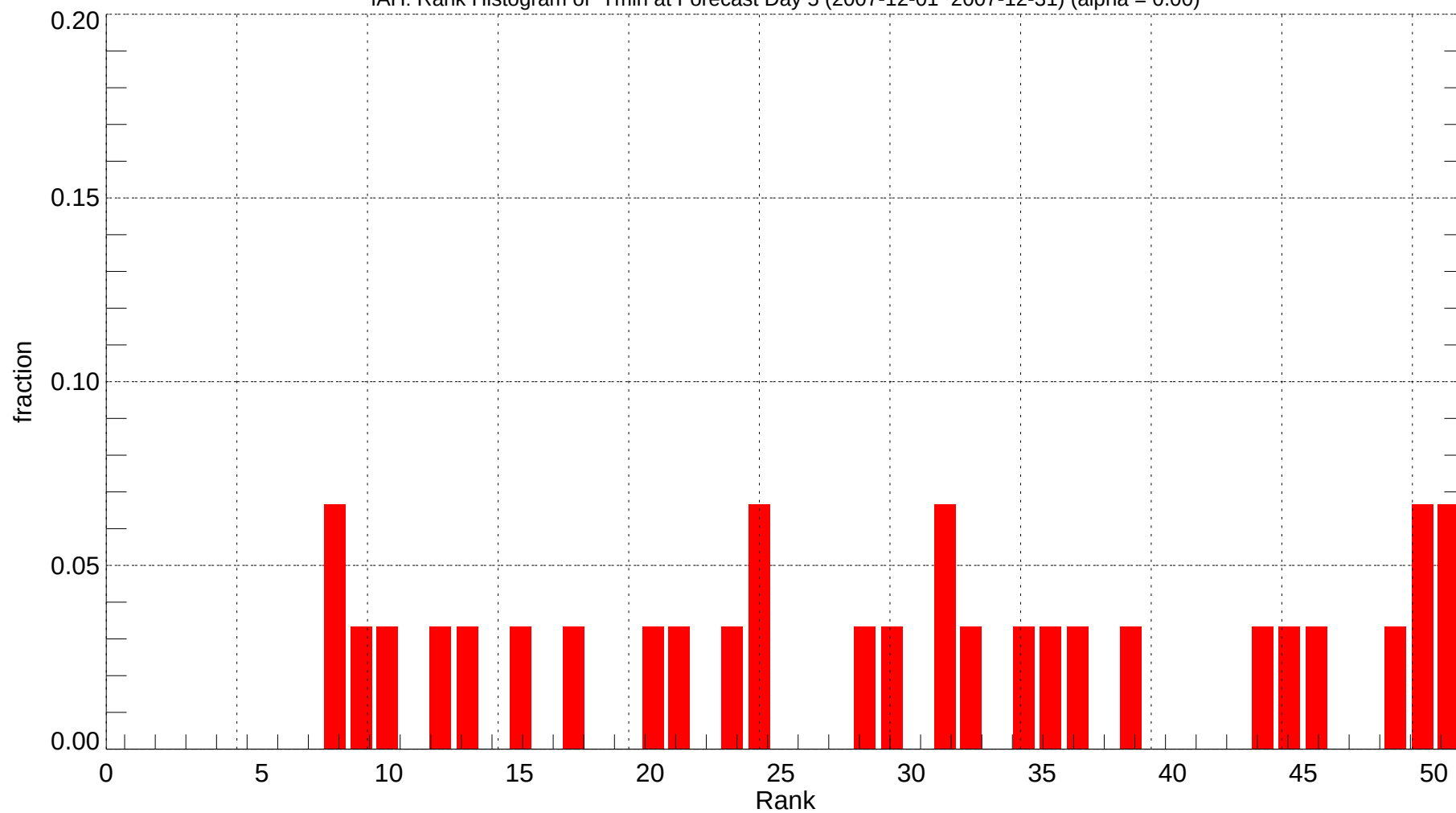
IAH: Rank Histogram of Tmin at Forecast Day 5 (2007-12-01~2007-12-31) (alpha = 0.00)
