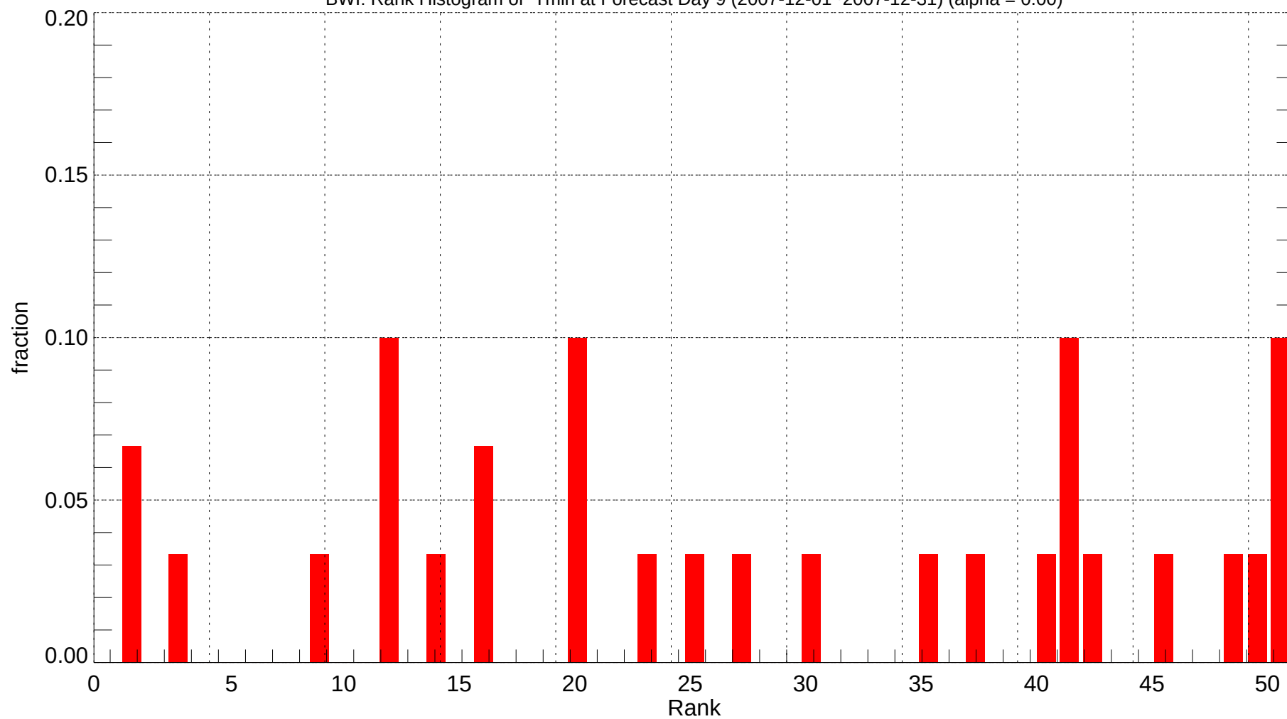
BWI: Rank Histogram of Tmin at Forecast Day 9 (2007-12-01~2007-12-31) (alpha = 0.00)
