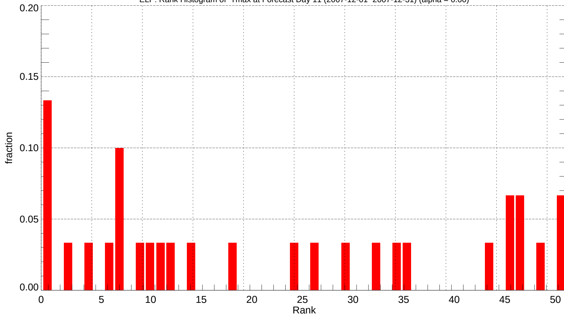
ELP: Rank Histogram of Tmax at Forecast Day 11 (2007-12-01~2007-12-31) (alpha = 0.00)
