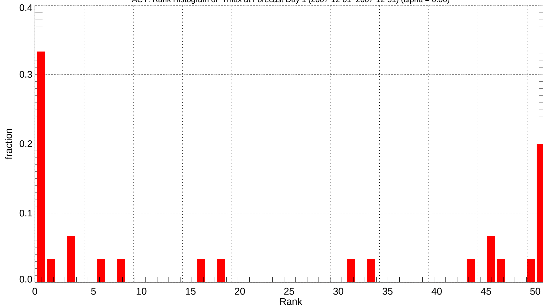
ACY: Rank Histogram of Tmax at Forecast Day 1 (2007-12-01~2007-12-31) (alpha = 0.00)
