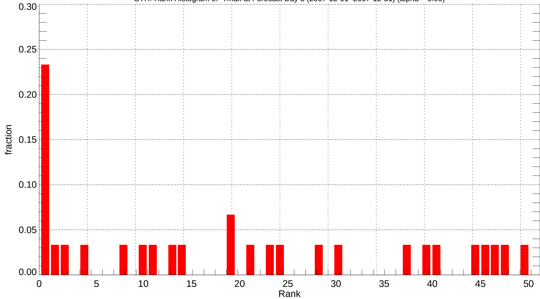
SYR: Rank Histogram of Tmax at Forecast Day 8 (2007-12-01~2007-12-31) (alpha = 0.00)
