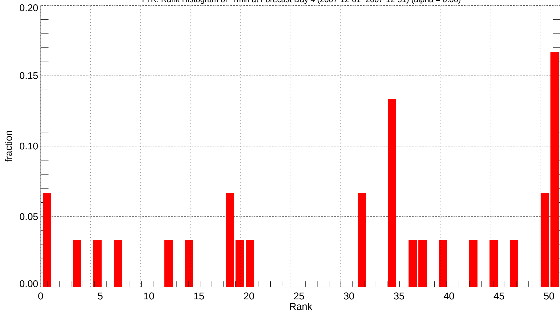
TYR: Rank Histogram of Tmin at Forecast Day 4 (2007-12-01~2007-12-31) (alpha = 0.00)
