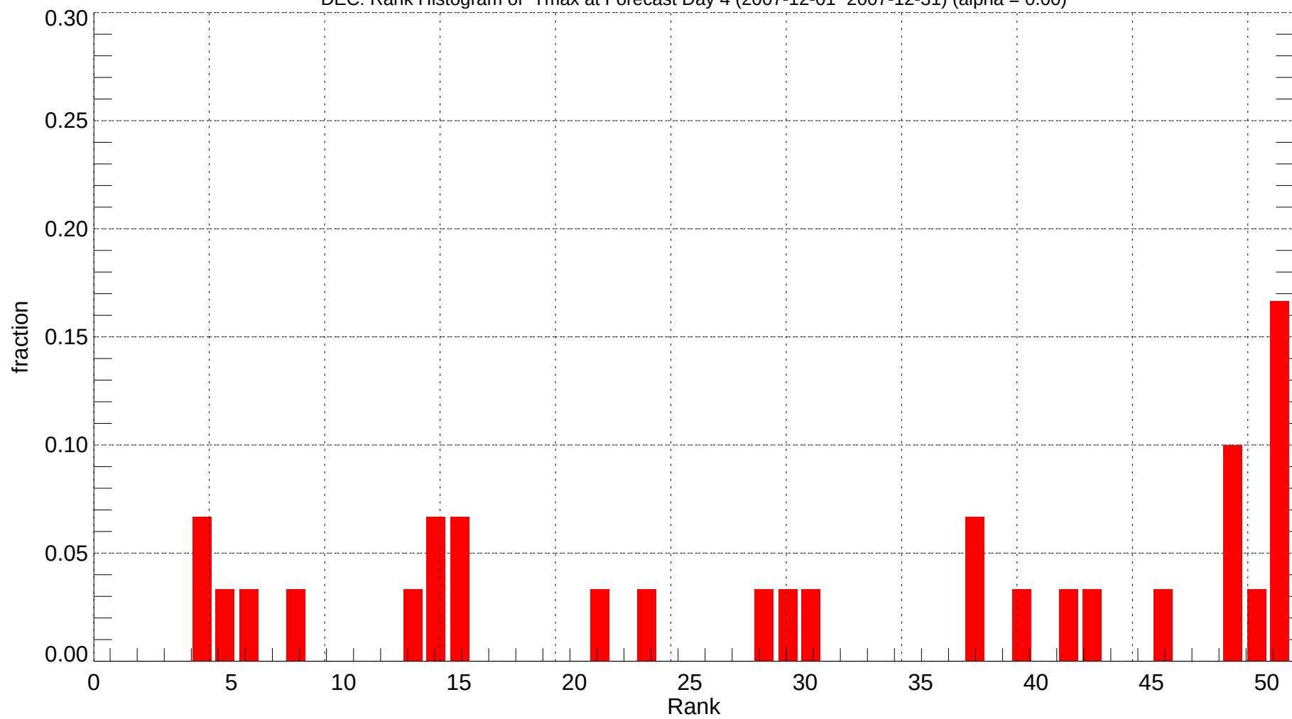
DEC: Rank Histogram of Tmax at Forecast Day 4 (2007-12-01~2007-12-31) (alpha = 0.00)
