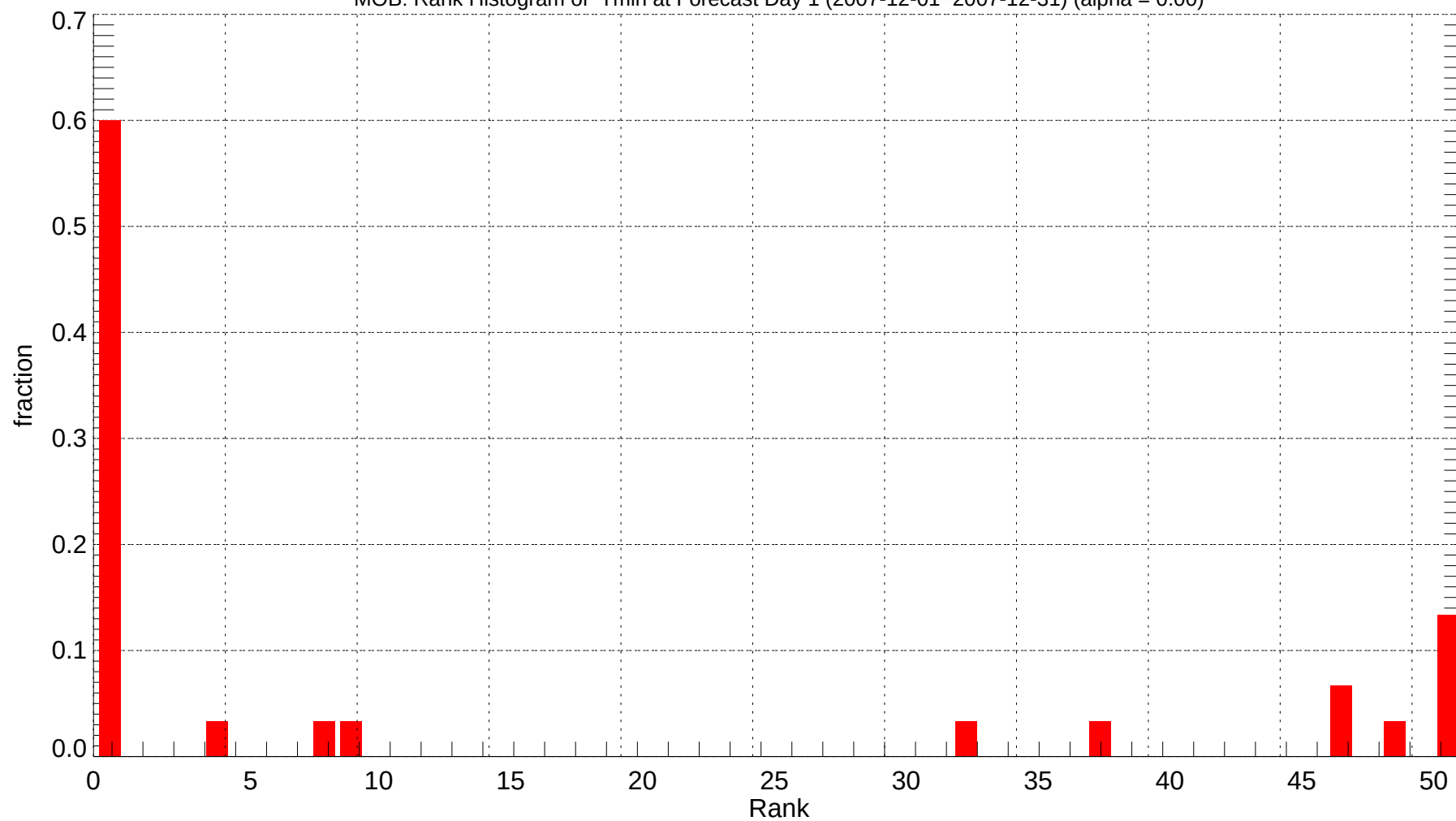
MOB: Rank Histogram of Tmin at Forecast Day 1 (2007-12-01~2007-12-31) (alpha = 0.00)
