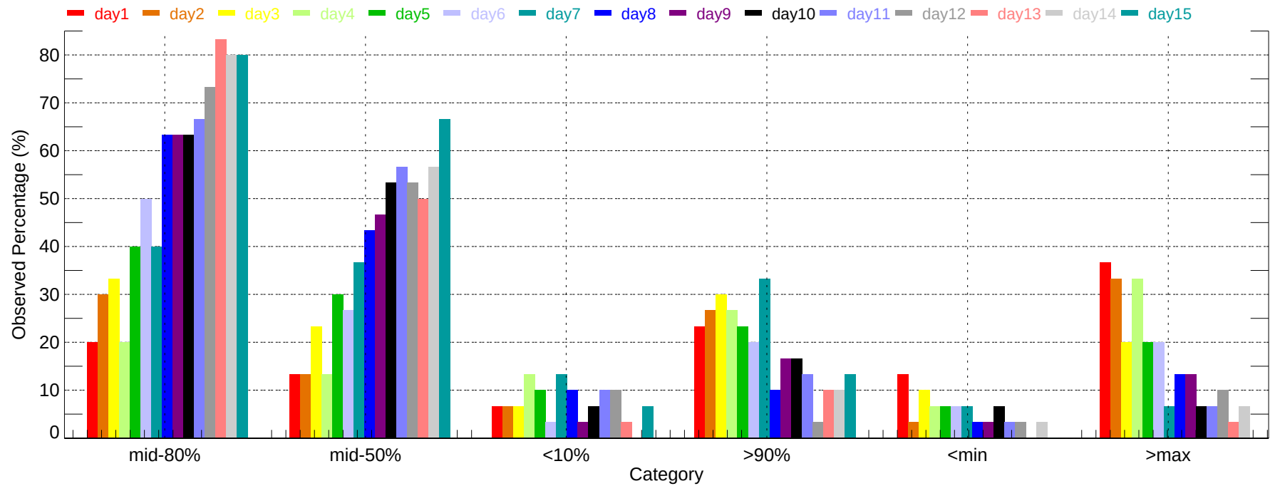
Observed Percentage of Ensembles - PDX: Max Temperature (2007-12-01~2007-12-31)
