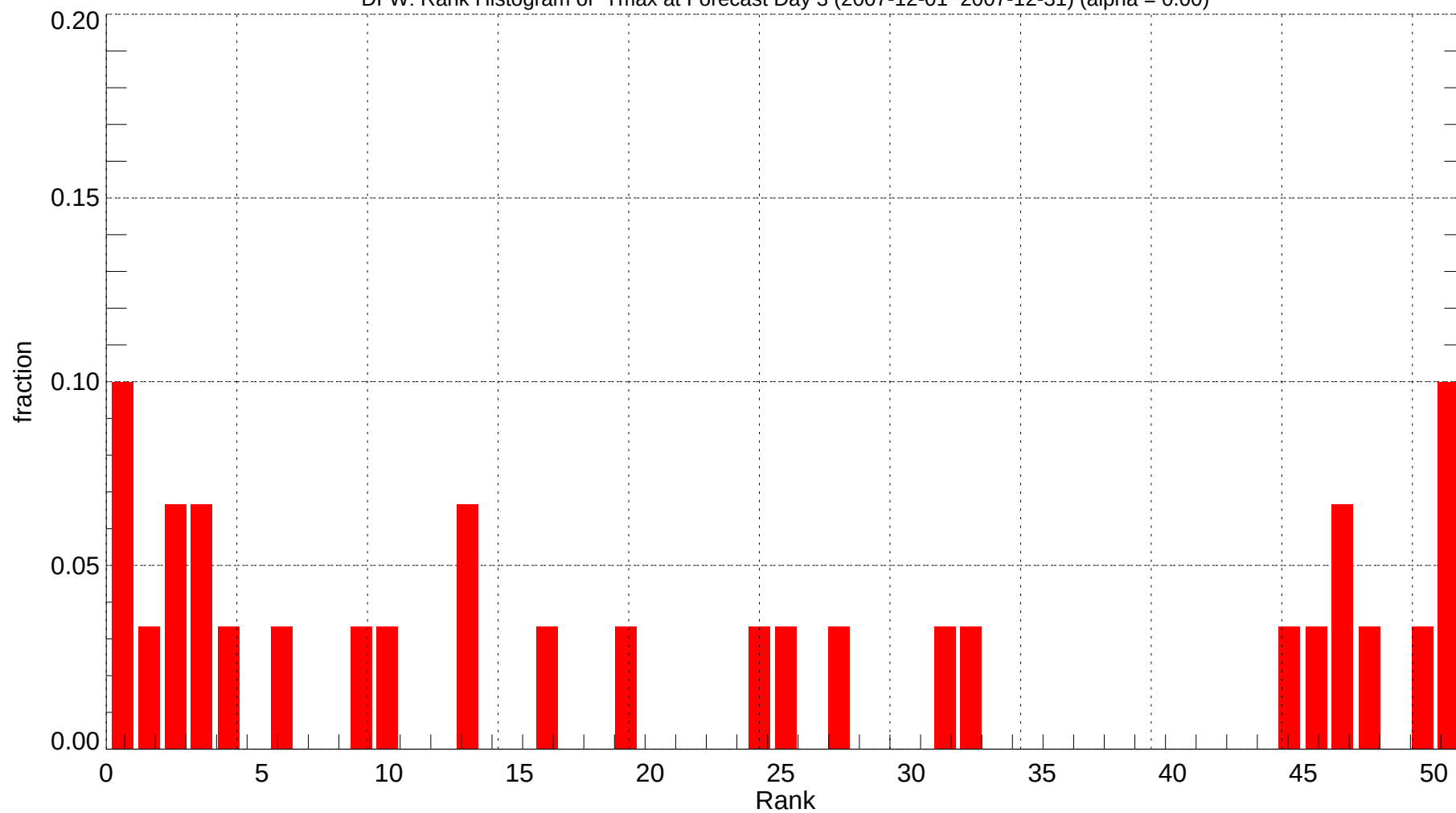
DFW: Rank Histogram of Tmax at Forecast Day 3 (2007-12-01~2007-12-31) (alpha = 0.00)
