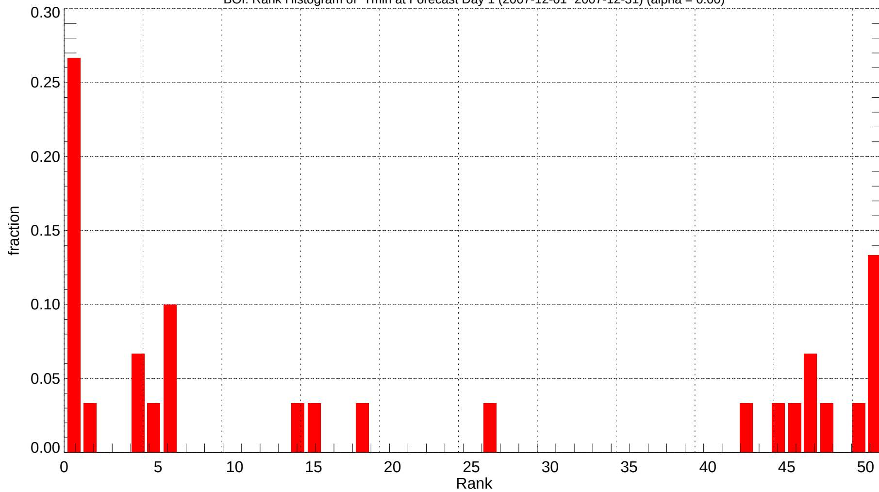
BOI: Rank Histogram of Tmin at Forecast Day 1 (2007-12-01~2007-12-31) (alpha = 0.00)
