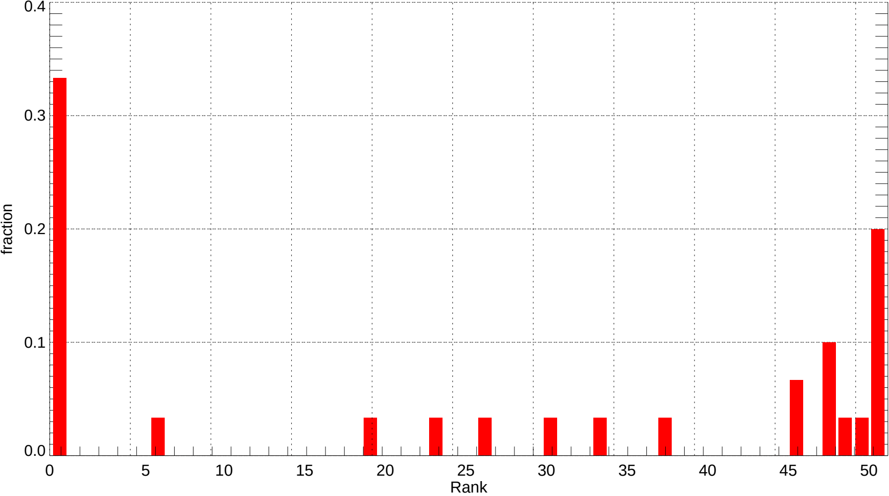
ATL: Rank Histogram of Tmin at Forecast Day 2 (2007-12-01~2007-12-31) (alpha = 0.00)
