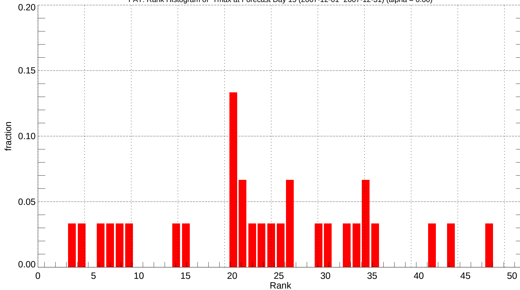
FAT: Rank Histogram of Tmax at Forecast Day 15 (2007-12-01~2007-12-31) (alpha = 0.00)
