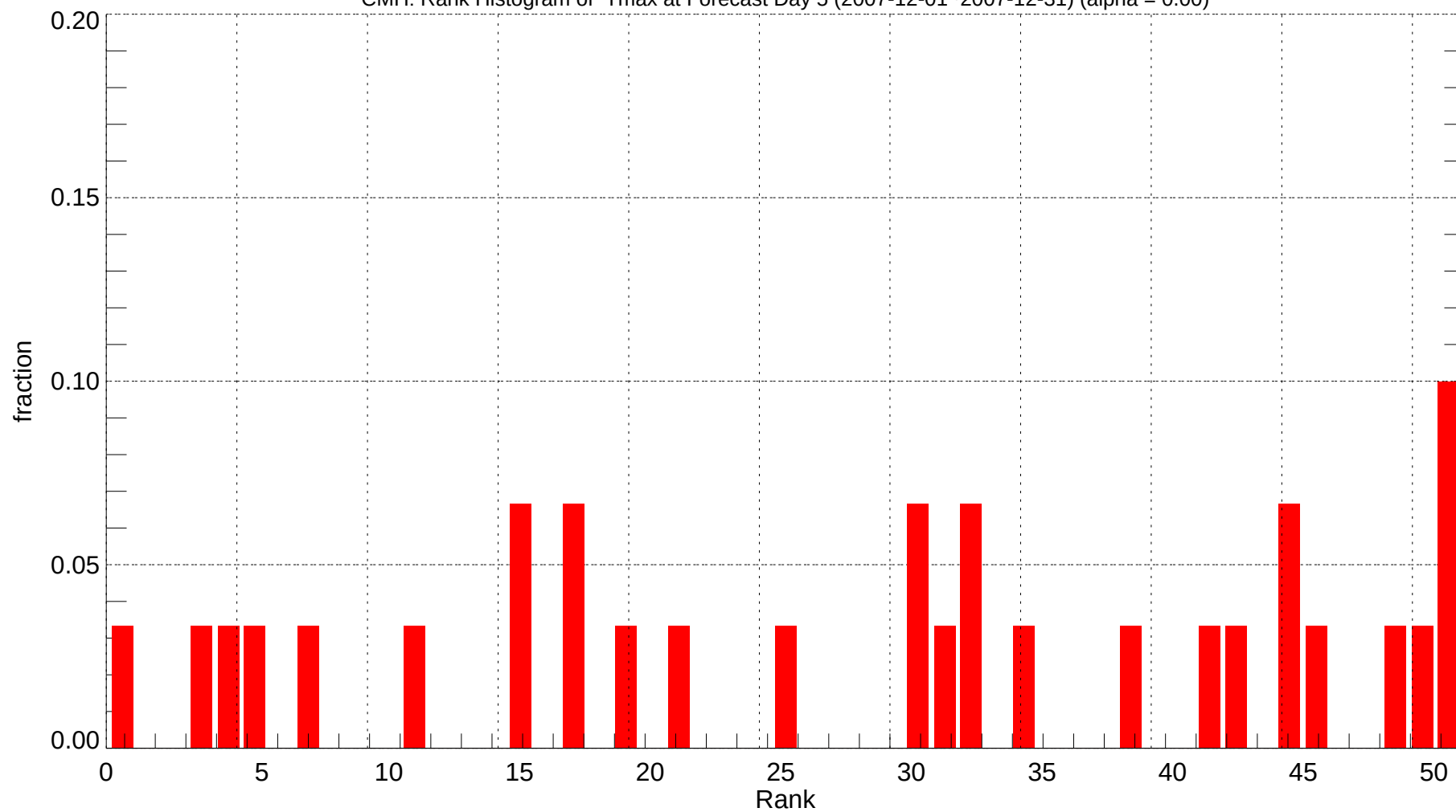
CMH: Rank Histogram of Tmax at Forecast Day 5 (2007-12-01~2007-12-31) (alpha = 0.00)
