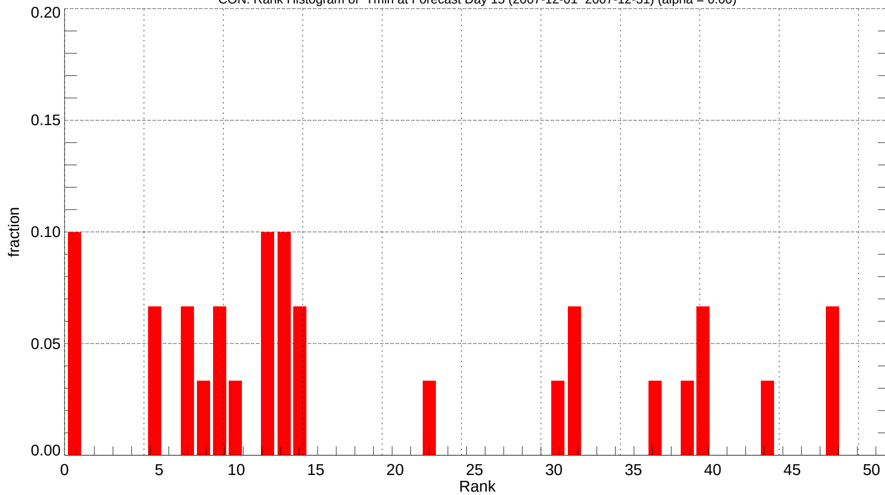
CON: Rank Histogram of Tmin at Forecast Day 15 (2007-12-01~2007-12-31) (alpha = 0.00)
