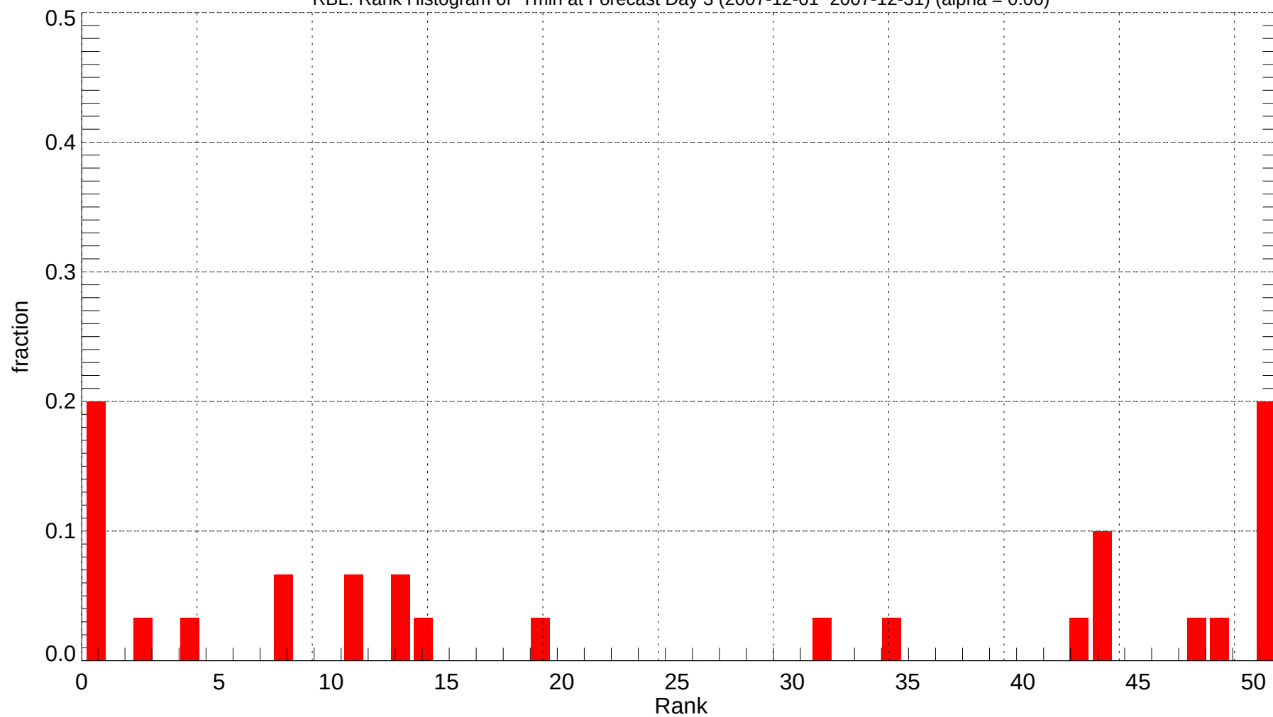
RBL: Rank Histogram of Tmin at Forecast Day 3 (2007-12-01~2007-12-31) (alpha = 0.00)
