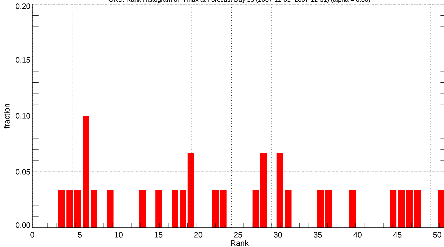
ORD: Rank Histogram of Tmax at Forecast Day 15 (2007-12-01~2007-12-31) (alpha = 0.00)
