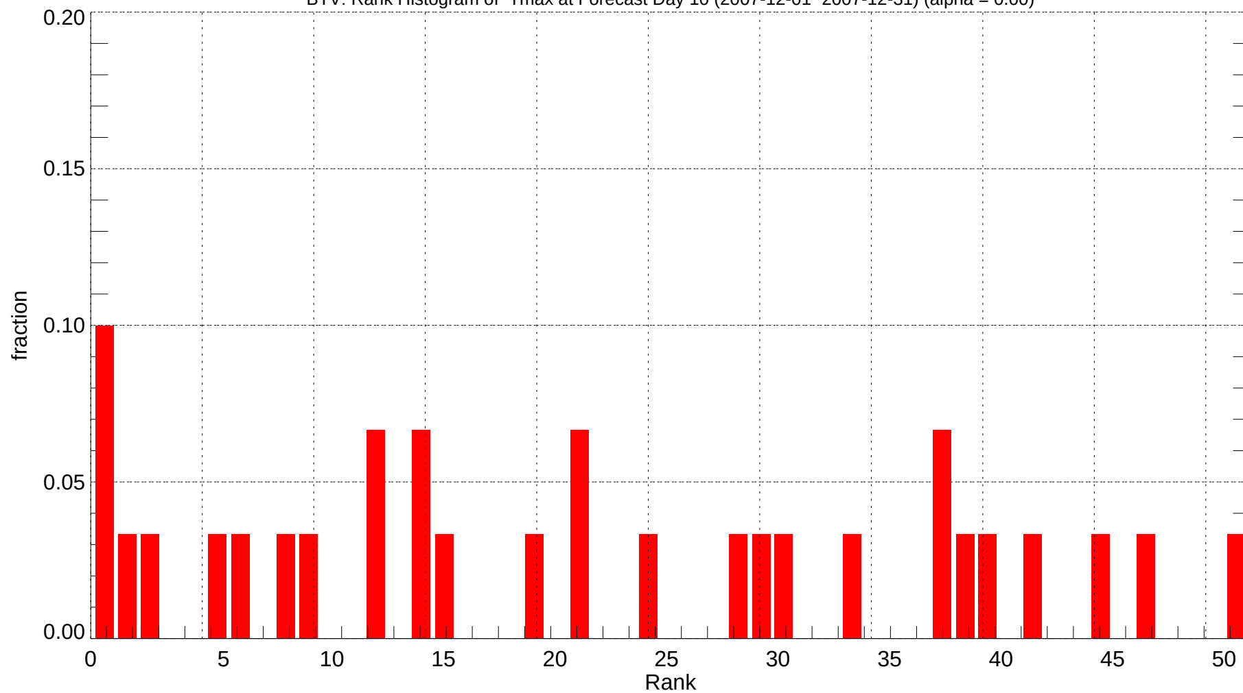
BTV: Rank Histogram of Tmax at Forecast Day 10 (2007-12-01~2007-12-31) (alpha = 0.00)
