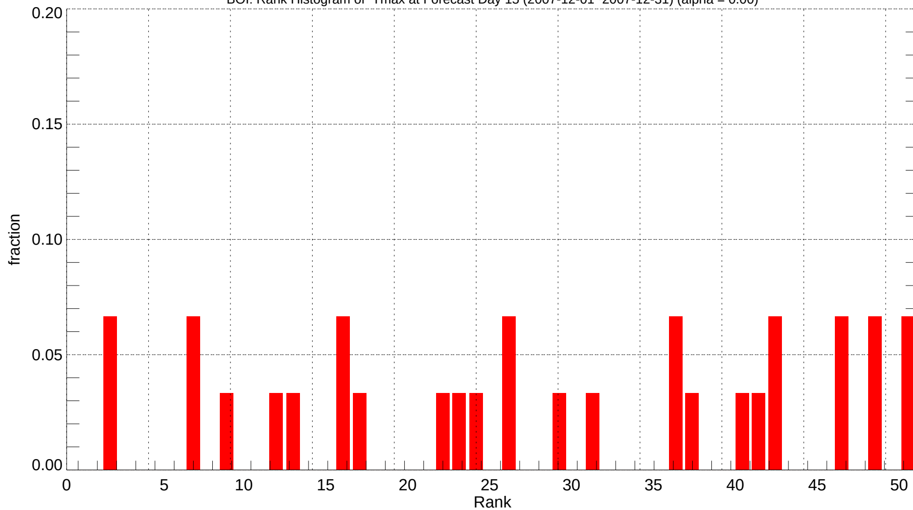
BOI: Rank Histogram of Tmax at Forecast Day 15 (2007-12-01~2007-12-31) (alpha = 0.00)
