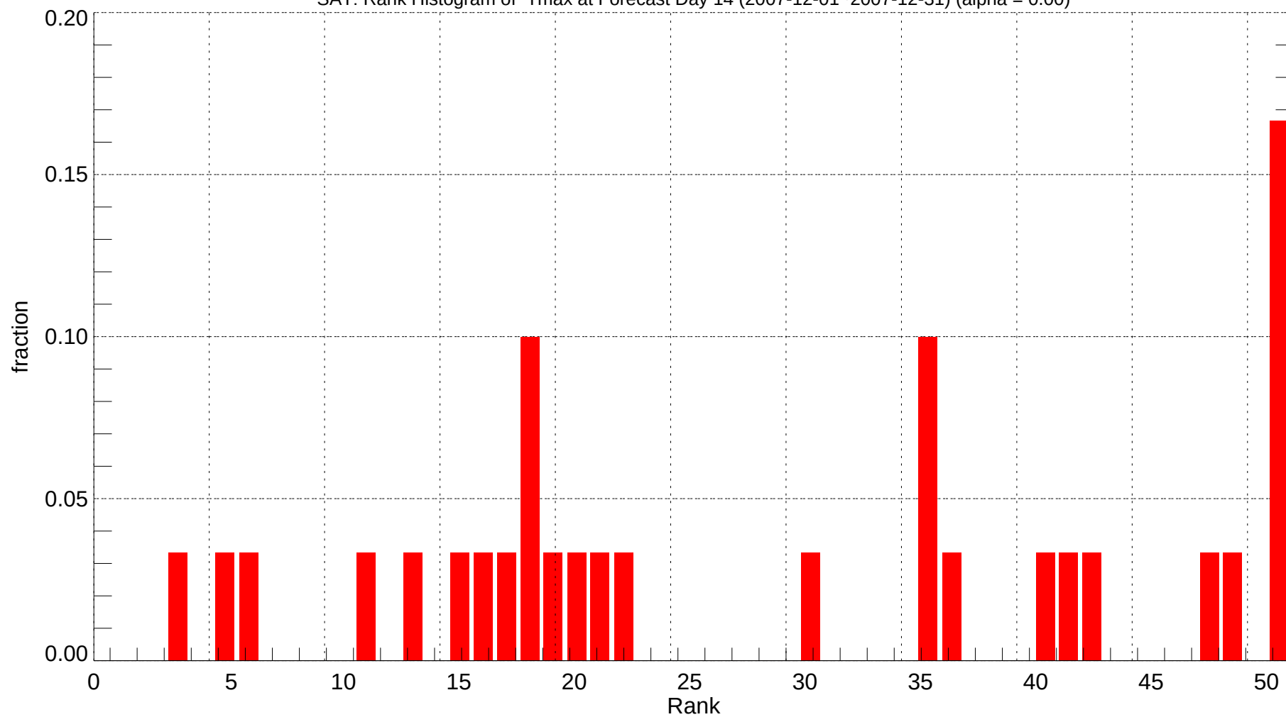
SAT: Rank Histogram of Tmax at Forecast Day 14 (2007-12-01~2007-12-31) (alpha = 0.00)
