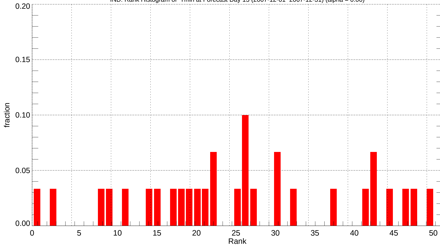
IND: Rank Histogram of Tmin at Forecast Day 13 (2007-12-01~2007-12-31) (alpha = 0.00)
