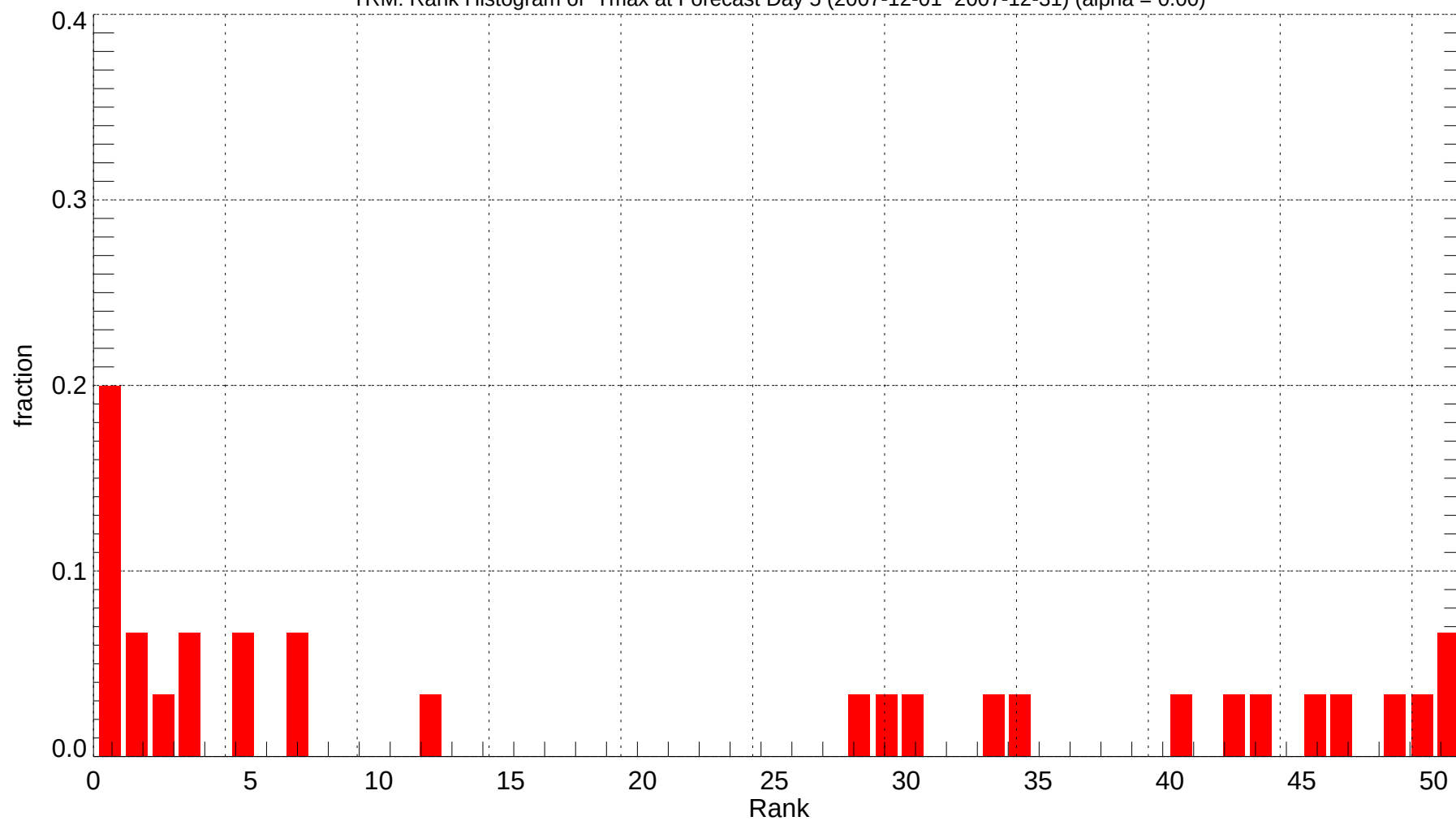
TRM: Rank Histogram of Tmax at Forecast Day 5 (2007-12-01~2007-12-31) (alpha = 0.00)
