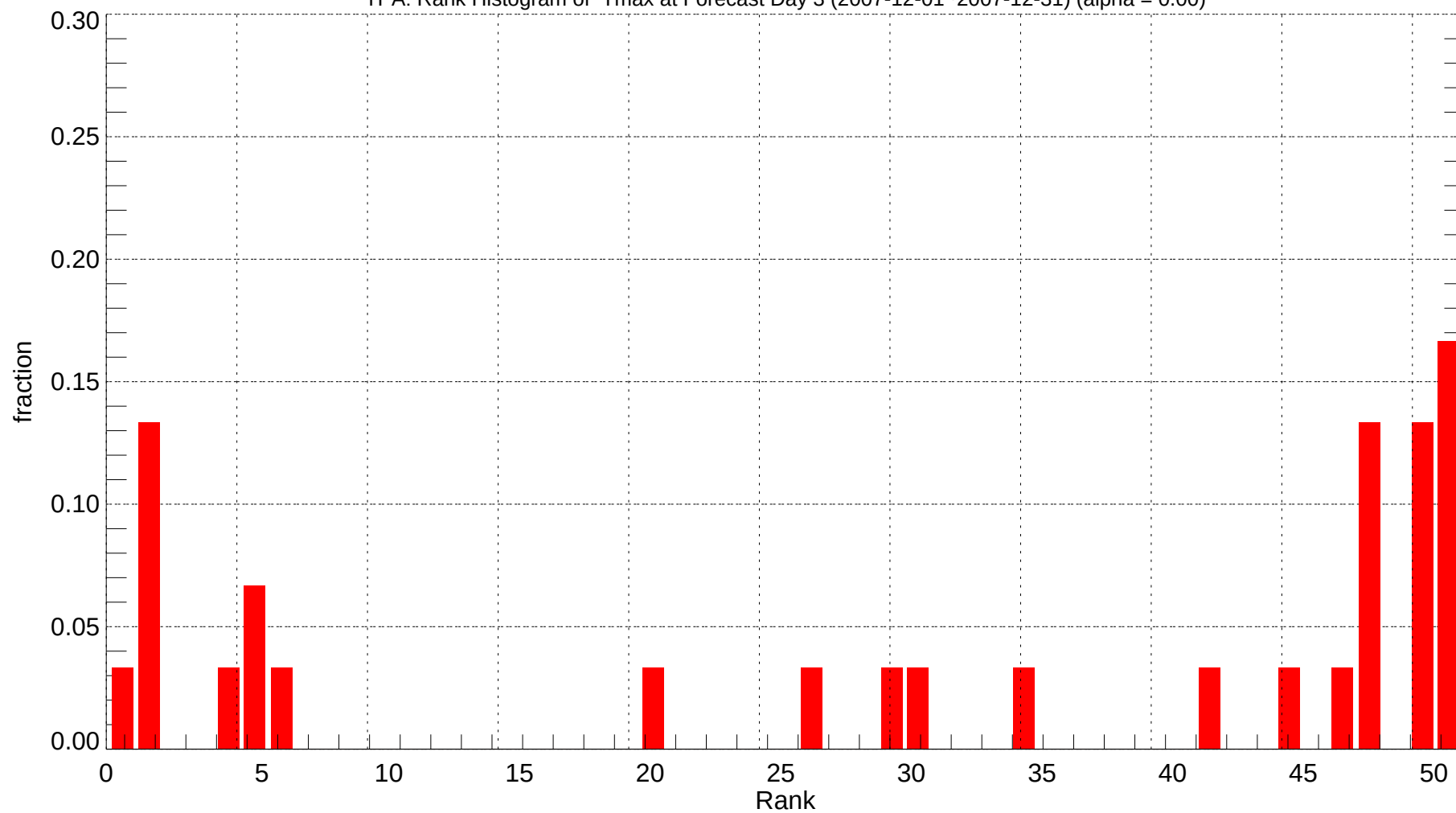
TPA: Rank Histogram of Tmax at Forecast Day 3 (2007-12-01~2007-12-31) (alpha = 0.00)
