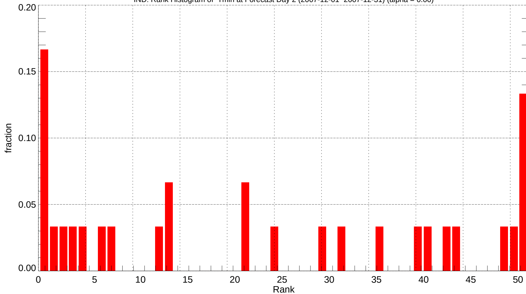
IND: Rank Histogram of Tmin at Forecast Day 2 (2007-12-01~2007-12-31) (alpha = 0.00)
