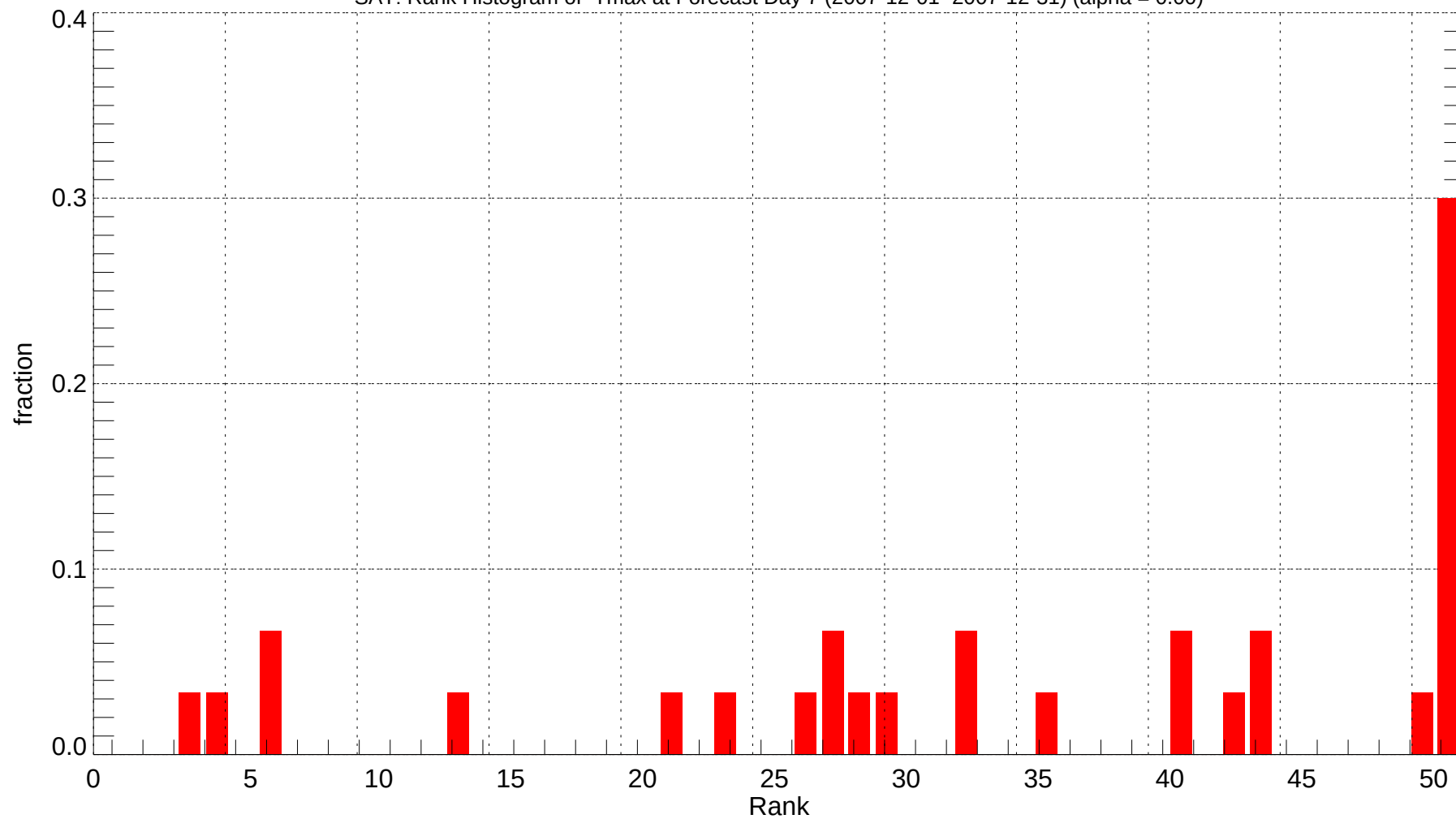
SAT: Rank Histogram of Tmax at Forecast Day 7 (2007-12-01~2007-12-31) (alpha = 0.00)
