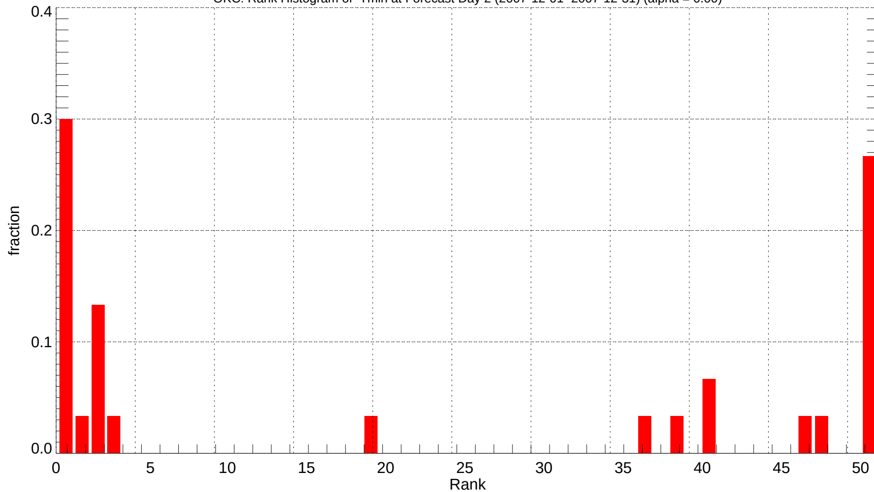
OKC: Rank Histogram of Tmin at Forecast Day 2 (2007-12-01~2007-12-31) (alpha = 0.00)
