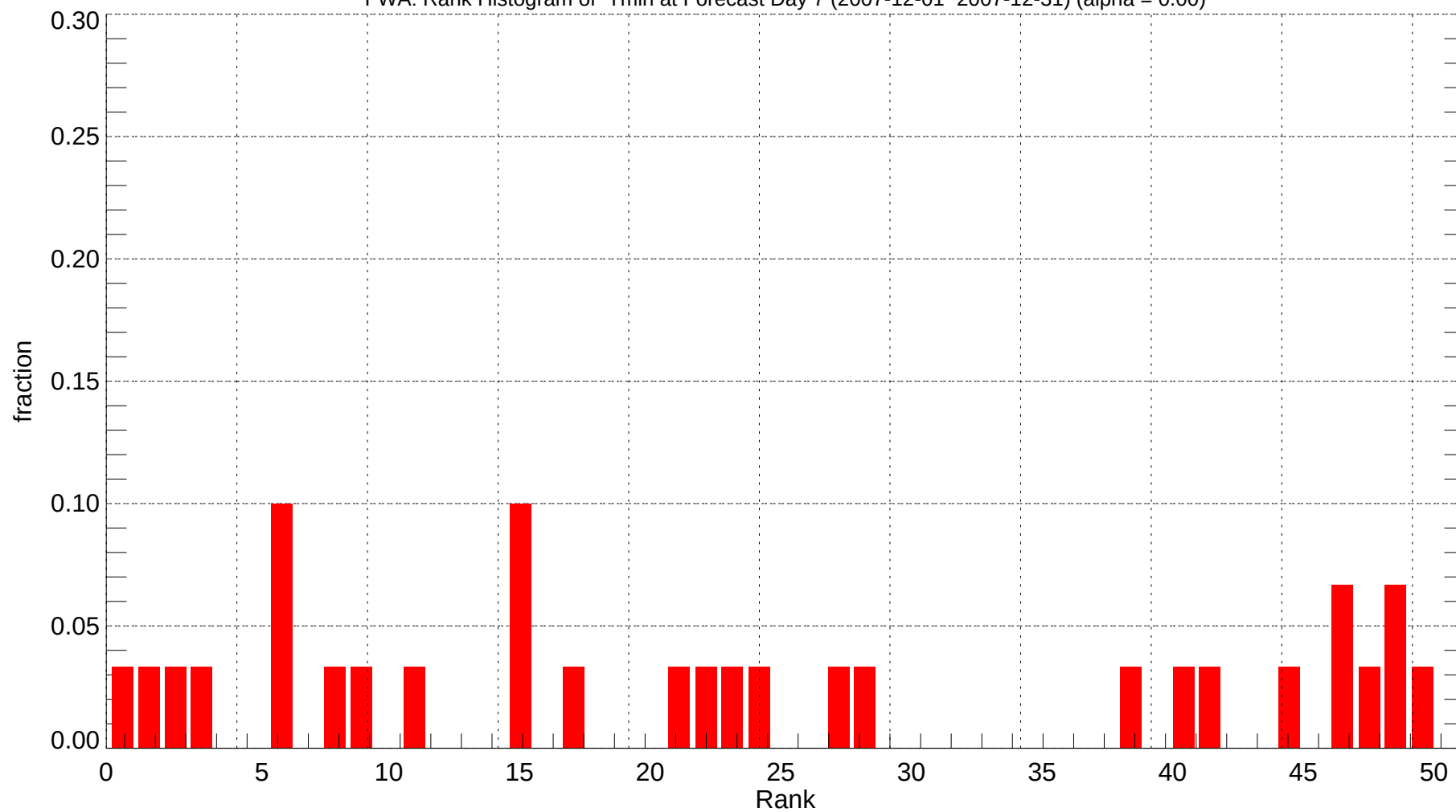
FWA: Rank Histogram of Tmin at Forecast Day 7 (2007-12-01~2007-12-31) (alpha = 0.00)
