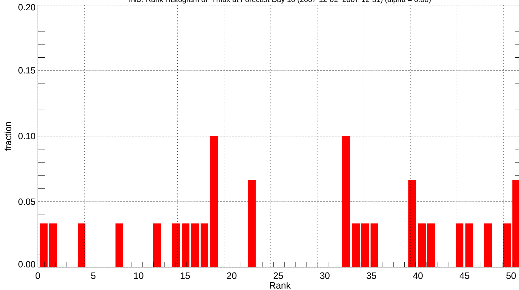
IND: Rank Histogram of Tmax at Forecast Day 10 (2007-12-01~2007-12-31) (alpha = 0.00)
