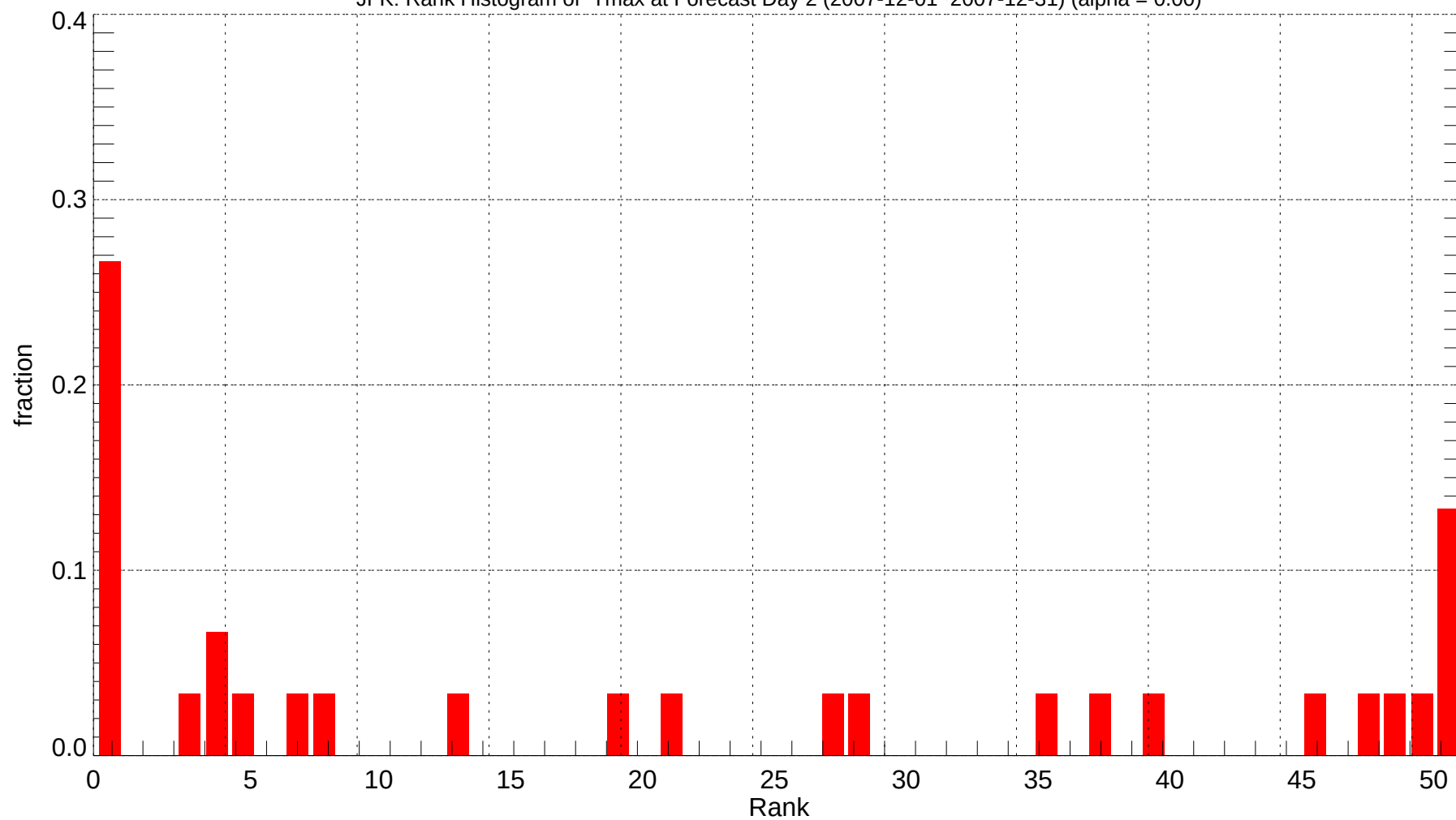
JFK: Rank Histogram of Tmax at Forecast Day 2 (2007-12-01~2007-12-31) (alpha = 0.00)
