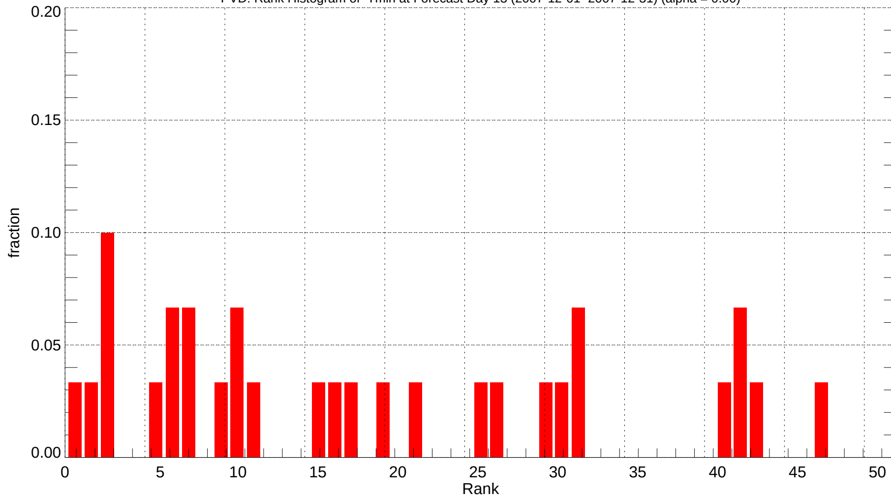
PVD: Rank Histogram of Tmin at Forecast Day 13 (2007-12-01~2007-12-31) (alpha = 0.00)
