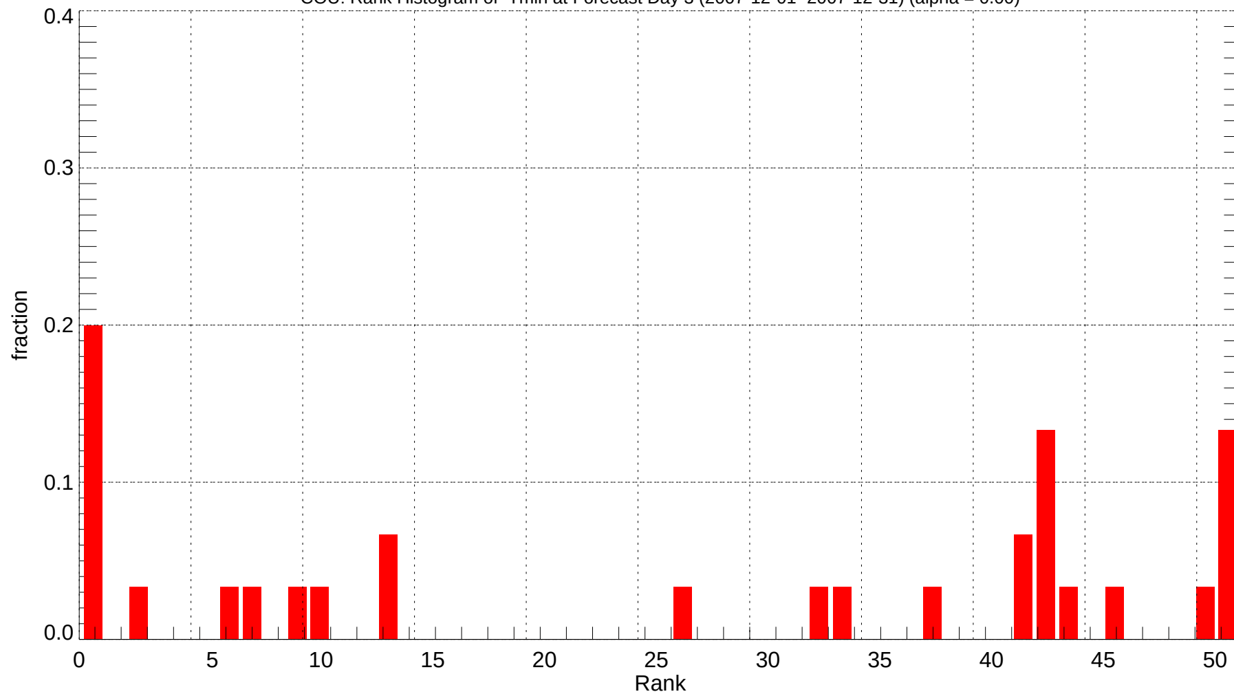
COU: Rank Histogram of Tmin at Forecast Day 3 (2007-12-01~2007-12-31) (alpha = 0.00)
