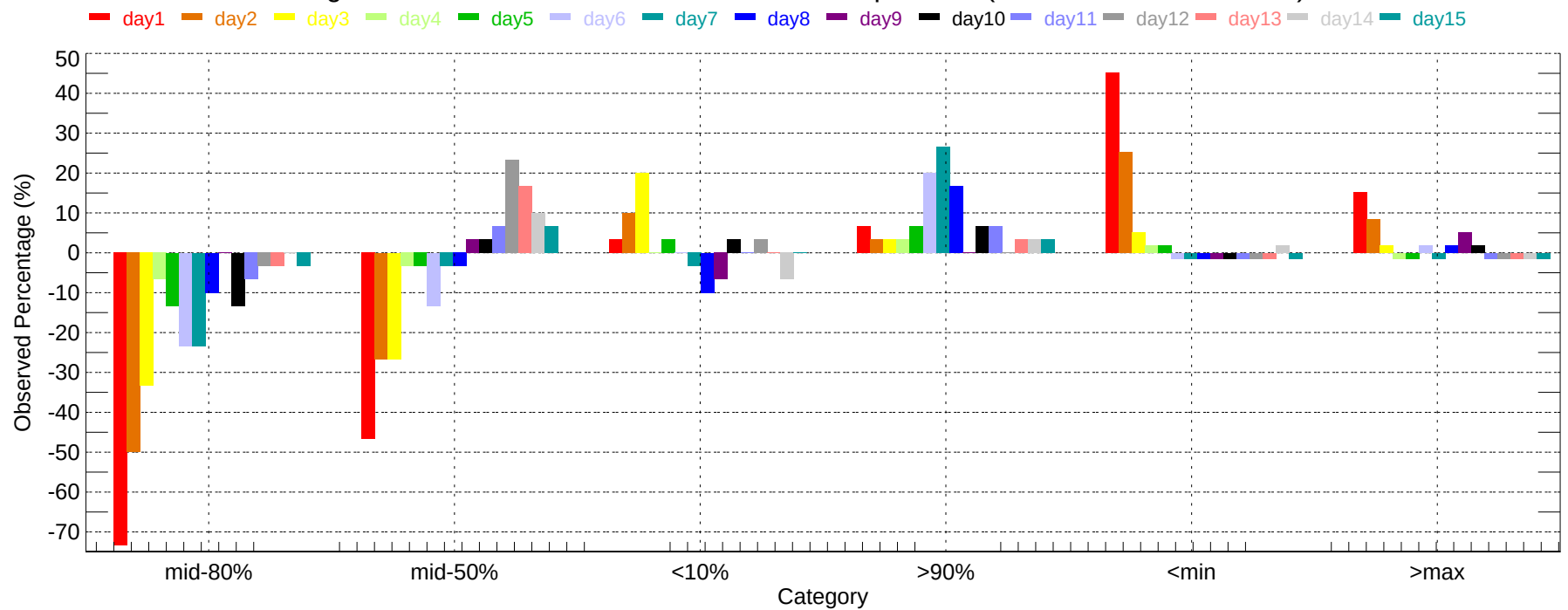
Observed Percentage Deviation of Ensembles - BOS: Max Temperature (2007-12-01~2007-12-31)
