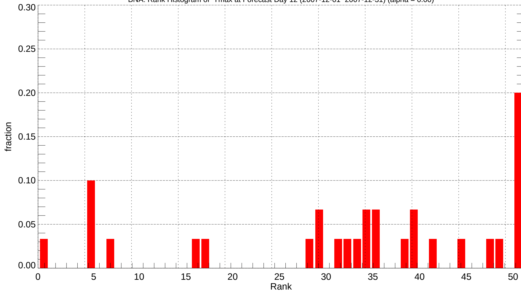
BNA: Rank Histogram of Tmax at Forecast Day 12 (2007-12-01~2007-12-31) (alpha = 0.00)
