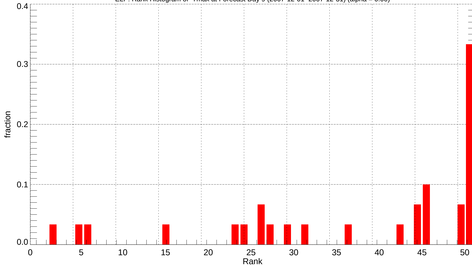
ELP: Rank Histogram of Tmax at Forecast Day 9 (2007-12-01~2007-12-31) (alpha = 0.00)
