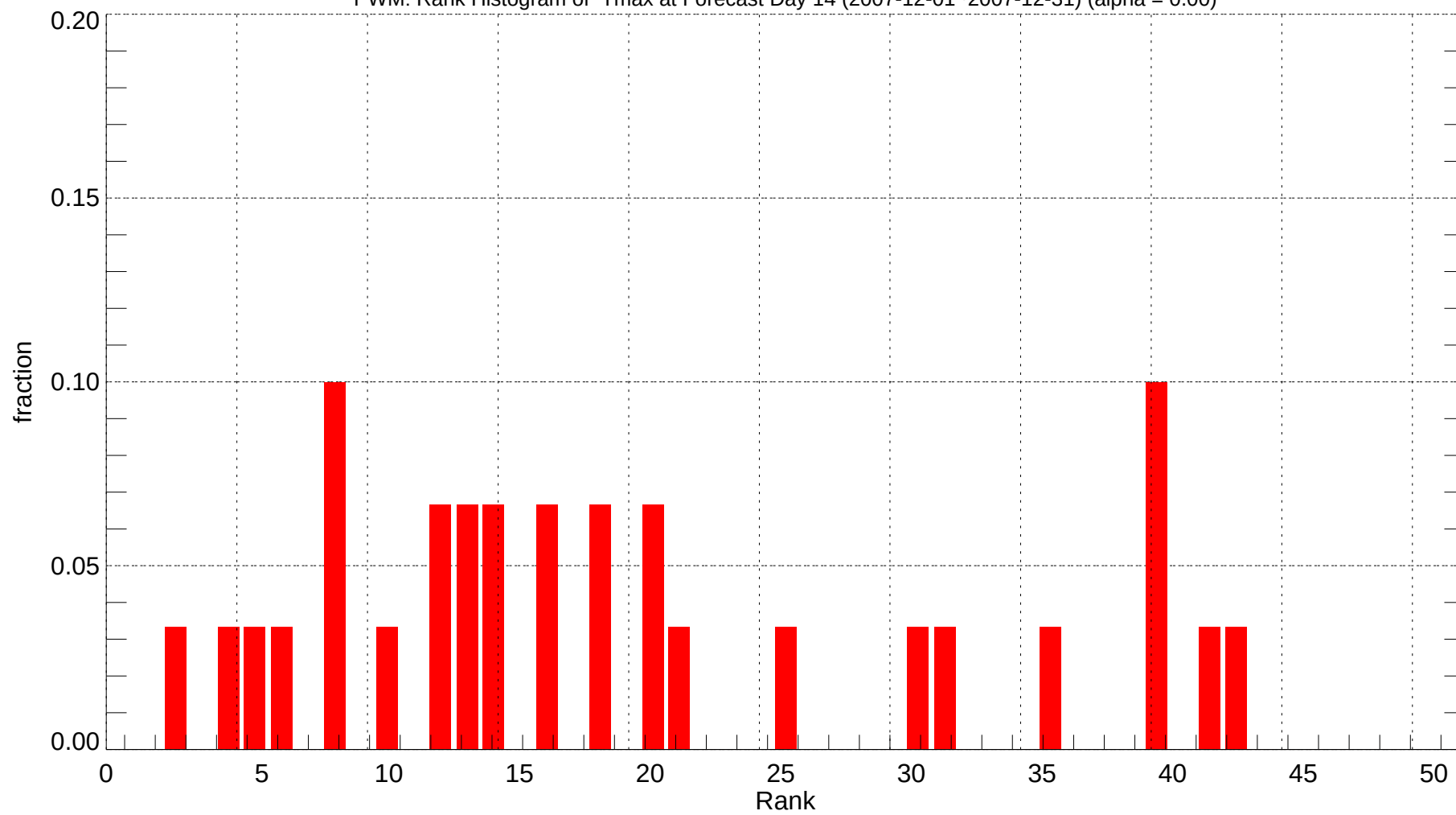
PWM: Rank Histogram of Tmax at Forecast Day 14 (2007-12-01~2007-12-31) (alpha = 0.00)
