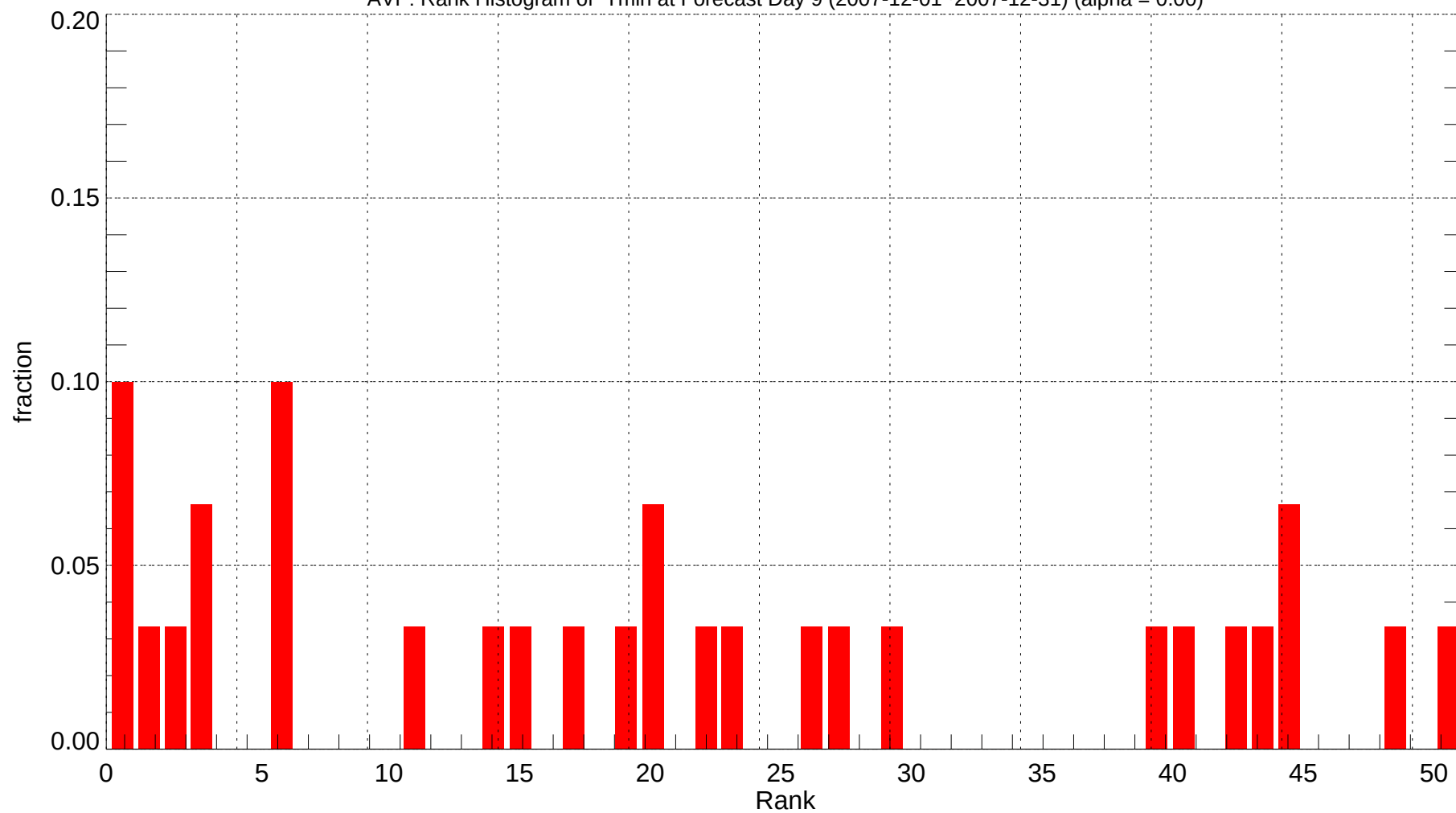
AVP: Rank Histogram of Tmin at Forecast Day 9 (2007-12-01~2007-12-31) (alpha = 0.00)
