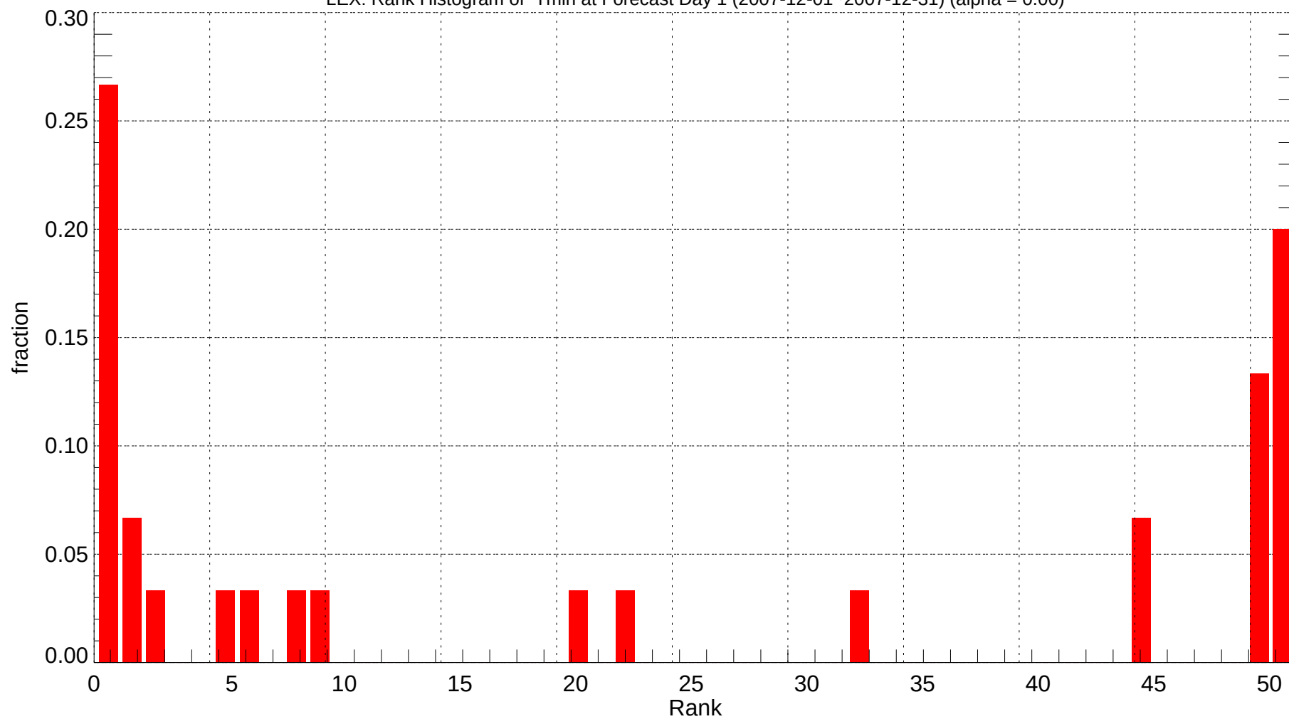
LEX: Rank Histogram of Tmin at Forecast Day 1 (2007-12-01~2007-12-31) (alpha = 0.00)
