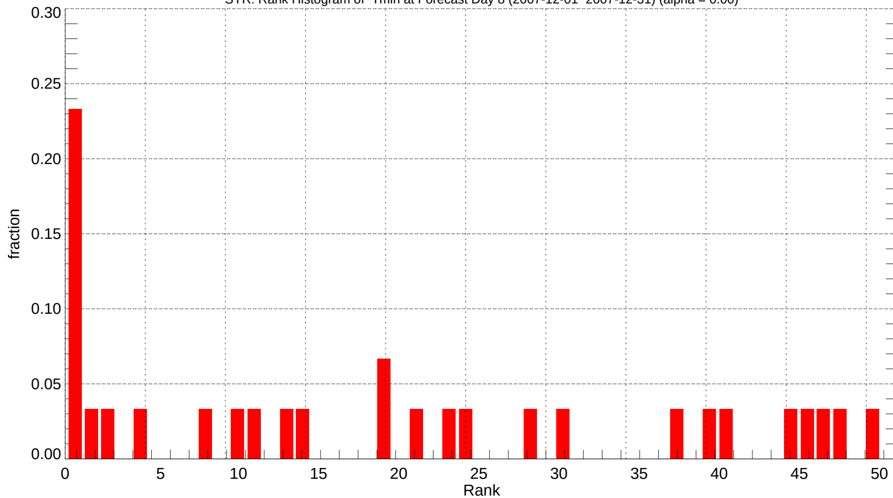
SYR: Rank Histogram of Tmin at Forecast Day 8 (2007-12-01~2007-12-31) (alpha = 0.00)
