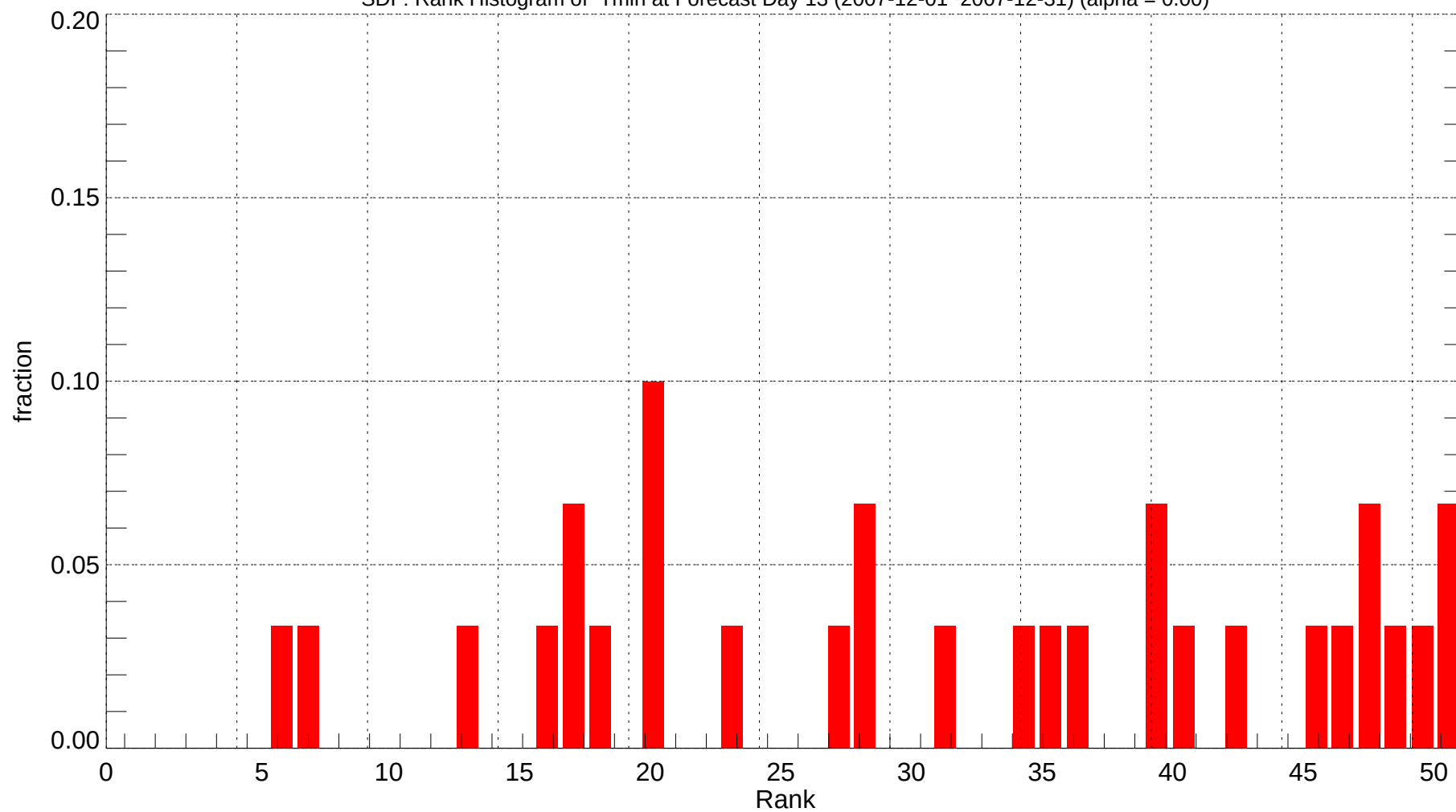
SDF: Rank Histogram of Tmin at Forecast Day 13 (2007-12-01~2007-12-31) (alpha = 0.00)
