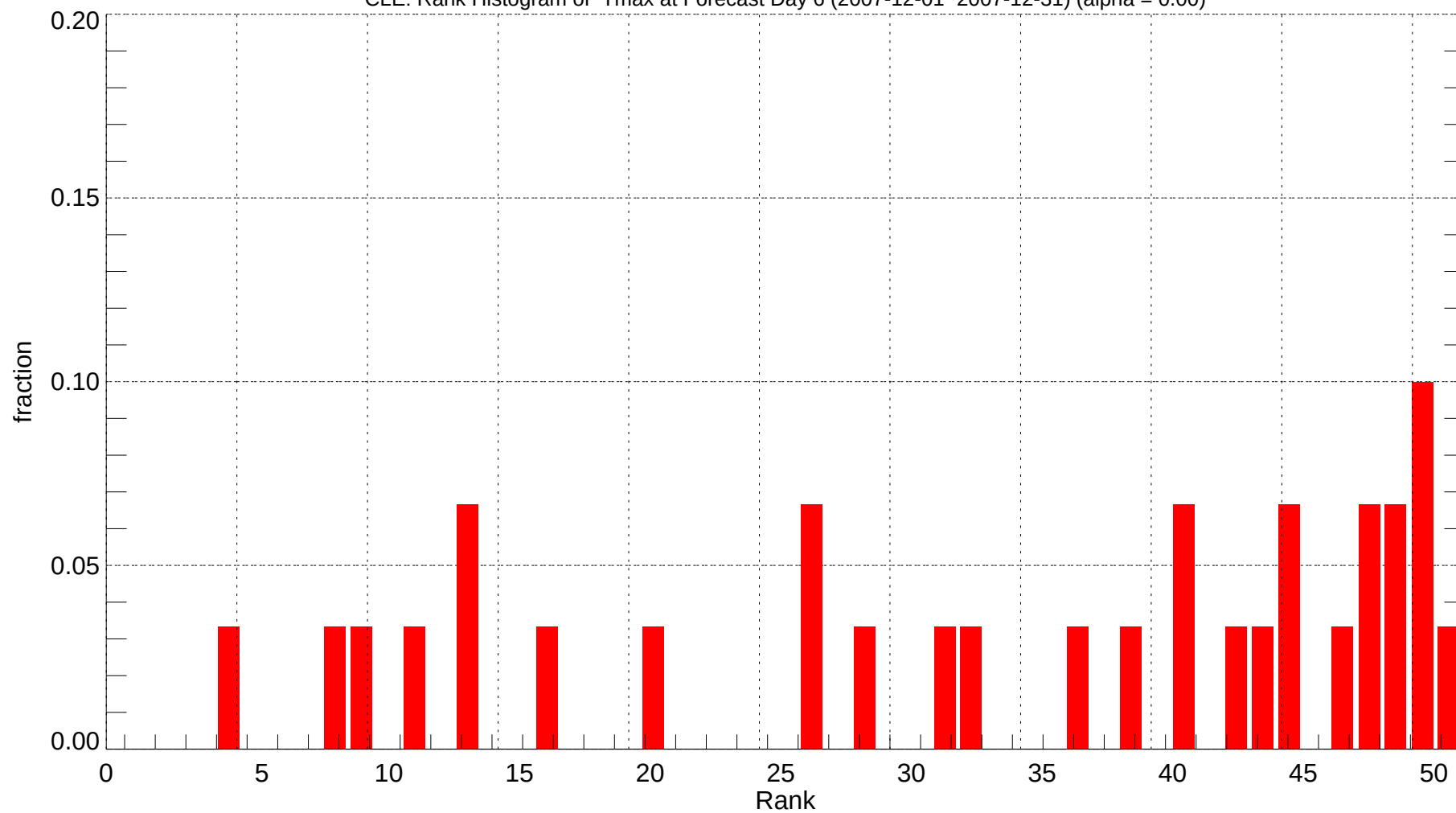
CLE: Rank Histogram of Tmax at Forecast Day 6 (2007-12-01~2007-12-31) (alpha = 0.00)
