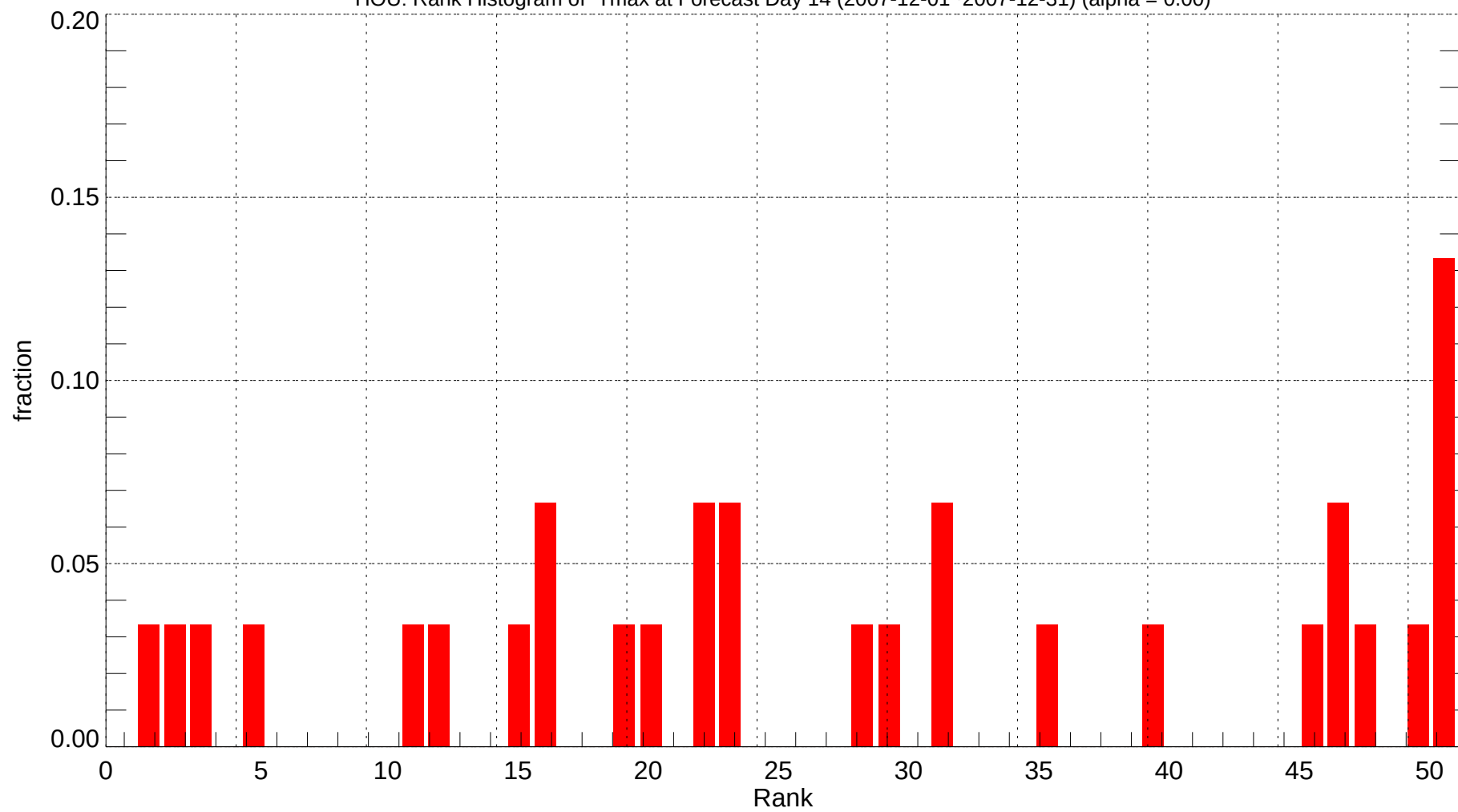
HOU: Rank Histogram of Tmax at Forecast Day 14 (2007-12-01~2007-12-31) (alpha = 0.00)
