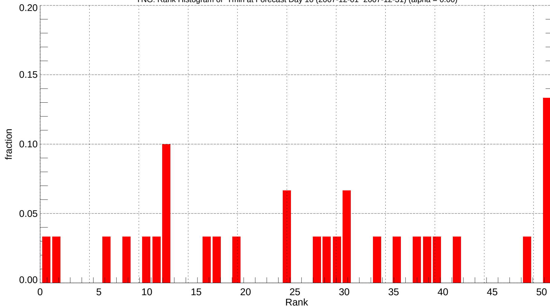
YNG: Rank Histogram of Tmin at Forecast Day 10 (2007-12-01~2007-12-31) (alpha = 0.00)
