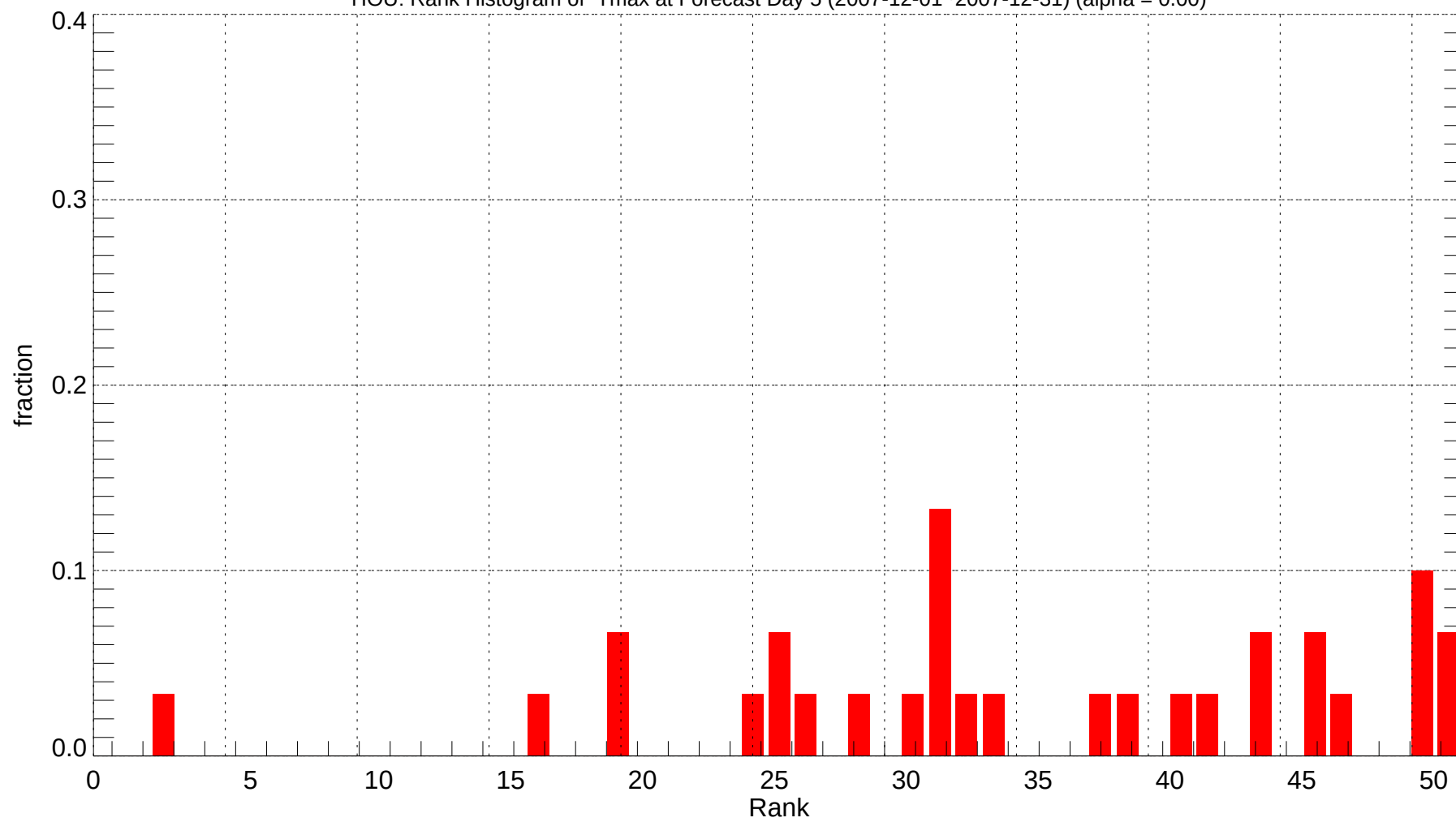
HOU: Rank Histogram of Tmax at Forecast Day 5 (2007-12-01~2007-12-31) (alpha = 0.00)
