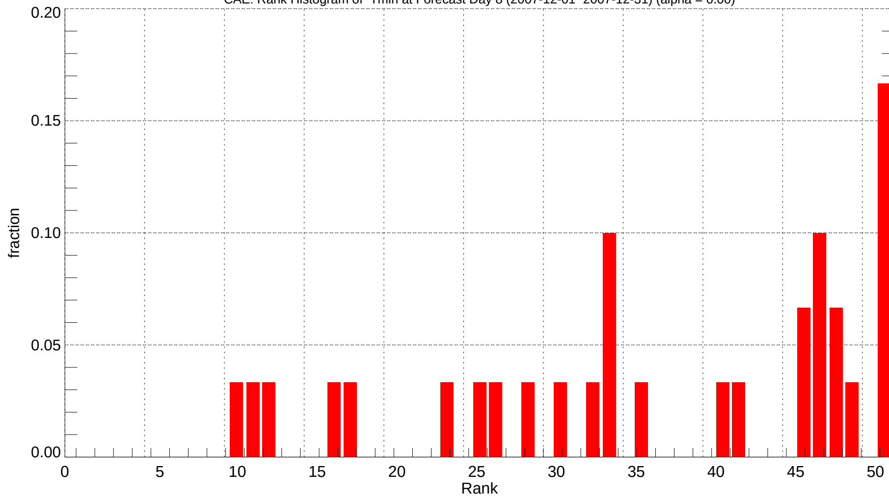
CAE: Rank Histogram of Tmin at Forecast Day 8 (2007-12-01~2007-12-31) (alpha = 0.00)
