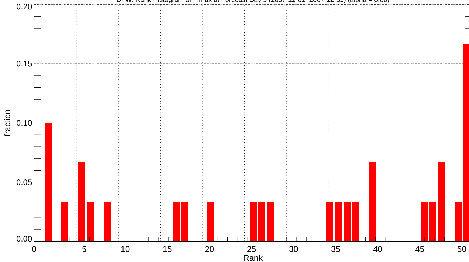
DFW: Rank Histogram of Tmax at Forecast Day 5 (2007-12-01~2007-12-31) (alpha = 0.00)
