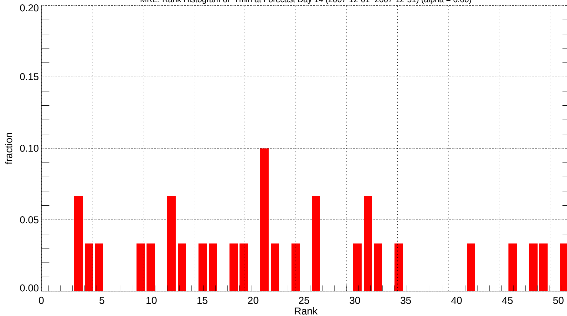
MKE: Rank Histogram of Tmin at Forecast Day 14 (2007-12-01~2007-12-31) (alpha = 0.00)
