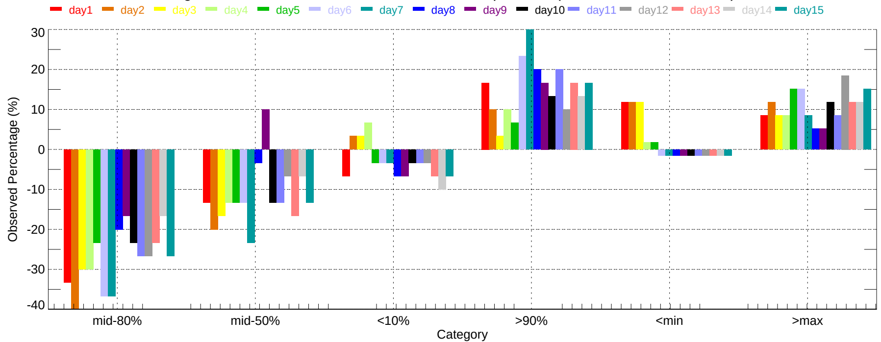
Observed Percentage Deviation of Ensembles - BHM: Max Temperature (2007-12-01~2007-12-31)
