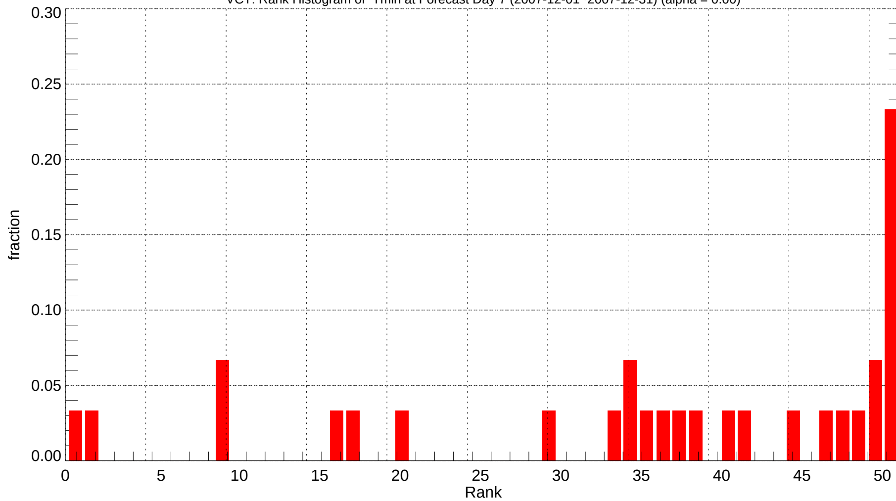
VCT: Rank Histogram of Tmin at Forecast Day 7 (2007-12-01~2007-12-31) (alpha = 0.00)
