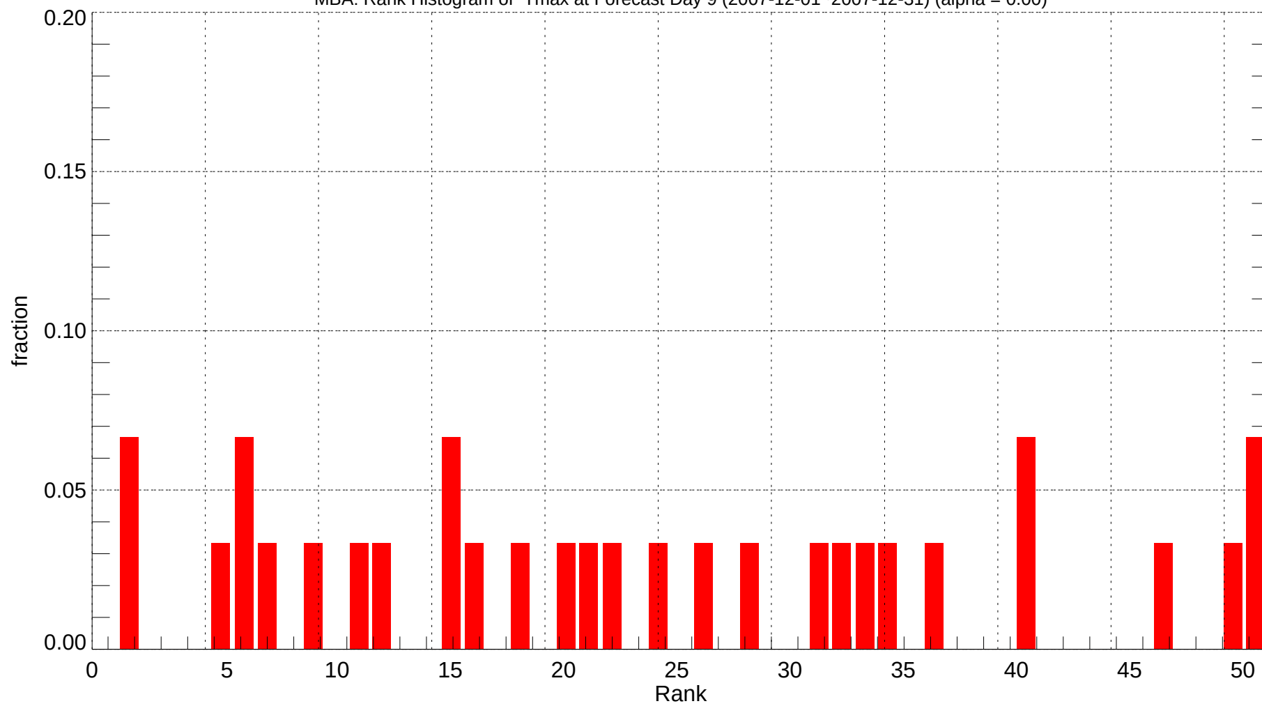
MBA: Rank Histogram of Tmax at Forecast Day 9 (2007-12-01~2007-12-31) (alpha = 0.00)
