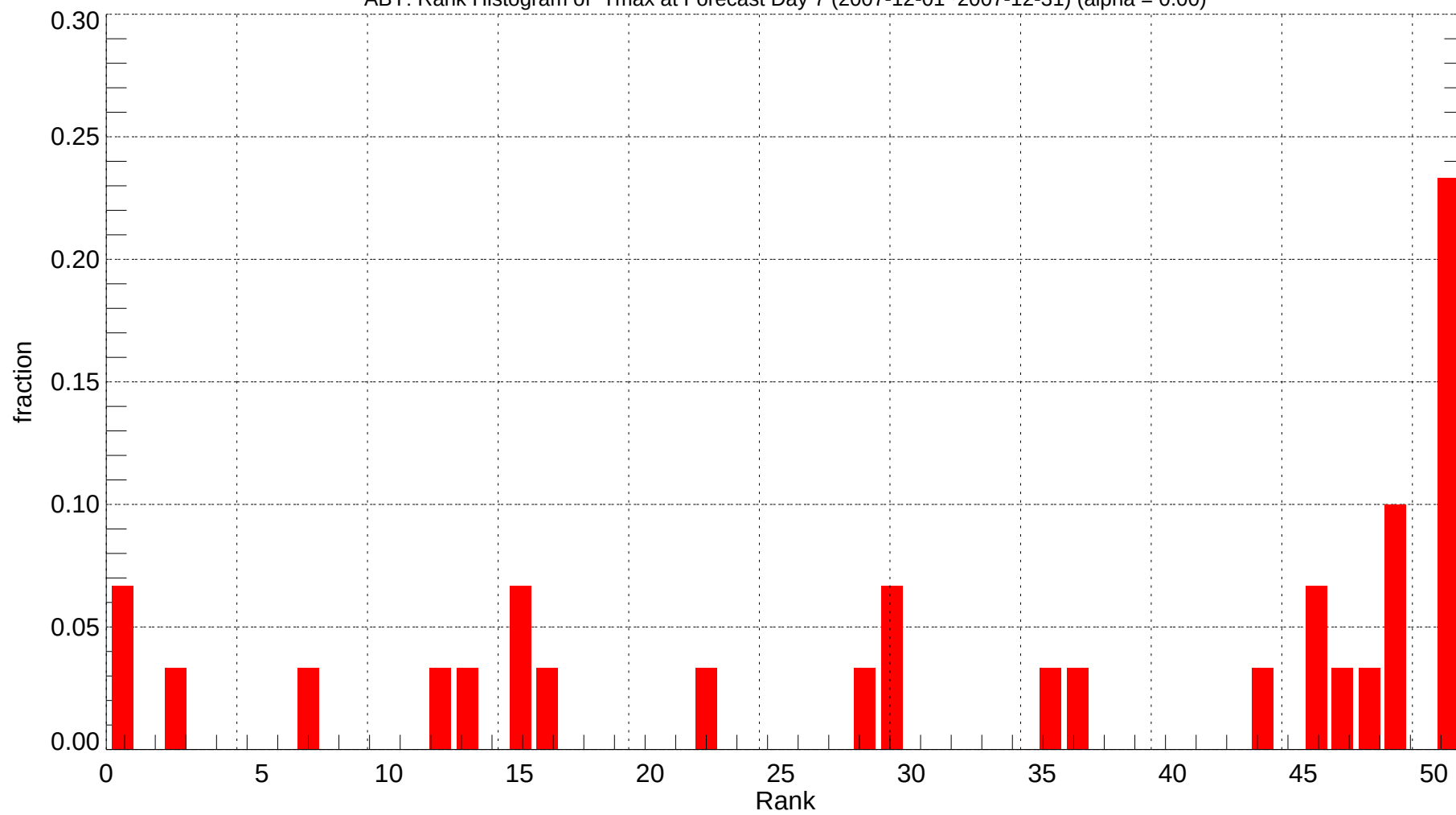
ABY: Rank Histogram of Tmax at Forecast Day 7 (2007-12-01~2007-12-31) (alpha = 0.00)
