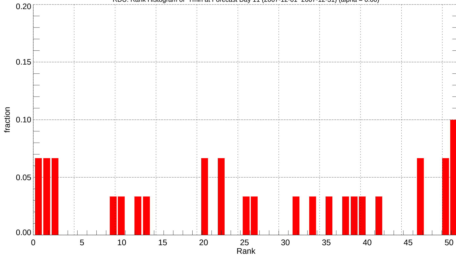
RDU: Rank Histogram of Tmin at Forecast Day 11 (2007-12-01~2007-12-31) (alpha = 0.00)
