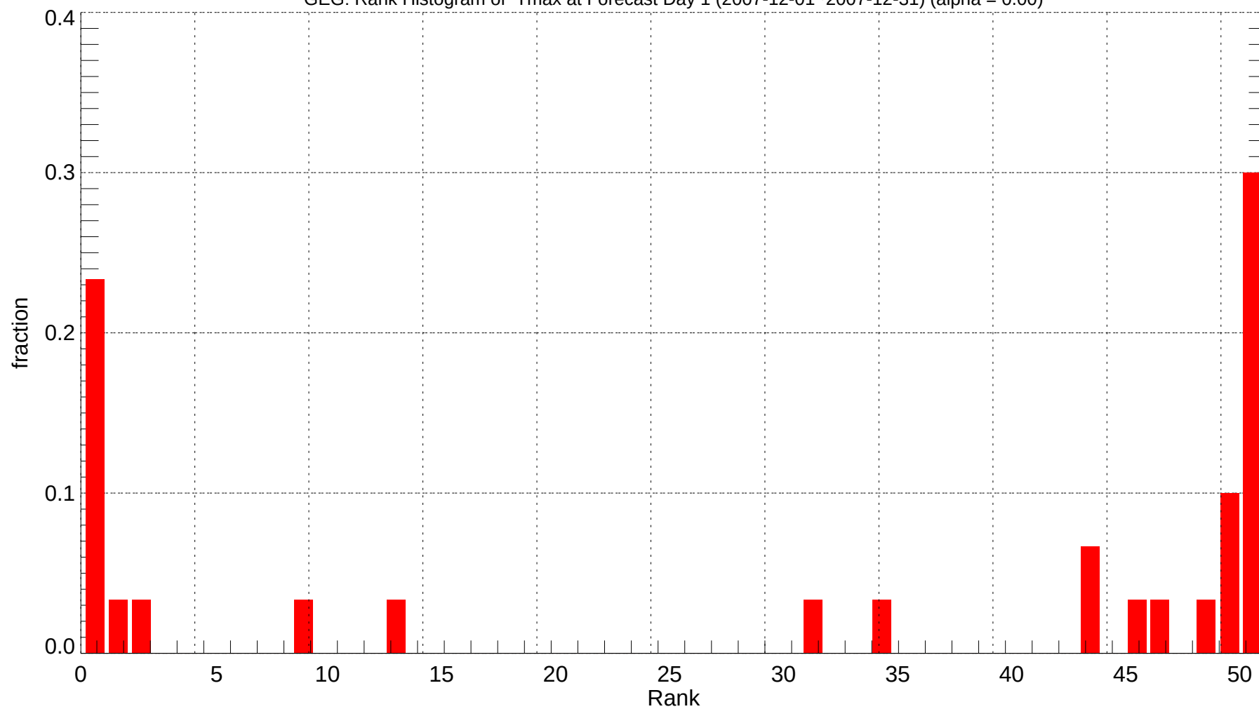
GEG: Rank Histogram of Tmax at Forecast Day 1 (2007-12-01~2007-12-31) (alpha = 0.00)
