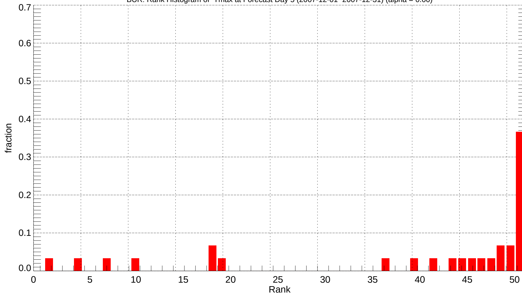
BUR: Rank Histogram of Tmax at Forecast Day 5 (2007-12-01~2007-12-31) (alpha = 0.00)
