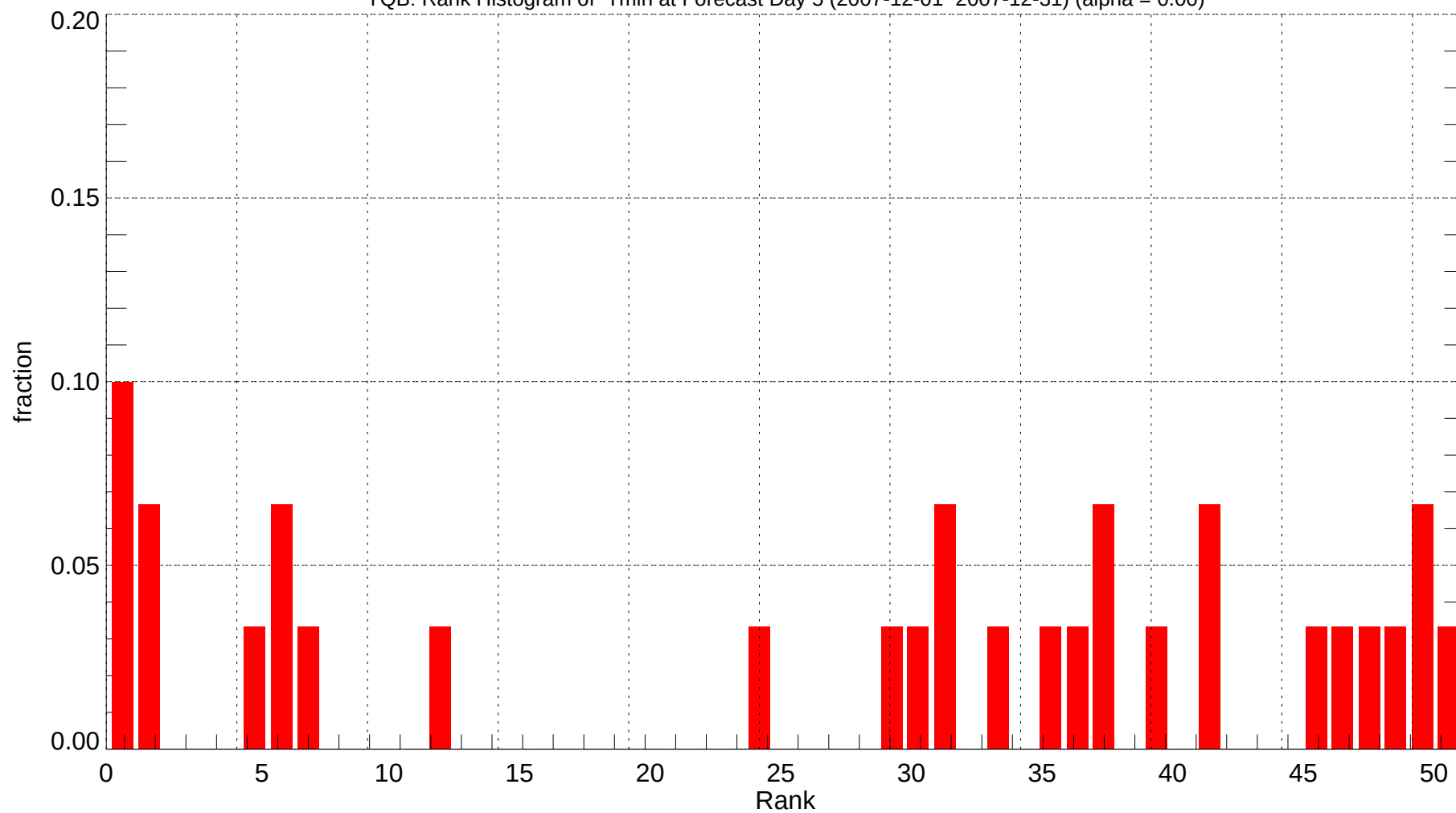
YQB: Rank Histogram of Tmin at Forecast Day 5 (2007-12-01~2007-12-31) (alpha = 0.00)
