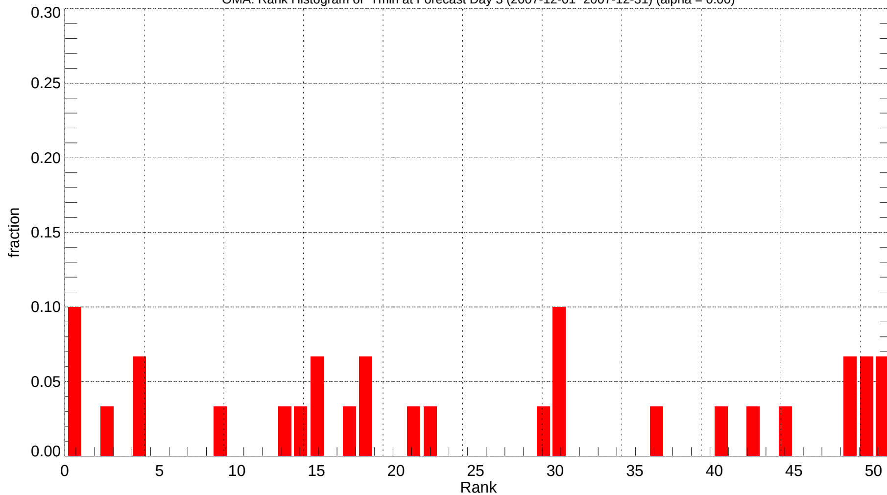
OMA: Rank Histogram of Tmin at Forecast Day 3 (2007-12-01~2007-12-31) (alpha = 0.00)
