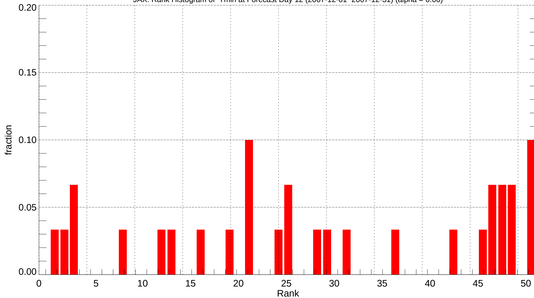
JAX: Rank Histogram of Tmin at Forecast Day 12 (2007-12-01~2007-12-31) (alpha = 0.00)
