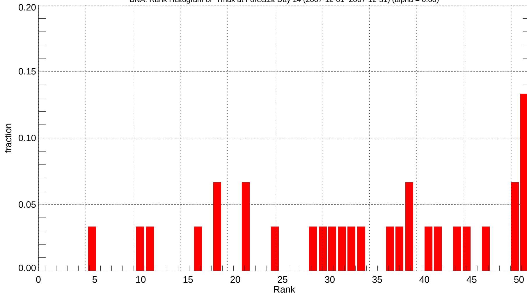
BNA: Rank Histogram of Tmax at Forecast Day 14 (2007-12-01~2007-12-31) (alpha = 0.00)
