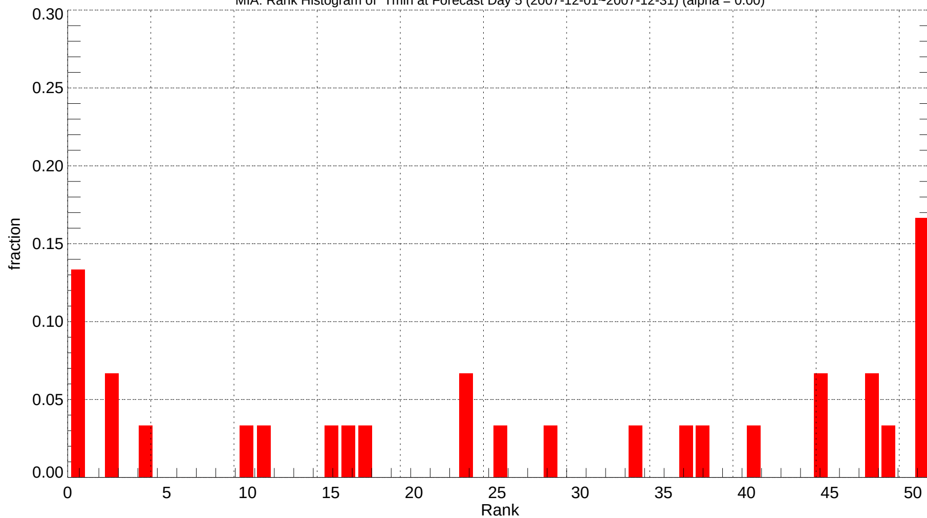
MIA: Rank Histogram of Tmin at Forecast Day 5 (2007-12-01~2007-12-31) (alpha = 0.00)
