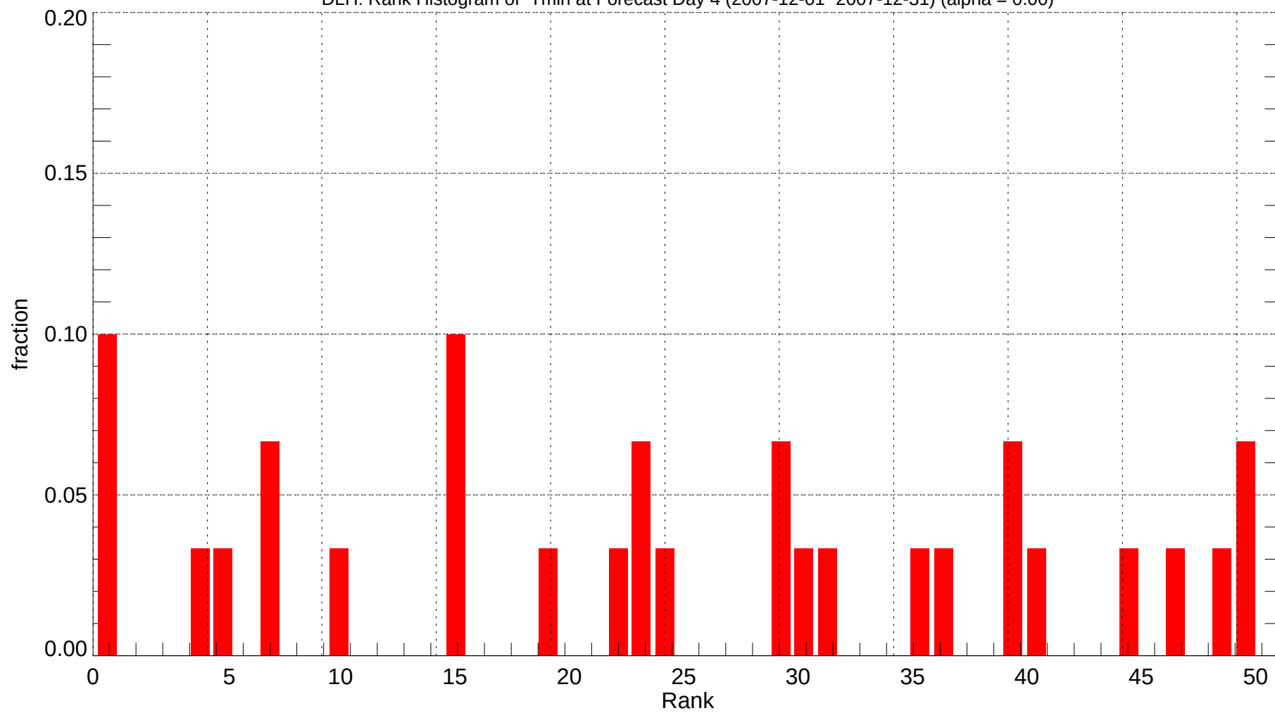
DLH: Rank Histogram of Tmin at Forecast Day 4 (2007-12-01~2007-12-31) (alpha = 0.00)
