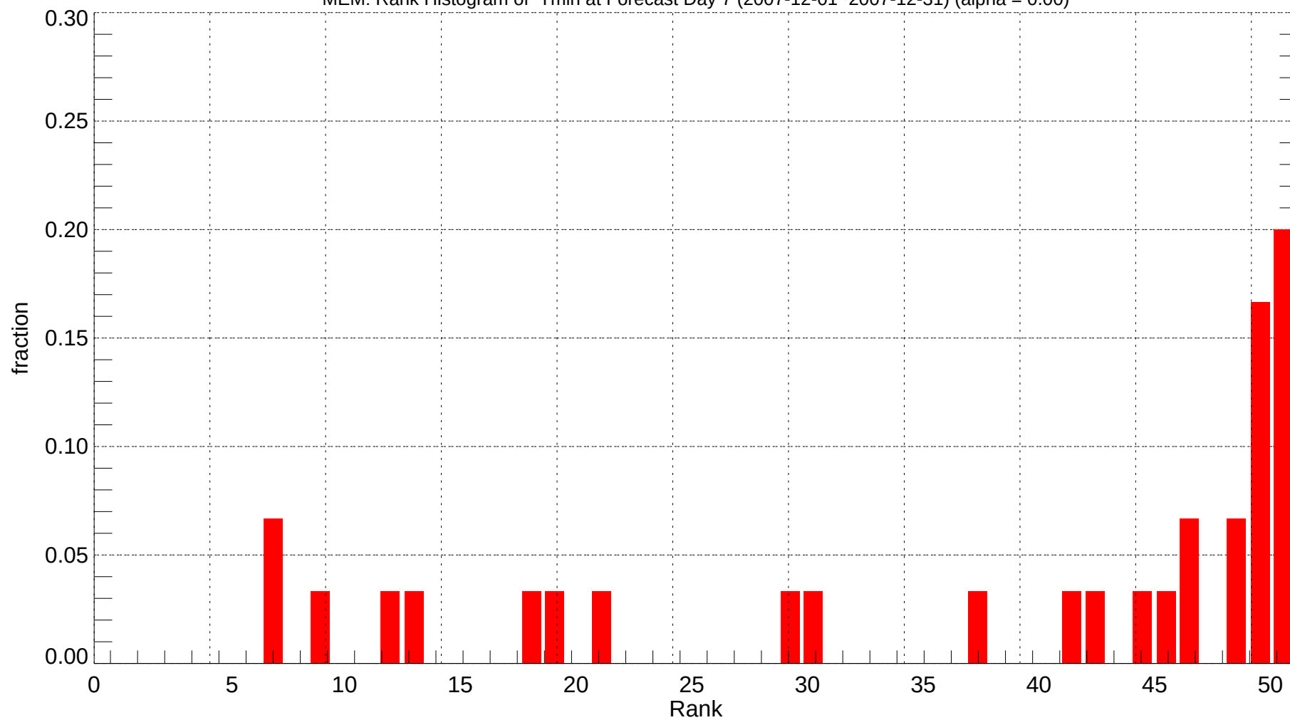
MEM: Rank Histogram of Tmin at Forecast Day 7 (2007-12-01~2007-12-31) (alpha = 0.00)
