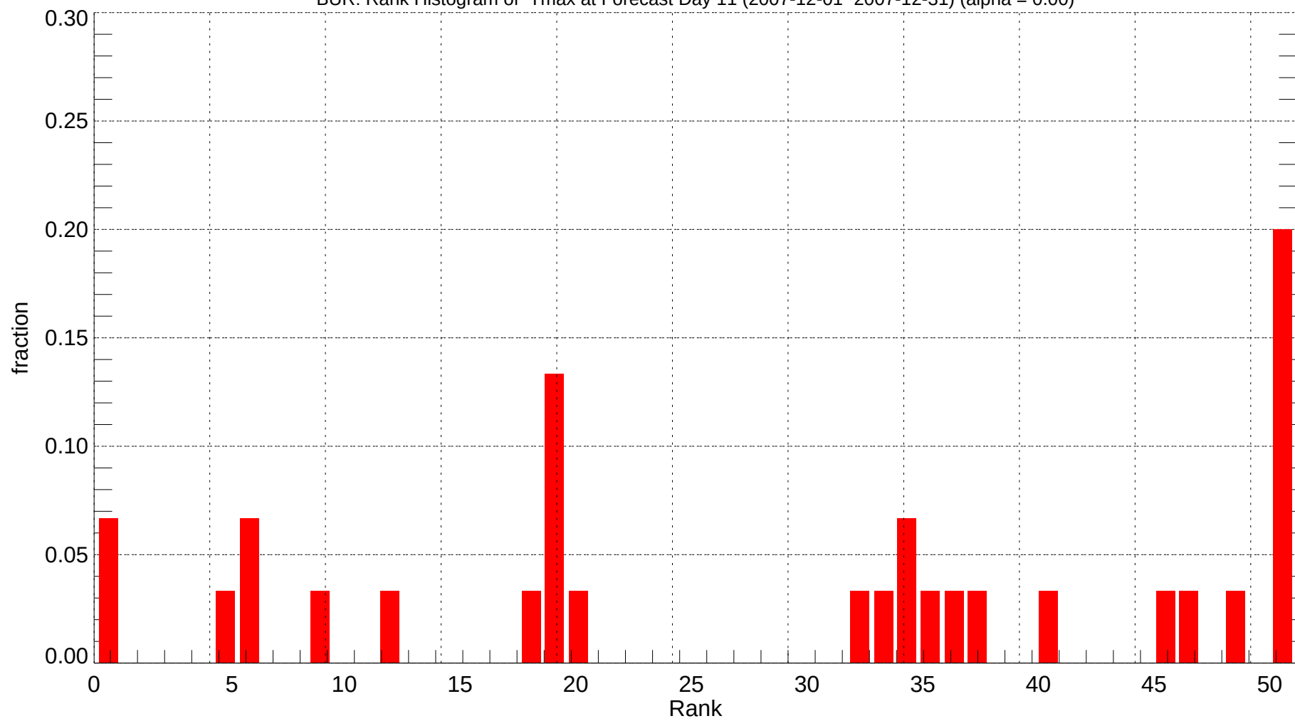
BUR: Rank Histogram of Tmax at Forecast Day 11 (2007-12-01~2007-12-31) (alpha = 0.00)
