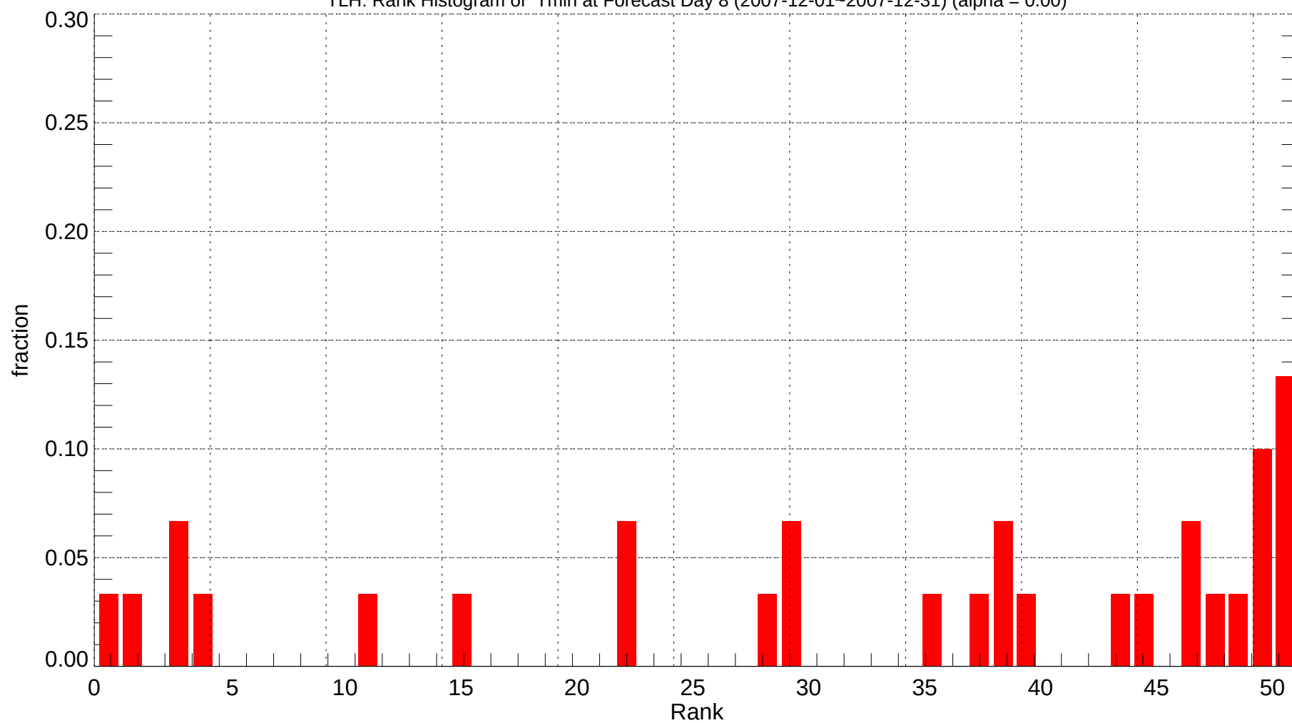
TLH: Rank Histogram of Tmin at Forecast Day 8 (2007-12-01~2007-12-31) (alpha = 0.00)
