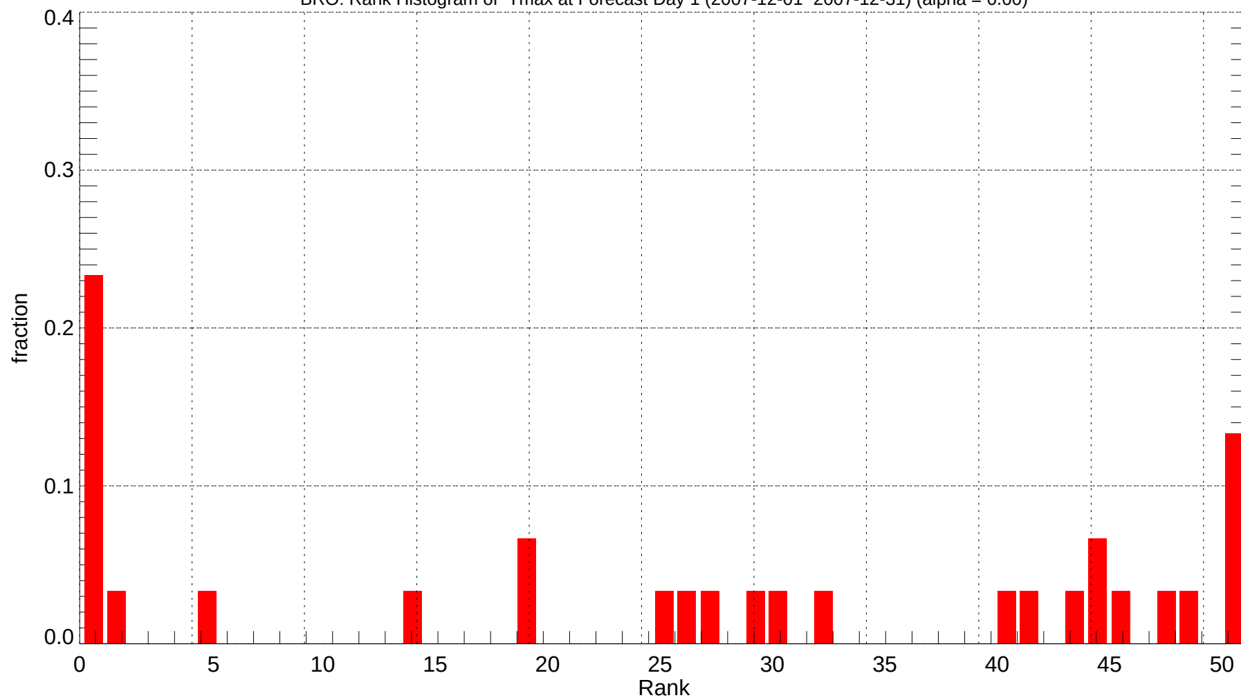
BRO: Rank Histogram of Tmax at Forecast Day 1 (2007-12-01~2007-12-31) (alpha = 0.00)
