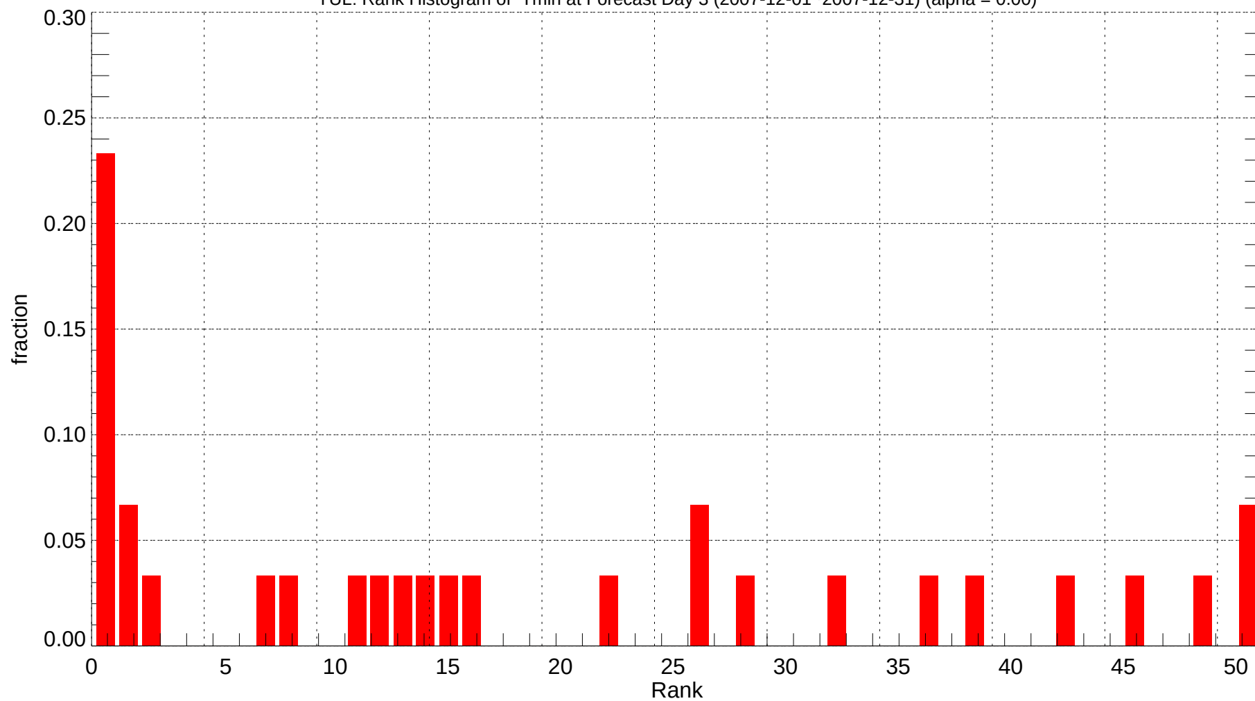
YUL: Rank Histogram of Tmin at Forecast Day 3 (2007-12-01~2007-12-31) (alpha = 0.00)
