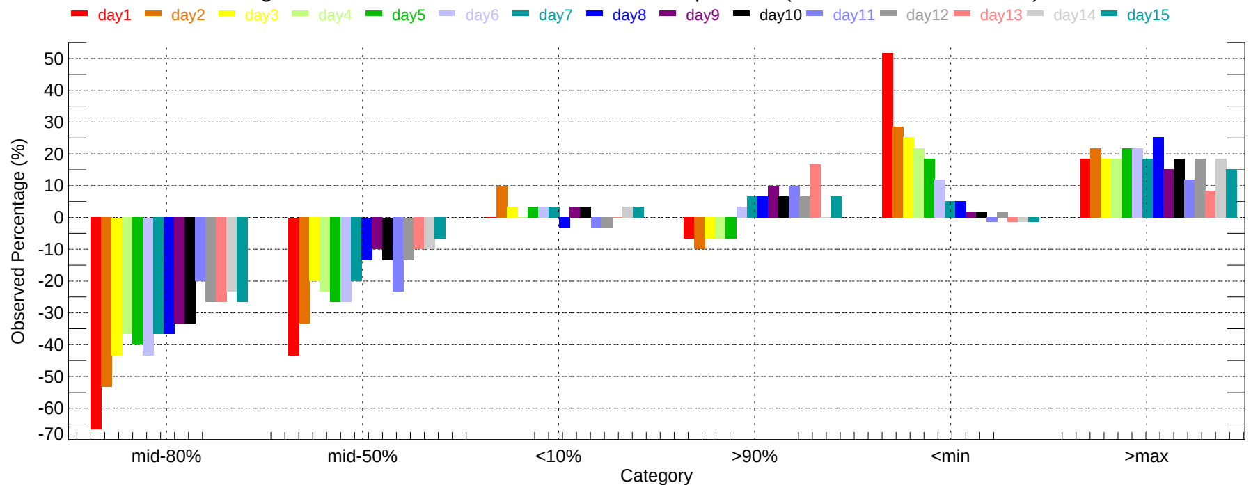
Observed Percentage Deviation of Ensembles - MOB: Min Temperature (2007-12-01~2007-12-31)
