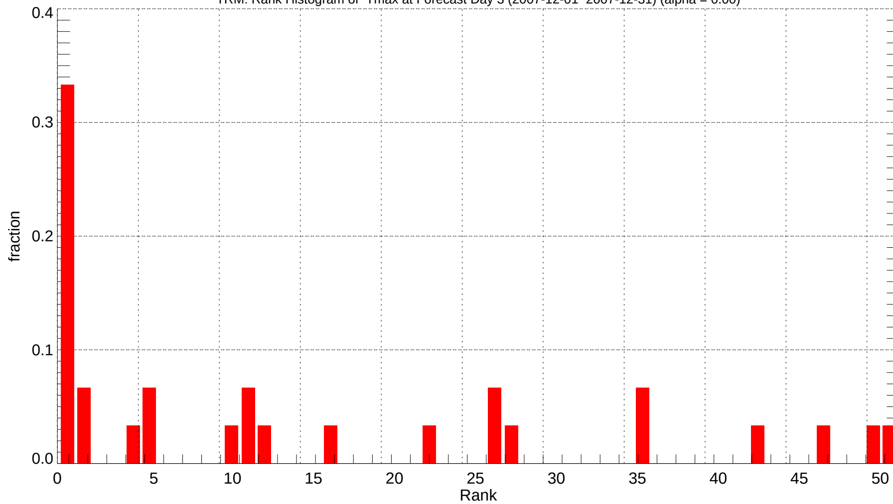
TRM: Rank Histogram of Tmax at Forecast Day 3 (2007-12-01~2007-12-31) (alpha = 0.00)
