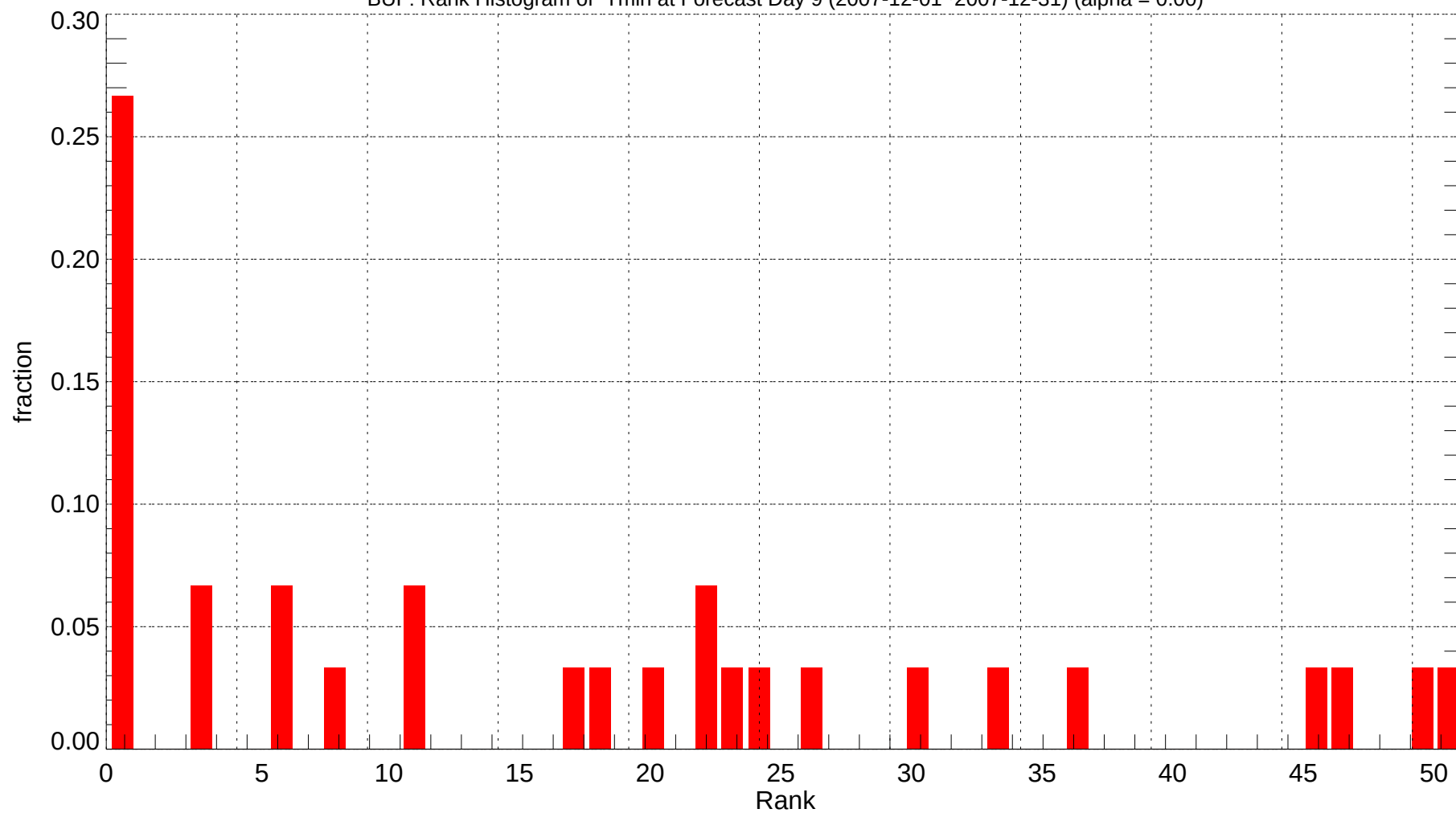
BUF: Rank Histogram of Tmin at Forecast Day 9 (2007-12-01~2007-12-31) (alpha = 0.00)
