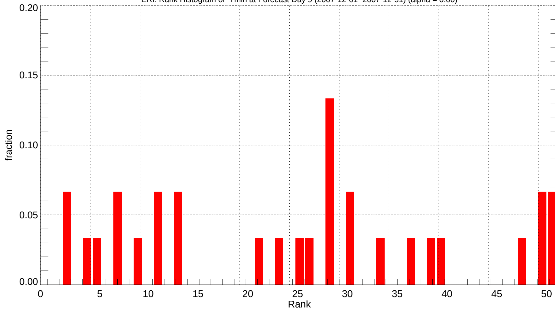
ERI: Rank Histogram of Tmin at Forecast Day 9 (2007-12-01~2007-12-31) (alpha = 0.00)
