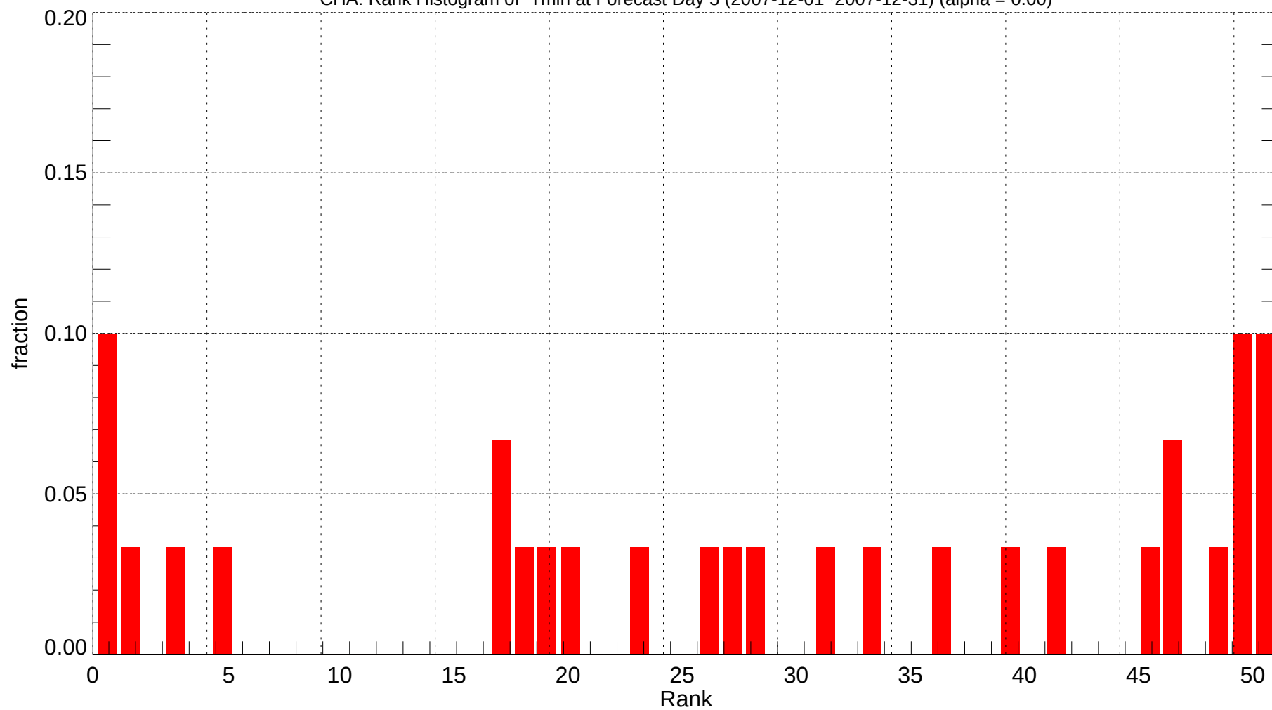
CHA: Rank Histogram of Tmin at Forecast Day 5 (2007-12-01~2007-12-31) (alpha = 0.00)
