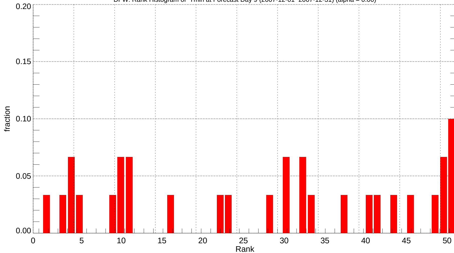
DFW: Rank Histogram of Tmin at Forecast Day 9 (2007-12-01~2007-12-31) (alpha = 0.00)
