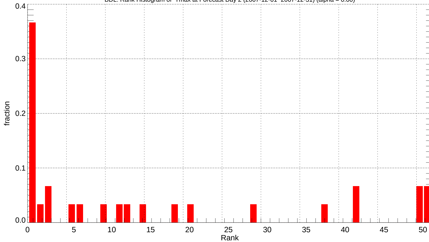
BDL: Rank Histogram of Tmax at Forecast Day 2 (2007-12-01~2007-12-31) (alpha = 0.00)
