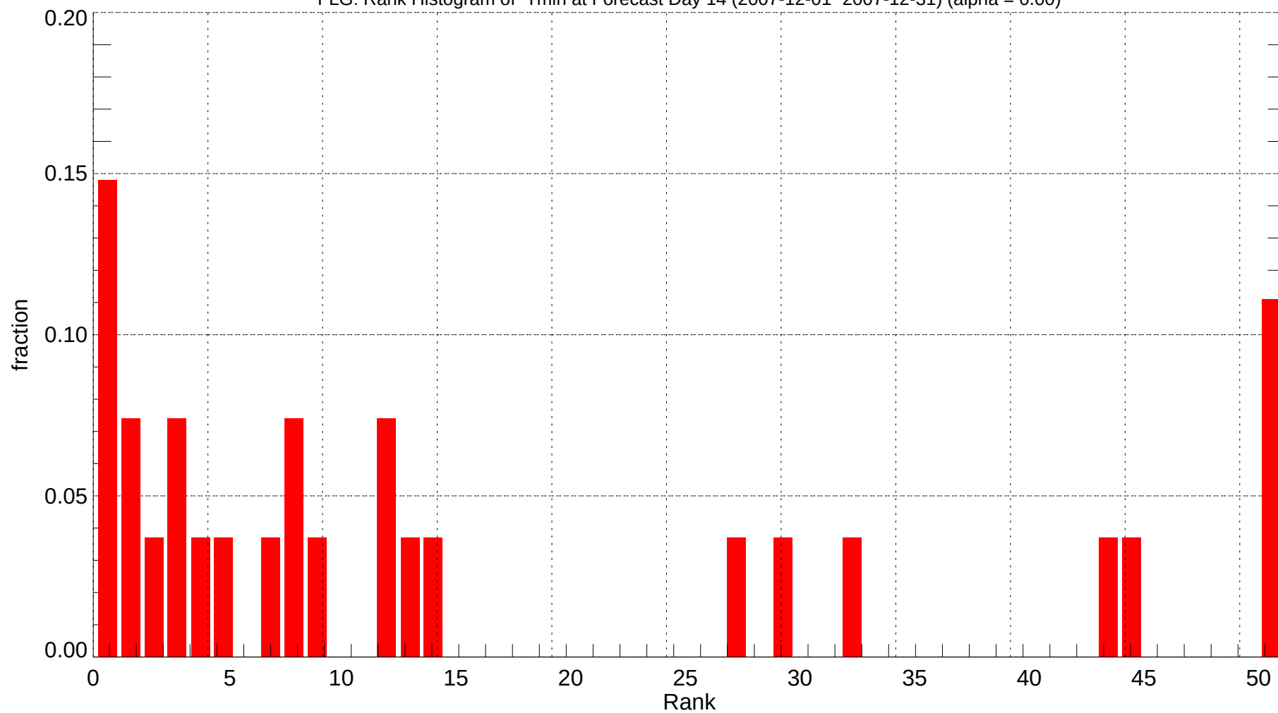
FLG: Rank Histogram of Tmin at Forecast Day 14 (2007-12-01~2007-12-31) (alpha = 0.00)
