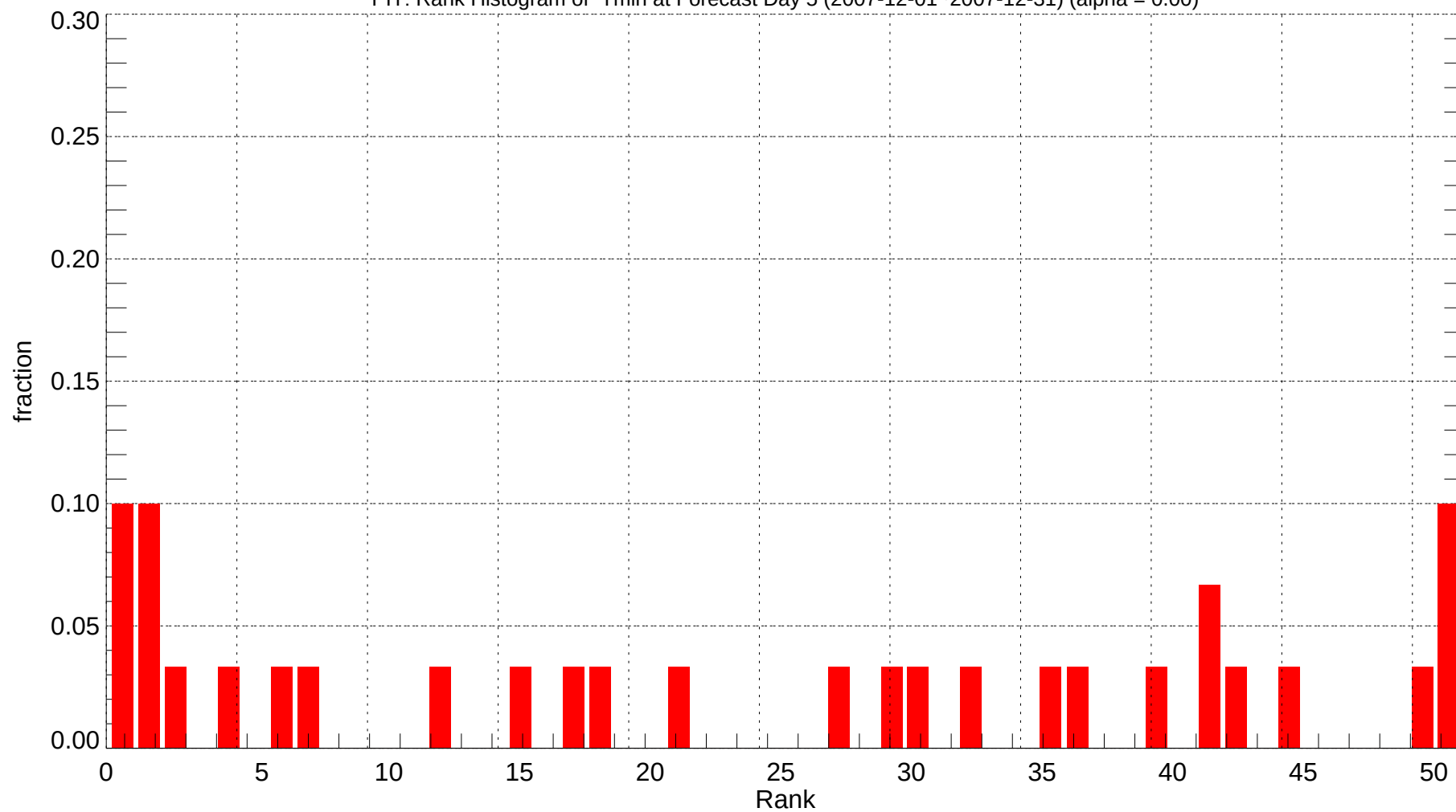
PIT: Rank Histogram of Tmin at Forecast Day 5 (2007-12-01~2007-12-31) (alpha = 0.00)
