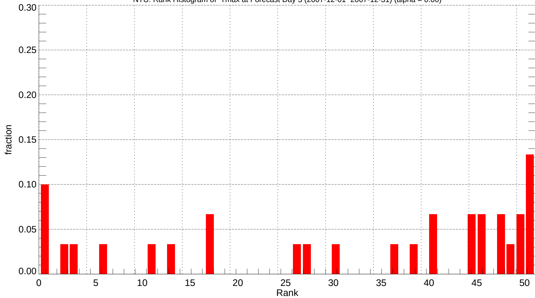
NTU: Rank Histogram of Tmax at Forecast Day 3 (2007-12-01~2007-12-31) (alpha = 0.00)
