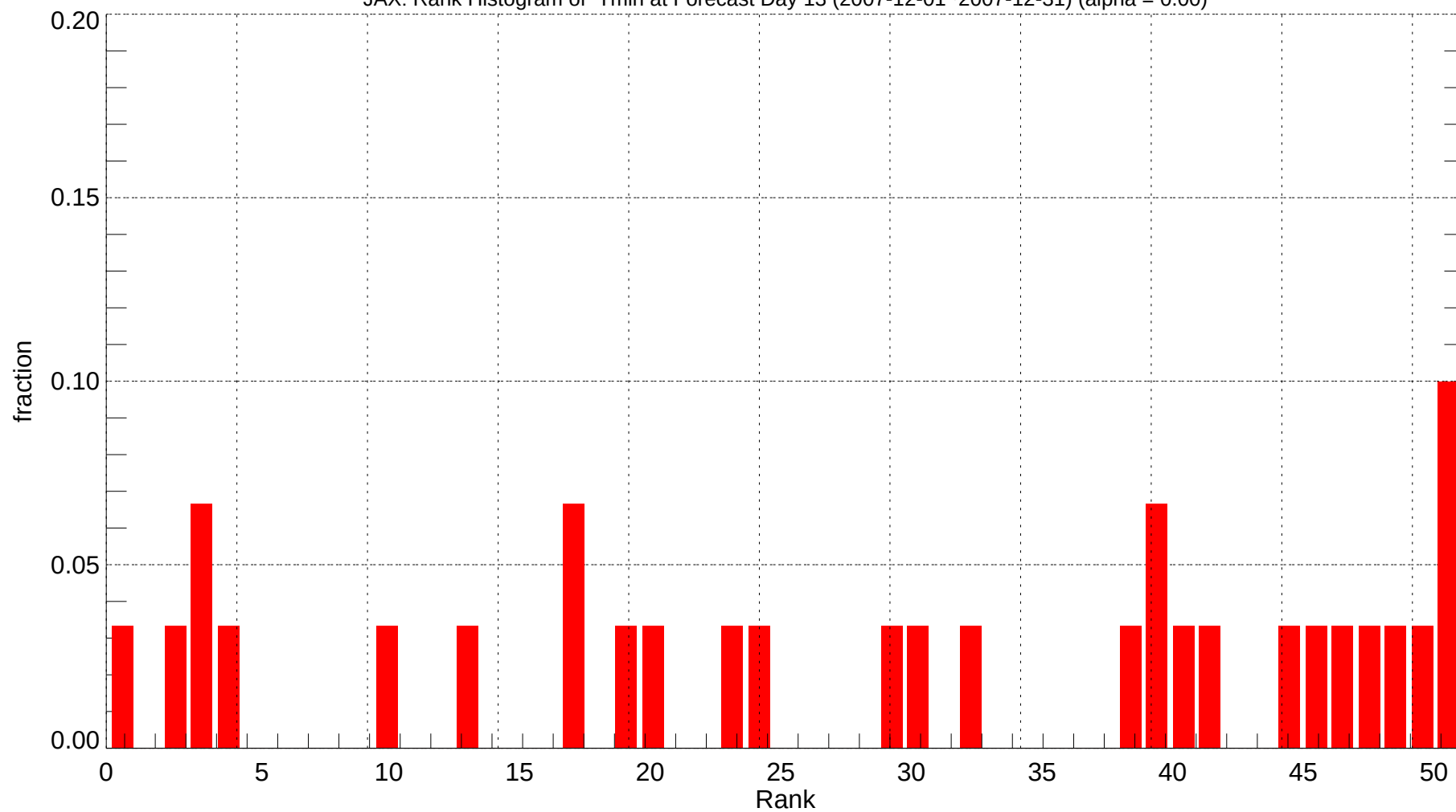
JAX: Rank Histogram of Tmin at Forecast Day 13 (2007-12-01~2007-12-31) (alpha = 0.00)
