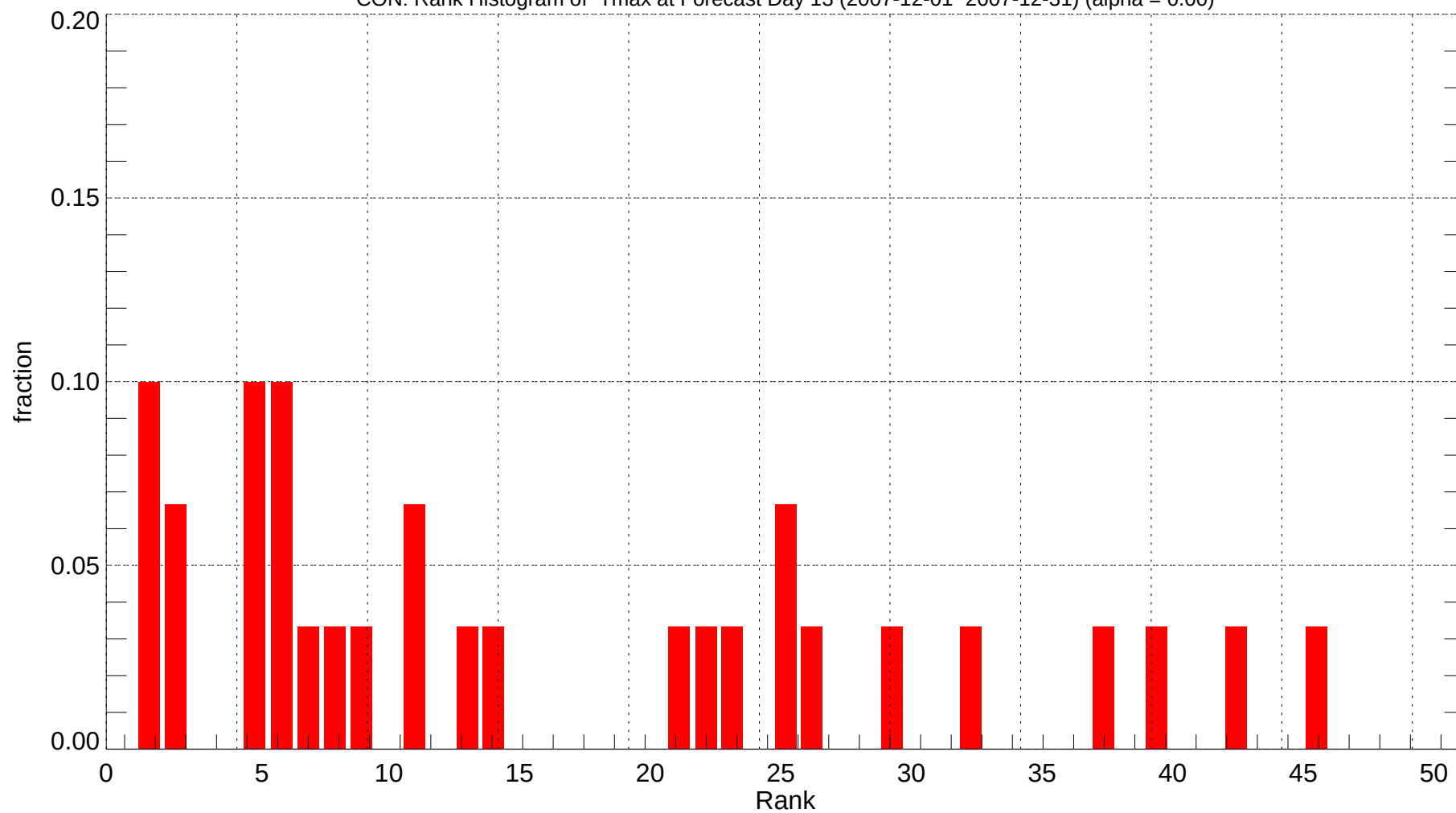
CON: Rank Histogram of Tmax at Forecast Day 13 (2007-12-01~2007-12-31) (alpha = 0.00)
