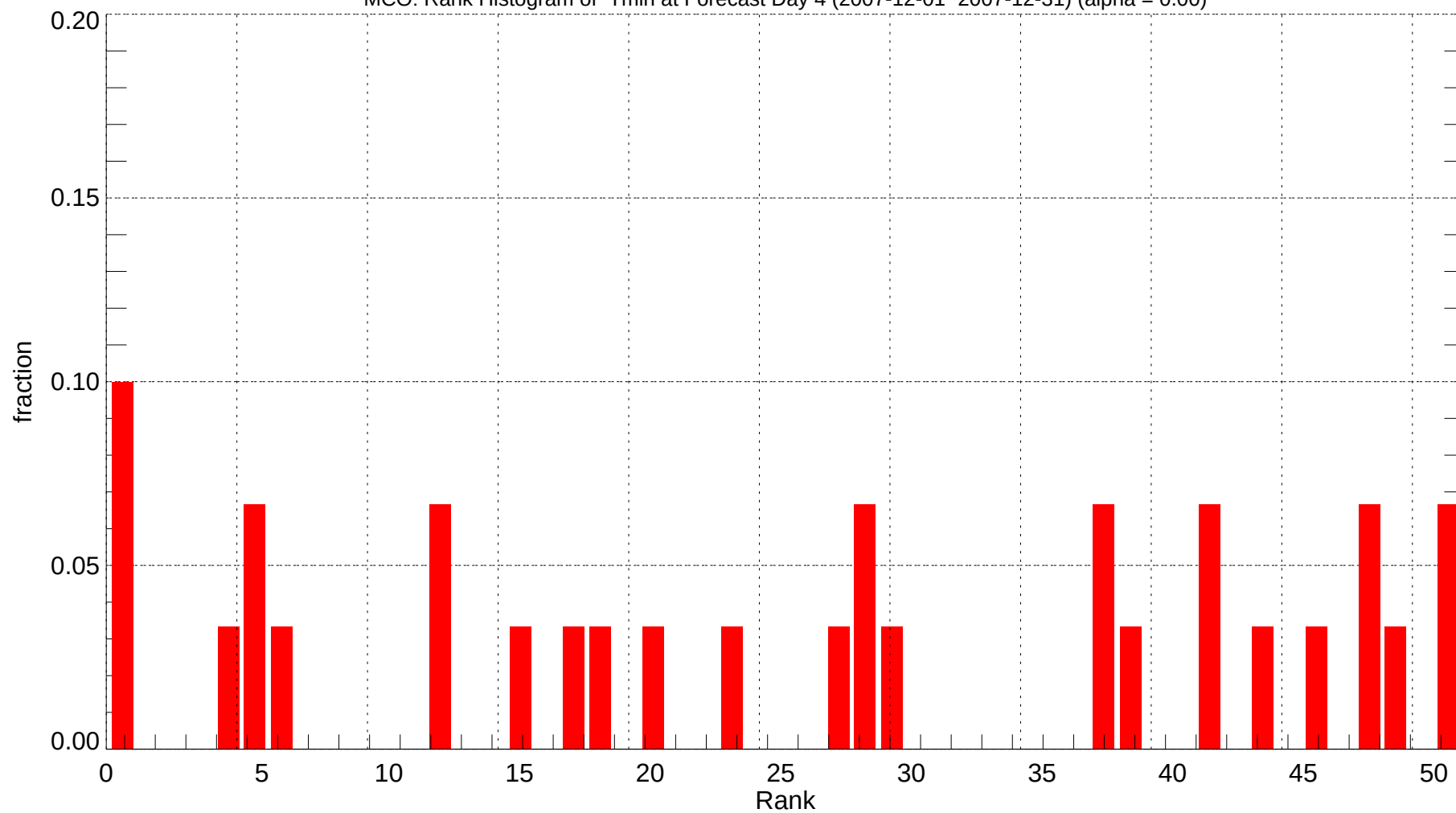
MCO: Rank Histogram of Tmin at Forecast Day 4 (2007-12-01~2007-12-31) (alpha = 0.00)
