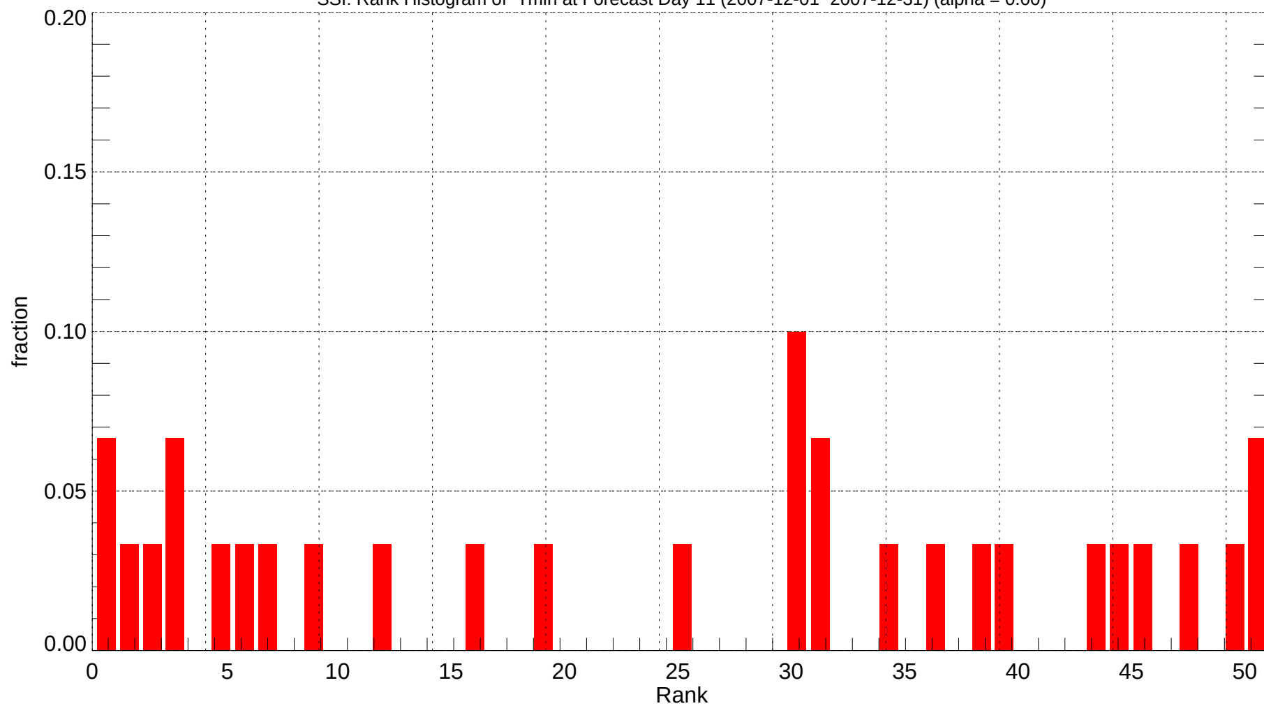
SSI: Rank Histogram of Tmin at Forecast Day 11 (2007-12-01~2007-12-31) (alpha = 0.00)
