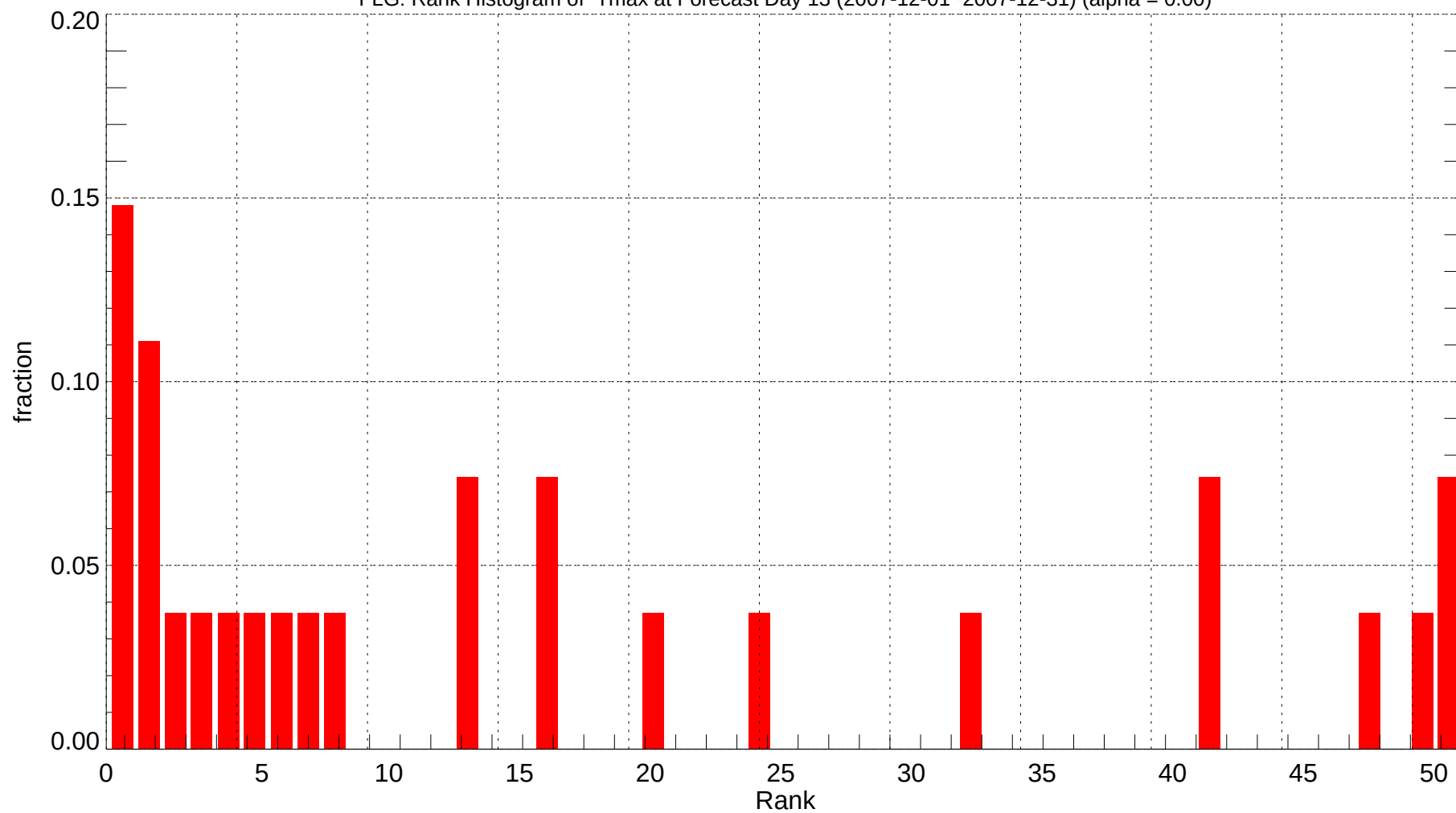
FLG: Rank Histogram of Tmax at Forecast Day 13 (2007-12-01~2007-12-31) (alpha = 0.00)
