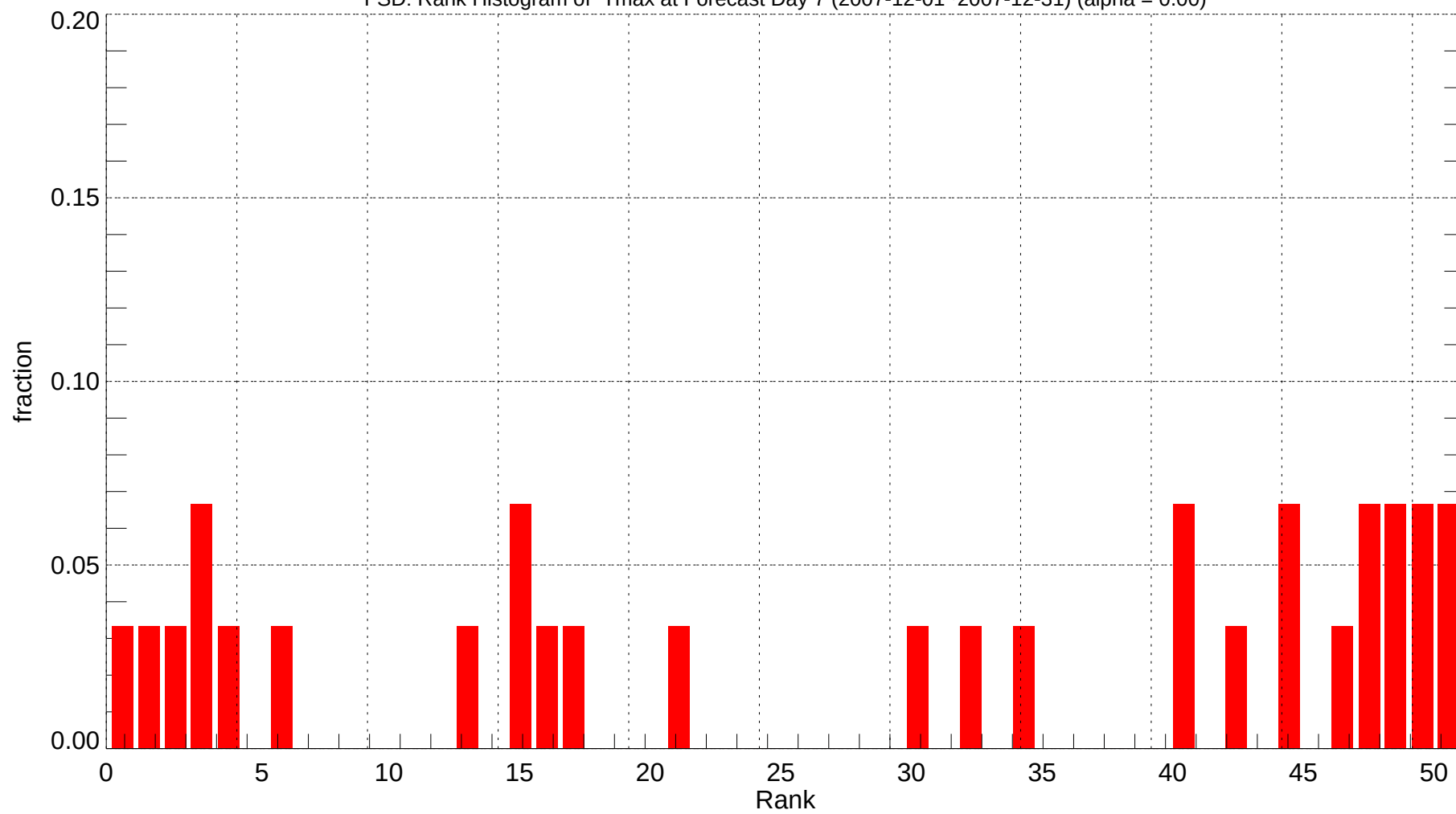
FSD: Rank Histogram of Tmax at Forecast Day 7 (2007-12-01~2007-12-31) (alpha = 0.00)
