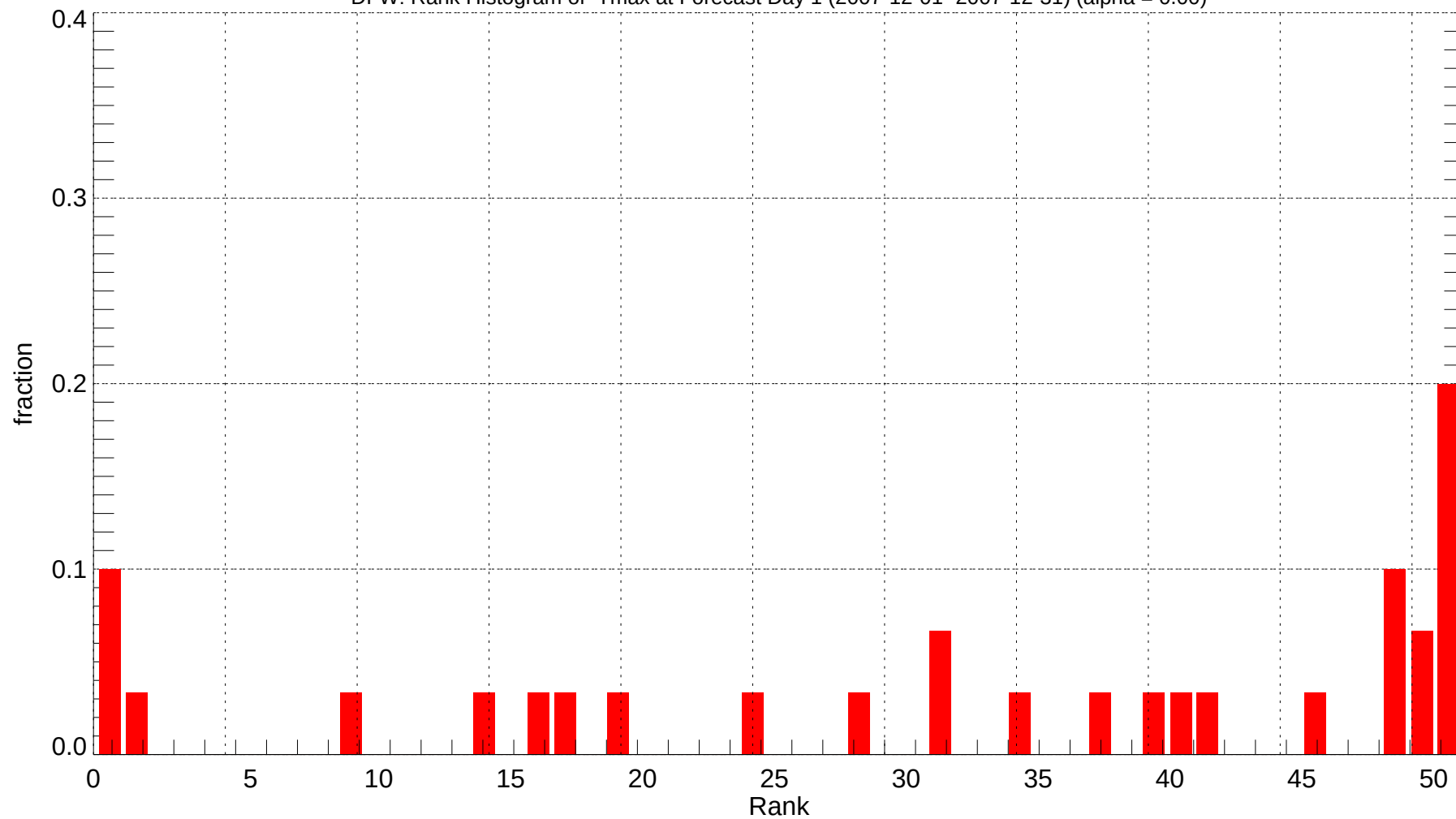
DFW: Rank Histogram of Tmax at Forecast Day 1 (2007-12-01~2007-12-31) (alpha = 0.00)
