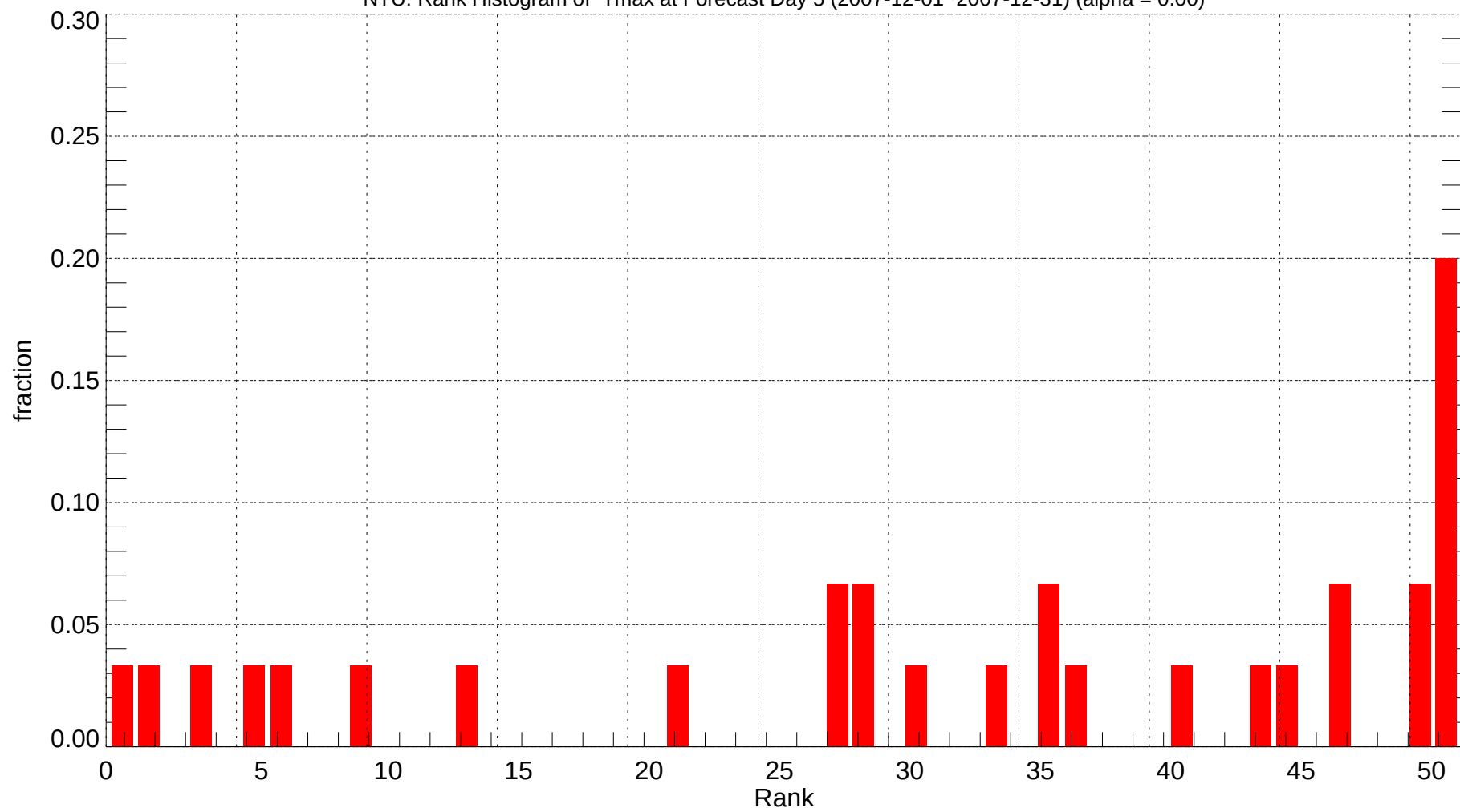
NTU: Rank Histogram of Tmax at Forecast Day 5 (2007-12-01~2007-12-31) (alpha = 0.00)
