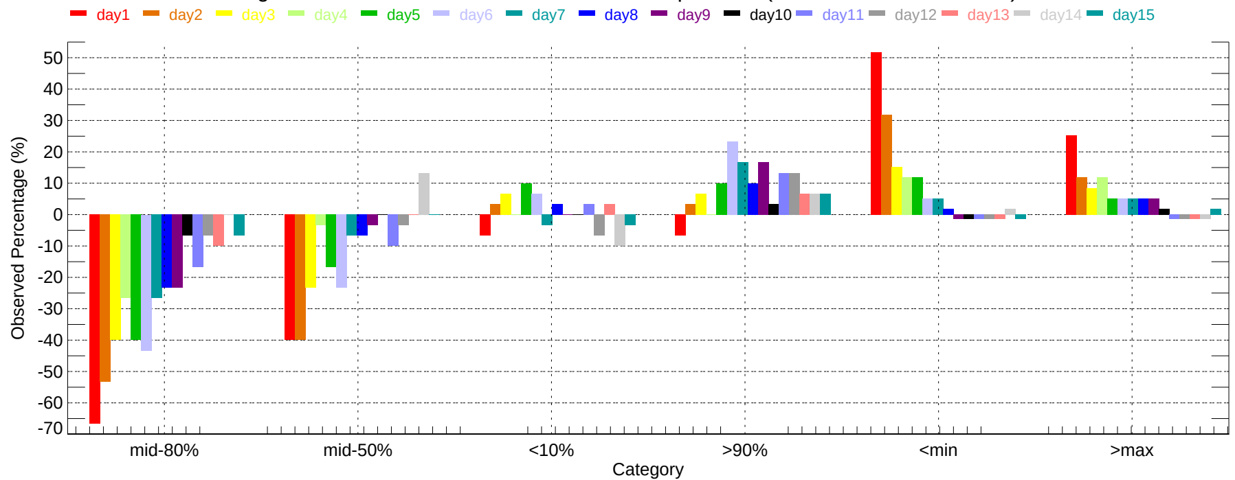
Observed Percentage Deviation of Ensembles - BWI: Min Temperature (2007-12-01~2007-12-31)
