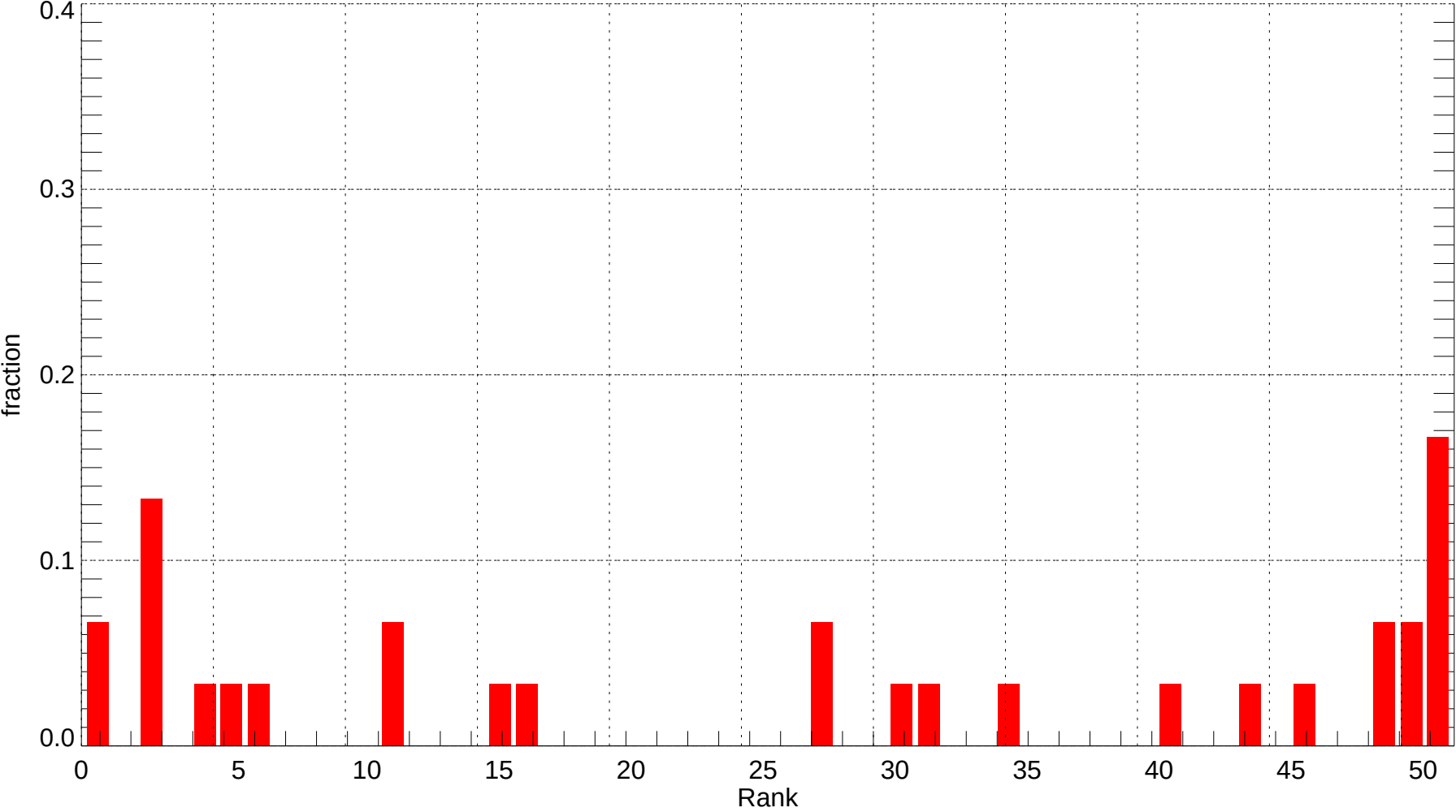
ELP: Rank Histogram of Tmin at Forecast Day 3 (2007-12-01~2007-12-31) (alpha = 0.00)
