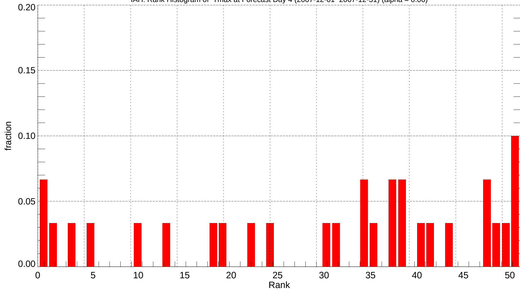
IAH: Rank Histogram of Tmax at Forecast Day 4 (2007-12-01~2007-12-31) (alpha = 0.00)
