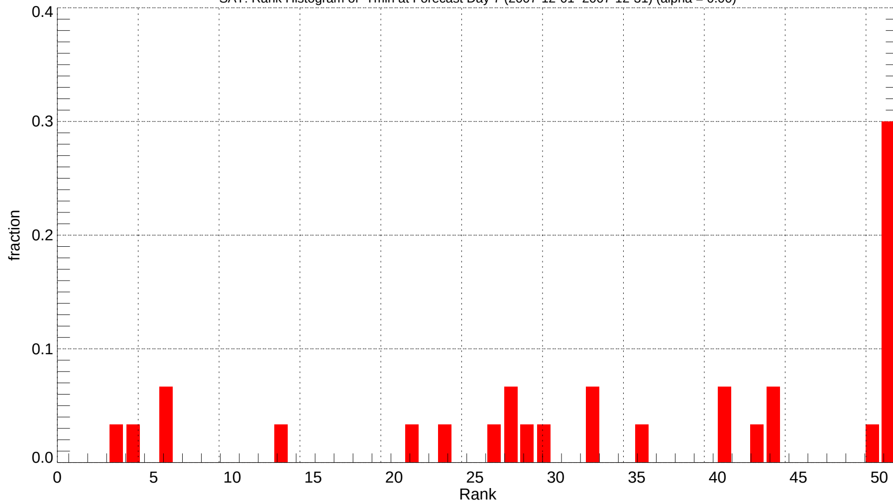
SAT: Rank Histogram of Tmin at Forecast Day 7 (2007-12-01~2007-12-31) (alpha = 0.00)
