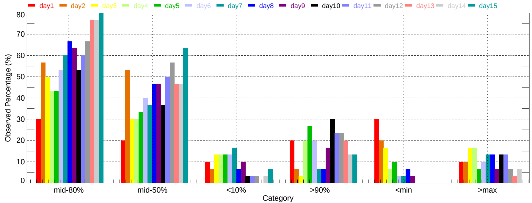
Observed Percentage of Ensembles - SEA: Max Temperature (2007-12-01~2007-12-31)
