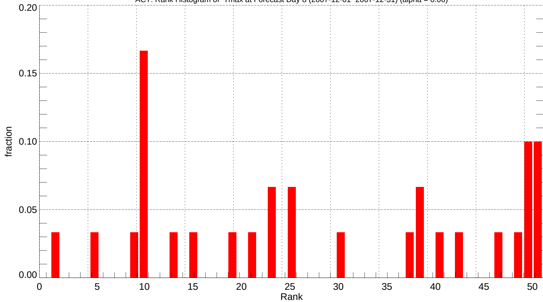
ACT: Rank Histogram of Tmax at Forecast Day 8 (2007-12-01~2007-12-31) (alpha = 0.00)
