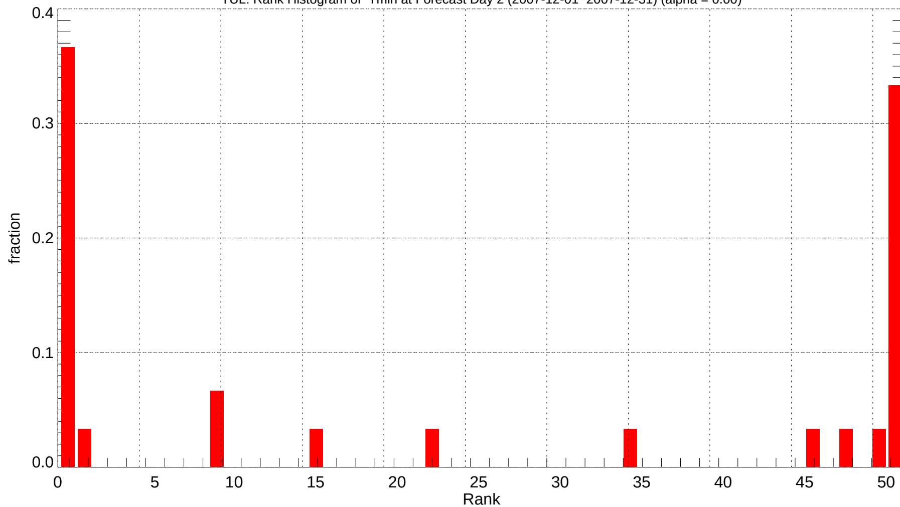
TUL: Rank Histogram of Tmin at Forecast Day 2 (2007-12-01~2007-12-31) (alpha = 0.00)
