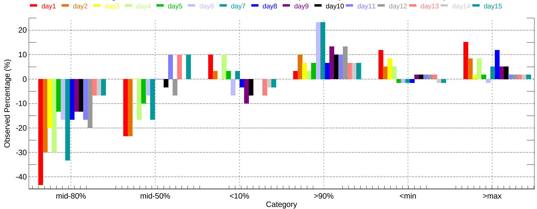
Observed Percentage Deviation of Ensembles - DAY: Max Temperature (2007-12-01~2007-12-31)
