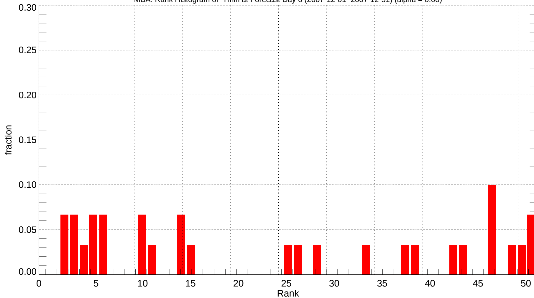
MBA: Rank Histogram of Tmin at Forecast Day 6 (2007-12-01~2007-12-31) (alpha = 0.00)
