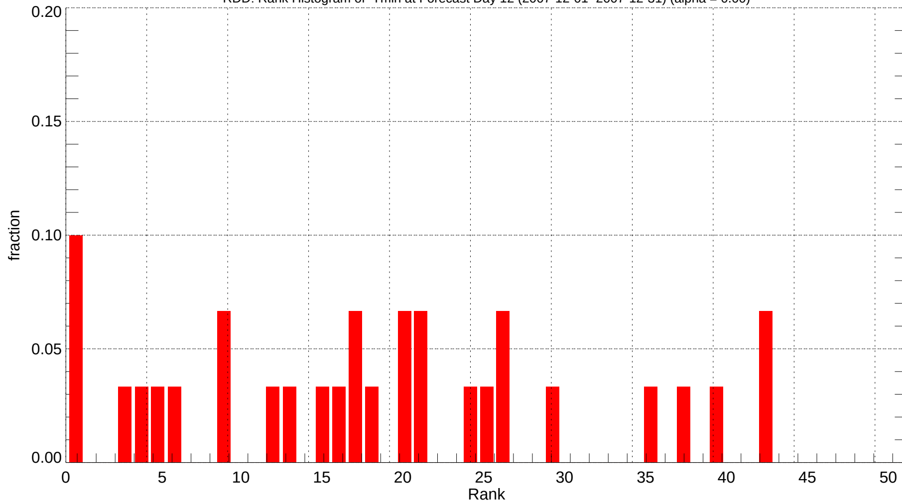
RDD: Rank Histogram of Tmin at Forecast Day 12 (2007-12-01~2007-12-31) (alpha = 0.00)
