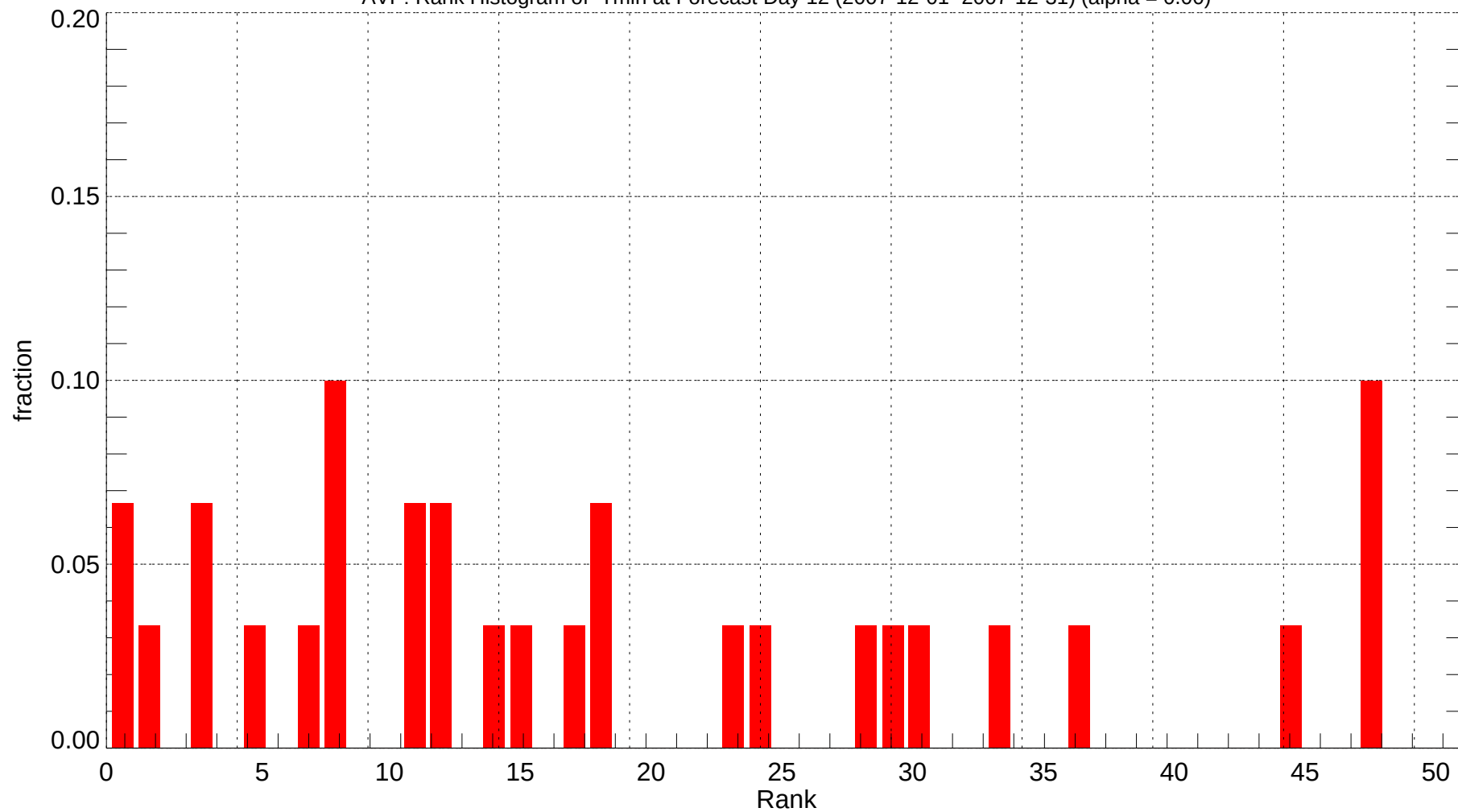
AVP: Rank Histogram of Tmin at Forecast Day 12 (2007-12-01~2007-12-31) (alpha = 0.00)
