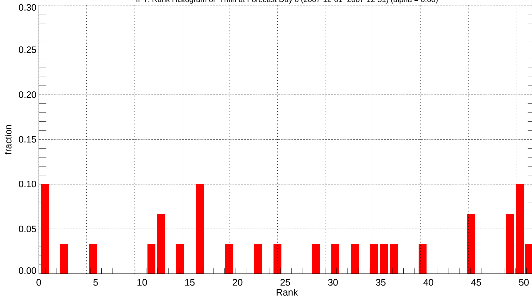
IPT: Rank Histogram of Tmin at Forecast Day 6 (2007-12-01~2007-12-31) (alpha = 0.00)
