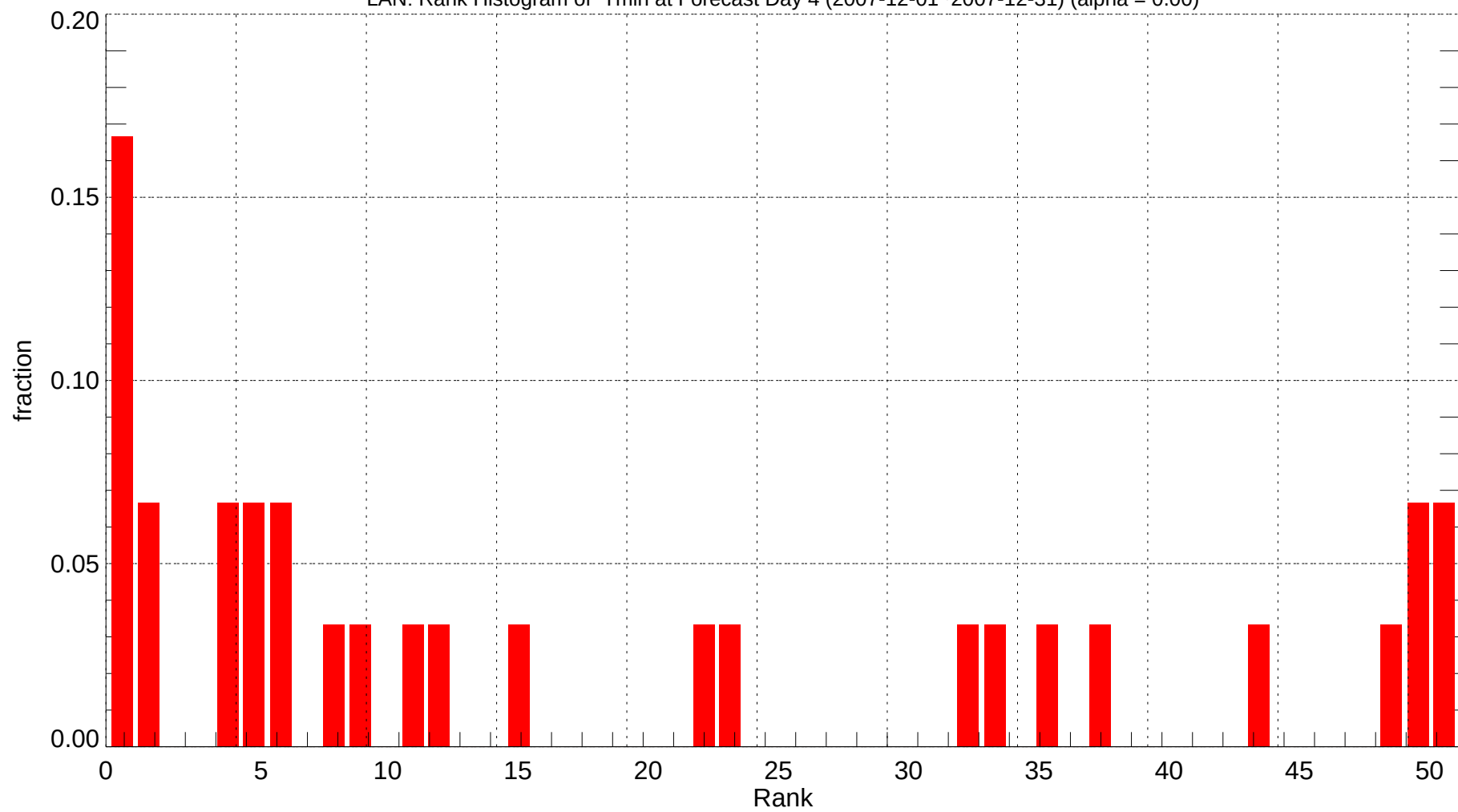
LAN: Rank Histogram of Tmin at Forecast Day 4 (2007-12-01~2007-12-31) (alpha = 0.00)
