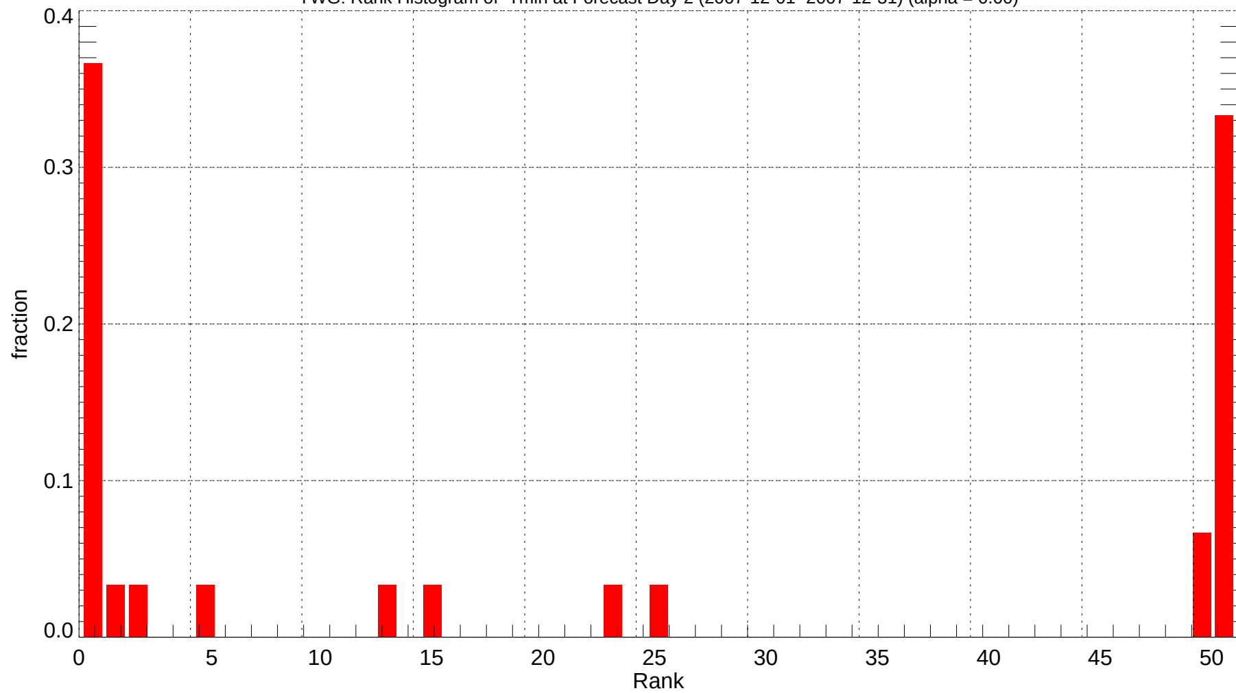
YWG: Rank Histogram of Tmin at Forecast Day 2 (2007-12-01~2007-12-31) (alpha = 0.00)
