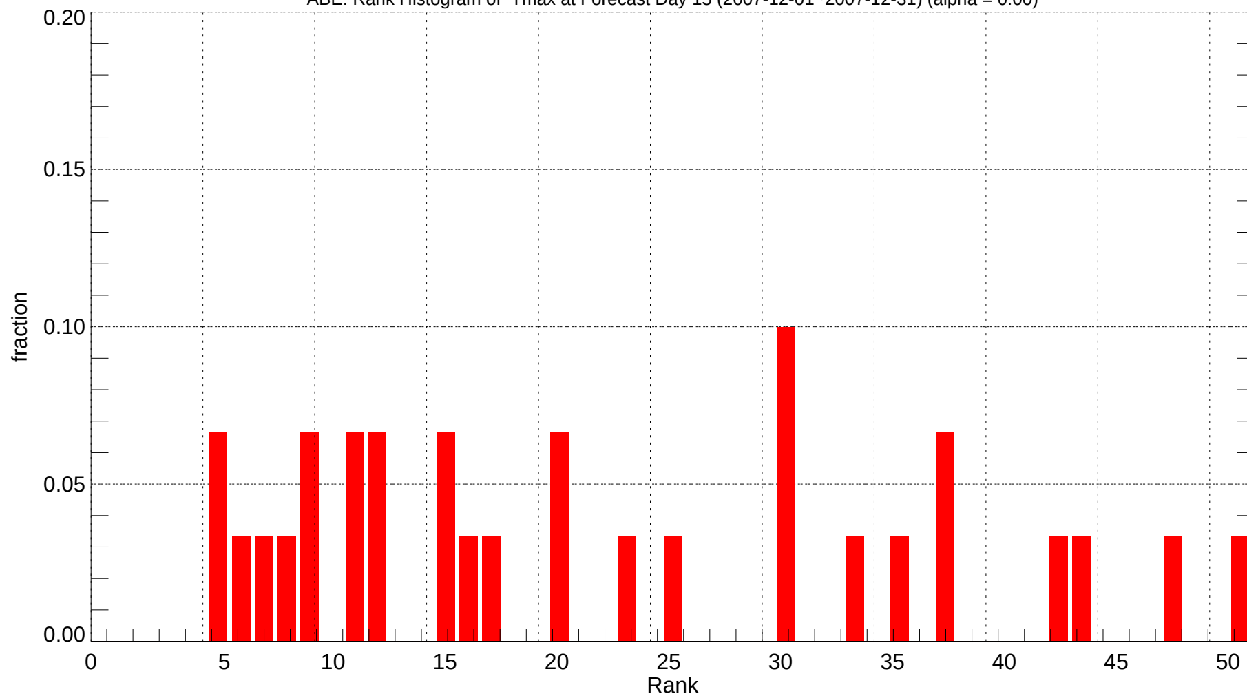
ABE: Rank Histogram of Tmax at Forecast Day 15 (2007-12-01~2007-12-31) (alpha = 0.00)
