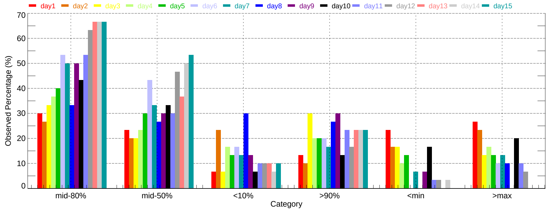
Observed Percentage of Ensembles - COU: Max Temperature (2007-12-01~2007-12-31)
