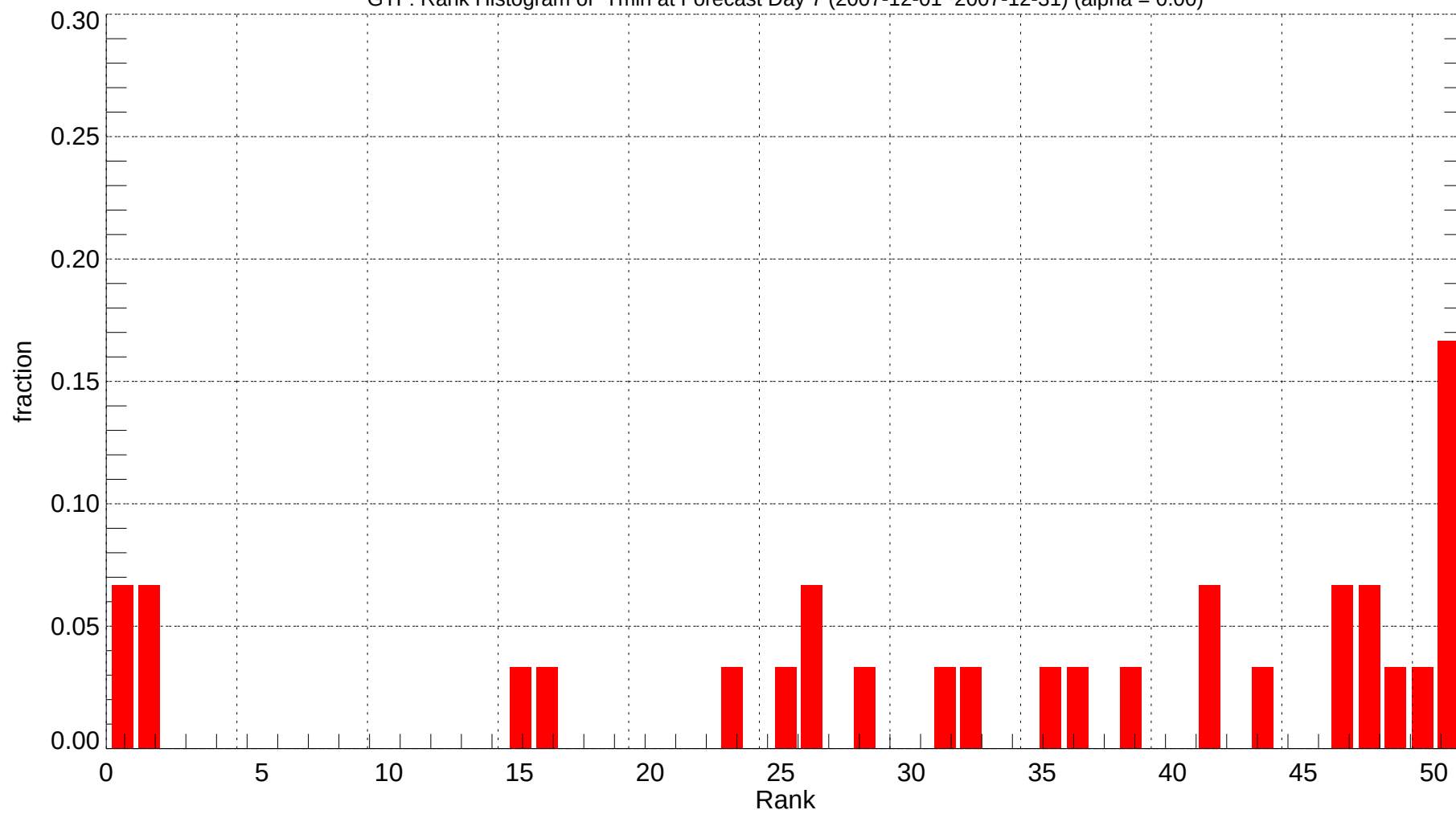
GTF: Rank Histogram of Tmin at Forecast Day 7 (2007-12-01~2007-12-31) (alpha = 0.00)
