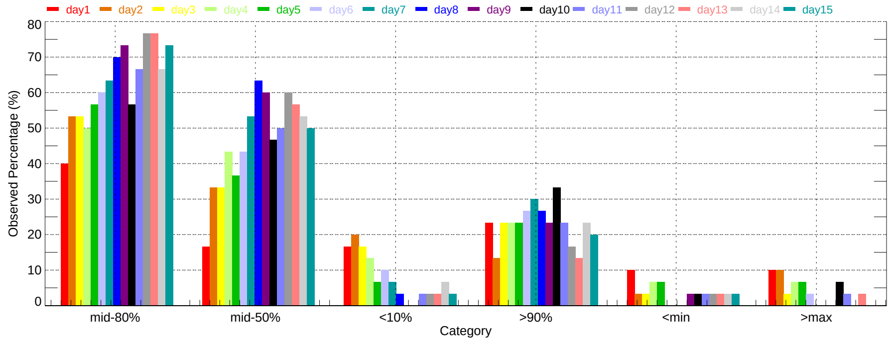
Observed Percentage of Ensembles - MCO: Max Temperature (2007-12-01~2007-12-31)
