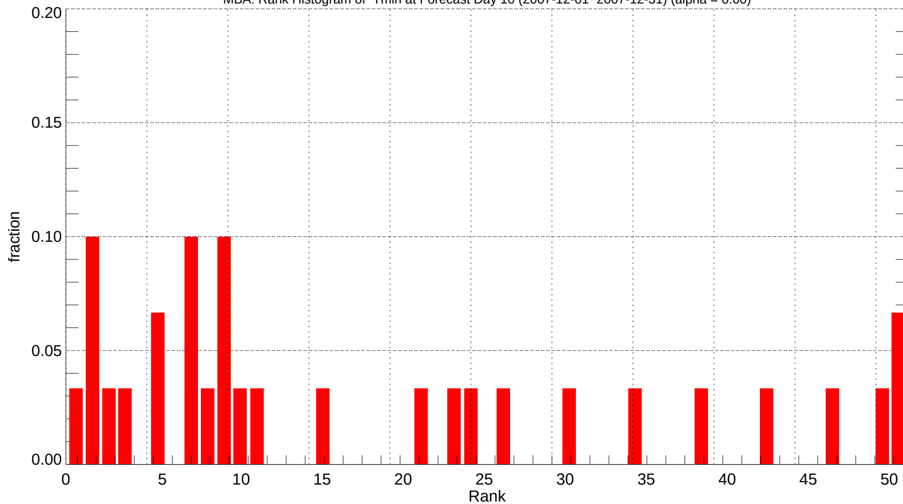
MBA: Rank Histogram of Tmin at Forecast Day 10 (2007-12-01~2007-12-31) (alpha = 0.00)
