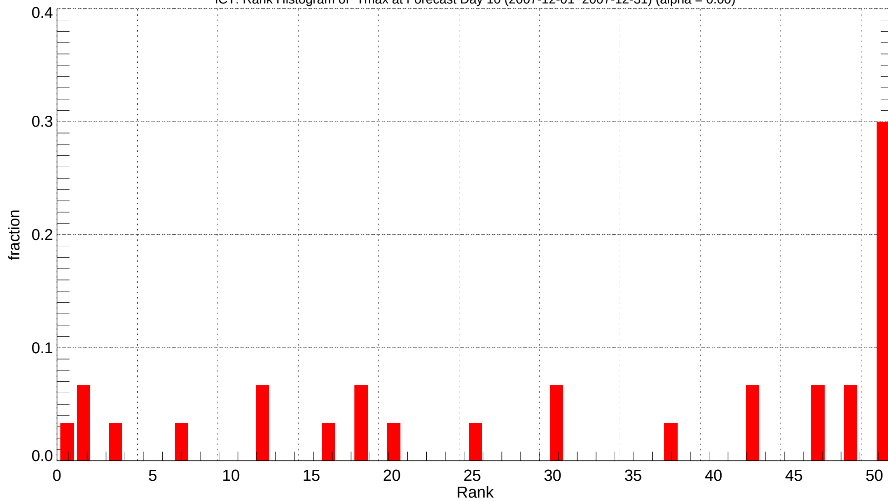
ICT: Rank Histogram of Tmax at Forecast Day 10 (2007-12-01~2007-12-31) (alpha = 0.00)
