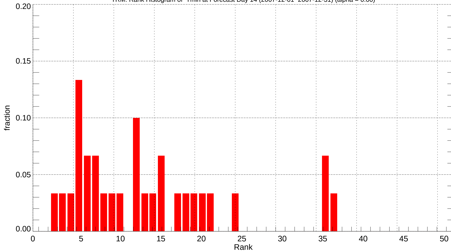
TRM: Rank Histogram of Tmin at Forecast Day 14 (2007-12-01~2007-12-31) (alpha = 0.00)
