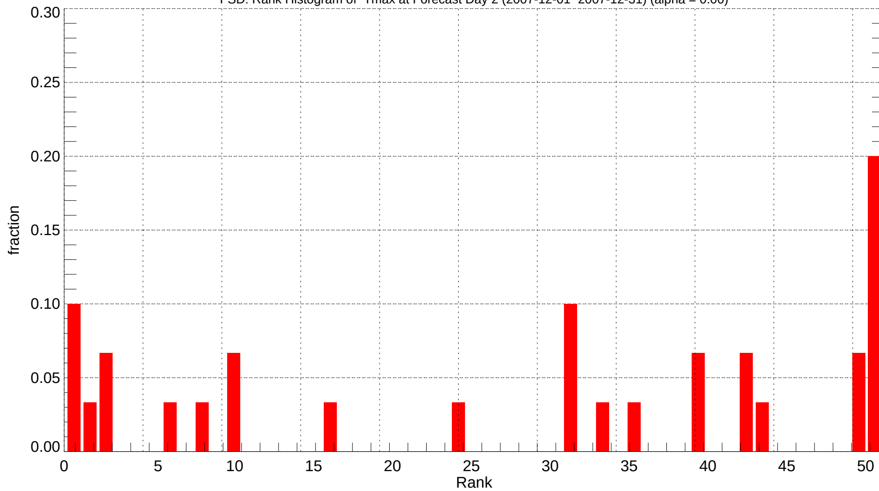
FSD: Rank Histogram of Tmax at Forecast Day 2 (2007-12-01~2007-12-31) (alpha = 0.00)
