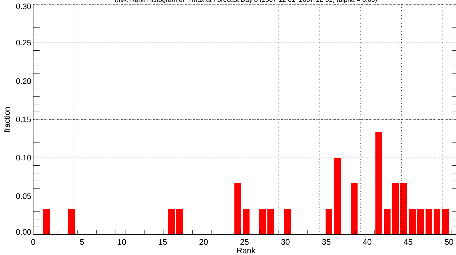
MIA: Rank Histogram of Tmax at Forecast Day 8 (2007-12-01~2007-12-31) (alpha = 0.00)
