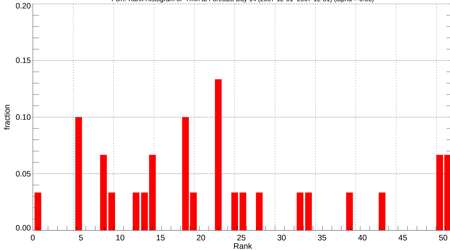
PDX: Rank Histogram of Tmin at Forecast Day 14 (2007-12-01~2007-12-31) (alpha = 0.00)
