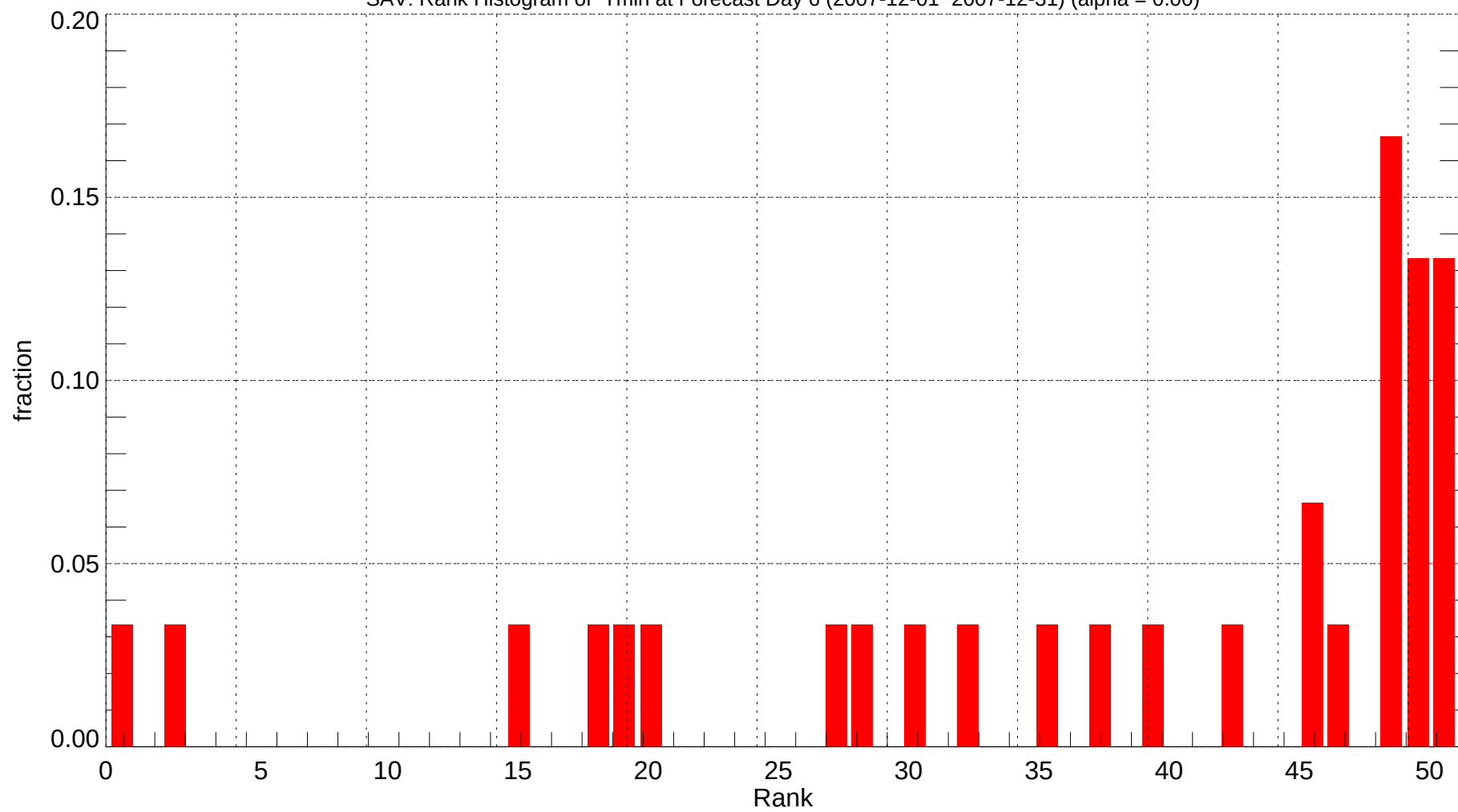
SAV: Rank Histogram of Tmin at Forecast Day 6 (2007-12-01~2007-12-31) (alpha = 0.00)
