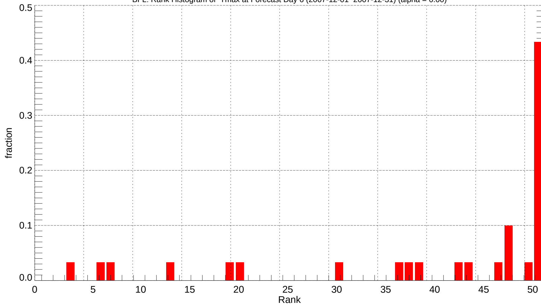
BFL: Rank Histogram of Tmax at Forecast Day 6 (2007-12-01~2007-12-31) (alpha = 0.00)
