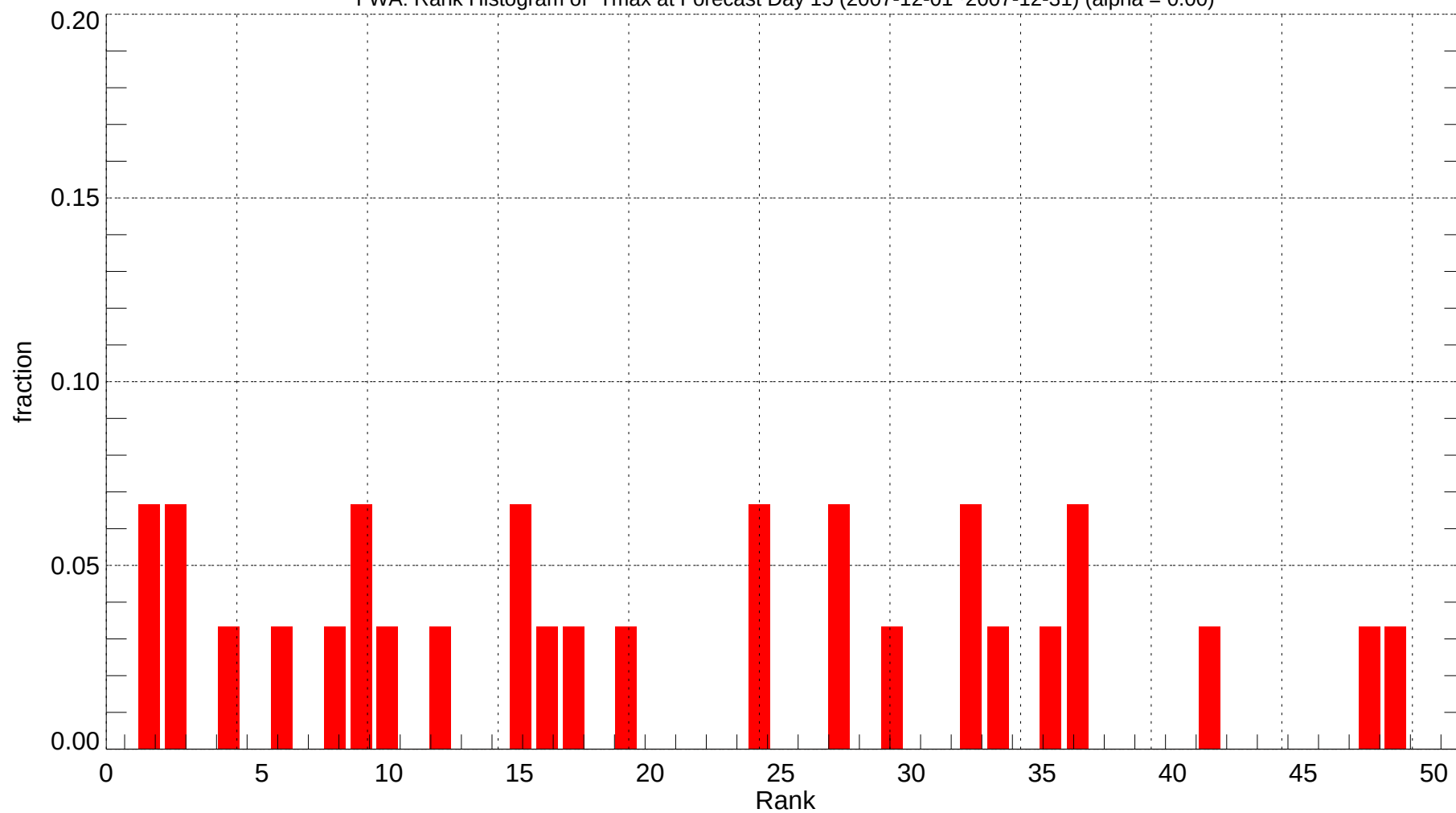
FWA: Rank Histogram of Tmax at Forecast Day 15 (2007-12-01~2007-12-31) (alpha = 0.00)
