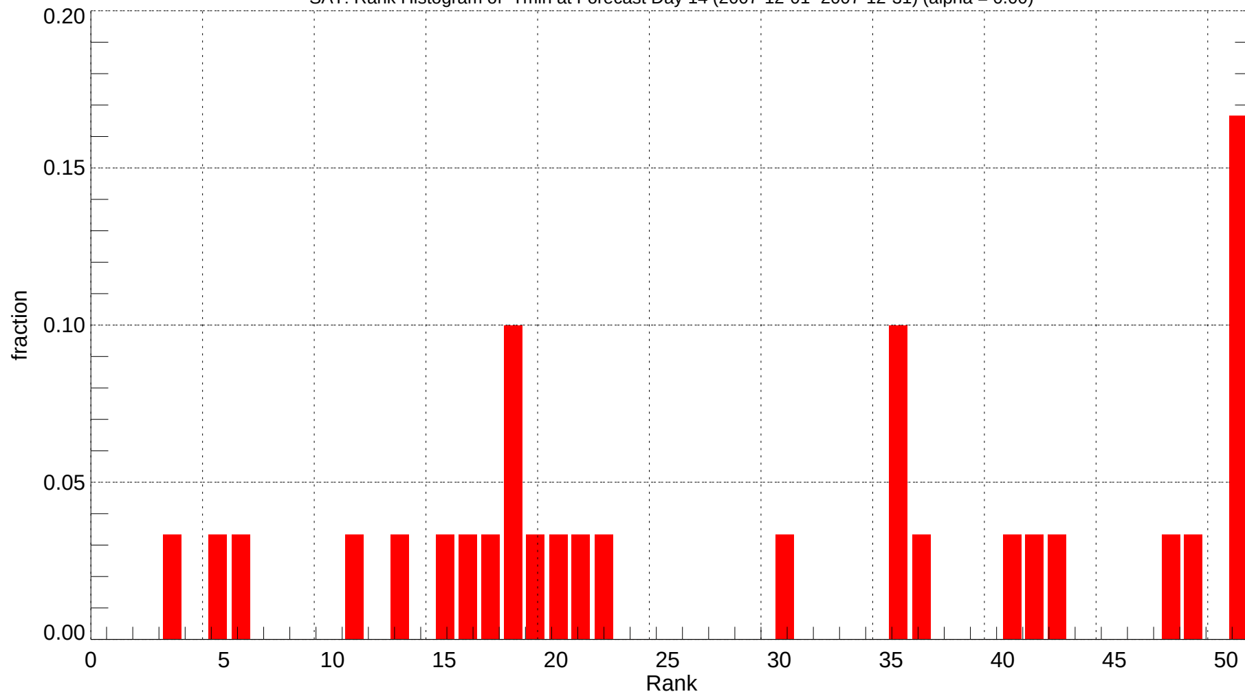
SAT: Rank Histogram of Tmin at Forecast Day 14 (2007-12-01~2007-12-31) (alpha = 0.00)
