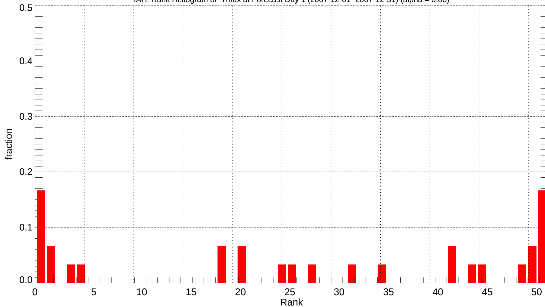
IAH: Rank Histogram of Tmax at Forecast Day 1 (2007-12-01~2007-12-31) (alpha = 0.00)
