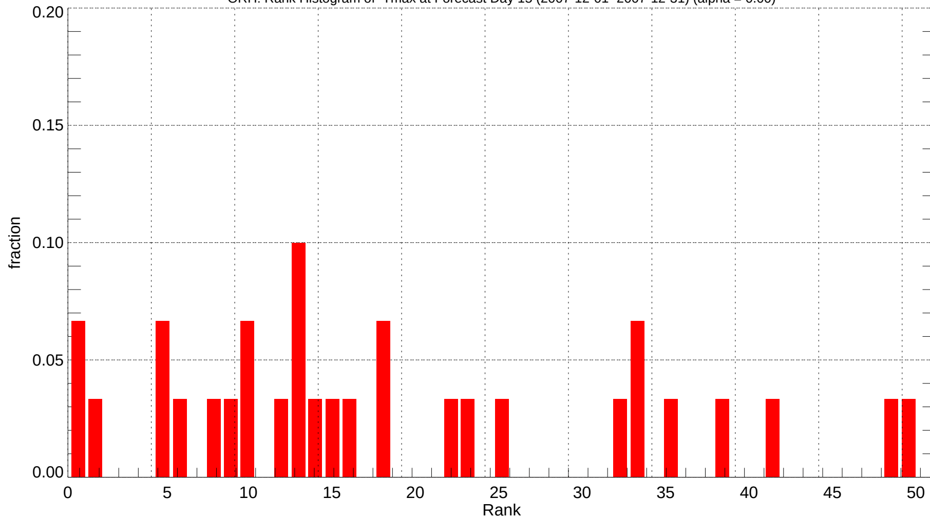
ORH: Rank Histogram of Tmax at Forecast Day 15 (2007-12-01~2007-12-31) (alpha = 0.00)
