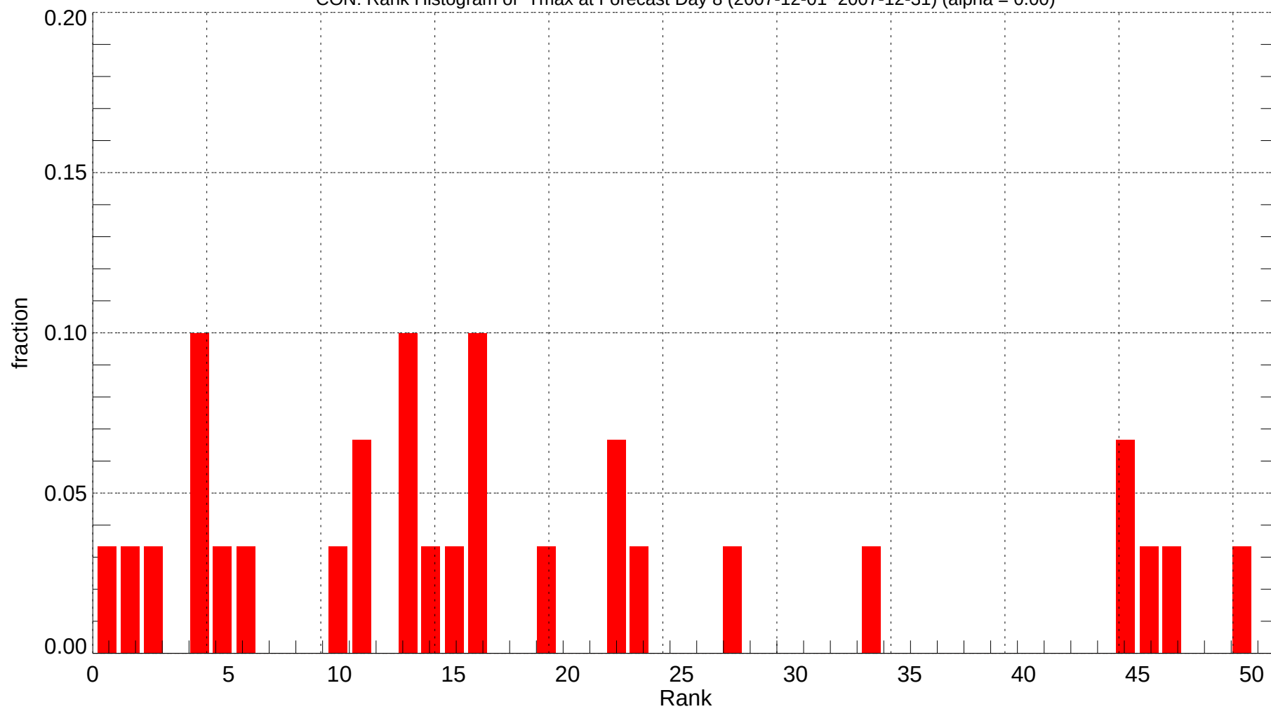
CON: Rank Histogram of Tmax at Forecast Day 8 (2007-12-01~2007-12-31) (alpha = 0.00)
