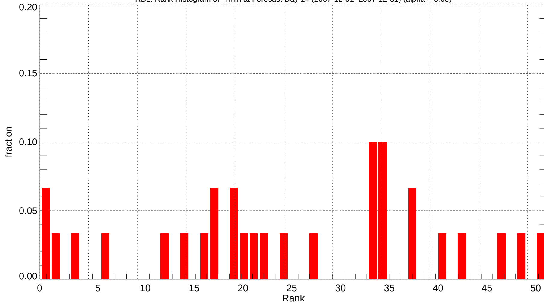
RBL: Rank Histogram of Tmin at Forecast Day 14 (2007-12-01~2007-12-31) (alpha = 0.00)
