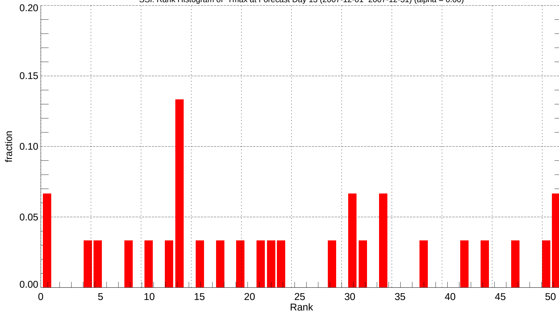
SSI: Rank Histogram of Tmax at Forecast Day 13 (2007-12-01~2007-12-31) (alpha = 0.00)
