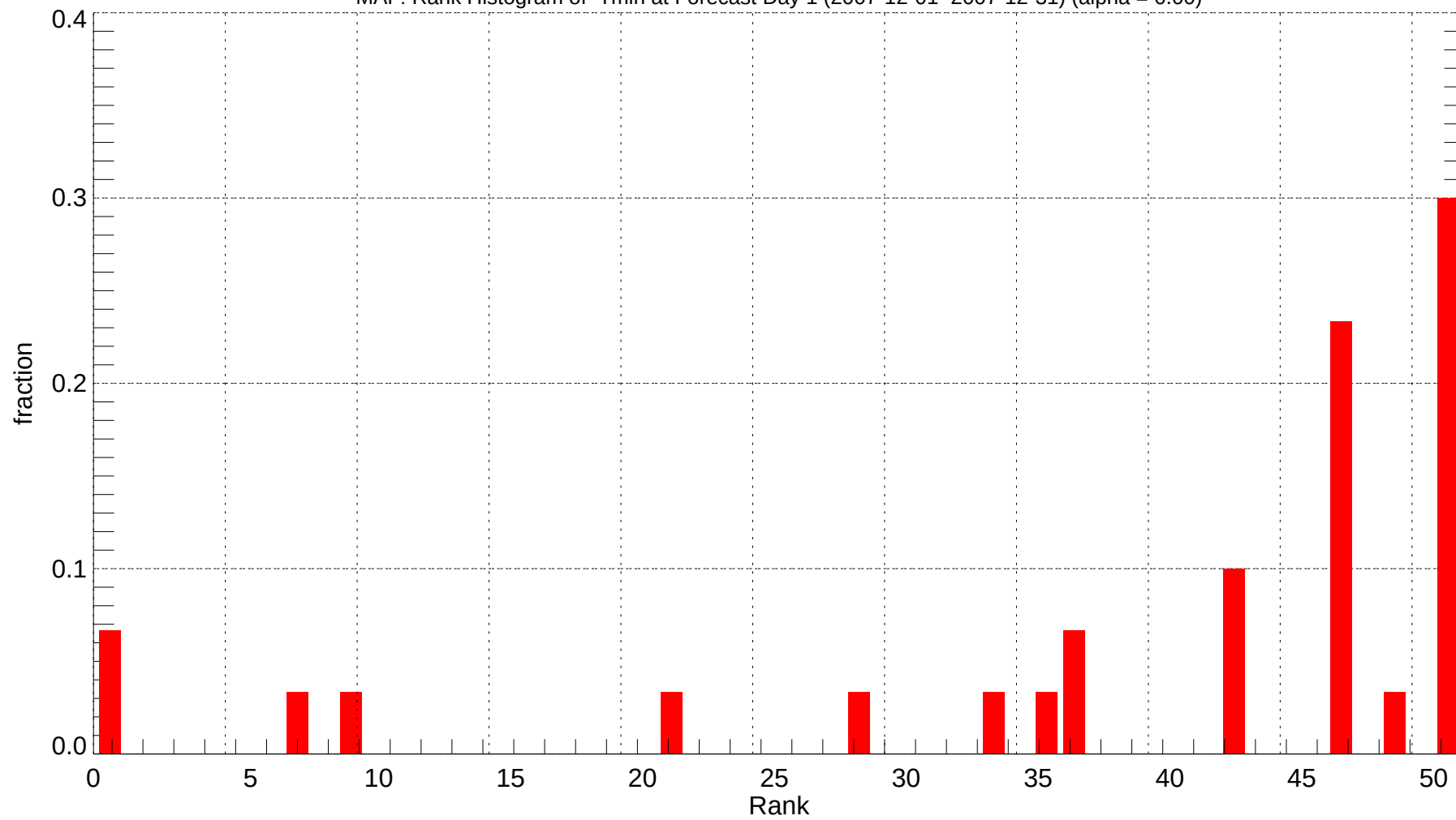
MAF: Rank Histogram of Tmin at Forecast Day 1 (2007-12-01~2007-12-31) (alpha = 0.00)
