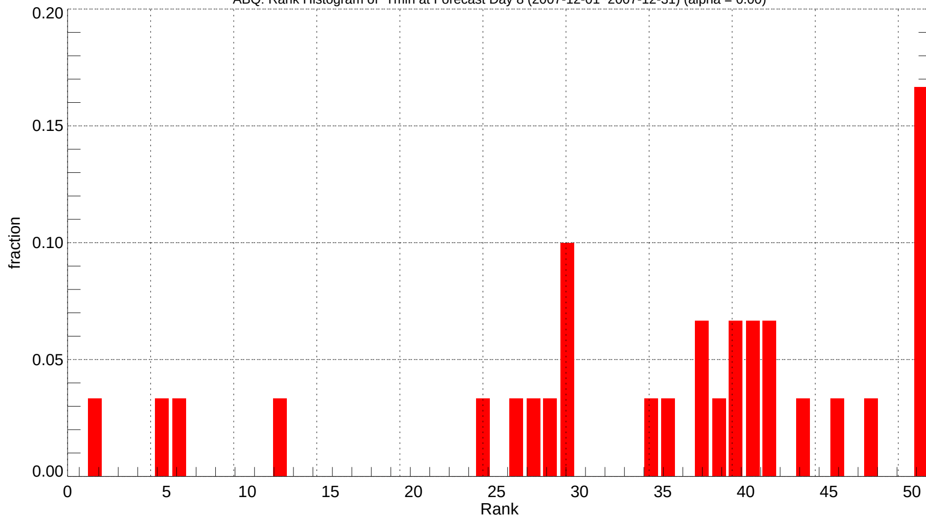
ABQ: Rank Histogram of Tmin at Forecast Day 8 (2007-12-01~2007-12-31) (alpha = 0.00)
