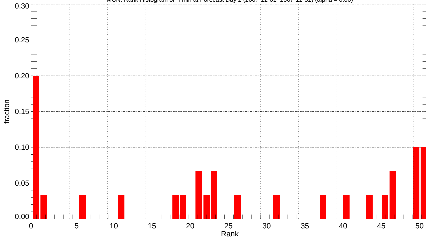
MCN: Rank Histogram of Tmin at Forecast Day 2 (2007-12-01~2007-12-31) (alpha = 0.00)
