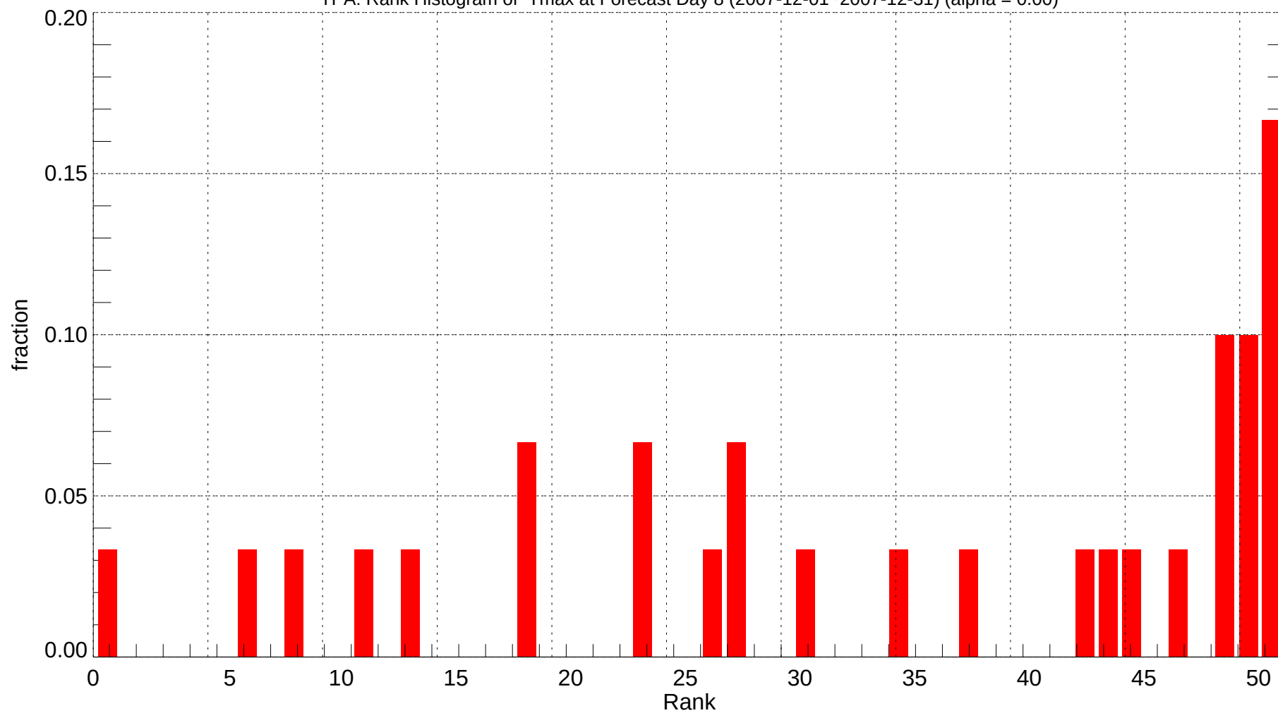
TPA: Rank Histogram of Tmax at Forecast Day 8 (2007-12-01~2007-12-31) (alpha = 0.00)
