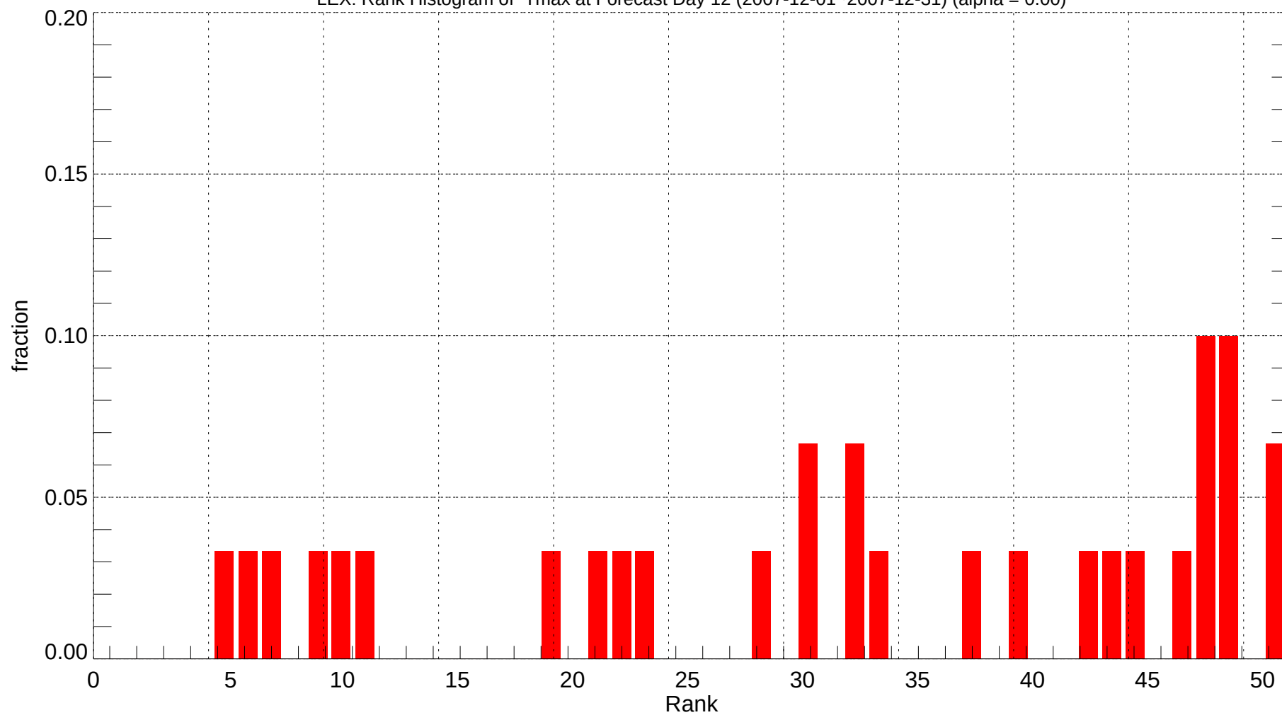
LEX: Rank Histogram of Tmax at Forecast Day 12 (2007-12-01~2007-12-31) (alpha = 0.00)
