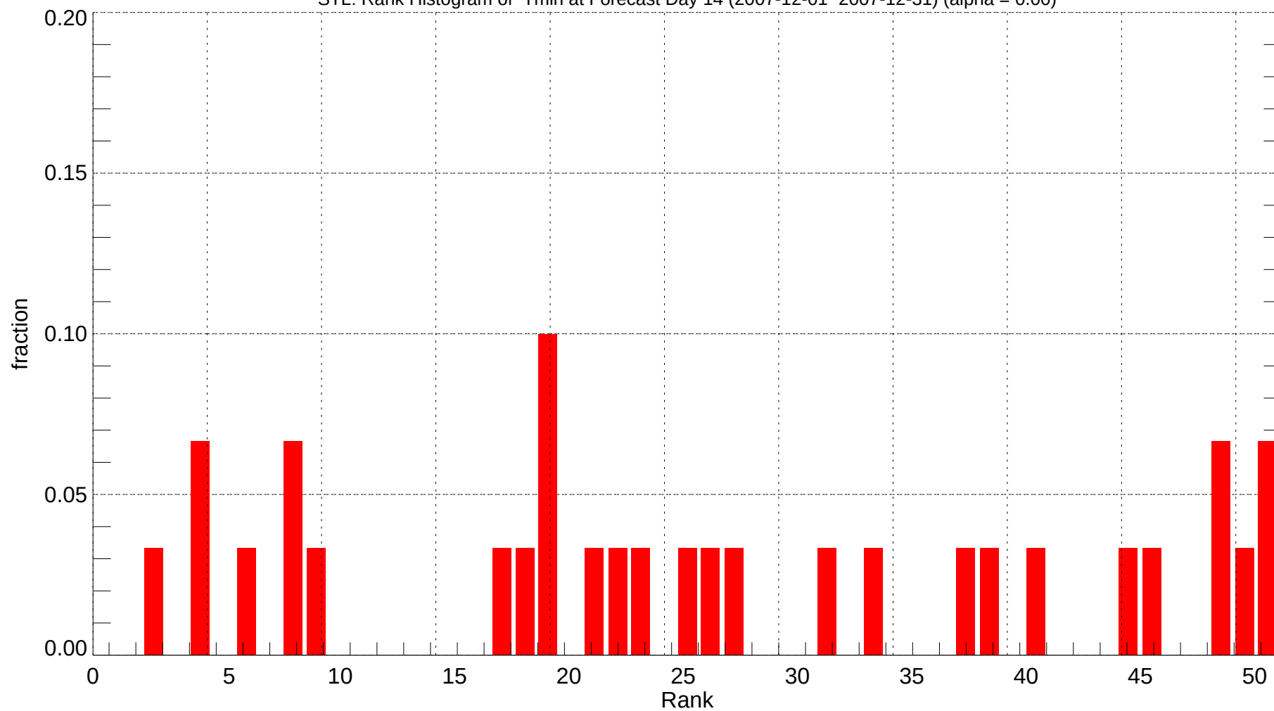
STL: Rank Histogram of Tmin at Forecast Day 14 (2007-12-01~2007-12-31) (alpha = 0.00)
