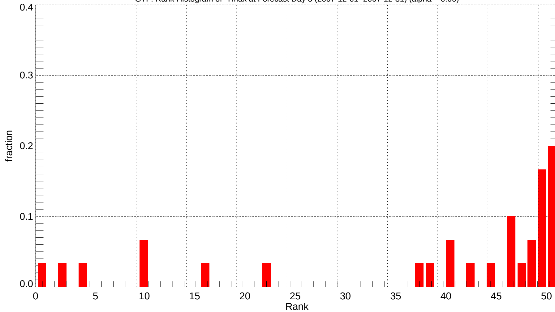
GTF: Rank Histogram of Tmax at Forecast Day 5 (2007-12-01~2007-12-31) (alpha = 0.00)
