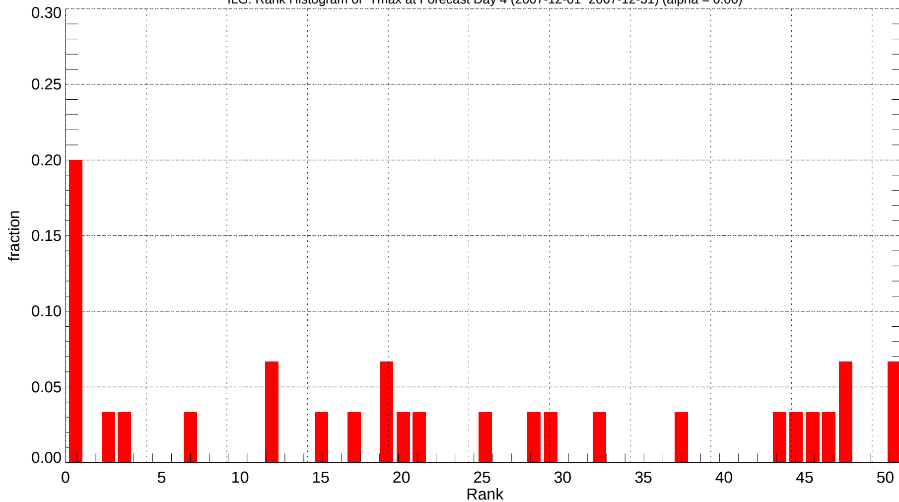
ILG: Rank Histogram of Tmax at Forecast Day 4 (2007-12-01~2007-12-31) (alpha = 0.00)
