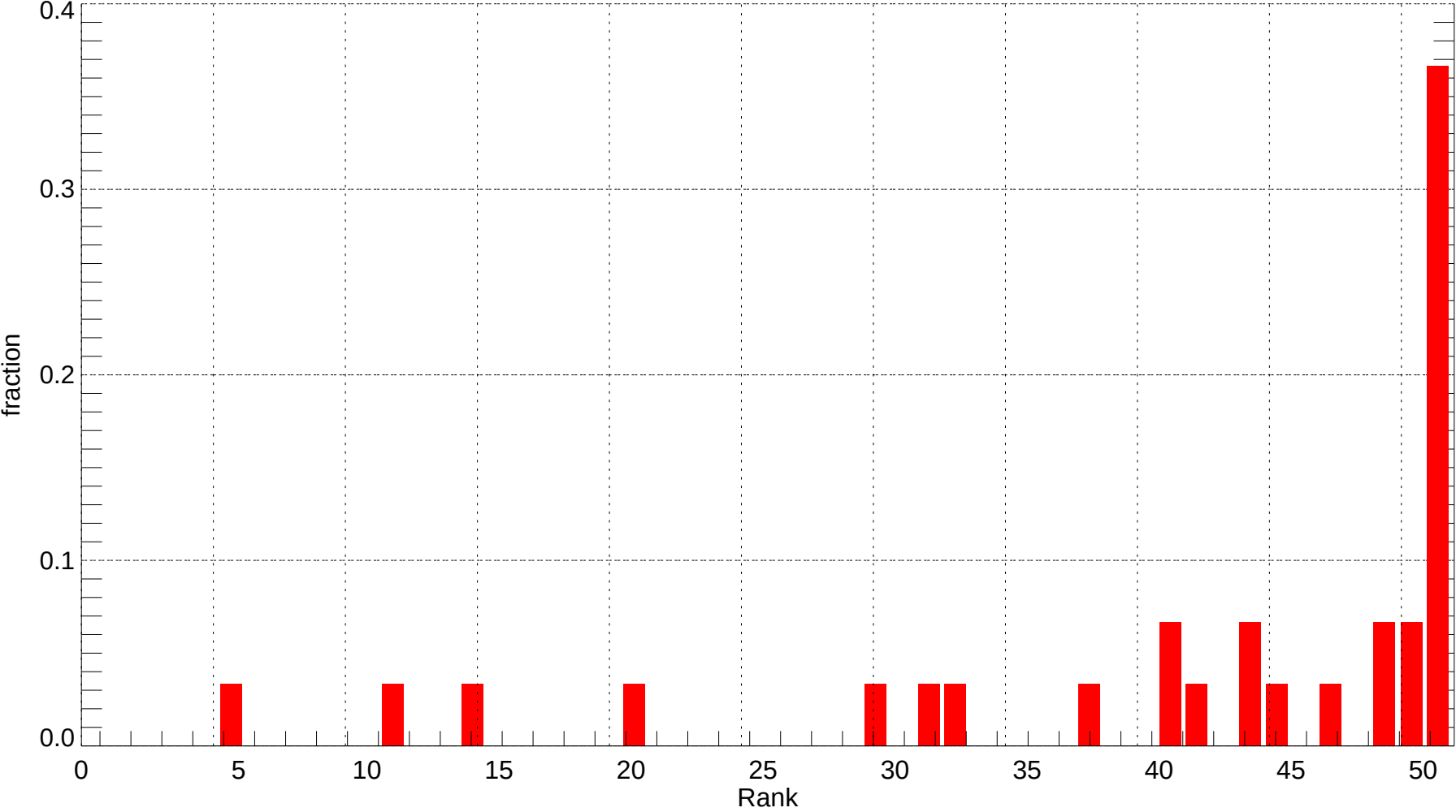
ELP: Rank Histogram of Tmin at Forecast Day 6 (2007-12-01~2007-12-31) (alpha = 0.00)
