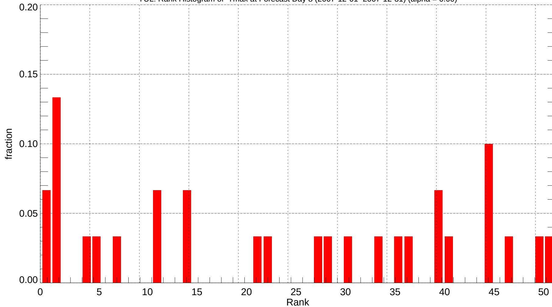
YUL: Rank Histogram of Tmax at Forecast Day 8 (2007-12-01~2007-12-31) (alpha = 0.00)
