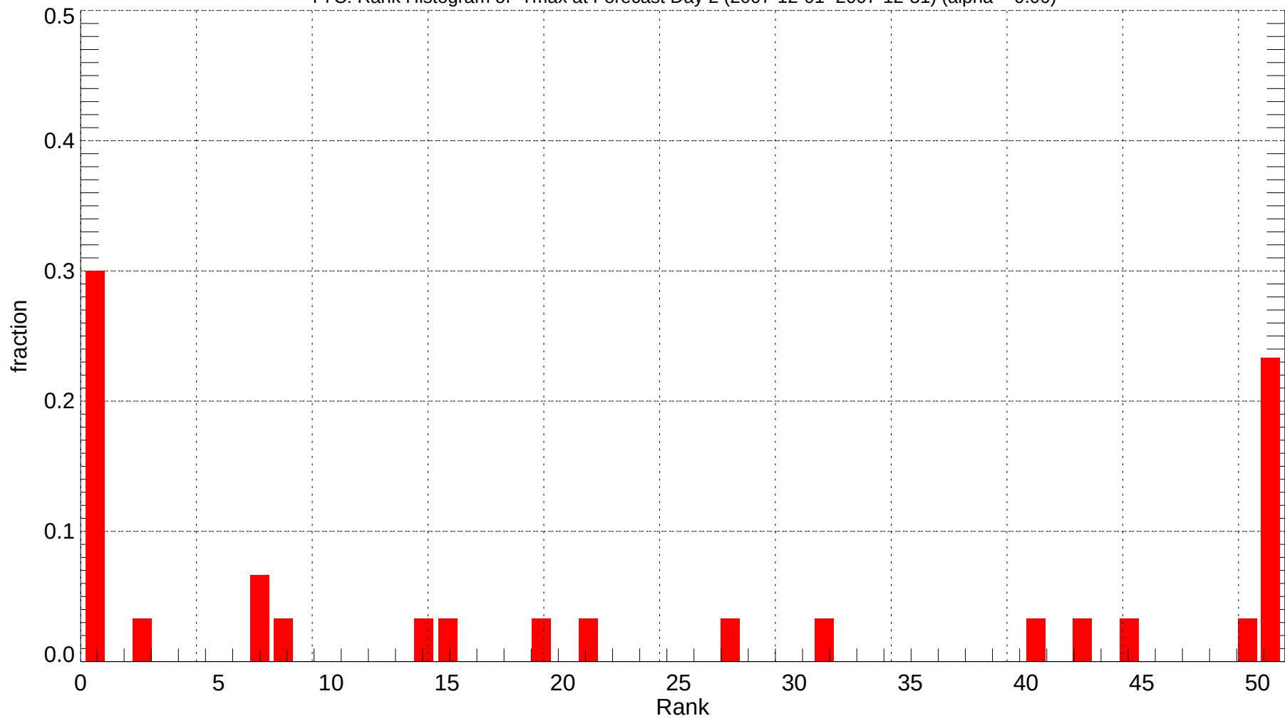
YYC: Rank Histogram of Tmax at Forecast Day 2 (2007-12-01~2007-12-31) (alpha = 0.00)
