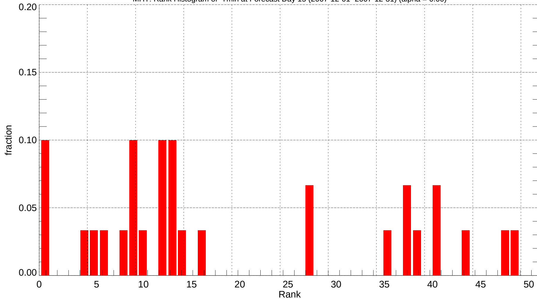
MHT: Rank Histogram of Tmin at Forecast Day 15 (2007-12-01~2007-12-31) (alpha = 0.00)
