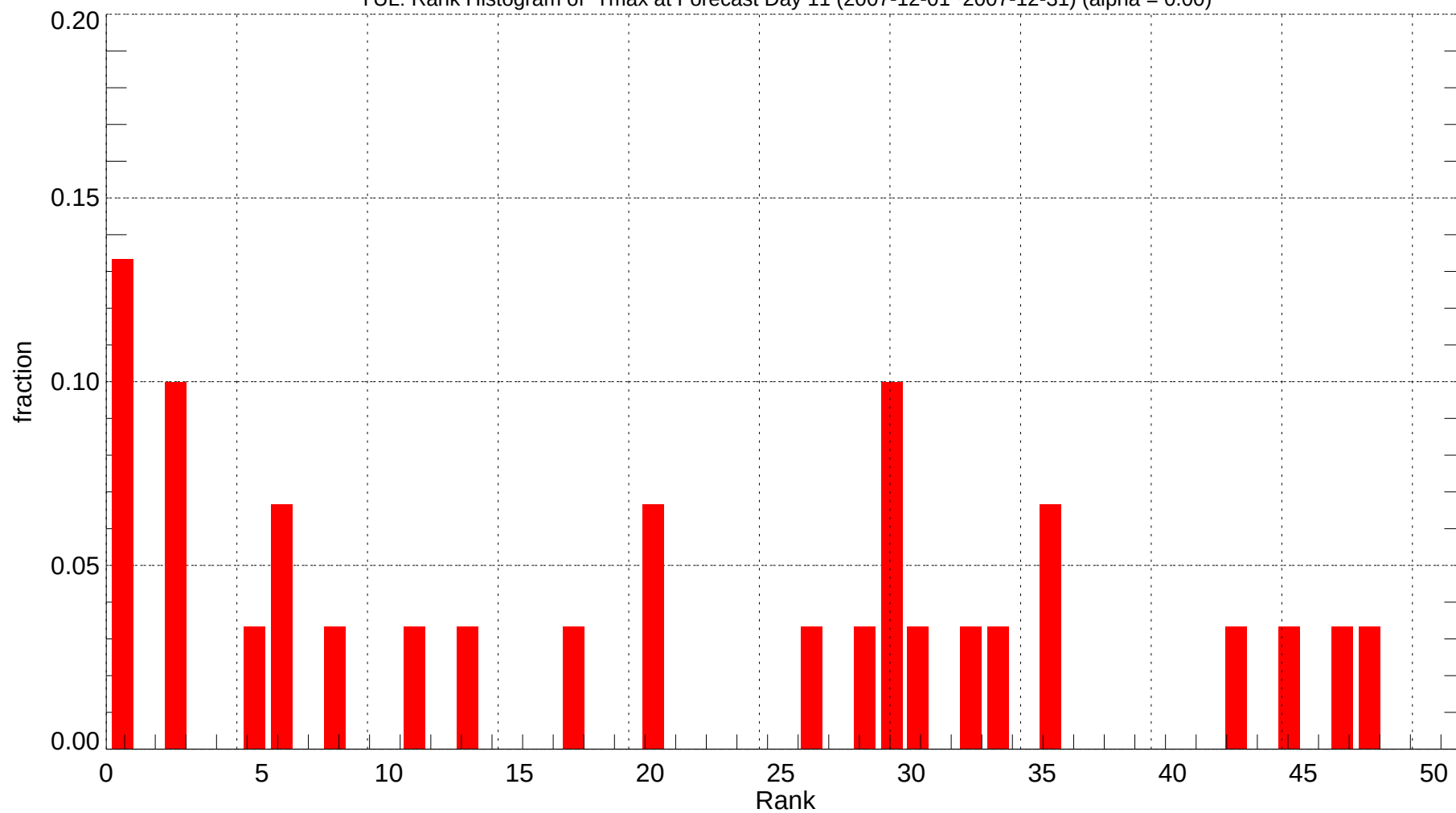
YUL: Rank Histogram of Tmax at Forecast Day 11 (2007-12-01~2007-12-31) (alpha = 0.00)
