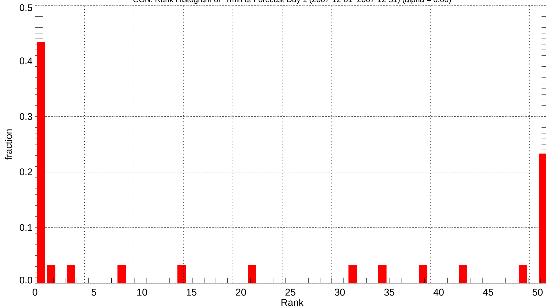
CON: Rank Histogram of Tmin at Forecast Day 1 (2007-12-01~2007-12-31) (alpha = 0.00)
