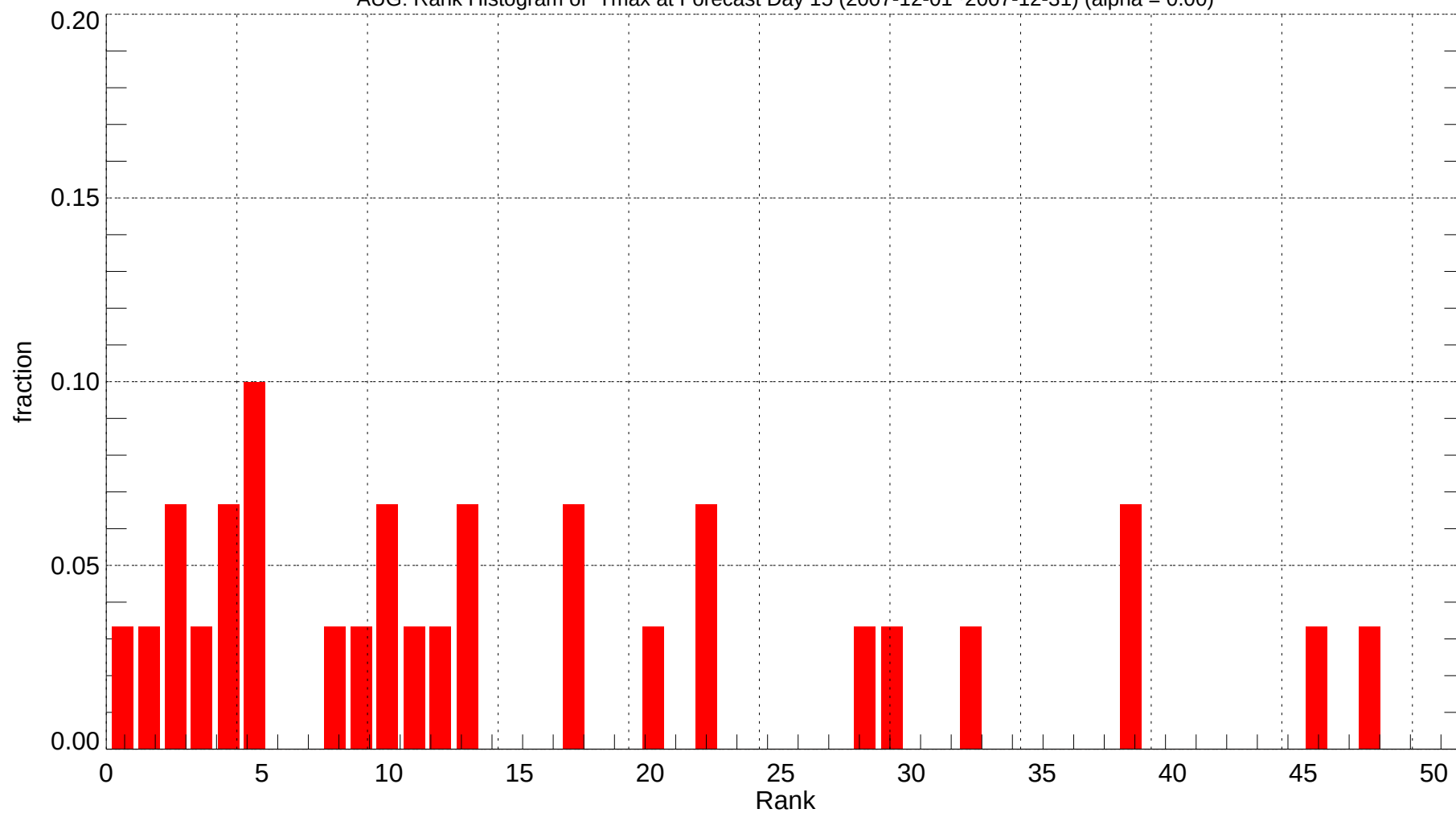
AUG: Rank Histogram of Tmax at Forecast Day 15 (2007-12-01~2007-12-31) (alpha = 0.00)
