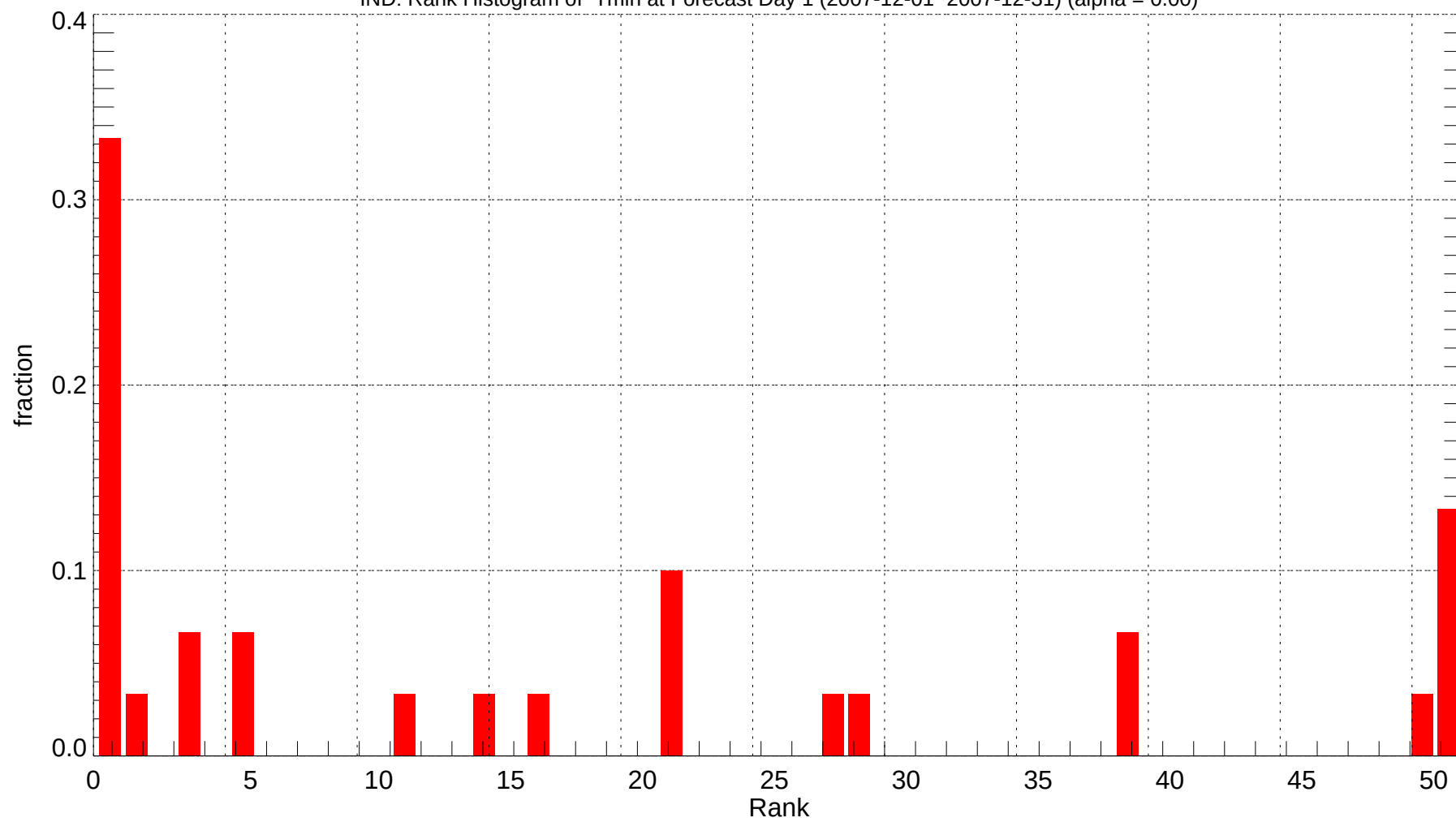
IND: Rank Histogram of Tmin at Forecast Day 1 (2007-12-01~2007-12-31) (alpha = 0.00)
