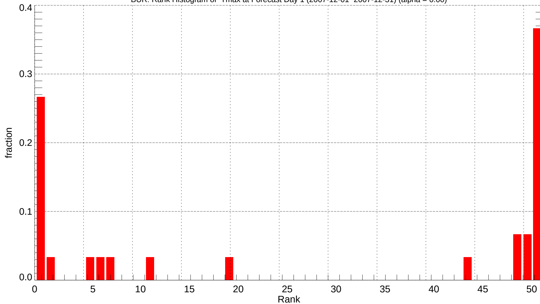
BUR: Rank Histogram of Tmax at Forecast Day 1 (2007-12-01~2007-12-31) (alpha = 0.00)
