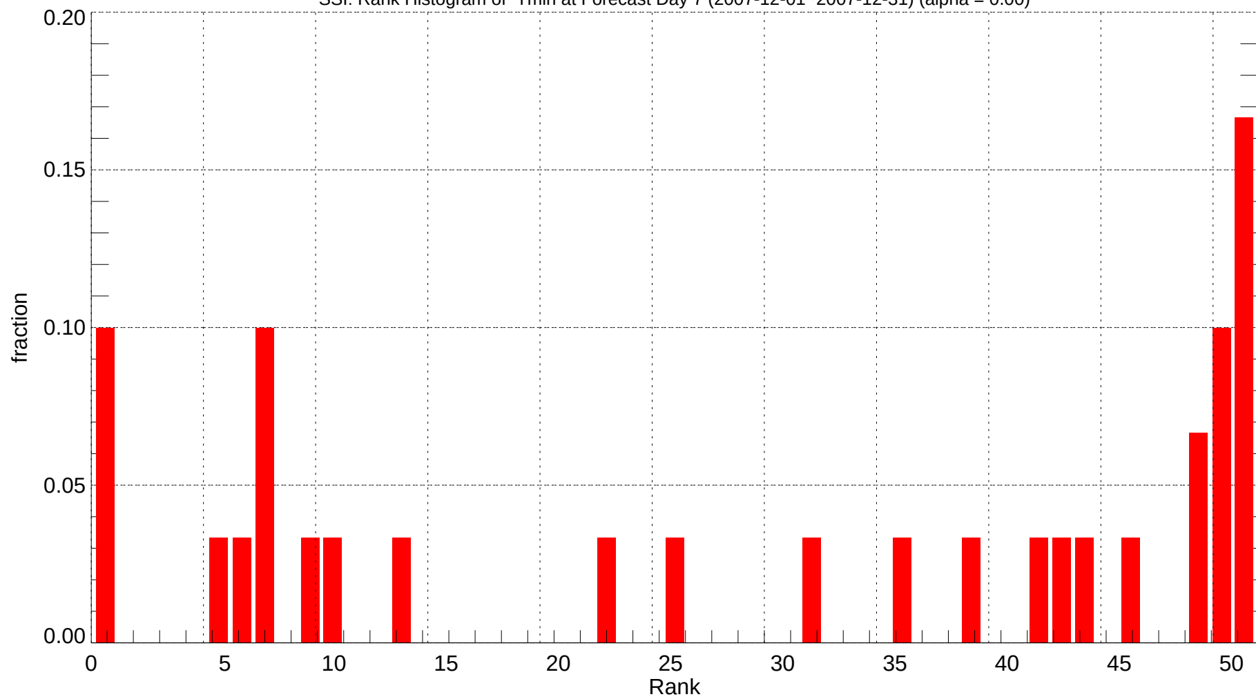
SSI: Rank Histogram of Tmin at Forecast Day 7 (2007-12-01~2007-12-31) (alpha = 0.00)
