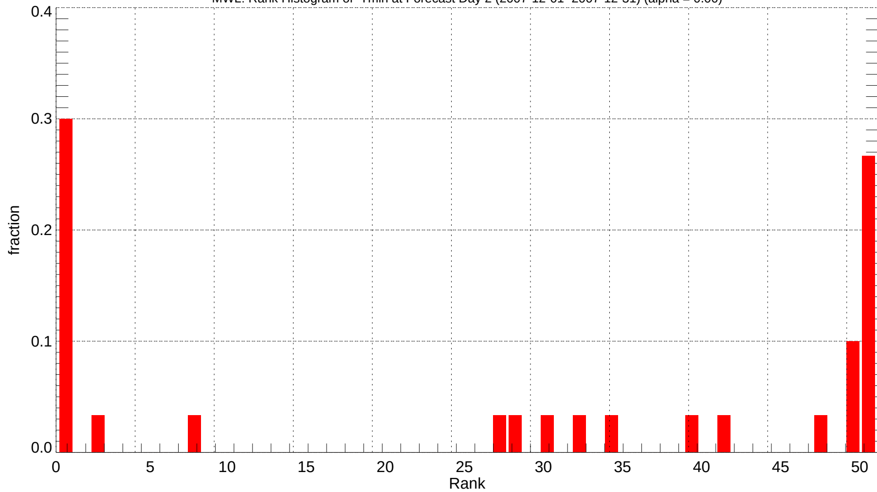
MWL: Rank Histogram of Tmin at Forecast Day 2 (2007-12-01~2007-12-31) (alpha = 0.00)
