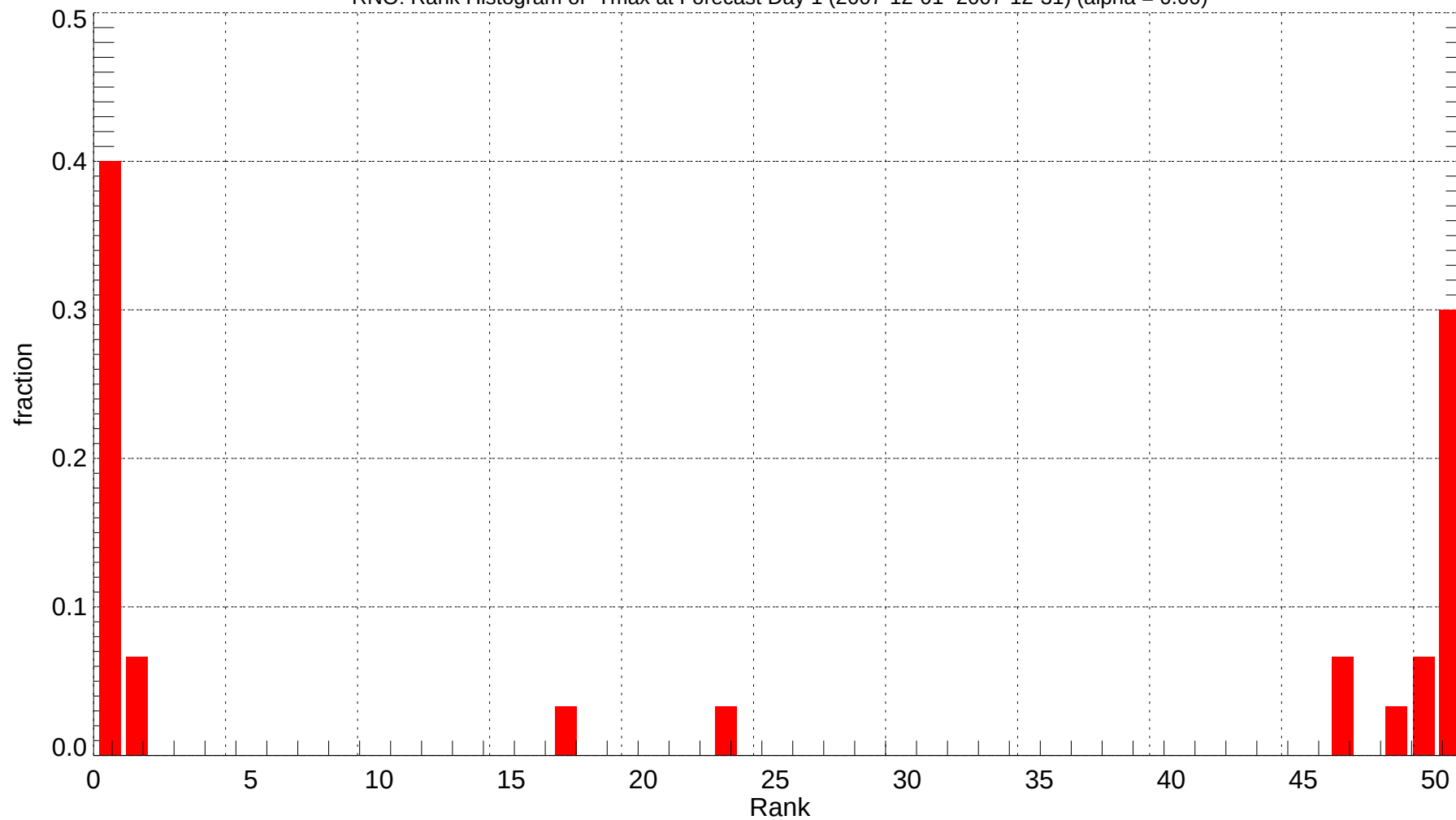
RNO: Rank Histogram of Tmax at Forecast Day 1 (2007-12-01~2007-12-31) (alpha = 0.00)
