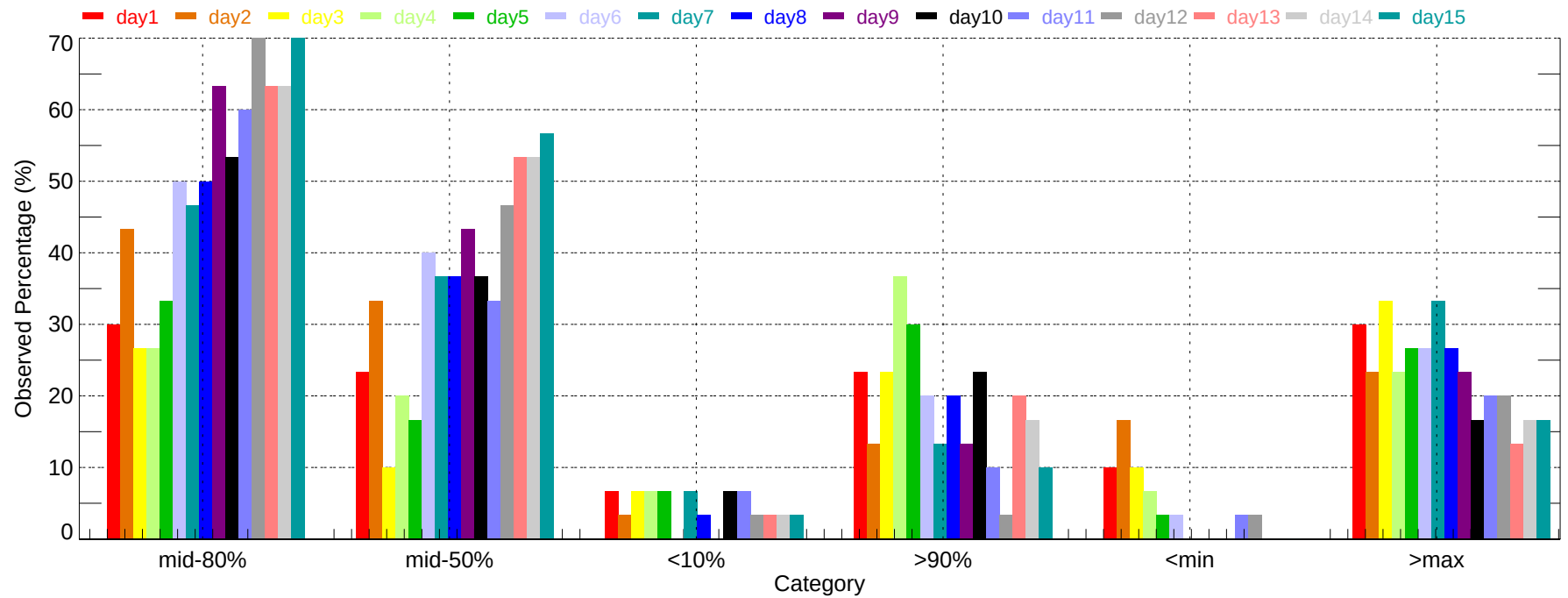
Observed Percentage of Ensembles - SAT: Min Temperature (2007-12-01~2007-12-31)
