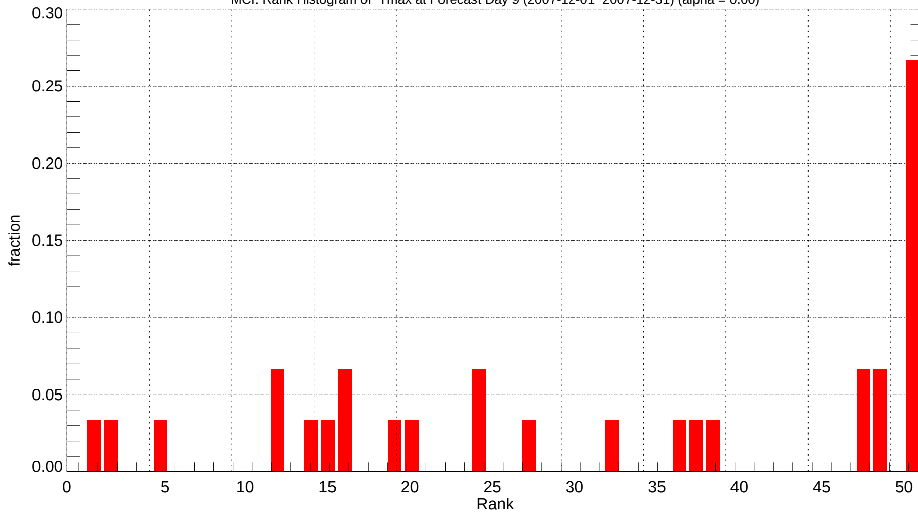
MCI: Rank Histogram of Tmax at Forecast Day 9 (2007-12-01~2007-12-31) (alpha = 0.00)
