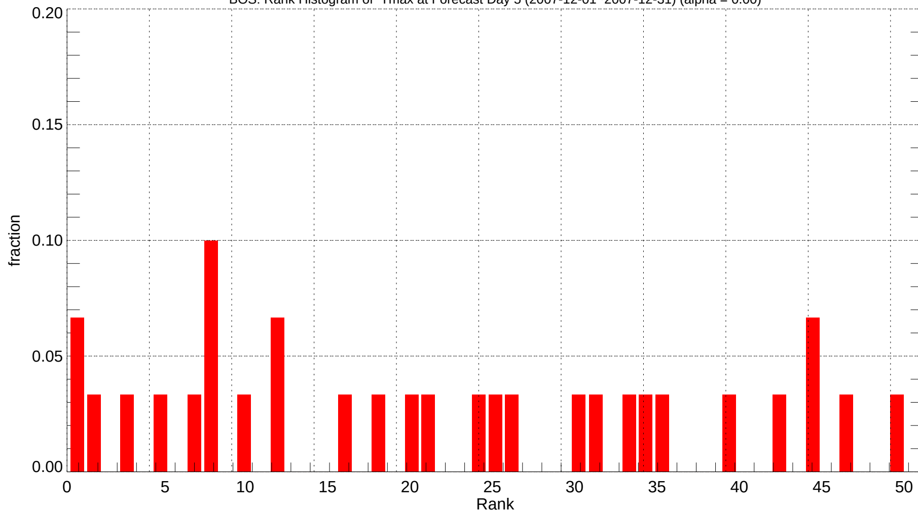
BOS: Rank Histogram of Tmax at Forecast Day 5 (2007-12-01~2007-12-31) (alpha = 0.00)
