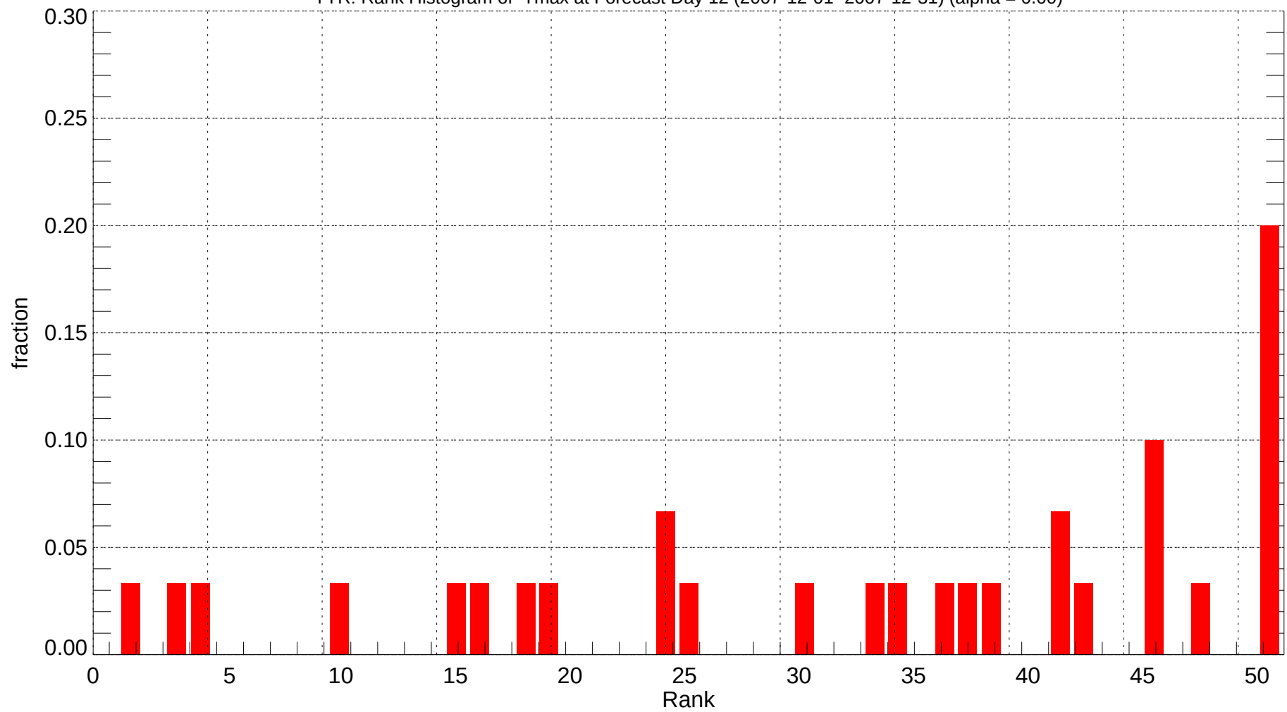
TYR: Rank Histogram of Tmax at Forecast Day 12 (2007-12-01~2007-12-31) (alpha = 0.00)
