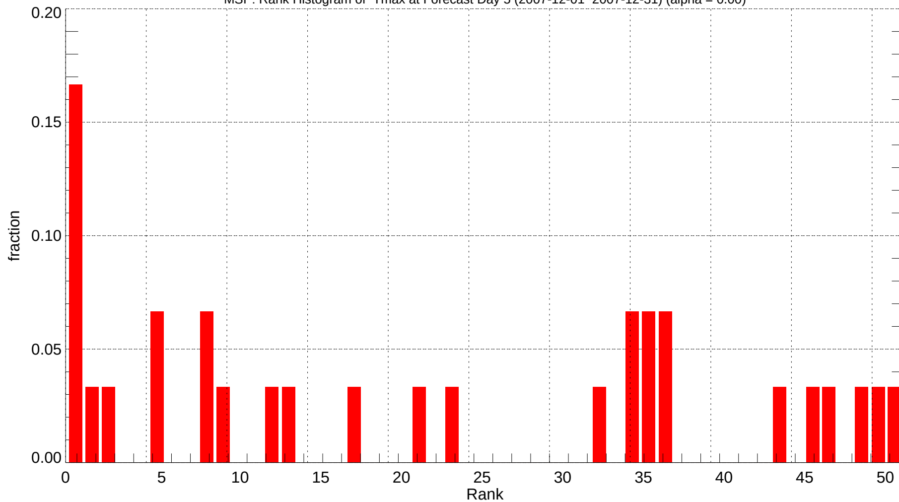
MSP: Rank Histogram of Tmax at Forecast Day 5 (2007-12-01~2007-12-31) (alpha = 0.00)
