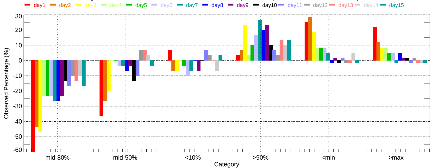
Observed Percentage Deviation of Ensembles - ACY: Max Temperature (2007-12-01~2007-12-31)
