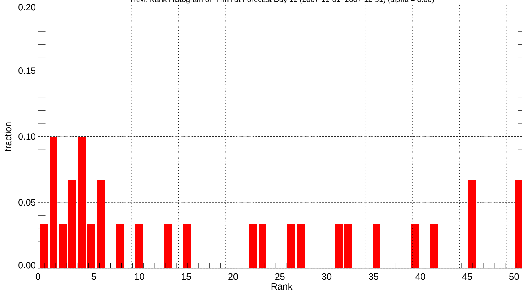
YKM: Rank Histogram of Tmin at Forecast Day 12 (2007-12-01~2007-12-31) (alpha = 0.00)
