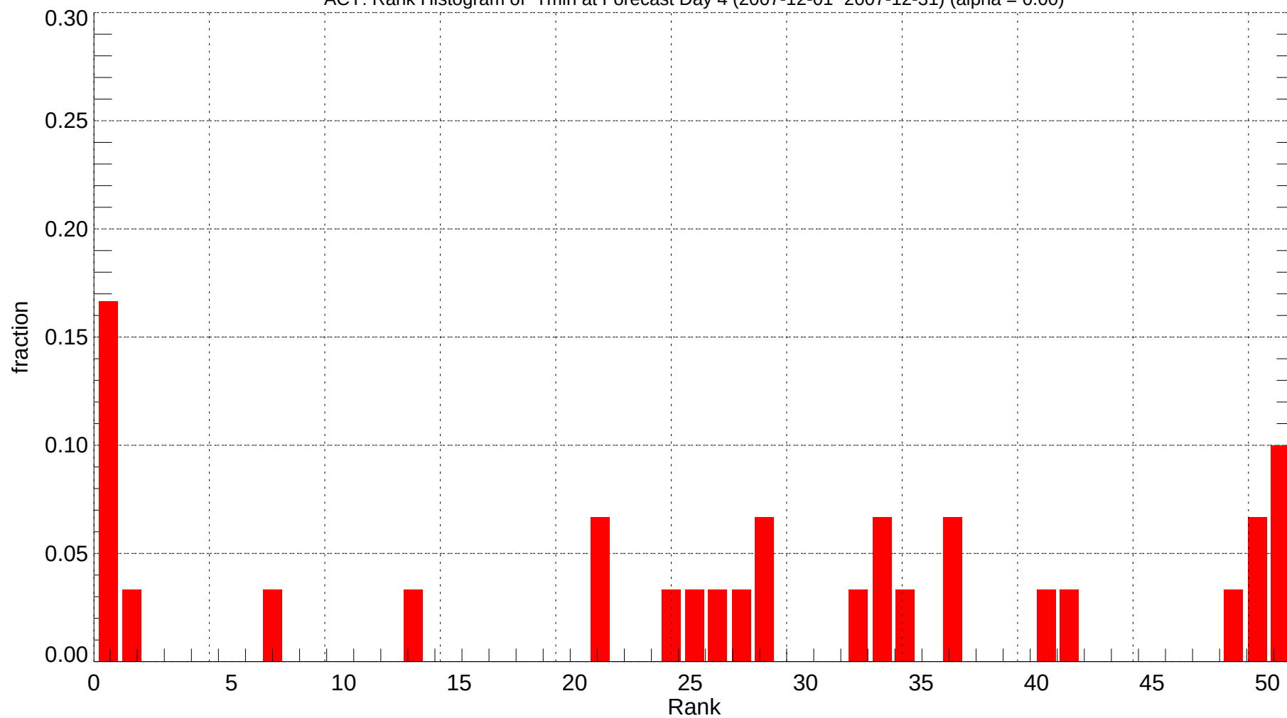
ACY: Rank Histogram of Tmin at Forecast Day 4 (2007-12-01~2007-12-31) (alpha = 0.00)
