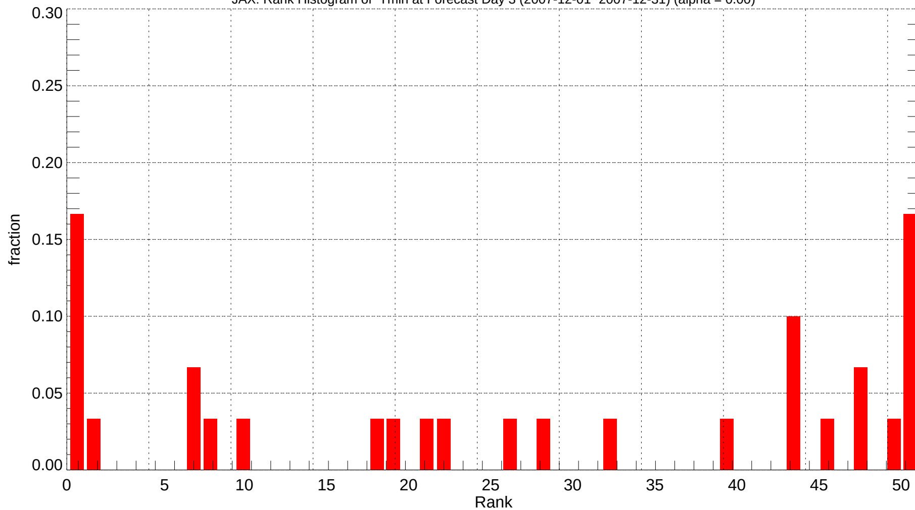
JAX: Rank Histogram of Tmin at Forecast Day 3 (2007-12-01~2007-12-31) (alpha = 0.00)
