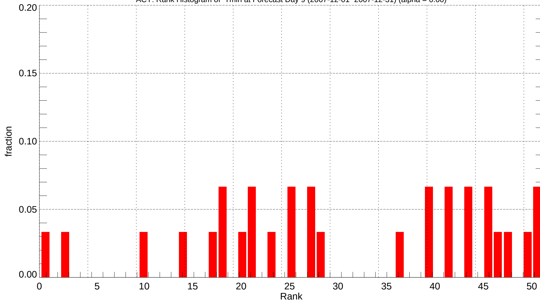
ACY: Rank Histogram of Tmin at Forecast Day 9 (2007-12-01~2007-12-31) (alpha = 0.00)
