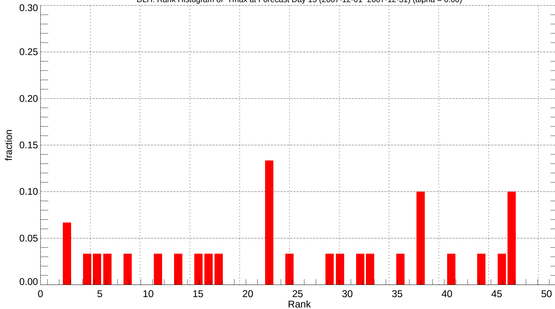
DLH: Rank Histogram of Tmax at Forecast Day 15 (2007-12-01~2007-12-31) (alpha = 0.00)
