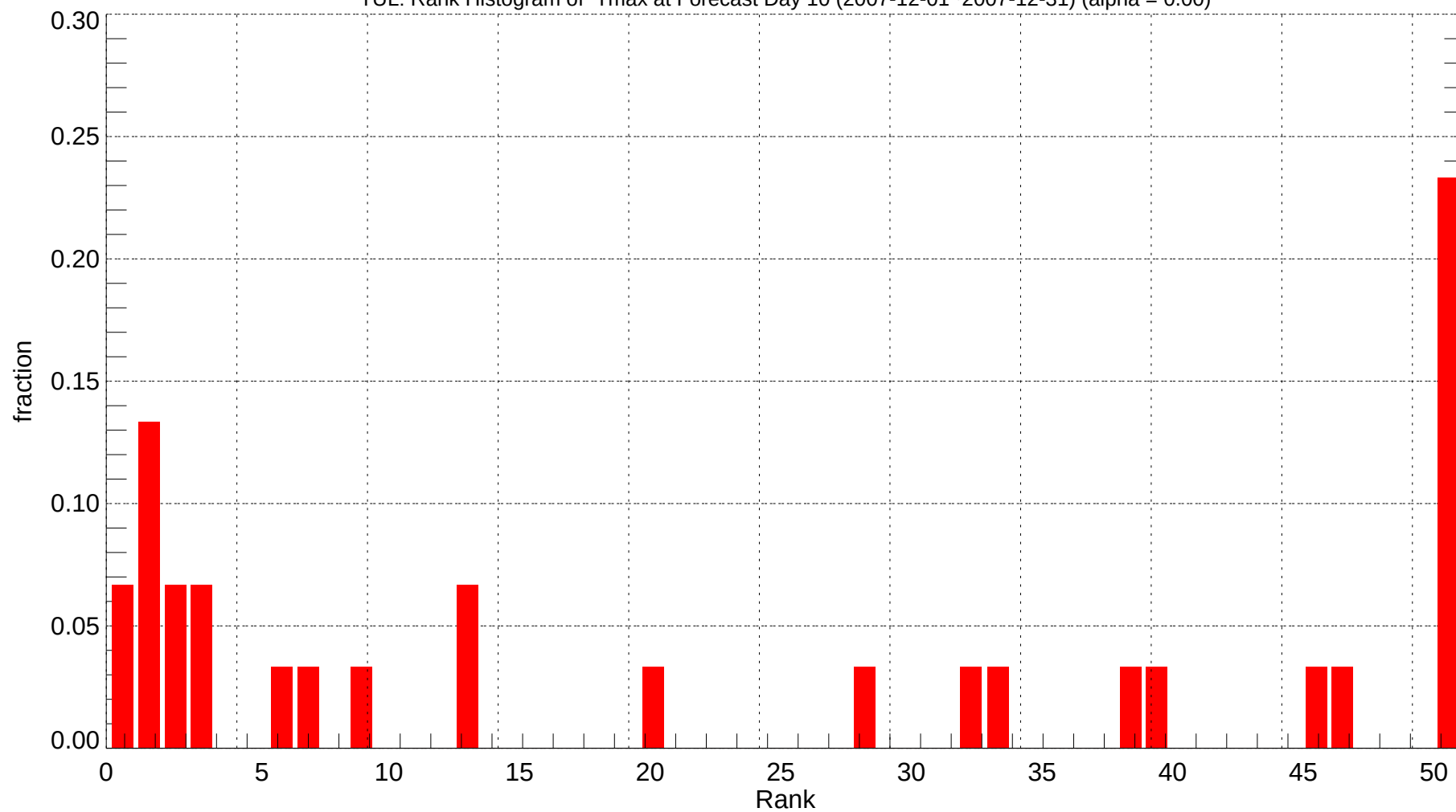
TUL: Rank Histogram of Tmax at Forecast Day 10 (2007-12-01~2007-12-31) (alpha = 0.00)
