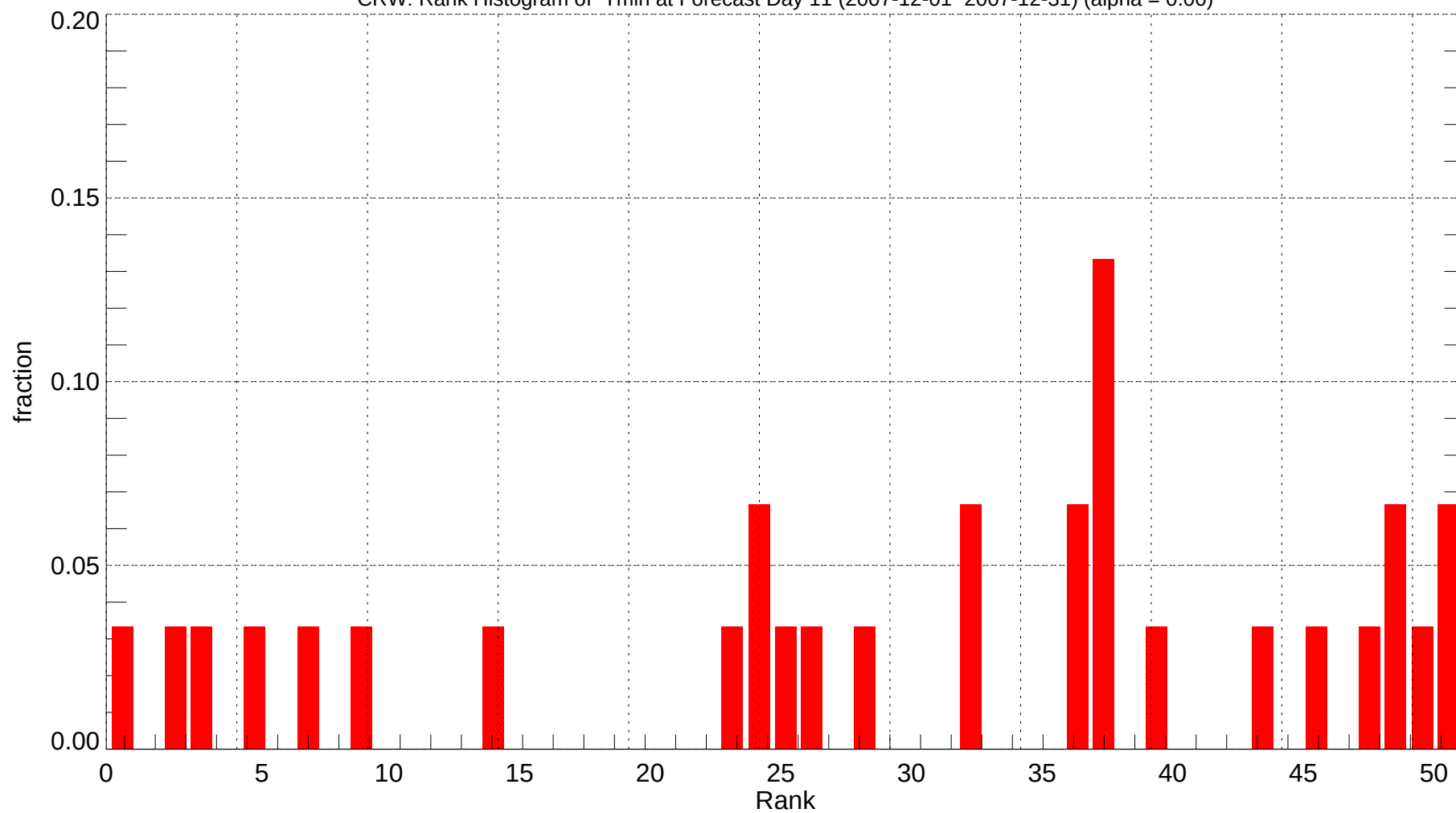
CRW: Rank Histogram of Tmin at Forecast Day 11 (2007-12-01~2007-12-31) (alpha = 0.00)
