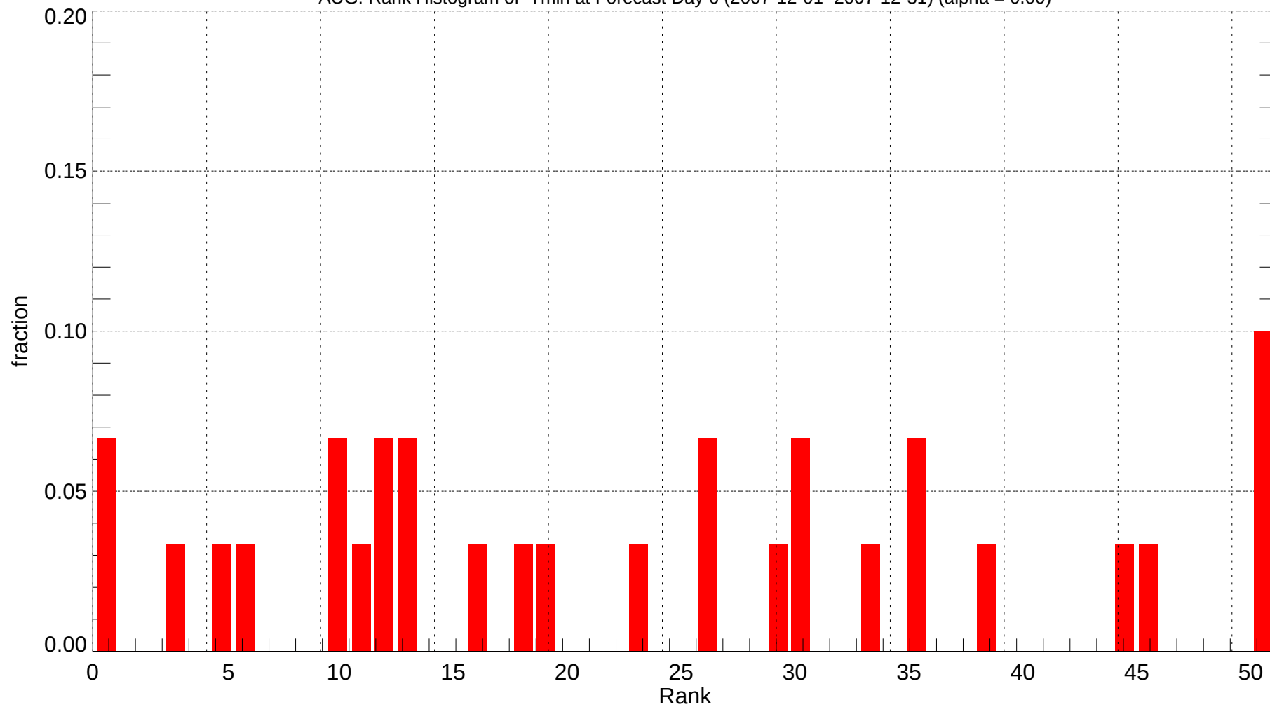
AUG: Rank Histogram of Tmin at Forecast Day 6 (2007-12-01~2007-12-31) (alpha = 0.00)
