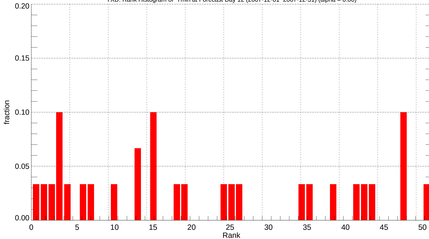
YXD: Rank Histogram of Tmin at Forecast Day 12 (2007-12-01~2007-12-31) (alpha = 0.00)
