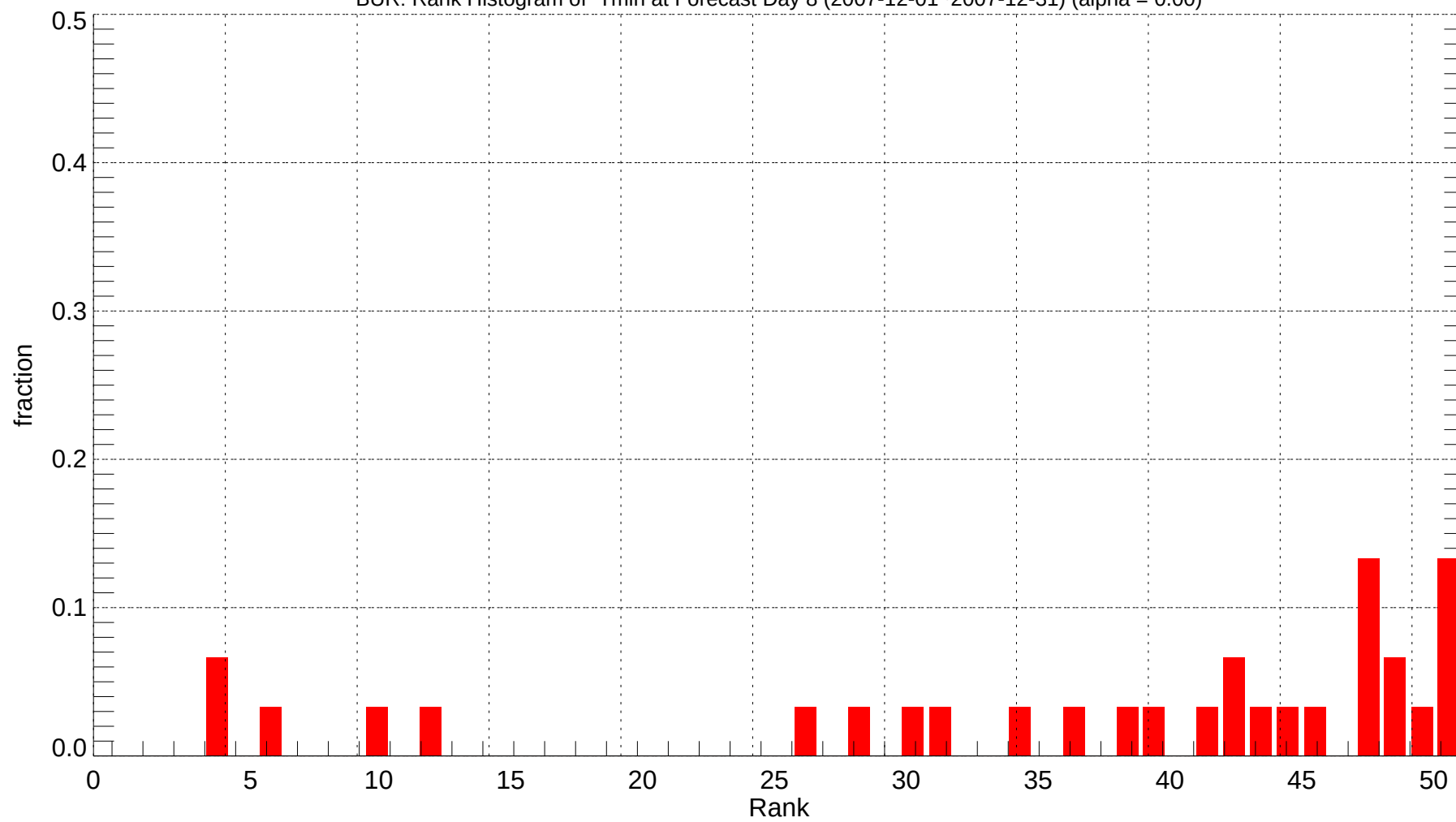
BUR: Rank Histogram of Tmin at Forecast Day 8 (2007-12-01~2007-12-31) (alpha = 0.00)
