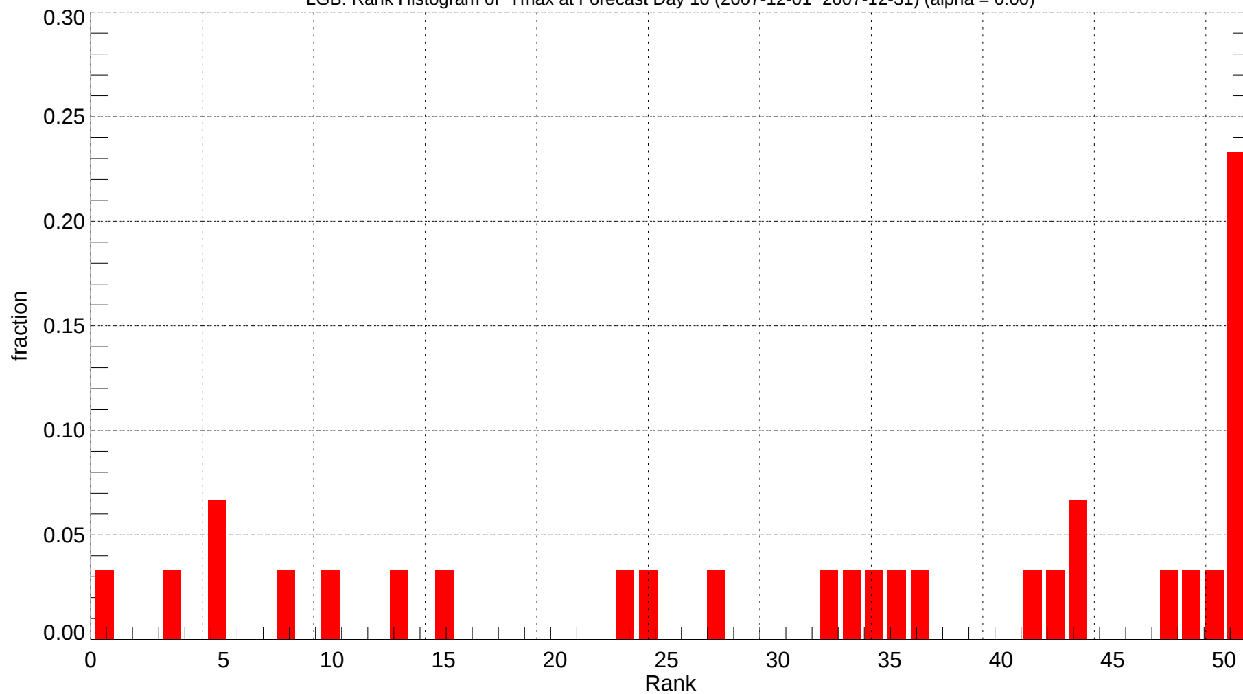
LGB: Rank Histogram of Tmax at Forecast Day 10 (2007-12-01~2007-12-31) (alpha = 0.00)
