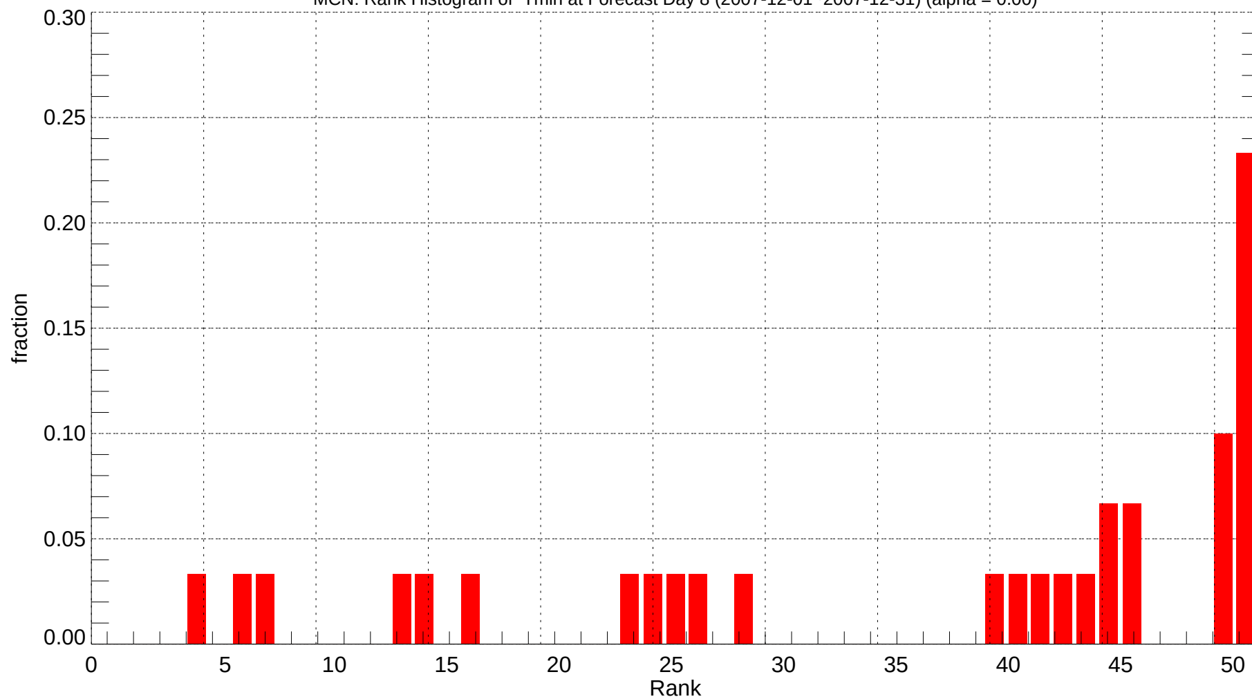
MCN: Rank Histogram of Tmin at Forecast Day 8 (2007-12-01~2007-12-31) (alpha = 0.00)
