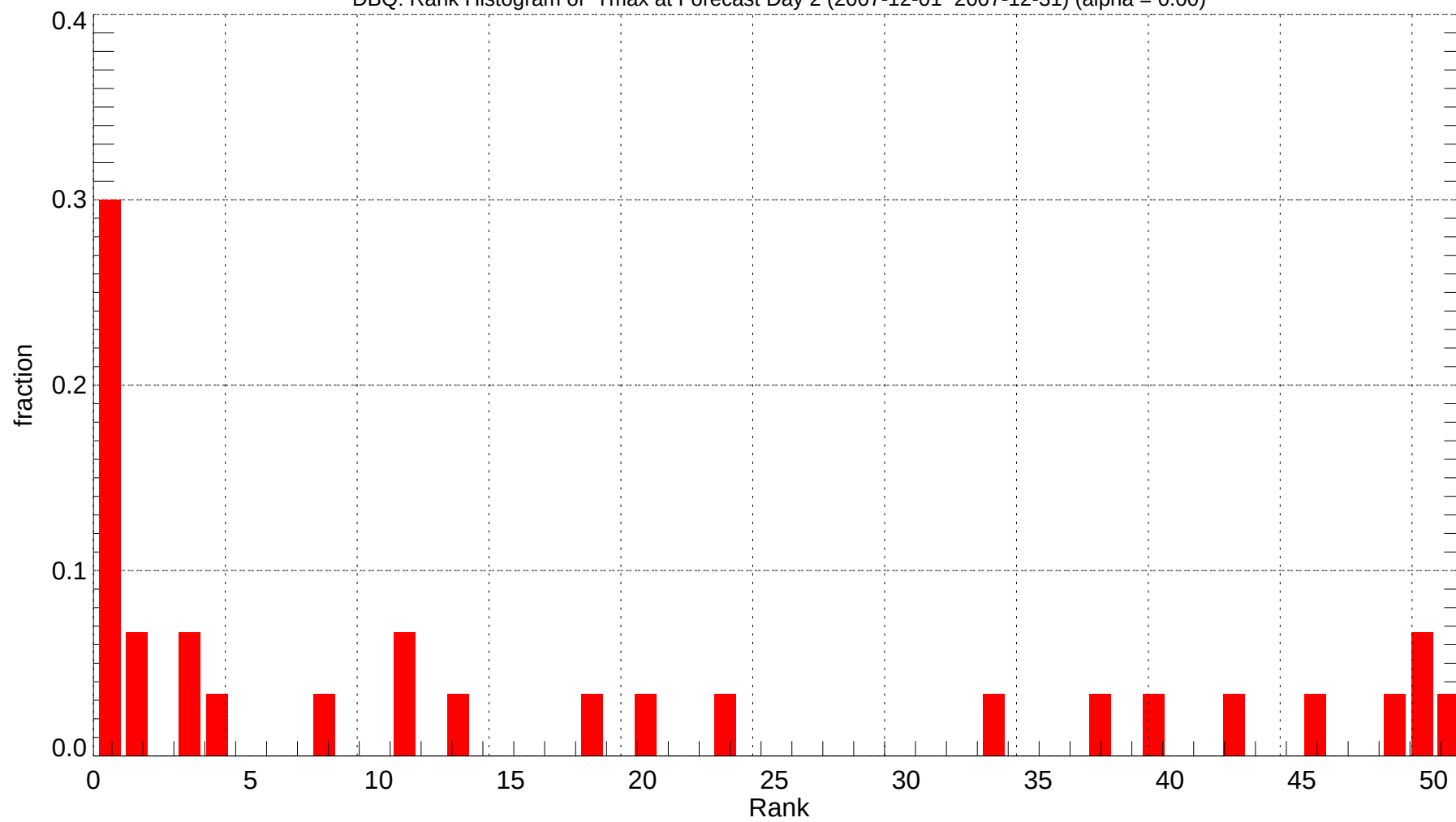
DBQ: Rank Histogram of Tmax at Forecast Day 2 (2007-12-01~2007-12-31) (alpha = 0.00)
