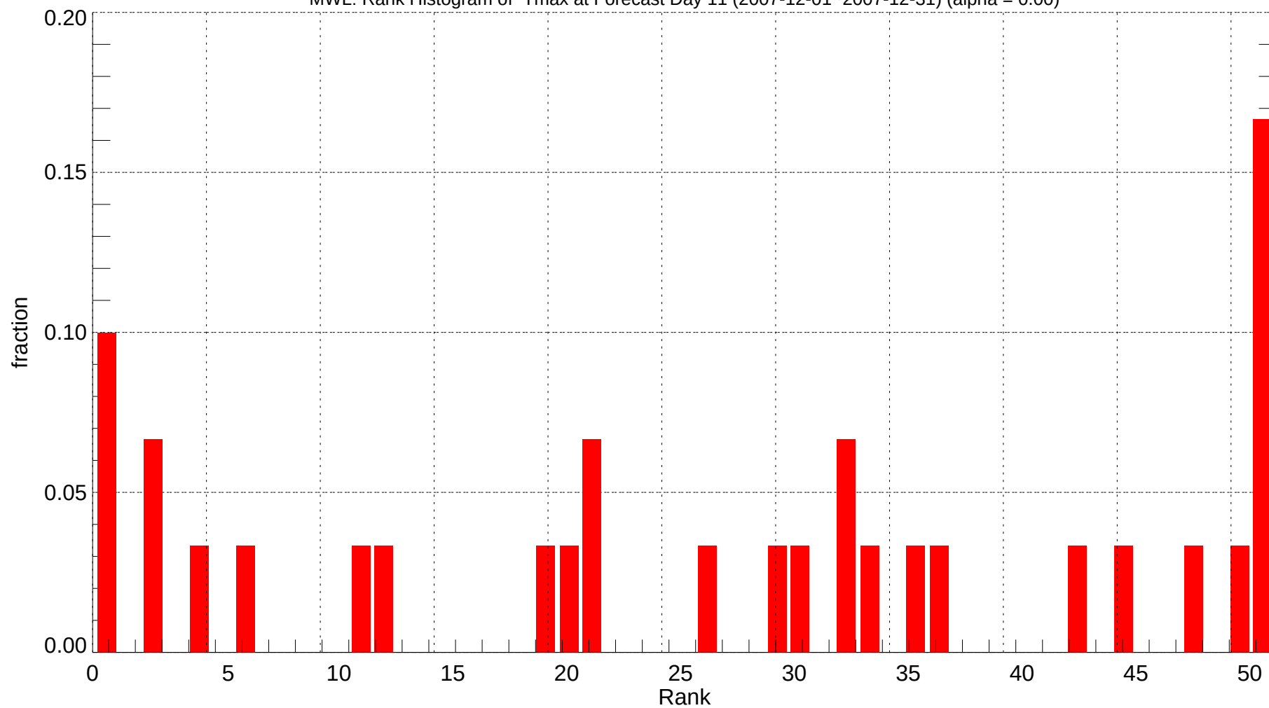
MWL: Rank Histogram of Tmax at Forecast Day 11 (2007-12-01~2007-12-31) (alpha = 0.00)
