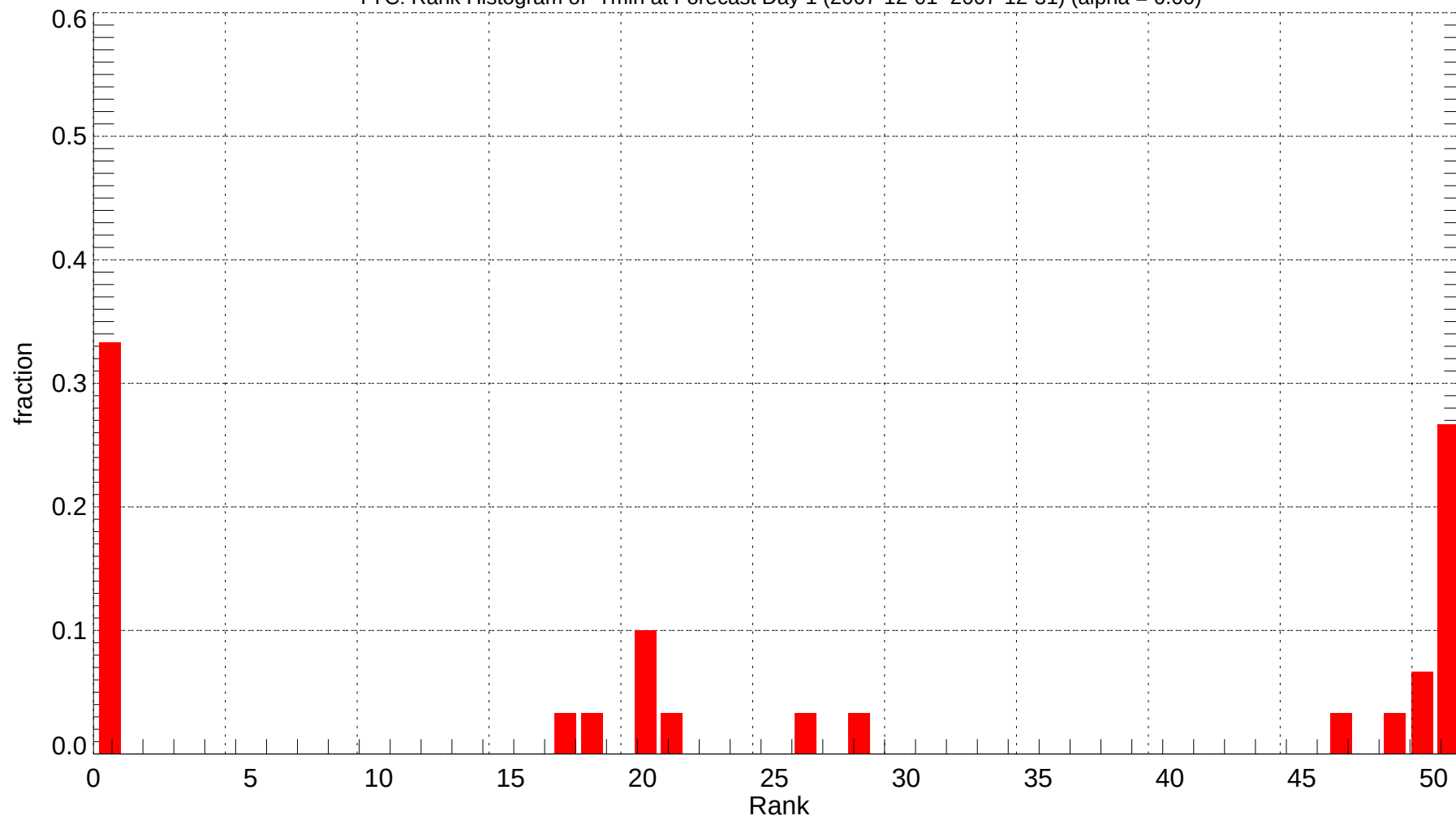
YYC: Rank Histogram of Tmin at Forecast Day 1 (2007-12-01~2007-12-31) (alpha = 0.00)
