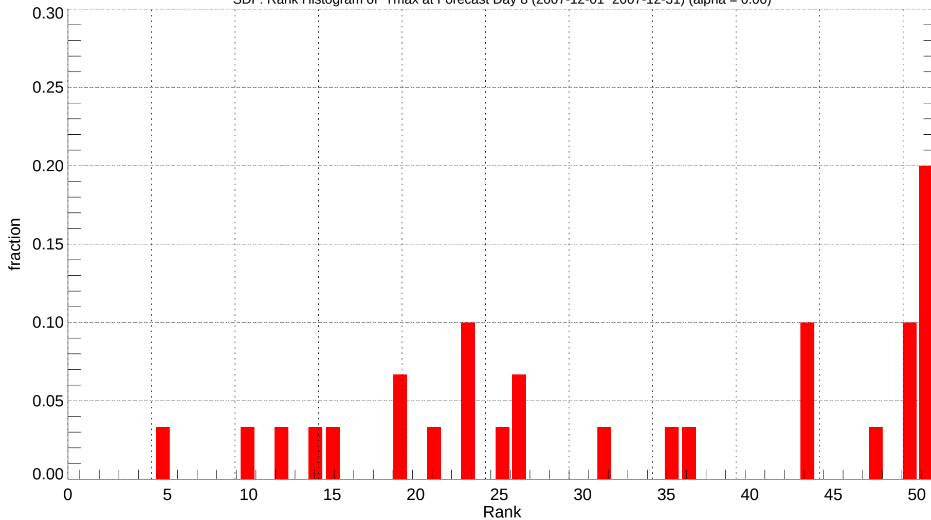
SDF: Rank Histogram of Tmax at Forecast Day 8 (2007-12-01~2007-12-31) (alpha = 0.00)
