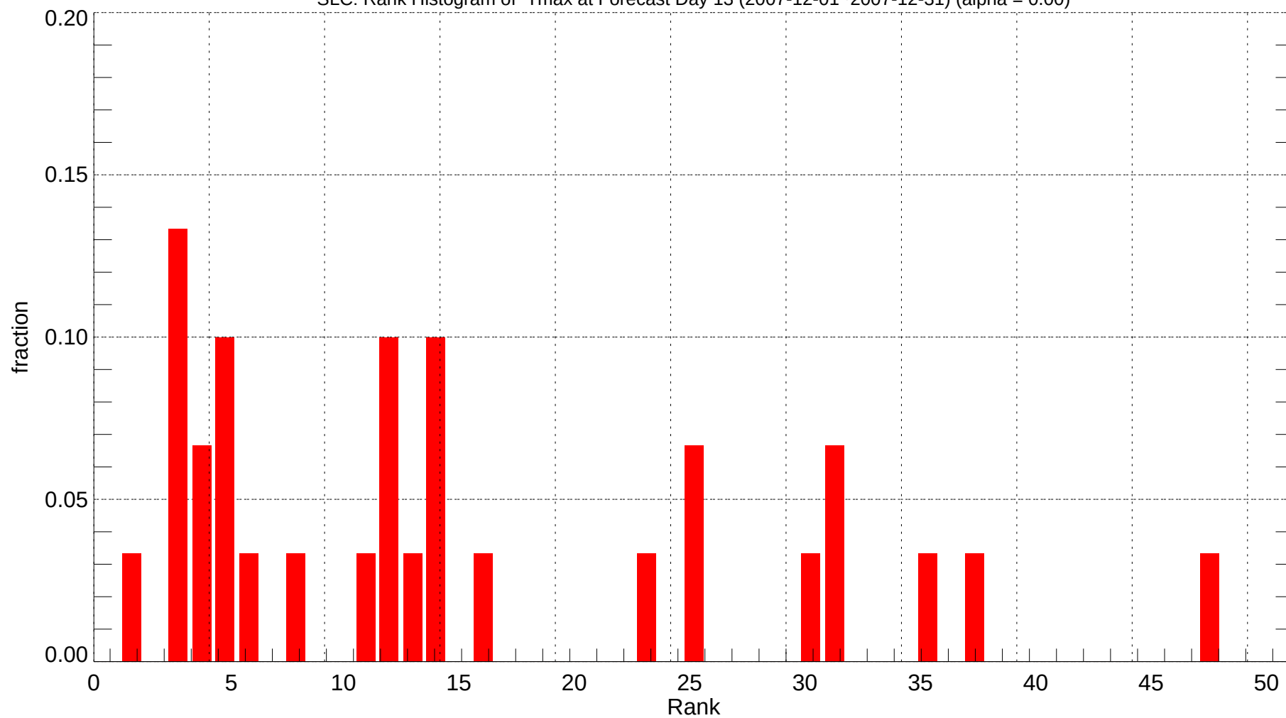
SLC: Rank Histogram of Tmax at Forecast Day 13 (2007-12-01~2007-12-31) (alpha = 0.00)
