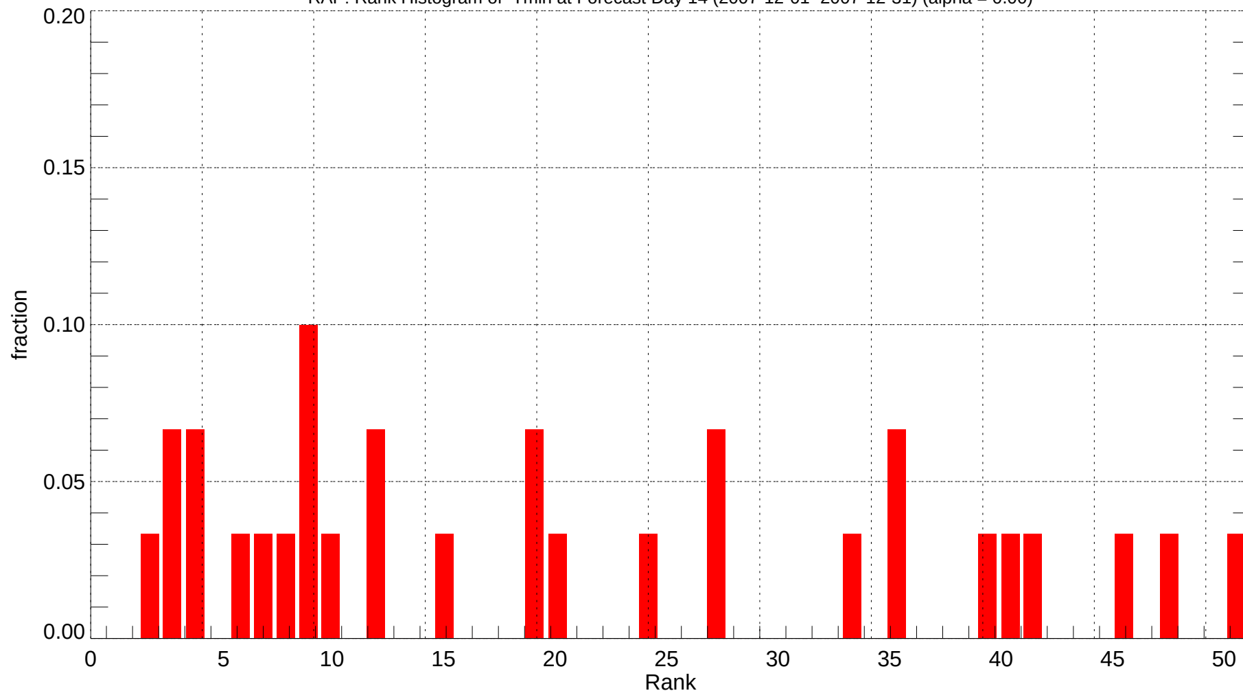
RAP: Rank Histogram of Tmin at Forecast Day 14 (2007-12-01~2007-12-31) (alpha = 0.00)
