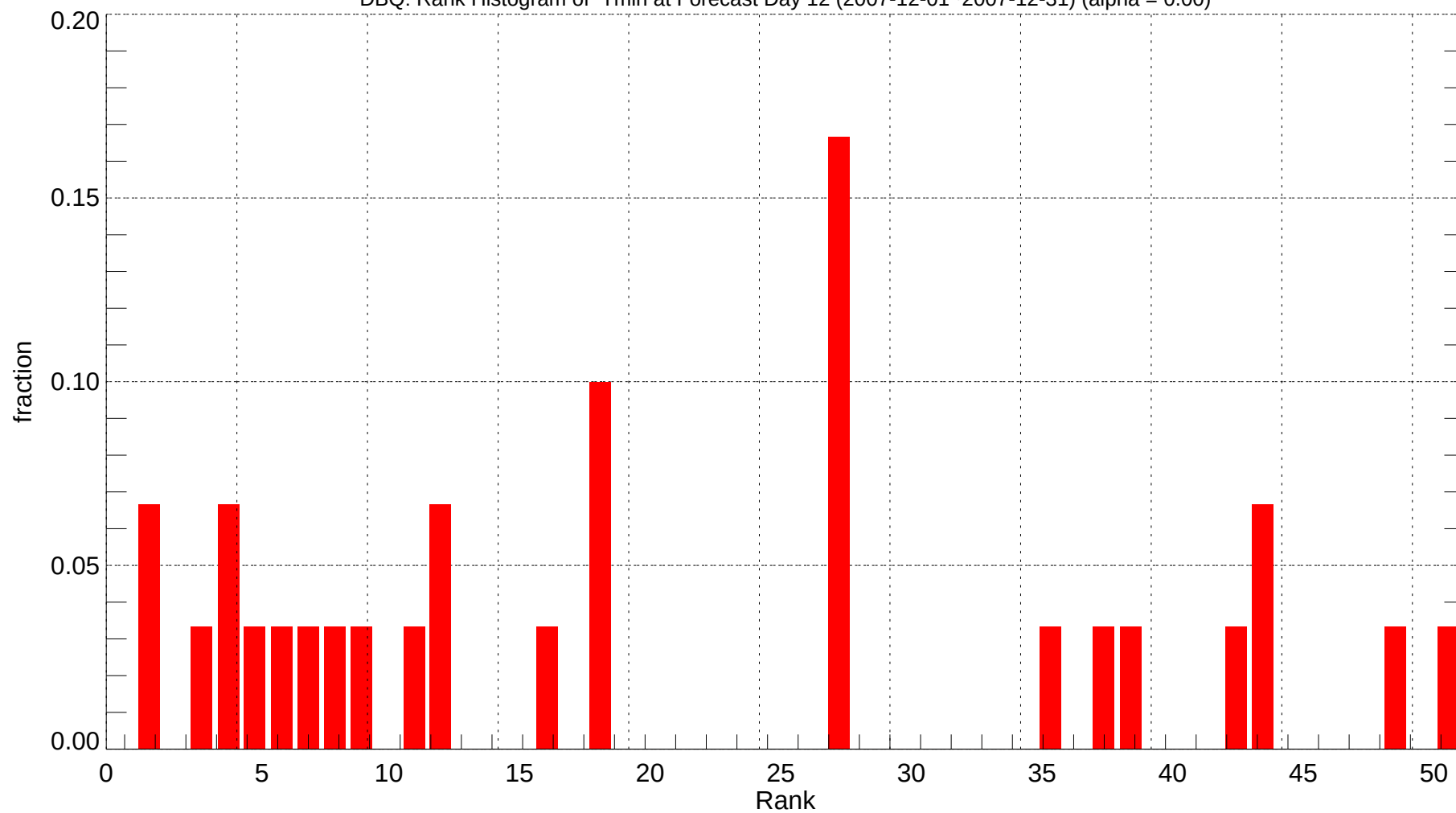
DBQ: Rank Histogram of Tmin at Forecast Day 12 (2007-12-01~2007-12-31) (alpha = 0.00)
