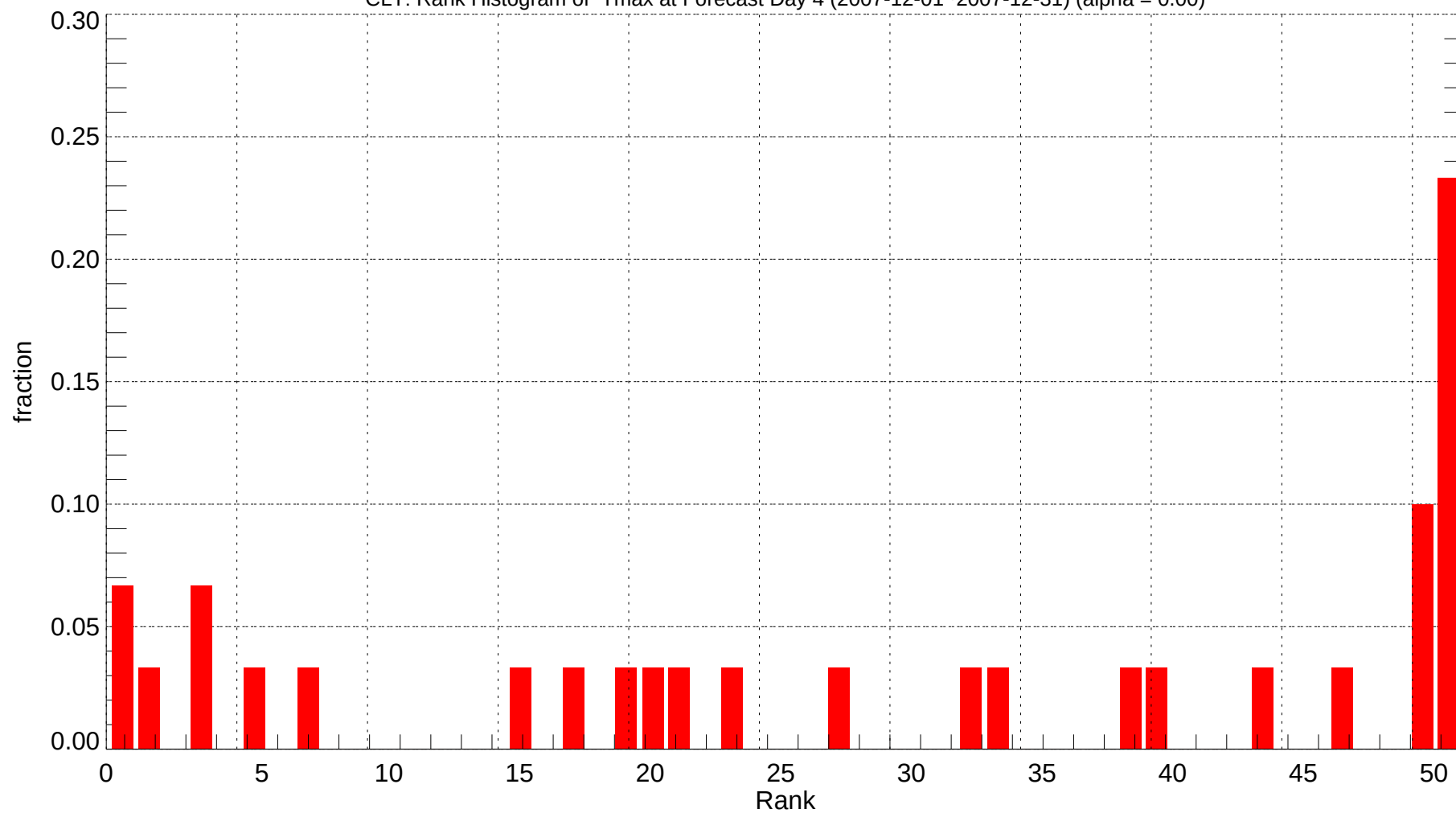
CLT: Rank Histogram of Tmax at Forecast Day 4 (2007-12-01~2007-12-31) (alpha = 0.00)
