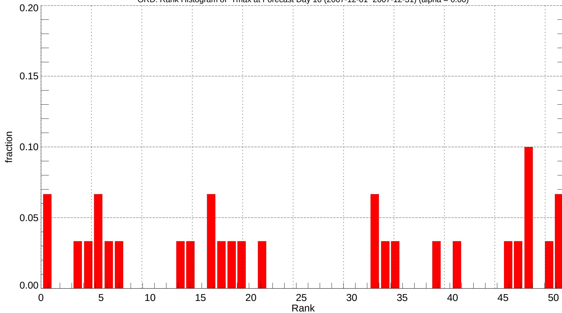
ORD: Rank Histogram of Tmax at Forecast Day 10 (2007-12-01~2007-12-31) (alpha = 0.00)
