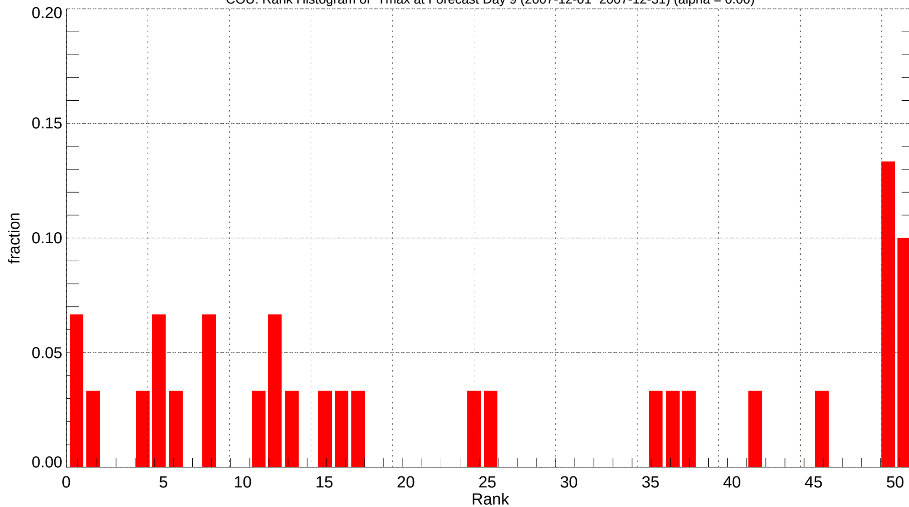
COU: Rank Histogram of Tmax at Forecast Day 9 (2007-12-01~2007-12-31) (alpha = 0.00)
