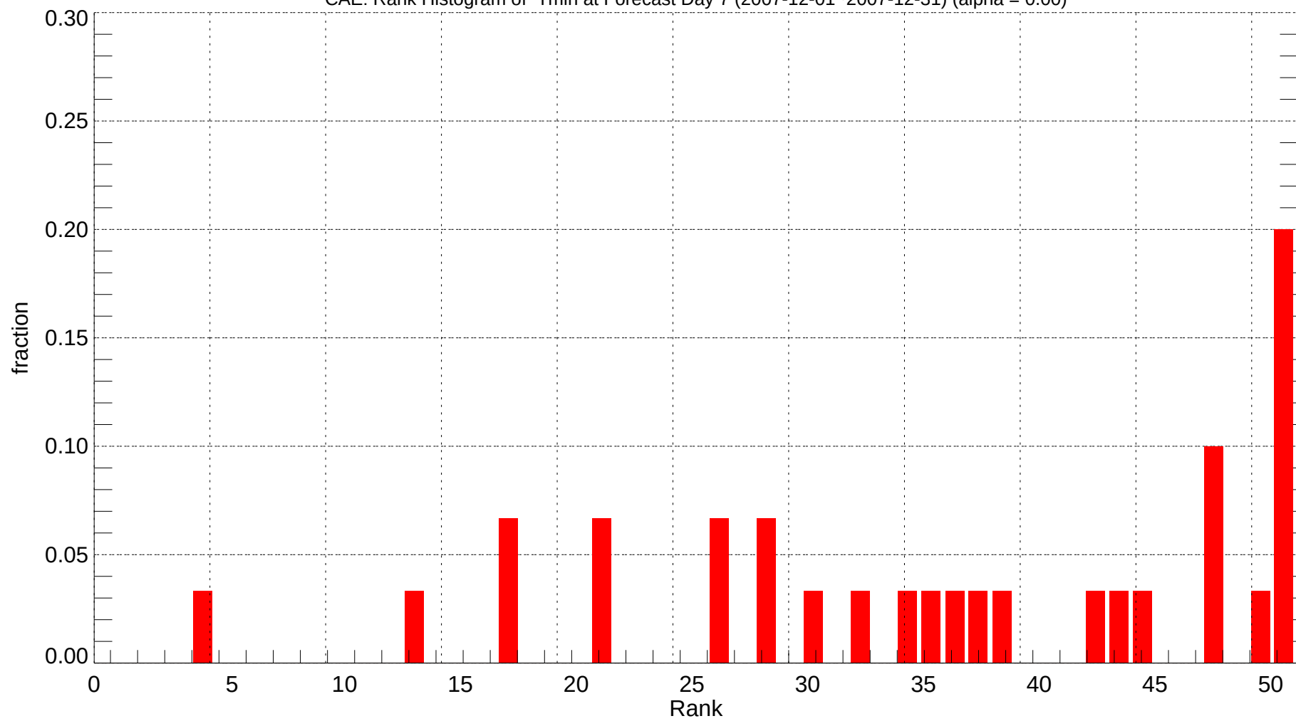
CAE: Rank Histogram of Tmin at Forecast Day 7 (2007-12-01~2007-12-31) (alpha = 0.00)
