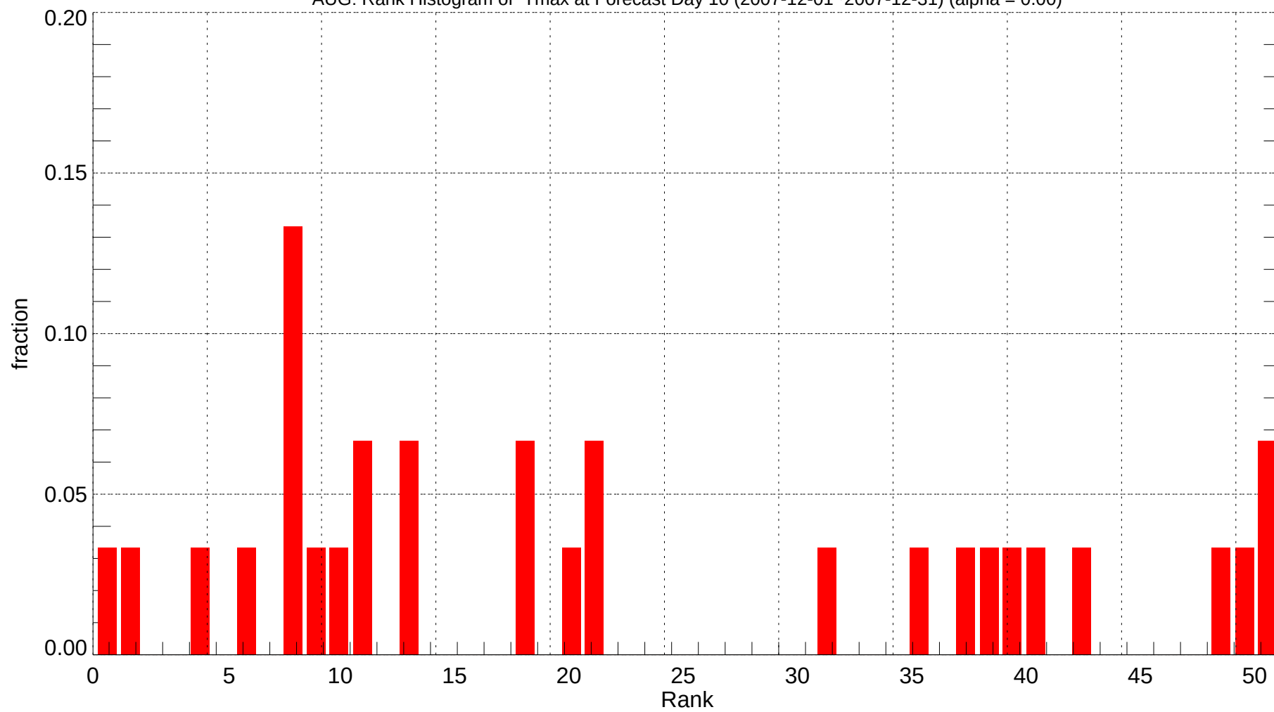
AUG: Rank Histogram of Tmax at Forecast Day 10 (2007-12-01~2007-12-31) (alpha = 0.00)
