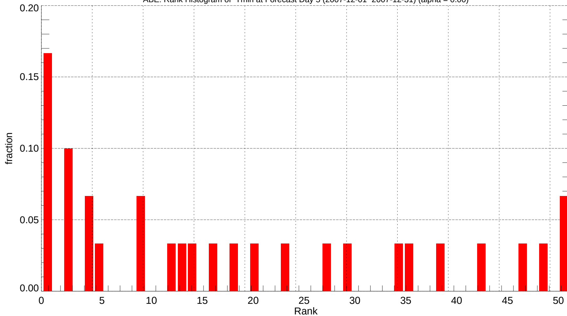
ABE: Rank Histogram of Tmin at Forecast Day 5 (2007-12-01~2007-12-31) (alpha = 0.00)
