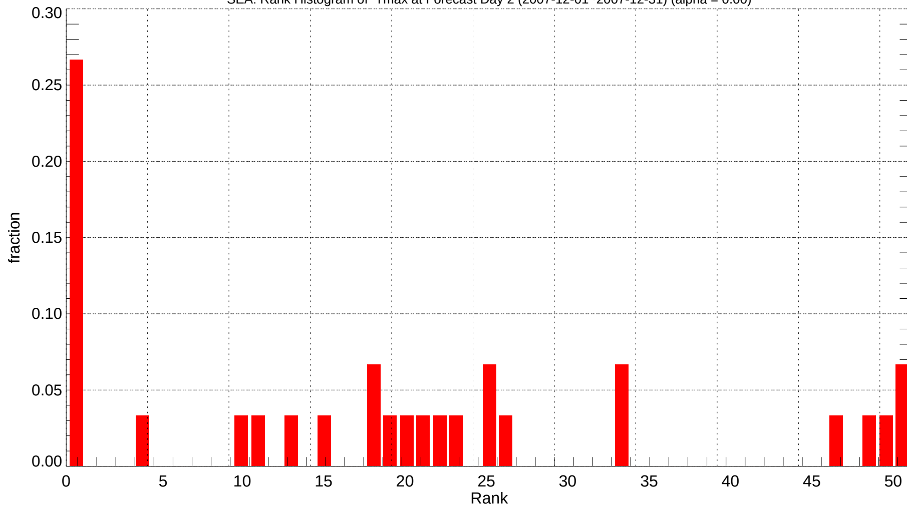
SEA: Rank Histogram of Tmax at Forecast Day 2 (2007-12-01~2007-12-31) (alpha = 0.00)
