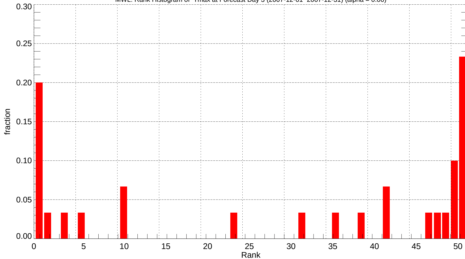
MWL: Rank Histogram of Tmax at Forecast Day 3 (2007-12-01~2007-12-31) (alpha = 0.00)
