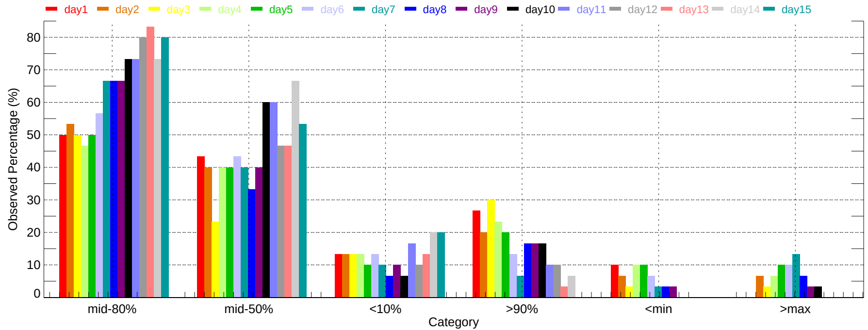
Observed Percentage of Ensembles - PHX: Min Temperature (2007-12-01~2007-12-31)
