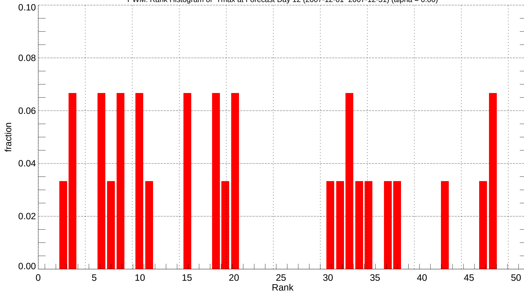
PWM: Rank Histogram of Tmax at Forecast Day 12 (2007-12-01~2007-12-31) (alpha = 0.00)
