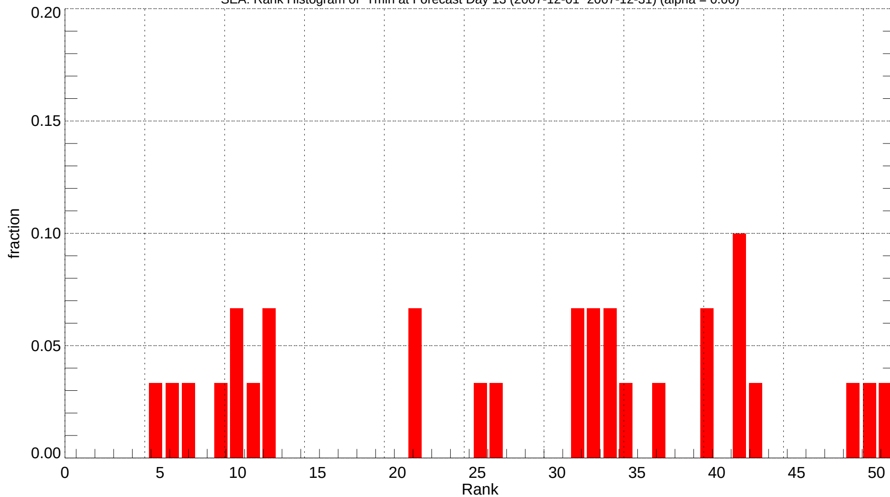
SEA: Rank Histogram of Tmin at Forecast Day 13 (2007-12-01~2007-12-31) (alpha = 0.00)
