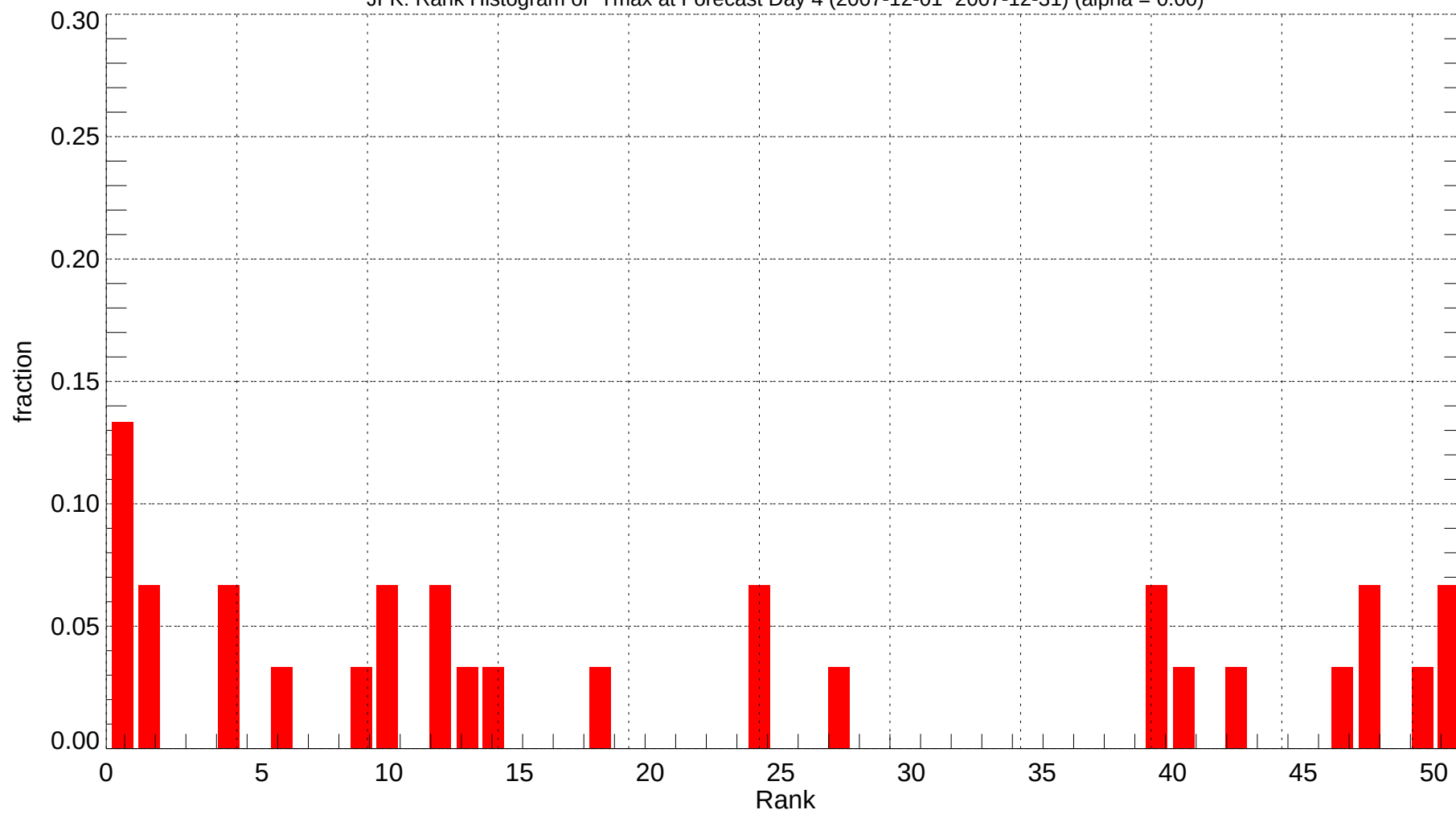
JFK: Rank Histogram of Tmax at Forecast Day 4 (2007-12-01~2007-12-31) (alpha = 0.00)
