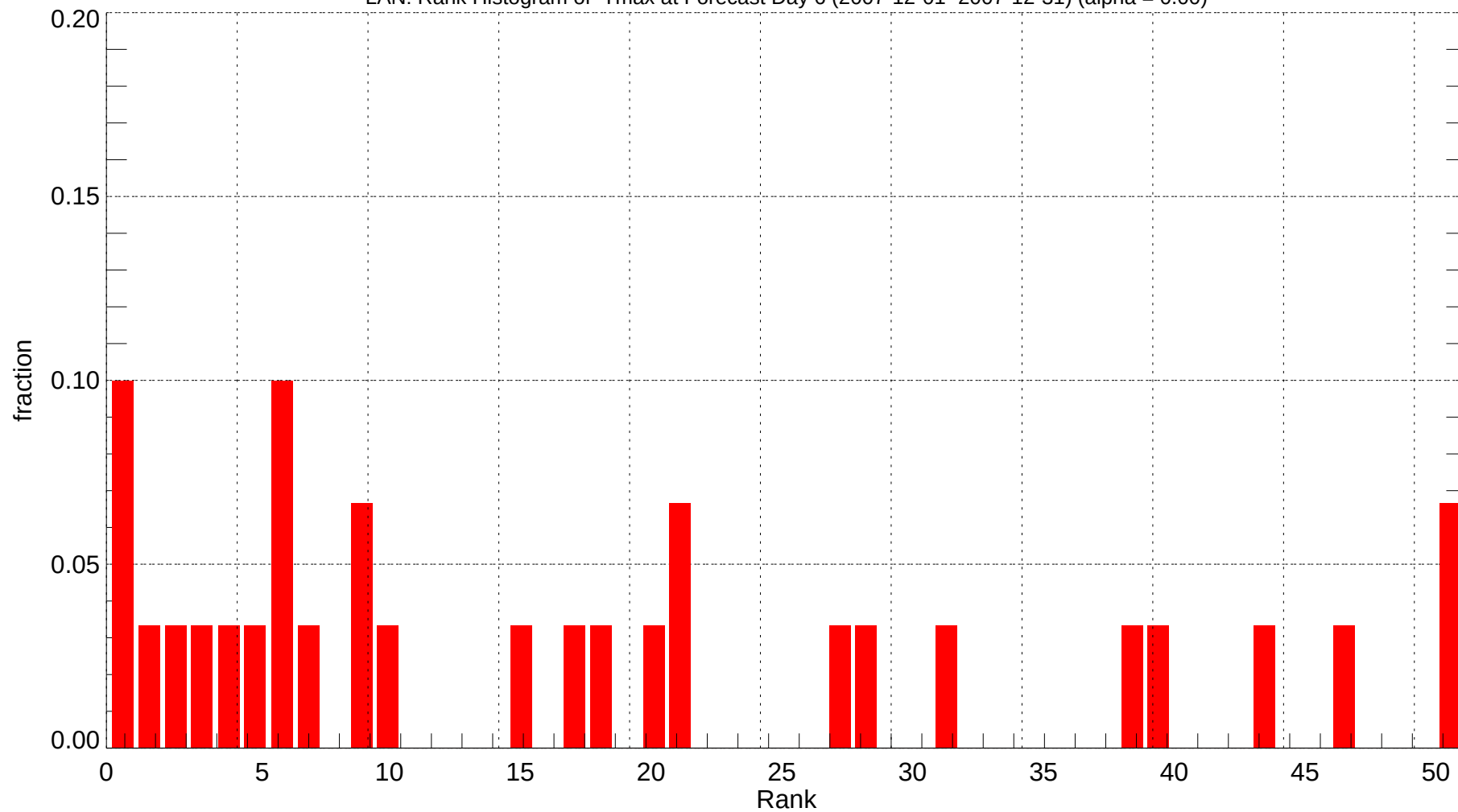
LAN: Rank Histogram of Tmax at Forecast Day 6 (2007-12-01~2007-12-31) (alpha = 0.00)
