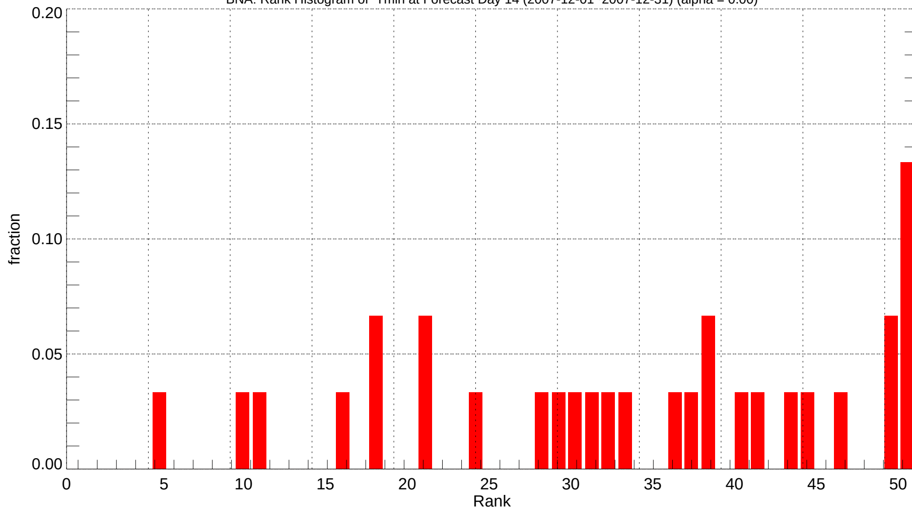
BNA: Rank Histogram of Tmin at Forecast Day 14 (2007-12-01~2007-12-31) (alpha = 0.00)
