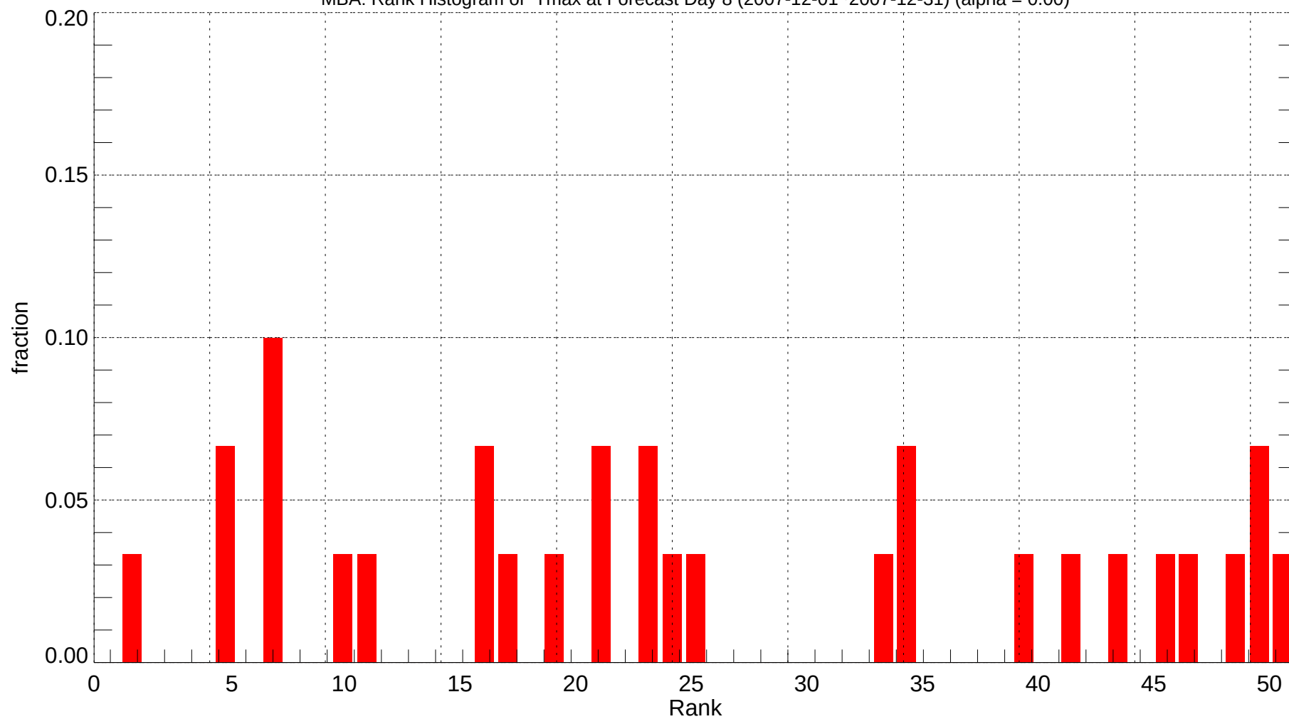
MBA: Rank Histogram of Tmax at Forecast Day 8 (2007-12-01~2007-12-31) (alpha = 0.00)
