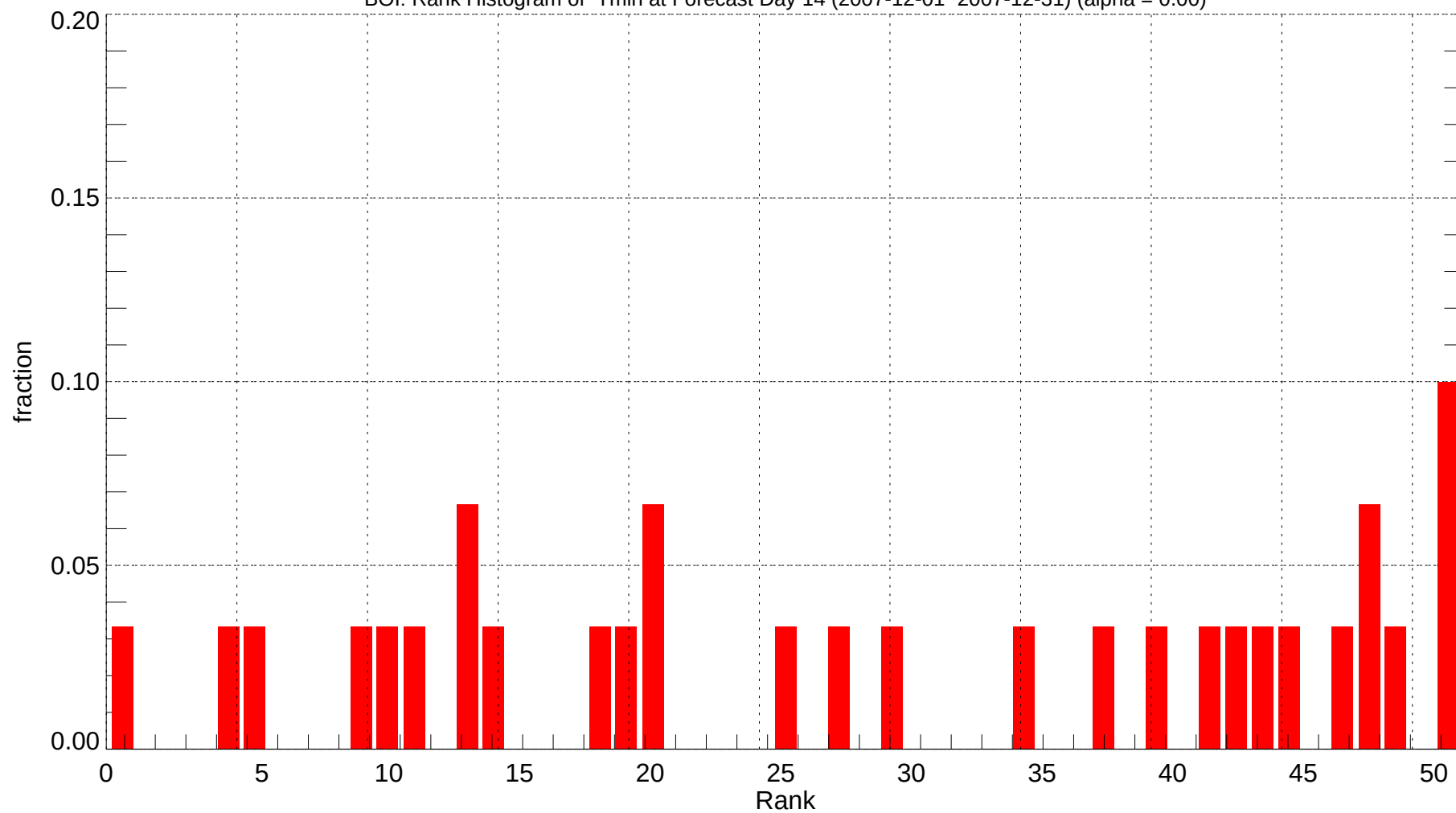
BOI: Rank Histogram of Tmin at Forecast Day 14 (2007-12-01~2007-12-31) (alpha = 0.00)
