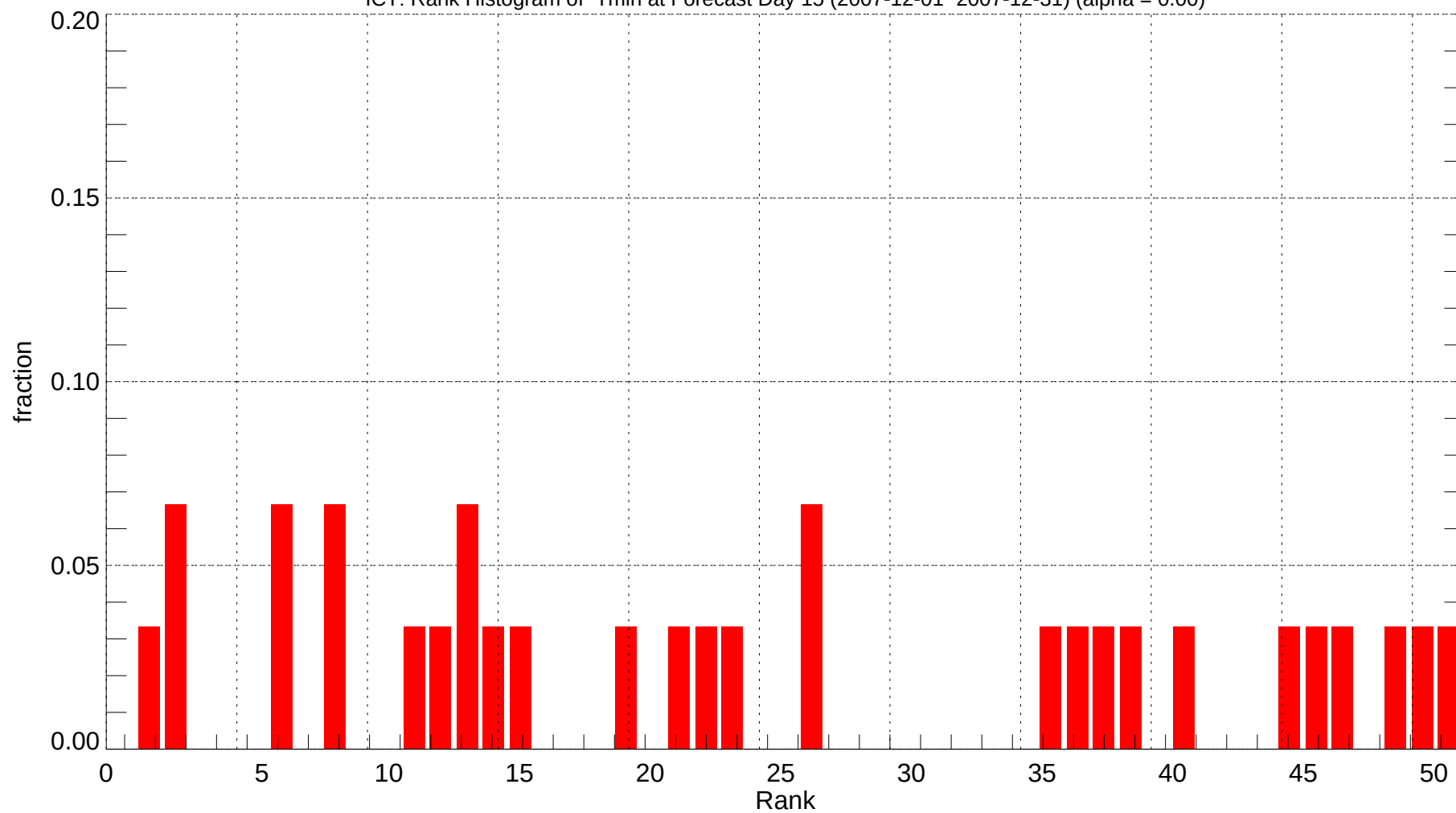
ICT: Rank Histogram of Tmin at Forecast Day 15 (2007-12-01~2007-12-31) (alpha = 0.00)
