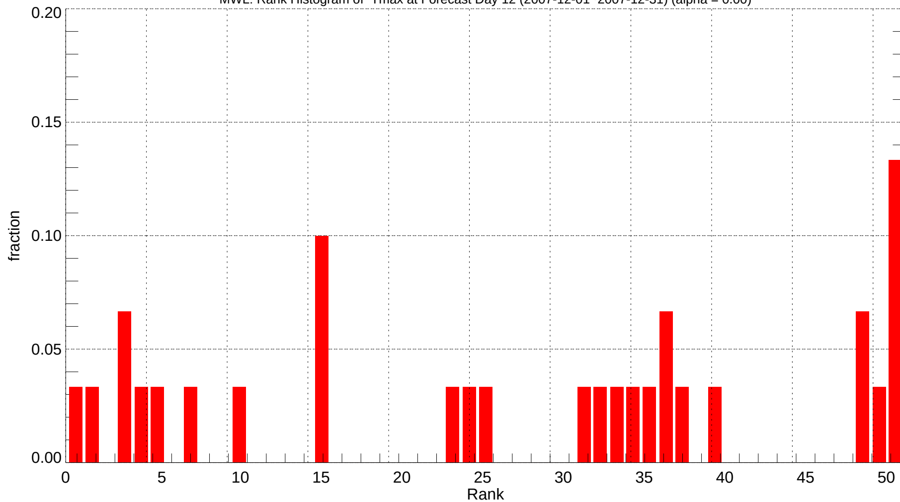
MWL: Rank Histogram of Tmax at Forecast Day 12 (2007-12-01~2007-12-31) (alpha = 0.00)
