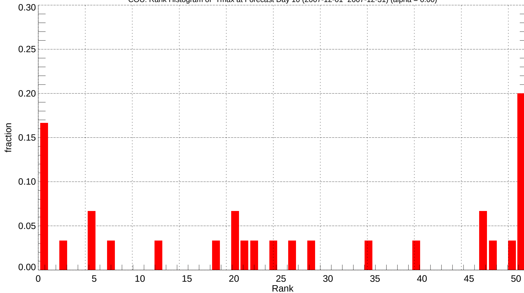
COU: Rank Histogram of Tmax at Forecast Day 10 (2007-12-01~2007-12-31) (alpha = 0.00)
