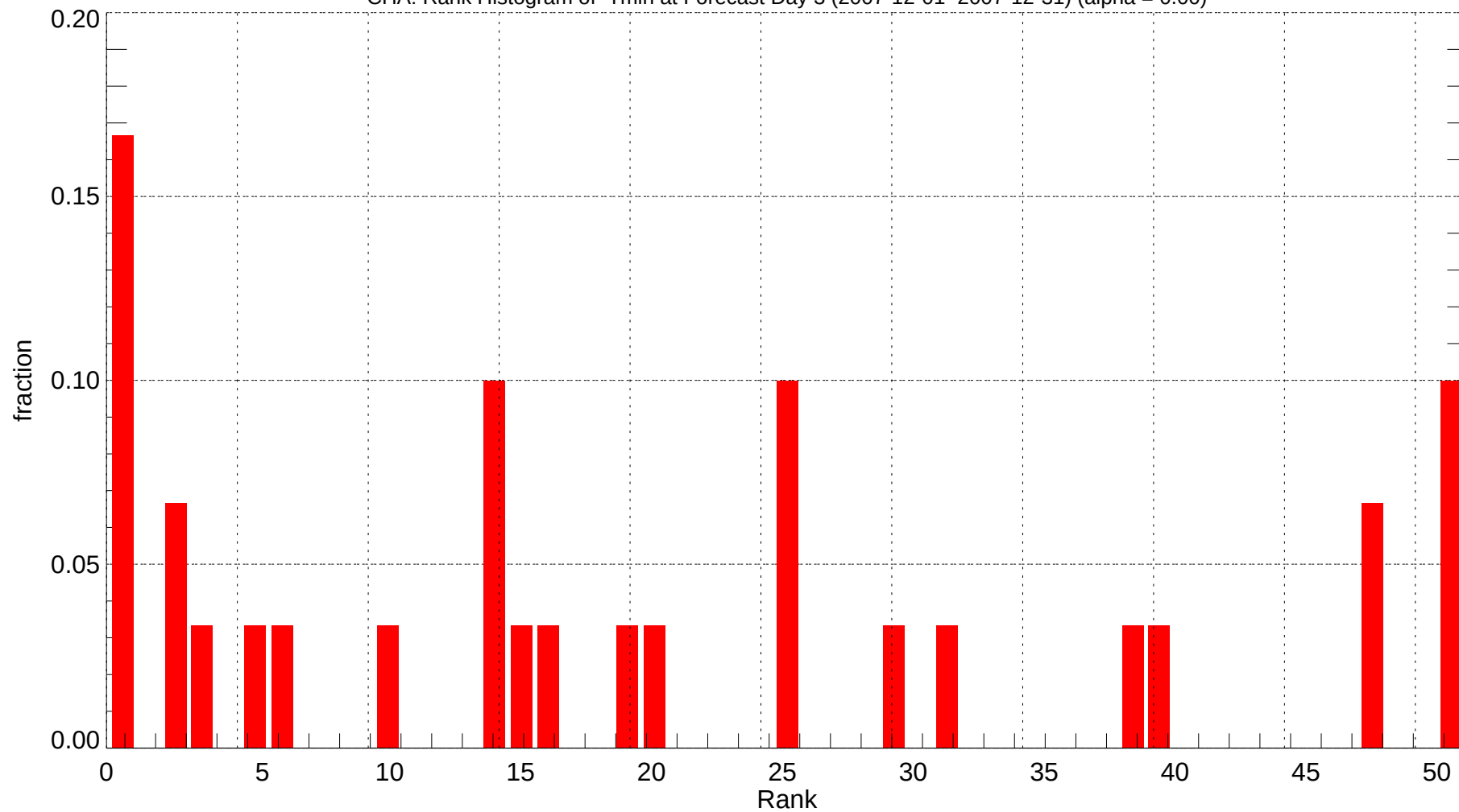
CHA: Rank Histogram of Tmin at Forecast Day 3 (2007-12-01~2007-12-31) (alpha = 0.00)
