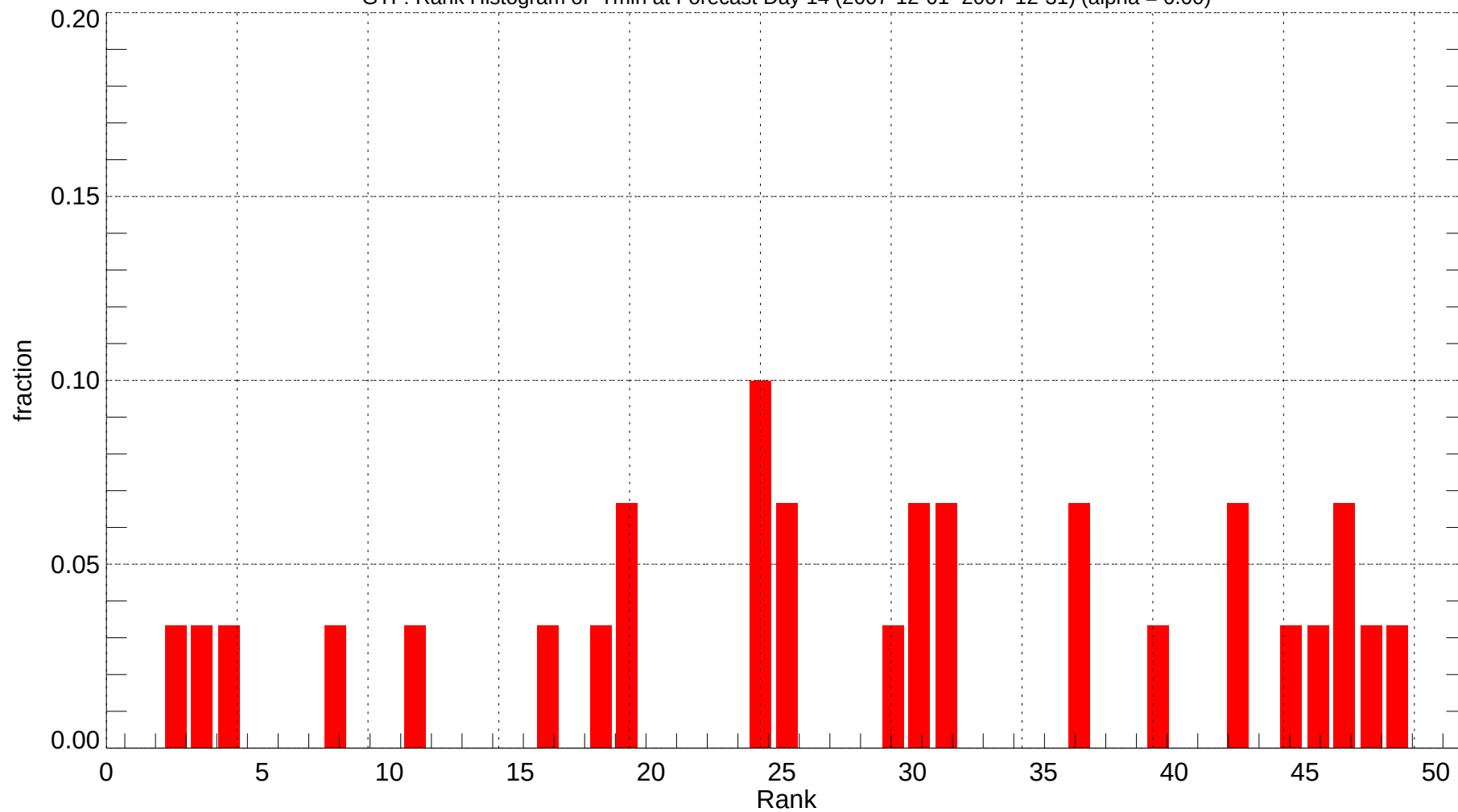
GTF: Rank Histogram of Tmin at Forecast Day 14 (2007-12-01~2007-12-31) (alpha = 0.00)
