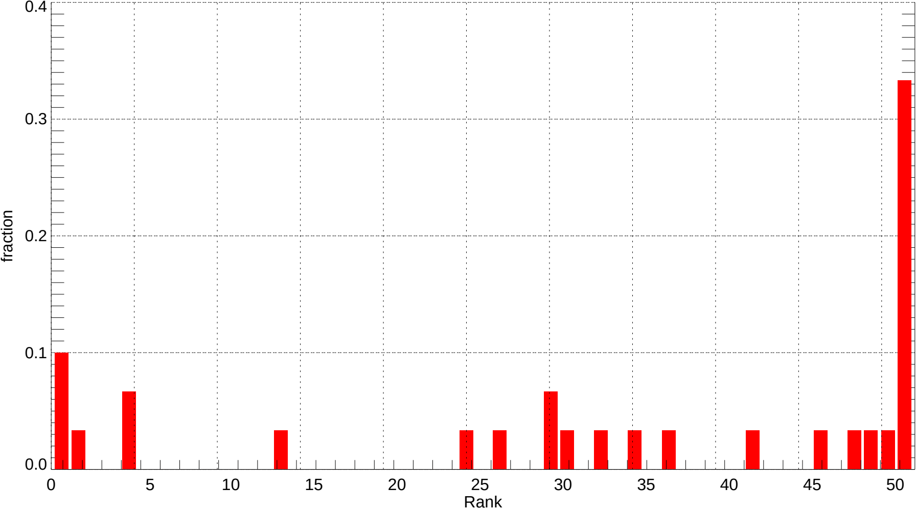
ATL: Rank Histogram of Tmin at Forecast Day 6 (2007-12-01~2007-12-31) (alpha = 0.00)
