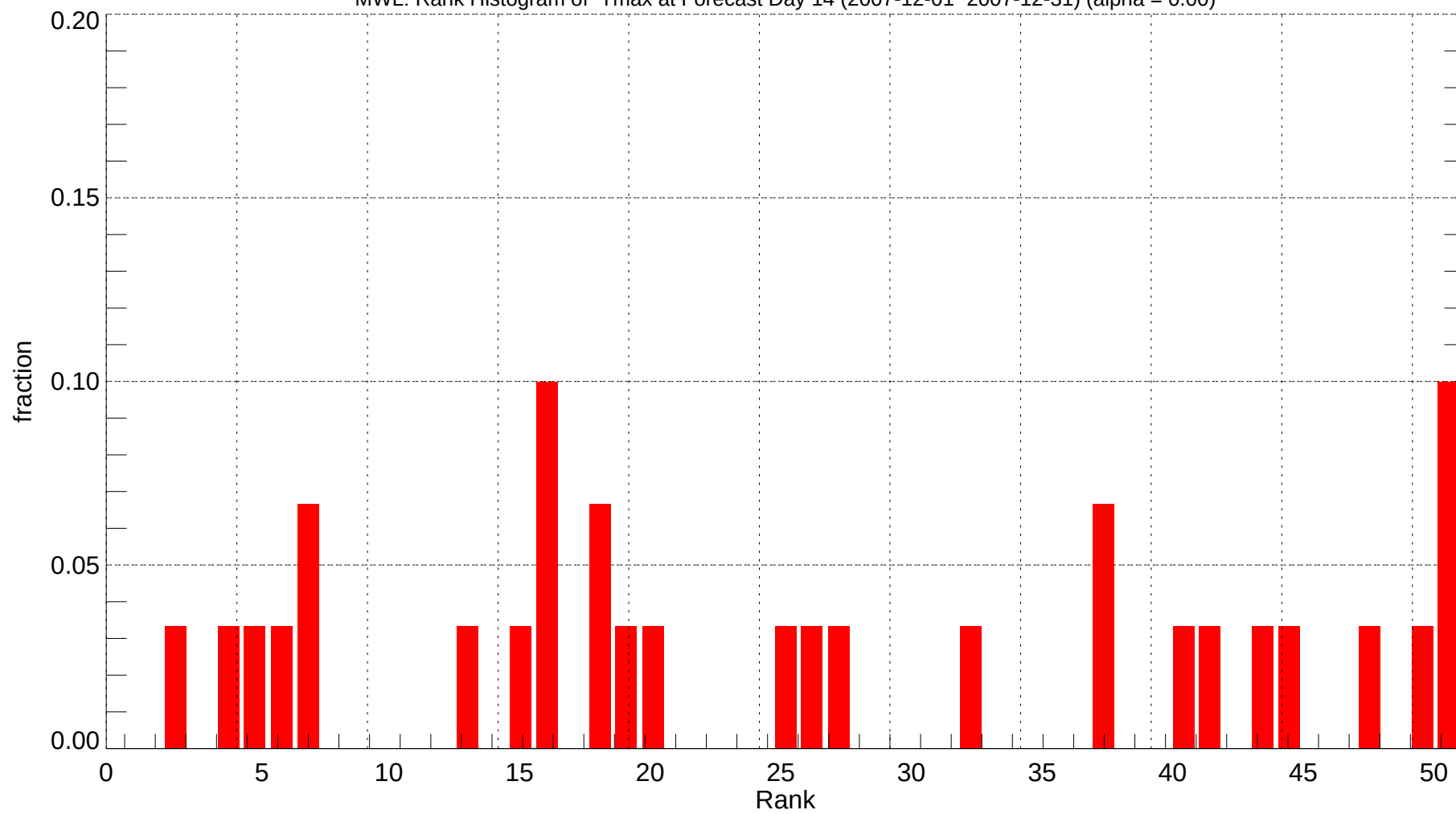
MWL: Rank Histogram of Tmax at Forecast Day 14 (2007-12-01~2007-12-31) (alpha = 0.00)
