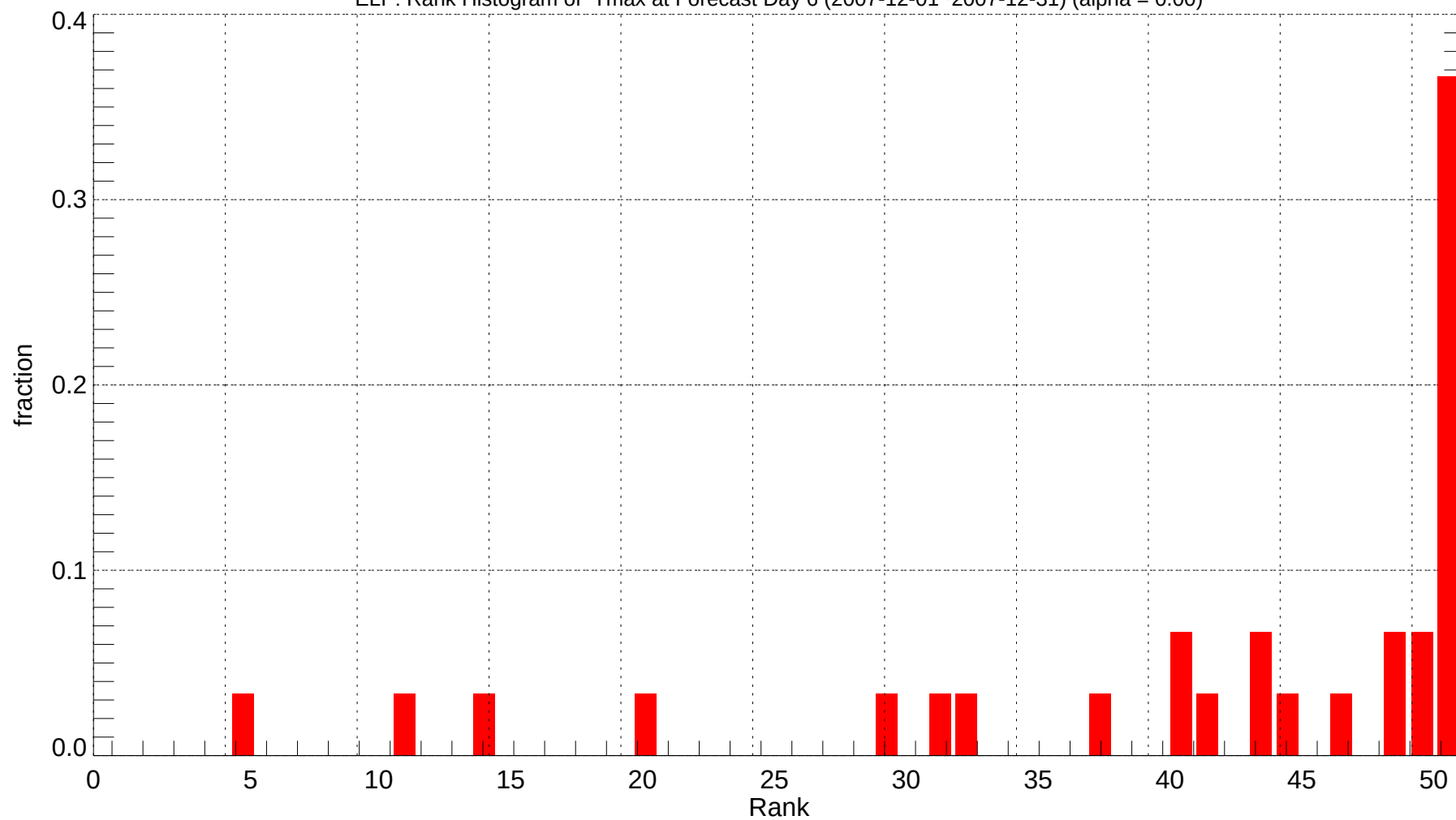
ELP: Rank Histogram of Tmax at Forecast Day 6 (2007-12-01~2007-12-31) (alpha = 0.00)
