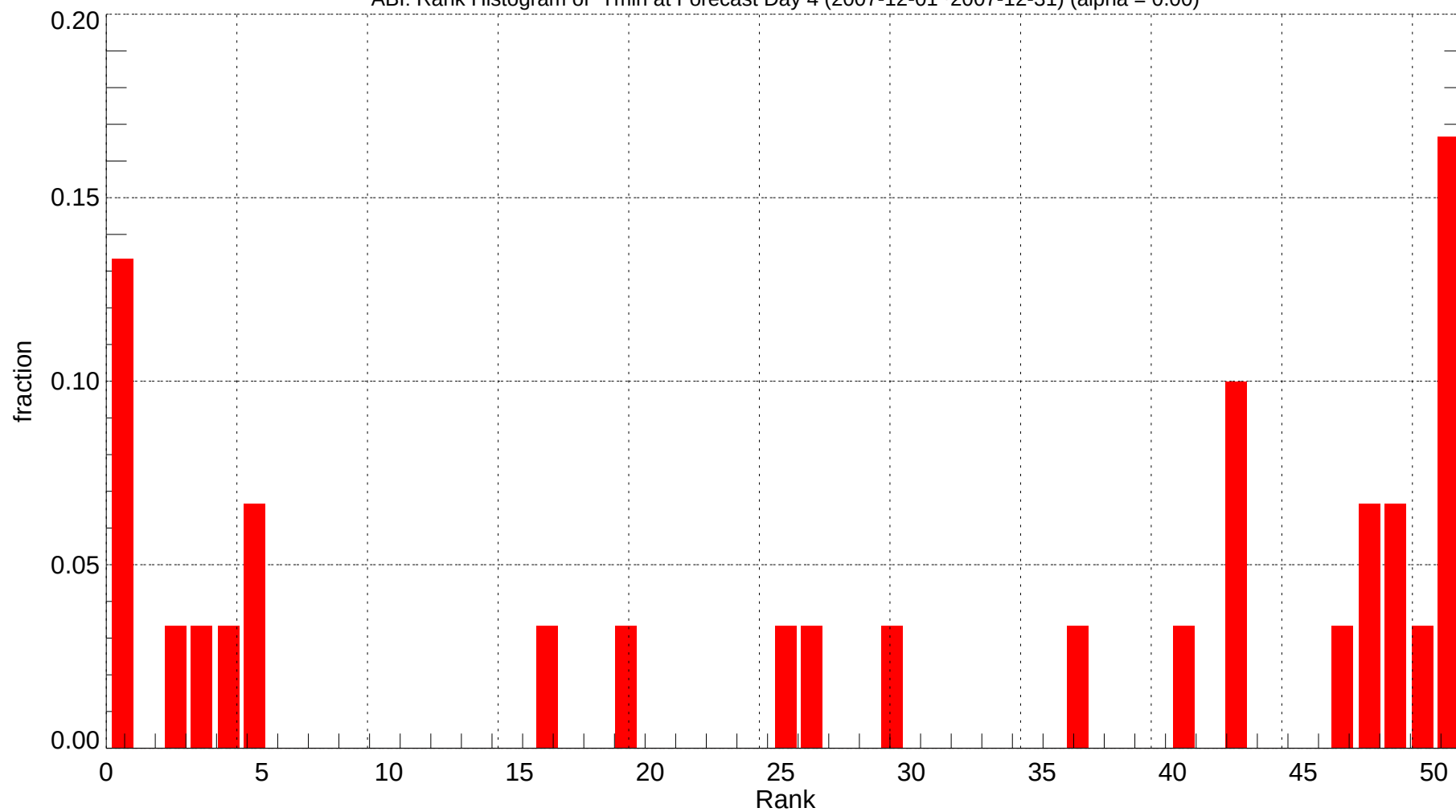
ABI: Rank Histogram of Tmin at Forecast Day 4 (2007-12-01~2007-12-31) (alpha = 0.00)
