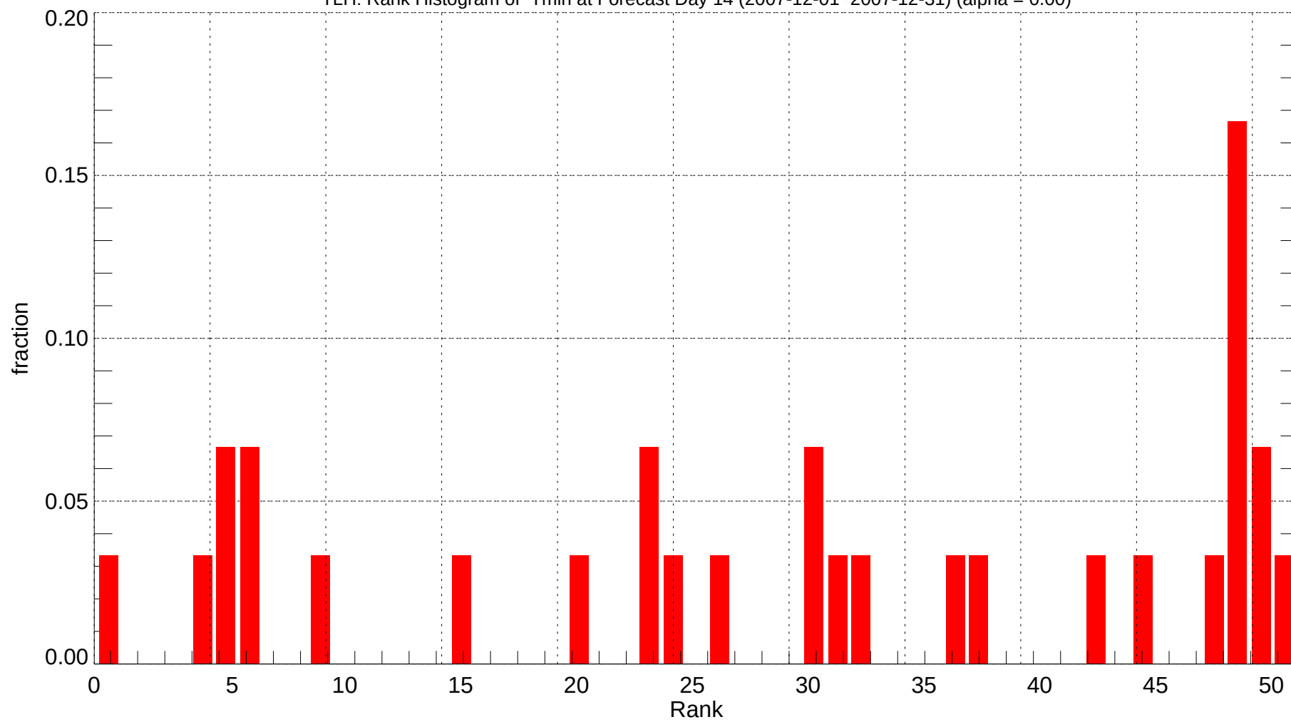
TLH: Rank Histogram of Tmin at Forecast Day 14 (2007-12-01~2007-12-31) (alpha = 0.00)
