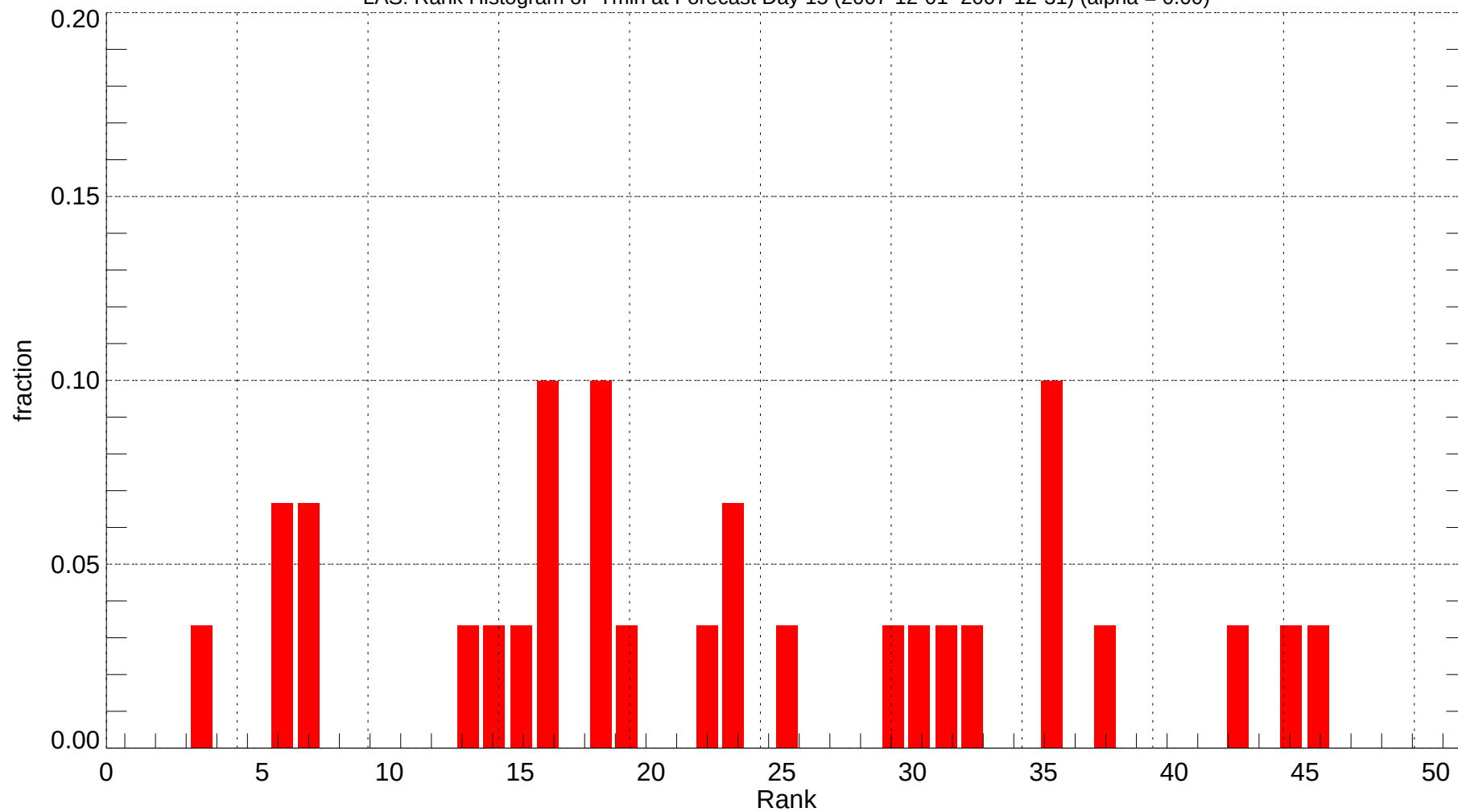
LAS: Rank Histogram of Tmin at Forecast Day 15 (2007-12-01~2007-12-31) (alpha = 0.00)
