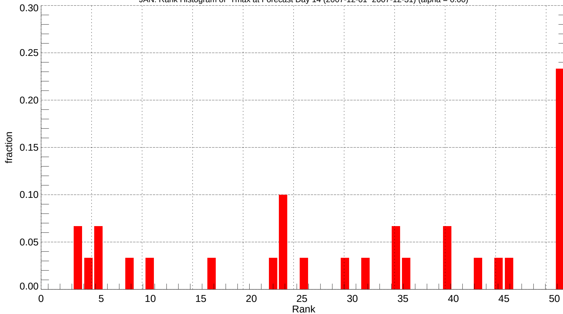
JAN: Rank Histogram of Tmax at Forecast Day 14 (2007-12-01~2007-12-31) (alpha = 0.00)
