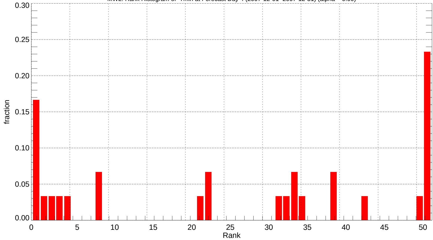
MWL: Rank Histogram of Tmin at Forecast Day 4 (2007-12-01~2007-12-31) (alpha = 0.00)
