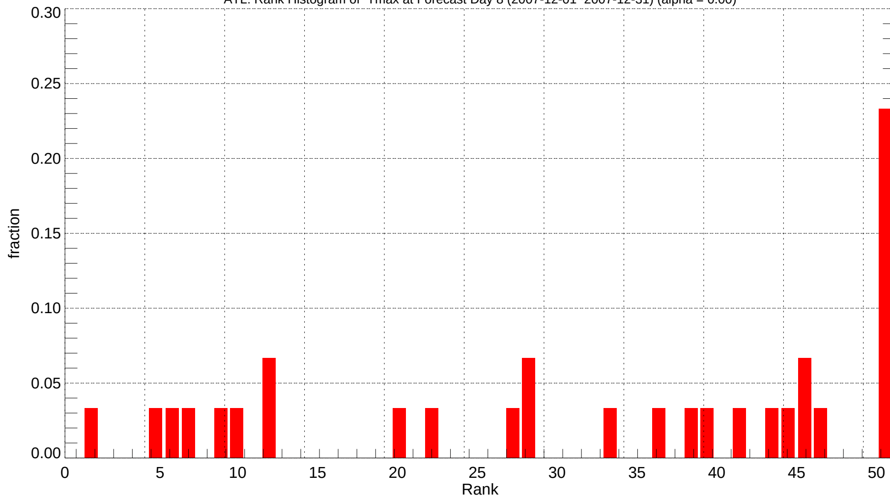
ATL: Rank Histogram of Tmax at Forecast Day 8 (2007-12-01~2007-12-31) (alpha = 0.00)
