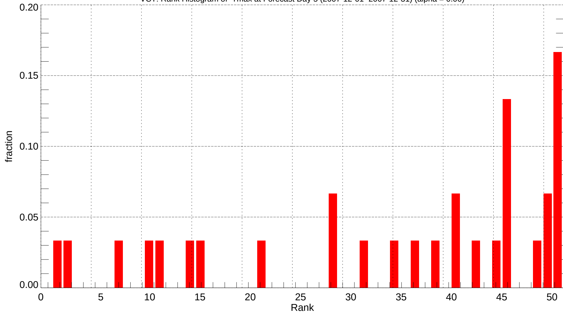
VCT: Rank Histogram of Tmax at Forecast Day 5 (2007-12-01~2007-12-31) (alpha = 0.00)
