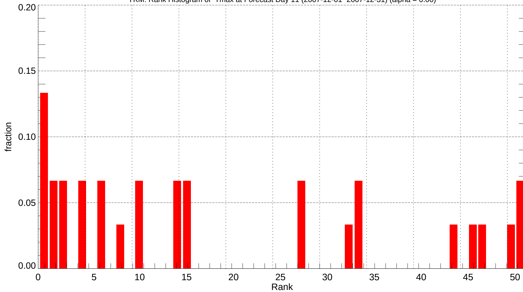
YKM: Rank Histogram of Tmax at Forecast Day 11 (2007-12-01~2007-12-31) (alpha = 0.00)
