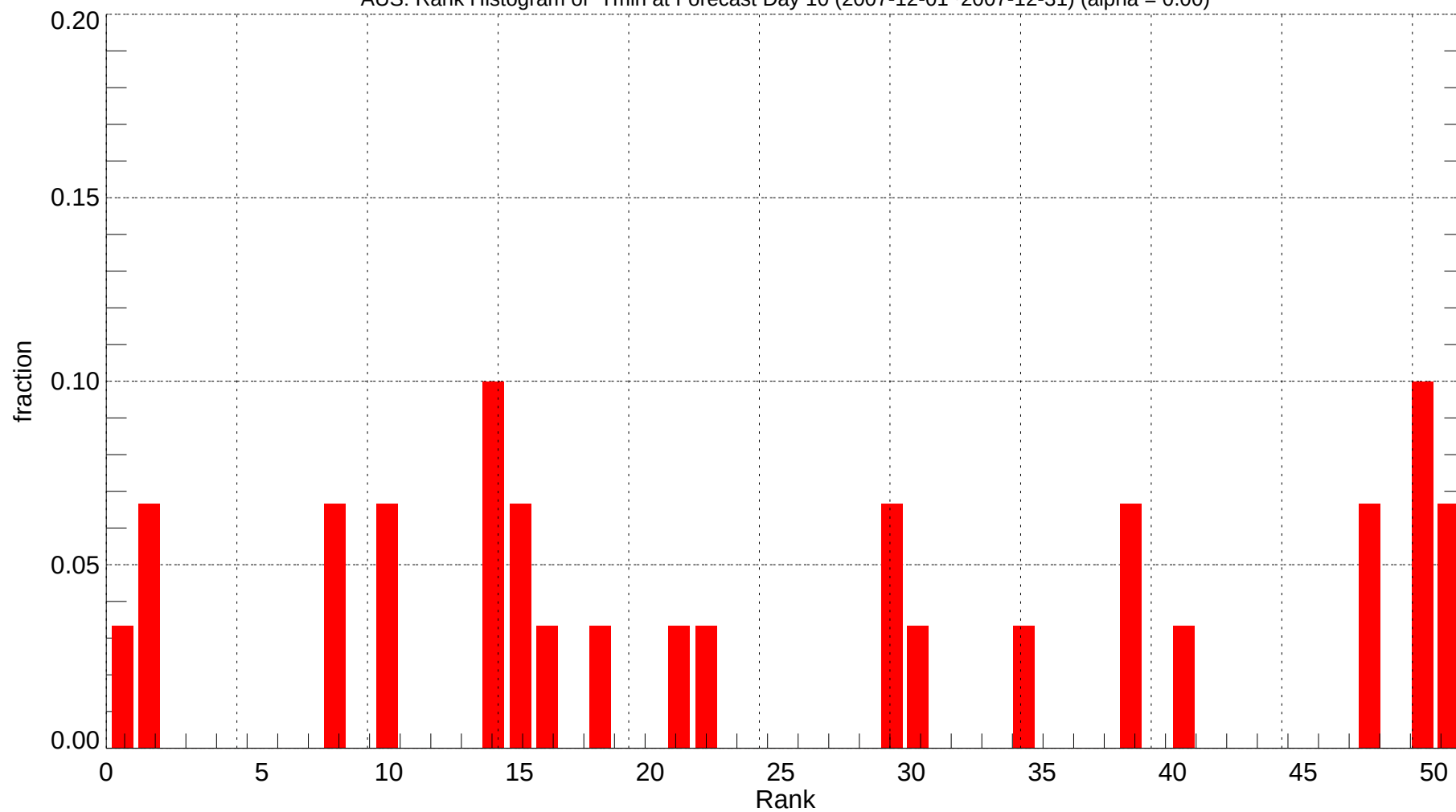
AUS: Rank Histogram of Tmin at Forecast Day 10 (2007-12-01~2007-12-31) (alpha = 0.00)
