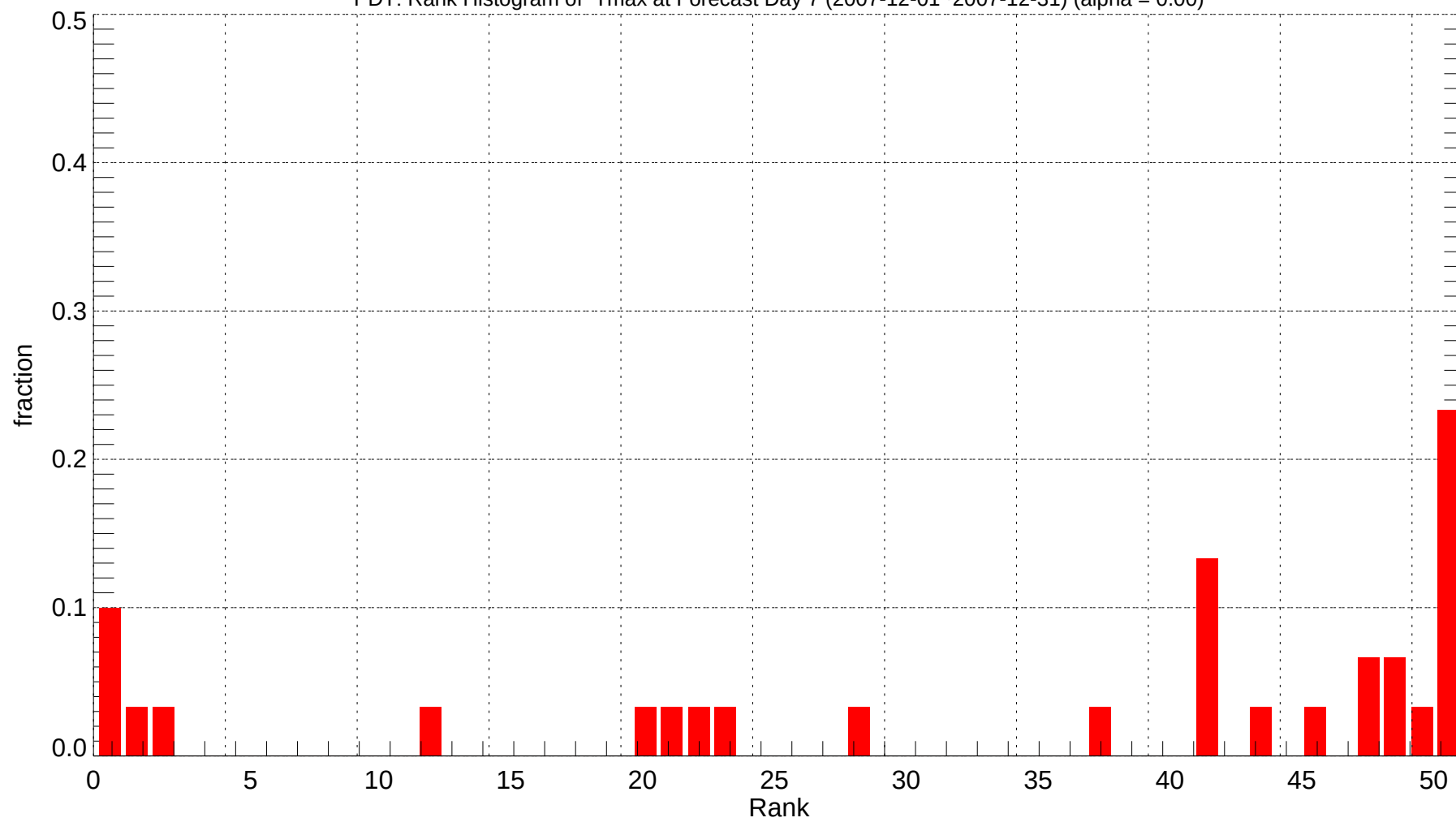
PDT: Rank Histogram of Tmax at Forecast Day 7 (2007-12-01~2007-12-31) (alpha = 0.00)
