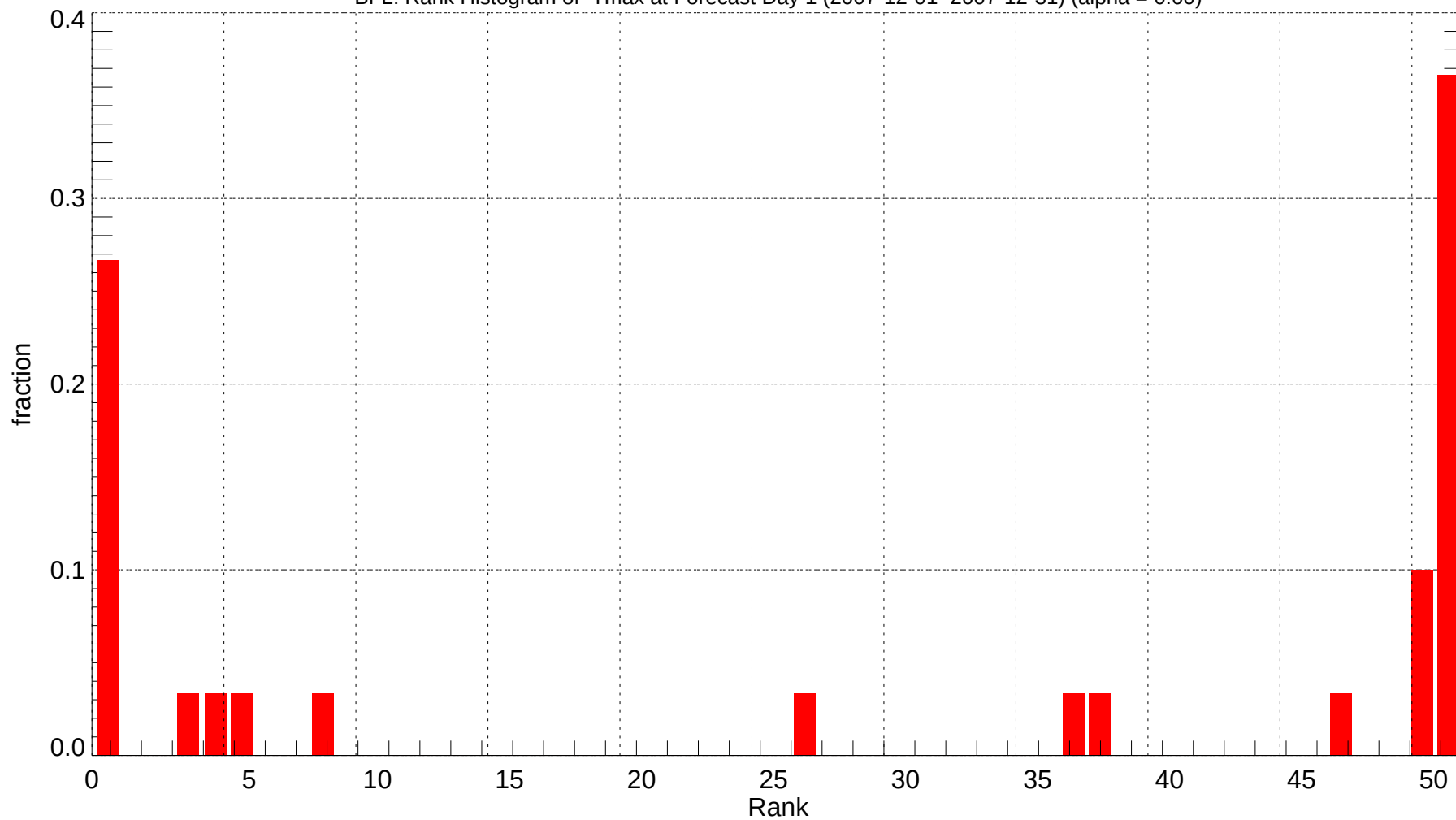
BFL: Rank Histogram of Tmax at Forecast Day 1 (2007-12-01~2007-12-31) (alpha = 0.00)
