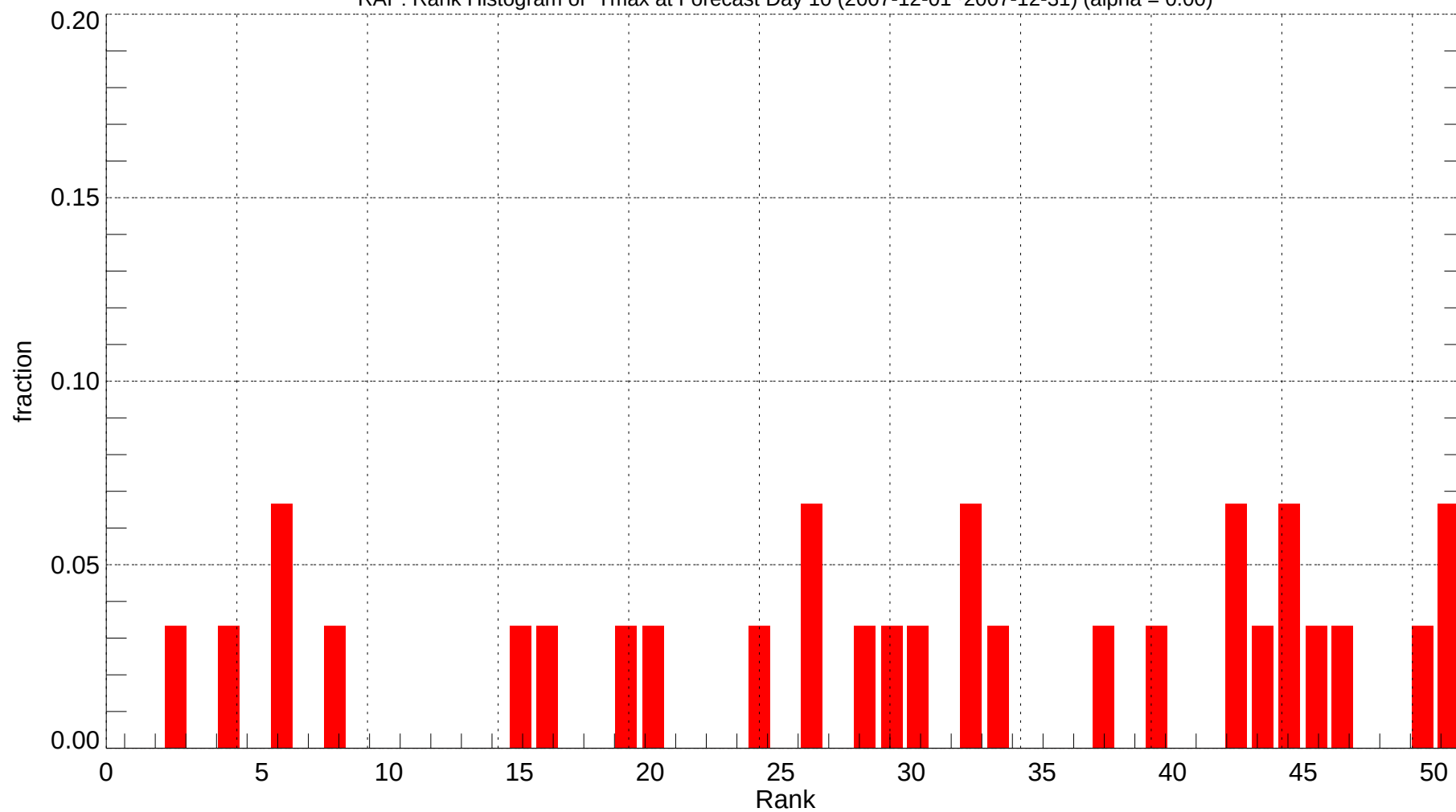
RAP: Rank Histogram of Tmax at Forecast Day 10 (2007-12-01~2007-12-31) (alpha = 0.00)
