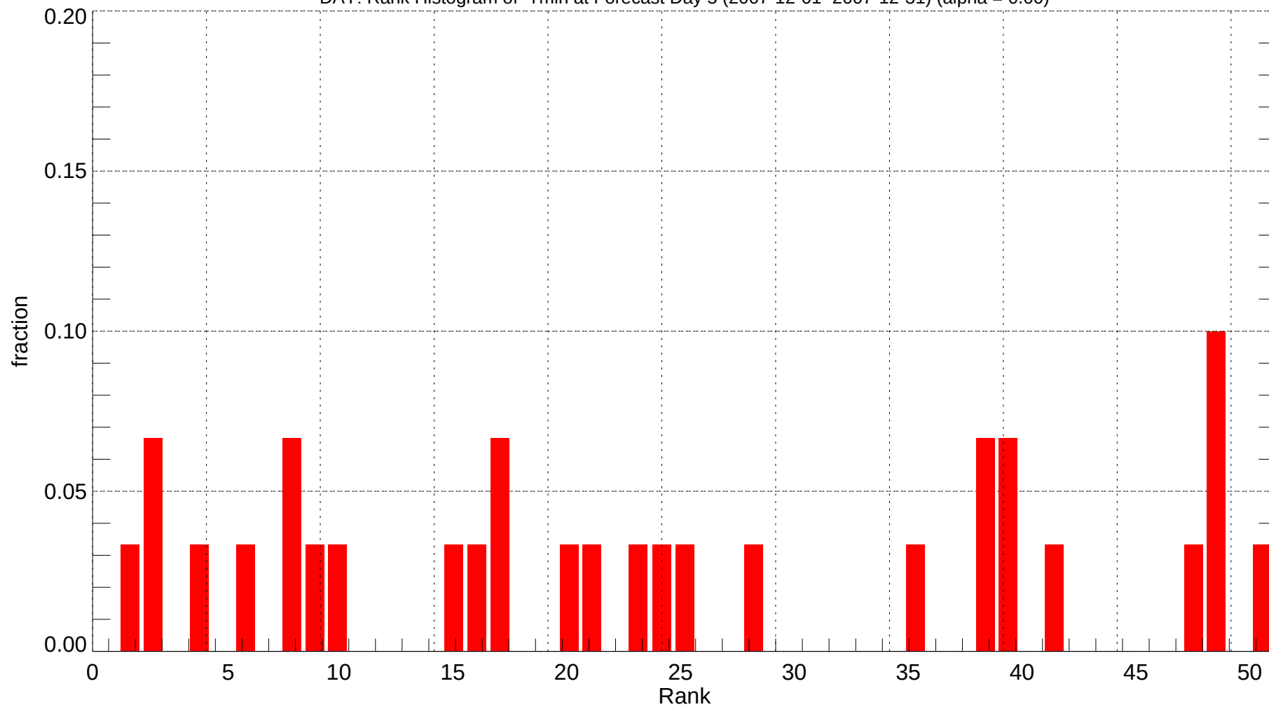
DAY: Rank Histogram of Tmin at Forecast Day 5 (2007-12-01~2007-12-31) (alpha = 0.00)
