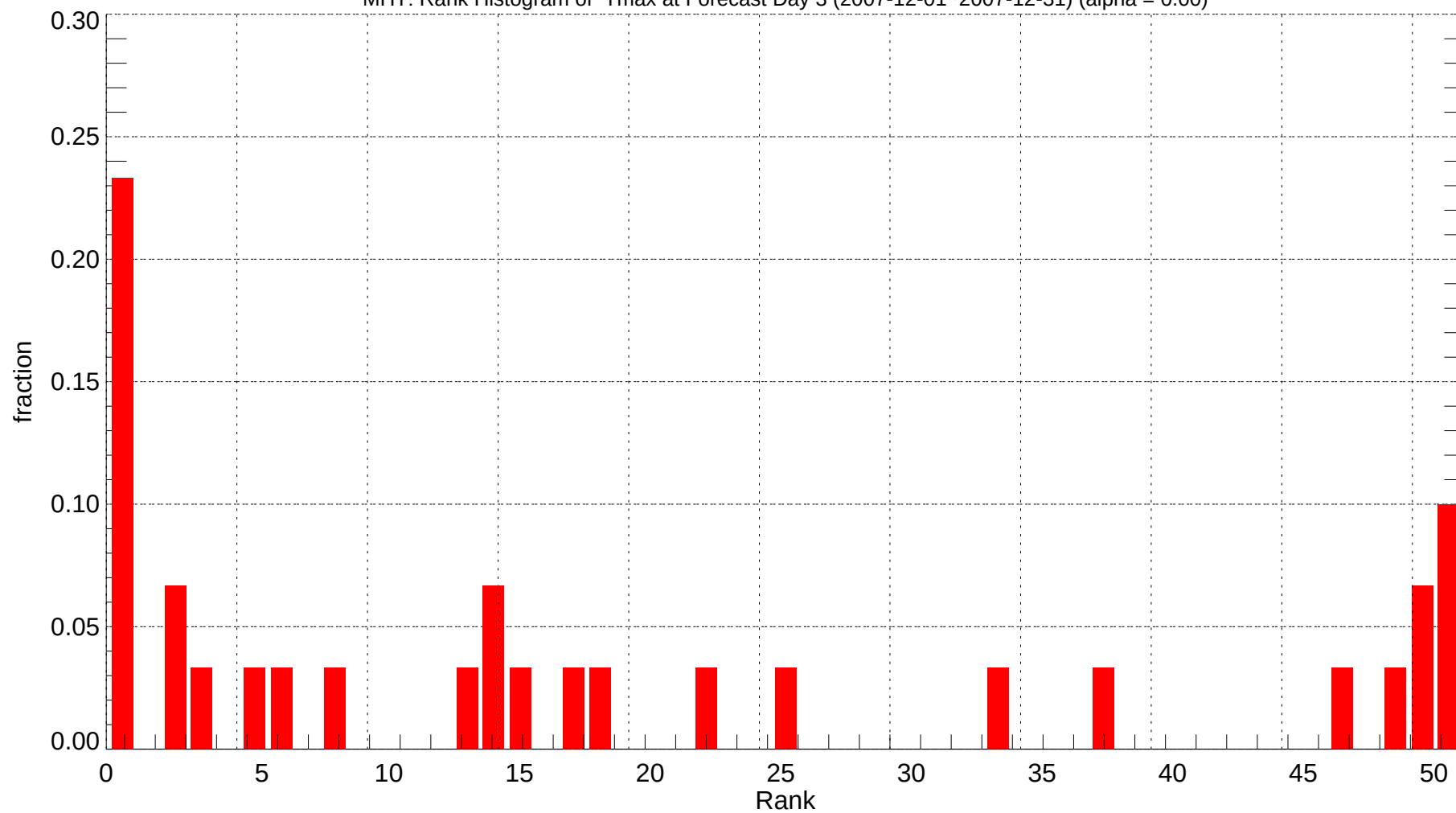
MHT: Rank Histogram of Tmax at Forecast Day 3 (2007-12-01~2007-12-31) (alpha = 0.00)
