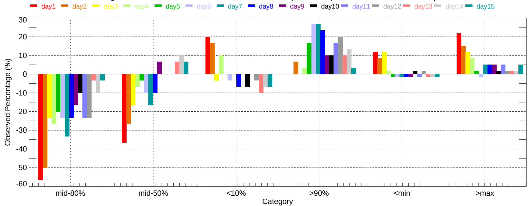
Observed Percentage Deviation of Ensembles - EVV: Min Temperature (2007-12-01~2007-12-31)
