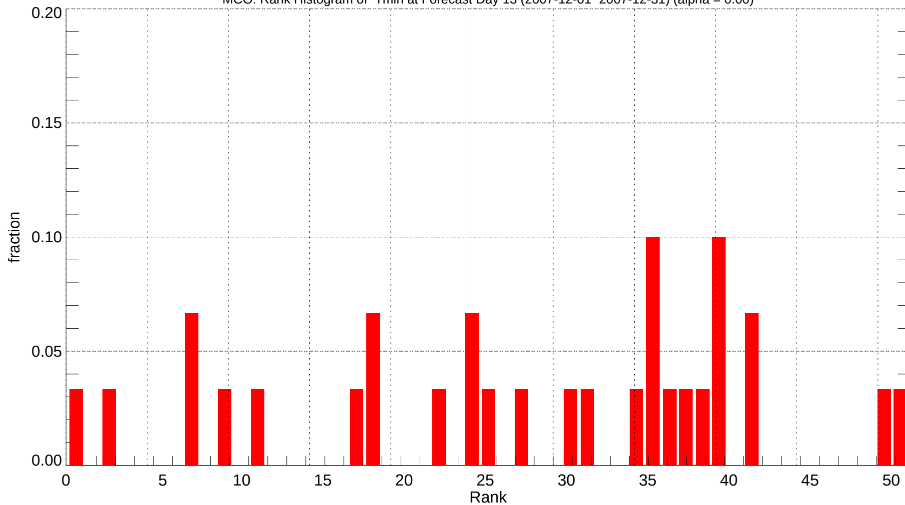
MCO: Rank Histogram of Tmin at Forecast Day 13 (2007-12-01~2007-12-31) (alpha = 0.00)
