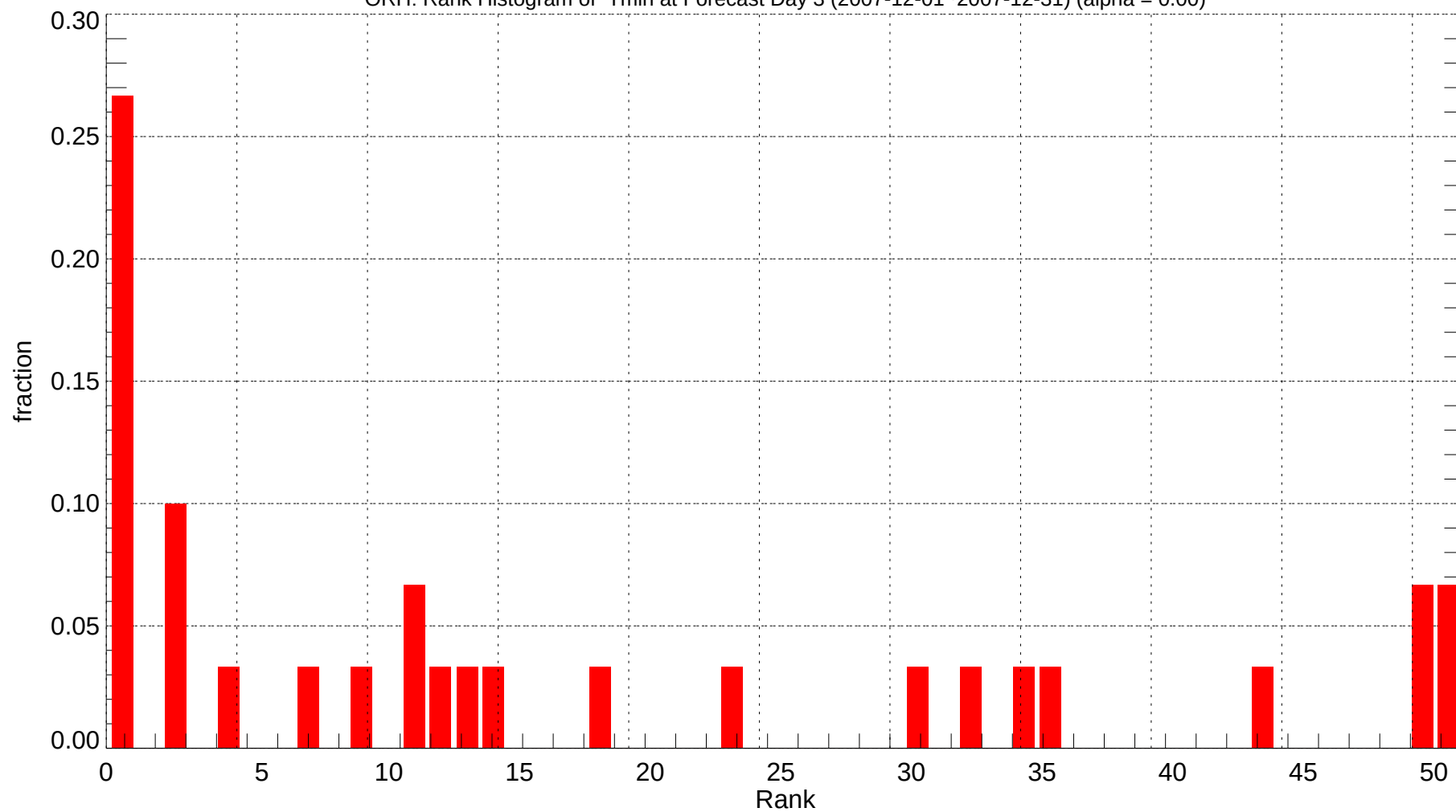
ORH: Rank Histogram of Tmin at Forecast Day 3 (2007-12-01~2007-12-31) (alpha = 0.00)
