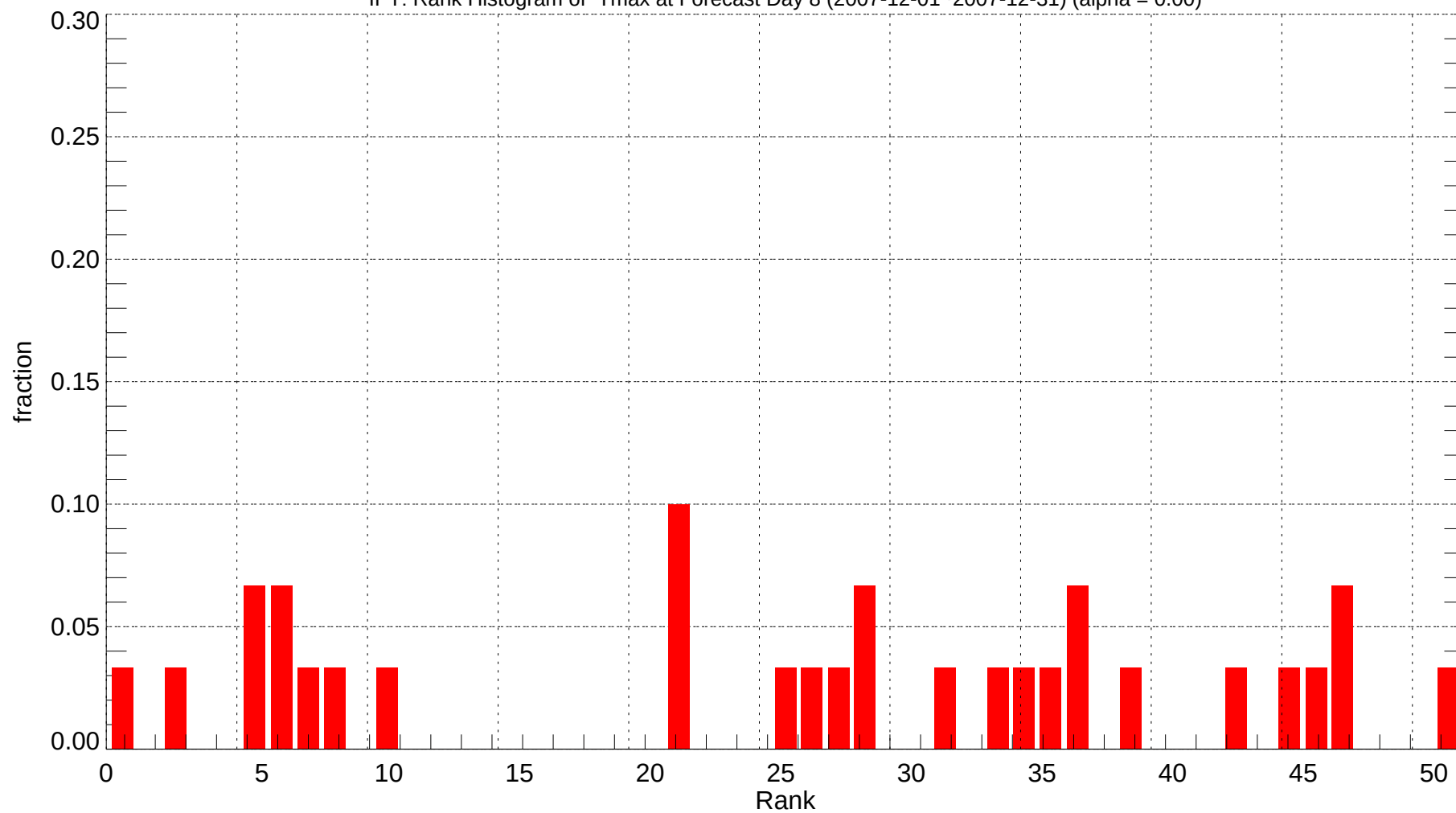
IPT: Rank Histogram of Tmax at Forecast Day 8 (2007-12-01~2007-12-31) (alpha = 0.00)
