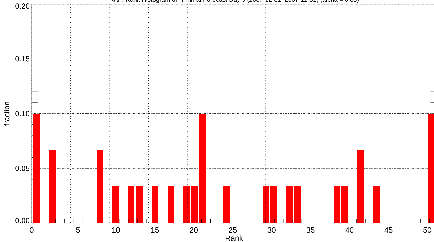
RAP: Rank Histogram of Tmin at Forecast Day 5 (2007-12-01~2007-12-31) (alpha = 0.00)
