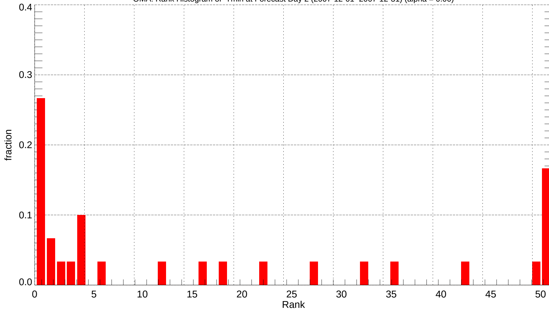
OMA: Rank Histogram of Tmin at Forecast Day 2 (2007-12-01~2007-12-31) (alpha = 0.00)
