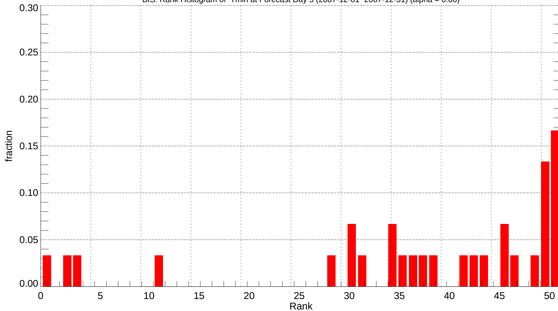
BIS: Rank Histogram of Tmin at Forecast Day 5 (2007-12-01~2007-12-31) (alpha = 0.00)
