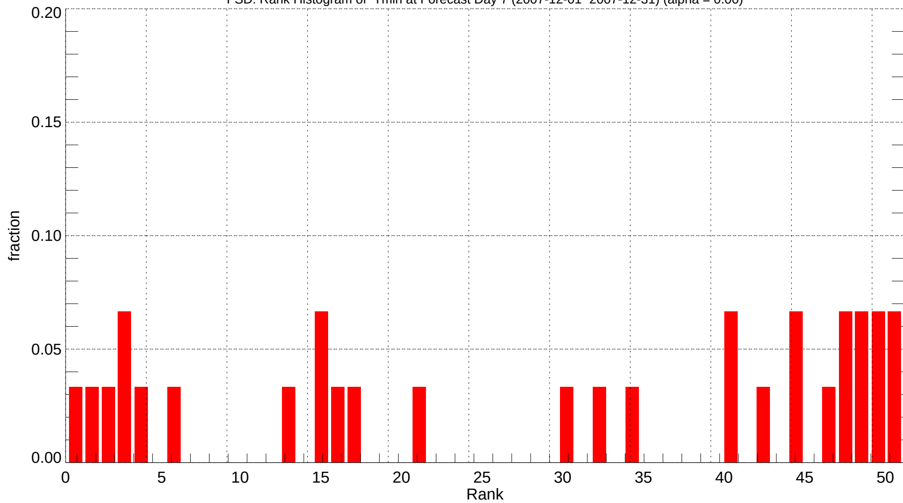
FSD: Rank Histogram of Tmin at Forecast Day 7 (2007-12-01~2007-12-31) (alpha = 0.00)
