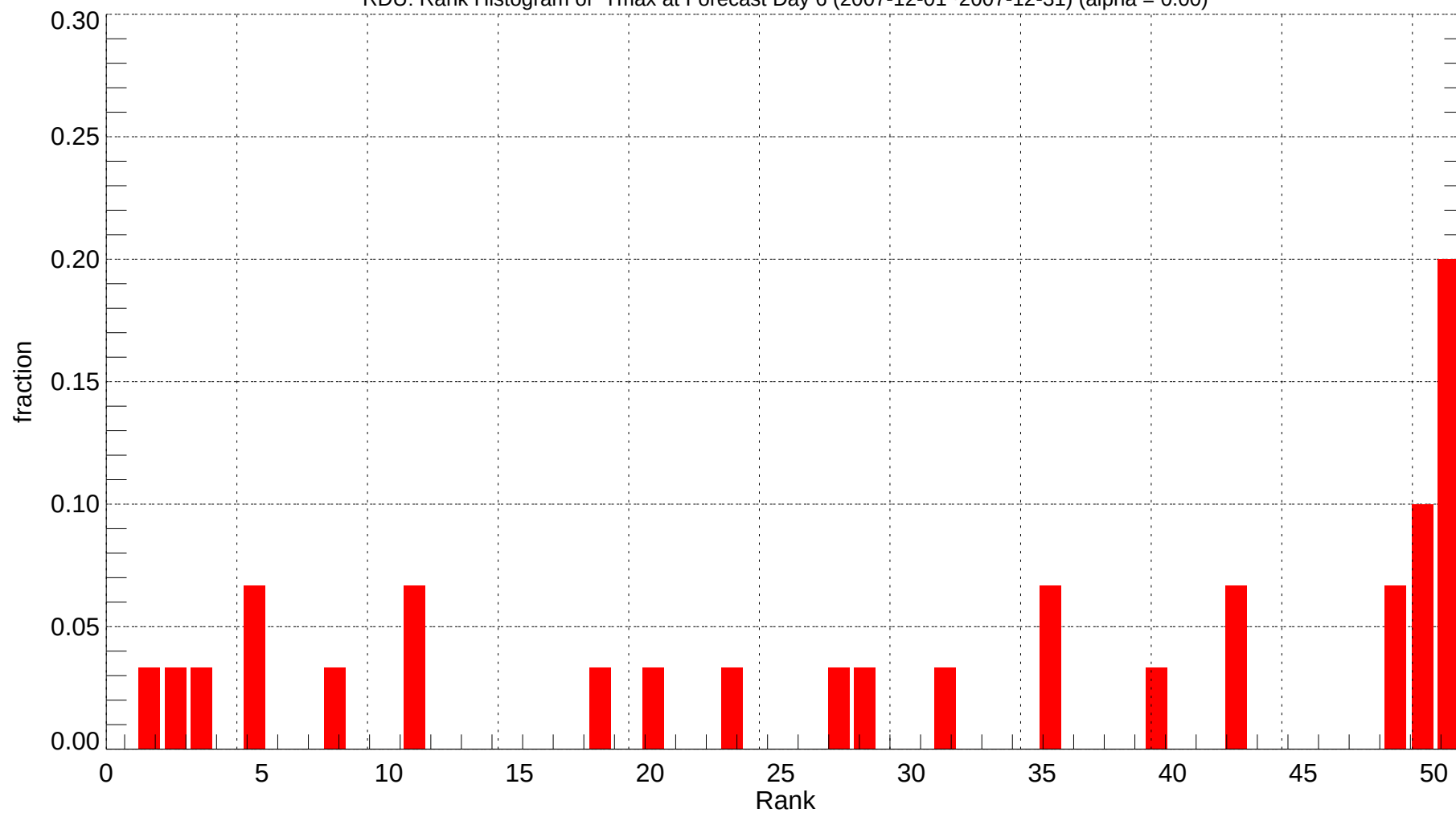
RDU: Rank Histogram of Tmax at Forecast Day 6 (2007-12-01~2007-12-31) (alpha = 0.00)
