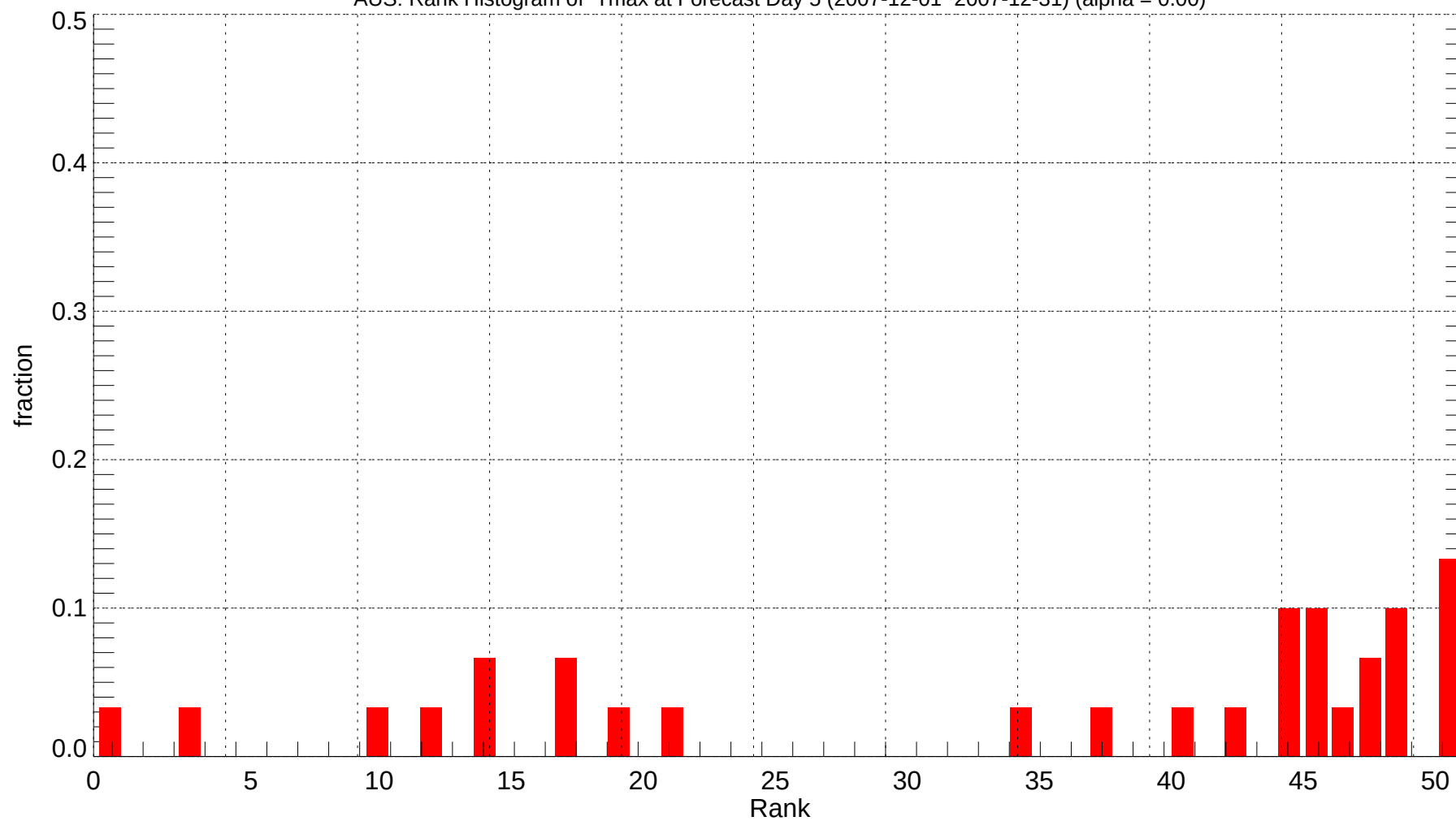
AUS: Rank Histogram of Tmax at Forecast Day 5 (2007-12-01~2007-12-31) (alpha = 0.00)
