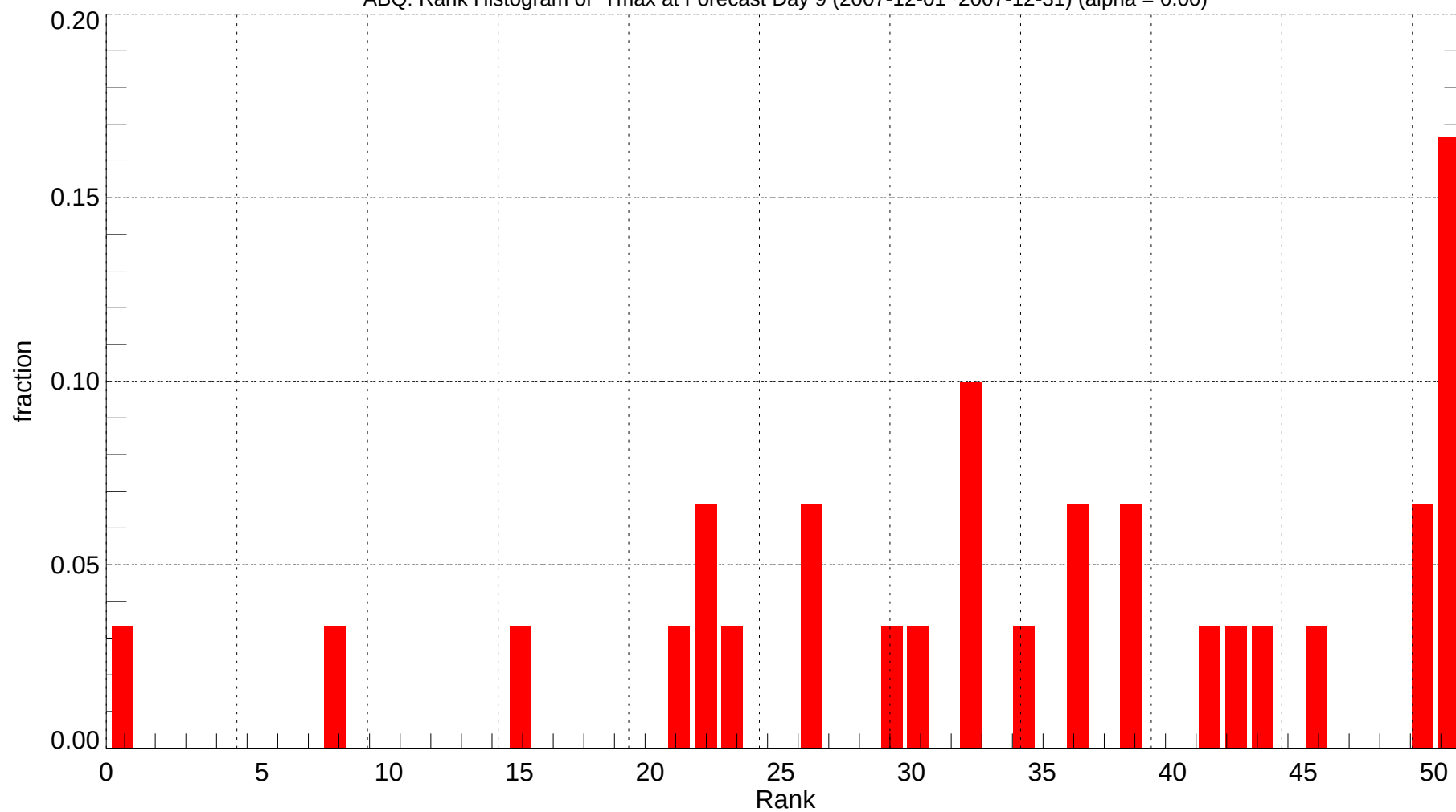
ABQ: Rank Histogram of Tmax at Forecast Day 9 (2007-12-01~2007-12-31) (alpha = 0.00)
