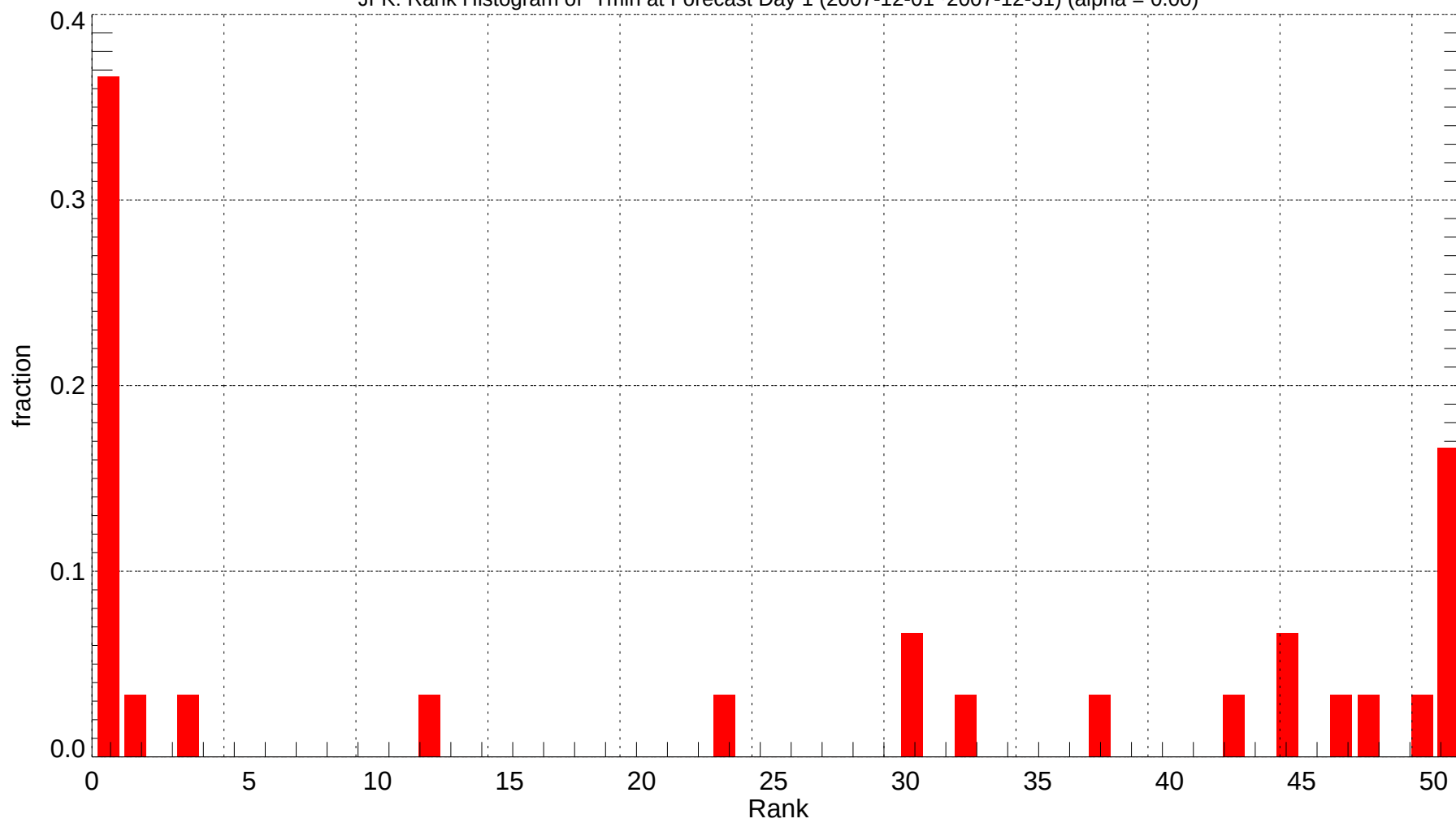
JFK: Rank Histogram of Tmin at Forecast Day 1 (2007-12-01~2007-12-31) (alpha = 0.00)
