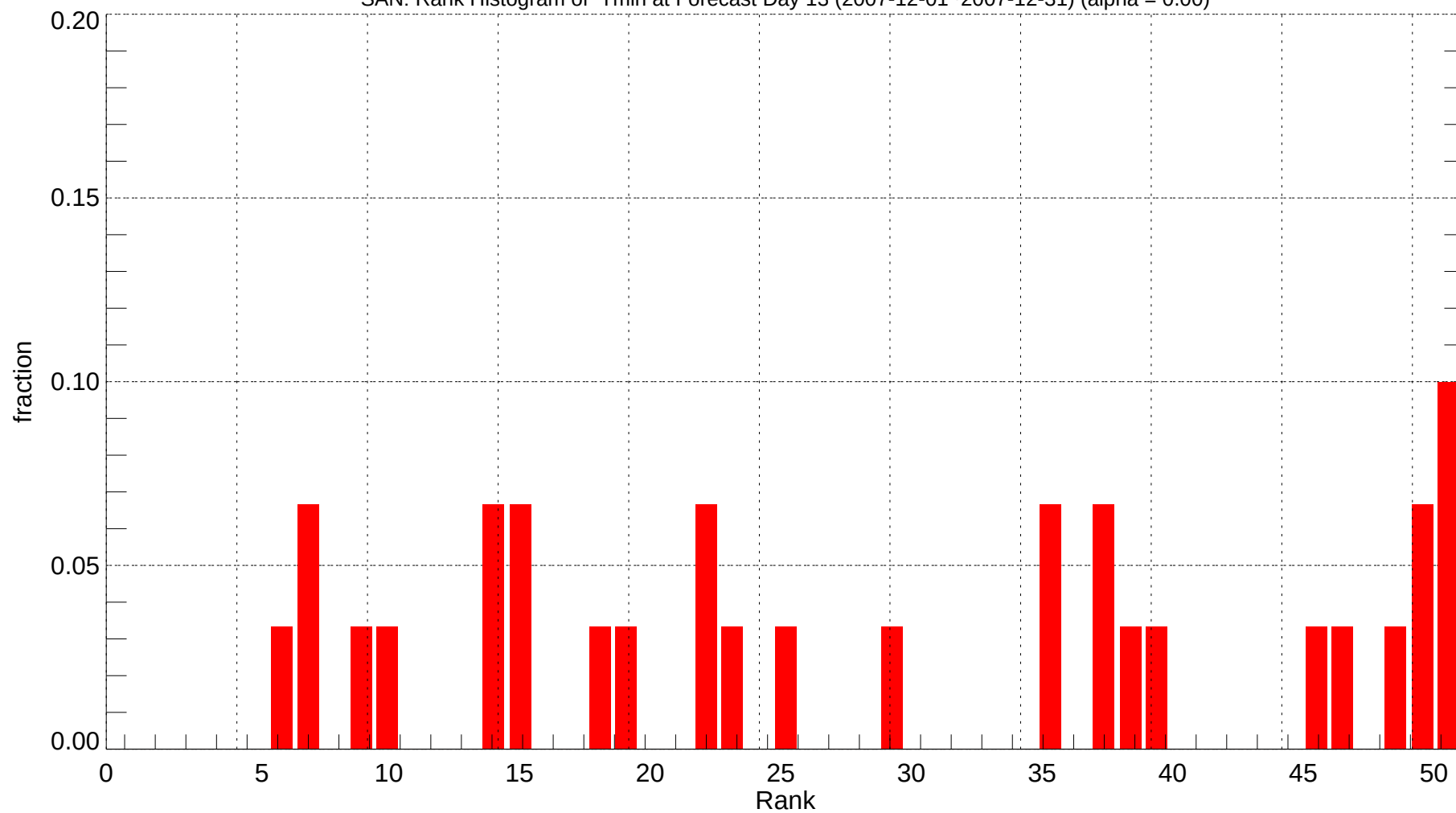
SAN: Rank Histogram of Tmin at Forecast Day 13 (2007-12-01~2007-12-31) (alpha = 0.00)
