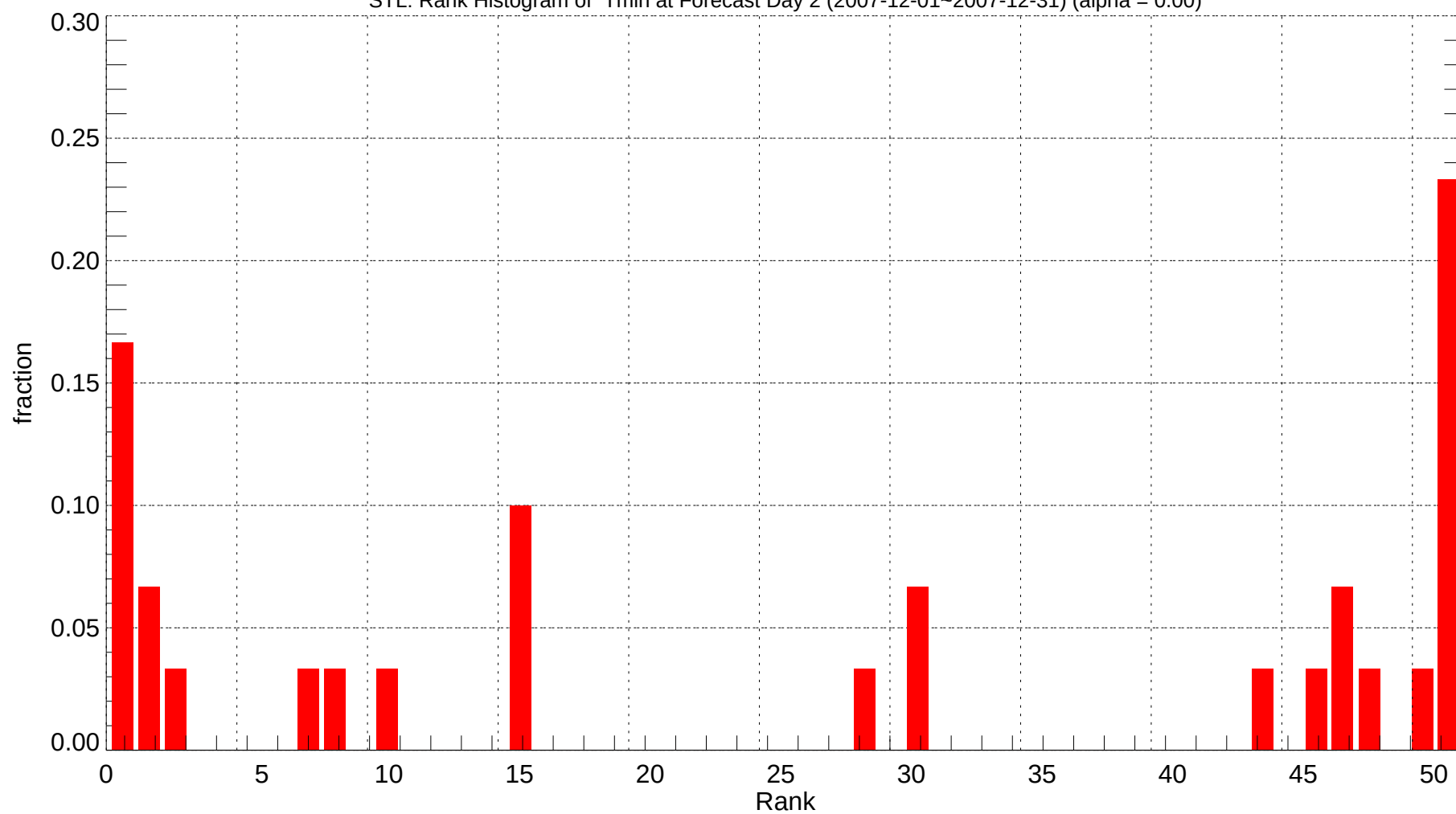
STL: Rank Histogram of Tmin at Forecast Day 2 (2007-12-01~2007-12-31) (alpha = 0.00)
