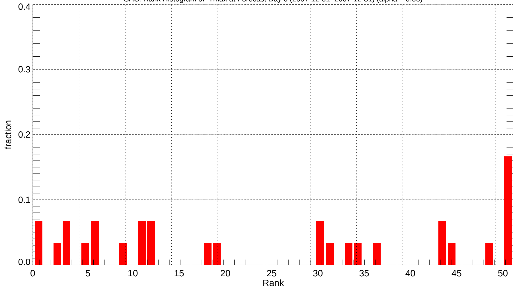
SAC: Rank Histogram of Tmax at Forecast Day 6 (2007-12-01~2007-12-31) (alpha = 0.00)
