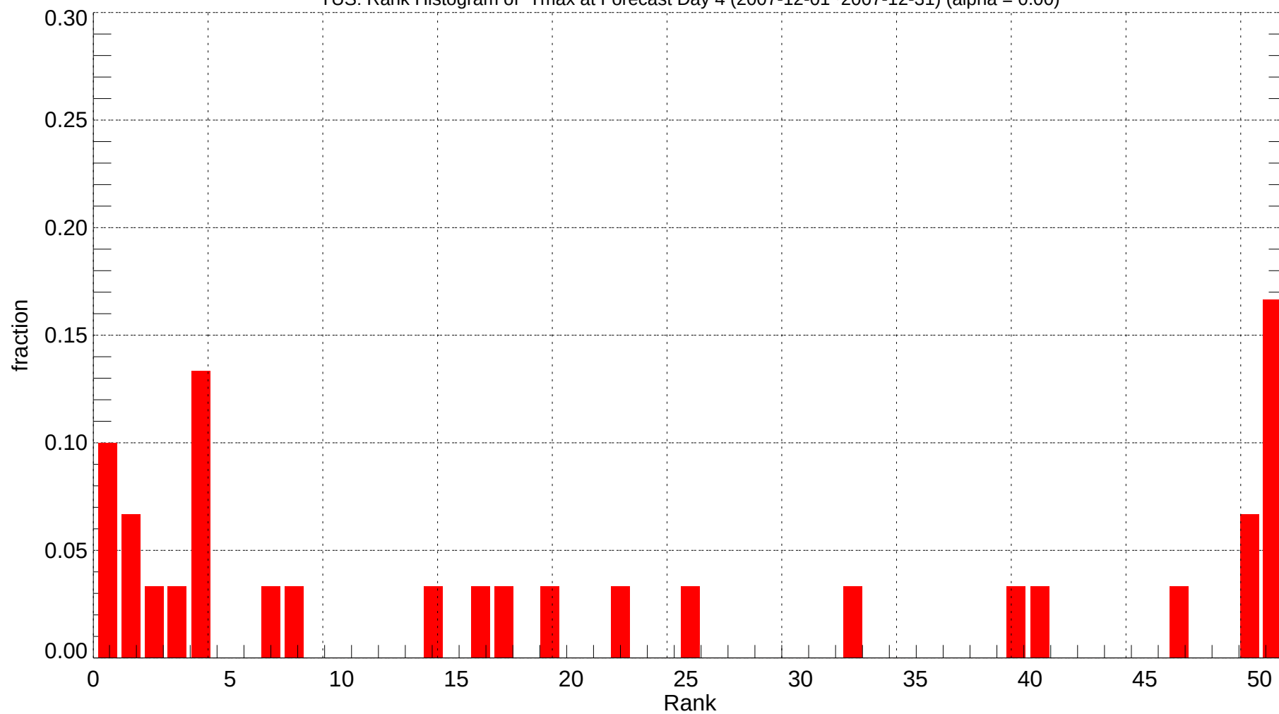
TUS: Rank Histogram of Tmax at Forecast Day 4 (2007-12-01~2007-12-31) (alpha = 0.00)
