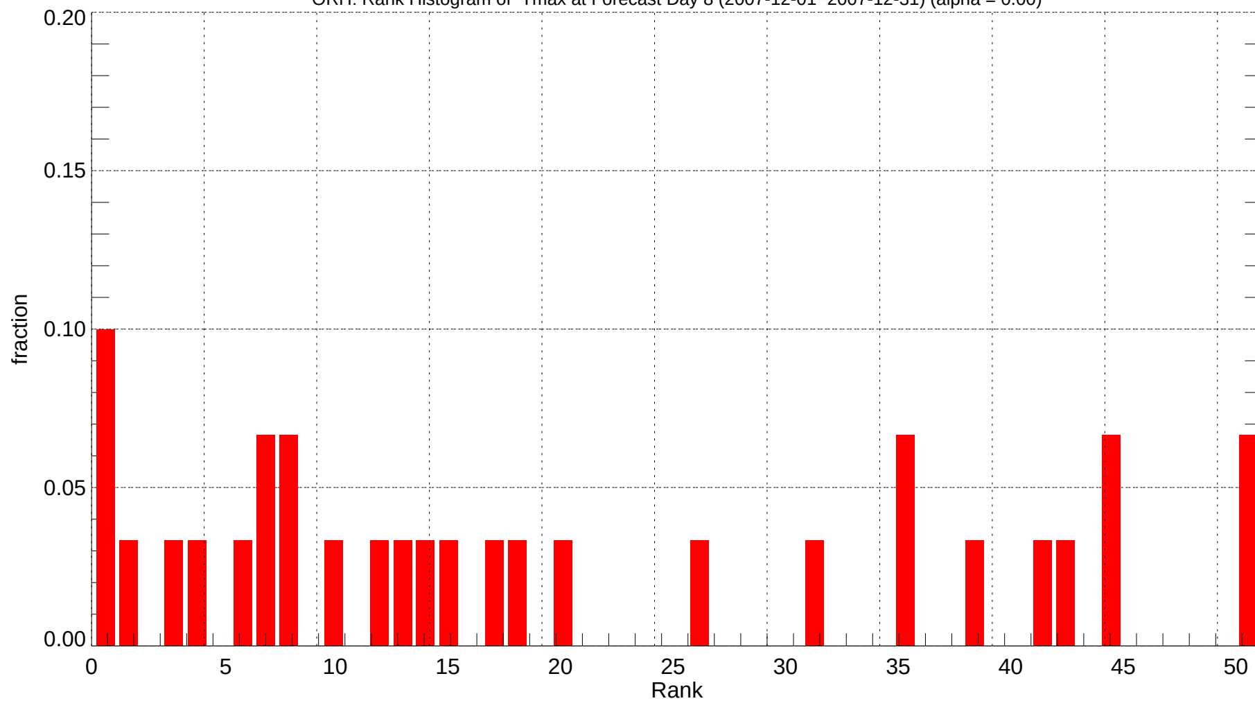
ORH: Rank Histogram of Tmax at Forecast Day 8 (2007-12-01~2007-12-31) (alpha = 0.00)
