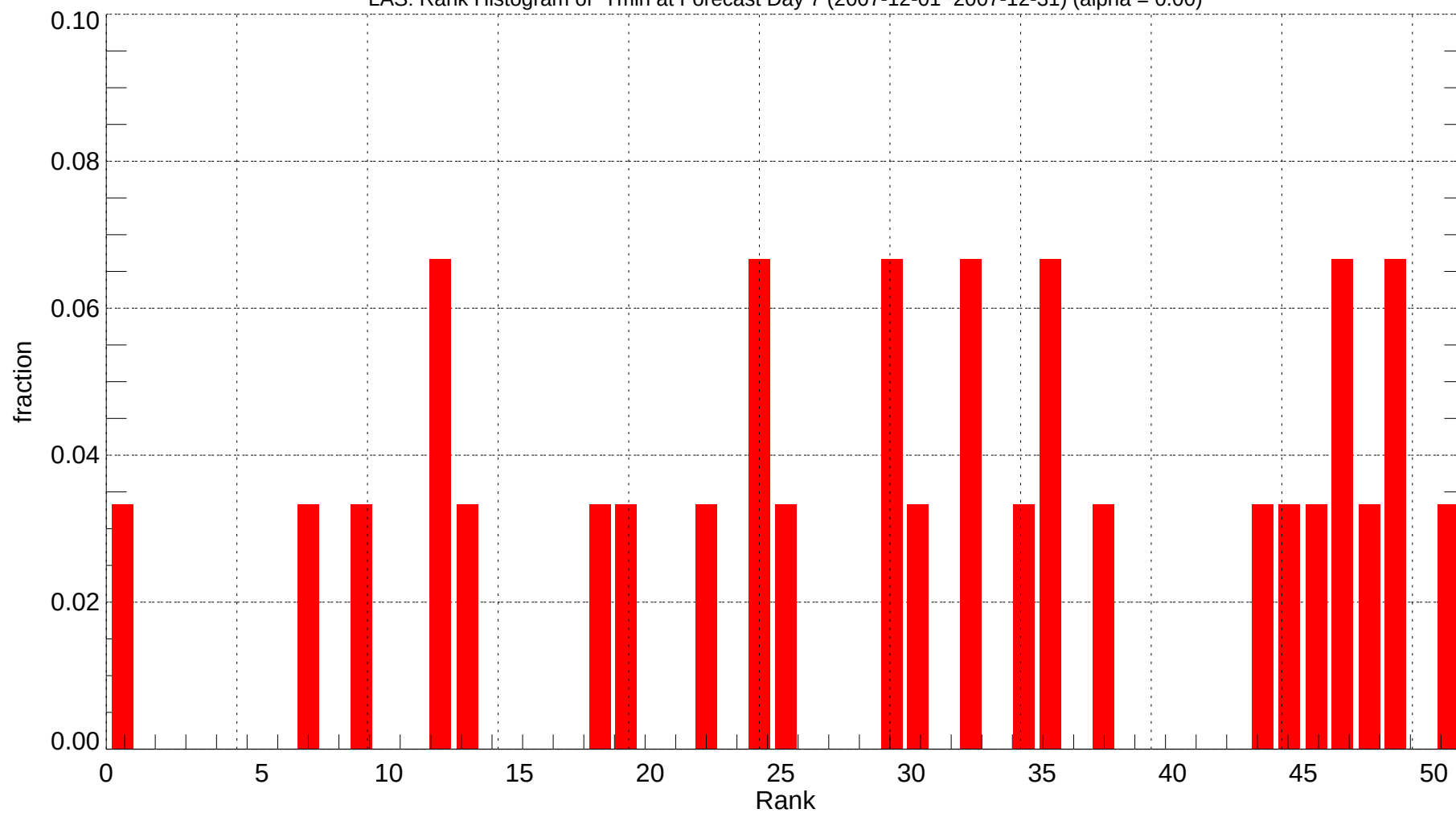
LAS: Rank Histogram of Tmin at Forecast Day 7 (2007-12-01~2007-12-31) (alpha = 0.00)
