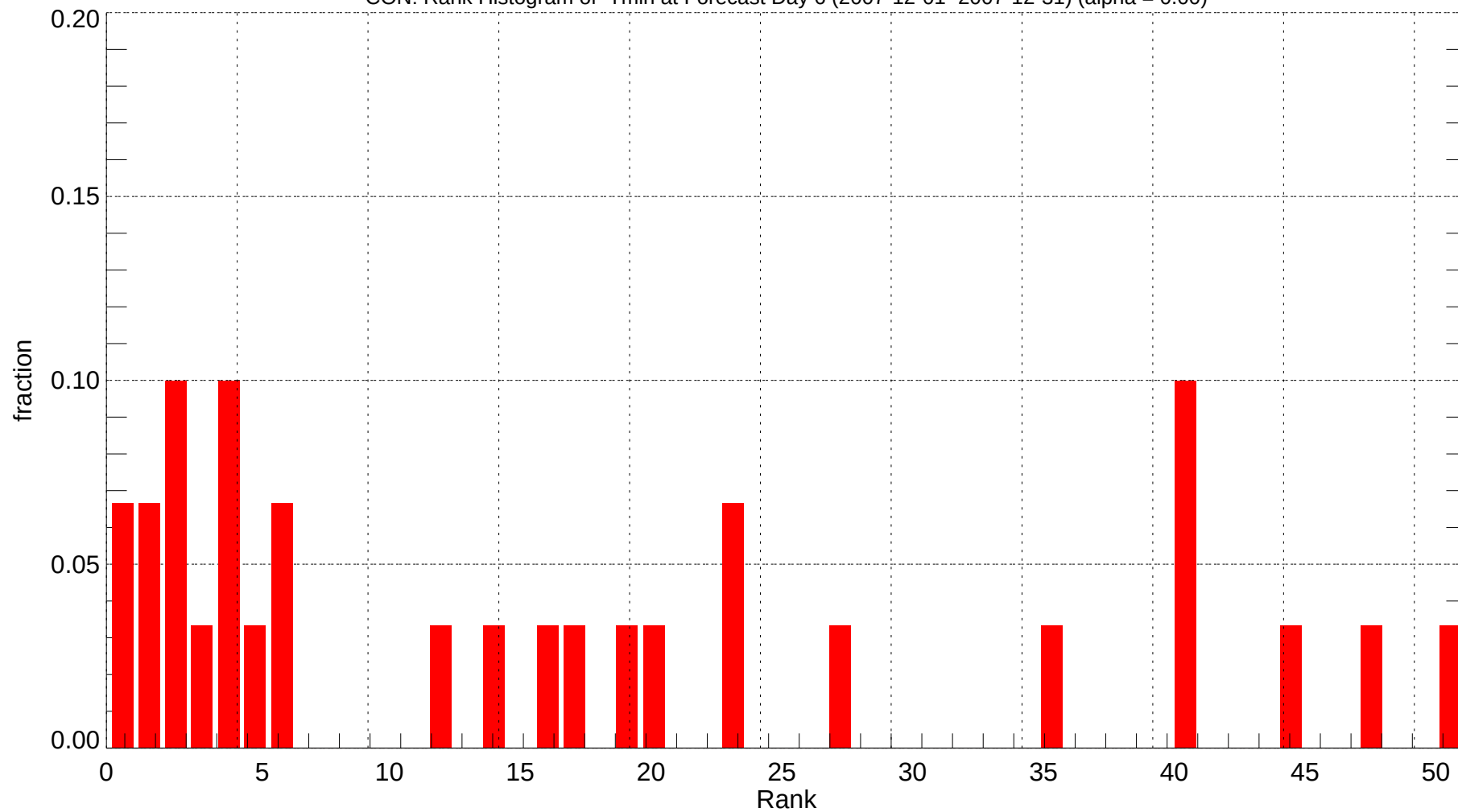
CON: Rank Histogram of Tmin at Forecast Day 6 (2007-12-01~2007-12-31) (alpha = 0.00)
