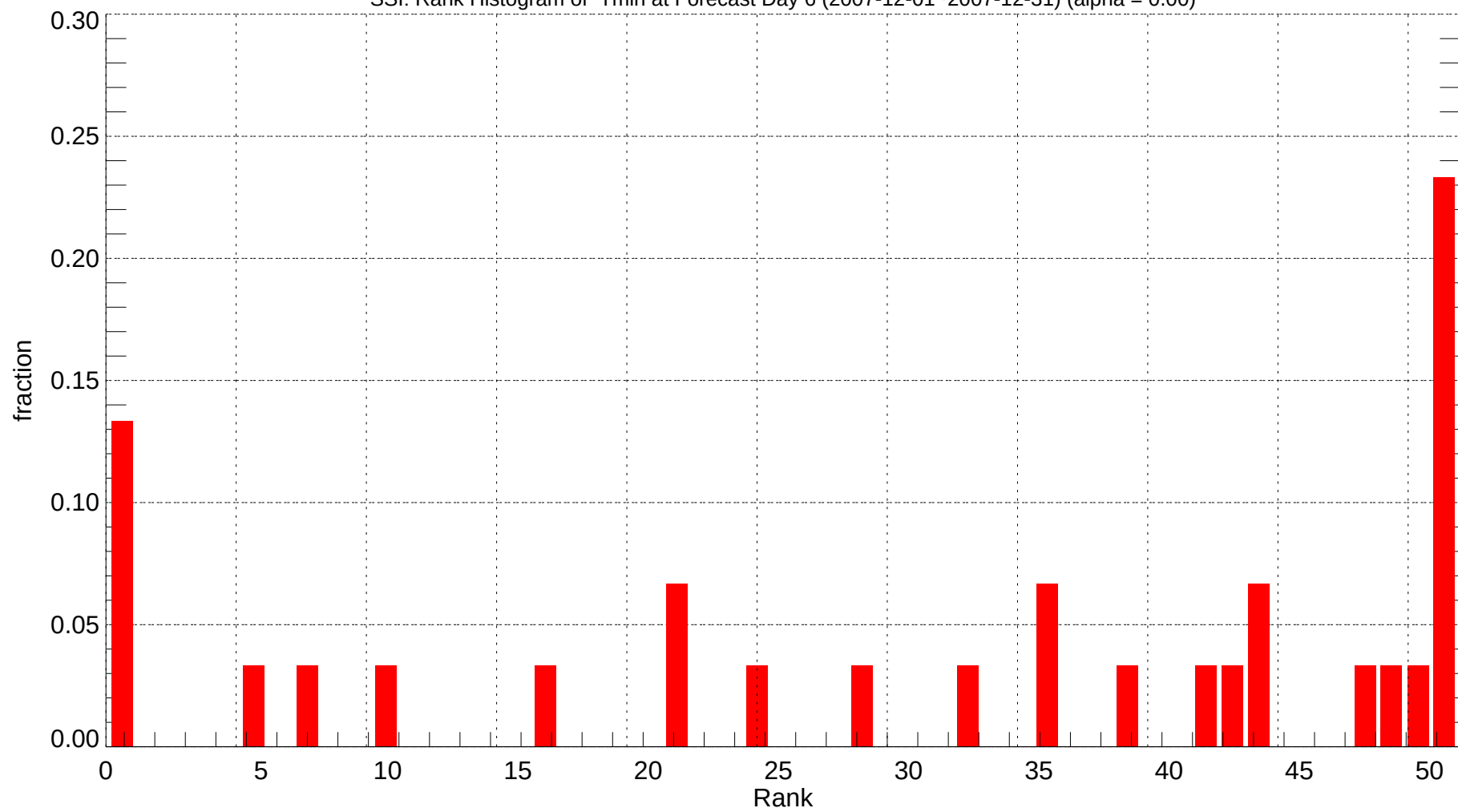
SSI: Rank Histogram of Tmin at Forecast Day 6 (2007-12-01~2007-12-31) (alpha = 0.00)
