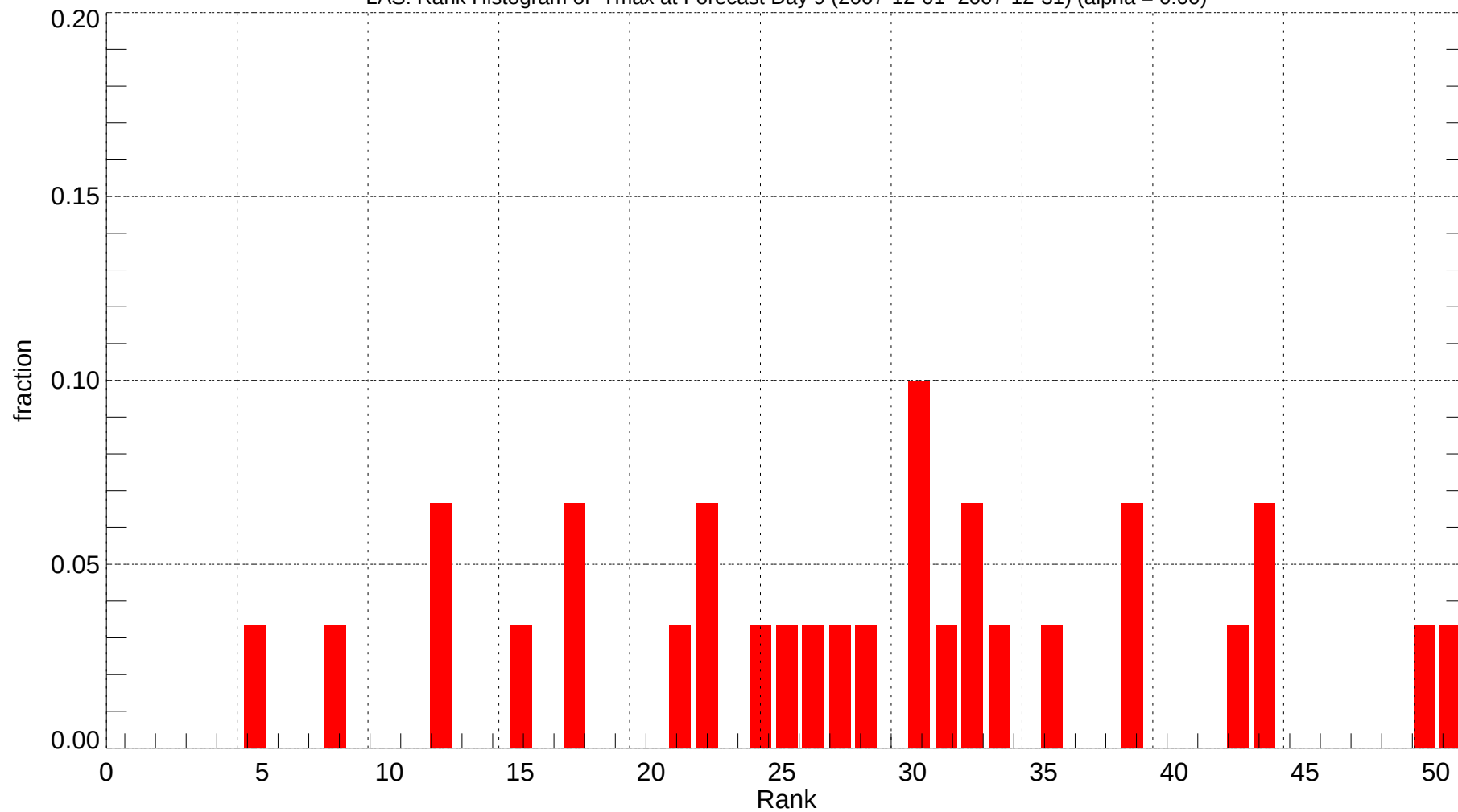
LAS: Rank Histogram of Tmax at Forecast Day 9 (2007-12-01~2007-12-31) (alpha = 0.00)
