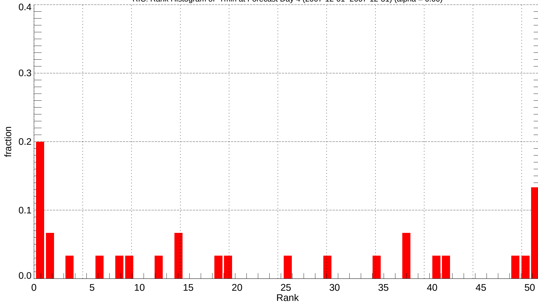
RIC: Rank Histogram of Tmin at Forecast Day 4 (2007-12-01~2007-12-31) (alpha = 0.00)
