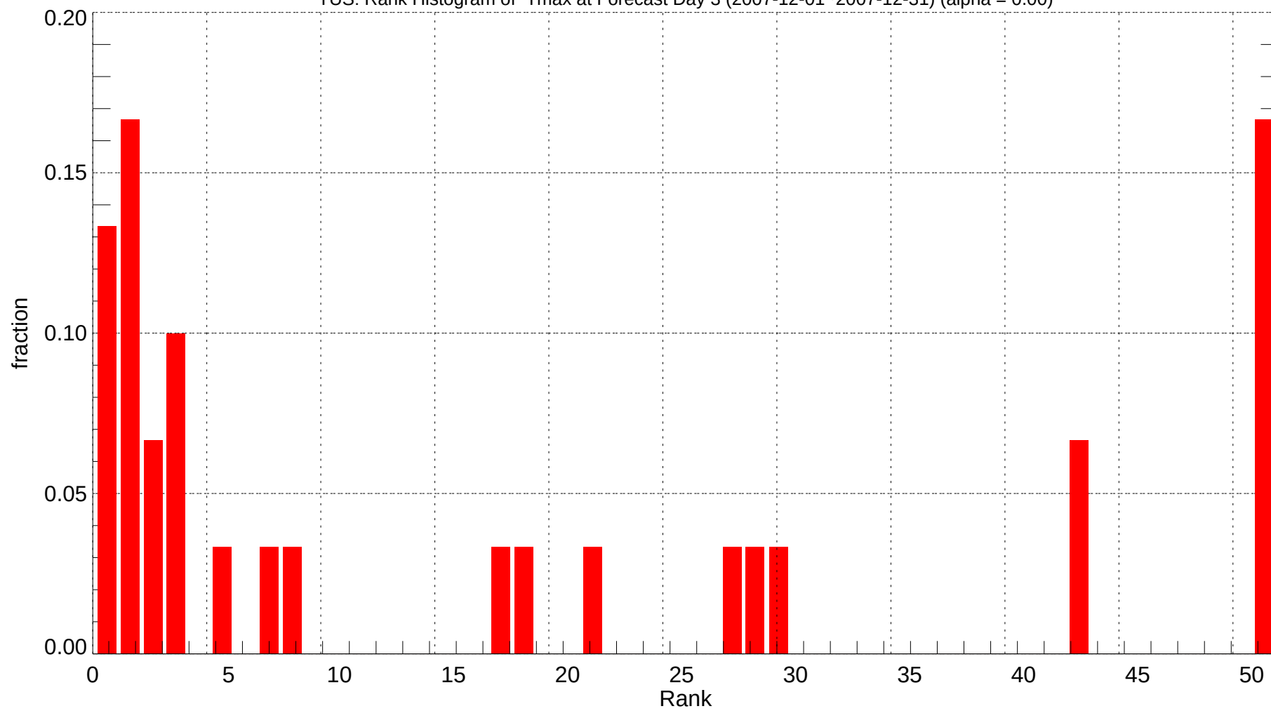
TUS: Rank Histogram of Tmax at Forecast Day 3 (2007-12-01~2007-12-31) (alpha = 0.00)
