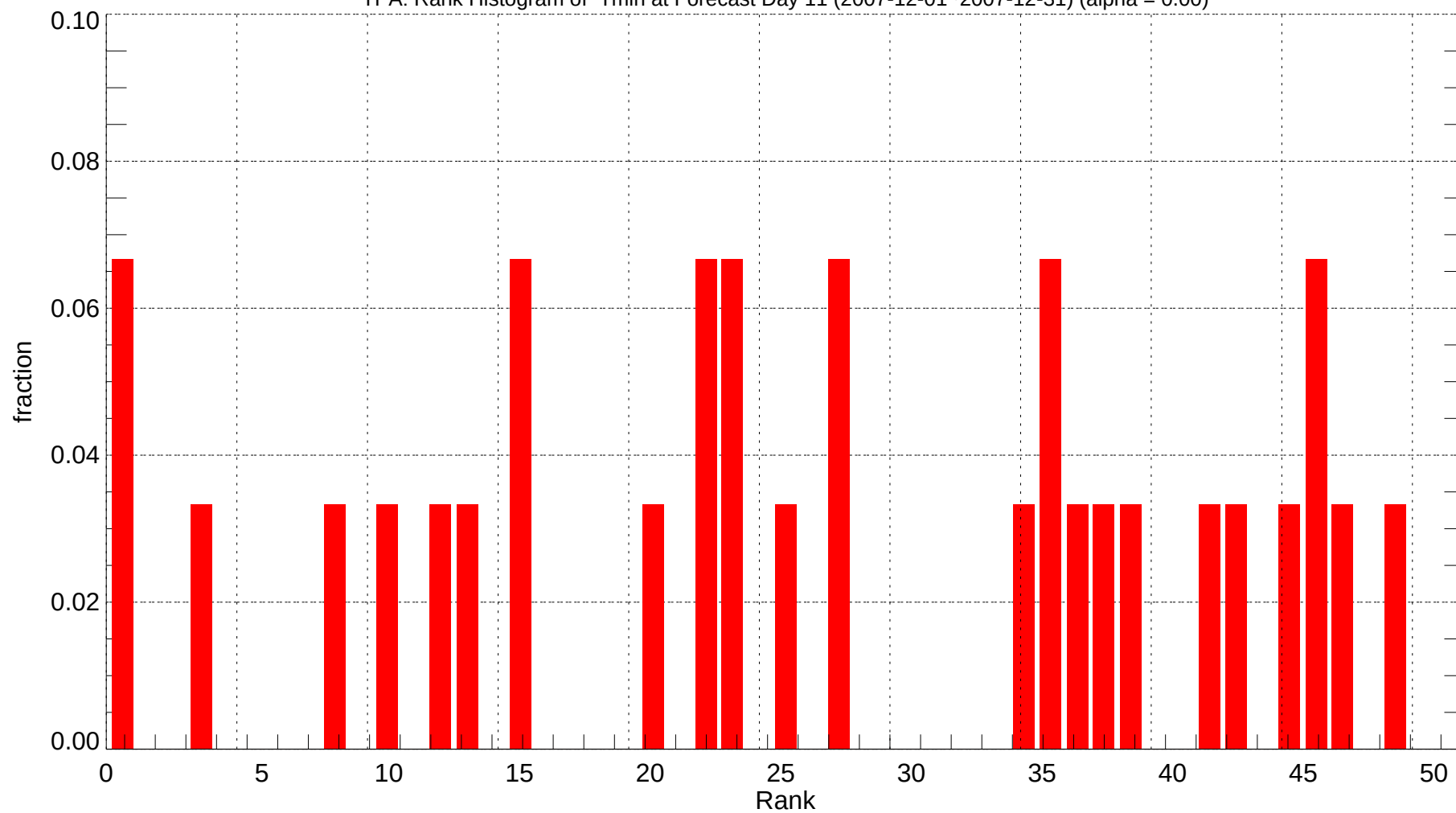
TPA: Rank Histogram of Tmin at Forecast Day 11 (2007-12-01~2007-12-31) (alpha = 0.00)
