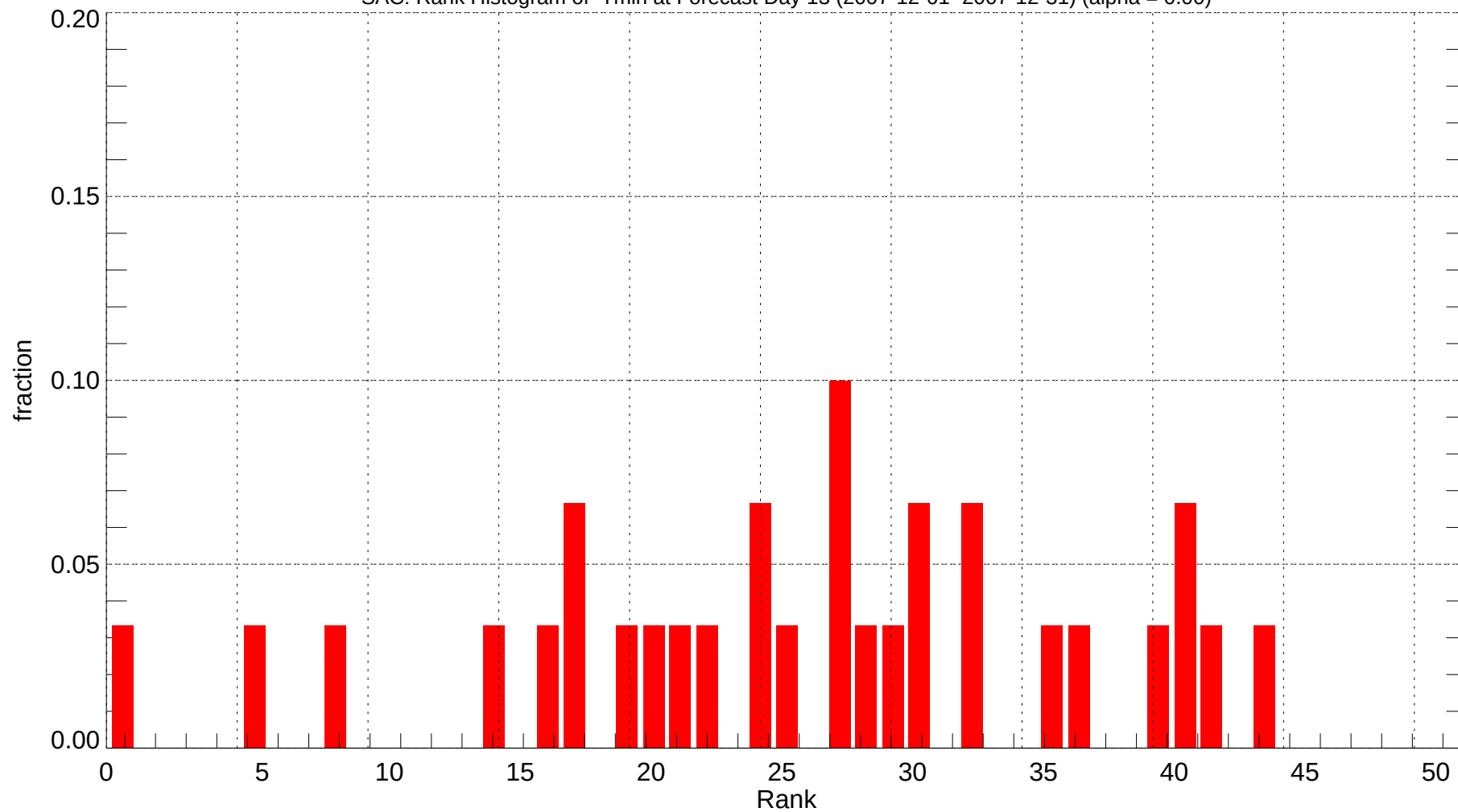
SAC: Rank Histogram of Tmin at Forecast Day 13 (2007-12-01~2007-12-31) (alpha = 0.00)
