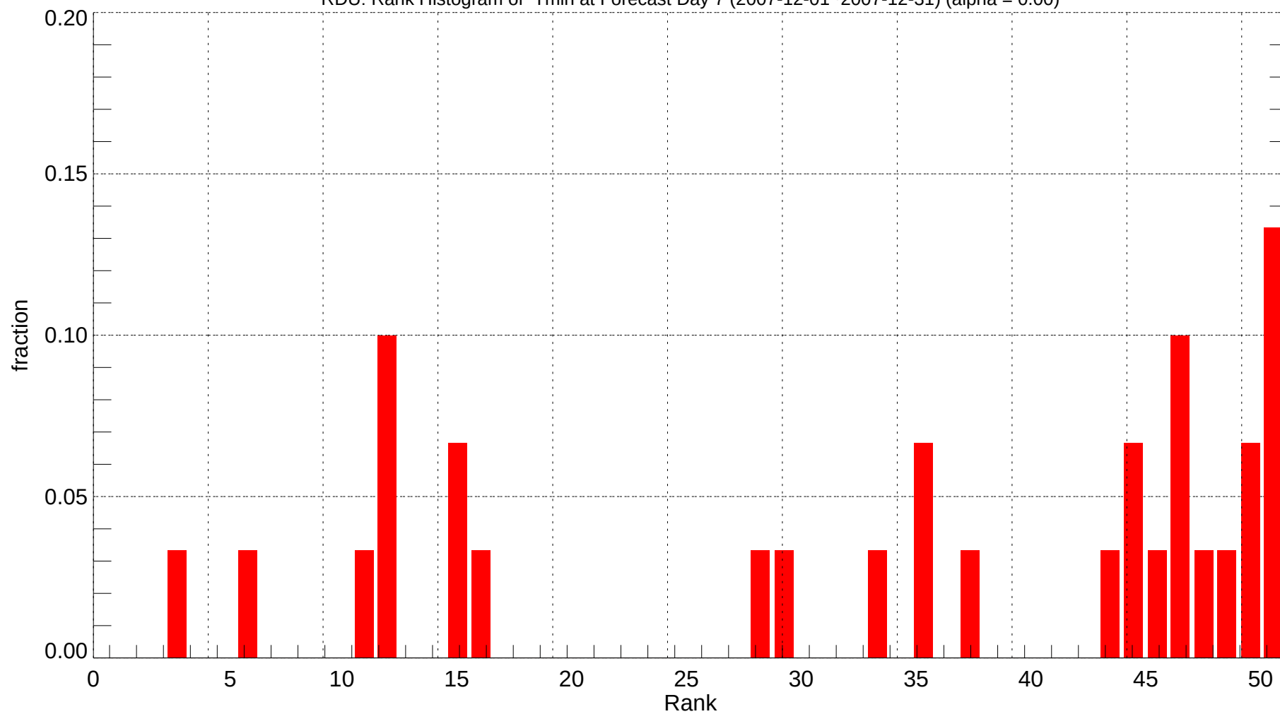
RDU: Rank Histogram of Tmin at Forecast Day 7 (2007-12-01~2007-12-31) (alpha = 0.00)
