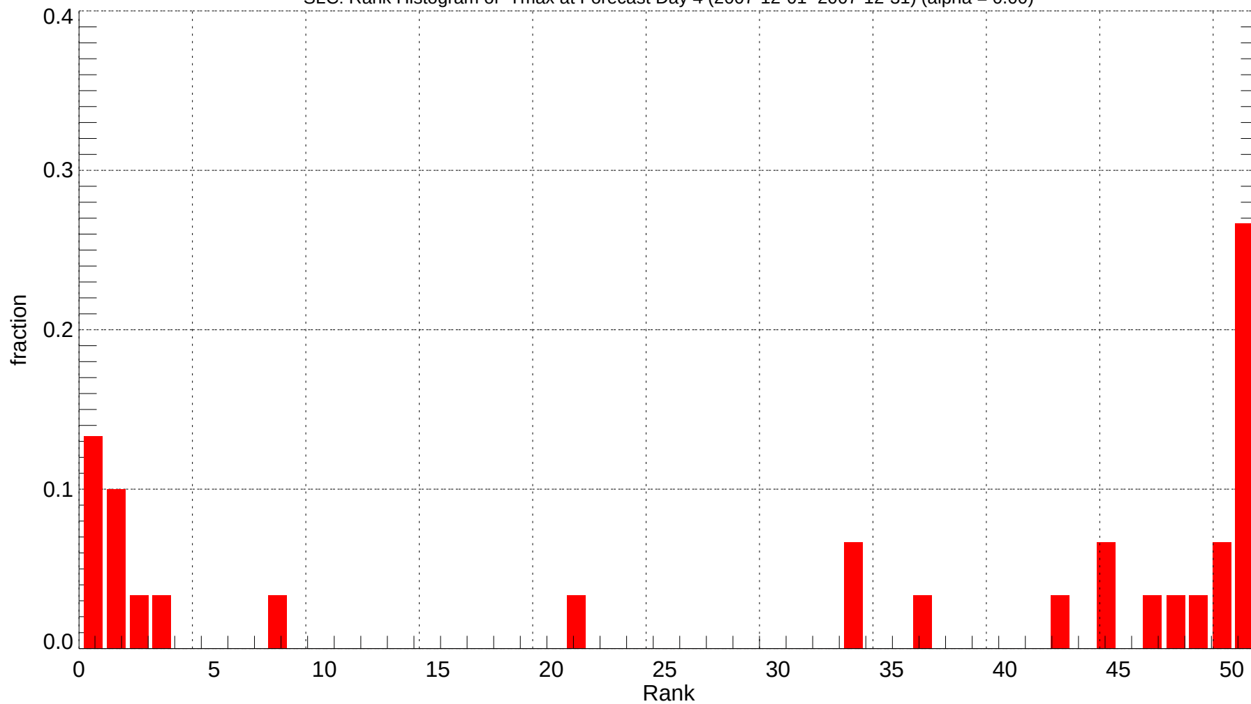
SLC: Rank Histogram of Tmax at Forecast Day 4 (2007-12-01~2007-12-31) (alpha = 0.00)
