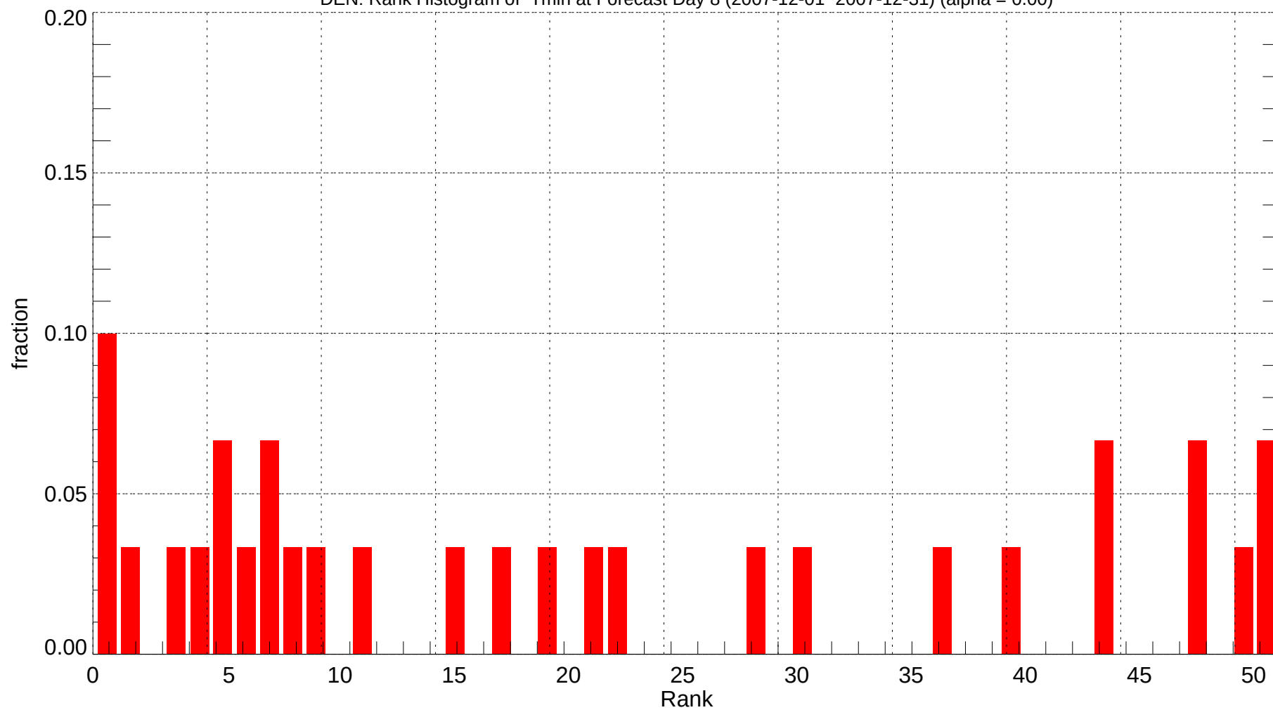
DEN: Rank Histogram of Tmin at Forecast Day 8 (2007-12-01~2007-12-31) (alpha = 0.00)
