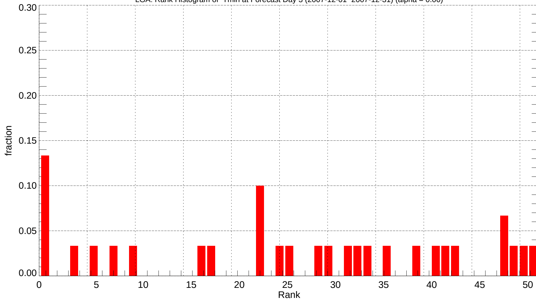
LGA: Rank Histogram of Tmin at Forecast Day 3 (2007-12-01~2007-12-31) (alpha = 0.00)
