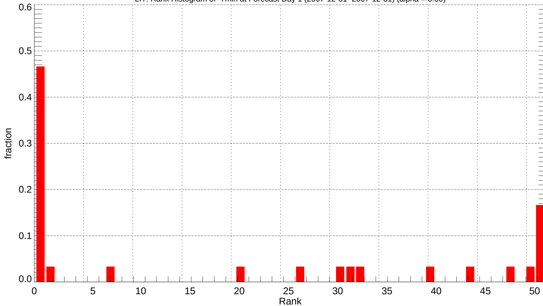
LIT: Rank Histogram of Tmin at Forecast Day 1 (2007-12-01~2007-12-31) (alpha = 0.00)
