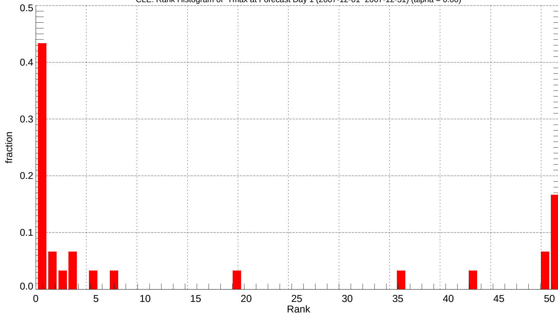
CLE: Rank Histogram of Tmax at Forecast Day 1 (2007-12-01~2007-12-31) (alpha = 0.00)
