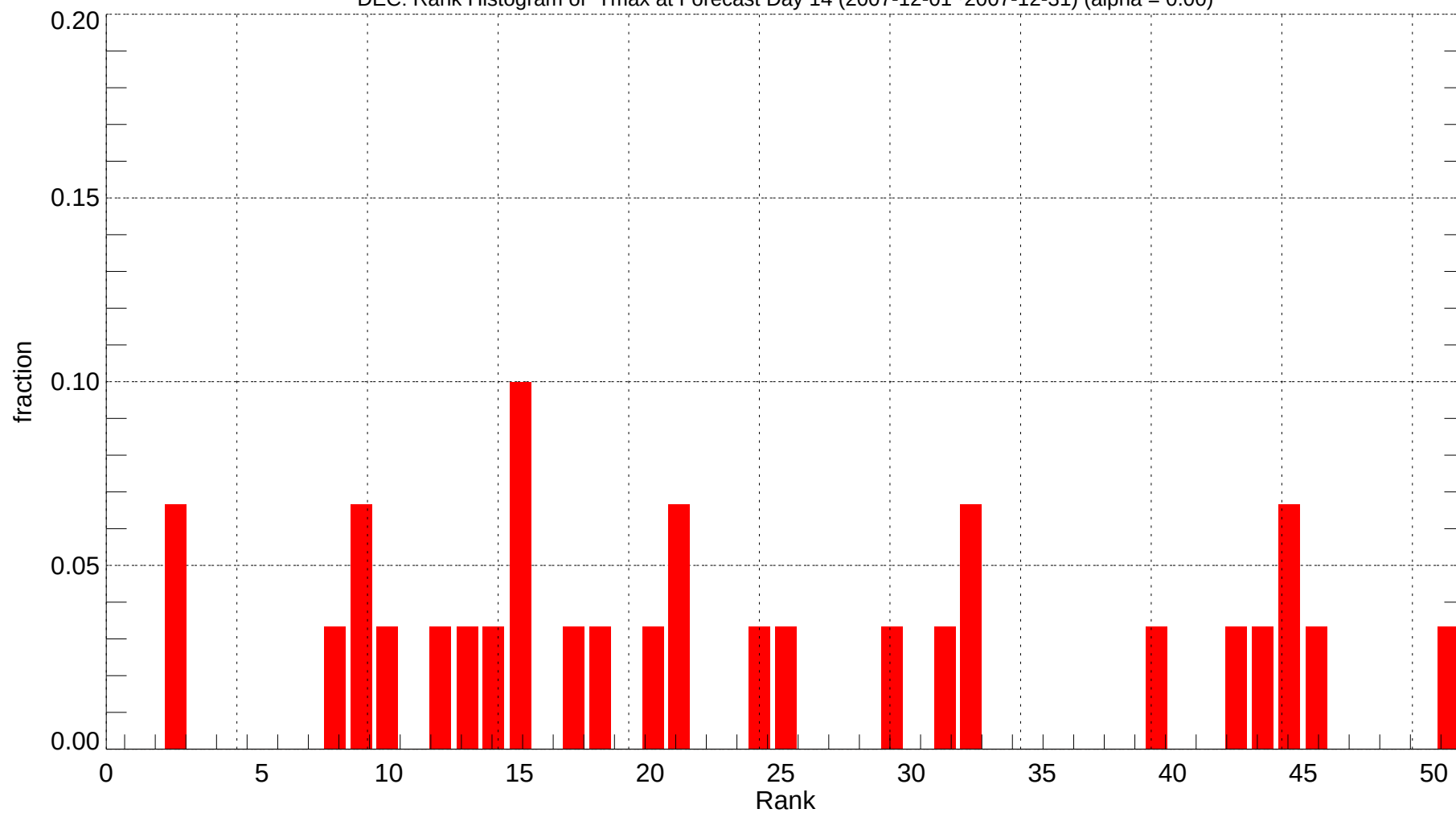
DEC: Rank Histogram of Tmax at Forecast Day 14 (2007-12-01~2007-12-31) (alpha = 0.00)
