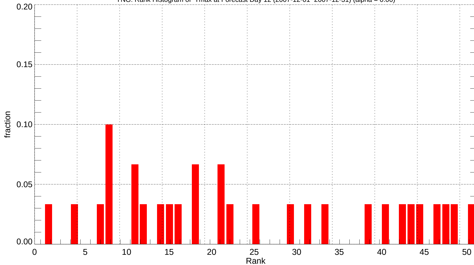
YNG: Rank Histogram of Tmax at Forecast Day 12 (2007-12-01~2007-12-31) (alpha = 0.00)
