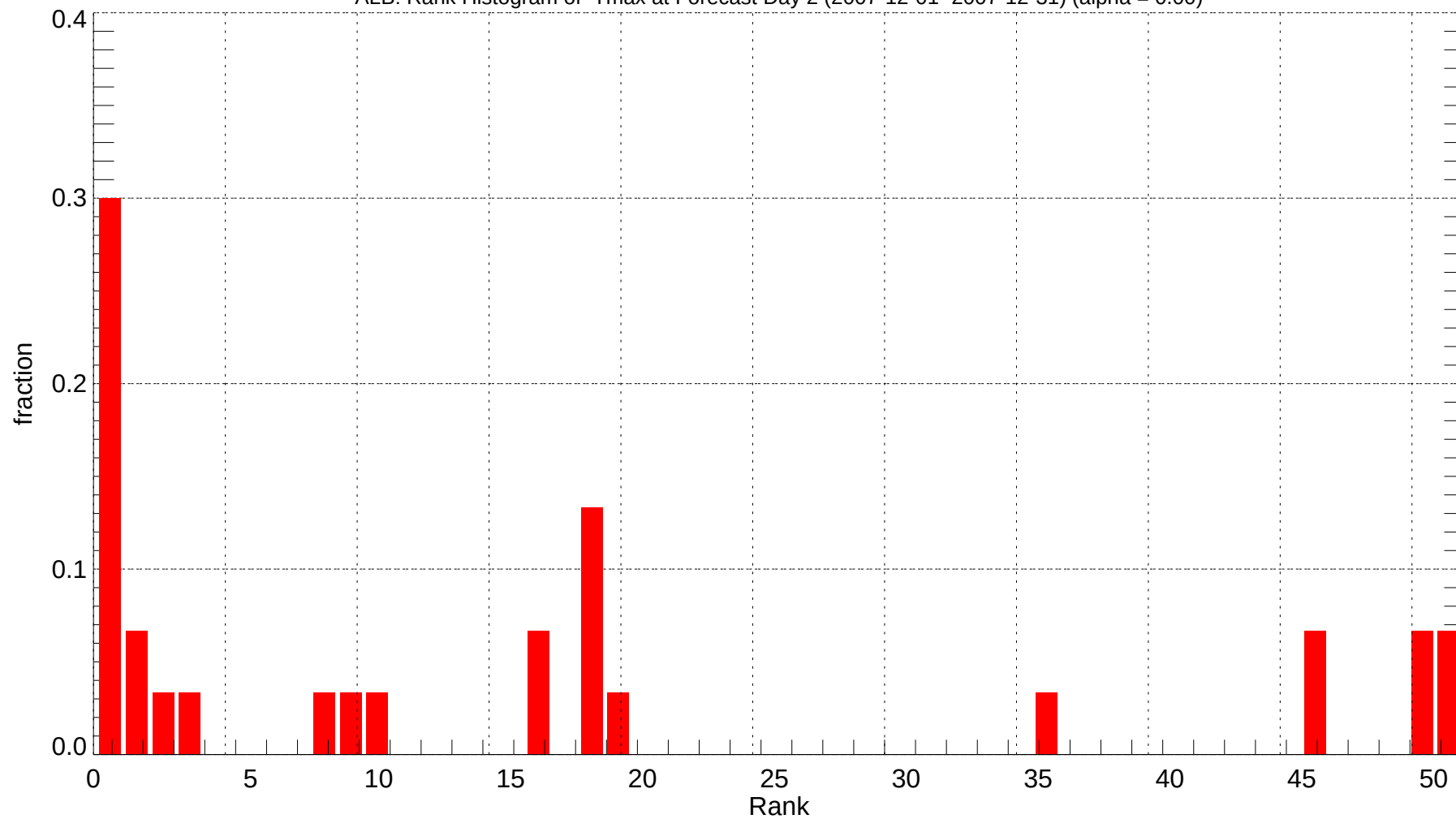
ALB: Rank Histogram of Tmax at Forecast Day 2 (2007-12-01~2007-12-31) (alpha = 0.00)
