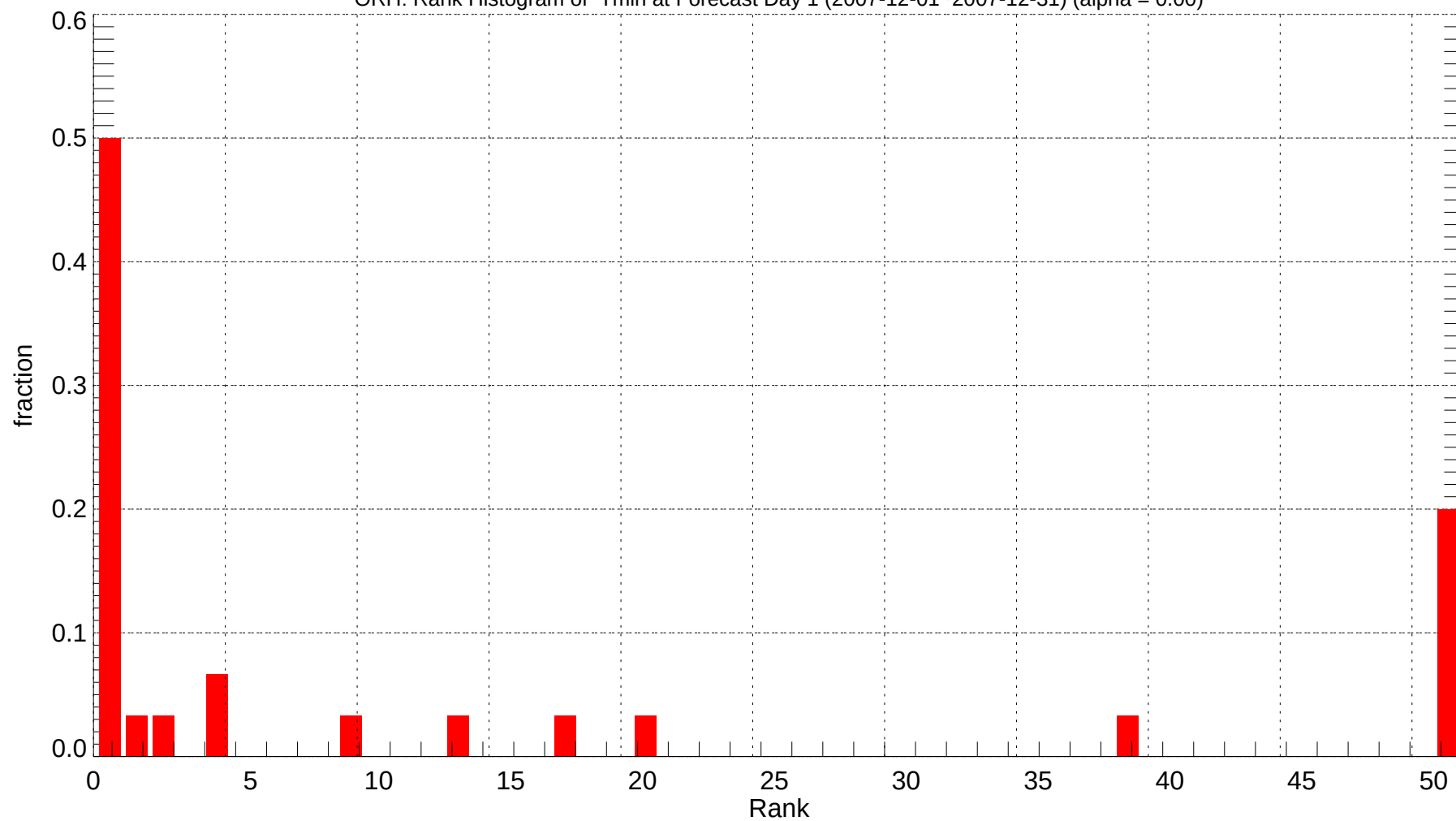
ORH: Rank Histogram of Tmin at Forecast Day 1 (2007-12-01~2007-12-31) (alpha = 0.00)
