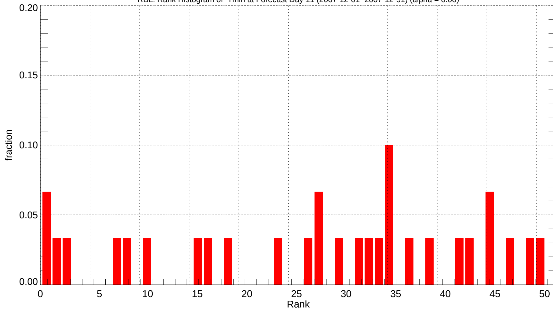
RBL: Rank Histogram of Tmin at Forecast Day 11 (2007-12-01~2007-12-31) (alpha = 0.00)
