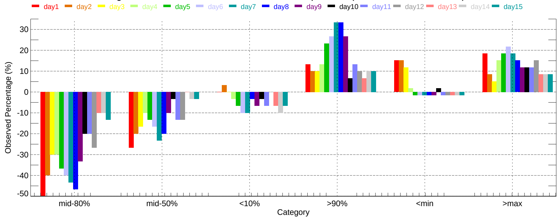
Observed Percentage Deviation of Ensembles - MEM: Min Temperature (2007-12-01~2007-12-31)
