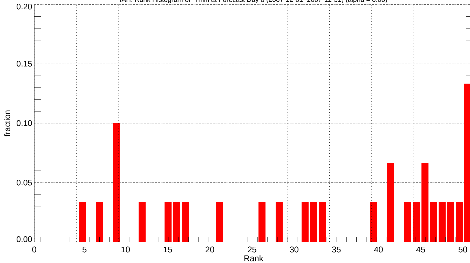
IAH: Rank Histogram of Tmin at Forecast Day 8 (2007-12-01~2007-12-31) (alpha = 0.00)
