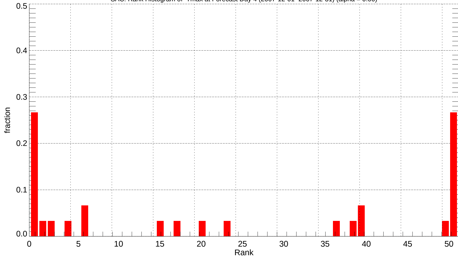
SAC: Rank Histogram of Tmax at Forecast Day 4 (2007-12-01~2007-12-31) (alpha = 0.00)
