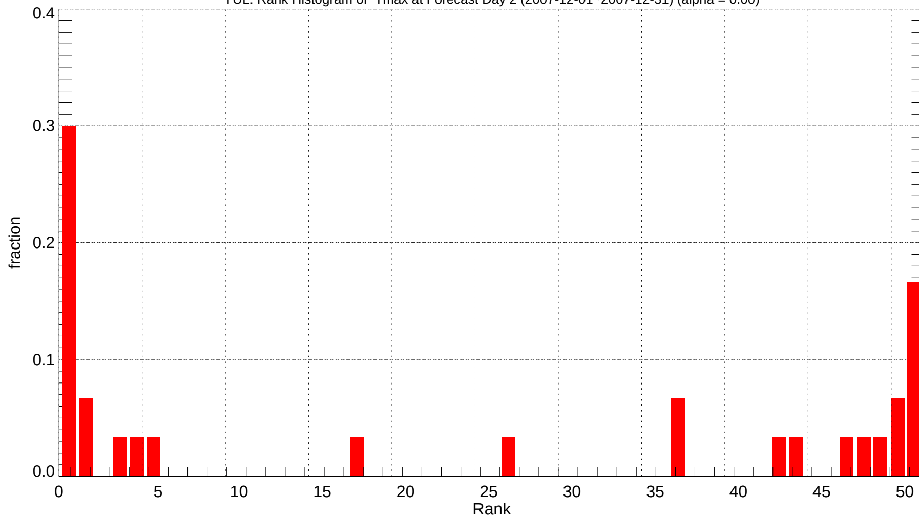
YUL: Rank Histogram of Tmax at Forecast Day 2 (2007-12-01~2007-12-31) (alpha = 0.00)
