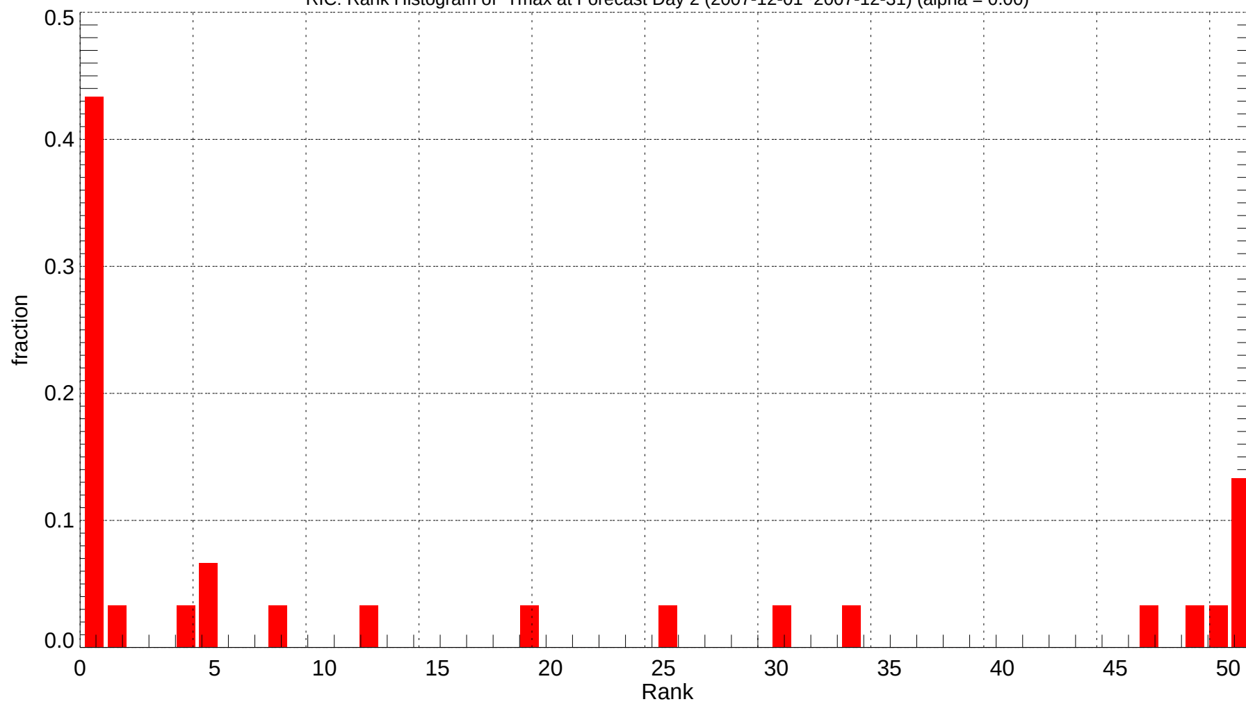
RIC: Rank Histogram of Tmax at Forecast Day 2 (2007-12-01~2007-12-31) (alpha = 0.00)
