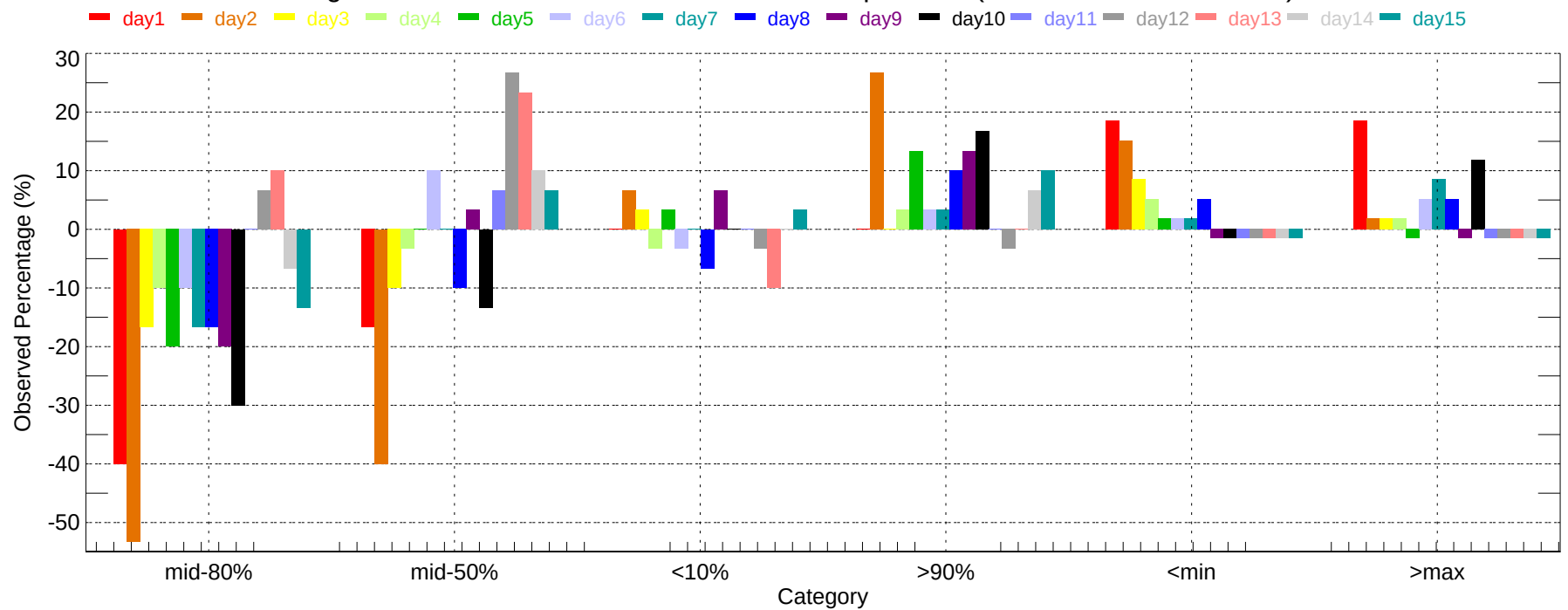
Observed Percentage Deviation of Ensembles - DLH: Min Temperature (2007-12-01~2007-12-31)
