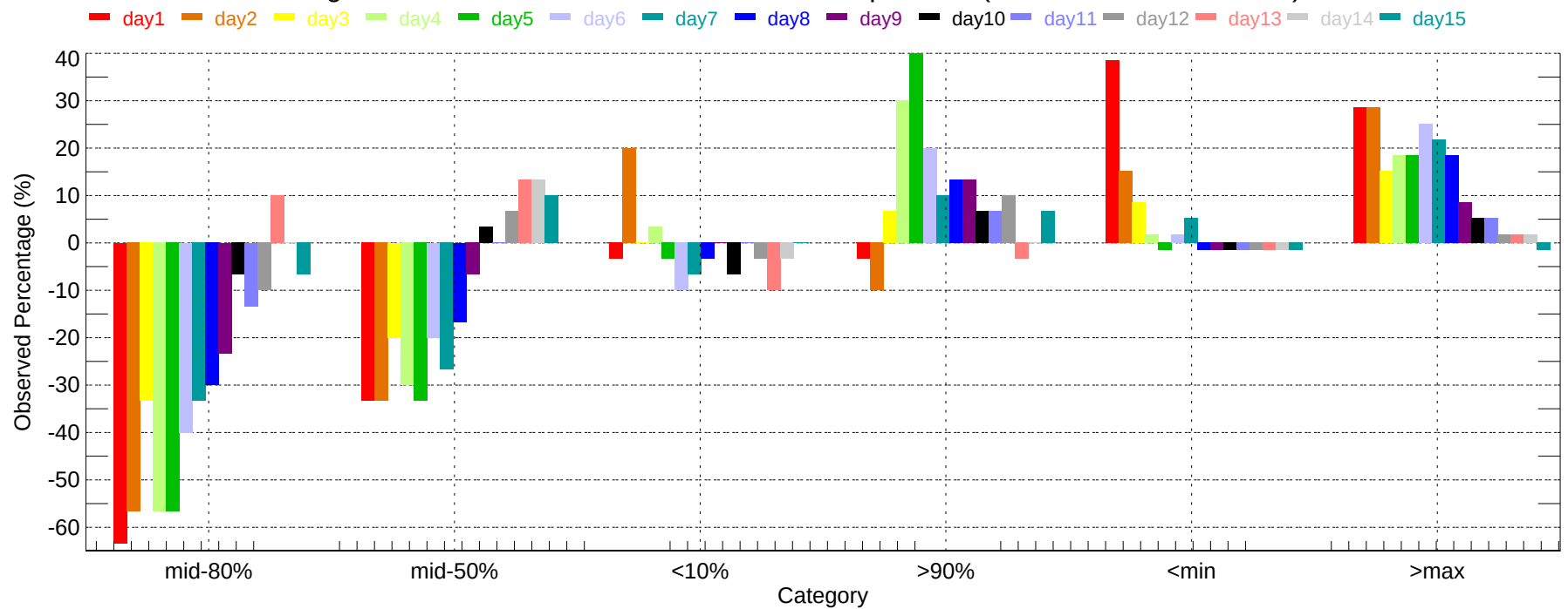
Observed Percentage Deviation of Ensembles - DSM: Min Temperature (2007-12-01~2007-12-31)
