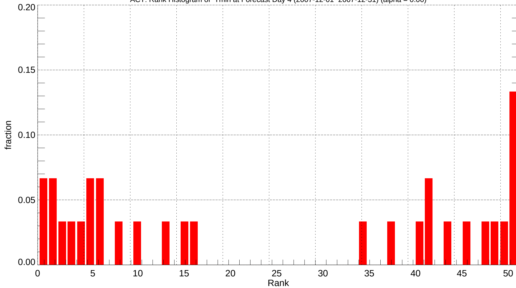
ACT: Rank Histogram of Tmin at Forecast Day 4 (2007-12-01~2007-12-31) (alpha = 0.00)
