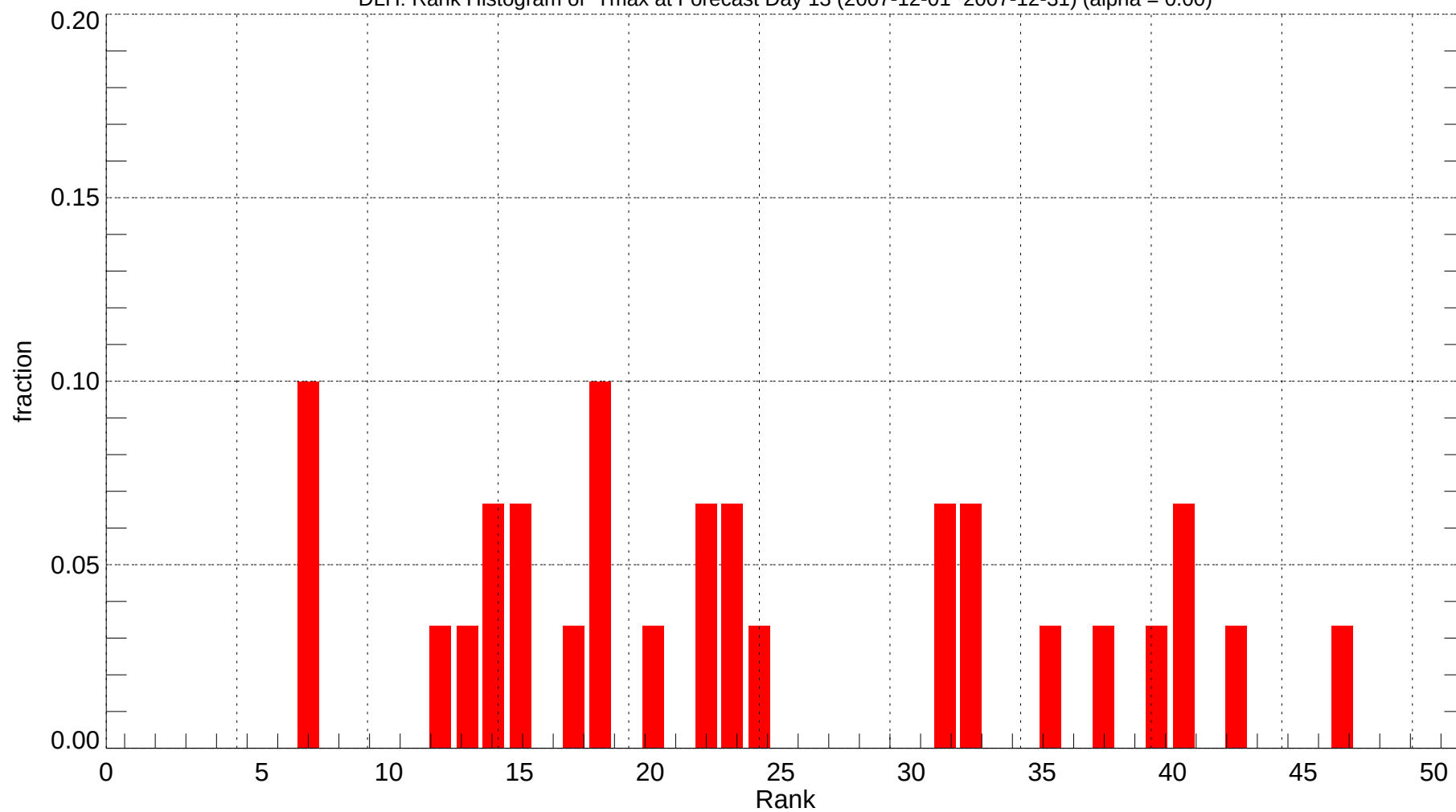
DLH: Rank Histogram of Tmax at Forecast Day 13 (2007-12-01~2007-12-31) (alpha = 0.00)
