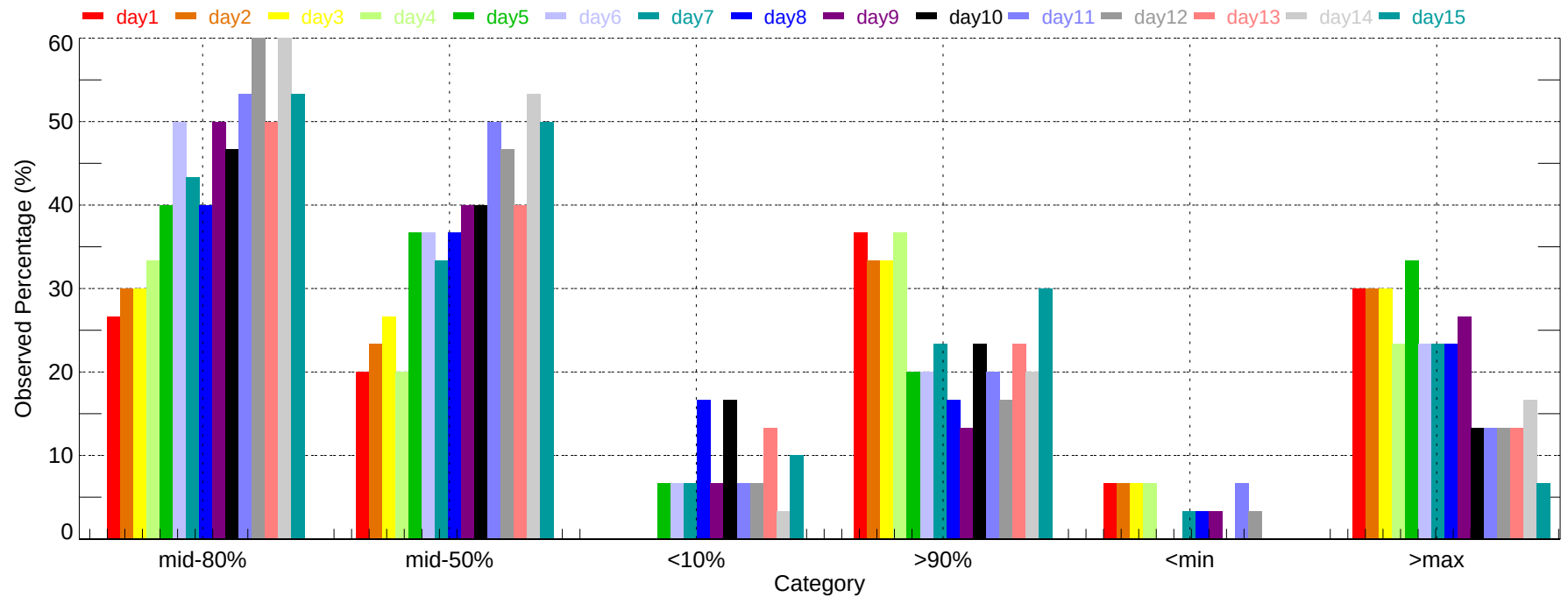
Observed Percentage of Ensembles - MAF: Min Temperature (2007-12-01~2007-12-31)
