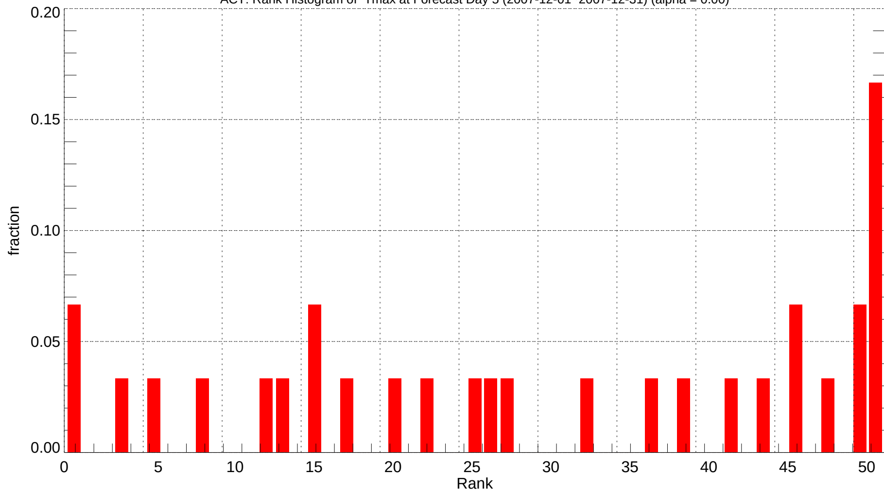
ACT: Rank Histogram of Tmax at Forecast Day 5 (2007-12-01~2007-12-31) (alpha = 0.00)
