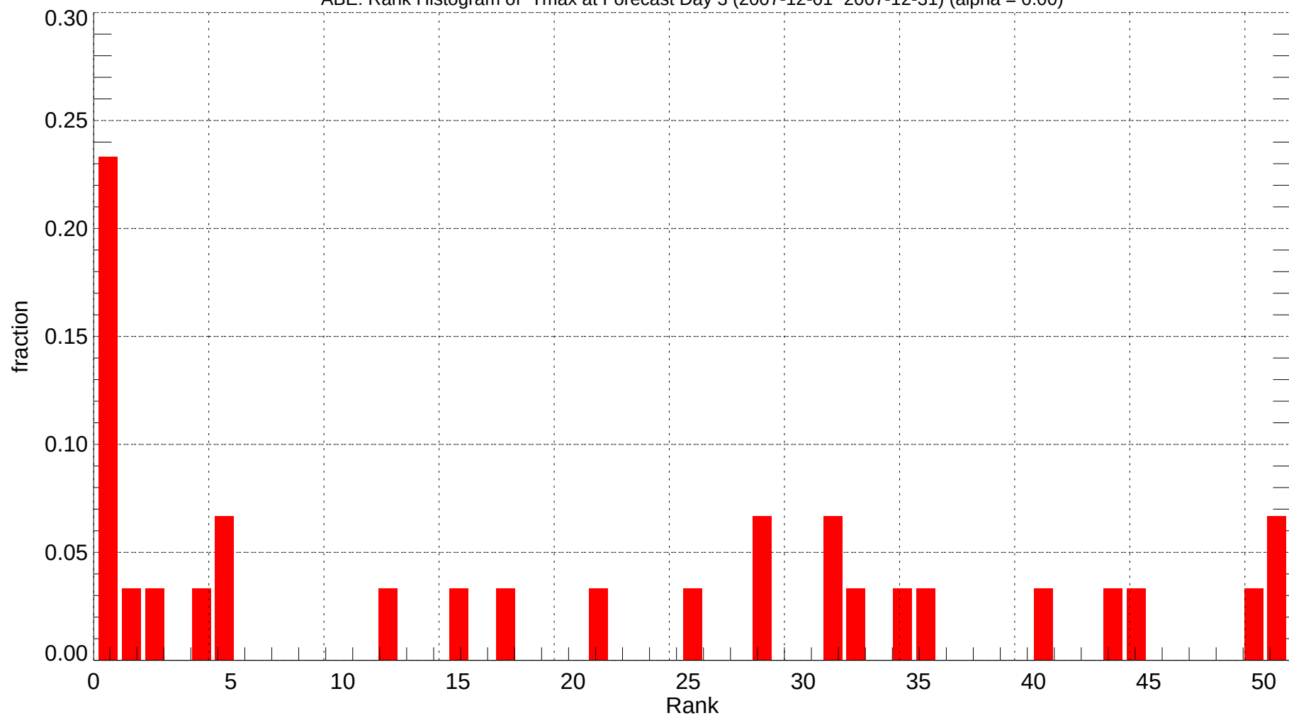
ABE: Rank Histogram of Tmax at Forecast Day 3 (2007-12-01~2007-12-31) (alpha = 0.00)
