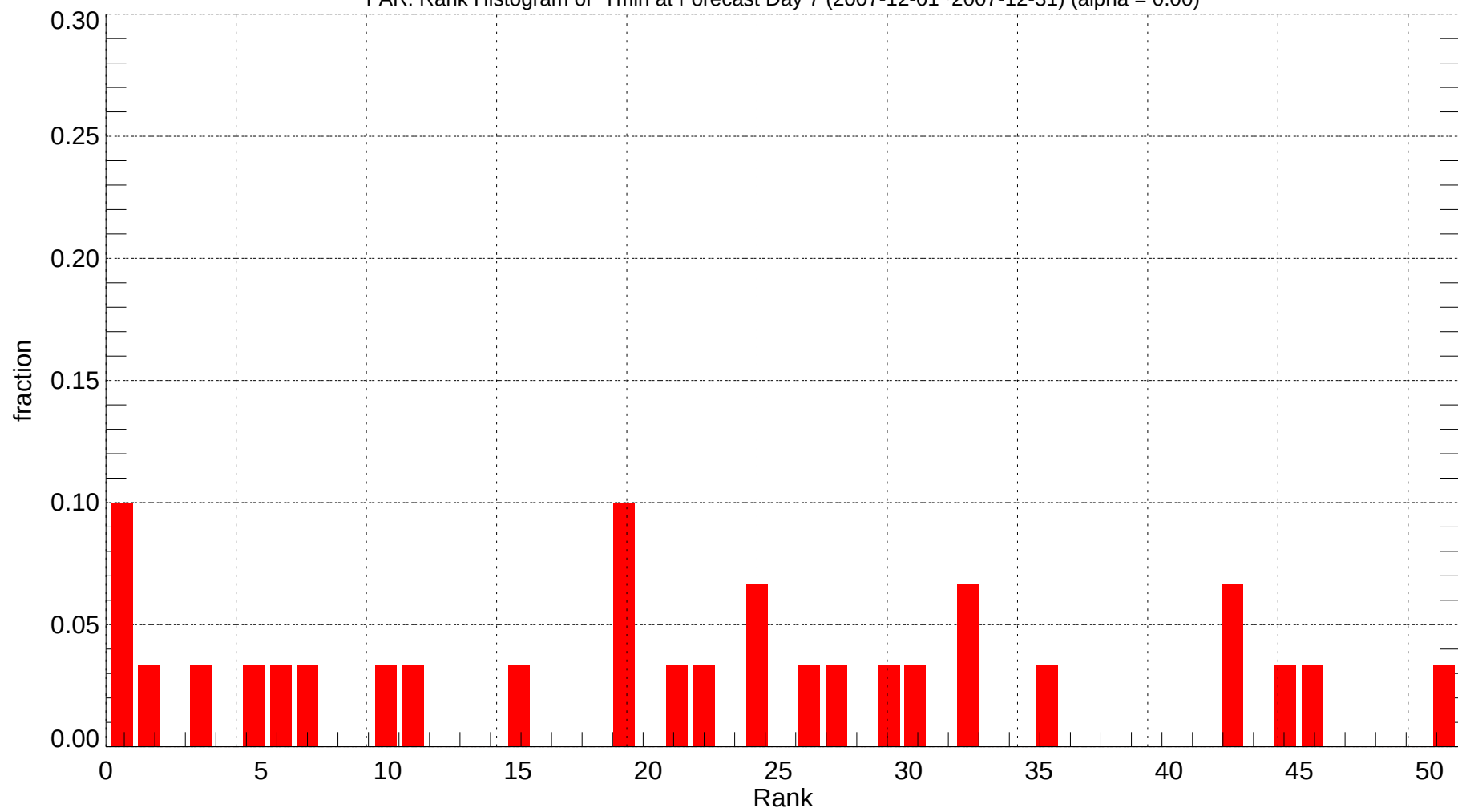
FAR: Rank Histogram of Tmin at Forecast Day 7 (2007-12-01~2007-12-31) (alpha = 0.00)
