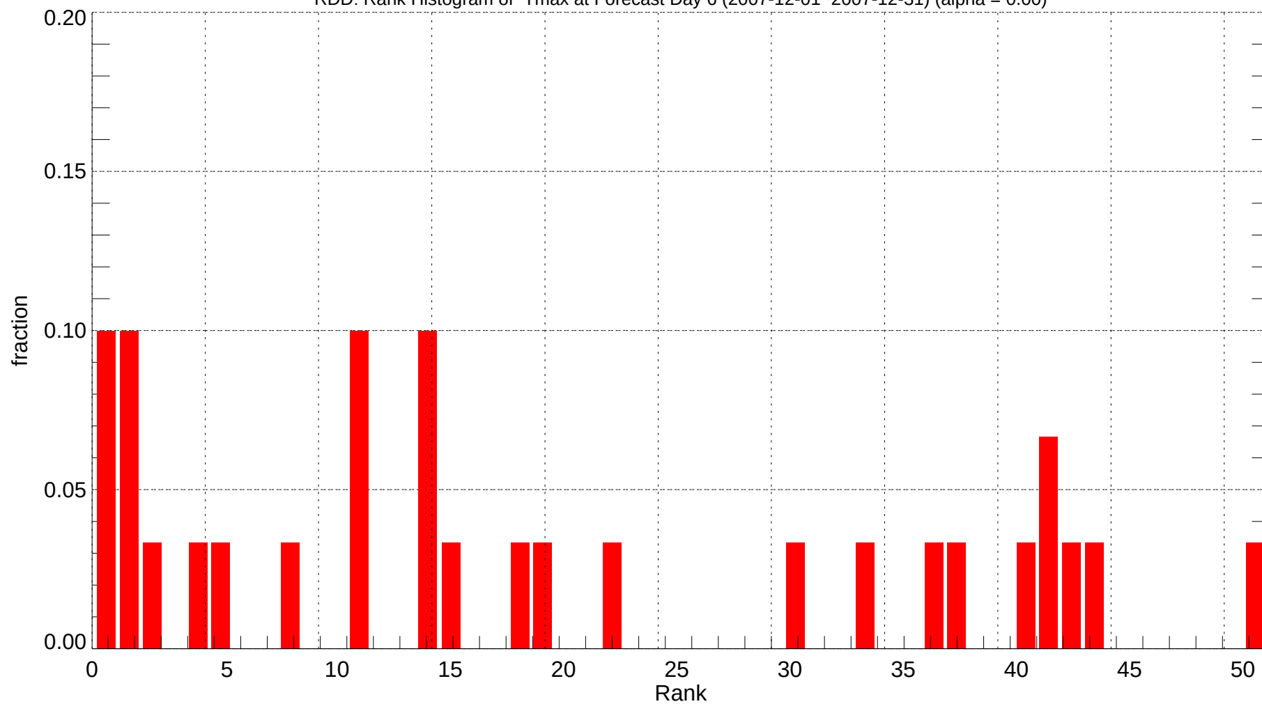
RDD: Rank Histogram of Tmax at Forecast Day 6 (2007-12-01~2007-12-31) (alpha = 0.00)
