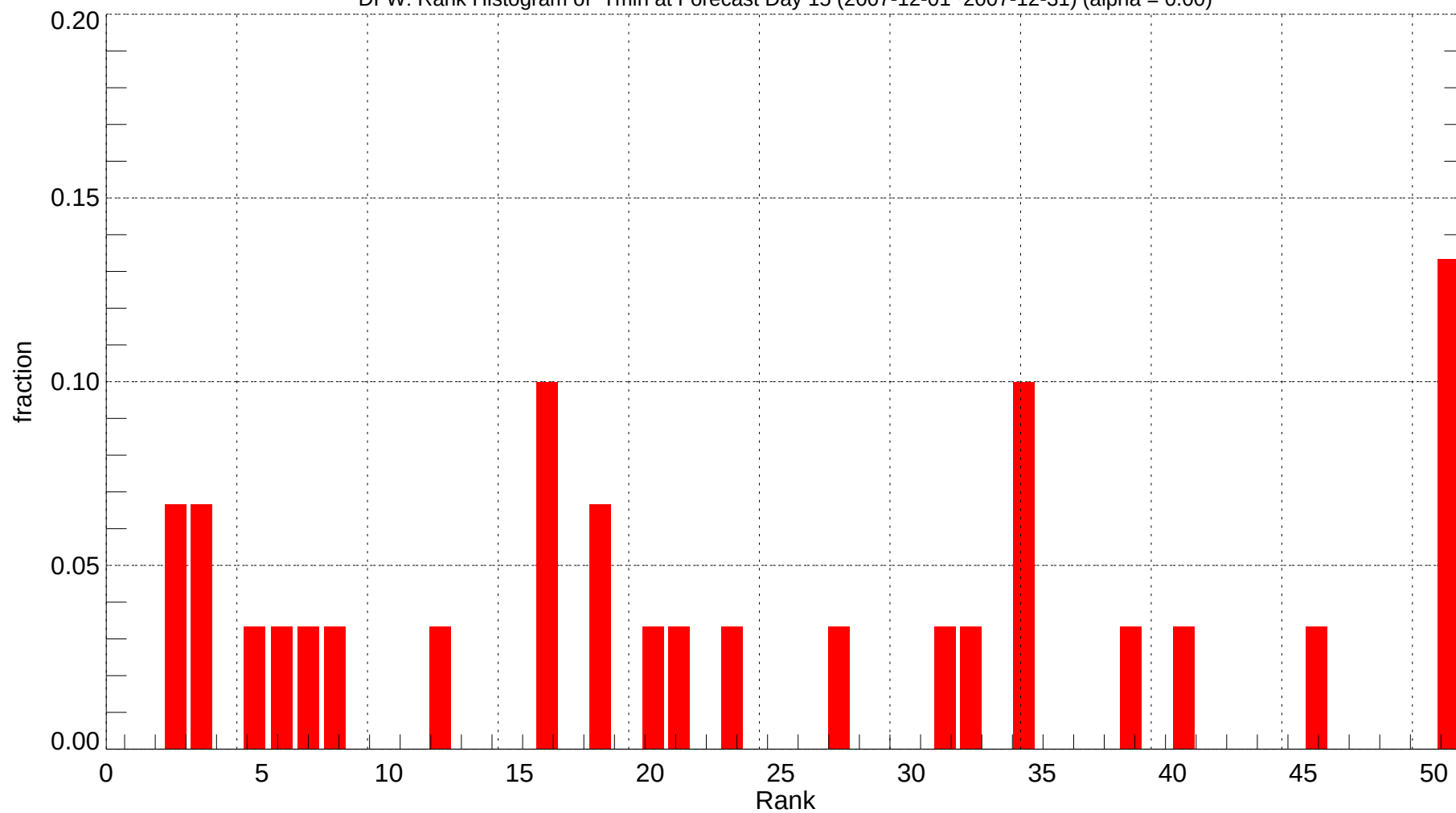
DFW: Rank Histogram of Tmin at Forecast Day 15 (2007-12-01~2007-12-31) (alpha = 0.00)
