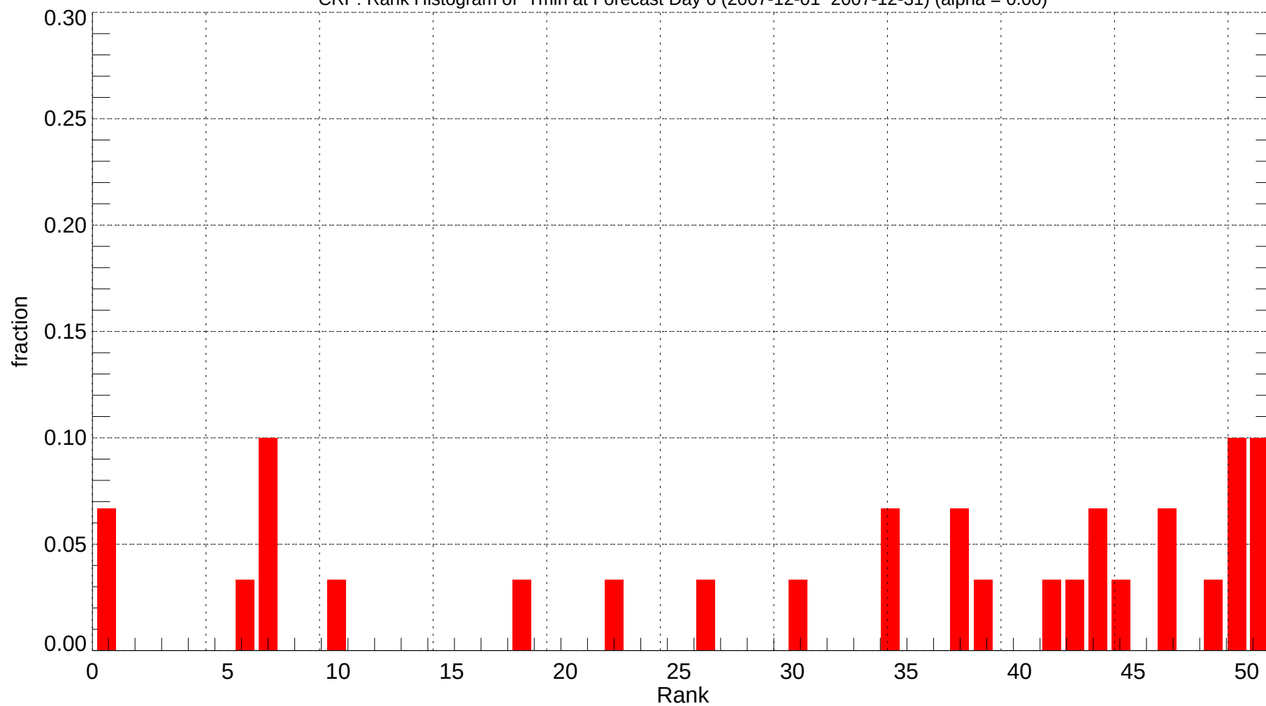
CRP: Rank Histogram of Tmin at Forecast Day 6 (2007-12-01~2007-12-31) (alpha = 0.00)
