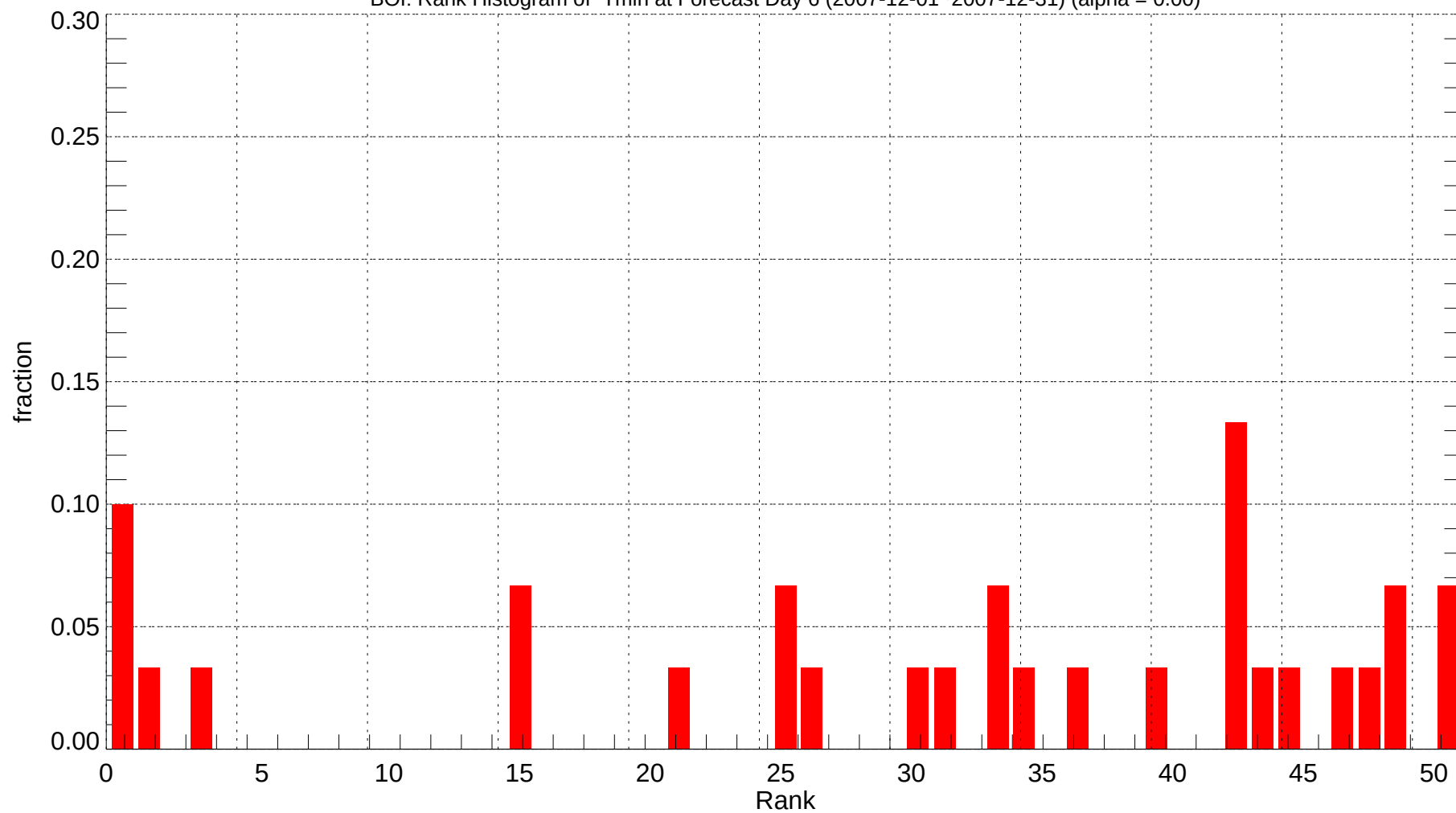
BOI: Rank Histogram of Tmin at Forecast Day 6 (2007-12-01~2007-12-31) (alpha = 0.00)
