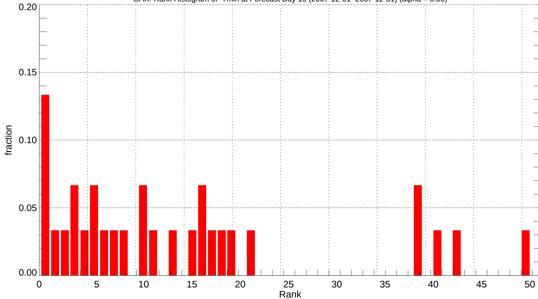
OAK: Rank Histogram of Tmin at Forecast Day 15 (2007-12-01~2007-12-31) (alpha = 0.00)
