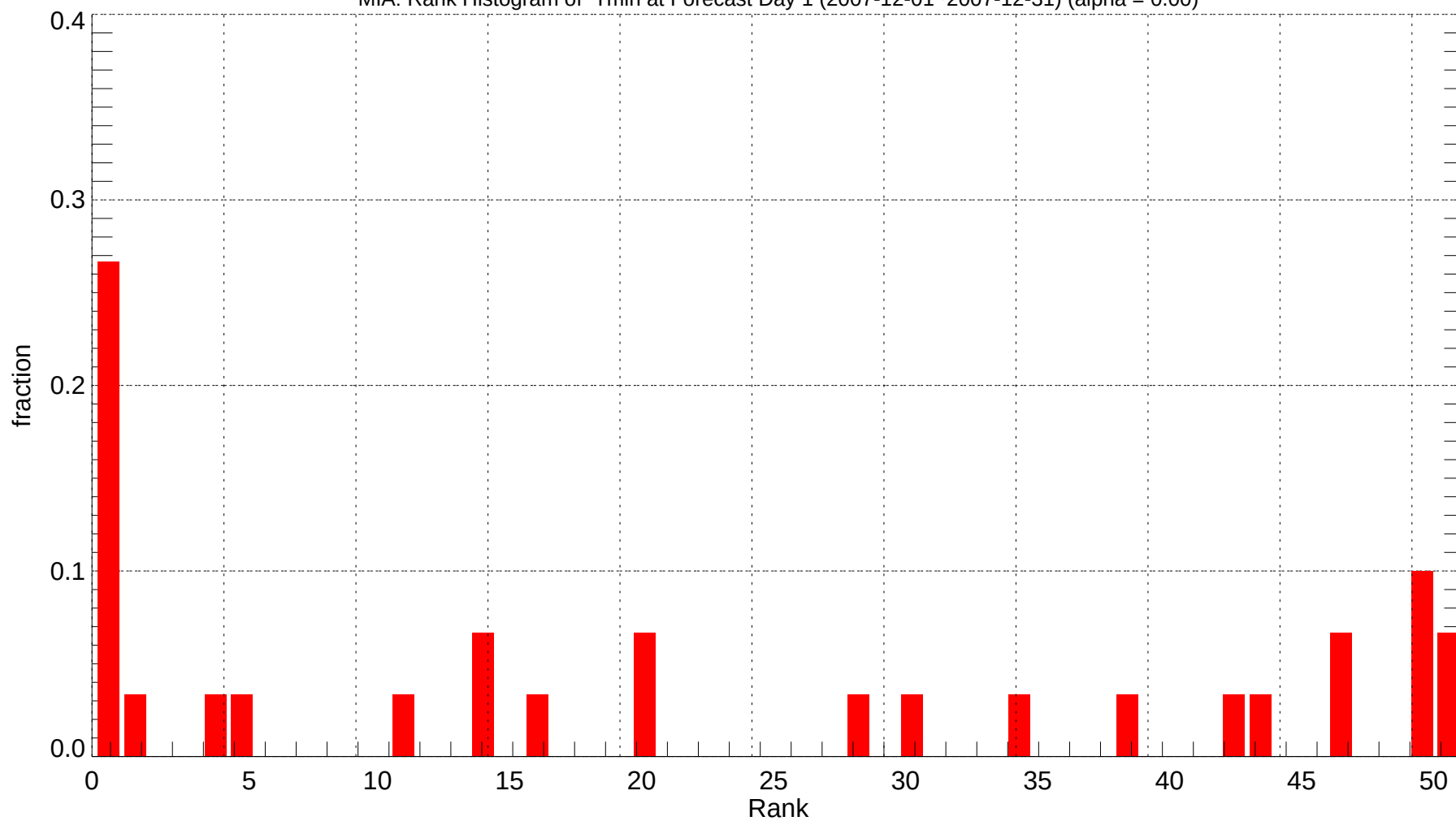
MIA: Rank Histogram of Tmin at Forecast Day 1 (2007-12-01~2007-12-31) (alpha = 0.00)
