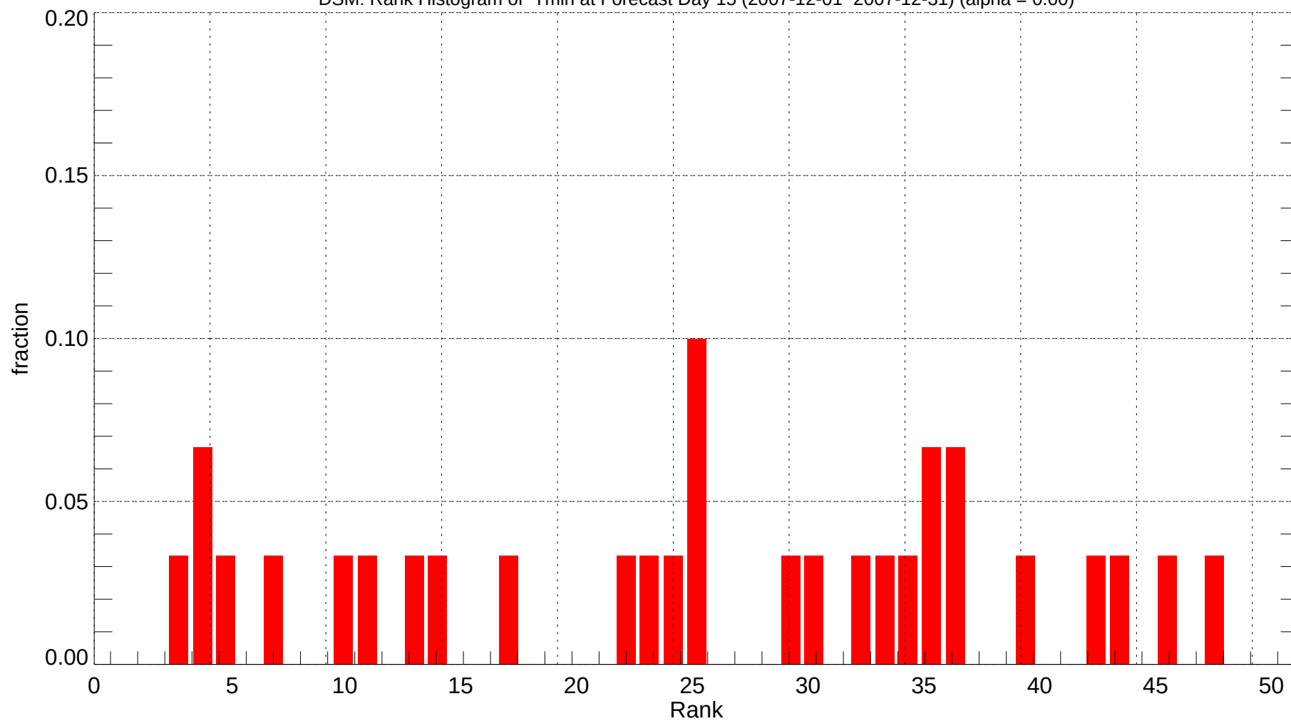
DSM: Rank Histogram of Tmin at Forecast Day 15 (2007-12-01~2007-12-31) (alpha = 0.00)
