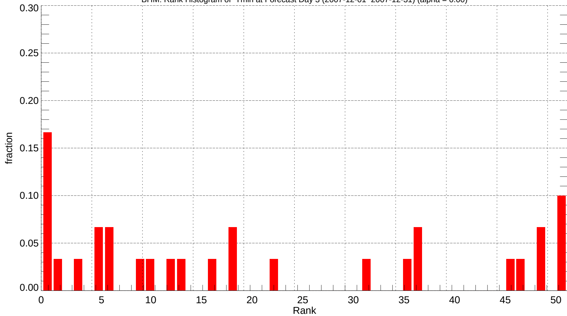
BHM: Rank Histogram of Tmin at Forecast Day 3 (2007-12-01~2007-12-31) (alpha = 0.00)
