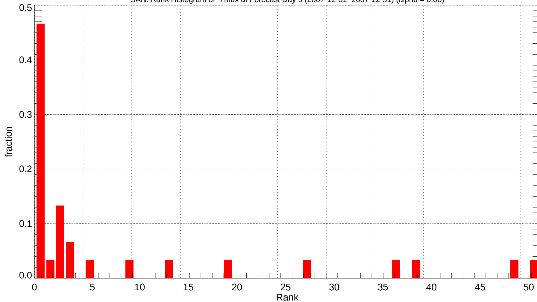
SAN: Rank Histogram of Tmax at Forecast Day 9 (2007-12-01~2007-12-31) (alpha = 0.00)
