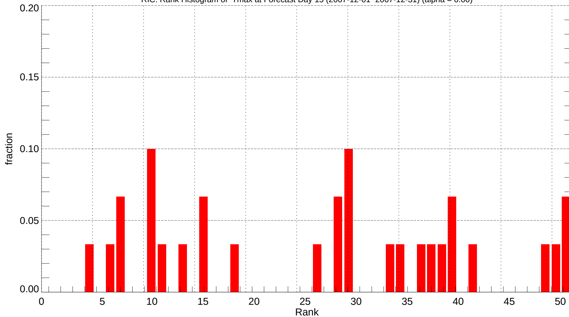
RIC: Rank Histogram of Tmax at Forecast Day 15 (2007-12-01~2007-12-31) (alpha = 0.00)
