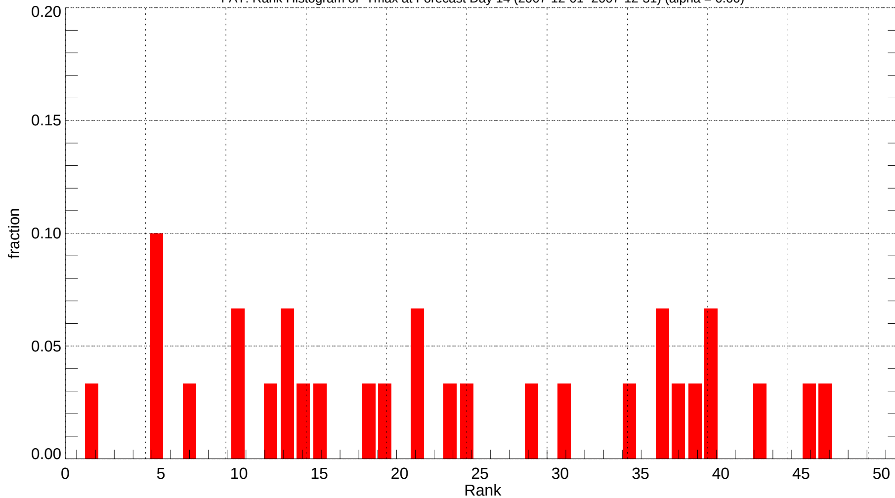
FAT: Rank Histogram of Tmax at Forecast Day 14 (2007-12-01~2007-12-31) (alpha = 0.00)
