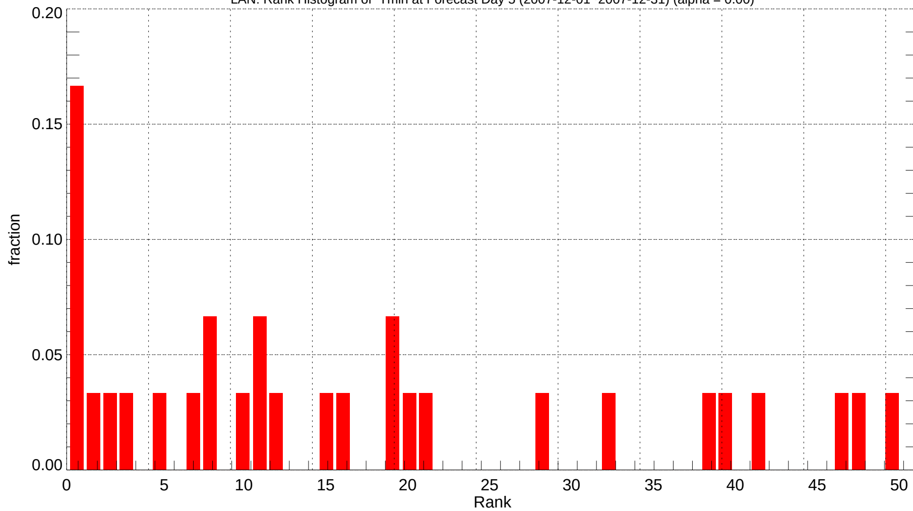
LAN: Rank Histogram of Tmin at Forecast Day 5 (2007-12-01~2007-12-31) (alpha = 0.00)
