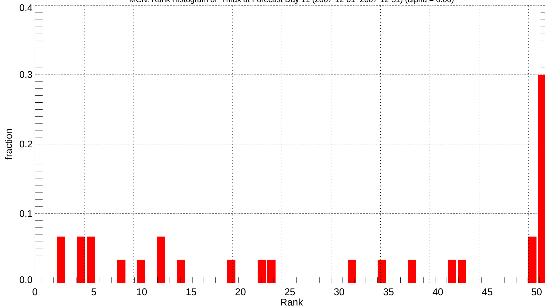
MCN: Rank Histogram of Tmax at Forecast Day 11 (2007-12-01~2007-12-31) (alpha = 0.00)
