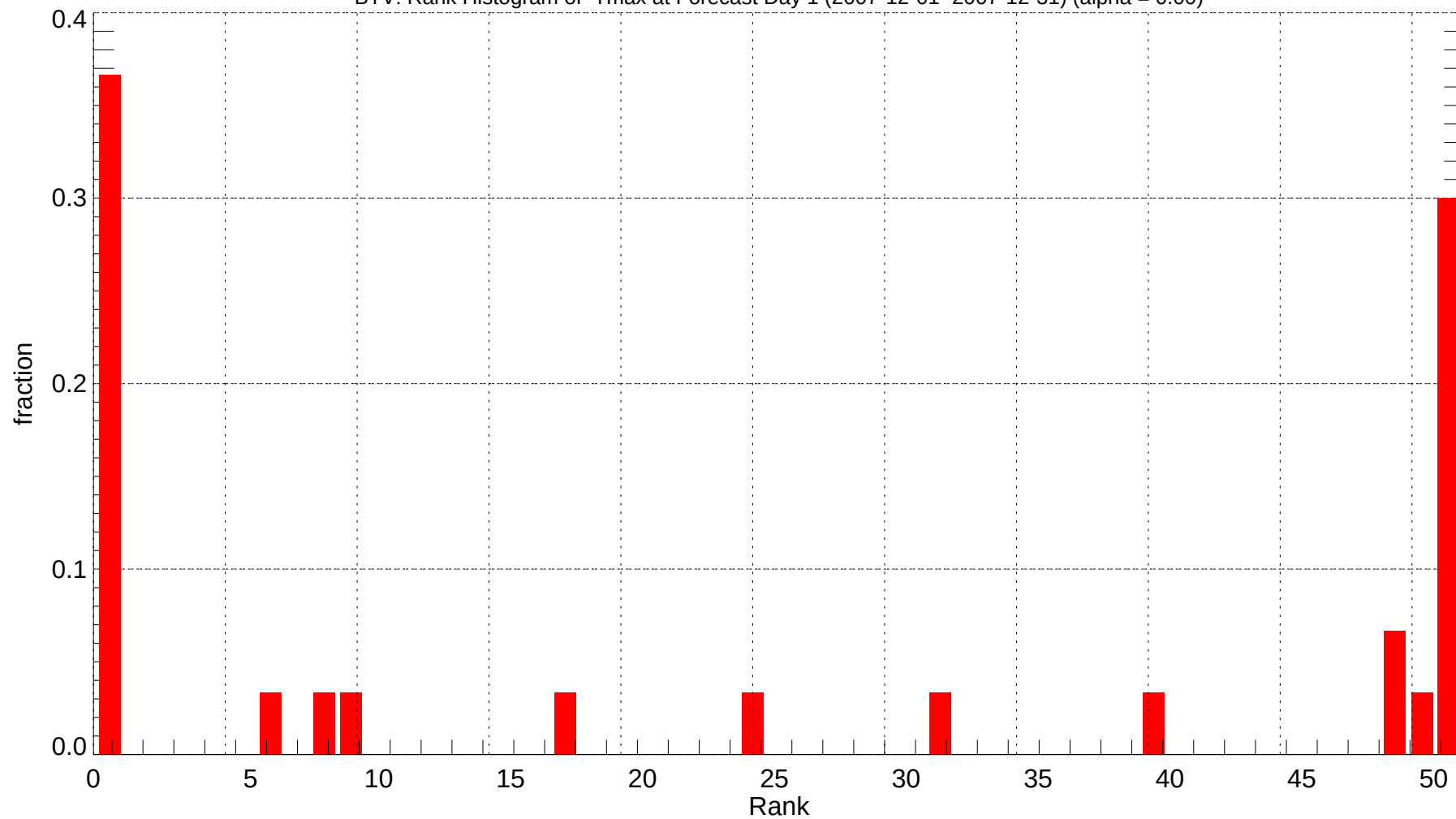
BTV: Rank Histogram of Tmax at Forecast Day 1 (2007-12-01~2007-12-31) (alpha = 0.00)
