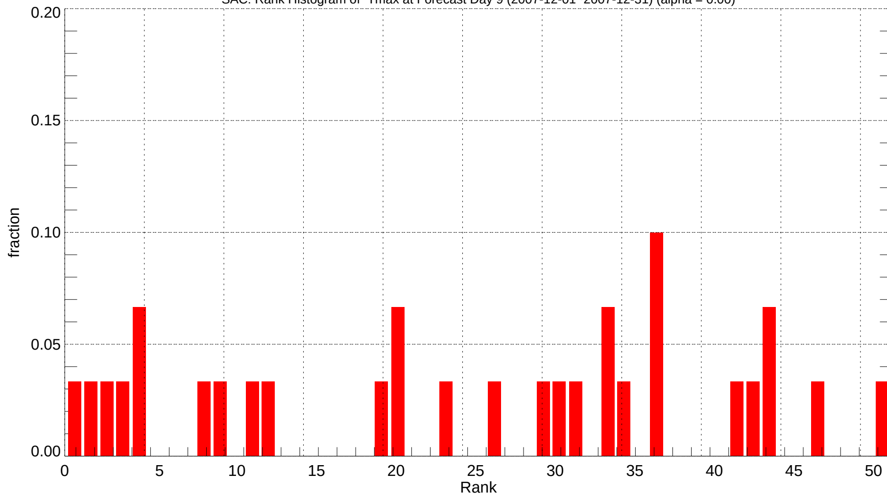
SAC: Rank Histogram of Tmax at Forecast Day 9 (2007-12-01~2007-12-31) (alpha = 0.00)
