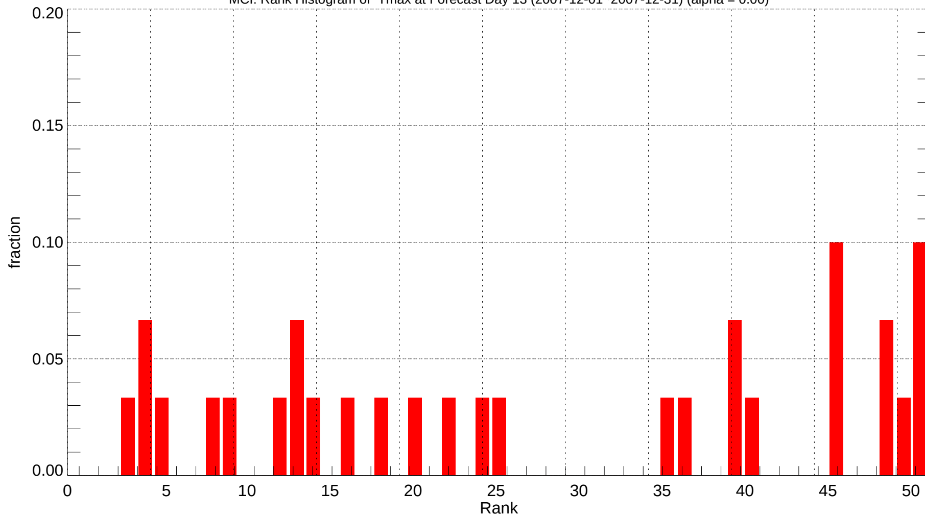
MCI: Rank Histogram of Tmax at Forecast Day 13 (2007-12-01~2007-12-31) (alpha = 0.00)
