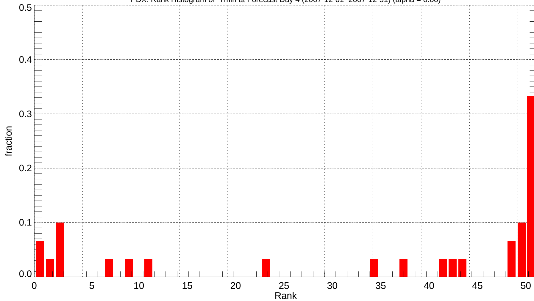
PDX: Rank Histogram of Tmin at Forecast Day 4 (2007-12-01~2007-12-31) (alpha = 0.00)
