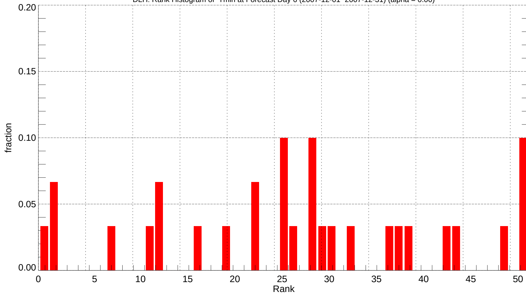
DLH: Rank Histogram of Tmin at Forecast Day 6 (2007-12-01~2007-12-31) (alpha = 0.00)
