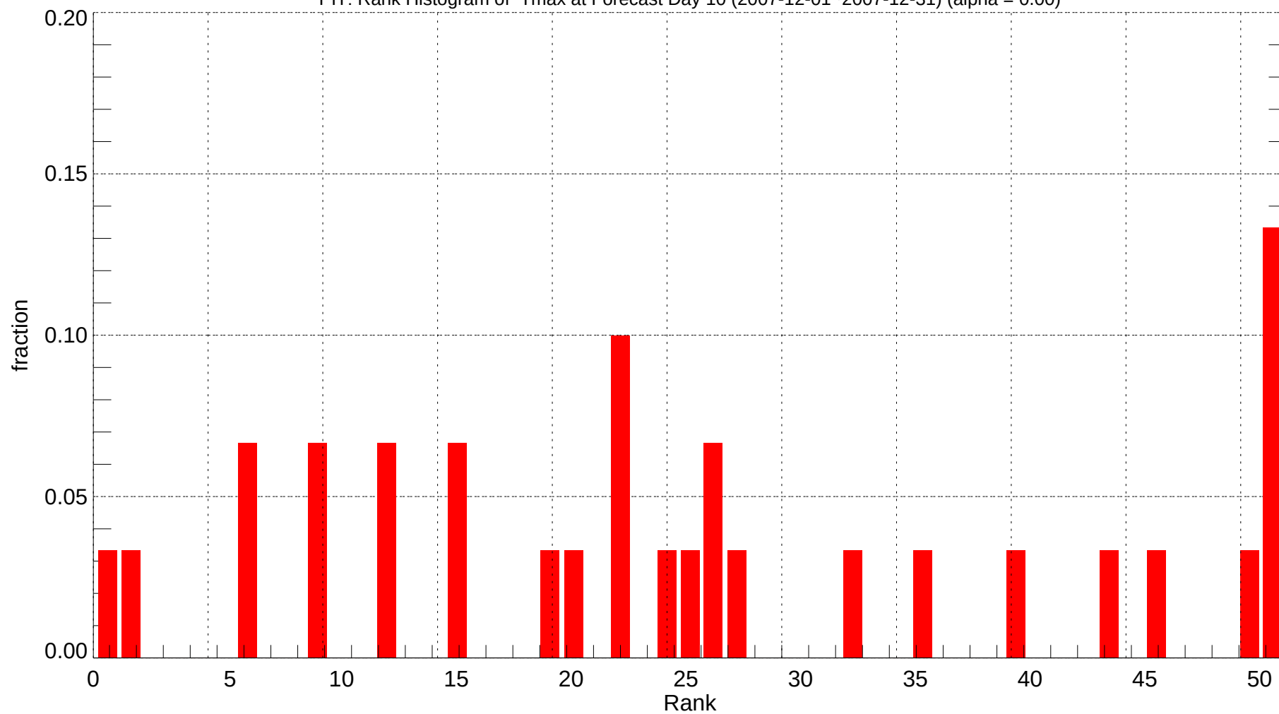
PIT: Rank Histogram of Tmax at Forecast Day 10 (2007-12-01~2007-12-31) (alpha = 0.00)
