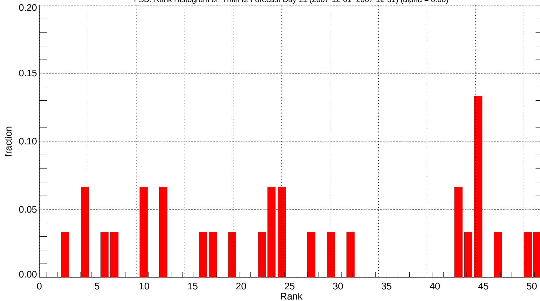
FSD: Rank Histogram of Tmin at Forecast Day 11 (2007-12-01~2007-12-31) (alpha = 0.00)
