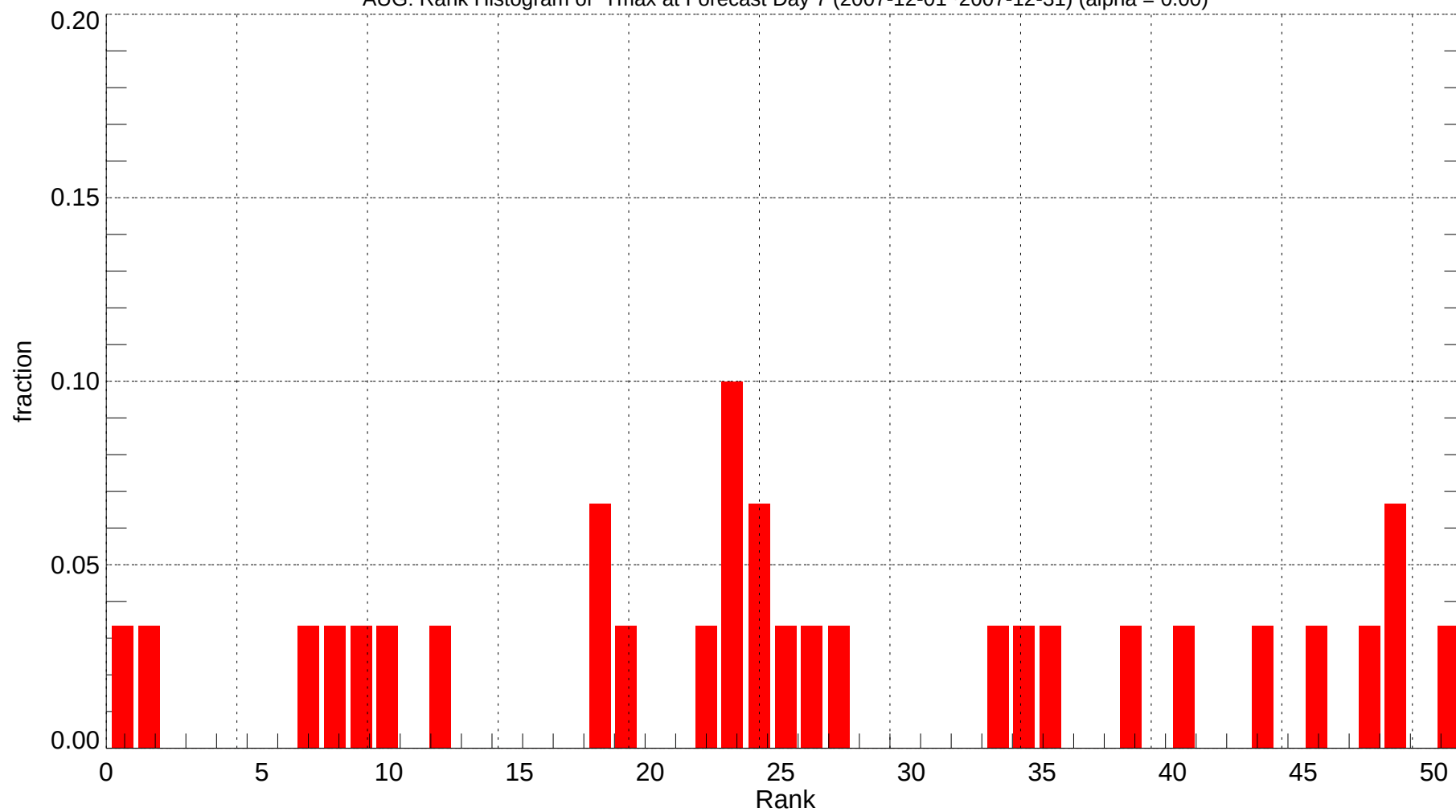
AUG: Rank Histogram of Tmax at Forecast Day 7 (2007-12-01~2007-12-31) (alpha = 0.00)
