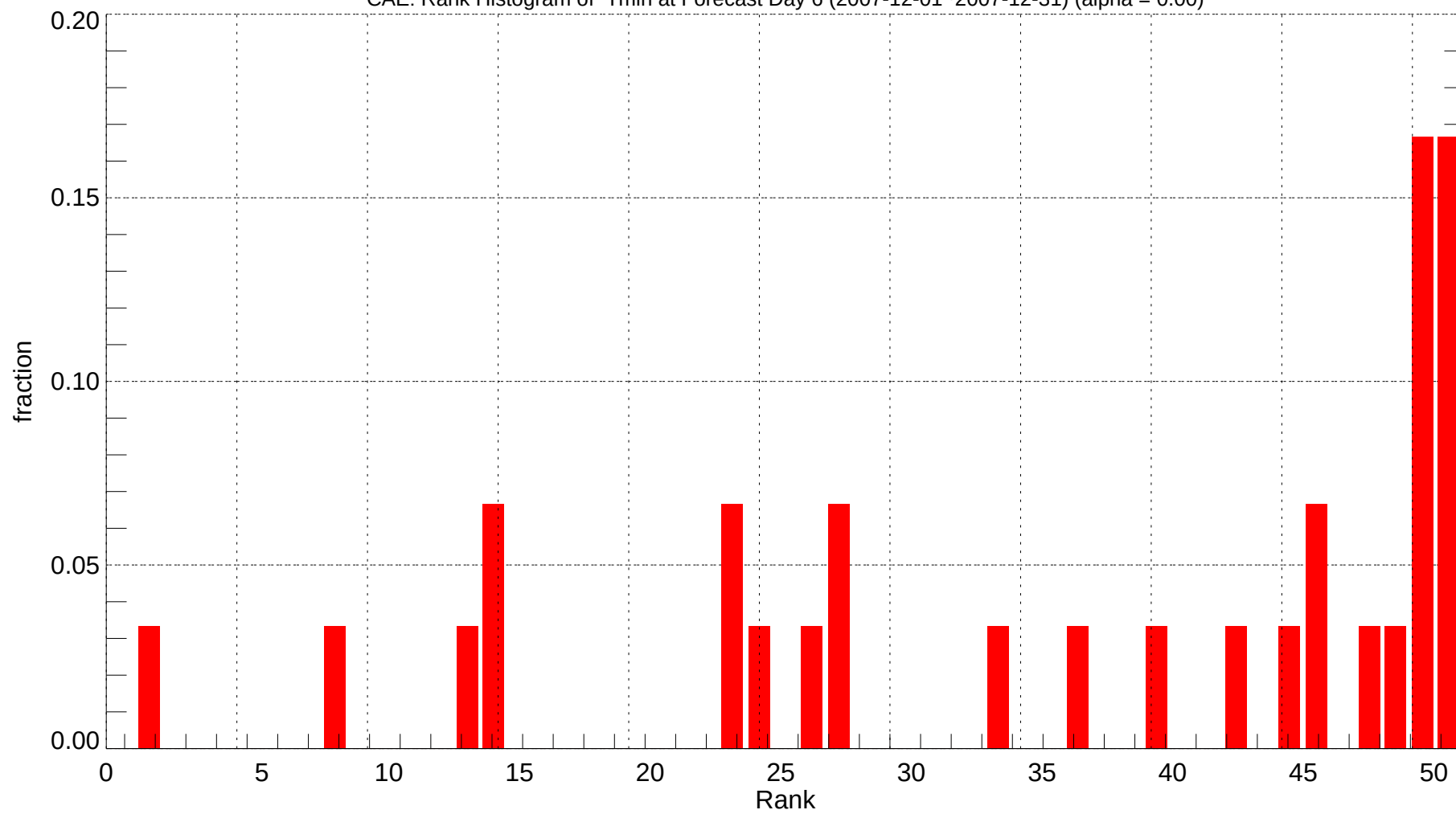
CAE: Rank Histogram of Tmin at Forecast Day 6 (2007-12-01~2007-12-31) (alpha = 0.00)
