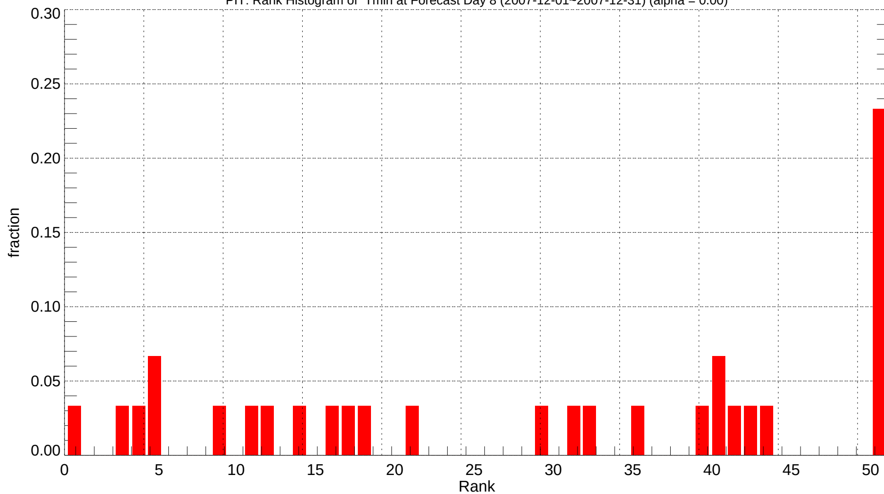
PIT: Rank Histogram of Tmin at Forecast Day 8 (2007-12-01~2007-12-31) (alpha = 0.00)
