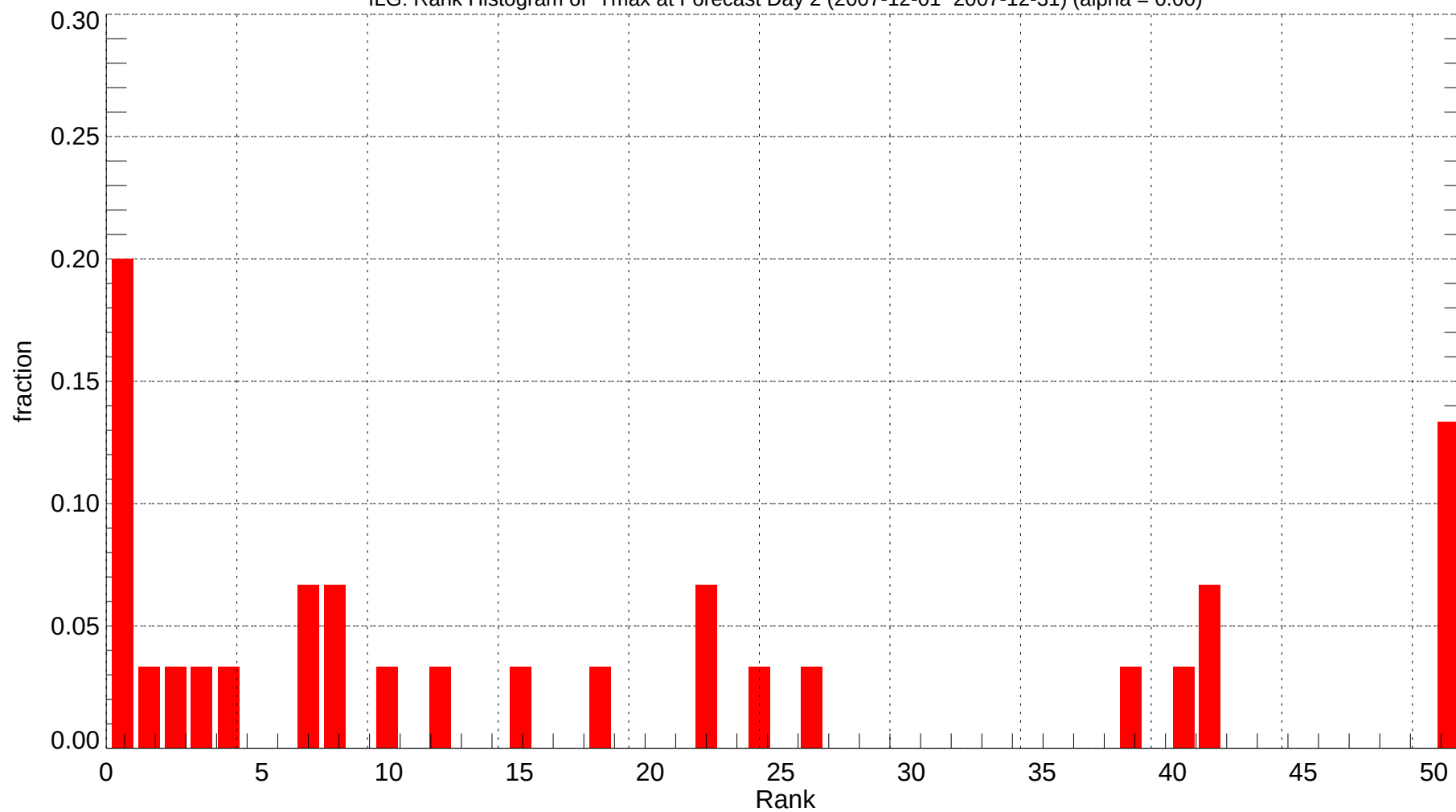
ILG: Rank Histogram of Tmax at Forecast Day 2 (2007-12-01~2007-12-31) (alpha = 0.00)
