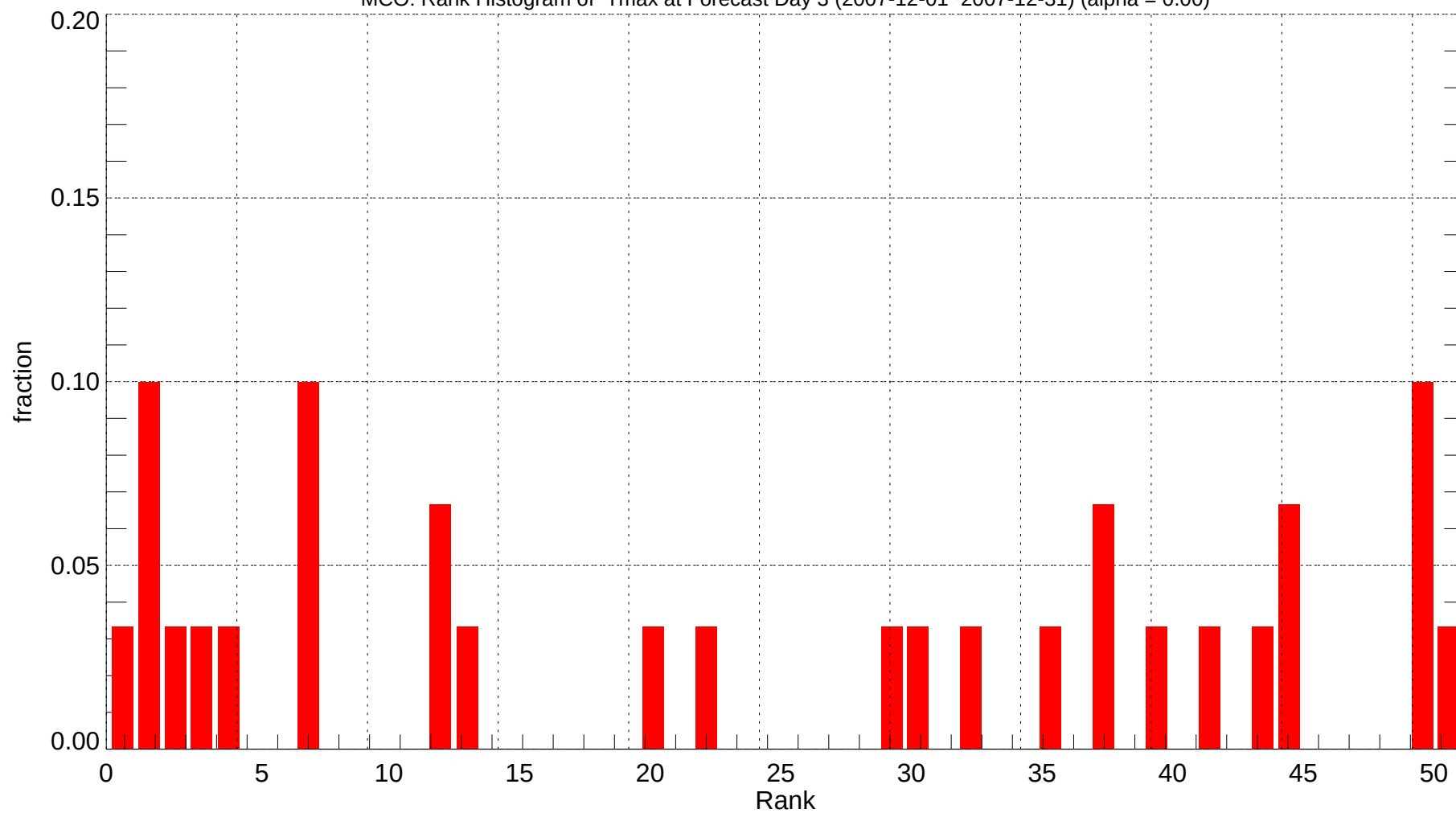
MCO: Rank Histogram of Tmax at Forecast Day 3 (2007-12-01~2007-12-31) (alpha = 0.00)
