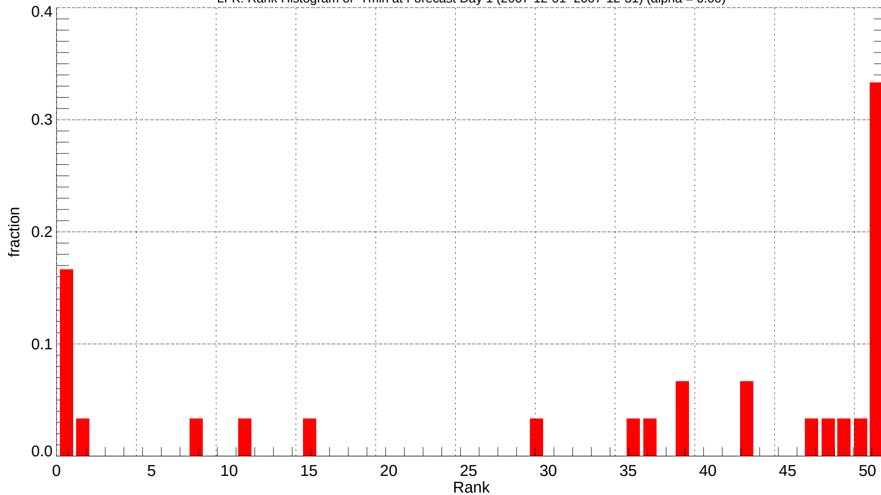
LFK: Rank Histogram of Tmin at Forecast Day 1 (2007-12-01~2007-12-31) (alpha = 0.00)
