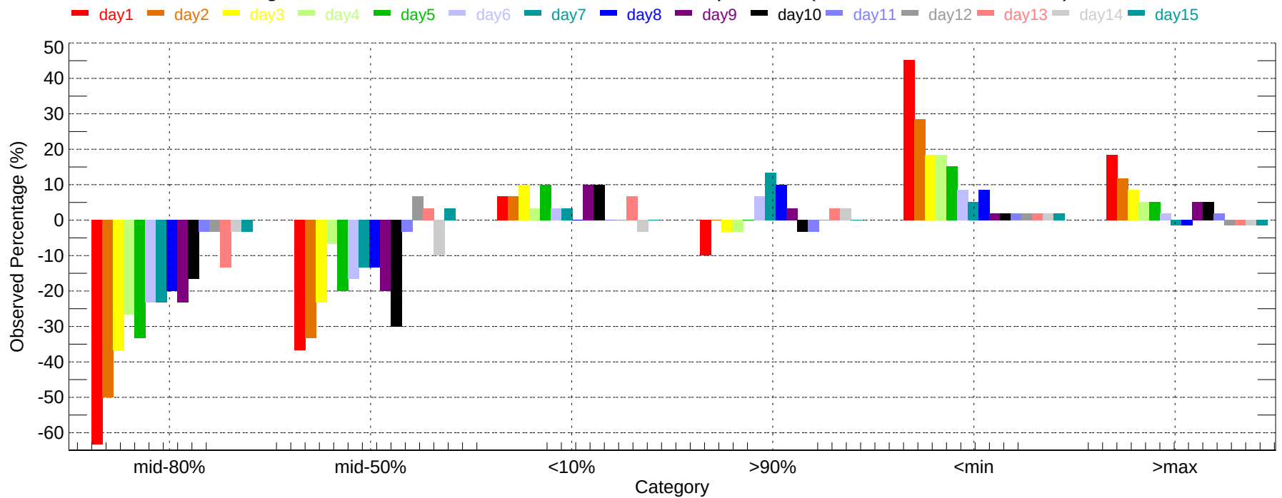
Observed Percentage Deviation of Ensembles - ORH: Max Temperature (2007-12-01~2007-12-31)
