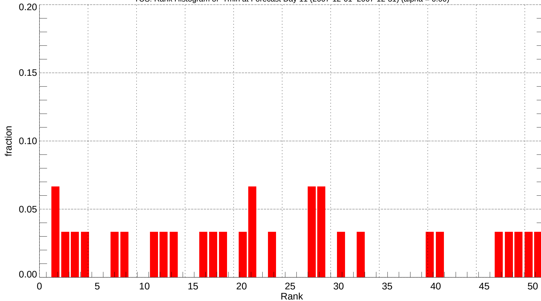
TUS: Rank Histogram of Tmin at Forecast Day 11 (2007-12-01~2007-12-31) (alpha = 0.00)
