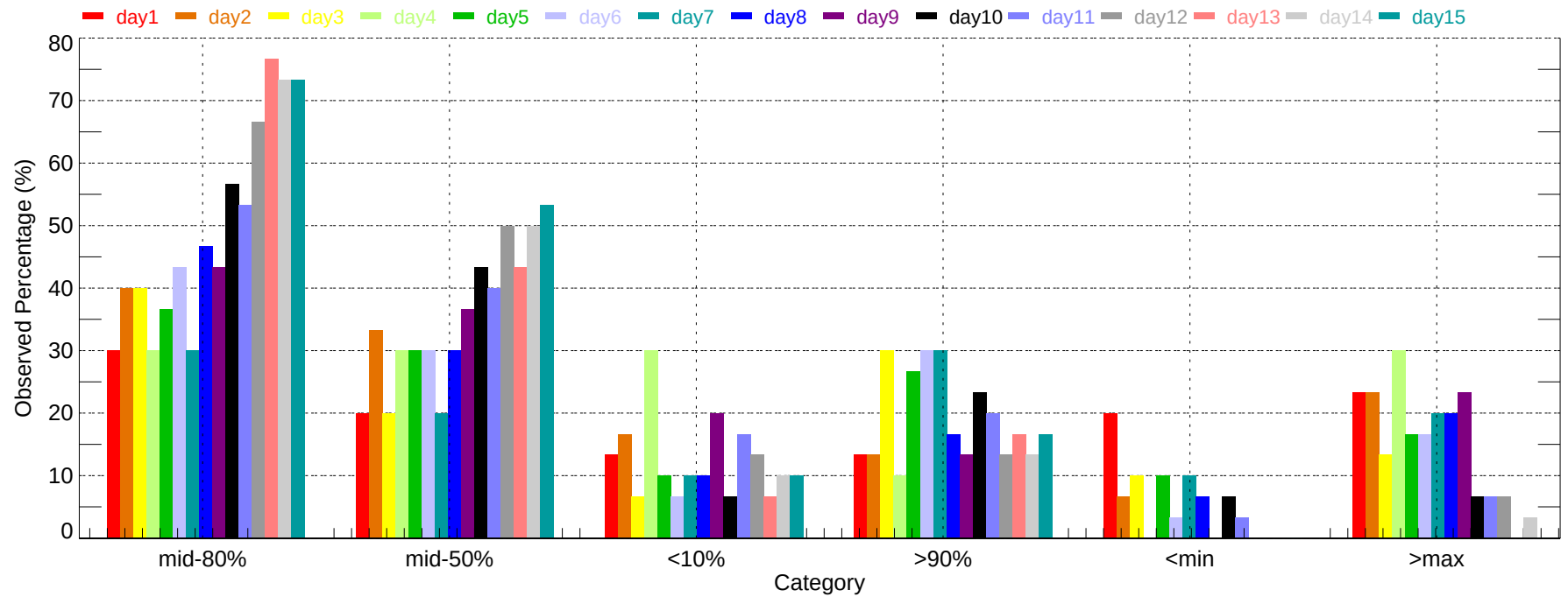
Observed Percentage of Ensembles - ORD: Min Temperature (2007-12-01~2007-12-31)
