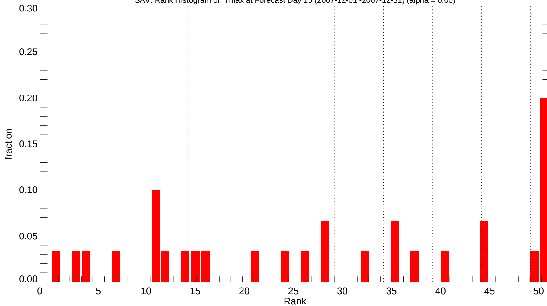
SAV: Rank Histogram of Tmax at Forecast Day 15 (2007-12-01~2007-12-31) (alpha = 0.00)
