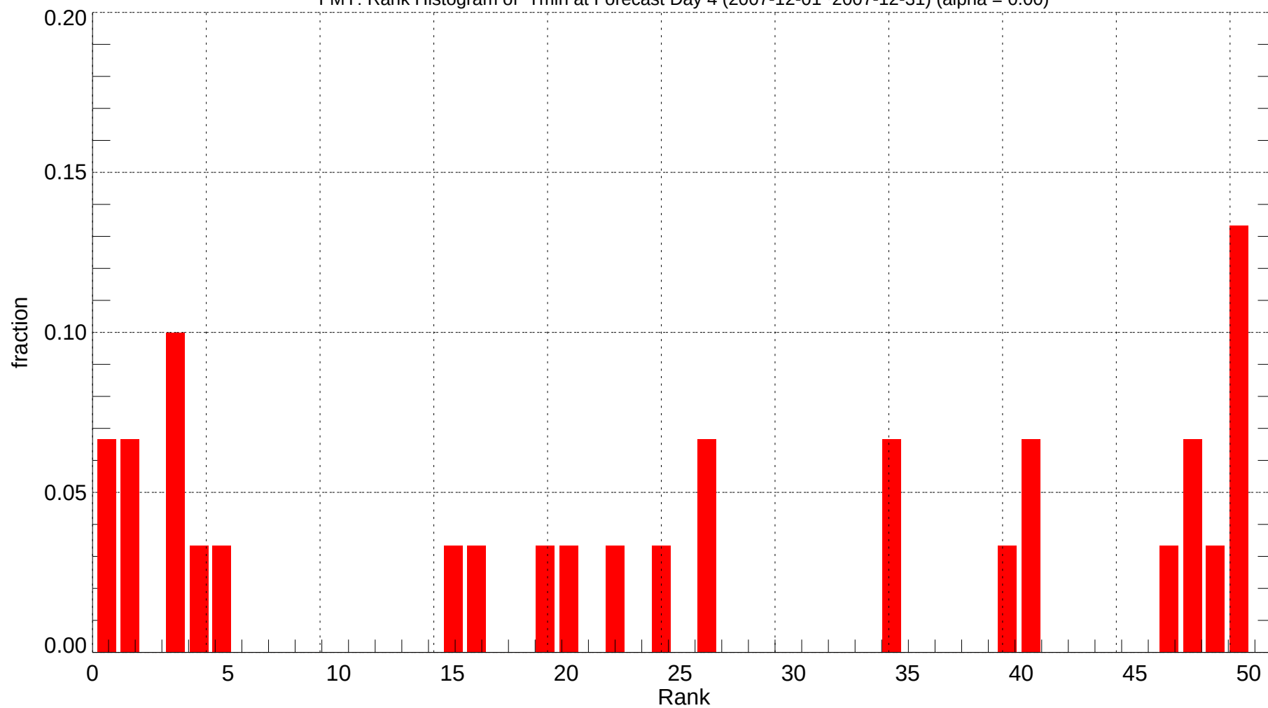
FMY: Rank Histogram of Tmin at Forecast Day 4 (2007-12-01~2007-12-31) (alpha = 0.00)
