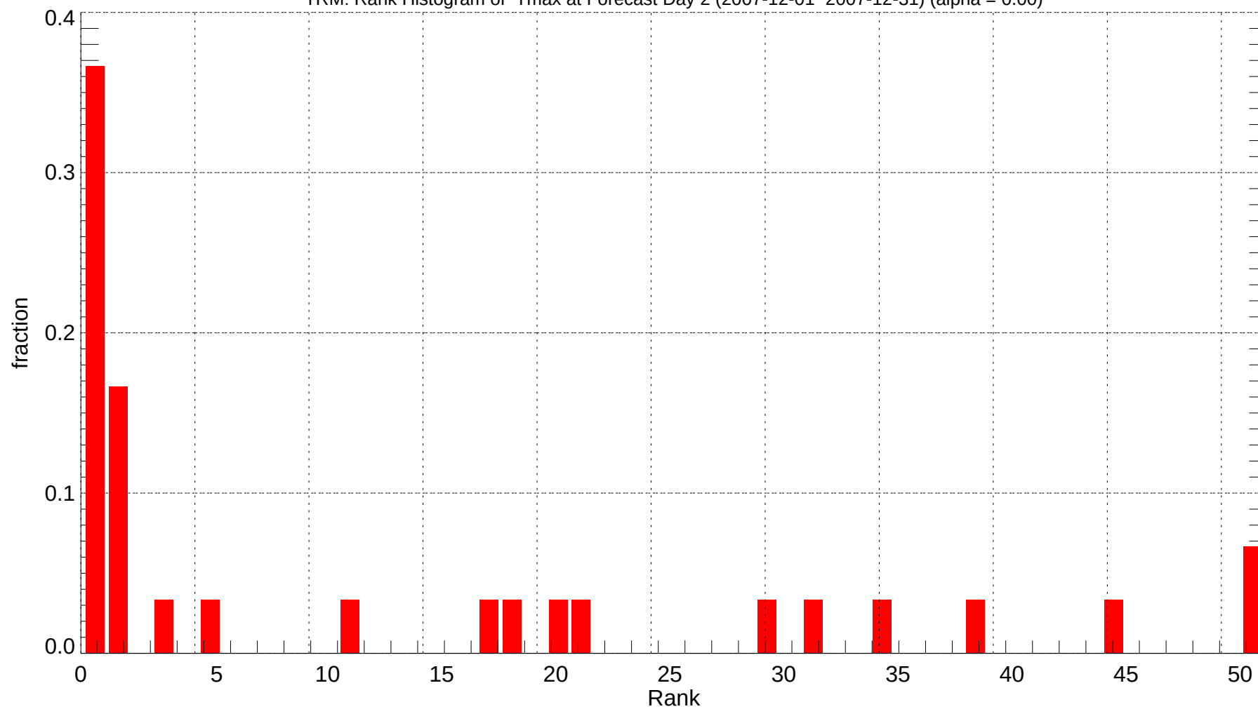
TRM: Rank Histogram of Tmax at Forecast Day 2 (2007-12-01~2007-12-31) (alpha = 0.00)
