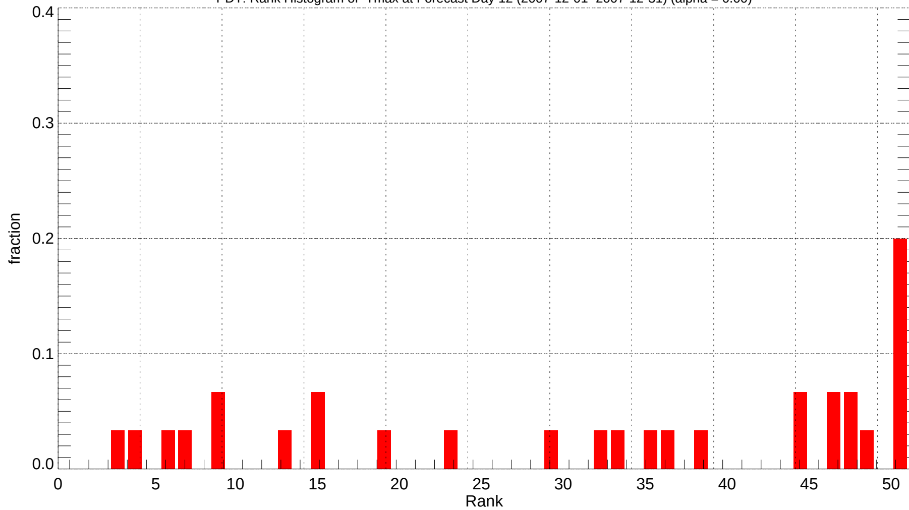
PDT: Rank Histogram of Tmax at Forecast Day 12 (2007-12-01~2007-12-31) (alpha = 0.00)
