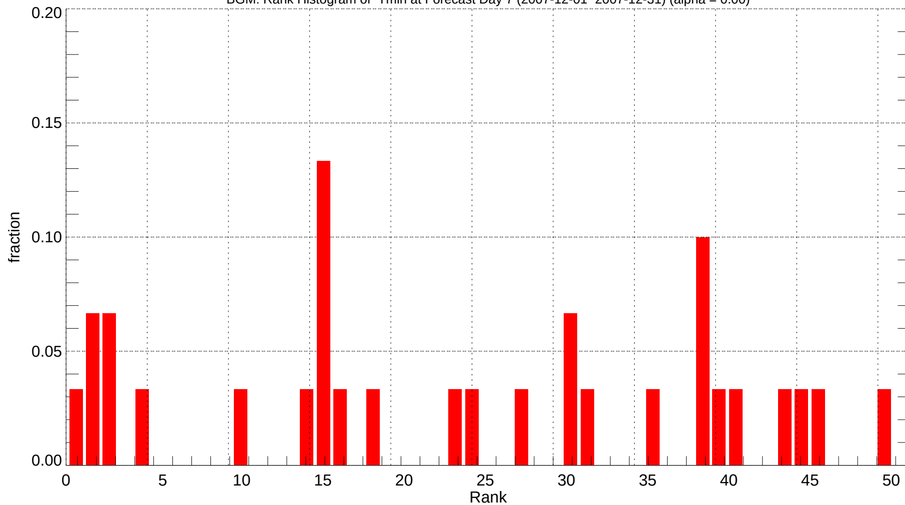
BGM: Rank Histogram of Tmin at Forecast Day 7 (2007-12-01~2007-12-31) (alpha = 0.00)
