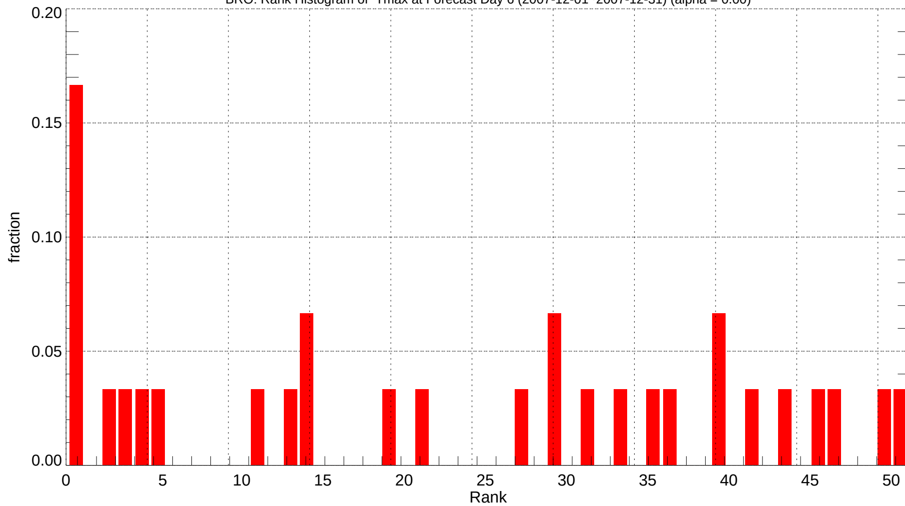
BRO: Rank Histogram of Tmax at Forecast Day 6 (2007-12-01~2007-12-31) (alpha = 0.00)
