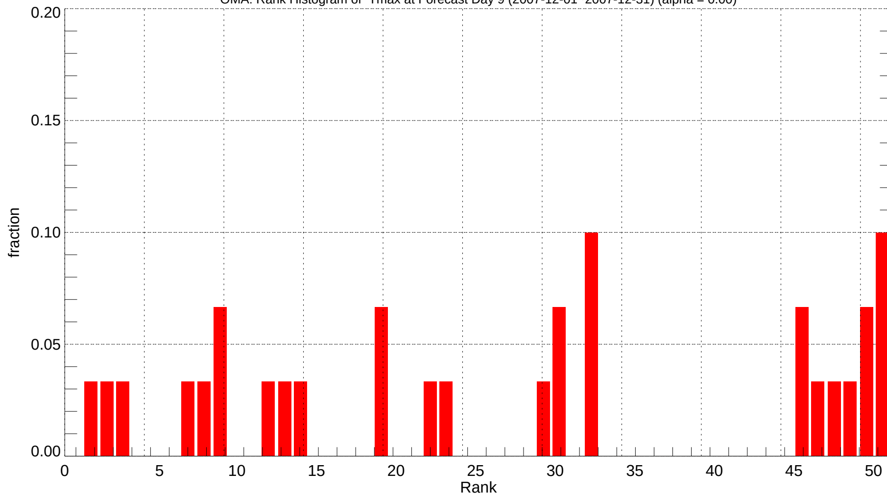
OMA: Rank Histogram of Tmax at Forecast Day 9 (2007-12-01~2007-12-31) (alpha = 0.00)
