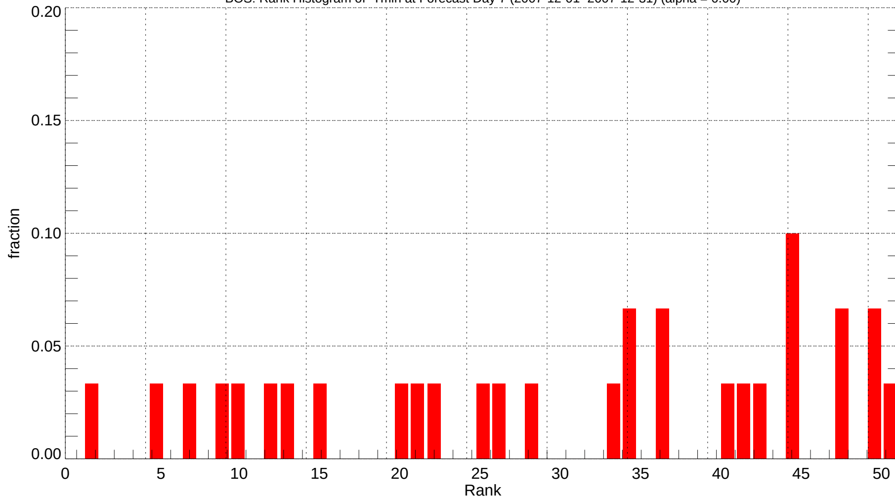
BOS: Rank Histogram of Tmin at Forecast Day 7 (2007-12-01~2007-12-31) (alpha = 0.00)
