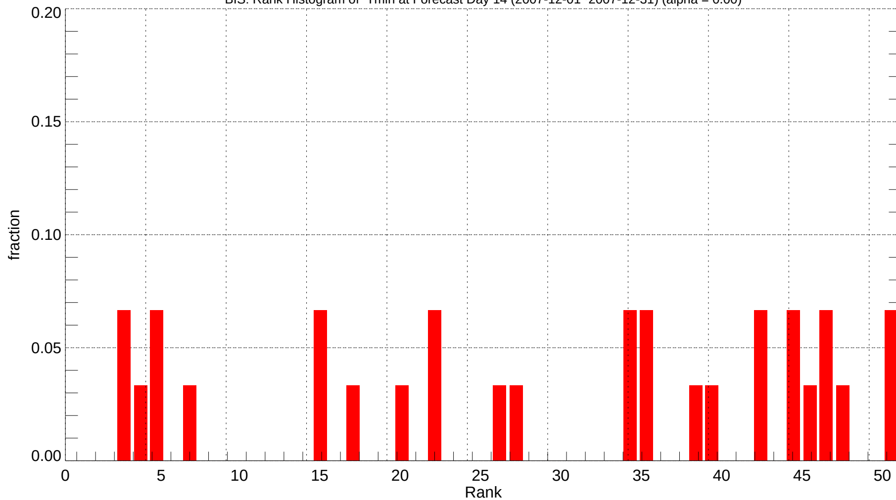
BIS: Rank Histogram of Tmin at Forecast Day 14 (2007-12-01~2007-12-31) (alpha = 0.00)
