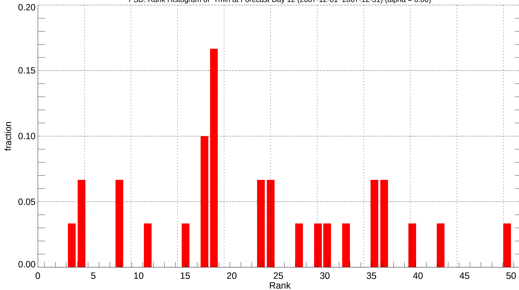
FSD: Rank Histogram of Tmin at Forecast Day 12 (2007-12-01~2007-12-31) (alpha = 0.00)
