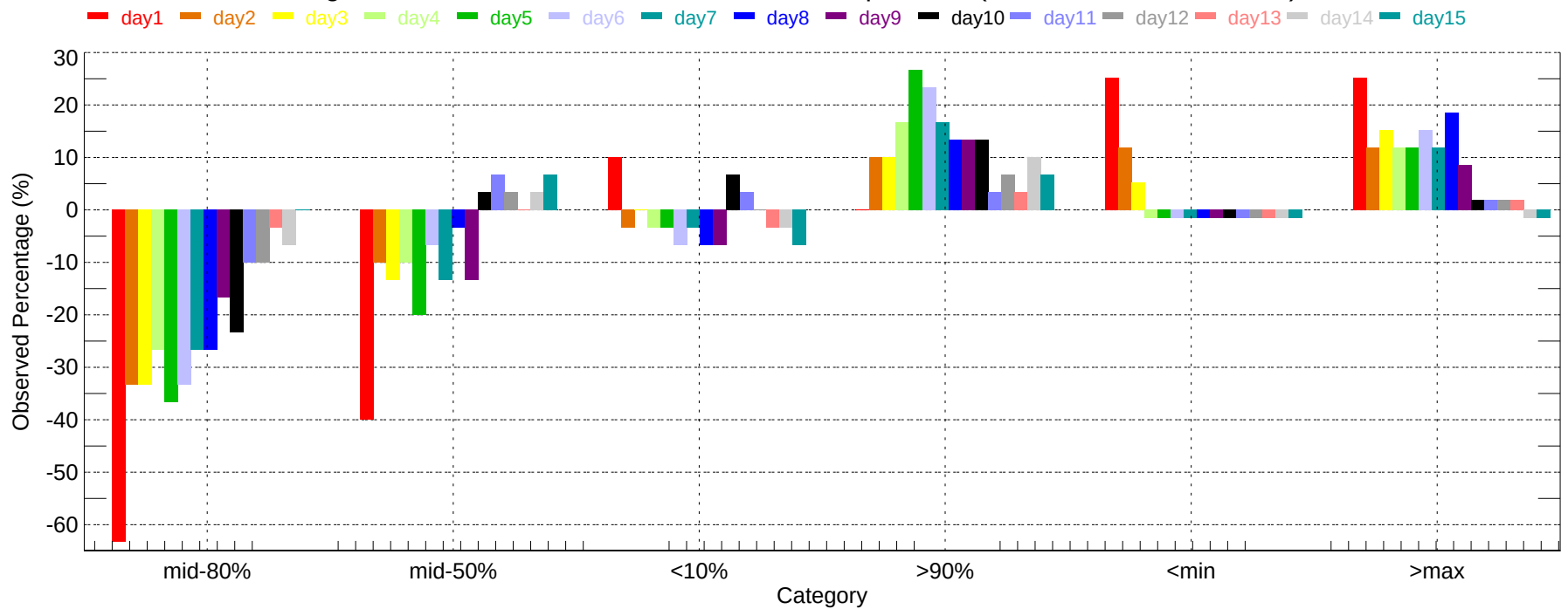
Observed Percentage Deviation of Ensembles - DEC: Min Temperature (2007-12-01~2007-12-31)
