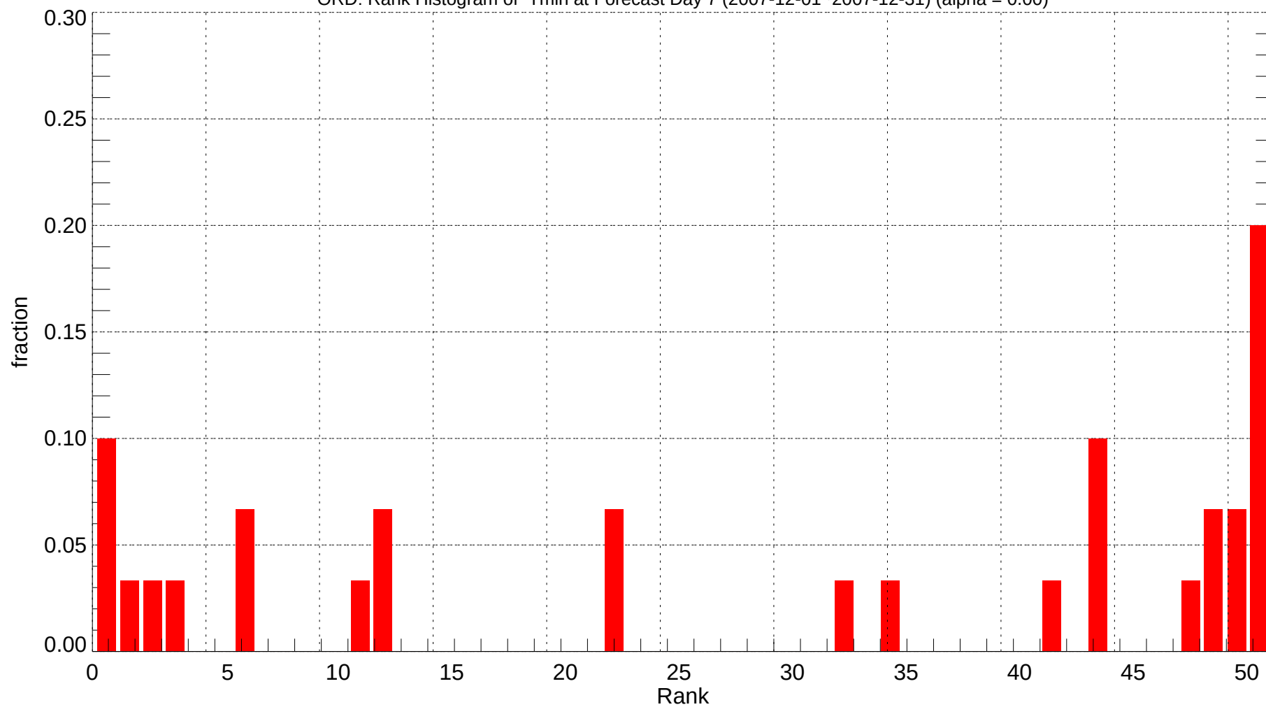
ORD: Rank Histogram of Tmin at Forecast Day 7 (2007-12-01~2007-12-31) (alpha = 0.00)
