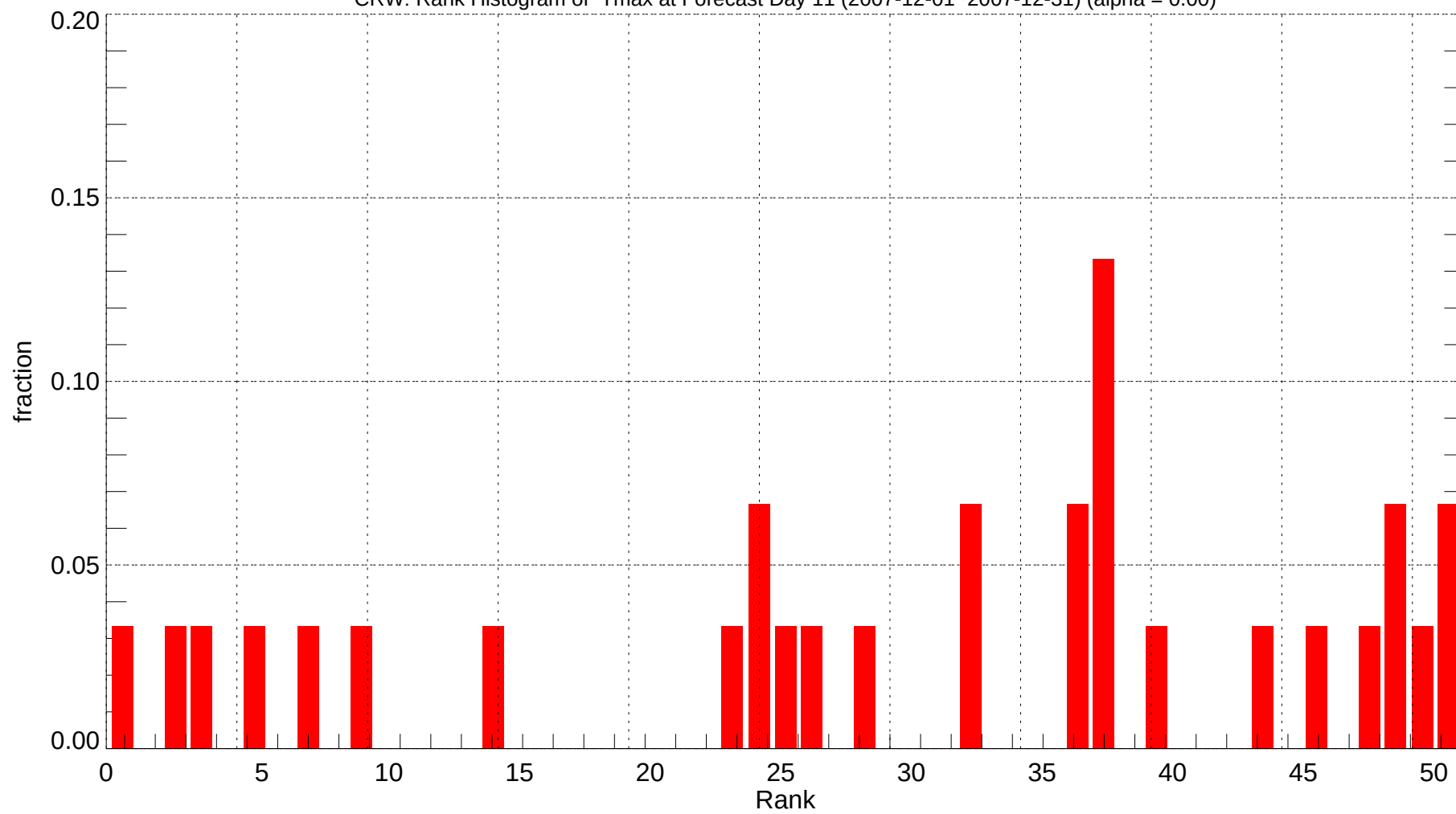
CRW: Rank Histogram of Tmax at Forecast Day 11 (2007-12-01~2007-12-31) (alpha = 0.00)
