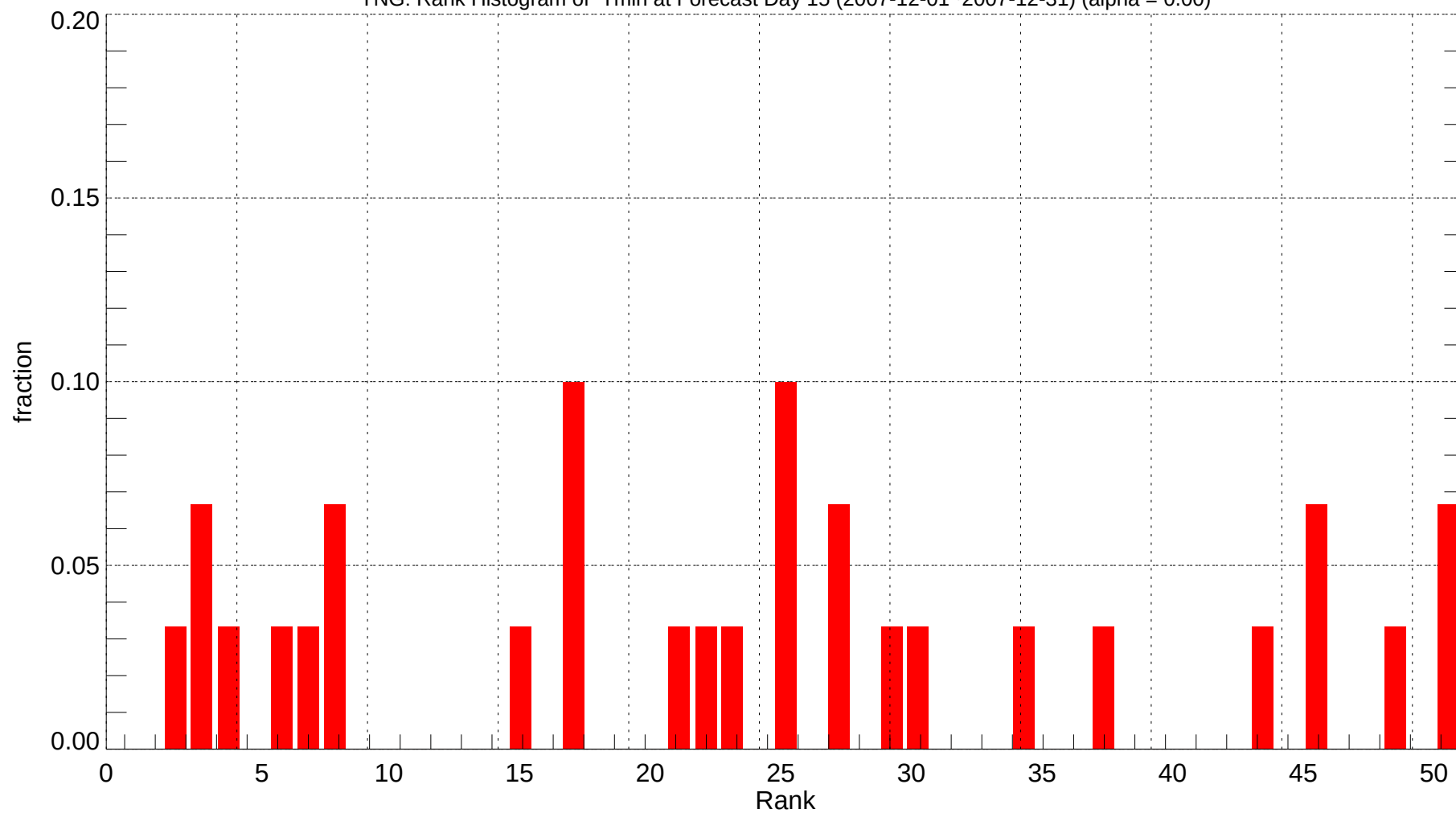
YNG: Rank Histogram of Tmin at Forecast Day 15 (2007-12-01~2007-12-31) (alpha = 0.00)
