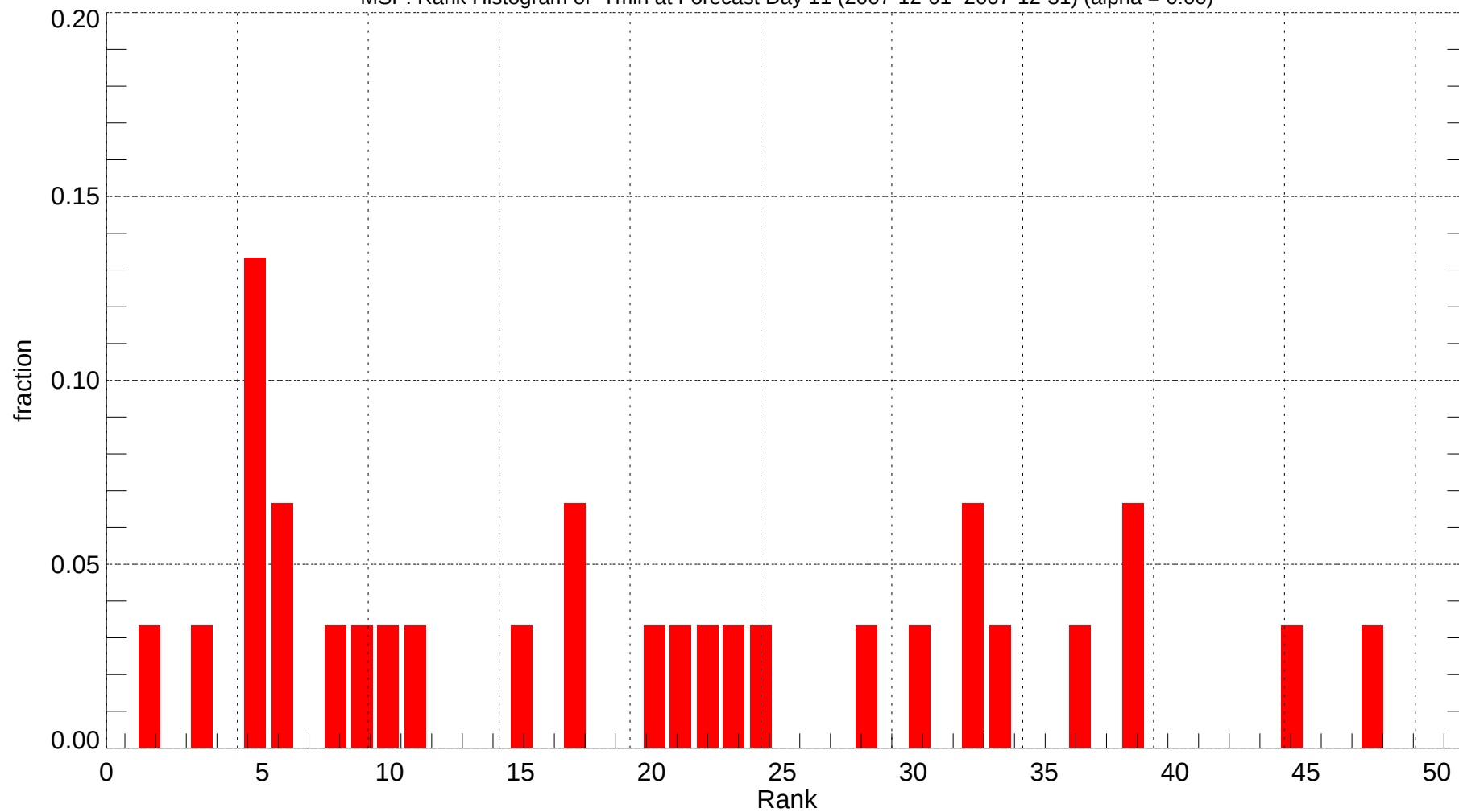
MSP: Rank Histogram of Tmin at Forecast Day 11 (2007-12-01~2007-12-31) (alpha = 0.00)
