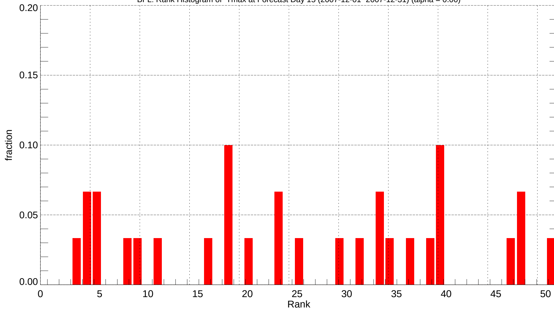
BFL: Rank Histogram of Tmax at Forecast Day 15 (2007-12-01~2007-12-31) (alpha = 0.00)
