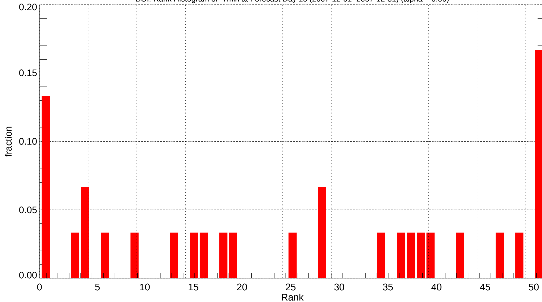
BOI: Rank Histogram of Tmin at Forecast Day 10 (2007-12-01~2007-12-31) (alpha = 0.00)
