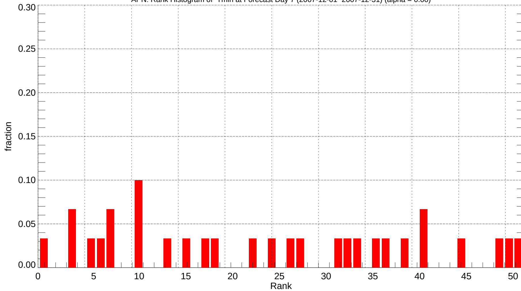
APN: Rank Histogram of Tmin at Forecast Day 7 (2007-12-01~2007-12-31) (alpha = 0.00)
