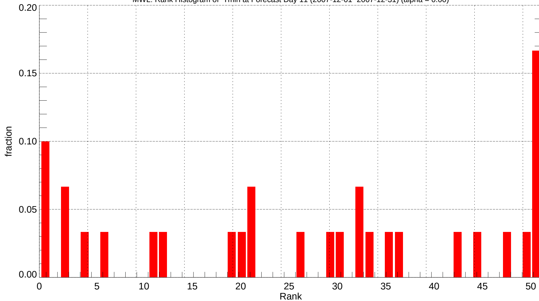
MWL: Rank Histogram of Tmin at Forecast Day 11 (2007-12-01~2007-12-31) (alpha = 0.00)
