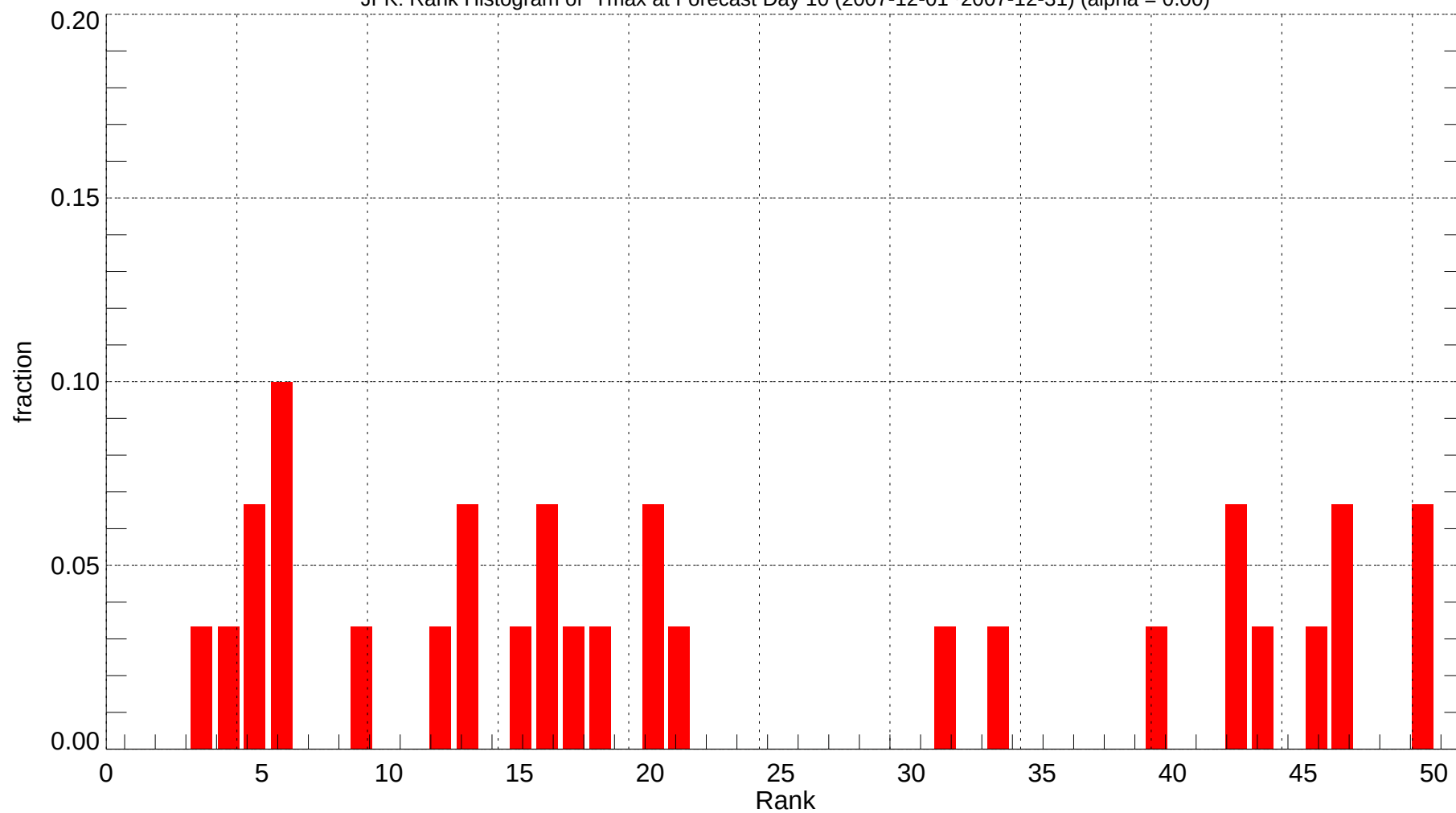
JFK: Rank Histogram of Tmax at Forecast Day 10 (2007-12-01~2007-12-31) (alpha = 0.00)
