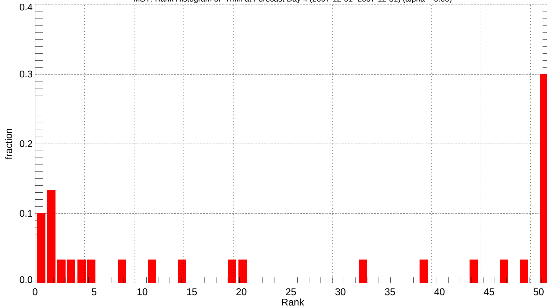
MSY: Rank Histogram of Tmin at Forecast Day 4 (2007-12-01~2007-12-31) (alpha = 0.00)
