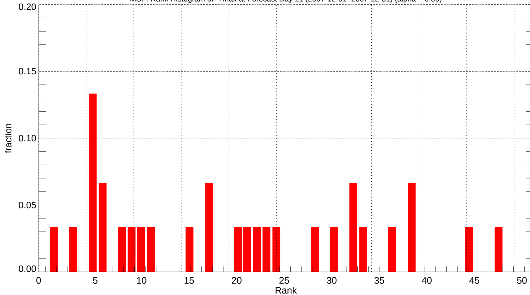
MSP: Rank Histogram of Tmax at Forecast Day 11 (2007-12-01~2007-12-31) (alpha = 0.00)
