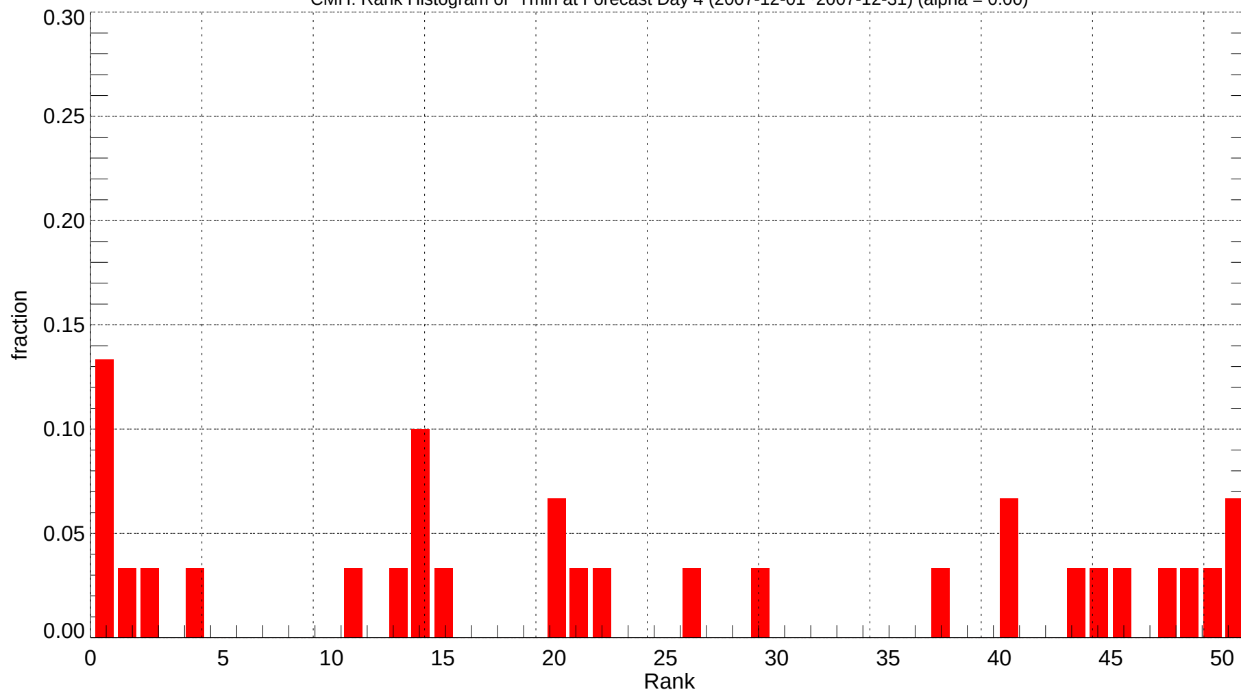
CMH: Rank Histogram of Tmin at Forecast Day 4 (2007-12-01~2007-12-31) (alpha = 0.00)
