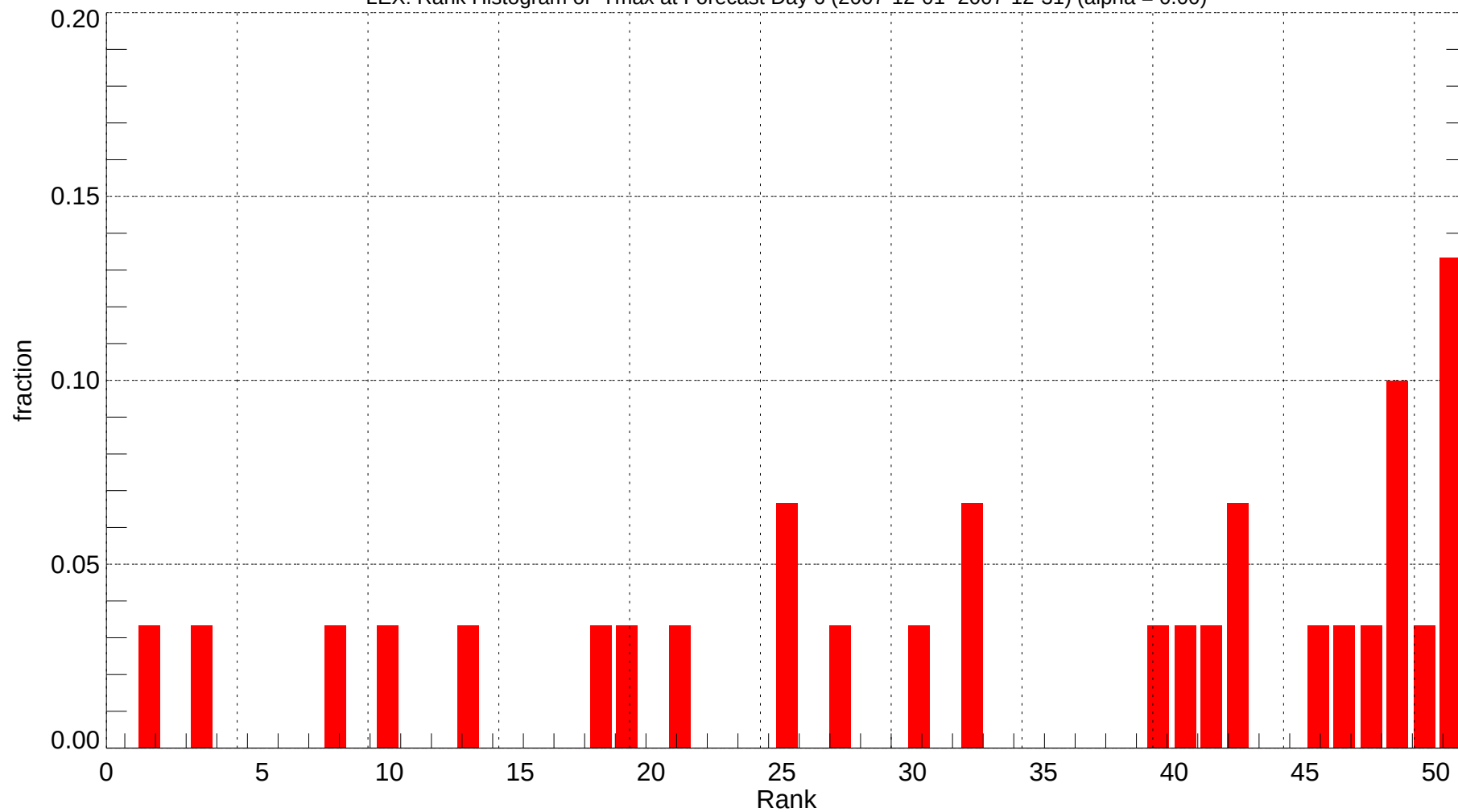
LEX: Rank Histogram of Tmax at Forecast Day 6 (2007-12-01~2007-12-31) (alpha = 0.00)
