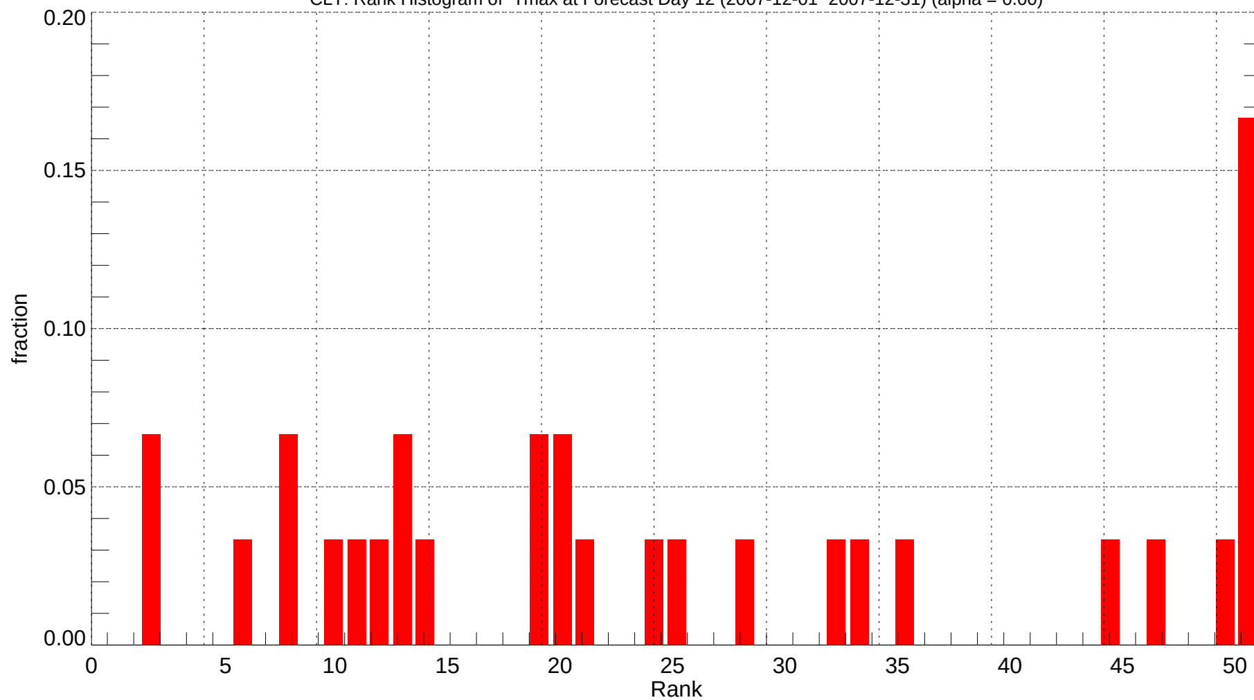
CLT: Rank Histogram of Tmax at Forecast Day 12 (2007-12-01~2007-12-31) (alpha = 0.00)
