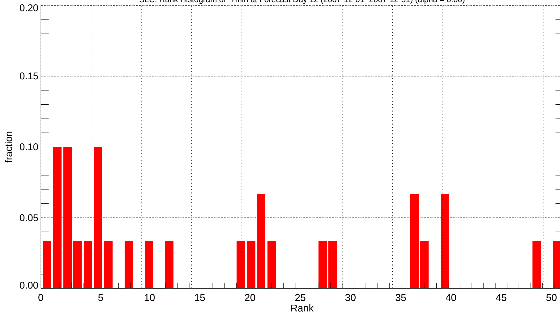
SLC: Rank Histogram of Tmin at Forecast Day 12 (2007-12-01~2007-12-31) (alpha = 0.00)
