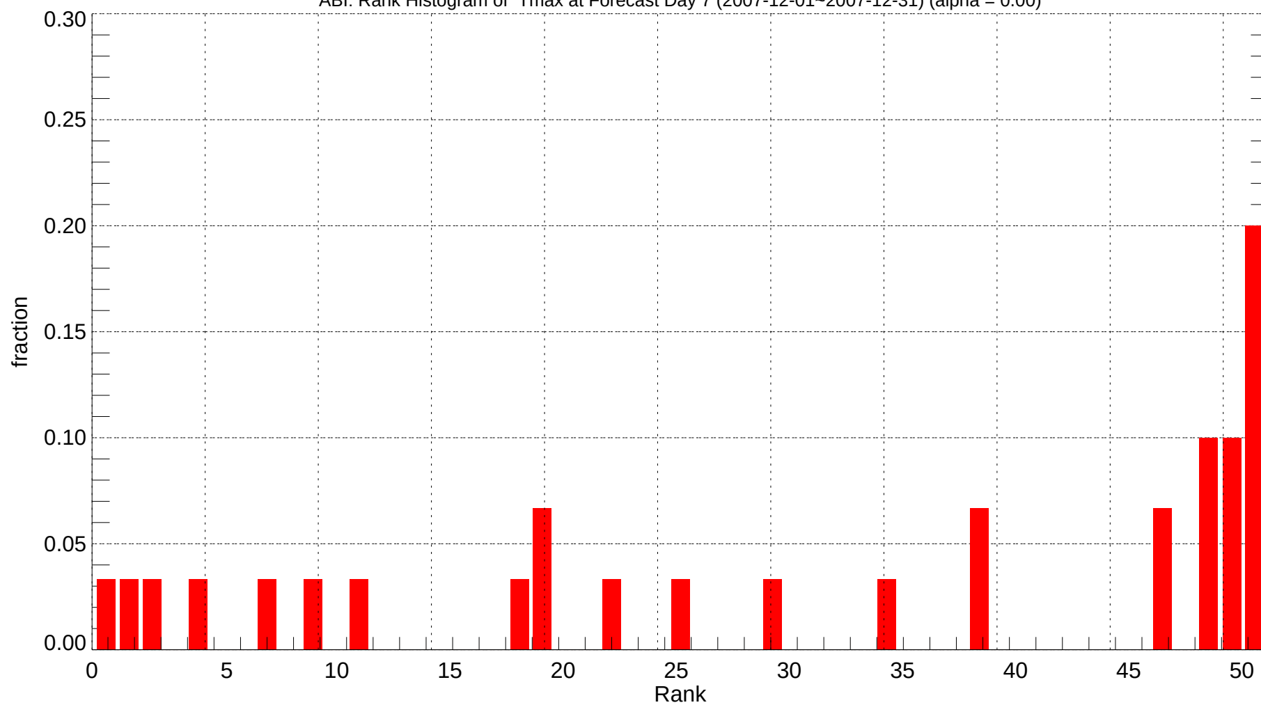
ABI: Rank Histogram of Tmax at Forecast Day 7 (2007-12-01~2007-12-31) (alpha = 0.00)
