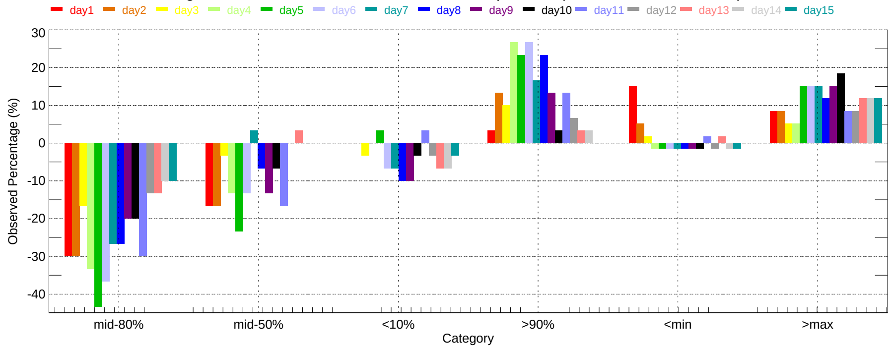
Observed Percentage Deviation of Ensembles - CAE: Max Temperature (2007-12-01~2007-12-31)
