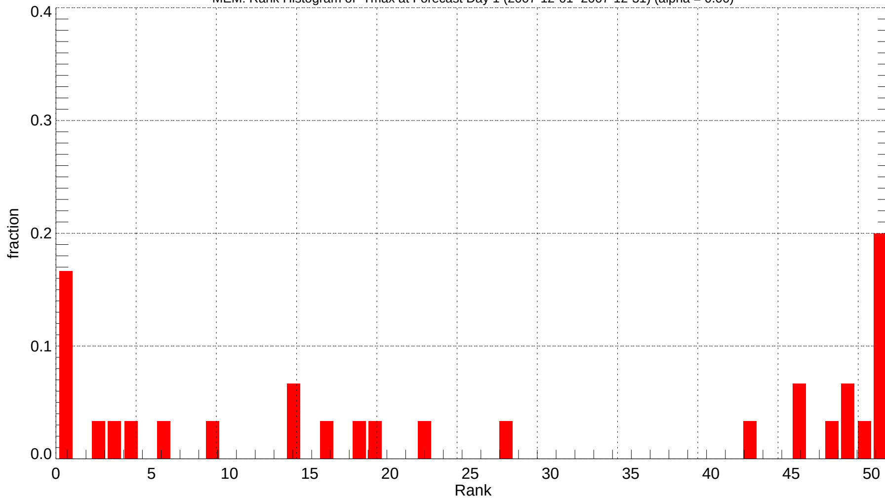
MEM: Rank Histogram of Tmax at Forecast Day 1 (2007-12-01~2007-12-31) (alpha = 0.00)
