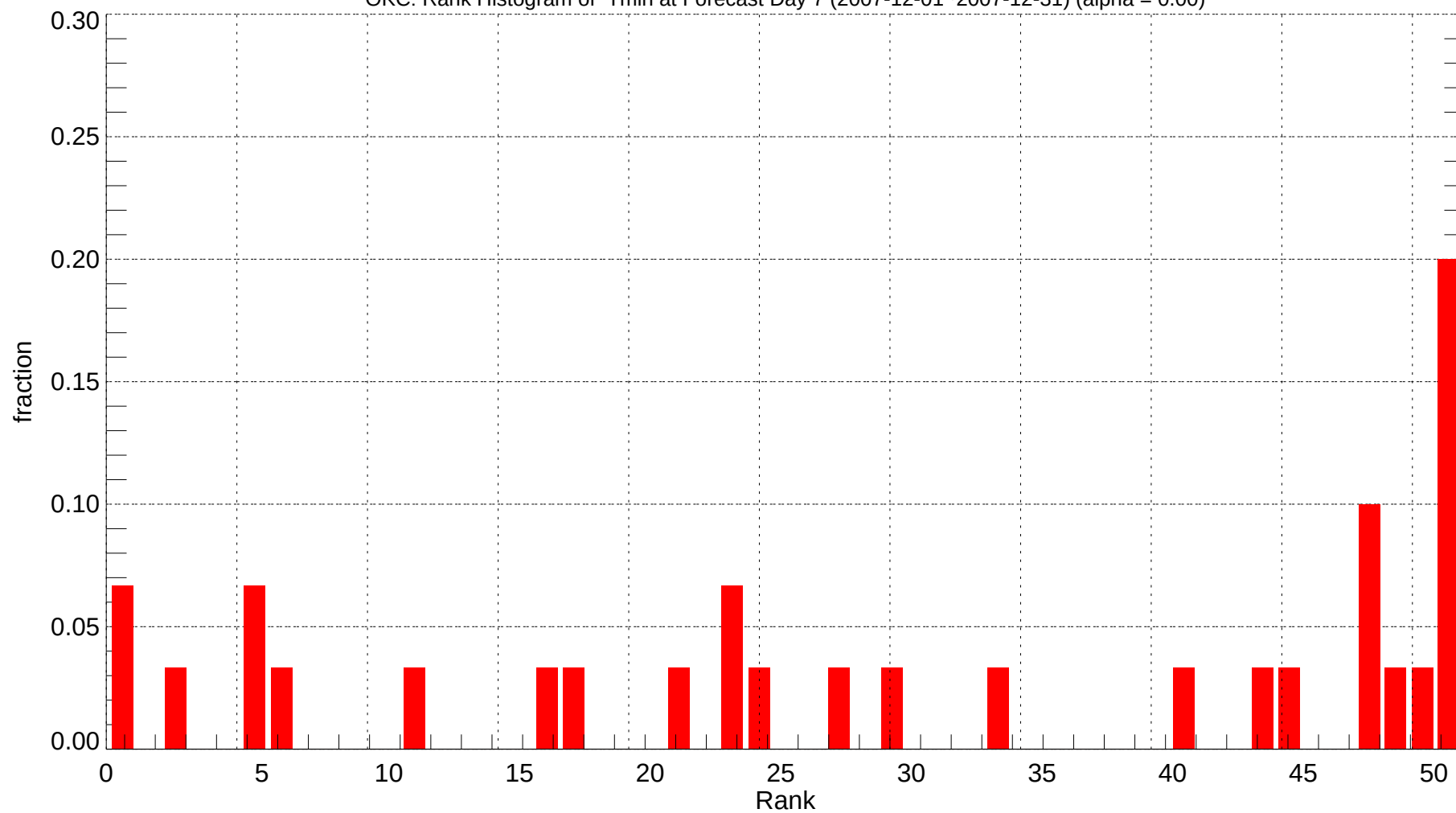
OKC: Rank Histogram of Tmin at Forecast Day 7 (2007-12-01~2007-12-31) (alpha = 0.00)
