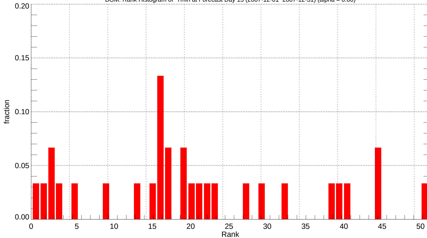
BGM: Rank Histogram of Tmin at Forecast Day 15 (2007-12-01~2007-12-31) (alpha = 0.00)
