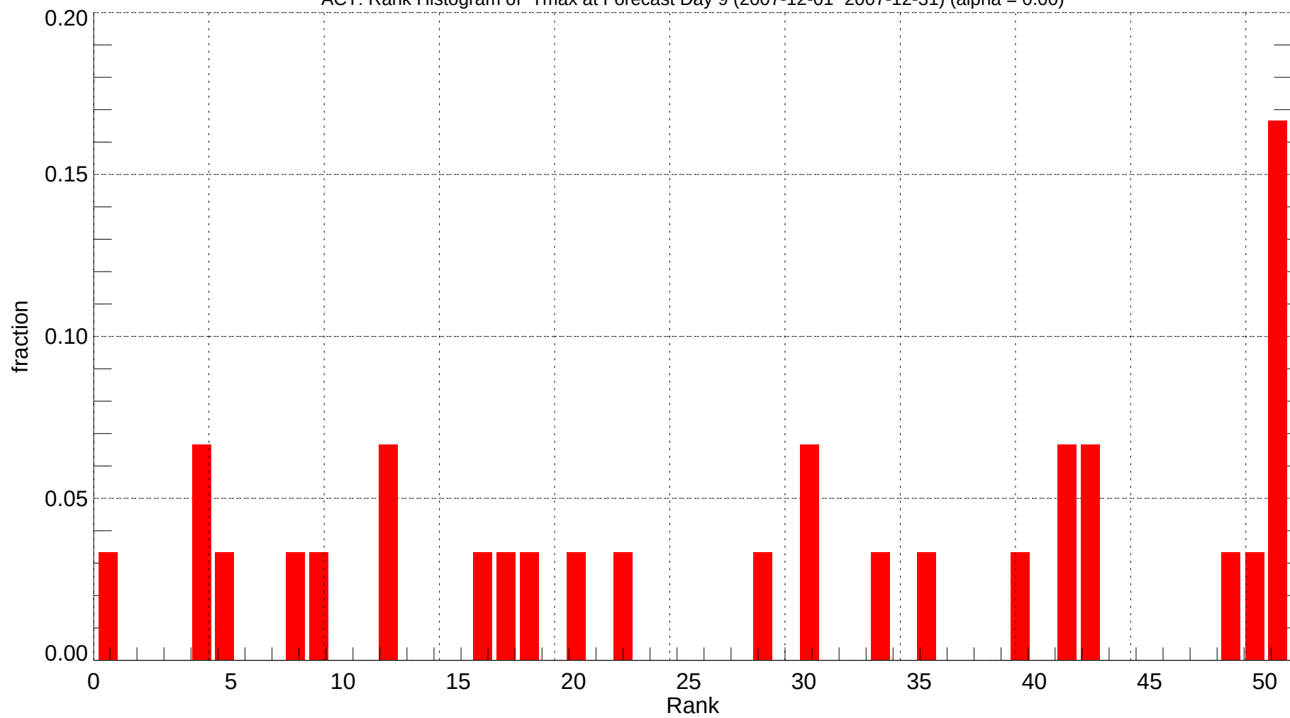
ACT: Rank Histogram of Tmax at Forecast Day 9 (2007-12-01~2007-12-31) (alpha = 0.00)
