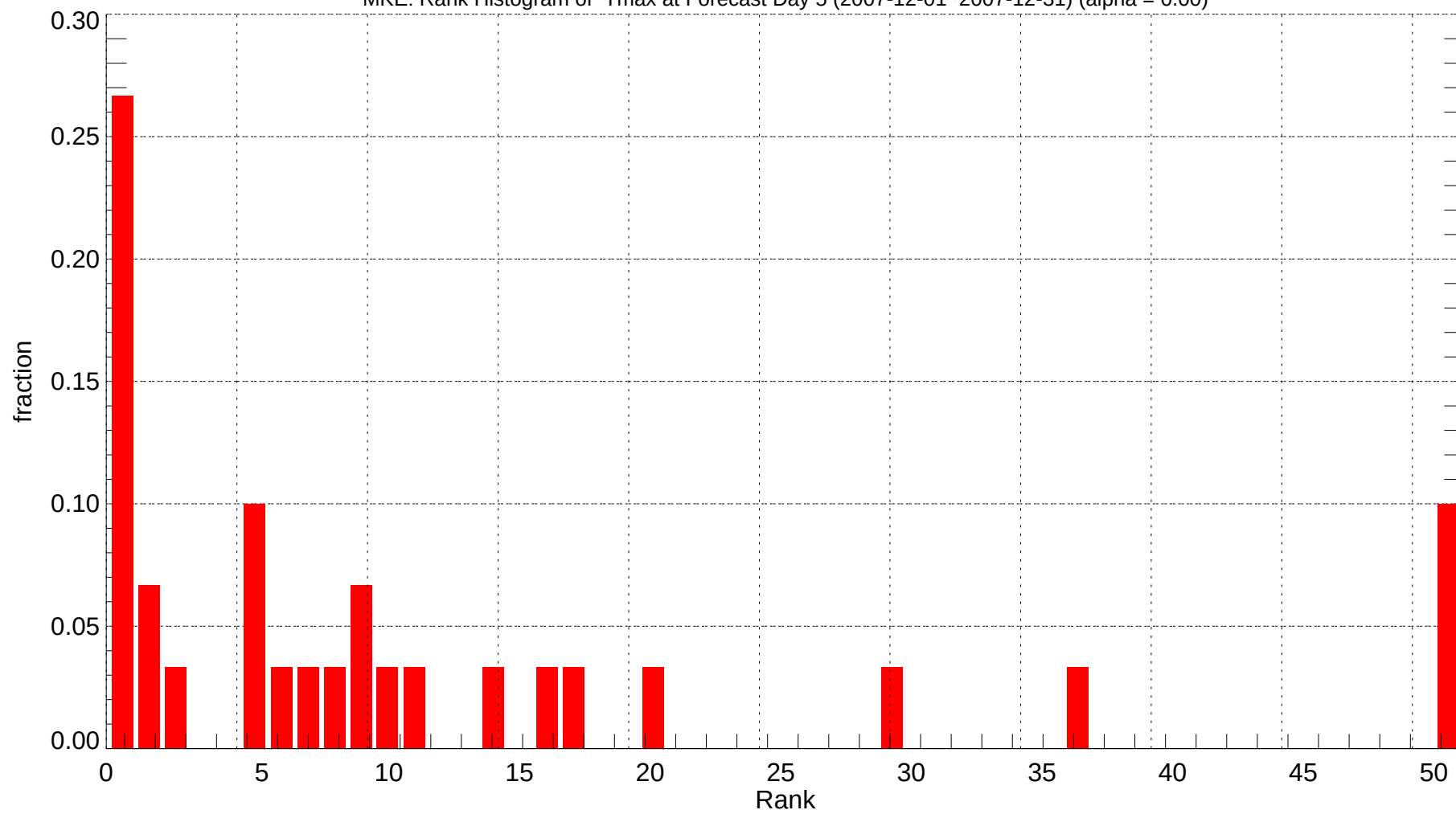
MKE: Rank Histogram of Tmax at Forecast Day 5 (2007-12-01~2007-12-31) (alpha = 0.00)
