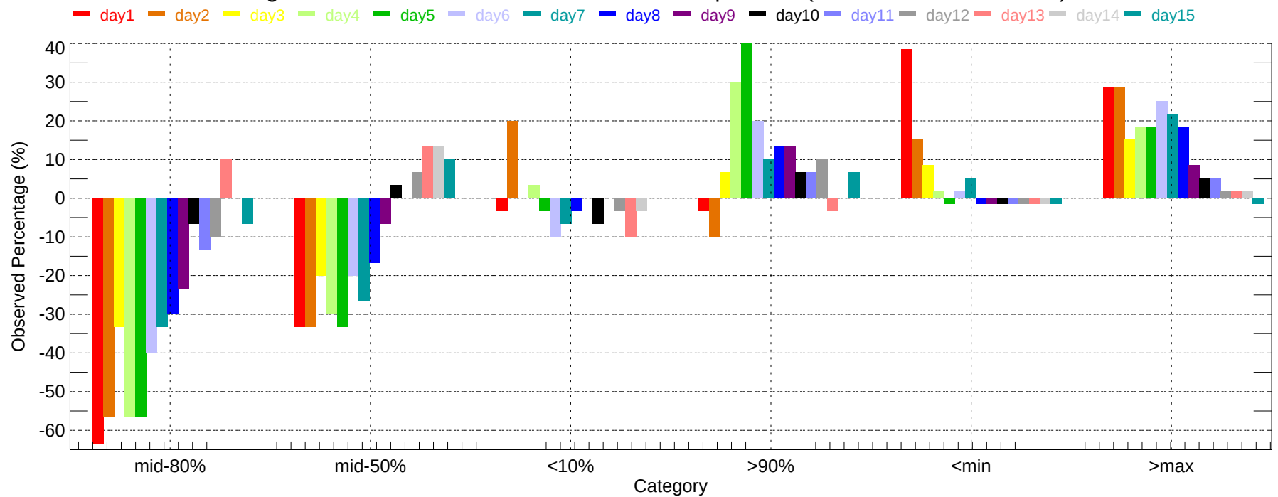
Observed Percentage Deviation of Ensembles - DSM: Max Temperature (2007-12-01~2007-12-31)
