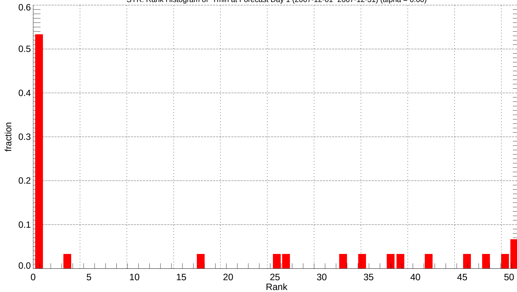
SYR: Rank Histogram of Tmin at Forecast Day 1 (2007-12-01~2007-12-31) (alpha = 0.00)
