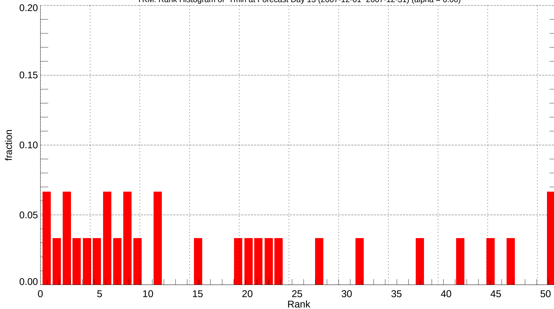
YKM: Rank Histogram of Tmin at Forecast Day 13 (2007-12-01~2007-12-31) (alpha = 0.00)
