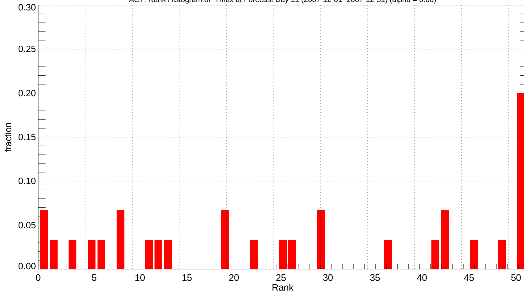
ACT: Rank Histogram of Tmax at Forecast Day 11 (2007-12-01~2007-12-31) (alpha = 0.00)
