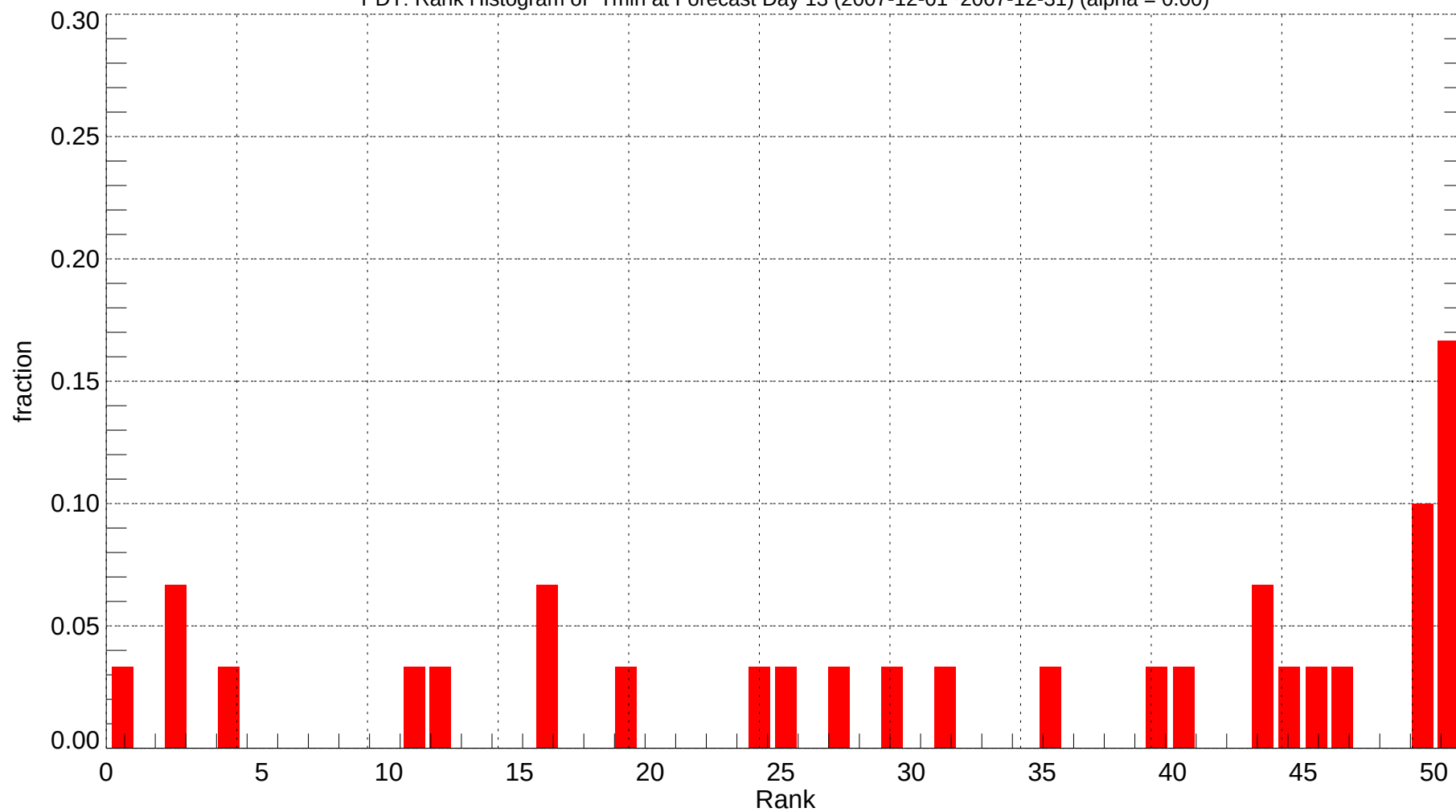
PDT: Rank Histogram of Tmin at Forecast Day 13 (2007-12-01~2007-12-31) (alpha = 0.00)
