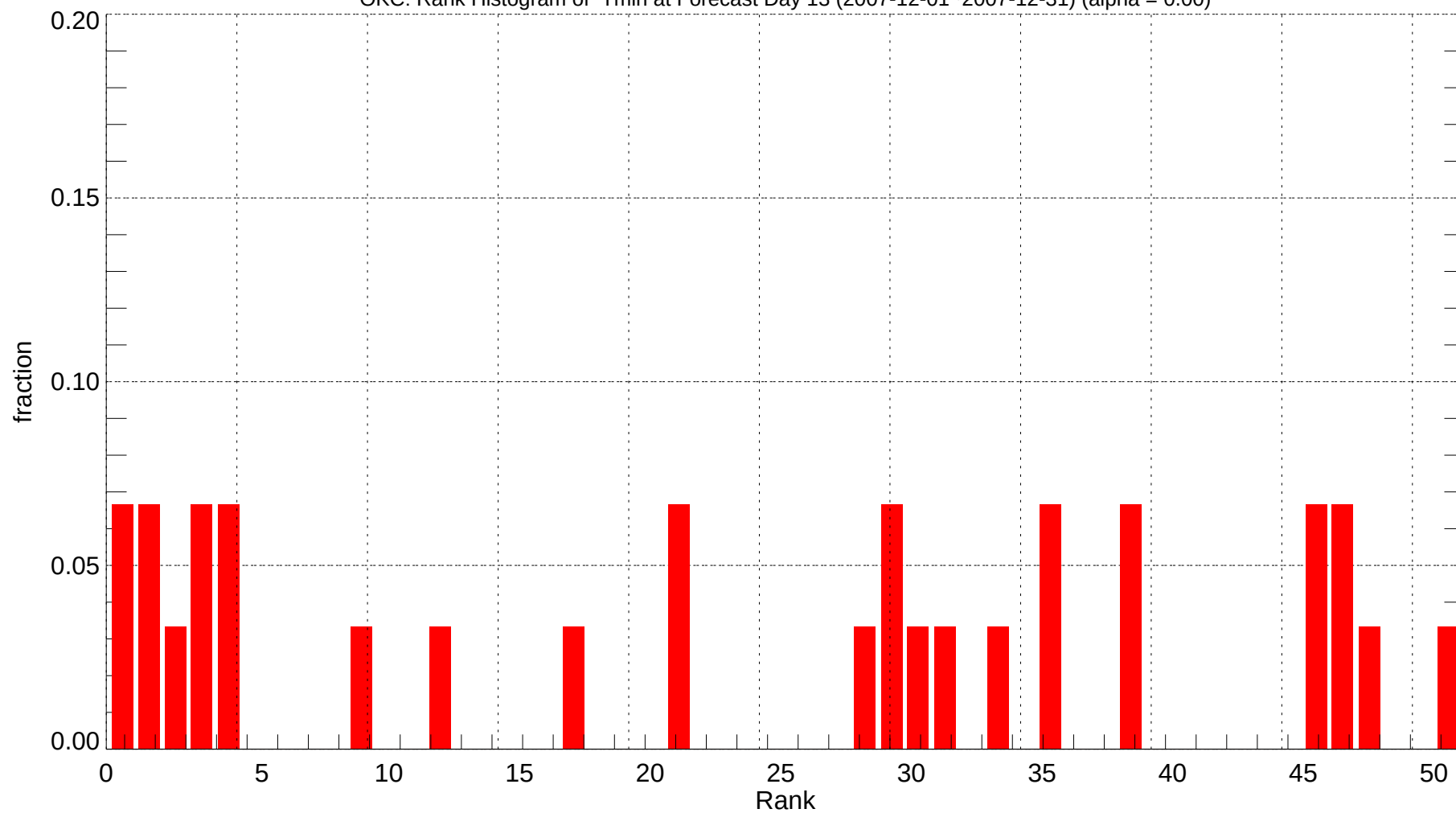
OKC: Rank Histogram of Tmin at Forecast Day 13 (2007-12-01~2007-12-31) (alpha = 0.00)
