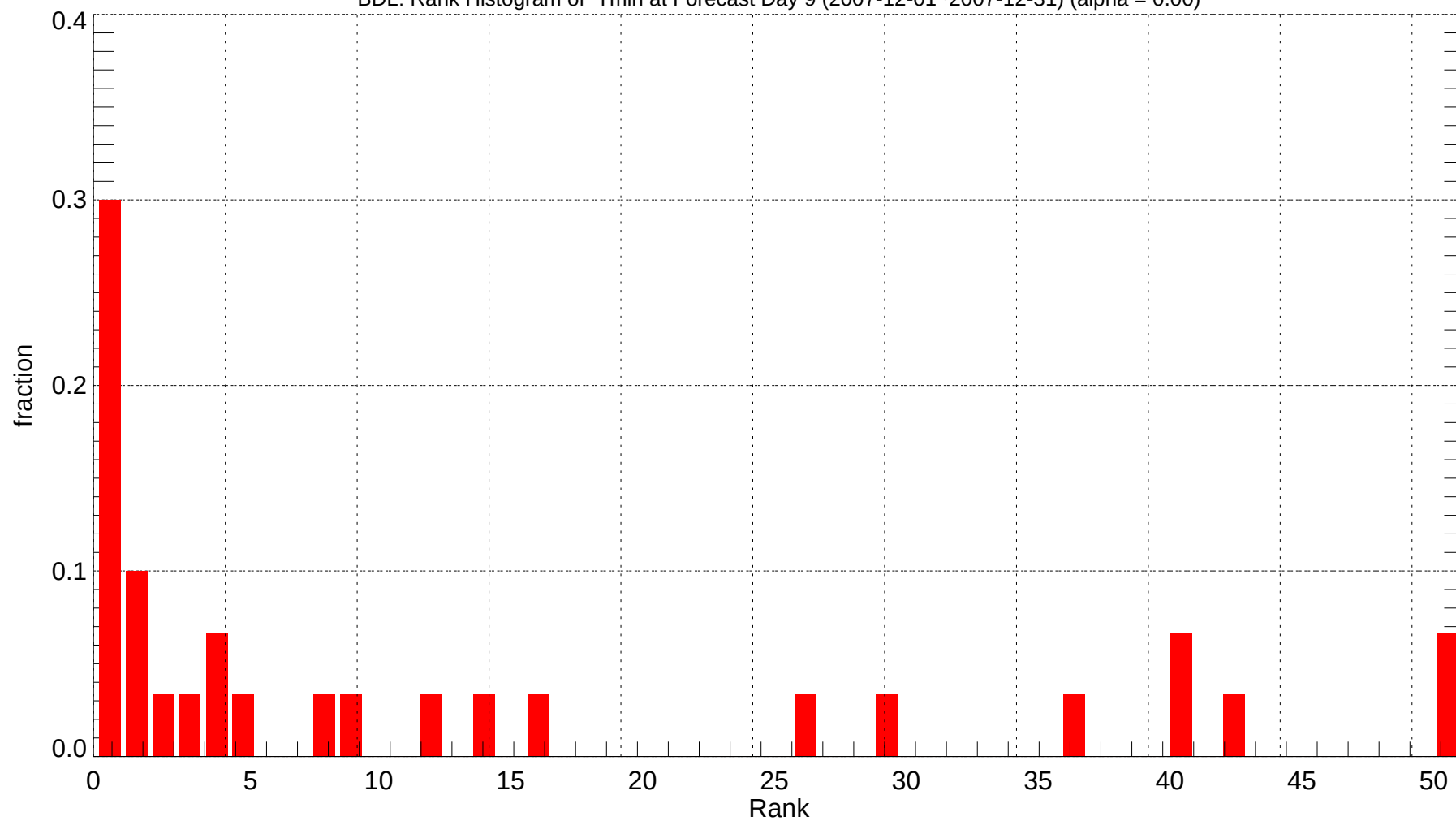
BDL: Rank Histogram of Tmin at Forecast Day 9 (2007-12-01~2007-12-31) (alpha = 0.00)
