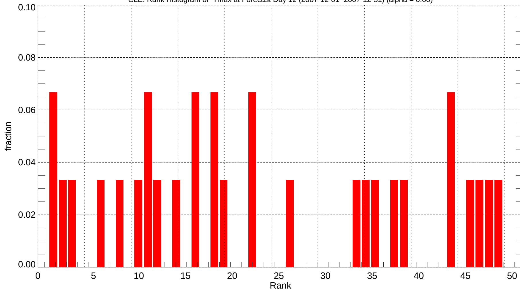
CLE: Rank Histogram of Tmax at Forecast Day 12 (2007-12-01~2007-12-31) (alpha = 0.00)
