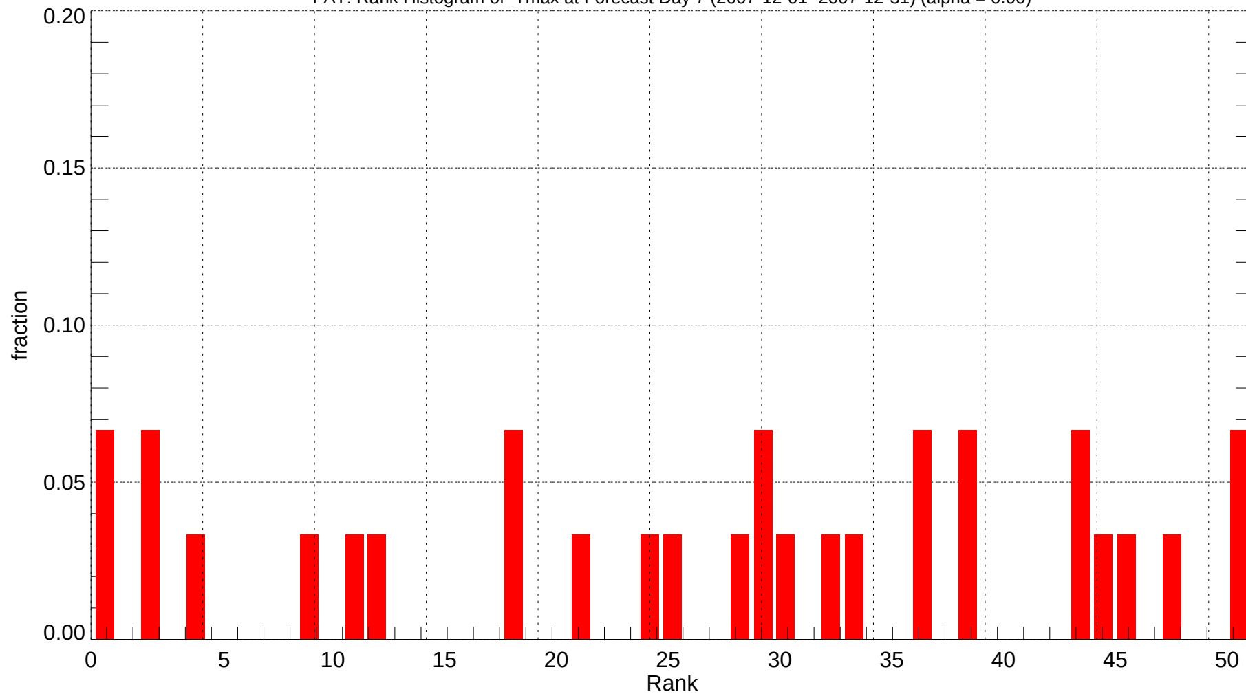
FAT: Rank Histogram of Tmax at Forecast Day 7 (2007-12-01~2007-12-31) (alpha = 0.00)
