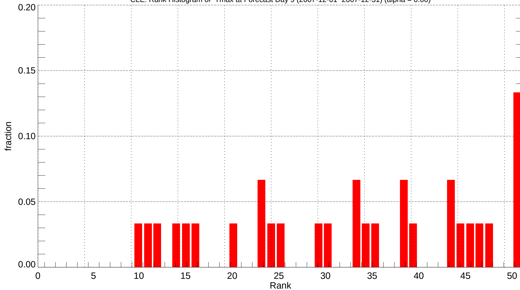
CLE: Rank Histogram of Tmax at Forecast Day 9 (2007-12-01~2007-12-31) (alpha = 0.00)
