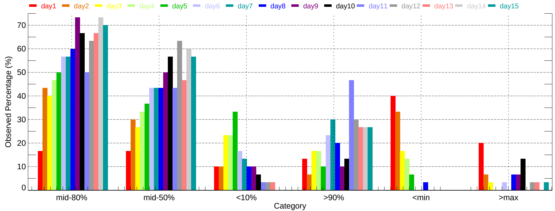
Observed Percentage of Ensembles - ERI: Max Temperature (2007-12-01~2007-12-31)
