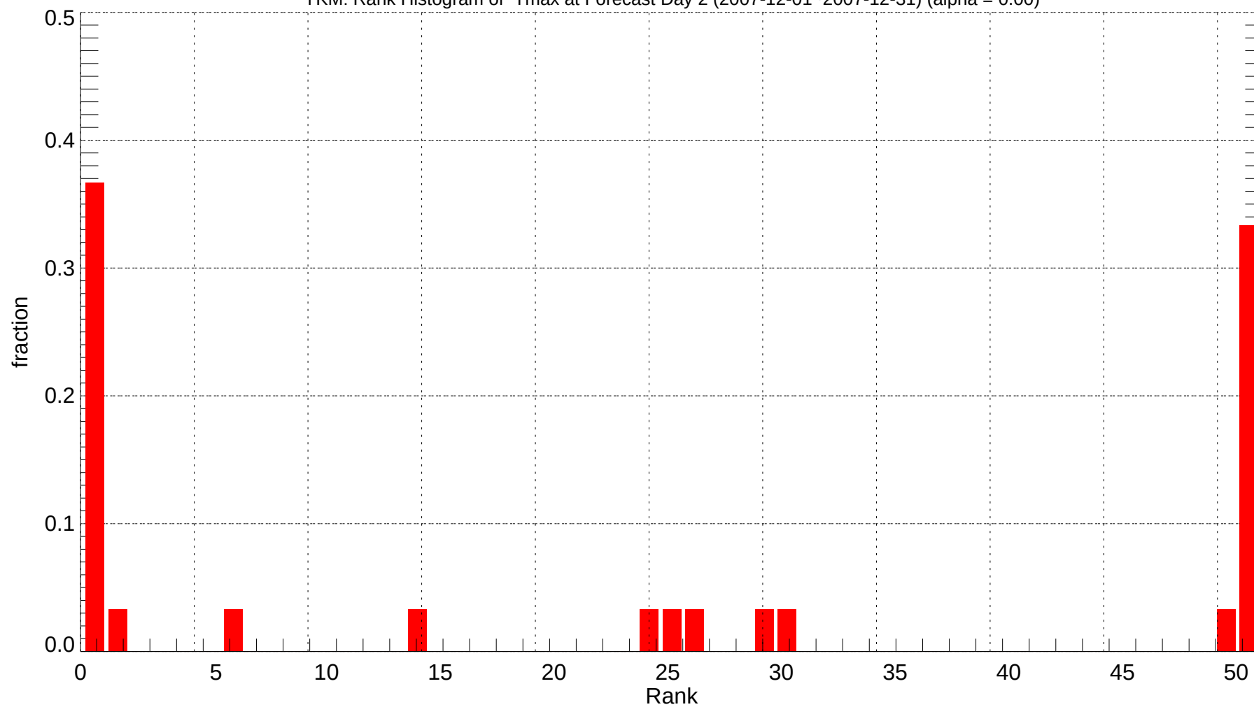
YKM: Rank Histogram of Tmax at Forecast Day 2 (2007-12-01~2007-12-31) (alpha = 0.00)
