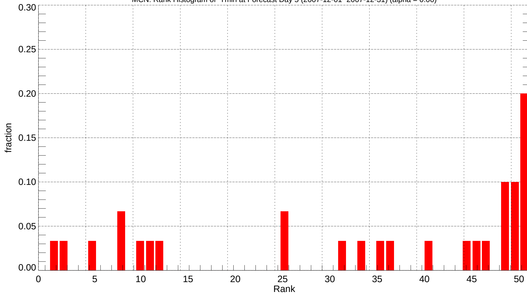
MCN: Rank Histogram of Tmin at Forecast Day 5 (2007-12-01~2007-12-31) (alpha = 0.00)
