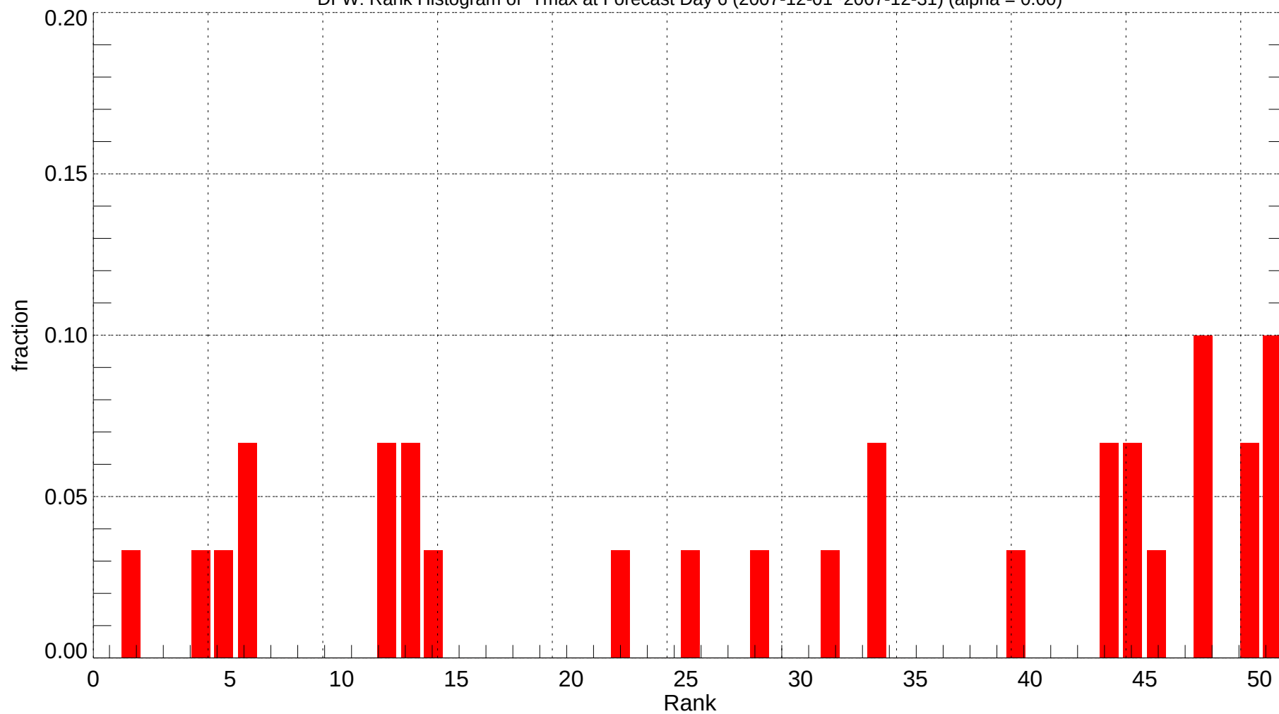
DFW: Rank Histogram of Tmax at Forecast Day 6 (2007-12-01~2007-12-31) (alpha = 0.00)
