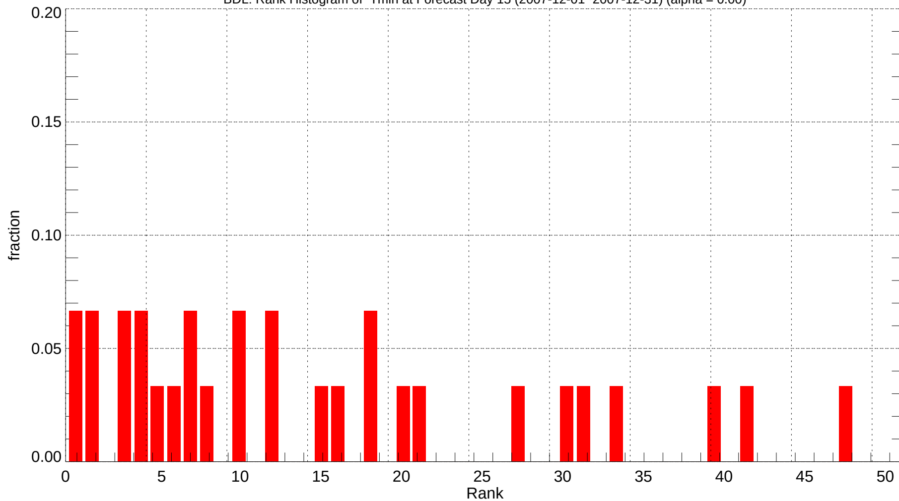
BDL: Rank Histogram of Tmin at Forecast Day 15 (2007-12-01~2007-12-31) (alpha = 0.00)
