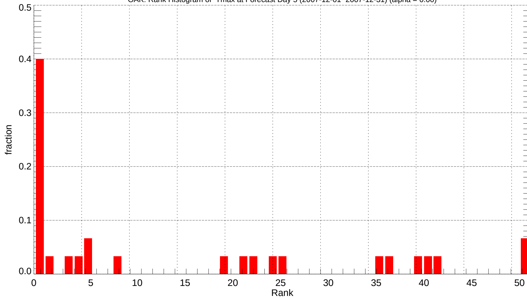
OAK: Rank Histogram of Tmax at Forecast Day 5 (2007-12-01~2007-12-31) (alpha = 0.00)
