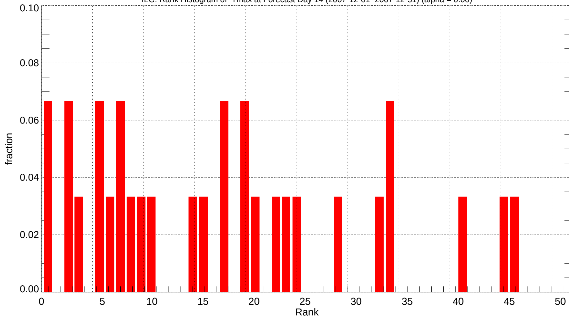
ILG: Rank Histogram of Tmax at Forecast Day 14 (2007-12-01~2007-12-31) (alpha = 0.00)
