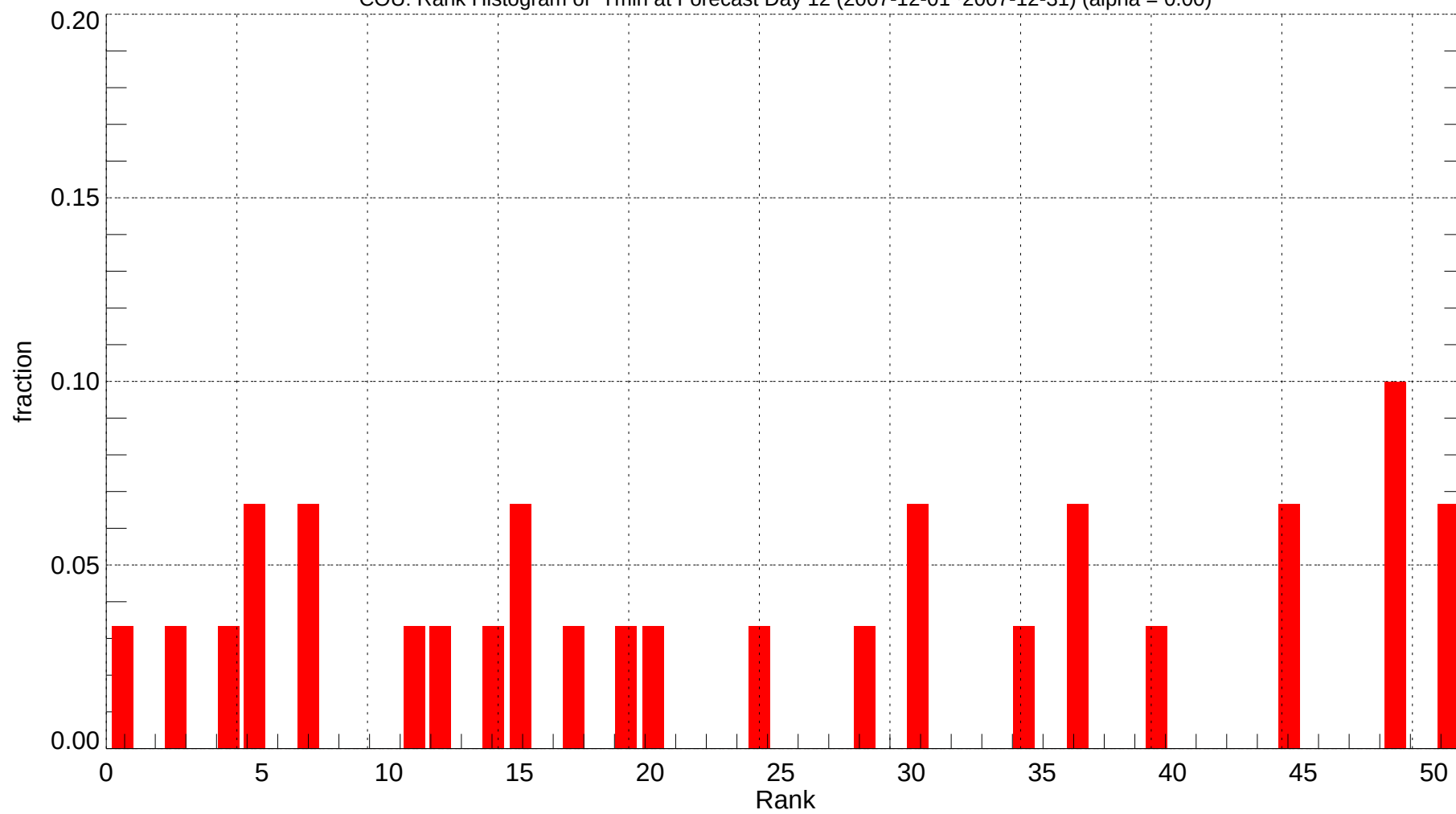
COU: Rank Histogram of Tmin at Forecast Day 12 (2007-12-01~2007-12-31) (alpha = 0.00)
