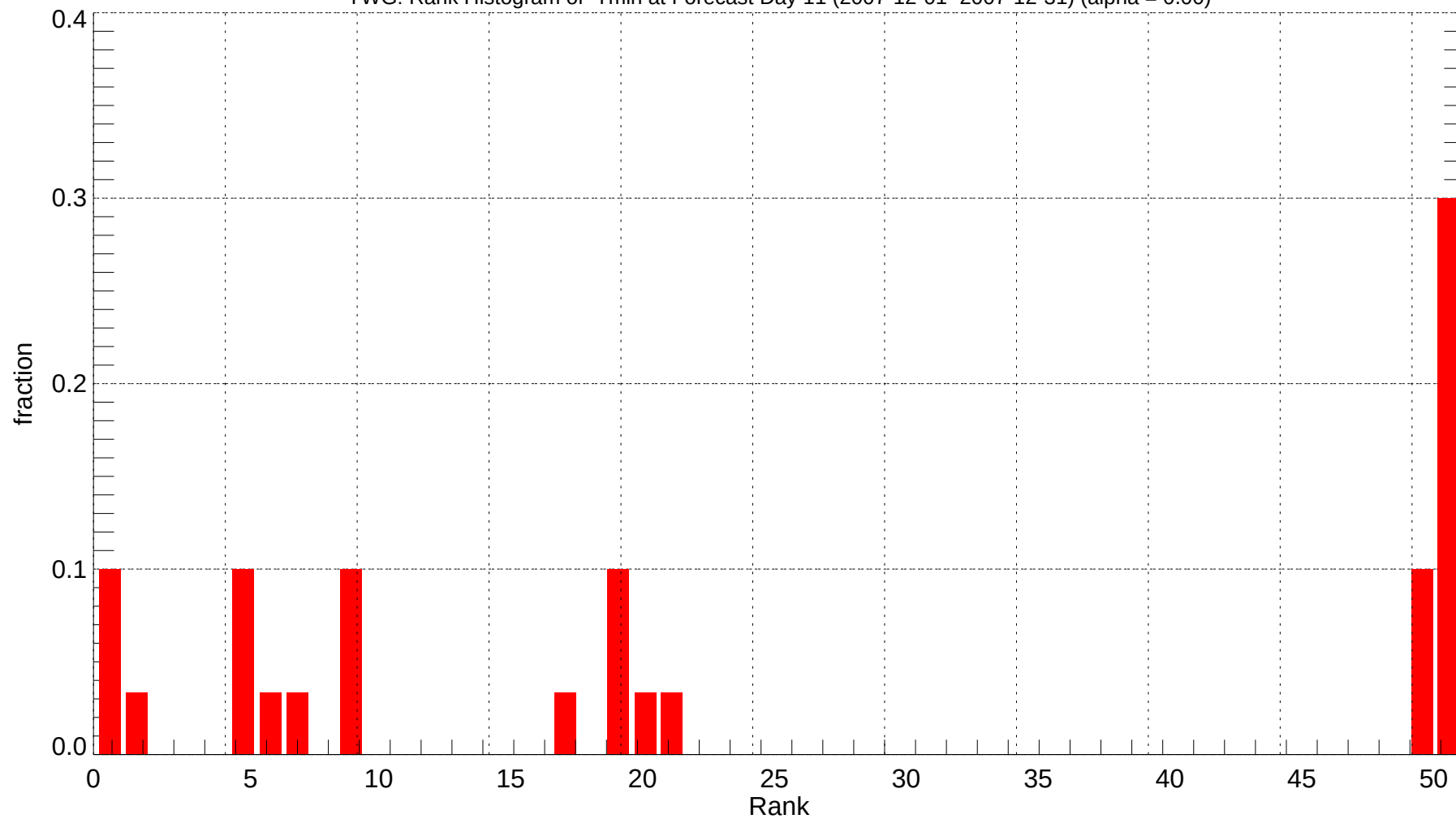
YWG: Rank Histogram of Tmin at Forecast Day 11 (2007-12-01~2007-12-31) (alpha = 0.00)
