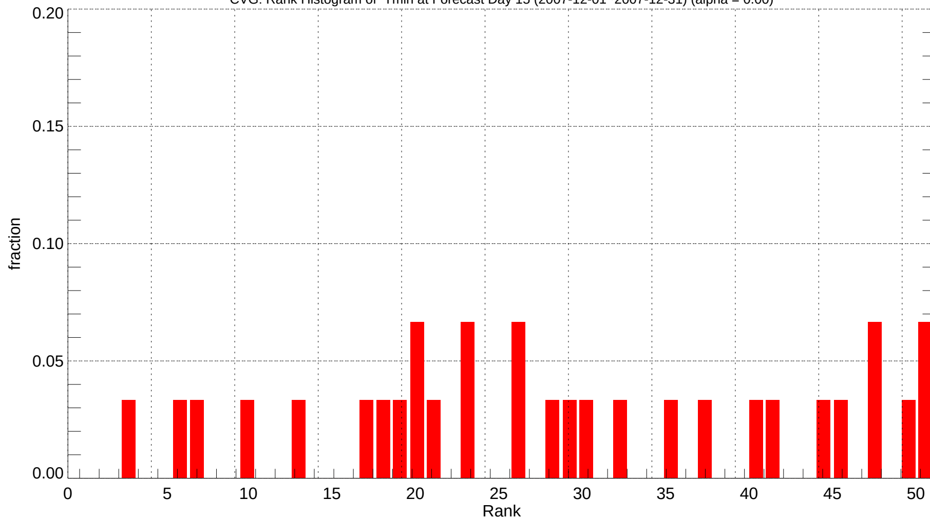
CVG: Rank Histogram of Tmin at Forecast Day 15 (2007-12-01~2007-12-31) (alpha = 0.00)
