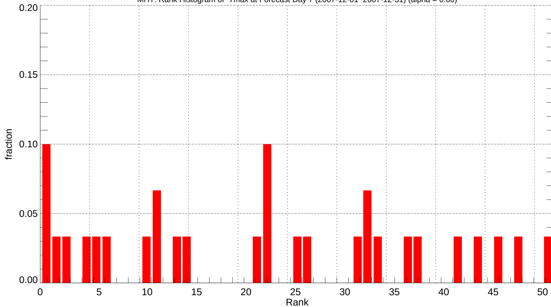
MHT: Rank Histogram of Tmax at Forecast Day 7 (2007-12-01~2007-12-31) (alpha = 0.00)
