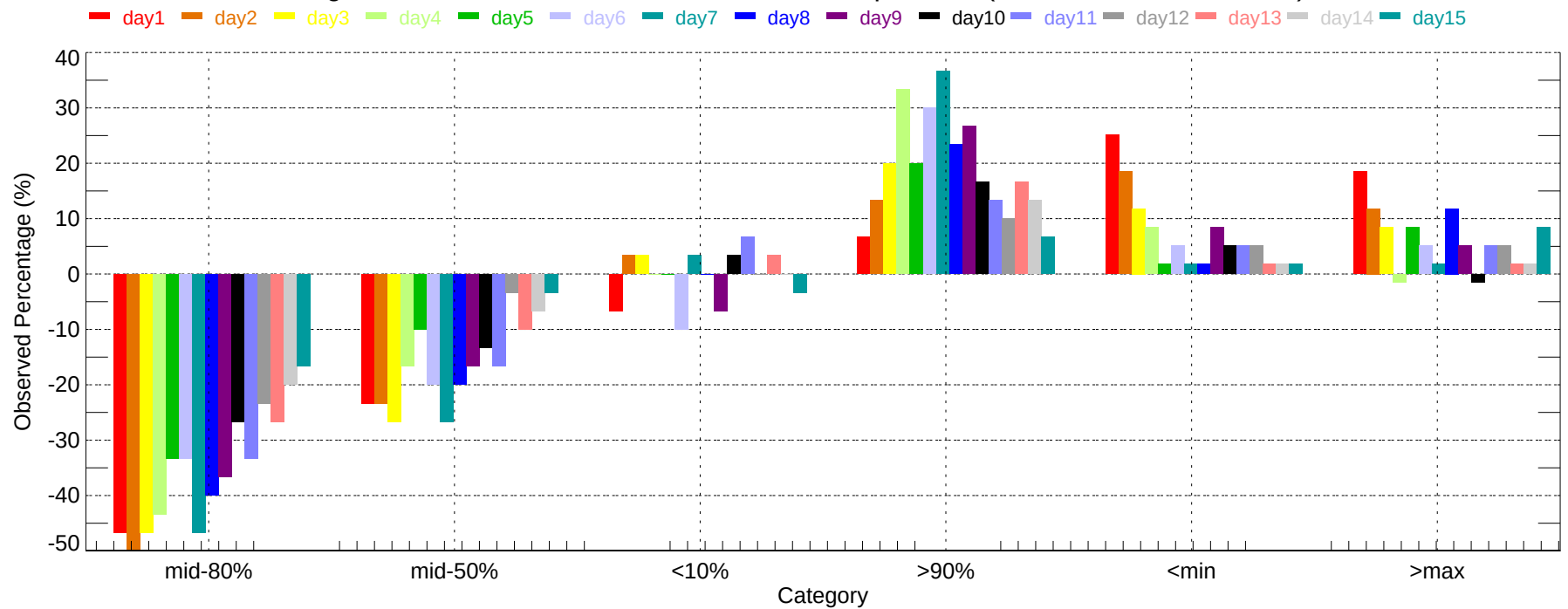
Observed Percentage Deviation of Ensembles - CRP: Max Temperature (2007-12-01~2007-12-31)
