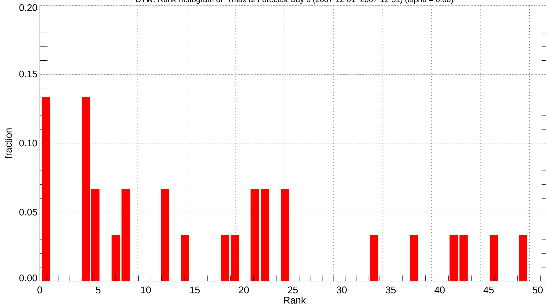
DTW: Rank Histogram of Tmax at Forecast Day 6 (2007-12-01~2007-12-31) (alpha = 0.00)
