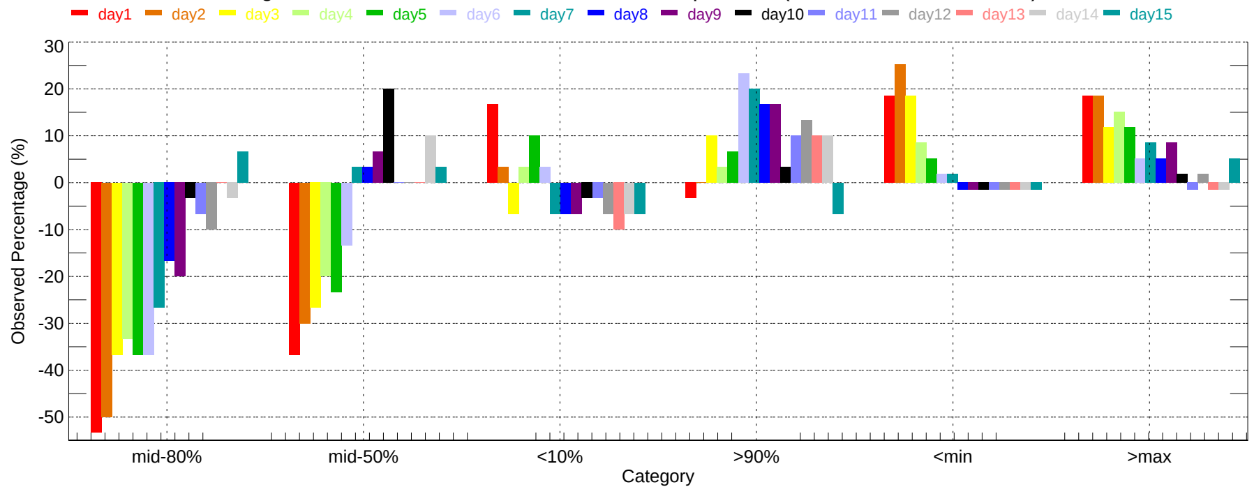
Observed Percentage Deviation of Ensembles - DCA: Min Temperature (2007-12-01~2007-12-31)
