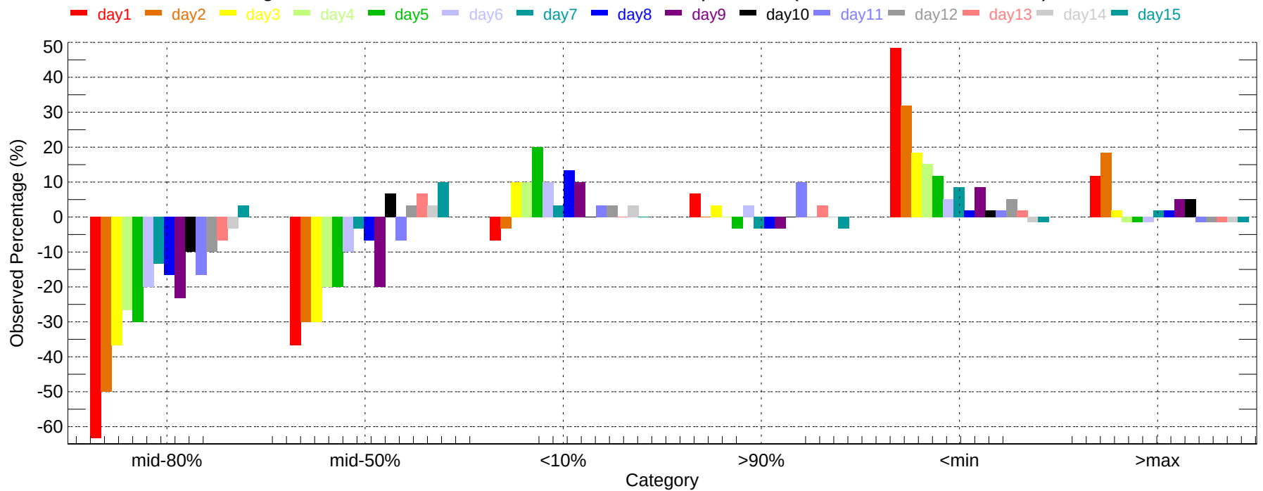
Observed Percentage Deviation of Ensembles - DTW: Min Temperature (2007-12-01~2007-12-31)
