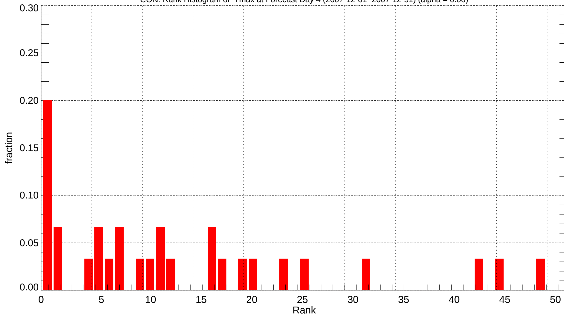
CON: Rank Histogram of Tmax at Forecast Day 4 (2007-12-01~2007-12-31) (alpha = 0.00)
