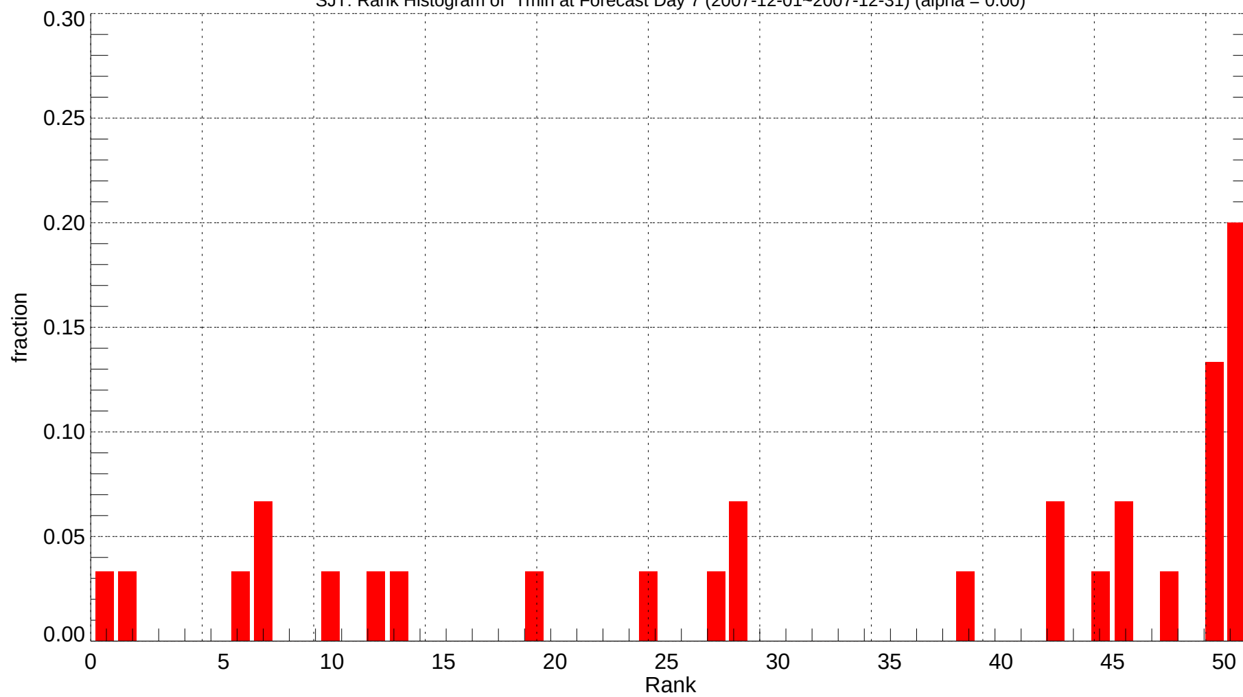
SJT: Rank Histogram of Tmin at Forecast Day 7 (2007-12-01~2007-12-31) (alpha = 0.00)
