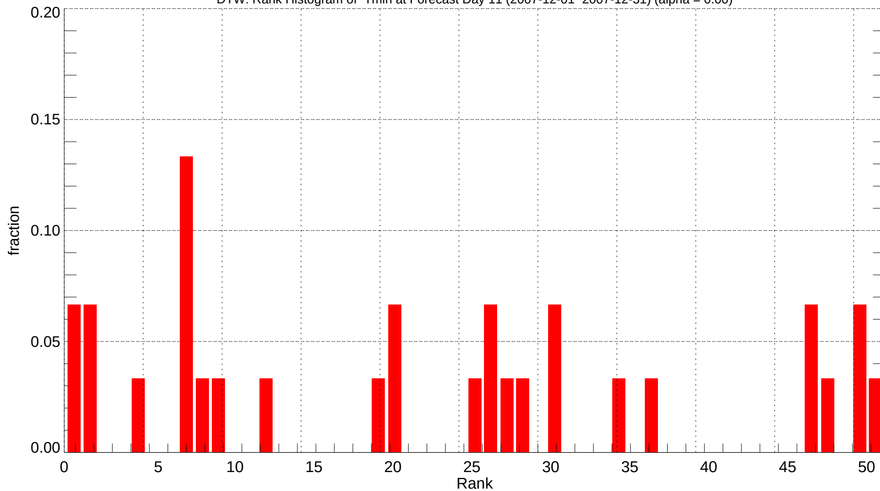
DTW: Rank Histogram of Tmin at Forecast Day 11 (2007-12-01~2007-12-31) (alpha = 0.00)
