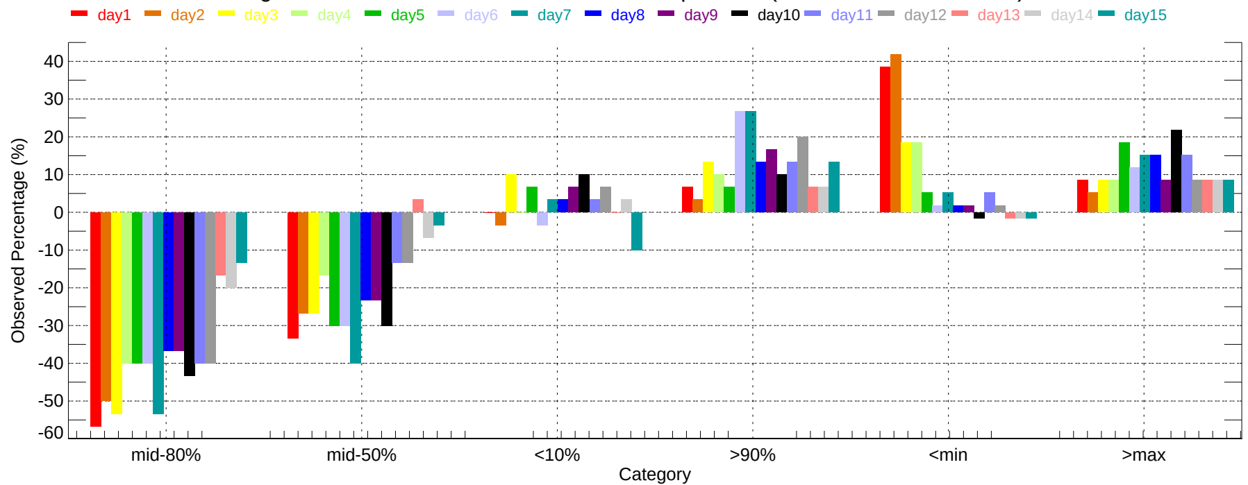
Observed Percentage Deviation of Ensembles - LIT: Max Temperature (2007-12-01~2007-12-31)
