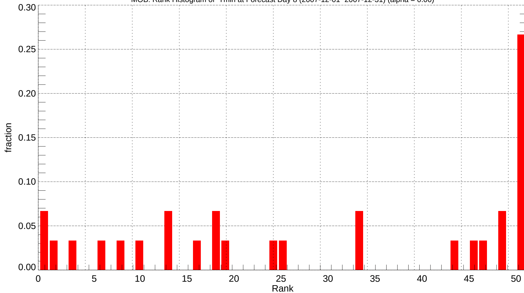
MOB: Rank Histogram of Tmin at Forecast Day 8 (2007-12-01~2007-12-31) (alpha = 0.00)
