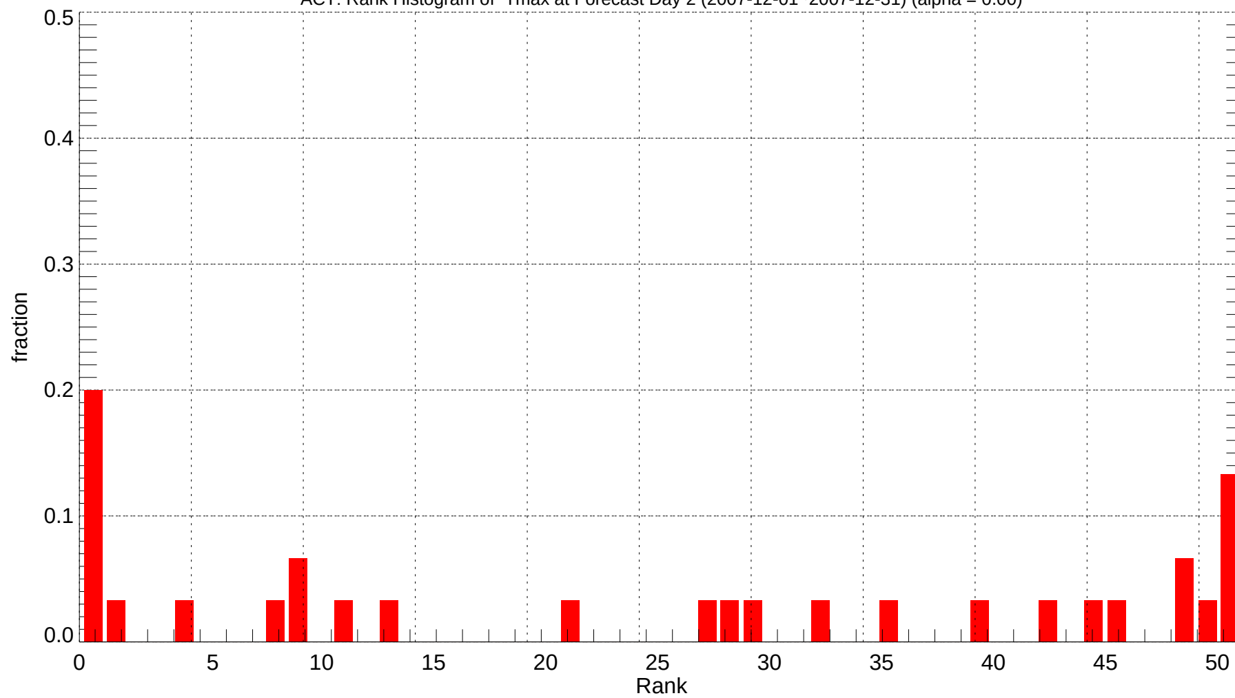
ACT: Rank Histogram of Tmax at Forecast Day 2 (2007-12-01~2007-12-31) (alpha = 0.00)
