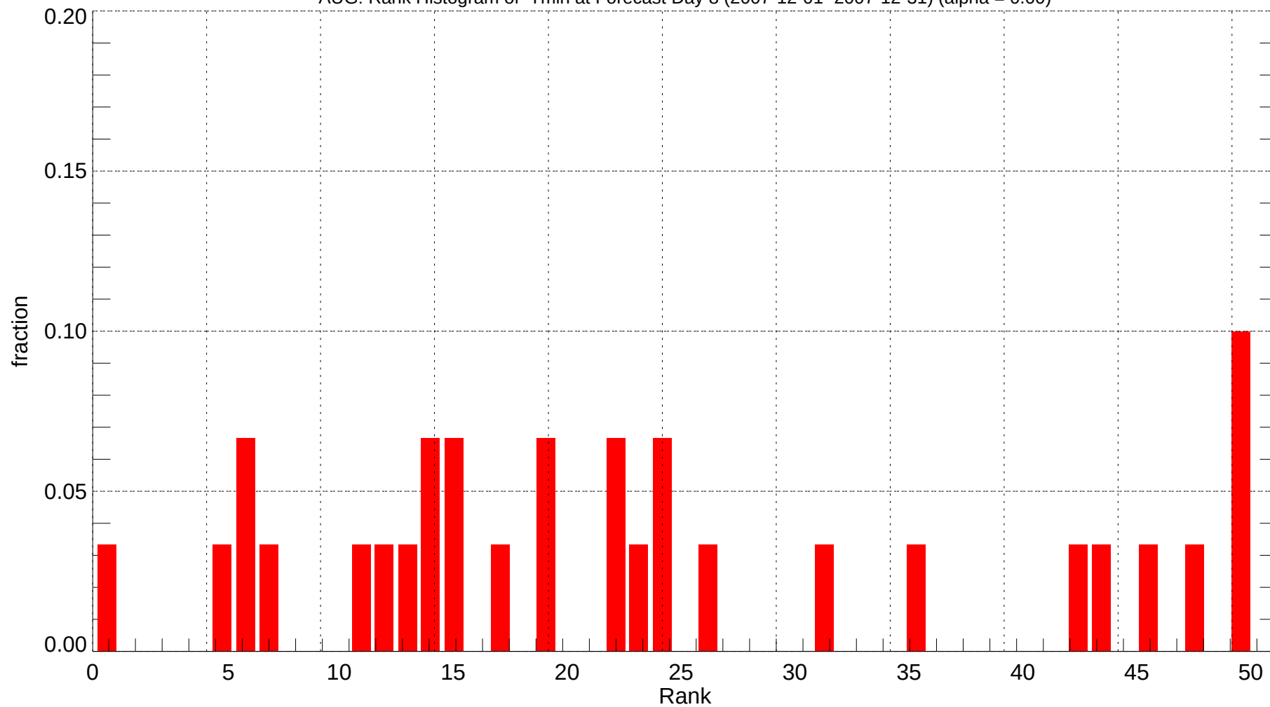
AUG: Rank Histogram of Tmin at Forecast Day 8 (2007-12-01~2007-12-31) (alpha = 0.00)
