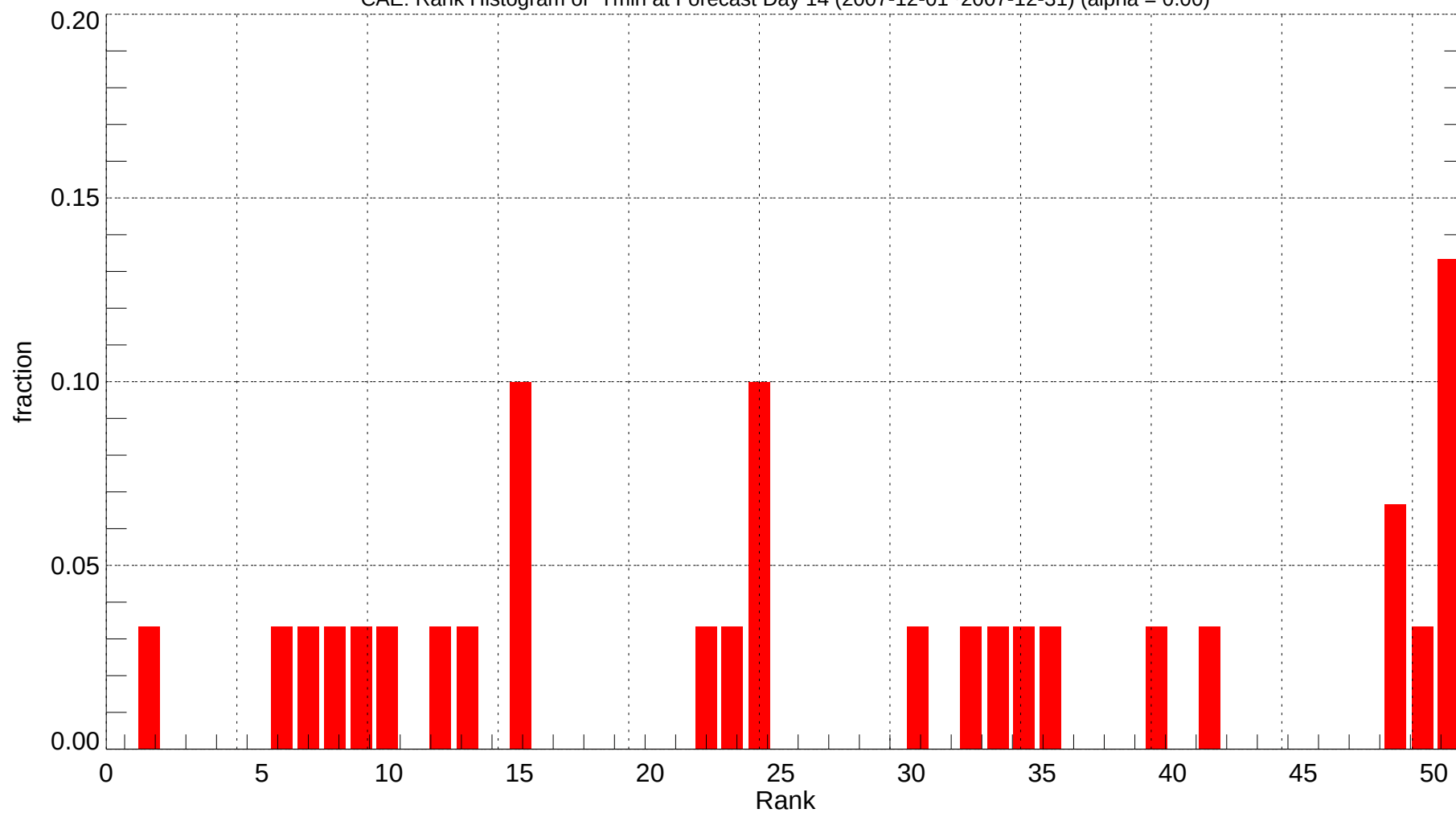
CAE: Rank Histogram of Tmin at Forecast Day 14 (2007-12-01~2007-12-31) (alpha = 0.00)
