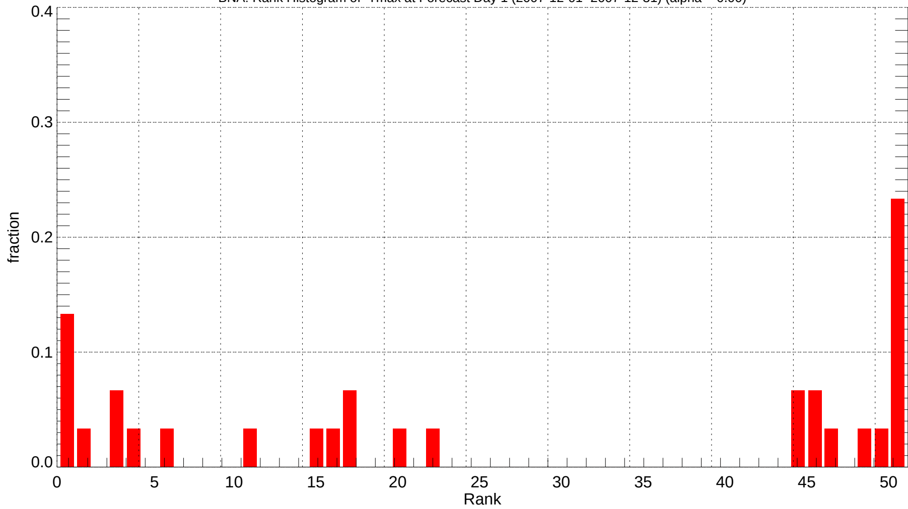
BNA: Rank Histogram of Tmax at Forecast Day 1 (2007-12-01~2007-12-31) (alpha = 0.00)
