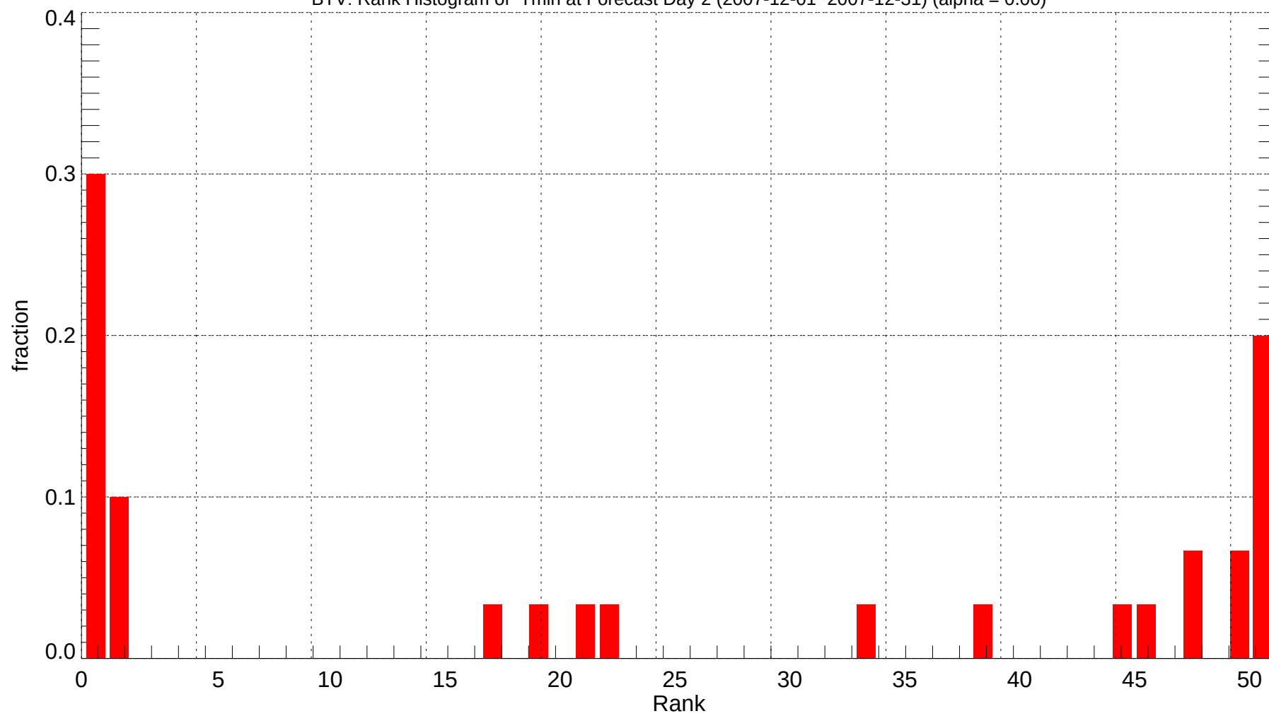
BTV: Rank Histogram of Tmin at Forecast Day 2 (2007-12-01~2007-12-31) (alpha = 0.00)
