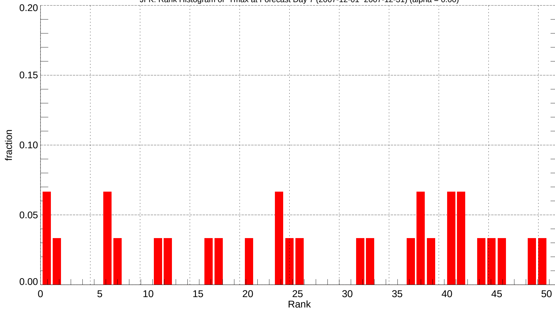
JFK: Rank Histogram of Tmax at Forecast Day 7 (2007-12-01~2007-12-31) (alpha = 0.00)
