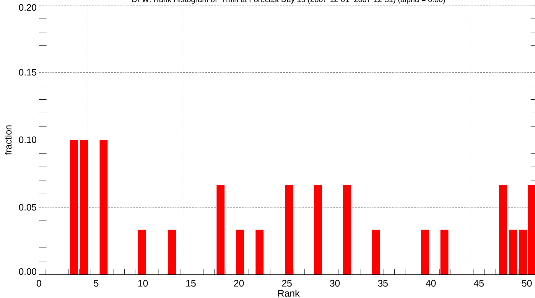
DFW: Rank Histogram of Tmin at Forecast Day 13 (2007-12-01~2007-12-31) (alpha = 0.00)
