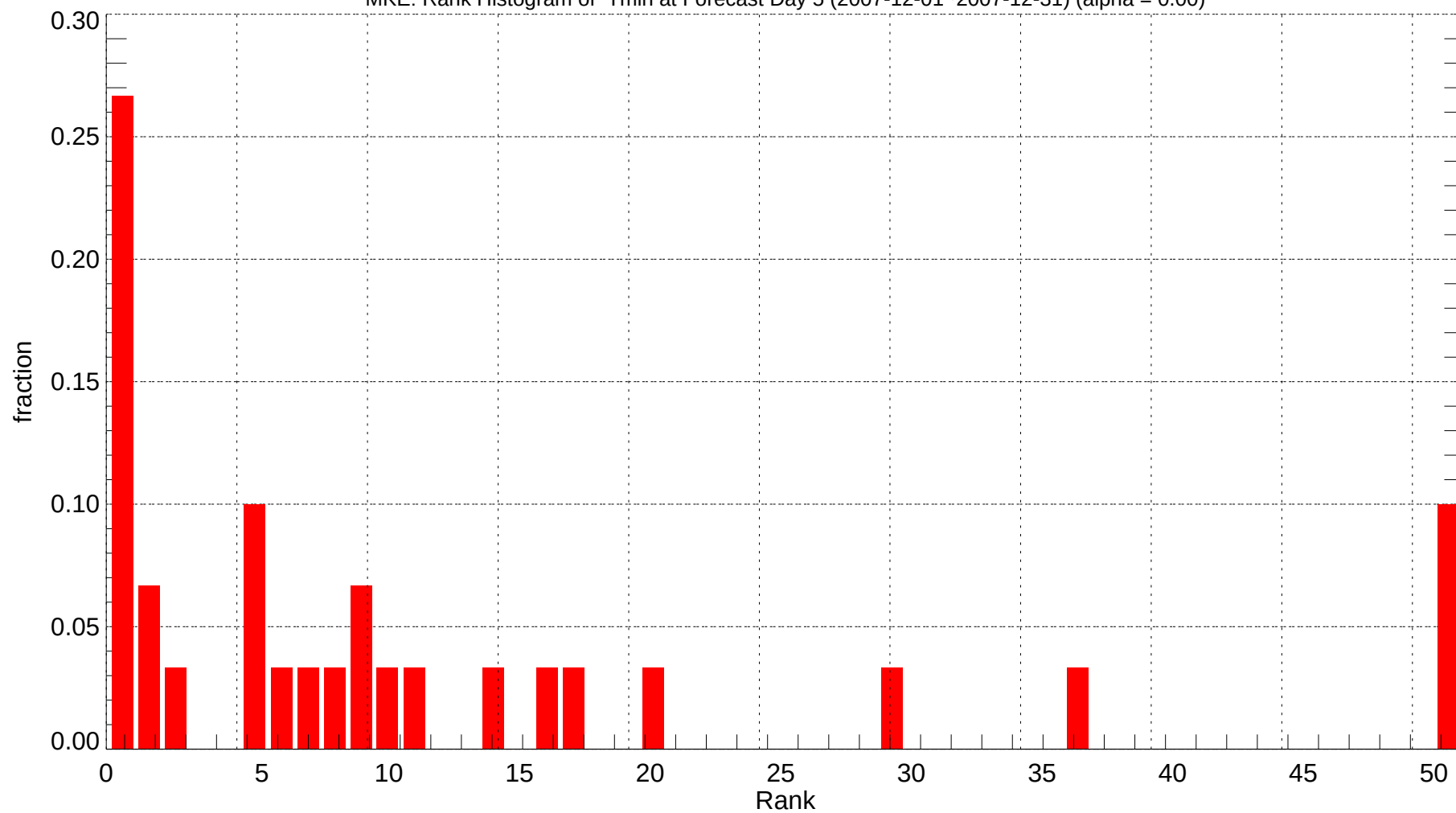
MKE: Rank Histogram of Tmin at Forecast Day 5 (2007-12-01~2007-12-31) (alpha = 0.00)
