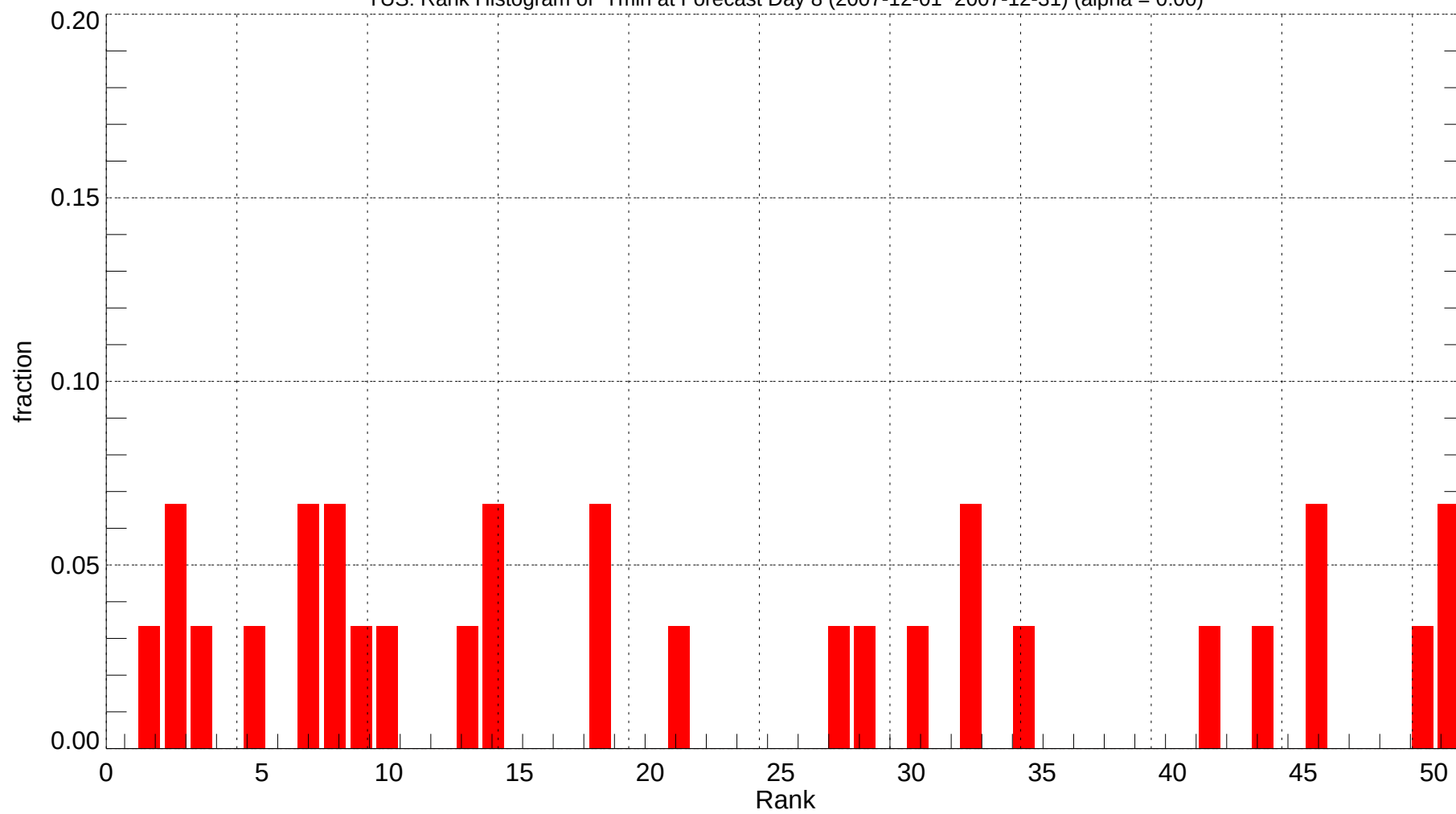
TUS: Rank Histogram of Tmin at Forecast Day 8 (2007-12-01~2007-12-31) (alpha = 0.00)
