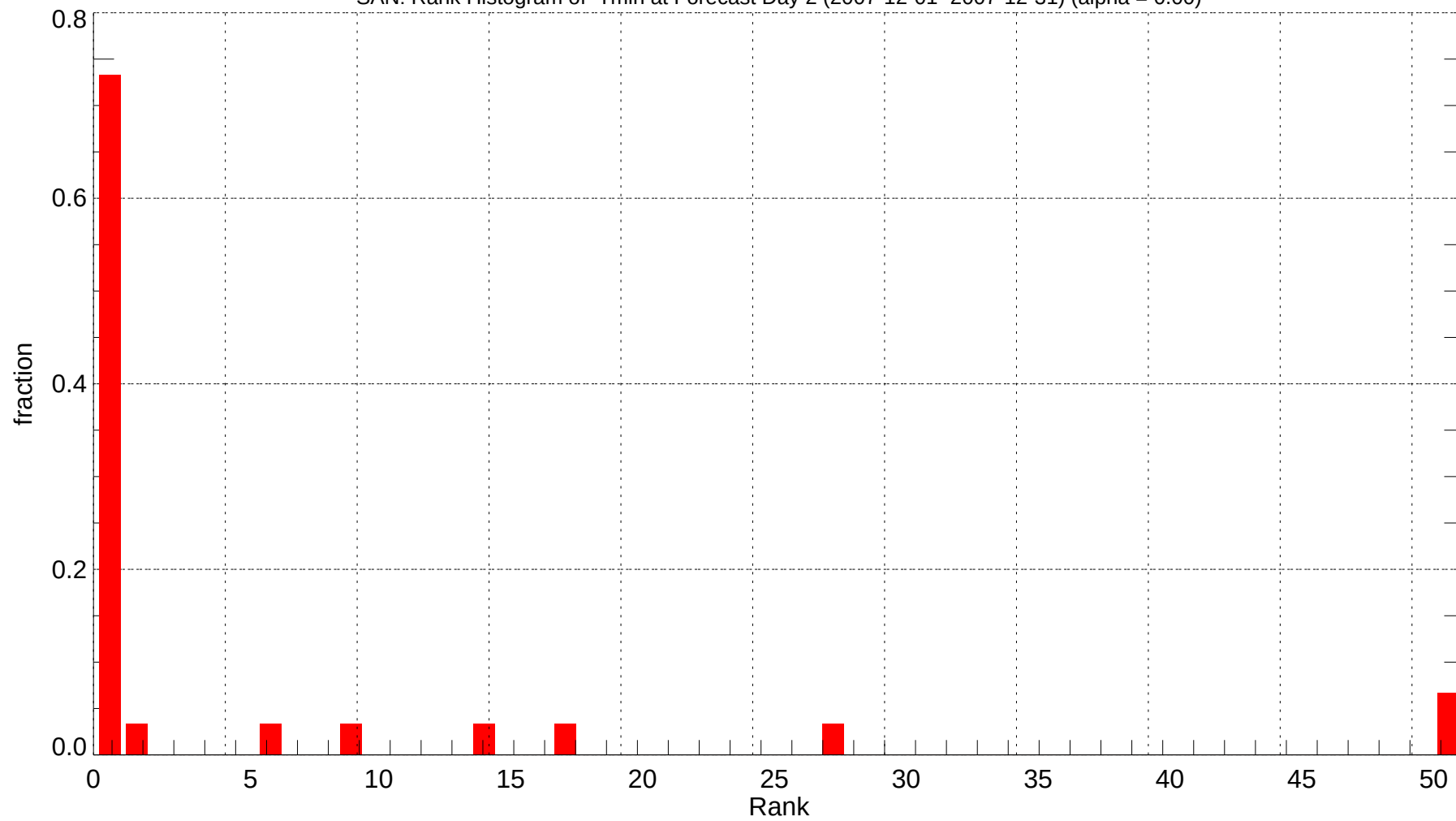
SAN: Rank Histogram of Tmin at Forecast Day 2 (2007-12-01~2007-12-31) (alpha = 0.00)
