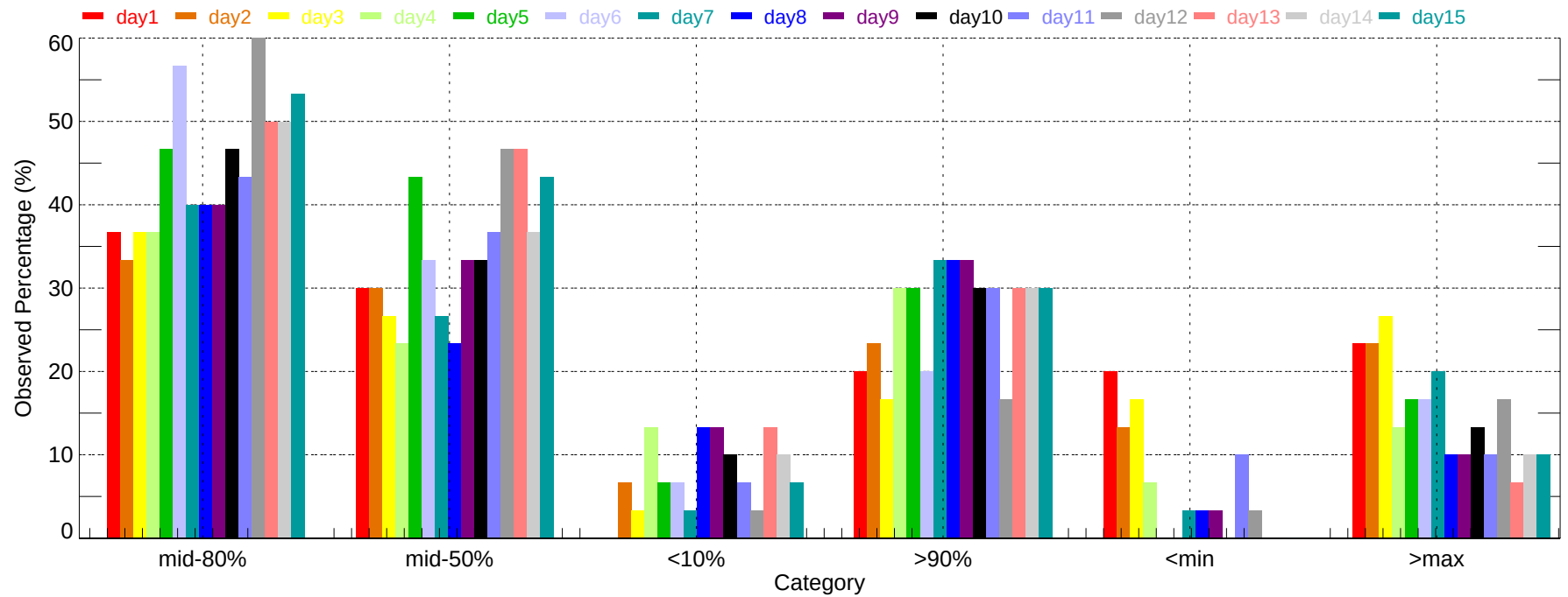
Observed Percentage of Ensembles - SJT: Min Temperature (2007-12-01~2007-12-31)
