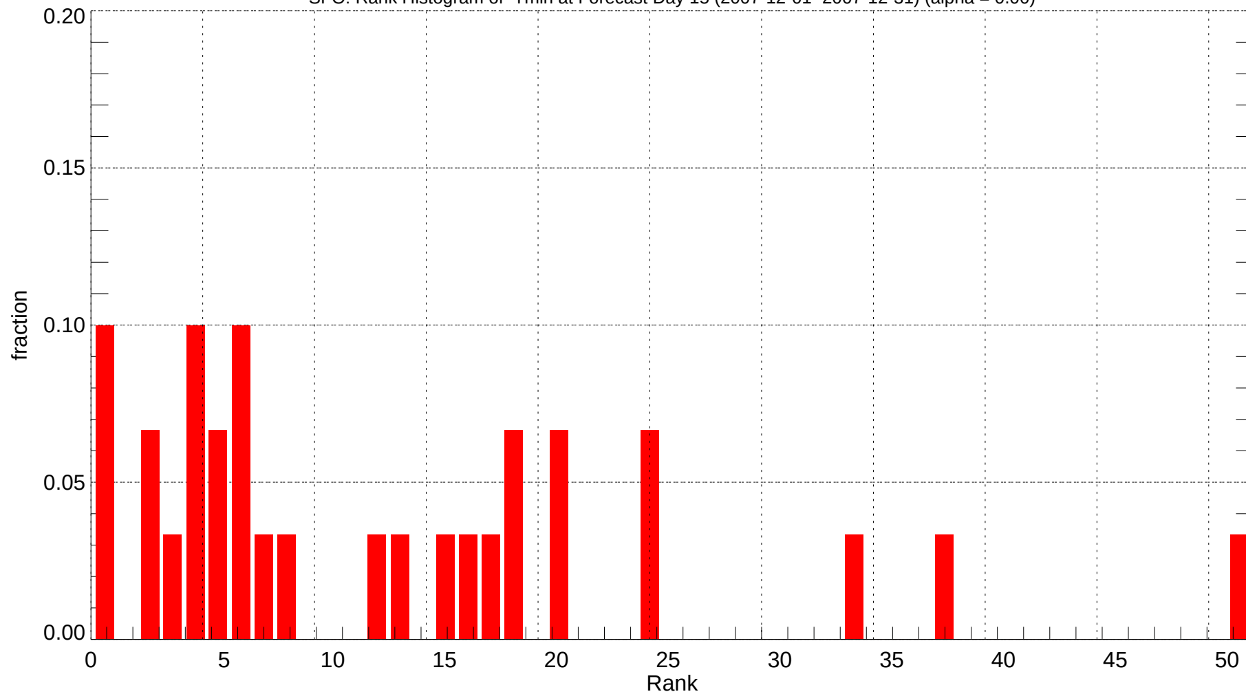
SFO: Rank Histogram of Tmin at Forecast Day 15 (2007-12-01~2007-12-31) (alpha = 0.00)
