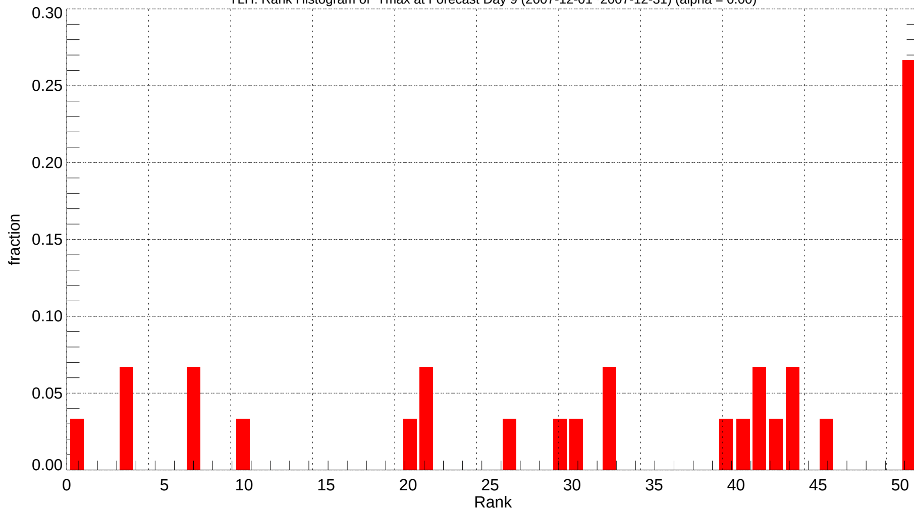
TLH: Rank Histogram of Tmax at Forecast Day 9 (2007-12-01~2007-12-31) (alpha = 0.00)
