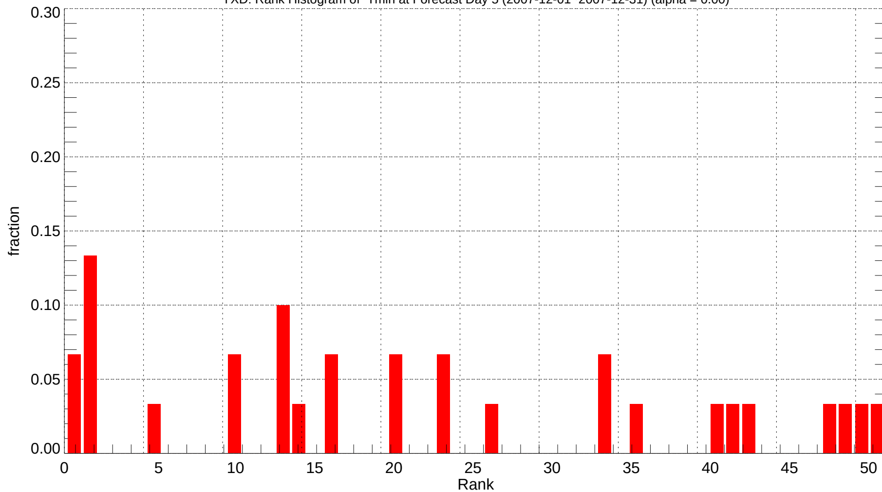
YXD: Rank Histogram of Tmin at Forecast Day 5 (2007-12-01~2007-12-31) (alpha = 0.00)
