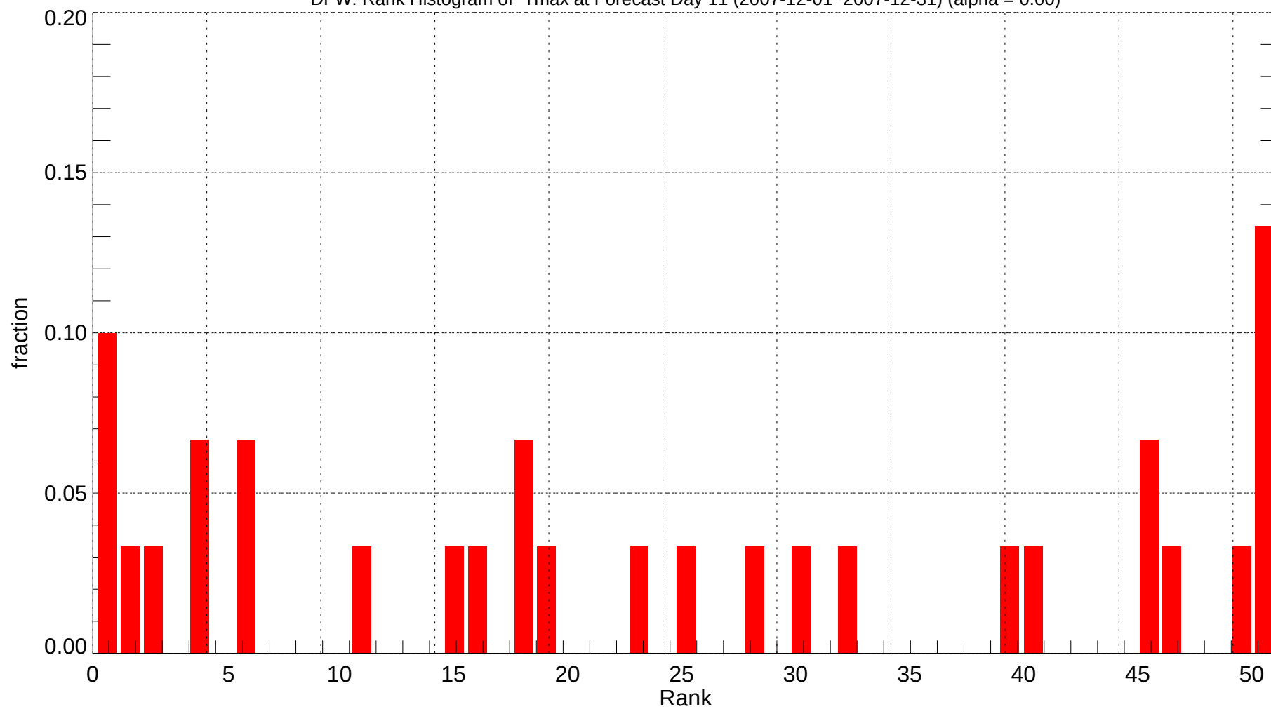
DFW: Rank Histogram of Tmax at Forecast Day 11 (2007-12-01~2007-12-31) (alpha = 0.00)
