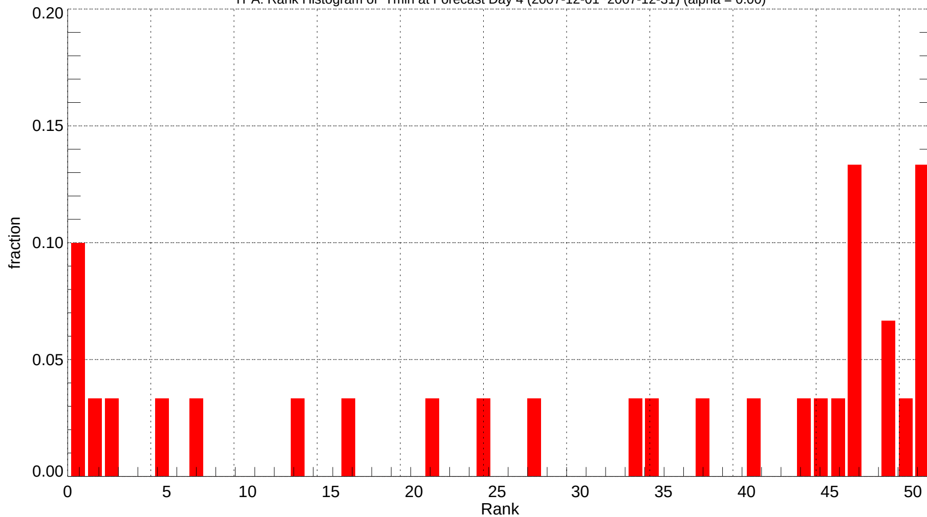
TPA: Rank Histogram of Tmin at Forecast Day 4 (2007-12-01~2007-12-31) (alpha = 0.00)
