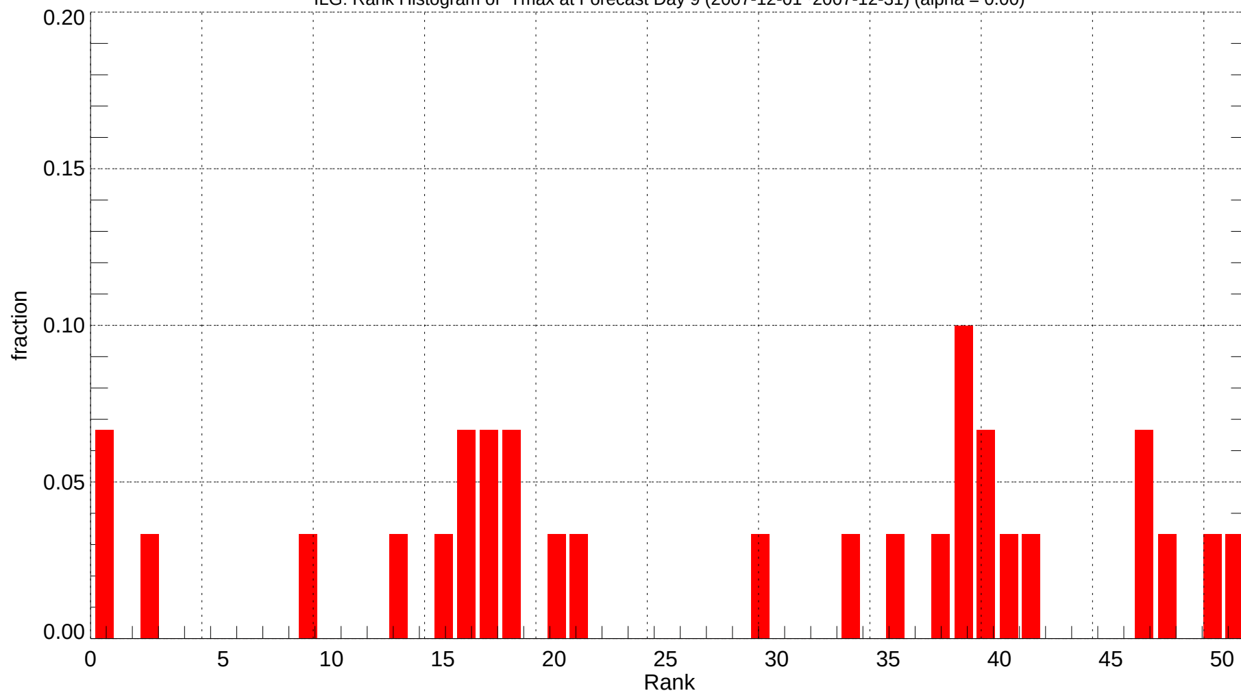
ILG: Rank Histogram of Tmax at Forecast Day 9 (2007-12-01~2007-12-31) (alpha = 0.00)
