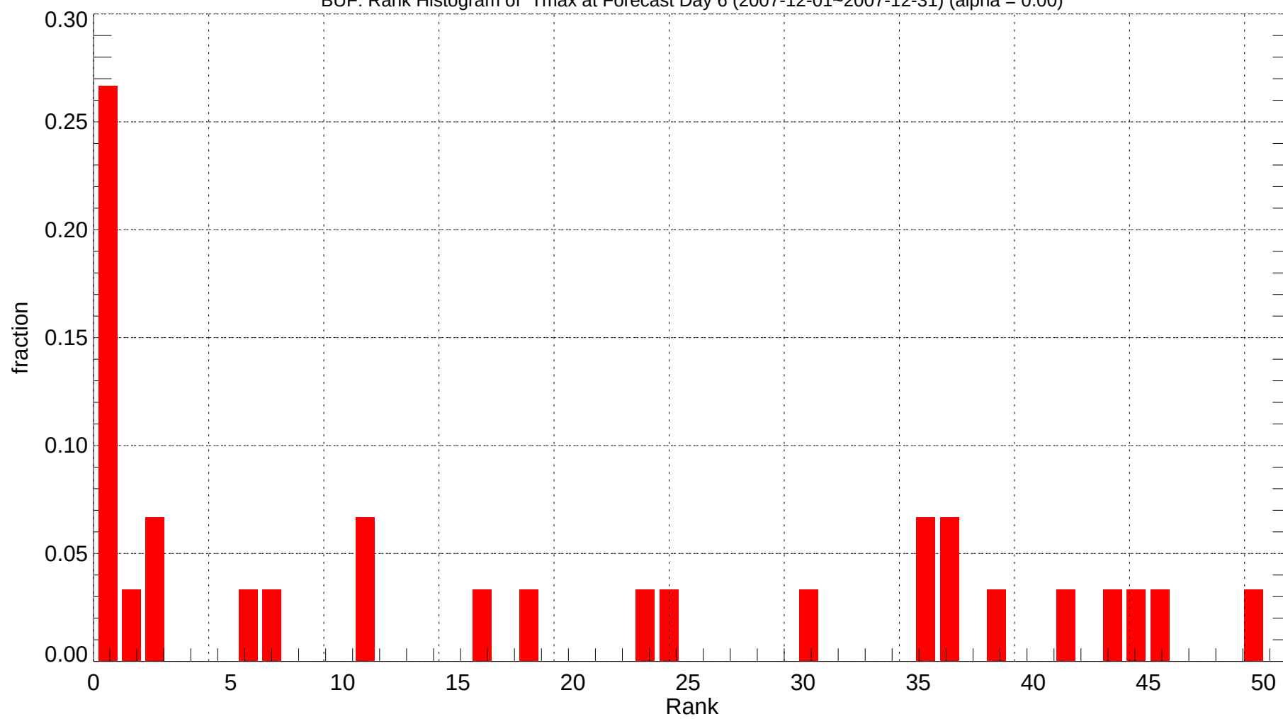
BUF: Rank Histogram of Tmax at Forecast Day 6 (2007-12-01~2007-12-31) (alpha = 0.00)
