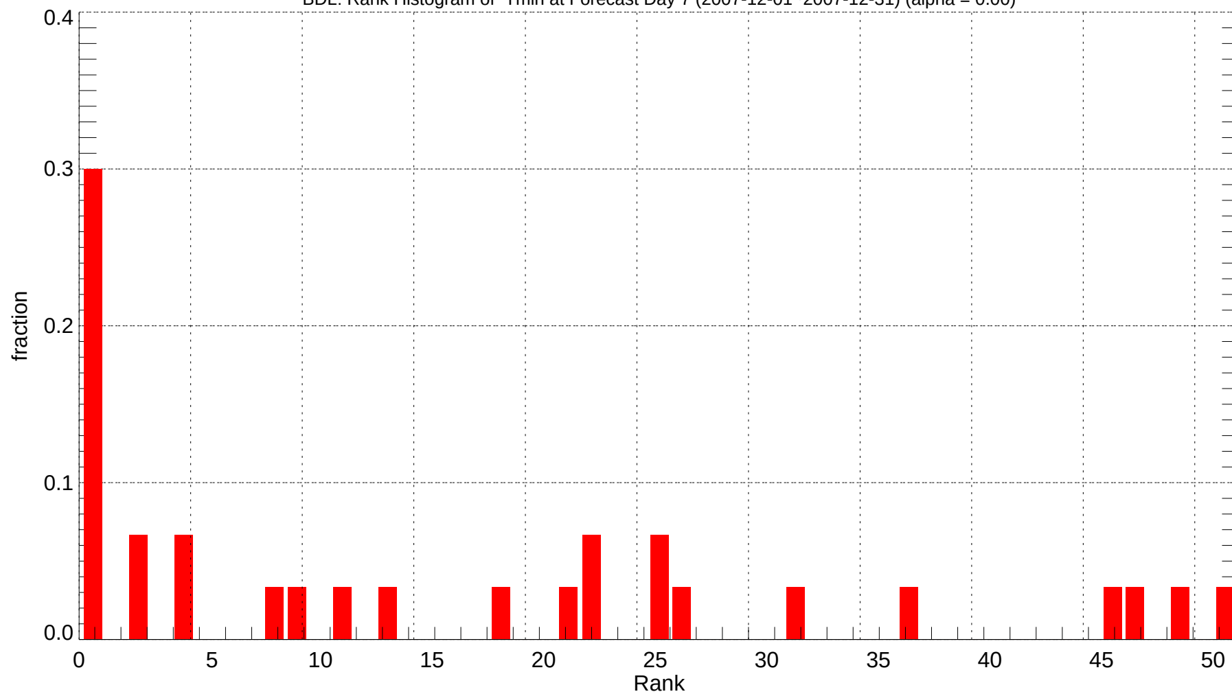
BDL: Rank Histogram of Tmin at Forecast Day 7 (2007-12-01~2007-12-31) (alpha = 0.00)
