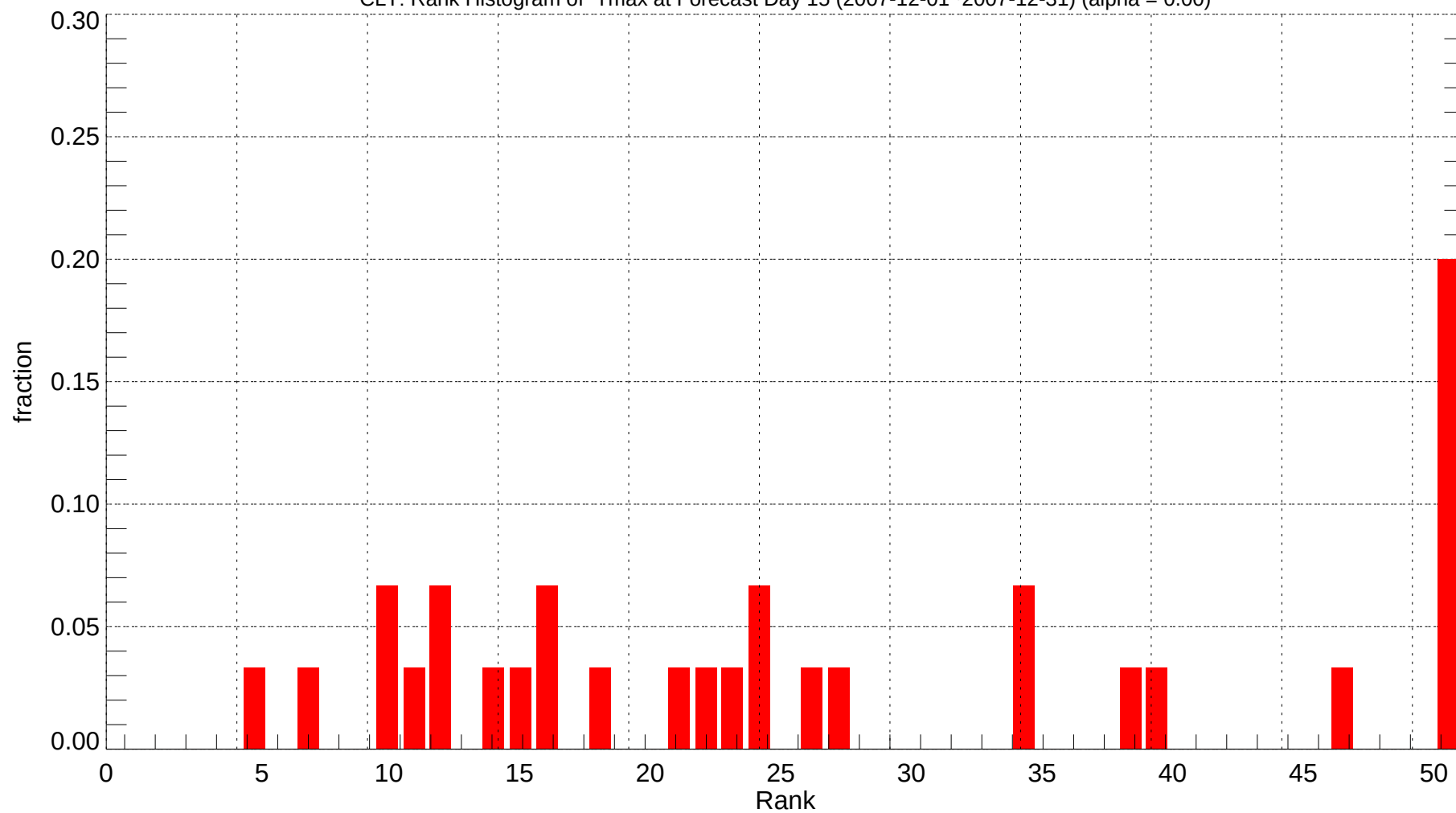
CLT: Rank Histogram of Tmax at Forecast Day 15 (2007-12-01~2007-12-31) (alpha = 0.00)
