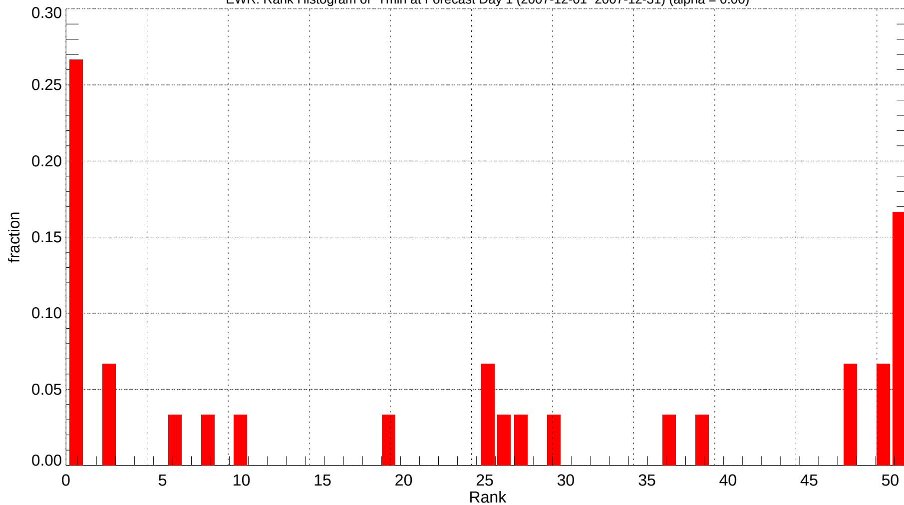
EWR: Rank Histogram of Tmin at Forecast Day 1 (2007-12-01~2007-12-31) (alpha = 0.00)
