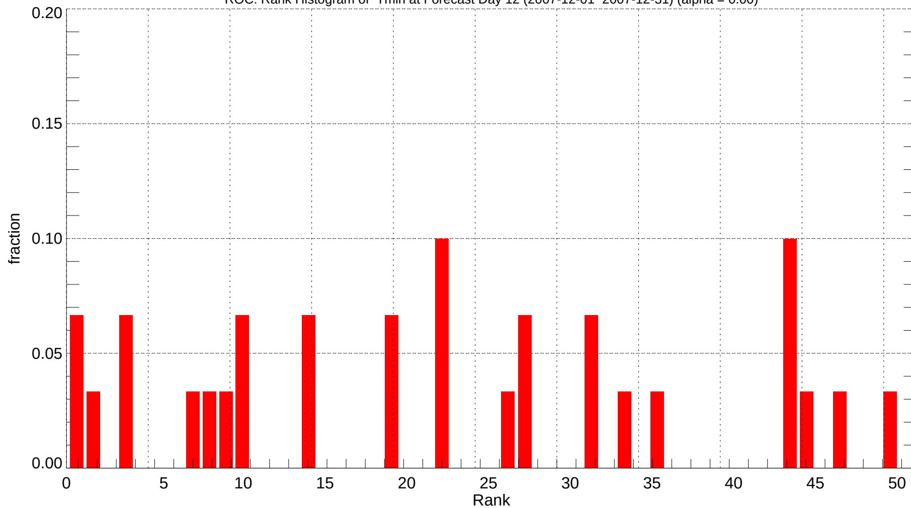
ROC: Rank Histogram of Tmin at Forecast Day 12 (2007-12-01~2007-12-31) (alpha = 0.00)
