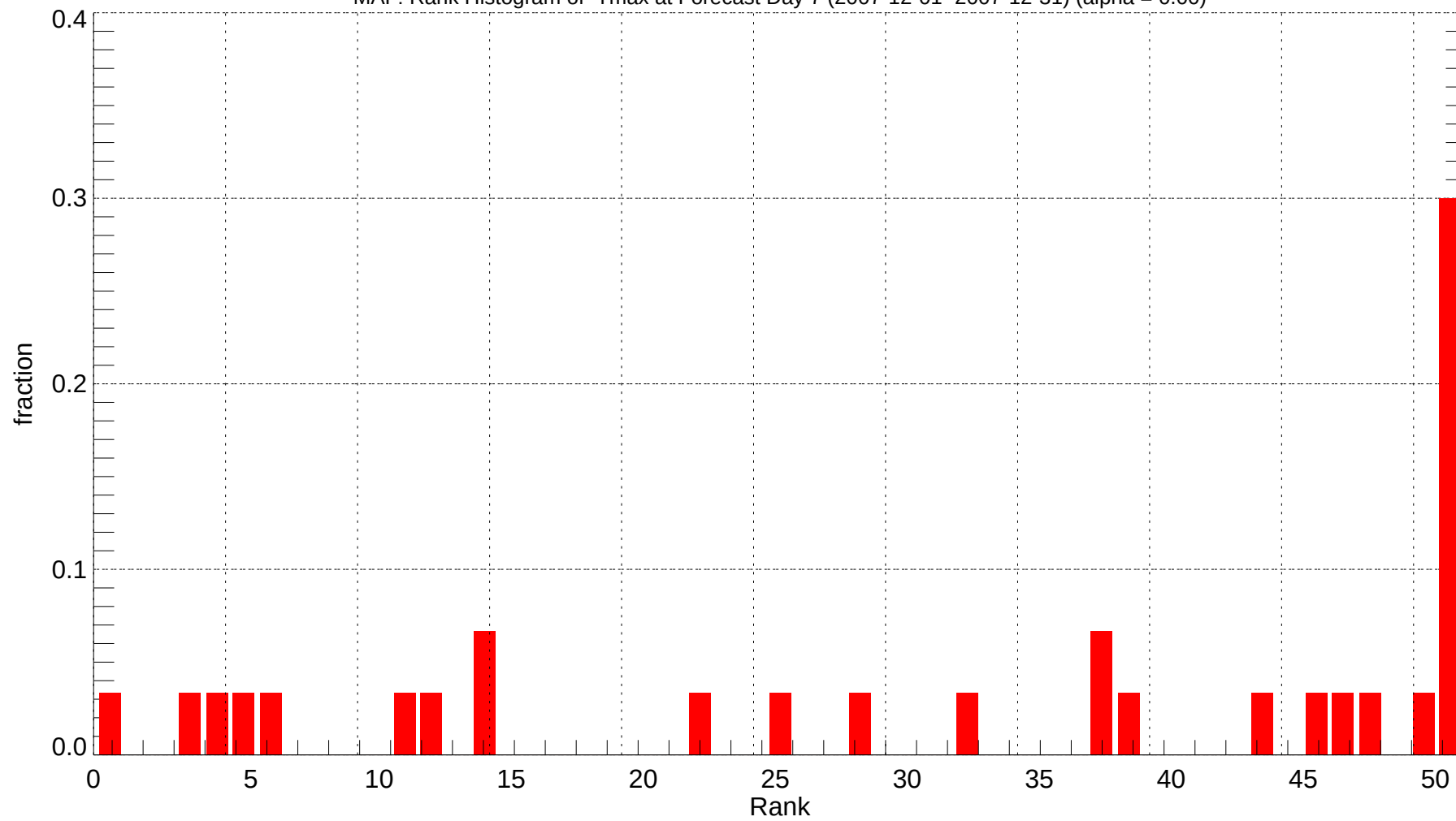
MAF: Rank Histogram of Tmax at Forecast Day 7 (2007-12-01~2007-12-31) (alpha = 0.00)
