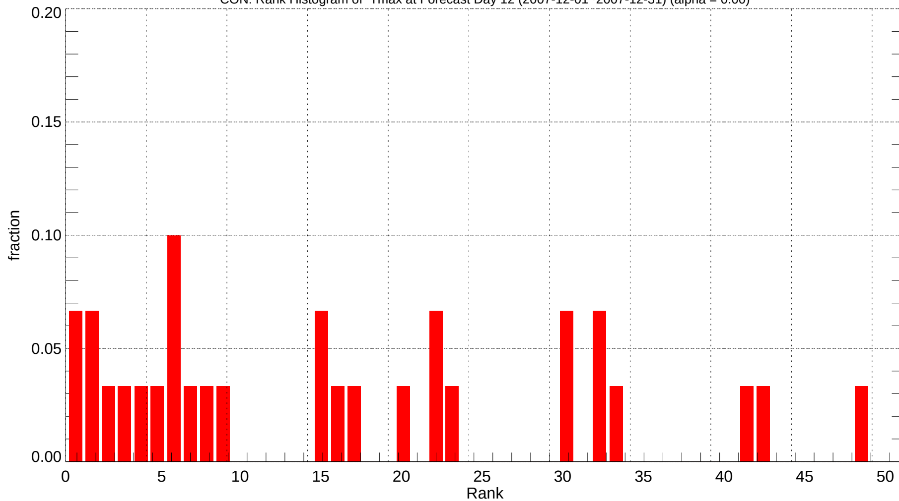
CON: Rank Histogram of Tmax at Forecast Day 12 (2007-12-01~2007-12-31) (alpha = 0.00)
