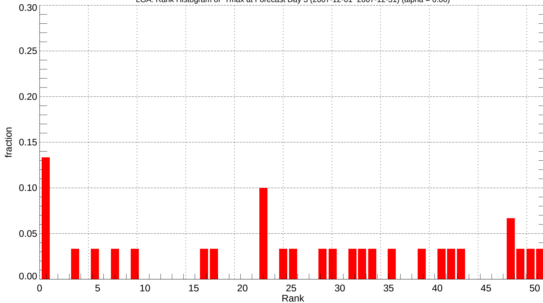
LGA: Rank Histogram of Tmax at Forecast Day 3 (2007-12-01~2007-12-31) (alpha = 0.00)
