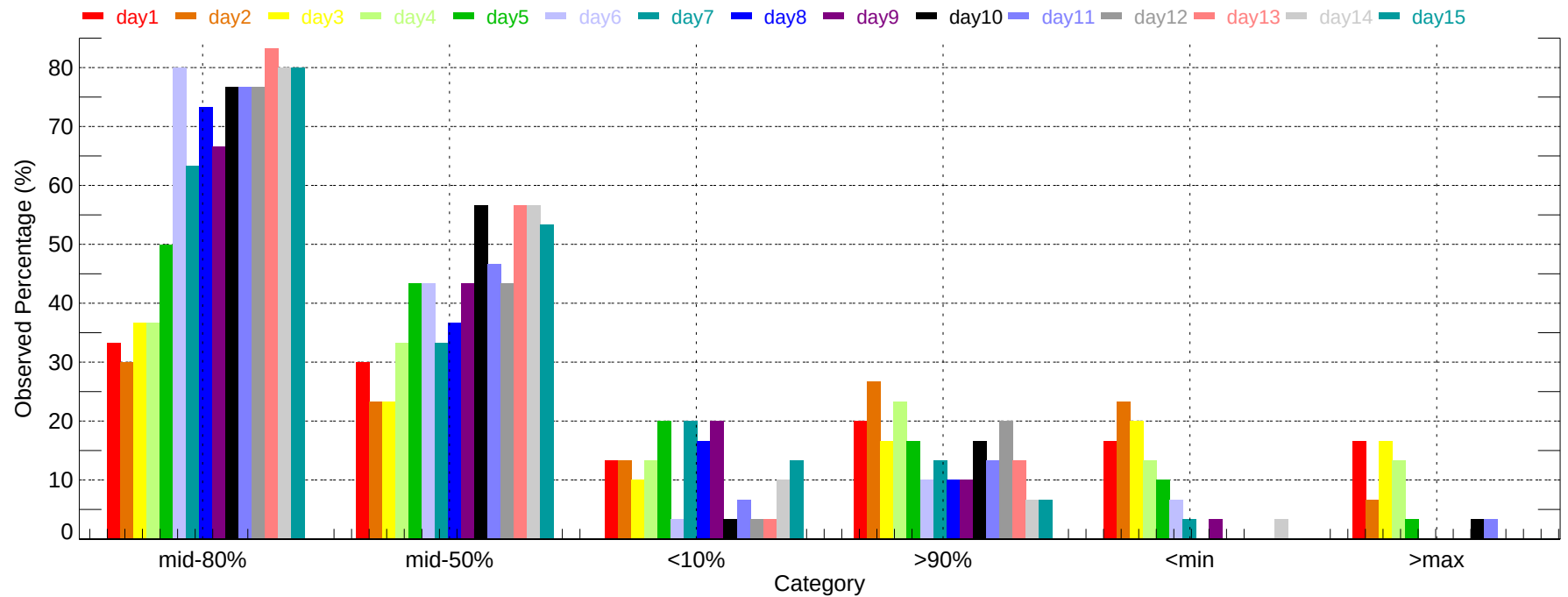
Observed Percentage of Ensembles - WJF: Max Temperature (2007-12-01~2007-12-31)
