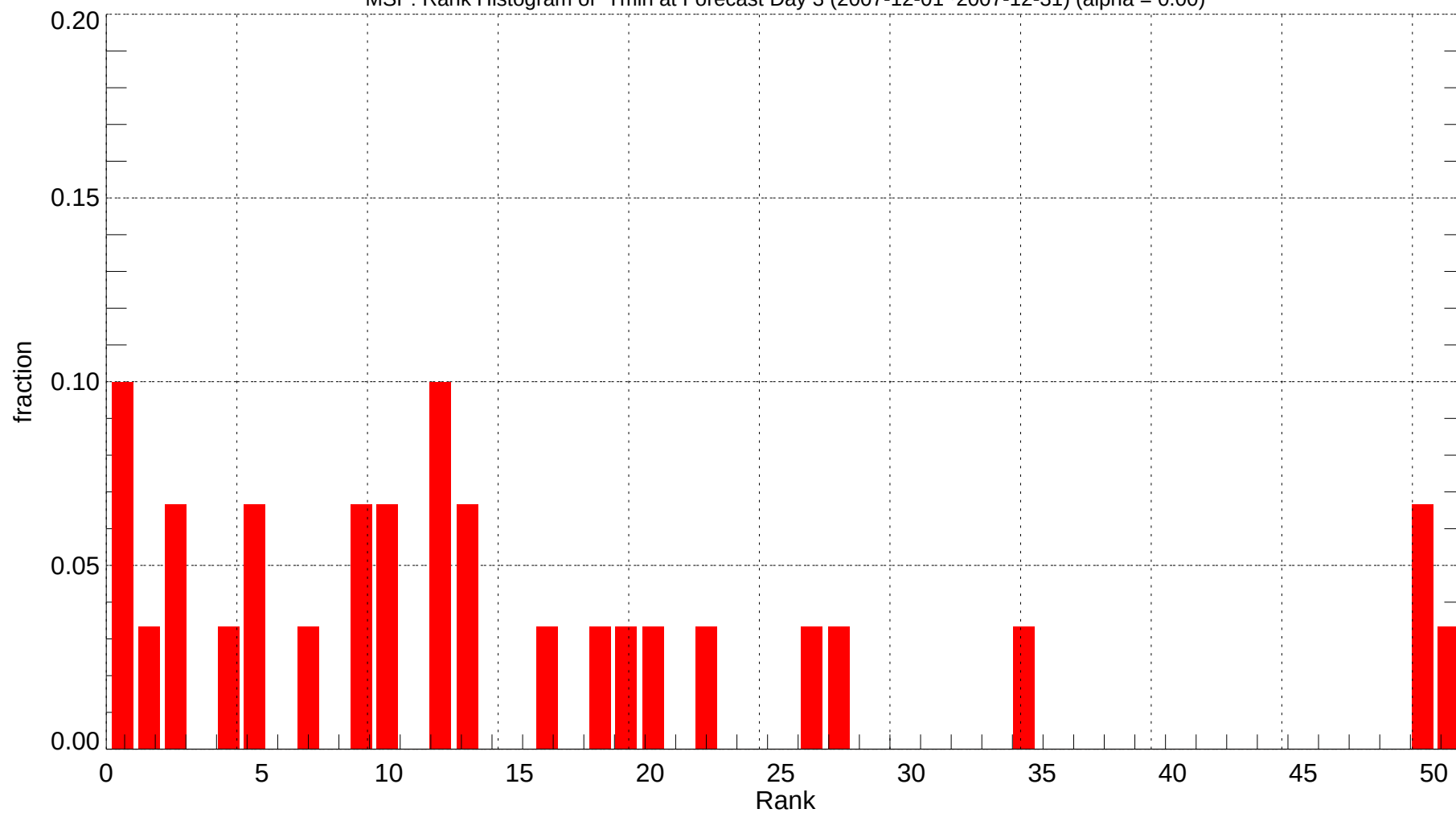
MSP: Rank Histogram of Tmin at Forecast Day 3 (2007-12-01~2007-12-31) (alpha = 0.00)
