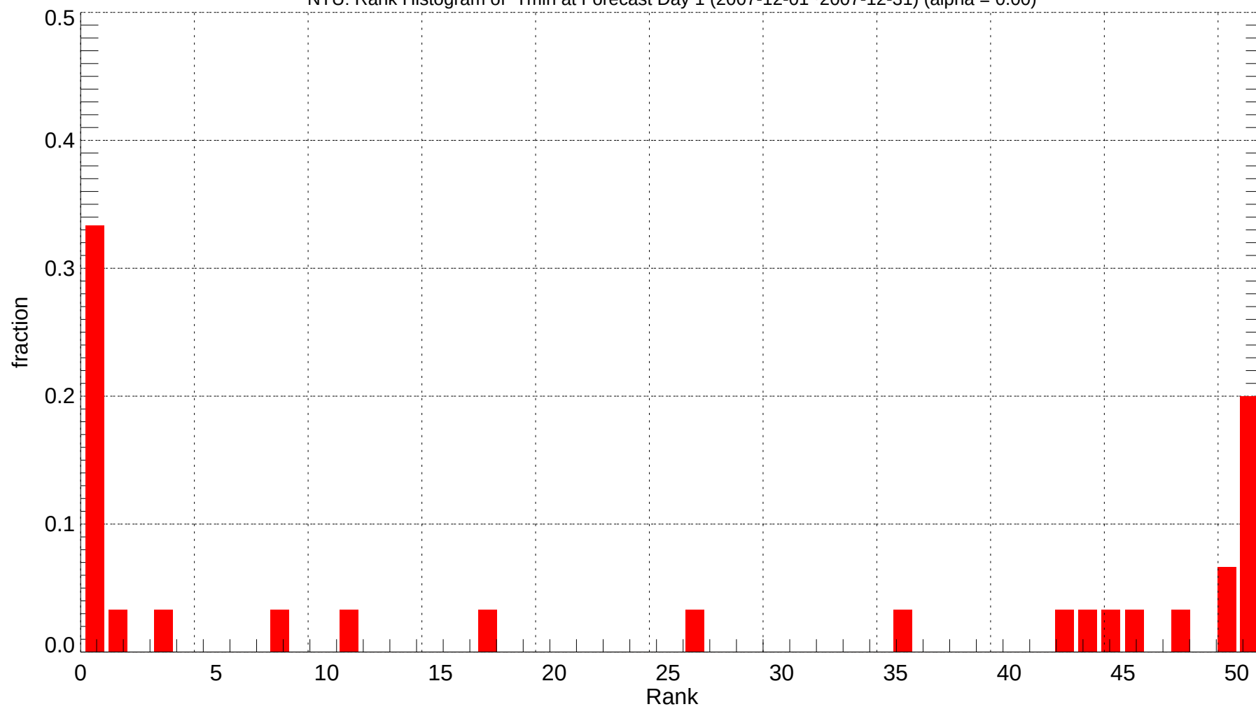
NTU: Rank Histogram of Tmin at Forecast Day 1 (2007-12-01~2007-12-31) (alpha = 0.00)
