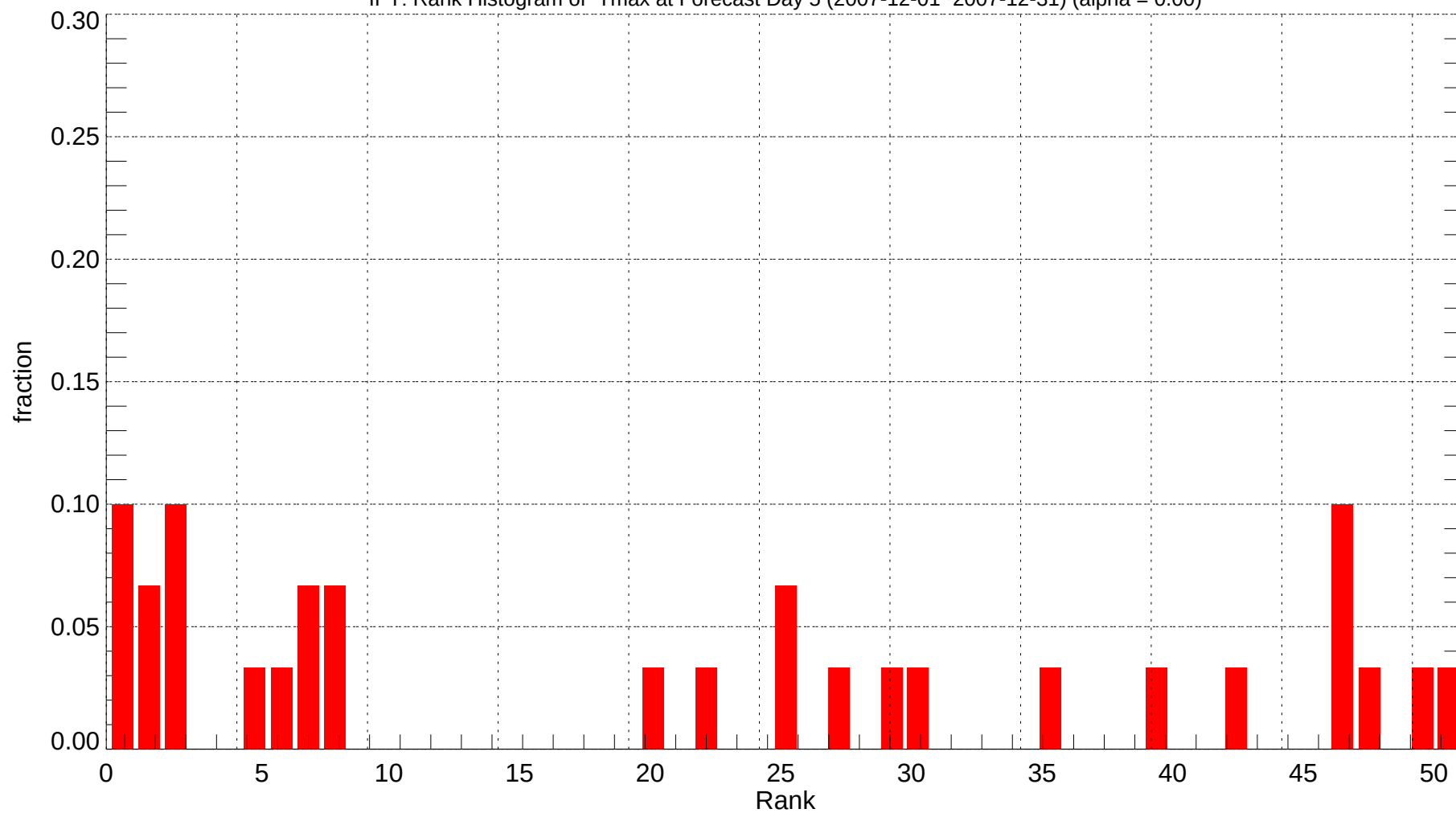
IPT: Rank Histogram of Tmax at Forecast Day 5 (2007-12-01~2007-12-31) (alpha = 0.00)
