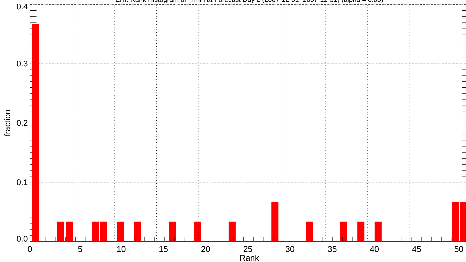
ERI: Rank Histogram of Tmin at Forecast Day 2 (2007-12-01~2007-12-31) (alpha = 0.00)
