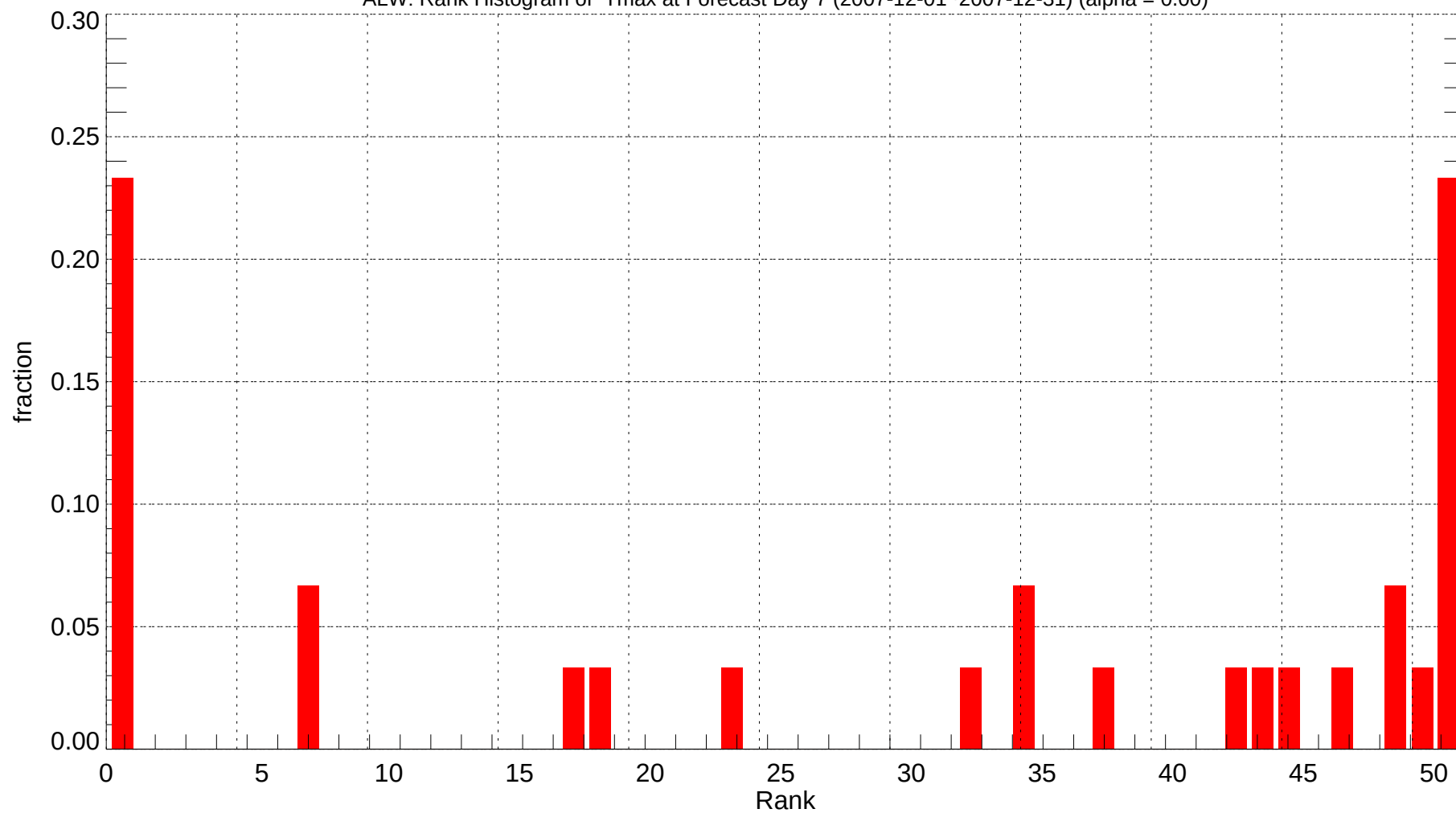
ALW: Rank Histogram of Tmax at Forecast Day 7 (2007-12-01~2007-12-31) (alpha = 0.00)
