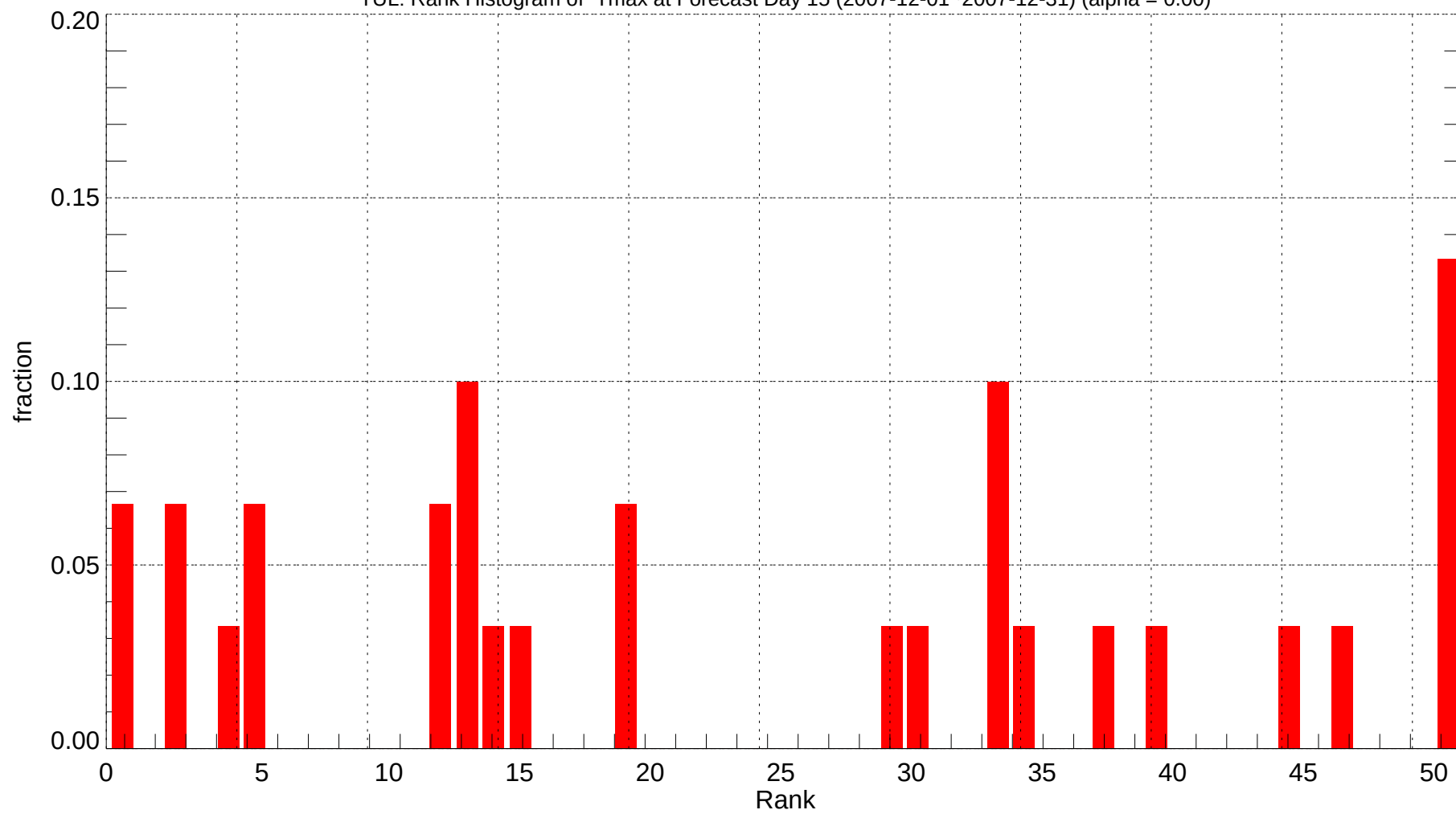
TUL: Rank Histogram of Tmax at Forecast Day 15 (2007-12-01~2007-12-31) (alpha = 0.00)
