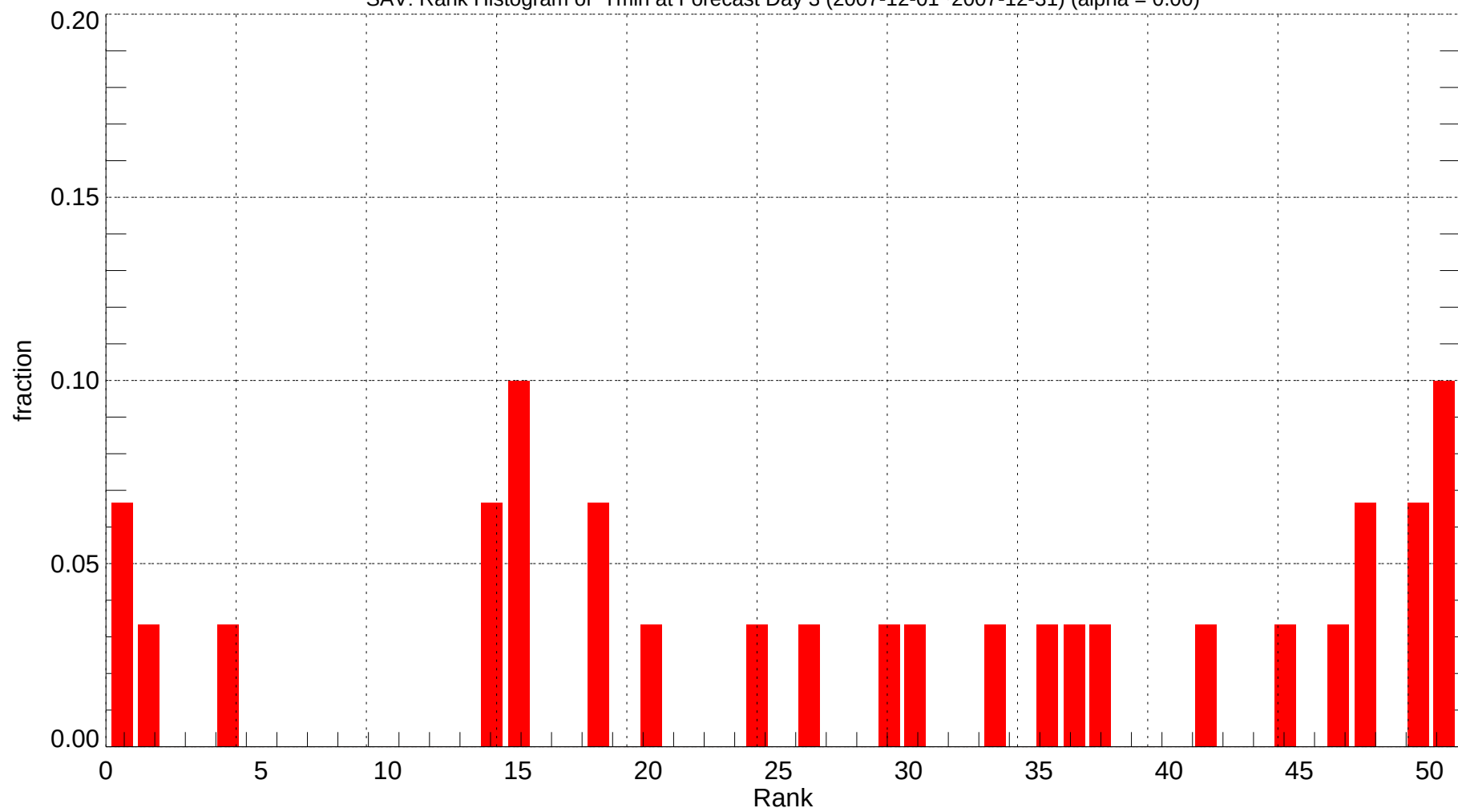
SAV: Rank Histogram of Tmin at Forecast Day 3 (2007-12-01~2007-12-31) (alpha = 0.00)
