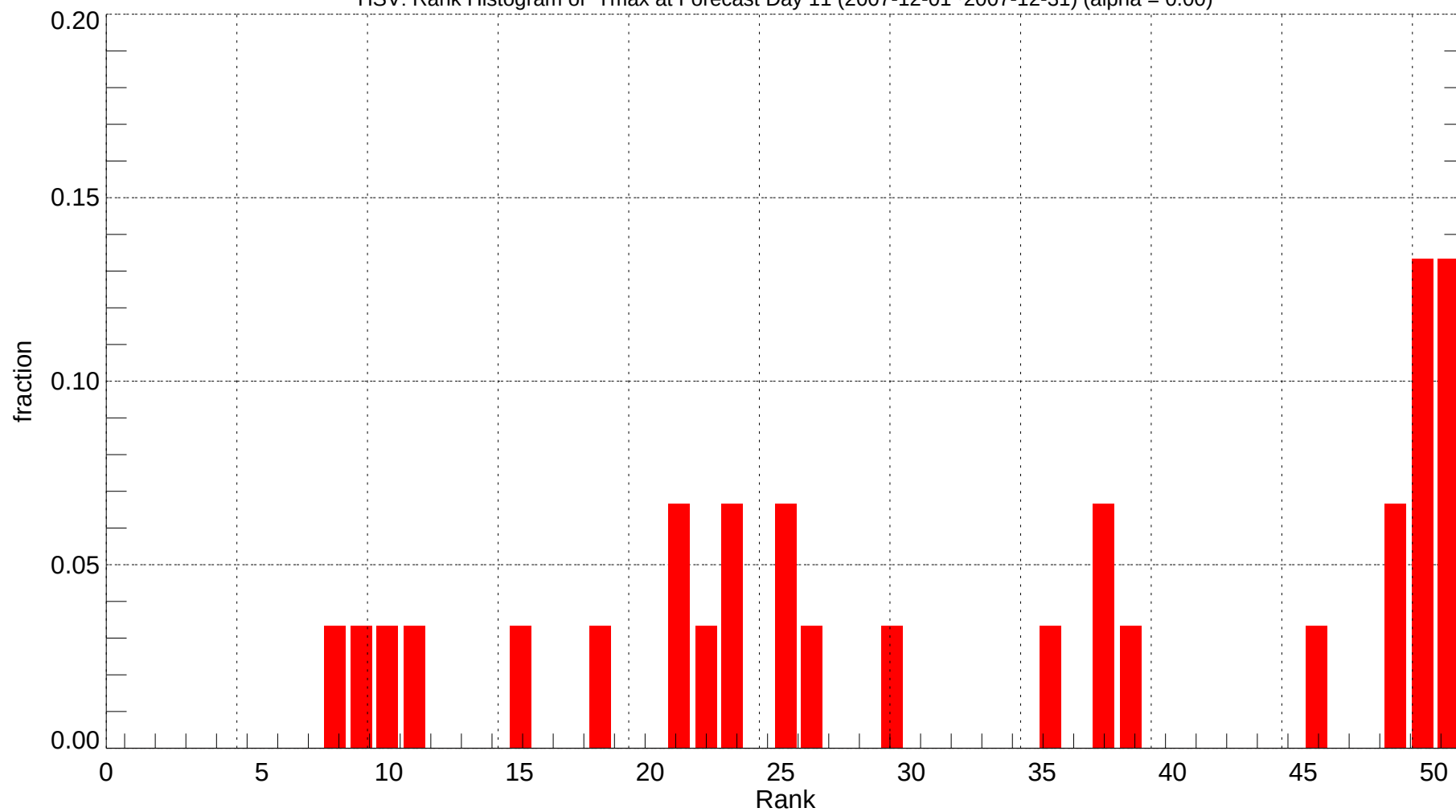
HSV: Rank Histogram of Tmax at Forecast Day 11 (2007-12-01~2007-12-31) (alpha = 0.00)
