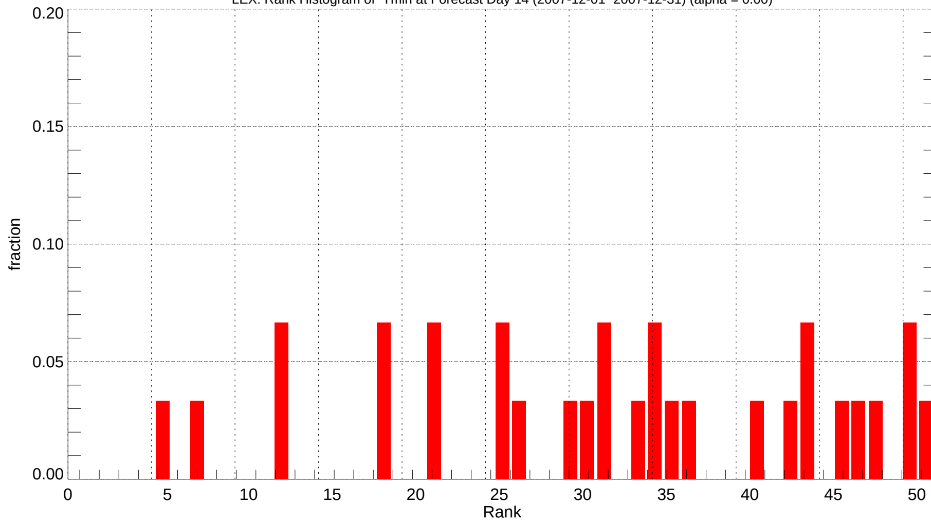
LEX: Rank Histogram of Tmin at Forecast Day 14 (2007-12-01~2007-12-31) (alpha = 0.00)
