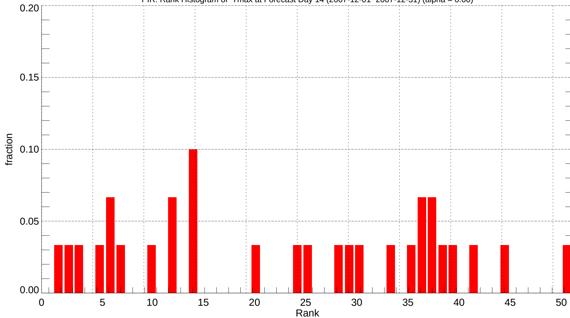
PIR: Rank Histogram of Tmax at Forecast Day 14 (2007-12-01~2007-12-31) (alpha = 0.00)
