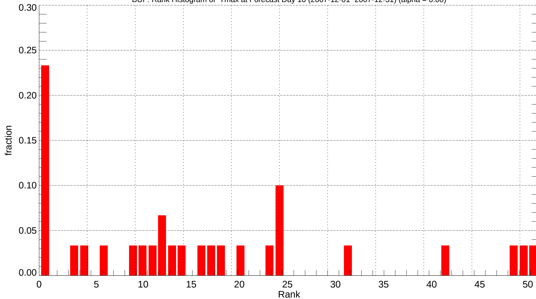
BUF: Rank Histogram of Tmax at Forecast Day 10 (2007-12-01~2007-12-31) (alpha = 0.00)
