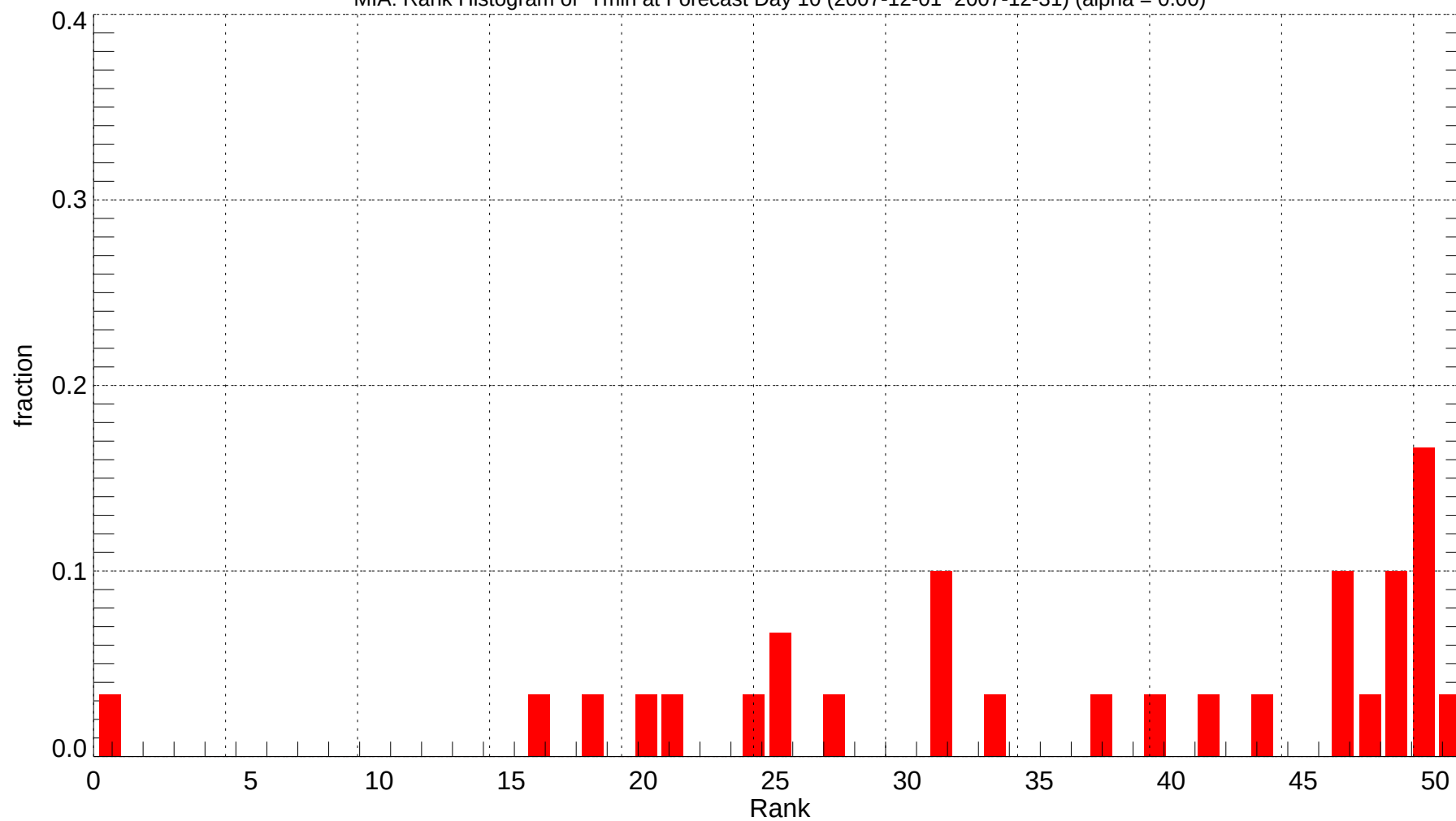
MIA: Rank Histogram of Tmin at Forecast Day 10 (2007-12-01~2007-12-31) (alpha = 0.00)
