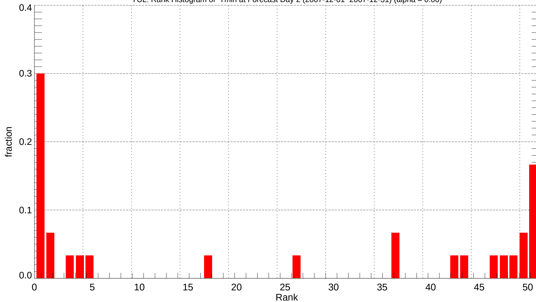
YUL: Rank Histogram of Tmin at Forecast Day 2 (2007-12-01~2007-12-31) (alpha = 0.00)
