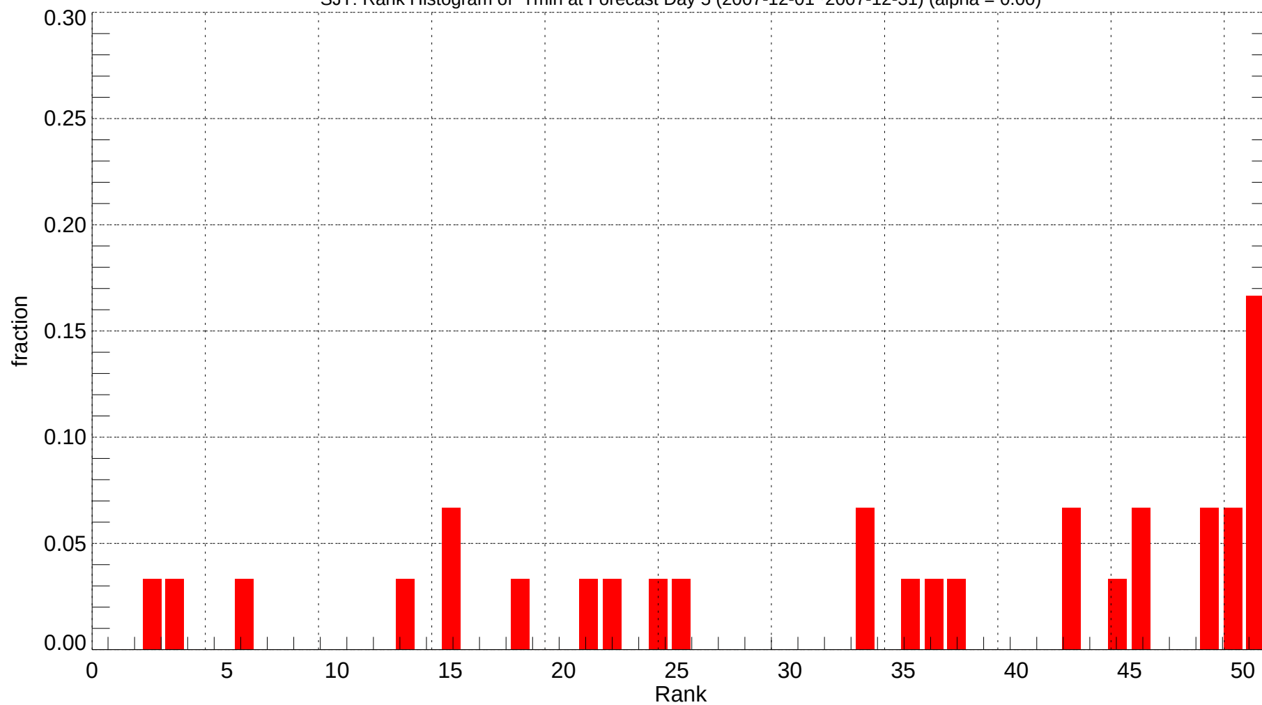
SJT: Rank Histogram of Tmin at Forecast Day 5 (2007-12-01~2007-12-31) (alpha = 0.00)
