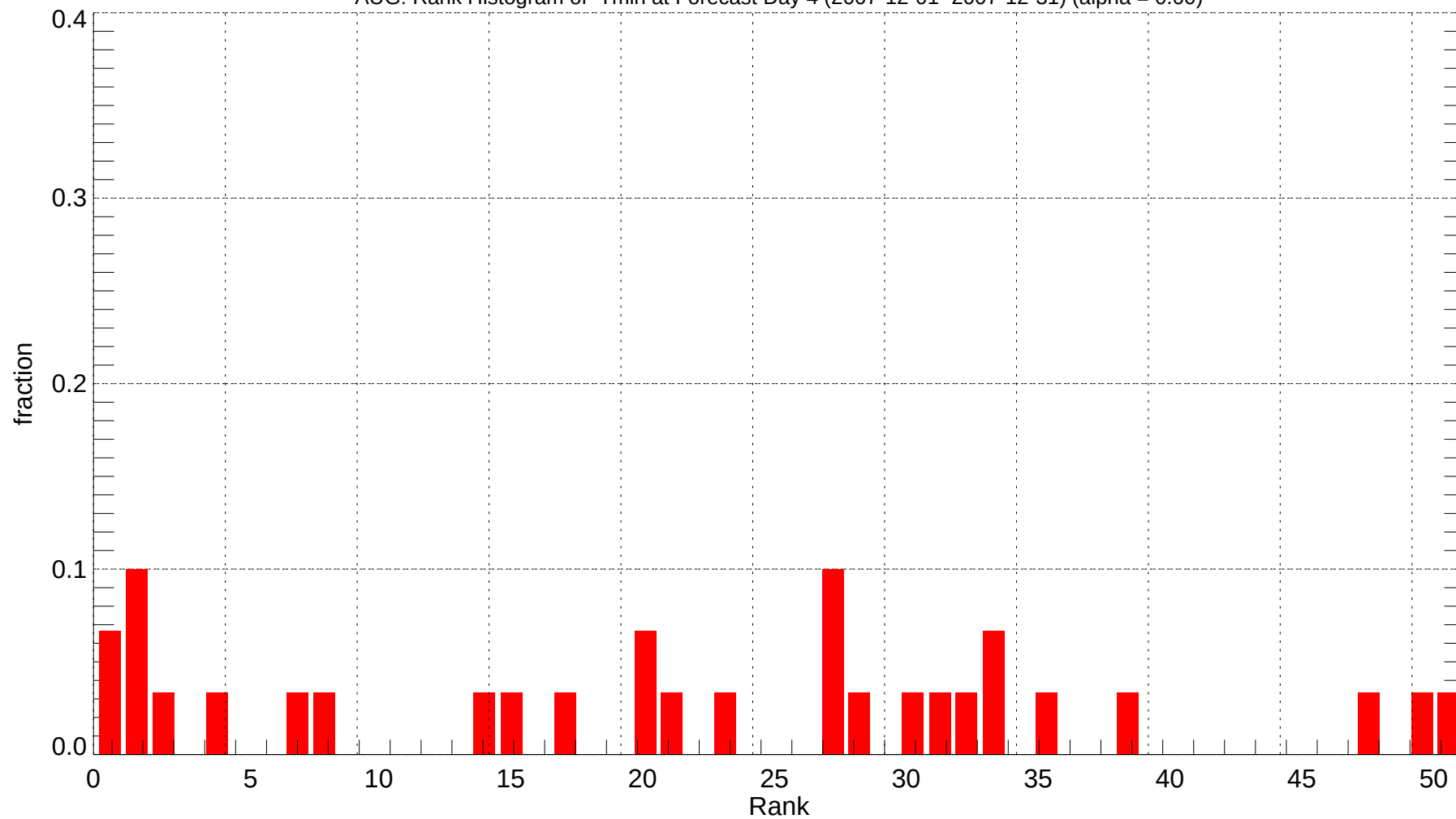
AUG: Rank Histogram of Tmin at Forecast Day 4 (2007-12-01~2007-12-31) (alpha = 0.00)
