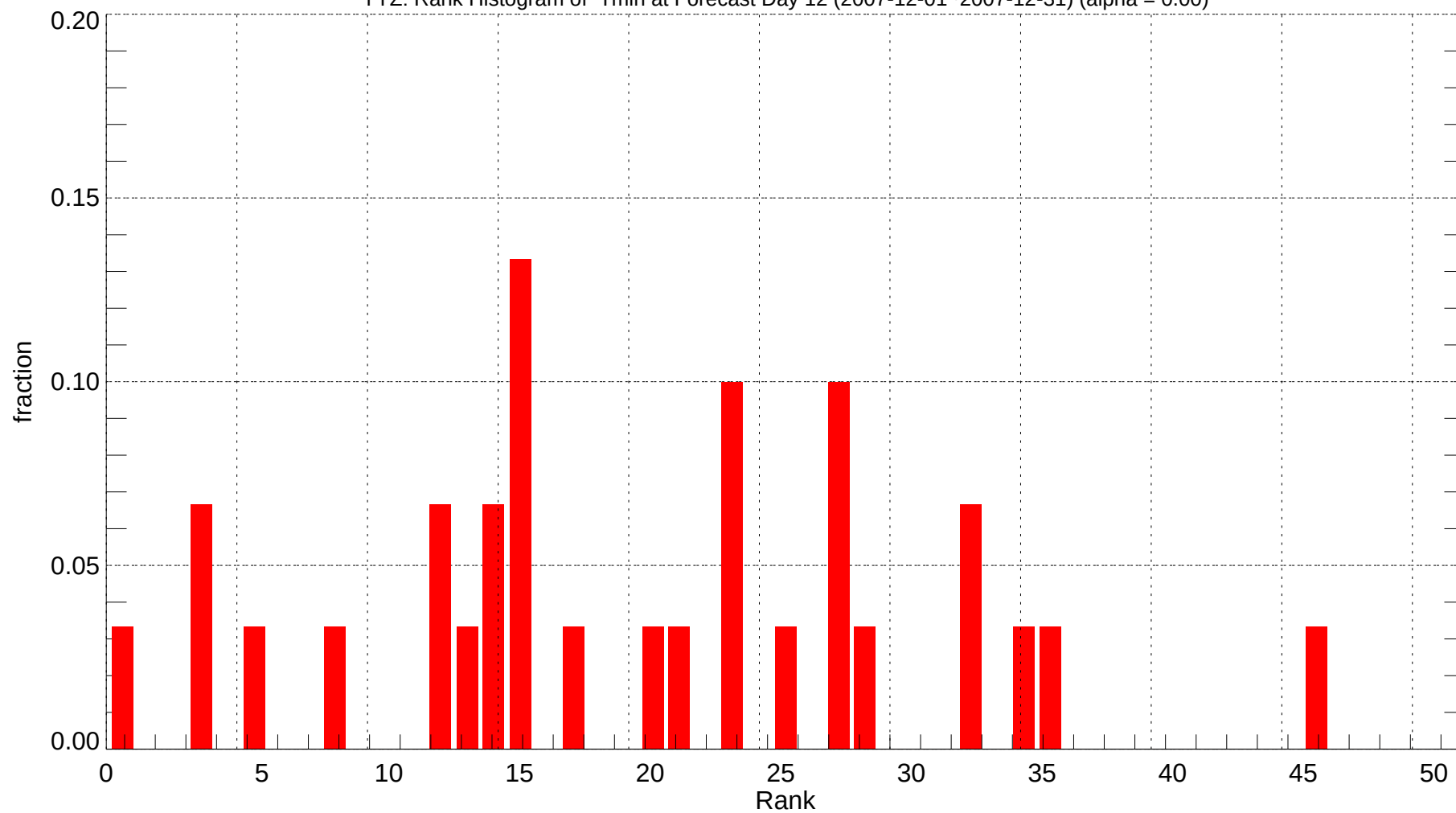
YYZ: Rank Histogram of Tmin at Forecast Day 12 (2007-12-01~2007-12-31) (alpha = 0.00)
