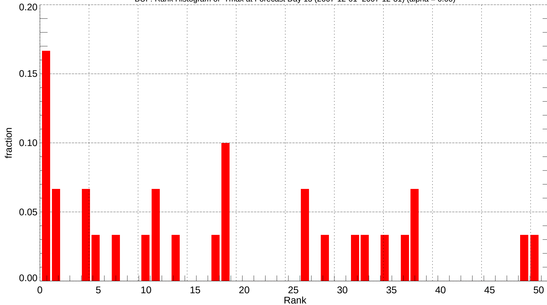
BUF: Rank Histogram of Tmax at Forecast Day 13 (2007-12-01~2007-12-31) (alpha = 0.00)
