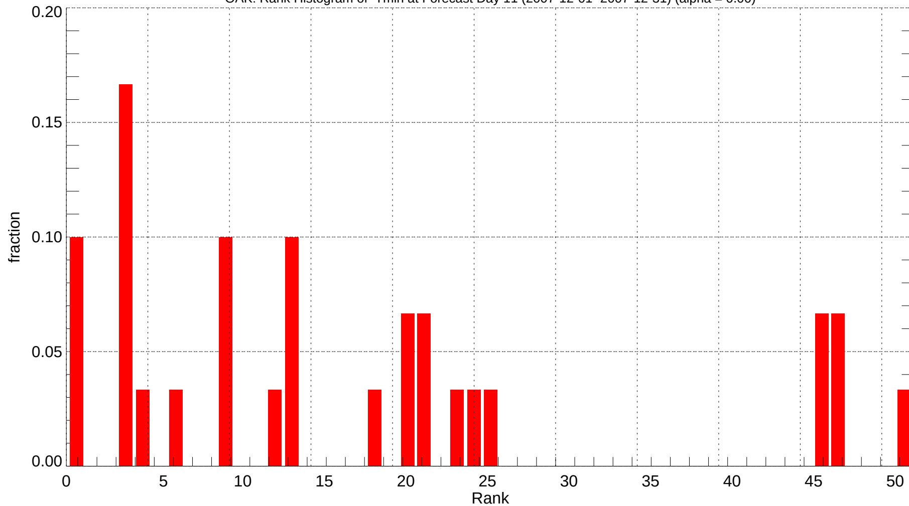
OAK: Rank Histogram of Tmin at Forecast Day 11 (2007-12-01~2007-12-31) (alpha = 0.00)
