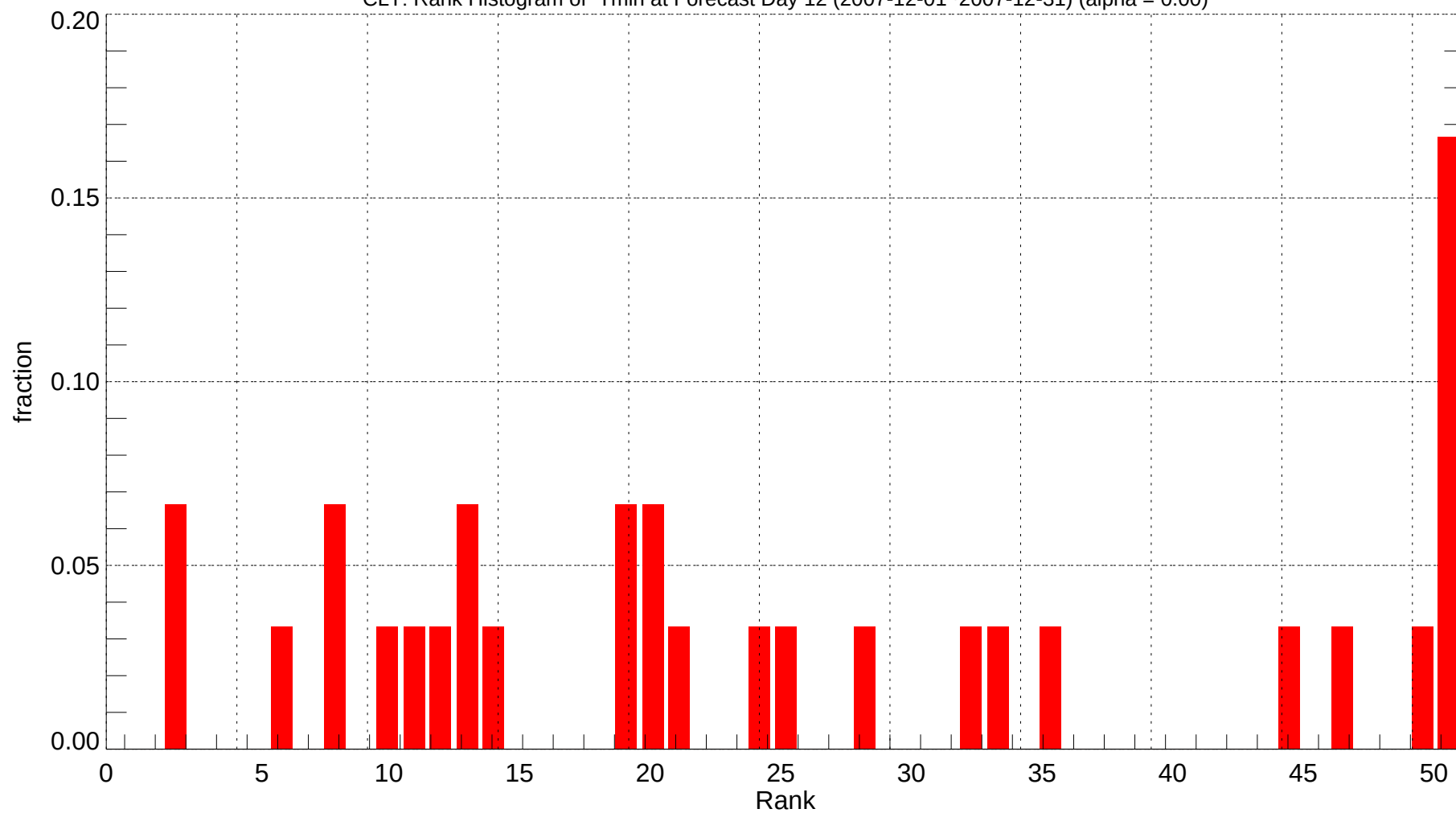
CLT: Rank Histogram of Tmin at Forecast Day 12 (2007-12-01~2007-12-31) (alpha = 0.00)
