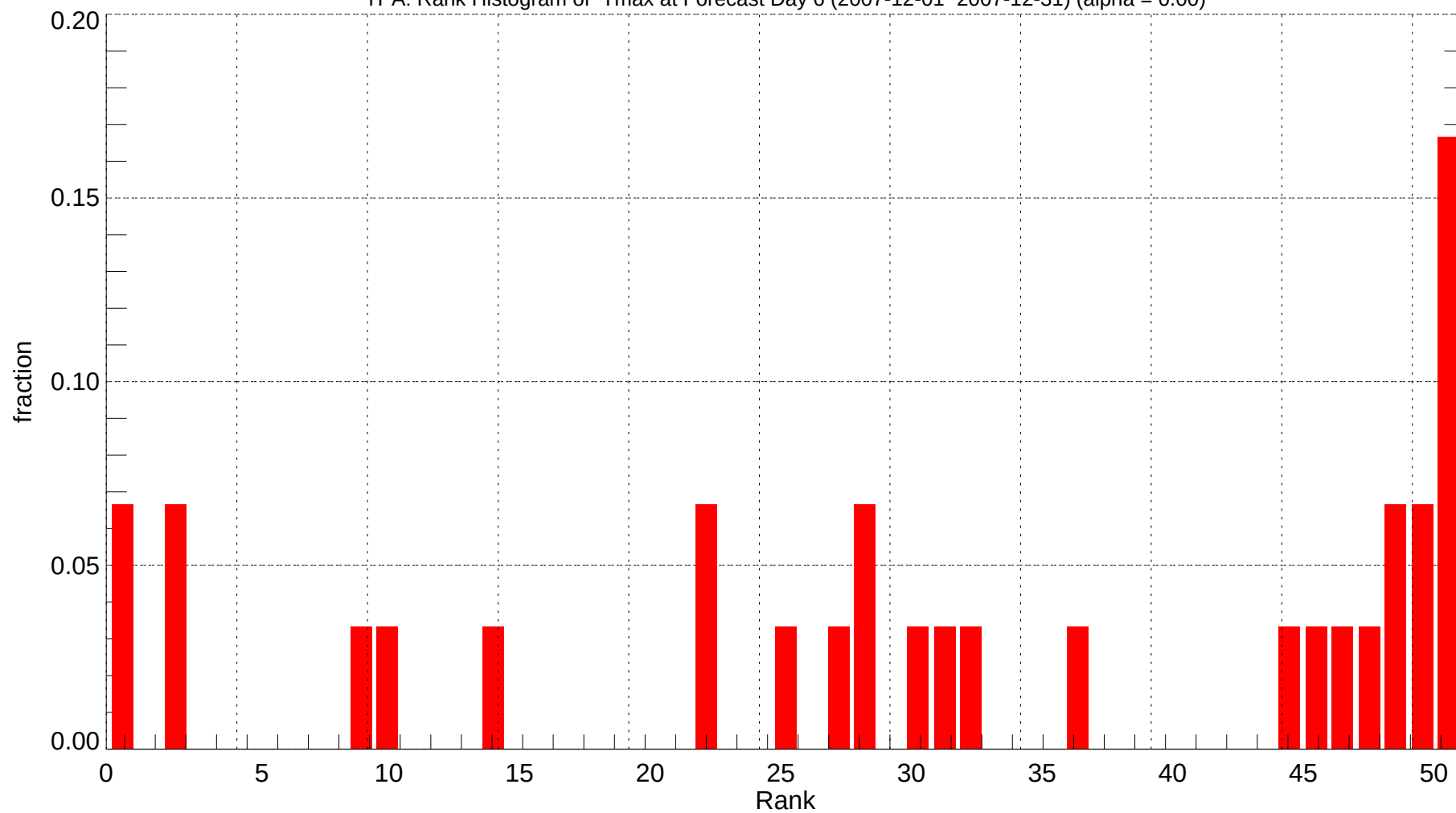
TPA: Rank Histogram of Tmax at Forecast Day 6 (2007-12-01~2007-12-31) (alpha = 0.00)
