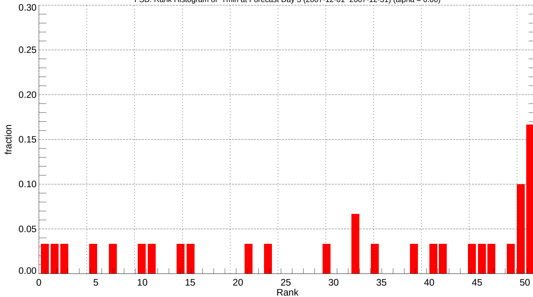
FSD: Rank Histogram of Tmin at Forecast Day 3 (2007-12-01~2007-12-31) (alpha = 0.00)
