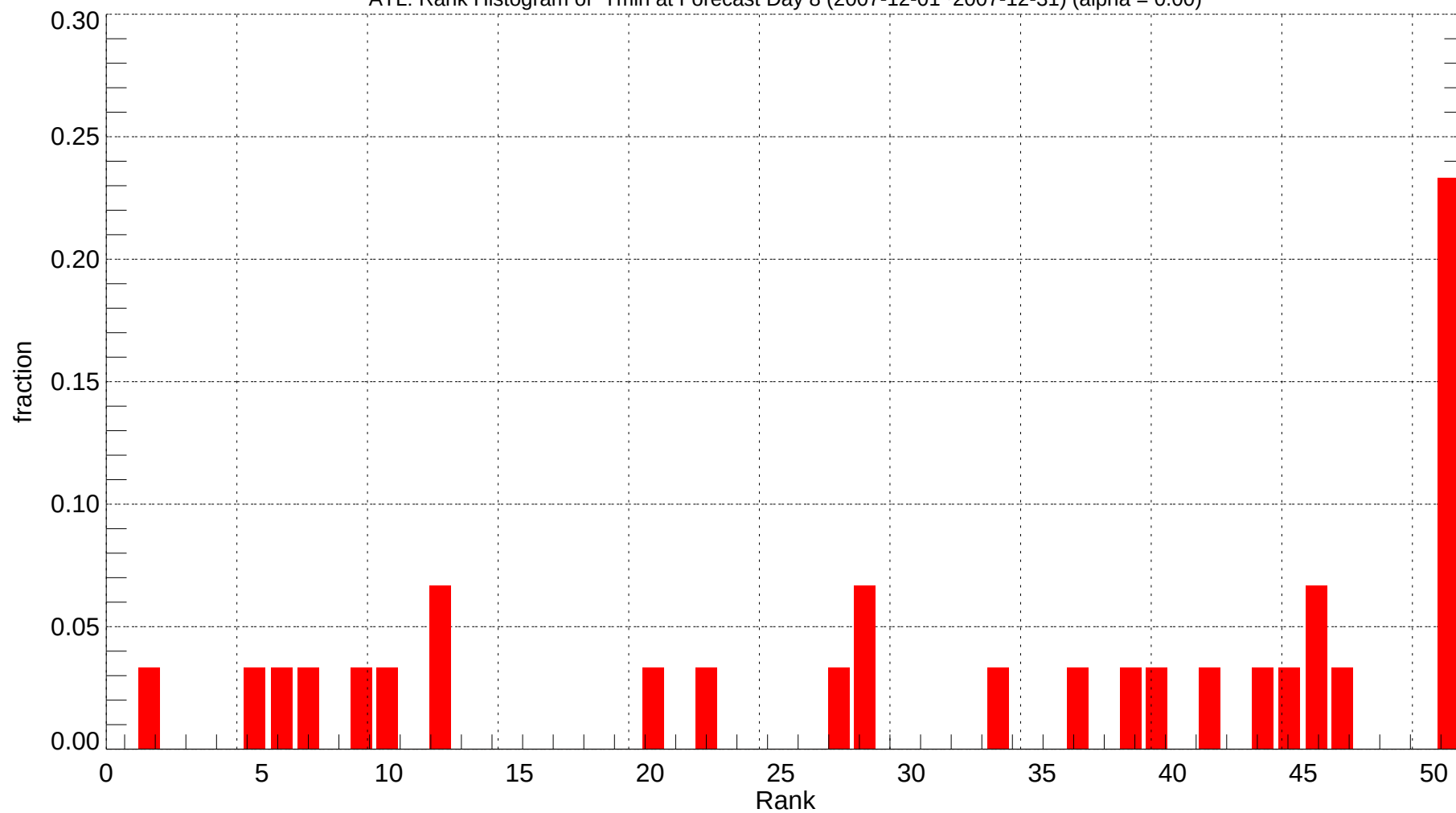
ATL: Rank Histogram of Tmin at Forecast Day 8 (2007-12-01~2007-12-31) (alpha = 0.00)
