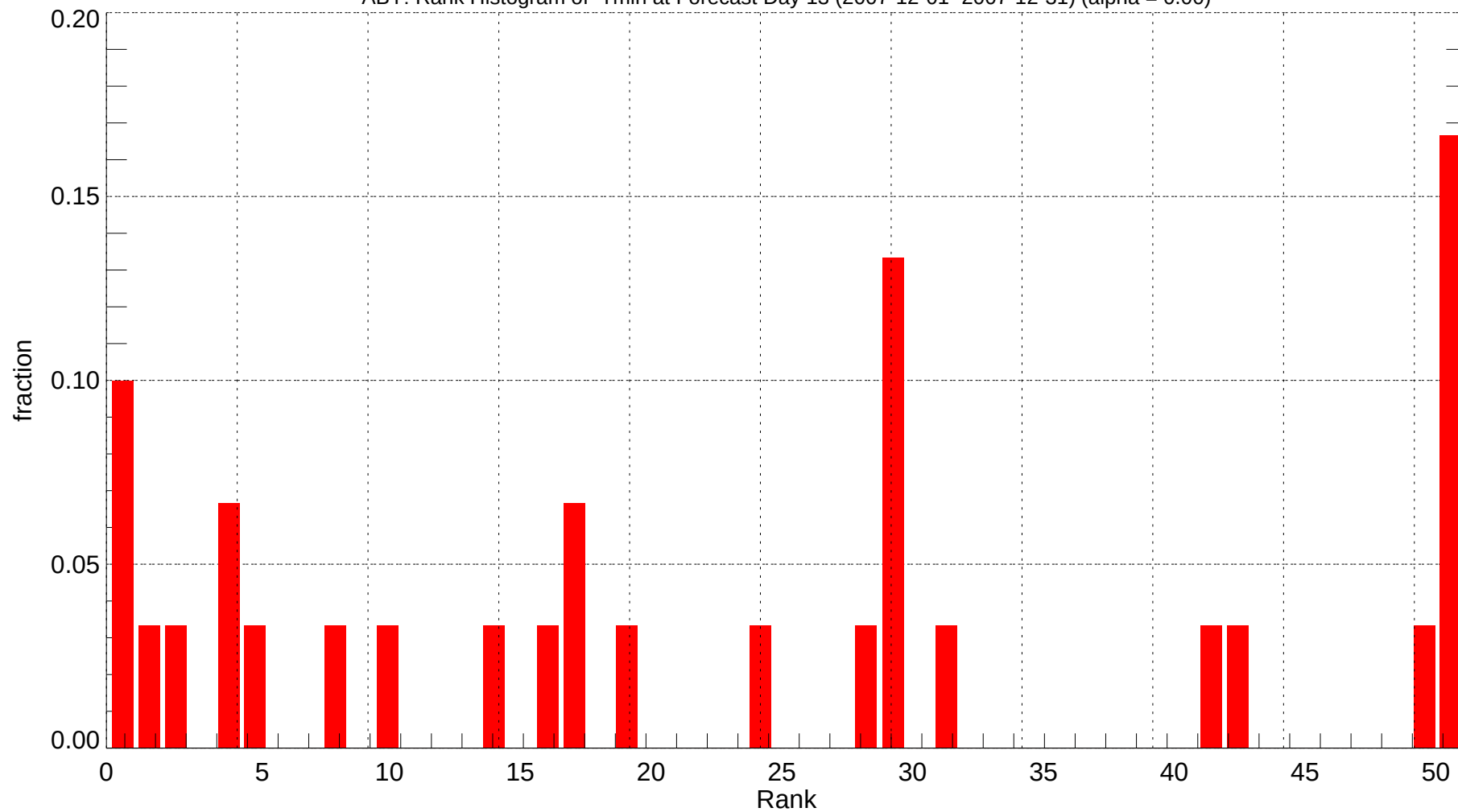
ABY: Rank Histogram of Tmin at Forecast Day 13 (2007-12-01~2007-12-31) (alpha = 0.00)
