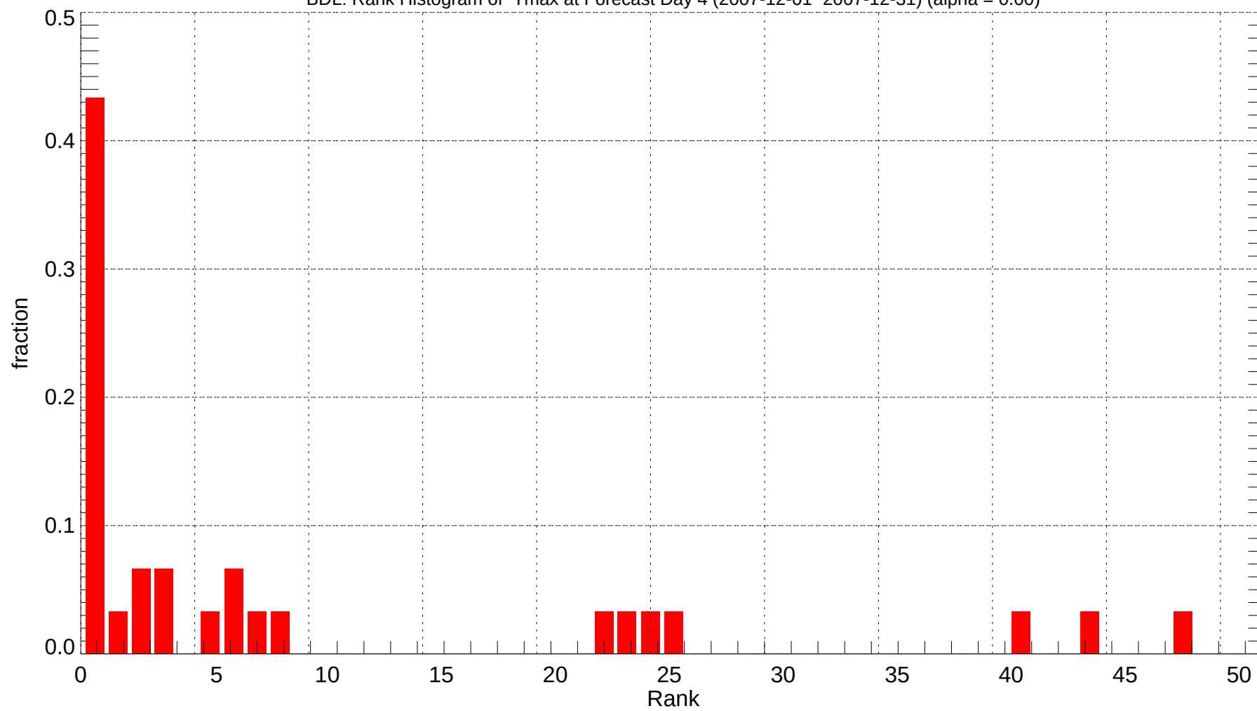
BDL: Rank Histogram of Tmax at Forecast Day 4 (2007-12-01~2007-12-31) (alpha = 0.00)
