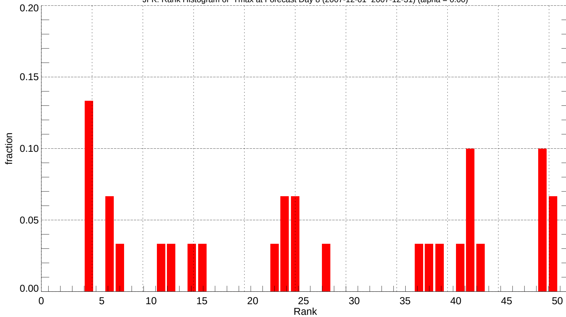
JFK: Rank Histogram of Tmax at Forecast Day 8 (2007-12-01~2007-12-31) (alpha = 0.00)
