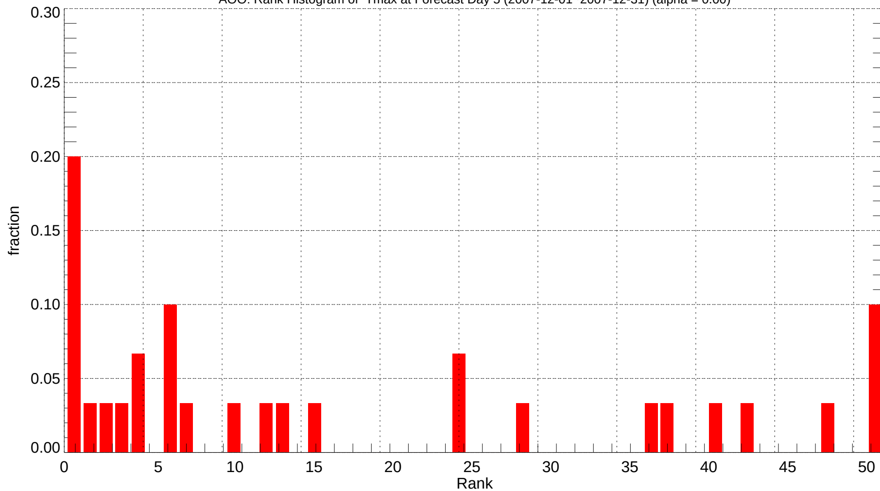
AOO: Rank Histogram of Tmax at Forecast Day 5 (2007-12-01~2007-12-31) (alpha = 0.00)
