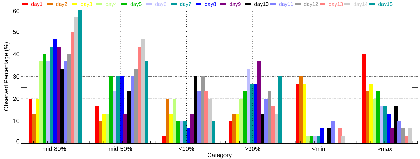
Observed Percentage of Ensembles - OKC: Max Temperature (2007-12-01~2007-12-31)
