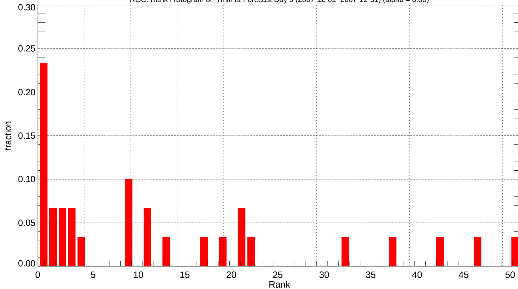
ROC: Rank Histogram of Tmin at Forecast Day 9 (2007-12-01~2007-12-31) (alpha = 0.00)
