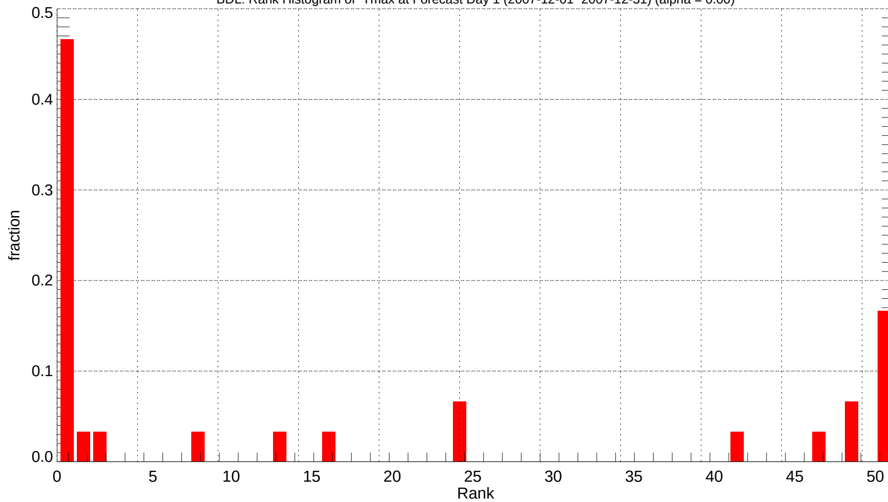
BDL: Rank Histogram of Tmax at Forecast Day 1 (2007-12-01~2007-12-31) (alpha = 0.00)
