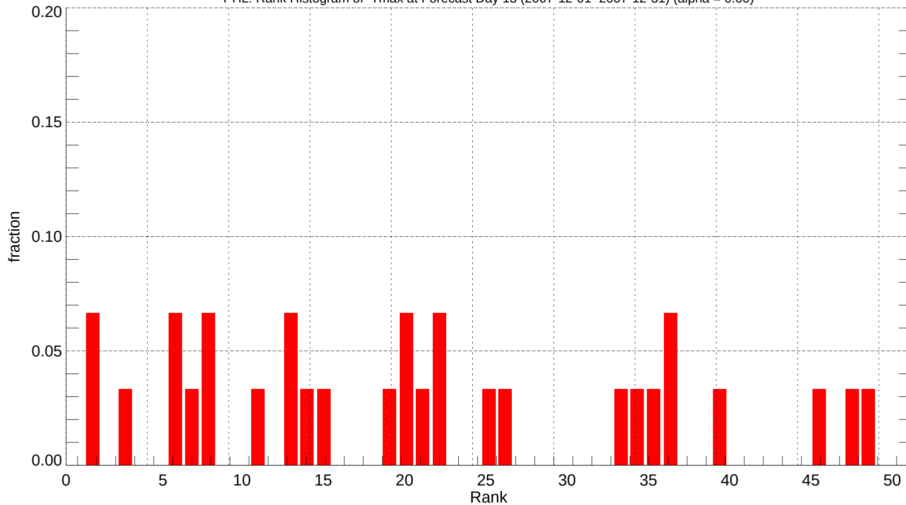
PHL: Rank Histogram of Tmax at Forecast Day 13 (2007-12-01~2007-12-31) (alpha = 0.00)
