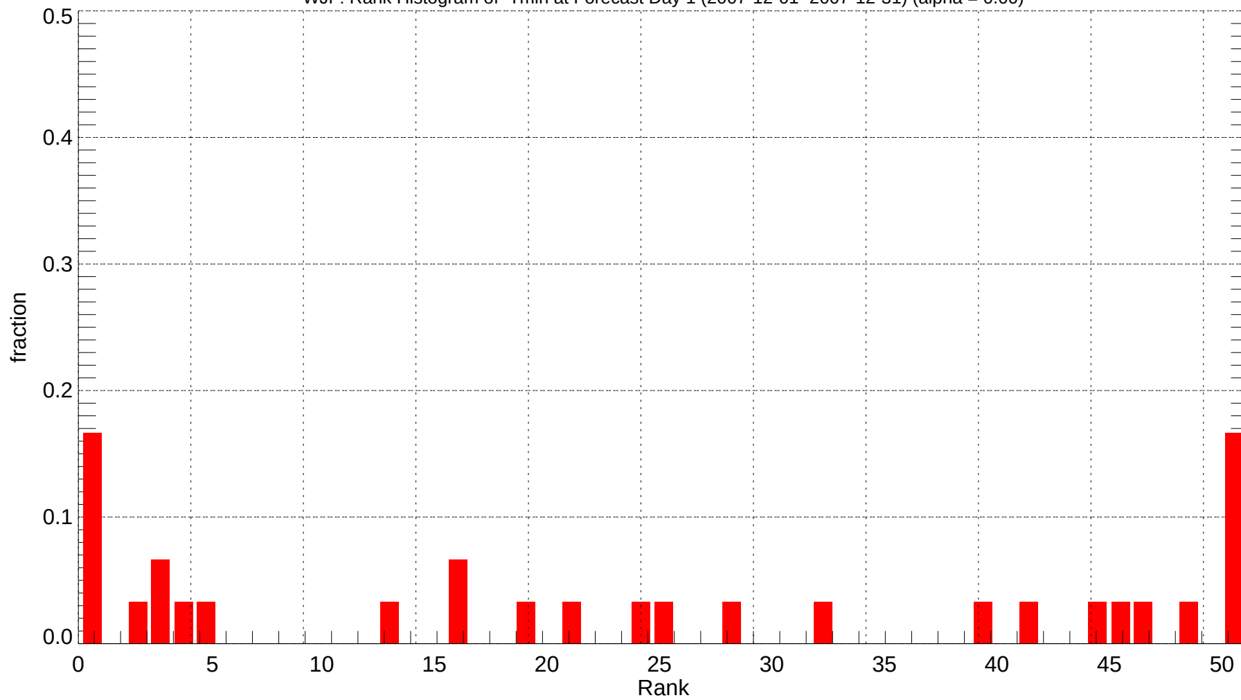
WJF: Rank Histogram of Tmin at Forecast Day 1 (2007-12-01~2007-12-31) (alpha = 0.00)
