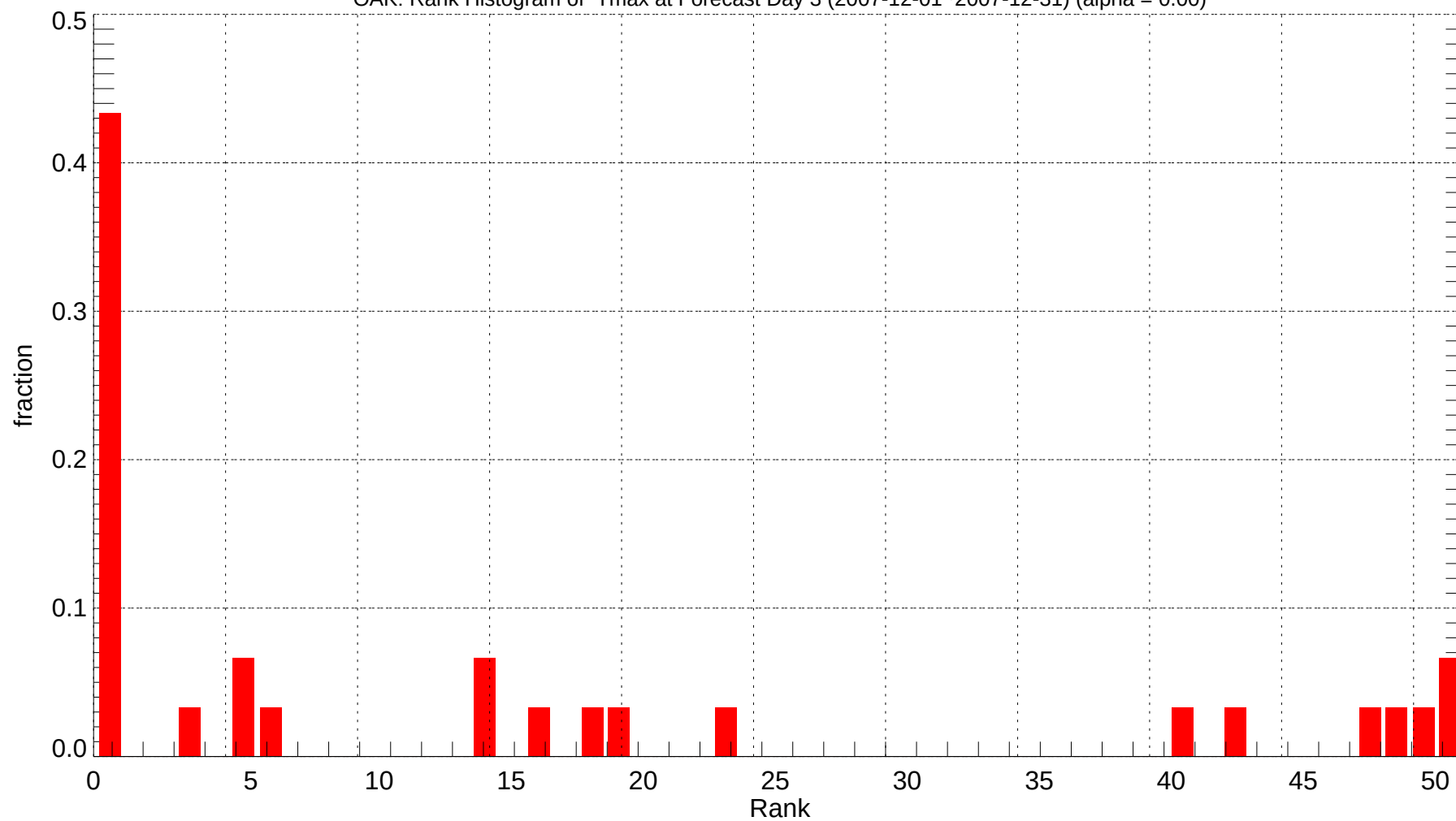
OAK: Rank Histogram of Tmax at Forecast Day 3 (2007-12-01~2007-12-31) (alpha = 0.00)
