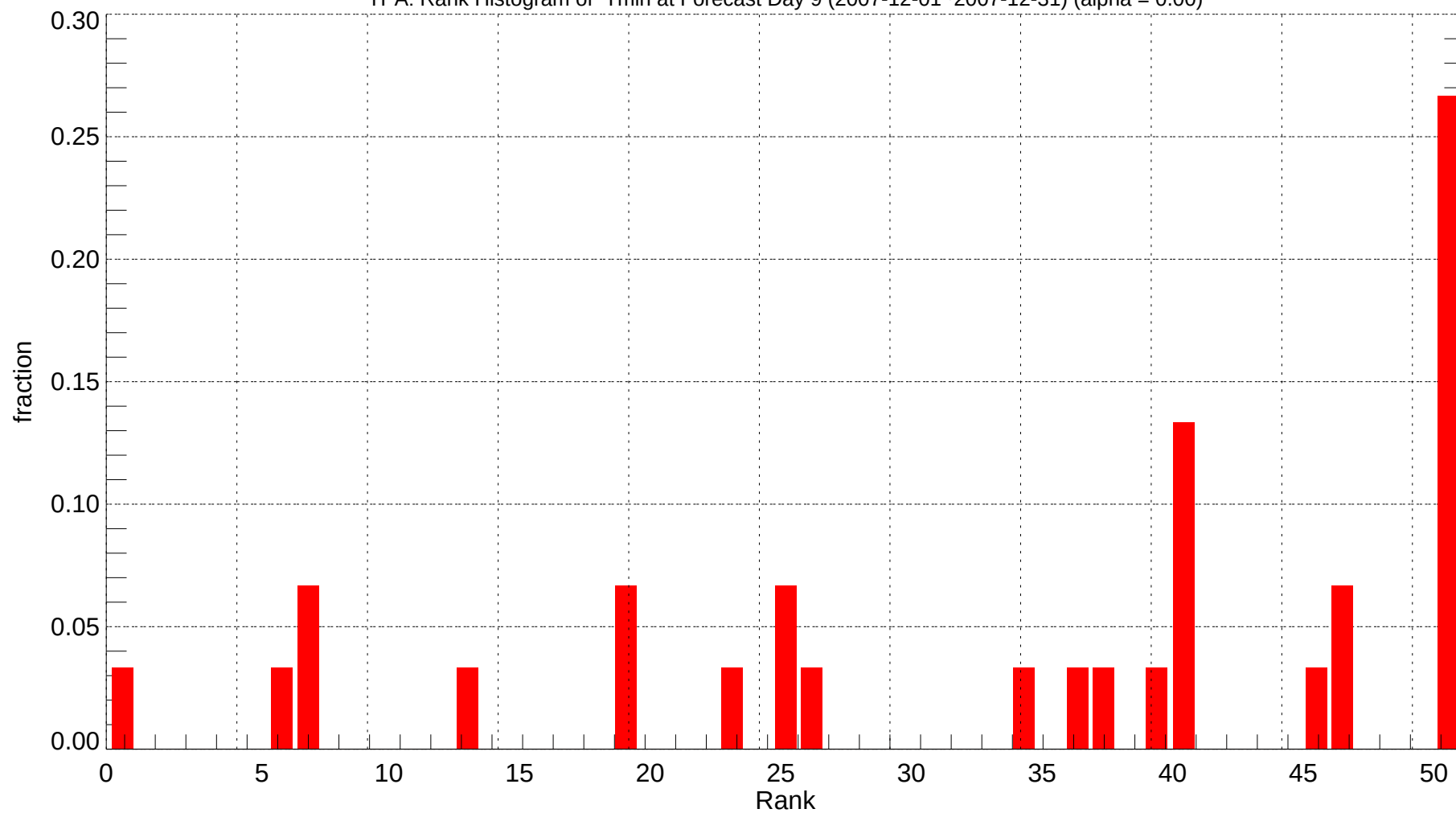
TPA: Rank Histogram of Tmin at Forecast Day 9 (2007-12-01~2007-12-31) (alpha = 0.00)
