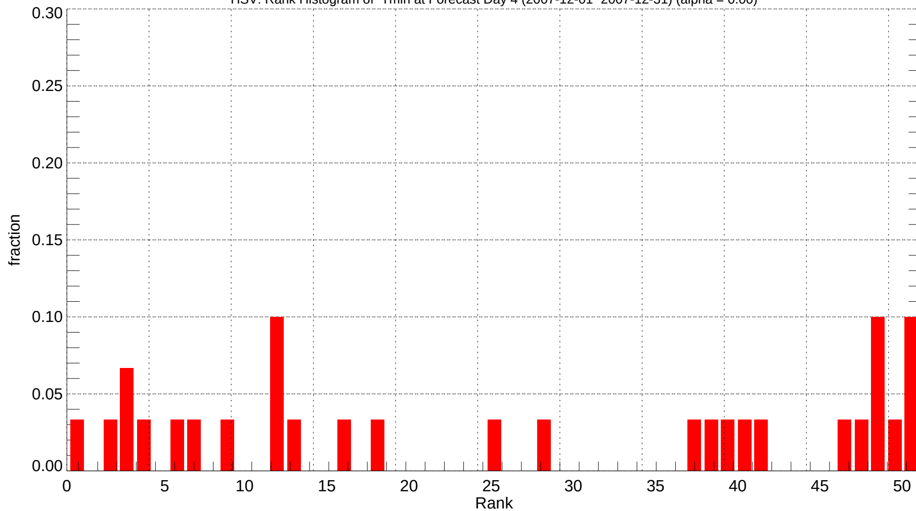
HSV: Rank Histogram of Tmin at Forecast Day 4 (2007-12-01~2007-12-31) (alpha = 0.00)
