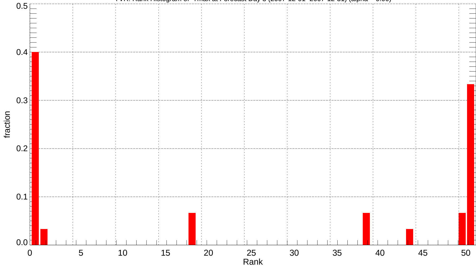
YVR: Rank Histogram of Tmax at Forecast Day 3 (2007-12-01~2007-12-31) (alpha = 0.00)
