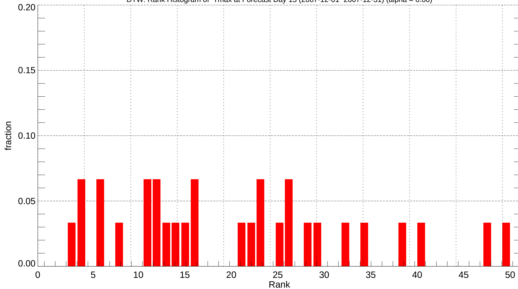
DTW: Rank Histogram of Tmax at Forecast Day 15 (2007-12-01~2007-12-31) (alpha = 0.00)
