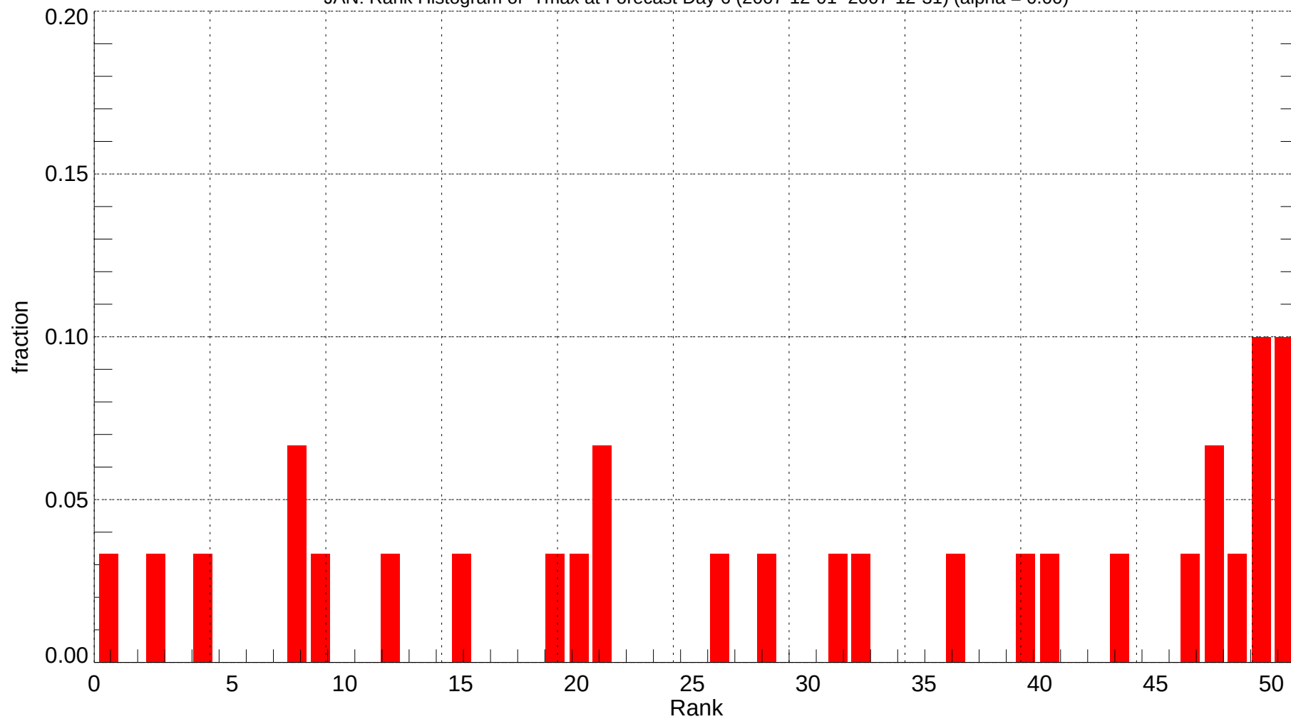
JAN: Rank Histogram of Tmax at Forecast Day 6 (2007-12-01~2007-12-31) (alpha = 0.00)
