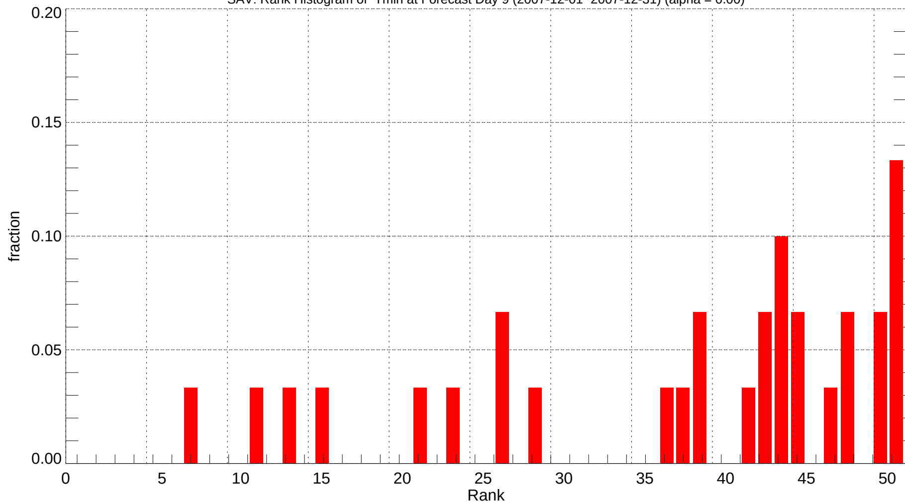
SAV: Rank Histogram of Tmin at Forecast Day 9 (2007-12-01~2007-12-31) (alpha = 0.00)
