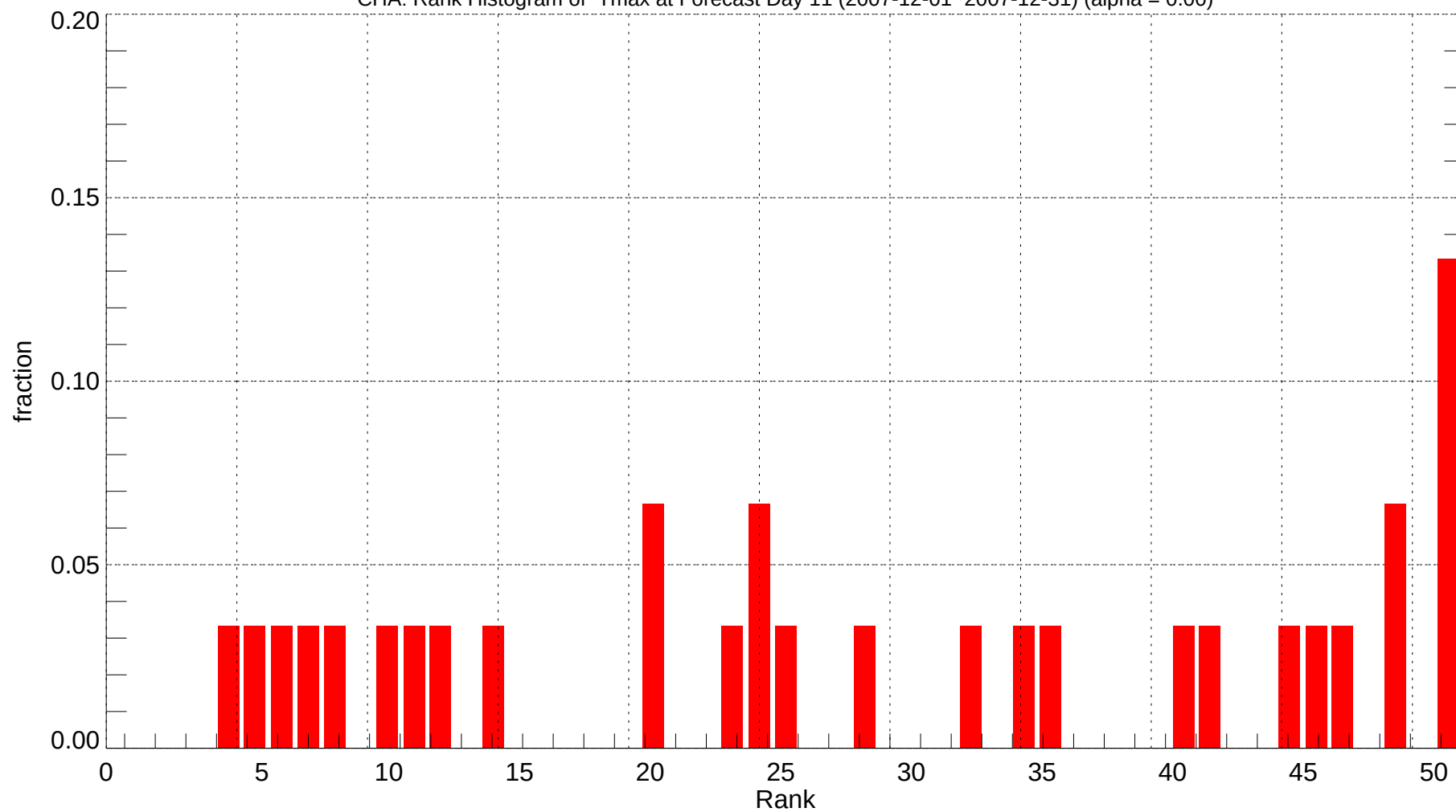
CHA: Rank Histogram of Tmax at Forecast Day 11 (2007-12-01~2007-12-31) (alpha = 0.00)
