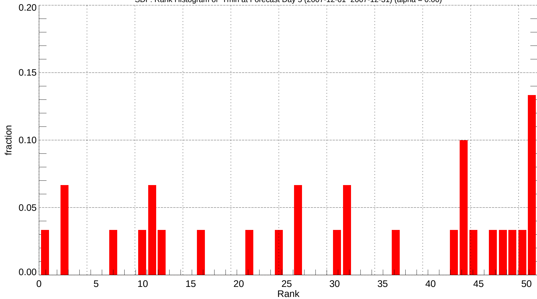
SDF: Rank Histogram of Tmin at Forecast Day 5 (2007-12-01~2007-12-31) (alpha = 0.00)
