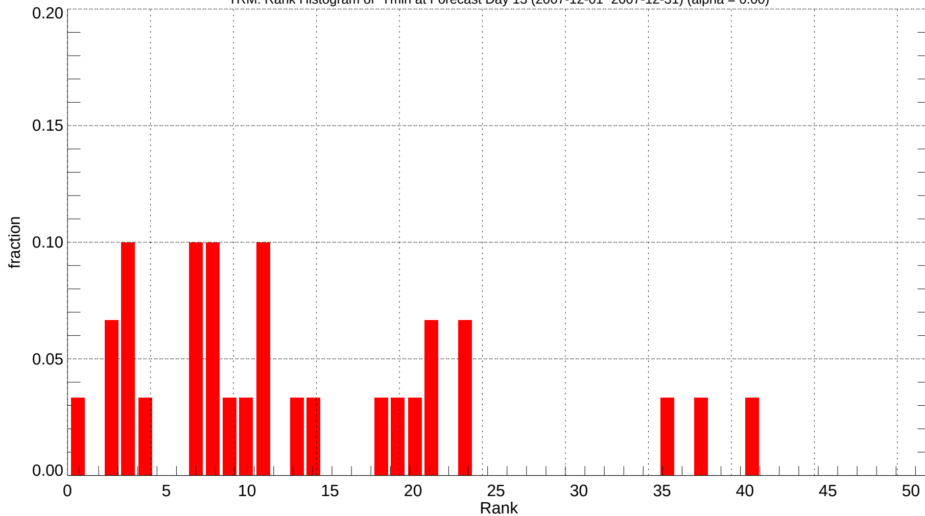
TRM: Rank Histogram of Tmin at Forecast Day 13 (2007-12-01~2007-12-31) (alpha = 0.00)
