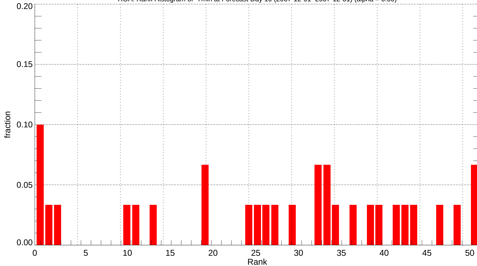
ROA: Rank Histogram of Tmin at Forecast Day 10 (2007-12-01~2007-12-31) (alpha = 0.00)
