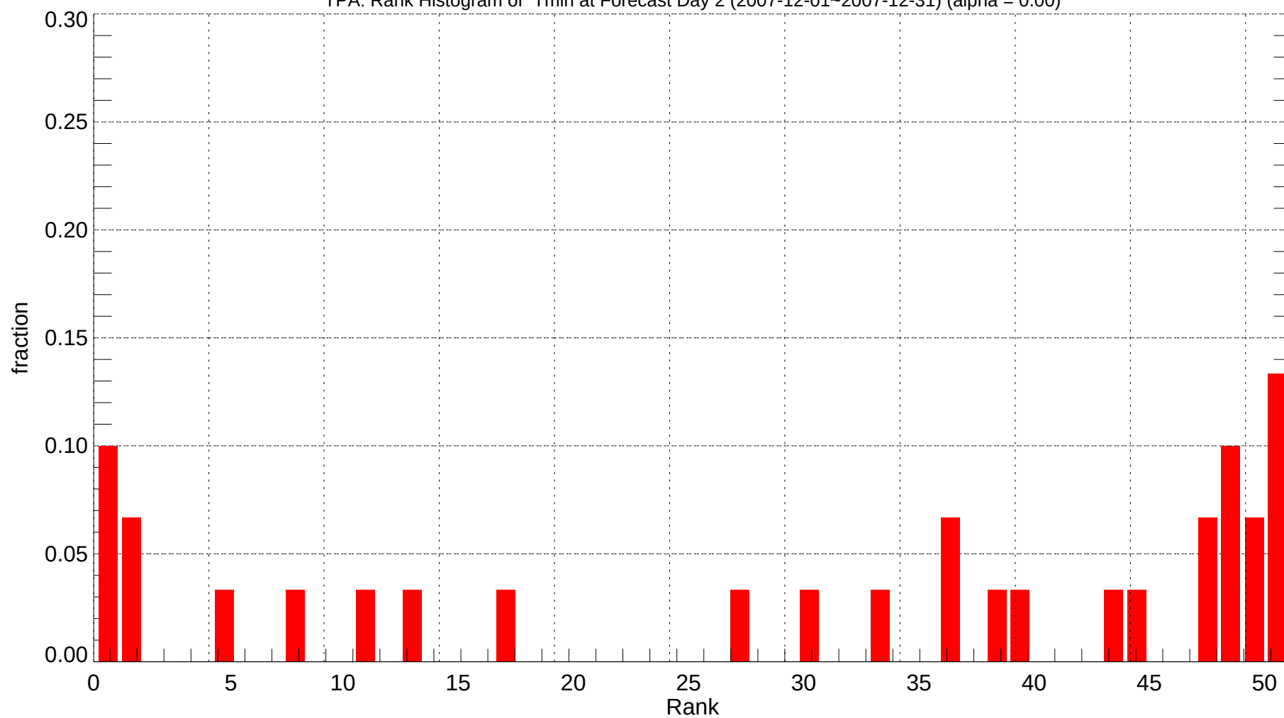
TPA: Rank Histogram of Tmin at Forecast Day 2 (2007-12-01~2007-12-31) (alpha = 0.00)
