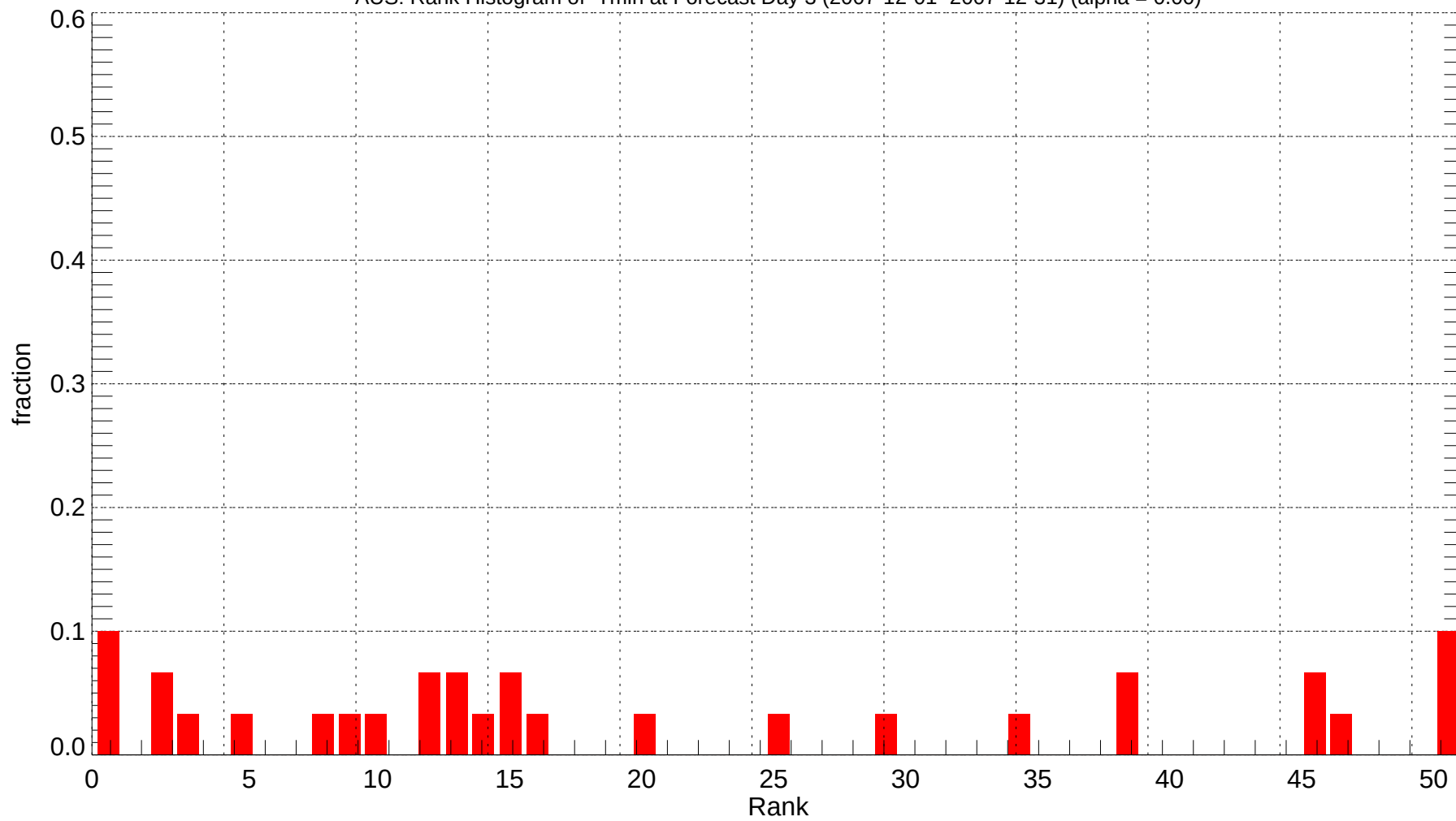
AUS: Rank Histogram of Tmin at Forecast Day 3 (2007-12-01~2007-12-31) (alpha = 0.00)
