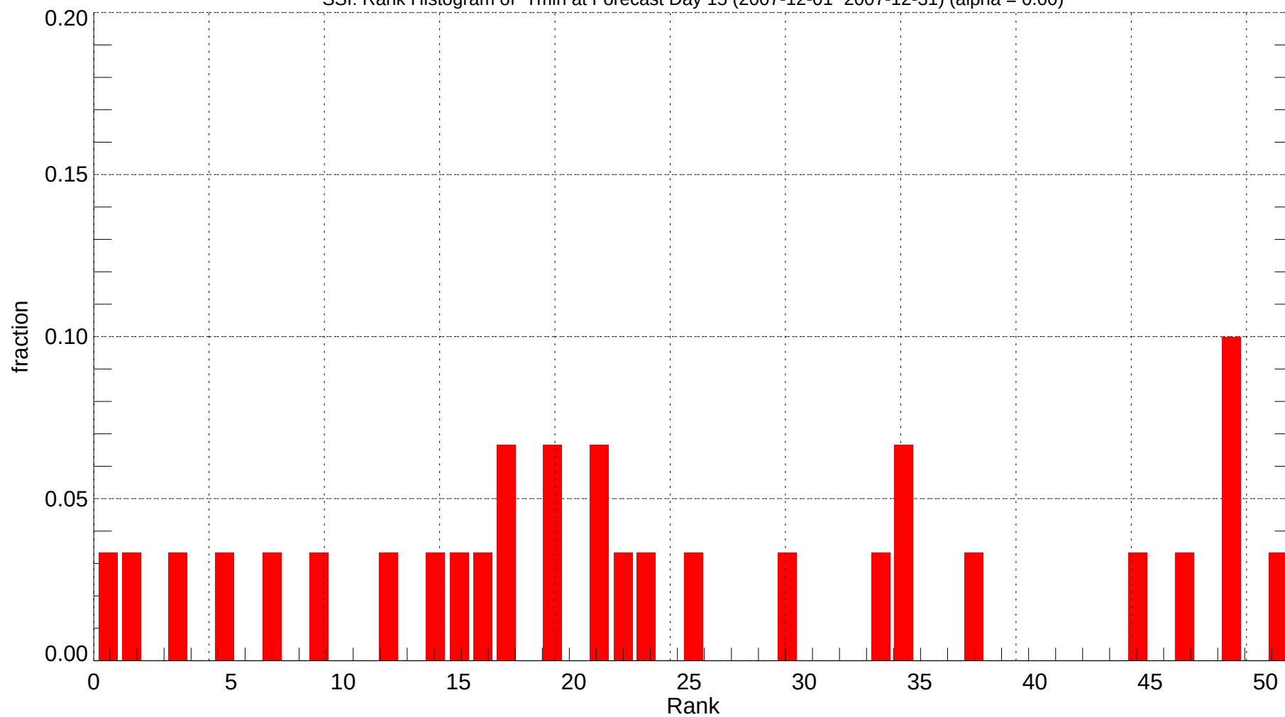
SSI: Rank Histogram of Tmin at Forecast Day 15 (2007-12-01~2007-12-31) (alpha = 0.00)
