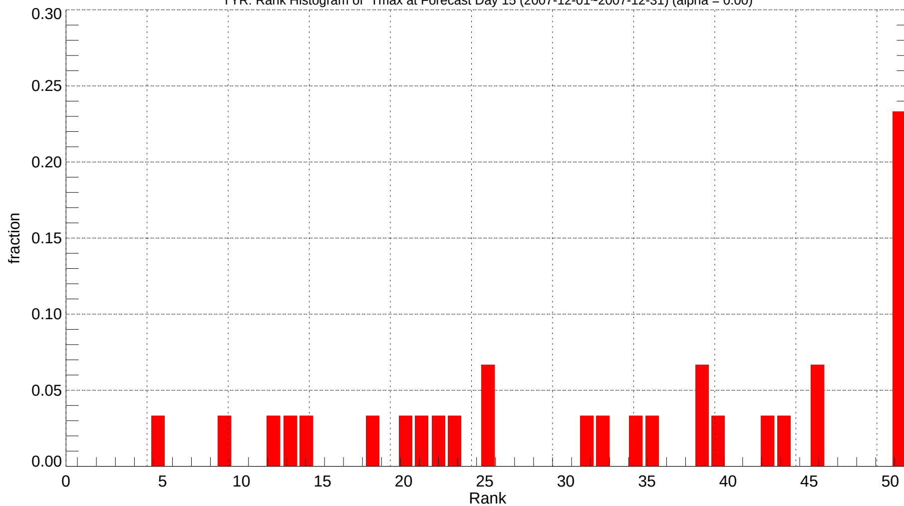
TYR: Rank Histogram of Tmax at Forecast Day 15 (2007-12-01~2007-12-31) (alpha = 0.00)
