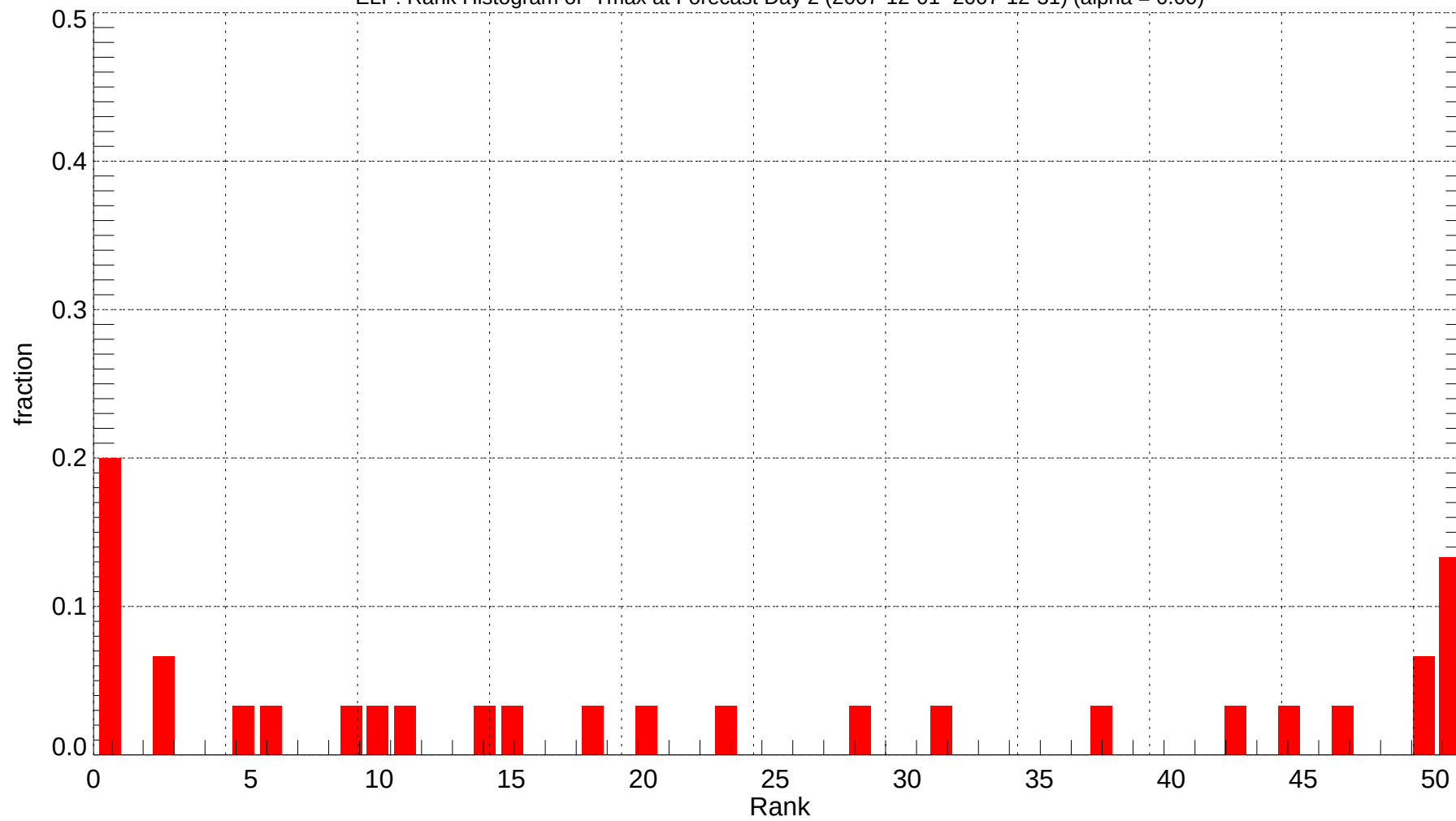
ELP: Rank Histogram of Tmax at Forecast Day 2 (2007-12-01~2007-12-31) (alpha = 0.00)
