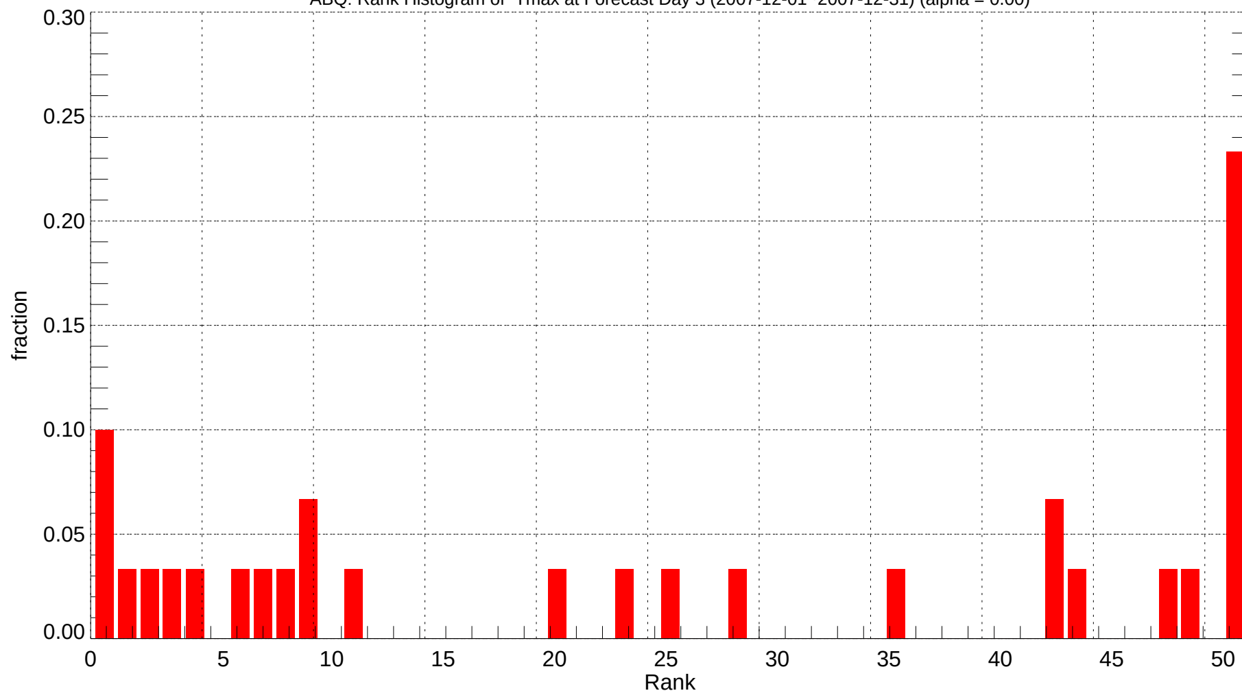
ABQ: Rank Histogram of Tmax at Forecast Day 3 (2007-12-01~2007-12-31) (alpha = 0.00)
