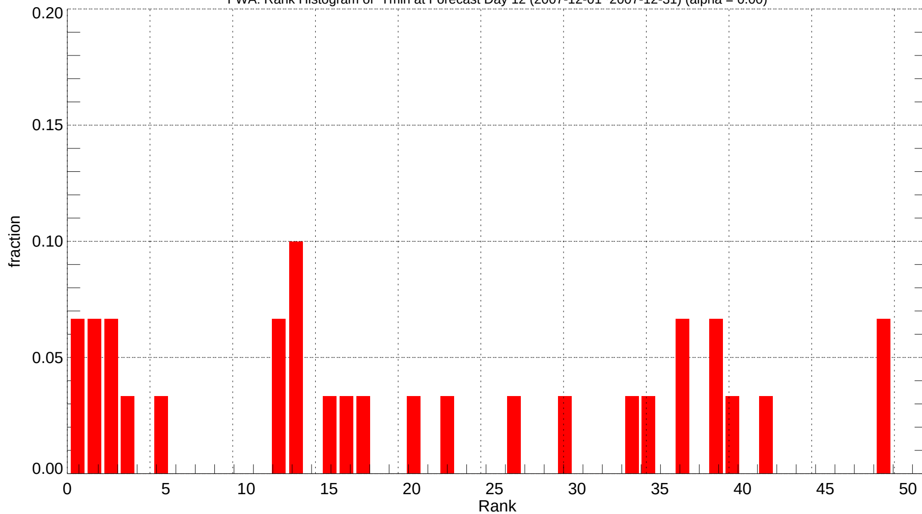
FWA: Rank Histogram of Tmin at Forecast Day 12 (2007-12-01~2007-12-31) (alpha = 0.00)
