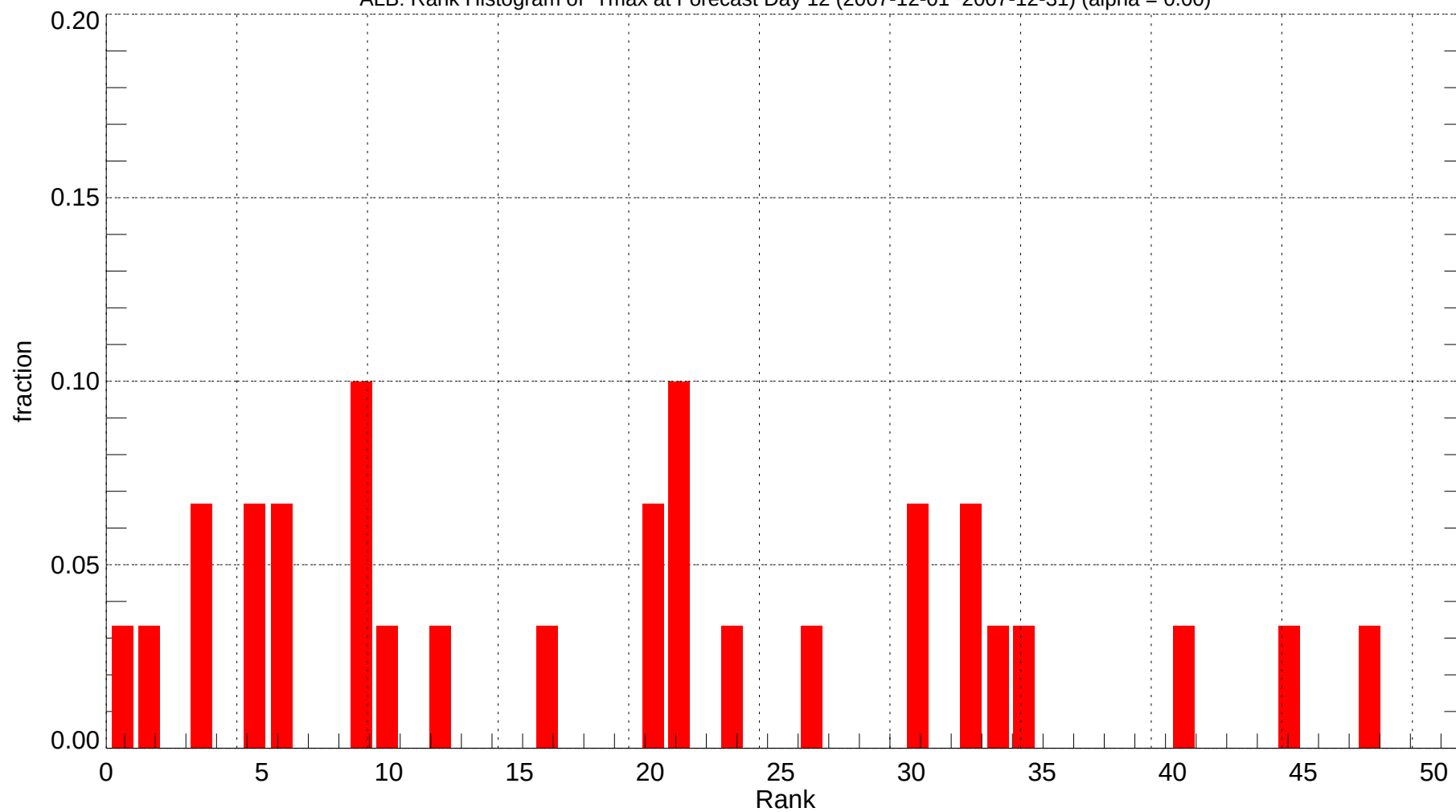
ALB: Rank Histogram of Tmax at Forecast Day 12 (2007-12-01~2007-12-31) (alpha = 0.00)
