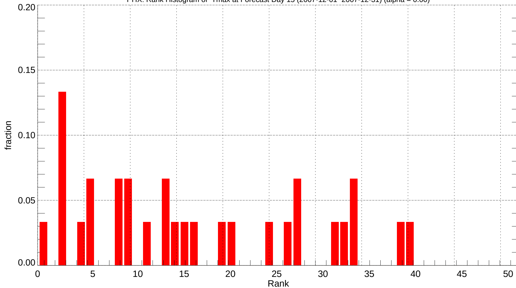
PHX: Rank Histogram of Tmax at Forecast Day 15 (2007-12-01~2007-12-31) (alpha = 0.00)
