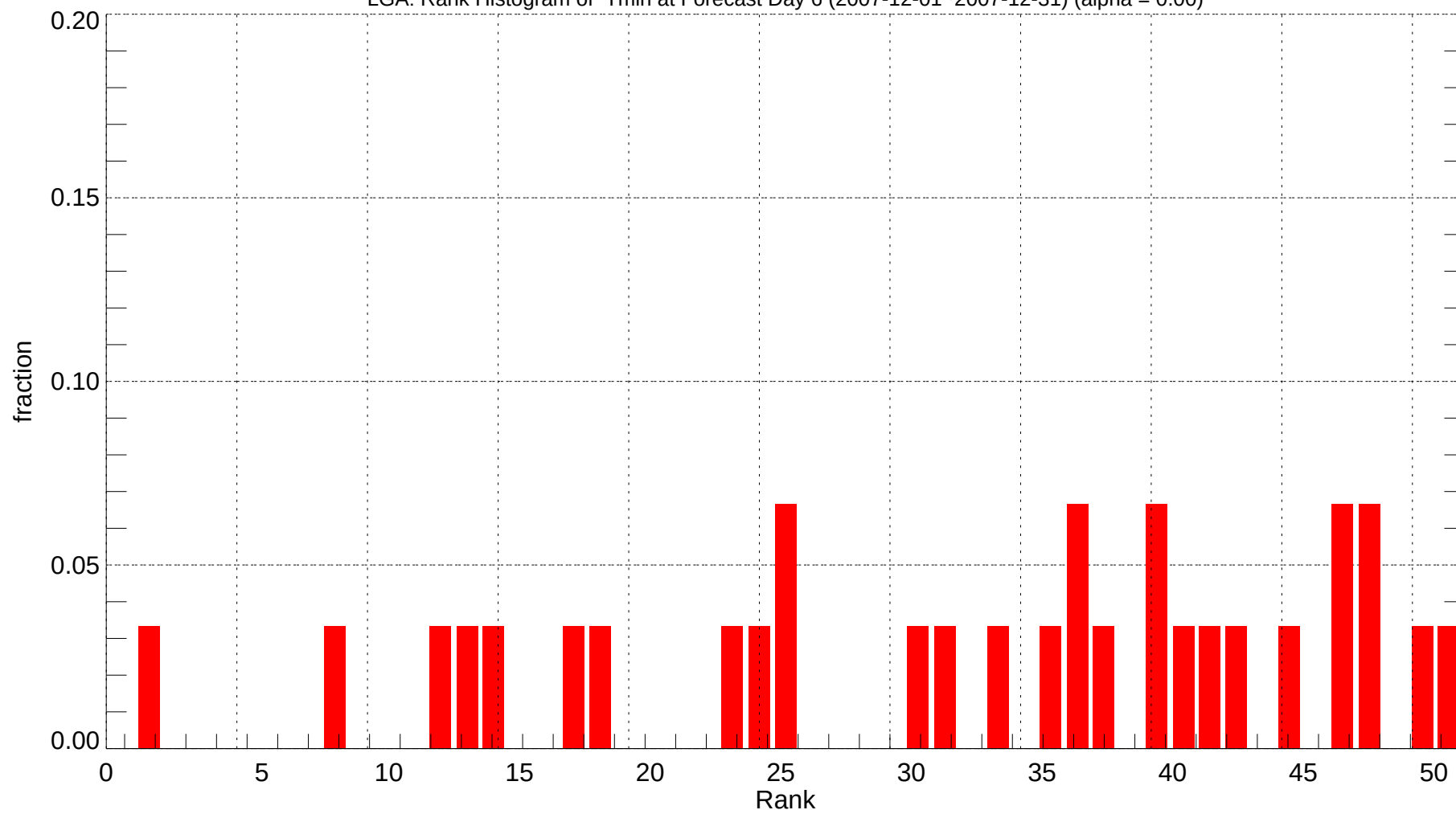
LGA: Rank Histogram of Tmin at Forecast Day 6 (2007-12-01~2007-12-31) (alpha = 0.00)
