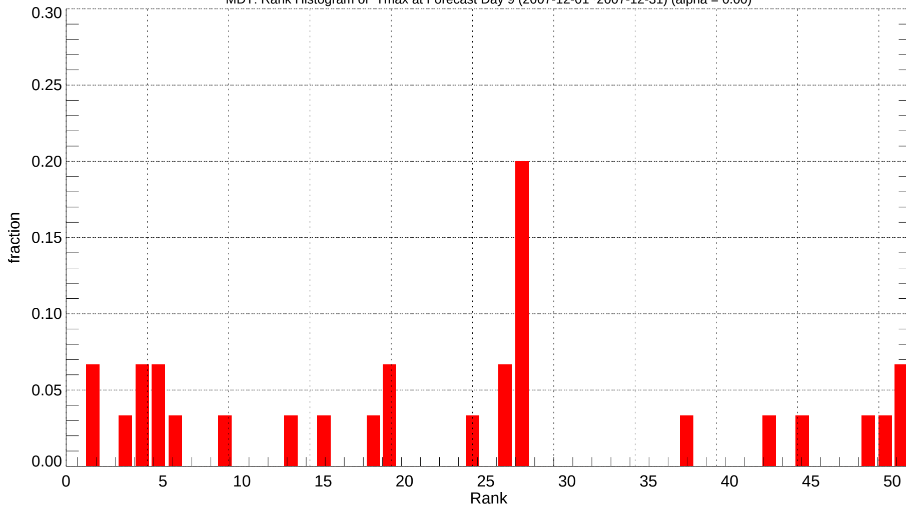
MDT: Rank Histogram of Tmax at Forecast Day 9 (2007-12-01~2007-12-31) (alpha = 0.00)
