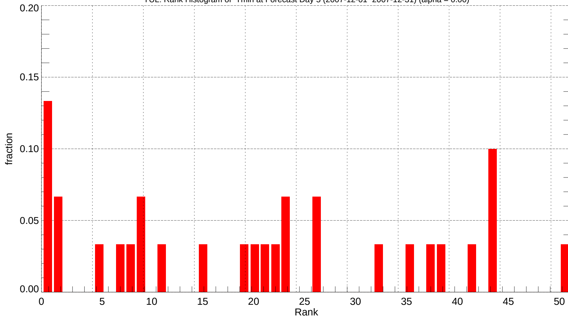
YUL: Rank Histogram of Tmin at Forecast Day 5 (2007-12-01~2007-12-31) (alpha = 0.00)
