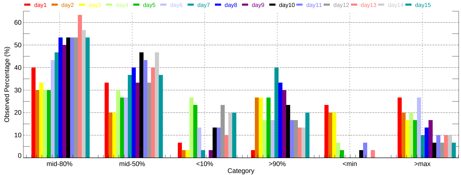
Observed Percentage of Ensembles - RDU: Min Temperature (2007-12-01~2007-12-31)
