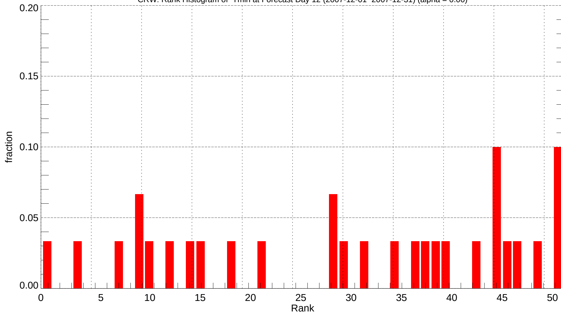
CRW: Rank Histogram of Tmin at Forecast Day 12 (2007-12-01~2007-12-31) (alpha = 0.00)
