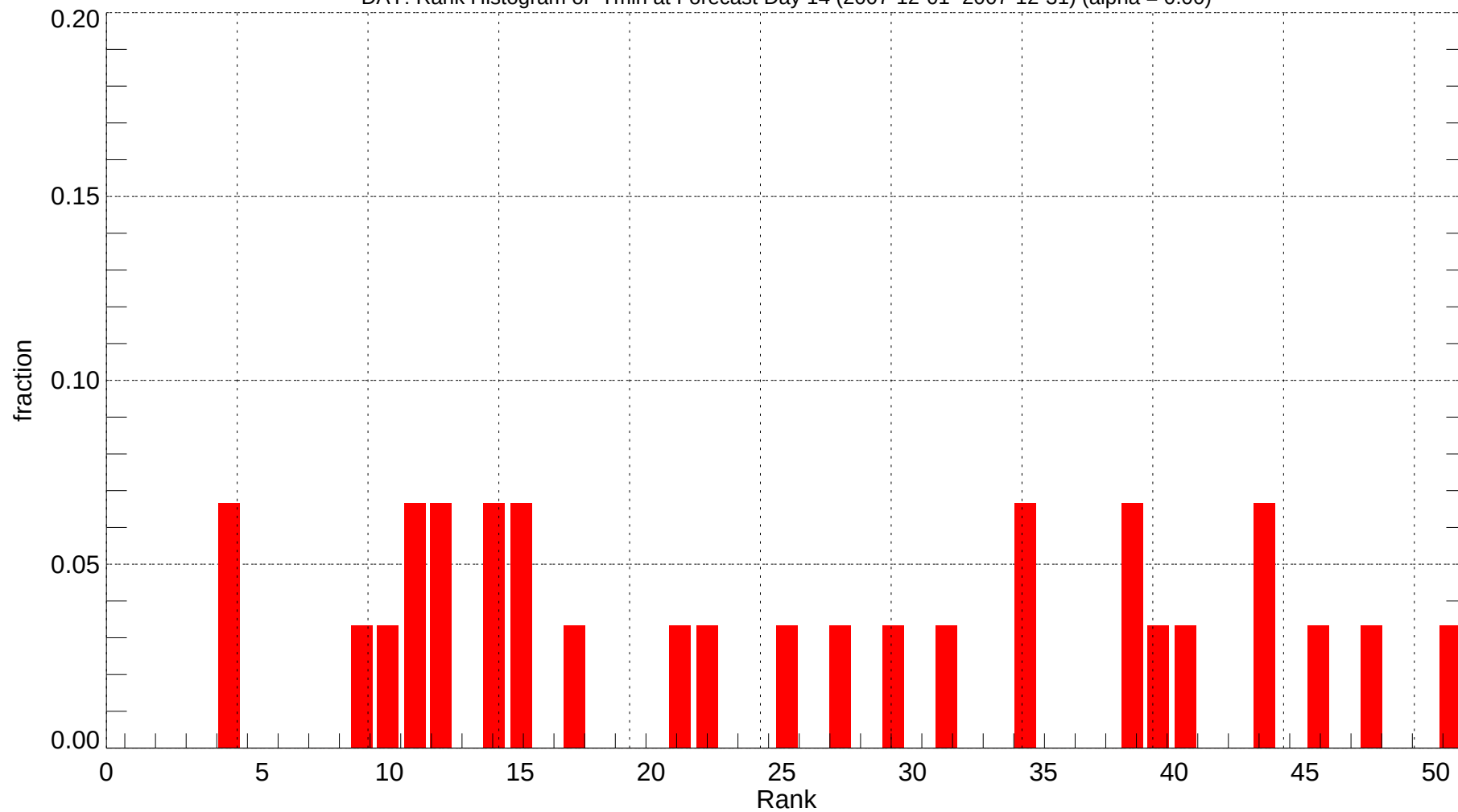
DAY: Rank Histogram of Tmin at Forecast Day 14 (2007-12-01~2007-12-31) (alpha = 0.00)
