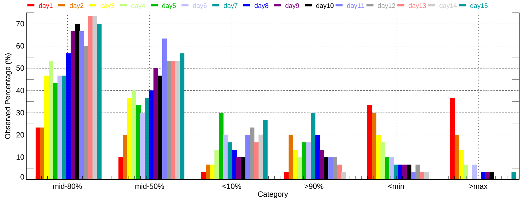
Observed Percentage of Ensembles - BTV: Max Temperature (2007-12-01~2007-12-31)
