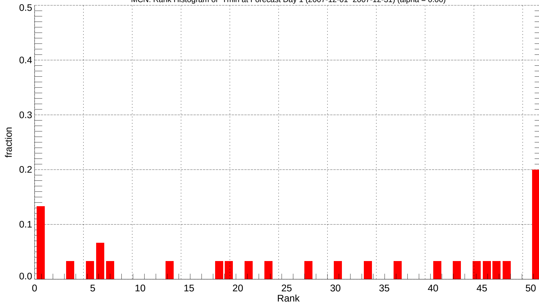
MCN: Rank Histogram of Tmin at Forecast Day 1 (2007-12-01~2007-12-31) (alpha = 0.00)
