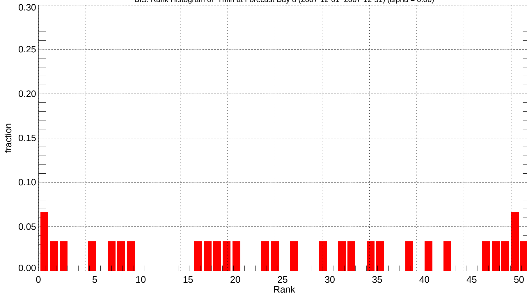
BIS: Rank Histogram of Tmin at Forecast Day 8 (2007-12-01~2007-12-31) (alpha = 0.00)
