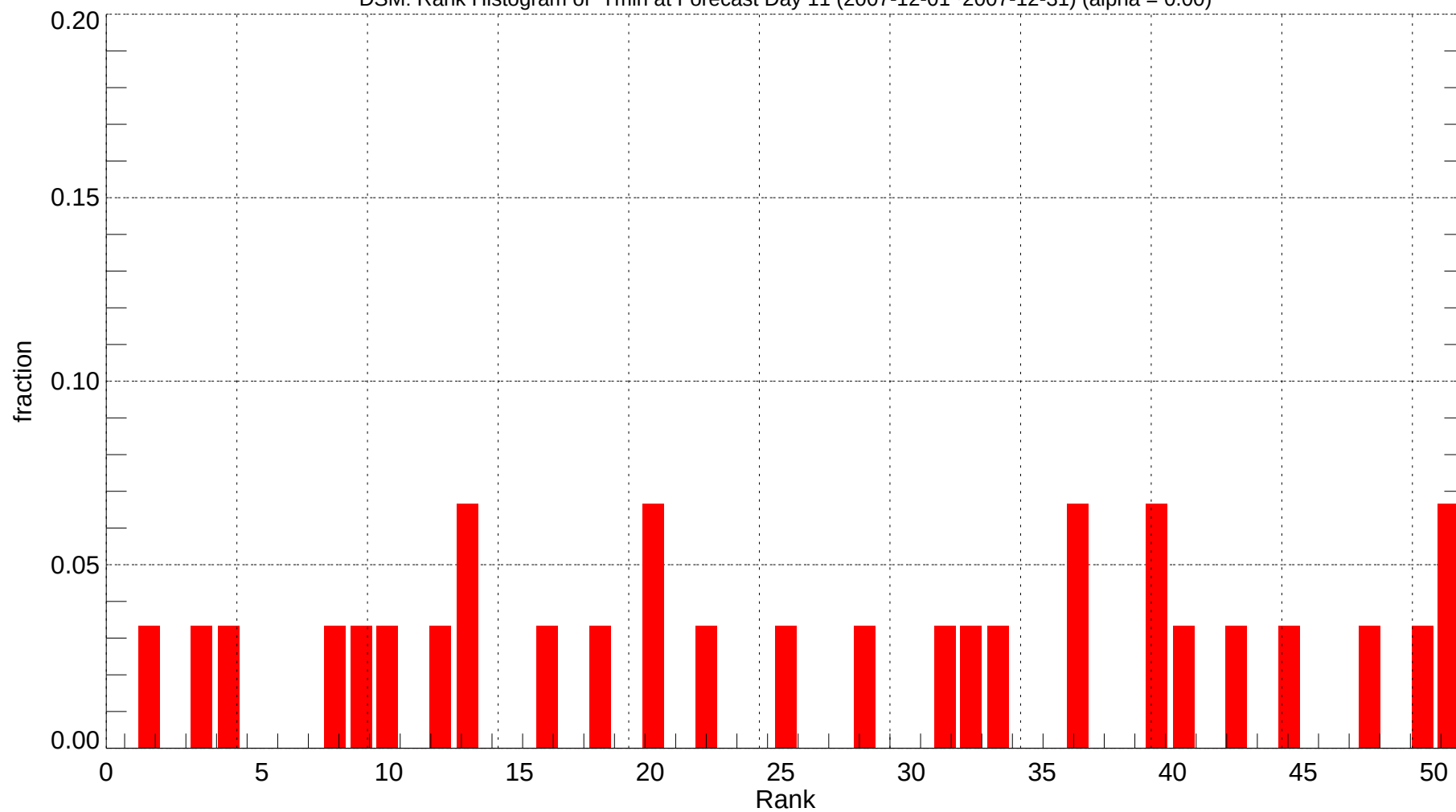
DSM: Rank Histogram of Tmin at Forecast Day 11 (2007-12-01~2007-12-31) (alpha = 0.00)
