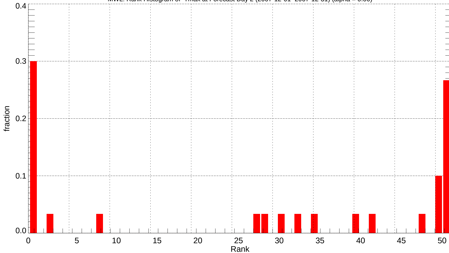
MWL: Rank Histogram of Tmax at Forecast Day 2 (2007-12-01~2007-12-31) (alpha = 0.00)
