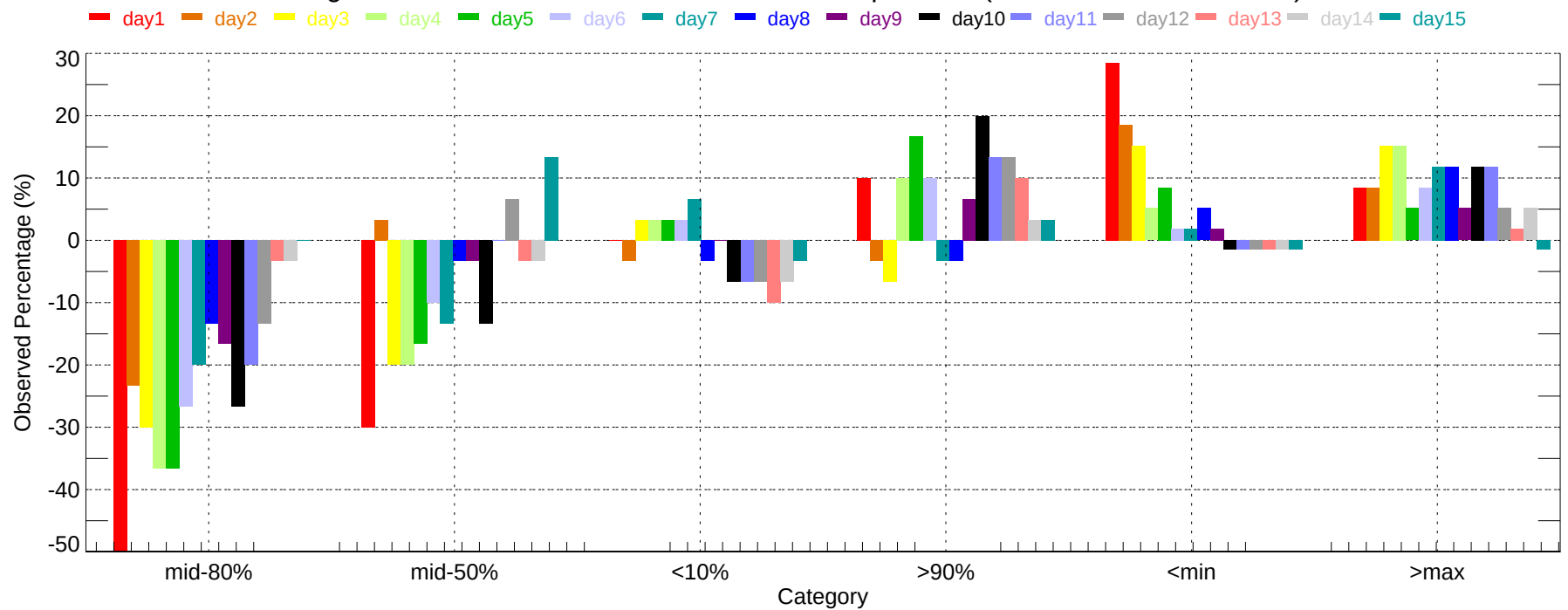
Observed Percentage Deviation of Ensembles - SEA: Max Temperature (2007-12-01~2007-12-31)
