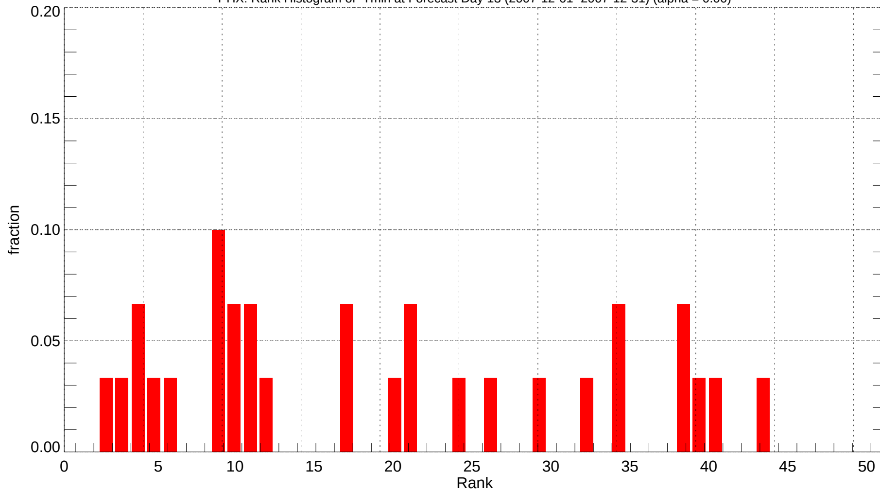
PHX: Rank Histogram of Tmin at Forecast Day 13 (2007-12-01~2007-12-31) (alpha = 0.00)
