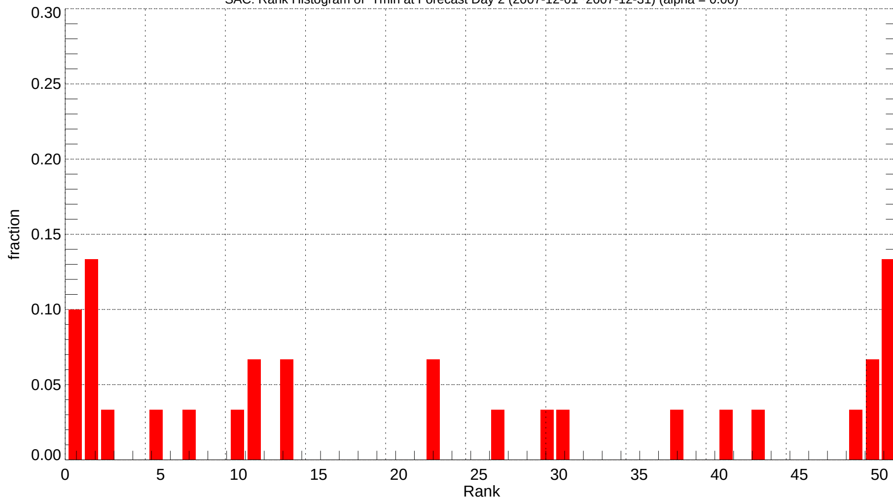
SAC: Rank Histogram of Tmin at Forecast Day 2 (2007-12-01~2007-12-31) (alpha = 0.00)
