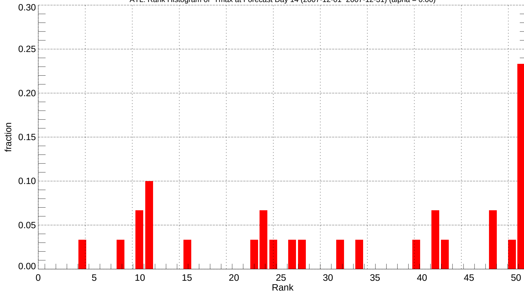
ATL: Rank Histogram of Tmax at Forecast Day 14 (2007-12-01~2007-12-31) (alpha = 0.00)
