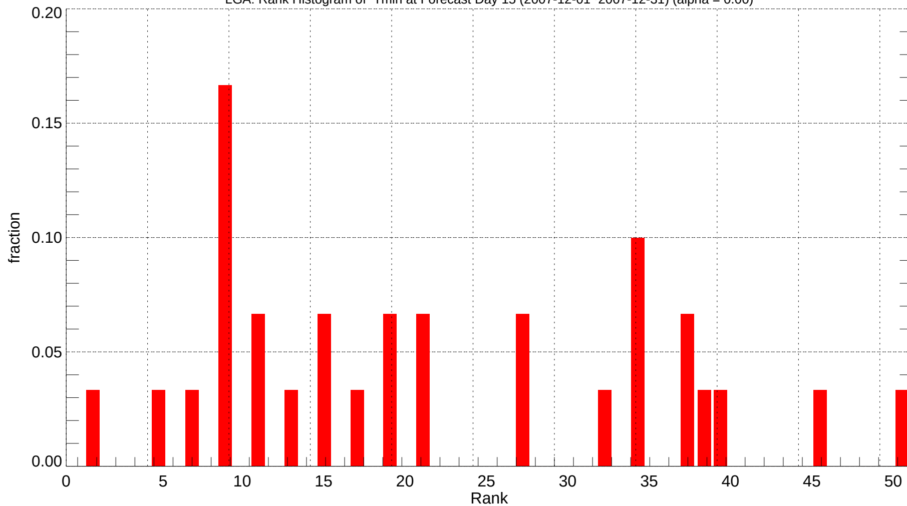
LGA: Rank Histogram of Tmin at Forecast Day 15 (2007-12-01~2007-12-31) (alpha = 0.00)
