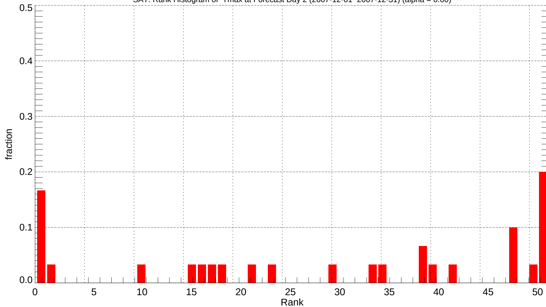
SAT: Rank Histogram of Tmax at Forecast Day 2 (2007-12-01~2007-12-31) (alpha = 0.00)
