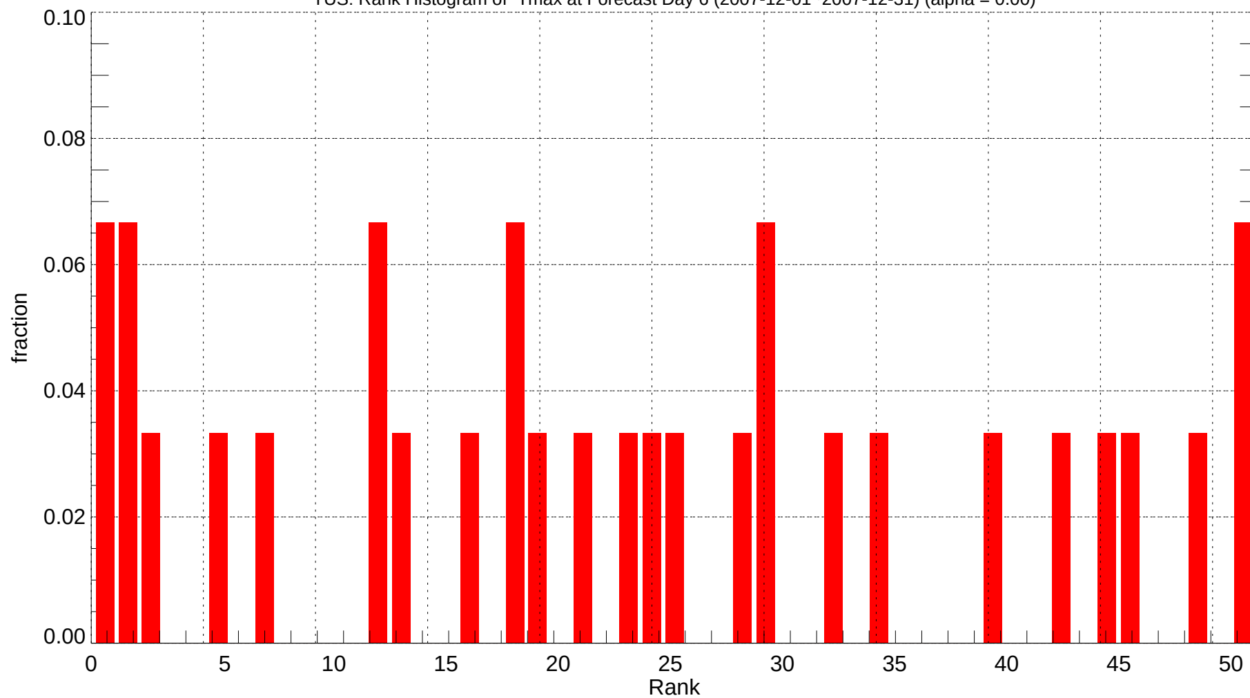
TUS: Rank Histogram of Tmax at Forecast Day 6 (2007-12-01~2007-12-31) (alpha = 0.00)
