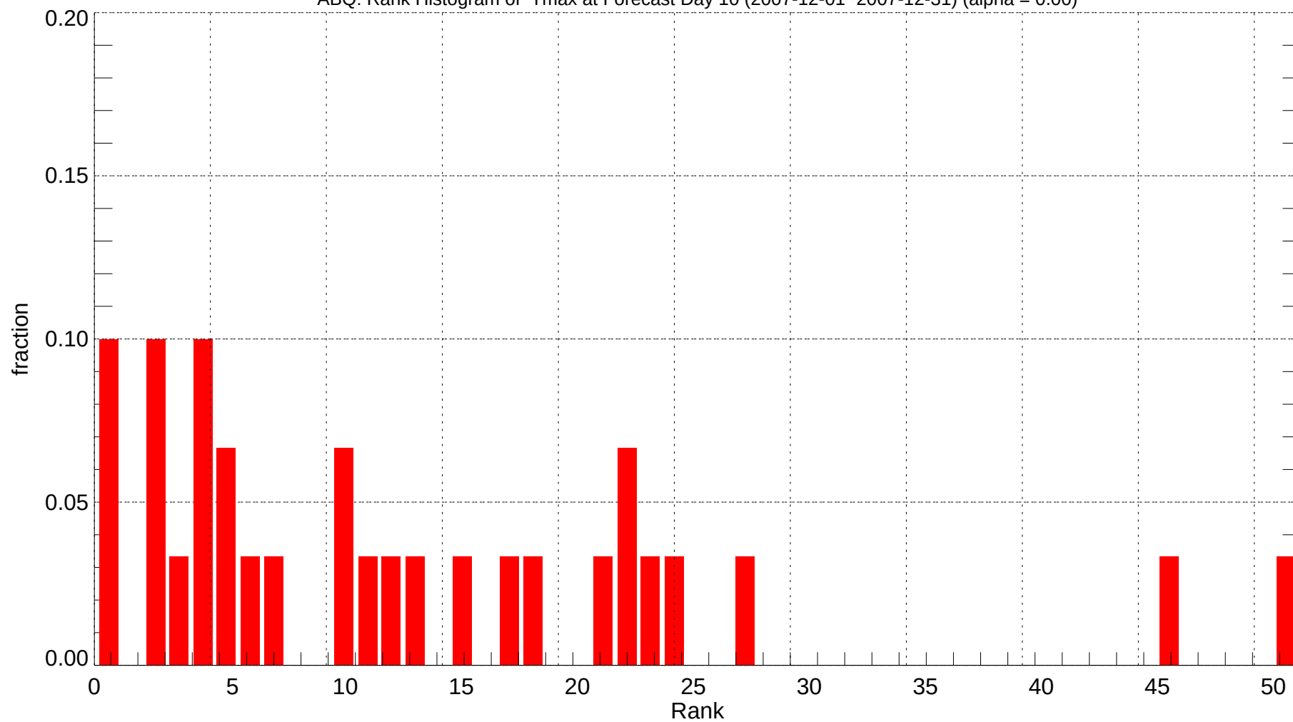
ABQ: Rank Histogram of Tmax at Forecast Day 10 (2007-12-01~2007-12-31) (alpha = 0.00)
