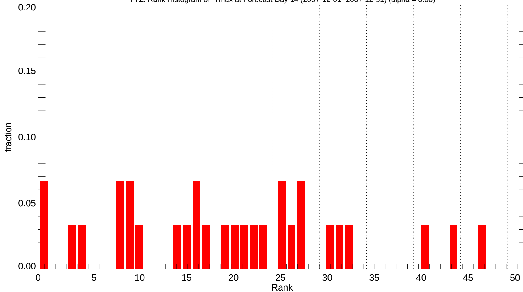
YYZ: Rank Histogram of Tmax at Forecast Day 14 (2007-12-01~2007-12-31) (alpha = 0.00)
