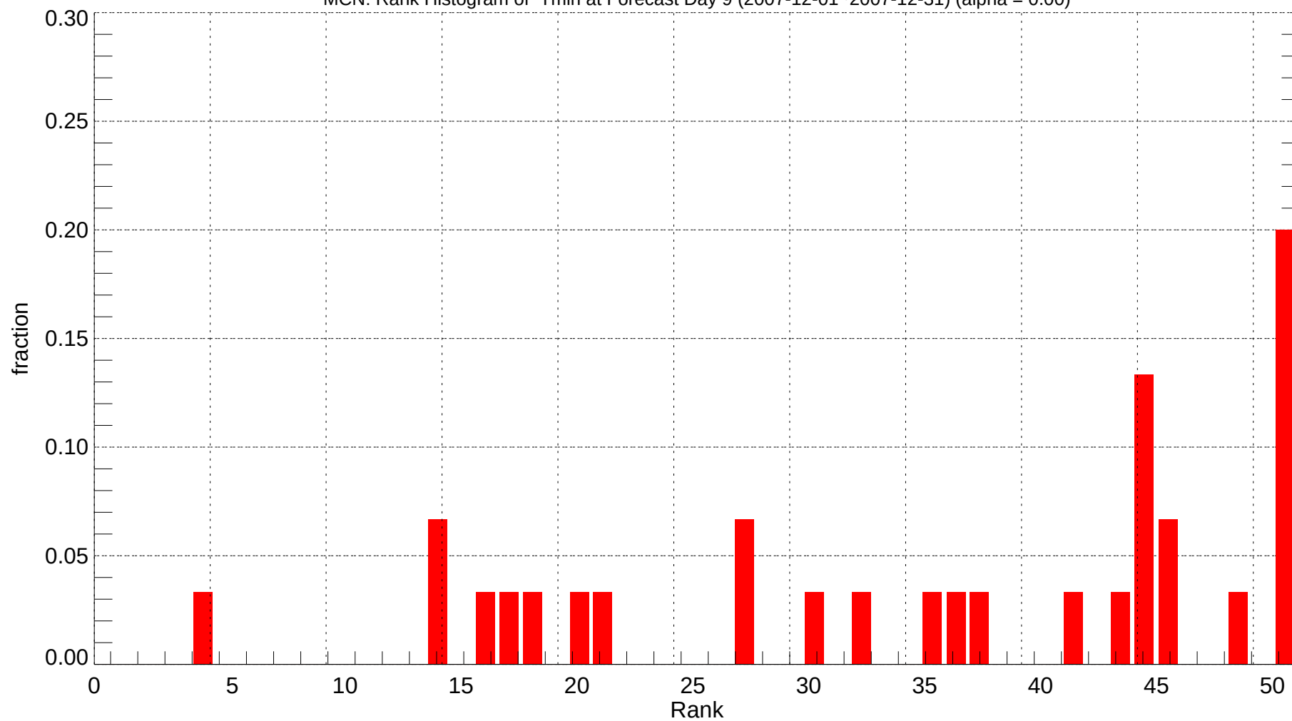
MCN: Rank Histogram of Tmin at Forecast Day 9 (2007-12-01~2007-12-31) (alpha = 0.00)
