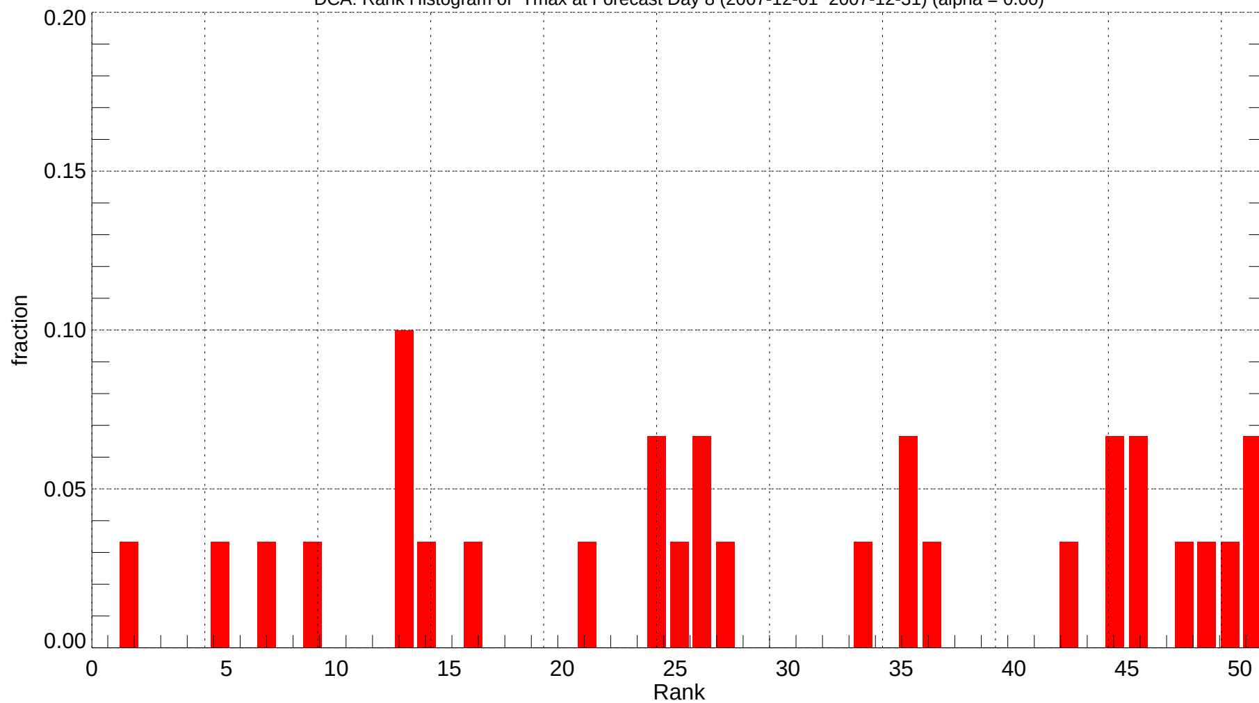
DCA: Rank Histogram of Tmax at Forecast Day 8 (2007-12-01~2007-12-31) (alpha = 0.00)
