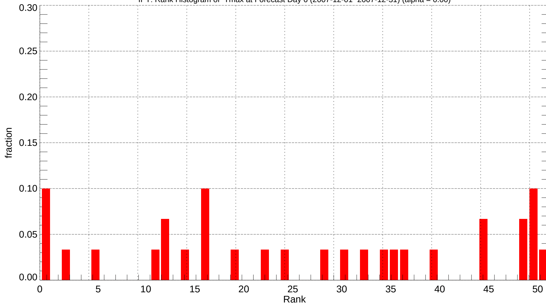
IPT: Rank Histogram of Tmax at Forecast Day 6 (2007-12-01~2007-12-31) (alpha = 0.00)
