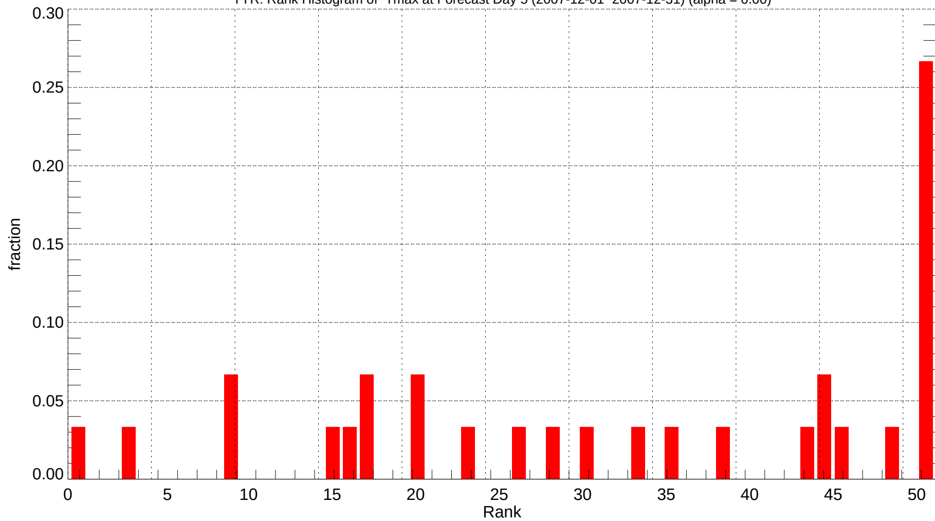
TYR: Rank Histogram of Tmax at Forecast Day 5 (2007-12-01~2007-12-31) (alpha = 0.00)
