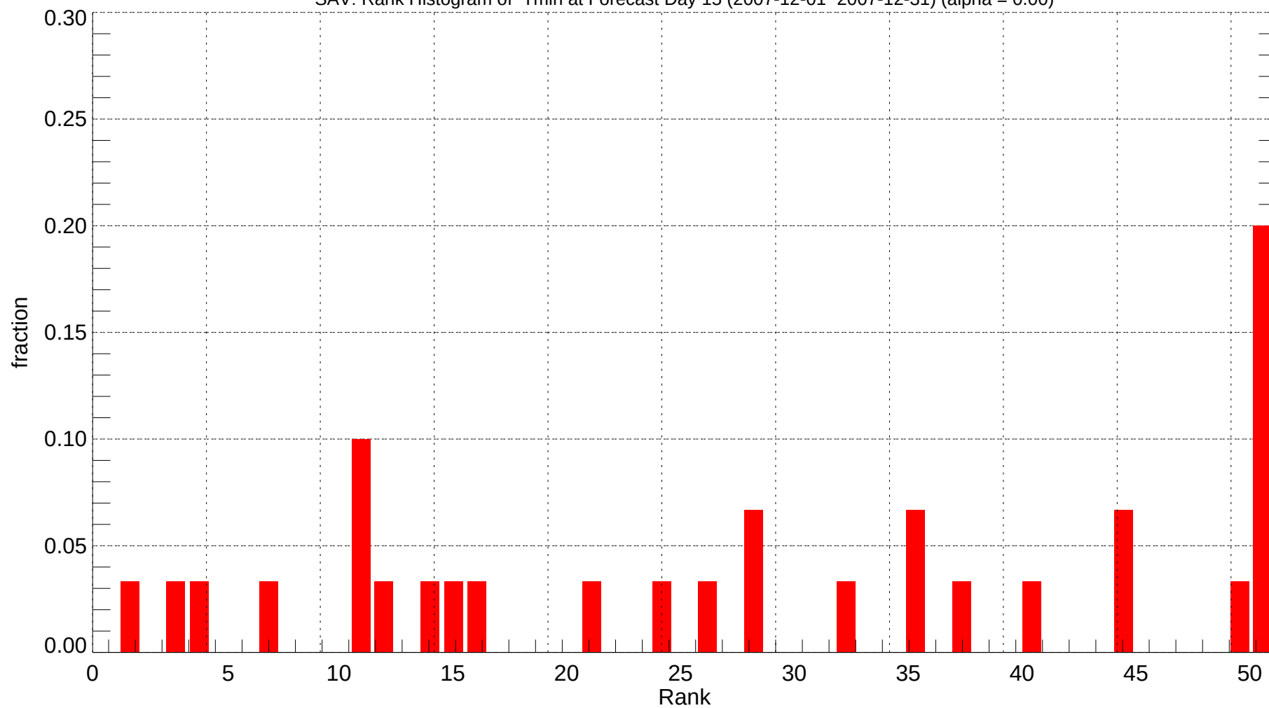
SAV: Rank Histogram of Tmin at Forecast Day 15 (2007-12-01~2007-12-31) (alpha = 0.00)
