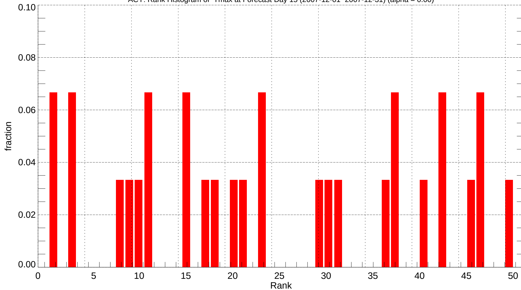
ACY: Rank Histogram of Tmax at Forecast Day 15 (2007-12-01~2007-12-31) (alpha = 0.00)
