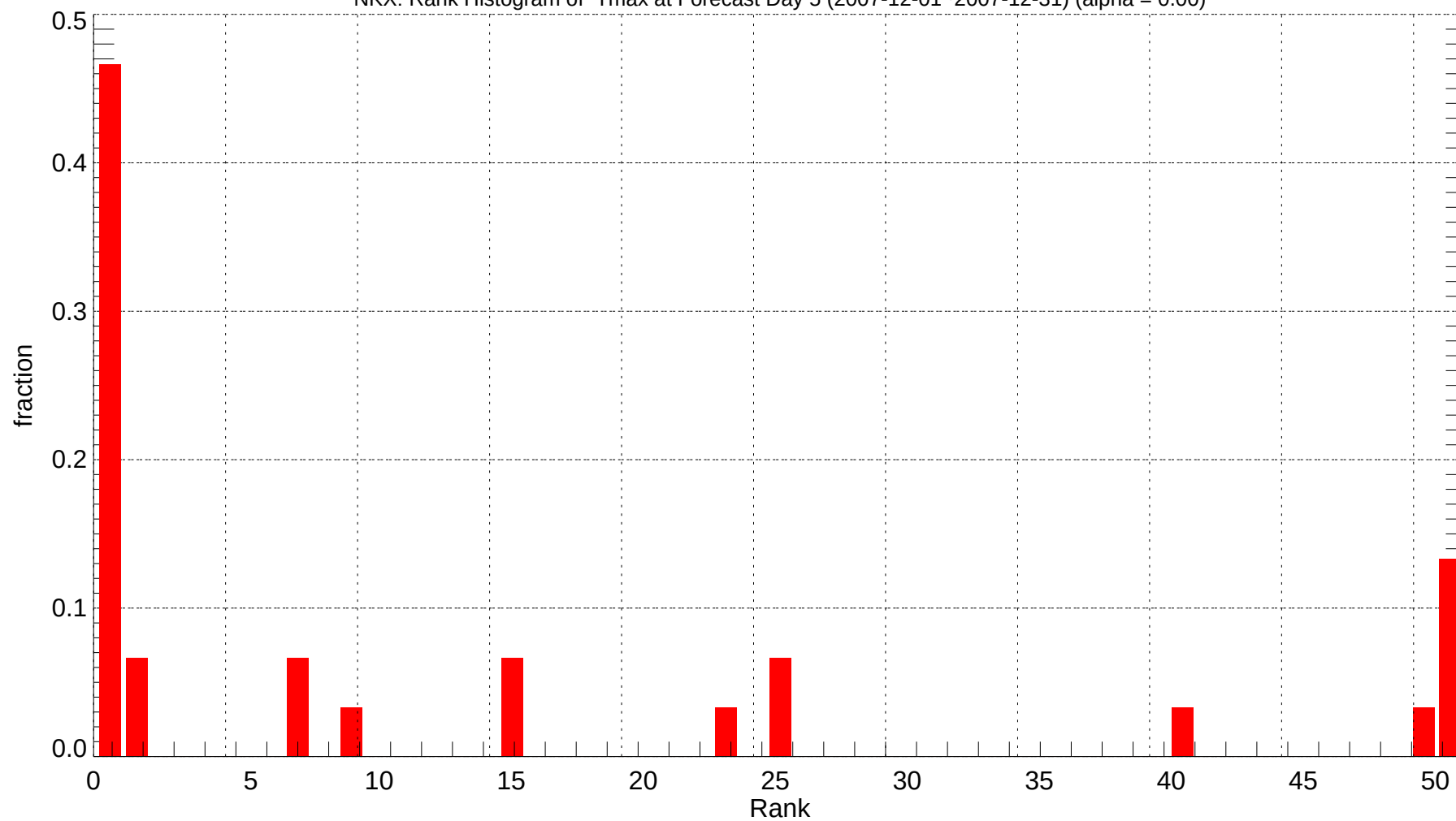
NKX: Rank Histogram of Tmax at Forecast Day 5 (2007-12-01~2007-12-31) (alpha = 0.00)
