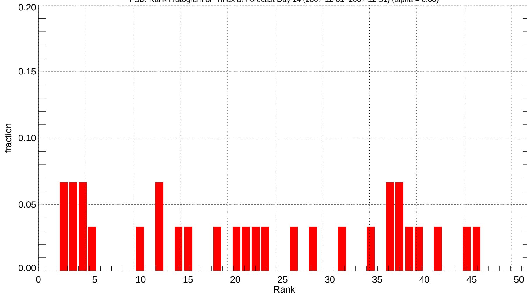
FSD: Rank Histogram of Tmax at Forecast Day 14 (2007-12-01~2007-12-31) (alpha = 0.00)
