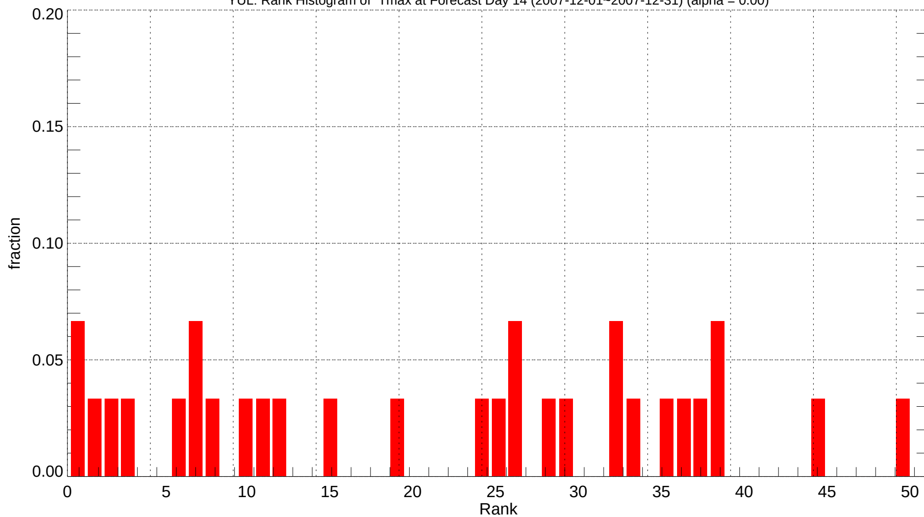
YUL: Rank Histogram of Tmax at Forecast Day 14 (2007-12-01~2007-12-31) (alpha = 0.00)
