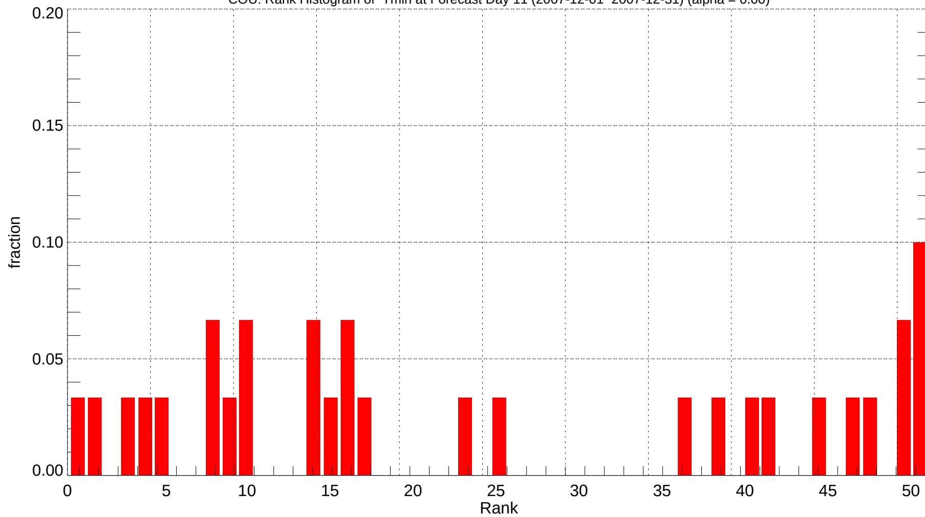
COU: Rank Histogram of Tmin at Forecast Day 11 (2007-12-01~2007-12-31) (alpha = 0.00)
