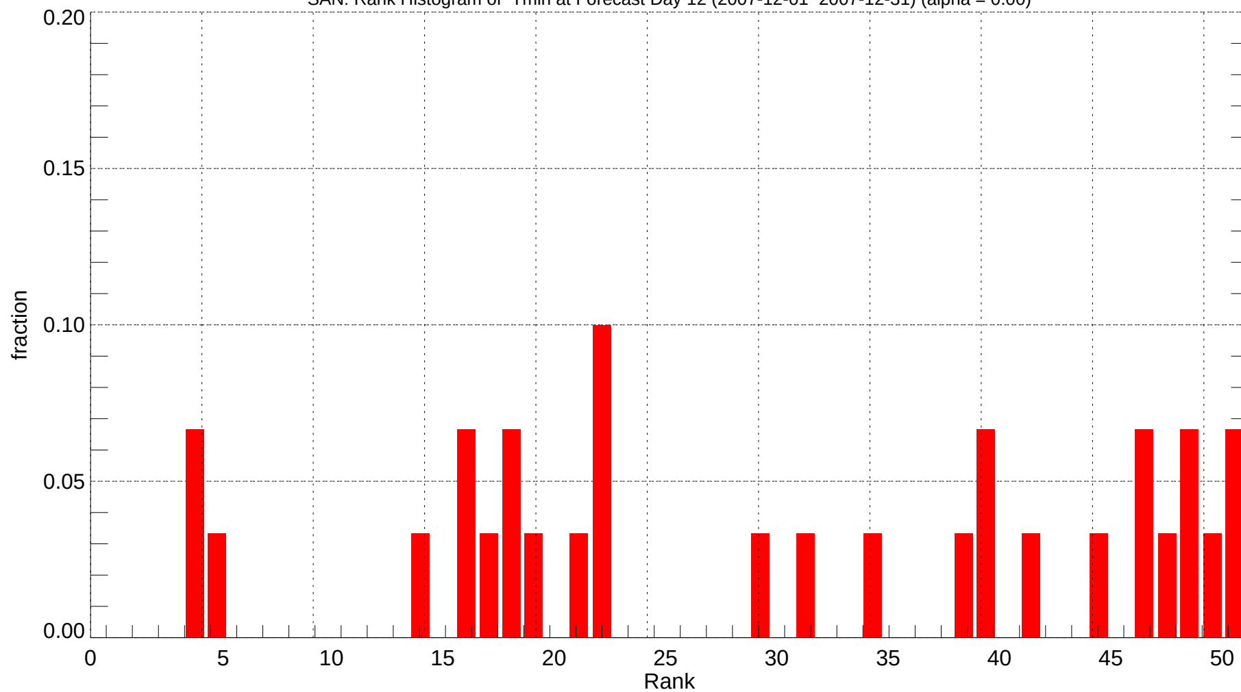
SAN: Rank Histogram of Tmin at Forecast Day 12 (2007-12-01~2007-12-31) (alpha = 0.00)
