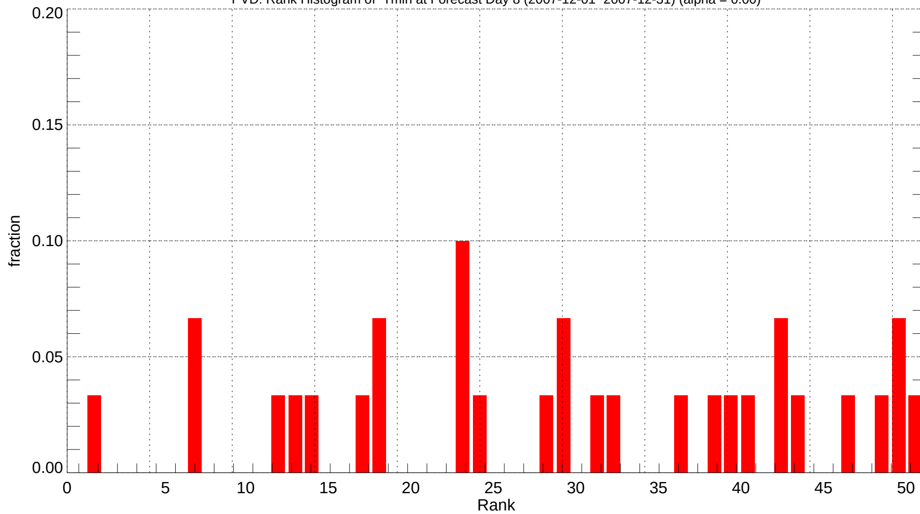
PVD: Rank Histogram of Tmin at Forecast Day 8 (2007-12-01~2007-12-31) (alpha = 0.00)
