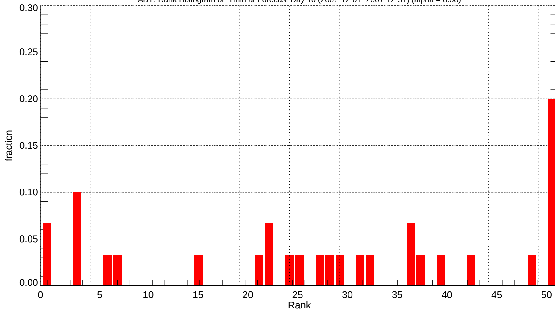
ABY: Rank Histogram of Tmin at Forecast Day 10 (2007-12-01~2007-12-31) (alpha = 0.00)
