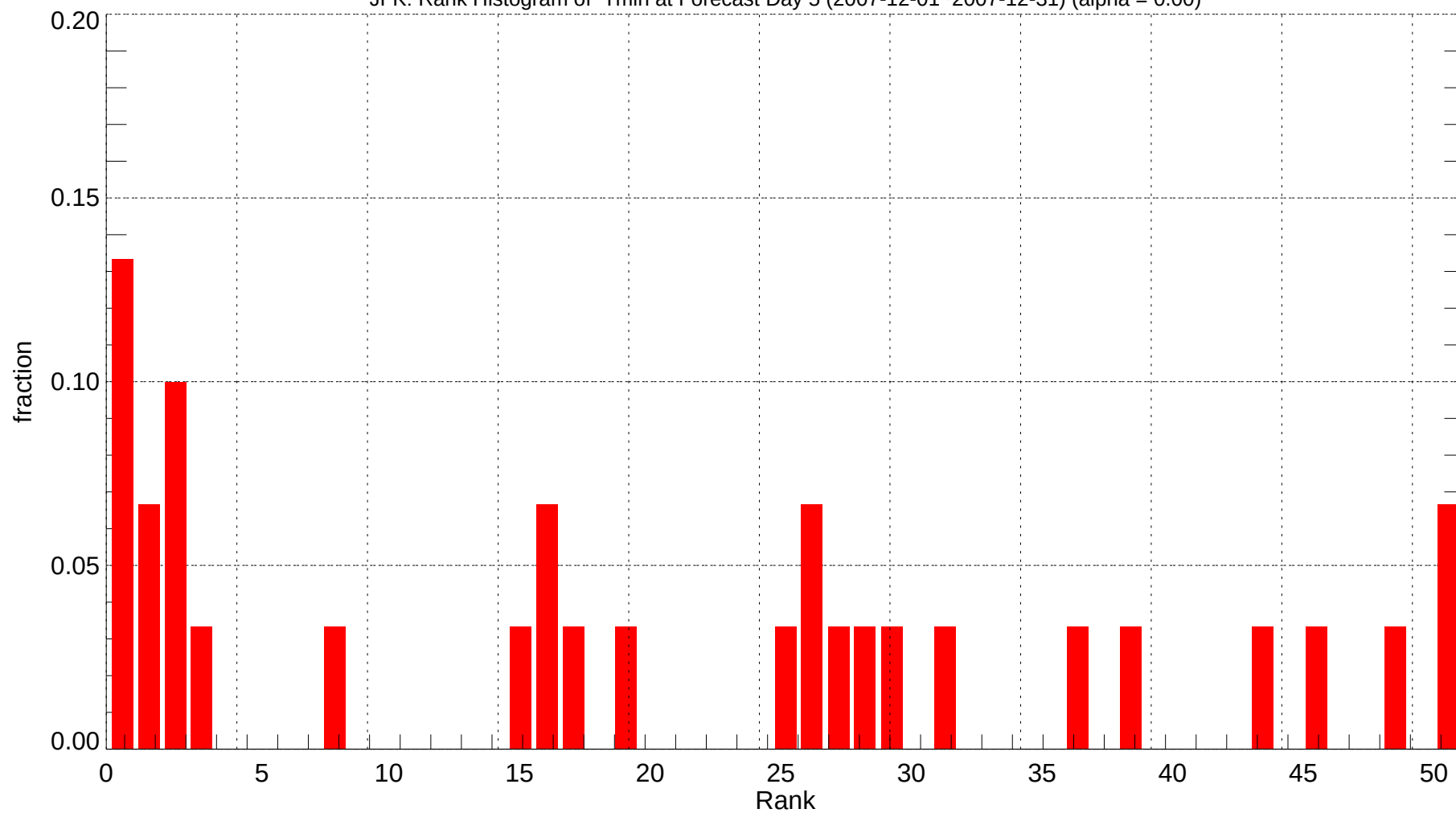
JFK: Rank Histogram of Tmin at Forecast Day 5 (2007-12-01~2007-12-31) (alpha = 0.00)
