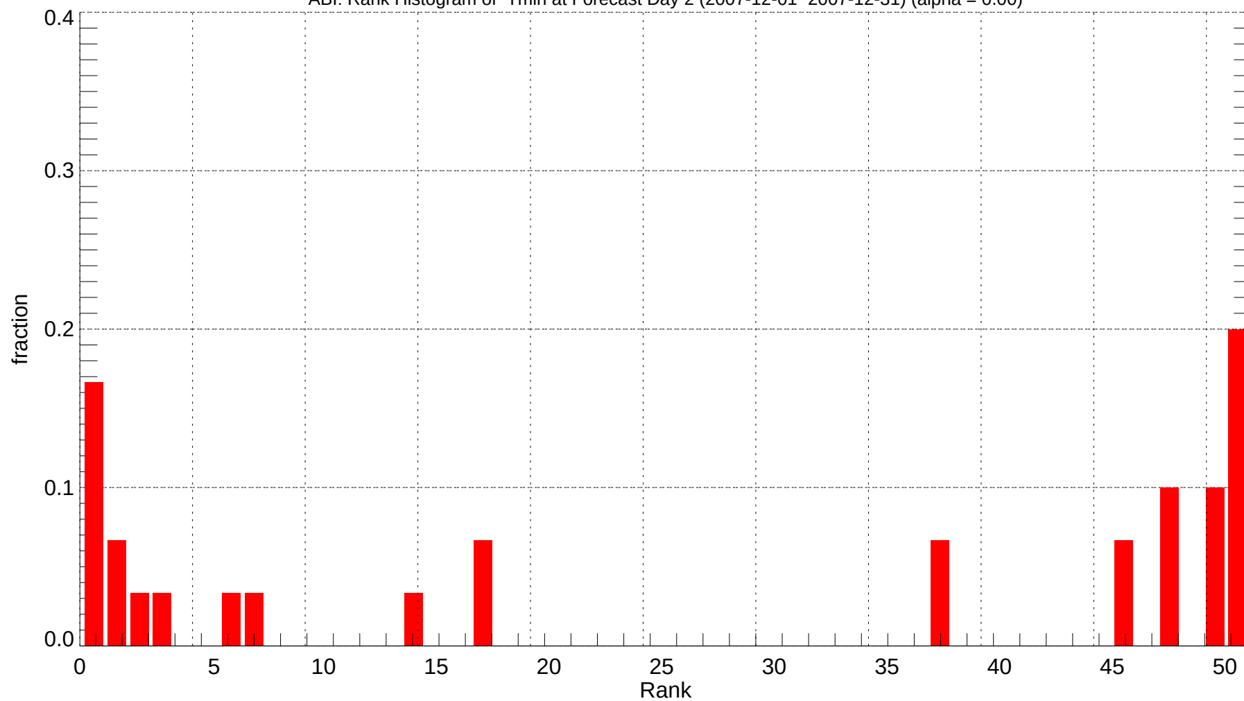
ABI: Rank Histogram of Tmin at Forecast Day 2 (2007-12-01~2007-12-31) (alpha = 0.00)
