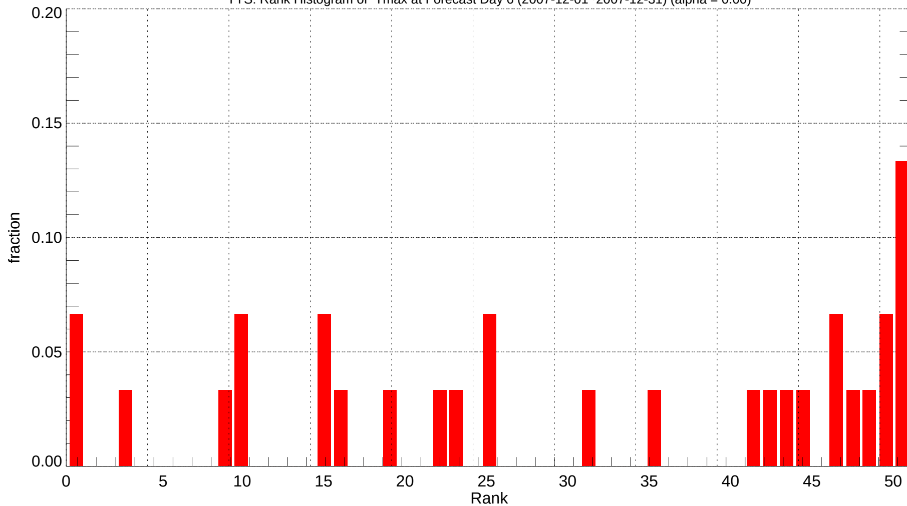
TYS: Rank Histogram of Tmax at Forecast Day 6 (2007-12-01~2007-12-31) (alpha = 0.00)
