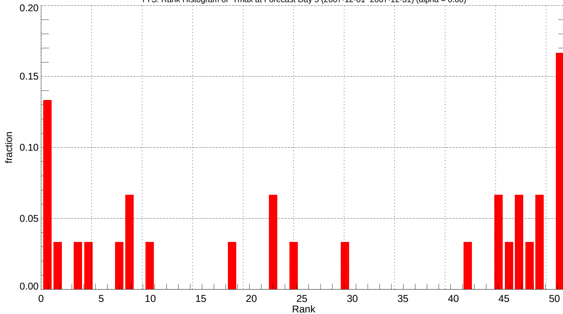
TYS: Rank Histogram of Tmax at Forecast Day 5 (2007-12-01~2007-12-31) (alpha = 0.00)
