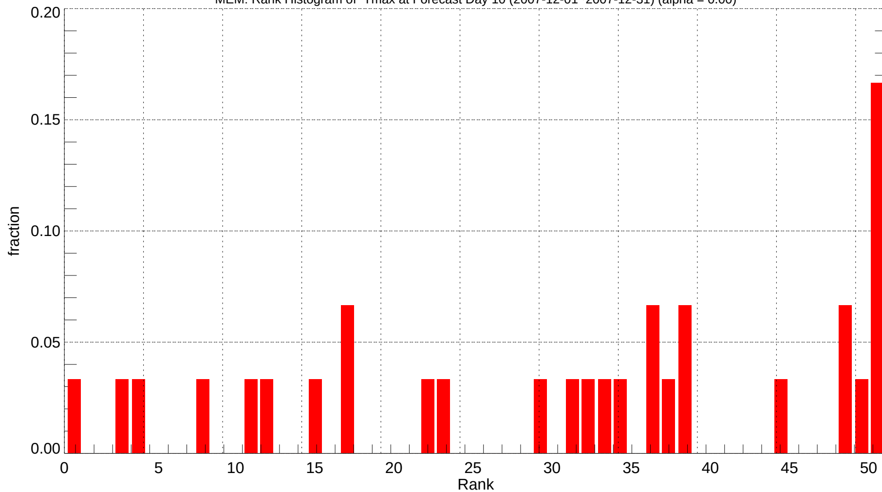
MEM: Rank Histogram of Tmax at Forecast Day 10 (2007-12-01~2007-12-31) (alpha = 0.00)
