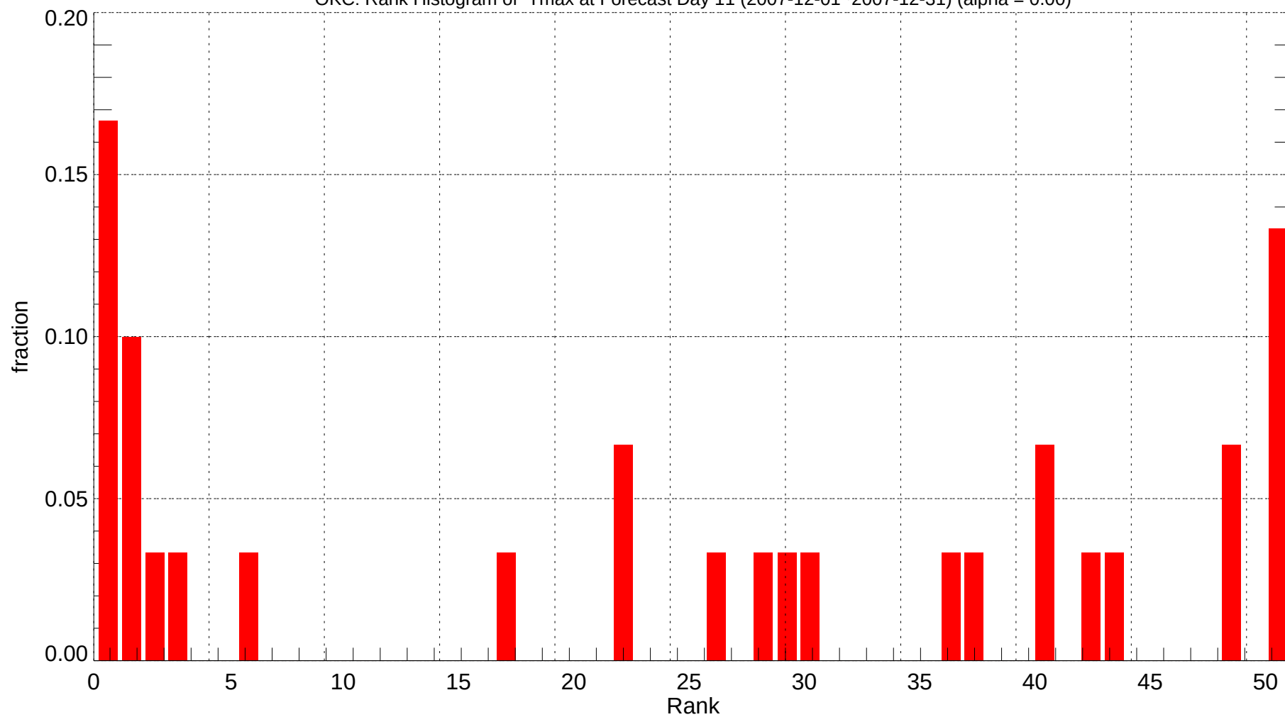
OKC: Rank Histogram of Tmax at Forecast Day 11 (2007-12-01~2007-12-31) (alpha = 0.00)
