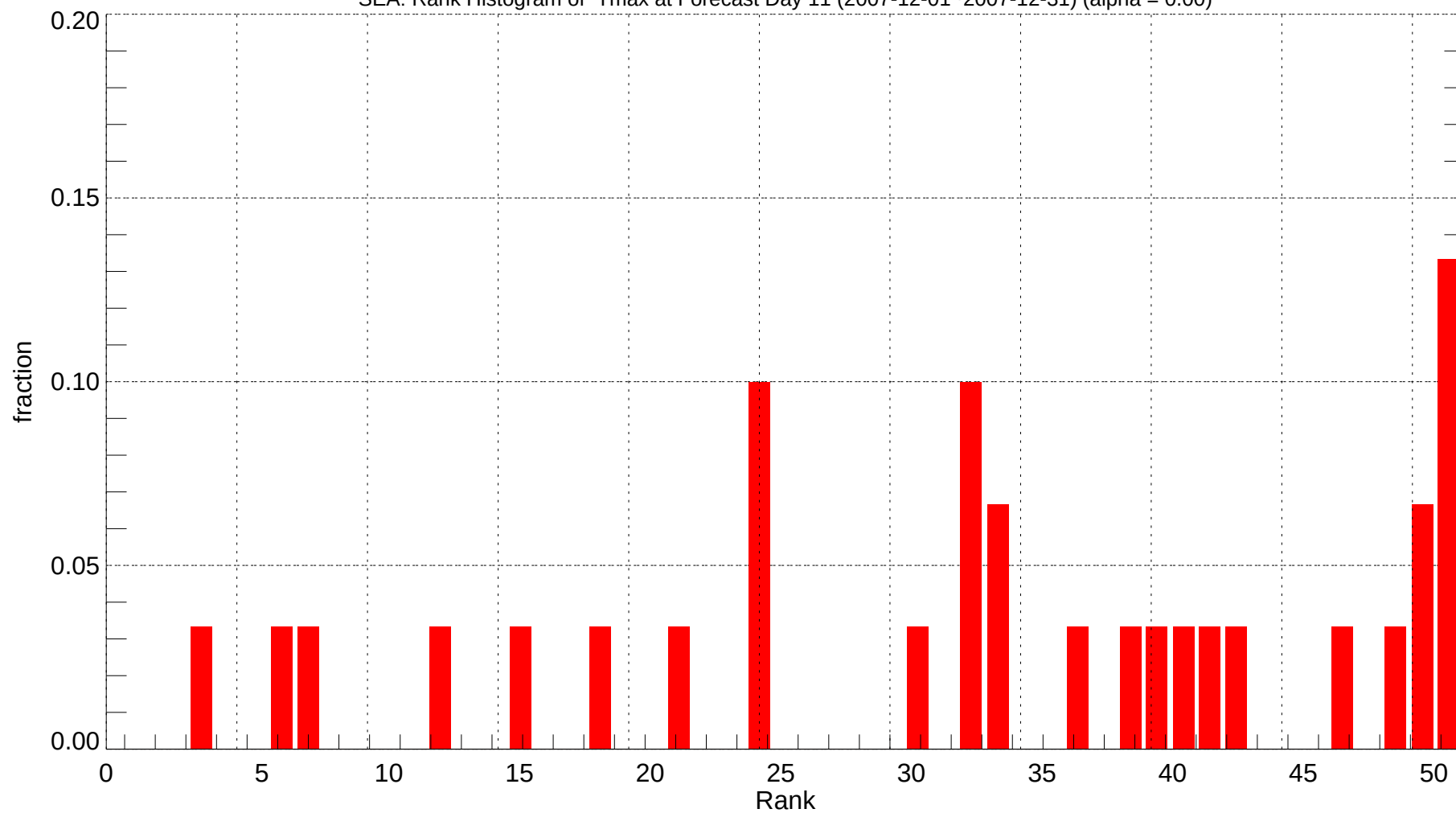
SEA: Rank Histogram of Tmax at Forecast Day 11 (2007-12-01~2007-12-31) (alpha = 0.00)
