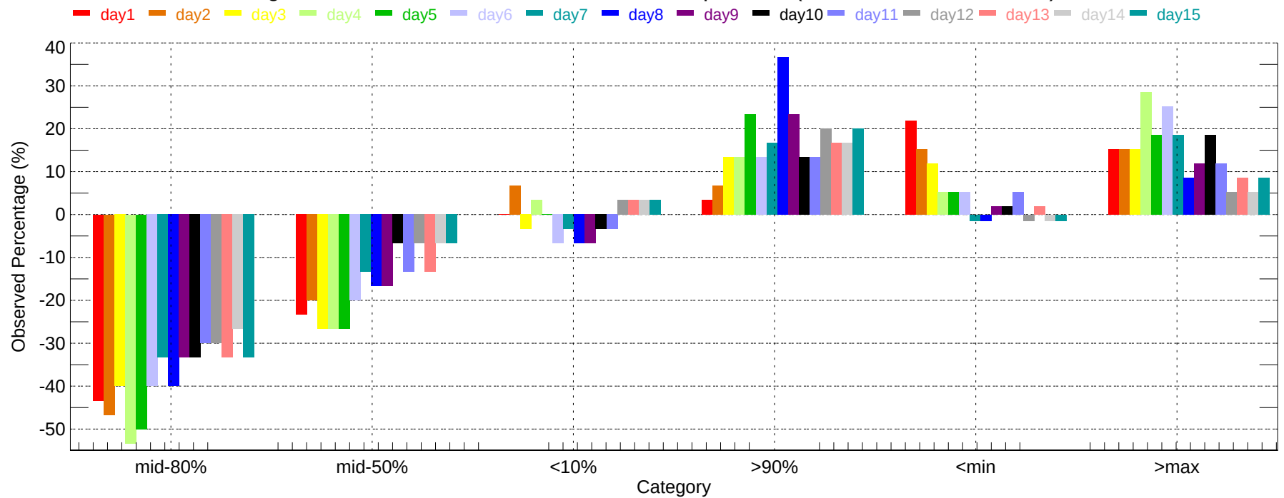
Observed Percentage Deviation of Ensembles - JAX: Min Temperature (2007-12-01~2007-12-31)
