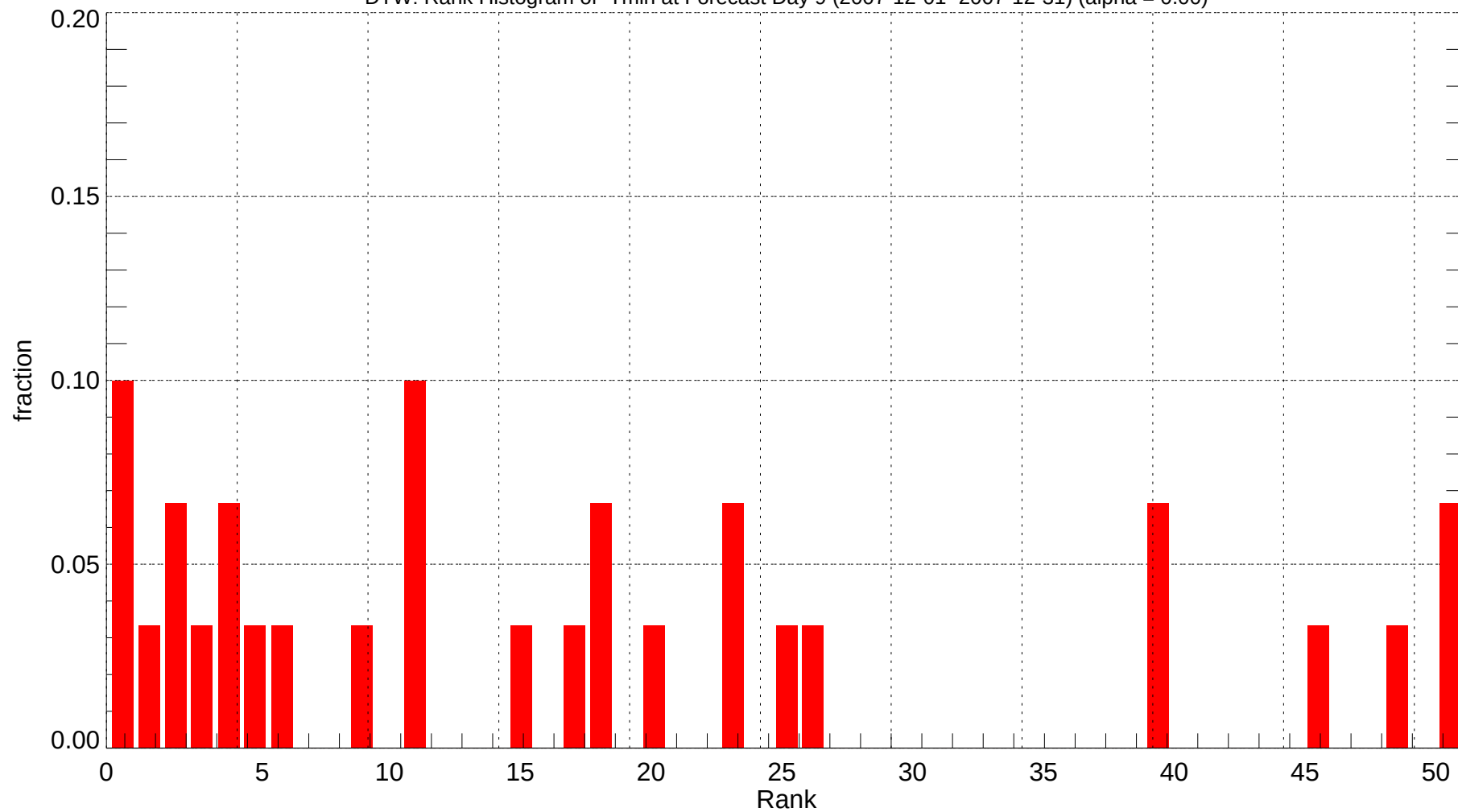
DTW: Rank Histogram of Tmin at Forecast Day 9 (2007-12-01~2007-12-31) (alpha = 0.00)
