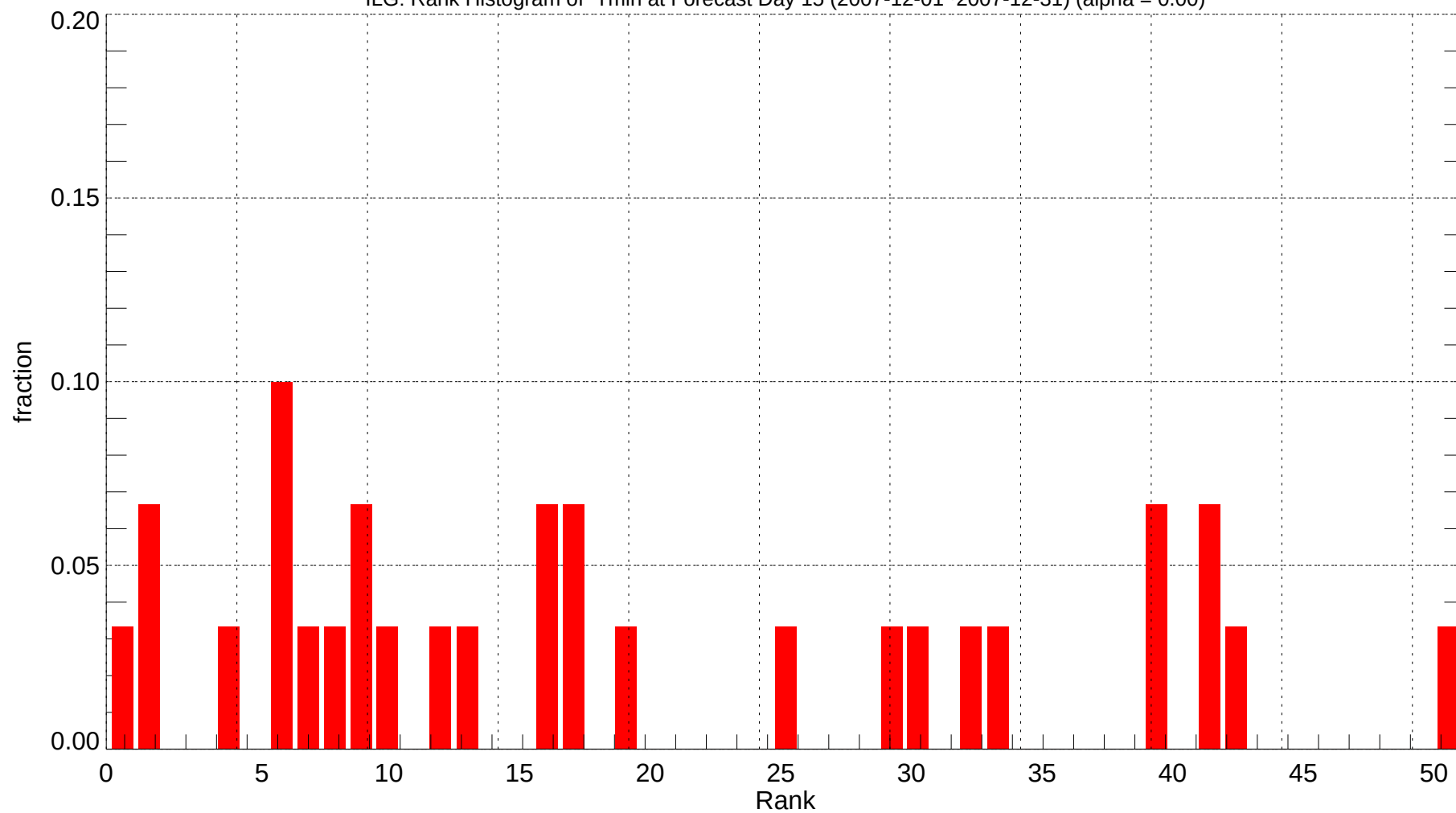
ILG: Rank Histogram of Tmin at Forecast Day 15 (2007-12-01~2007-12-31) (alpha = 0.00)
