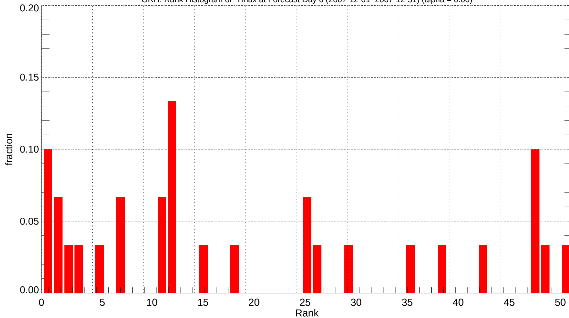
ORH: Rank Histogram of Tmax at Forecast Day 6 (2007-12-01~2007-12-31) (alpha = 0.00)
