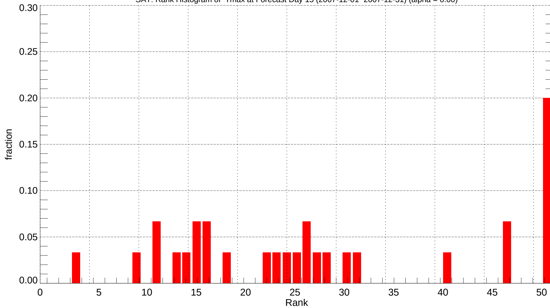
SAT: Rank Histogram of Tmax at Forecast Day 15 (2007-12-01~2007-12-31) (alpha = 0.00)
