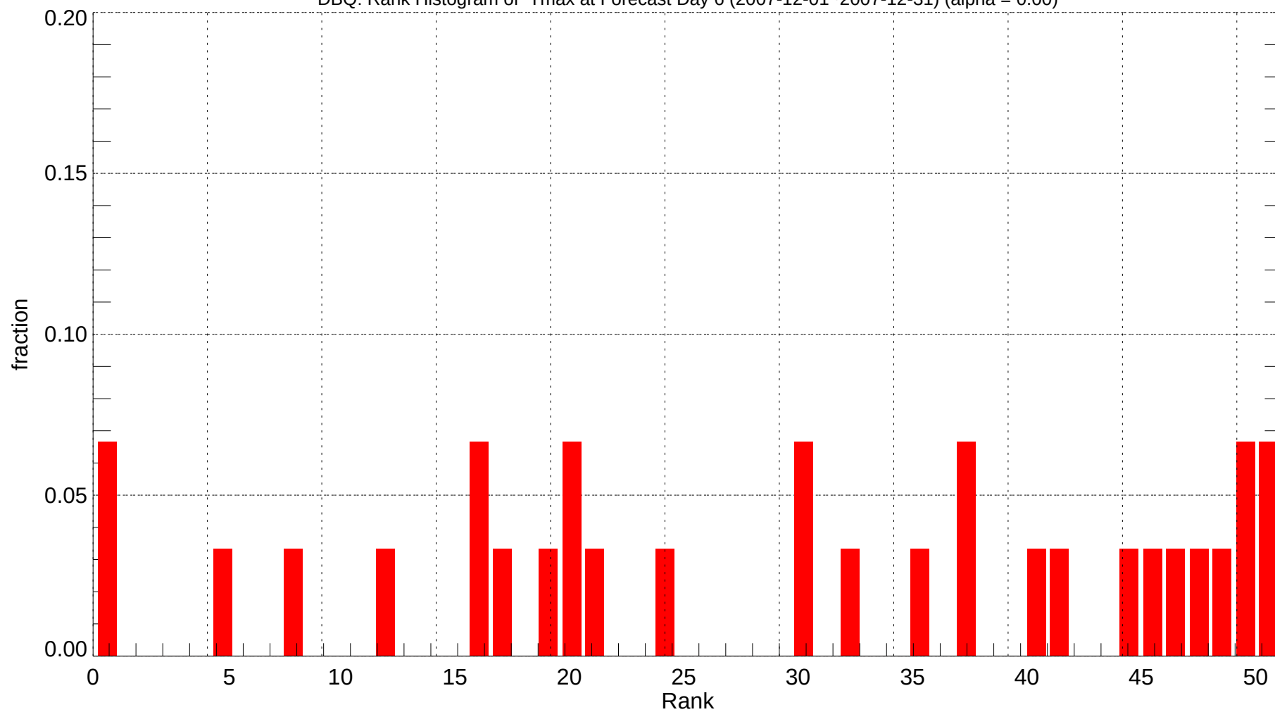
DBQ: Rank Histogram of Tmax at Forecast Day 6 (2007-12-01~2007-12-31) (alpha = 0.00)
