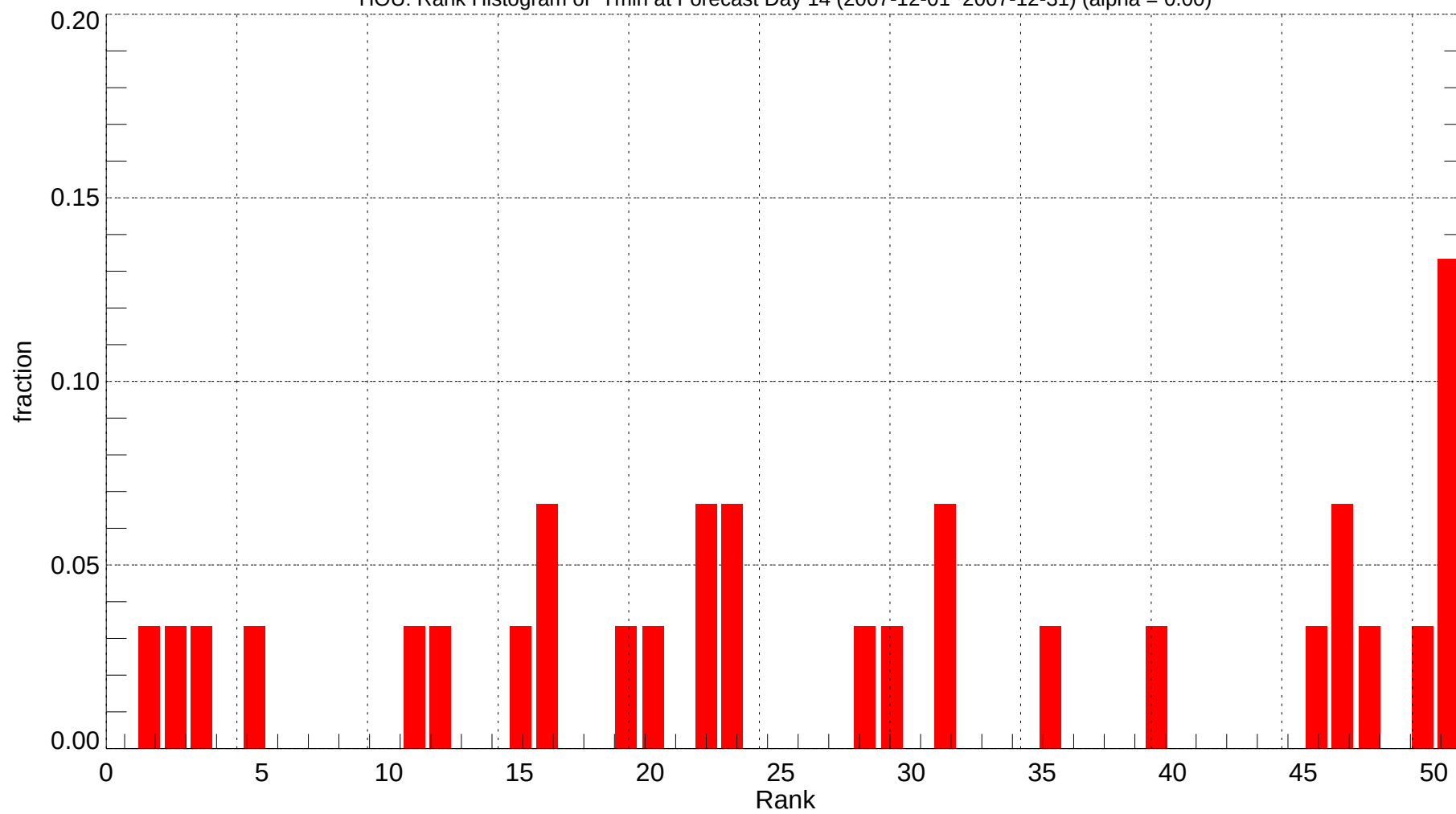
HOU: Rank Histogram of Tmin at Forecast Day 14 (2007-12-01~2007-12-31) (alpha = 0.00)
