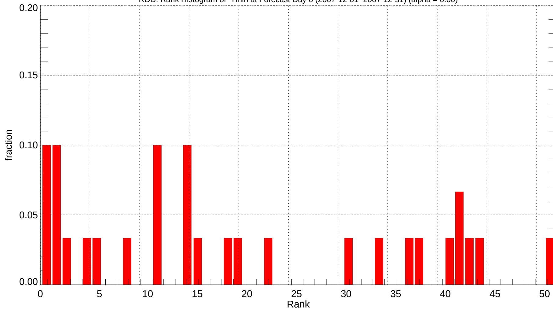
RDD: Rank Histogram of Tmin at Forecast Day 6 (2007-12-01~2007-12-31) (alpha = 0.00)
