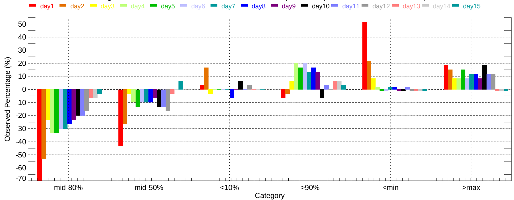
Observed Percentage Deviation of Ensembles - OMA: Min Temperature (2007-12-01~2007-12-31)
