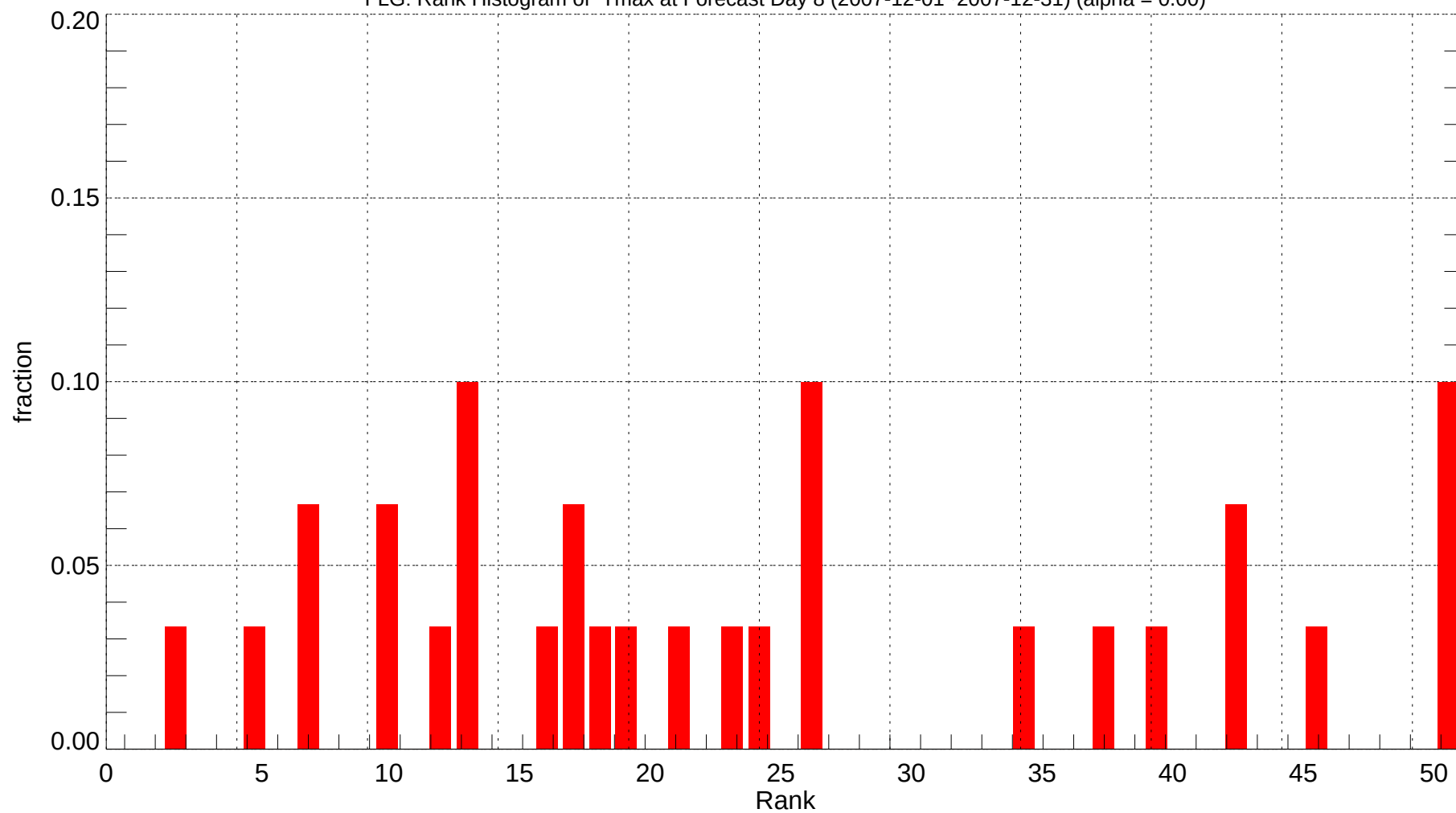
FLG: Rank Histogram of Tmax at Forecast Day 8 (2007-12-01~2007-12-31) (alpha = 0.00)
