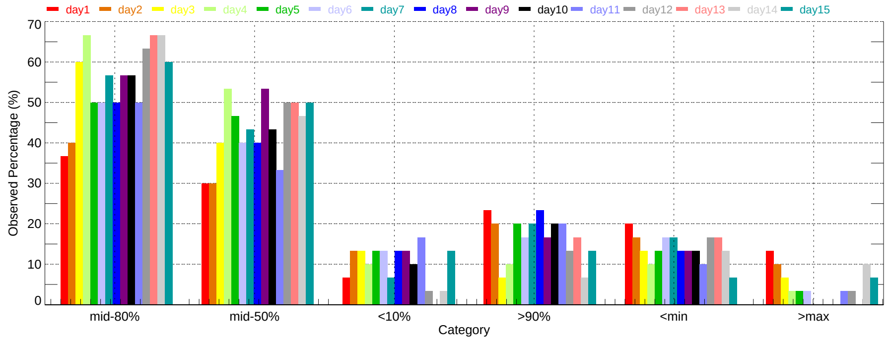
Observed Percentage of Ensembles - BRO: Max Temperature (2007-12-01~2007-12-31)
