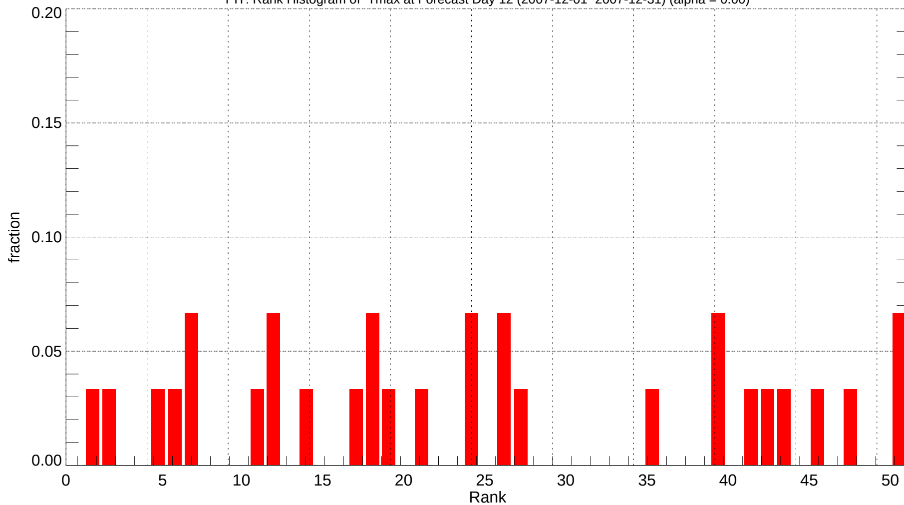
PIT: Rank Histogram of Tmax at Forecast Day 12 (2007-12-01~2007-12-31) (alpha = 0.00)
