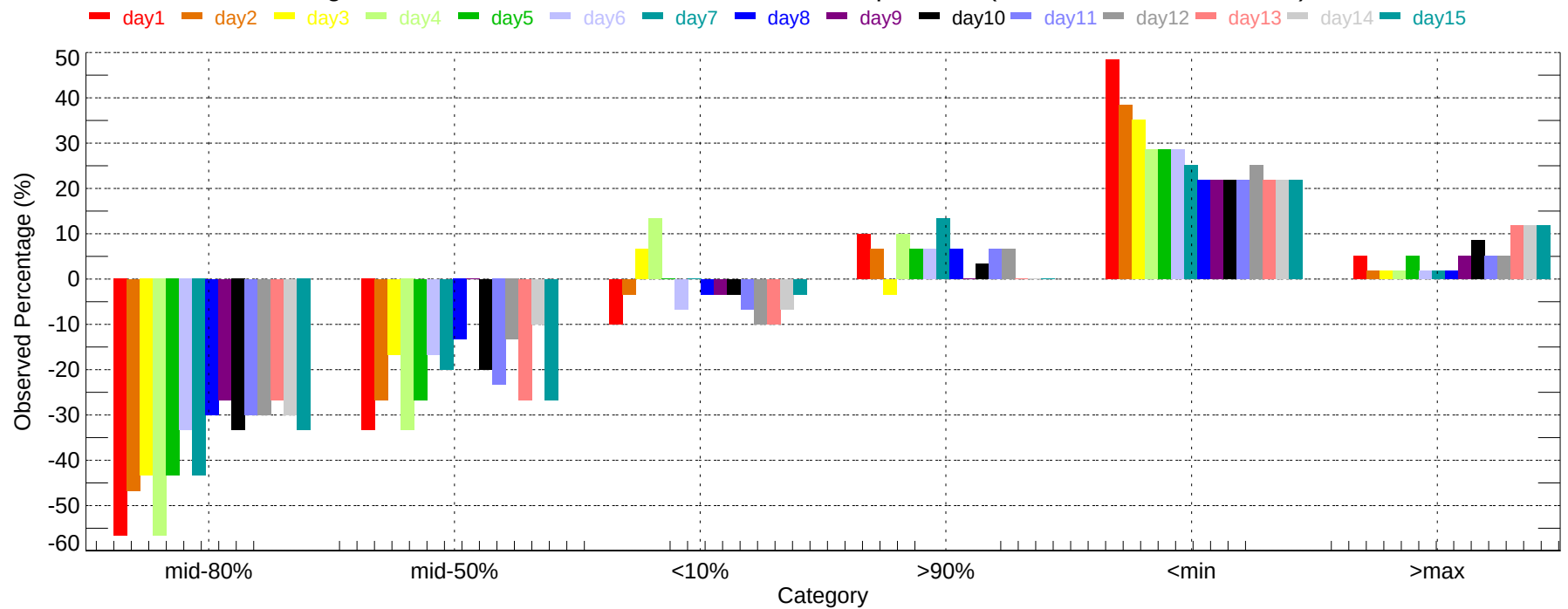
Observed Percentage Deviation of Ensembles - GAD: Max Temperature (2007-12-01~2007-12-31)
