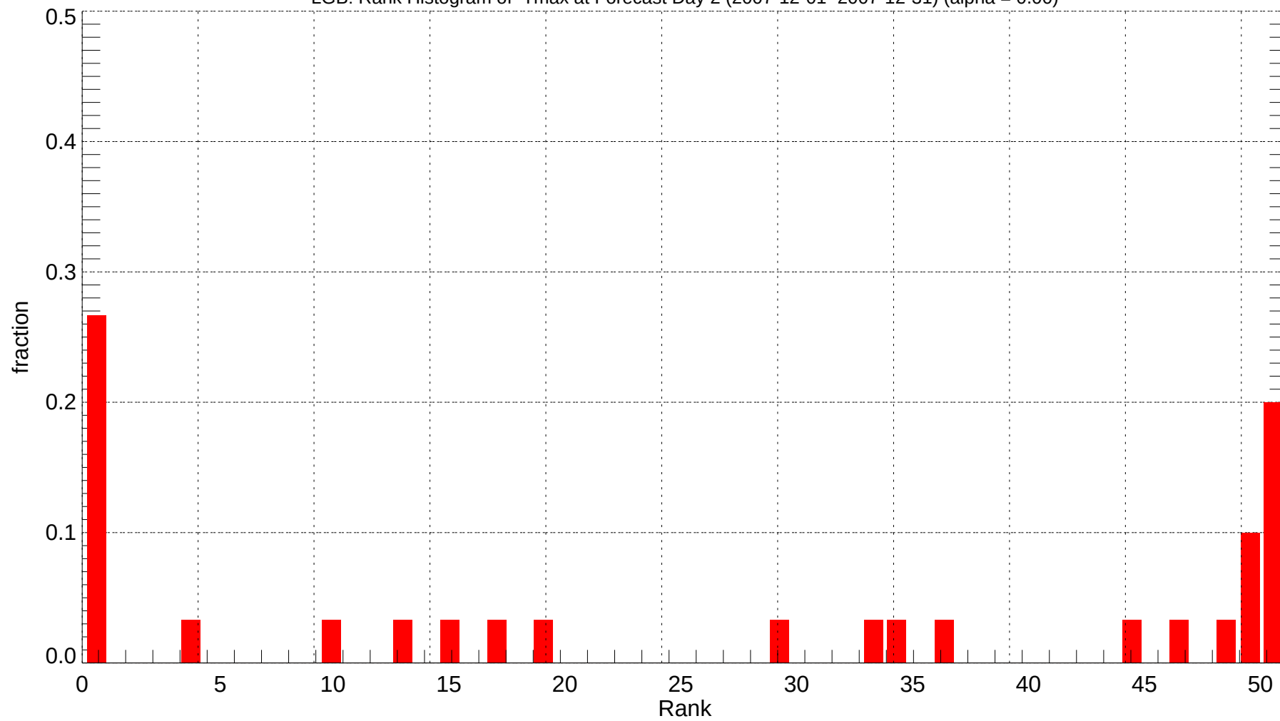
LGB: Rank Histogram of Tmax at Forecast Day 2 (2007-12-01~2007-12-31) (alpha = 0.00)
