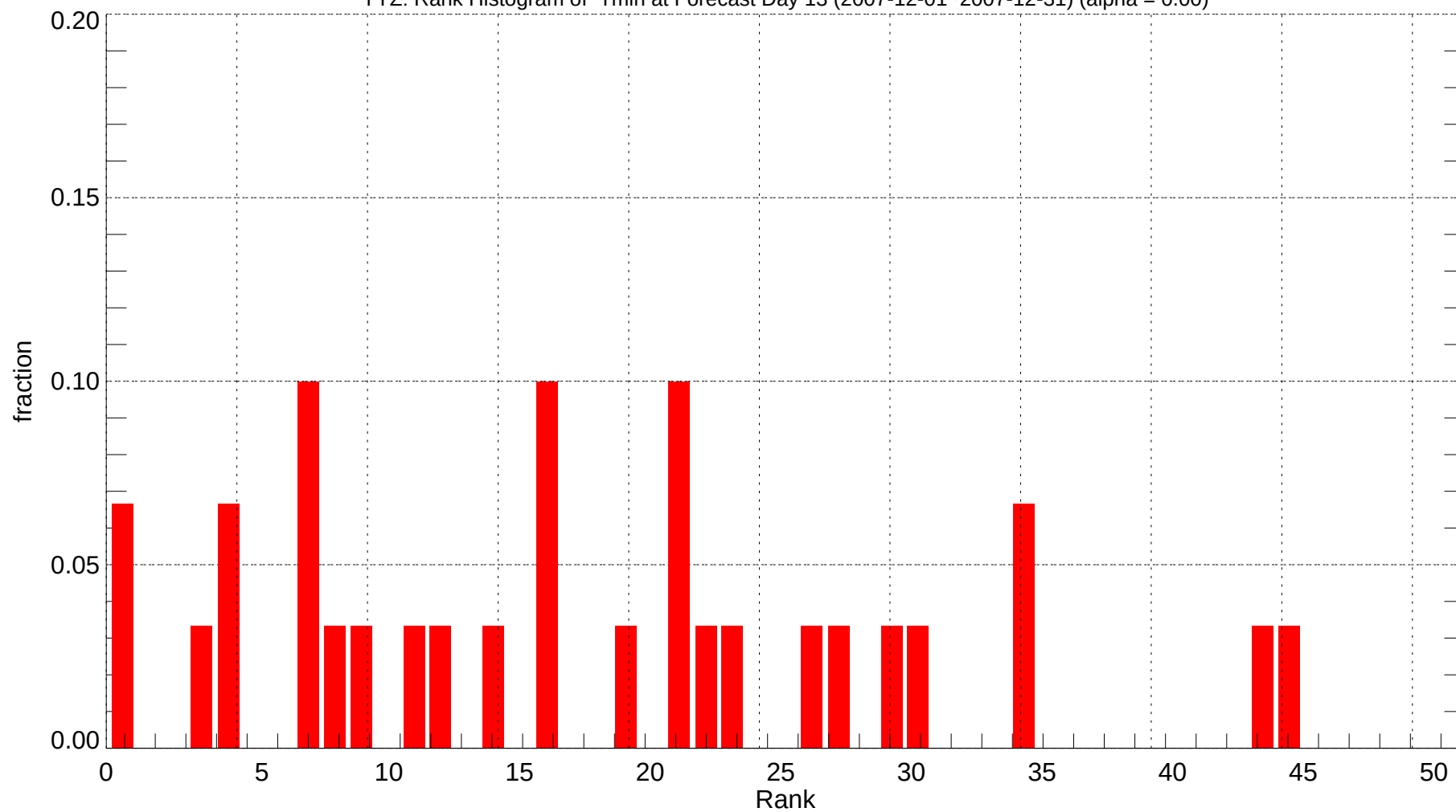
YYZ: Rank Histogram of Tmin at Forecast Day 13 (2007-12-01~2007-12-31) (alpha = 0.00)
