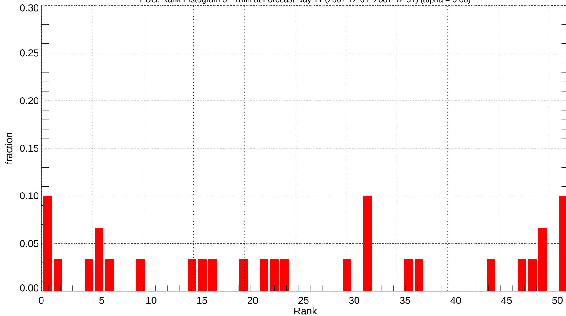
EUG: Rank Histogram of Tmin at Forecast Day 11 (2007-12-01~2007-12-31) (alpha = 0.00)
