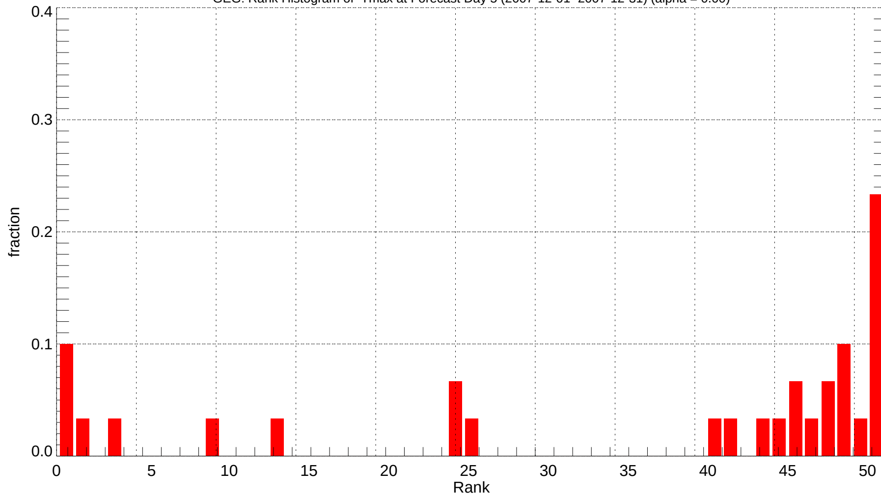
GEG: Rank Histogram of Tmax at Forecast Day 5 (2007-12-01~2007-12-31) (alpha = 0.00)
