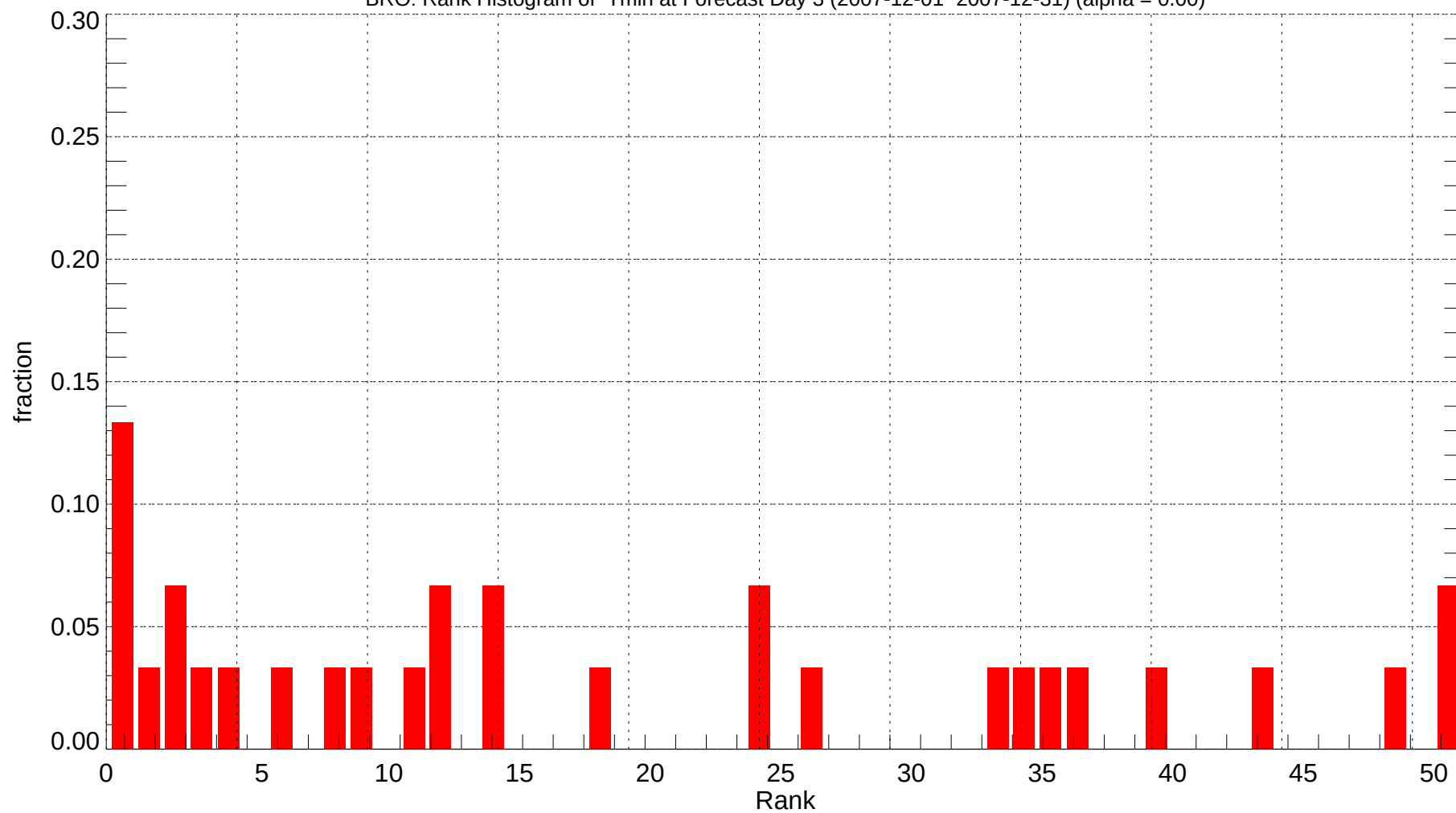
BRO: Rank Histogram of Tmin at Forecast Day 3 (2007-12-01~2007-12-31) (alpha = 0.00)
