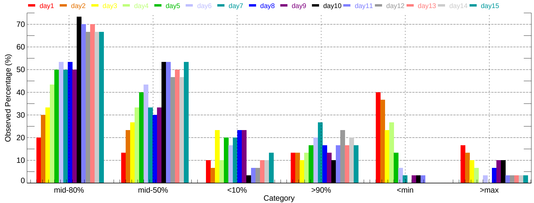
Observed Percentage of Ensembles - YNG: Min Temperature (2007-12-01~2007-12-31)
