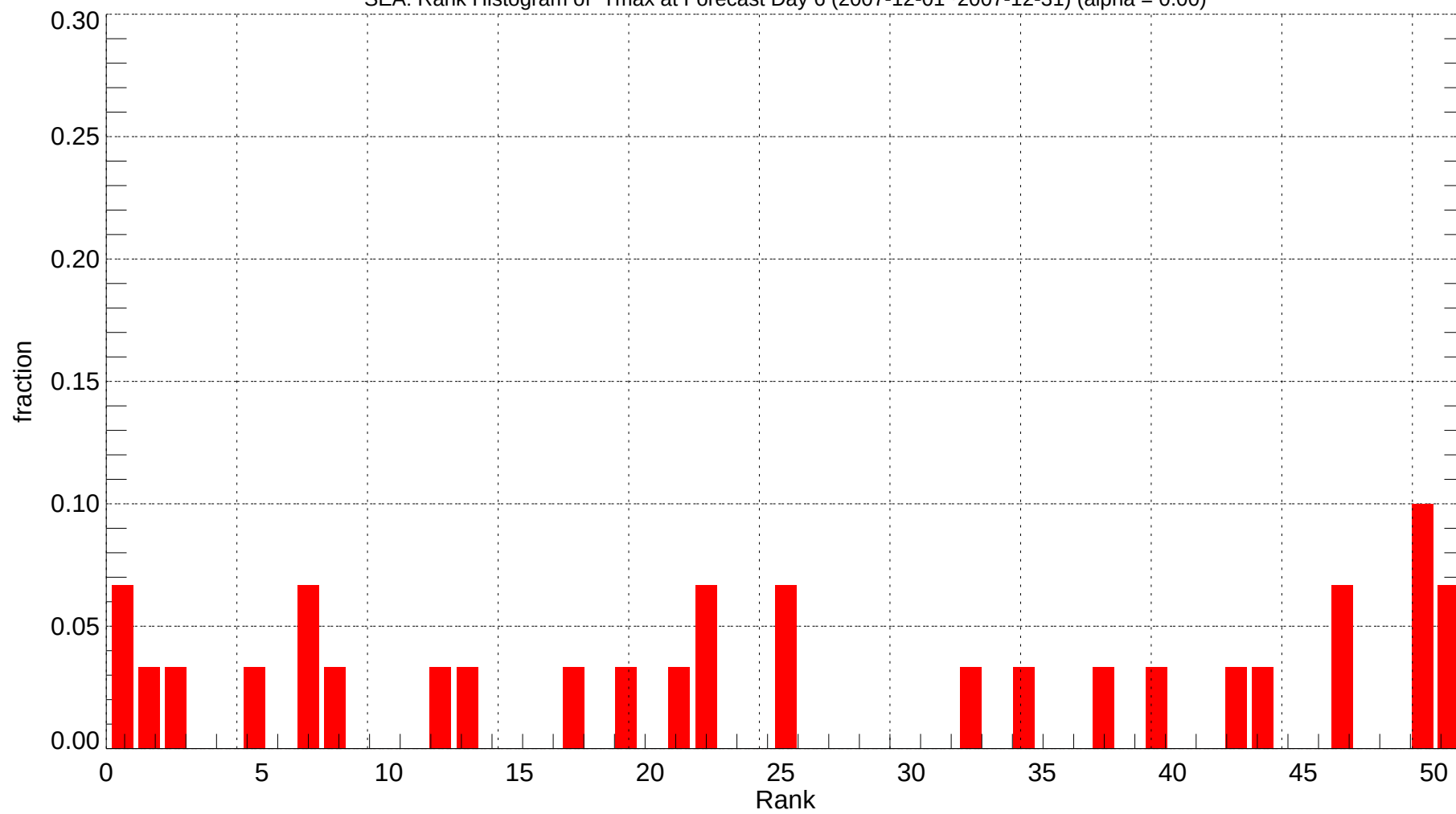
SEA: Rank Histogram of Tmax at Forecast Day 6 (2007-12-01~2007-12-31) (alpha = 0.00)
