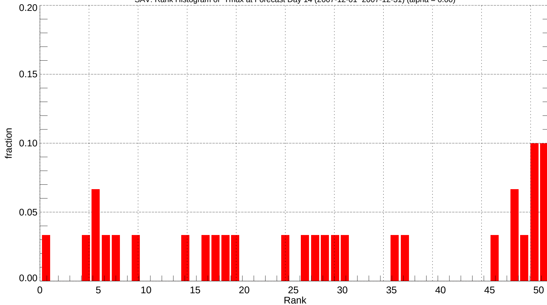
SAV: Rank Histogram of Tmax at Forecast Day 14 (2007-12-01~2007-12-31) (alpha = 0.00)
