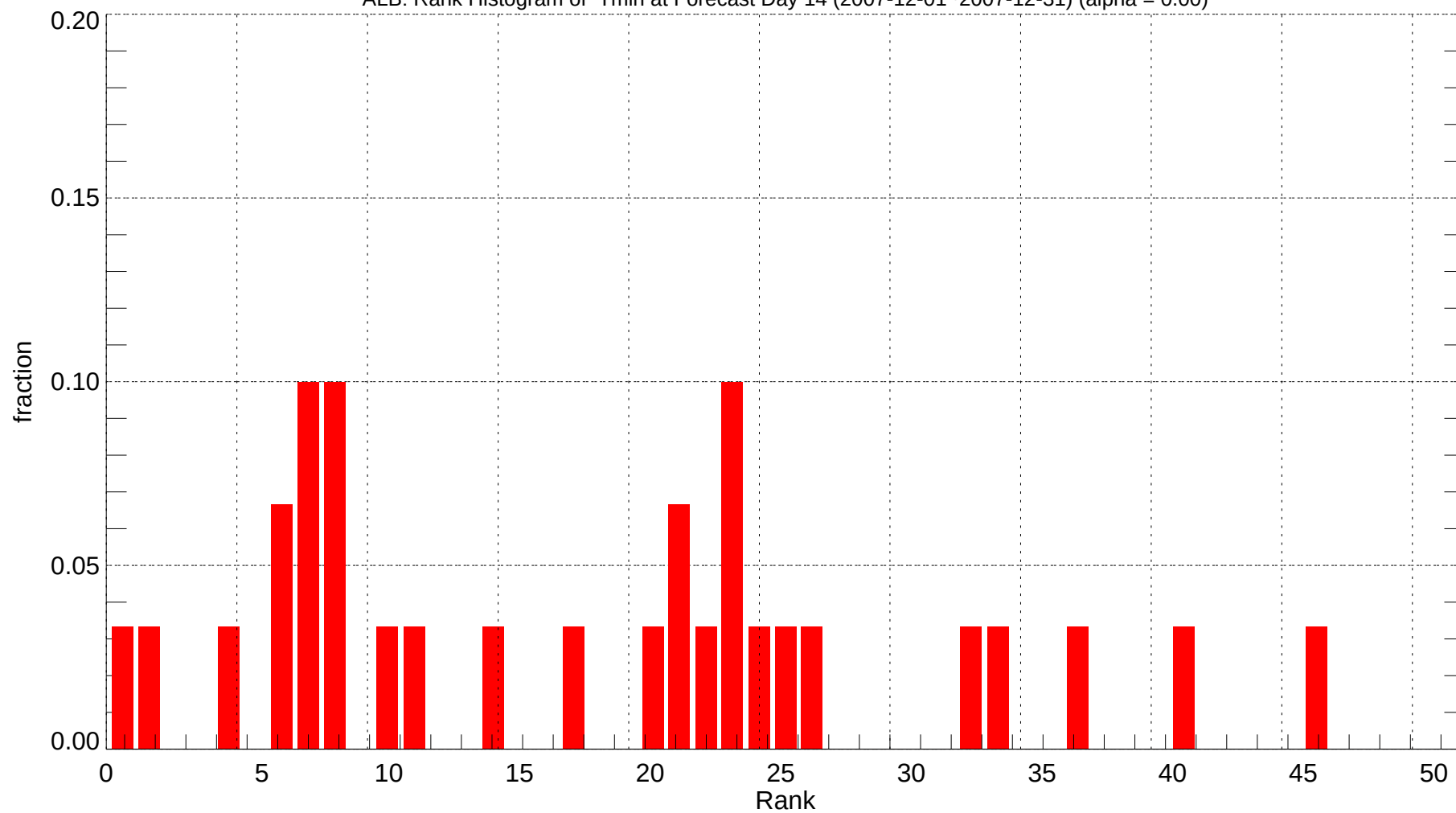
ALB: Rank Histogram of Tmin at Forecast Day 14 (2007-12-01~2007-12-31) (alpha = 0.00)
