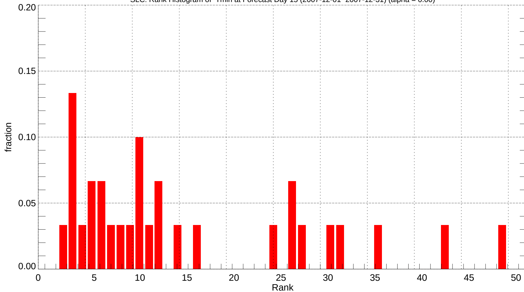
SLC: Rank Histogram of Tmin at Forecast Day 15 (2007-12-01~2007-12-31) (alpha = 0.00)
