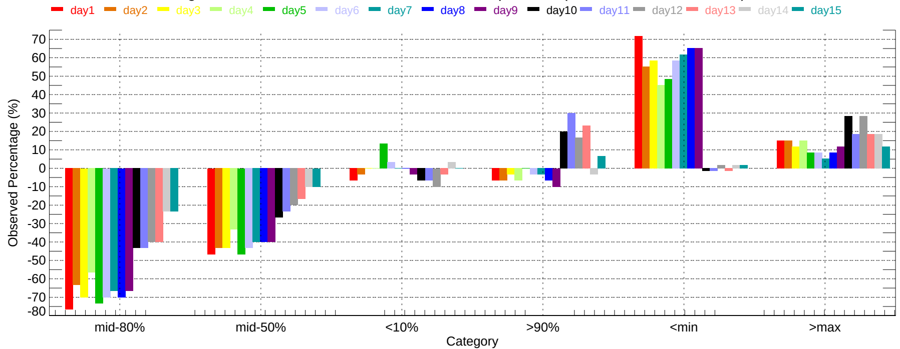
Observed Percentage Deviation of Ensembles - LAX: Max Temperature (2007-12-01~2007-12-31)
