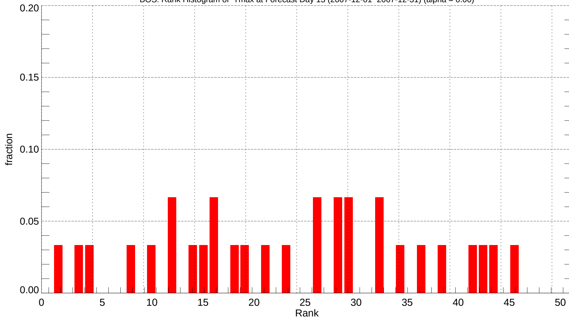
BOS: Rank Histogram of Tmax at Forecast Day 13 (2007-12-01~2007-12-31) (alpha = 0.00)
