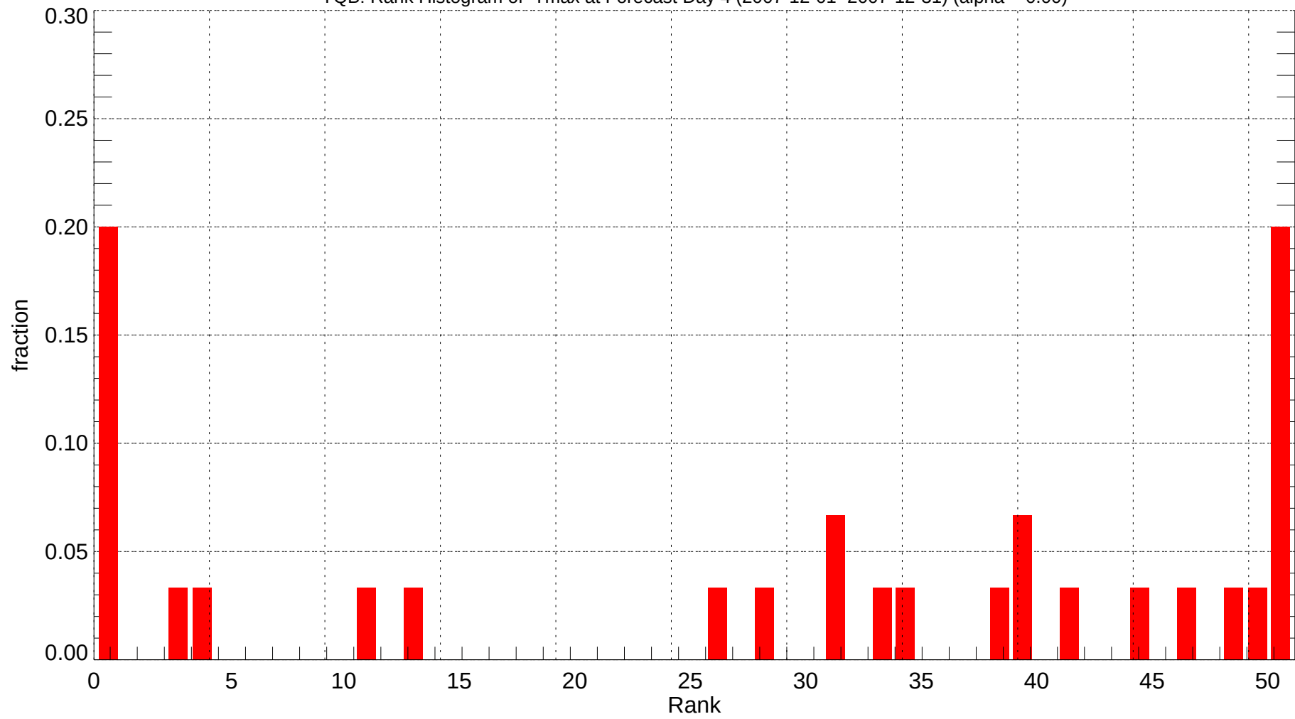
YQB: Rank Histogram of Tmax at Forecast Day 4 (2007-12-01~2007-12-31) (alpha = 0.00)
