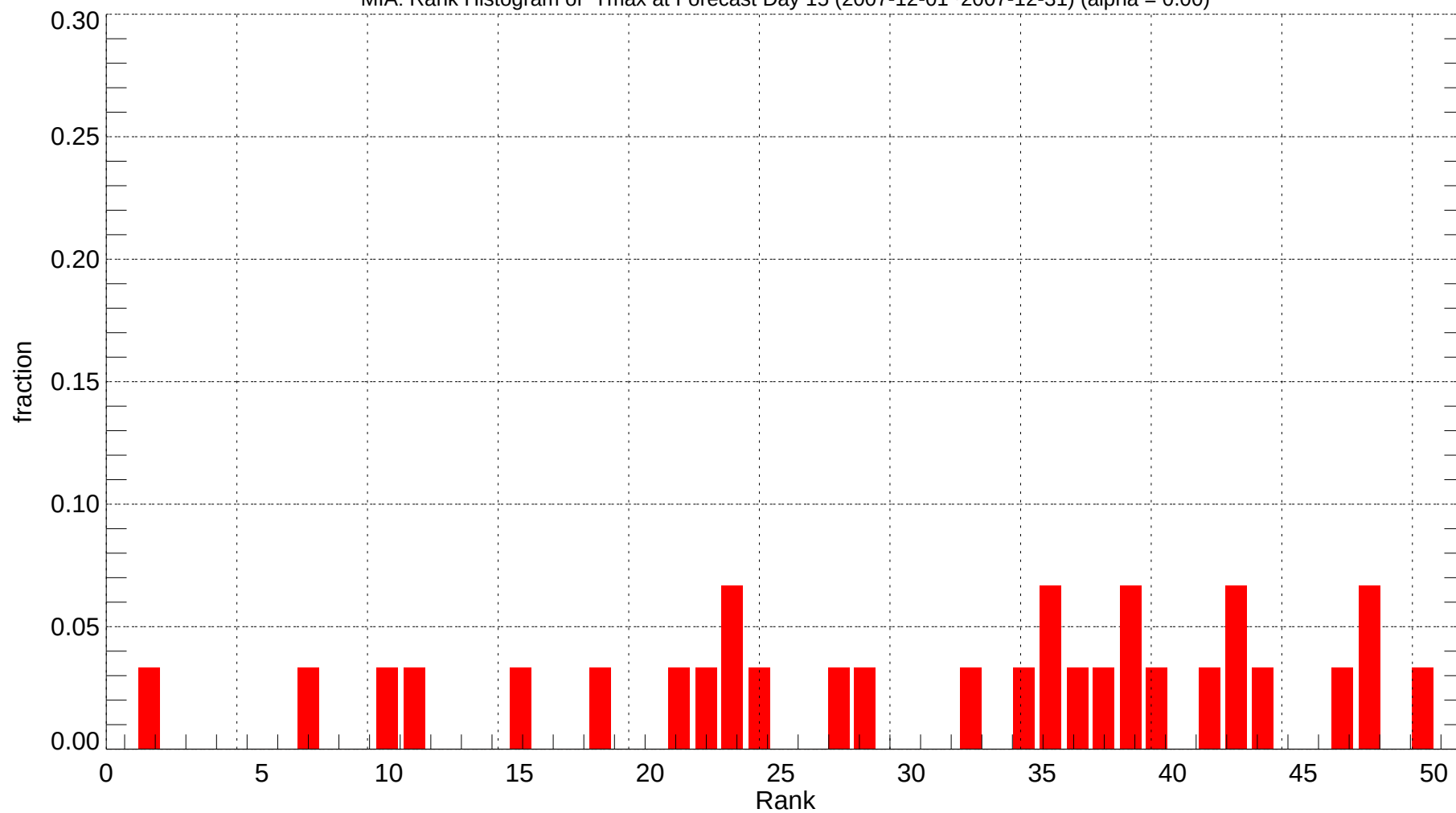
MIA: Rank Histogram of Tmax at Forecast Day 15 (2007-12-01~2007-12-31) (alpha = 0.00)
