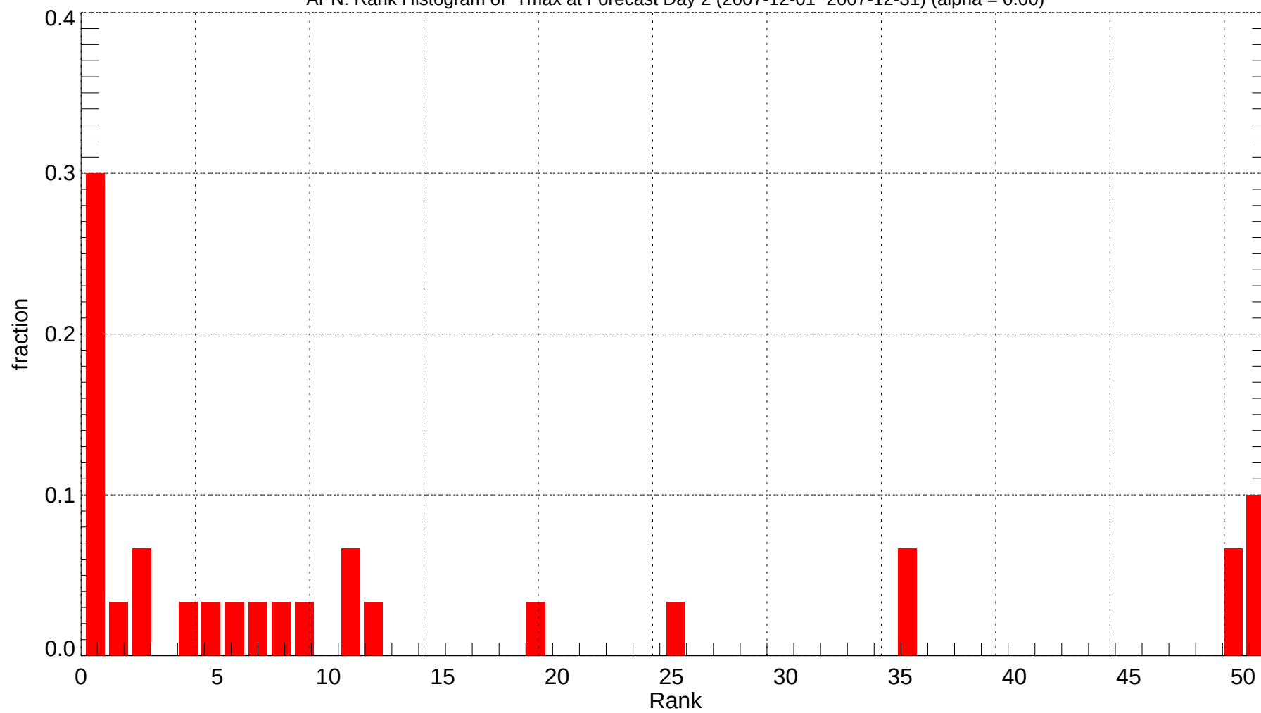
APN: Rank Histogram of Tmax at Forecast Day 2 (2007-12-01~2007-12-31) (alpha = 0.00)
