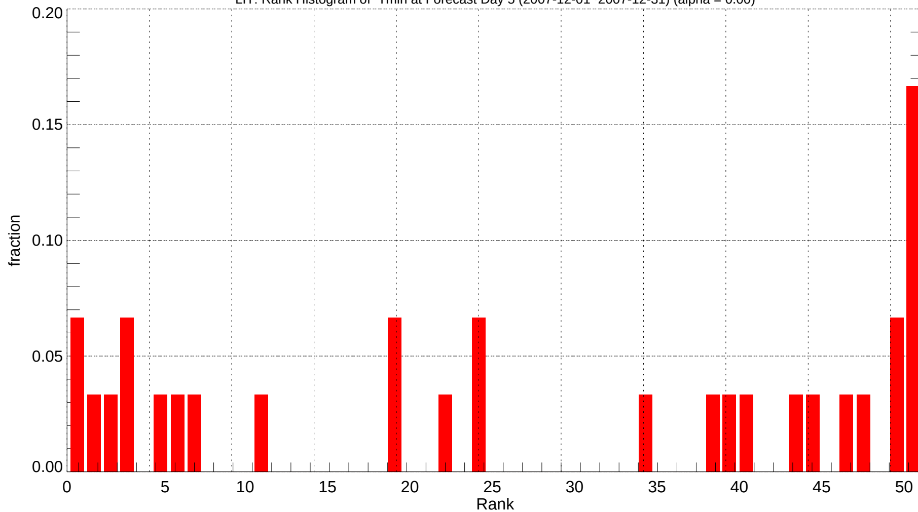
LIT: Rank Histogram of Tmin at Forecast Day 5 (2007-12-01~2007-12-31) (alpha = 0.00)
