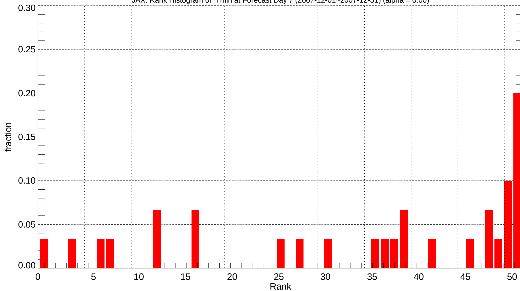
JAX: Rank Histogram of Tmin at Forecast Day 7 (2007-12-01~2007-12-31) (alpha = 0.00)
