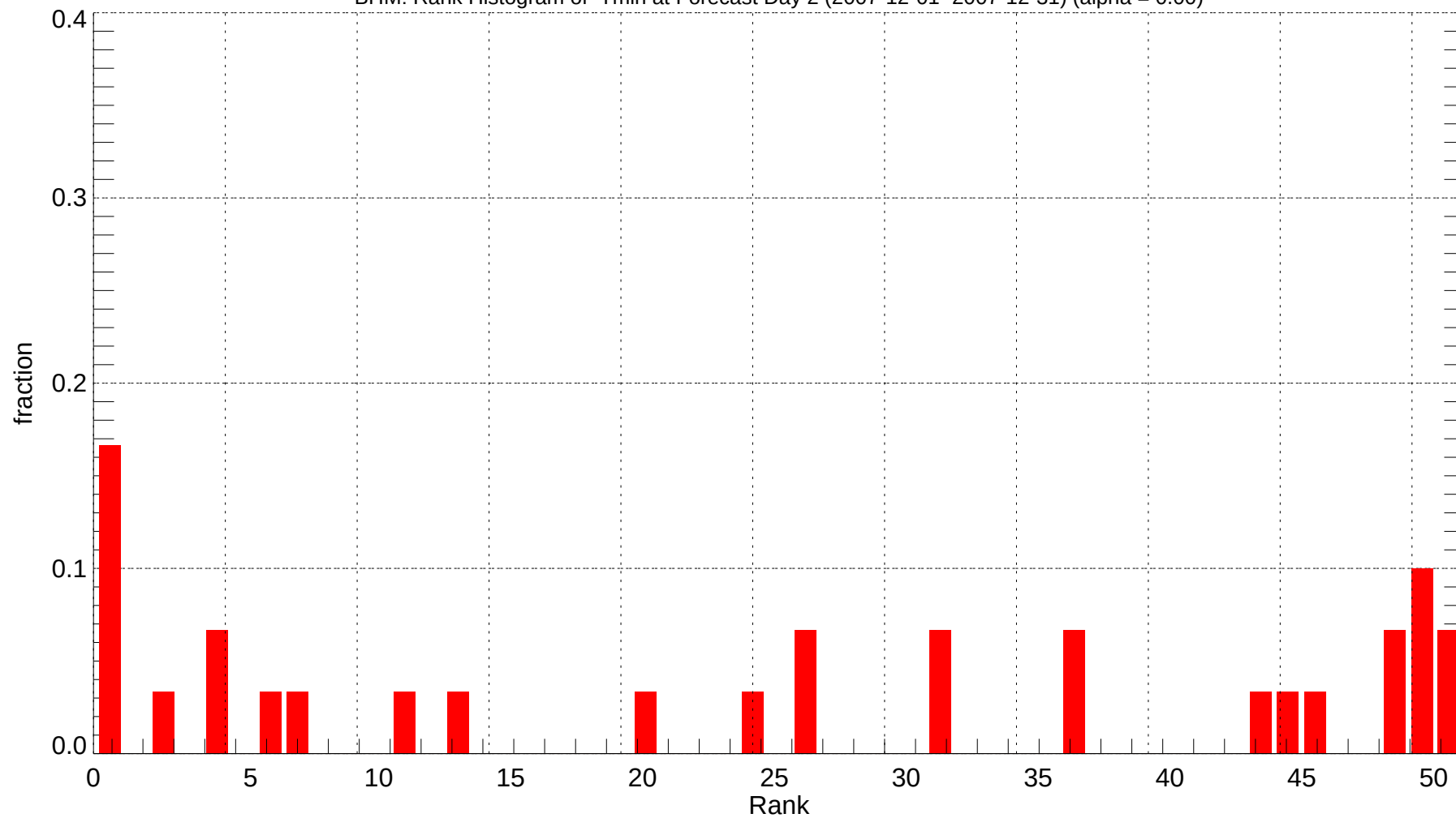
BHM: Rank Histogram of Tmin at Forecast Day 2 (2007-12-01~2007-12-31) (alpha = 0.00)
