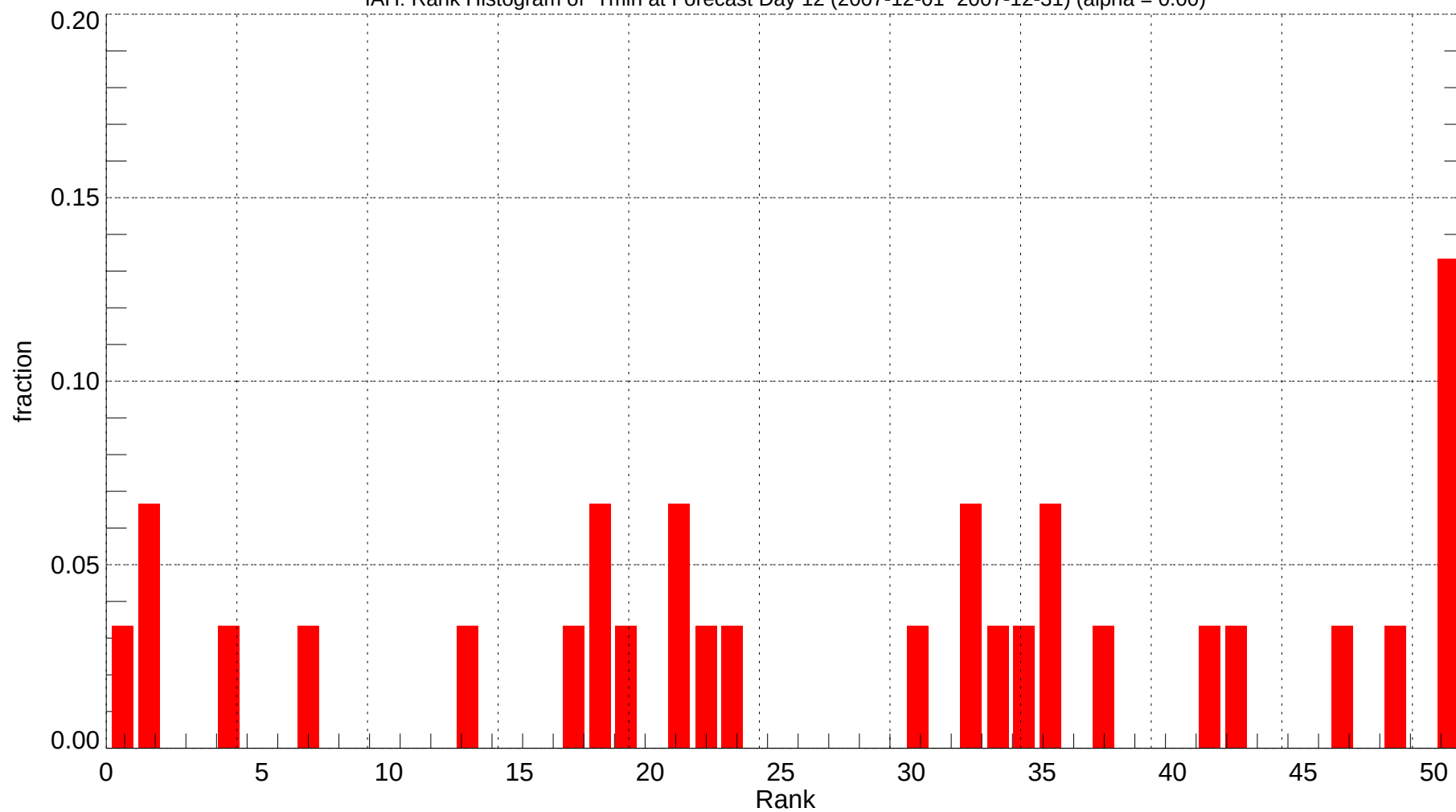
IAH: Rank Histogram of Tmin at Forecast Day 12 (2007-12-01~2007-12-31) (alpha = 0.00)
