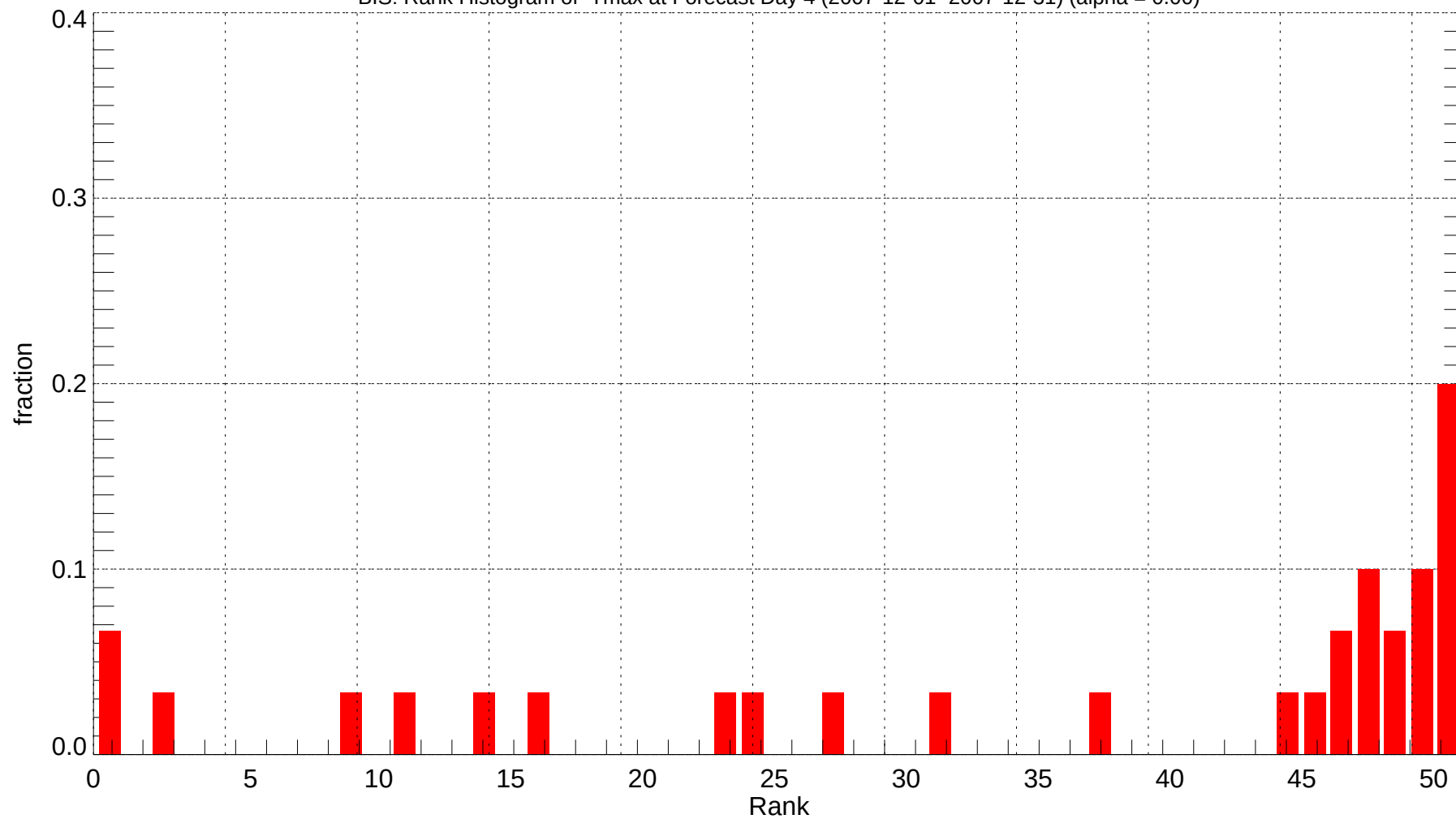
BIS: Rank Histogram of Tmax at Forecast Day 4 (2007-12-01~2007-12-31) (alpha = 0.00)
