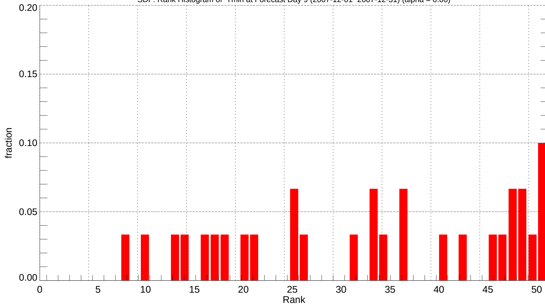
SDF: Rank Histogram of Tmin at Forecast Day 9 (2007-12-01~2007-12-31) (alpha = 0.00)
