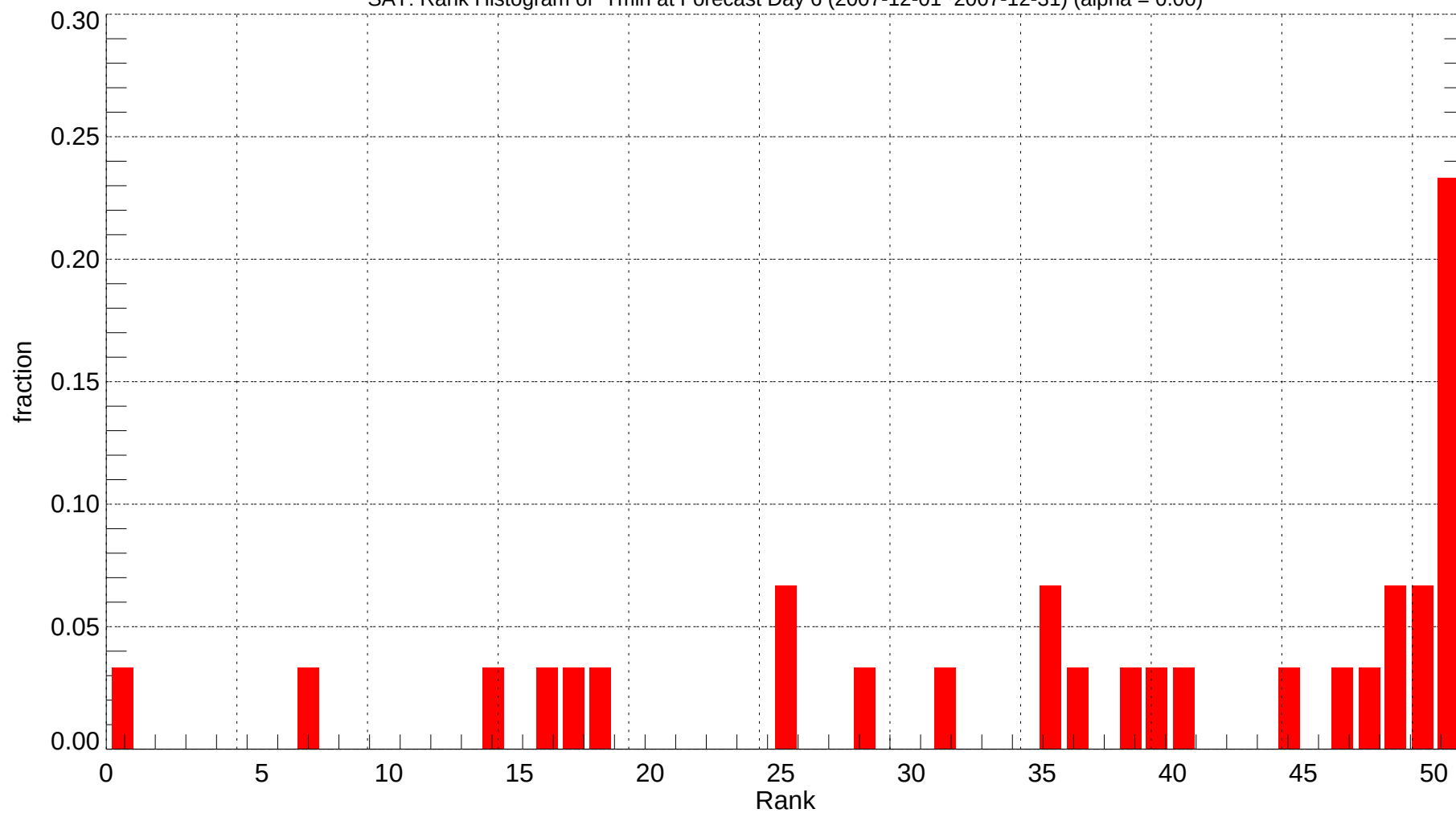
SAT: Rank Histogram of Tmin at Forecast Day 6 (2007-12-01~2007-12-31) (alpha = 0.00)
