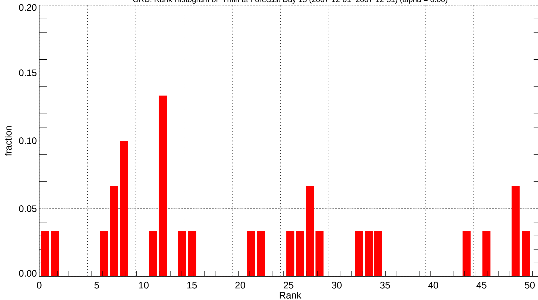
ORD: Rank Histogram of Tmin at Forecast Day 13 (2007-12-01~2007-12-31) (alpha = 0.00)
