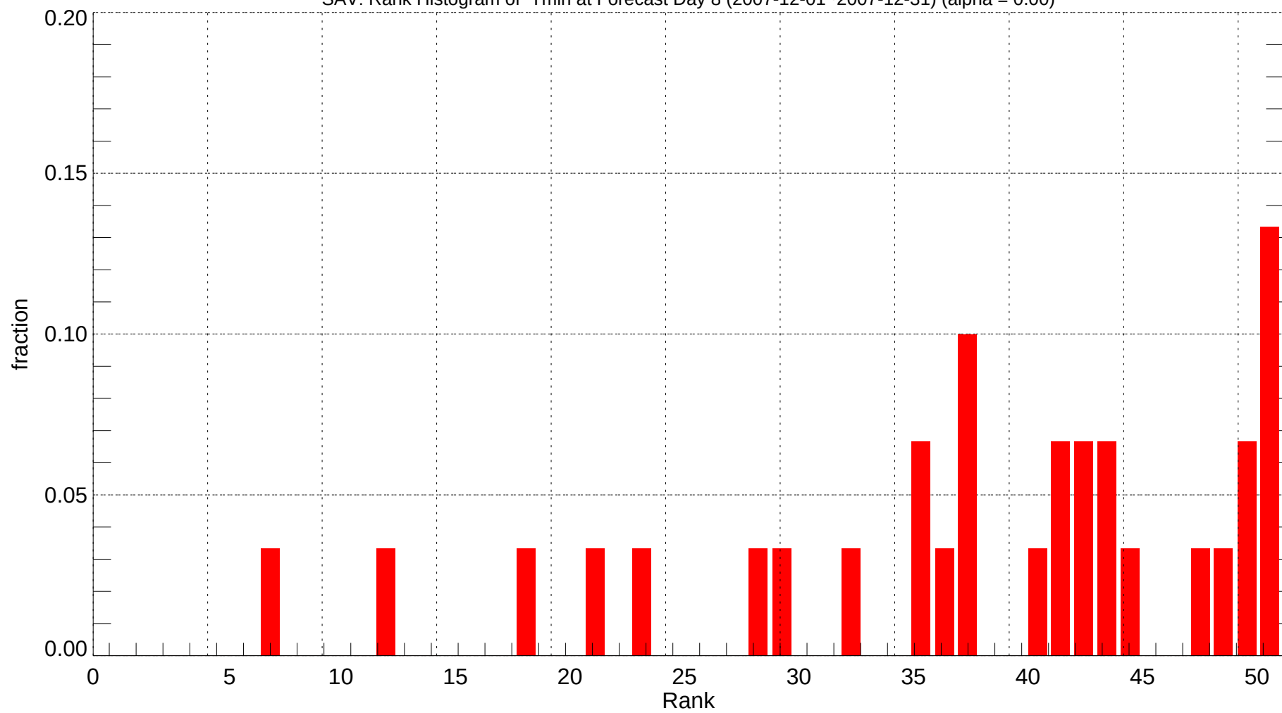
SAV: Rank Histogram of Tmin at Forecast Day 8 (2007-12-01~2007-12-31) (alpha = 0.00)
