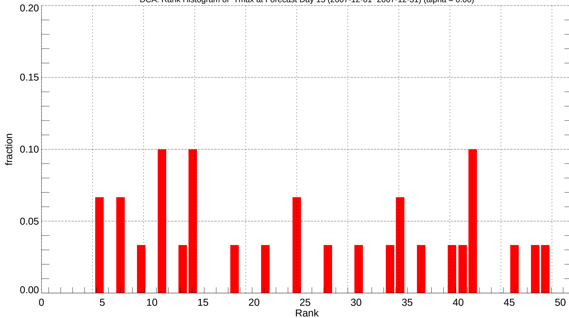
DCA: Rank Histogram of Tmax at Forecast Day 13 (2007-12-01~2007-12-31) (alpha = 0.00)
