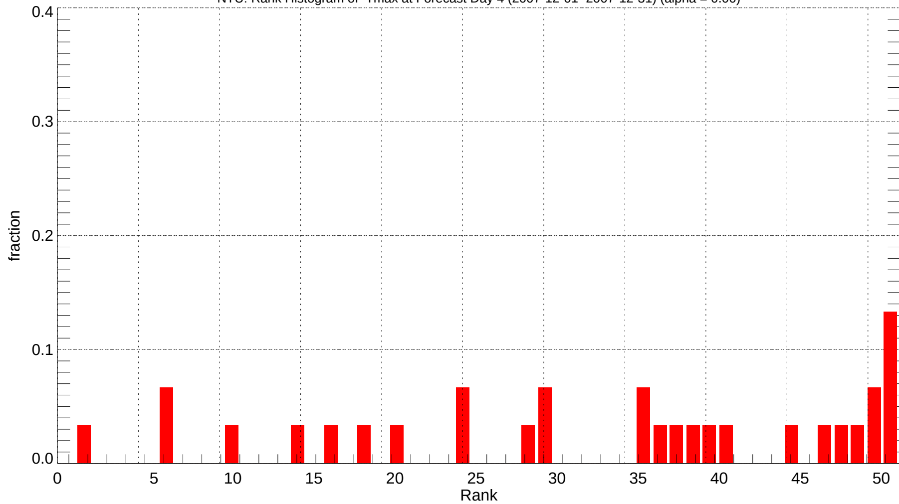
NTU: Rank Histogram of Tmax at Forecast Day 4 (2007-12-01~2007-12-31) (alpha = 0.00)
