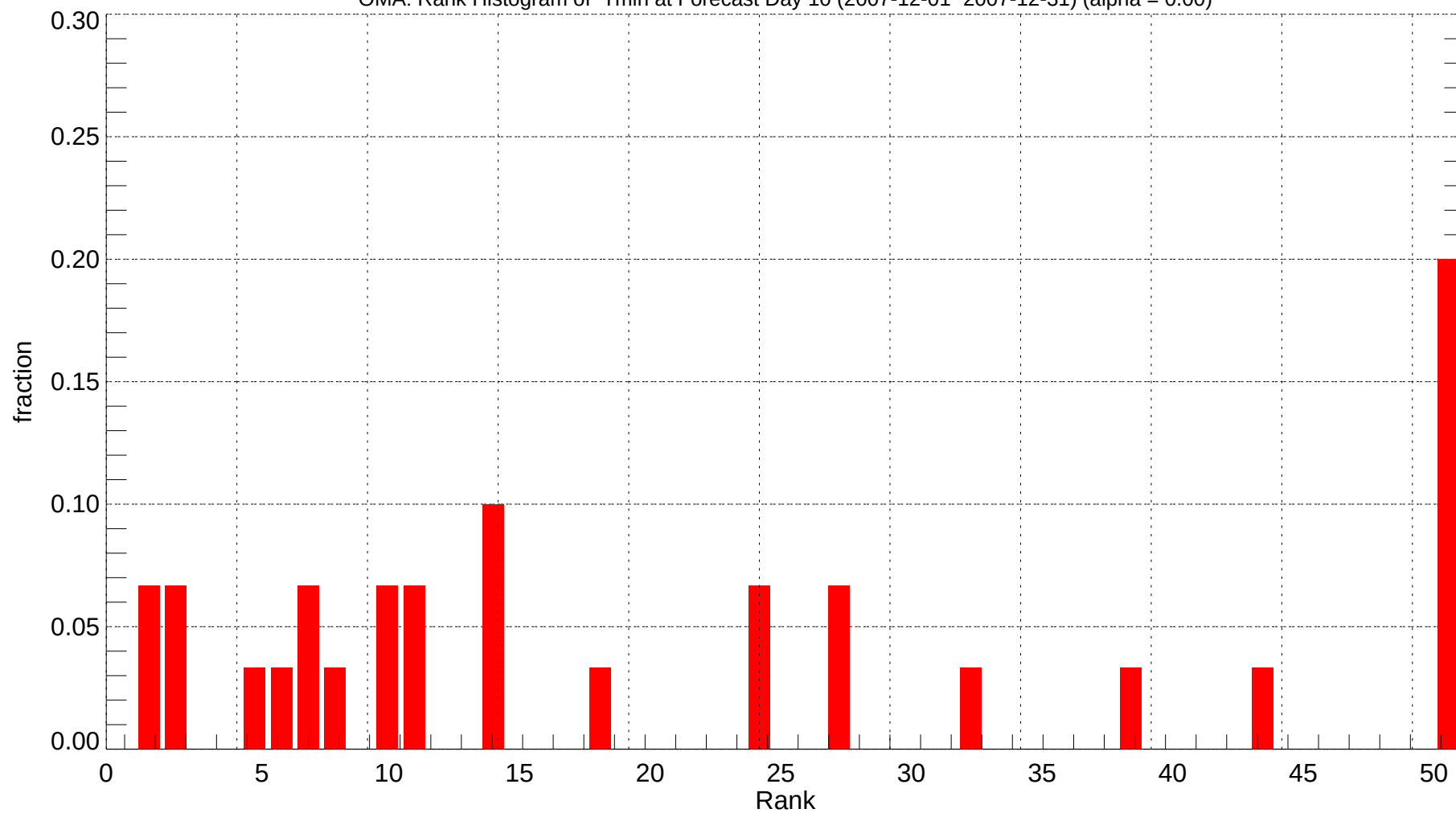
OMA: Rank Histogram of Tmin at Forecast Day 10 (2007-12-01~2007-12-31) (alpha = 0.00)
