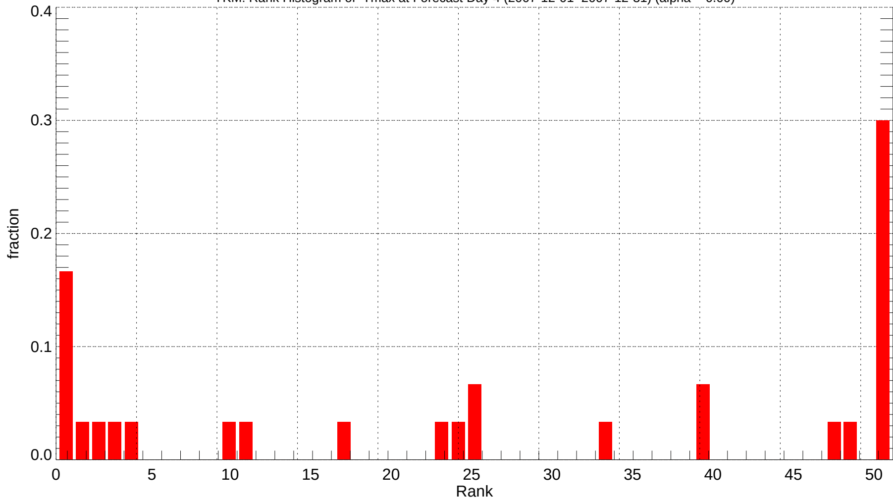
YKM: Rank Histogram of Tmax at Forecast Day 4 (2007-12-01~2007-12-31) (alpha = 0.00)
