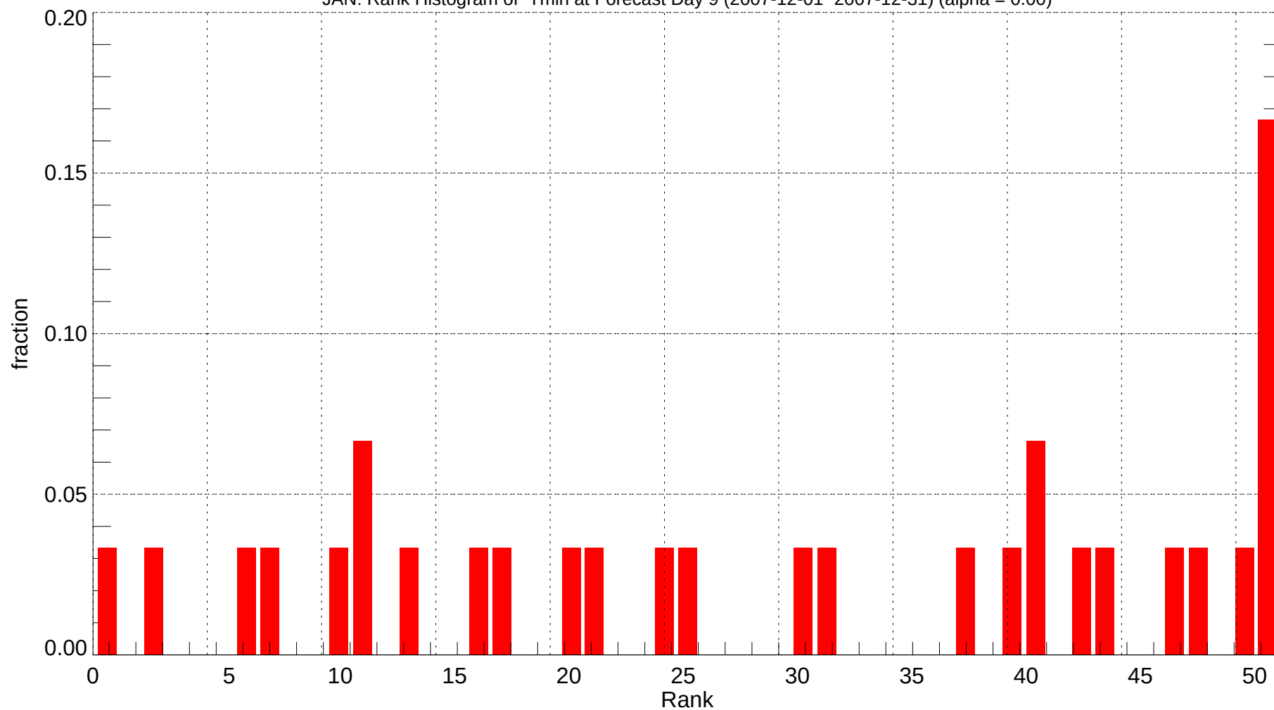
JAN: Rank Histogram of Tmin at Forecast Day 9 (2007-12-01~2007-12-31) (alpha = 0.00)
