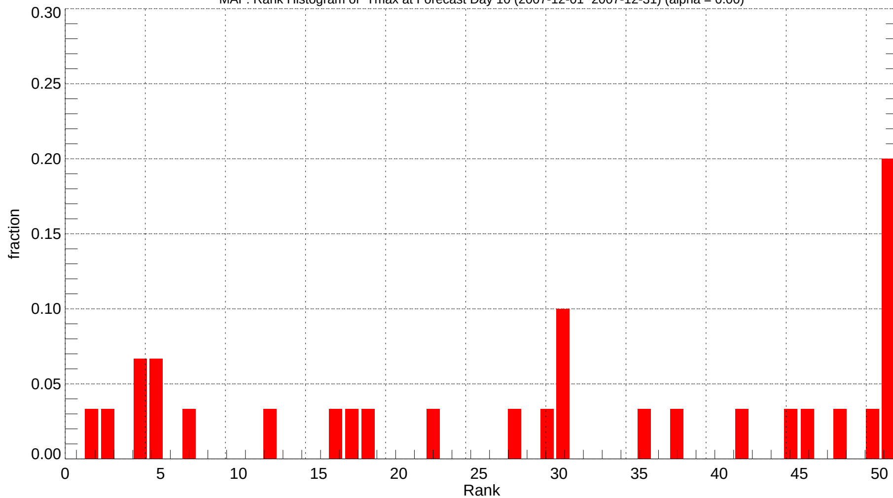
MAF: Rank Histogram of Tmax at Forecast Day 10 (2007-12-01~2007-12-31) (alpha = 0.00)
