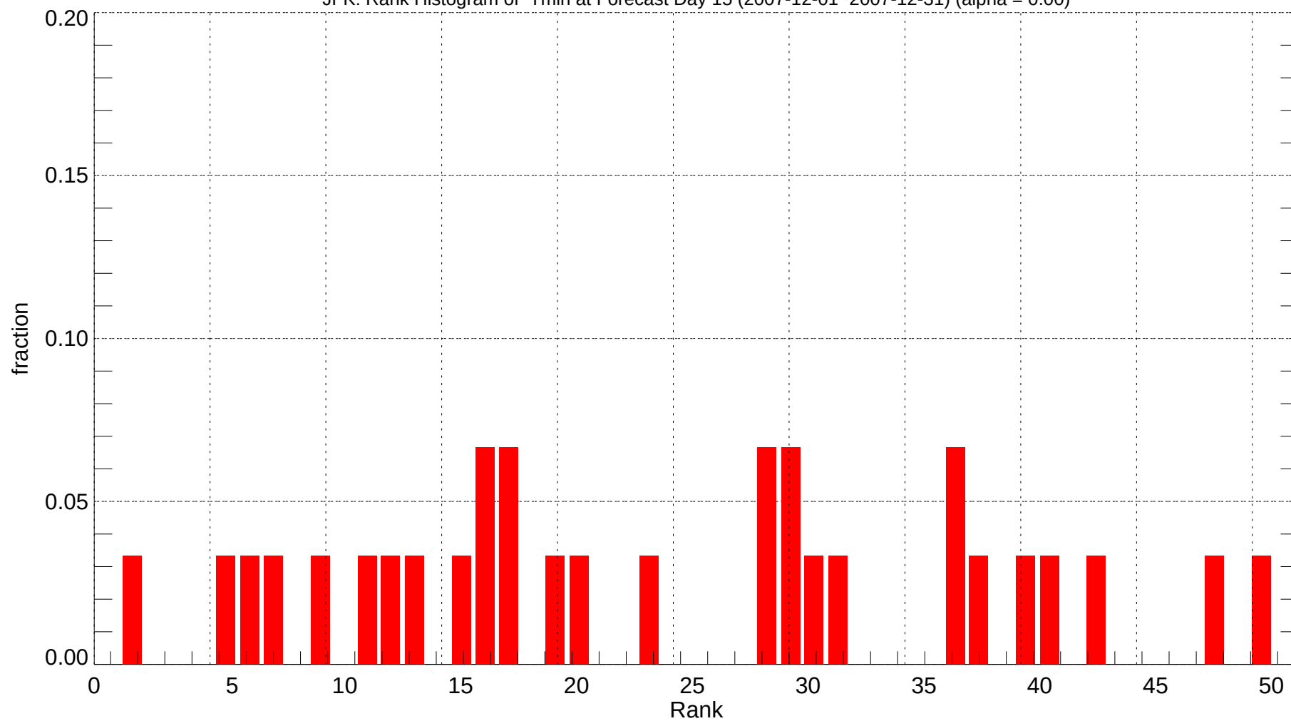
JFK: Rank Histogram of Tmin at Forecast Day 15 (2007-12-01~2007-12-31) (alpha = 0.00)
