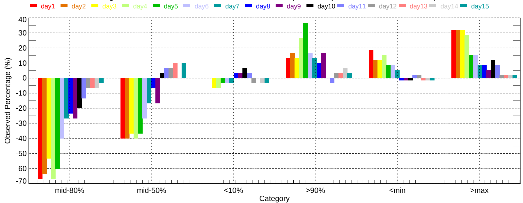
Observed Percentage Deviation of Ensembles - GEG: Max Temperature (2007-12-01~2007-12-31)
