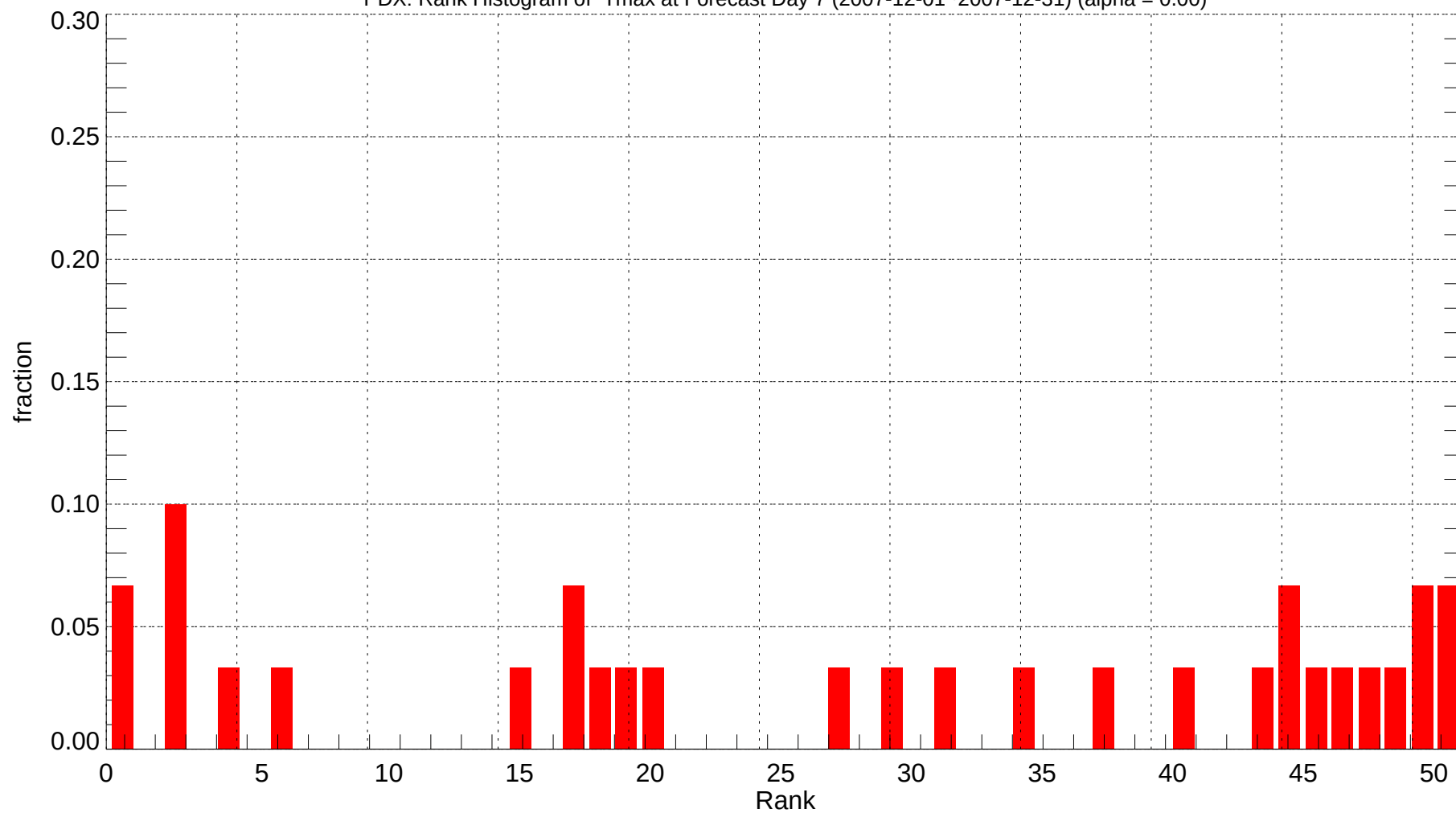
PDX: Rank Histogram of Tmax at Forecast Day 7 (2007-12-01~2007-12-31) (alpha = 0.00)
