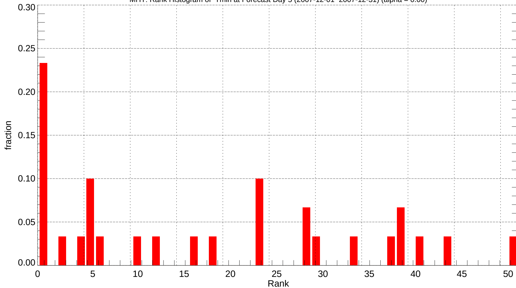
MHT: Rank Histogram of Tmin at Forecast Day 5 (2007-12-01~2007-12-31) (alpha = 0.00)
