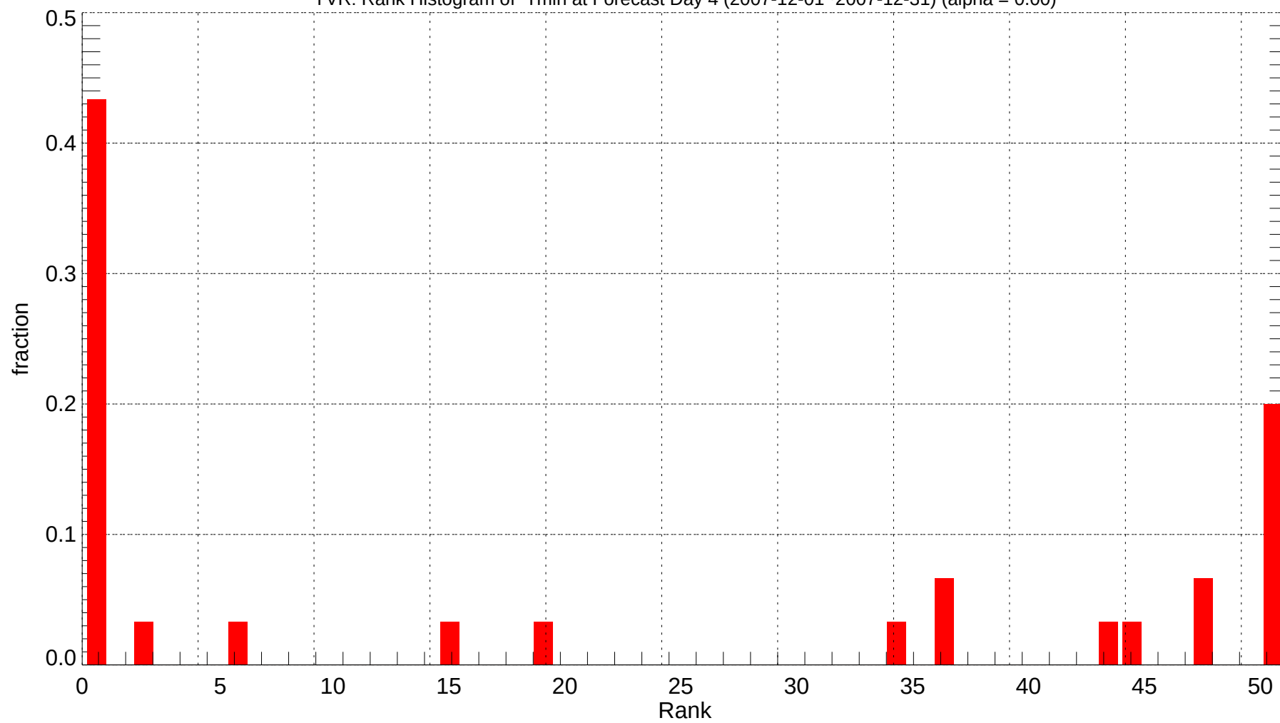
YVR: Rank Histogram of Tmin at Forecast Day 4 (2007-12-01~2007-12-31) (alpha = 0.00)
