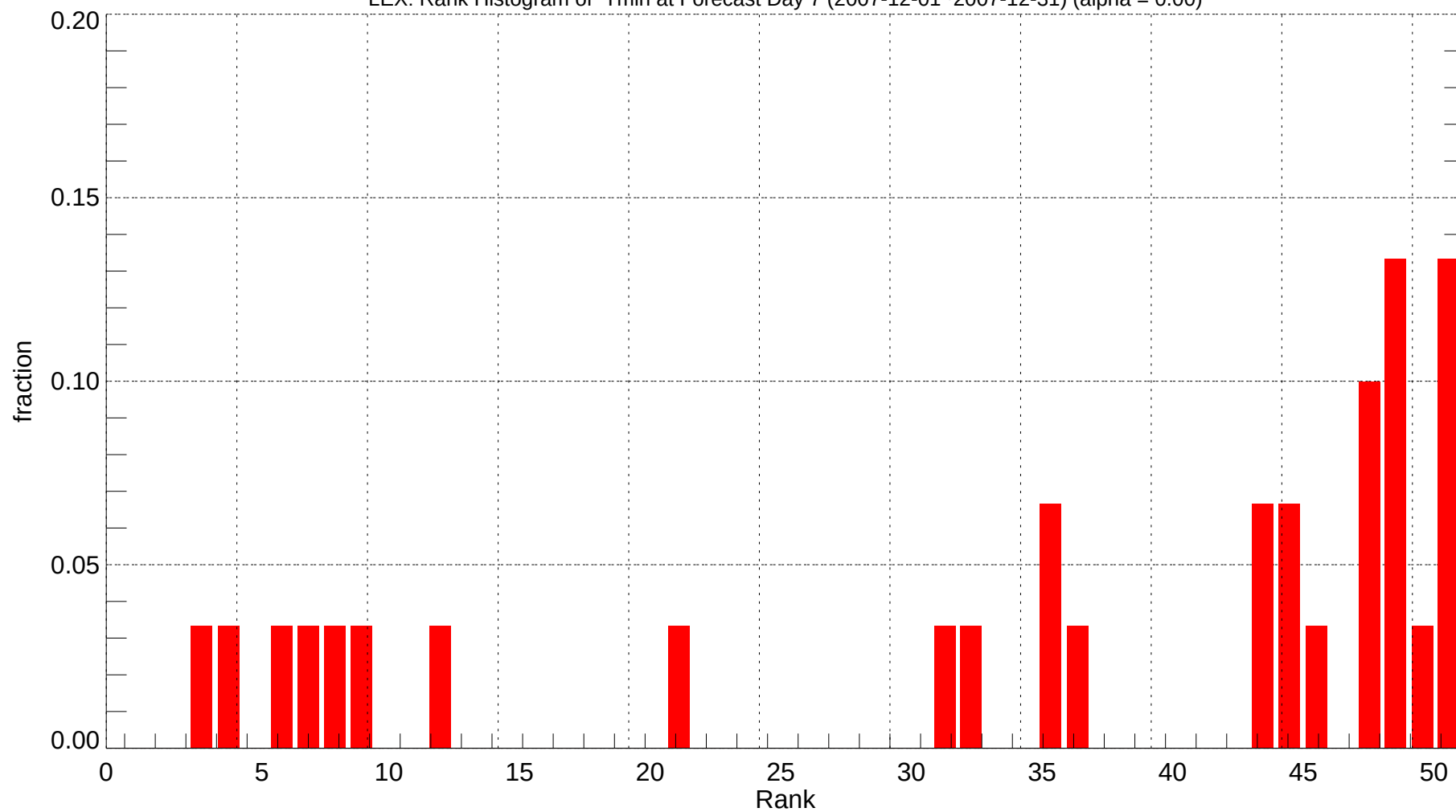
LEX: Rank Histogram of Tmin at Forecast Day 7 (2007-12-01~2007-12-31) (alpha = 0.00)
