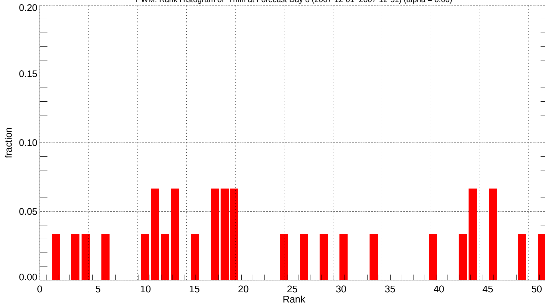
PWM: Rank Histogram of Tmin at Forecast Day 8 (2007-12-01~2007-12-31) (alpha = 0.00)
