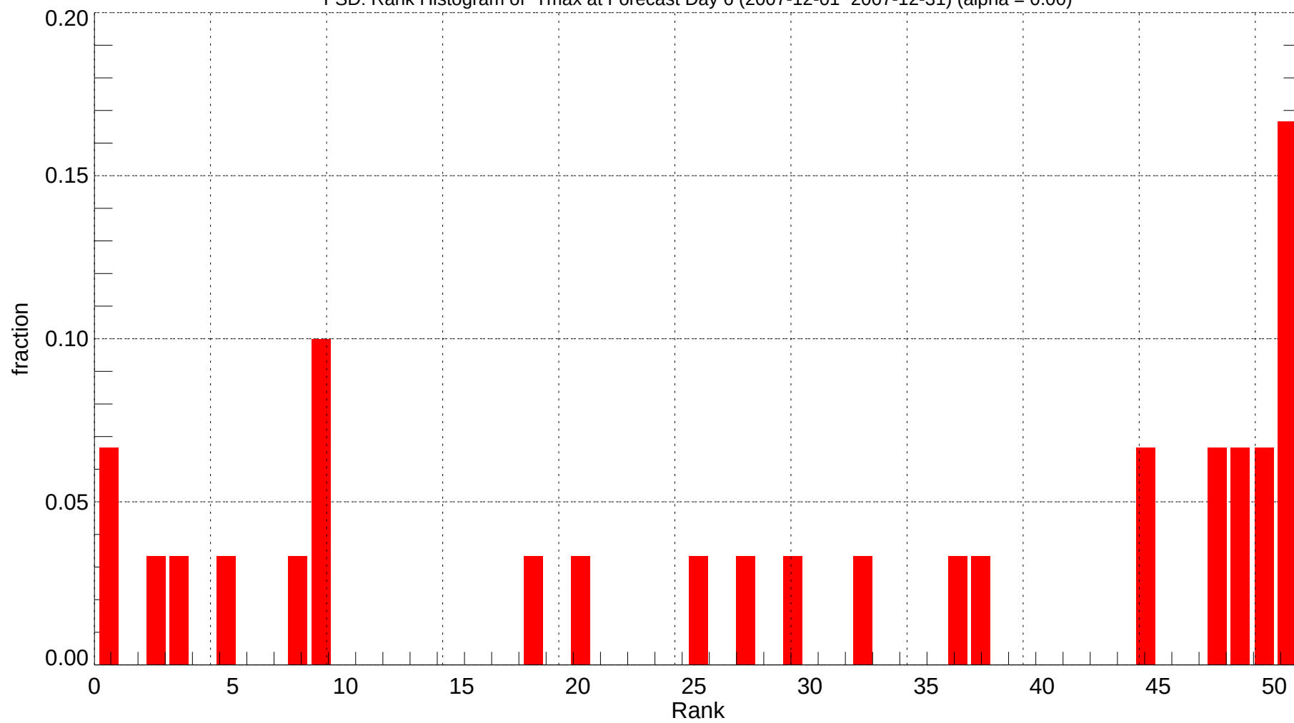
FSD: Rank Histogram of Tmax at Forecast Day 6 (2007-12-01~2007-12-31) (alpha = 0.00)
