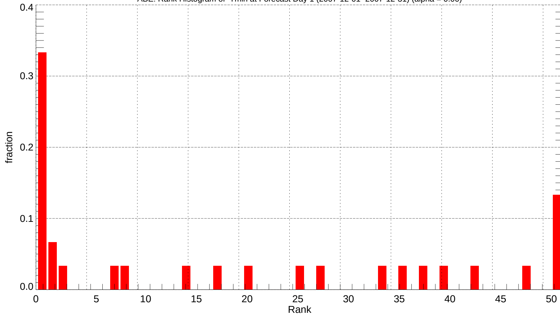
ABE: Rank Histogram of Tmin at Forecast Day 1 (2007-12-01~2007-12-31) (alpha = 0.00)
