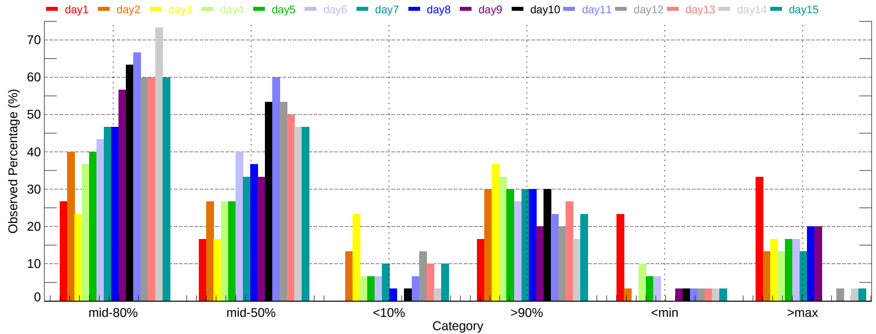
Observed Percentage of Ensembles - TPA: Max Temperature (2007-12-01~2007-12-31)
