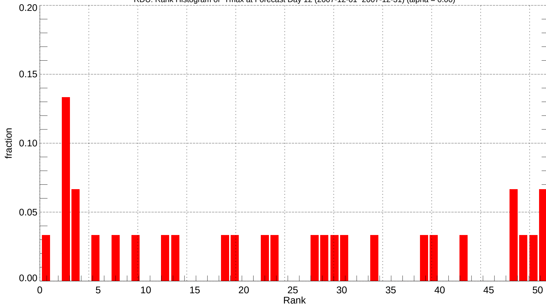
RDU: Rank Histogram of Tmax at Forecast Day 12 (2007-12-01~2007-12-31) (alpha = 0.00)
