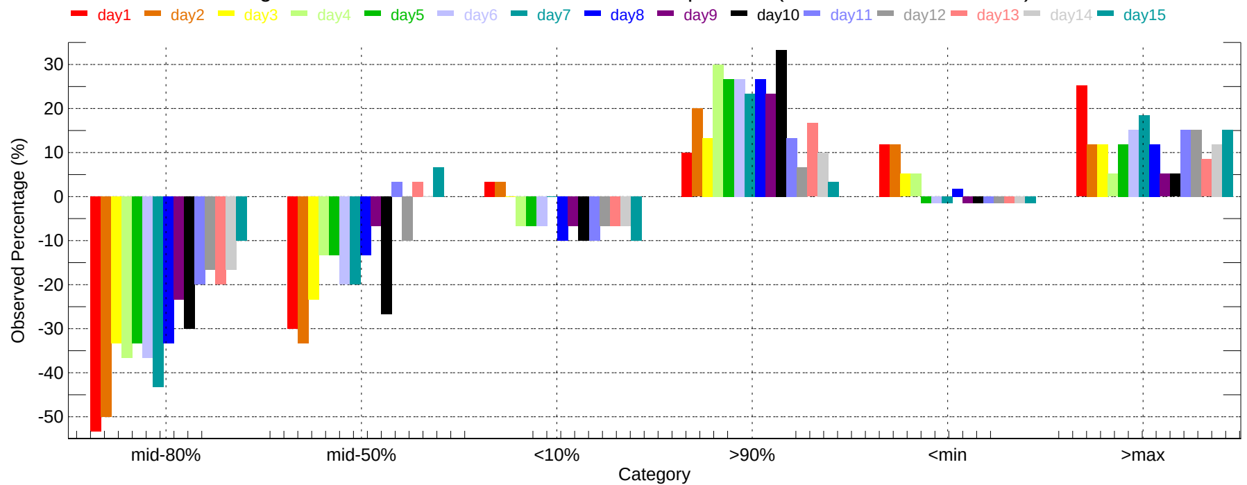
Observed Percentage Deviation of Ensembles - BNA: Min Temperature (2007-12-01~2007-12-31)
