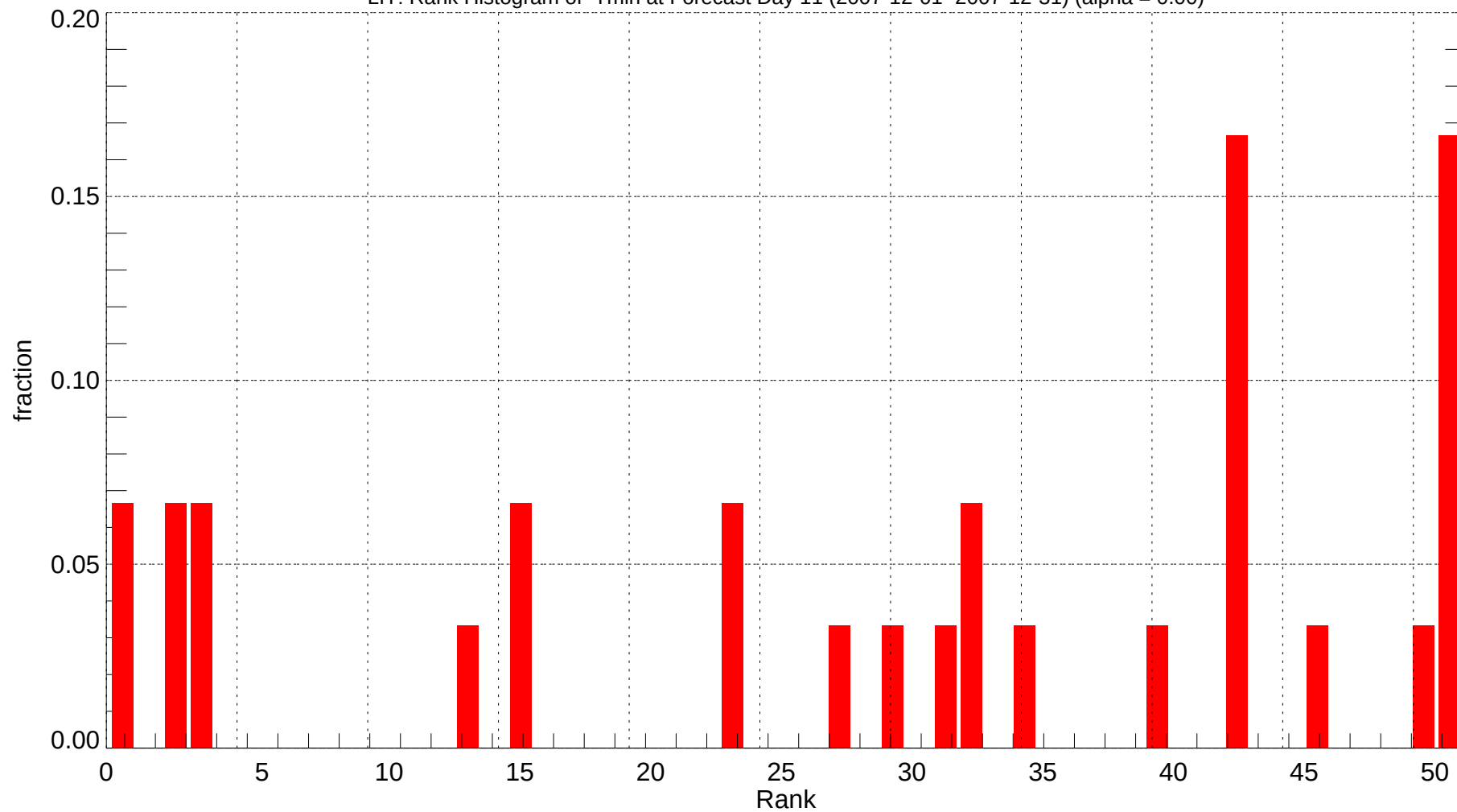
LIT: Rank Histogram of Tmin at Forecast Day 11 (2007-12-01~2007-12-31) (alpha = 0.00)
