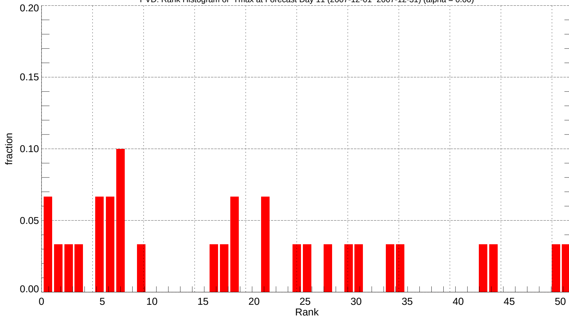
PVD: Rank Histogram of Tmax at Forecast Day 11 (2007-12-01~2007-12-31) (alpha = 0.00)
