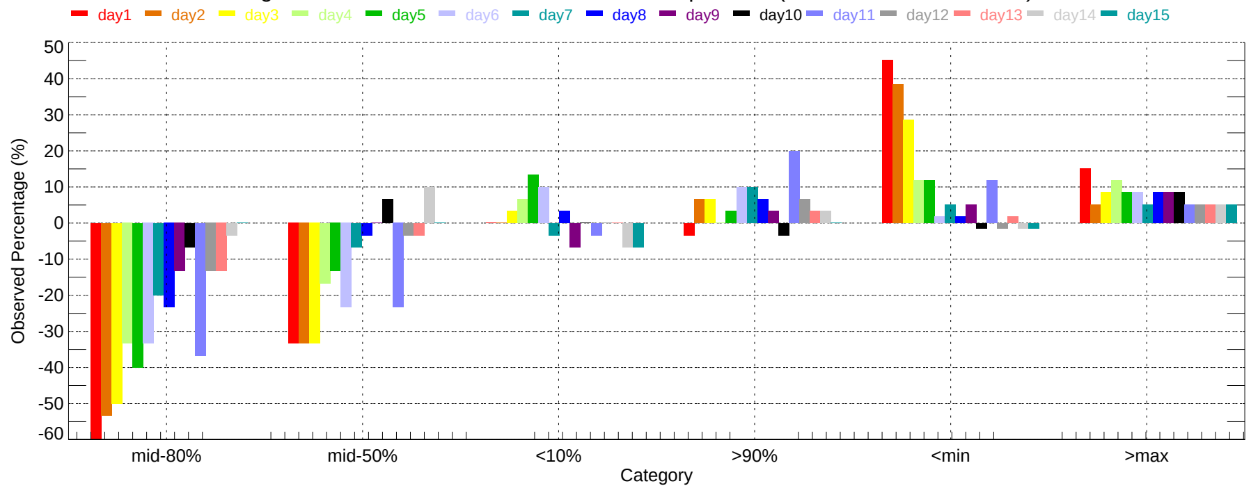
Observed Percentage Deviation of Ensembles - RIC: Max Temperature (2007-12-01~2007-12-31)
