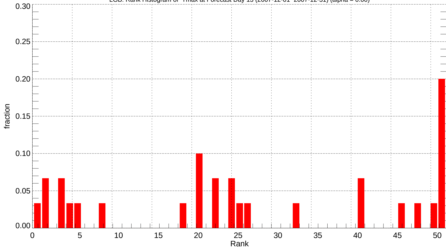
LGB: Rank Histogram of Tmax at Forecast Day 13 (2007-12-01~2007-12-31) (alpha = 0.00)
