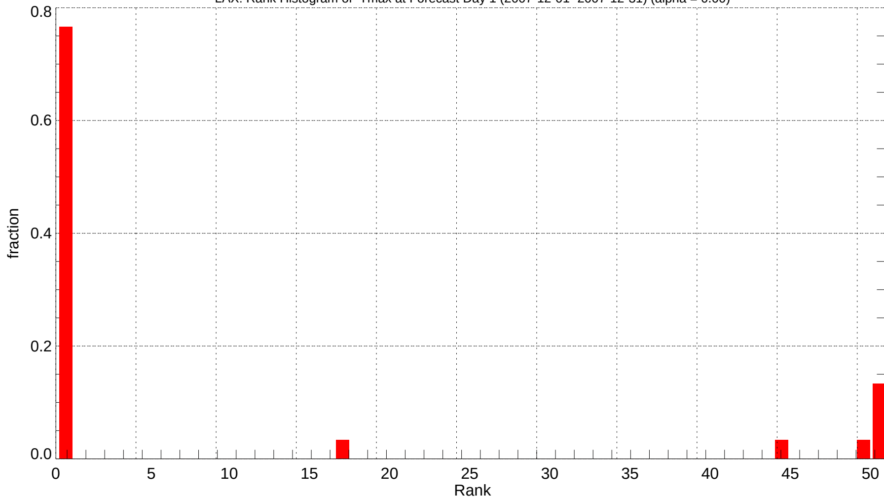
LAX: Rank Histogram of Tmax at Forecast Day 1 (2007-12-01~2007-12-31) (alpha = 0.00)
