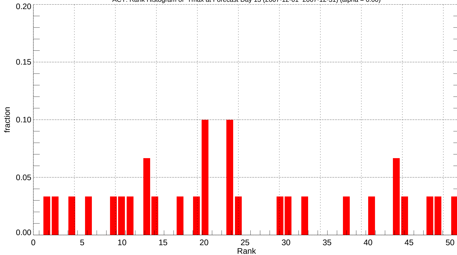
ACY: Rank Histogram of Tmax at Forecast Day 13 (2007-12-01~2007-12-31) (alpha = 0.00)
