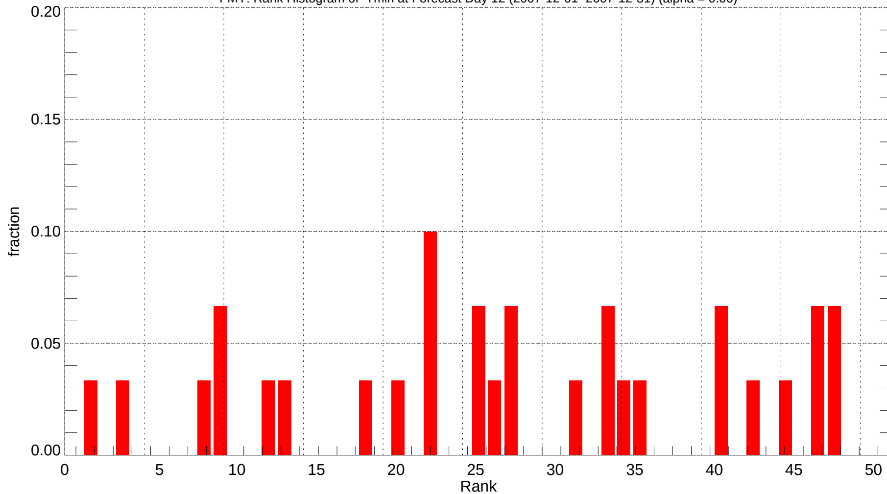
FMY: Rank Histogram of Tmin at Forecast Day 12 (2007-12-01~2007-12-31) (alpha = 0.00)
