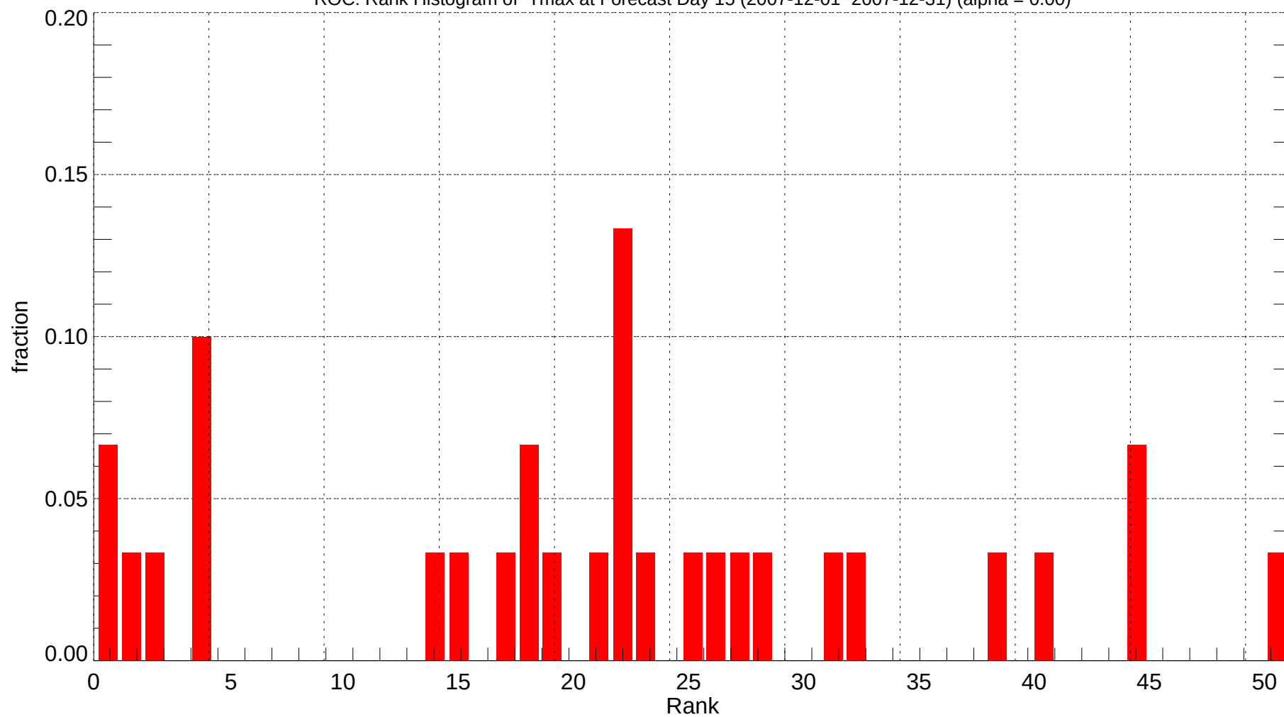
ROC: Rank Histogram of Tmax at Forecast Day 15 (2007-12-01~2007-12-31) (alpha = 0.00)
