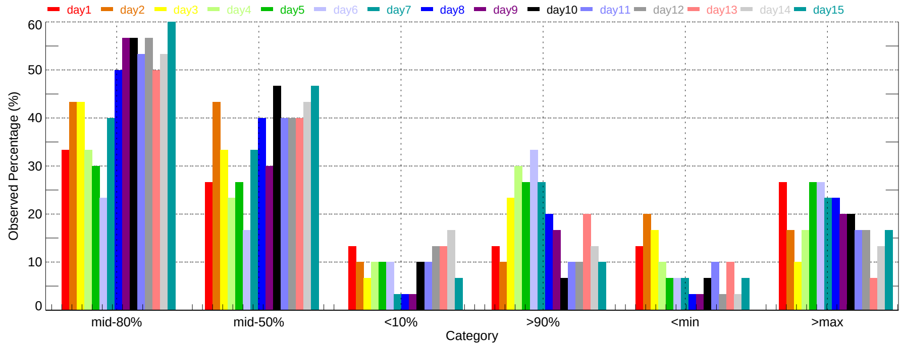
Observed Percentage of Ensembles - ABY: Min Temperature (2007-12-01~2007-12-31)
