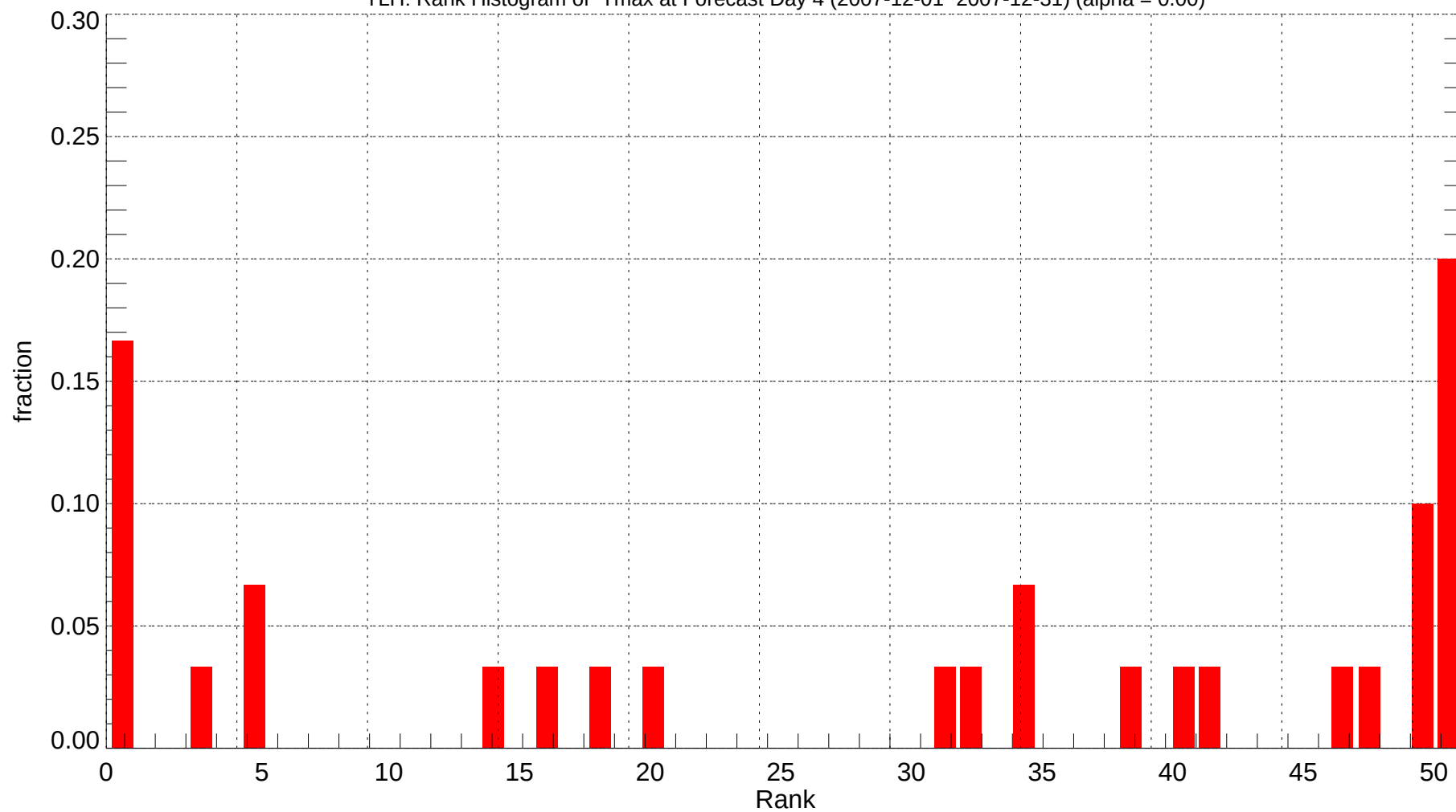
TLH: Rank Histogram of Tmax at Forecast Day 4 (2007-12-01~2007-12-31) (alpha = 0.00)
