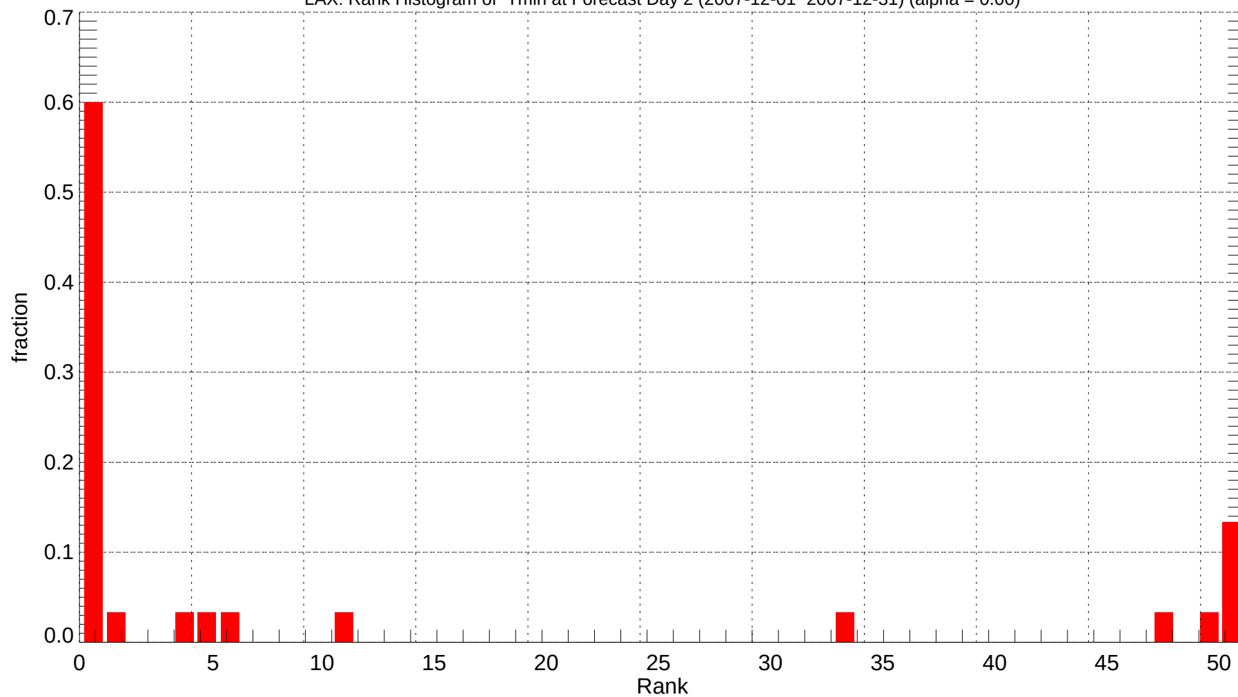
LAX: Rank Histogram of Tmin at Forecast Day 2 (2007-12-01~2007-12-31) (alpha = 0.00)
