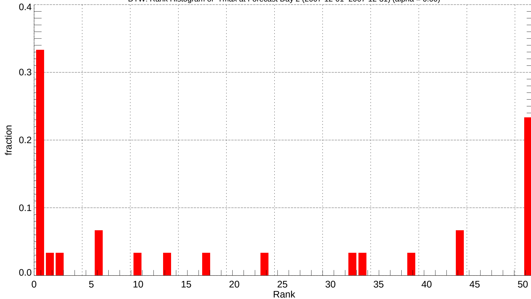
DTW: Rank Histogram of Tmax at Forecast Day 2 (2007-12-01~2007-12-31) (alpha = 0.00)
