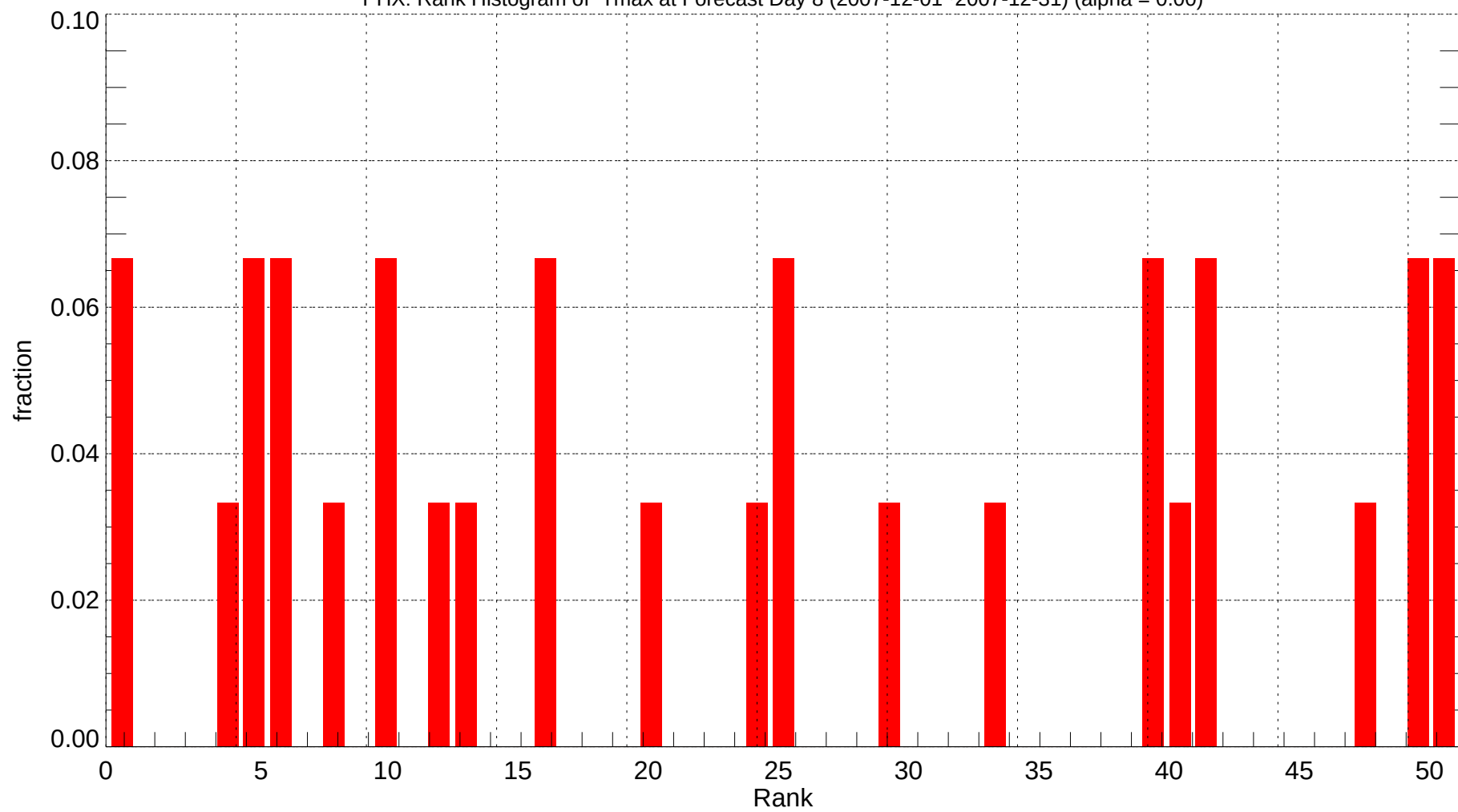
PHX: Rank Histogram of Tmax at Forecast Day 8 (2007-12-01~2007-12-31) (alpha = 0.00)
