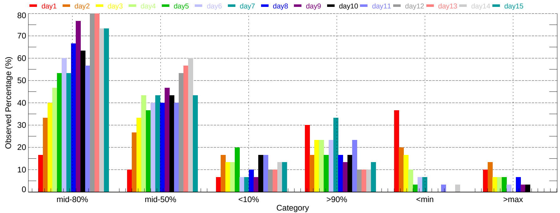
Observed Percentage of Ensembles - PHL: Max Temperature (2007-12-01~2007-12-31)
