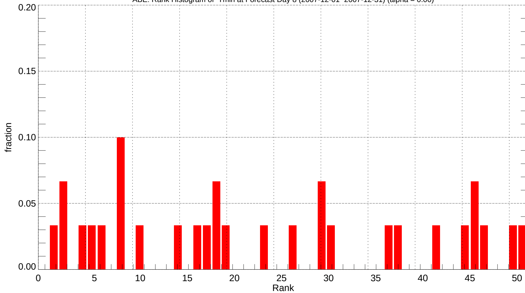
ABE: Rank Histogram of Tmin at Forecast Day 8 (2007-12-01~2007-12-31) (alpha = 0.00)
