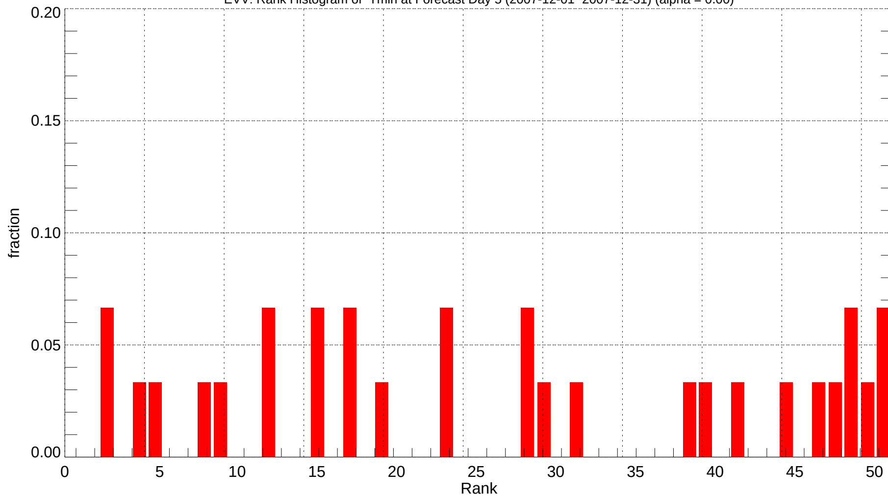
EVV: Rank Histogram of Tmin at Forecast Day 5 (2007-12-01~2007-12-31) (alpha = 0.00)
