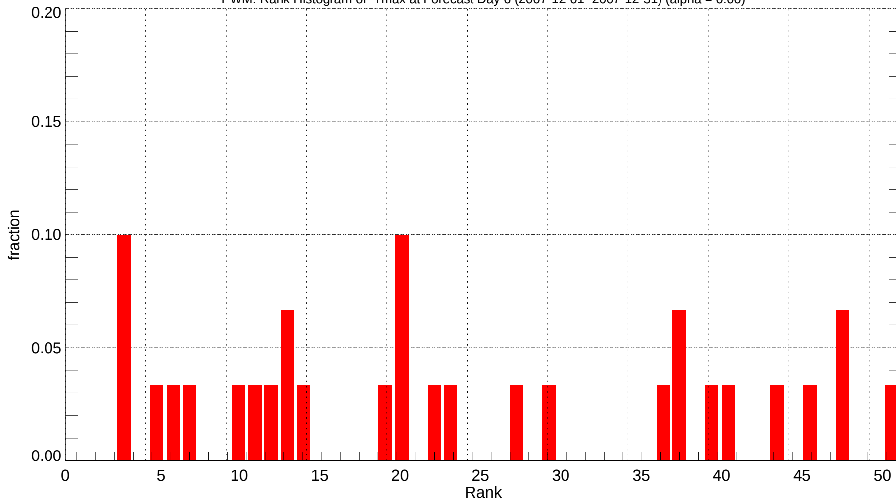
PWM: Rank Histogram of Tmax at Forecast Day 6 (2007-12-01~2007-12-31) (alpha = 0.00)
