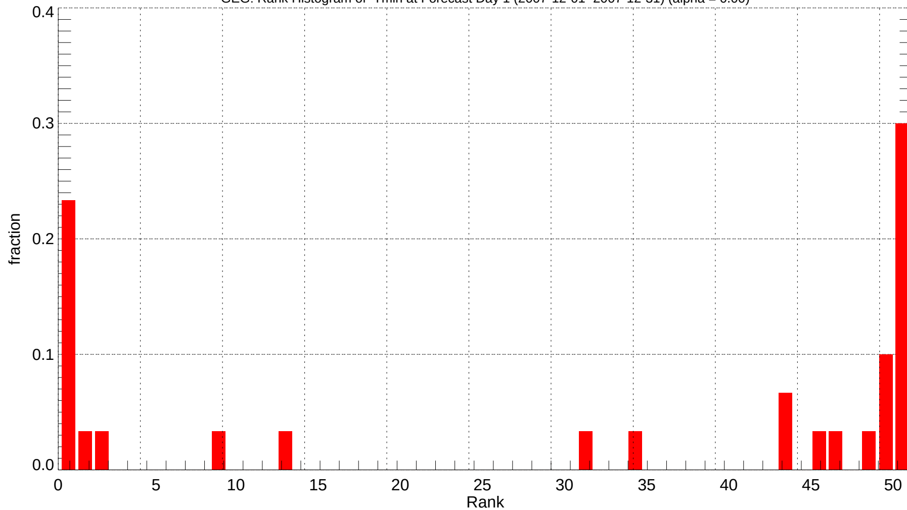
GEG: Rank Histogram of Tmin at Forecast Day 1 (2007-12-01~2007-12-31) (alpha = 0.00)
