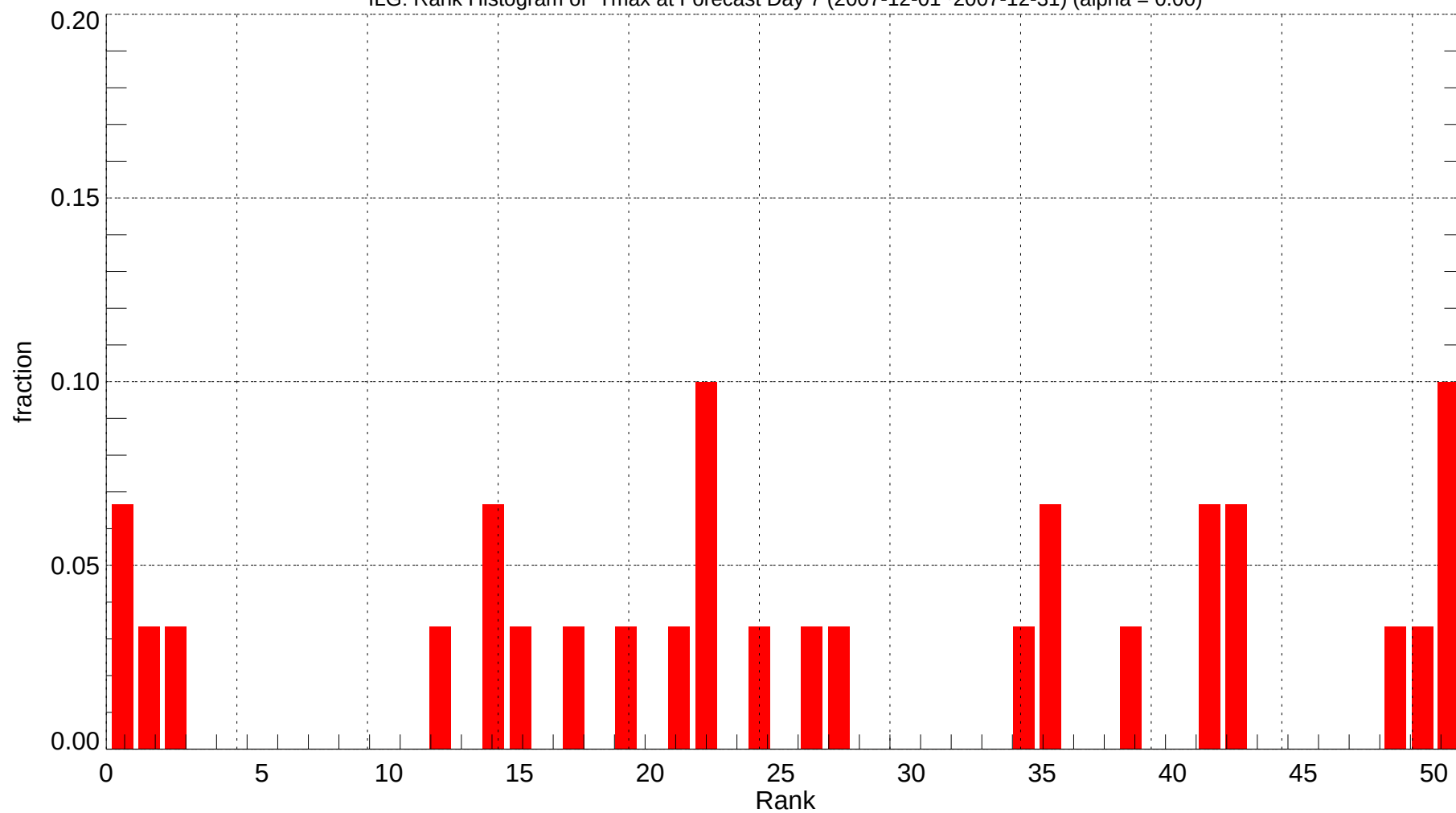
ILG: Rank Histogram of Tmax at Forecast Day 7 (2007-12-01~2007-12-31) (alpha = 0.00)
