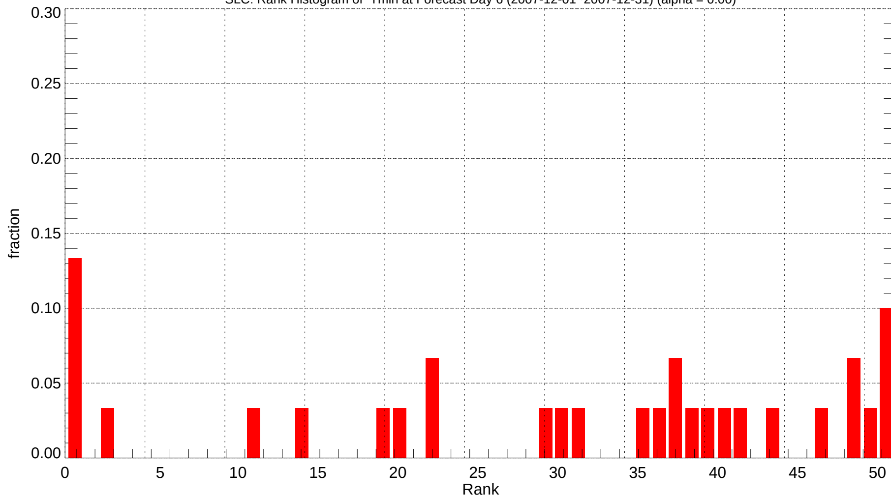
SLC: Rank Histogram of Tmin at Forecast Day 6 (2007-12-01~2007-12-31) (alpha = 0.00)
