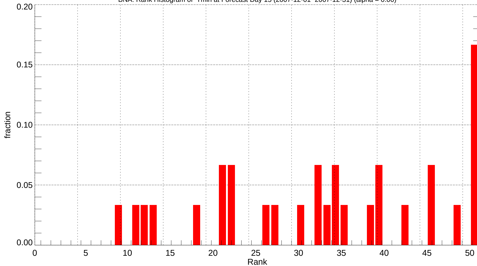
BNA: Rank Histogram of Tmin at Forecast Day 15 (2007-12-01~2007-12-31) (alpha = 0.00)
