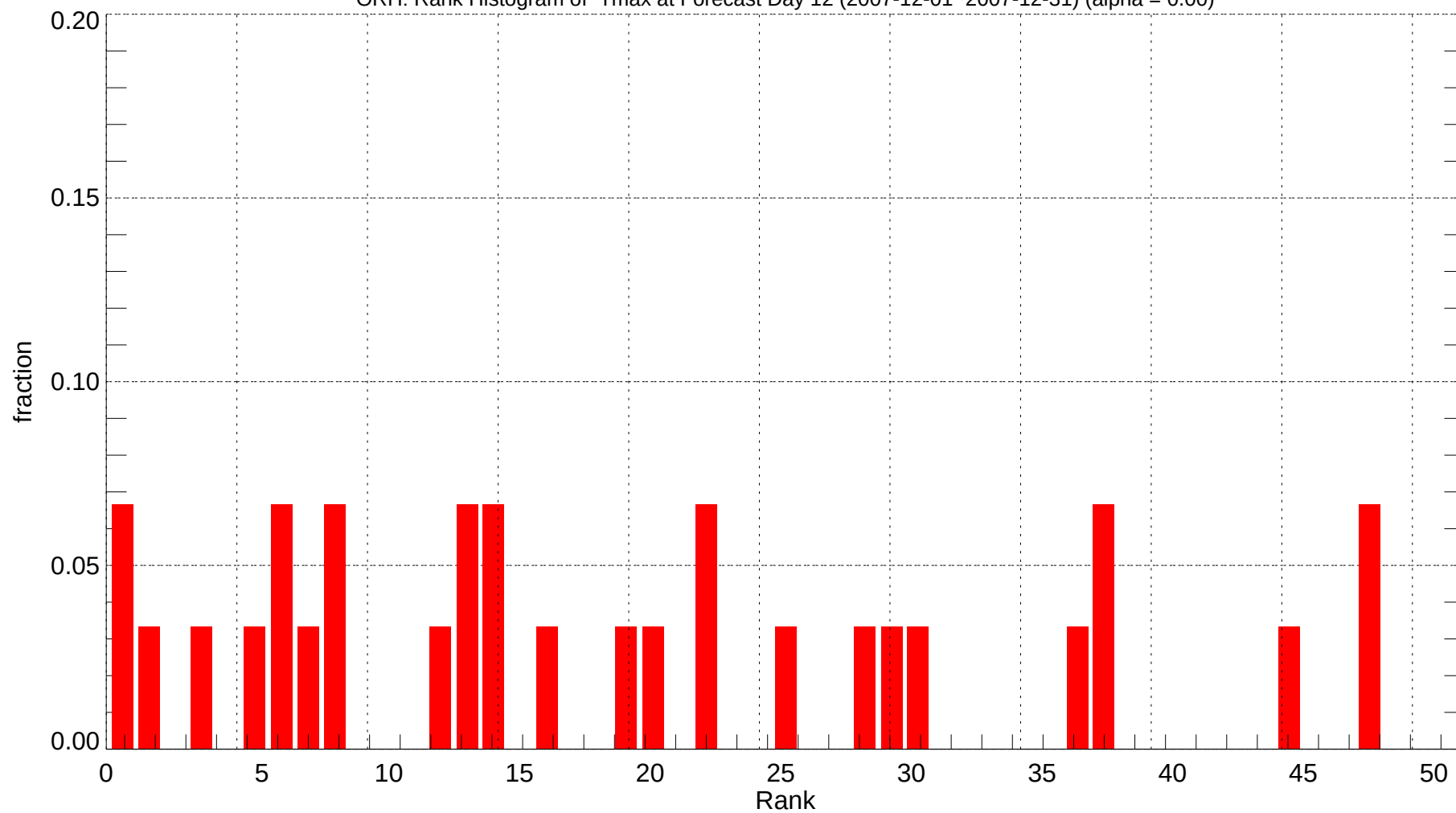
ORH: Rank Histogram of Tmax at Forecast Day 12 (2007-12-01~2007-12-31) (alpha = 0.00)
