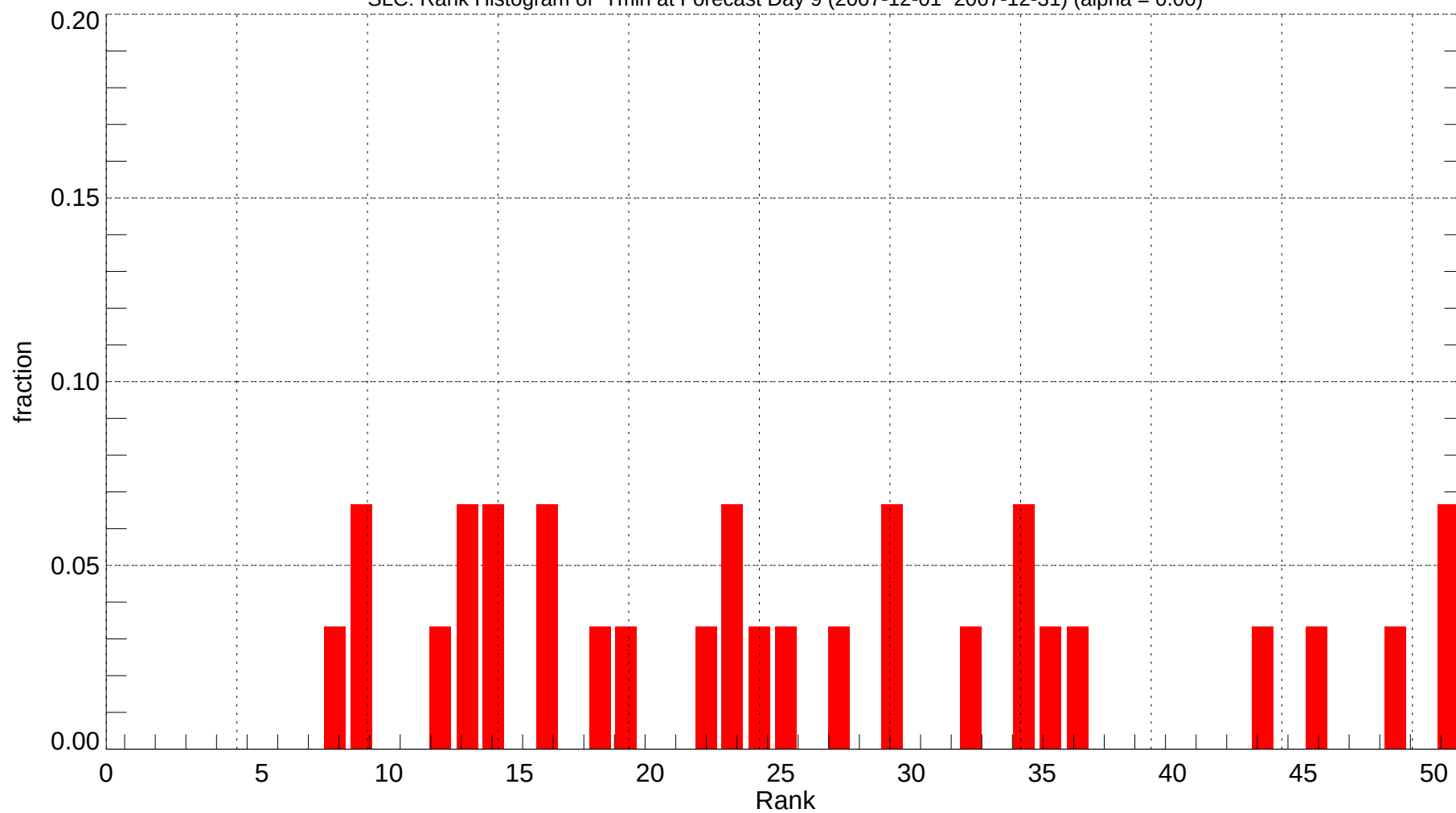
SLC: Rank Histogram of Tmin at Forecast Day 9 (2007-12-01~2007-12-31) (alpha = 0.00)
