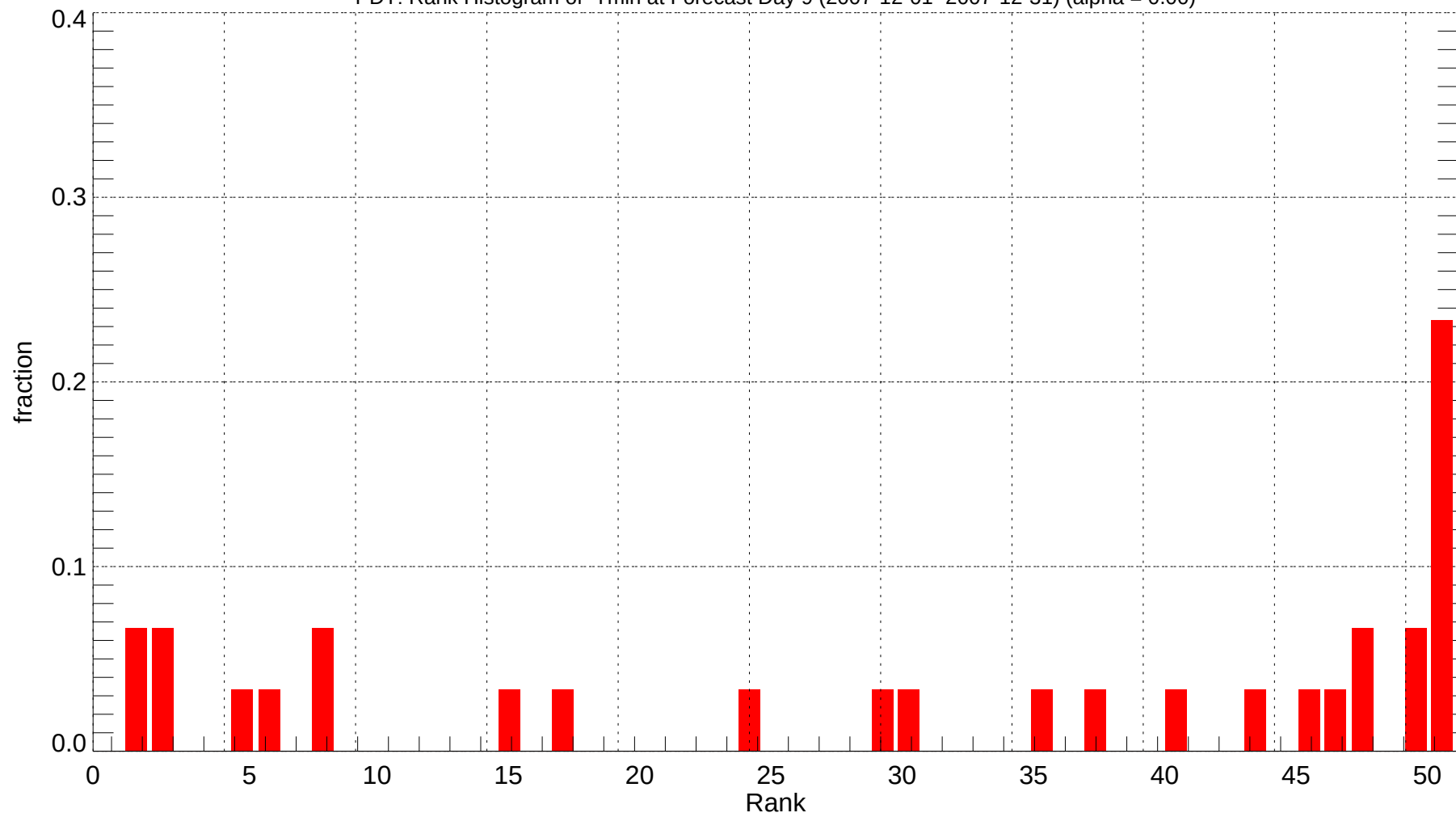
PDT: Rank Histogram of Tmin at Forecast Day 9 (2007-12-01~2007-12-31) (alpha = 0.00)
