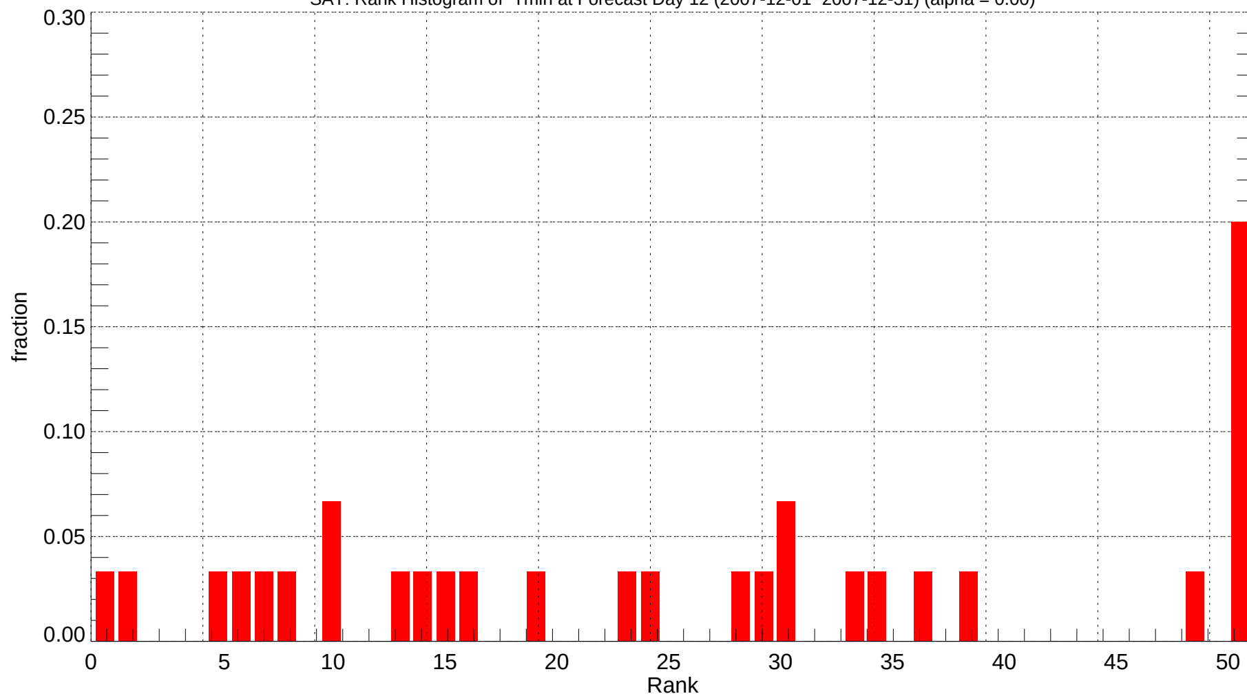
SAT: Rank Histogram of Tmin at Forecast Day 12 (2007-12-01~2007-12-31) (alpha = 0.00)
