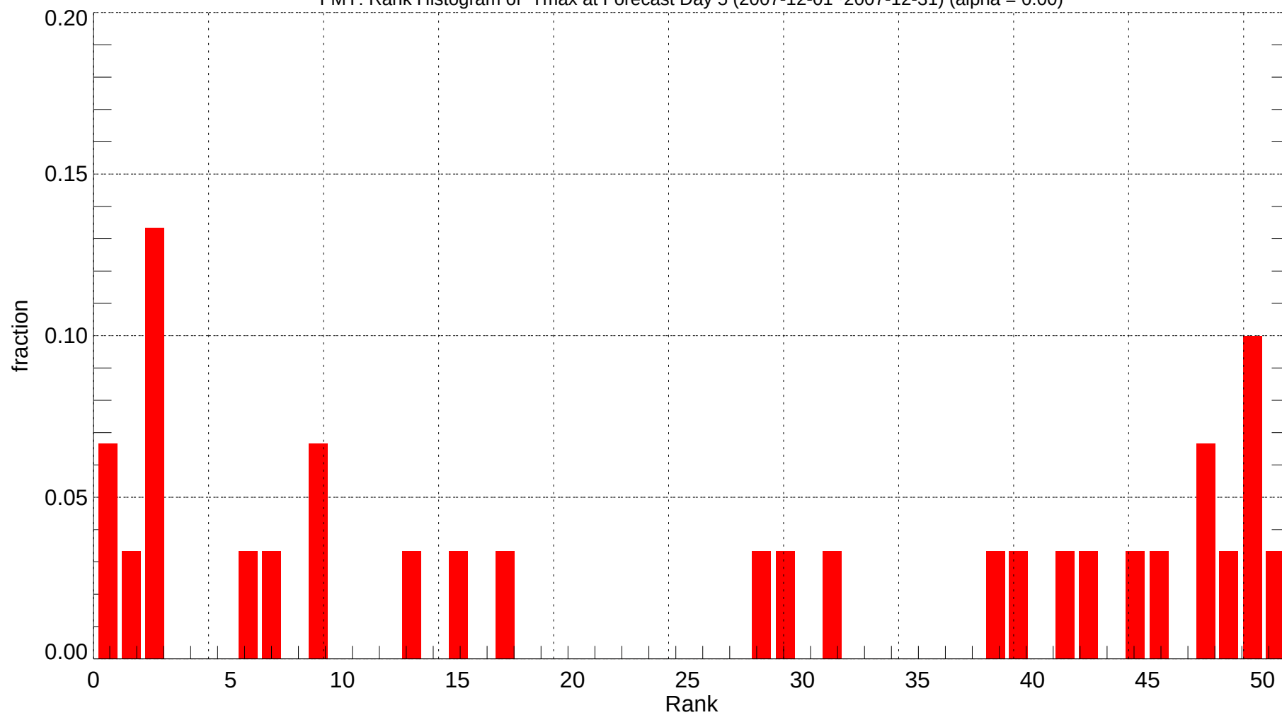
FMY: Rank Histogram of Tmax at Forecast Day 5 (2007-12-01~2007-12-31) (alpha = 0.00)
