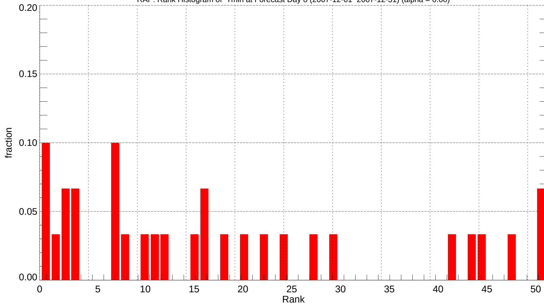
RAP: Rank Histogram of Tmin at Forecast Day 8 (2007-12-01~2007-12-31) (alpha = 0.00)
