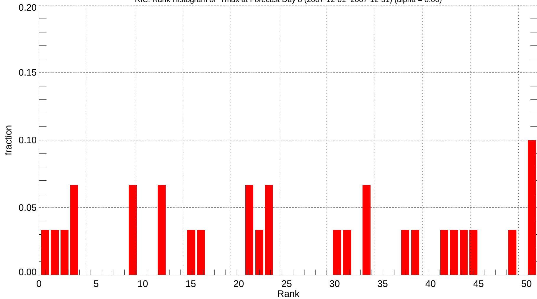
RIC: Rank Histogram of Tmax at Forecast Day 8 (2007-12-01~2007-12-31) (alpha = 0.00)
