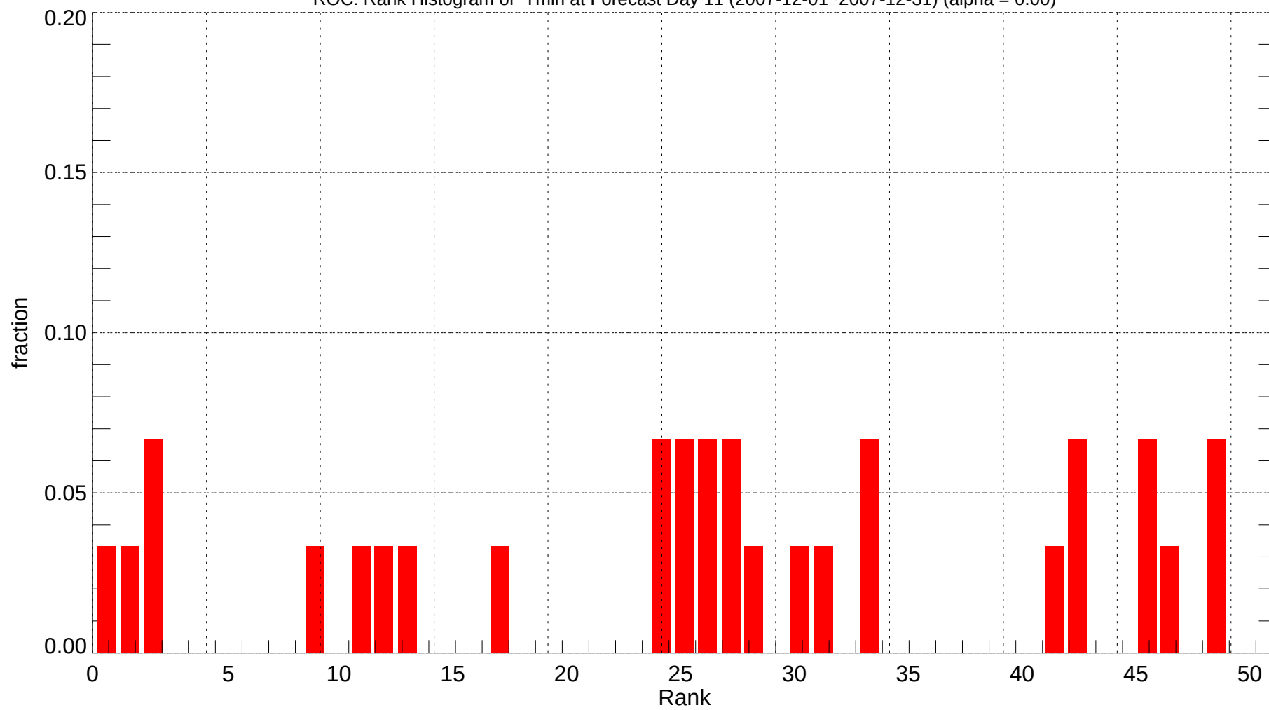
ROC: Rank Histogram of Tmin at Forecast Day 11 (2007-12-01~2007-12-31) (alpha = 0.00)
