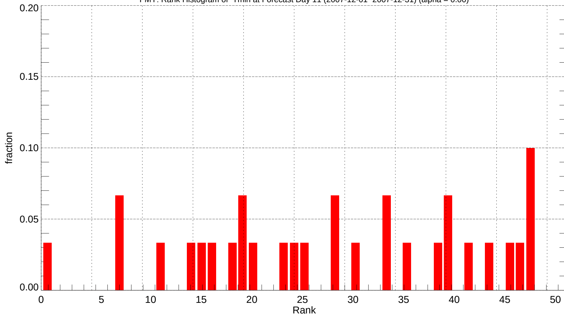
FMY: Rank Histogram of Tmin at Forecast Day 11 (2007-12-01~2007-12-31) (alpha = 0.00)
