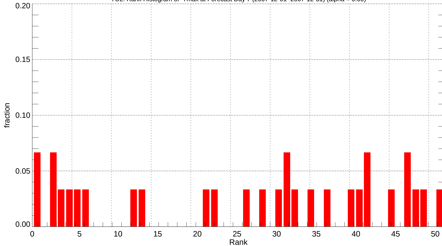
YUL: Rank Histogram of Tmax at Forecast Day 7 (2007-12-01~2007-12-31) (alpha = 0.00)
