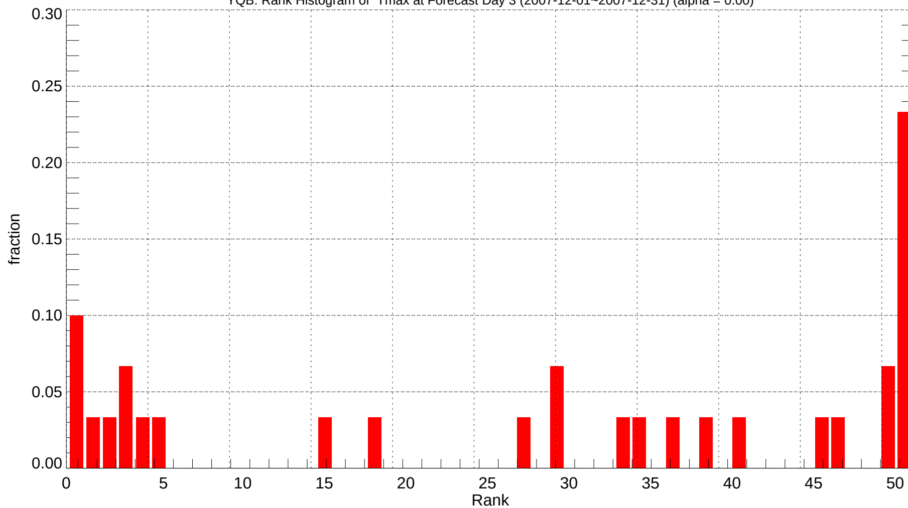
YQB: Rank Histogram of Tmax at Forecast Day 3 (2007-12-01~2007-12-31) (alpha = 0.00)
