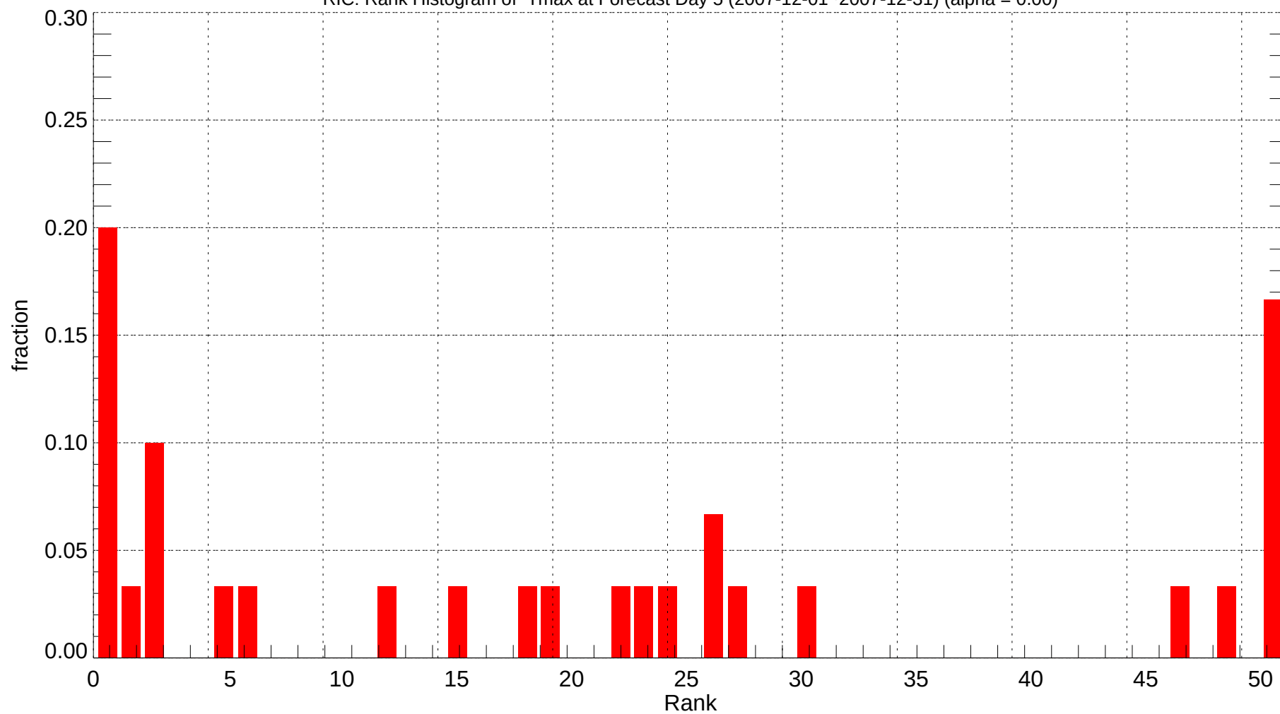
RIC: Rank Histogram of Tmax at Forecast Day 5 (2007-12-01~2007-12-31) (alpha = 0.00)
