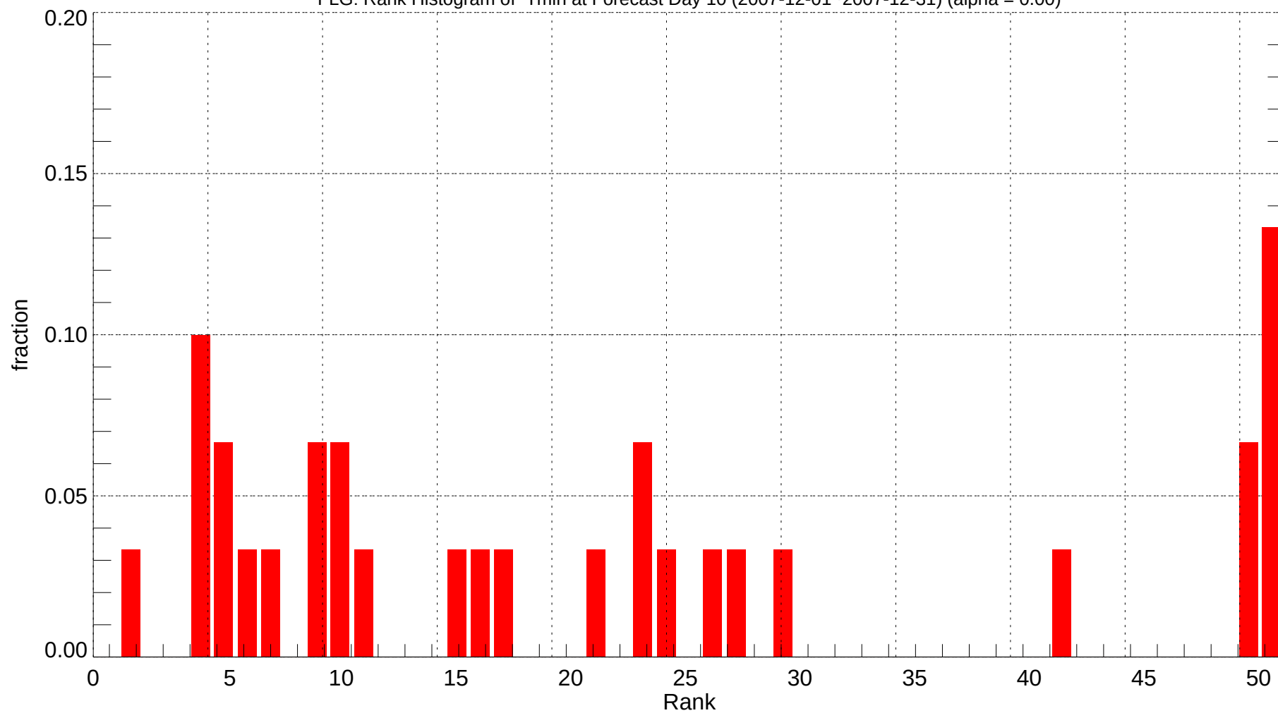
FLG: Rank Histogram of Tmin at Forecast Day 10 (2007-12-01~2007-12-31) (alpha = 0.00)
