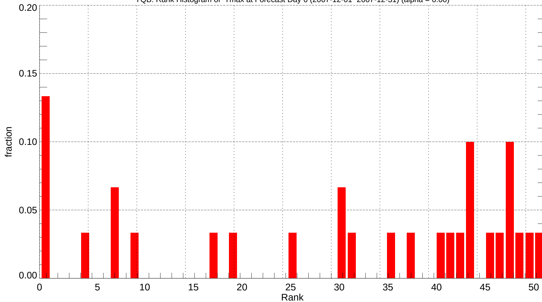
YQB: Rank Histogram of Tmax at Forecast Day 6 (2007-12-01~2007-12-31) (alpha = 0.00)
