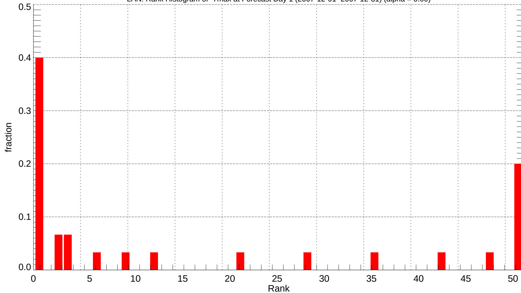
LAN: Rank Histogram of Tmax at Forecast Day 1 (2007-12-01~2007-12-31) (alpha = 0.00)
