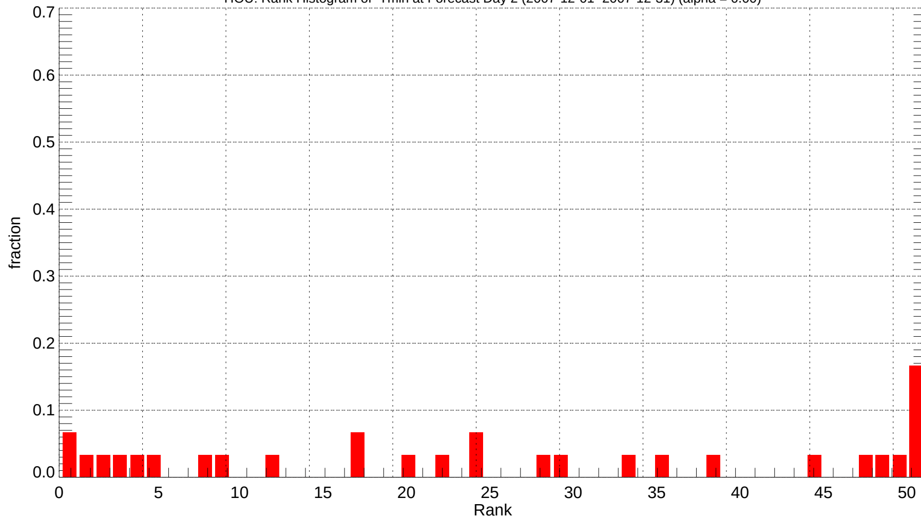
HOU: Rank Histogram of Tmin at Forecast Day 2 (2007-12-01~2007-12-31) (alpha = 0.00)
