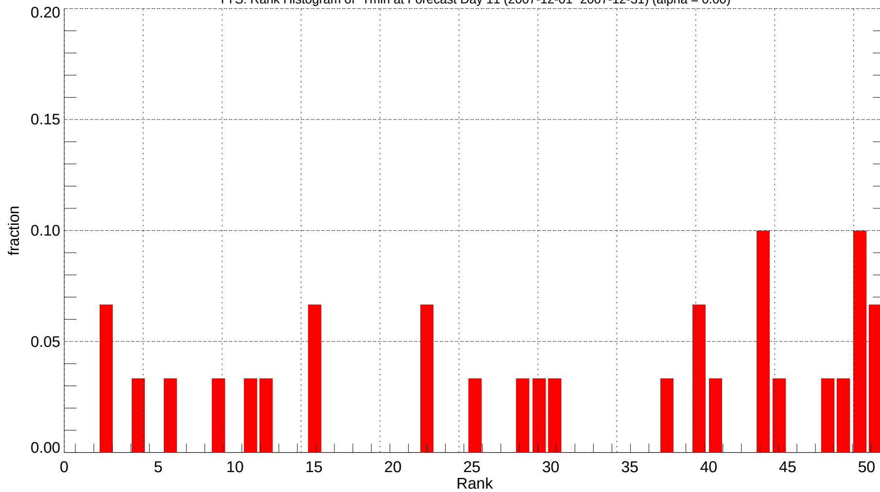
TYS: Rank Histogram of Tmin at Forecast Day 11 (2007-12-01~2007-12-31) (alpha = 0.00)
