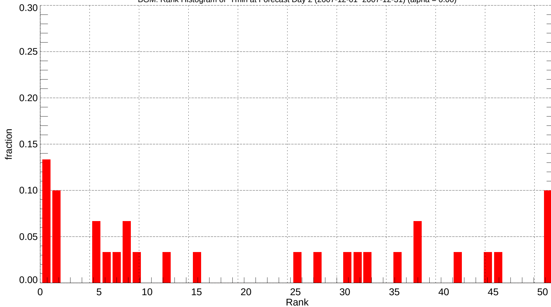
BGM: Rank Histogram of Tmin at Forecast Day 2 (2007-12-01~2007-12-31) (alpha = 0.00)
