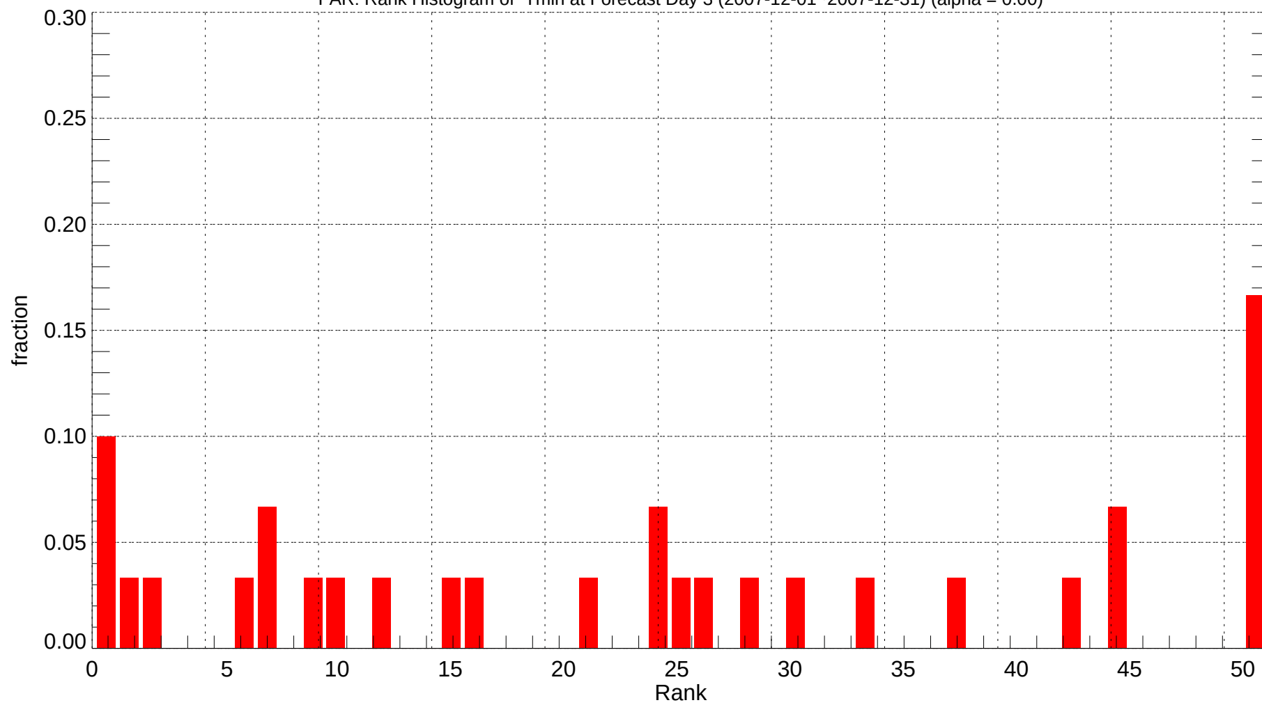
FAR: Rank Histogram of Tmin at Forecast Day 3 (2007-12-01~2007-12-31) (alpha = 0.00)
