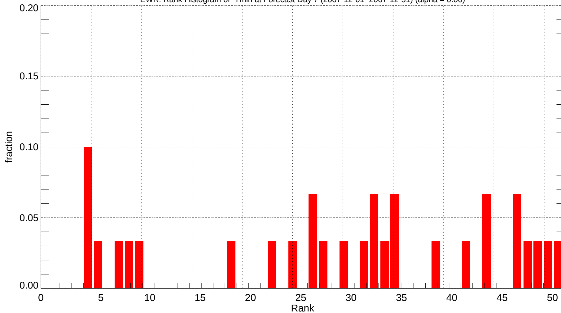
EWR: Rank Histogram of Tmin at Forecast Day 7 (2007-12-01~2007-12-31) (alpha = 0.00)
