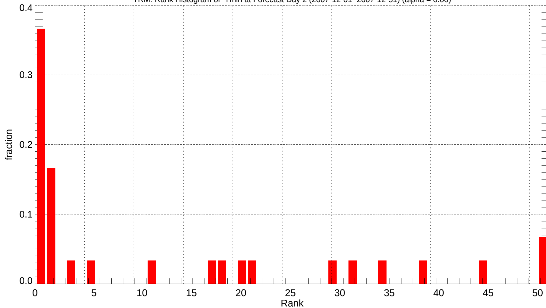
TRM: Rank Histogram of Tmin at Forecast Day 2 (2007-12-01~2007-12-31) (alpha = 0.00)
