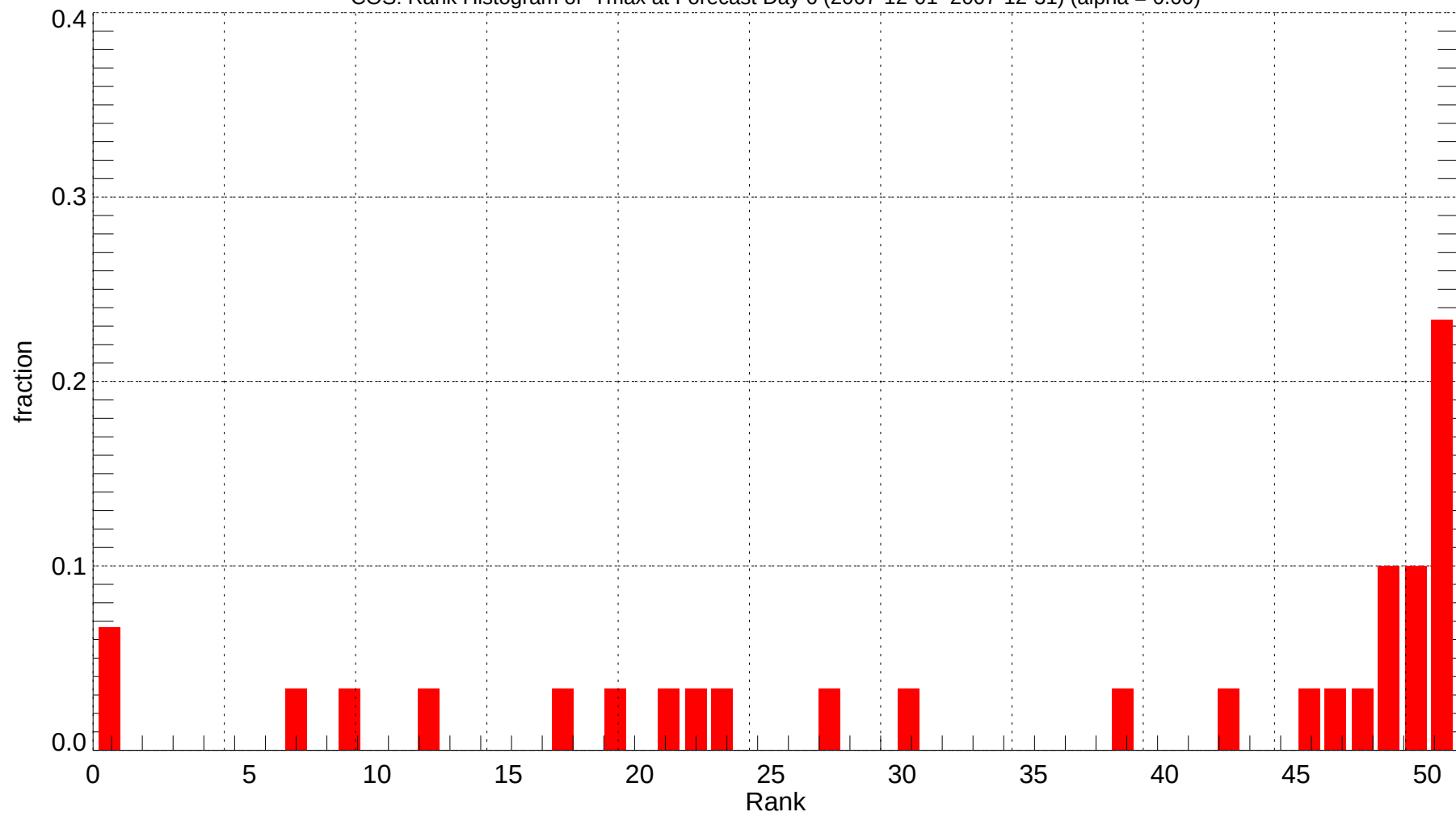
COS: Rank Histogram of Tmax at Forecast Day 6 (2007-12-01~2007-12-31) (alpha = 0.00)
