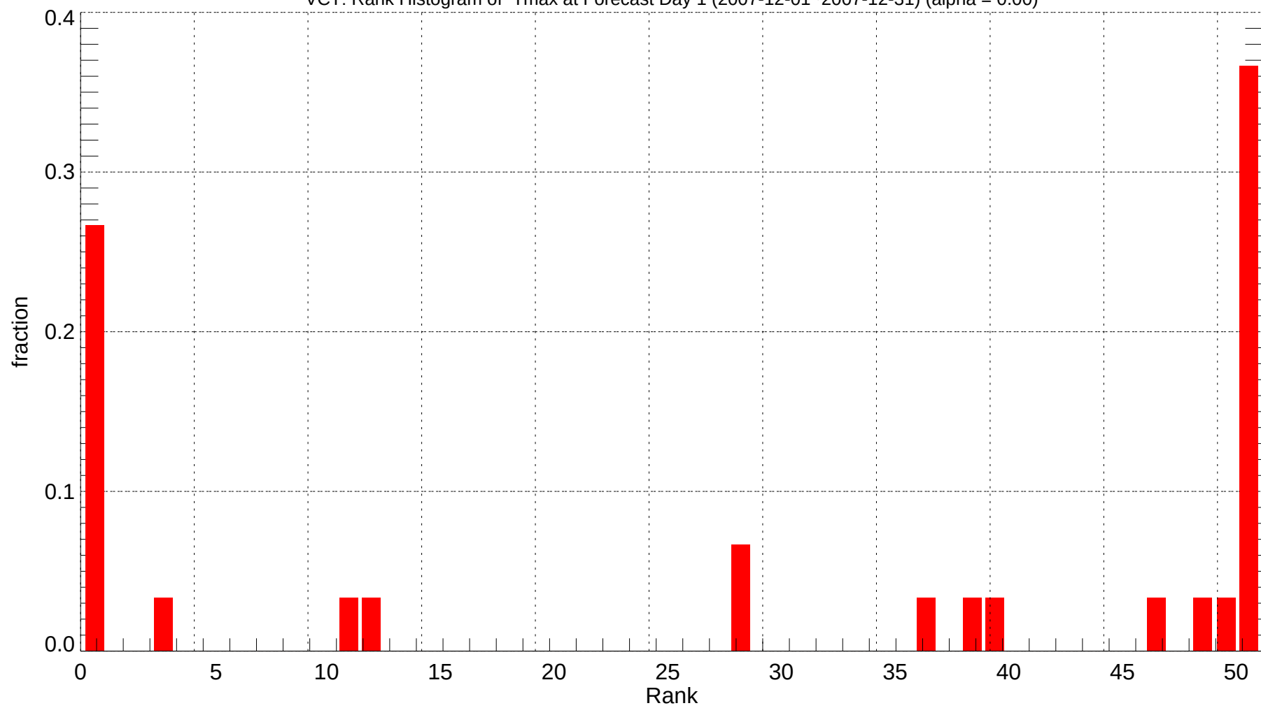
VCT: Rank Histogram of Tmax at Forecast Day 1 (2007-12-01~2007-12-31) (alpha = 0.00)
