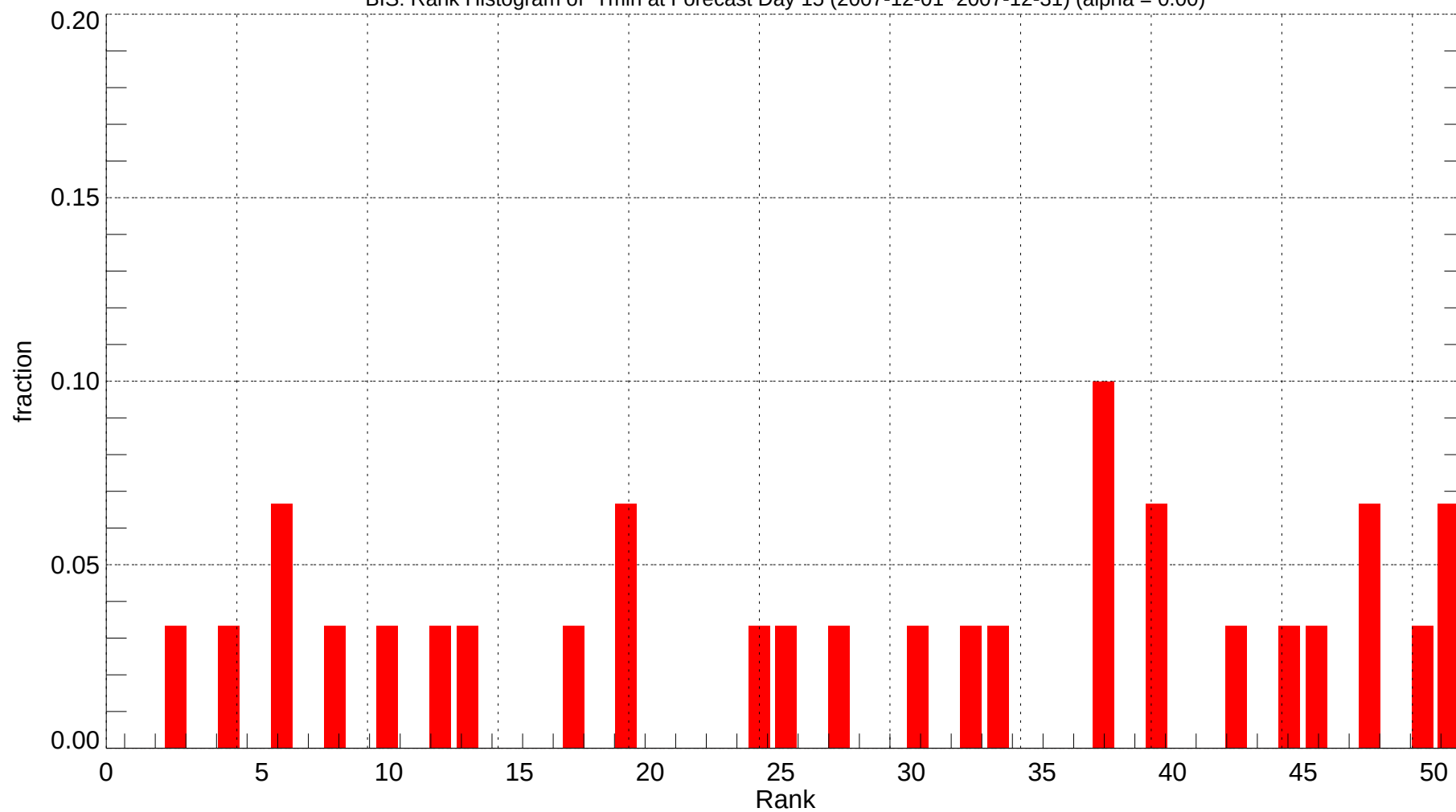
BIS: Rank Histogram of Tmin at Forecast Day 15 (2007-12-01~2007-12-31) (alpha = 0.00)
