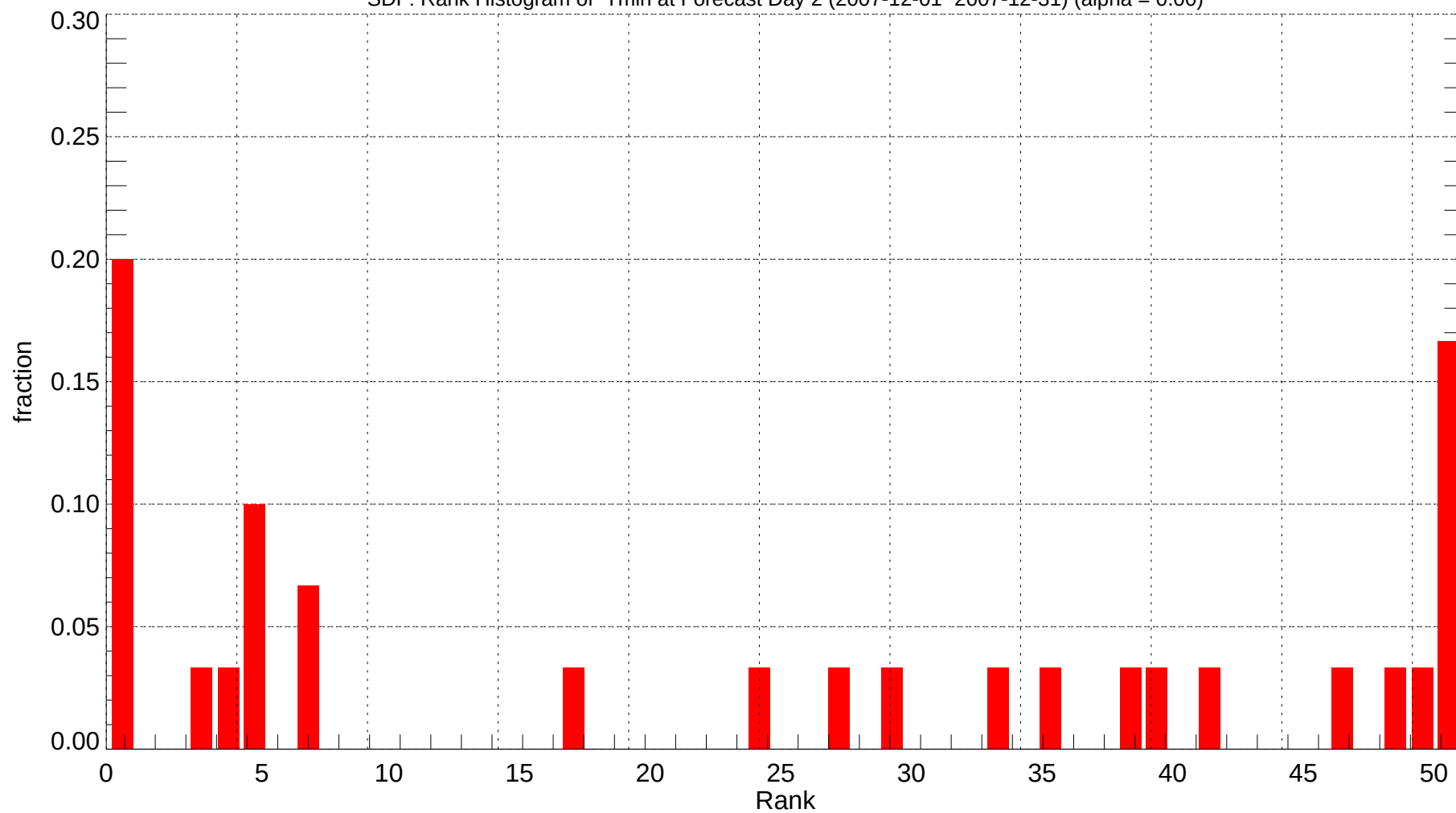
SDF: Rank Histogram of Tmin at Forecast Day 2 (2007-12-01~2007-12-31) (alpha = 0.00)
