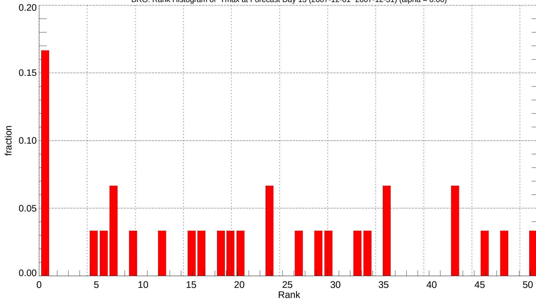
BRO: Rank Histogram of Tmax at Forecast Day 13 (2007-12-01~2007-12-31) (alpha = 0.00)
