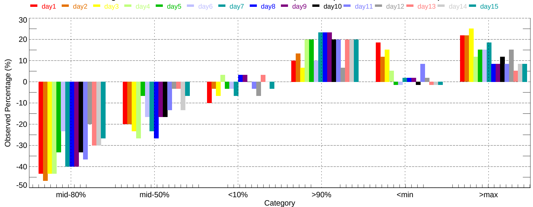
Observed Percentage Deviation of Ensembles - SJT: Max Temperature (2007-12-01~2007-12-31)
