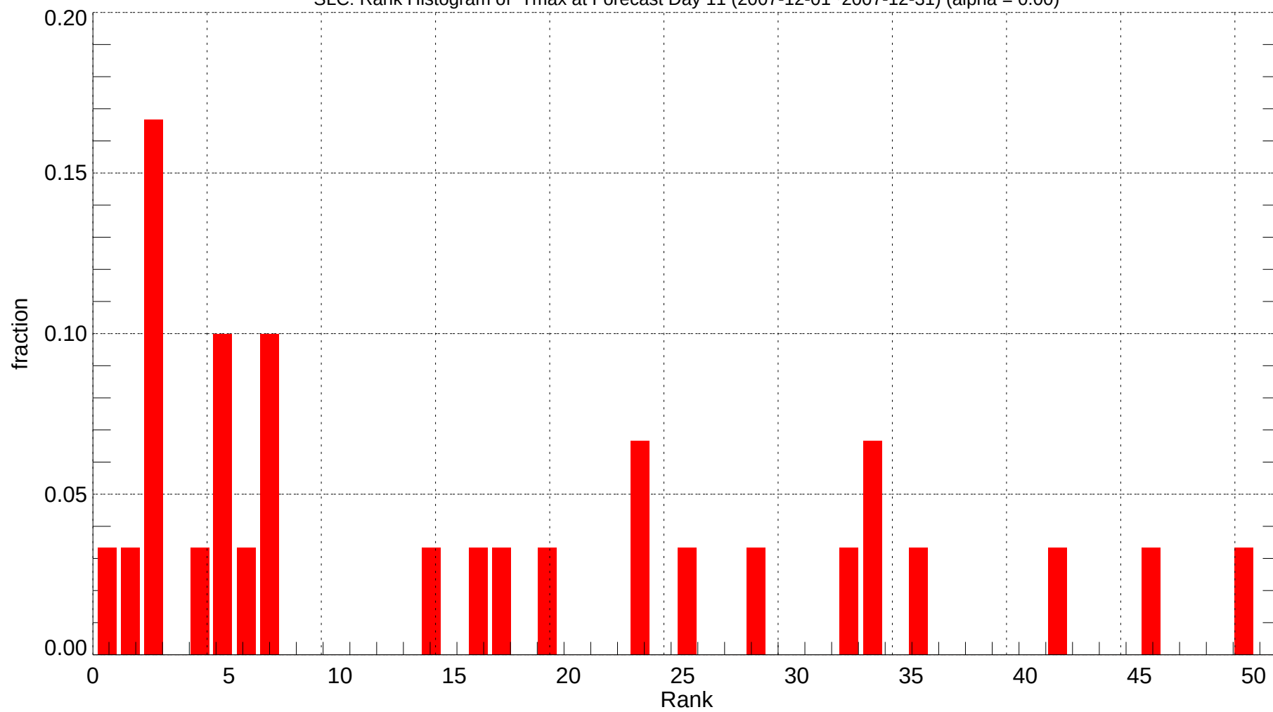
SLC: Rank Histogram of Tmax at Forecast Day 11 (2007-12-01~2007-12-31) (alpha = 0.00)
