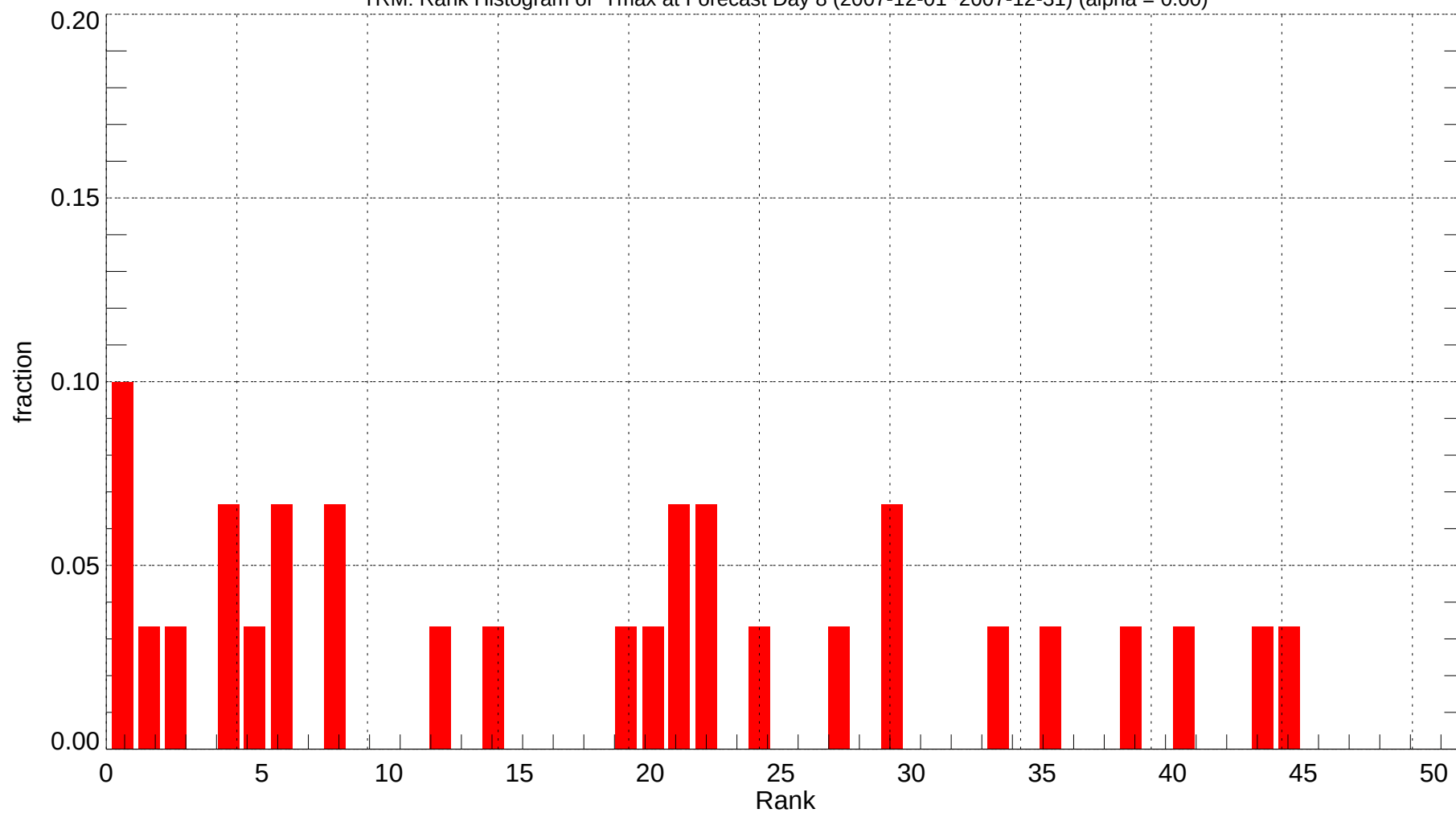
TRM: Rank Histogram of Tmax at Forecast Day 8 (2007-12-01~2007-12-31) (alpha = 0.00)
