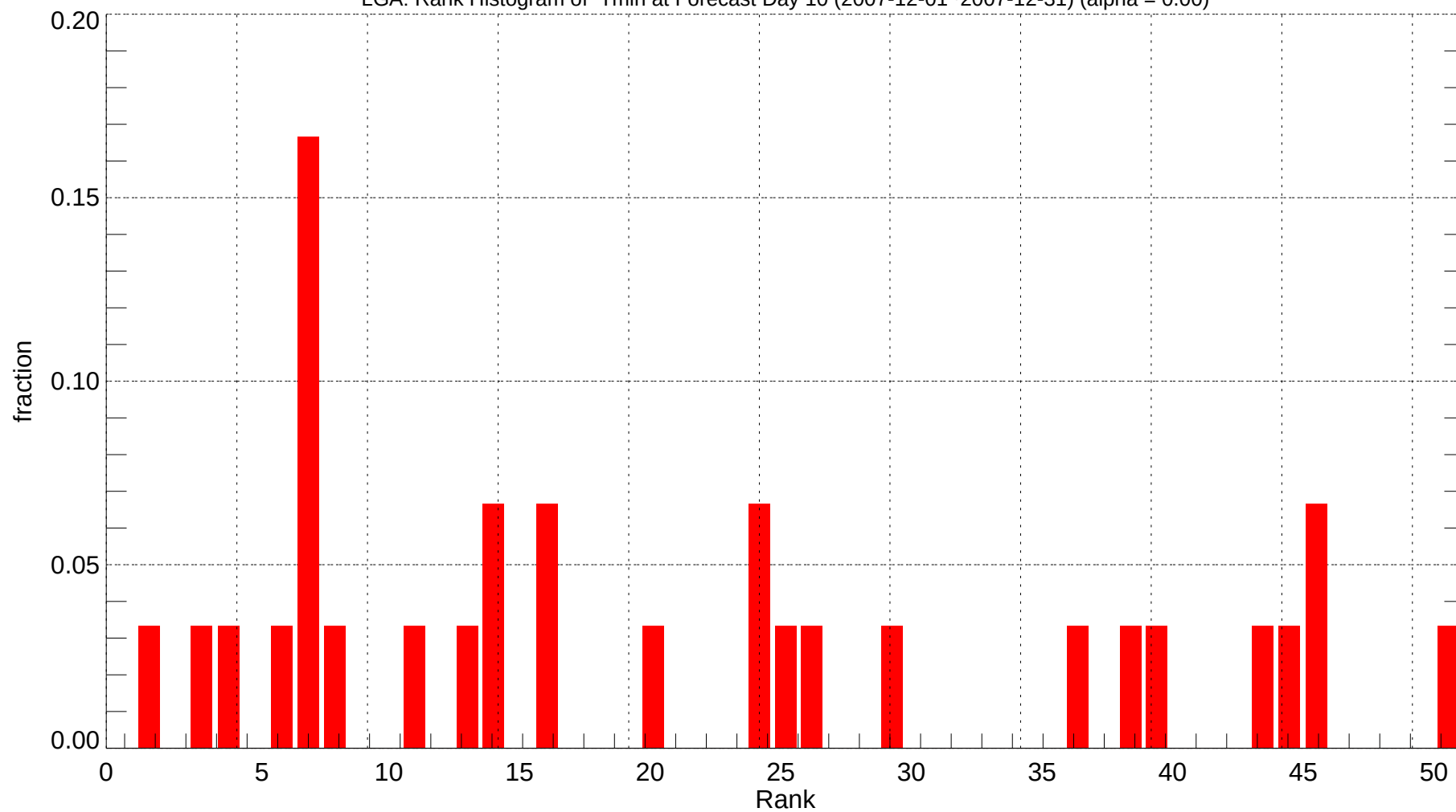
LGA: Rank Histogram of Tmin at Forecast Day 10 (2007-12-01~2007-12-31) (alpha = 0.00)
