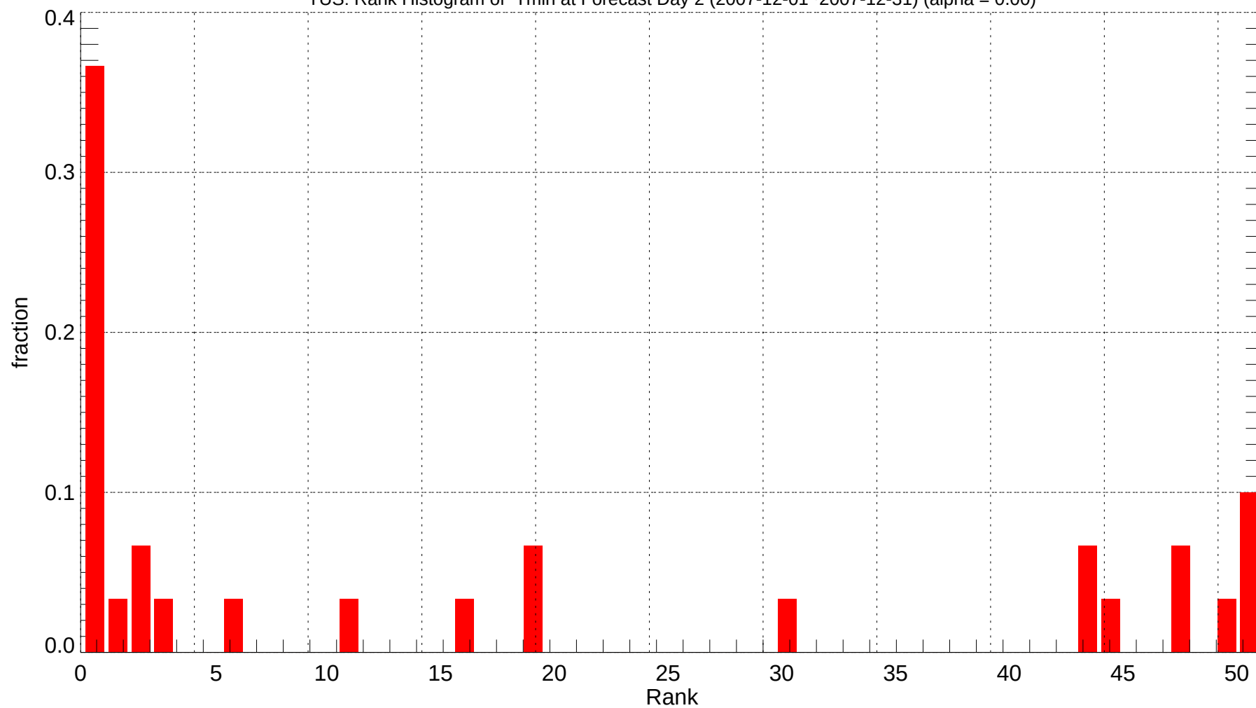
TUS: Rank Histogram of Tmin at Forecast Day 2 (2007-12-01~2007-12-31) (alpha = 0.00)
