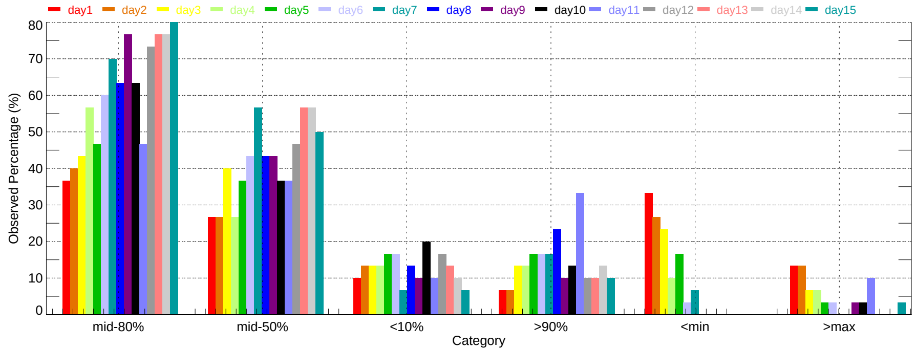
Observed Percentage of Ensembles - ABE: Max Temperature (2007-12-01~2007-12-31)
