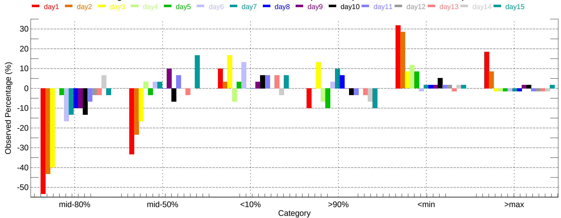
Observed Percentage Deviation of Ensembles - ALB: Max Temperature (2007-12-01~2007-12-31)
