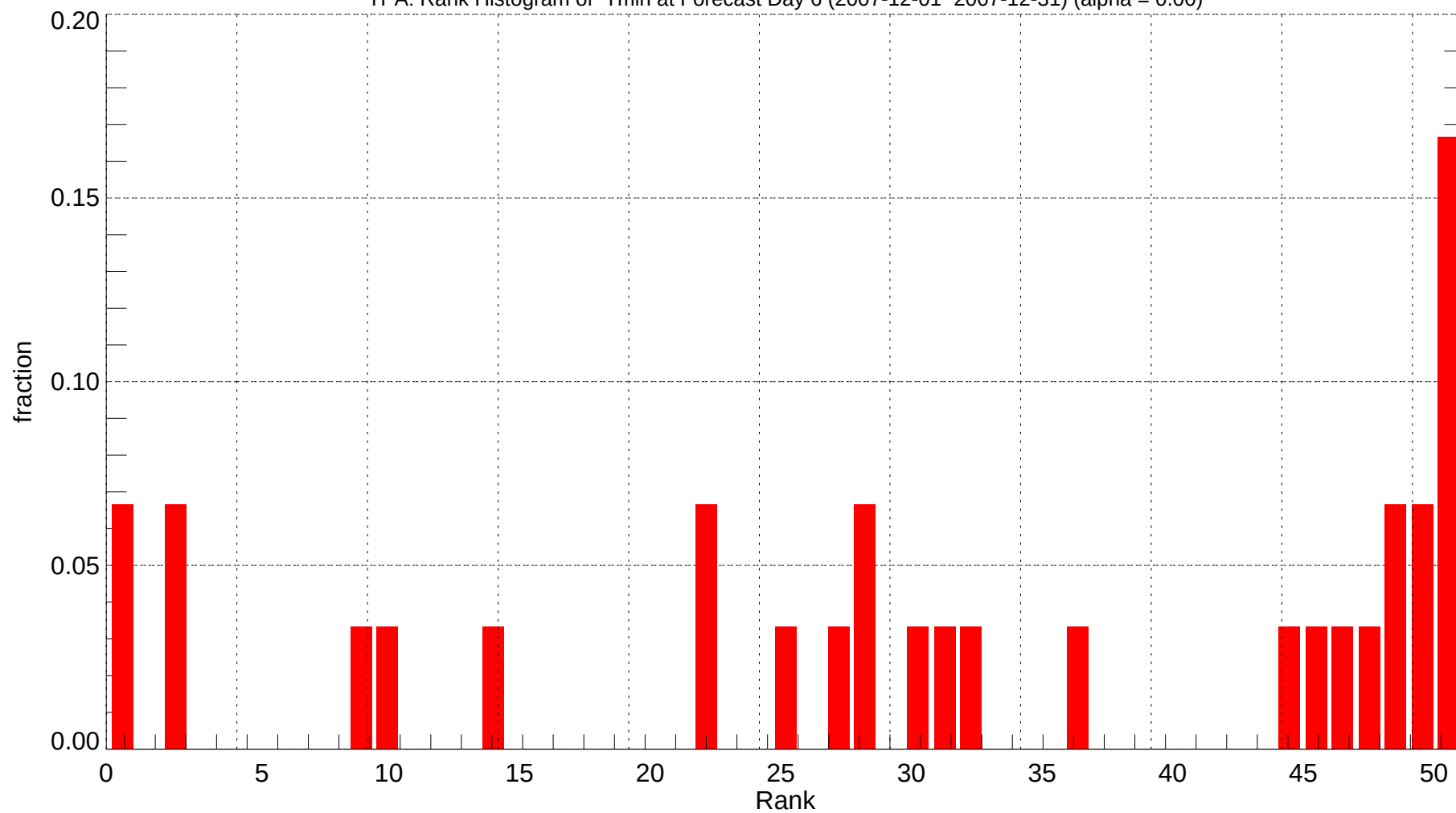
TPA: Rank Histogram of Tmin at Forecast Day 6 (2007-12-01~2007-12-31) (alpha = 0.00)
