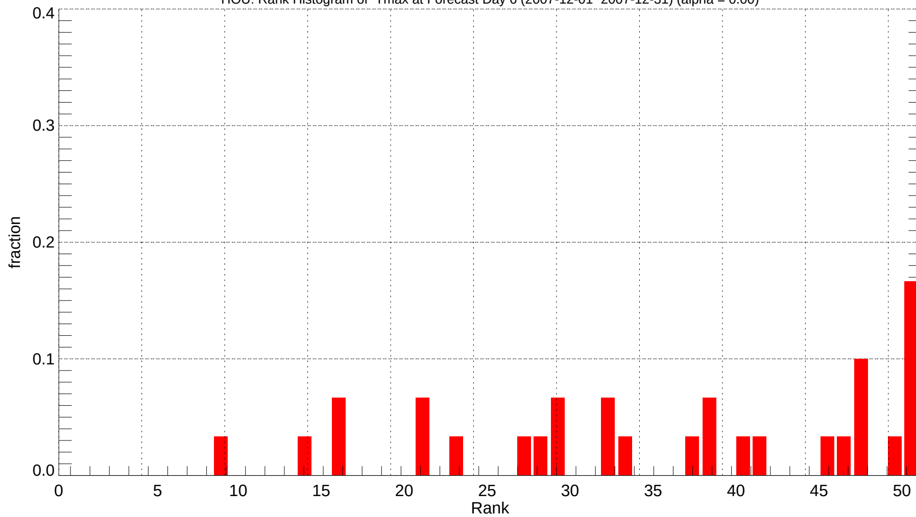
HOU: Rank Histogram of Tmax at Forecast Day 6 (2007-12-01~2007-12-31) (alpha = 0.00)
