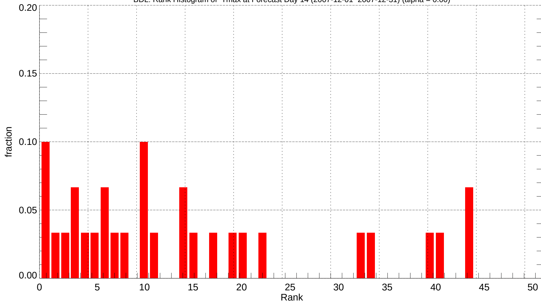
BDL: Rank Histogram of Tmax at Forecast Day 14 (2007-12-01~2007-12-31) (alpha = 0.00)
