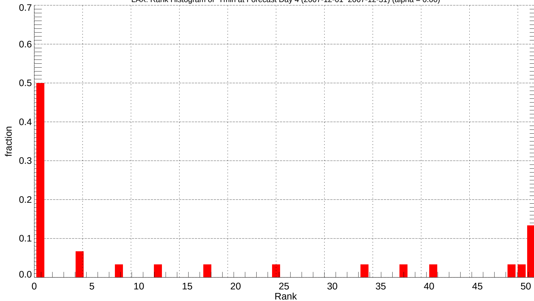
LAX: Rank Histogram of Tmin at Forecast Day 4 (2007-12-01~2007-12-31) (alpha = 0.00)
