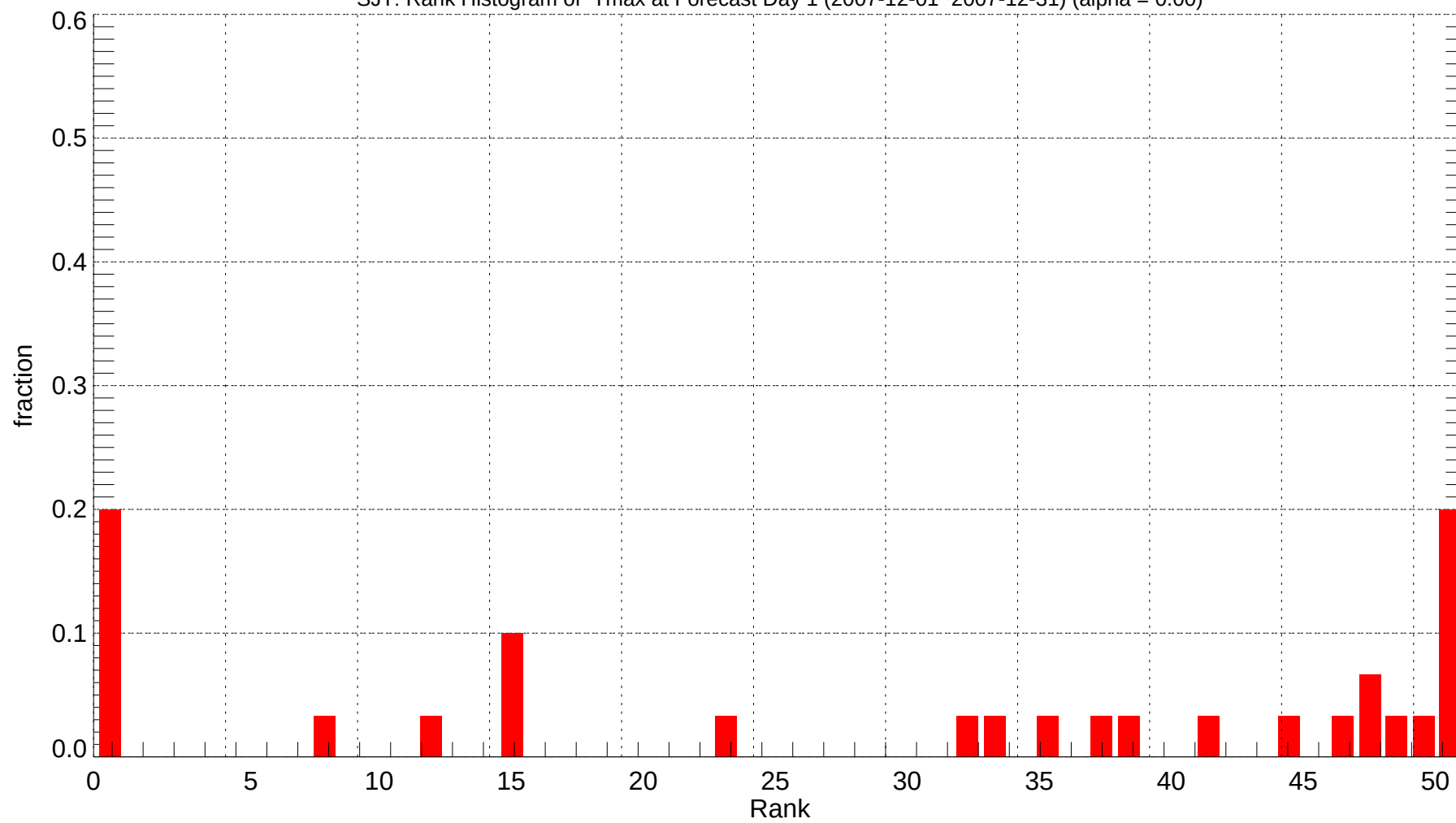
SJT: Rank Histogram of Tmax at Forecast Day 1 (2007-12-01~2007-12-31) (alpha = 0.00)
