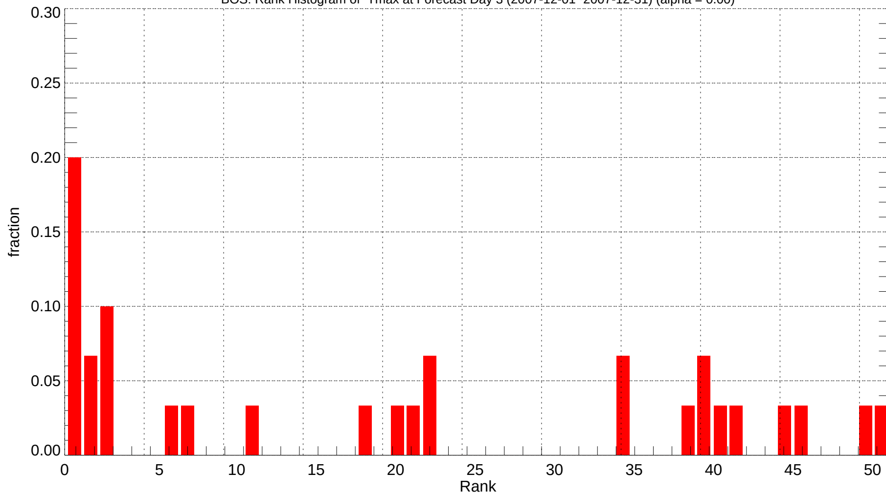
BOS: Rank Histogram of Tmax at Forecast Day 3 (2007-12-01~2007-12-31) (alpha = 0.00)
