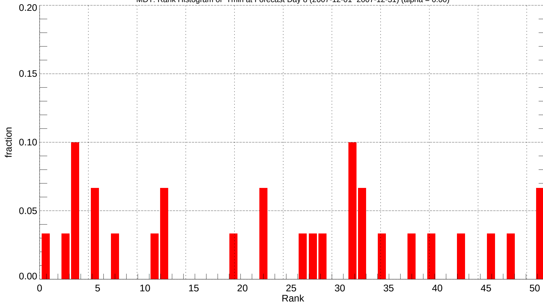
MDT: Rank Histogram of Tmin at Forecast Day 8 (2007-12-01~2007-12-31) (alpha = 0.00)
