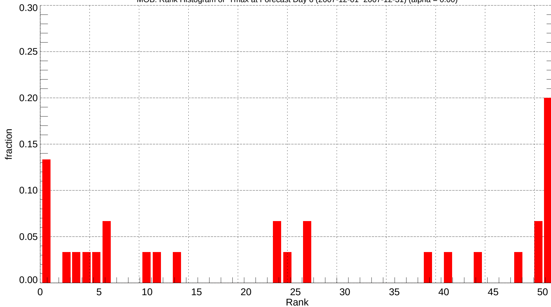
MOB: Rank Histogram of Tmax at Forecast Day 6 (2007-12-01~2007-12-31) (alpha = 0.00)
