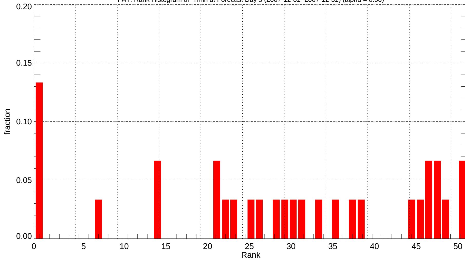
FAT: Rank Histogram of Tmin at Forecast Day 5 (2007-12-01~2007-12-31) (alpha = 0.00)
