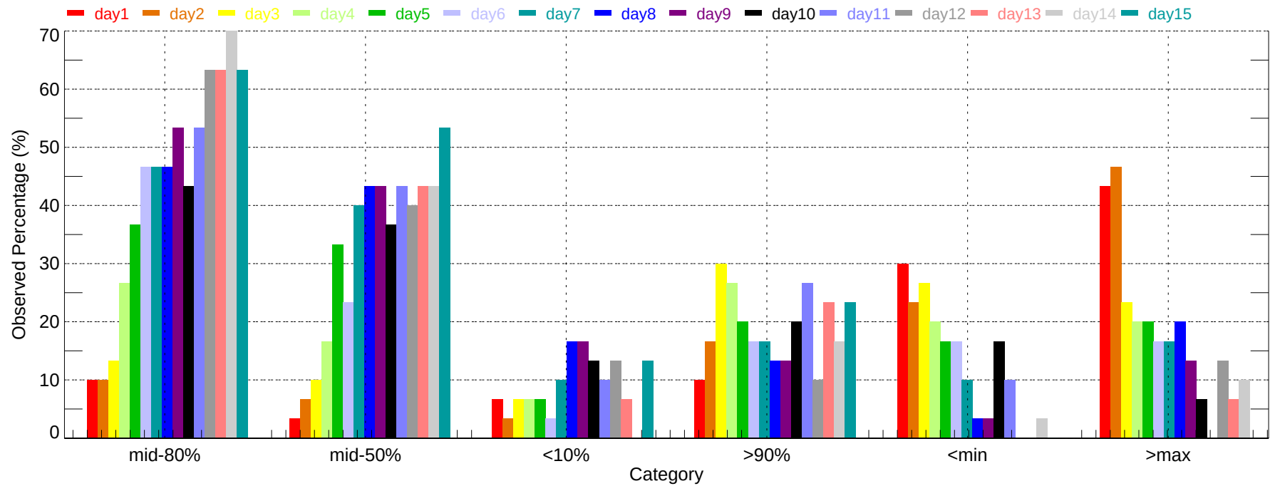
Observed Percentage of Ensembles - EUG: Max Temperature (2007-12-01~2007-12-31)
