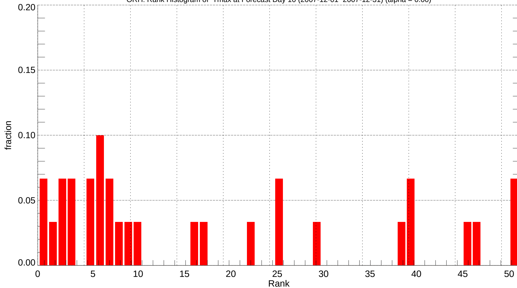
ORH: Rank Histogram of Tmax at Forecast Day 10 (2007-12-01~2007-12-31) (alpha = 0.00)
