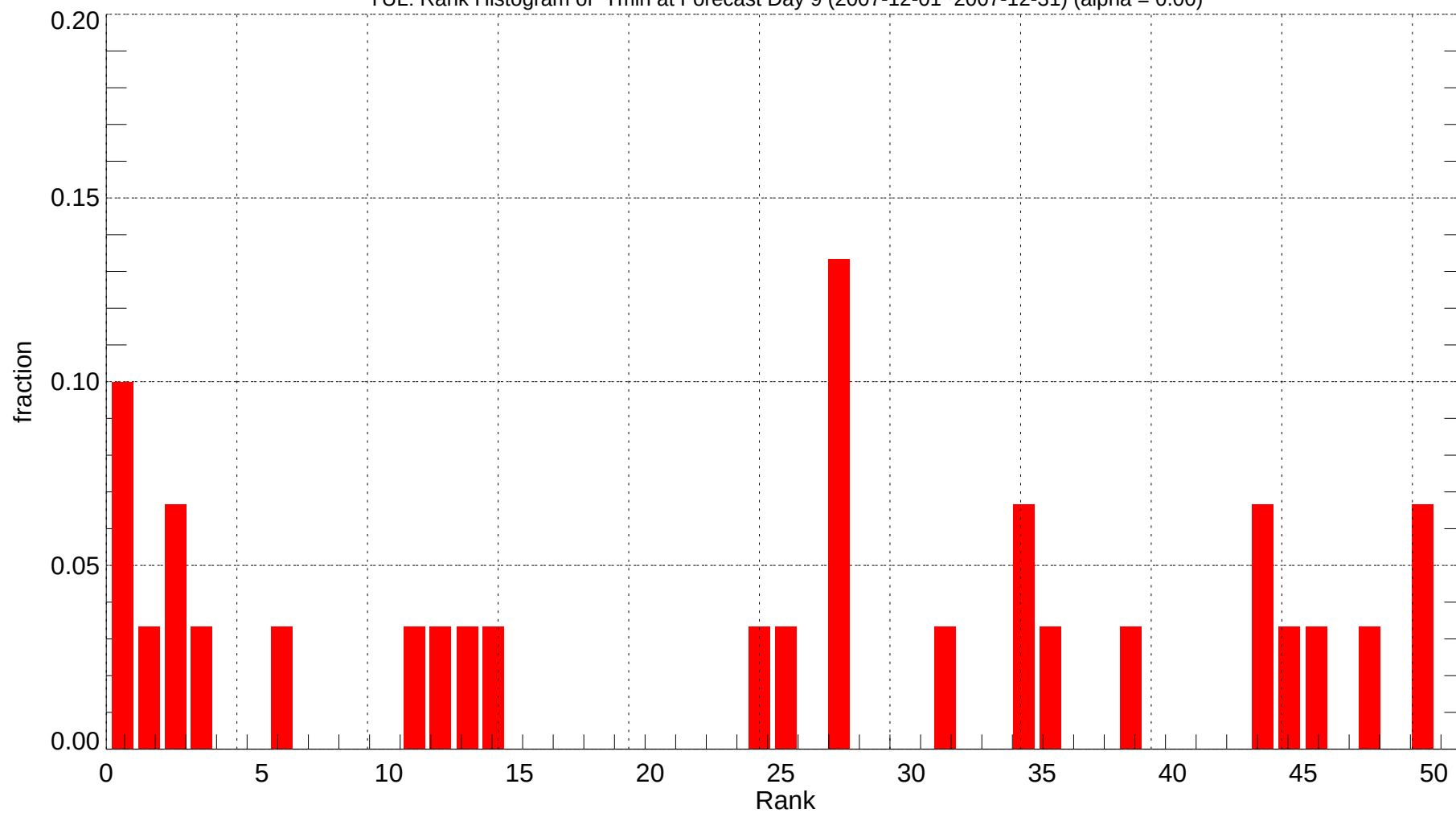
YUL: Rank Histogram of Tmin at Forecast Day 9 (2007-12-01~2007-12-31) (alpha = 0.00)
