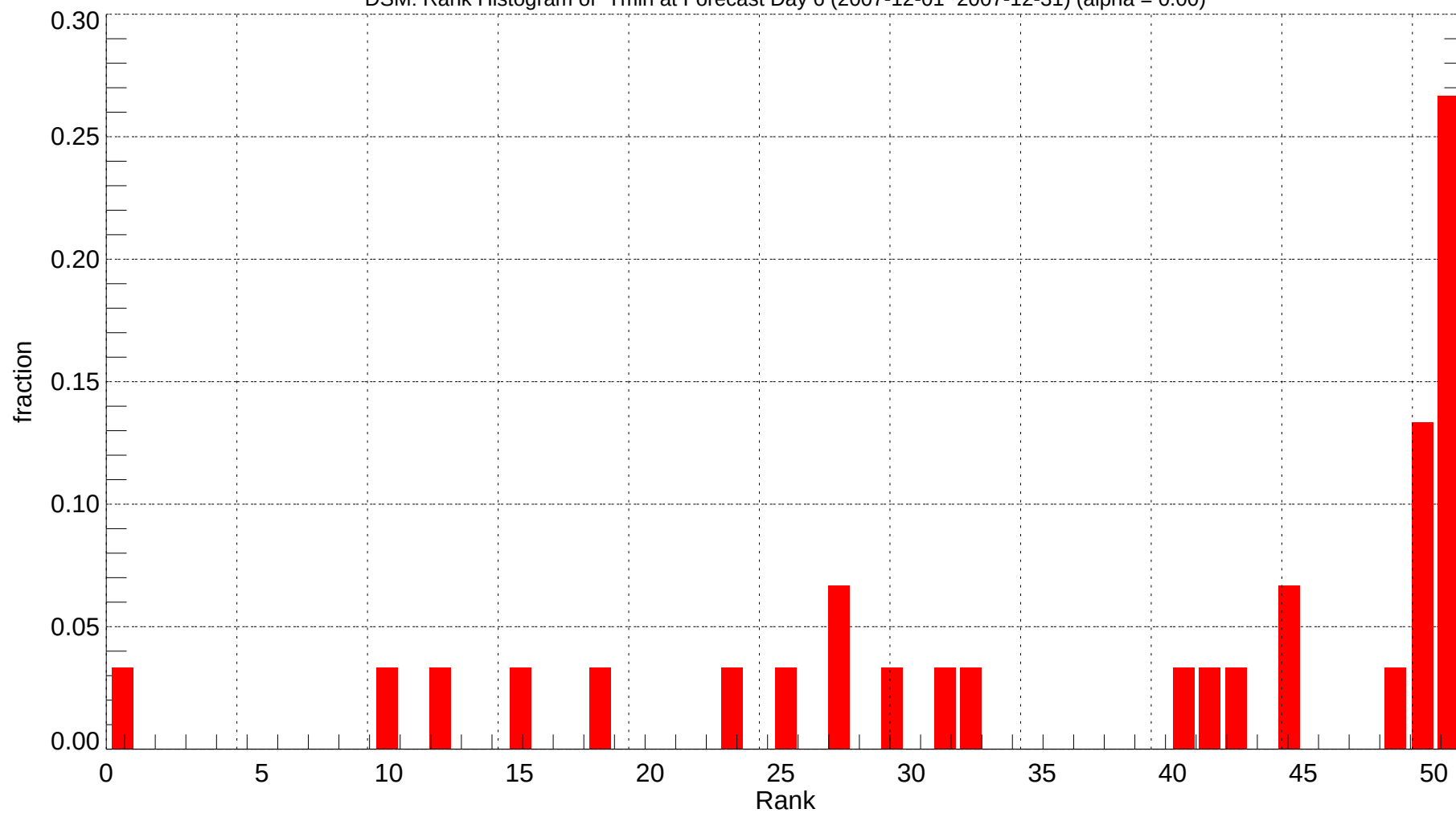
DSM: Rank Histogram of Tmin at Forecast Day 6 (2007-12-01~2007-12-31) (alpha = 0.00)
