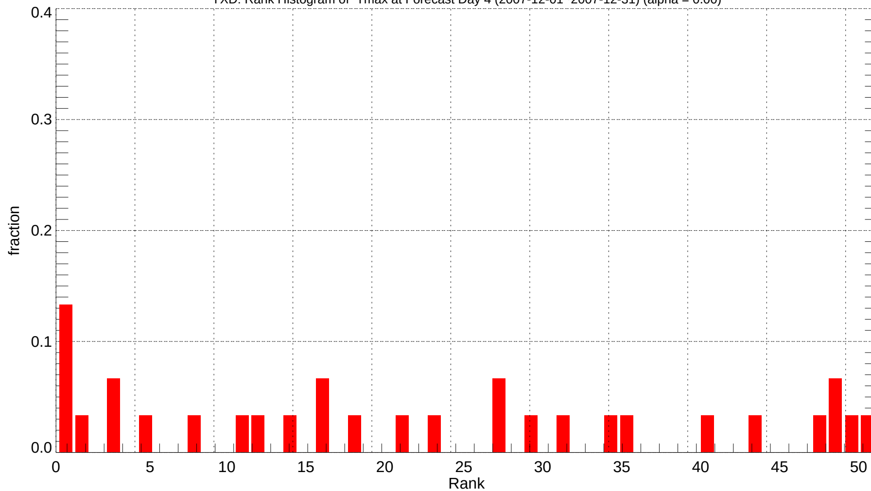
YXD: Rank Histogram of Tmax at Forecast Day 4 (2007-12-01~2007-12-31) (alpha = 0.00)
