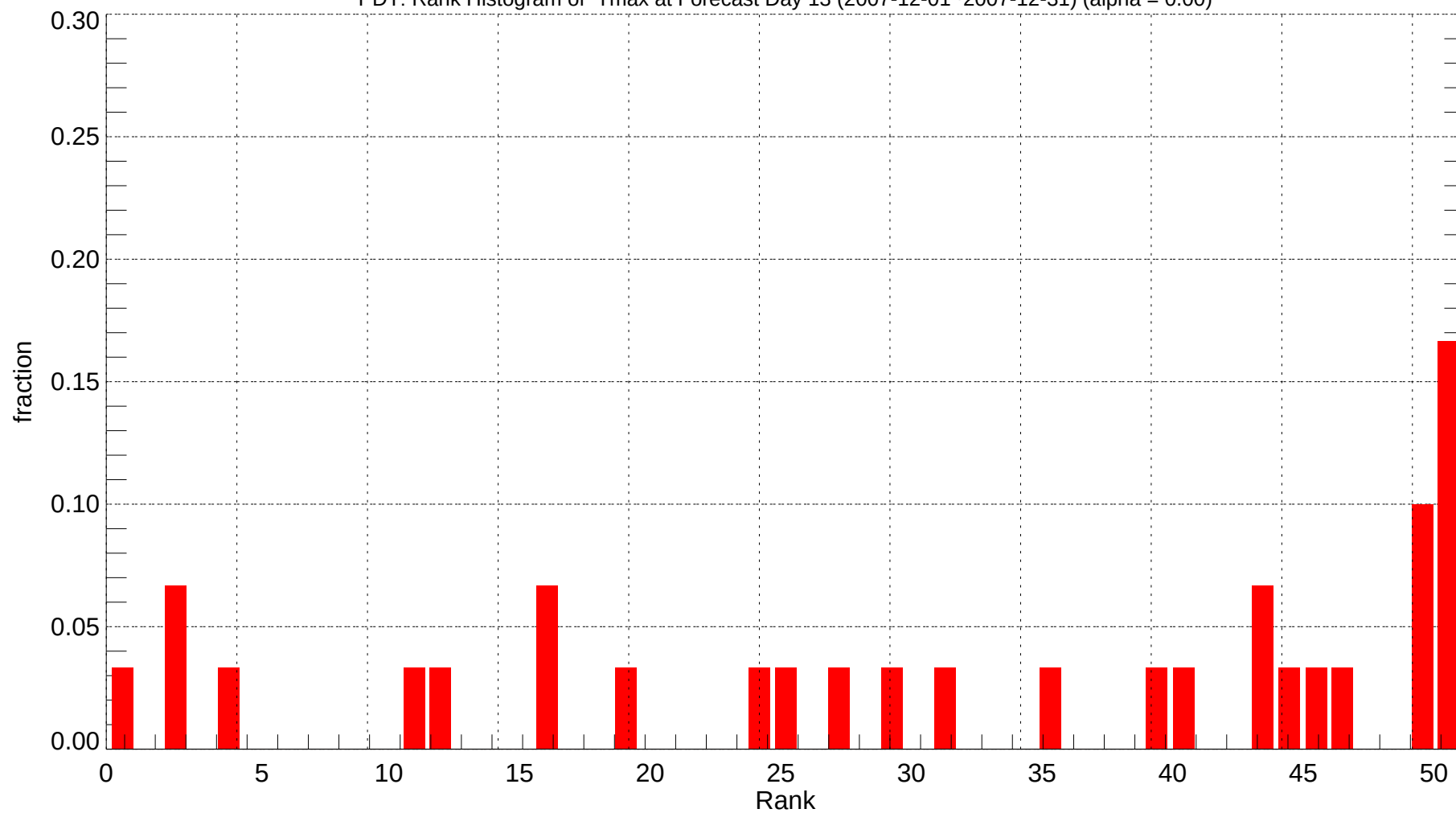
PDT: Rank Histogram of Tmax at Forecast Day 13 (2007-12-01~2007-12-31) (alpha = 0.00)
