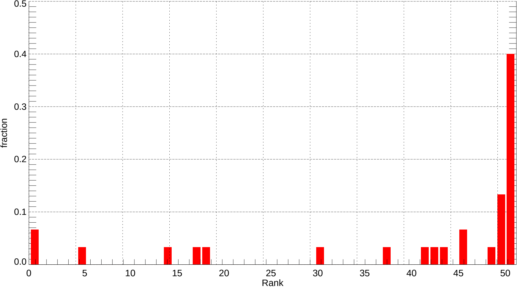
BFL: Rank Histogram of Tmin at Forecast Day 5 (2007-12-01~2007-12-31) (alpha = 0.00)
