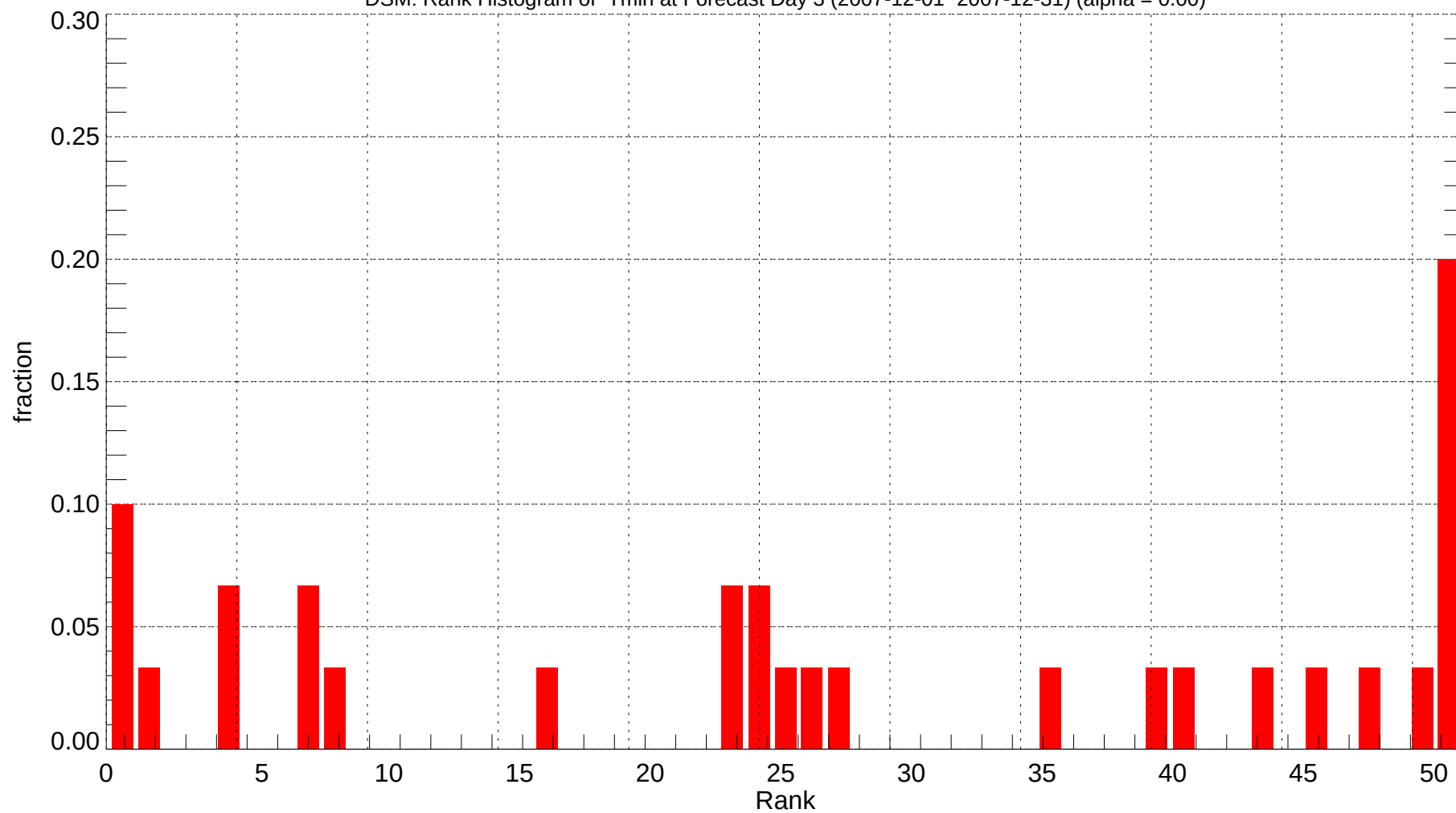
DSM: Rank Histogram of Tmin at Forecast Day 3 (2007-12-01~2007-12-31) (alpha = 0.00)
