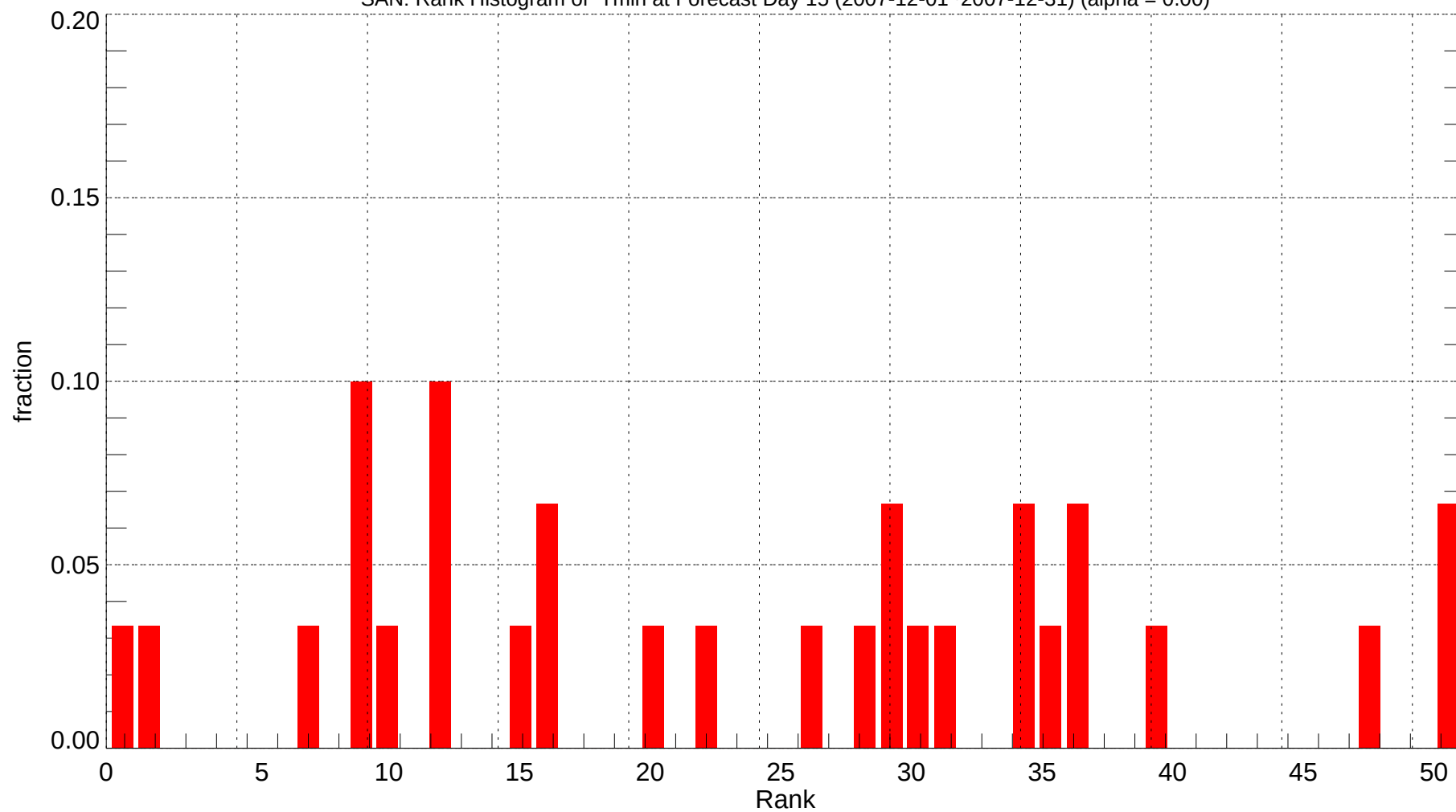
SAN: Rank Histogram of Tmin at Forecast Day 15 (2007-12-01~2007-12-31) (alpha = 0.00)
