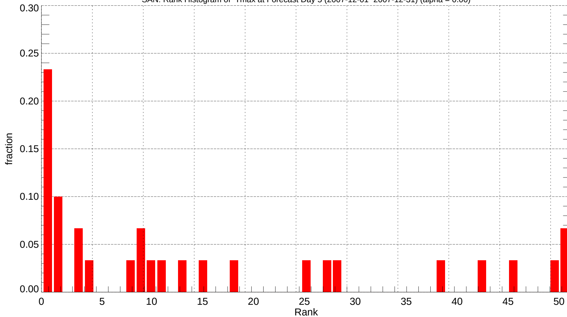
SAN: Rank Histogram of Tmax at Forecast Day 5 (2007-12-01~2007-12-31) (alpha = 0.00)
