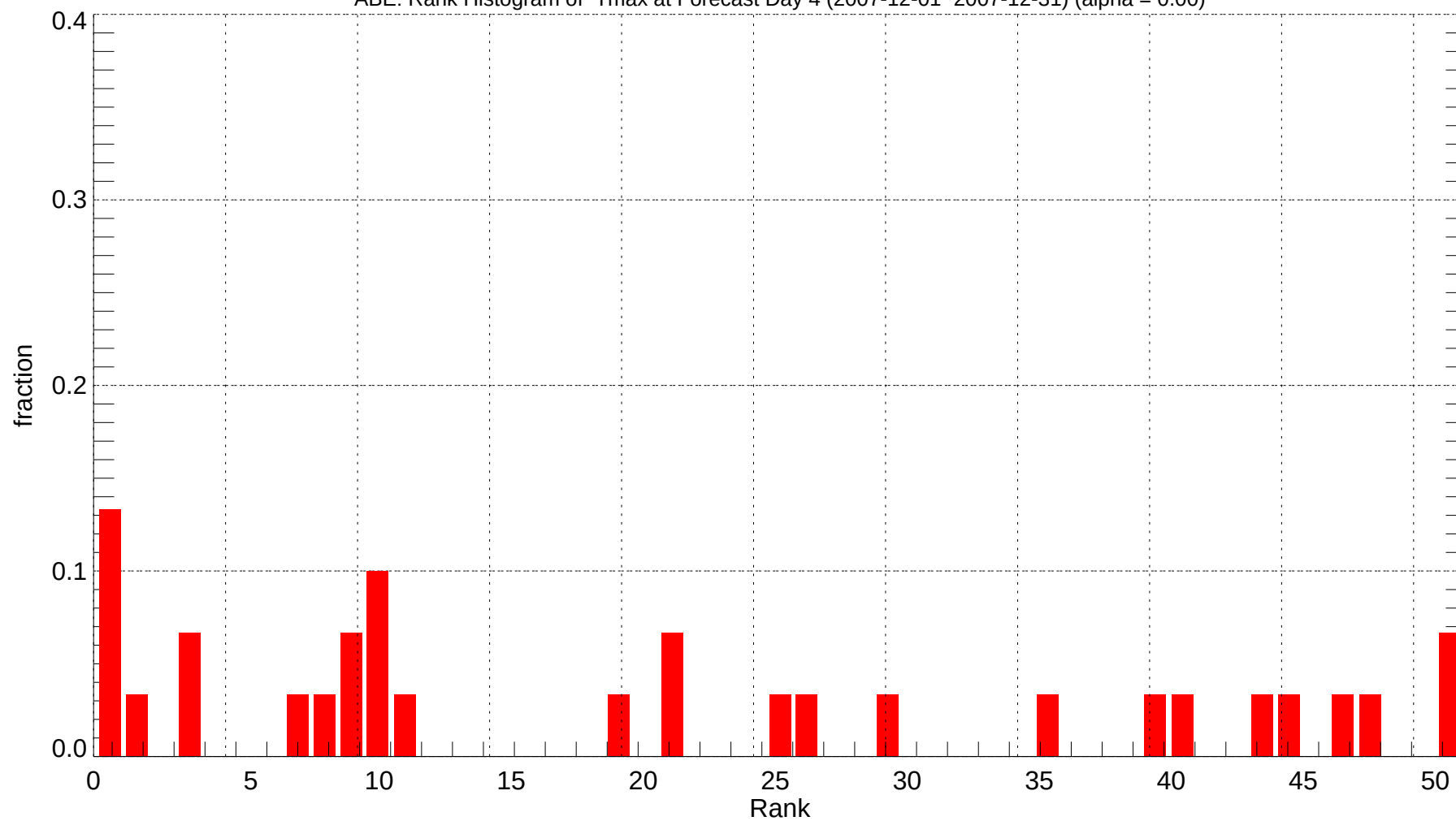
ABE: Rank Histogram of Tmax at Forecast Day 4 (2007-12-01~2007-12-31) (alpha = 0.00)
