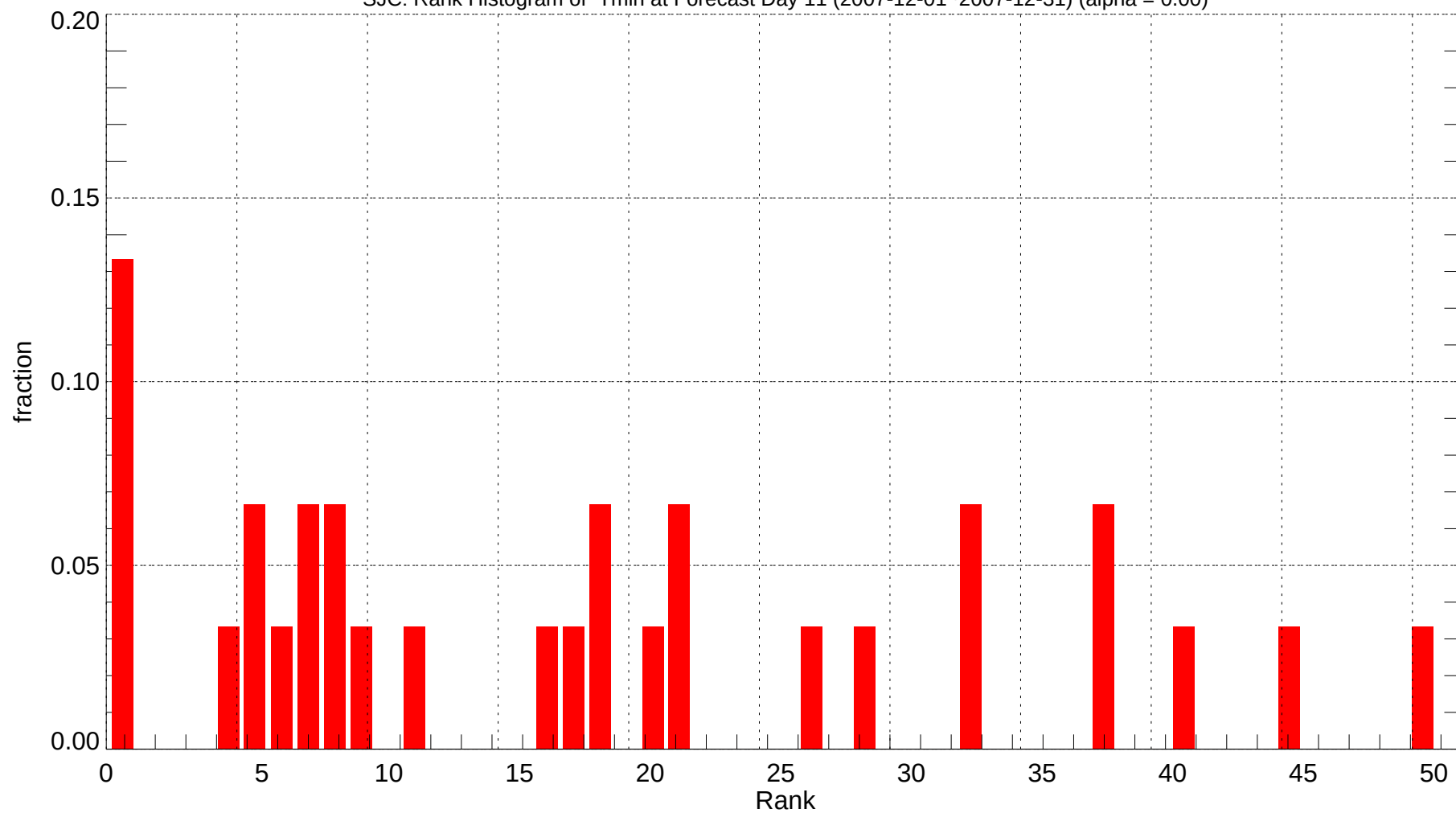
SJC: Rank Histogram of Tmin at Forecast Day 11 (2007-12-01~2007-12-31) (alpha = 0.00)
