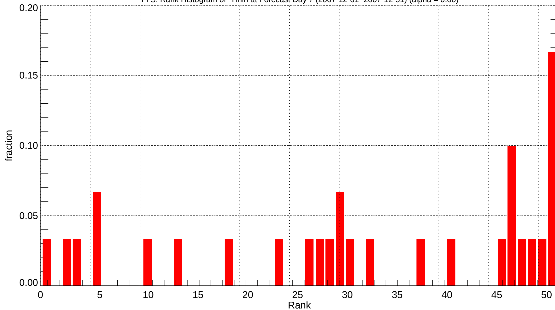
TYS: Rank Histogram of Tmin at Forecast Day 7 (2007-12-01~2007-12-31) (alpha = 0.00)
