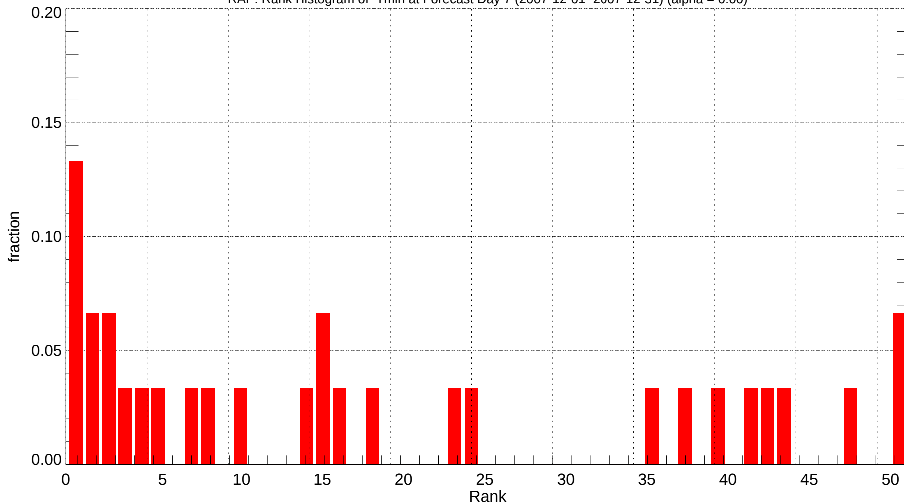
RAP: Rank Histogram of Tmin at Forecast Day 7 (2007-12-01~2007-12-31) (alpha = 0.00)
