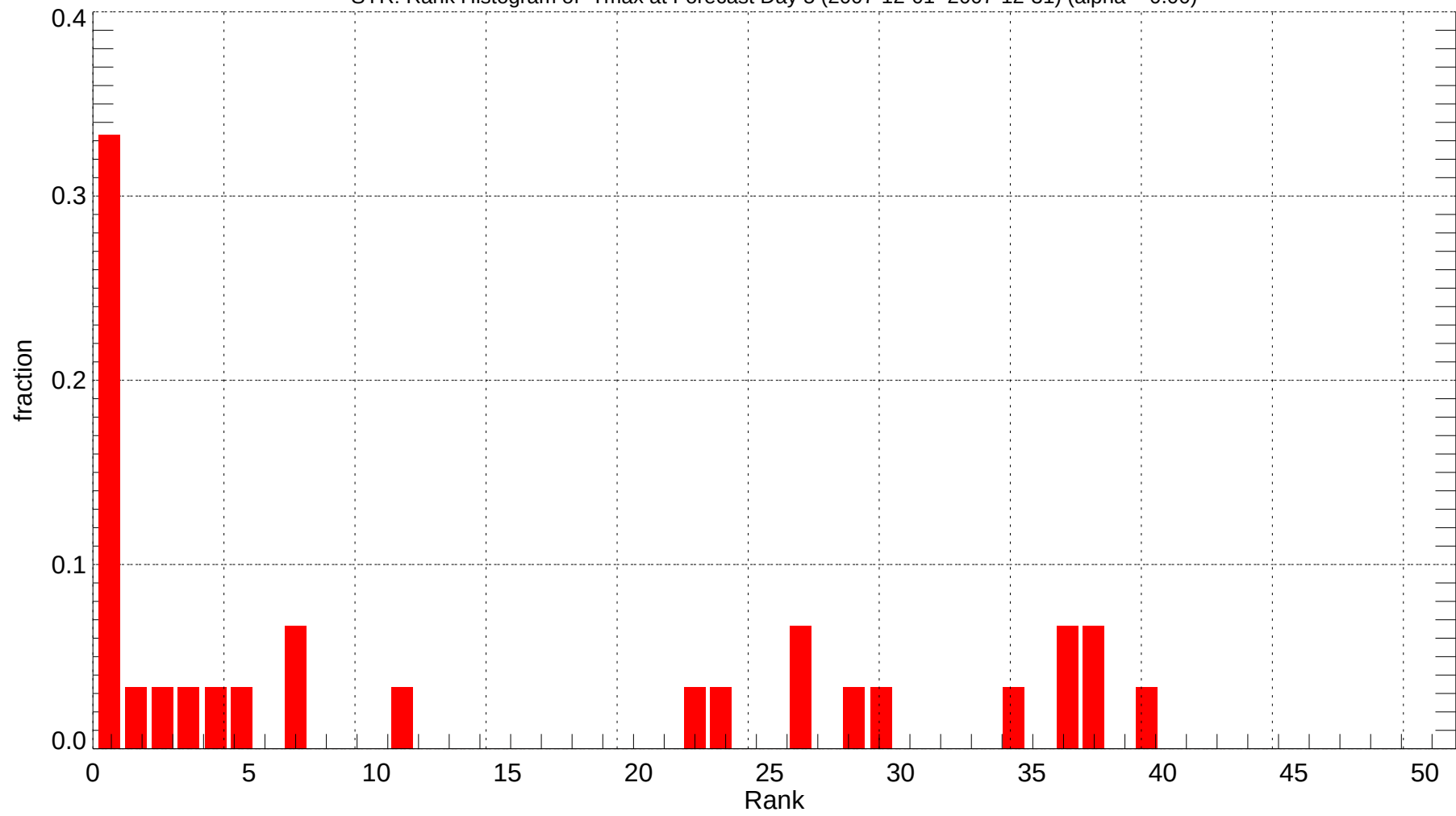
SYR: Rank Histogram of Tmax at Forecast Day 5 (2007-12-01~2007-12-31) (alpha = 0.00)
