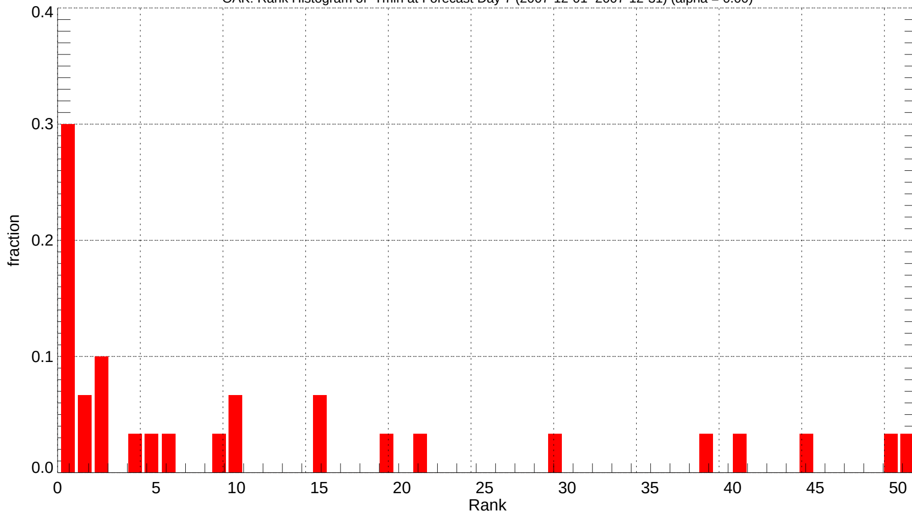
OAK: Rank Histogram of Tmin at Forecast Day 7 (2007-12-01~2007-12-31) (alpha = 0.00)
