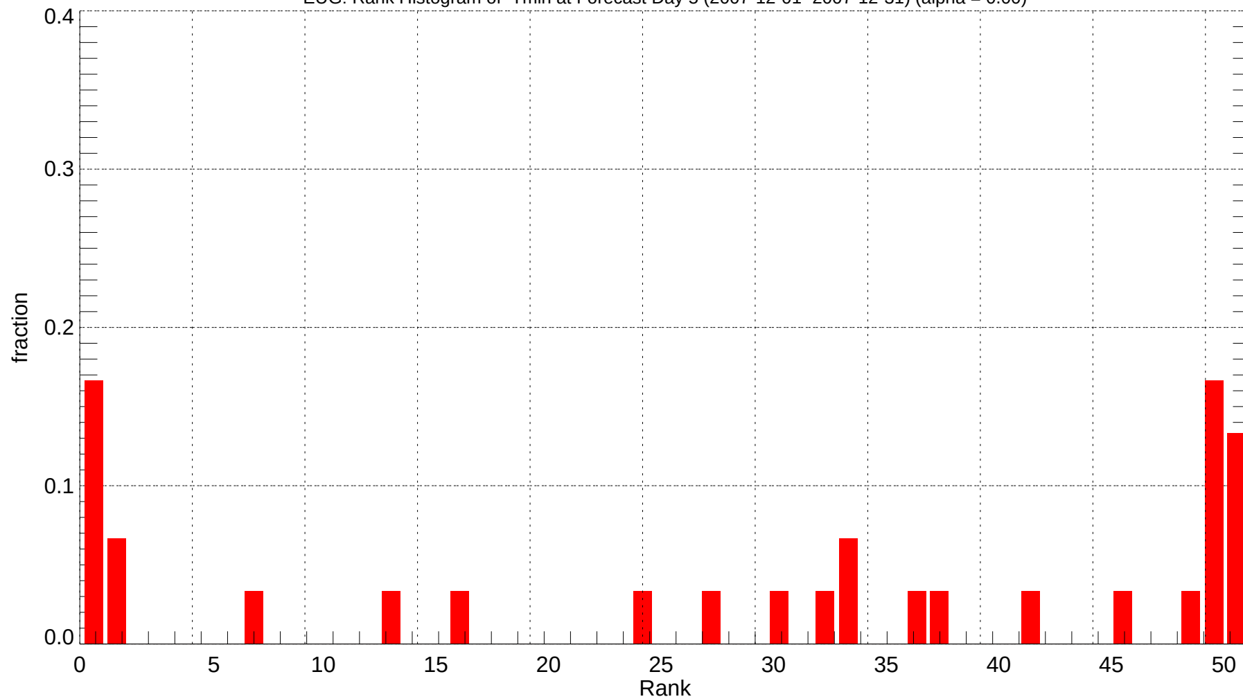
EUG: Rank Histogram of Tmin at Forecast Day 5 (2007-12-01~2007-12-31) (alpha = 0.00)
