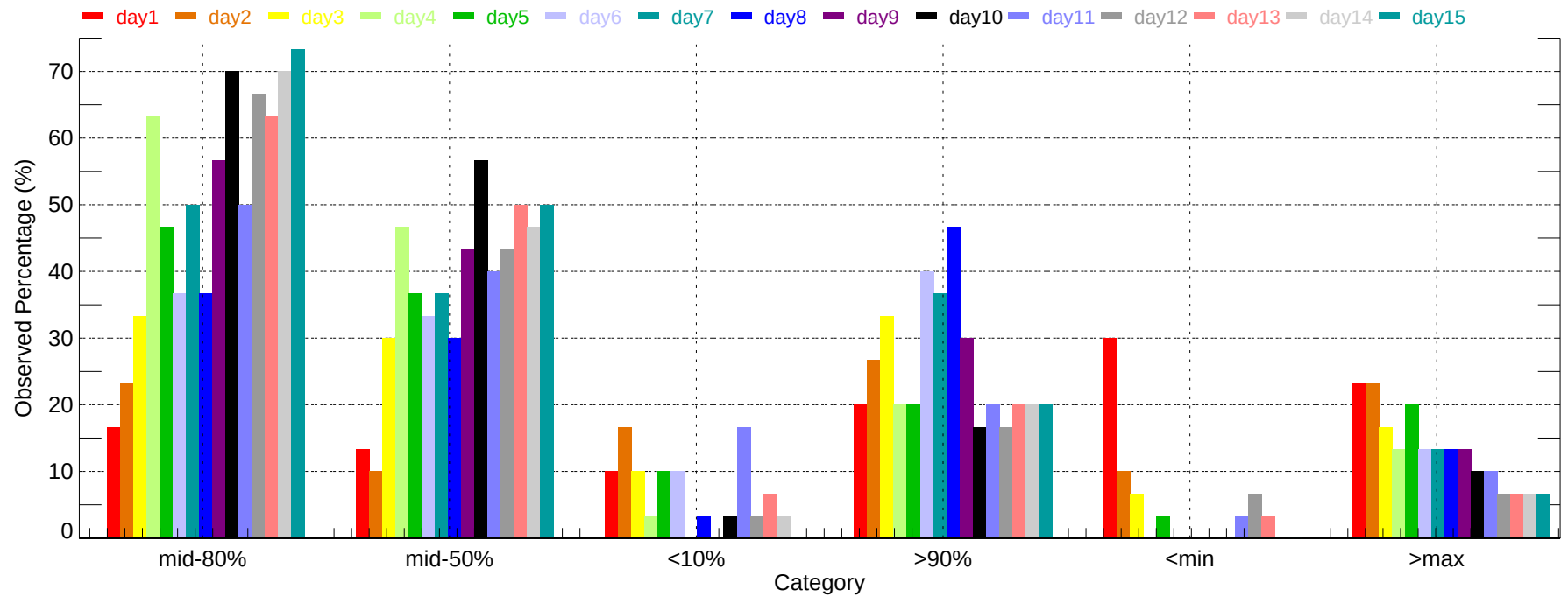
Observed Percentage of Ensembles - NTU: Min Temperature (2007-12-01~2007-12-31)
