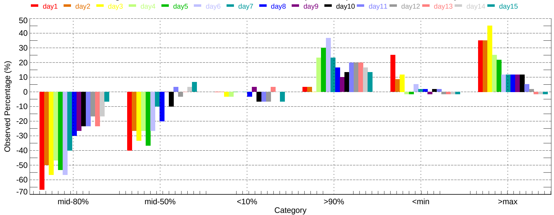
Observed Percentage Deviation of Ensembles - GTF: Min Temperature (2007-12-01~2007-12-31)
