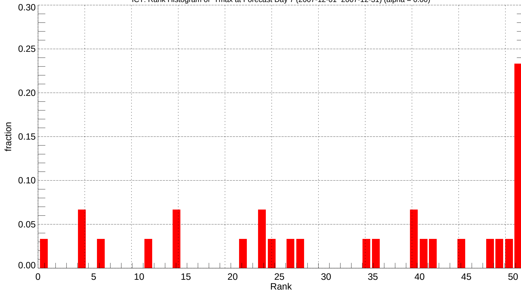
ICT: Rank Histogram of Tmax at Forecast Day 7 (2007-12-01~2007-12-31) (alpha = 0.00)
