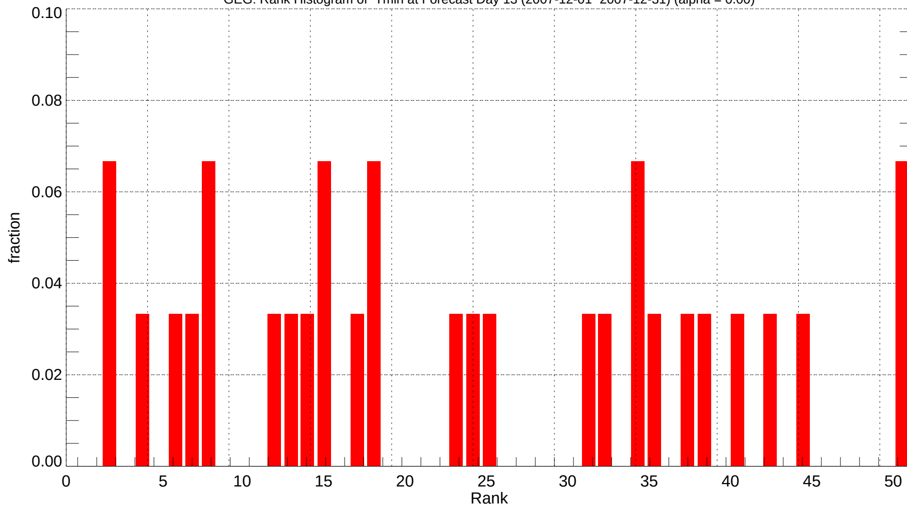
GEG: Rank Histogram of Tmin at Forecast Day 13 (2007-12-01~2007-12-31) (alpha = 0.00)
