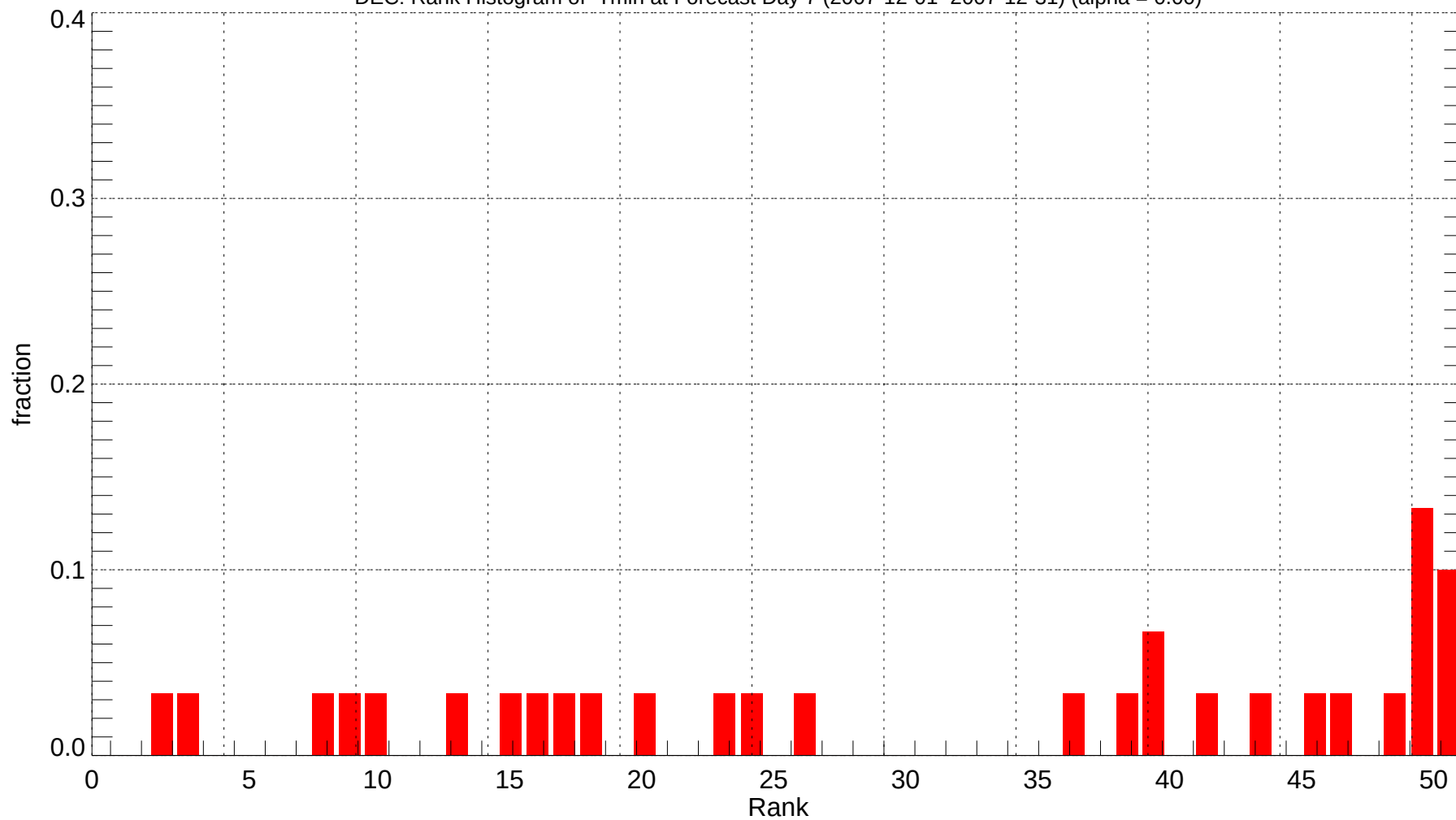
DEC: Rank Histogram of Tmin at Forecast Day 7 (2007-12-01~2007-12-31) (alpha = 0.00)
