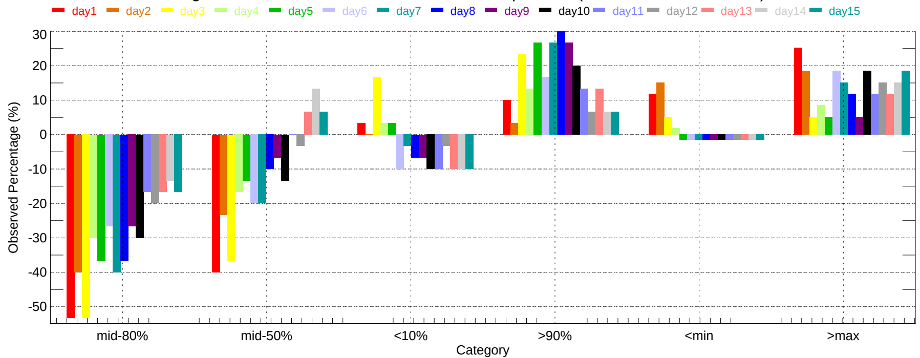
Observed Percentage Deviation of Ensembles - HSV: Max Temperature (2007-12-01~2007-12-31)
