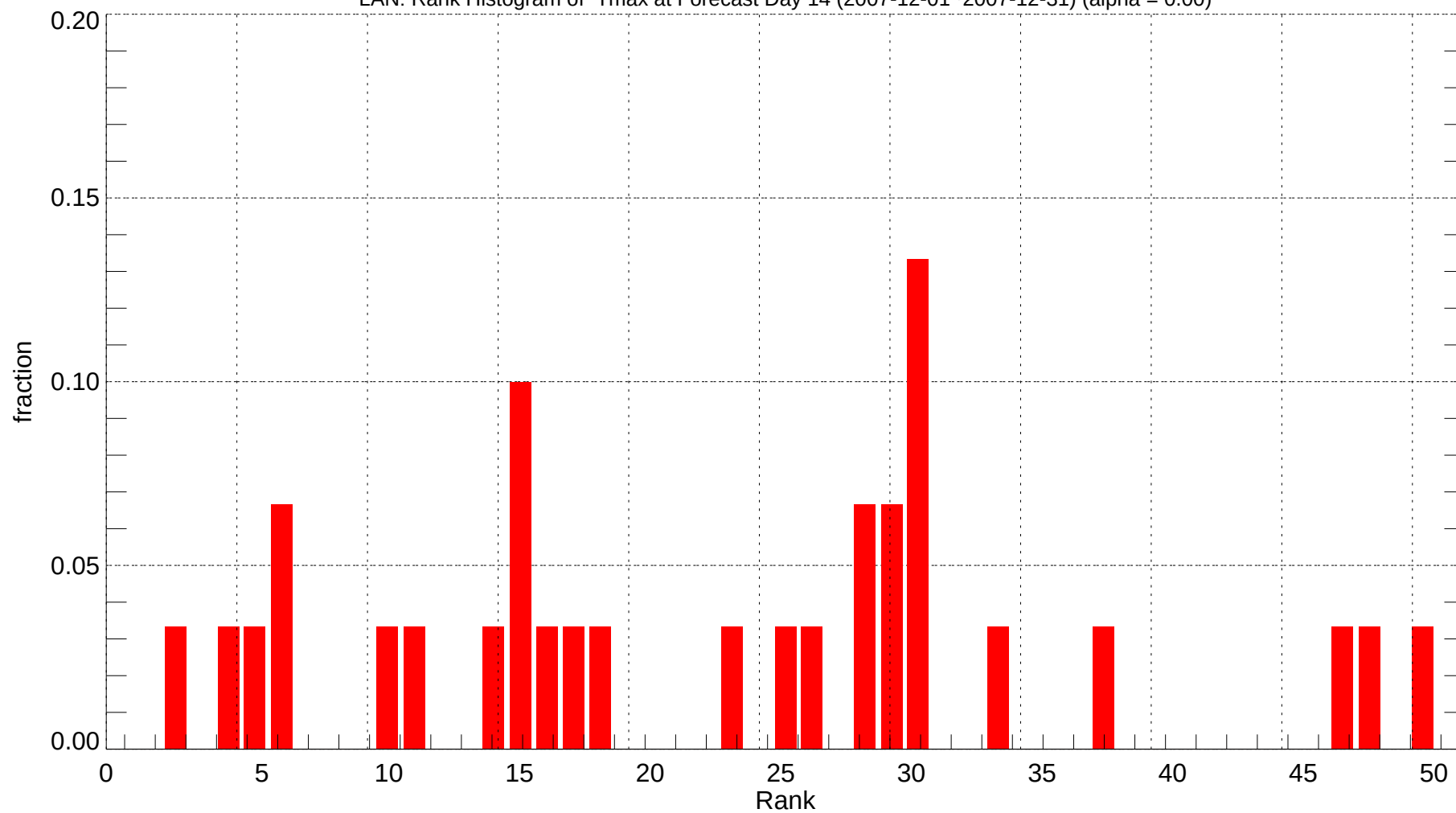
LAN: Rank Histogram of Tmax at Forecast Day 14 (2007-12-01~2007-12-31) (alpha = 0.00)
