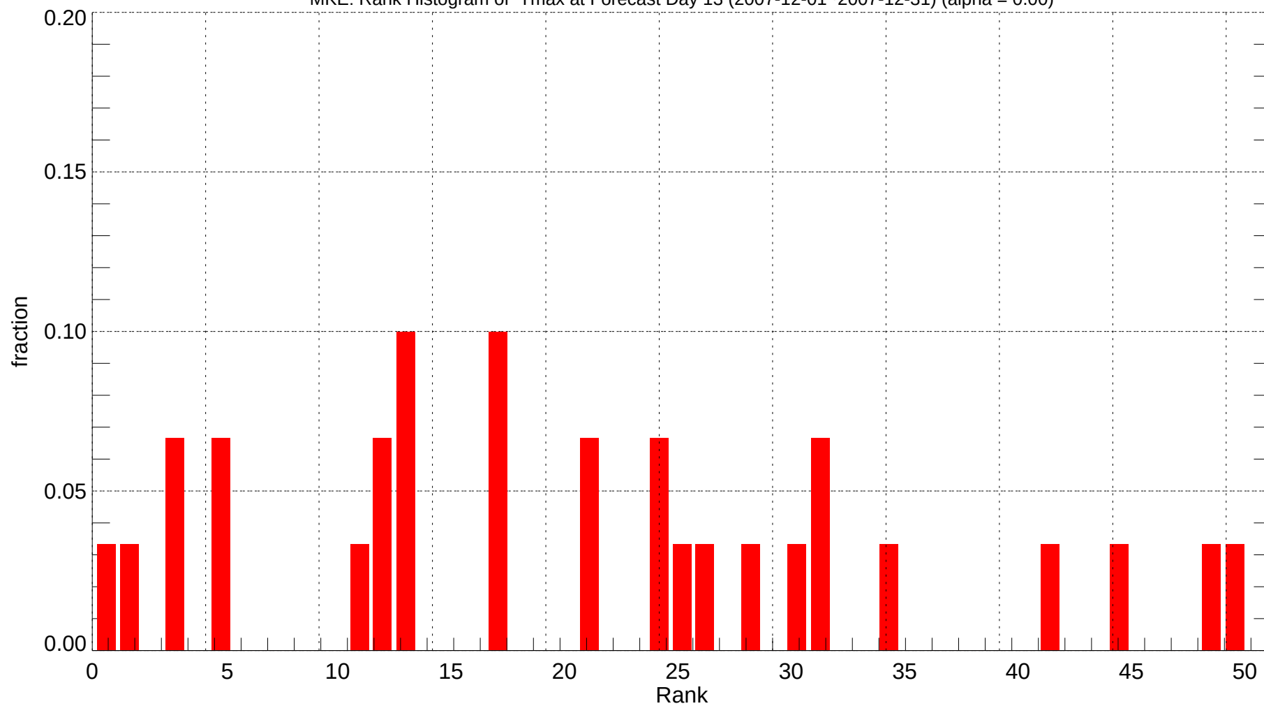
MKE: Rank Histogram of Tmax at Forecast Day 13 (2007-12-01~2007-12-31) (alpha = 0.00)
