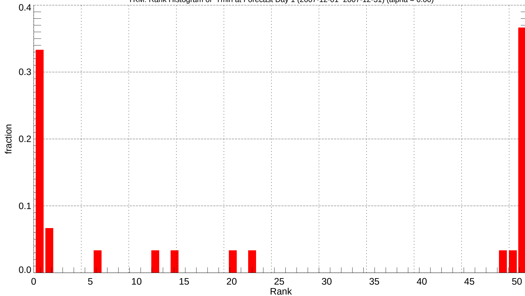
YKM: Rank Histogram of Tmin at Forecast Day 1 (2007-12-01~2007-12-31) (alpha = 0.00)
