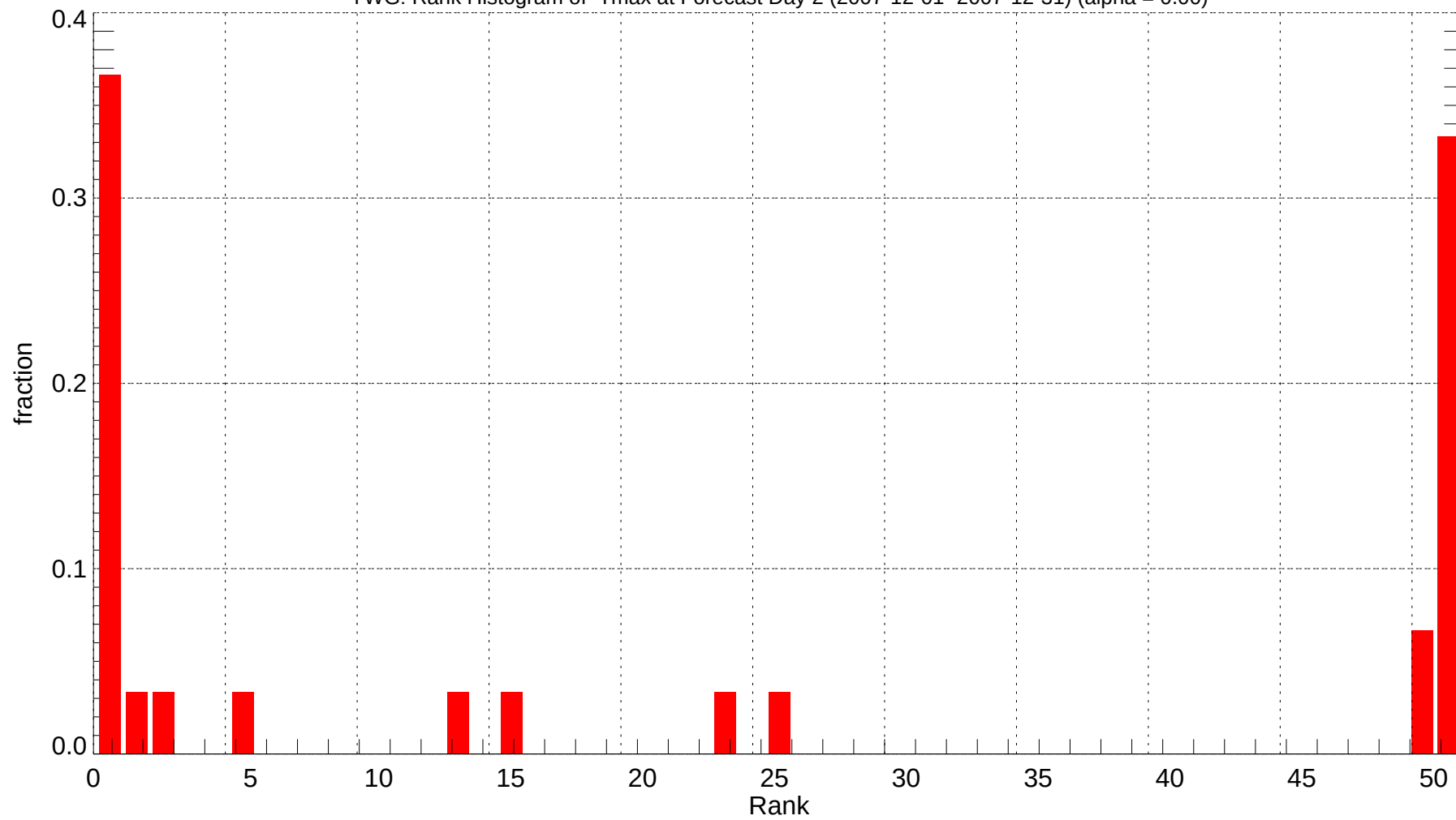
YWG: Rank Histogram of Tmax at Forecast Day 2 (2007-12-01~2007-12-31) (alpha = 0.00)
