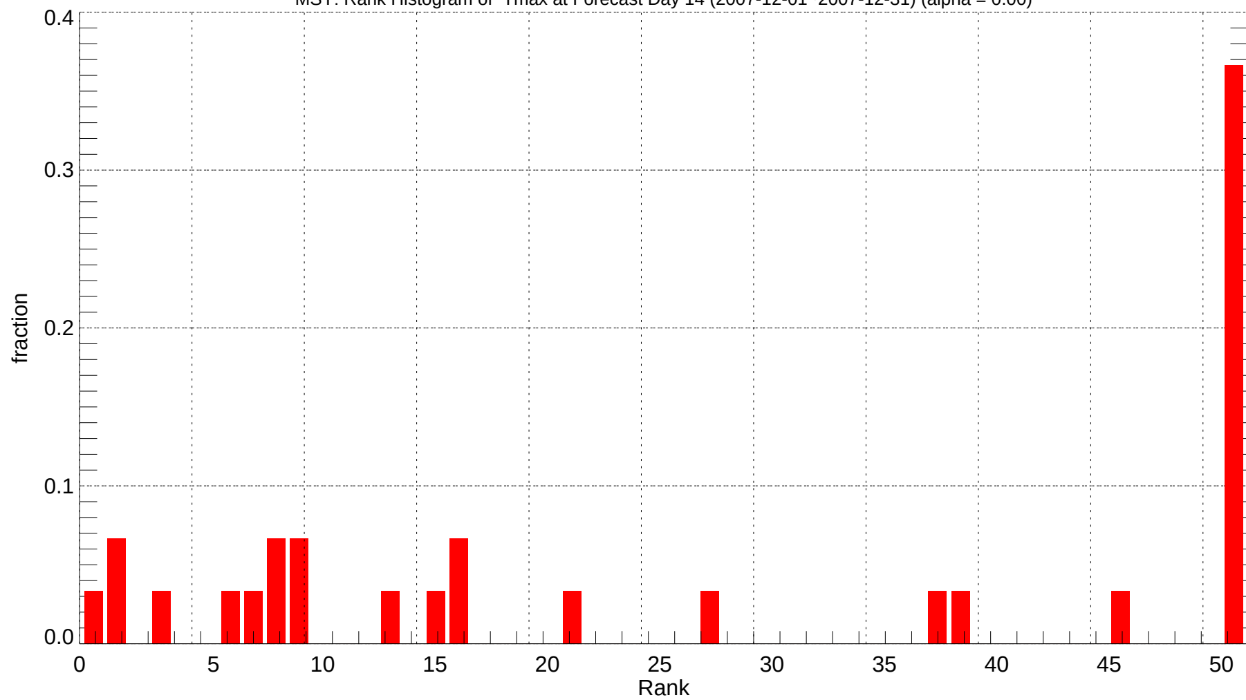
MSY: Rank Histogram of Tmax at Forecast Day 14 (2007-12-01~2007-12-31) (alpha = 0.00)
