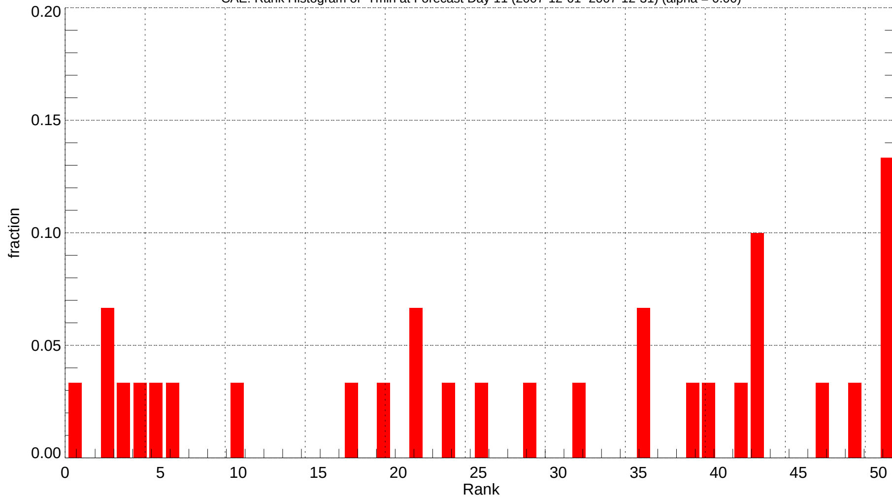
CAE: Rank Histogram of Tmin at Forecast Day 11 (2007-12-01~2007-12-31) (alpha = 0.00)
