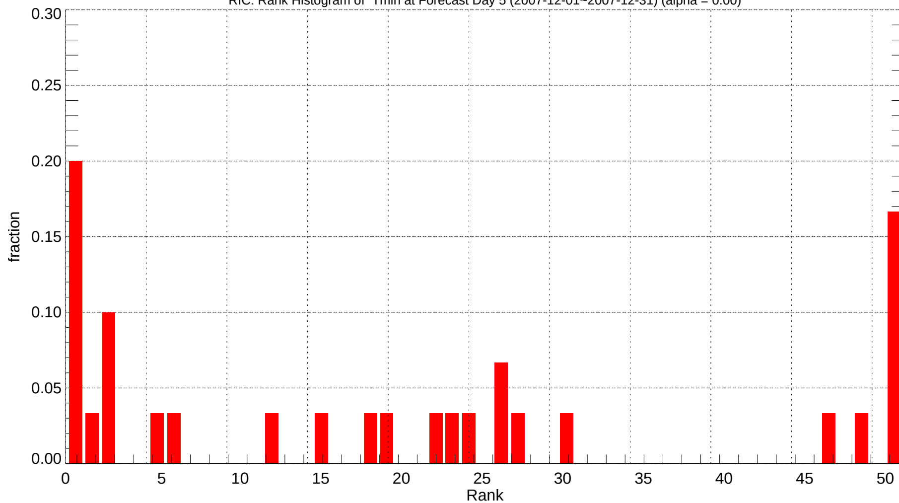
RIC: Rank Histogram of Tmin at Forecast Day 5 (2007-12-01~2007-12-31) (alpha = 0.00)
