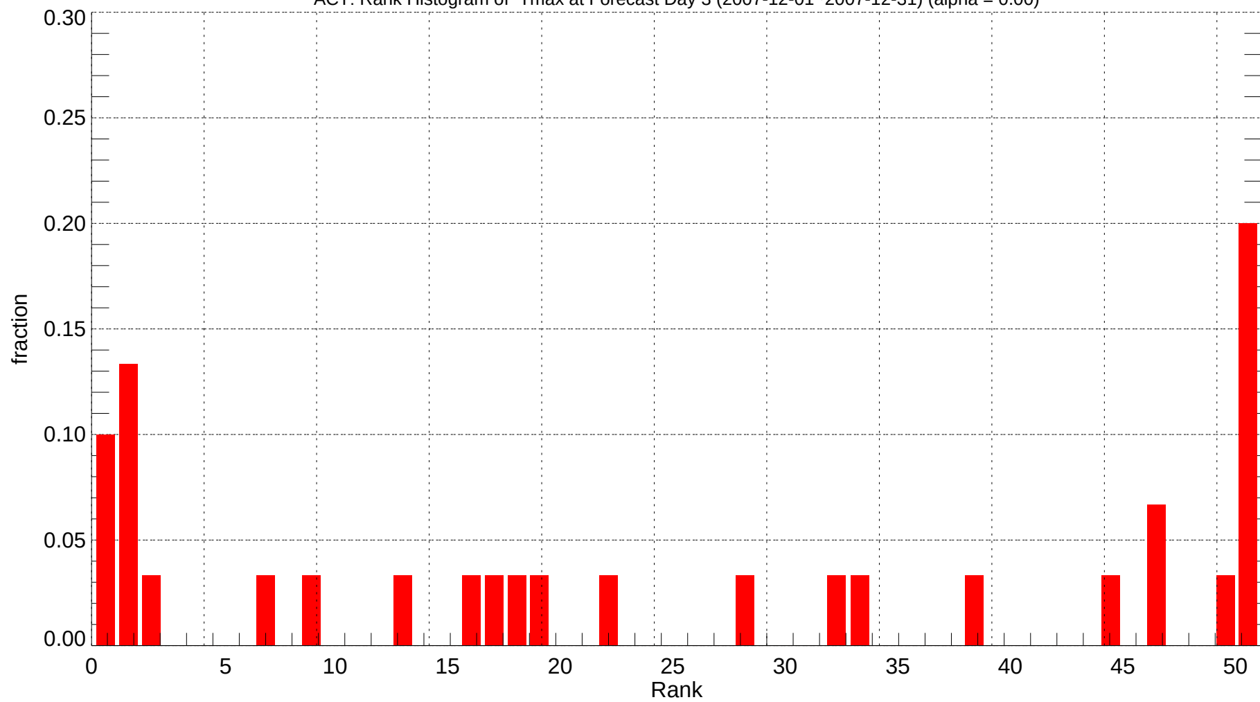
ACT: Rank Histogram of Tmax at Forecast Day 3 (2007-12-01~2007-12-31) (alpha = 0.00)
