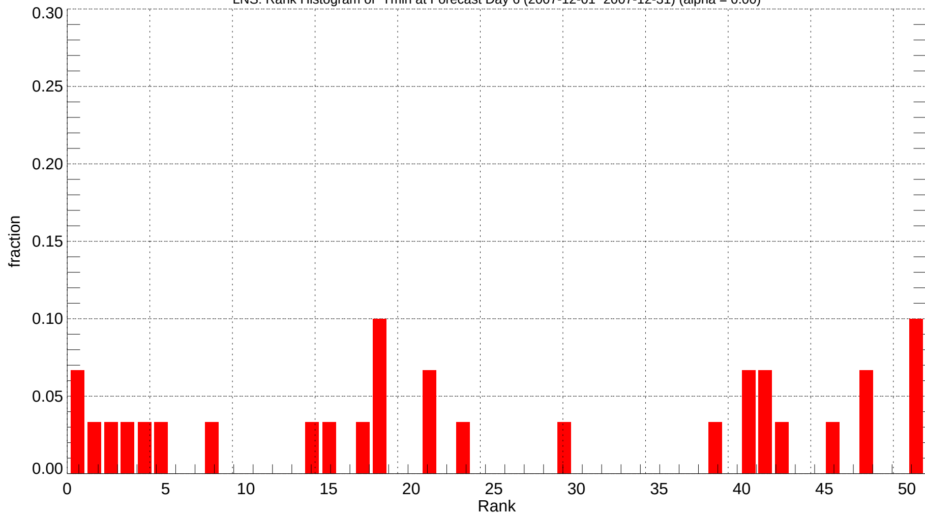
LNS: Rank Histogram of Tmin at Forecast Day 6 (2007-12-01~2007-12-31) (alpha = 0.00)
