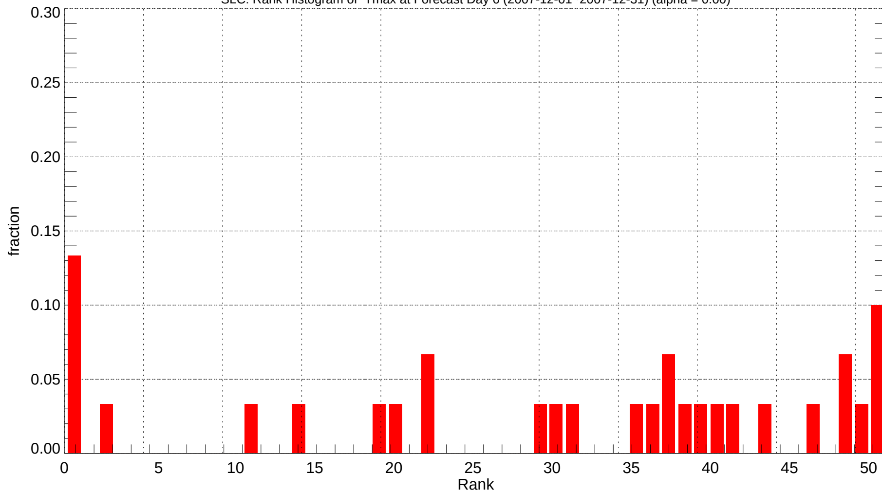
SLC: Rank Histogram of Tmax at Forecast Day 6 (2007-12-01~2007-12-31) (alpha = 0.00)
