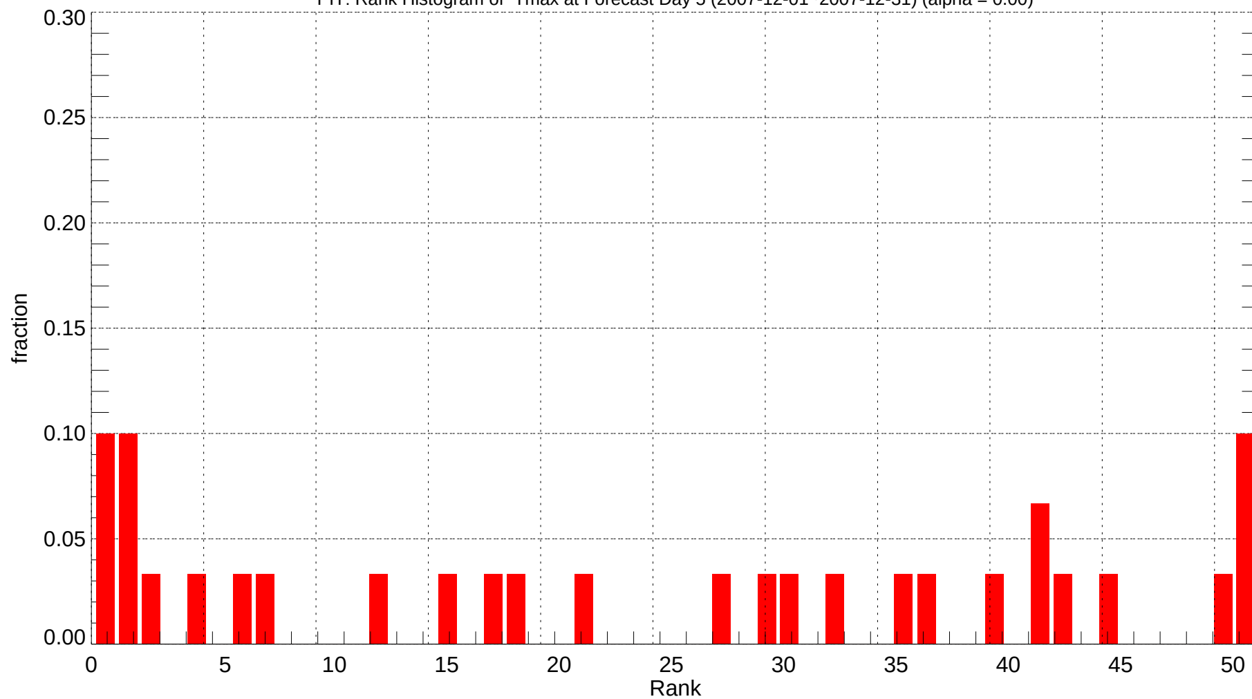
PIT: Rank Histogram of Tmax at Forecast Day 5 (2007-12-01~2007-12-31) (alpha = 0.00)
