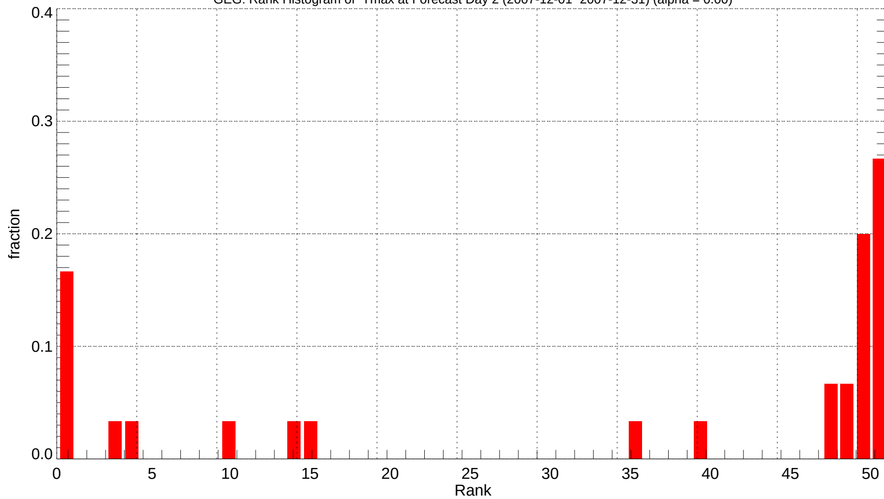
GEG: Rank Histogram of Tmax at Forecast Day 2 (2007-12-01~2007-12-31) (alpha = 0.00)
