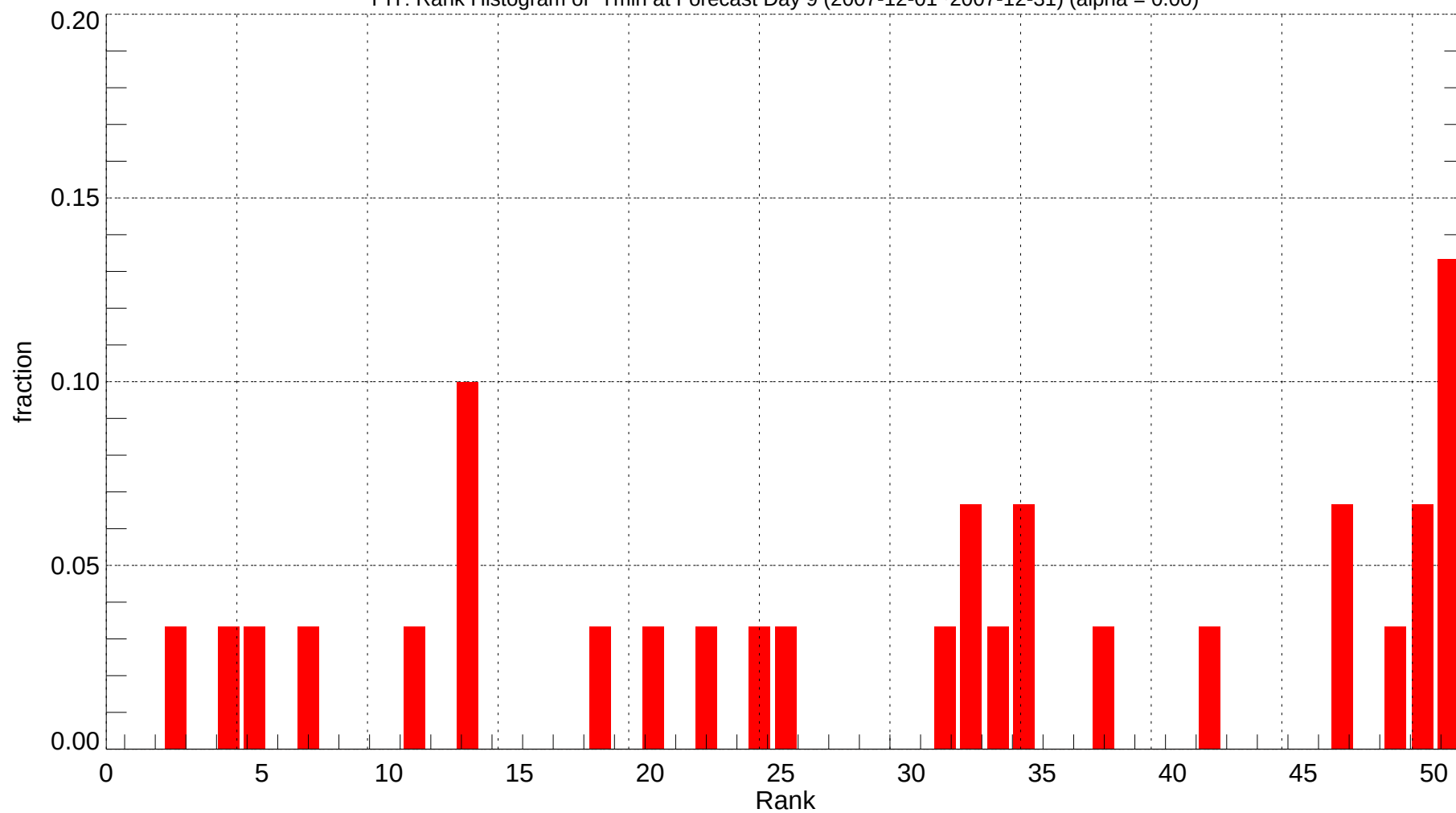
PIT: Rank Histogram of Tmin at Forecast Day 9 (2007-12-01~2007-12-31) (alpha = 0.00)
