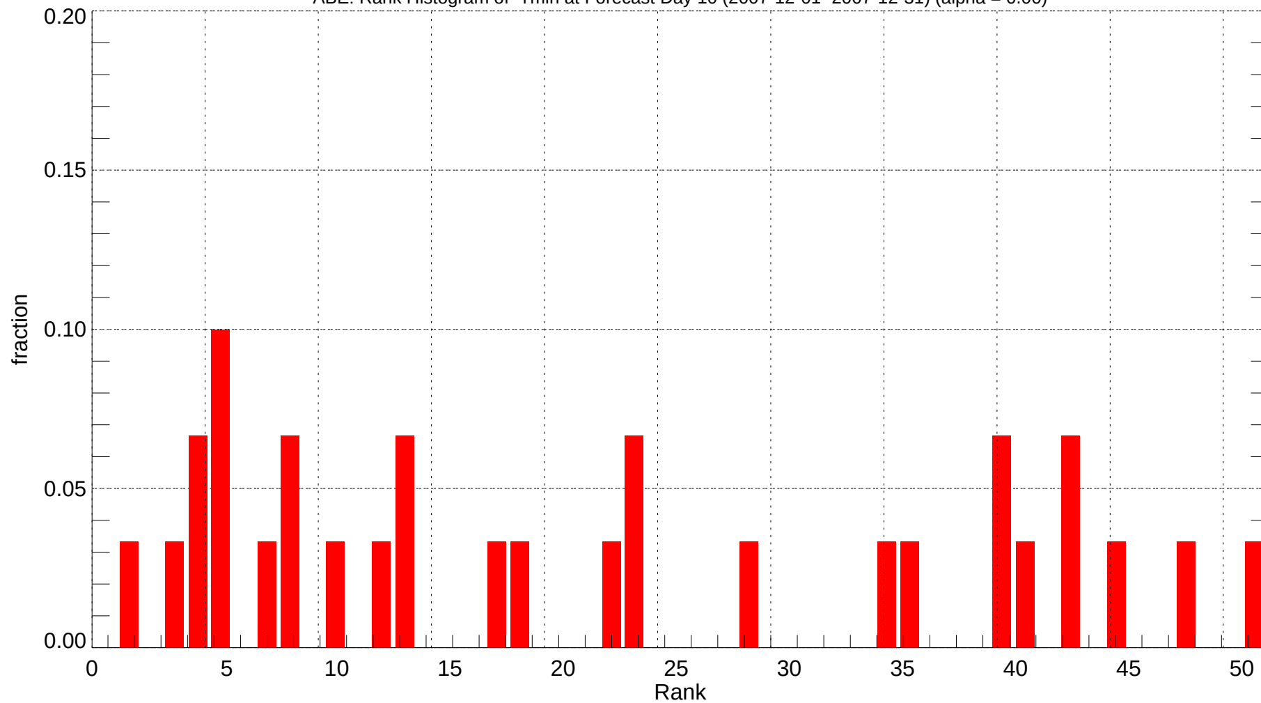
ABE: Rank Histogram of Tmin at Forecast Day 10 (2007-12-01~2007-12-31) (alpha = 0.00)
