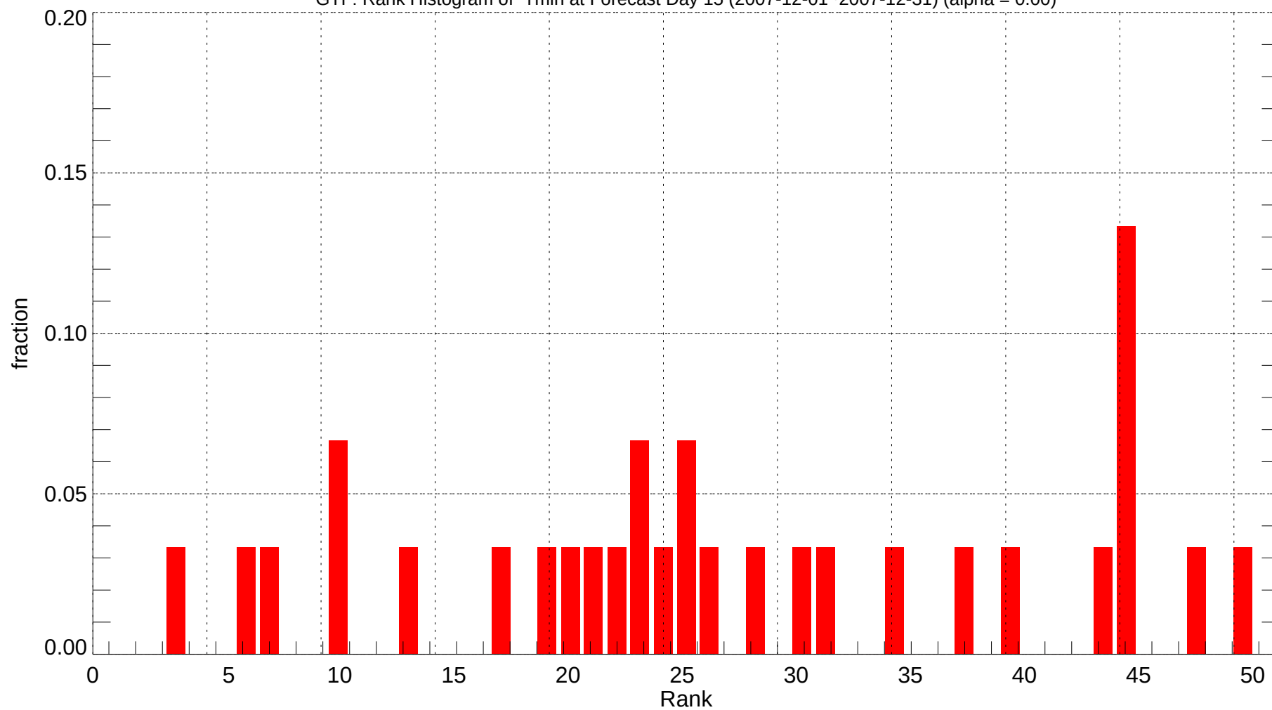
GTF: Rank Histogram of Tmin at Forecast Day 15 (2007-12-01~2007-12-31) (alpha = 0.00)
