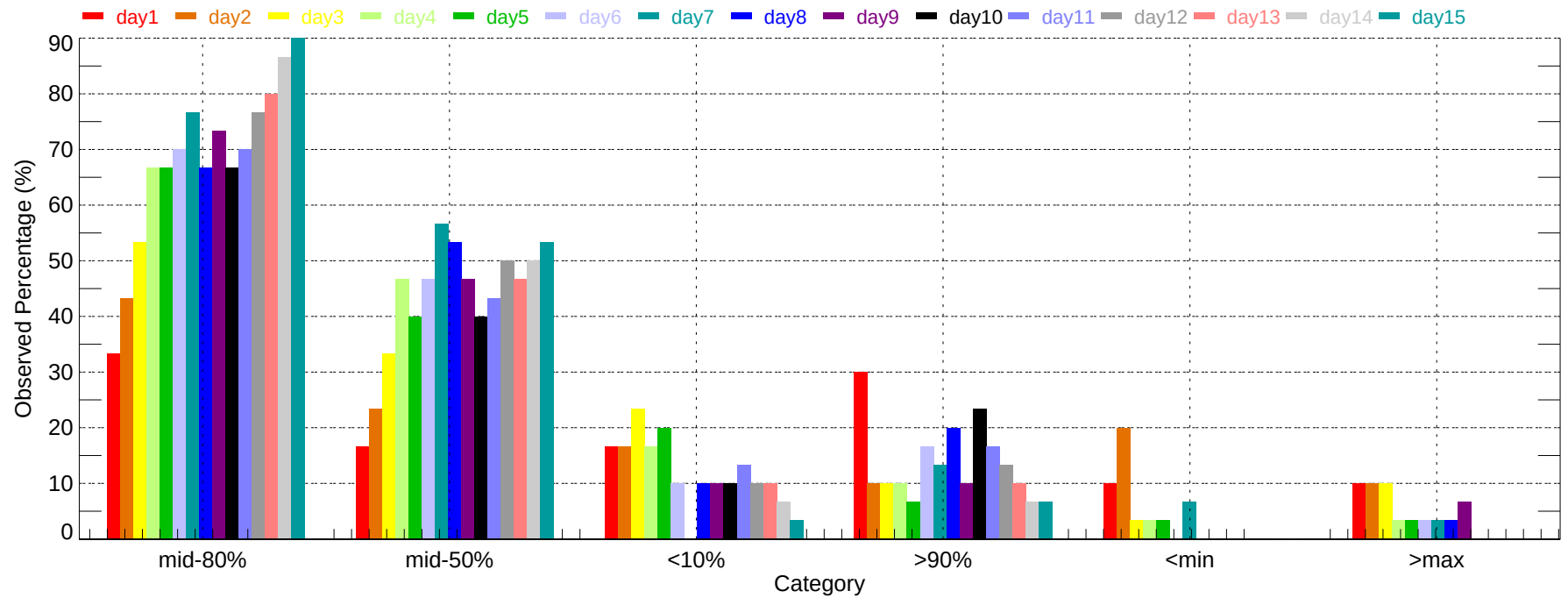
Observed Percentage of Ensembles - PWM: Max Temperature (2007-12-01~2007-12-31)
