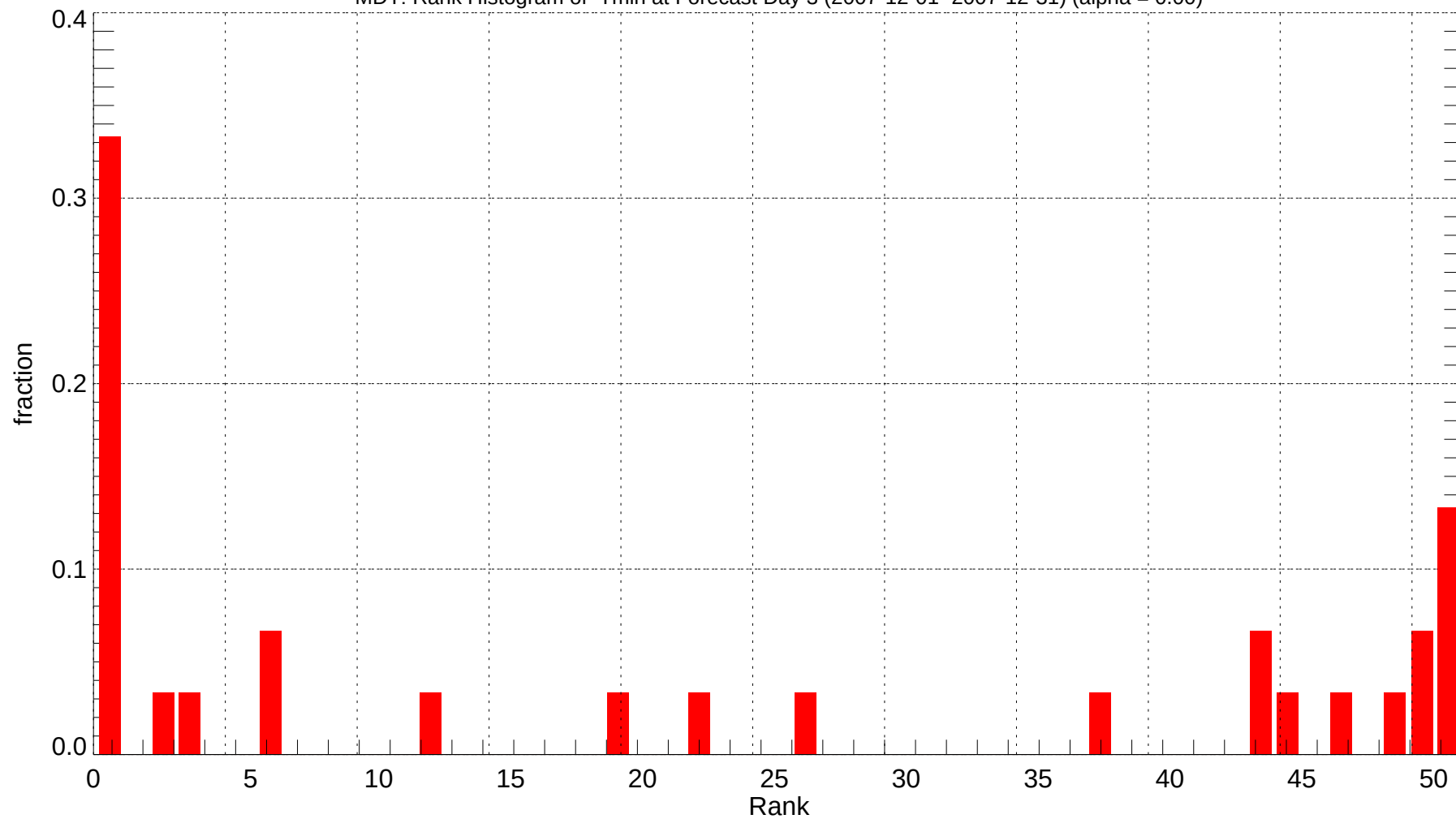
MDT: Rank Histogram of Tmin at Forecast Day 3 (2007-12-01~2007-12-31) (alpha = 0.00)
