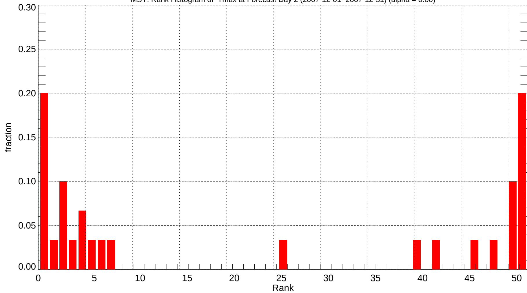
MSY: Rank Histogram of Tmax at Forecast Day 2 (2007-12-01~2007-12-31) (alpha = 0.00)
