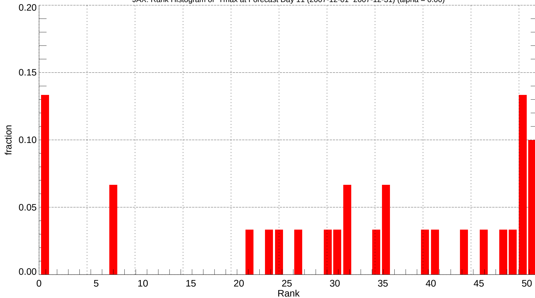
JAX: Rank Histogram of Tmax at Forecast Day 11 (2007-12-01~2007-12-31) (alpha = 0.00)
