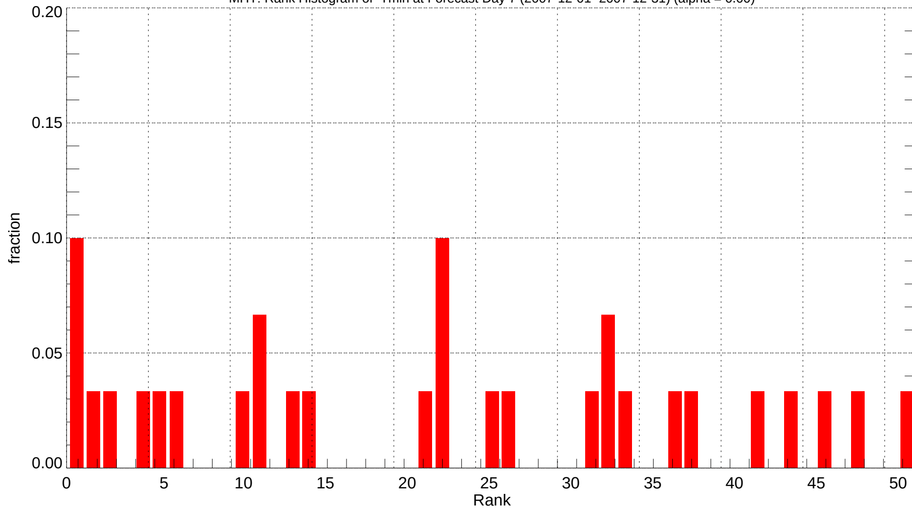
MHT: Rank Histogram of Tmin at Forecast Day 7 (2007-12-01~2007-12-31) (alpha = 0.00)
