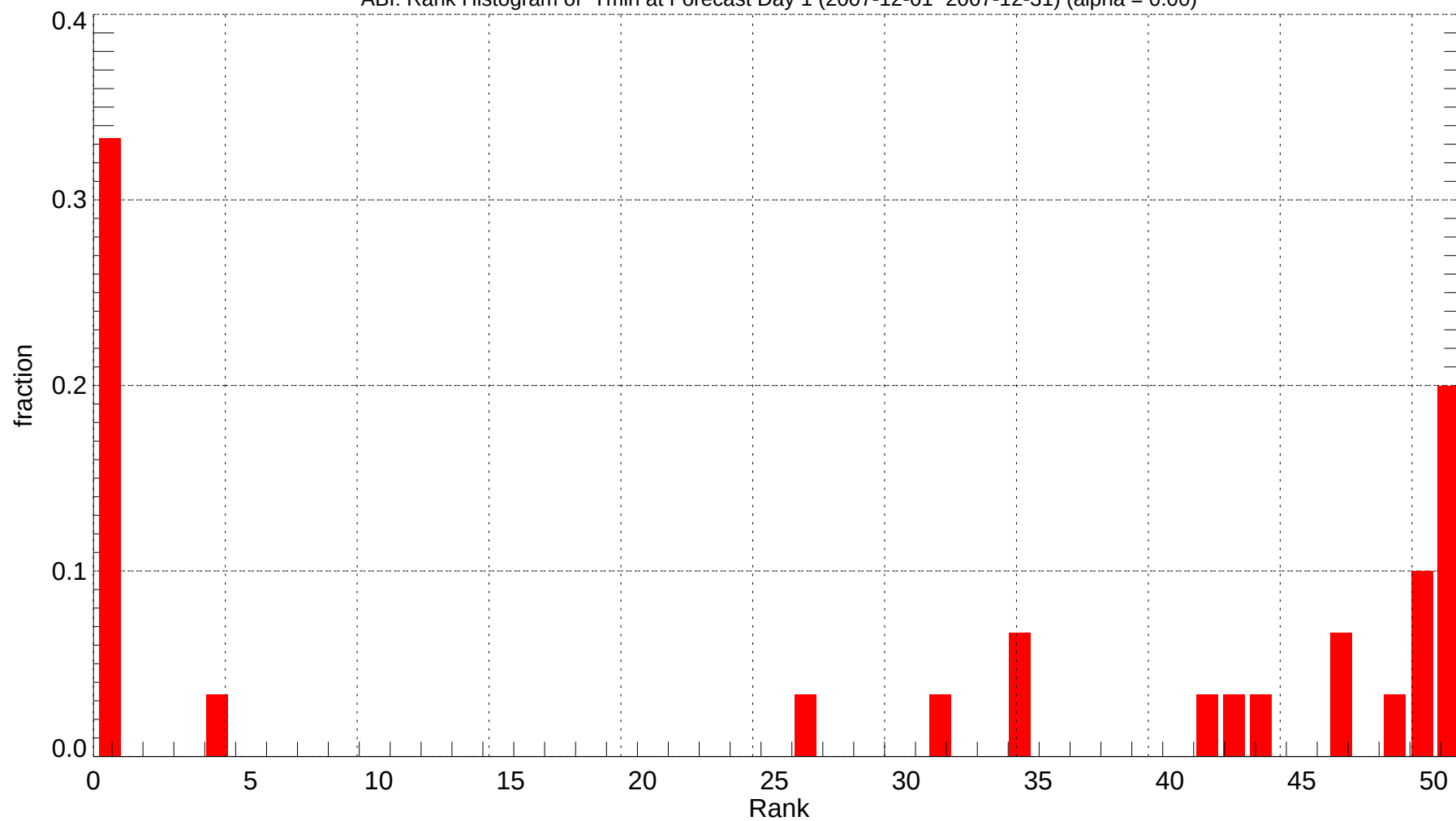
ABI: Rank Histogram of Tmin at Forecast Day 1 (2007-12-01~2007-12-31) (alpha = 0.00)
