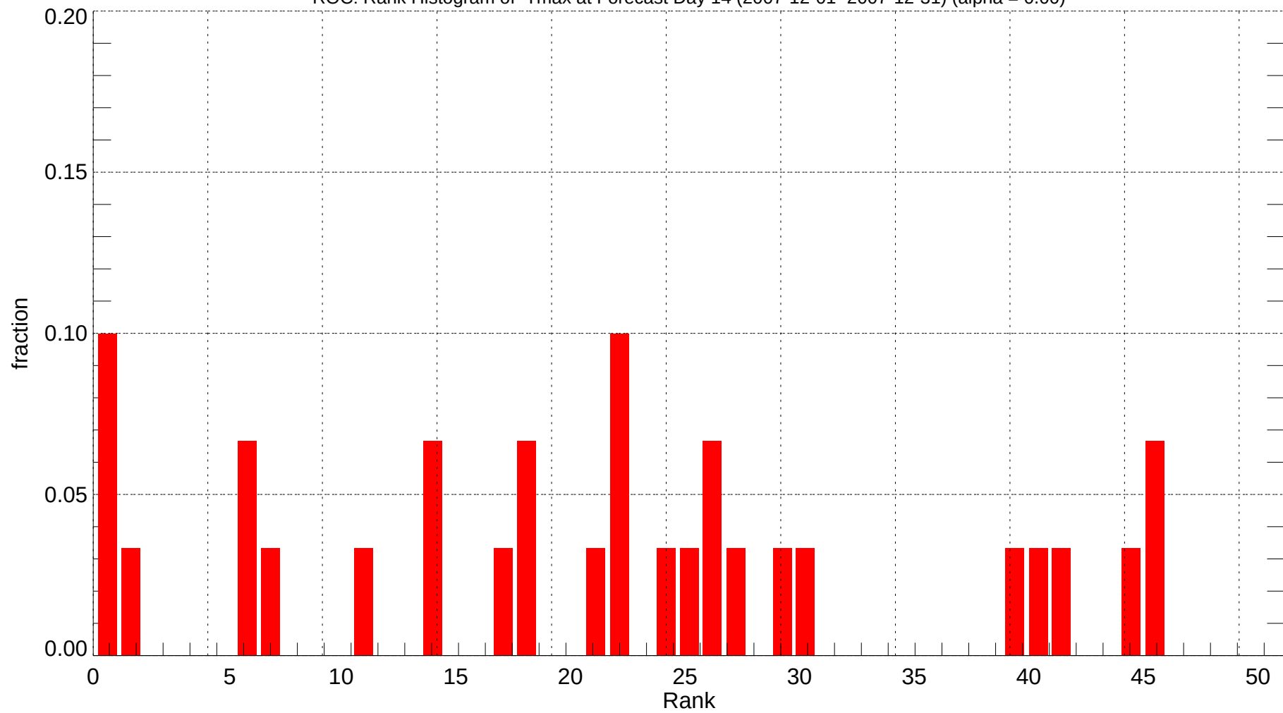
ROC: Rank Histogram of Tmax at Forecast Day 14 (2007-12-01~2007-12-31) (alpha = 0.00)
