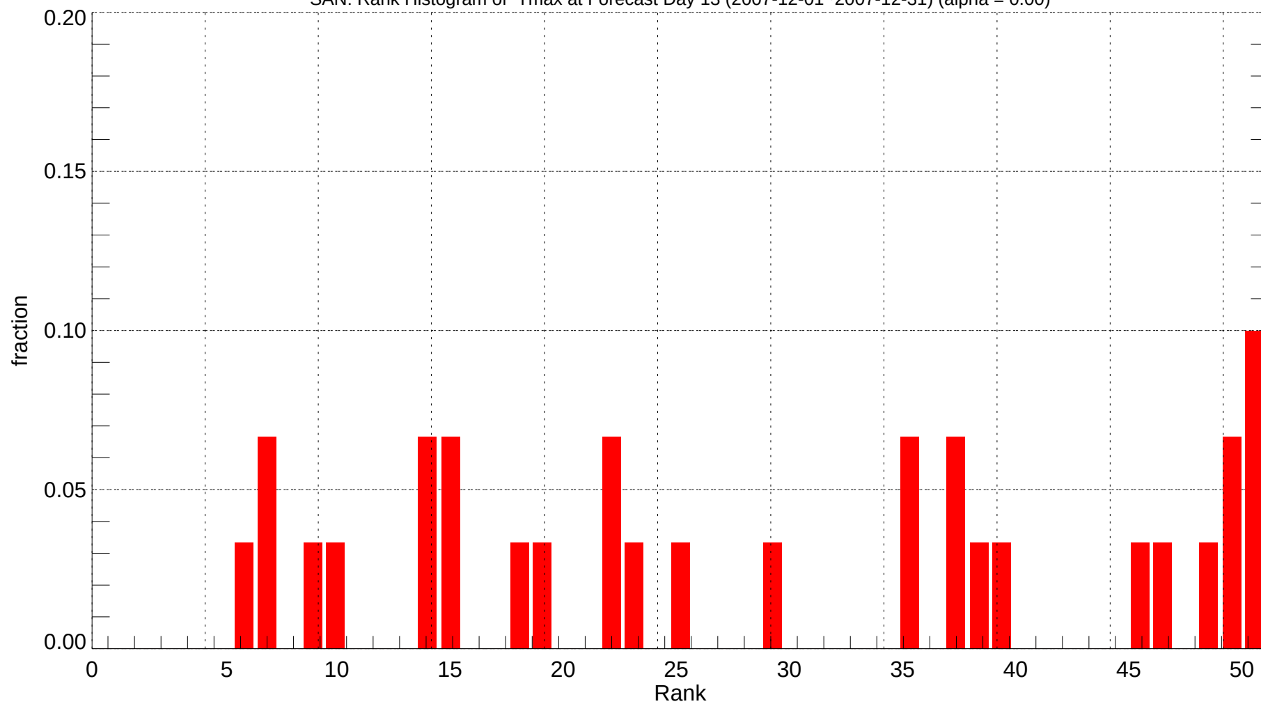
SAN: Rank Histogram of Tmax at Forecast Day 13 (2007-12-01~2007-12-31) (alpha = 0.00)
