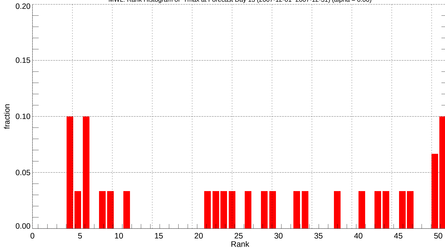
MWL: Rank Histogram of Tmax at Forecast Day 13 (2007-12-01~2007-12-31) (alpha = 0.00)
