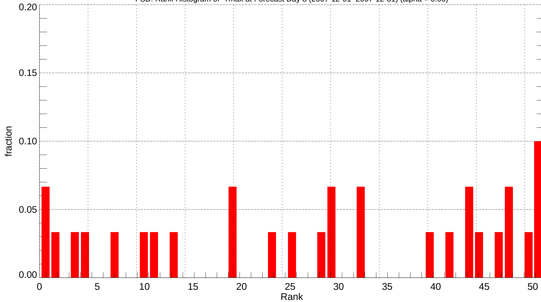
FSD: Rank Histogram of Tmax at Forecast Day 8 (2007-12-01~2007-12-31) (alpha = 0.00)
