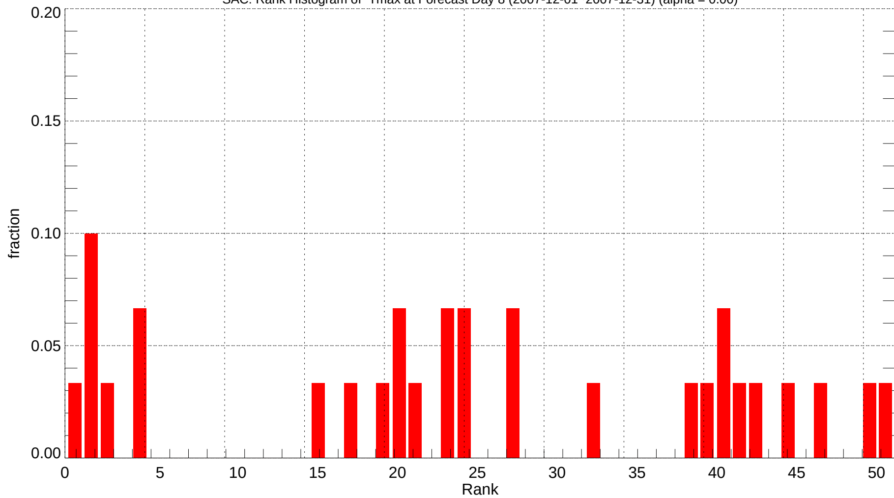
SAC: Rank Histogram of Tmax at Forecast Day 8 (2007-12-01~2007-12-31) (alpha = 0.00)
