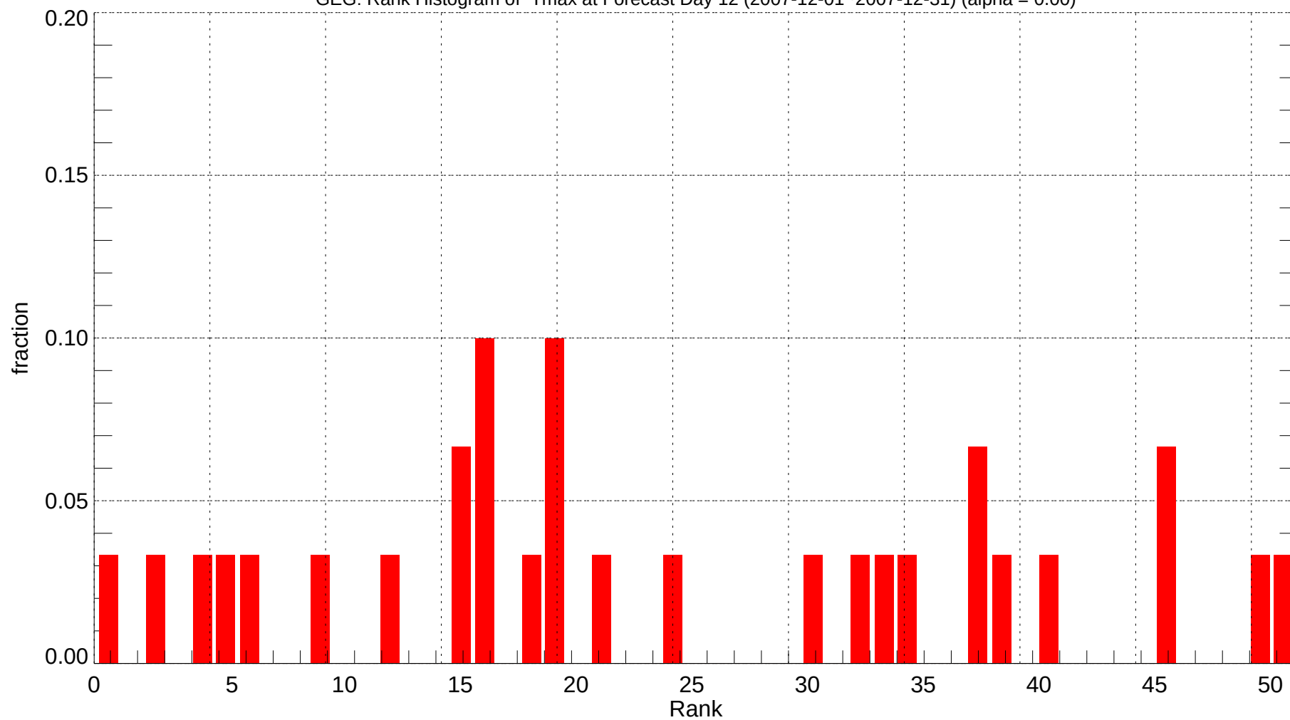
GEG: Rank Histogram of Tmax at Forecast Day 12 (2007-12-01~2007-12-31) (alpha = 0.00)
