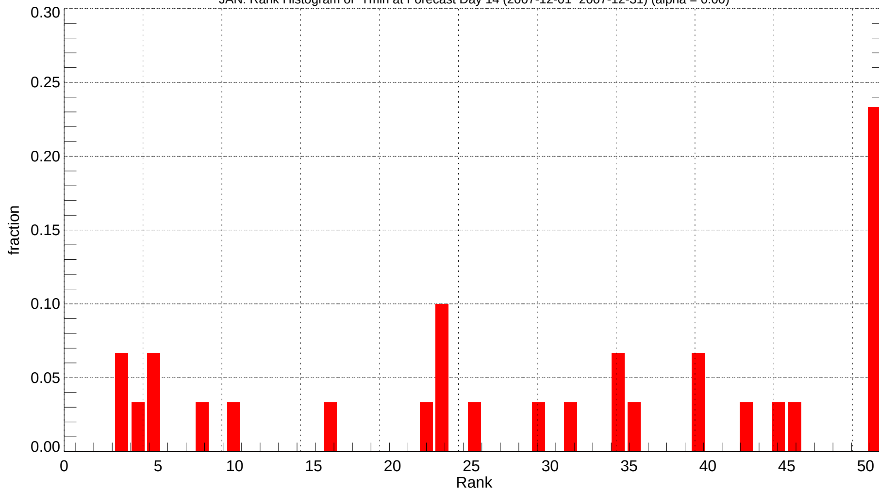
JAN: Rank Histogram of Tmin at Forecast Day 14 (2007-12-01~2007-12-31) (alpha = 0.00)
