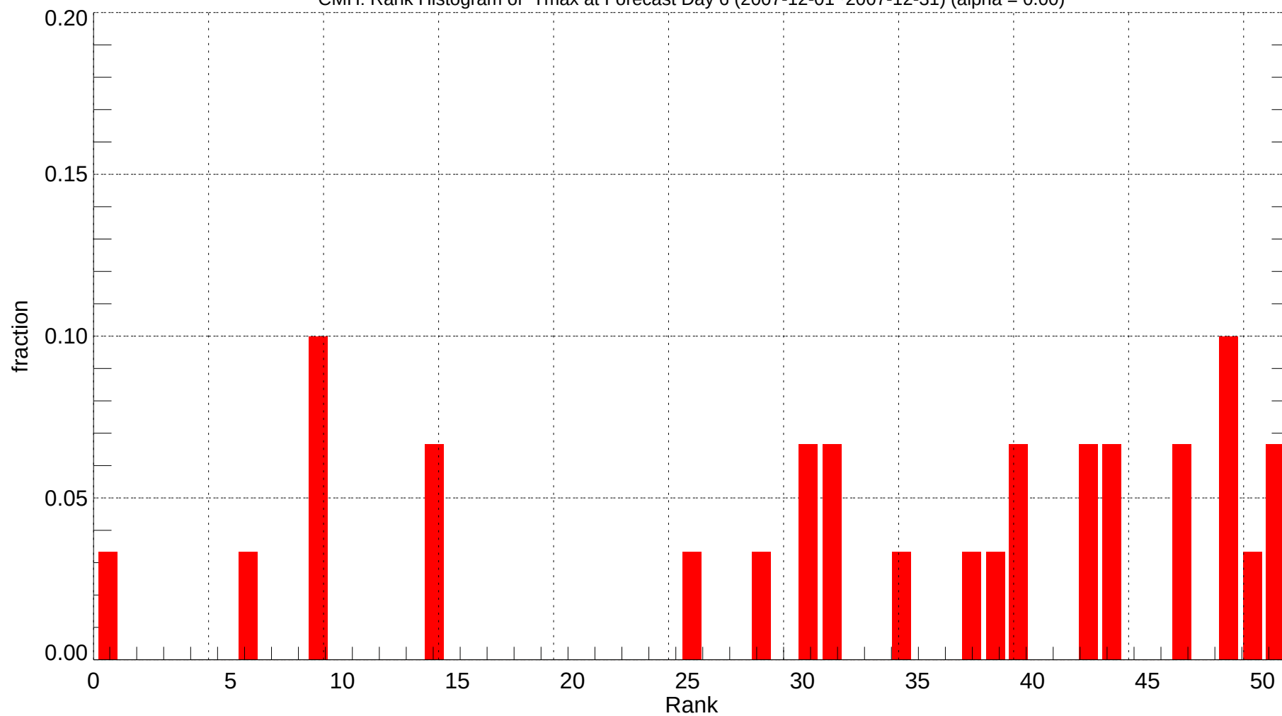
CMH: Rank Histogram of Tmax at Forecast Day 6 (2007-12-01~2007-12-31) (alpha = 0.00)
