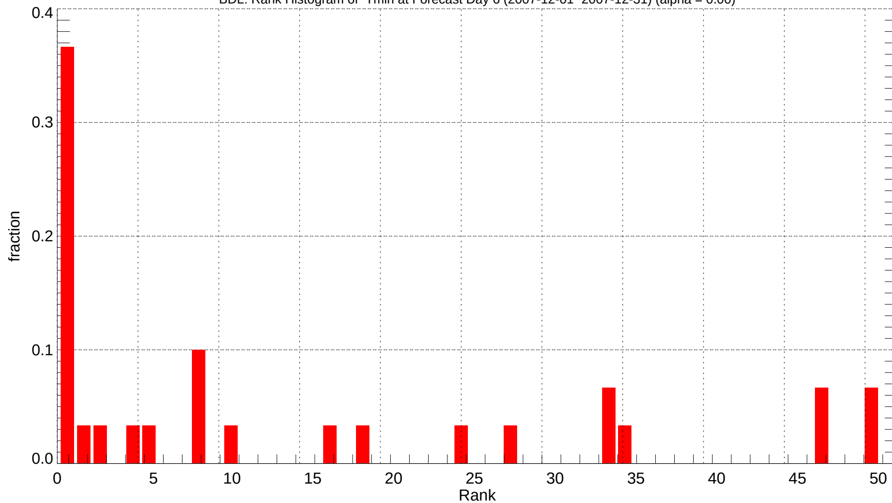
BDL: Rank Histogram of Tmin at Forecast Day 6 (2007-12-01~2007-12-31) (alpha = 0.00)
