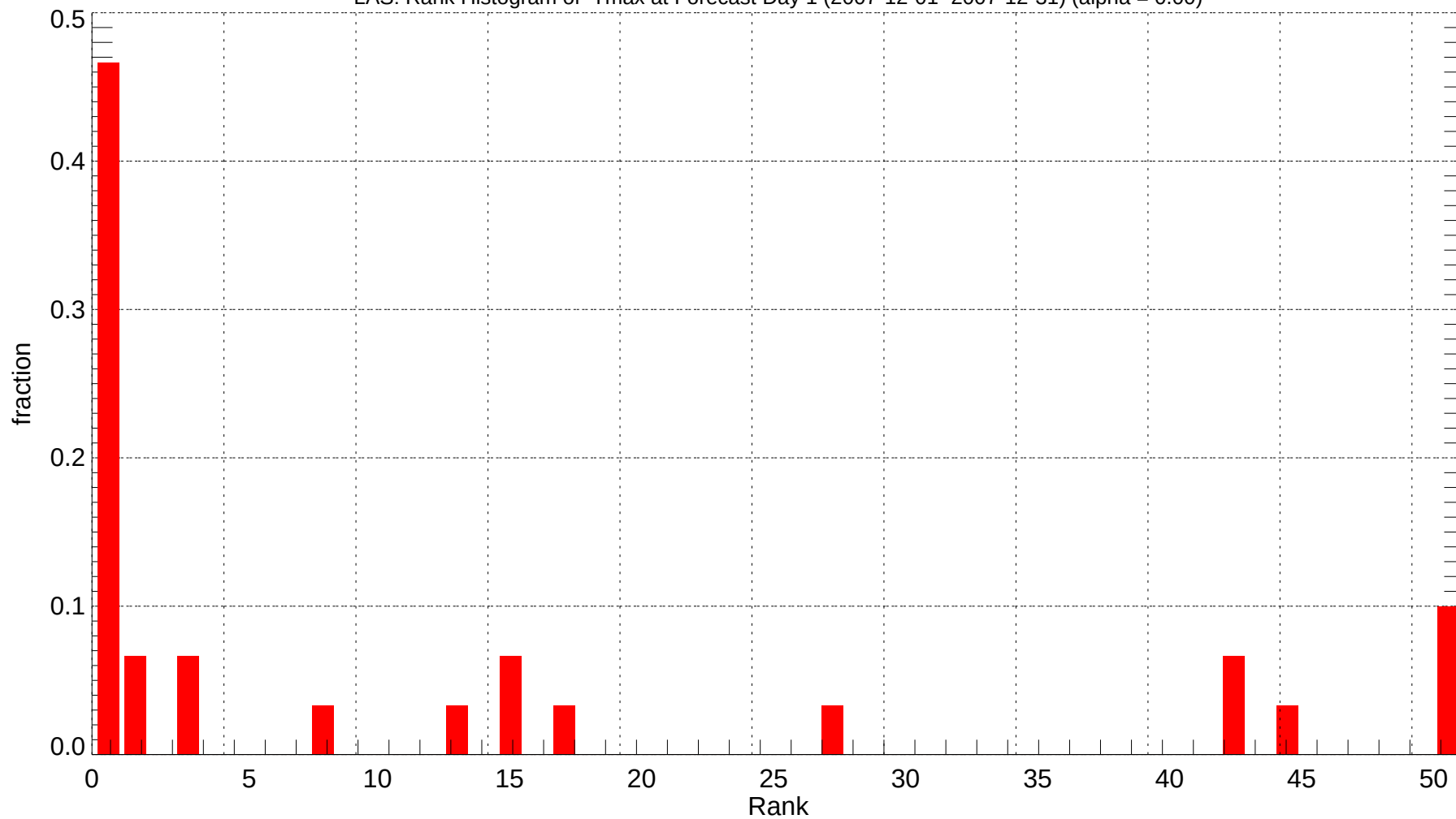
LAS: Rank Histogram of Tmax at Forecast Day 1 (2007-12-01~2007-12-31) (alpha = 0.00)
