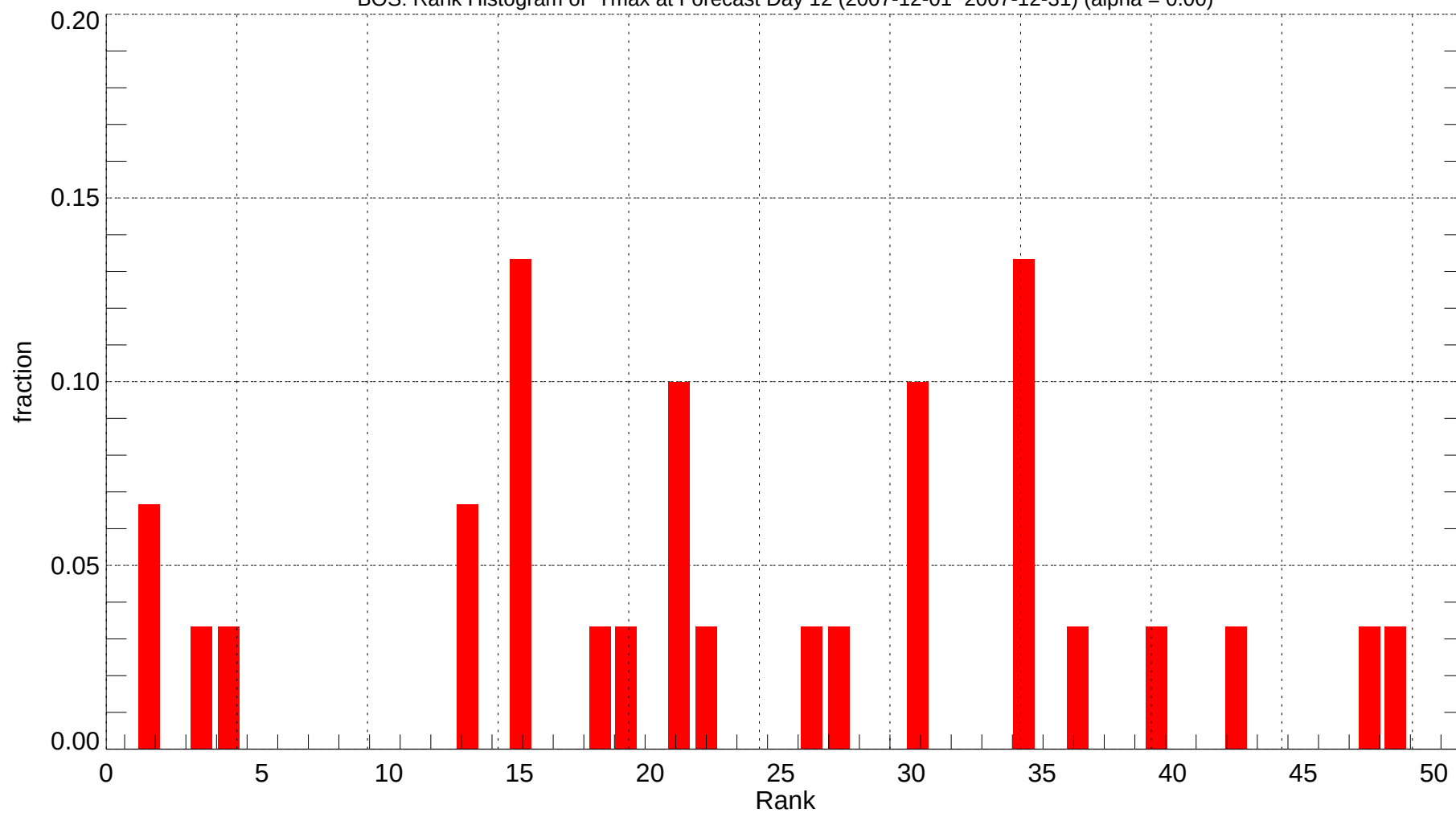
BOS: Rank Histogram of Tmax at Forecast Day 12 (2007-12-01~2007-12-31) (alpha = 0.00)
