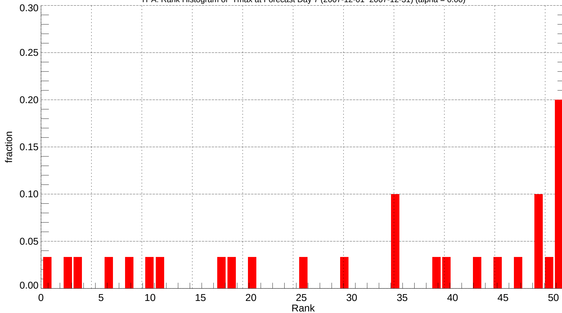
TPA: Rank Histogram of Tmax at Forecast Day 7 (2007-12-01~2007-12-31) (alpha = 0.00)
