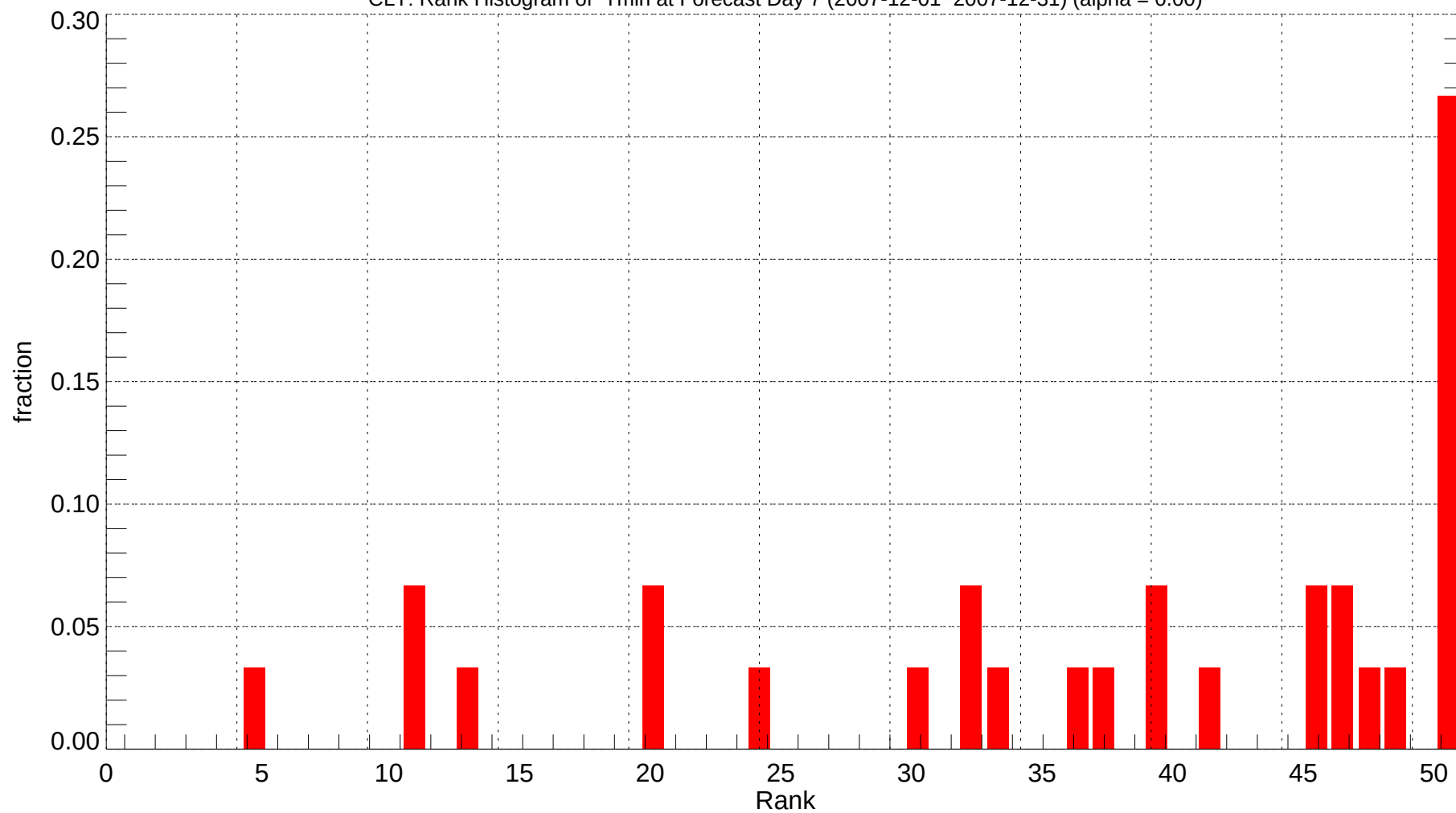
CLT: Rank Histogram of Tmin at Forecast Day 7 (2007-12-01~2007-12-31) (alpha = 0.00)
