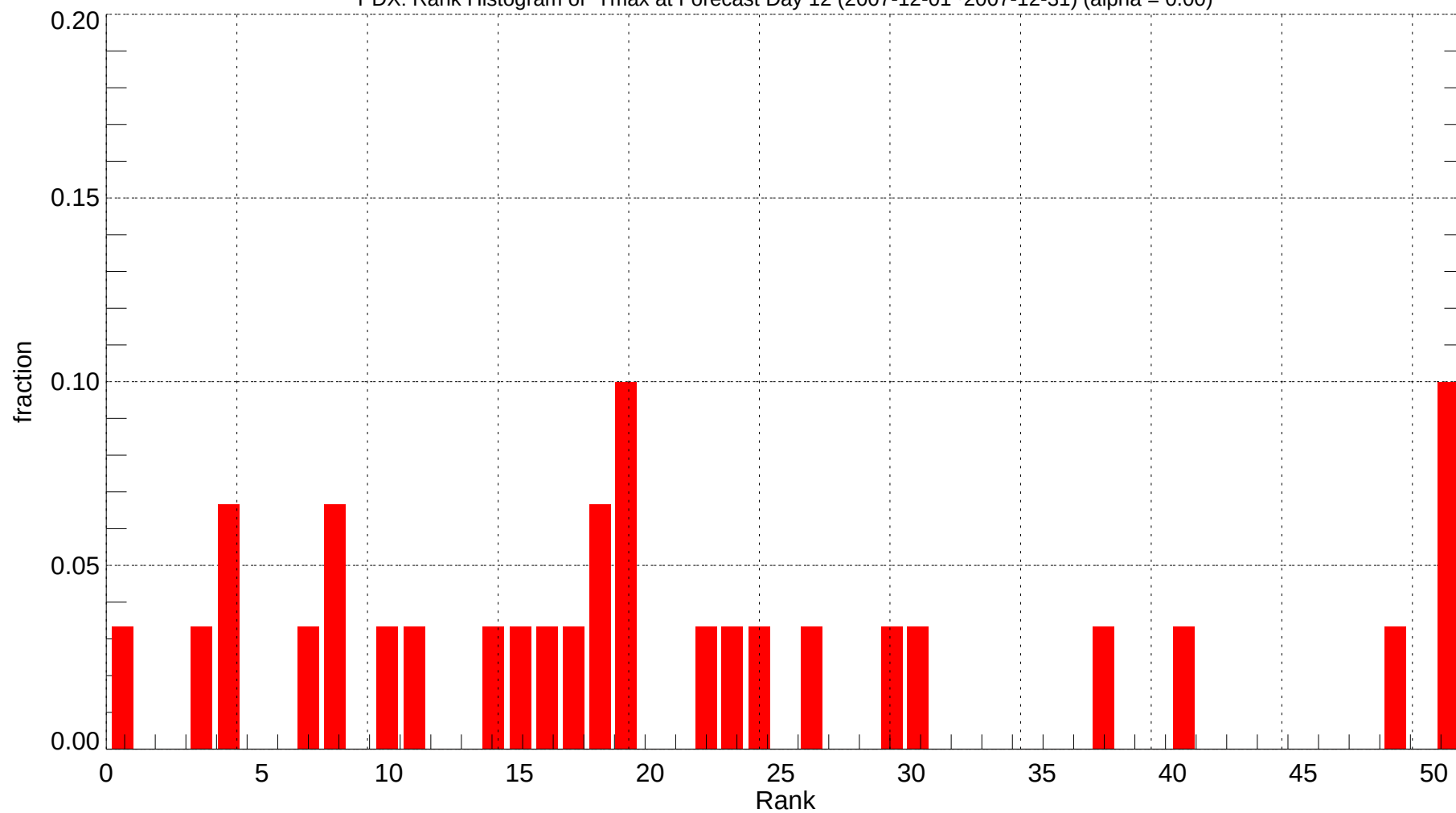
PDX: Rank Histogram of Tmax at Forecast Day 12 (2007-12-01~2007-12-31) (alpha = 0.00)
