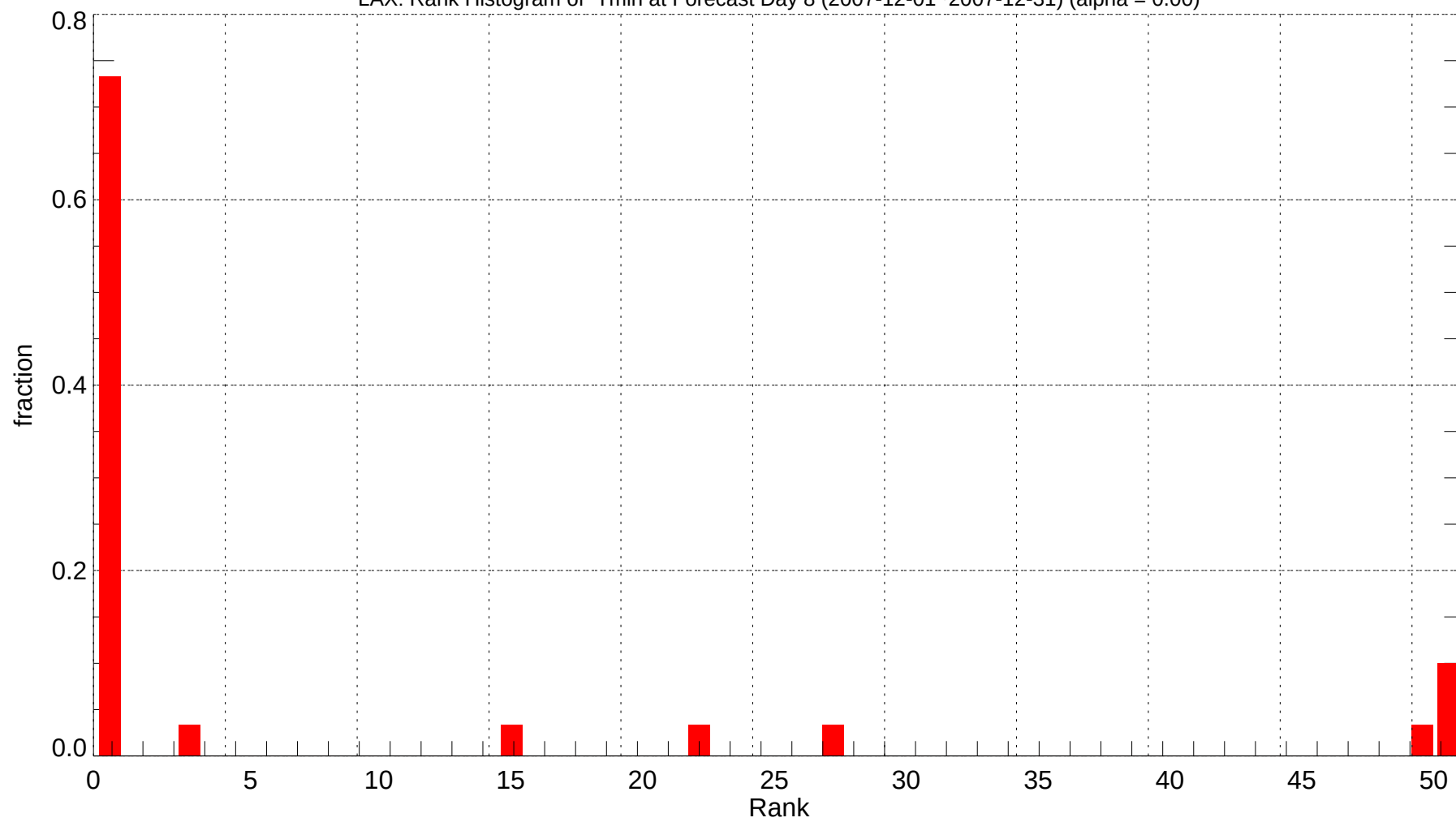
LAX: Rank Histogram of Tmin at Forecast Day 8 (2007-12-01~2007-12-31) (alpha = 0.00)
