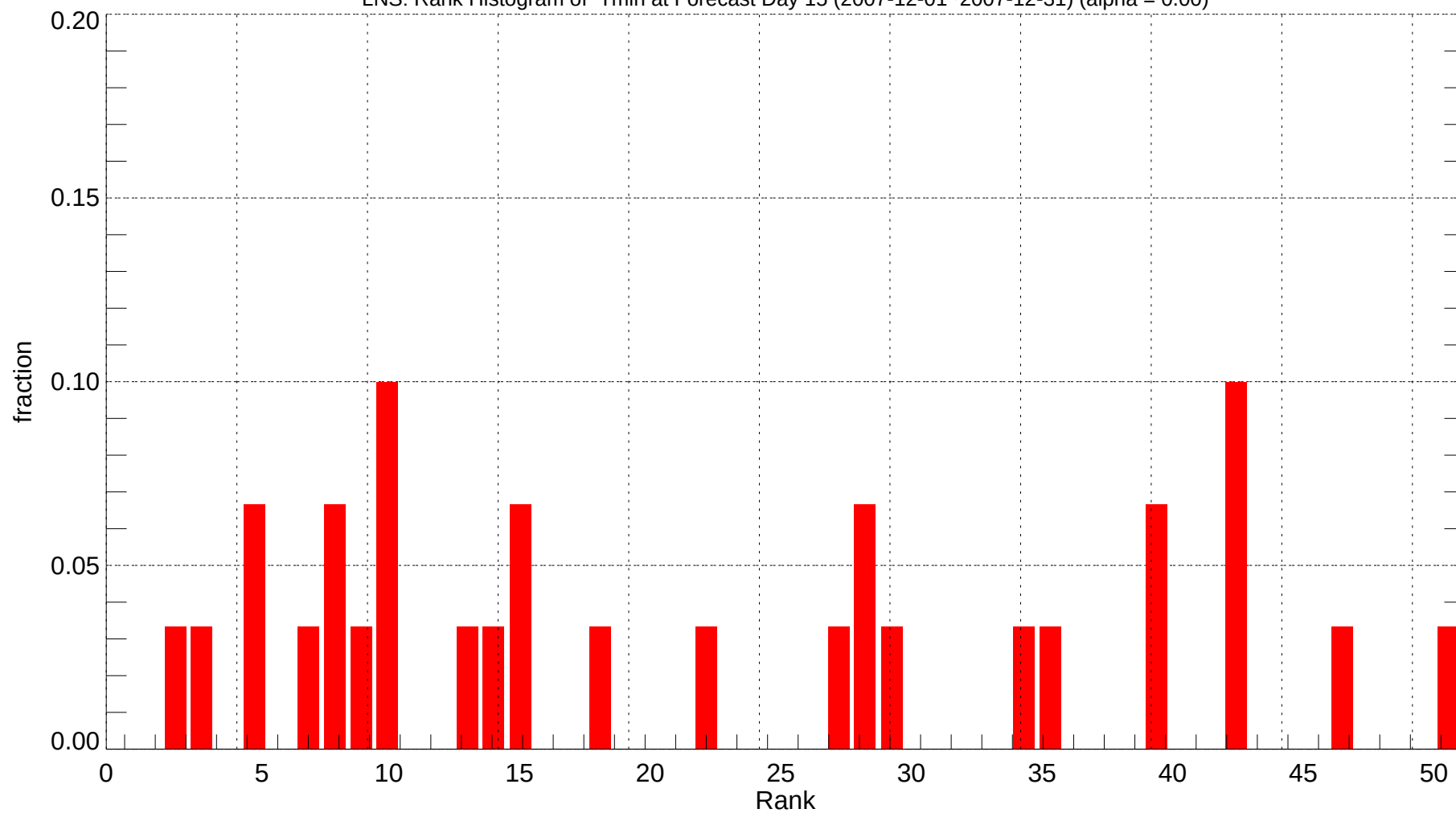
LNS: Rank Histogram of Tmin at Forecast Day 15 (2007-12-01~2007-12-31) (alpha = 0.00)
