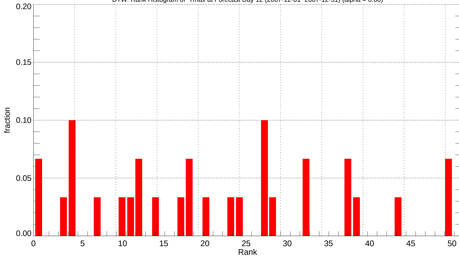
DTW: Rank Histogram of Tmax at Forecast Day 12 (2007-12-01~2007-12-31) (alpha = 0.00)
