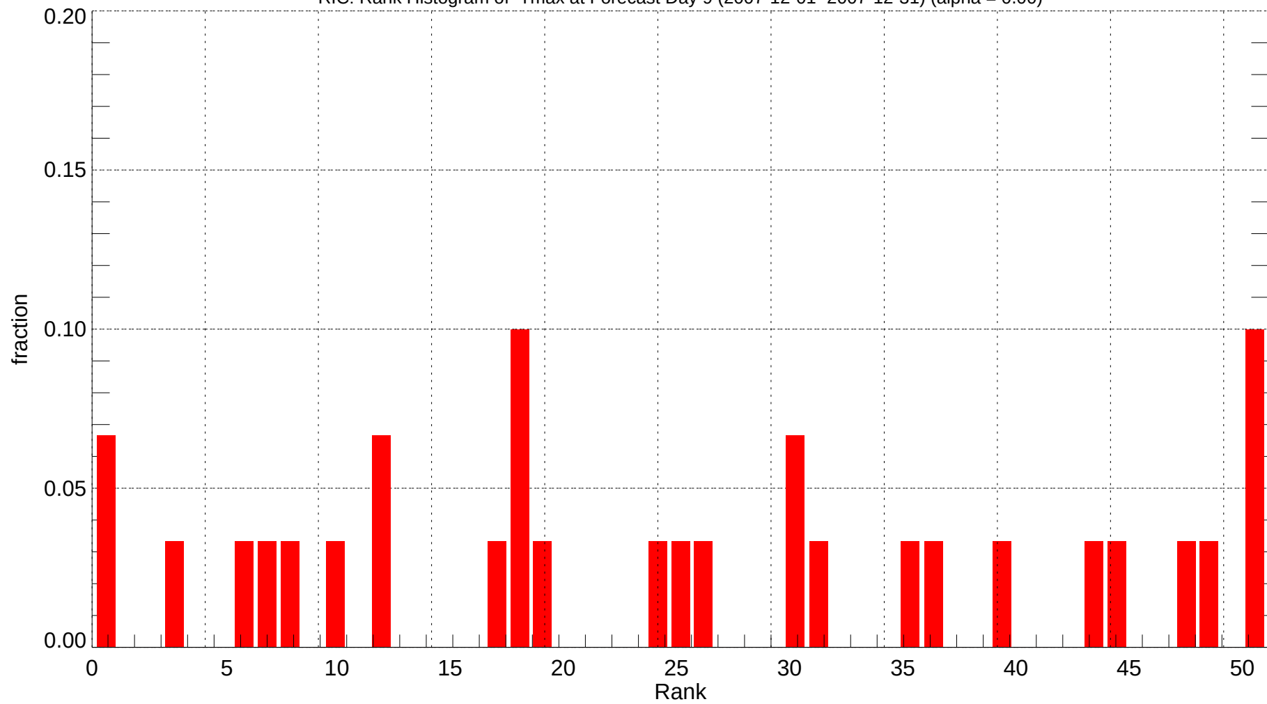
RIC: Rank Histogram of Tmax at Forecast Day 9 (2007-12-01~2007-12-31) (alpha = 0.00)
