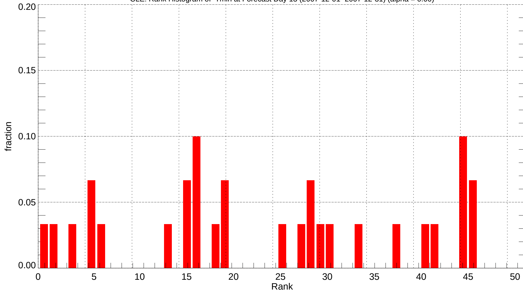
CLE: Rank Histogram of Tmin at Forecast Day 13 (2007-12-01~2007-12-31) (alpha = 0.00)
