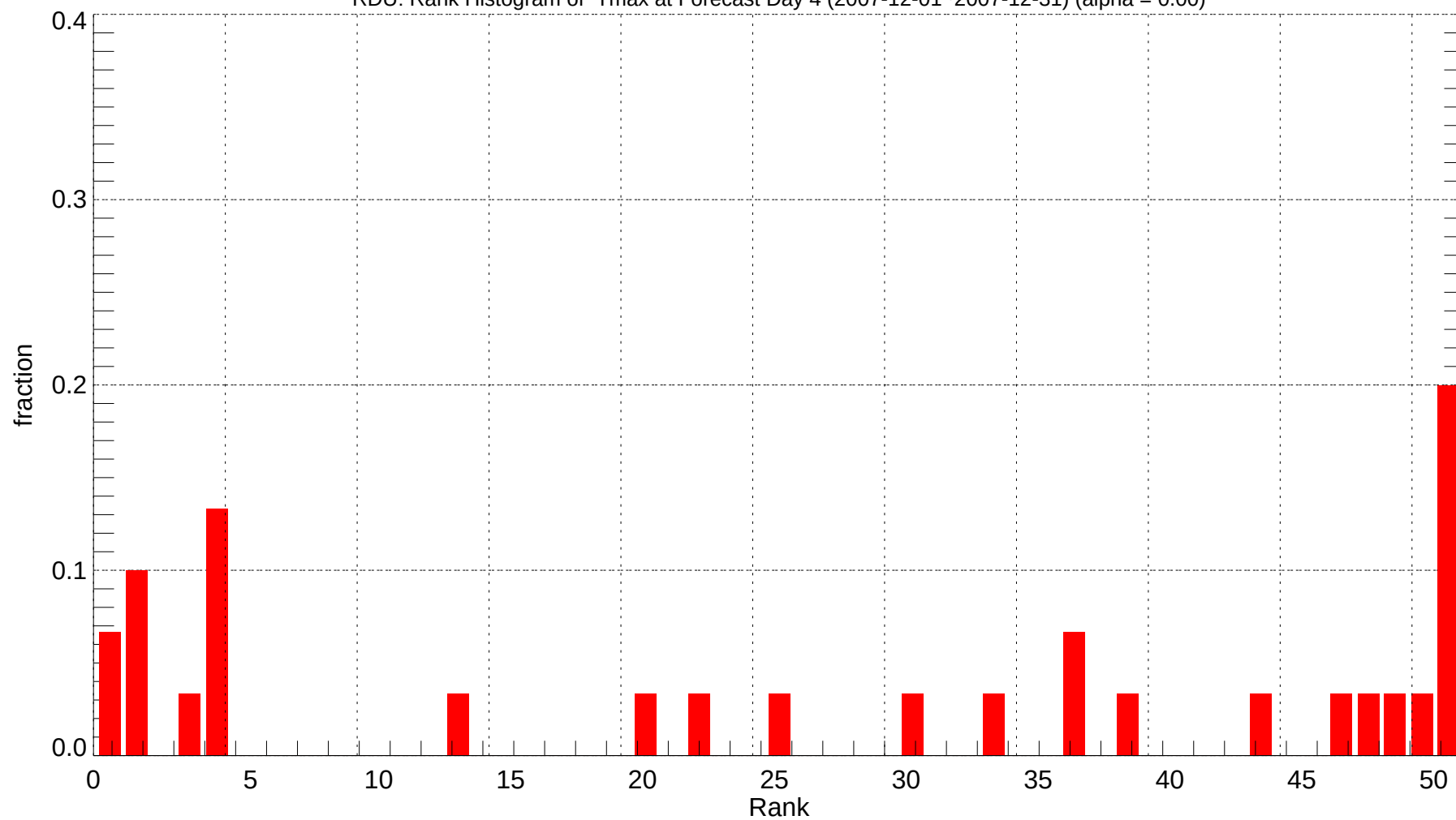
RDU: Rank Histogram of Tmax at Forecast Day 4 (2007-12-01~2007-12-31) (alpha = 0.00)
