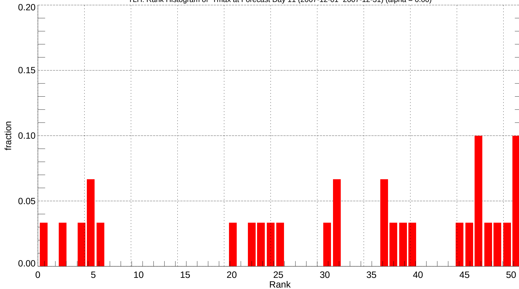
TLH: Rank Histogram of Tmax at Forecast Day 11 (2007-12-01~2007-12-31) (alpha = 0.00)
