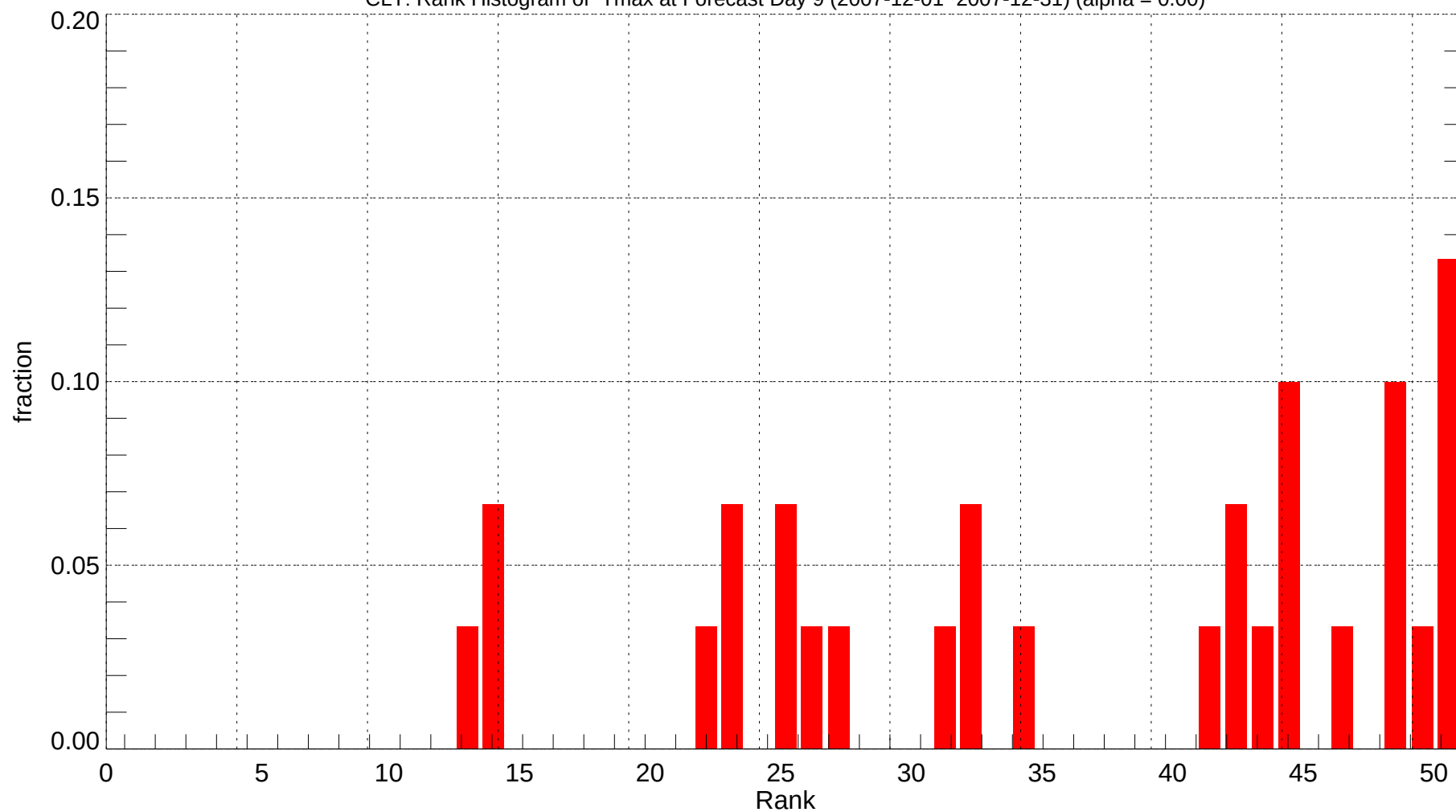
CLT: Rank Histogram of Tmax at Forecast Day 9 (2007-12-01~2007-12-31) (alpha = 0.00)
