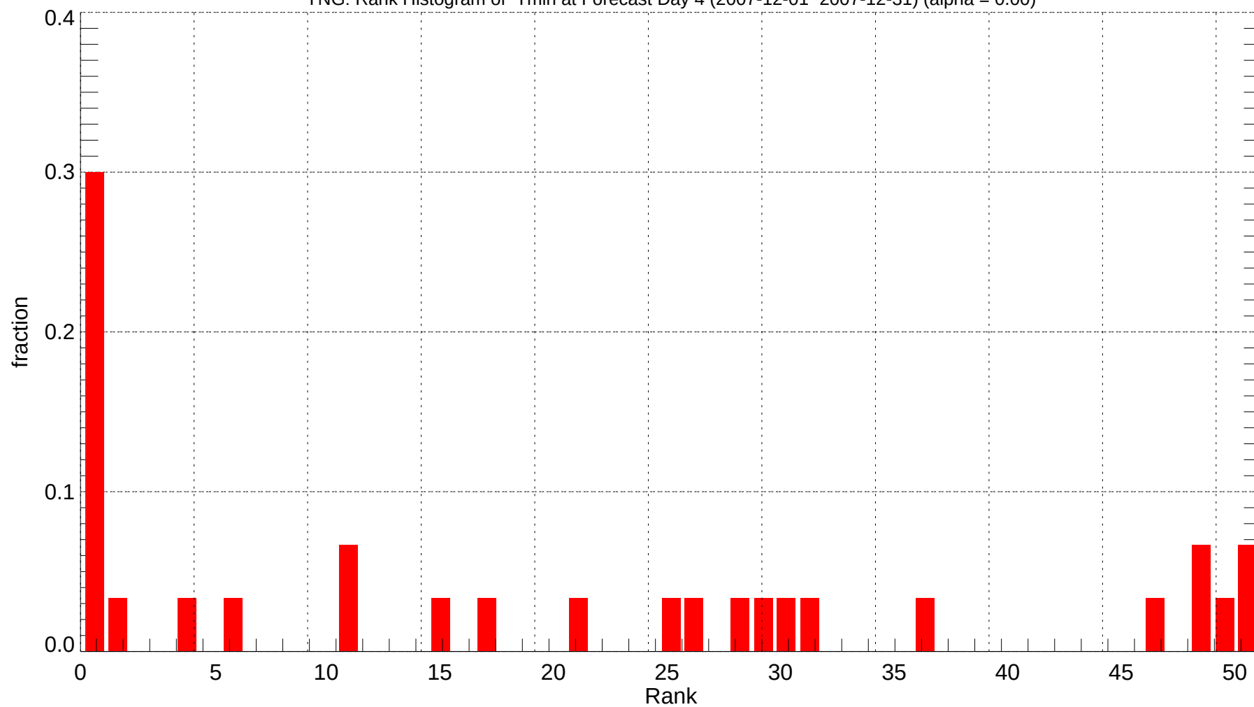
YNG: Rank Histogram of Tmin at Forecast Day 4 (2007-12-01~2007-12-31) (alpha = 0.00)
