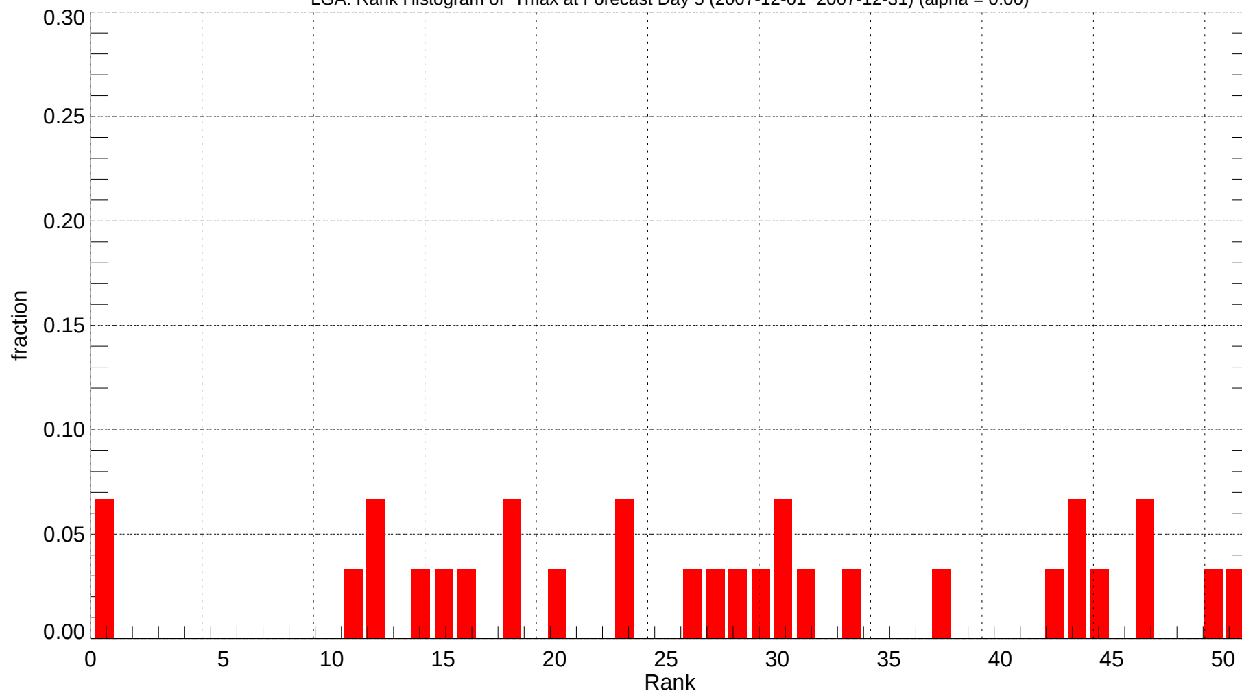
LGA: Rank Histogram of Tmax at Forecast Day 5 (2007-12-01~2007-12-31) (alpha = 0.00)
