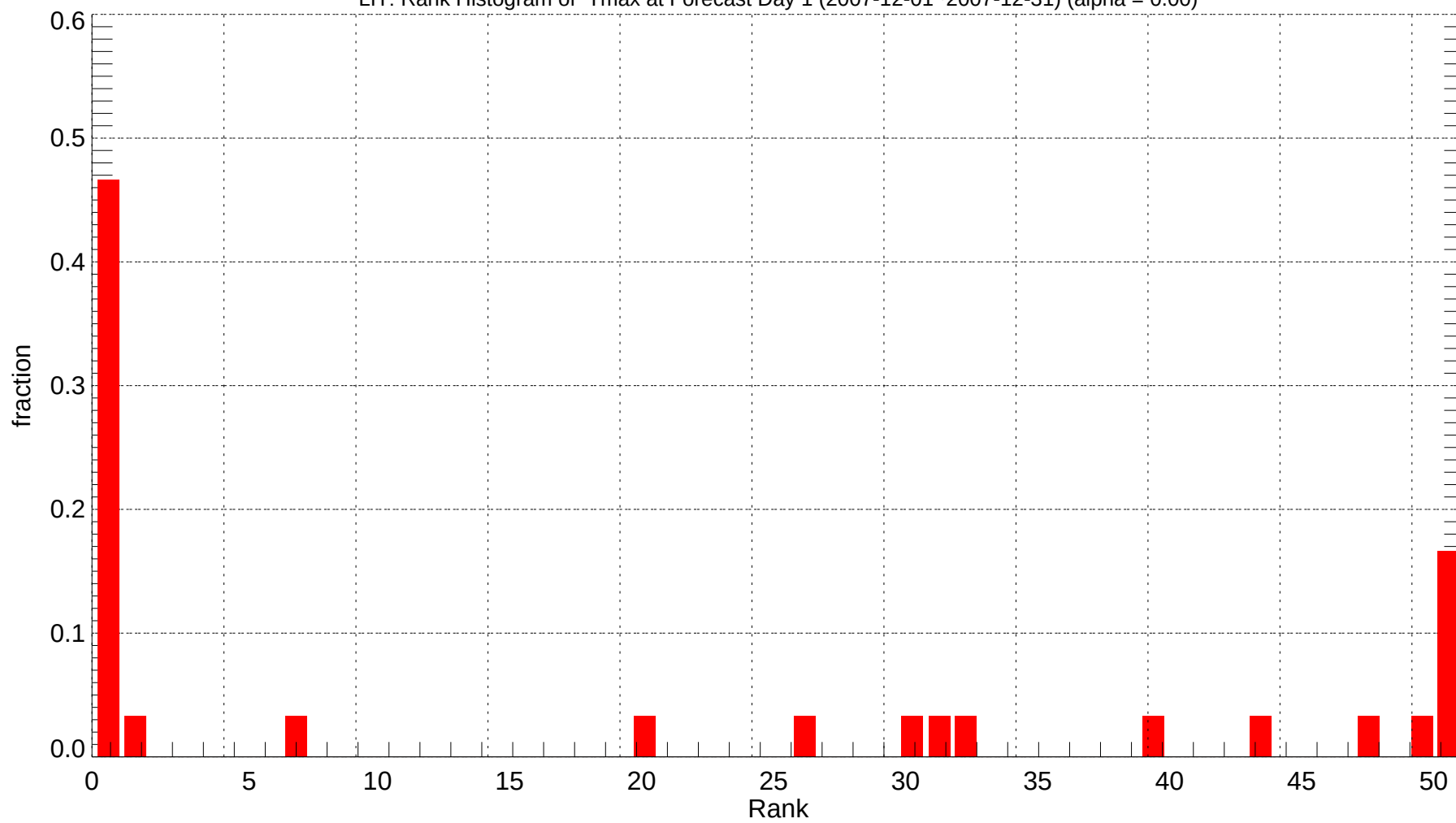
LIT: Rank Histogram of Tmax at Forecast Day 1 (2007-12-01~2007-12-31) (alpha = 0.00)
