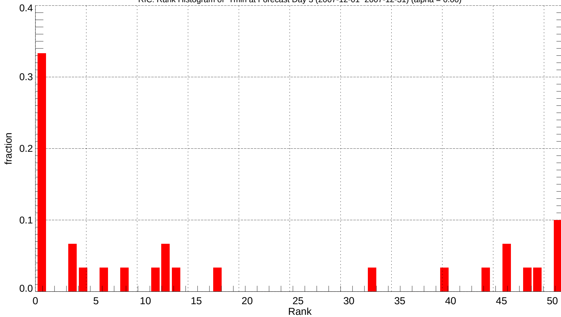
RIC: Rank Histogram of Tmin at Forecast Day 3 (2007-12-01~2007-12-31) (alpha = 0.00)
