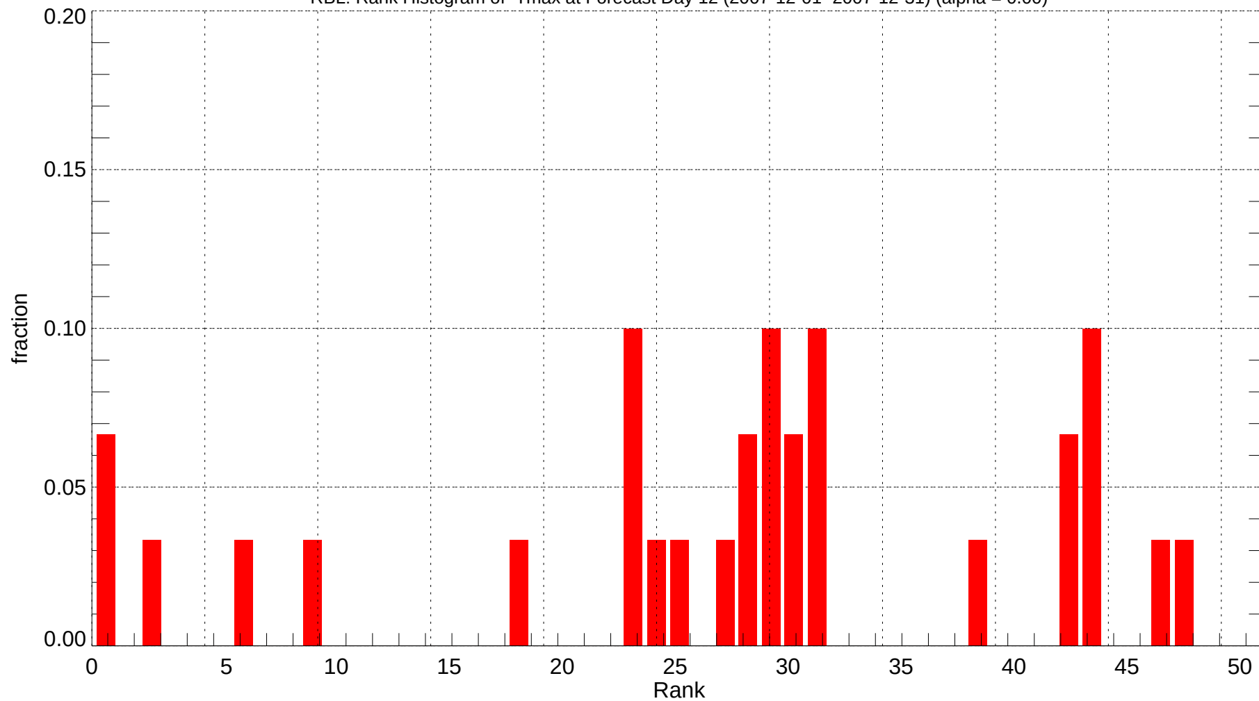
RBL: Rank Histogram of Tmax at Forecast Day 12 (2007-12-01~2007-12-31) (alpha = 0.00)
