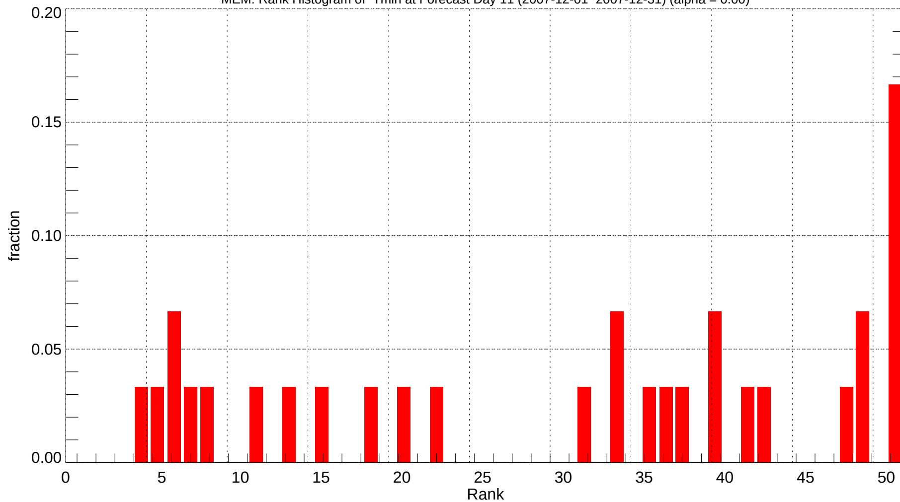
MEM: Rank Histogram of Tmin at Forecast Day 11 (2007-12-01~2007-12-31) (alpha = 0.00)
