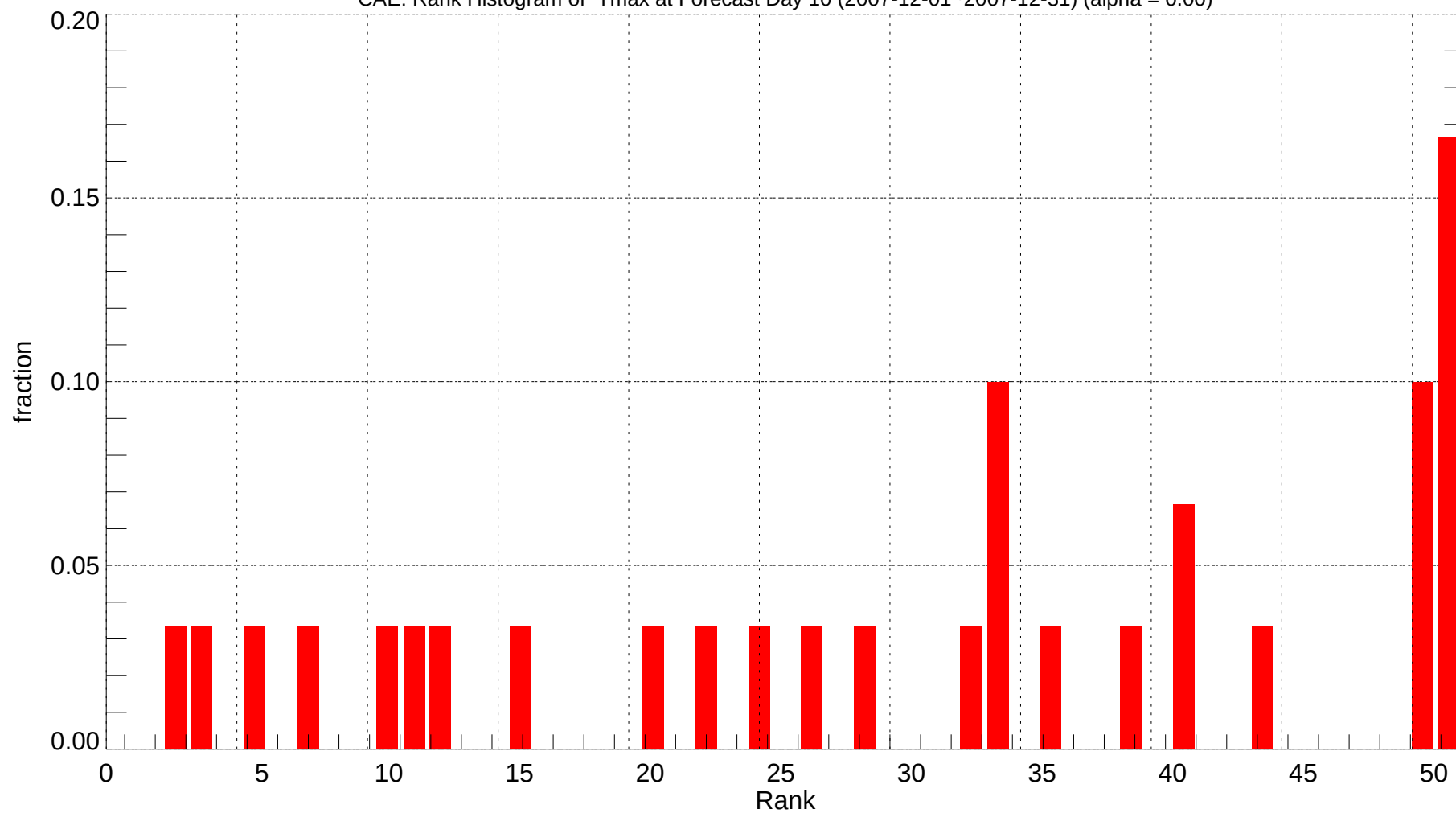
CAE: Rank Histogram of Tmax at Forecast Day 10 (2007-12-01~2007-12-31) (alpha = 0.00)
