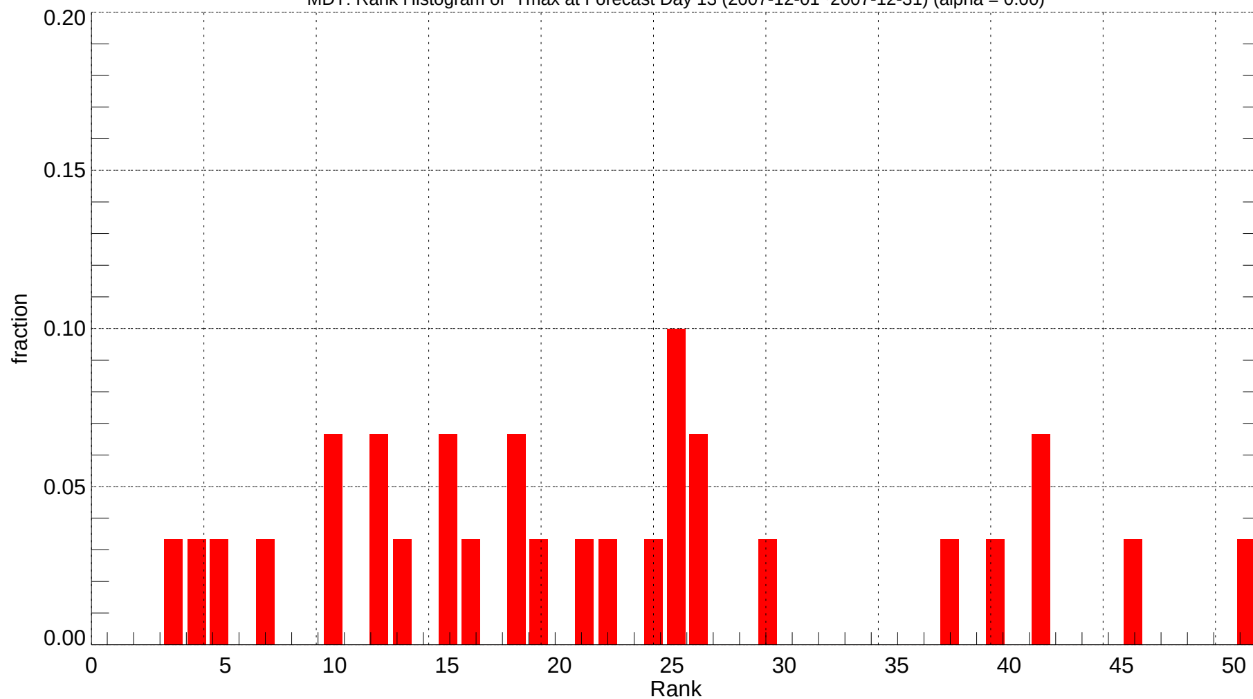
MDT: Rank Histogram of Tmax at Forecast Day 13 (2007-12-01~2007-12-31) (alpha = 0.00)
