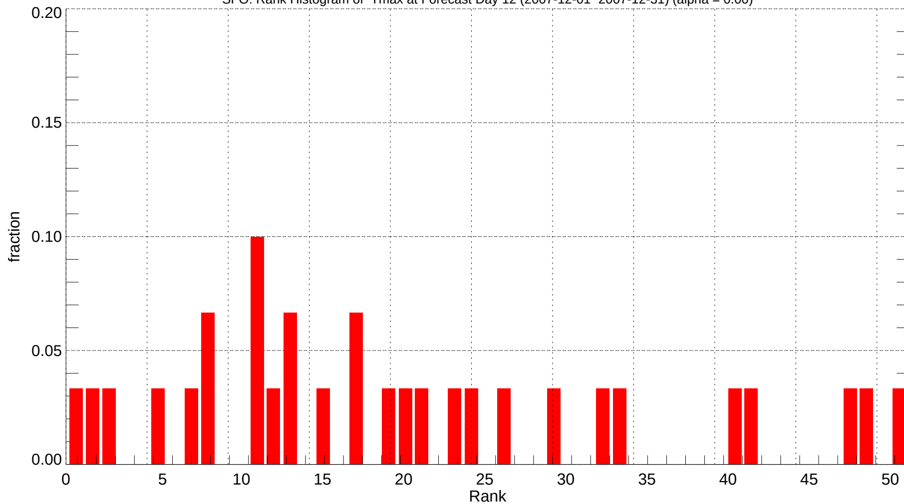
SFO: Rank Histogram of Tmax at Forecast Day 12 (2007-12-01~2007-12-31) (alpha = 0.00)
