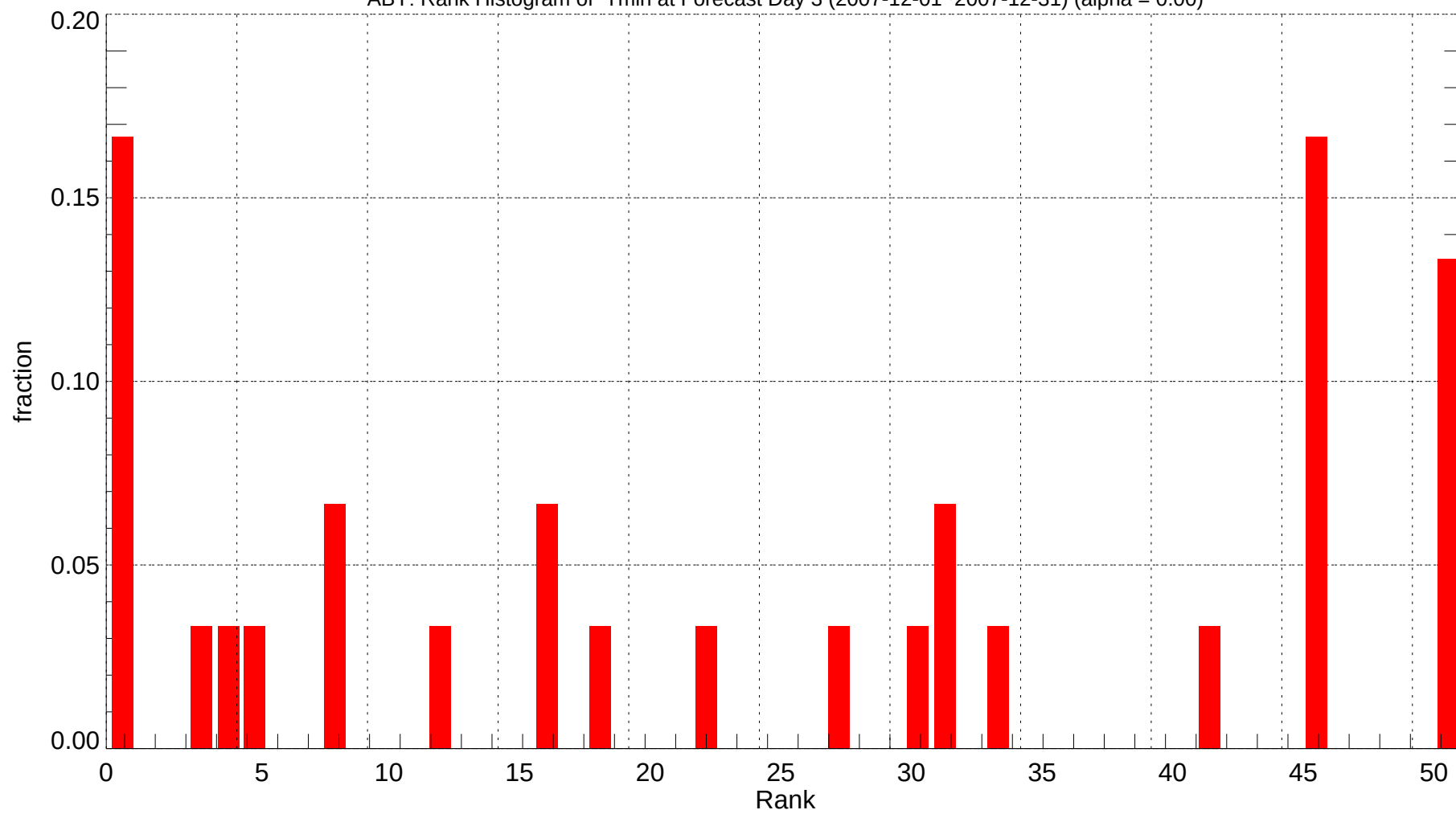
ABY: Rank Histogram of Tmin at Forecast Day 3 (2007-12-01~2007-12-31) (alpha = 0.00)
