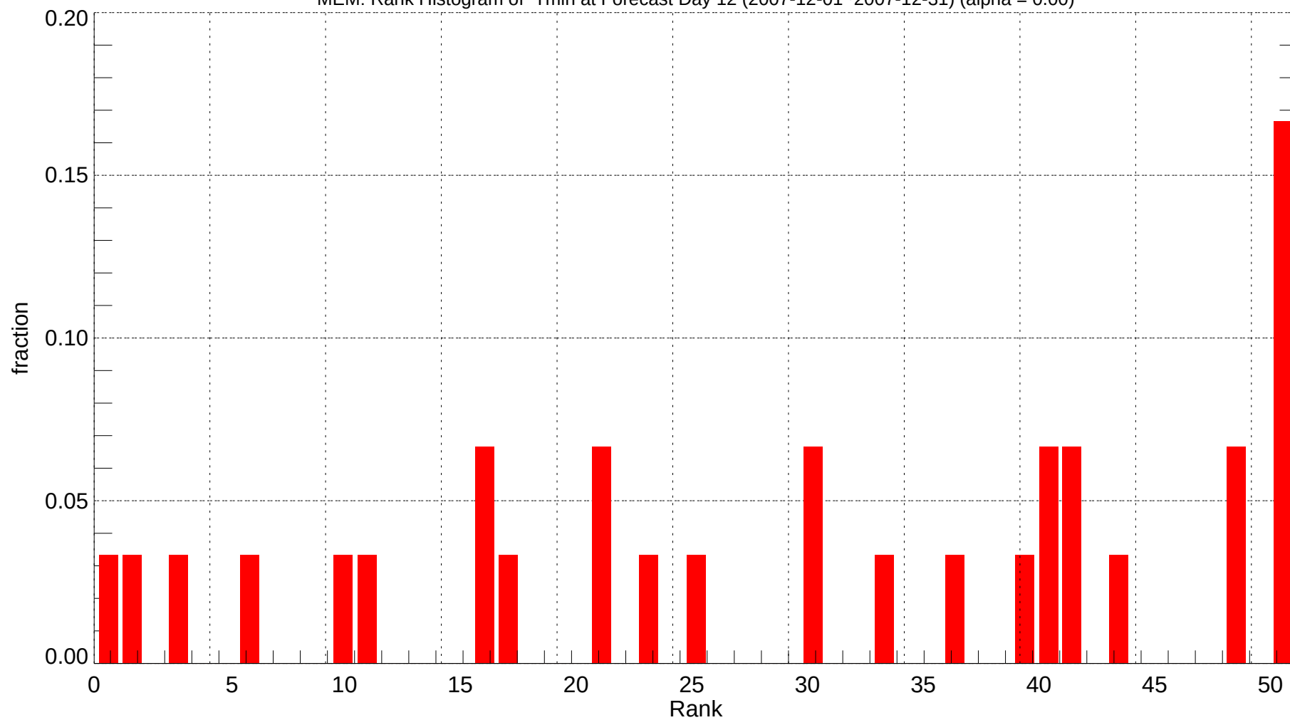
MEM: Rank Histogram of Tmin at Forecast Day 12 (2007-12-01~2007-12-31) (alpha = 0.00)
