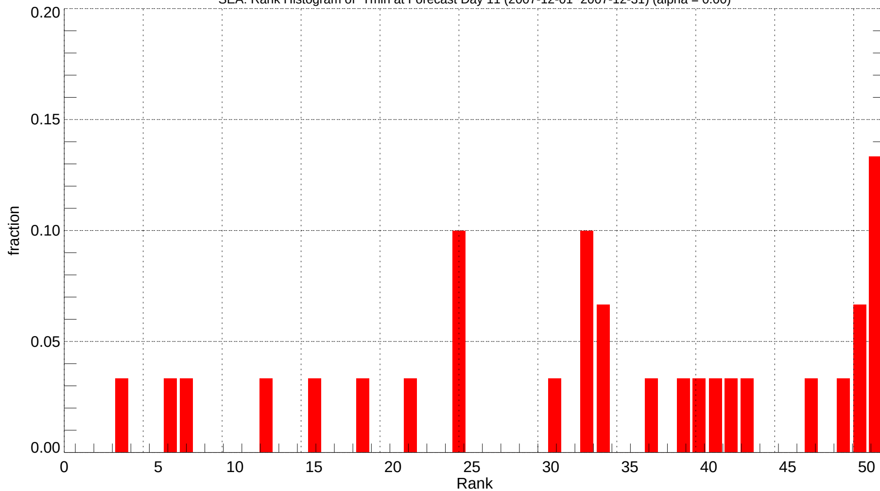
SEA: Rank Histogram of Tmin at Forecast Day 11 (2007-12-01~2007-12-31) (alpha = 0.00)
