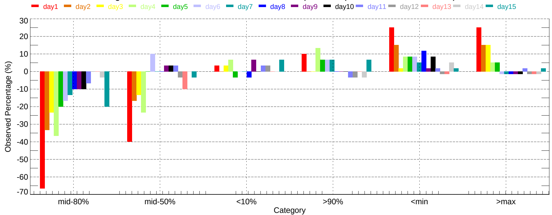
Observed Percentage Deviation of Ensembles - FAR: Min Temperature (2007-12-01~2007-12-31)
