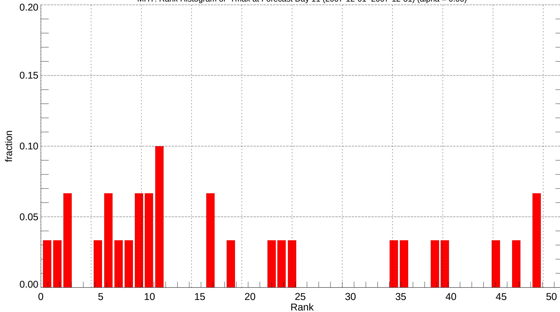
MHT: Rank Histogram of Tmax at Forecast Day 11 (2007-12-01~2007-12-31) (alpha = 0.00)
