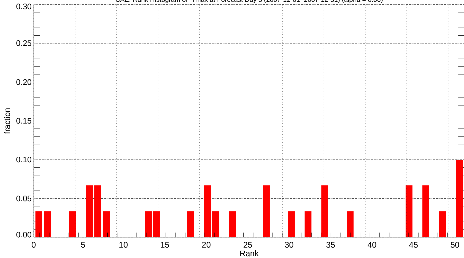
CAE: Rank Histogram of Tmax at Forecast Day 3 (2007-12-01~2007-12-31) (alpha = 0.00)
