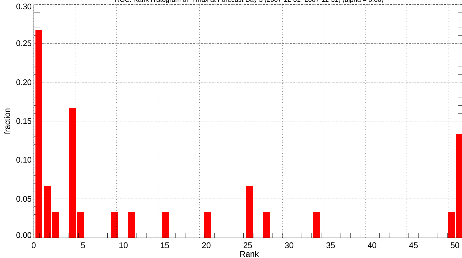
ROC: Rank Histogram of Tmax at Forecast Day 3 (2007-12-01~2007-12-31) (alpha = 0.00)
