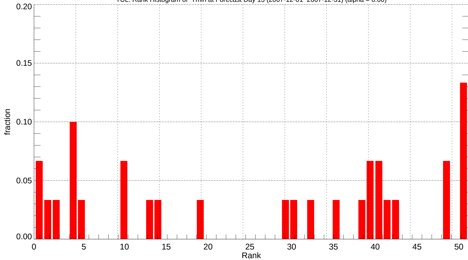
TUL: Rank Histogram of Tmin at Forecast Day 13 (2007-12-01~2007-12-31) (alpha = 0.00)
