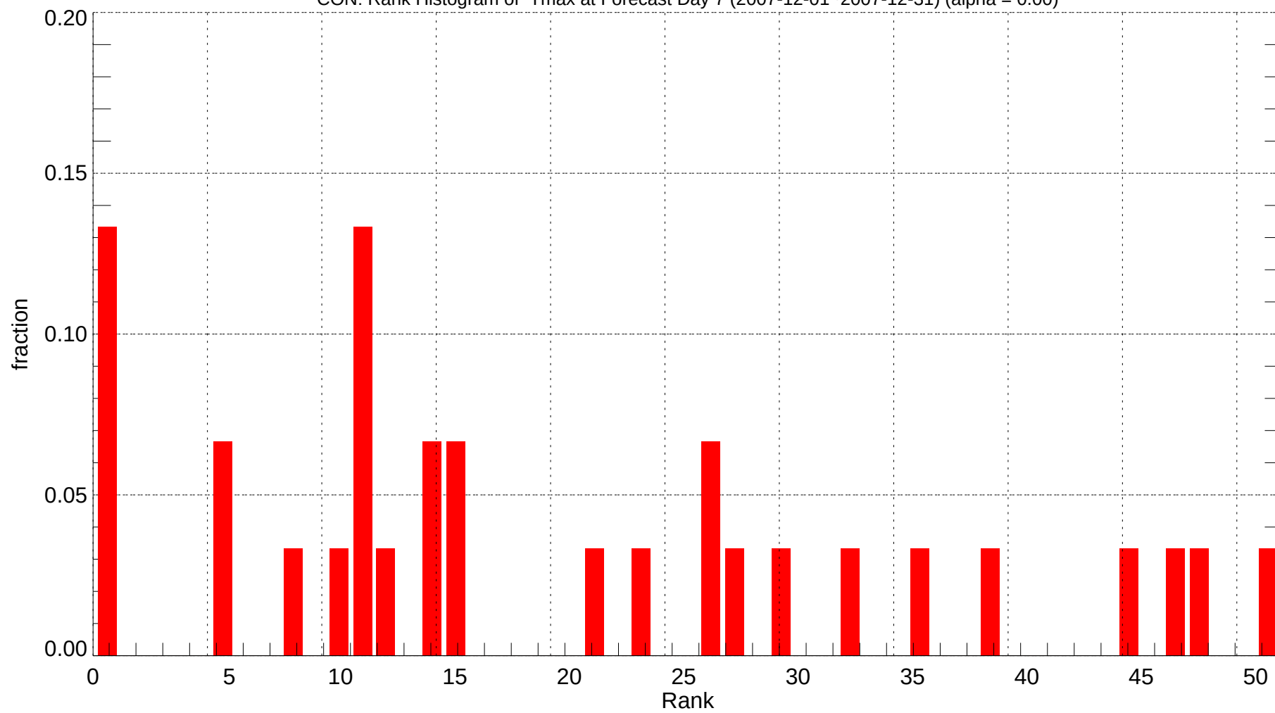
CON: Rank Histogram of Tmax at Forecast Day 7 (2007-12-01~2007-12-31) (alpha = 0.00)
