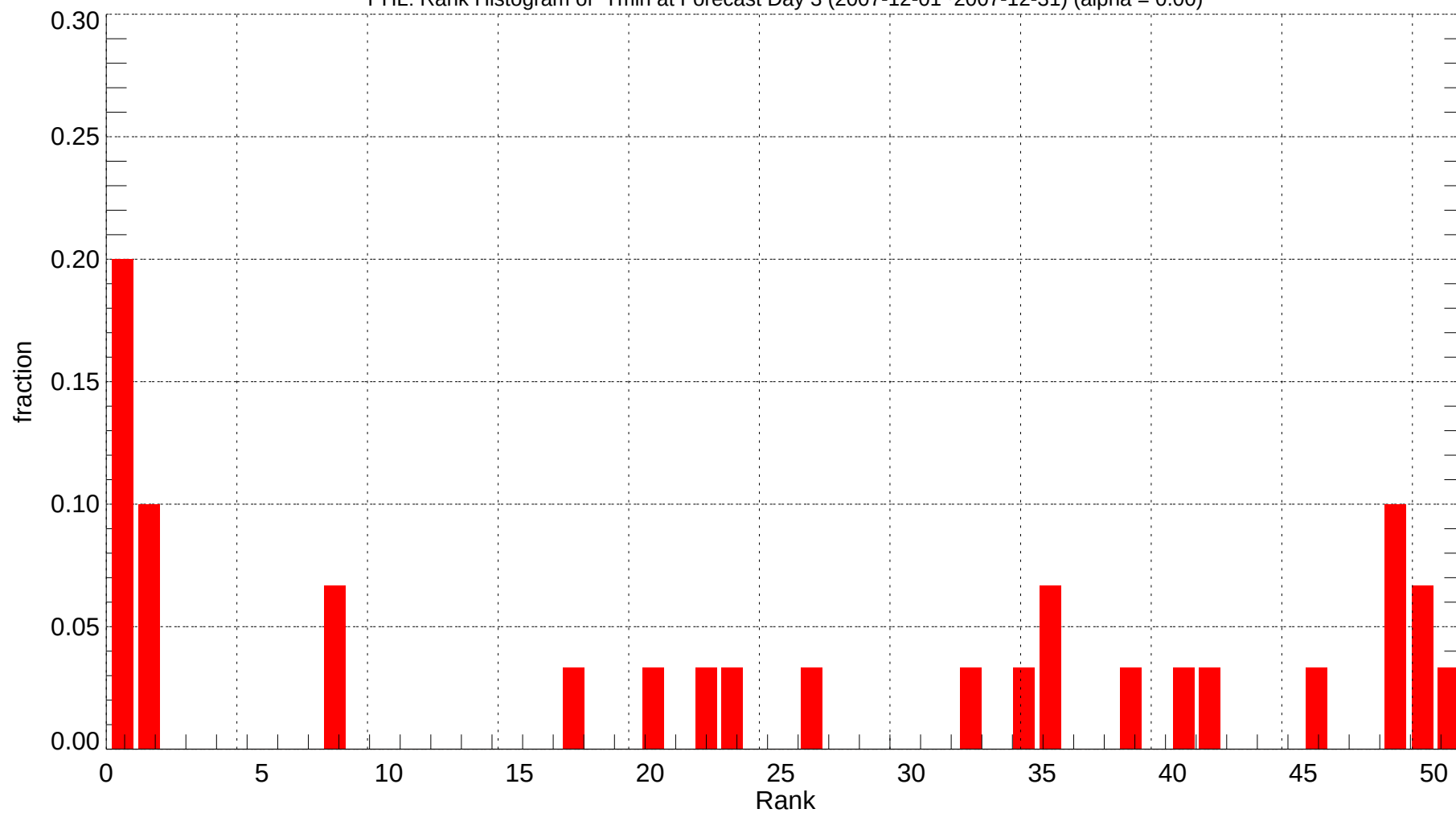
PHL: Rank Histogram of Tmin at Forecast Day 3 (2007-12-01~2007-12-31) (alpha = 0.00)
