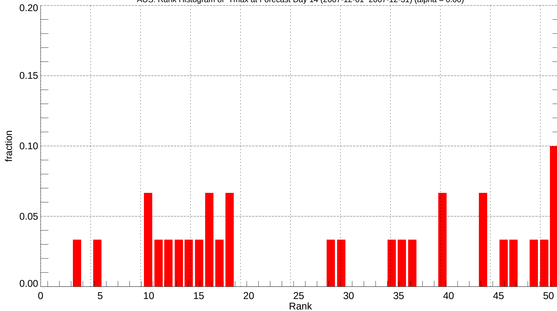
AUS: Rank Histogram of Tmax at Forecast Day 14 (2007-12-01~2007-12-31) (alpha = 0.00)
