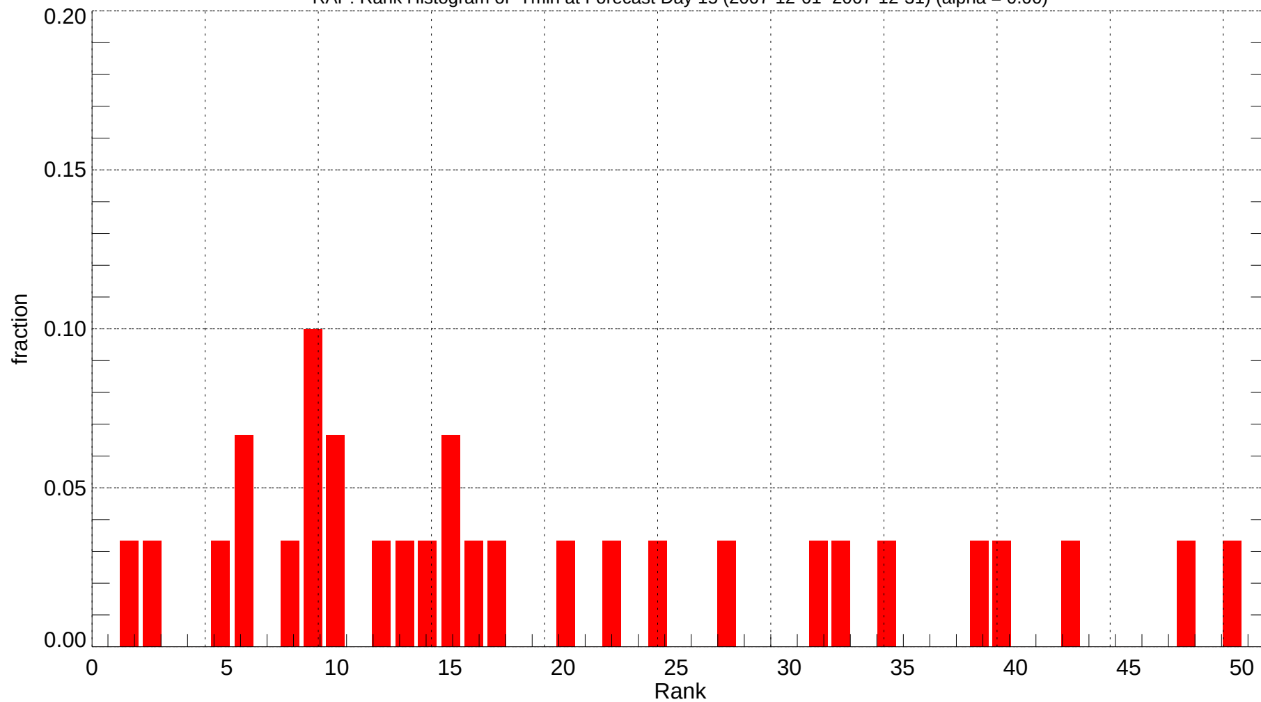
RAP: Rank Histogram of Tmin at Forecast Day 15 (2007-12-01~2007-12-31) (alpha = 0.00)
