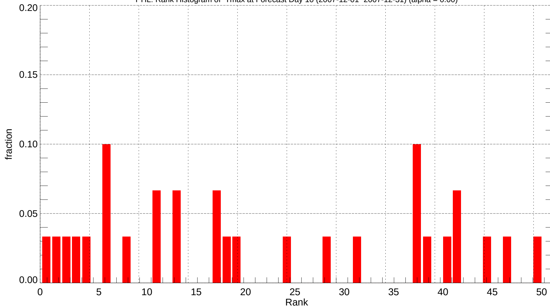
PHL: Rank Histogram of Tmax at Forecast Day 10 (2007-12-01~2007-12-31) (alpha = 0.00)
