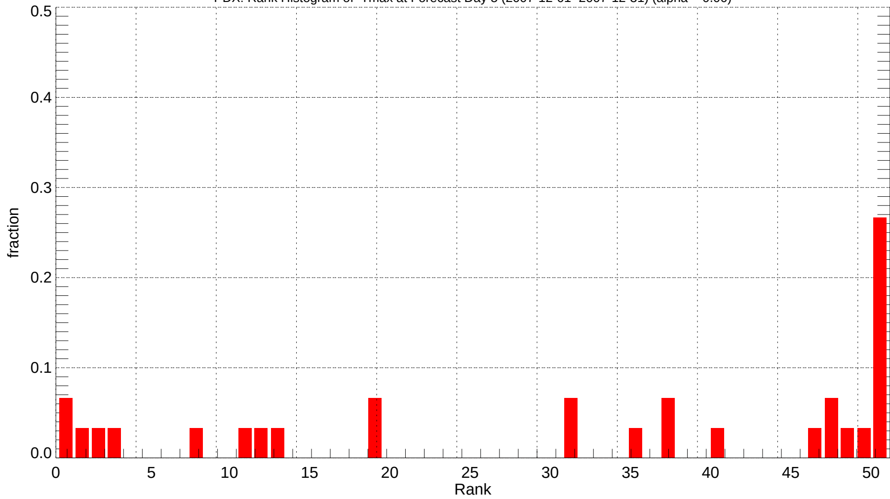
PDX: Rank Histogram of Tmax at Forecast Day 5 (2007-12-01~2007-12-31) (alpha = 0.00)
