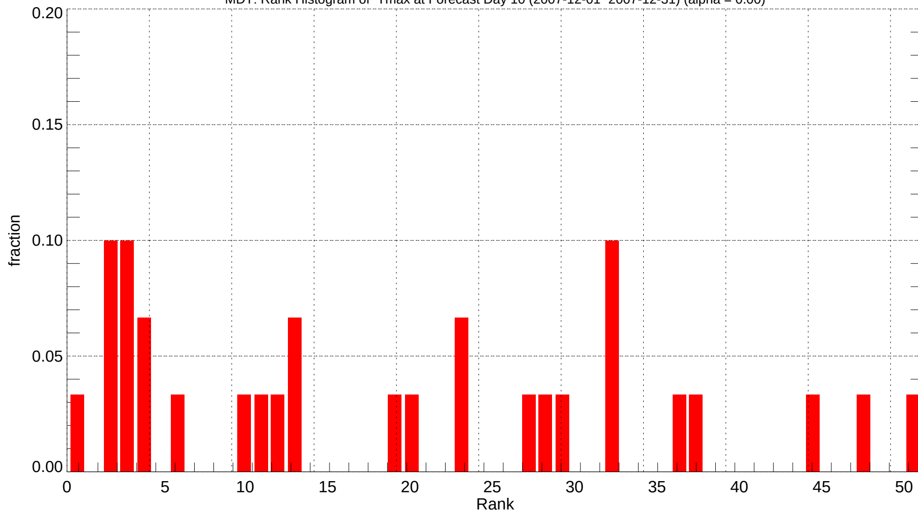
MDT: Rank Histogram of Tmax at Forecast Day 10 (2007-12-01~2007-12-31) (alpha = 0.00)
