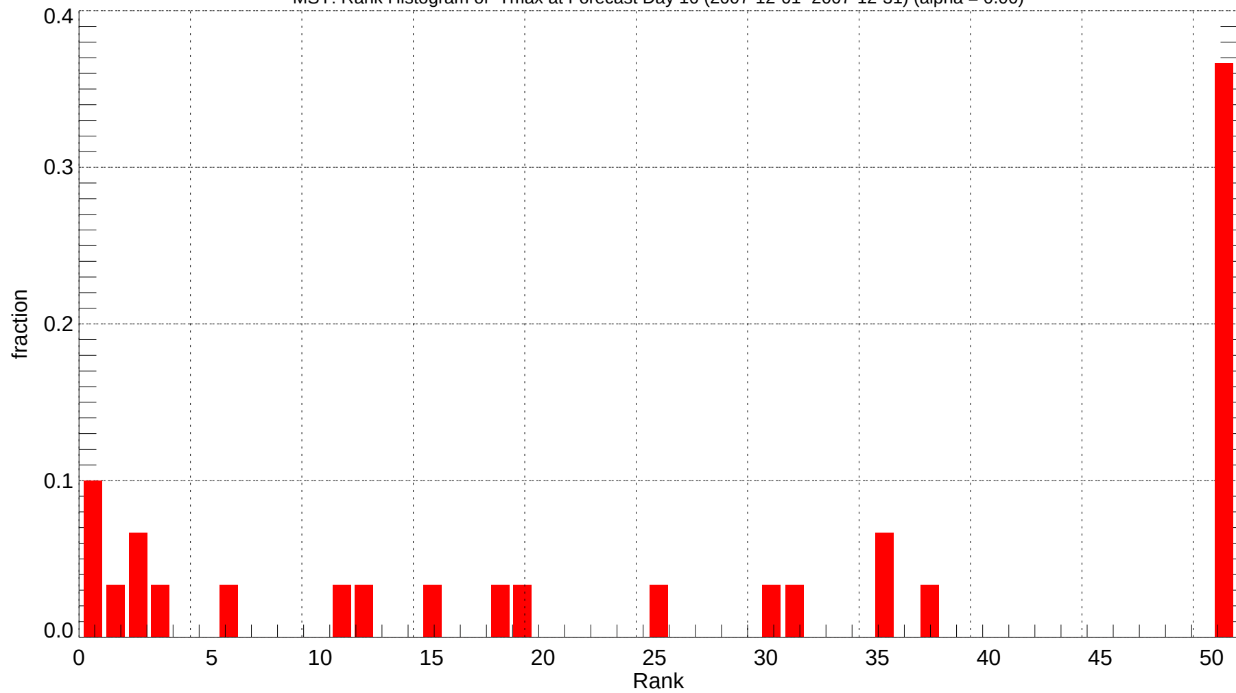
MSY: Rank Histogram of Tmax at Forecast Day 10 (2007-12-01~2007-12-31) (alpha = 0.00)
