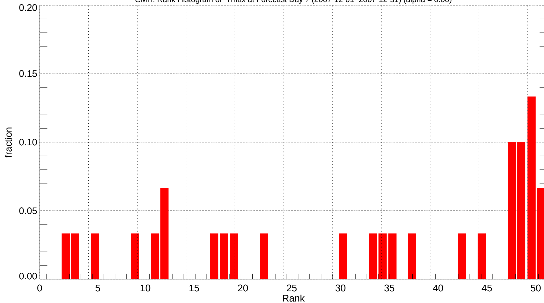
CMH: Rank Histogram of Tmax at Forecast Day 7 (2007-12-01~2007-12-31) (alpha = 0.00)
