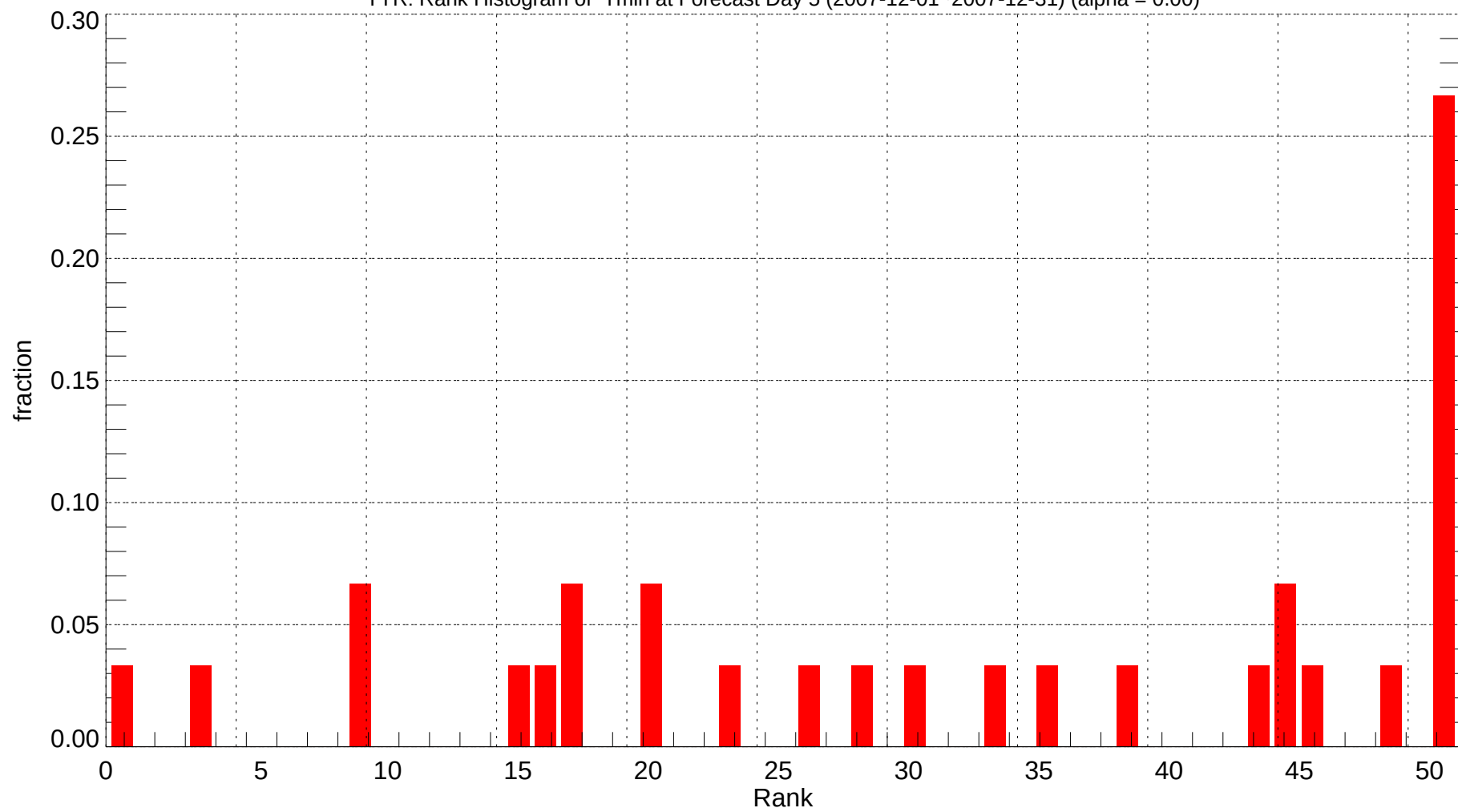
TYR: Rank Histogram of Tmin at Forecast Day 5 (2007-12-01~2007-12-31) (alpha = 0.00)
