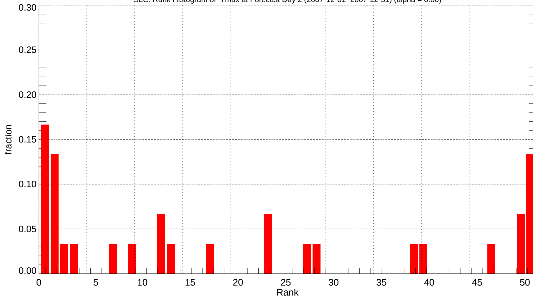
SLC: Rank Histogram of Tmax at Forecast Day 2 (2007-12-01~2007-12-31) (alpha = 0.00)
