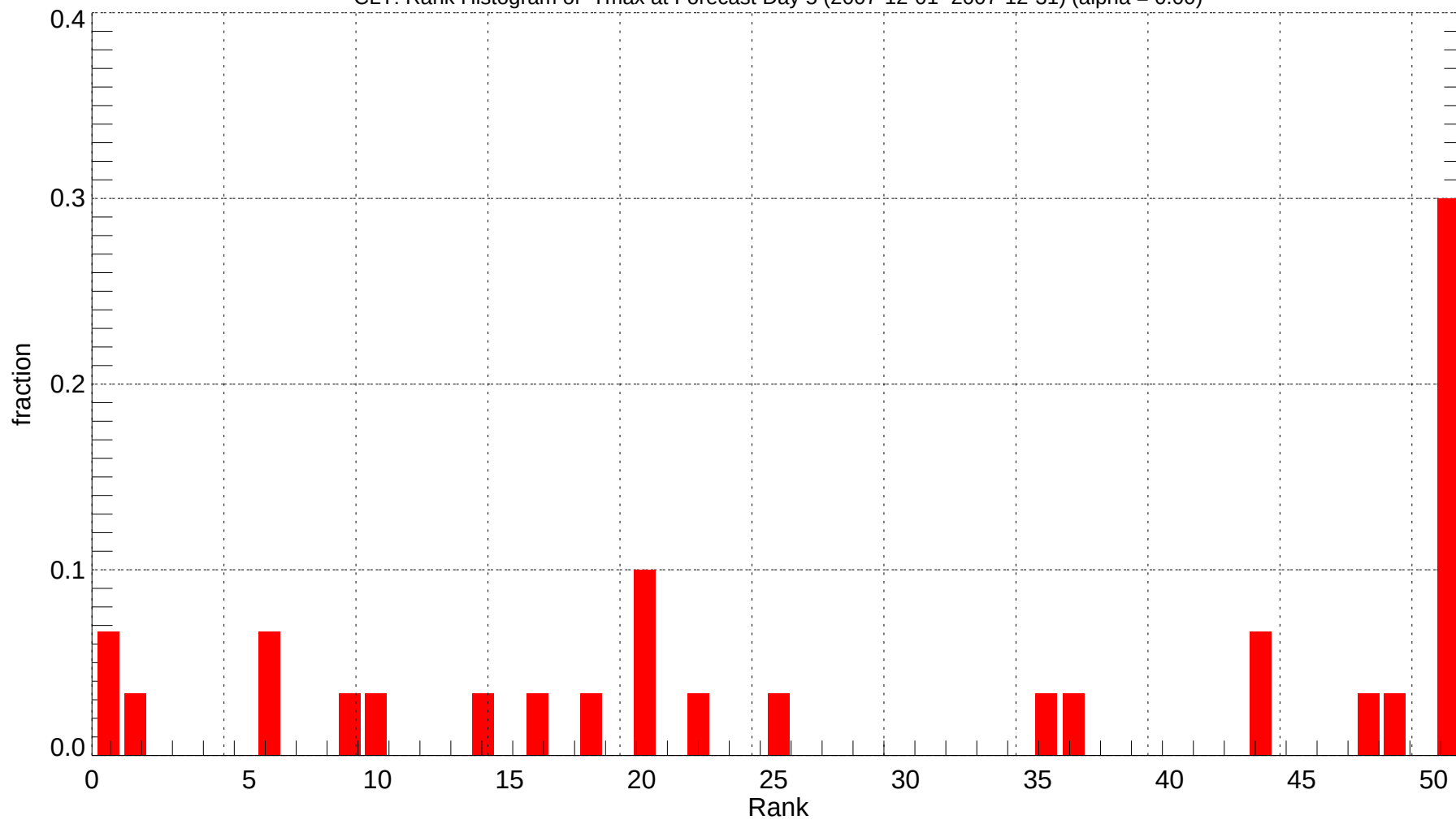
CLT: Rank Histogram of Tmax at Forecast Day 5 (2007-12-01~2007-12-31) (alpha = 0.00)
