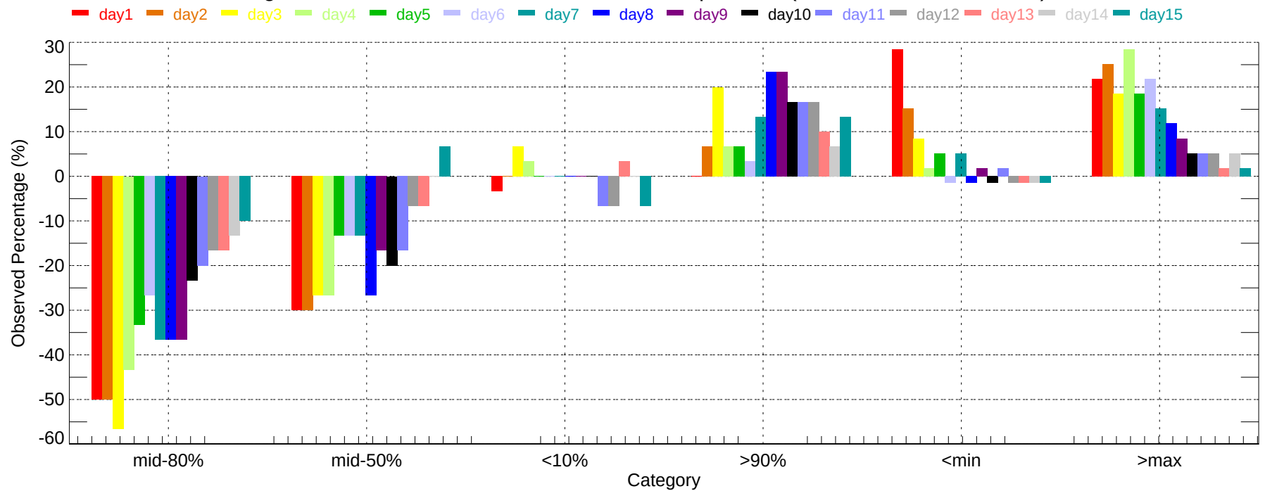
Observed Percentage Deviation of Ensembles - STL: Max Temperature (2007-12-01~2007-12-31)
