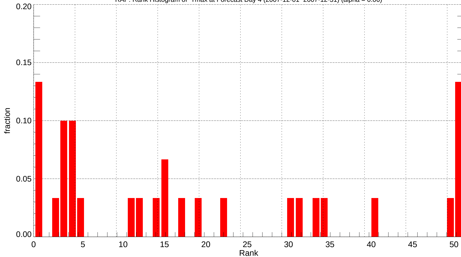
RAP: Rank Histogram of Tmax at Forecast Day 4 (2007-12-01~2007-12-31) (alpha = 0.00)
