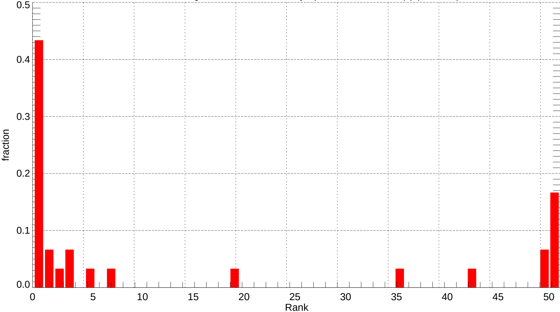
CLE: Rank Histogram of Tmin at Forecast Day 1 (2007-12-01~2007-12-31) (alpha = 0.00)
