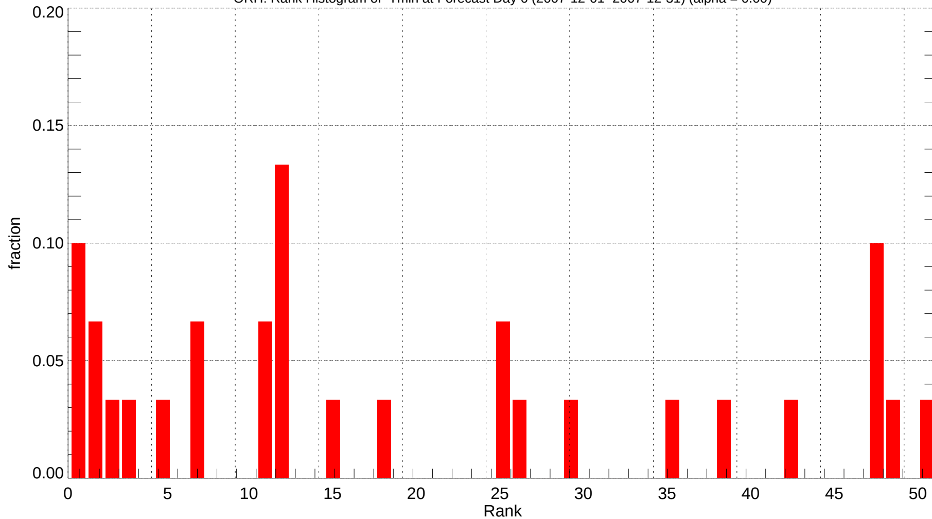
ORH: Rank Histogram of Tmin at Forecast Day 6 (2007-12-01~2007-12-31) (alpha = 0.00)
