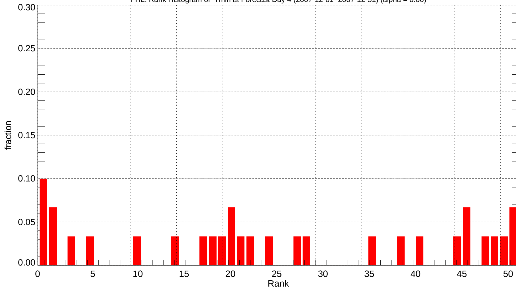
PHL: Rank Histogram of Tmin at Forecast Day 4 (2007-12-01~2007-12-31) (alpha = 0.00)
