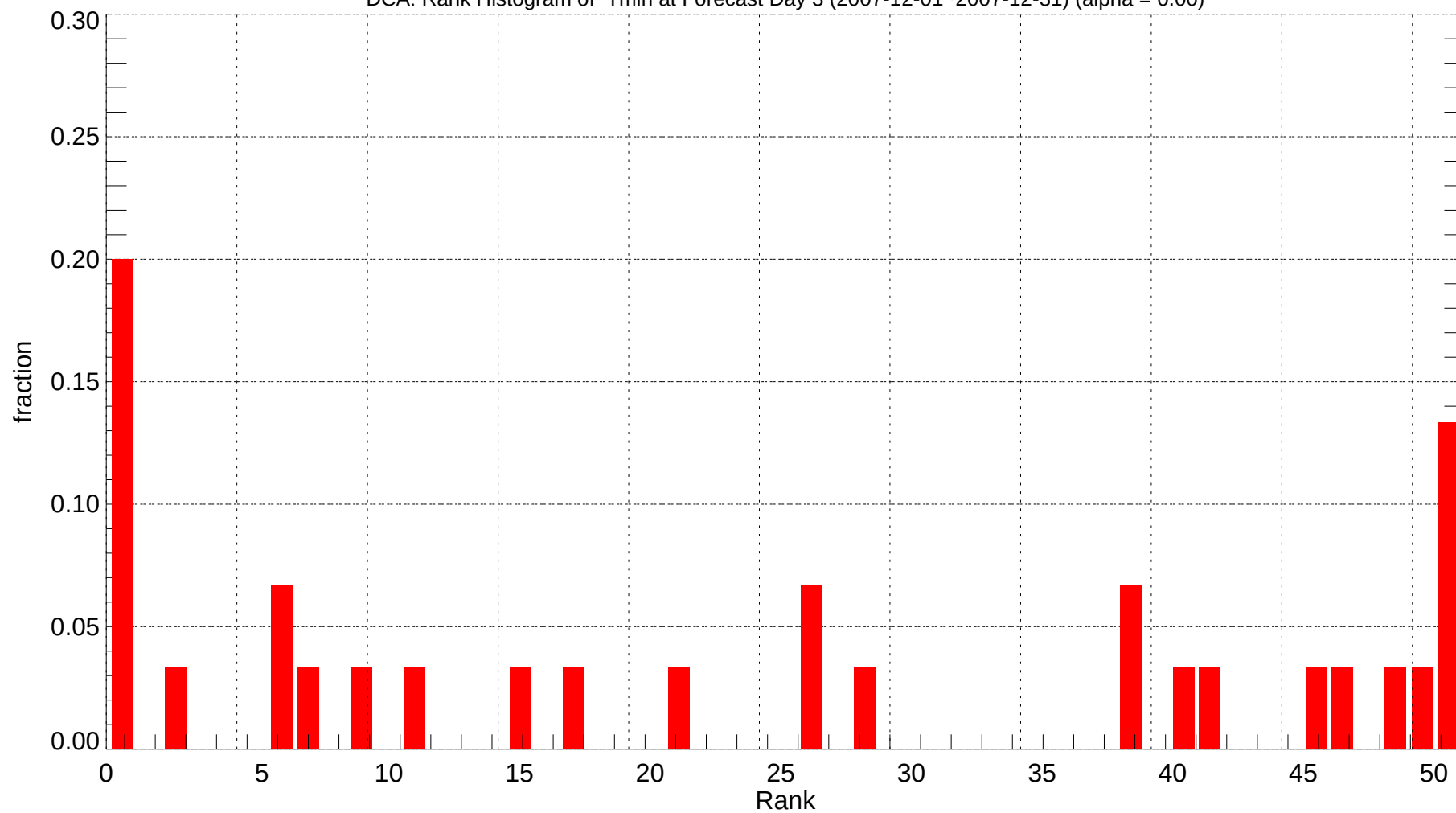
DCA: Rank Histogram of Tmin at Forecast Day 3 (2007-12-01~2007-12-31) (alpha = 0.00)
