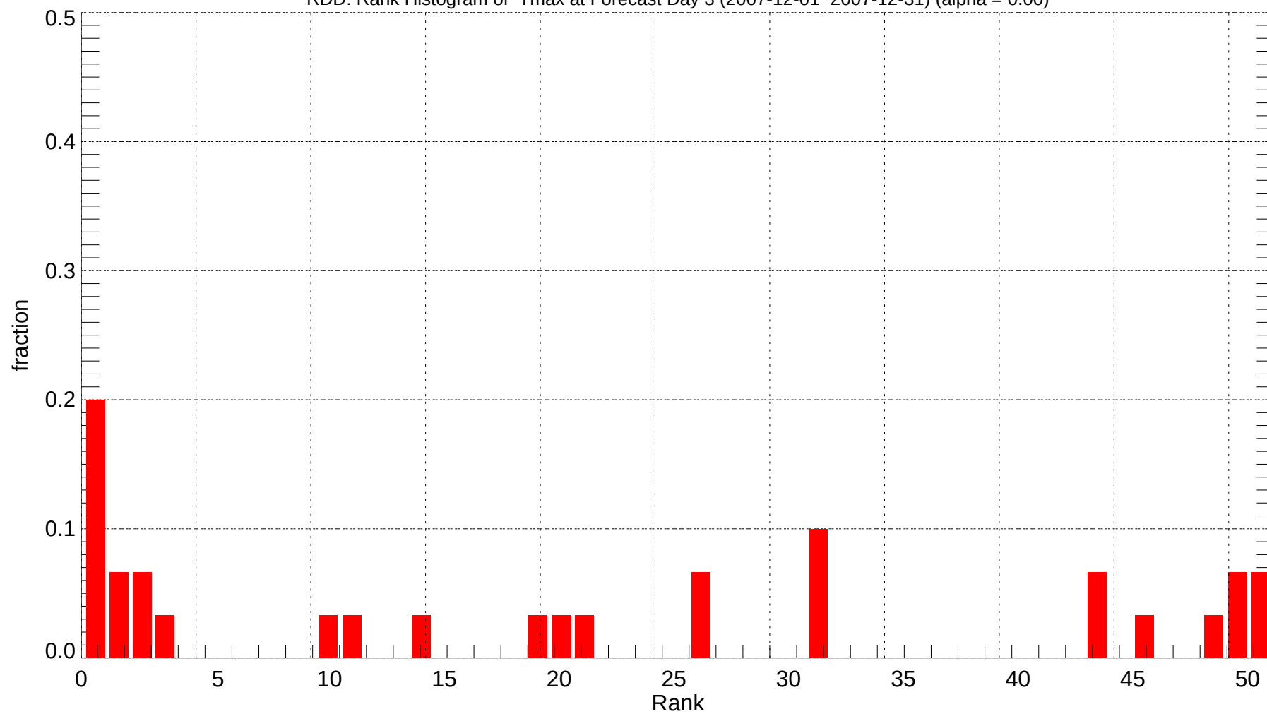
RDD: Rank Histogram of Tmax at Forecast Day 3 (2007-12-01~2007-12-31) (alpha = 0.00)
