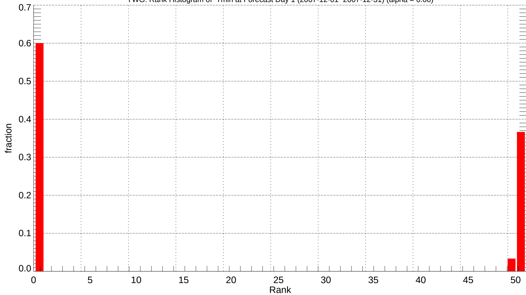
YWG: Rank Histogram of Tmin at Forecast Day 1 (2007-12-01~2007-12-31) (alpha = 0.00)
