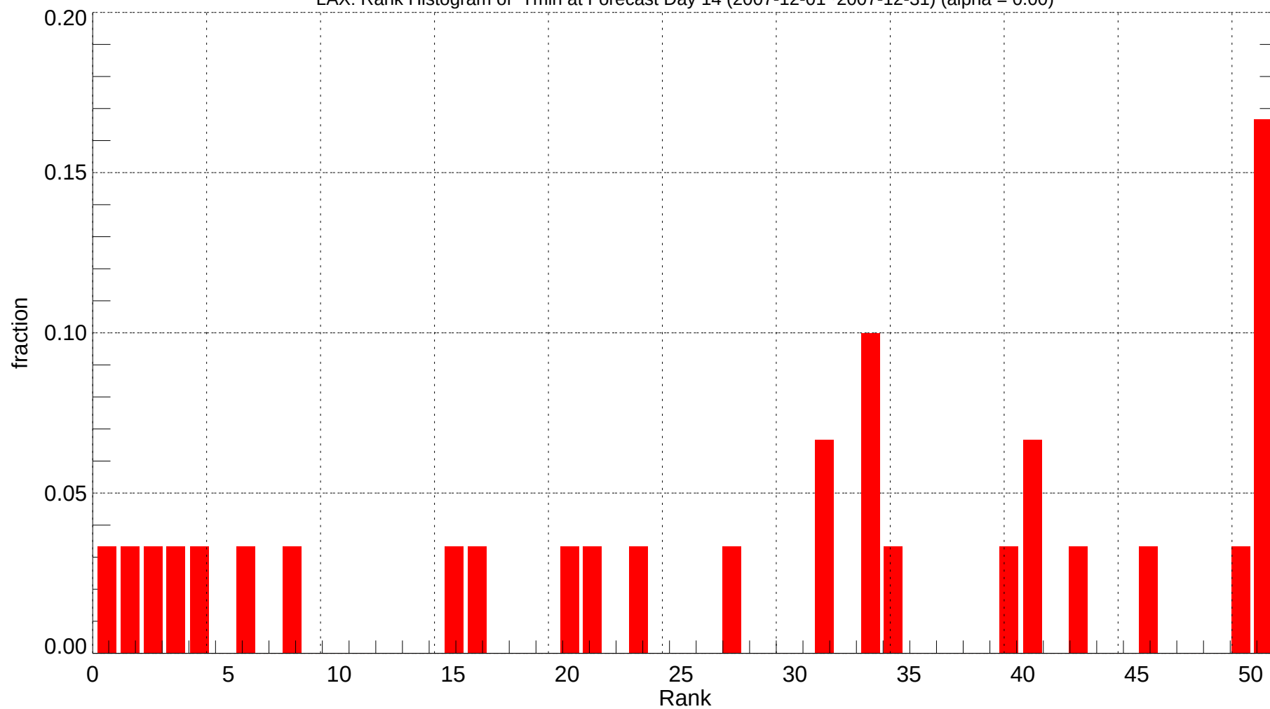
LAX: Rank Histogram of Tmin at Forecast Day 14 (2007-12-01~2007-12-31) (alpha = 0.00)
