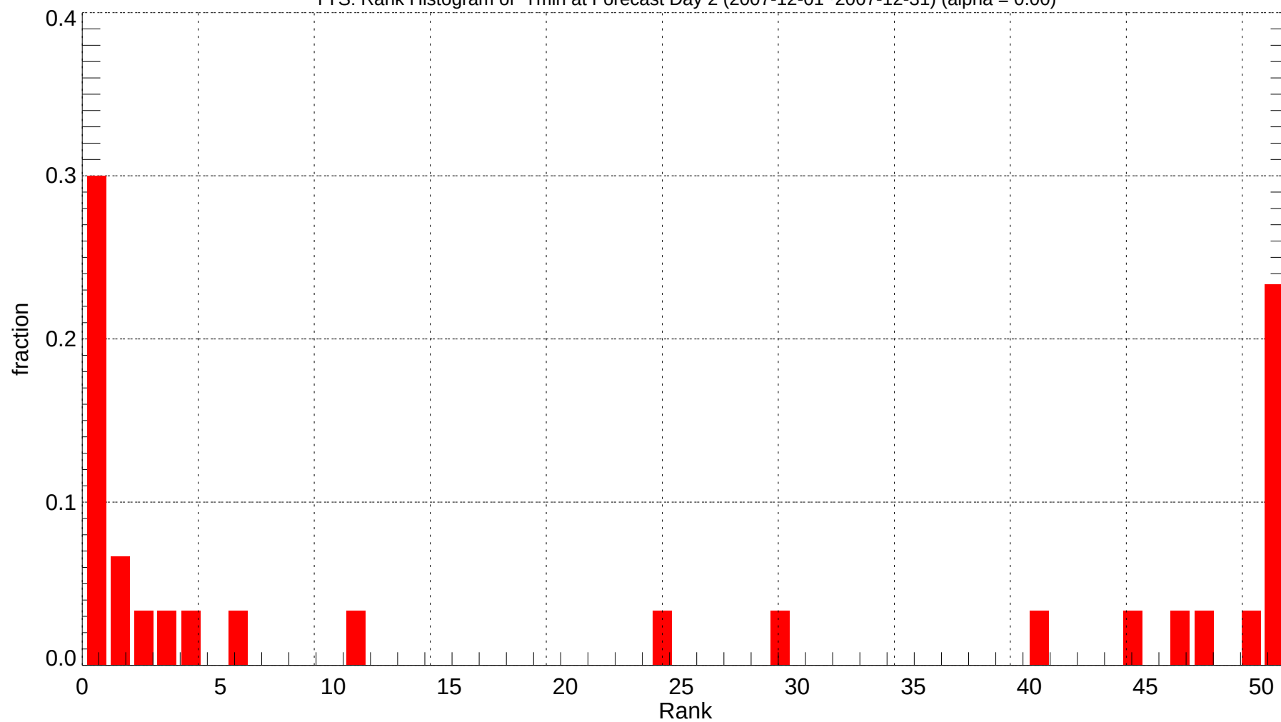
TYS: Rank Histogram of Tmin at Forecast Day 2 (2007-12-01~2007-12-31) (alpha = 0.00)
