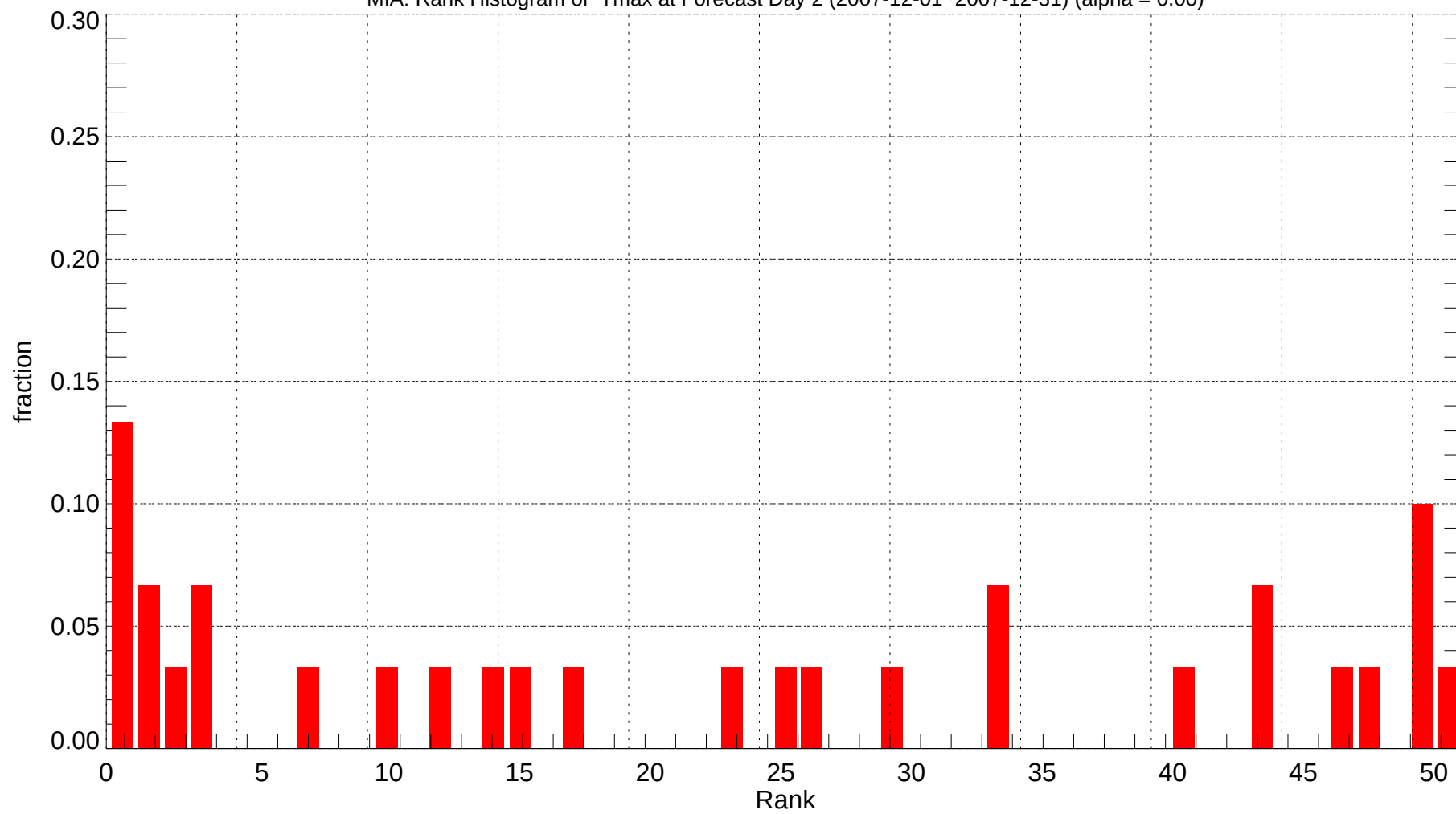
MIA: Rank Histogram of Tmax at Forecast Day 2 (2007-12-01~2007-12-31) (alpha = 0.00)
