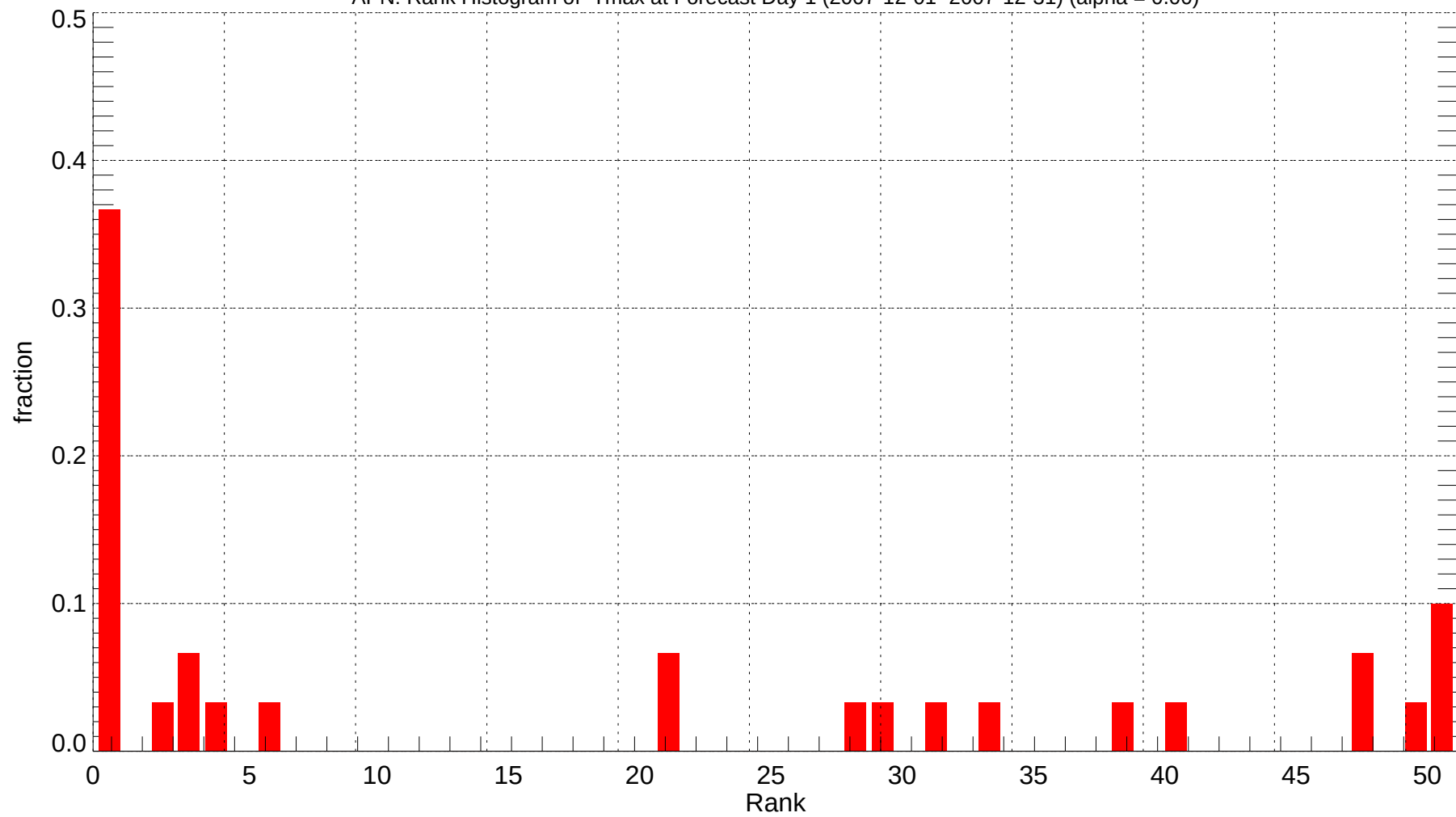
APN: Rank Histogram of Tmax at Forecast Day 1 (2007-12-01~2007-12-31) (alpha = 0.00)
