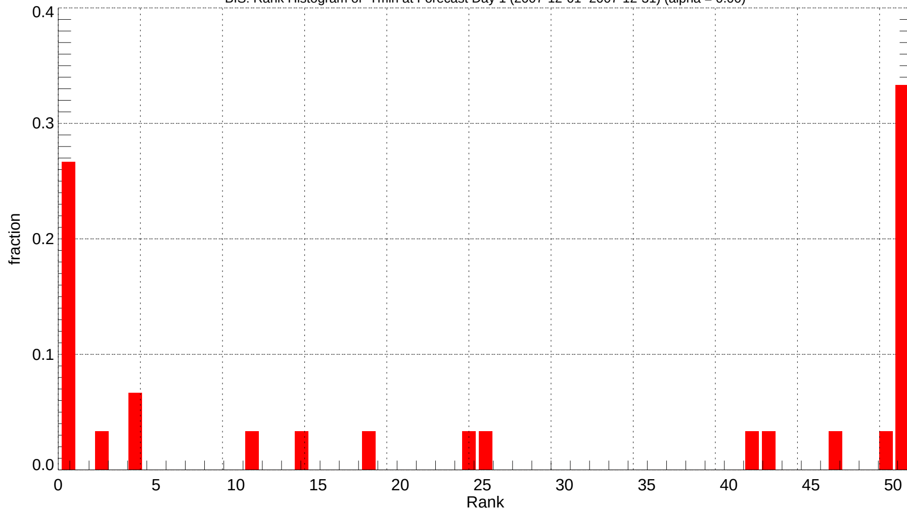
BIS: Rank Histogram of Tmin at Forecast Day 1 (2007-12-01~2007-12-31) (alpha = 0.00)
