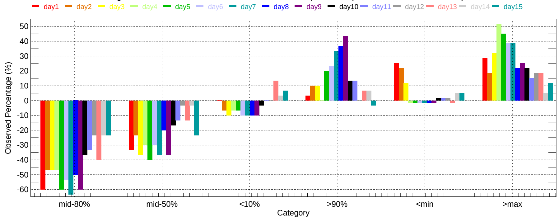
Observed Percentage Deviation of Ensembles - LGB: Max Temperature (2007-12-01~2007-12-31)
