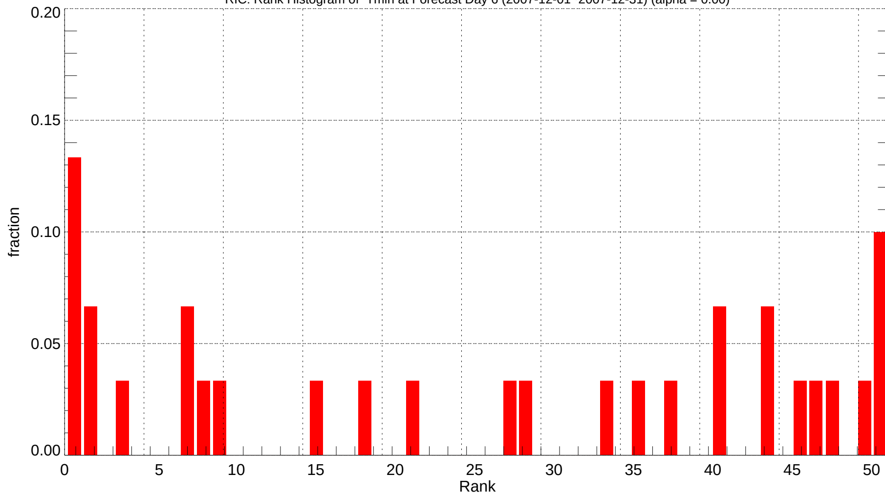
RIC: Rank Histogram of Tmin at Forecast Day 6 (2007-12-01~2007-12-31) (alpha = 0.00)
