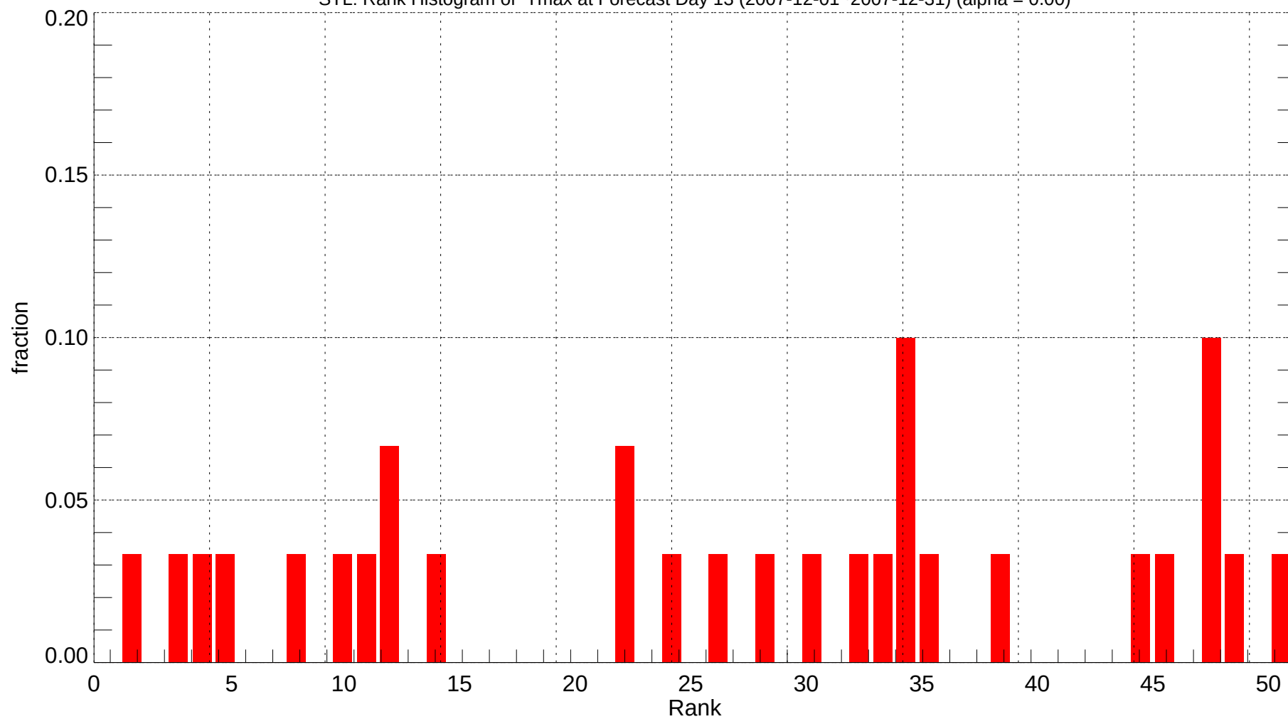
STL: Rank Histogram of Tmax at Forecast Day 13 (2007-12-01~2007-12-31) (alpha = 0.00)
