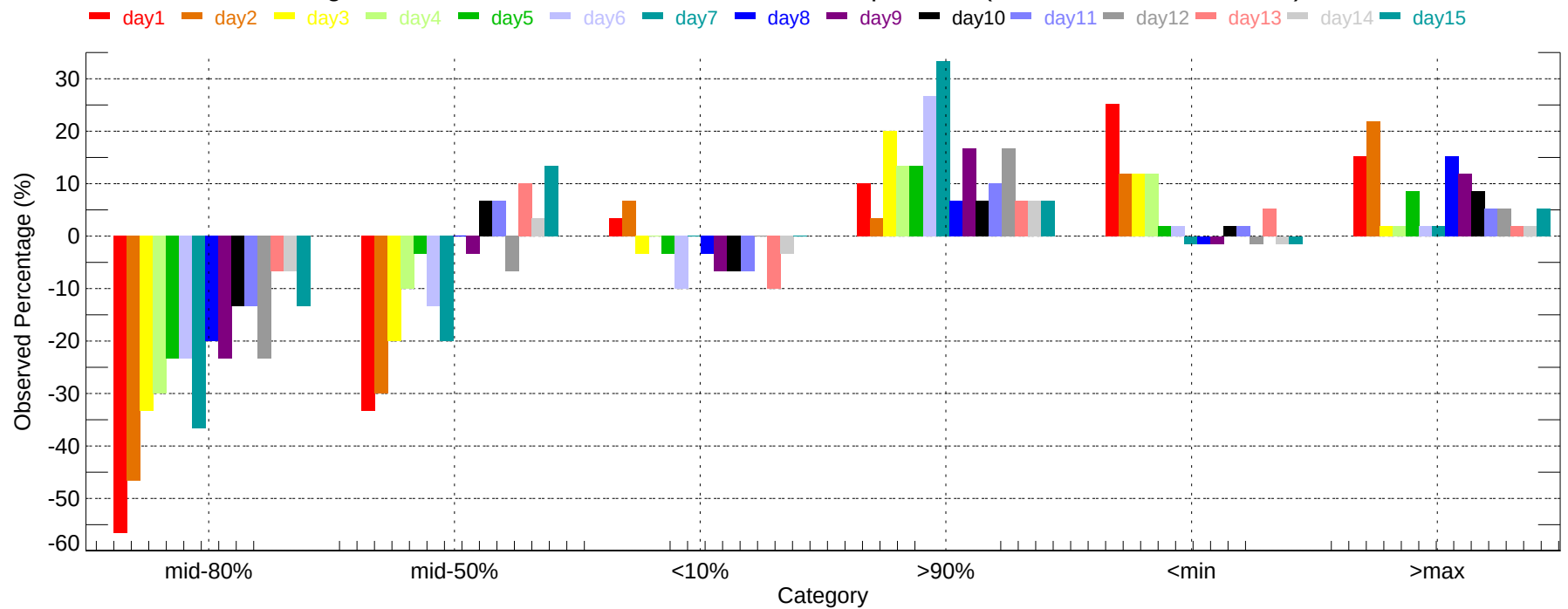
Observed Percentage Deviation of Ensembles - CMH: Min Temperature (2007-12-01~2007-12-31)
