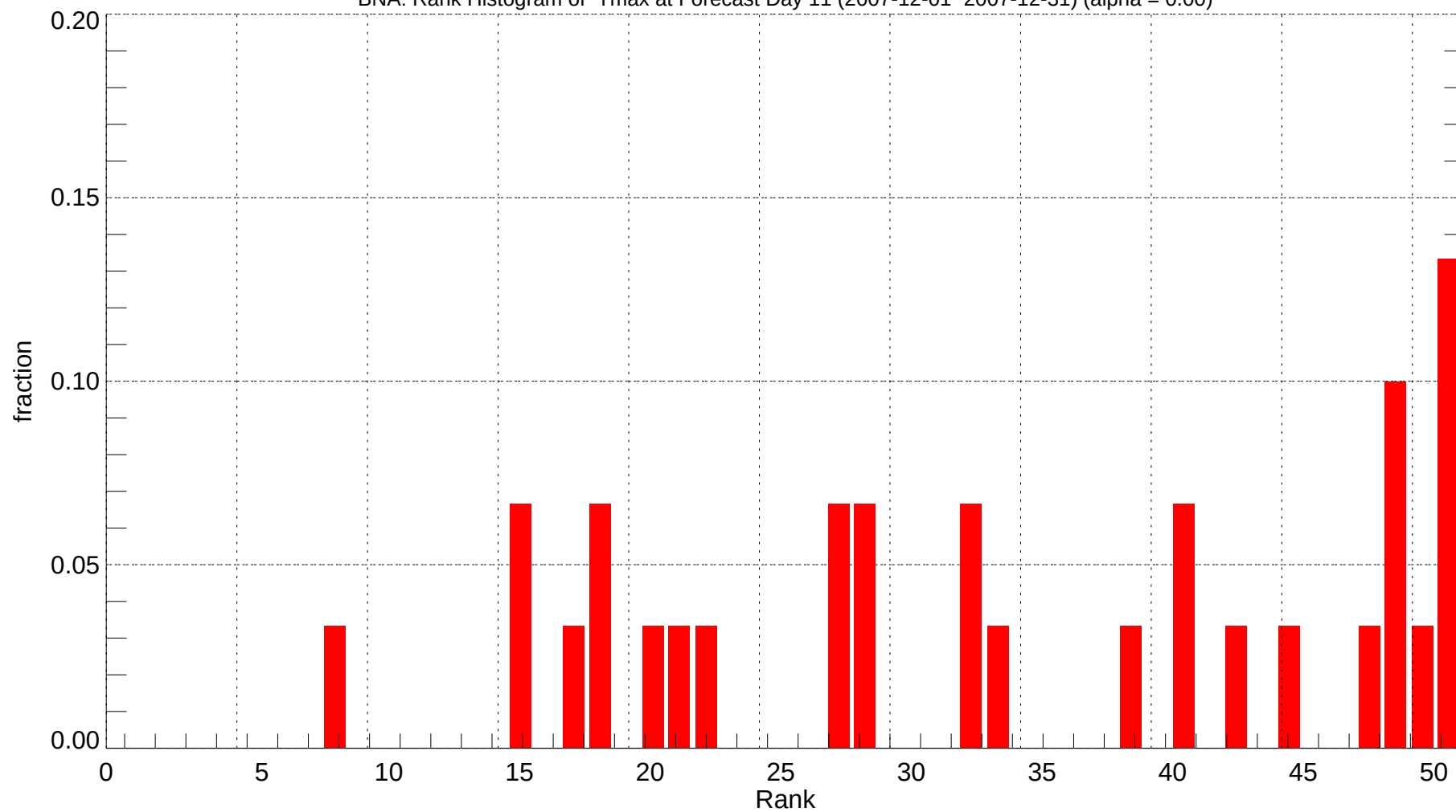
BNA: Rank Histogram of Tmax at Forecast Day 11 (2007-12-01~2007-12-31) (alpha = 0.00)
