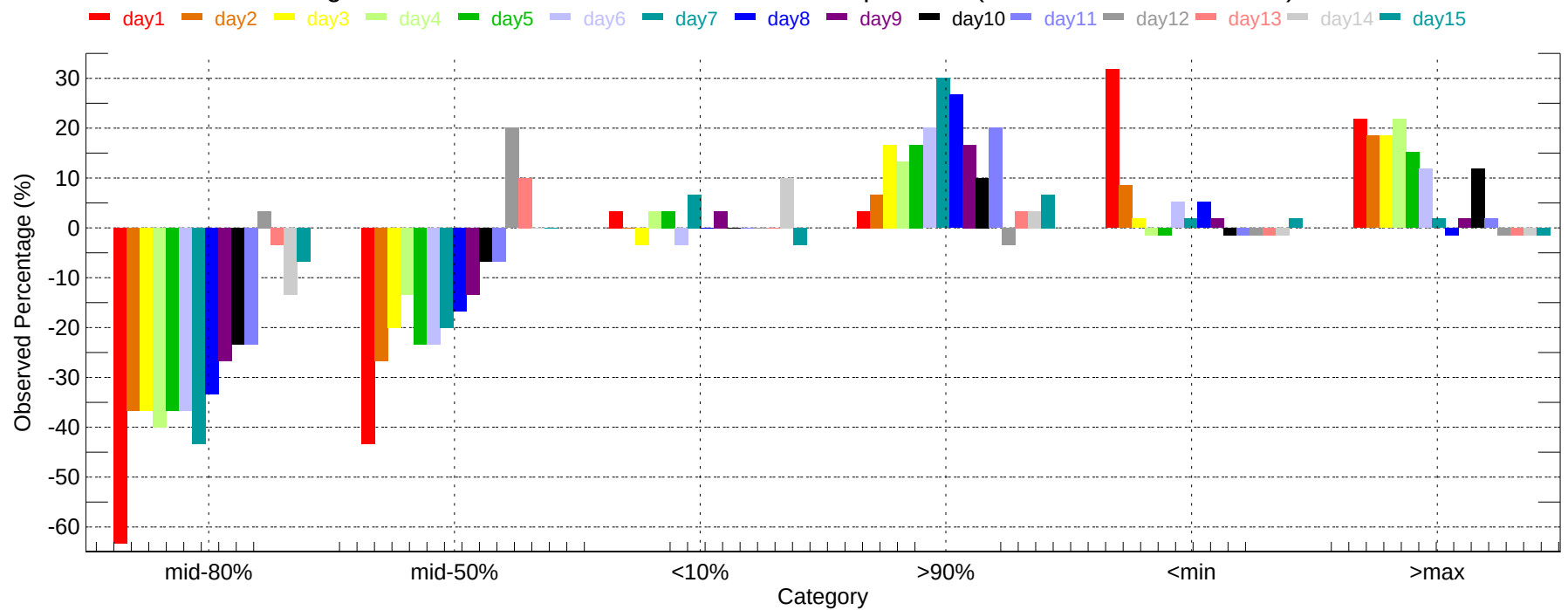
Observed Percentage Deviation of Ensembles - FSD: Min Temperature (2007-12-01~2007-12-31)
