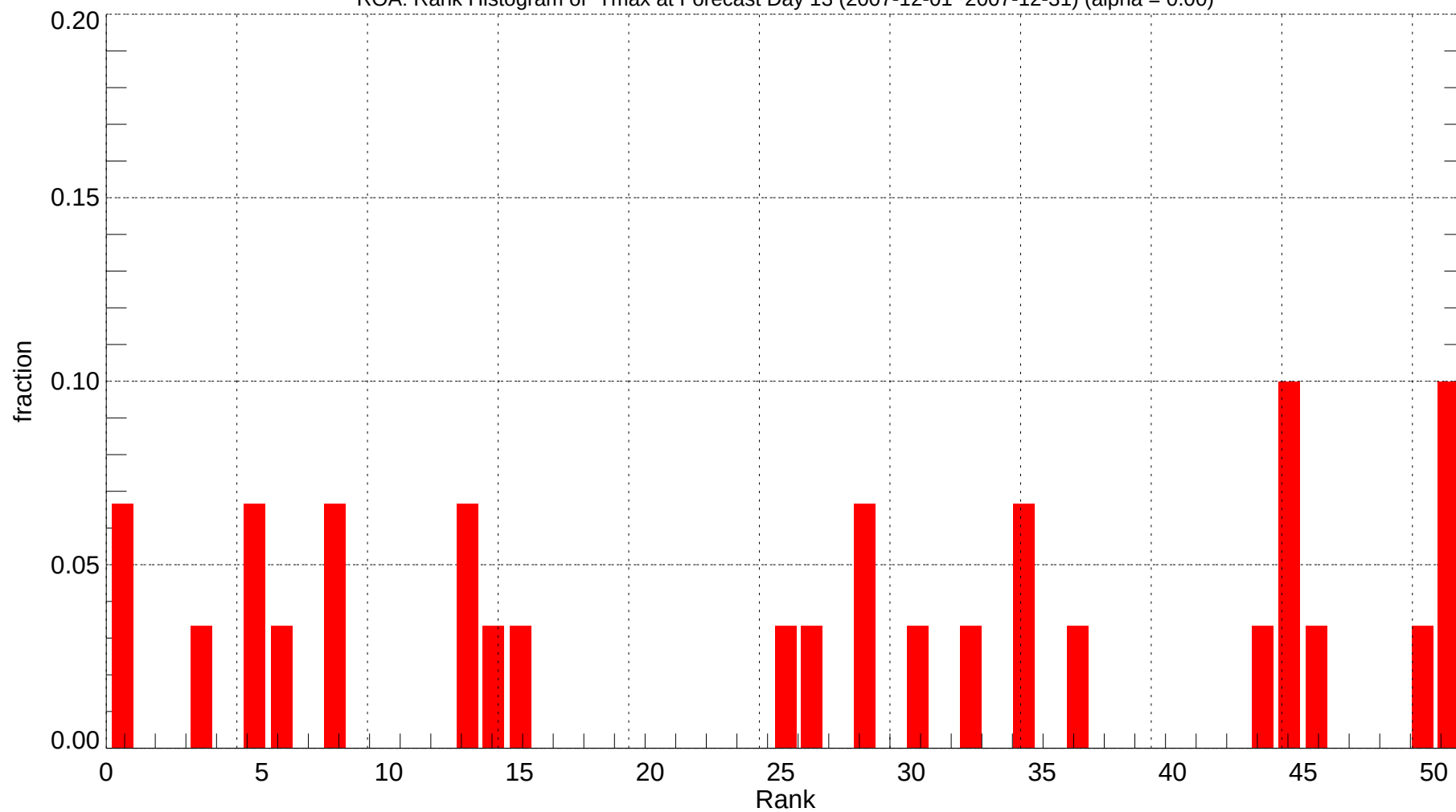
ROA: Rank Histogram of Tmax at Forecast Day 13 (2007-12-01~2007-12-31) (alpha = 0.00)
