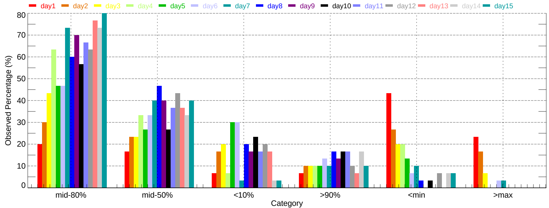
Observed Percentage of Ensembles - CON: Max Temperature (2007-12-01~2007-12-31)
