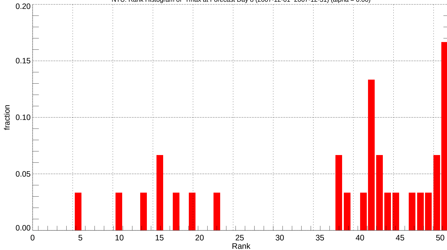
NTU: Rank Histogram of Tmax at Forecast Day 8 (2007-12-01~2007-12-31) (alpha = 0.00)
