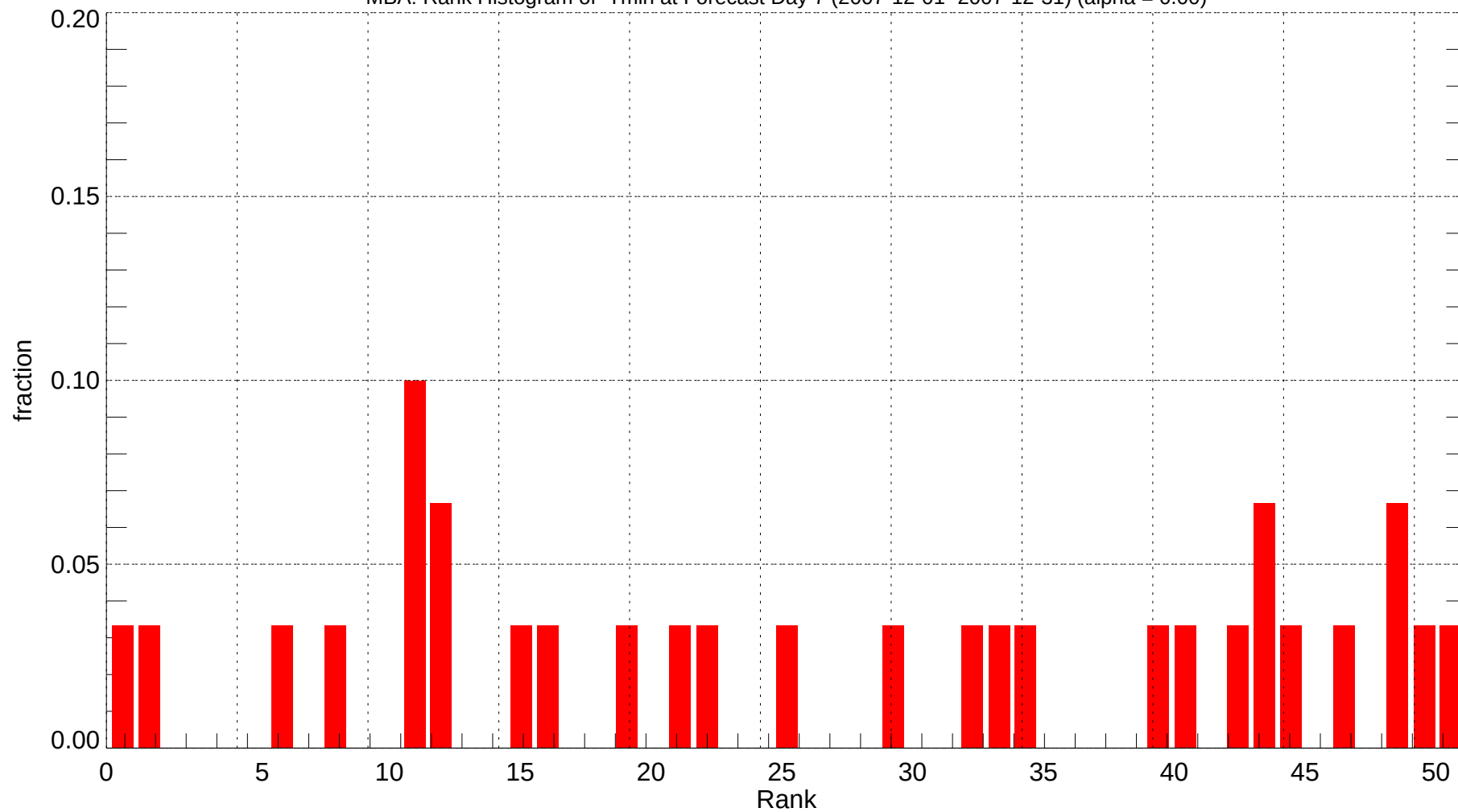
MBA: Rank Histogram of Tmin at Forecast Day 7 (2007-12-01~2007-12-31) (alpha = 0.00)
