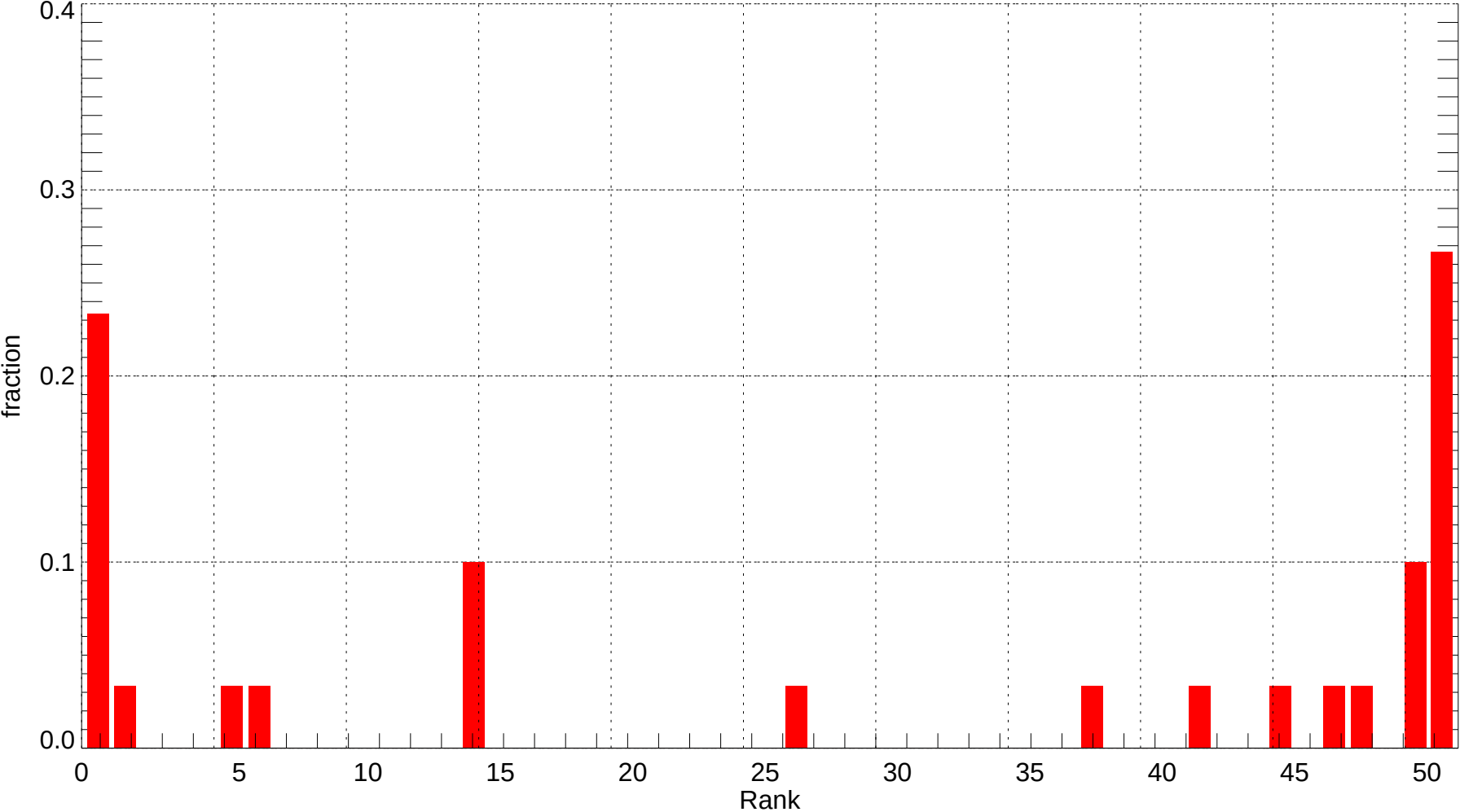
SSI: Rank Histogram of Tmax at Forecast Day 2 (2007-12-01~2007-12-31) (alpha = 0.00)
