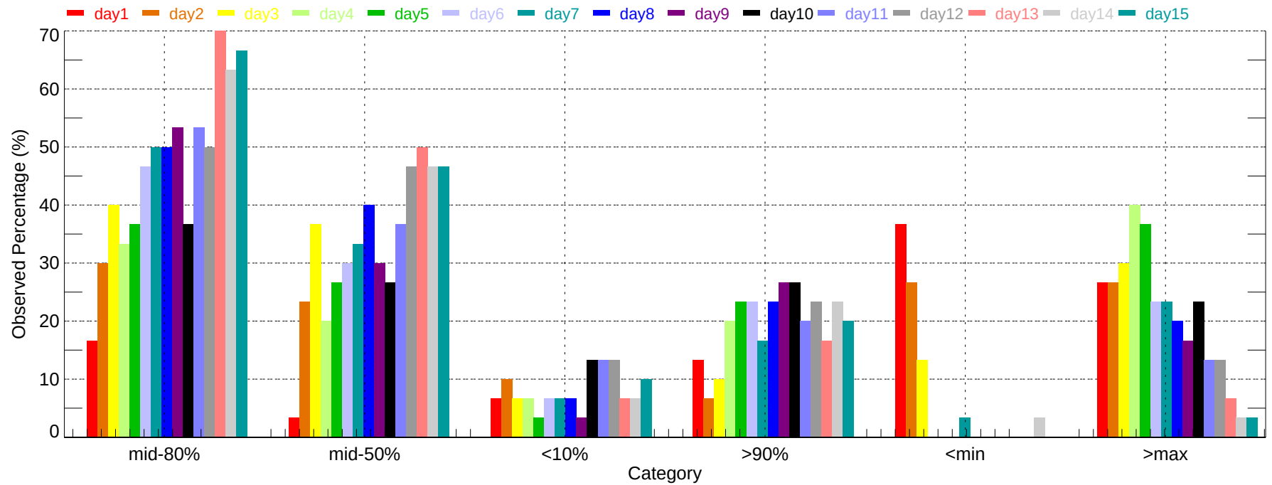
Observed Percentage of Ensembles - ICT: Min Temperature (2007-12-01~2007-12-31)
