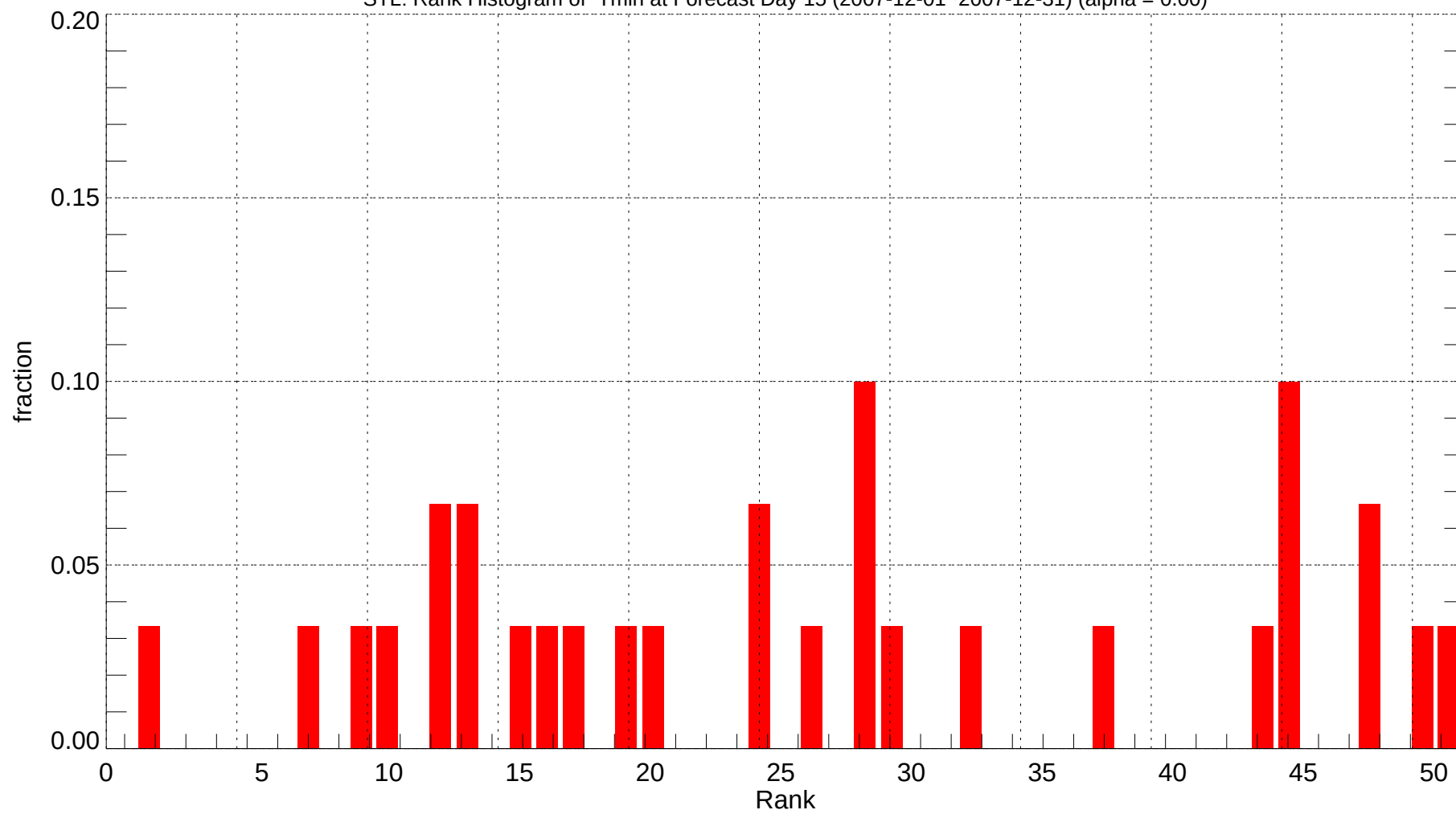
STL: Rank Histogram of Tmin at Forecast Day 15 (2007-12-01~2007-12-31) (alpha = 0.00)
