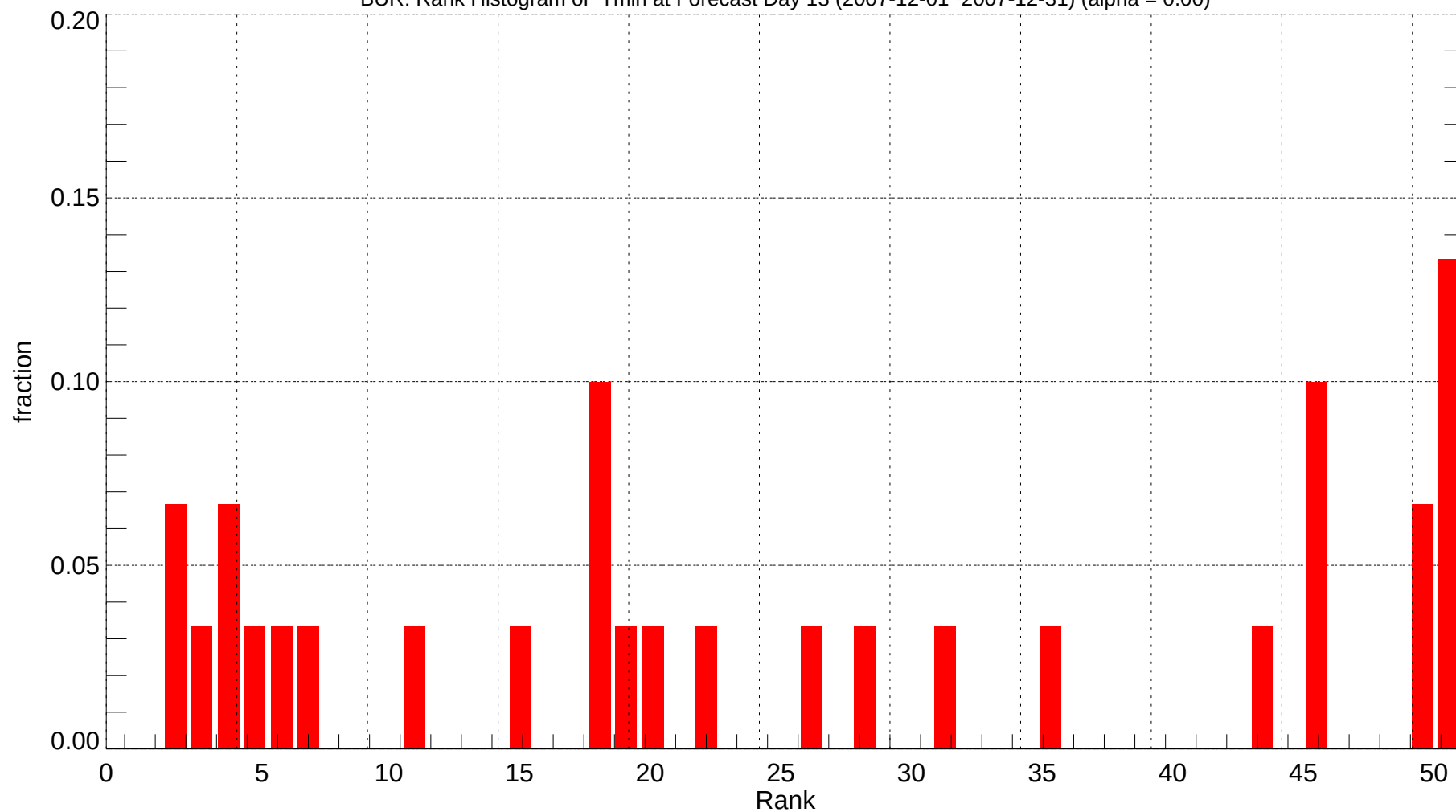
BUR: Rank Histogram of Tmin at Forecast Day 13 (2007-12-01~2007-12-31) (alpha = 0.00)
