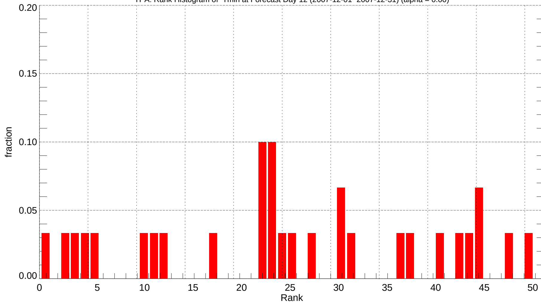
TPA: Rank Histogram of Tmin at Forecast Day 12 (2007-12-01~2007-12-31) (alpha = 0.00)
