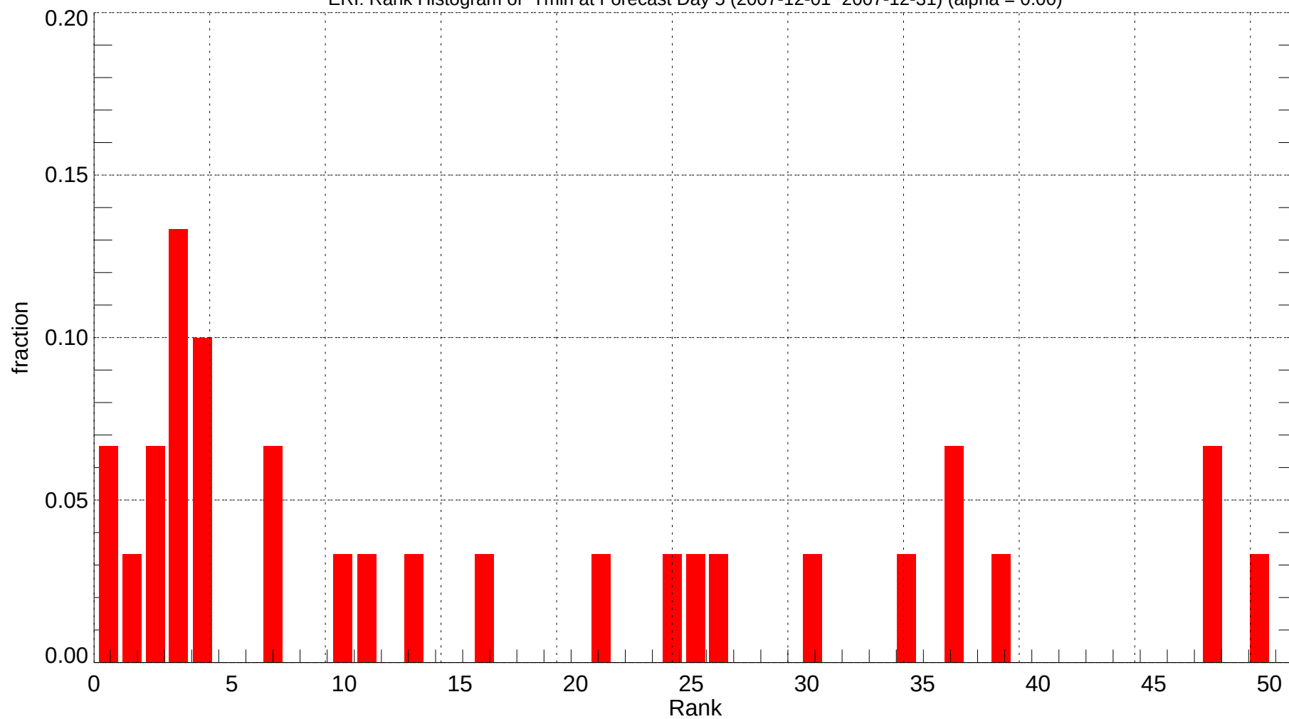
ERI: Rank Histogram of Tmin at Forecast Day 5 (2007-12-01~2007-12-31) (alpha = 0.00)
