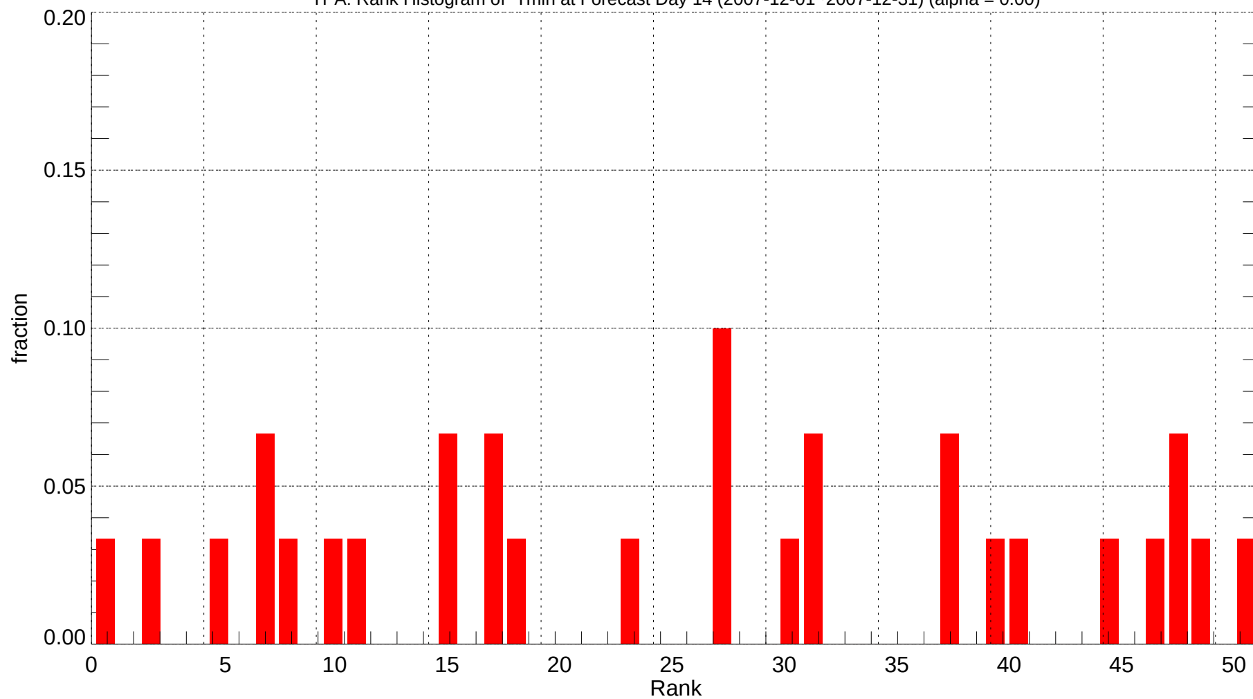
TPA: Rank Histogram of Tmin at Forecast Day 14 (2007-12-01~2007-12-31) (alpha = 0.00)
