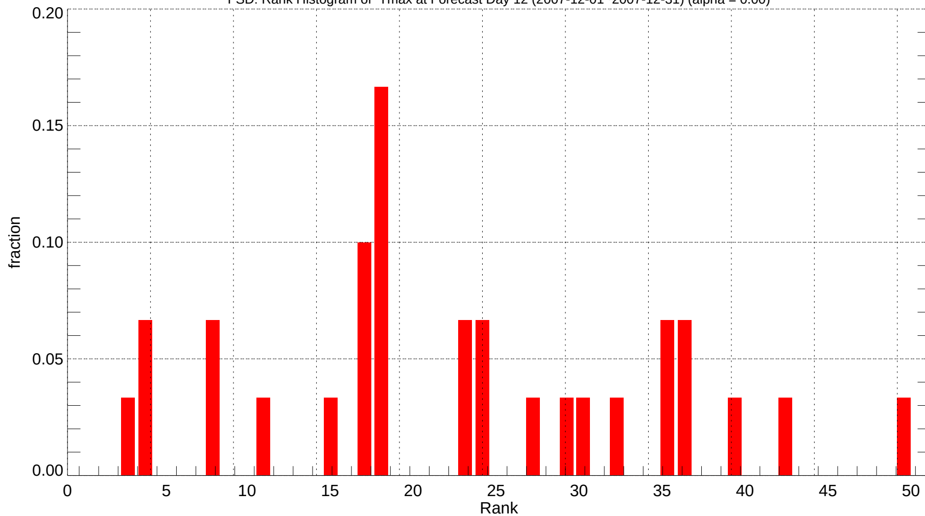
FSD: Rank Histogram of Tmax at Forecast Day 12 (2007-12-01~2007-12-31) (alpha = 0.00)
