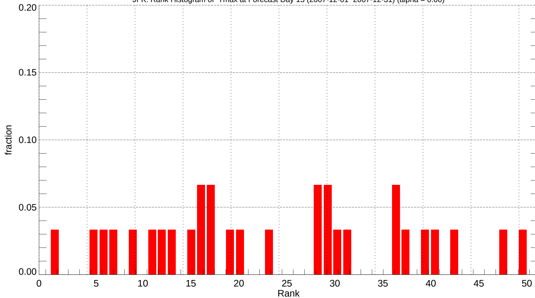
JFK: Rank Histogram of Tmax at Forecast Day 15 (2007-12-01~2007-12-31) (alpha = 0.00)
