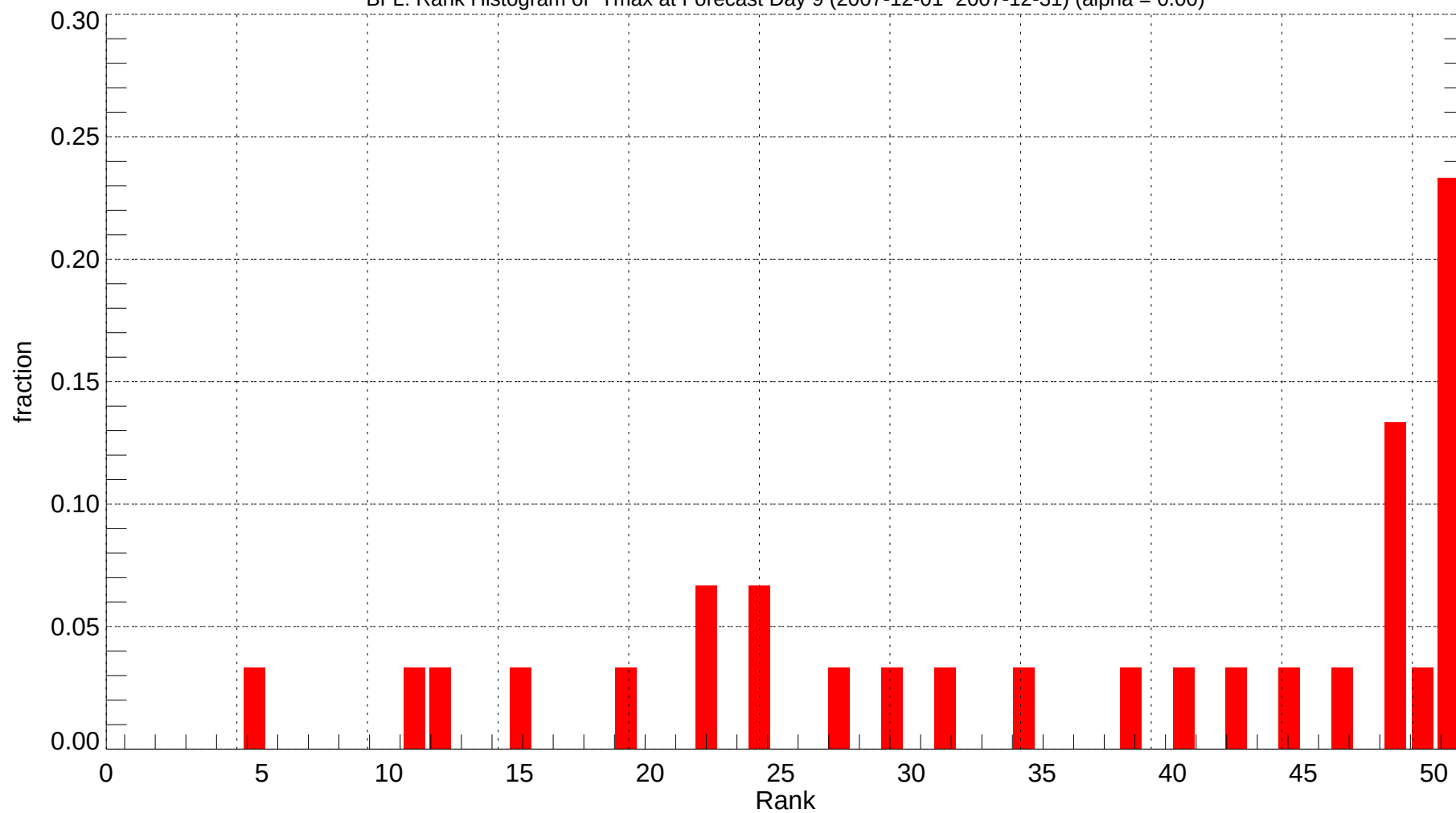
BFL: Rank Histogram of Tmax at Forecast Day 9 (2007-12-01~2007-12-31) (alpha = 0.00)
