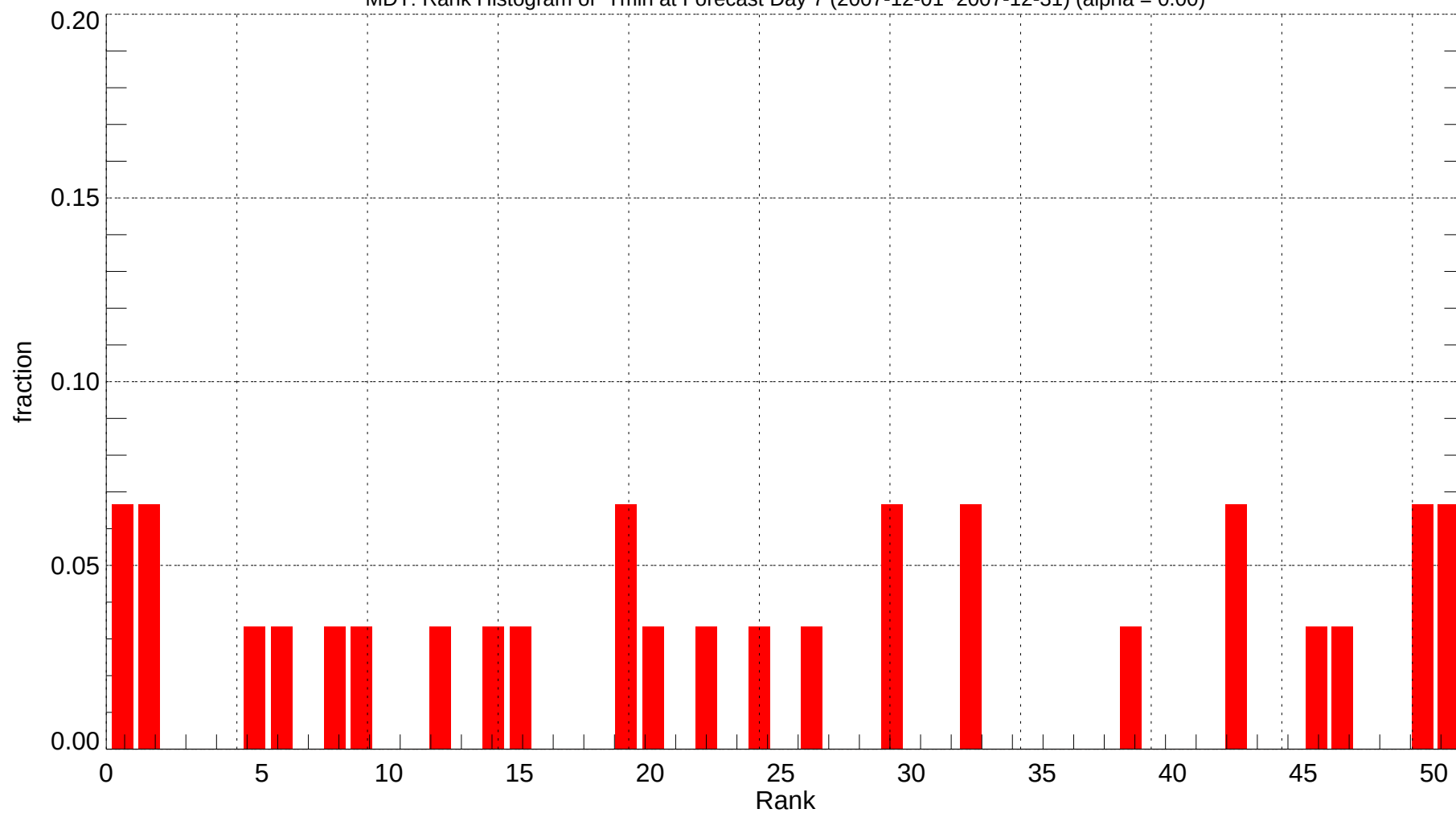
MDT: Rank Histogram of Tmin at Forecast Day 7 (2007-12-01~2007-12-31) (alpha = 0.00)
