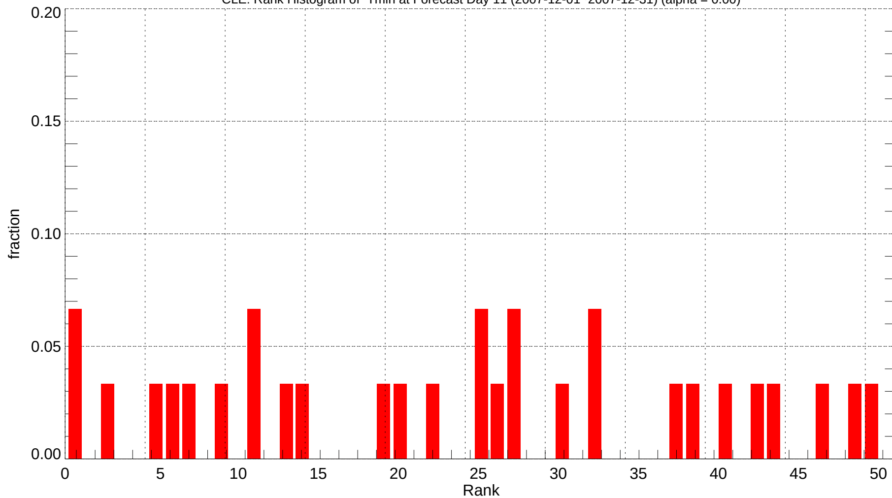
CLE: Rank Histogram of Tmin at Forecast Day 11 (2007-12-01~2007-12-31) (alpha = 0.00)
