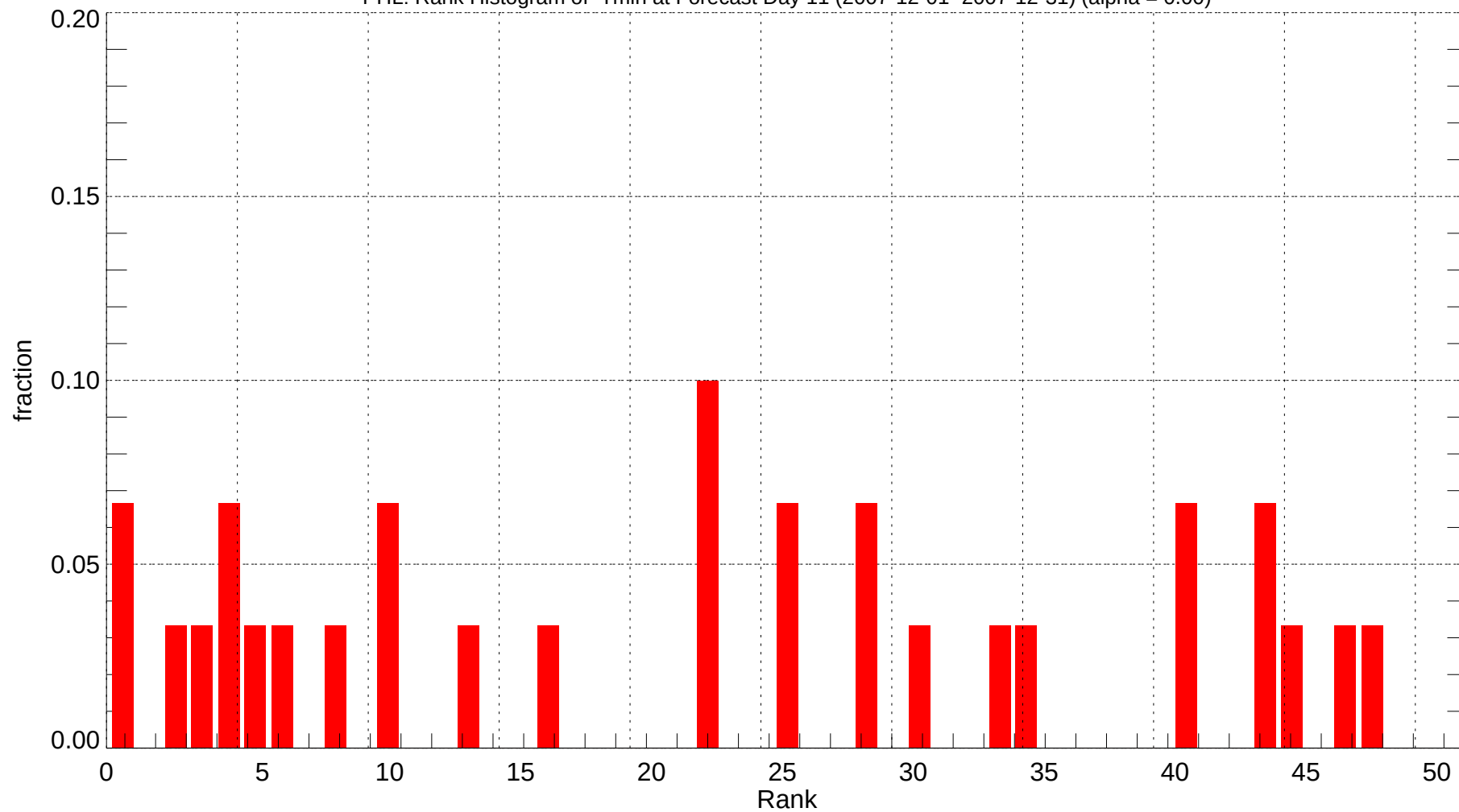
PHL: Rank Histogram of Tmin at Forecast Day 11 (2007-12-01~2007-12-31) (alpha = 0.00)
