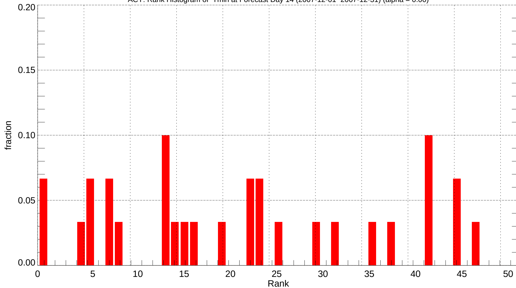
ACY: Rank Histogram of Tmin at Forecast Day 14 (2007-12-01~2007-12-31) (alpha = 0.00)
