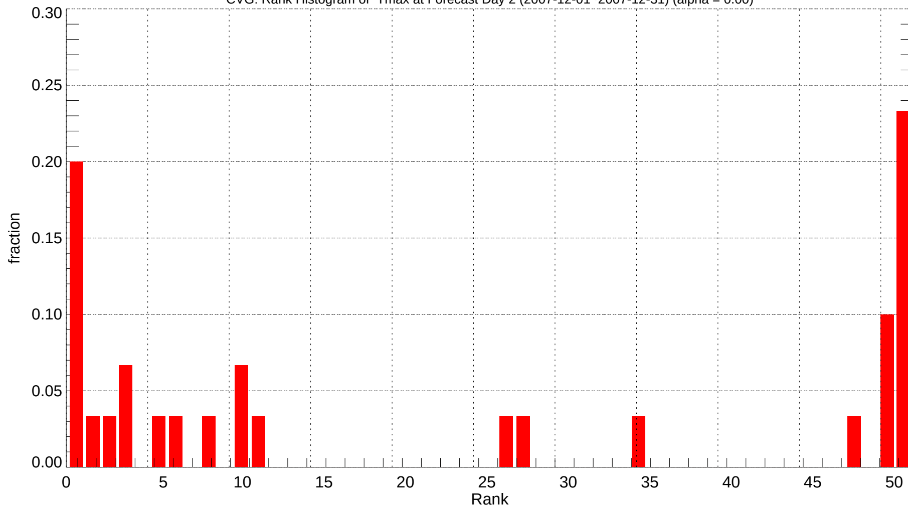
CVG: Rank Histogram of Tmax at Forecast Day 2 (2007-12-01~2007-12-31) (alpha = 0.00)
