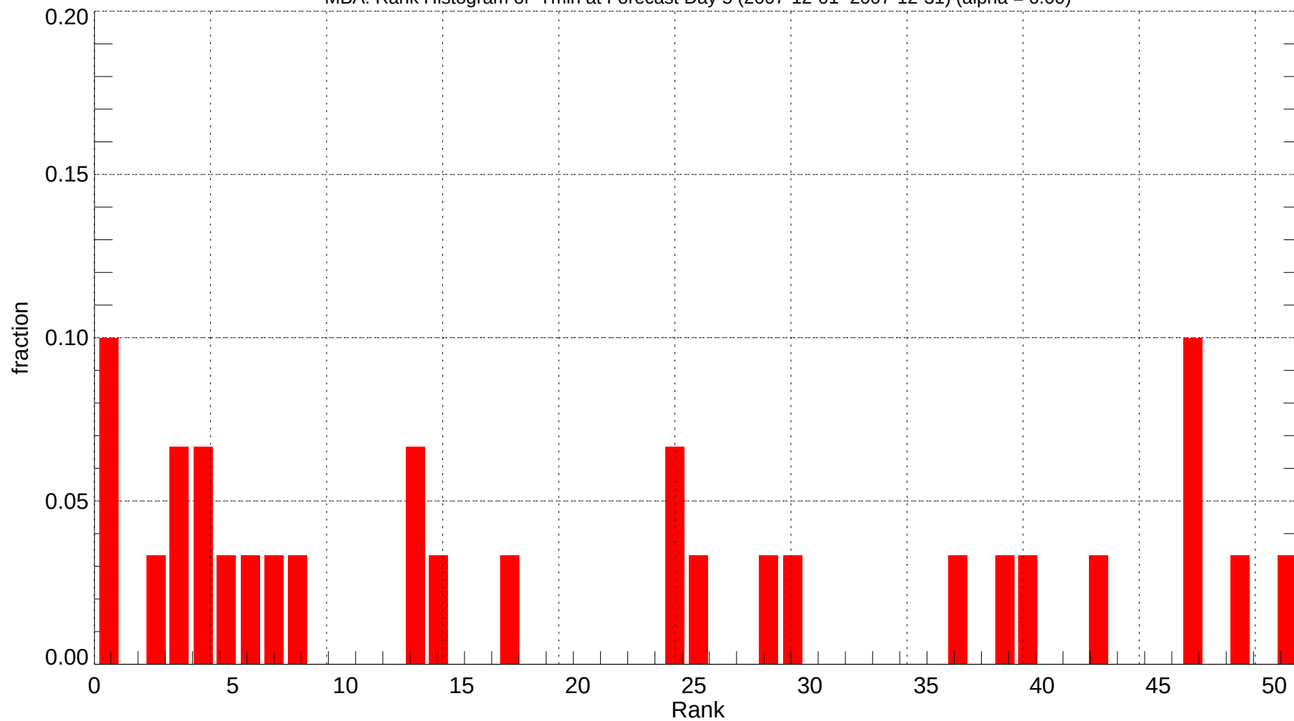
MBA: Rank Histogram of Tmin at Forecast Day 5 (2007-12-01~2007-12-31) (alpha = 0.00)
