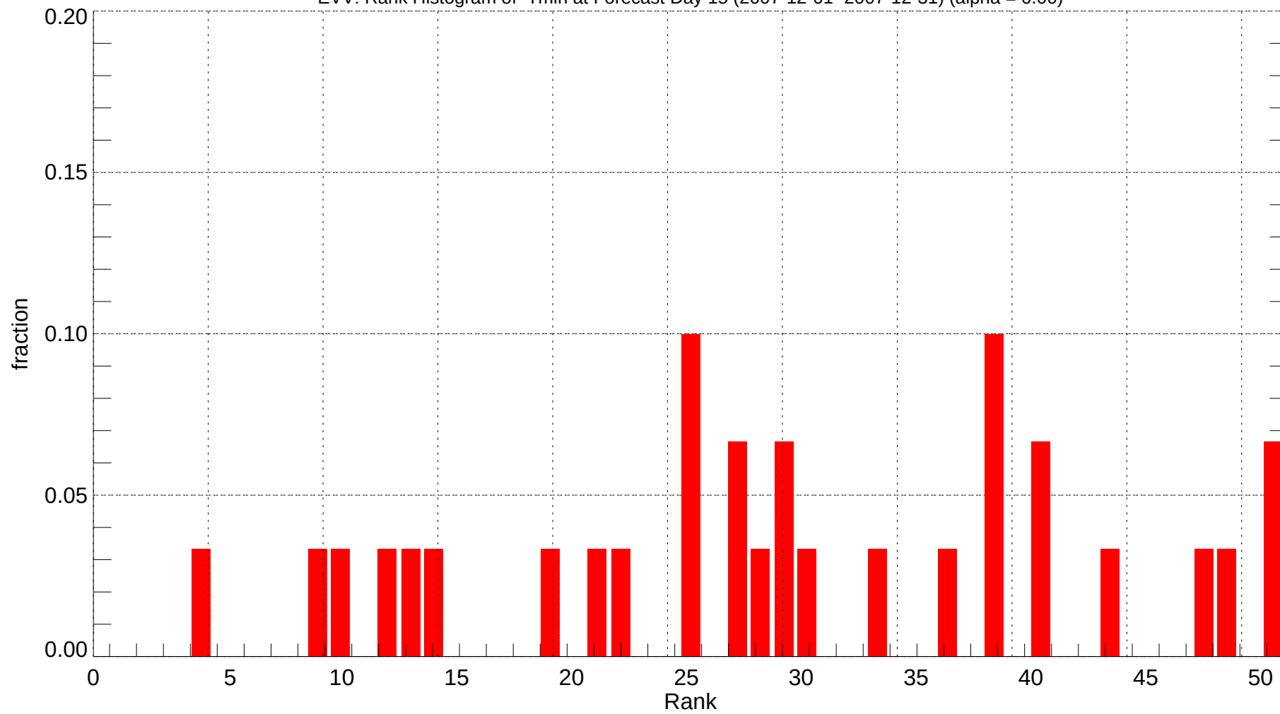
EVV: Rank Histogram of Tmin at Forecast Day 15 (2007-12-01~2007-12-31) (alpha = 0.00)
