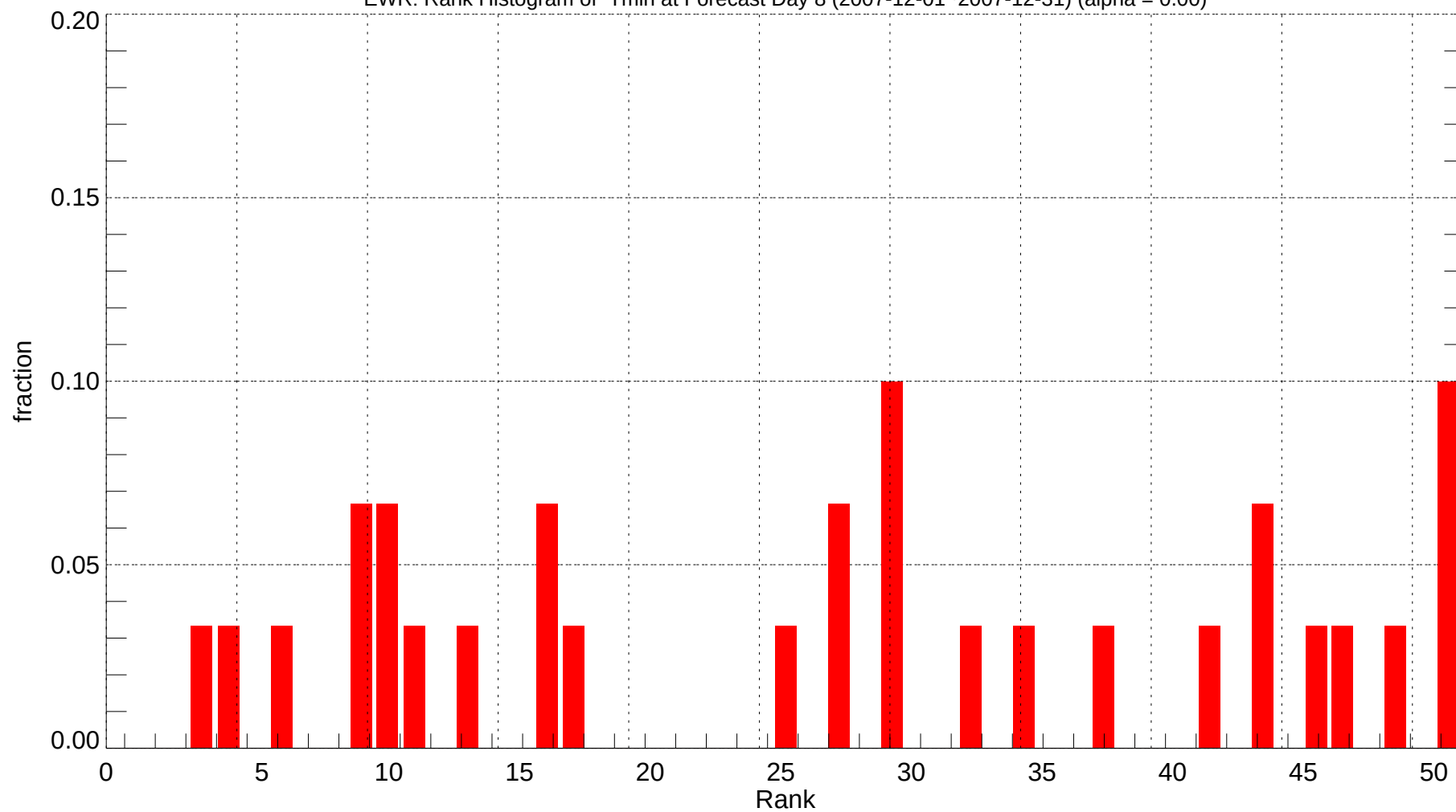
EWR: Rank Histogram of Tmin at Forecast Day 8 (2007-12-01~2007-12-31) (alpha = 0.00)
