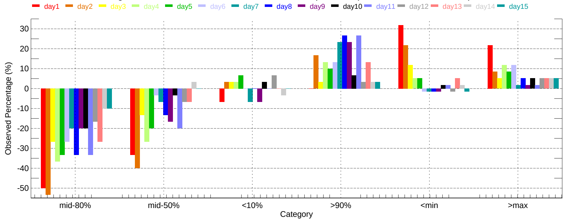
Observed Percentage Deviation of Ensembles - ROA: Max Temperature (2007-12-01~2007-12-31)
