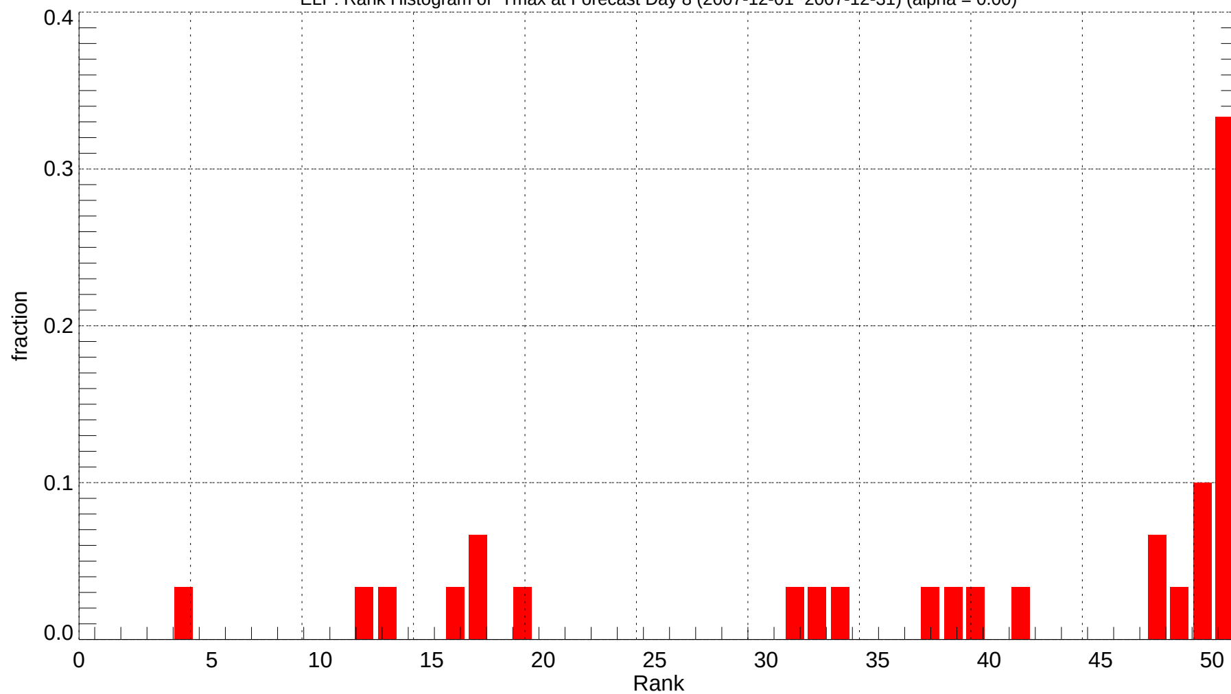
ELP: Rank Histogram of Tmax at Forecast Day 8 (2007-12-01~2007-12-31) (alpha = 0.00)
