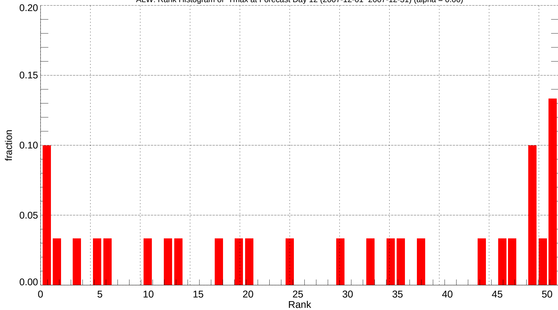
ALW: Rank Histogram of Tmax at Forecast Day 12 (2007-12-01~2007-12-31) (alpha = 0.00)
