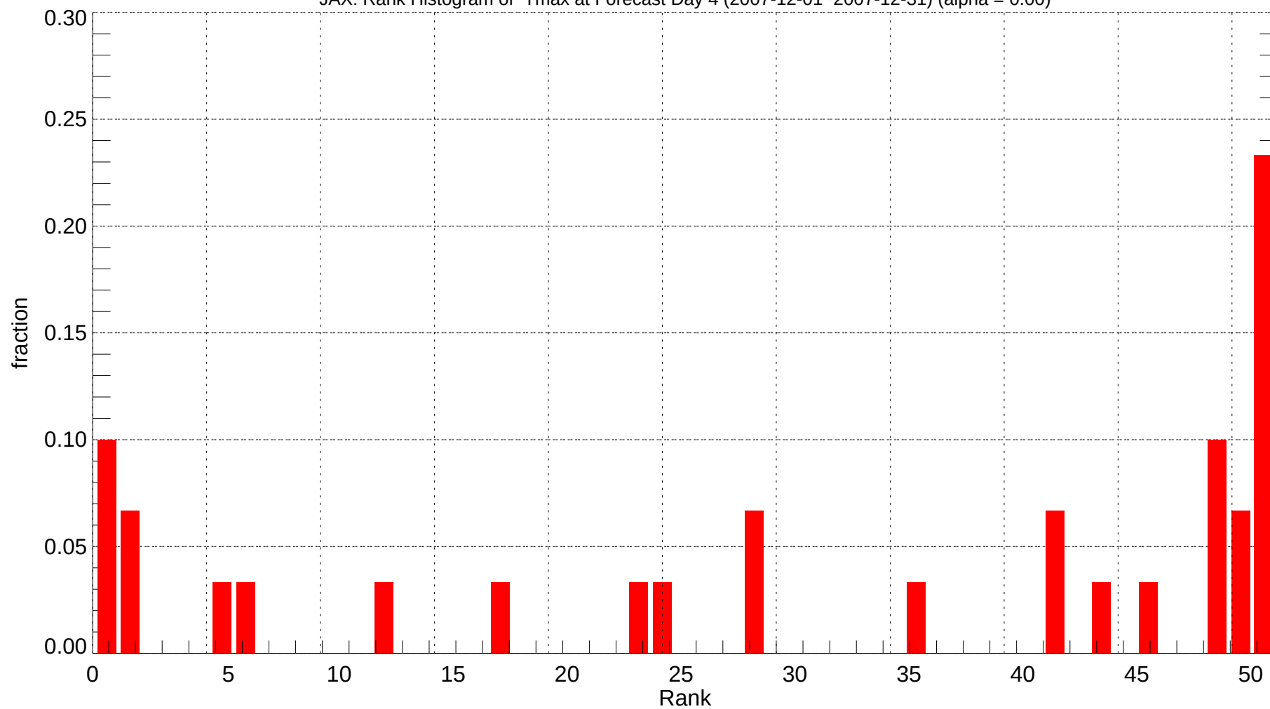
JAX: Rank Histogram of Tmax at Forecast Day 4 (2007-12-01~2007-12-31) (alpha = 0.00)
