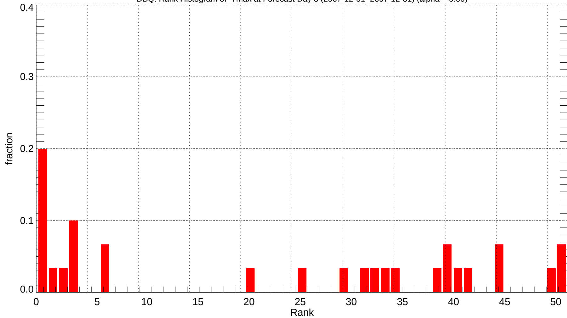
DBQ: Rank Histogram of Tmax at Forecast Day 3 (2007-12-01~2007-12-31) (alpha = 0.00)
