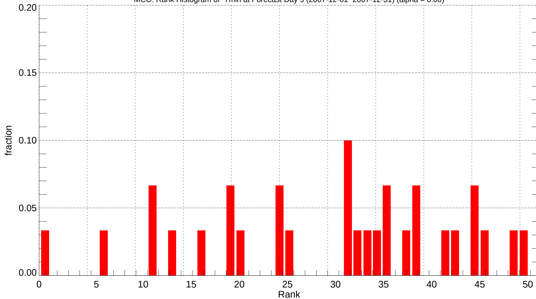
MCO: Rank Histogram of Tmin at Forecast Day 9 (2007-12-01~2007-12-31) (alpha = 0.00)
