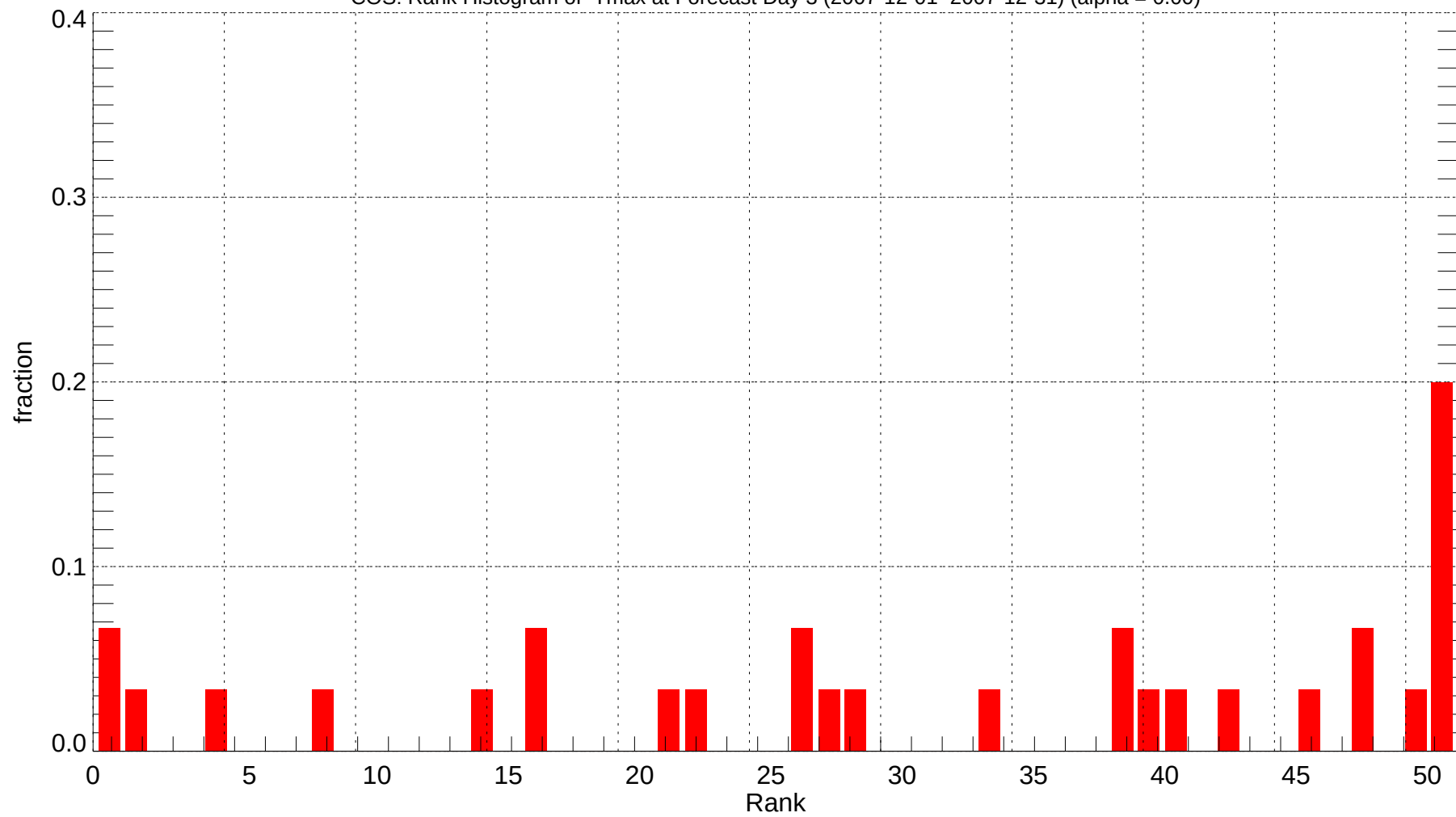
COS: Rank Histogram of Tmax at Forecast Day 3 (2007-12-01~2007-12-31) (alpha = 0.00)
