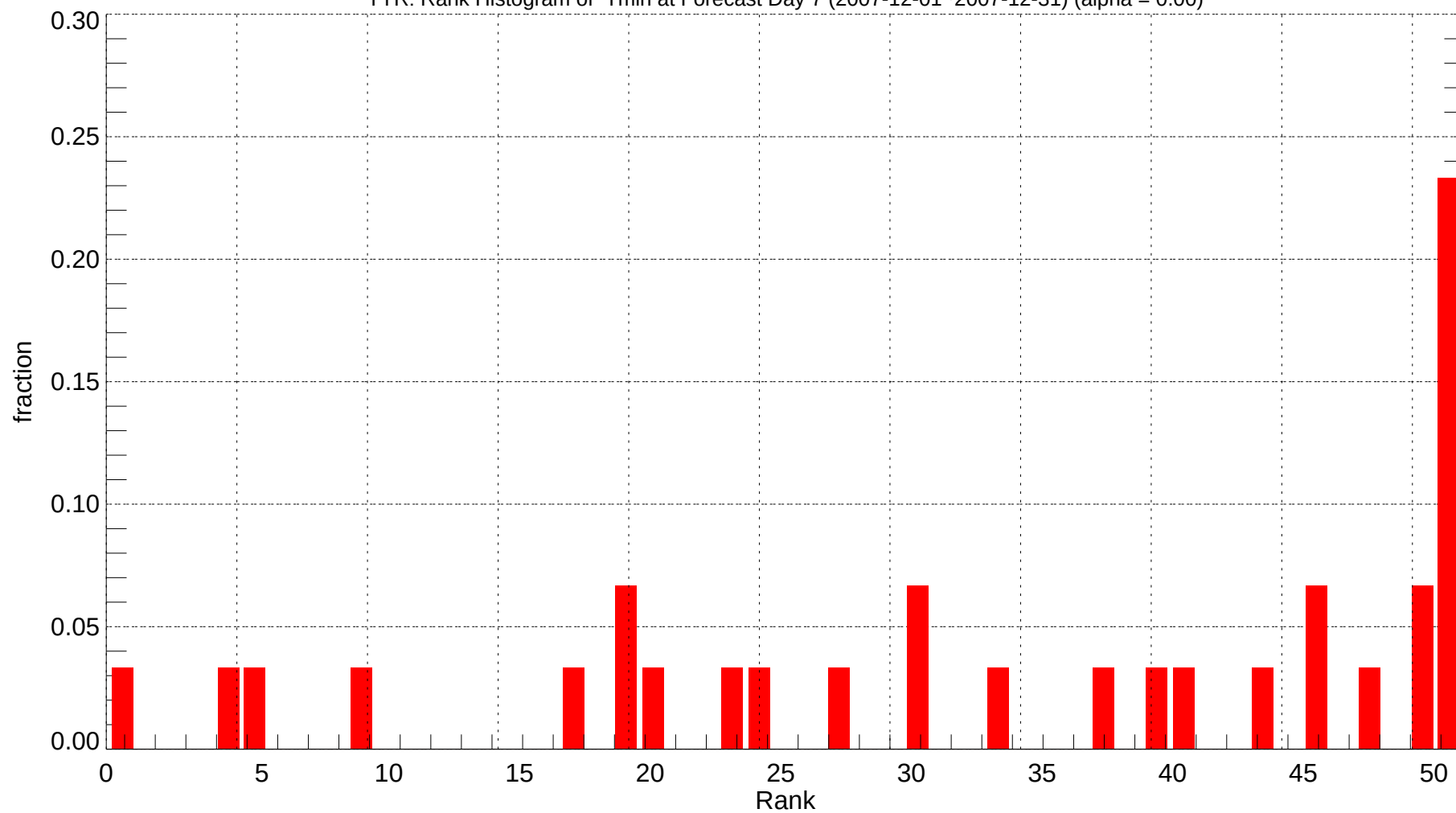
TYR: Rank Histogram of Tmin at Forecast Day 7 (2007-12-01~2007-12-31) (alpha = 0.00)
