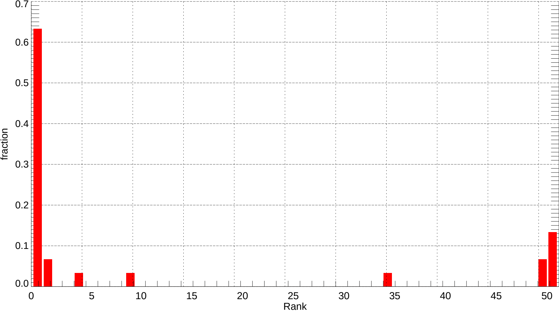
LAX: Rank Histogram of Tmin at Forecast Day 3 (2007-12-01~2007-12-31) (alpha = 0.00)
