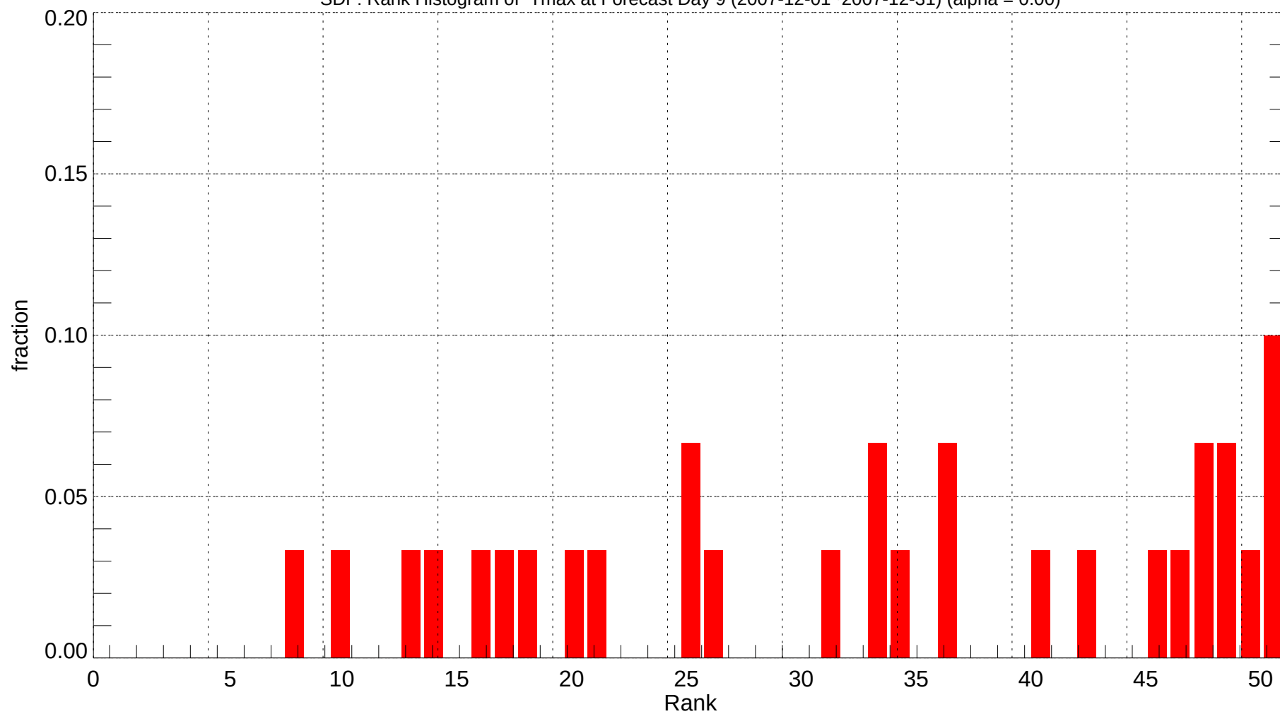
SDF: Rank Histogram of Tmax at Forecast Day 9 (2007-12-01~2007-12-31) (alpha = 0.00)
