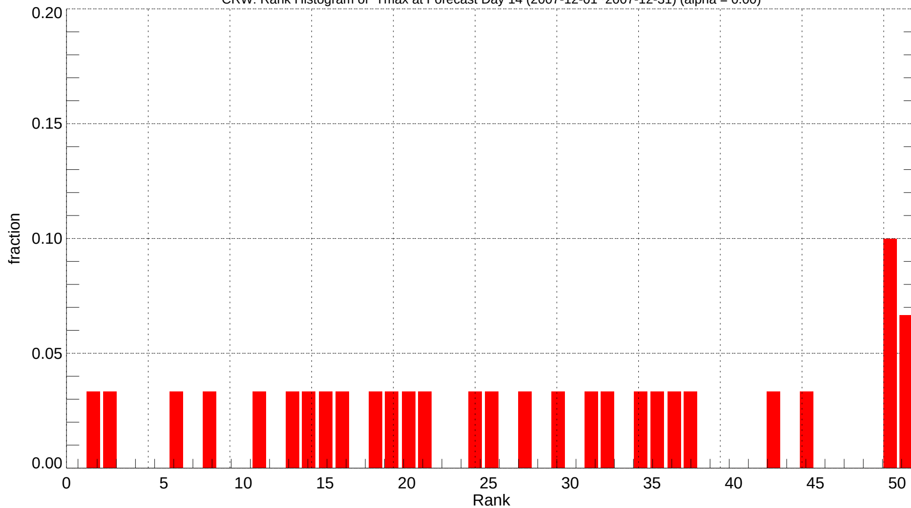
CRW: Rank Histogram of Tmax at Forecast Day 14 (2007-12-01~2007-12-31) (alpha = 0.00)
