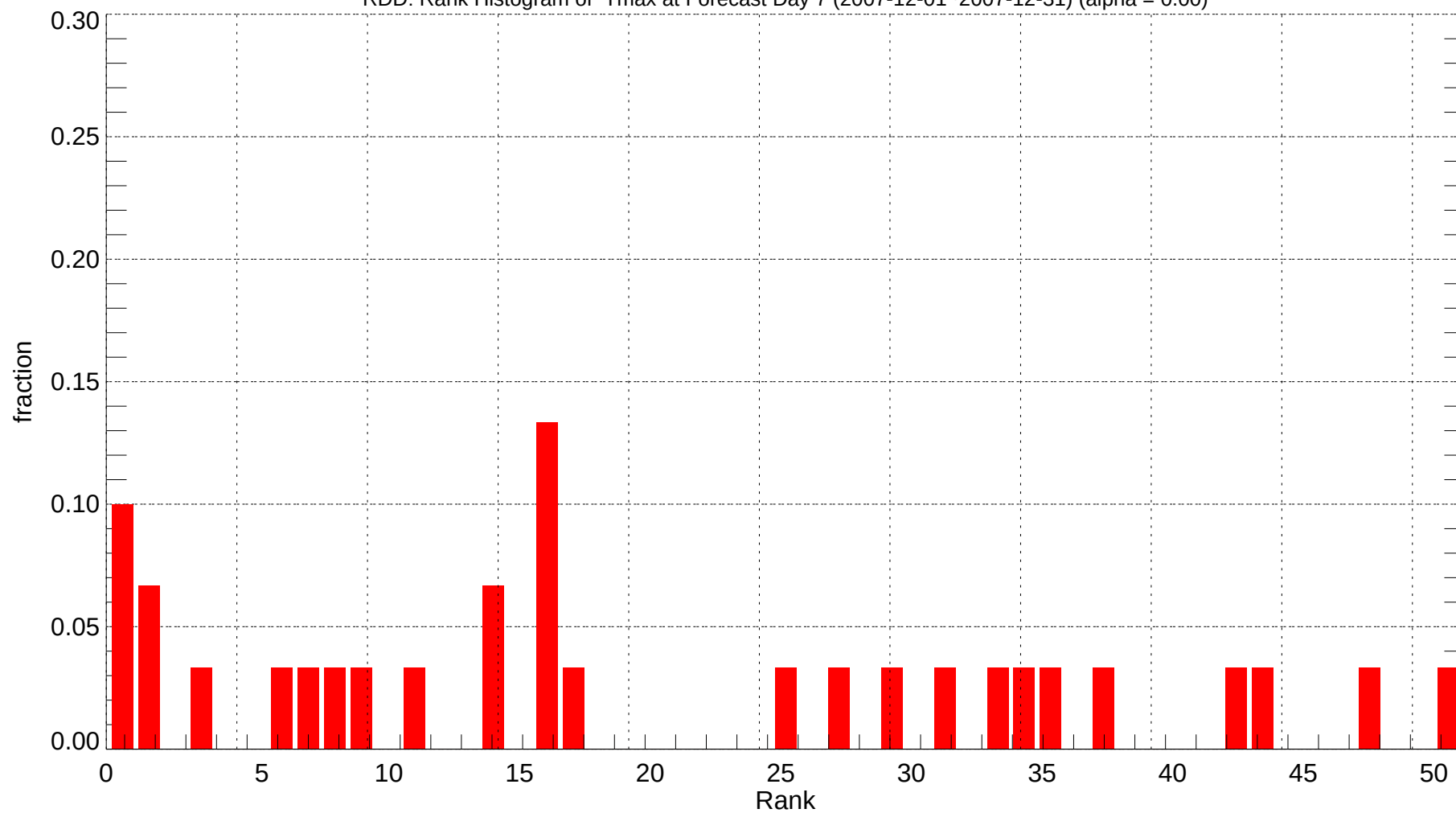
RDD: Rank Histogram of Tmax at Forecast Day 7 (2007-12-01~2007-12-31) (alpha = 0.00)
