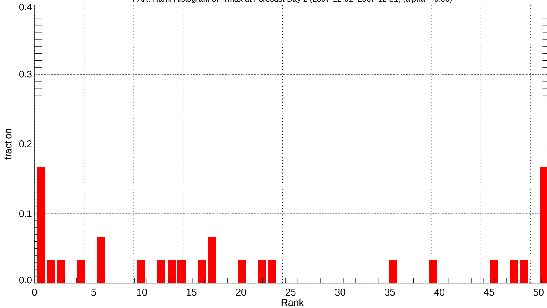
FAR: Rank Histogram of Tmax at Forecast Day 2 (2007-12-01~2007-12-31) (alpha = 0.00)
