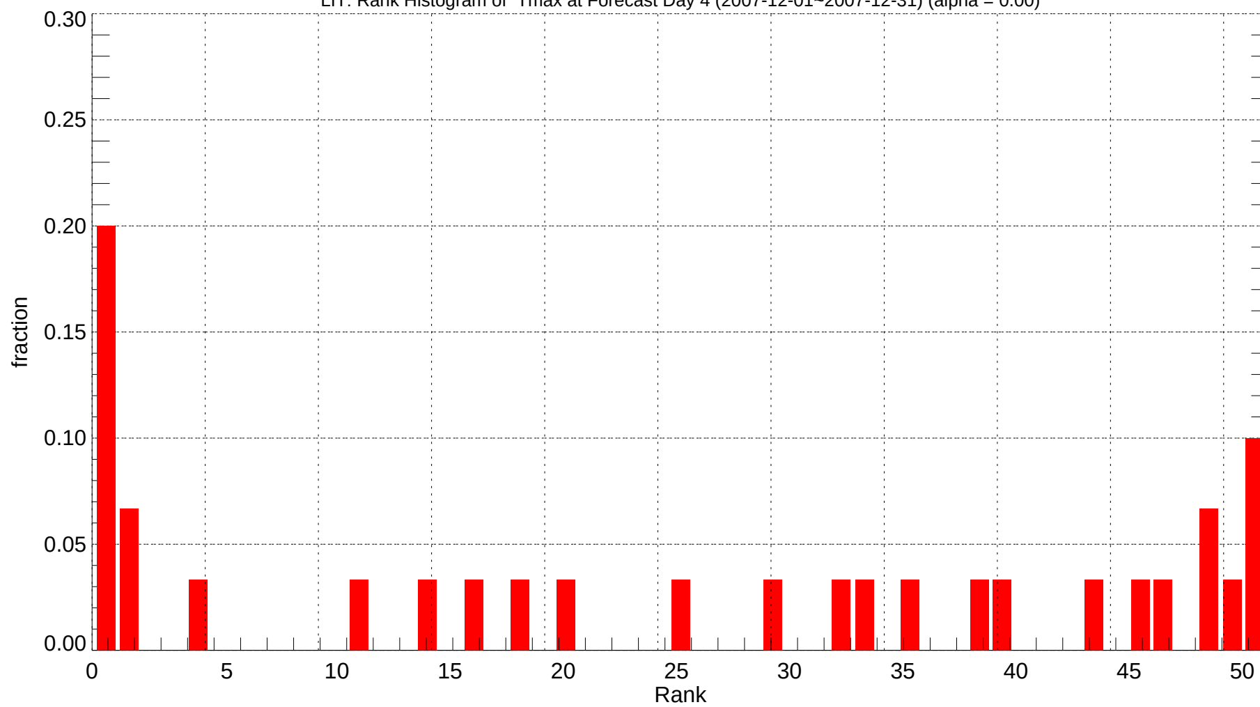
LIT: Rank Histogram of Tmax at Forecast Day 4 (2007-12-01~2007-12-31) (alpha = 0.00)
