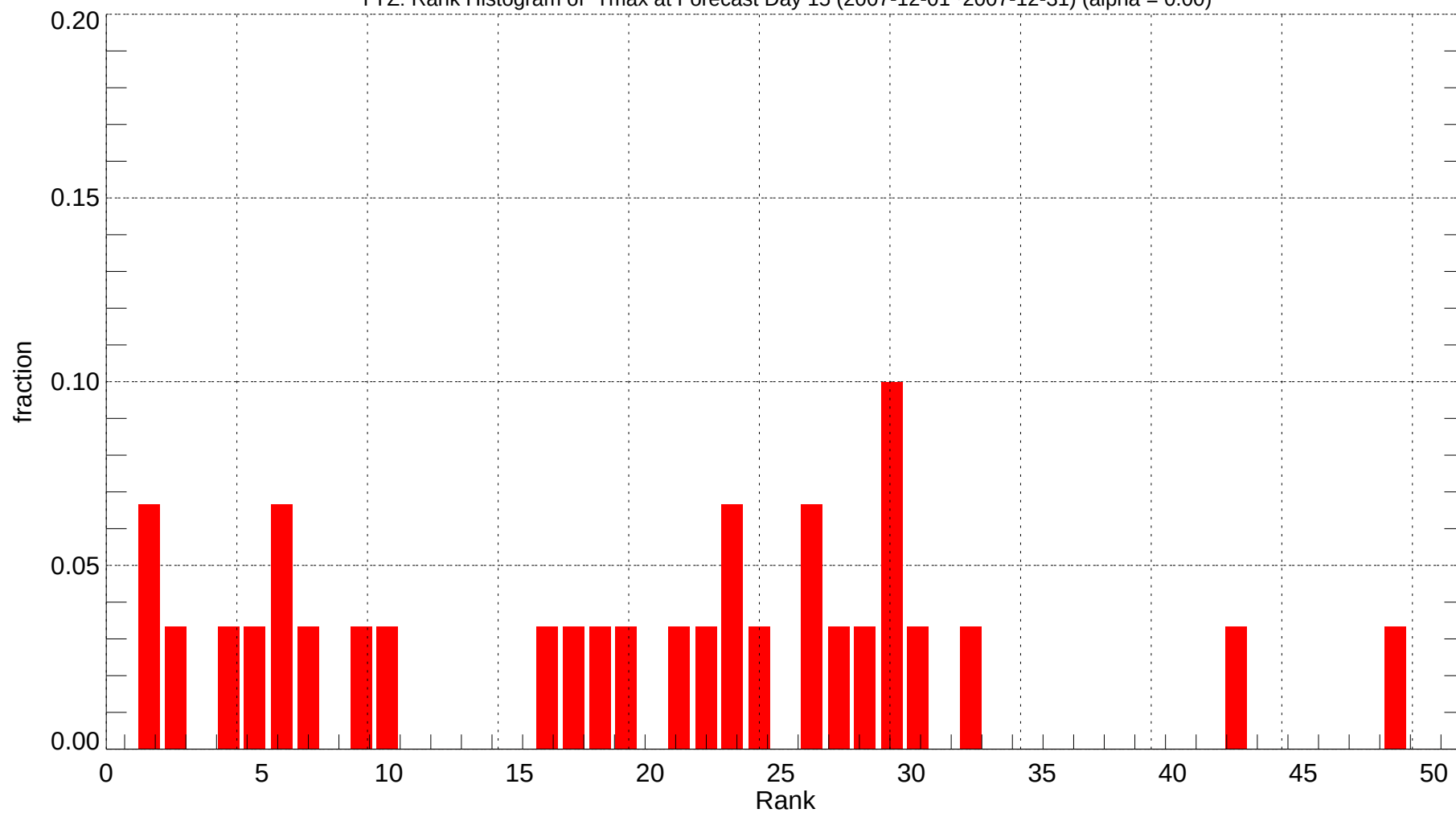
YYZ: Rank Histogram of Tmax at Forecast Day 15 (2007-12-01~2007-12-31) (alpha = 0.00)
