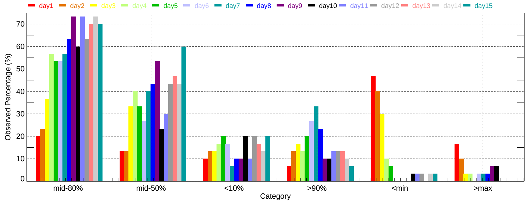
Observed Percentage of Ensembles - MBA: Max Temperature (2007-12-01~2007-12-31)
