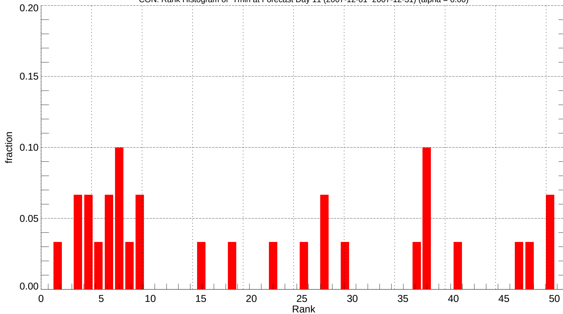
CON: Rank Histogram of Tmin at Forecast Day 11 (2007-12-01~2007-12-31) (alpha = 0.00)
