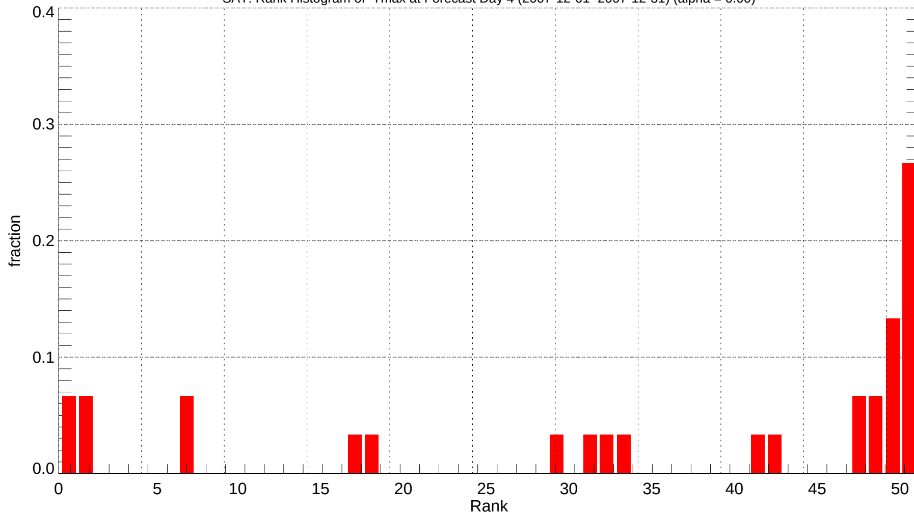
SAT: Rank Histogram of Tmax at Forecast Day 4 (2007-12-01~2007-12-31) (alpha = 0.00)
