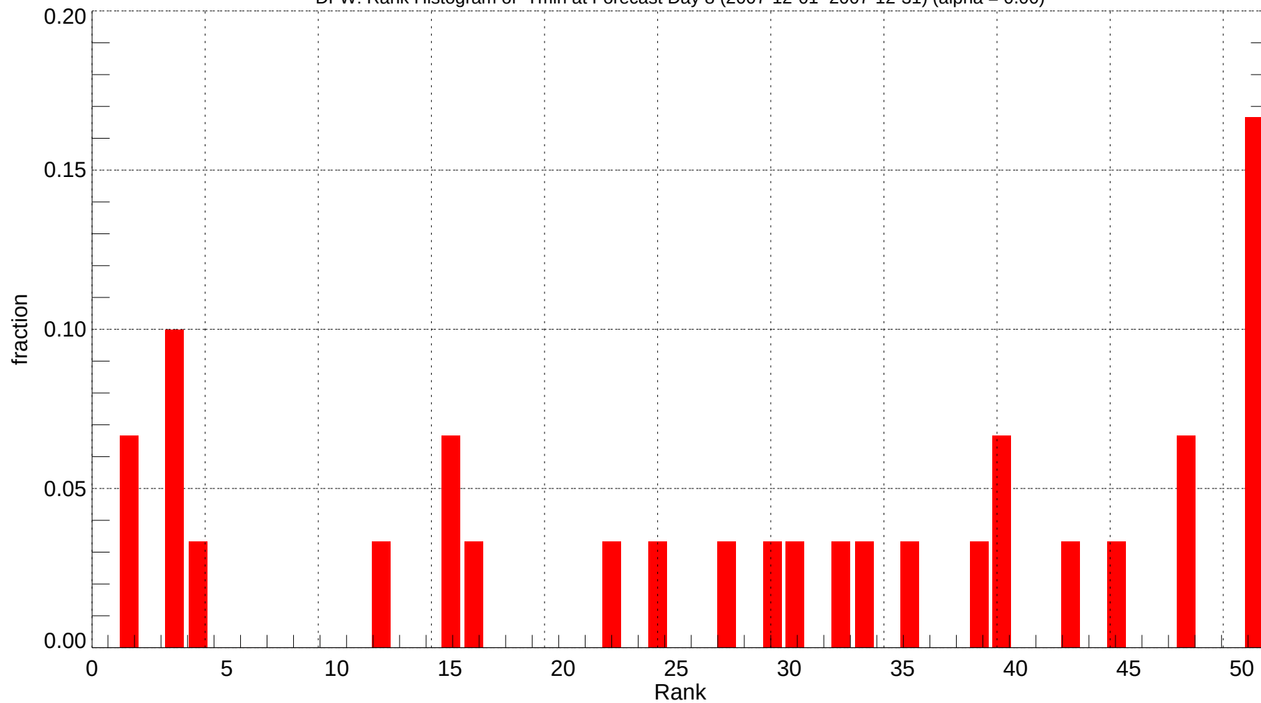
DFW: Rank Histogram of Tmin at Forecast Day 8 (2007-12-01~2007-12-31) (alpha = 0.00)
