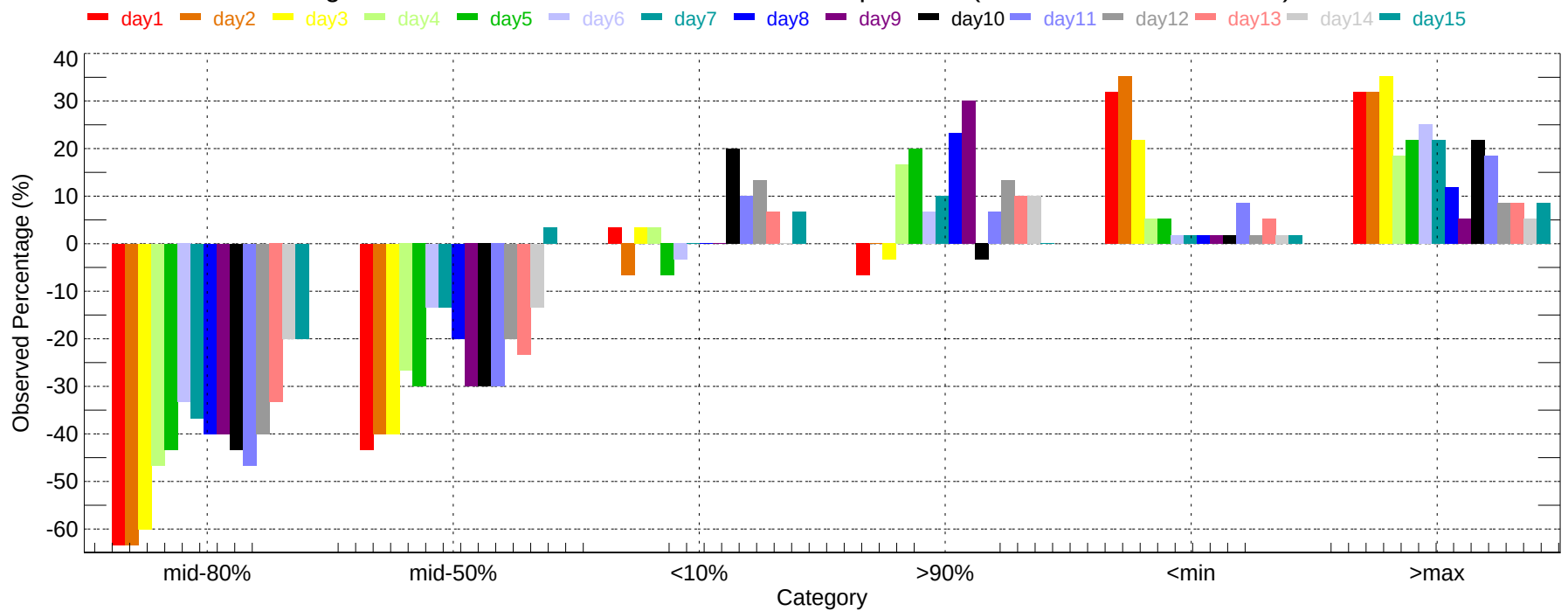
Observed Percentage Deviation of Ensembles - TUL: Min Temperature (2007-12-01~2007-12-31)
