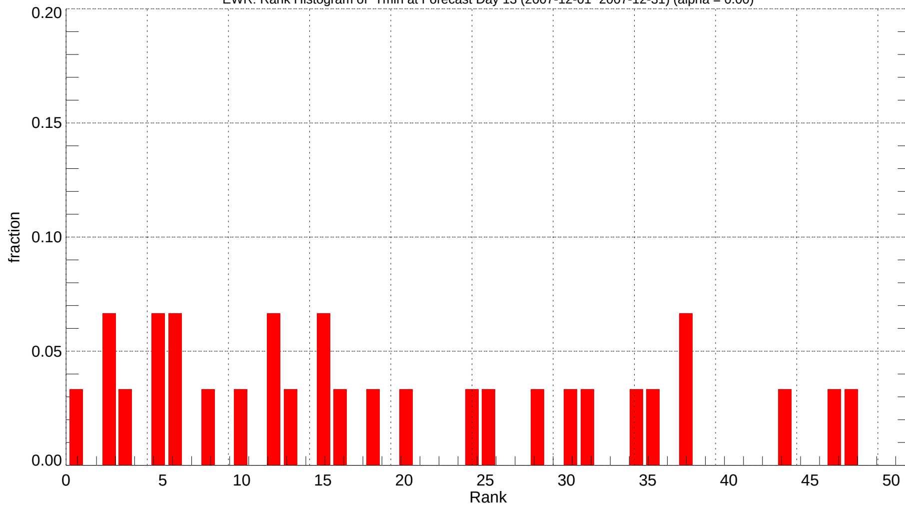
EWR: Rank Histogram of Tmin at Forecast Day 13 (2007-12-01~2007-12-31) (alpha = 0.00)
