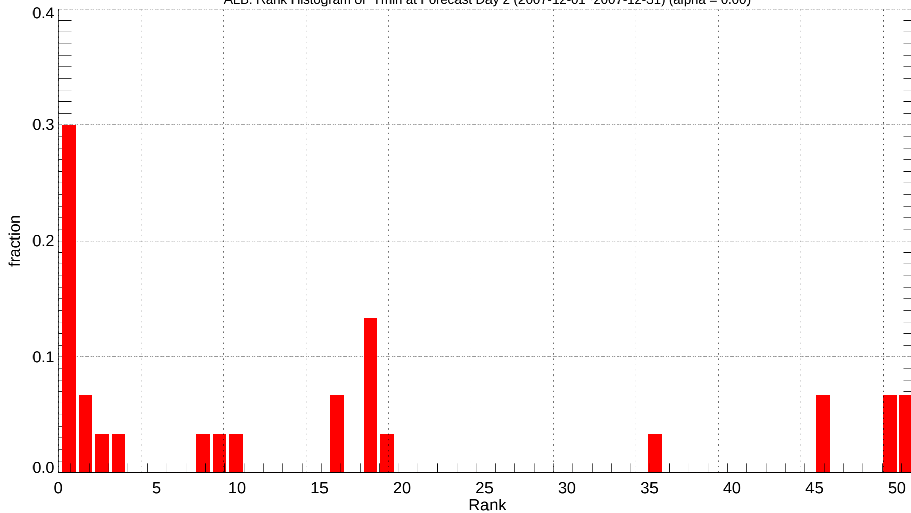
ALB: Rank Histogram of Tmin at Forecast Day 2 (2007-12-01~2007-12-31) (alpha = 0.00)
