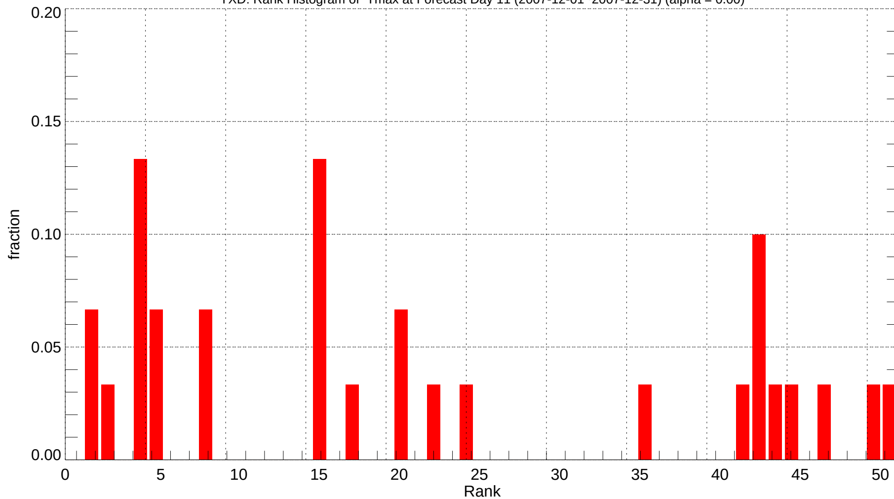
YXD: Rank Histogram of Tmax at Forecast Day 11 (2007-12-01~2007-12-31) (alpha = 0.00)
