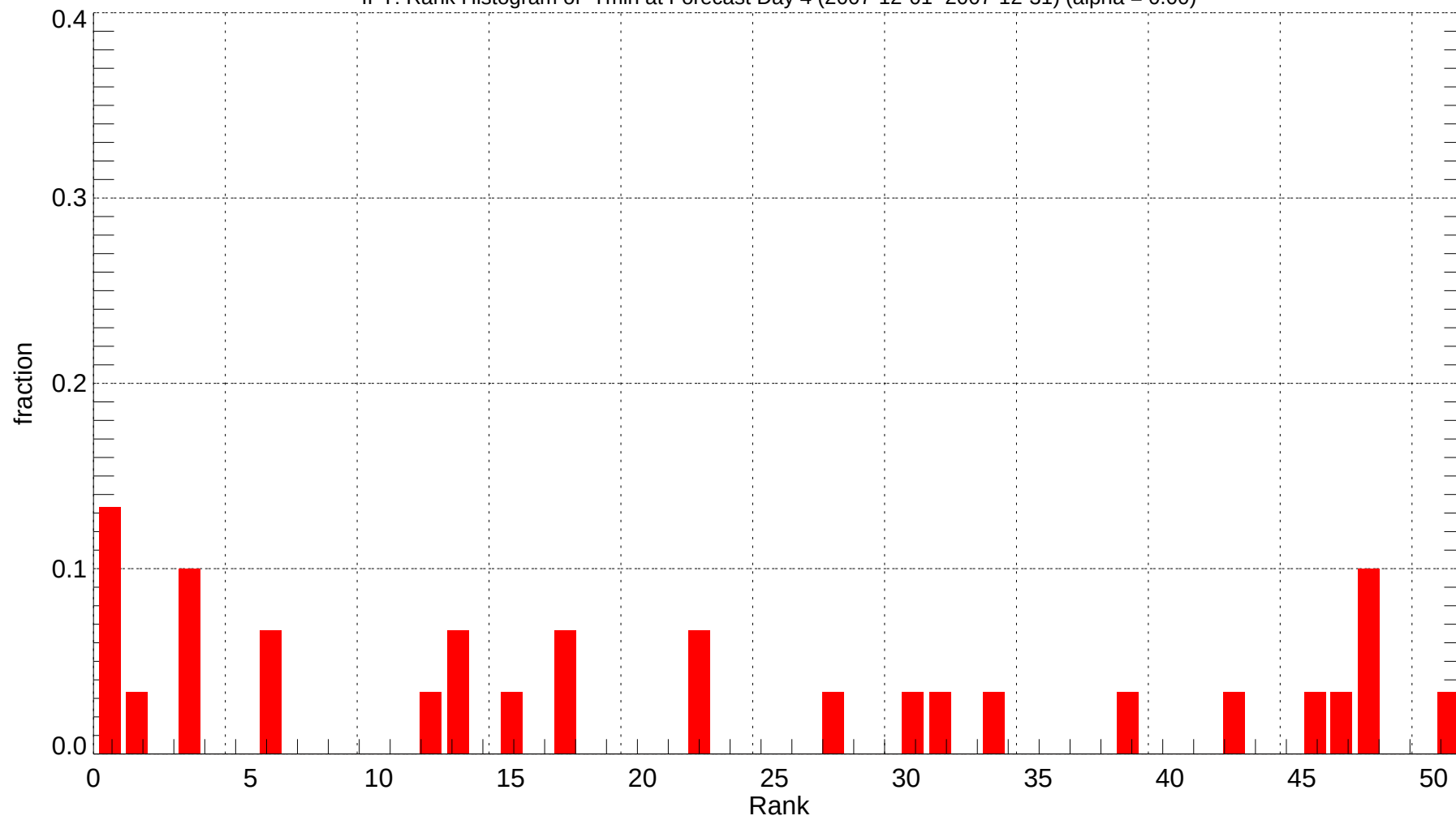
IPT: Rank Histogram of Tmin at Forecast Day 4 (2007-12-01~2007-12-31) (alpha = 0.00)
