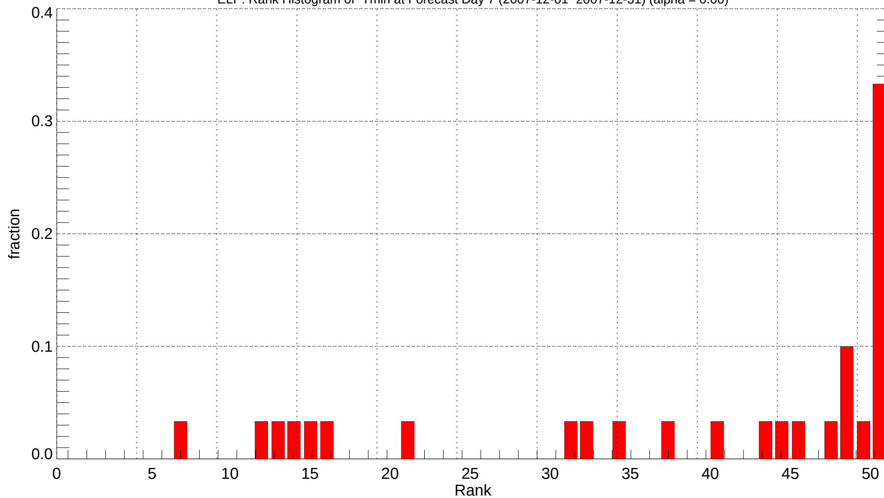
ELP: Rank Histogram of Tmin at Forecast Day 7 (2007-12-01~2007-12-31) (alpha = 0.00)
