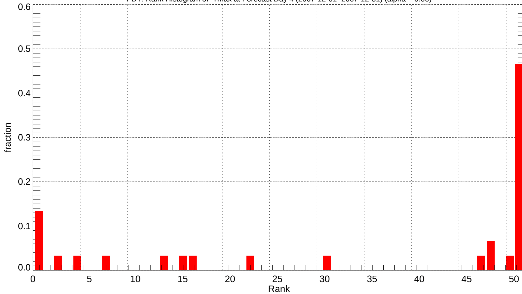
PDT: Rank Histogram of Tmax at Forecast Day 4 (2007-12-01~2007-12-31) (alpha = 0.00)
