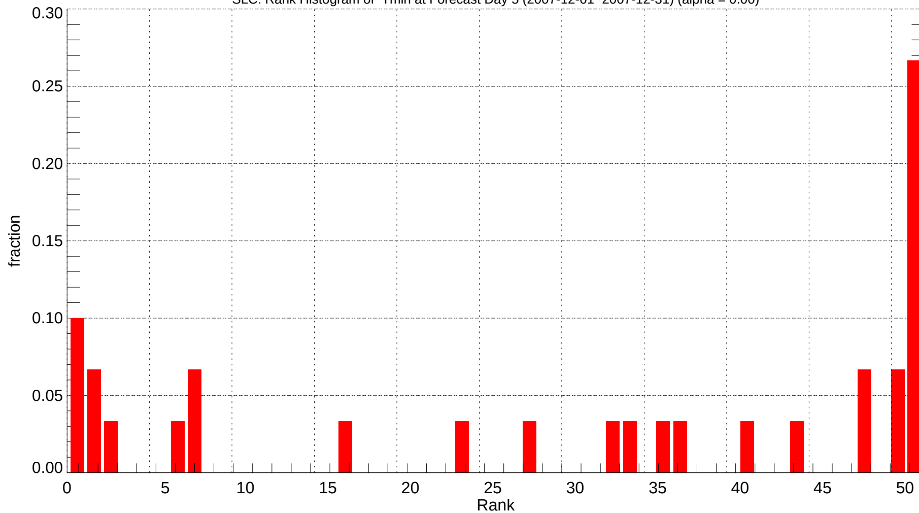
SLC: Rank Histogram of Tmin at Forecast Day 5 (2007-12-01~2007-12-31) (alpha = 0.00)
