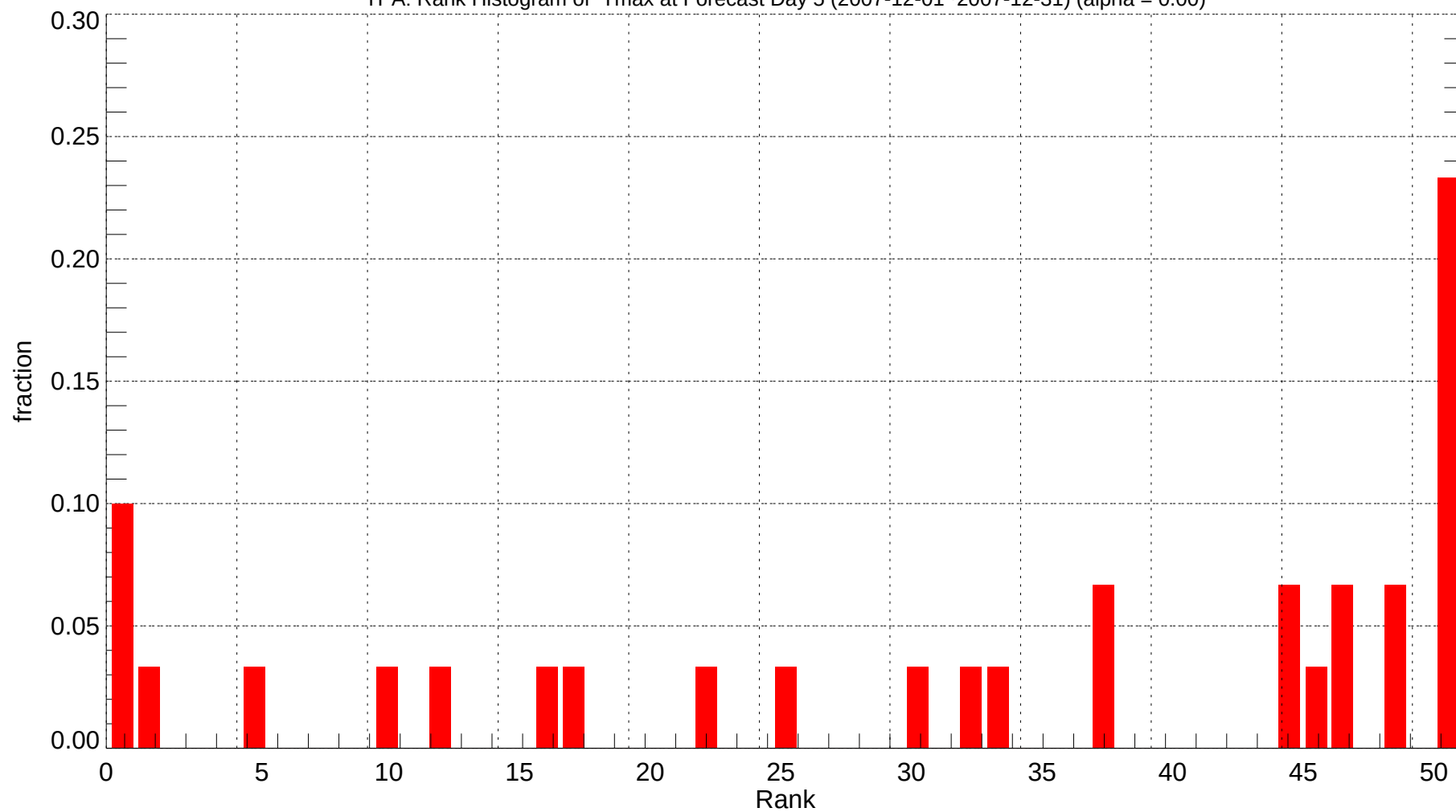
TPA: Rank Histogram of Tmax at Forecast Day 5 (2007-12-01~2007-12-31) (alpha = 0.00)
