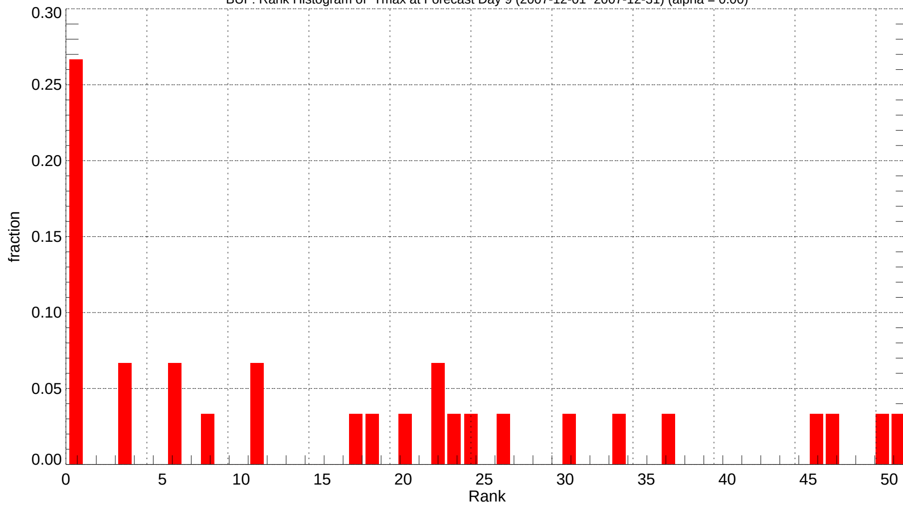
BUF: Rank Histogram of Tmax at Forecast Day 9 (2007-12-01~2007-12-31) (alpha = 0.00)
