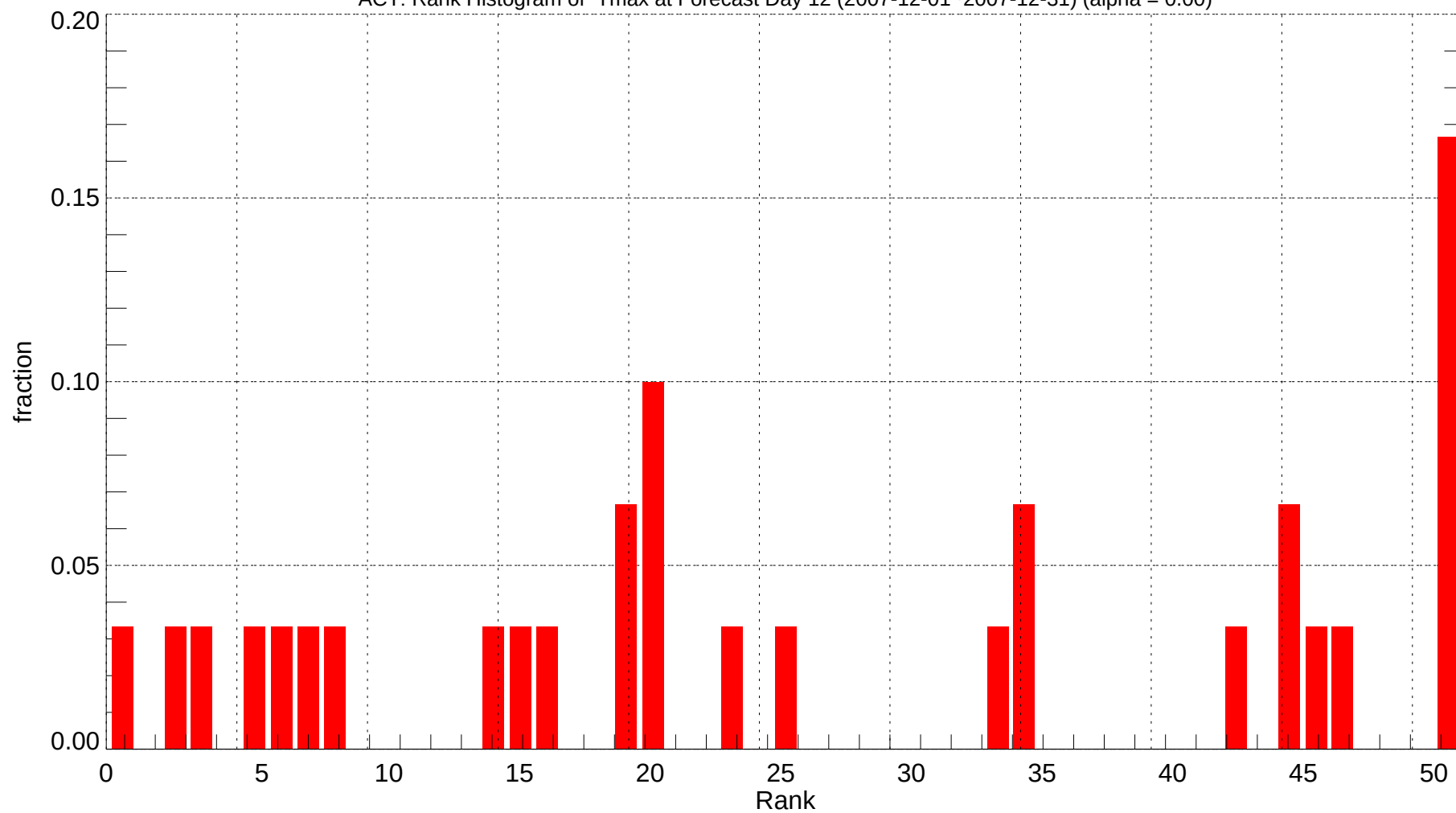
ACT: Rank Histogram of Tmax at Forecast Day 12 (2007-12-01~2007-12-31) (alpha = 0.00)
