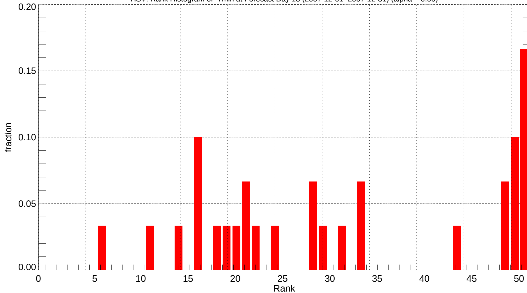
HSV: Rank Histogram of Tmin at Forecast Day 13 (2007-12-01~2007-12-31) (alpha = 0.00)
