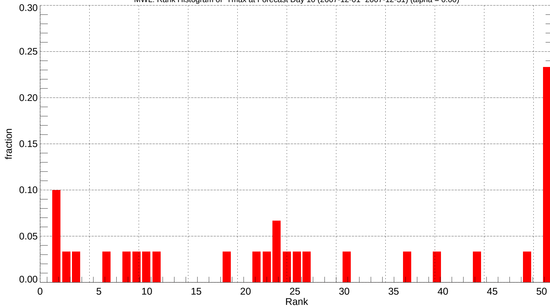
MWL: Rank Histogram of Tmax at Forecast Day 10 (2007-12-01~2007-12-31) (alpha = 0.00)
