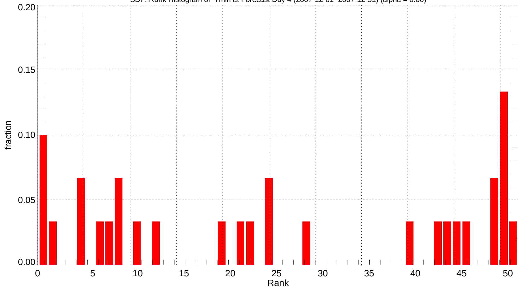
SDF: Rank Histogram of Tmin at Forecast Day 4 (2007-12-01~2007-12-31) (alpha = 0.00)
