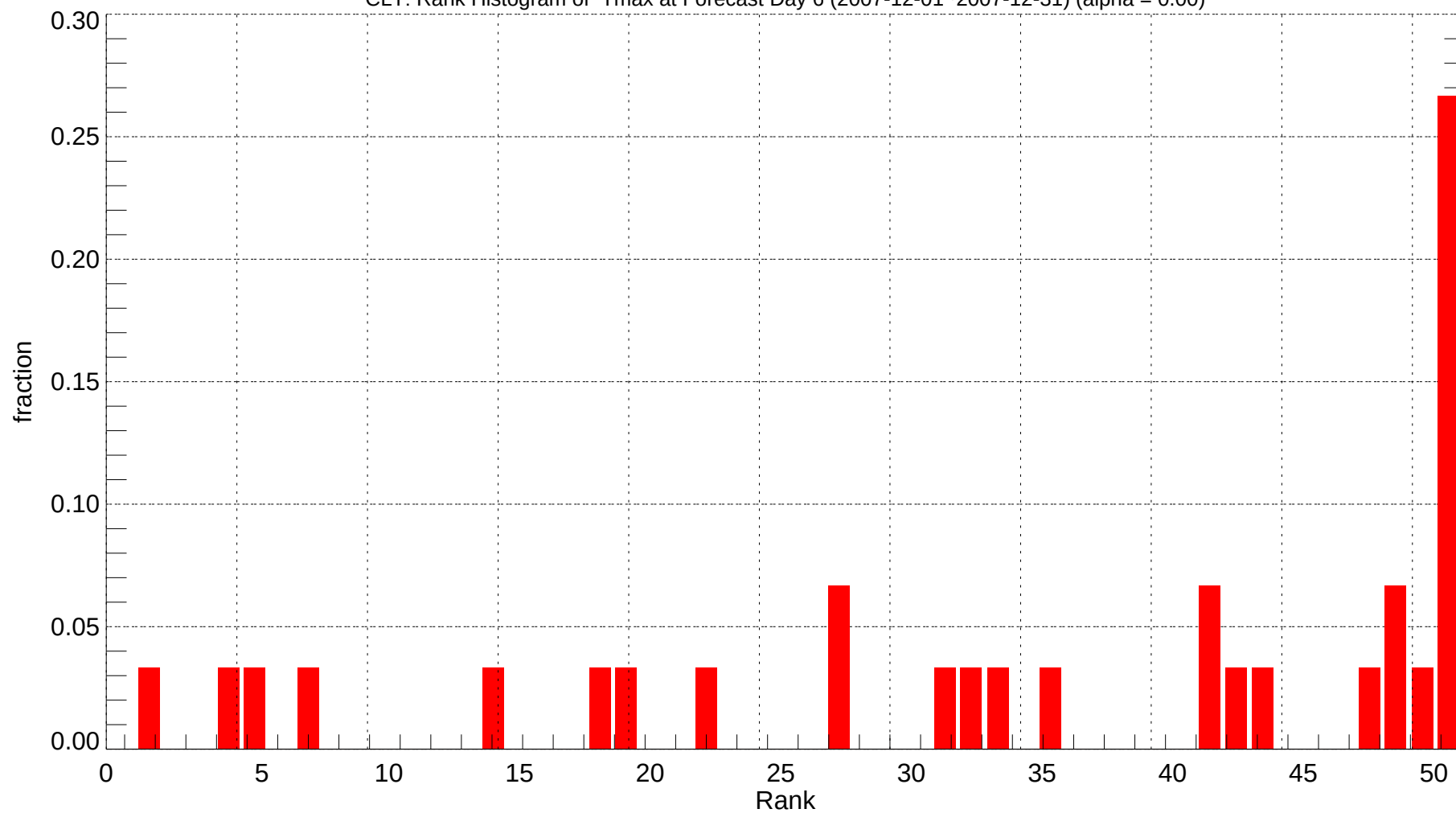
CLT: Rank Histogram of Tmax at Forecast Day 6 (2007-12-01~2007-12-31) (alpha = 0.00)
