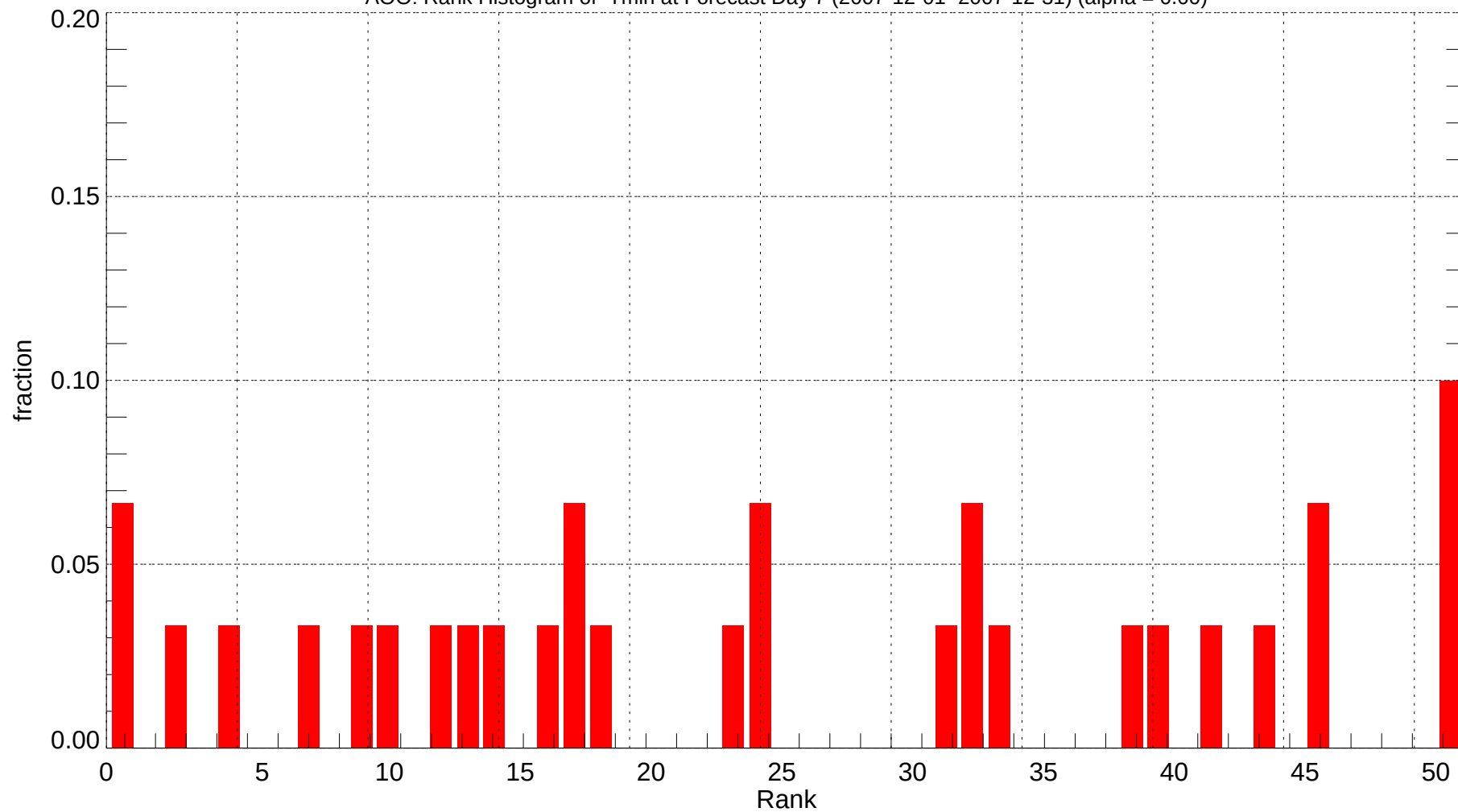
AOO: Rank Histogram of Tmin at Forecast Day 7 (2007-12-01~2007-12-31) (alpha = 0.00)
