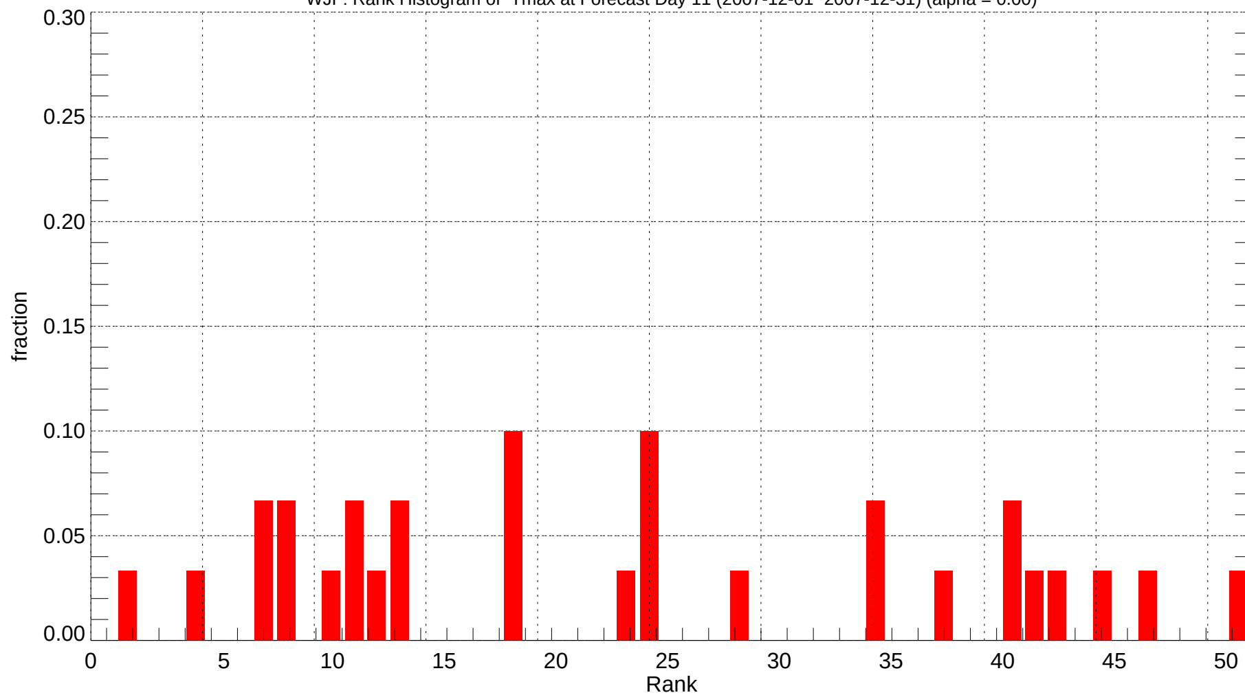
WJF: Rank Histogram of Tmax at Forecast Day 11 (2007-12-01~2007-12-31) (alpha = 0.00)
