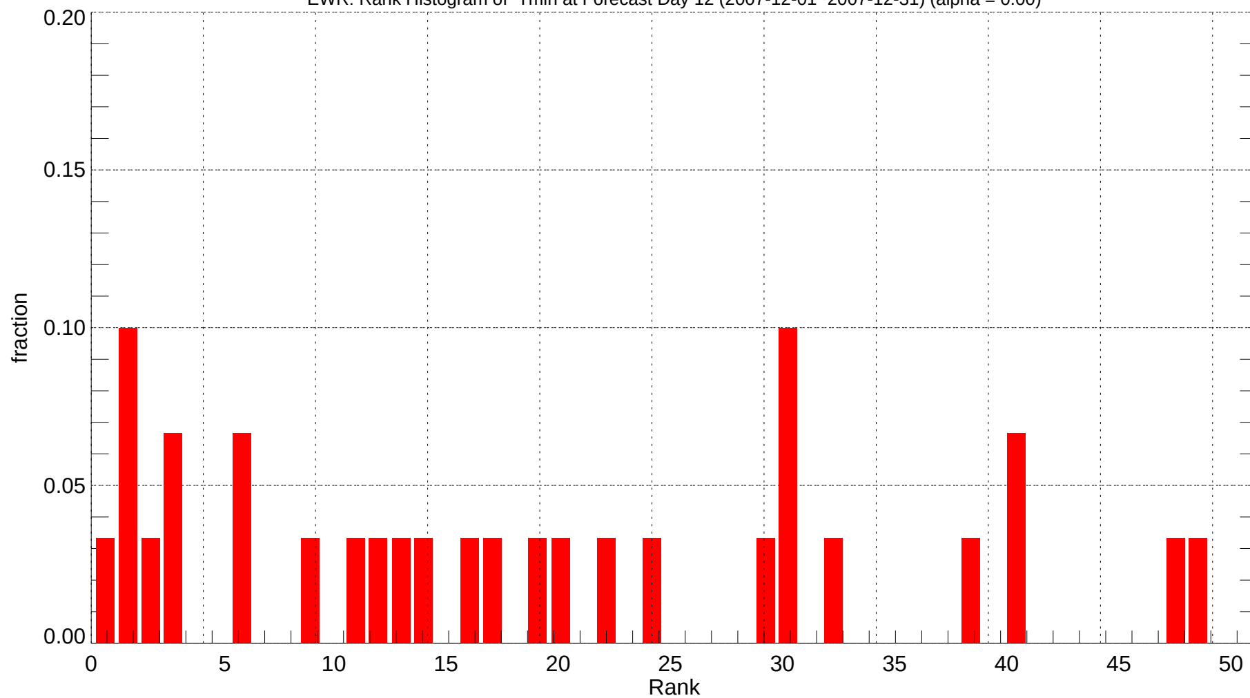
EWR: Rank Histogram of Tmin at Forecast Day 12 (2007-12-01~2007-12-31) (alpha = 0.00)
