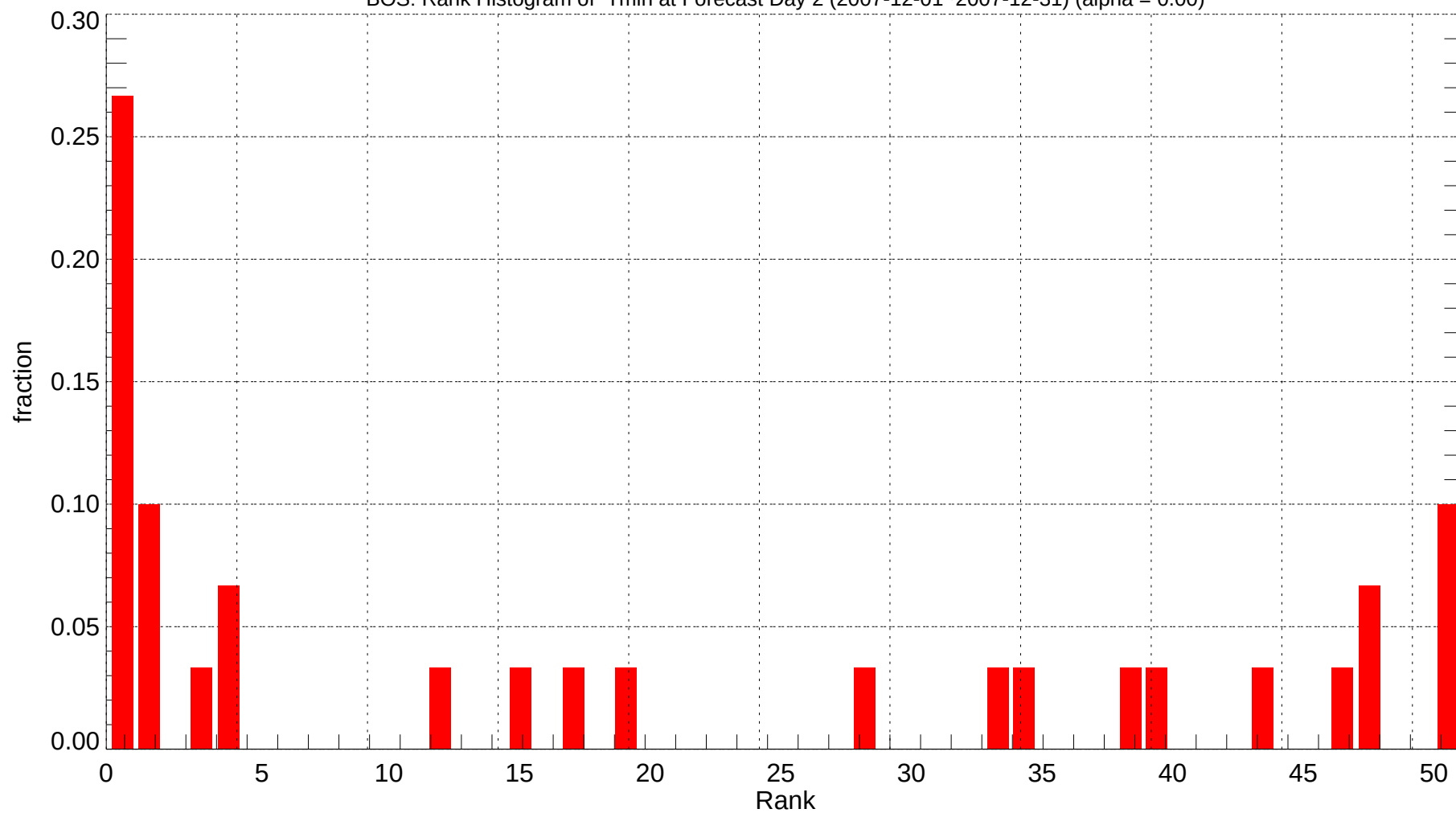
BOS: Rank Histogram of Tmin at Forecast Day 2 (2007-12-01~2007-12-31) (alpha = 0.00)
