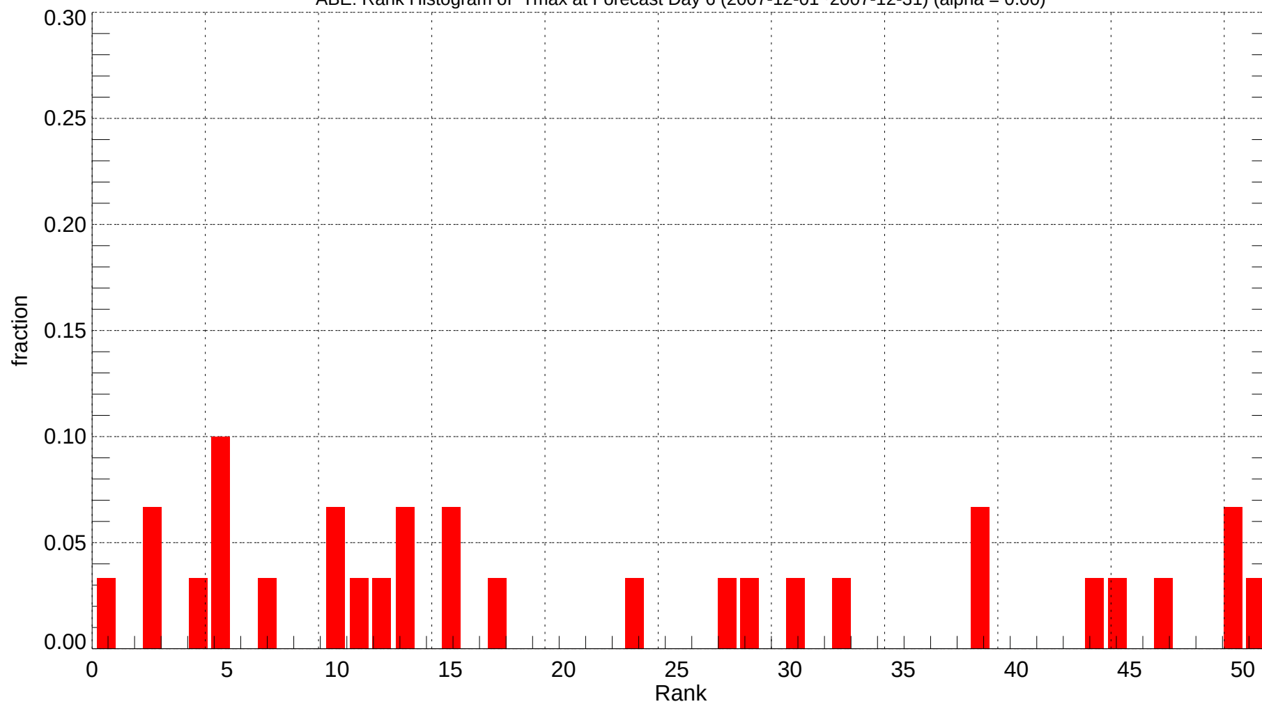
ABE: Rank Histogram of Tmax at Forecast Day 6 (2007-12-01~2007-12-31) (alpha = 0.00)
