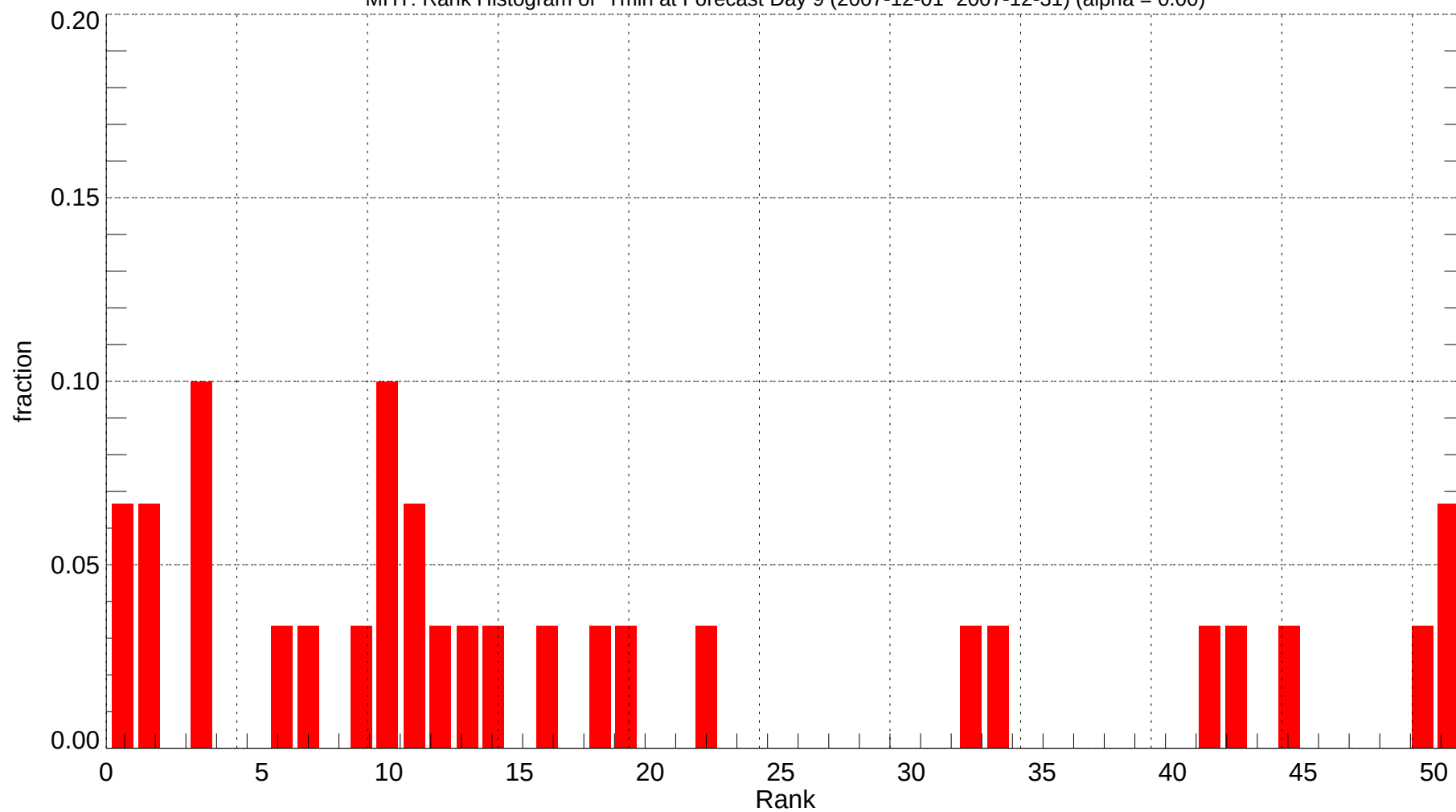
MHT: Rank Histogram of Tmin at Forecast Day 9 (2007-12-01~2007-12-31) (alpha = 0.00)
