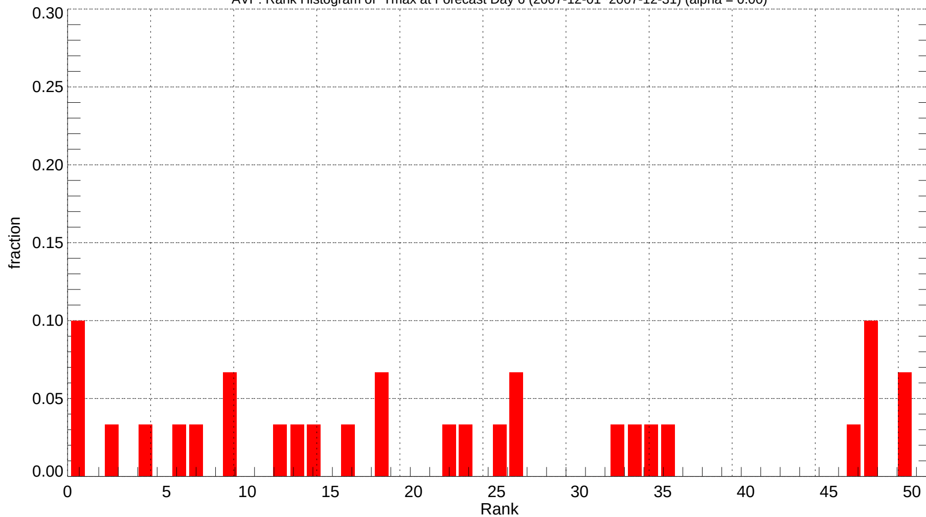
AVP: Rank Histogram of Tmax at Forecast Day 6 (2007-12-01~2007-12-31) (alpha = 0.00)
