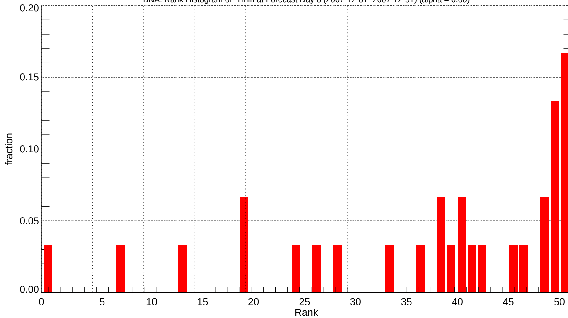
BNA: Rank Histogram of Tmin at Forecast Day 6 (2007-12-01~2007-12-31) (alpha = 0.00)
