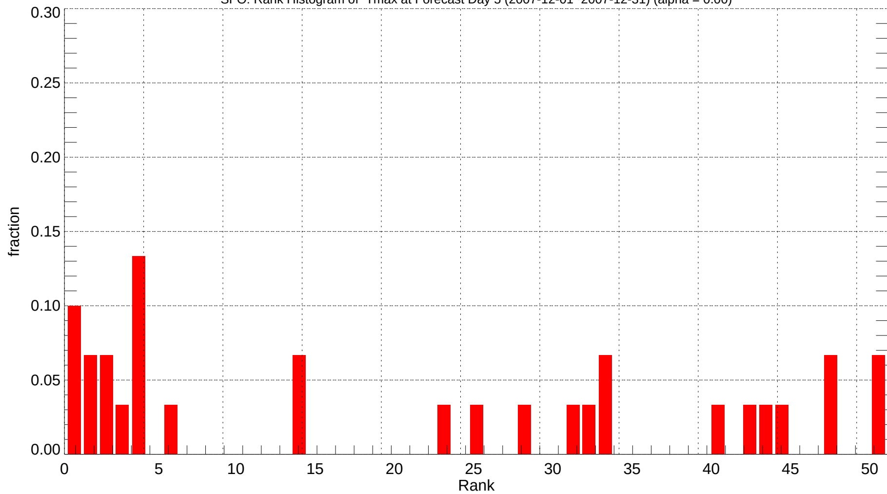
SFO: Rank Histogram of Tmax at Forecast Day 5 (2007-12-01~2007-12-31) (alpha = 0.00)
