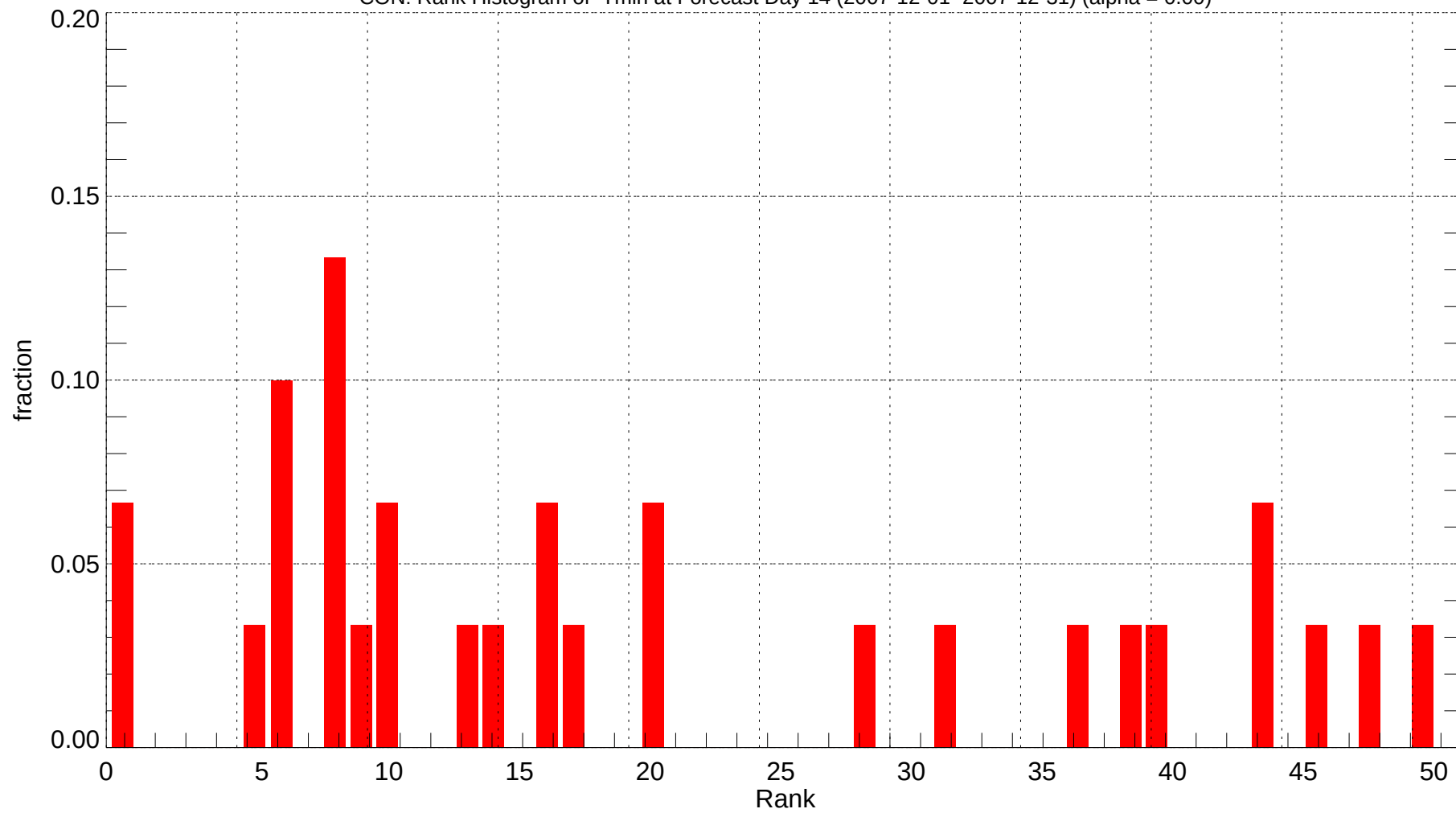
CON: Rank Histogram of Tmin at Forecast Day 14 (2007-12-01~2007-12-31) (alpha = 0.00)
