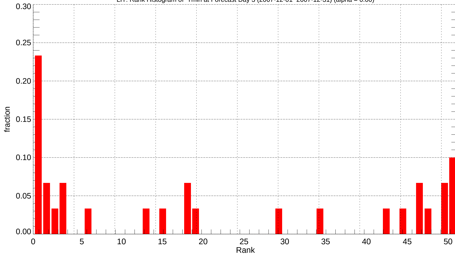
LIT: Rank Histogram of Tmin at Forecast Day 3 (2007-12-01~2007-12-31) (alpha = 0.00)
