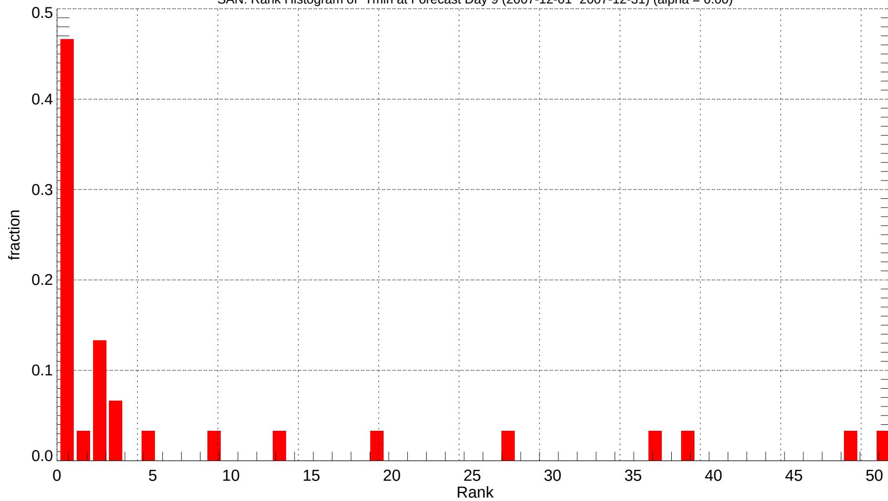
SAN: Rank Histogram of Tmin at Forecast Day 9 (2007-12-01~2007-12-31) (alpha = 0.00)
