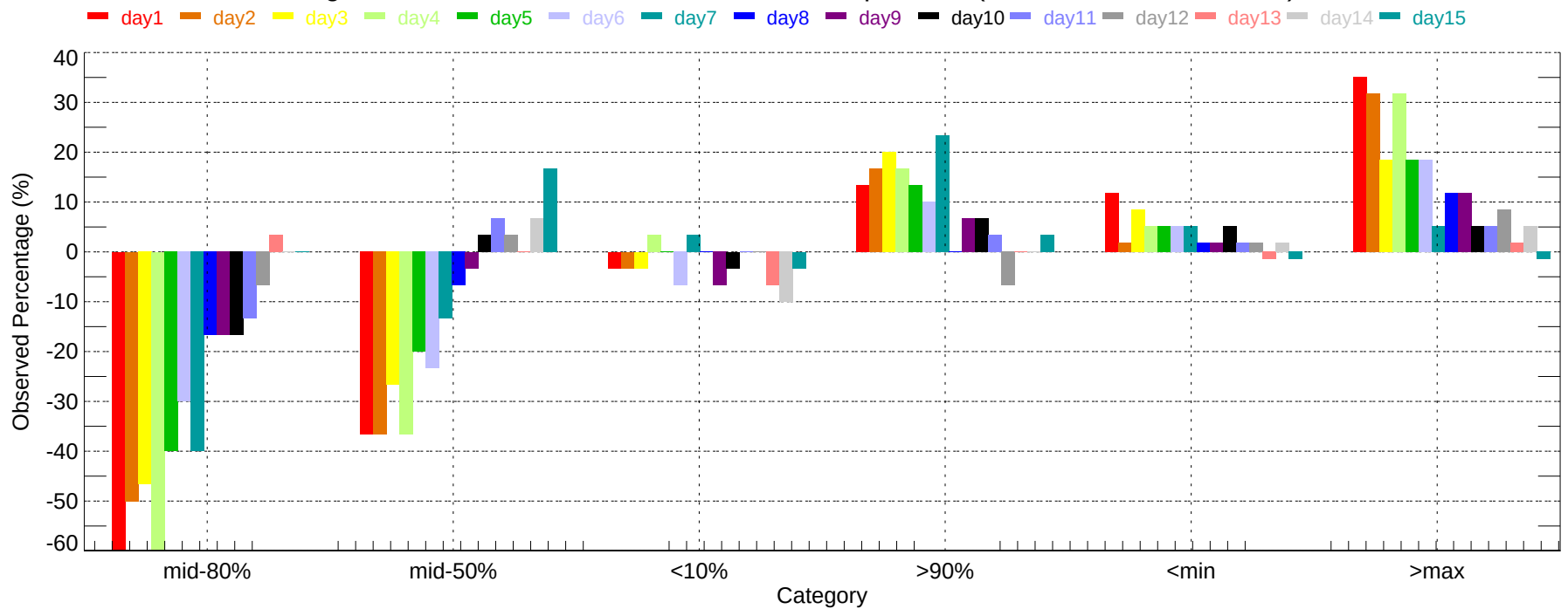
Observed Percentage Deviation of Ensembles - PDX: Min Temperature (2007-12-01~2007-12-31)
