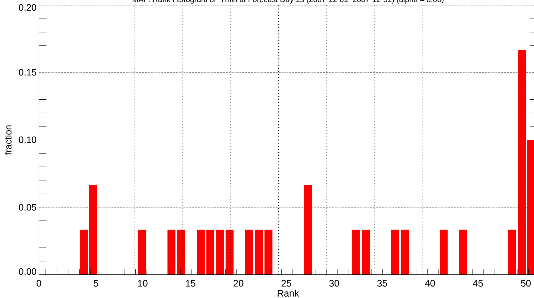
MAF: Rank Histogram of Tmin at Forecast Day 15 (2007-12-01~2007-12-31) (alpha = 0.00)
