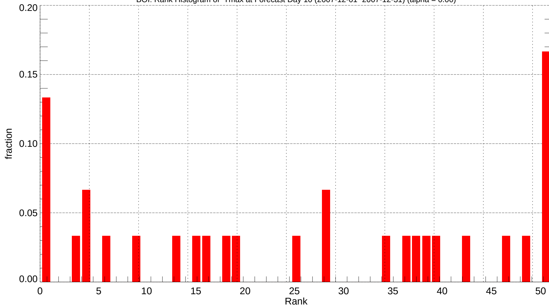
BOI: Rank Histogram of Tmax at Forecast Day 10 (2007-12-01~2007-12-31) (alpha = 0.00)
