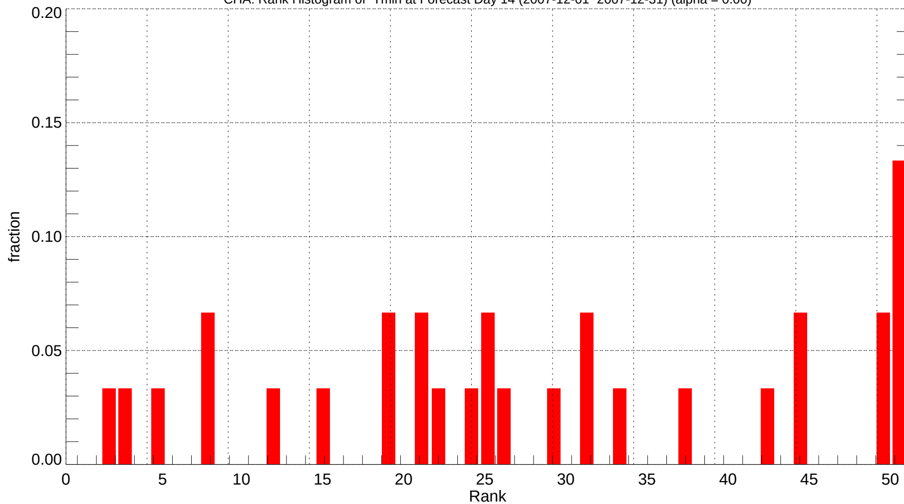
CHA: Rank Histogram of Tmin at Forecast Day 14 (2007-12-01~2007-12-31) (alpha = 0.00)
