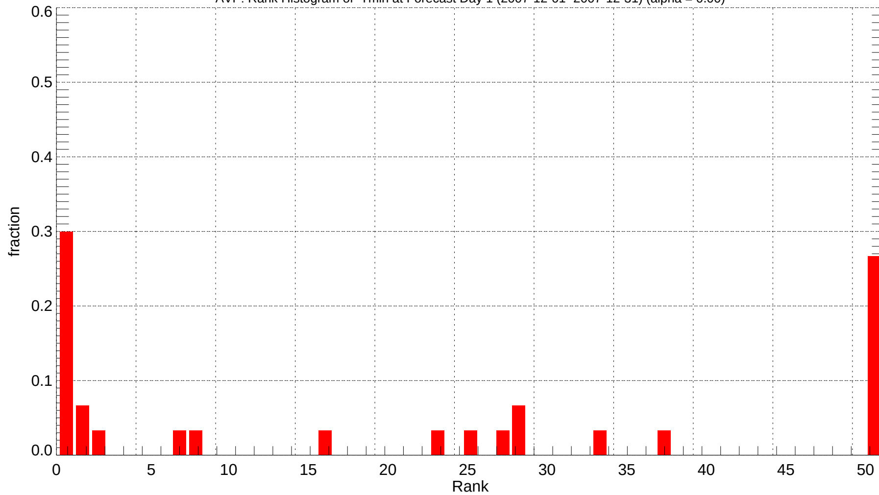
AVP: Rank Histogram of Tmin at Forecast Day 1 (2007-12-01~2007-12-31) (alpha = 0.00)
