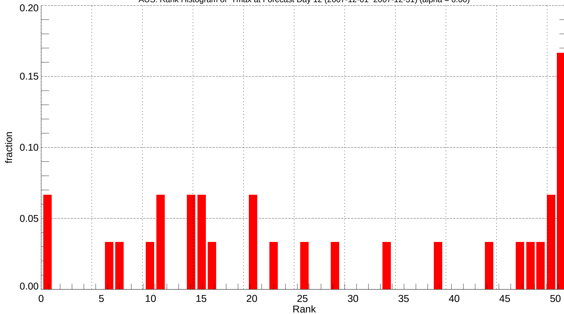
AUS: Rank Histogram of Tmax at Forecast Day 12 (2007-12-01~2007-12-31) (alpha = 0.00)
