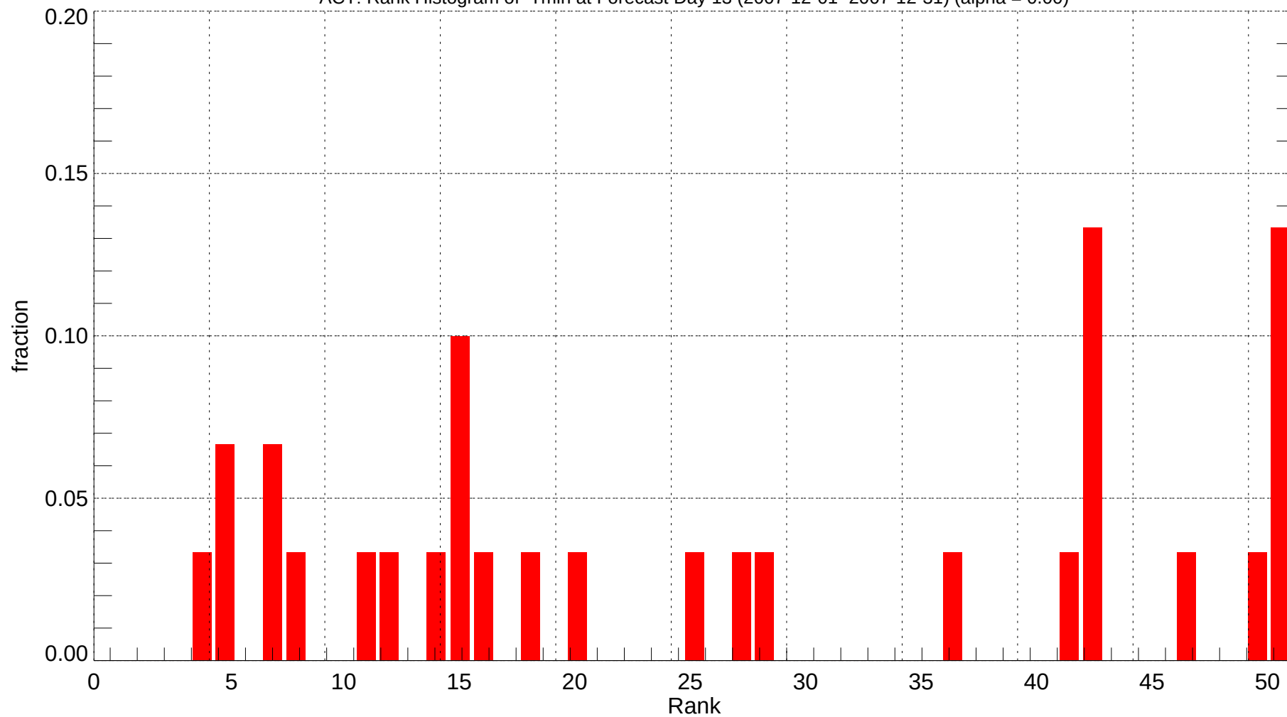
ACT: Rank Histogram of Tmin at Forecast Day 13 (2007-12-01~2007-12-31) (alpha = 0.00)
