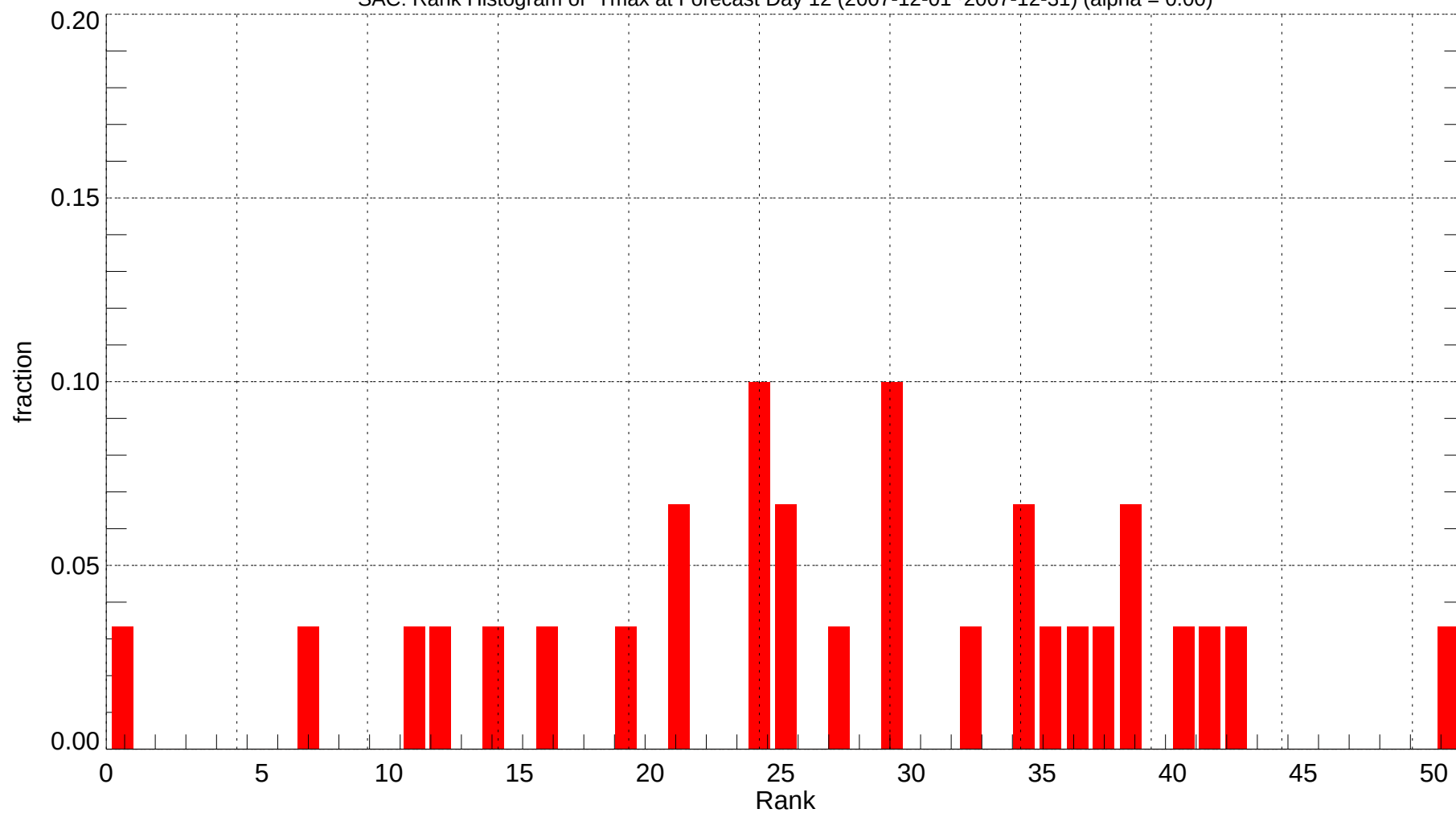
SAC: Rank Histogram of Tmax at Forecast Day 12 (2007-12-01~2007-12-31) (alpha = 0.00)
