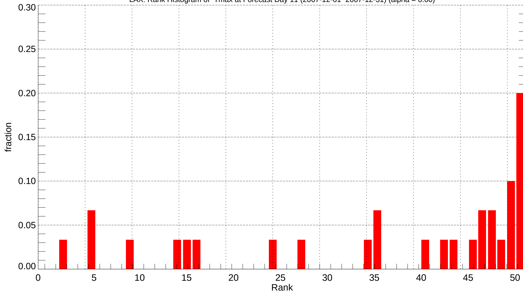
LAX: Rank Histogram of Tmax at Forecast Day 11 (2007-12-01~2007-12-31) (alpha = 0.00)
