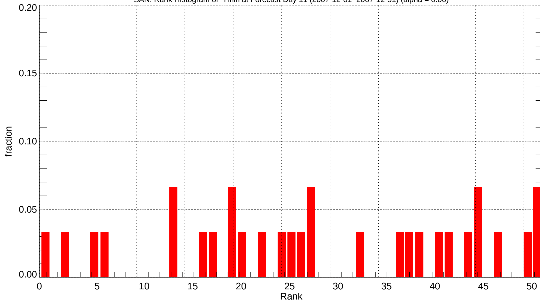
SAN: Rank Histogram of Tmin at Forecast Day 11 (2007-12-01~2007-12-31) (alpha = 0.00)
