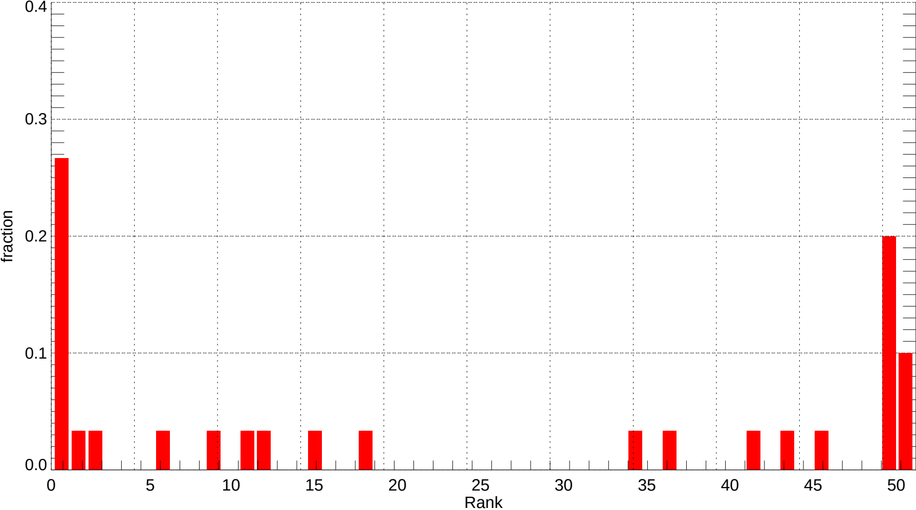
CLT: Rank Histogram of Tmin at Forecast Day 1 (2007-12-01~2007-12-31) (alpha = 0.00)
