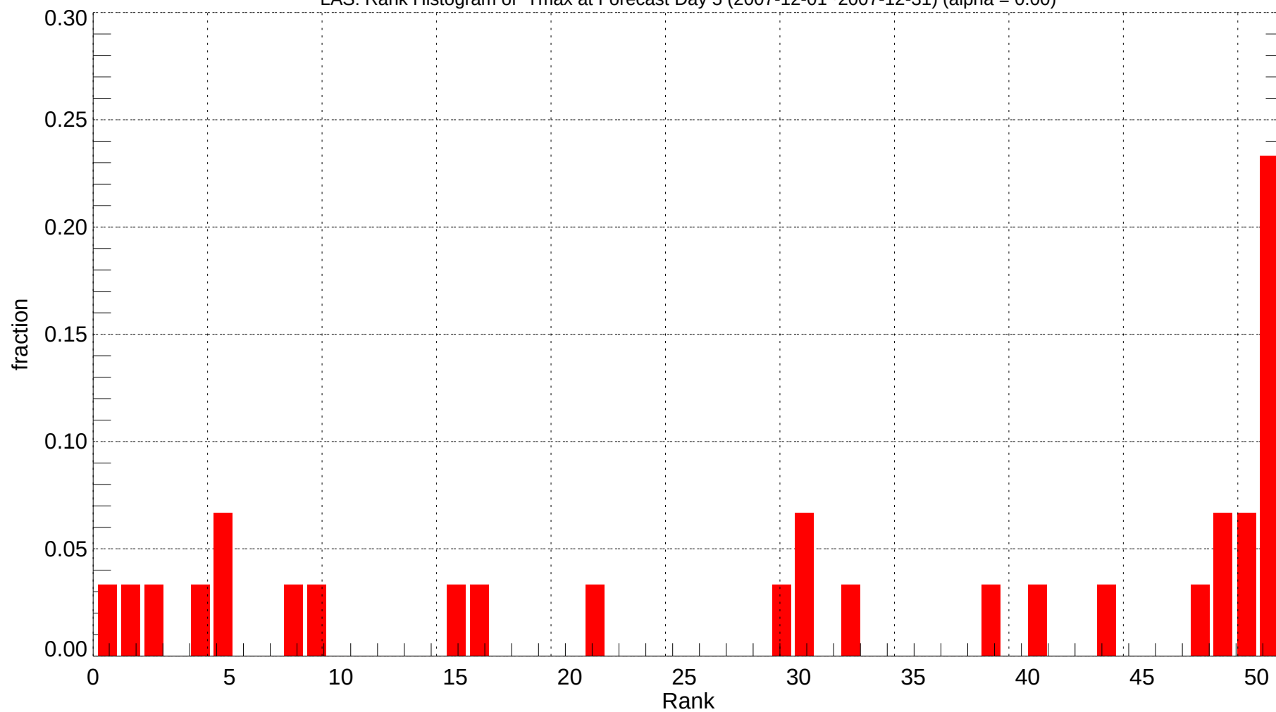
LAS: Rank Histogram of Tmax at Forecast Day 5 (2007-12-01~2007-12-31) (alpha = 0.00)
