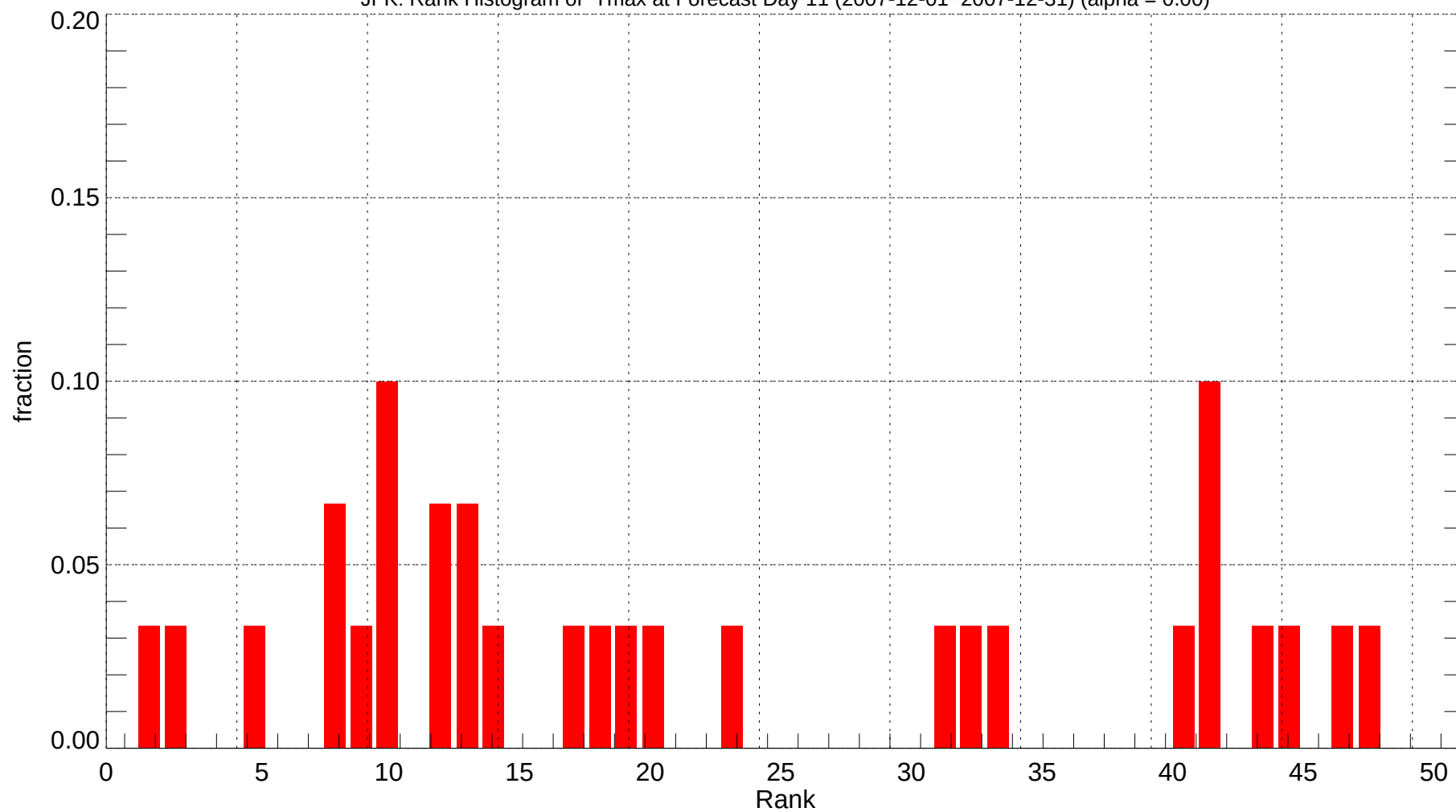
JFK: Rank Histogram of Tmax at Forecast Day 11 (2007-12-01~2007-12-31) (alpha = 0.00)
