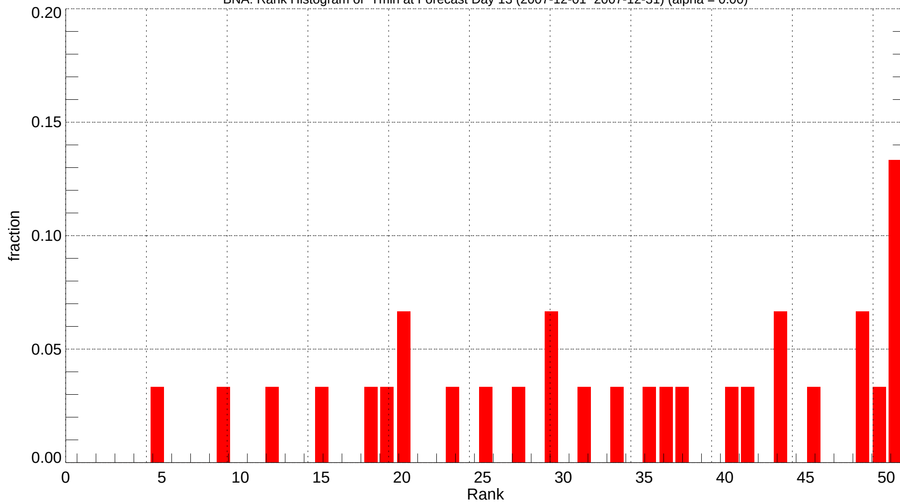
BNA: Rank Histogram of Tmin at Forecast Day 13 (2007-12-01~2007-12-31) (alpha = 0.00)
