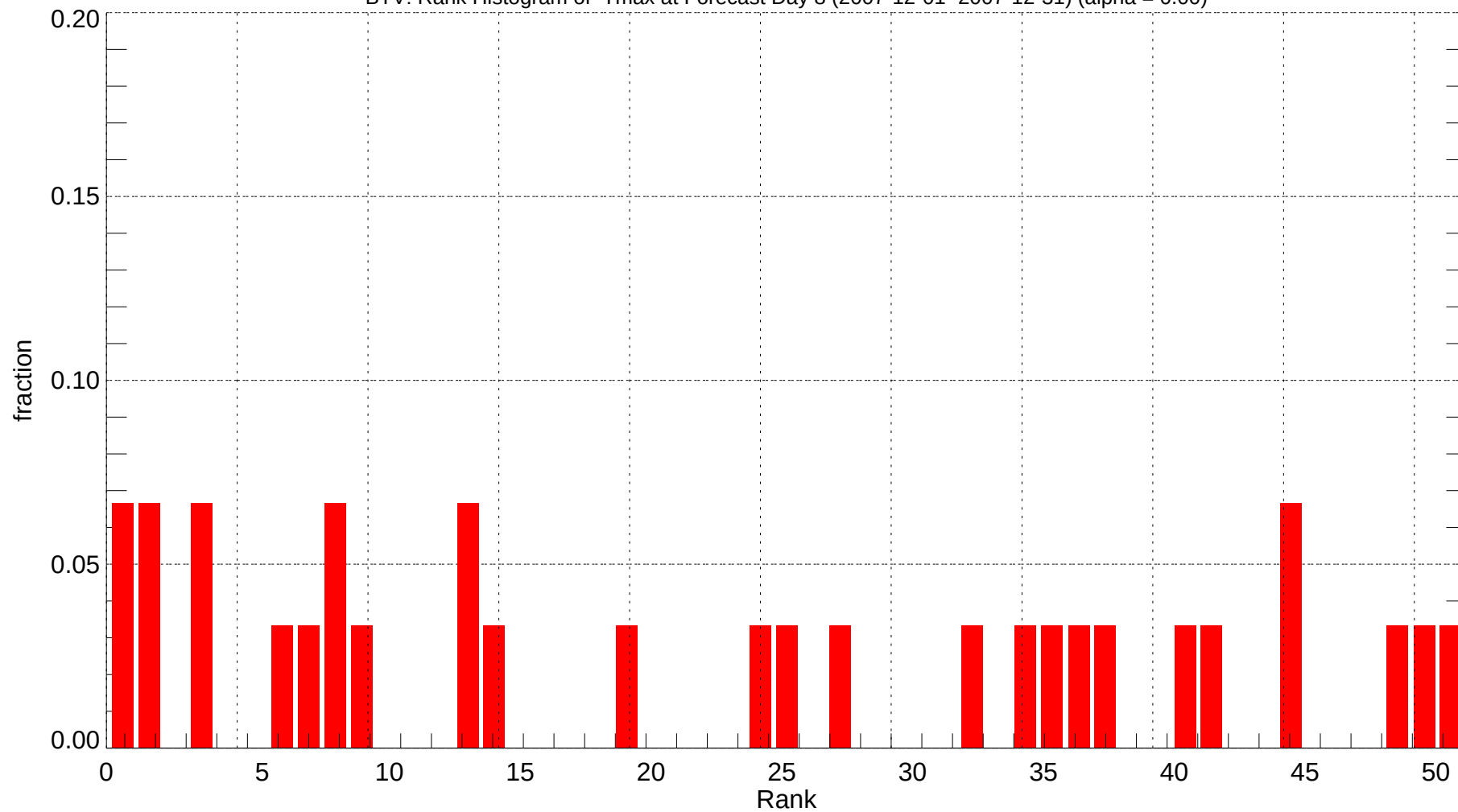
BTV: Rank Histogram of Tmax at Forecast Day 8 (2007-12-01~2007-12-31) (alpha = 0.00)
