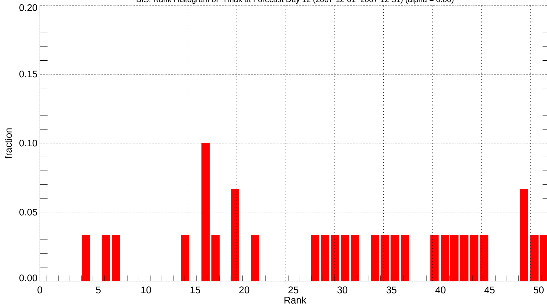
BIS: Rank Histogram of Tmax at Forecast Day 12 (2007-12-01~2007-12-31) (alpha = 0.00)
