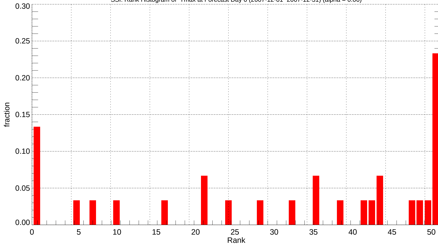
SSI: Rank Histogram of Tmax at Forecast Day 6 (2007-12-01~2007-12-31) (alpha = 0.00)
