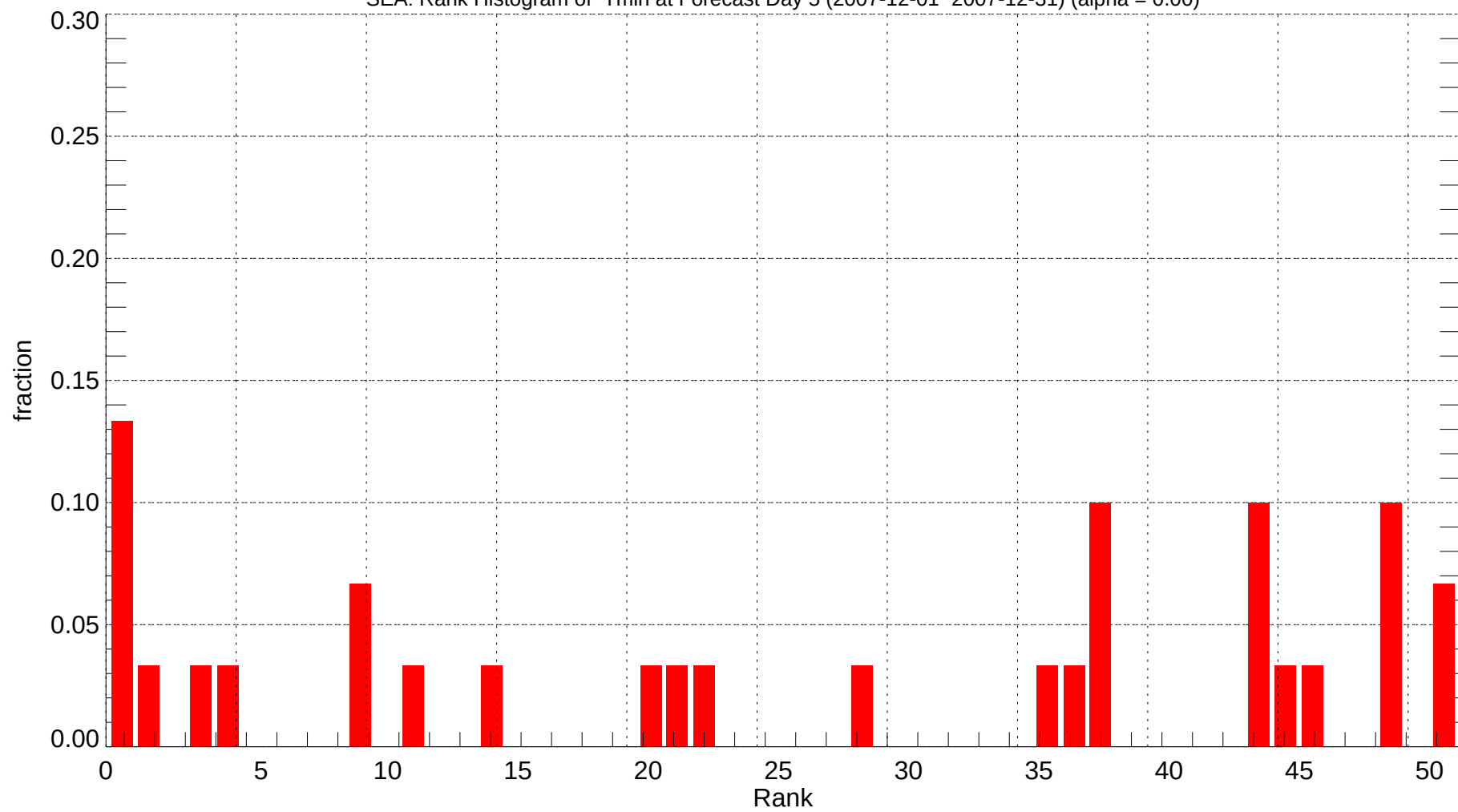
SEA: Rank Histogram of Tmin at Forecast Day 5 (2007-12-01~2007-12-31) (alpha = 0.00)
