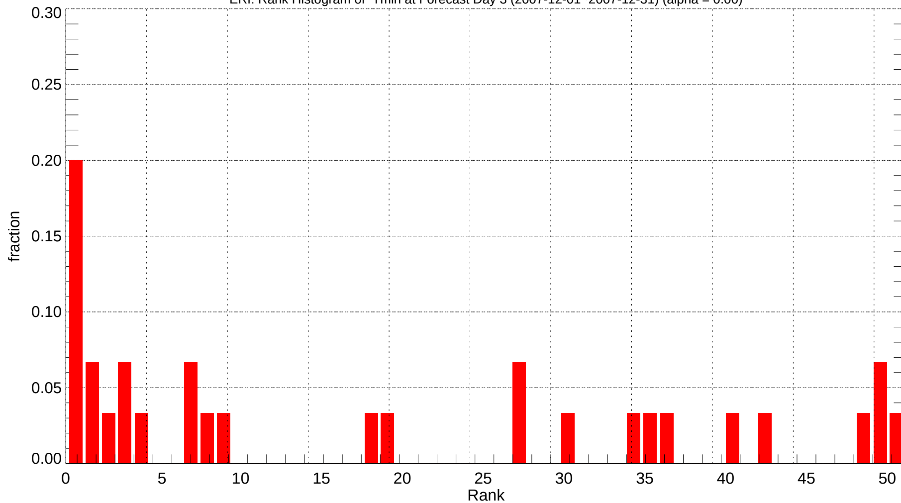
ERI: Rank Histogram of Tmin at Forecast Day 3 (2007-12-01~2007-12-31) (alpha = 0.00)
