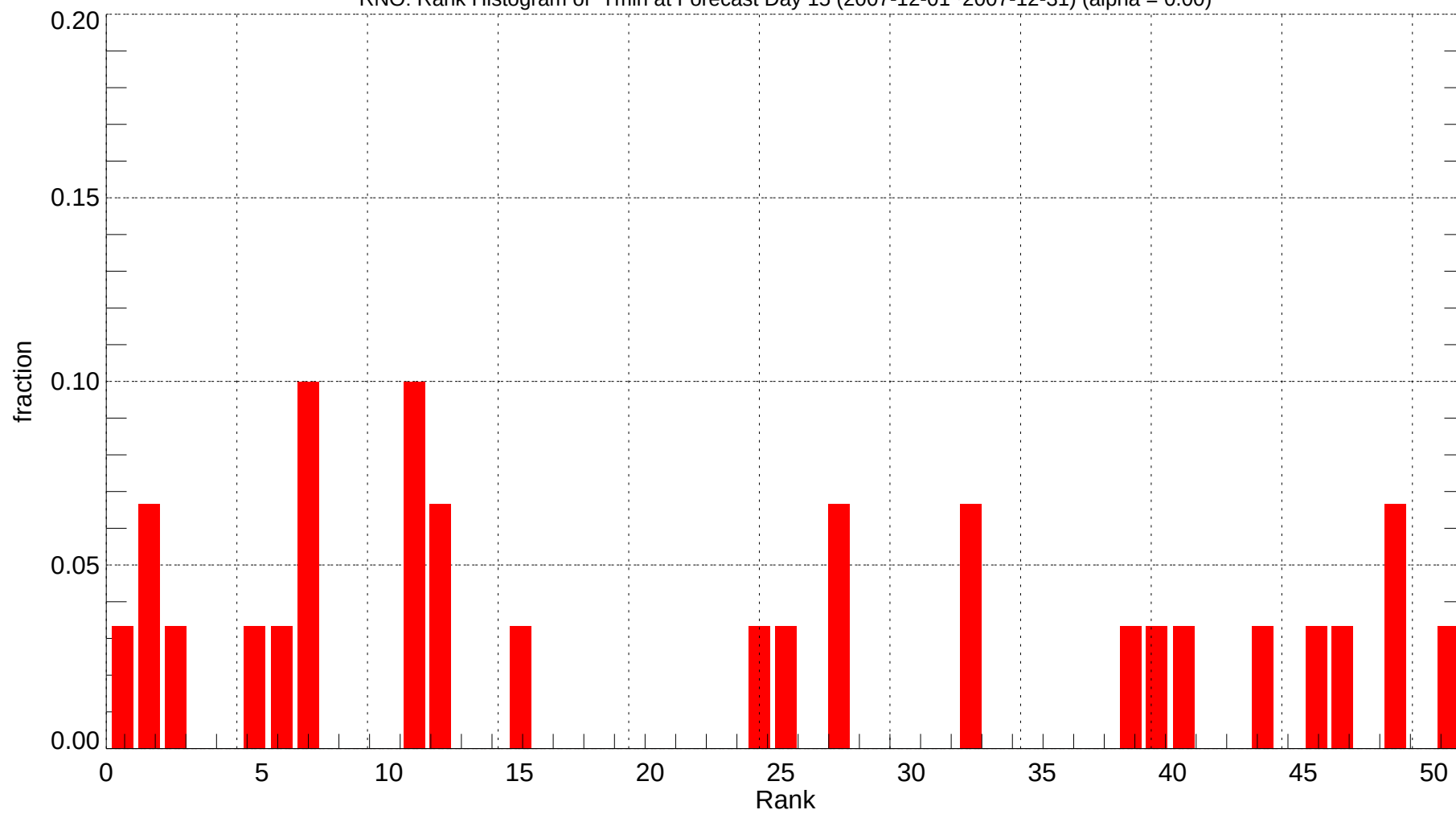
RNO: Rank Histogram of Tmin at Forecast Day 15 (2007-12-01~2007-12-31) (alpha = 0.00)
