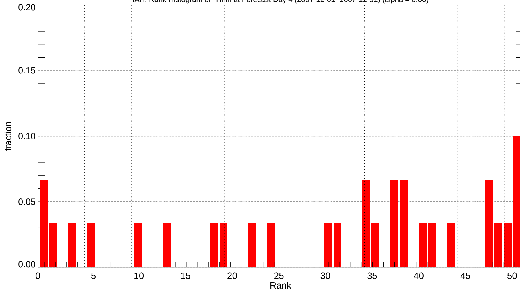
IAH: Rank Histogram of Tmin at Forecast Day 4 (2007-12-01~2007-12-31) (alpha = 0.00)
