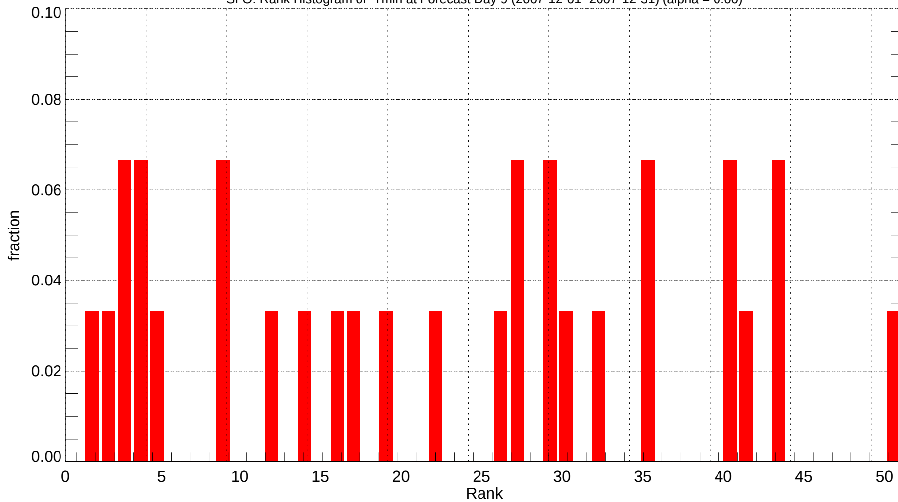
SFO: Rank Histogram of Tmin at Forecast Day 9 (2007-12-01~2007-12-31) (alpha = 0.00)
