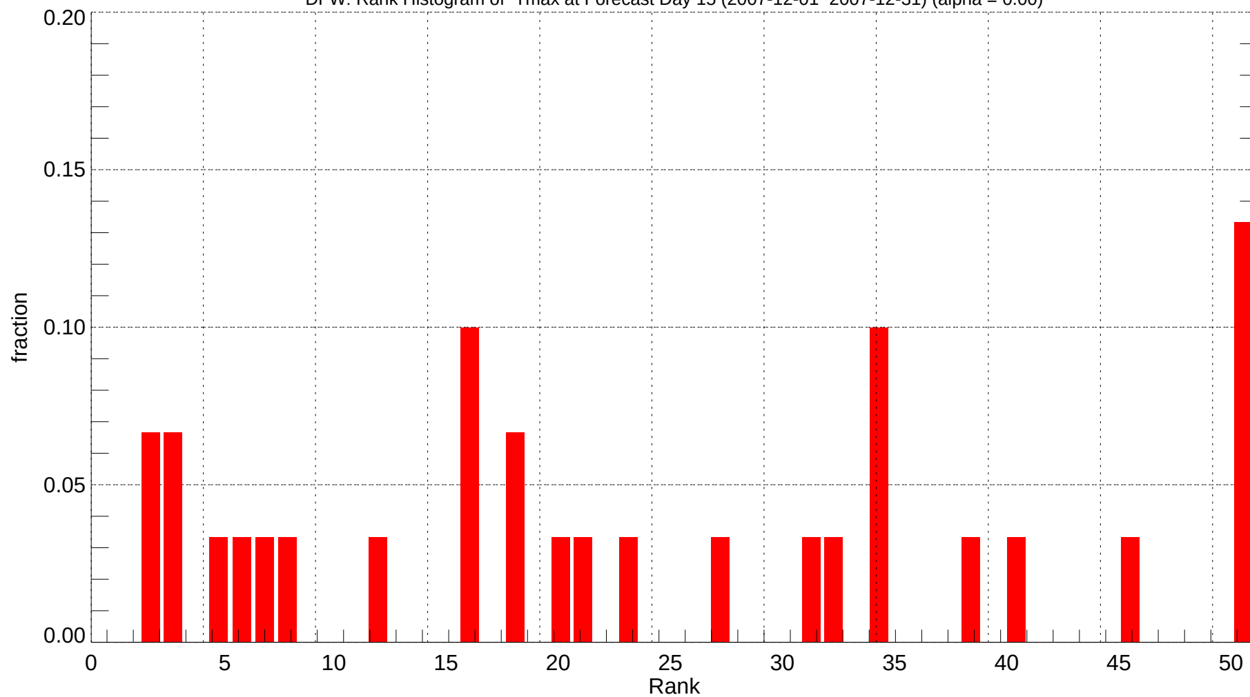
DFW: Rank Histogram of Tmax at Forecast Day 15 (2007-12-01~2007-12-31) (alpha = 0.00)
