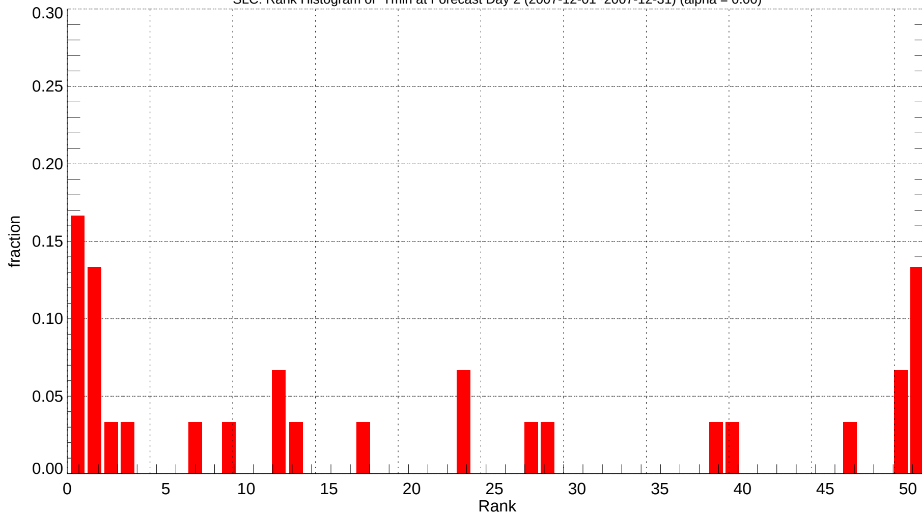
SLC: Rank Histogram of Tmin at Forecast Day 2 (2007-12-01~2007-12-31) (alpha = 0.00)
