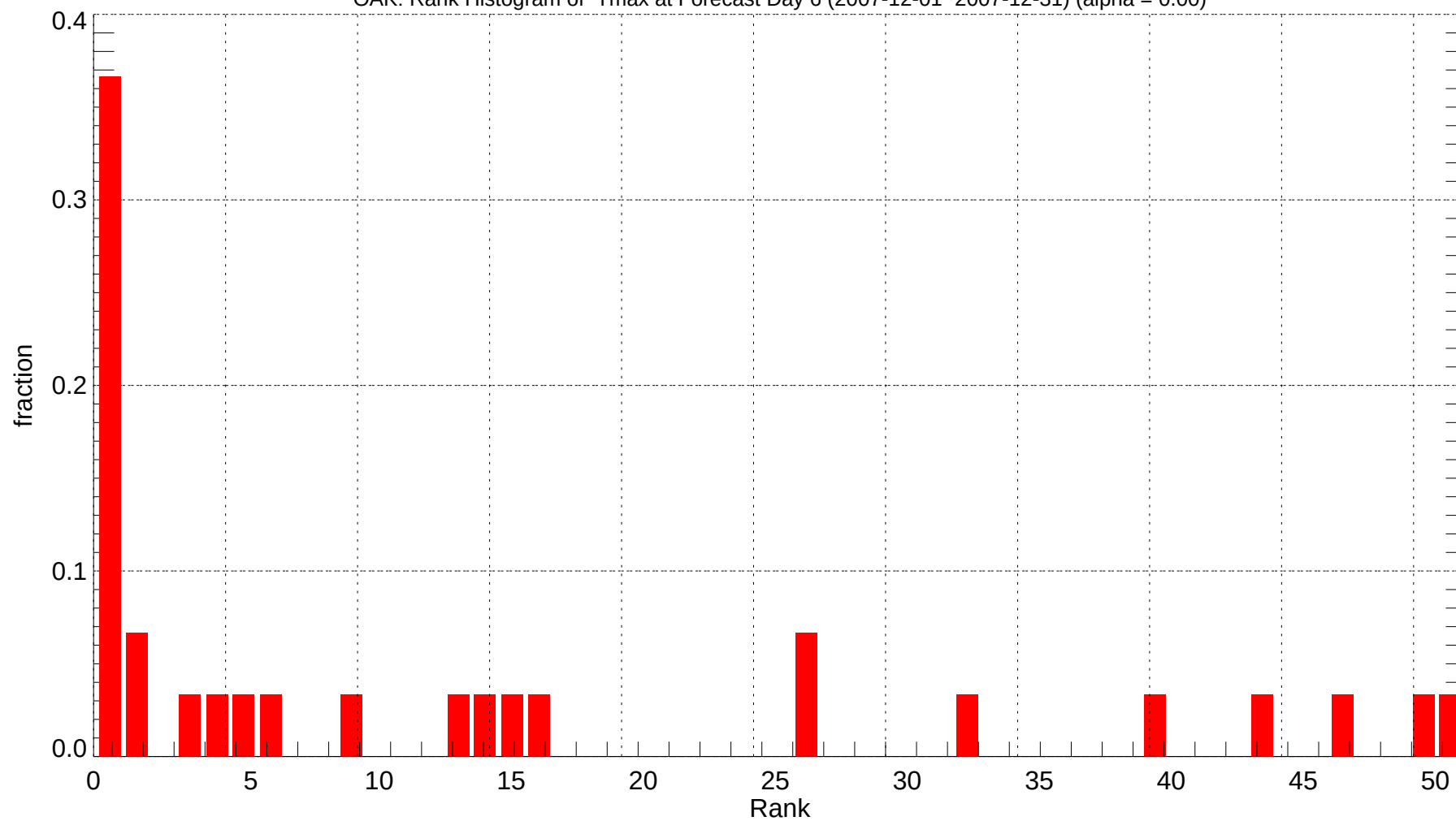
OAK: Rank Histogram of Tmax at Forecast Day 6 (2007-12-01~2007-12-31) (alpha = 0.00)
