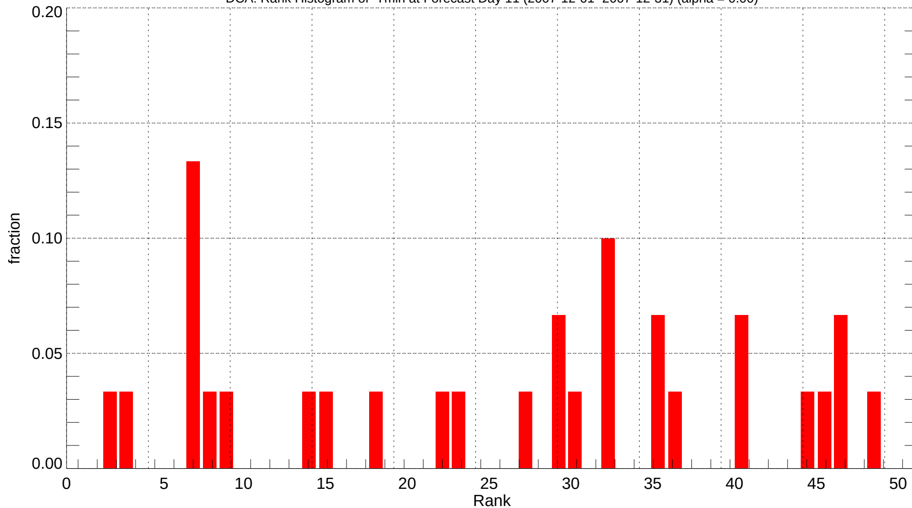
DCA: Rank Histogram of Tmin at Forecast Day 11 (2007-12-01~2007-12-31) (alpha = 0.00)
