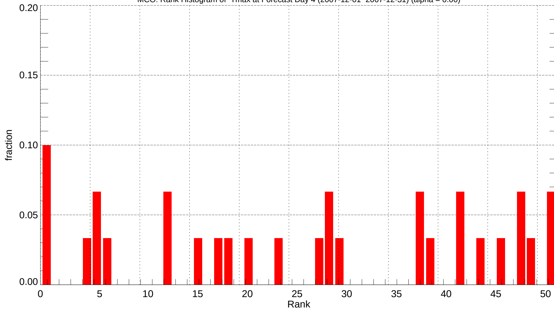
MCO: Rank Histogram of Tmax at Forecast Day 4 (2007-12-01~2007-12-31) (alpha = 0.00)
