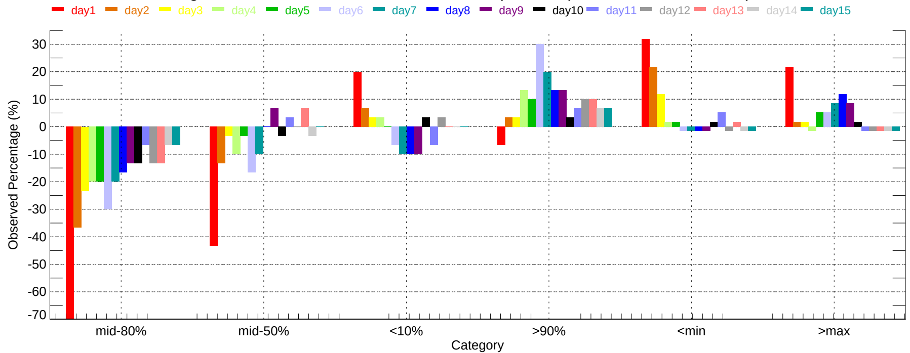
Observed Percentage Deviation of Ensembles - CLE: Min Temperature (2007-12-01~2007-12-31)
