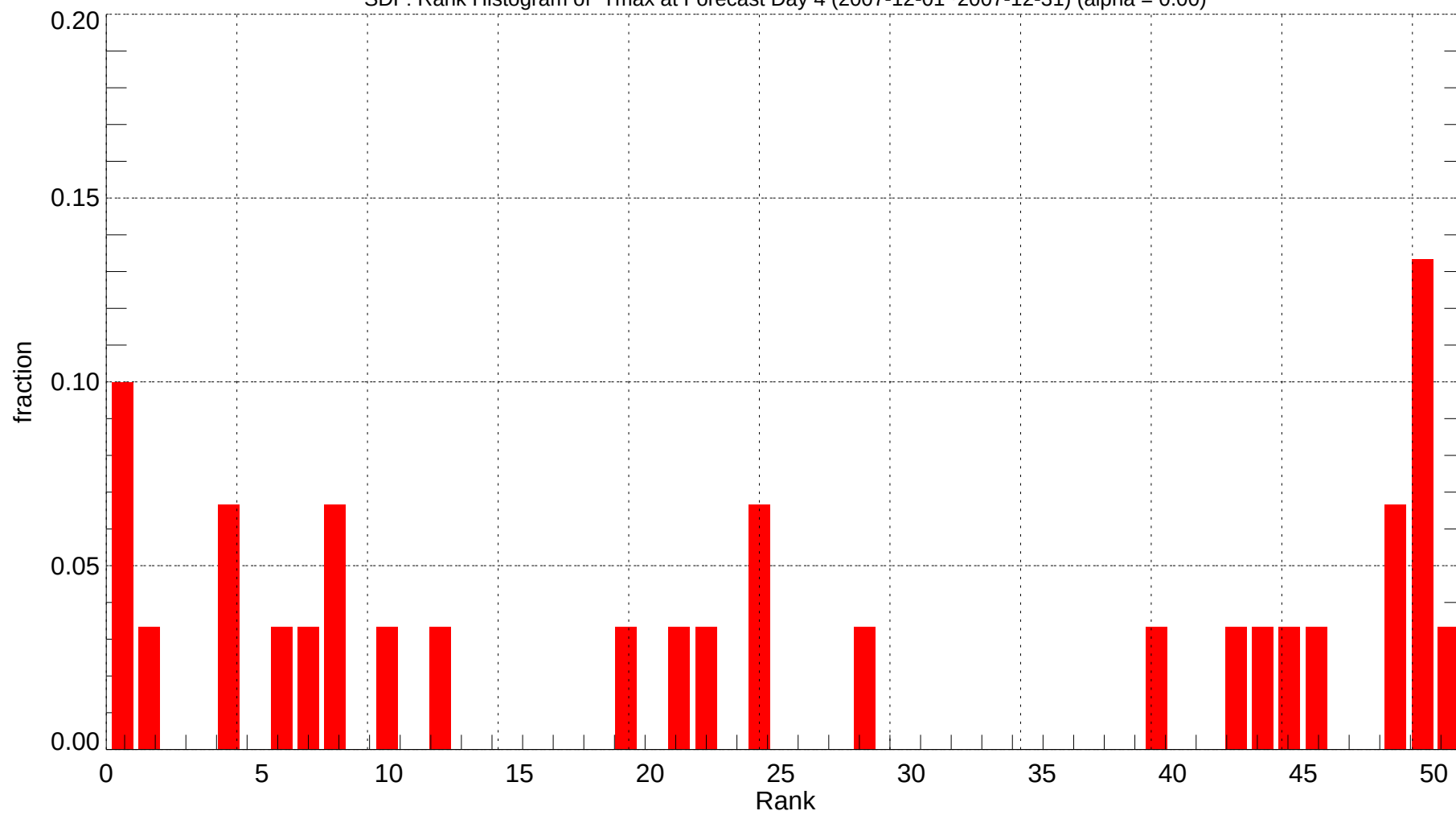
SDF: Rank Histogram of Tmax at Forecast Day 4 (2007-12-01~2007-12-31) (alpha = 0.00)
