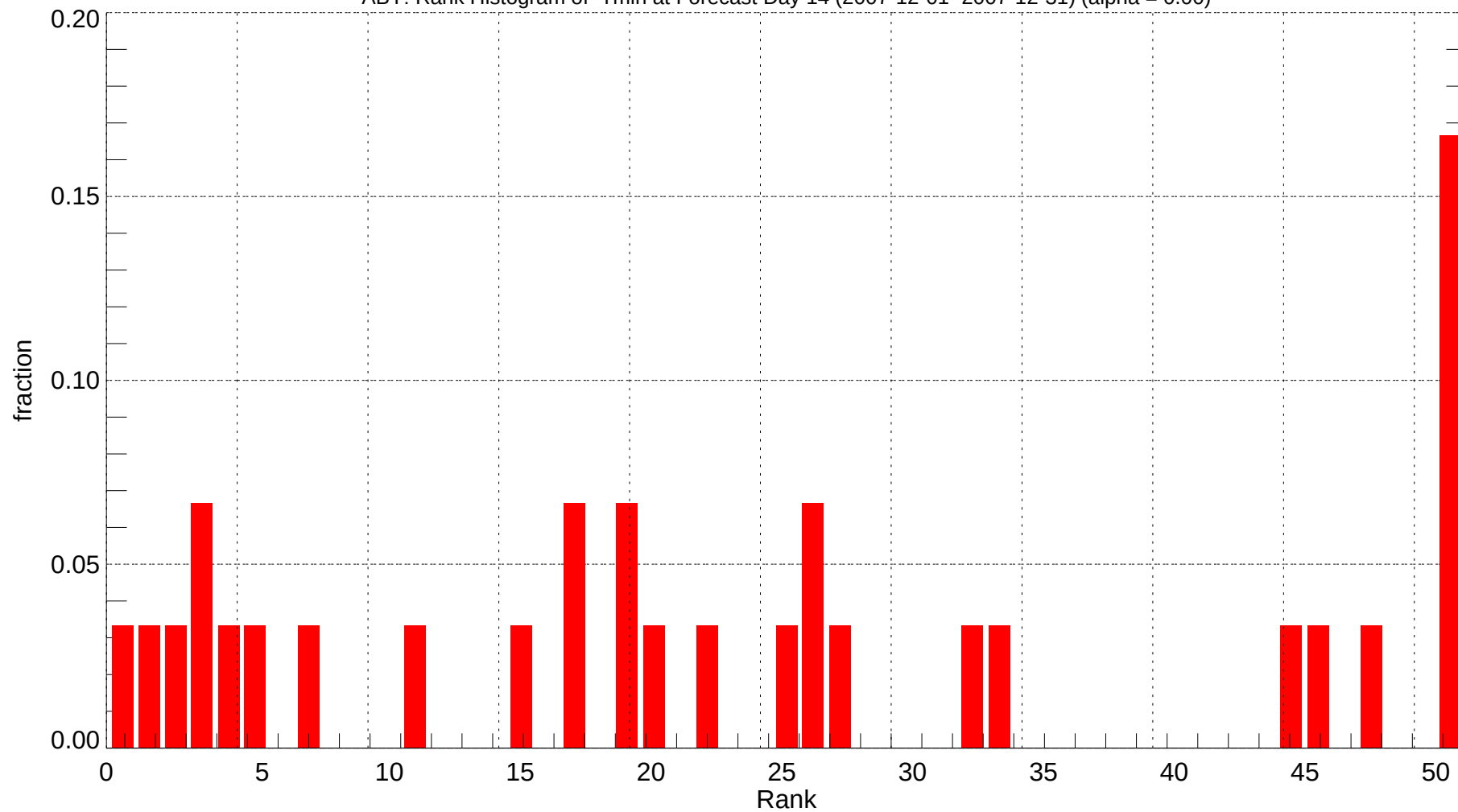
ABY: Rank Histogram of Tmin at Forecast Day 14 (2007-12-01~2007-12-31) (alpha = 0.00)
