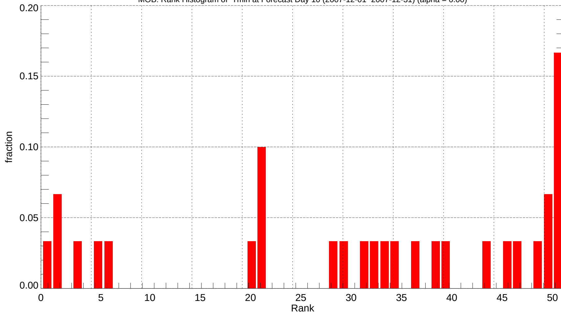
MOB: Rank Histogram of Tmin at Forecast Day 10 (2007-12-01~2007-12-31) (alpha = 0.00)
