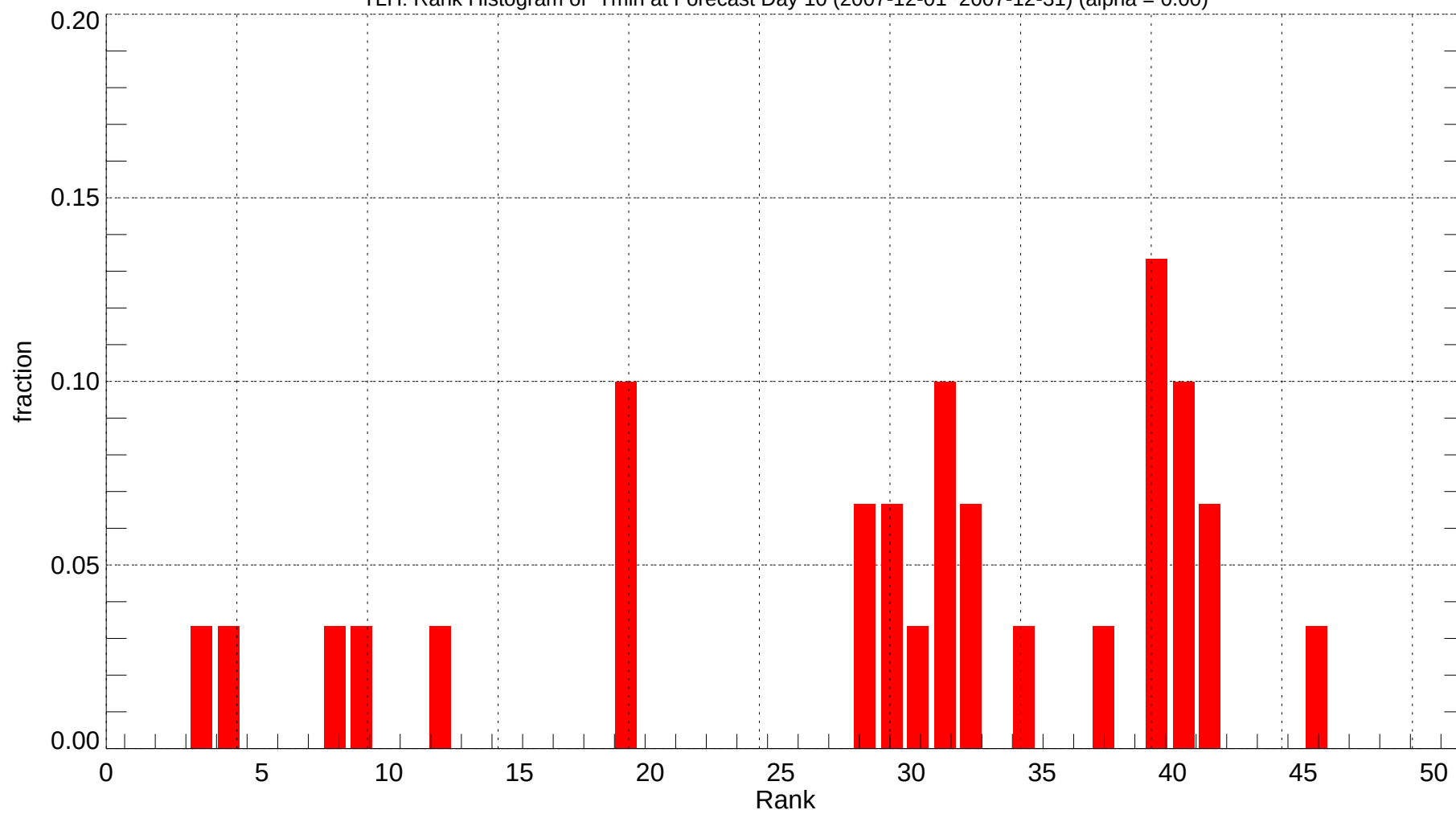
TLH: Rank Histogram of Tmin at Forecast Day 10 (2007-12-01~2007-12-31) (alpha = 0.00)
