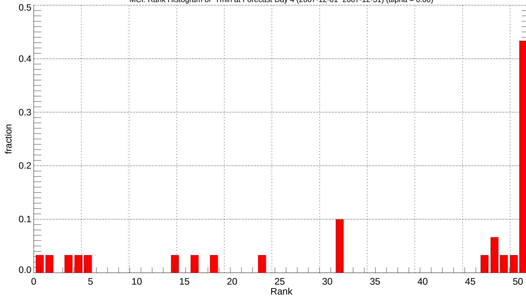
MCI: Rank Histogram of Tmin at Forecast Day 4 (2007-12-01~2007-12-31) (alpha = 0.00)
