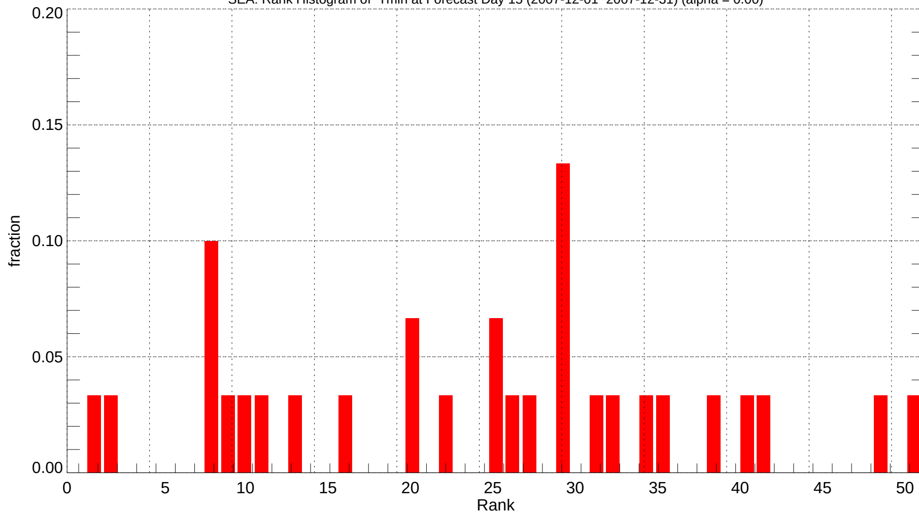
SEA: Rank Histogram of Tmin at Forecast Day 15 (2007-12-01~2007-12-31) (alpha = 0.00)
