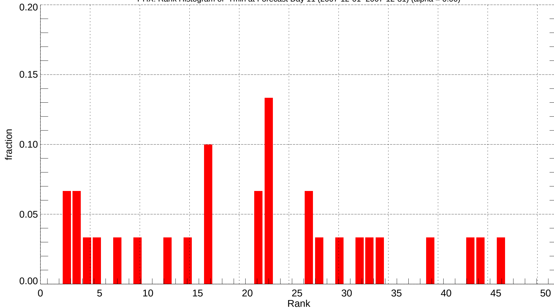
PHX: Rank Histogram of Tmin at Forecast Day 11 (2007-12-01~2007-12-31) (alpha = 0.00)
