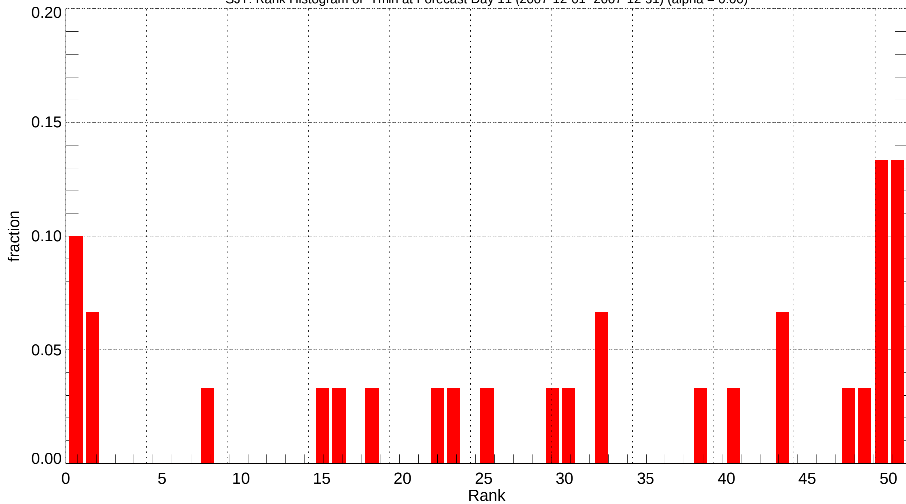
SJT: Rank Histogram of Tmin at Forecast Day 11 (2007-12-01~2007-12-31) (alpha = 0.00)
