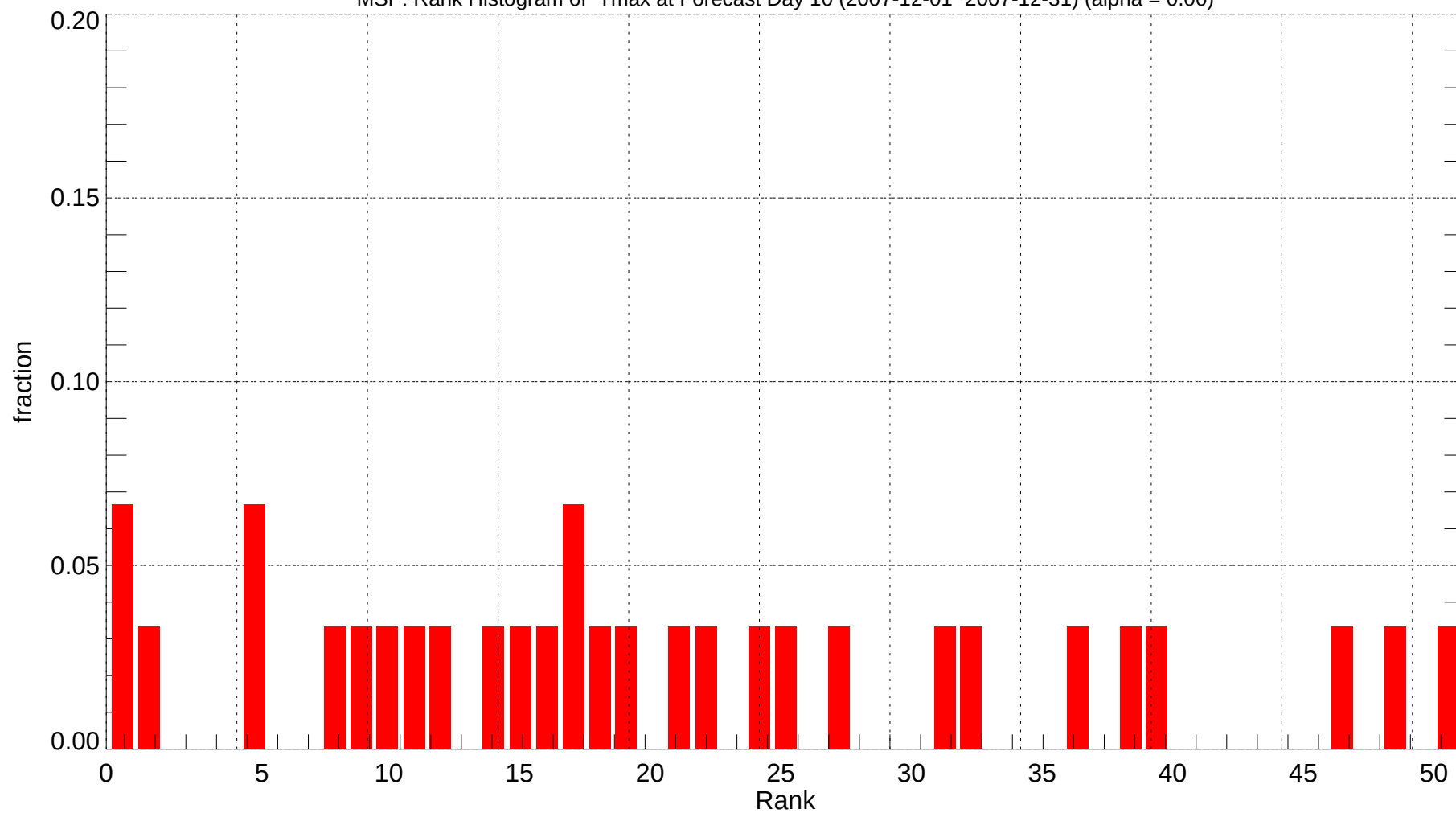
MSP: Rank Histogram of Tmax at Forecast Day 10 (2007-12-01~2007-12-31) (alpha = 0.00)
