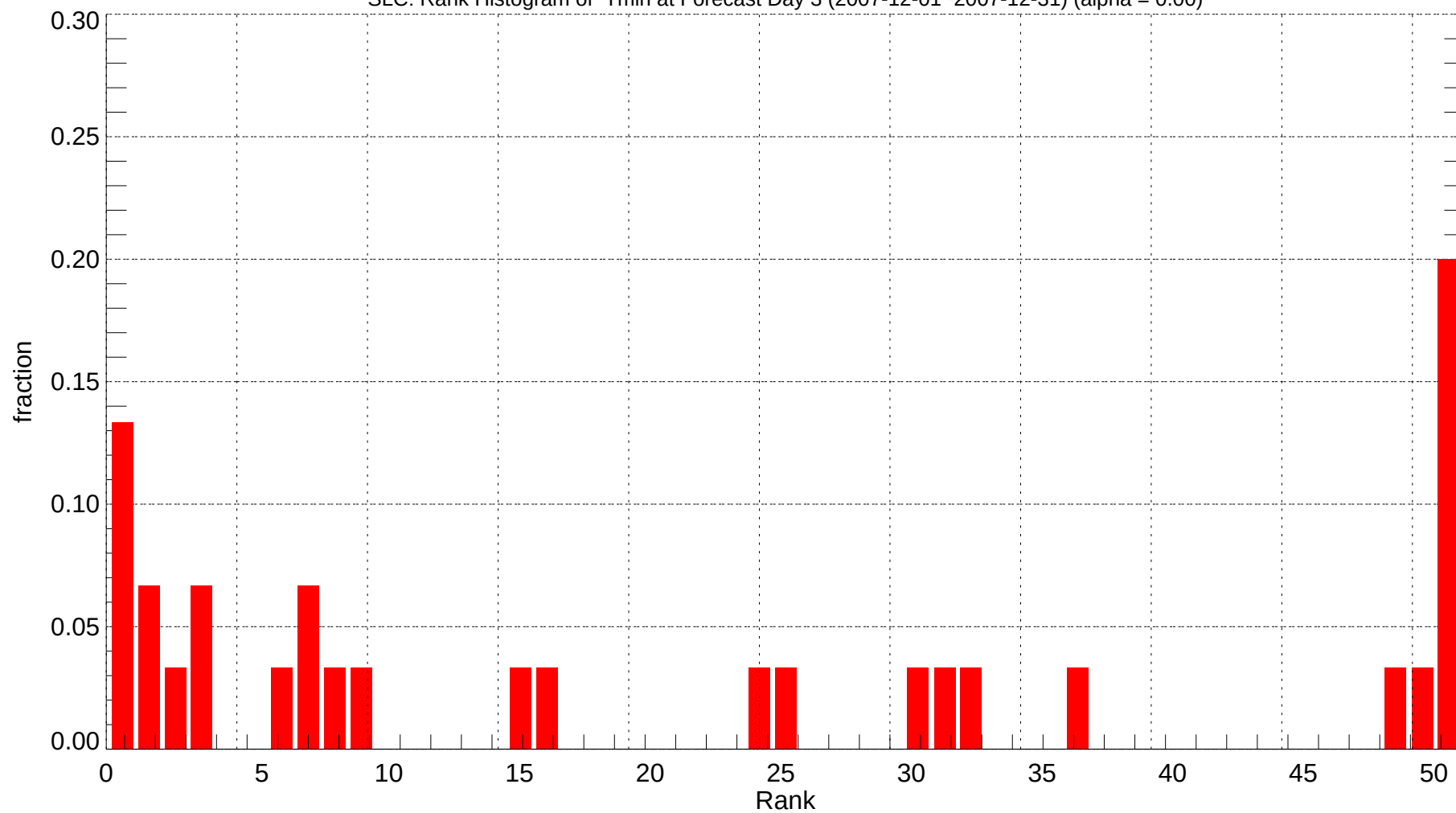
SLC: Rank Histogram of Tmin at Forecast Day 3 (2007-12-01~2007-12-31) (alpha = 0.00)
