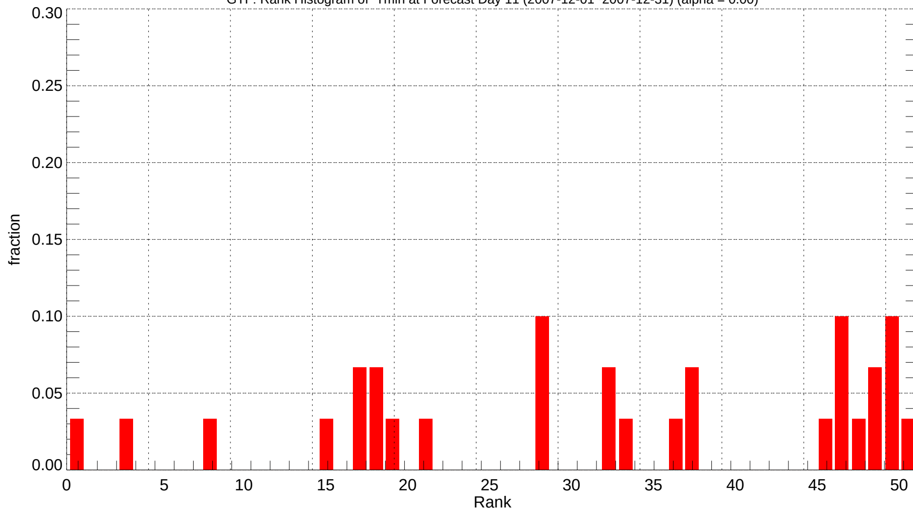
GTF: Rank Histogram of Tmin at Forecast Day 11 (2007-12-01~2007-12-31) (alpha = 0.00)
