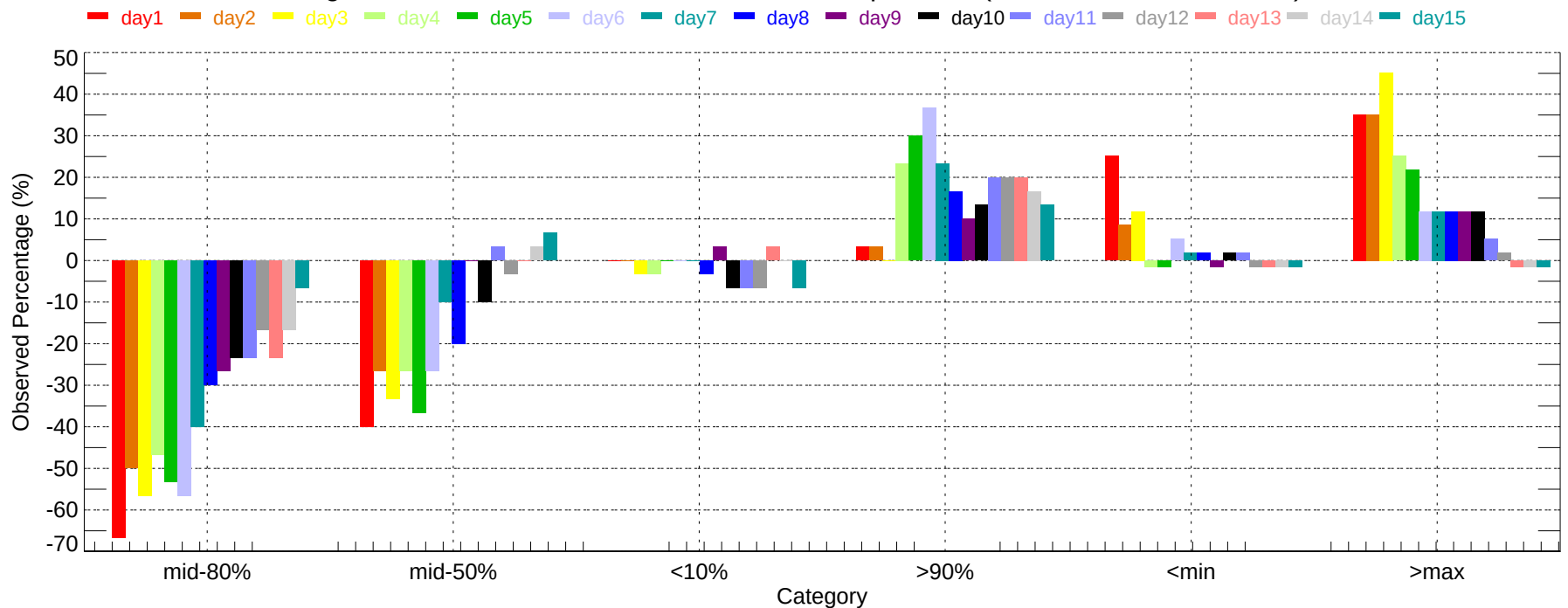
Observed Percentage Deviation of Ensembles - GTF: Max Temperature (2007-12-01~2007-12-31)
