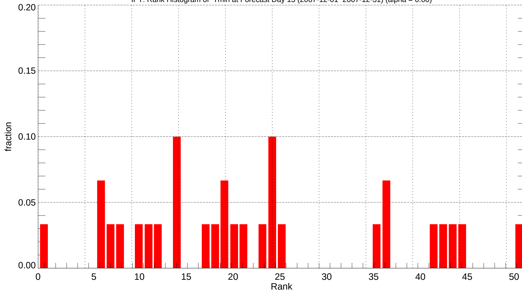
IPT: Rank Histogram of Tmin at Forecast Day 13 (2007-12-01~2007-12-31) (alpha = 0.00)
