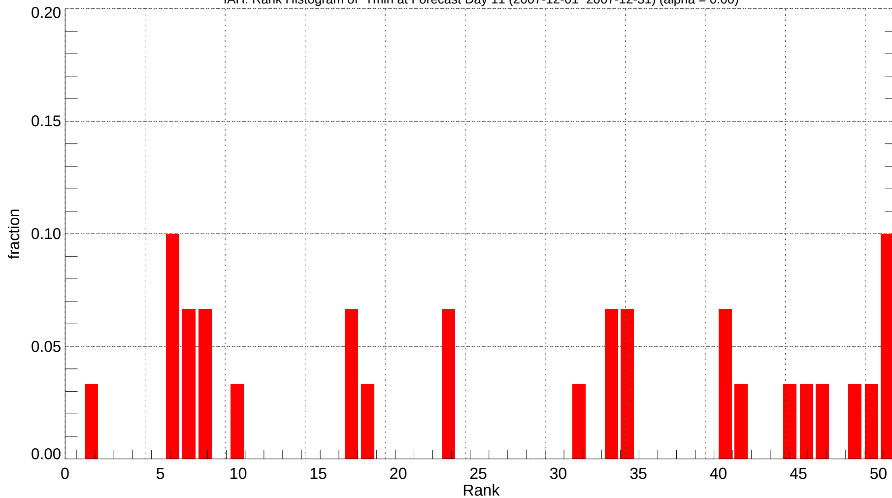
IAH: Rank Histogram of Tmin at Forecast Day 11 (2007-12-01~2007-12-31) (alpha = 0.00)
