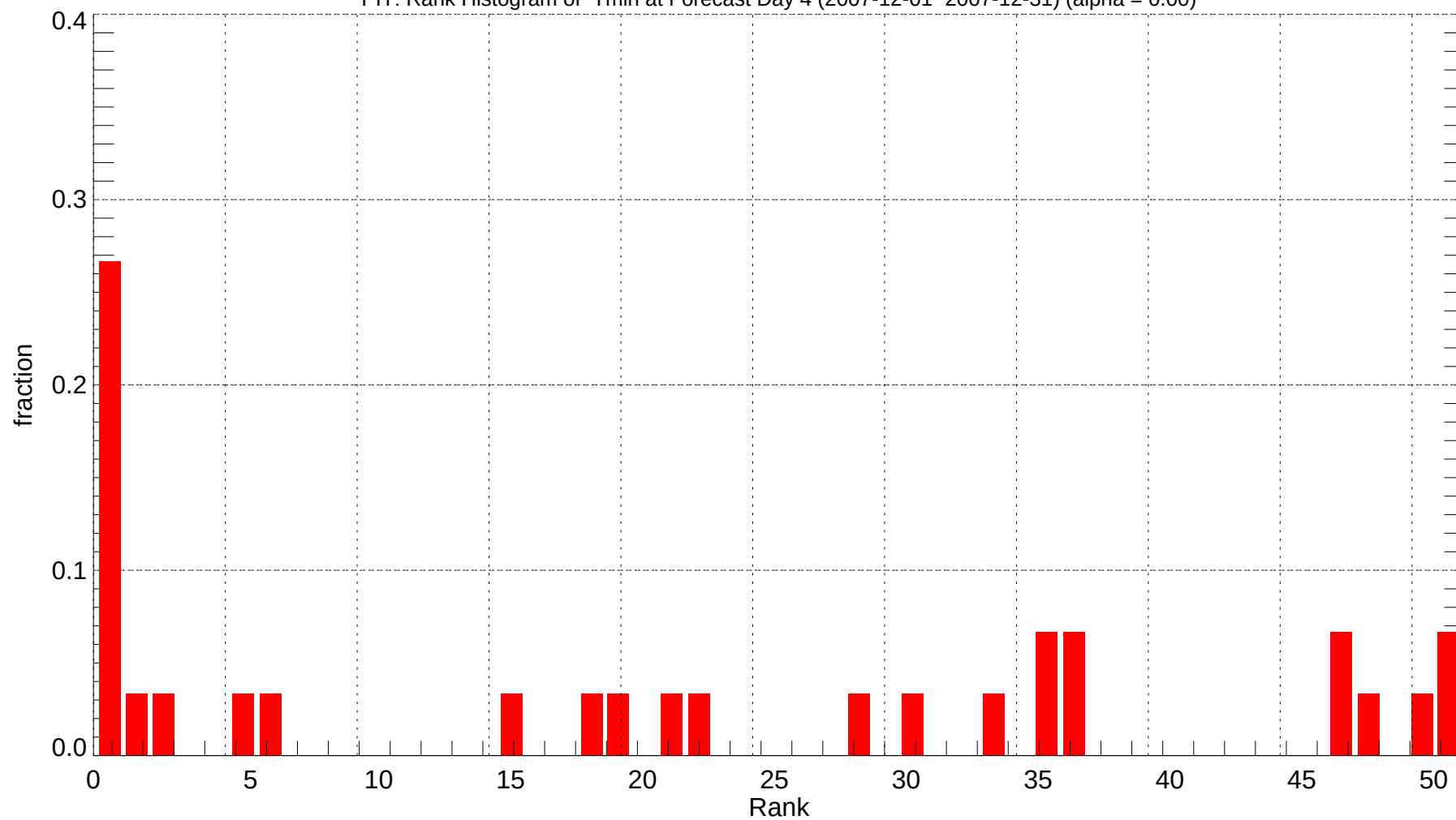
PIT: Rank Histogram of Tmin at Forecast Day 4 (2007-12-01~2007-12-31) (alpha = 0.00)
