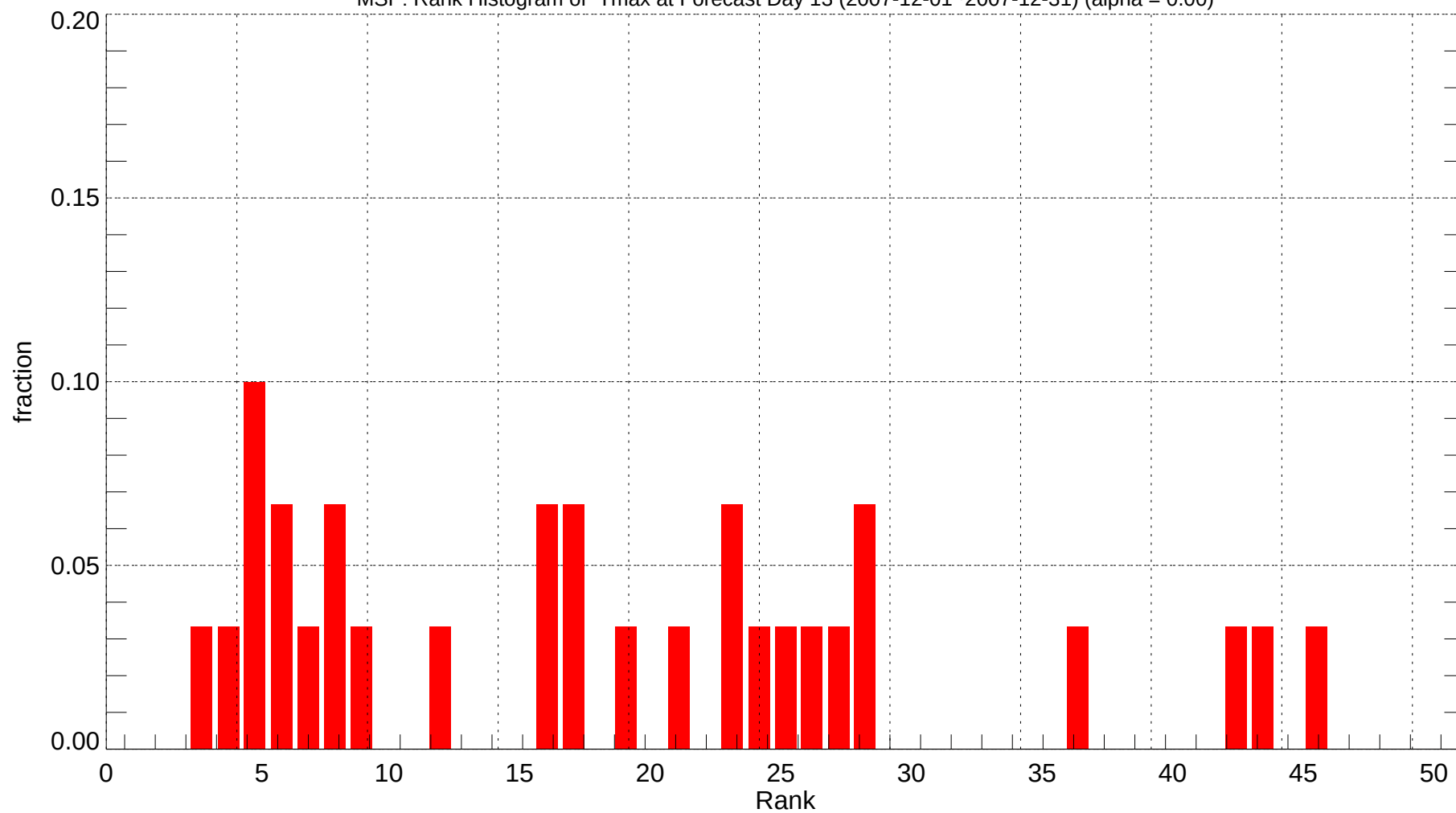
MSP: Rank Histogram of Tmax at Forecast Day 13 (2007-12-01~2007-12-31) (alpha = 0.00)
