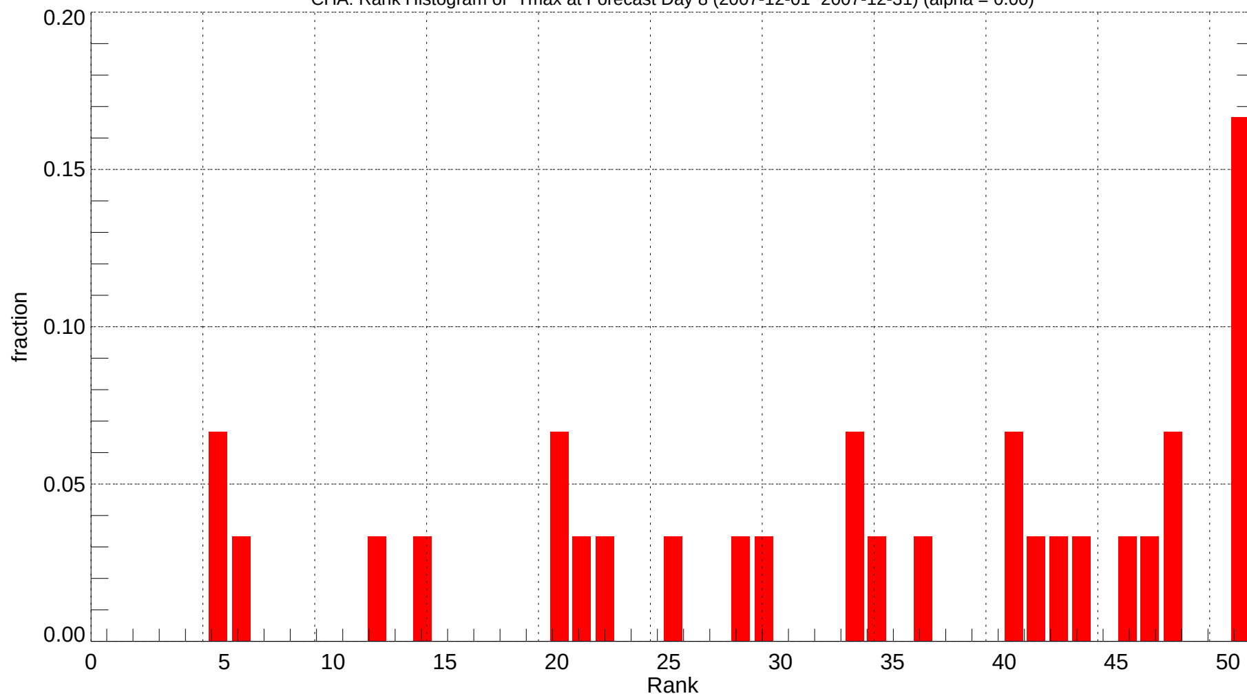
CHA: Rank Histogram of Tmax at Forecast Day 8 (2007-12-01~2007-12-31) (alpha = 0.00)
