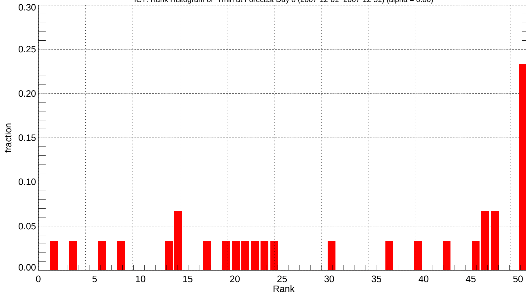
ICT: Rank Histogram of Tmin at Forecast Day 8 (2007-12-01~2007-12-31) (alpha = 0.00)
