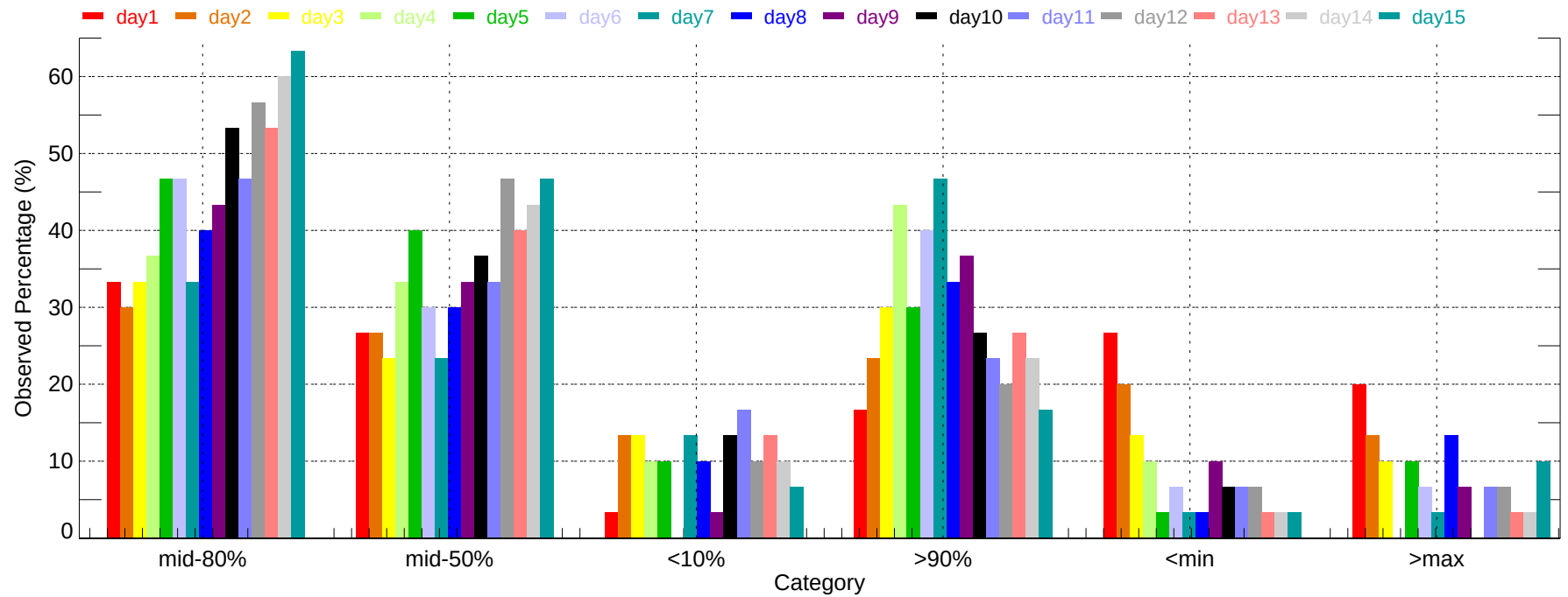
Observed Percentage of Ensembles - CRP: Min Temperature (2007-12-01~2007-12-31)
