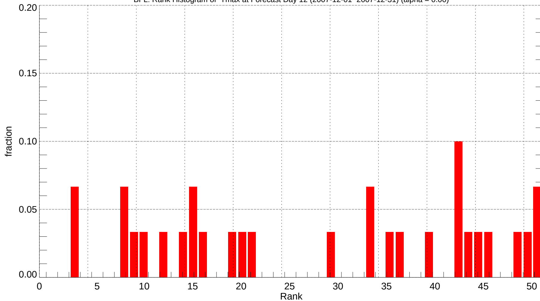
BFL: Rank Histogram of Tmax at Forecast Day 12 (2007-12-01~2007-12-31) (alpha = 0.00)
