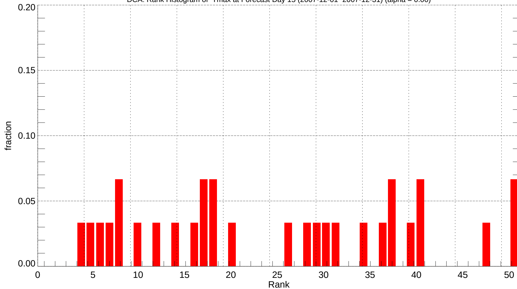
DCA: Rank Histogram of Tmax at Forecast Day 15 (2007-12-01~2007-12-31) (alpha = 0.00)
