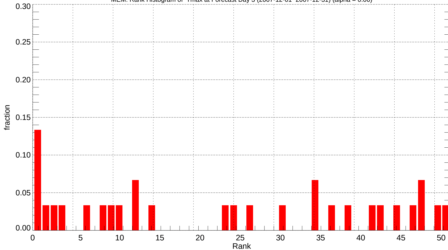
MEM: Rank Histogram of Tmax at Forecast Day 3 (2007-12-01~2007-12-31) (alpha = 0.00)
