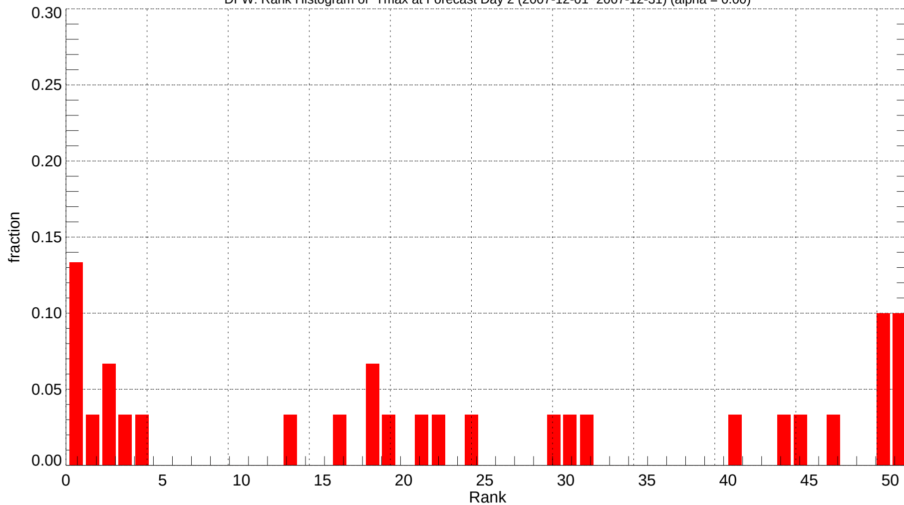
DFW: Rank Histogram of Tmax at Forecast Day 2 (2007-12-01~2007-12-31) (alpha = 0.00)
