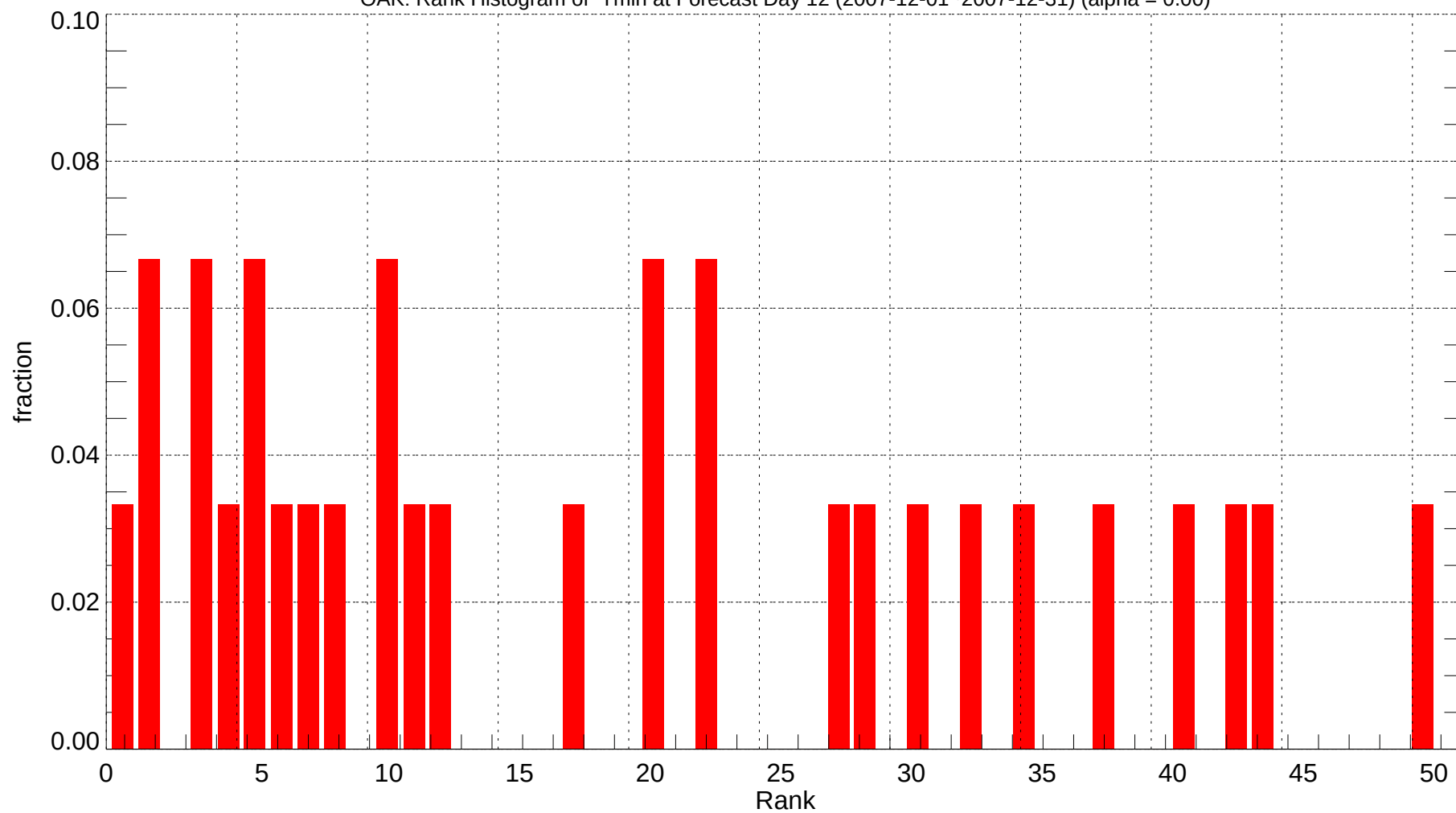
OAK: Rank Histogram of Tmin at Forecast Day 12 (2007-12-01~2007-12-31) (alpha = 0.00)
