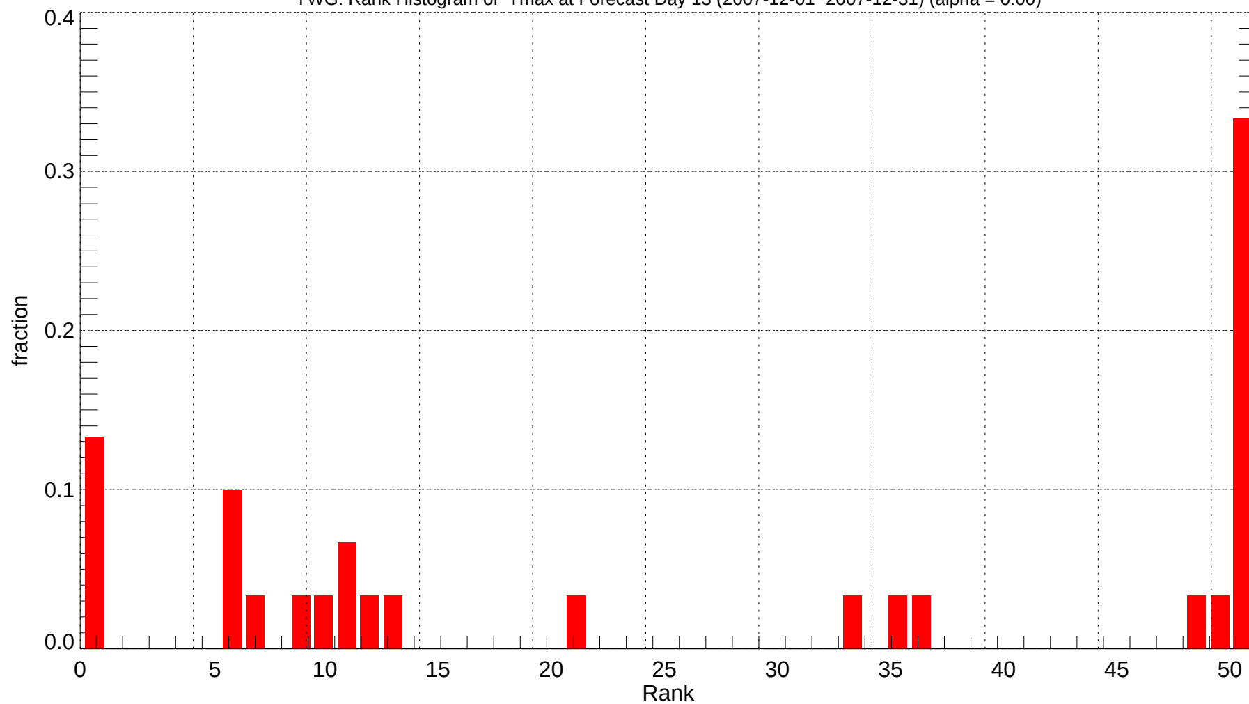
YWG: Rank Histogram of Tmax at Forecast Day 13 (2007-12-01~2007-12-31) (alpha = 0.00)
