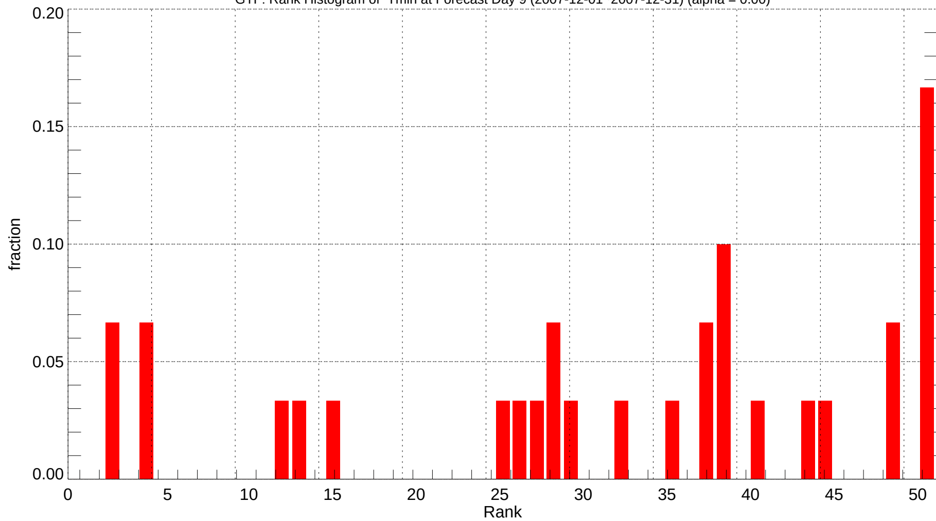
GTF: Rank Histogram of Tmin at Forecast Day 9 (2007-12-01~2007-12-31) (alpha = 0.00)
