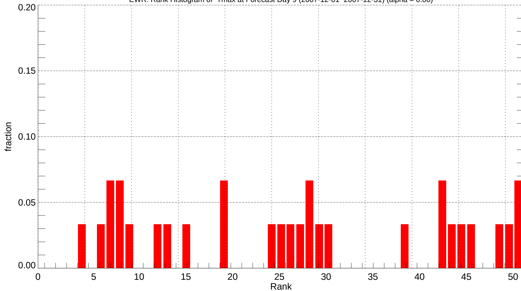
EWR: Rank Histogram of Tmax at Forecast Day 9 (2007-12-01~2007-12-31) (alpha = 0.00)
