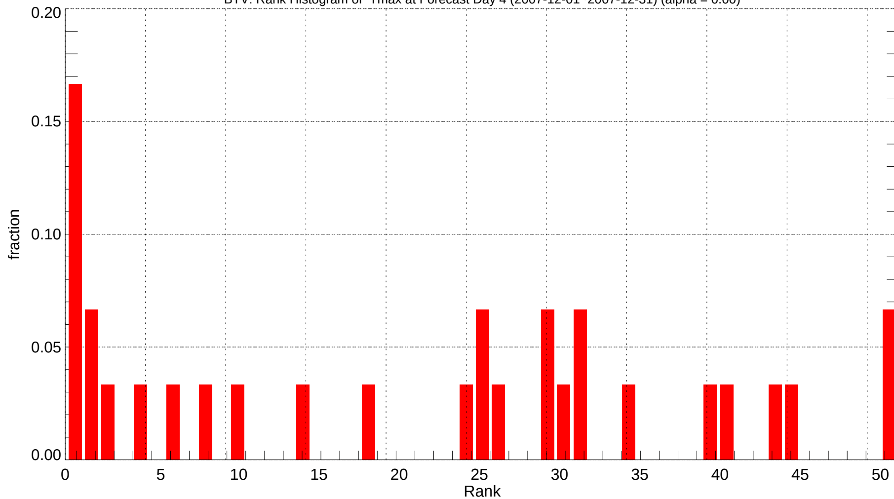
BTV: Rank Histogram of Tmax at Forecast Day 4 (2007-12-01~2007-12-31) (alpha = 0.00)
