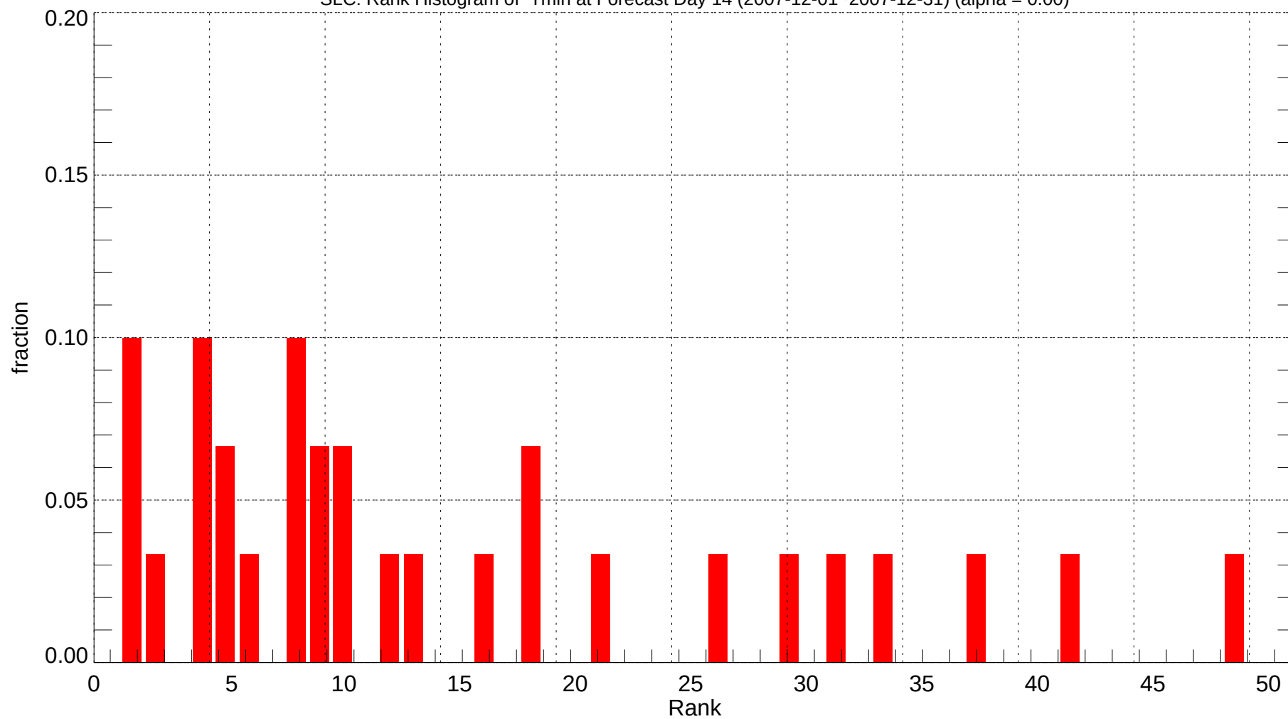
SLC: Rank Histogram of Tmin at Forecast Day 14 (2007-12-01~2007-12-31) (alpha = 0.00)
