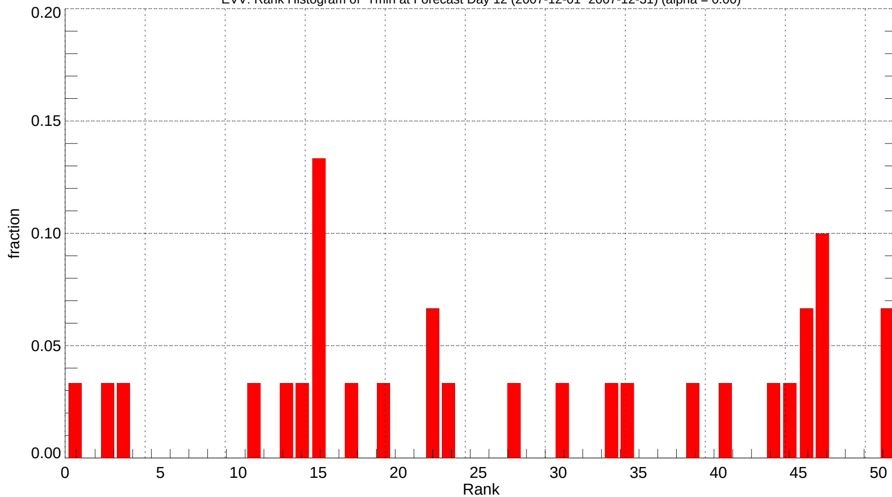
EVV: Rank Histogram of Tmin at Forecast Day 12 (2007-12-01~2007-12-31) (alpha = 0.00)
