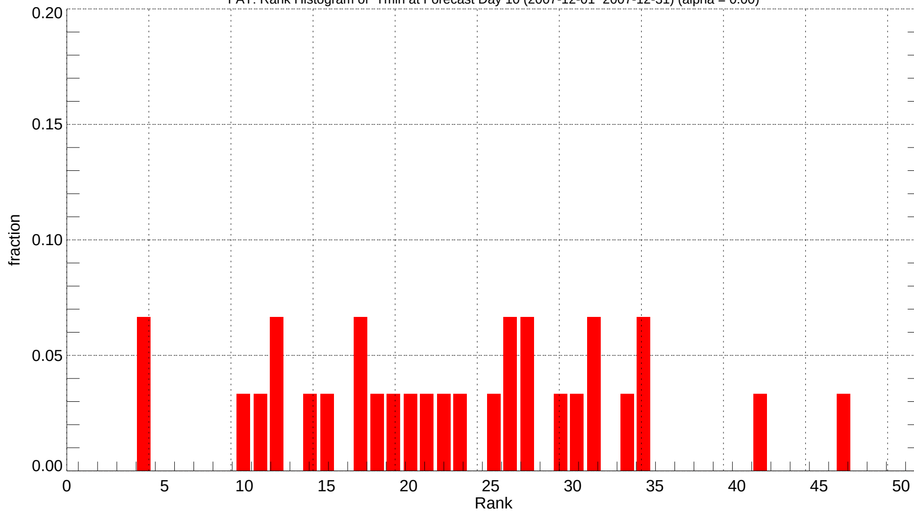
FAT: Rank Histogram of Tmin at Forecast Day 10 (2007-12-01~2007-12-31) (alpha = 0.00)
