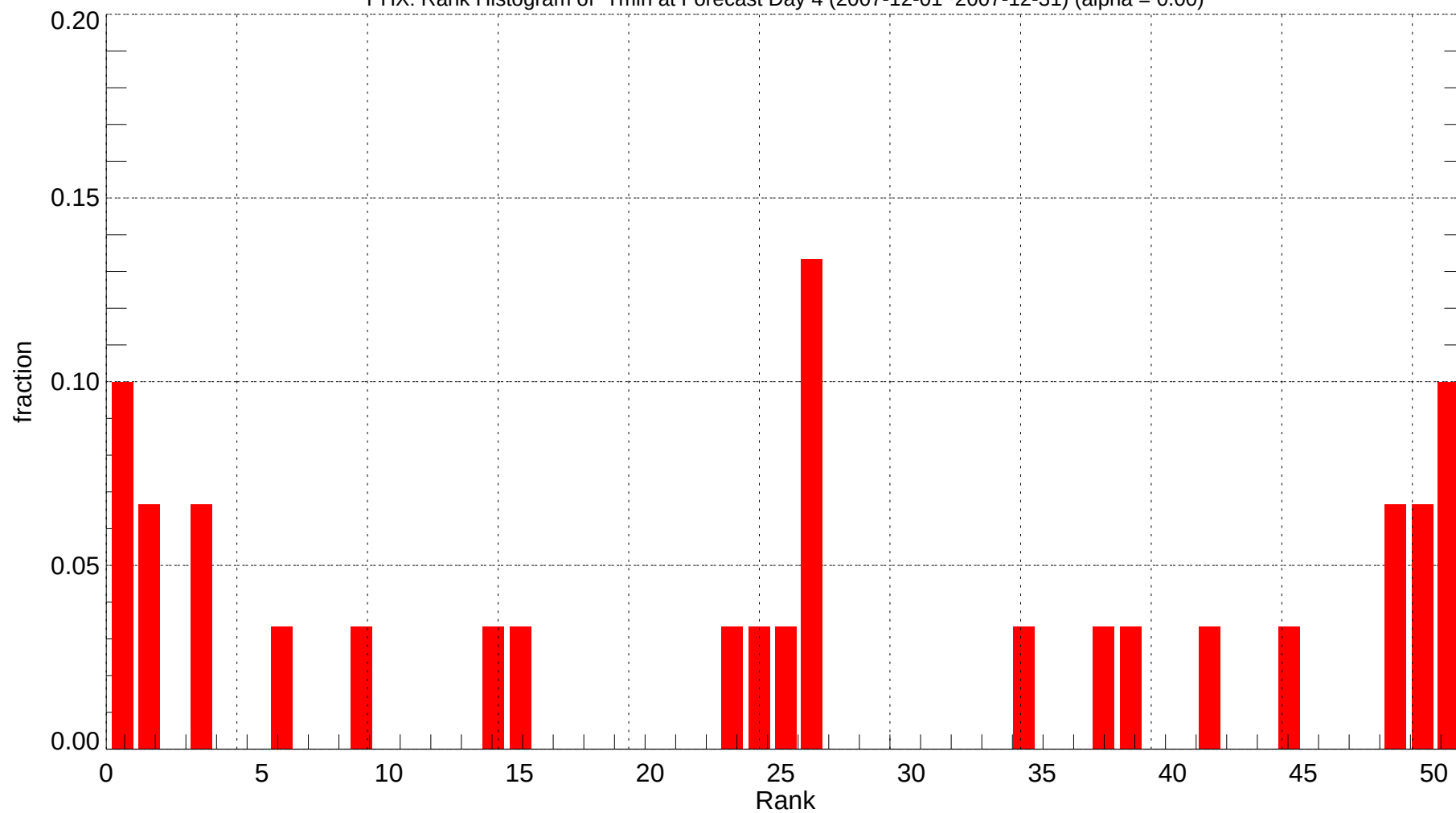
PHX: Rank Histogram of Tmin at Forecast Day 4 (2007-12-01~2007-12-31) (alpha = 0.00)
