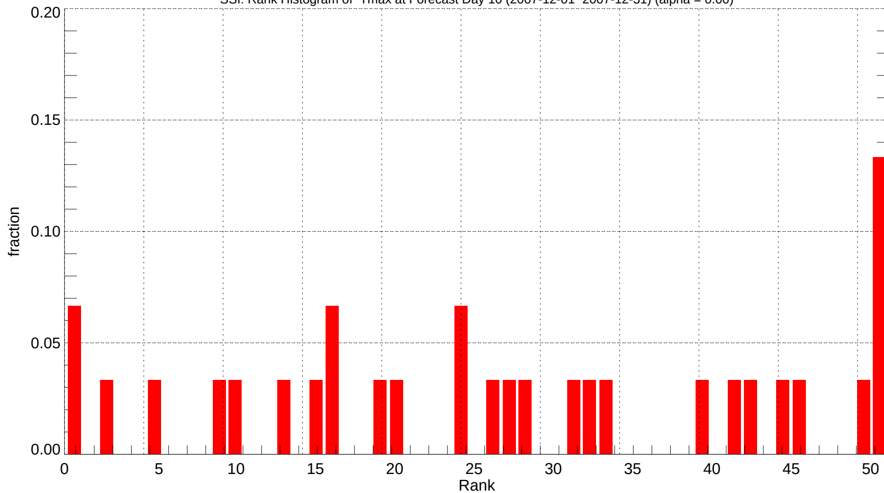
SSI: Rank Histogram of Tmax at Forecast Day 10 (2007-12-01~2007-12-31) (alpha = 0.00)
