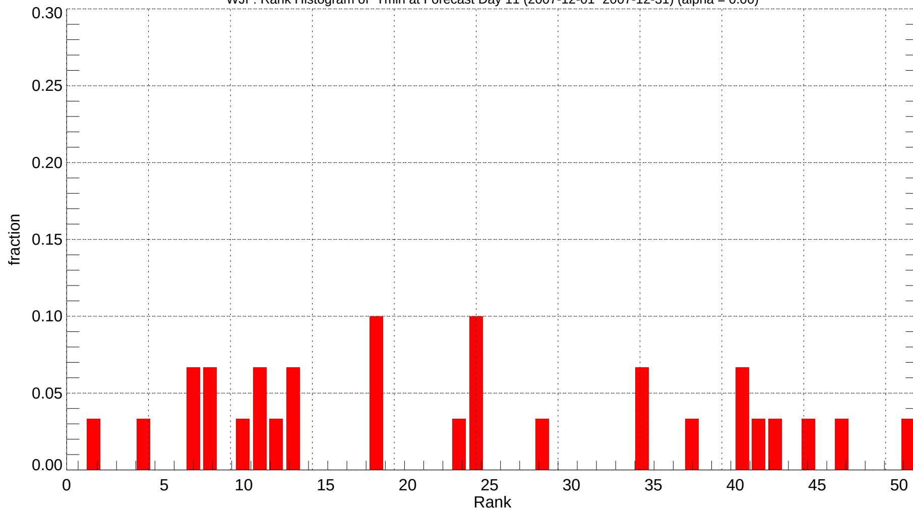
WJF: Rank Histogram of Tmin at Forecast Day 11 (2007-12-01~2007-12-31) (alpha = 0.00)
