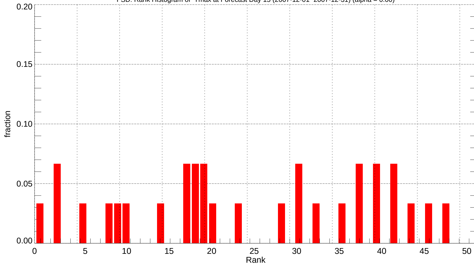
FSD: Rank Histogram of Tmax at Forecast Day 15 (2007-12-01~2007-12-31) (alpha = 0.00)
