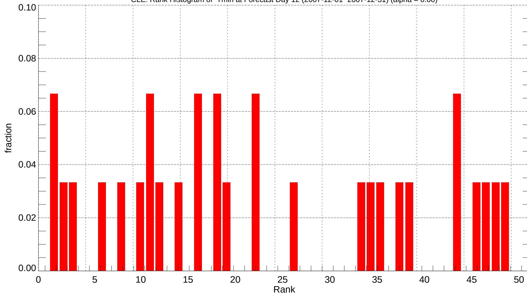
CLE: Rank Histogram of Tmin at Forecast Day 12 (2007-12-01~2007-12-31) (alpha = 0.00)
