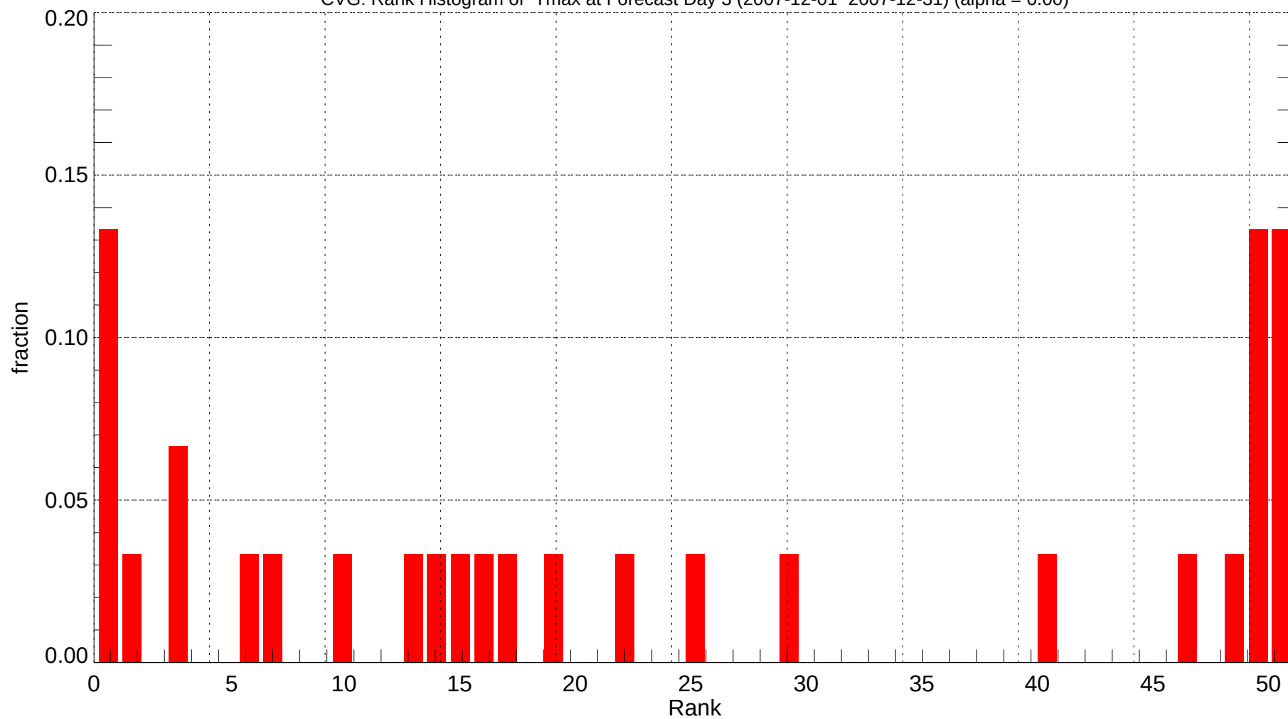
CVG: Rank Histogram of Tmax at Forecast Day 3 (2007-12-01~2007-12-31) (alpha = 0.00)
