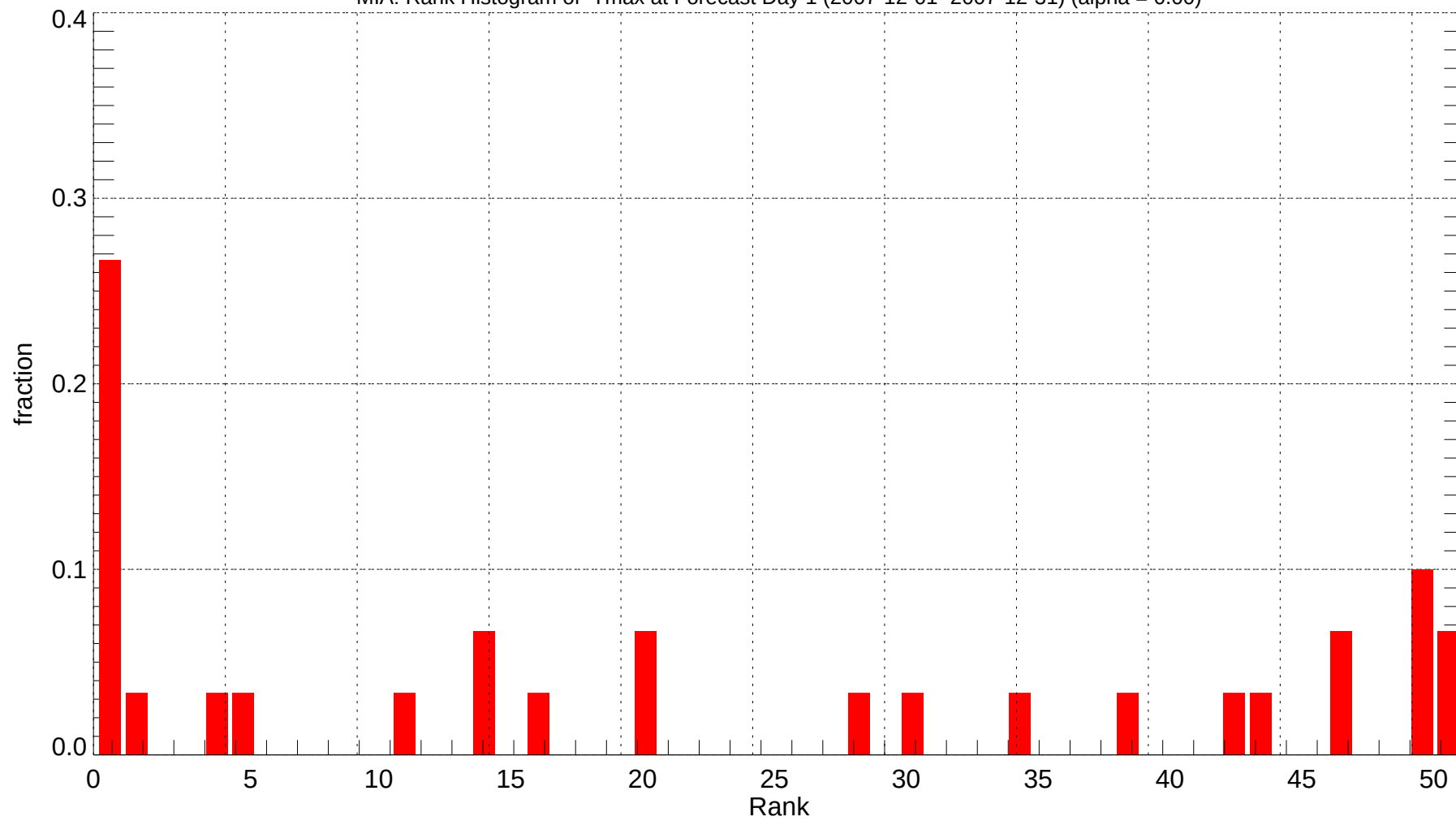
MIA: Rank Histogram of Tmax at Forecast Day 1 (2007-12-01~2007-12-31) (alpha = 0.00)
