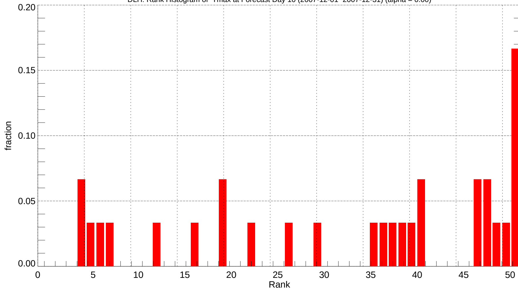
DLH: Rank Histogram of Tmax at Forecast Day 10 (2007-12-01~2007-12-31) (alpha = 0.00)
