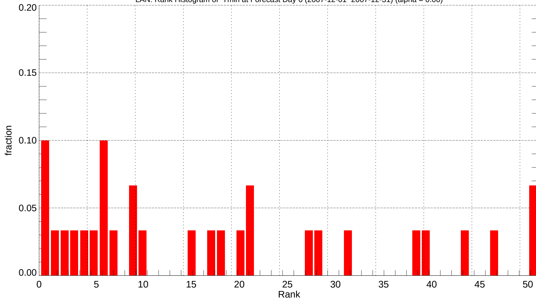
LAN: Rank Histogram of Tmin at Forecast Day 6 (2007-12-01~2007-12-31) (alpha = 0.00)
