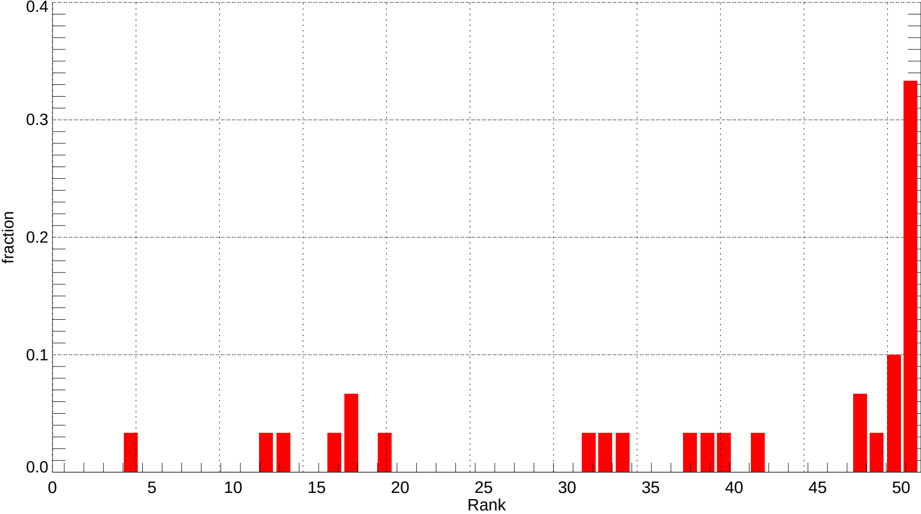
ELP: Rank Histogram of Tmin at Forecast Day 8 (2007-12-01~2007-12-31) (alpha = 0.00)
