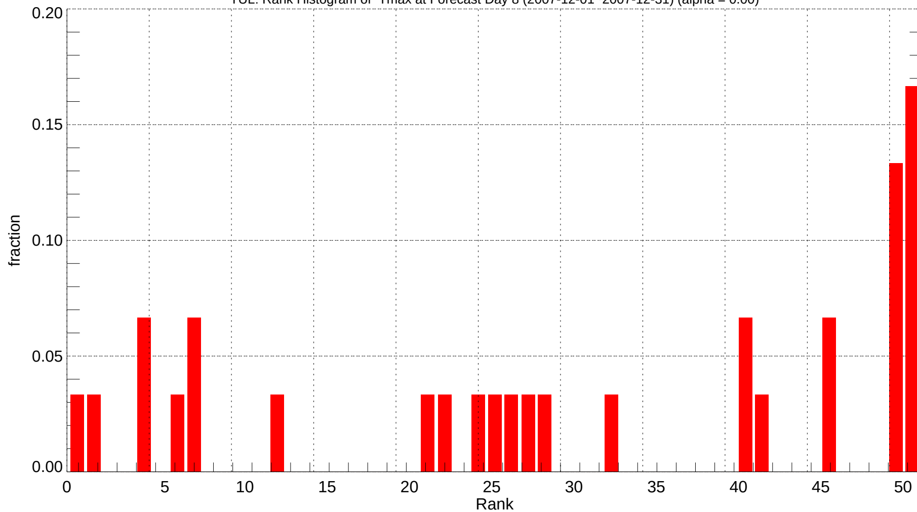
TUL: Rank Histogram of Tmax at Forecast Day 8 (2007-12-01~2007-12-31) (alpha = 0.00)
