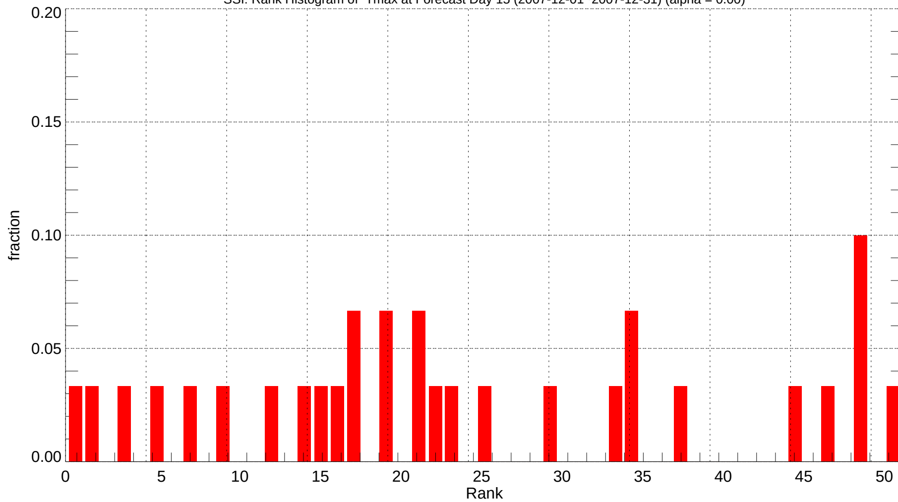
SSI: Rank Histogram of Tmax at Forecast Day 15 (2007-12-01~2007-12-31) (alpha = 0.00)
