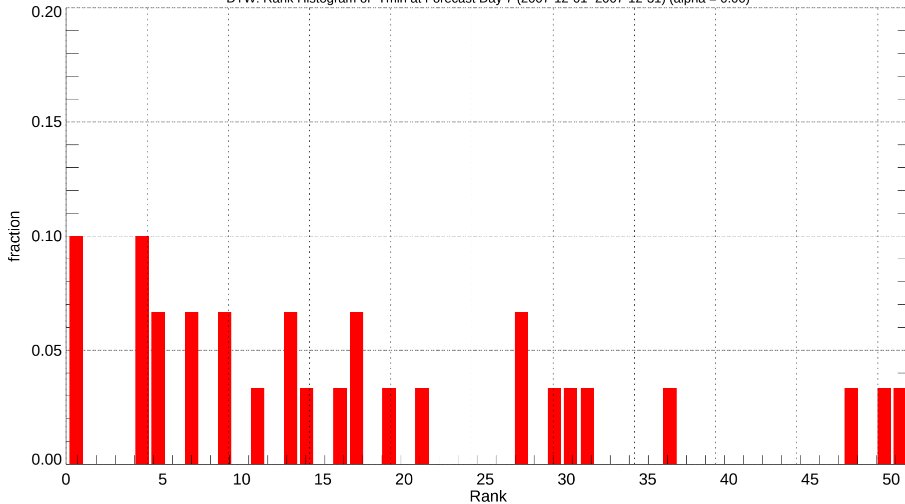
DTW: Rank Histogram of Tmin at Forecast Day 7 (2007-12-01~2007-12-31) (alpha = 0.00)
