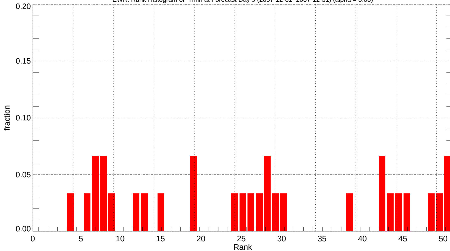
EWR: Rank Histogram of Tmin at Forecast Day 9 (2007-12-01~2007-12-31) (alpha = 0.00)
