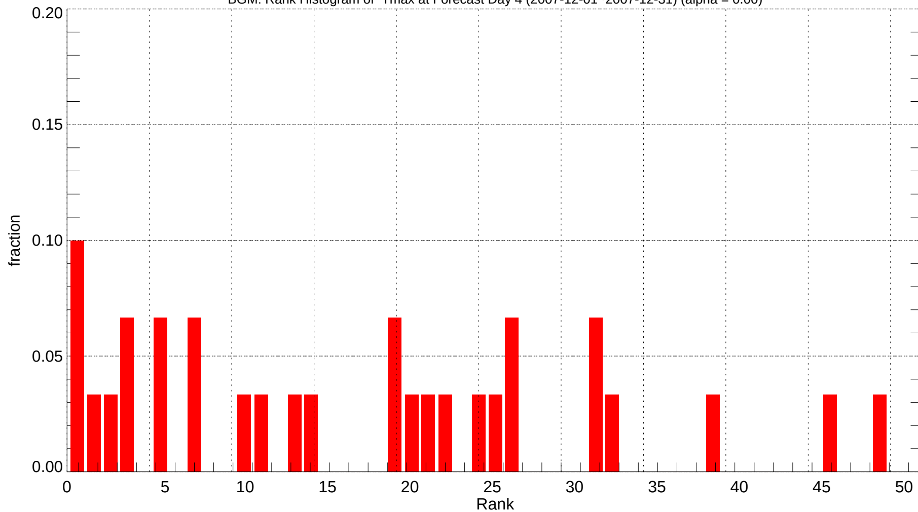
BGM: Rank Histogram of Tmax at Forecast Day 4 (2007-12-01~2007-12-31) (alpha = 0.00)
