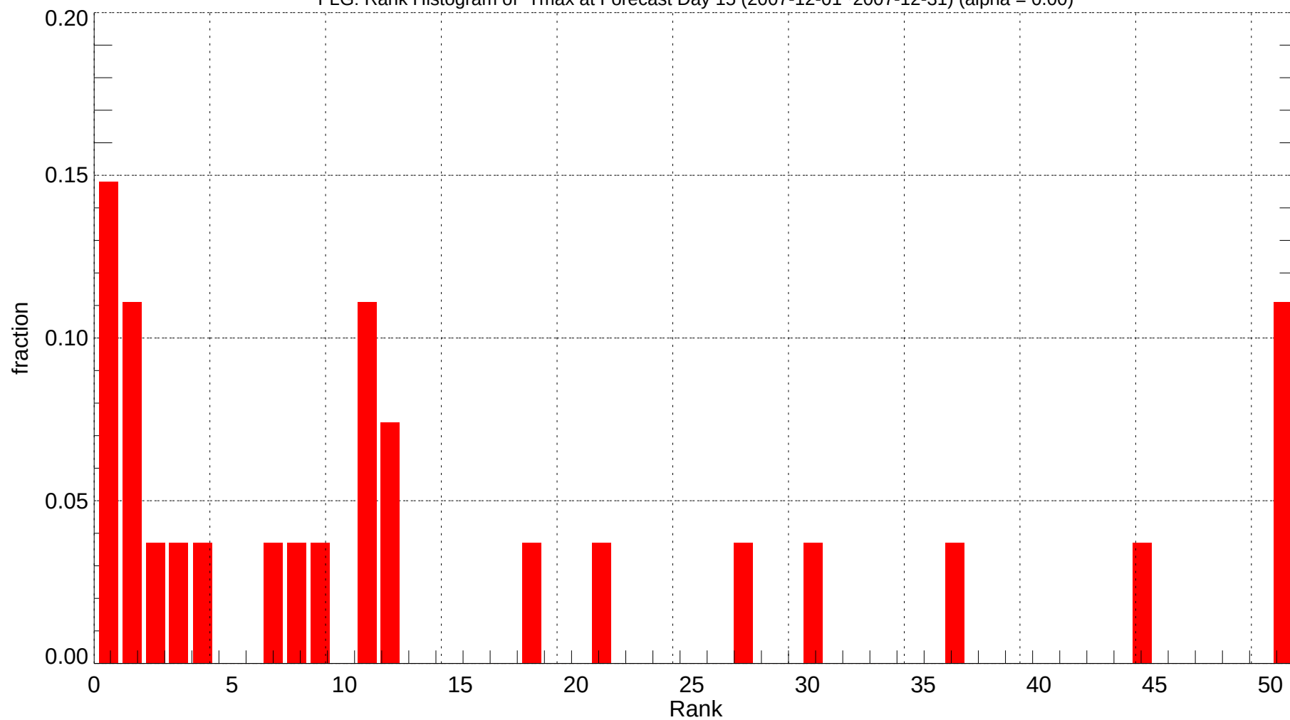
FLG: Rank Histogram of Tmax at Forecast Day 15 (2007-12-01~2007-12-31) (alpha = 0.00)
