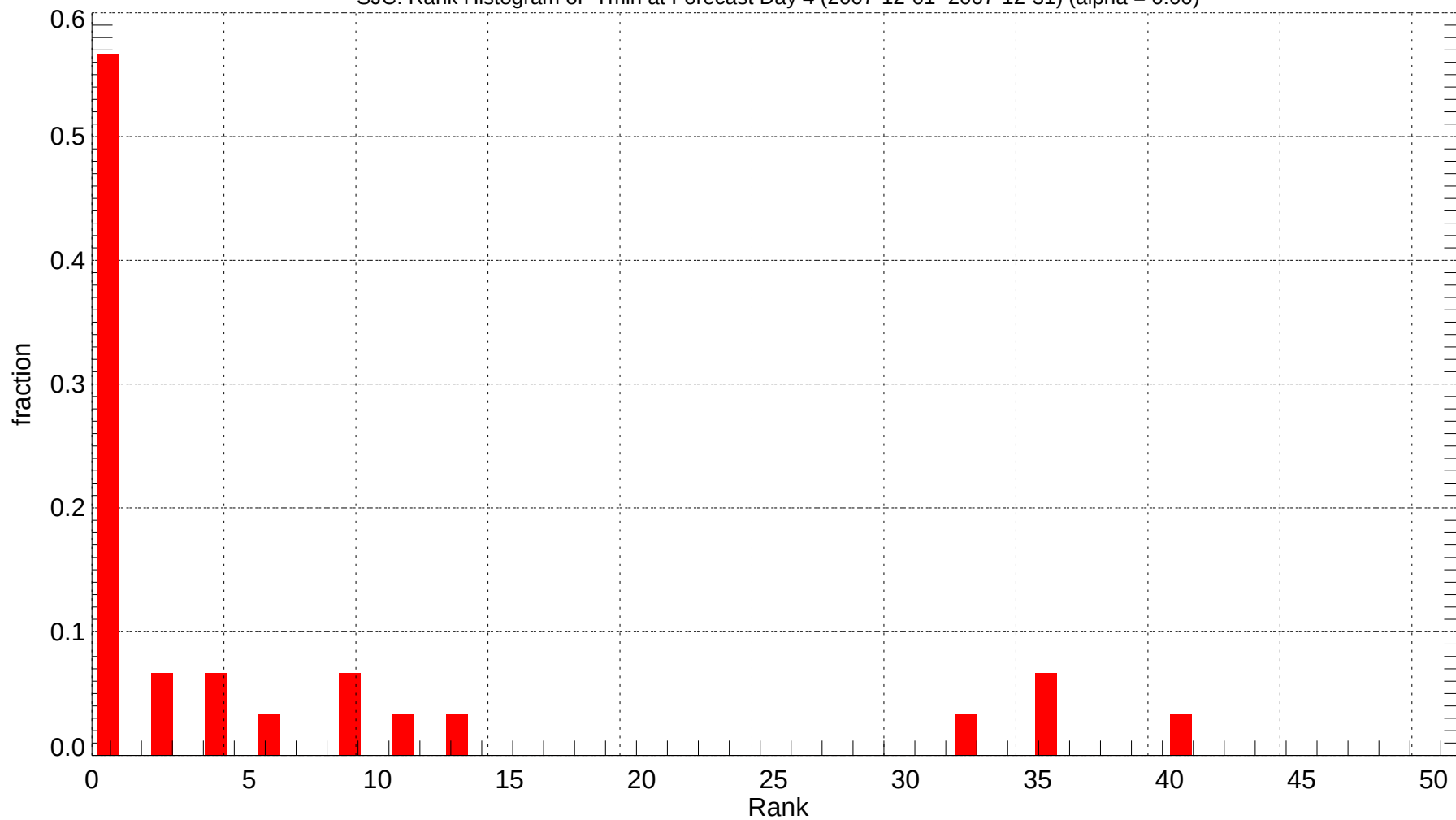
SJC: Rank Histogram of Tmin at Forecast Day 4 (2007-12-01~2007-12-31) (alpha = 0.00)
