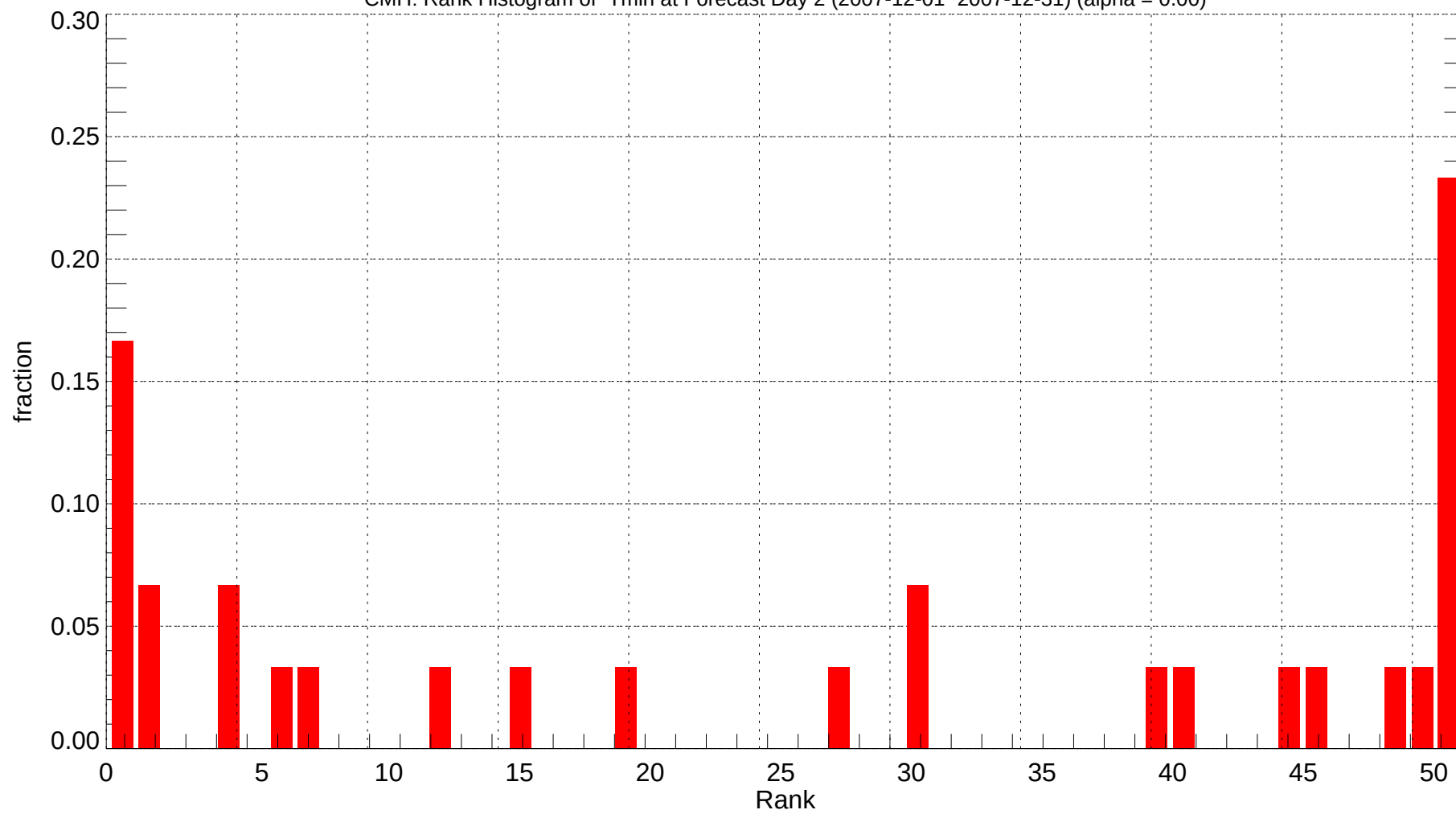
CMH: Rank Histogram of Tmin at Forecast Day 2 (2007-12-01~2007-12-31) (alpha = 0.00)
