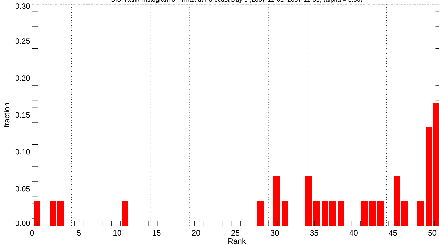
BIS: Rank Histogram of Tmax at Forecast Day 5 (2007-12-01~2007-12-31) (alpha = 0.00)
