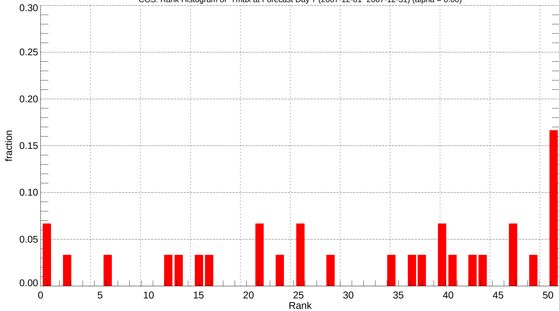
COS: Rank Histogram of Tmax at Forecast Day 7 (2007-12-01~2007-12-31) (alpha = 0.00)
