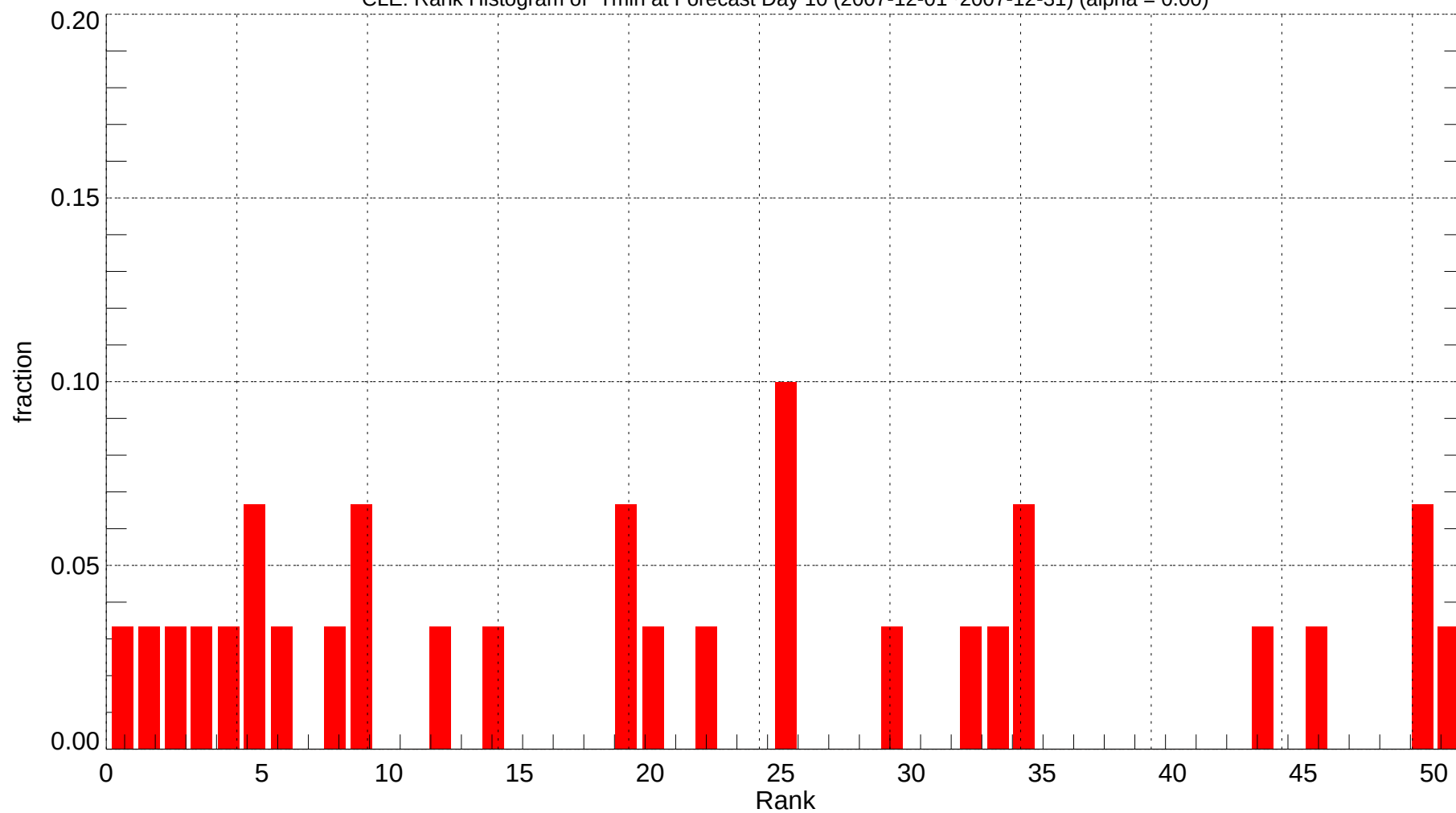
CLE: Rank Histogram of Tmin at Forecast Day 10 (2007-12-01~2007-12-31) (alpha = 0.00)
