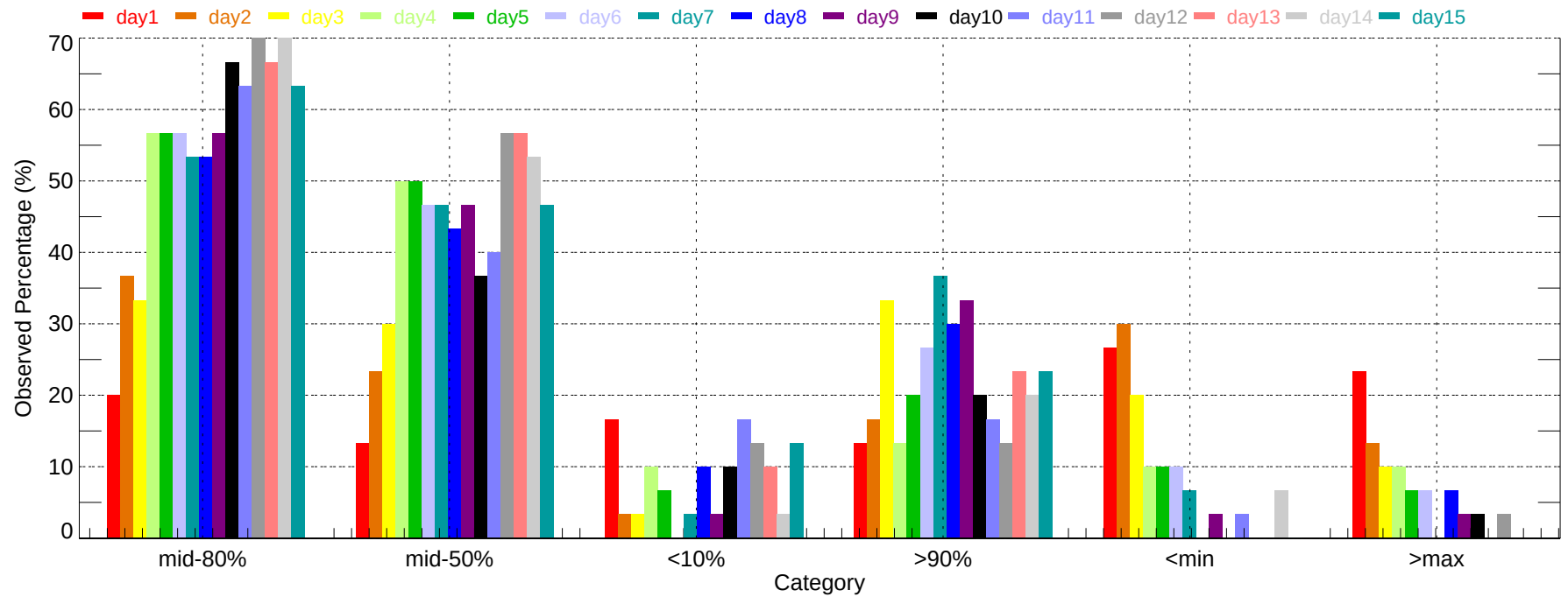
Observed Percentage of Ensembles - ACY: Min Temperature (2007-12-01~2007-12-31)
