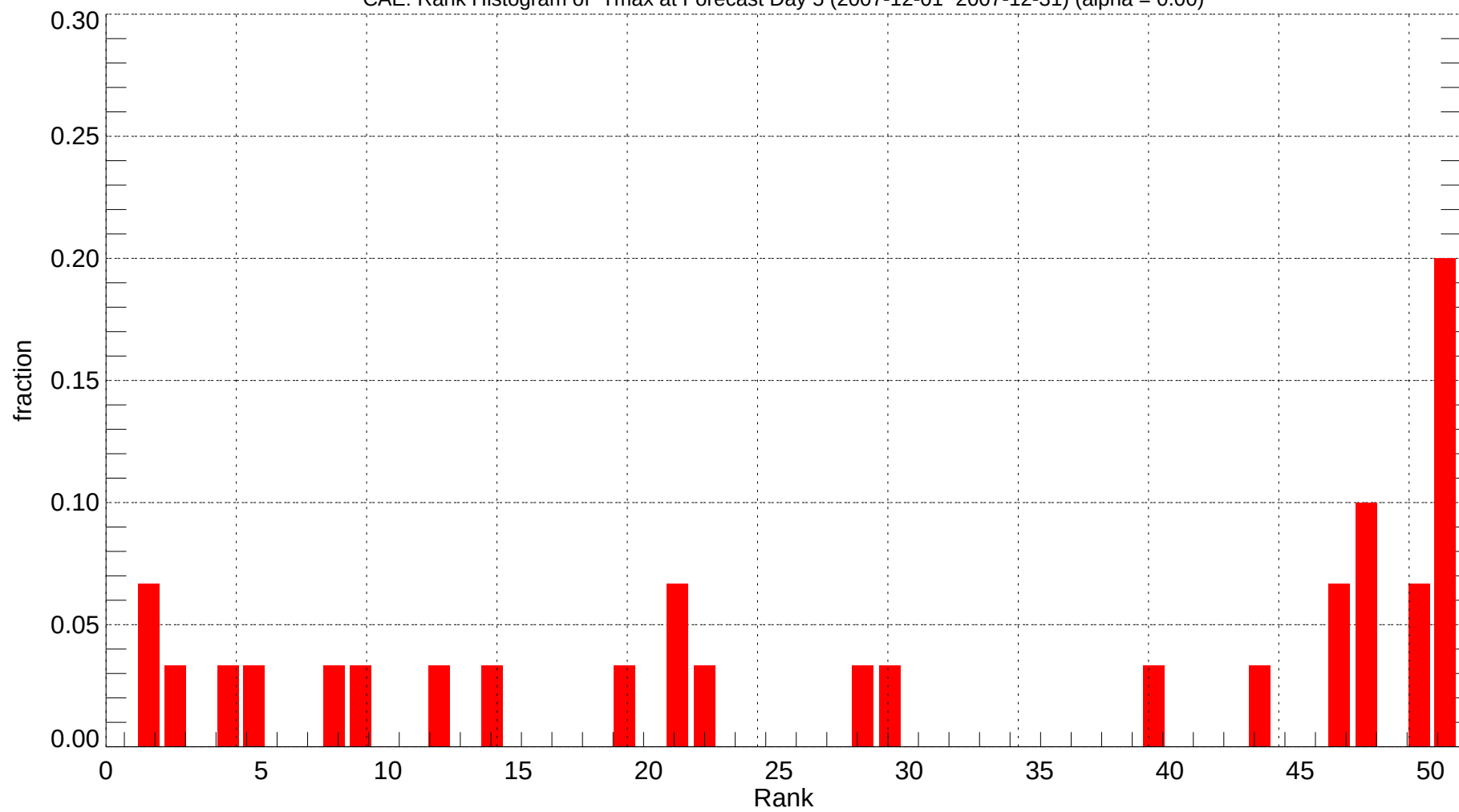
CAE: Rank Histogram of Tmax at Forecast Day 5 (2007-12-01~2007-12-31) (alpha = 0.00)
