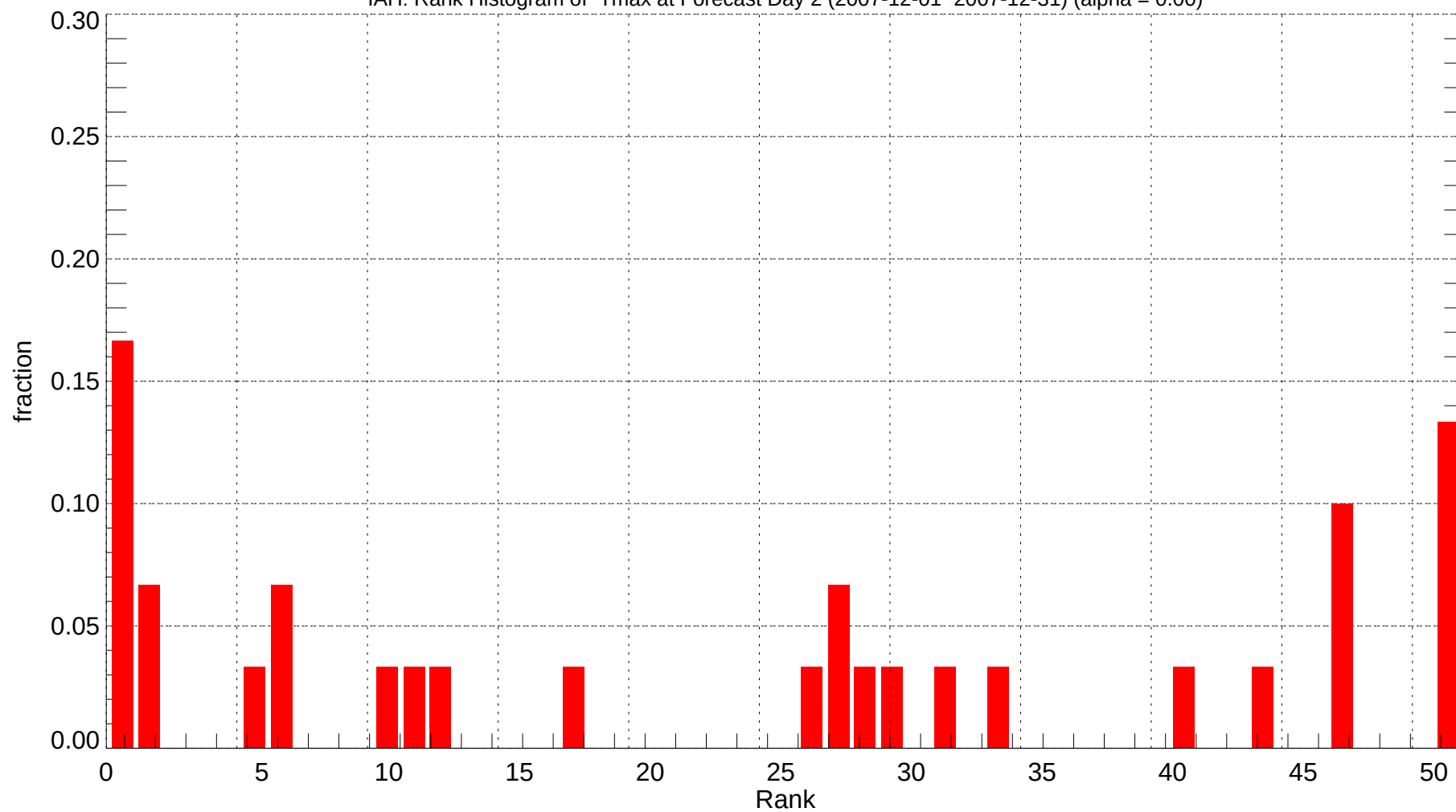
IAH: Rank Histogram of Tmax at Forecast Day 2 (2007-12-01~2007-12-31) (alpha = 0.00)
