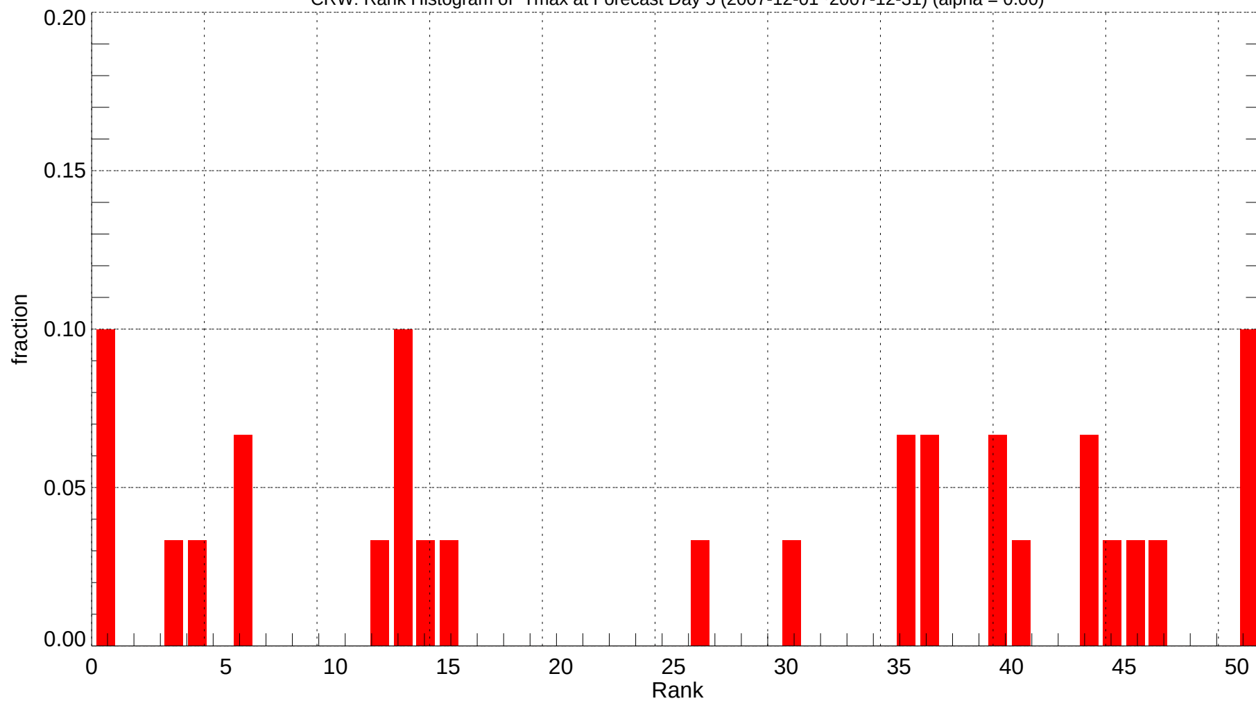
CRW: Rank Histogram of Tmax at Forecast Day 5 (2007-12-01~2007-12-31) (alpha = 0.00)
