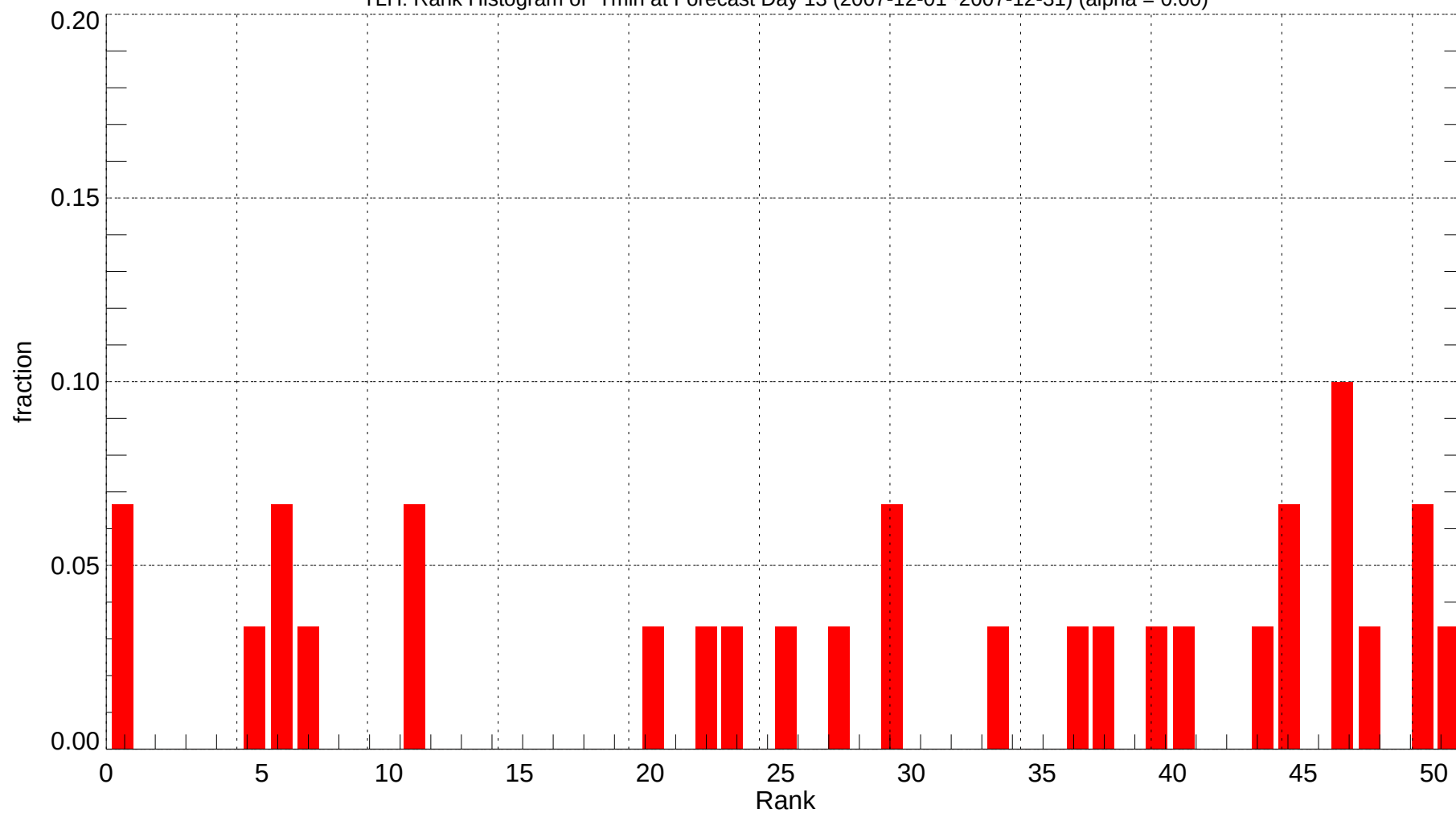
TLH: Rank Histogram of Tmin at Forecast Day 13 (2007-12-01~2007-12-31) (alpha = 0.00)
