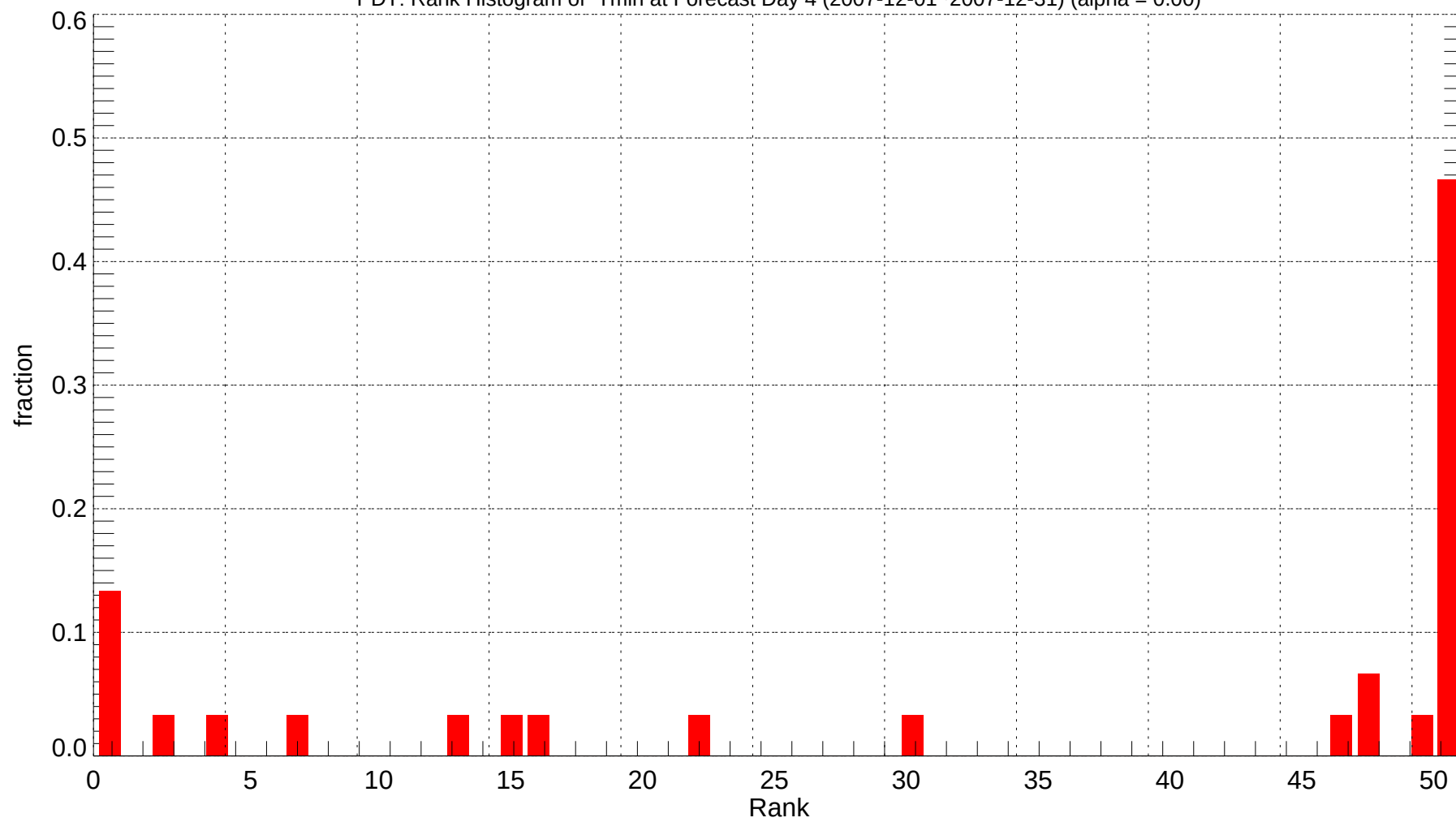
PDT: Rank Histogram of Tmin at Forecast Day 4 (2007-12-01~2007-12-31) (alpha = 0.00)
