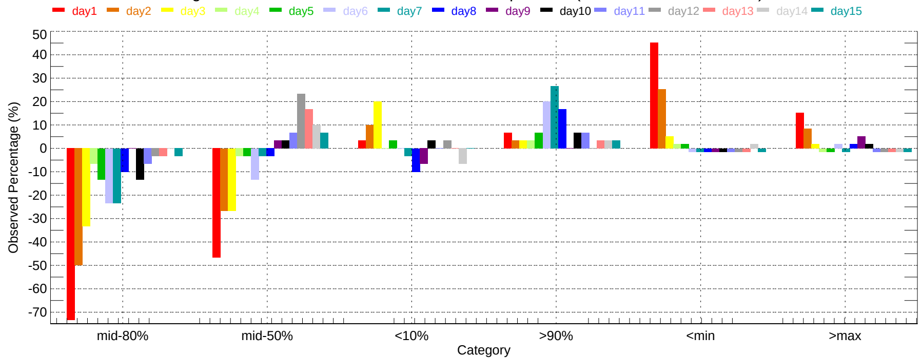
Observed Percentage Deviation of Ensembles - BOS: Min Temperature (2007-12-01~2007-12-31)
