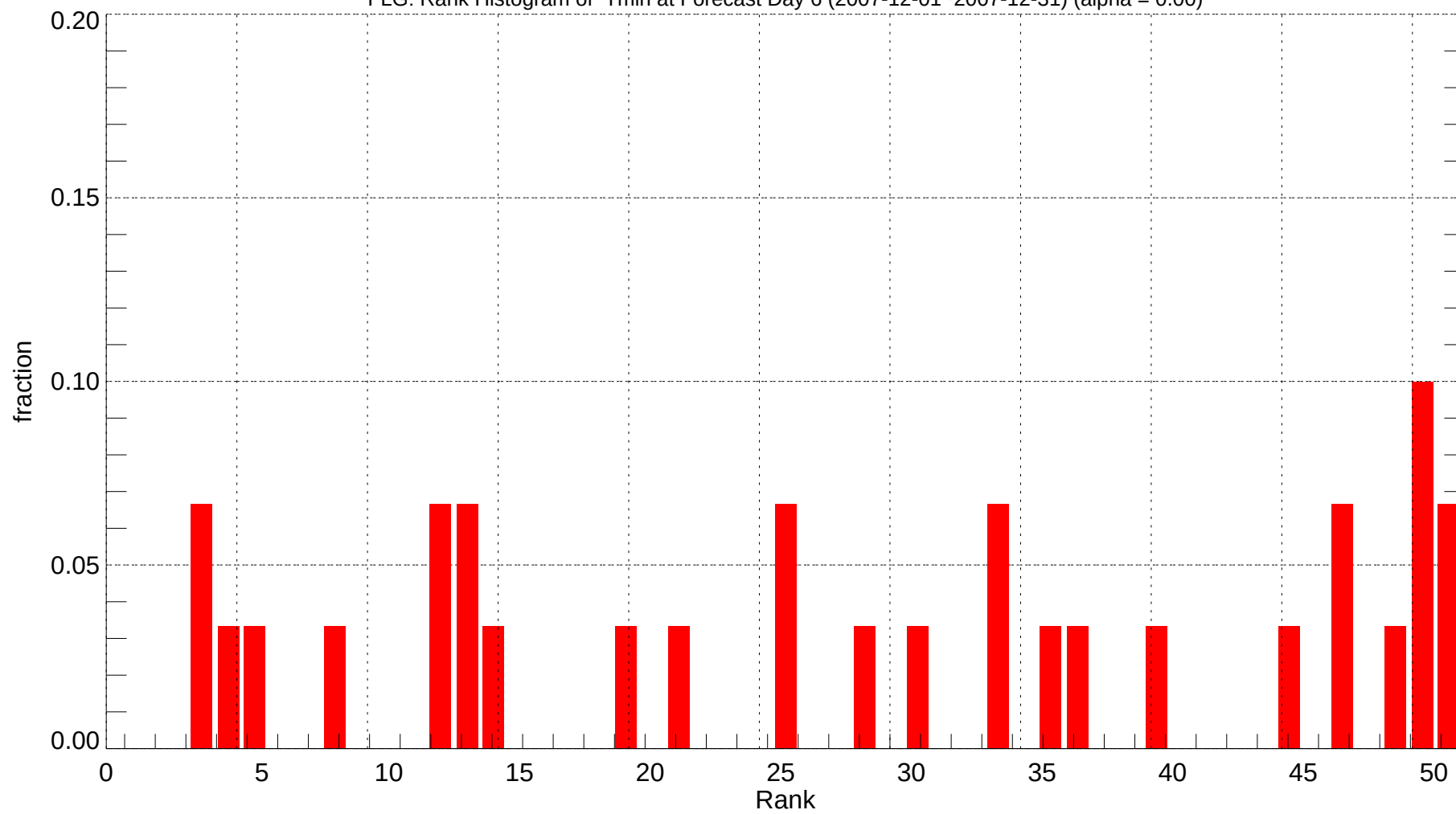
FLG: Rank Histogram of Tmin at Forecast Day 6 (2007-12-01~2007-12-31) (alpha = 0.00)
