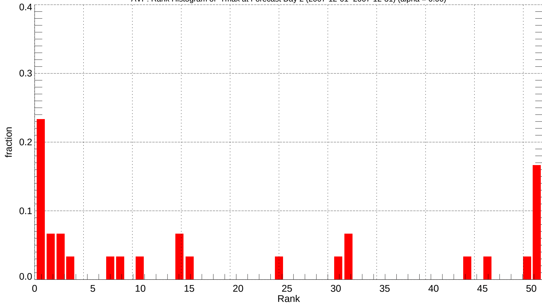
AVP: Rank Histogram of Tmax at Forecast Day 2 (2007-12-01~2007-12-31) (alpha = 0.00)
