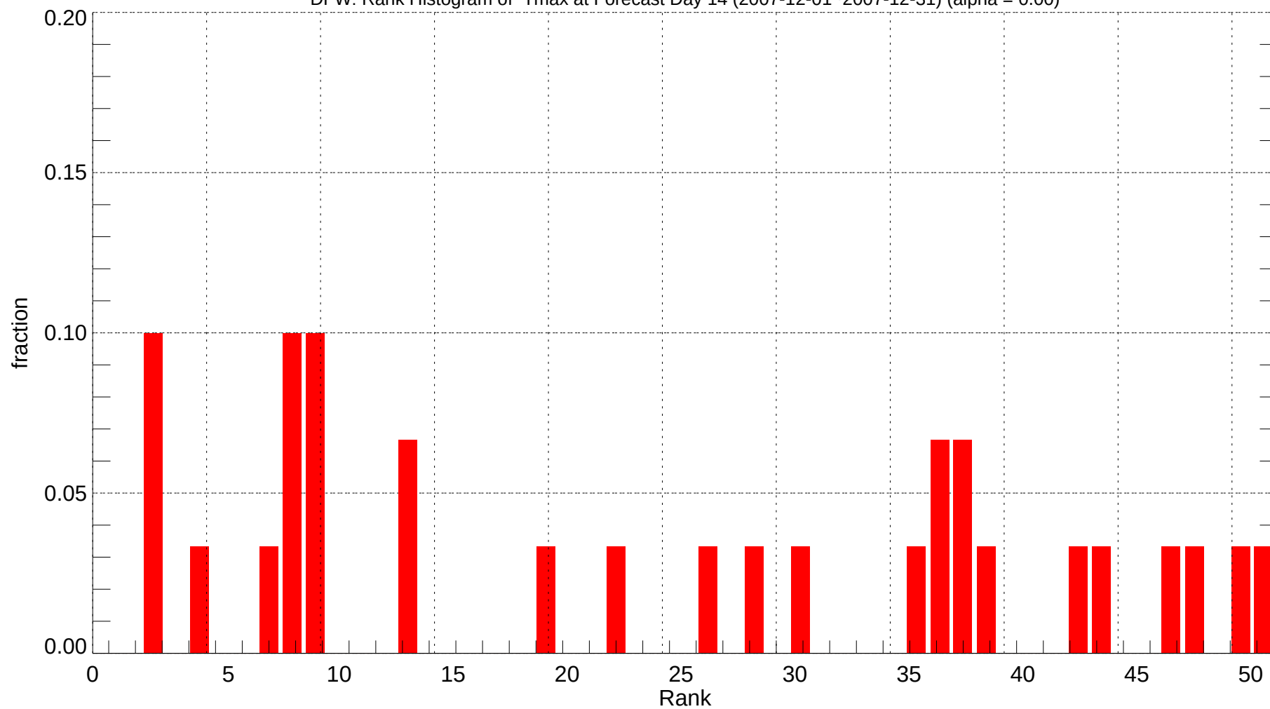
DFW: Rank Histogram of Tmax at Forecast Day 14 (2007-12-01~2007-12-31) (alpha = 0.00)
