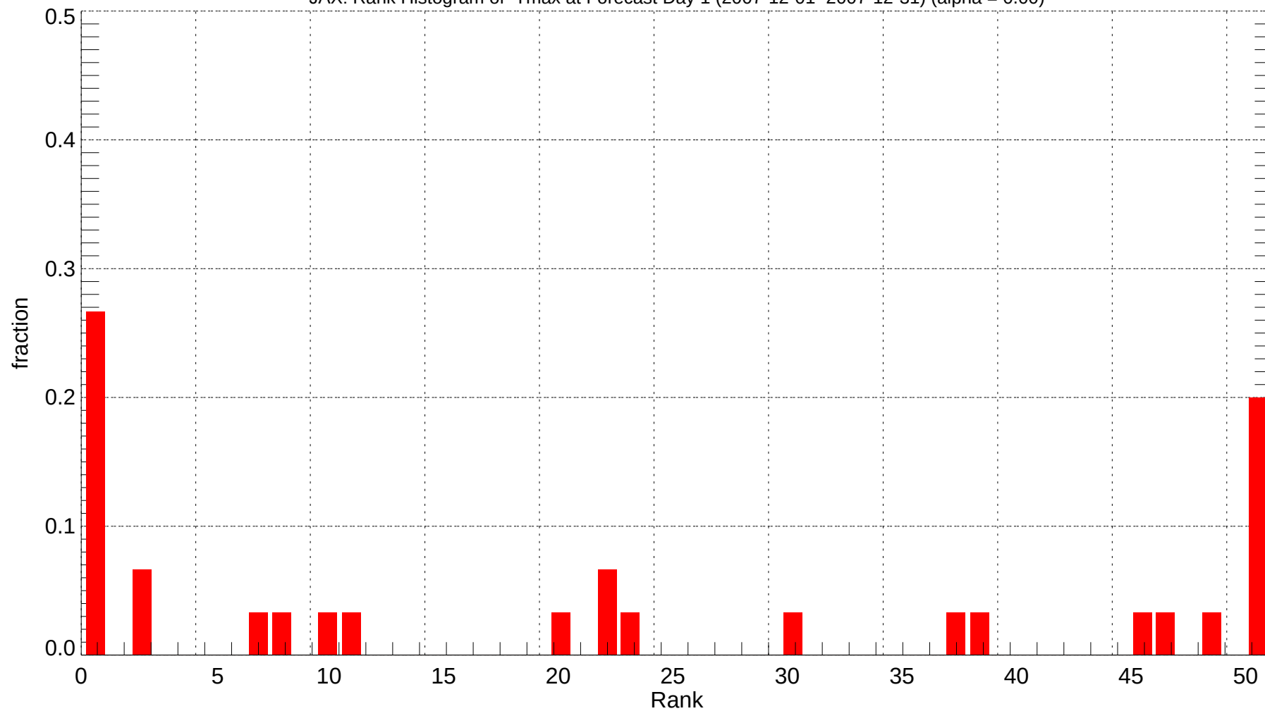
JAX: Rank Histogram of Tmax at Forecast Day 1 (2007-12-01~2007-12-31) (alpha = 0.00)
