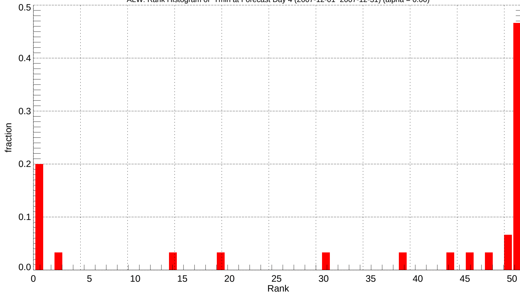
ALW: Rank Histogram of Tmin at Forecast Day 4 (2007-12-01~2007-12-31) (alpha = 0.00)
