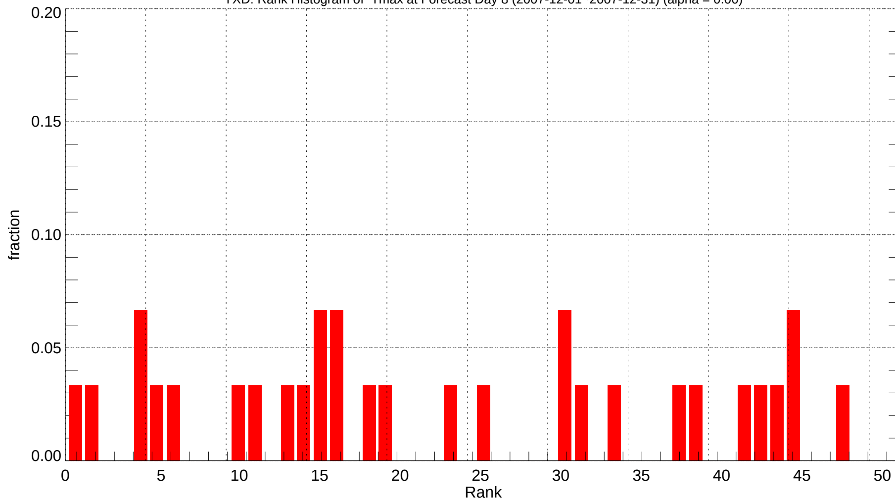
YXD: Rank Histogram of Tmax at Forecast Day 8 (2007-12-01~2007-12-31) (alpha = 0.00)
