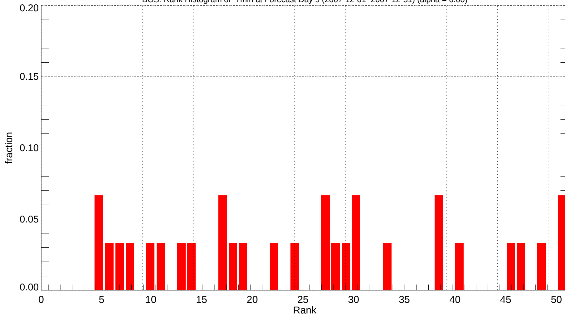
BOS: Rank Histogram of Tmin at Forecast Day 9 (2007-12-01~2007-12-31) (alpha = 0.00)
