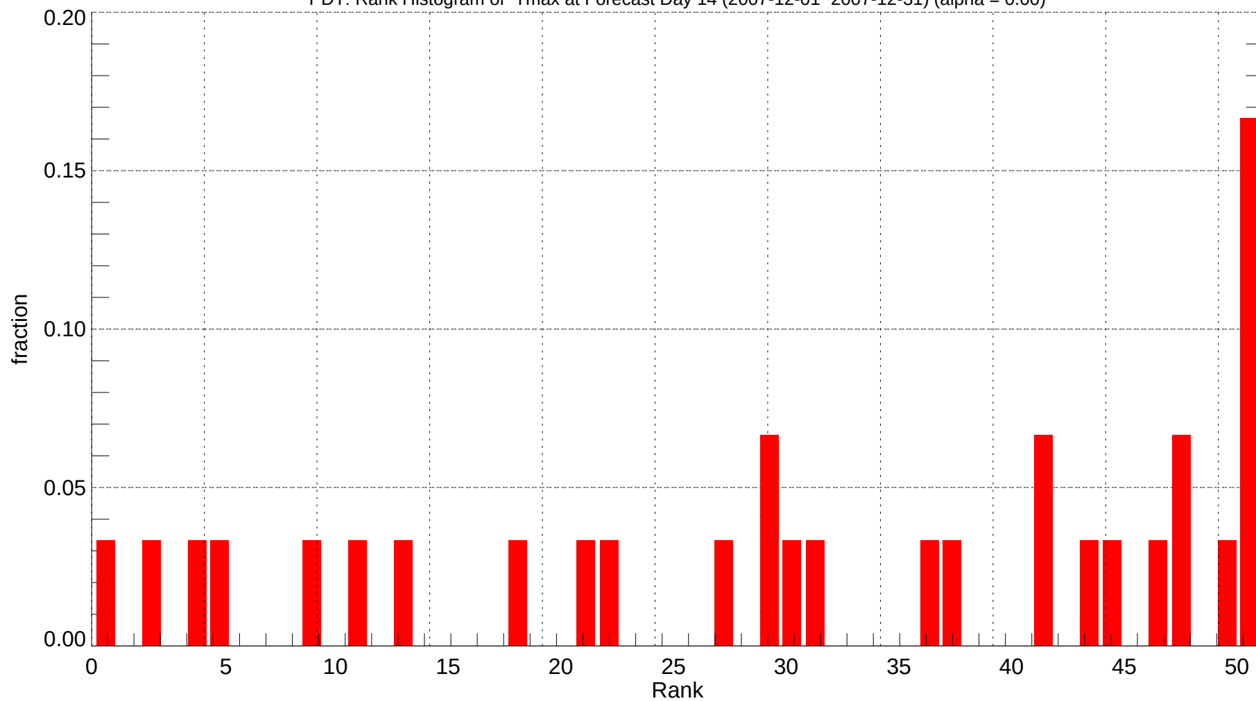
PDT: Rank Histogram of Tmax at Forecast Day 14 (2007-12-01~2007-12-31) (alpha = 0.00)
