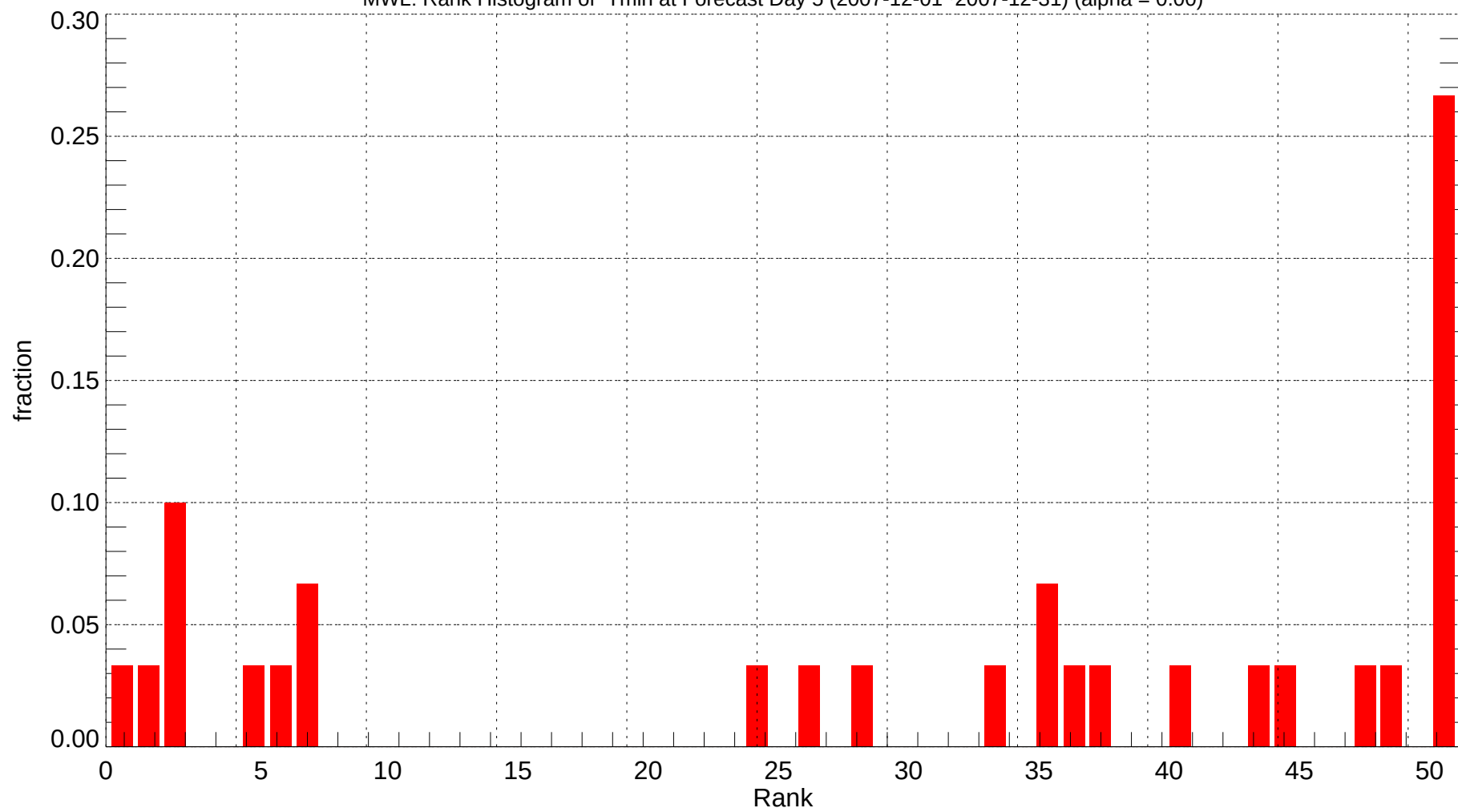
MWL: Rank Histogram of Tmin at Forecast Day 5 (2007-12-01~2007-12-31) (alpha = 0.00)
