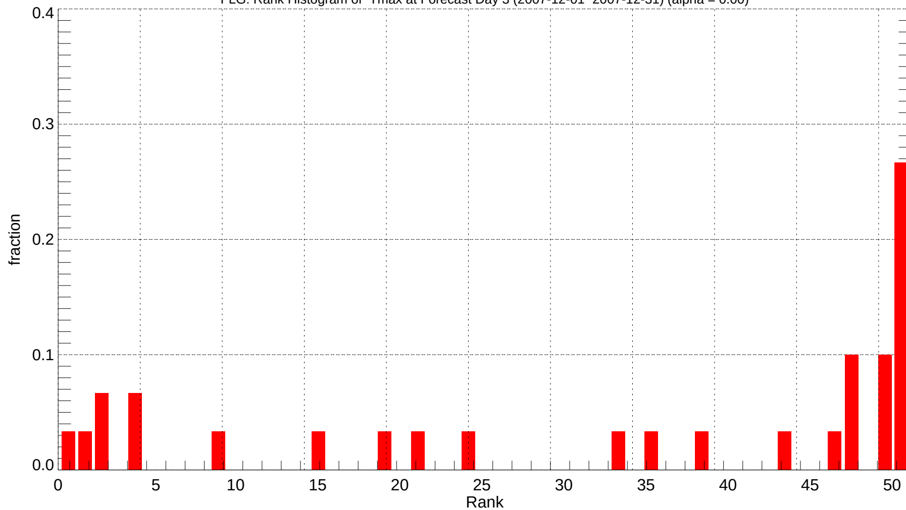
FLG: Rank Histogram of Tmax at Forecast Day 3 (2007-12-01~2007-12-31) (alpha = 0.00)
