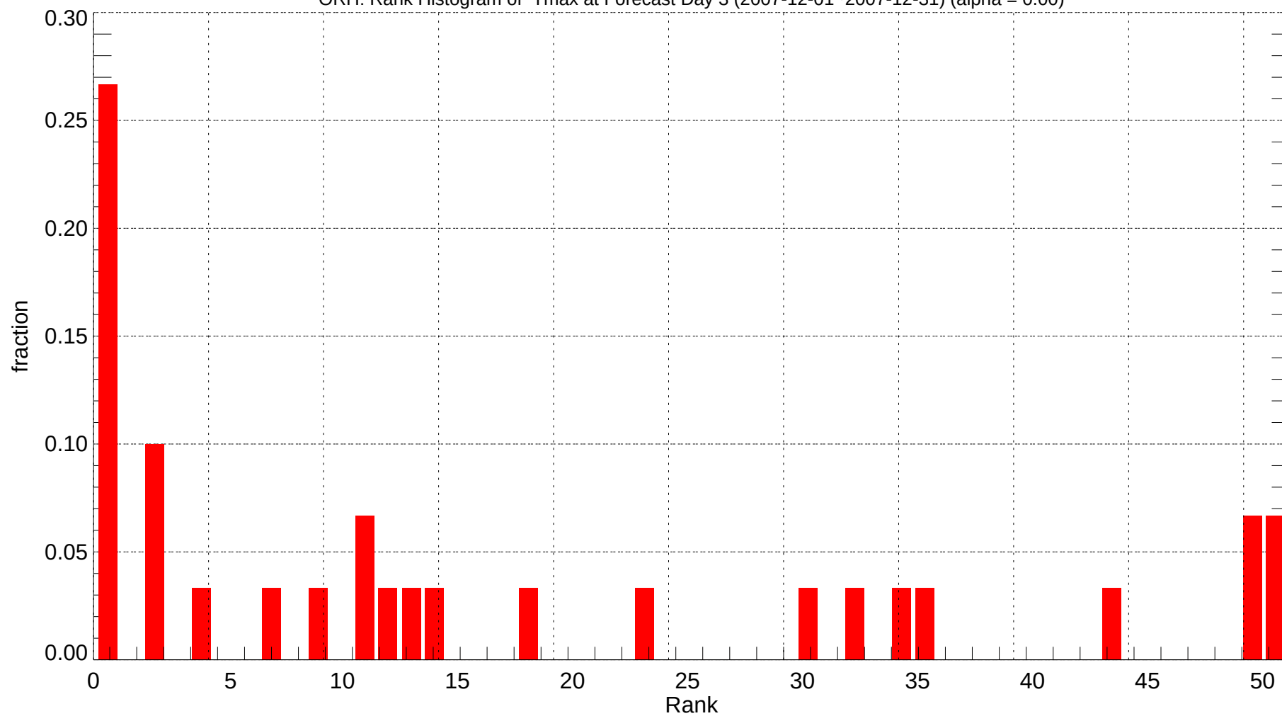
ORH: Rank Histogram of Tmax at Forecast Day 3 (2007-12-01~2007-12-31) (alpha = 0.00)
