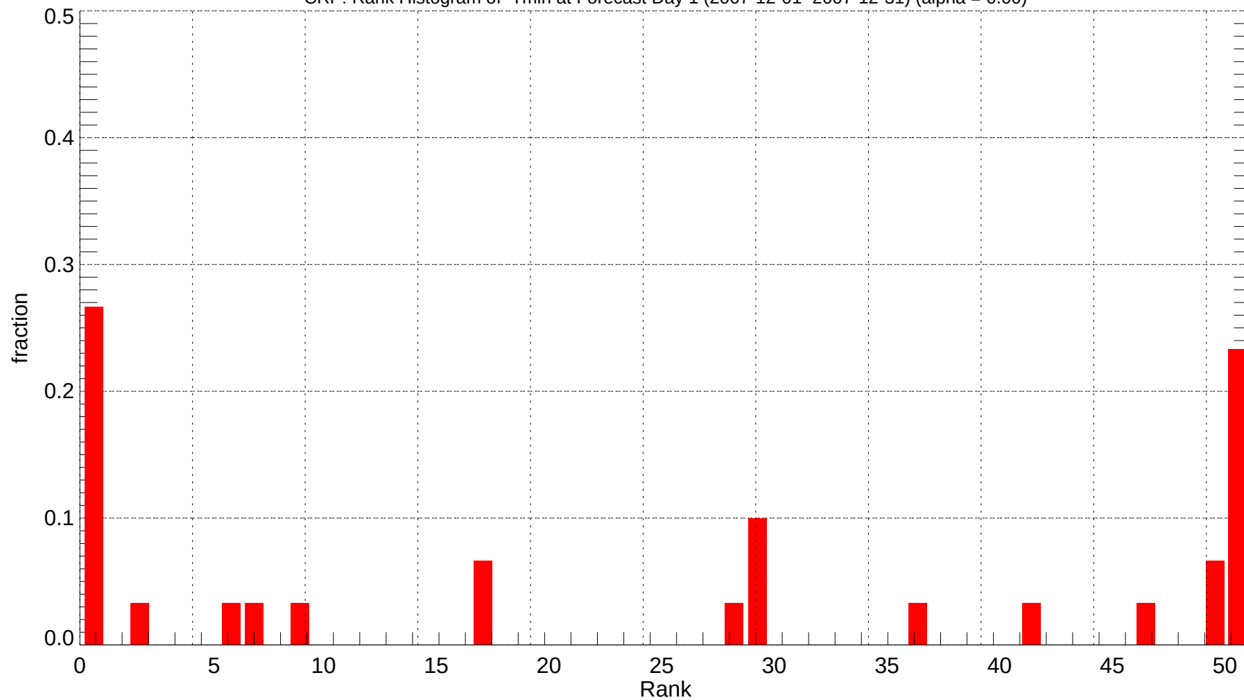
CRP: Rank Histogram of Tmin at Forecast Day 1 (2007-12-01~2007-12-31) (alpha = 0.00)
