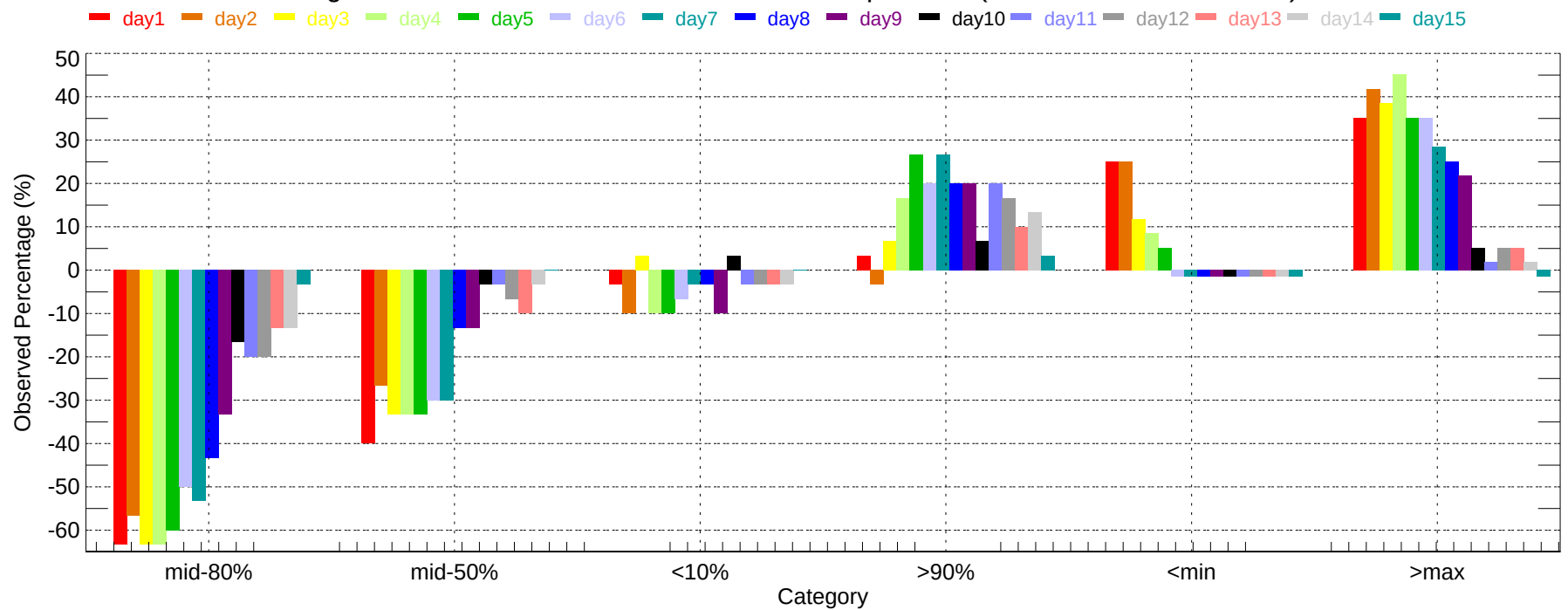
Observed Percentage Deviation of Ensembles - BFL: Max Temperature (2007-12-01~2007-12-31)
