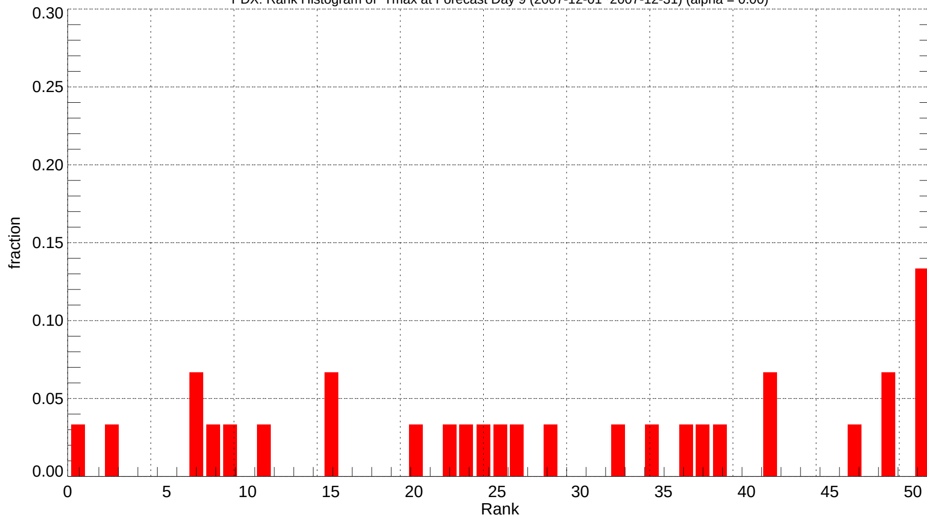
PDX: Rank Histogram of Tmax at Forecast Day 9 (2007-12-01~2007-12-31) (alpha = 0.00)
