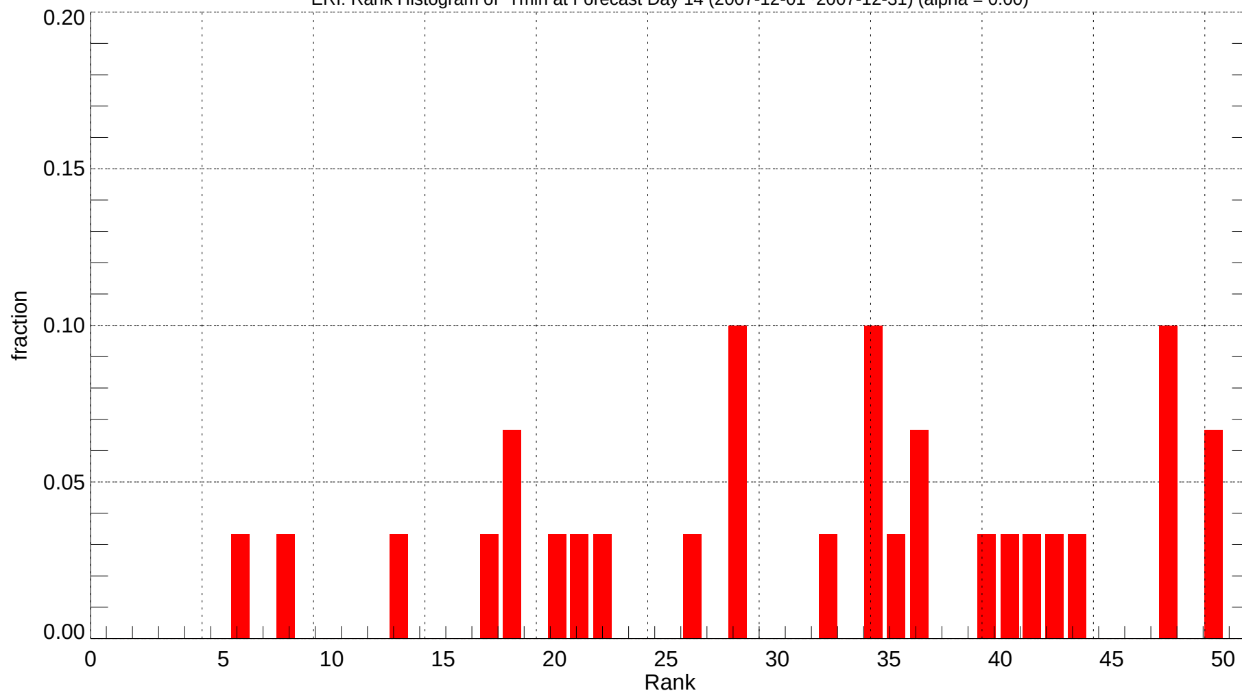
ERI: Rank Histogram of Tmin at Forecast Day 14 (2007-12-01~2007-12-31) (alpha = 0.00)
