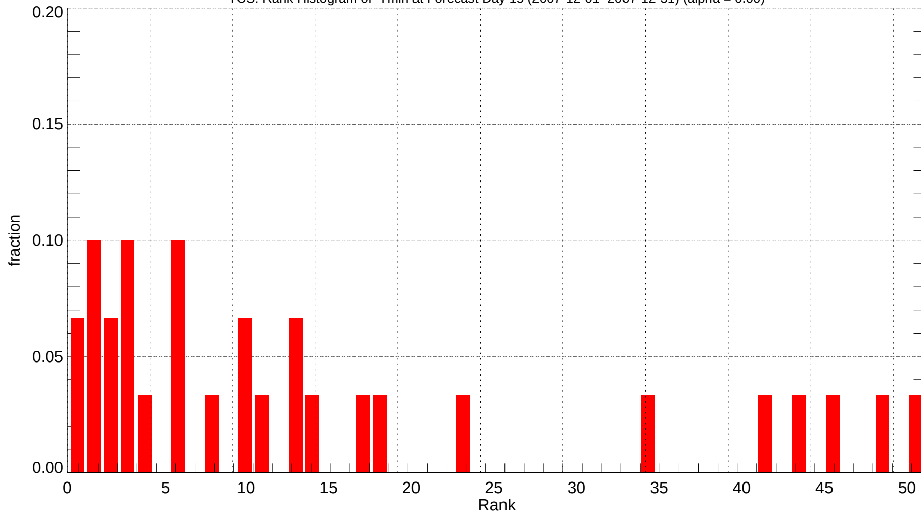
TUS: Rank Histogram of Tmin at Forecast Day 15 (2007-12-01~2007-12-31) (alpha = 0.00)
