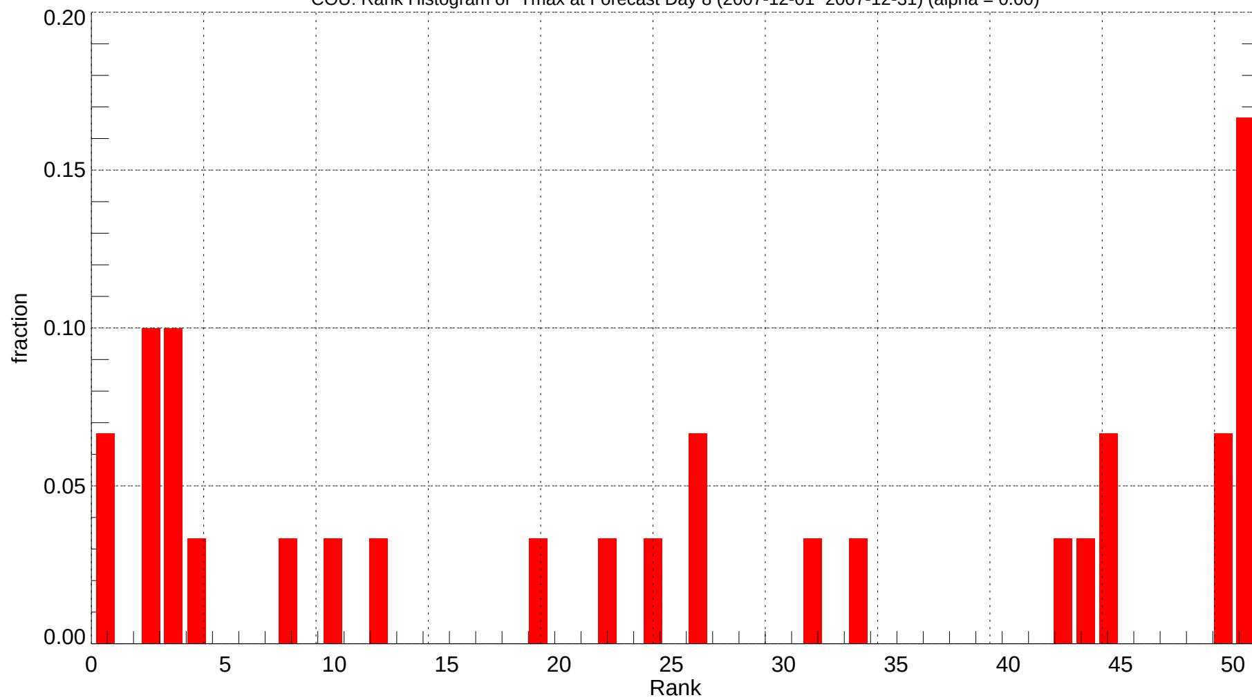
COU: Rank Histogram of Tmax at Forecast Day 8 (2007-12-01~2007-12-31) (alpha = 0.00)
