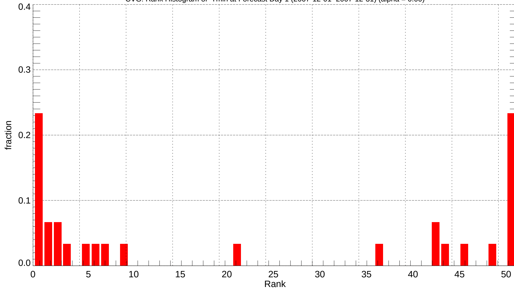
CVG: Rank Histogram of Tmin at Forecast Day 1 (2007-12-01~2007-12-31) (alpha = 0.00)
