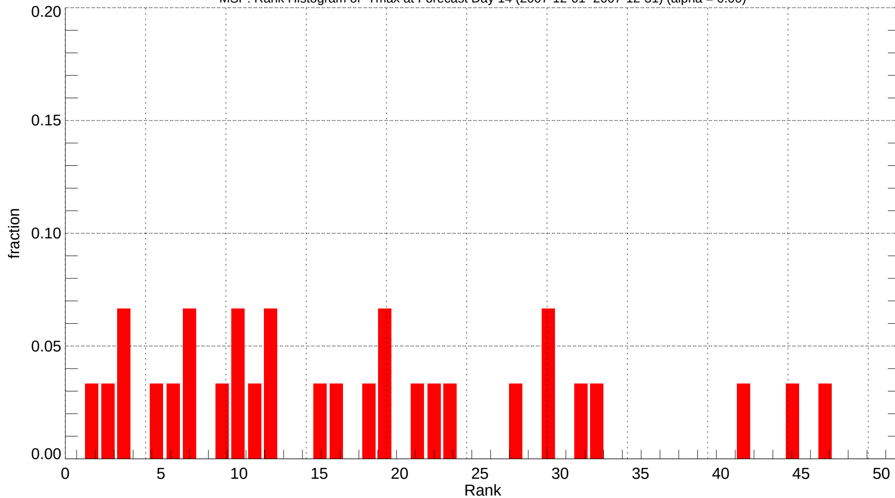
MSP: Rank Histogram of Tmax at Forecast Day 14 (2007-12-01~2007-12-31) (alpha = 0.00)
