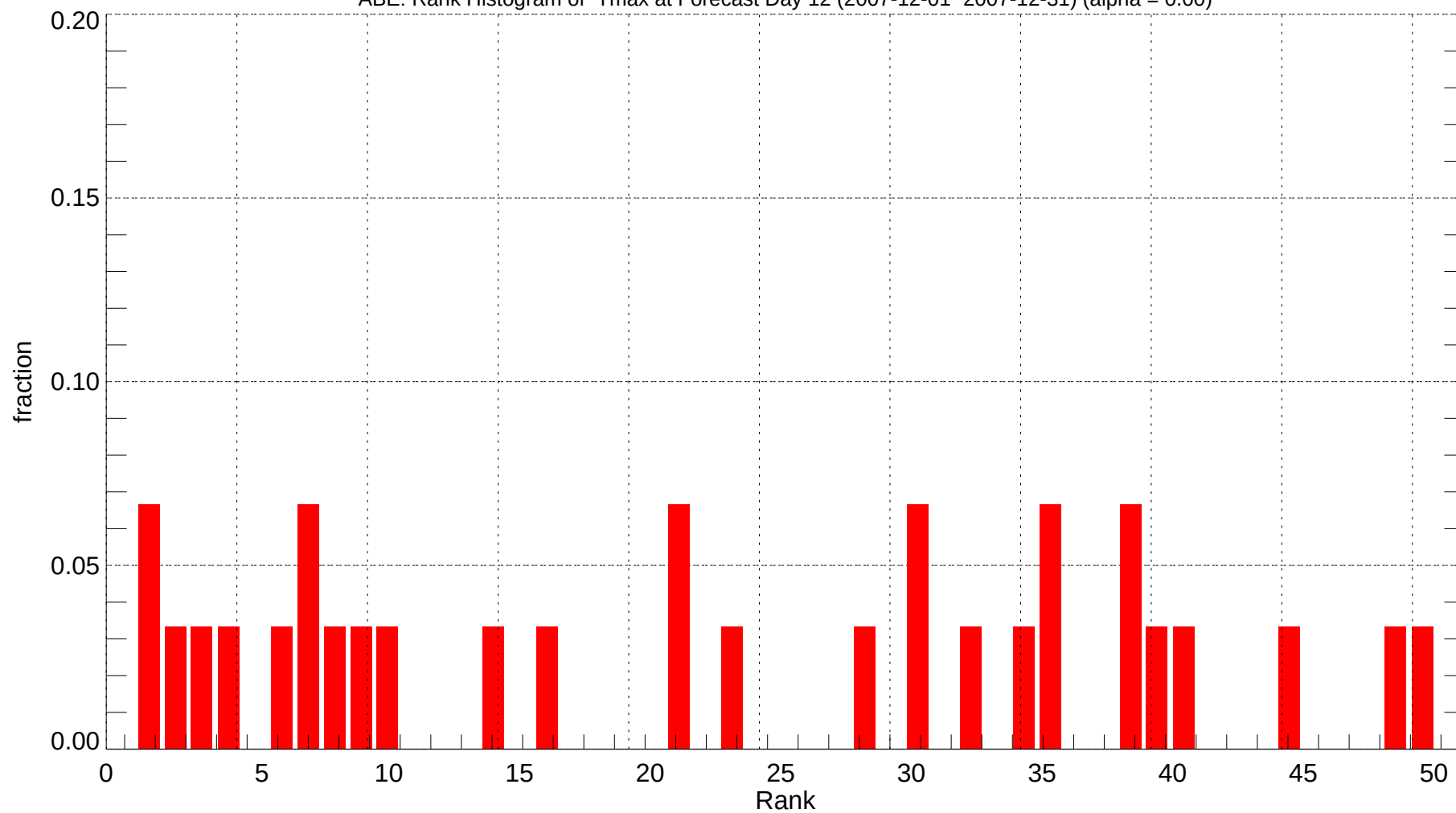
ABE: Rank Histogram of Tmax at Forecast Day 12 (2007-12-01~2007-12-31) (alpha = 0.00)
