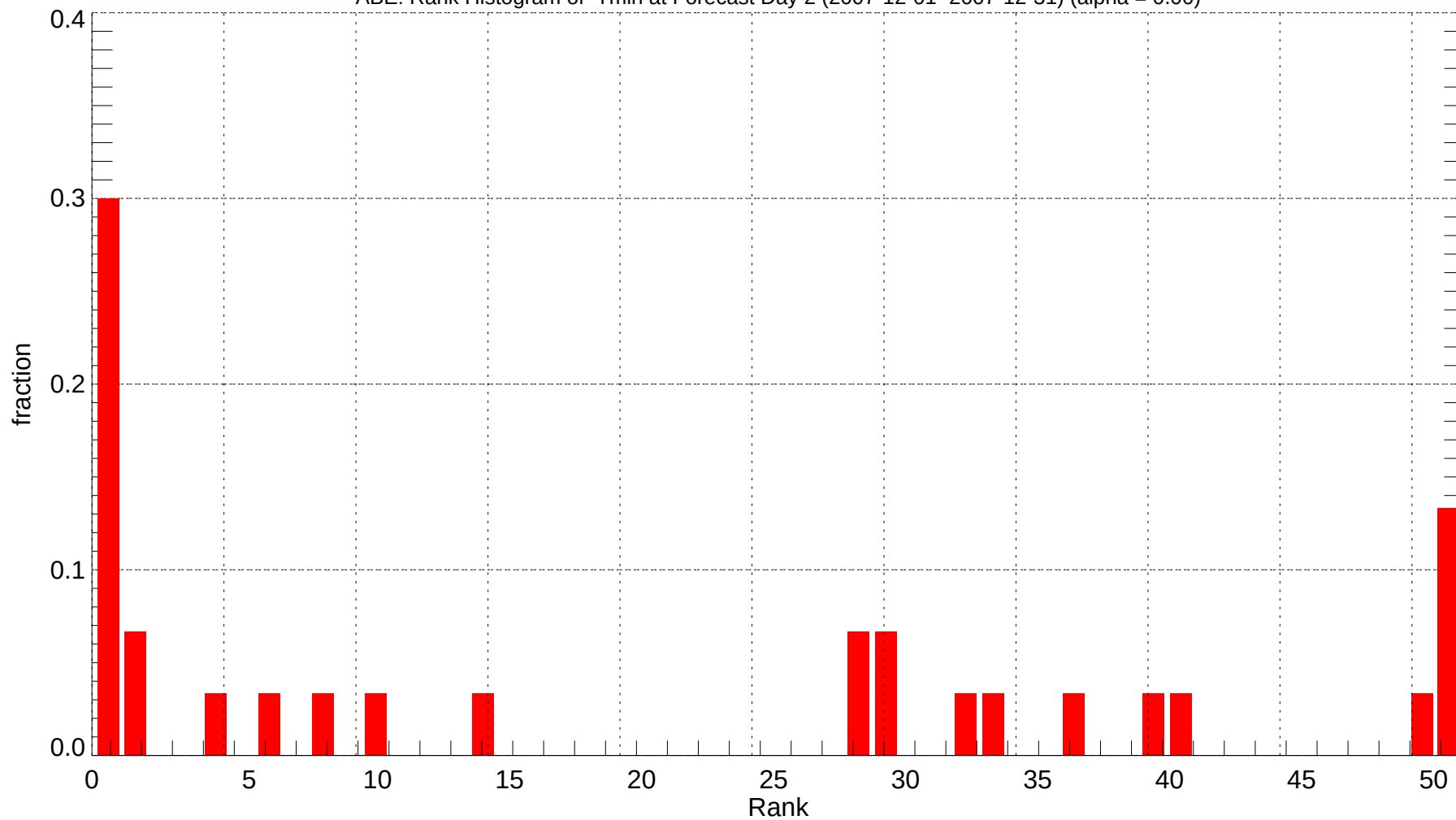
ABE: Rank Histogram of Tmin at Forecast Day 2 (2007-12-01~2007-12-31) (alpha = 0.00)
