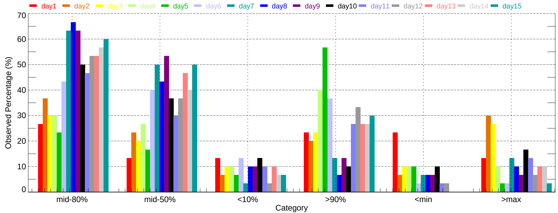
Observed Percentage of Ensembles - BOI: Min Temperature (2007-12-01~2007-12-31)
