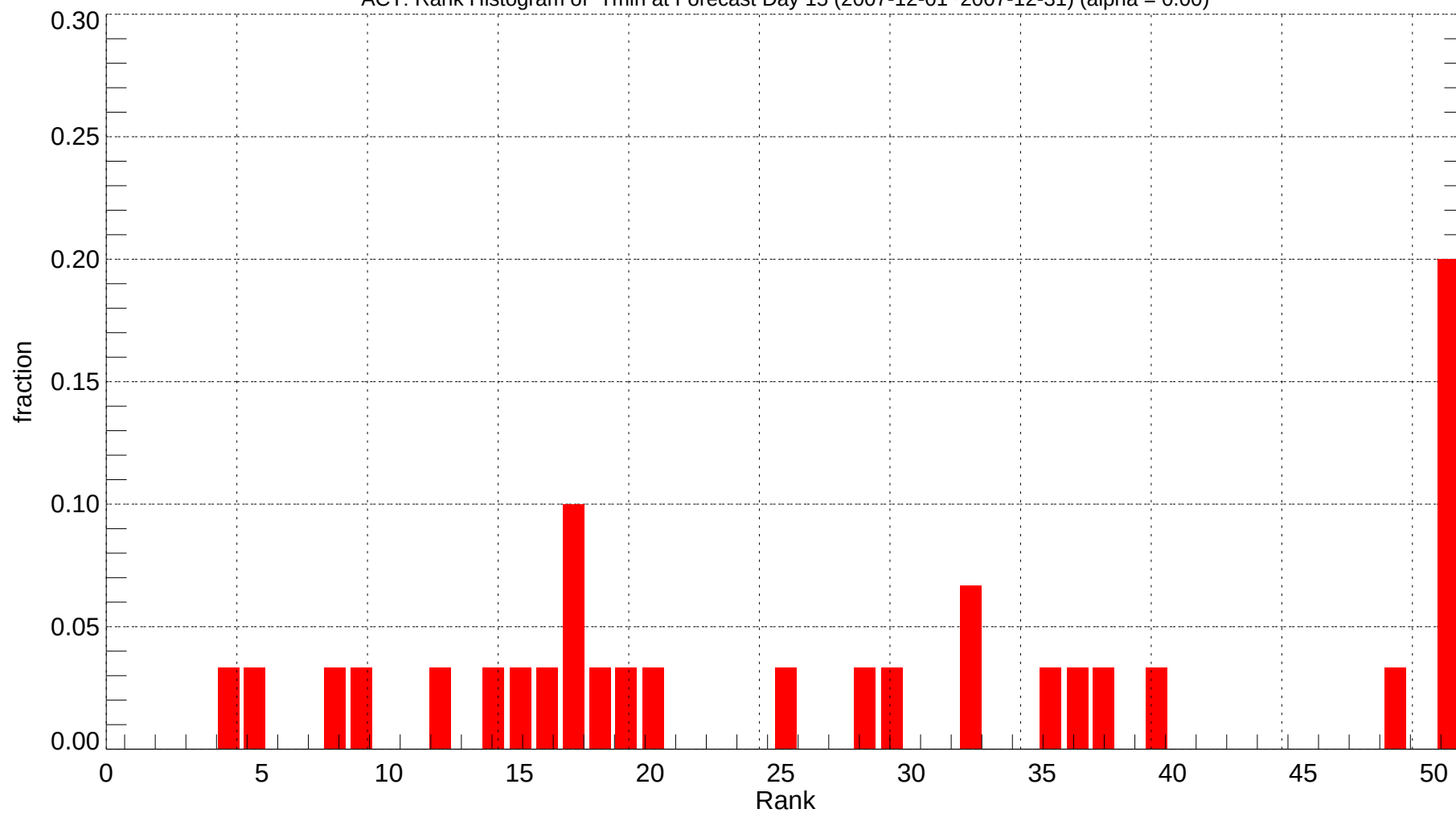
ACT: Rank Histogram of Tmin at Forecast Day 15 (2007-12-01~2007-12-31) (alpha = 0.00)
