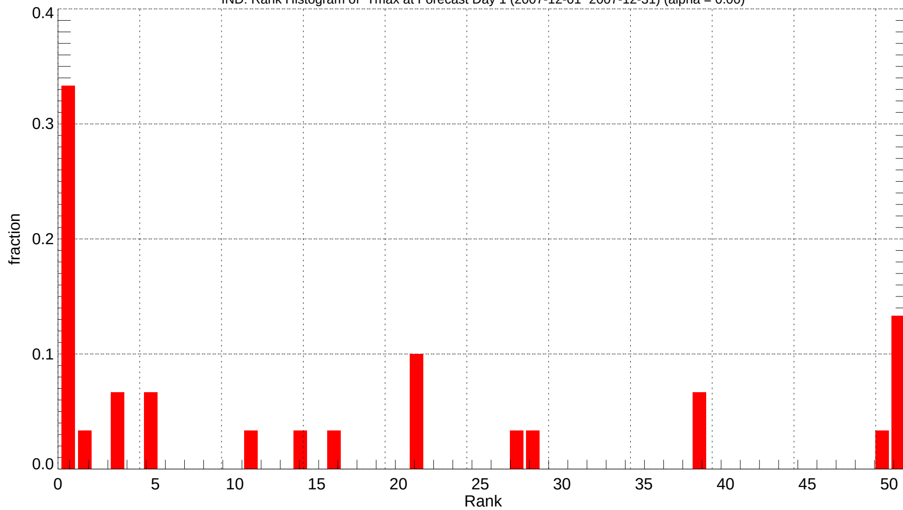
IND: Rank Histogram of Tmax at Forecast Day 1 (2007-12-01~2007-12-31) (alpha = 0.00)
