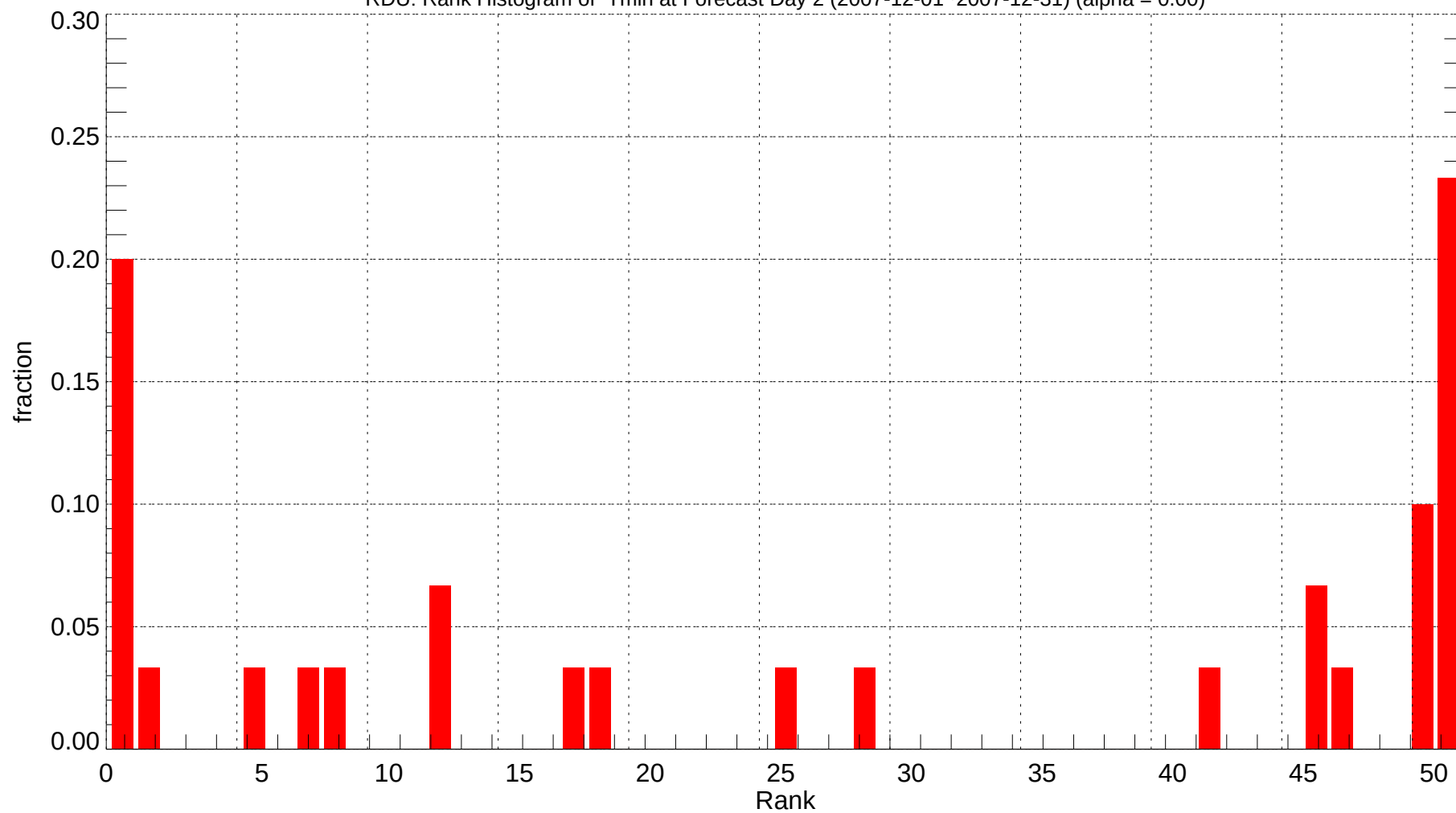
RDU: Rank Histogram of Tmin at Forecast Day 2 (2007-12-01~2007-12-31) (alpha = 0.00)
