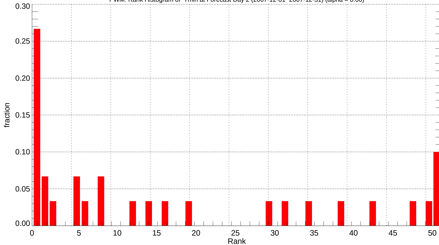
PWM: Rank Histogram of Tmin at Forecast Day 2 (2007-12-01~2007-12-31) (alpha = 0.00)
