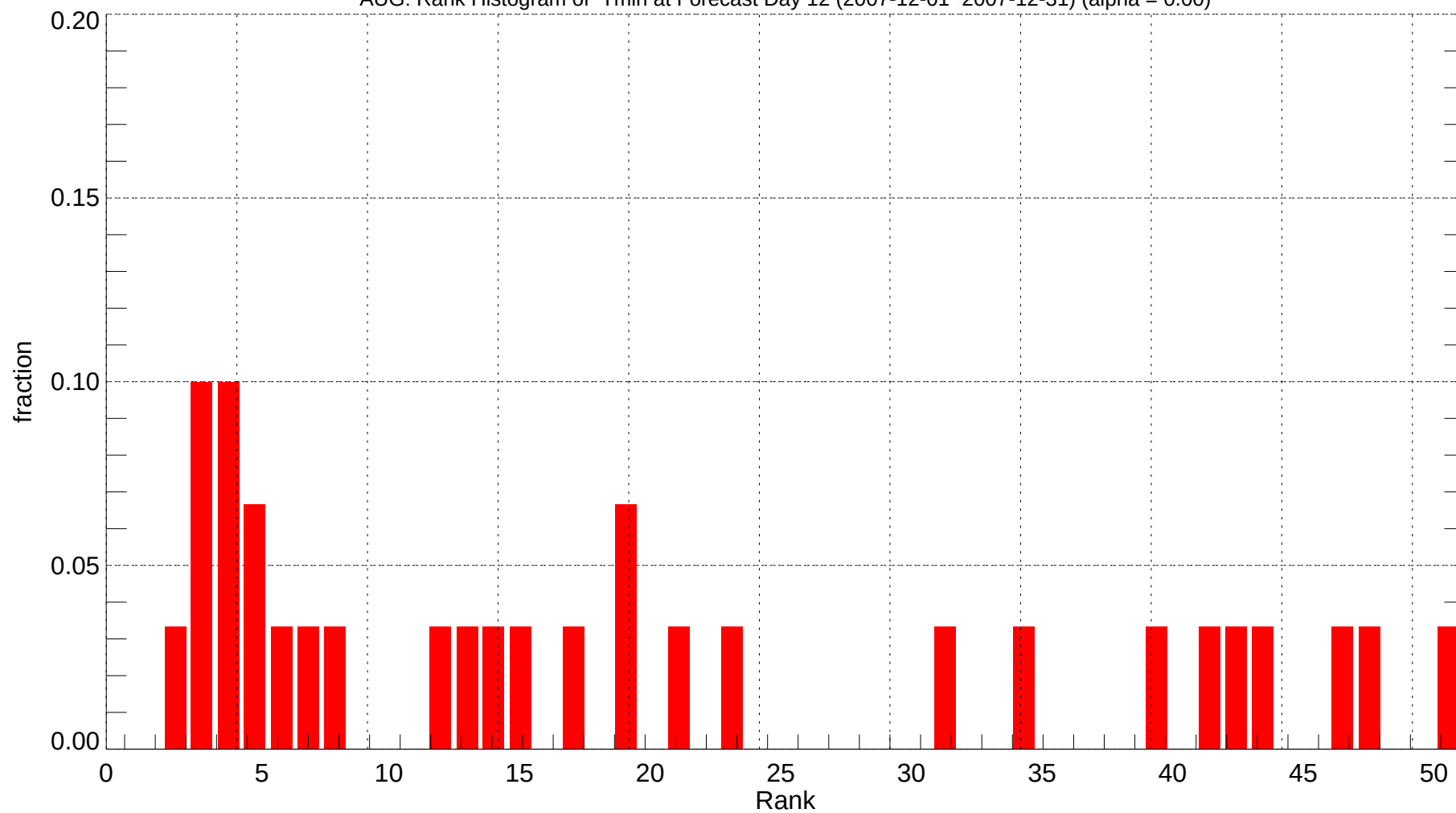
AUG: Rank Histogram of Tmin at Forecast Day 12 (2007-12-01~2007-12-31) (alpha = 0.00)
