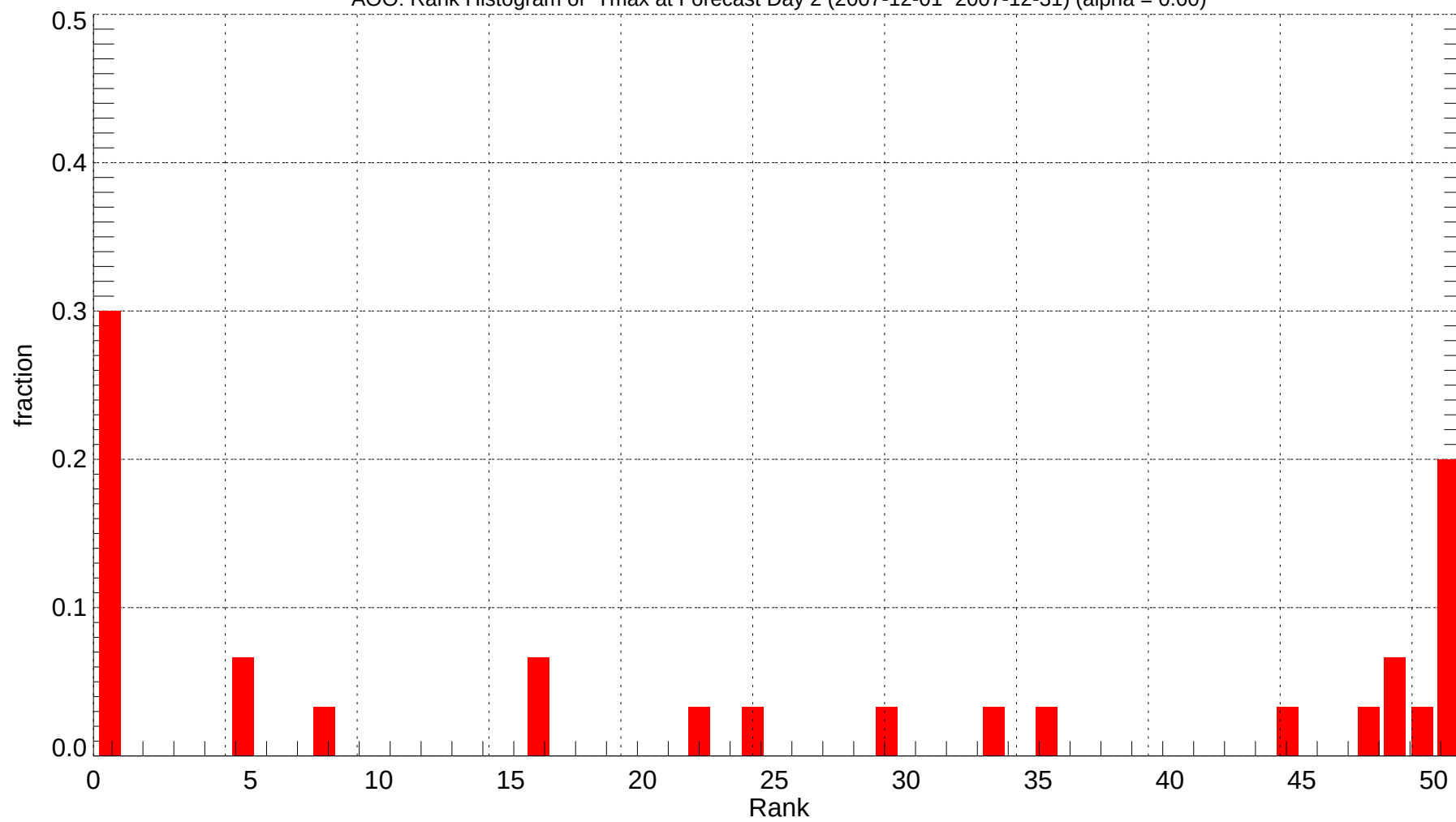
AOO: Rank Histogram of Tmax at Forecast Day 2 (2007-12-01~2007-12-31) (alpha = 0.00)
