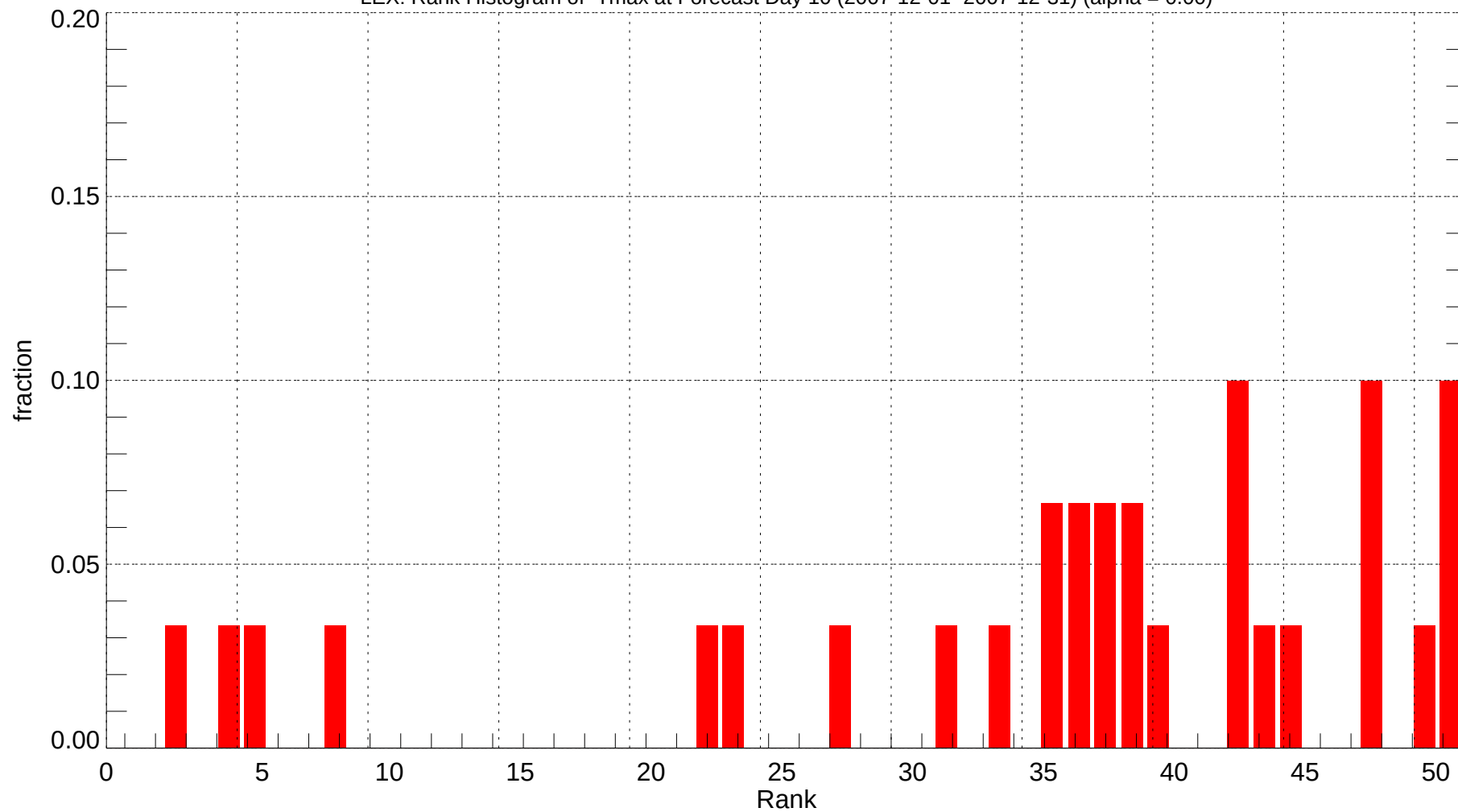
LEX: Rank Histogram of Tmax at Forecast Day 10 (2007-12-01~2007-12-31) (alpha = 0.00)
