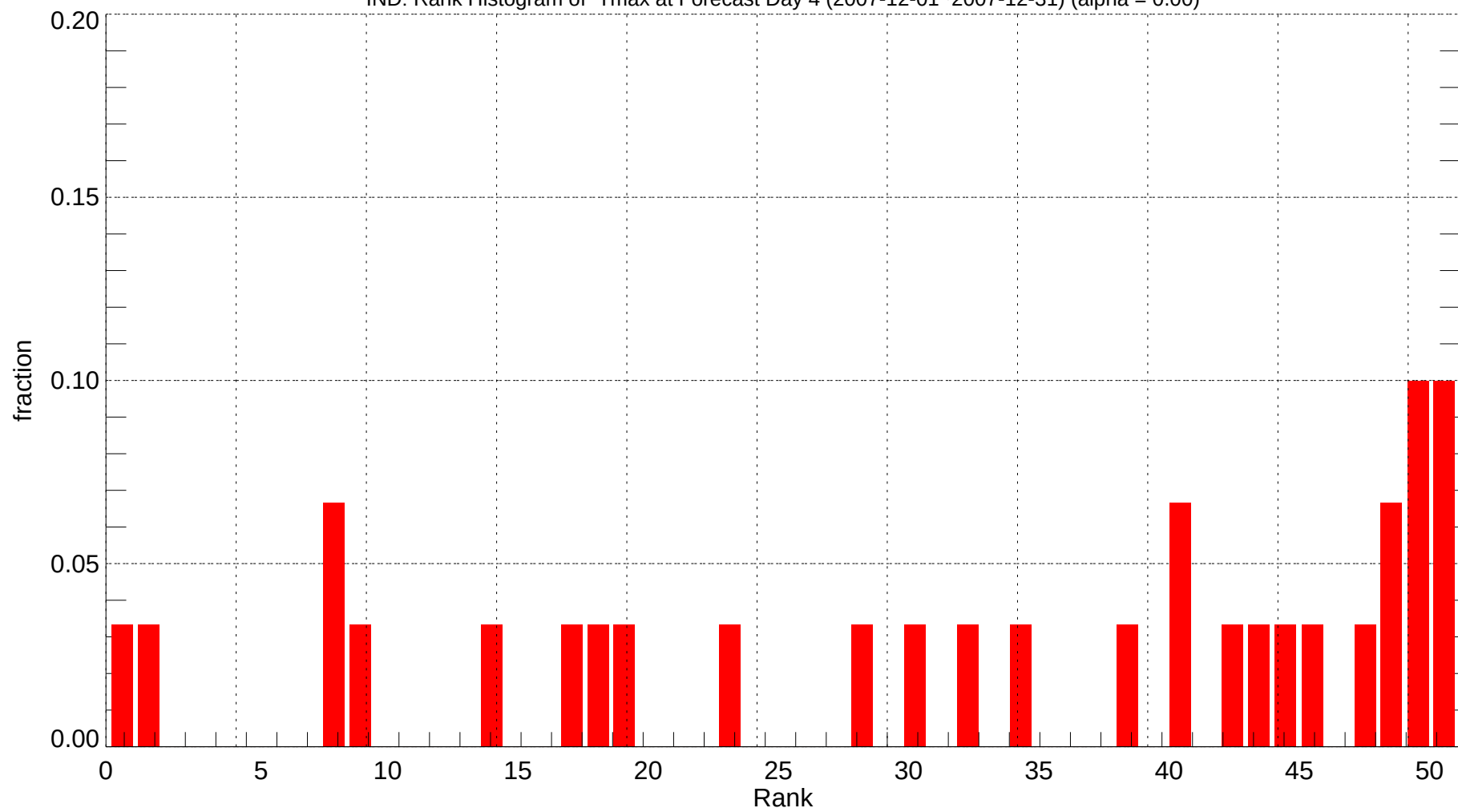
IND: Rank Histogram of Tmax at Forecast Day 4 (2007-12-01~2007-12-31) (alpha = 0.00)
