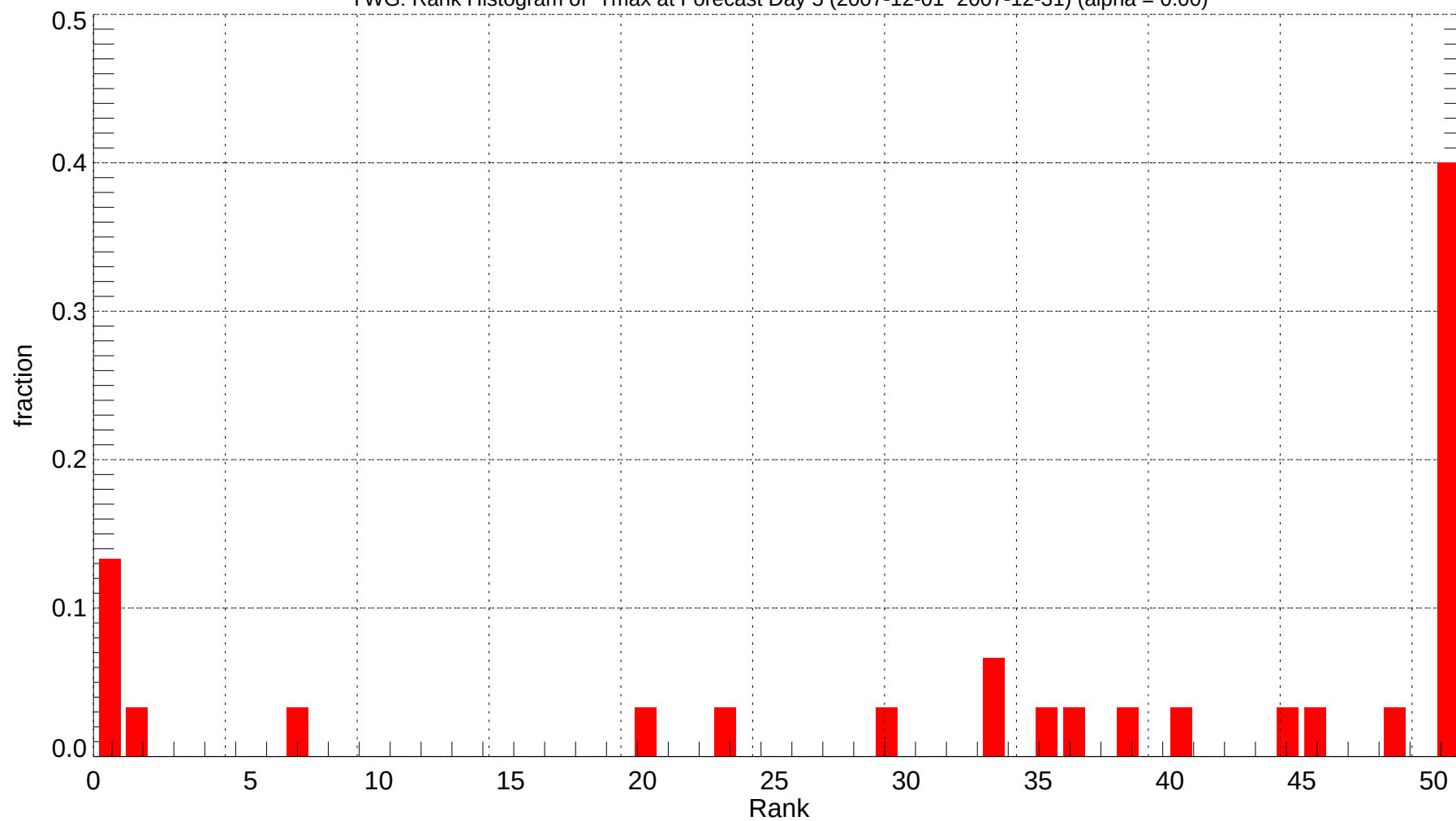
YWG: Rank Histogram of Tmax at Forecast Day 5 (2007-12-01~2007-12-31) (alpha = 0.00)
