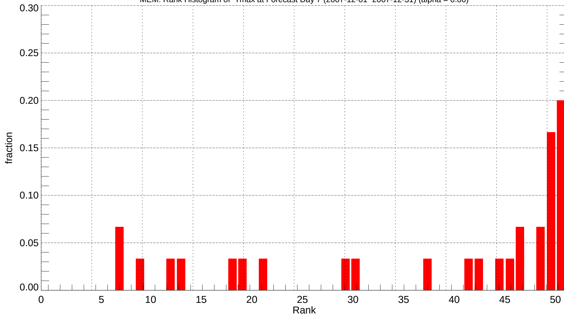
MEM: Rank Histogram of Tmax at Forecast Day 7 (2007-12-01~2007-12-31) (alpha = 0.00)
