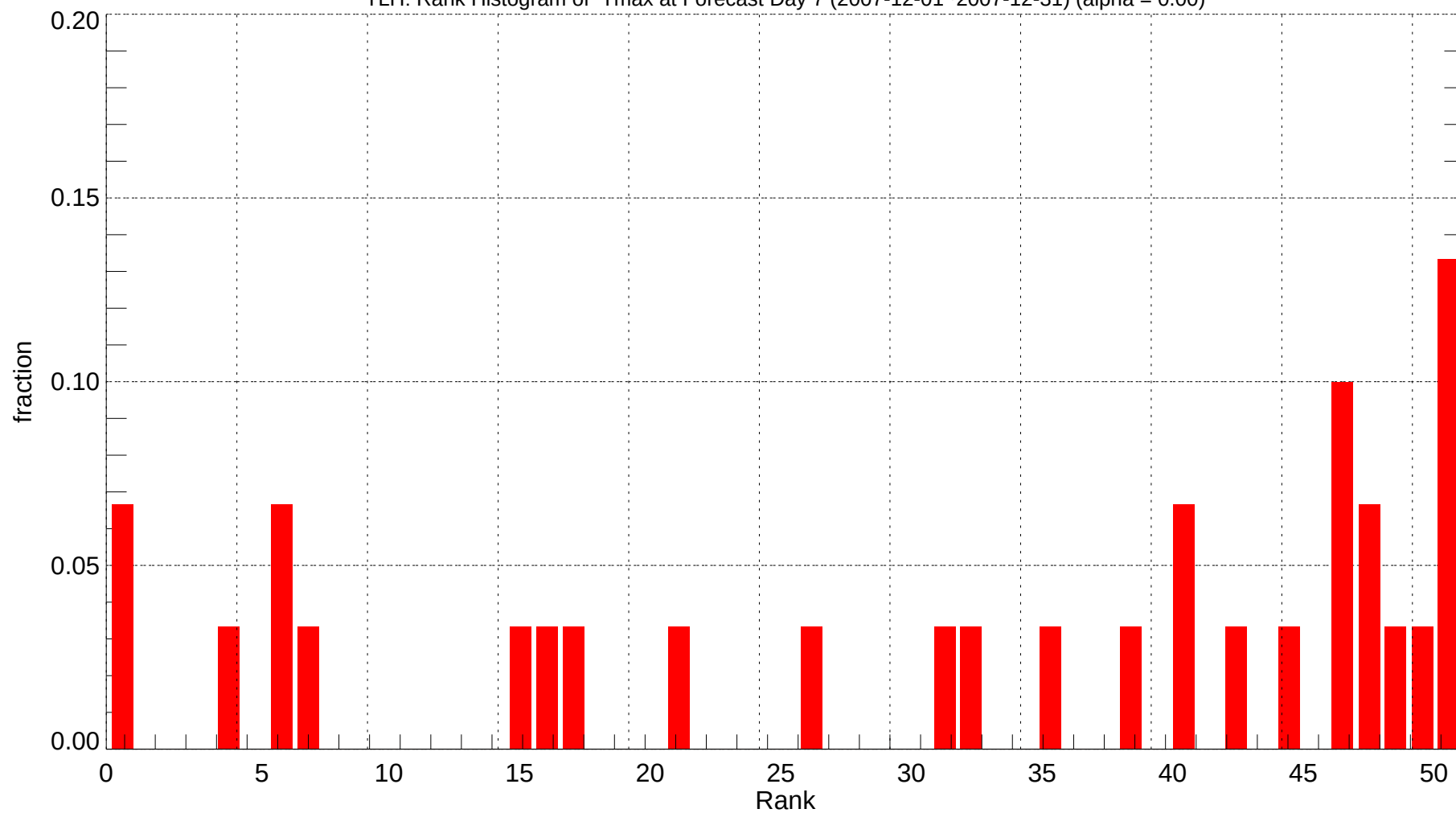
TLH: Rank Histogram of Tmax at Forecast Day 7 (2007-12-01~2007-12-31) (alpha = 0.00)
