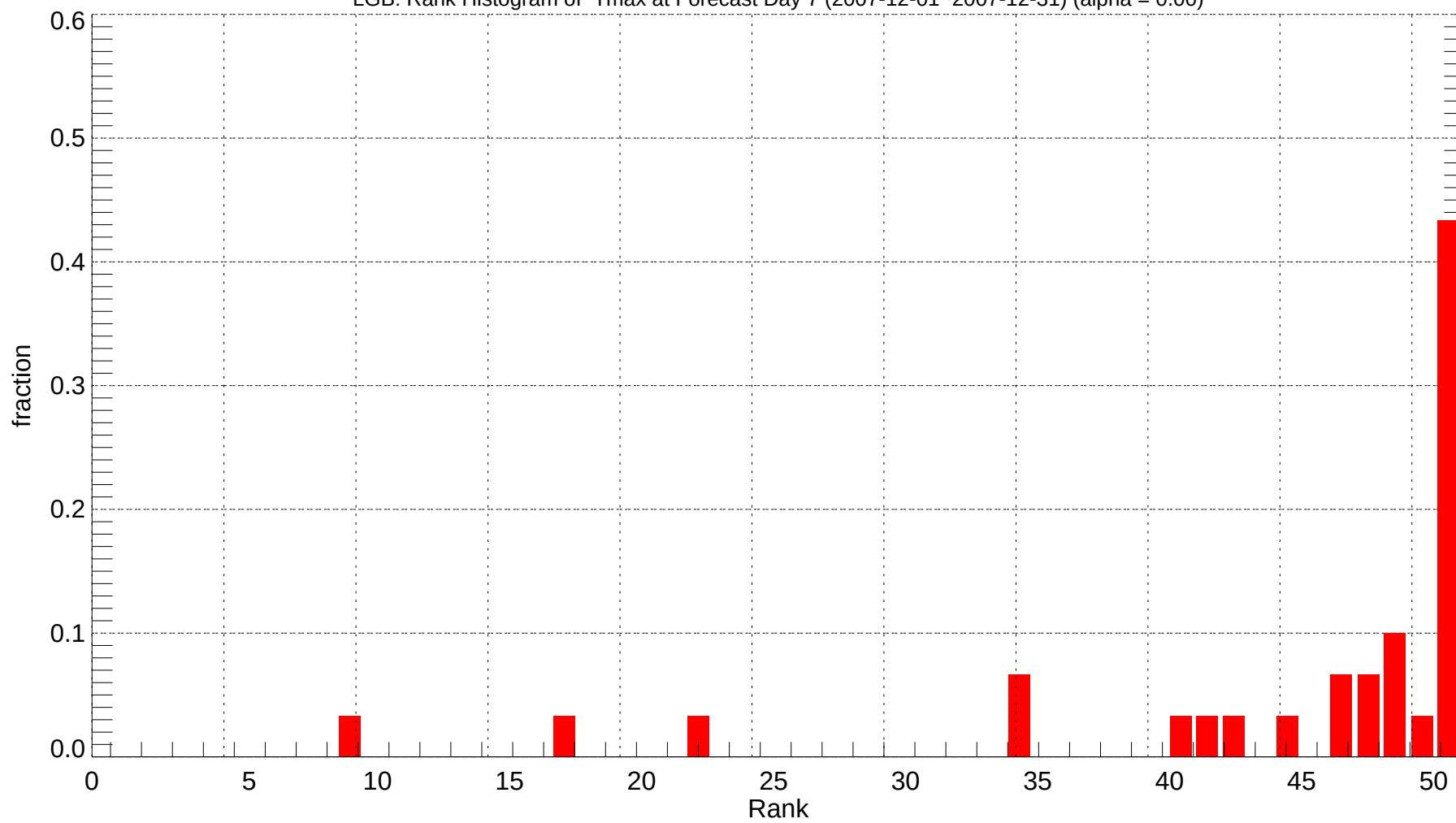
LGB: Rank Histogram of Tmax at Forecast Day 7 (2007-12-01~2007-12-31) (alpha = 0.00)
