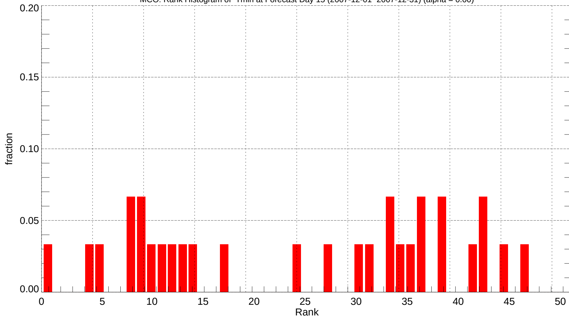
MCO: Rank Histogram of Tmin at Forecast Day 15 (2007-12-01~2007-12-31) (alpha = 0.00)
