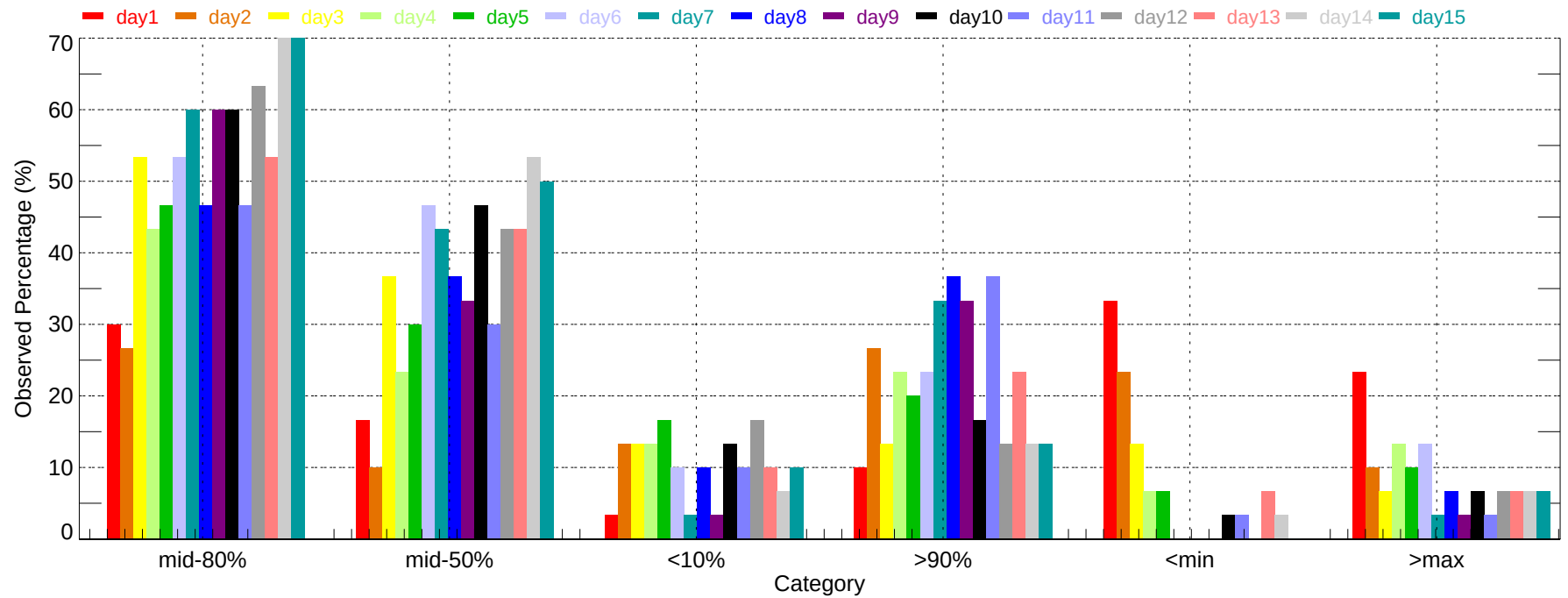
Observed Percentage of Ensembles - ROA: Max Temperature (2007-12-01~2007-12-31)
