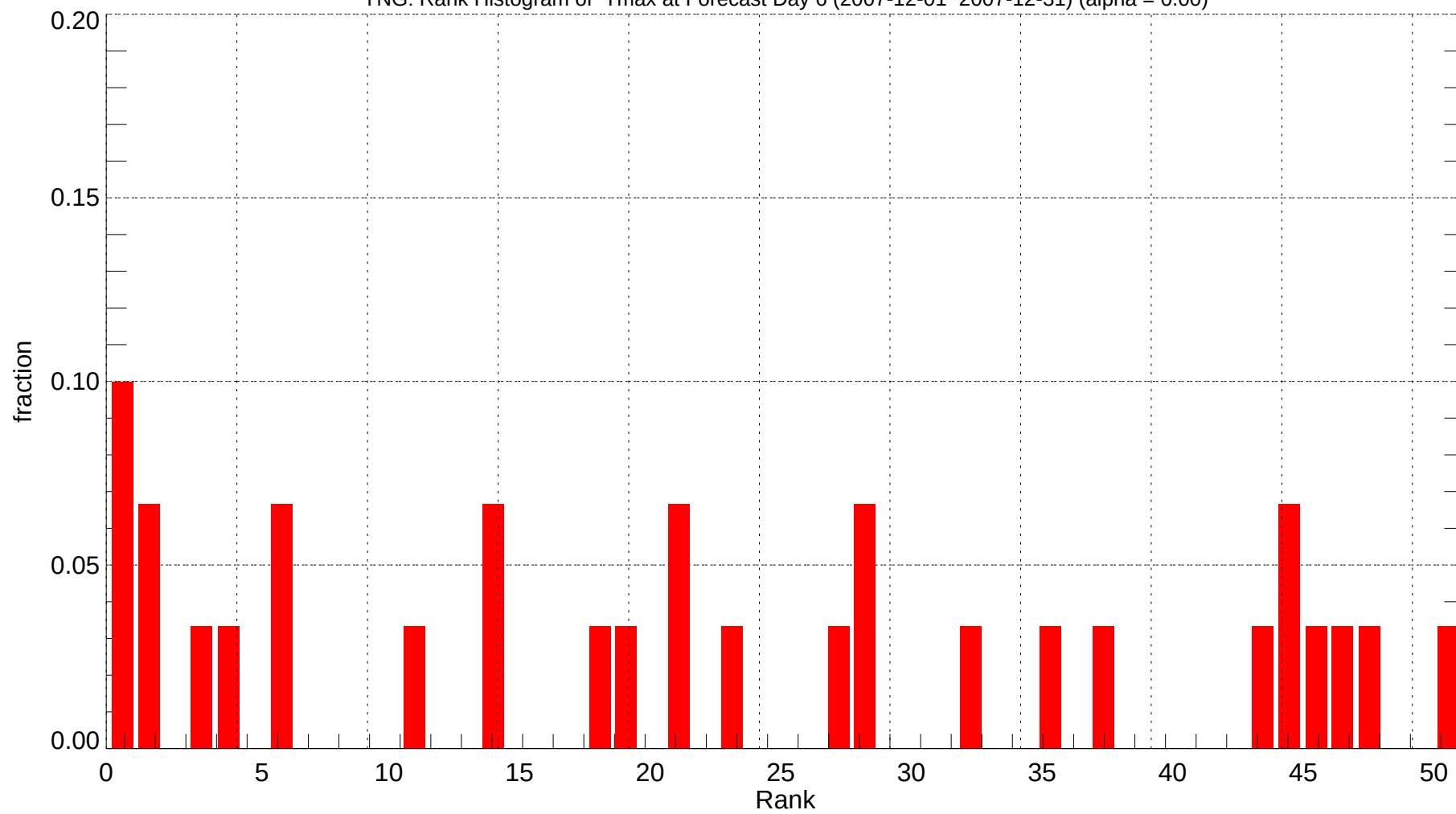
YNG: Rank Histogram of Tmax at Forecast Day 6 (2007-12-01~2007-12-31) (alpha = 0.00)
