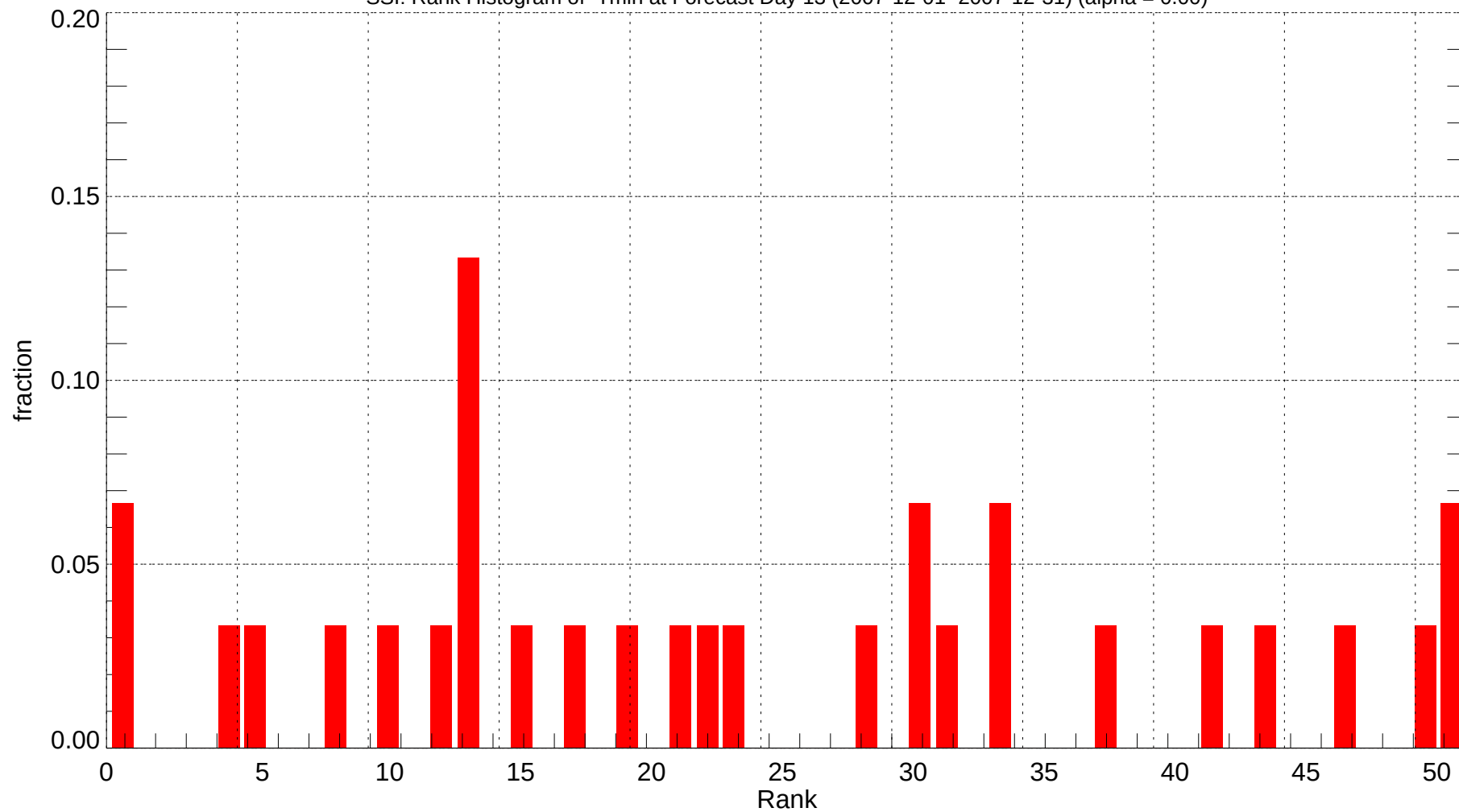
SSI: Rank Histogram of Tmin at Forecast Day 13 (2007-12-01~2007-12-31) (alpha = 0.00)
