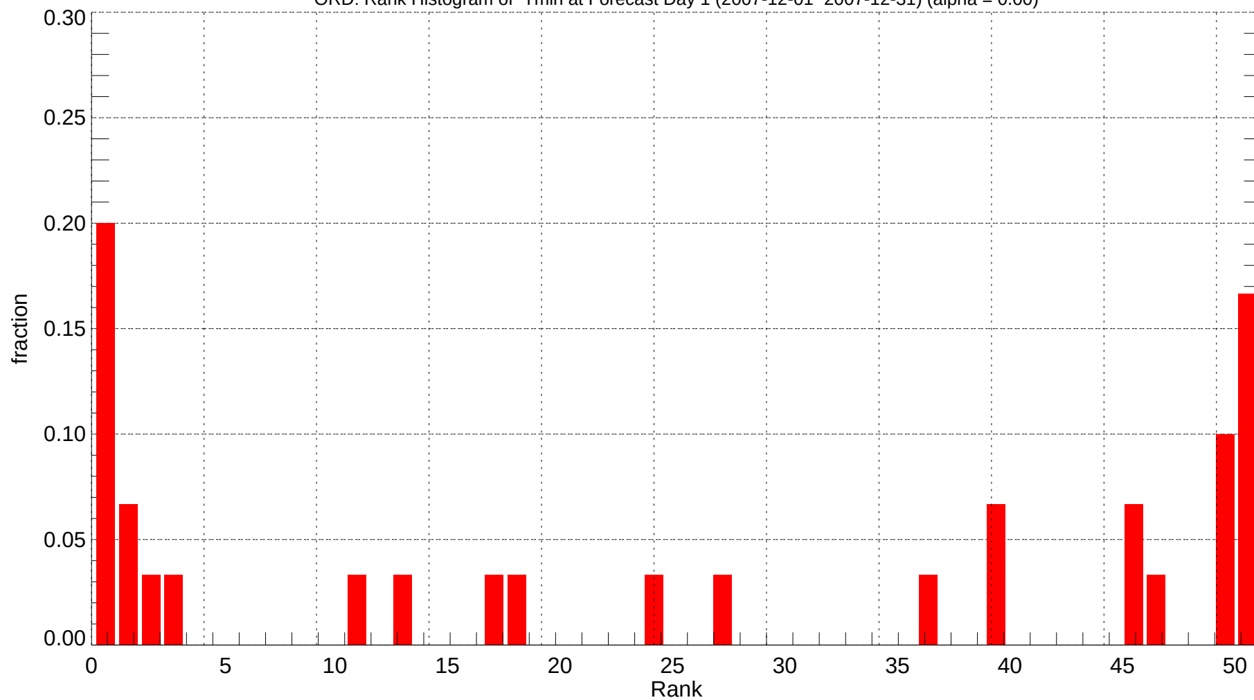
ORD: Rank Histogram of Tmin at Forecast Day 1 (2007-12-01~2007-12-31) (alpha = 0.00)
