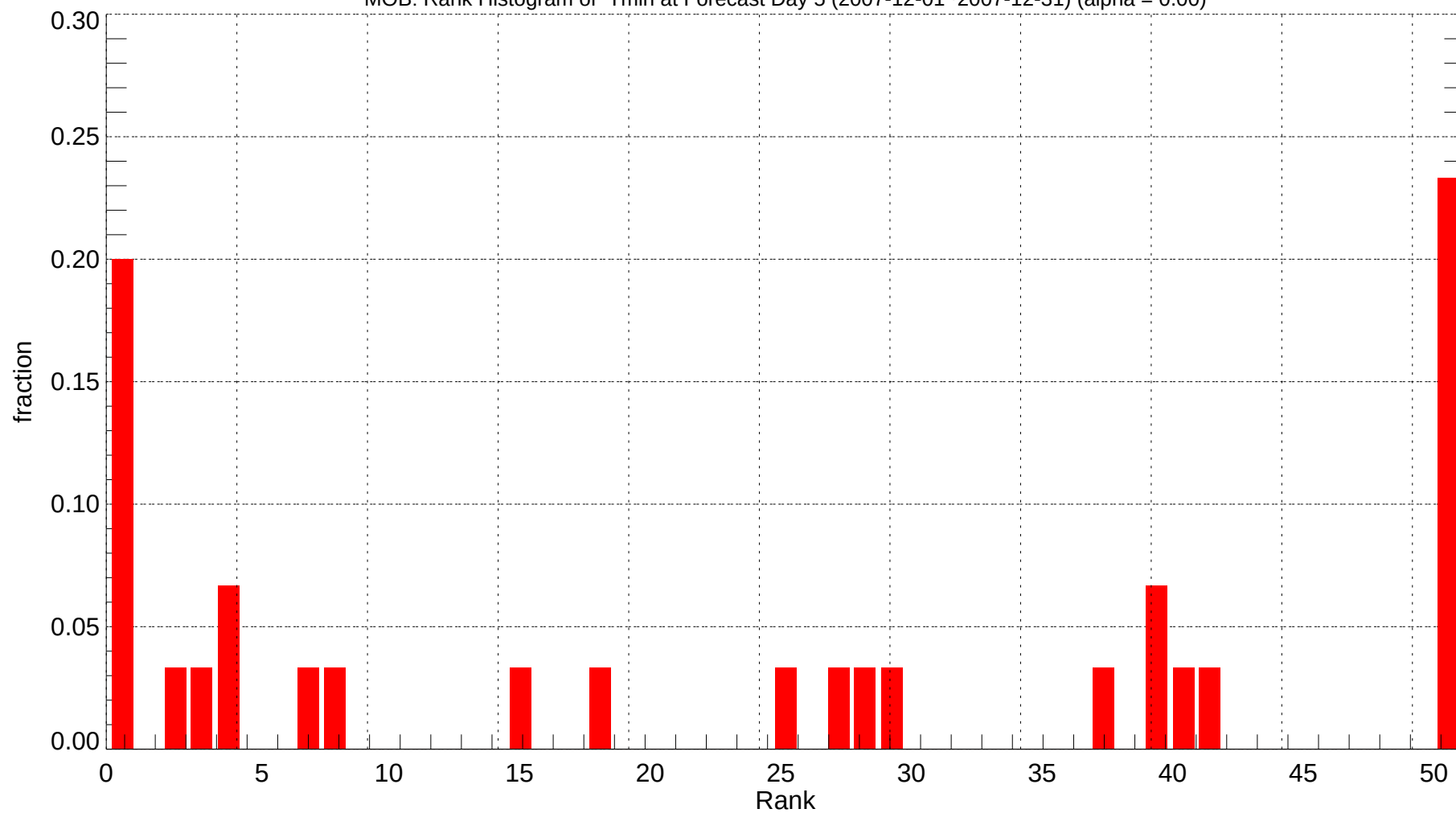
MOB: Rank Histogram of Tmin at Forecast Day 5 (2007-12-01~2007-12-31) (alpha = 0.00)
