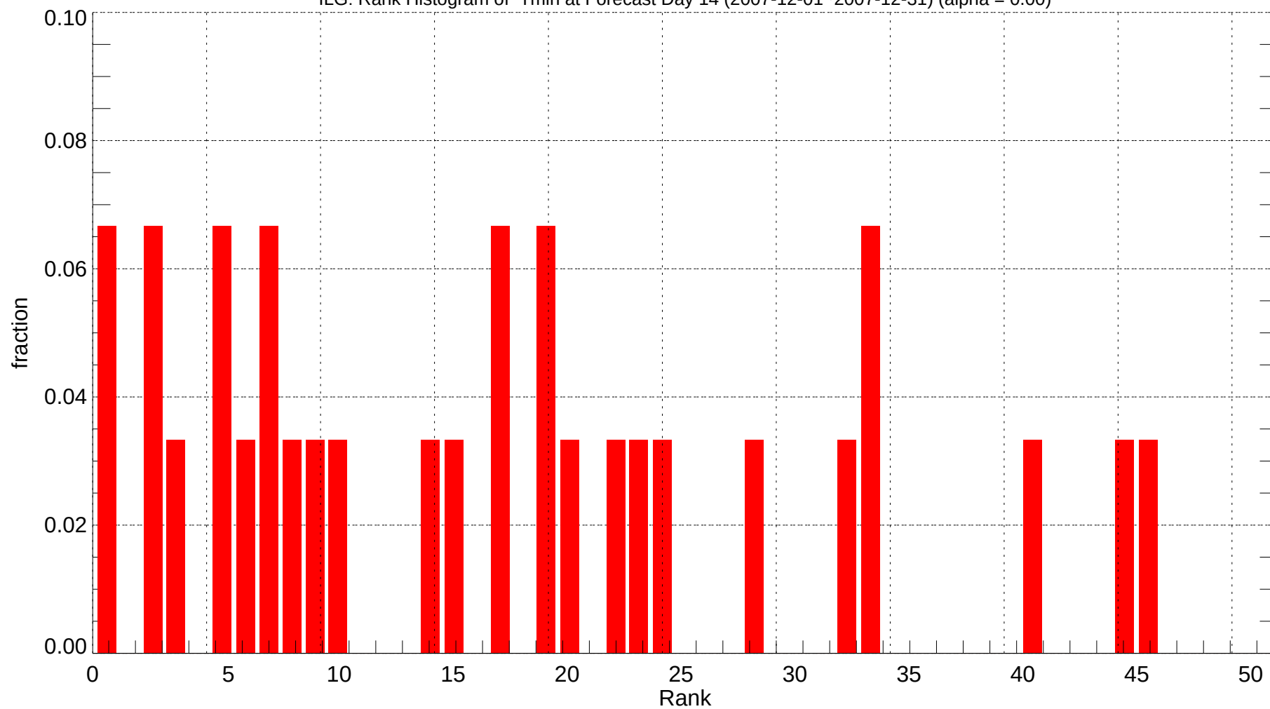
ILG: Rank Histogram of Tmin at Forecast Day 14 (2007-12-01~2007-12-31) (alpha = 0.00)
