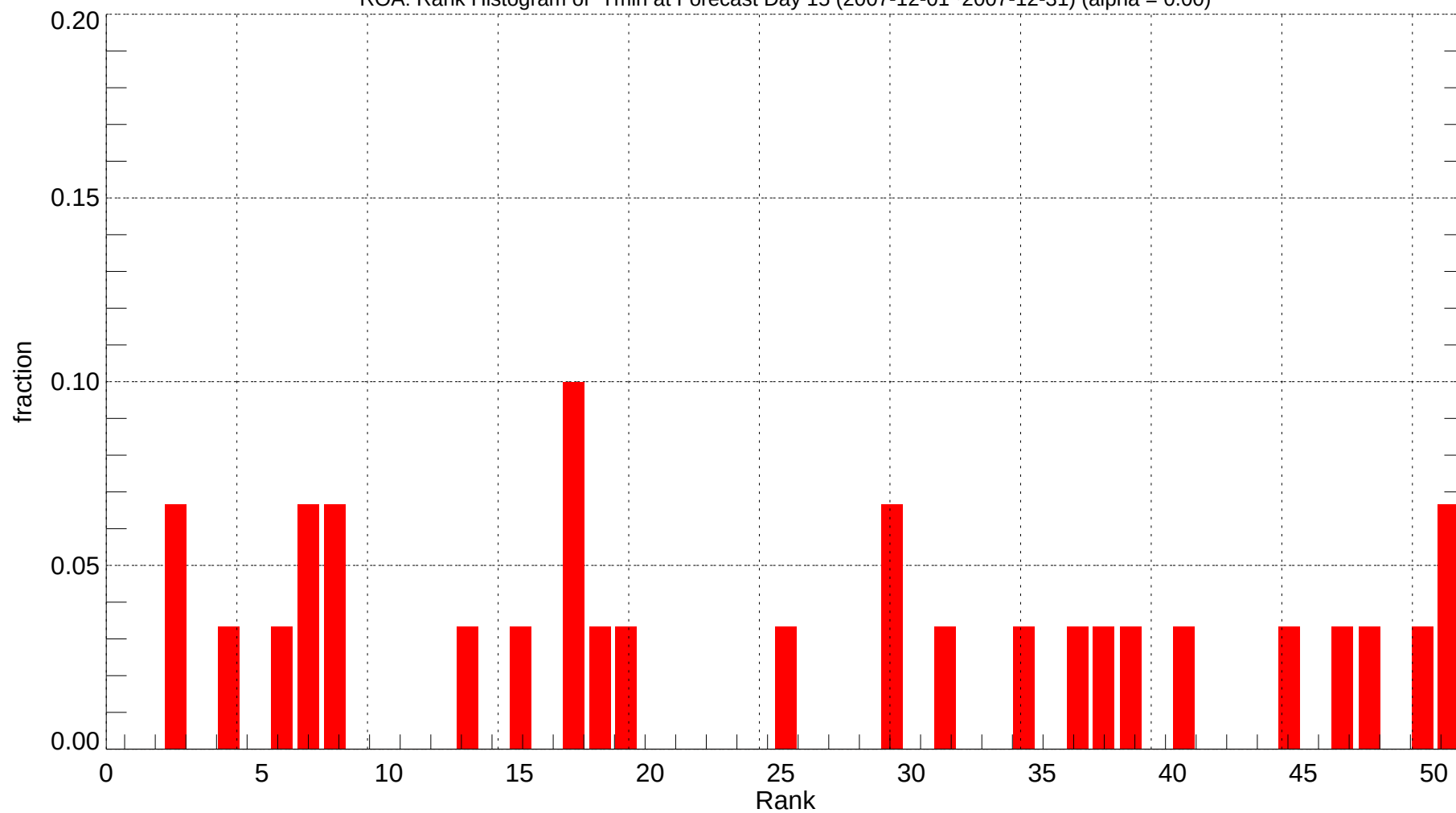
ROA: Rank Histogram of Tmin at Forecast Day 15 (2007-12-01~2007-12-31) (alpha = 0.00)
