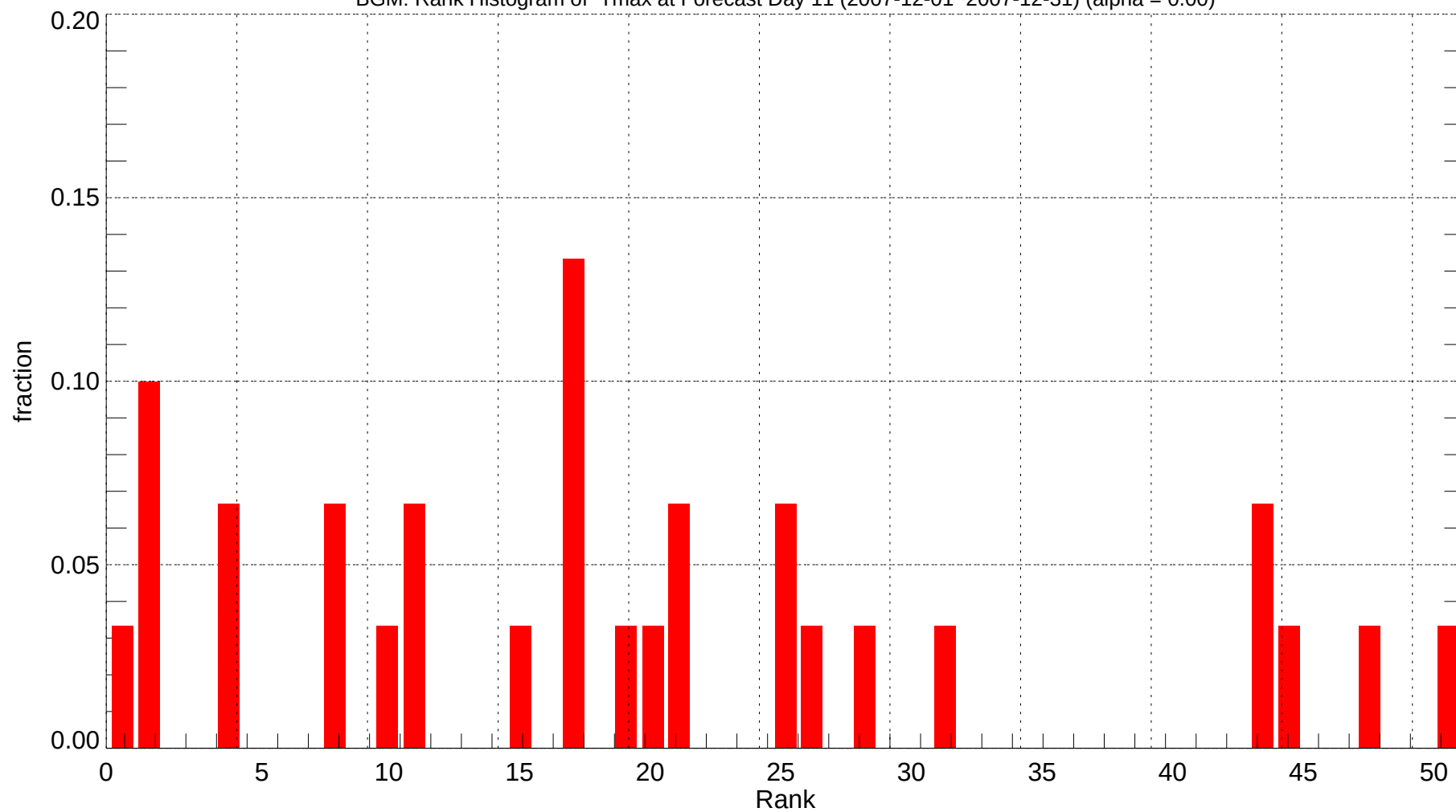
BGM: Rank Histogram of Tmax at Forecast Day 11 (2007-12-01~2007-12-31) (alpha = 0.00)
