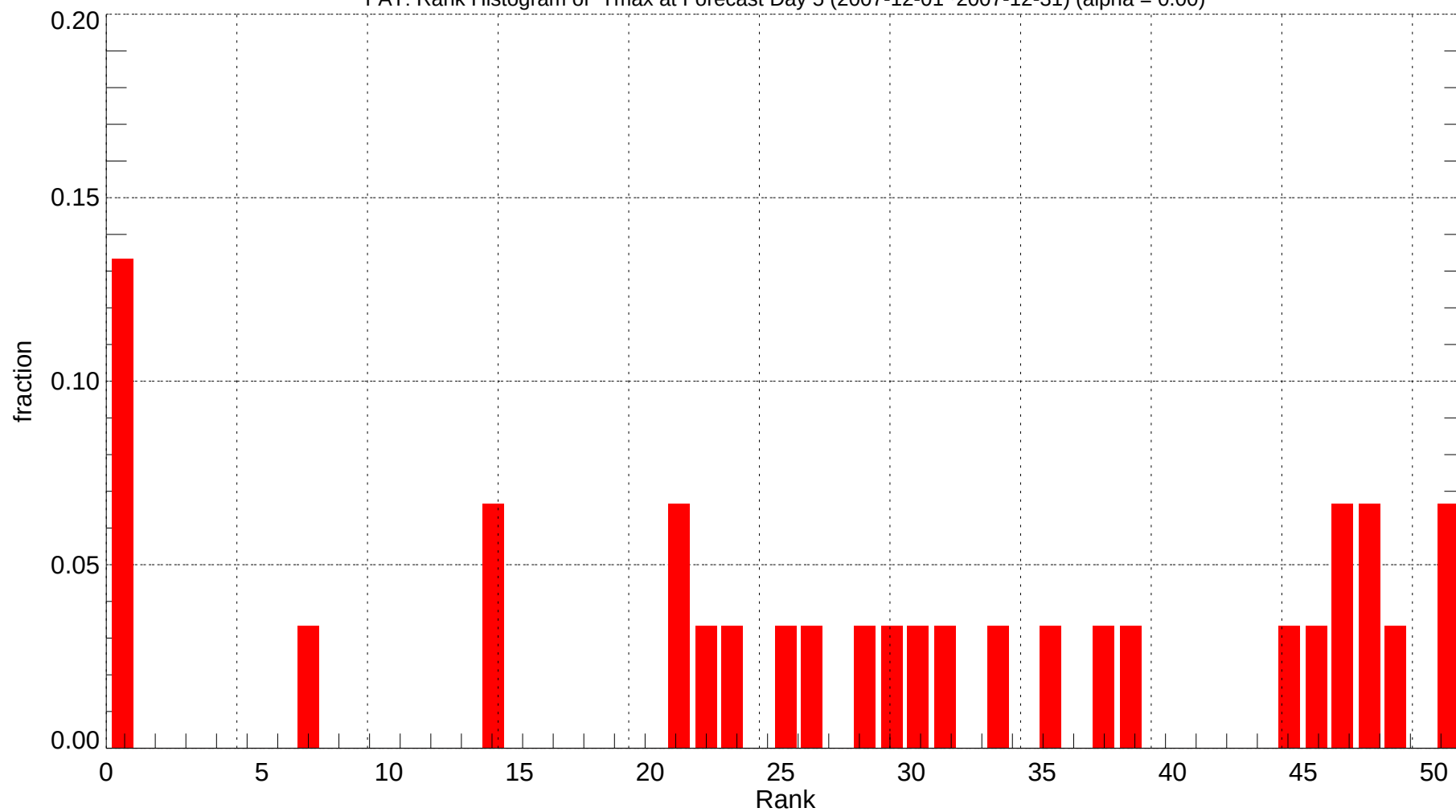
FAT: Rank Histogram of Tmax at Forecast Day 5 (2007-12-01~2007-12-31) (alpha = 0.00)
