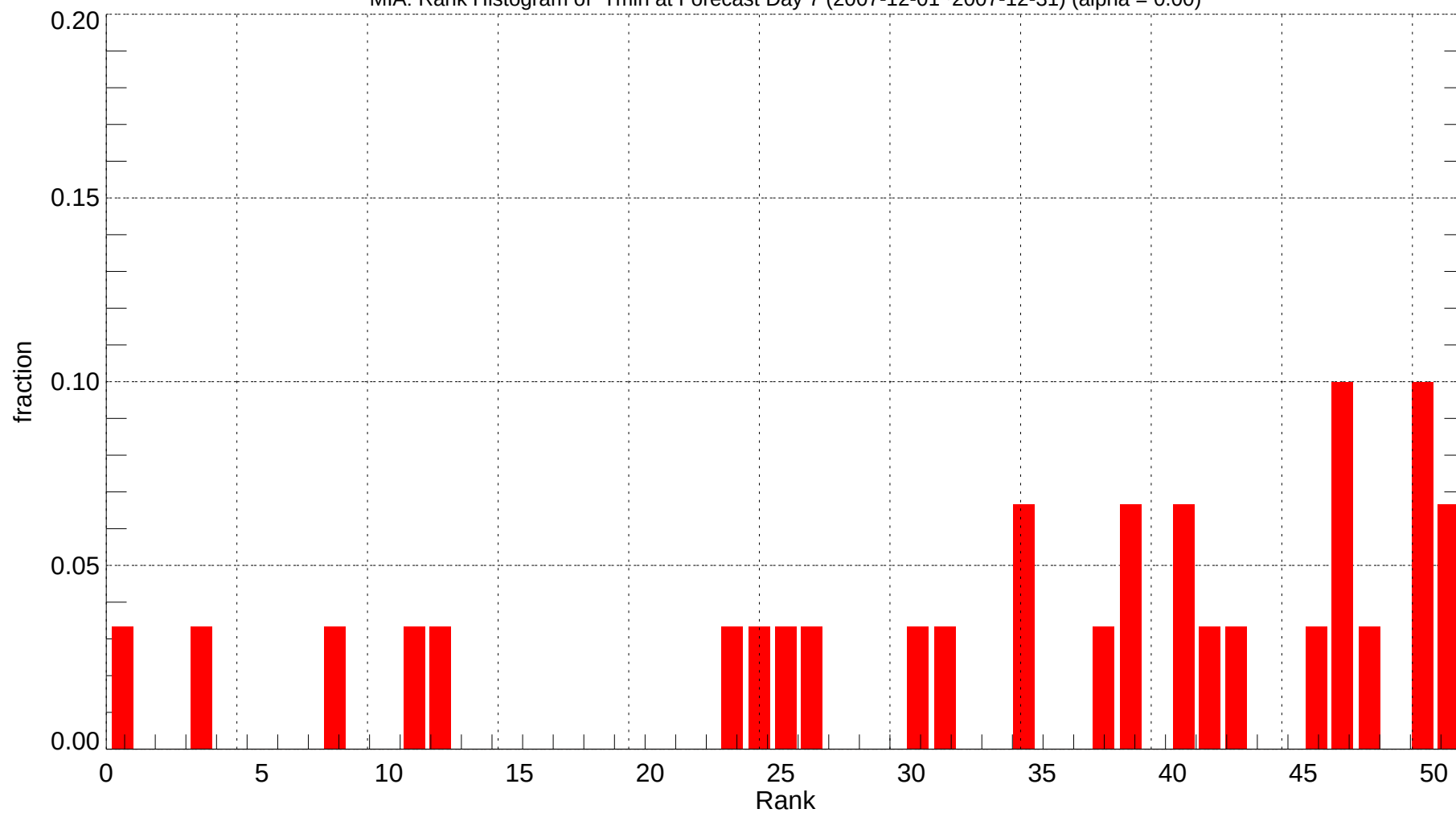
MIA: Rank Histogram of Tmin at Forecast Day 7 (2007-12-01~2007-12-31) (alpha = 0.00)
