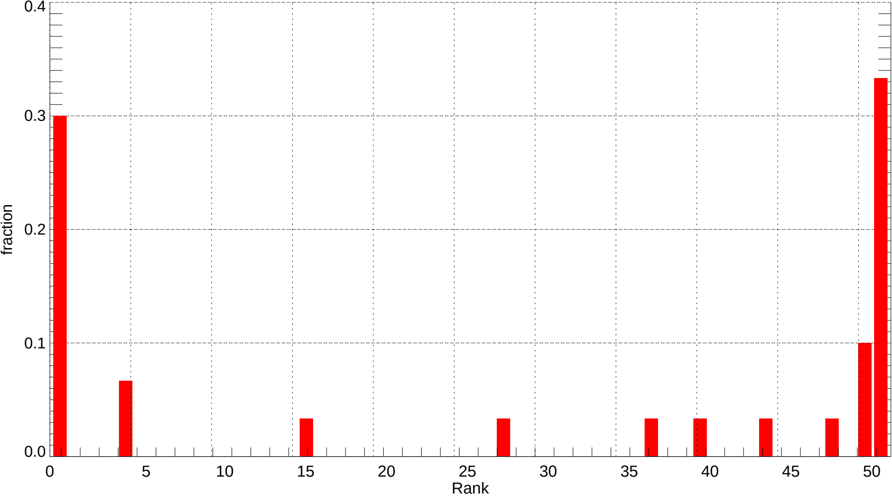
SSI: Rank Histogram of Tmax at Forecast Day 1 (2007-12-01~2007-12-31) (alpha = 0.00)
