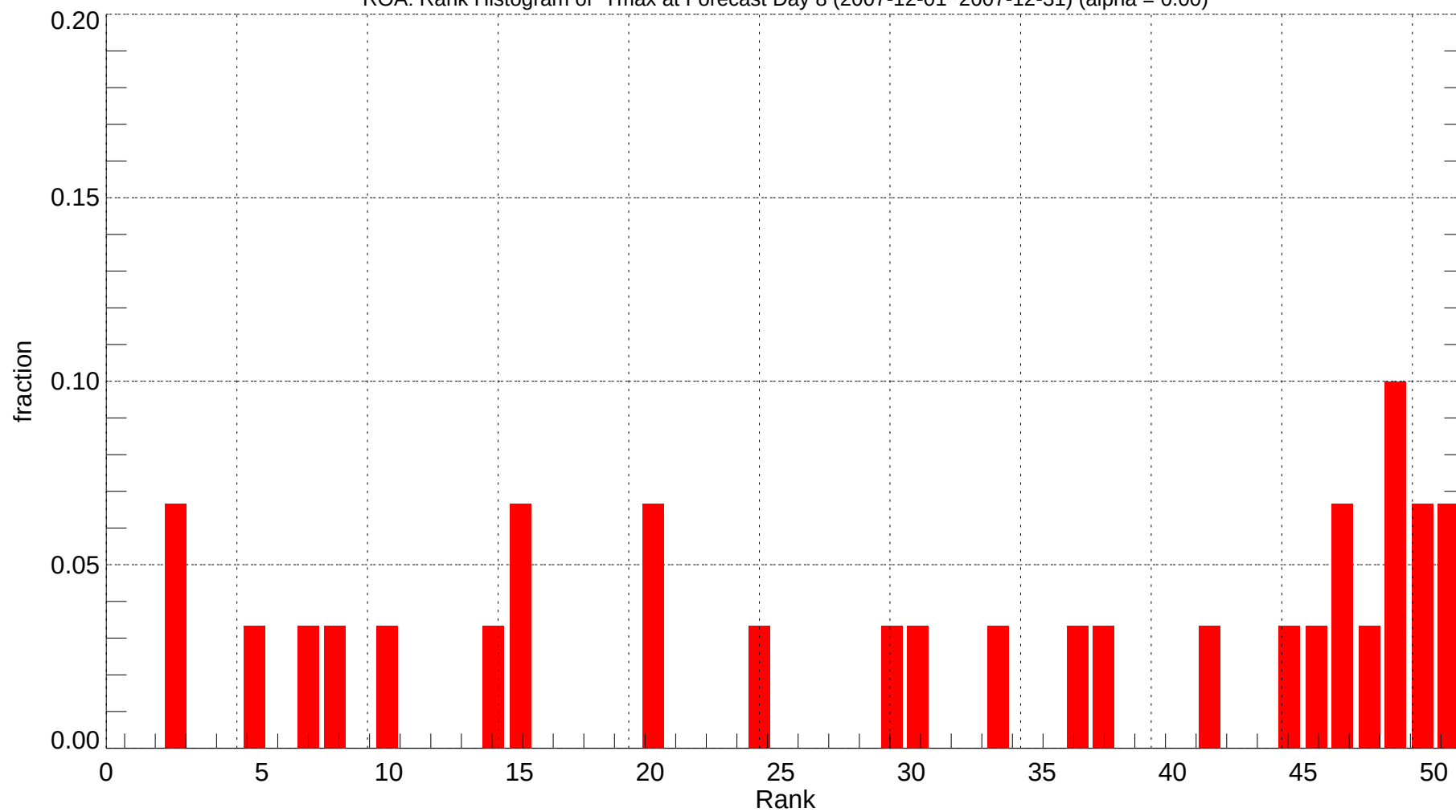
ROA: Rank Histogram of Tmax at Forecast Day 8 (2007-12-01~2007-12-31) (alpha = 0.00)
