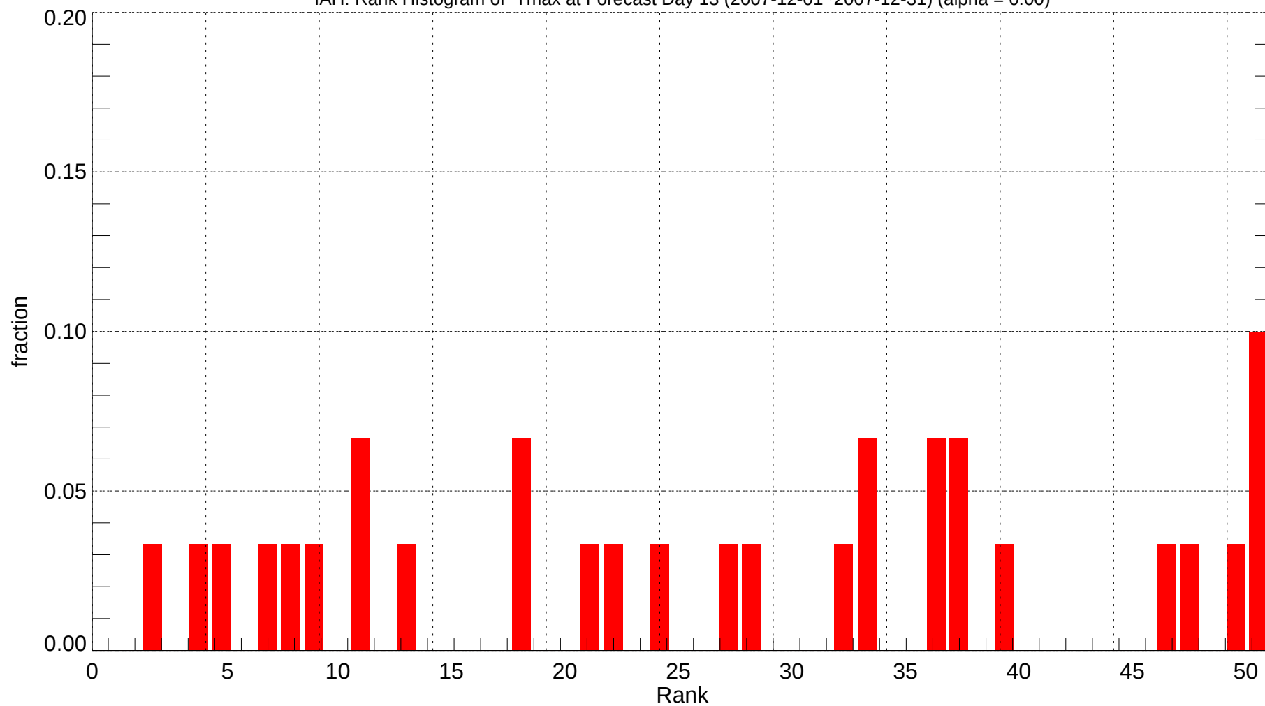
IAH: Rank Histogram of Tmax at Forecast Day 13 (2007-12-01~2007-12-31) (alpha = 0.00)
