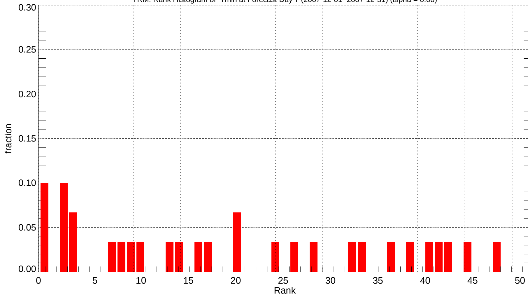
TRM: Rank Histogram of Tmin at Forecast Day 7 (2007-12-01~2007-12-31) (alpha = 0.00)
