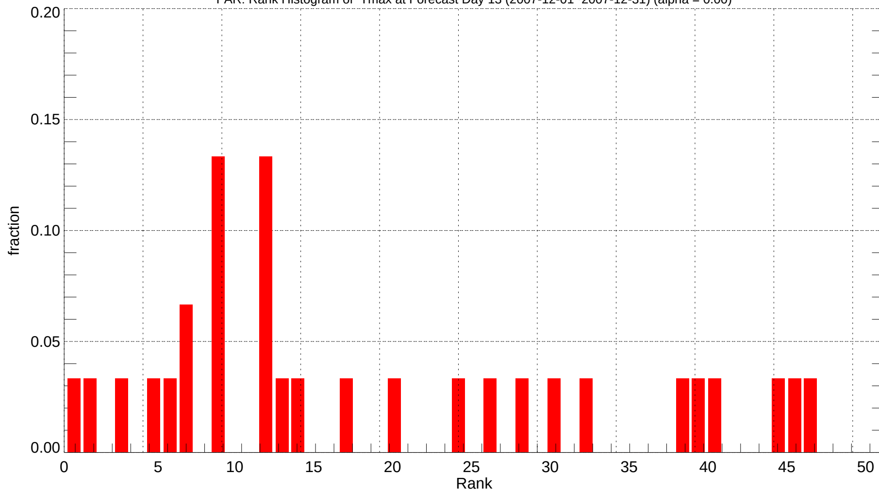
FAR: Rank Histogram of Tmax at Forecast Day 13 (2007-12-01~2007-12-31) (alpha = 0.00)
