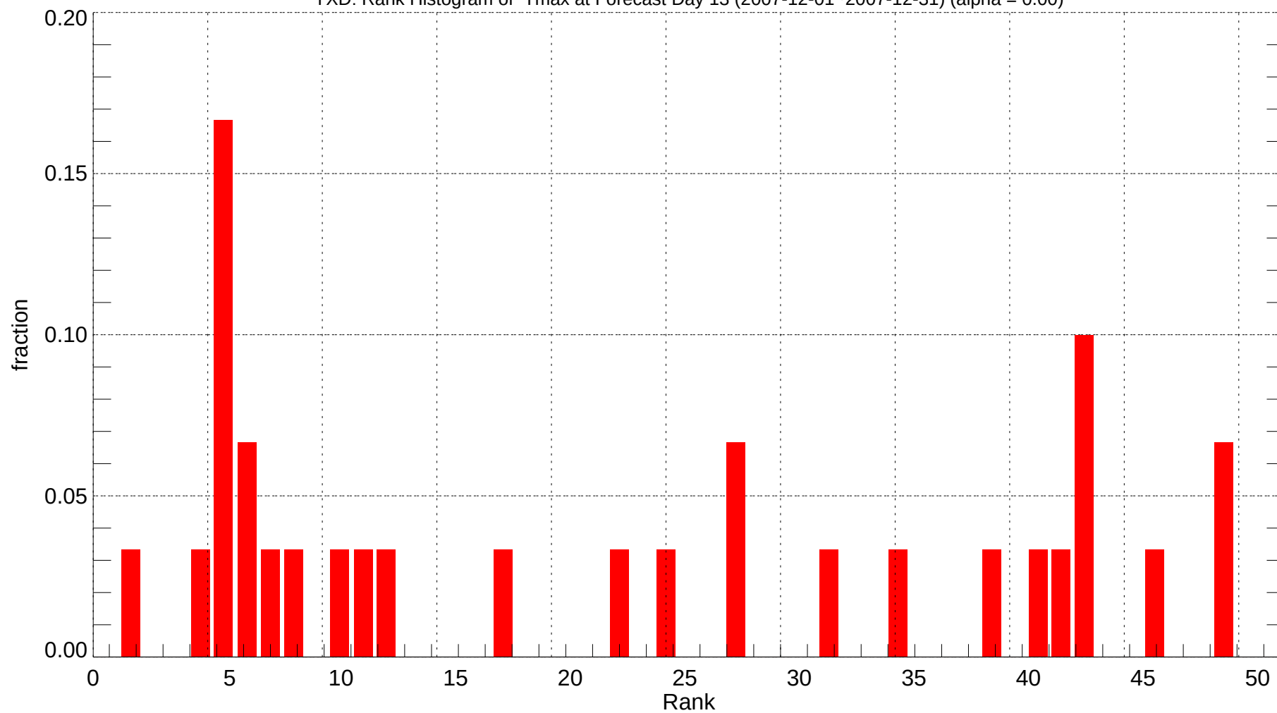
YXD: Rank Histogram of Tmax at Forecast Day 13 (2007-12-01~2007-12-31) (alpha = 0.00)
