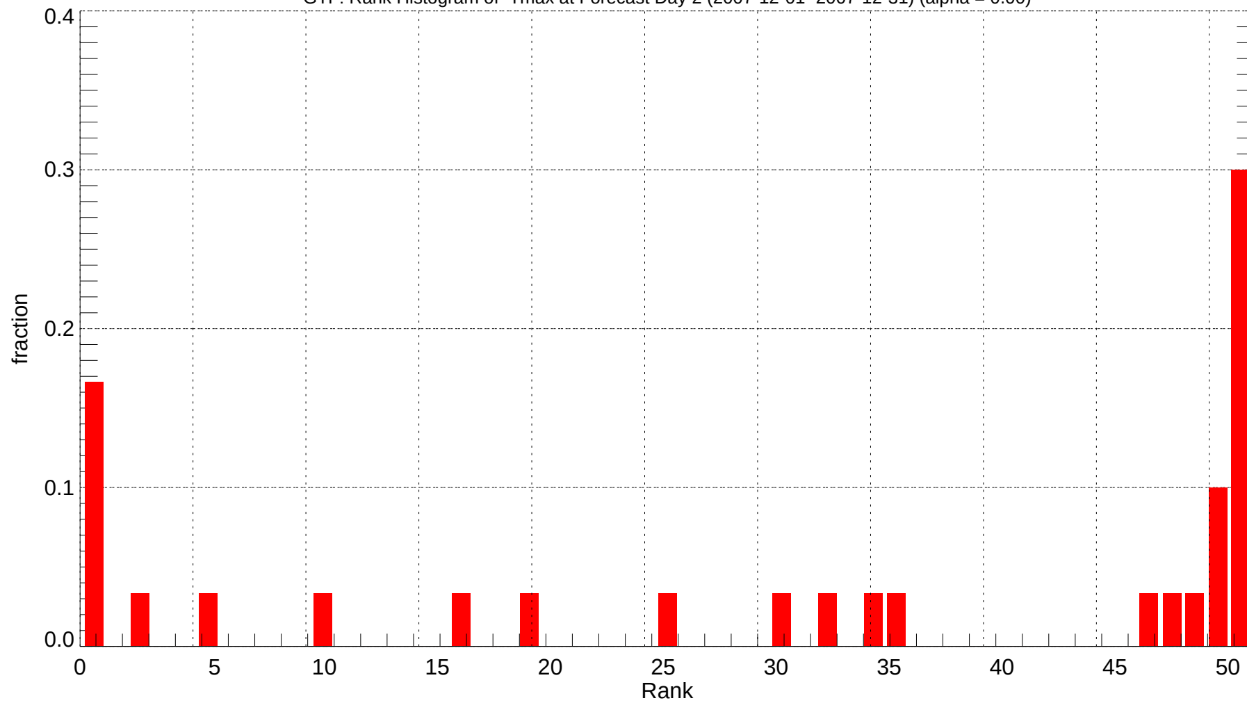
GTF: Rank Histogram of Tmax at Forecast Day 2 (2007-12-01~2007-12-31) (alpha = 0.00)
