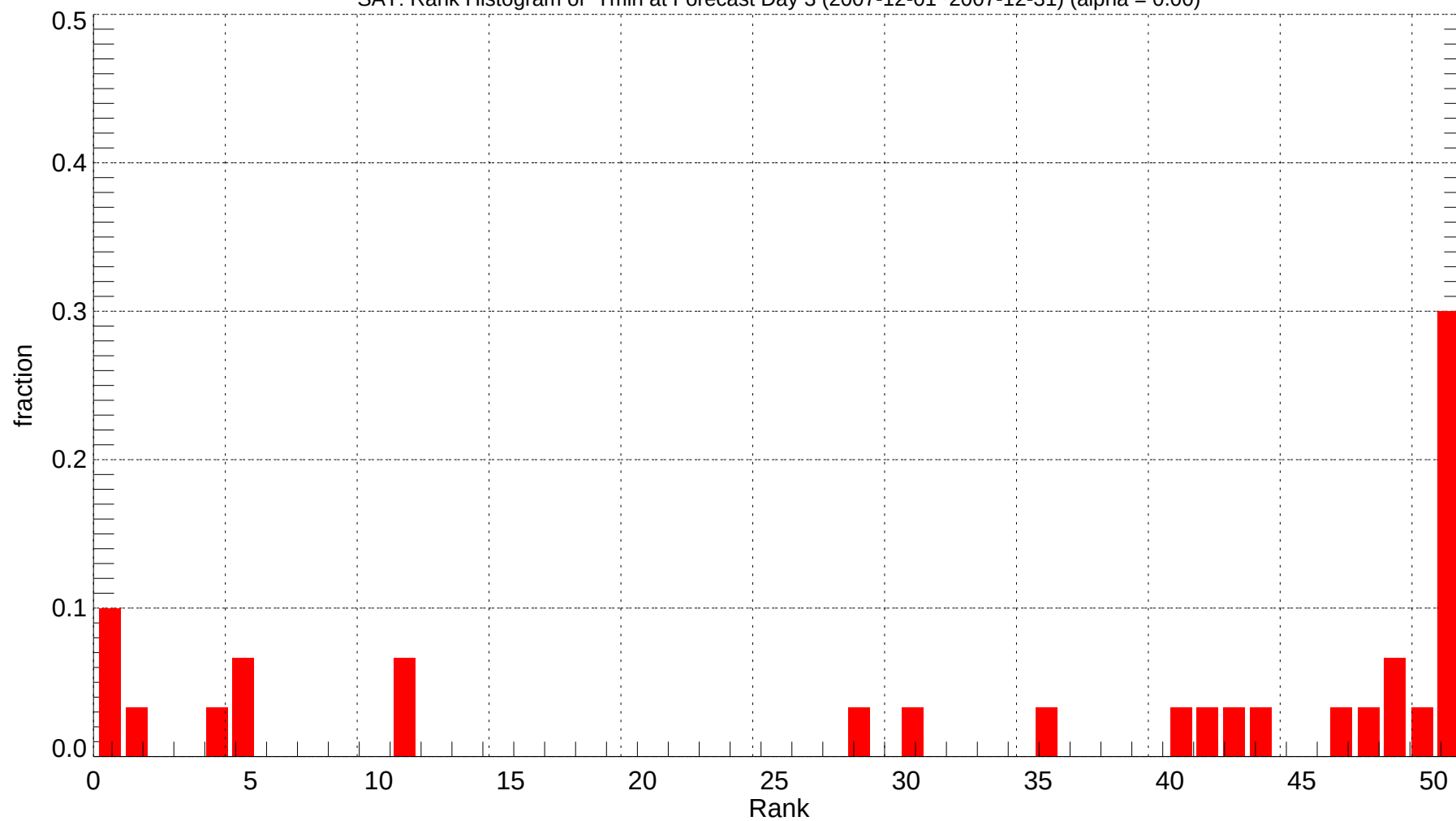
SAT: Rank Histogram of Tmin at Forecast Day 3 (2007-12-01~2007-12-31) (alpha = 0.00)
