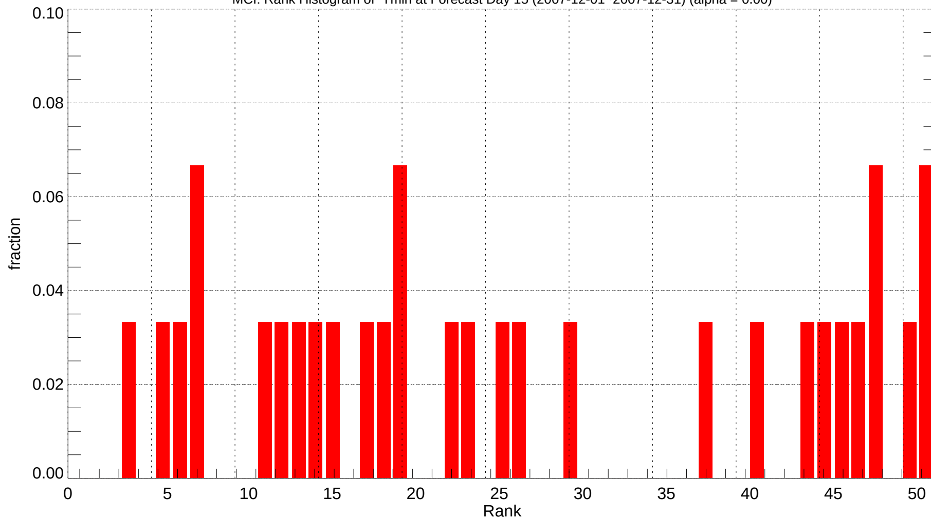
MCI: Rank Histogram of Tmin at Forecast Day 15 (2007-12-01~2007-12-31) (alpha = 0.00)
