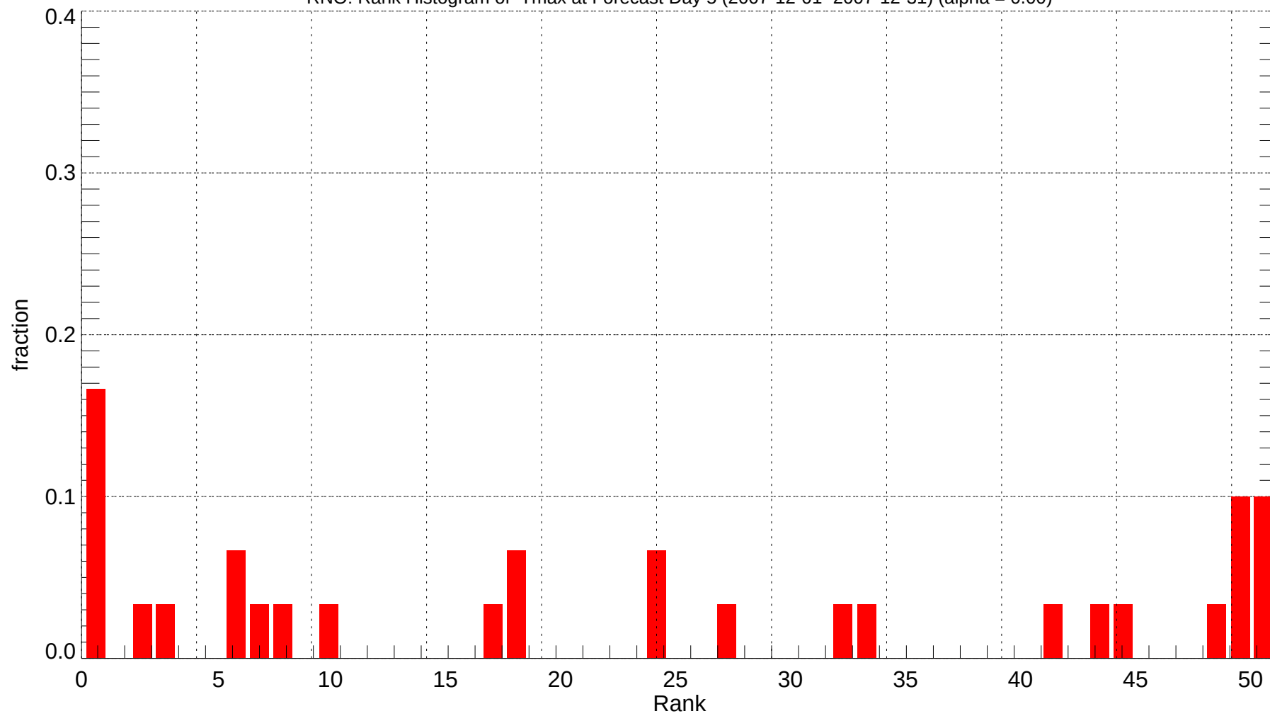
RNO: Rank Histogram of Tmax at Forecast Day 5 (2007-12-01~2007-12-31) (alpha = 0.00)
