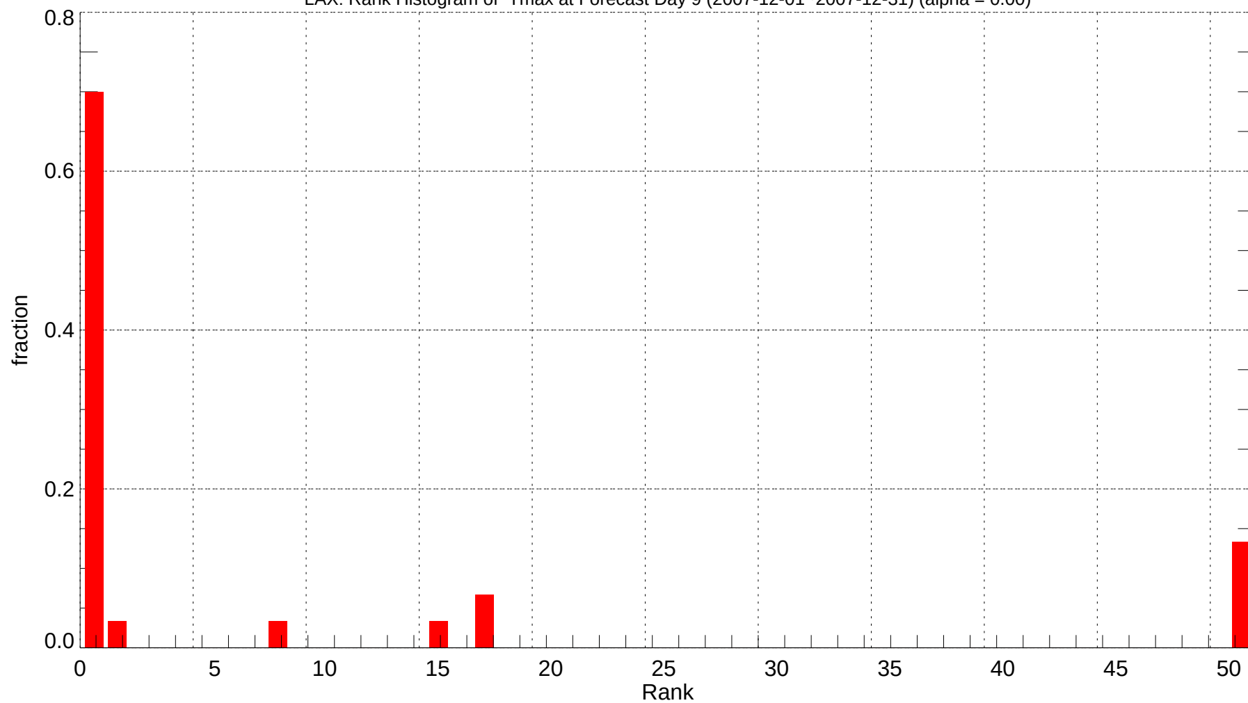
LAX: Rank Histogram of Tmax at Forecast Day 9 (2007-12-01~2007-12-31) (alpha = 0.00)
