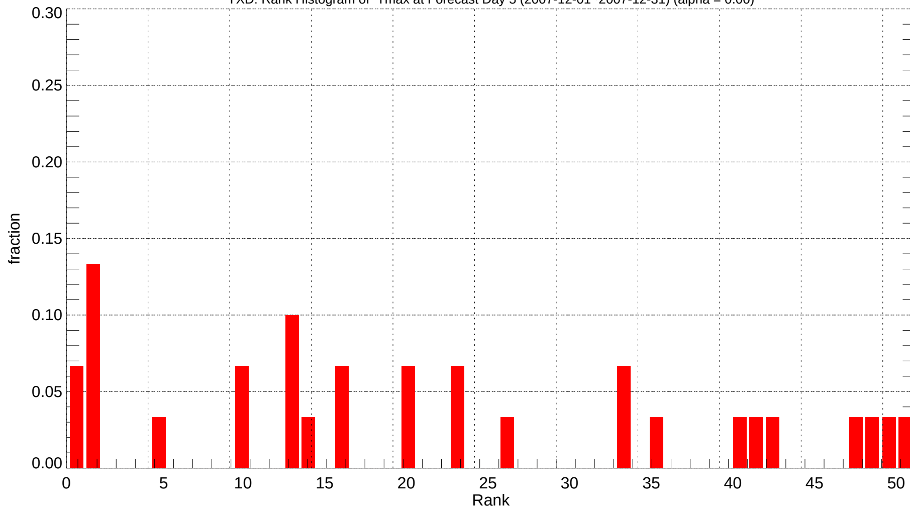
YXD: Rank Histogram of Tmax at Forecast Day 5 (2007-12-01~2007-12-31) (alpha = 0.00)
