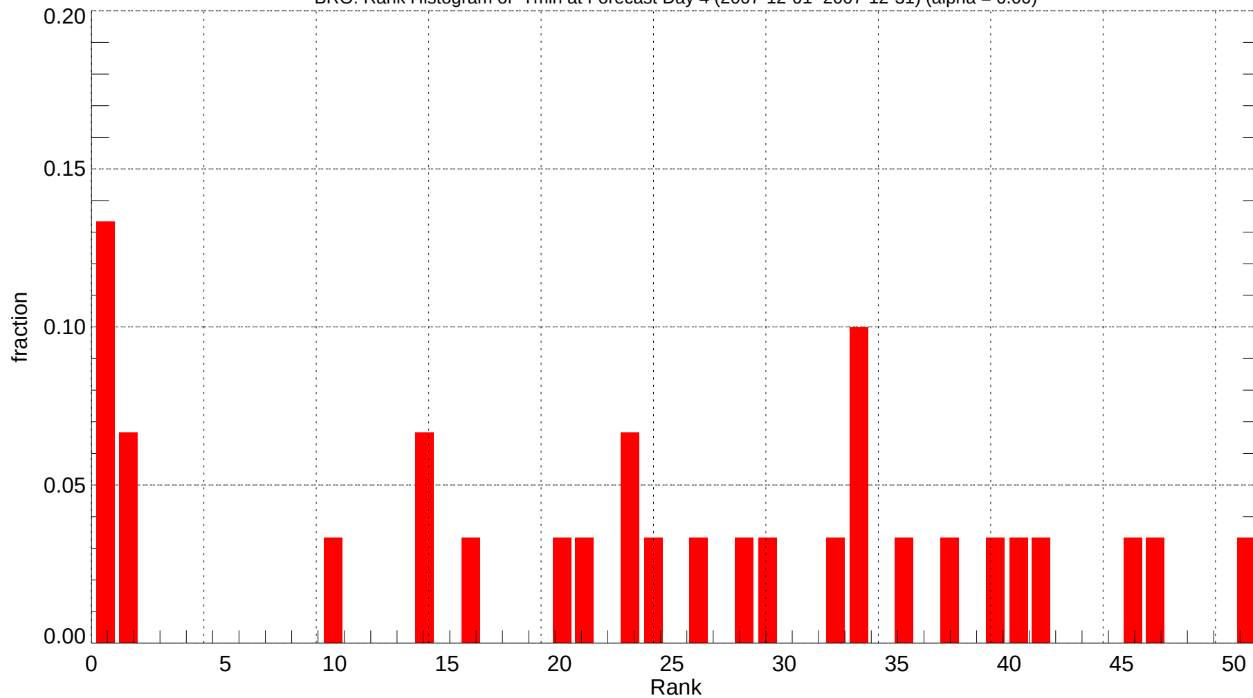
BRO: Rank Histogram of Tmin at Forecast Day 4 (2007-12-01~2007-12-31) (alpha = 0.00)
