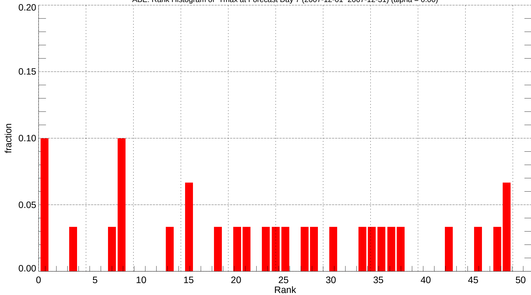
ABE: Rank Histogram of Tmax at Forecast Day 7 (2007-12-01~2007-12-31) (alpha = 0.00)
