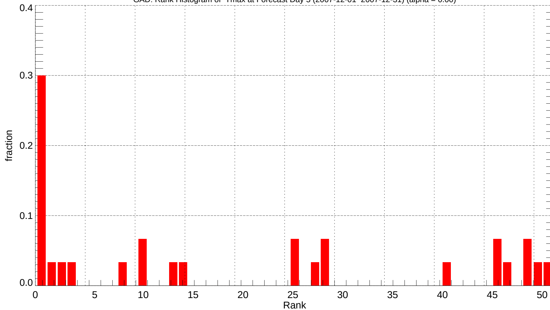
GAD: Rank Histogram of Tmax at Forecast Day 5 (2007-12-01~2007-12-31) (alpha = 0.00)
