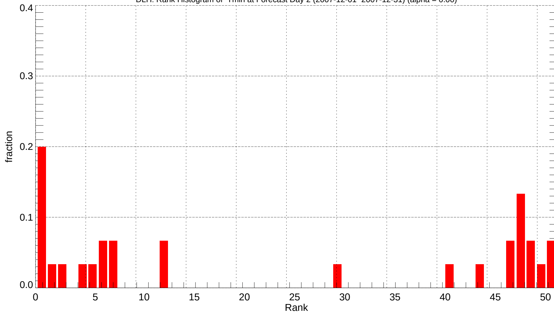
DLH: Rank Histogram of Tmin at Forecast Day 2 (2007-12-01~2007-12-31) (alpha = 0.00)
