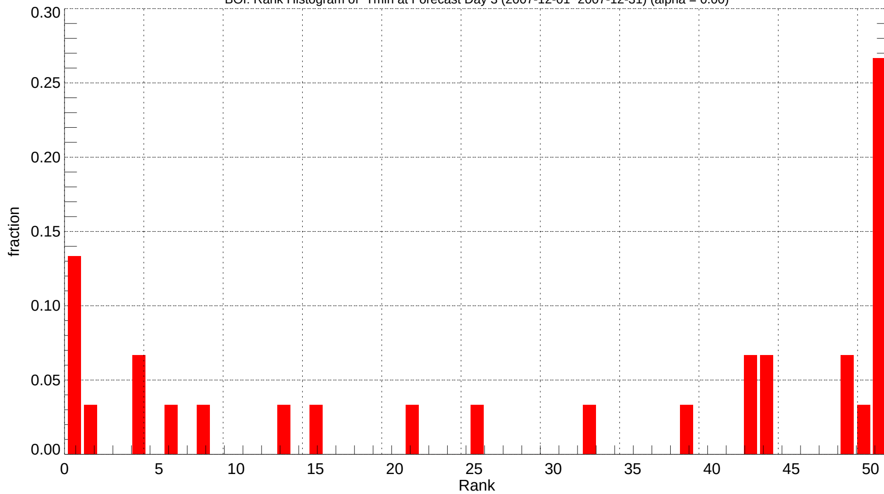
BOI: Rank Histogram of Tmin at Forecast Day 3 (2007-12-01~2007-12-31) (alpha = 0.00)
