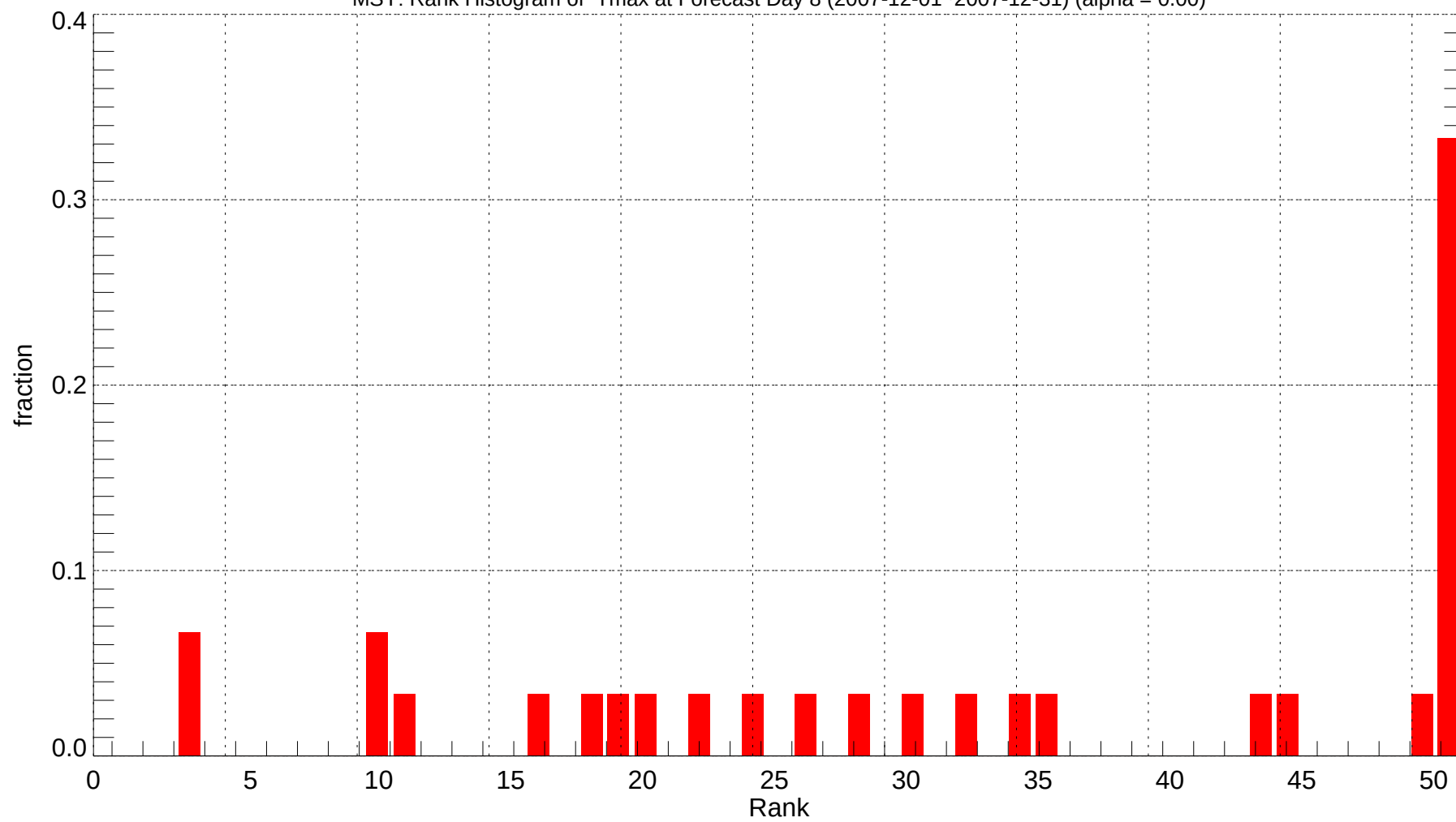
MSY: Rank Histogram of Tmax at Forecast Day 8 (2007-12-01~2007-12-31) (alpha = 0.00)
