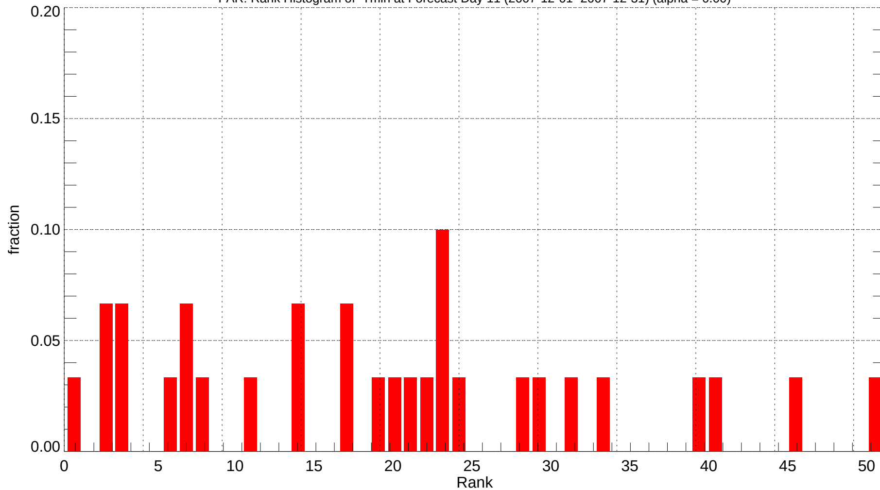
FAR: Rank Histogram of Tmin at Forecast Day 11 (2007-12-01~2007-12-31) (alpha = 0.00)
