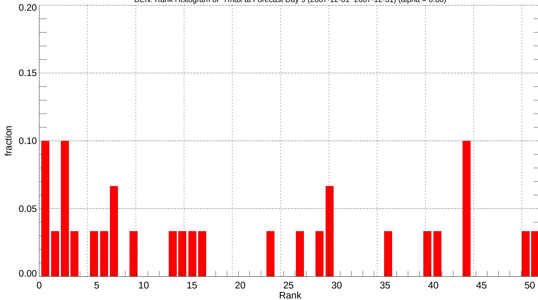
DEN: Rank Histogram of Tmax at Forecast Day 9 (2007-12-01~2007-12-31) (alpha = 0.00)
