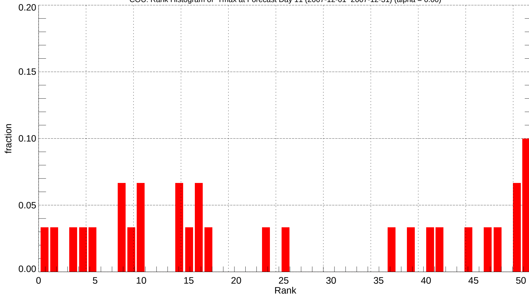
COU: Rank Histogram of Tmax at Forecast Day 11 (2007-12-01~2007-12-31) (alpha = 0.00)
