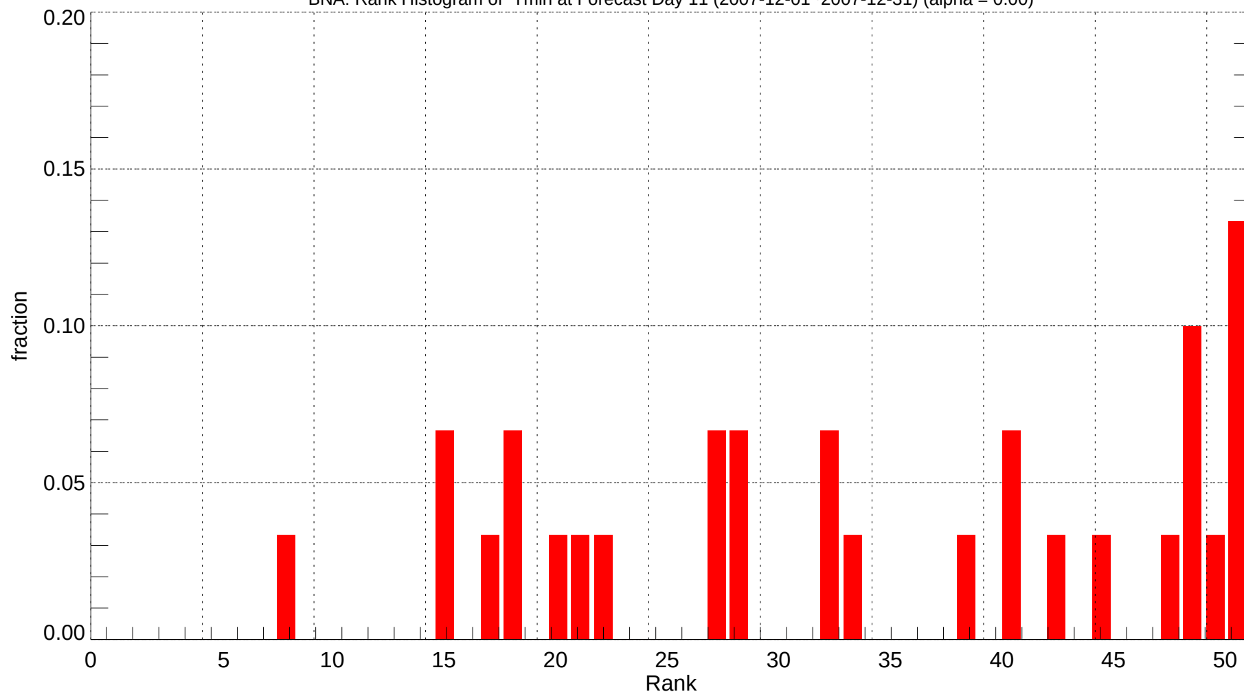
BNA: Rank Histogram of Tmin at Forecast Day 11 (2007-12-01~2007-12-31) (alpha = 0.00)
