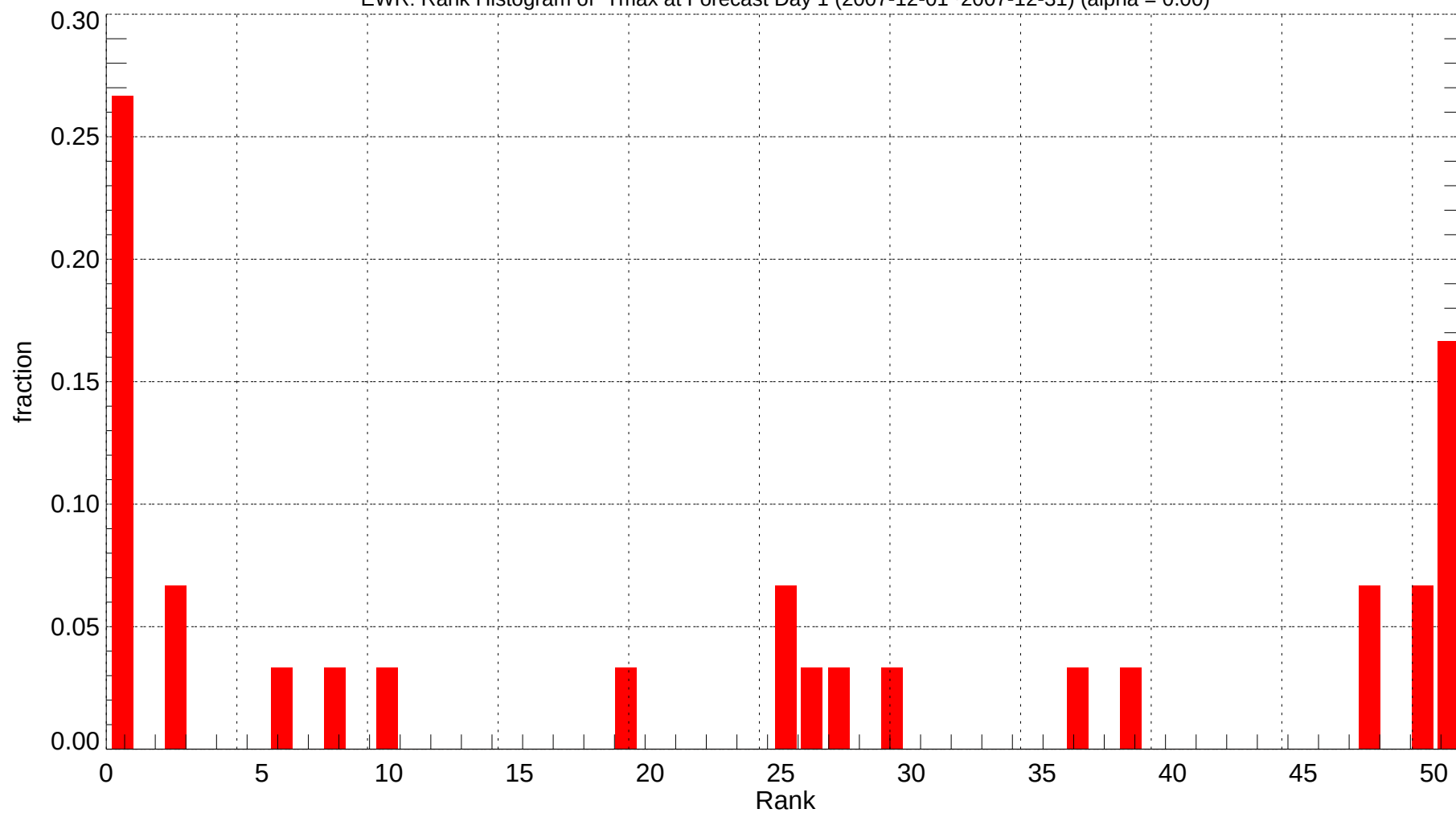
EWR: Rank Histogram of Tmax at Forecast Day 1 (2007-12-01~2007-12-31) (alpha = 0.00)
