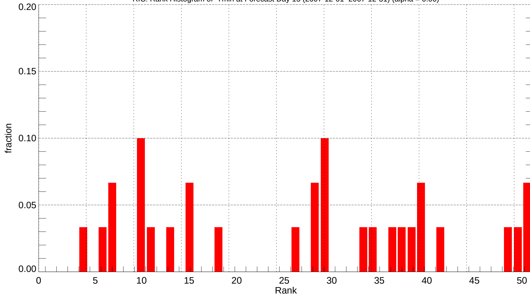
RIC: Rank Histogram of Tmin at Forecast Day 15 (2007-12-01~2007-12-31) (alpha = 0.00)
