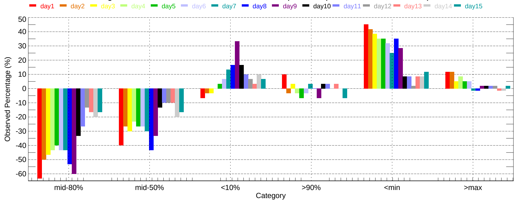
Observed Percentage Deviation of Ensembles - OAK: Max Temperature (2007-12-01~2007-12-31)
