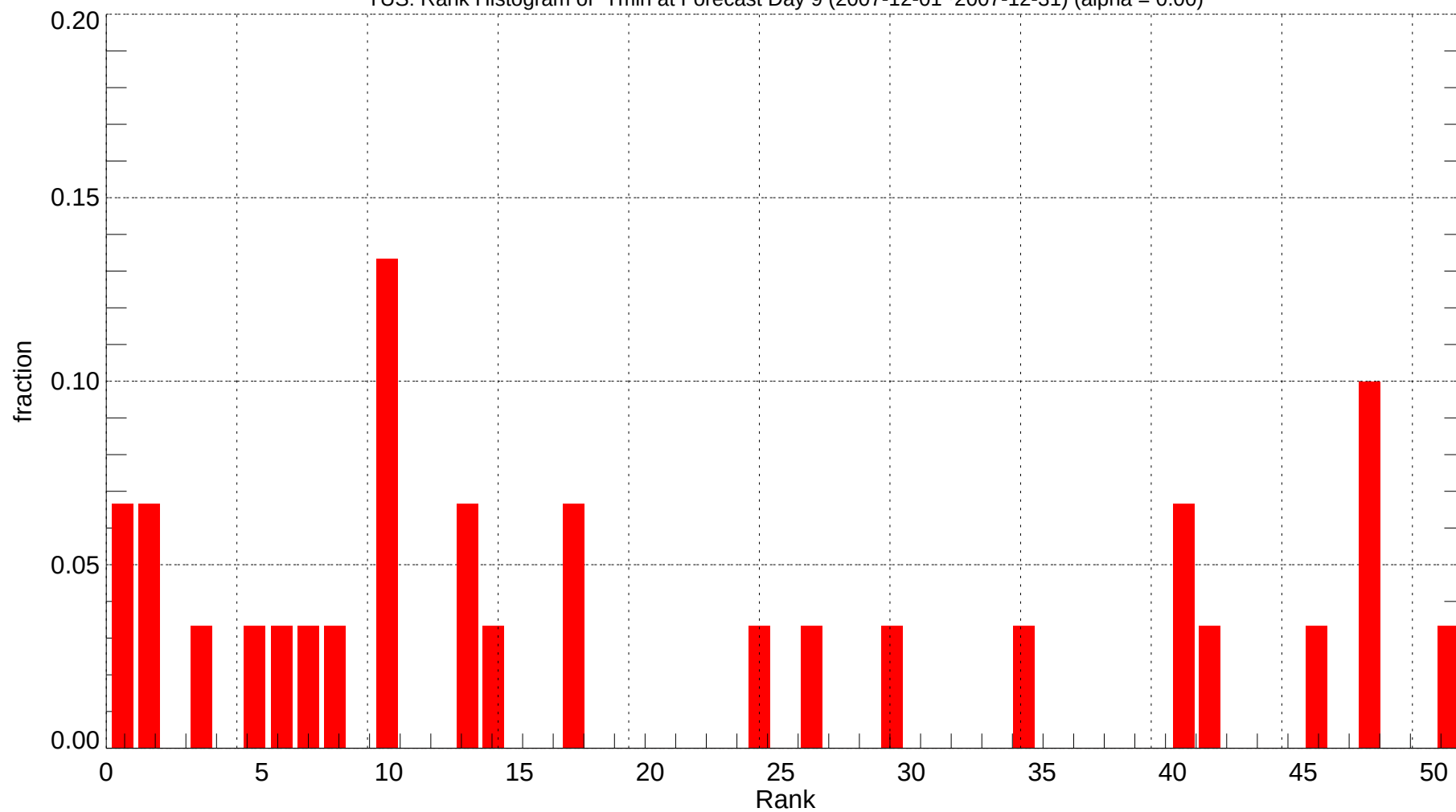
TUS: Rank Histogram of Tmin at Forecast Day 9 (2007-12-01~2007-12-31) (alpha = 0.00)
