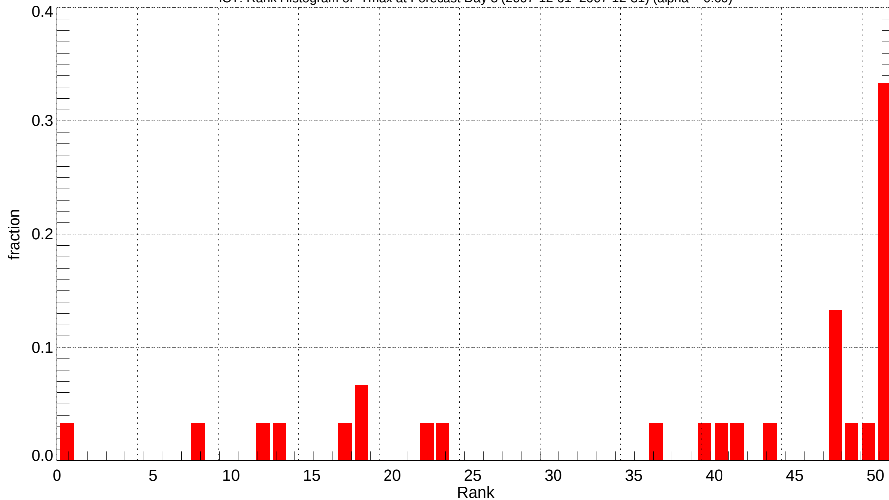
ICT: Rank Histogram of Tmax at Forecast Day 5 (2007-12-01~2007-12-31) (alpha = 0.00)
