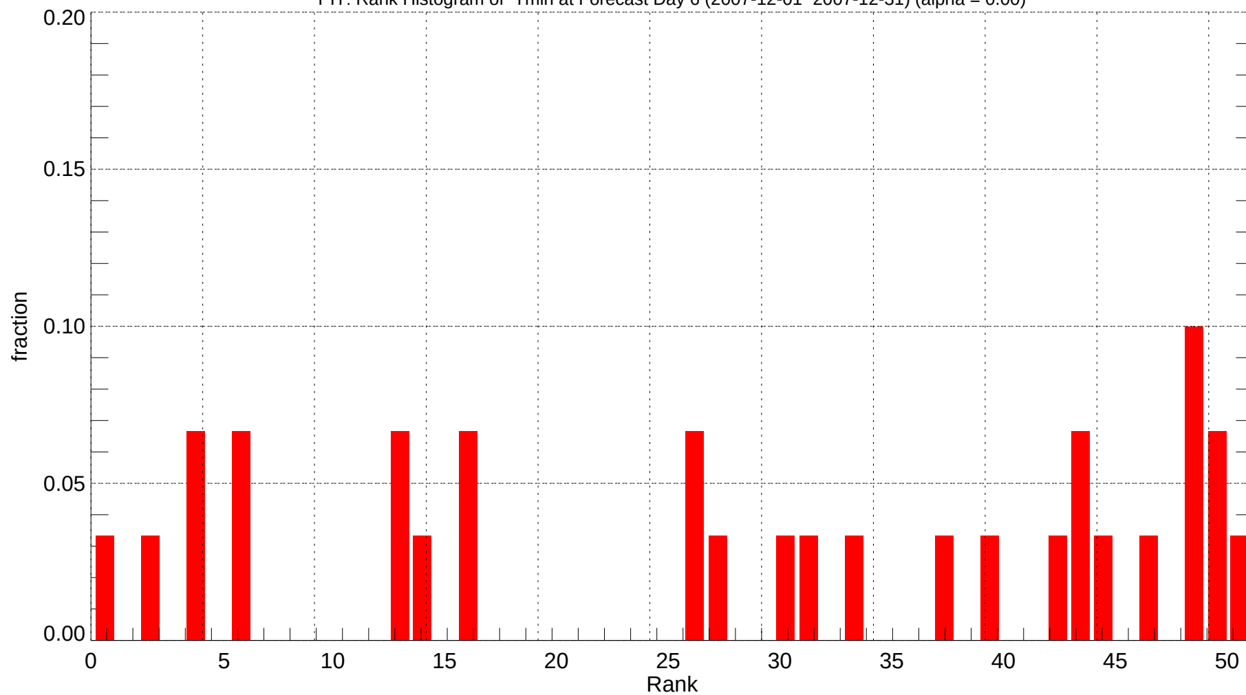
PIT: Rank Histogram of Tmin at Forecast Day 6 (2007-12-01~2007-12-31) (alpha = 0.00)
