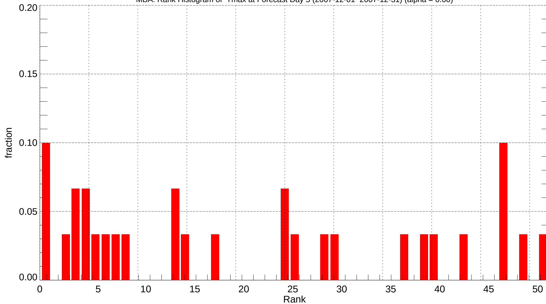
MBA: Rank Histogram of Tmax at Forecast Day 5 (2007-12-01~2007-12-31) (alpha = 0.00)
