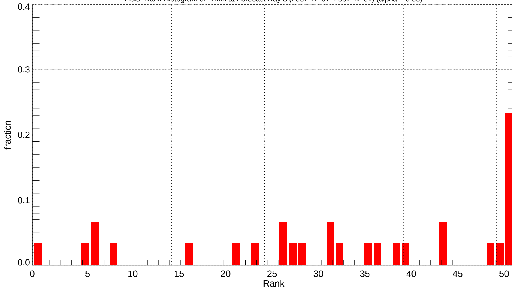
AUS: Rank Histogram of Tmin at Forecast Day 8 (2007-12-01~2007-12-31) (alpha = 0.00)
