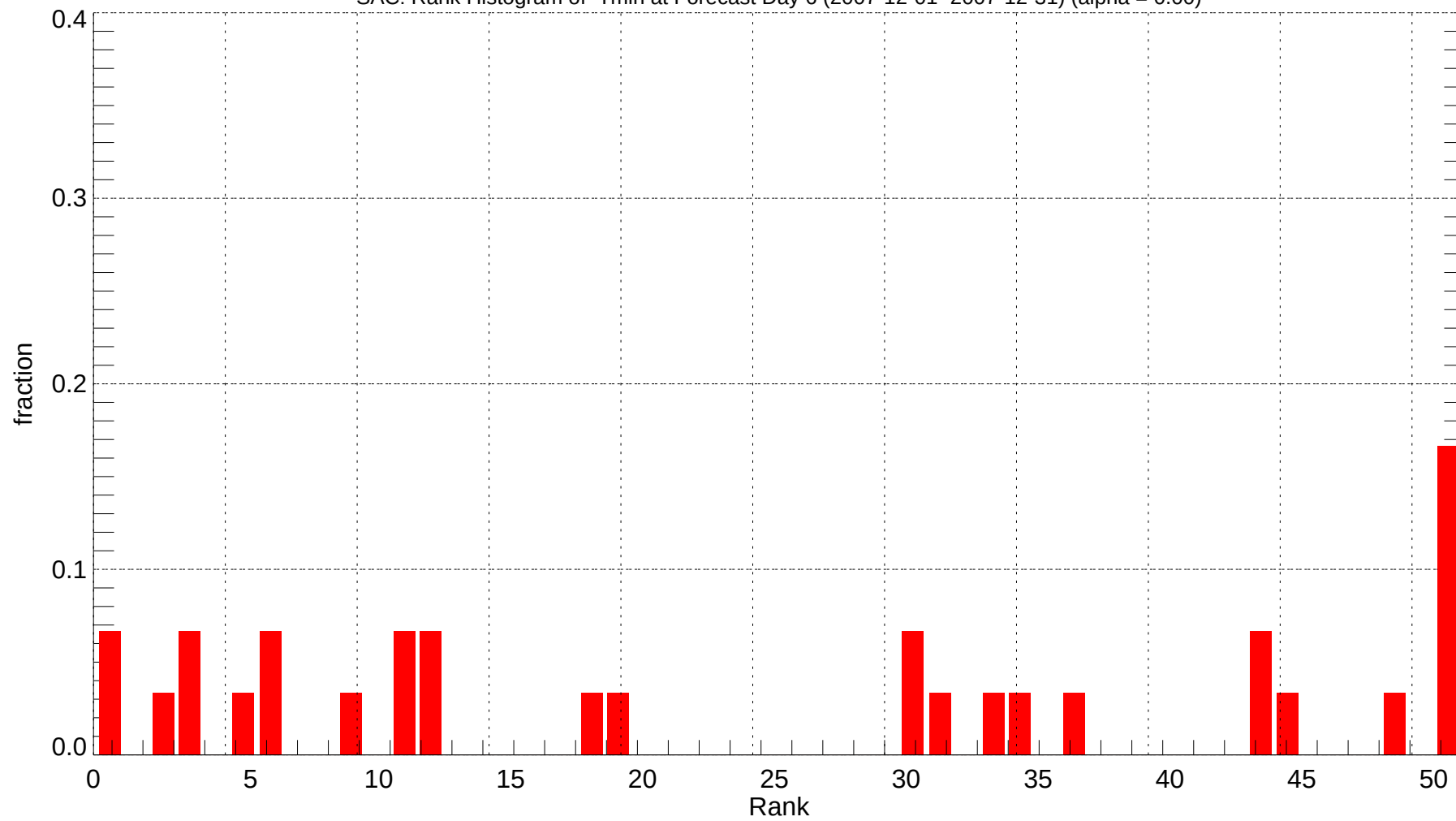
SAC: Rank Histogram of Tmin at Forecast Day 6 (2007-12-01~2007-12-31) (alpha = 0.00)
