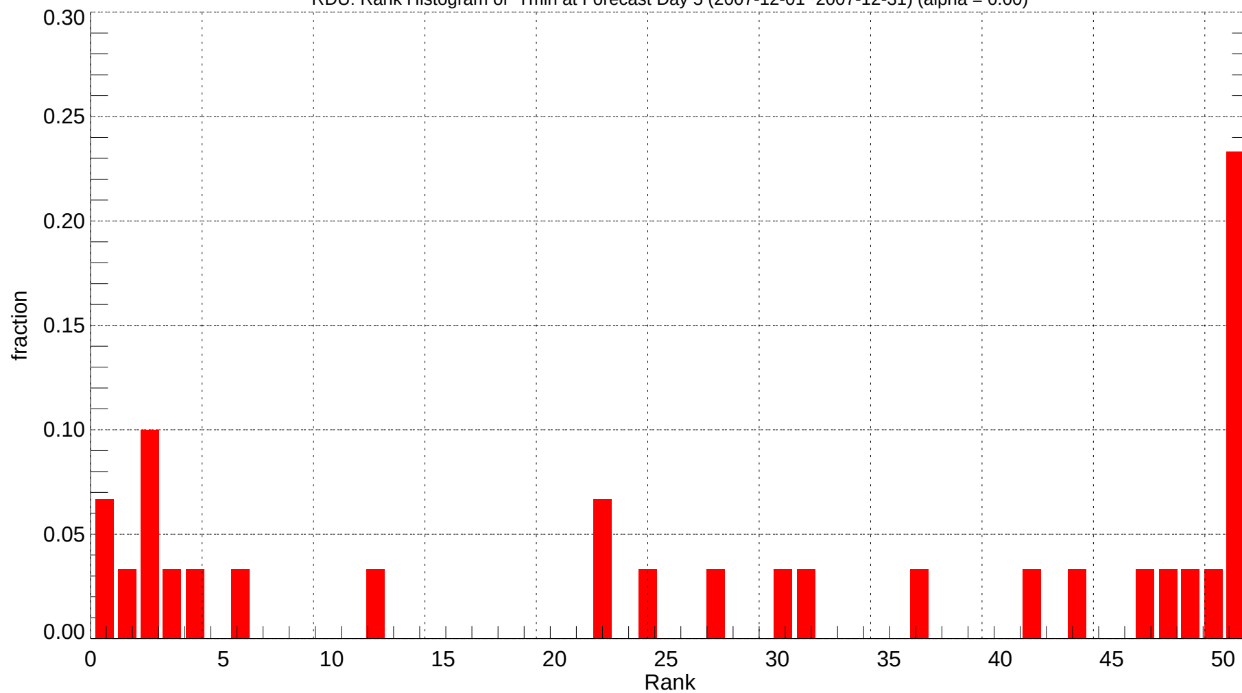
RDU: Rank Histogram of Tmin at Forecast Day 5 (2007-12-01~2007-12-31) (alpha = 0.00)
