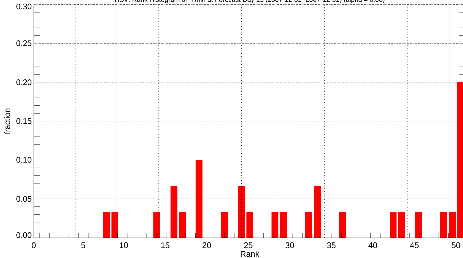
HSV: Rank Histogram of Tmin at Forecast Day 15 (2007-12-01~2007-12-31) (alpha = 0.00)
