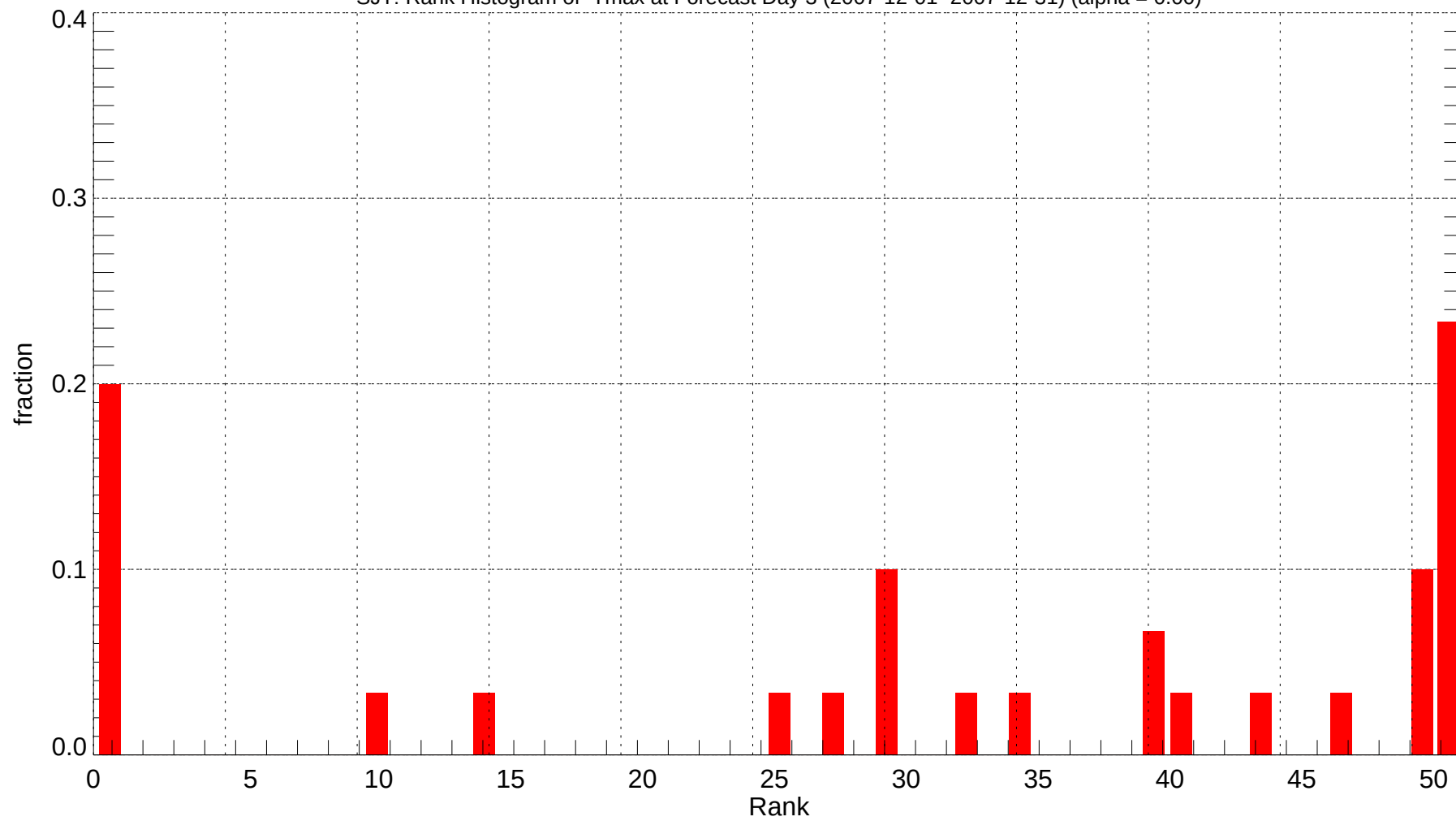
SJT: Rank Histogram of Tmax at Forecast Day 3 (2007-12-01~2007-12-31) (alpha = 0.00)
