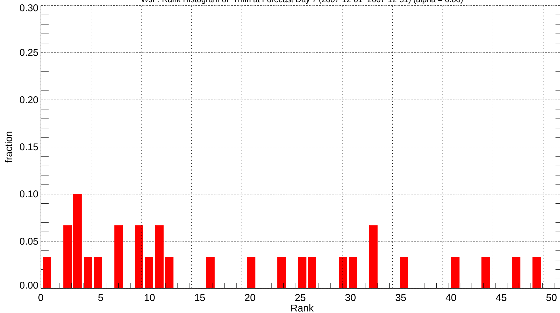
WJF: Rank Histogram of Tmin at Forecast Day 7 (2007-12-01~2007-12-31) (alpha = 0.00)
