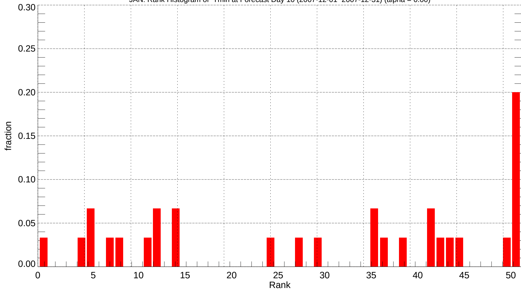
JAN: Rank Histogram of Tmin at Forecast Day 10 (2007-12-01~2007-12-31) (alpha = 0.00)
