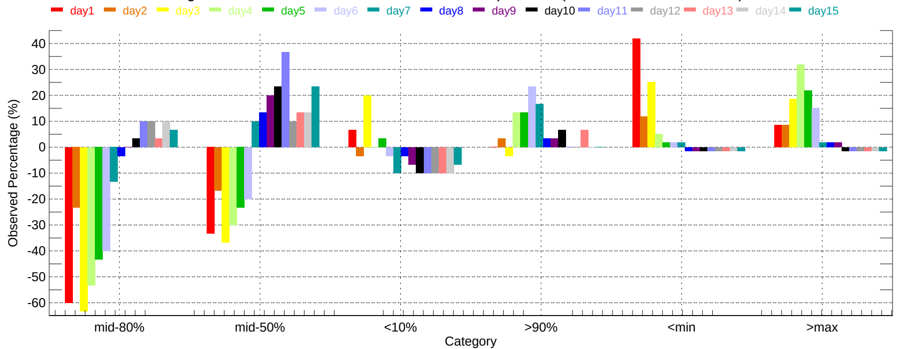
Observed Percentage Deviation of Ensembles - LAS: Max Temperature (2007-12-01~2007-12-31)
