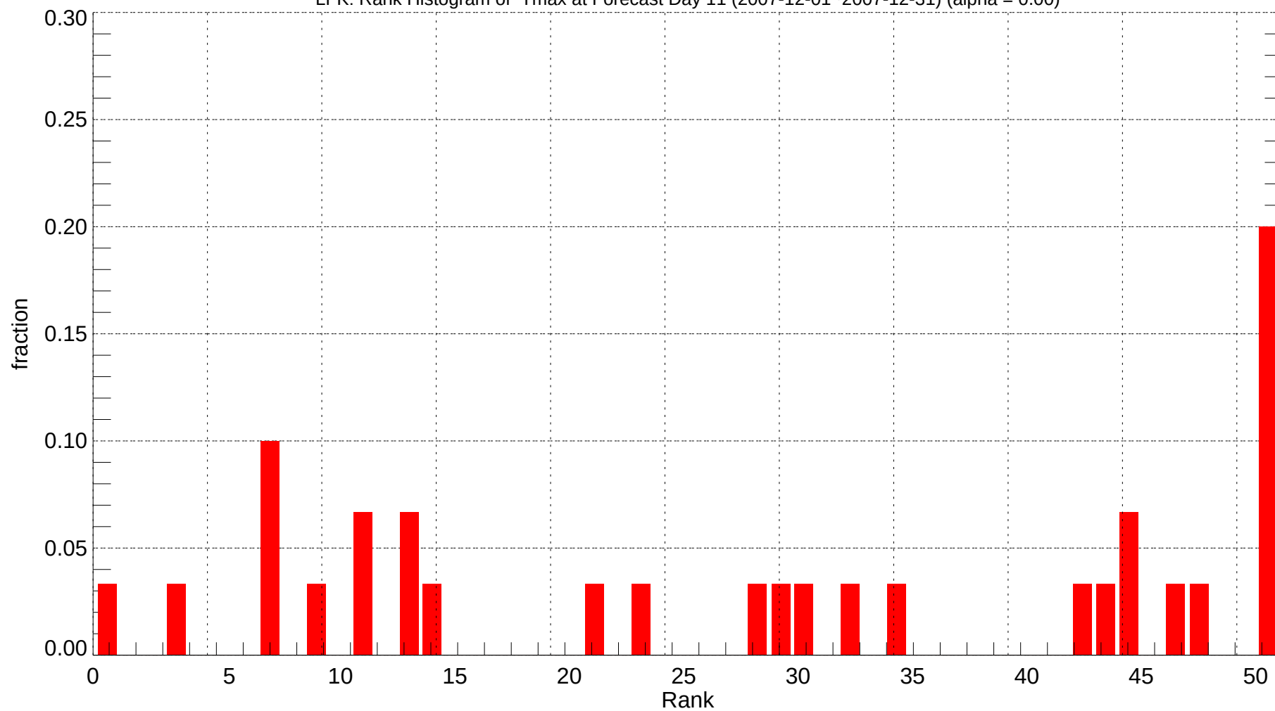
LFK: Rank Histogram of Tmax at Forecast Day 11 (2007-12-01~2007-12-31) (alpha = 0.00)
