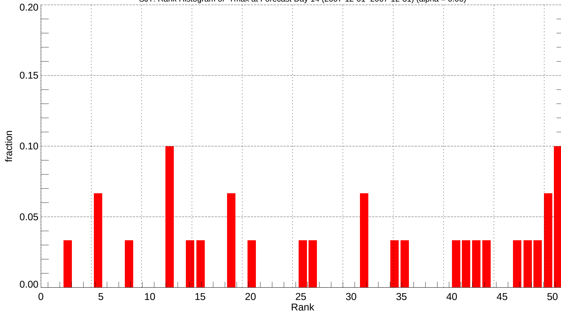
SJT: Rank Histogram of Tmax at Forecast Day 14 (2007-12-01~2007-12-31) (alpha = 0.00)
