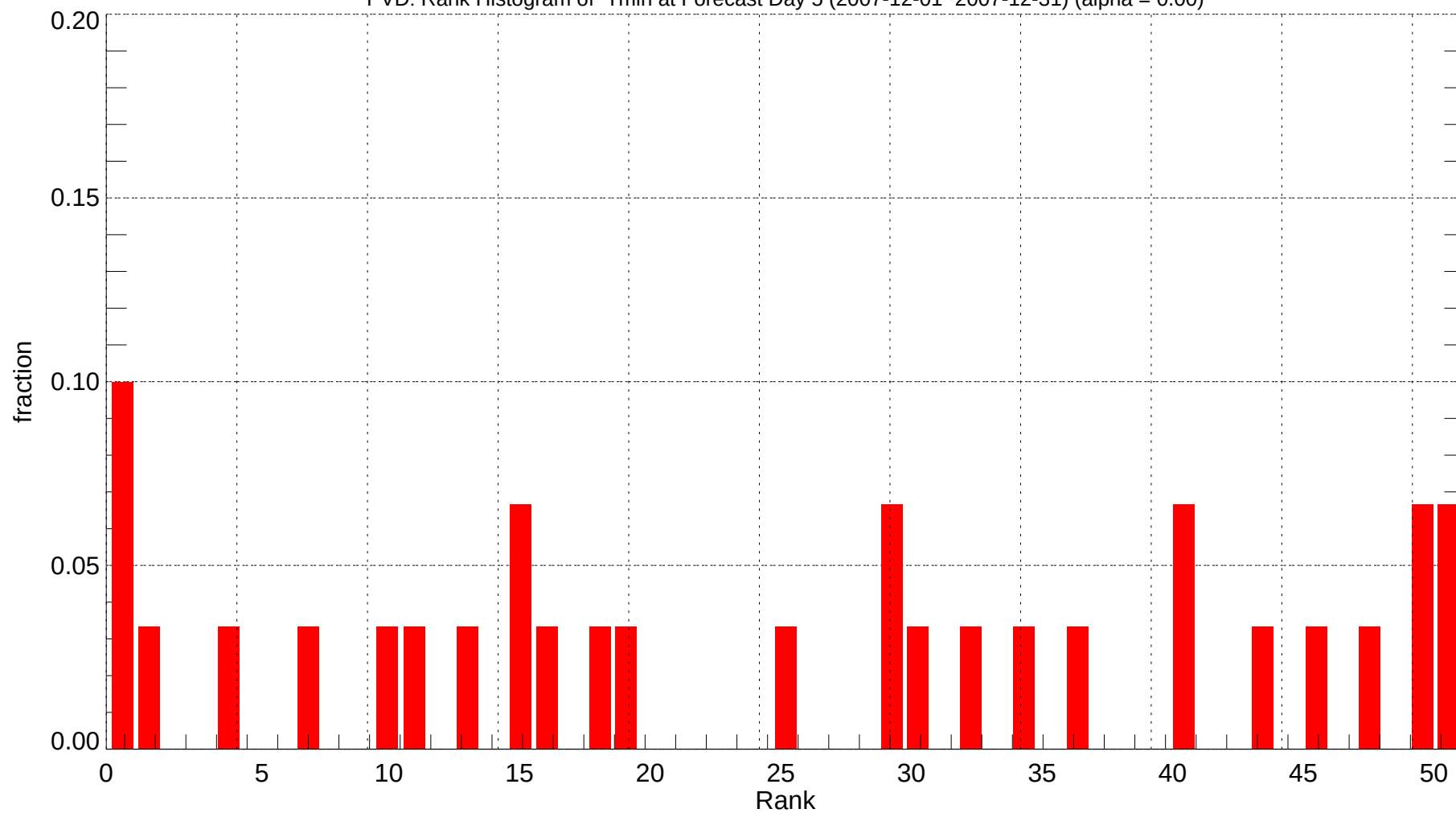
PVD: Rank Histogram of Tmin at Forecast Day 5 (2007-12-01~2007-12-31) (alpha = 0.00)
