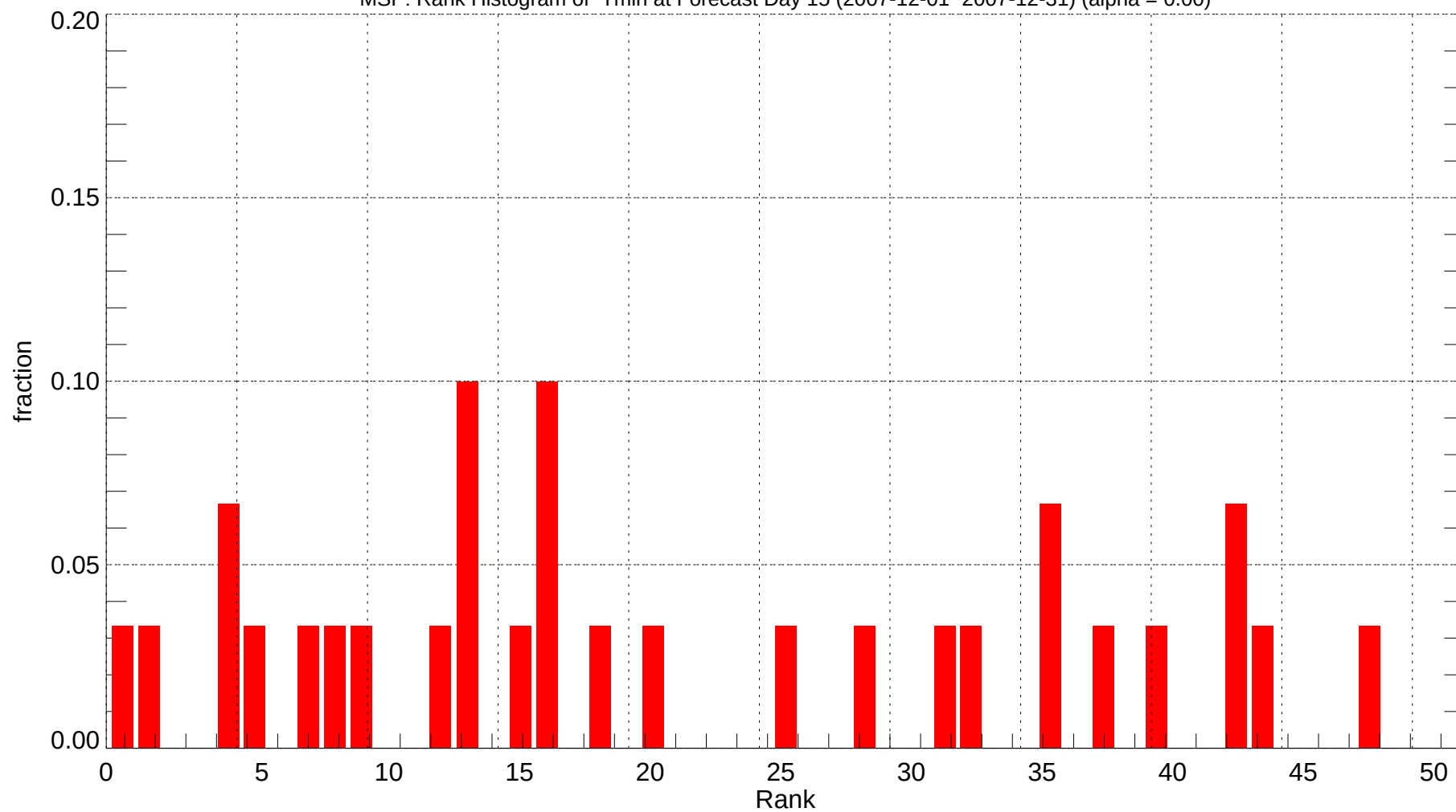
MSP: Rank Histogram of Tmin at Forecast Day 15 (2007-12-01~2007-12-31) (alpha = 0.00)
