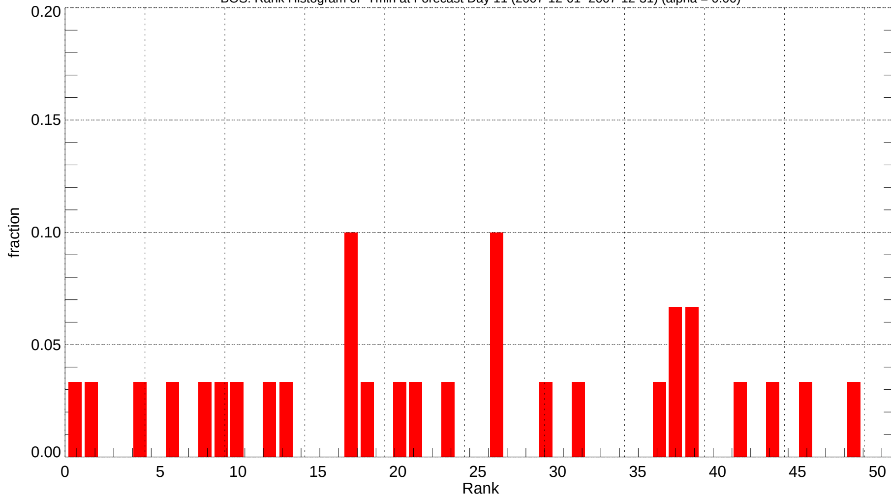
BOS: Rank Histogram of Tmin at Forecast Day 11 (2007-12-01~2007-12-31) (alpha = 0.00)
