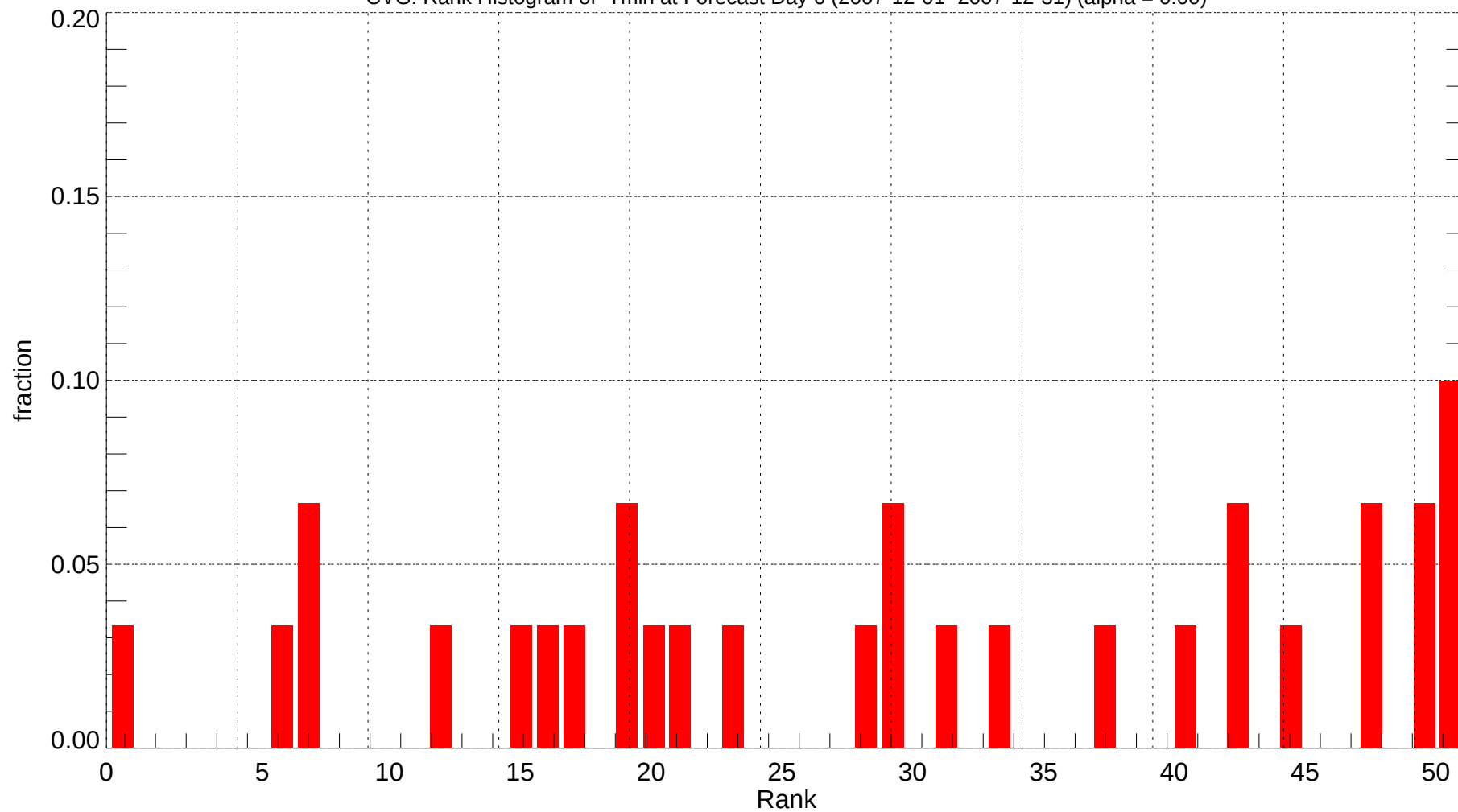
CVG: Rank Histogram of Tmin at Forecast Day 6 (2007-12-01~2007-12-31) (alpha = 0.00)
