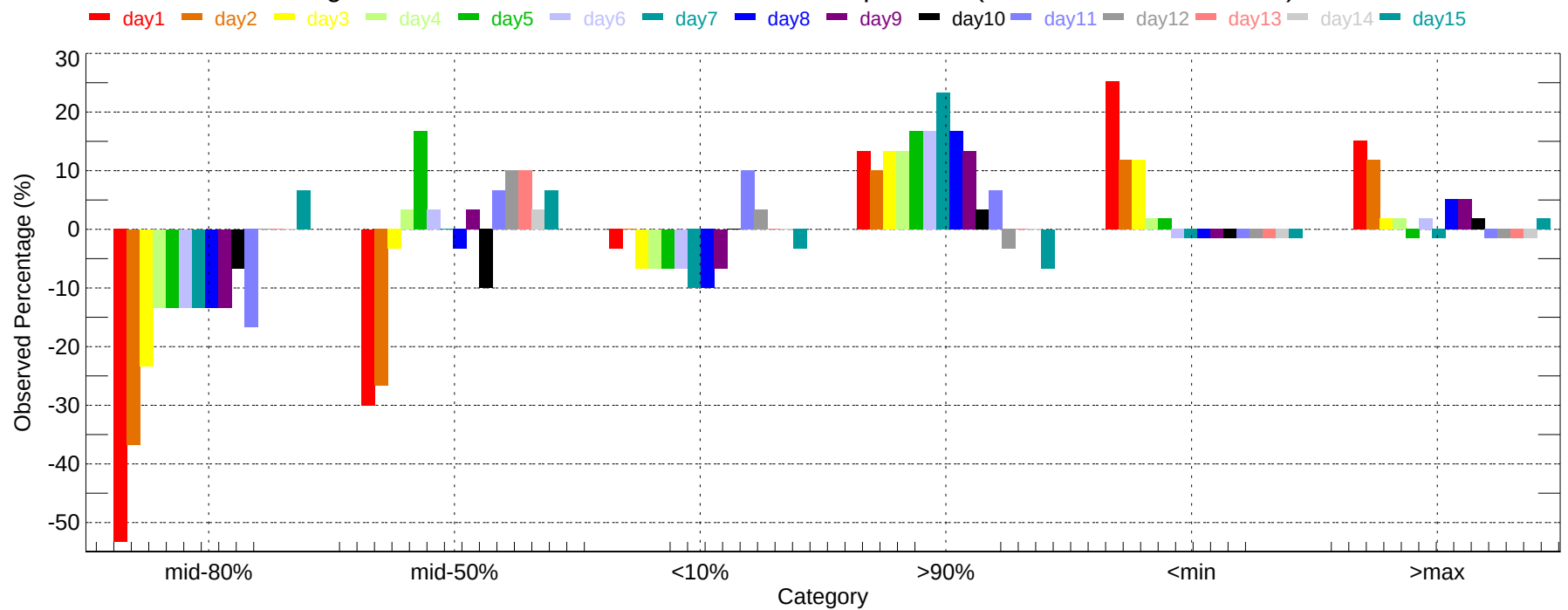
Observed Percentage Deviation of Ensembles - LGA: Min Temperature (2007-12-01~2007-12-31)
