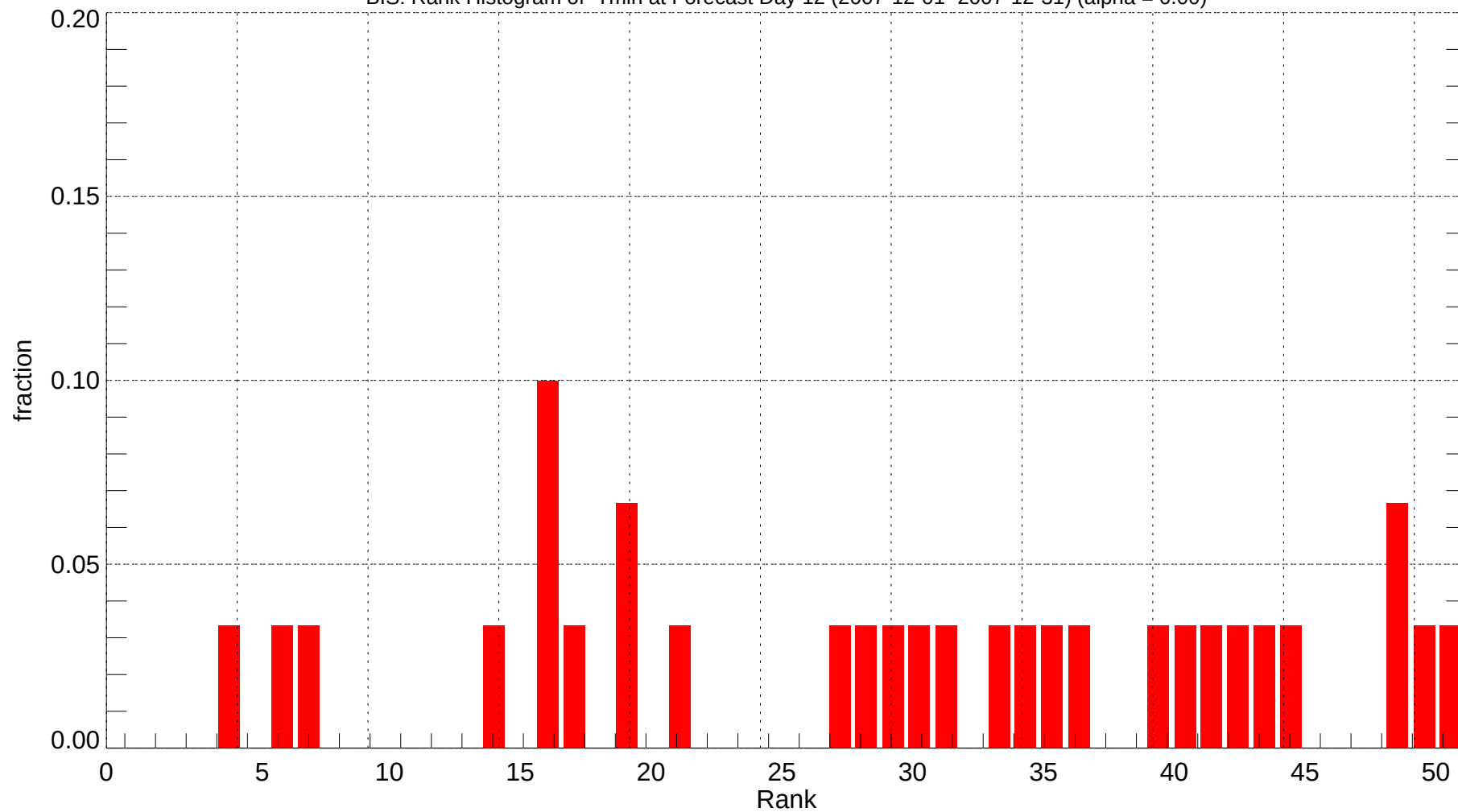
BIS: Rank Histogram of Tmin at Forecast Day 12 (2007-12-01~2007-12-31) (alpha = 0.00)
