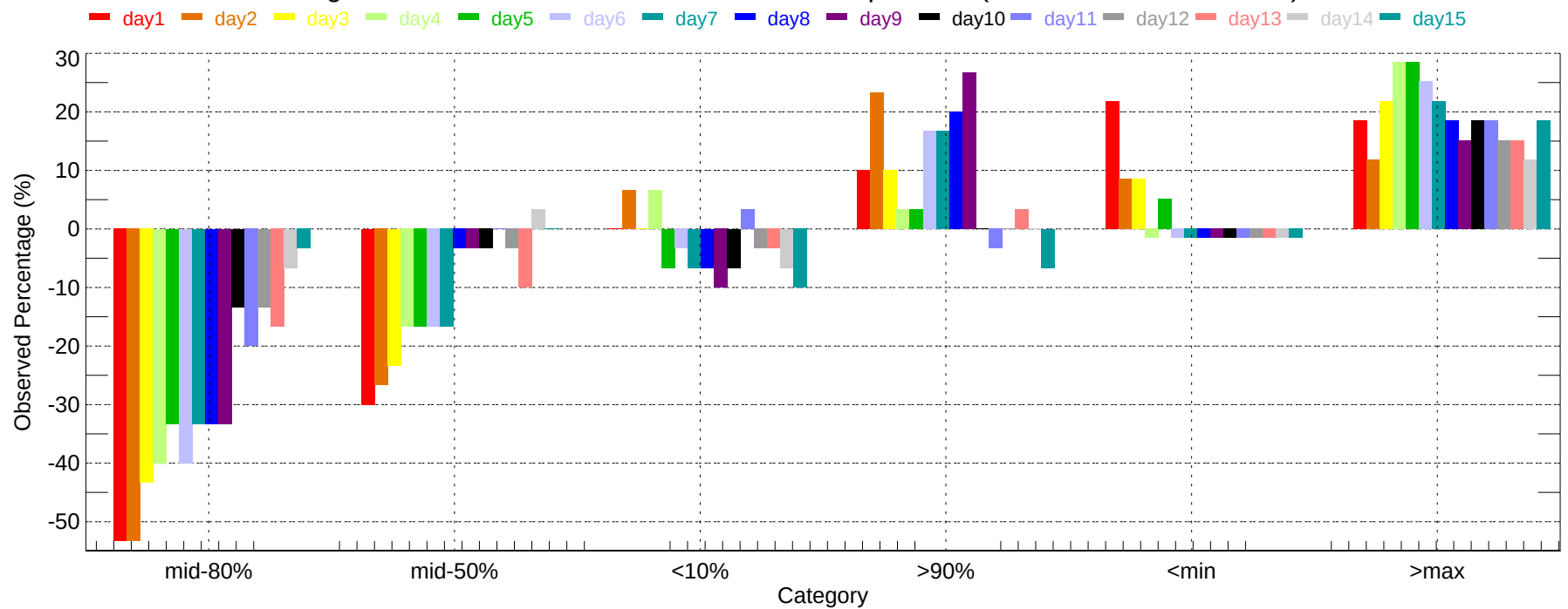
Observed Percentage Deviation of Ensembles - CLT: Max Temperature (2007-12-01~2007-12-31)
