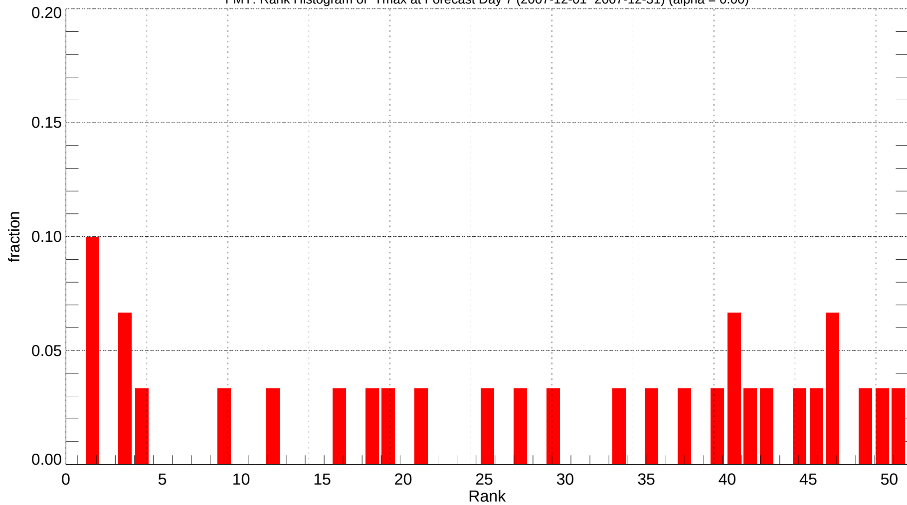
FMY: Rank Histogram of Tmax at Forecast Day 7 (2007-12-01~2007-12-31) (alpha = 0.00)
