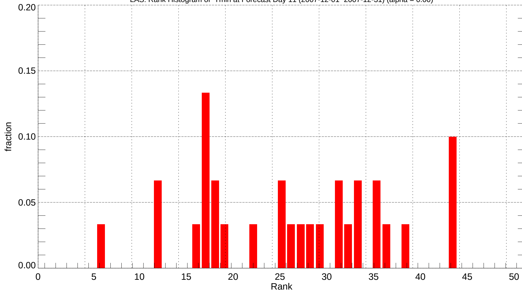
LAS: Rank Histogram of Tmin at Forecast Day 11 (2007-12-01~2007-12-31) (alpha = 0.00)
