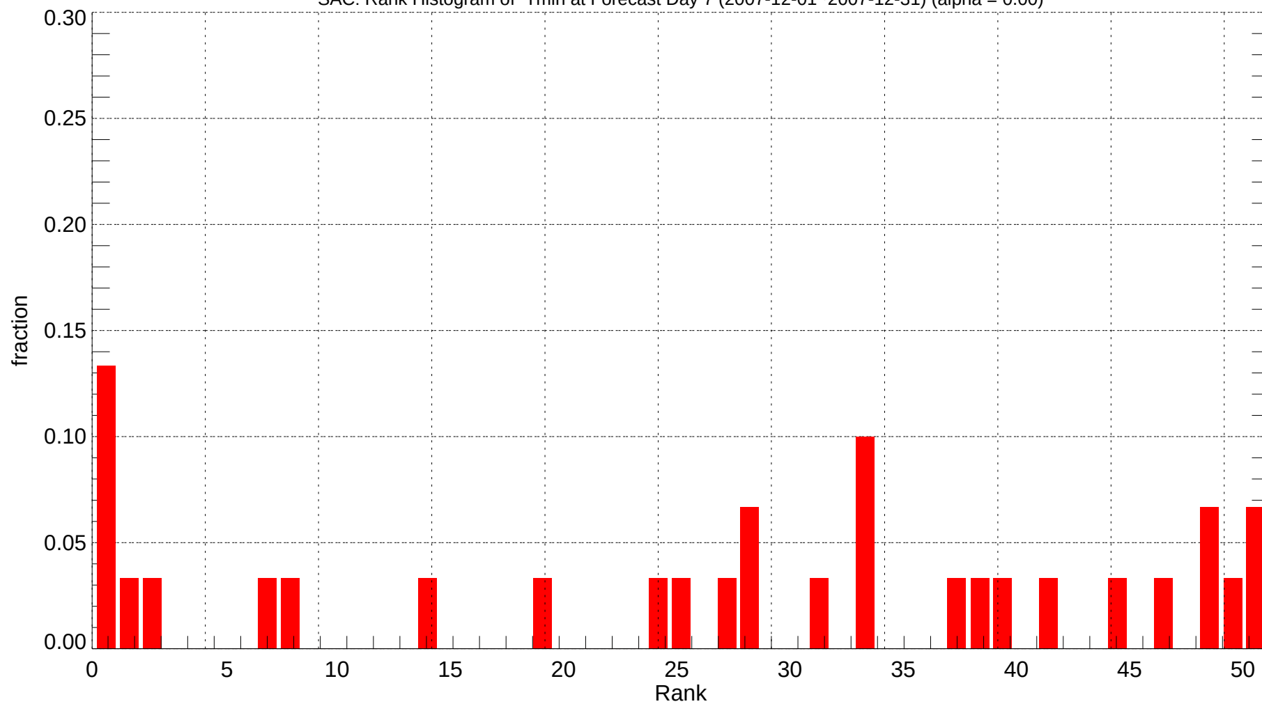
SAC: Rank Histogram of Tmin at Forecast Day 7 (2007-12-01~2007-12-31) (alpha = 0.00)
