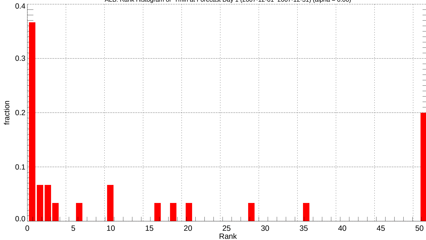
ALB: Rank Histogram of Tmin at Forecast Day 1 (2007-12-01~2007-12-31) (alpha = 0.00)
