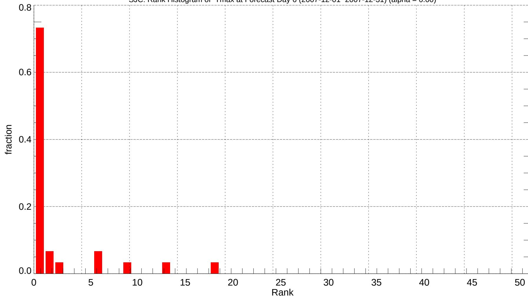
SJC: Rank Histogram of Tmax at Forecast Day 6 (2007-12-01~2007-12-31) (alpha = 0.00)
