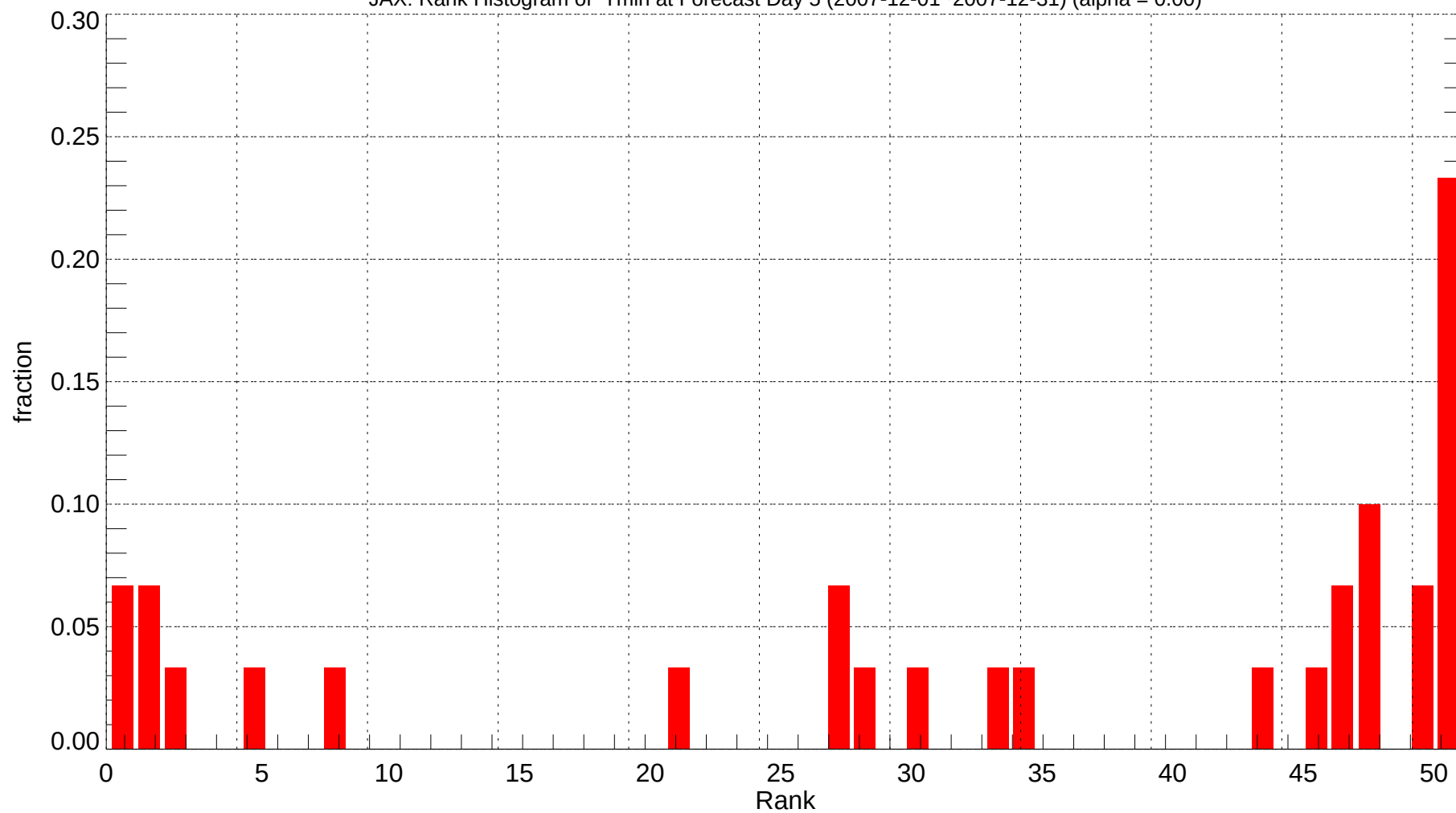
JAX: Rank Histogram of Tmin at Forecast Day 5 (2007-12-01~2007-12-31) (alpha = 0.00)
