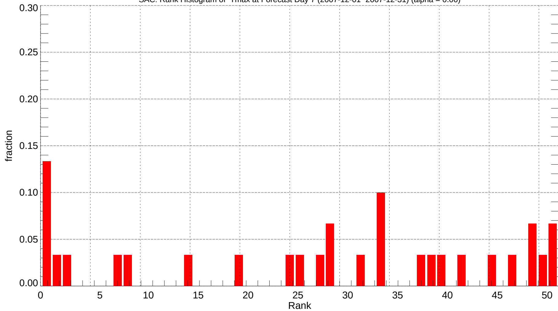
SAC: Rank Histogram of Tmax at Forecast Day 7 (2007-12-01~2007-12-31) (alpha = 0.00)
