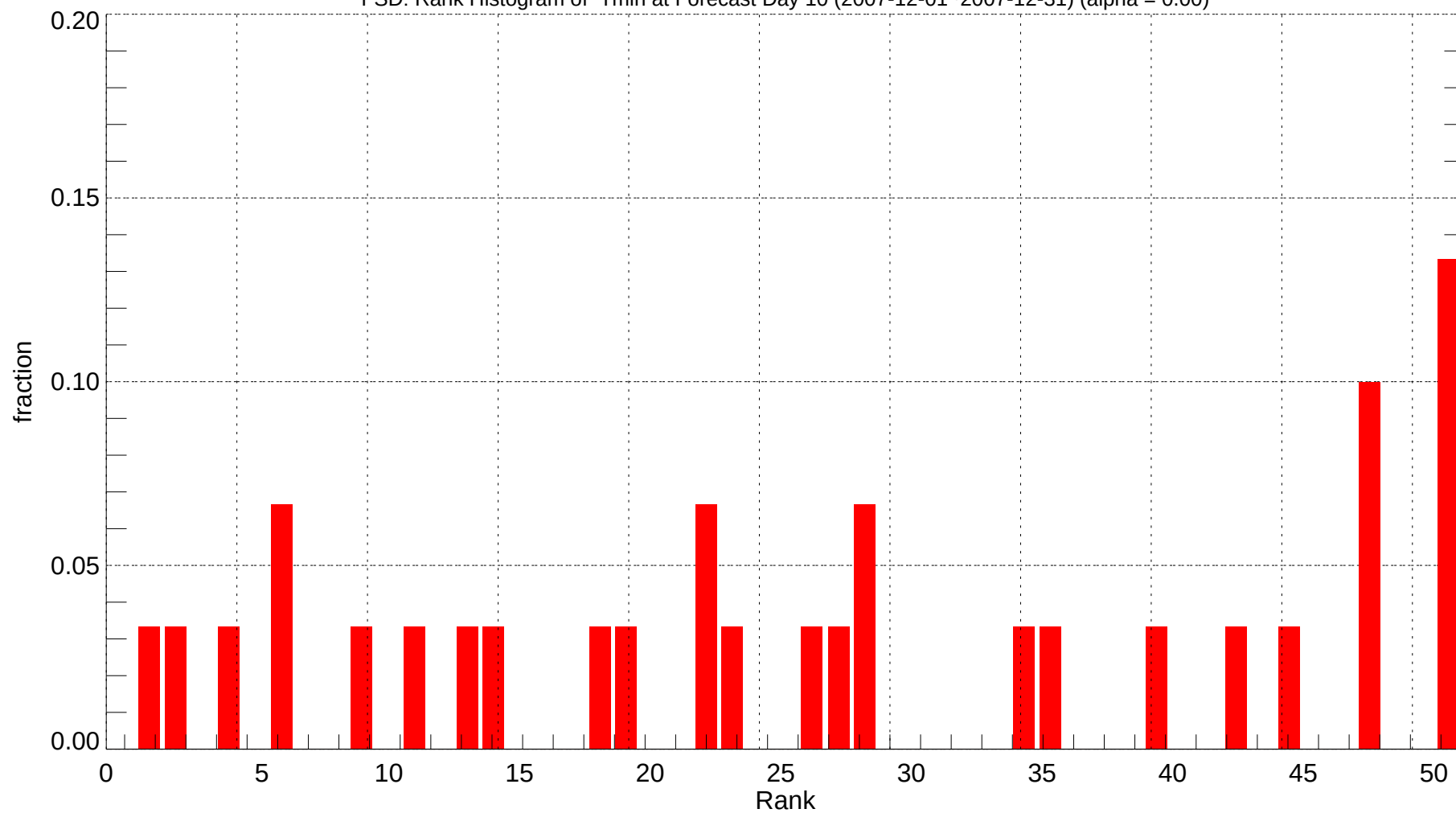
FSD: Rank Histogram of Tmin at Forecast Day 10 (2007-12-01~2007-12-31) (alpha = 0.00)
