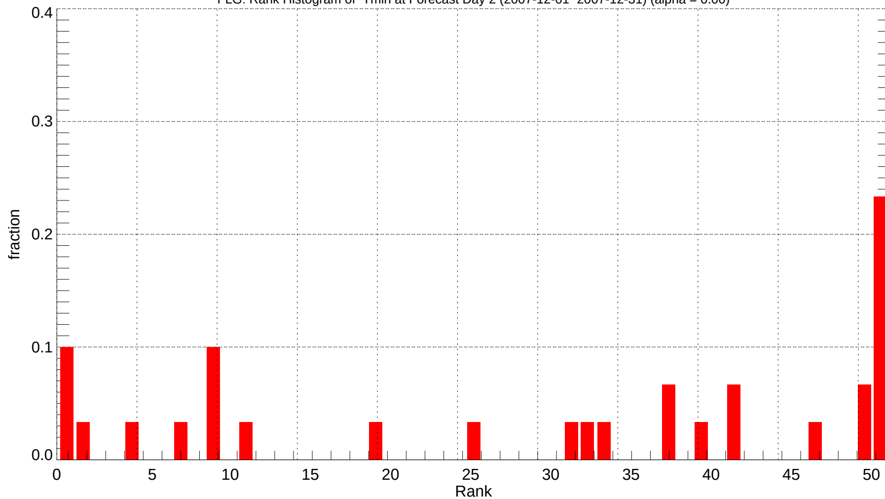
FLG: Rank Histogram of Tmin at Forecast Day 2 (2007-12-01~2007-12-31) (alpha = 0.00)
