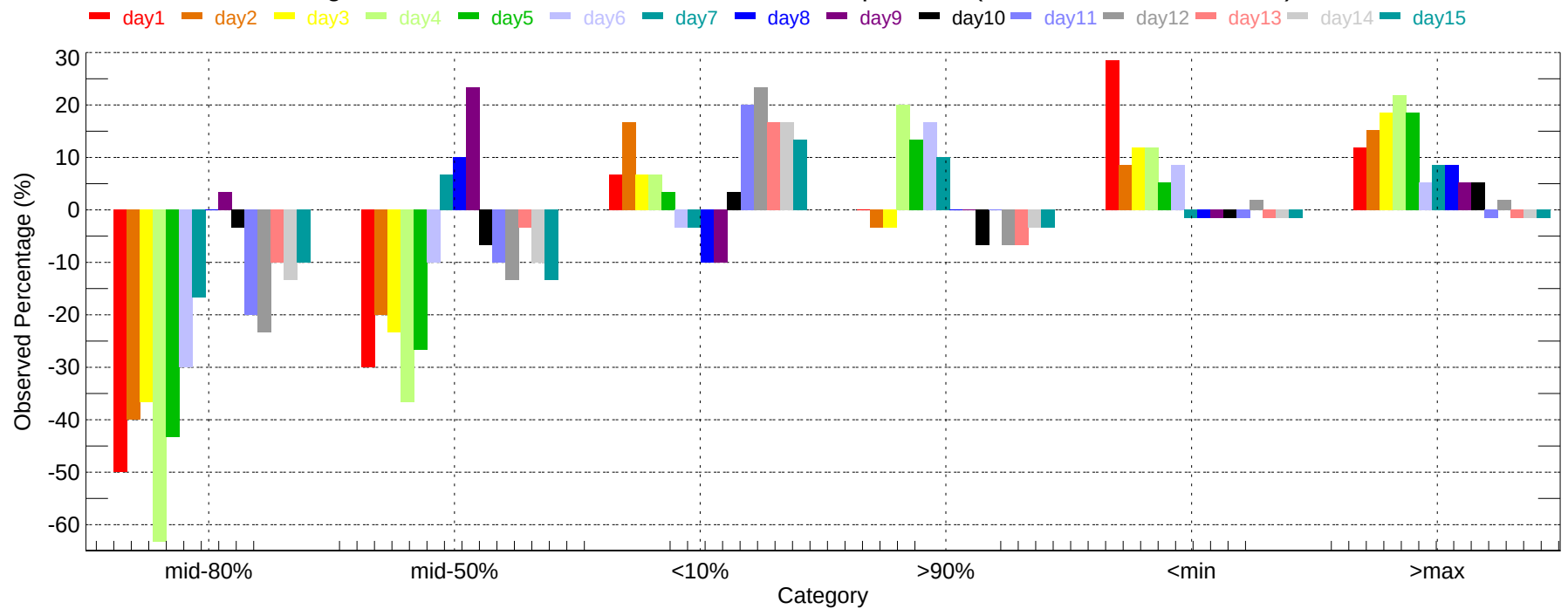
Observed Percentage Deviation of Ensembles - SLC: Min Temperature (2007-12-01~2007-12-31)
