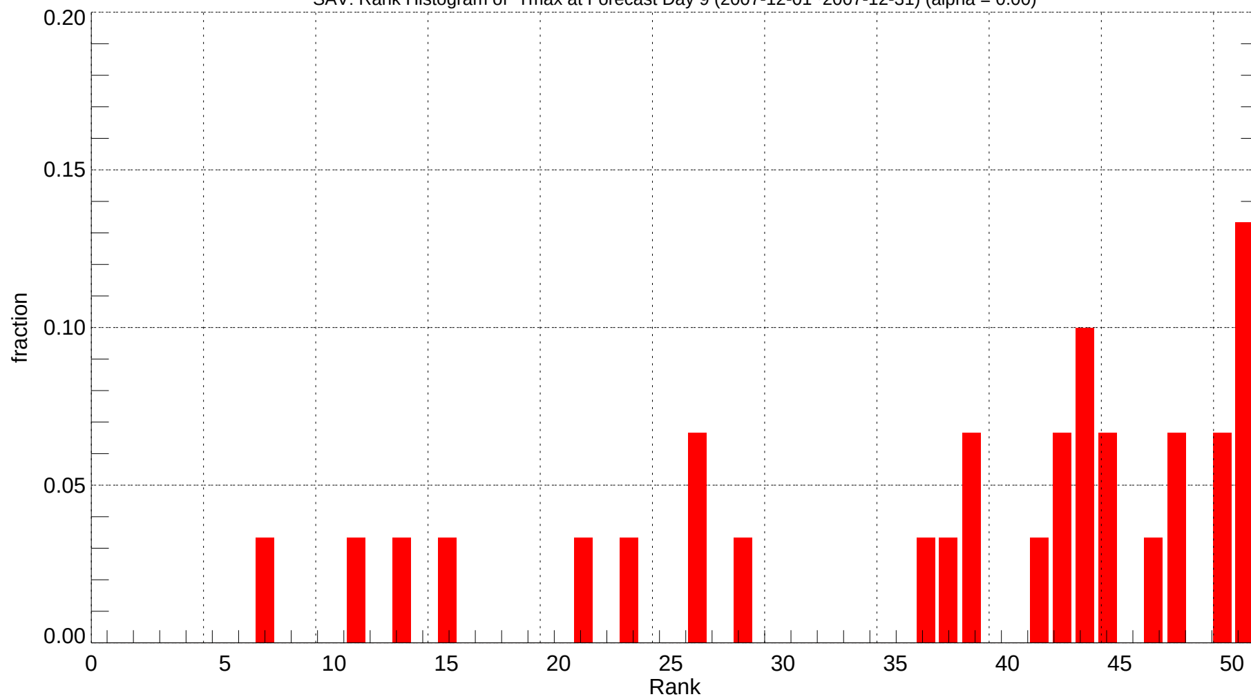
SAV: Rank Histogram of Tmax at Forecast Day 9 (2007-12-01~2007-12-31) (alpha = 0.00)
