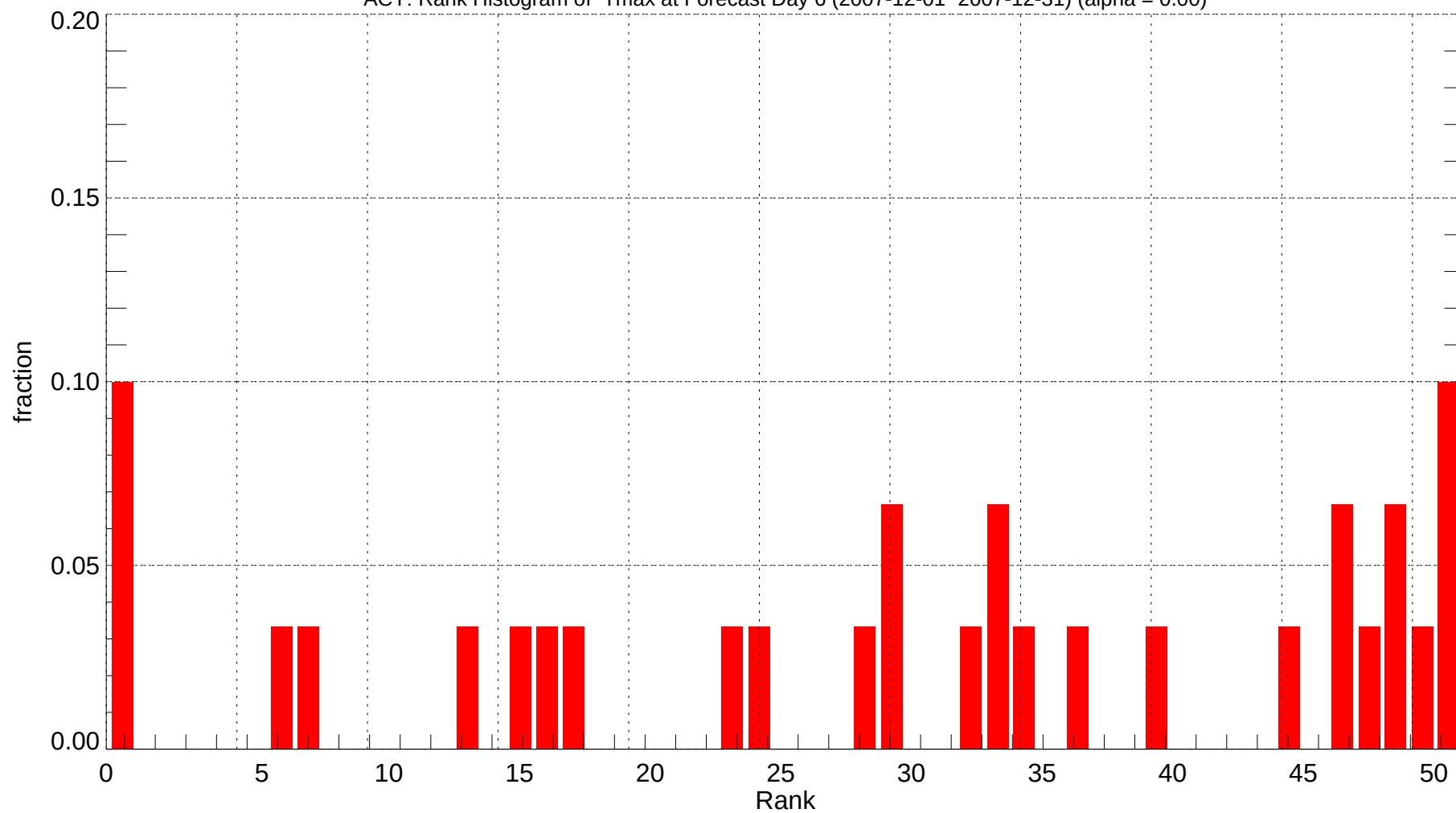
ACY: Rank Histogram of Tmax at Forecast Day 6 (2007-12-01~2007-12-31) (alpha = 0.00)
