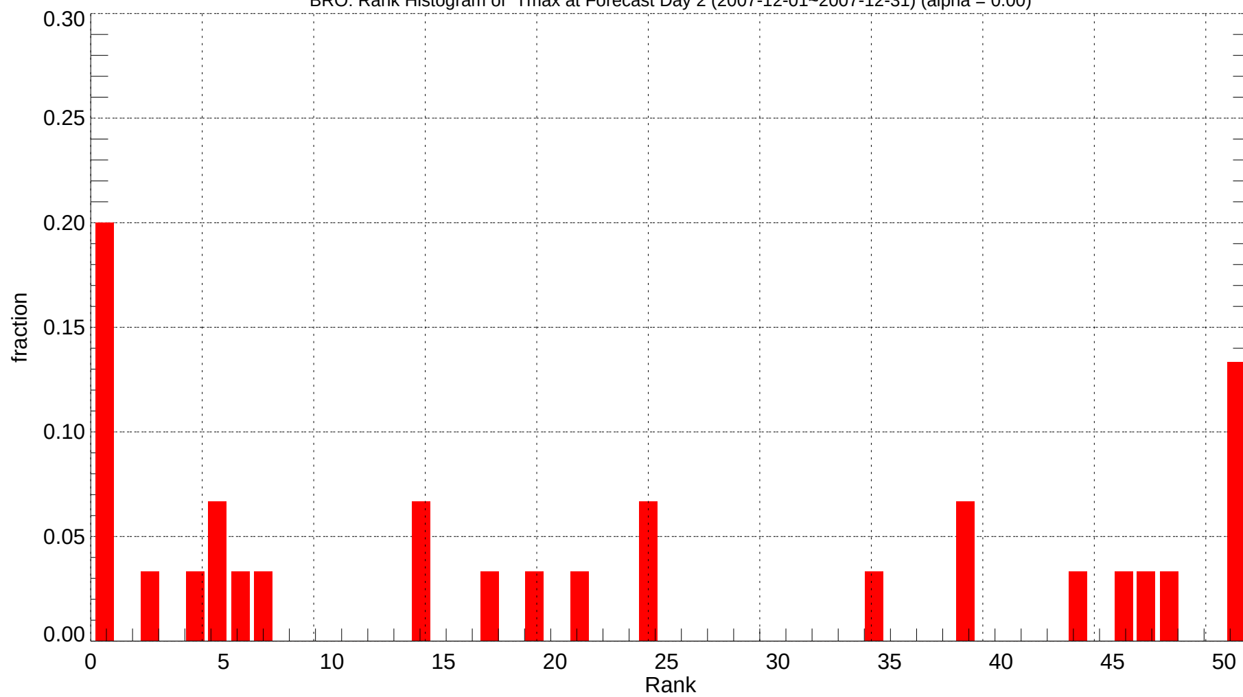
BRO: Rank Histogram of Tmax at Forecast Day 2 (2007-12-01~2007-12-31) (alpha = 0.00)
