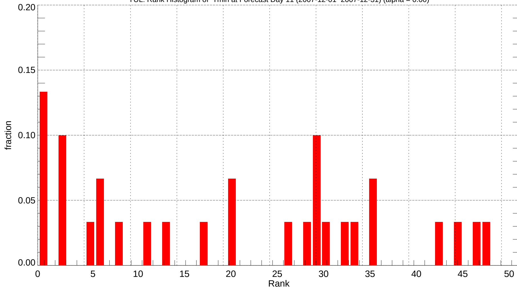
YUL: Rank Histogram of Tmin at Forecast Day 11 (2007-12-01~2007-12-31) (alpha = 0.00)
