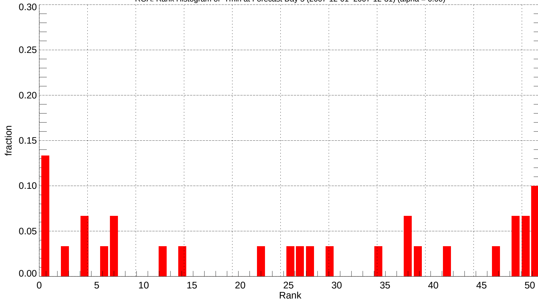
ROA: Rank Histogram of Tmin at Forecast Day 5 (2007-12-01~2007-12-31) (alpha = 0.00)
