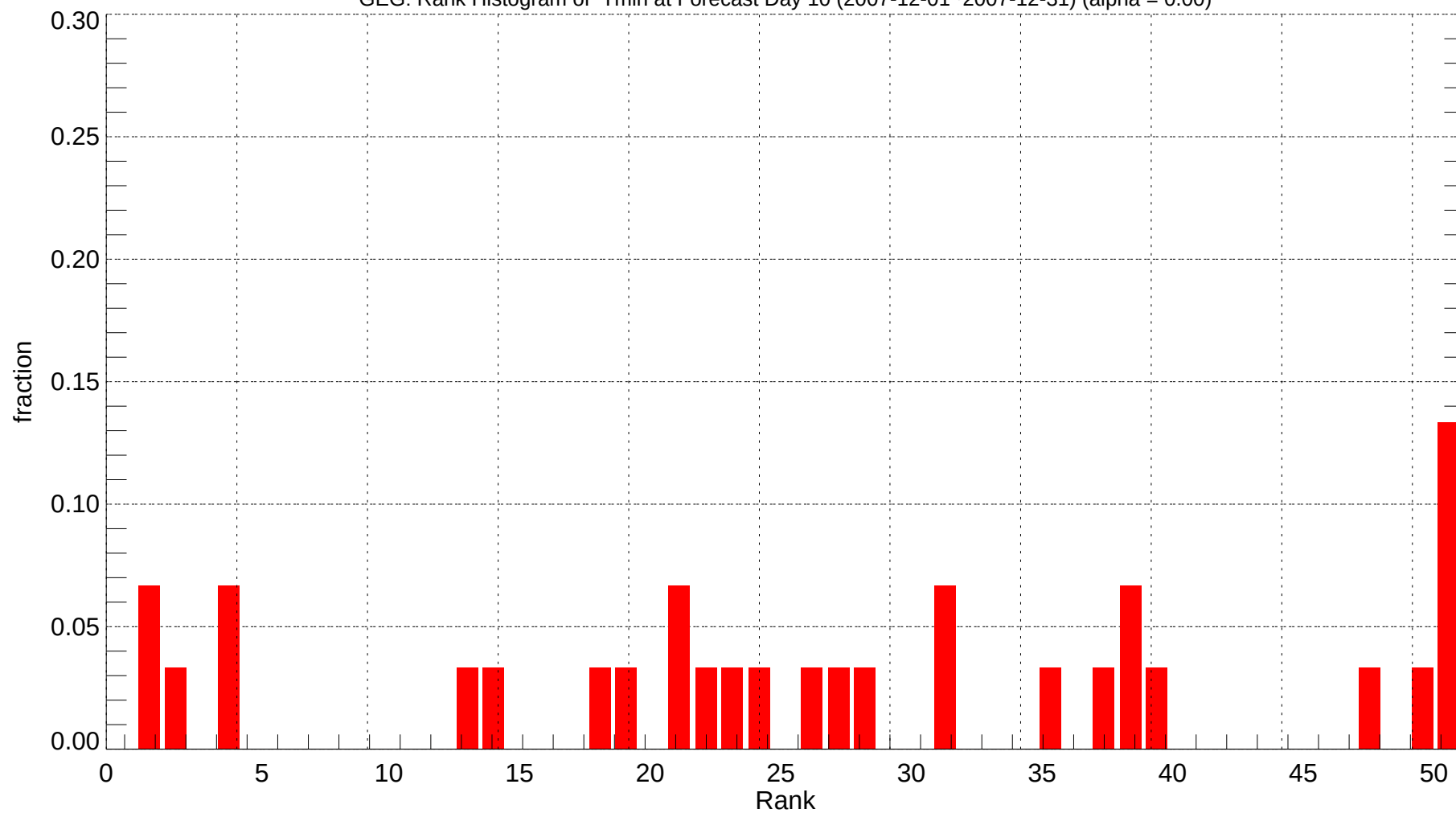
GEG: Rank Histogram of Tmin at Forecast Day 10 (2007-12-01~2007-12-31) (alpha = 0.00)
