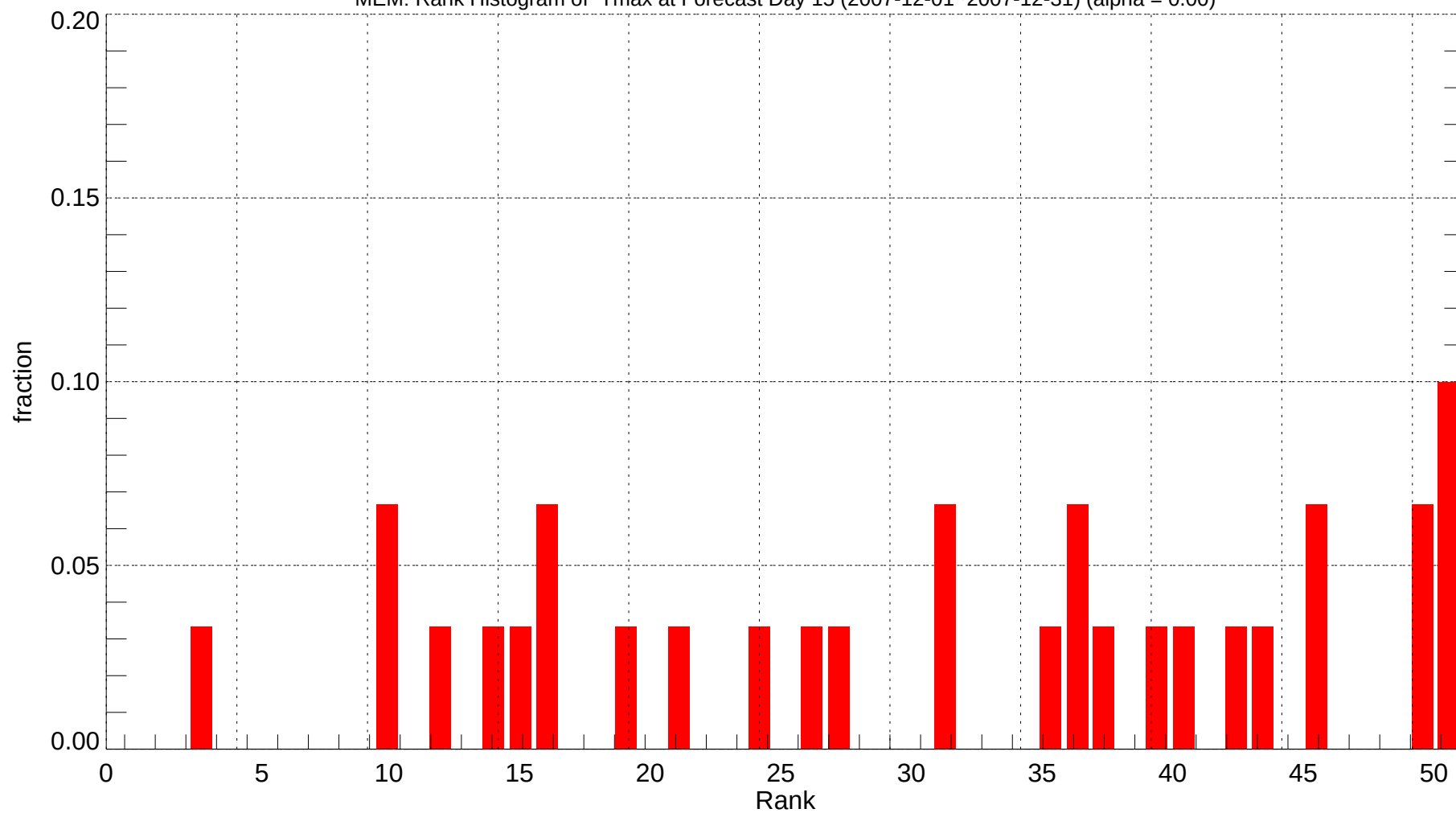
MEM: Rank Histogram of Tmax at Forecast Day 15 (2007-12-01~2007-12-31) (alpha = 0.00)
