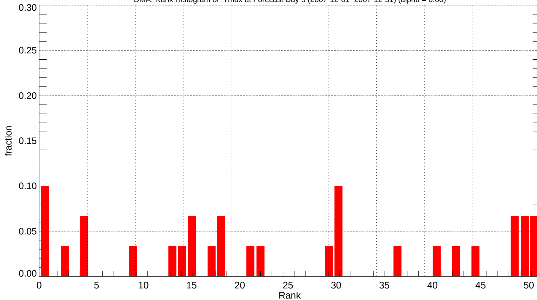
OMA: Rank Histogram of Tmax at Forecast Day 3 (2007-12-01~2007-12-31) (alpha = 0.00)
