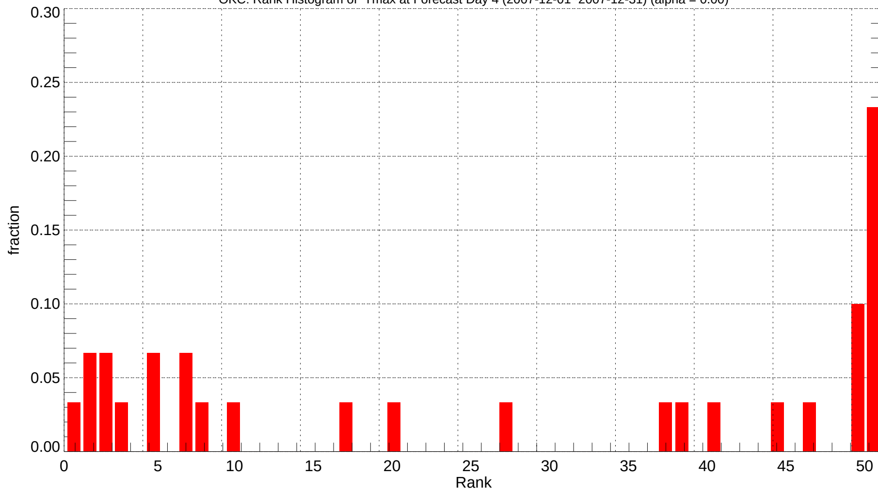
OKC: Rank Histogram of Tmax at Forecast Day 4 (2007-12-01~2007-12-31) (alpha = 0.00)
