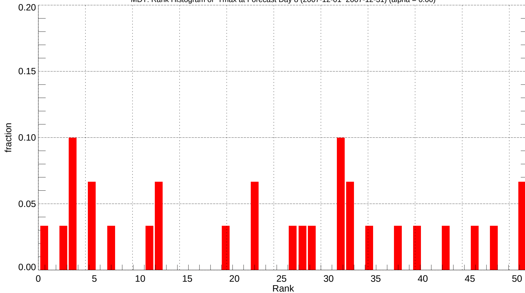
MDT: Rank Histogram of Tmax at Forecast Day 8 (2007-12-01~2007-12-31) (alpha = 0.00)
