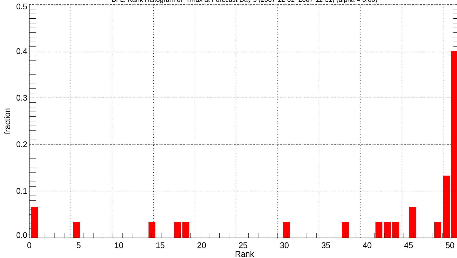
BFL: Rank Histogram of Tmax at Forecast Day 5 (2007-12-01~2007-12-31) (alpha = 0.00)
