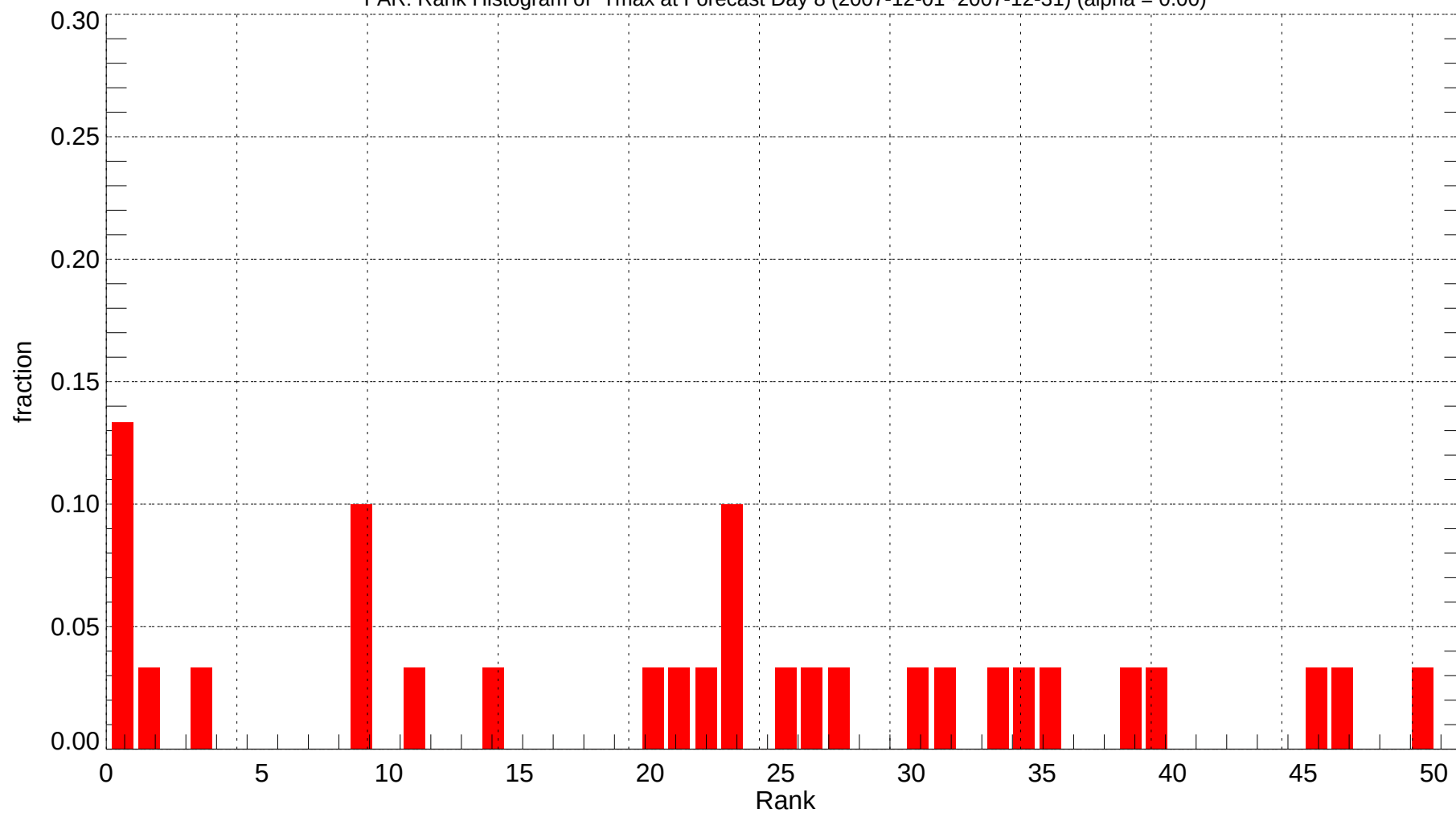
FAR: Rank Histogram of Tmax at Forecast Day 8 (2007-12-01~2007-12-31) (alpha = 0.00)
