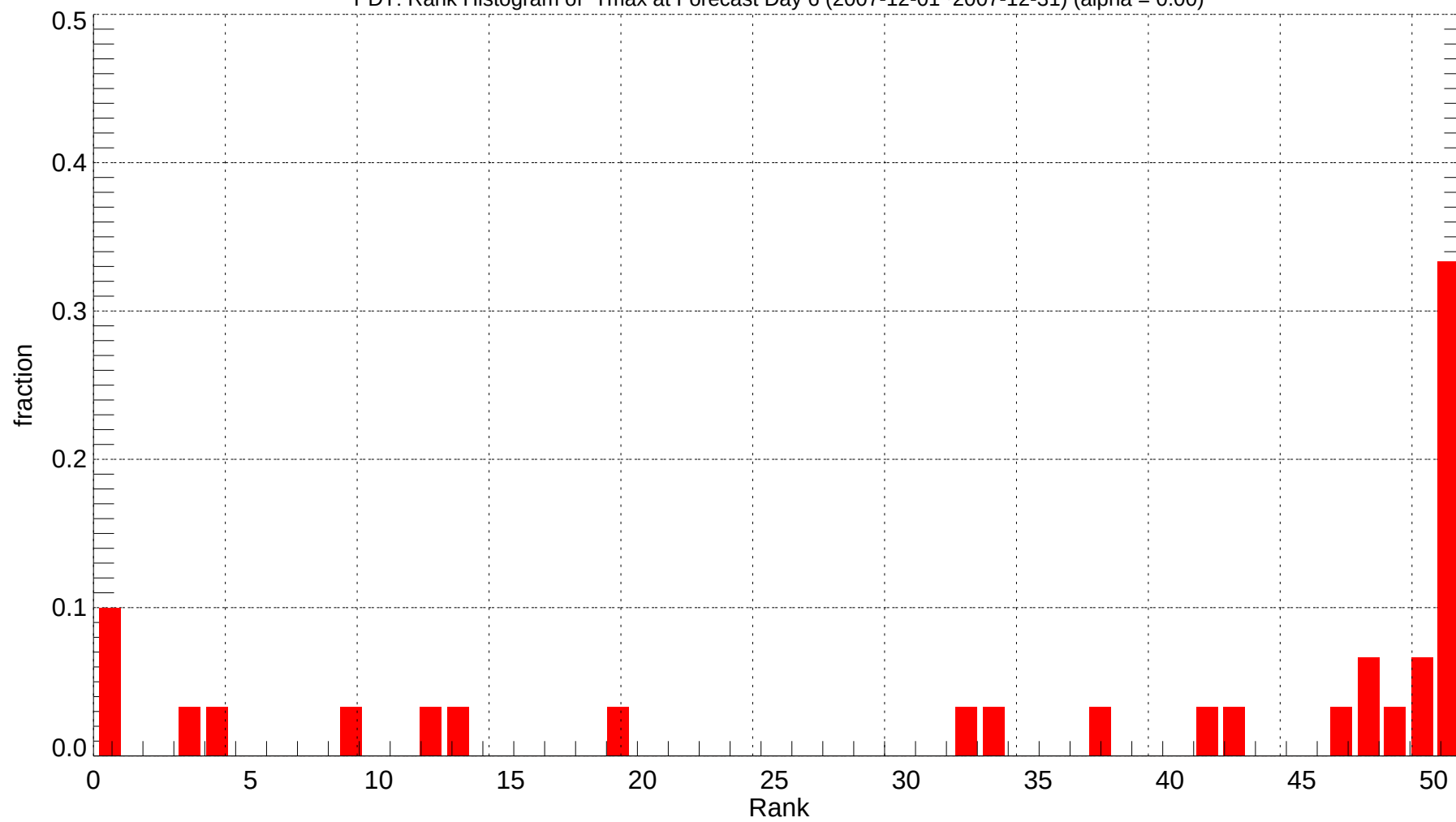
PDT: Rank Histogram of Tmax at Forecast Day 6 (2007-12-01~2007-12-31) (alpha = 0.00)
