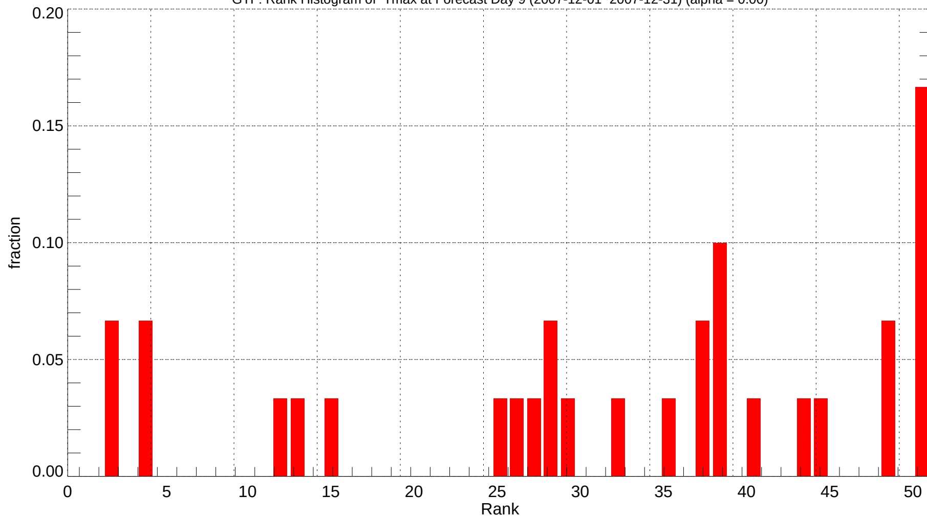
GTF: Rank Histogram of Tmax at Forecast Day 9 (2007-12-01~2007-12-31) (alpha = 0.00)
