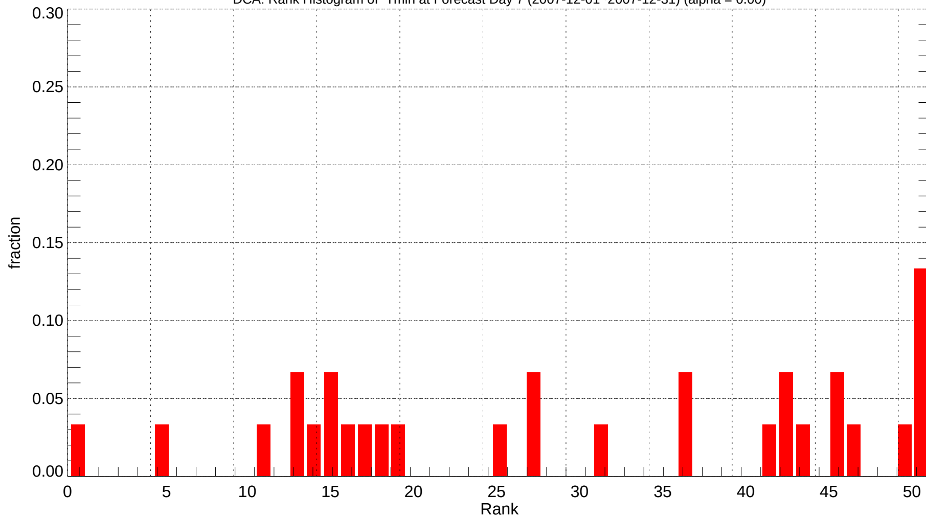
DCA: Rank Histogram of Tmin at Forecast Day 7 (2007-12-01~2007-12-31) (alpha = 0.00)
