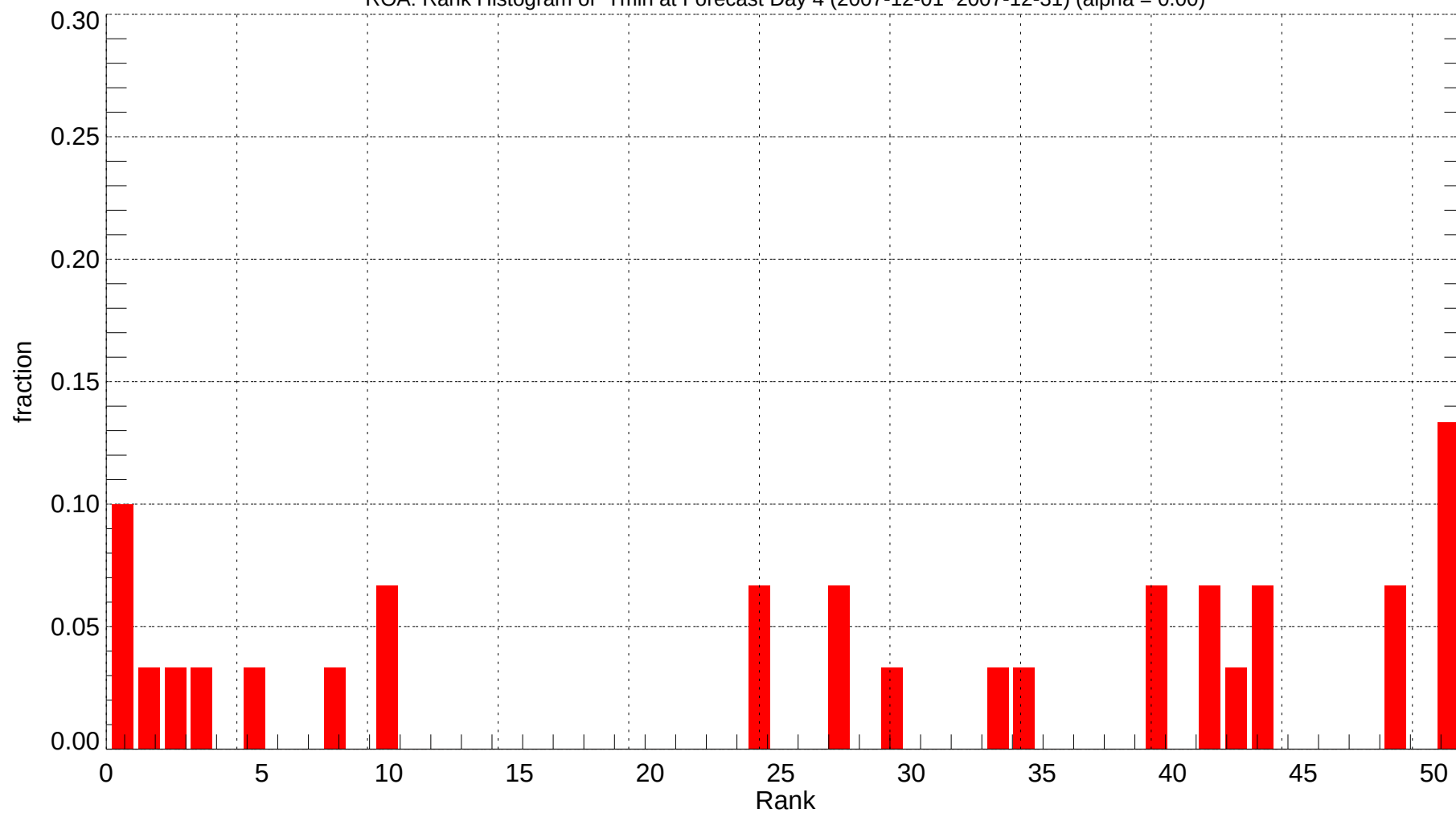
ROA: Rank Histogram of Tmin at Forecast Day 4 (2007-12-01~2007-12-31) (alpha = 0.00)
