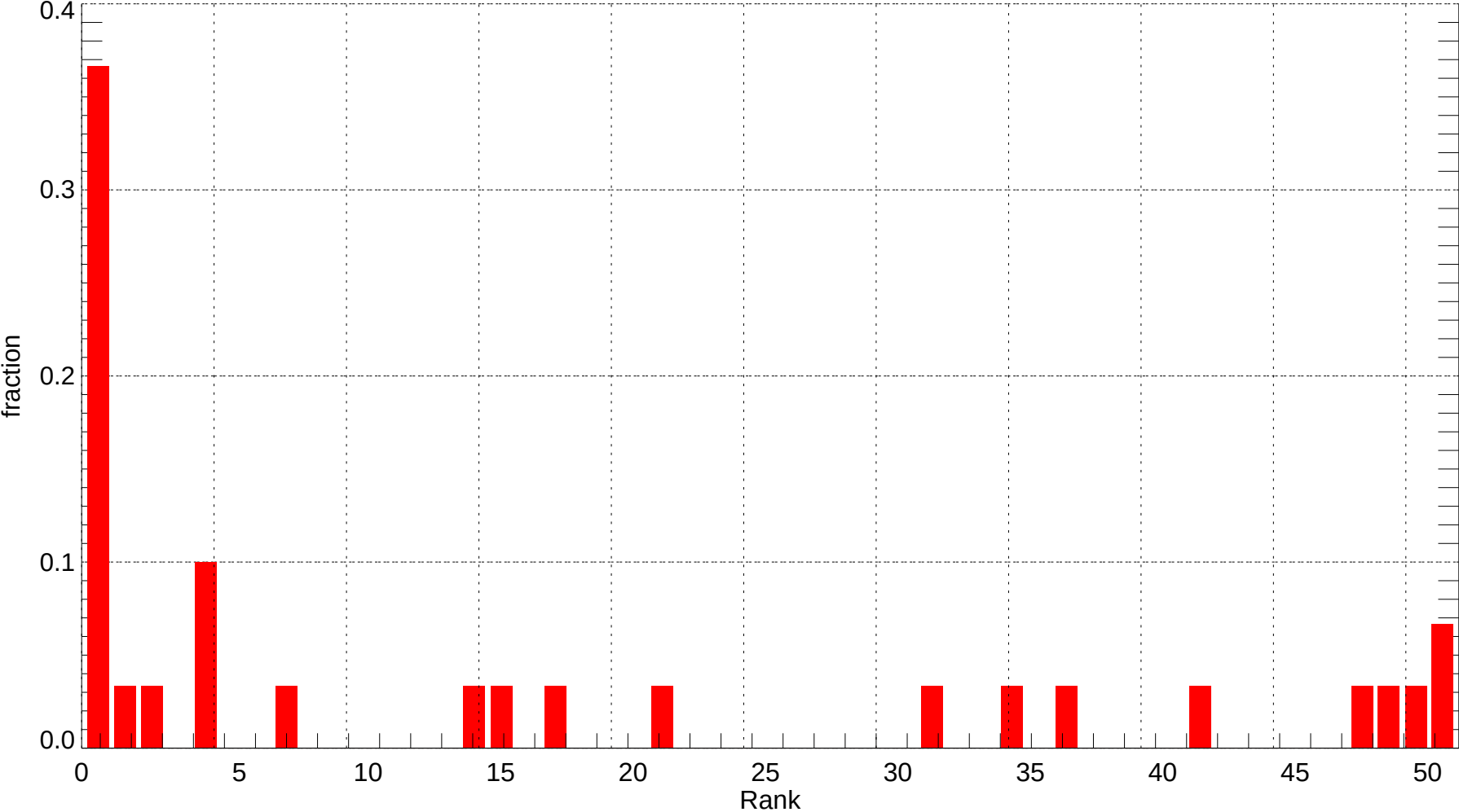
SJC: Rank Histogram of Tmin at Forecast Day 1 (2007-12-01~2007-12-31) (alpha = 0.00)
