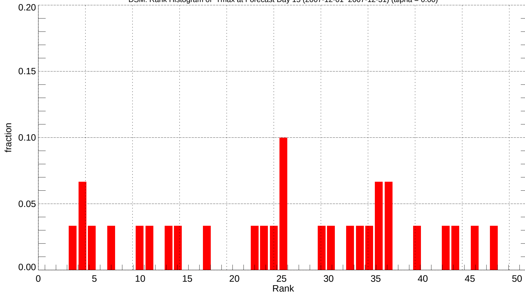
DSM: Rank Histogram of Tmax at Forecast Day 15 (2007-12-01~2007-12-31) (alpha = 0.00)
