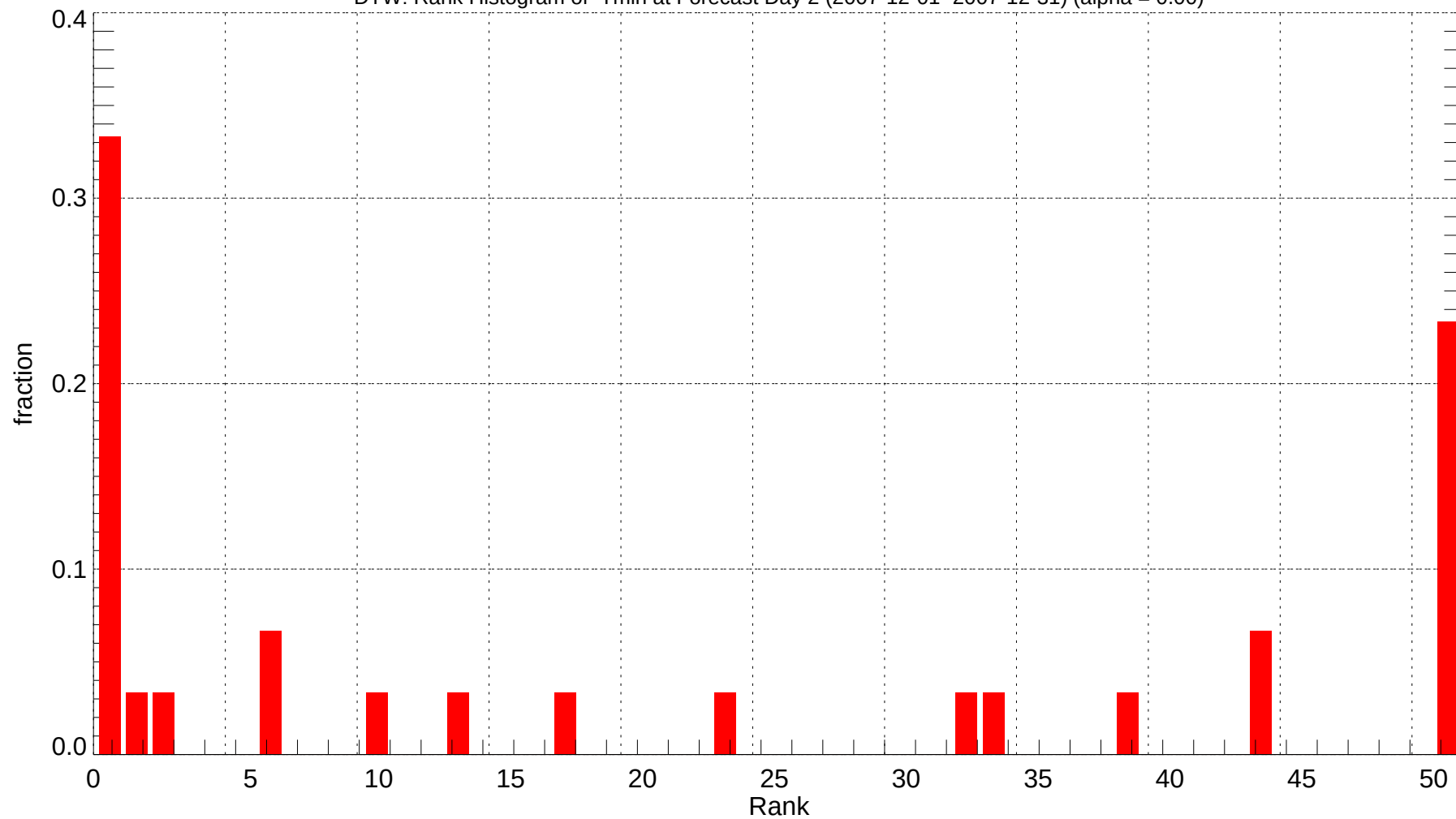
DTW: Rank Histogram of Tmin at Forecast Day 2 (2007-12-01~2007-12-31) (alpha = 0.00)
