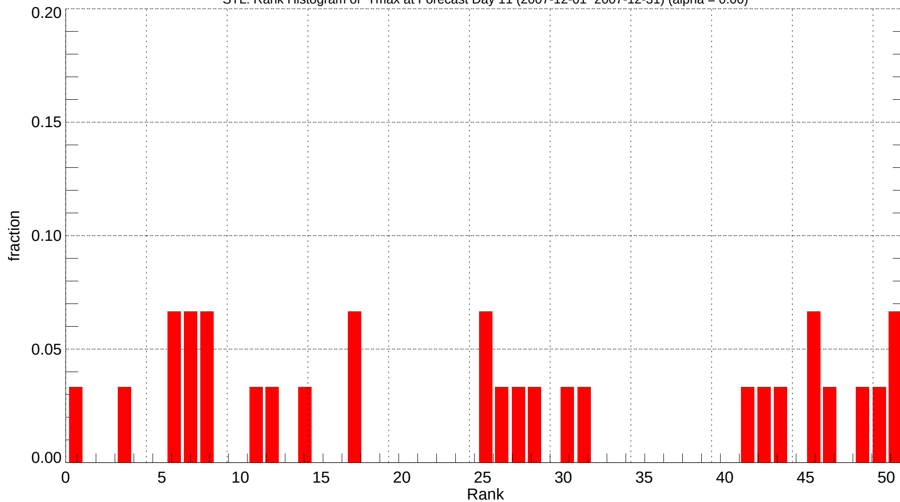
STL: Rank Histogram of Tmax at Forecast Day 11 (2007-12-01~2007-12-31) (alpha = 0.00)
