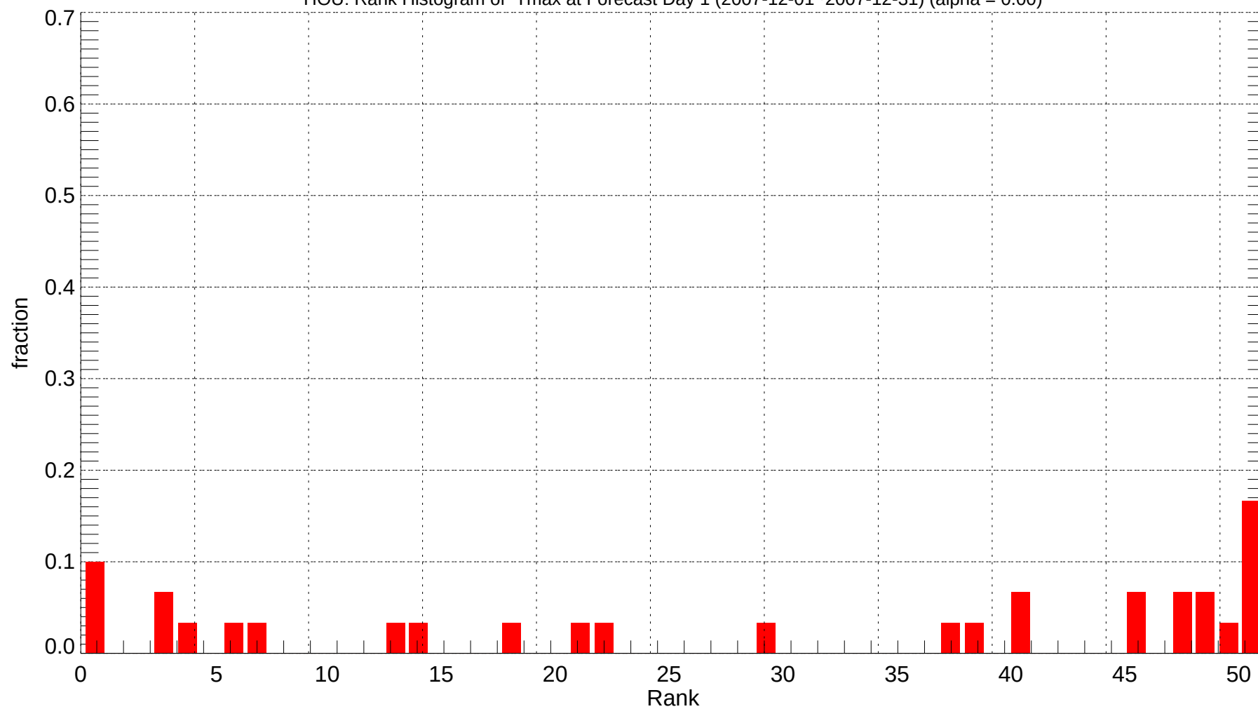
HOU: Rank Histogram of Tmax at Forecast Day 1 (2007-12-01~2007-12-31) (alpha = 0.00)
