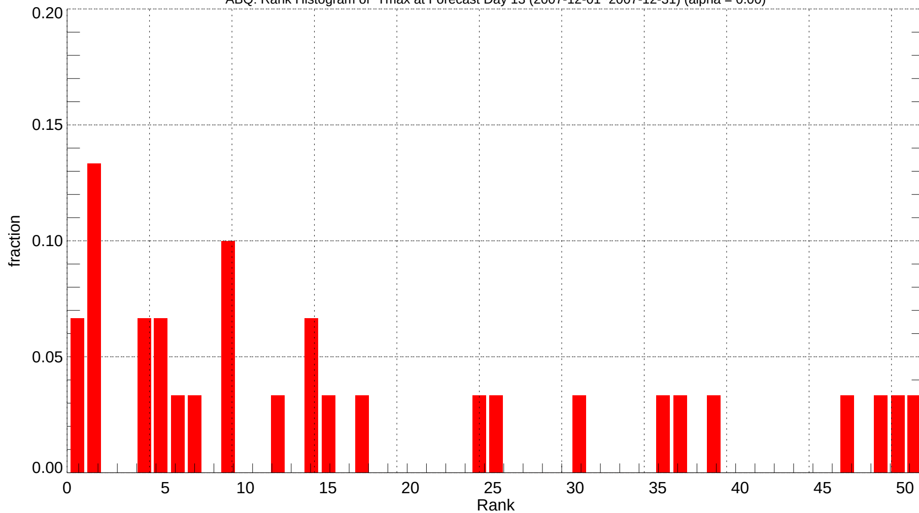
ABQ: Rank Histogram of Tmax at Forecast Day 13 (2007-12-01~2007-12-31) (alpha = 0.00)
