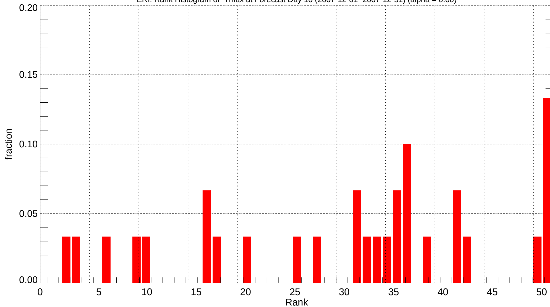
ERI: Rank Histogram of Tmax at Forecast Day 10 (2007-12-01~2007-12-31) (alpha = 0.00)
