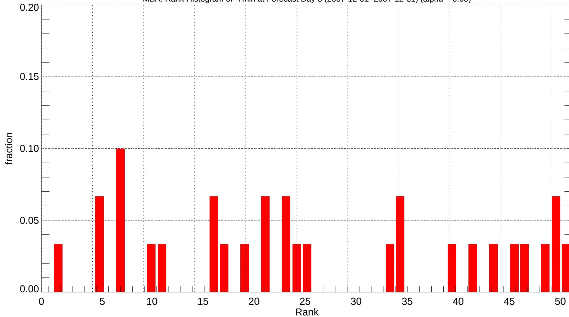
MBA: Rank Histogram of Tmin at Forecast Day 8 (2007-12-01~2007-12-31) (alpha = 0.00)
