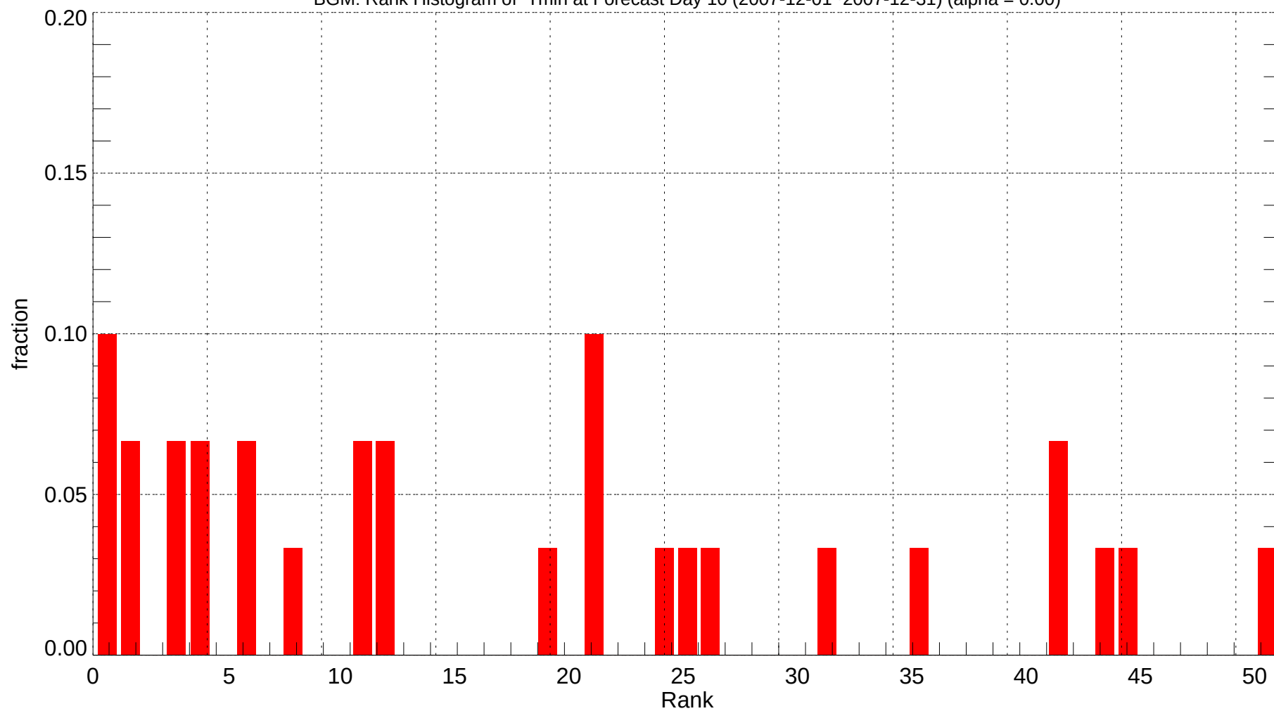
BGM: Rank Histogram of Tmin at Forecast Day 10 (2007-12-01~2007-12-31) (alpha = 0.00)
