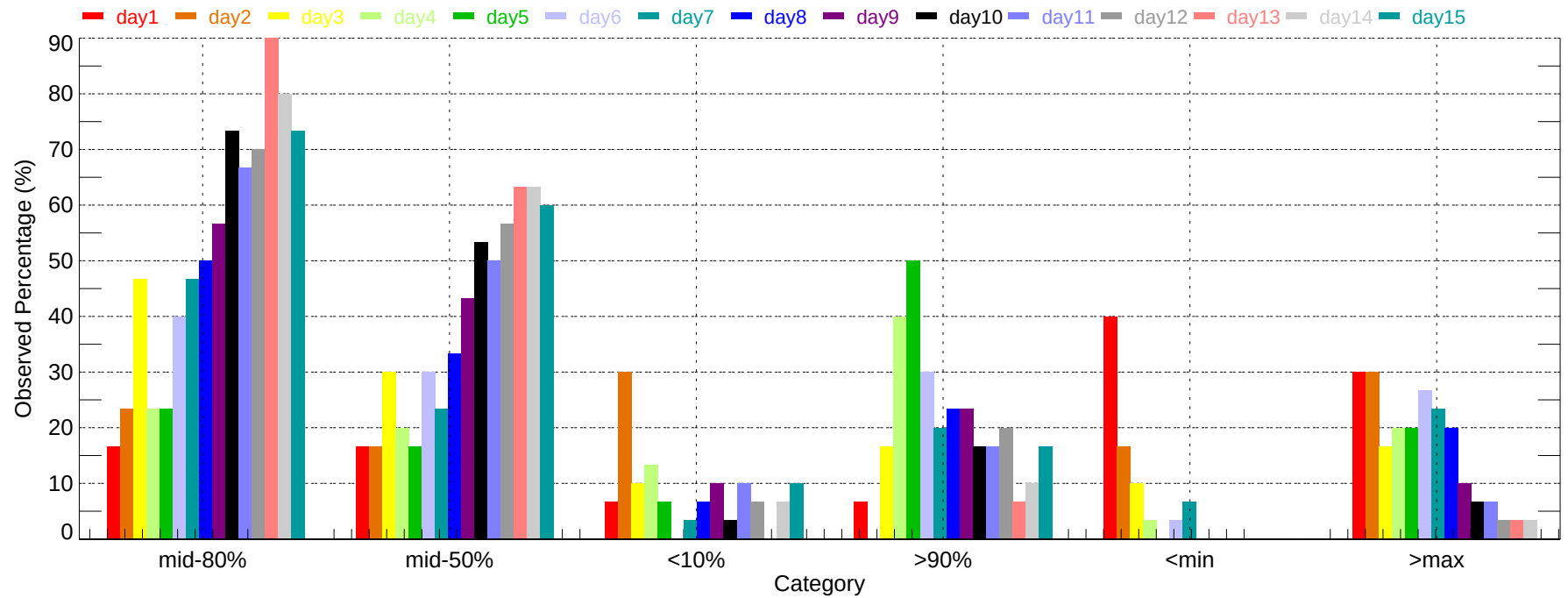
Observed Percentage of Ensembles - DSM: Min Temperature (2007-12-01~2007-12-31)
