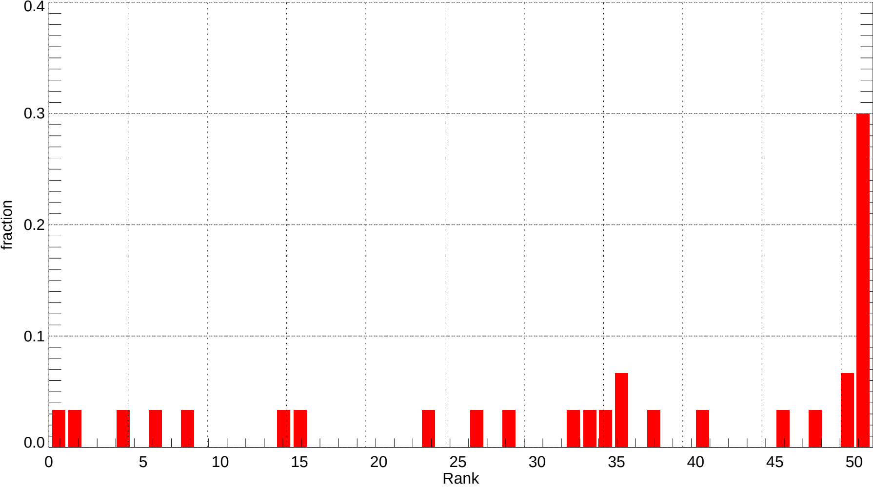
MCI: Rank Histogram of Tmin at Forecast Day 7 (2007-12-01~2007-12-31) (alpha = 0.00)
