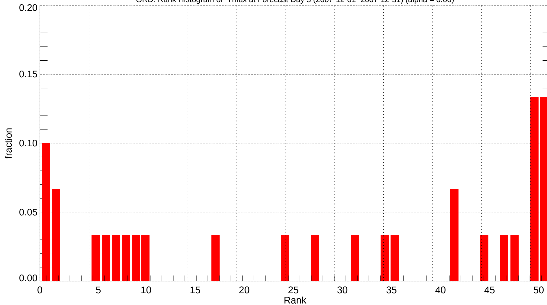
ORD: Rank Histogram of Tmax at Forecast Day 3 (2007-12-01~2007-12-31) (alpha = 0.00)
