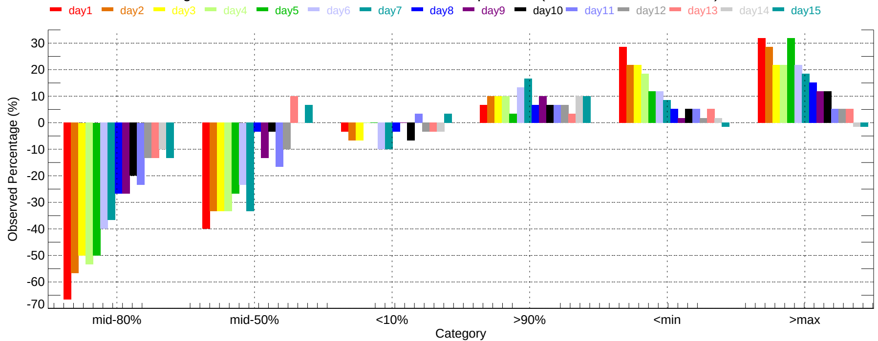
Observed Percentage Deviation of Ensembles - SSI: Min Temperature (2007-12-01~2007-12-31)
