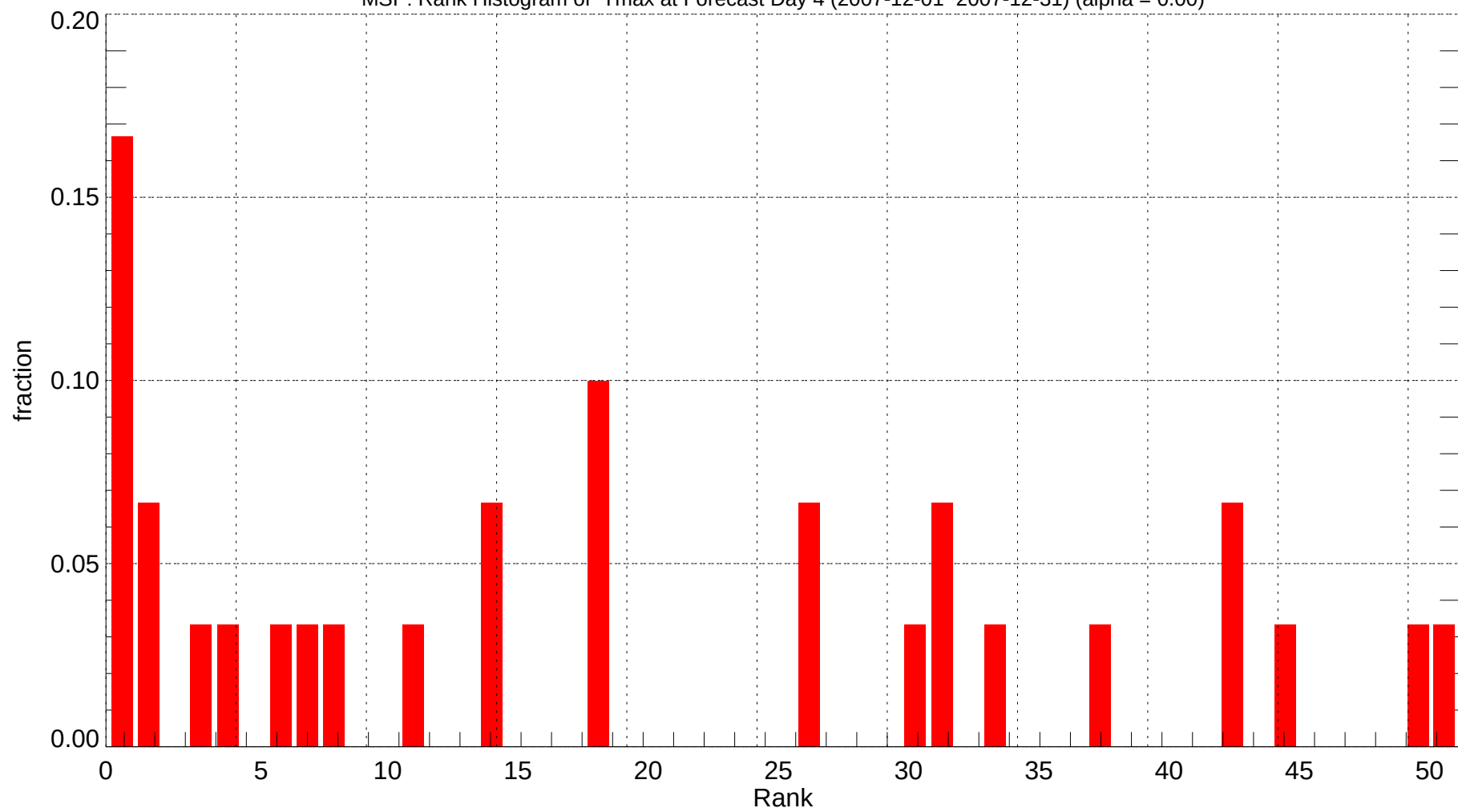
MSP: Rank Histogram of Tmax at Forecast Day 4 (2007-12-01~2007-12-31) (alpha = 0.00)
