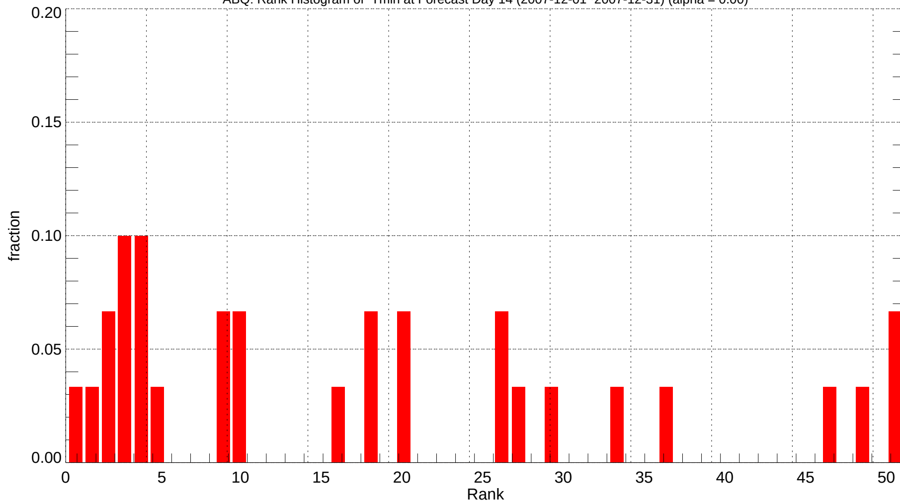
ABQ: Rank Histogram of Tmin at Forecast Day 14 (2007-12-01~2007-12-31) (alpha = 0.00)
