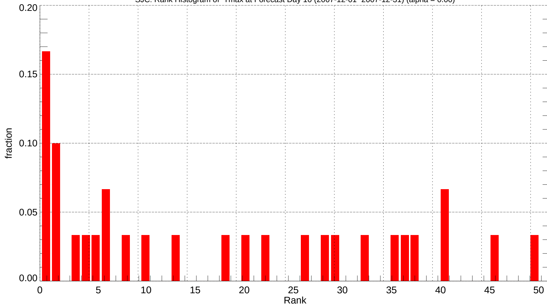
SJC: Rank Histogram of Tmax at Forecast Day 10 (2007-12-01~2007-12-31) (alpha = 0.00)
