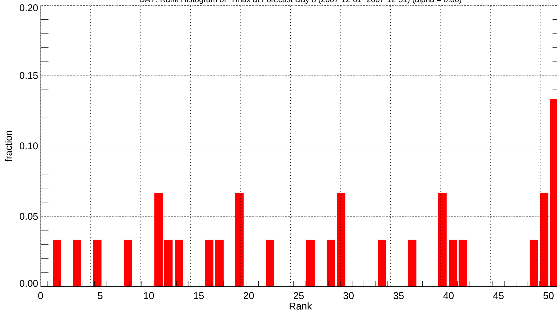
DAY: Rank Histogram of Tmax at Forecast Day 8 (2007-12-01~2007-12-31) (alpha = 0.00)
