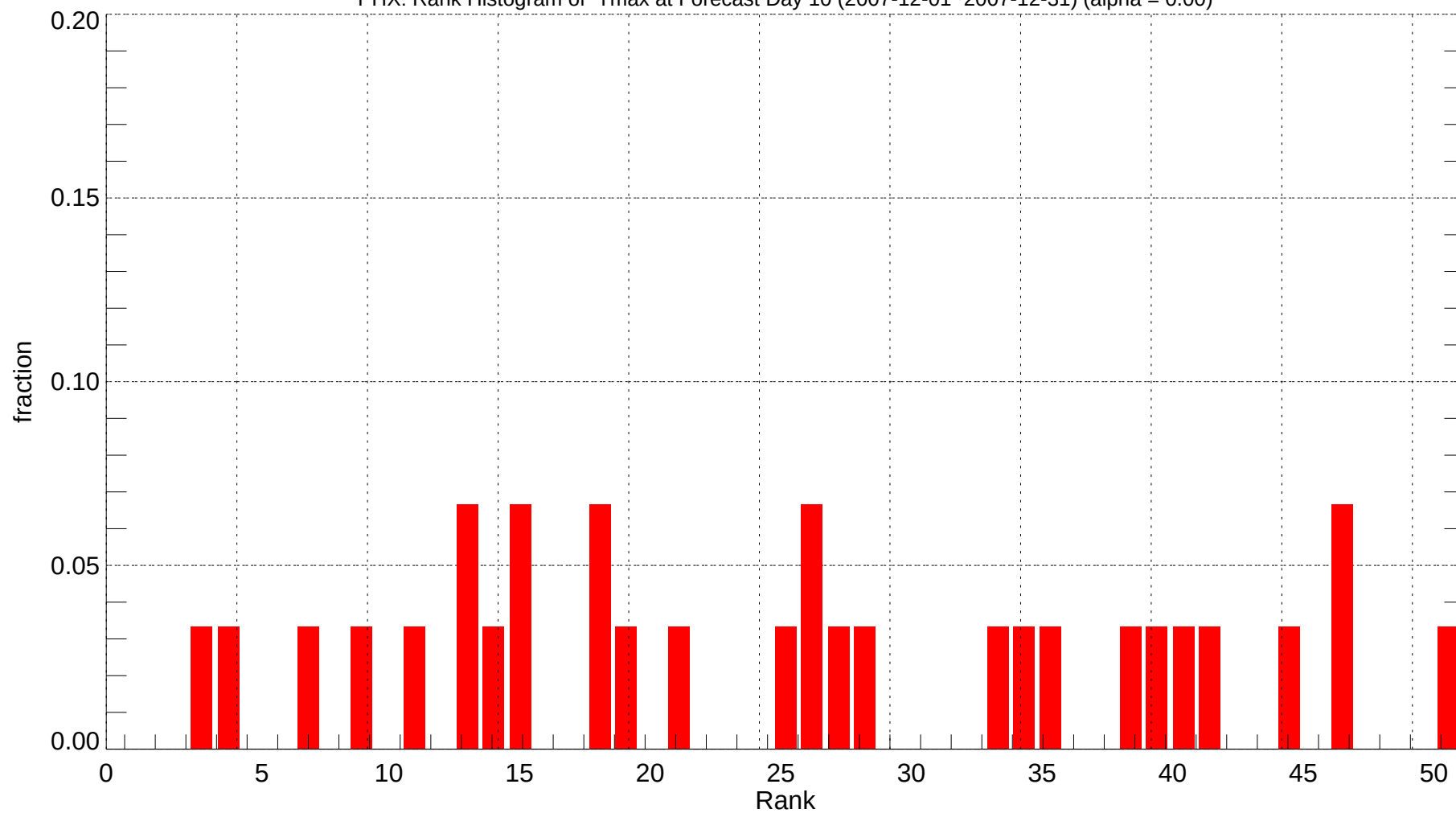
PHX: Rank Histogram of Tmax at Forecast Day 10 (2007-12-01~2007-12-31) (alpha = 0.00)
