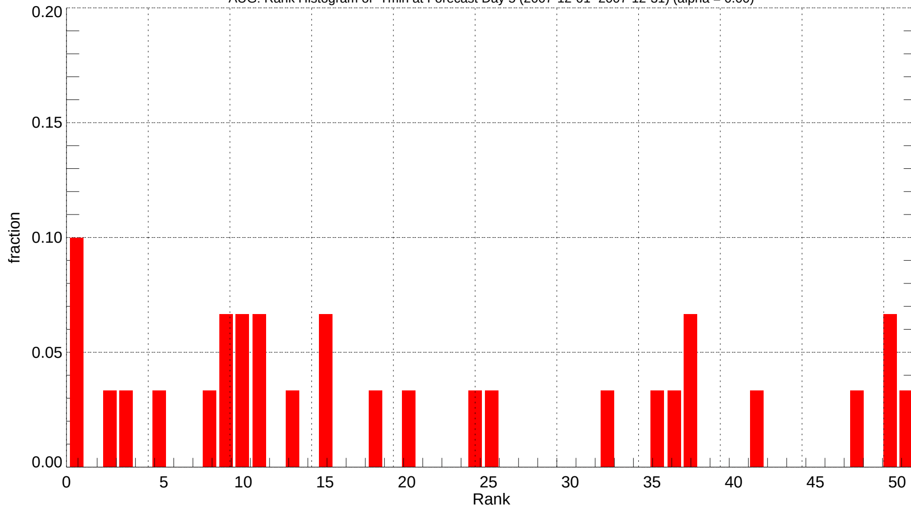
AUG: Rank Histogram of Tmin at Forecast Day 5 (2007-12-01~2007-12-31) (alpha = 0.00)
