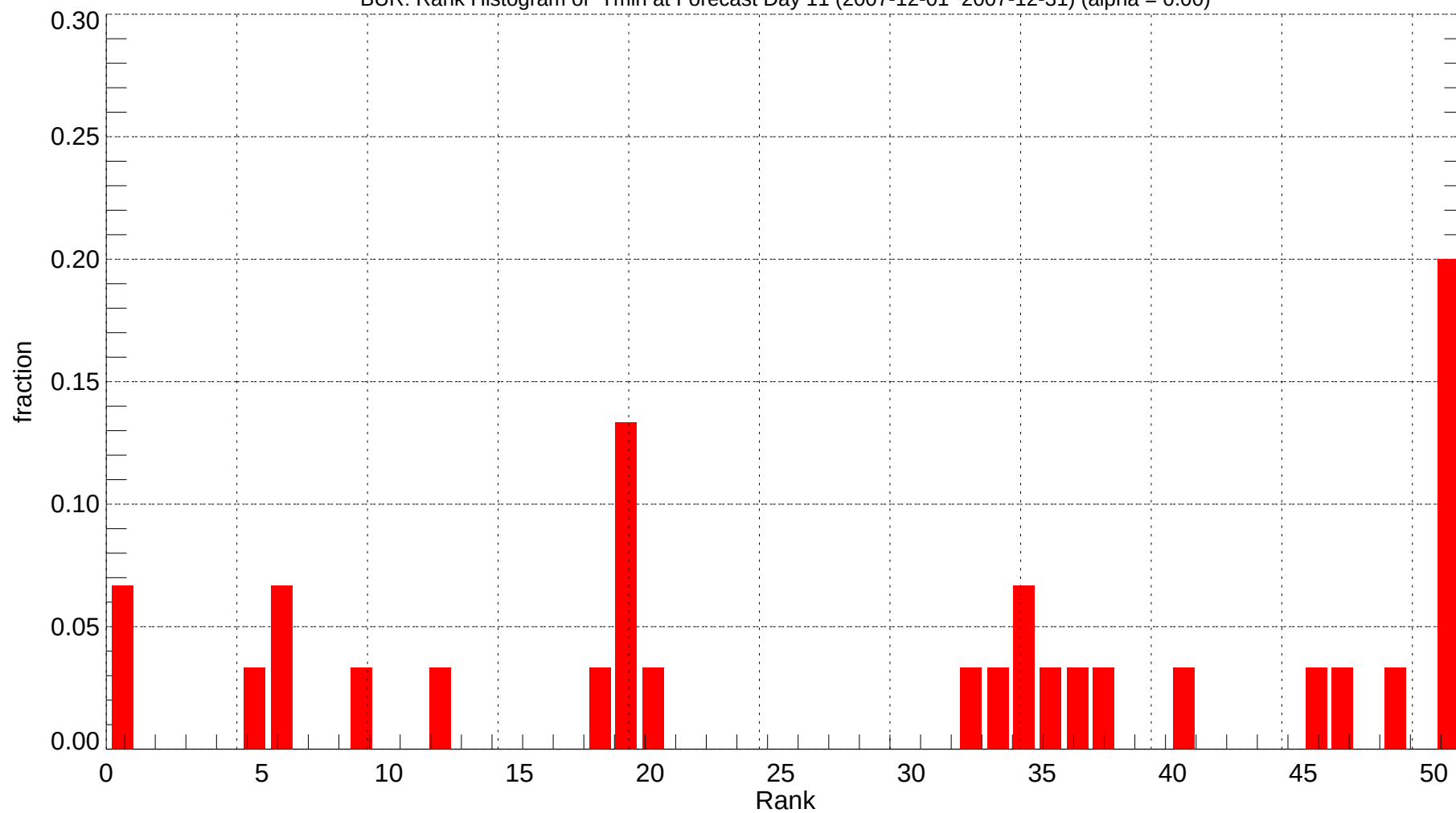
BUR: Rank Histogram of Tmin at Forecast Day 11 (2007-12-01~2007-12-31) (alpha = 0.00)
