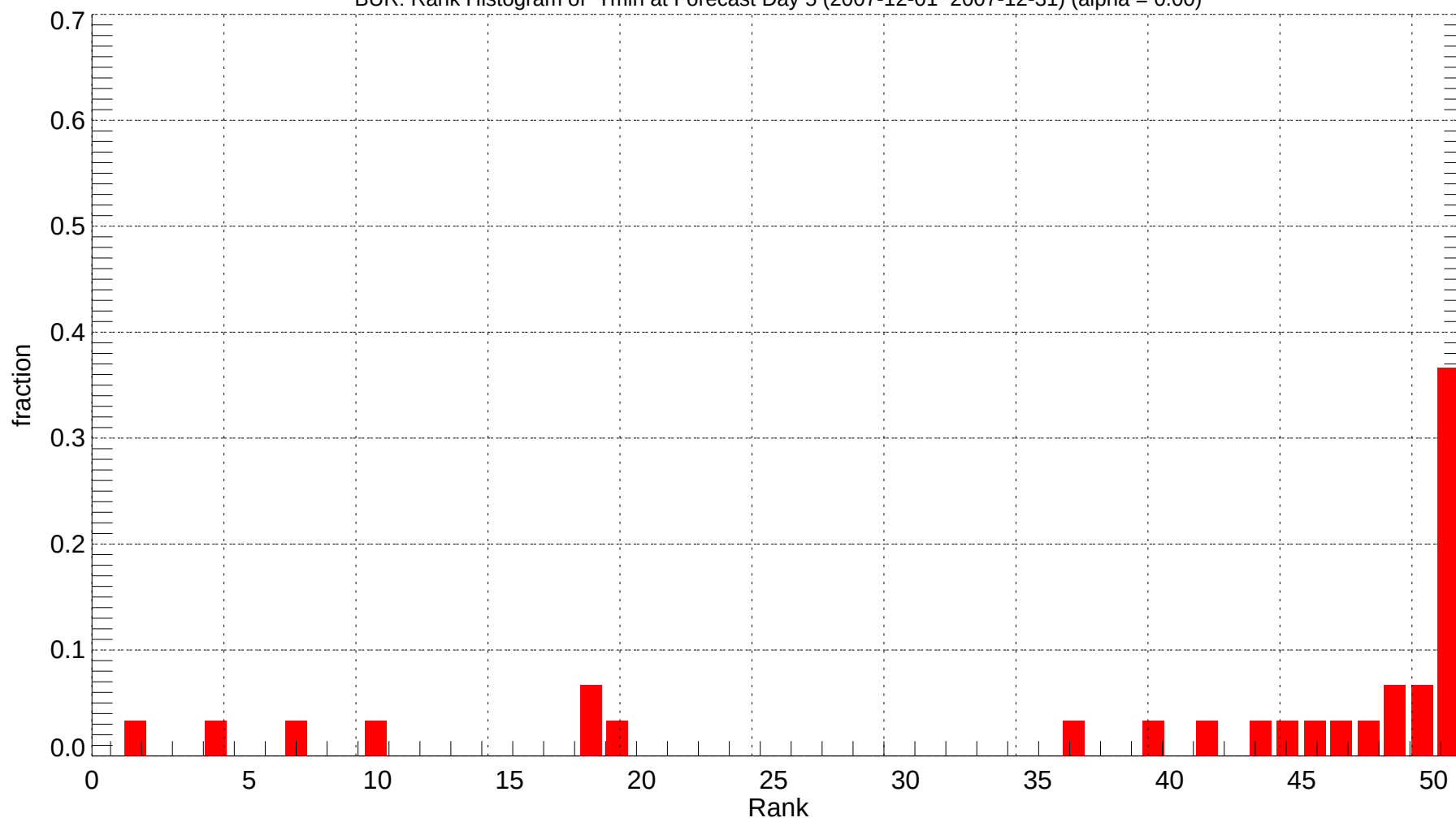
BUR: Rank Histogram of Tmin at Forecast Day 5 (2007-12-01~2007-12-31) (alpha = 0.00)
