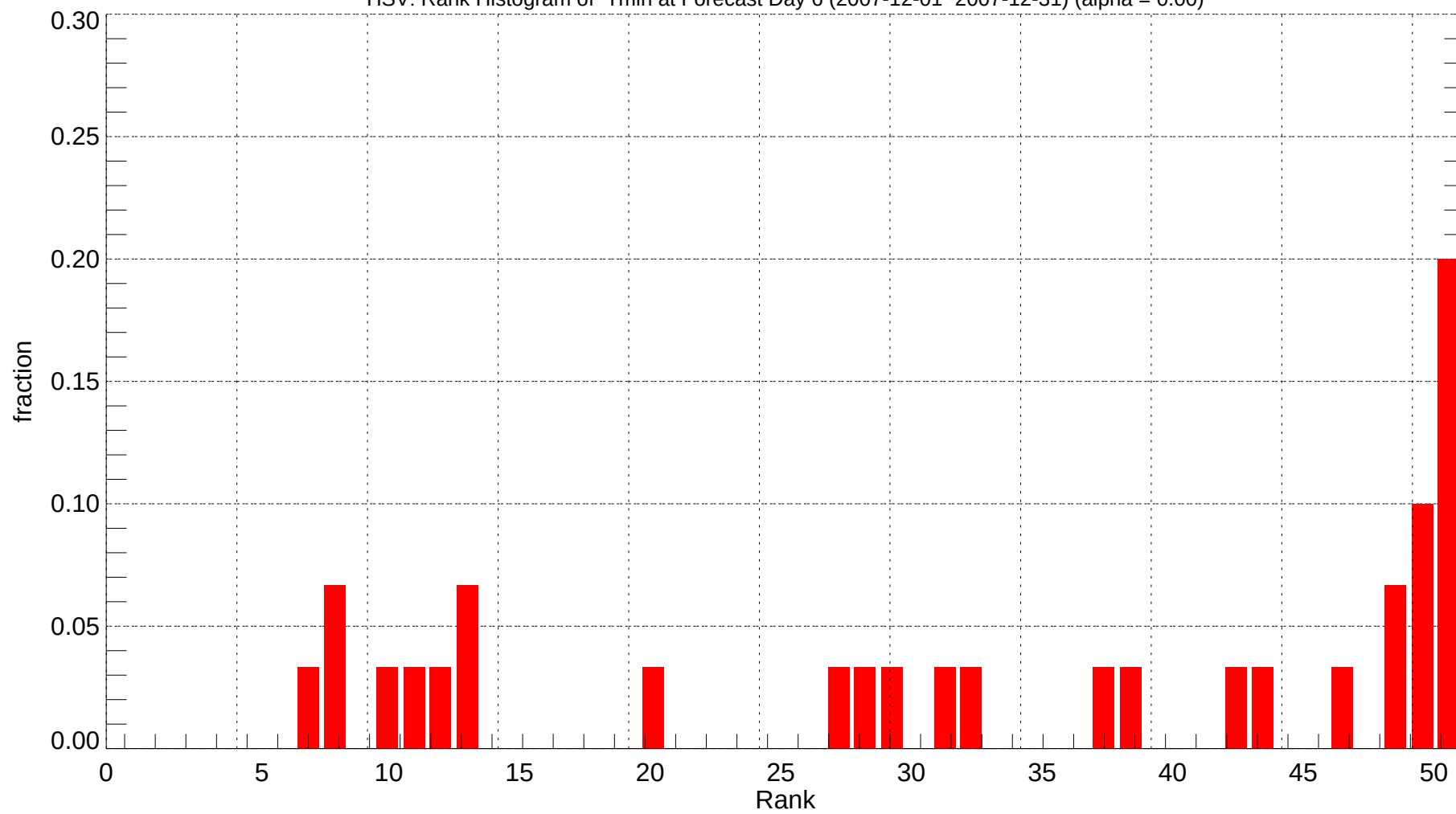
HSV: Rank Histogram of Tmin at Forecast Day 6 (2007-12-01~2007-12-31) (alpha = 0.00)
