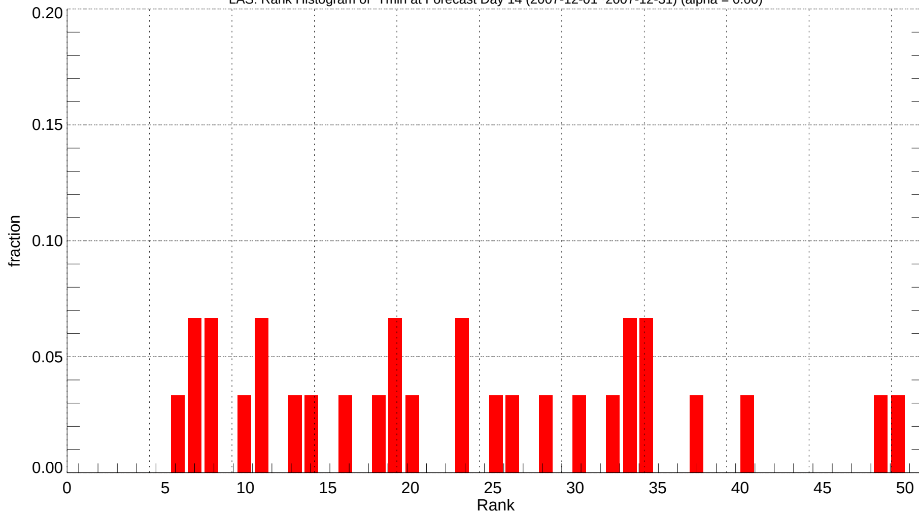
LAS: Rank Histogram of Tmin at Forecast Day 14 (2007-12-01~2007-12-31) (alpha = 0.00)
