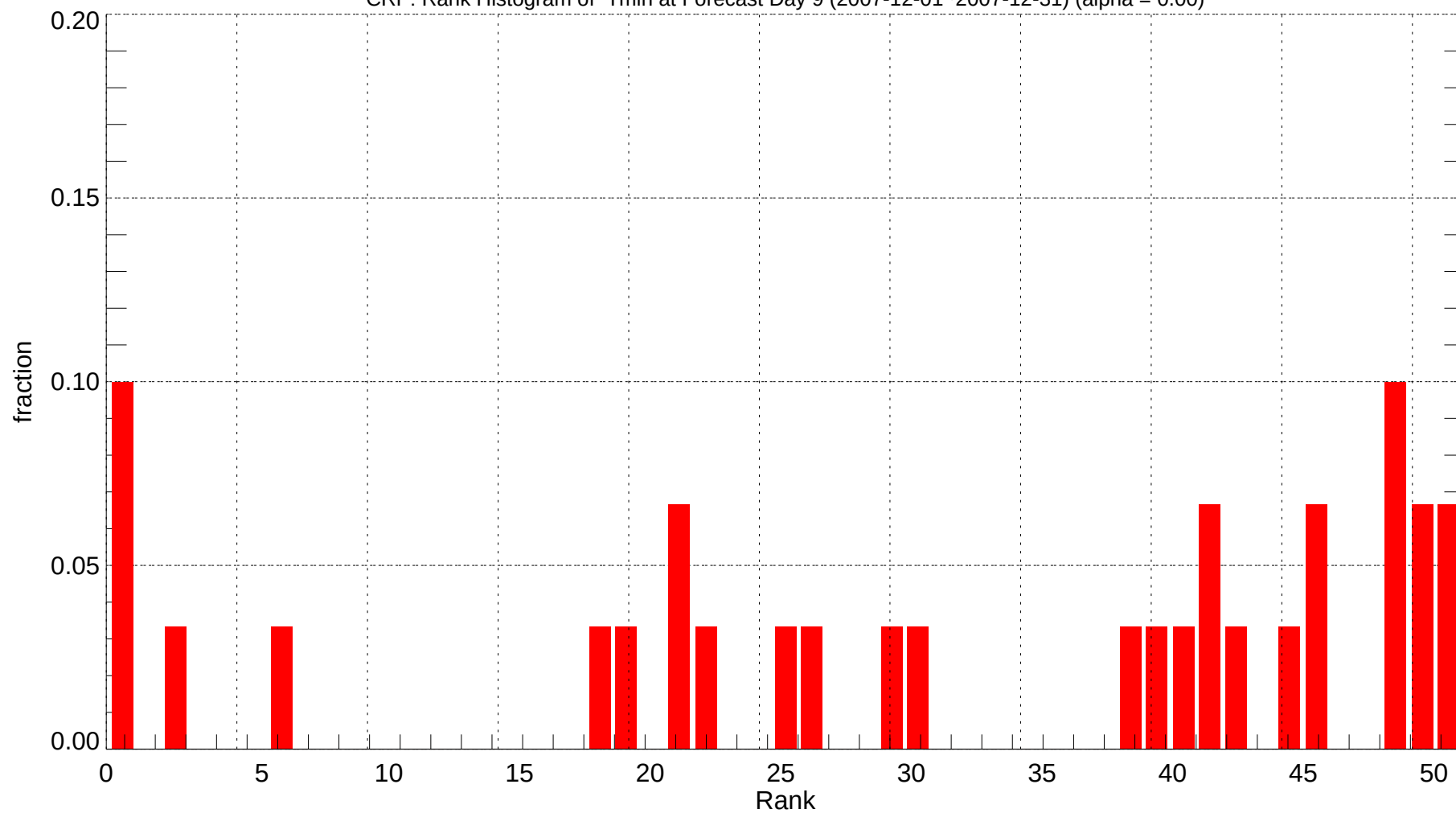
CRP: Rank Histogram of Tmin at Forecast Day 9 (2007-12-01~2007-12-31) (alpha = 0.00)
