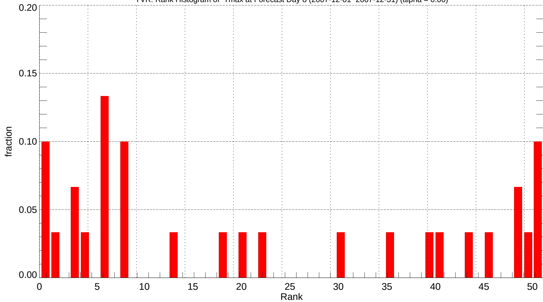
YVR: Rank Histogram of Tmax at Forecast Day 8 (2007-12-01~2007-12-31) (alpha = 0.00)
