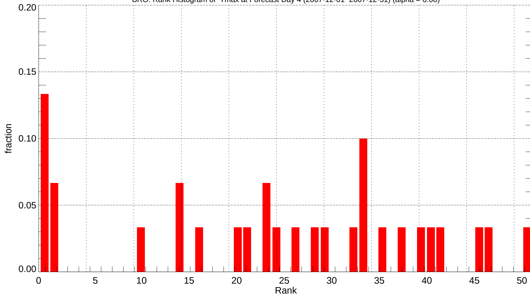
BRO: Rank Histogram of Tmax at Forecast Day 4 (2007-12-01~2007-12-31) (alpha = 0.00)
