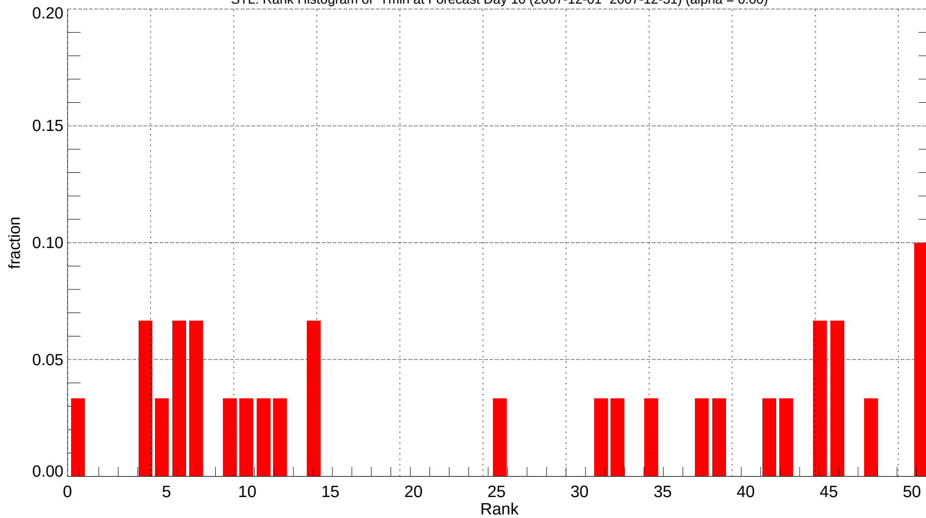
STL: Rank Histogram of Tmin at Forecast Day 10 (2007-12-01~2007-12-31) (alpha = 0.00)
