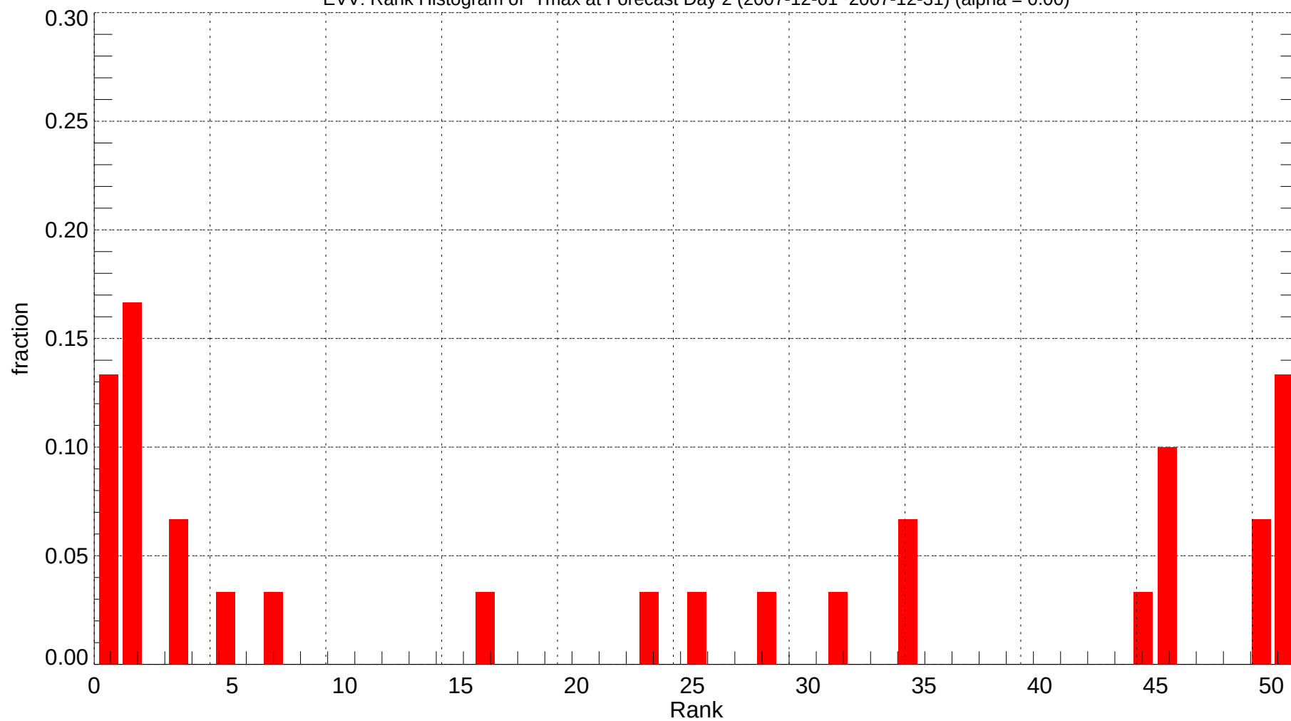
EVV: Rank Histogram of Tmax at Forecast Day 2 (2007-12-01~2007-12-31) (alpha = 0.00)
