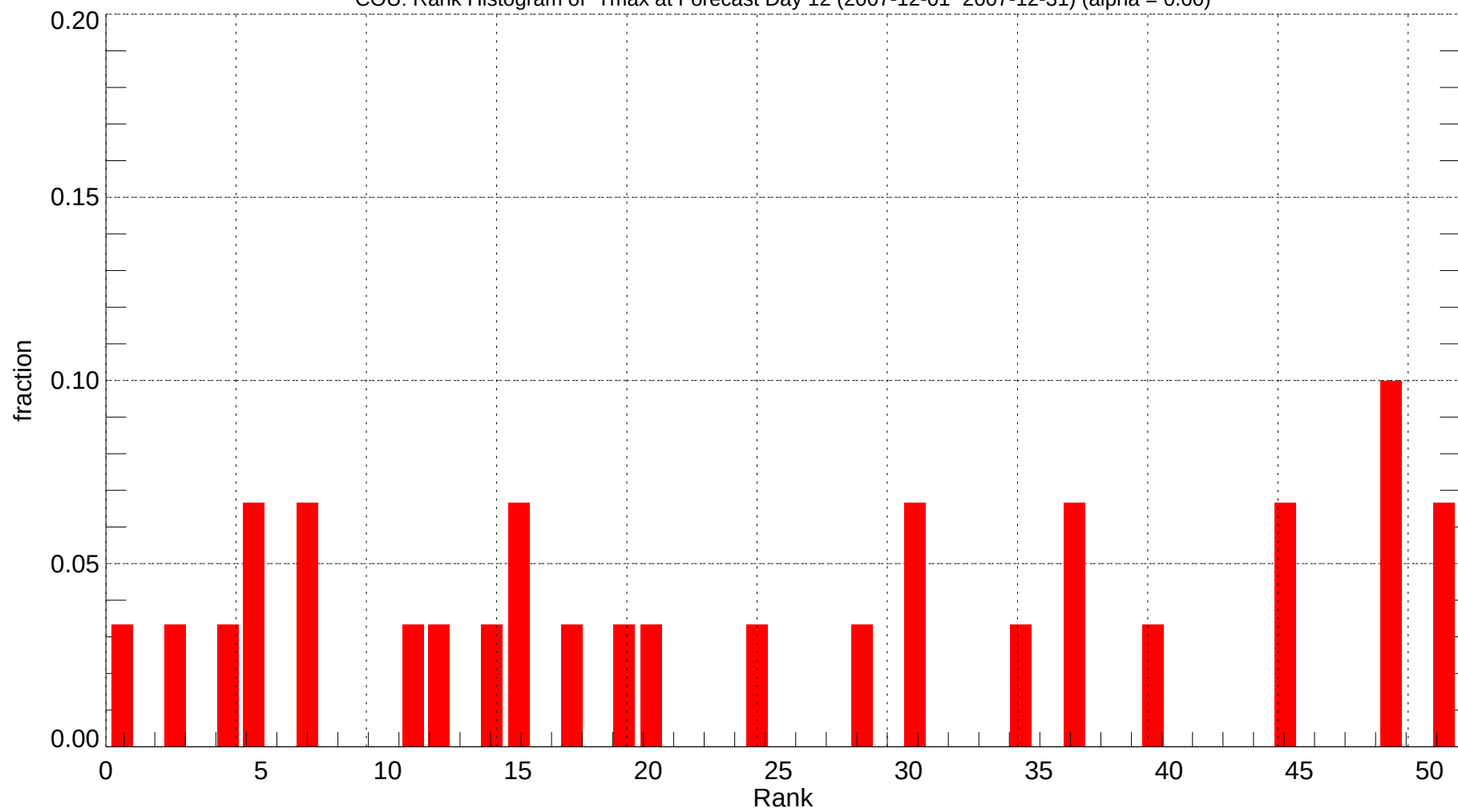
COU: Rank Histogram of Tmax at Forecast Day 12 (2007-12-01~2007-12-31) (alpha = 0.00)
