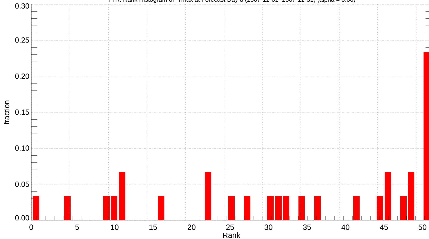
TYR: Rank Histogram of Tmax at Forecast Day 8 (2007-12-01~2007-12-31) (alpha = 0.00)
