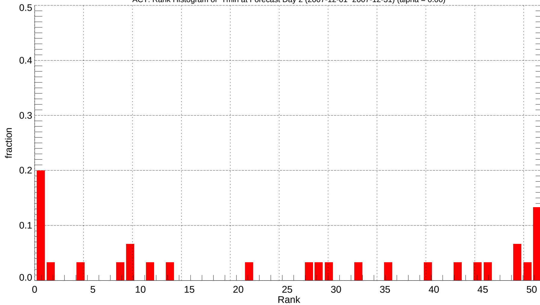
ACT: Rank Histogram of Tmin at Forecast Day 2 (2007-12-01~2007-12-31) (alpha = 0.00)
