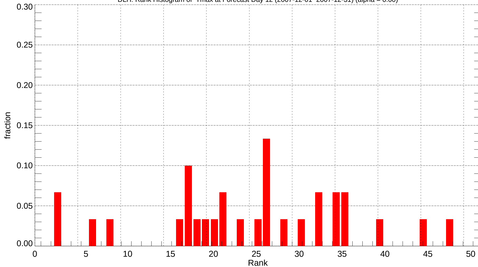
DLH: Rank Histogram of Tmax at Forecast Day 12 (2007-12-01~2007-12-31) (alpha = 0.00)
