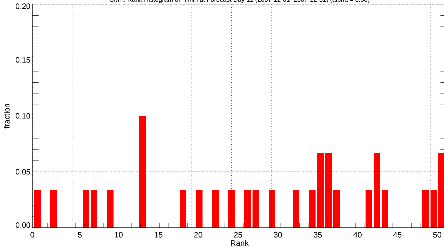
CMH: Rank Histogram of Tmin at Forecast Day 11 (2007-12-01~2007-12-31) (alpha = 0.00)
