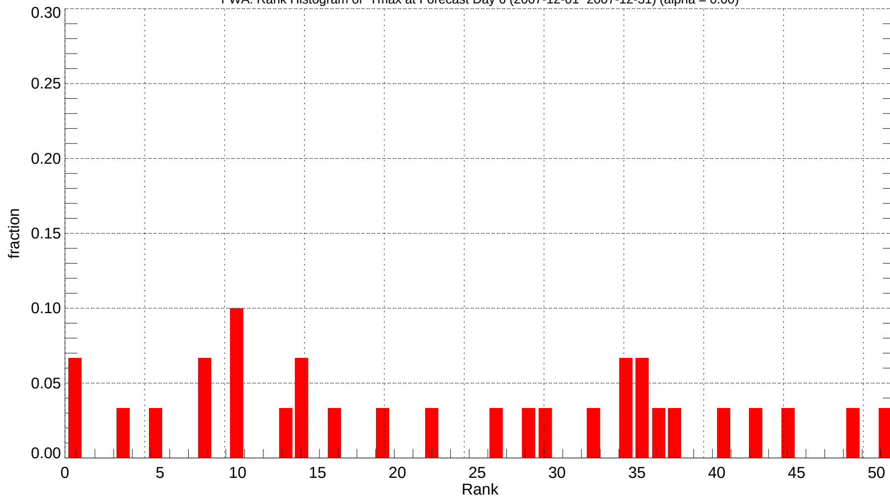
FWA: Rank Histogram of Tmax at Forecast Day 6 (2007-12-01~2007-12-31) (alpha = 0.00)
