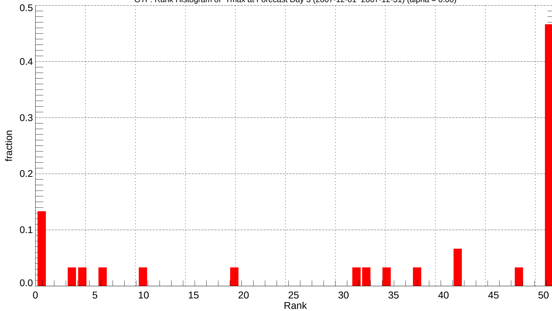
GTF: Rank Histogram of Tmax at Forecast Day 3 (2007-12-01~2007-12-31) (alpha = 0.00)
