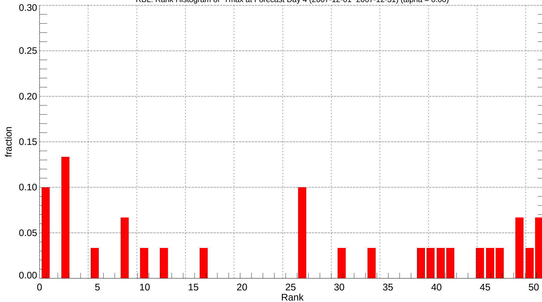
RBL: Rank Histogram of Tmax at Forecast Day 4 (2007-12-01~2007-12-31) (alpha = 0.00)
