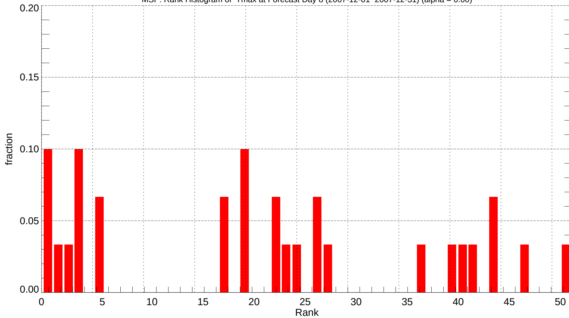
MSP: Rank Histogram of Tmax at Forecast Day 8 (2007-12-01~2007-12-31) (alpha = 0.00)
