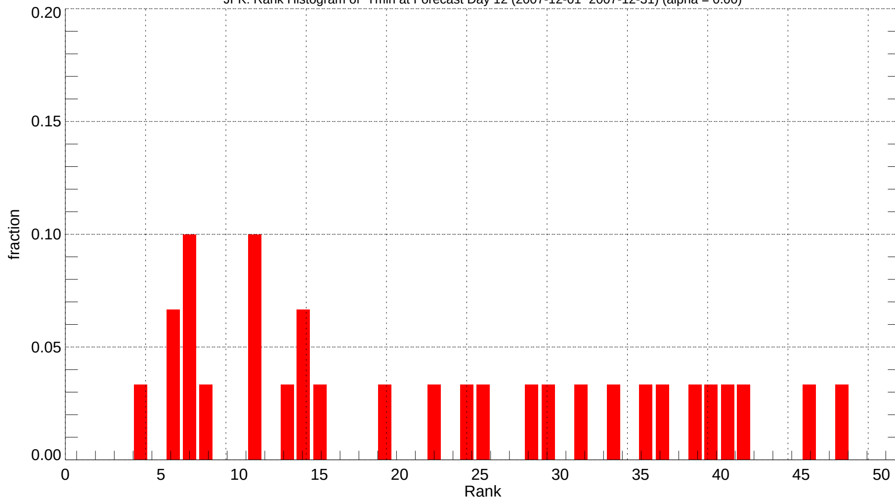
JFK: Rank Histogram of Tmin at Forecast Day 12 (2007-12-01~2007-12-31) (alpha = 0.00)
