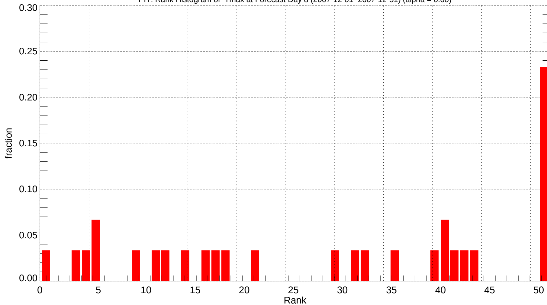
PIT: Rank Histogram of Tmax at Forecast Day 8 (2007-12-01~2007-12-31) (alpha = 0.00)
