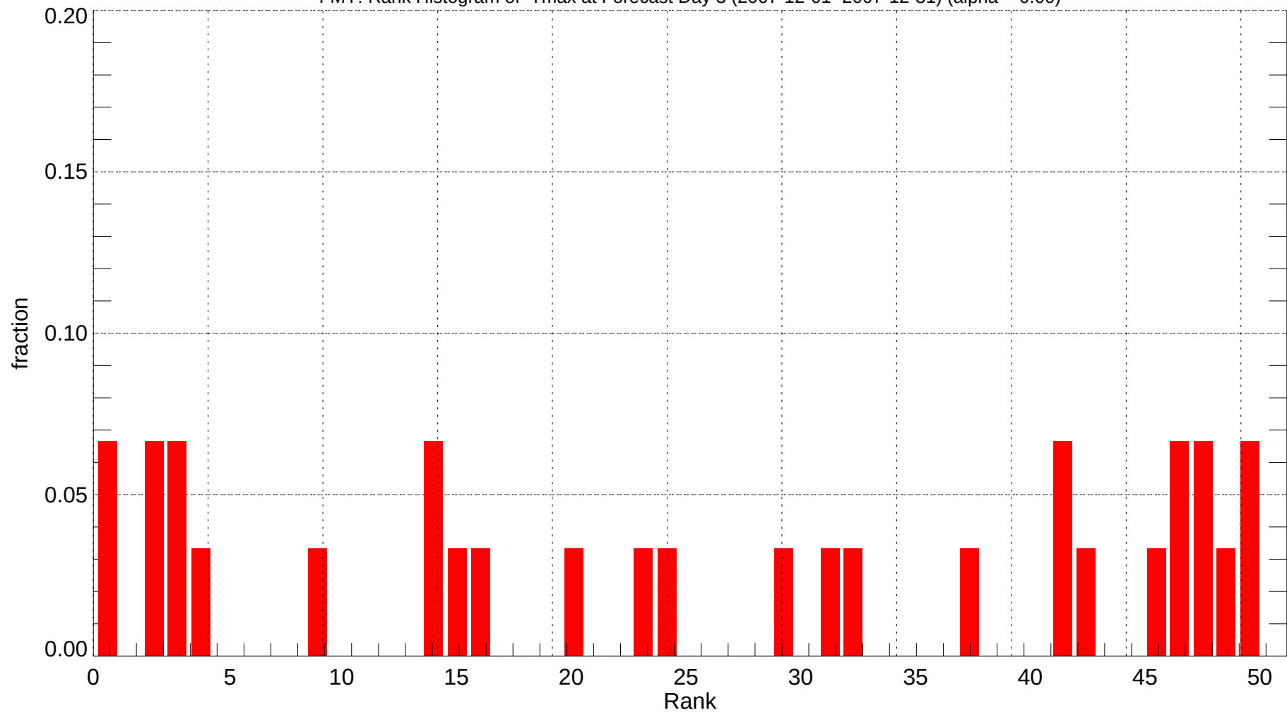
FMY: Rank Histogram of Tmax at Forecast Day 3 (2007-12-01~2007-12-31) (alpha = 0.00)
