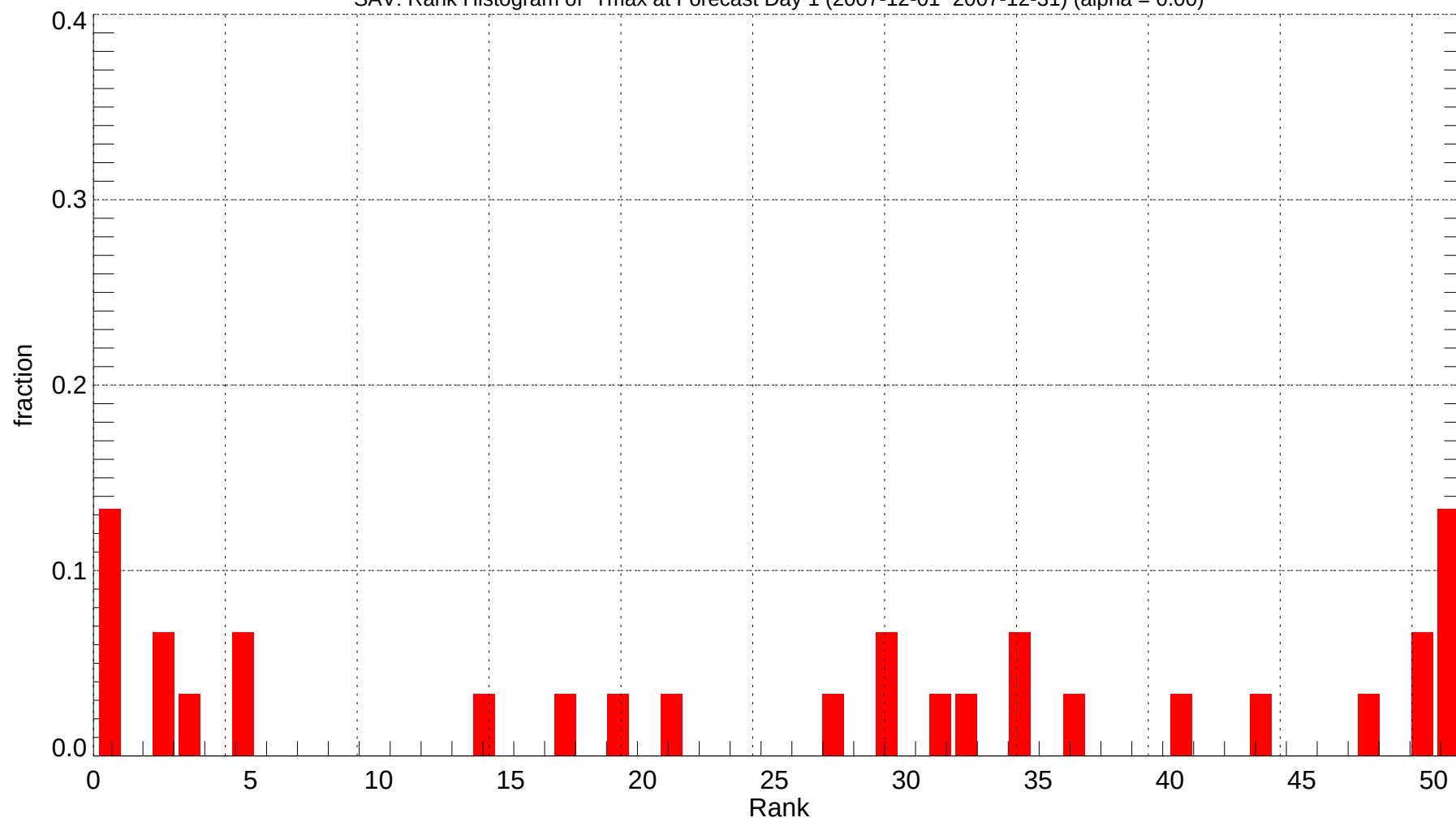
SAV: Rank Histogram of Tmax at Forecast Day 1 (2007-12-01~2007-12-31) (alpha = 0.00)
