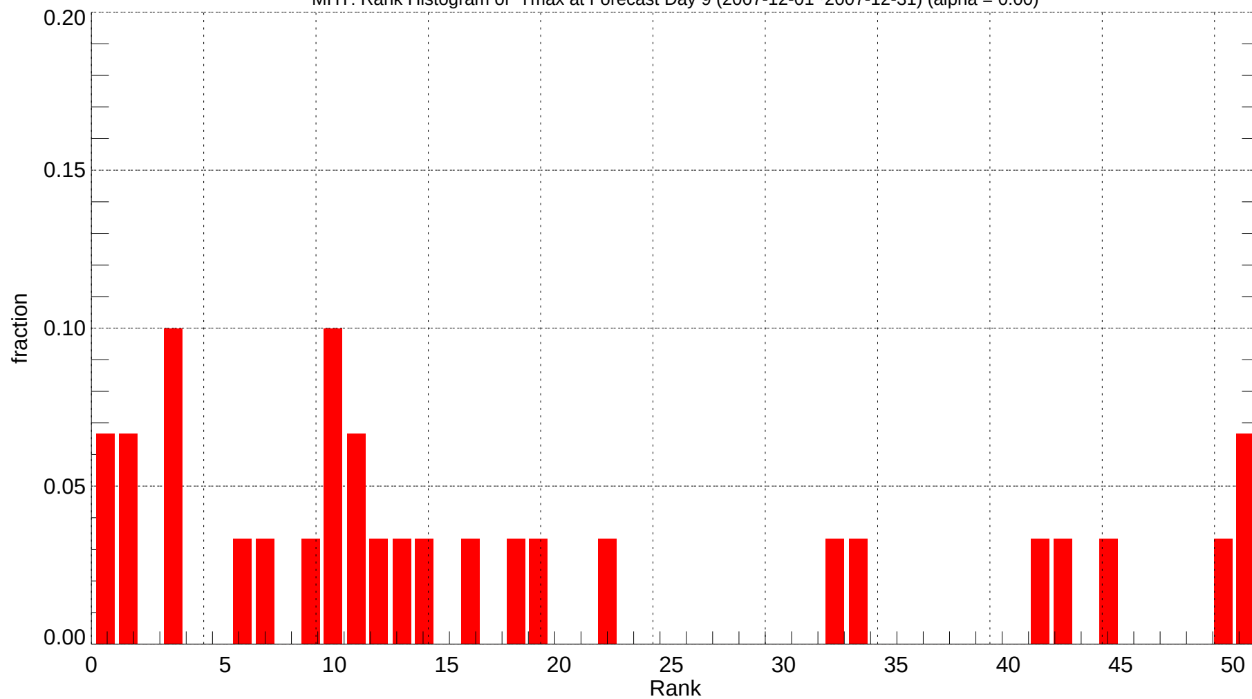
MHT: Rank Histogram of Tmax at Forecast Day 9 (2007-12-01~2007-12-31) (alpha = 0.00)
