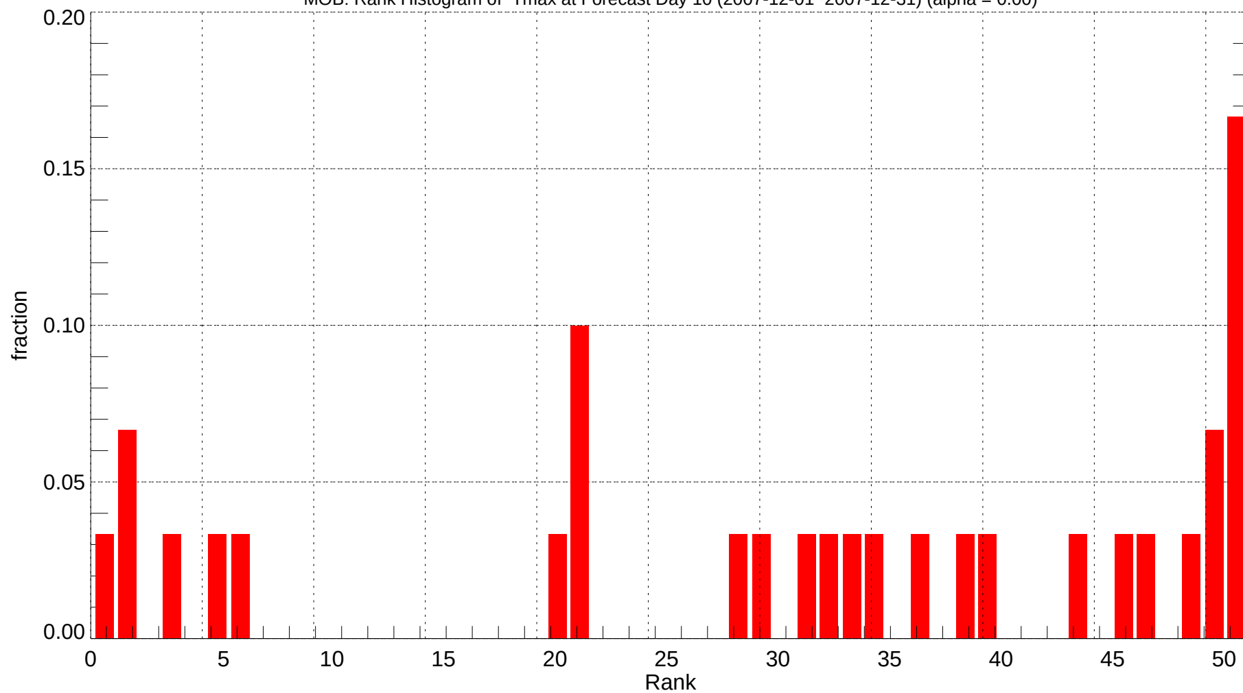
MOB: Rank Histogram of Tmax at Forecast Day 10 (2007-12-01~2007-12-31) (alpha = 0.00)
