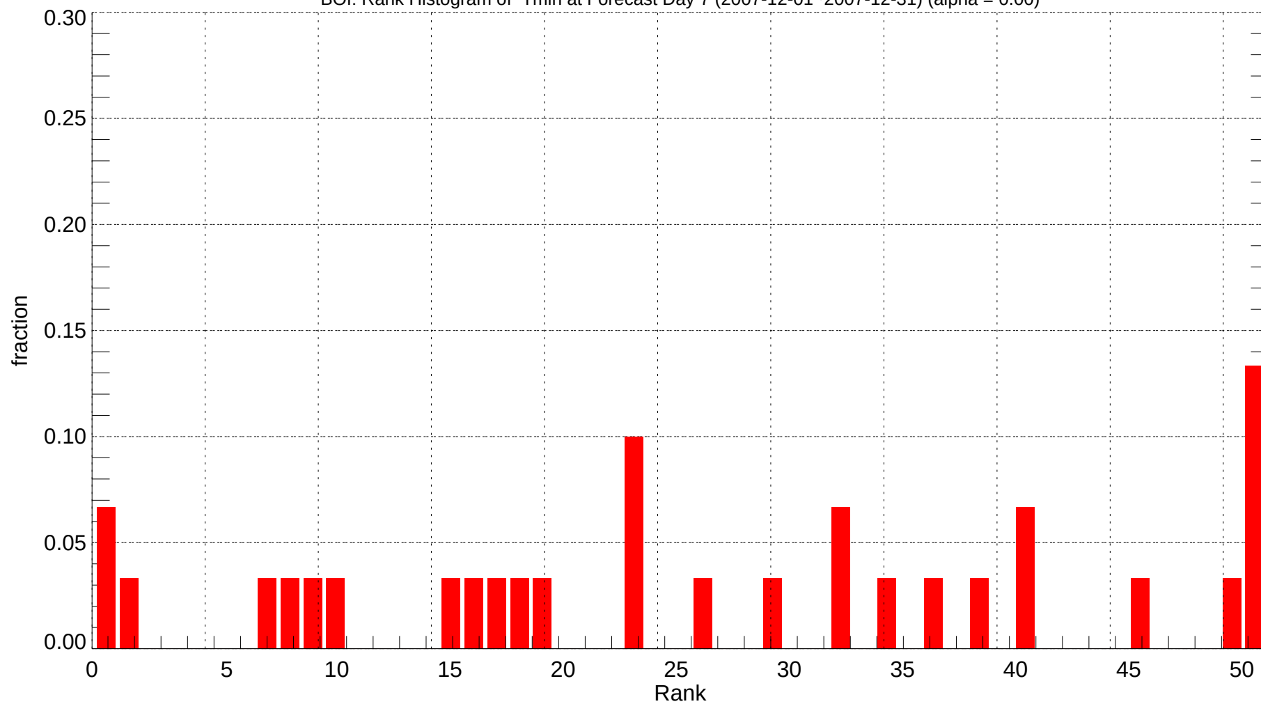
BOI: Rank Histogram of Tmin at Forecast Day 7 (2007-12-01~2007-12-31) (alpha = 0.00)
