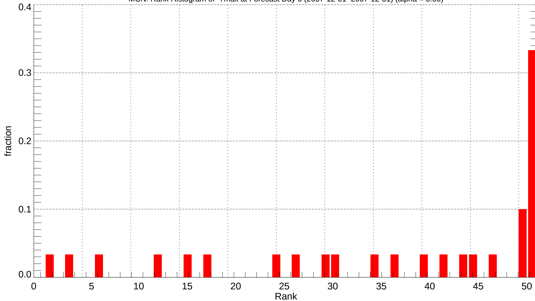
MCN: Rank Histogram of Tmax at Forecast Day 6 (2007-12-01~2007-12-31) (alpha = 0.00)
