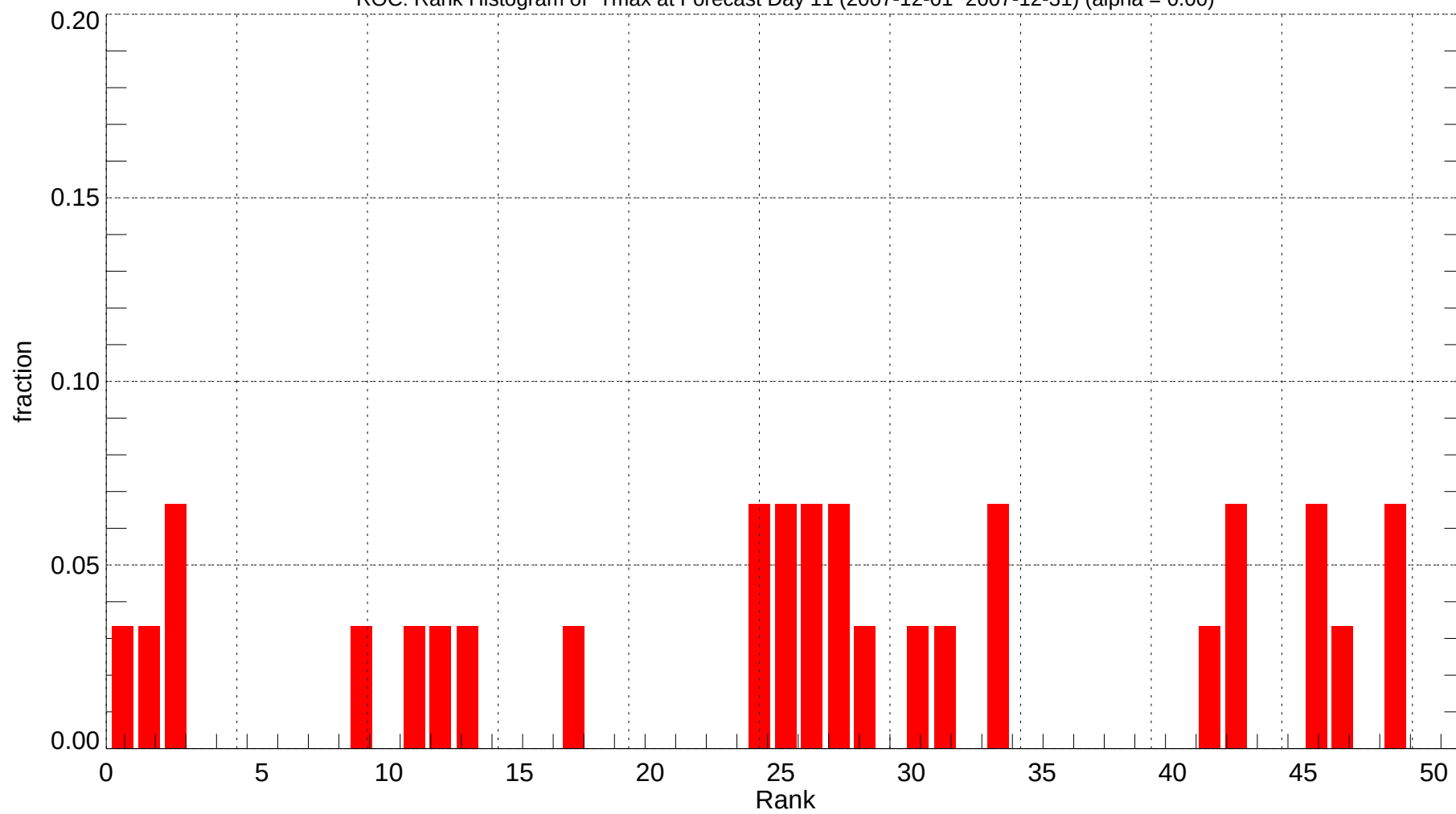
ROC: Rank Histogram of Tmax at Forecast Day 11 (2007-12-01~2007-12-31) (alpha = 0.00)
