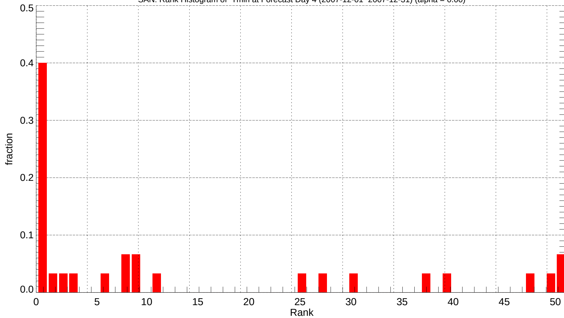
SAN: Rank Histogram of Tmin at Forecast Day 4 (2007-12-01~2007-12-31) (alpha = 0.00)
