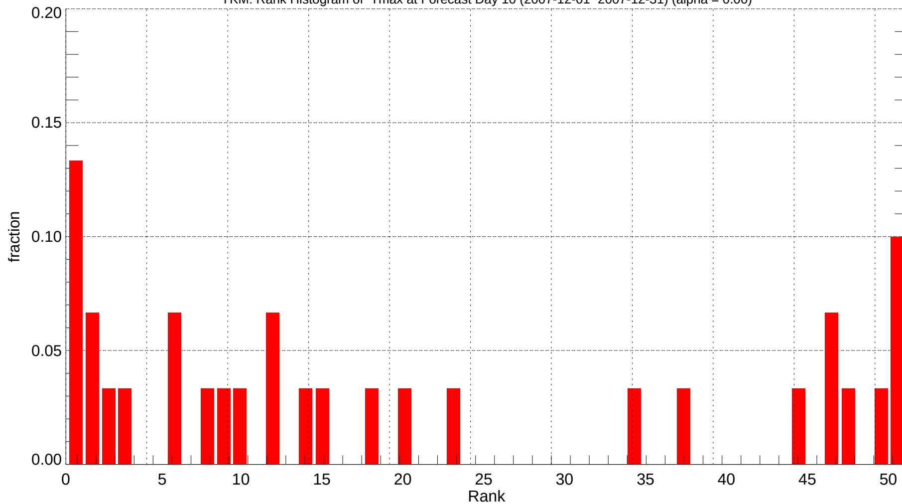
YKM: Rank Histogram of Tmax at Forecast Day 10 (2007-12-01~2007-12-31) (alpha = 0.00)
