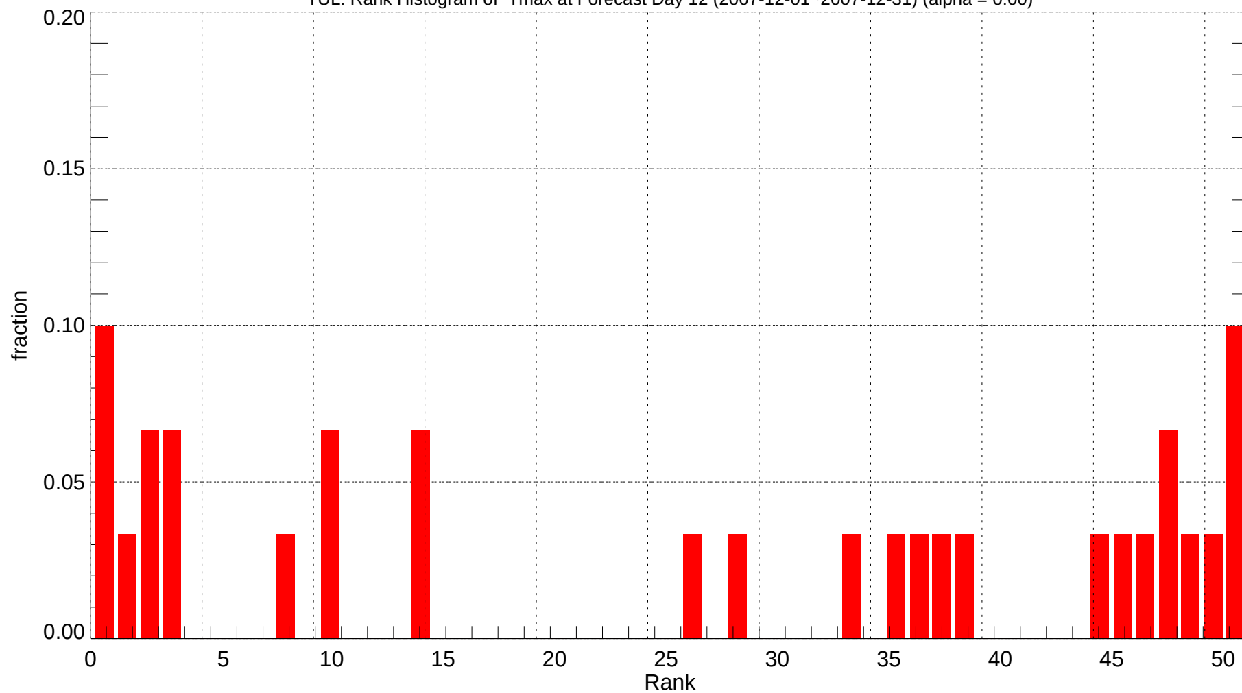
TUL: Rank Histogram of Tmax at Forecast Day 12 (2007-12-01~2007-12-31) (alpha = 0.00)
