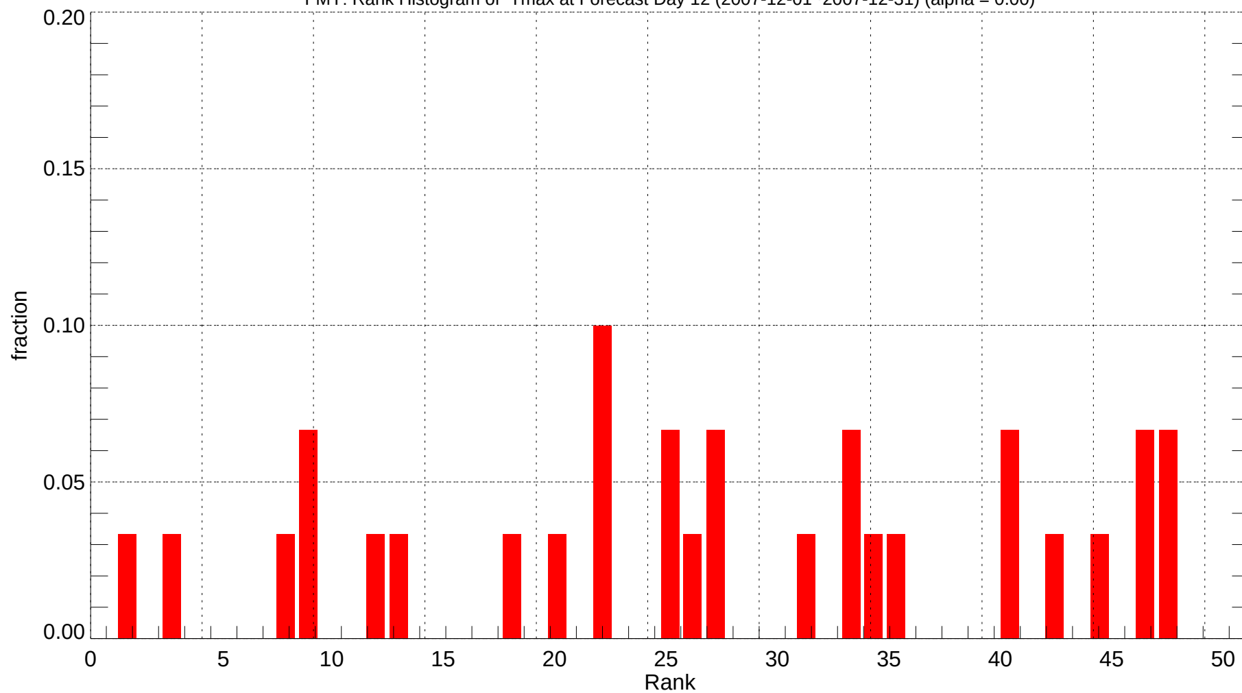
FMY: Rank Histogram of Tmax at Forecast Day 12 (2007-12-01~2007-12-31) (alpha = 0.00)
