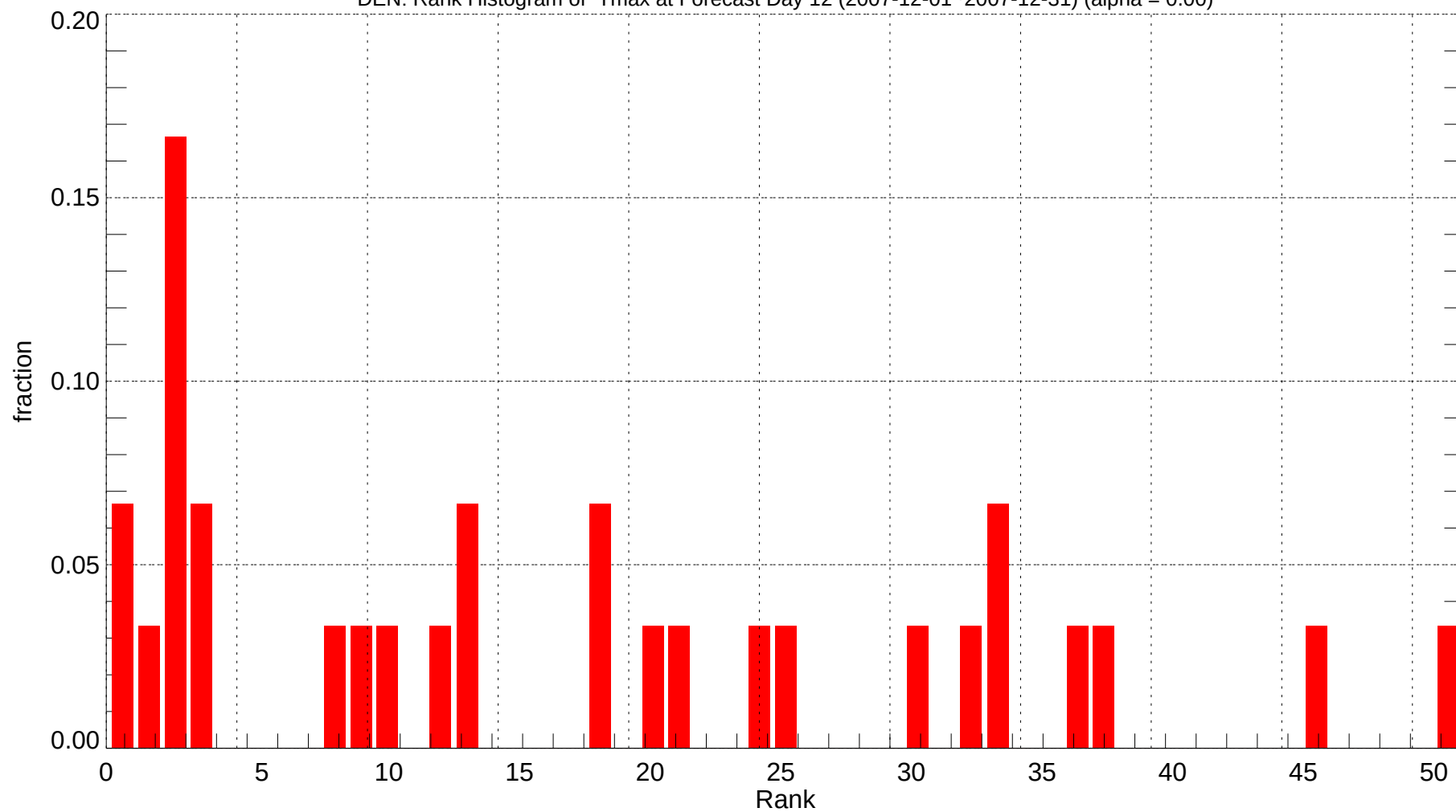
DEN: Rank Histogram of Tmax at Forecast Day 12 (2007-12-01~2007-12-31) (alpha = 0.00)
