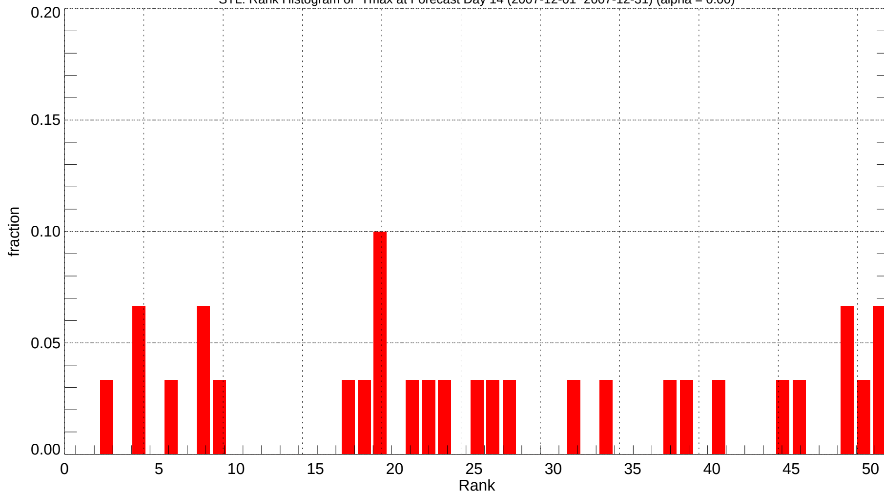
STL: Rank Histogram of Tmax at Forecast Day 14 (2007-12-01~2007-12-31) (alpha = 0.00)
