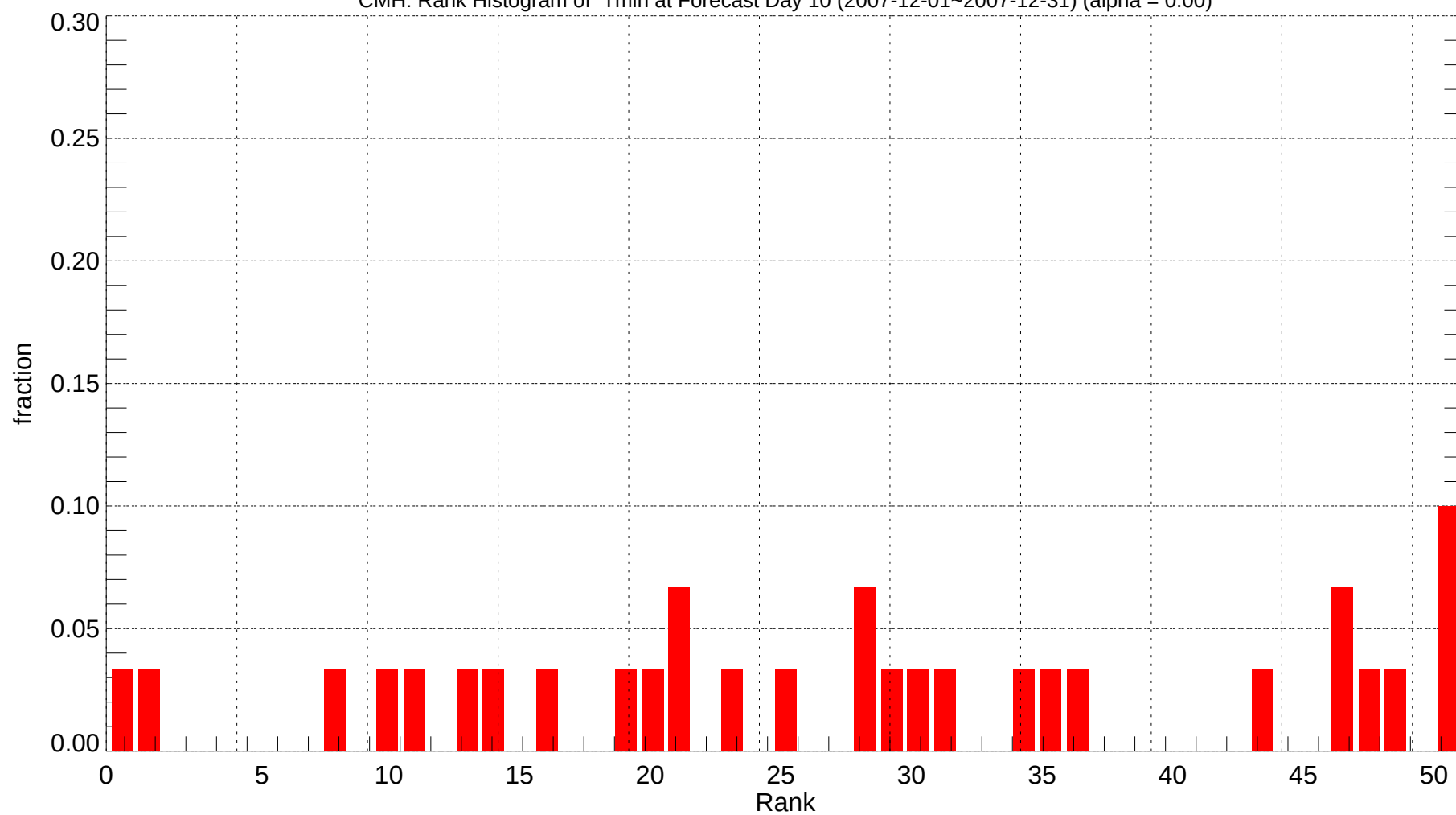
CMH: Rank Histogram of Tmin at Forecast Day 10 (2007-12-01~2007-12-31) (alpha = 0.00)
