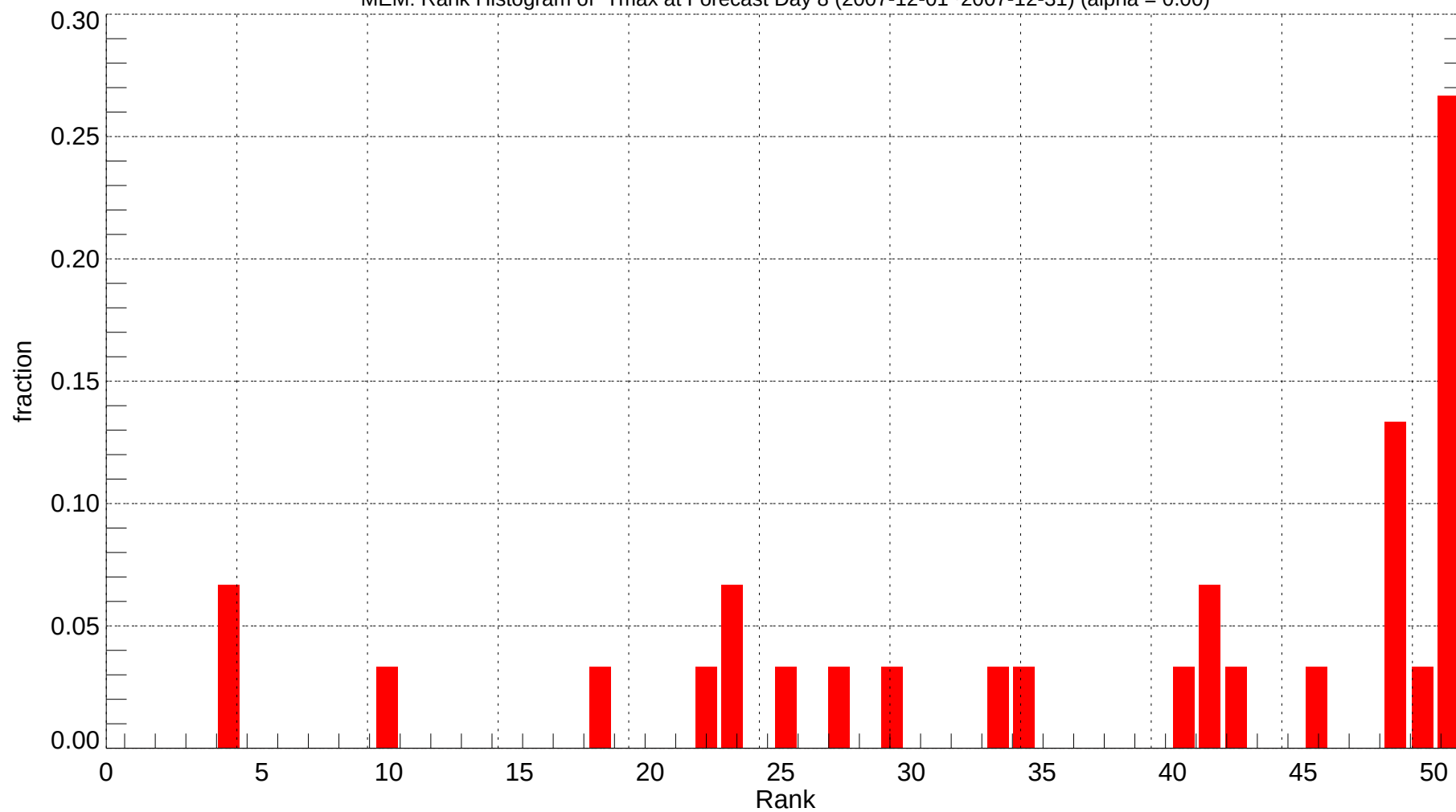
MEM: Rank Histogram of Tmax at Forecast Day 8 (2007-12-01~2007-12-31) (alpha = 0.00)
