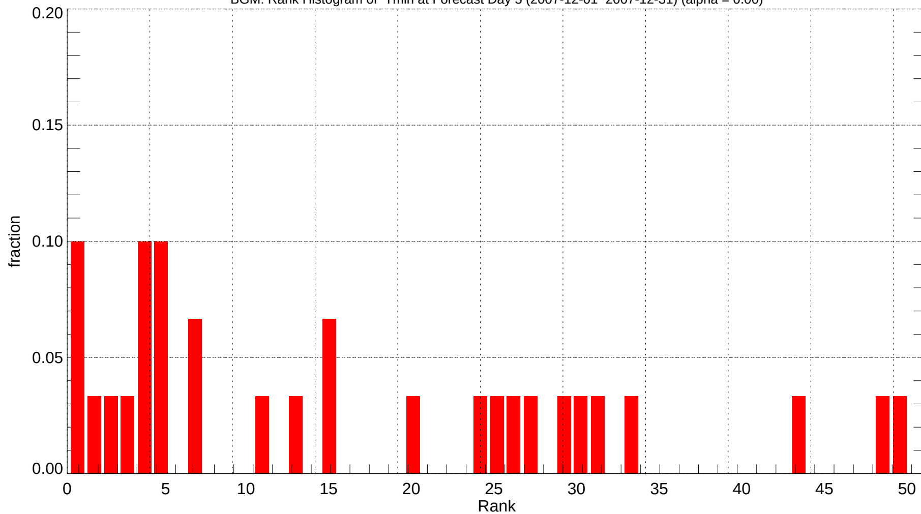
BGM: Rank Histogram of Tmin at Forecast Day 5 (2007-12-01~2007-12-31) (alpha = 0.00)
