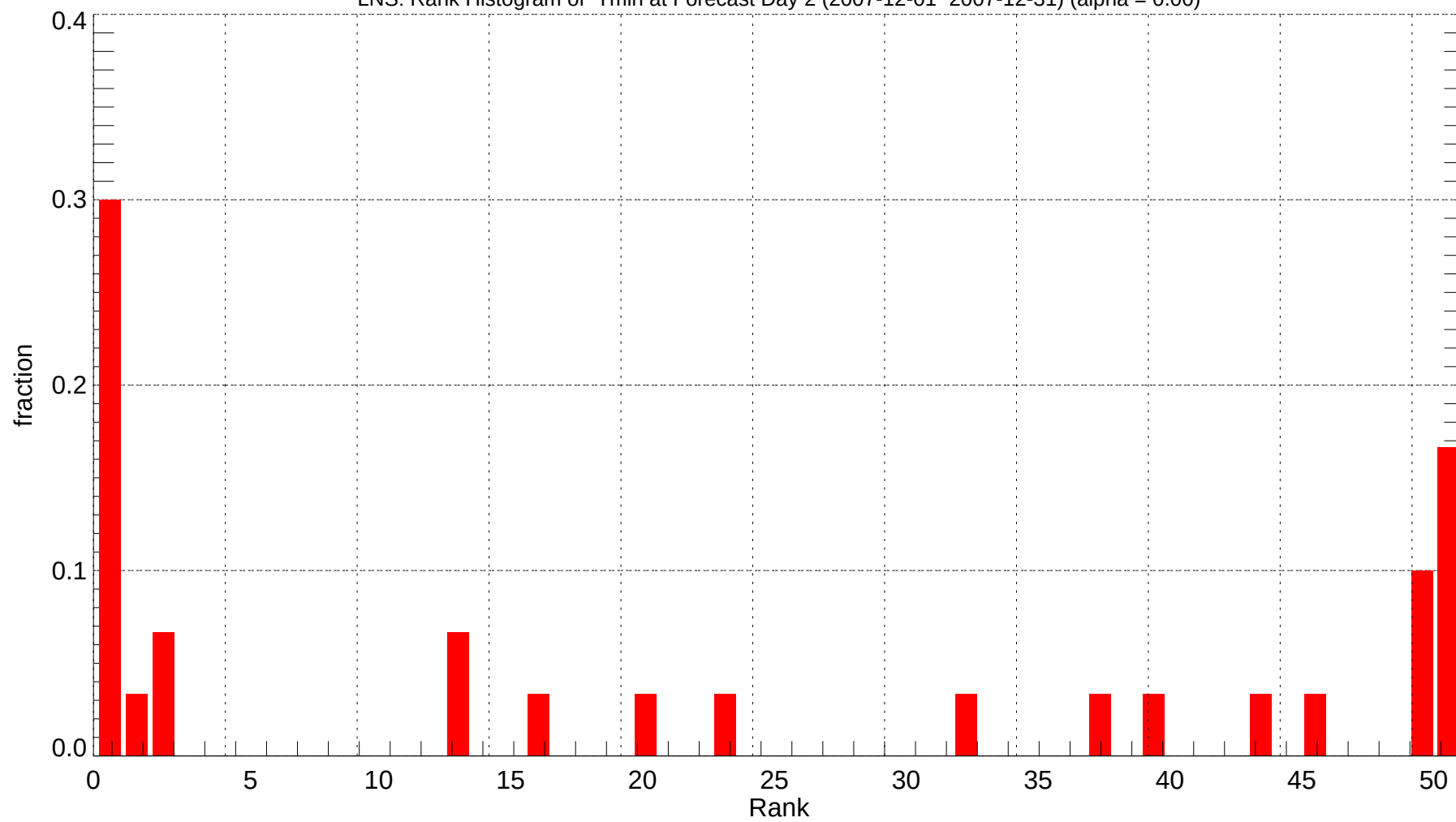
LNS: Rank Histogram of Tmin at Forecast Day 2 (2007-12-01~2007-12-31) (alpha = 0.00)
