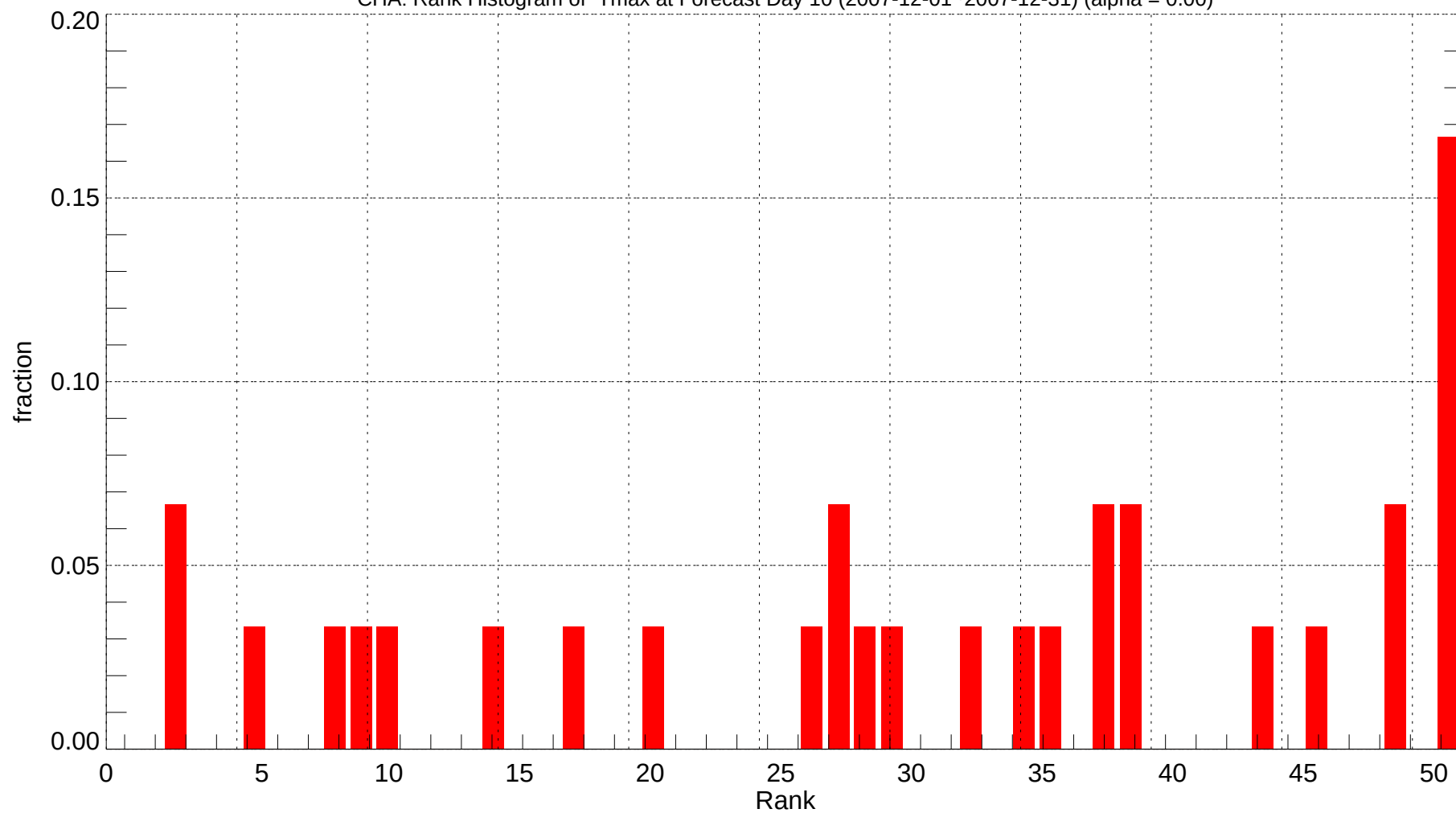
CHA: Rank Histogram of Tmax at Forecast Day 10 (2007-12-01~2007-12-31) (alpha = 0.00)
