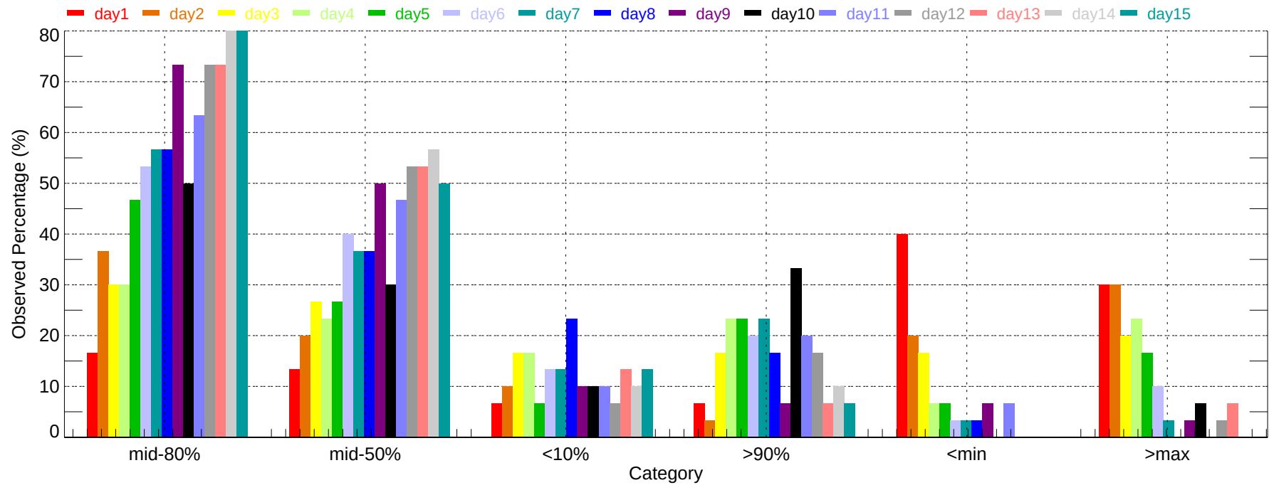
Observed Percentage of Ensembles - PIR: Max Temperature (2007-12-01~2007-12-31)
