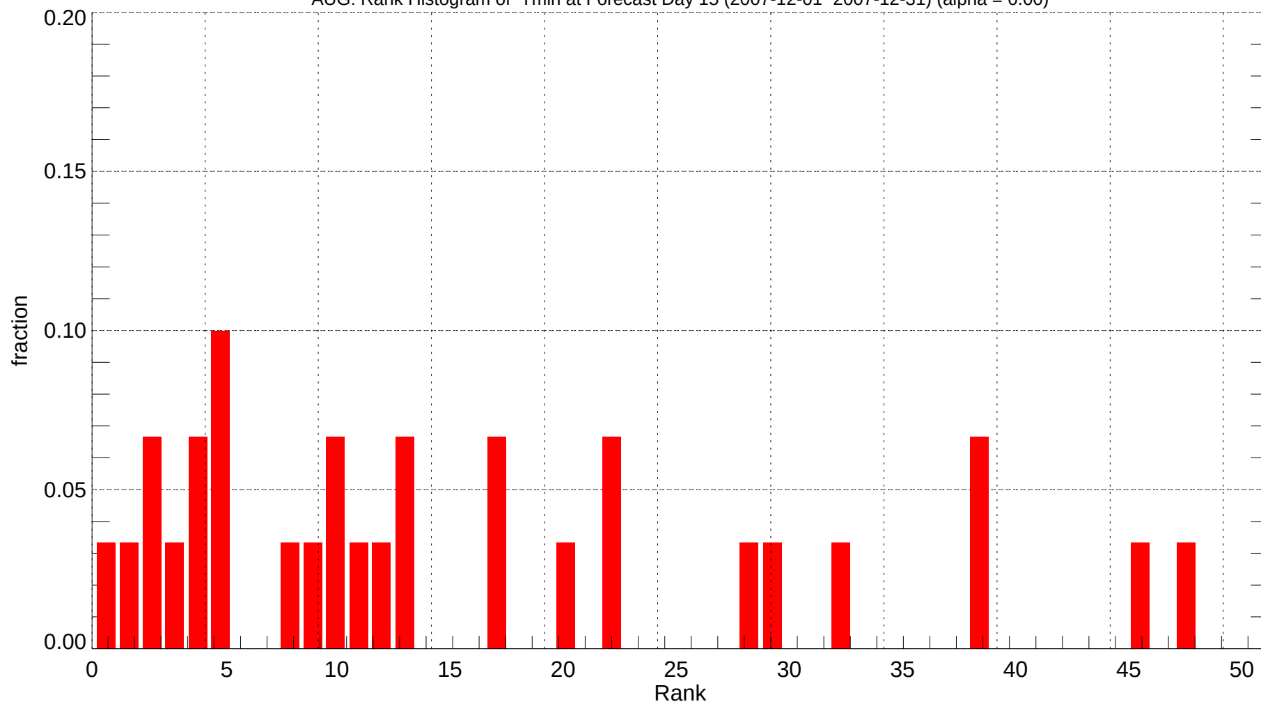
AUG: Rank Histogram of Tmin at Forecast Day 15 (2007-12-01~2007-12-31) (alpha = 0.00)
