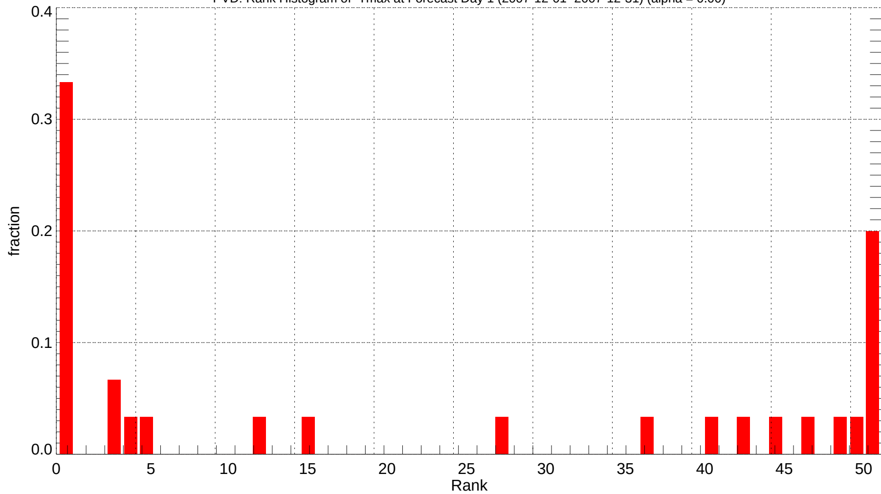
PVD: Rank Histogram of Tmax at Forecast Day 1 (2007-12-01~2007-12-31) (alpha = 0.00)
