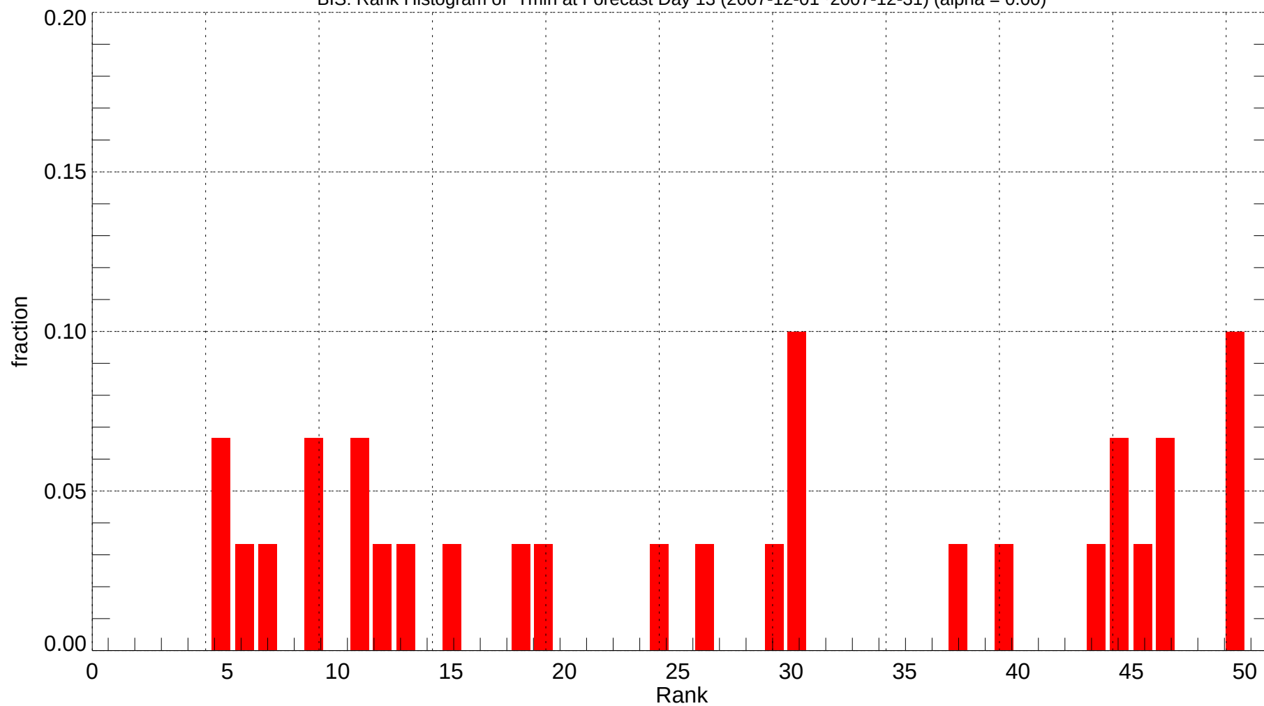
BIS: Rank Histogram of Tmin at Forecast Day 13 (2007-12-01~2007-12-31) (alpha = 0.00)
