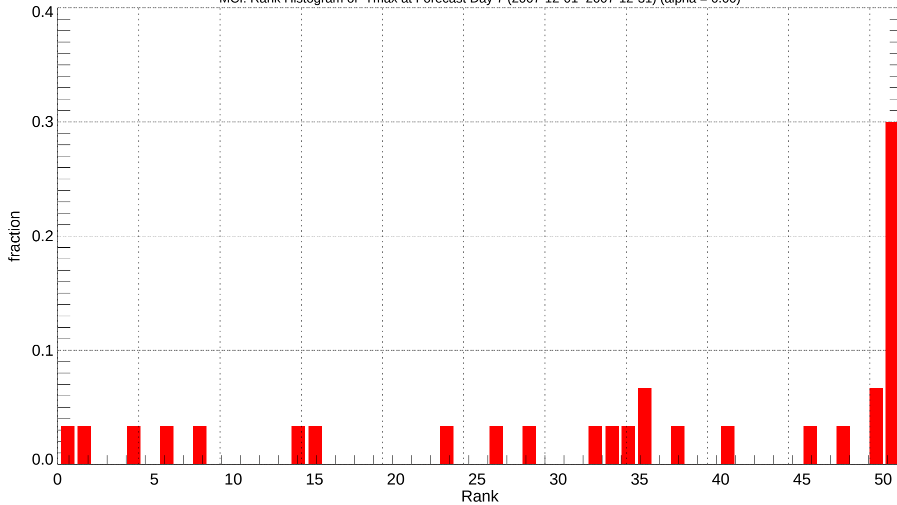
MCI: Rank Histogram of Tmax at Forecast Day 7 (2007-12-01~2007-12-31) (alpha = 0.00)
