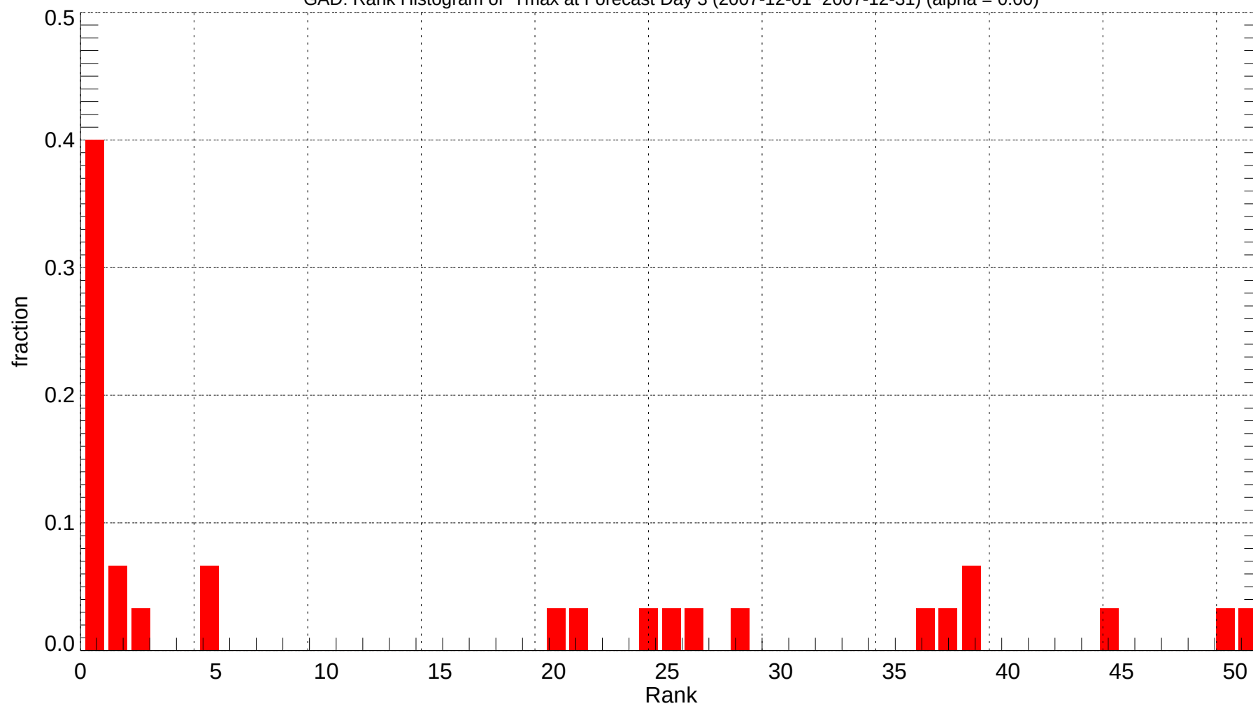
GAD: Rank Histogram of Tmax at Forecast Day 3 (2007-12-01~2007-12-31) (alpha = 0.00)
