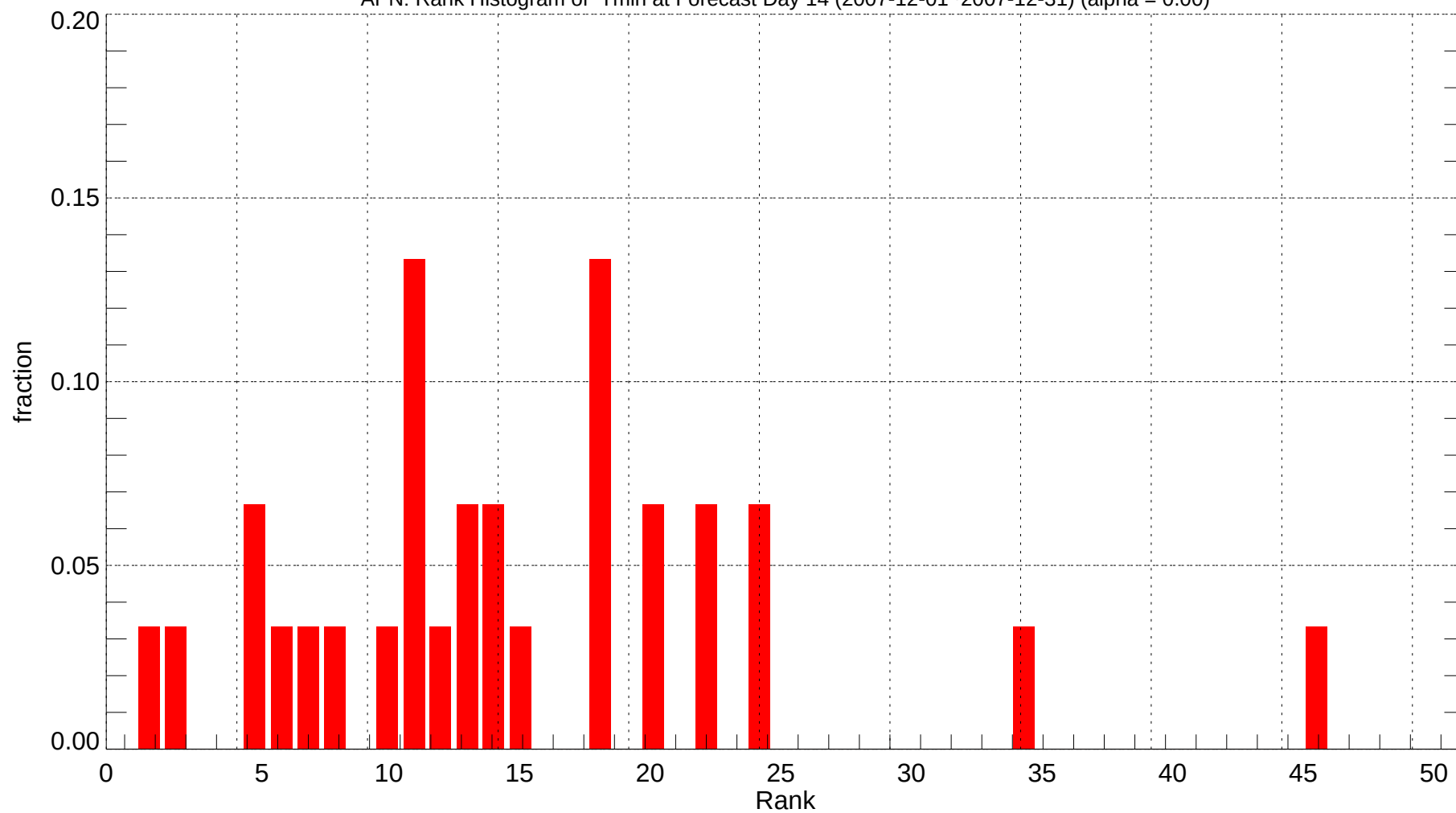
APN: Rank Histogram of Tmin at Forecast Day 14 (2007-12-01~2007-12-31) (alpha = 0.00)
