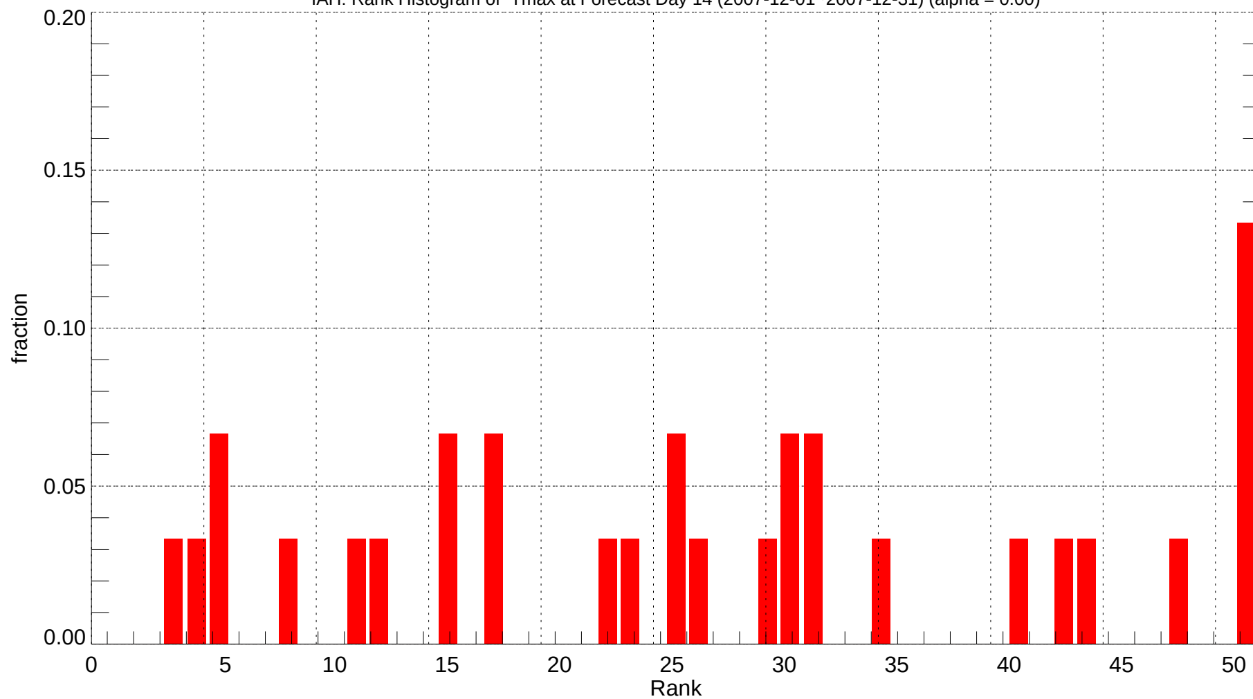
IAH: Rank Histogram of Tmax at Forecast Day 14 (2007-12-01~2007-12-31) (alpha = 0.00)
