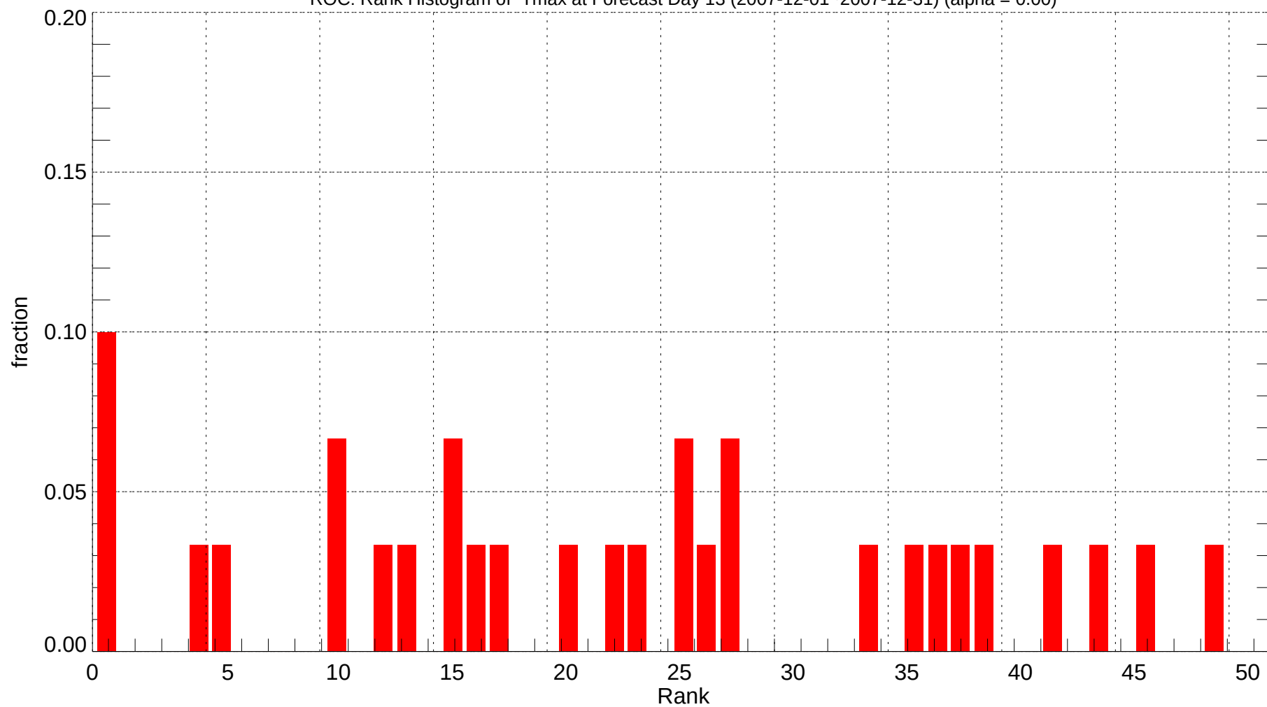
ROC: Rank Histogram of Tmax at Forecast Day 13 (2007-12-01~2007-12-31) (alpha = 0.00)
