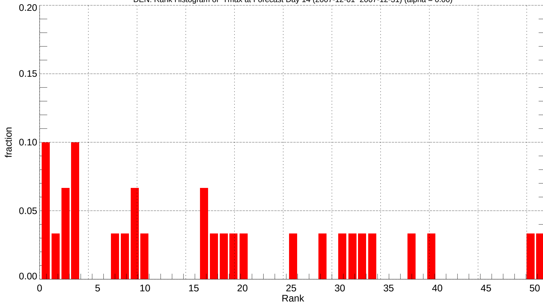
DEN: Rank Histogram of Tmax at Forecast Day 14 (2007-12-01~2007-12-31) (alpha = 0.00)
