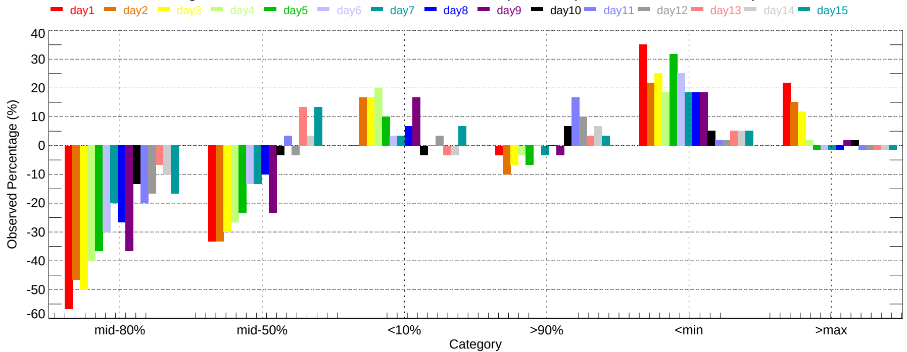
Observed Percentage Deviation of Ensembles - ROC: Max Temperature (2007-12-01~2007-12-31)
