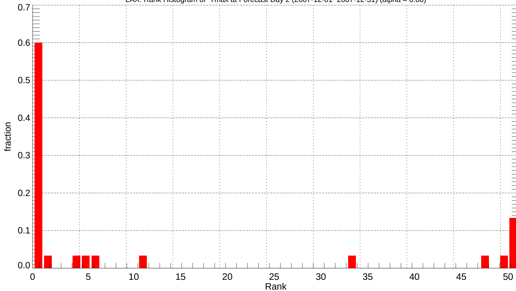
LAX: Rank Histogram of Tmax at Forecast Day 2 (2007-12-01~2007-12-31) (alpha = 0.00)
