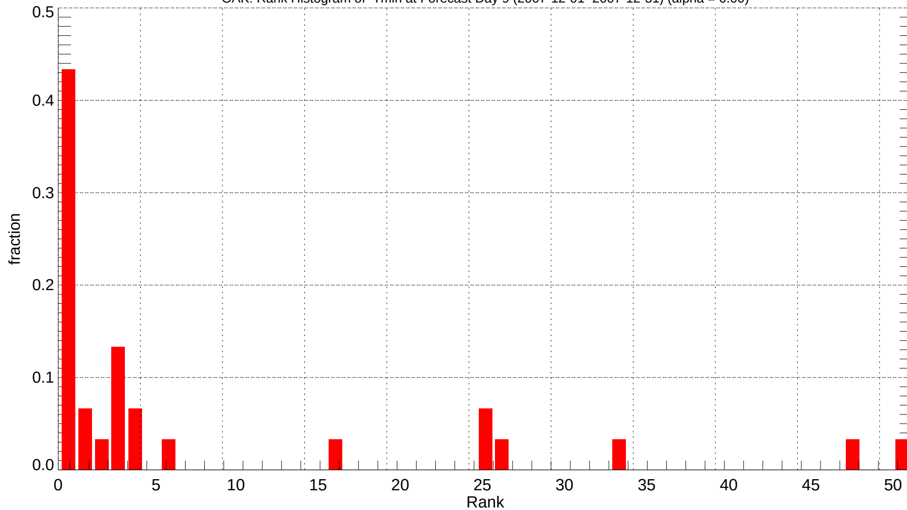
OAK: Rank Histogram of Tmin at Forecast Day 9 (2007-12-01~2007-12-31) (alpha = 0.00)
