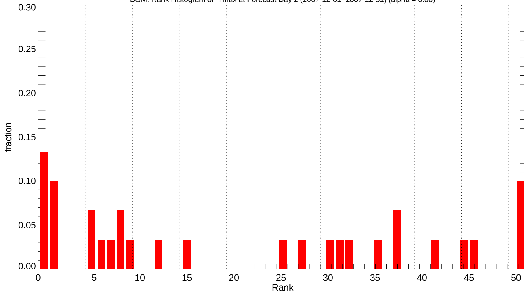
BGM: Rank Histogram of Tmax at Forecast Day 2 (2007-12-01~2007-12-31) (alpha = 0.00)
