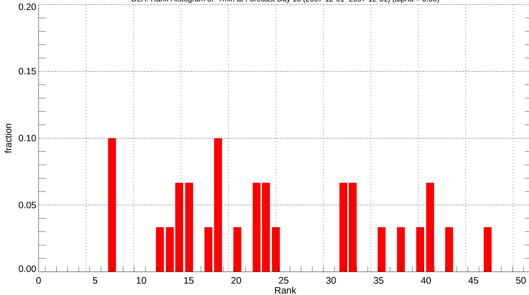
DLH: Rank Histogram of Tmin at Forecast Day 13 (2007-12-01~2007-12-31) (alpha = 0.00)
