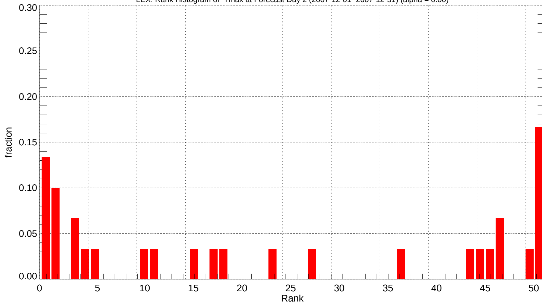
LEX: Rank Histogram of Tmax at Forecast Day 2 (2007-12-01~2007-12-31) (alpha = 0.00)
