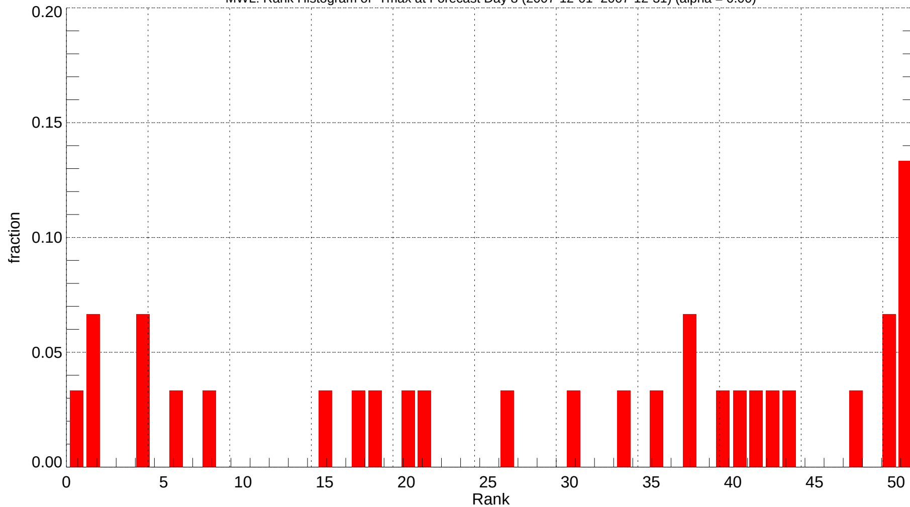
MWL: Rank Histogram of Tmax at Forecast Day 8 (2007-12-01~2007-12-31) (alpha = 0.00)
