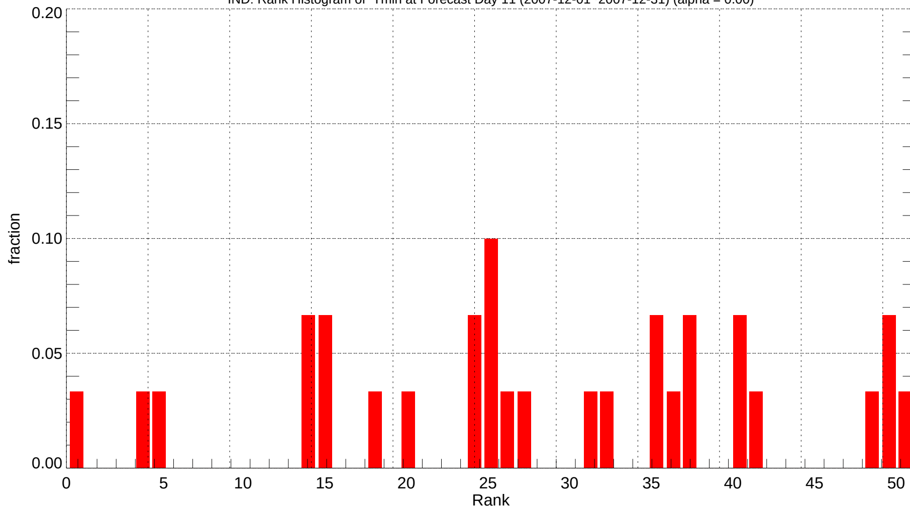
IND: Rank Histogram of Tmin at Forecast Day 11 (2007-12-01~2007-12-31) (alpha = 0.00)
