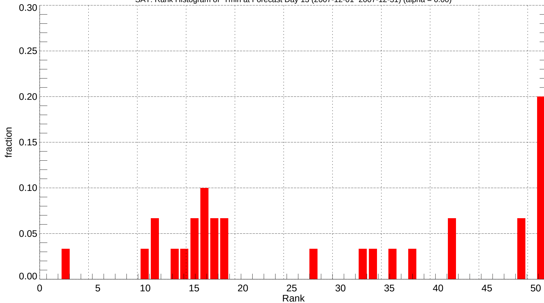
SAT: Rank Histogram of Tmin at Forecast Day 13 (2007-12-01~2007-12-31) (alpha = 0.00)
