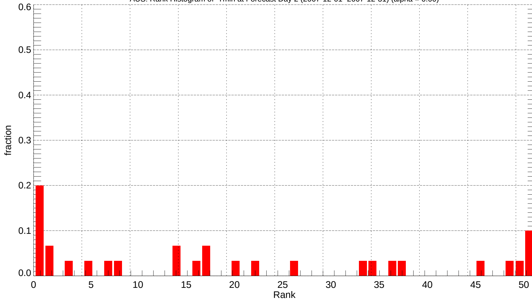
AUS: Rank Histogram of Tmin at Forecast Day 2 (2007-12-01~2007-12-31) (alpha = 0.00)
