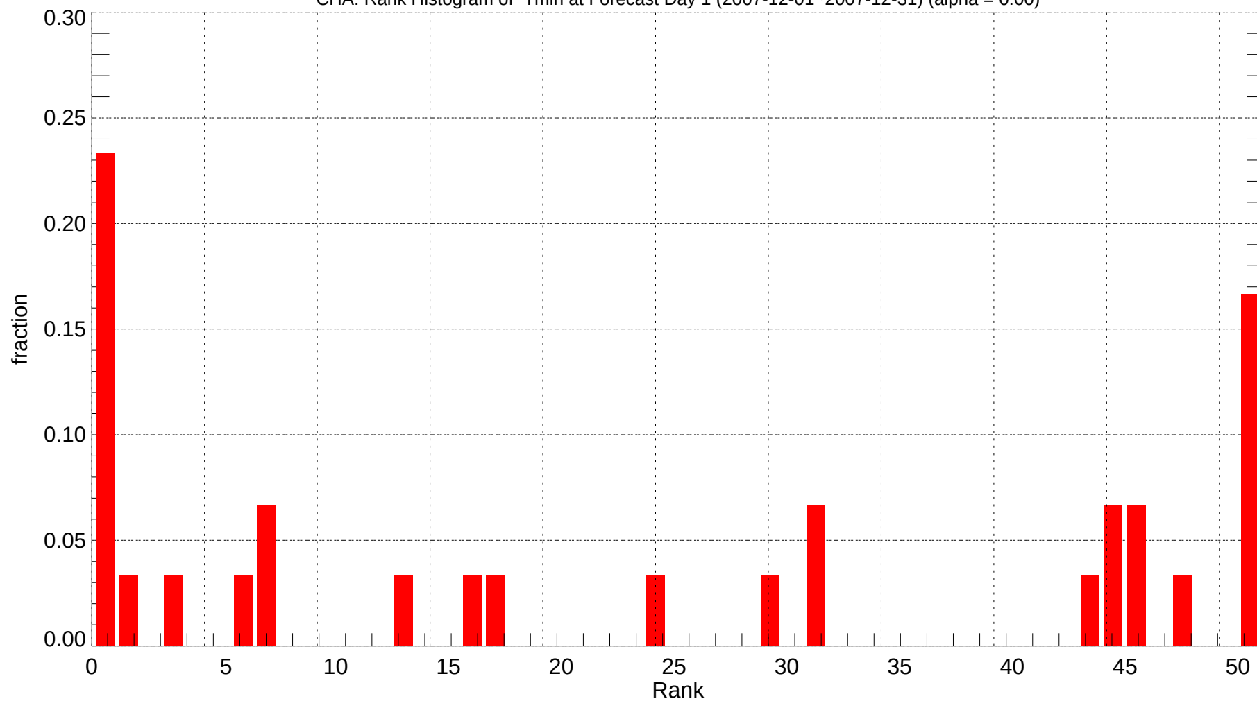
CHA: Rank Histogram of Tmin at Forecast Day 1 (2007-12-01~2007-12-31) (alpha = 0.00)
