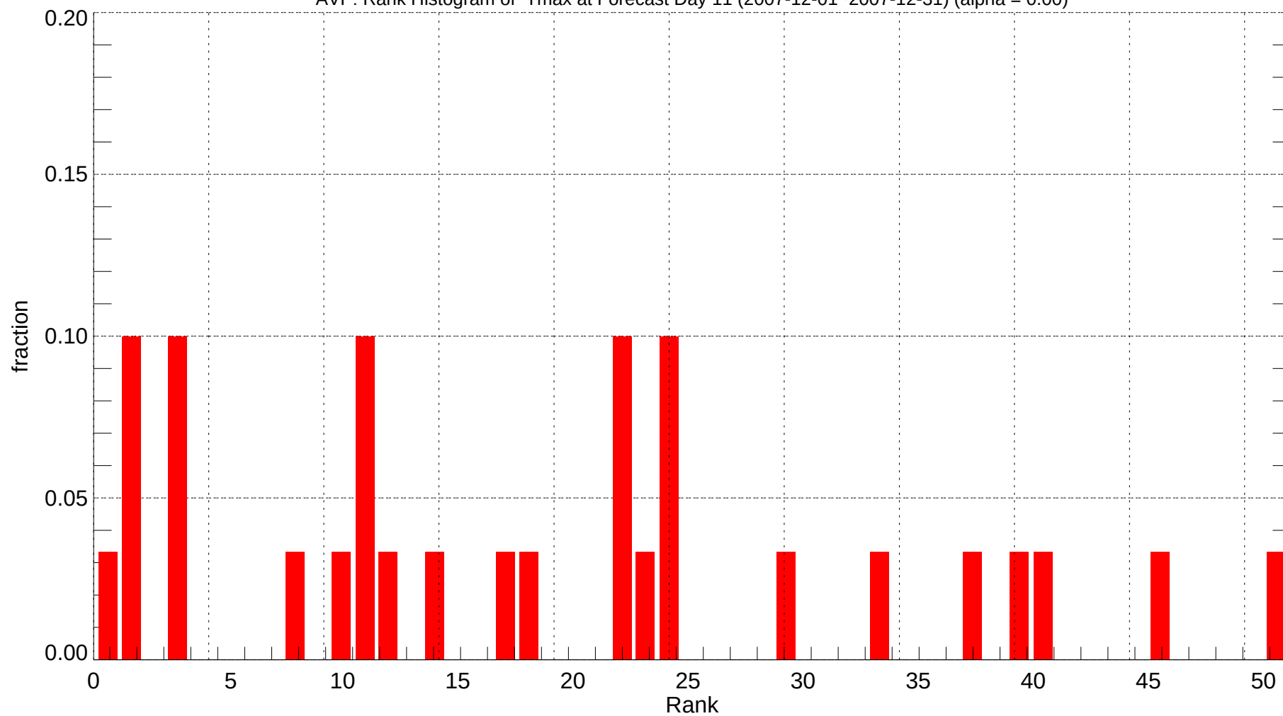
AVP: Rank Histogram of Tmax at Forecast Day 11 (2007-12-01~2007-12-31) (alpha = 0.00)
