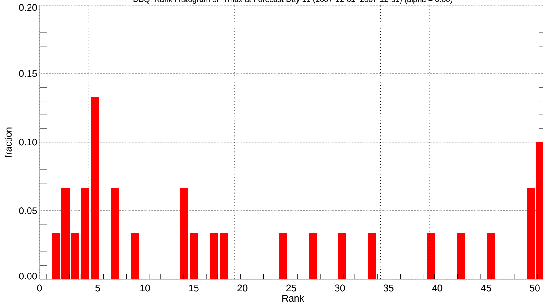
DBQ: Rank Histogram of Tmax at Forecast Day 11 (2007-12-01~2007-12-31) (alpha = 0.00)
