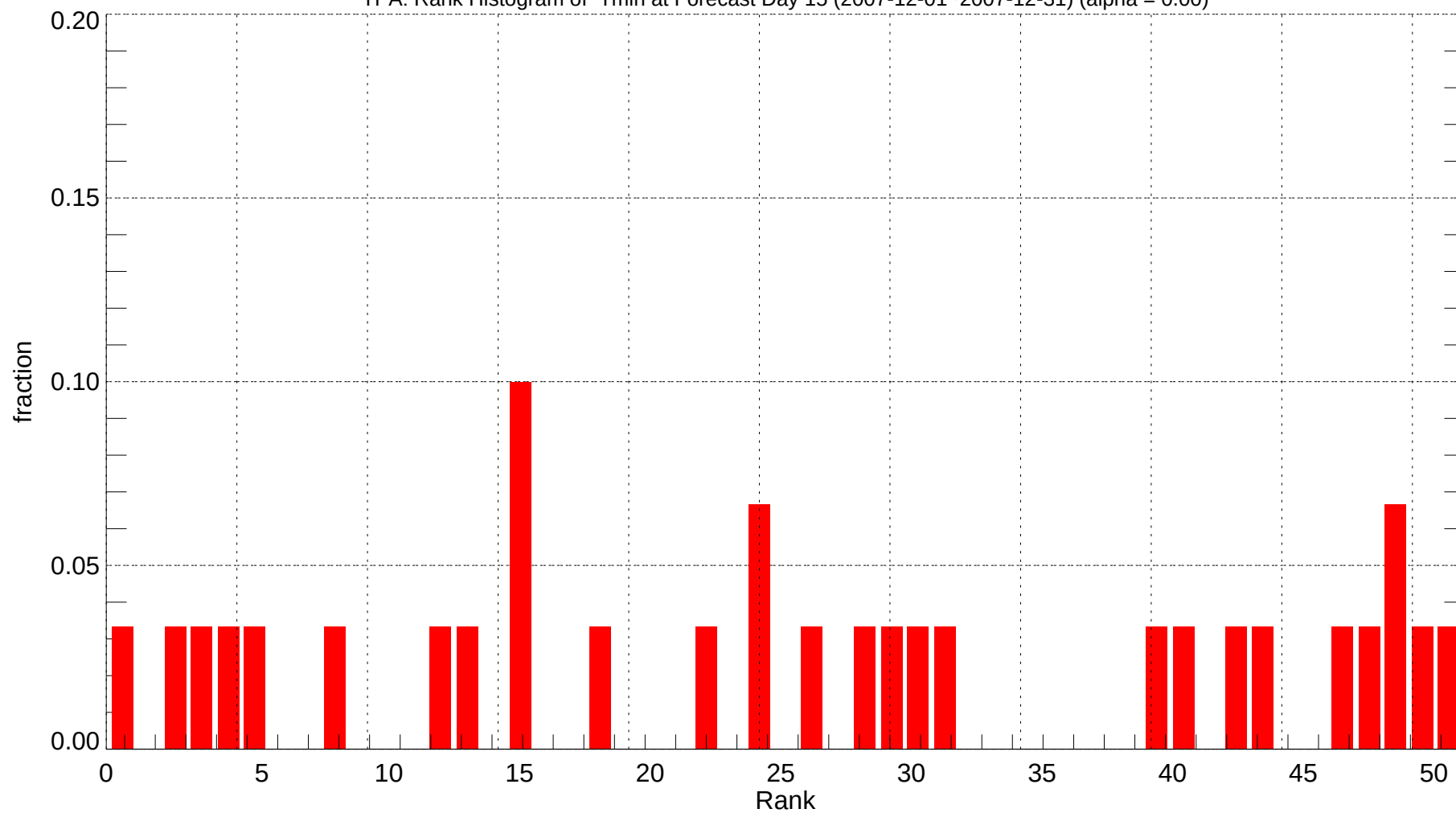
TPA: Rank Histogram of Tmin at Forecast Day 15 (2007-12-01~2007-12-31) (alpha = 0.00)
