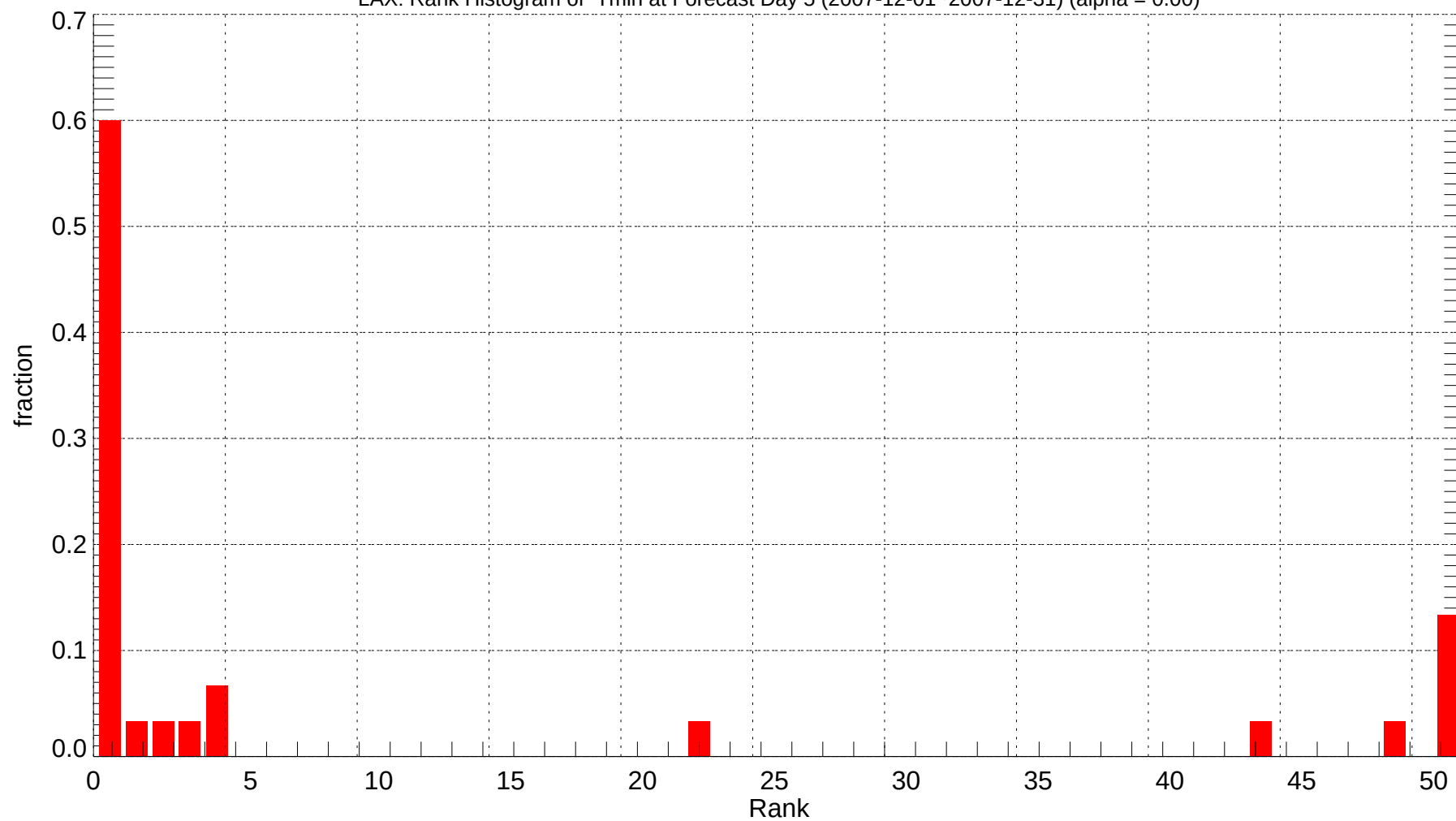
LAX: Rank Histogram of Tmin at Forecast Day 5 (2007-12-01~2007-12-31) (alpha = 0.00)
