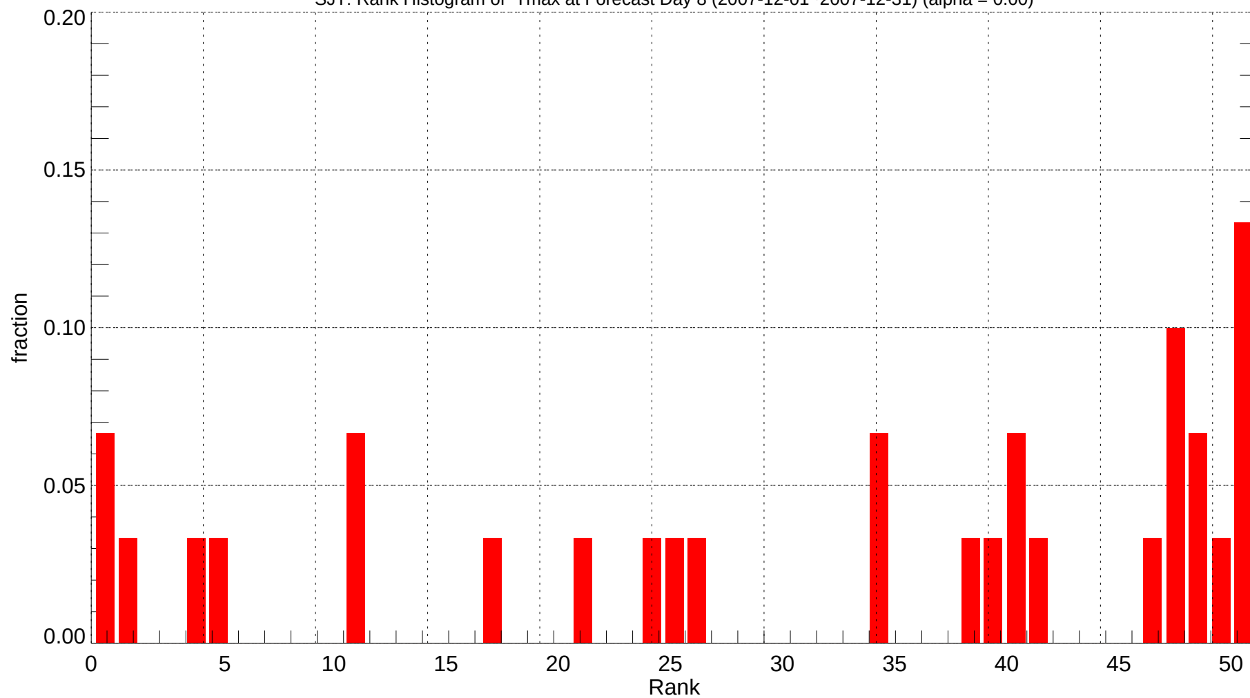
SJT: Rank Histogram of Tmax at Forecast Day 8 (2007-12-01~2007-12-31) (alpha = 0.00)
