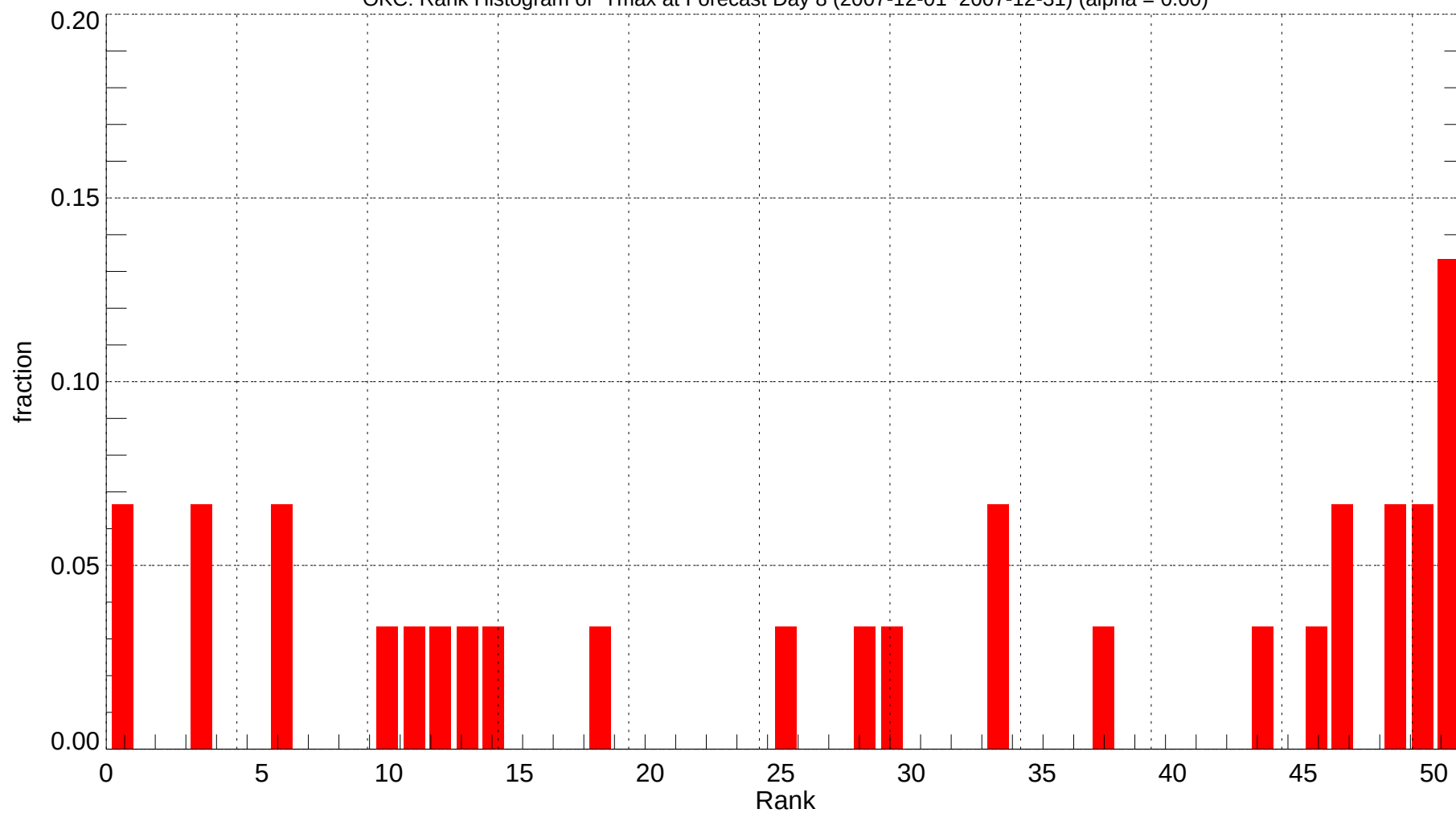
OKC: Rank Histogram of Tmax at Forecast Day 8 (2007-12-01~2007-12-31) (alpha = 0.00)
