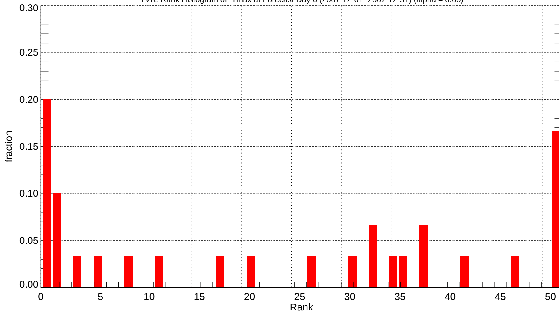
YVR: Rank Histogram of Tmax at Forecast Day 6 (2007-12-01~2007-12-31) (alpha = 0.00)
