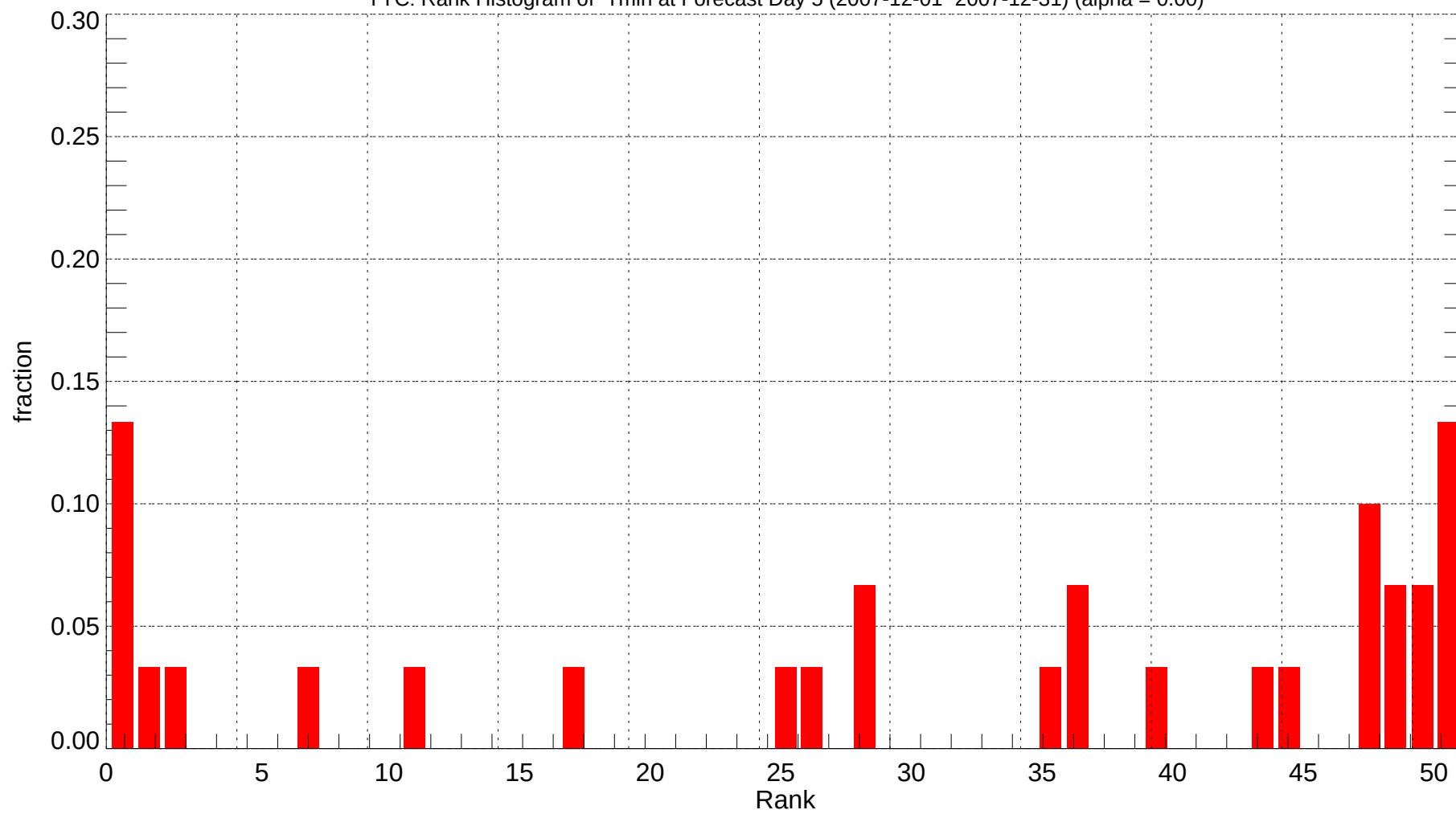
YYC: Rank Histogram of Tmin at Forecast Day 5 (2007-12-01~2007-12-31) (alpha = 0.00)
