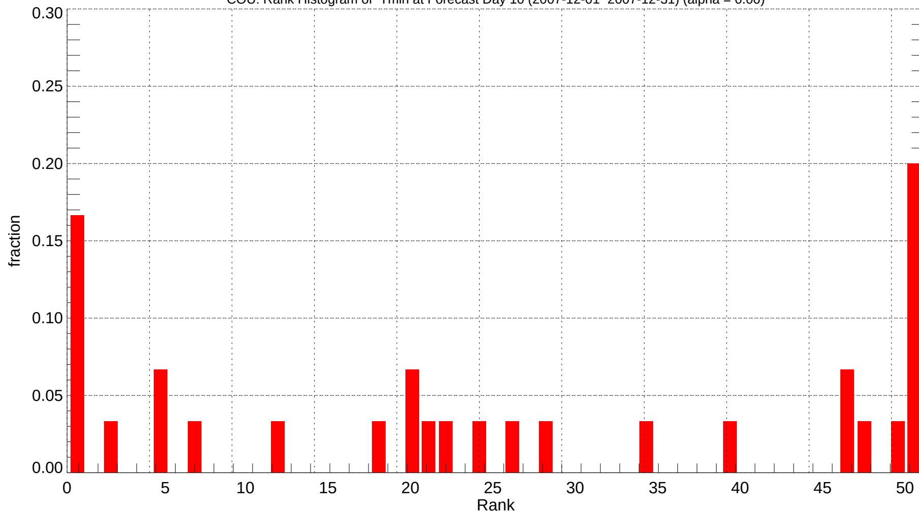
COU: Rank Histogram of Tmin at Forecast Day 10 (2007-12-01~2007-12-31) (alpha = 0.00)
