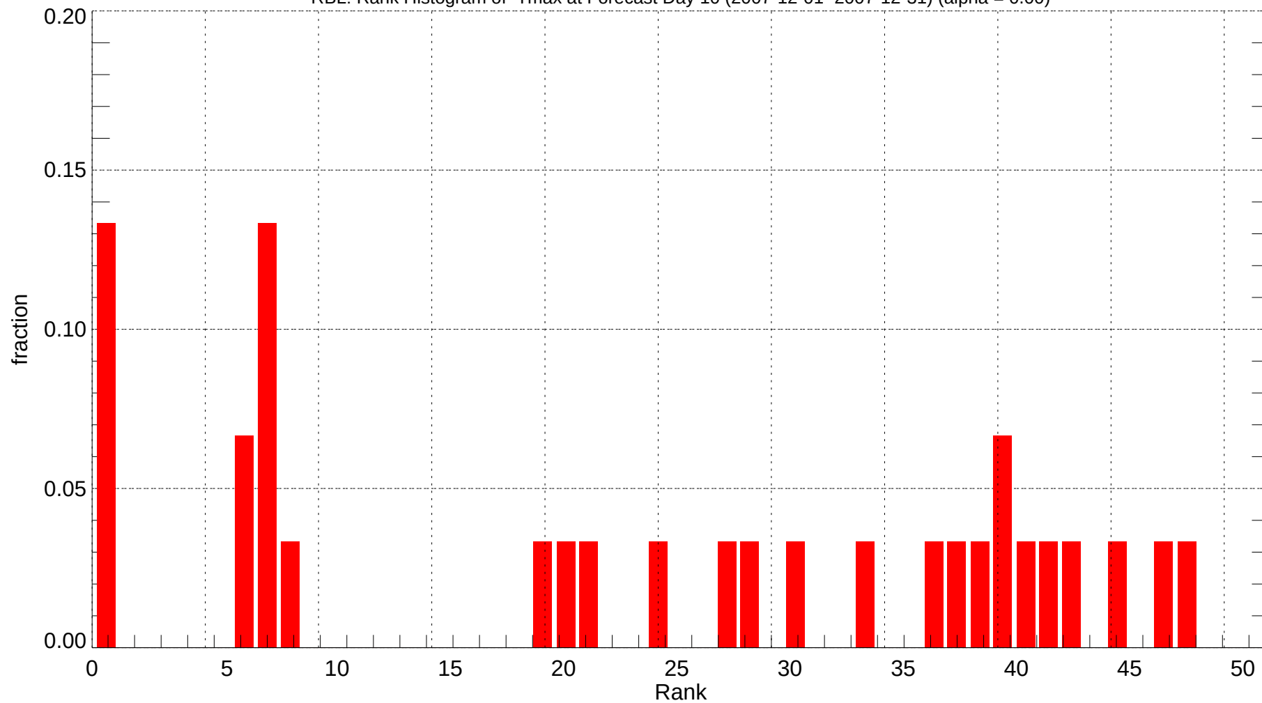
RBL: Rank Histogram of Tmax at Forecast Day 10 (2007-12-01~2007-12-31) (alpha = 0.00)
