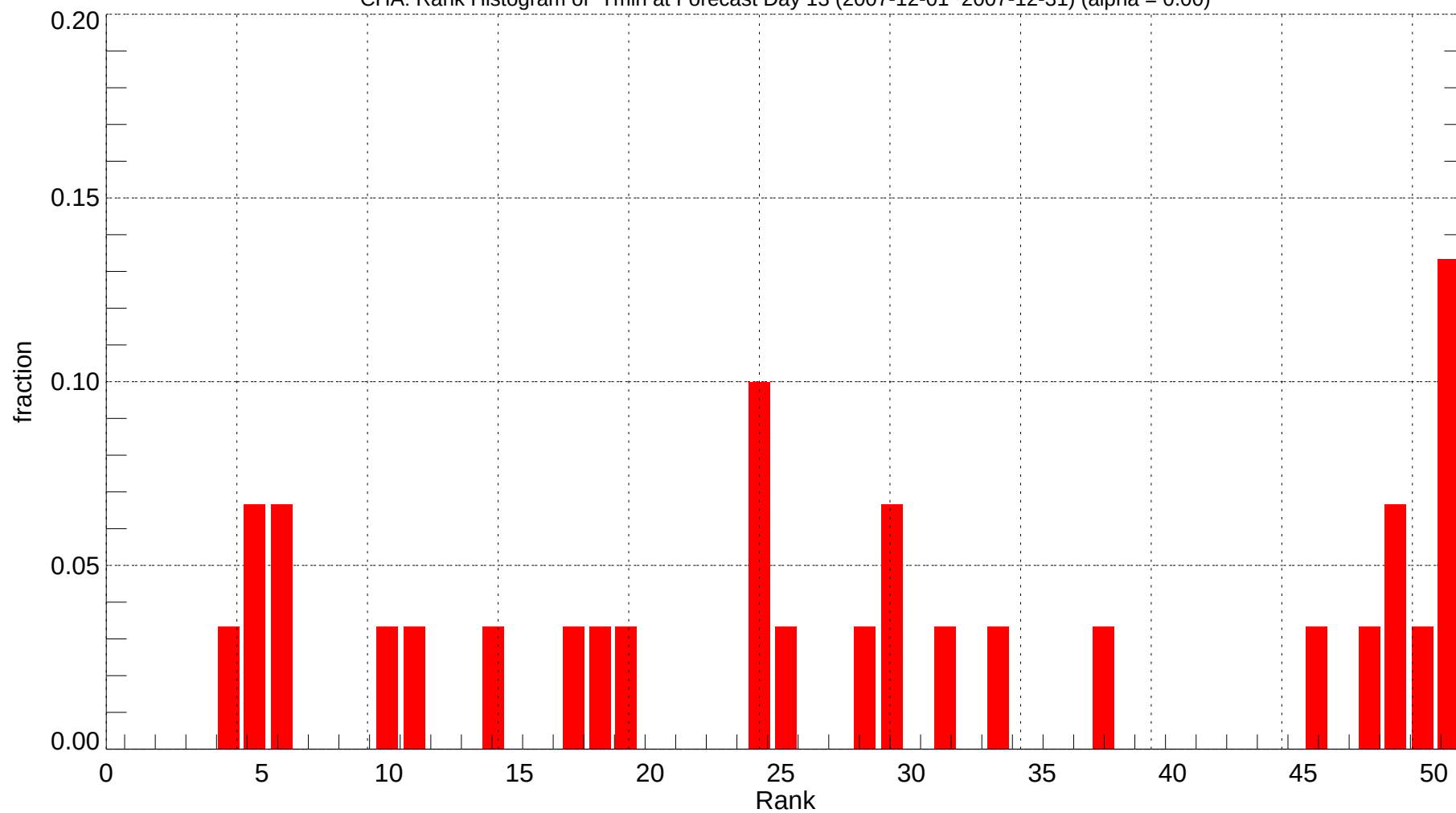
CHA: Rank Histogram of Tmin at Forecast Day 13 (2007-12-01~2007-12-31) (alpha = 0.00)
