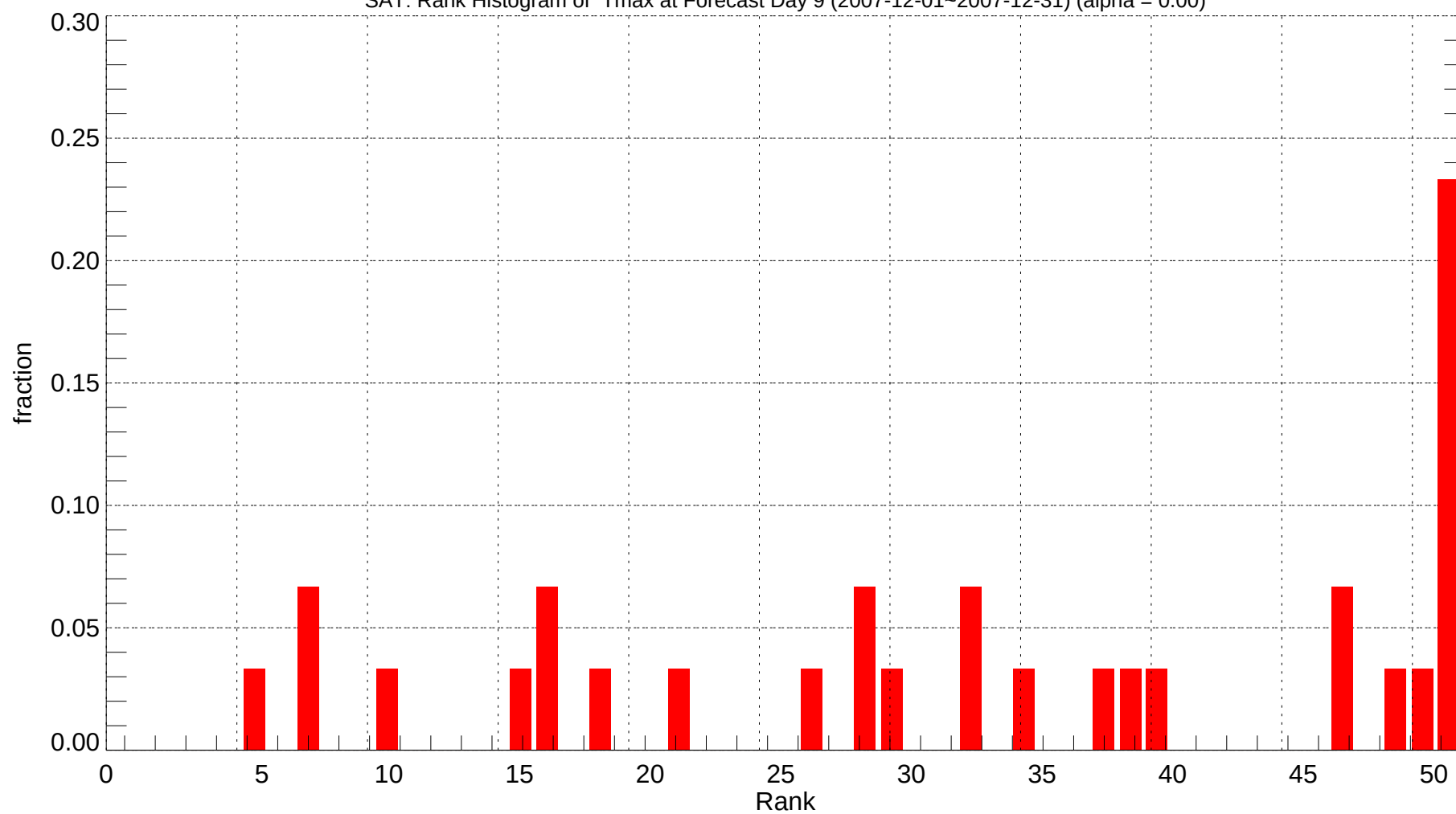
SAT: Rank Histogram of Tmax at Forecast Day 9 (2007-12-01~2007-12-31) (alpha = 0.00)
