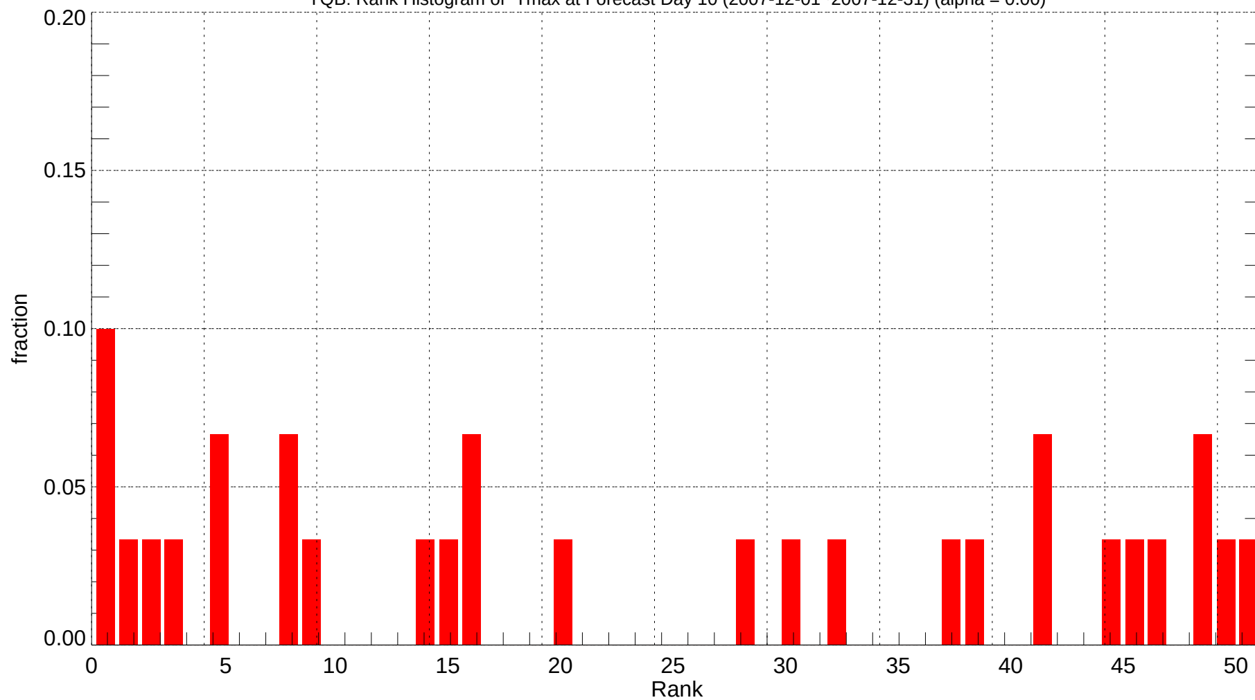
YQB: Rank Histogram of Tmax at Forecast Day 10 (2007-12-01~2007-12-31) (alpha = 0.00)
