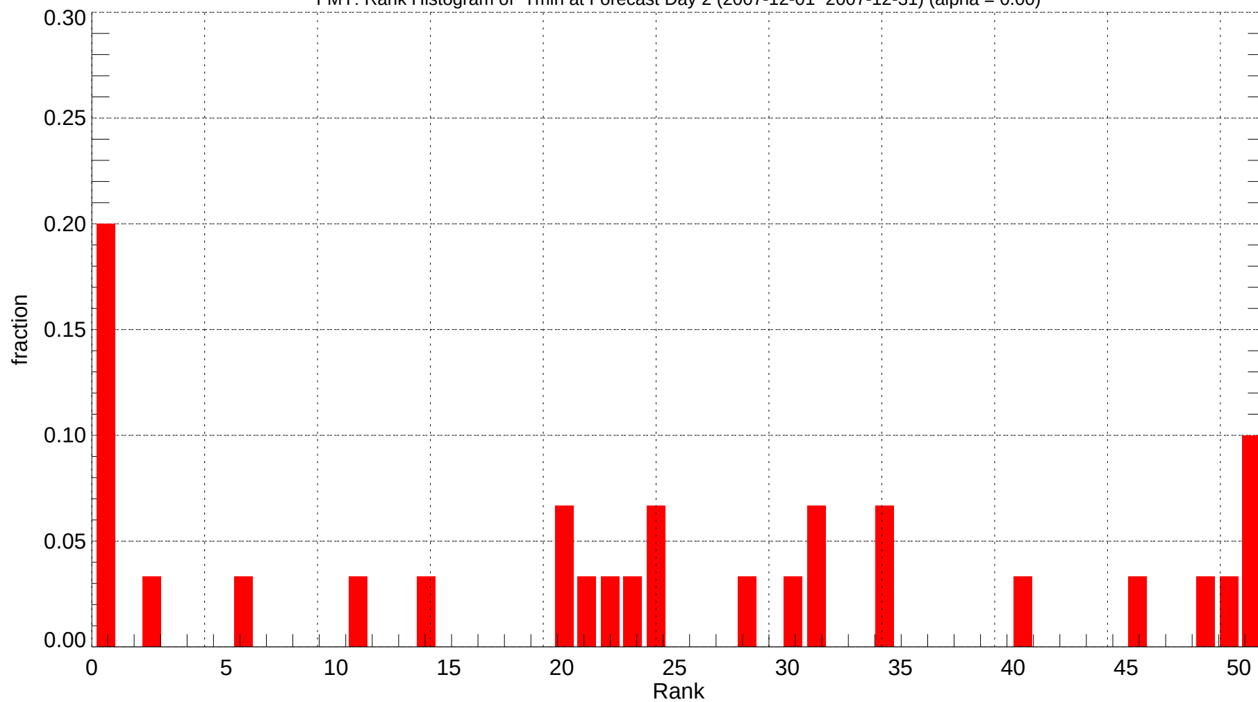
FMY: Rank Histogram of Tmin at Forecast Day 2 (2007-12-01~2007-12-31) (alpha = 0.00)
