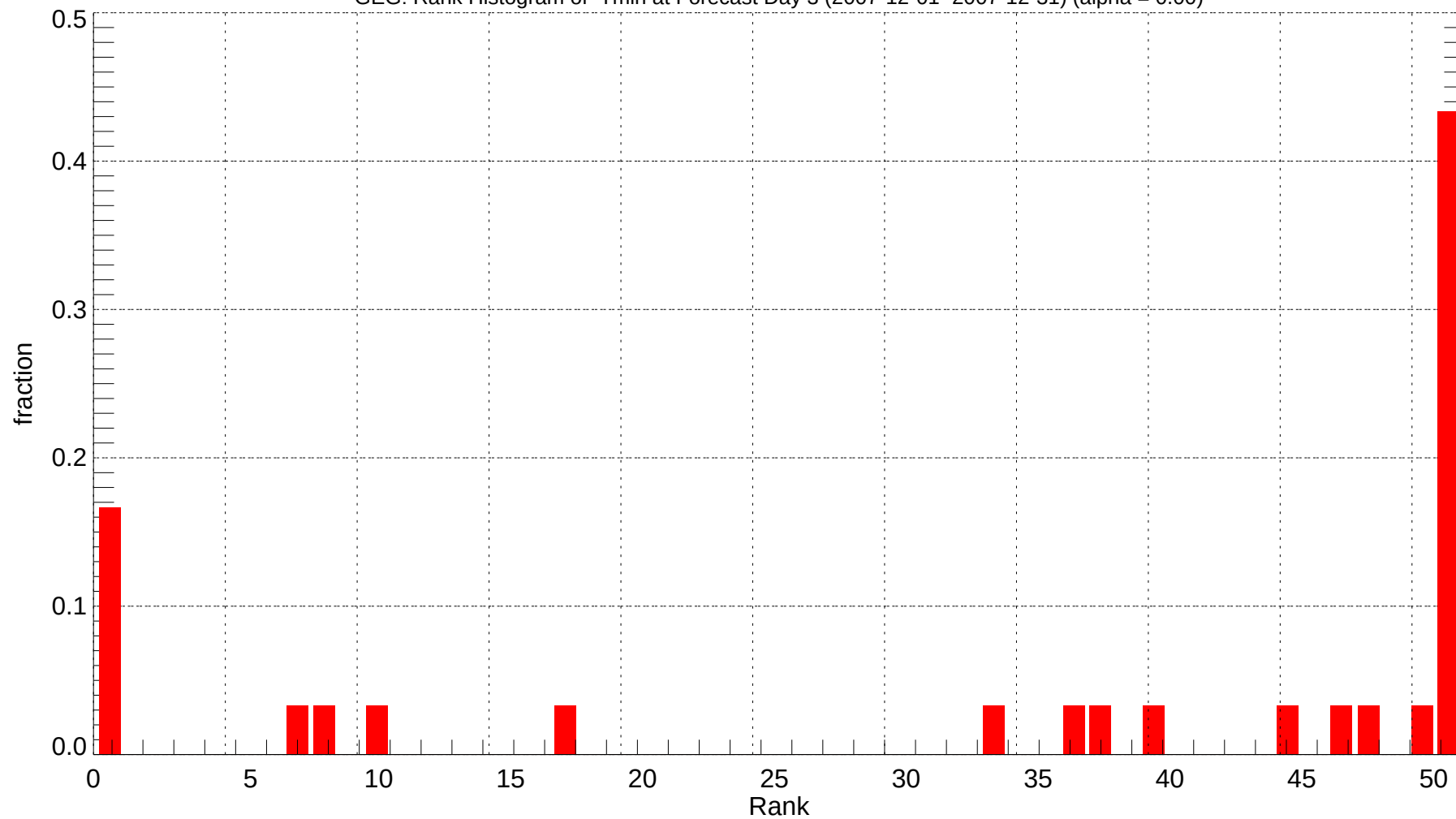
GEG: Rank Histogram of Tmin at Forecast Day 3 (2007-12-01~2007-12-31) (alpha = 0.00)
