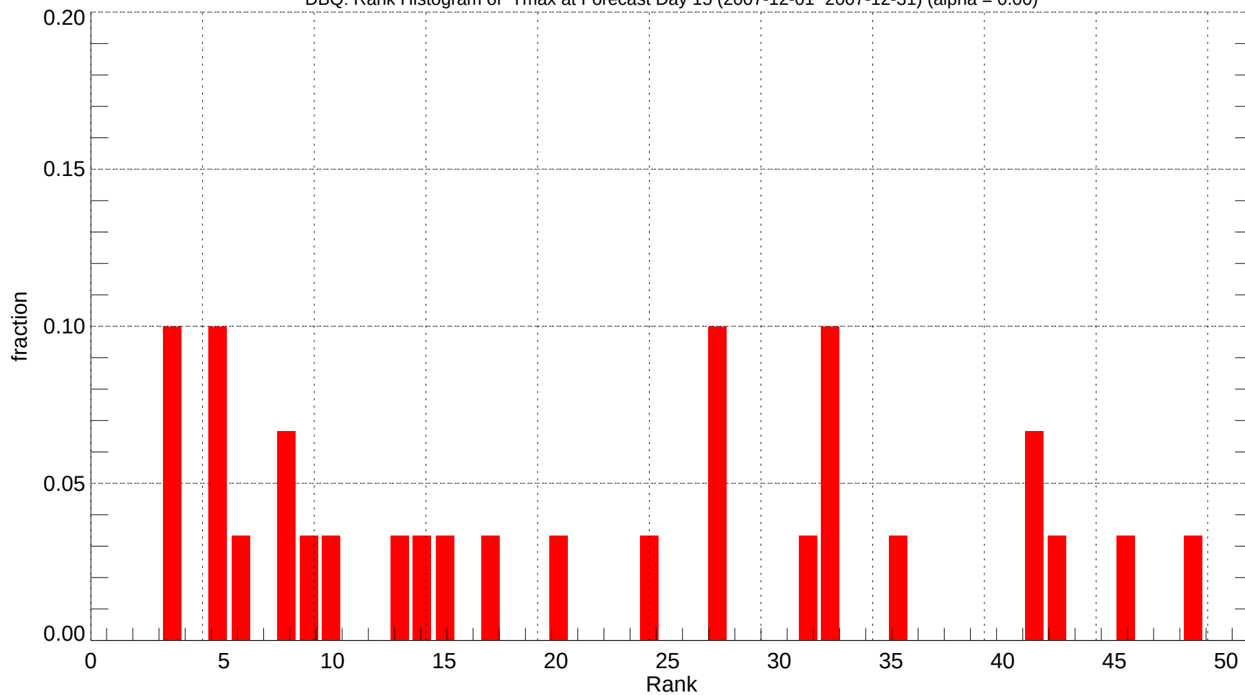
DBQ: Rank Histogram of Tmax at Forecast Day 15 (2007-12-01~2007-12-31) (alpha = 0.00)
