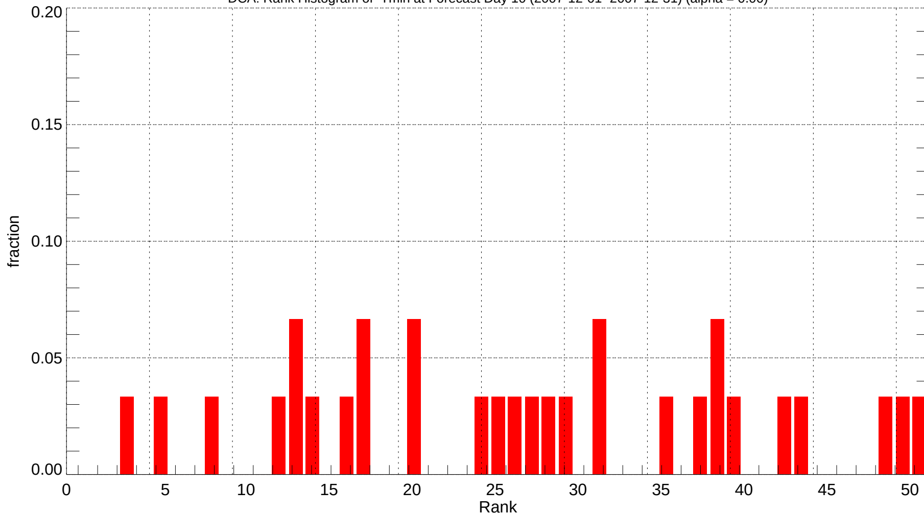
DCA: Rank Histogram of Tmin at Forecast Day 10 (2007-12-01~2007-12-31) (alpha = 0.00)
