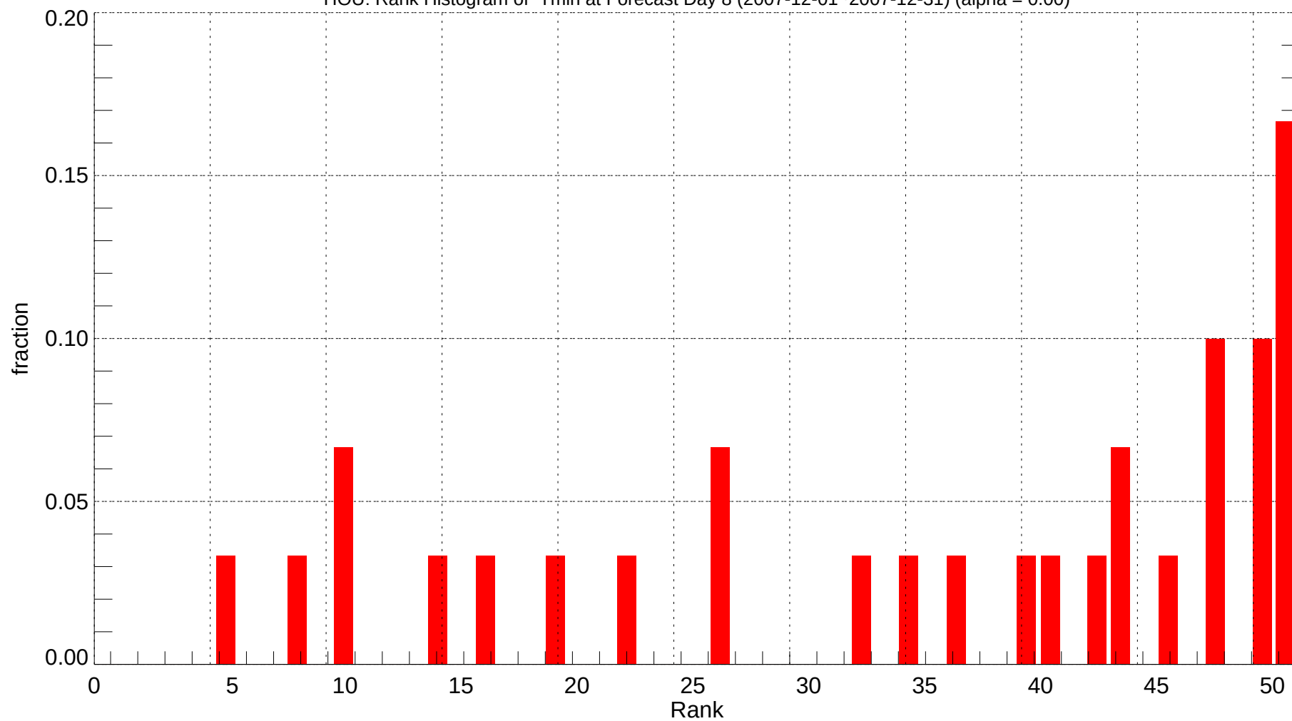
HOU: Rank Histogram of Tmin at Forecast Day 8 (2007-12-01~2007-12-31) (alpha = 0.00)
