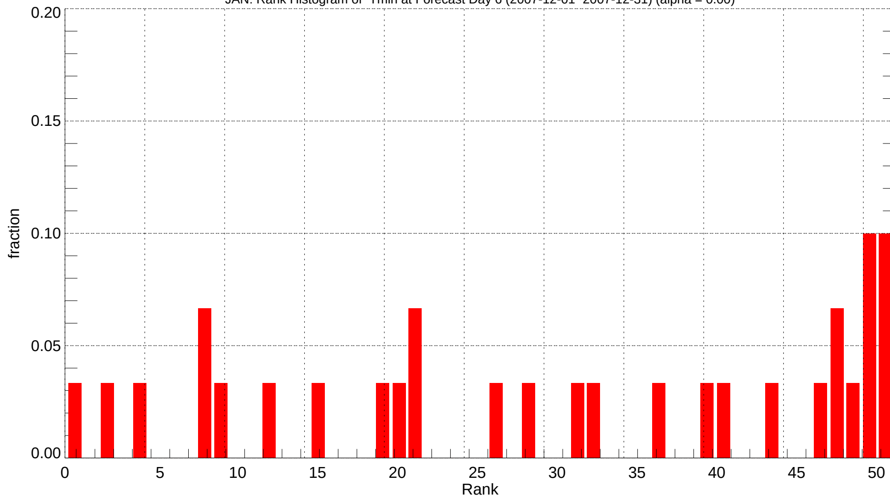
JAN: Rank Histogram of Tmin at Forecast Day 6 (2007-12-01~2007-12-31) (alpha = 0.00)
