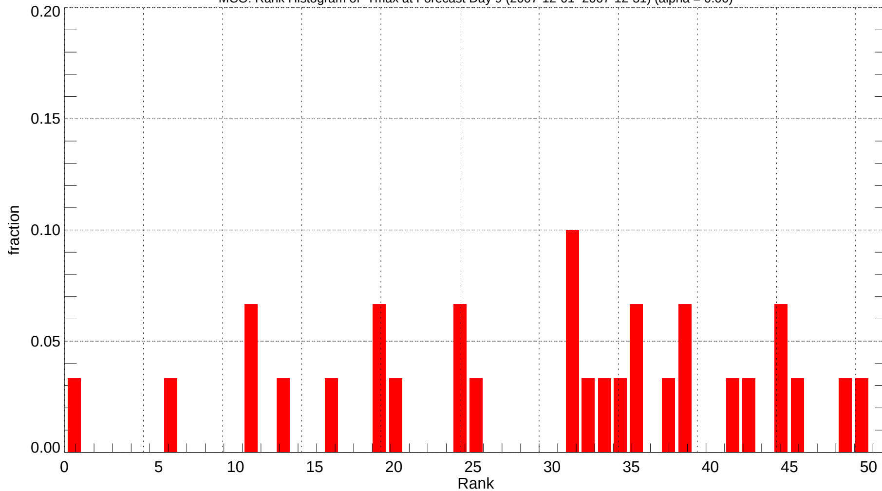
MCO: Rank Histogram of Tmax at Forecast Day 9 (2007-12-01~2007-12-31) (alpha = 0.00)
