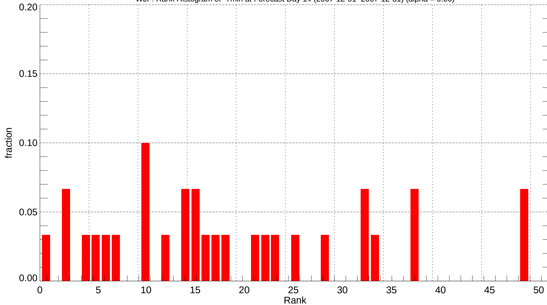
WJF: Rank Histogram of Tmin at Forecast Day 14 (2007-12-01~2007-12-31) (alpha = 0.00)
