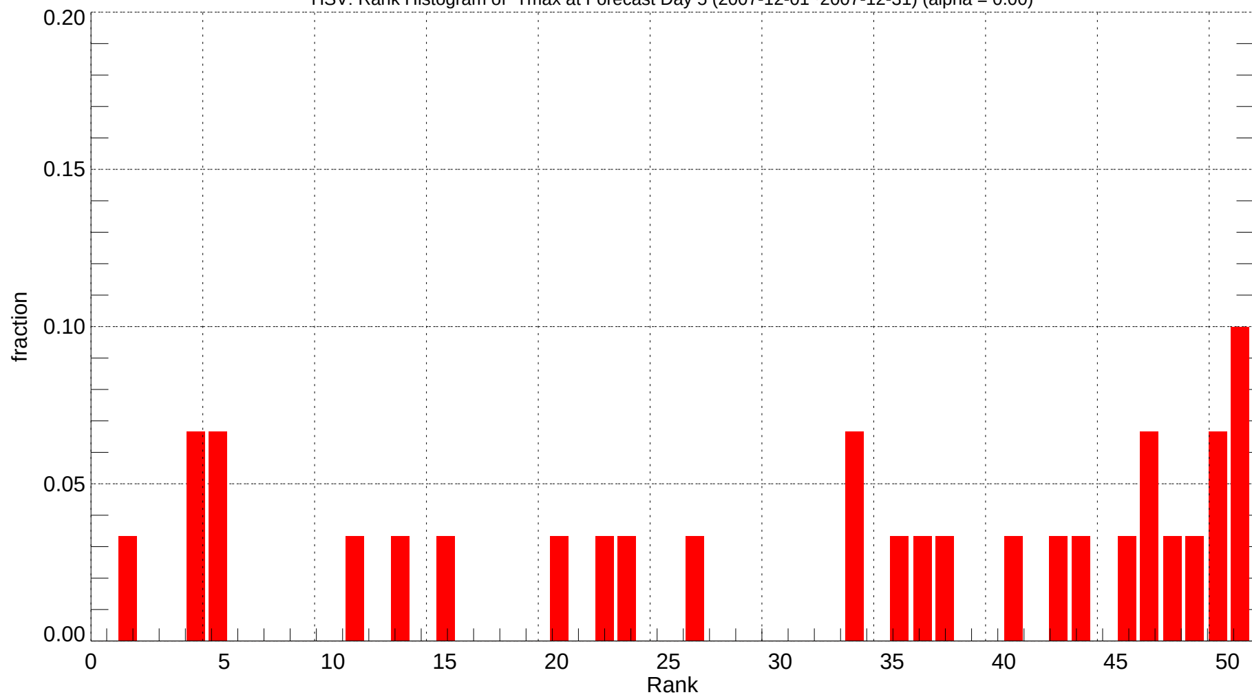
HSV: Rank Histogram of Tmax at Forecast Day 5 (2007-12-01~2007-12-31) (alpha = 0.00)
