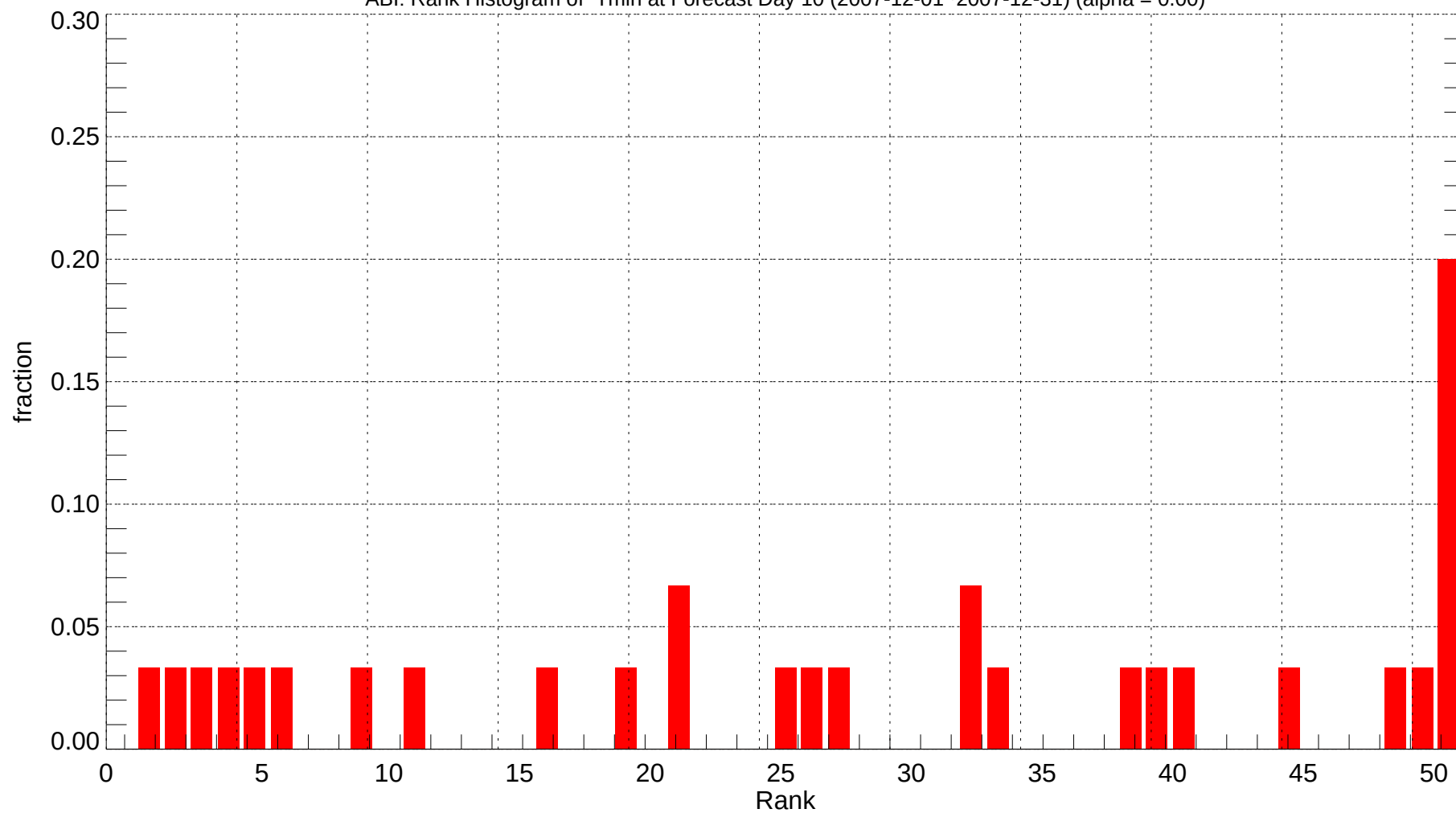
ABI: Rank Histogram of Tmin at Forecast Day 10 (2007-12-01~2007-12-31) (alpha = 0.00)
