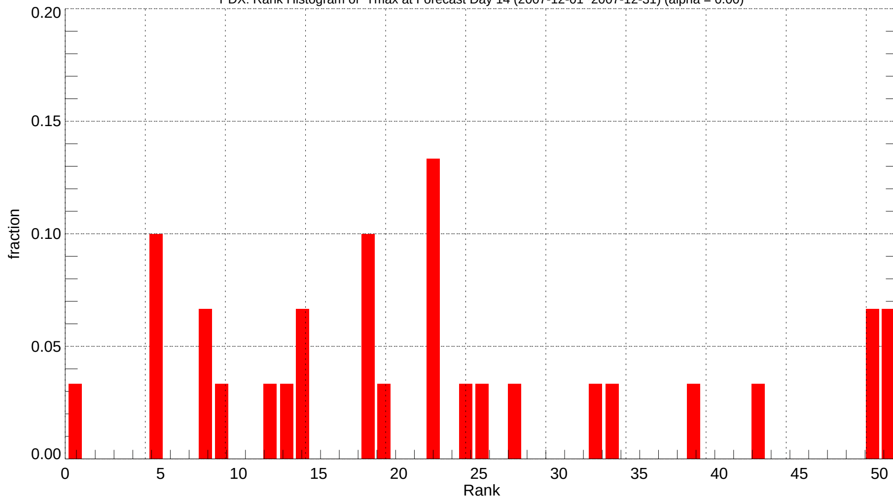
PDX: Rank Histogram of Tmax at Forecast Day 14 (2007-12-01~2007-12-31) (alpha = 0.00)
