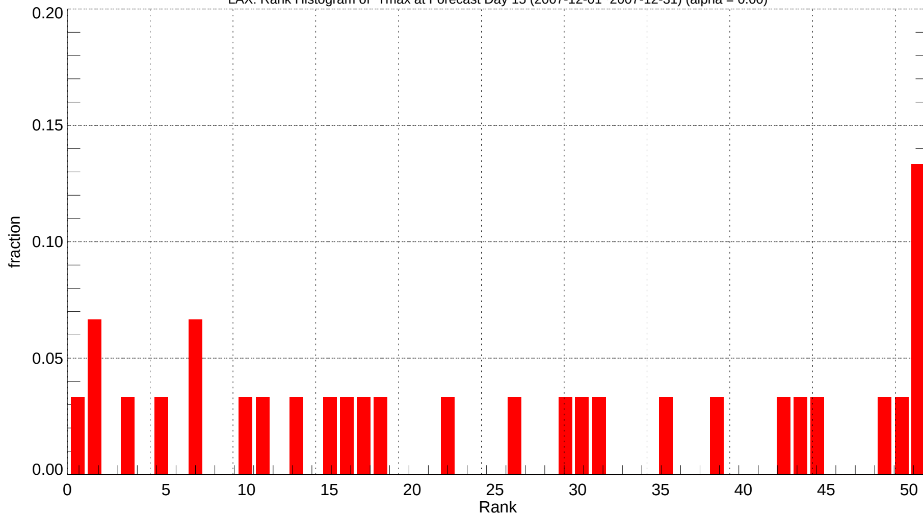
LAX: Rank Histogram of Tmax at Forecast Day 15 (2007-12-01~2007-12-31) (alpha = 0.00)
