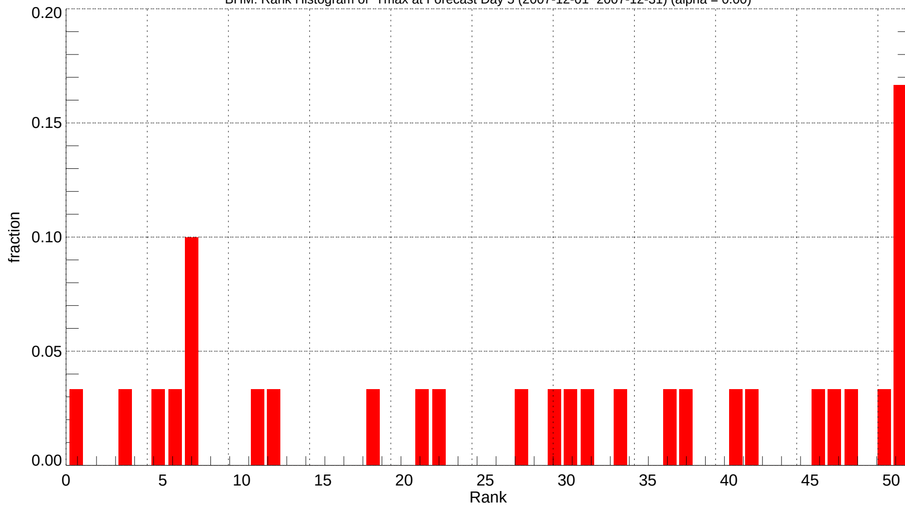
BHM: Rank Histogram of Tmax at Forecast Day 5 (2007-12-01~2007-12-31) (alpha = 0.00)
