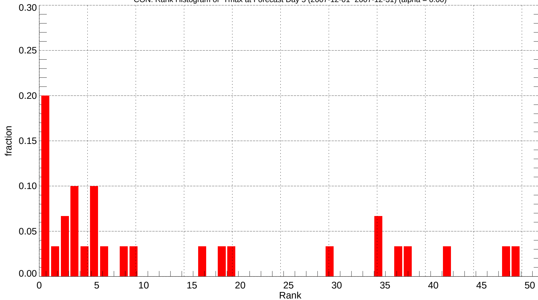
CON: Rank Histogram of Tmax at Forecast Day 5 (2007-12-01~2007-12-31) (alpha = 0.00)
