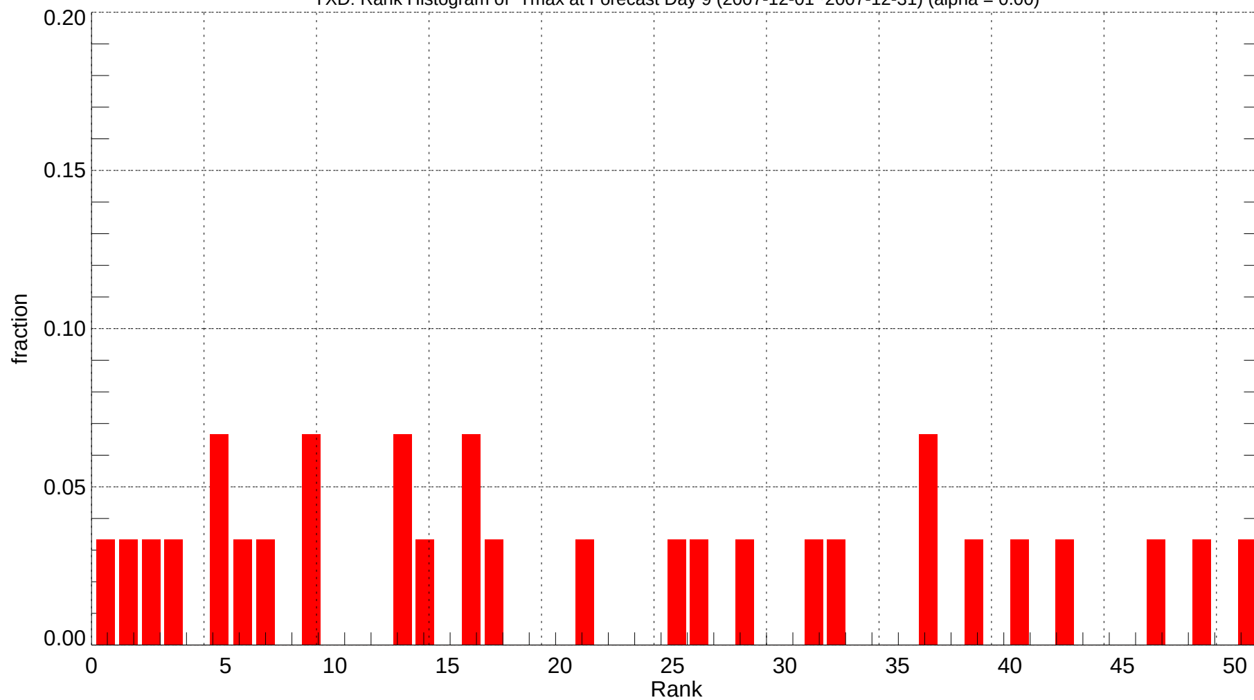
YXD: Rank Histogram of Tmax at Forecast Day 9 (2007-12-01~2007-12-31) (alpha = 0.00)
