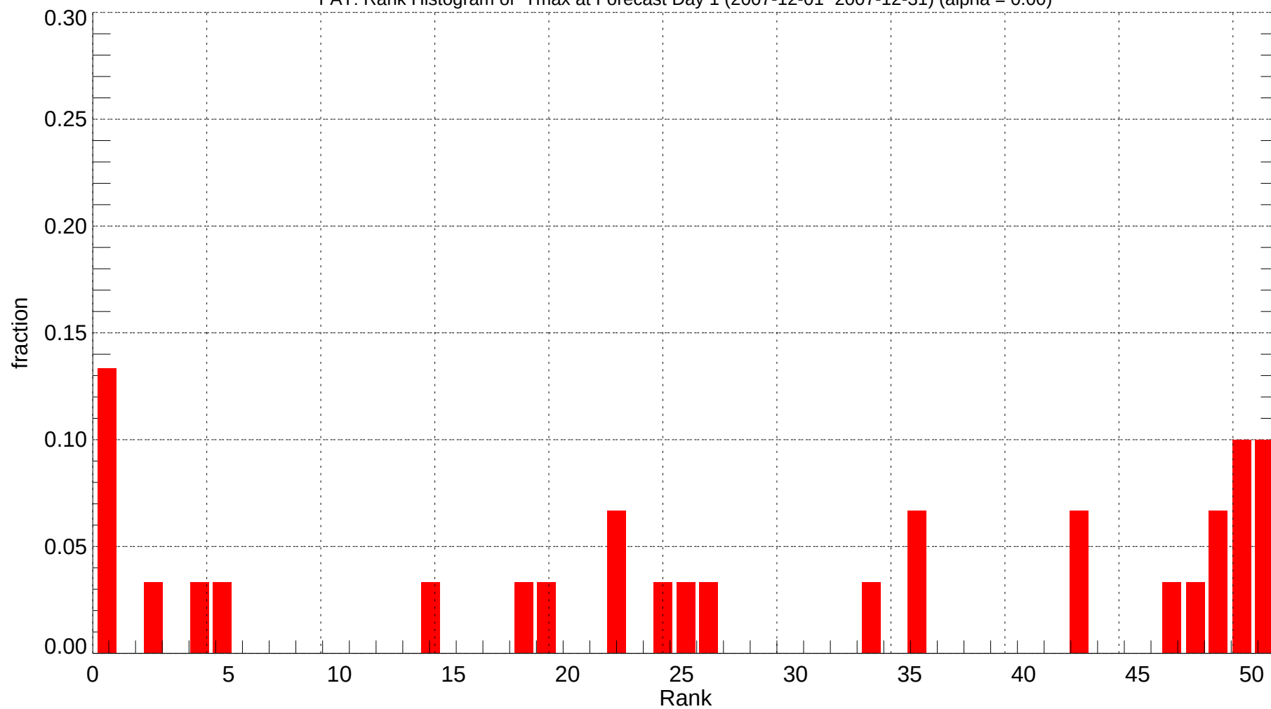
FAT: Rank Histogram of Tmax at Forecast Day 1 (2007-12-01~2007-12-31) (alpha = 0.00)
