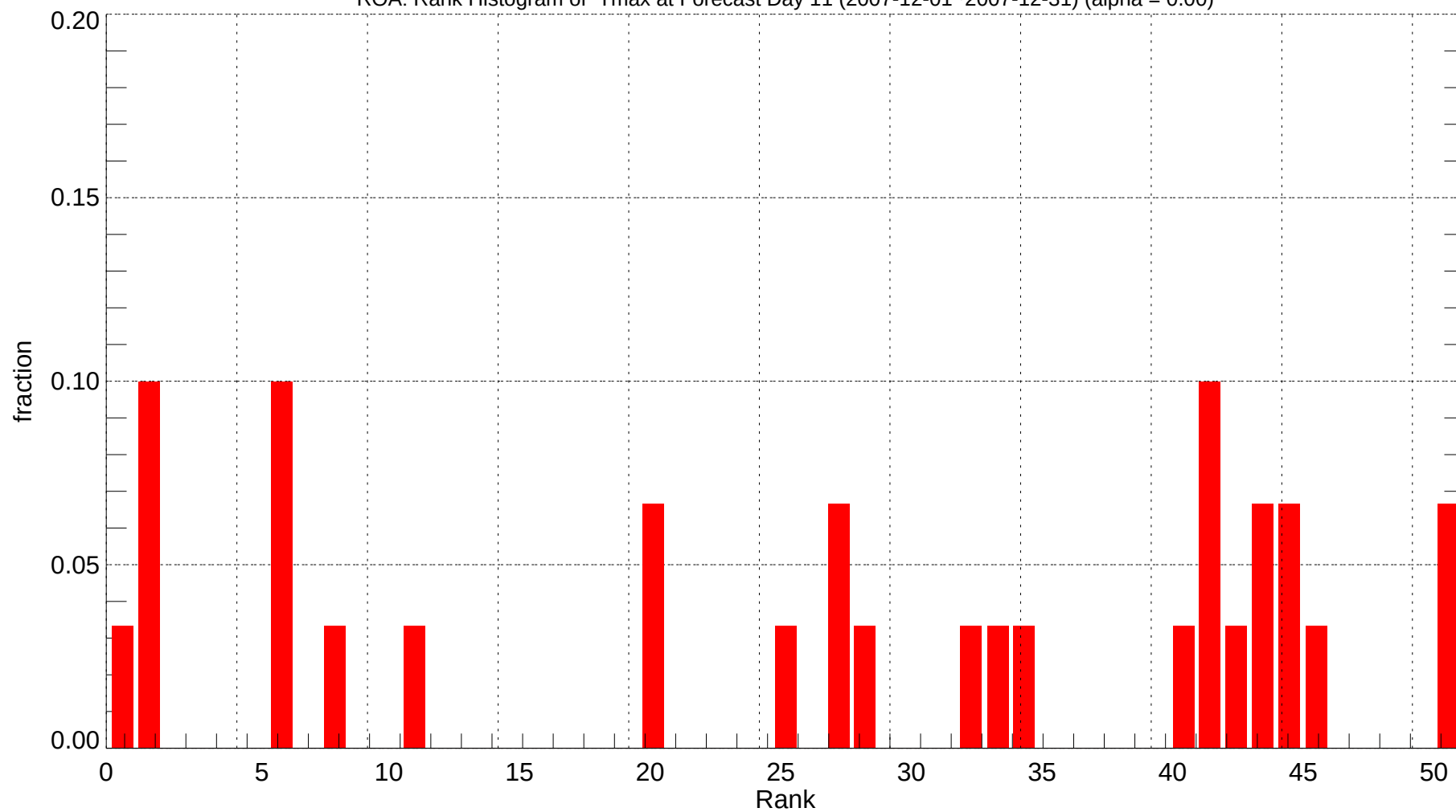
ROA: Rank Histogram of Tmax at Forecast Day 11 (2007-12-01~2007-12-31) (alpha = 0.00)
