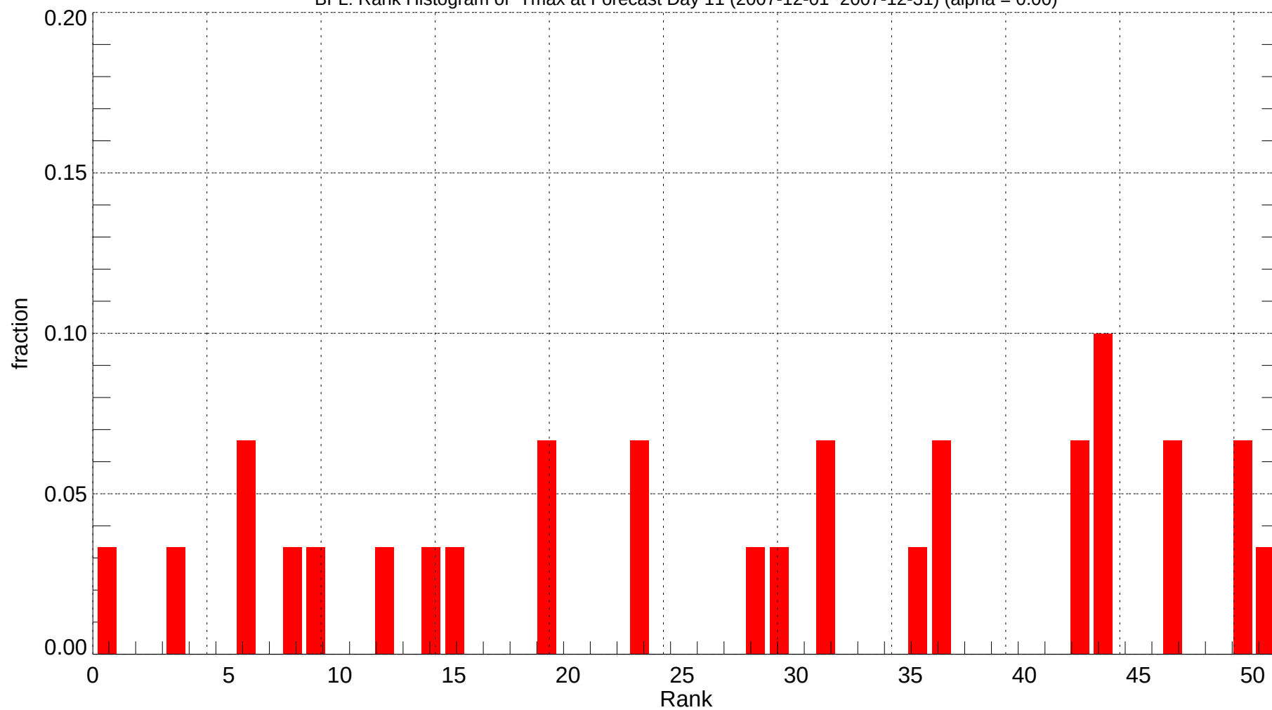
BFL: Rank Histogram of Tmax at Forecast Day 11 (2007-12-01~2007-12-31) (alpha = 0.00)
