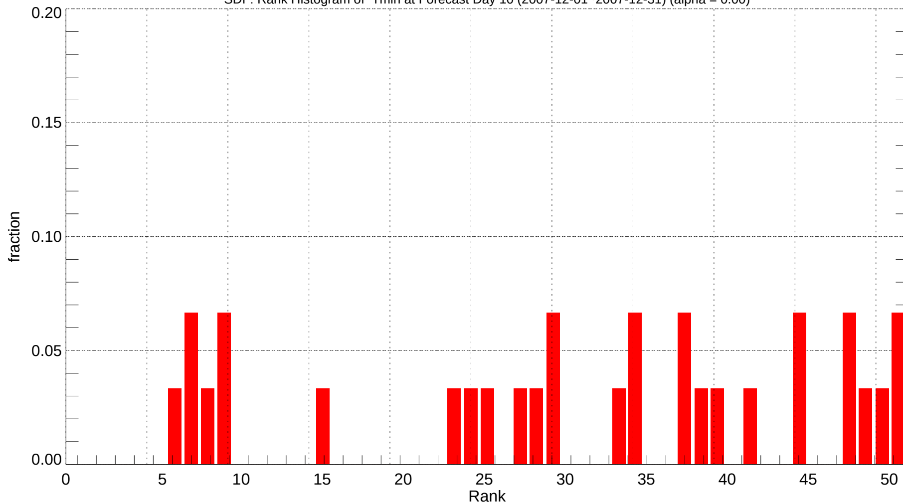
SDF: Rank Histogram of Tmin at Forecast Day 10 (2007-12-01~2007-12-31) (alpha = 0.00)
