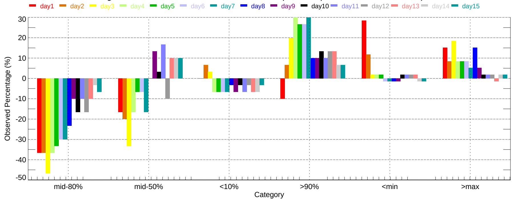
Observed Percentage Deviation of Ensembles - IND: Max Temperature (2007-12-01~2007-12-31)
