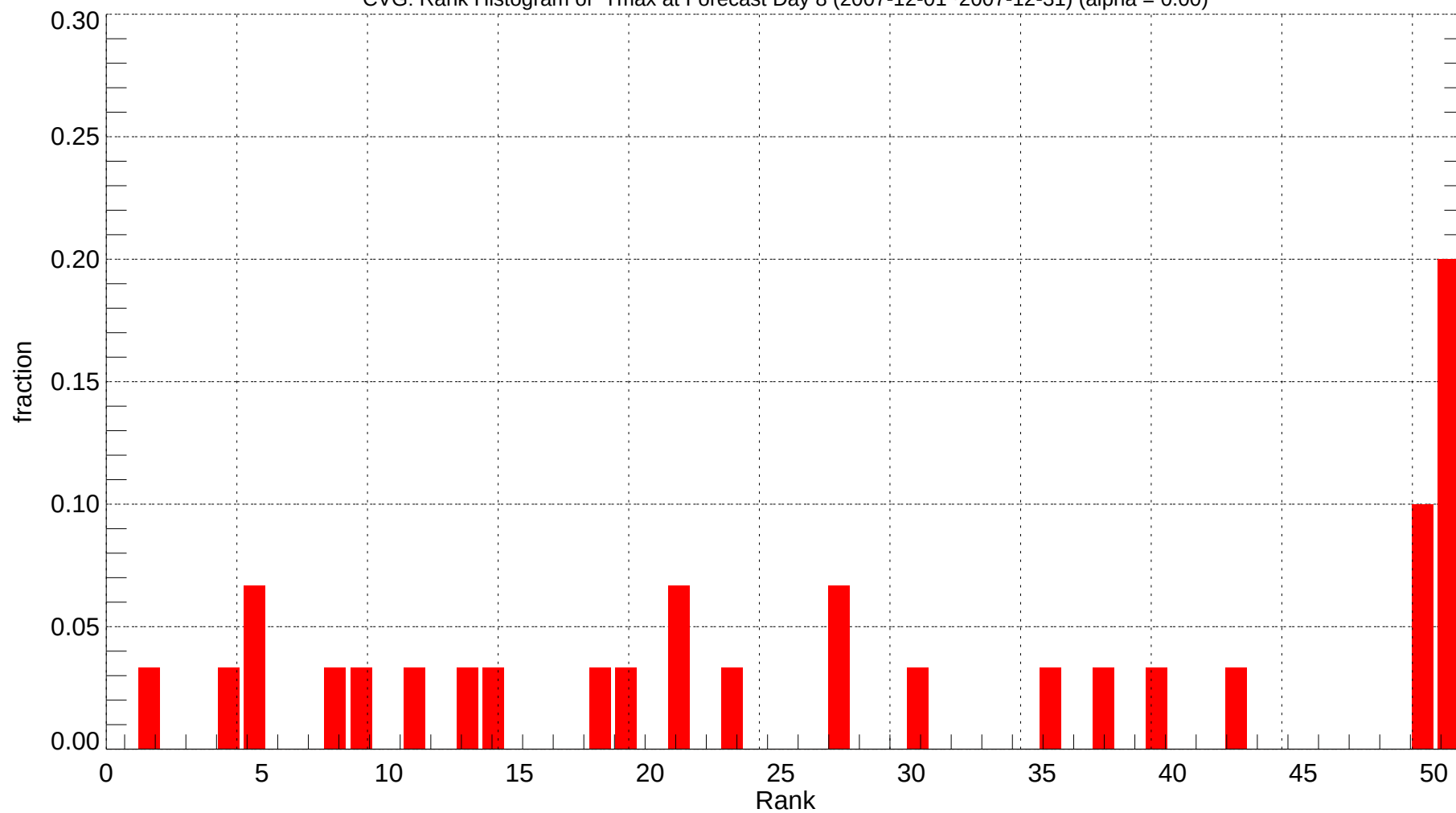
CVG: Rank Histogram of Tmax at Forecast Day 8 (2007-12-01~2007-12-31) (alpha = 0.00)
