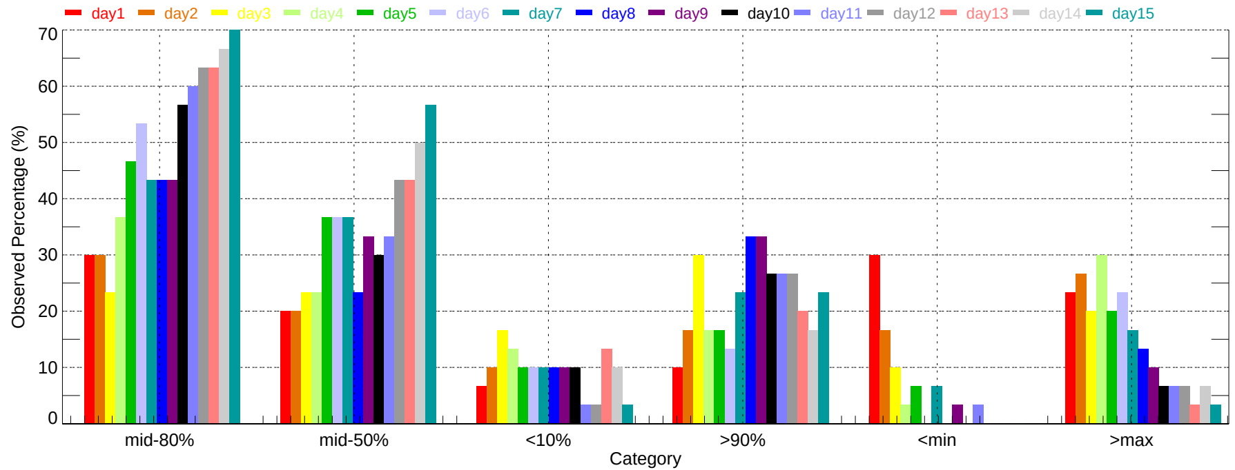
Observed Percentage of Ensembles - STL: Min Temperature (2007-12-01~2007-12-31)
