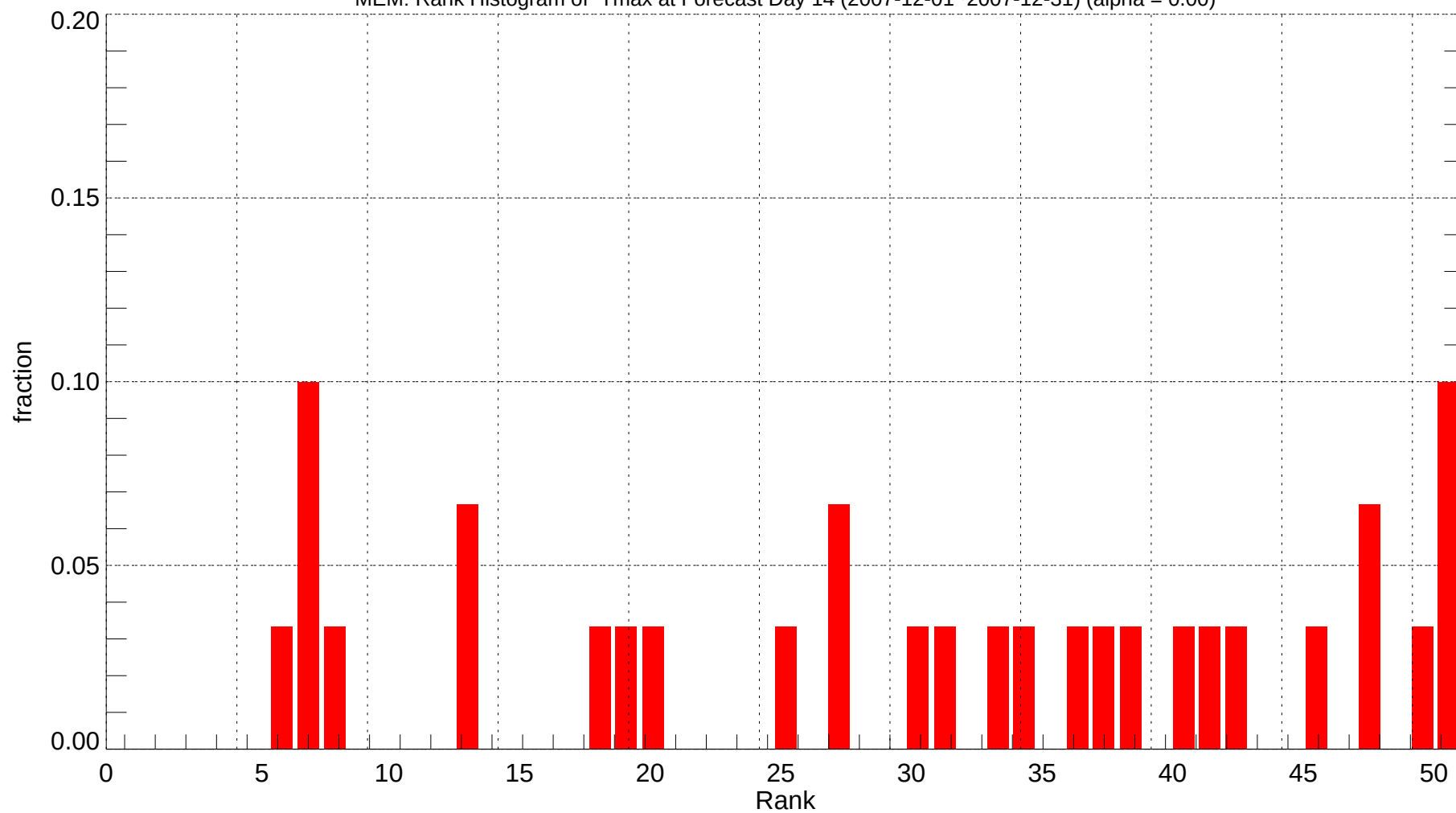
MEM: Rank Histogram of Tmax at Forecast Day 14 (2007-12-01~2007-12-31) (alpha = 0.00)
