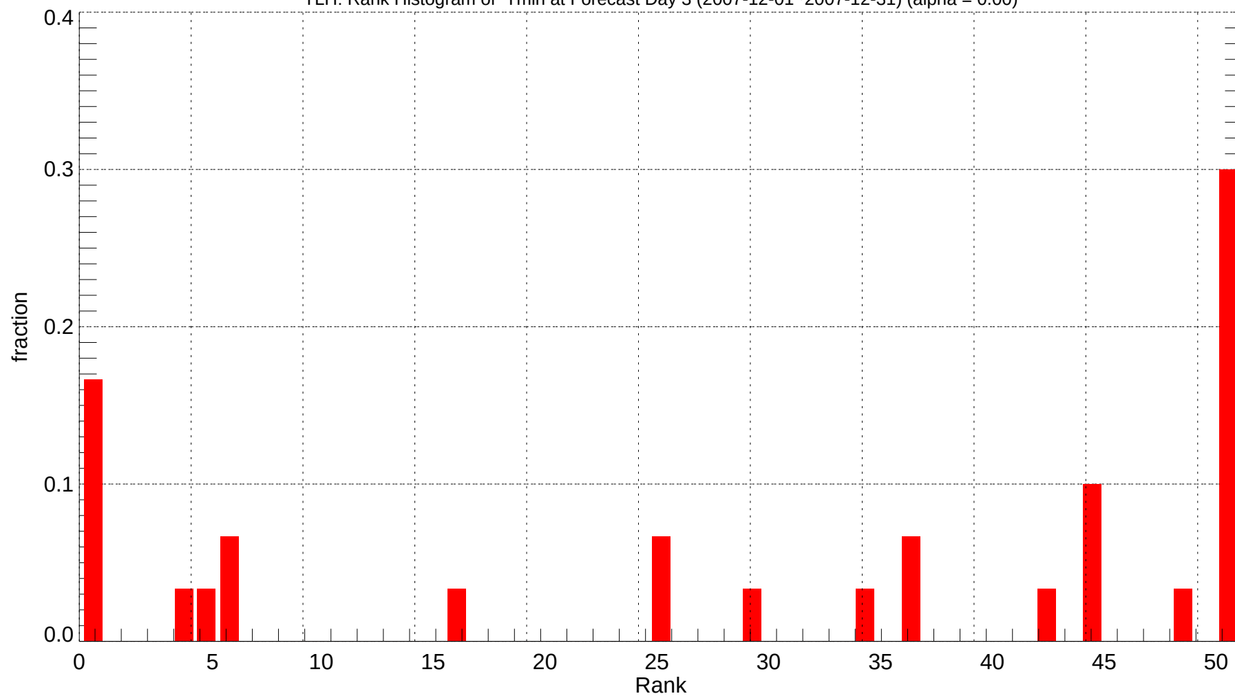
TLH: Rank Histogram of Tmin at Forecast Day 3 (2007-12-01~2007-12-31) (alpha = 0.00)
