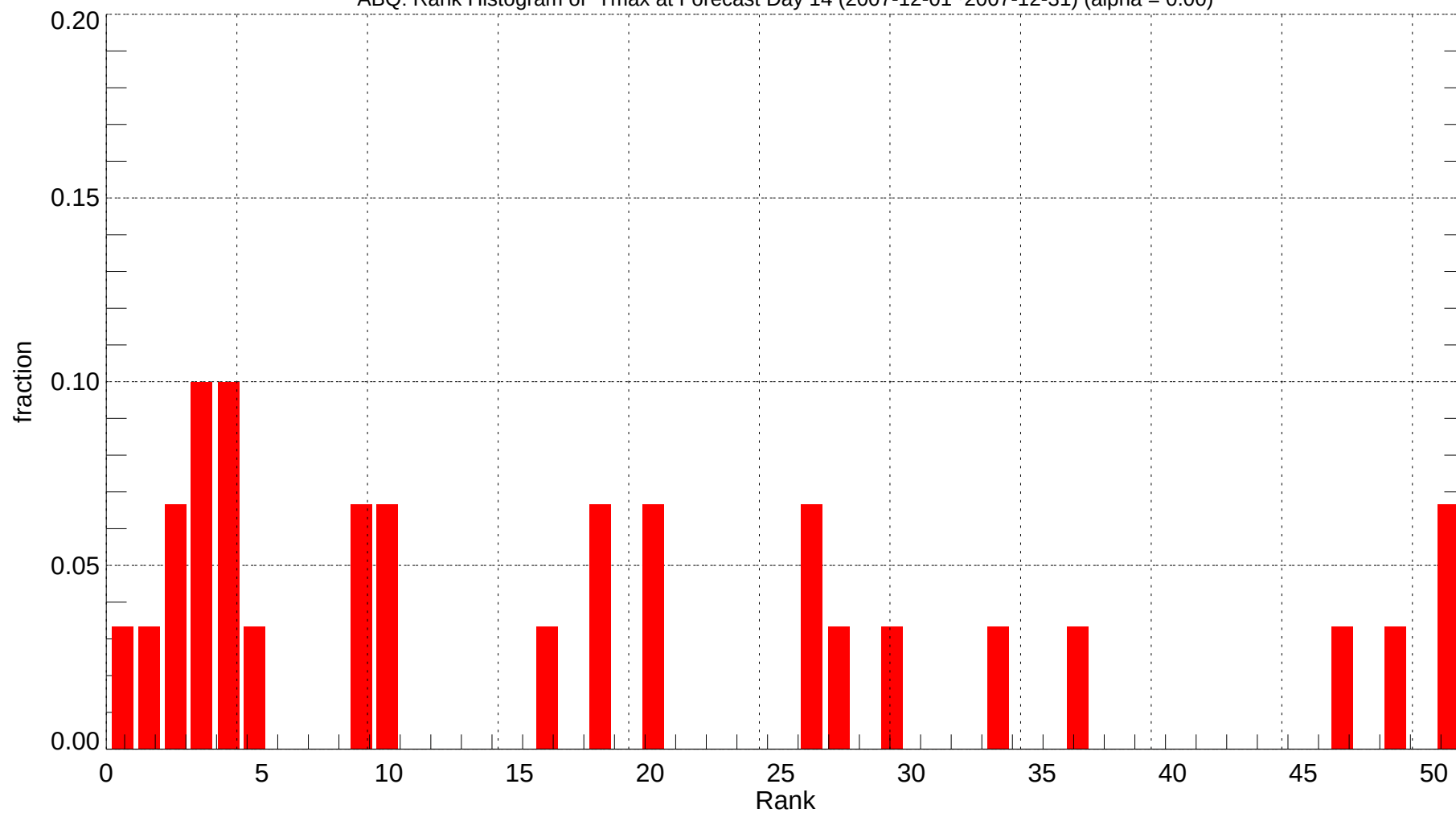
ABQ: Rank Histogram of Tmax at Forecast Day 14 (2007-12-01~2007-12-31) (alpha = 0.00)
