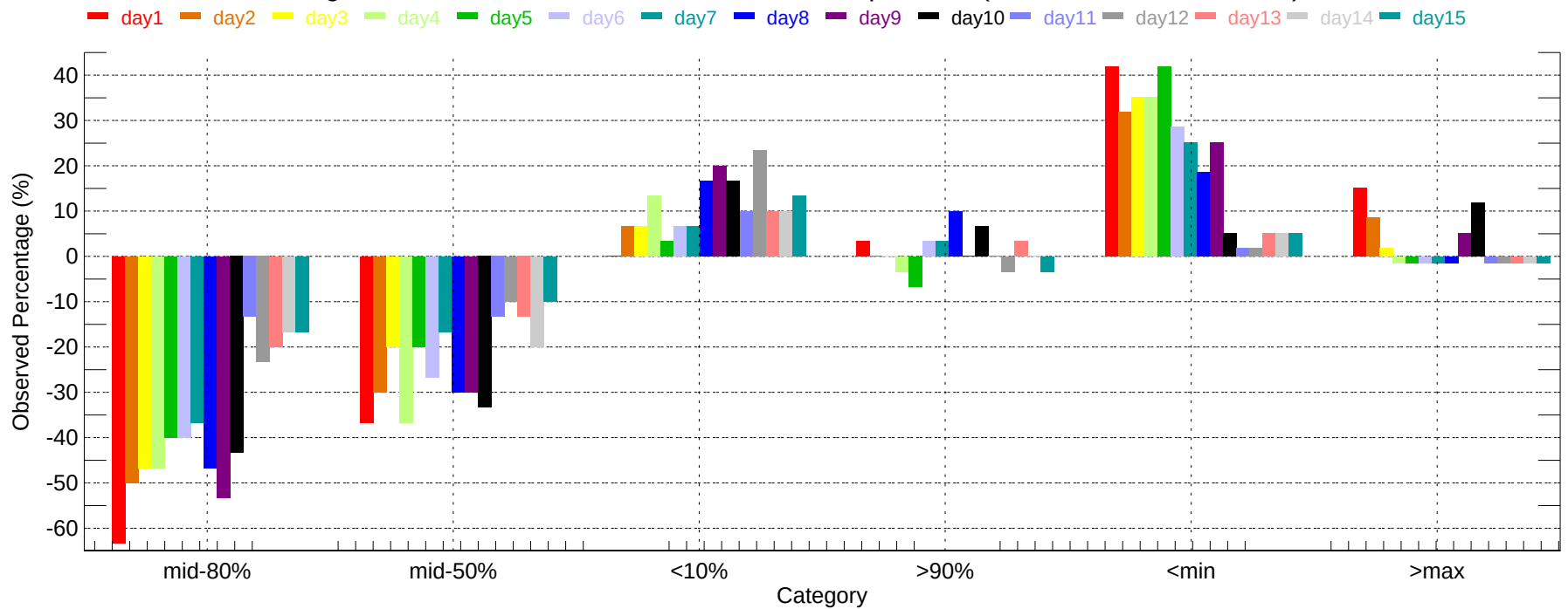
Observed Percentage Deviation of Ensembles - BDL: Max Temperature (2007-12-01~2007-12-31)
