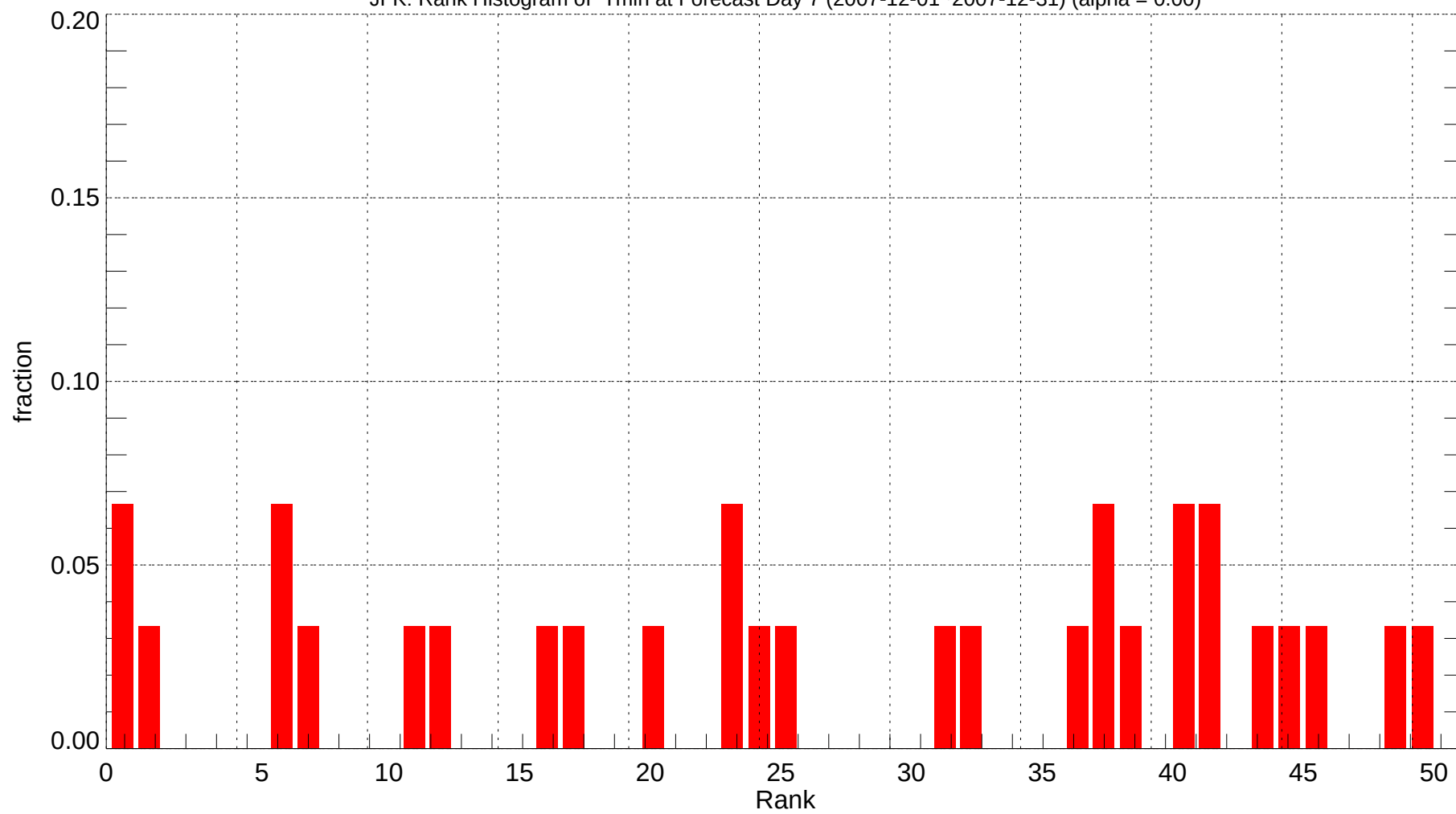
JFK: Rank Histogram of Tmin at Forecast Day 7 (2007-12-01~2007-12-31) (alpha = 0.00)
