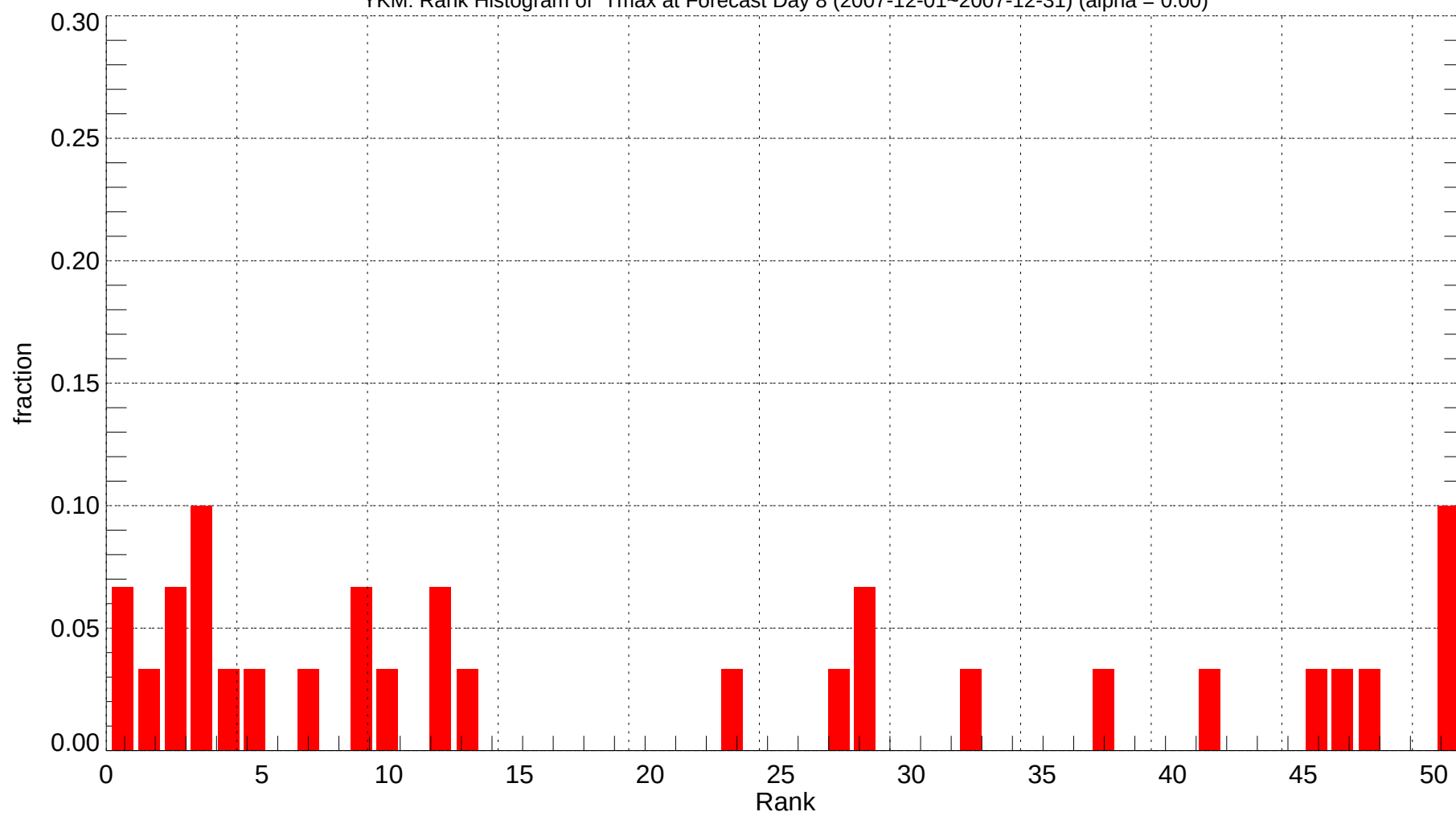
YKM: Rank Histogram of Tmax at Forecast Day 8 (2007-12-01~2007-12-31) (alpha = 0.00)
