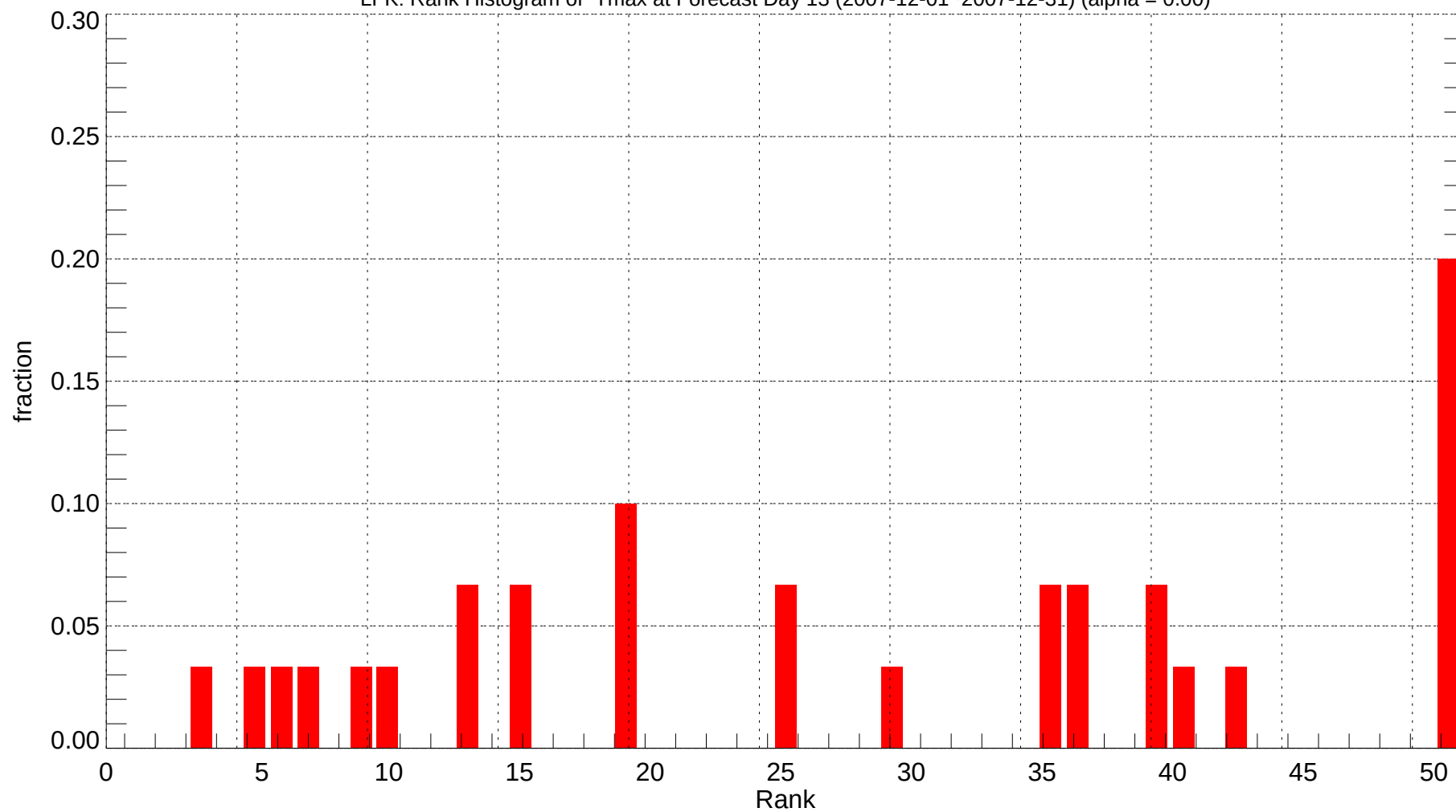
LFK: Rank Histogram of Tmax at Forecast Day 13 (2007-12-01~2007-12-31) (alpha = 0.00)
