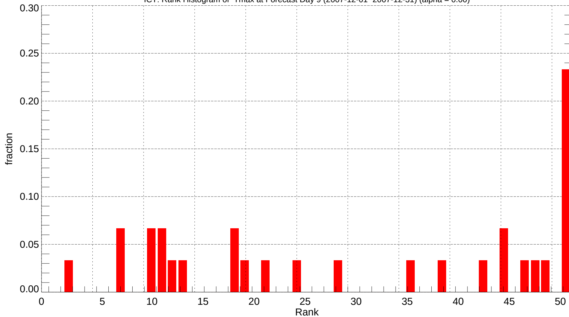
ICT: Rank Histogram of Tmax at Forecast Day 9 (2007-12-01~2007-12-31) (alpha = 0.00)
