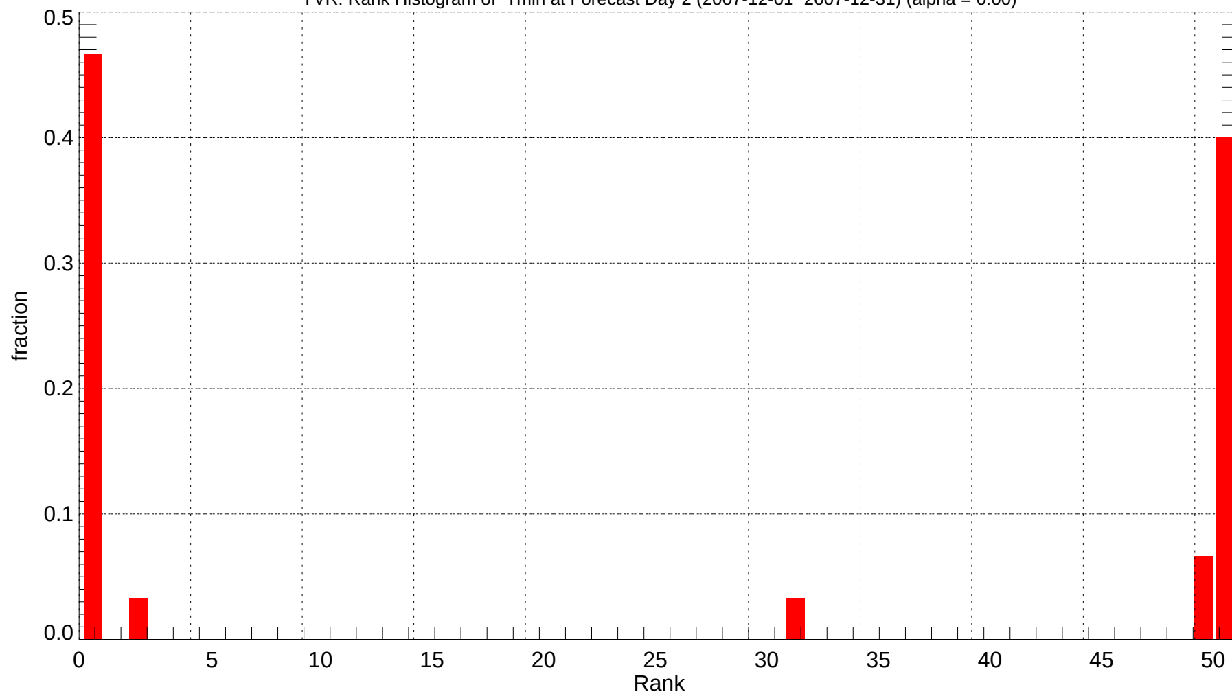
YVR: Rank Histogram of Tmin at Forecast Day 2 (2007-12-01~2007-12-31) (alpha = 0.00)
