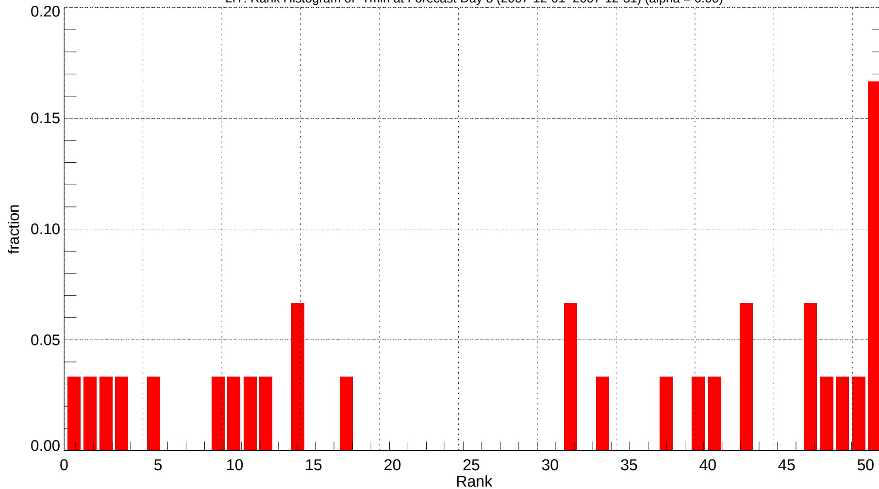
LIT: Rank Histogram of Tmin at Forecast Day 8 (2007-12-01~2007-12-31) (alpha = 0.00)
