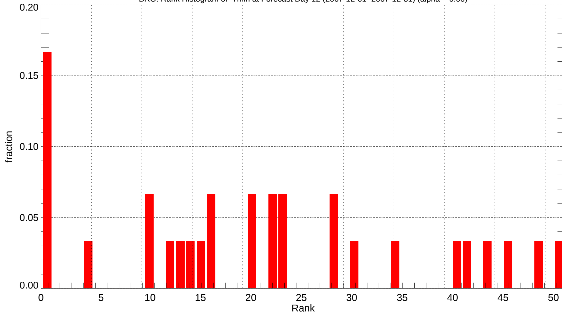
BRO: Rank Histogram of Tmin at Forecast Day 12 (2007-12-01~2007-12-31) (alpha = 0.00)
