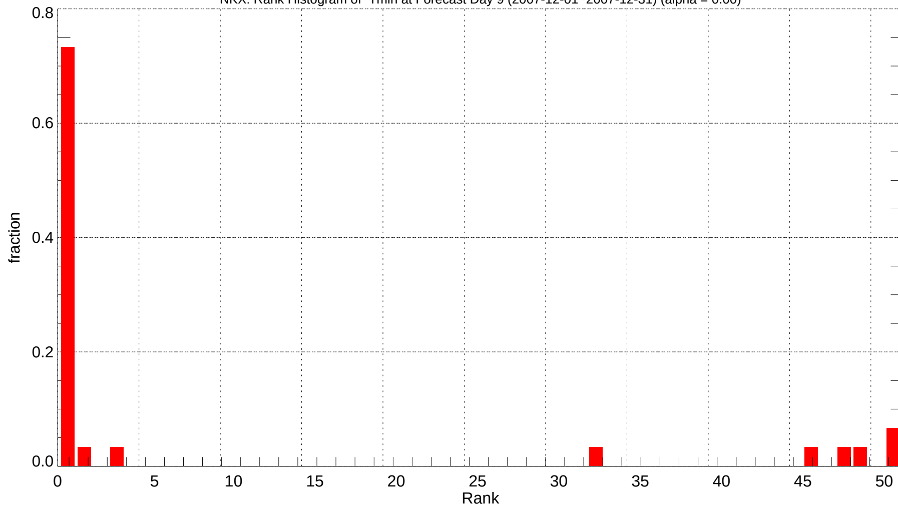
NKX: Rank Histogram of Tmin at Forecast Day 9 (2007-12-01~2007-12-31) (alpha = 0.00)
