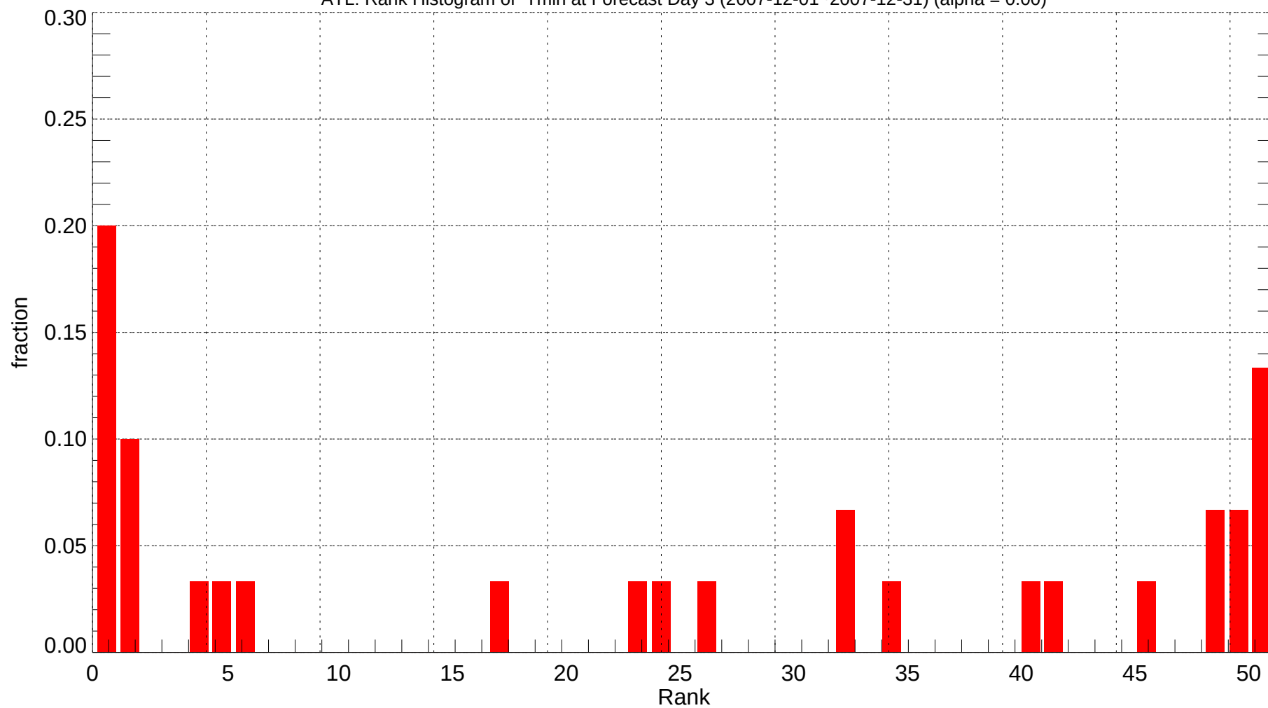
ATL: Rank Histogram of Tmin at Forecast Day 3 (2007-12-01~2007-12-31) (alpha = 0.00)
