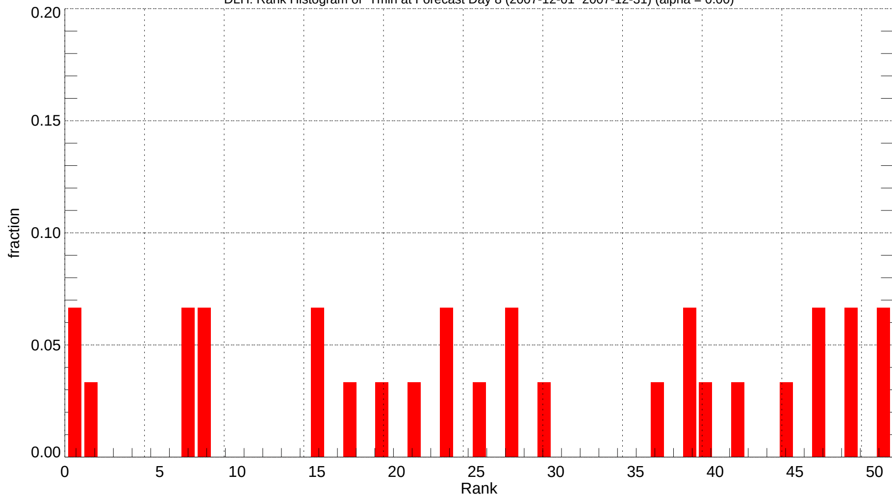
DLH: Rank Histogram of Tmin at Forecast Day 8 (2007-12-01~2007-12-31) (alpha = 0.00)
