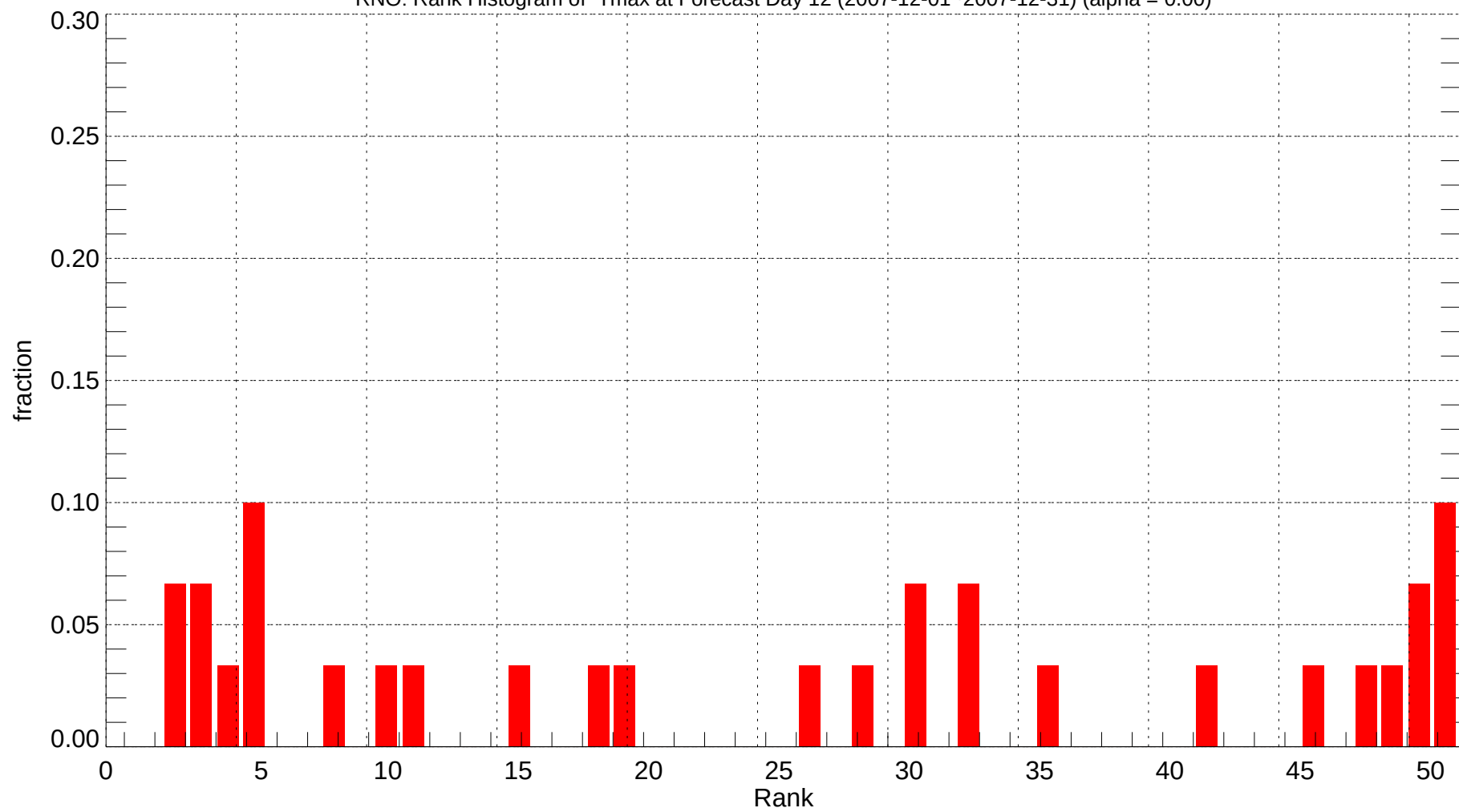
RNO: Rank Histogram of Tmax at Forecast Day 12 (2007-12-01~2007-12-31) (alpha = 0.00)
