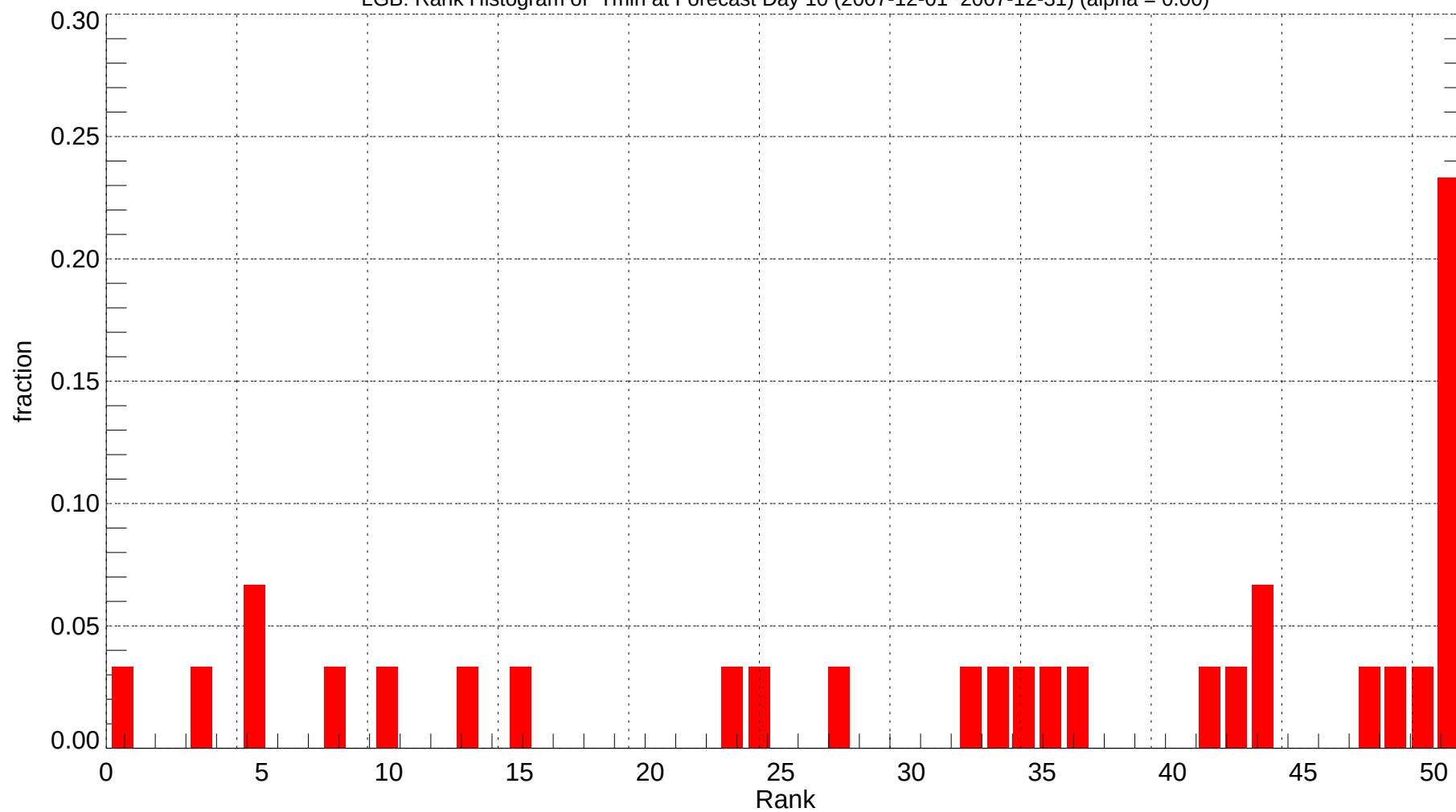
LGB: Rank Histogram of Tmin at Forecast Day 10 (2007-12-01~2007-12-31) (alpha = 0.00)
