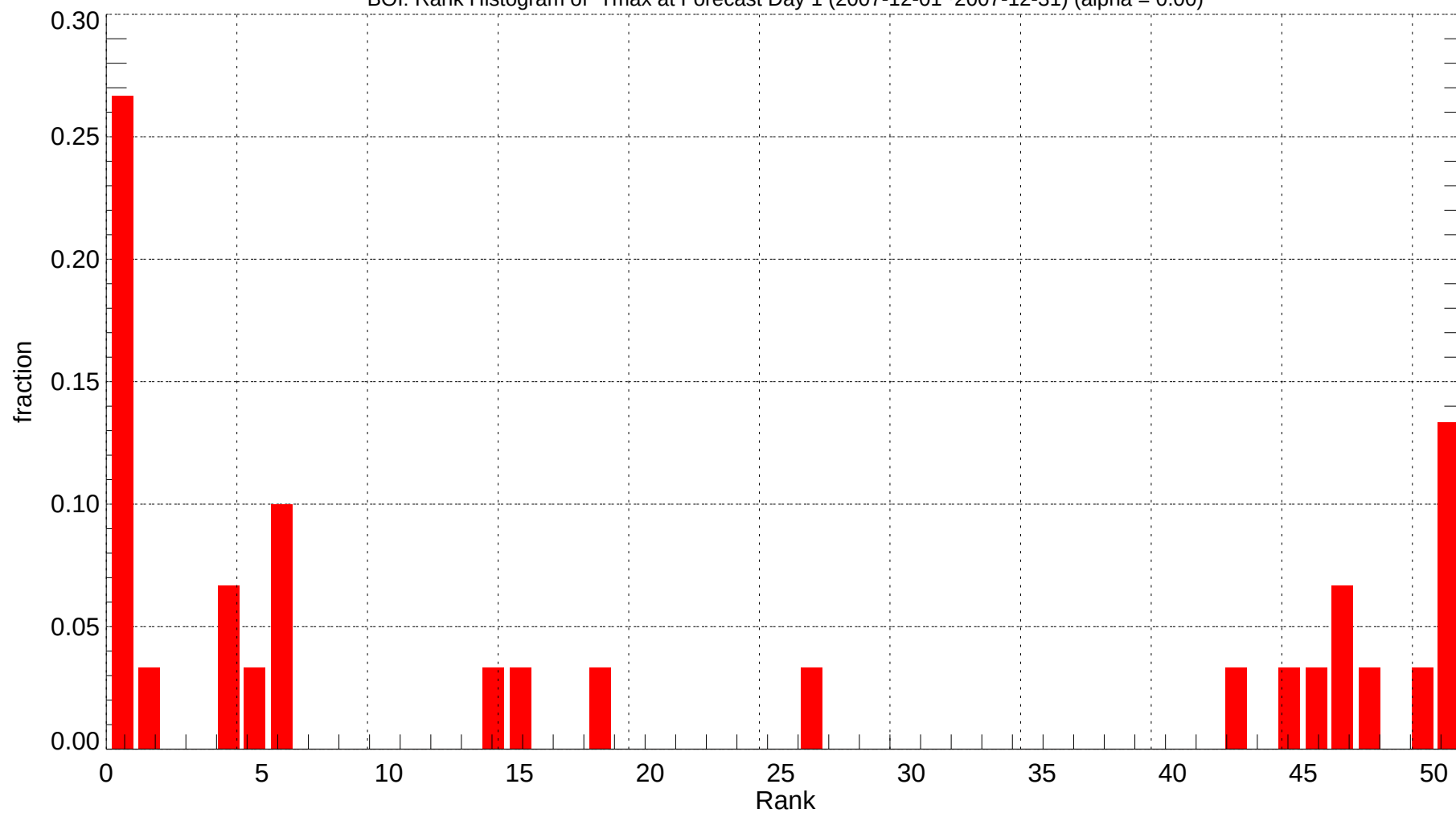
BOI: Rank Histogram of Tmax at Forecast Day 1 (2007-12-01~2007-12-31) (alpha = 0.00)
