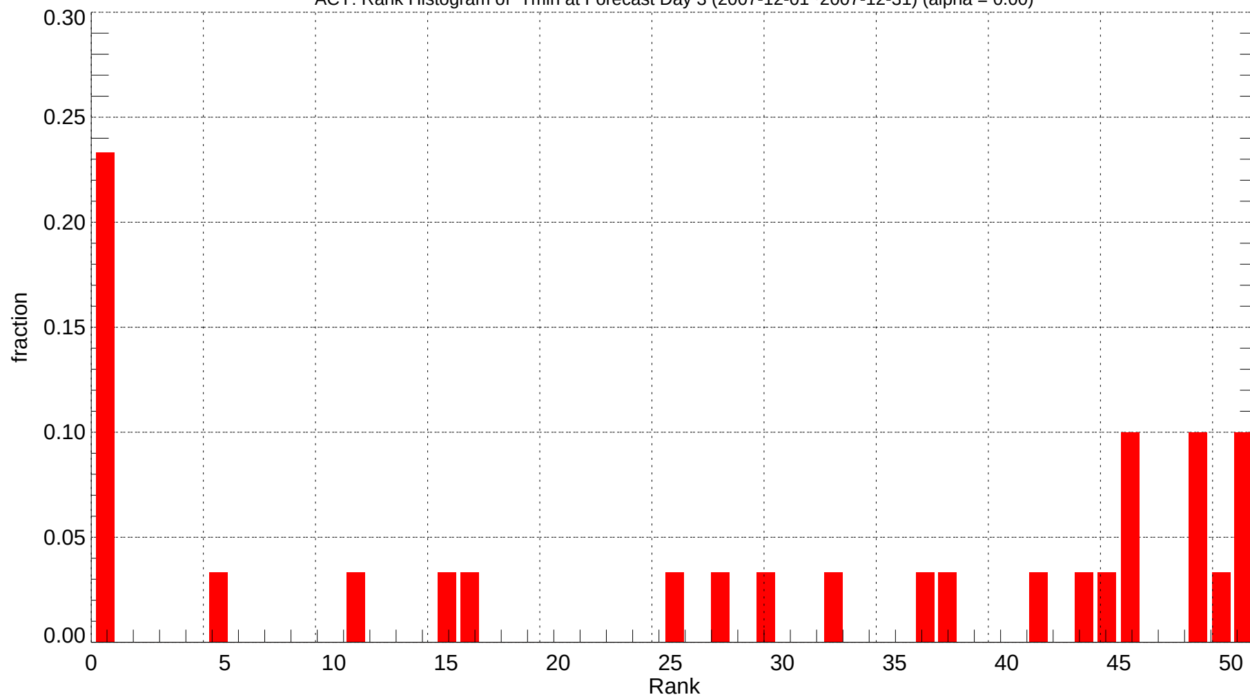
ACY: Rank Histogram of Tmin at Forecast Day 3 (2007-12-01~2007-12-31) (alpha = 0.00)
