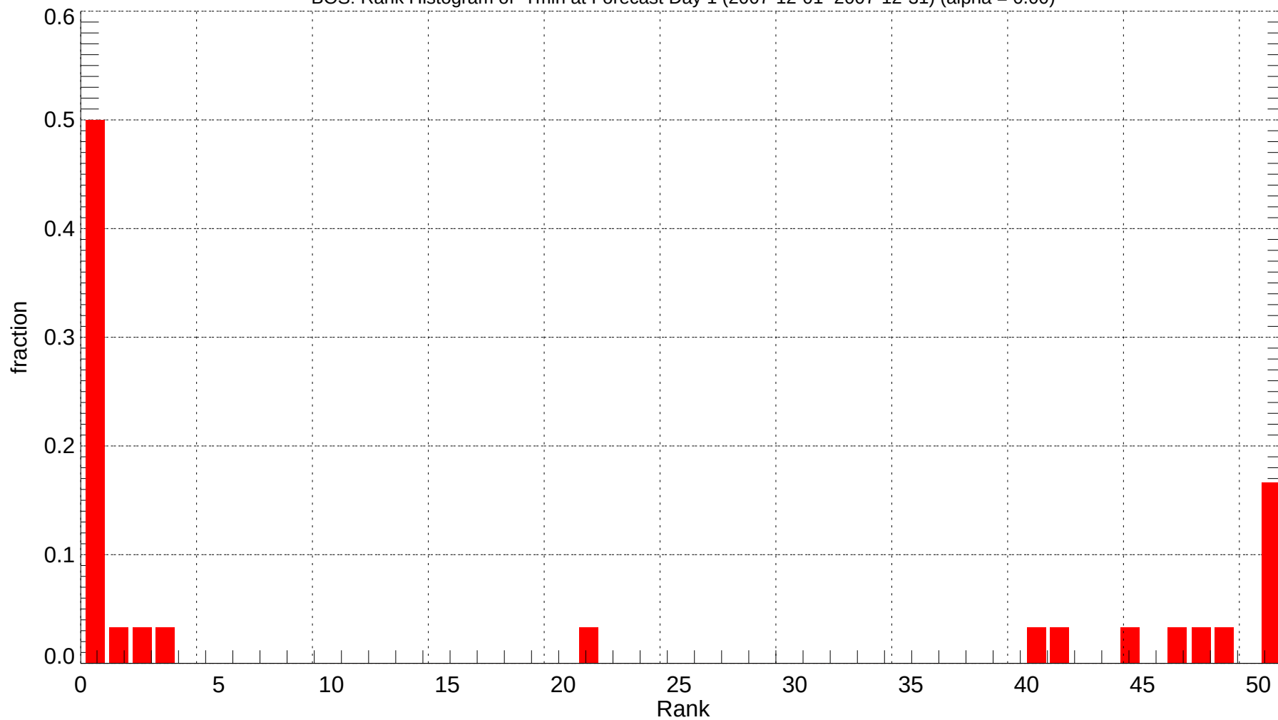
BOS: Rank Histogram of Tmin at Forecast Day 1 (2007-12-01~2007-12-31) (alpha = 0.00)
