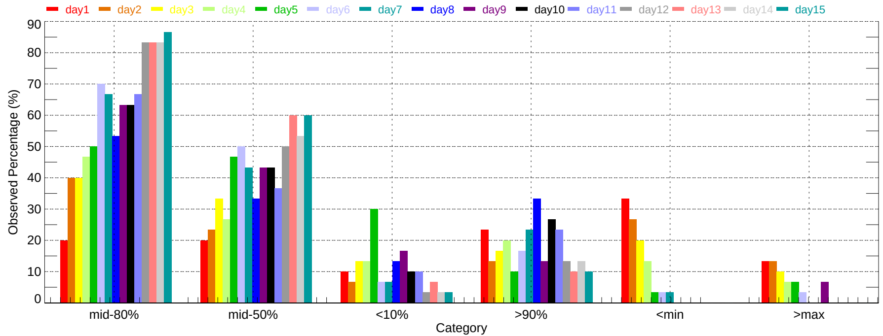
Observed Percentage of Ensembles - JFK: Min Temperature (2007-12-01~2007-12-31)
