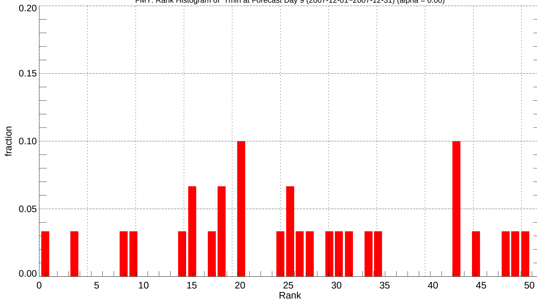
FMY: Rank Histogram of Tmin at Forecast Day 9 (2007-12-01~2007-12-31) (alpha = 0.00)
