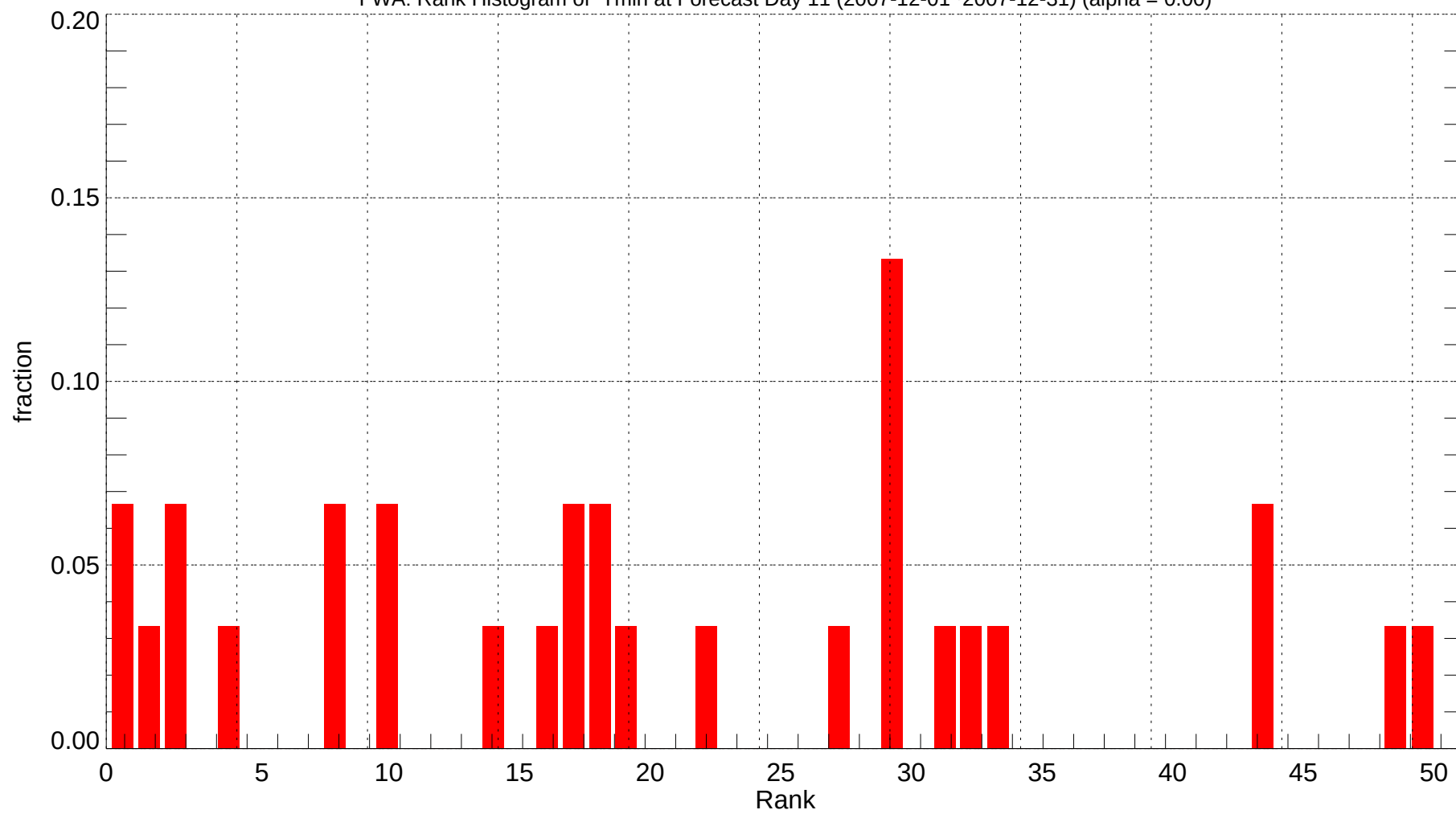
FWA: Rank Histogram of Tmin at Forecast Day 11 (2007-12-01~2007-12-31) (alpha = 0.00)
