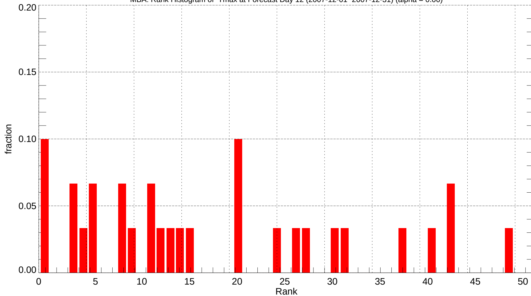
MBA: Rank Histogram of Tmax at Forecast Day 12 (2007-12-01~2007-12-31) (alpha = 0.00)
