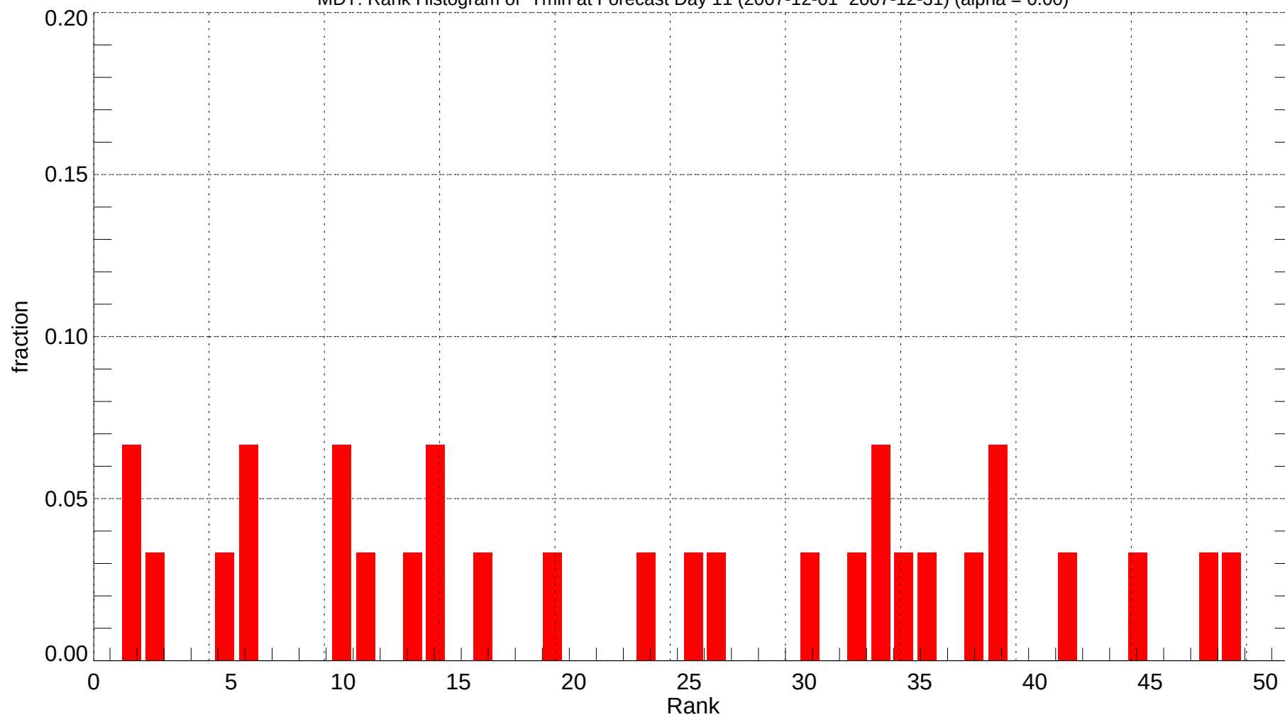
MDT: Rank Histogram of Tmin at Forecast Day 11 (2007-12-01~2007-12-31) (alpha = 0.00)
