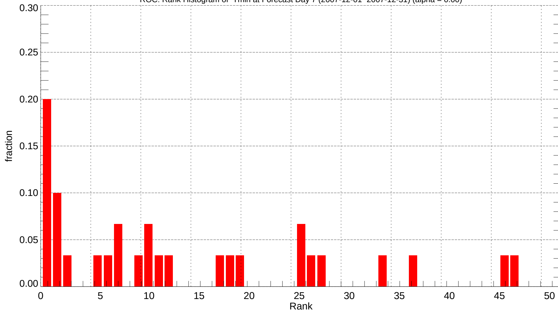
ROC: Rank Histogram of Tmin at Forecast Day 7 (2007-12-01~2007-12-31) (alpha = 0.00)
