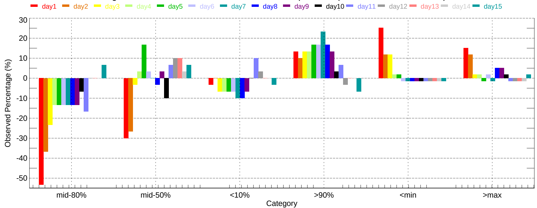
Observed Percentage Deviation of Ensembles - LGA: Max Temperature (2007-12-01~2007-12-31)
