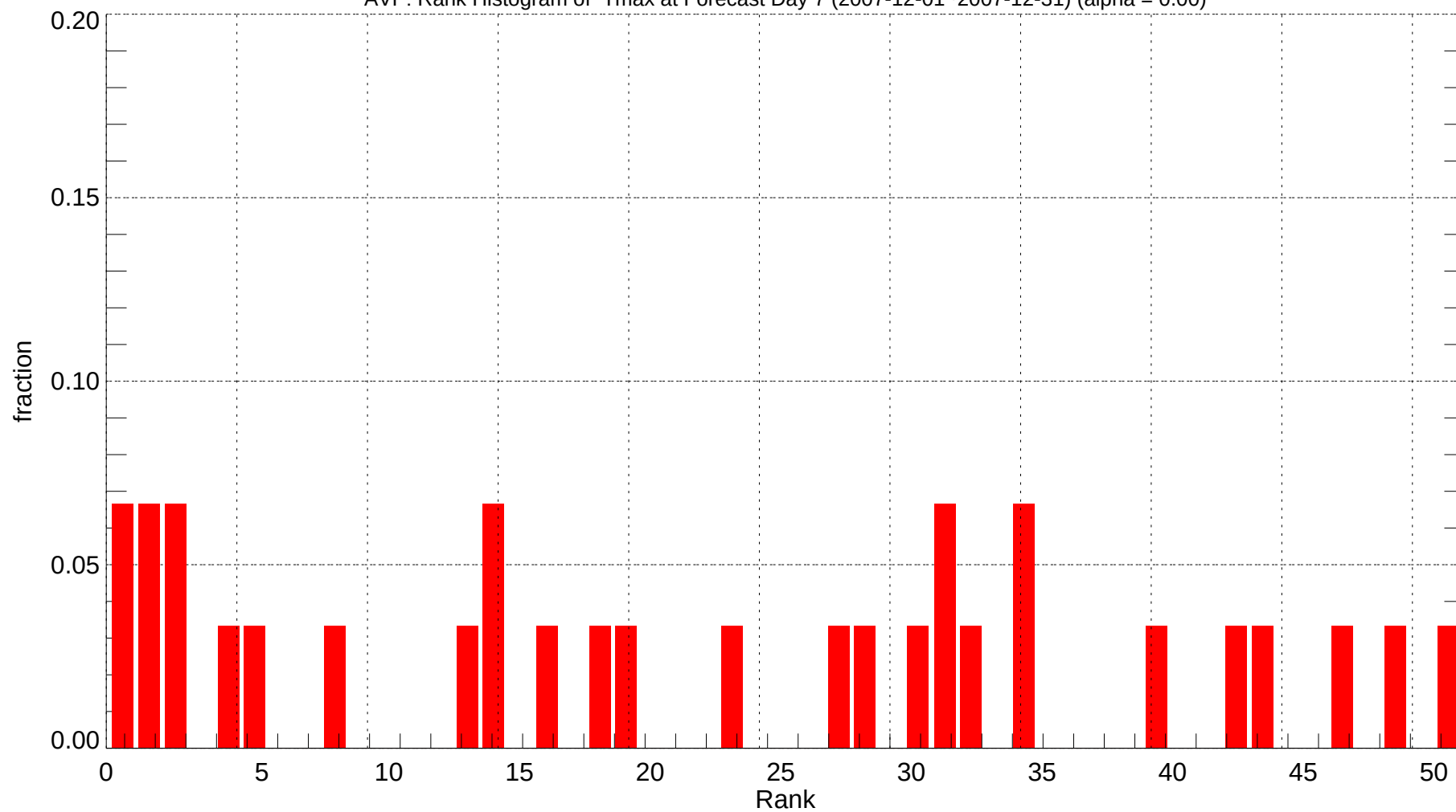
AVP: Rank Histogram of Tmax at Forecast Day 7 (2007-12-01~2007-12-31) (alpha = 0.00)
