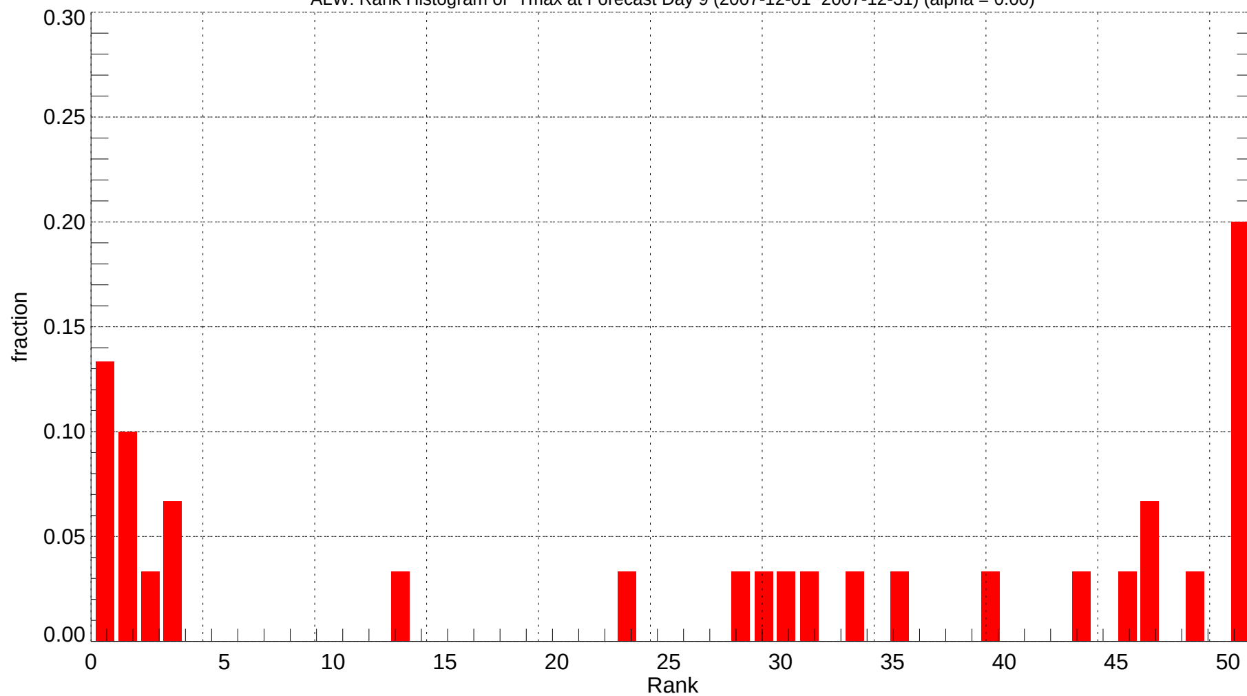
ALW: Rank Histogram of Tmax at Forecast Day 9 (2007-12-01~2007-12-31) (alpha = 0.00)
