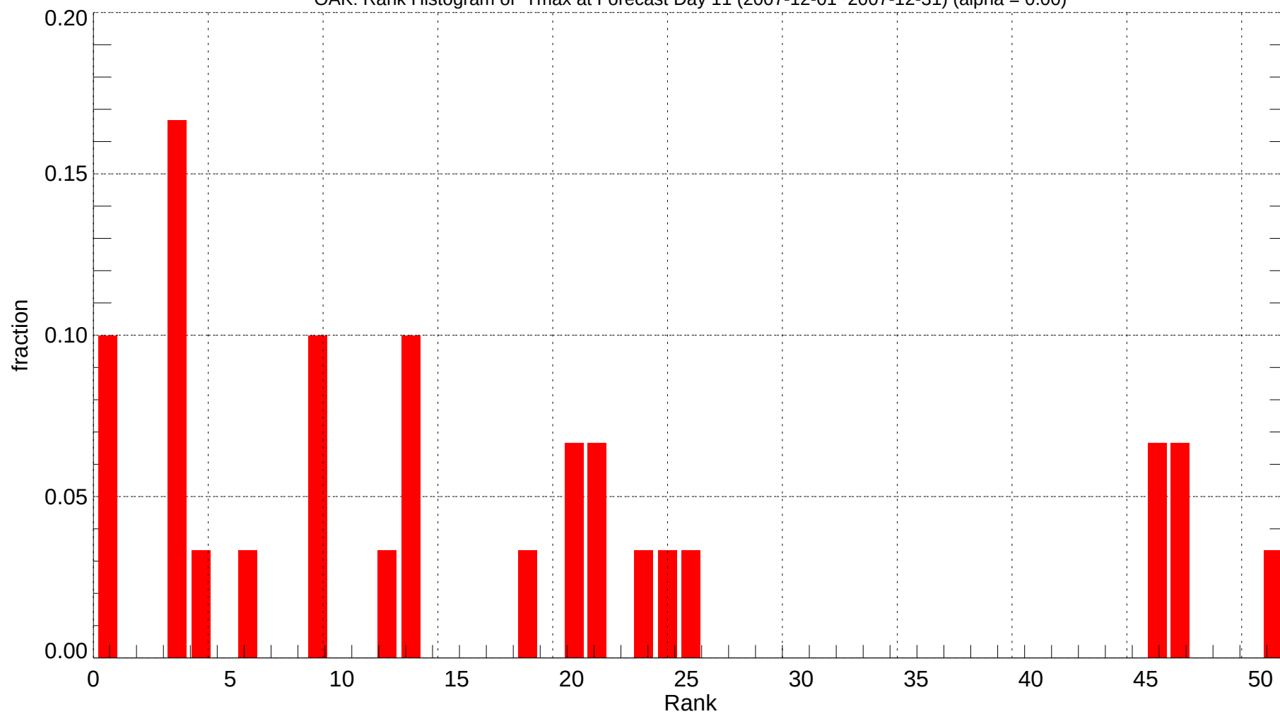
OAK: Rank Histogram of Tmax at Forecast Day 11 (2007-12-01~2007-12-31) (alpha = 0.00)
