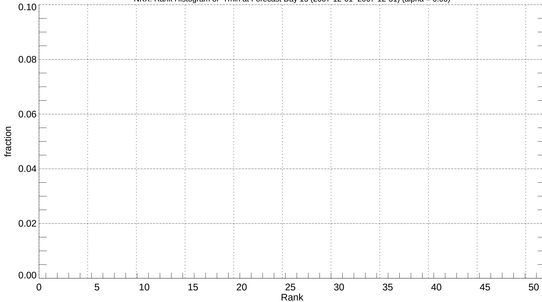
NKX: Rank Histogram of Tmin at Forecast Day 15 (2007-12-01~2007-12-31) (alpha = 0.00)
