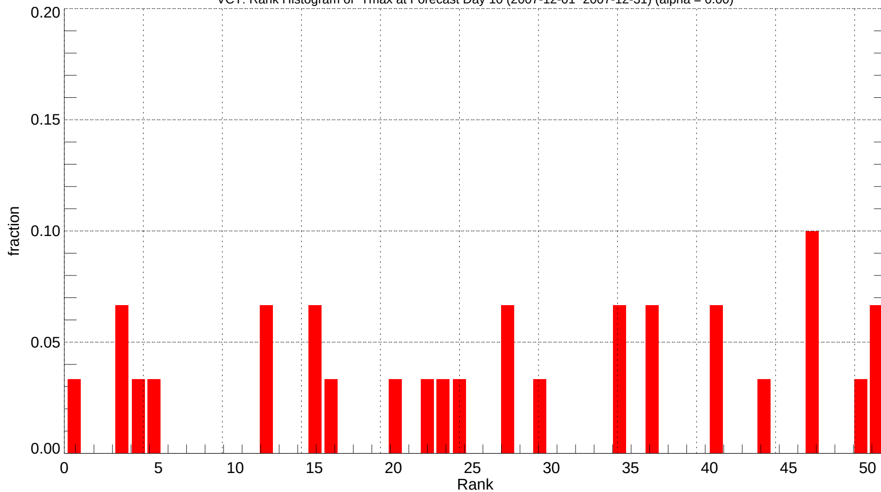
VCT: Rank Histogram of Tmax at Forecast Day 10 (2007-12-01~2007-12-31) (alpha = 0.00)
