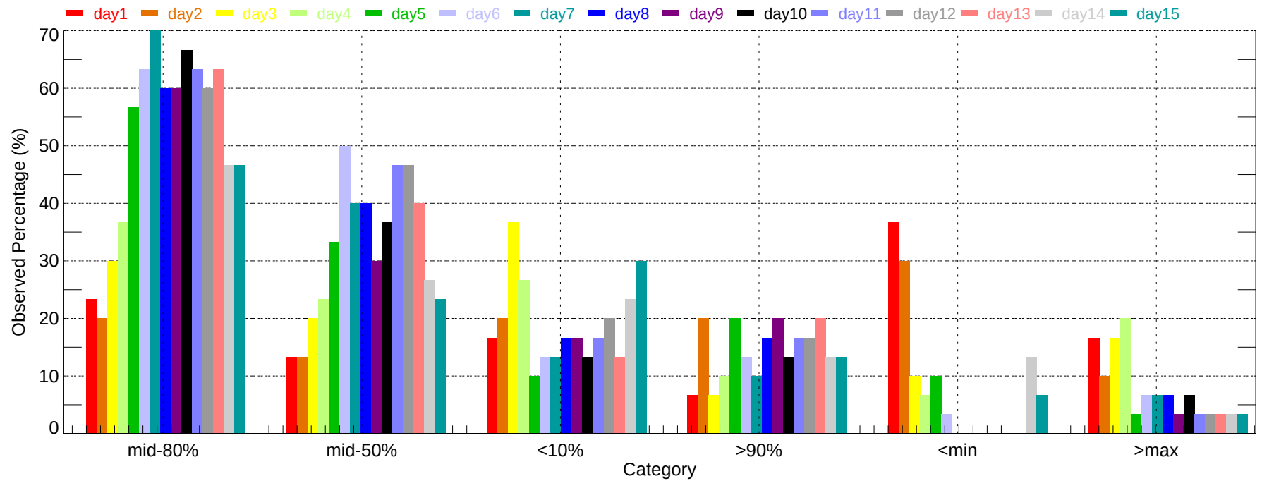
Observed Percentage of Ensembles - TUS: Max Temperature (2007-12-01~2007-12-31)
