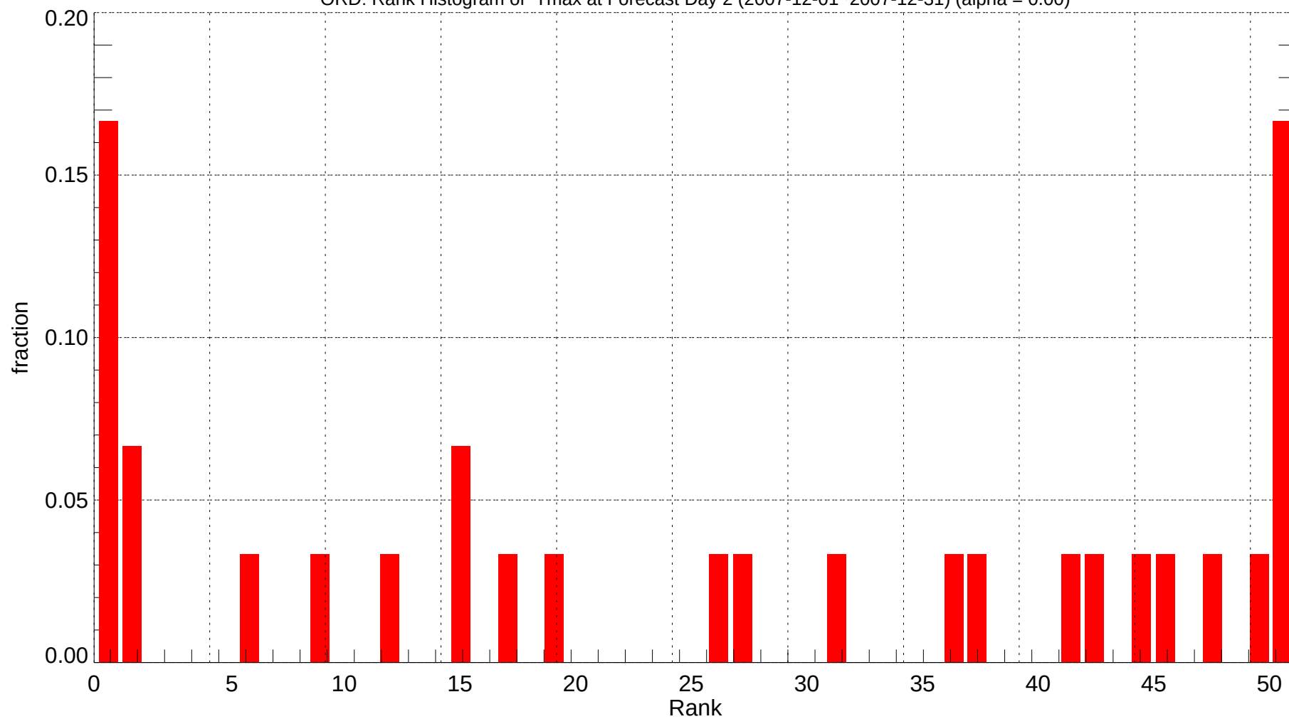
ORD: Rank Histogram of Tmax at Forecast Day 2 (2007-12-01~2007-12-31) (alpha = 0.00)
