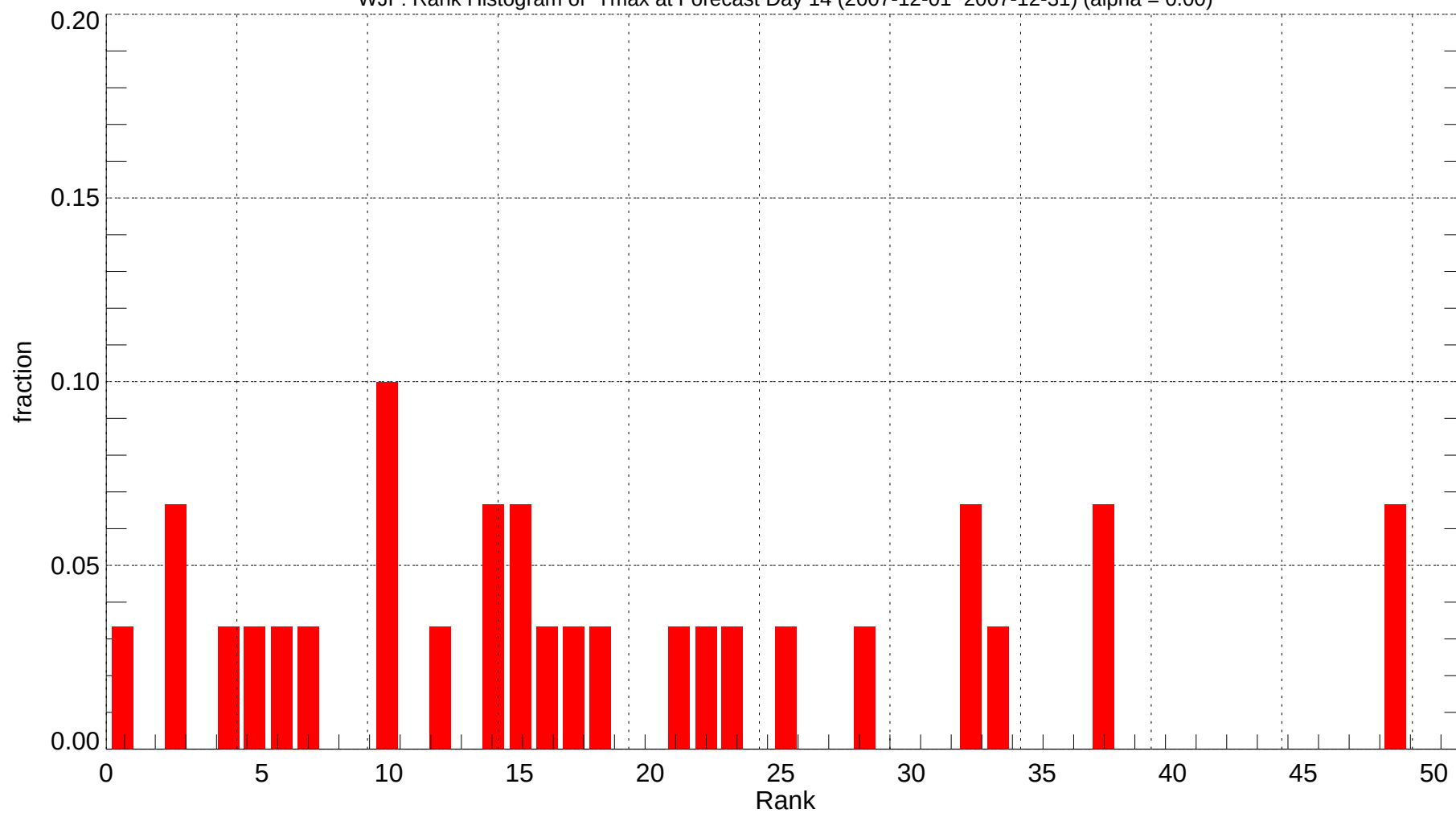
WJF: Rank Histogram of Tmax at Forecast Day 14 (2007-12-01~2007-12-31) (alpha = 0.00)
