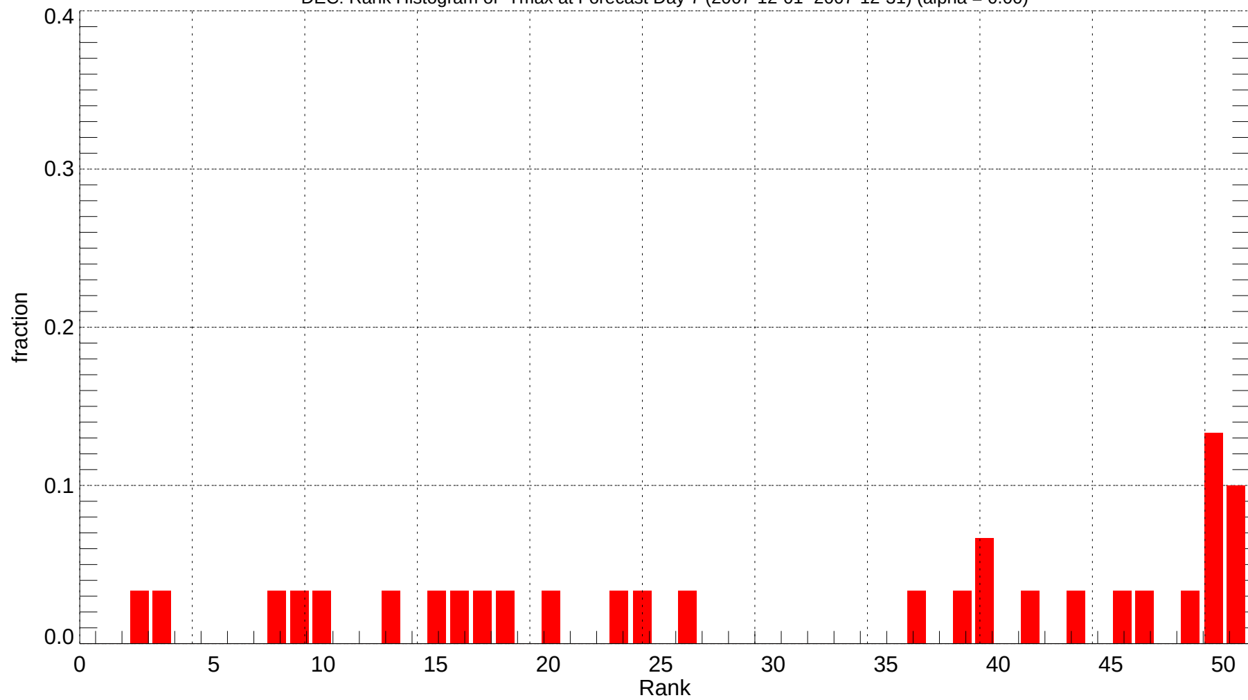
DEC: Rank Histogram of Tmax at Forecast Day 7 (2007-12-01~2007-12-31) (alpha = 0.00)
