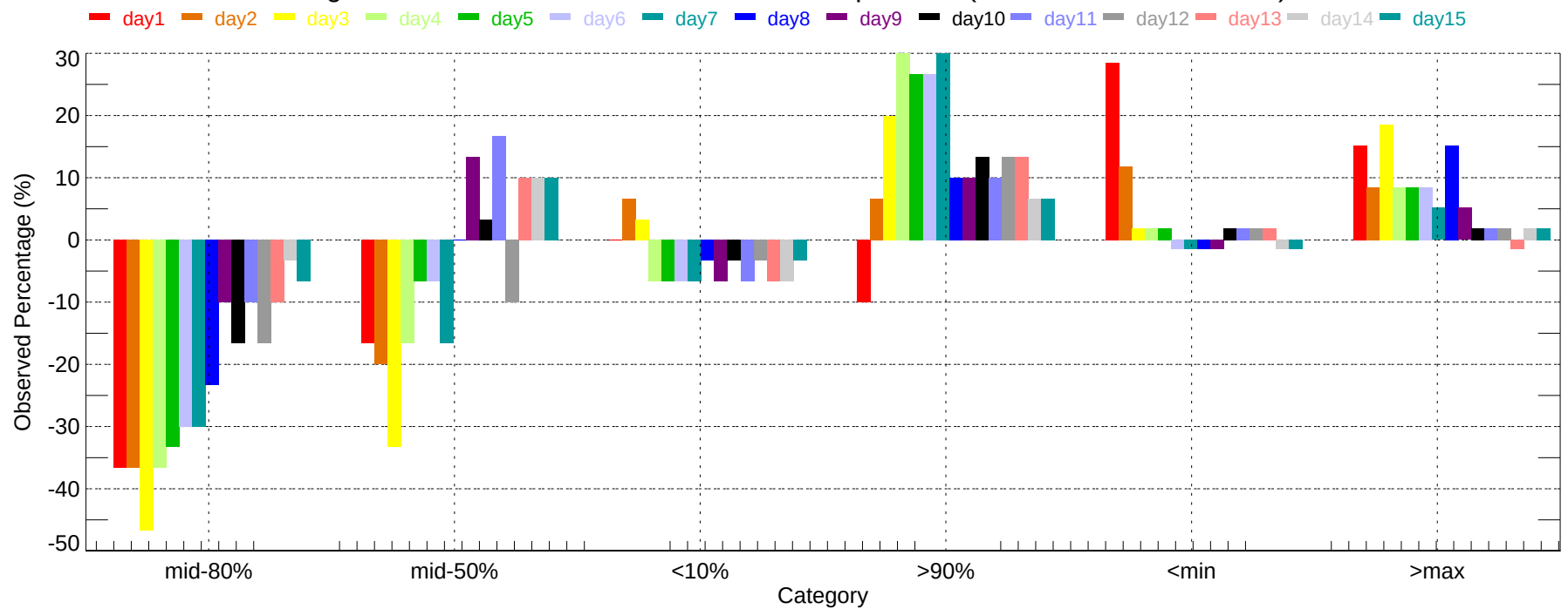
Observed Percentage Deviation of Ensembles - IND: Min Temperature (2007-12-01~2007-12-31)
