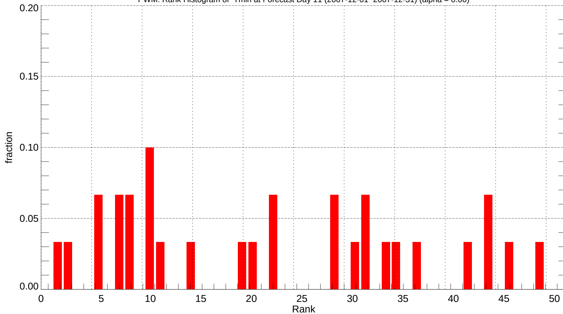
PWM: Rank Histogram of Tmin at Forecast Day 11 (2007-12-01~2007-12-31) (alpha = 0.00)
