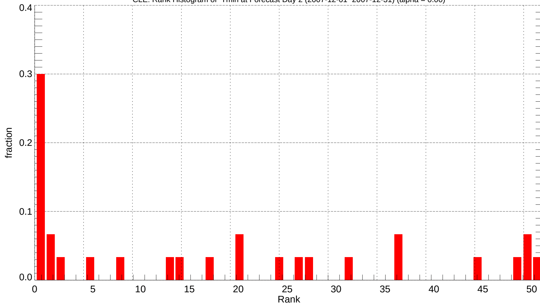
CLE: Rank Histogram of Tmin at Forecast Day 2 (2007-12-01~2007-12-31) (alpha = 0.00)
