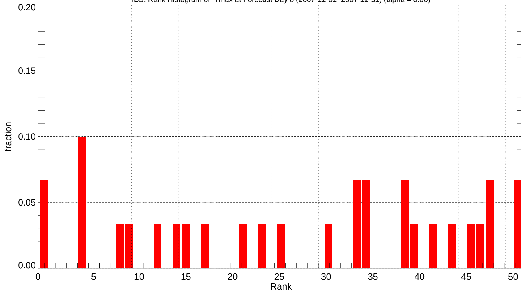
ILG: Rank Histogram of Tmax at Forecast Day 8 (2007-12-01~2007-12-31) (alpha = 0.00)
