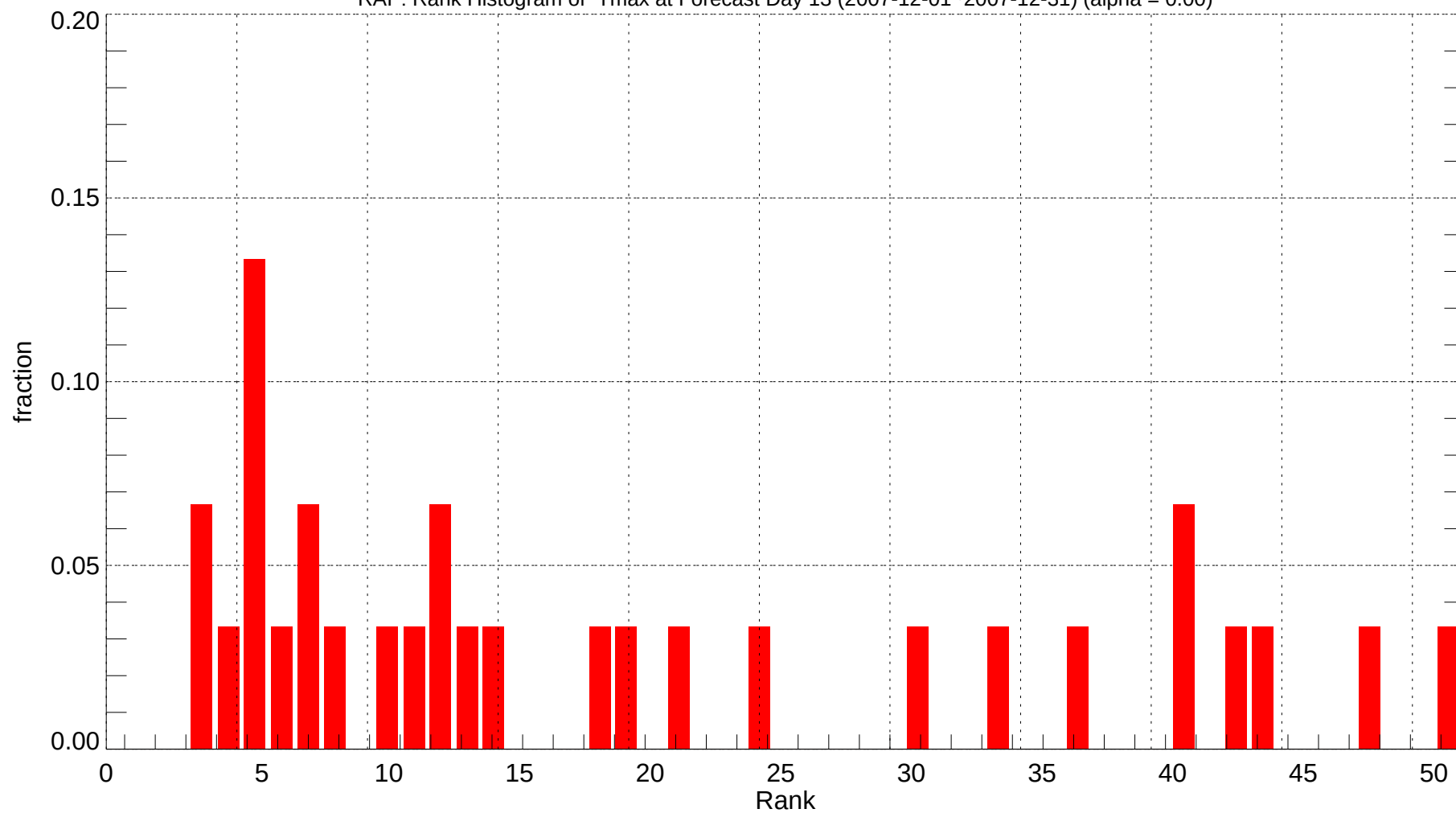
RAP: Rank Histogram of Tmax at Forecast Day 13 (2007-12-01~2007-12-31) (alpha = 0.00)
