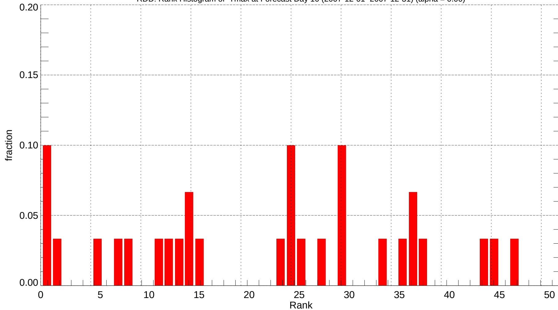
RDD: Rank Histogram of Tmax at Forecast Day 10 (2007-12-01~2007-12-31) (alpha = 0.00)
