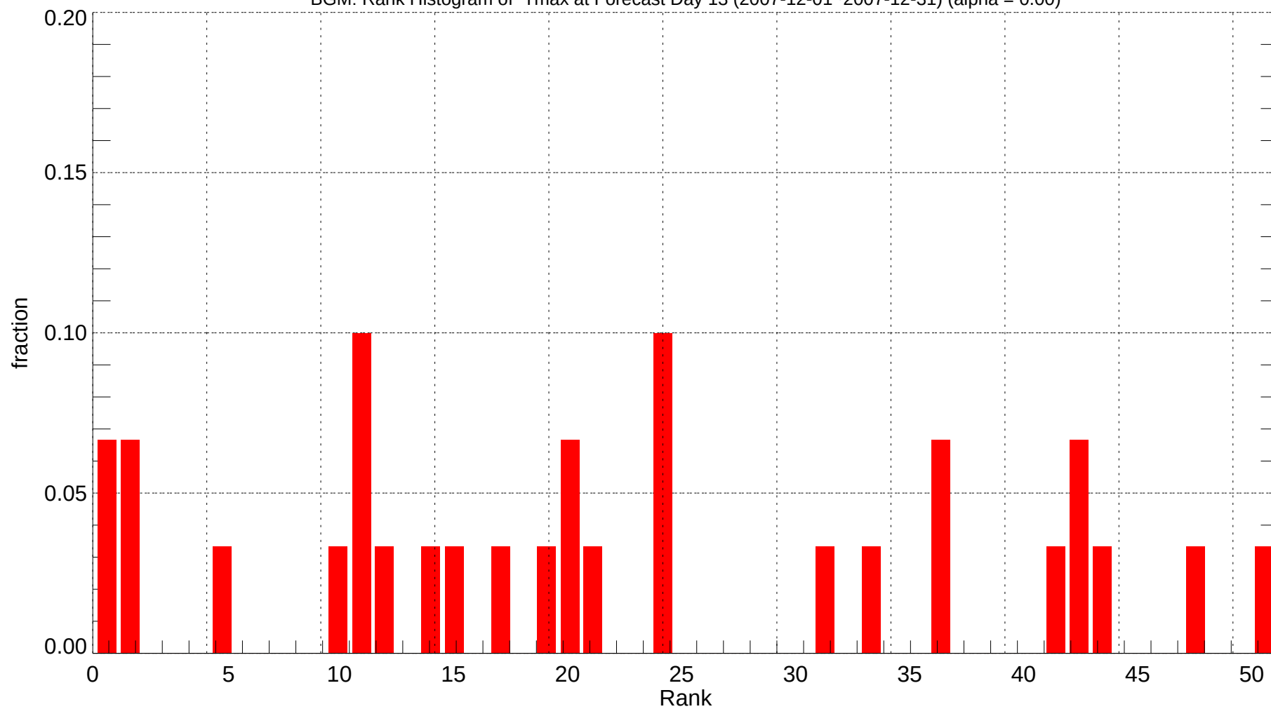
BGM: Rank Histogram of Tmax at Forecast Day 13 (2007-12-01~2007-12-31) (alpha = 0.00)
