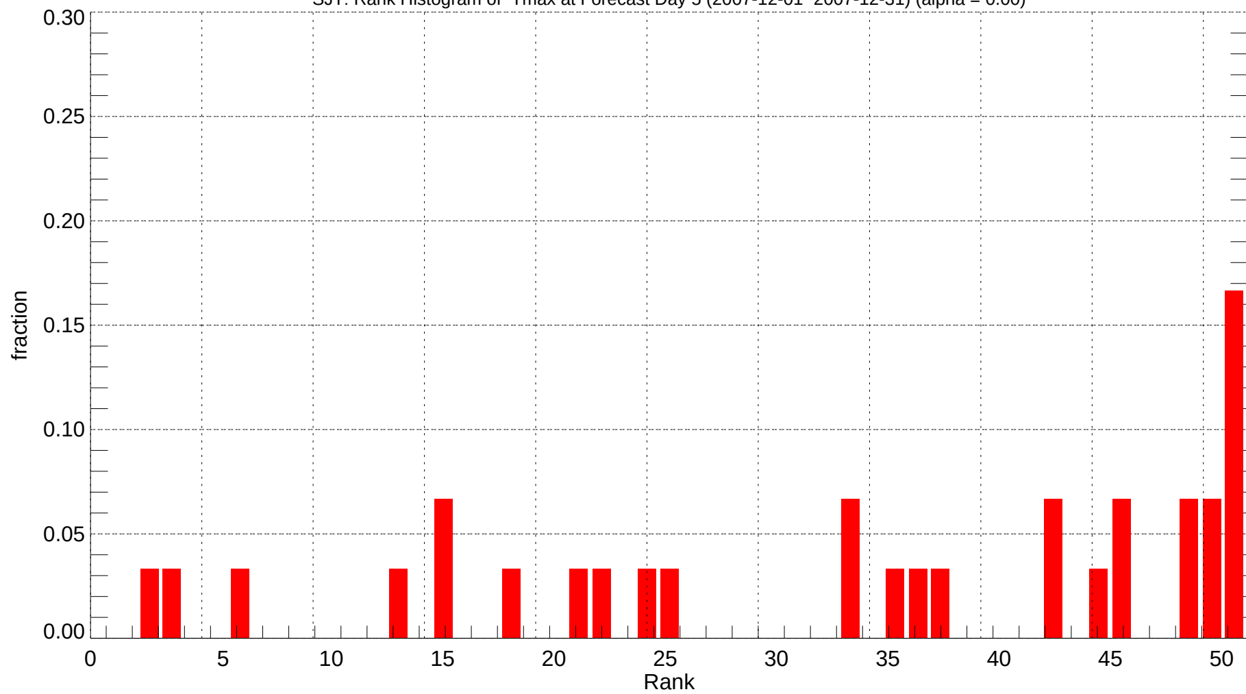
SJT: Rank Histogram of Tmax at Forecast Day 5 (2007-12-01~2007-12-31) (alpha = 0.00)
