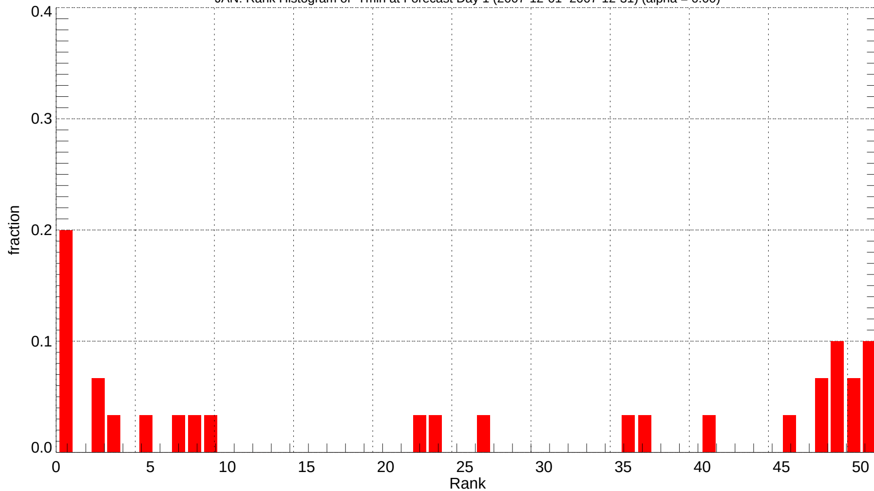
JAN: Rank Histogram of Tmin at Forecast Day 1 (2007-12-01~2007-12-31) (alpha = 0.00)
