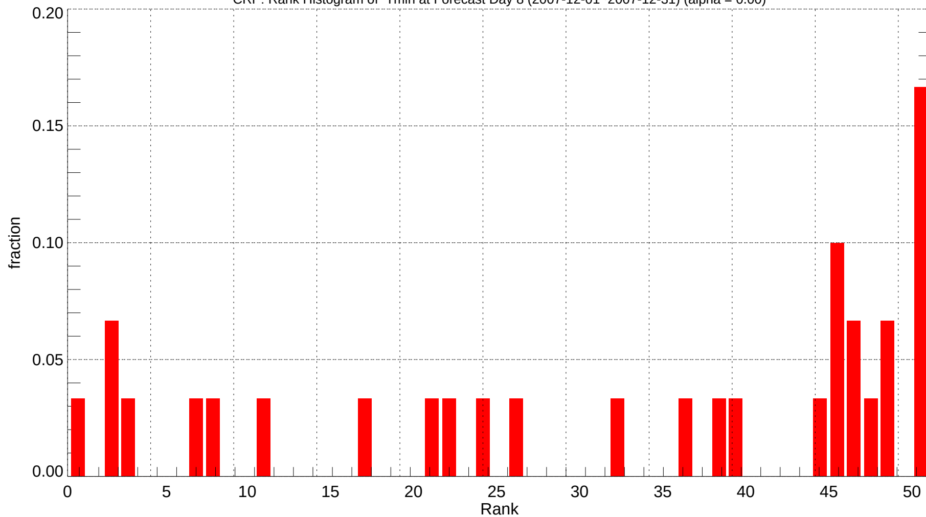
CRP: Rank Histogram of Tmin at Forecast Day 8 (2007-12-01~2007-12-31) (alpha = 0.00)
