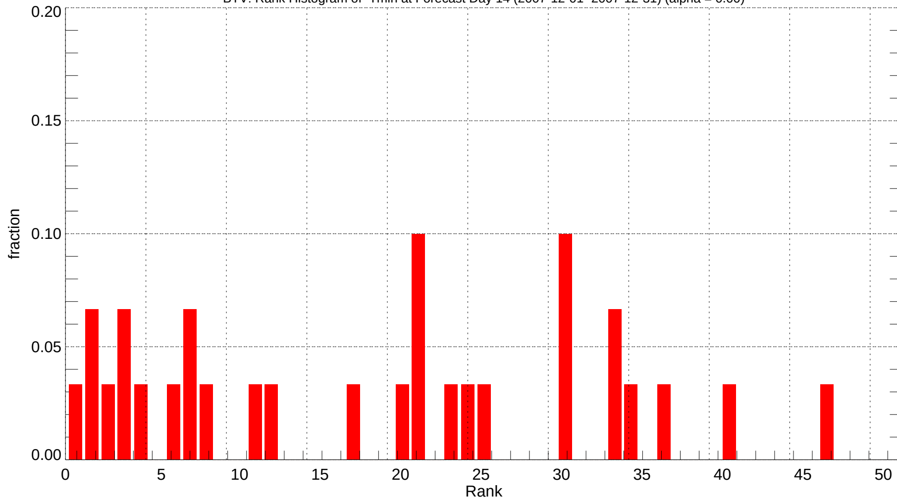
BTV: Rank Histogram of Tmin at Forecast Day 14 (2007-12-01~2007-12-31) (alpha = 0.00)
