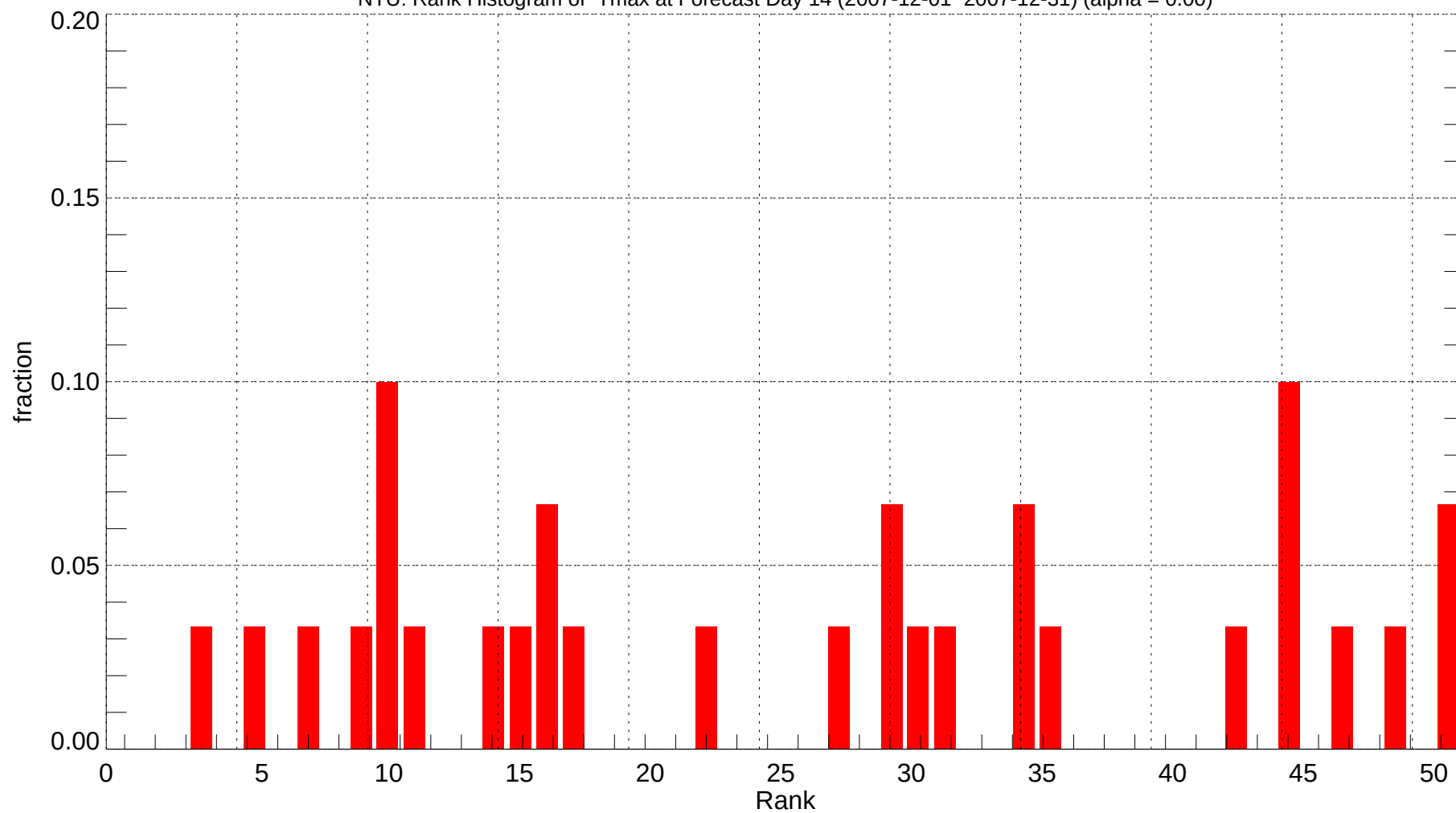
NTU: Rank Histogram of Tmax at Forecast Day 14 (2007-12-01~2007-12-31) (alpha = 0.00)
