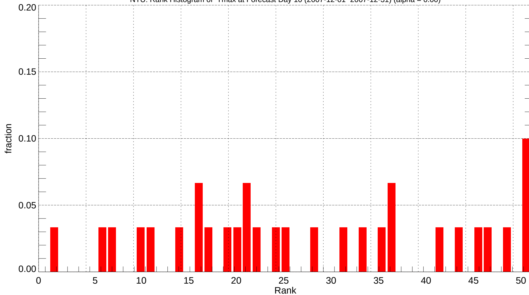
NTU: Rank Histogram of Tmax at Forecast Day 10 (2007-12-01~2007-12-31) (alpha = 0.00)
