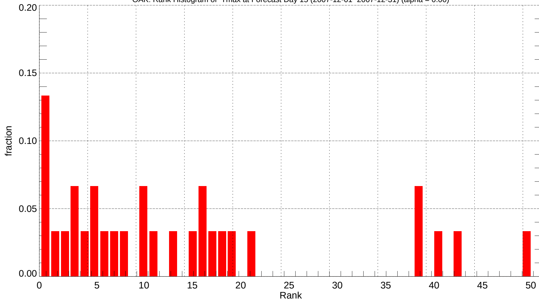
OAK: Rank Histogram of Tmax at Forecast Day 15 (2007-12-01~2007-12-31) (alpha = 0.00)
