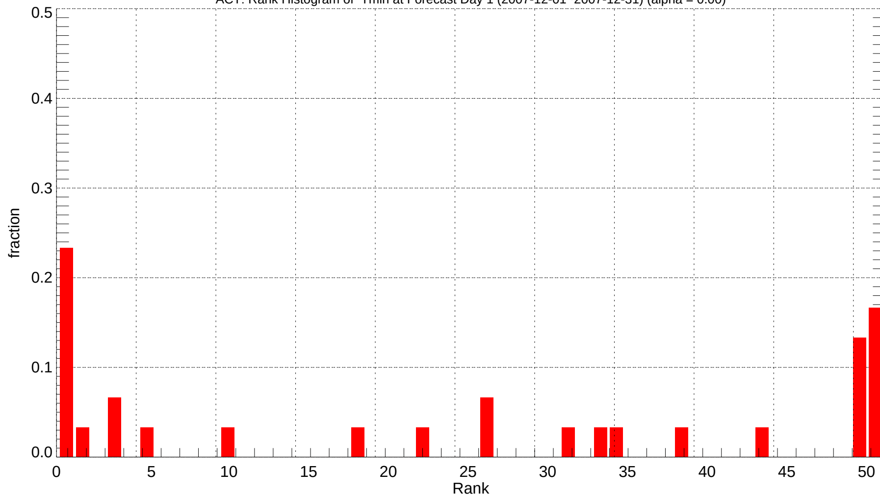
ACT: Rank Histogram of Tmin at Forecast Day 1 (2007-12-01~2007-12-31) (alpha = 0.00)
