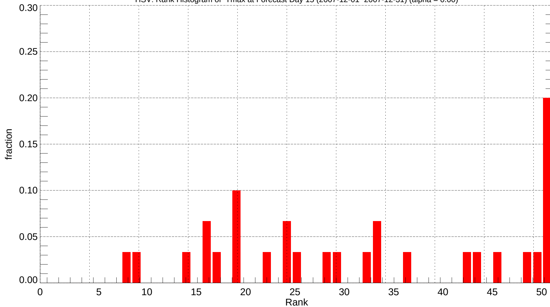
HSV: Rank Histogram of Tmax at Forecast Day 15 (2007-12-01~2007-12-31) (alpha = 0.00)
