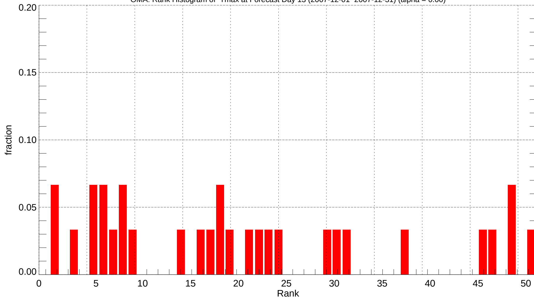
OMA: Rank Histogram of Tmax at Forecast Day 13 (2007-12-01~2007-12-31) (alpha = 0.00)
