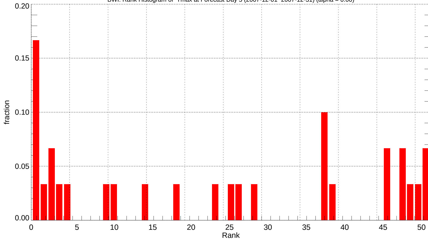
BWI: Rank Histogram of Tmax at Forecast Day 5 (2007-12-01~2007-12-31) (alpha = 0.00)
