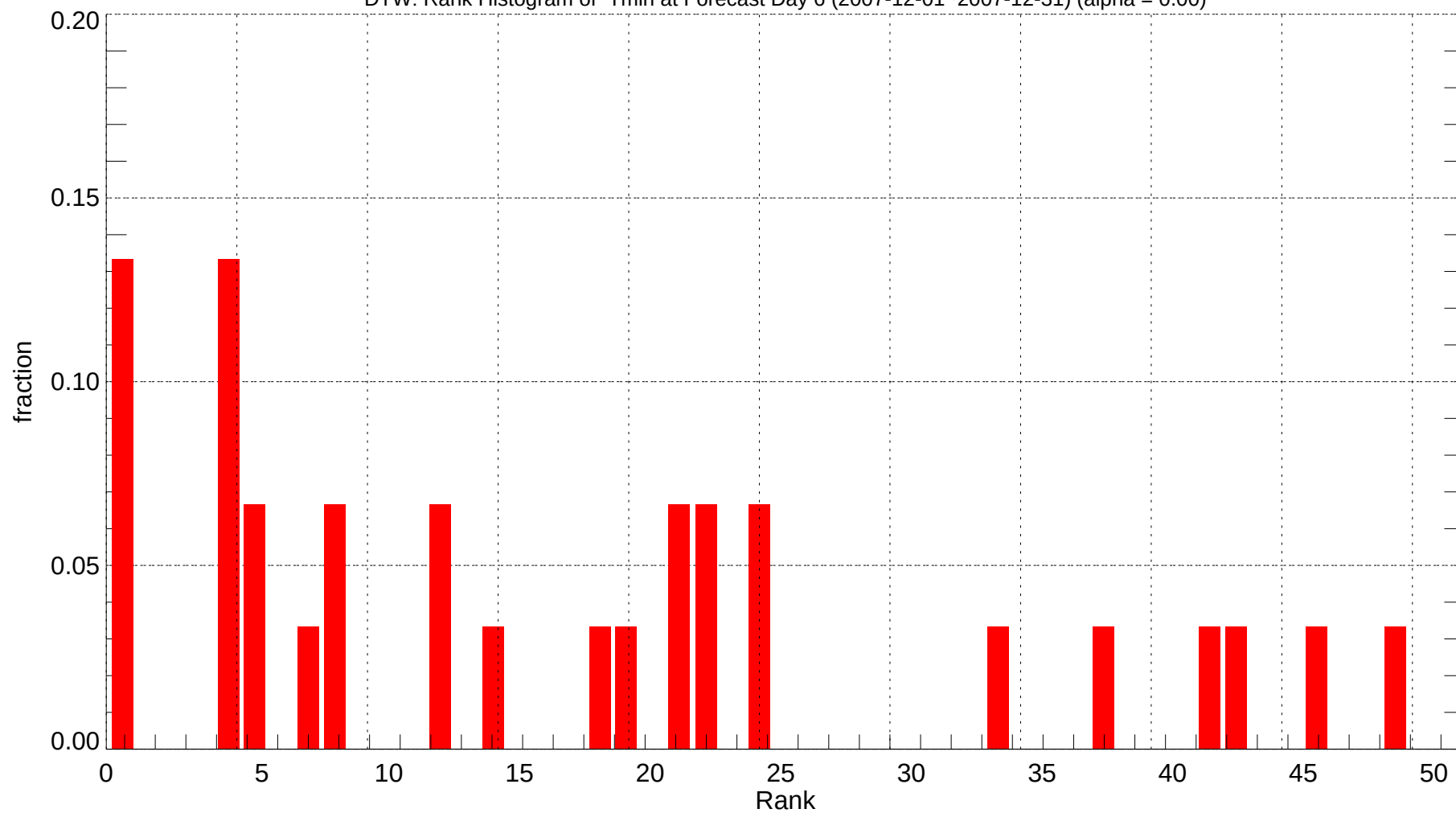
DTW: Rank Histogram of Tmin at Forecast Day 6 (2007-12-01~2007-12-31) (alpha = 0.00)
