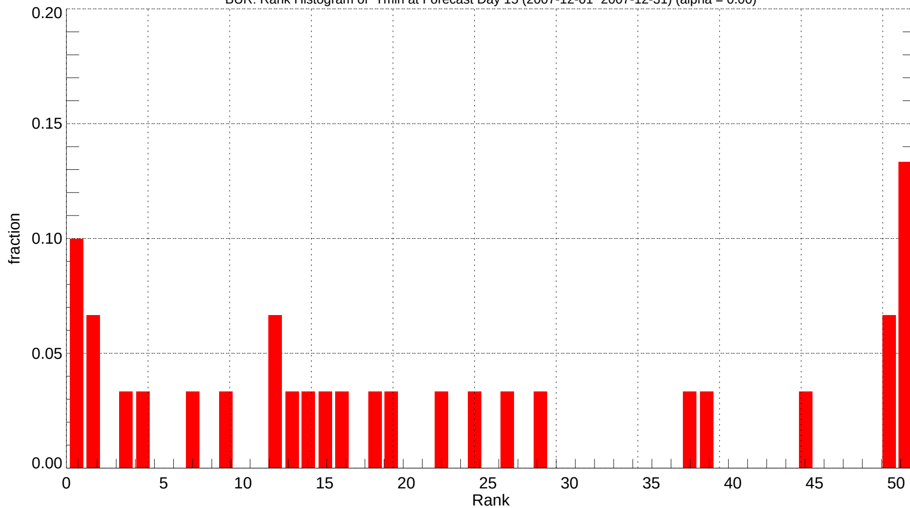
BUR: Rank Histogram of Tmin at Forecast Day 15 (2007-12-01~2007-12-31) (alpha = 0.00)
