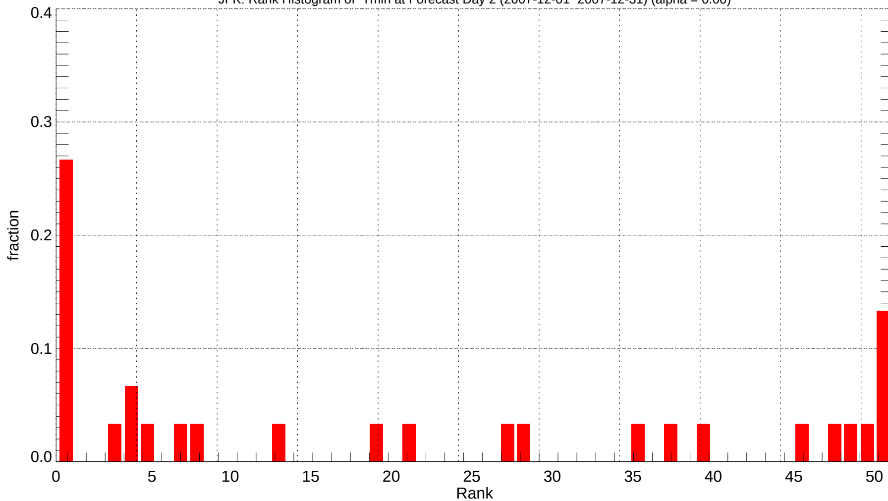
JFK: Rank Histogram of Tmin at Forecast Day 2 (2007-12-01~2007-12-31) (alpha = 0.00)
