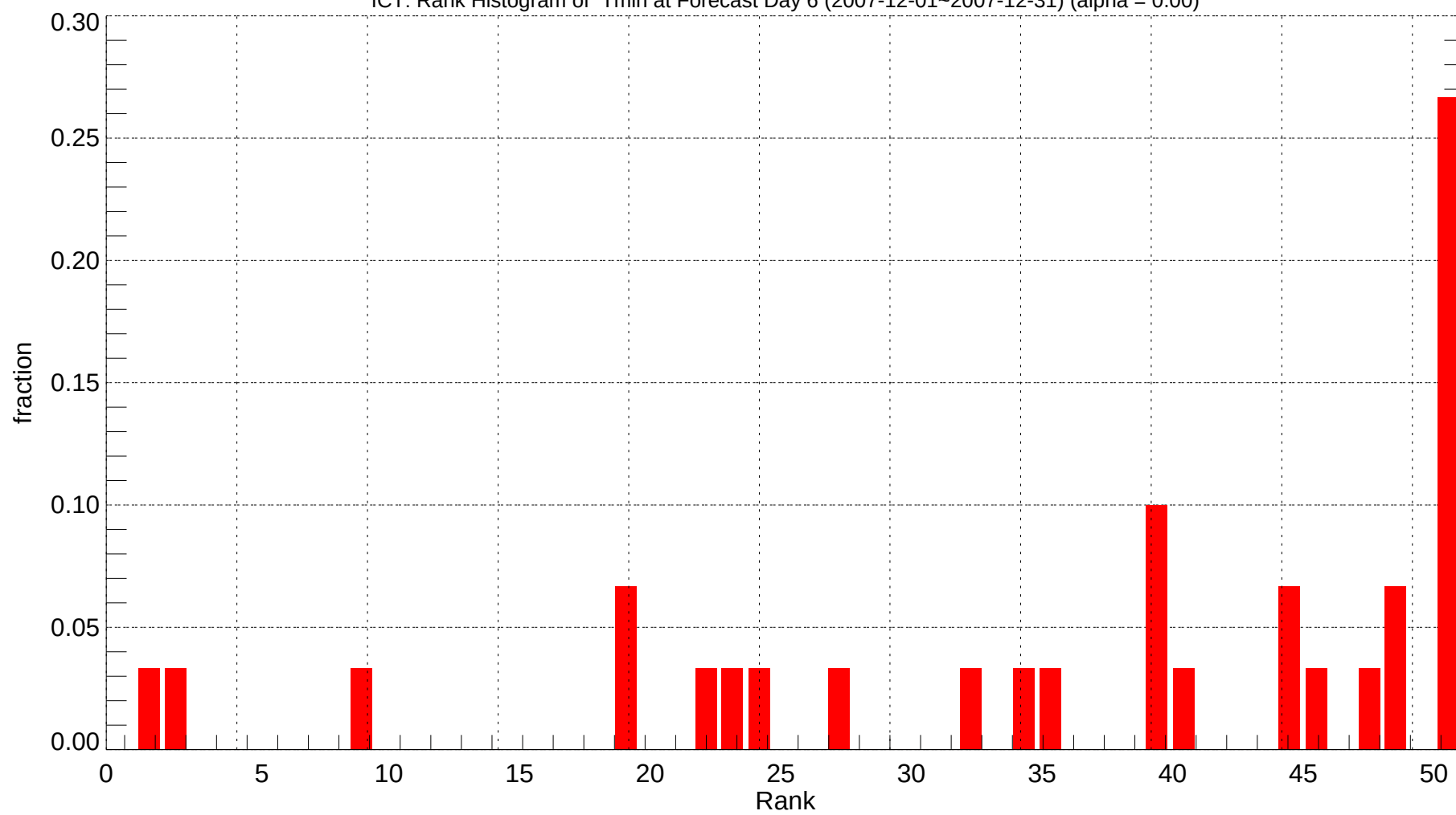
ICT: Rank Histogram of Tmin at Forecast Day 6 (2007-12-01~2007-12-31) (alpha = 0.00)
