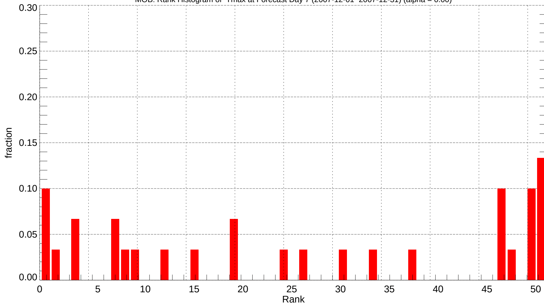
MOB: Rank Histogram of Tmax at Forecast Day 7 (2007-12-01~2007-12-31) (alpha = 0.00)
