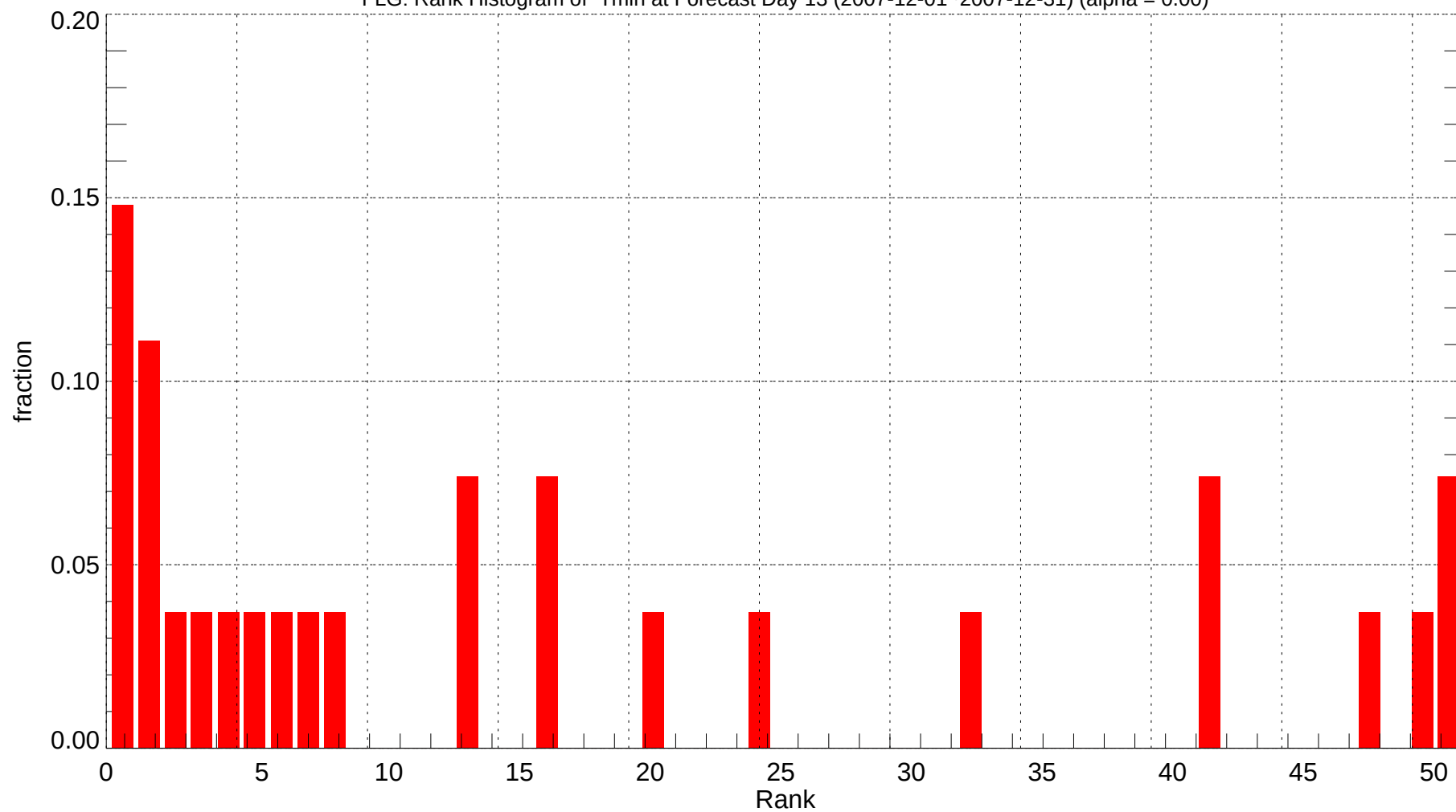
FLG: Rank Histogram of Tmin at Forecast Day 13 (2007-12-01~2007-12-31) (alpha = 0.00)
