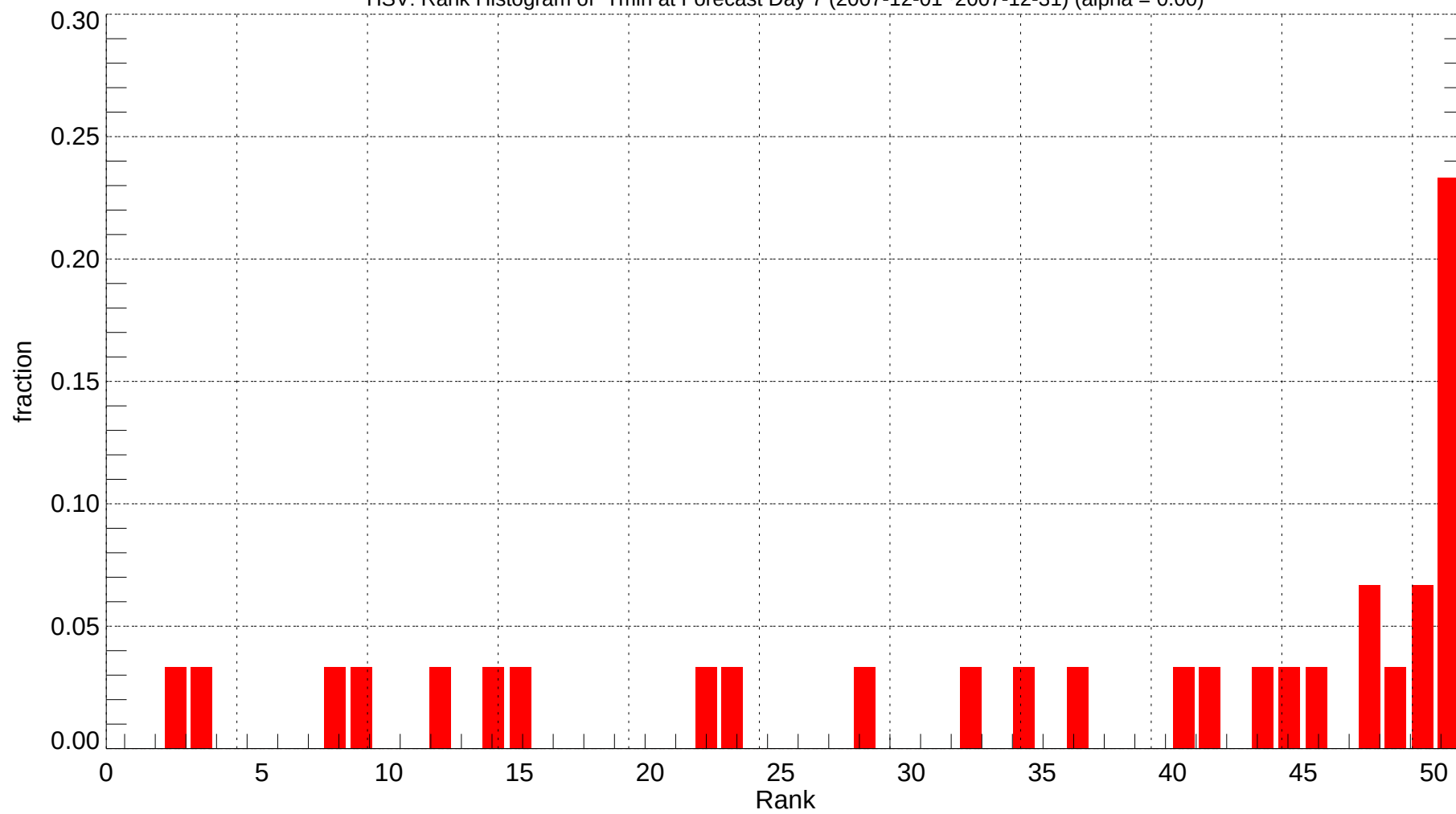
HSV: Rank Histogram of Tmin at Forecast Day 7 (2007-12-01~2007-12-31) (alpha = 0.00)
