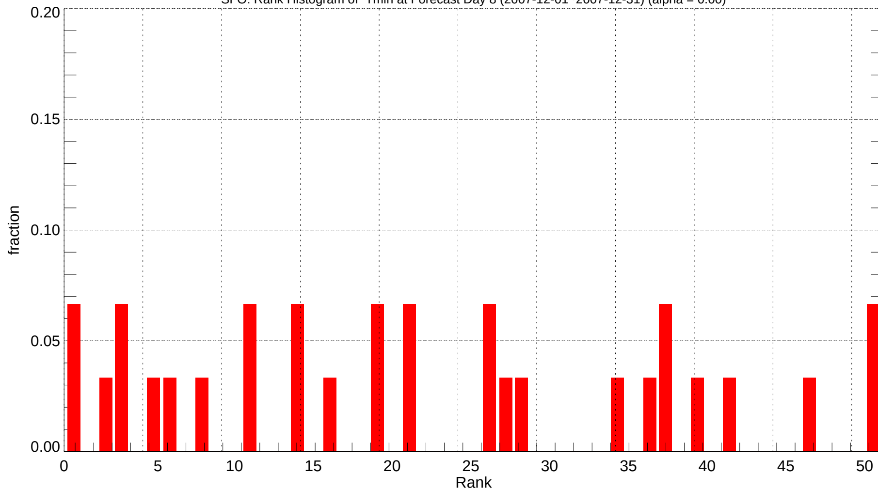
SFO: Rank Histogram of Tmin at Forecast Day 8 (2007-12-01~2007-12-31) (alpha = 0.00)
