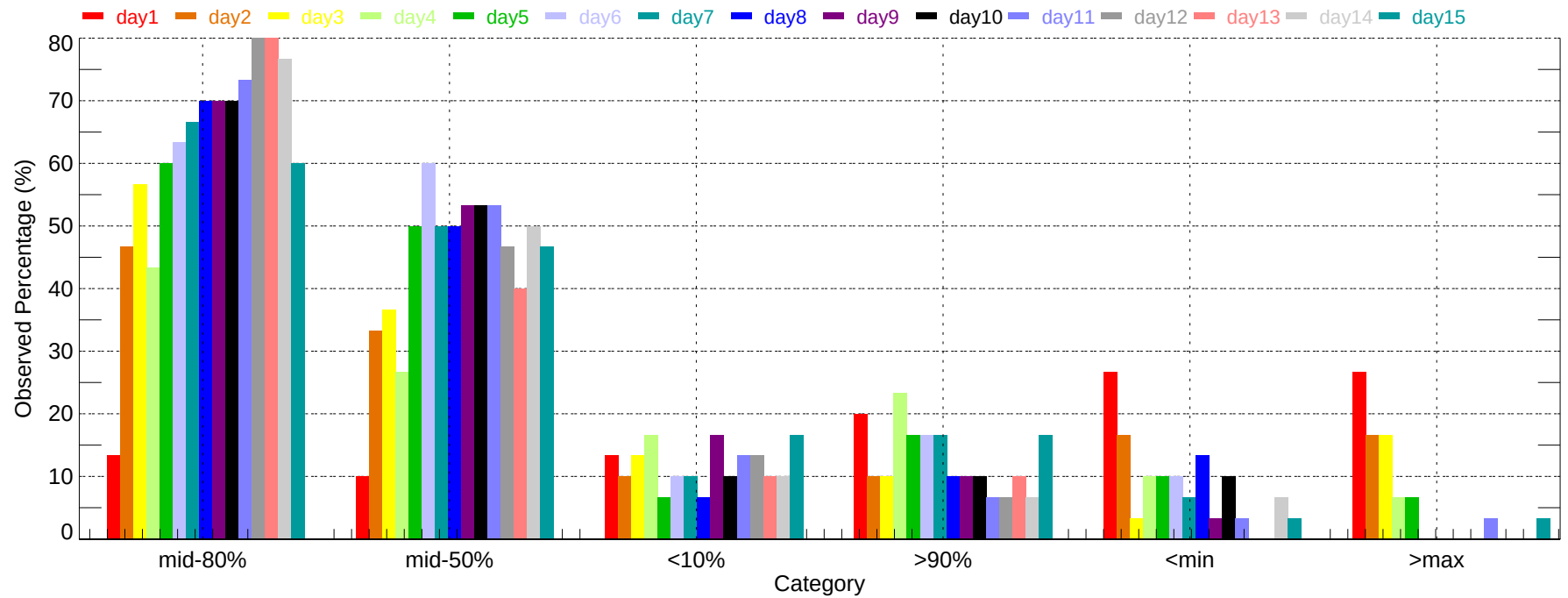
Observed Percentage of Ensembles - FAR: Min Temperature (2007-12-01~2007-12-31)
