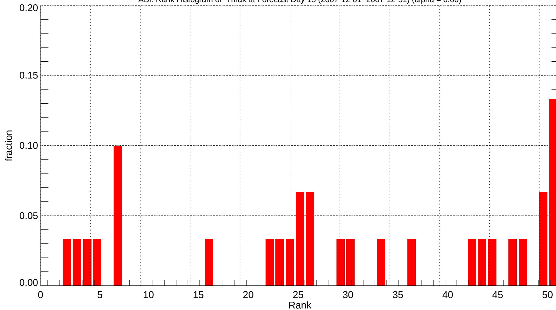
ABI: Rank Histogram of Tmax at Forecast Day 13 (2007-12-01~2007-12-31) (alpha = 0.00)
