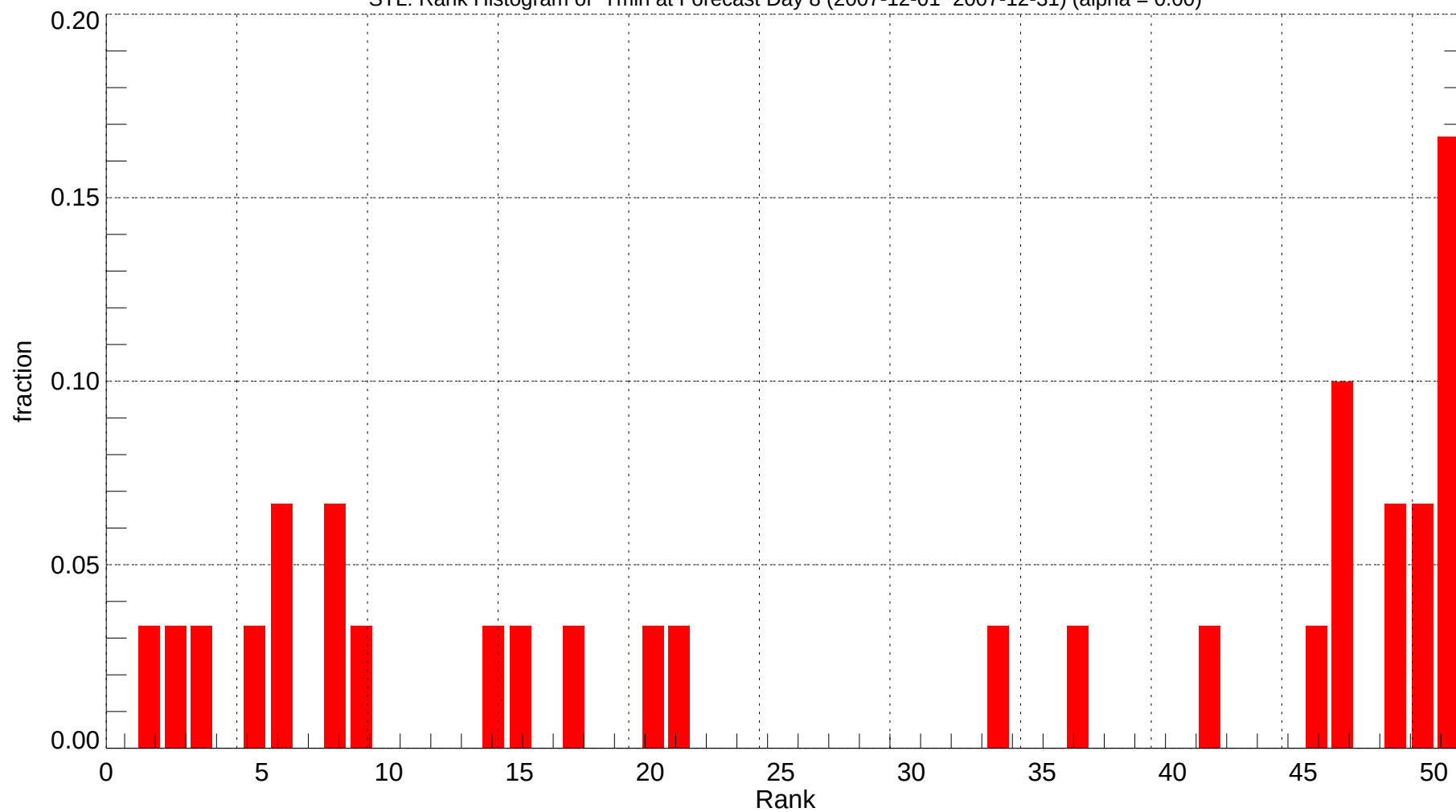
STL: Rank Histogram of Tmin at Forecast Day 8 (2007-12-01~2007-12-31) (alpha = 0.00)
