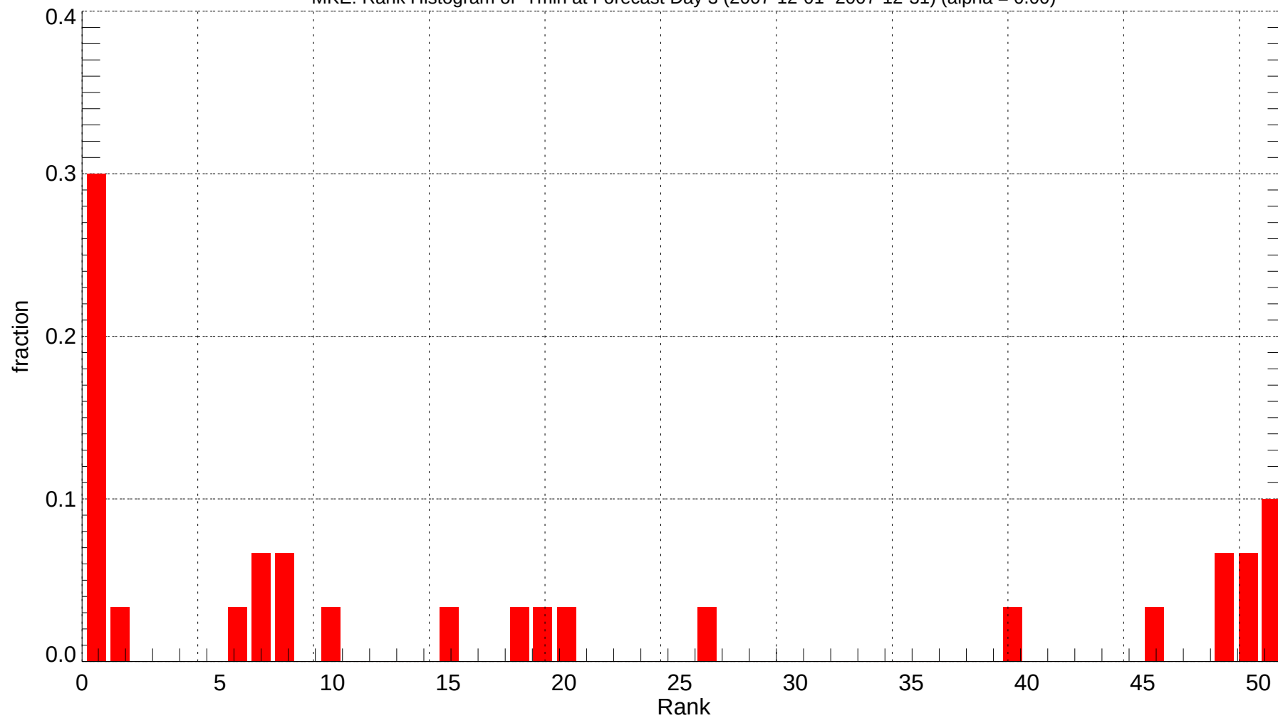
MKE: Rank Histogram of Tmin at Forecast Day 3 (2007-12-01~2007-12-31) (alpha = 0.00)
