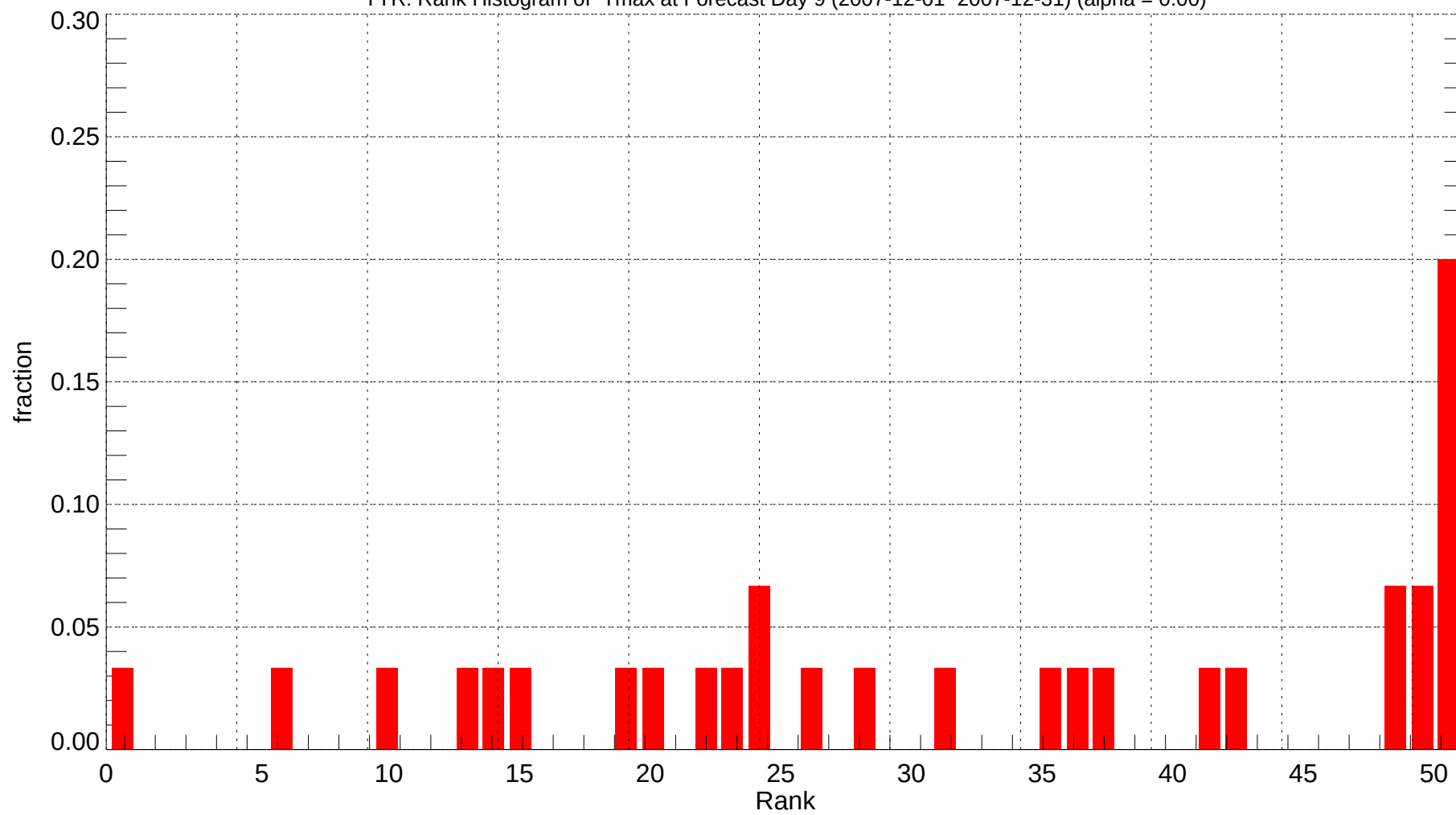
TYR: Rank Histogram of Tmax at Forecast Day 9 (2007-12-01~2007-12-31) (alpha = 0.00)
