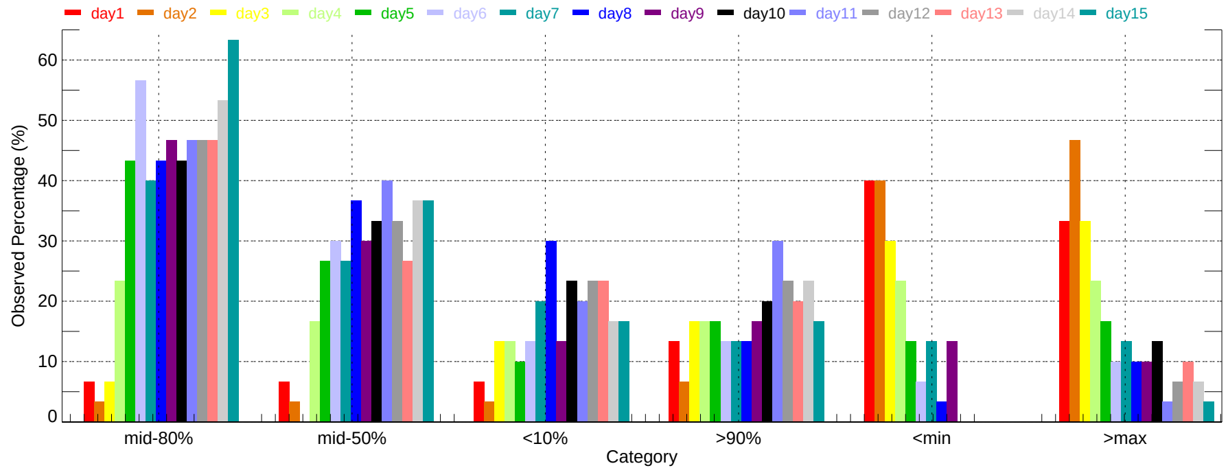
Observed Percentage of Ensembles - RNO: Min Temperature (2007-12-01~2007-12-31)
