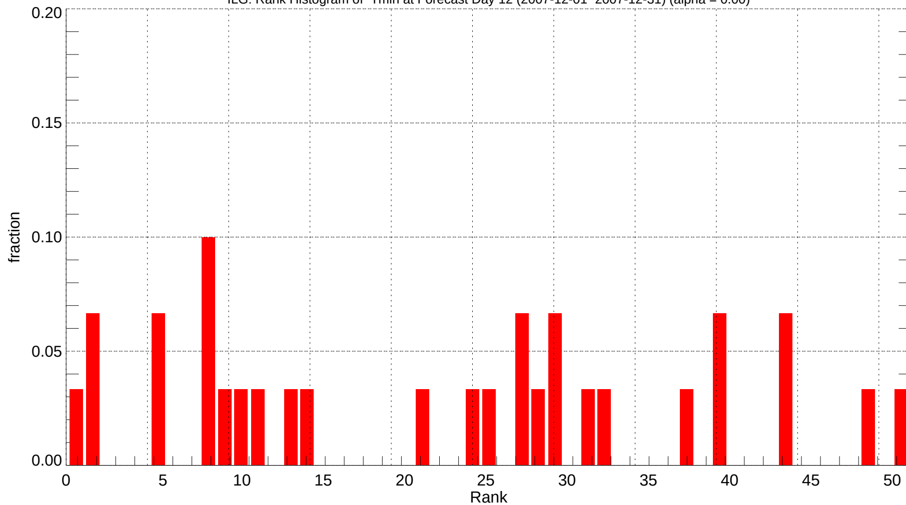
ILG: Rank Histogram of Tmin at Forecast Day 12 (2007-12-01~2007-12-31) (alpha = 0.00)
