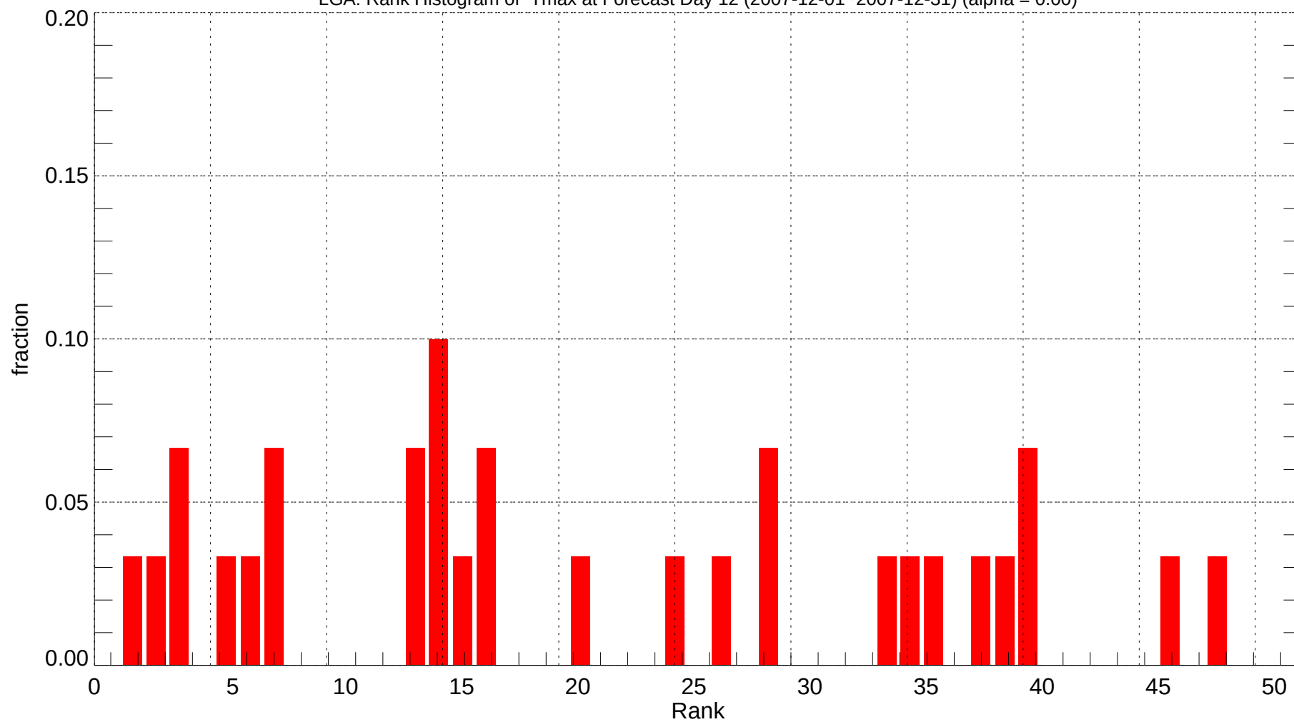
LGA: Rank Histogram of Tmax at Forecast Day 12 (2007-12-01~2007-12-31) (alpha = 0.00)
