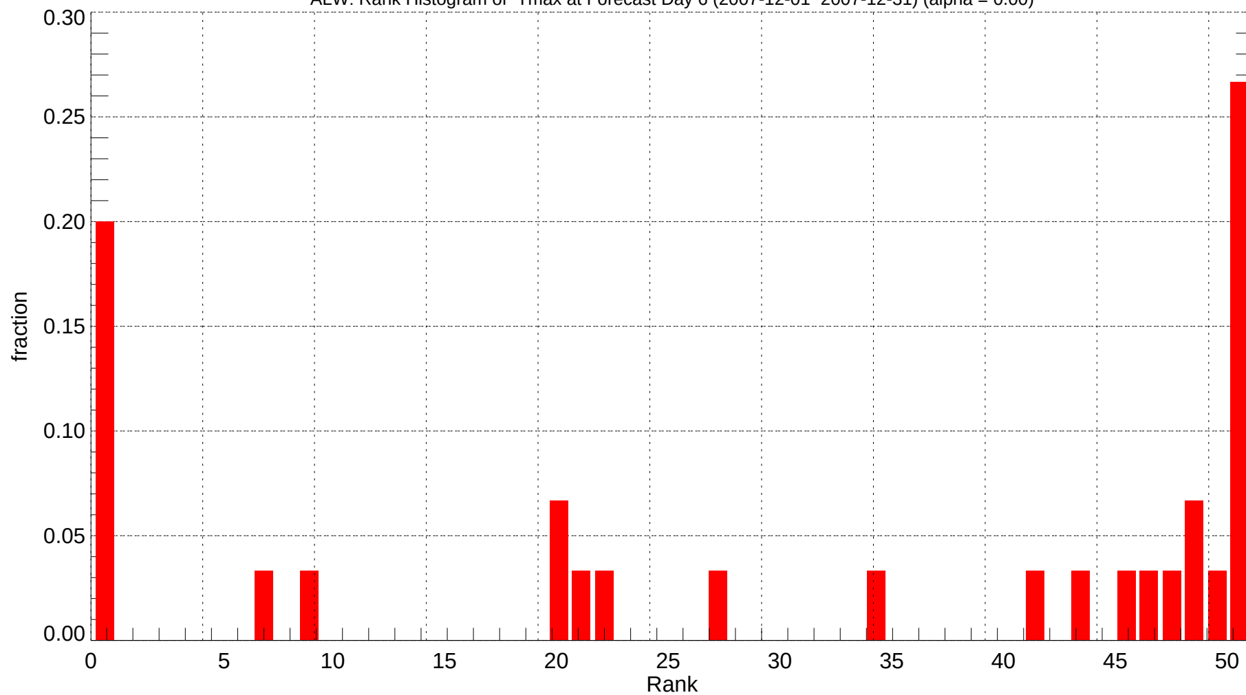
ALW: Rank Histogram of Tmax at Forecast Day 6 (2007-12-01~2007-12-31) (alpha = 0.00)
