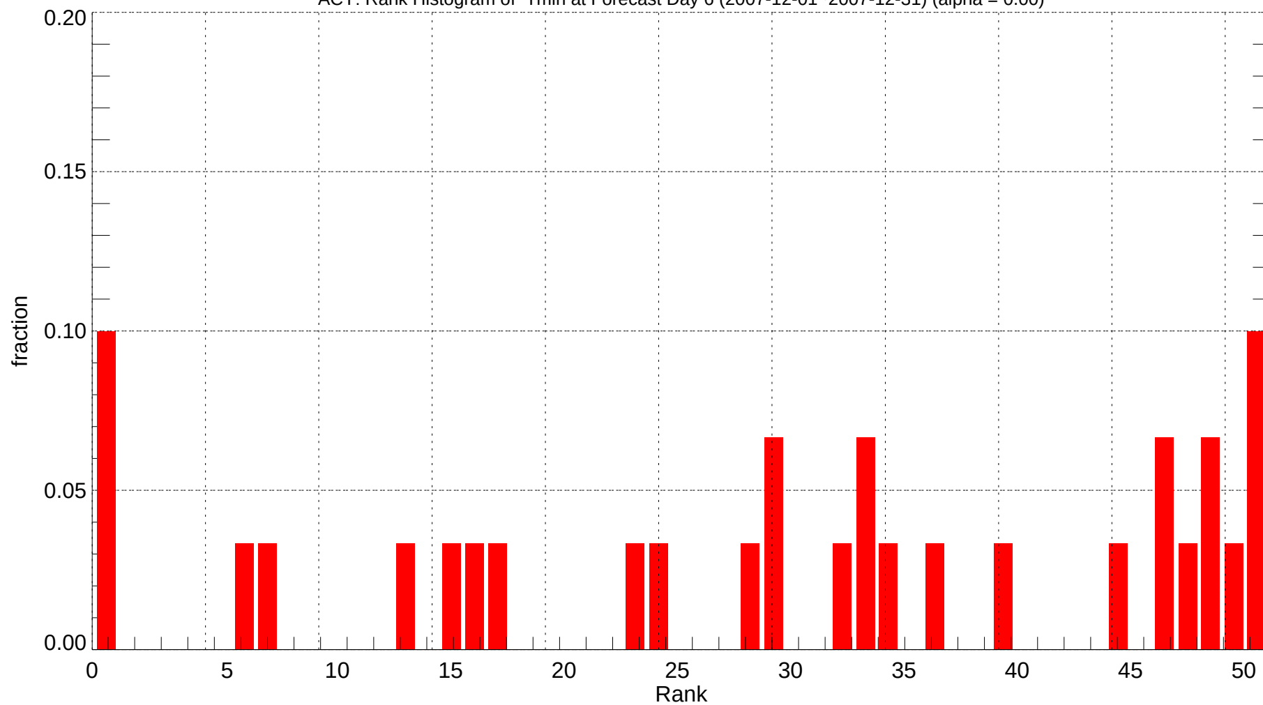
ACY: Rank Histogram of Tmin at Forecast Day 6 (2007-12-01~2007-12-31) (alpha = 0.00)
