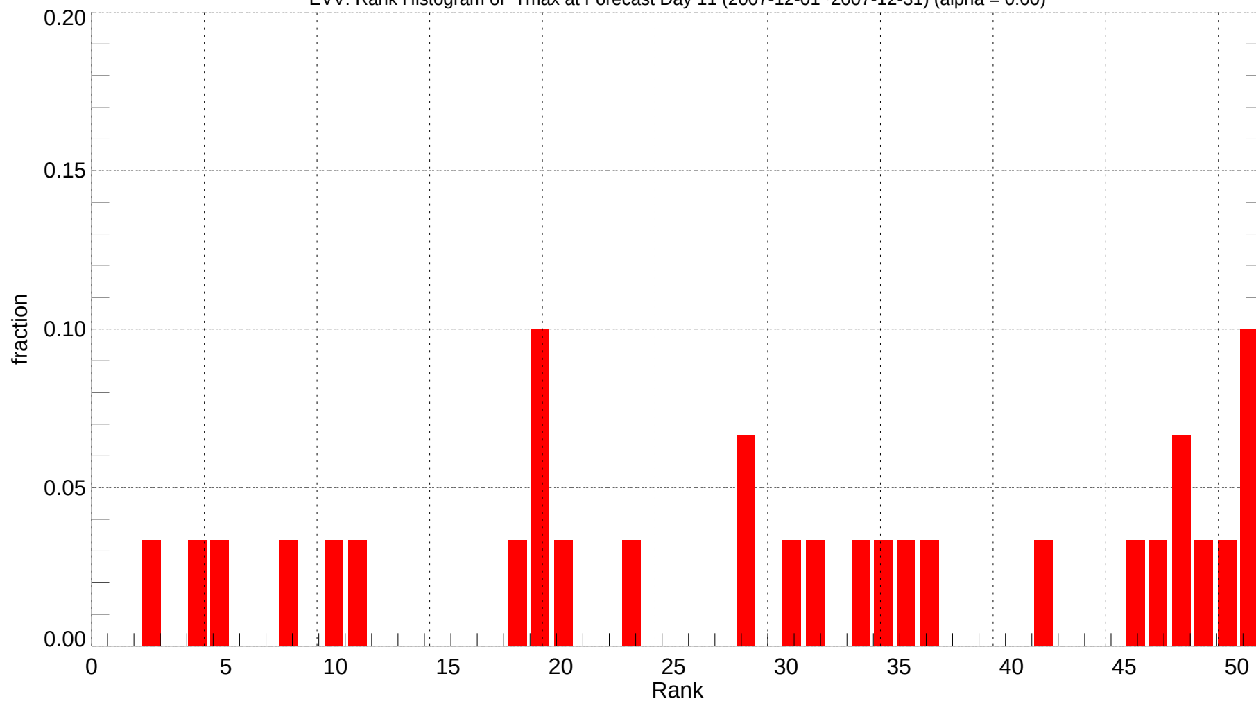
EVV: Rank Histogram of Tmax at Forecast Day 11 (2007-12-01~2007-12-31) (alpha = 0.00)
