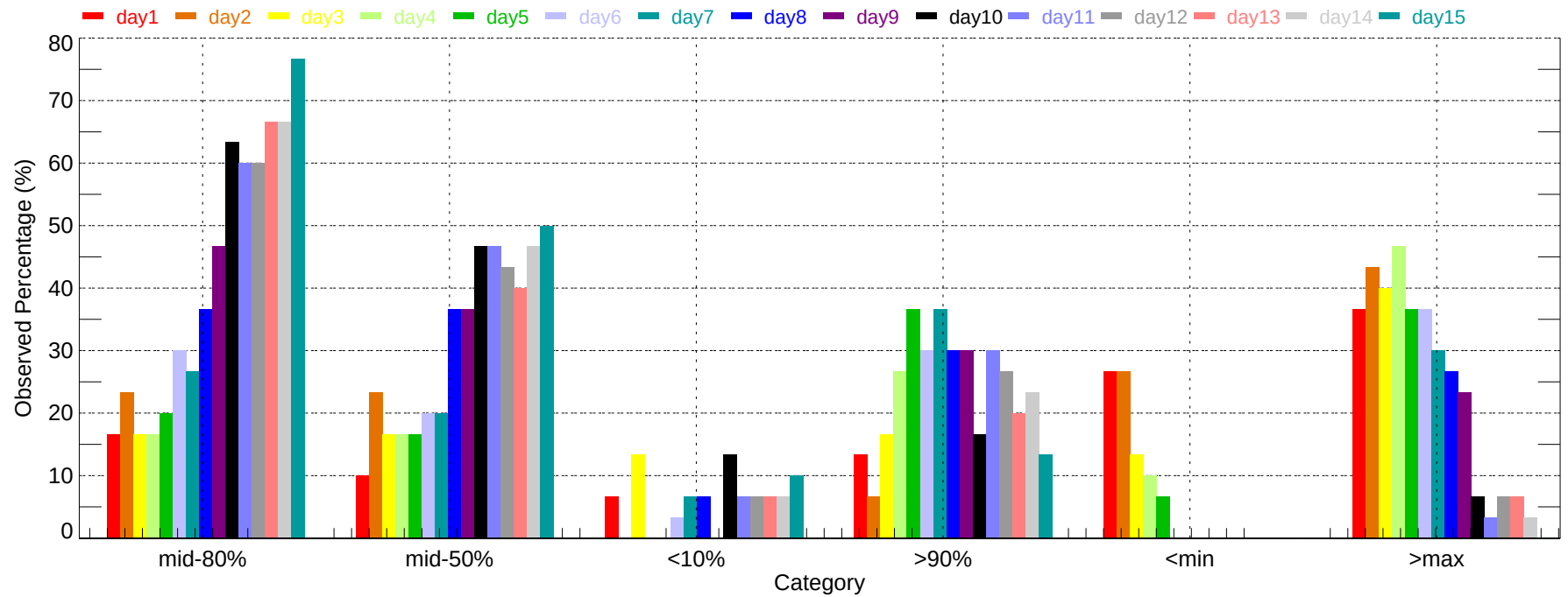
Observed Percentage of Ensembles - BFL: Max Temperature (2007-12-01~2007-12-31)
