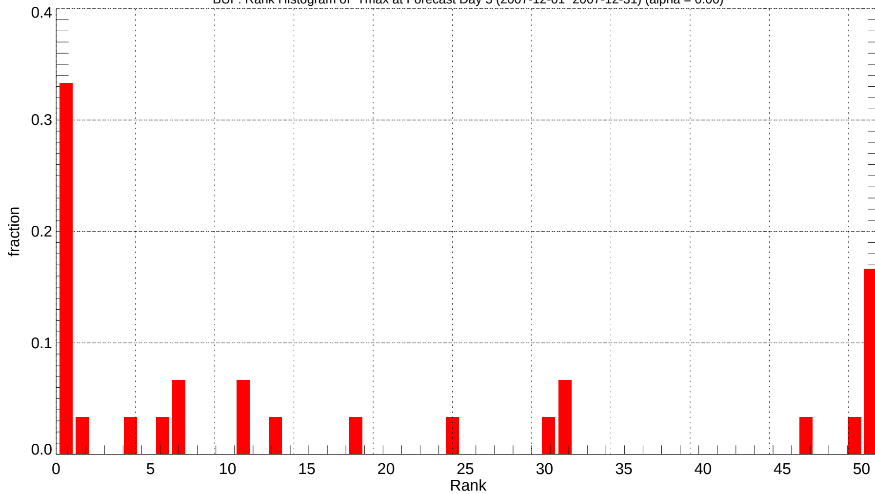
BUF: Rank Histogram of Tmax at Forecast Day 3 (2007-12-01~2007-12-31) (alpha = 0.00)
