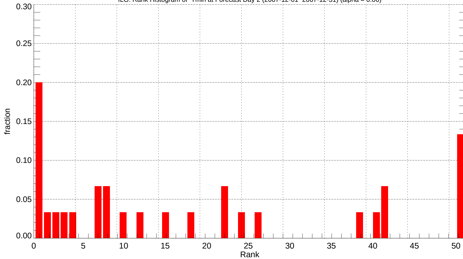
ILG: Rank Histogram of Tmin at Forecast Day 2 (2007-12-01~2007-12-31) (alpha = 0.00)
