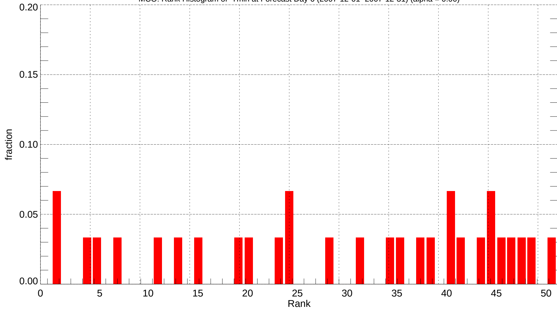
MCO: Rank Histogram of Tmin at Forecast Day 6 (2007-12-01~2007-12-31) (alpha = 0.00)
