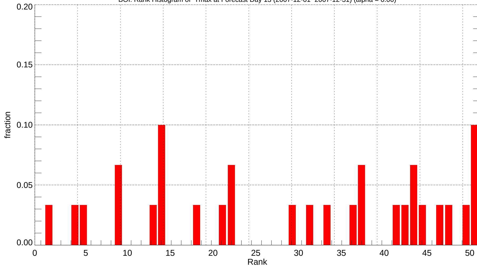
BOI: Rank Histogram of Tmax at Forecast Day 13 (2007-12-01~2007-12-31) (alpha = 0.00)
