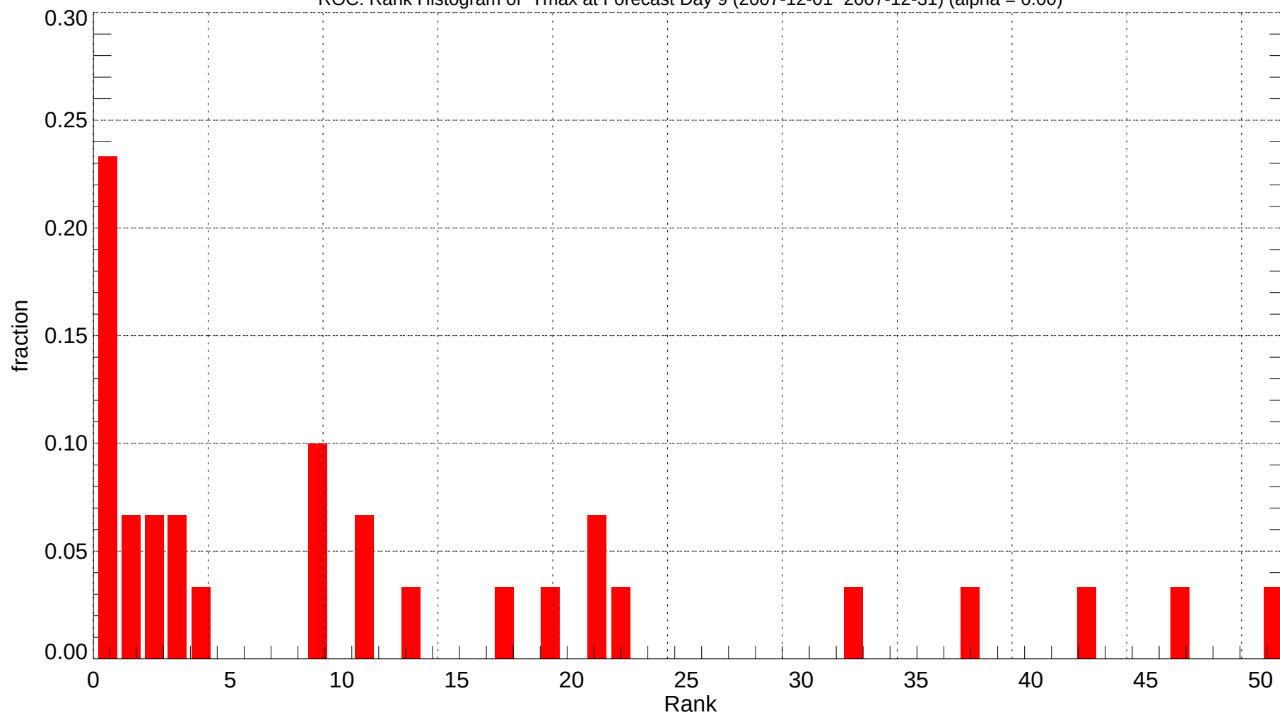
ROC: Rank Histogram of Tmax at Forecast Day 9 (2007-12-01~2007-12-31) (alpha = 0.00)
