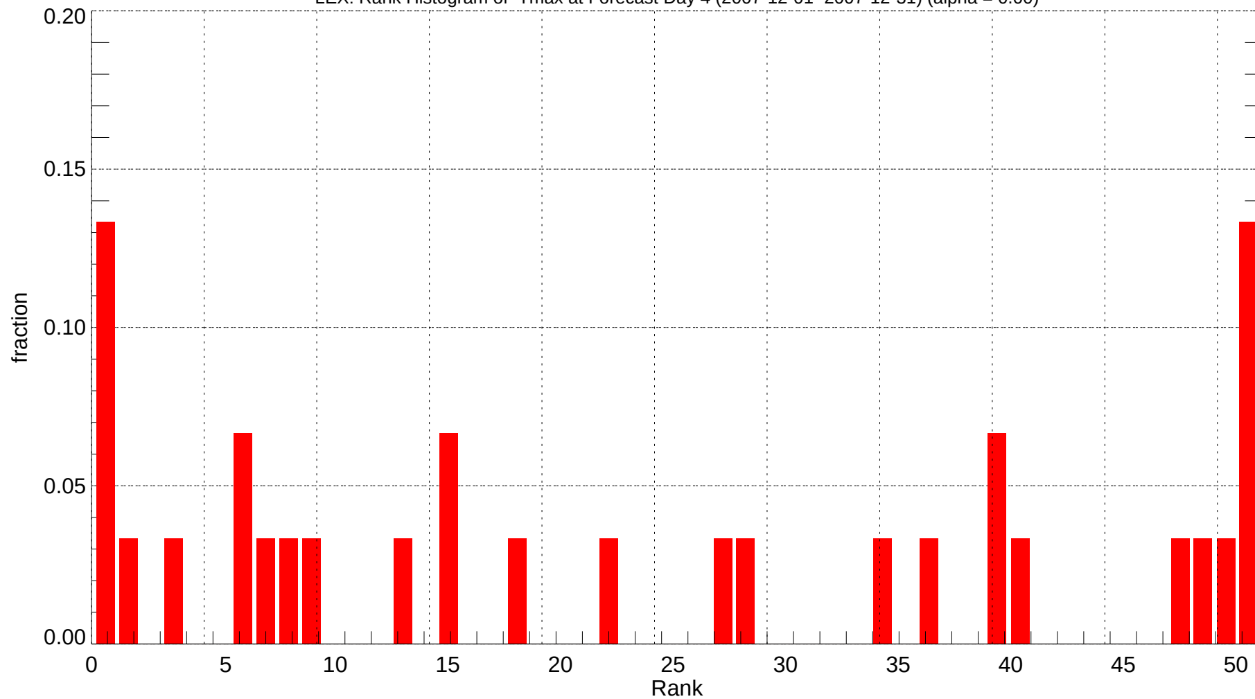
LEX: Rank Histogram of Tmax at Forecast Day 4 (2007-12-01~2007-12-31) (alpha = 0.00)
