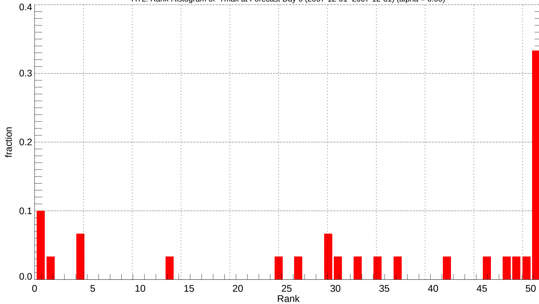
ATL: Rank Histogram of Tmax at Forecast Day 6 (2007-12-01~2007-12-31) (alpha = 0.00)
