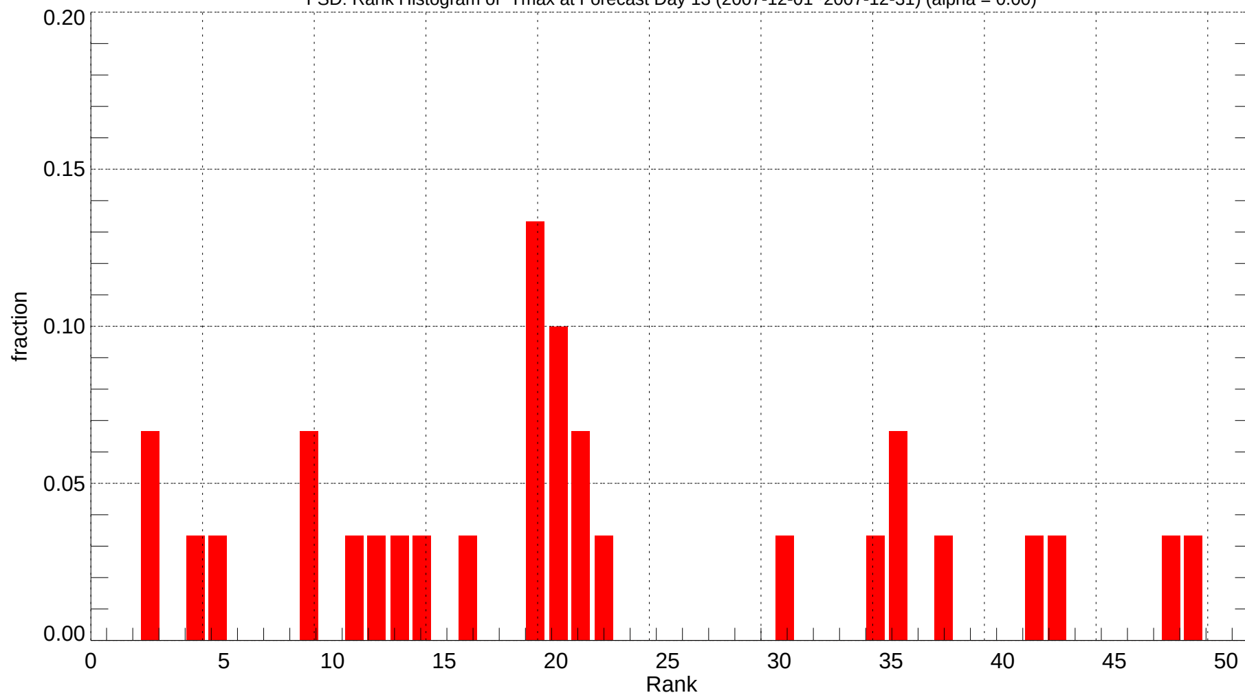
FSD: Rank Histogram of Tmax at Forecast Day 13 (2007-12-01~2007-12-31) (alpha = 0.00)
