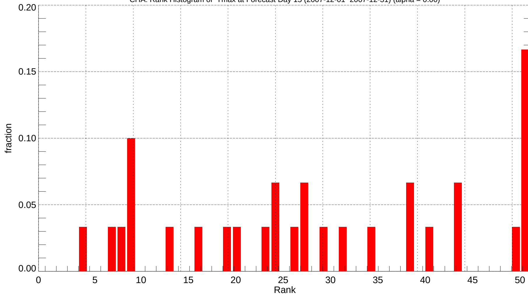
CHA: Rank Histogram of Tmax at Forecast Day 15 (2007-12-01~2007-12-31) (alpha = 0.00)
