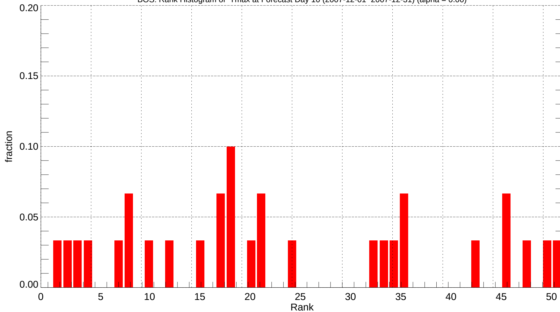
BOS: Rank Histogram of Tmax at Forecast Day 10 (2007-12-01~2007-12-31) (alpha = 0.00)
