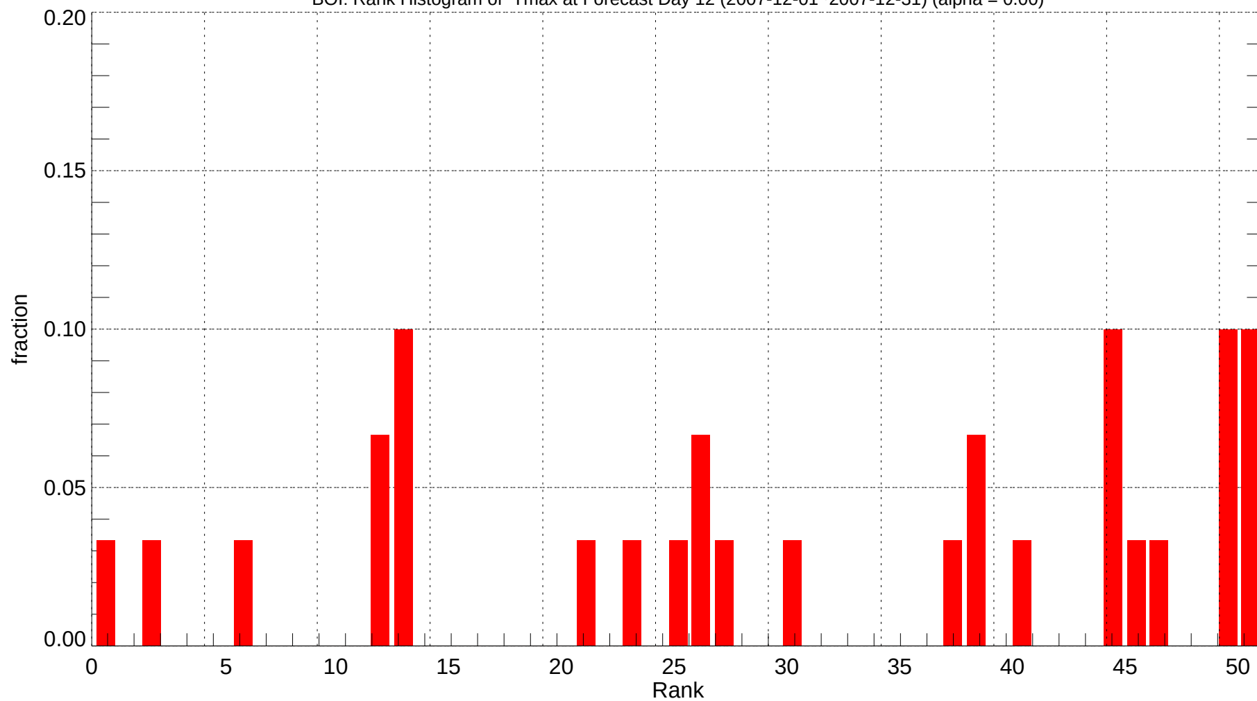
BOI: Rank Histogram of Tmax at Forecast Day 12 (2007-12-01~2007-12-31) (alpha = 0.00)
