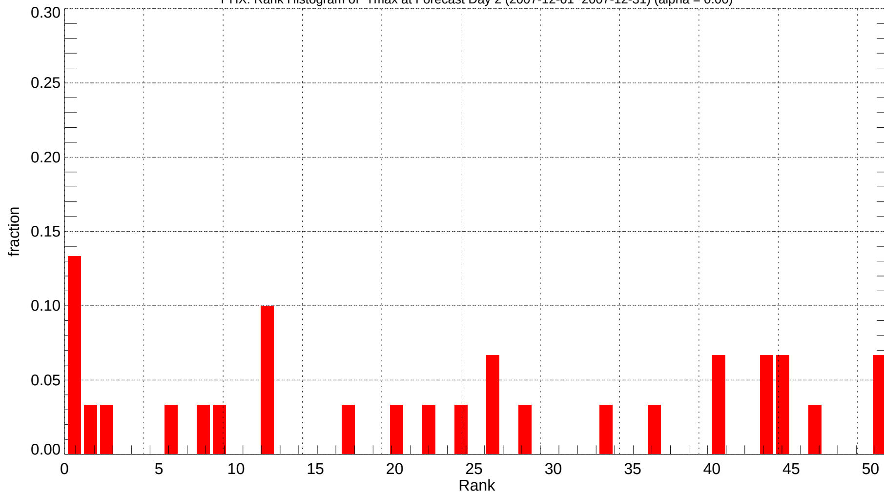
PHX: Rank Histogram of Tmax at Forecast Day 2 (2007-12-01~2007-12-31) (alpha = 0.00)
