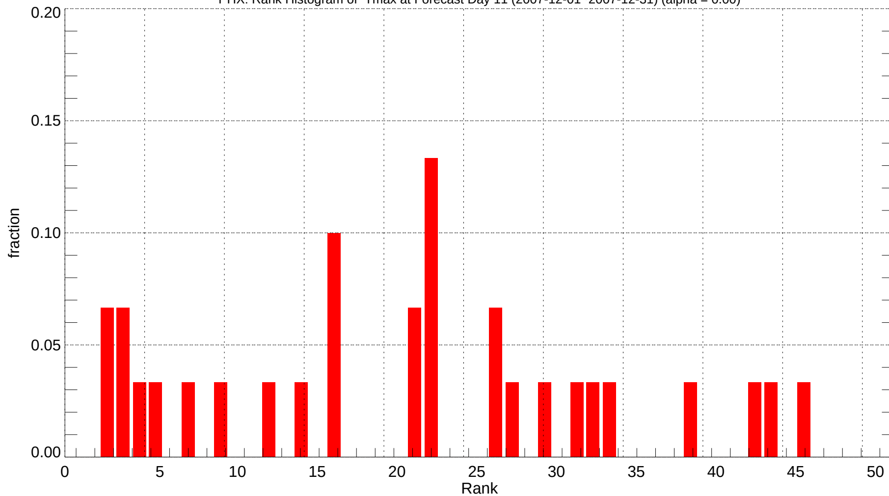
PHX: Rank Histogram of Tmax at Forecast Day 11 (2007-12-01~2007-12-31) (alpha = 0.00)
