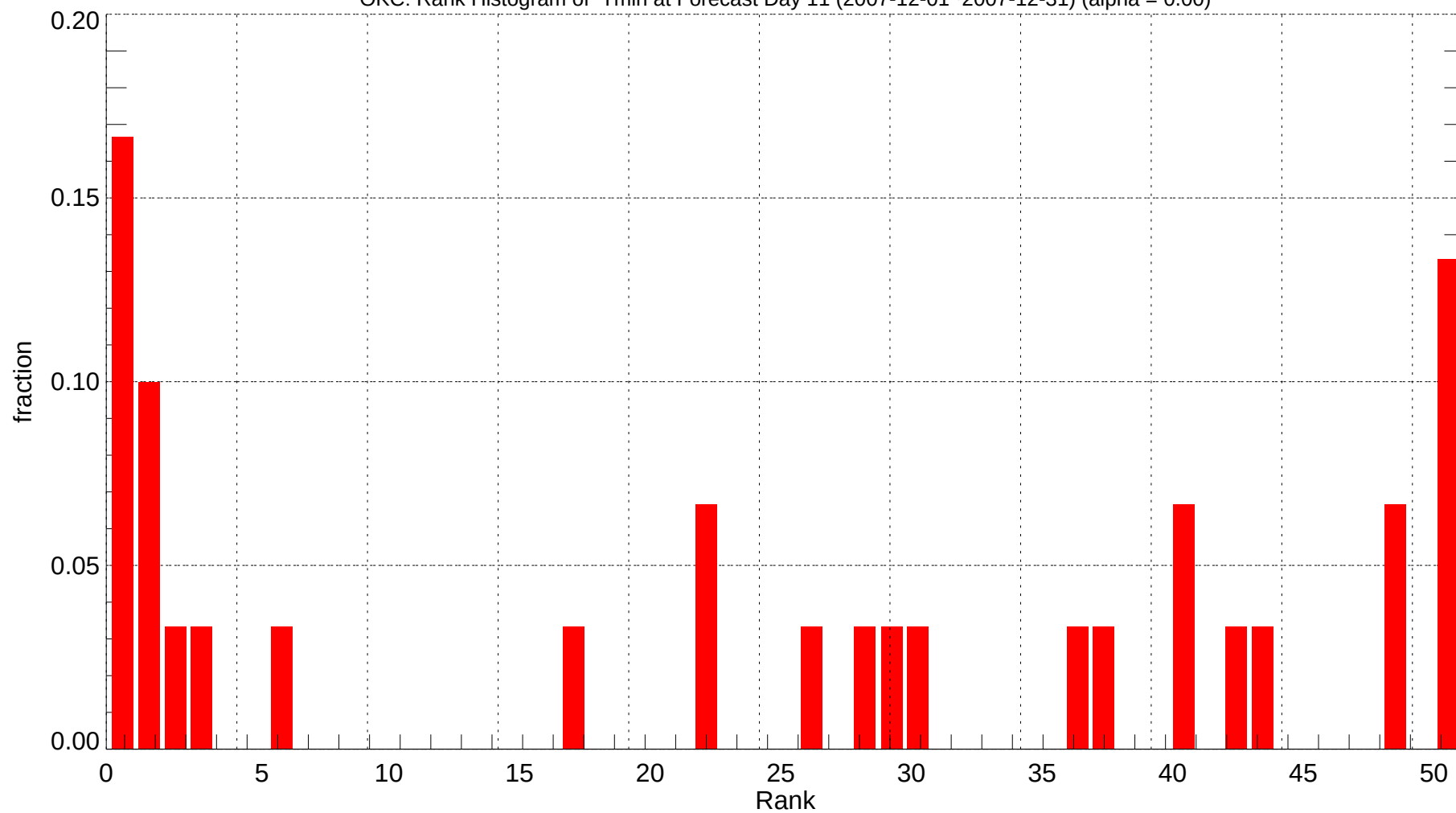
OKC: Rank Histogram of Tmin at Forecast Day 11 (2007-12-01~2007-12-31) (alpha = 0.00)
