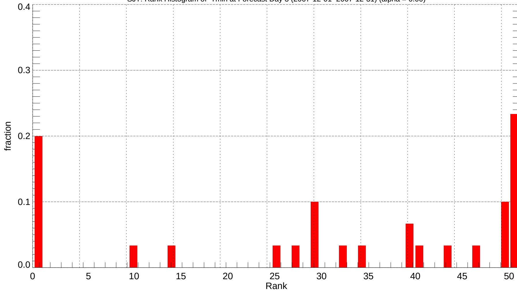
SJT: Rank Histogram of Tmin at Forecast Day 3 (2007-12-01~2007-12-31) (alpha = 0.00)
