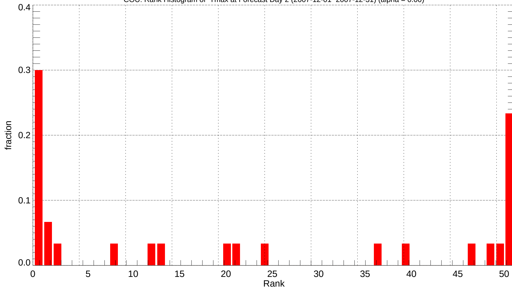
COU: Rank Histogram of Tmax at Forecast Day 2 (2007-12-01~2007-12-31) (alpha = 0.00)
