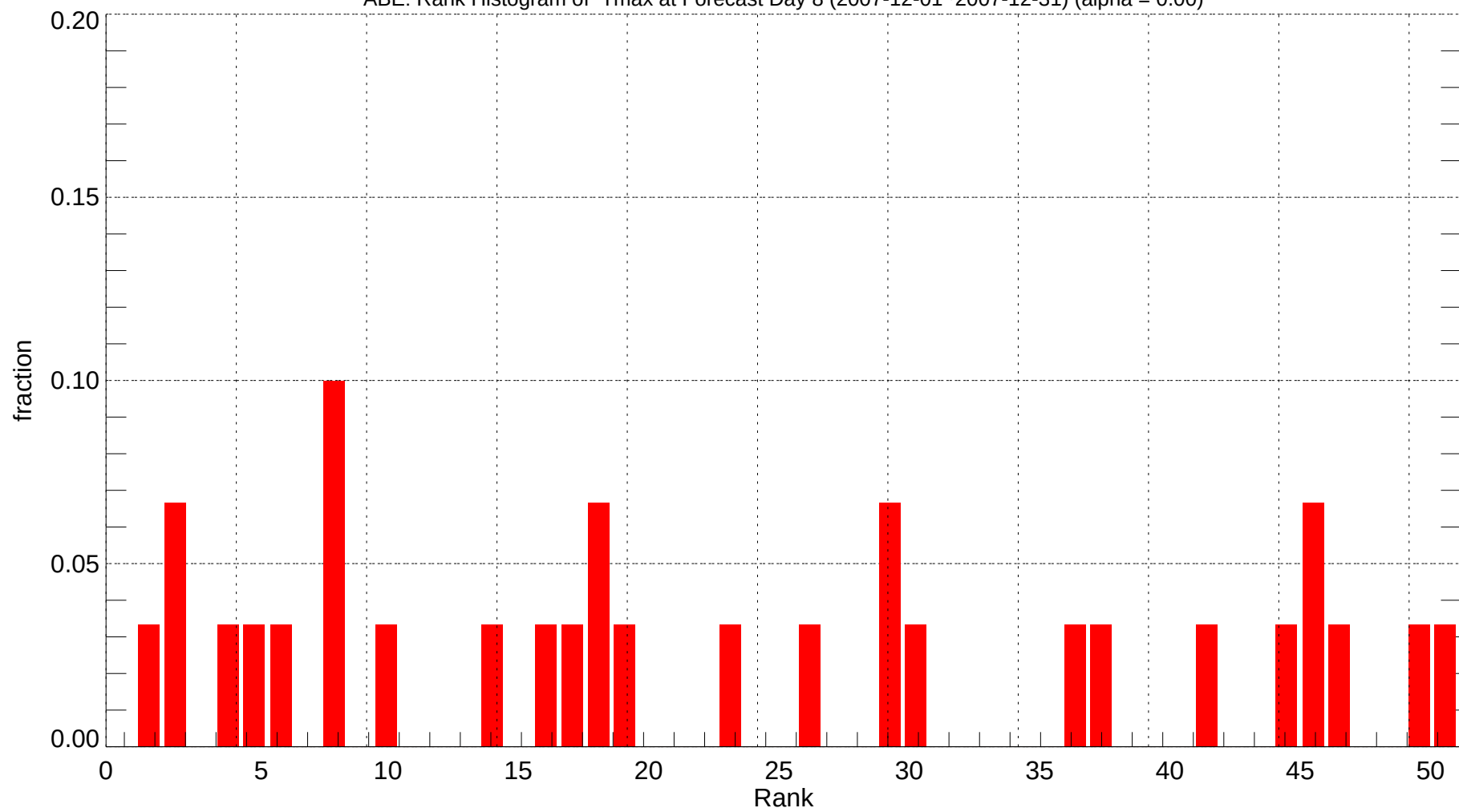
ABE: Rank Histogram of Tmax at Forecast Day 8 (2007-12-01~2007-12-31) (alpha = 0.00)
