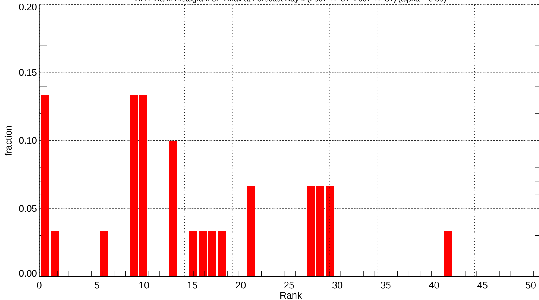
ALB: Rank Histogram of Tmax at Forecast Day 4 (2007-12-01~2007-12-31) (alpha = 0.00)
