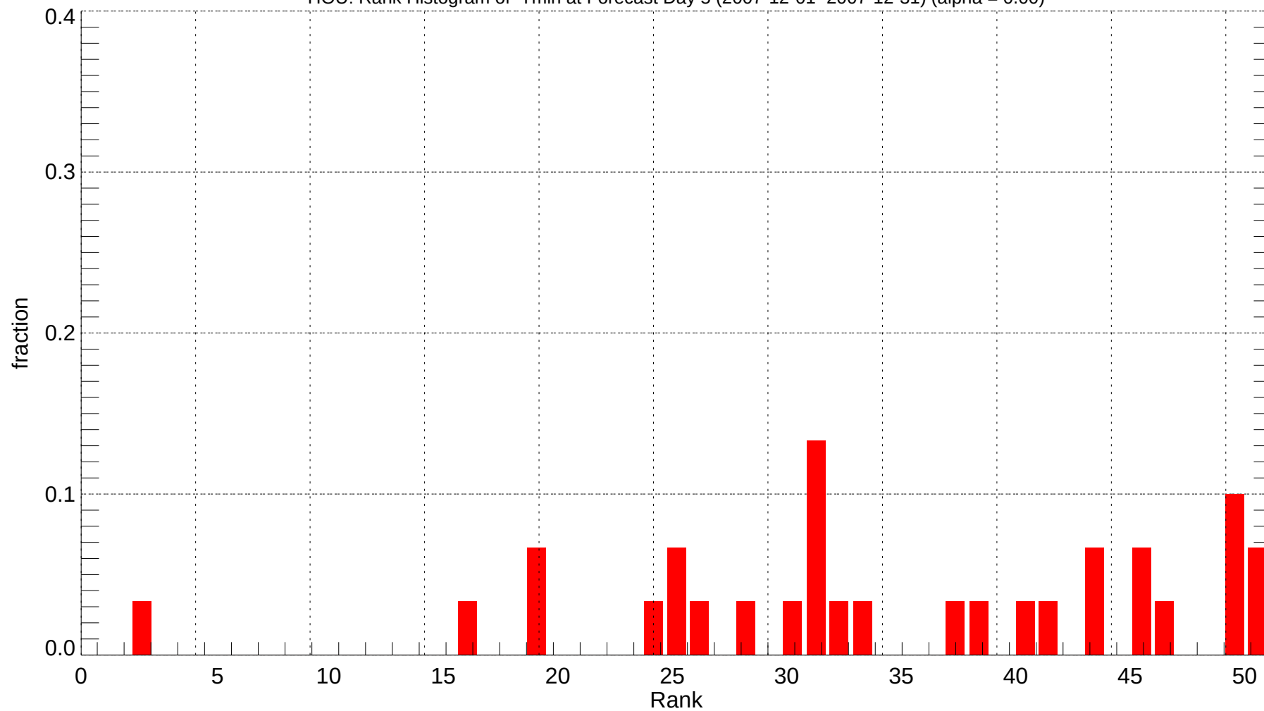
HOU: Rank Histogram of Tmin at Forecast Day 5 (2007-12-01~2007-12-31) (alpha = 0.00)
