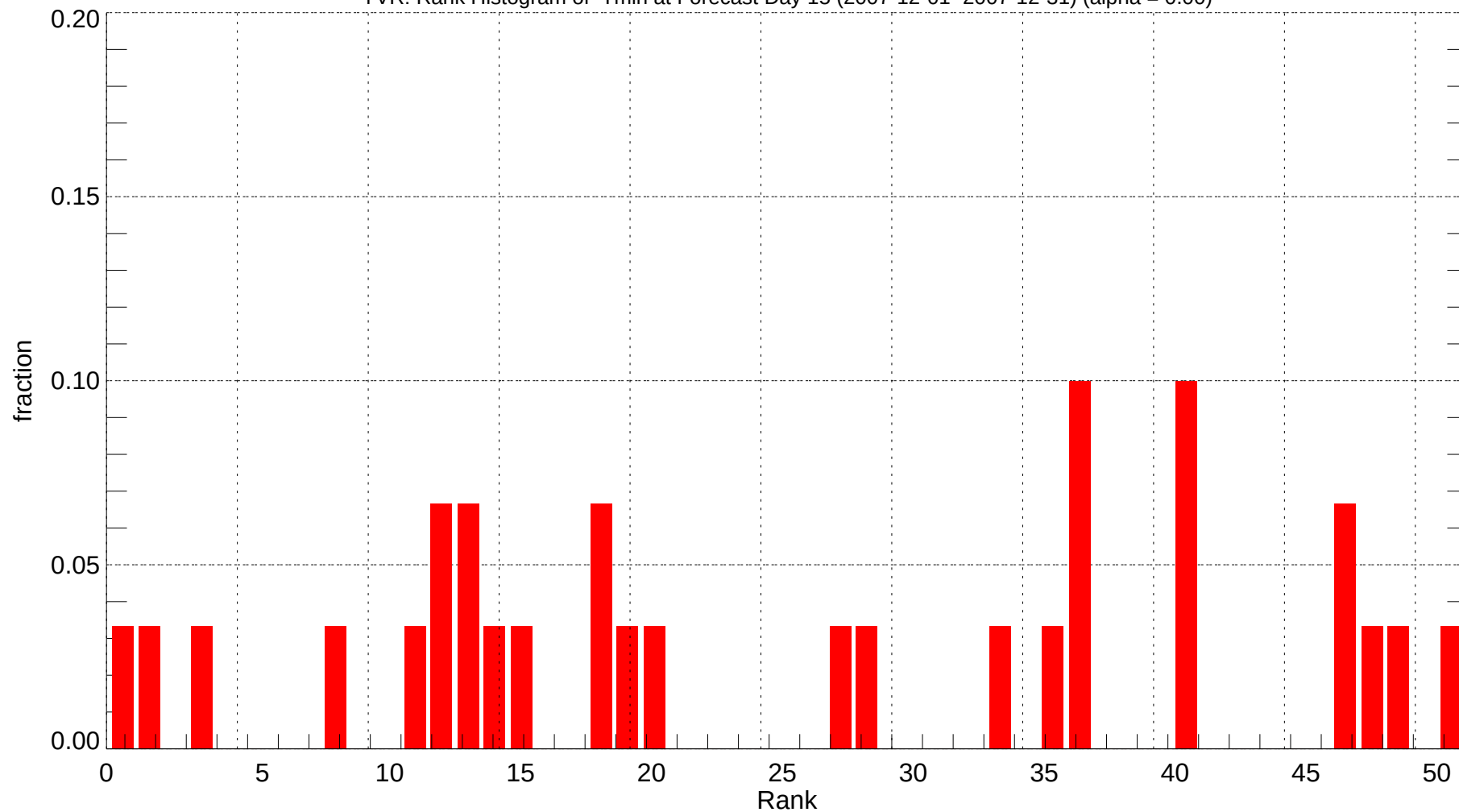
YVR: Rank Histogram of Tmin at Forecast Day 15 (2007-12-01~2007-12-31) (alpha = 0.00)
