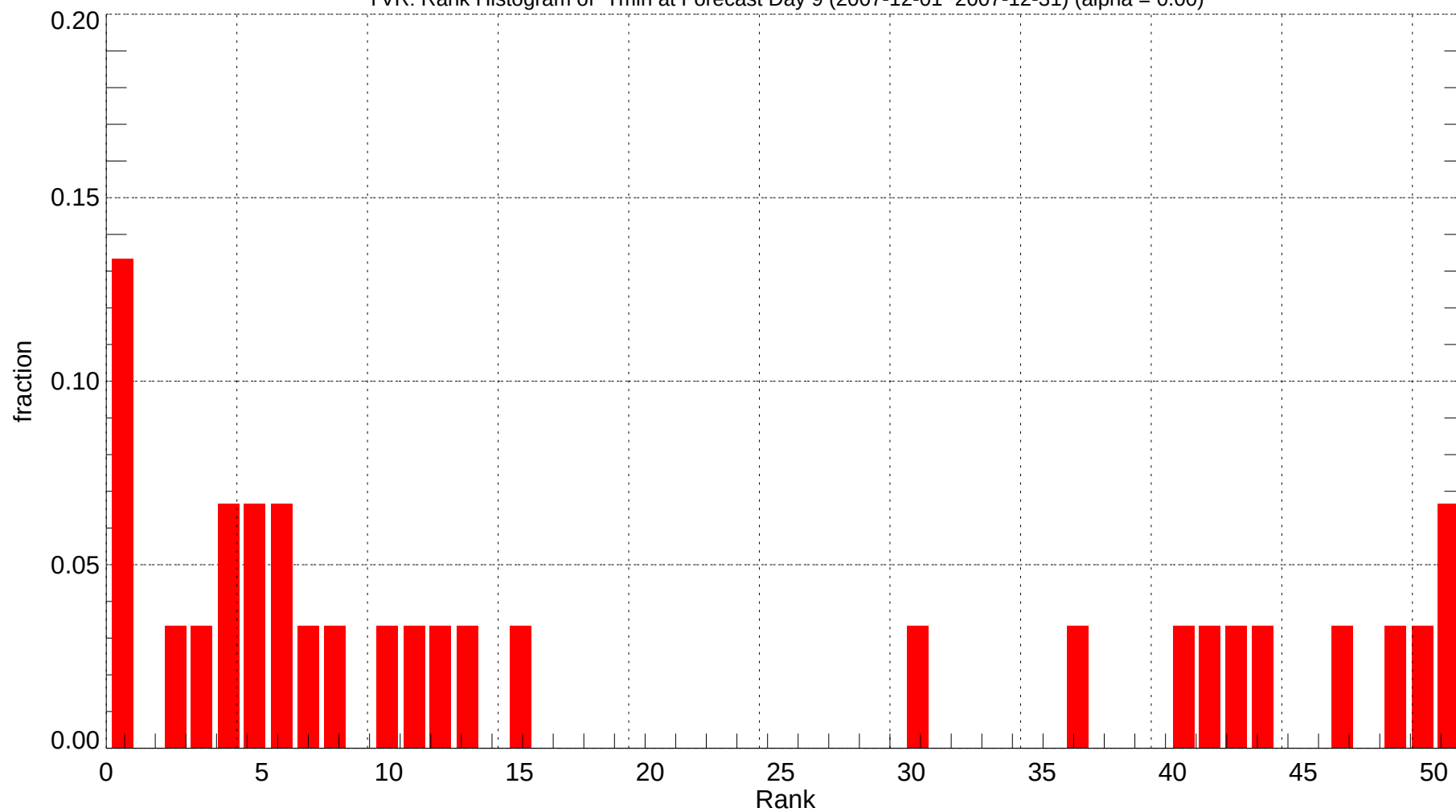
YVR: Rank Histogram of Tmin at Forecast Day 9 (2007-12-01~2007-12-31) (alpha = 0.00)
