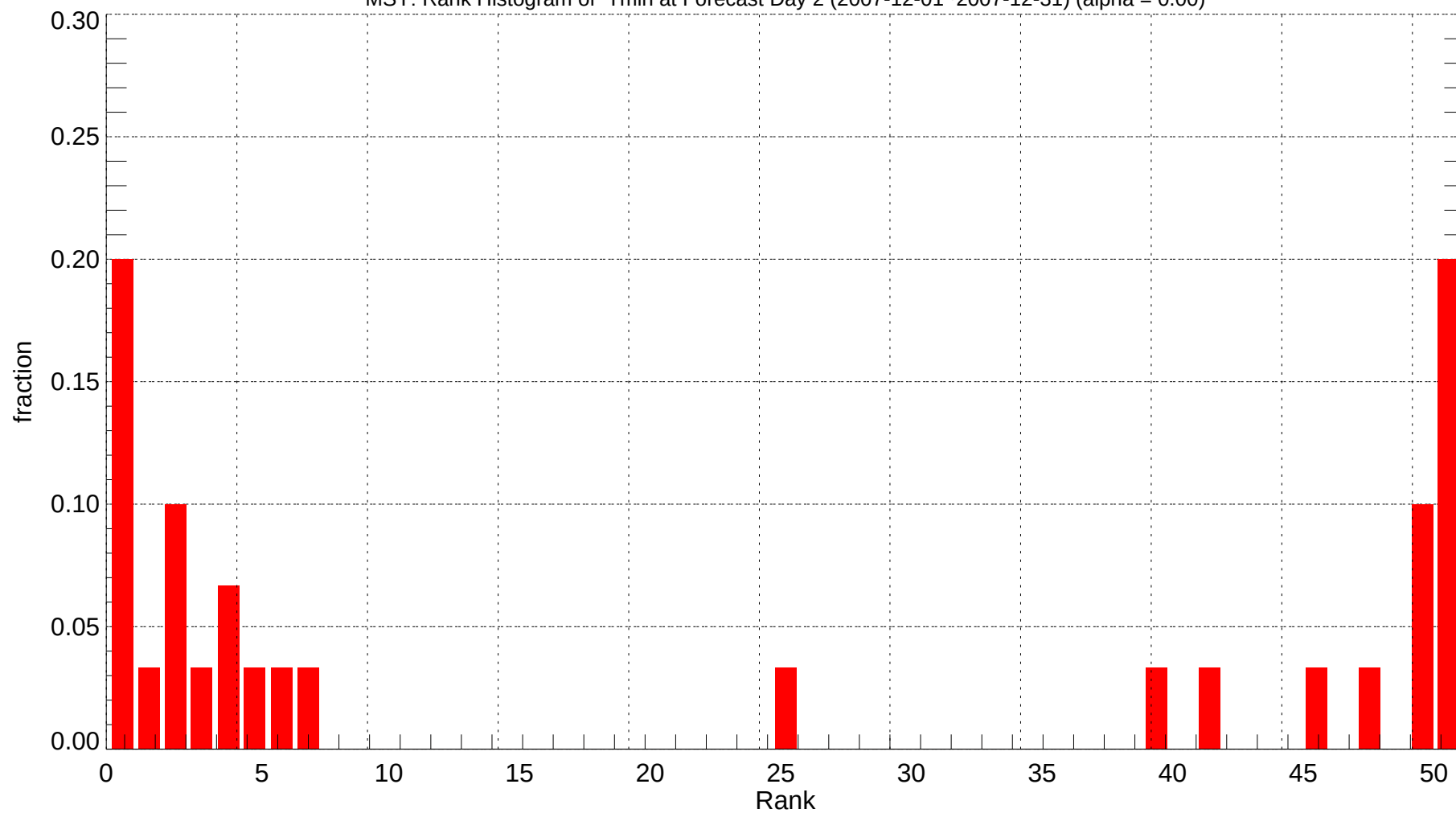
MSY: Rank Histogram of Tmin at Forecast Day 2 (2007-12-01~2007-12-31) (alpha = 0.00)
