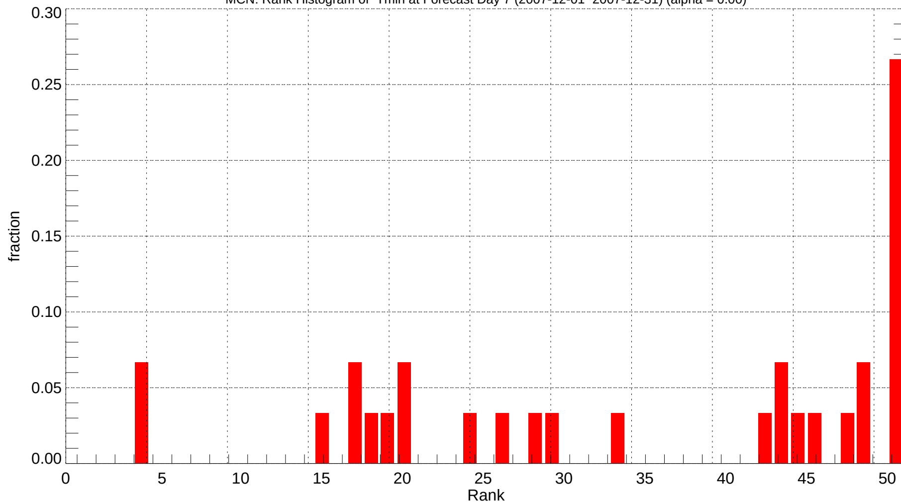
MCN: Rank Histogram of Tmin at Forecast Day 7 (2007-12-01~2007-12-31) (alpha = 0.00)
