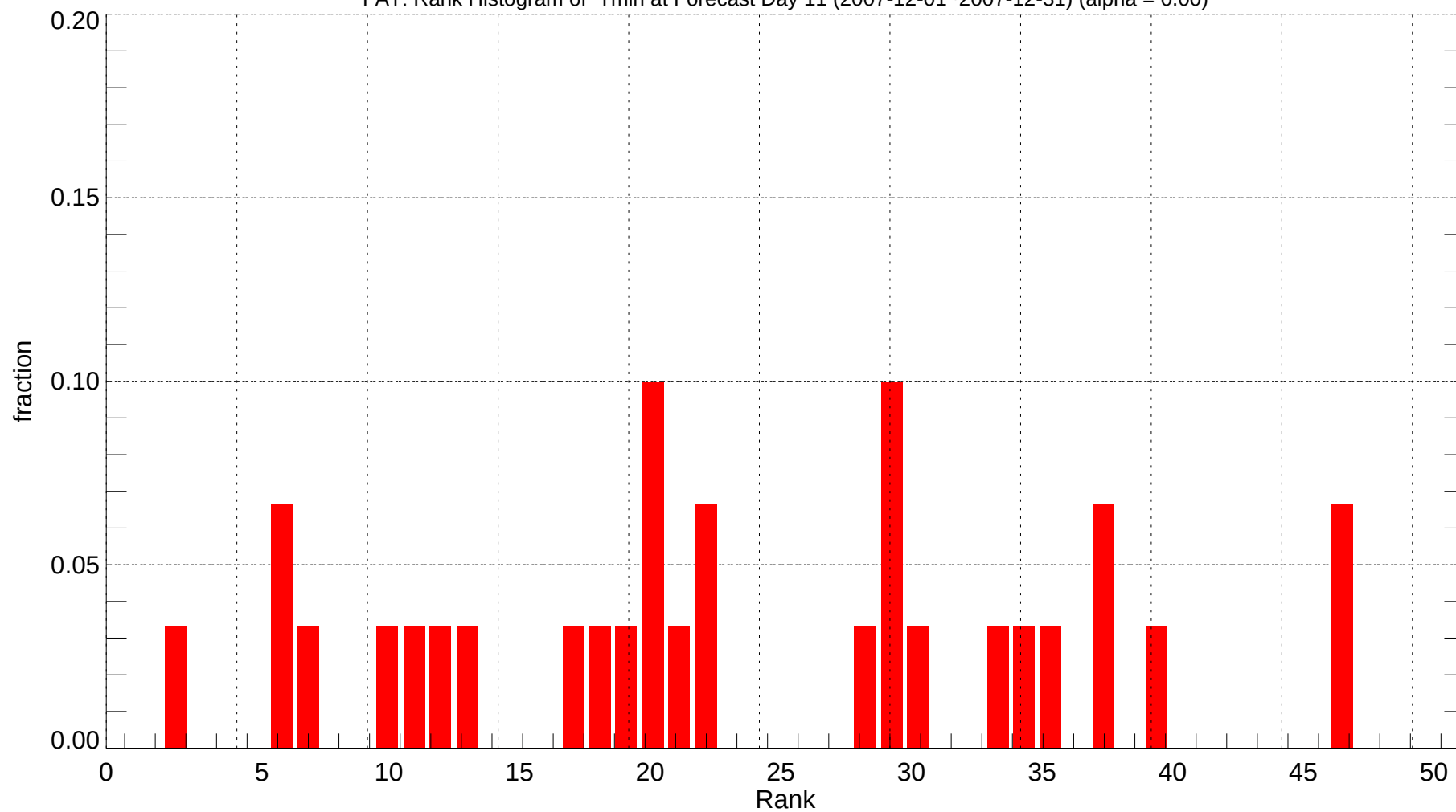
FAT: Rank Histogram of Tmin at Forecast Day 11 (2007-12-01~2007-12-31) (alpha = 0.00)
