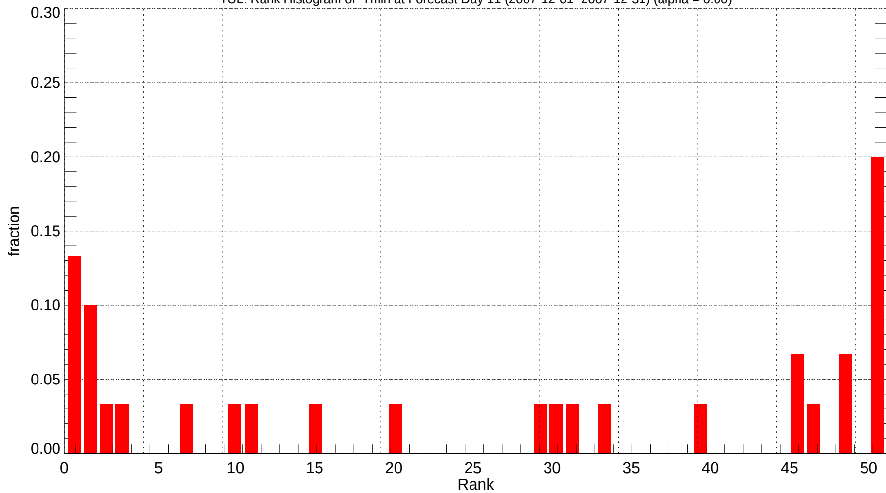
TUL: Rank Histogram of Tmin at Forecast Day 11 (2007-12-01~2007-12-31) (alpha = 0.00)
