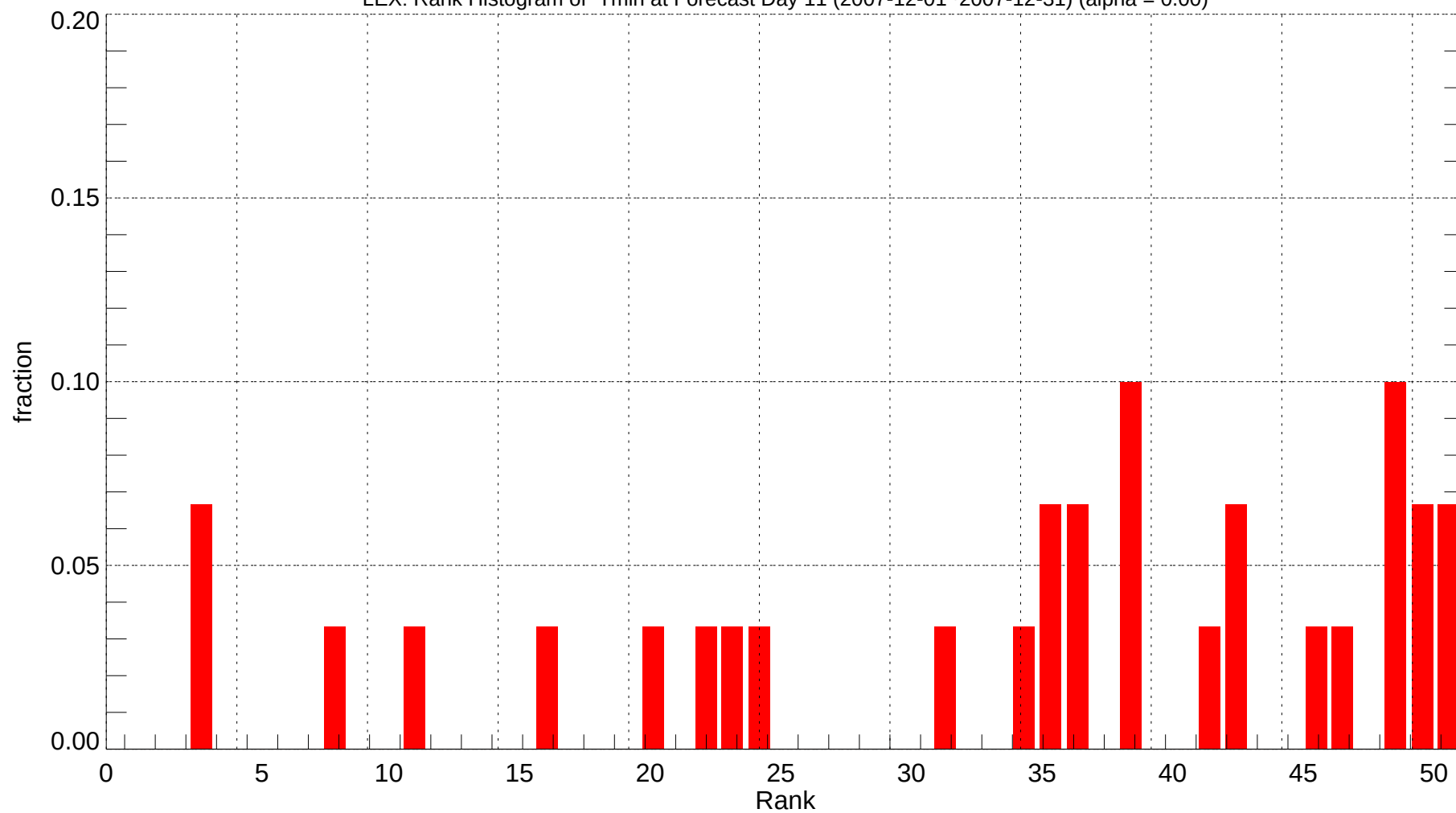
LEX: Rank Histogram of Tmin at Forecast Day 11 (2007-12-01~2007-12-31) (alpha = 0.00)
