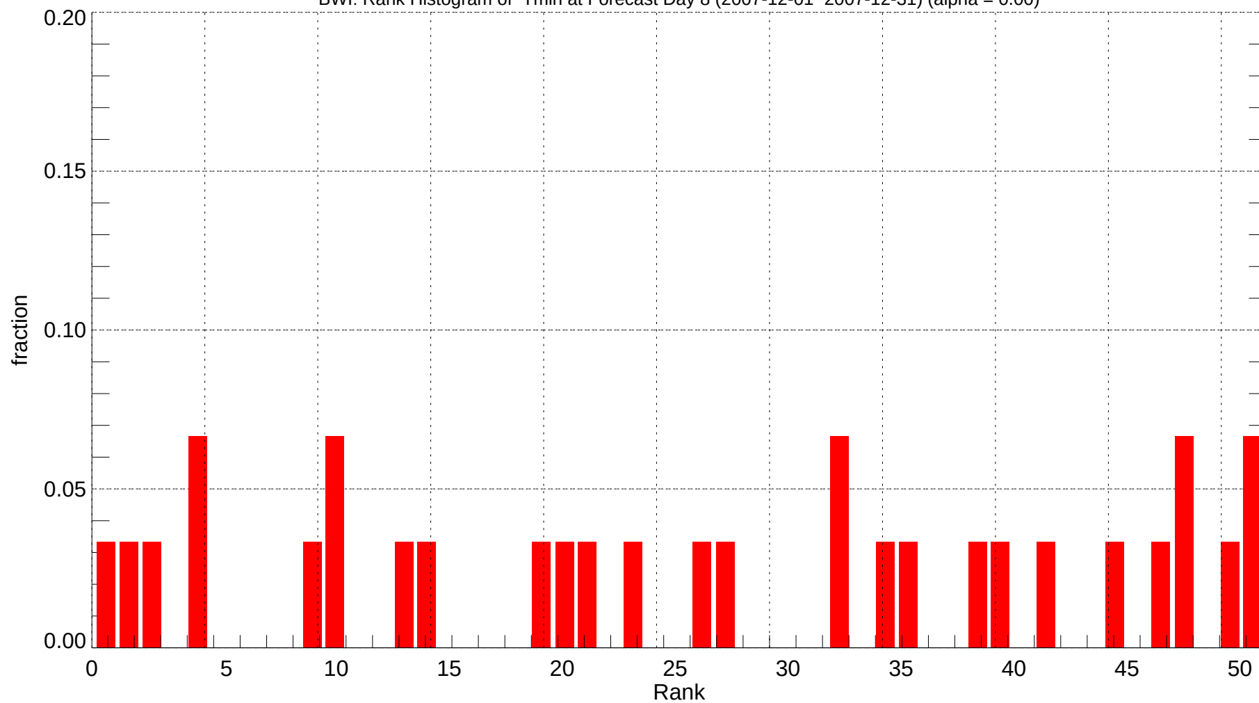
BWI: Rank Histogram of Tmin at Forecast Day 8 (2007-12-01~2007-12-31) (alpha = 0.00)
