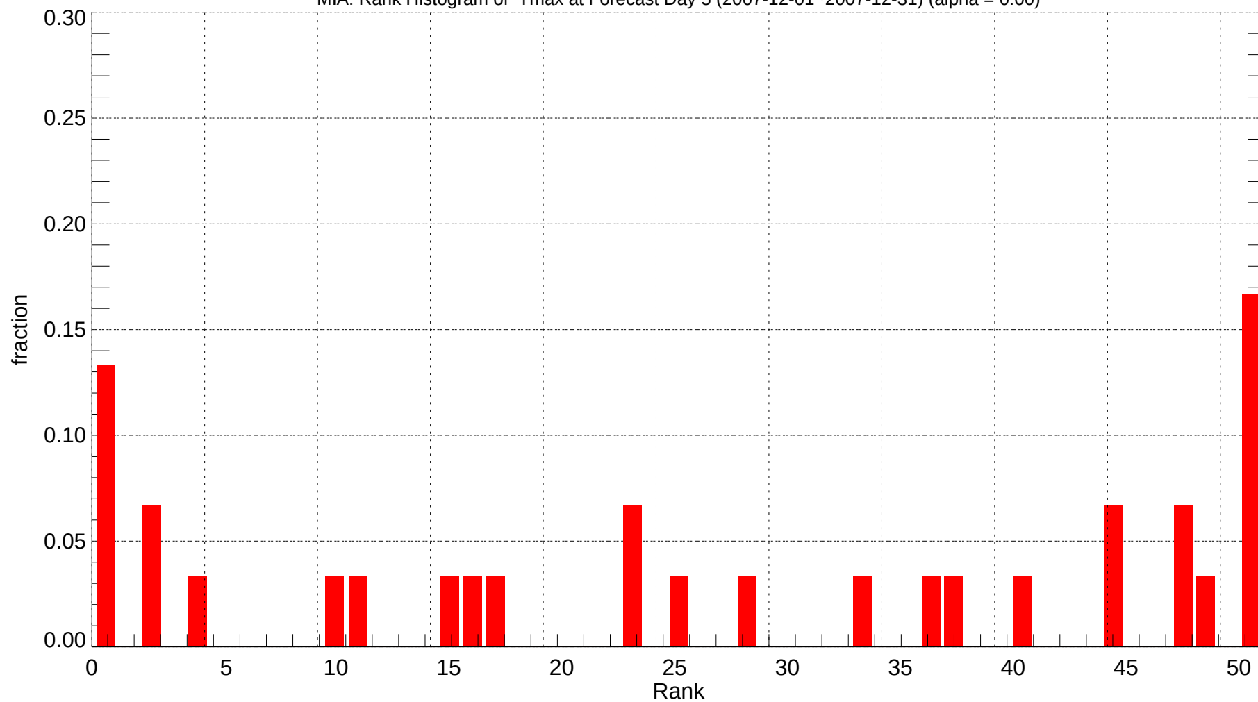
MIA: Rank Histogram of Tmax at Forecast Day 5 (2007-12-01~2007-12-31) (alpha = 0.00)
