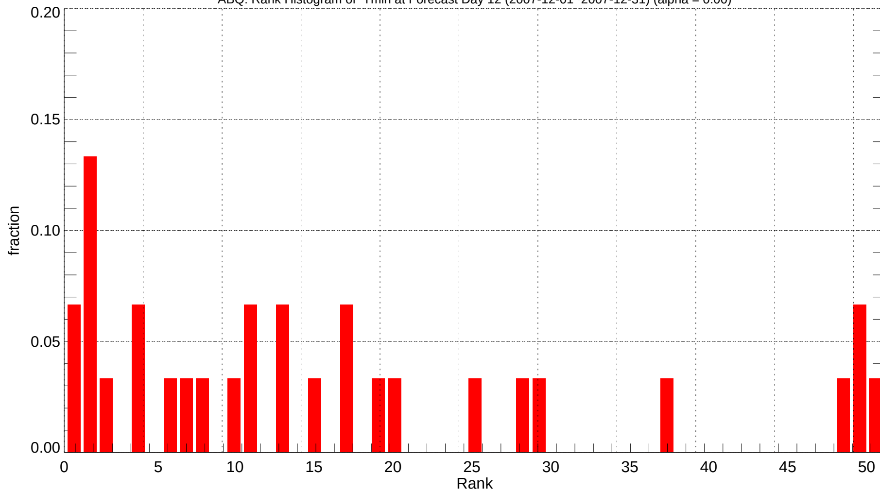
ABQ: Rank Histogram of Tmin at Forecast Day 12 (2007-12-01~2007-12-31) (alpha = 0.00)
