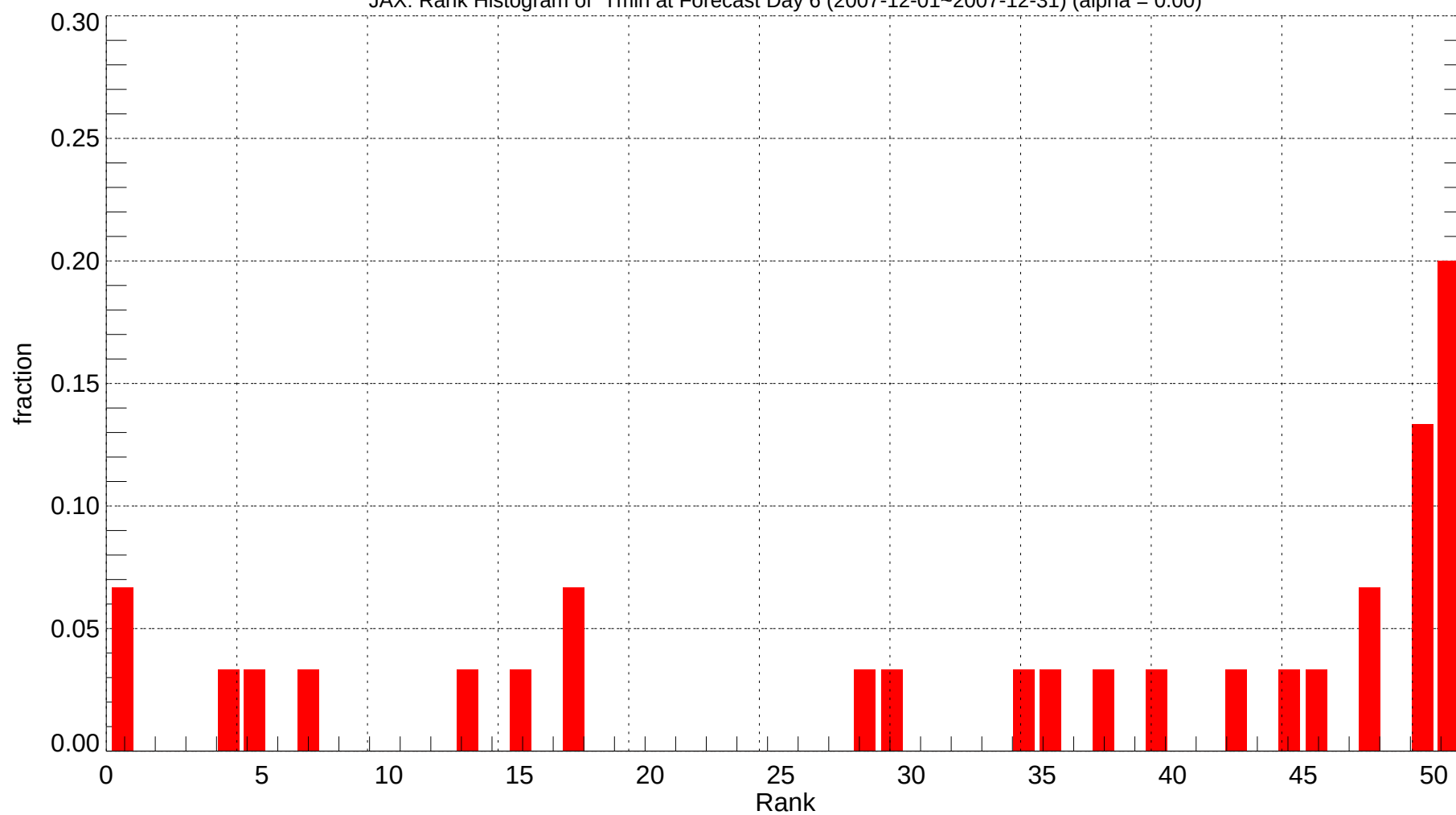
JAX: Rank Histogram of Tmin at Forecast Day 6 (2007-12-01~2007-12-31) (alpha = 0.00)
