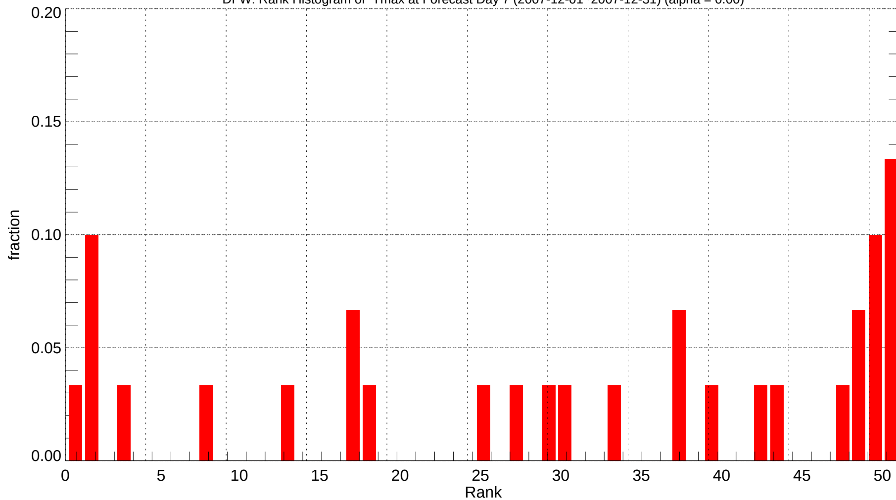
DFW: Rank Histogram of Tmax at Forecast Day 7 (2007-12-01~2007-12-31) (alpha = 0.00)
