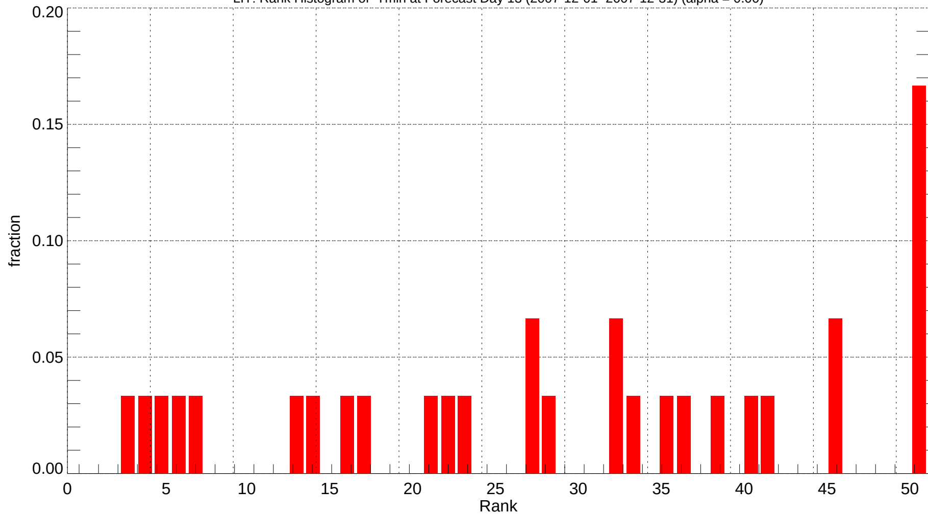
LIT: Rank Histogram of Tmin at Forecast Day 13 (2007-12-01~2007-12-31) (alpha = 0.00)
