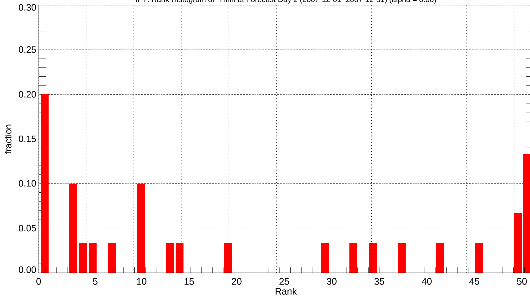
IPT: Rank Histogram of Tmin at Forecast Day 2 (2007-12-01~2007-12-31) (alpha = 0.00)
