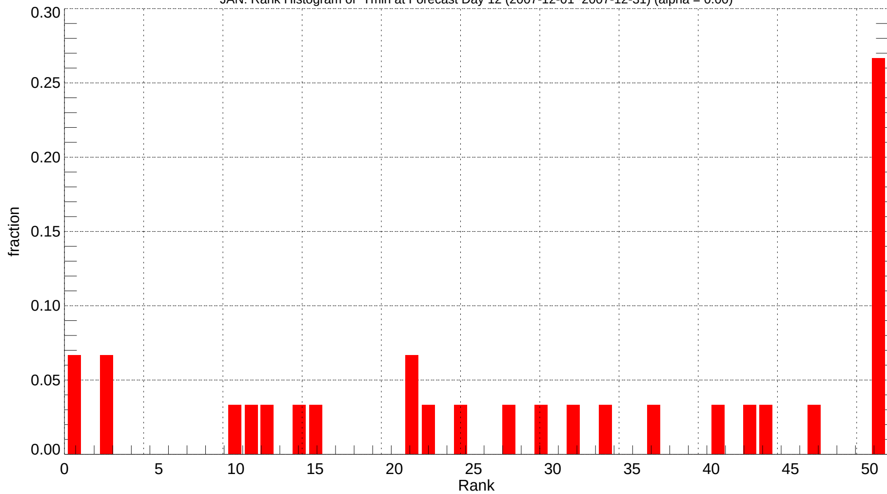
JAN: Rank Histogram of Tmin at Forecast Day 12 (2007-12-01~2007-12-31) (alpha = 0.00)
