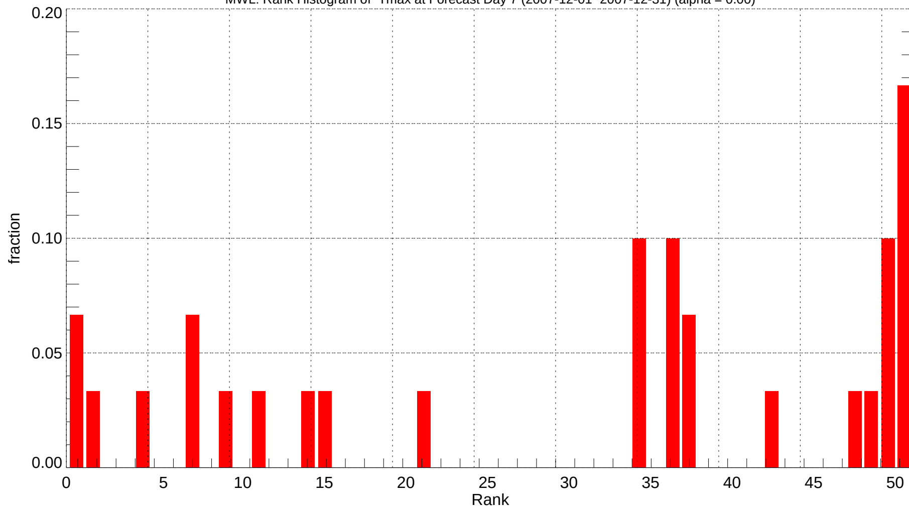
MWL: Rank Histogram of Tmax at Forecast Day 7 (2007-12-01~2007-12-31) (alpha = 0.00)
