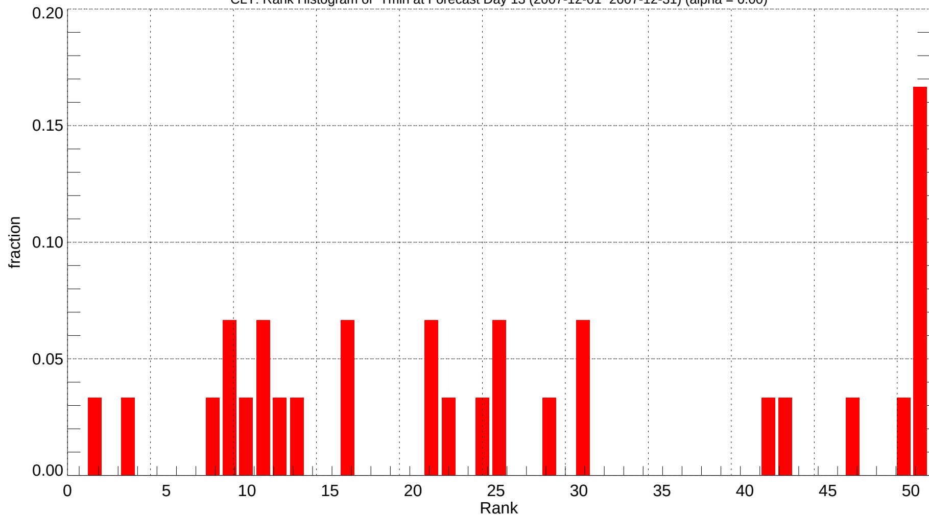
CLT: Rank Histogram of Tmin at Forecast Day 13 (2007-12-01~2007-12-31) (alpha = 0.00)
