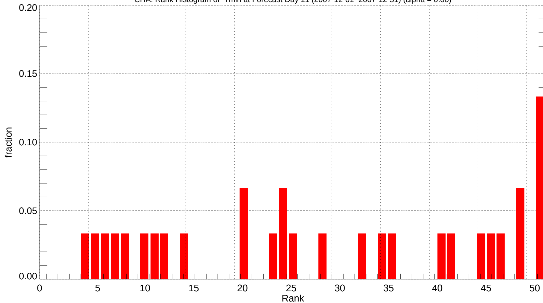
CHA: Rank Histogram of Tmin at Forecast Day 11 (2007-12-01~2007-12-31) (alpha = 0.00)
