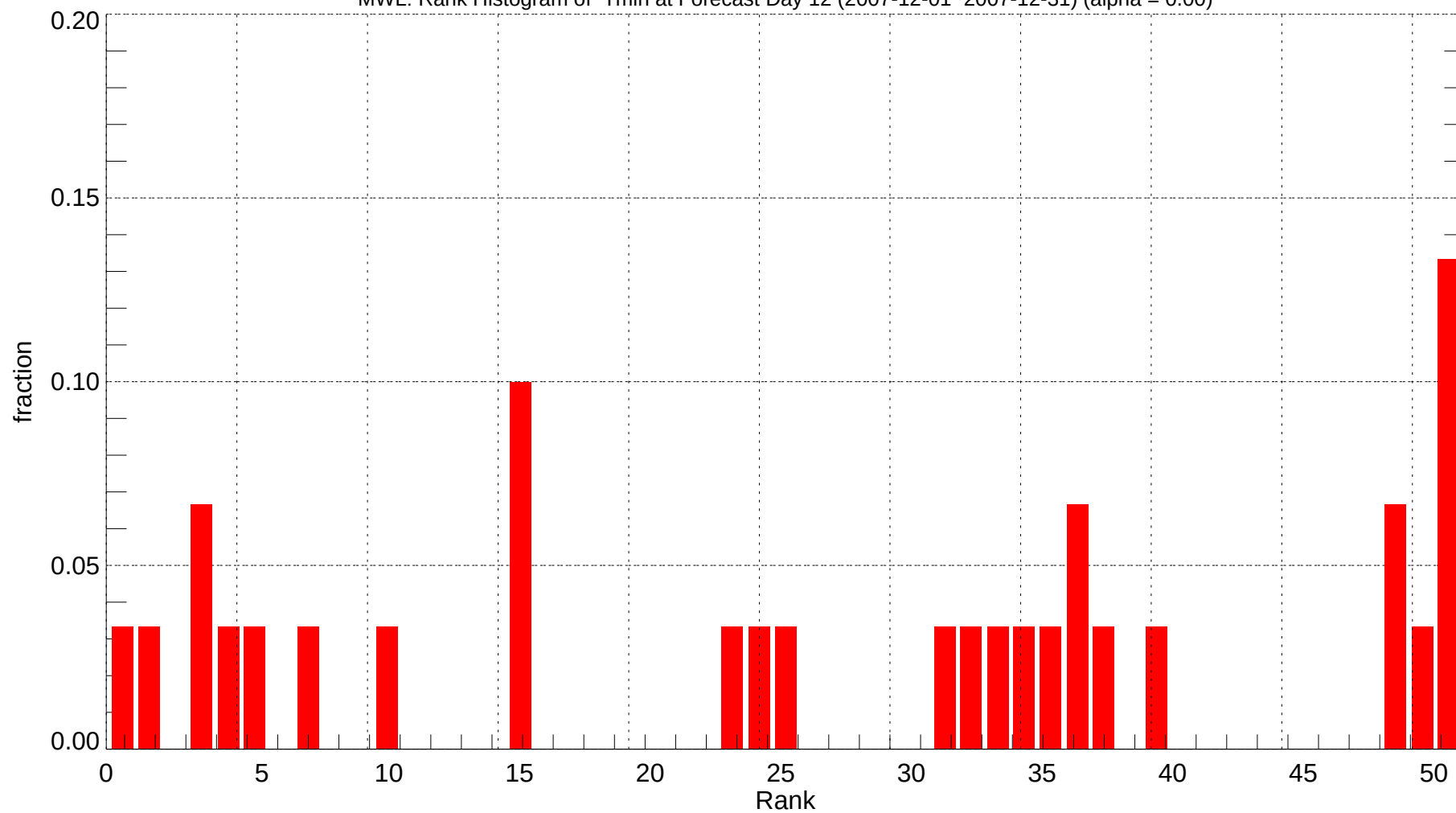
MWL: Rank Histogram of Tmin at Forecast Day 12 (2007-12-01~2007-12-31) (alpha = 0.00)
