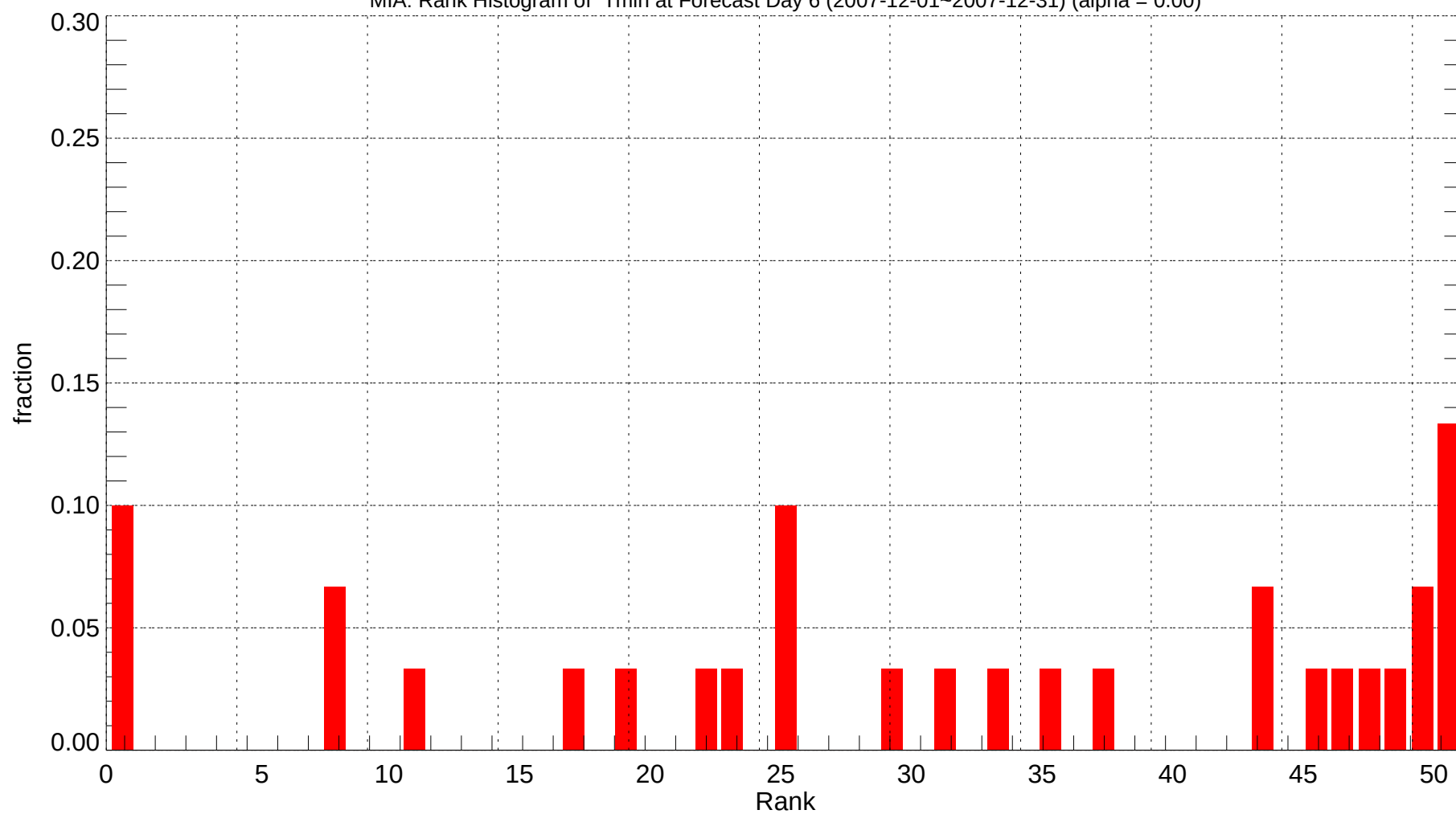
MIA: Rank Histogram of Tmin at Forecast Day 6 (2007-12-01~2007-12-31) (alpha = 0.00)
