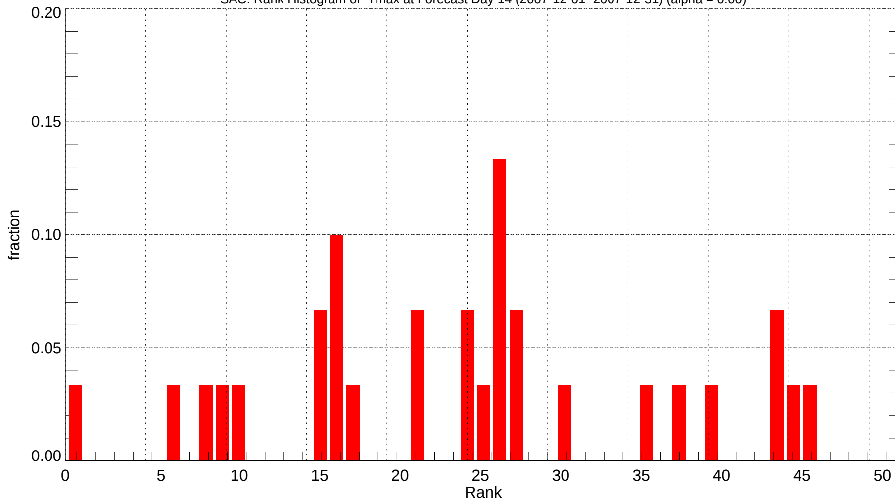
SAC: Rank Histogram of Tmax at Forecast Day 14 (2007-12-01~2007-12-31) (alpha = 0.00)
