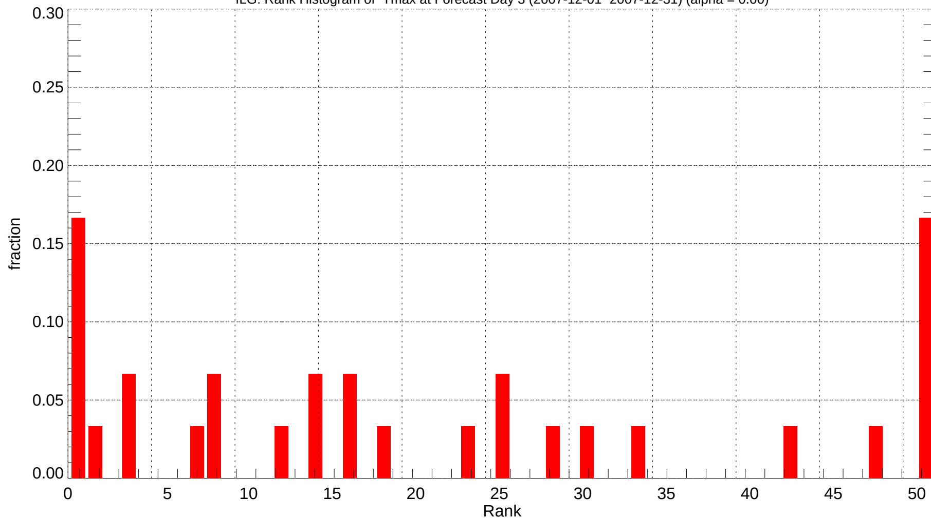
ILG: Rank Histogram of Tmax at Forecast Day 3 (2007-12-01~2007-12-31) (alpha = 0.00)
