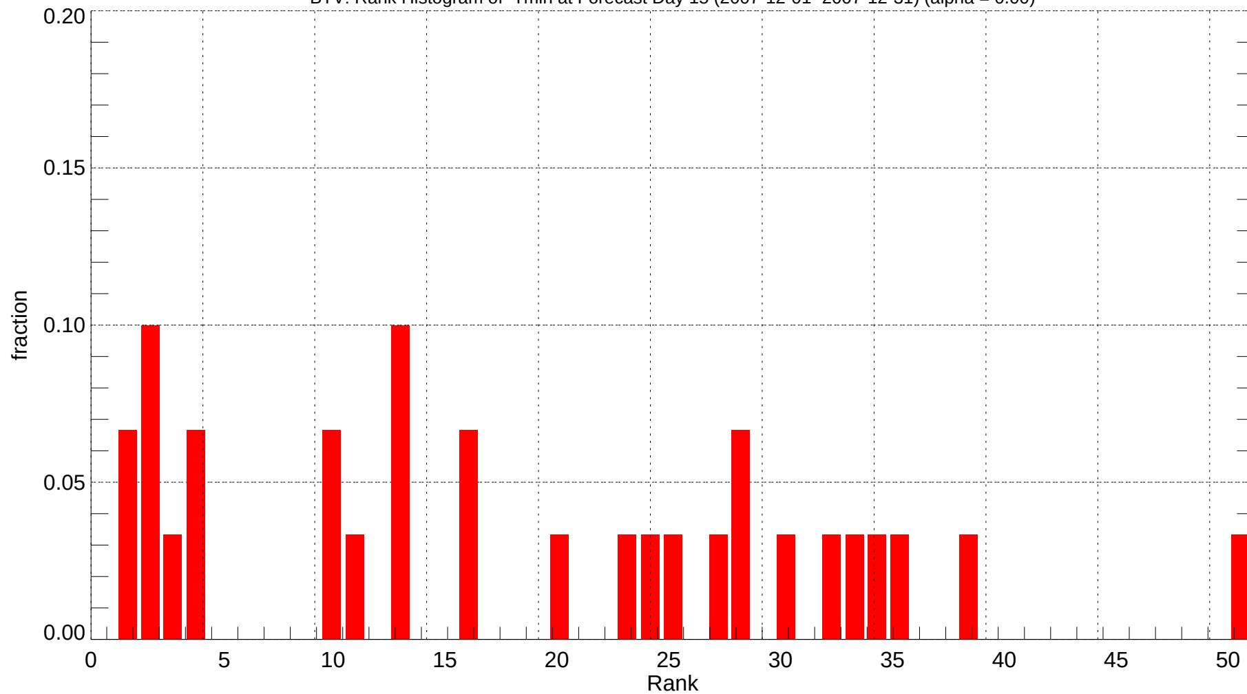
BTV: Rank Histogram of Tmin at Forecast Day 15 (2007-12-01~2007-12-31) (alpha = 0.00)
