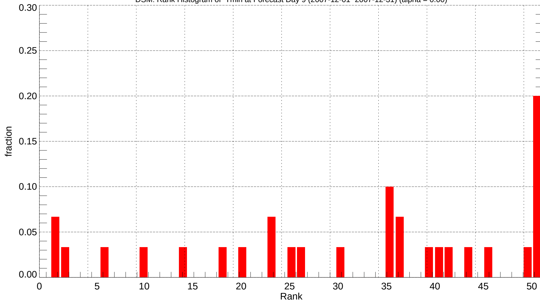
DSM: Rank Histogram of Tmin at Forecast Day 9 (2007-12-01~2007-12-31) (alpha = 0.00)
