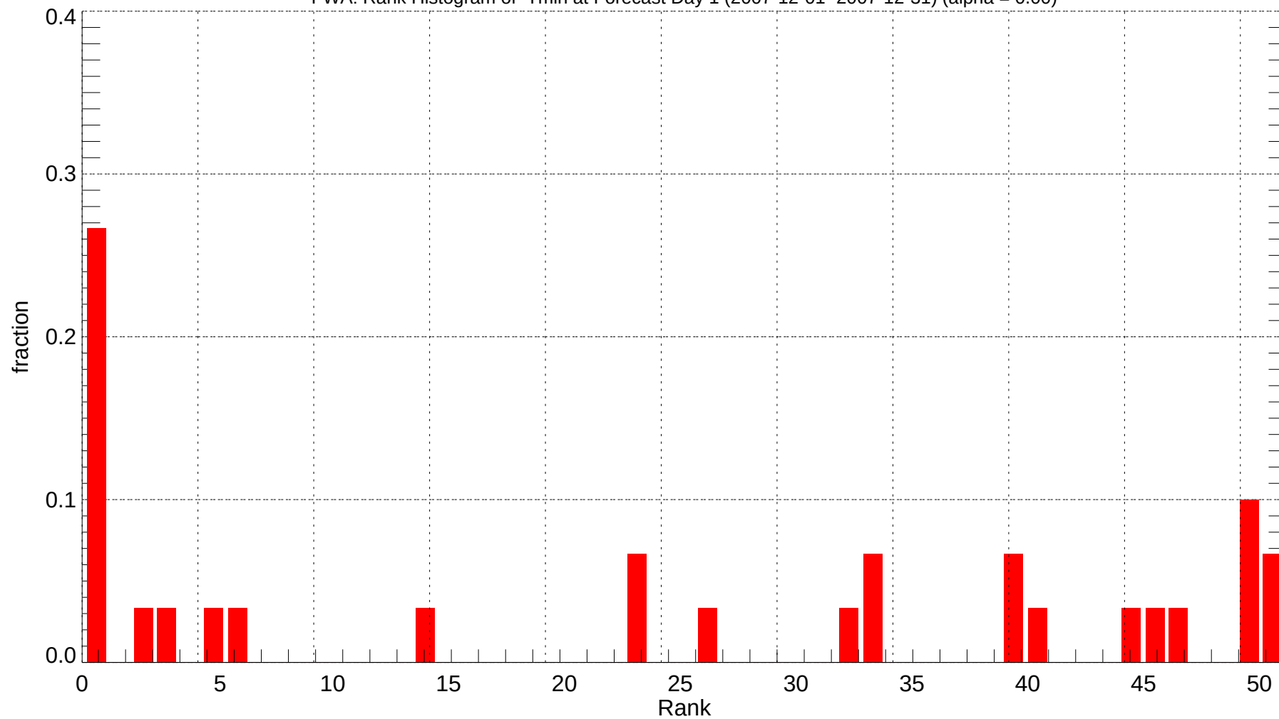
FWA: Rank Histogram of Tmin at Forecast Day 1 (2007-12-01~2007-12-31) (alpha = 0.00)
