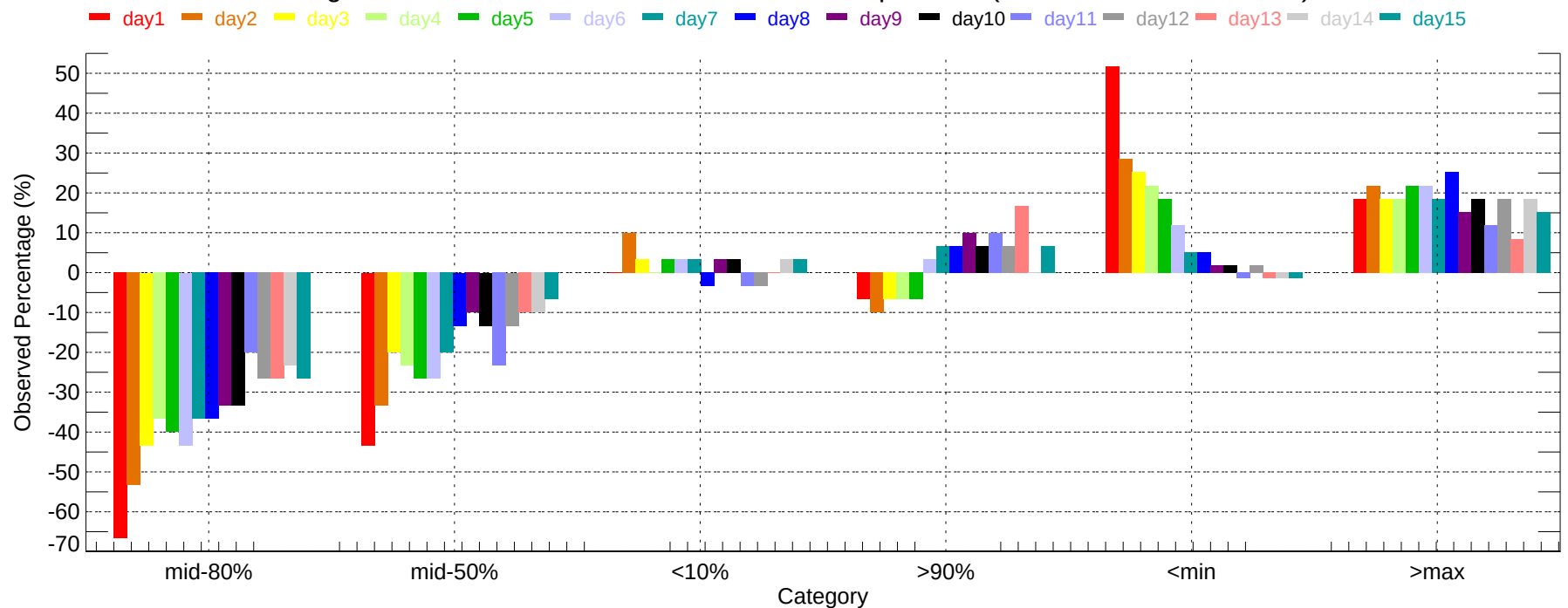
Observed Percentage Deviation of Ensembles - MOB: Max Temperature (2007-12-01~2007-12-31)
