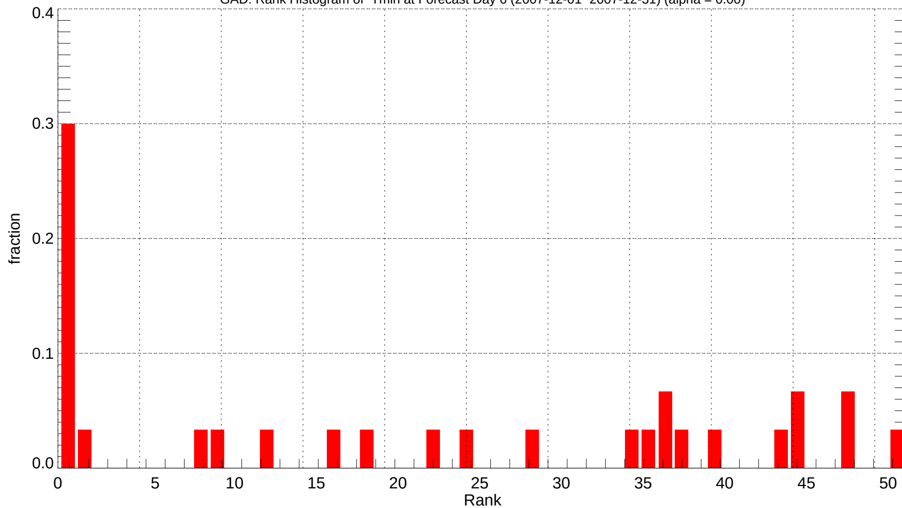
GAD: Rank Histogram of Tmin at Forecast Day 6 (2007-12-01~2007-12-31) (alpha = 0.00)
