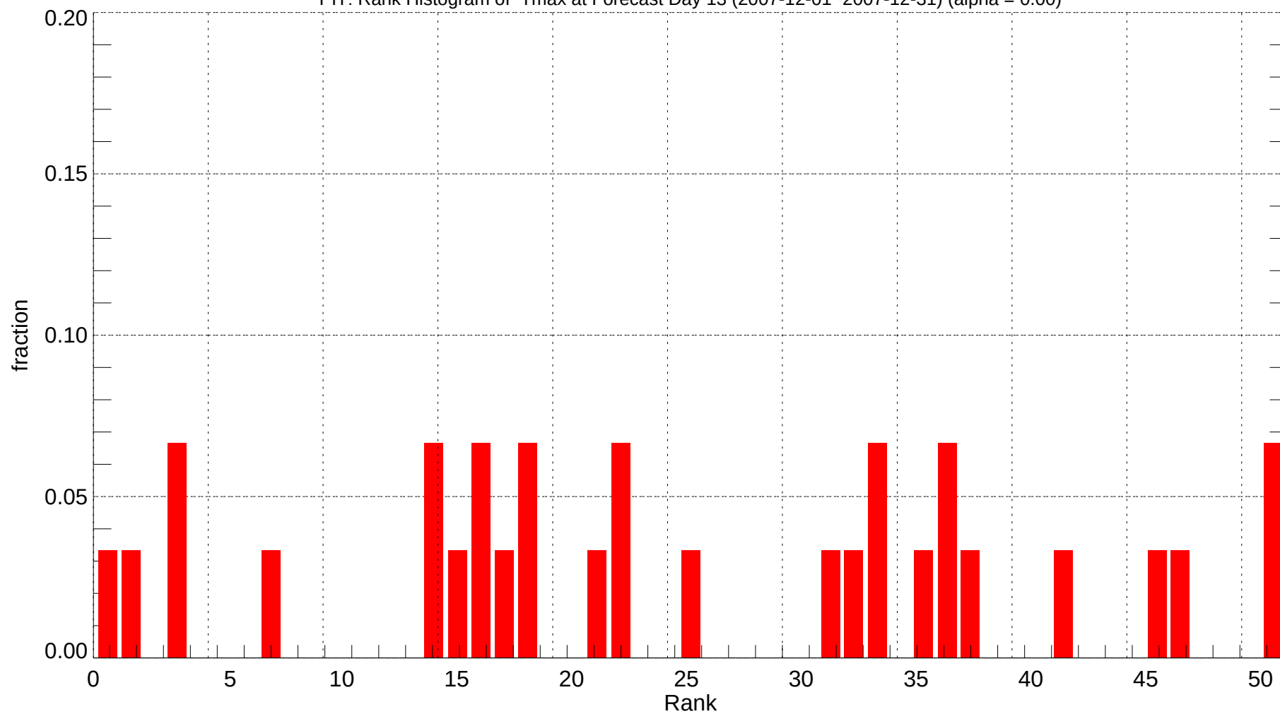
PIT: Rank Histogram of Tmax at Forecast Day 13 (2007-12-01~2007-12-31) (alpha = 0.00)
