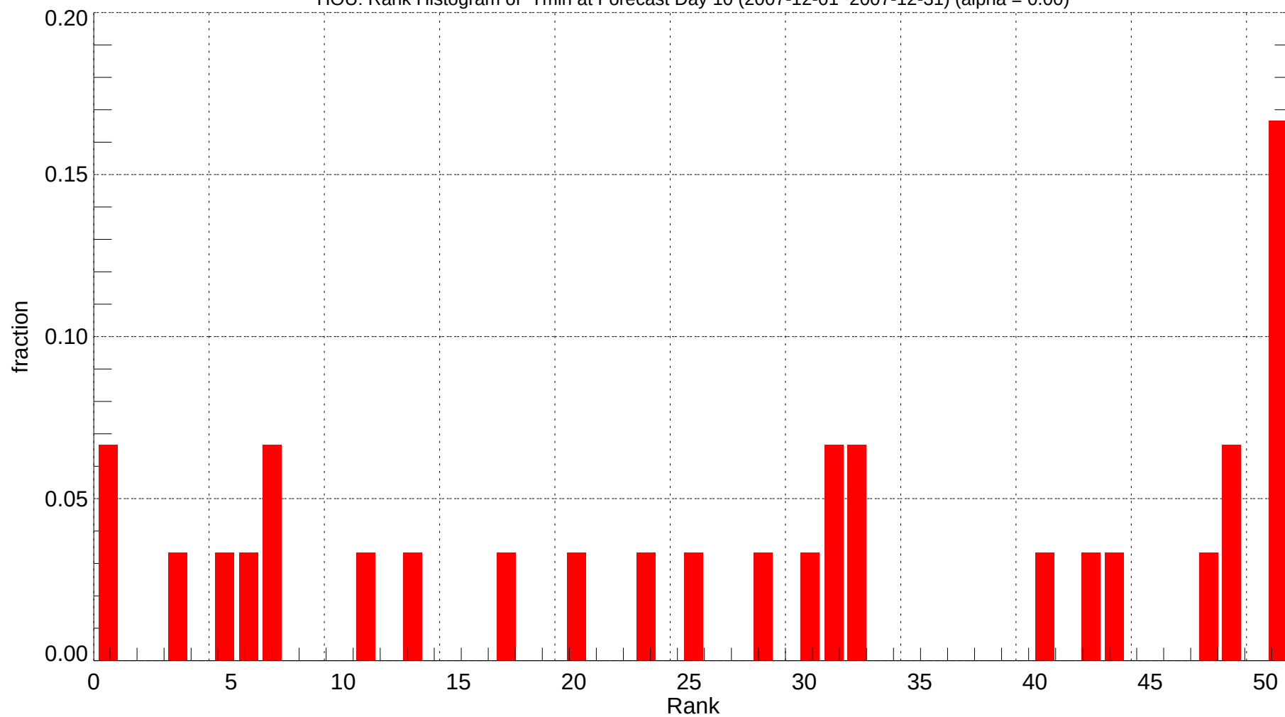
HOU: Rank Histogram of Tmin at Forecast Day 10 (2007-12-01~2007-12-31) (alpha = 0.00)
