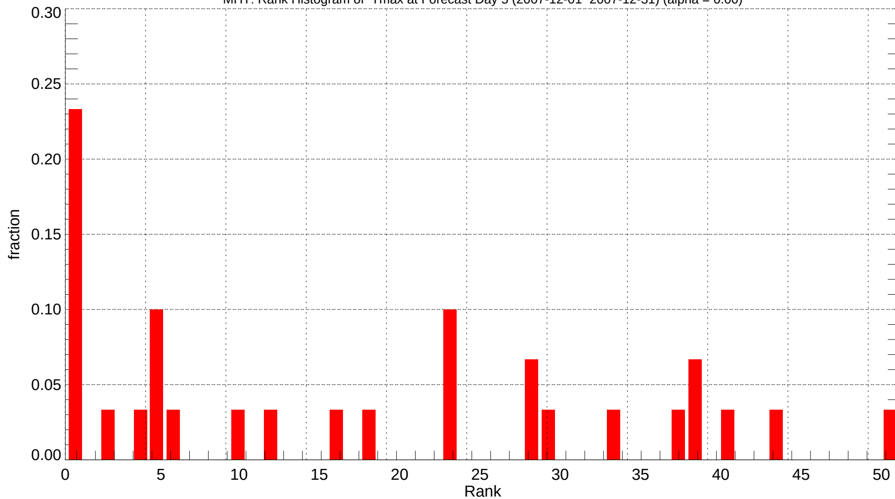
MHT: Rank Histogram of Tmax at Forecast Day 5 (2007-12-01~2007-12-31) (alpha = 0.00)
