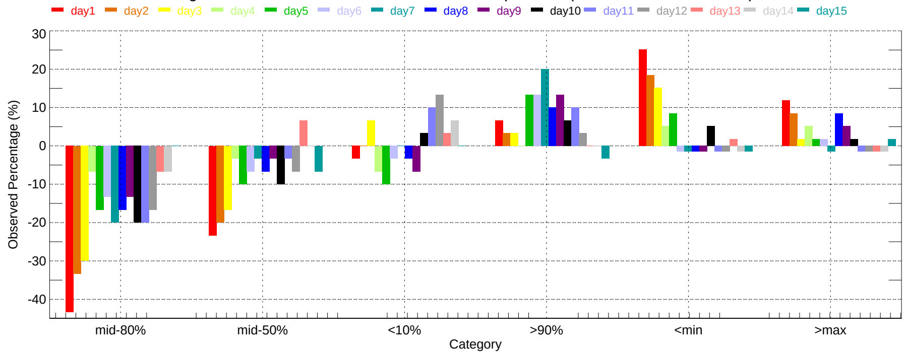
Observed Percentage Deviation of Ensembles - EWR: Min Temperature (2007-12-01~2007-12-31)
