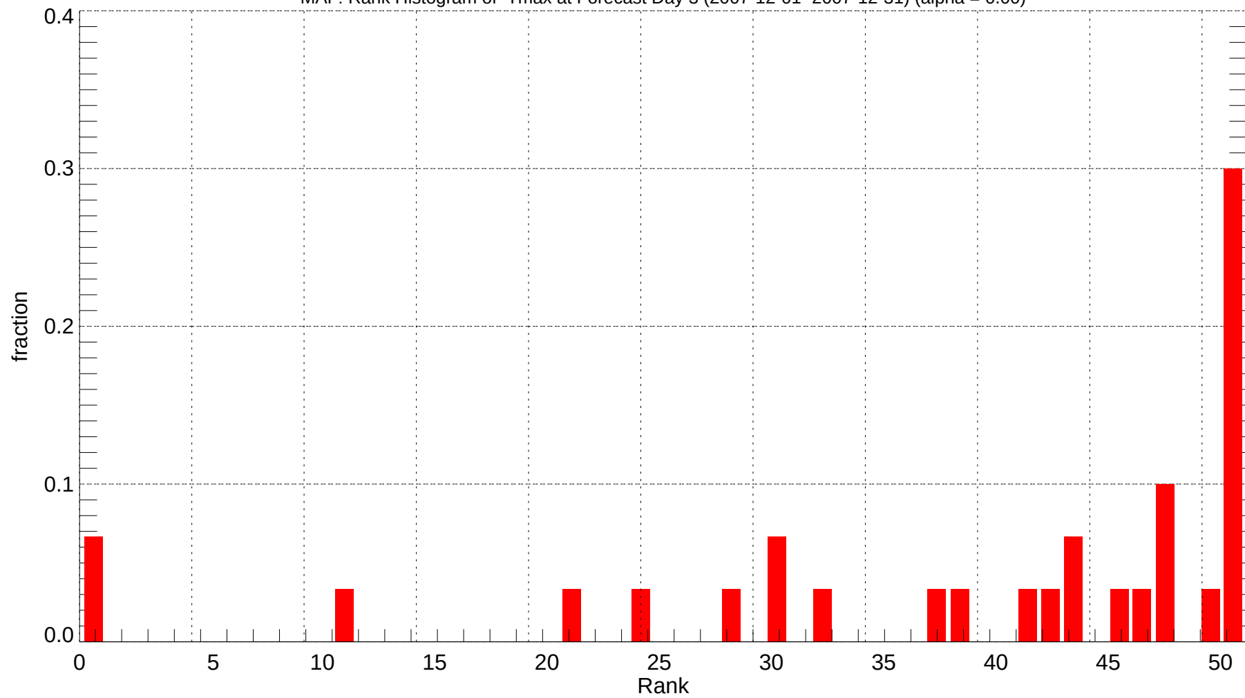
MAF: Rank Histogram of Tmax at Forecast Day 3 (2007-12-01~2007-12-31) (alpha = 0.00)
