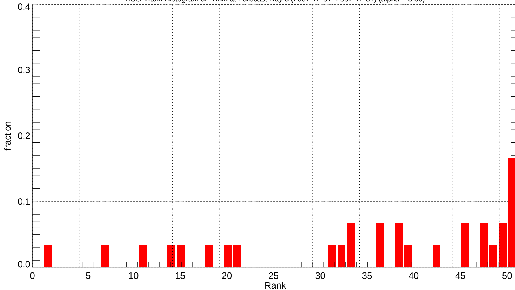
AUS: Rank Histogram of Tmin at Forecast Day 6 (2007-12-01~2007-12-31) (alpha = 0.00)
