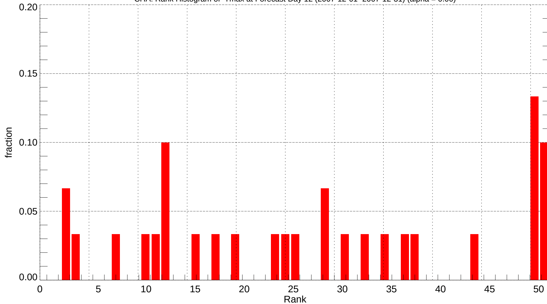
CHA: Rank Histogram of Tmax at Forecast Day 12 (2007-12-01~2007-12-31) (alpha = 0.00)
