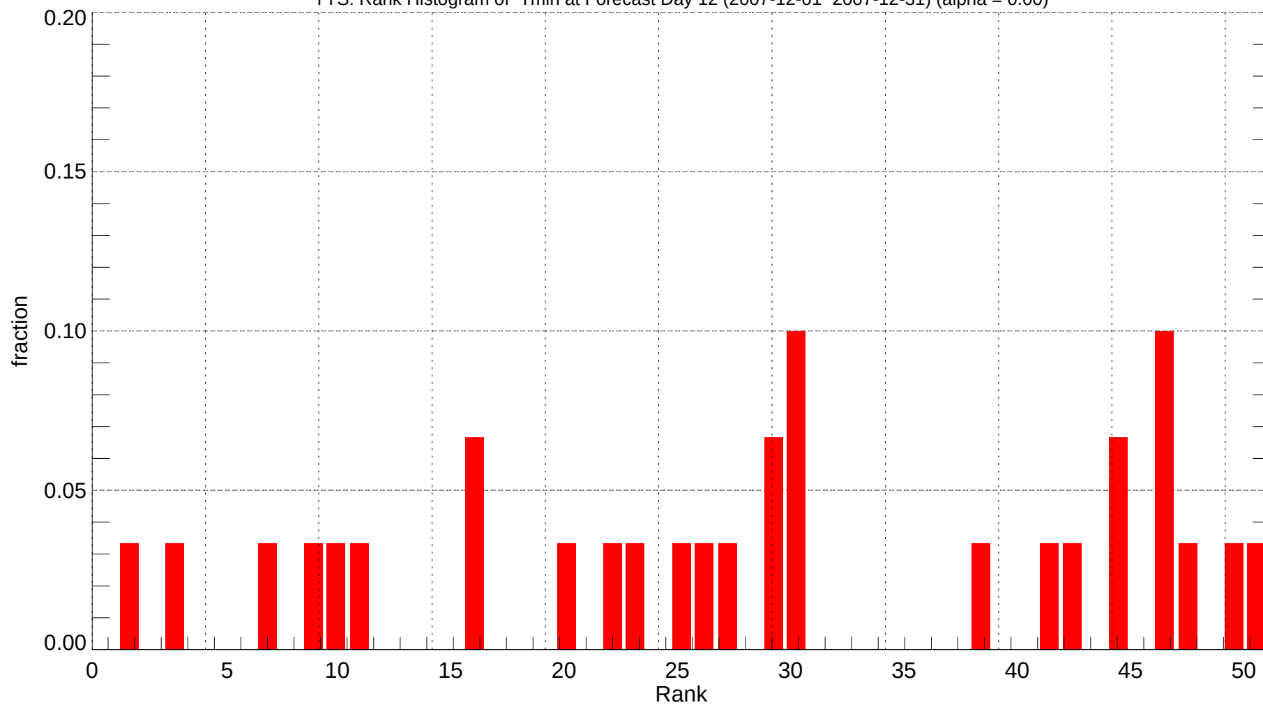
TYS: Rank Histogram of Tmin at Forecast Day 12 (2007-12-01~2007-12-31) (alpha = 0.00)
