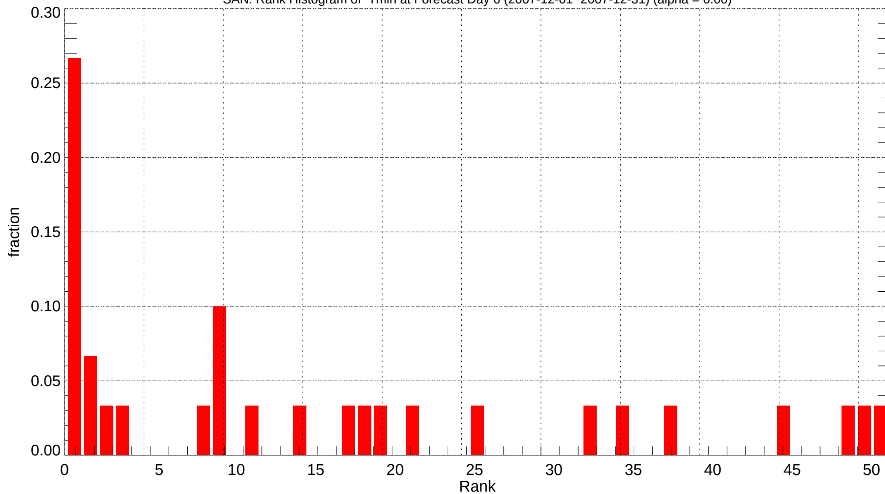
SAN: Rank Histogram of Tmin at Forecast Day 6 (2007-12-01~2007-12-31) (alpha = 0.00)
