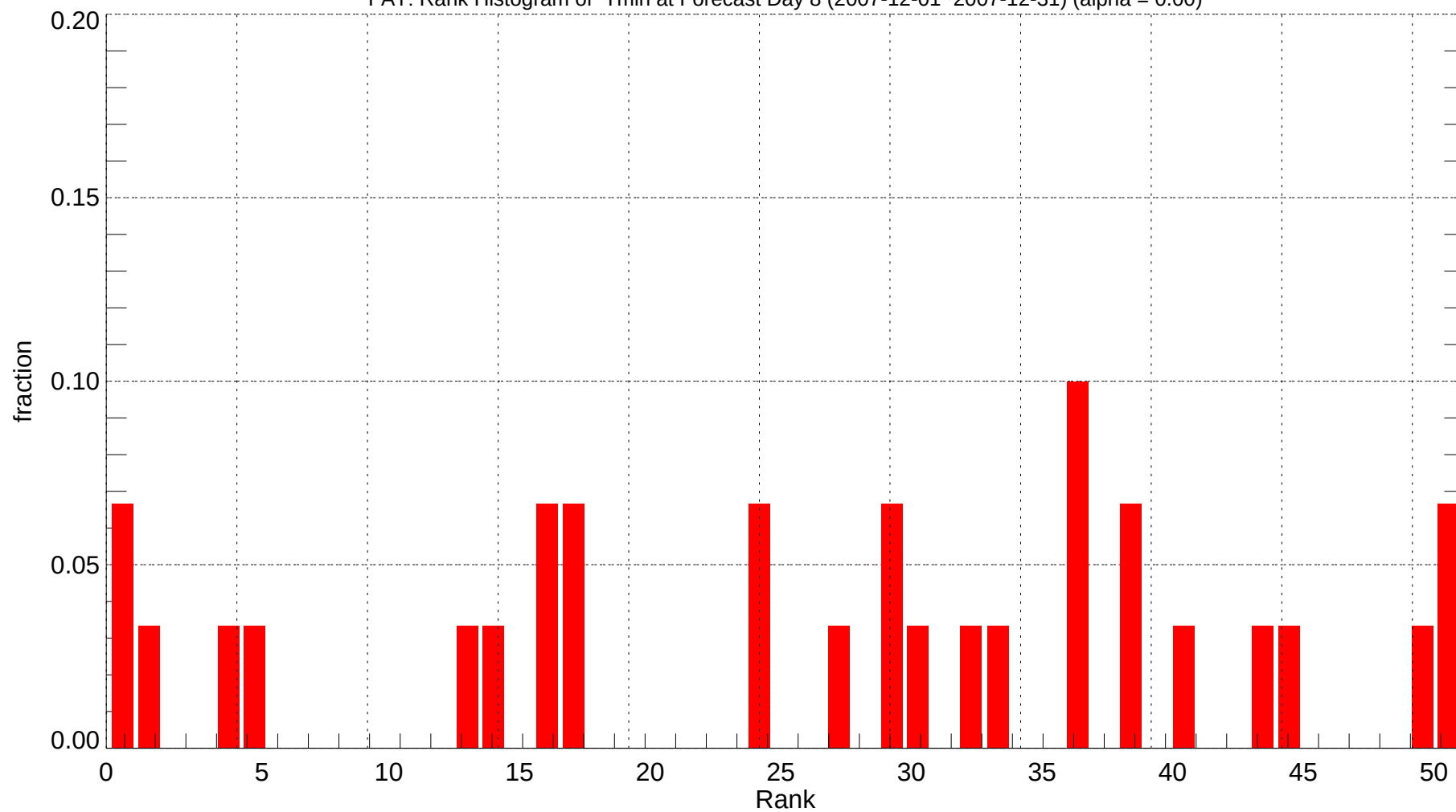
FAT: Rank Histogram of Tmin at Forecast Day 8 (2007-12-01~2007-12-31) (alpha = 0.00)
