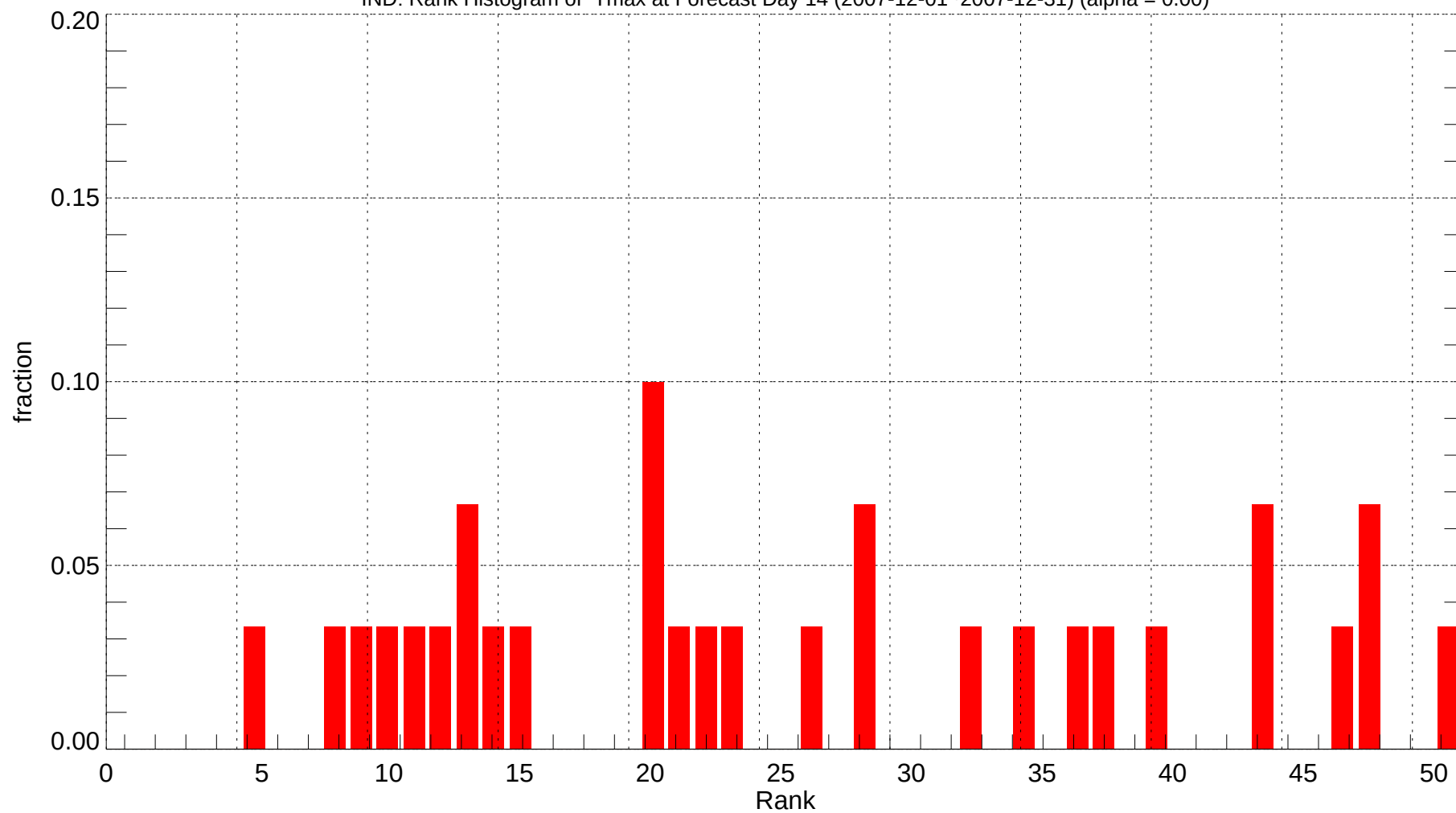
IND: Rank Histogram of Tmax at Forecast Day 14 (2007-12-01~2007-12-31) (alpha = 0.00)
