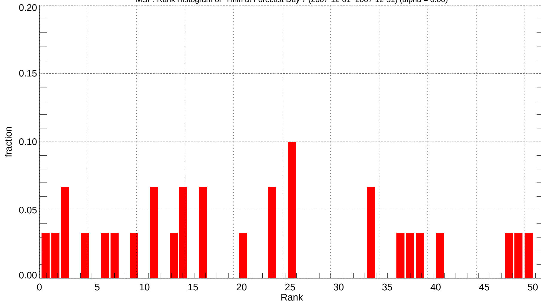
MSP: Rank Histogram of Tmin at Forecast Day 7 (2007-12-01~2007-12-31) (alpha = 0.00)
