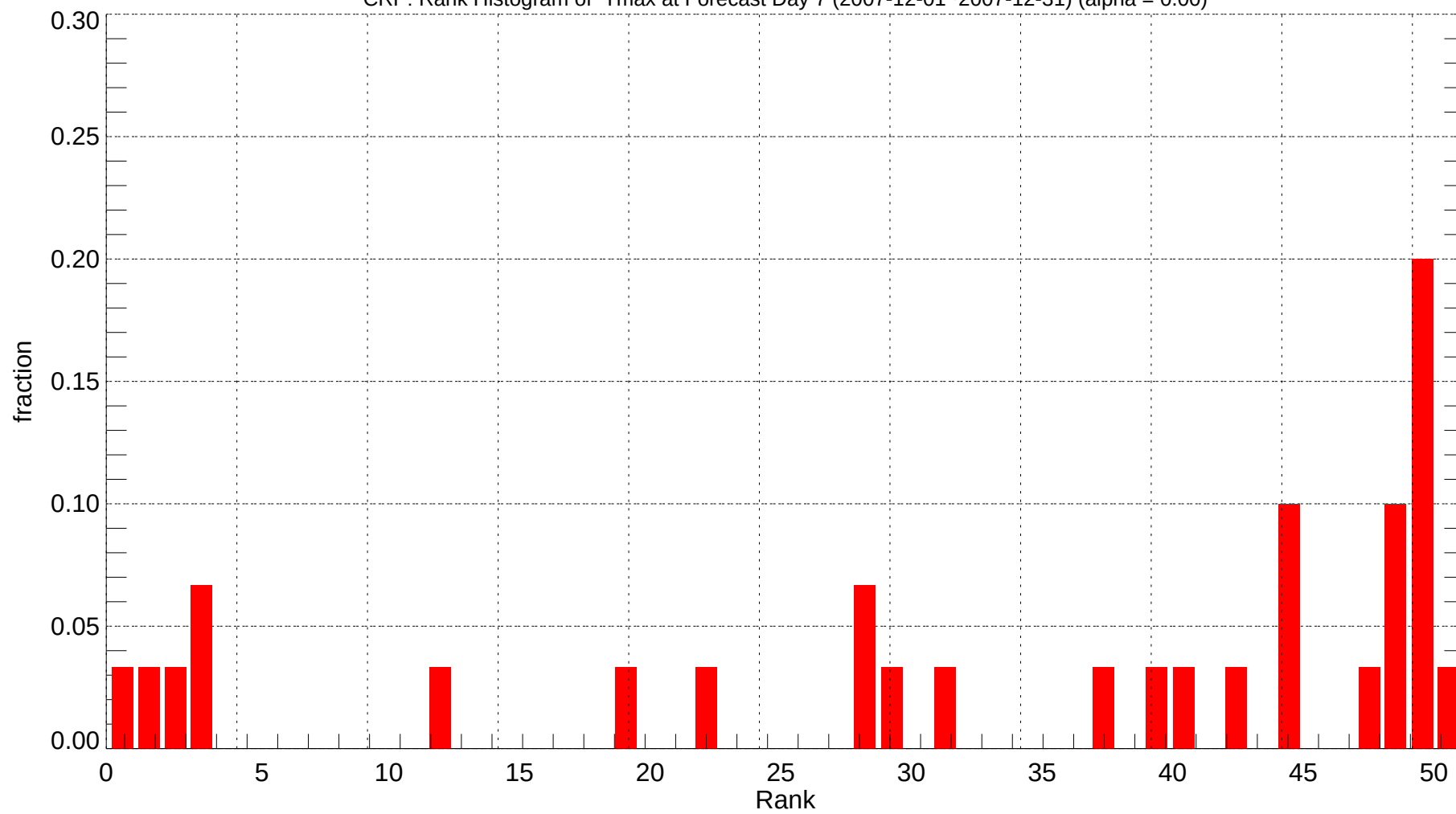
CRP: Rank Histogram of Tmax at Forecast Day 7 (2007-12-01~2007-12-31) (alpha = 0.00)
