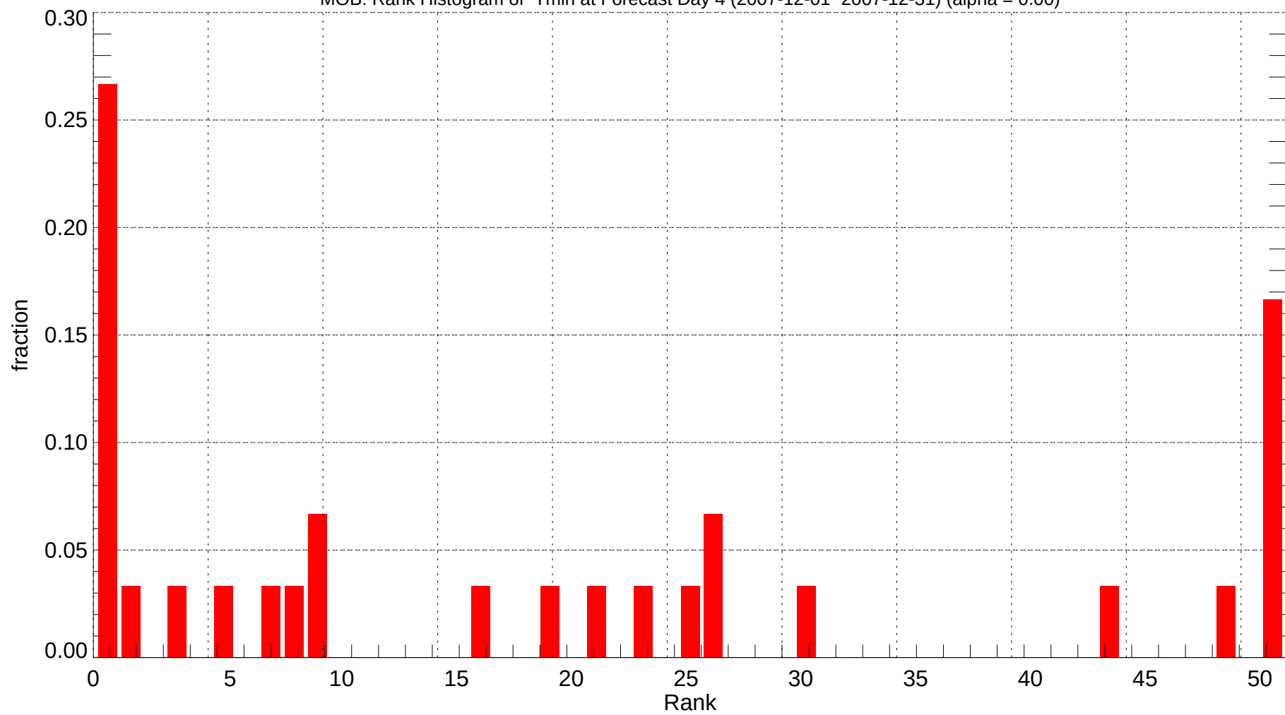
MOB: Rank Histogram of Tmin at Forecast Day 4 (2007-12-01~2007-12-31) (alpha = 0.00)
