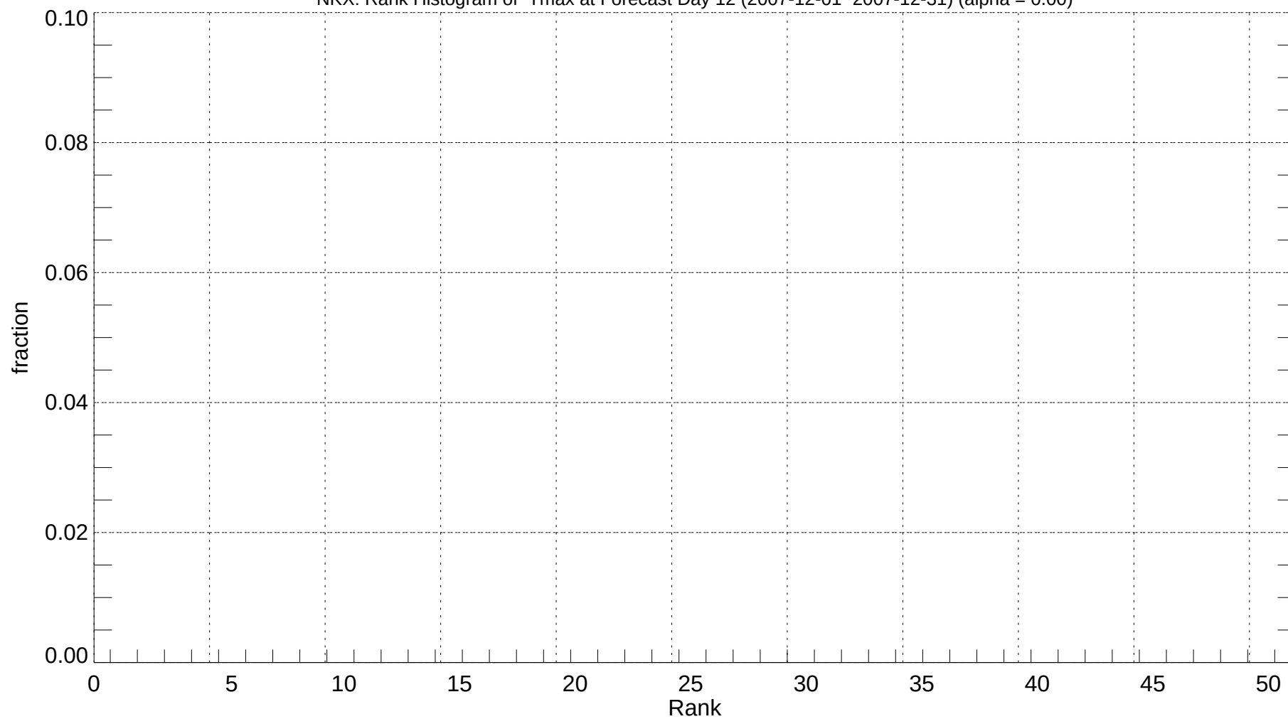
NKX: Rank Histogram of Tmax at Forecast Day 12 (2007-12-01~2007-12-31) (alpha = 0.00)
