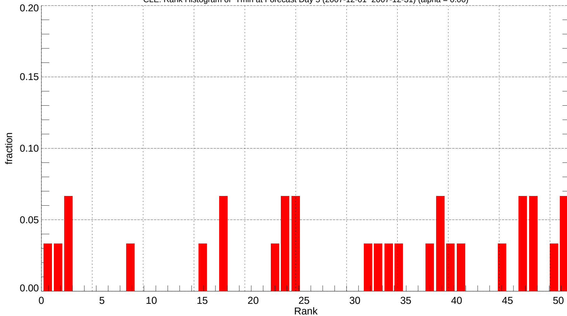
CLE: Rank Histogram of Tmin at Forecast Day 5 (2007-12-01~2007-12-31) (alpha = 0.00)
