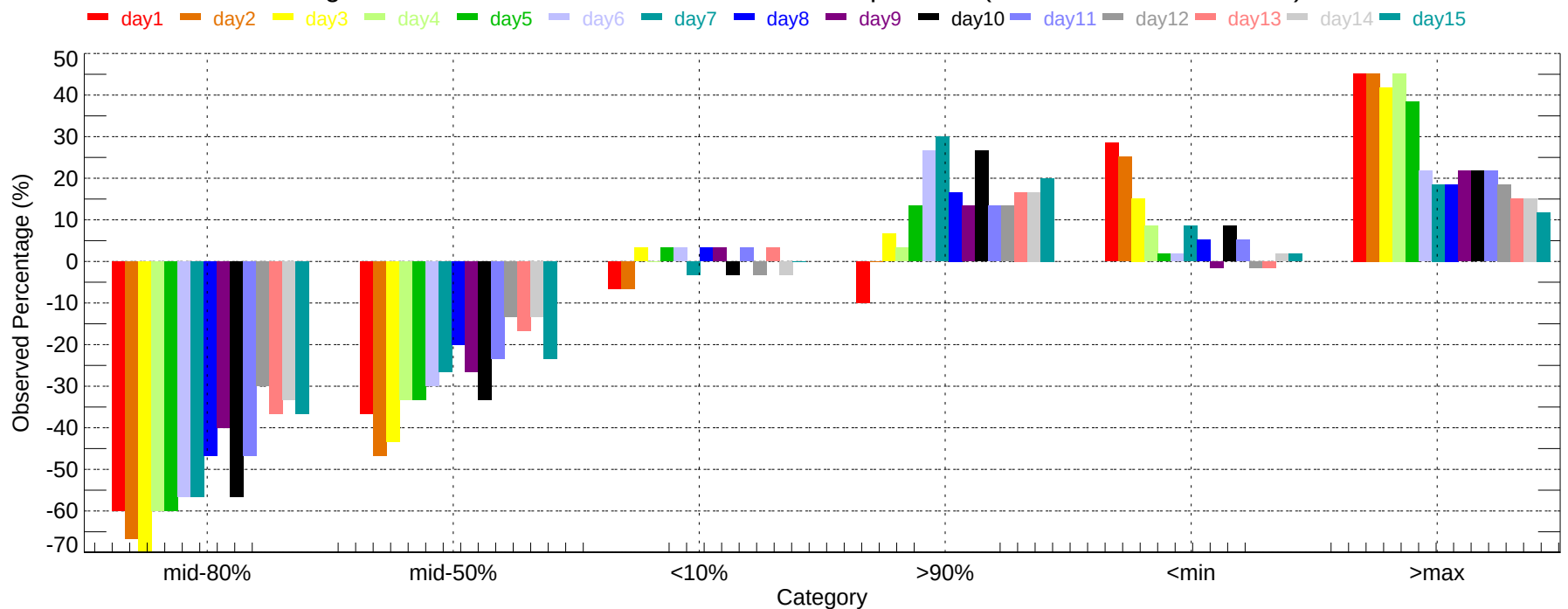
Observed Percentage Deviation of Ensembles - PDT: Max Temperature (2007-12-01~2007-12-31)
