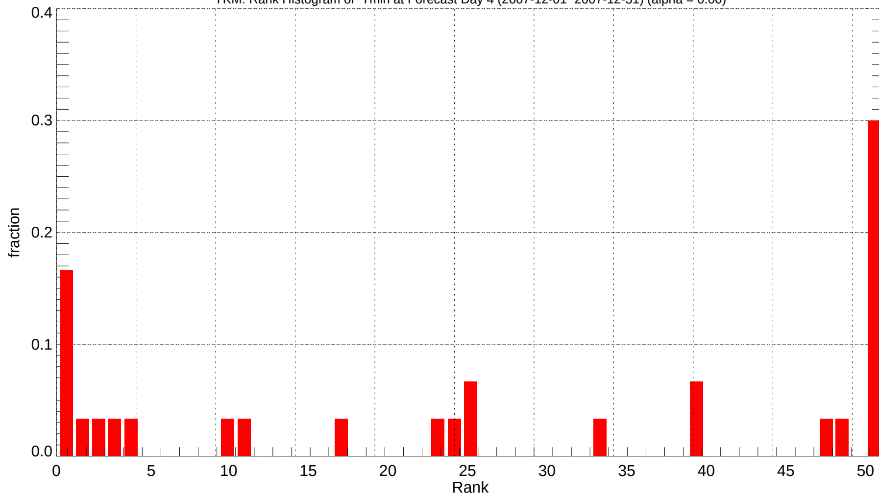
YKM: Rank Histogram of Tmin at Forecast Day 4 (2007-12-01~2007-12-31) (alpha = 0.00)
