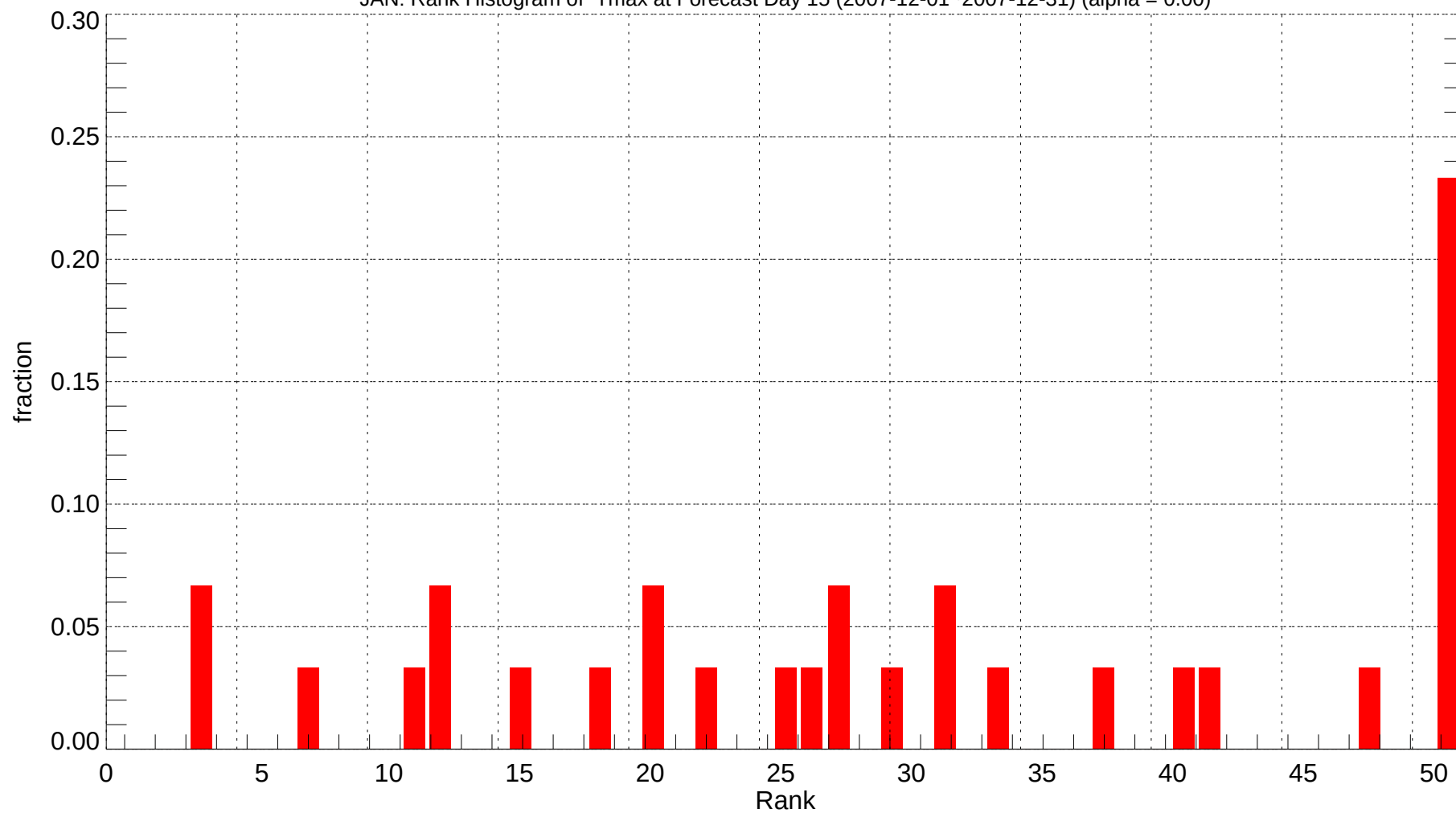
JAN: Rank Histogram of Tmax at Forecast Day 15 (2007-12-01~2007-12-31) (alpha = 0.00)
