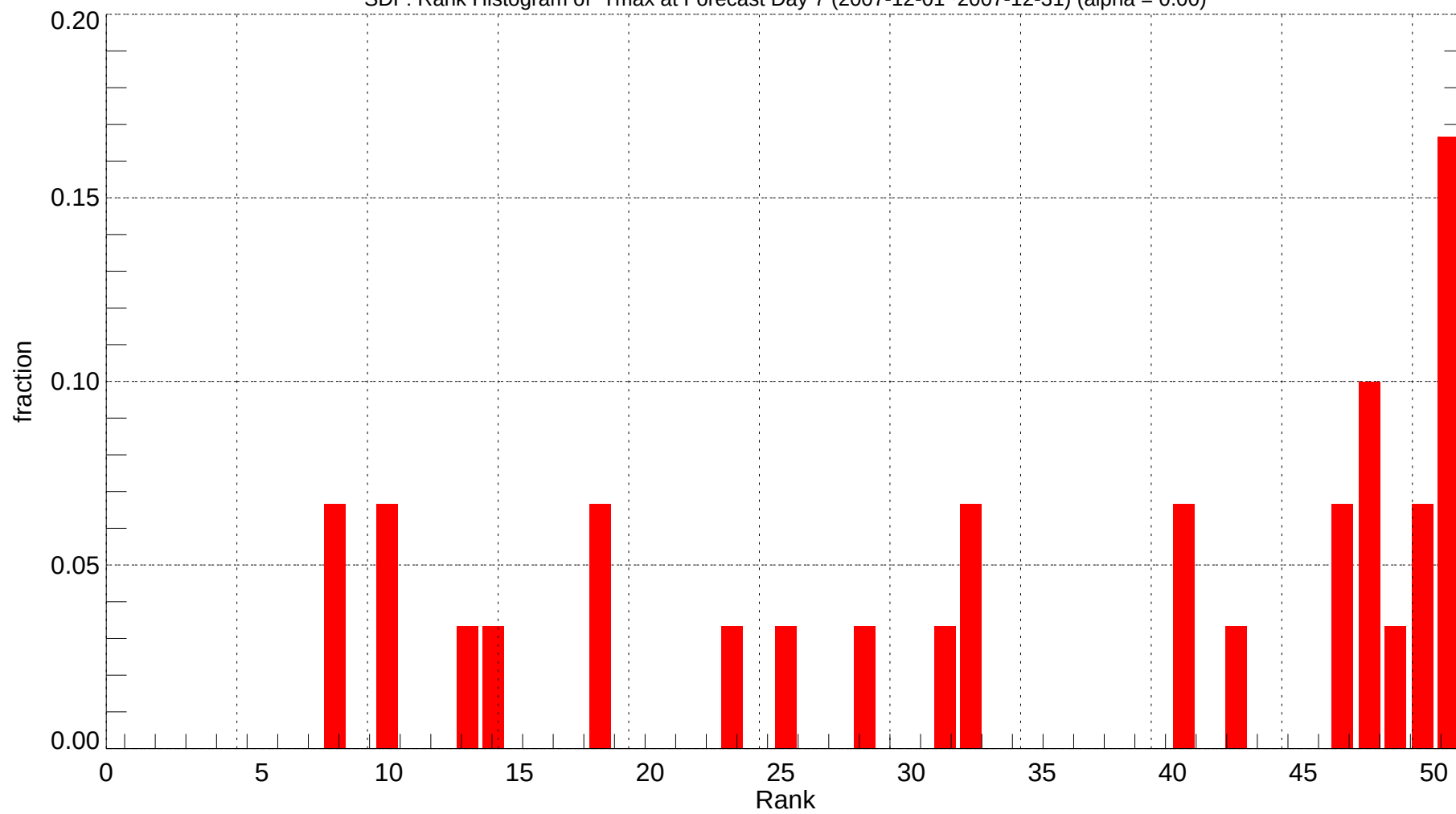
SDF: Rank Histogram of Tmax at Forecast Day 7 (2007-12-01~2007-12-31) (alpha = 0.00)
