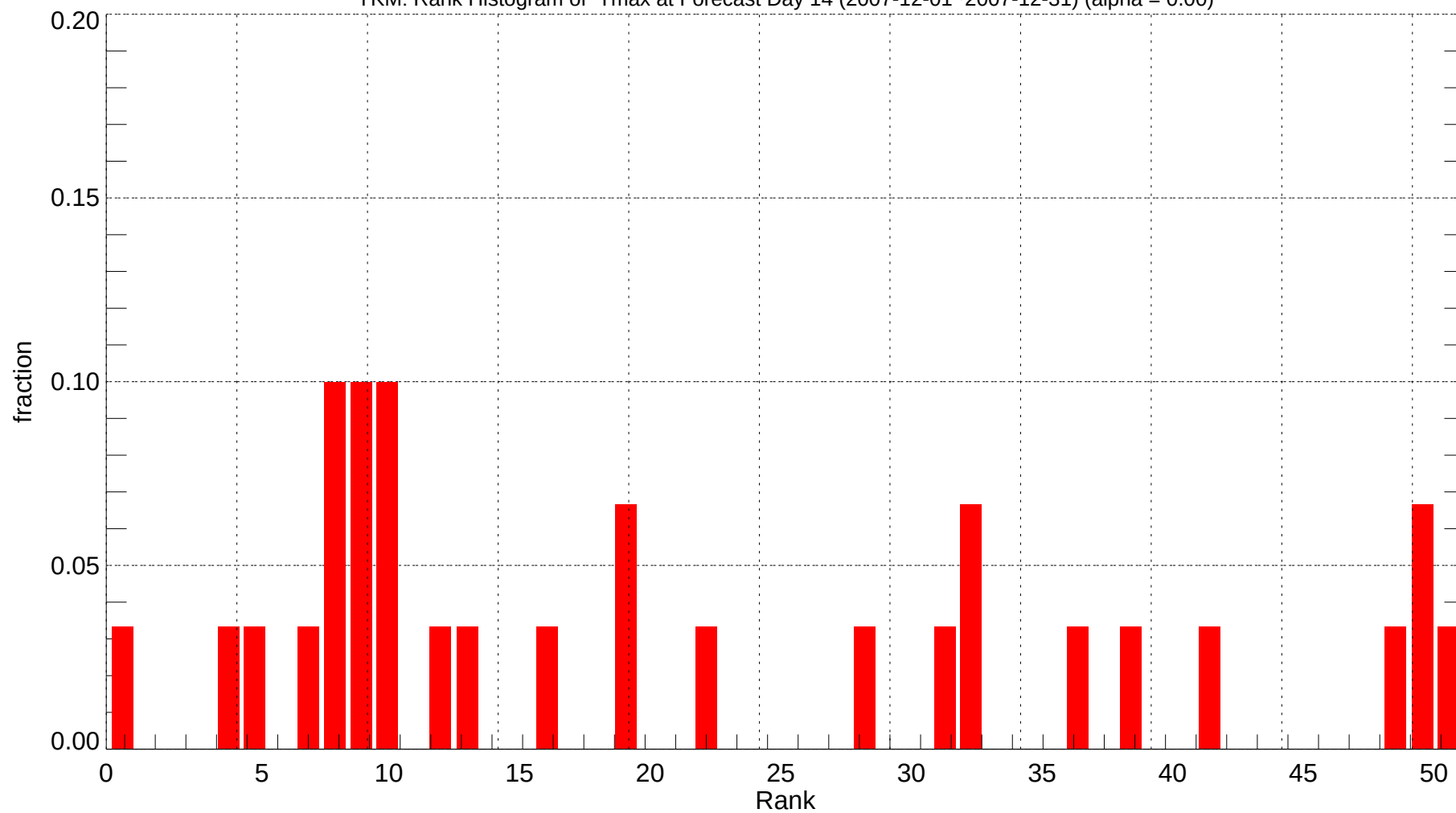
YKM: Rank Histogram of Tmax at Forecast Day 14 (2007-12-01~2007-12-31) (alpha = 0.00)
