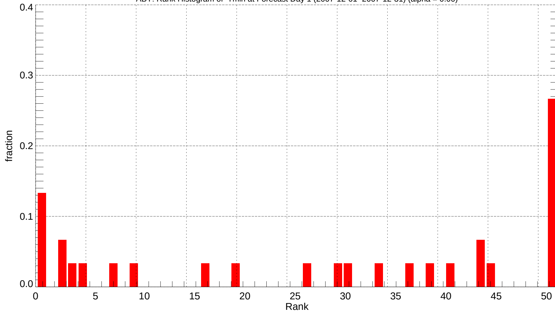
ABY: Rank Histogram of Tmin at Forecast Day 1 (2007-12-01~2007-12-31) (alpha = 0.00)
