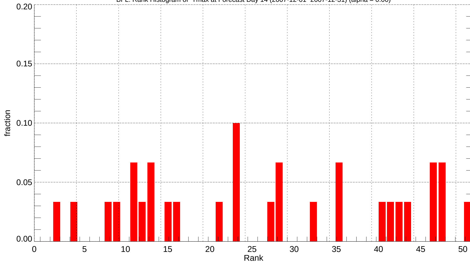
BFL: Rank Histogram of Tmax at Forecast Day 14 (2007-12-01~2007-12-31) (alpha = 0.00)
