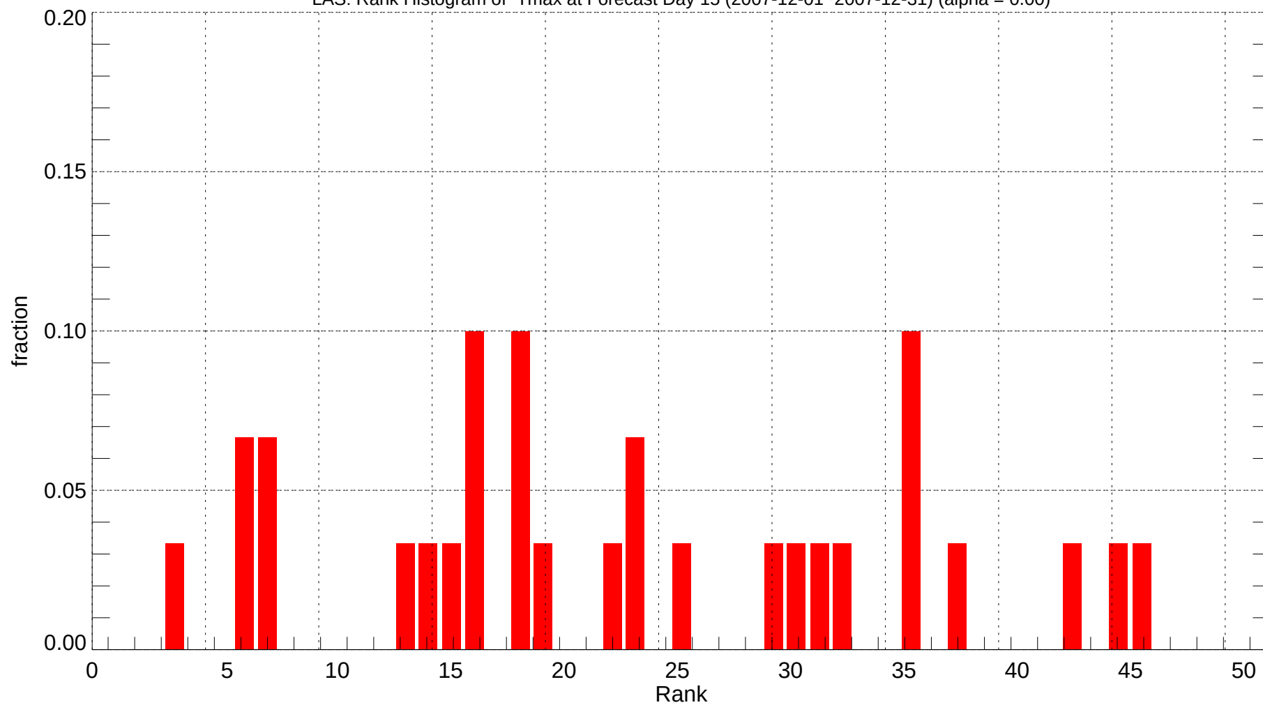
LAS: Rank Histogram of Tmax at Forecast Day 15 (2007-12-01~2007-12-31) (alpha = 0.00)
