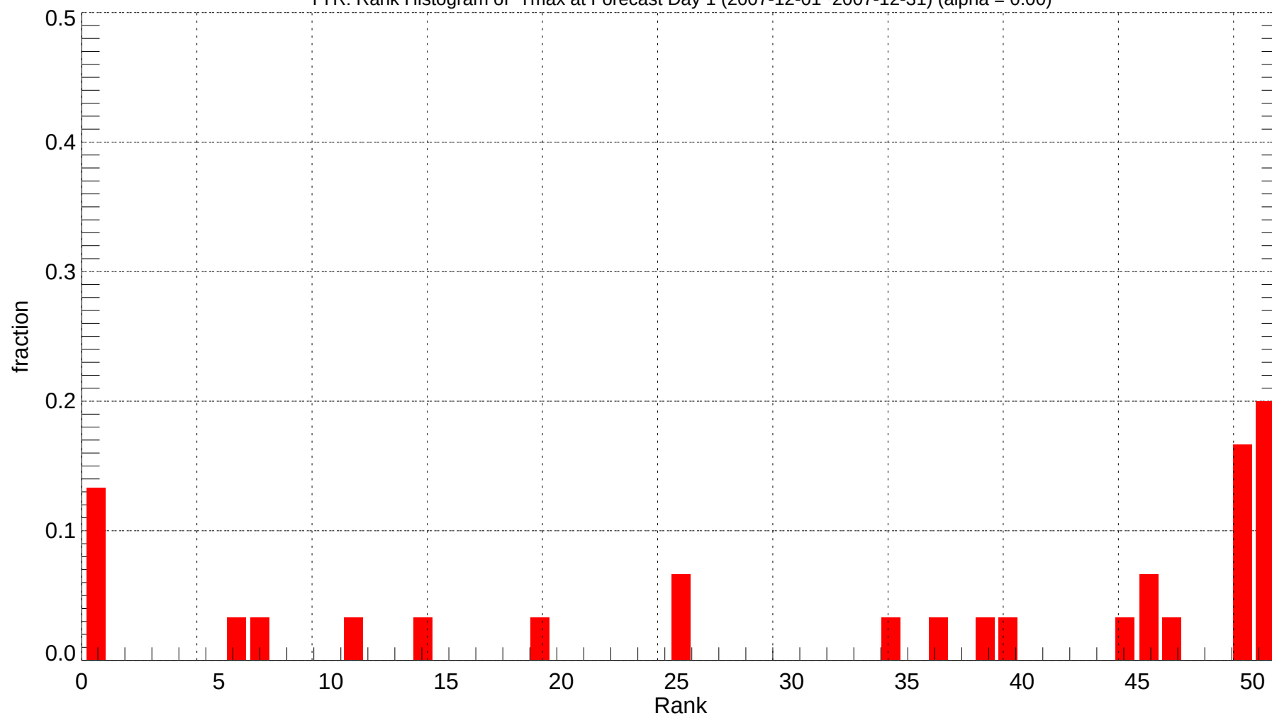
TYR: Rank Histogram of Tmax at Forecast Day 1 (2007-12-01~2007-12-31) (alpha = 0.00)
