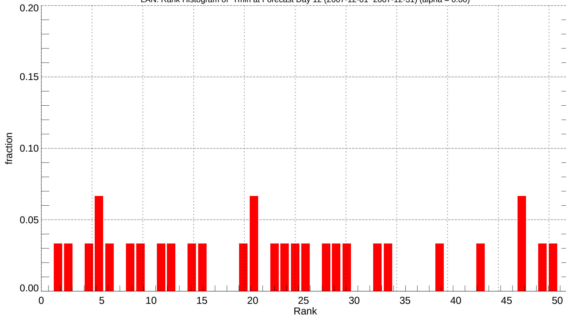
LAN: Rank Histogram of Tmin at Forecast Day 12 (2007-12-01~2007-12-31) (alpha = 0.00)
