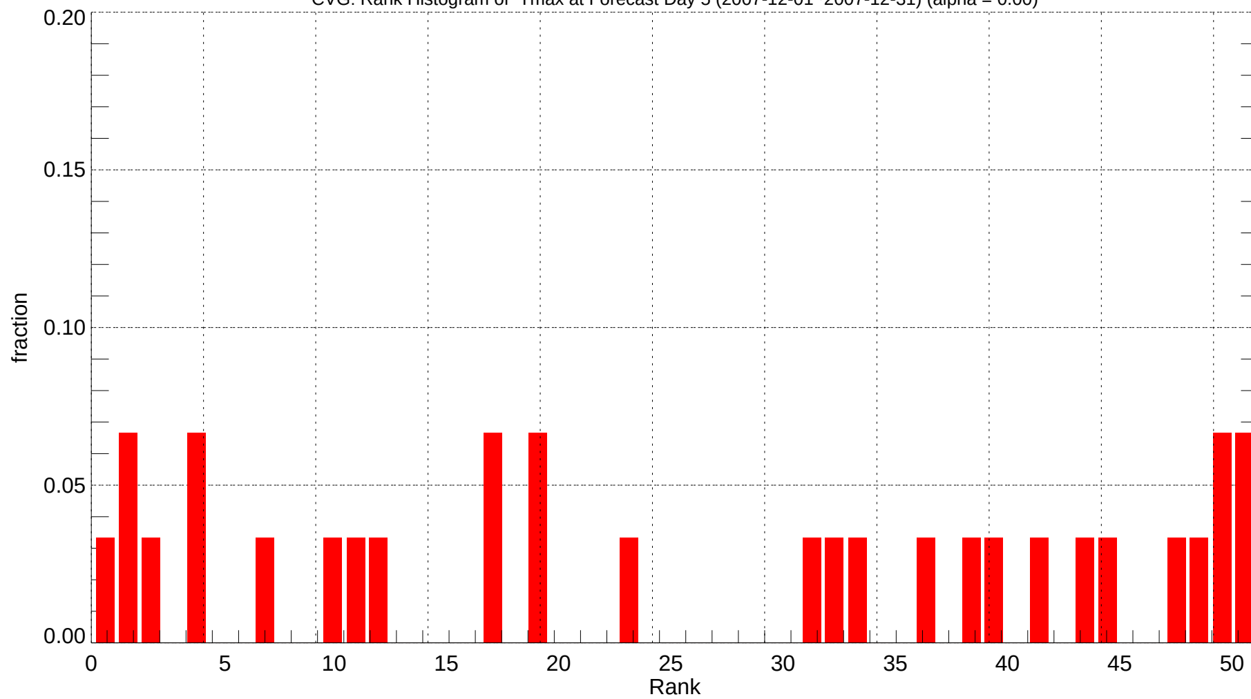
CVG: Rank Histogram of Tmax at Forecast Day 5 (2007-12-01~2007-12-31) (alpha = 0.00)
