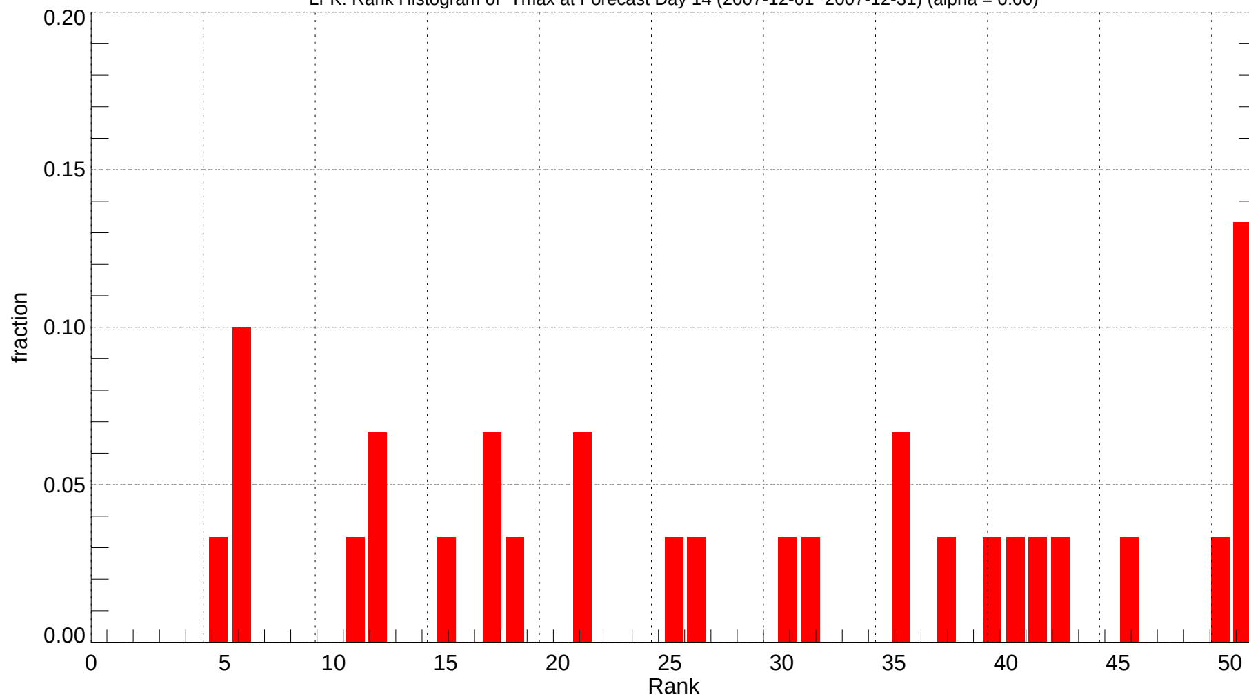
LFK: Rank Histogram of Tmax at Forecast Day 14 (2007-12-01~2007-12-31) (alpha = 0.00)
