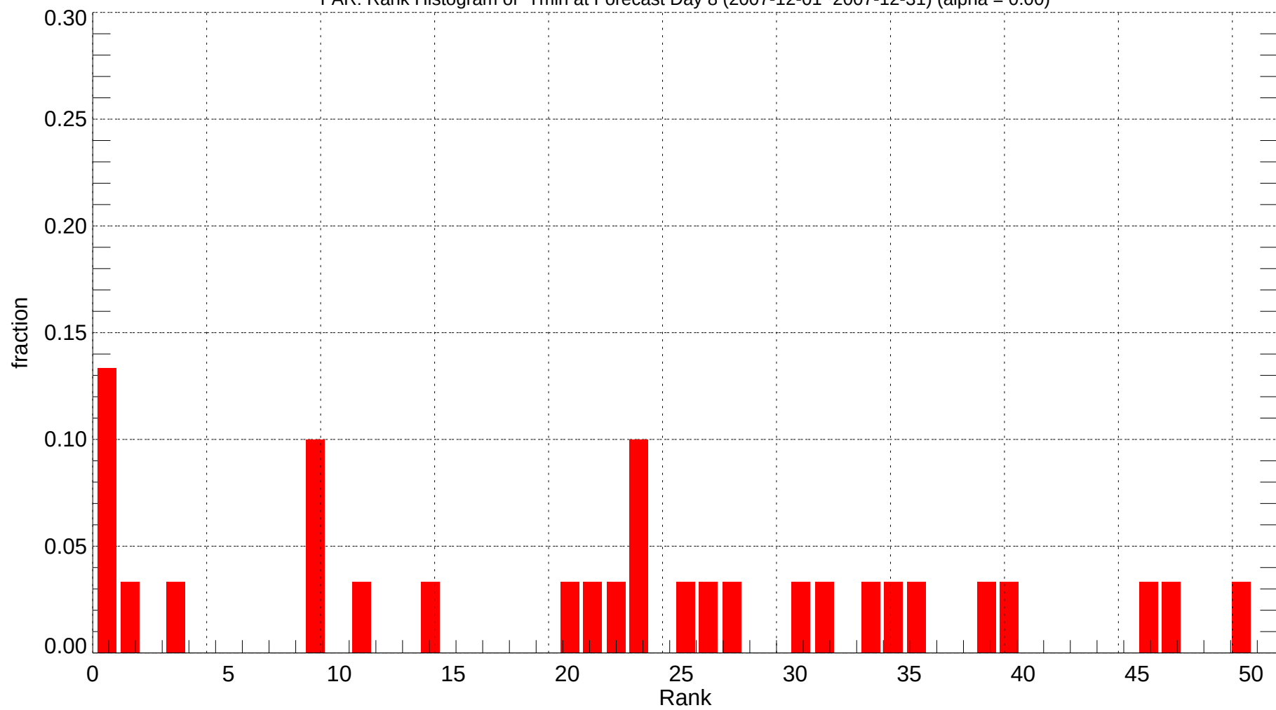
FAR: Rank Histogram of Tmin at Forecast Day 8 (2007-12-01~2007-12-31) (alpha = 0.00)
