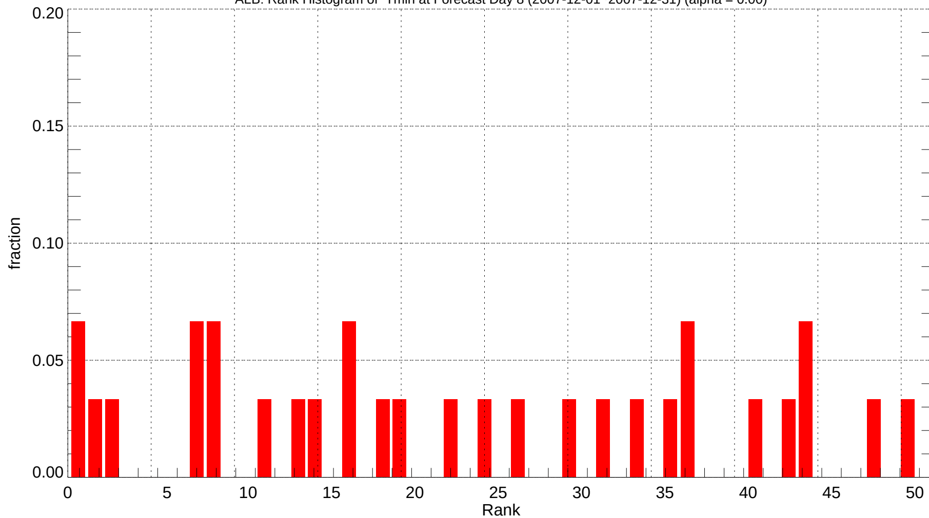
ALB: Rank Histogram of Tmin at Forecast Day 8 (2007-12-01~2007-12-31) (alpha = 0.00)
