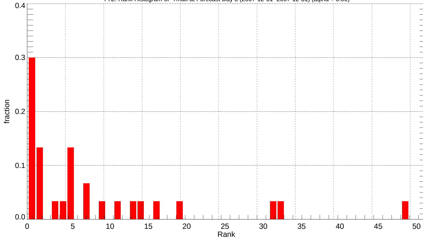
YYZ: Rank Histogram of Tmax at Forecast Day 8 (2007-12-01~2007-12-31) (alpha = 0.00)
