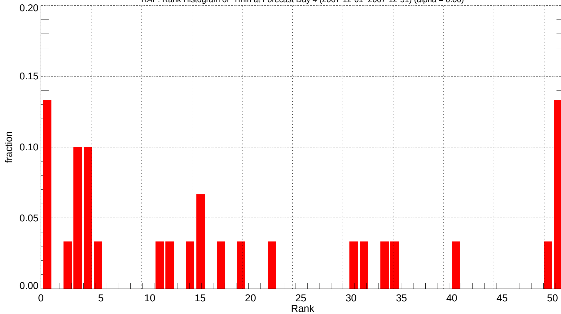
RAP: Rank Histogram of Tmin at Forecast Day 4 (2007-12-01~2007-12-31) (alpha = 0.00)
