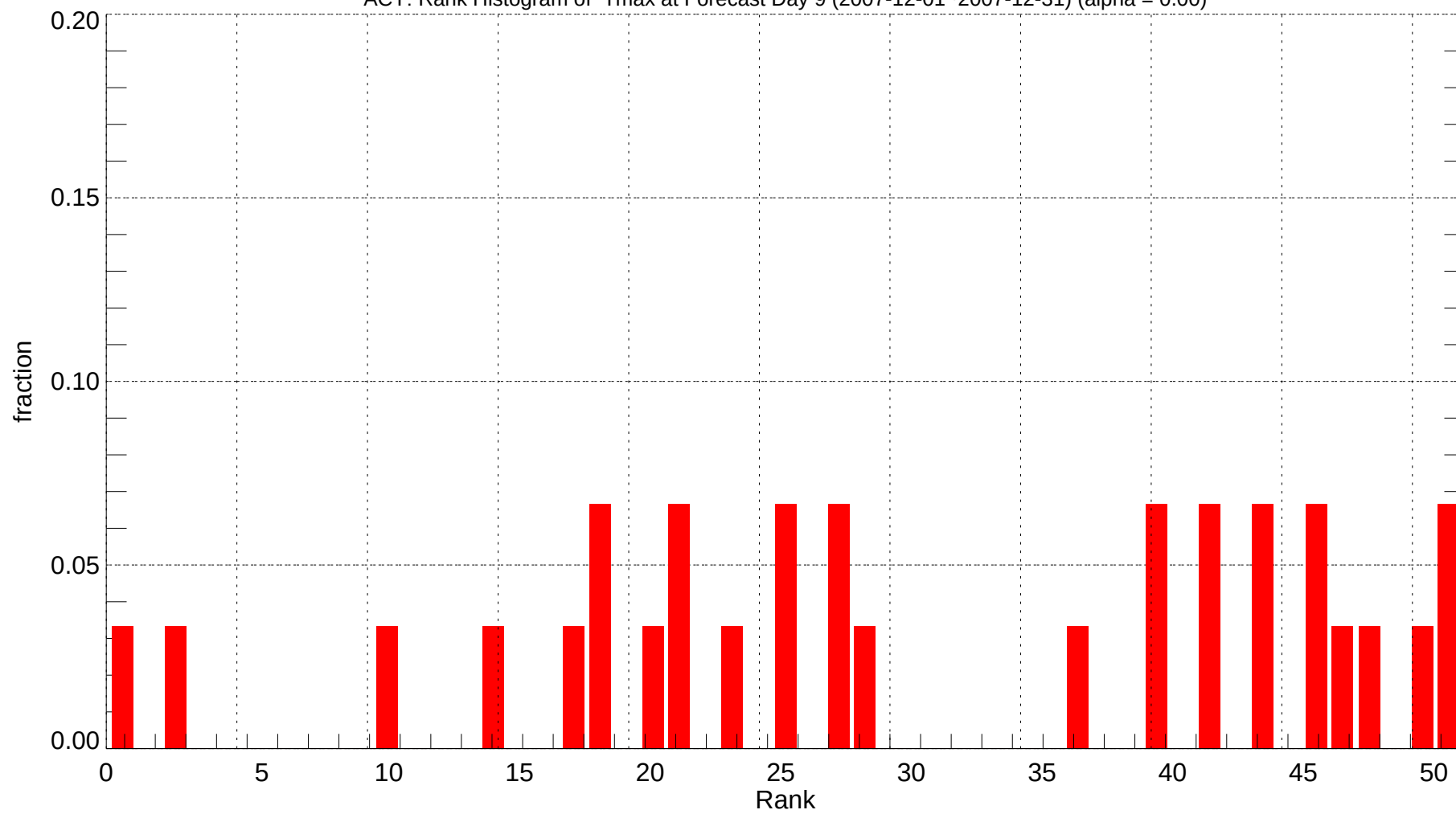
ACY: Rank Histogram of Tmax at Forecast Day 9 (2007-12-01~2007-12-31) (alpha = 0.00)
