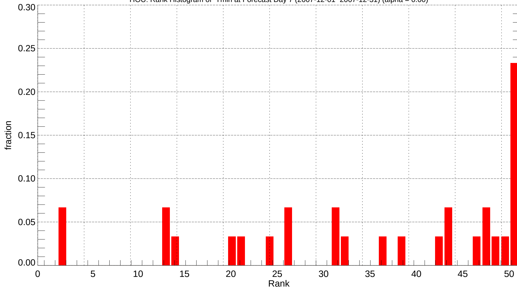
HOU: Rank Histogram of Tmin at Forecast Day 7 (2007-12-01~2007-12-31) (alpha = 0.00)
