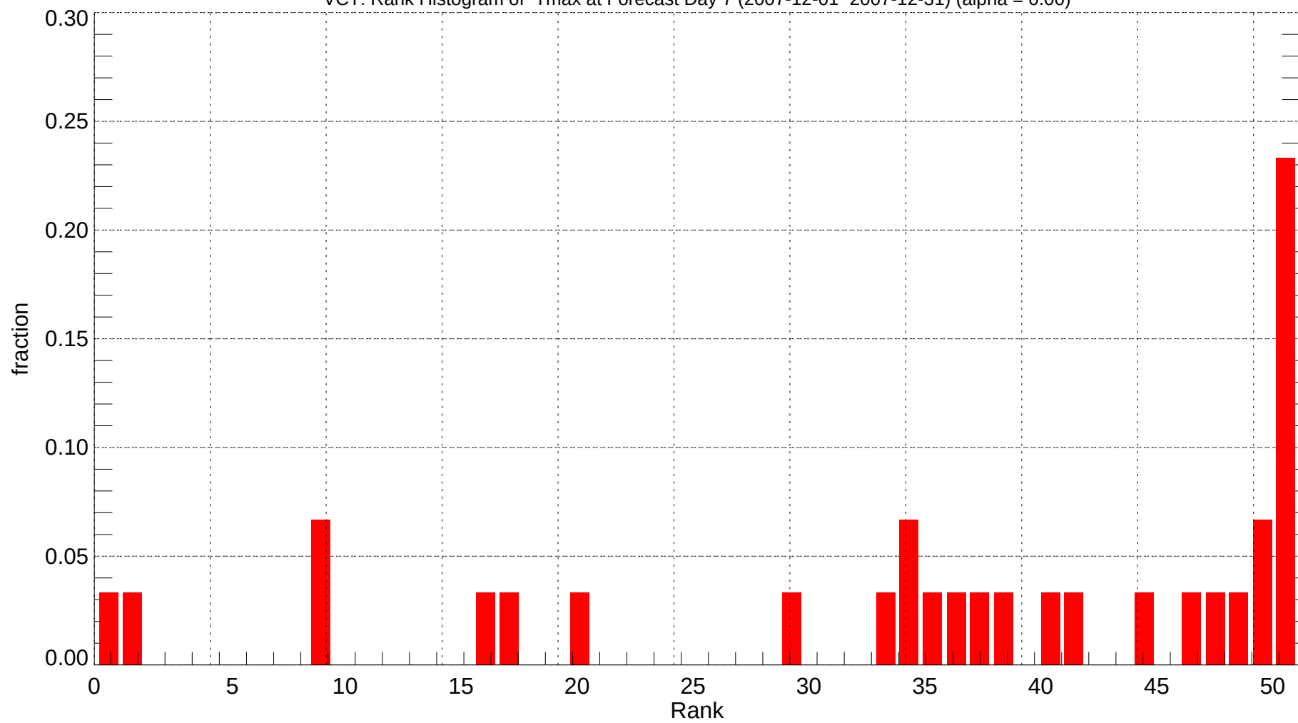
VCT: Rank Histogram of Tmax at Forecast Day 7 (2007-12-01~2007-12-31) (alpha = 0.00)
