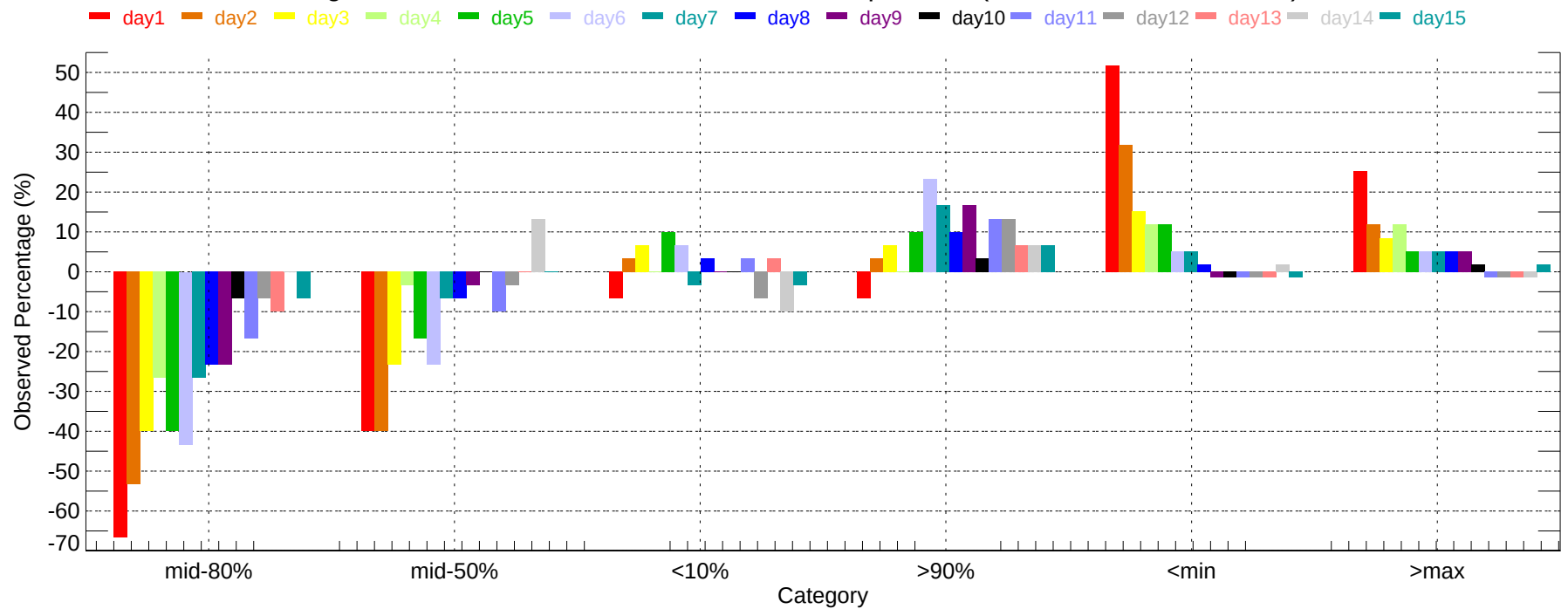
Observed Percentage Deviation of Ensembles - BWI: Max Temperature (2007-12-01~2007-12-31)
