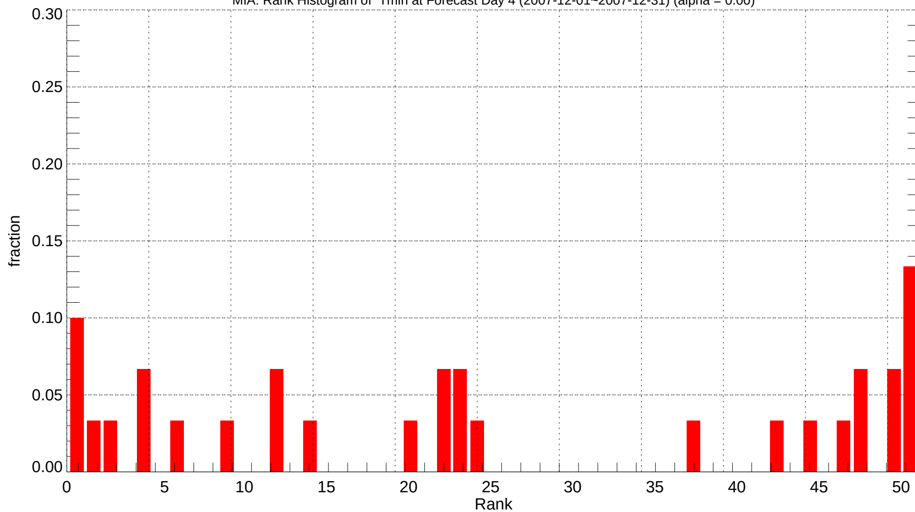
MIA: Rank Histogram of Tmin at Forecast Day 4 (2007-12-01~2007-12-31) (alpha = 0.00)
