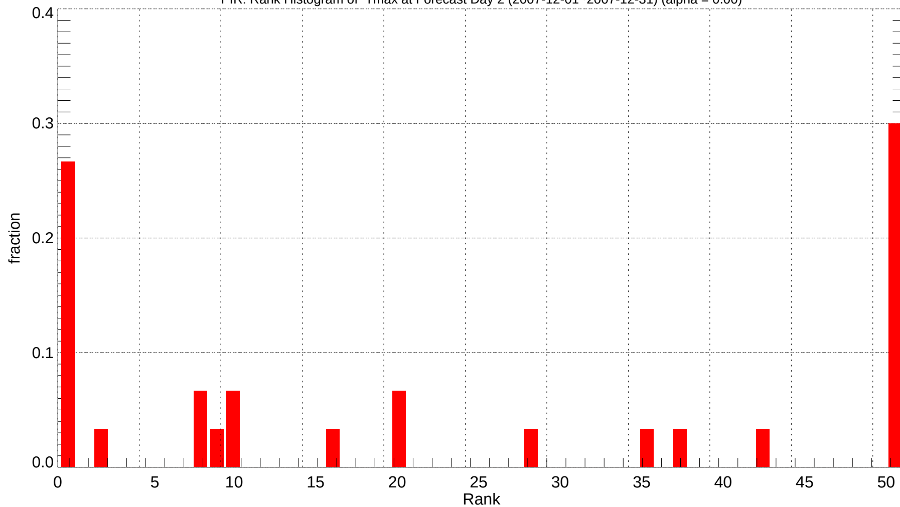
PIR: Rank Histogram of Tmax at Forecast Day 2 (2007-12-01~2007-12-31) (alpha = 0.00)
