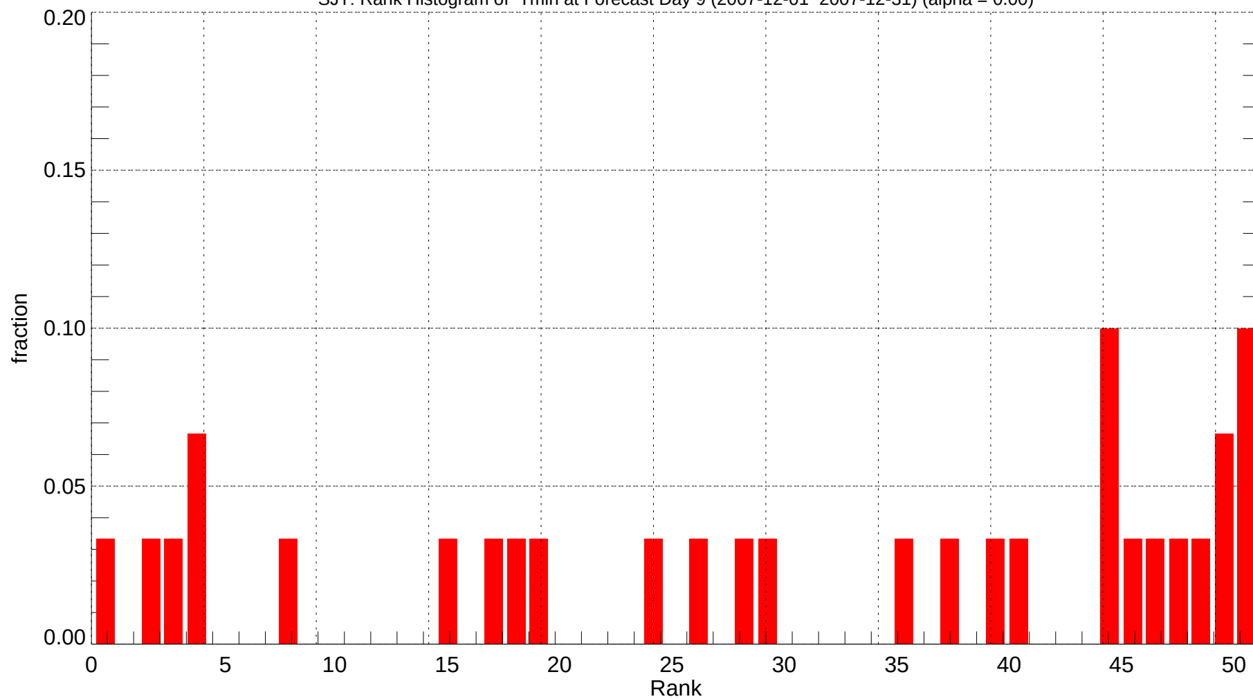
SJT: Rank Histogram of Tmin at Forecast Day 9 (2007-12-01~2007-12-31) (alpha = 0.00)
