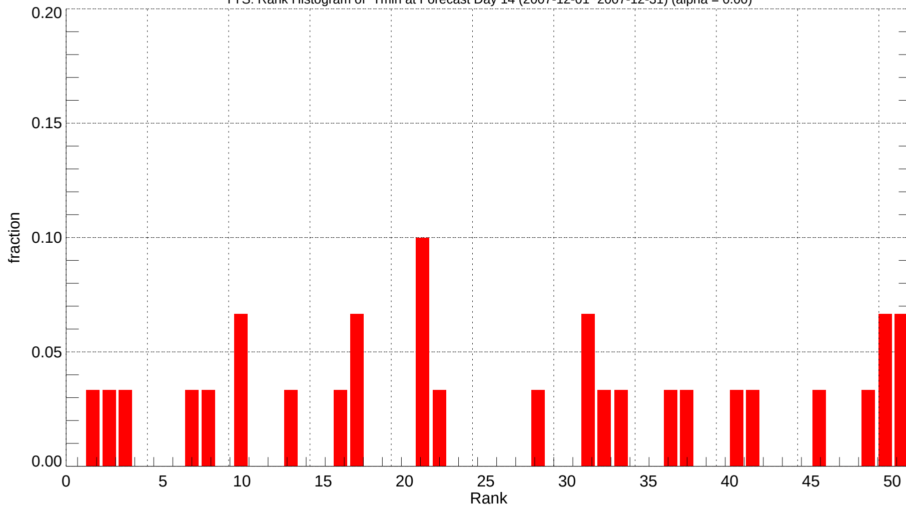
TYS: Rank Histogram of Tmin at Forecast Day 14 (2007-12-01~2007-12-31) (alpha = 0.00)
