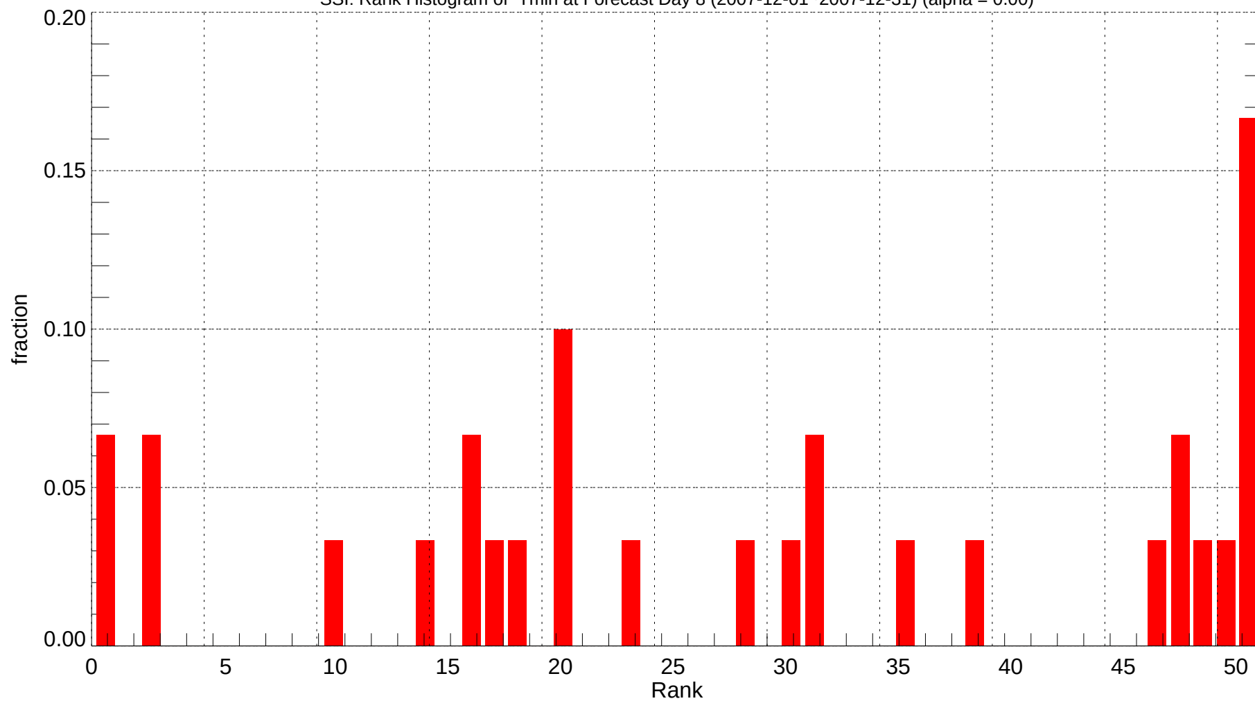
SSI: Rank Histogram of Tmin at Forecast Day 8 (2007-12-01~2007-12-31) (alpha = 0.00)
