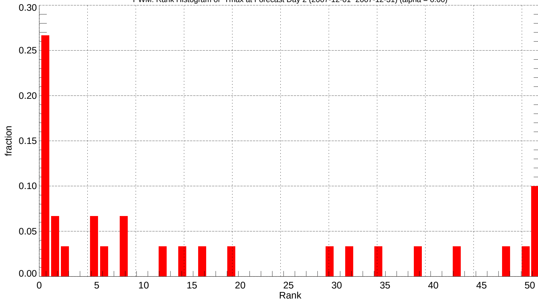
PWM: Rank Histogram of Tmax at Forecast Day 2 (2007-12-01~2007-12-31) (alpha = 0.00)
