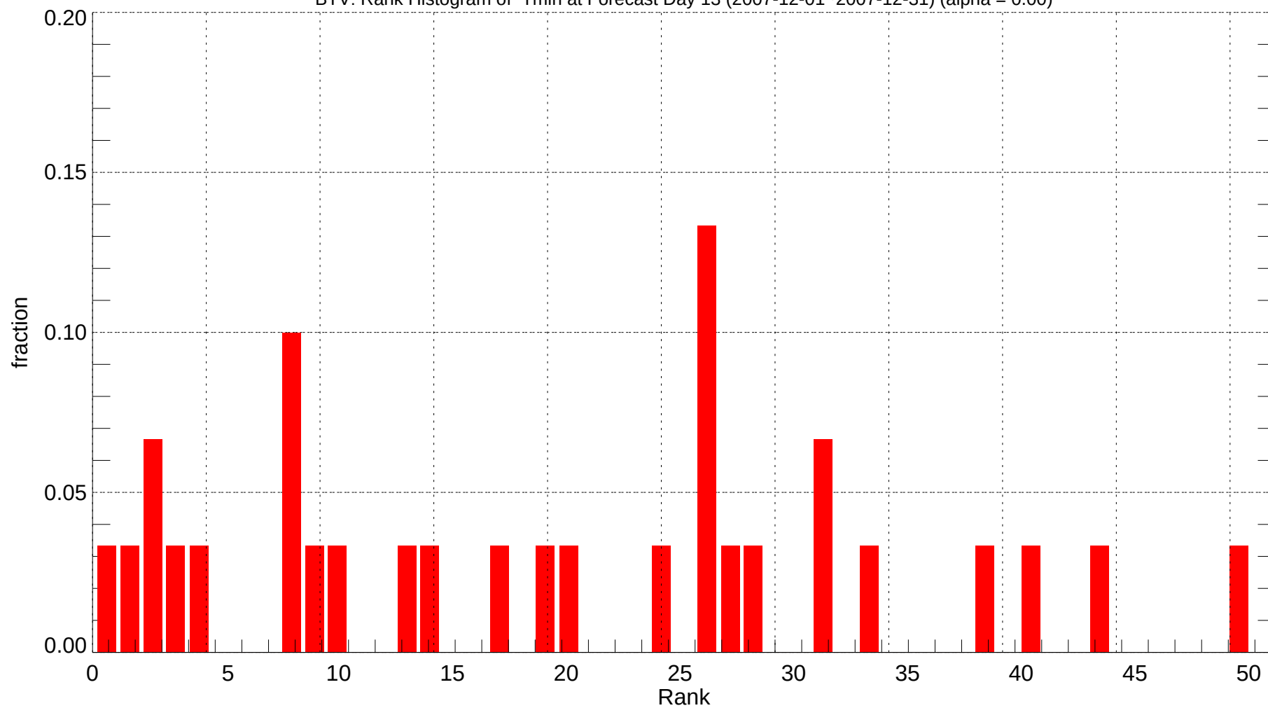
BTV: Rank Histogram of Tmin at Forecast Day 13 (2007-12-01~2007-12-31) (alpha = 0.00)
