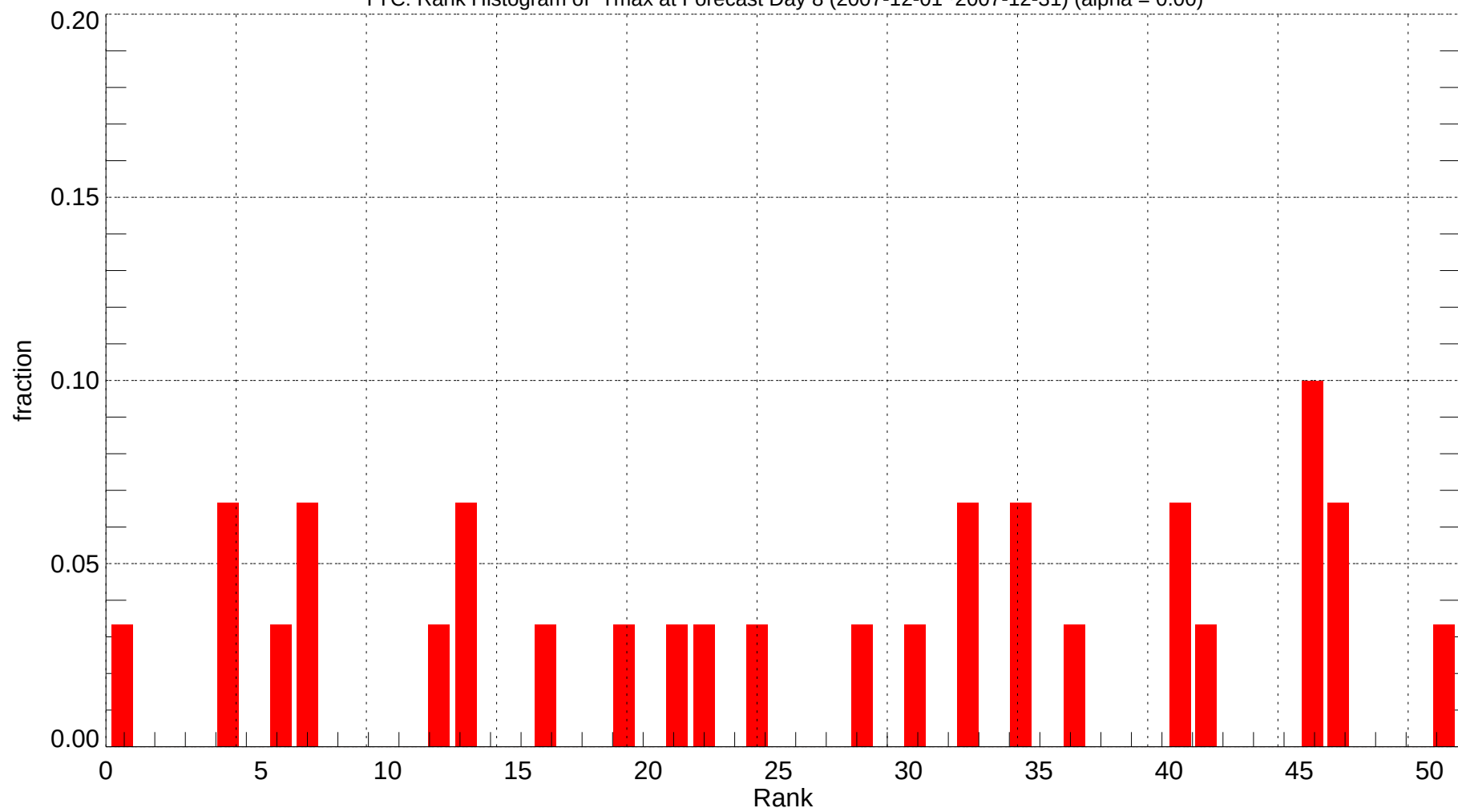
YYC: Rank Histogram of Tmax at Forecast Day 8 (2007-12-01~2007-12-31) (alpha = 0.00)
