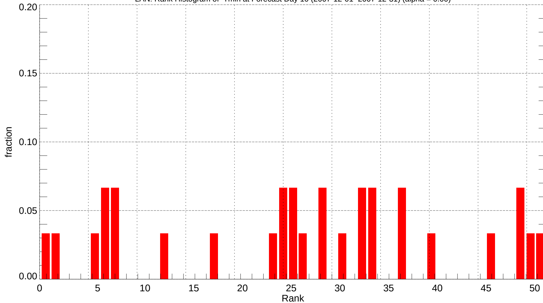
LAN: Rank Histogram of Tmin at Forecast Day 10 (2007-12-01~2007-12-31) (alpha = 0.00)
