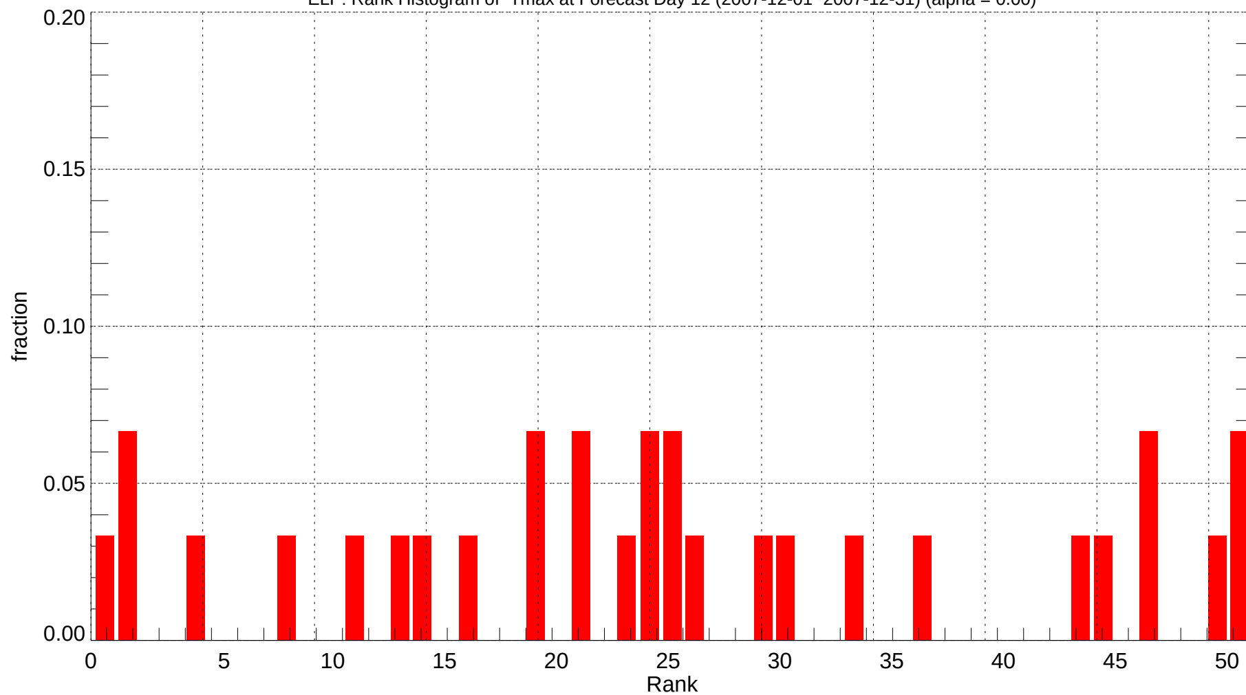
ELP: Rank Histogram of Tmax at Forecast Day 12 (2007-12-01~2007-12-31) (alpha = 0.00)
