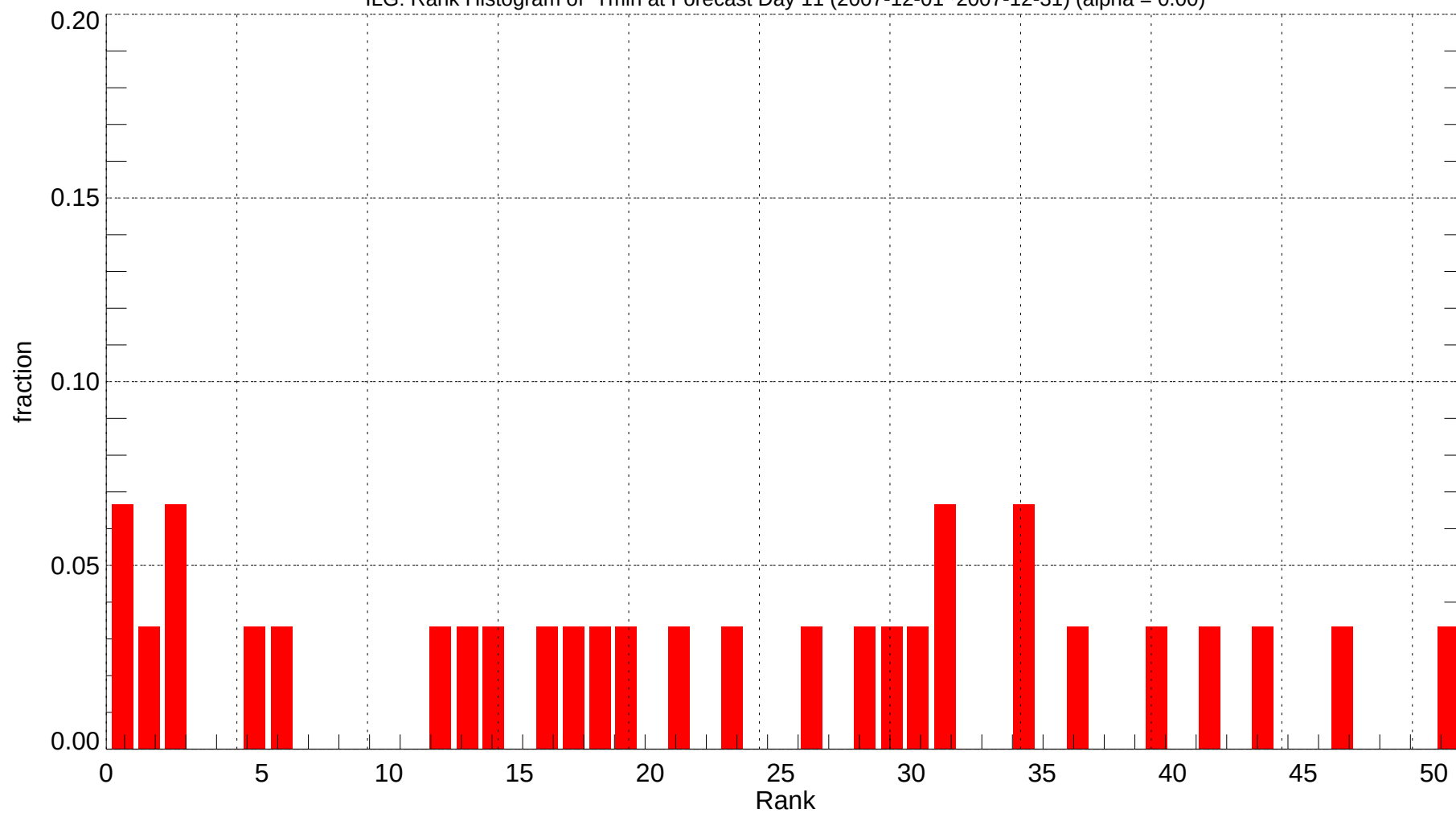
ILG: Rank Histogram of Tmin at Forecast Day 11 (2007-12-01~2007-12-31) (alpha = 0.00)
