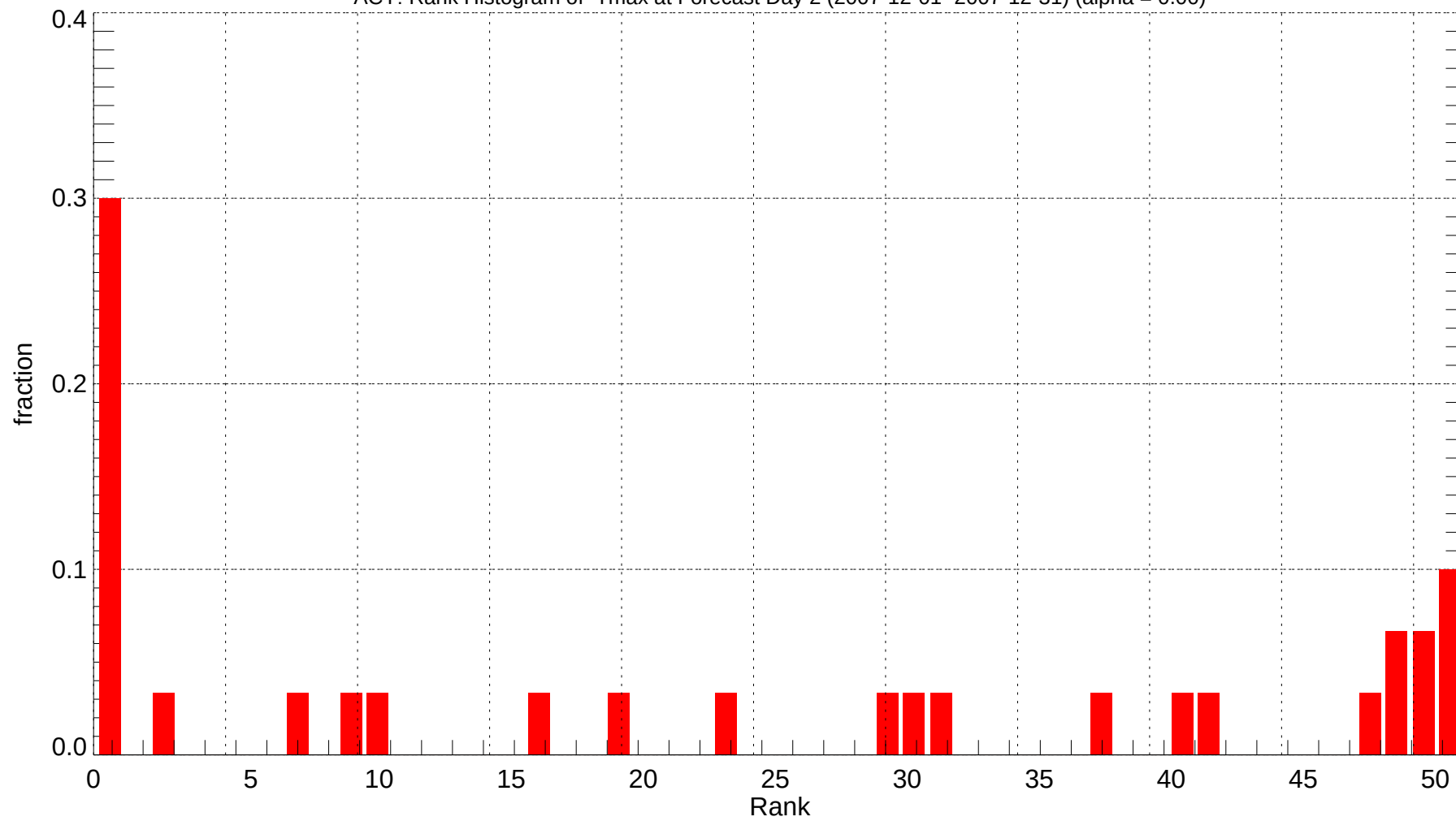
ACY: Rank Histogram of Tmax at Forecast Day 2 (2007-12-01~2007-12-31) (alpha = 0.00)
