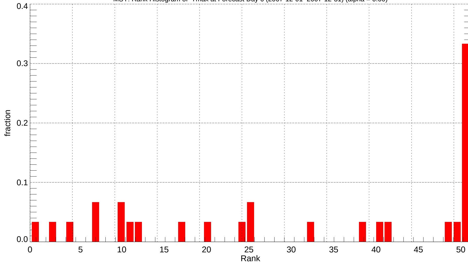
MSY: Rank Histogram of Tmax at Forecast Day 6 (2007-12-01~2007-12-31) (alpha = 0.00)
