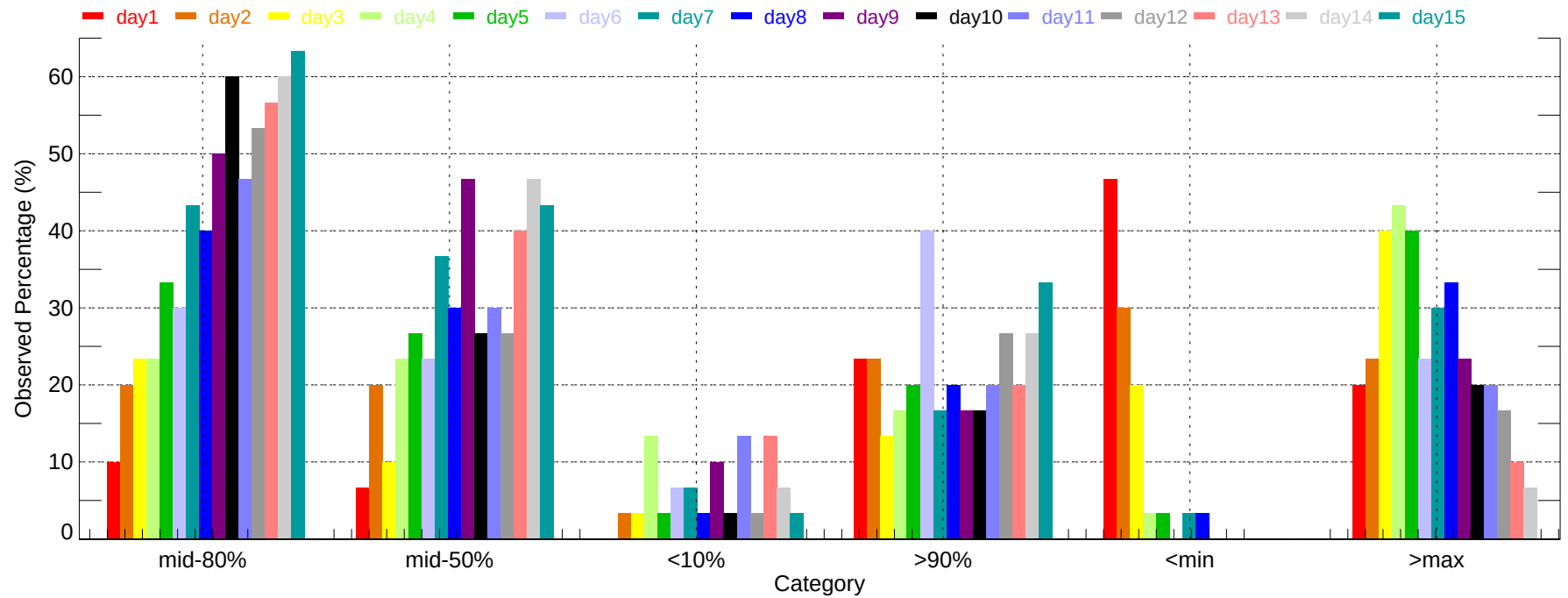
Observed Percentage of Ensembles - MCI: Max Temperature (2007-12-01~2007-12-31)
