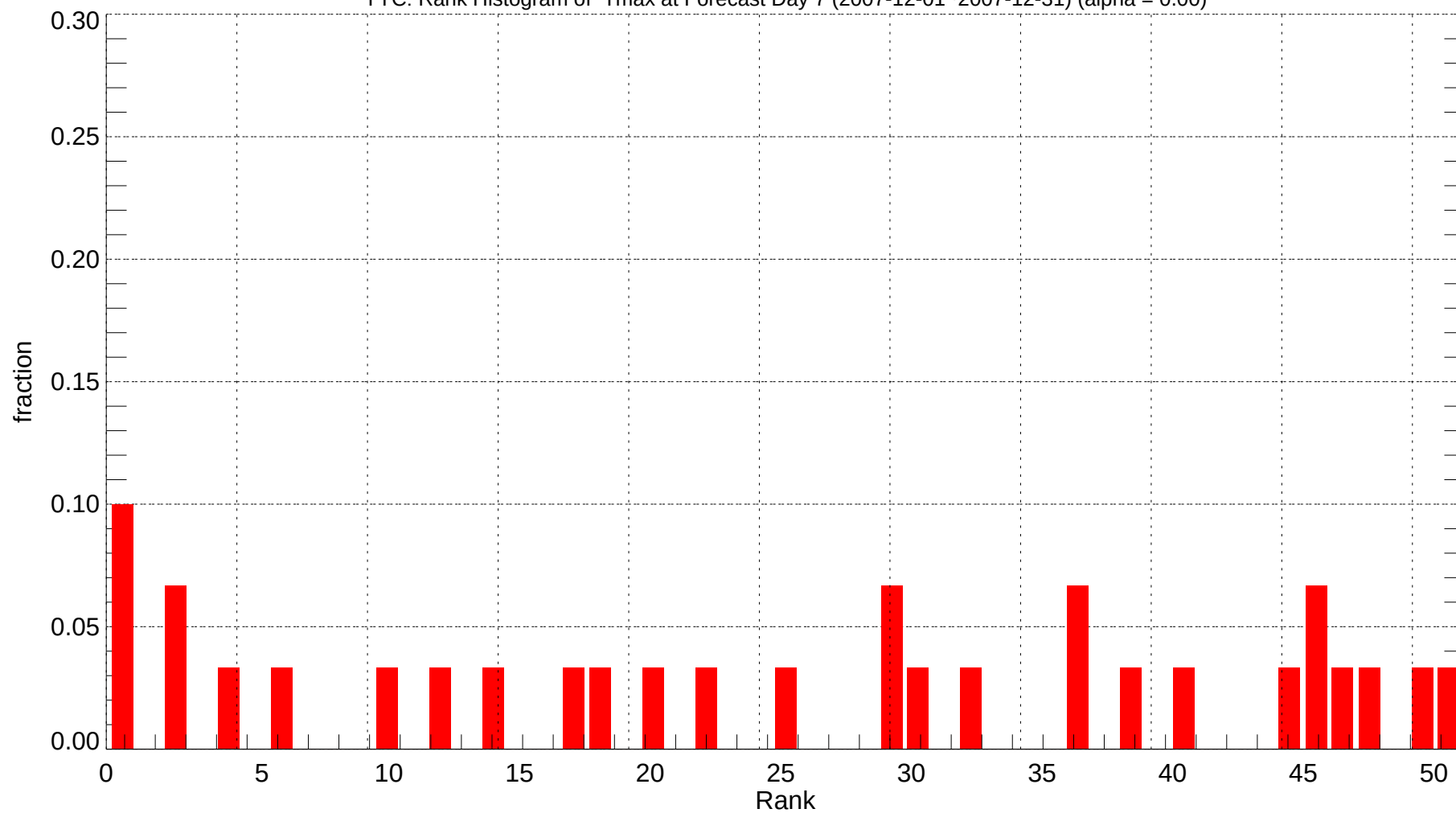
YYC: Rank Histogram of Tmax at Forecast Day 7 (2007-12-01~2007-12-31) (alpha = 0.00)
