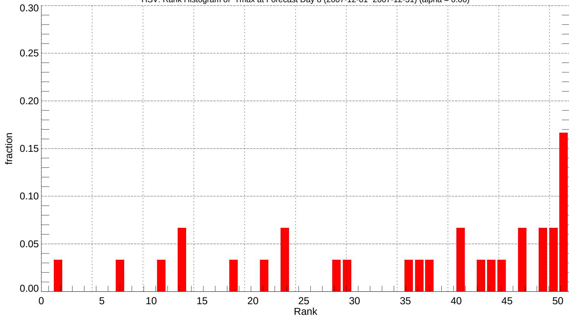
HSV: Rank Histogram of Tmax at Forecast Day 8 (2007-12-01~2007-12-31) (alpha = 0.00)
