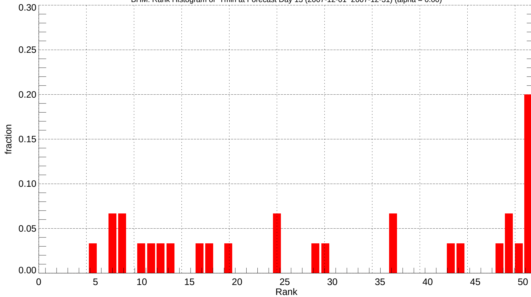
BHM: Rank Histogram of Tmin at Forecast Day 13 (2007-12-01~2007-12-31) (alpha = 0.00)
