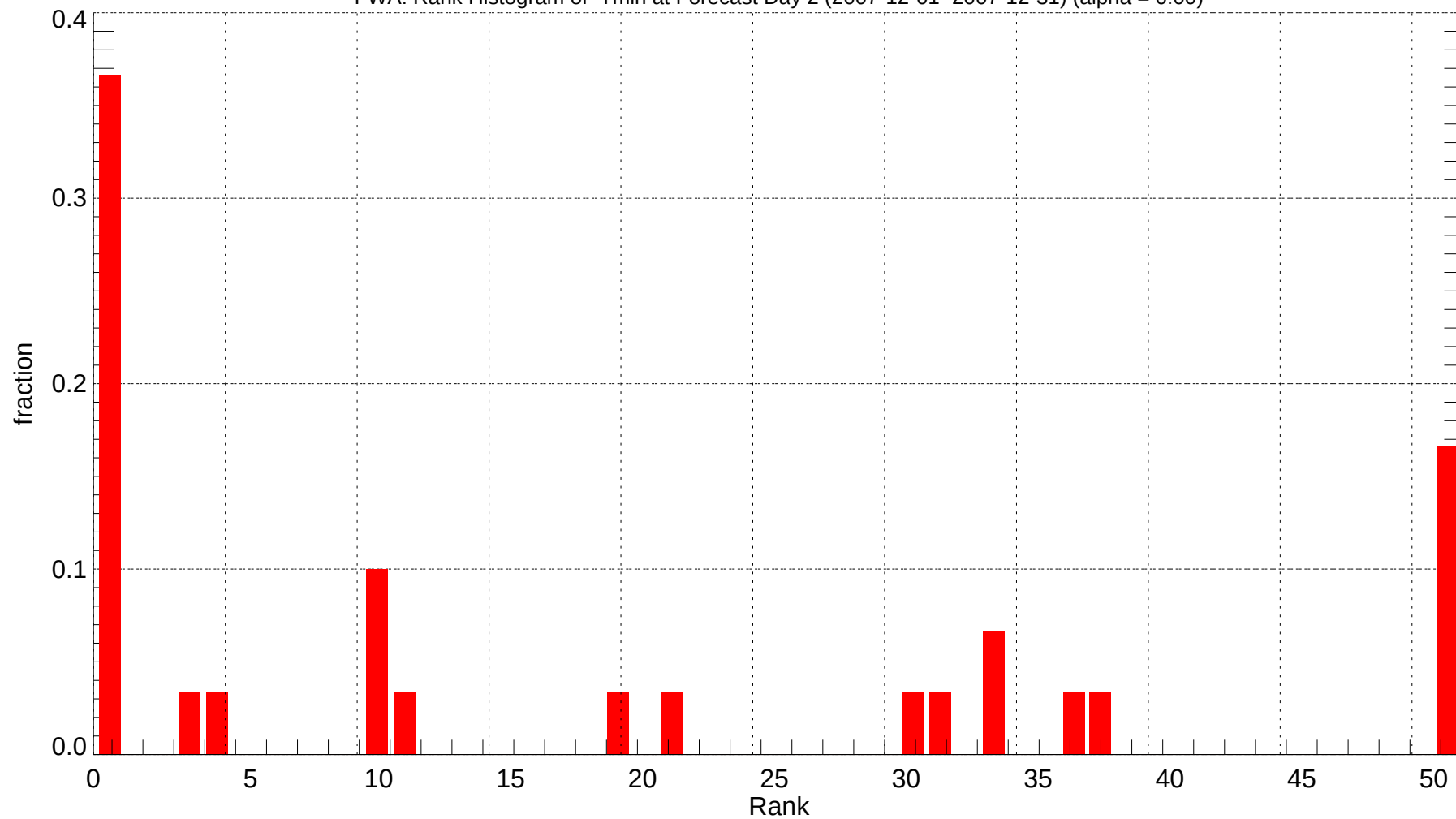
FWA: Rank Histogram of Tmin at Forecast Day 2 (2007-12-01~2007-12-31) (alpha = 0.00)
