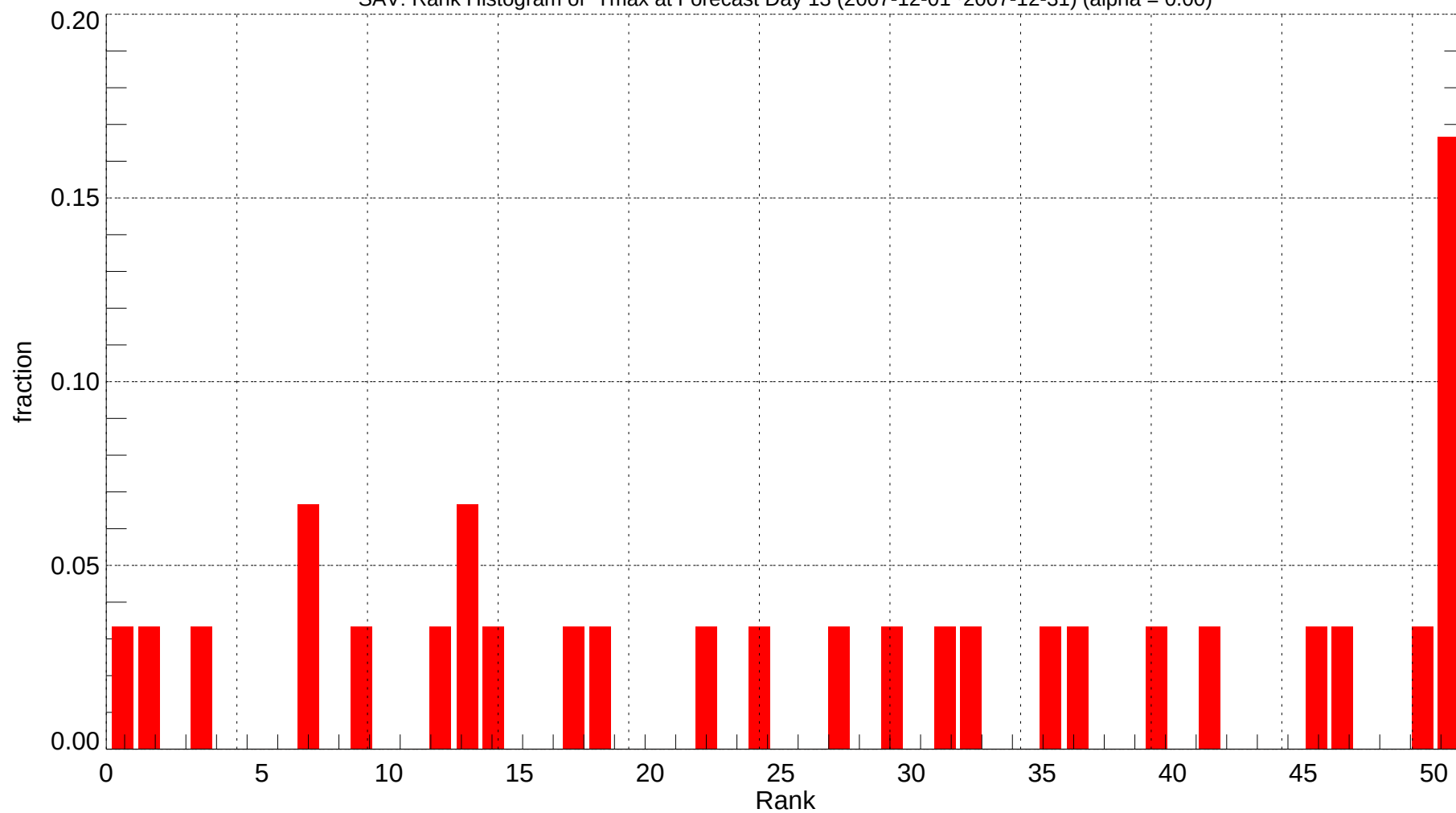
SAV: Rank Histogram of Tmax at Forecast Day 13 (2007-12-01~2007-12-31) (alpha = 0.00)
