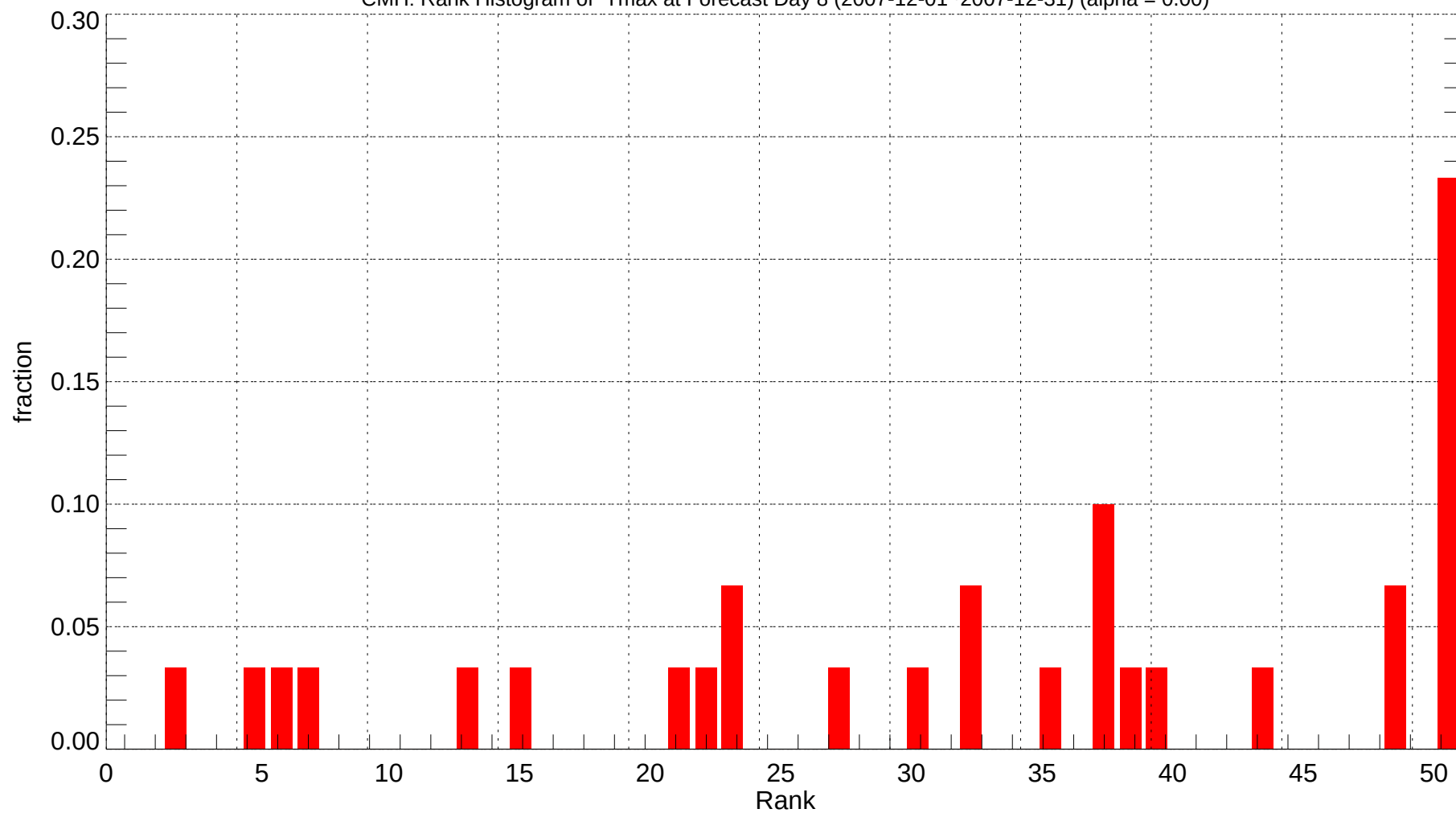
CMH: Rank Histogram of Tmax at Forecast Day 8 (2007-12-01~2007-12-31) (alpha = 0.00)
