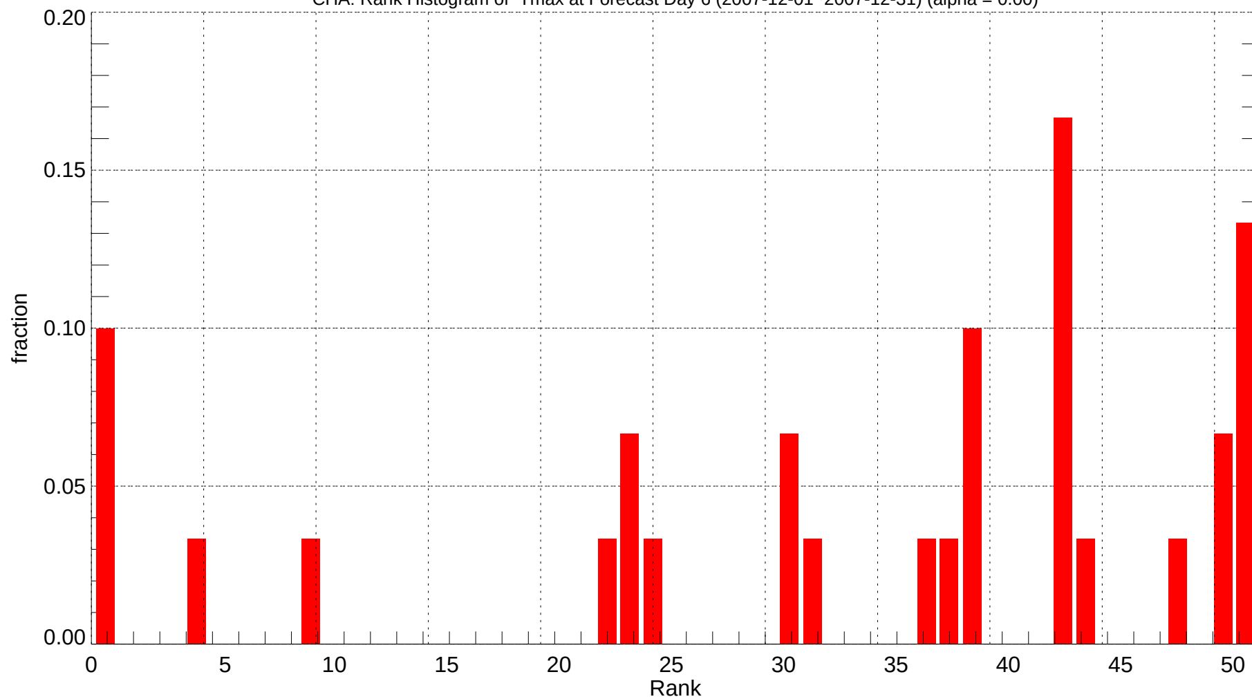
CHA: Rank Histogram of Tmax at Forecast Day 6 (2007-12-01~2007-12-31) (alpha = 0.00)
