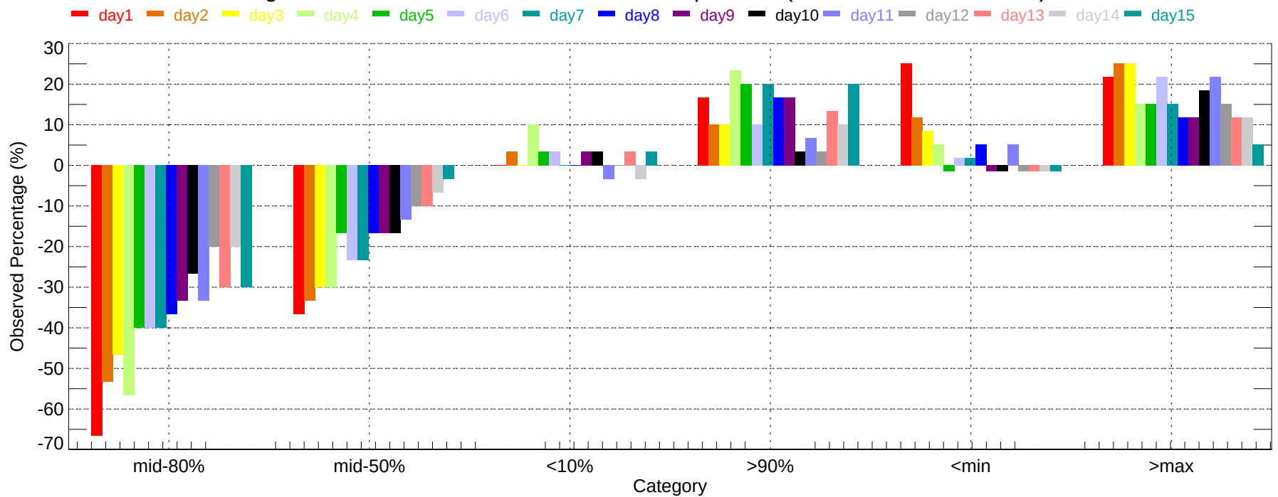
Observed Percentage Deviation of Ensembles - ABI: Min Temperature (2007-12-01~2007-12-31)
