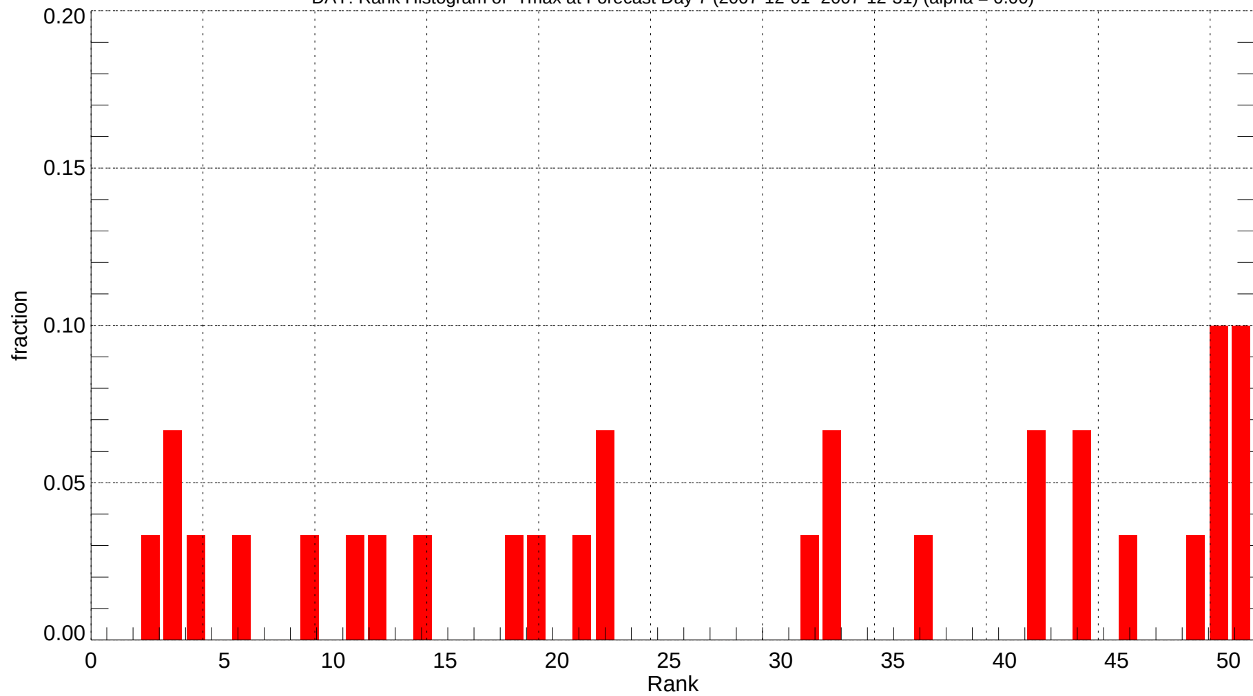
DAY: Rank Histogram of Tmax at Forecast Day 7 (2007-12-01~2007-12-31) (alpha = 0.00)
