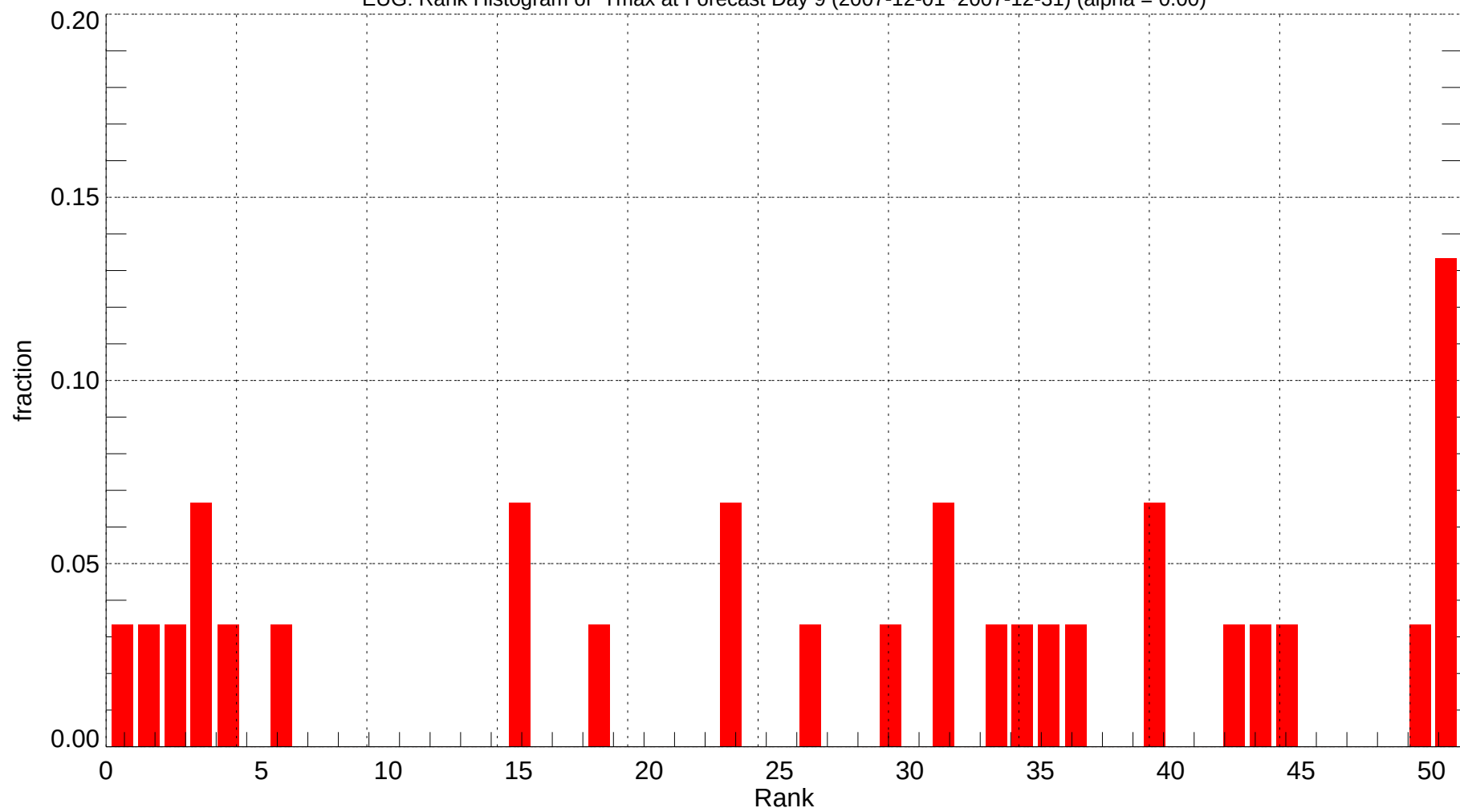
EUG: Rank Histogram of Tmax at Forecast Day 9 (2007-12-01~2007-12-31) (alpha = 0.00)
