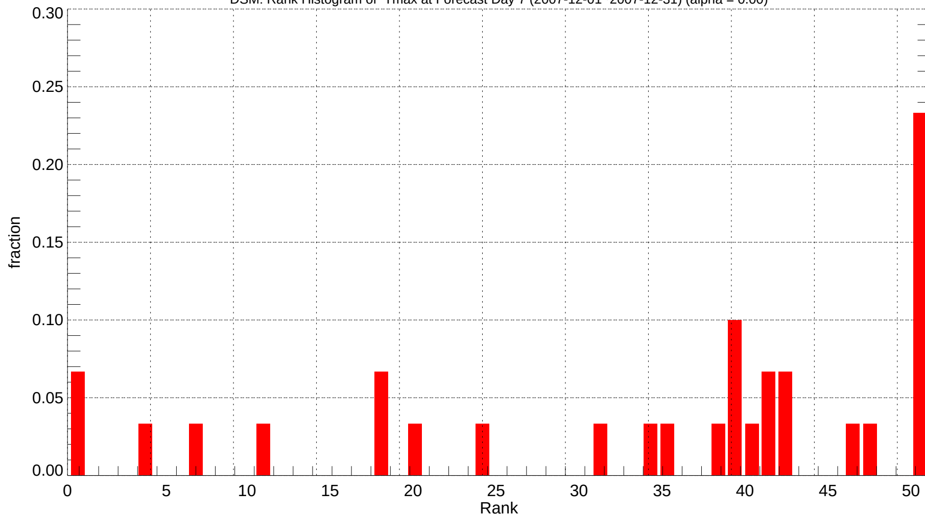
DSM: Rank Histogram of Tmax at Forecast Day 7 (2007-12-01~2007-12-31) (alpha = 0.00)
