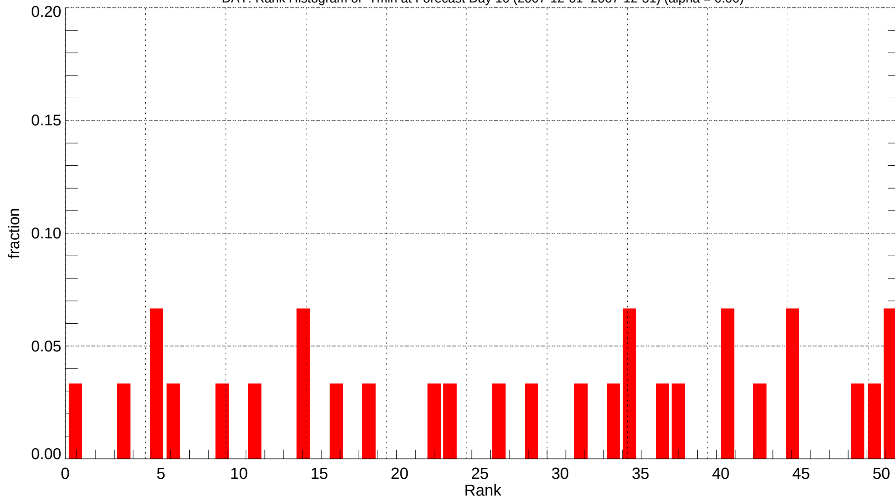
DAY: Rank Histogram of Tmin at Forecast Day 10 (2007-12-01~2007-12-31) (alpha = 0.00)
