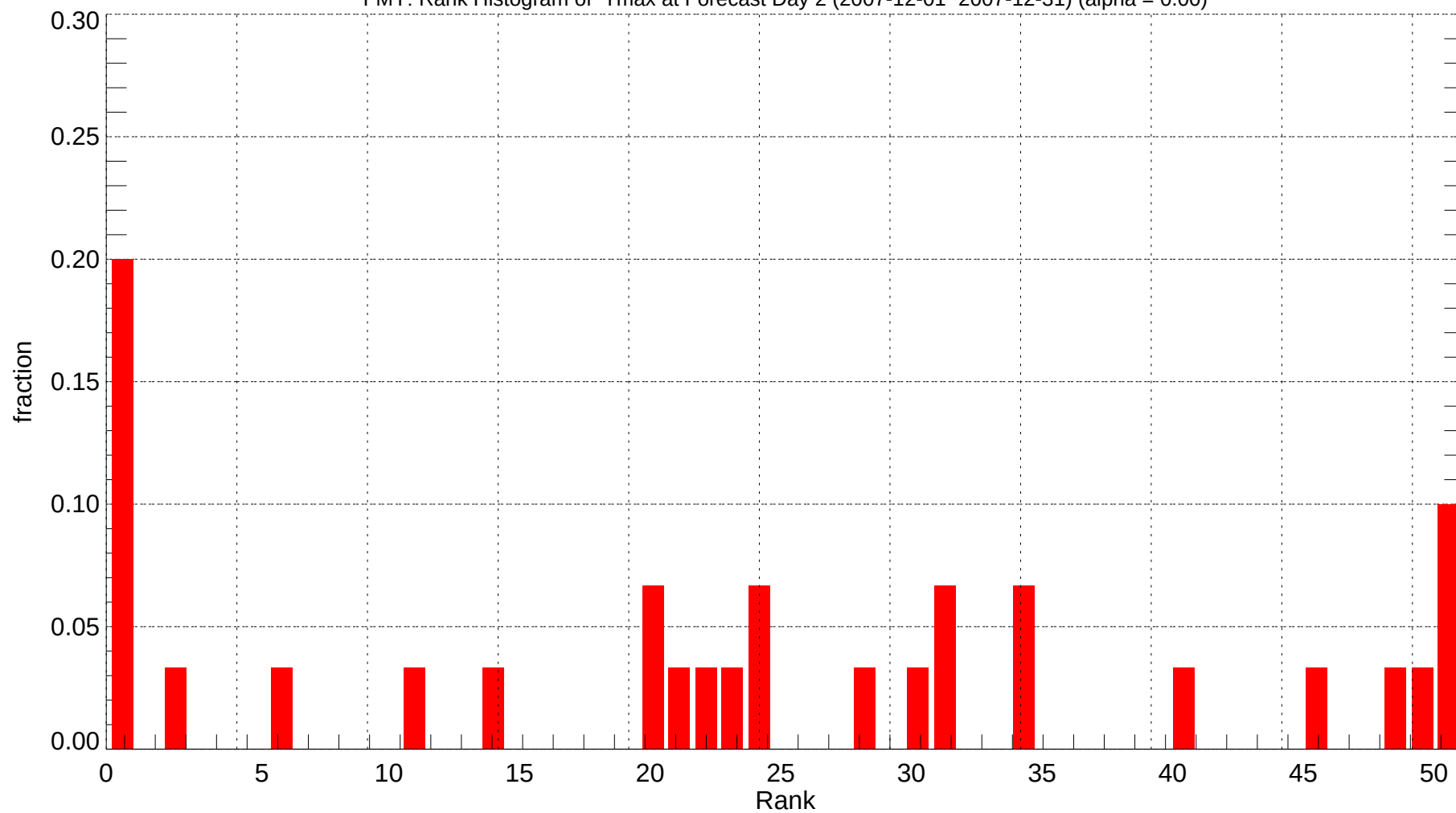
FMY: Rank Histogram of Tmax at Forecast Day 2 (2007-12-01~2007-12-31) (alpha = 0.00)
