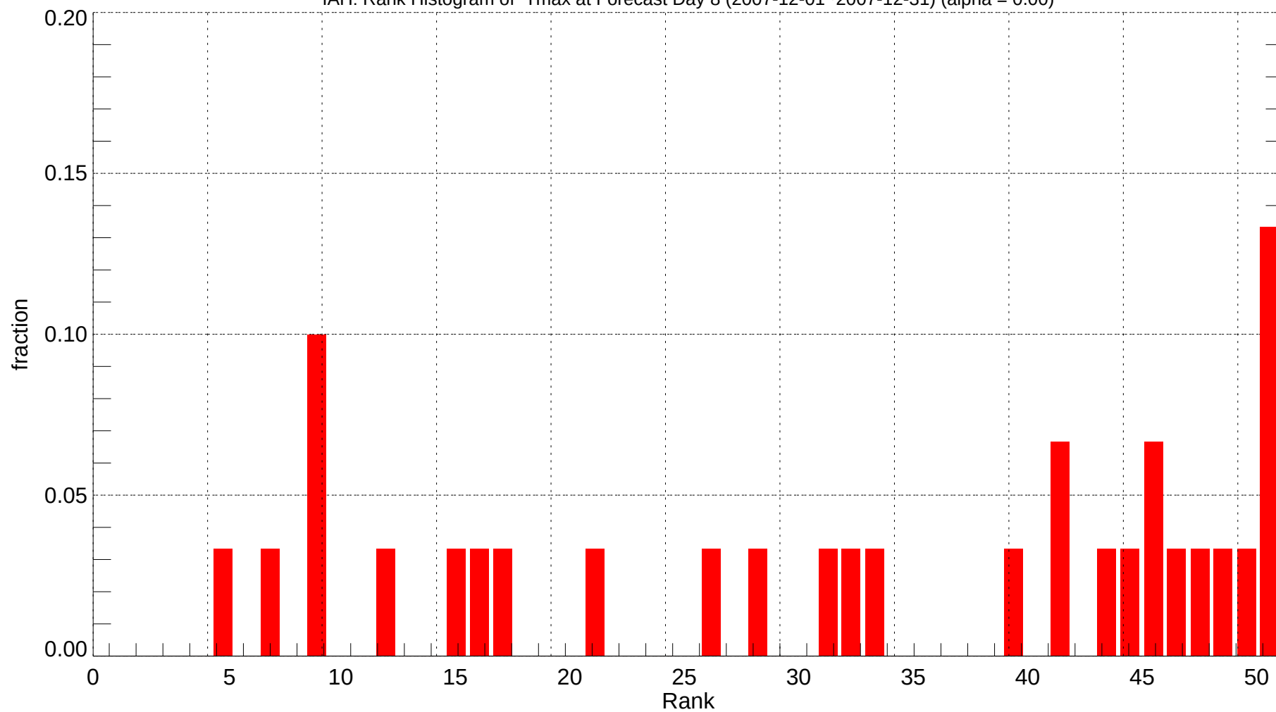
IAH: Rank Histogram of Tmax at Forecast Day 8 (2007-12-01~2007-12-31) (alpha = 0.00)
