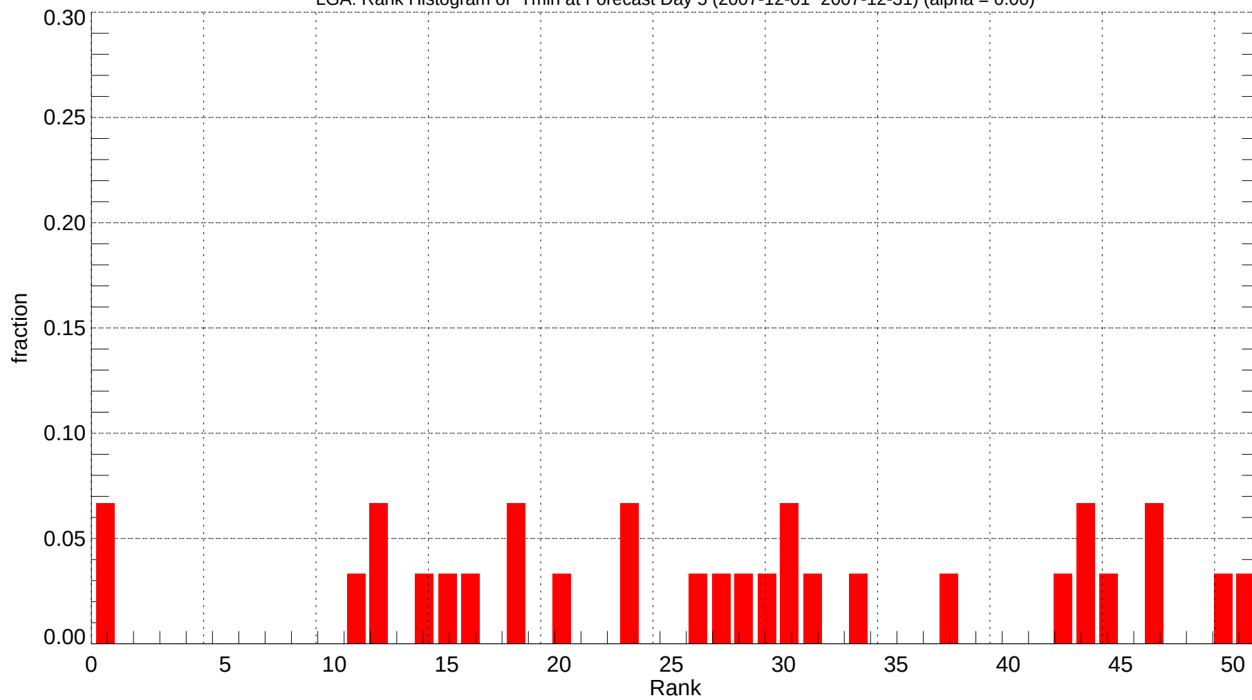
LGA: Rank Histogram of Tmin at Forecast Day 5 (2007-12-01~2007-12-31) (alpha = 0.00)
