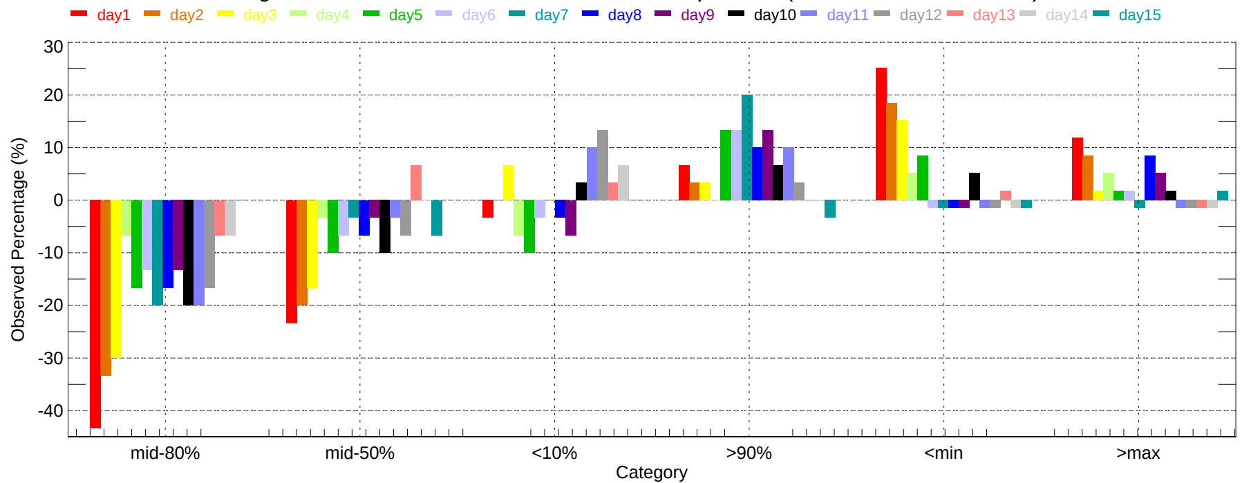
Observed Percentage Deviation of Ensembles - EWR: Max Temperature (2007-12-01~2007-12-31)
