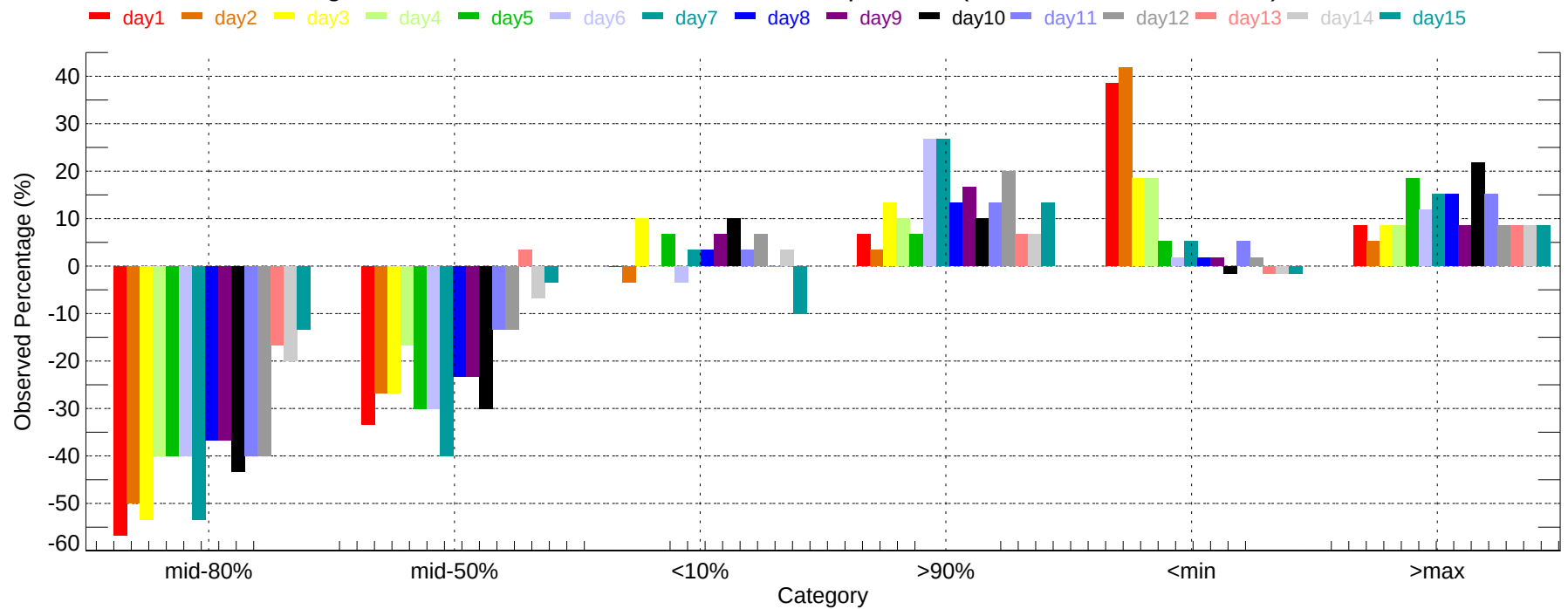
Observed Percentage Deviation of Ensembles - LIT: Min Temperature (2007-12-01~2007-12-31)
