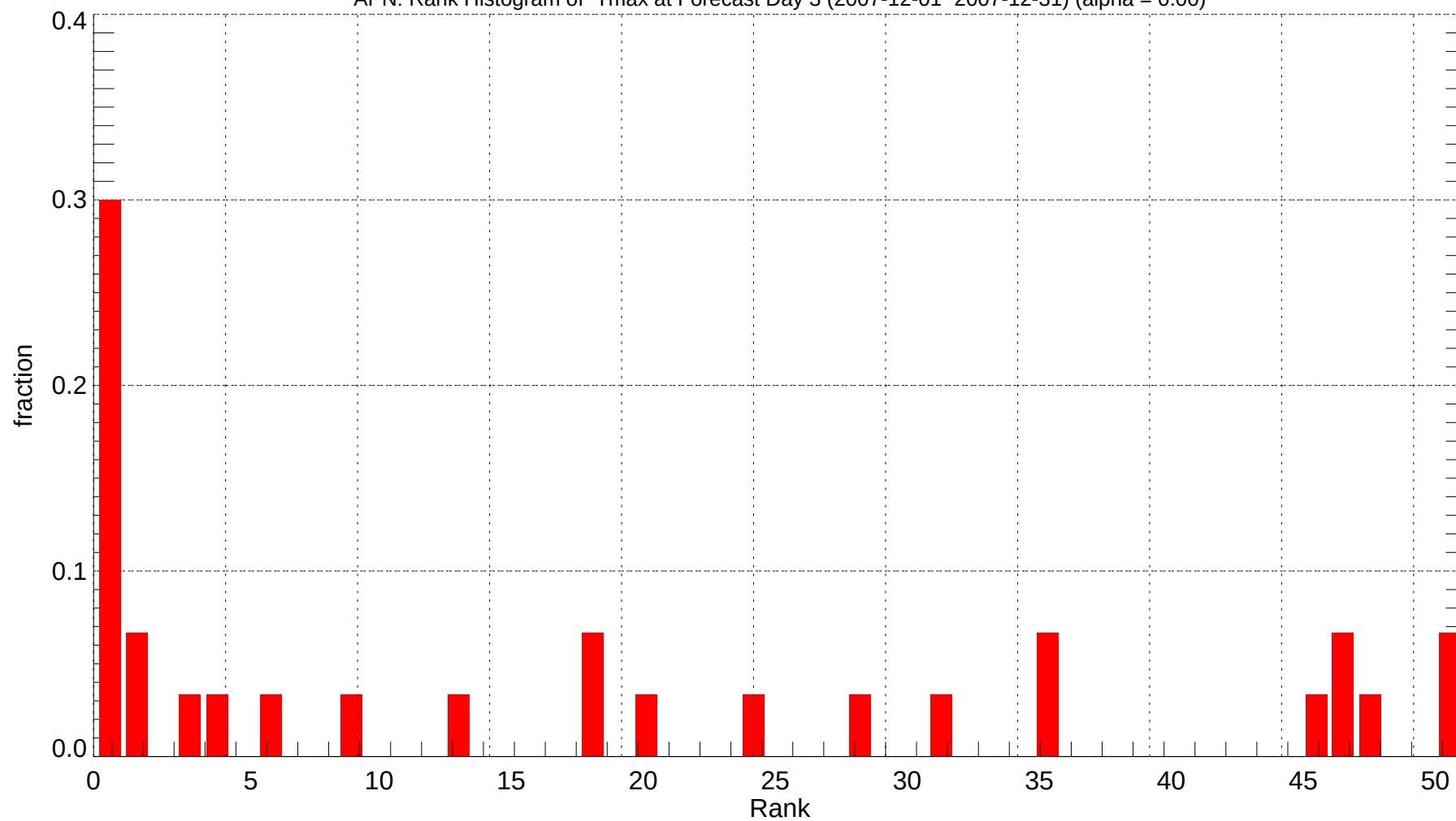
APN: Rank Histogram of Tmax at Forecast Day 3 (2007-12-01~2007-12-31) (alpha = 0.00)
