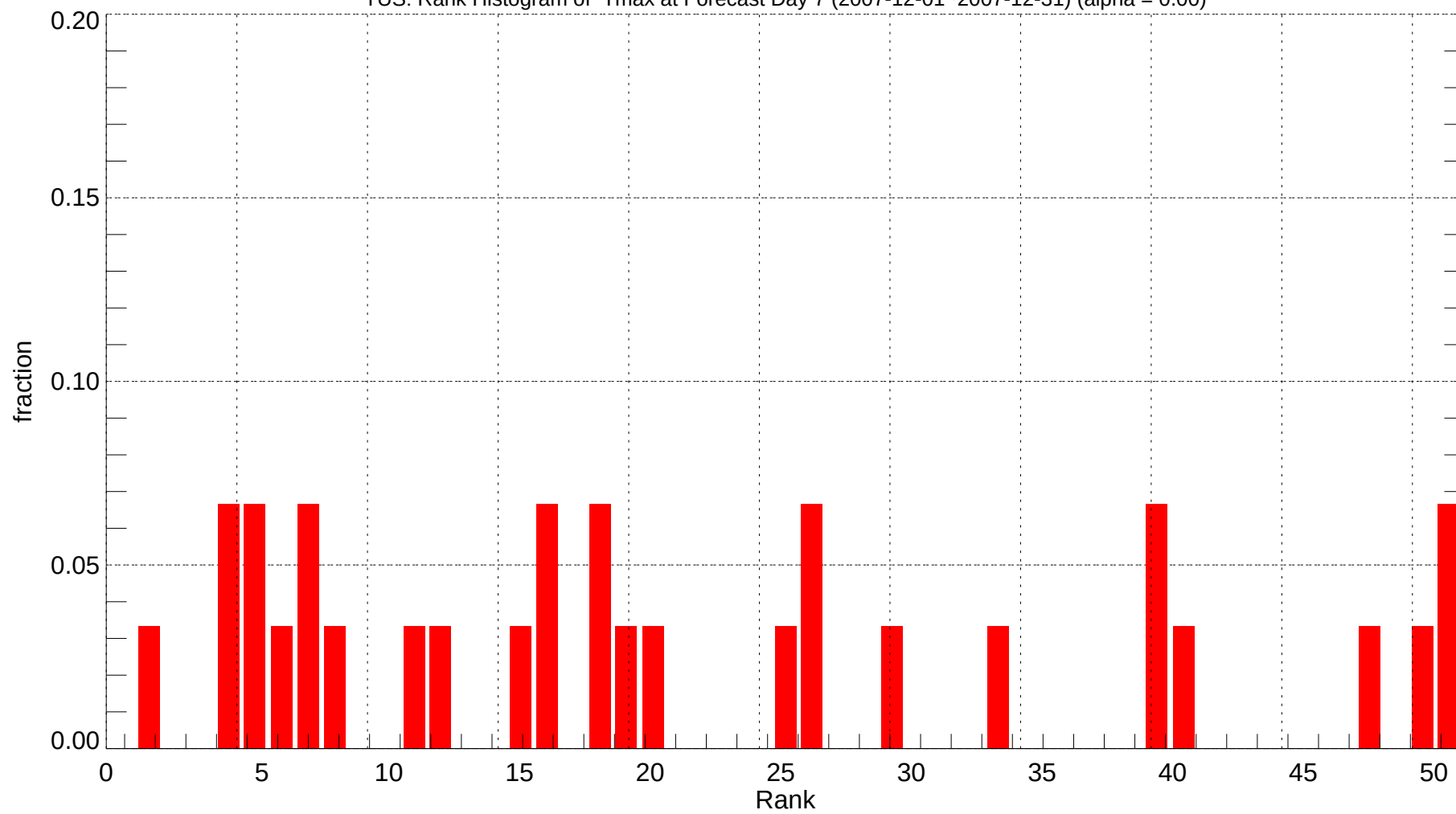
TUS: Rank Histogram of Tmax at Forecast Day 7 (2007-12-01~2007-12-31) (alpha = 0.00)
