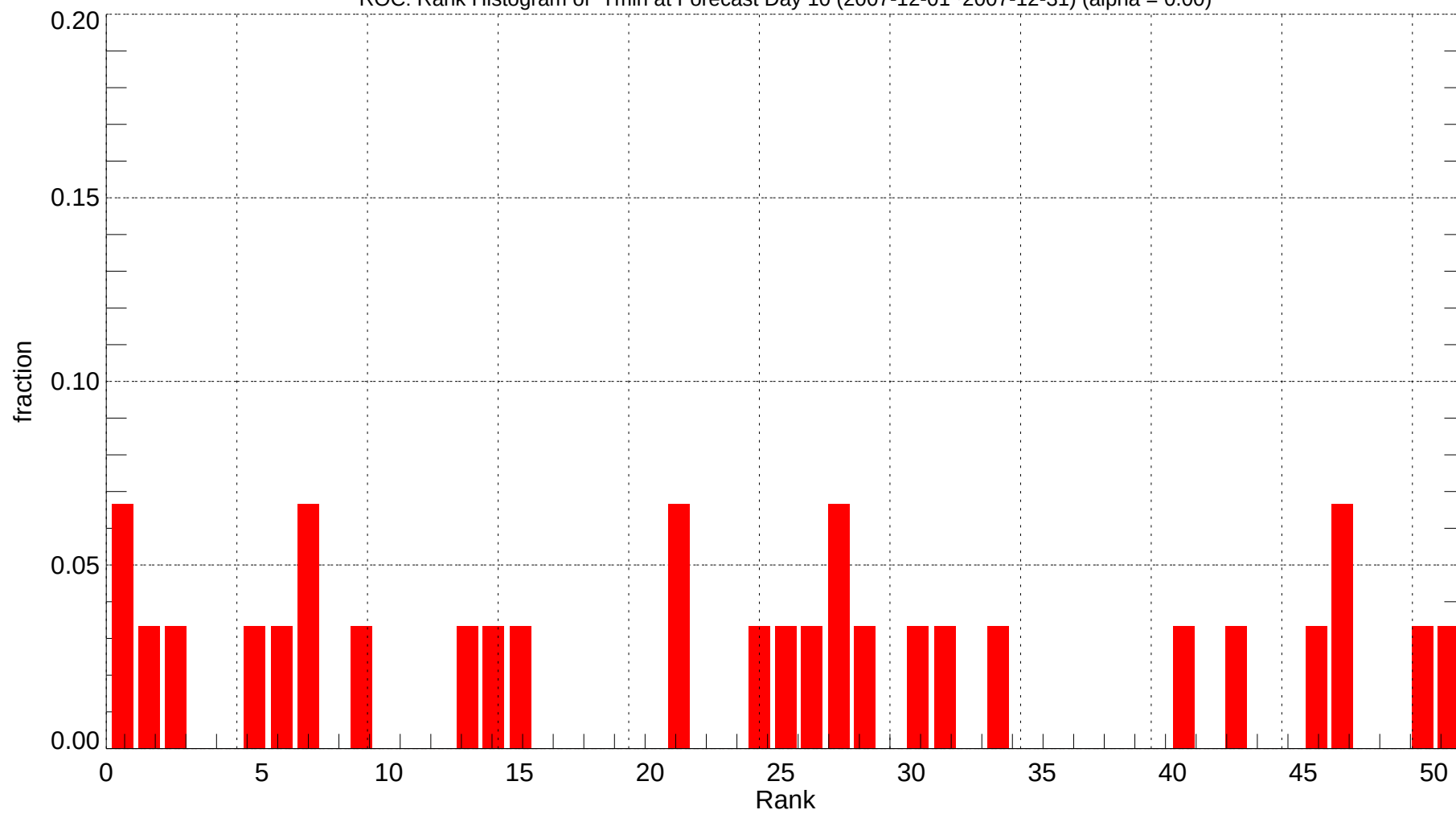
ROC: Rank Histogram of Tmin at Forecast Day 10 (2007-12-01~2007-12-31) (alpha = 0.00)
