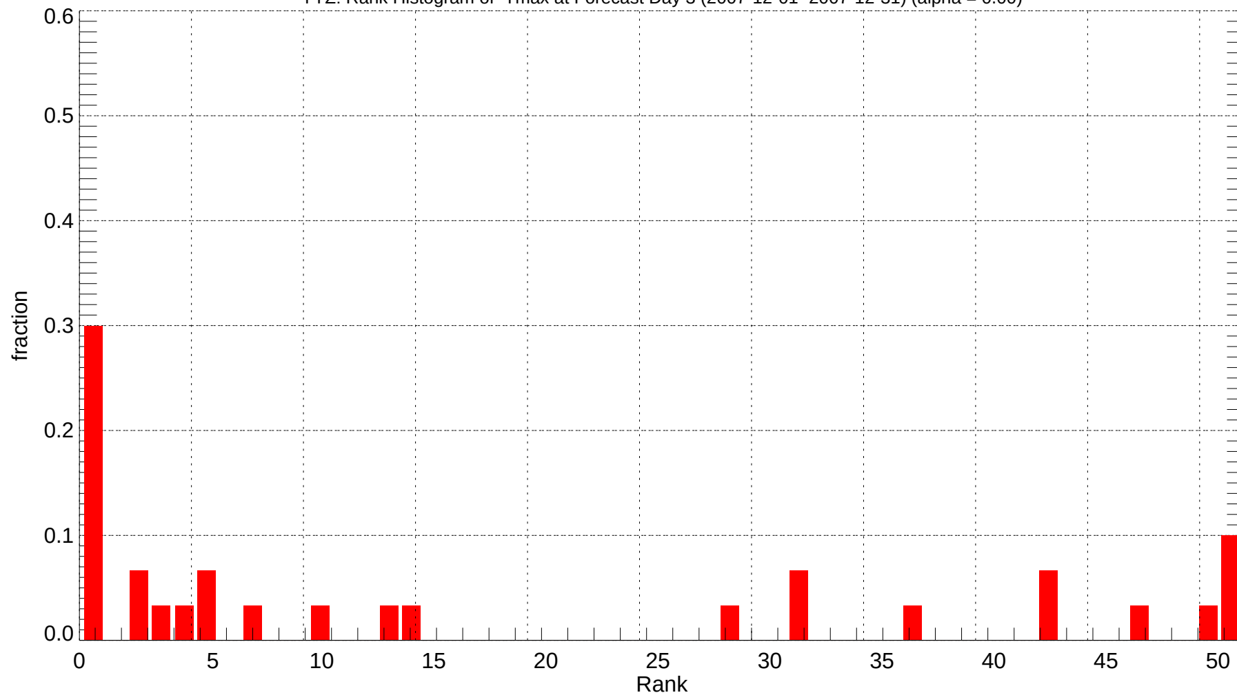
YYZ: Rank Histogram of Tmax at Forecast Day 3 (2007-12-01~2007-12-31) (alpha = 0.00)
