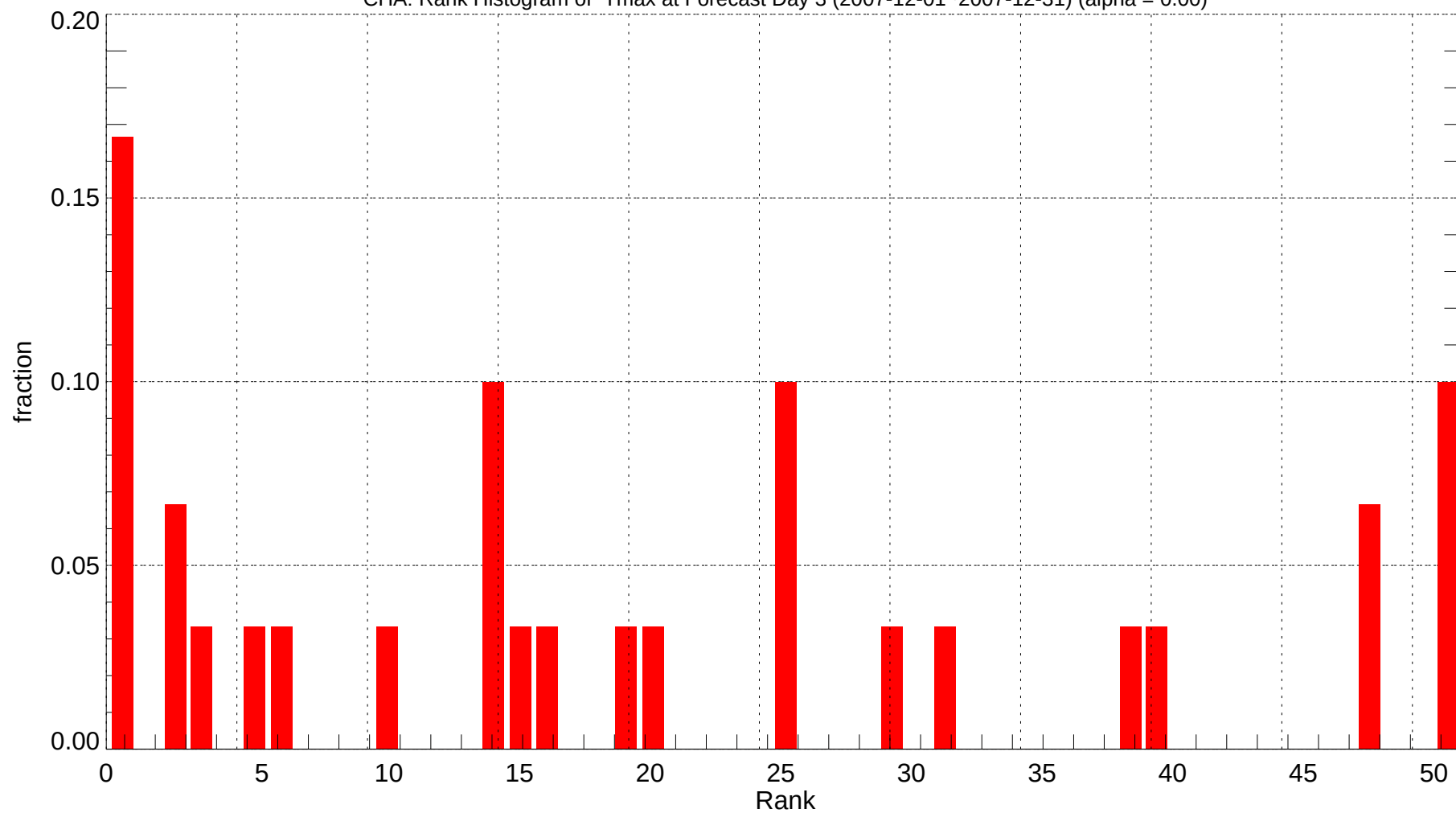
CHA: Rank Histogram of Tmax at Forecast Day 3 (2007-12-01~2007-12-31) (alpha = 0.00)
