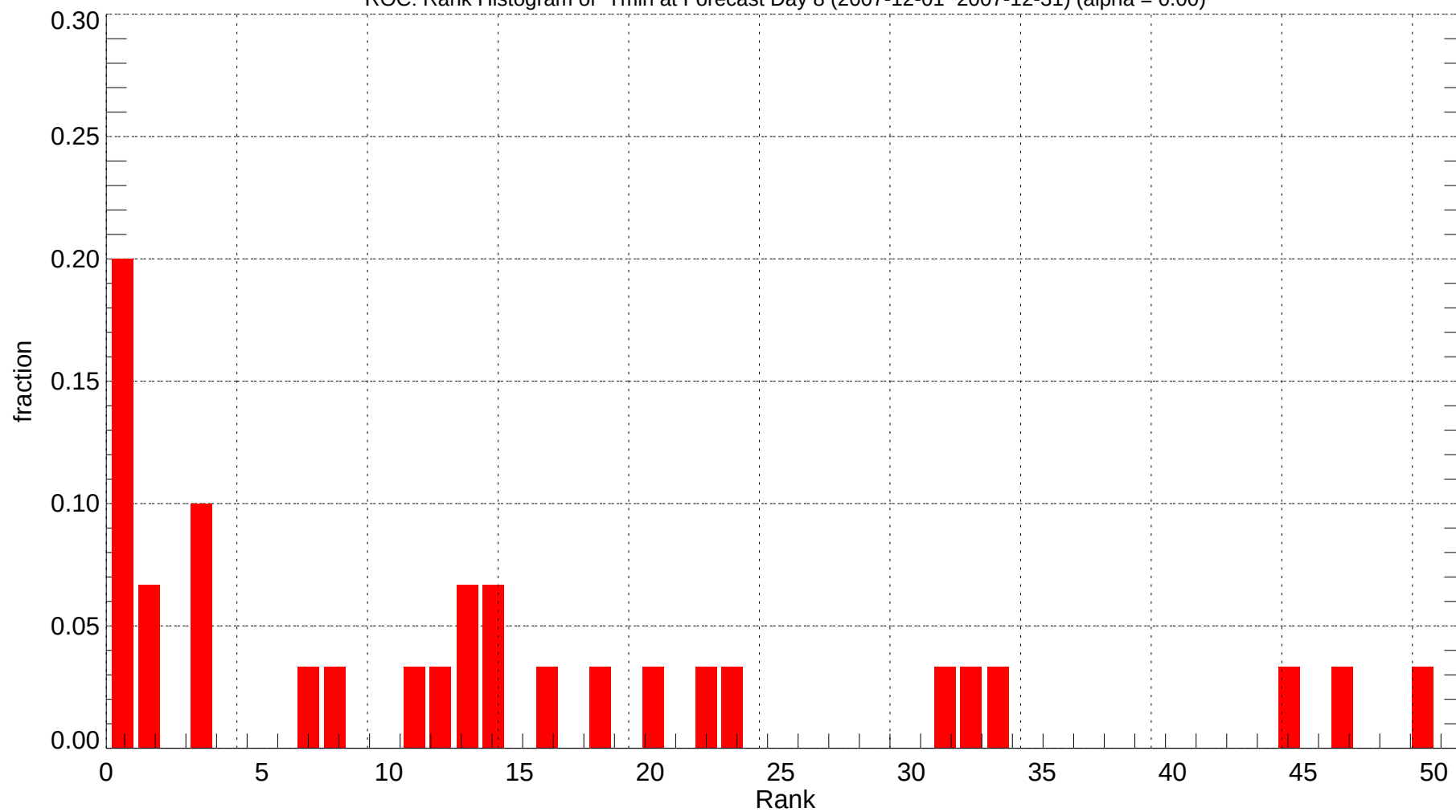
ROC: Rank Histogram of Tmin at Forecast Day 8 (2007-12-01~2007-12-31) (alpha = 0.00)
