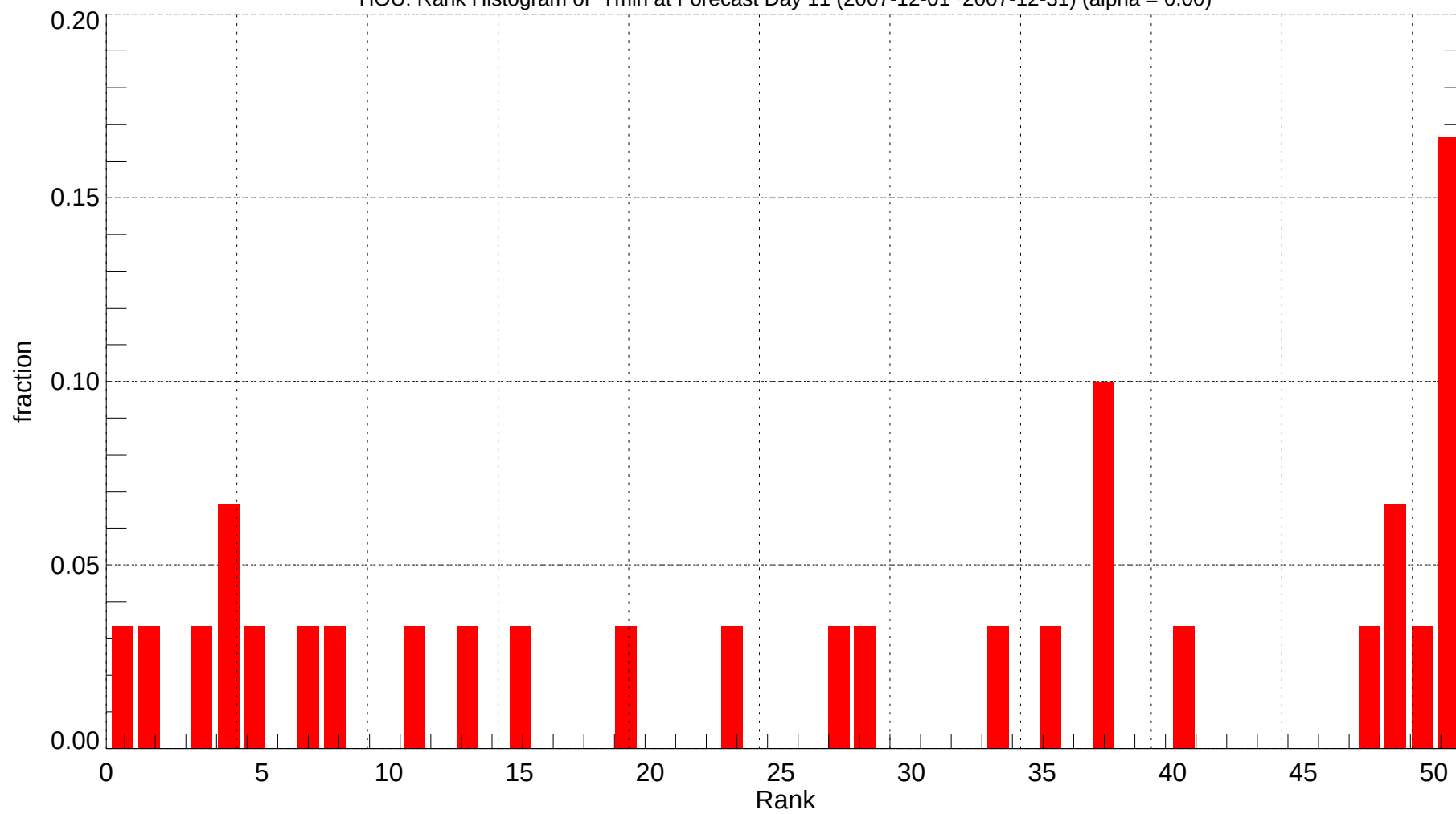
HOU: Rank Histogram of Tmin at Forecast Day 11 (2007-12-01~2007-12-31) (alpha = 0.00)
