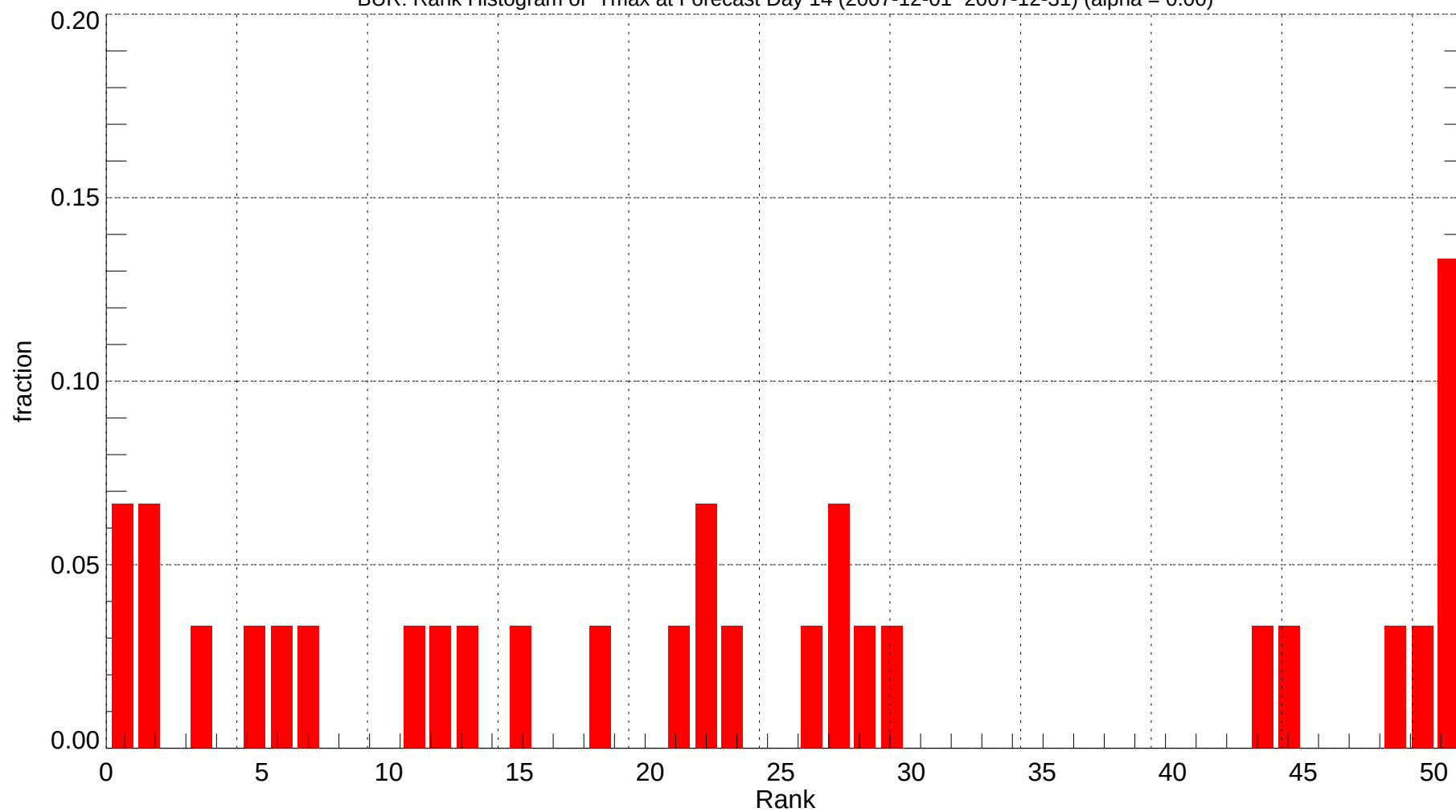
BUR: Rank Histogram of Tmax at Forecast Day 14 (2007-12-01~2007-12-31) (alpha = 0.00)
