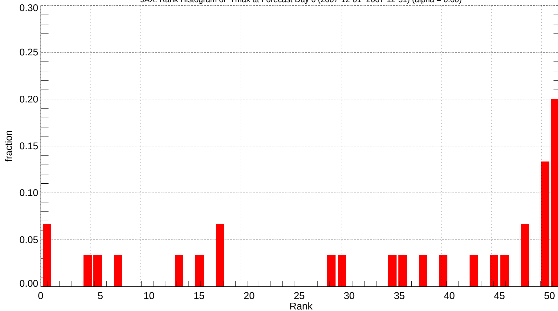
JAX: Rank Histogram of Tmax at Forecast Day 6 (2007-12-01~2007-12-31) (alpha = 0.00)
