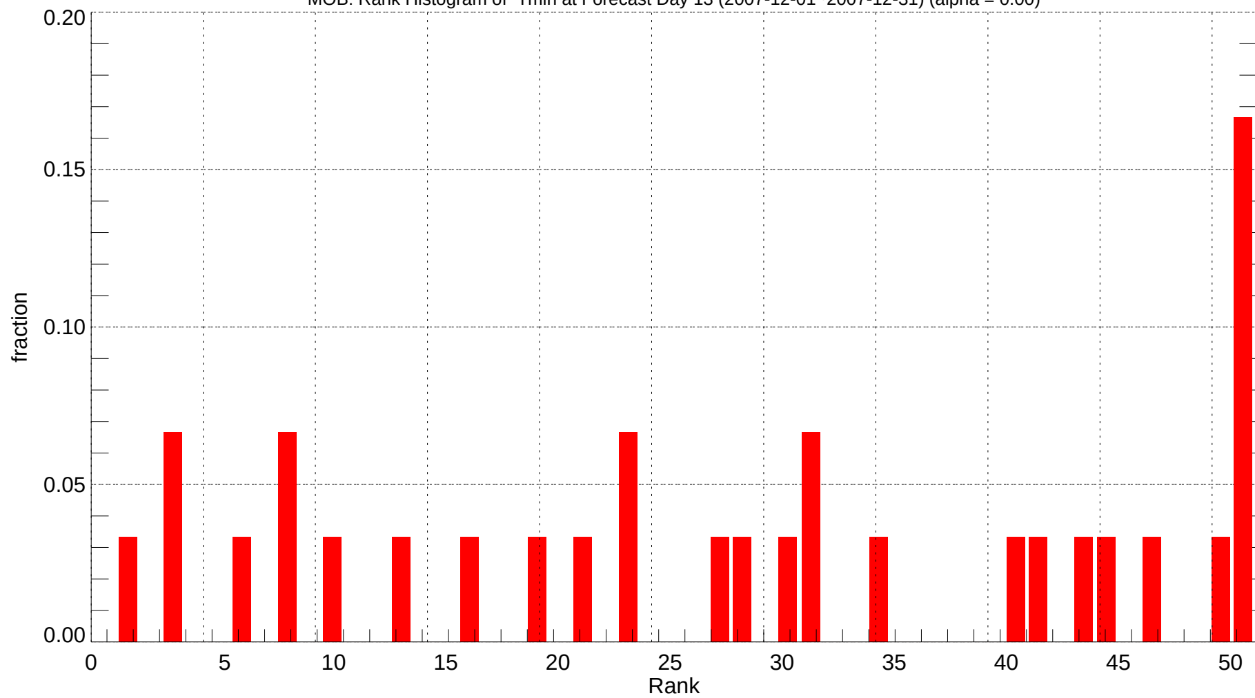
MOB: Rank Histogram of Tmin at Forecast Day 13 (2007-12-01~2007-12-31) (alpha = 0.00)
