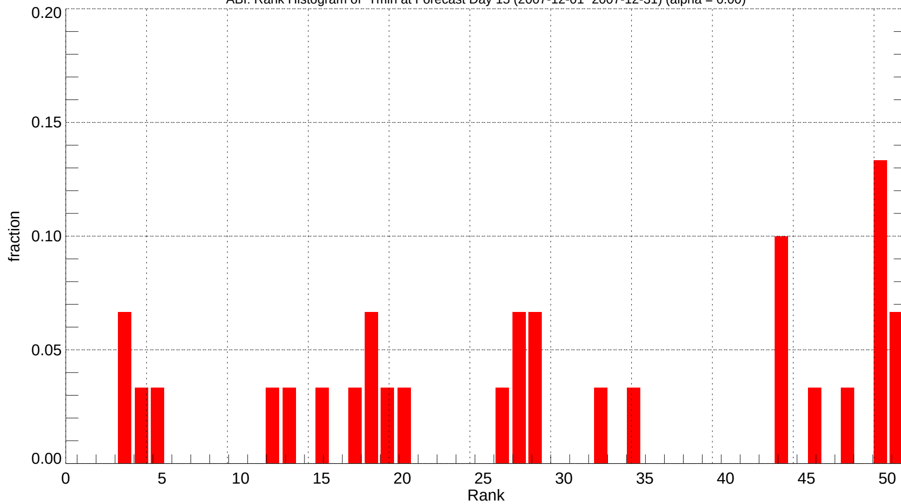
ABI: Rank Histogram of Tmin at Forecast Day 15 (2007-12-01~2007-12-31) (alpha = 0.00)
