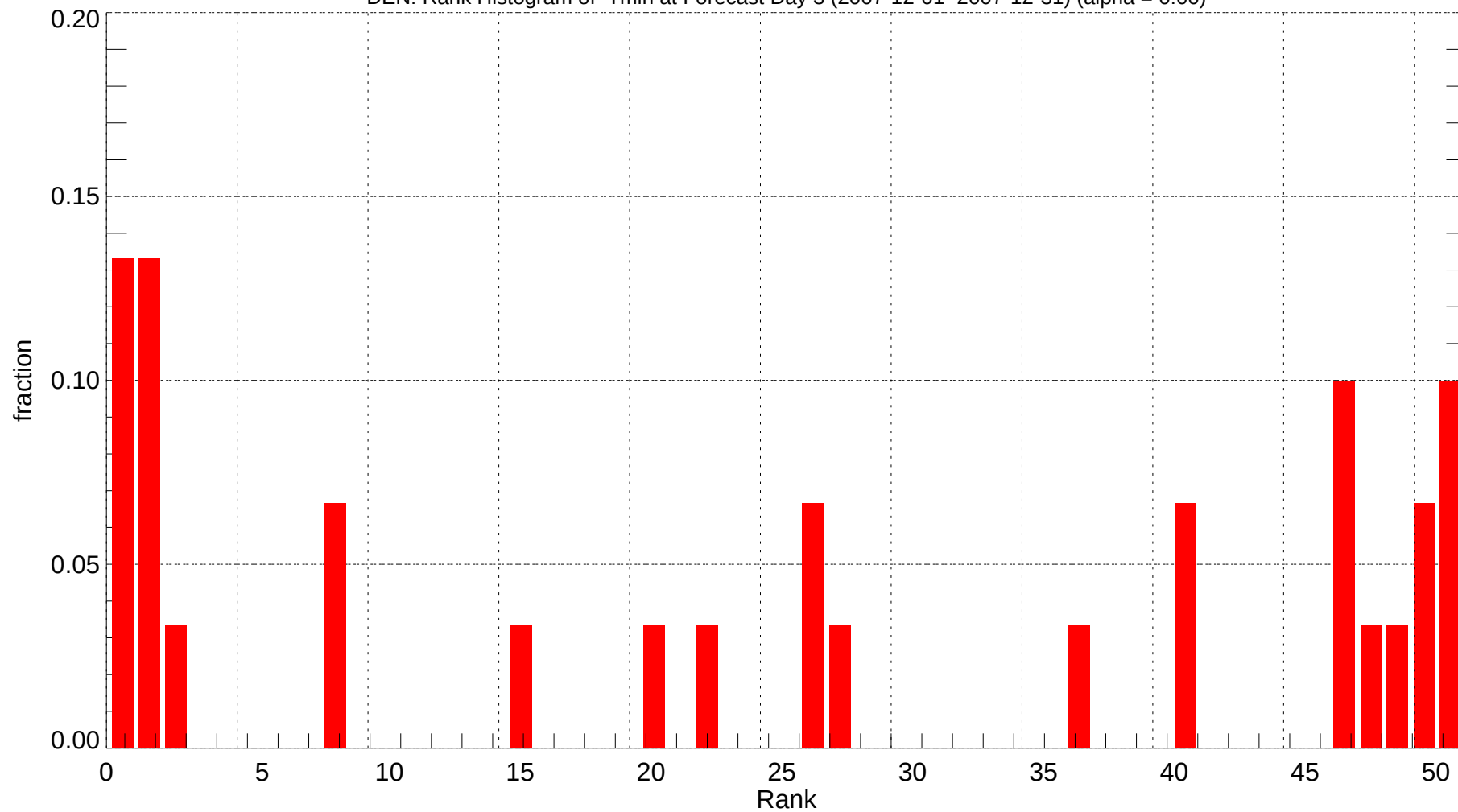
DEN: Rank Histogram of Tmin at Forecast Day 3 (2007-12-01~2007-12-31) (alpha = 0.00)
