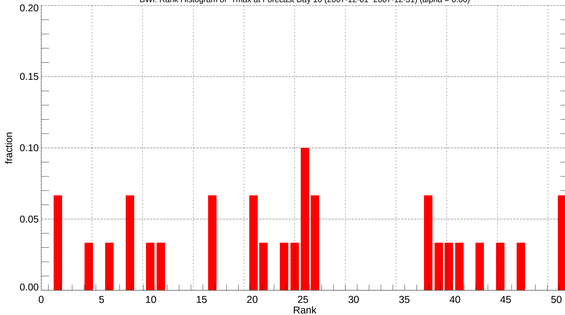
BWI: Rank Histogram of Tmax at Forecast Day 10 (2007-12-01~2007-12-31) (alpha = 0.00)
