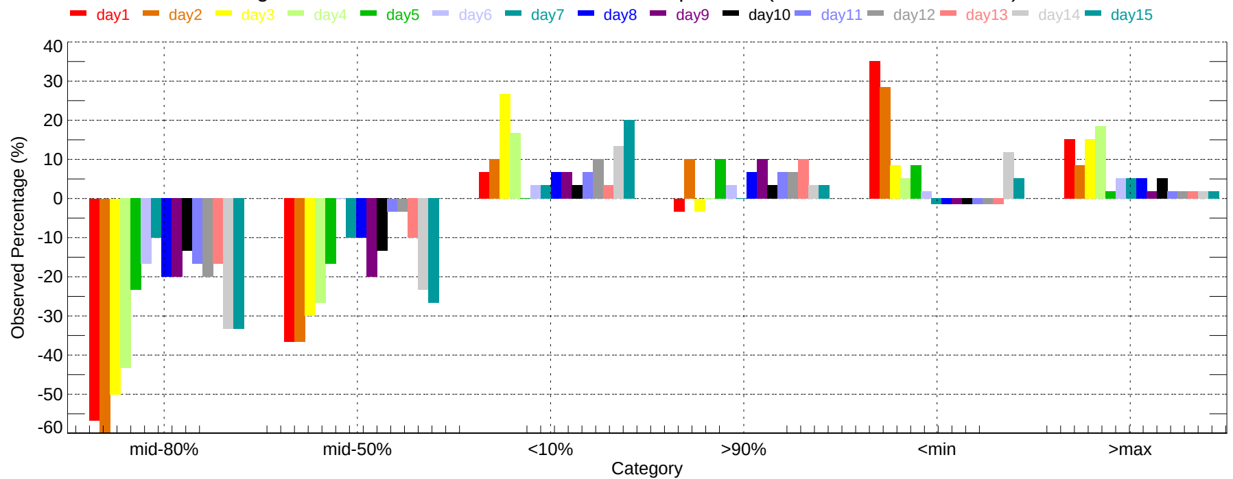
Observed Percentage Deviation of Ensembles - TUS: Min Temperature (2007-12-01~2007-12-31)
