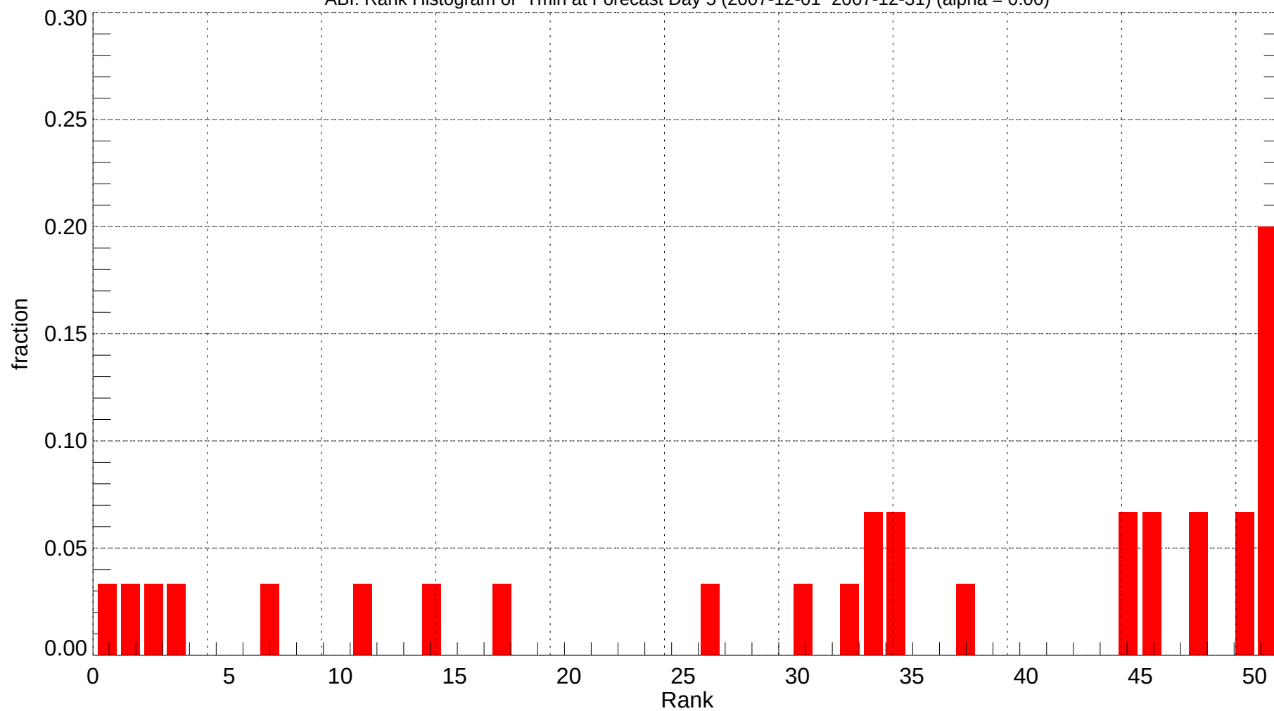
ABI: Rank Histogram of Tmin at Forecast Day 5 (2007-12-01~2007-12-31) (alpha = 0.00)
