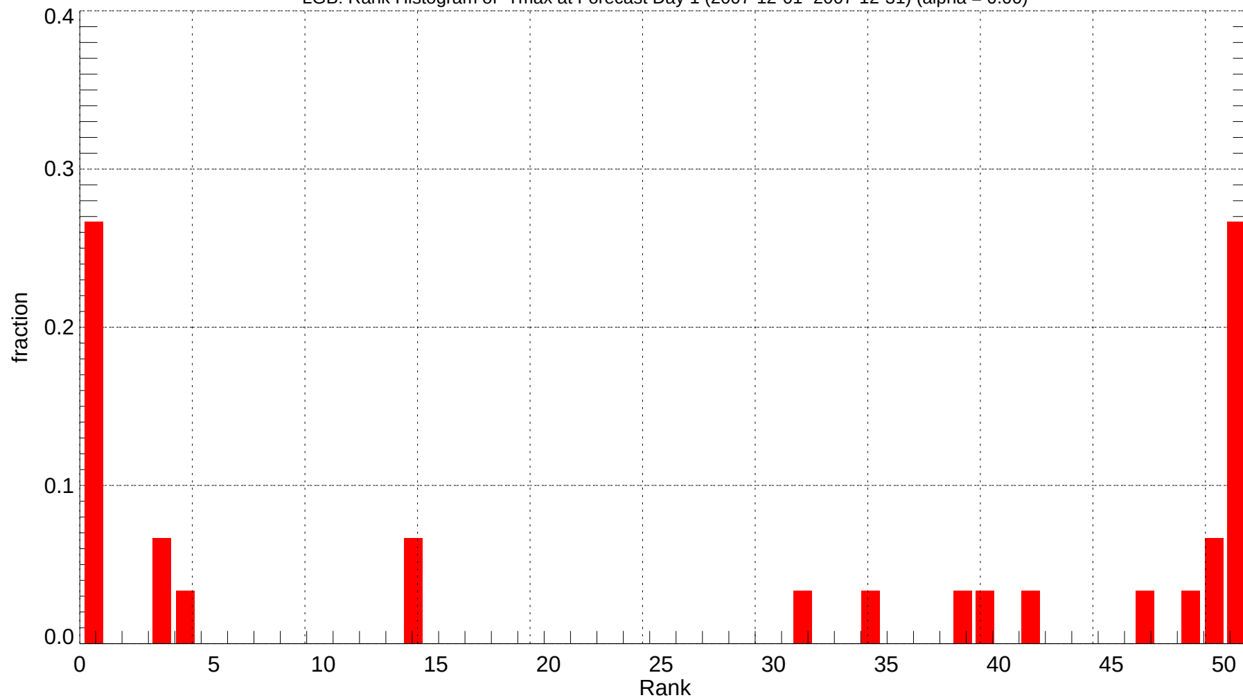
LGB: Rank Histogram of Tmax at Forecast Day 1 (2007-12-01~2007-12-31) (alpha = 0.00)
