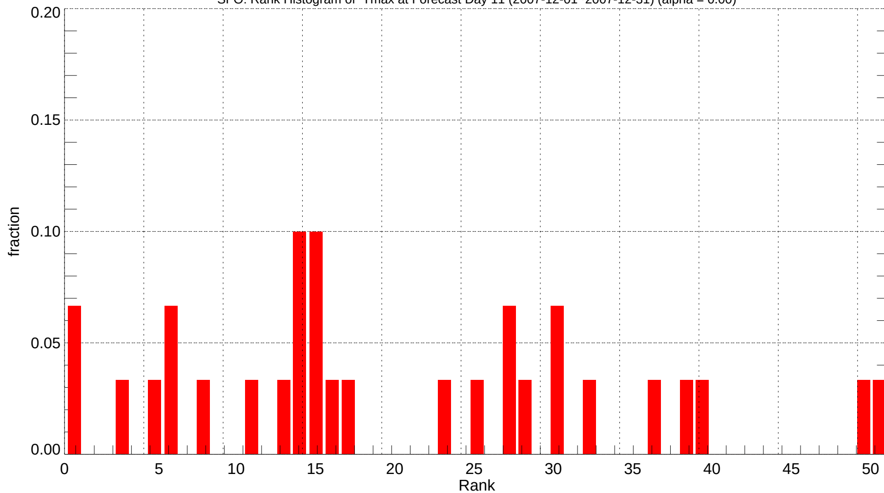
SFO: Rank Histogram of Tmax at Forecast Day 11 (2007-12-01~2007-12-31) (alpha = 0.00)
