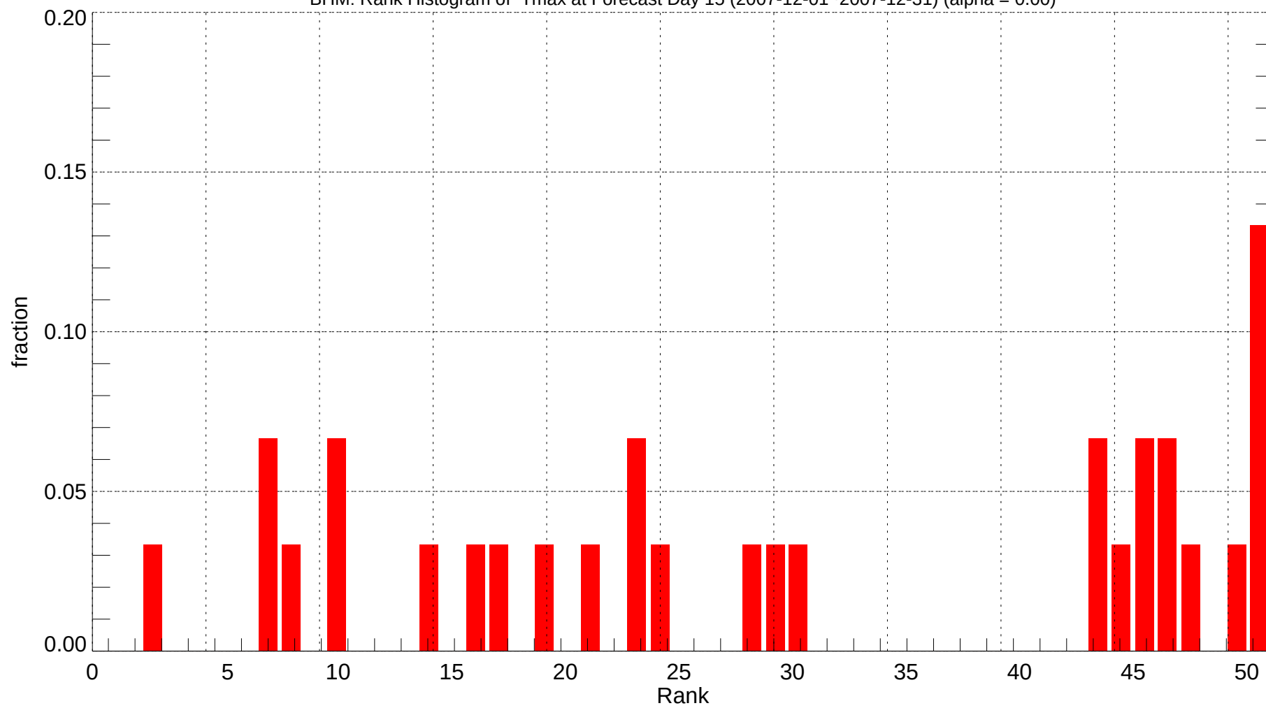
BHM: Rank Histogram of Tmax at Forecast Day 15 (2007-12-01~2007-12-31) (alpha = 0.00)
