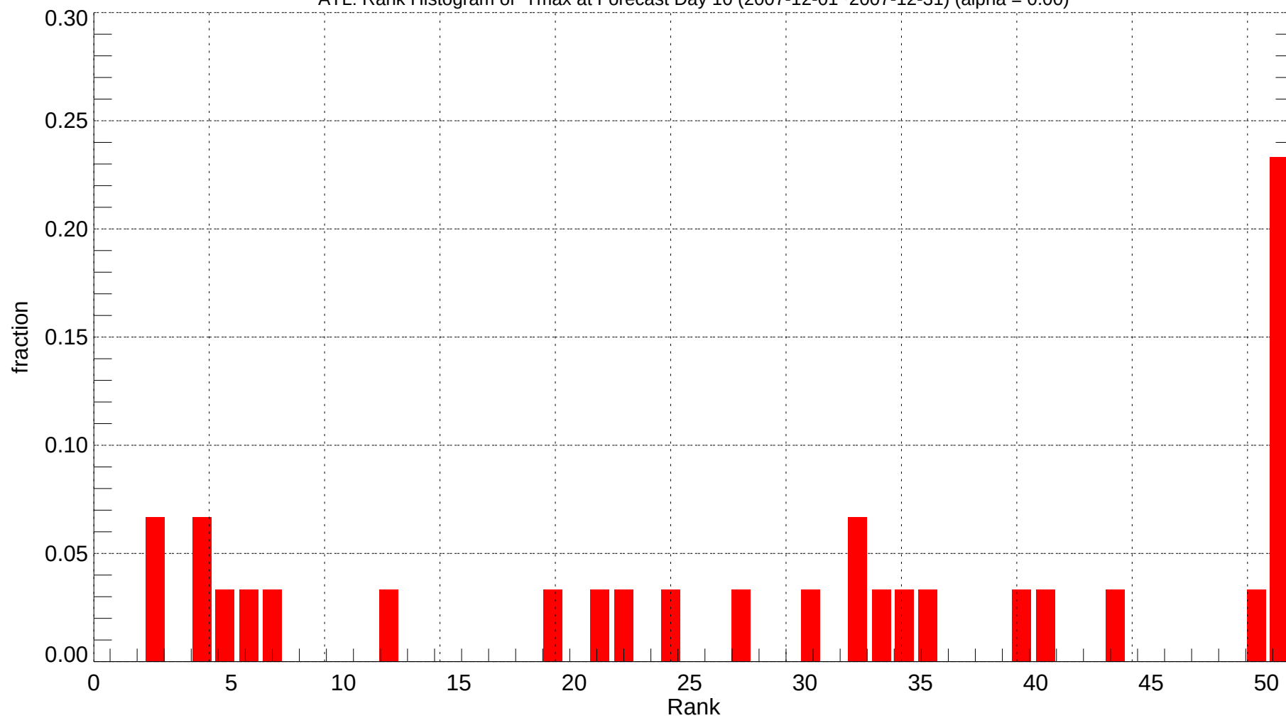
ATL: Rank Histogram of Tmax at Forecast Day 10 (2007-12-01~2007-12-31) (alpha = 0.00)
