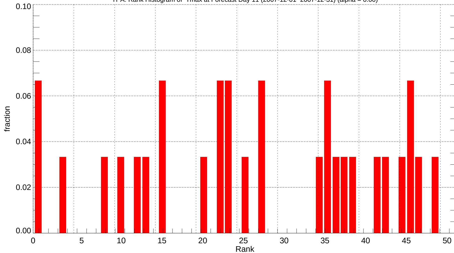
TPA: Rank Histogram of Tmax at Forecast Day 11 (2007-12-01~2007-12-31) (alpha = 0.00)
