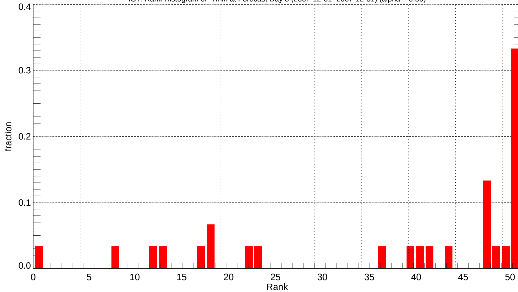
ICT: Rank Histogram of Tmin at Forecast Day 5 (2007-12-01~2007-12-31) (alpha = 0.00)
