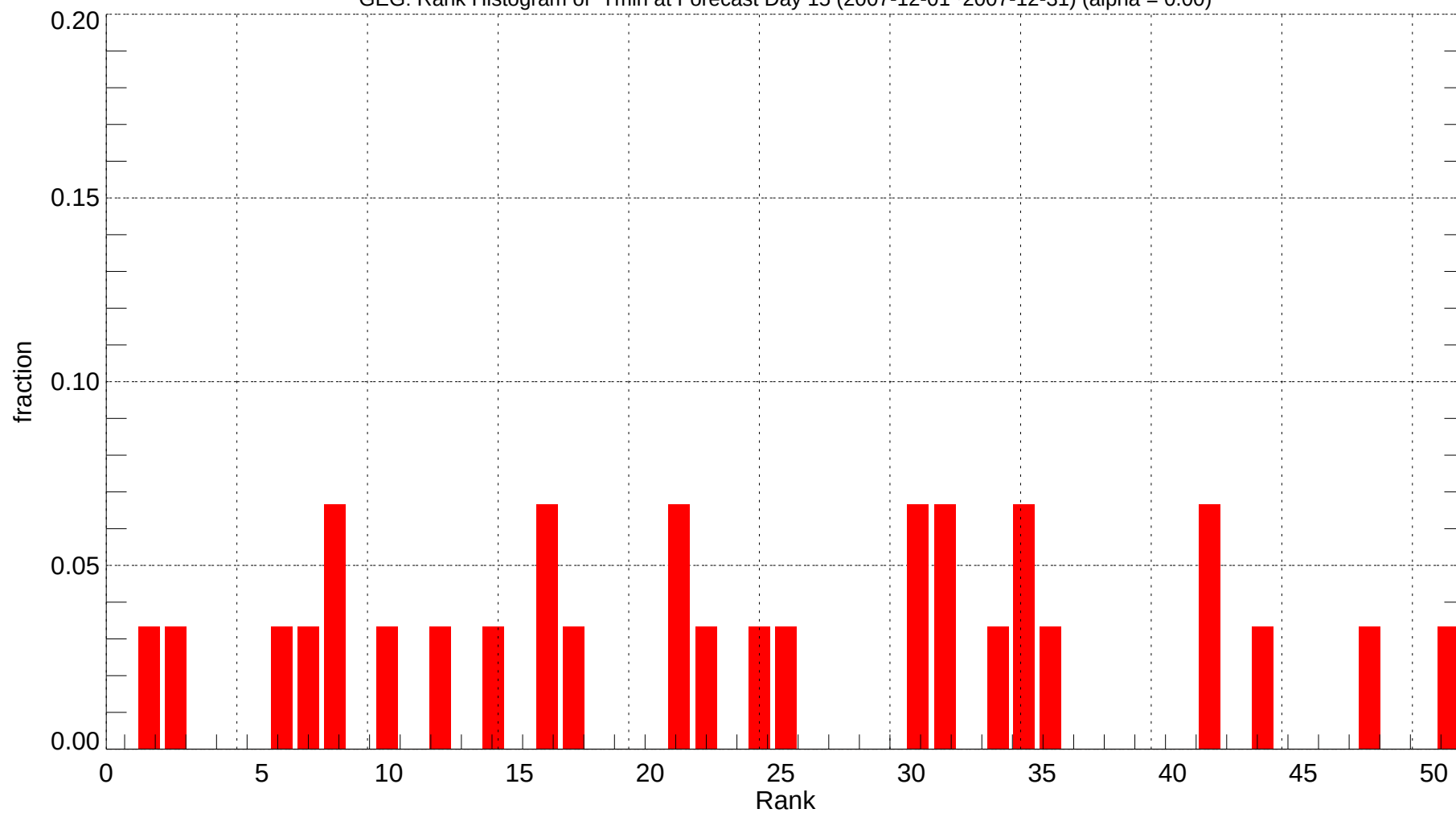
GEG: Rank Histogram of Tmin at Forecast Day 15 (2007-12-01~2007-12-31) (alpha = 0.00)
