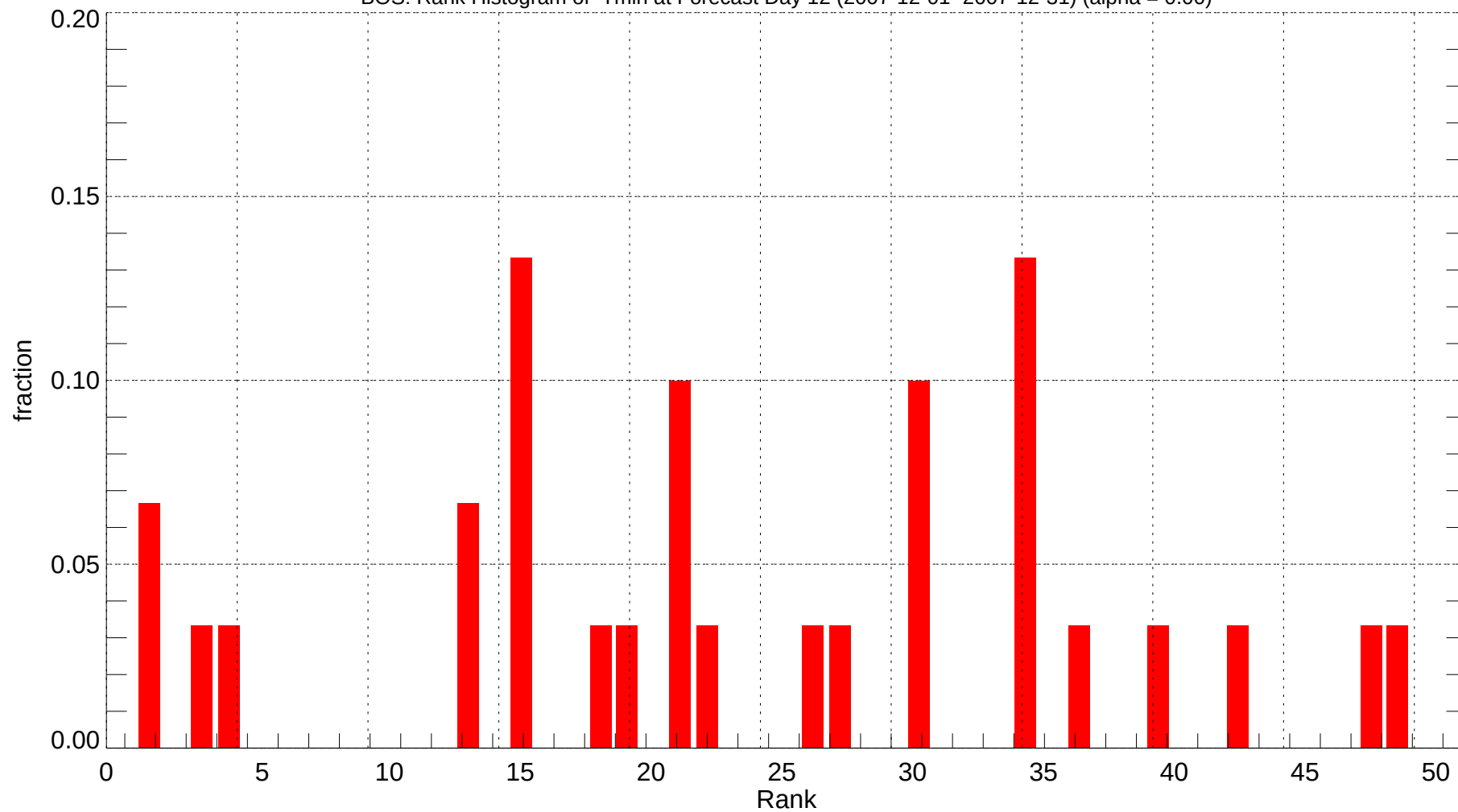
BOS: Rank Histogram of Tmin at Forecast Day 12 (2007-12-01~2007-12-31) (alpha = 0.00)
