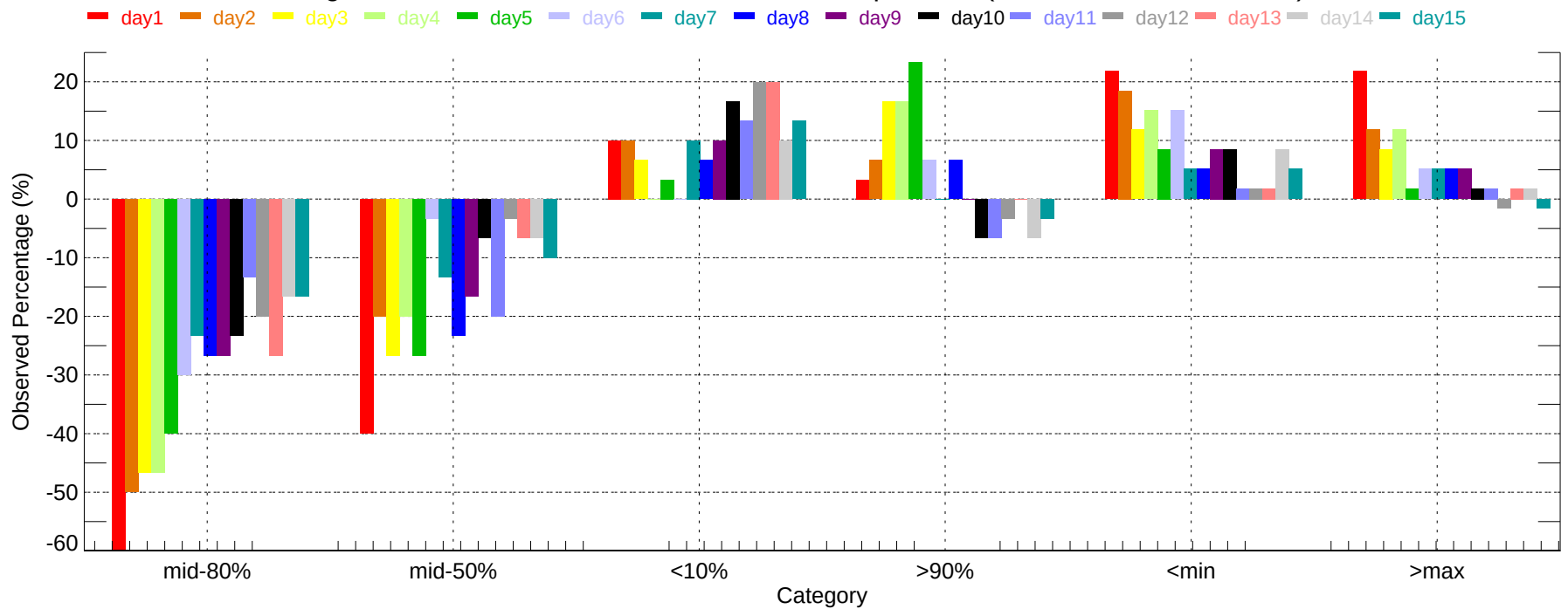
Observed Percentage Deviation of Ensembles - DEN: Max Temperature (2007-12-01~2007-12-31)
