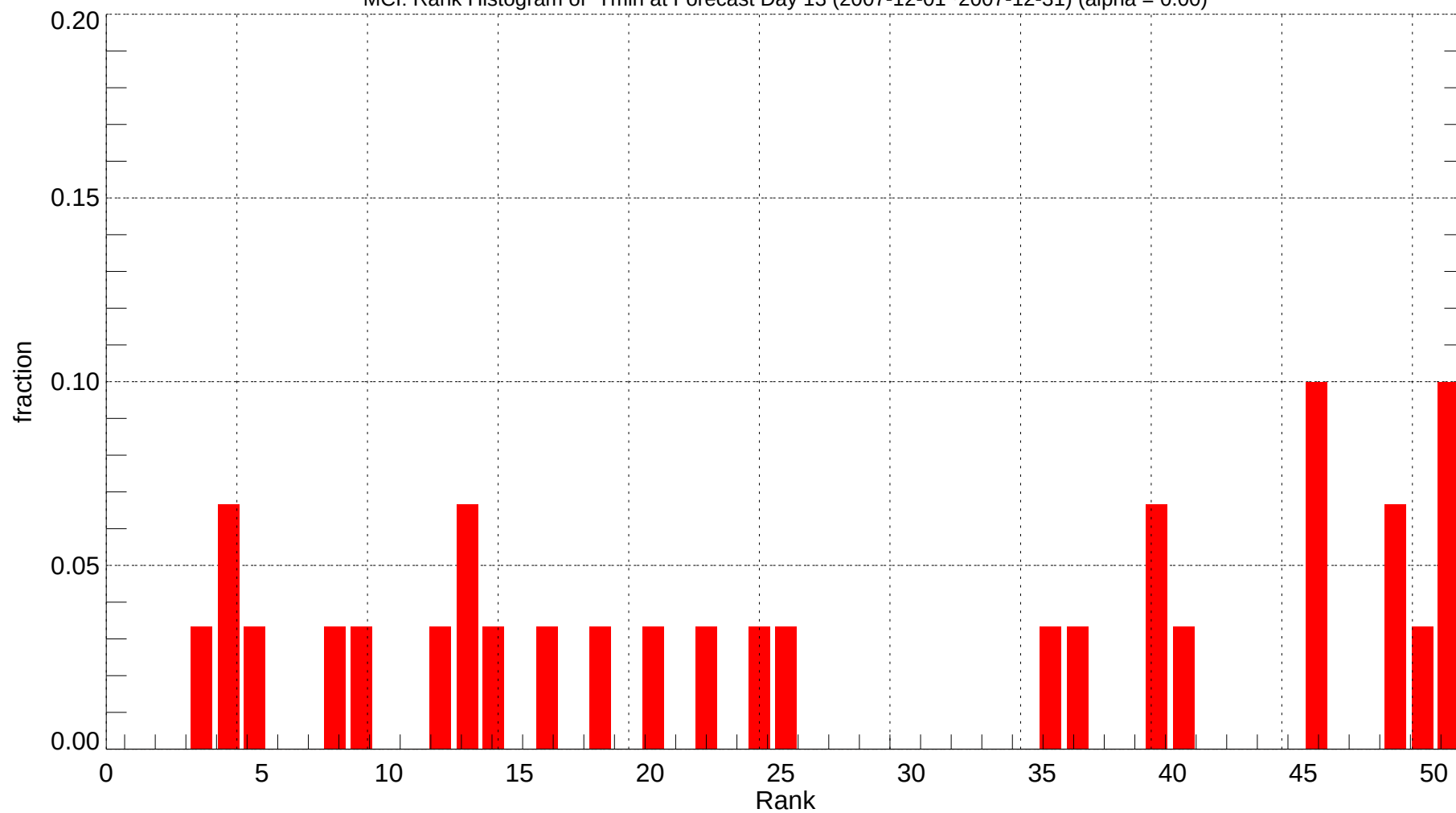
MCI: Rank Histogram of Tmin at Forecast Day 13 (2007-12-01~2007-12-31) (alpha = 0.00)
