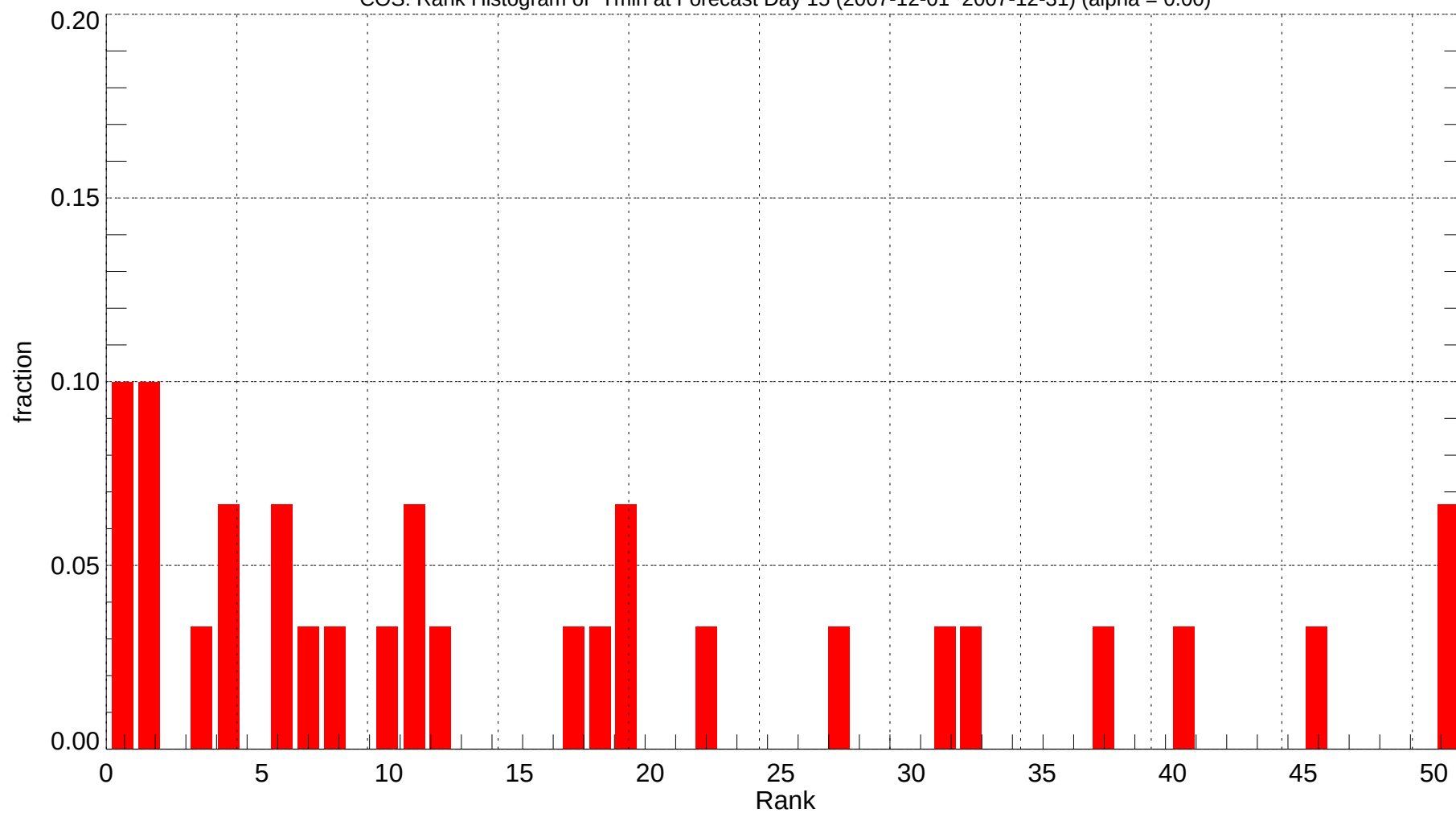
COS: Rank Histogram of Tmin at Forecast Day 15 (2007-12-01~2007-12-31) (alpha = 0.00)
