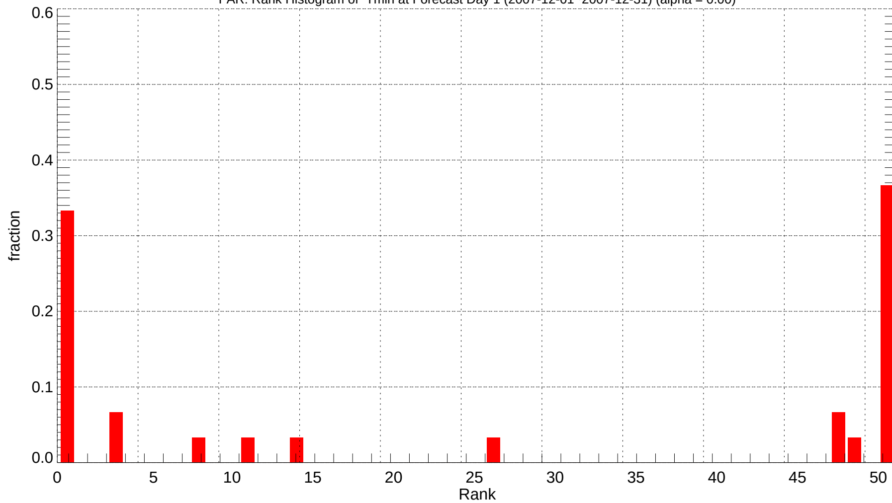
FAR: Rank Histogram of Tmin at Forecast Day 1 (2007-12-01~2007-12-31) (alpha = 0.00)
