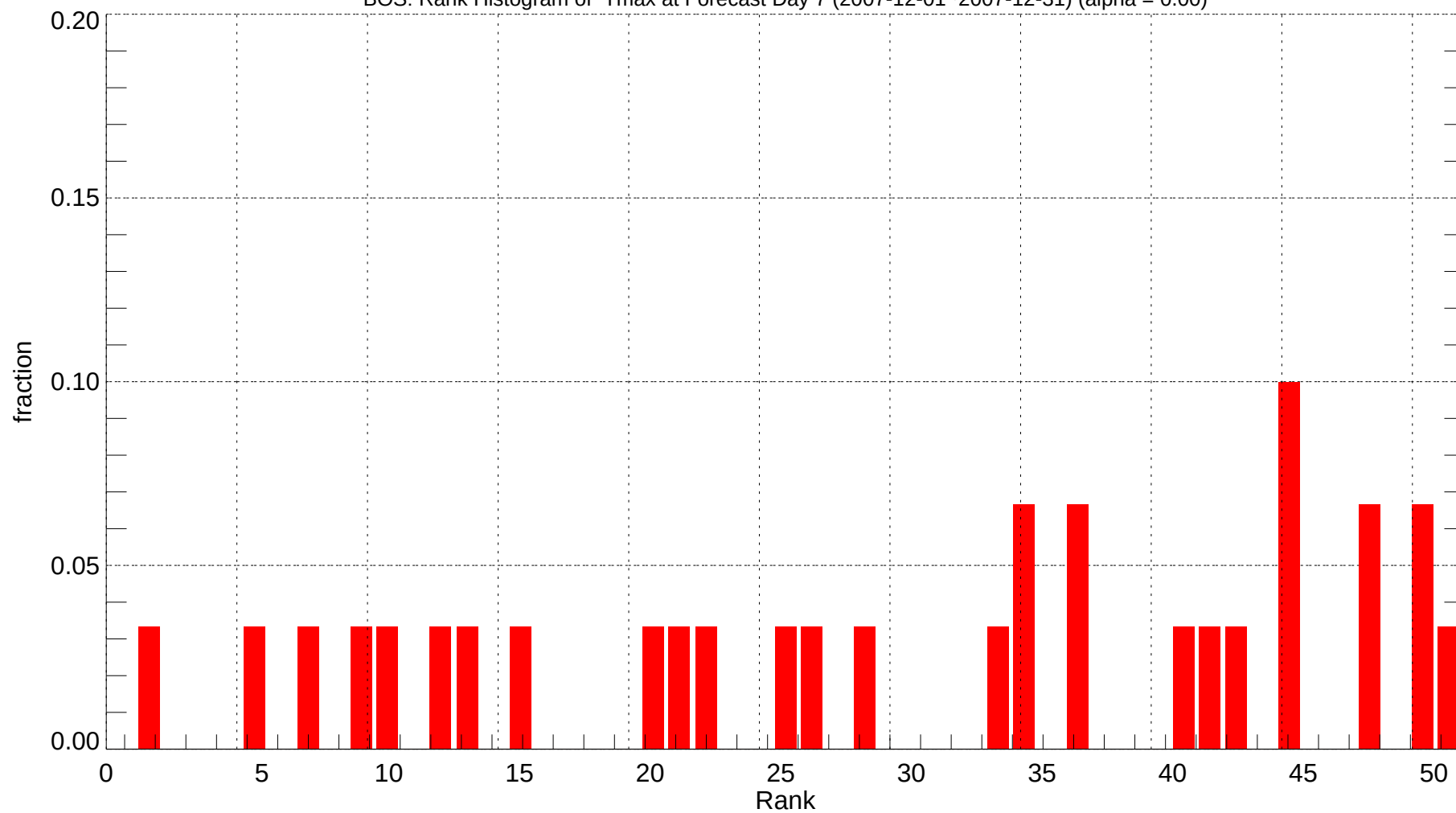
BOS: Rank Histogram of Tmax at Forecast Day 7 (2007-12-01~2007-12-31) (alpha = 0.00)
