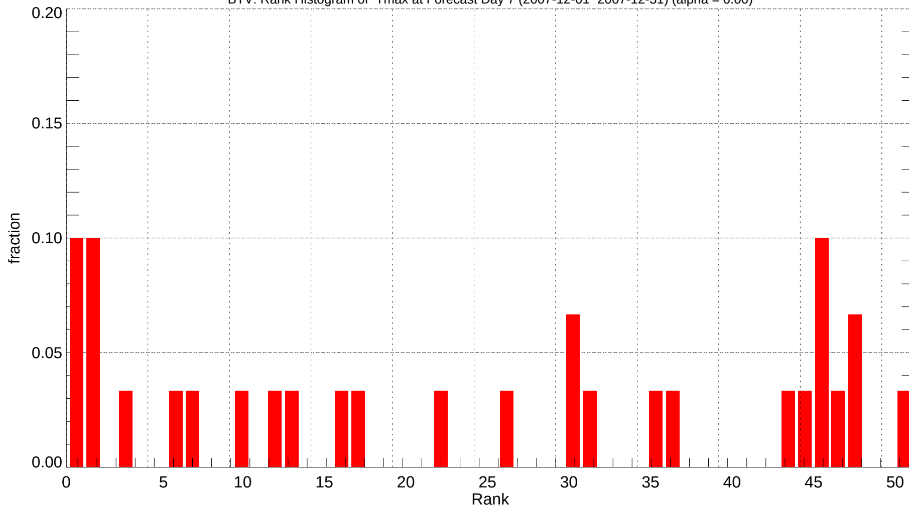
BTV: Rank Histogram of Tmax at Forecast Day 7 (2007-12-01~2007-12-31) (alpha = 0.00)
