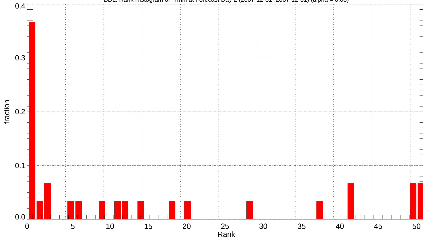
BDL: Rank Histogram of Tmin at Forecast Day 2 (2007-12-01~2007-12-31) (alpha = 0.00)
