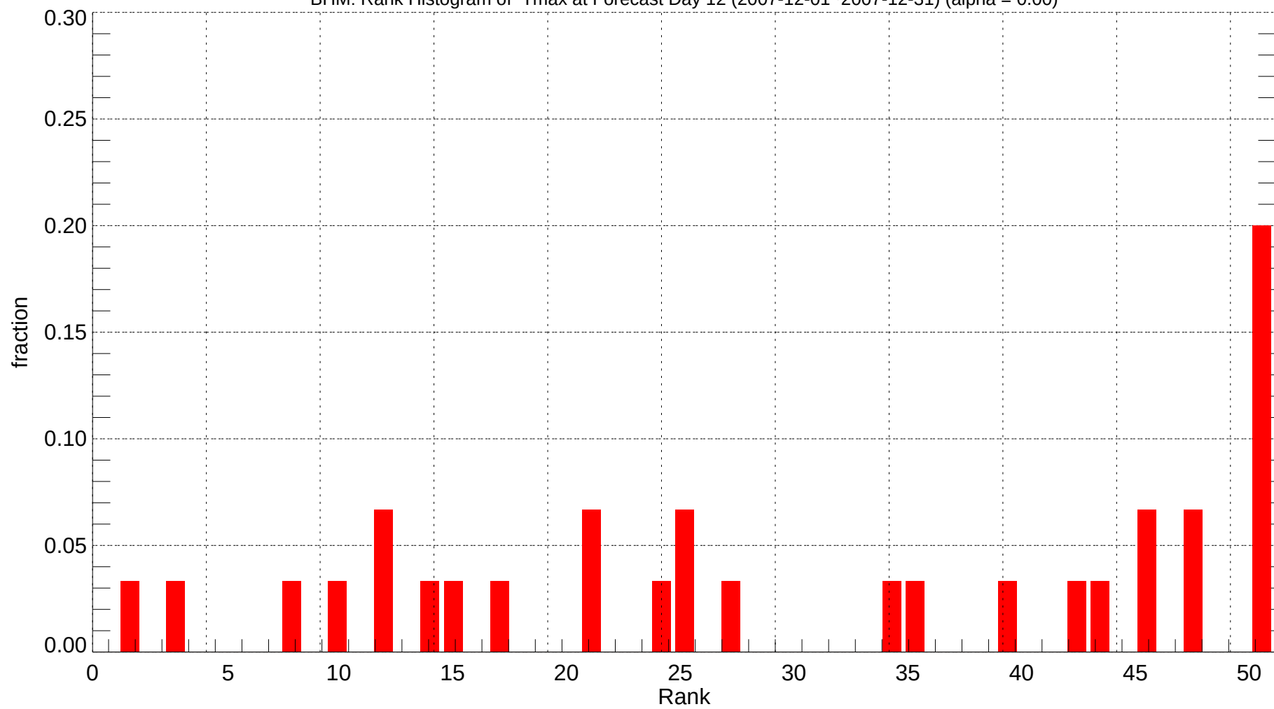
BHM: Rank Histogram of Tmax at Forecast Day 12 (2007-12-01~2007-12-31) (alpha = 0.00)
