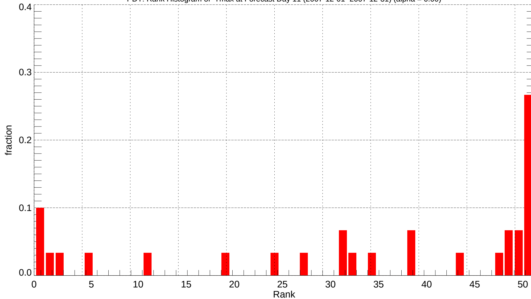
PDT: Rank Histogram of Tmax at Forecast Day 11 (2007-12-01~2007-12-31) (alpha = 0.00)
