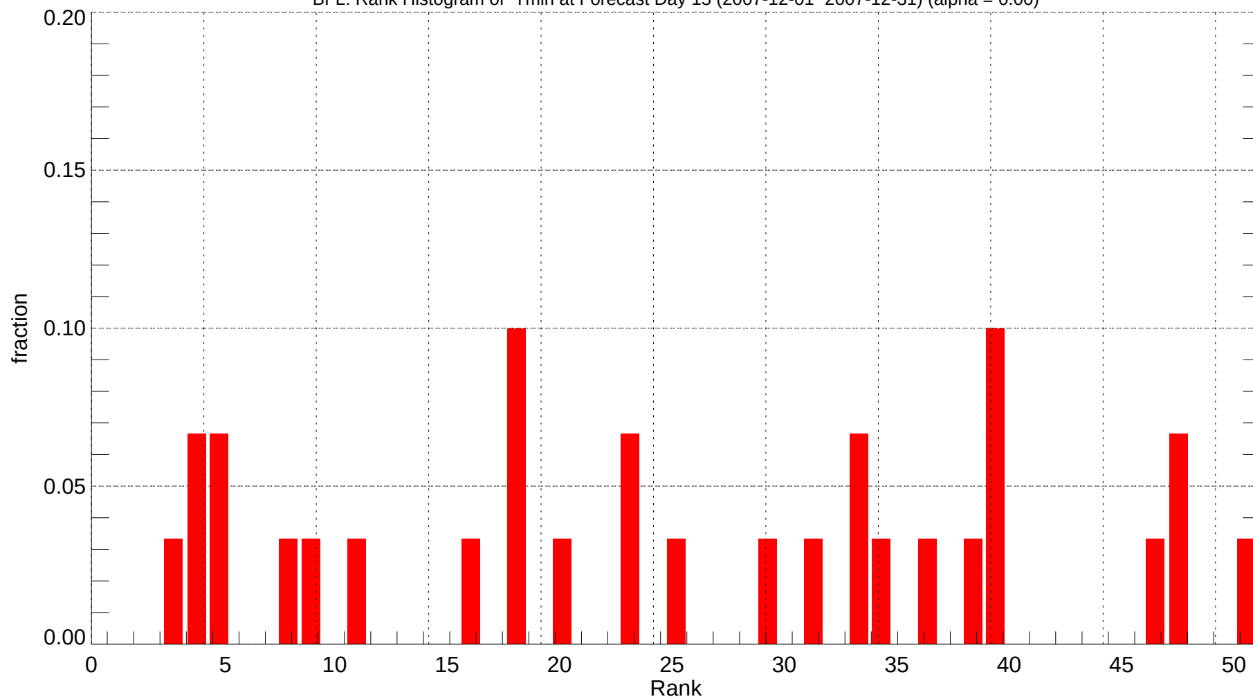
BFL: Rank Histogram of Tmin at Forecast Day 15 (2007-12-01~2007-12-31) (alpha = 0.00)
