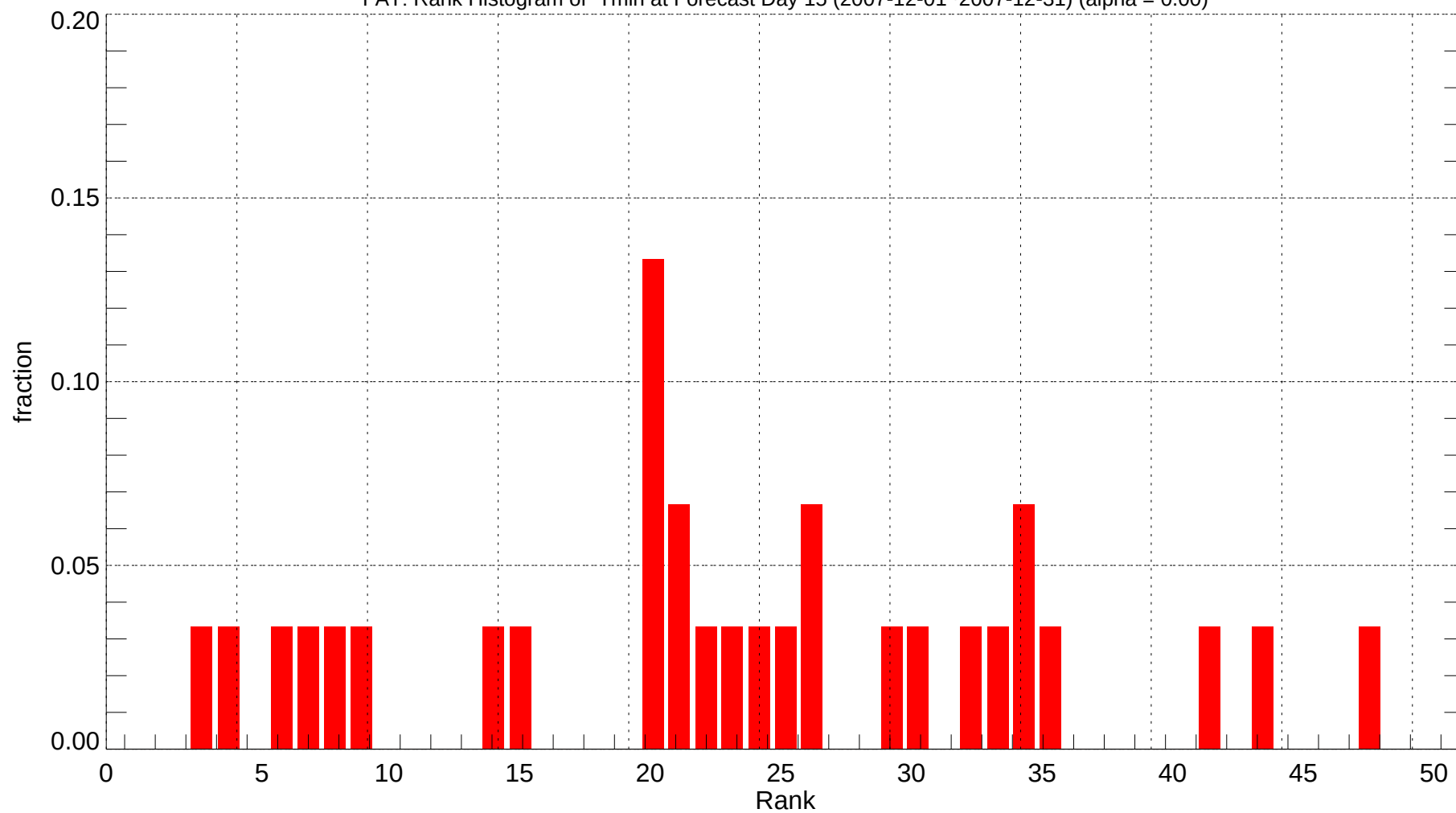
FAT: Rank Histogram of Tmin at Forecast Day 15 (2007-12-01~2007-12-31) (alpha = 0.00)
