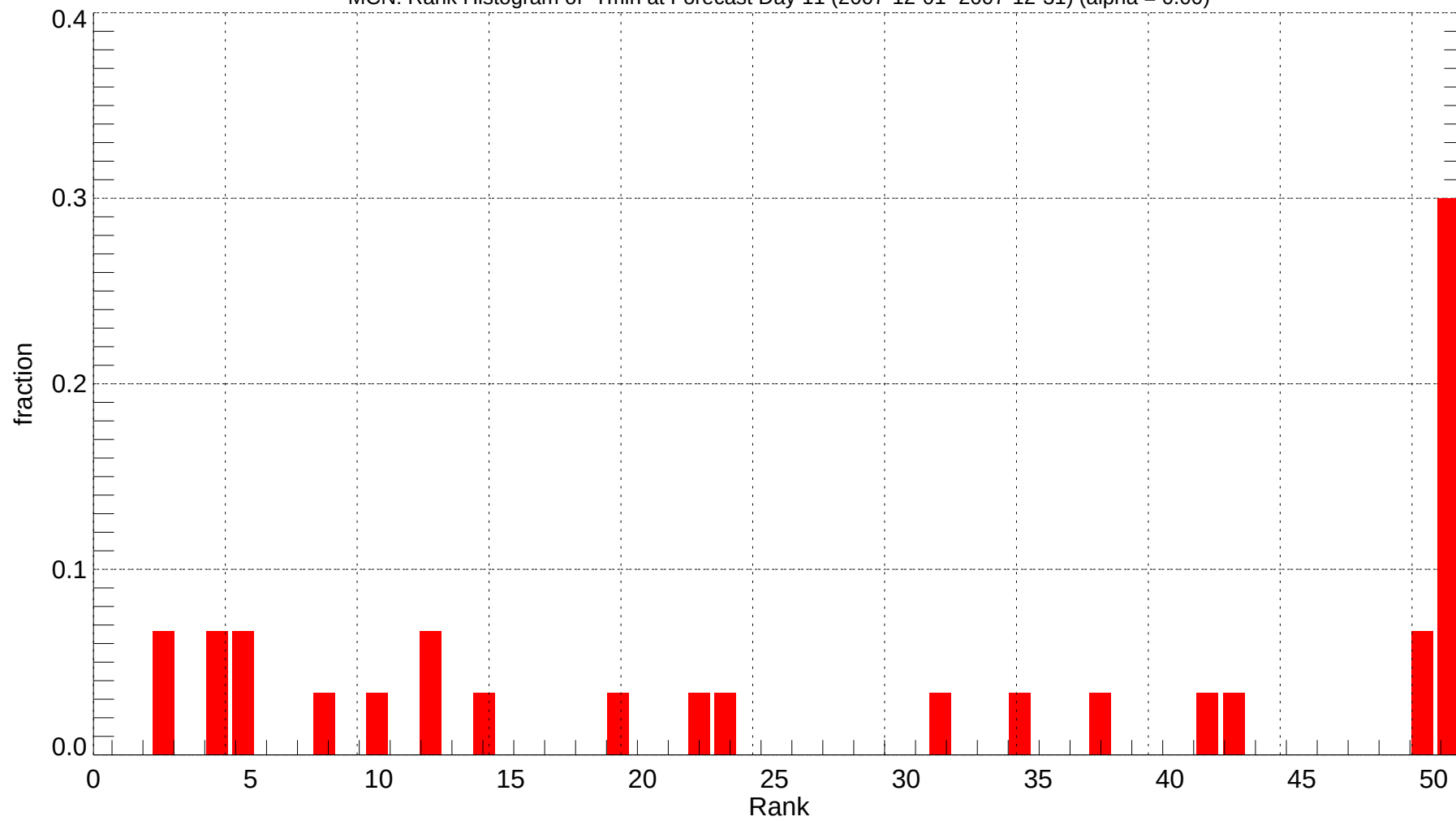
MCN: Rank Histogram of Tmin at Forecast Day 11 (2007-12-01~2007-12-31) (alpha = 0.00)
