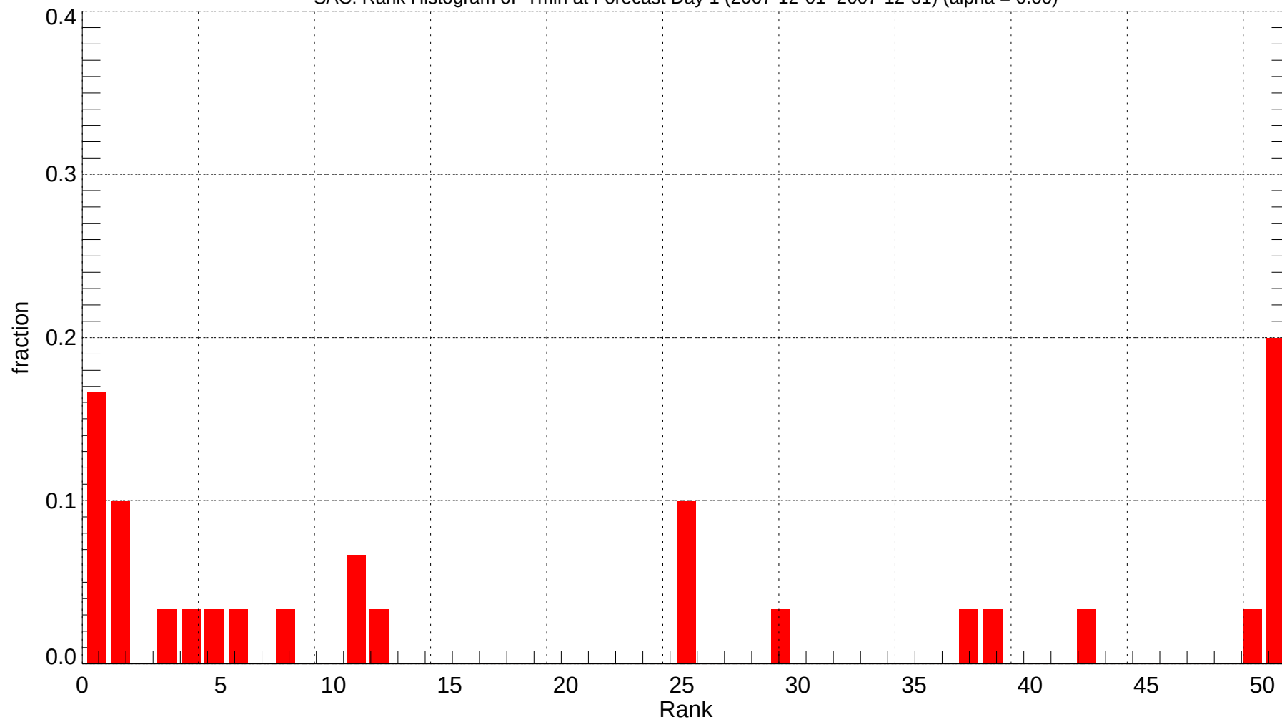
SAC: Rank Histogram of Tmin at Forecast Day 1 (2007-12-01~2007-12-31) (alpha = 0.00)
