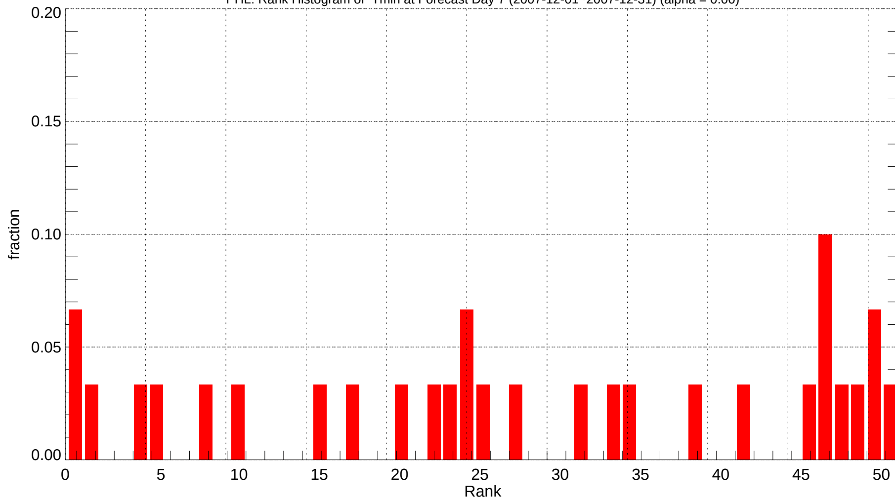
PHL: Rank Histogram of Tmin at Forecast Day 7 (2007-12-01~2007-12-31) (alpha = 0.00)
