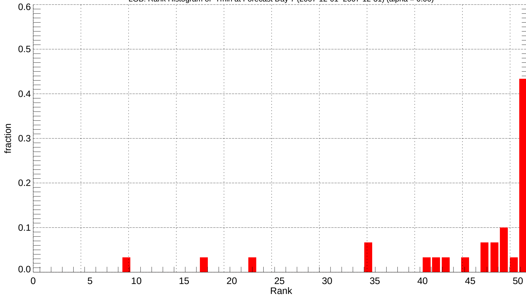
LGB: Rank Histogram of Tmin at Forecast Day 7 (2007-12-01~2007-12-31) (alpha = 0.00)
