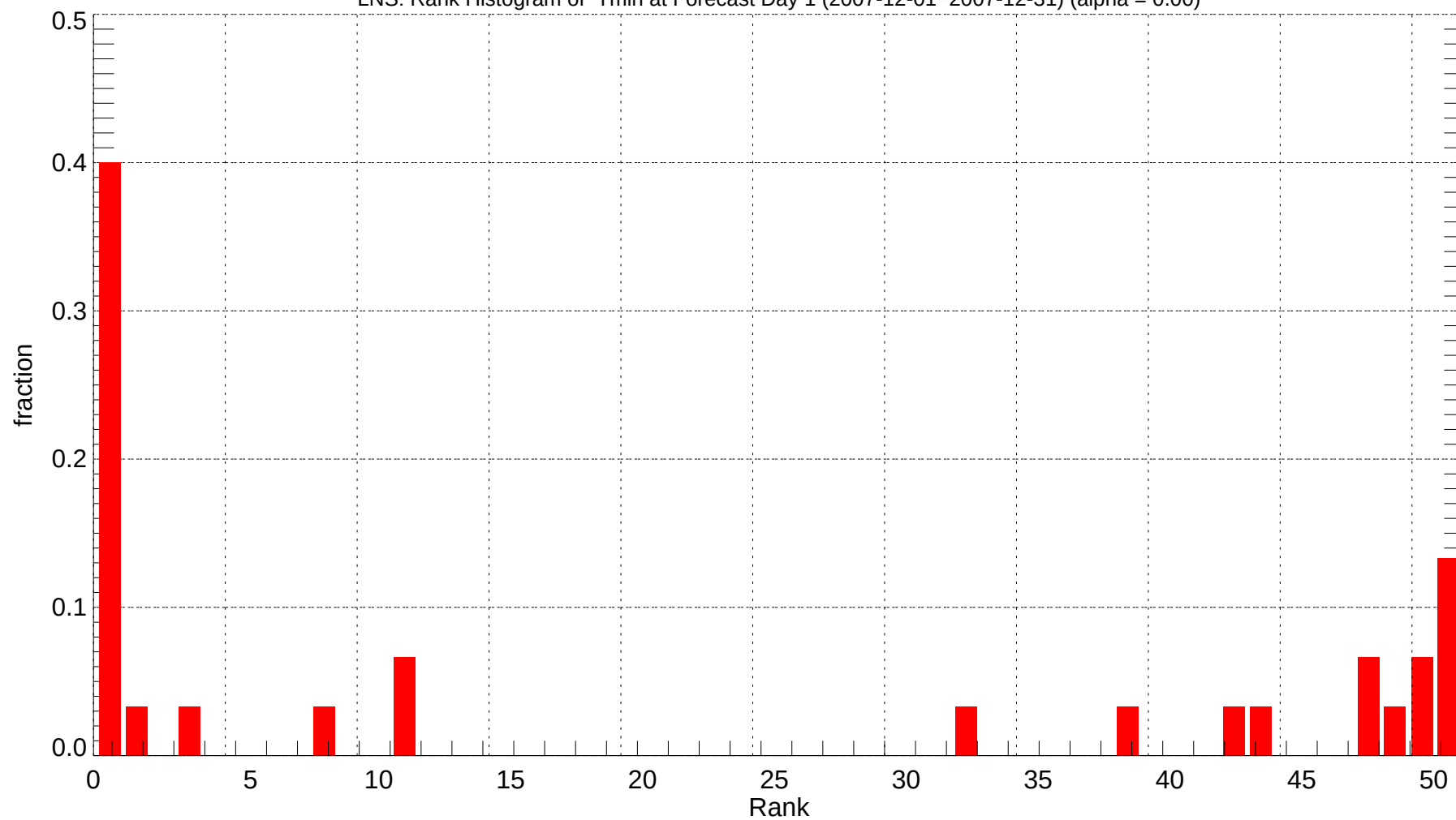
LNS: Rank Histogram of Tmin at Forecast Day 1 (2007-12-01~2007-12-31) (alpha = 0.00)
