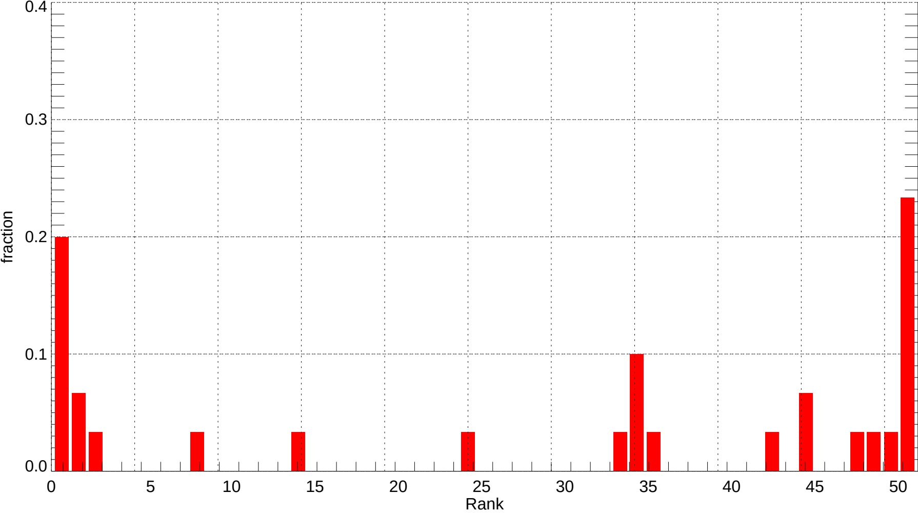
ATL: Rank Histogram of Tmin at Forecast Day 1 (2007-12-01~2007-12-31) (alpha = 0.00)
