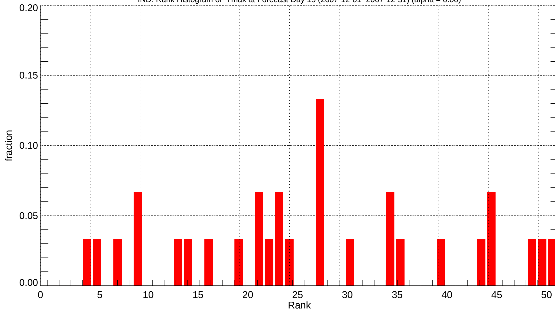
IND: Rank Histogram of Tmax at Forecast Day 15 (2007-12-01~2007-12-31) (alpha = 0.00)
