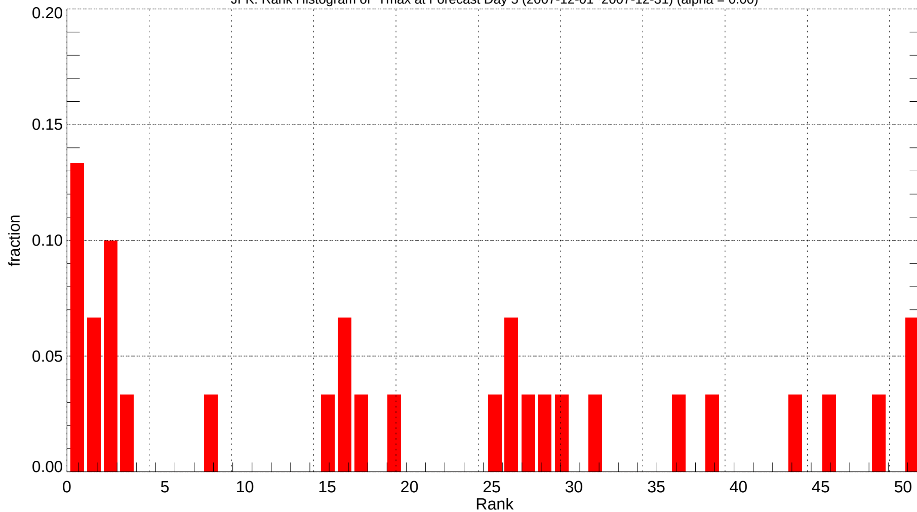
JFK: Rank Histogram of Tmax at Forecast Day 5 (2007-12-01~2007-12-31) (alpha = 0.00)
