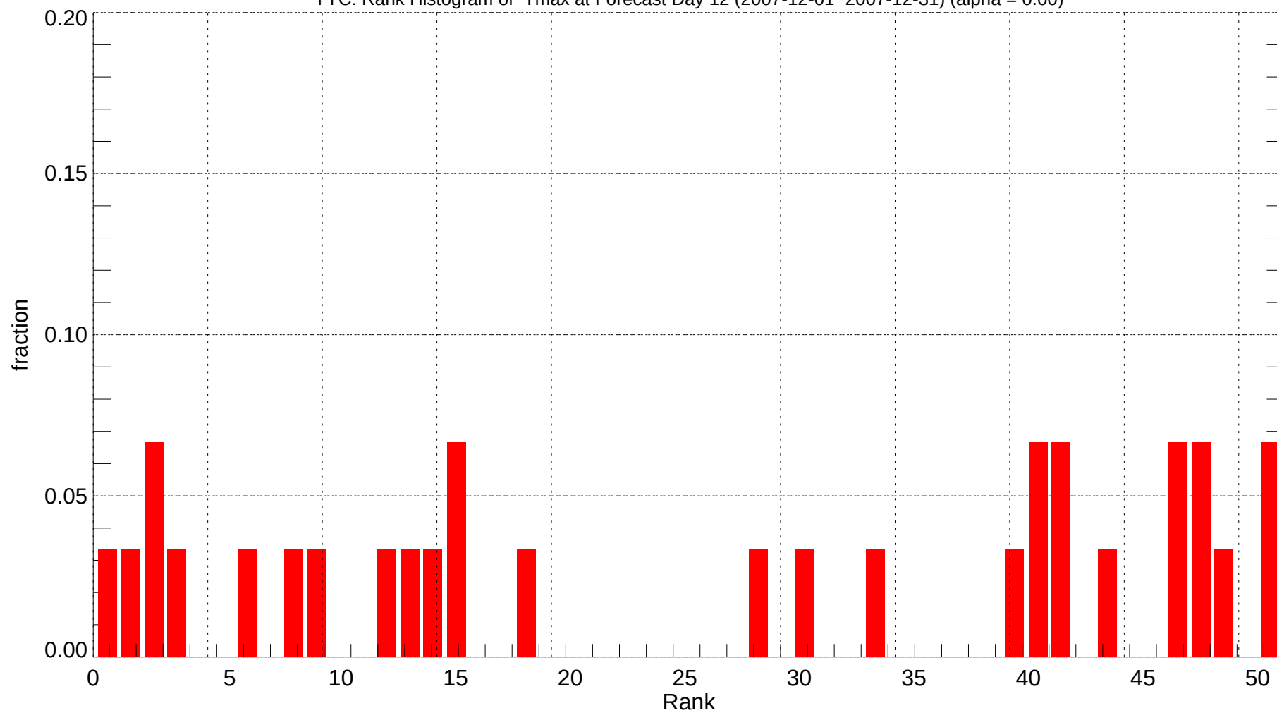
YYC: Rank Histogram of Tmax at Forecast Day 12 (2007-12-01~2007-12-31) (alpha = 0.00)
