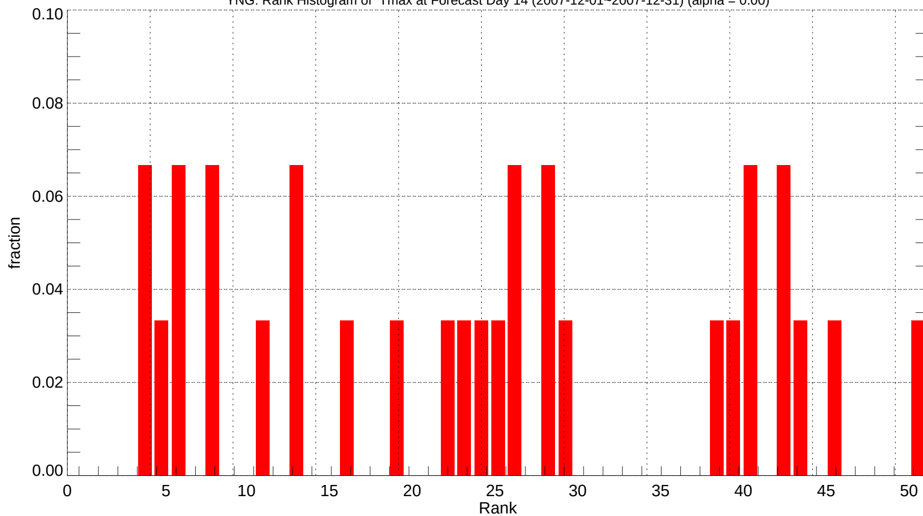
YNG: Rank Histogram of Tmax at Forecast Day 14 (2007-12-01~2007-12-31) (alpha = 0.00)
