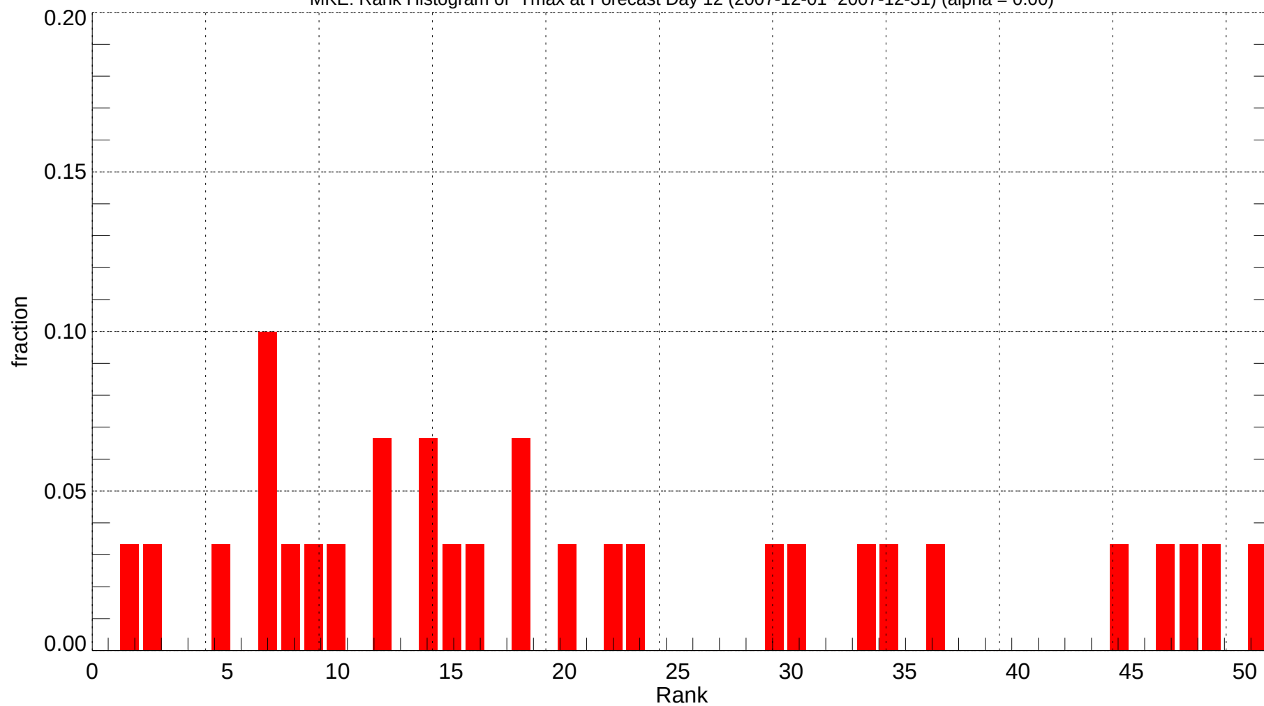
MKE: Rank Histogram of Tmax at Forecast Day 12 (2007-12-01~2007-12-31) (alpha = 0.00)
