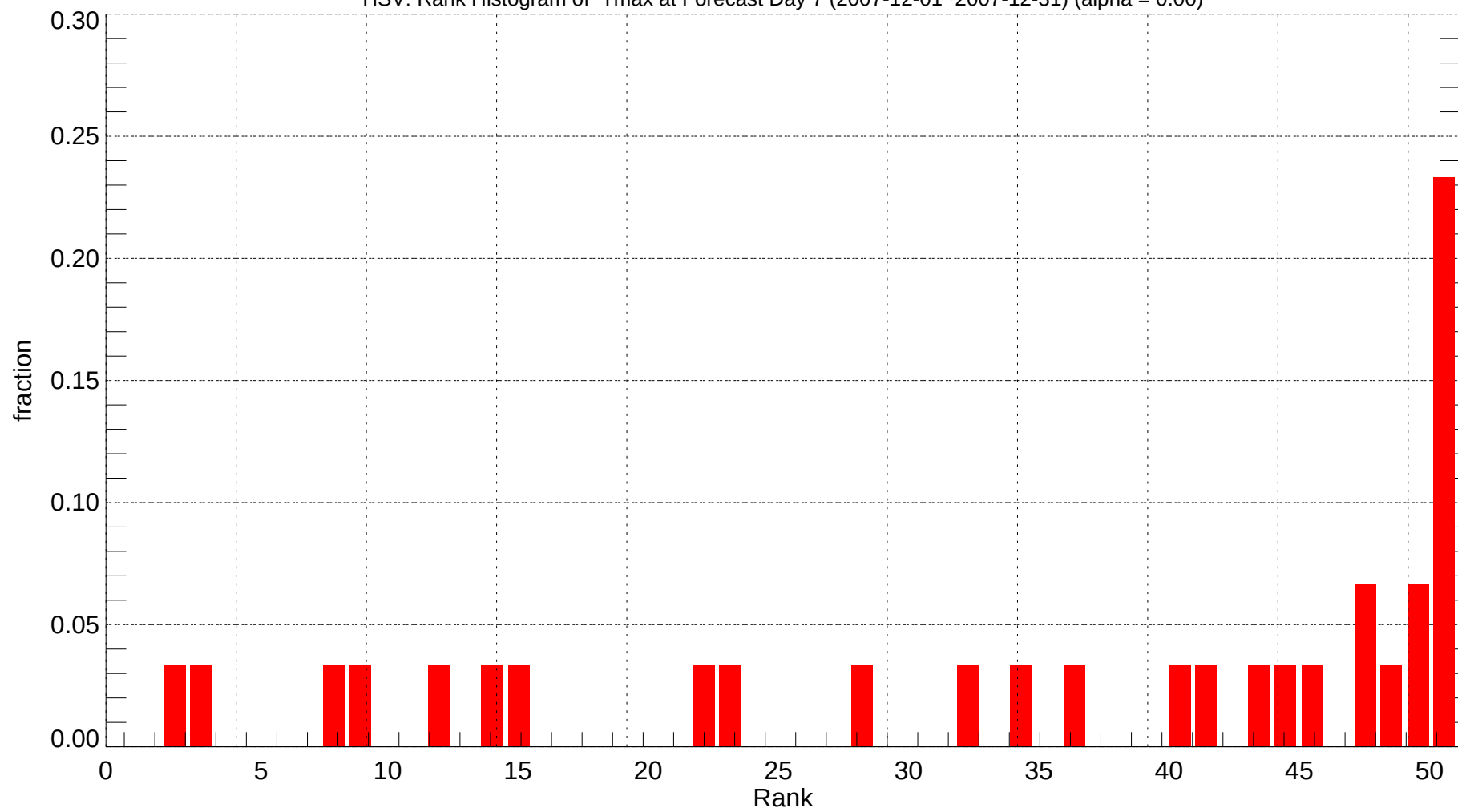
HSV: Rank Histogram of Tmax at Forecast Day 7 (2007-12-01~2007-12-31) (alpha = 0.00)
