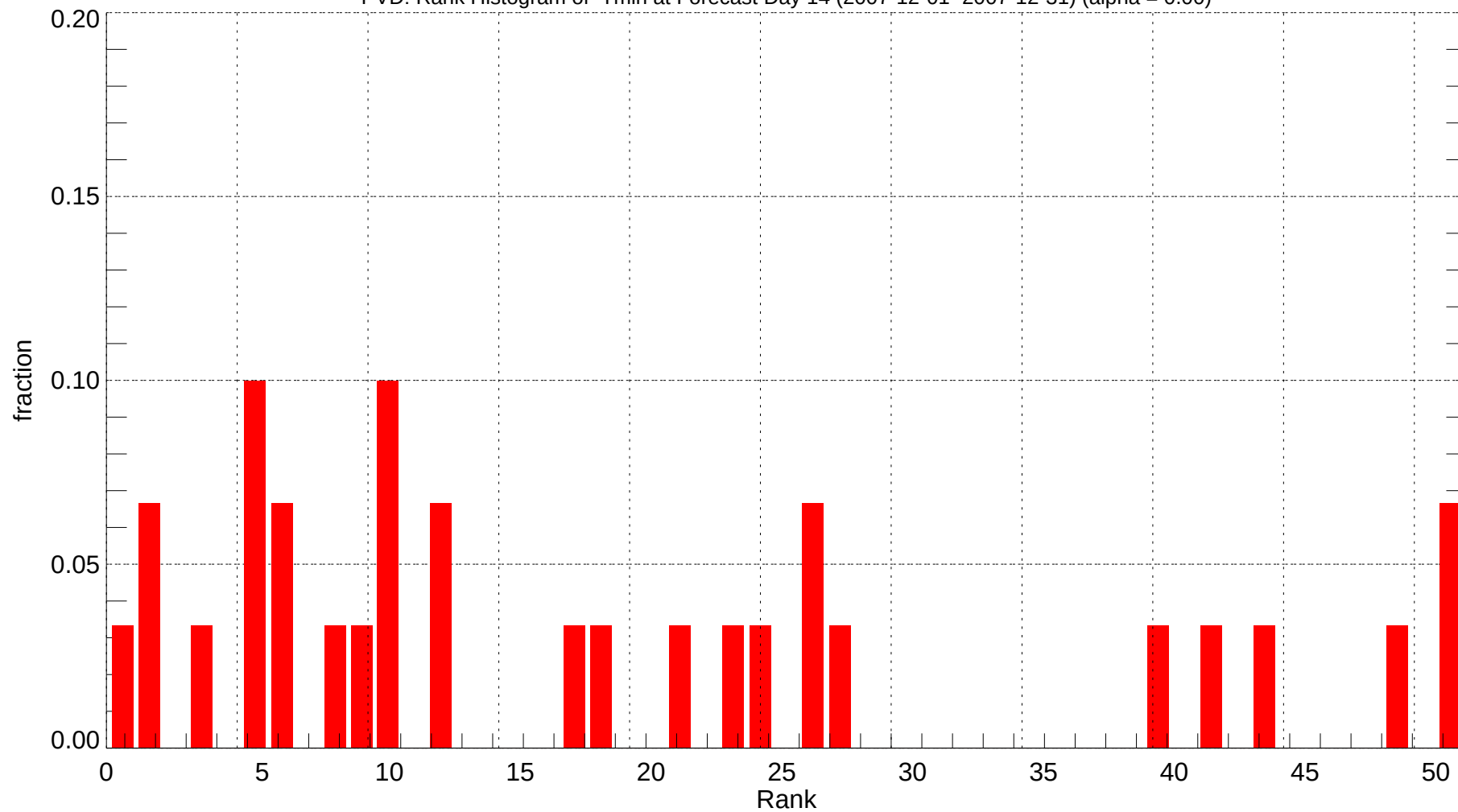
PVD: Rank Histogram of Tmin at Forecast Day 14 (2007-12-01~2007-12-31) (alpha = 0.00)
