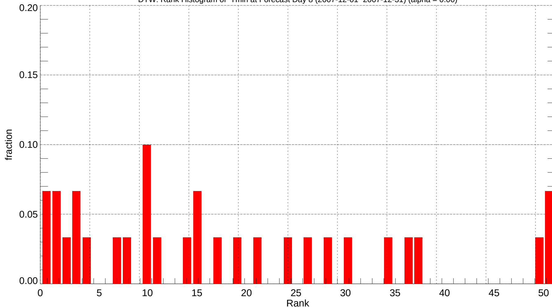
DTW: Rank Histogram of Tmin at Forecast Day 8 (2007-12-01~2007-12-31) (alpha = 0.00)
