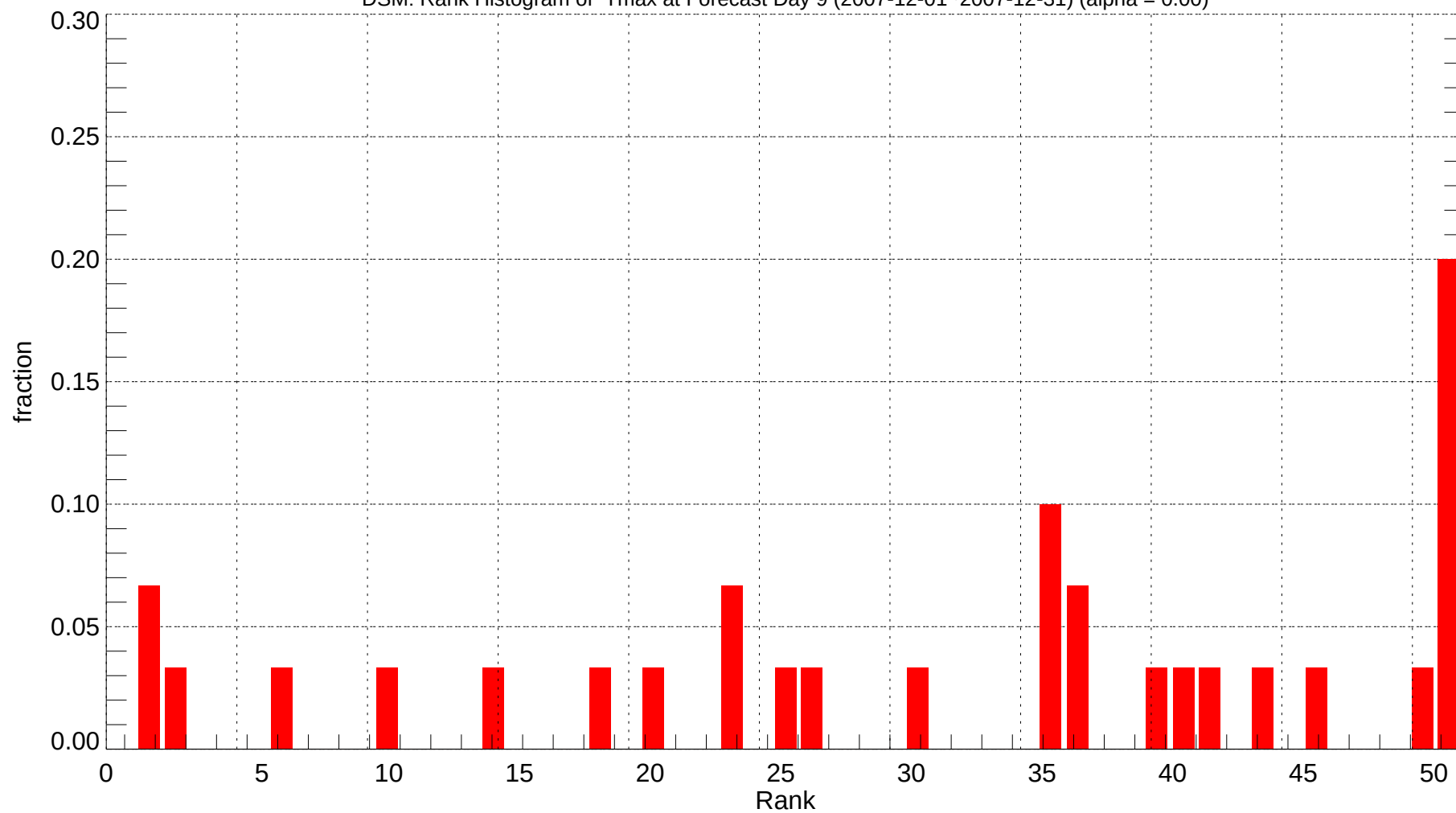
DSM: Rank Histogram of Tmax at Forecast Day 9 (2007-12-01~2007-12-31) (alpha = 0.00)
