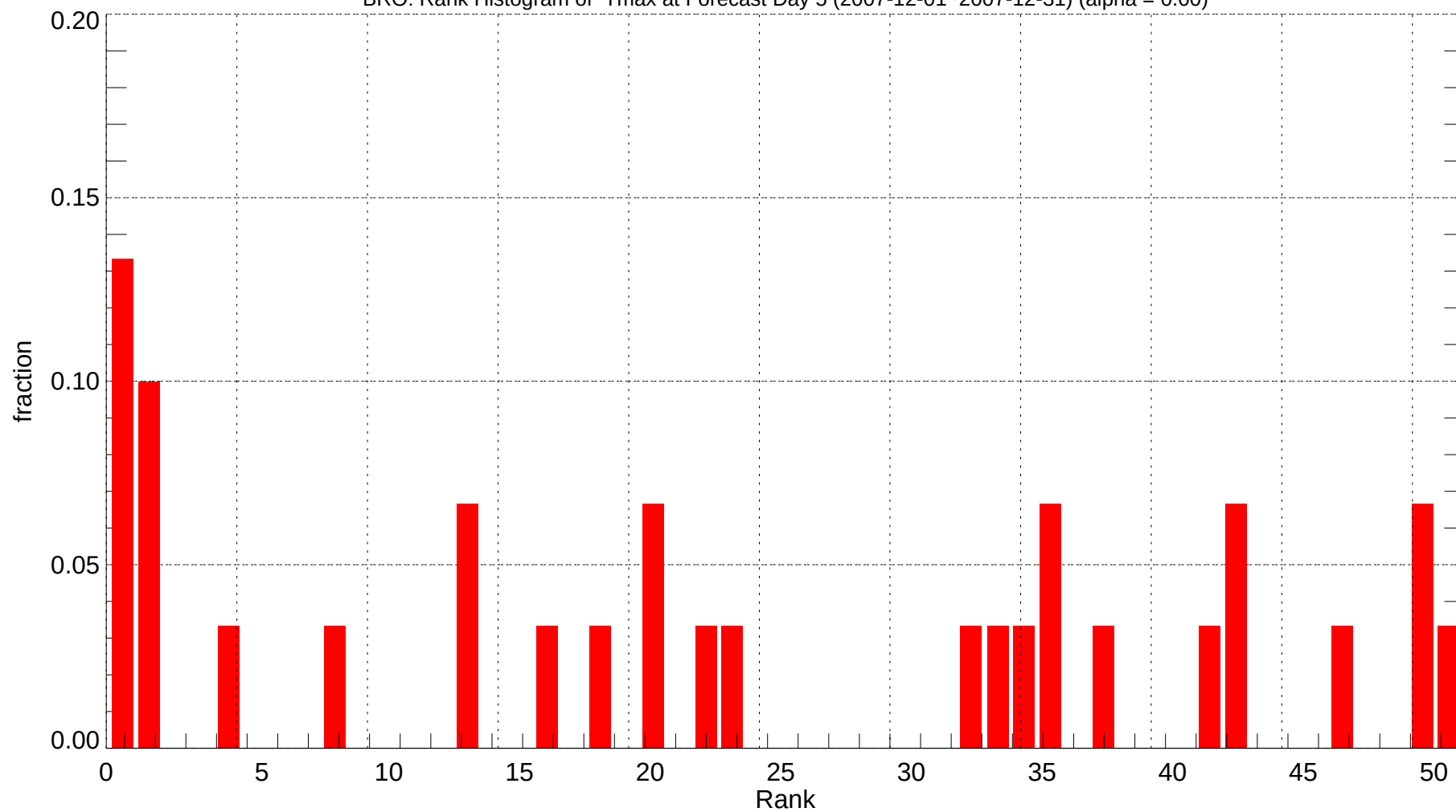
BRO: Rank Histogram of Tmax at Forecast Day 5 (2007-12-01~2007-12-31) (alpha = 0.00)
