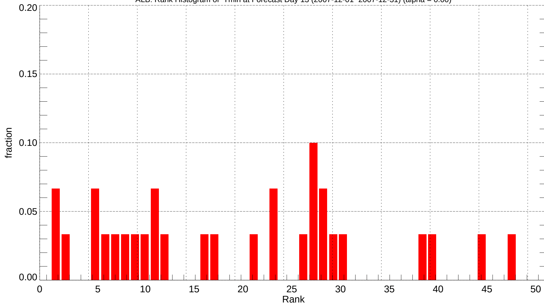
ALB: Rank Histogram of Tmin at Forecast Day 13 (2007-12-01~2007-12-31) (alpha = 0.00)
