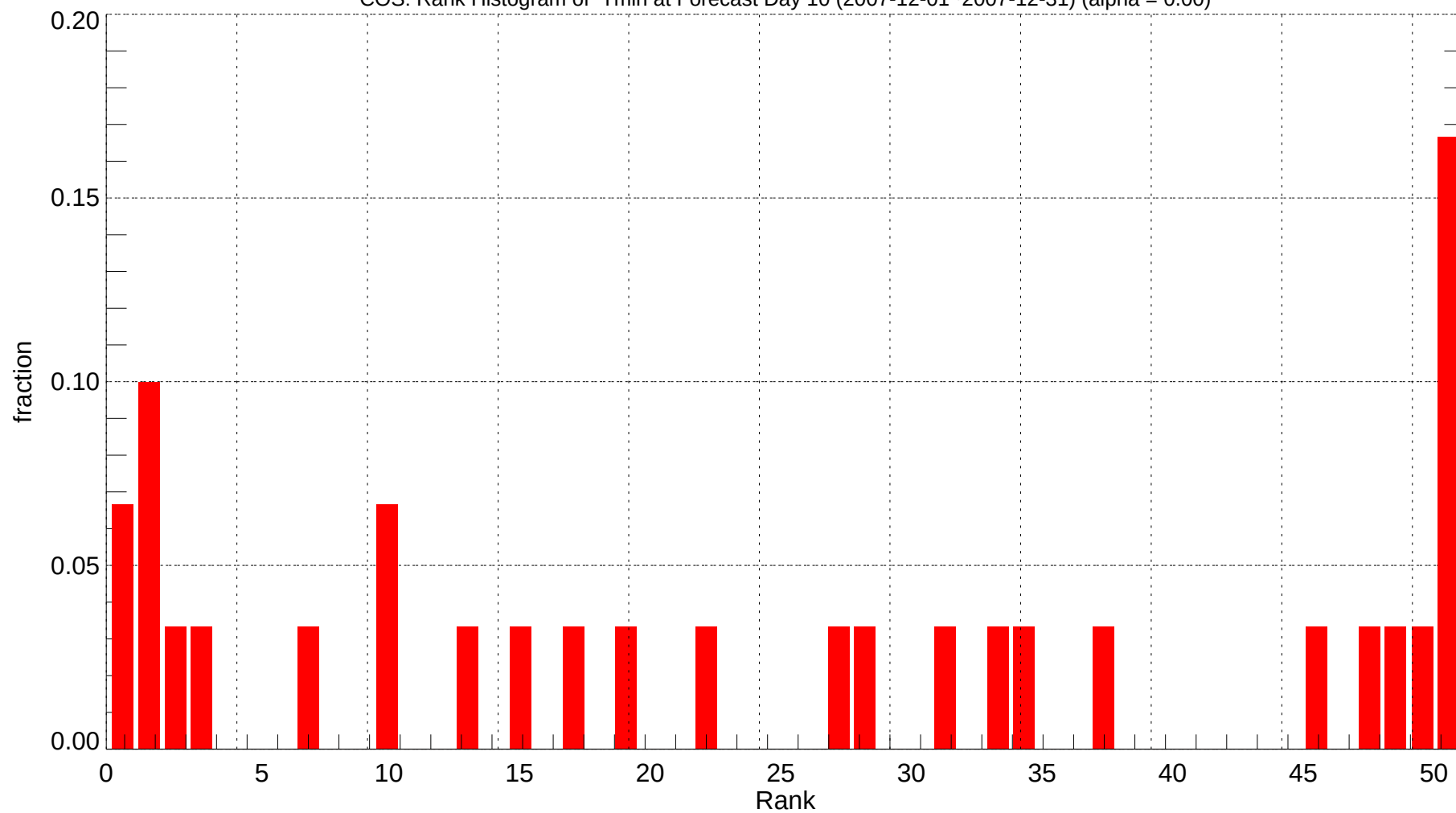
COS: Rank Histogram of Tmin at Forecast Day 10 (2007-12-01~2007-12-31) (alpha = 0.00)
