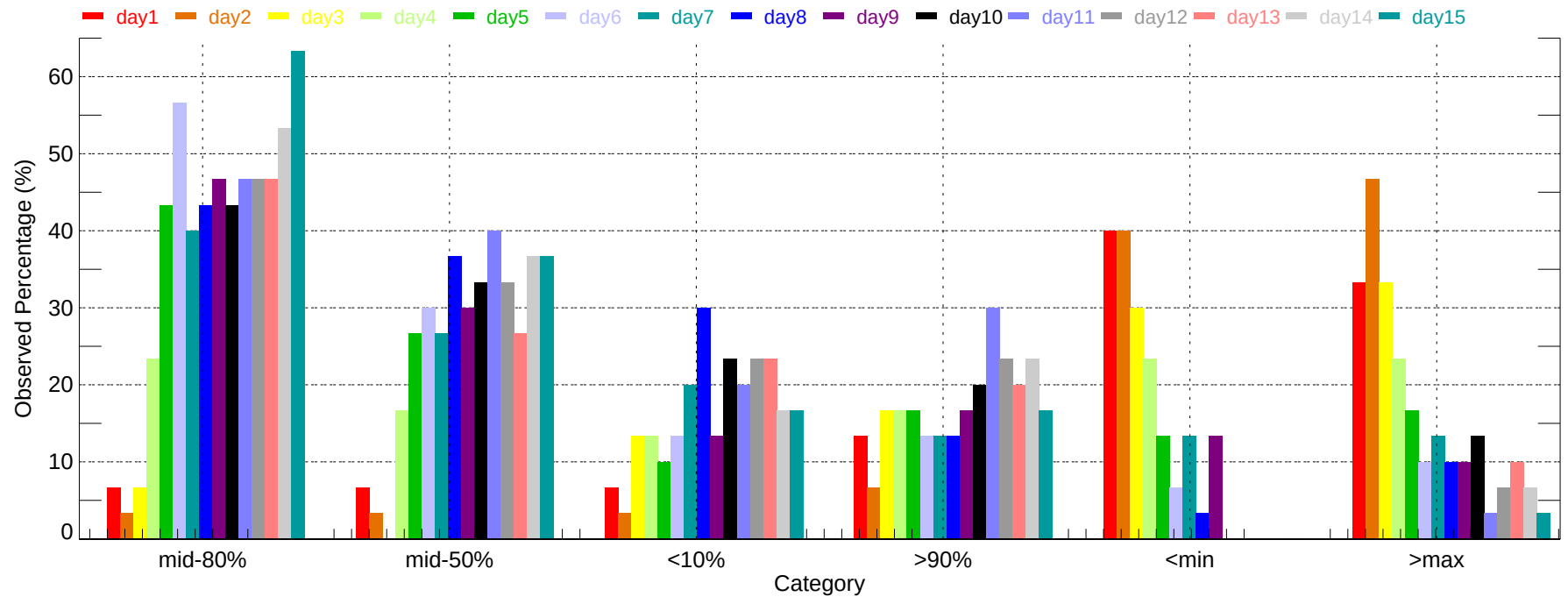
Observed Percentage of Ensembles - RNO: Max Temperature (2007-12-01~2007-12-31)
