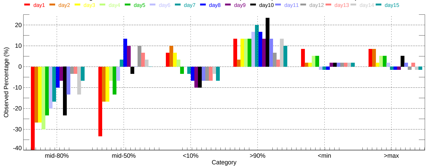
Observed Percentage Deviation of Ensembles - MCO: Max Temperature (2007-12-01~2007-12-31)
