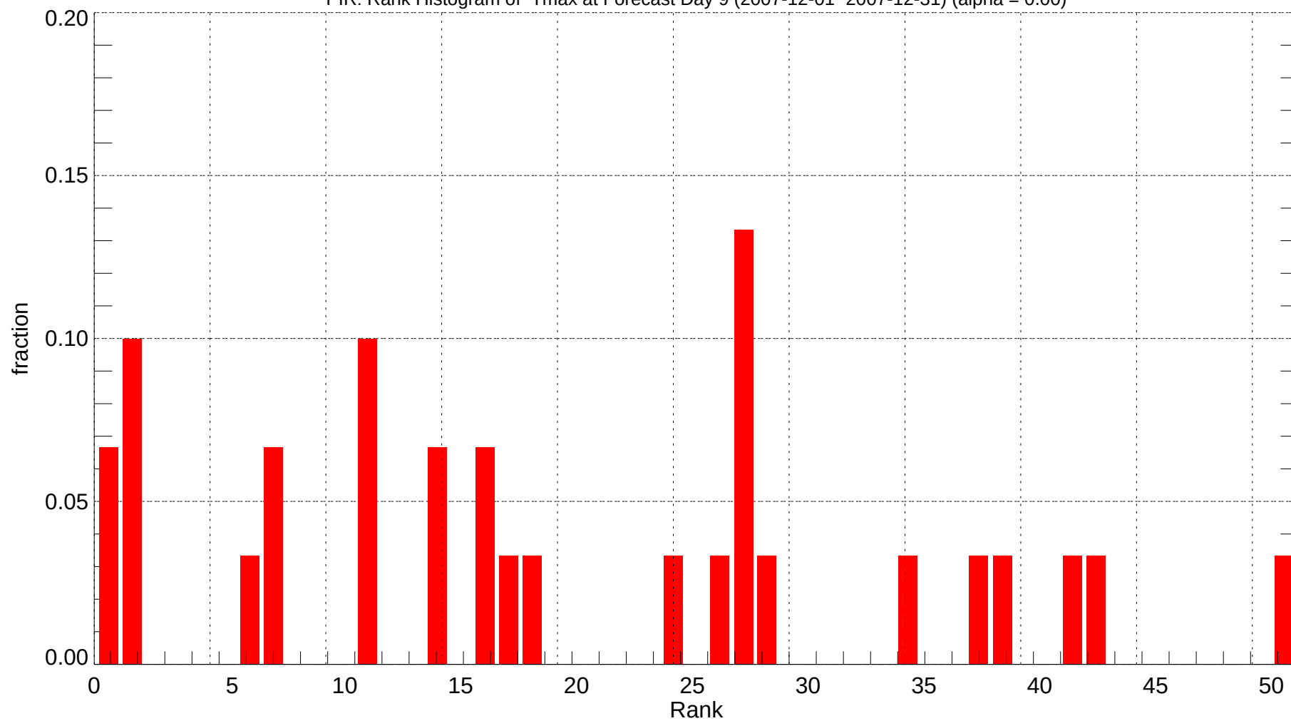
PIR: Rank Histogram of Tmax at Forecast Day 9 (2007-12-01~2007-12-31) (alpha = 0.00)
