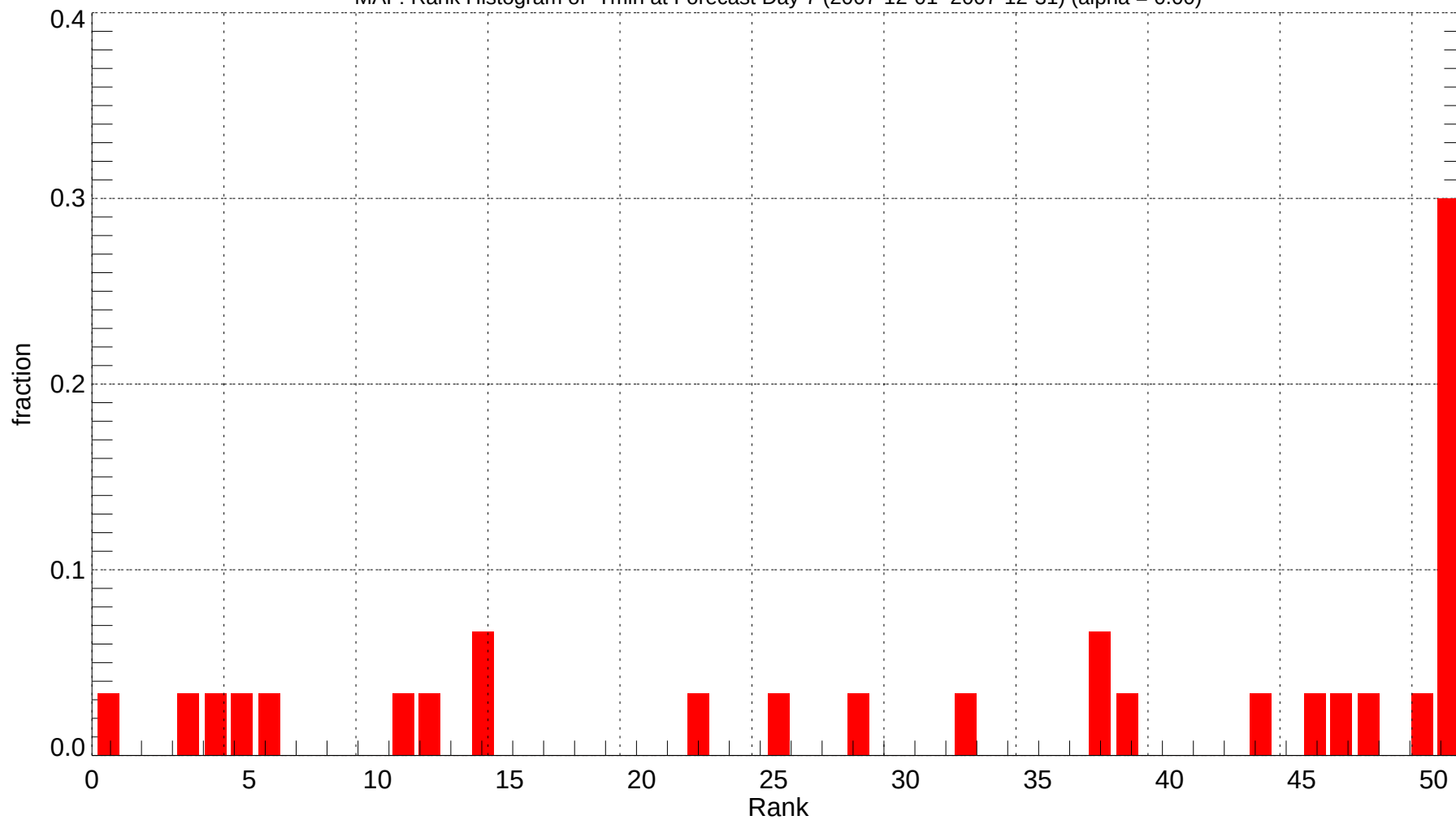
MAF: Rank Histogram of Tmin at Forecast Day 7 (2007-12-01~2007-12-31) (alpha = 0.00)
