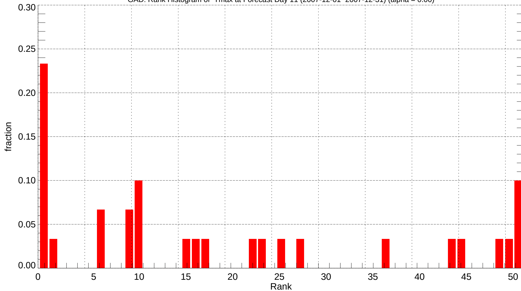
GAD: Rank Histogram of Tmax at Forecast Day 11 (2007-12-01~2007-12-31) (alpha = 0.00)
