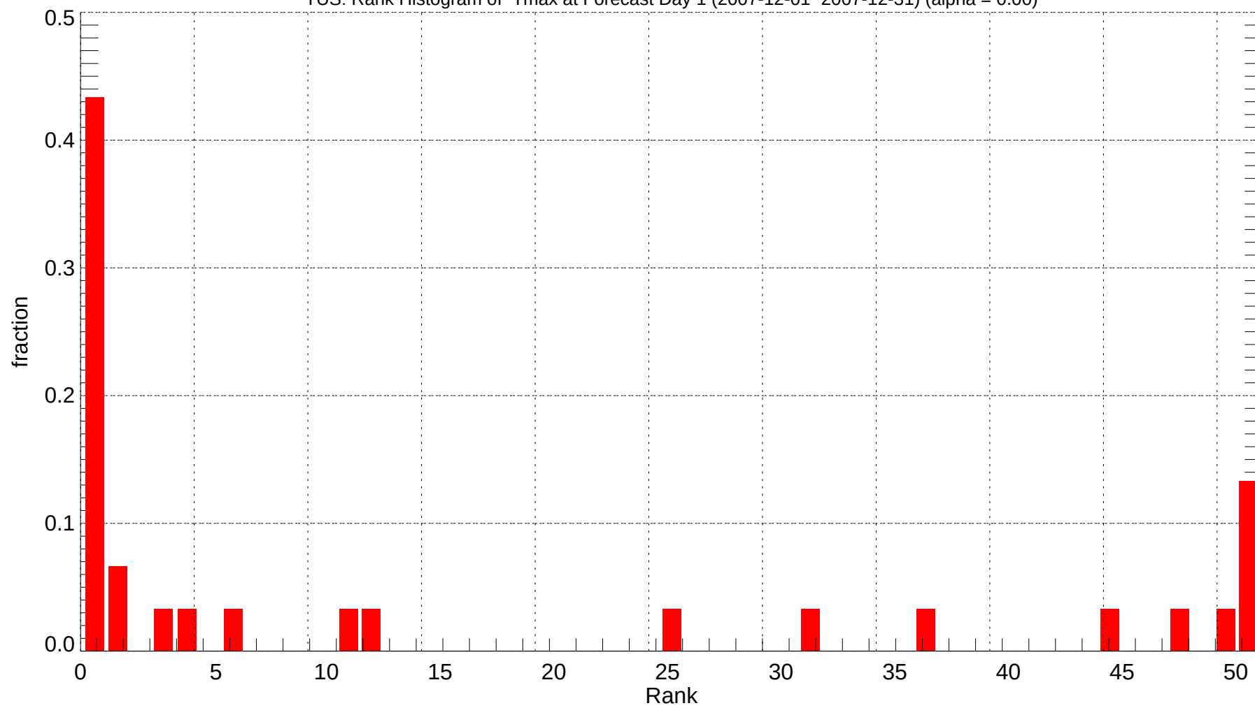
TUS: Rank Histogram of Tmax at Forecast Day 1 (2007-12-01~2007-12-31) (alpha = 0.00)
