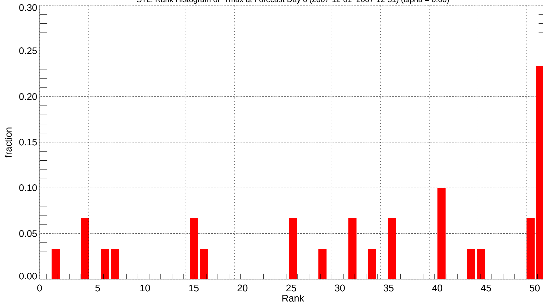
STL: Rank Histogram of Tmax at Forecast Day 6 (2007-12-01~2007-12-31) (alpha = 0.00)
