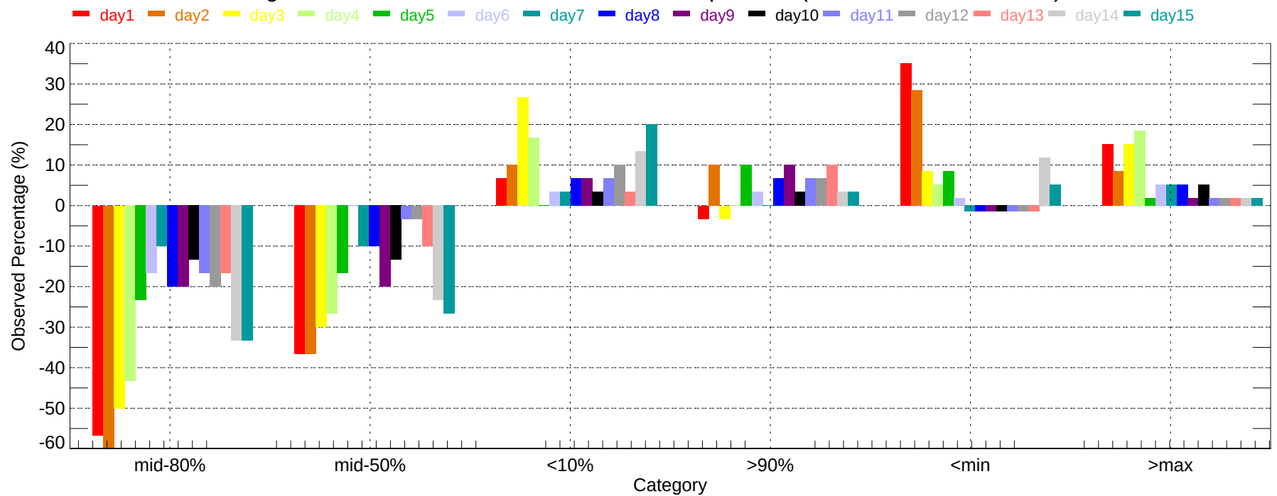
Observed Percentage Deviation of Ensembles - TUS: Max Temperature (2007-12-01~2007-12-31)
