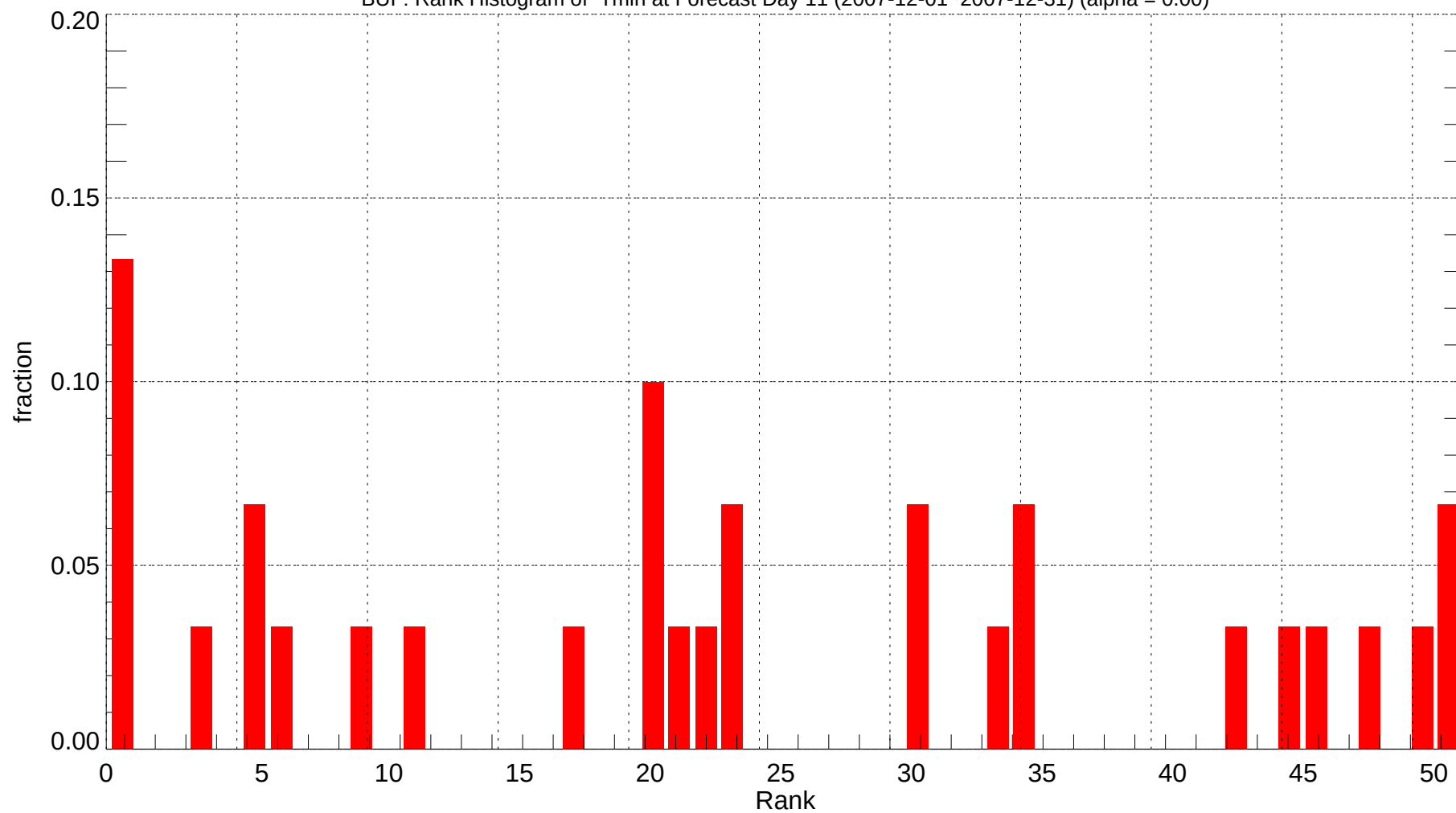
BUF: Rank Histogram of Tmin at Forecast Day 11 (2007-12-01~2007-12-31) (alpha = 0.00)
