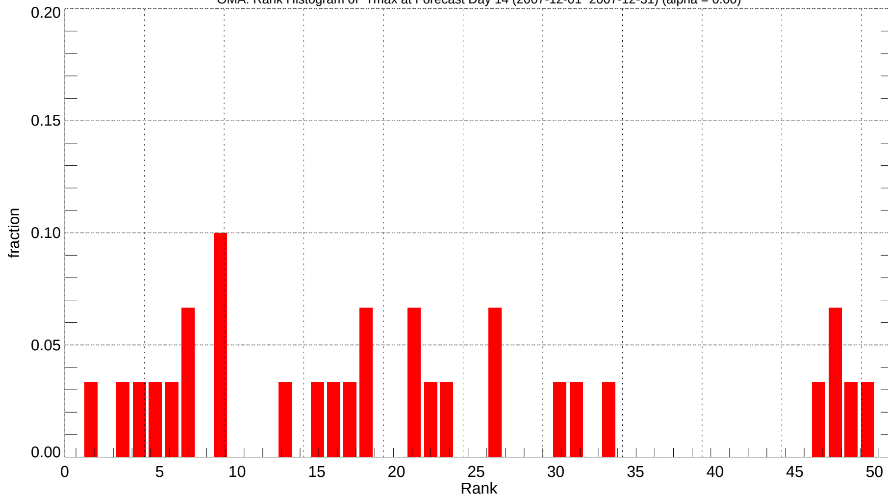
OMA: Rank Histogram of Tmax at Forecast Day 14 (2007-12-01~2007-12-31) (alpha = 0.00)
