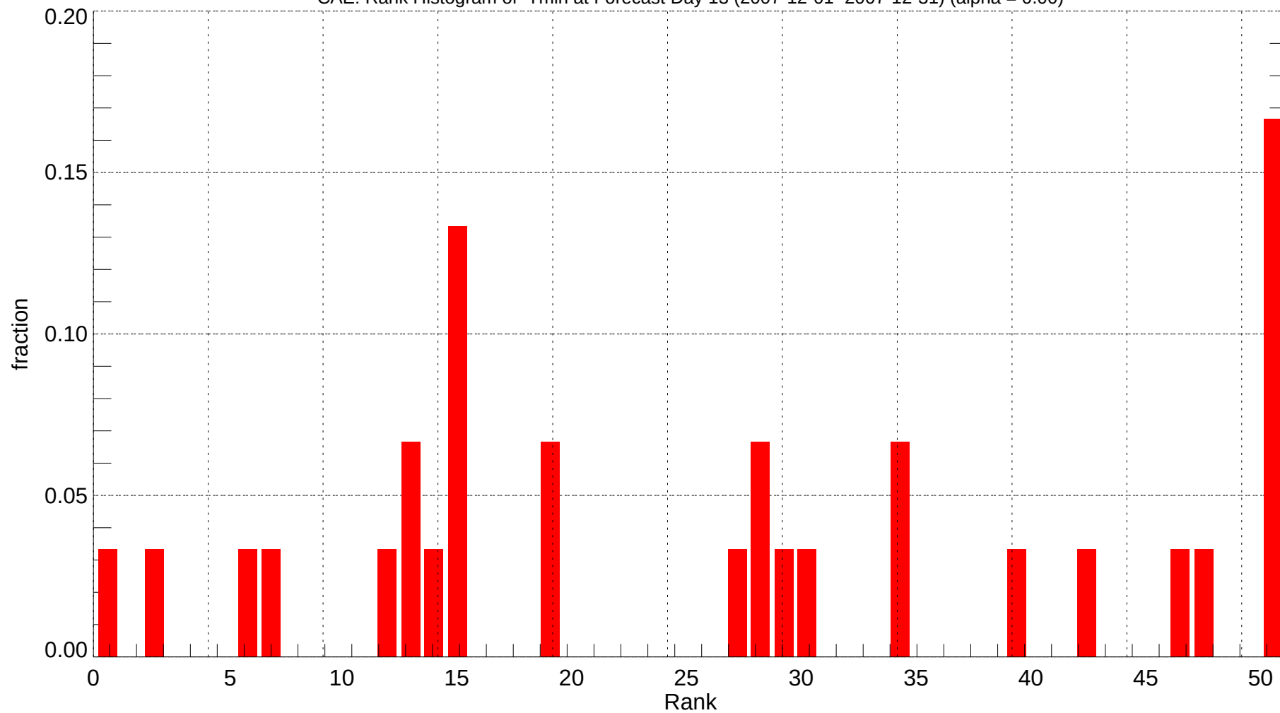
CAE: Rank Histogram of Tmin at Forecast Day 13 (2007-12-01~2007-12-31) (alpha = 0.00)
