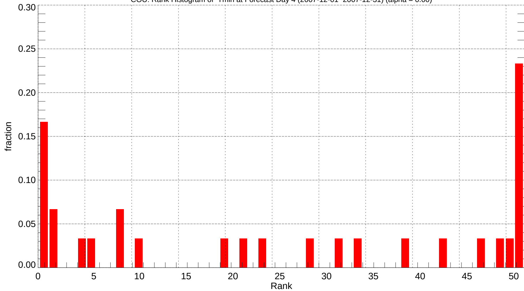
COU: Rank Histogram of Tmin at Forecast Day 4 (2007-12-01~2007-12-31) (alpha = 0.00)
