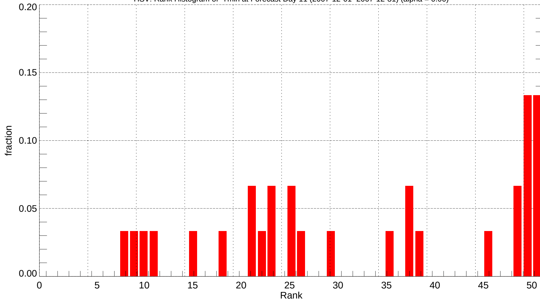
HSV: Rank Histogram of Tmin at Forecast Day 11 (2007-12-01~2007-12-31) (alpha = 0.00)
