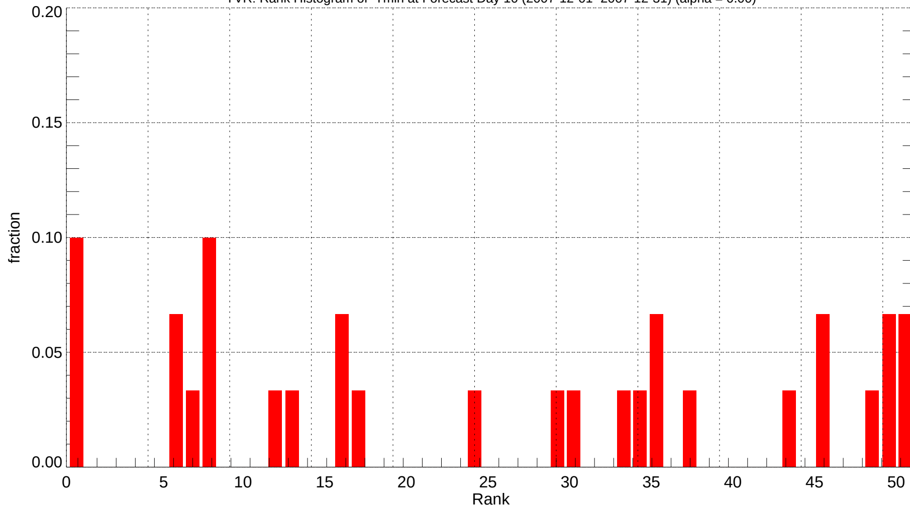
YVR: Rank Histogram of Tmin at Forecast Day 10 (2007-12-01~2007-12-31) (alpha = 0.00)
