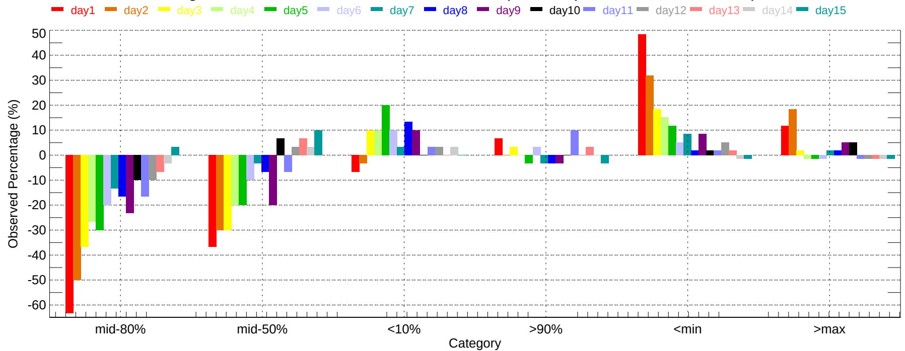
Observed Percentage Deviation of Ensembles - DTW: Max Temperature (2007-12-01~2007-12-31)
