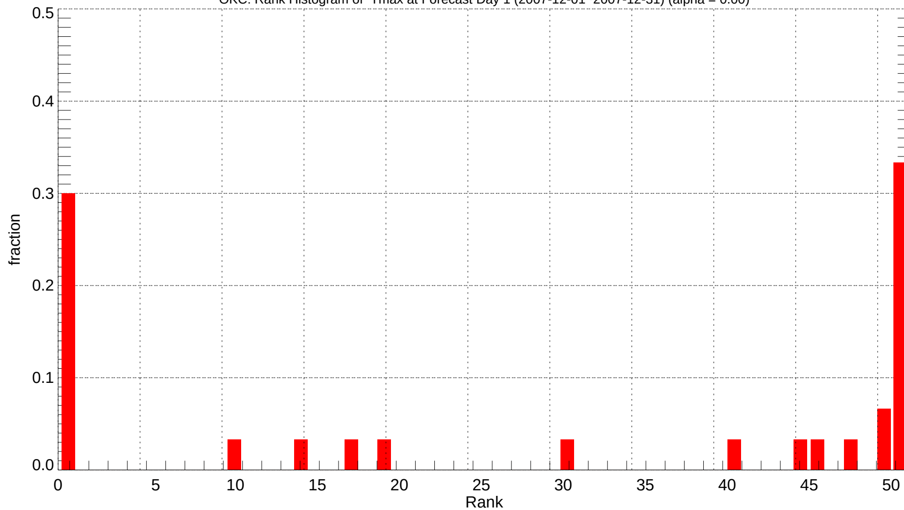
OKC: Rank Histogram of Tmax at Forecast Day 1 (2007-12-01~2007-12-31) (alpha = 0.00)
