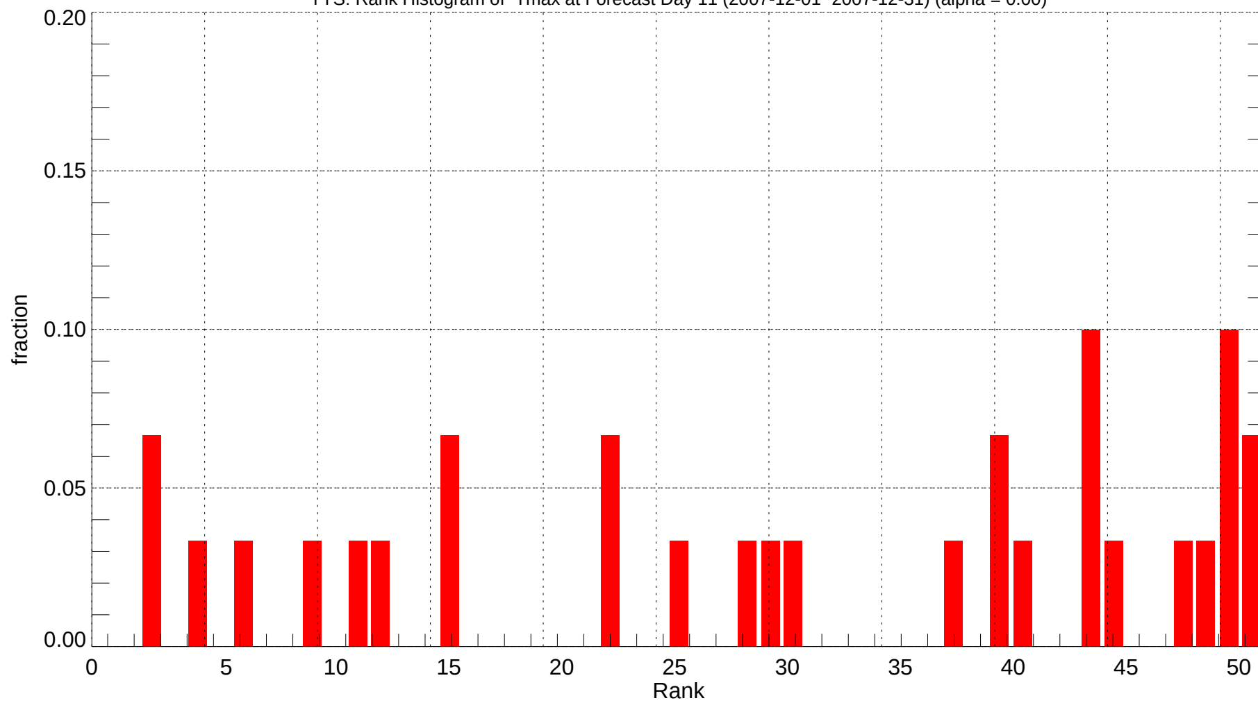
TYS: Rank Histogram of Tmax at Forecast Day 11 (2007-12-01~2007-12-31) (alpha = 0.00)
