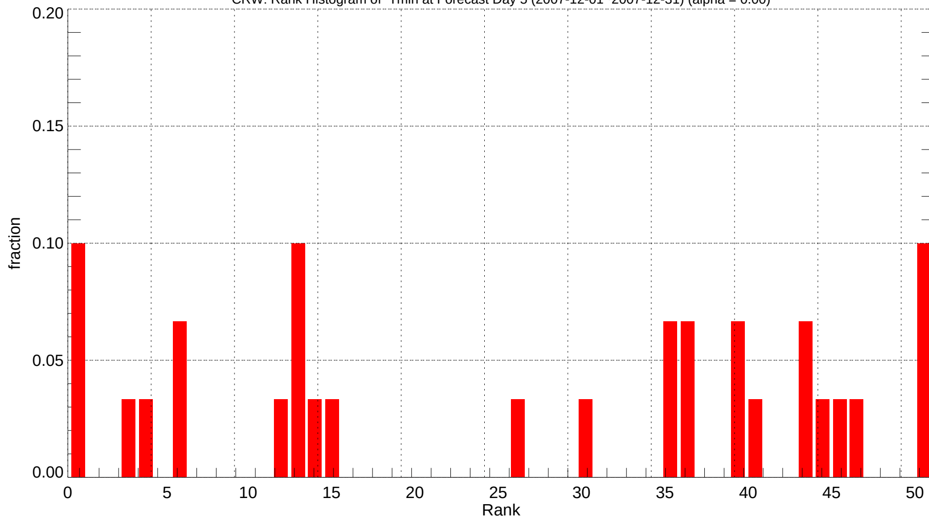
CRW: Rank Histogram of Tmin at Forecast Day 5 (2007-12-01~2007-12-31) (alpha = 0.00)
