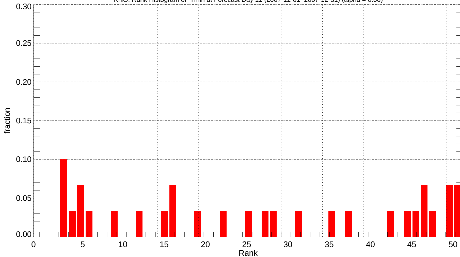
RNO: Rank Histogram of Tmin at Forecast Day 11 (2007-12-01~2007-12-31) (alpha = 0.00)
