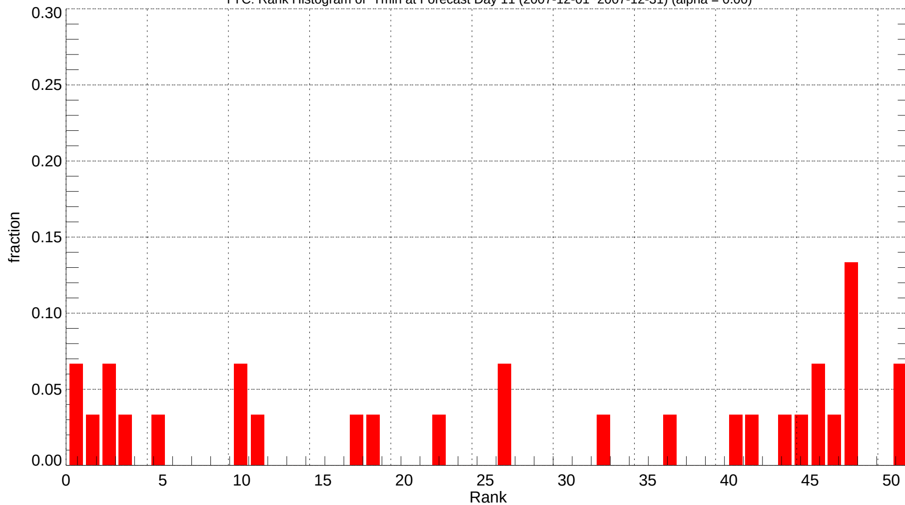
YYC: Rank Histogram of Tmin at Forecast Day 11 (2007-12-01~2007-12-31) (alpha = 0.00)
