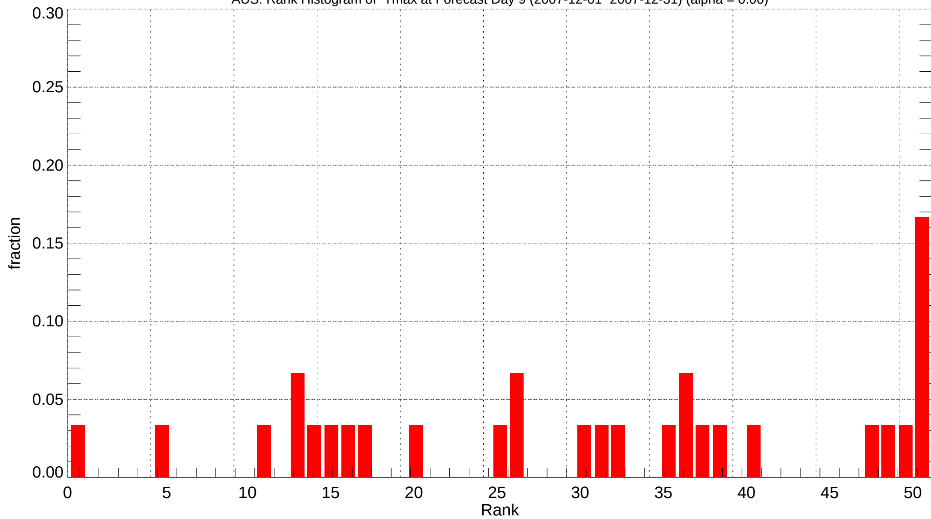
AUS: Rank Histogram of Tmax at Forecast Day 9 (2007-12-01~2007-12-31) (alpha = 0.00)
