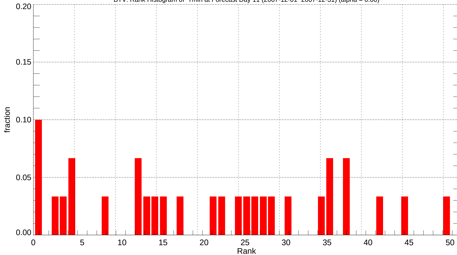
BTV: Rank Histogram of Tmin at Forecast Day 11 (2007-12-01~2007-12-31) (alpha = 0.00)
