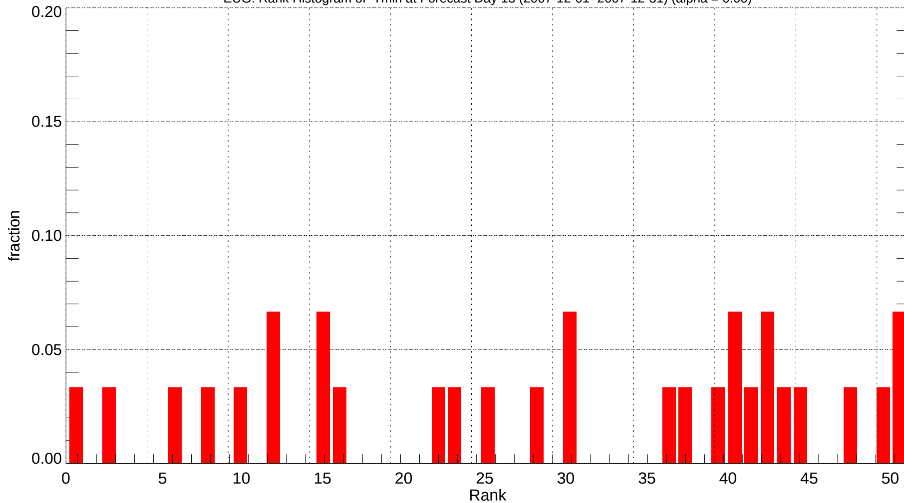
EUG: Rank Histogram of Tmin at Forecast Day 13 (2007-12-01~2007-12-31) (alpha = 0.00)
