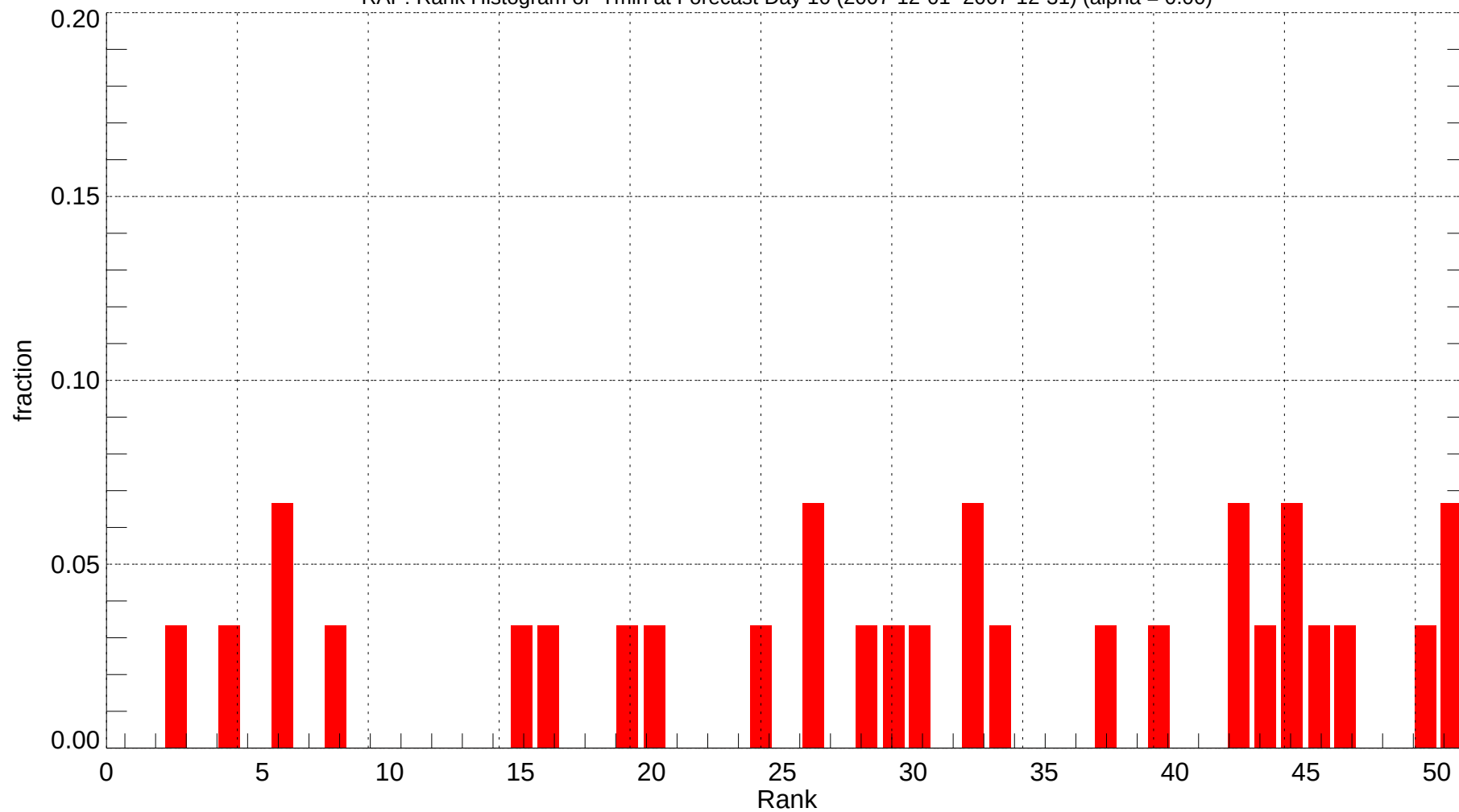
RAP: Rank Histogram of Tmin at Forecast Day 10 (2007-12-01~2007-12-31) (alpha = 0.00)
