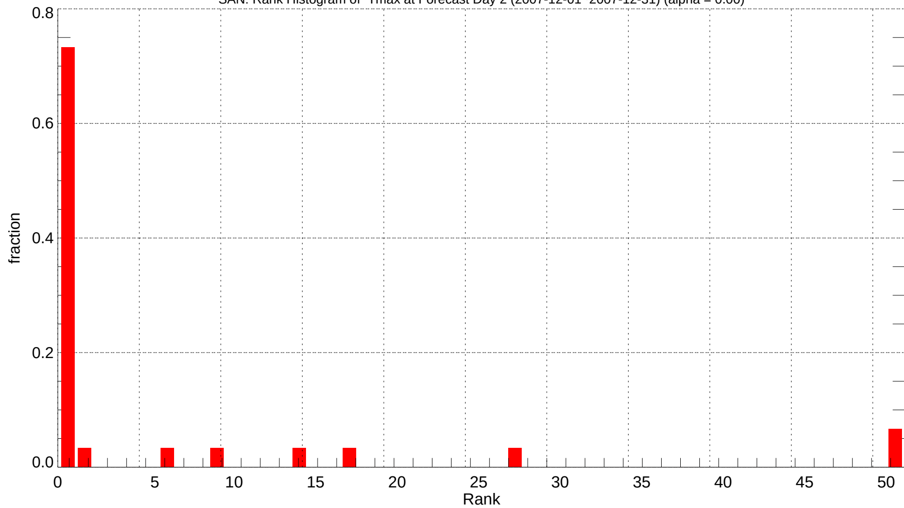
SAN: Rank Histogram of Tmax at Forecast Day 2 (2007-12-01~2007-12-31) (alpha = 0.00)
