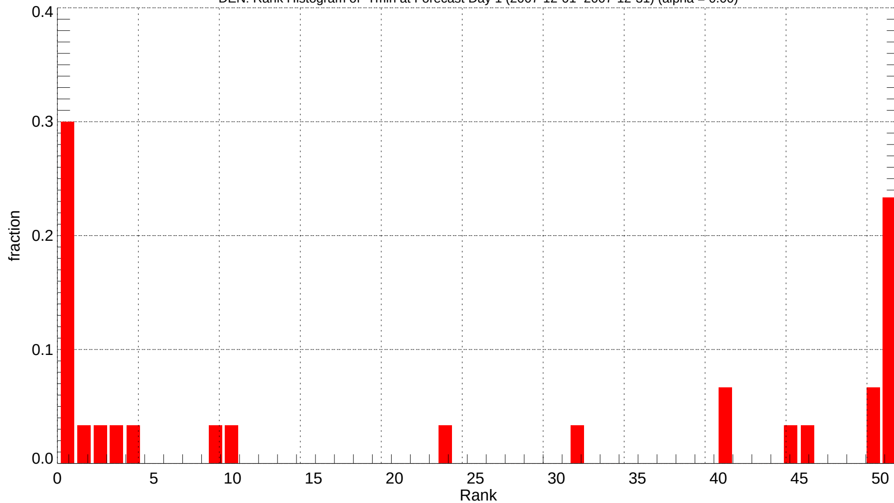
DEN: Rank Histogram of Tmin at Forecast Day 1 (2007-12-01~2007-12-31) (alpha = 0.00)
