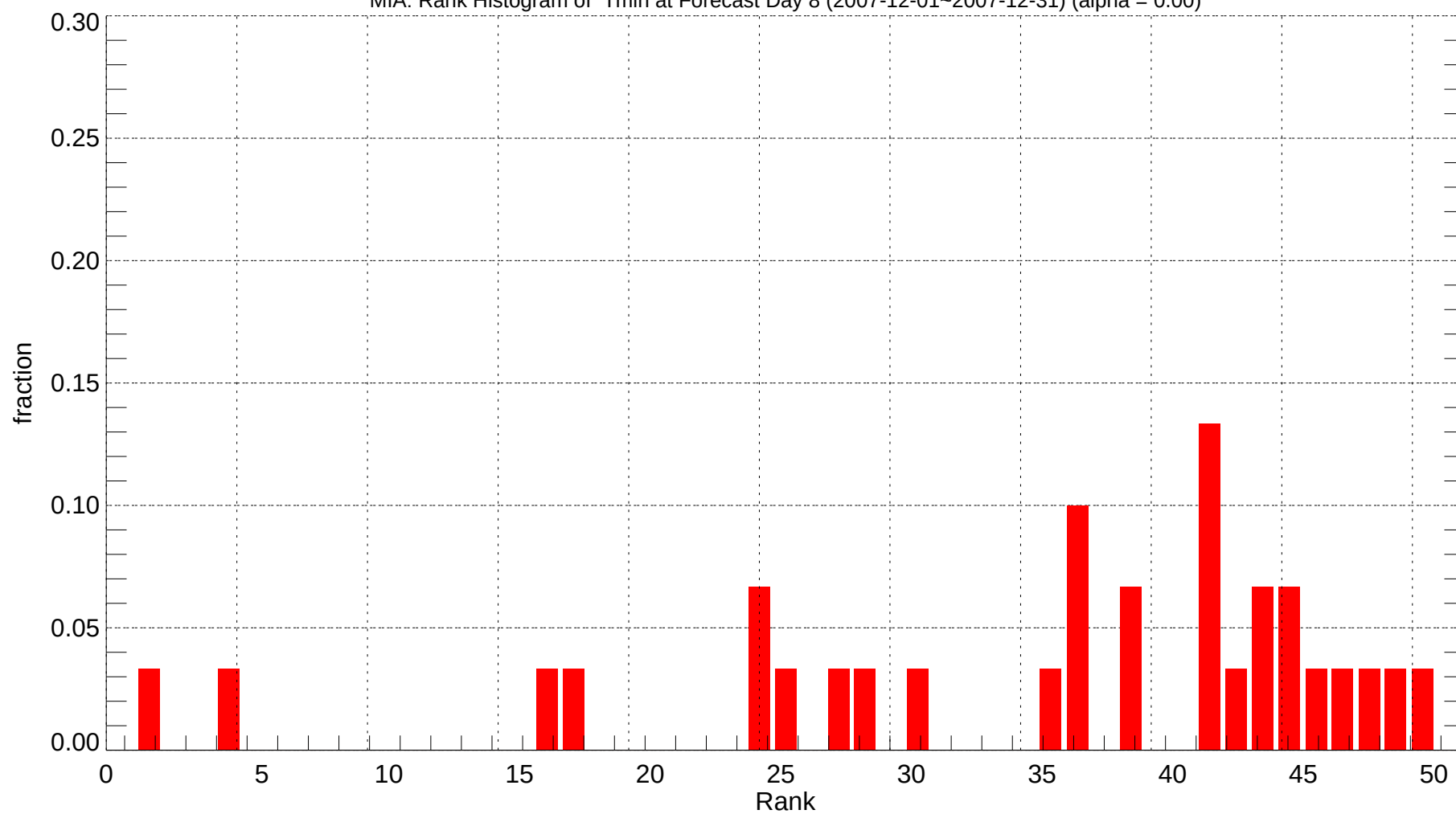
MIA: Rank Histogram of Tmin at Forecast Day 8 (2007-12-01~2007-12-31) (alpha = 0.00)
