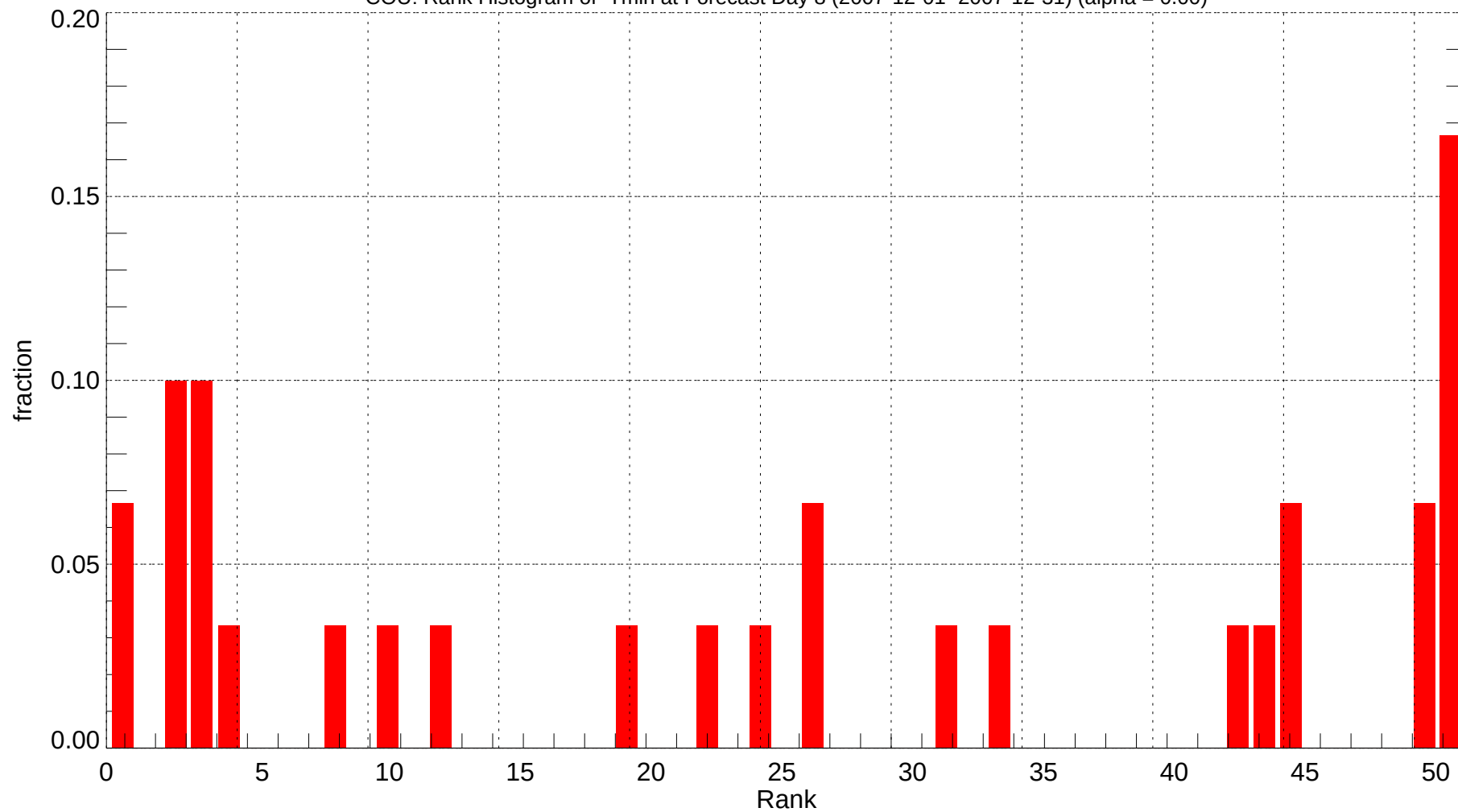
COU: Rank Histogram of Tmin at Forecast Day 8 (2007-12-01~2007-12-31) (alpha = 0.00)
