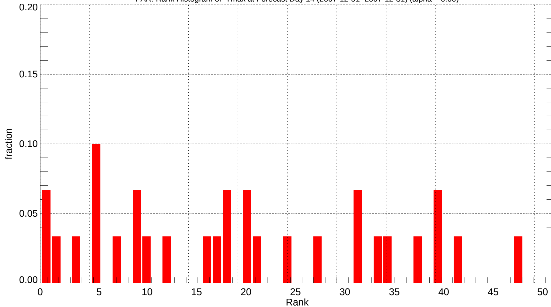
FAR: Rank Histogram of Tmax at Forecast Day 14 (2007-12-01~2007-12-31) (alpha = 0.00)
