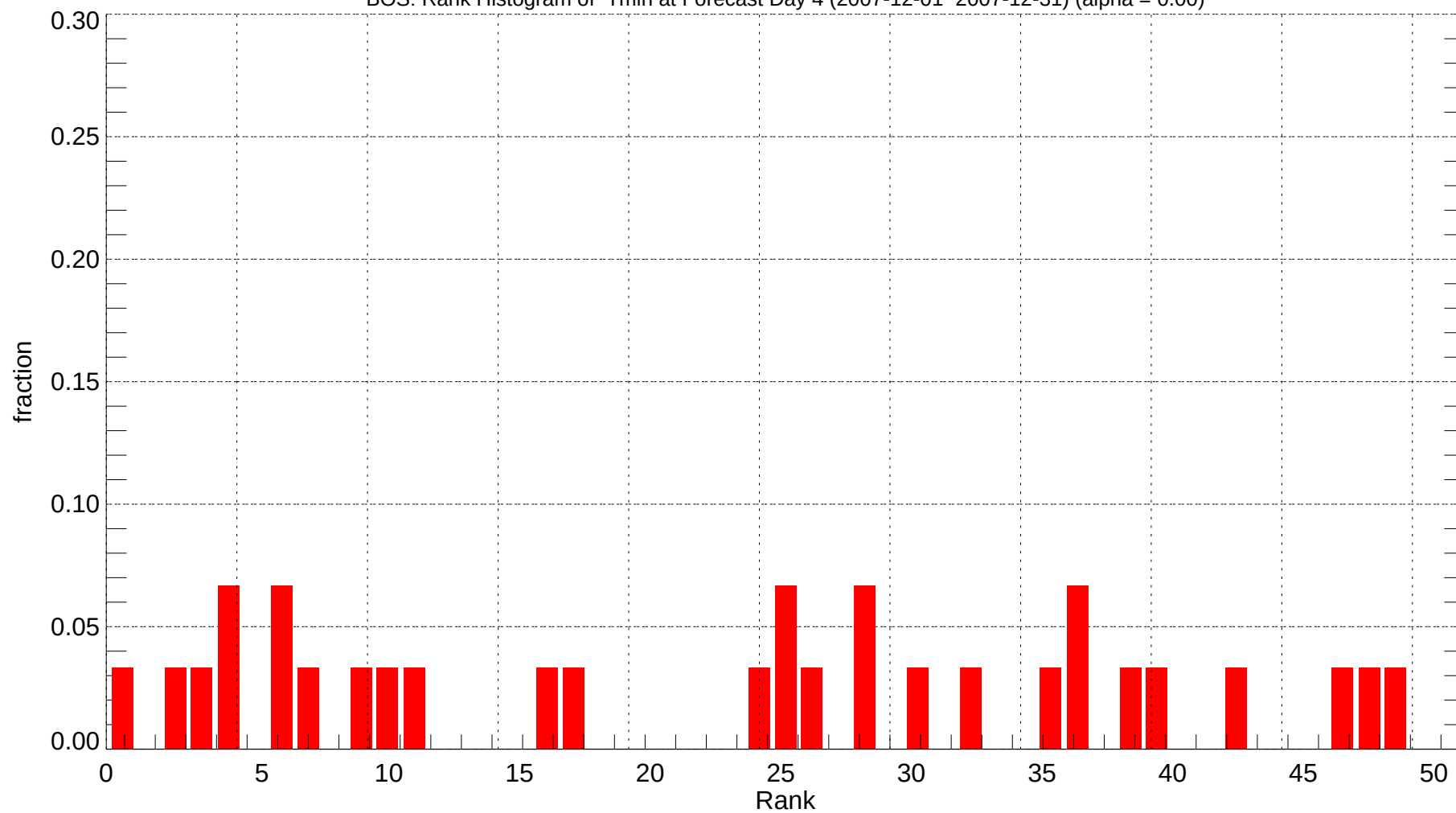
BOS: Rank Histogram of Tmin at Forecast Day 4 (2007-12-01~2007-12-31) (alpha = 0.00)
