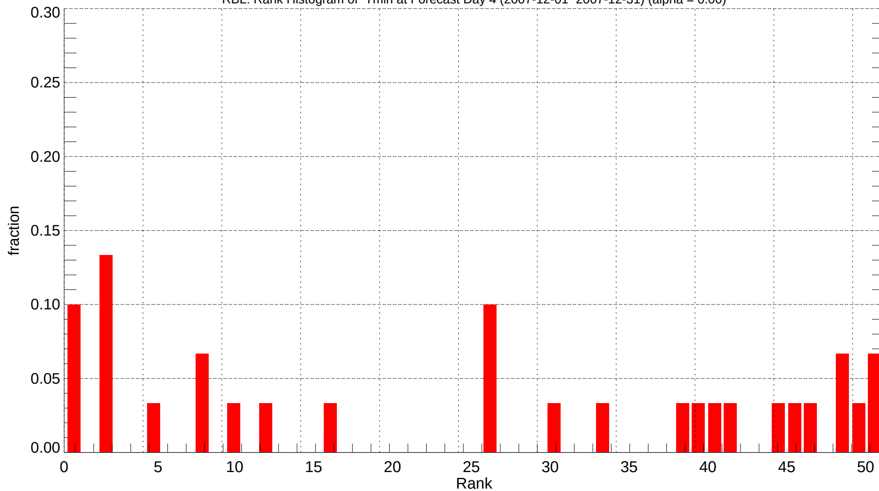
RBL: Rank Histogram of Tmin at Forecast Day 4 (2007-12-01~2007-12-31) (alpha = 0.00)
