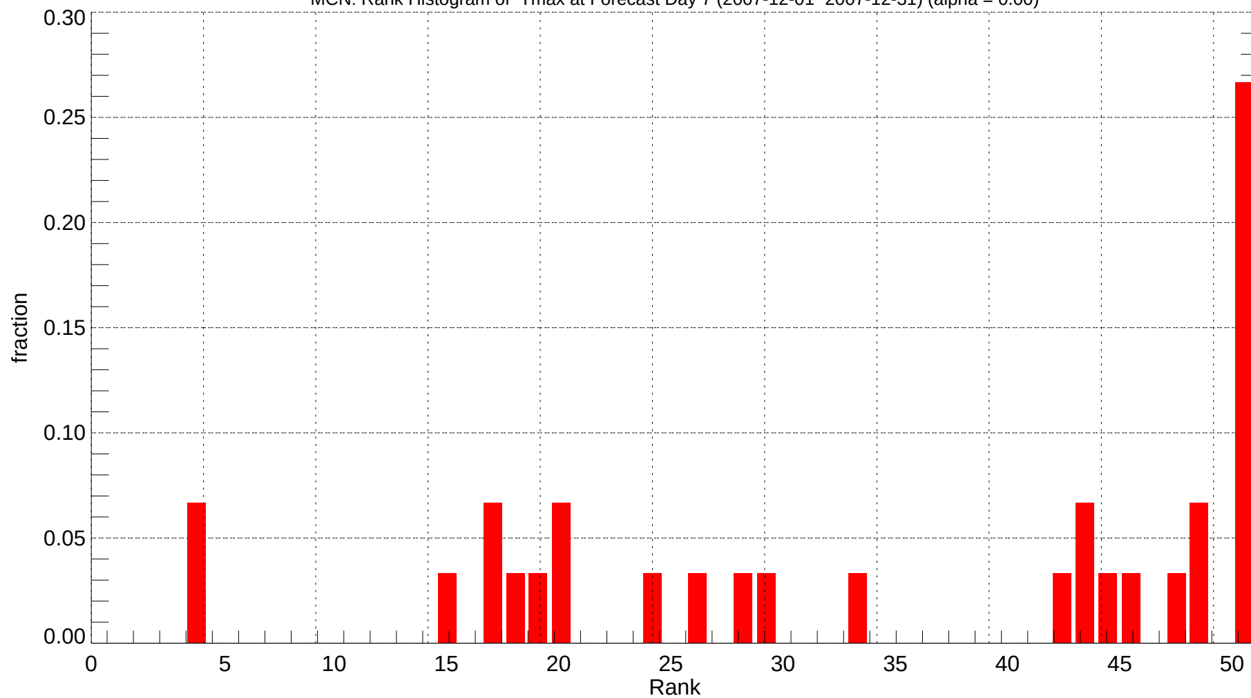
MCN: Rank Histogram of Tmax at Forecast Day 7 (2007-12-01~2007-12-31) (alpha = 0.00)
