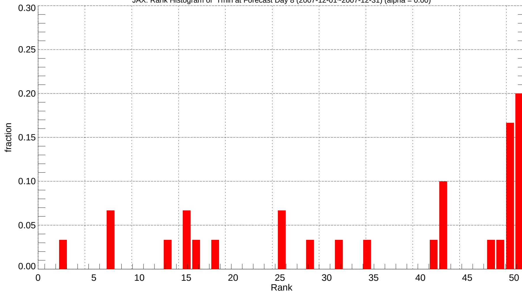
JAX: Rank Histogram of Tmin at Forecast Day 8 (2007-12-01~2007-12-31) (alpha = 0.00)
