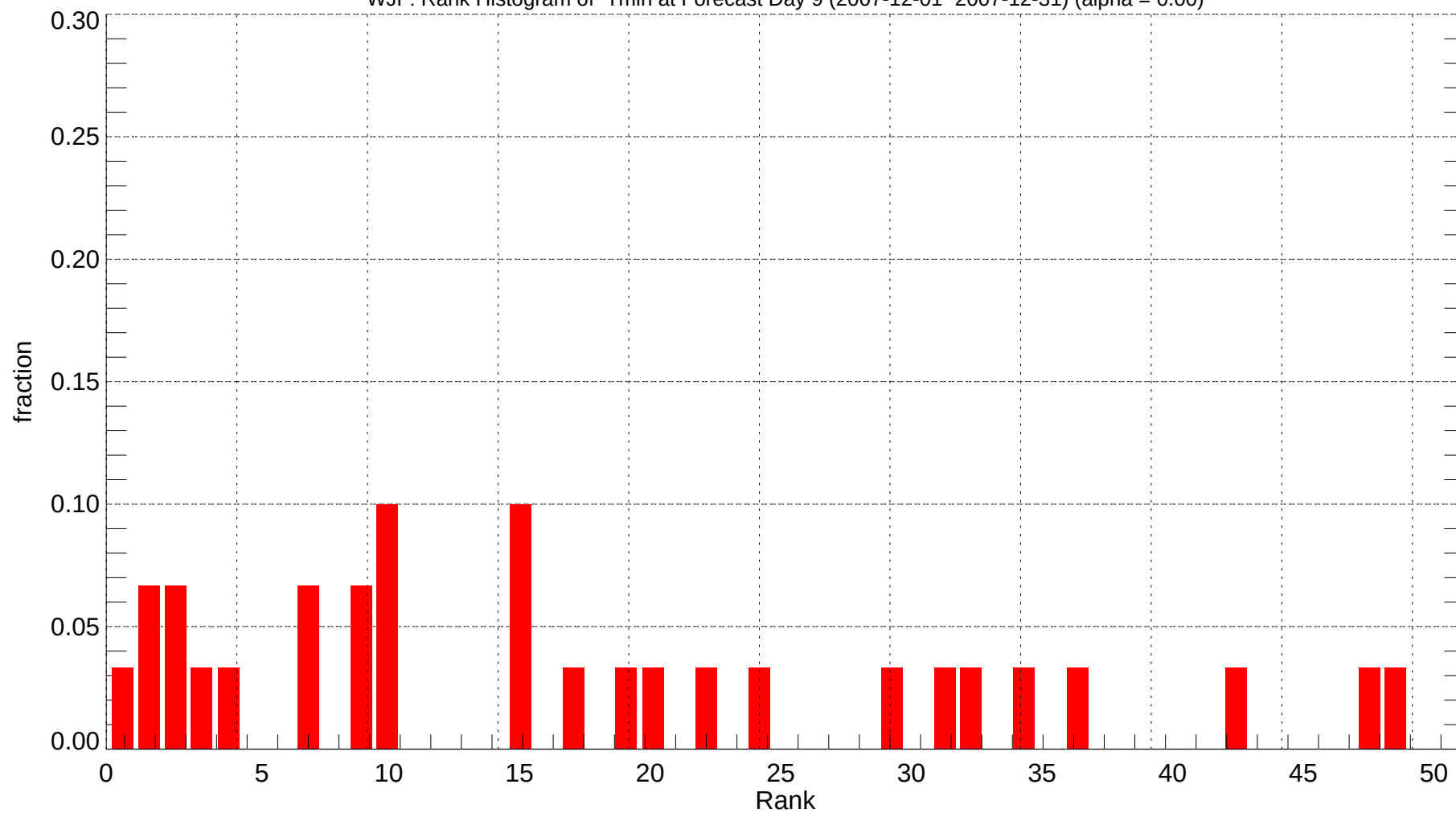
WJF: Rank Histogram of Tmin at Forecast Day 9 (2007-12-01~2007-12-31) (alpha = 0.00)
