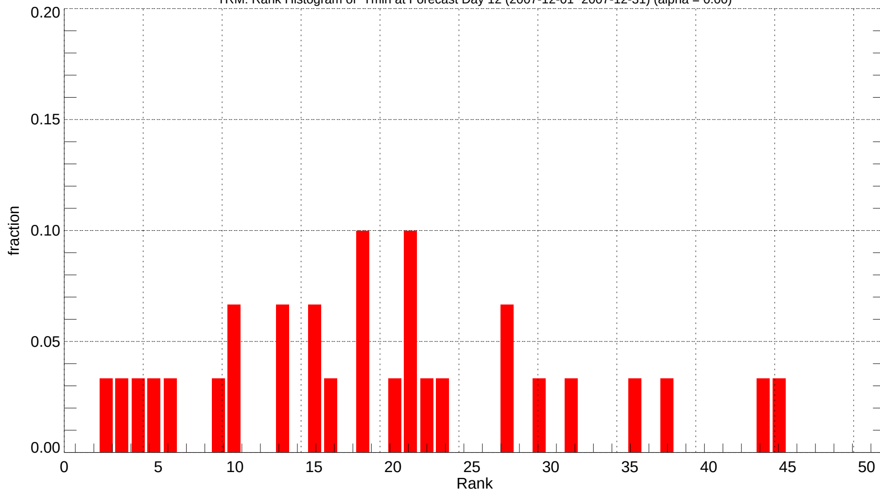
TRM: Rank Histogram of Tmin at Forecast Day 12 (2007-12-01~2007-12-31) (alpha = 0.00)
