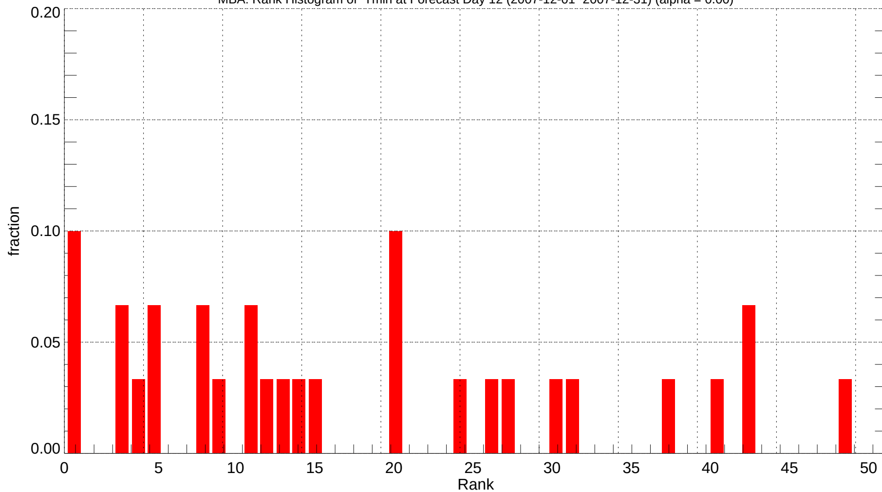
MBA: Rank Histogram of Tmin at Forecast Day 12 (2007-12-01~2007-12-31) (alpha = 0.00)
