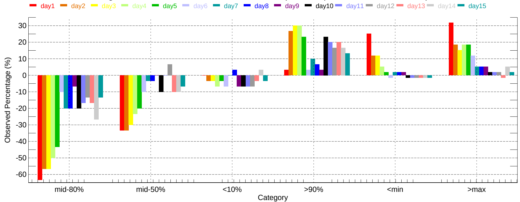
Observed Percentage Deviation of Ensembles - BIS: Max Temperature (2007-12-01~2007-12-31)
