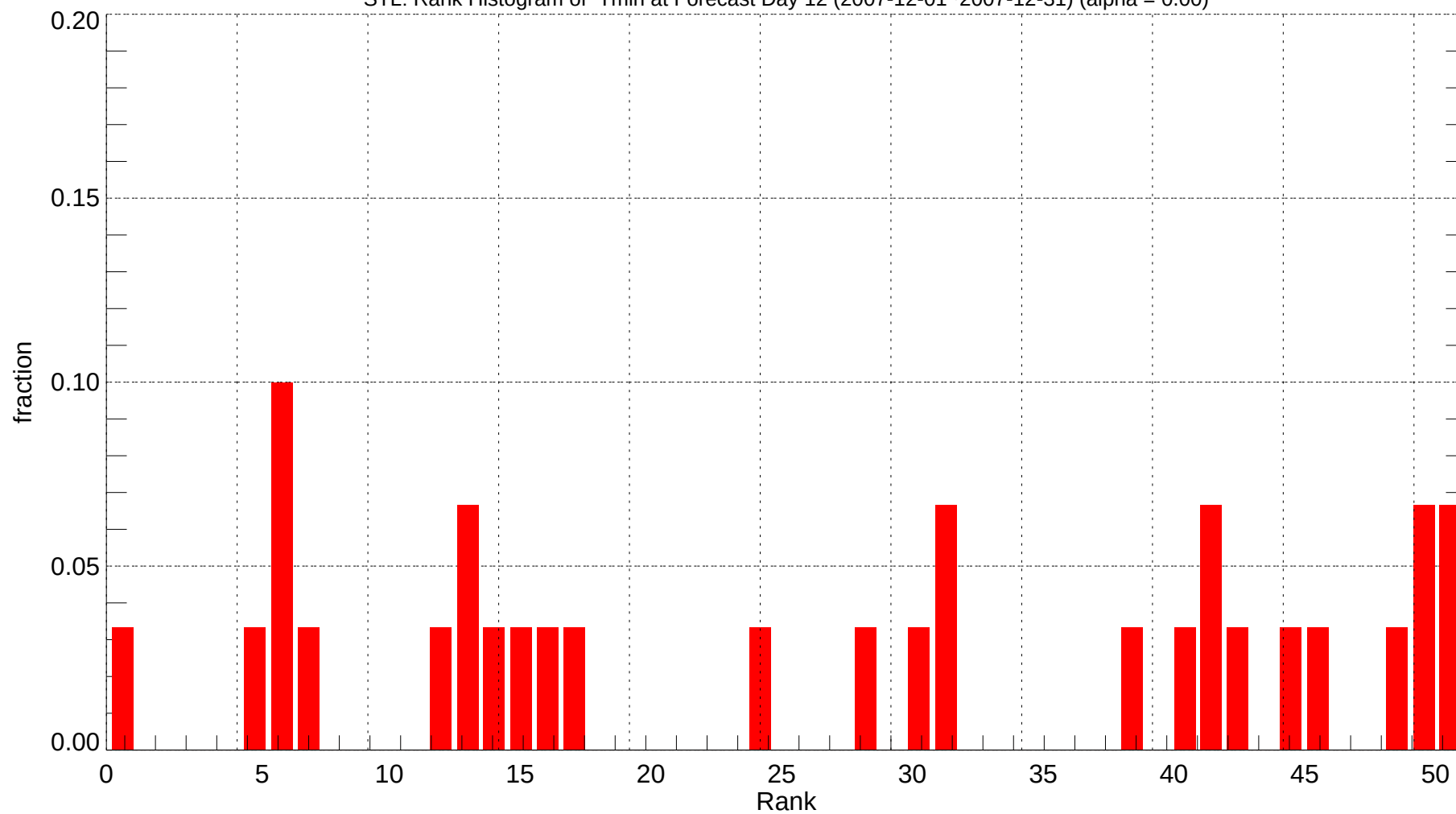
STL: Rank Histogram of Tmin at Forecast Day 12 (2007-12-01~2007-12-31) (alpha = 0.00)
