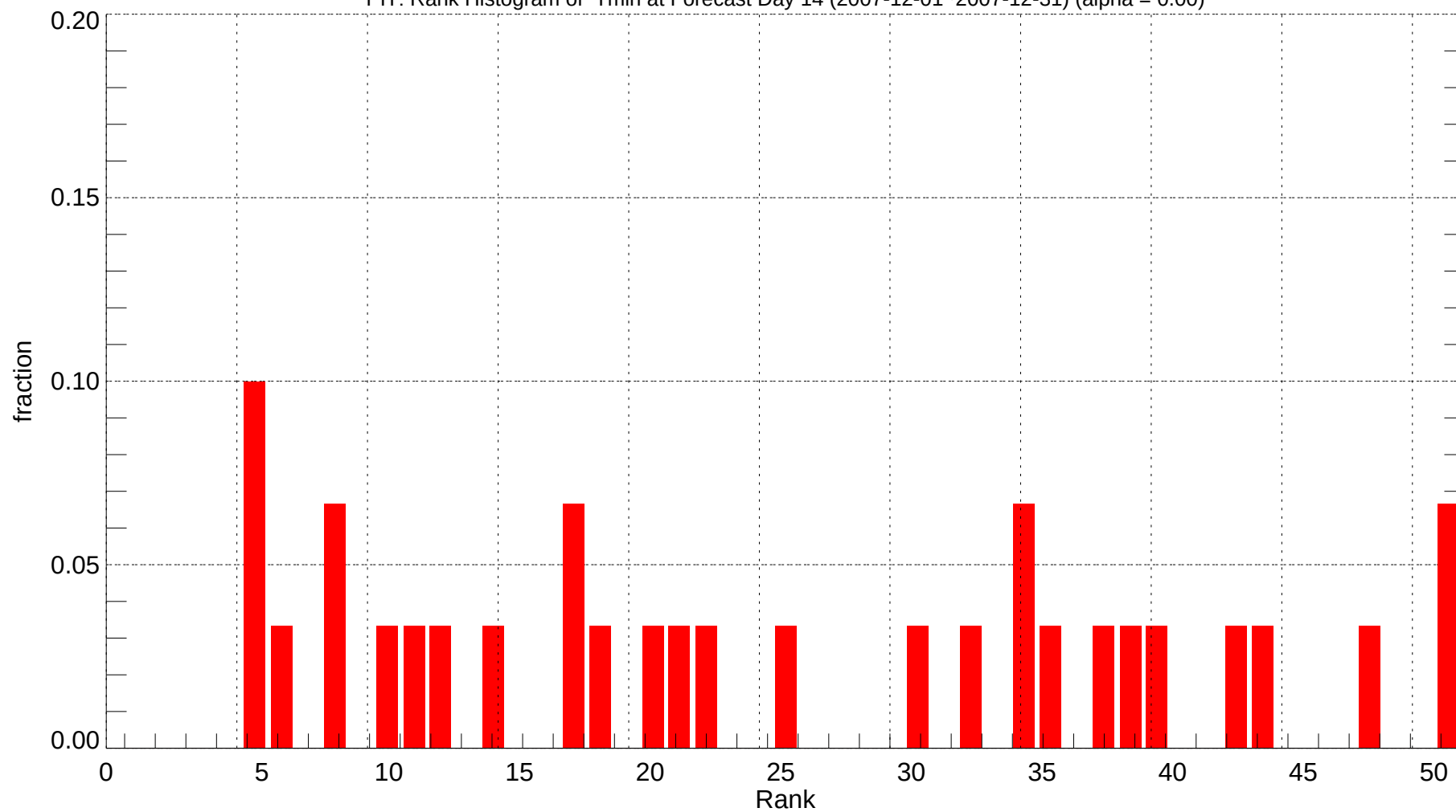
PIT: Rank Histogram of Tmin at Forecast Day 14 (2007-12-01~2007-12-31) (alpha = 0.00)
