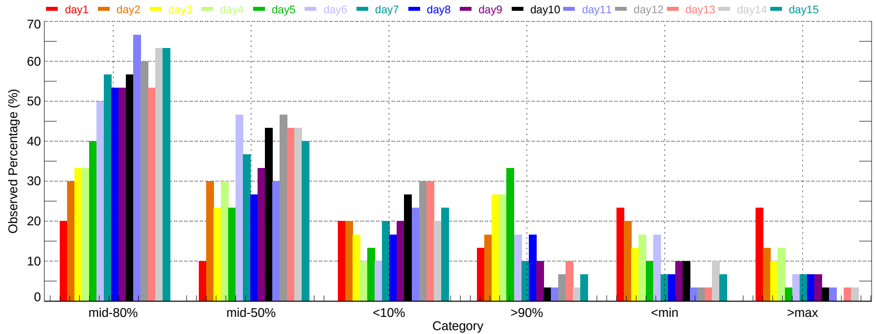
Observed Percentage of Ensembles - DEN: Min Temperature (2007-12-01~2007-12-31)
