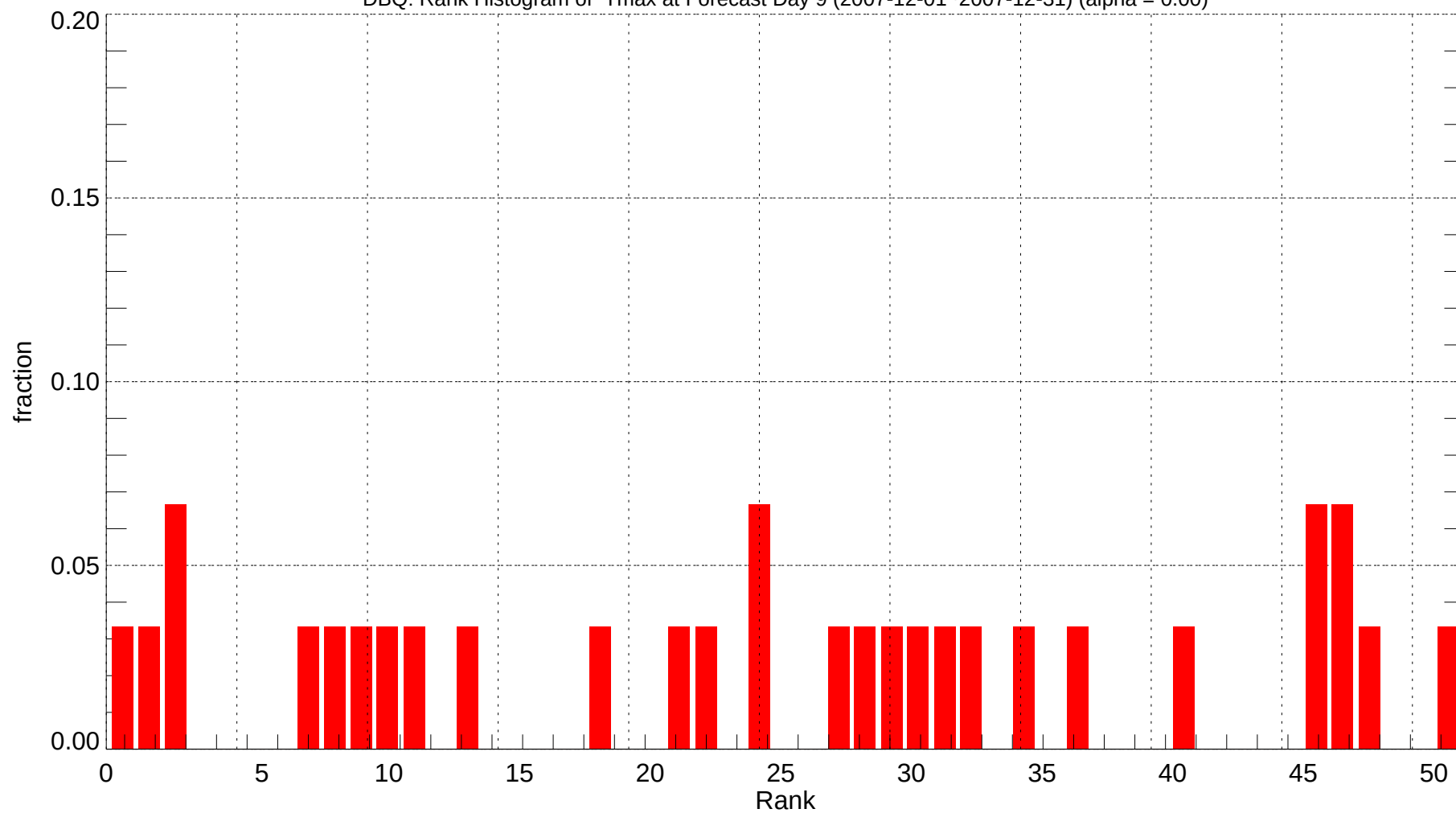
DBQ: Rank Histogram of Tmax at Forecast Day 9 (2007-12-01~2007-12-31) (alpha = 0.00)
