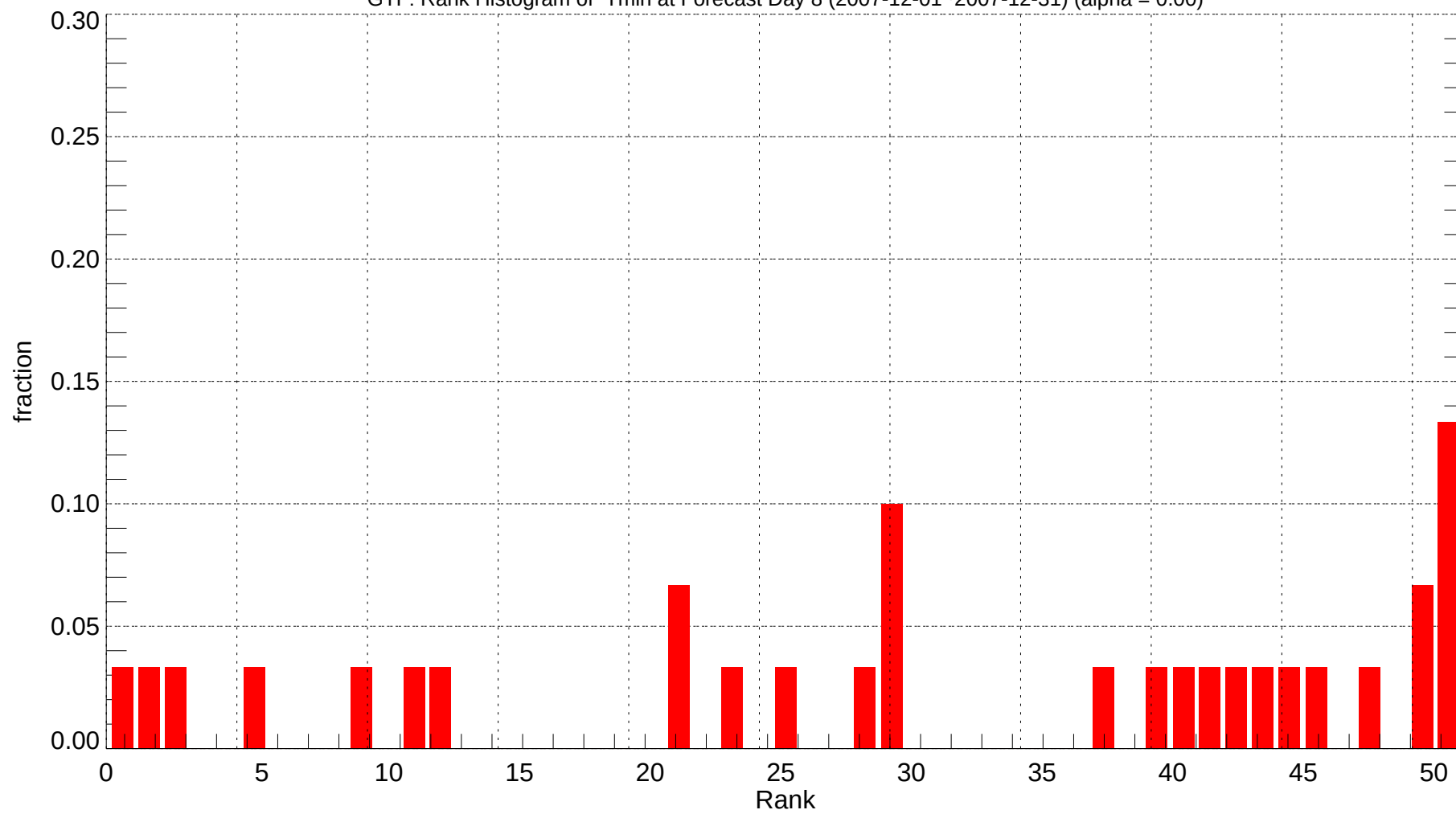
GTF: Rank Histogram of Tmin at Forecast Day 8 (2007-12-01~2007-12-31) (alpha = 0.00)
