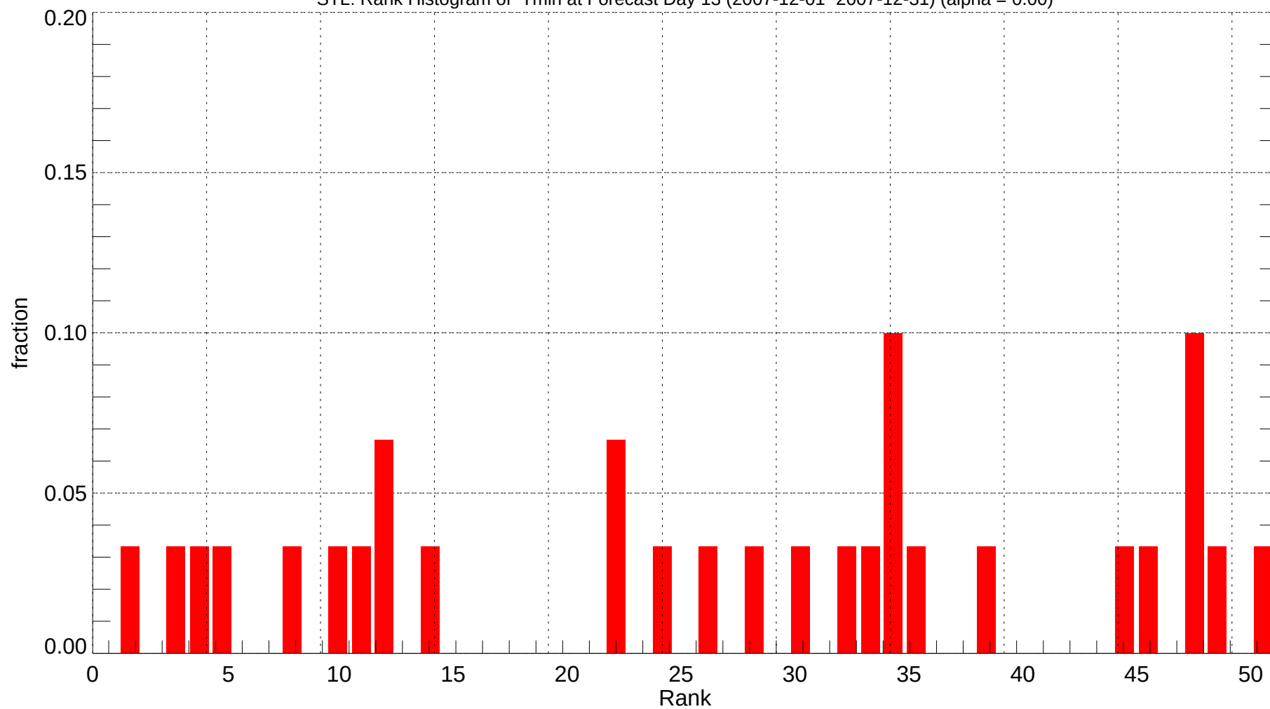
STL: Rank Histogram of Tmin at Forecast Day 13 (2007-12-01~2007-12-31) (alpha = 0.00)
