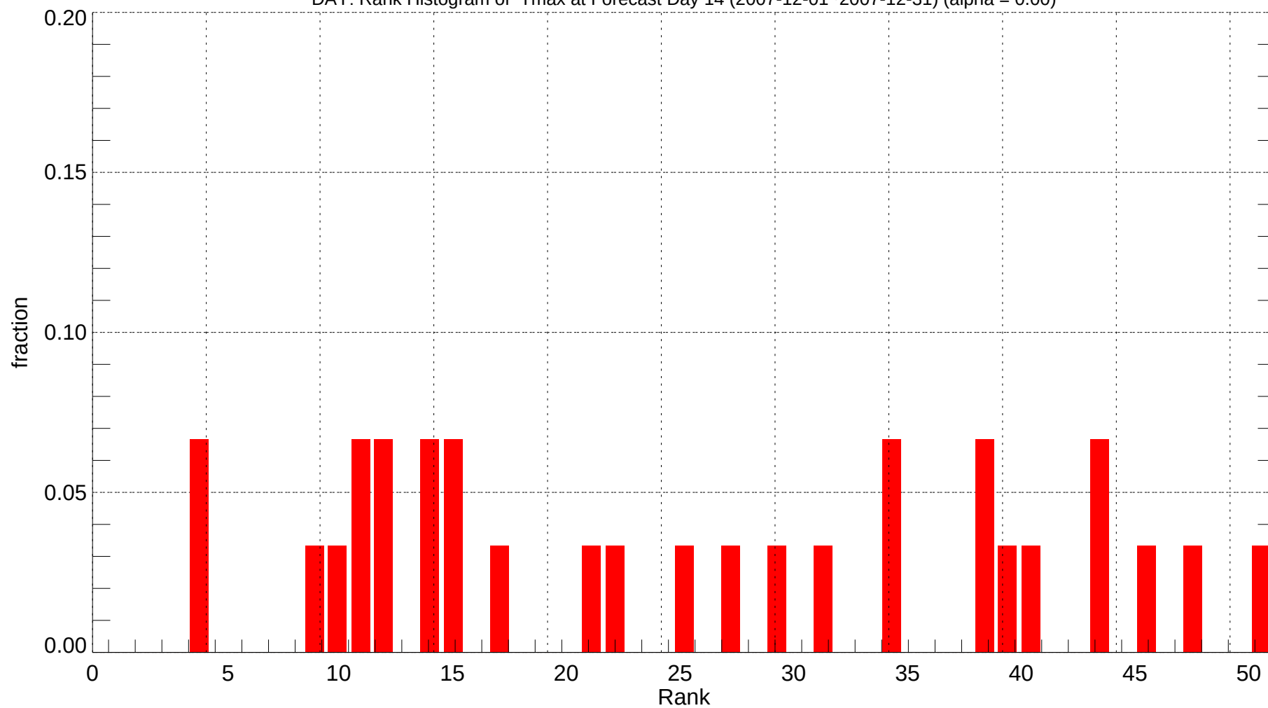
DAY: Rank Histogram of Tmax at Forecast Day 14 (2007-12-01~2007-12-31) (alpha = 0.00)
