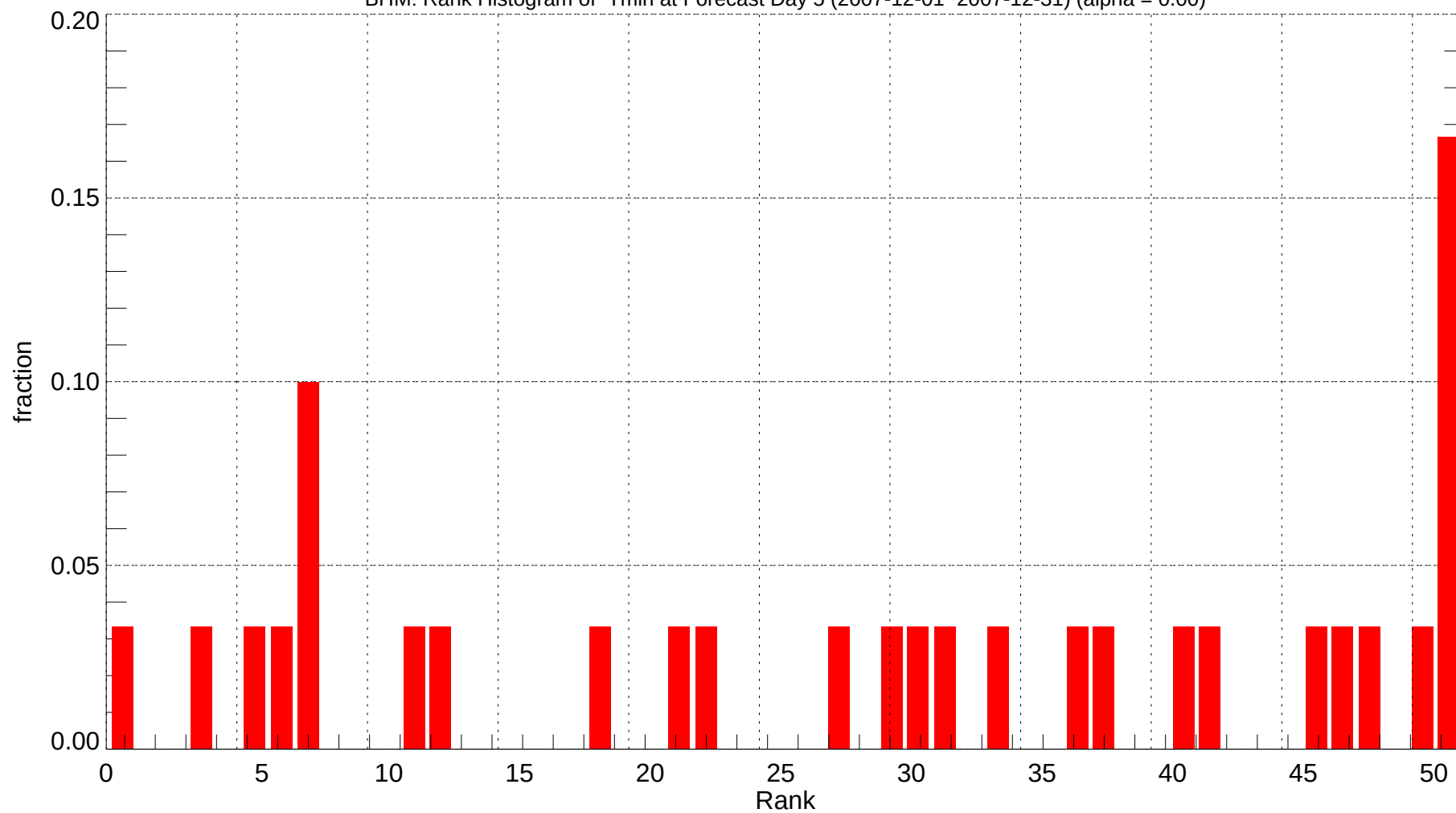
BHM: Rank Histogram of Tmin at Forecast Day 5 (2007-12-01~2007-12-31) (alpha = 0.00)
