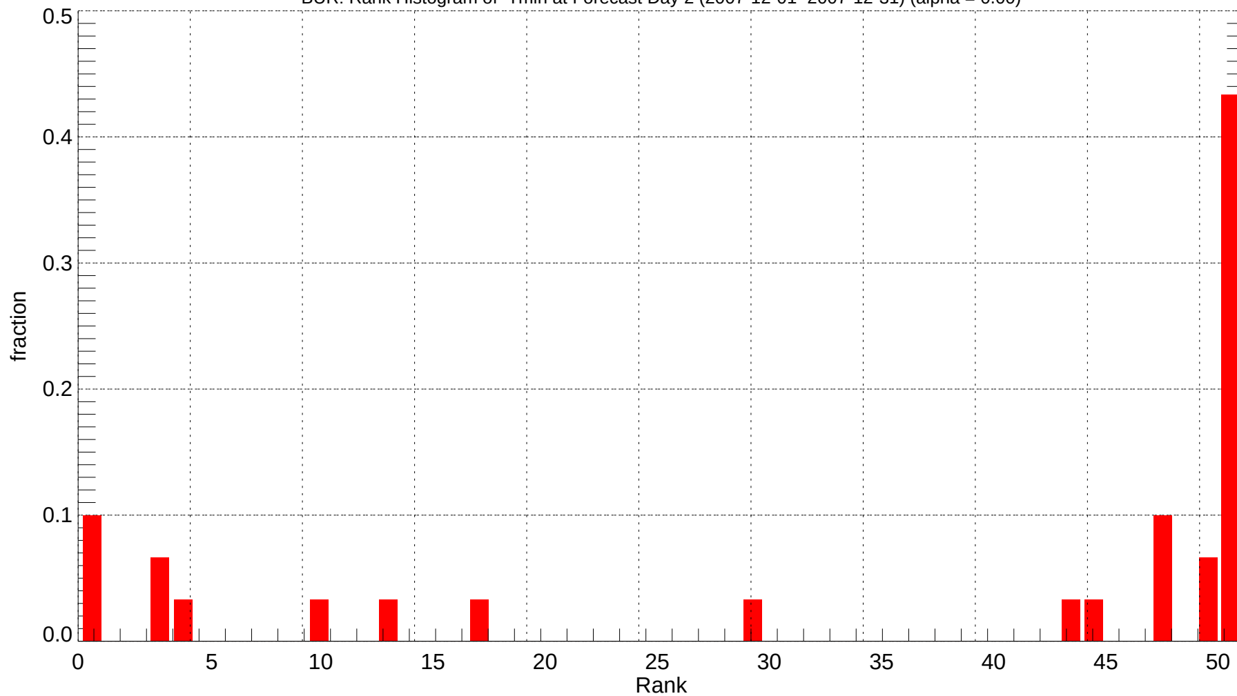
BUR: Rank Histogram of Tmin at Forecast Day 2 (2007-12-01~2007-12-31) (alpha = 0.00)
