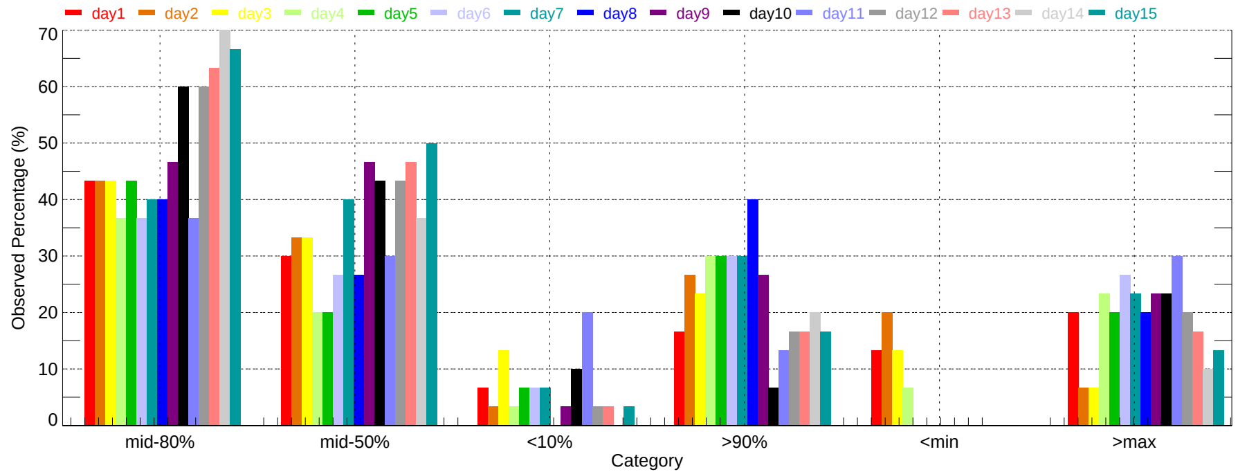
Observed Percentage of Ensembles - MCN: Max Temperature (2007-12-01~2007-12-31)
