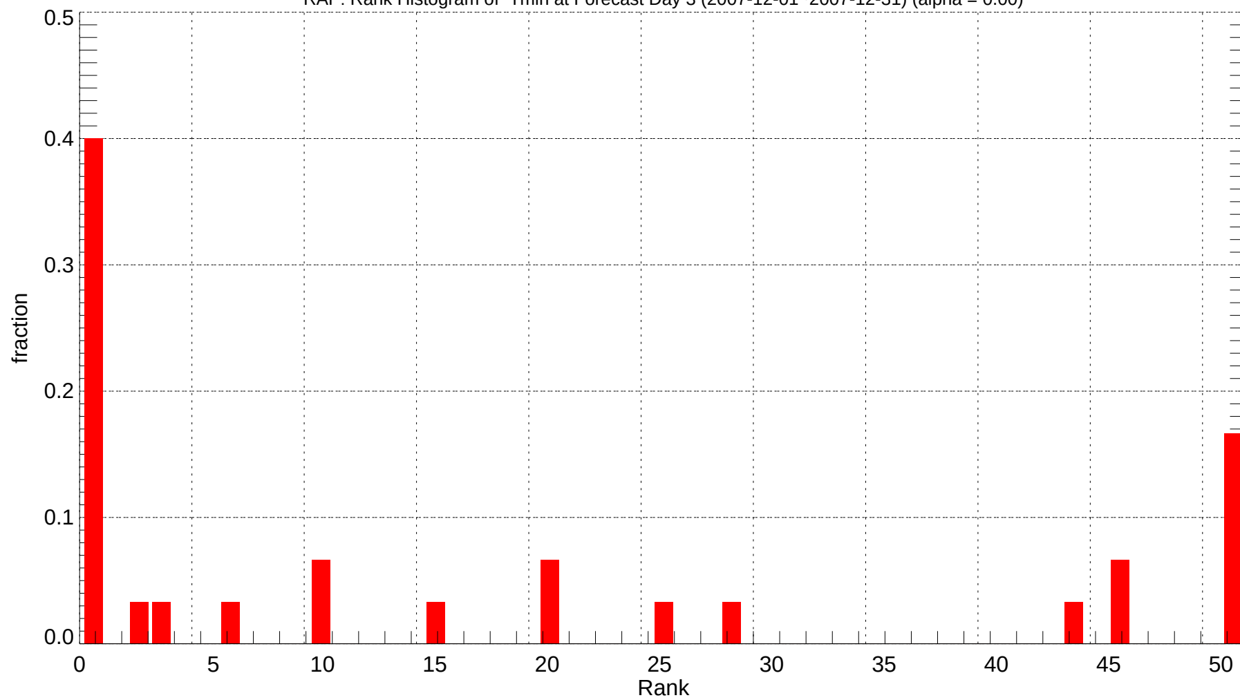
RAP: Rank Histogram of Tmin at Forecast Day 3 (2007-12-01~2007-12-31) (alpha = 0.00)
