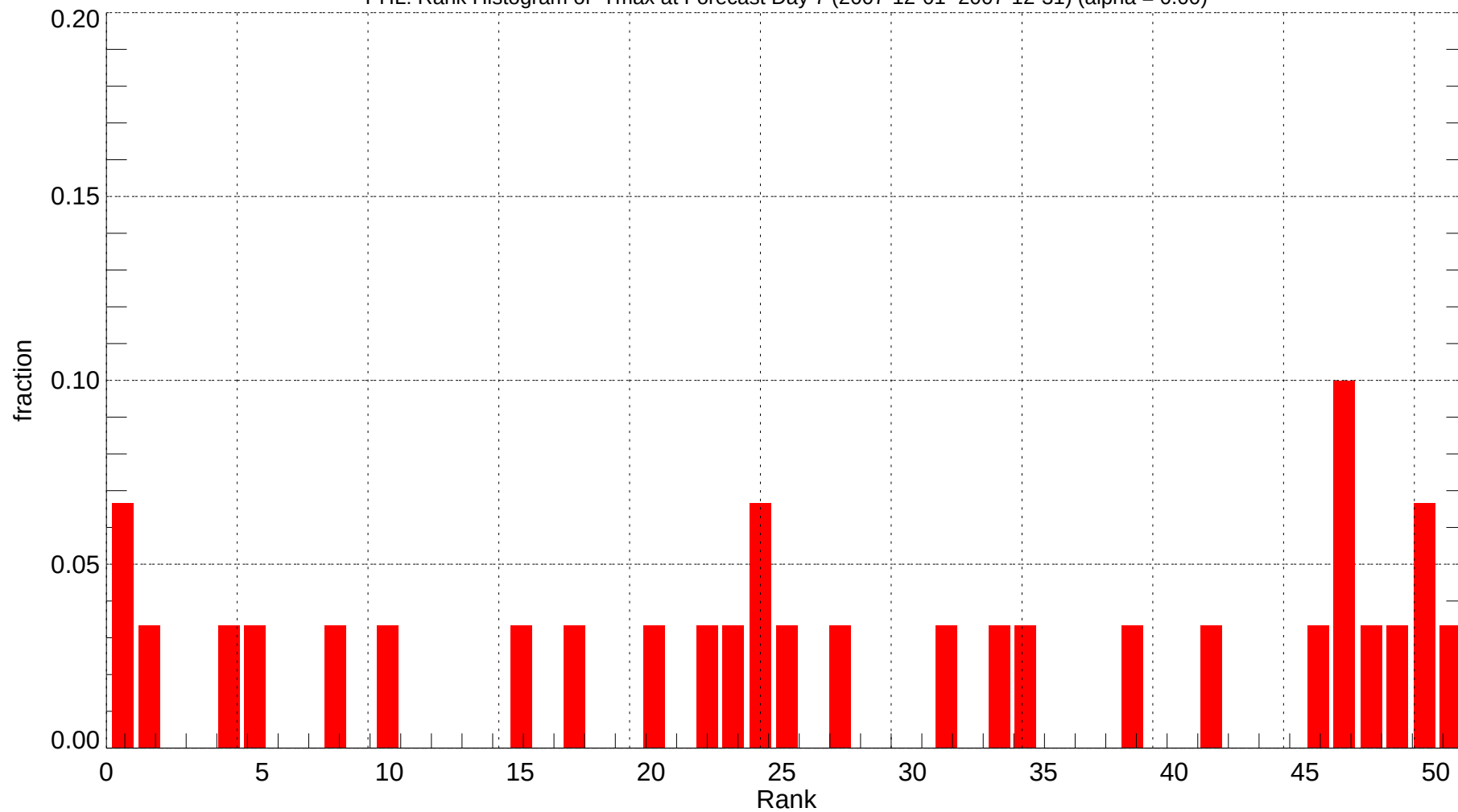
PHL: Rank Histogram of Tmax at Forecast Day 7 (2007-12-01~2007-12-31) (alpha = 0.00)
