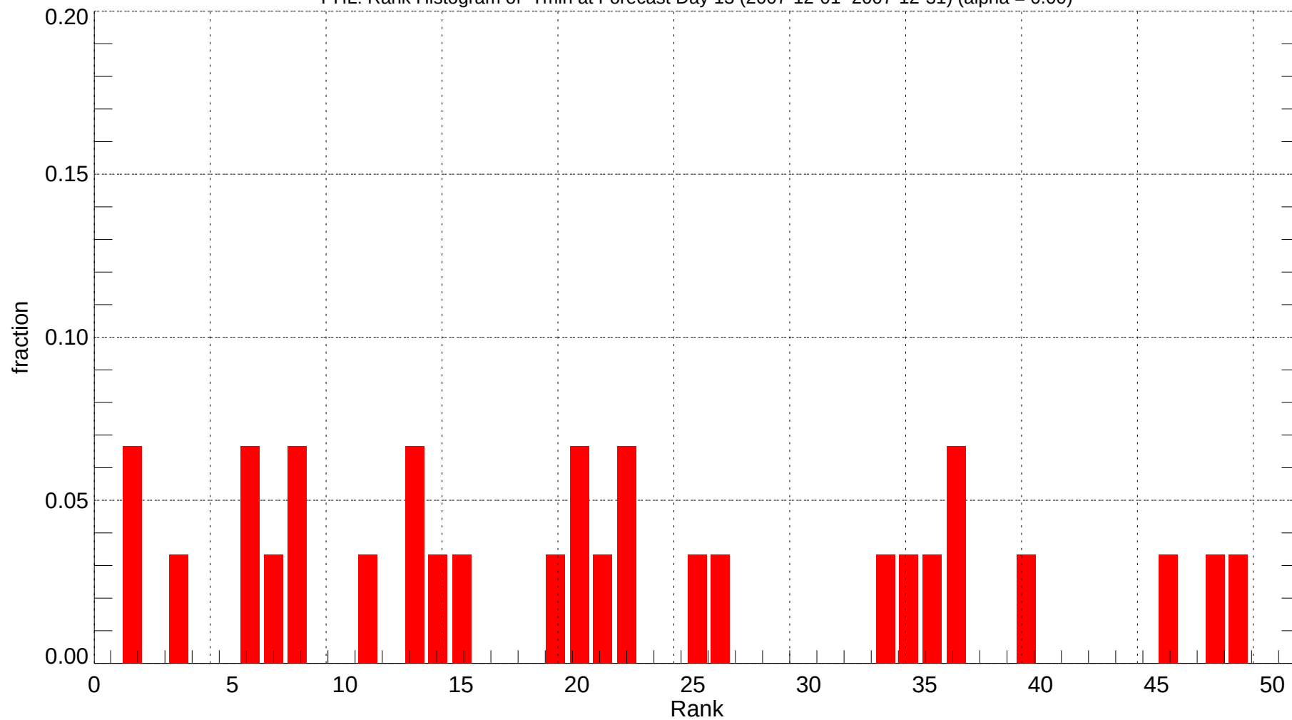
PHL: Rank Histogram of Tmin at Forecast Day 13 (2007-12-01~2007-12-31) (alpha = 0.00)
