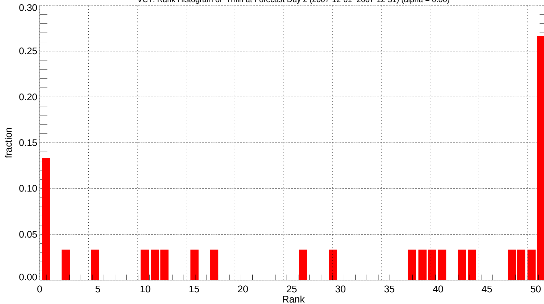
VCT: Rank Histogram of Tmin at Forecast Day 2 (2007-12-01~2007-12-31) (alpha = 0.00)
