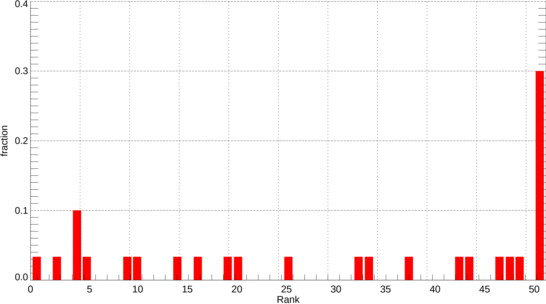
STL: Rank Histogram of Tmin at Forecast Day 4 (2007-12-01~2007-12-31) (alpha = 0.00)
