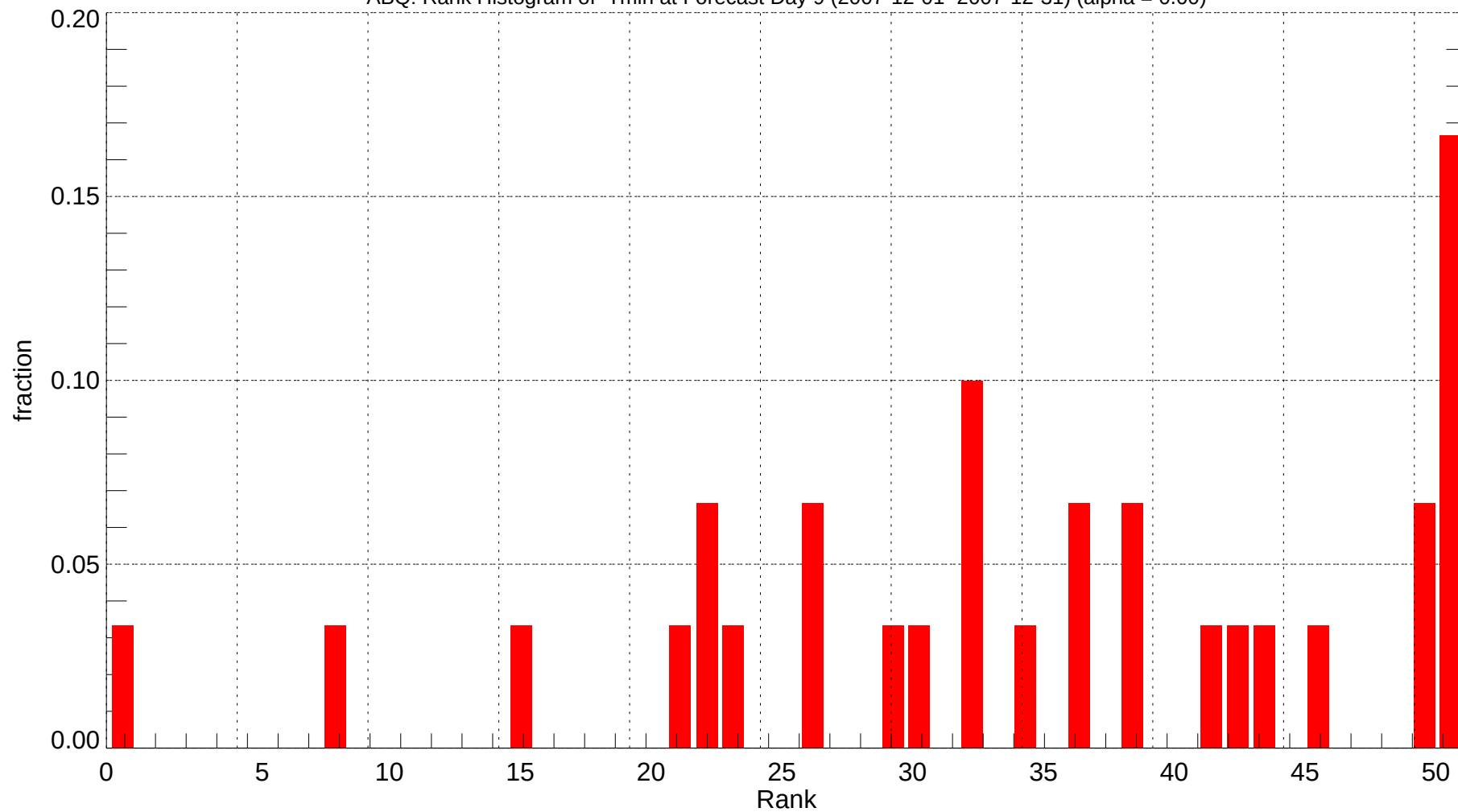
ABQ: Rank Histogram of Tmin at Forecast Day 9 (2007-12-01~2007-12-31) (alpha = 0.00)
