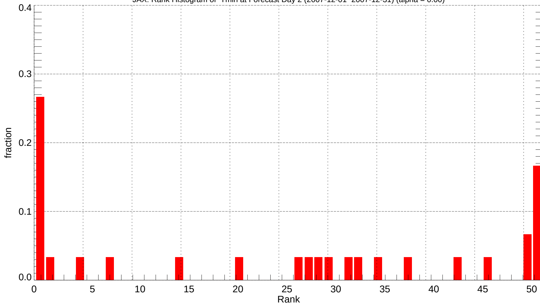
JAX: Rank Histogram of Tmin at Forecast Day 2 (2007-12-01~2007-12-31) (alpha = 0.00)
