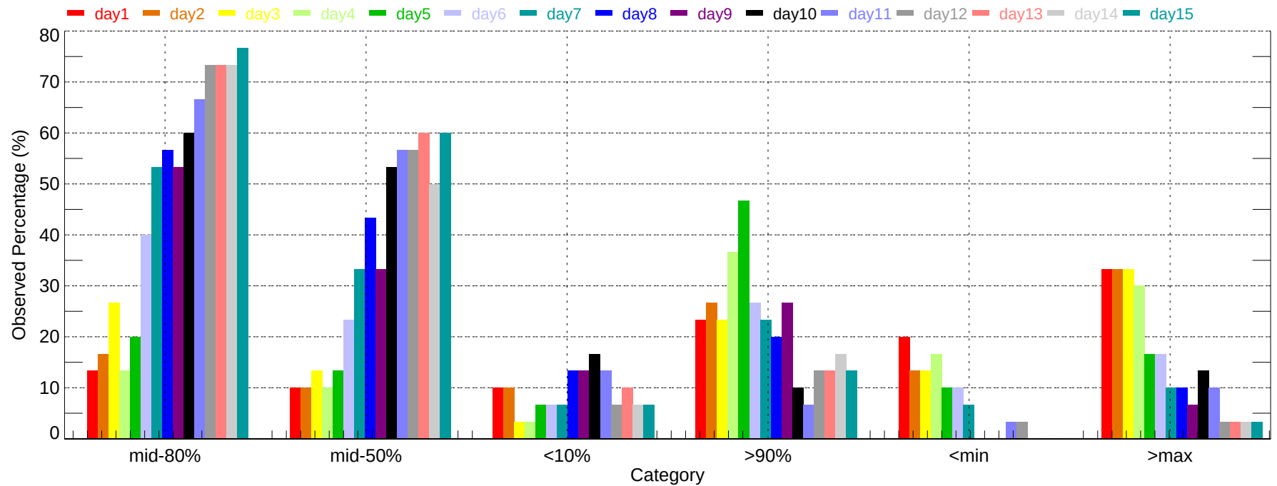
Observed Percentage of Ensembles - GEG: Max Temperature (2007-12-01~2007-12-31)
