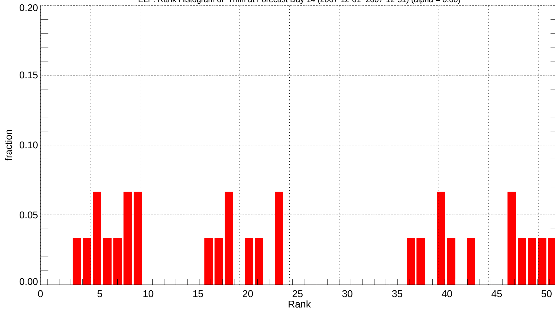
ELP: Rank Histogram of Tmin at Forecast Day 14 (2007-12-01~2007-12-31) (alpha = 0.00)
