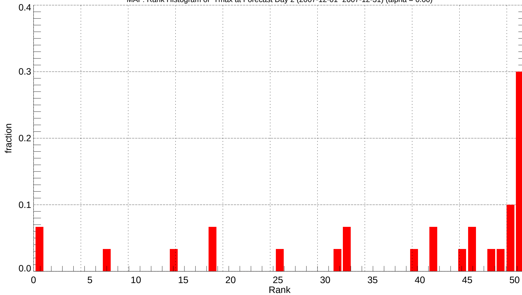
MAF: Rank Histogram of Tmax at Forecast Day 2 (2007-12-01~2007-12-31) (alpha = 0.00)
