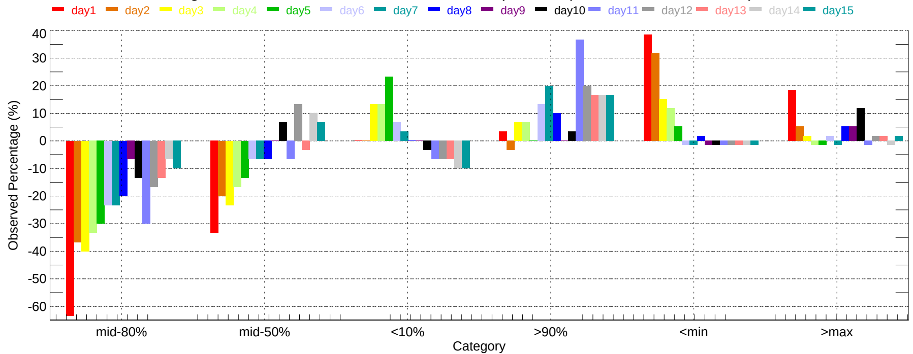
Observed Percentage Deviation of Ensembles - ERI: Max Temperature (2007-12-01~2007-12-31)
