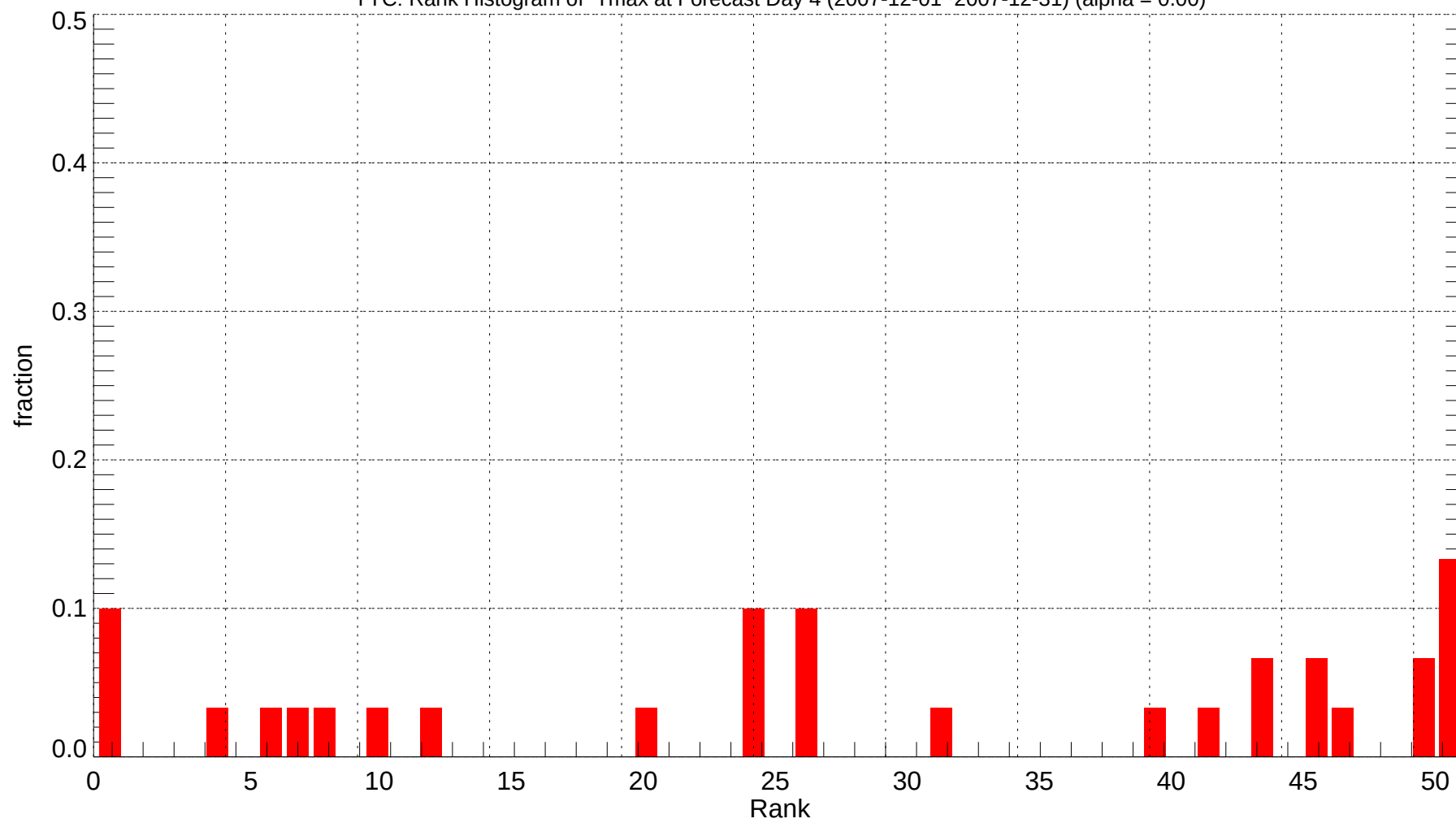
YYC: Rank Histogram of Tmax at Forecast Day 4 (2007-12-01~2007-12-31) (alpha = 0.00)
