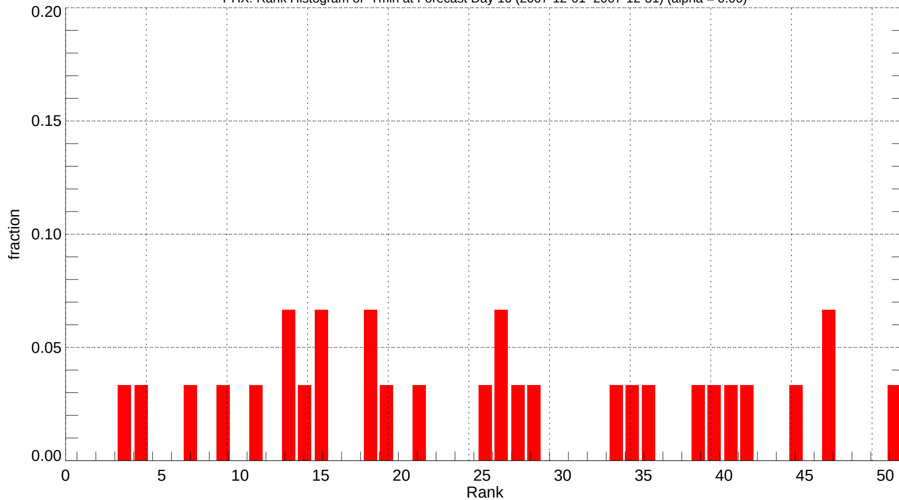
PHX: Rank Histogram of Tmin at Forecast Day 10 (2007-12-01~2007-12-31) (alpha = 0.00)
