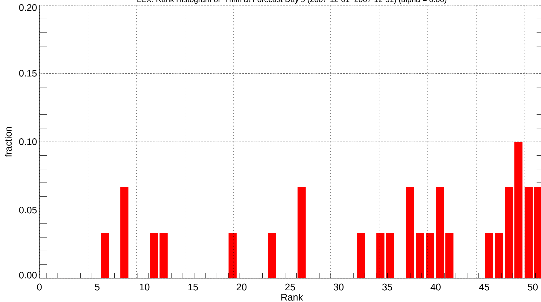
LEX: Rank Histogram of Tmin at Forecast Day 9 (2007-12-01~2007-12-31) (alpha = 0.00)
