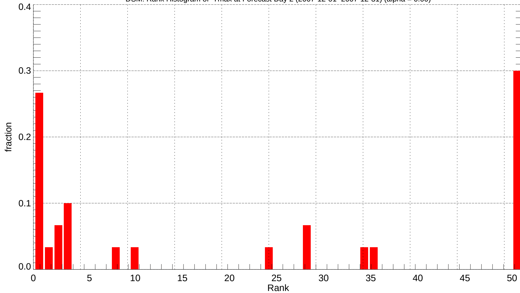
DSM: Rank Histogram of Tmax at Forecast Day 2 (2007-12-01~2007-12-31) (alpha = 0.00)
