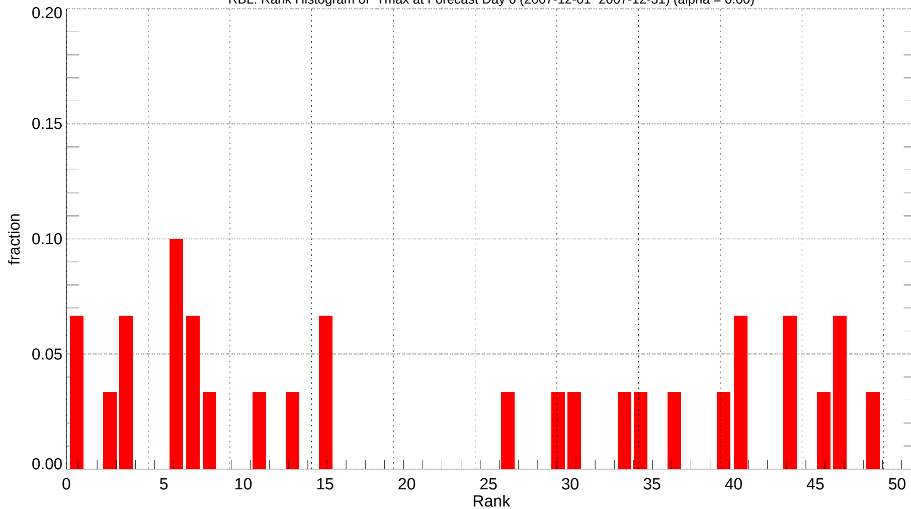
RBL: Rank Histogram of Tmax at Forecast Day 6 (2007-12-01~2007-12-31) (alpha = 0.00)
