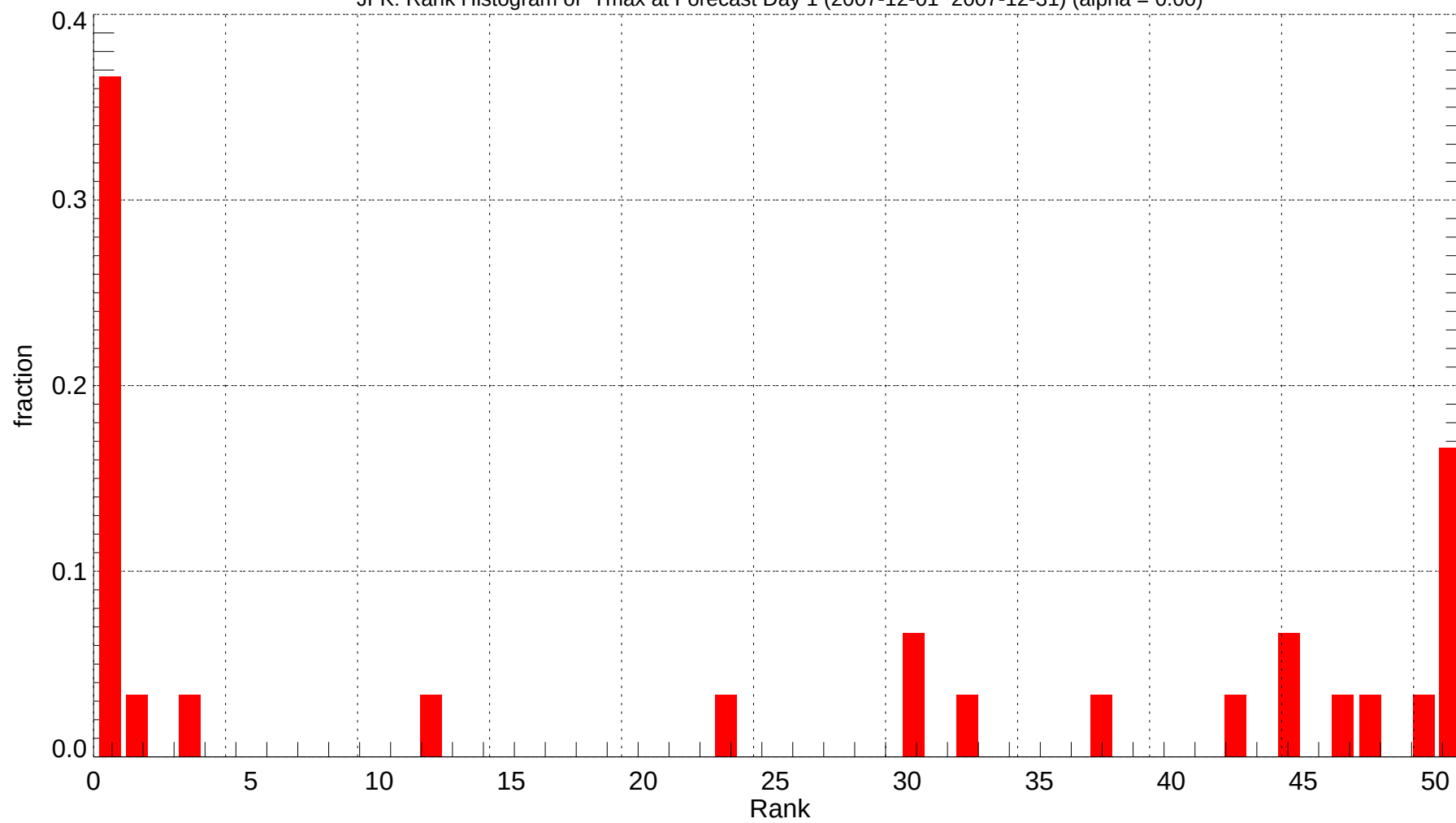
JFK: Rank Histogram of Tmax at Forecast Day 1 (2007-12-01~2007-12-31) (alpha = 0.00)
