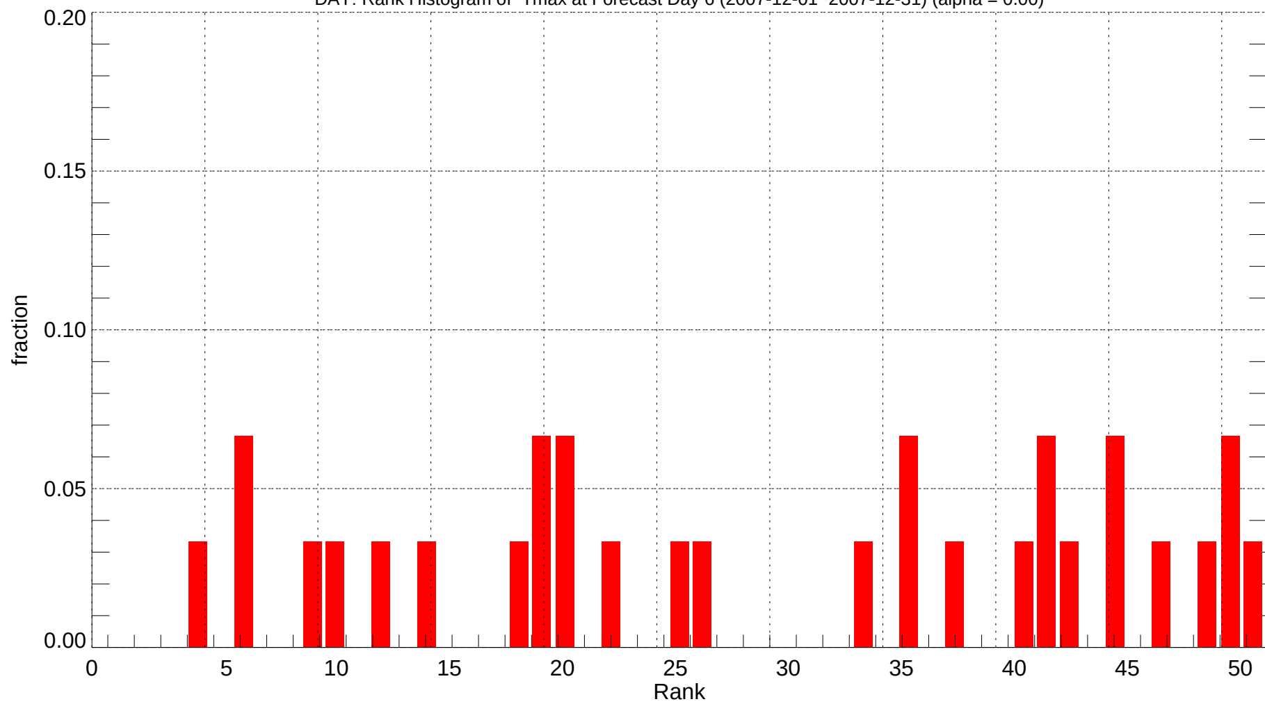
DAY: Rank Histogram of Tmax at Forecast Day 6 (2007-12-01~2007-12-31) (alpha = 0.00)
