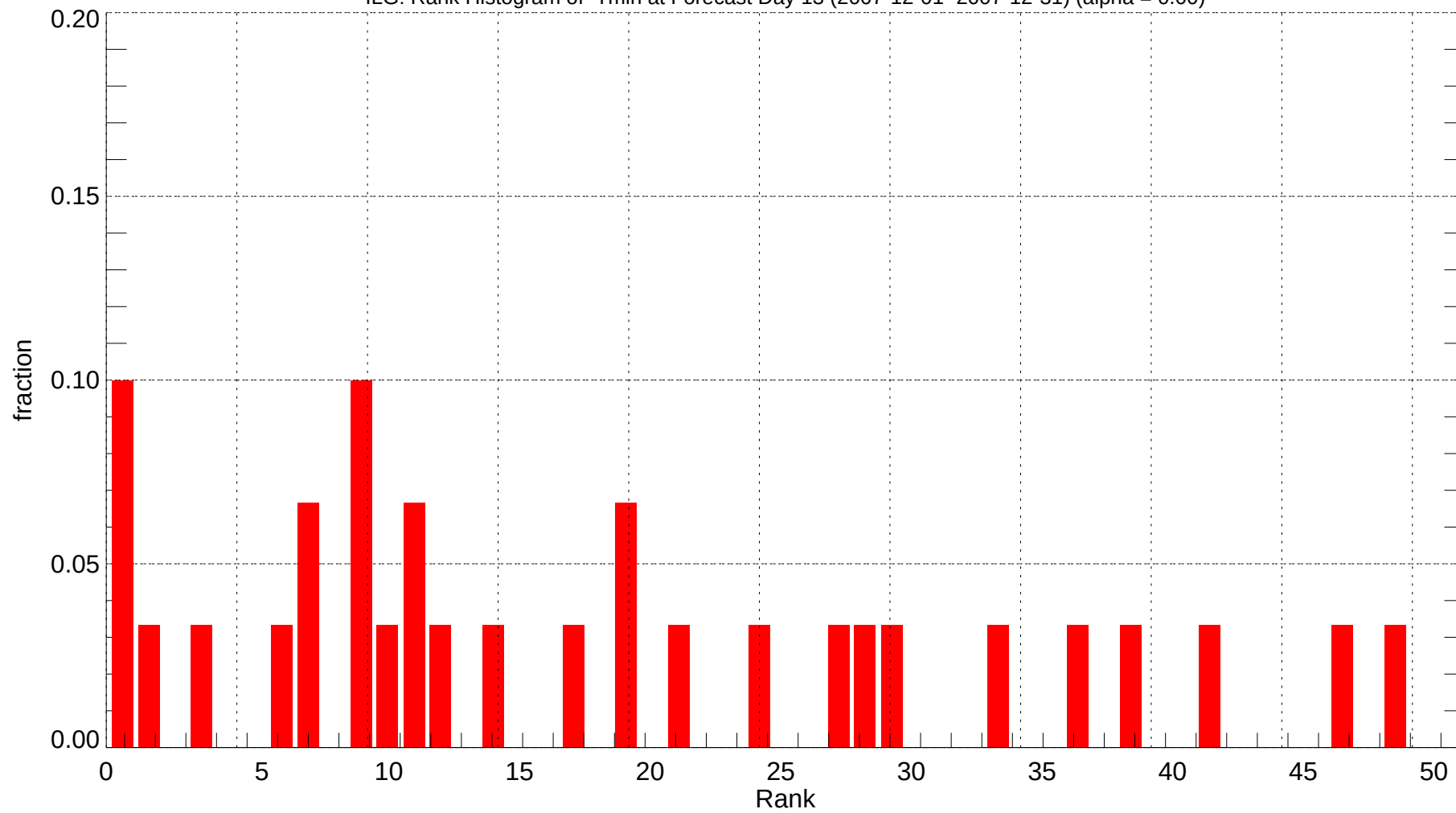
ILG: Rank Histogram of Tmin at Forecast Day 13 (2007-12-01~2007-12-31) (alpha = 0.00)
