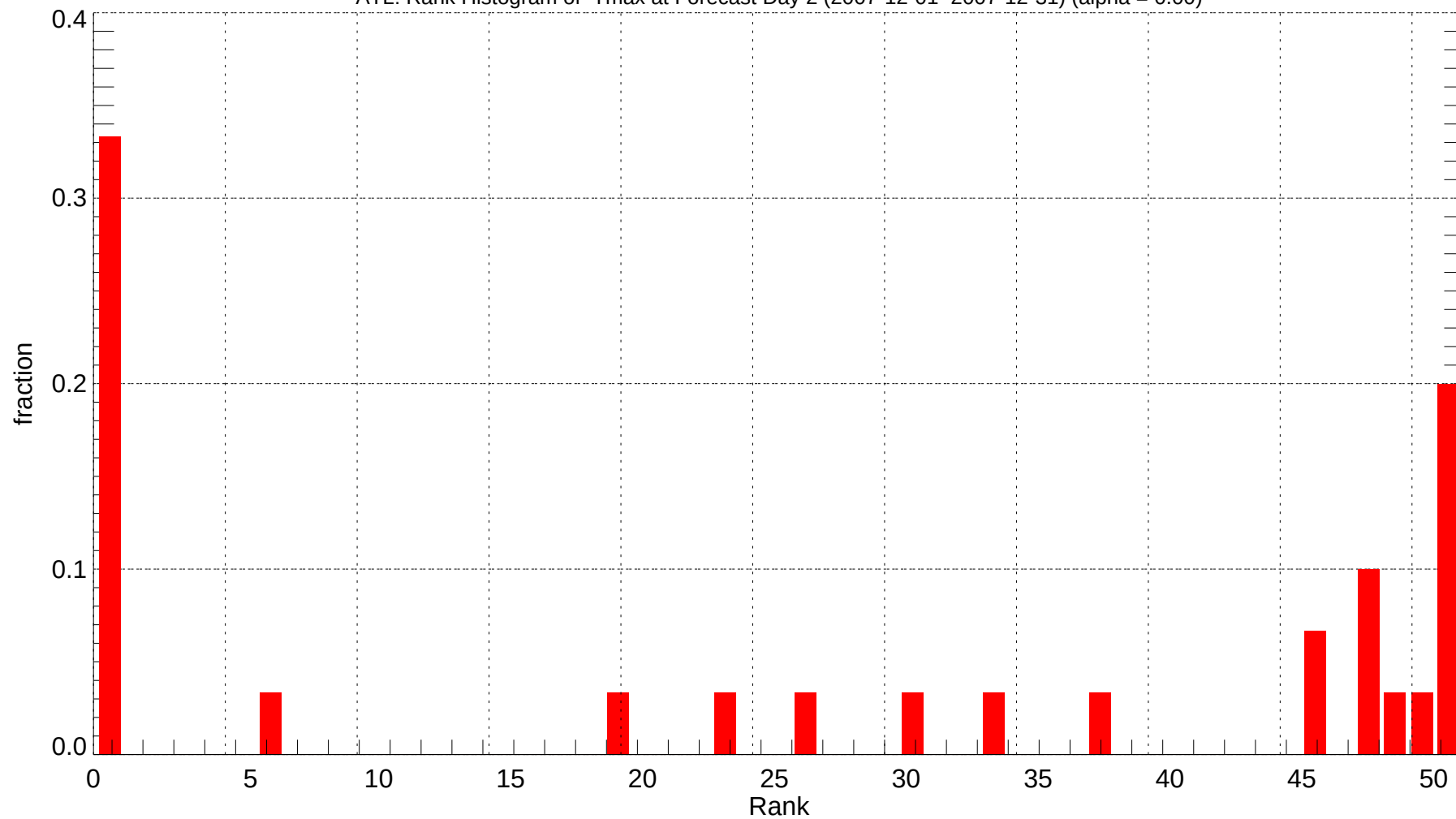
ATL: Rank Histogram of Tmax at Forecast Day 2 (2007-12-01~2007-12-31) (alpha = 0.00)
