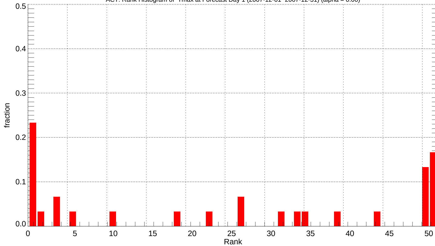
ACT: Rank Histogram of Tmax at Forecast Day 1 (2007-12-01~2007-12-31) (alpha = 0.00)
