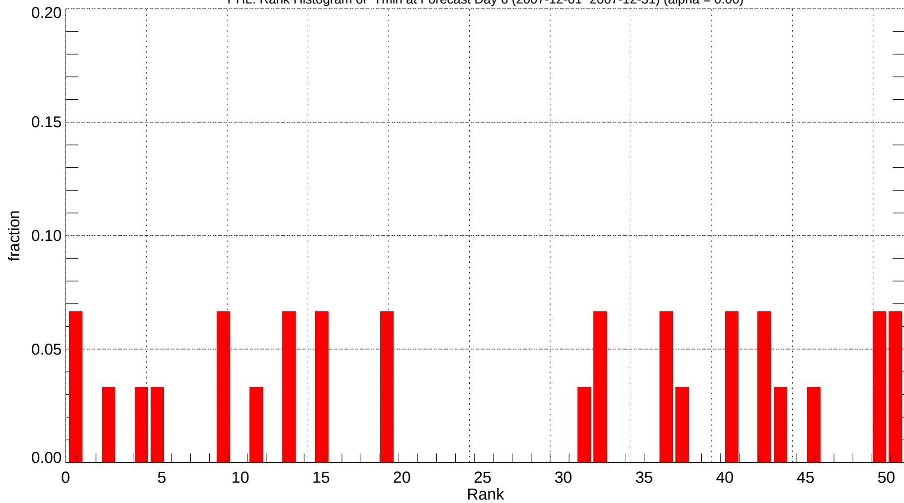
PHL: Rank Histogram of Tmin at Forecast Day 6 (2007-12-01~2007-12-31) (alpha = 0.00)
