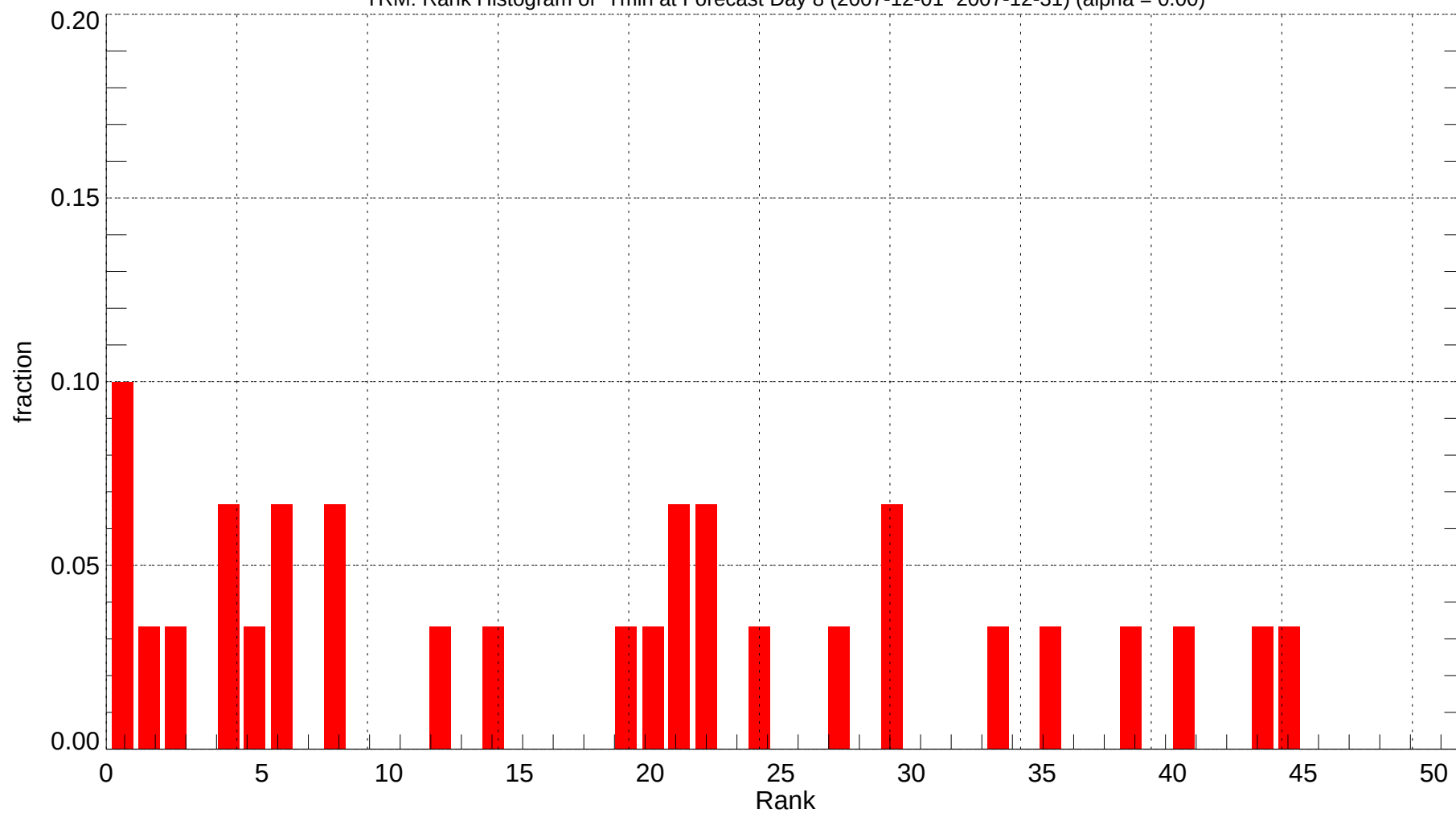
TRM: Rank Histogram of Tmin at Forecast Day 8 (2007-12-01~2007-12-31) (alpha = 0.00)
