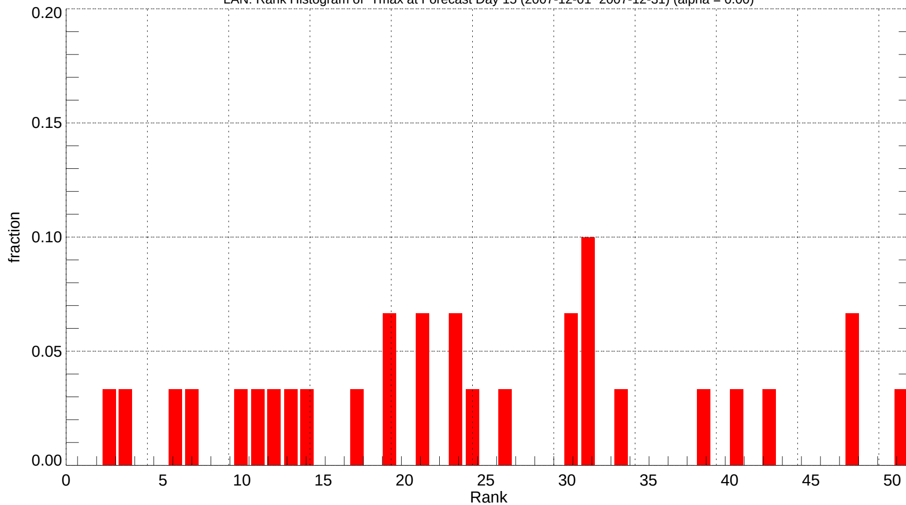
LAN: Rank Histogram of Tmax at Forecast Day 15 (2007-12-01~2007-12-31) (alpha = 0.00)
