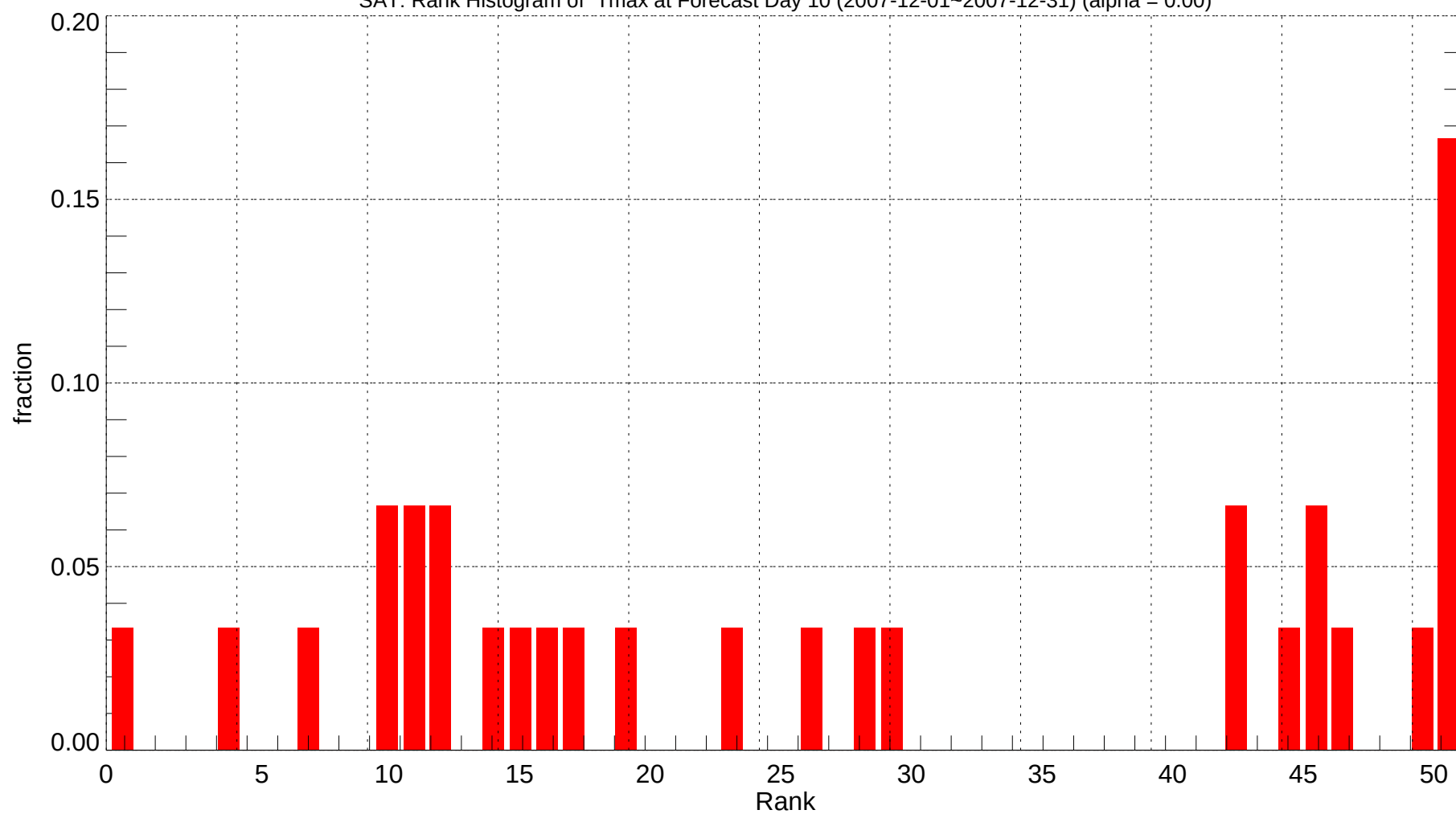
SAT: Rank Histogram of Tmax at Forecast Day 10 (2007-12-01~2007-12-31) (alpha = 0.00)
