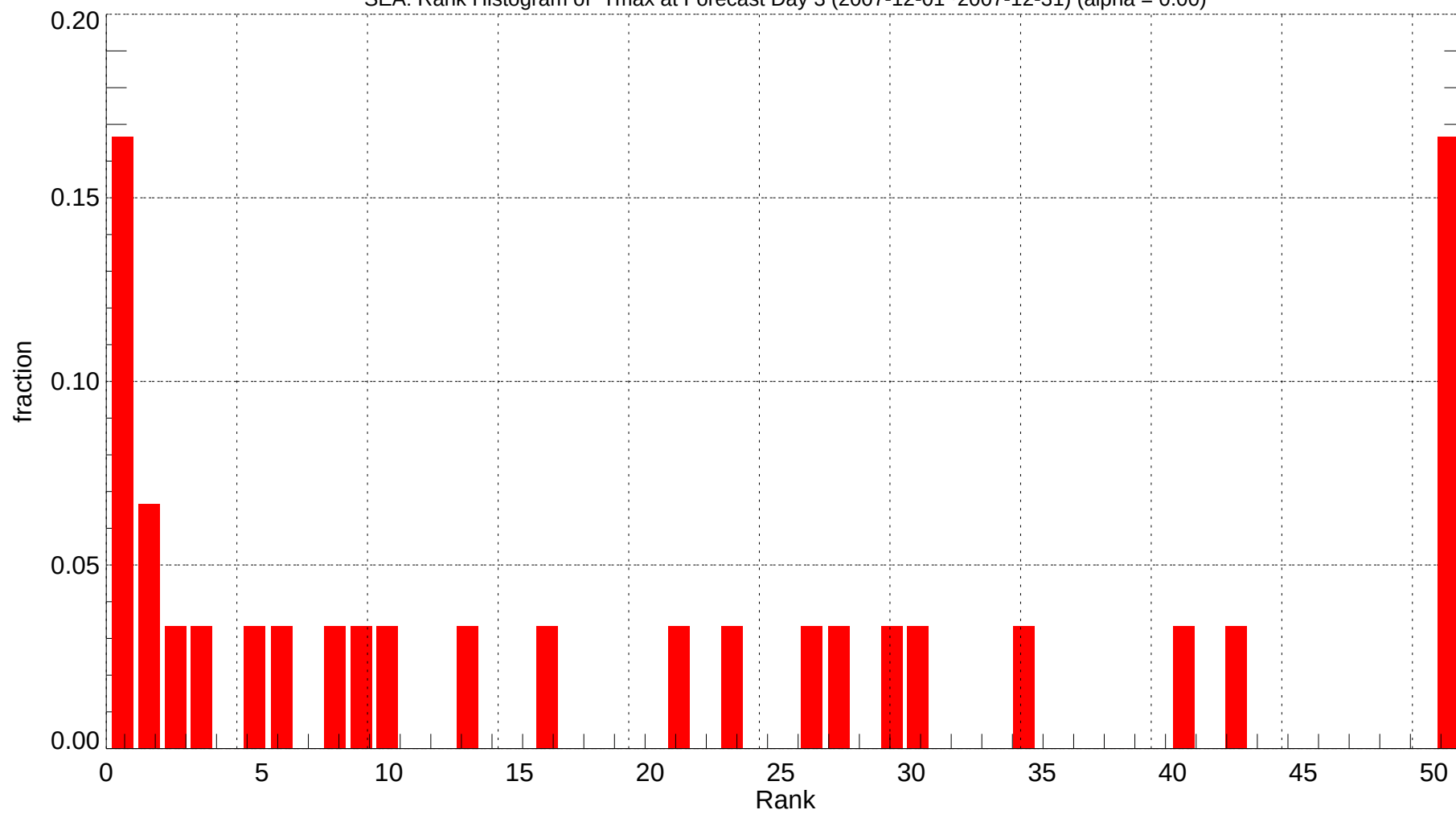
SEA: Rank Histogram of Tmax at Forecast Day 3 (2007-12-01~2007-12-31) (alpha = 0.00)
