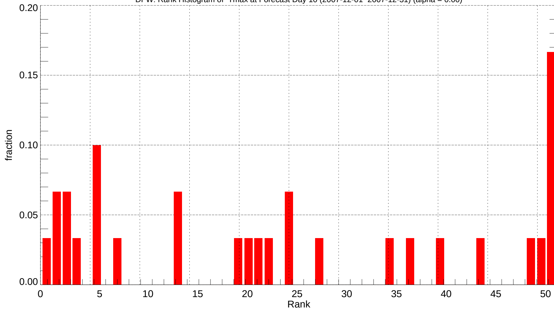
DFW: Rank Histogram of Tmax at Forecast Day 10 (2007-12-01~2007-12-31) (alpha = 0.00)
