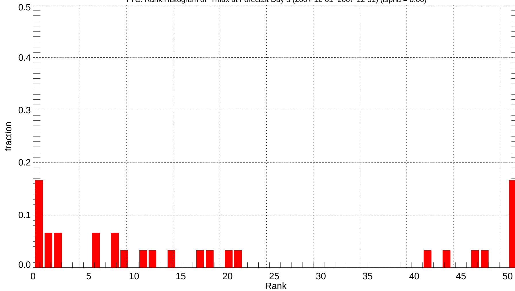
YYC: Rank Histogram of Tmax at Forecast Day 3 (2007-12-01~2007-12-31) (alpha = 0.00)
