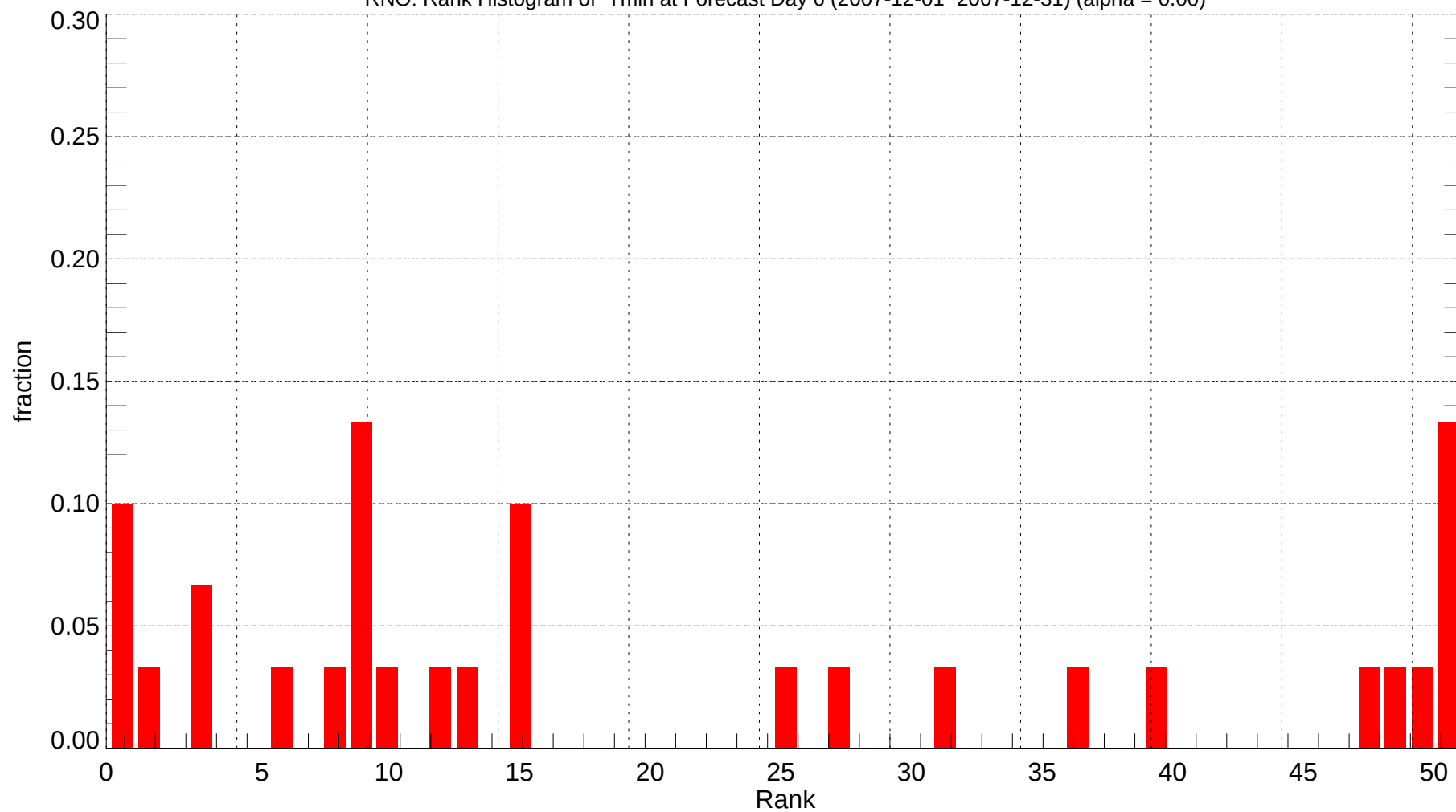
RNO: Rank Histogram of Tmin at Forecast Day 6 (2007-12-01~2007-12-31) (alpha = 0.00)
