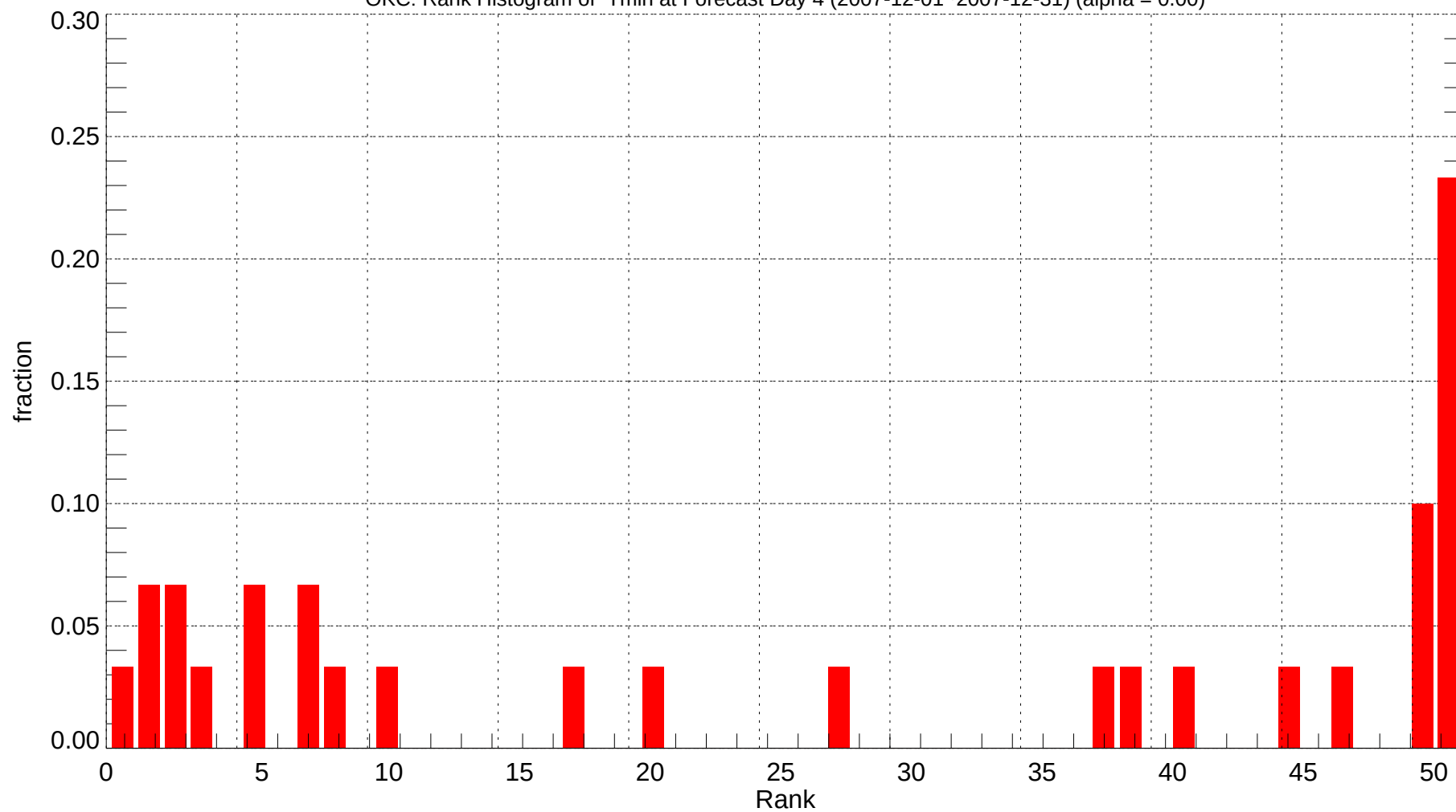
OKC: Rank Histogram of Tmin at Forecast Day 4 (2007-12-01~2007-12-31) (alpha = 0.00)
