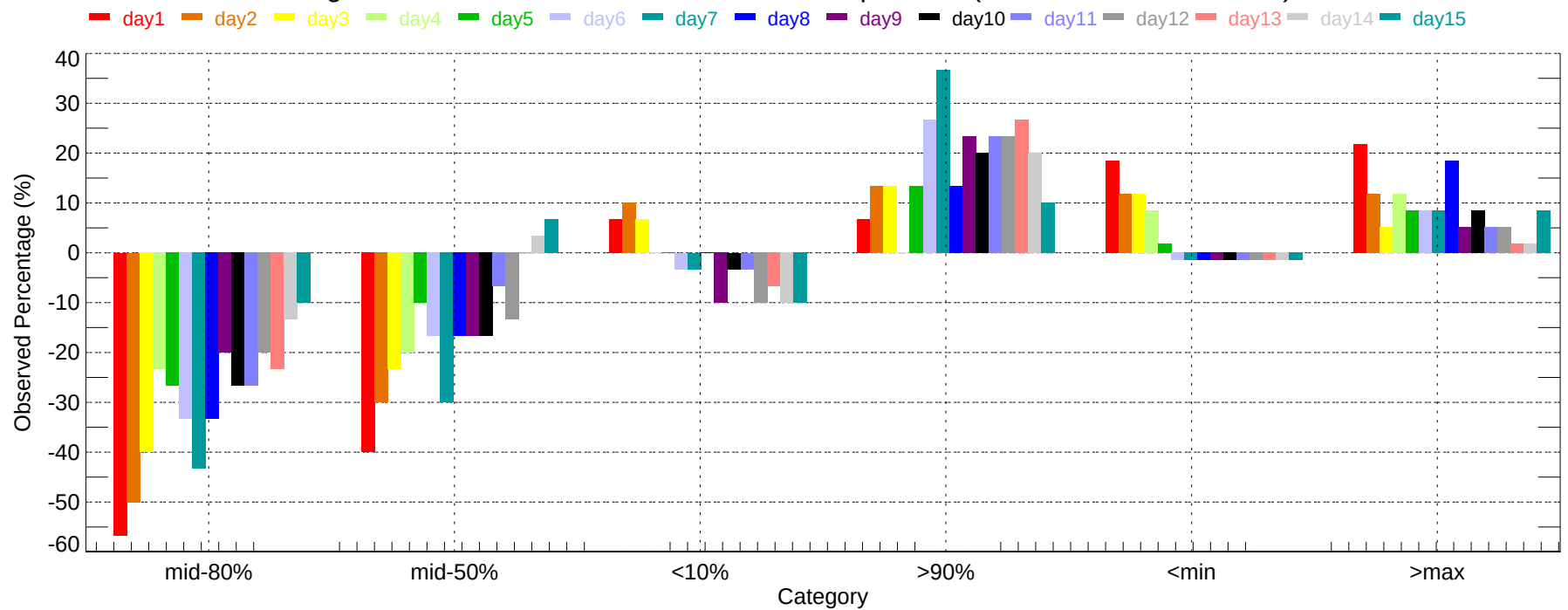
Observed Percentage Deviation of Ensembles - LEX: Min Temperature (2007-12-01~2007-12-31)
