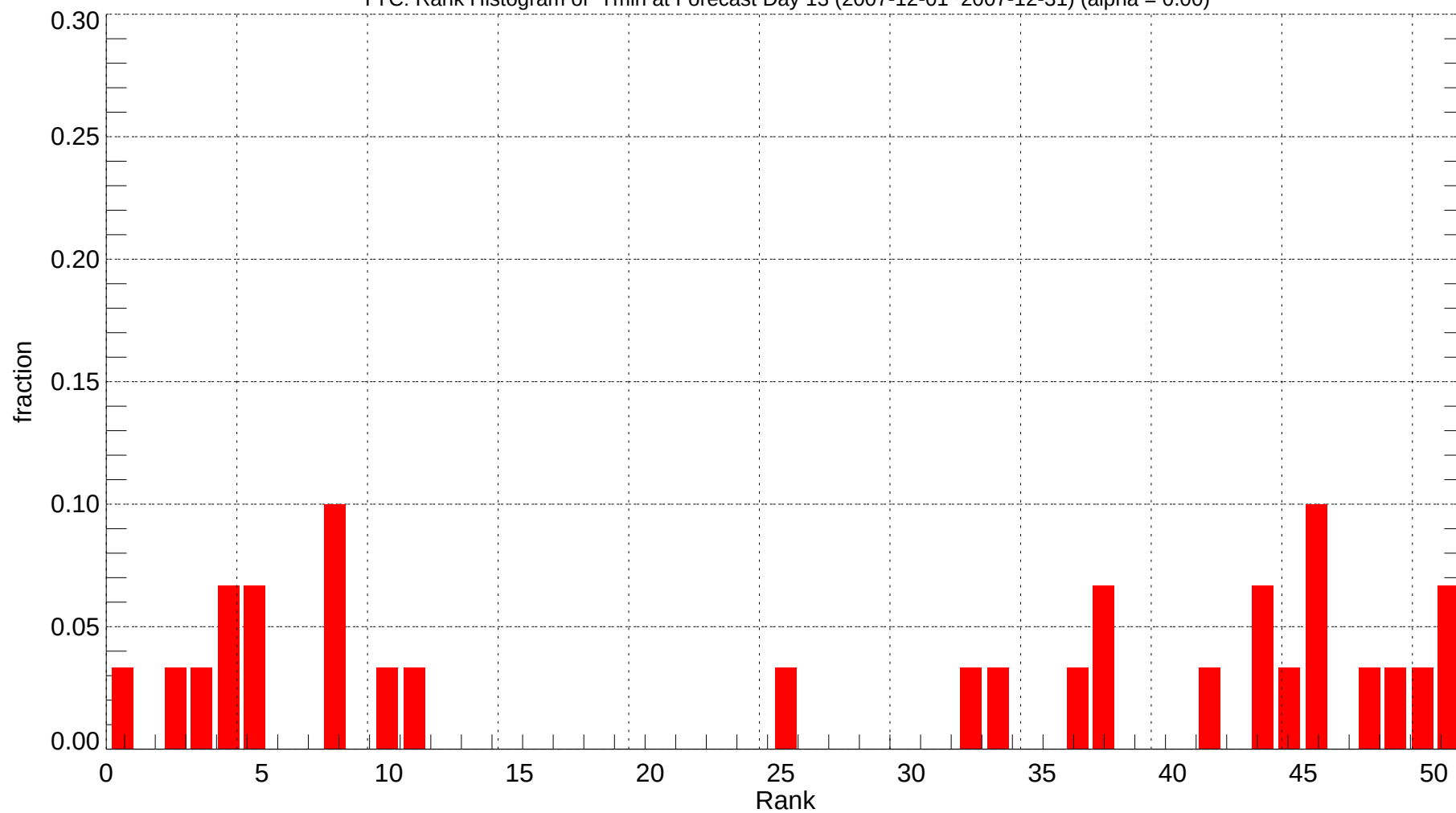
YYC: Rank Histogram of Tmin at Forecast Day 13 (2007-12-01~2007-12-31) (alpha = 0.00)
