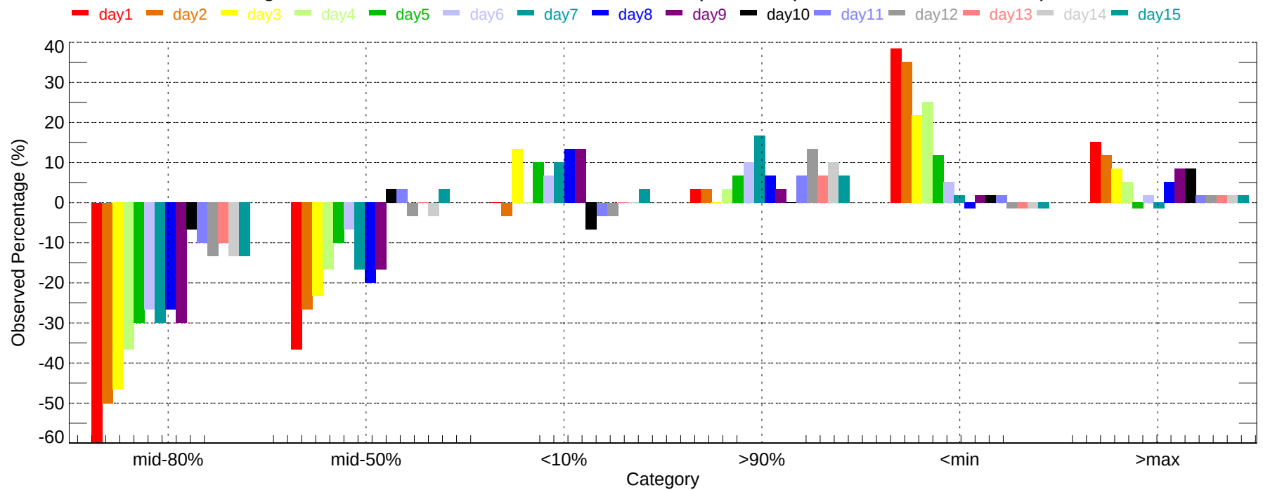
Observed Percentage Deviation of Ensembles - YNG: Min Temperature (2007-12-01~2007-12-31)
