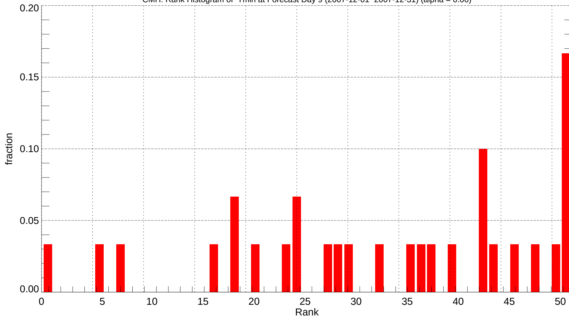
CMH: Rank Histogram of Tmin at Forecast Day 9 (2007-12-01~2007-12-31) (alpha = 0.00)
