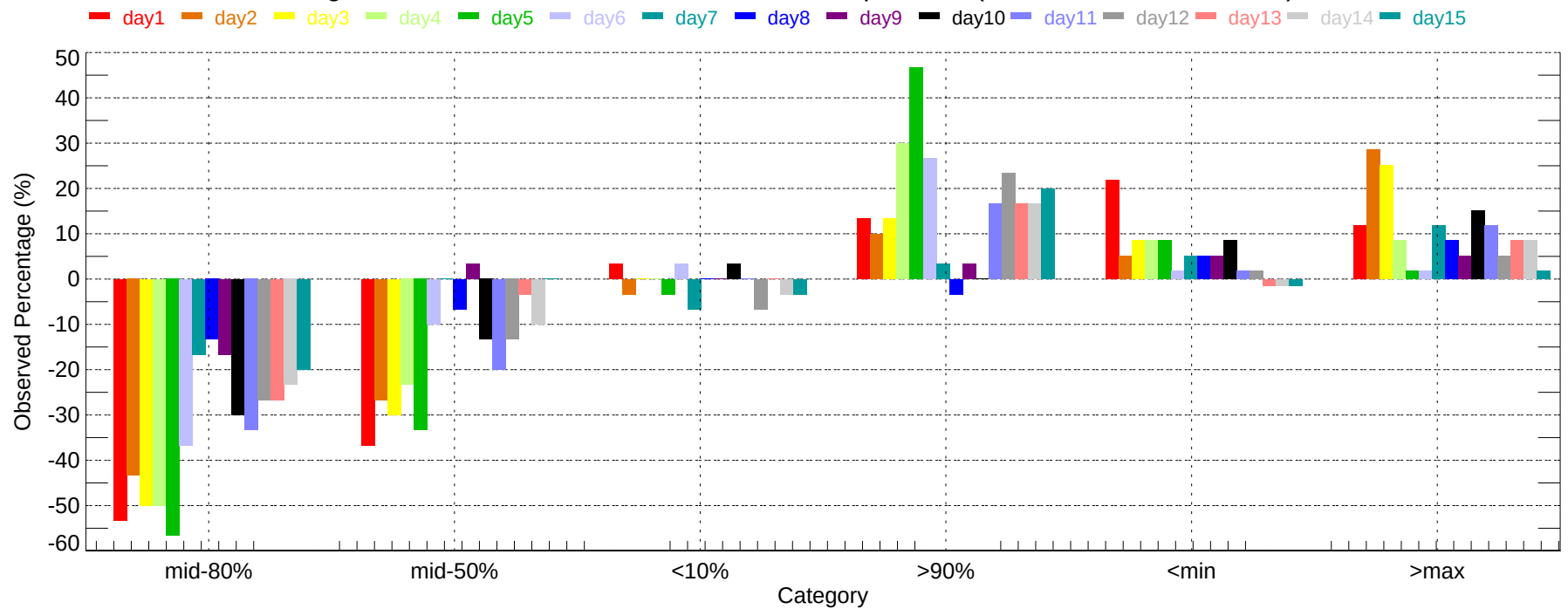
Observed Percentage Deviation of Ensembles - BOI: Max Temperature (2007-12-01~2007-12-31)
