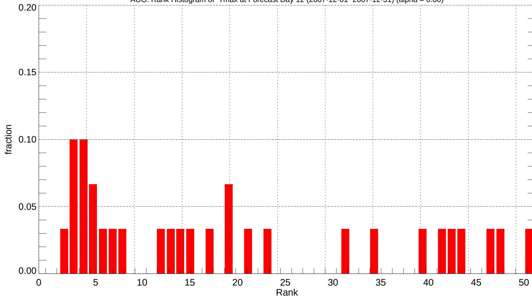
AUG: Rank Histogram of Tmax at Forecast Day 12 (2007-12-01~2007-12-31) (alpha = 0.00)
