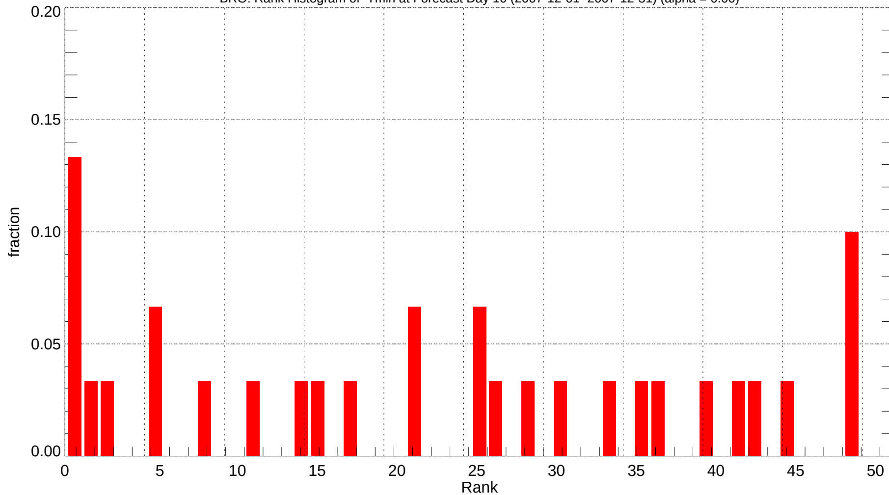
BRO: Rank Histogram of Tmin at Forecast Day 10 (2007-12-01~2007-12-31) (alpha = 0.00)
