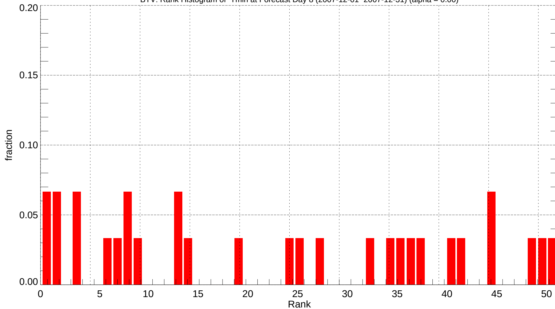
BTV: Rank Histogram of Tmin at Forecast Day 8 (2007-12-01~2007-12-31) (alpha = 0.00)
