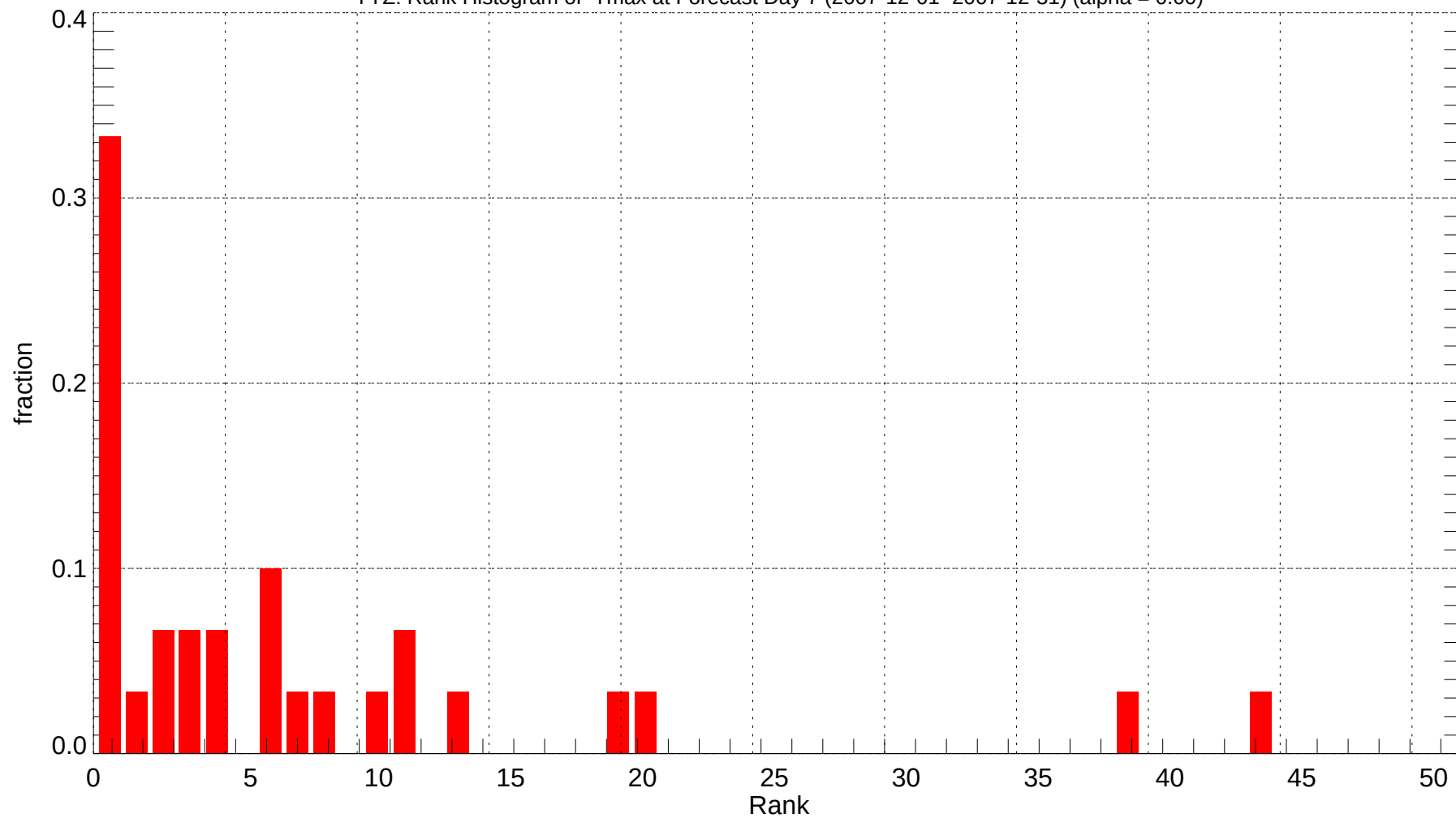
YYZ: Rank Histogram of Tmax at Forecast Day 7 (2007-12-01~2007-12-31) (alpha = 0.00)
