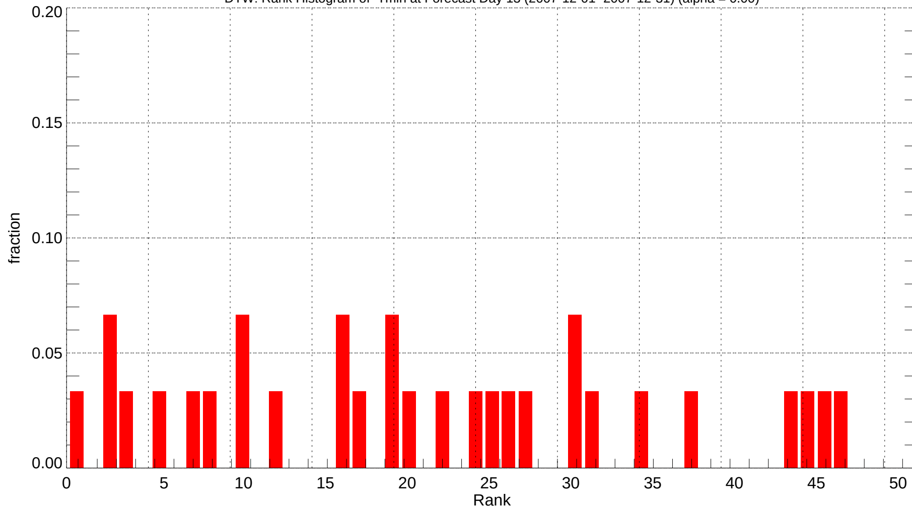
DTW: Rank Histogram of Tmin at Forecast Day 13 (2007-12-01~2007-12-31) (alpha = 0.00)
