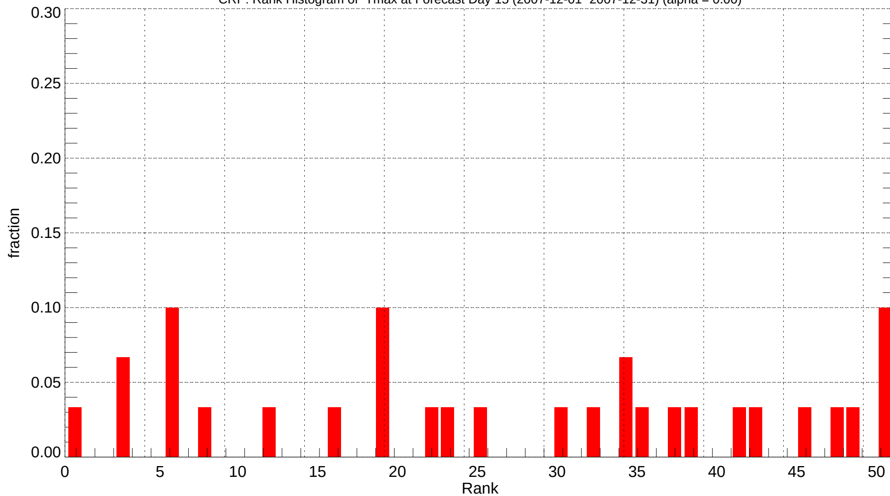
CRP: Rank Histogram of Tmax at Forecast Day 15 (2007-12-01~2007-12-31) (alpha = 0.00)
