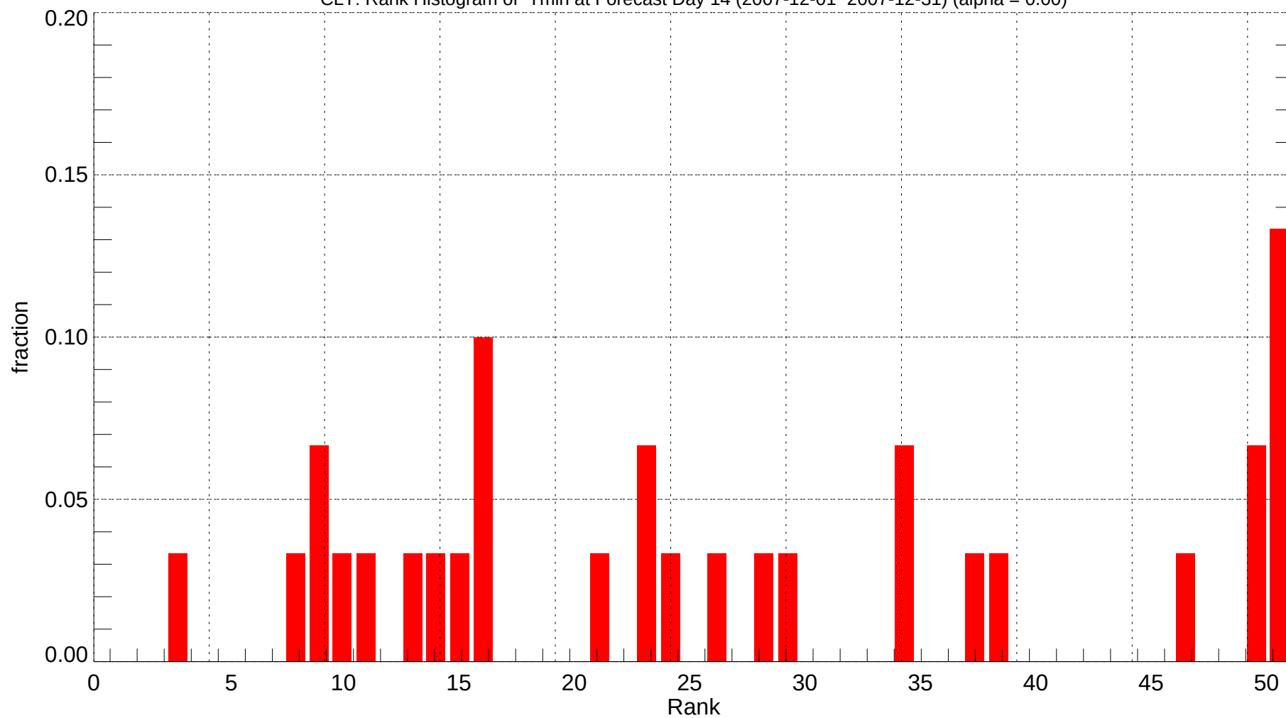
CLT: Rank Histogram of Tmin at Forecast Day 14 (2007-12-01~2007-12-31) (alpha = 0.00)
