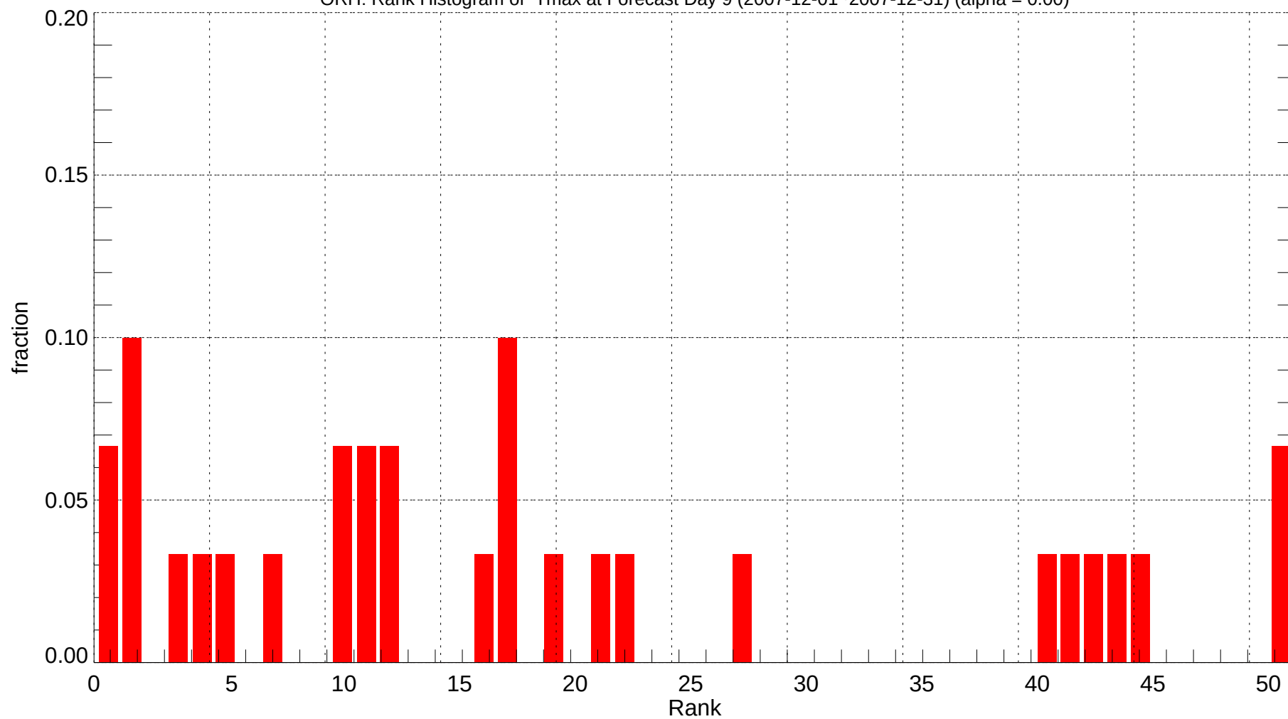
ORH: Rank Histogram of Tmax at Forecast Day 9 (2007-12-01~2007-12-31) (alpha = 0.00)
