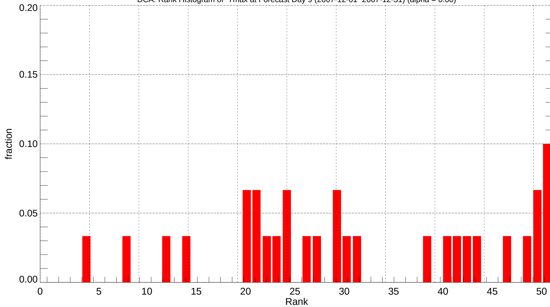
DCA: Rank Histogram of Tmax at Forecast Day 9 (2007-12-01~2007-12-31) (alpha = 0.00)
