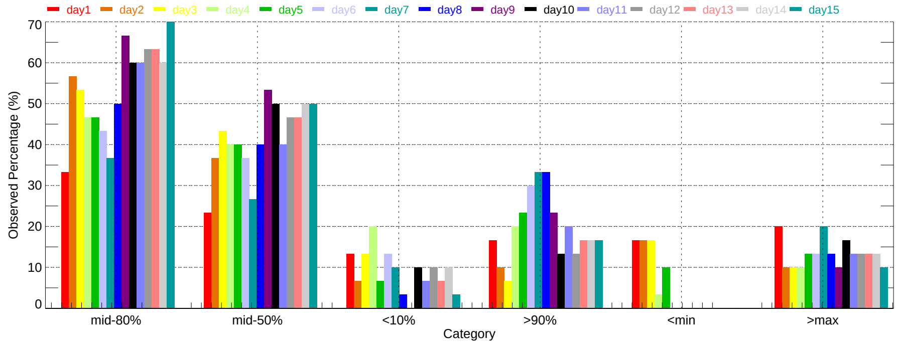
Observed Percentage of Ensembles - CHA: Min Temperature (2007-12-01~2007-12-31)
