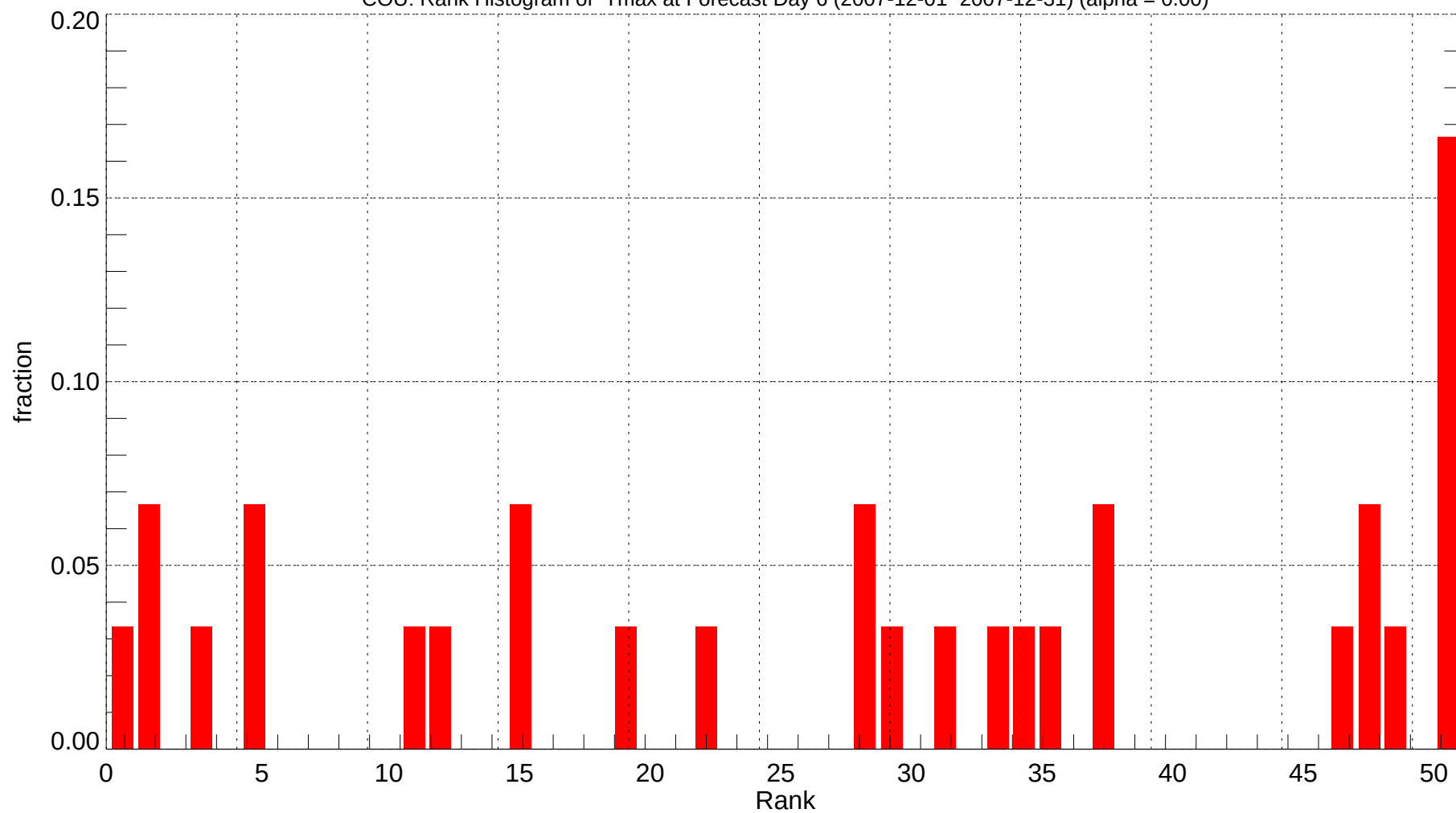
COU: Rank Histogram of Tmax at Forecast Day 6 (2007-12-01~2007-12-31) (alpha = 0.00)
