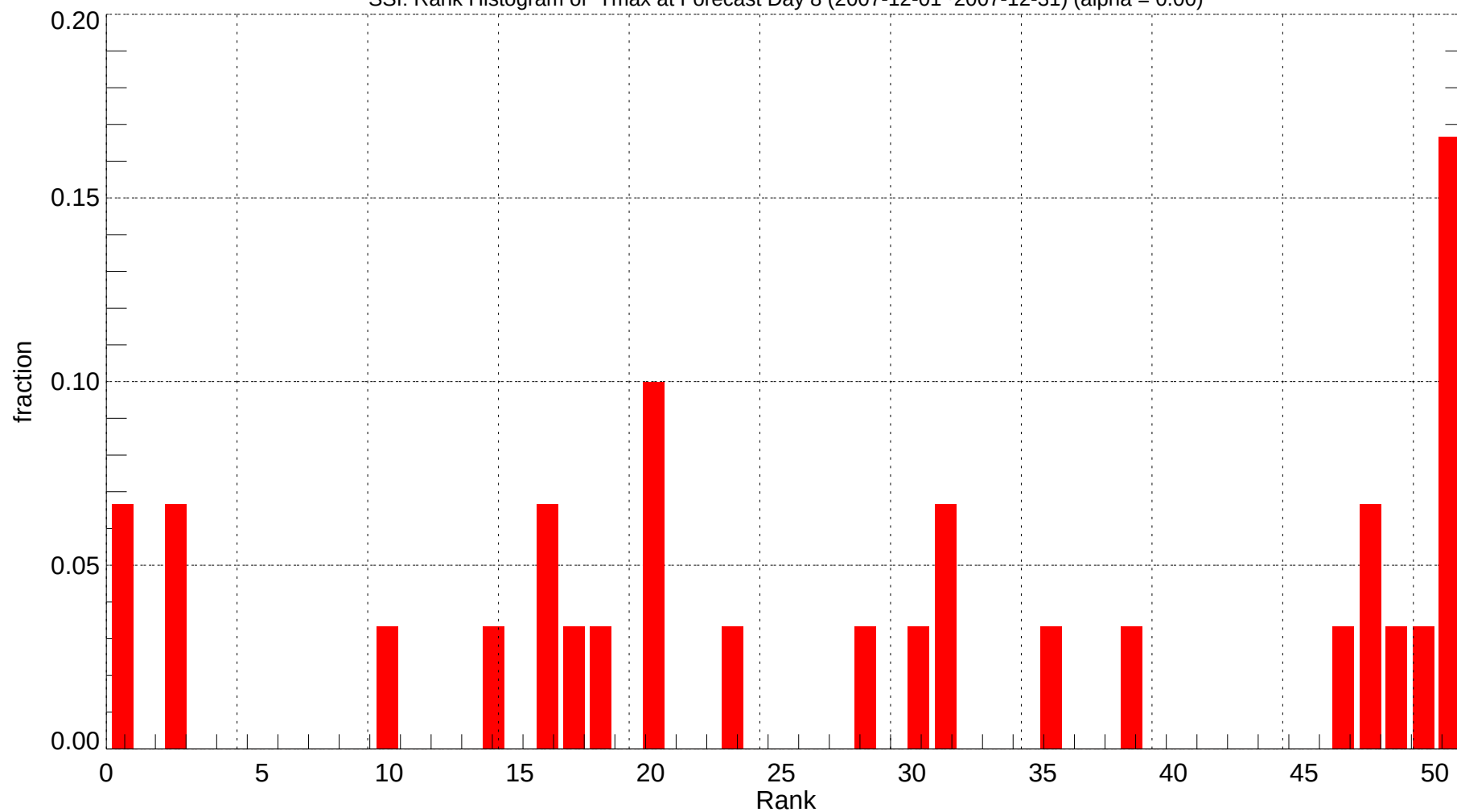
SSI: Rank Histogram of Tmax at Forecast Day 8 (2007-12-01~2007-12-31) (alpha = 0.00)
