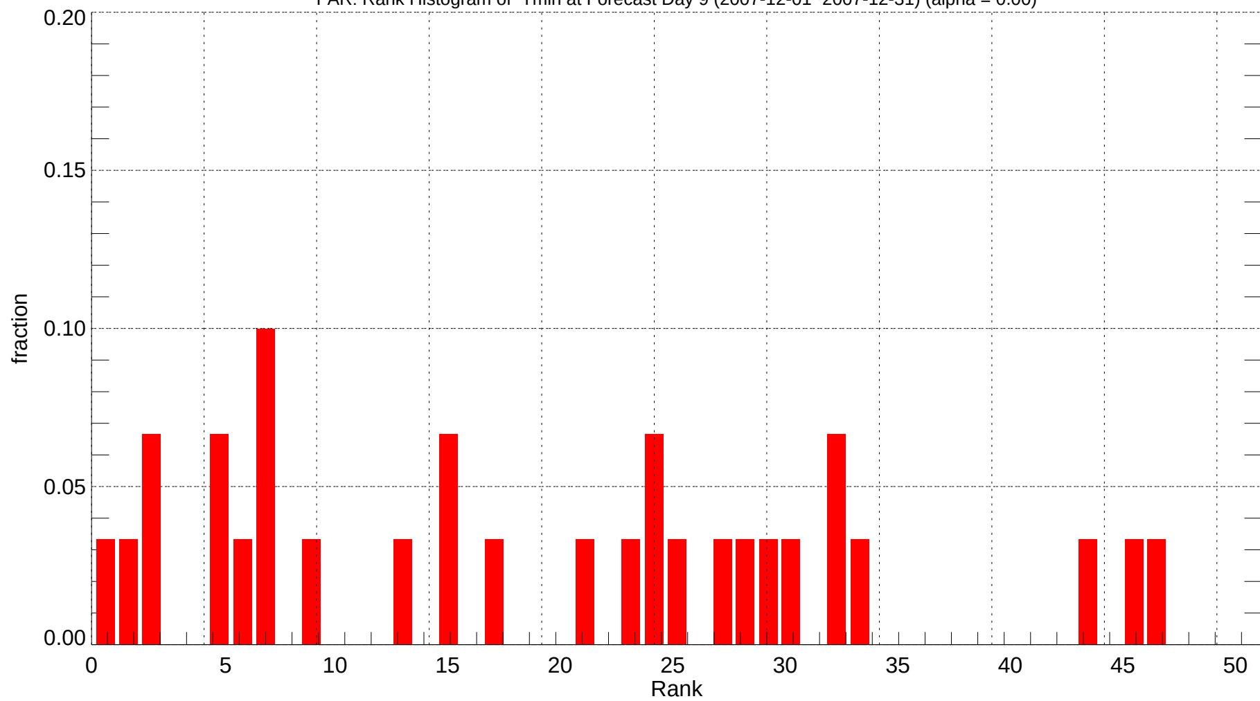
FAR: Rank Histogram of Tmin at Forecast Day 9 (2007-12-01~2007-12-31) (alpha = 0.00)
