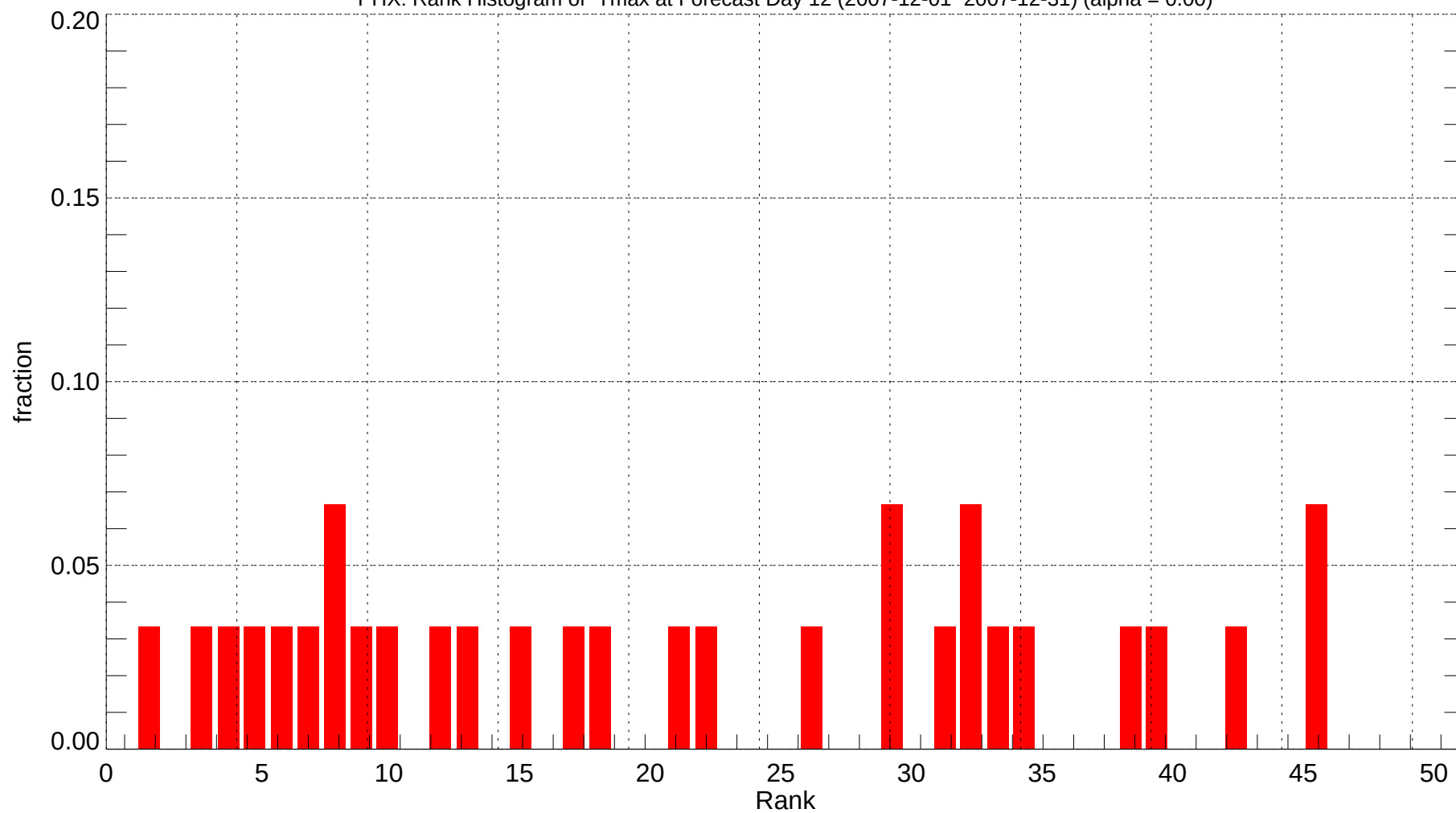
PHX: Rank Histogram of Tmax at Forecast Day 12 (2007-12-01~2007-12-31) (alpha = 0.00)
