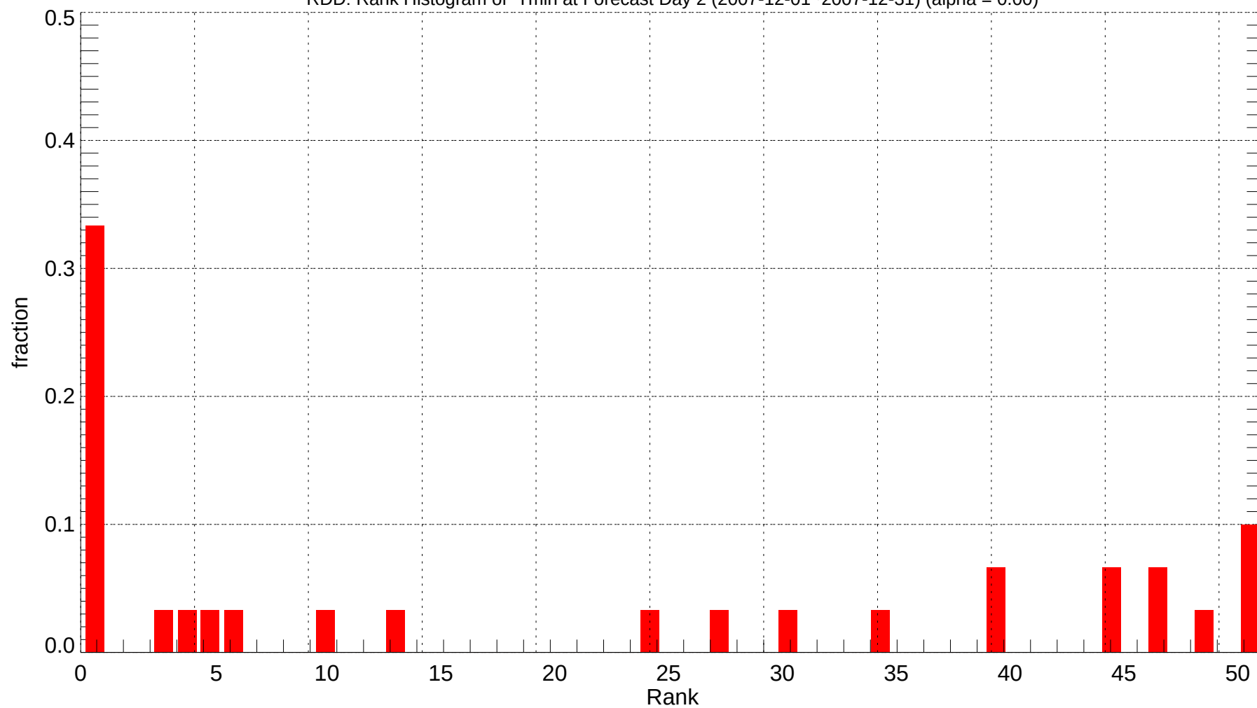
RDD: Rank Histogram of Tmin at Forecast Day 2 (2007-12-01~2007-12-31) (alpha = 0.00)
