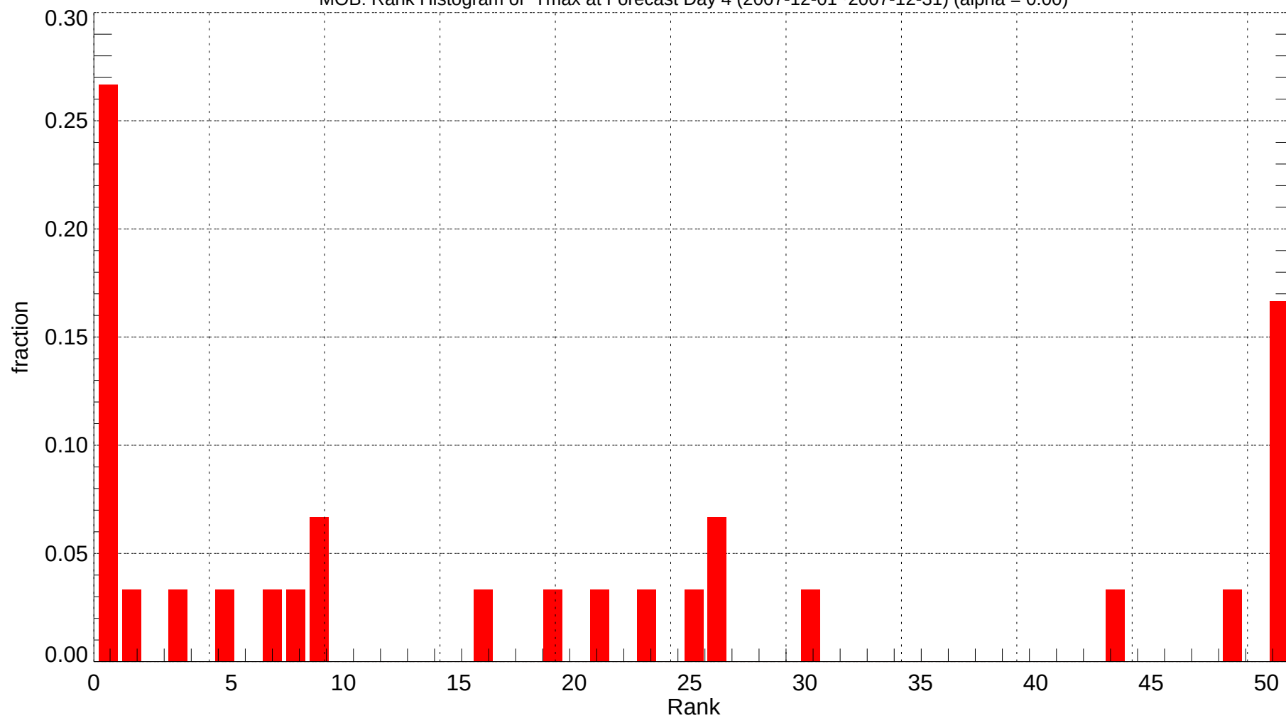
MOB: Rank Histogram of Tmax at Forecast Day 4 (2007-12-01~2007-12-31) (alpha = 0.00)
