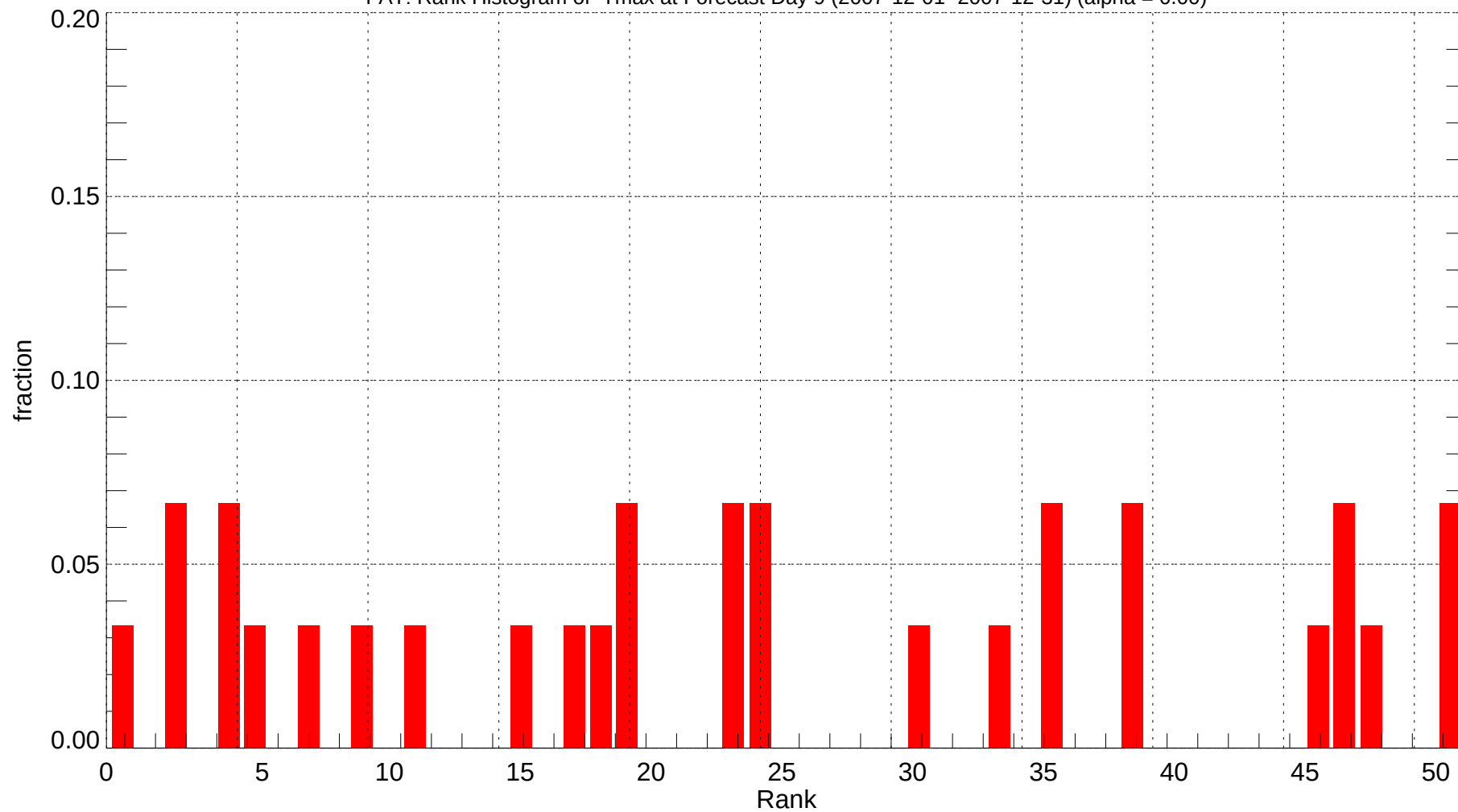
FAT: Rank Histogram of Tmax at Forecast Day 9 (2007-12-01~2007-12-31) (alpha = 0.00)
