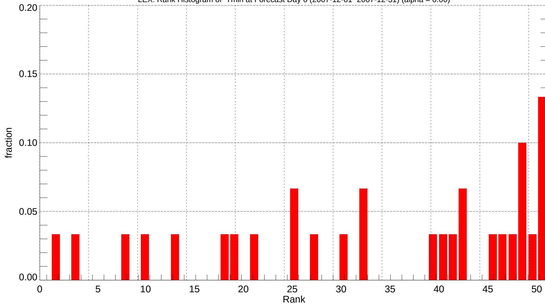
LEX: Rank Histogram of Tmin at Forecast Day 6 (2007-12-01~2007-12-31) (alpha = 0.00)
