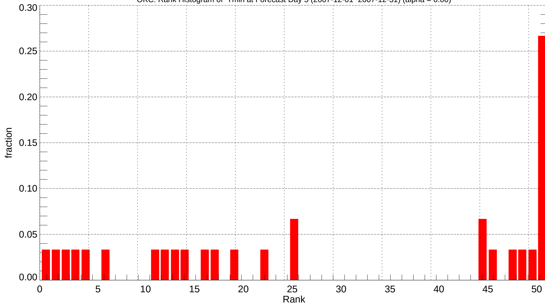
OKC: Rank Histogram of Tmin at Forecast Day 5 (2007-12-01~2007-12-31) (alpha = 0.00)
