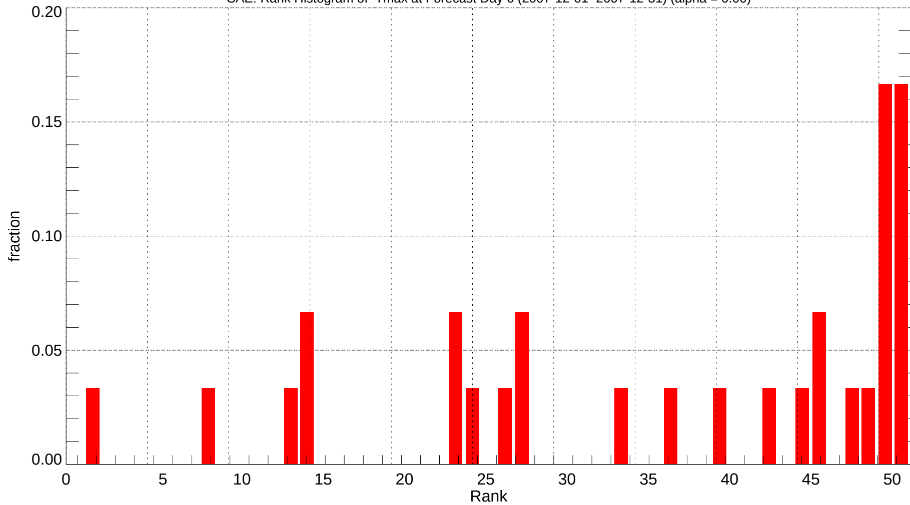
CAE: Rank Histogram of Tmax at Forecast Day 6 (2007-12-01~2007-12-31) (alpha = 0.00)
