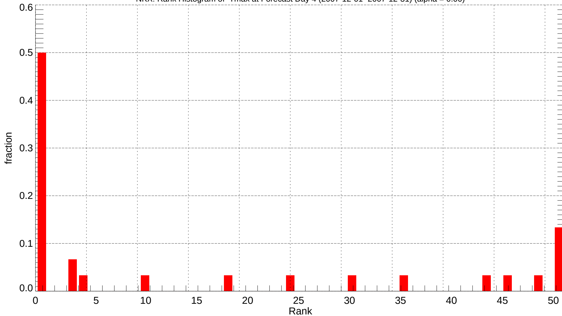
NKX: Rank Histogram of Tmax at Forecast Day 4 (2007-12-01~2007-12-31) (alpha = 0.00)
