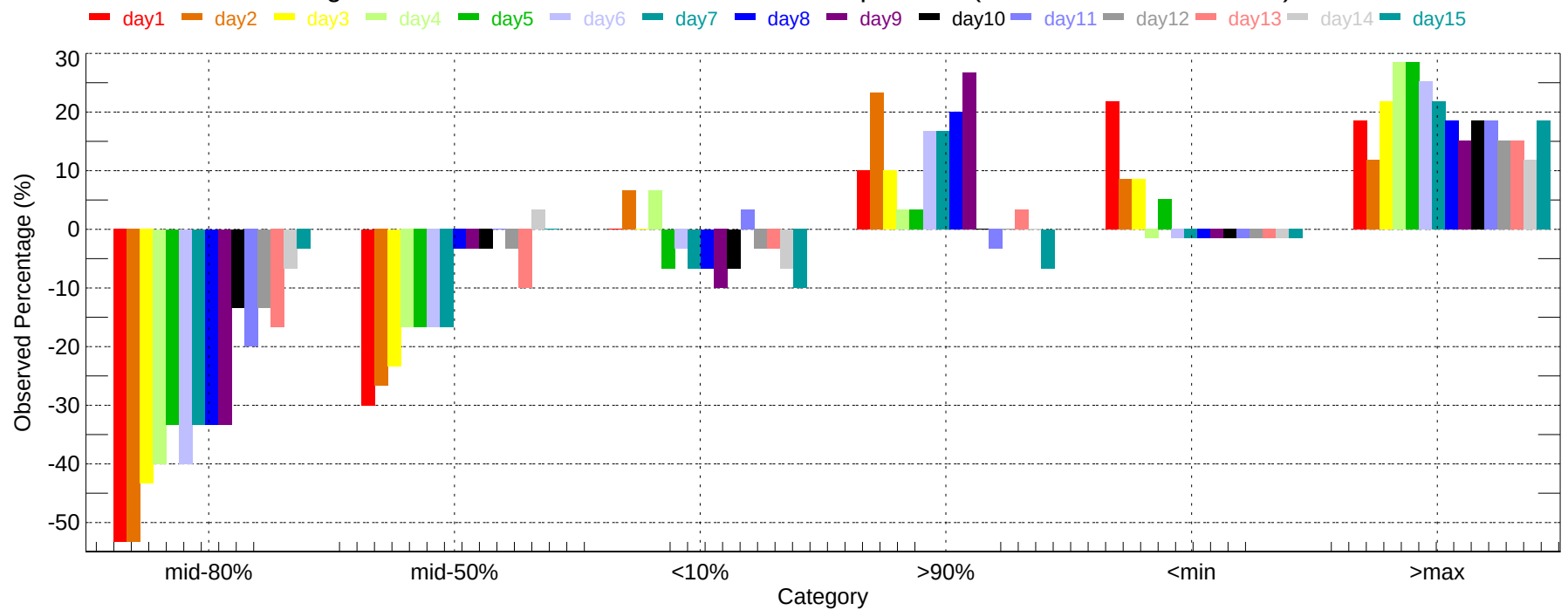
Observed Percentage Deviation of Ensembles - CLT: Min Temperature (2007-12-01~2007-12-31)
