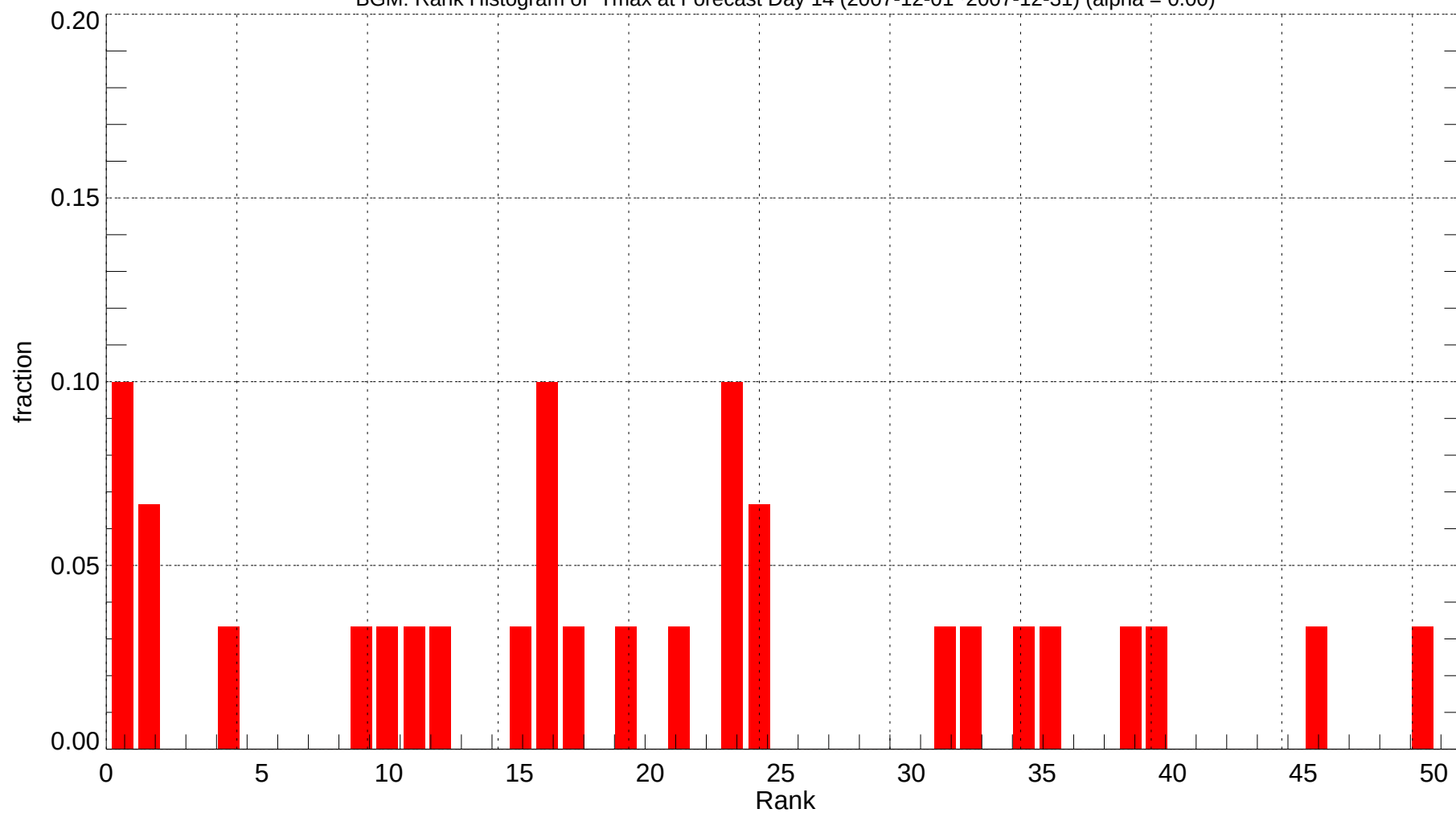
BGM: Rank Histogram of Tmax at Forecast Day 14 (2007-12-01~2007-12-31) (alpha = 0.00)
