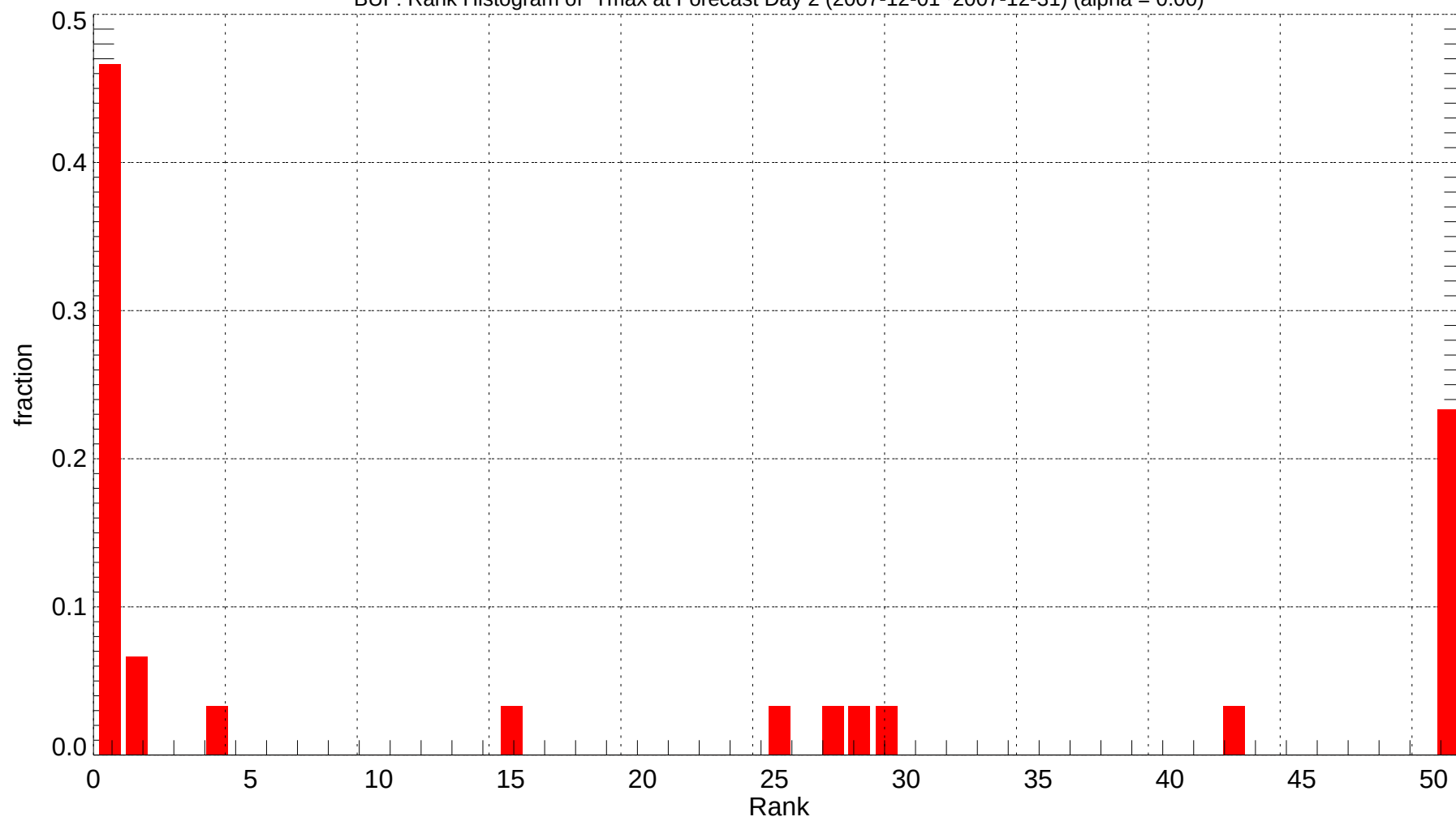
BUF: Rank Histogram of Tmax at Forecast Day 2 (2007-12-01~2007-12-31) (alpha = 0.00)
