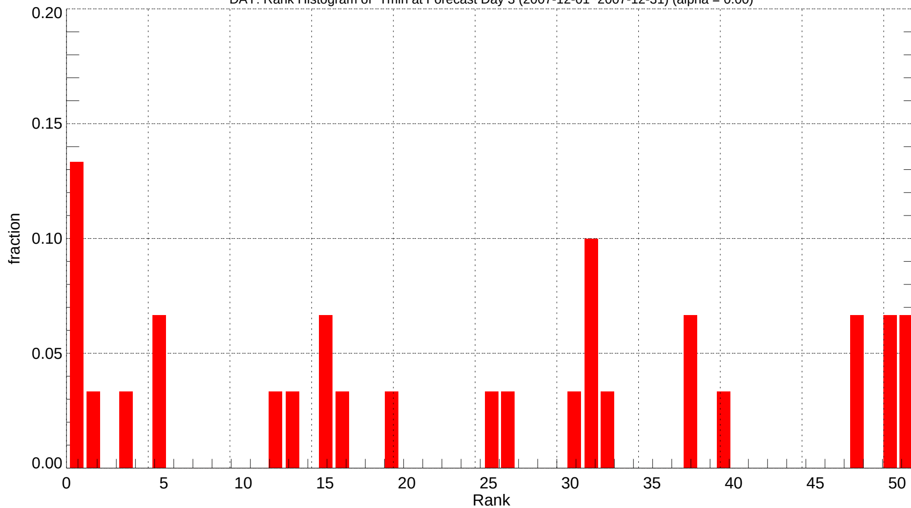
DAY: Rank Histogram of Tmin at Forecast Day 3 (2007-12-01~2007-12-31) (alpha = 0.00)
