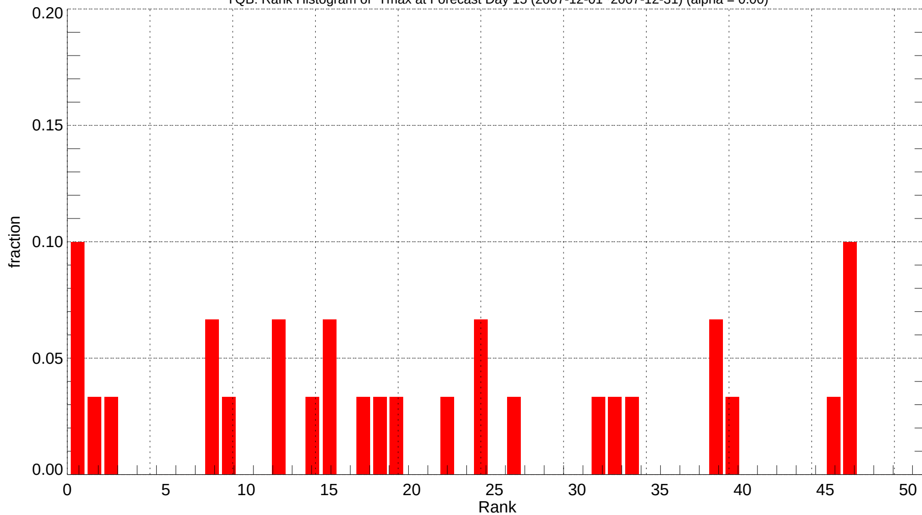
YQB: Rank Histogram of Tmax at Forecast Day 15 (2007-12-01~2007-12-31) (alpha = 0.00)
