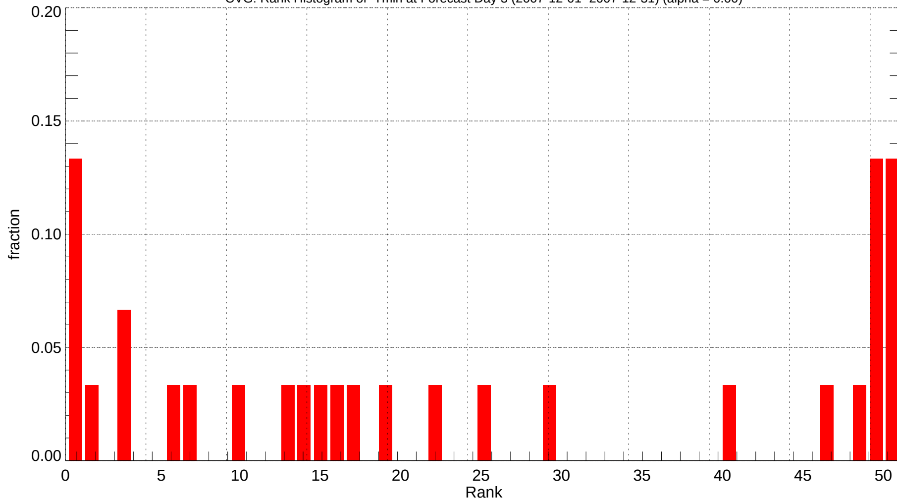
CVG: Rank Histogram of Tmin at Forecast Day 3 (2007-12-01~2007-12-31) (alpha = 0.00)
