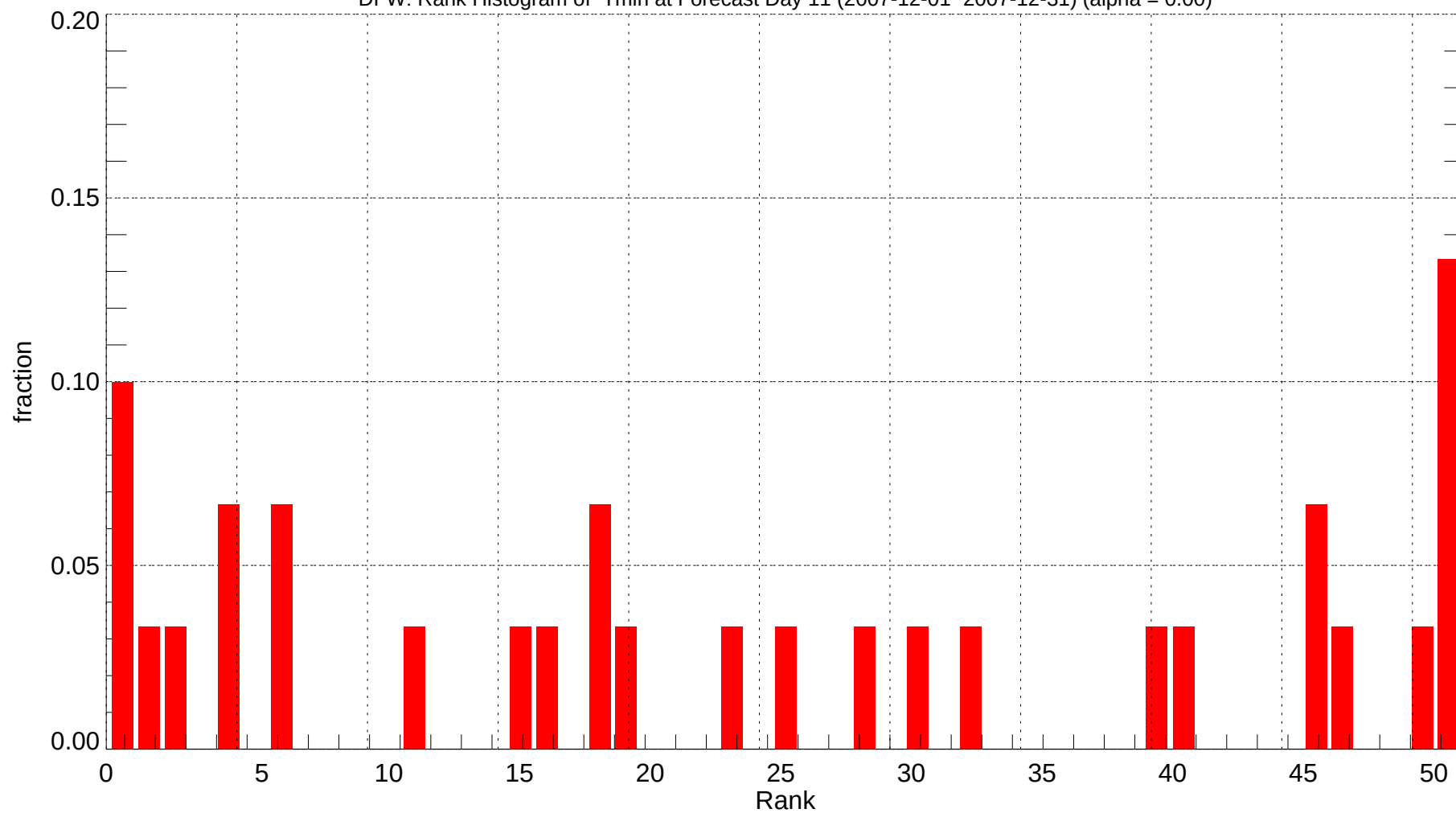
DFW: Rank Histogram of Tmin at Forecast Day 11 (2007-12-01~2007-12-31) (alpha = 0.00)
