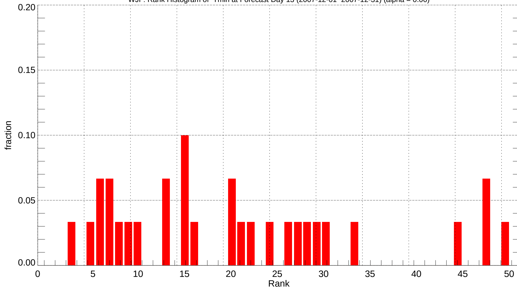
WJF: Rank Histogram of Tmin at Forecast Day 13 (2007-12-01~2007-12-31) (alpha = 0.00)
