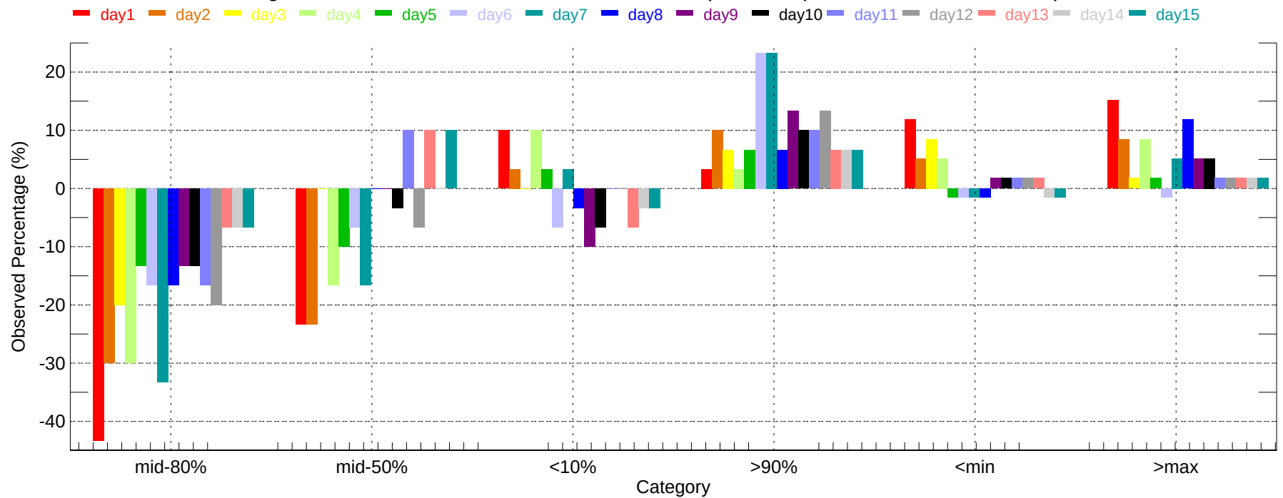
Observed Percentage Deviation of Ensembles - DAY: Min Temperature (2007-12-01~2007-12-31)
