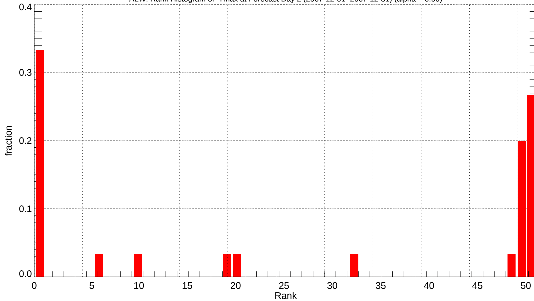
ALW: Rank Histogram of Tmax at Forecast Day 2 (2007-12-01~2007-12-31) (alpha = 0.00)
