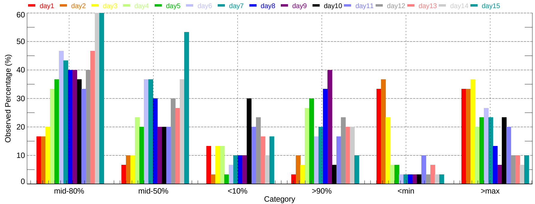
Observed Percentage of Ensembles - TUL: Max Temperature (2007-12-01~2007-12-31)
