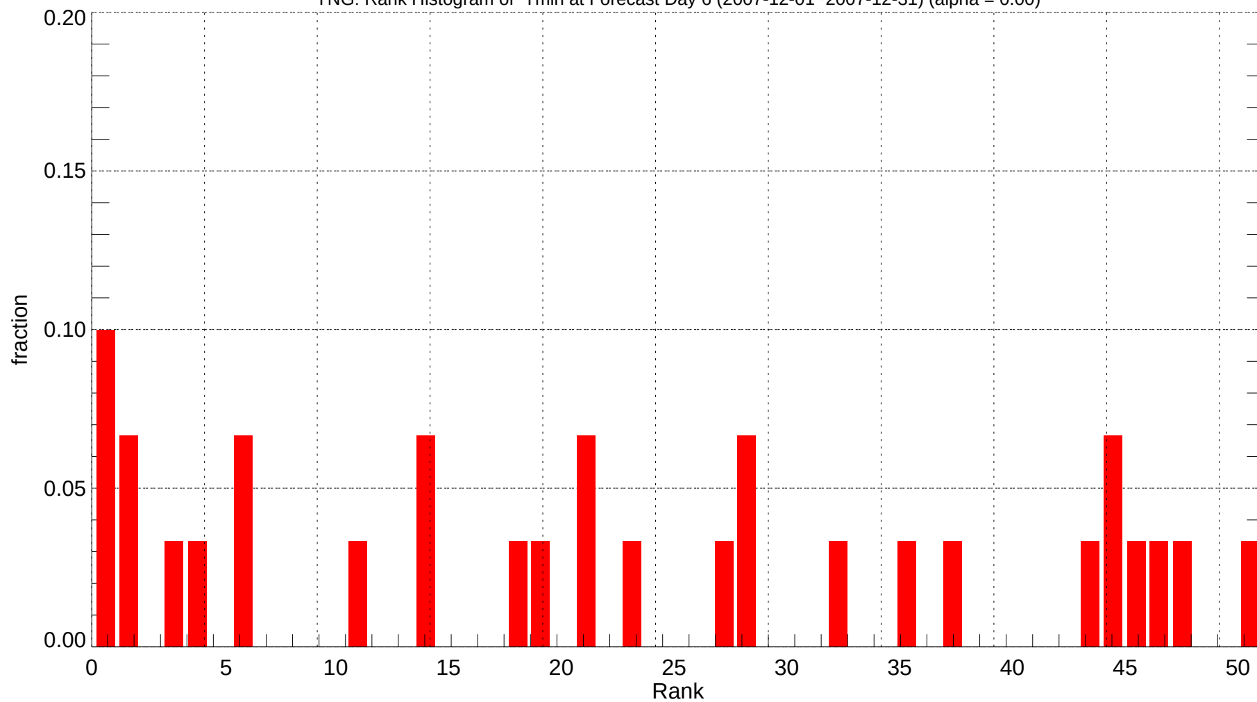
YNG: Rank Histogram of Tmin at Forecast Day 6 (2007-12-01~2007-12-31) (alpha = 0.00)
