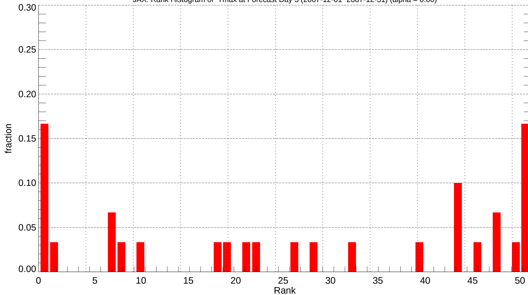
JAX: Rank Histogram of Tmax at Forecast Day 3 (2007-12-01~2007-12-31) (alpha = 0.00)
