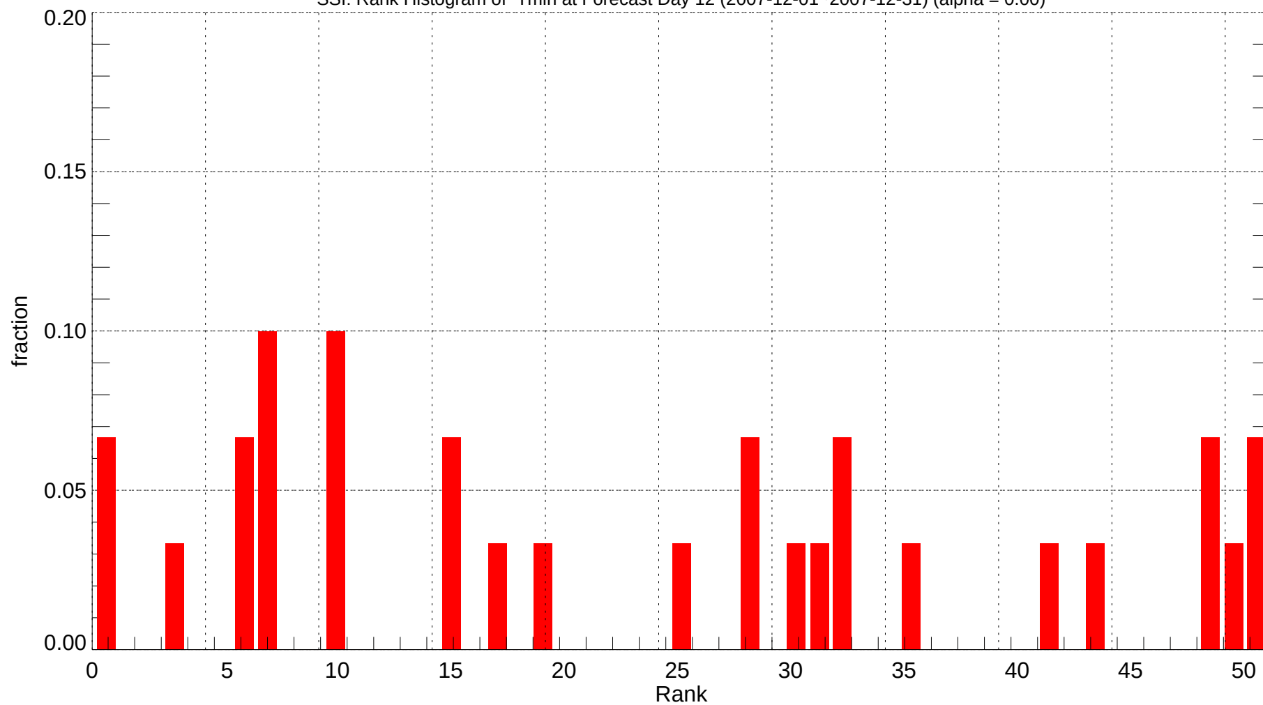
SSI: Rank Histogram of Tmin at Forecast Day 12 (2007-12-01~2007-12-31) (alpha = 0.00)
