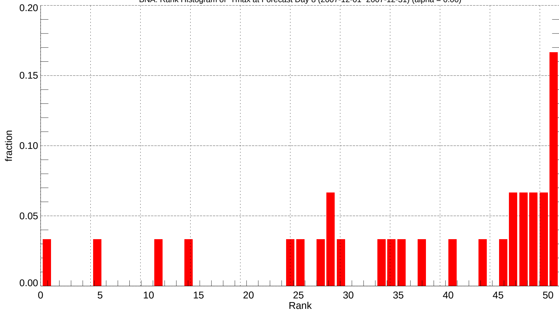
BNA: Rank Histogram of Tmax at Forecast Day 8 (2007-12-01~2007-12-31) (alpha = 0.00)
