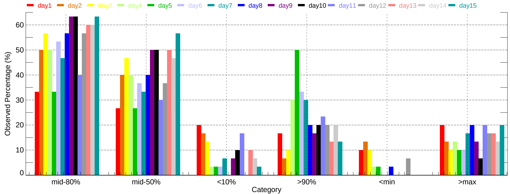
Observed Percentage of Ensembles - AUS: Min Temperature (2007-12-01~2007-12-31)
