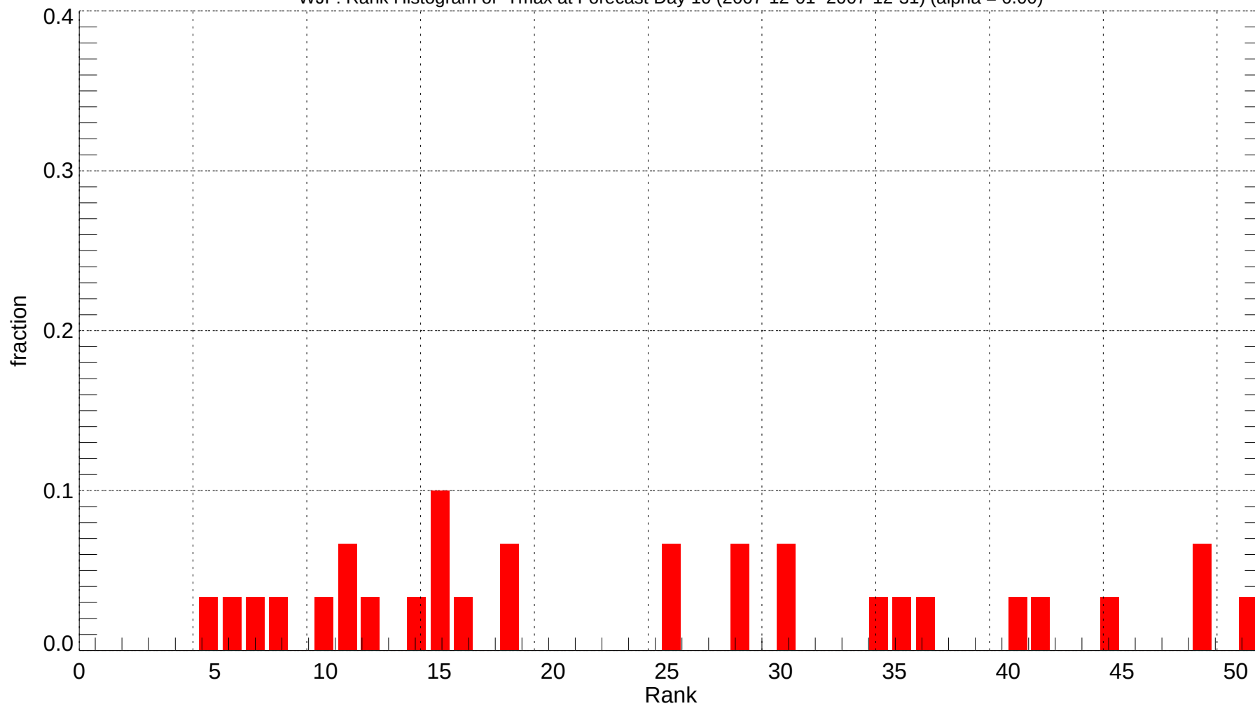
WJF: Rank Histogram of Tmax at Forecast Day 10 (2007-12-01~2007-12-31) (alpha = 0.00)
