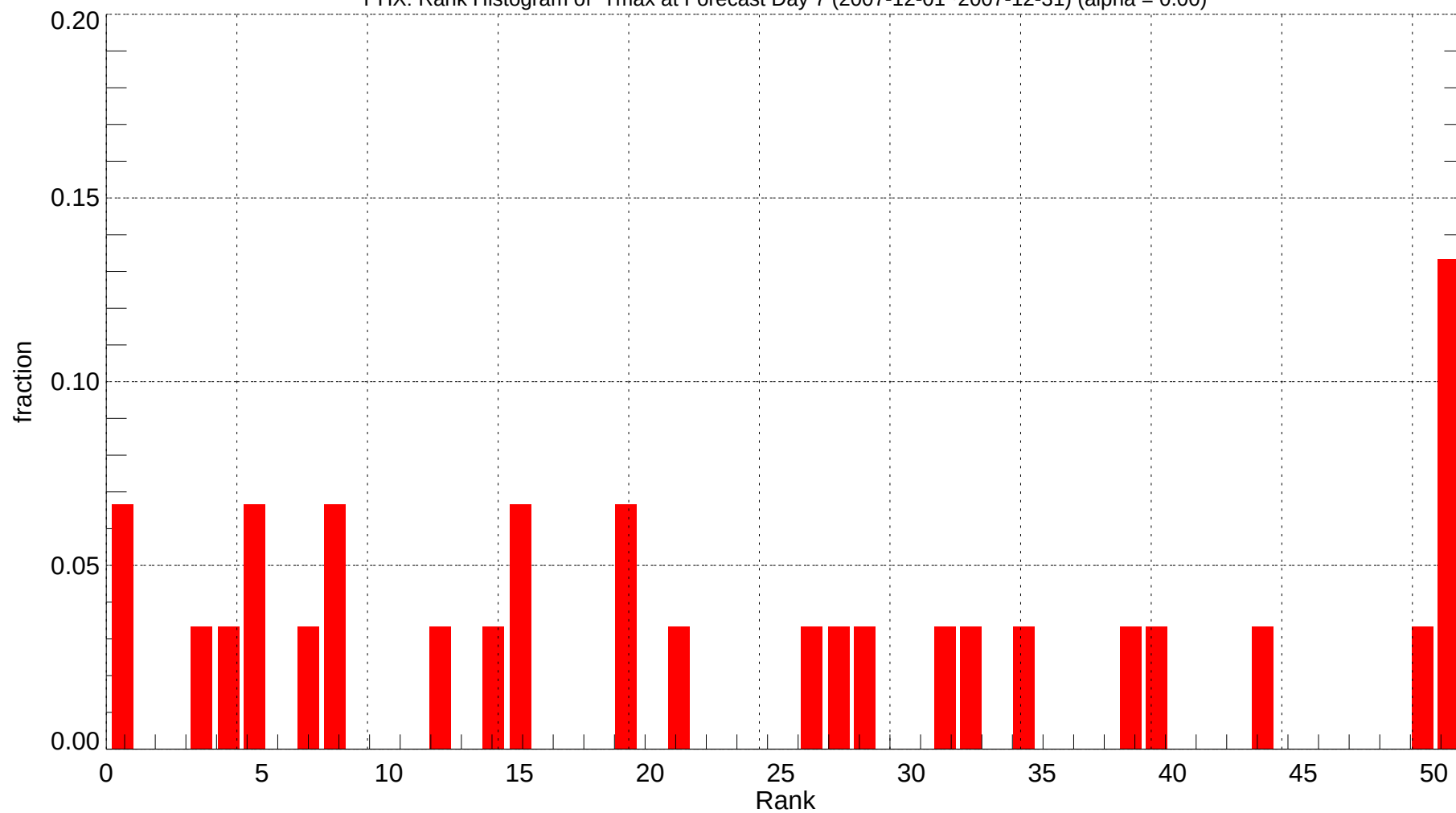
PHX: Rank Histogram of Tmax at Forecast Day 7 (2007-12-01~2007-12-31) (alpha = 0.00)
