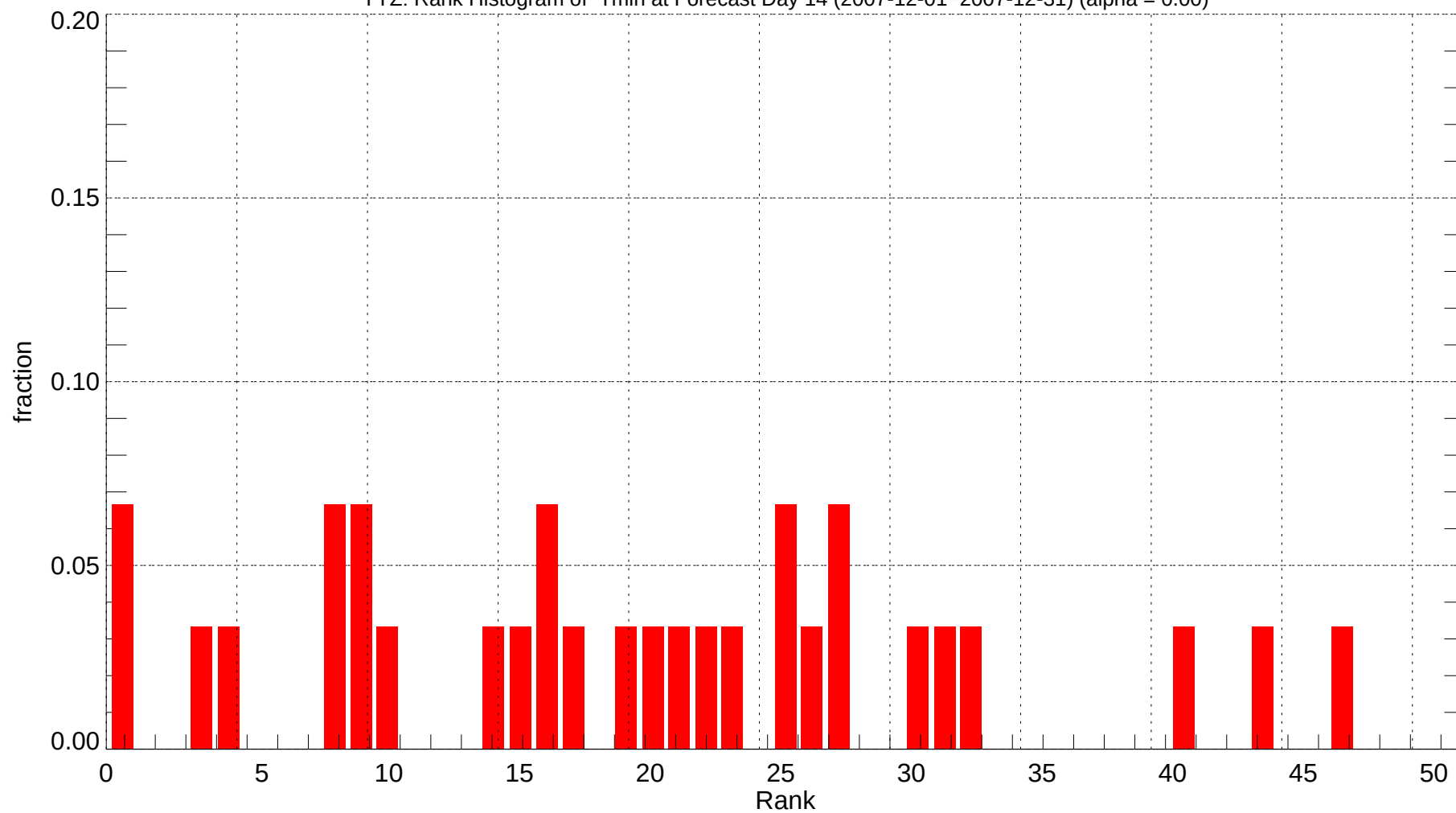
YYZ: Rank Histogram of Tmin at Forecast Day 14 (2007-12-01~2007-12-31) (alpha = 0.00)
