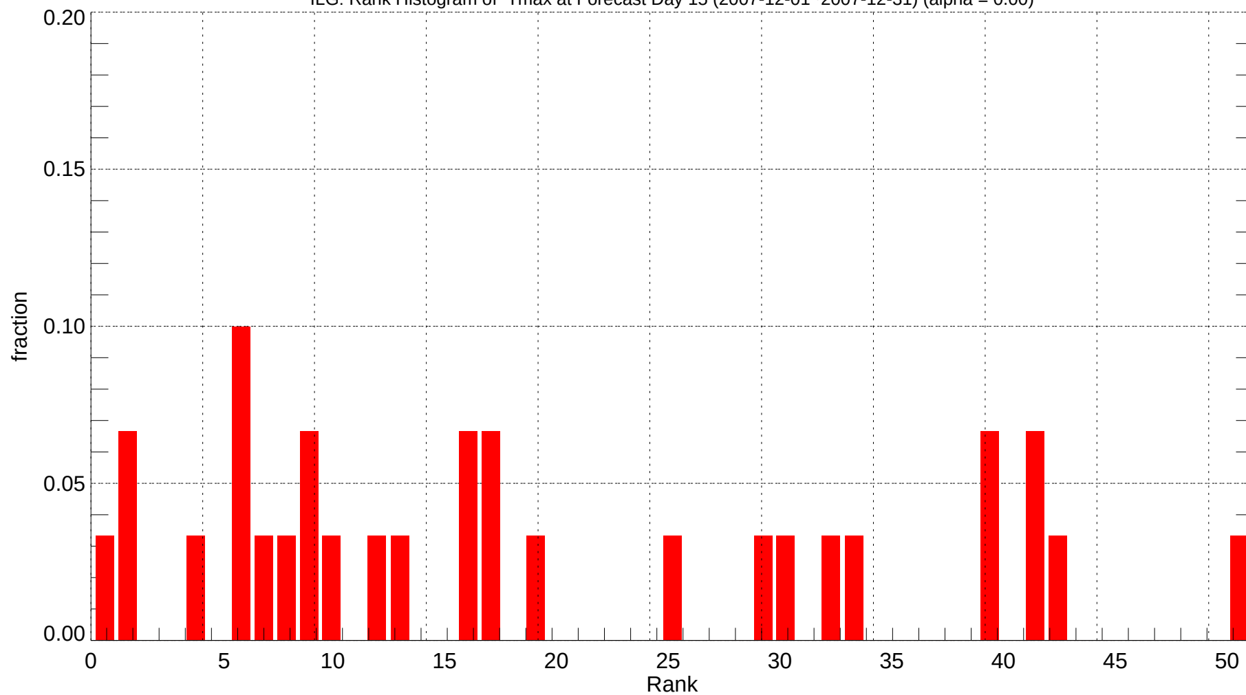
ILG: Rank Histogram of Tmax at Forecast Day 15 (2007-12-01~2007-12-31) (alpha = 0.00)
