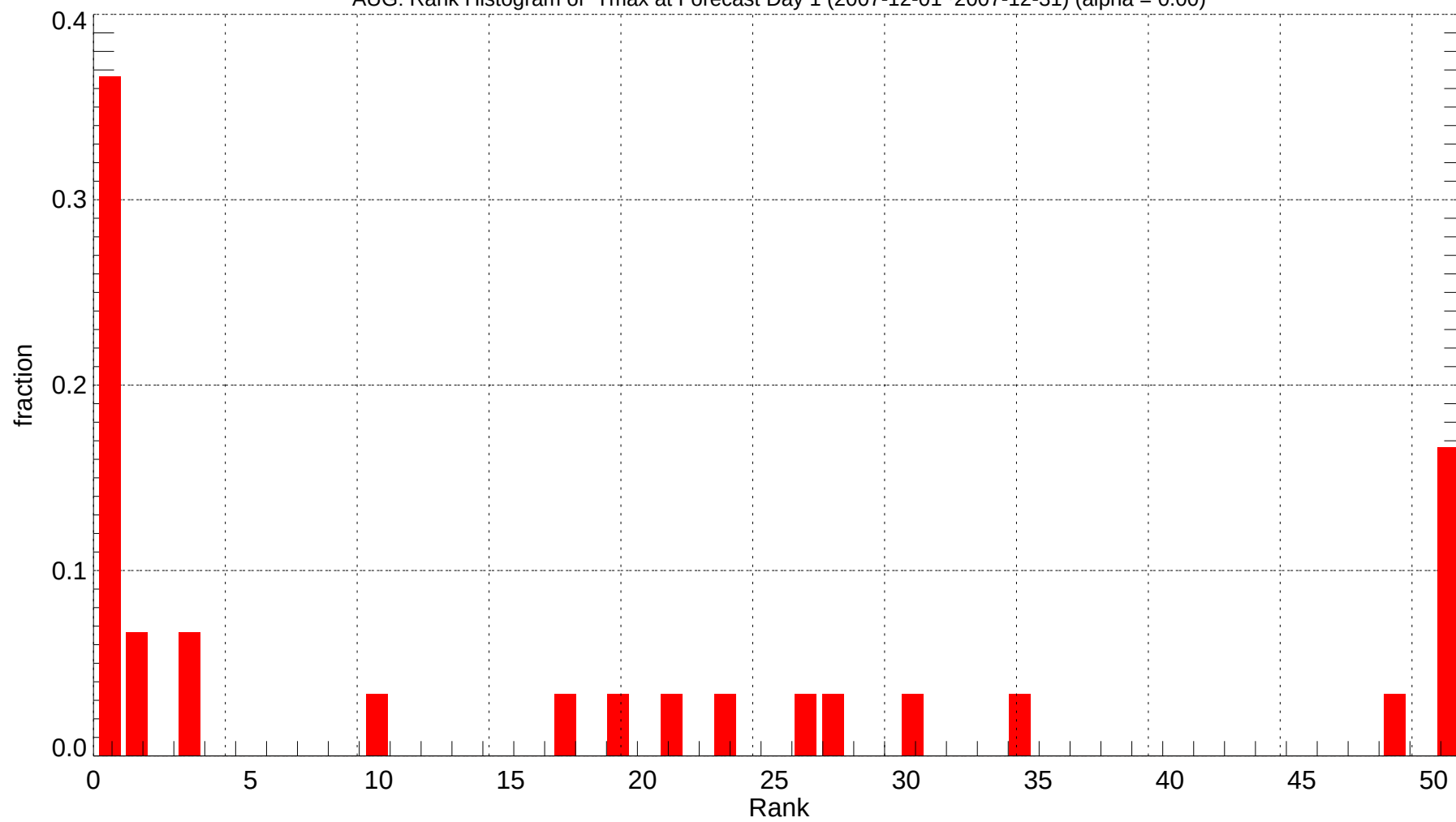
AUG: Rank Histogram of Tmax at Forecast Day 1 (2007-12-01~2007-12-31) (alpha = 0.00)
