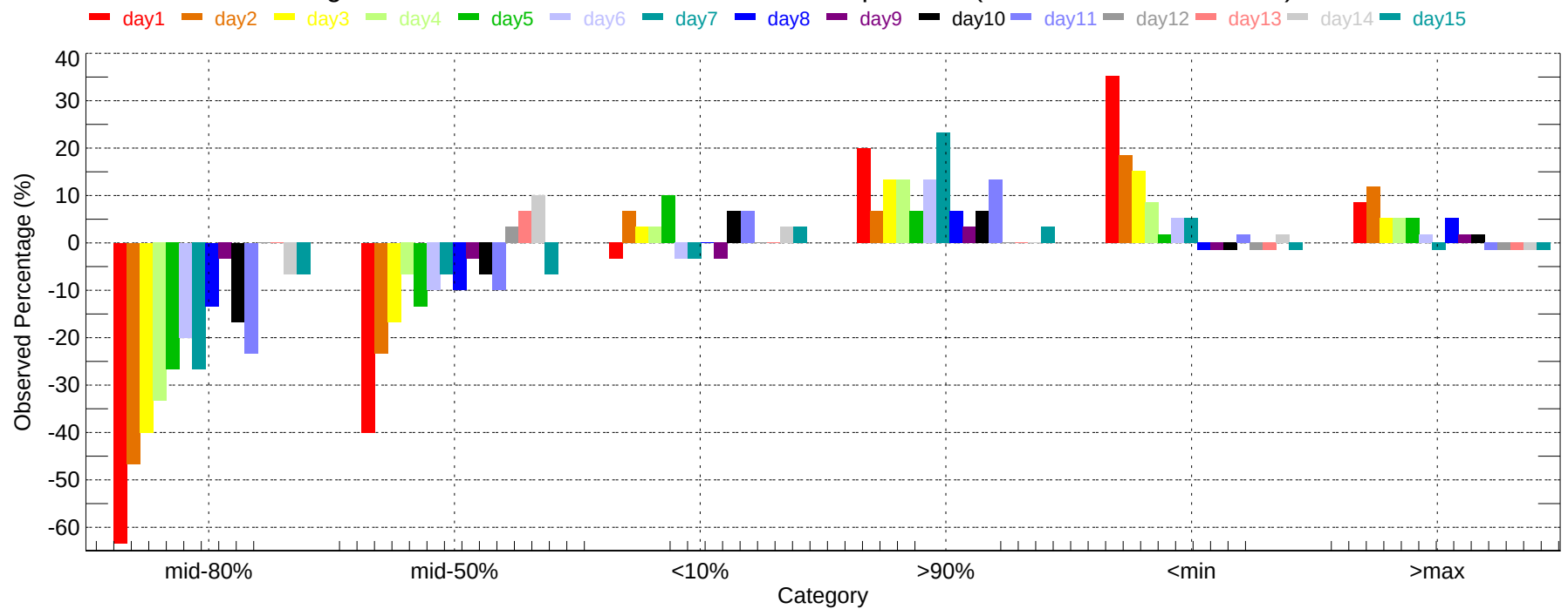
Observed Percentage Deviation of Ensembles - PHL: Min Temperature (2007-12-01~2007-12-31)
