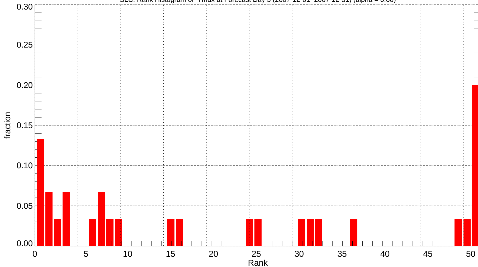
SLC: Rank Histogram of Tmax at Forecast Day 3 (2007-12-01~2007-12-31) (alpha = 0.00)
