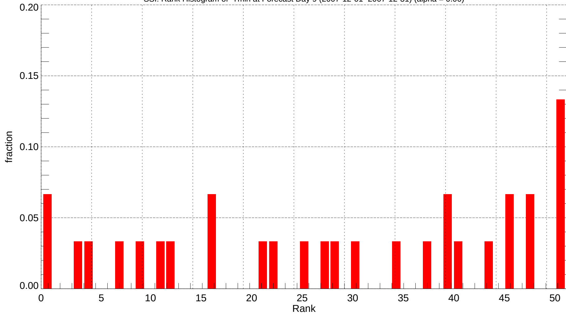
SSI: Rank Histogram of Tmin at Forecast Day 9 (2007-12-01~2007-12-31) (alpha = 0.00)
