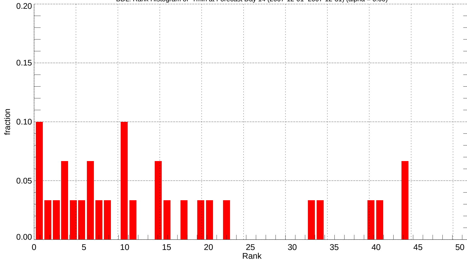
BDL: Rank Histogram of Tmin at Forecast Day 14 (2007-12-01~2007-12-31) (alpha = 0.00)
