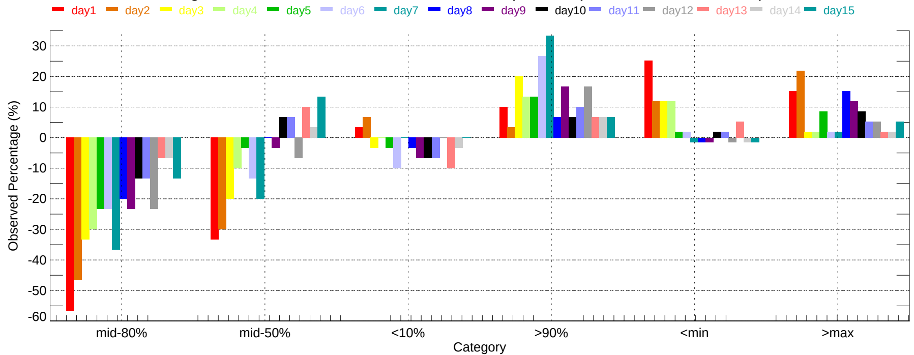
Observed Percentage Deviation of Ensembles - CMH: Max Temperature (2007-12-01~2007-12-31)
