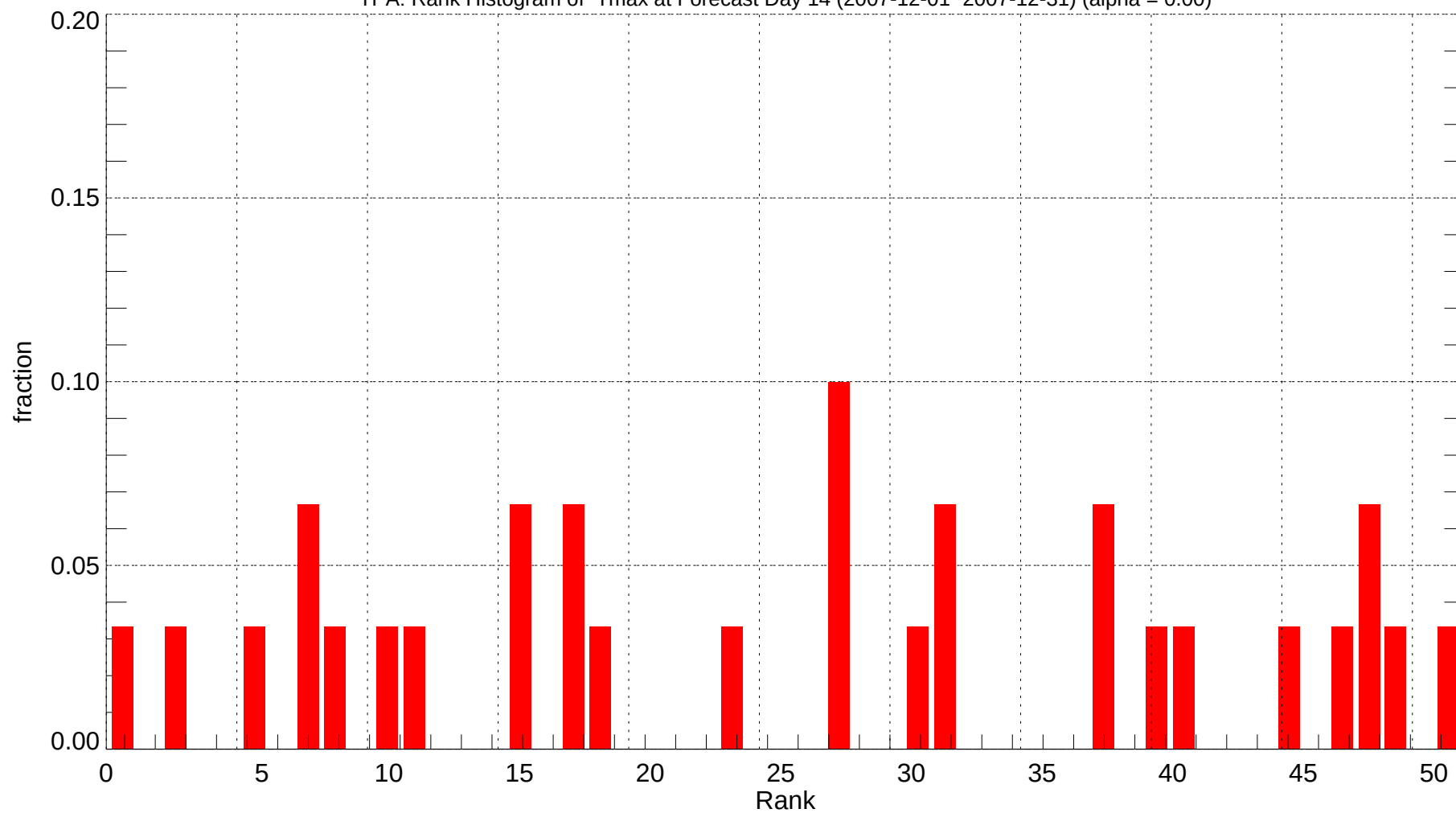
TPA: Rank Histogram of Tmax at Forecast Day 14 (2007-12-01~2007-12-31) (alpha = 0.00)
