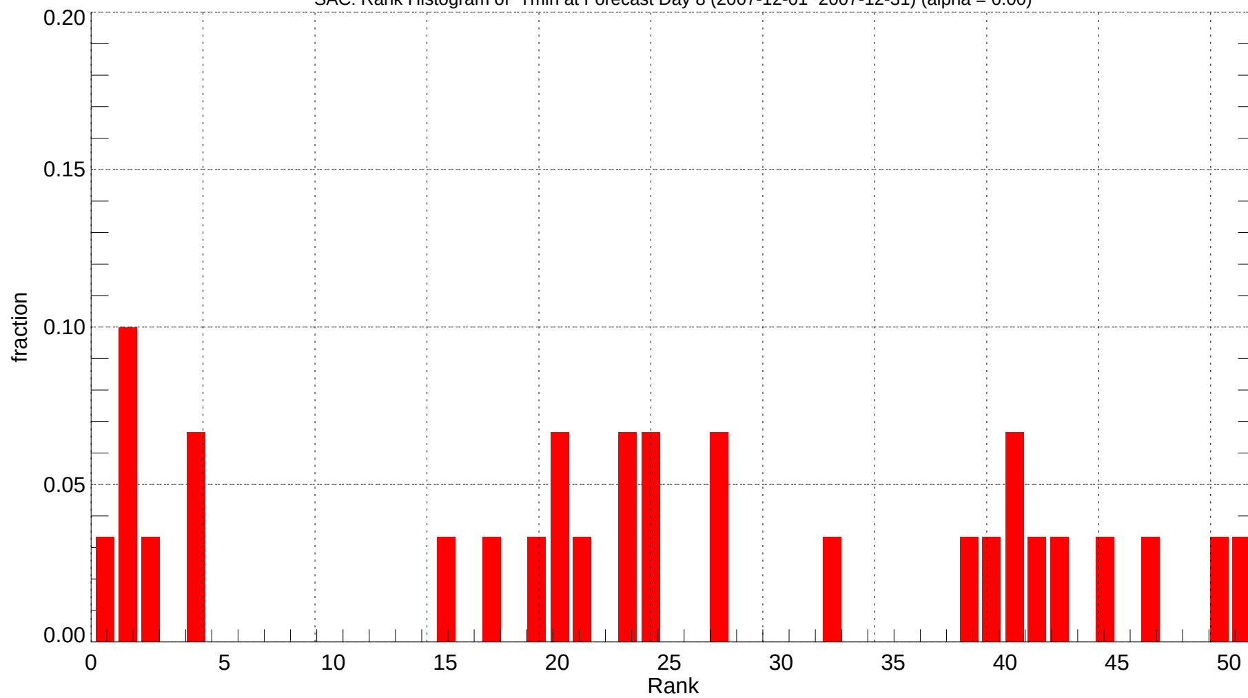
SAC: Rank Histogram of Tmin at Forecast Day 8 (2007-12-01~2007-12-31) (alpha = 0.00)
