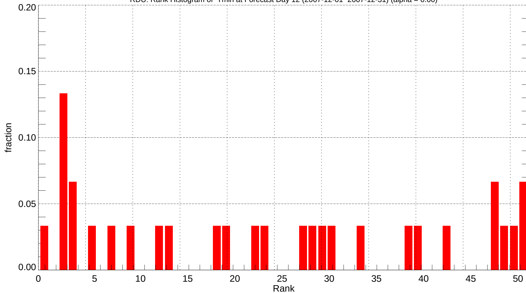
RDU: Rank Histogram of Tmin at Forecast Day 12 (2007-12-01~2007-12-31) (alpha = 0.00)
