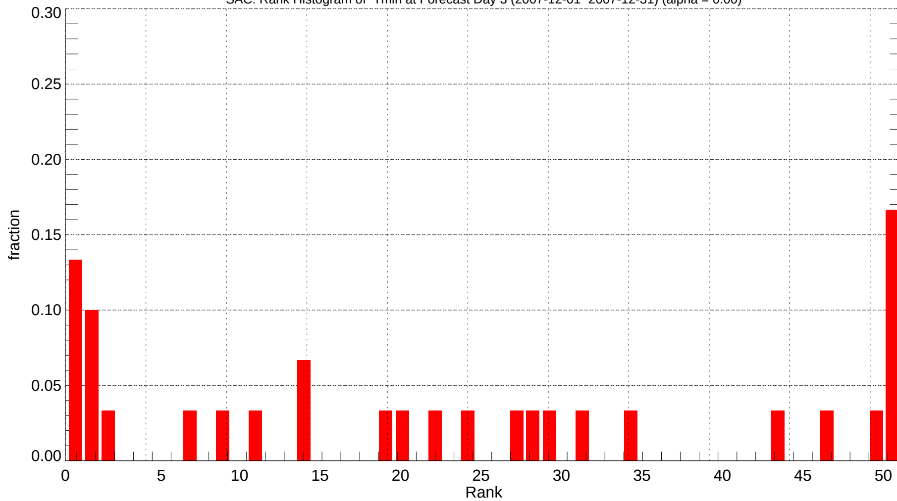
SAC: Rank Histogram of Tmin at Forecast Day 3 (2007-12-01~2007-12-31) (alpha = 0.00)
