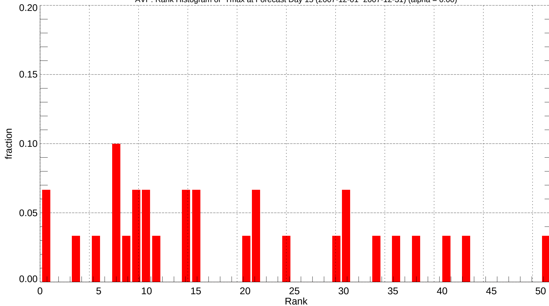
AVP: Rank Histogram of Tmax at Forecast Day 15 (2007-12-01~2007-12-31) (alpha = 0.00)
