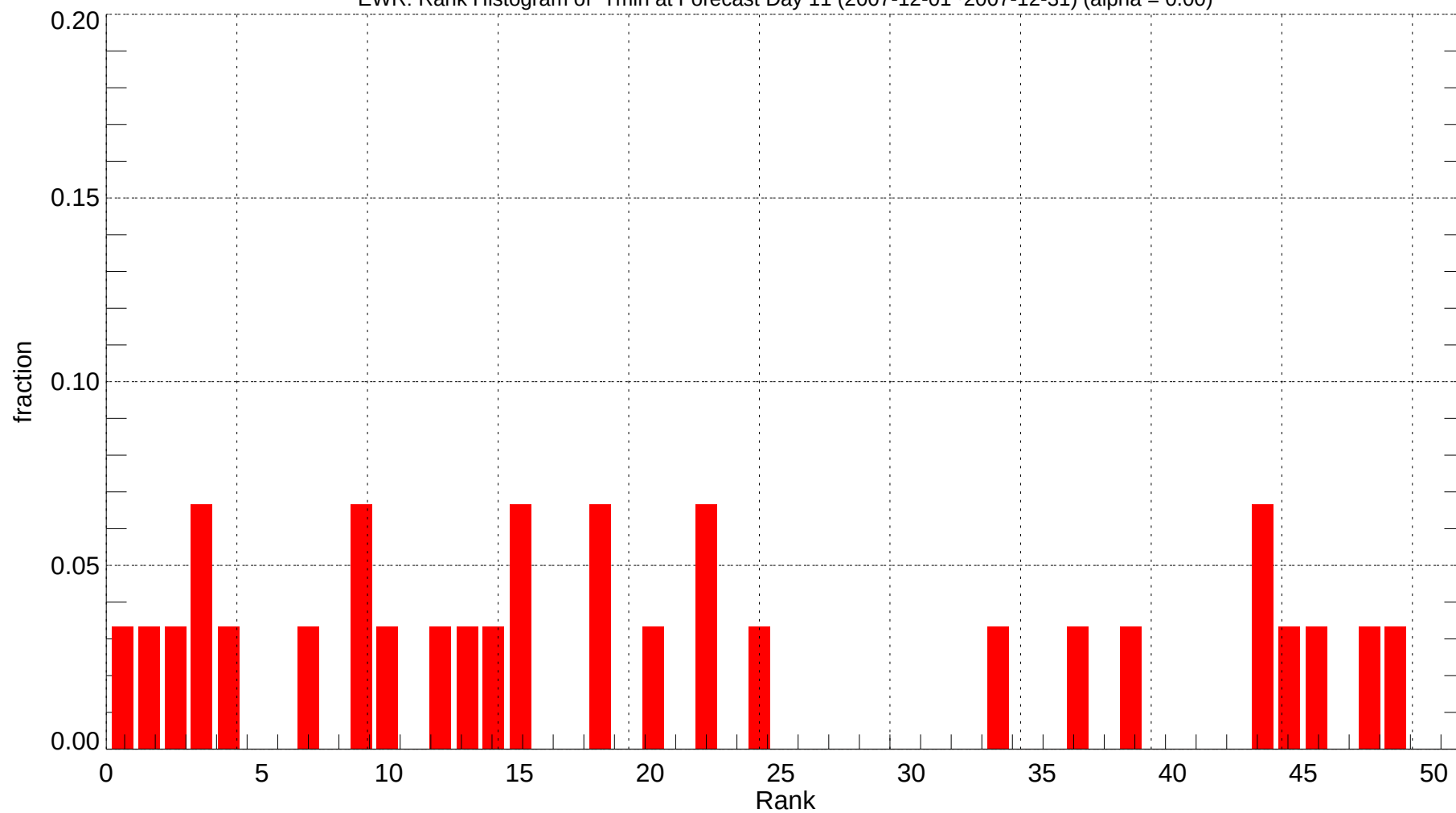
EWR: Rank Histogram of Tmin at Forecast Day 11 (2007-12-01~2007-12-31) (alpha = 0.00)
