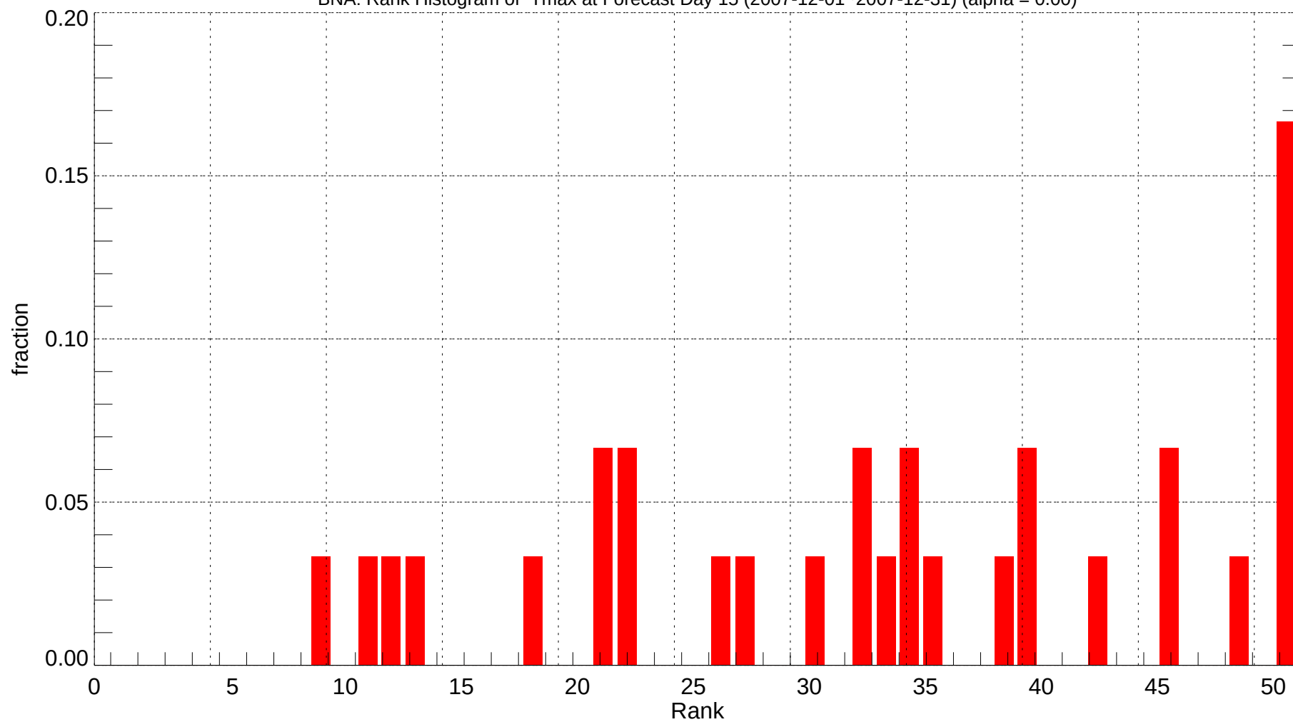
BNA: Rank Histogram of Tmax at Forecast Day 15 (2007-12-01~2007-12-31) (alpha = 0.00)
