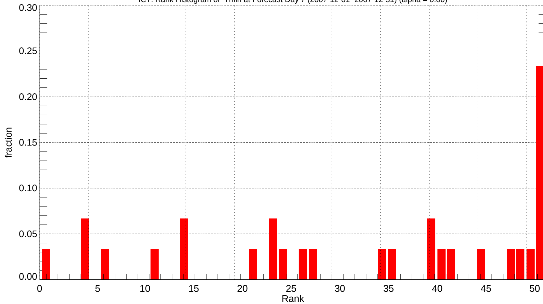
ICT: Rank Histogram of Tmin at Forecast Day 7 (2007-12-01~2007-12-31) (alpha = 0.00)
