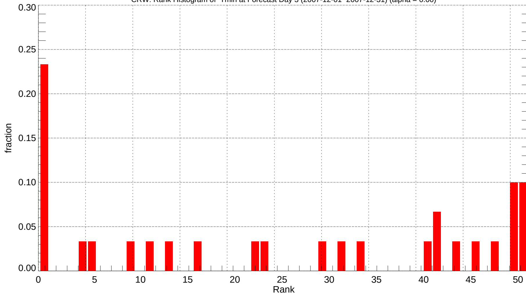
CRW: Rank Histogram of Tmin at Forecast Day 3 (2007-12-01~2007-12-31) (alpha = 0.00)
