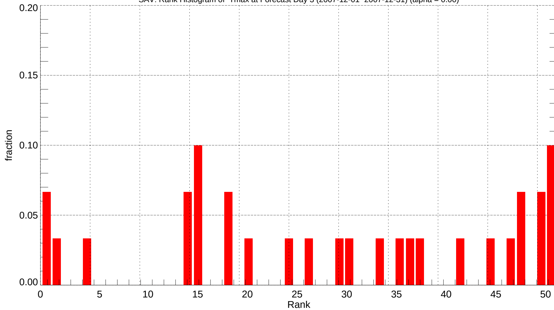
SAV: Rank Histogram of Tmax at Forecast Day 3 (2007-12-01~2007-12-31) (alpha = 0.00)
