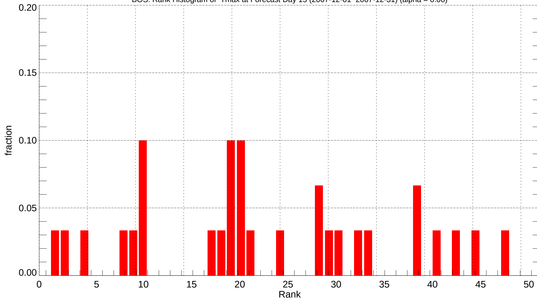
BOS: Rank Histogram of Tmax at Forecast Day 15 (2007-12-01~2007-12-31) (alpha = 0.00)
