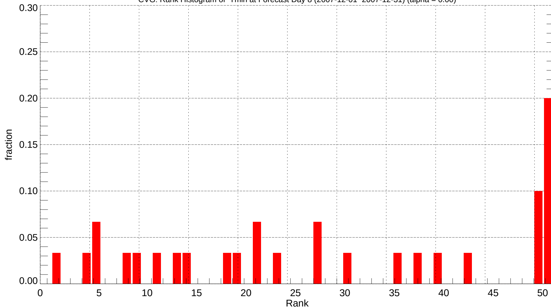
CVG: Rank Histogram of Tmin at Forecast Day 8 (2007-12-01~2007-12-31) (alpha = 0.00)
