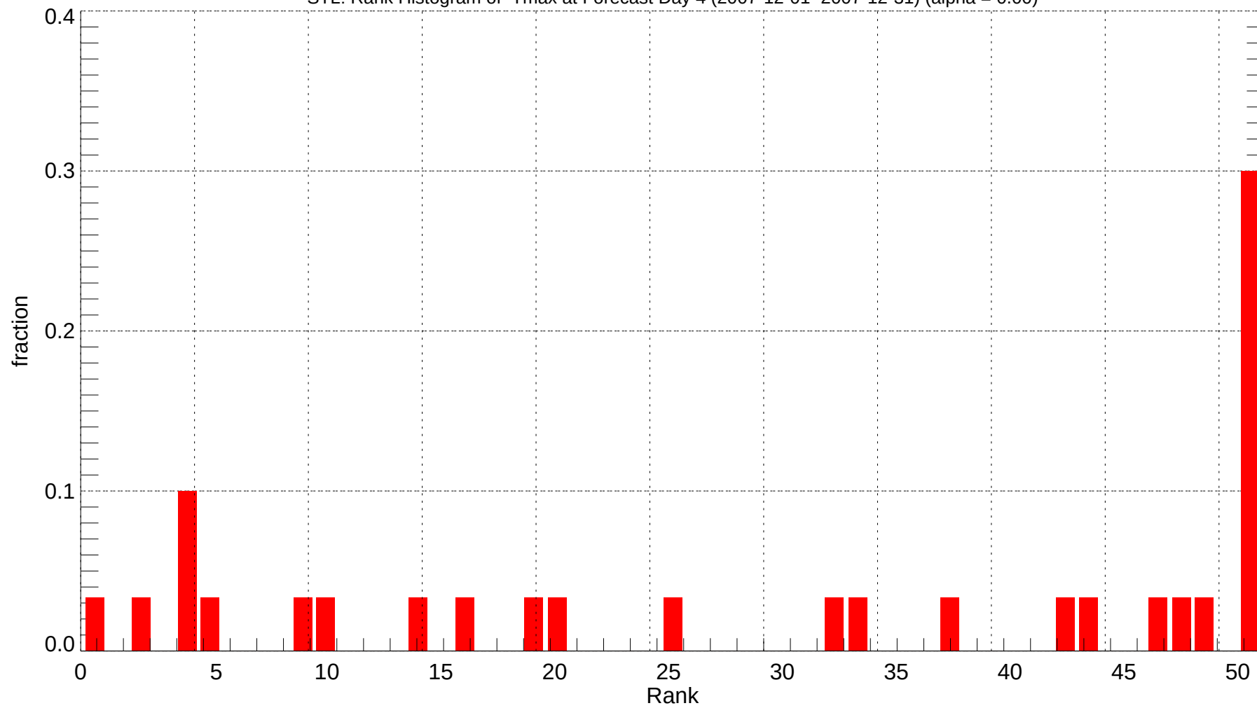
STL: Rank Histogram of Tmax at Forecast Day 4 (2007-12-01~2007-12-31) (alpha = 0.00)
