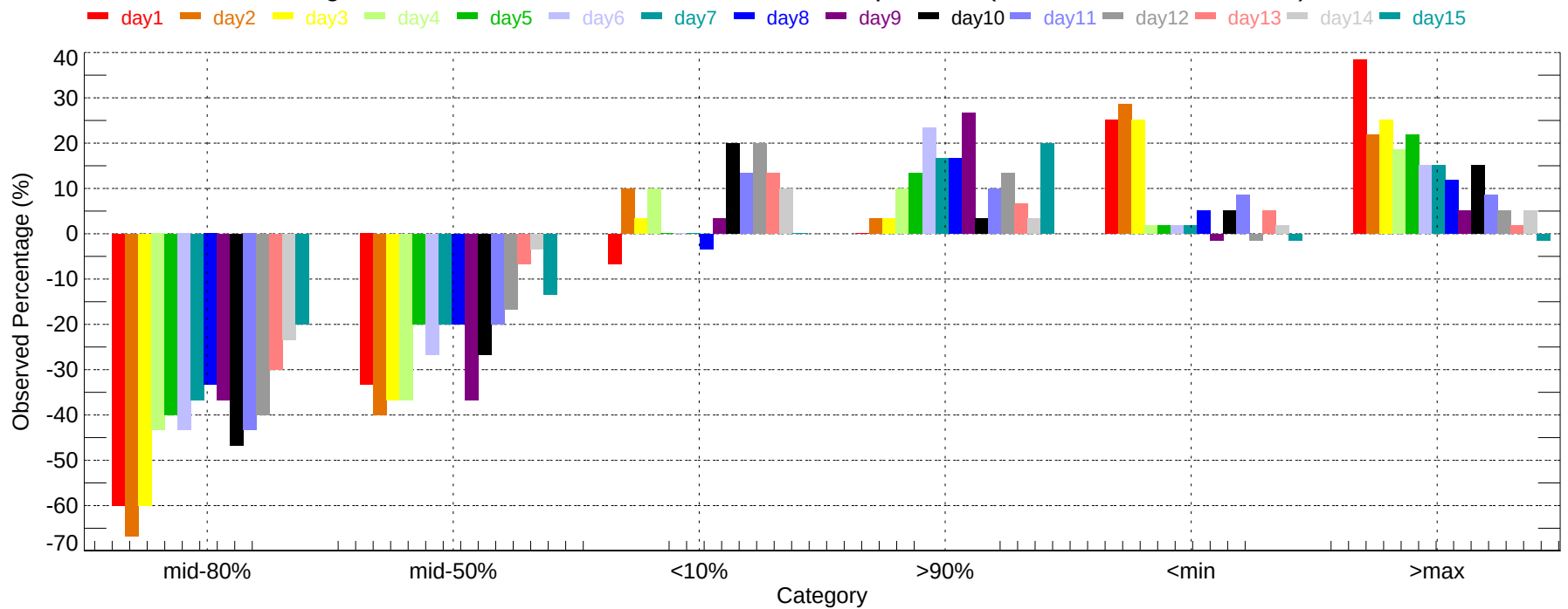
Observed Percentage Deviation of Ensembles - OKC: Max Temperature (2007-12-01~2007-12-31)
