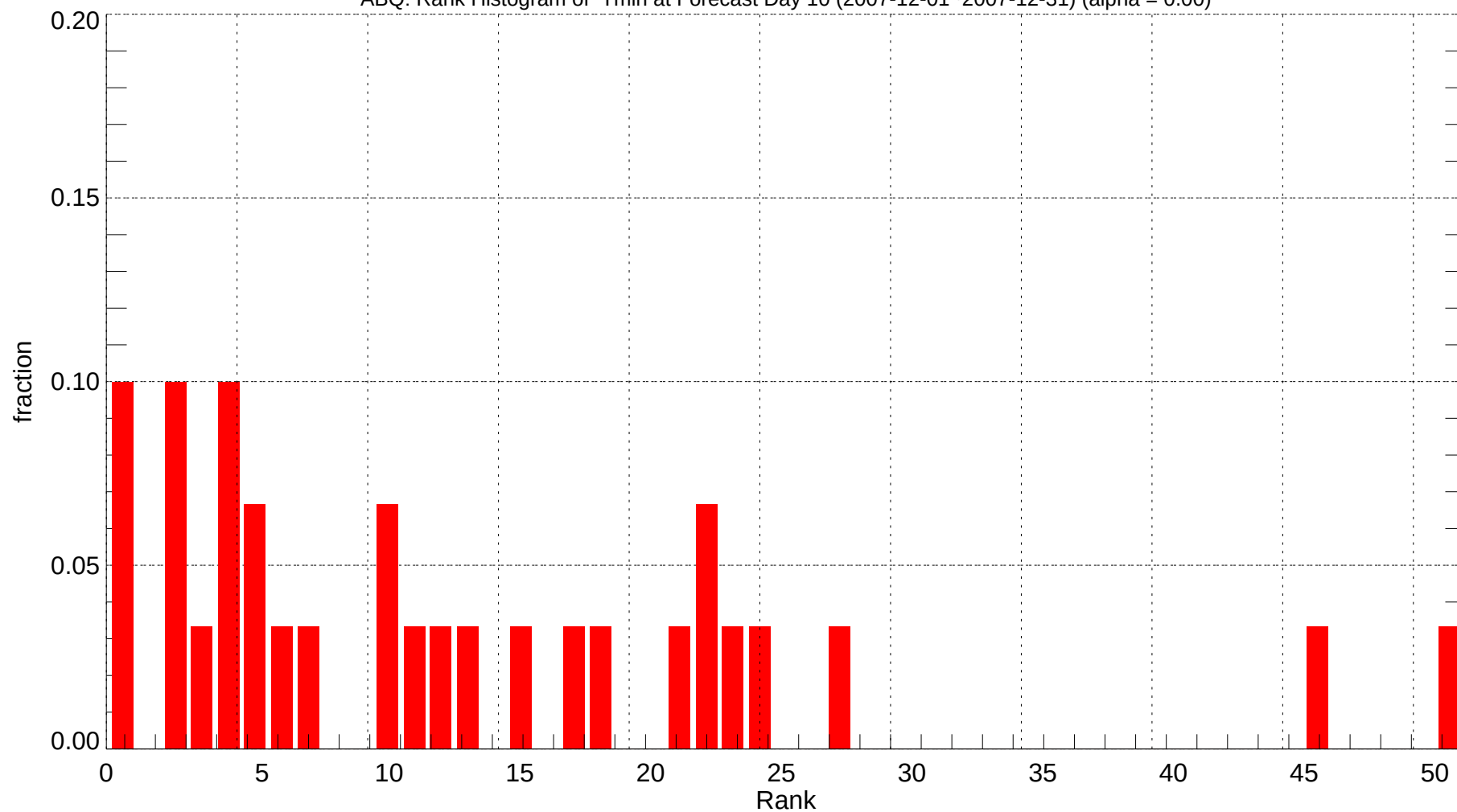
ABQ: Rank Histogram of Tmin at Forecast Day 10 (2007-12-01~2007-12-31) (alpha = 0.00)
