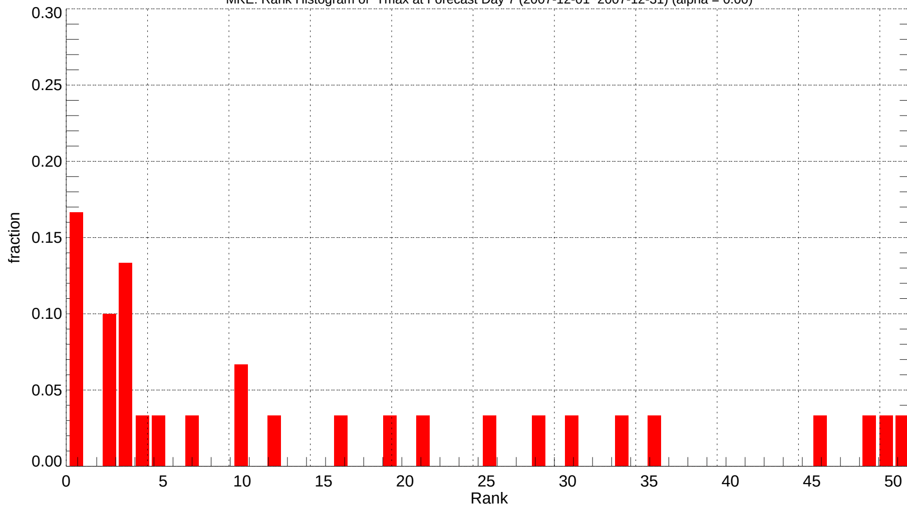
MKE: Rank Histogram of Tmax at Forecast Day 7 (2007-12-01~2007-12-31) (alpha = 0.00)
