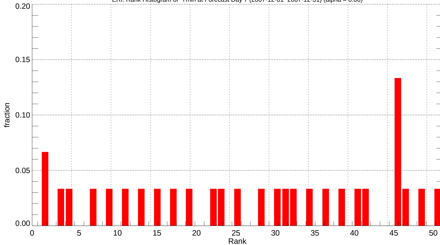
ERI: Rank Histogram of Tmin at Forecast Day 7 (2007-12-01~2007-12-31) (alpha = 0.00)
