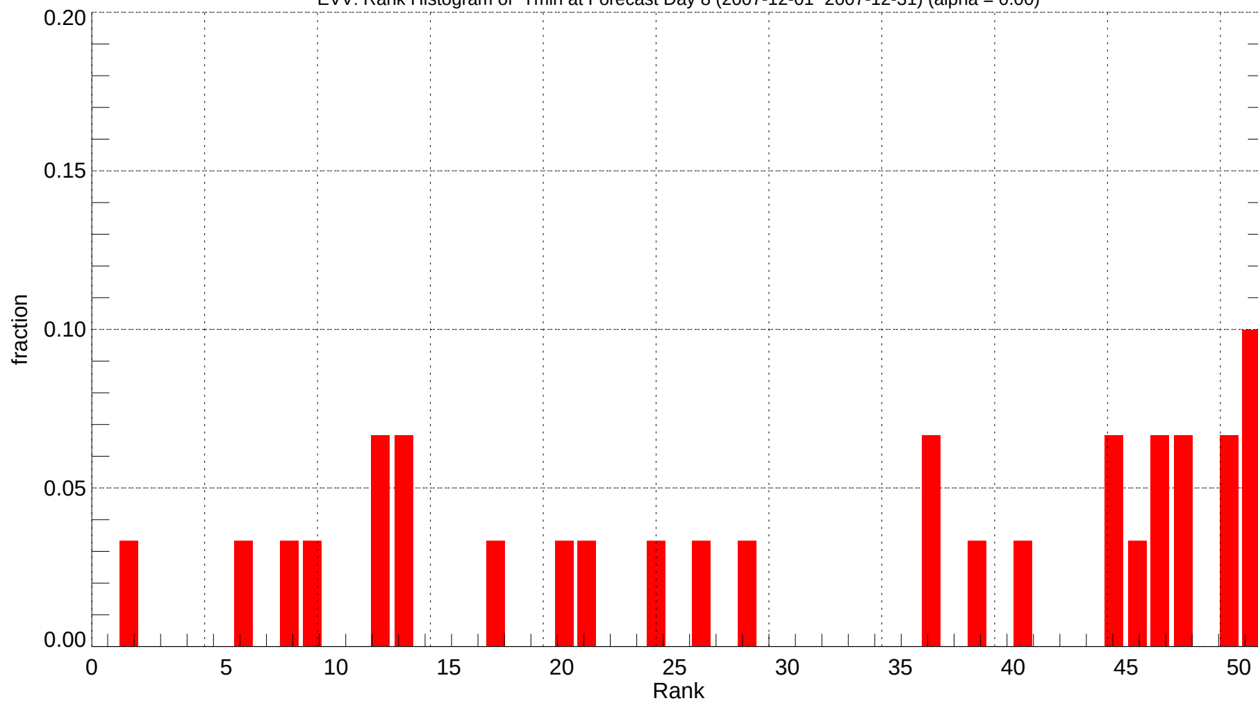
EVV: Rank Histogram of Tmin at Forecast Day 8 (2007-12-01~2007-12-31) (alpha = 0.00)
