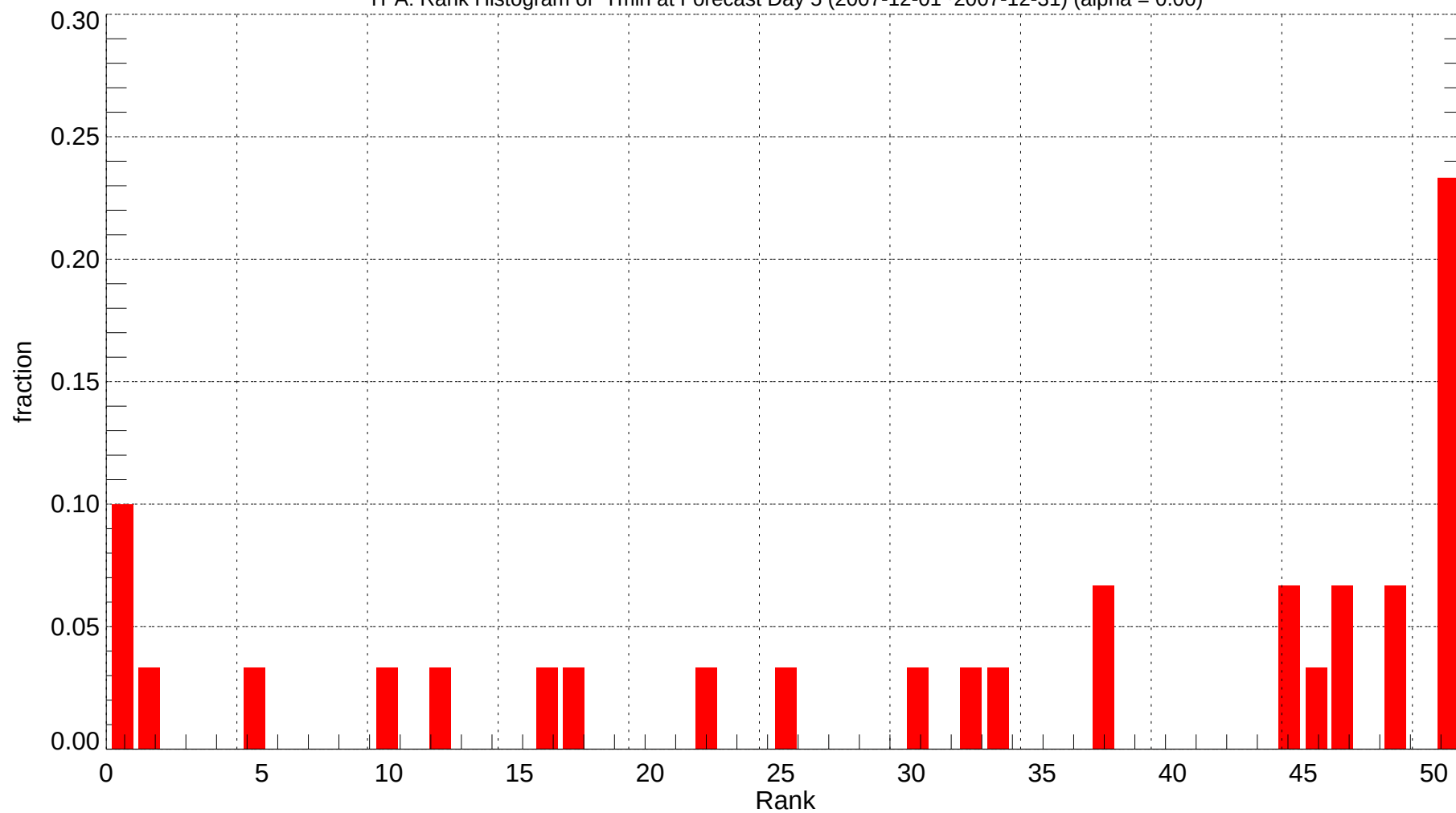
TPA: Rank Histogram of Tmin at Forecast Day 5 (2007-12-01~2007-12-31) (alpha = 0.00)
