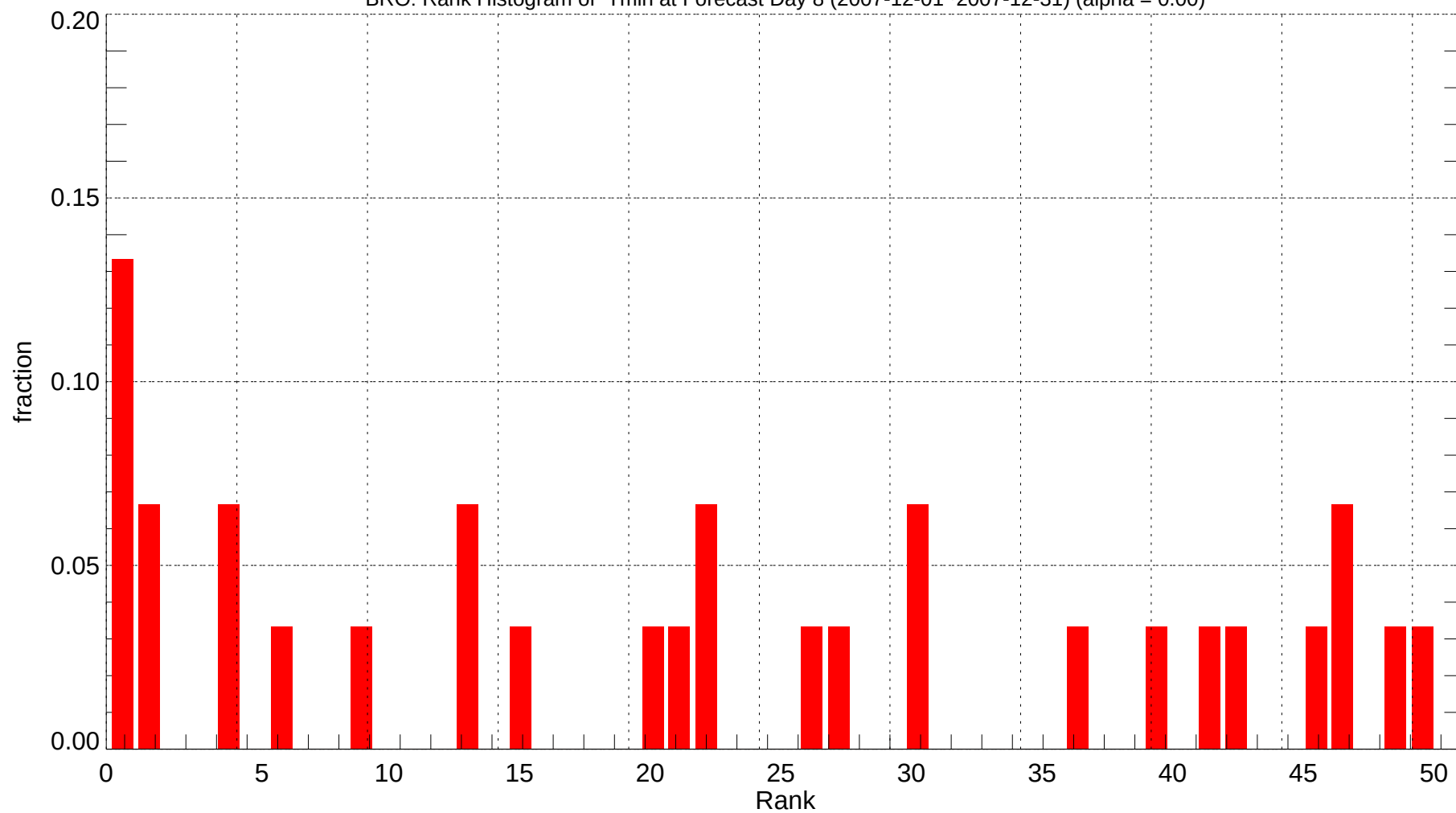
BRO: Rank Histogram of Tmin at Forecast Day 8 (2007-12-01~2007-12-31) (alpha = 0.00)
