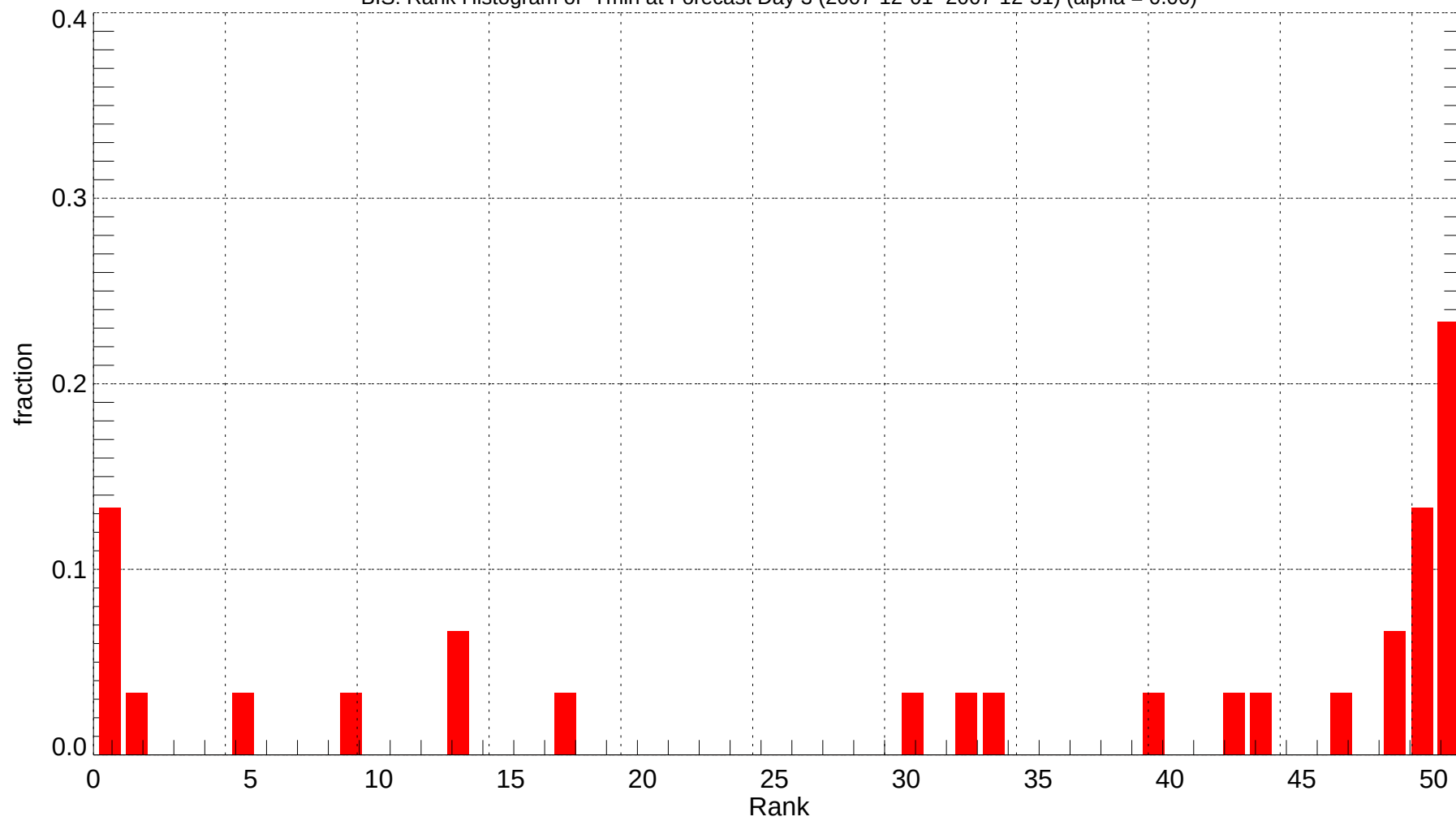
BIS: Rank Histogram of Tmin at Forecast Day 3 (2007-12-01~2007-12-31) (alpha = 0.00)
