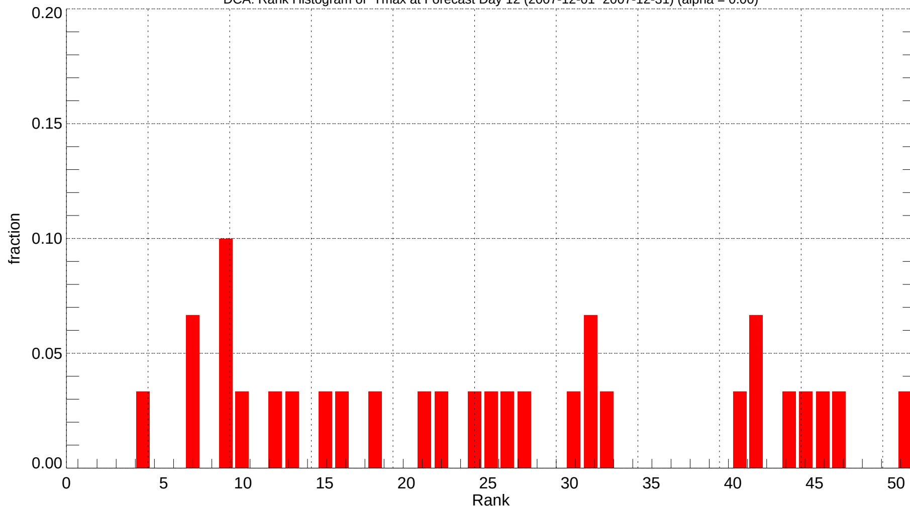
DCA: Rank Histogram of Tmax at Forecast Day 12 (2007-12-01~2007-12-31) (alpha = 0.00)
