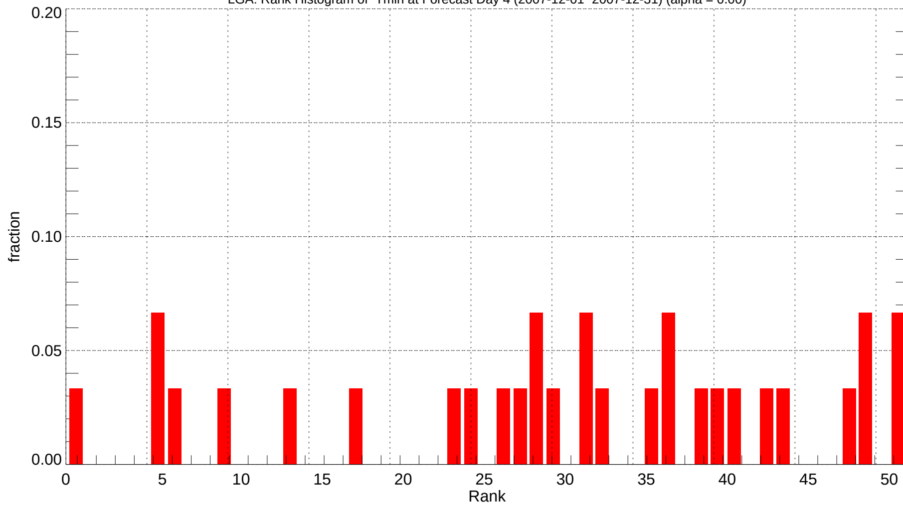
LGA: Rank Histogram of Tmin at Forecast Day 4 (2007-12-01~2007-12-31) (alpha = 0.00)
