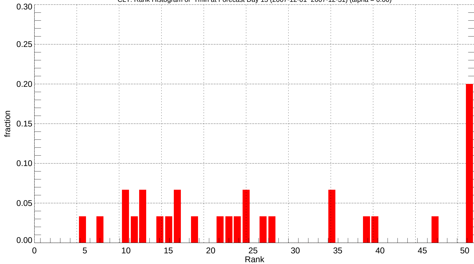
CLT: Rank Histogram of Tmin at Forecast Day 15 (2007-12-01~2007-12-31) (alpha = 0.00)
