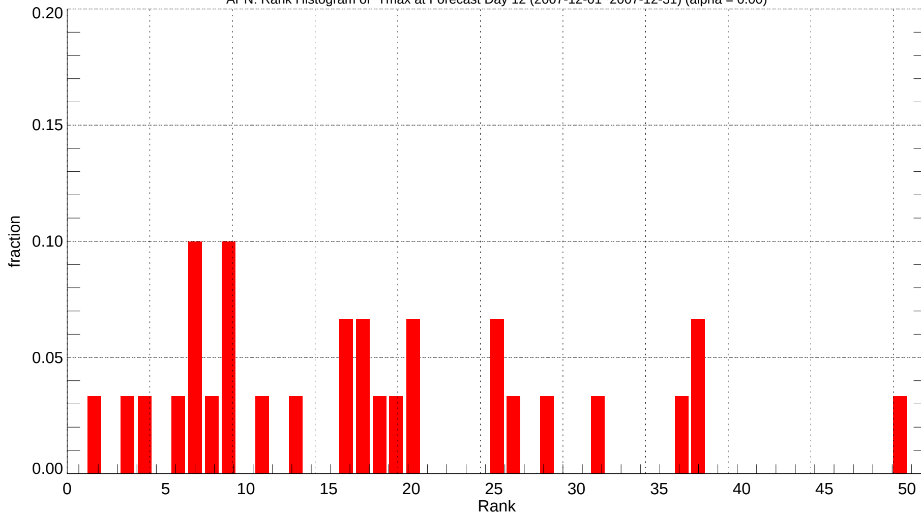
APN: Rank Histogram of Tmax at Forecast Day 12 (2007-12-01~2007-12-31) (alpha = 0.00)
