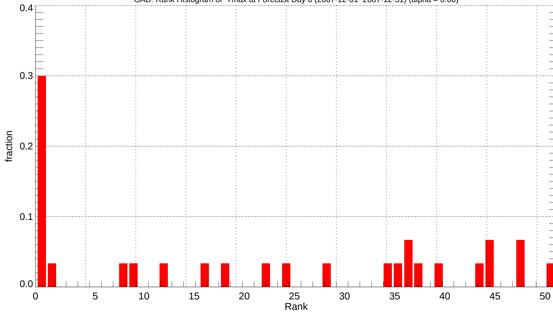
GAD: Rank Histogram of Tmax at Forecast Day 6 (2007-12-01~2007-12-31) (alpha = 0.00)
