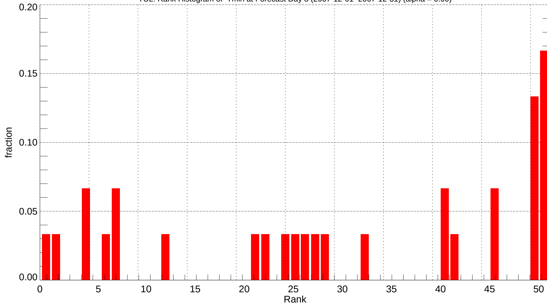
TUL: Rank Histogram of Tmin at Forecast Day 8 (2007-12-01~2007-12-31) (alpha = 0.00)
