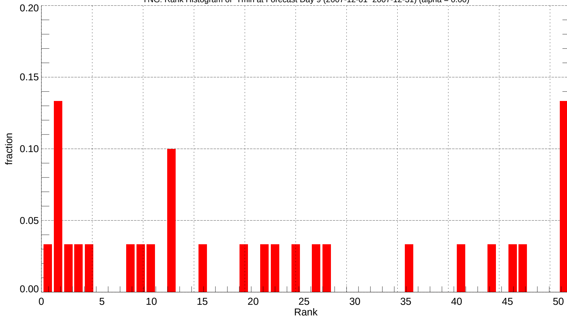
YNG: Rank Histogram of Tmin at Forecast Day 9 (2007-12-01~2007-12-31) (alpha = 0.00)
