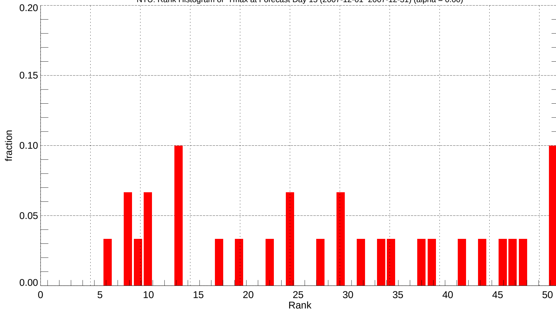
NTU: Rank Histogram of Tmax at Forecast Day 15 (2007-12-01~2007-12-31) (alpha = 0.00)
