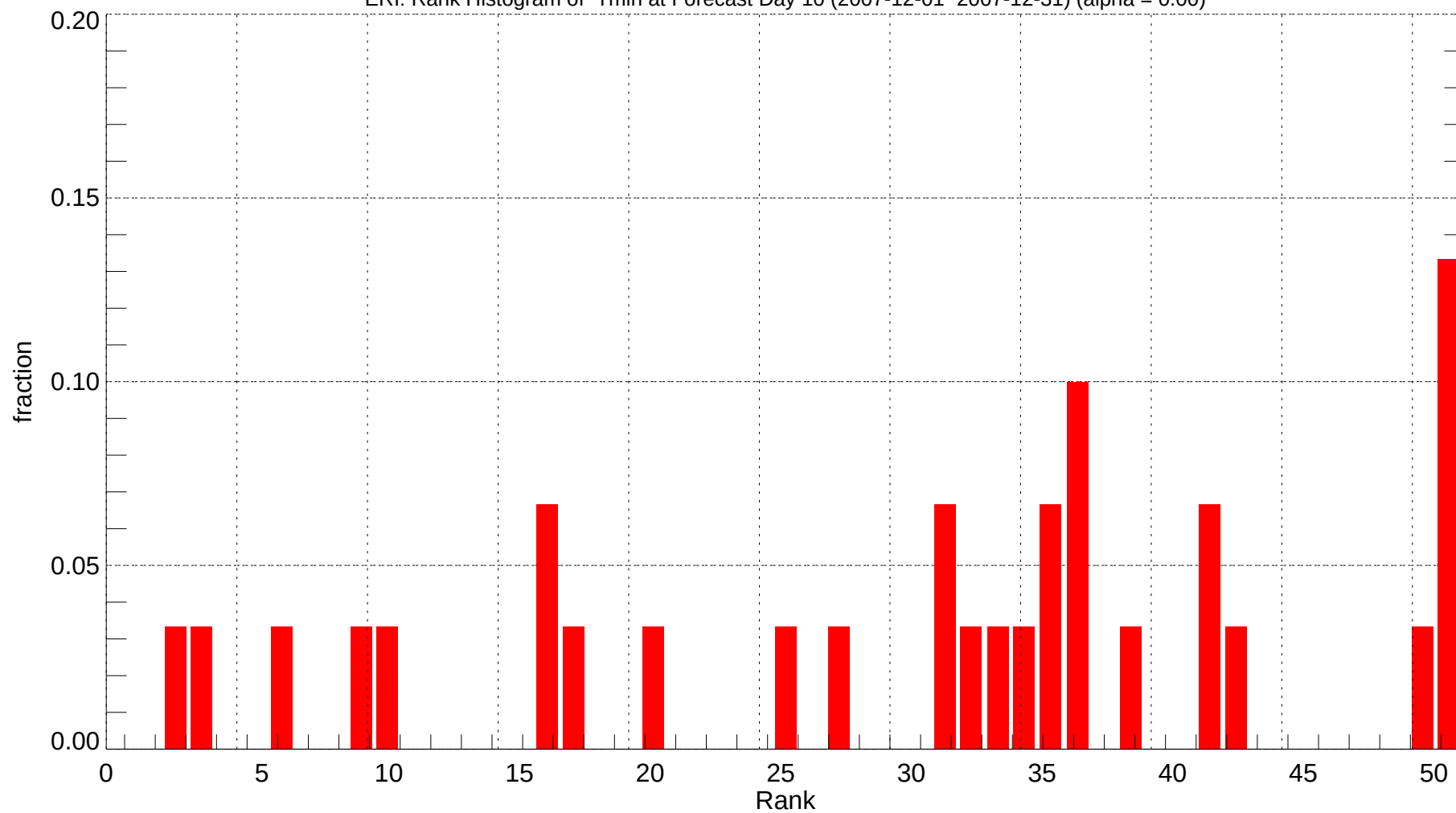
ERI: Rank Histogram of Tmin at Forecast Day 10 (2007-12-01~2007-12-31) (alpha = 0.00)
