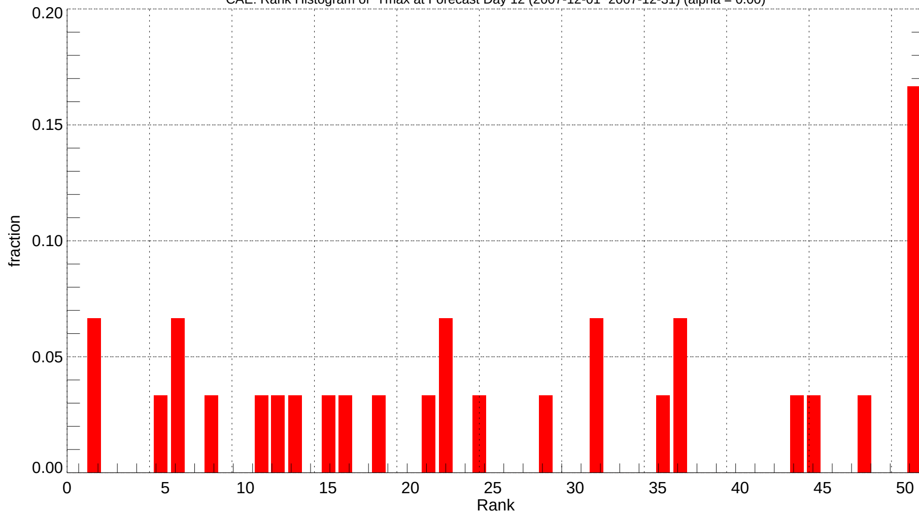
CAE: Rank Histogram of Tmax at Forecast Day 12 (2007-12-01~2007-12-31) (alpha = 0.00)
