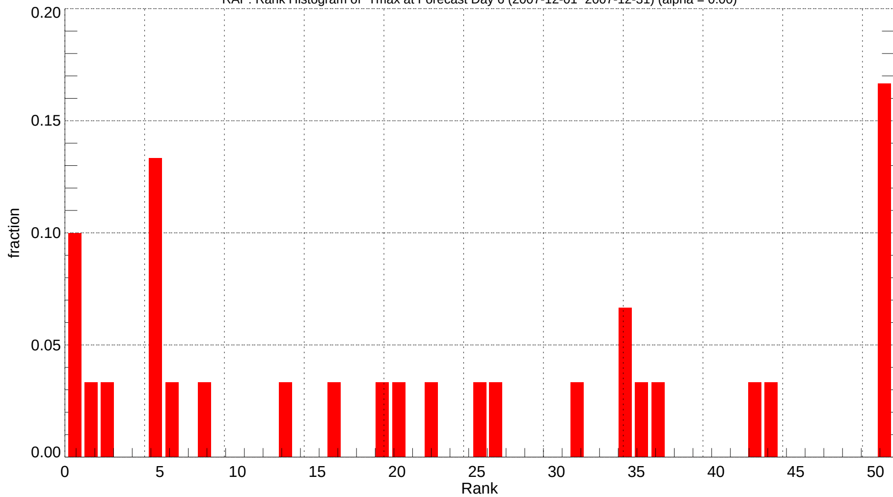
RAP: Rank Histogram of Tmax at Forecast Day 6 (2007-12-01~2007-12-31) (alpha = 0.00)
