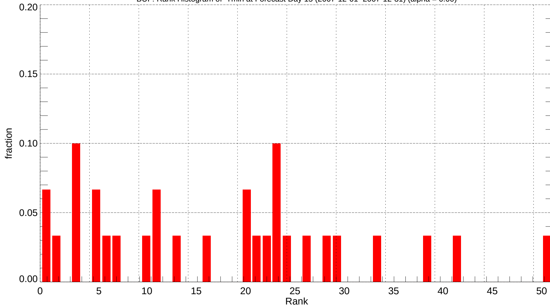
BUF: Rank Histogram of Tmin at Forecast Day 15 (2007-12-01~2007-12-31) (alpha = 0.00)
