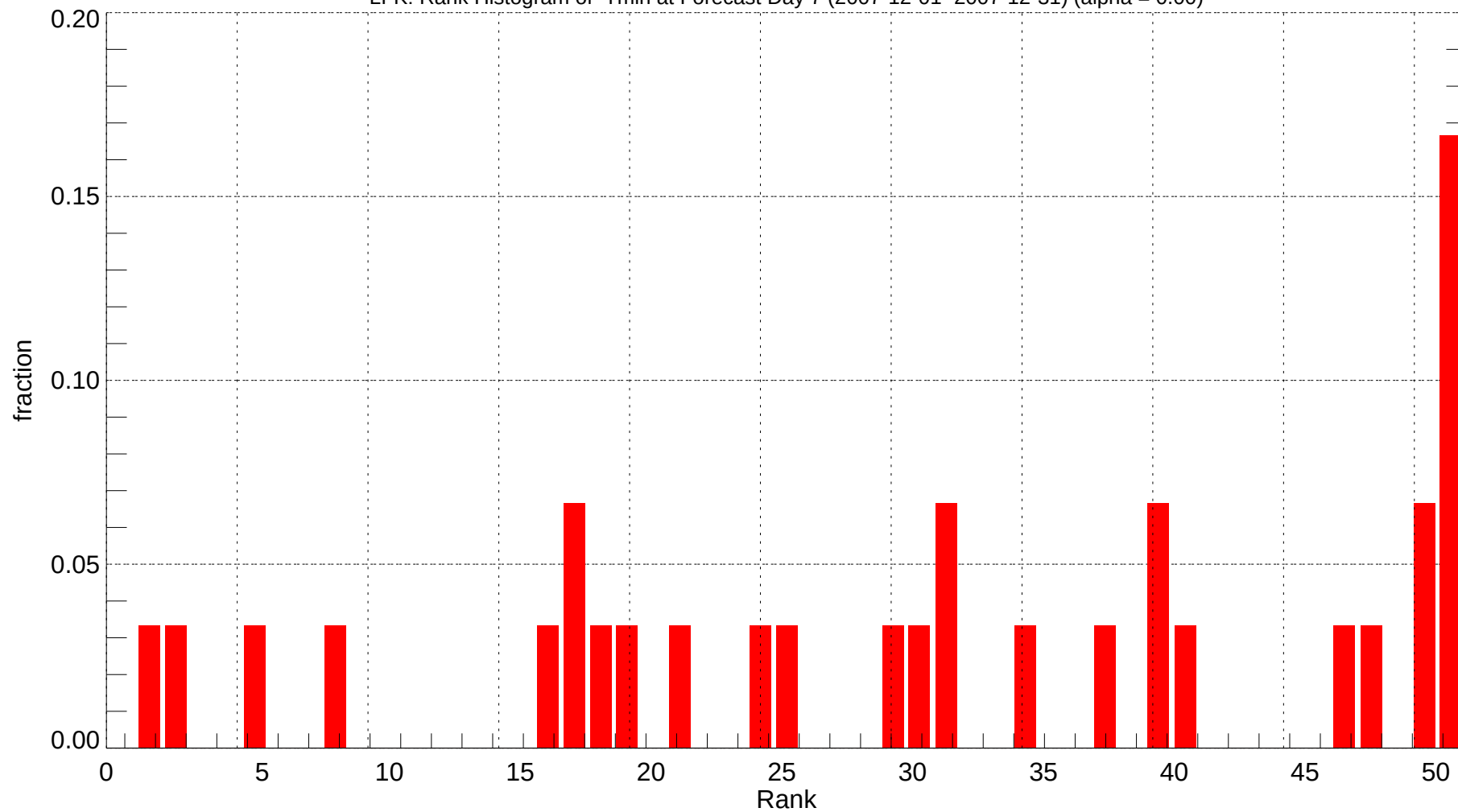
LFK: Rank Histogram of Tmin at Forecast Day 7 (2007-12-01~2007-12-31) (alpha = 0.00)
