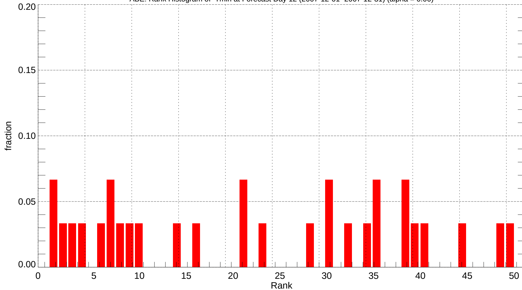
ABE: Rank Histogram of Tmin at Forecast Day 12 (2007-12-01~2007-12-31) (alpha = 0.00)
