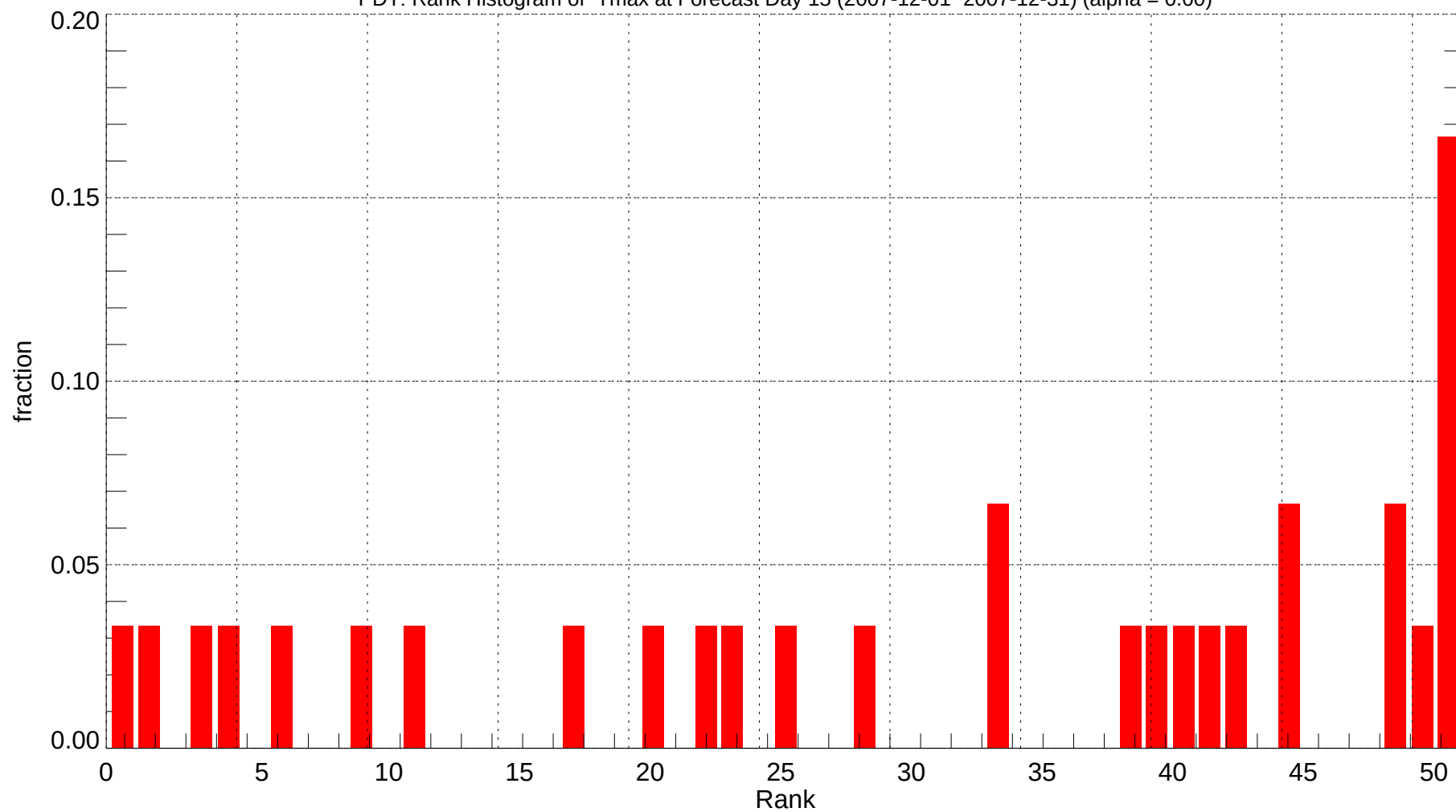
PDT: Rank Histogram of Tmax at Forecast Day 15 (2007-12-01~2007-12-31) (alpha = 0.00)
