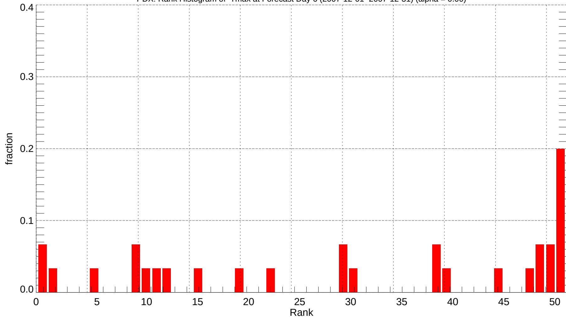
PDX: Rank Histogram of Tmax at Forecast Day 6 (2007-12-01~2007-12-31) (alpha = 0.00)
