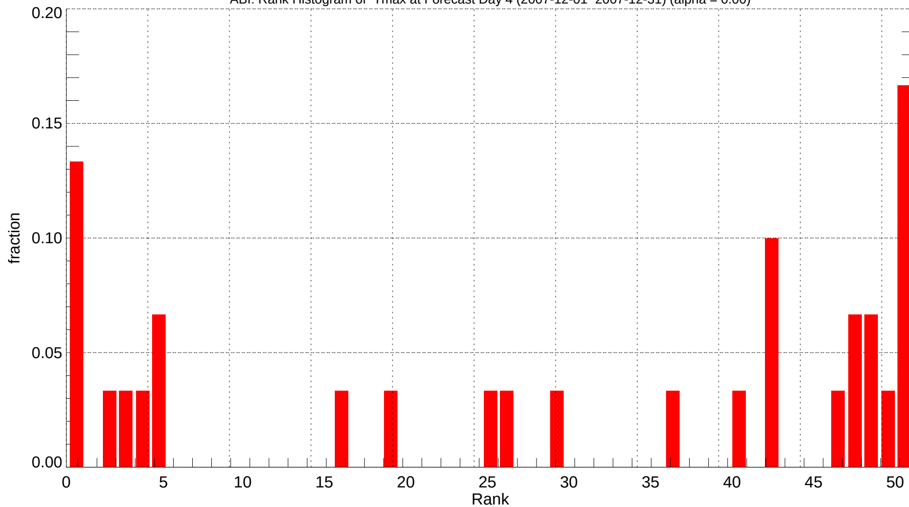
ABI: Rank Histogram of Tmax at Forecast Day 4 (2007-12-01~2007-12-31) (alpha = 0.00)
