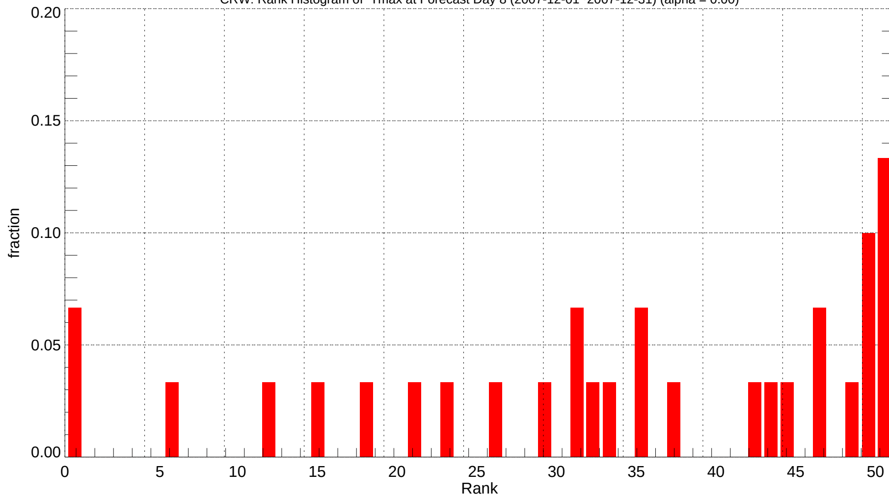
CRW: Rank Histogram of Tmax at Forecast Day 8 (2007-12-01~2007-12-31) (alpha = 0.00)
