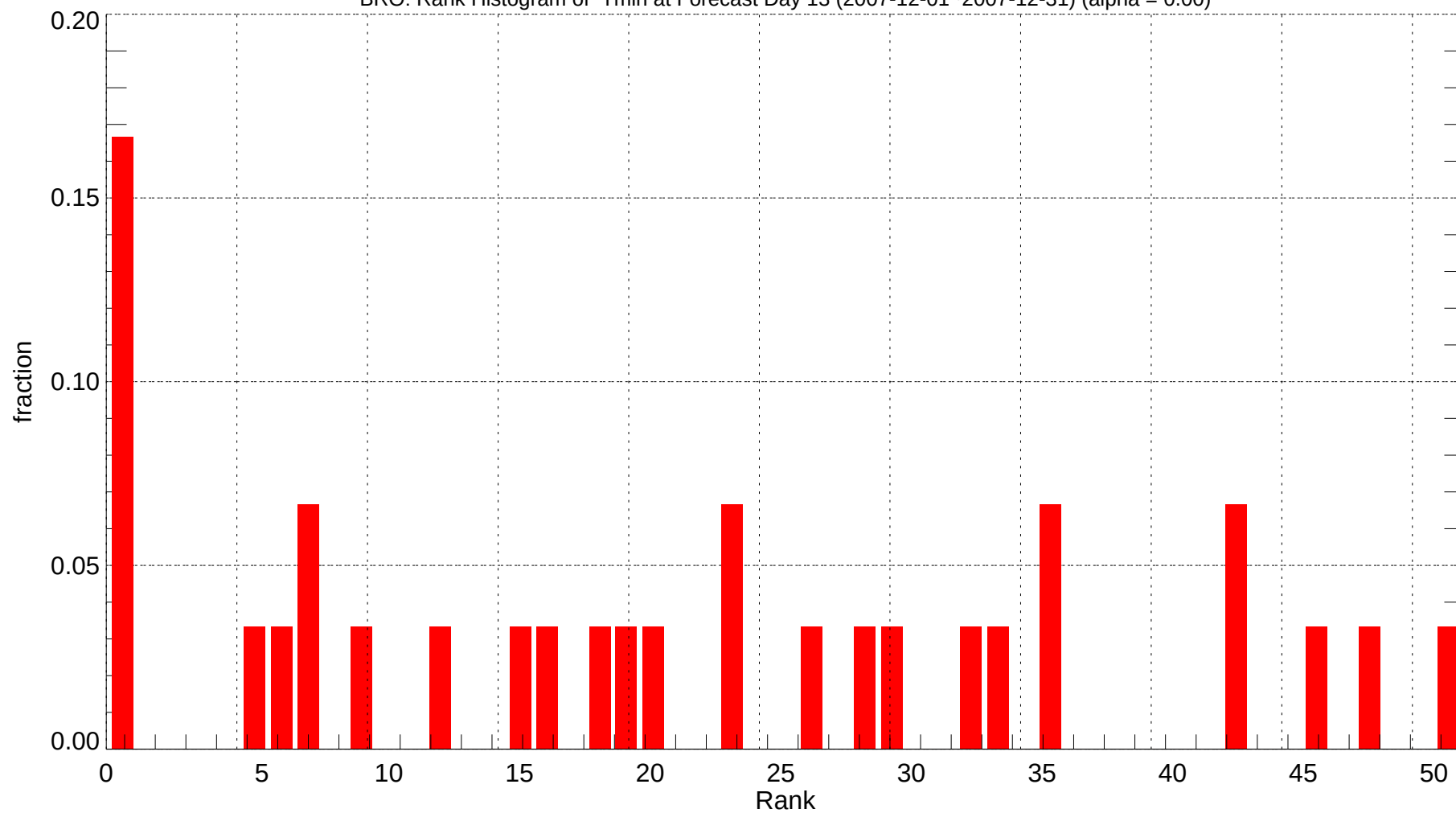
BRO: Rank Histogram of Tmin at Forecast Day 13 (2007-12-01~2007-12-31) (alpha = 0.00)
