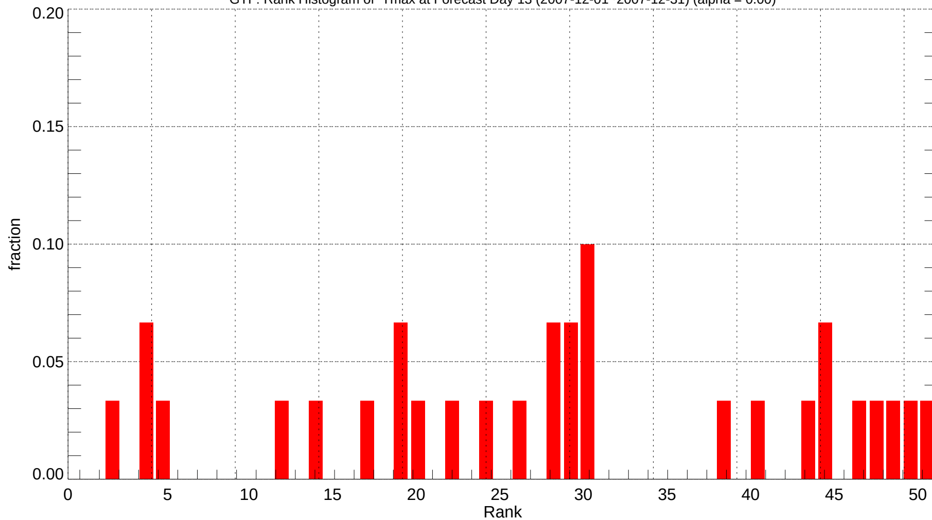
GTF: Rank Histogram of Tmax at Forecast Day 13 (2007-12-01~2007-12-31) (alpha = 0.00)
