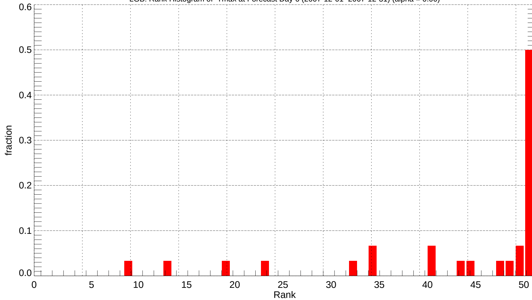
LGB: Rank Histogram of Tmax at Forecast Day 6 (2007-12-01~2007-12-31) (alpha = 0.00)
