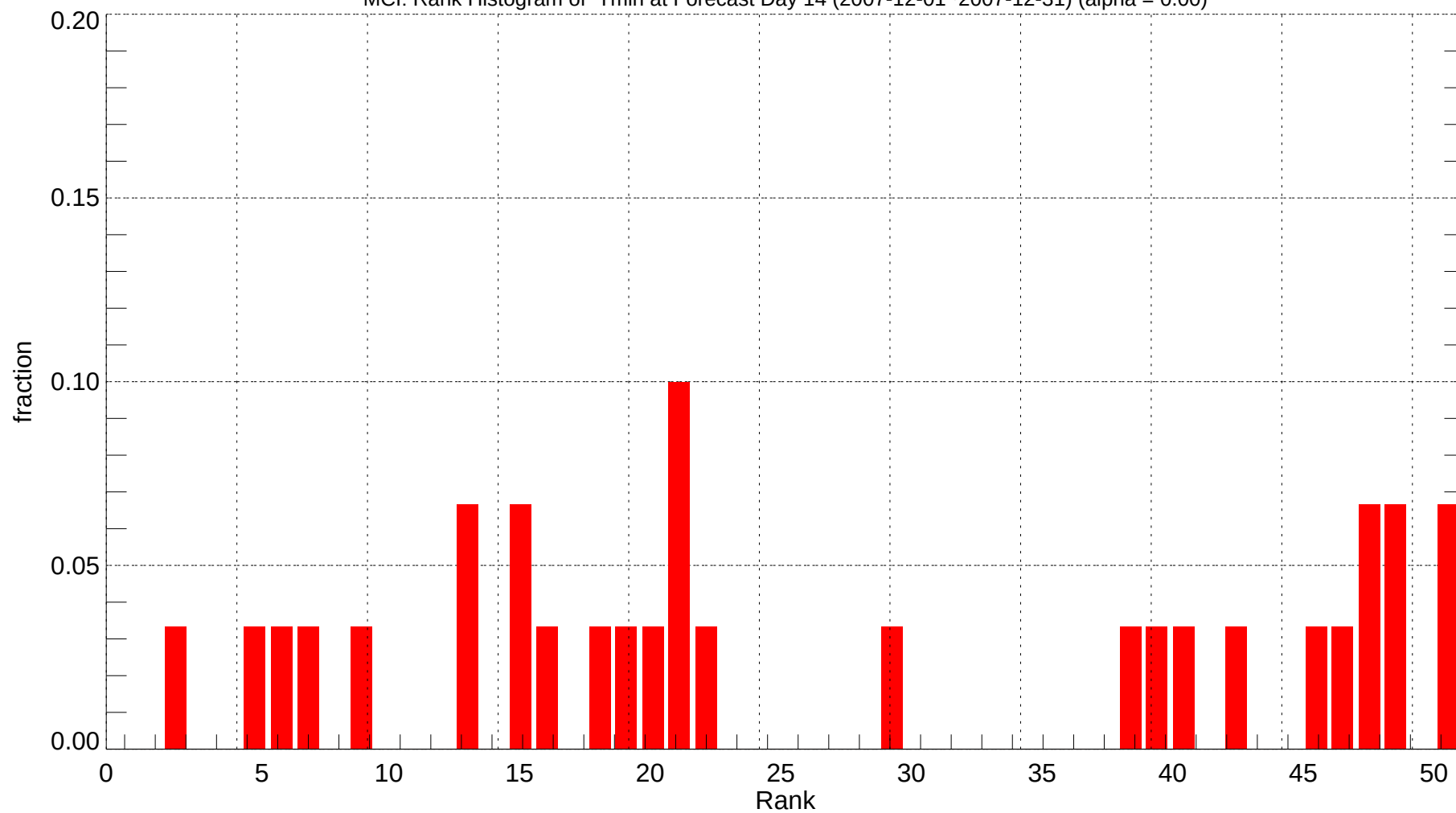
MCI: Rank Histogram of Tmin at Forecast Day 14 (2007-12-01~2007-12-31) (alpha = 0.00)
