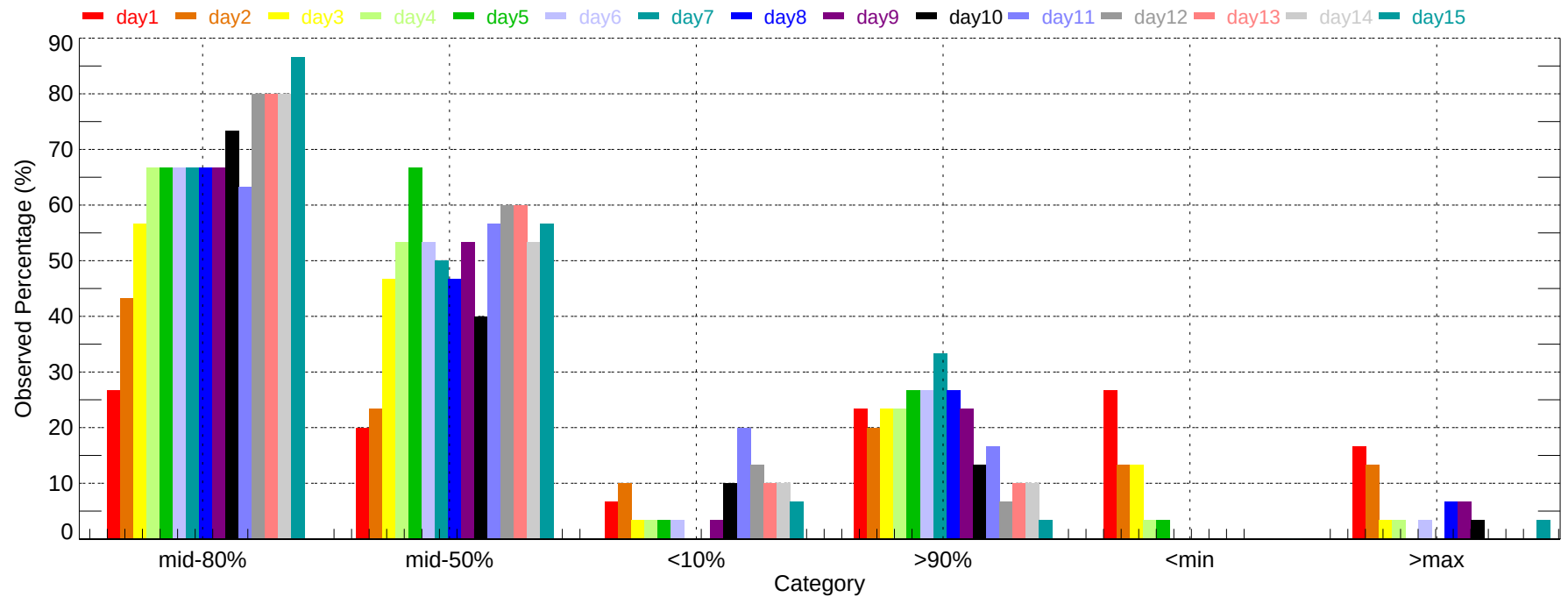
Observed Percentage of Ensembles - LGA: Max Temperature (2007-12-01~2007-12-31)
