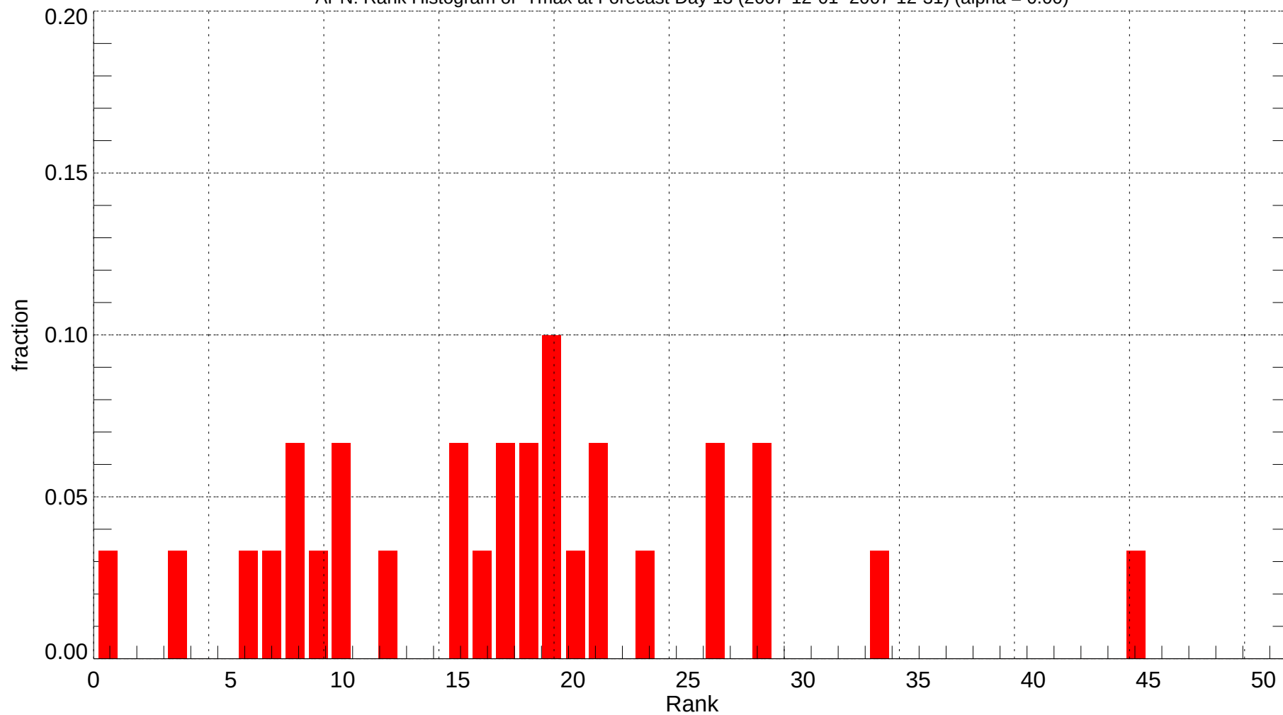
APN: Rank Histogram of Tmax at Forecast Day 13 (2007-12-01~2007-12-31) (alpha = 0.00)
