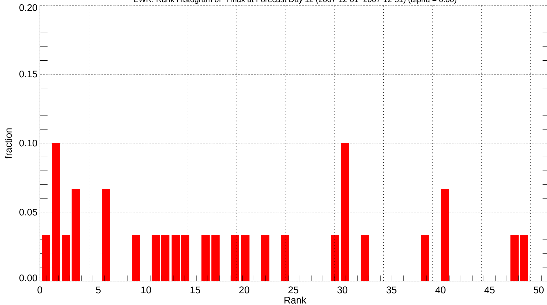
EWR: Rank Histogram of Tmax at Forecast Day 12 (2007-12-01~2007-12-31) (alpha = 0.00)
