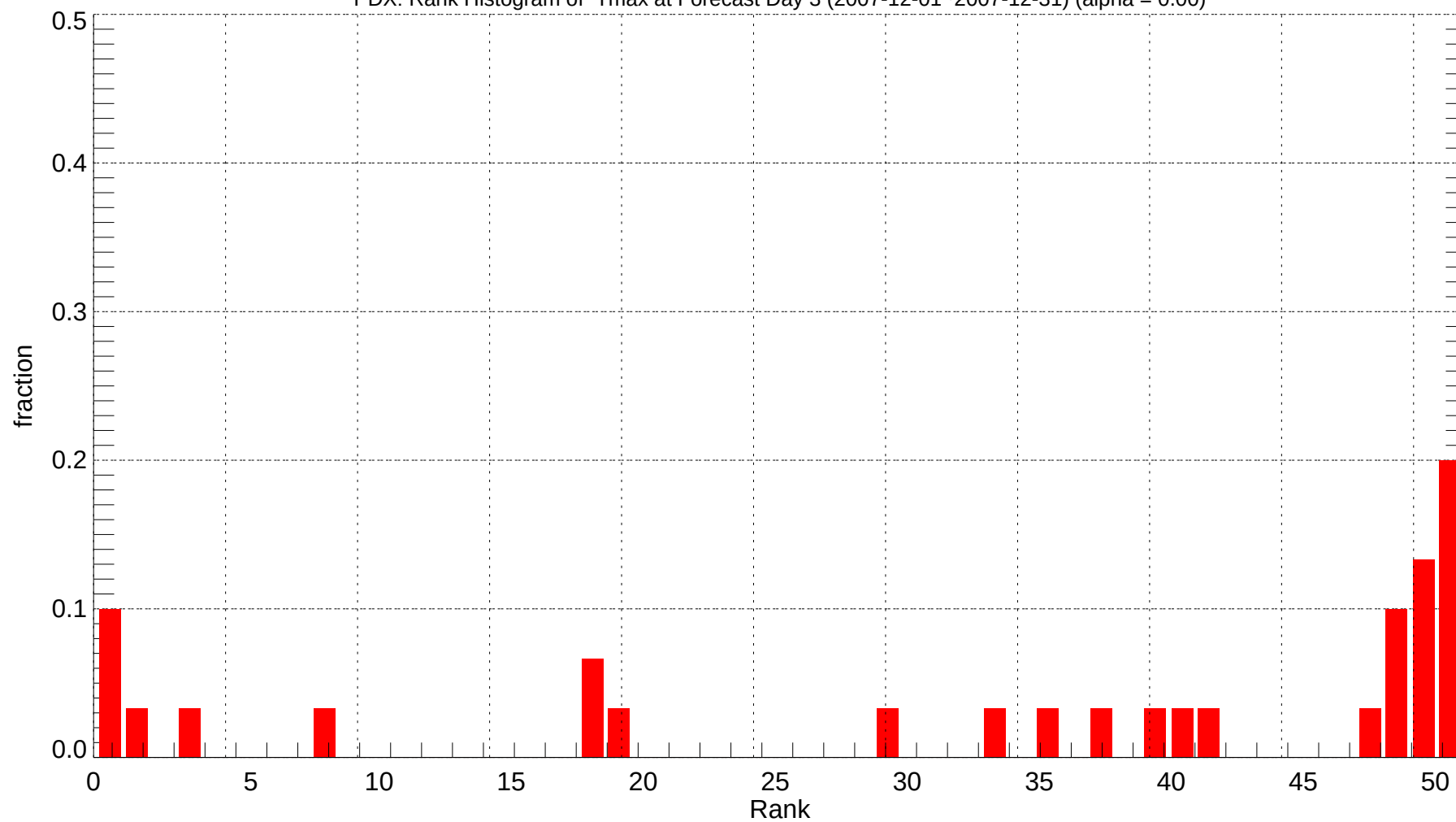
PDX: Rank Histogram of Tmax at Forecast Day 3 (2007-12-01~2007-12-31) (alpha = 0.00)
