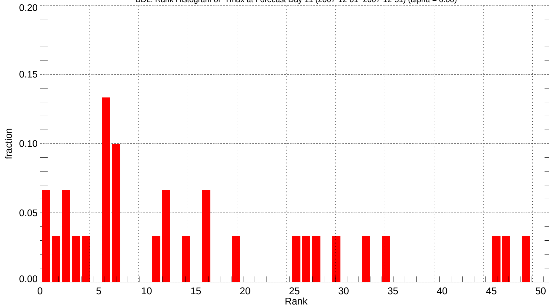
BDL: Rank Histogram of Tmax at Forecast Day 11 (2007-12-01~2007-12-31) (alpha = 0.00)
