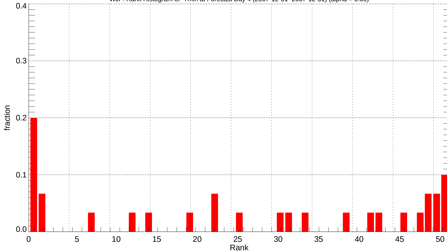
WJF: Rank Histogram of Tmin at Forecast Day 4 (2007-12-01~2007-12-31) (alpha = 0.00)
