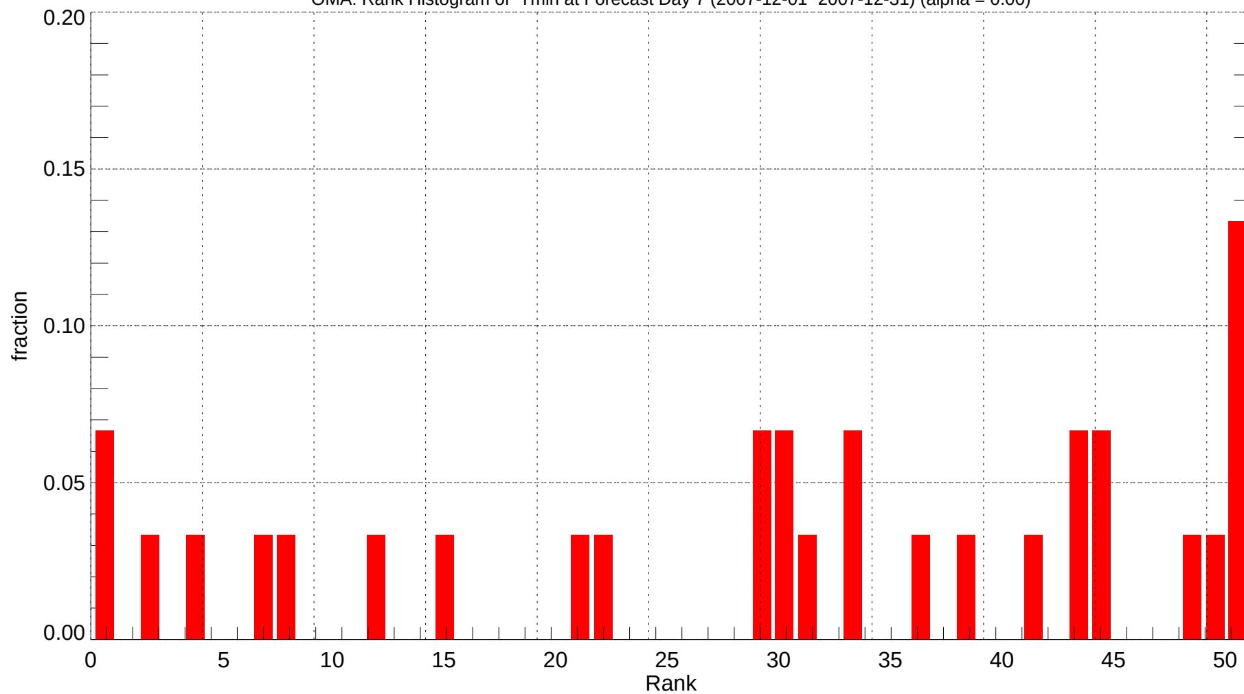
OMA: Rank Histogram of Tmin at Forecast Day 7 (2007-12-01~2007-12-31) (alpha = 0.00)
