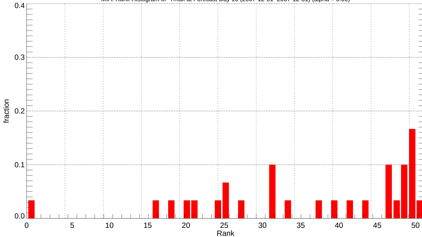
MIA: Rank Histogram of Tmax at Forecast Day 10 (2007-12-01~2007-12-31) (alpha = 0.00)
