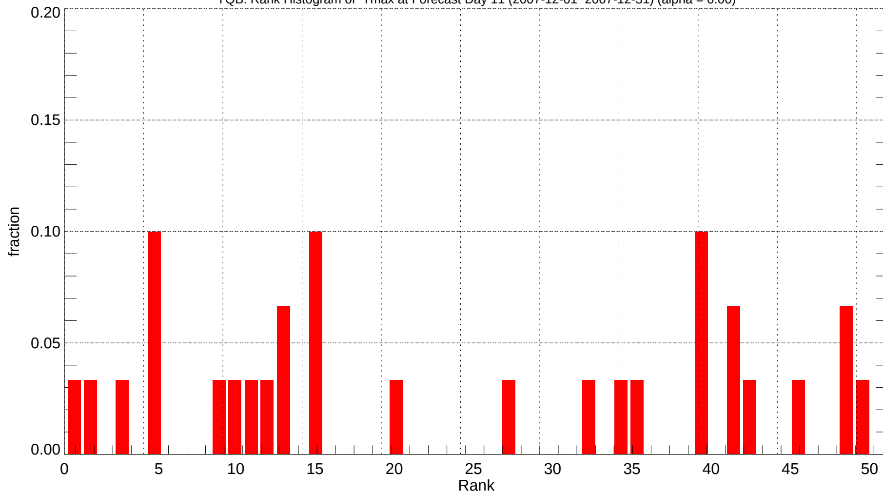
YQB: Rank Histogram of Tmax at Forecast Day 11 (2007-12-01~2007-12-31) (alpha = 0.00)
