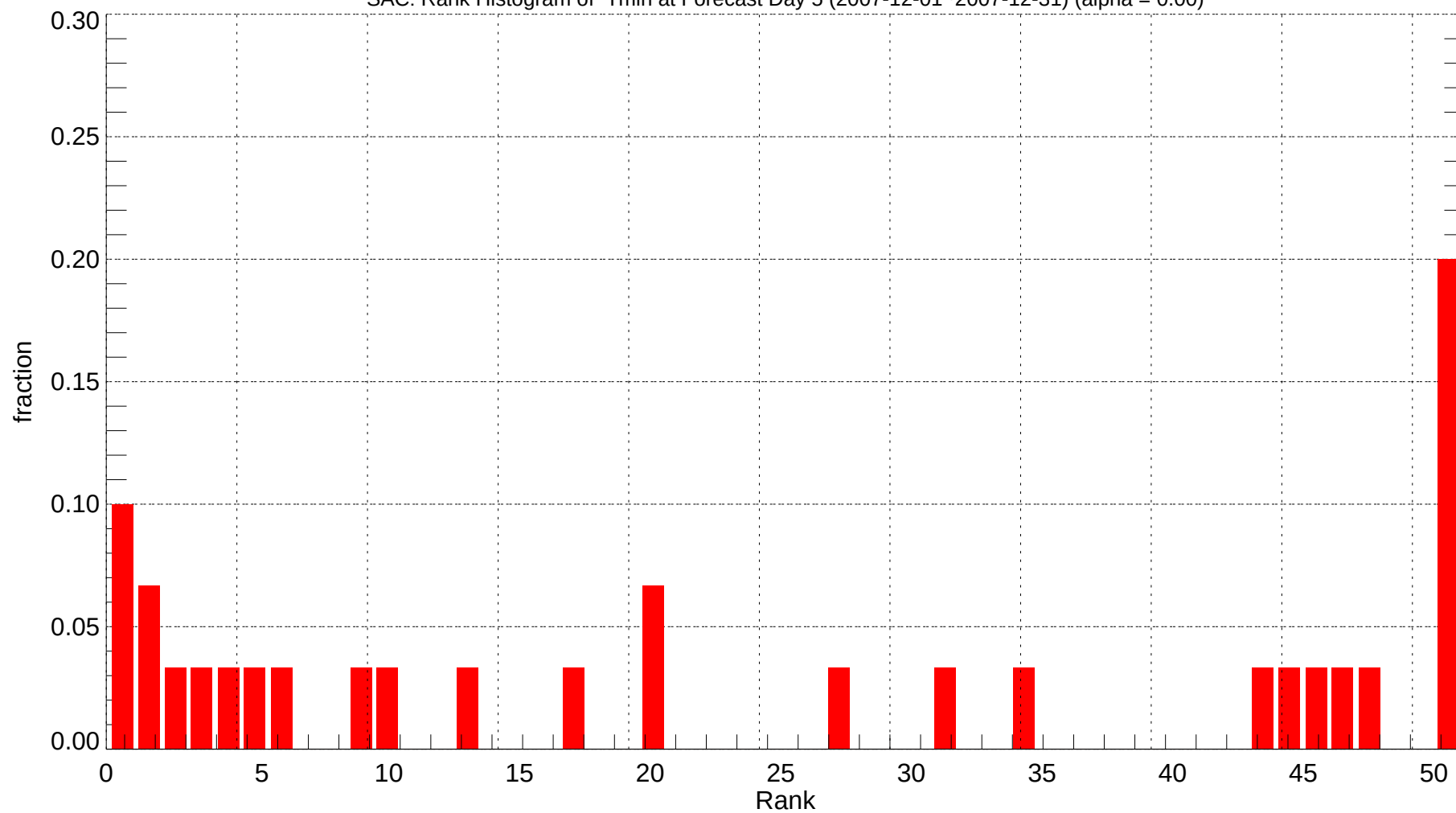
SAC: Rank Histogram of Tmin at Forecast Day 5 (2007-12-01~2007-12-31) (alpha = 0.00)
