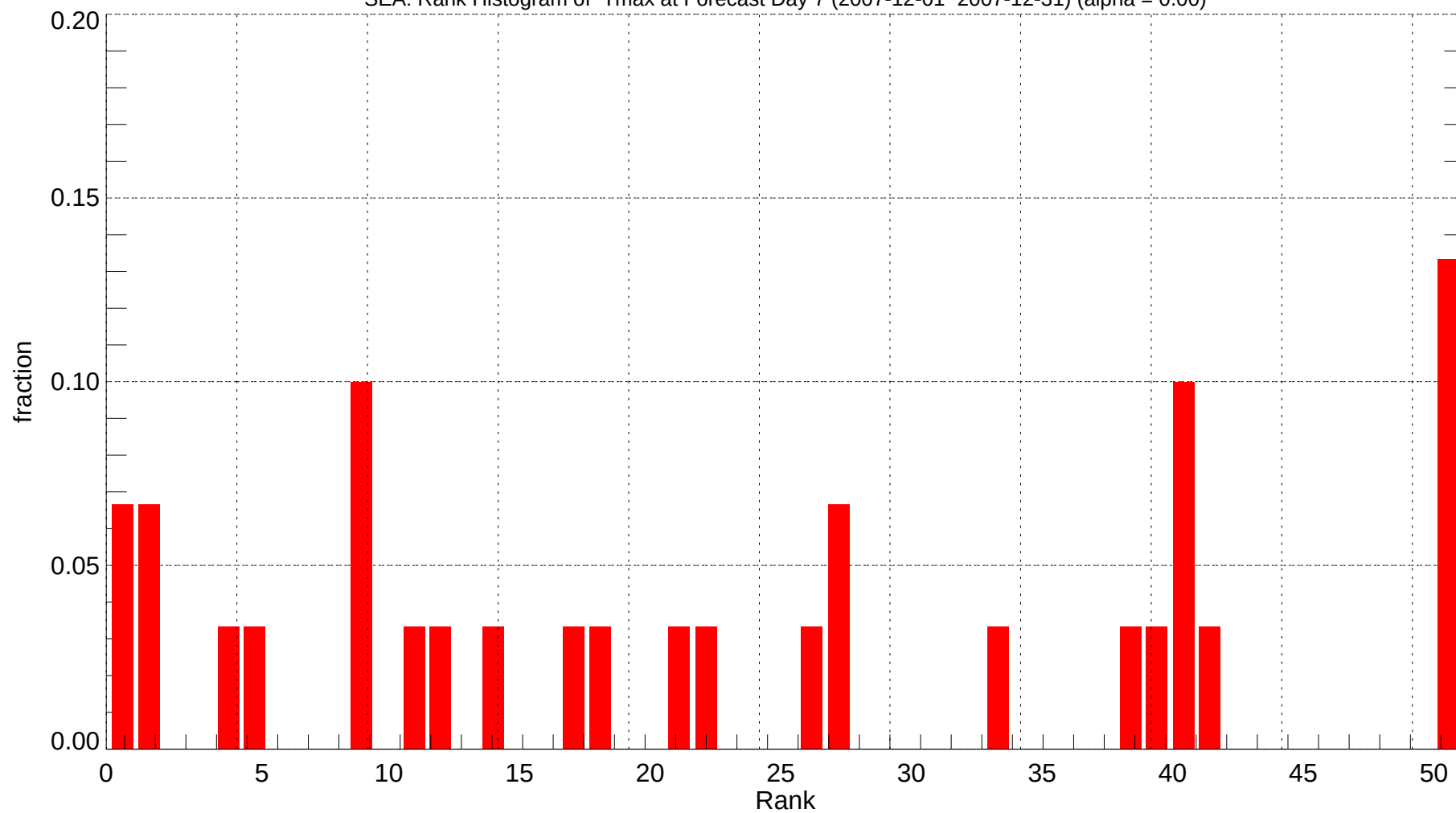
SEA: Rank Histogram of Tmax at Forecast Day 7 (2007-12-01~2007-12-31) (alpha = 0.00)
