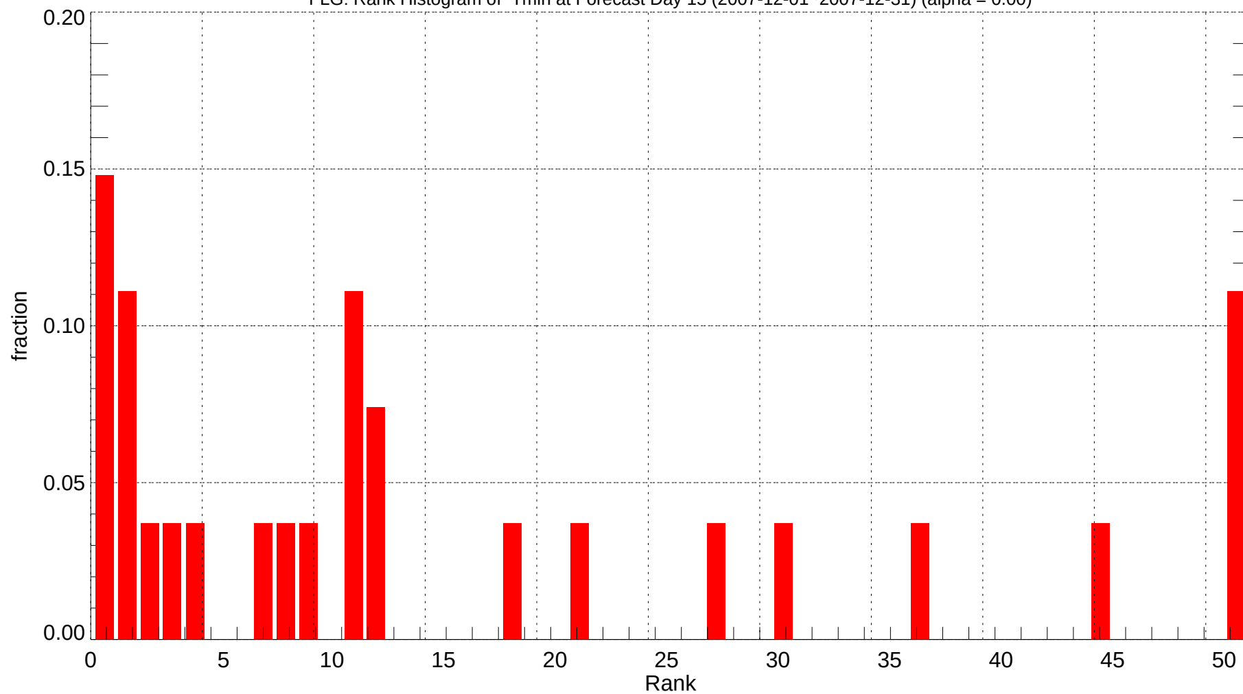
FLG: Rank Histogram of Tmin at Forecast Day 15 (2007-12-01~2007-12-31) (alpha = 0.00)
