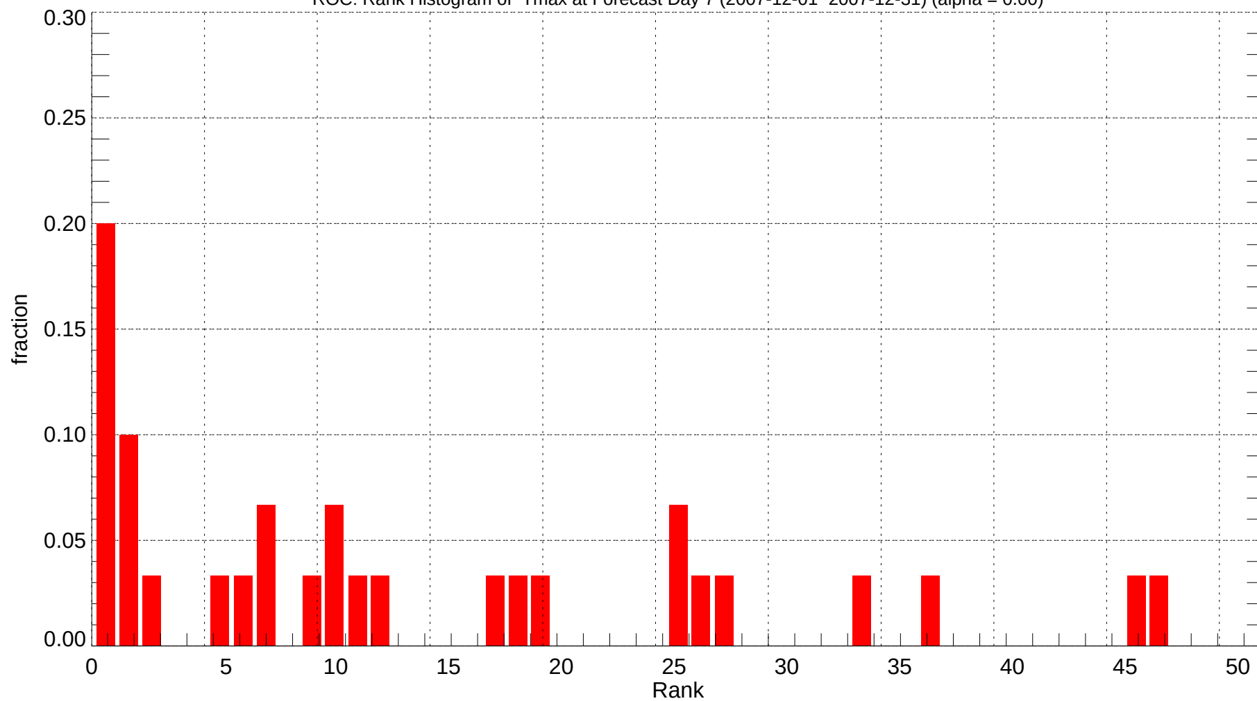
ROC: Rank Histogram of Tmax at Forecast Day 7 (2007-12-01~2007-12-31) (alpha = 0.00)
