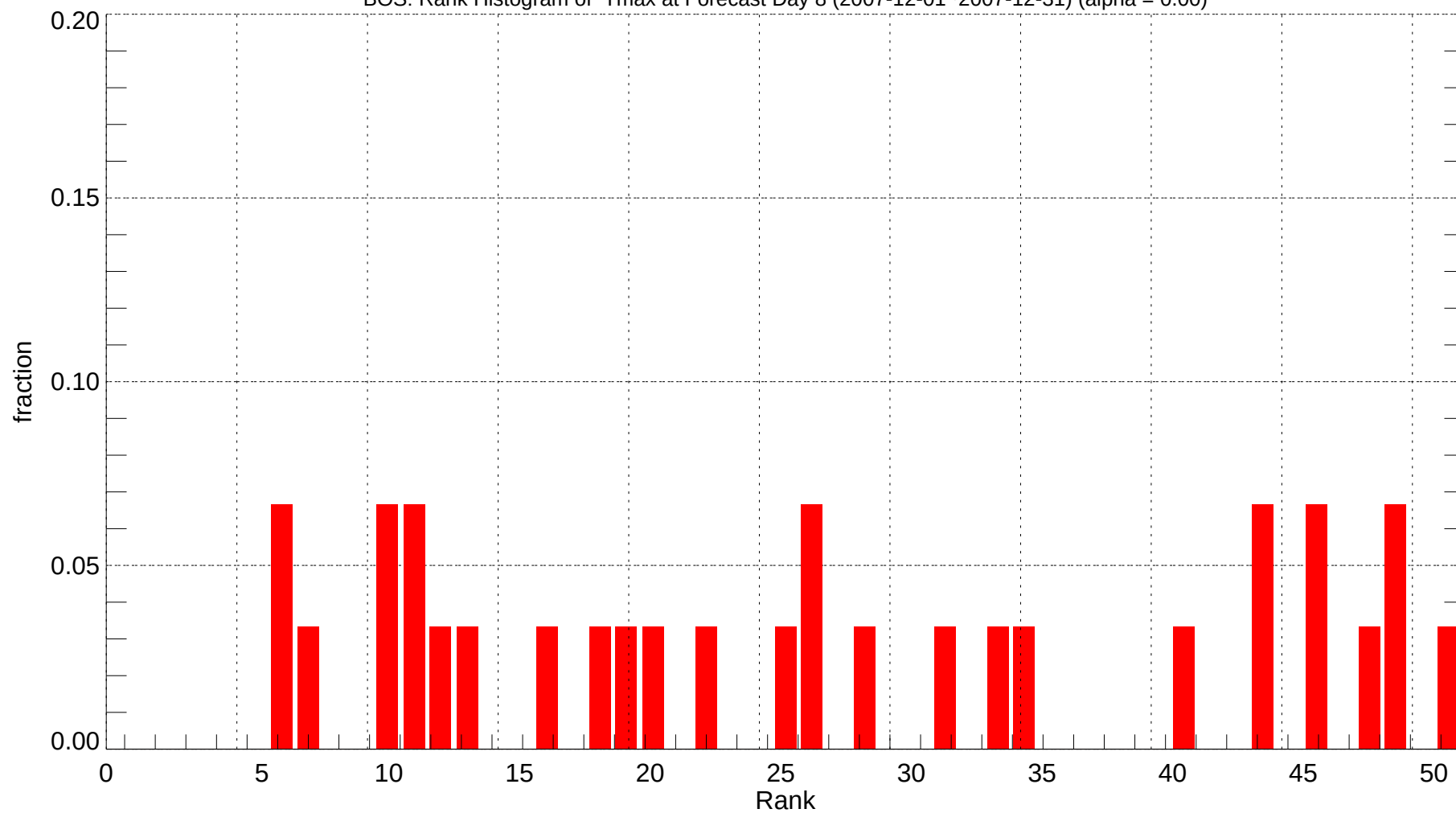
BOS: Rank Histogram of Tmax at Forecast Day 8 (2007-12-01~2007-12-31) (alpha = 0.00)
