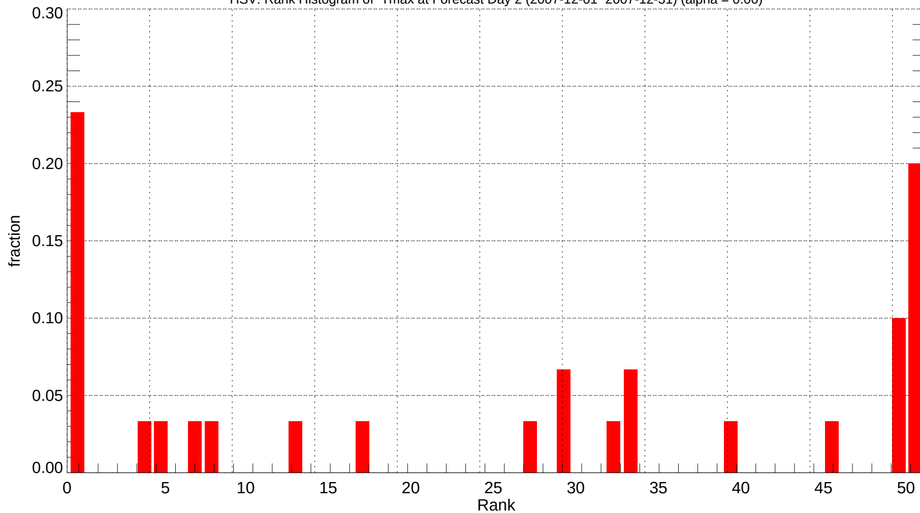
HSV: Rank Histogram of Tmax at Forecast Day 2 (2007-12-01~2007-12-31) (alpha = 0.00)
