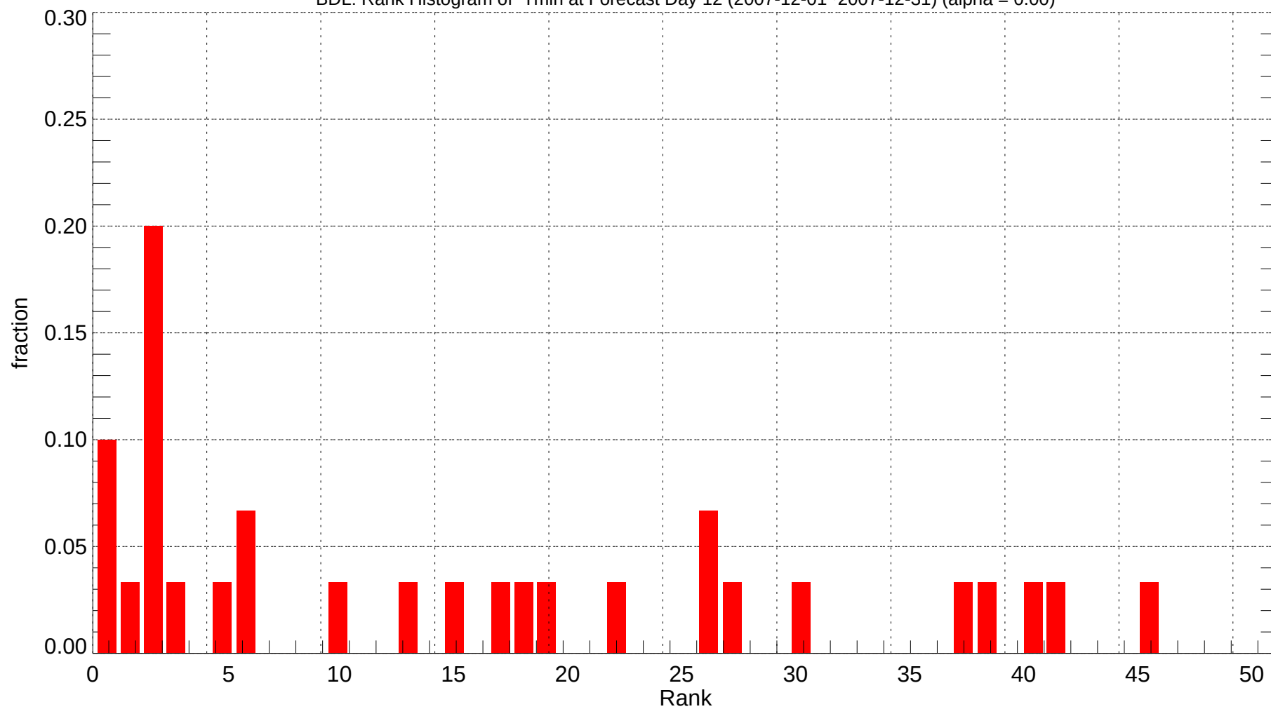
BDL: Rank Histogram of Tmin at Forecast Day 12 (2007-12-01~2007-12-31) (alpha = 0.00)
