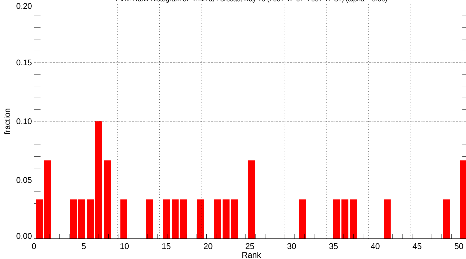
PVD: Rank Histogram of Tmin at Forecast Day 15 (2007-12-01~2007-12-31) (alpha = 0.00)
