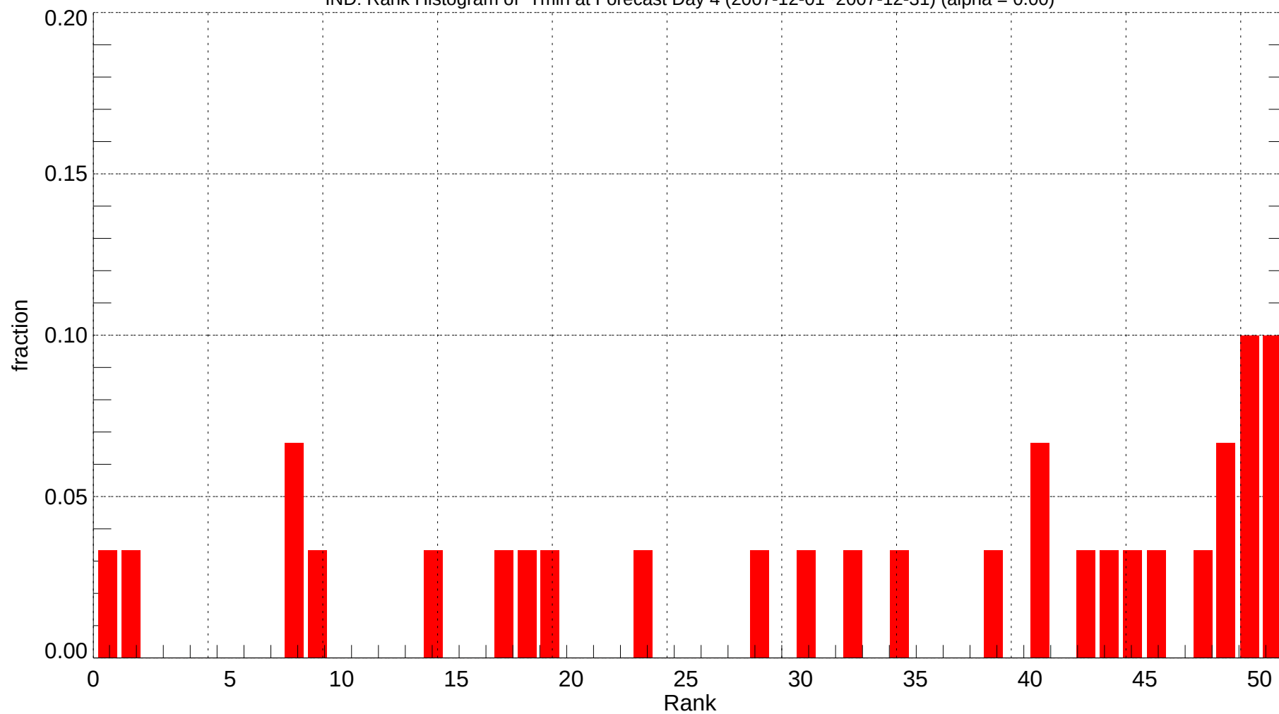
IND: Rank Histogram of Tmin at Forecast Day 4 (2007-12-01~2007-12-31) (alpha = 0.00)
