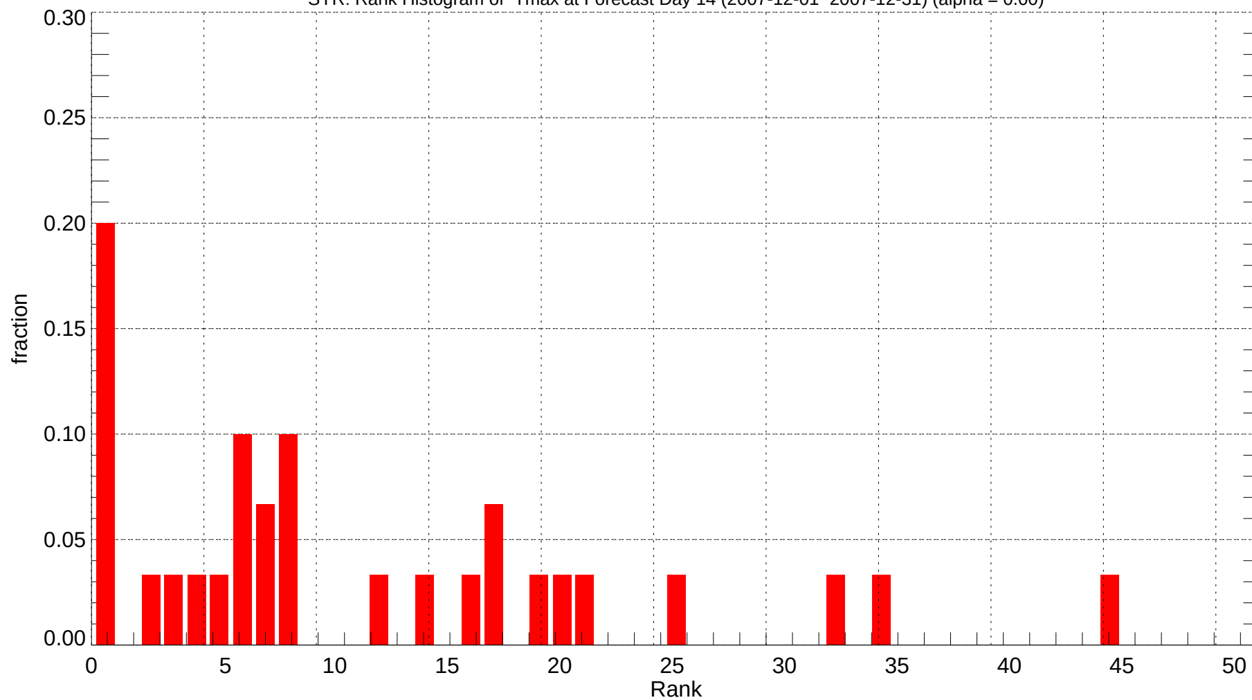
SYR: Rank Histogram of Tmax at Forecast Day 14 (2007-12-01~2007-12-31) (alpha = 0.00)
