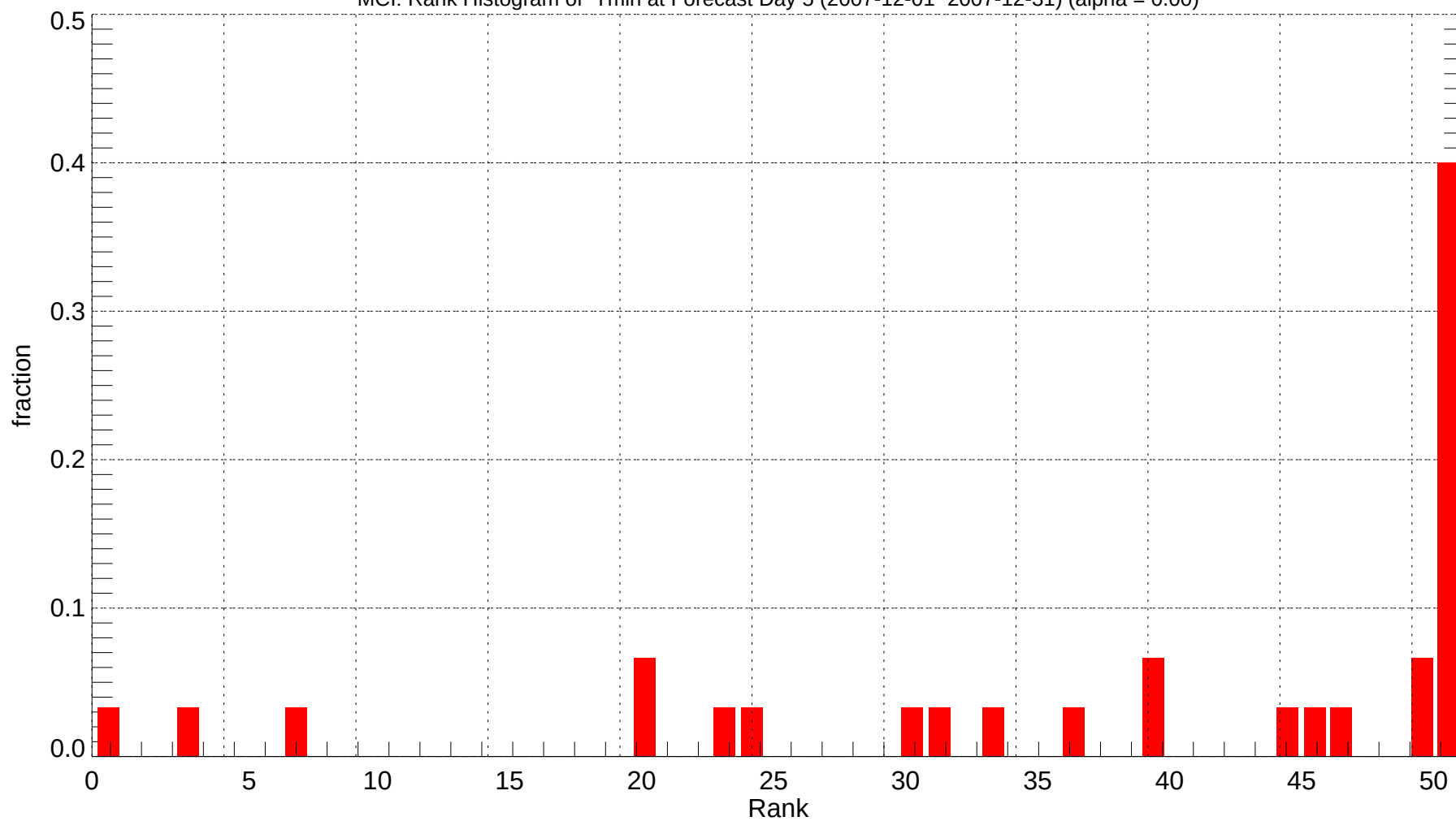
MCI: Rank Histogram of Tmin at Forecast Day 5 (2007-12-01~2007-12-31) (alpha = 0.00)
