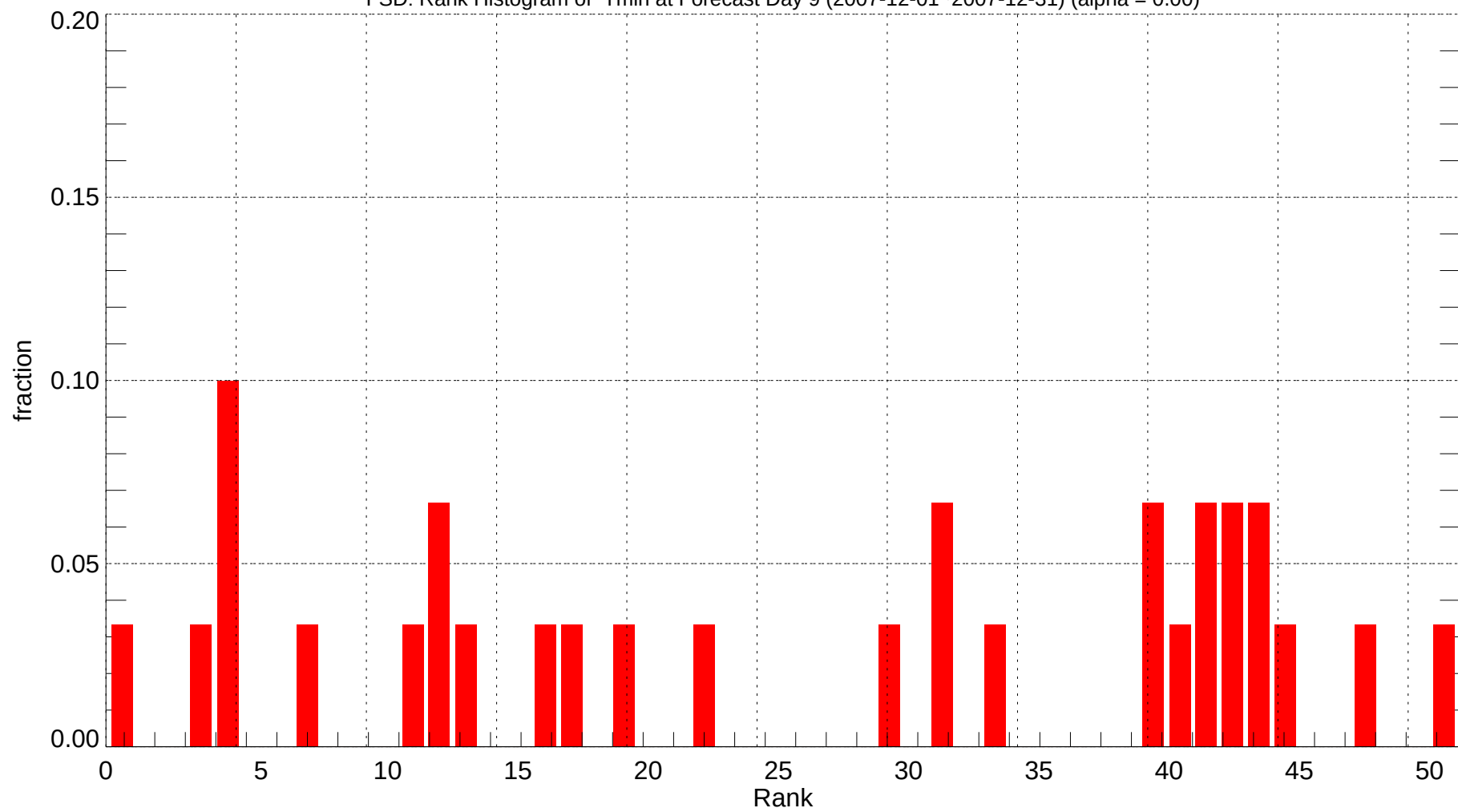
FSD: Rank Histogram of Tmin at Forecast Day 9 (2007-12-01~2007-12-31) (alpha = 0.00)
