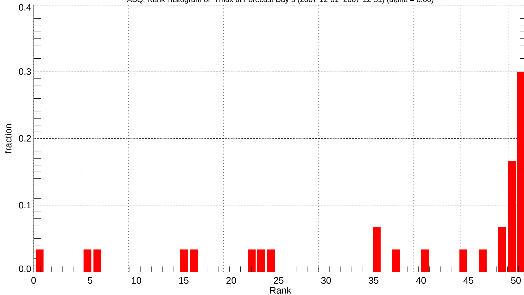
ABQ: Rank Histogram of Tmax at Forecast Day 5 (2007-12-01~2007-12-31) (alpha = 0.00)
