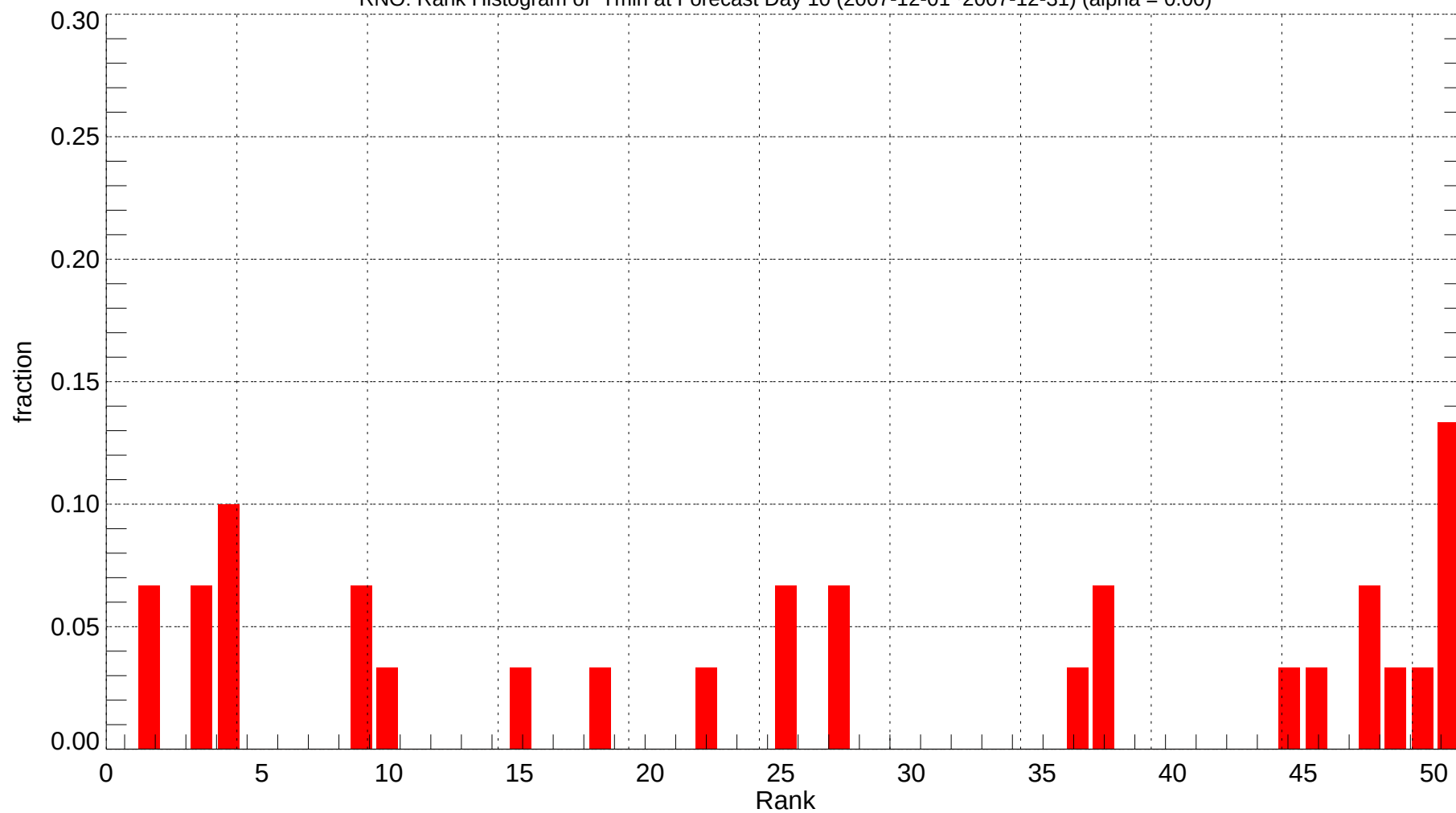
RNO: Rank Histogram of Tmin at Forecast Day 10 (2007-12-01~2007-12-31) (alpha = 0.00)
