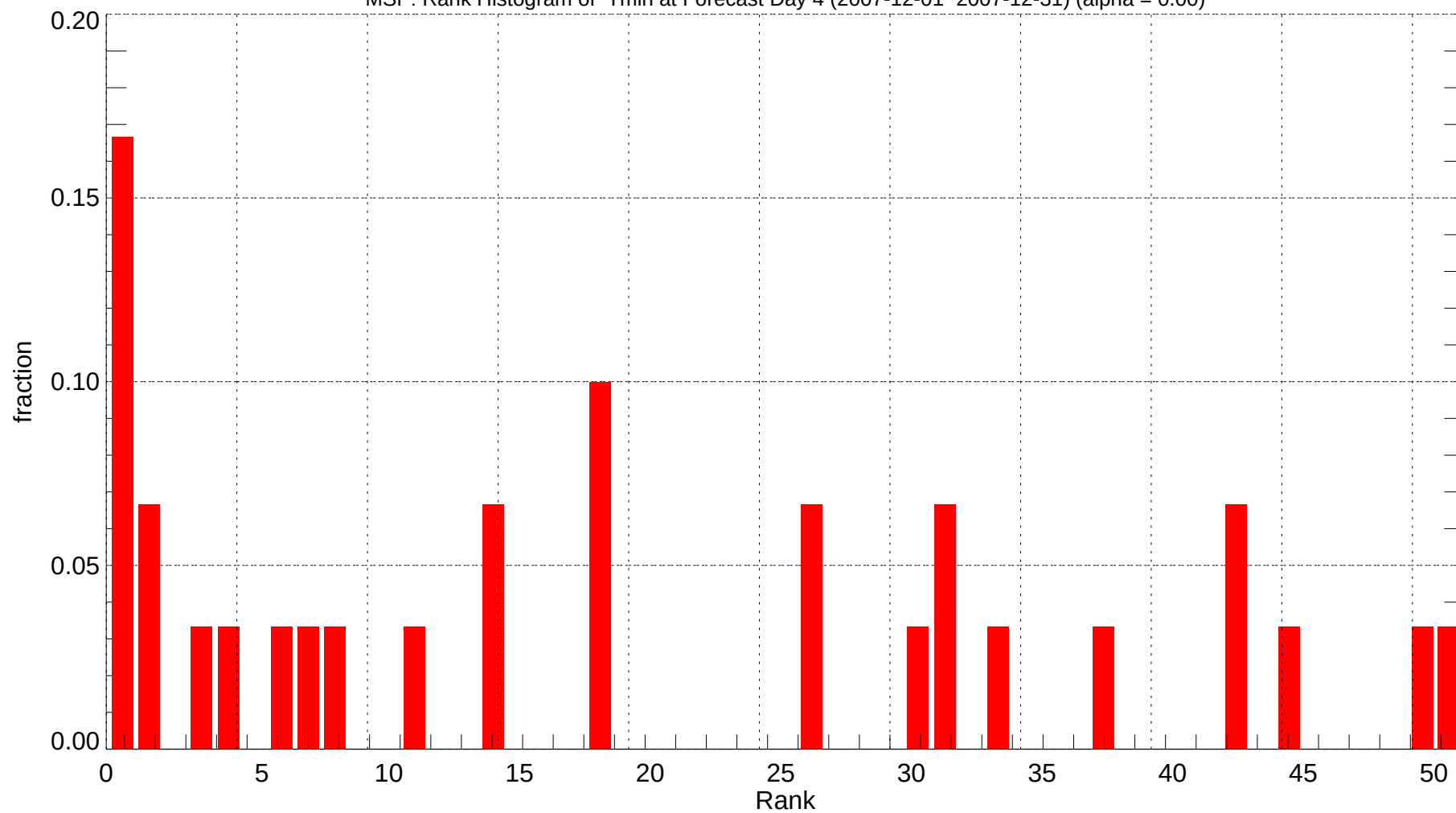
MSP: Rank Histogram of Tmin at Forecast Day 4 (2007-12-01~2007-12-31) (alpha = 0.00)
