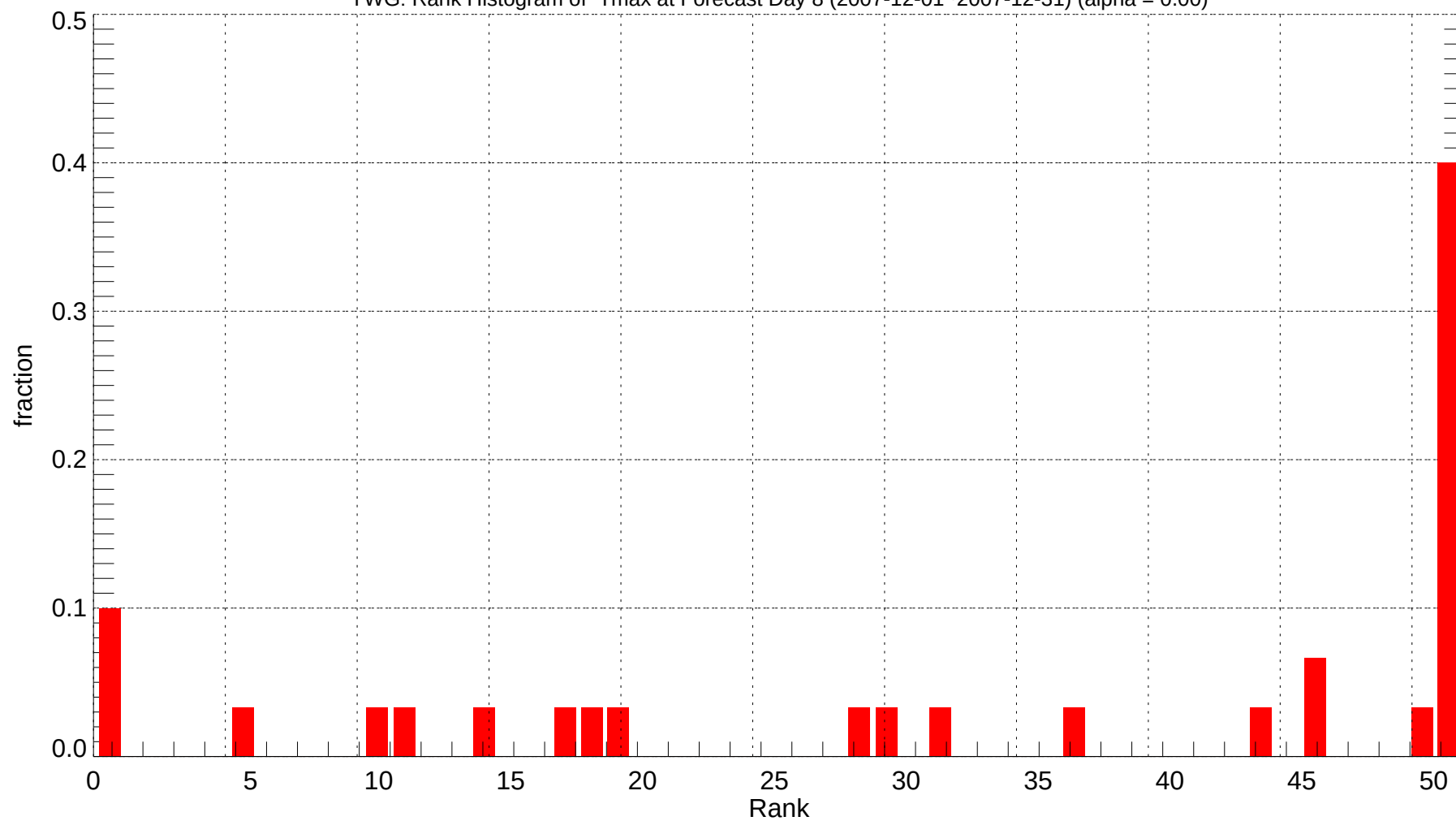
YWG: Rank Histogram of Tmax at Forecast Day 8 (2007-12-01~2007-12-31) (alpha = 0.00)
