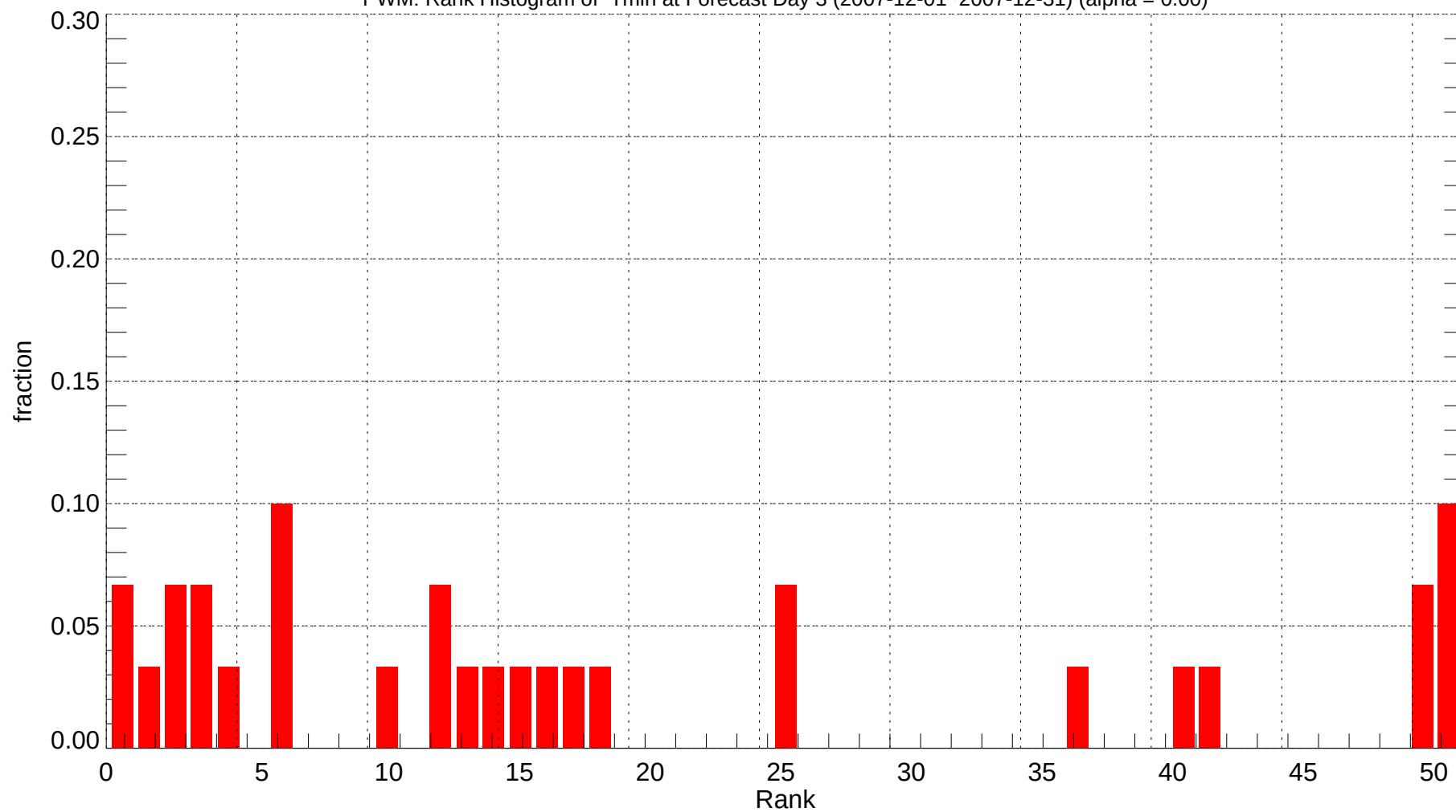
PWM: Rank Histogram of Tmin at Forecast Day 3 (2007-12-01~2007-12-31) (alpha = 0.00)
