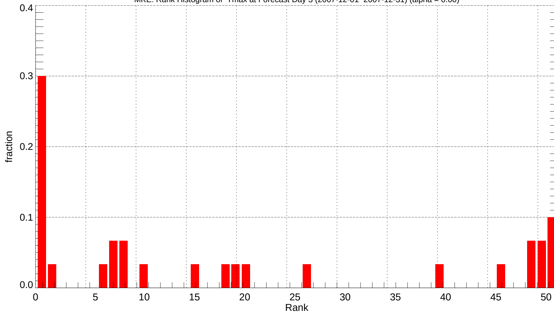
MKE: Rank Histogram of Tmax at Forecast Day 3 (2007-12-01~2007-12-31) (alpha = 0.00)
