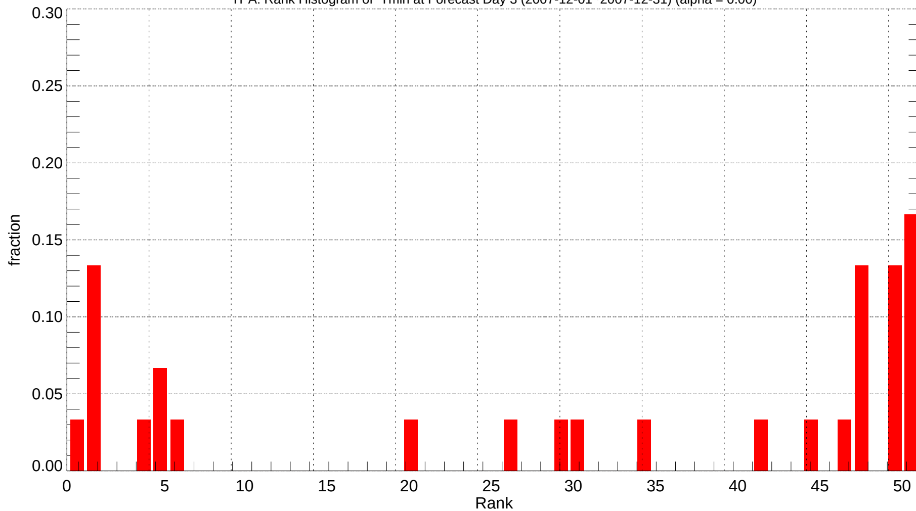
TPA: Rank Histogram of Tmin at Forecast Day 3 (2007-12-01~2007-12-31) (alpha = 0.00)
