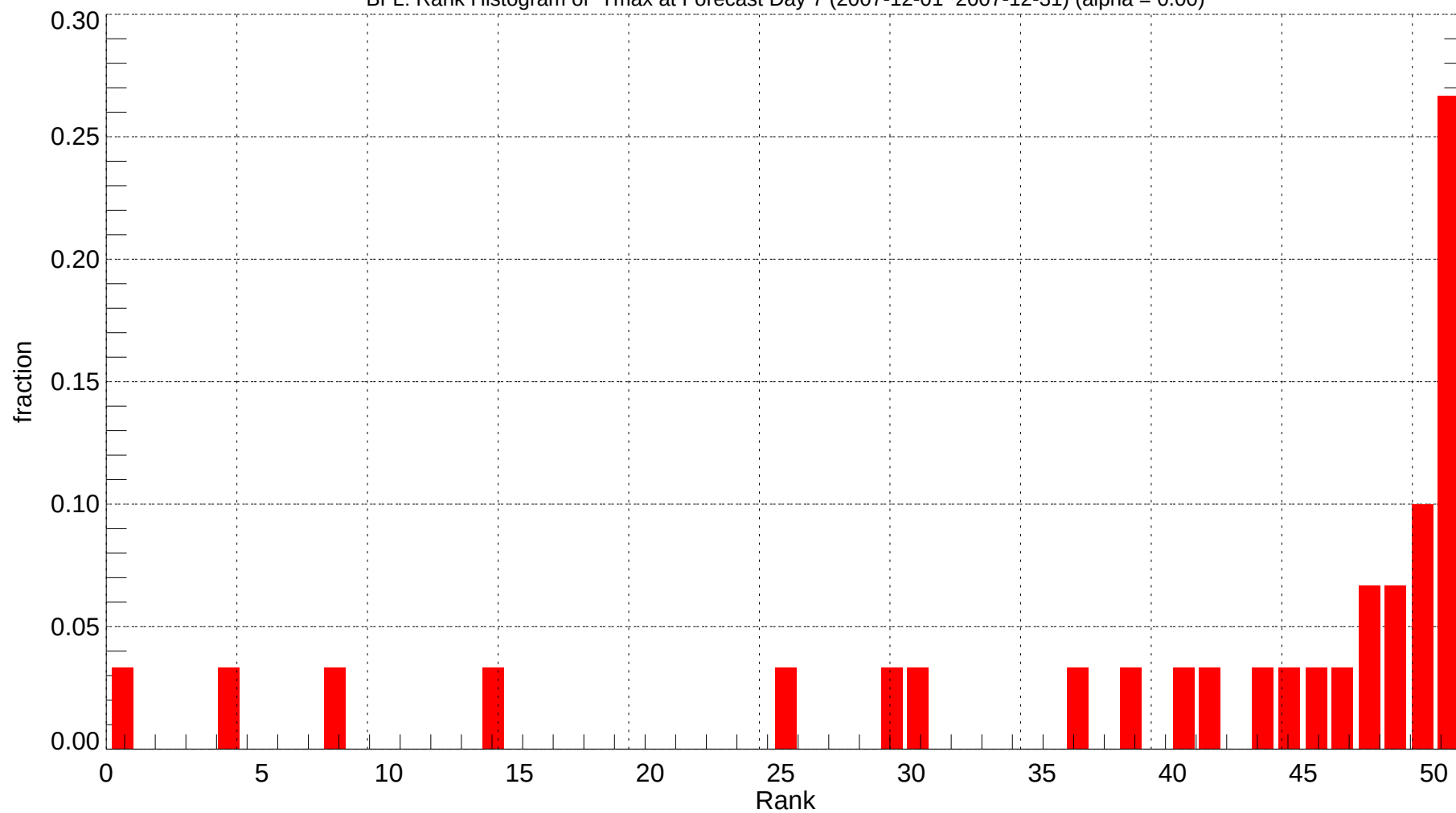
BFL: Rank Histogram of Tmax at Forecast Day 7 (2007-12-01~2007-12-31) (alpha = 0.00)
