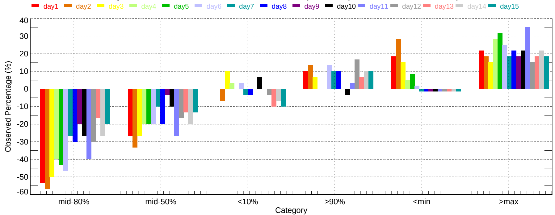
Observed Percentage Deviation of Ensembles - ATL: Max Temperature (2007-12-01~2007-12-31)
