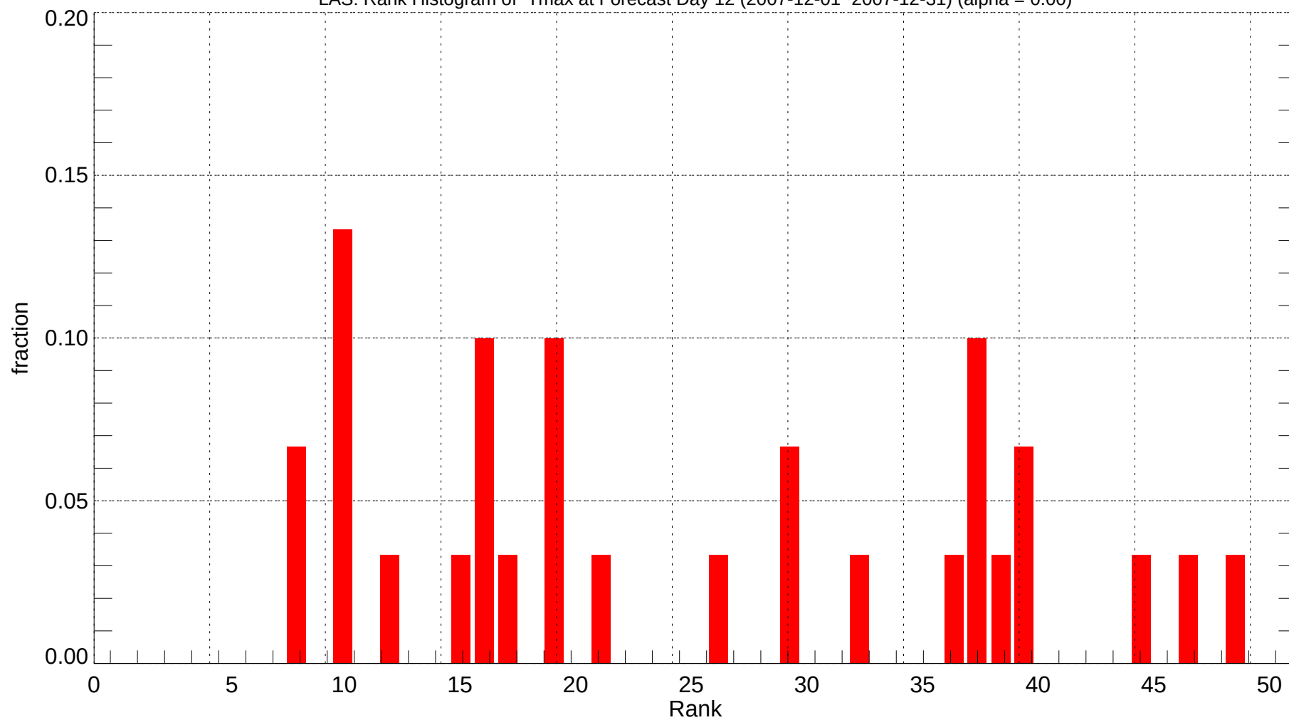
LAS: Rank Histogram of Tmax at Forecast Day 12 (2007-12-01~2007-12-31) (alpha = 0.00)
