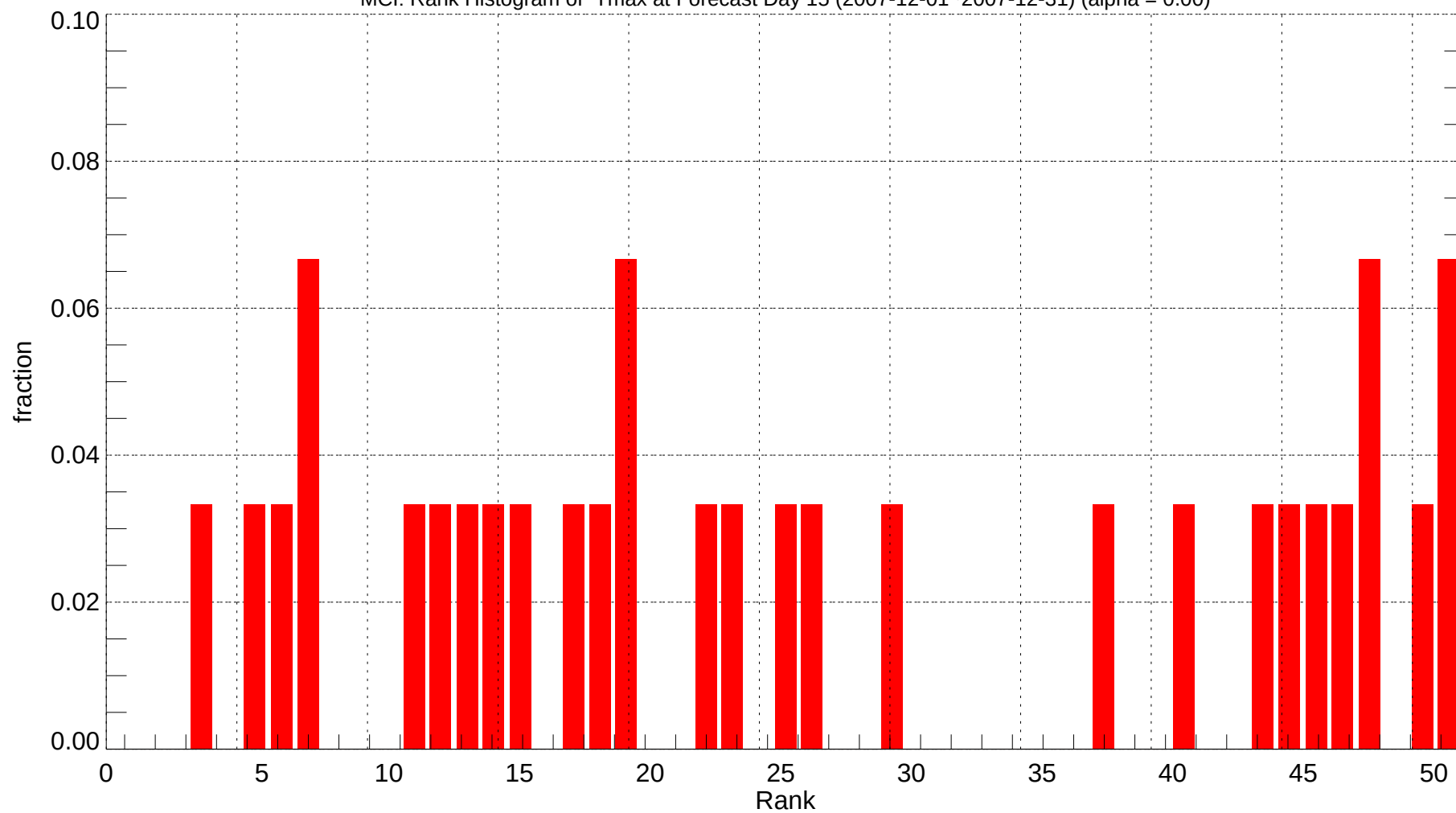
MCI: Rank Histogram of Tmax at Forecast Day 15 (2007-12-01~2007-12-31) (alpha = 0.00)
