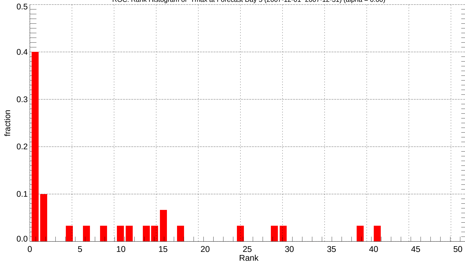
ROC: Rank Histogram of Tmax at Forecast Day 5 (2007-12-01~2007-12-31) (alpha = 0.00)
