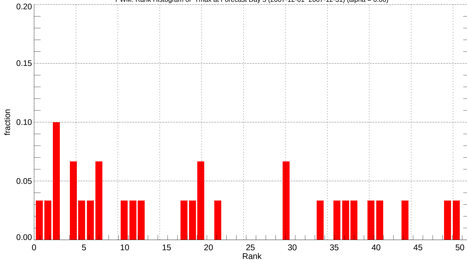
PWM: Rank Histogram of Tmax at Forecast Day 5 (2007-12-01~2007-12-31) (alpha = 0.00)
