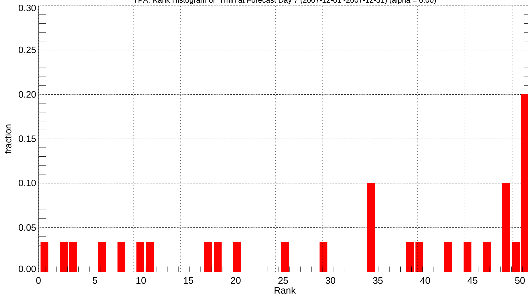
TPA: Rank Histogram of Tmin at Forecast Day 7 (2007-12-01~2007-12-31) (alpha = 0.00)
