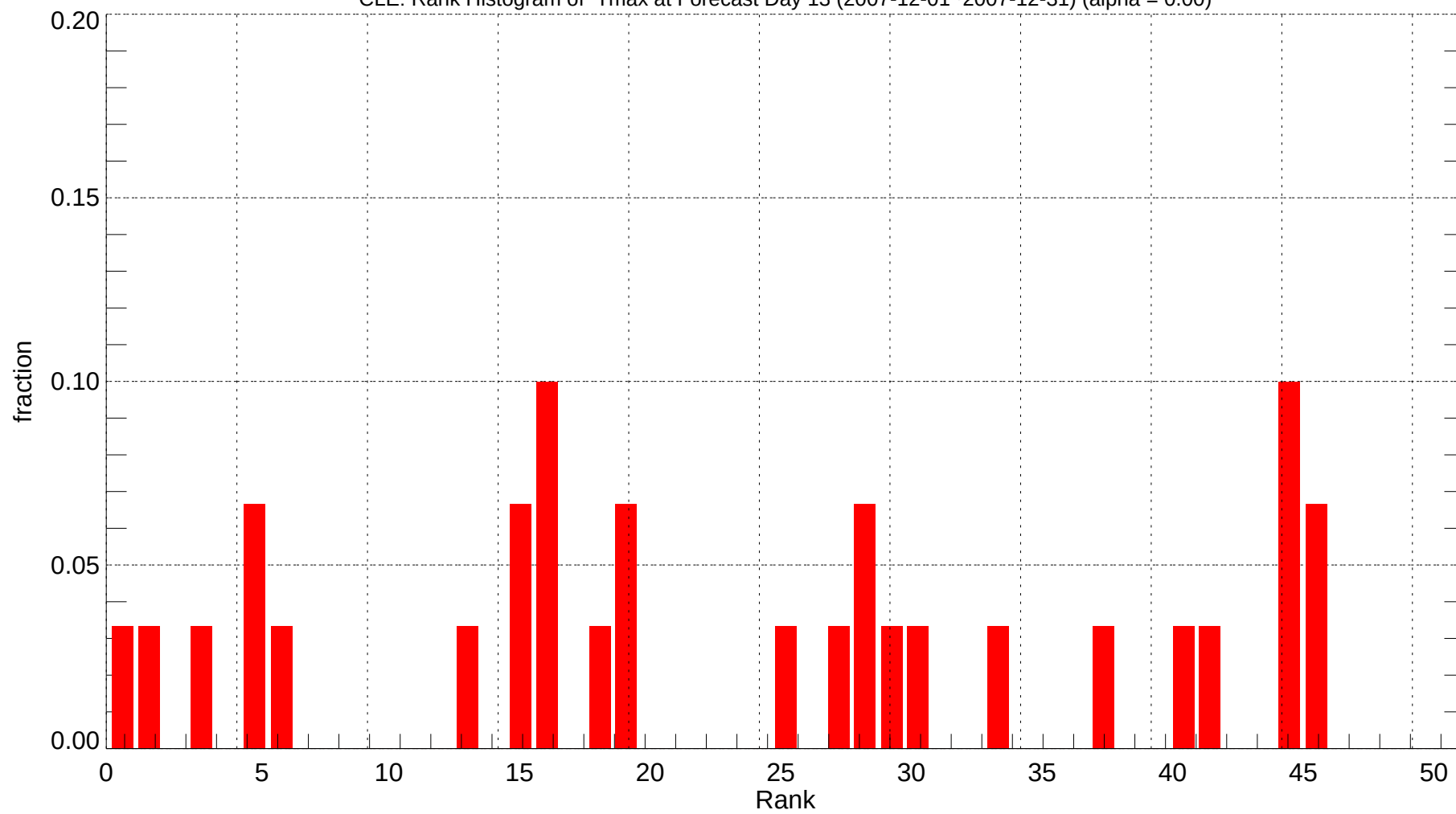
CLE: Rank Histogram of Tmax at Forecast Day 13 (2007-12-01~2007-12-31) (alpha = 0.00)
