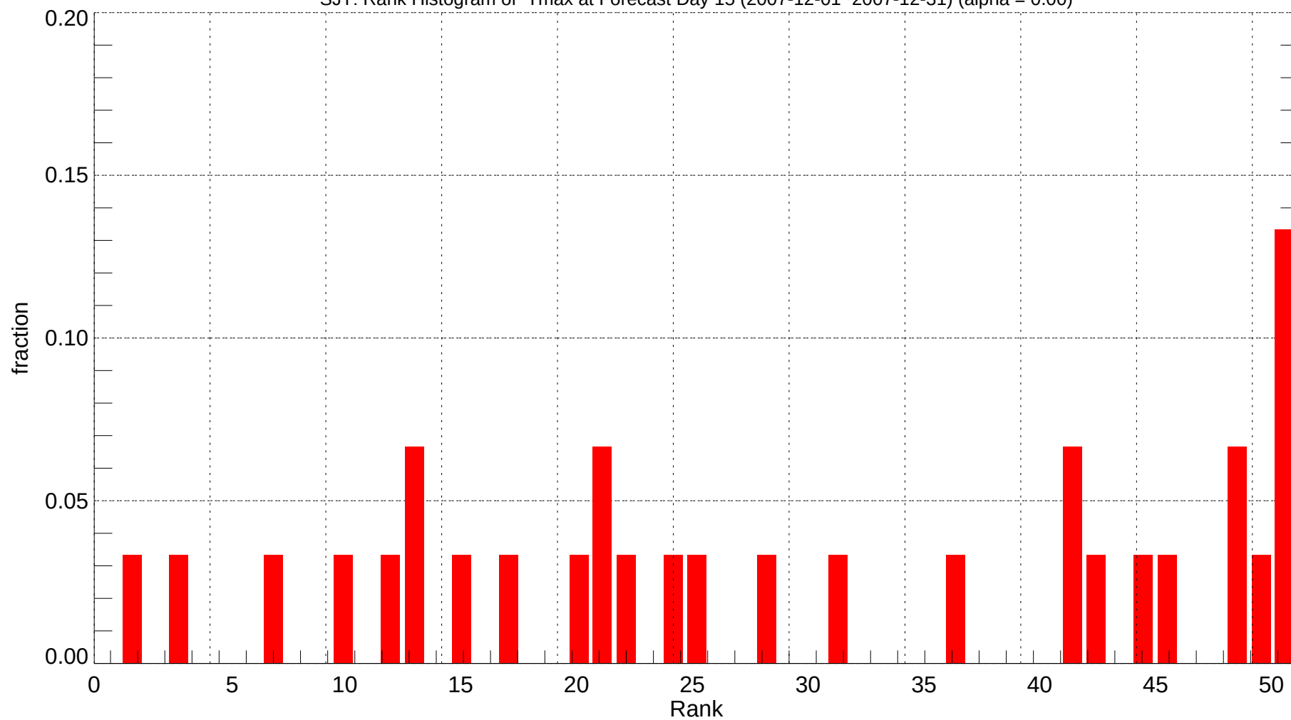
SJT: Rank Histogram of Tmax at Forecast Day 15 (2007-12-01~2007-12-31) (alpha = 0.00)
