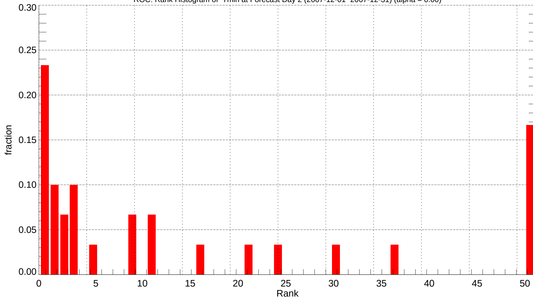
ROC: Rank Histogram of Tmin at Forecast Day 2 (2007-12-01~2007-12-31) (alpha = 0.00)
