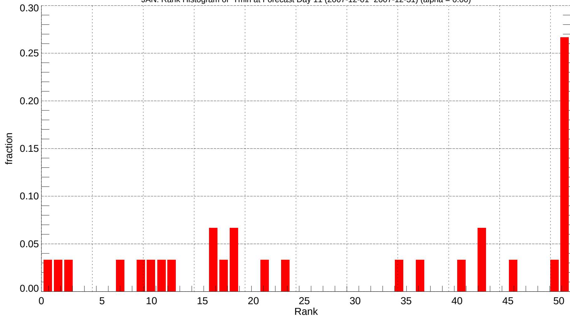
JAN: Rank Histogram of Tmin at Forecast Day 11 (2007-12-01~2007-12-31) (alpha = 0.00)
