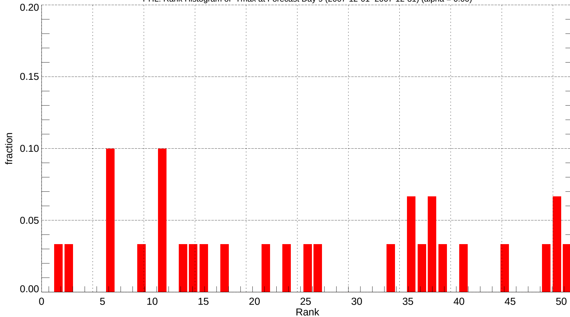
PHL: Rank Histogram of Tmax at Forecast Day 9 (2007-12-01~2007-12-31) (alpha = 0.00)
