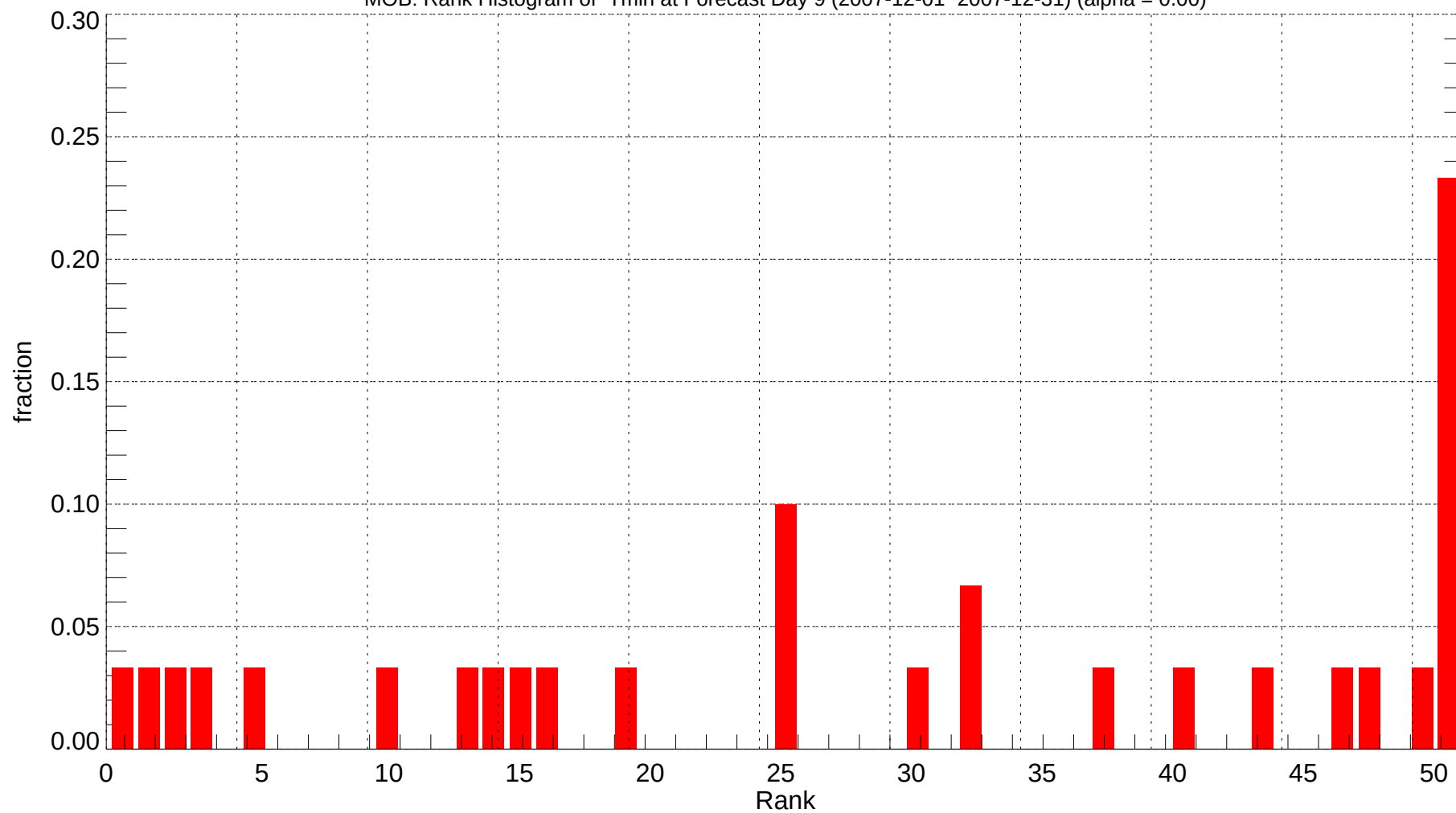
MOB: Rank Histogram of Tmin at Forecast Day 9 (2007-12-01~2007-12-31) (alpha = 0.00)
