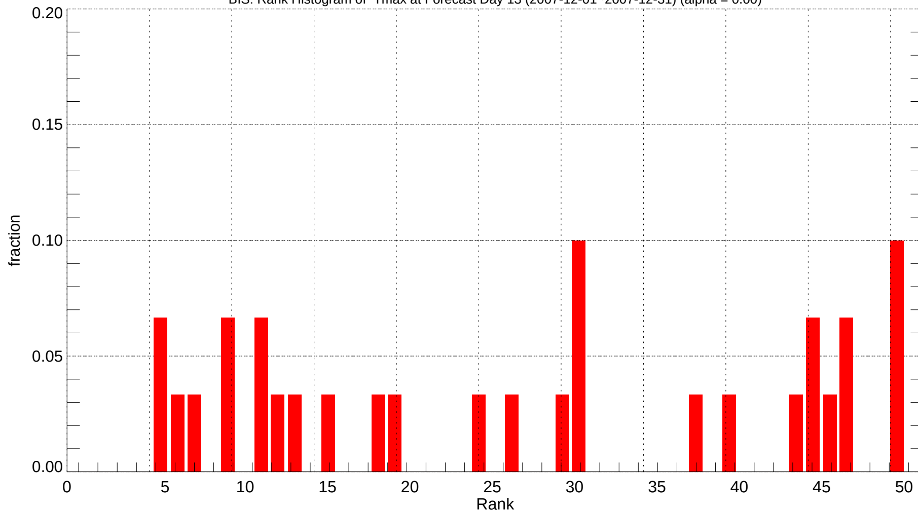
BIS: Rank Histogram of Tmax at Forecast Day 13 (2007-12-01~2007-12-31) (alpha = 0.00)
