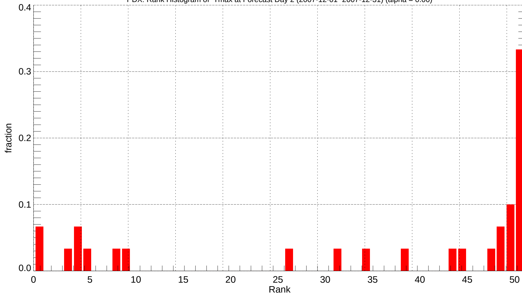
PDX: Rank Histogram of Tmax at Forecast Day 2 (2007-12-01~2007-12-31) (alpha = 0.00)
