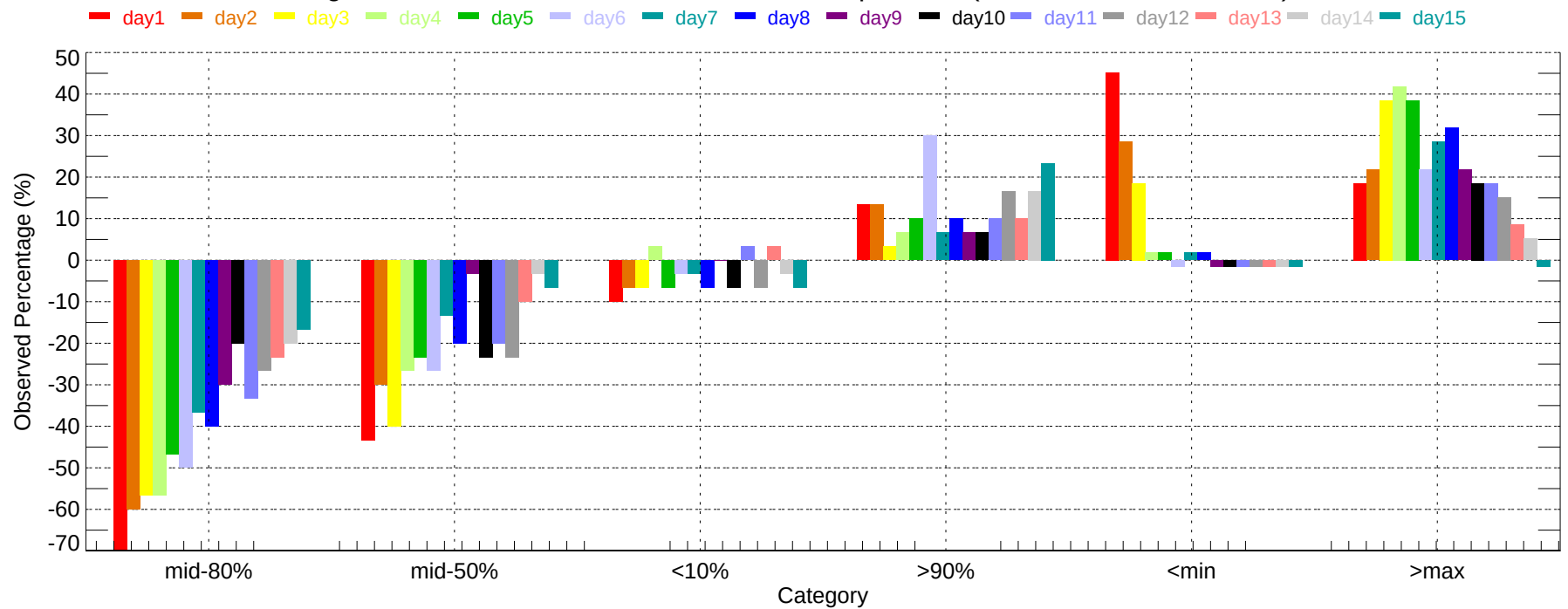
Observed Percentage Deviation of Ensembles - MCI: Min Temperature (2007-12-01~2007-12-31)
