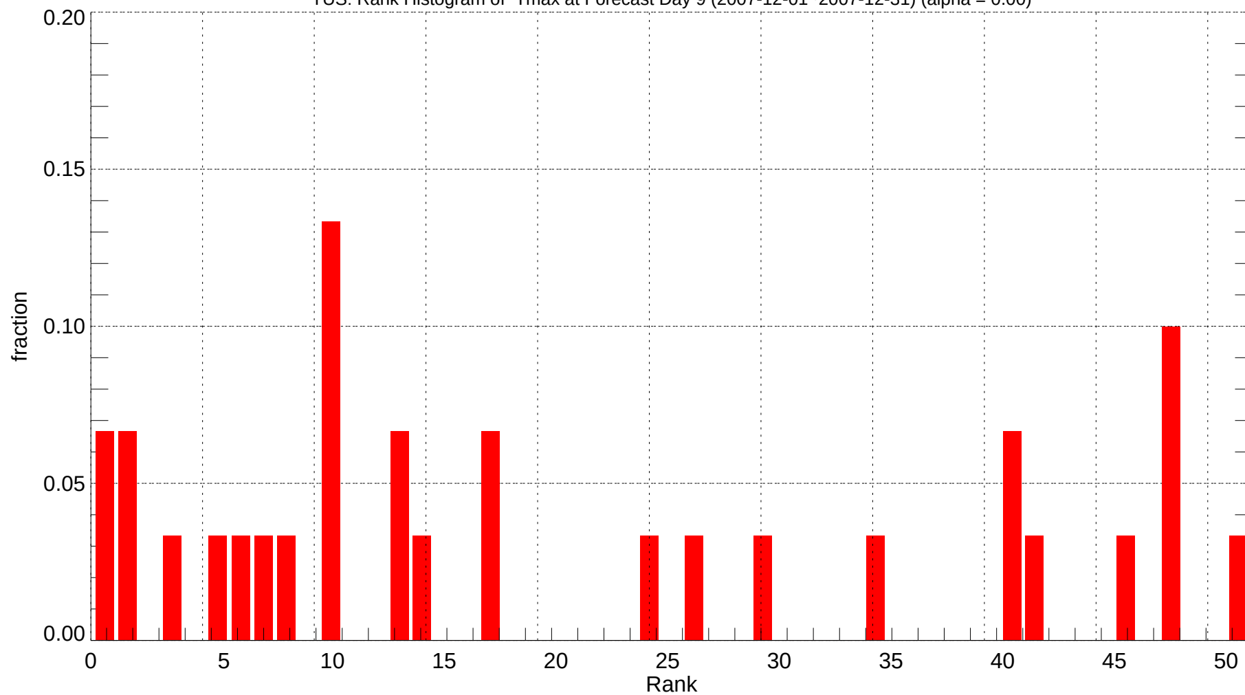
TUS: Rank Histogram of Tmax at Forecast Day 9 (2007-12-01~2007-12-31) (alpha = 0.00)
