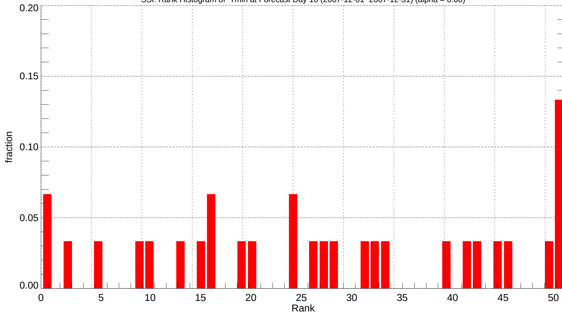
SSI: Rank Histogram of Tmin at Forecast Day 10 (2007-12-01~2007-12-31) (alpha = 0.00)
