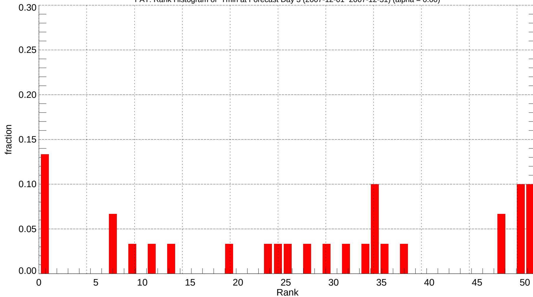
FAT: Rank Histogram of Tmin at Forecast Day 3 (2007-12-01~2007-12-31) (alpha = 0.00)
