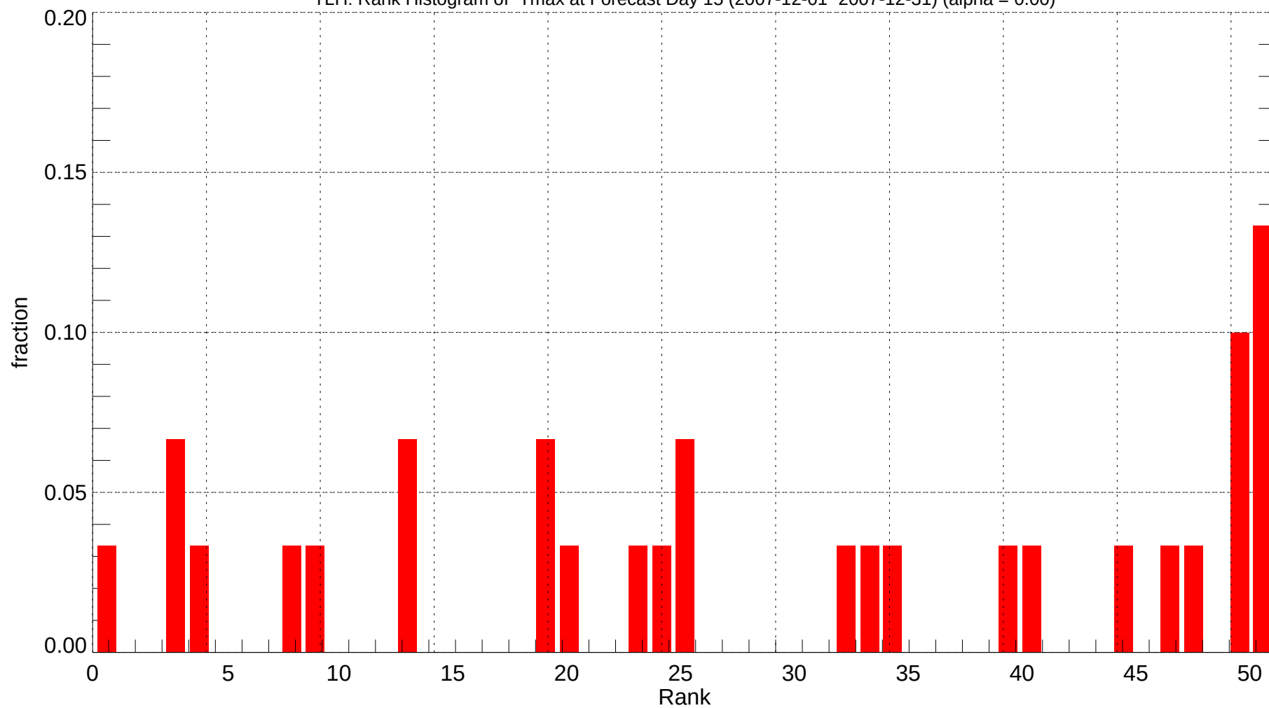
TLH: Rank Histogram of Tmax at Forecast Day 15 (2007-12-01~2007-12-31) (alpha = 0.00)
