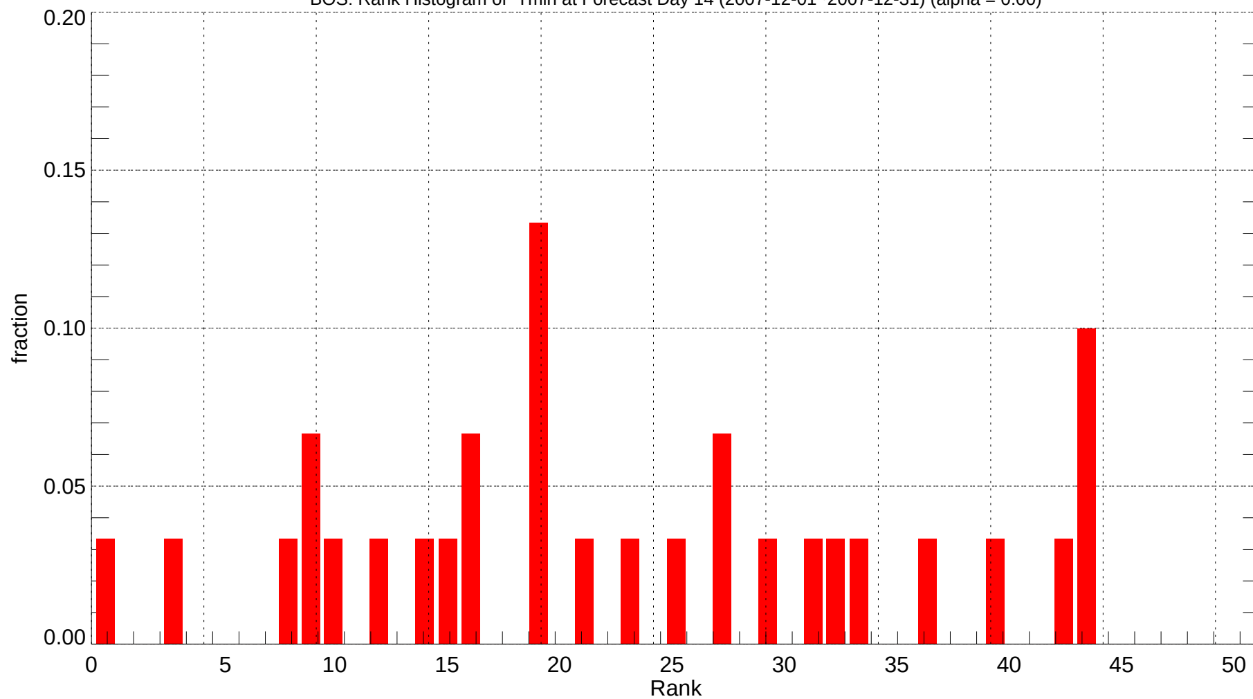
BOS: Rank Histogram of Tmin at Forecast Day 14 (2007-12-01~2007-12-31) (alpha = 0.00)
