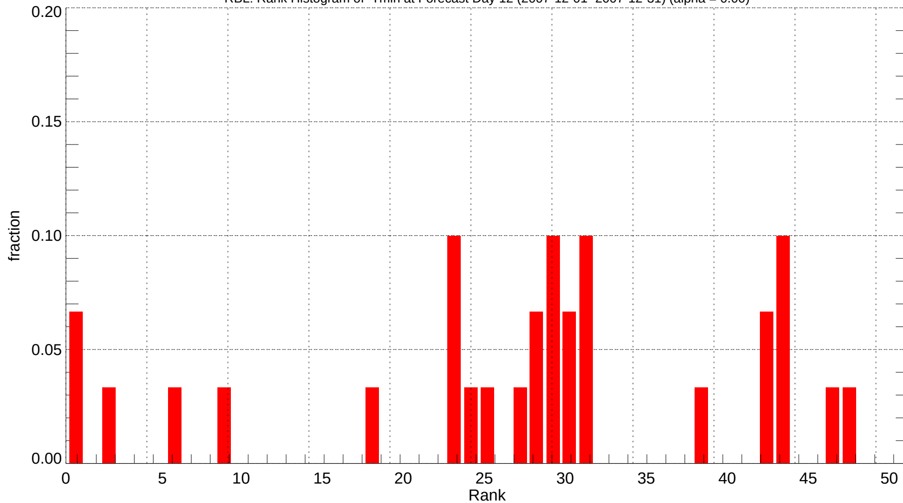
RBL: Rank Histogram of Tmin at Forecast Day 12 (2007-12-01~2007-12-31) (alpha = 0.00)
