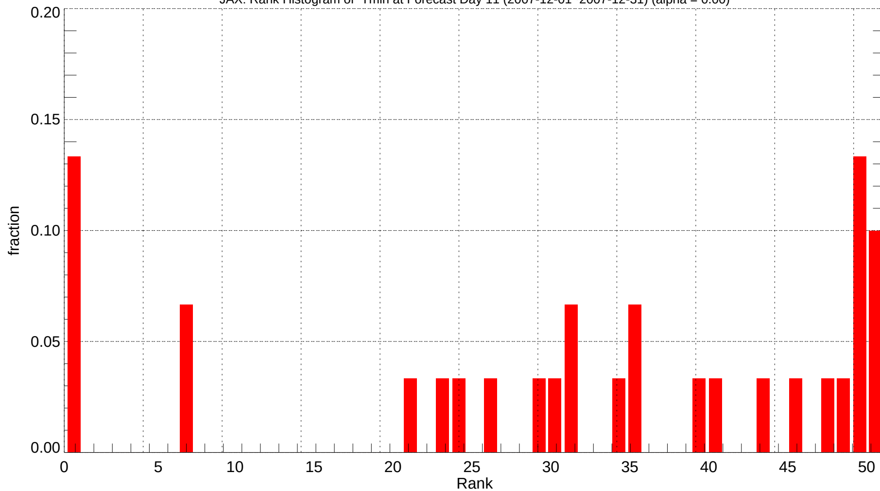
JAX: Rank Histogram of Tmin at Forecast Day 11 (2007-12-01~2007-12-31) (alpha = 0.00)
