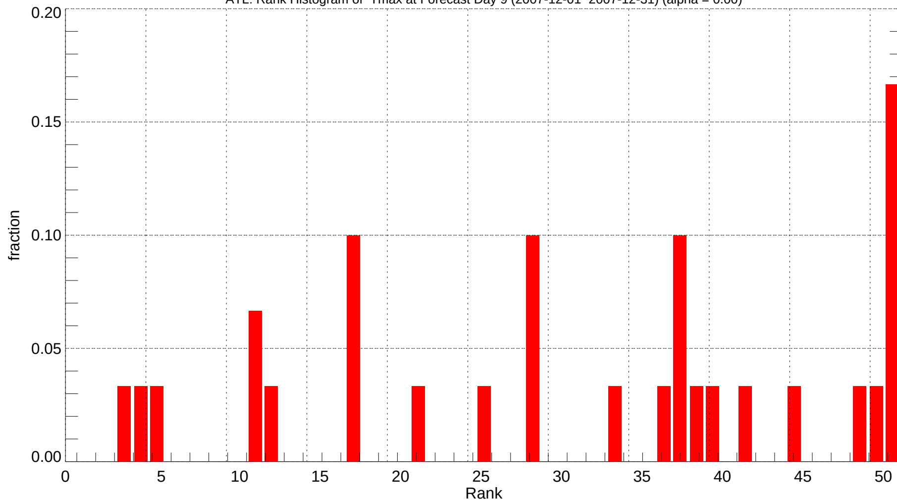
ATL: Rank Histogram of Tmax at Forecast Day 9 (2007-12-01~2007-12-31) (alpha = 0.00)
