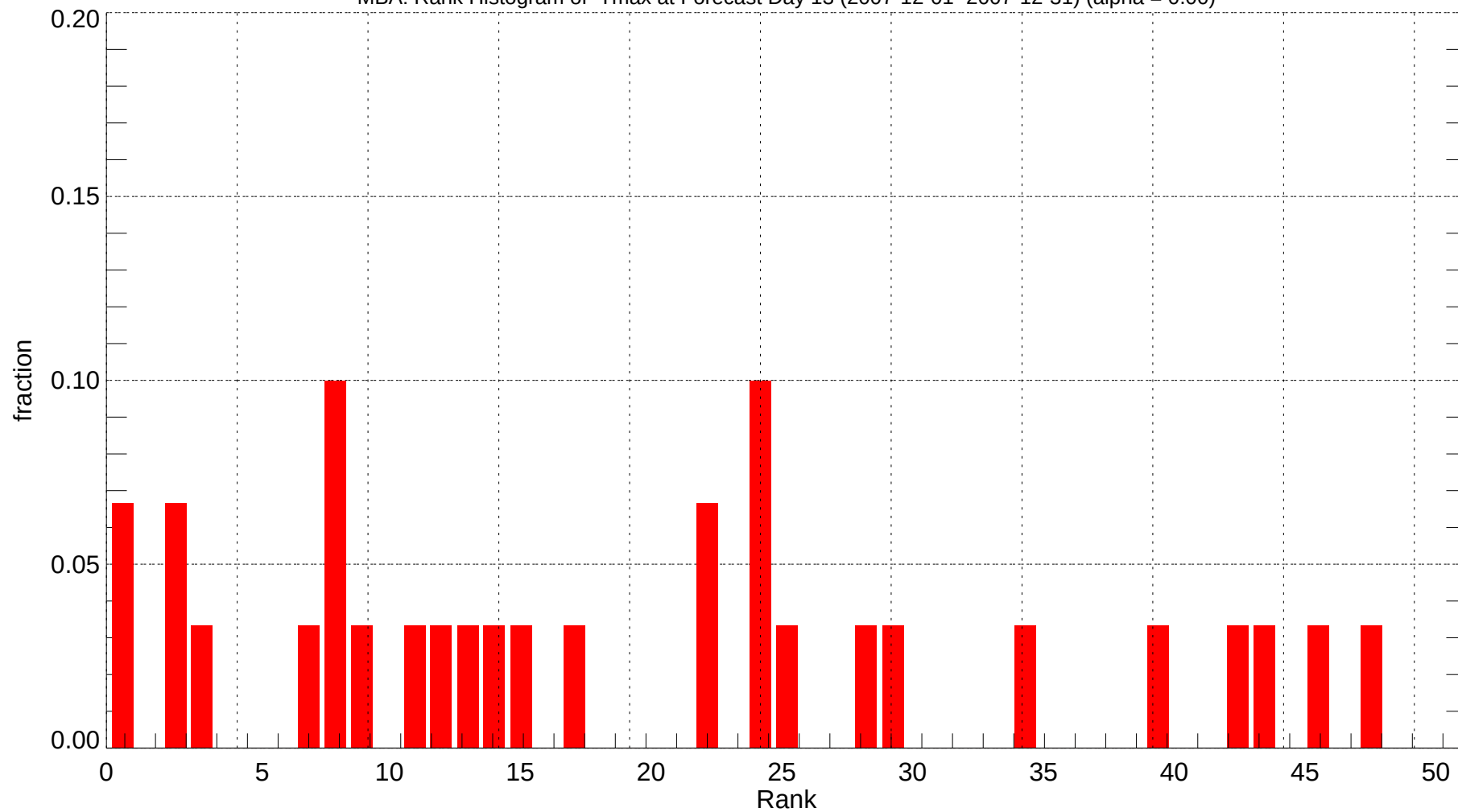
MBA: Rank Histogram of Tmax at Forecast Day 13 (2007-12-01~2007-12-31) (alpha = 0.00)
