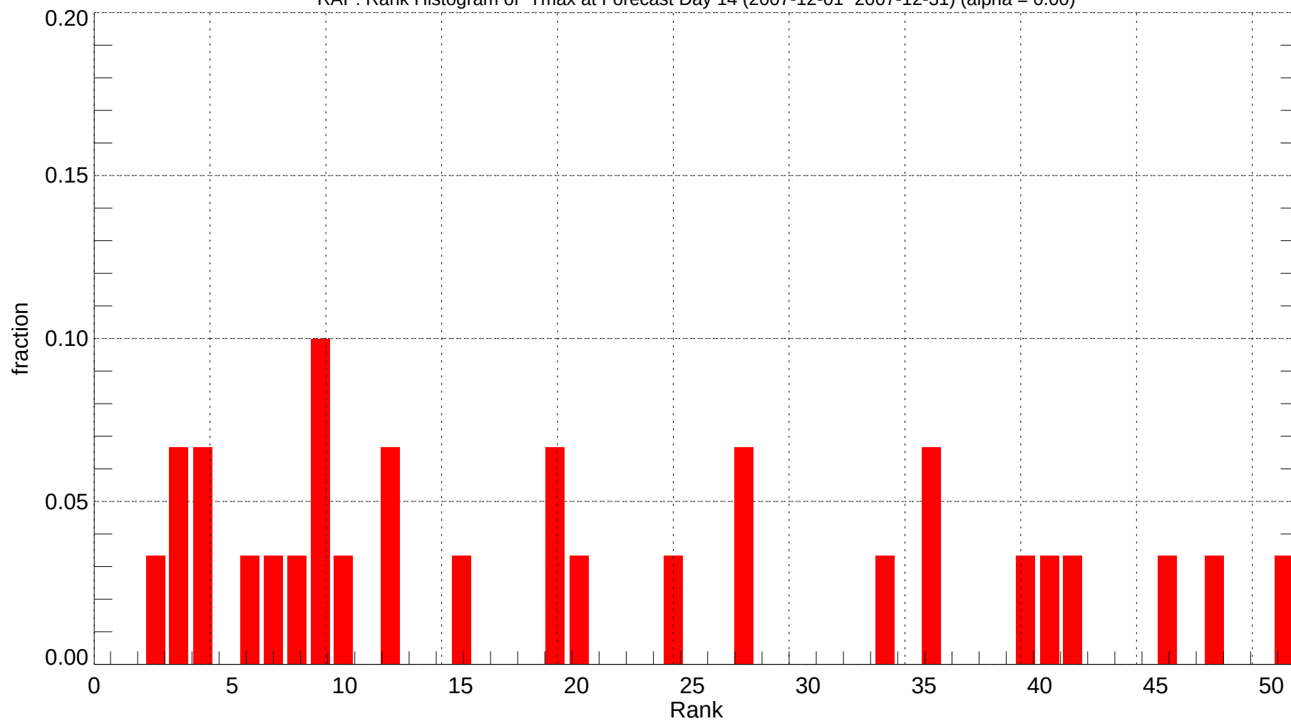
RAP: Rank Histogram of Tmax at Forecast Day 14 (2007-12-01~2007-12-31) (alpha = 0.00)
