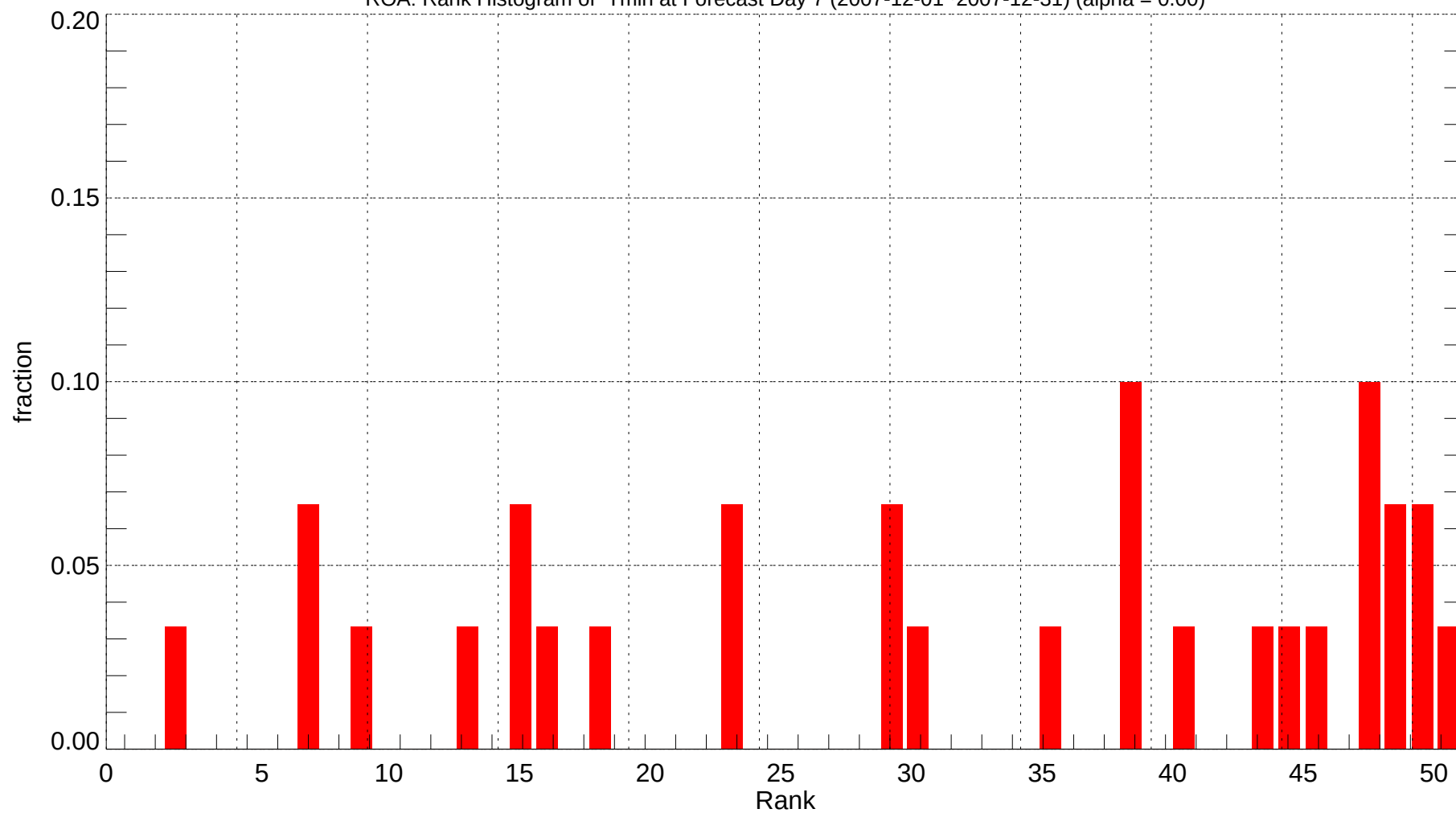
ROA: Rank Histogram of Tmin at Forecast Day 7 (2007-12-01~2007-12-31) (alpha = 0.00)
