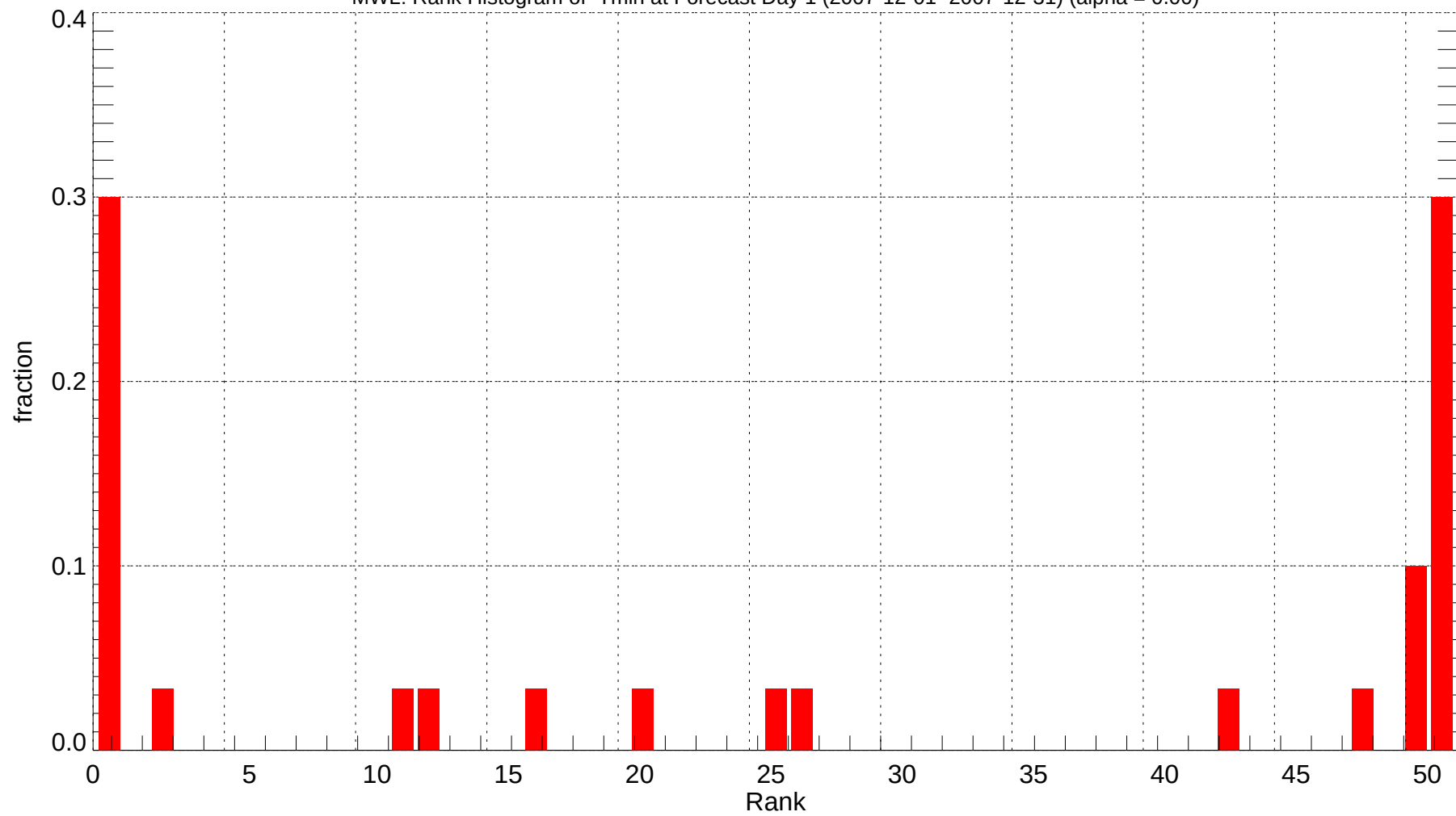
MWL: Rank Histogram of Tmin at Forecast Day 1 (2007-12-01~2007-12-31) (alpha = 0.00)
