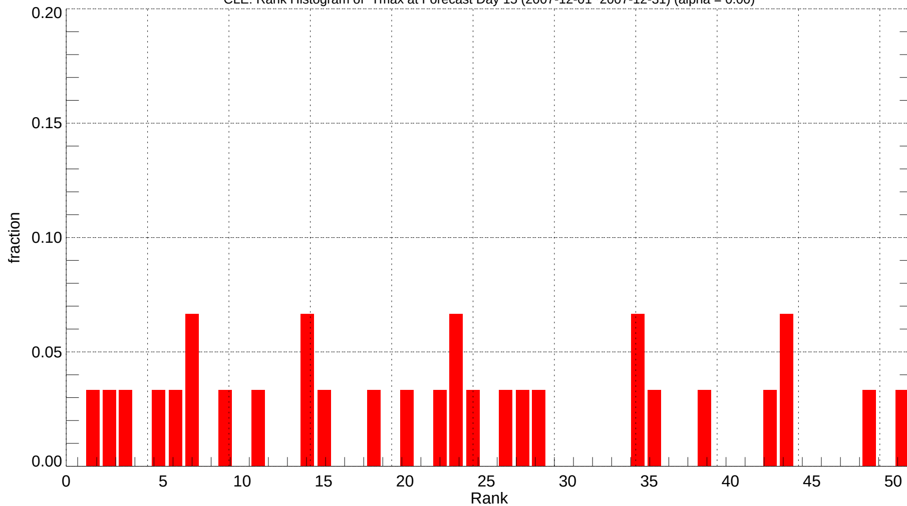
CLE: Rank Histogram of Tmax at Forecast Day 15 (2007-12-01~2007-12-31) (alpha = 0.00)
