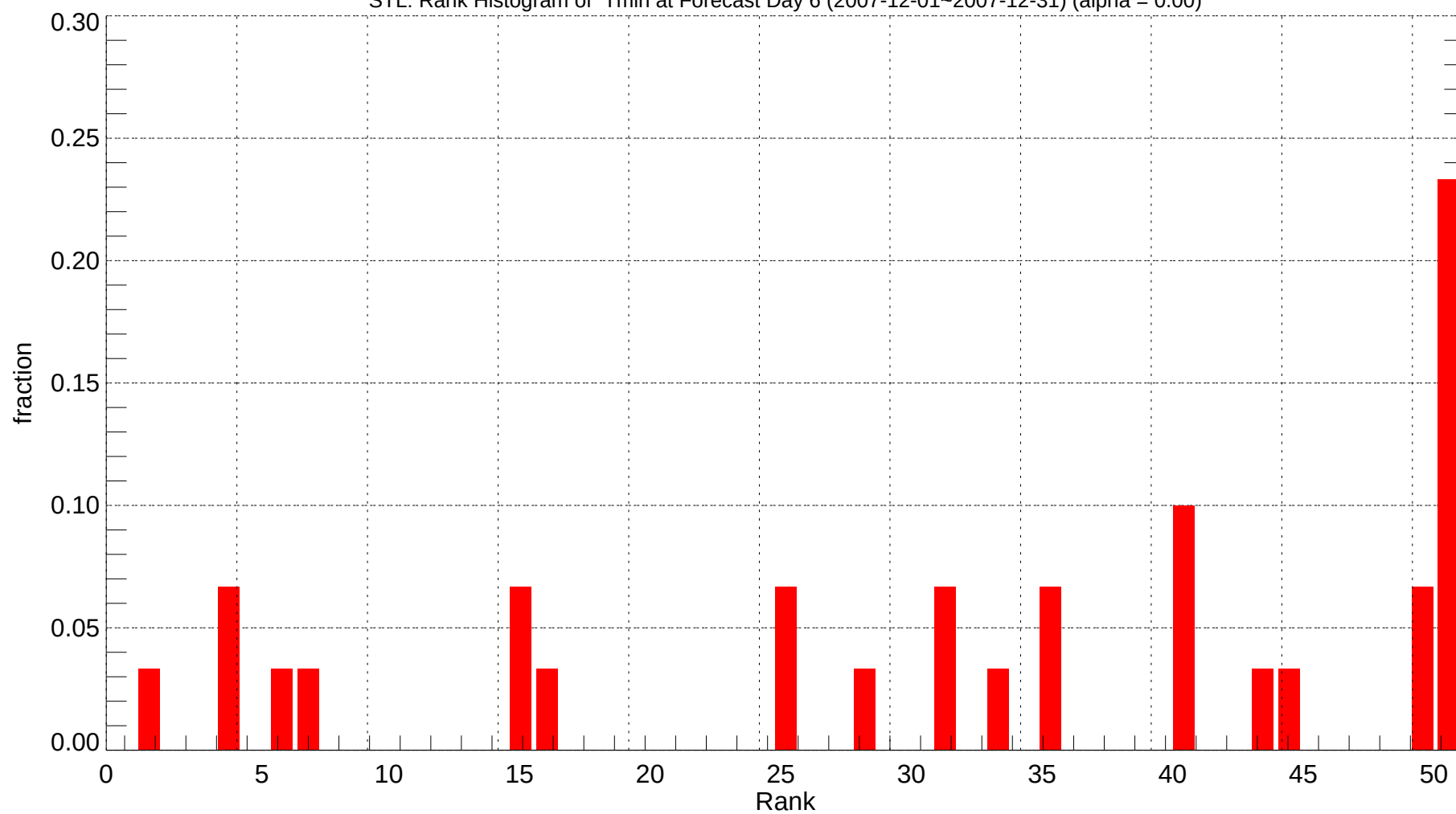
STL: Rank Histogram of Tmin at Forecast Day 6 (2007-12-01~2007-12-31) (alpha = 0.00)
