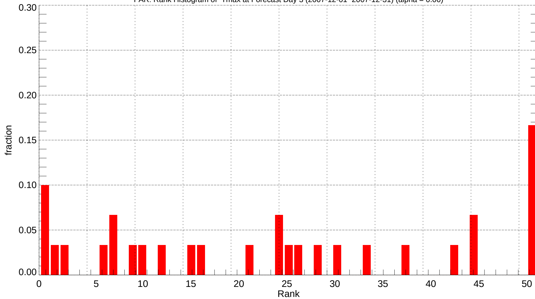
FAR: Rank Histogram of Tmax at Forecast Day 3 (2007-12-01~2007-12-31) (alpha = 0.00)
