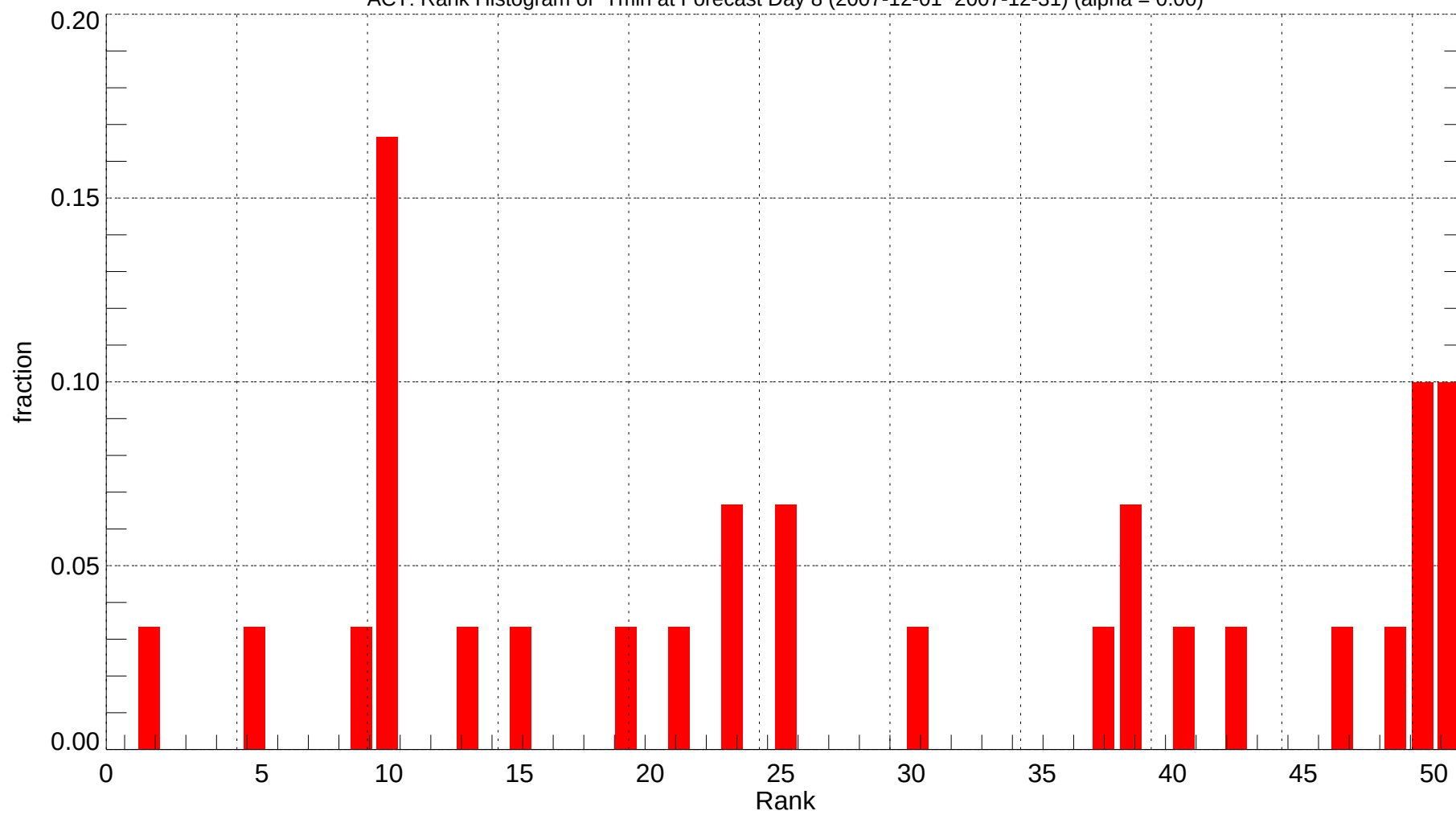
ACT: Rank Histogram of Tmin at Forecast Day 8 (2007-12-01~2007-12-31) (alpha = 0.00)
