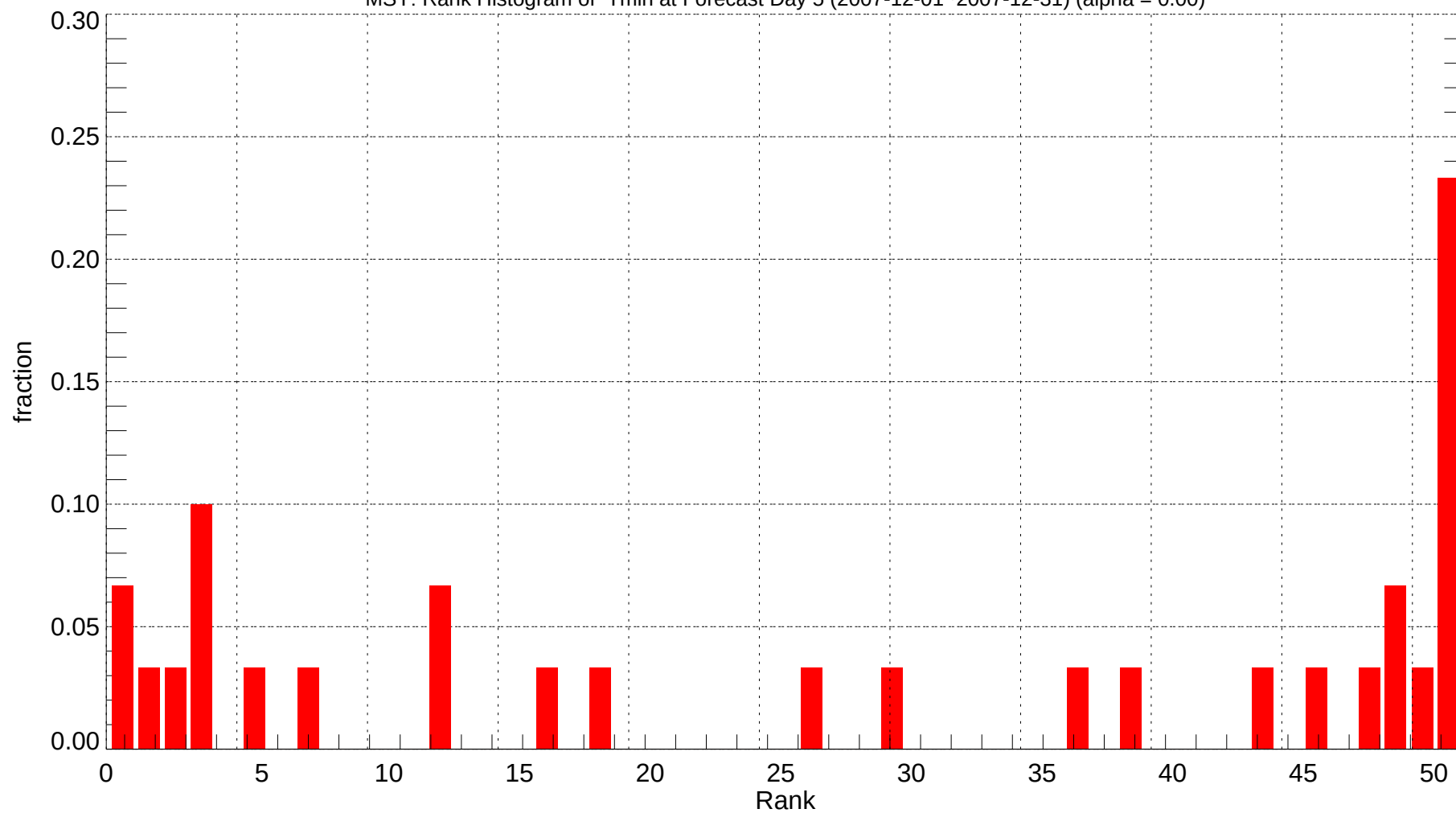
MSY: Rank Histogram of Tmin at Forecast Day 5 (2007-12-01~2007-12-31) (alpha = 0.00)
