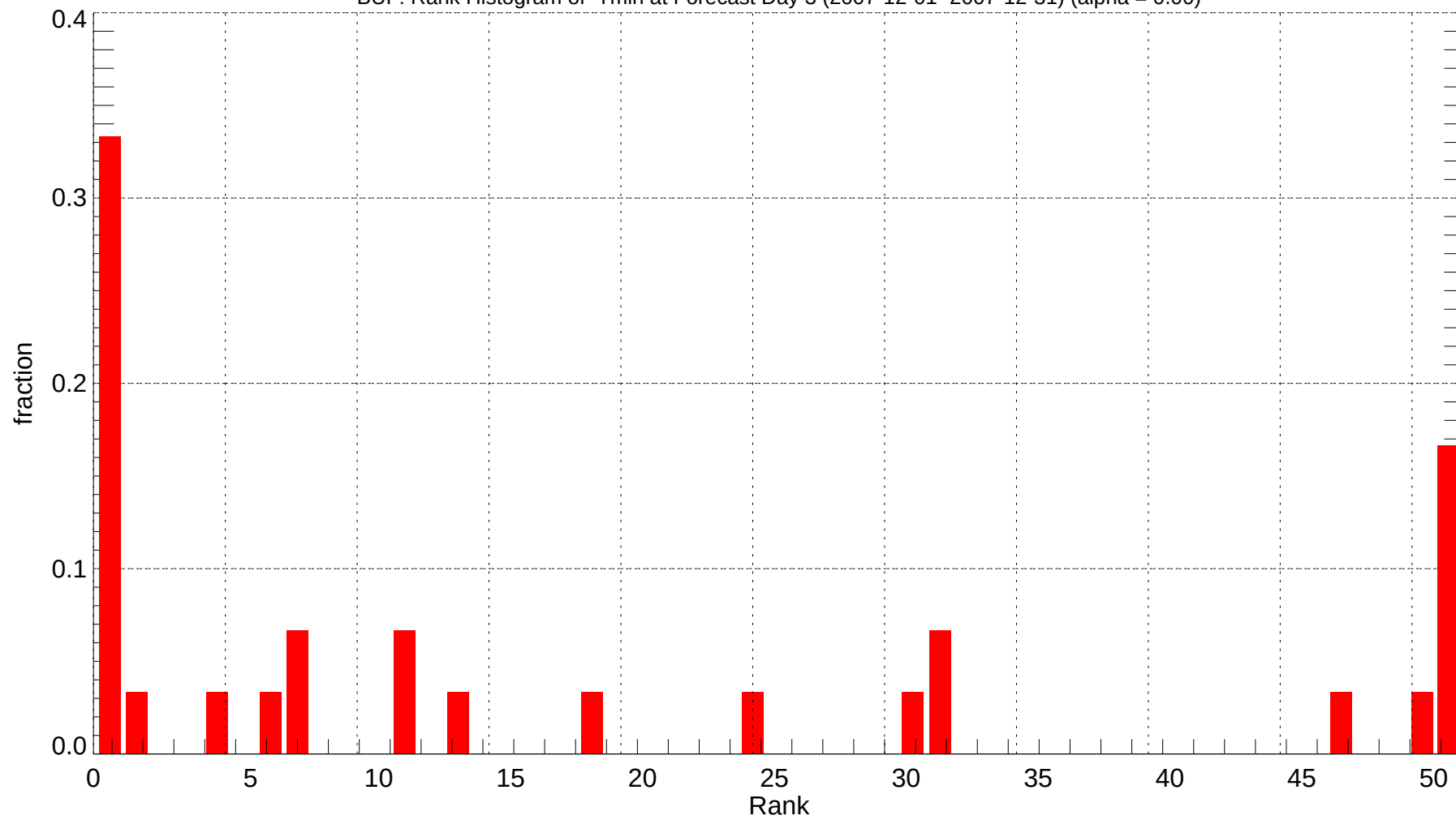
BUF: Rank Histogram of Tmin at Forecast Day 3 (2007-12-01~2007-12-31) (alpha = 0.00)
