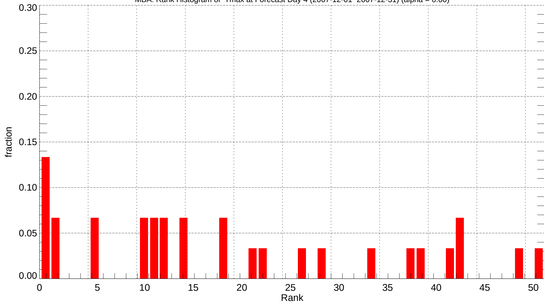
MBA: Rank Histogram of Tmax at Forecast Day 4 (2007-12-01~2007-12-31) (alpha = 0.00)
