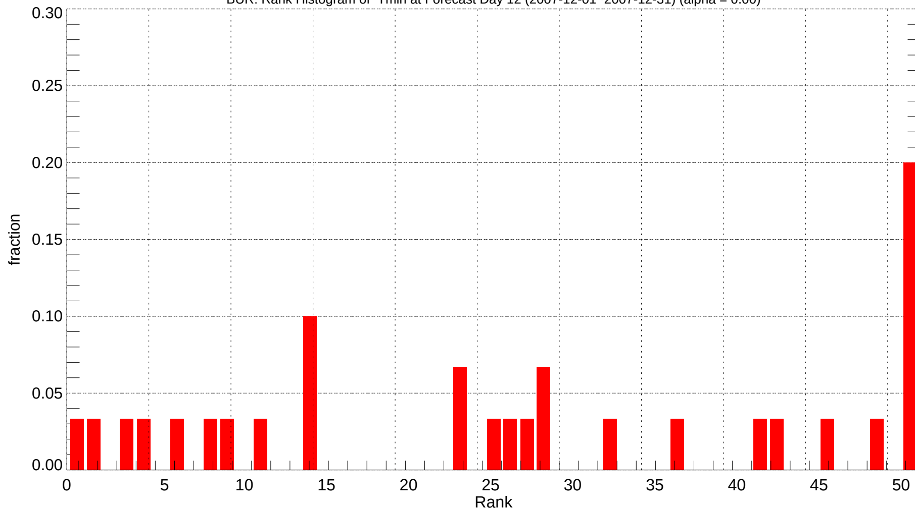
BUR: Rank Histogram of Tmin at Forecast Day 12 (2007-12-01~2007-12-31) (alpha = 0.00)
