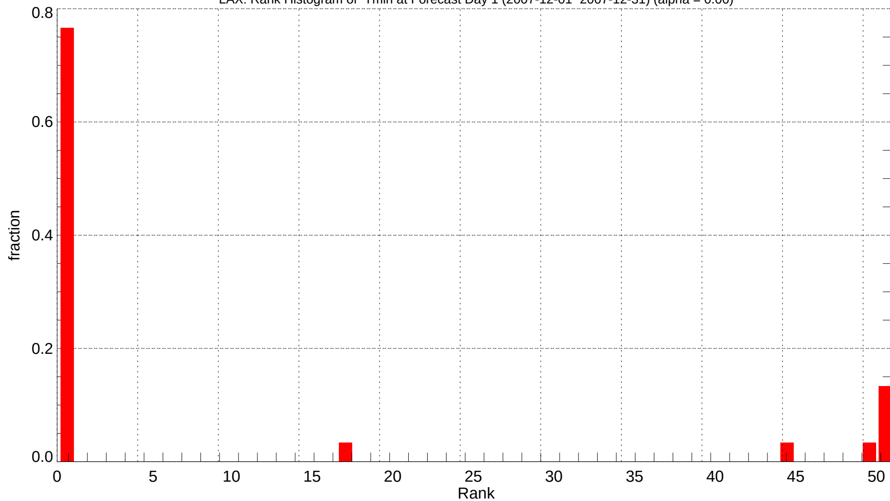
LAX: Rank Histogram of Tmin at Forecast Day 1 (2007-12-01~2007-12-31) (alpha = 0.00)
