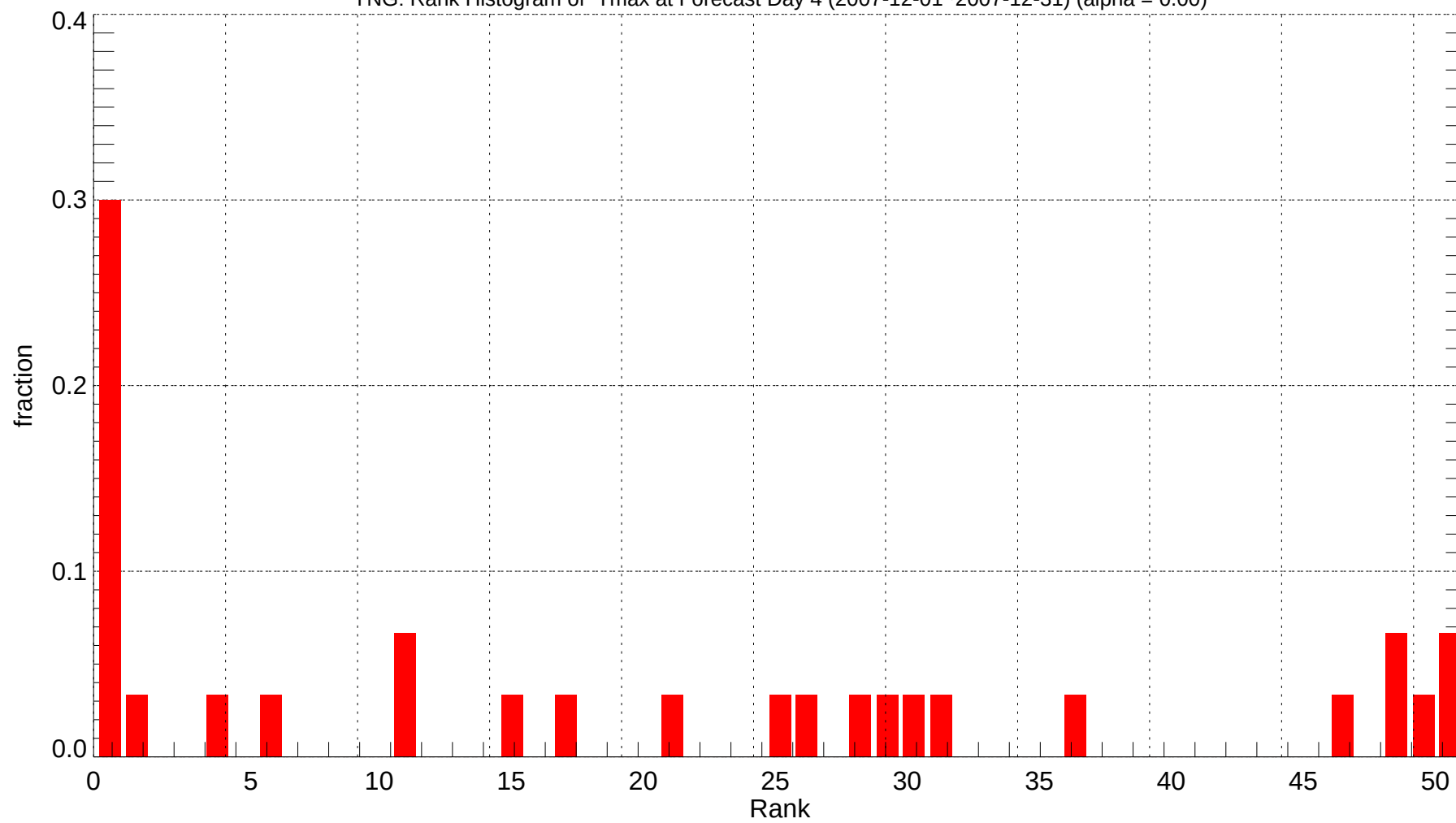
YNG: Rank Histogram of Tmax at Forecast Day 4 (2007-12-01~2007-12-31) (alpha = 0.00)
