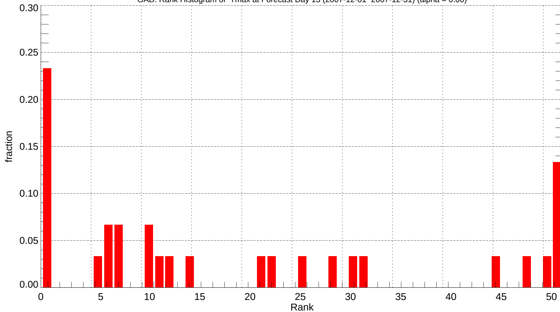
GAD: Rank Histogram of Tmax at Forecast Day 13 (2007-12-01~2007-12-31) (alpha = 0.00)
