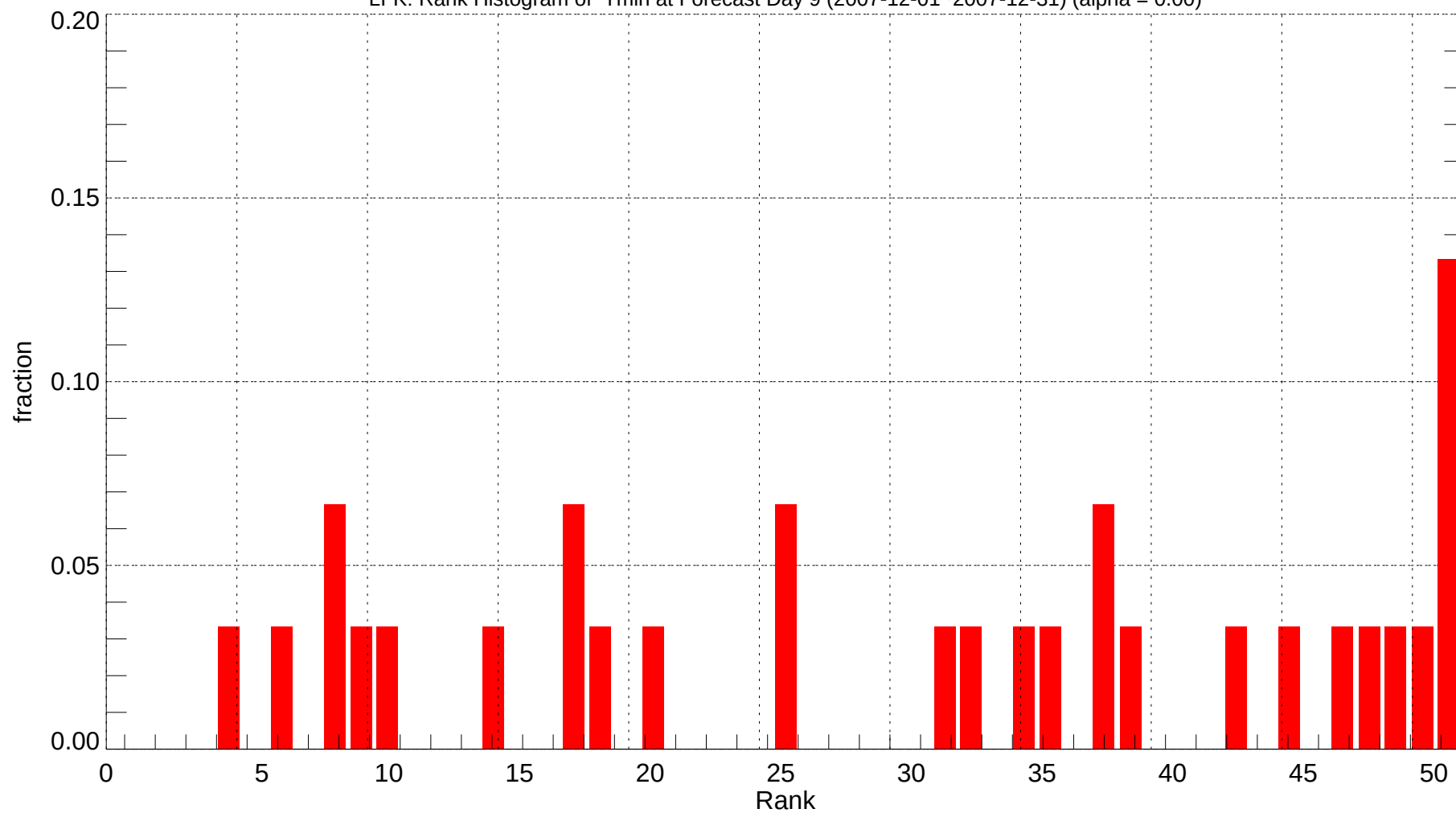
LFK: Rank Histogram of Tmin at Forecast Day 9 (2007-12-01~2007-12-31) (alpha = 0.00)
