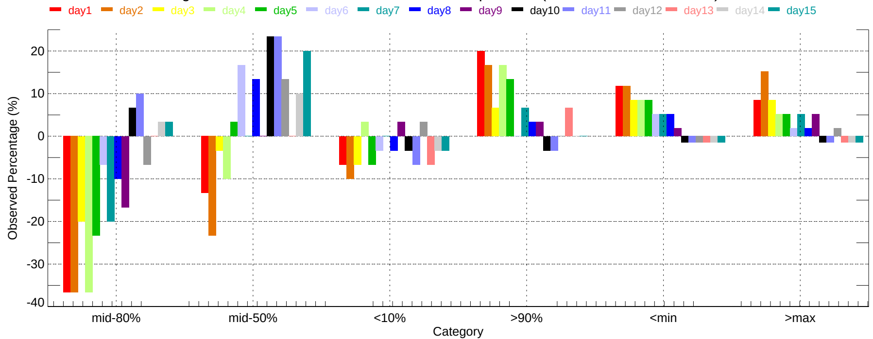
Observed Percentage Deviation of Ensembles - FAT: Min Temperature (2007-12-01~2007-12-31)
