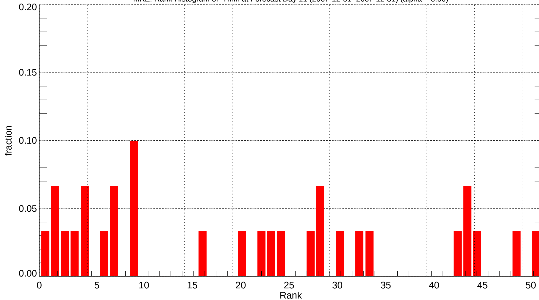
MKE: Rank Histogram of Tmin at Forecast Day 11 (2007-12-01~2007-12-31) (alpha = 0.00)
