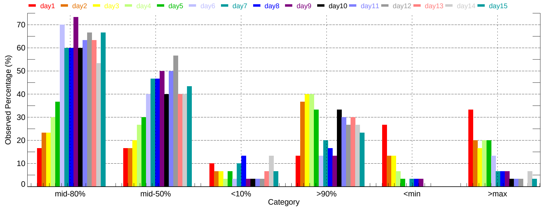
Observed Percentage of Ensembles - BIS: Max Temperature (2007-12-01~2007-12-31)
