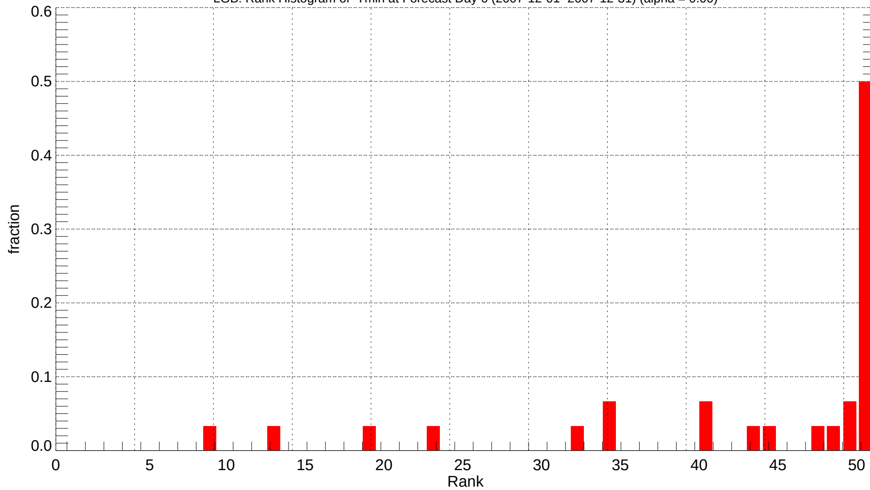
LGB: Rank Histogram of Tmin at Forecast Day 6 (2007-12-01~2007-12-31) (alpha = 0.00)
