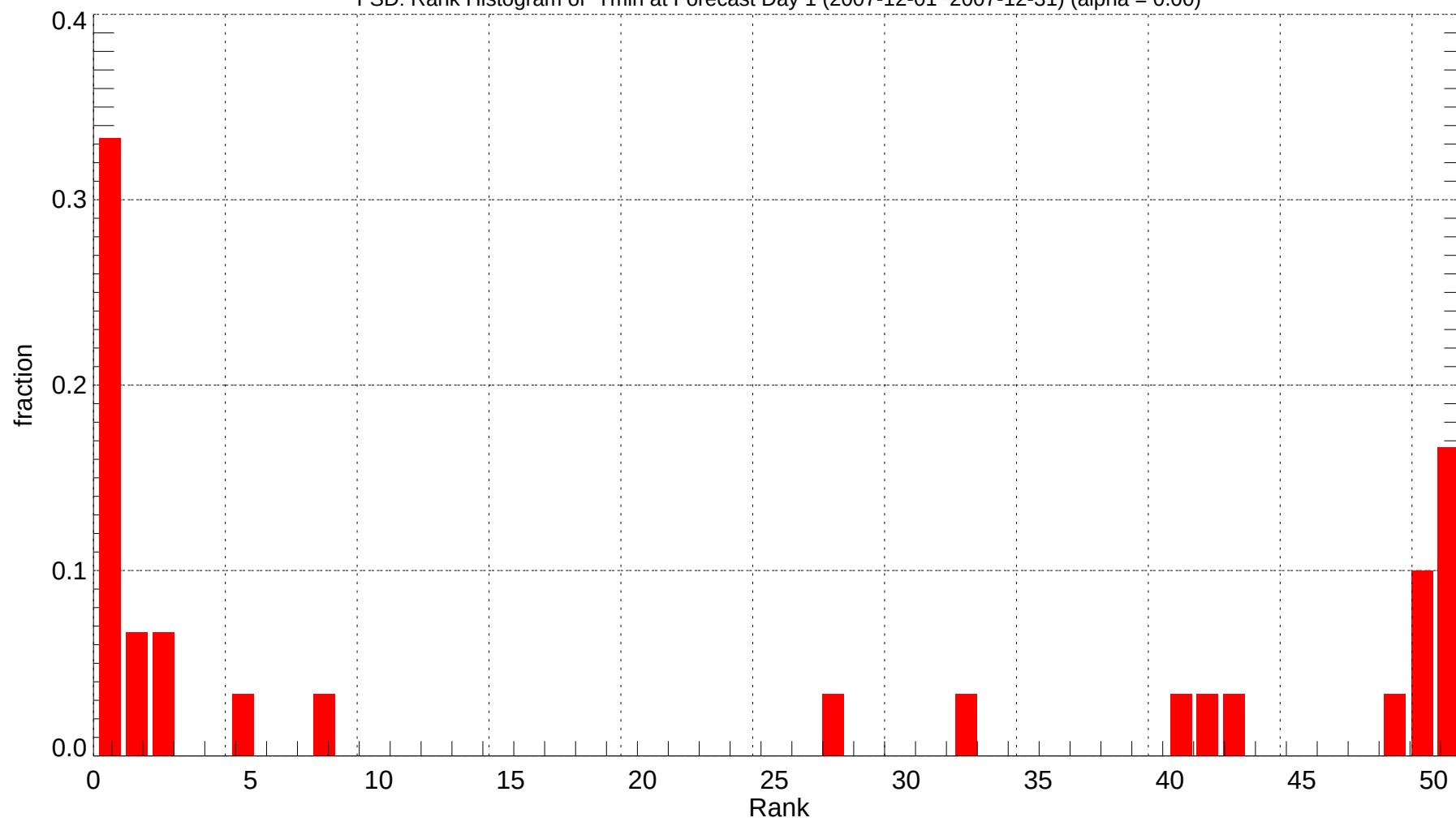
FSD: Rank Histogram of Tmin at Forecast Day 1 (2007-12-01~2007-12-31) (alpha = 0.00)
