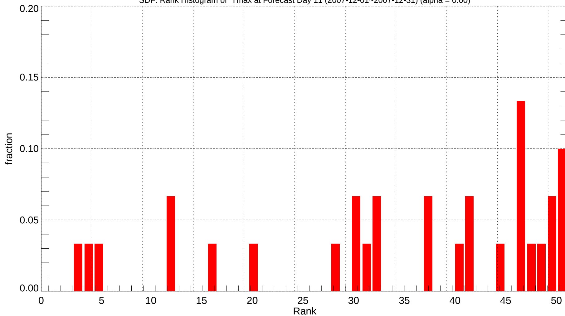
SDF: Rank Histogram of Tmax at Forecast Day 11 (2007-12-01~2007-12-31) (alpha = 0.00)
