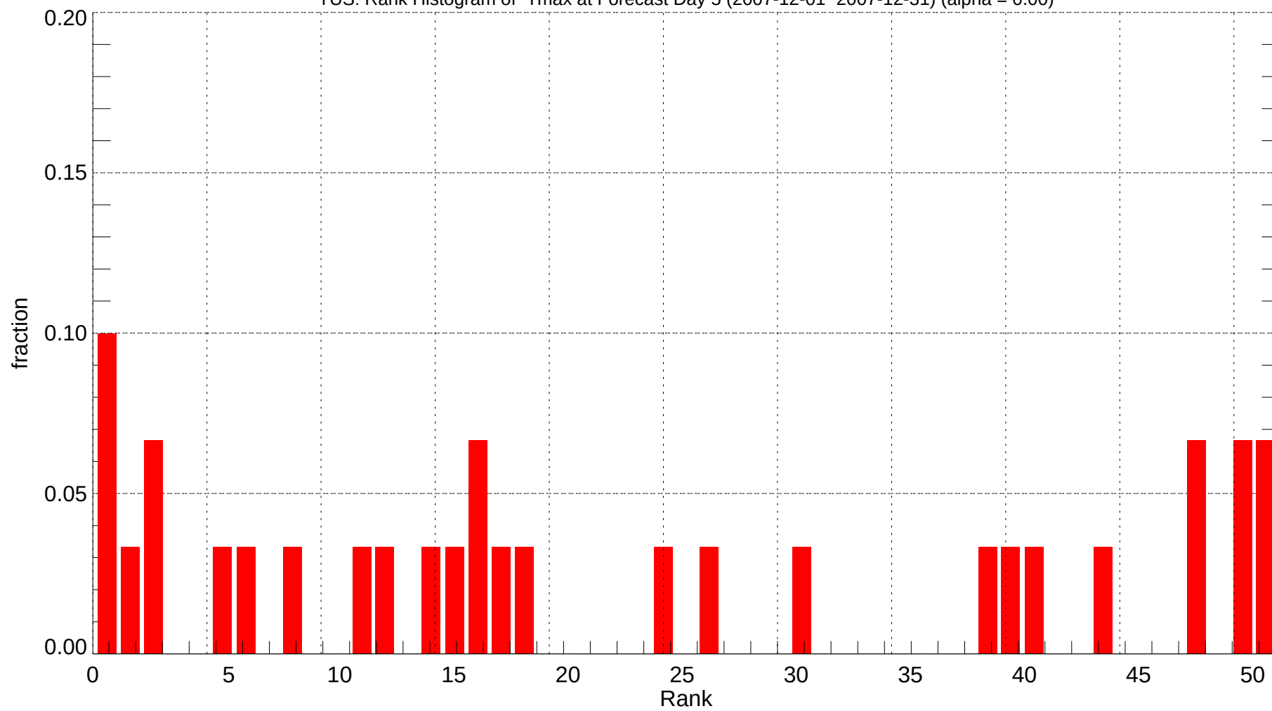
TUS: Rank Histogram of Tmax at Forecast Day 5 (2007-12-01~2007-12-31) (alpha = 0.00)
