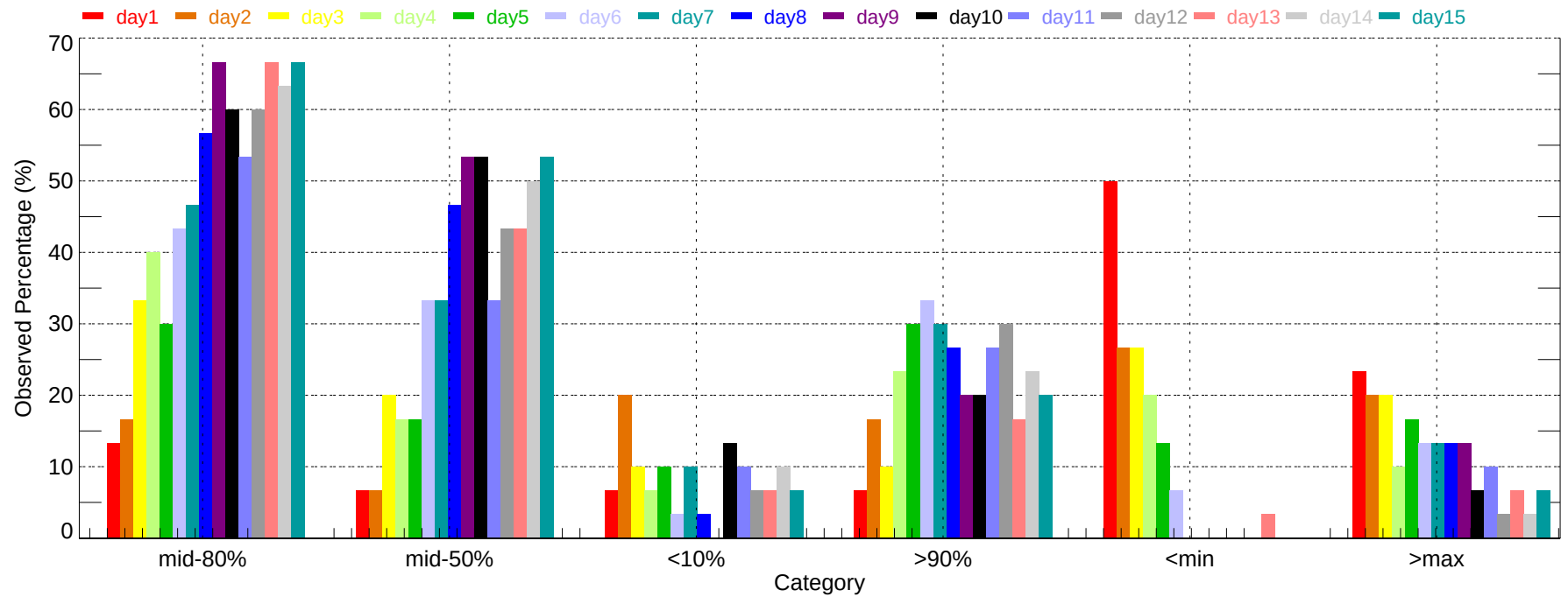
Observed Percentage of Ensembles - TYS: Max Temperature (2007-12-01~2007-12-31)
