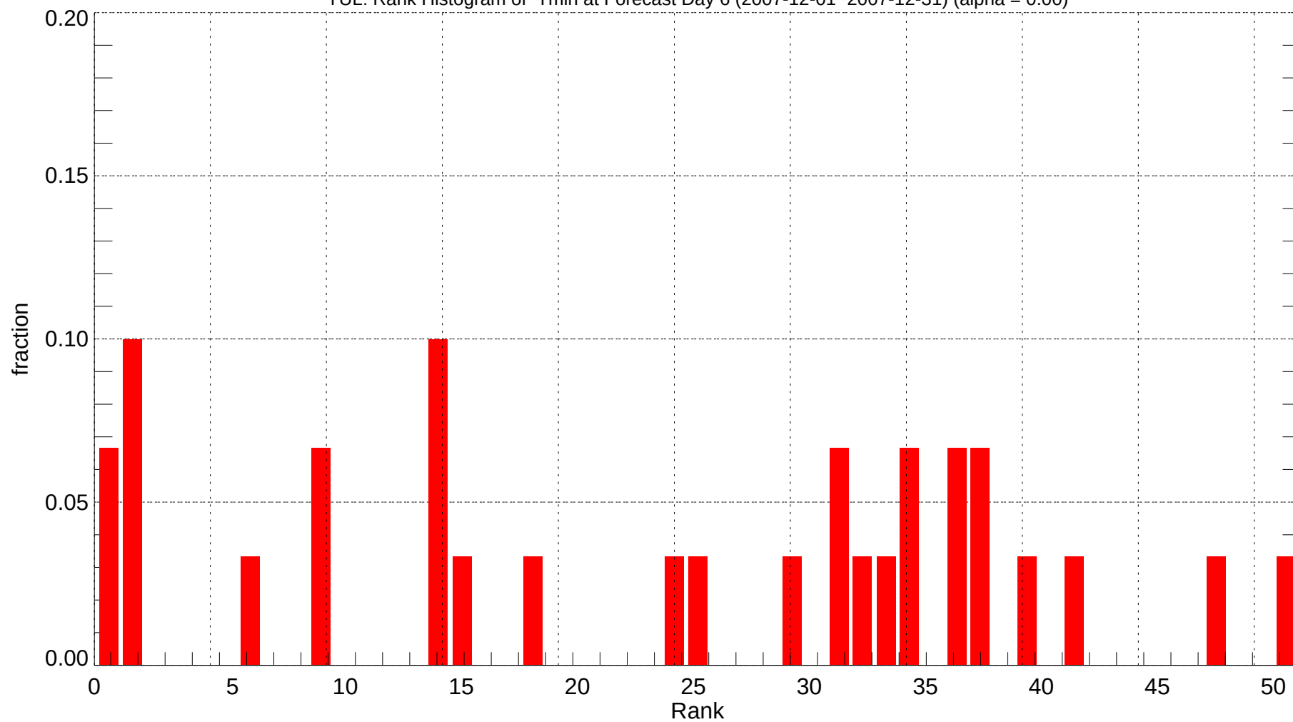
YUL: Rank Histogram of Tmin at Forecast Day 6 (2007-12-01~2007-12-31) (alpha = 0.00)
