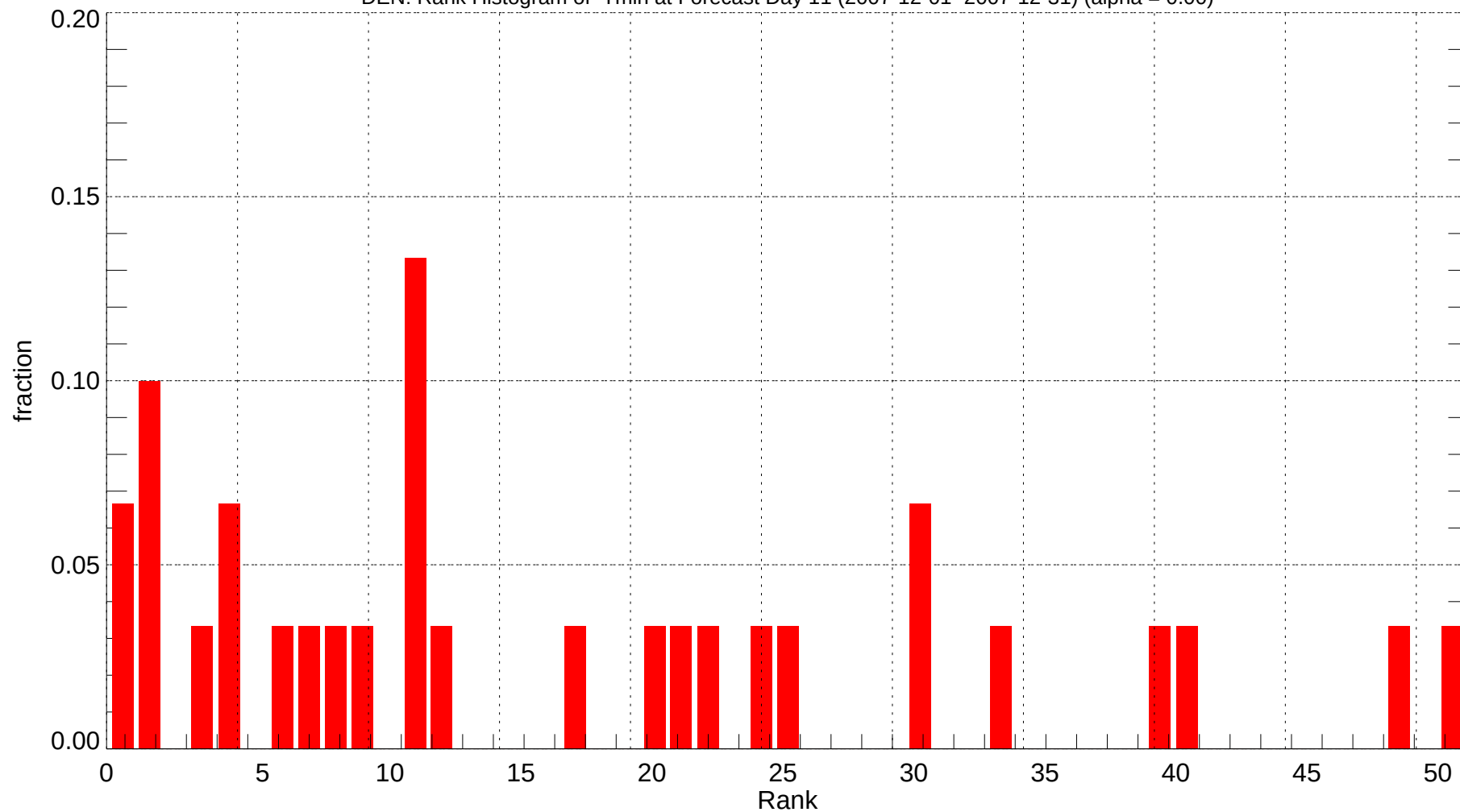
DEN: Rank Histogram of Tmin at Forecast Day 11 (2007-12-01~2007-12-31) (alpha = 0.00)
