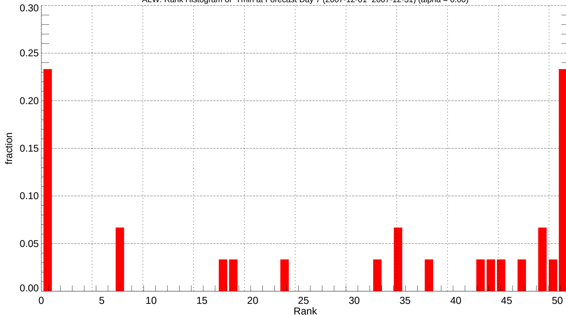
ALW: Rank Histogram of Tmin at Forecast Day 7 (2007-12-01~2007-12-31) (alpha = 0.00)
