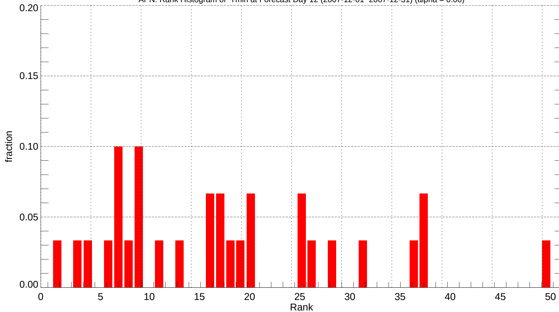
APN: Rank Histogram of Tmin at Forecast Day 12 (2007-12-01~2007-12-31) (alpha = 0.00)
