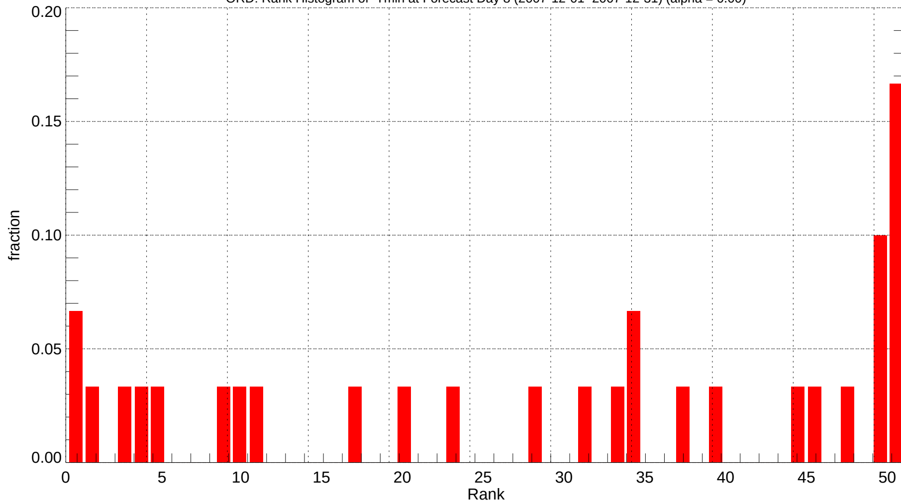
ORD: Rank Histogram of Tmin at Forecast Day 8 (2007-12-01~2007-12-31) (alpha = 0.00)
