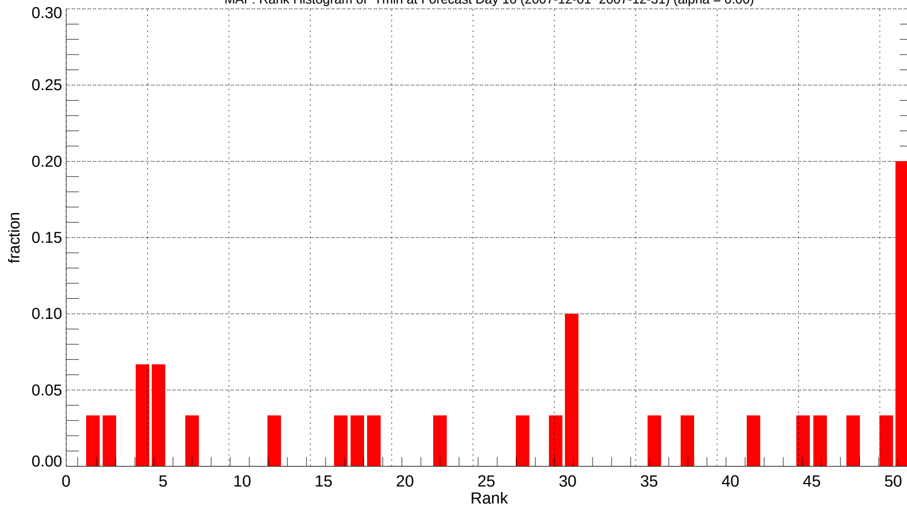
MAF: Rank Histogram of Tmin at Forecast Day 10 (2007-12-01~2007-12-31) (alpha = 0.00)
