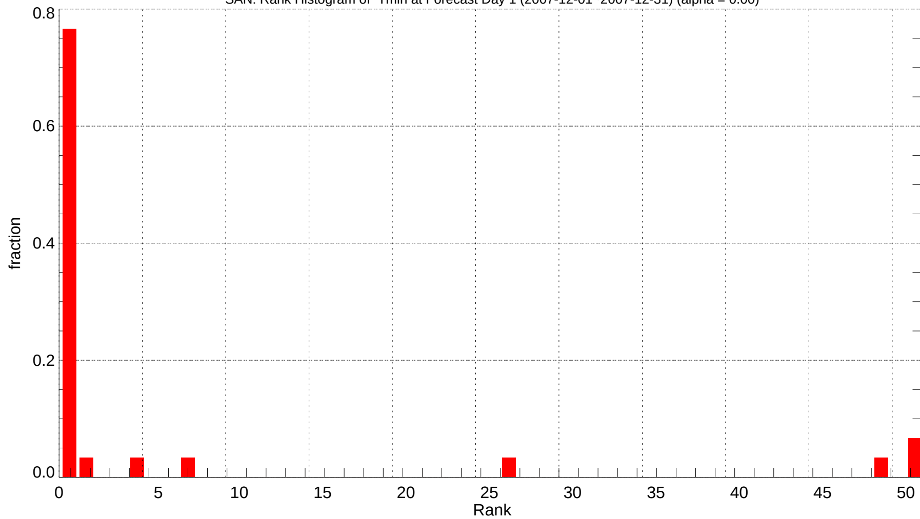
SAN: Rank Histogram of Tmin at Forecast Day 1 (2007-12-01~2007-12-31) (alpha = 0.00)
