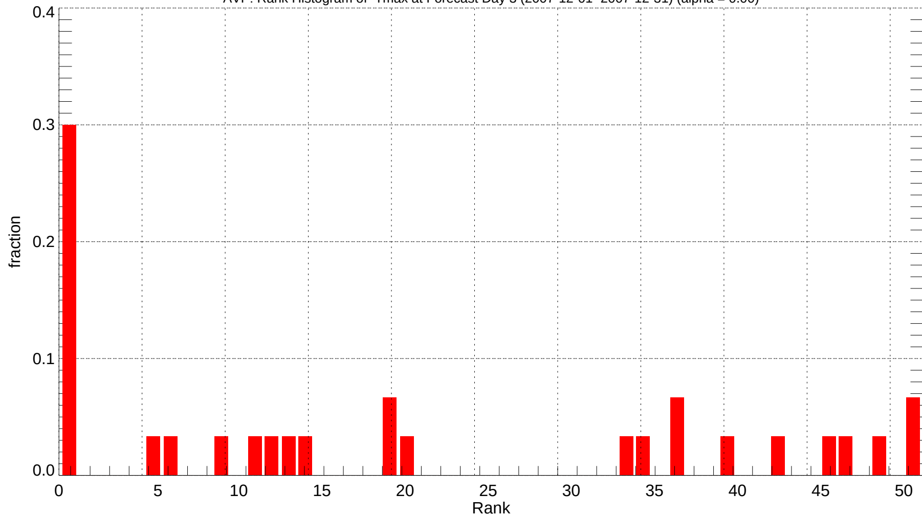
AVP: Rank Histogram of Tmax at Forecast Day 3 (2007-12-01~2007-12-31) (alpha = 0.00)
