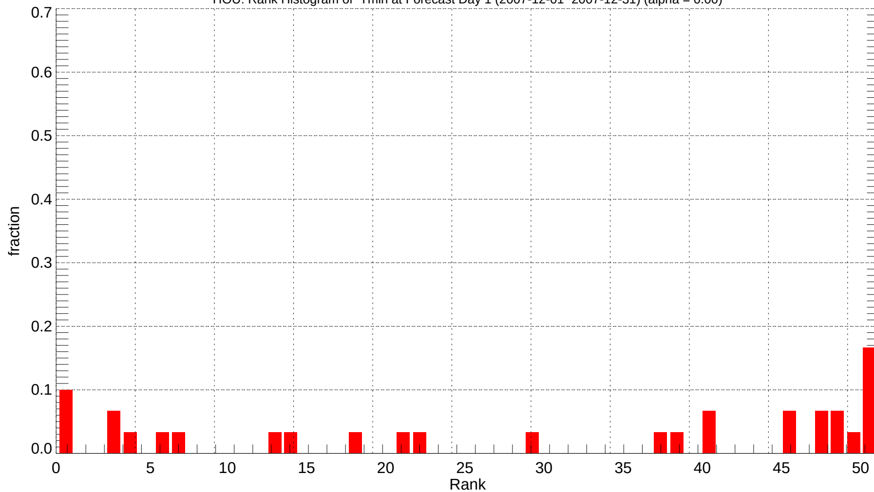
HOU: Rank Histogram of Tmin at Forecast Day 1 (2007-12-01~2007-12-31) (alpha = 0.00)
