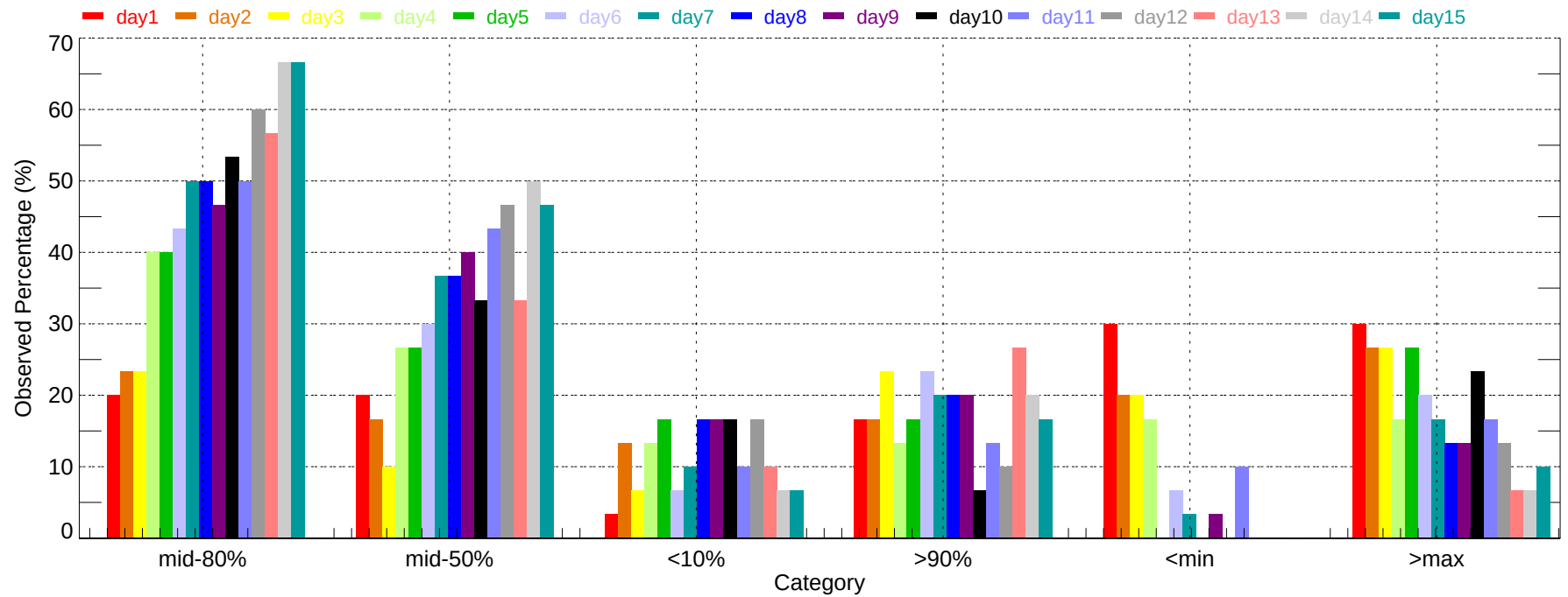
Observed Percentage of Ensembles - MWL: Max Temperature (2007-12-01~2007-12-31)
