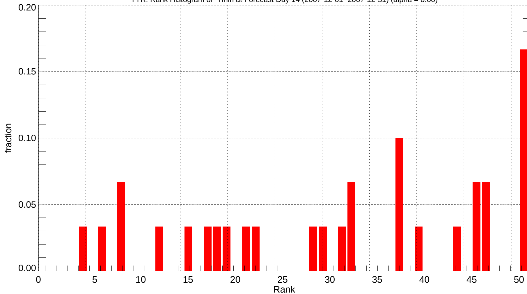
TYR: Rank Histogram of Tmin at Forecast Day 14 (2007-12-01~2007-12-31) (alpha = 0.00)
