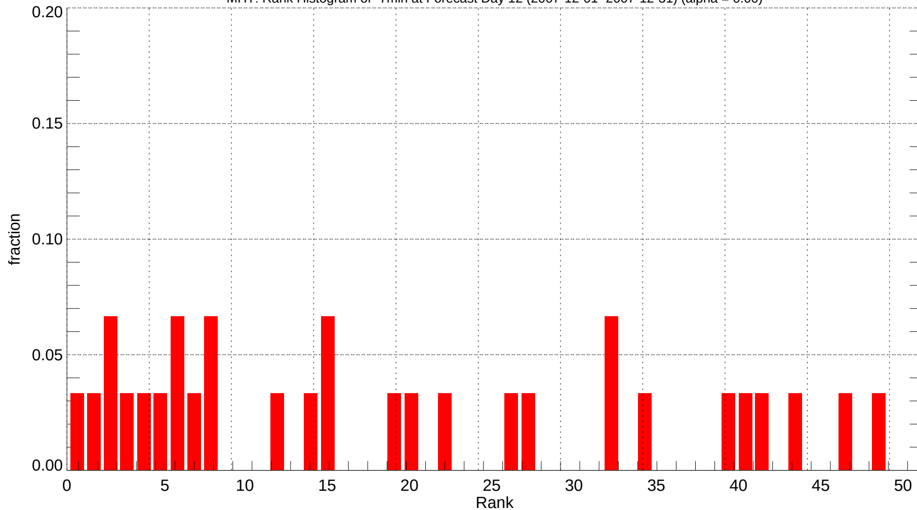
MHT: Rank Histogram of Tmin at Forecast Day 12 (2007-12-01~2007-12-31) (alpha = 0.00)
