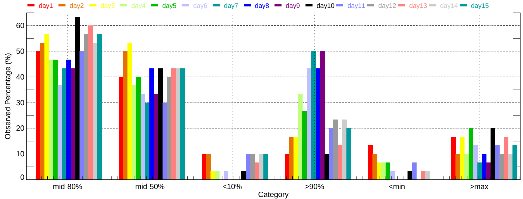
Observed Percentage of Ensembles - SAV: Max Temperature (2007-12-01~2007-12-31)
