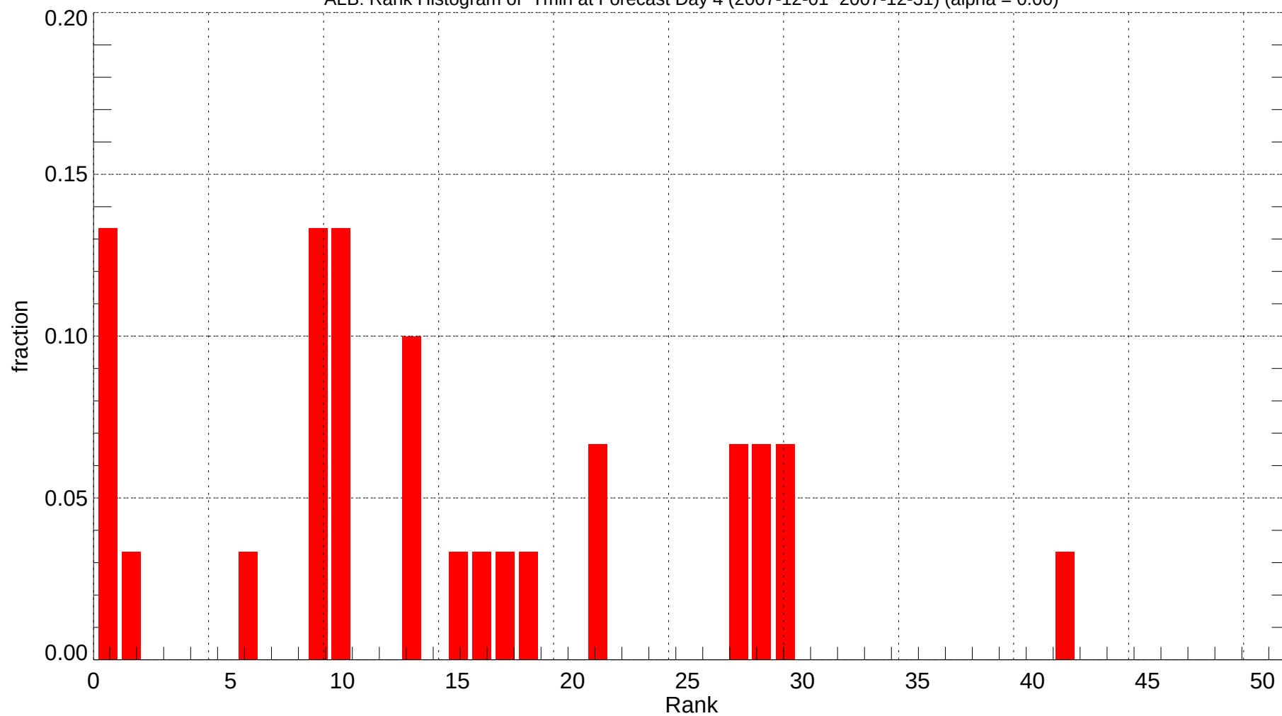
ALB: Rank Histogram of Tmin at Forecast Day 4 (2007-12-01~2007-12-31) (alpha = 0.00)
