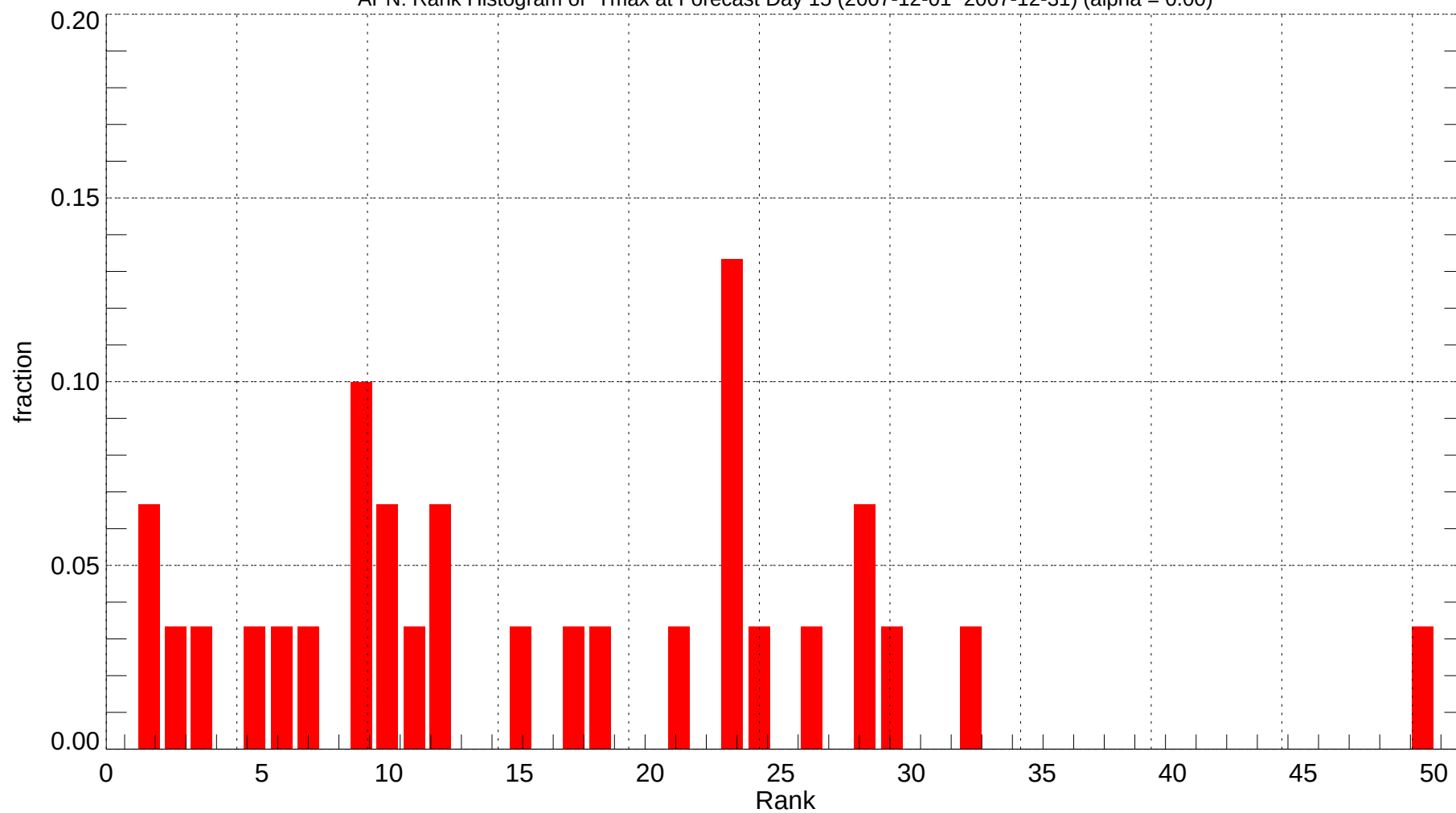
APN: Rank Histogram of Tmax at Forecast Day 15 (2007-12-01~2007-12-31) (alpha = 0.00)
