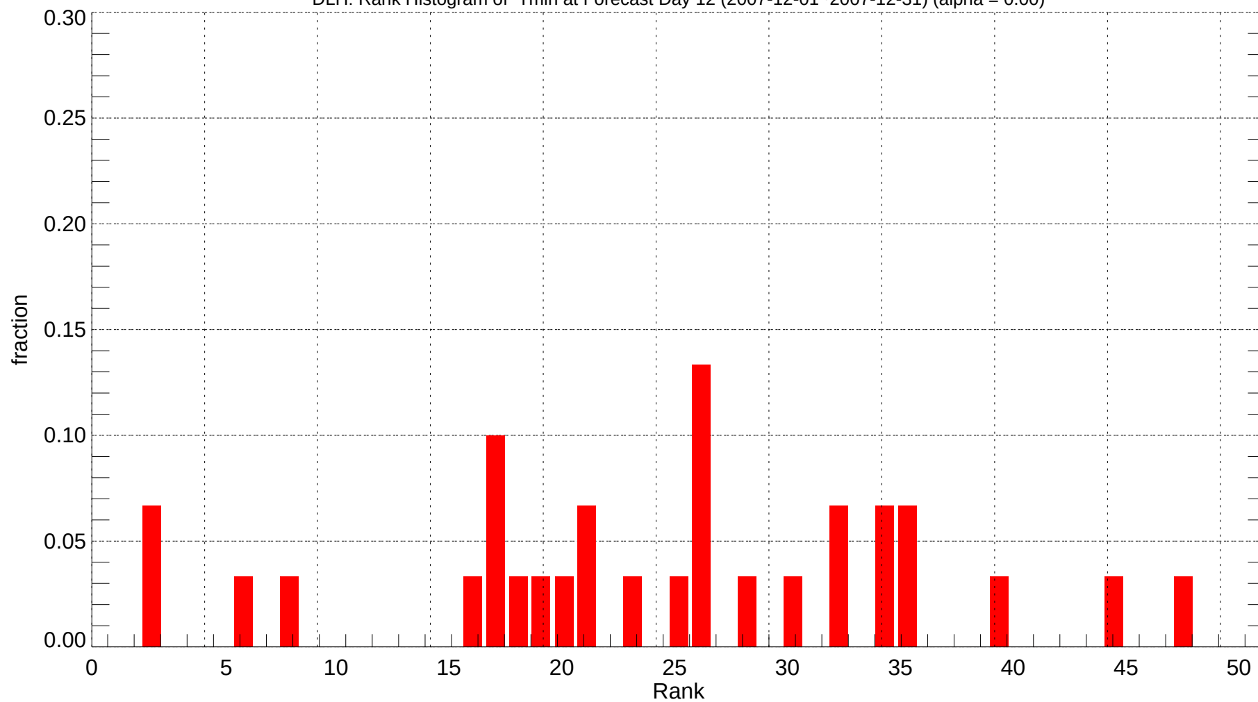
DLH: Rank Histogram of Tmin at Forecast Day 12 (2007-12-01~2007-12-31) (alpha = 0.00)
