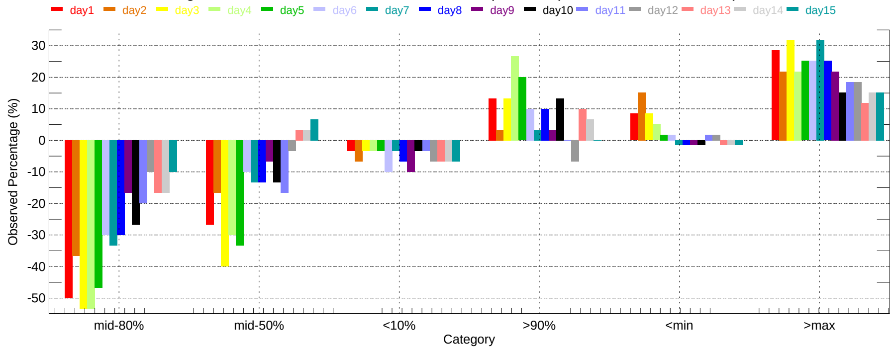
Observed Percentage Deviation of Ensembles - SAT: Min Temperature (2007-12-01~2007-12-31)
