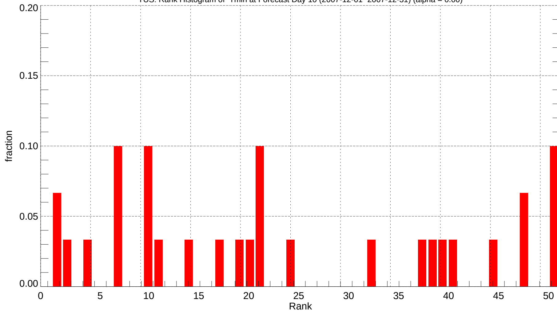
TUS: Rank Histogram of Tmin at Forecast Day 10 (2007-12-01~2007-12-31) (alpha = 0.00)
