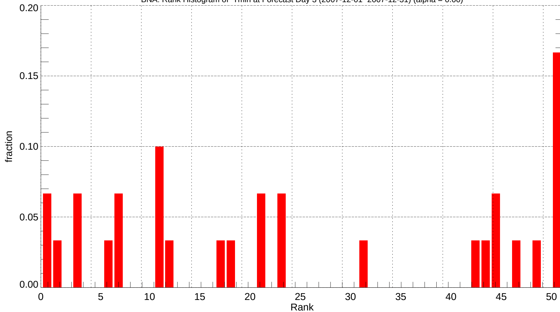
BNA: Rank Histogram of Tmin at Forecast Day 3 (2007-12-01~2007-12-31) (alpha = 0.00)
