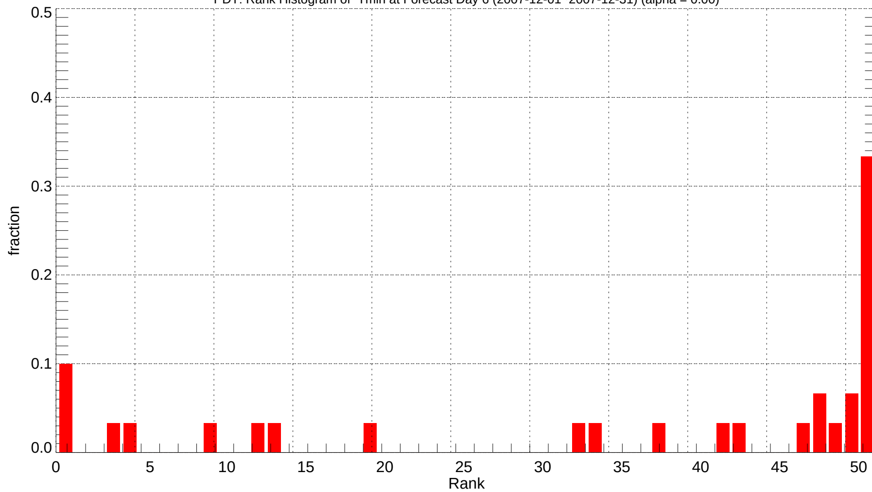
PDT: Rank Histogram of Tmin at Forecast Day 6 (2007-12-01~2007-12-31) (alpha = 0.00)
