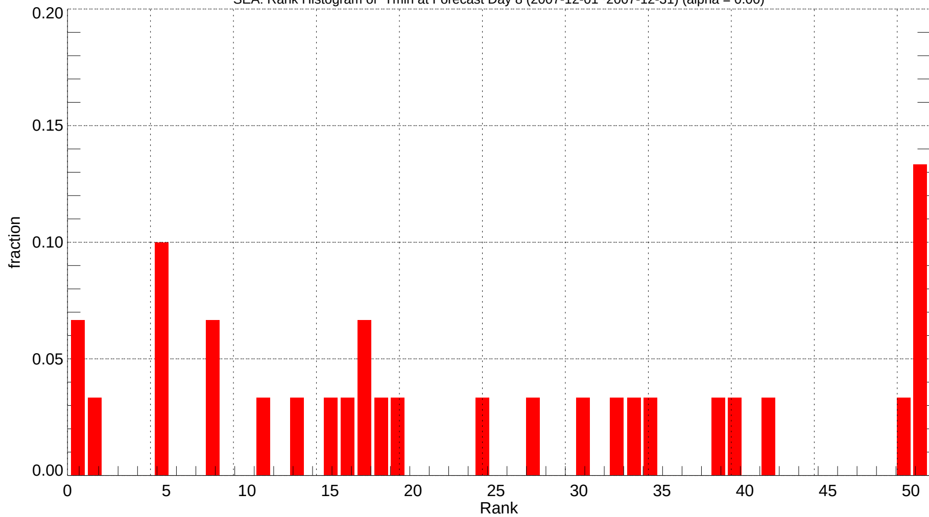
SEA: Rank Histogram of Tmin at Forecast Day 8 (2007-12-01~2007-12-31) (alpha = 0.00)
