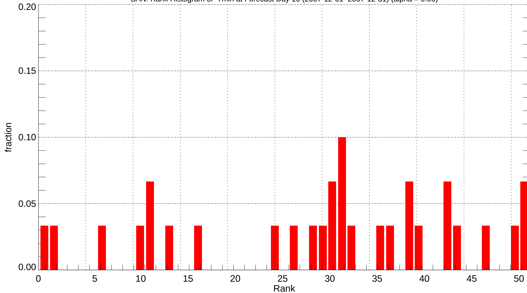
SAN: Rank Histogram of Tmin at Forecast Day 10 (2007-12-01~2007-12-31) (alpha = 0.00)
