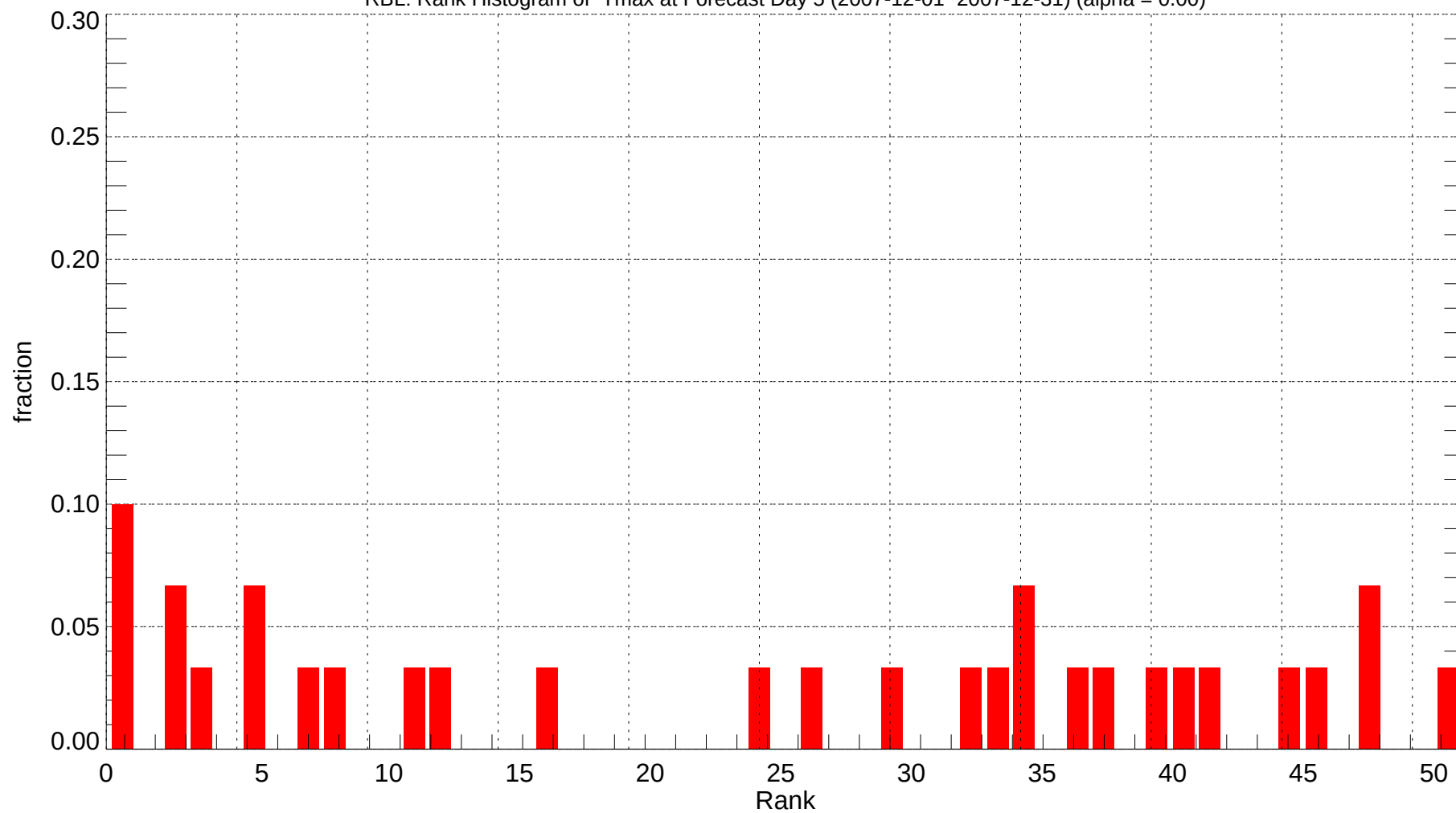
RBL: Rank Histogram of Tmax at Forecast Day 5 (2007-12-01~2007-12-31) (alpha = 0.00)
