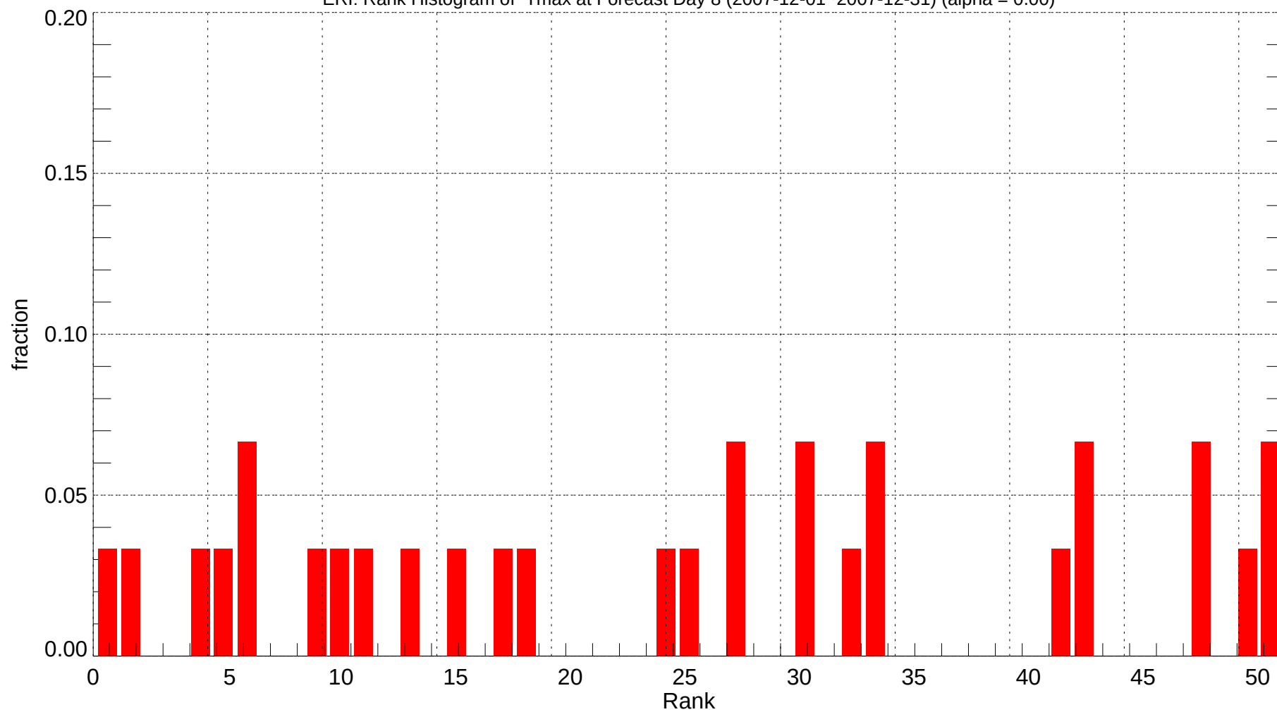
ERI: Rank Histogram of Tmax at Forecast Day 8 (2007-12-01~2007-12-31) (alpha = 0.00)
