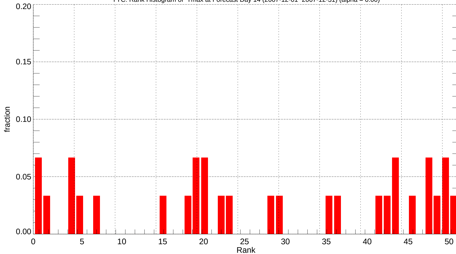
YYC: Rank Histogram of Tmax at Forecast Day 14 (2007-12-01~2007-12-31) (alpha = 0.00)
