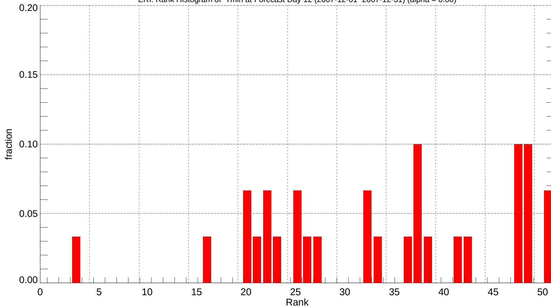
ERI: Rank Histogram of Tmin at Forecast Day 12 (2007-12-01~2007-12-31) (alpha = 0.00)
