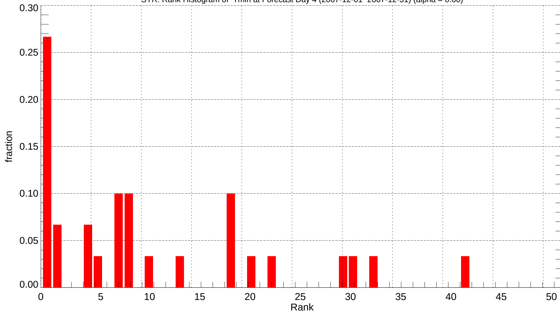
SYR: Rank Histogram of Tmin at Forecast Day 4 (2007-12-01~2007-12-31) (alpha = 0.00)
