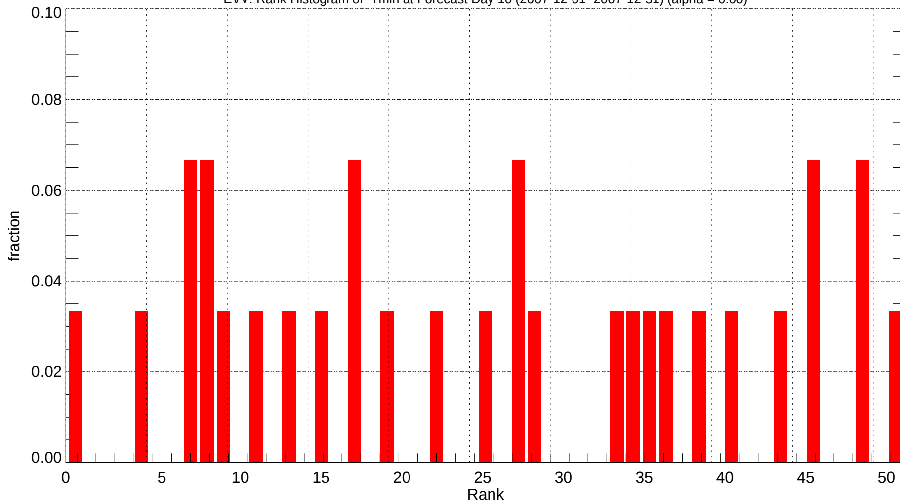
EVV: Rank Histogram of Tmin at Forecast Day 10 (2007-12-01~2007-12-31) (alpha = 0.00)
