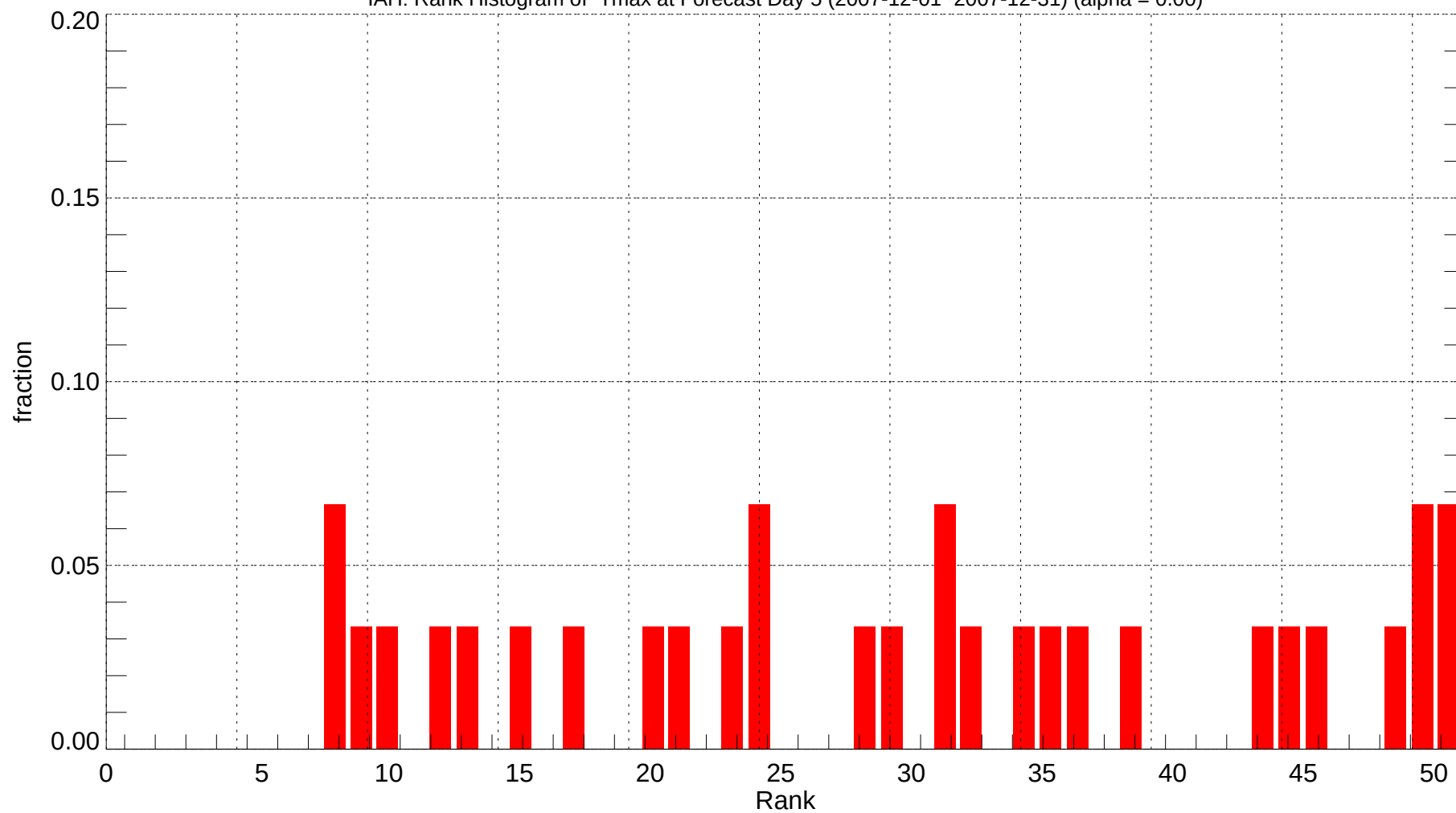
IAH: Rank Histogram of Tmax at Forecast Day 5 (2007-12-01~2007-12-31) (alpha = 0.00)
