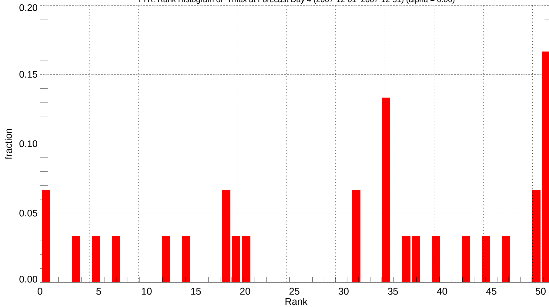
TYR: Rank Histogram of Tmax at Forecast Day 4 (2007-12-01~2007-12-31) (alpha = 0.00)
