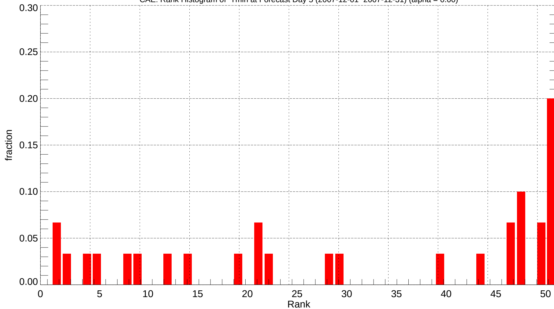
CAE: Rank Histogram of Tmin at Forecast Day 5 (2007-12-01~2007-12-31) (alpha = 0.00)
