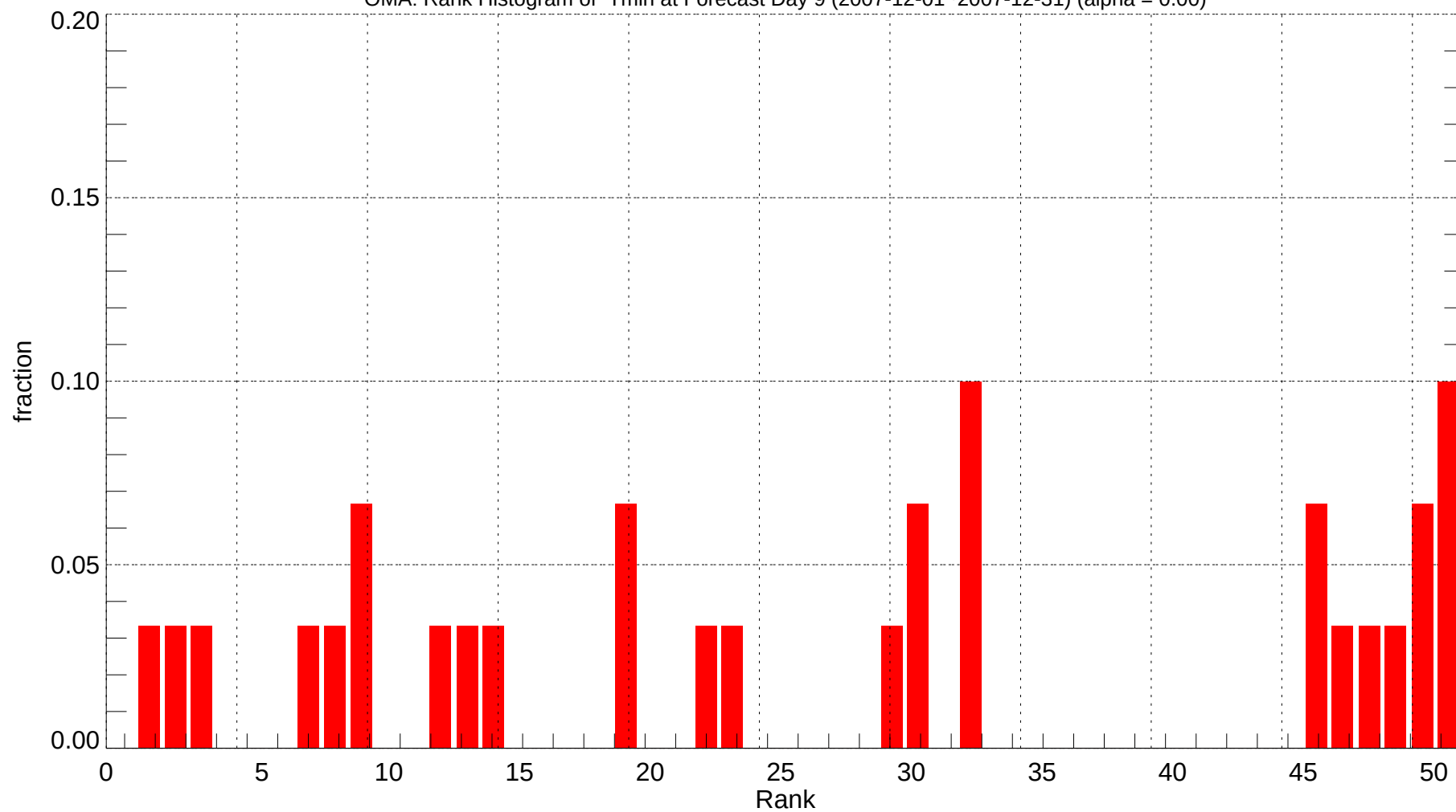
OMA: Rank Histogram of Tmin at Forecast Day 9 (2007-12-01~2007-12-31) (alpha = 0.00)
