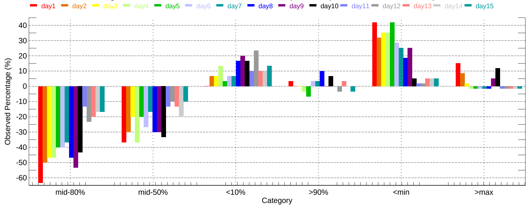
Observed Percentage Deviation of Ensembles - BDL: Min Temperature (2007-12-01~2007-12-31)
