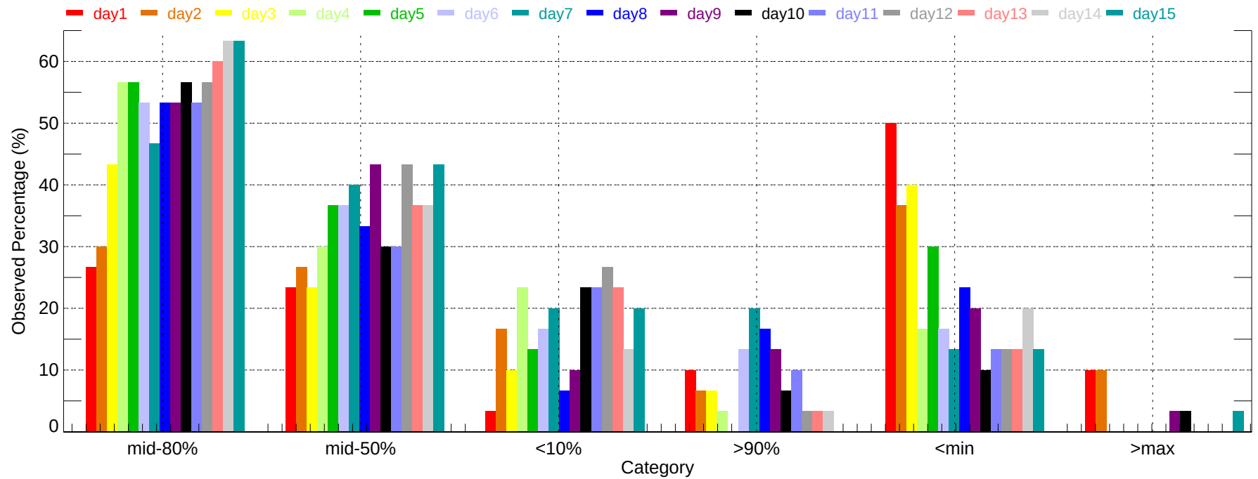
Observed Percentage of Ensembles - SYR: Min Temperature (2007-12-01~2007-12-31)
