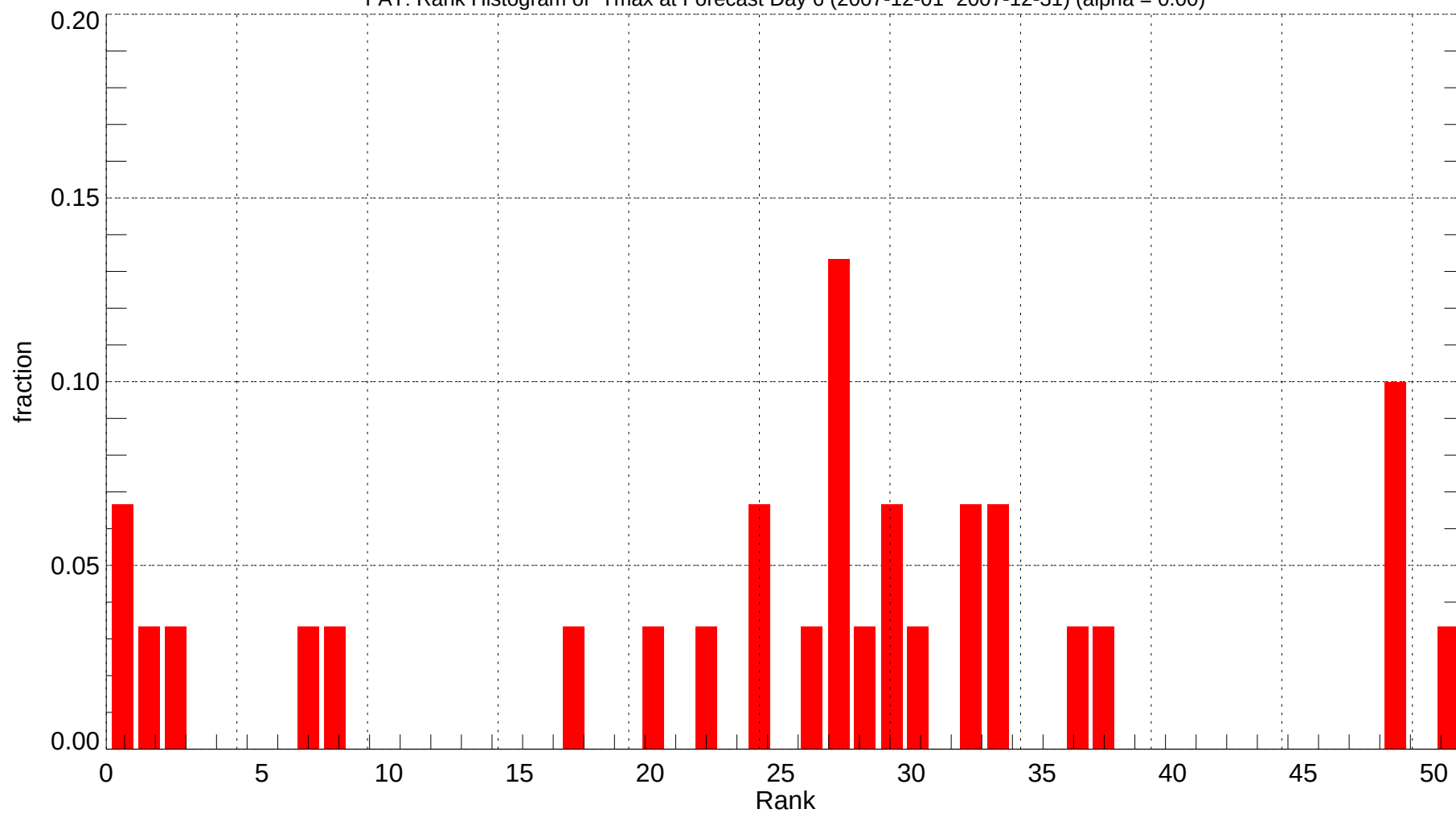
FAT: Rank Histogram of Tmax at Forecast Day 6 (2007-12-01~2007-12-31) (alpha = 0.00)
