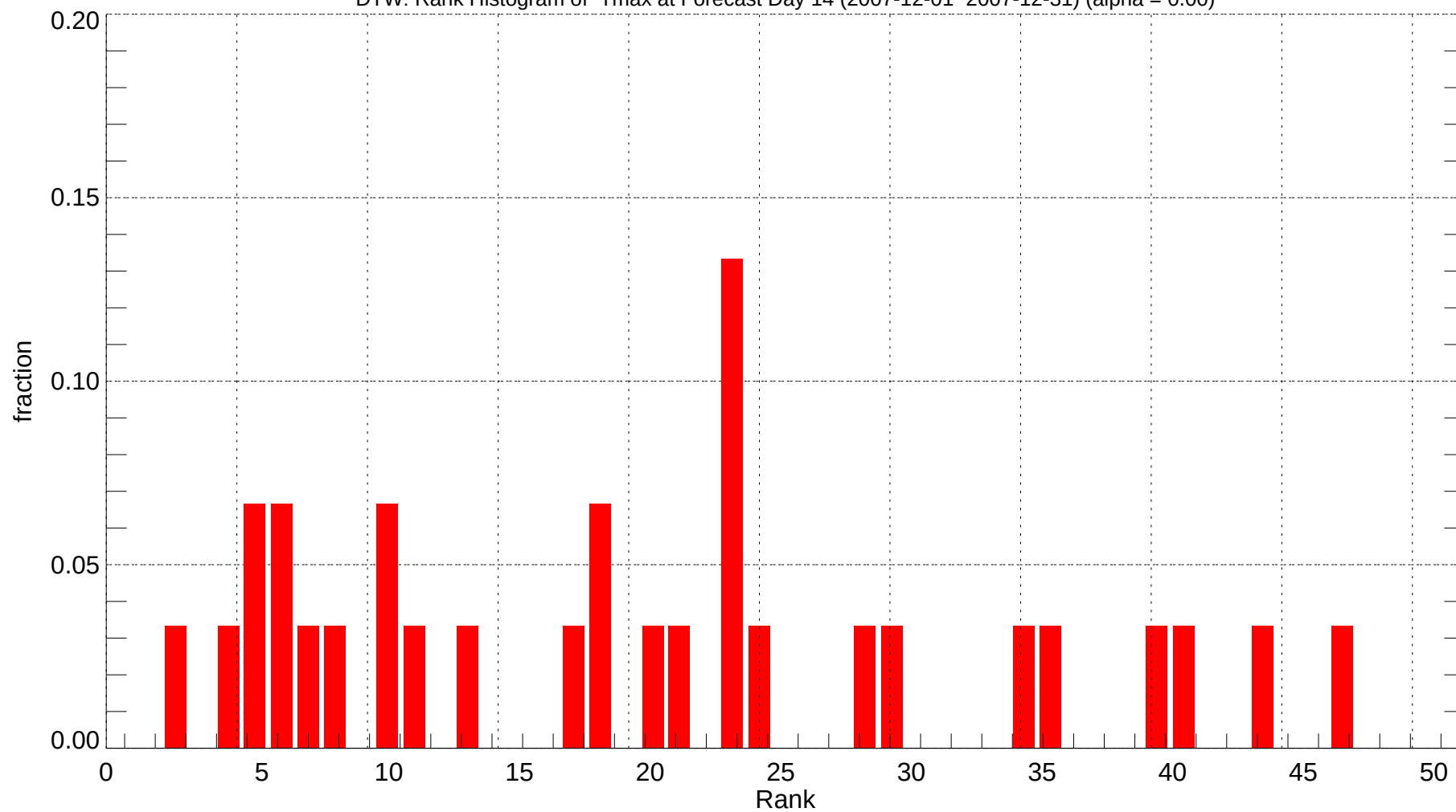
DTW: Rank Histogram of Tmax at Forecast Day 14 (2007-12-01~2007-12-31) (alpha = 0.00)
