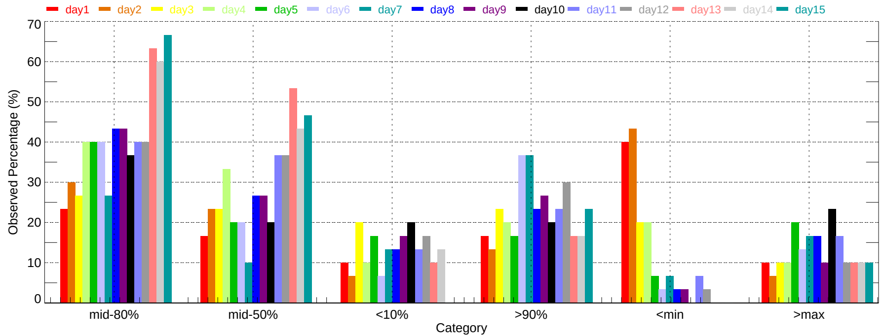
Observed Percentage of Ensembles - LIT: Min Temperature (2007-12-01~2007-12-31)
