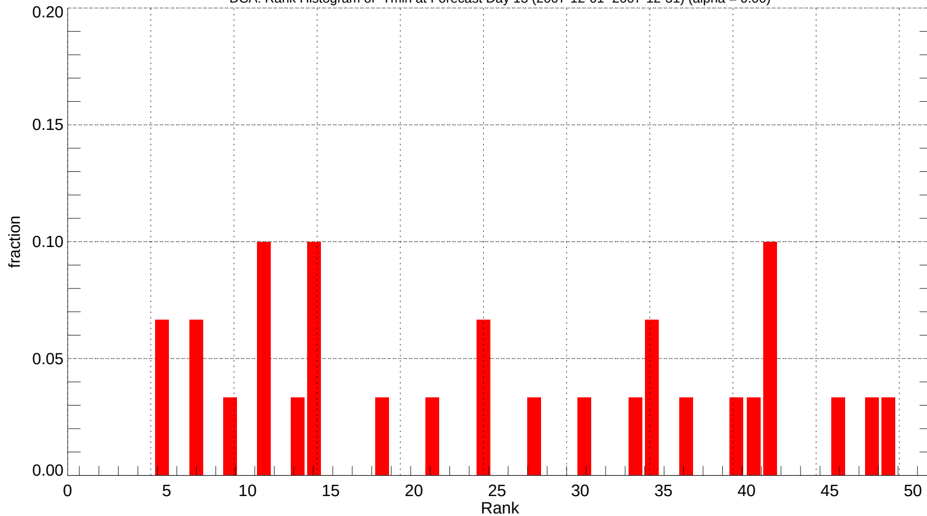
DCA: Rank Histogram of Tmin at Forecast Day 13 (2007-12-01~2007-12-31) (alpha = 0.00)
