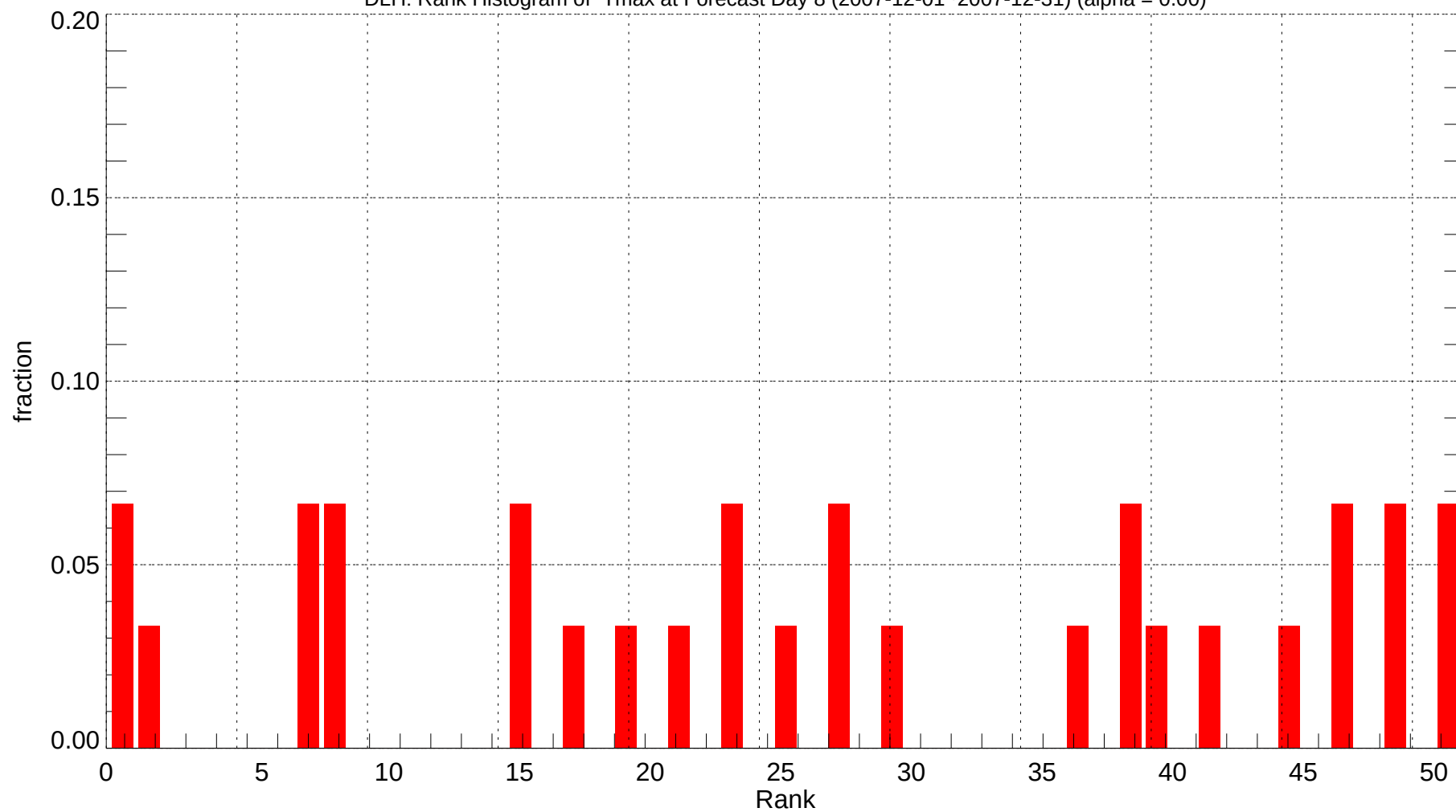
DLH: Rank Histogram of Tmax at Forecast Day 8 (2007-12-01~2007-12-31) (alpha = 0.00)
