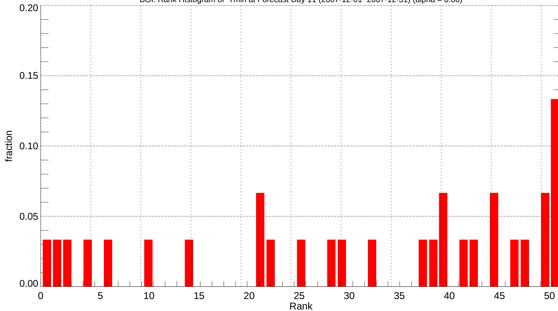
BOI: Rank Histogram of Tmin at Forecast Day 11 (2007-12-01~2007-12-31) (alpha = 0.00)
