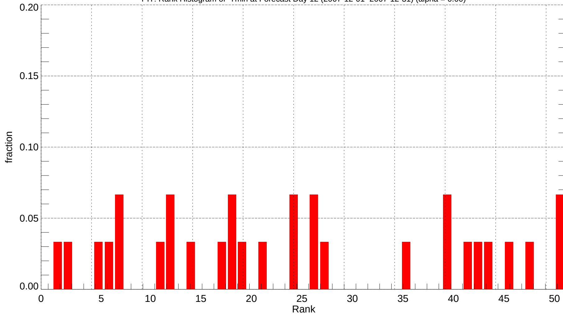
PIT: Rank Histogram of Tmin at Forecast Day 12 (2007-12-01~2007-12-31) (alpha = 0.00)
