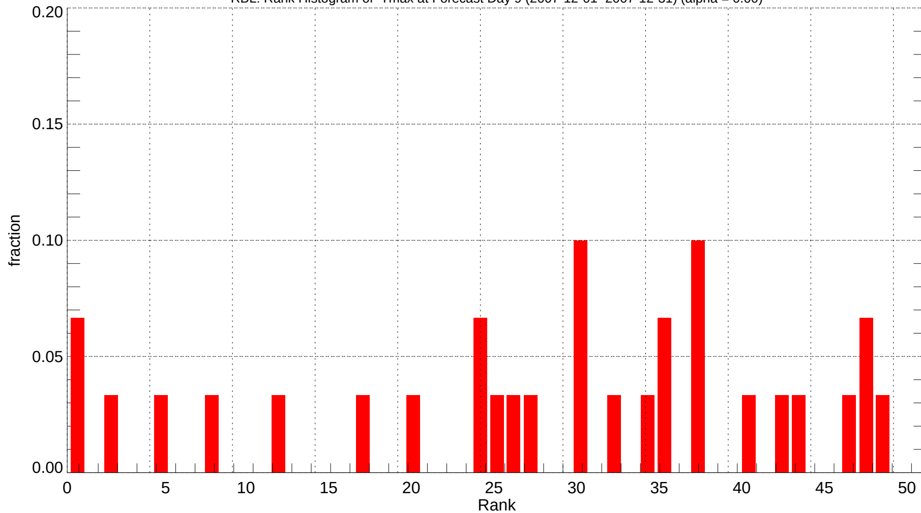
RBL: Rank Histogram of Tmax at Forecast Day 9 (2007-12-01~2007-12-31) (alpha = 0.00)
