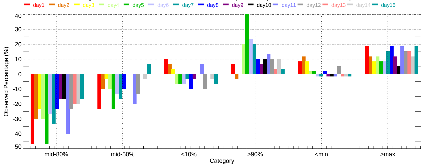
Observed Percentage Deviation of Ensembles - AUS: Max Temperature (2007-12-01~2007-12-31)
