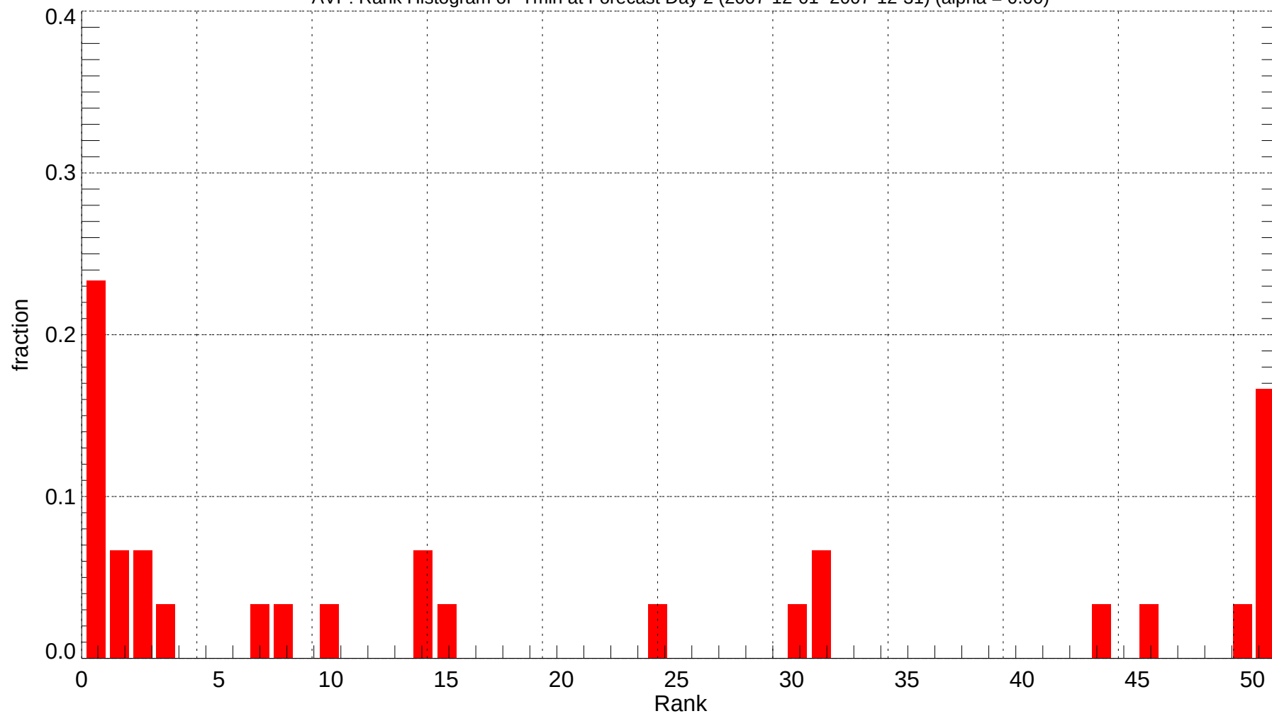
AVP: Rank Histogram of Tmin at Forecast Day 2 (2007-12-01~2007-12-31) (alpha = 0.00)
