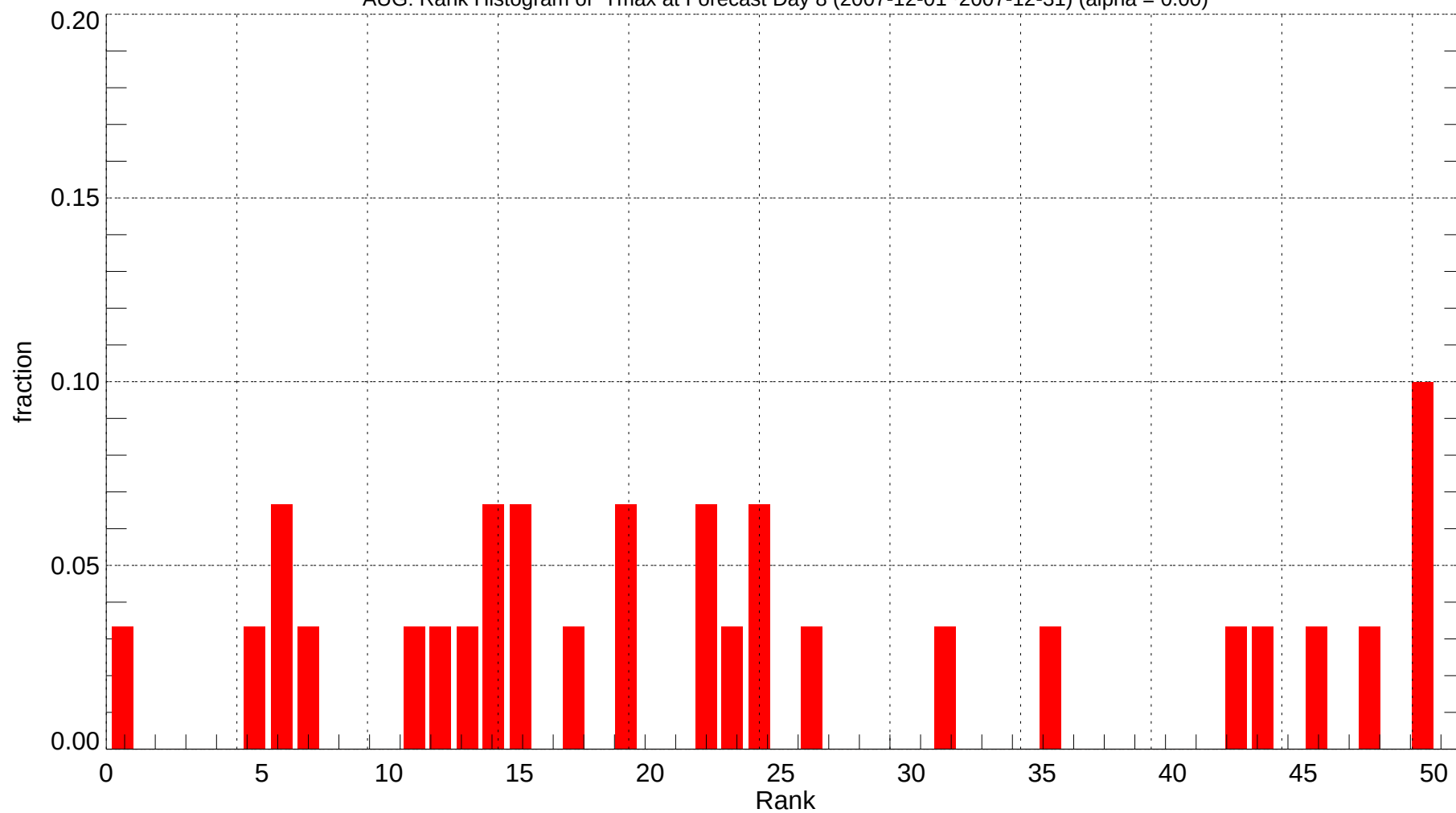
AUG: Rank Histogram of Tmax at Forecast Day 8 (2007-12-01~2007-12-31) (alpha = 0.00)
