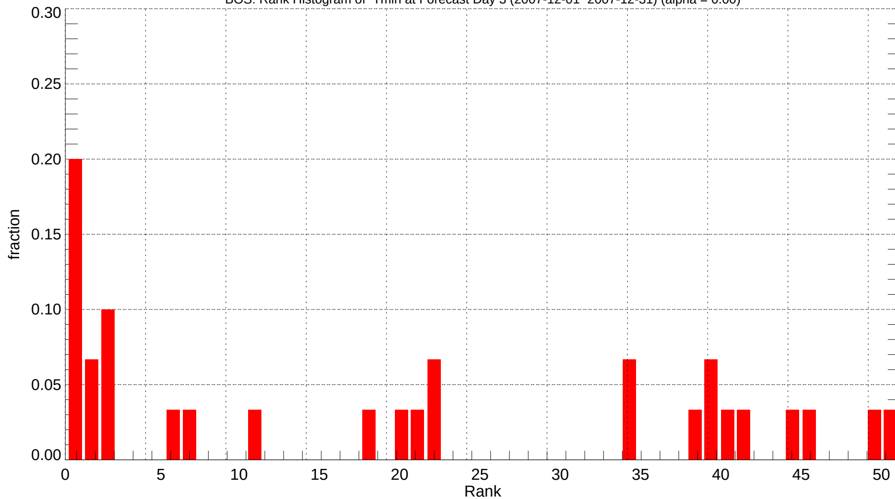
BOS: Rank Histogram of Tmin at Forecast Day 3 (2007-12-01~2007-12-31) (alpha = 0.00)
