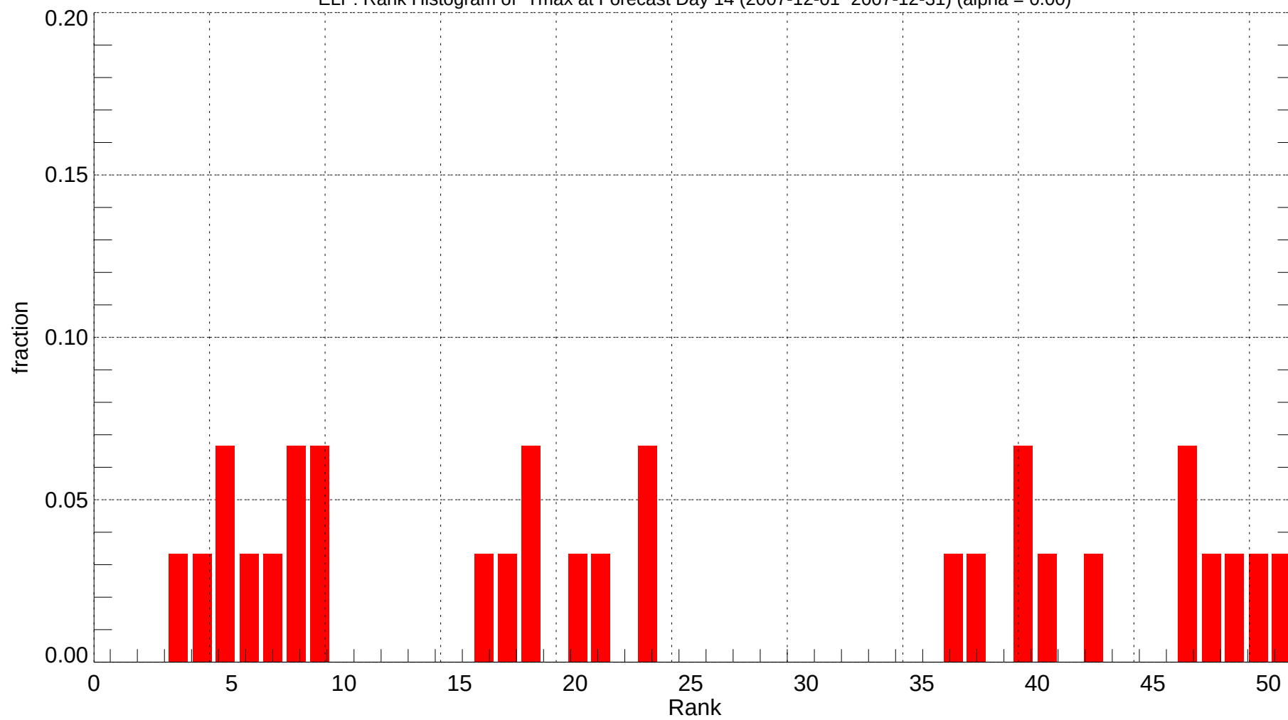
ELP: Rank Histogram of Tmax at Forecast Day 14 (2007-12-01~2007-12-31) (alpha = 0.00)
