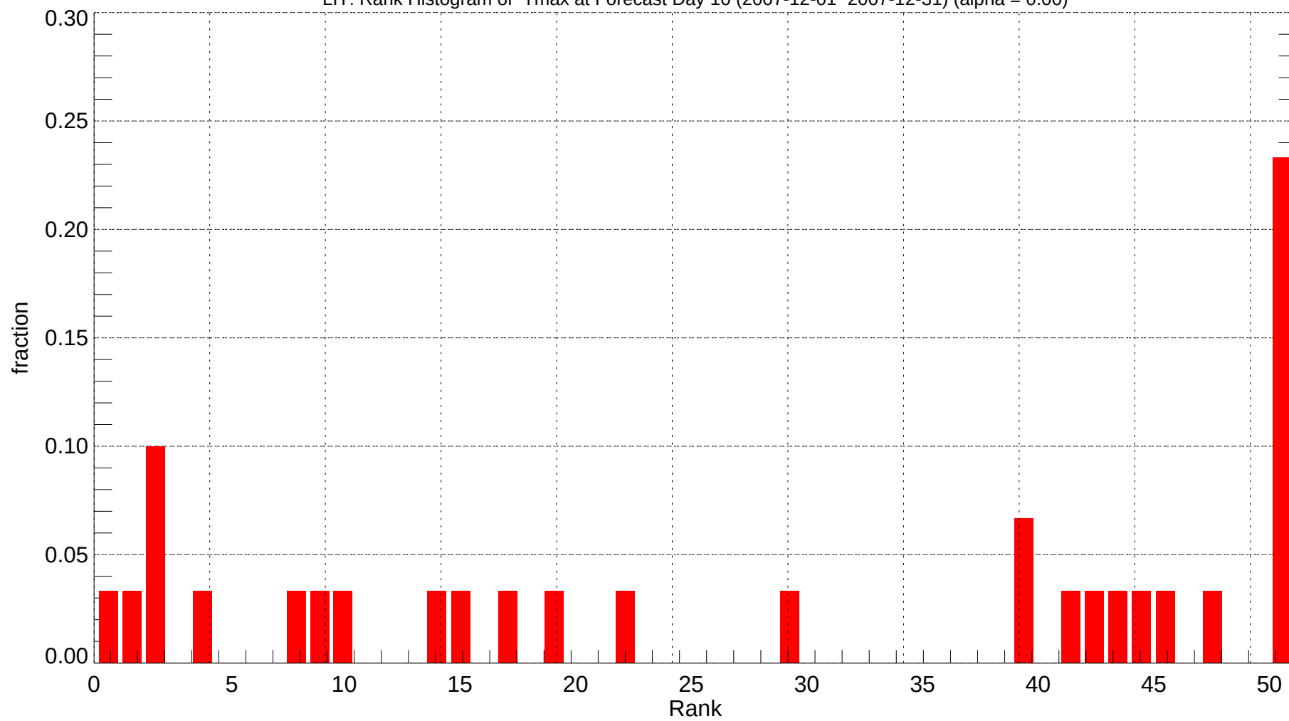
LIT: Rank Histogram of Tmax at Forecast Day 10 (2007-12-01~2007-12-31) (alpha = 0.00)
