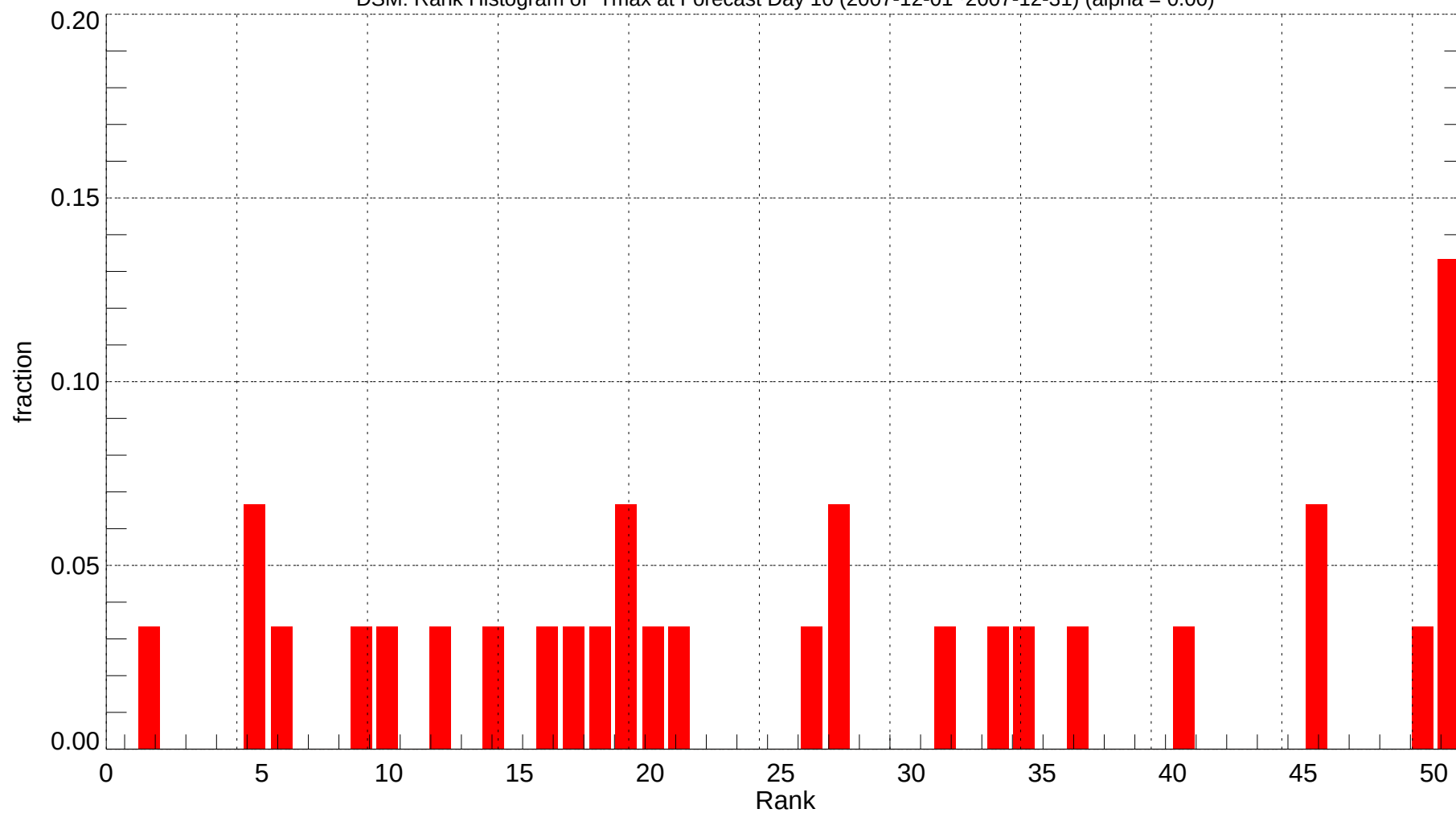
DSM: Rank Histogram of Tmax at Forecast Day 10 (2007-12-01~2007-12-31) (alpha = 0.00)
