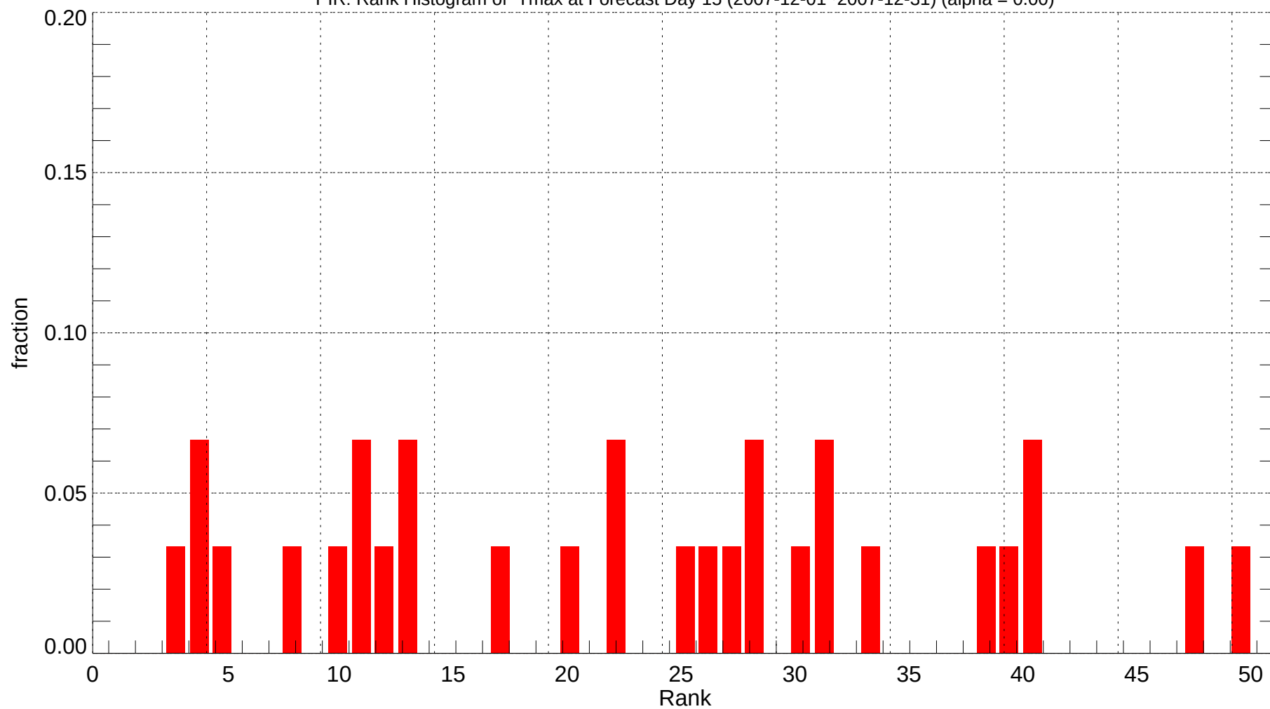
PIR: Rank Histogram of Tmax at Forecast Day 15 (2007-12-01~2007-12-31) (alpha = 0.00)
