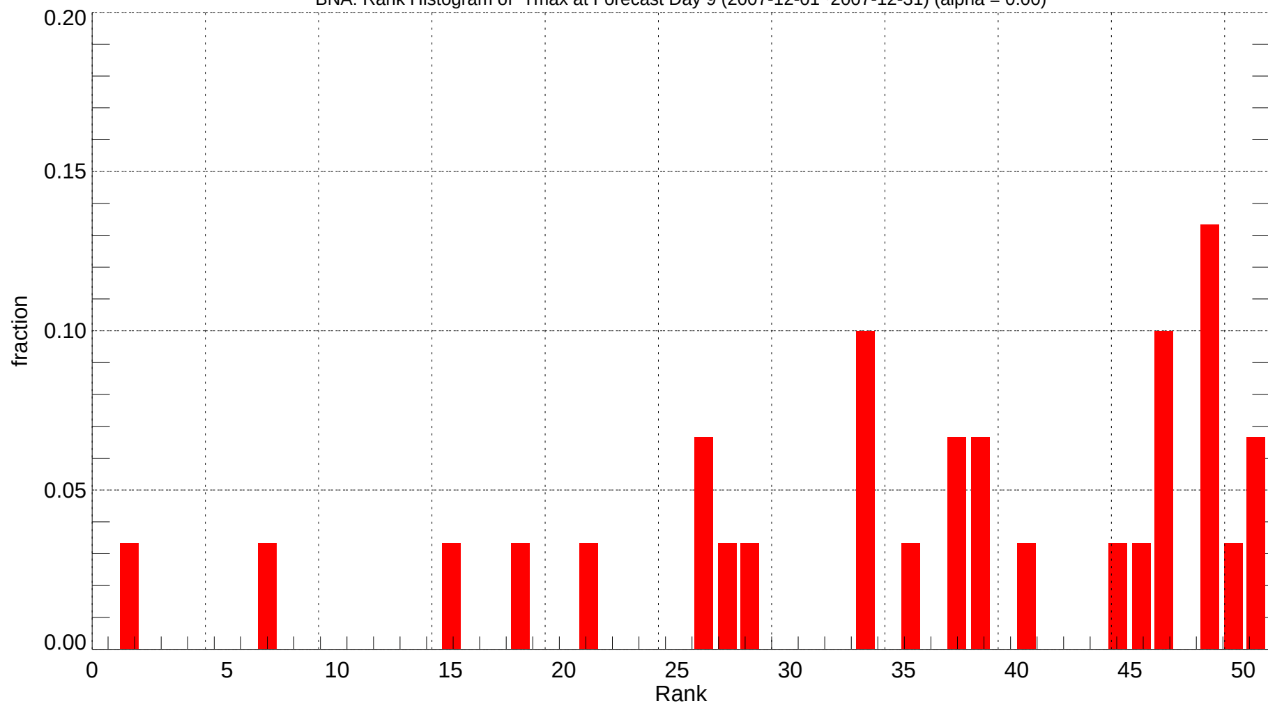
BNA: Rank Histogram of Tmax at Forecast Day 9 (2007-12-01~2007-12-31) (alpha = 0.00)
