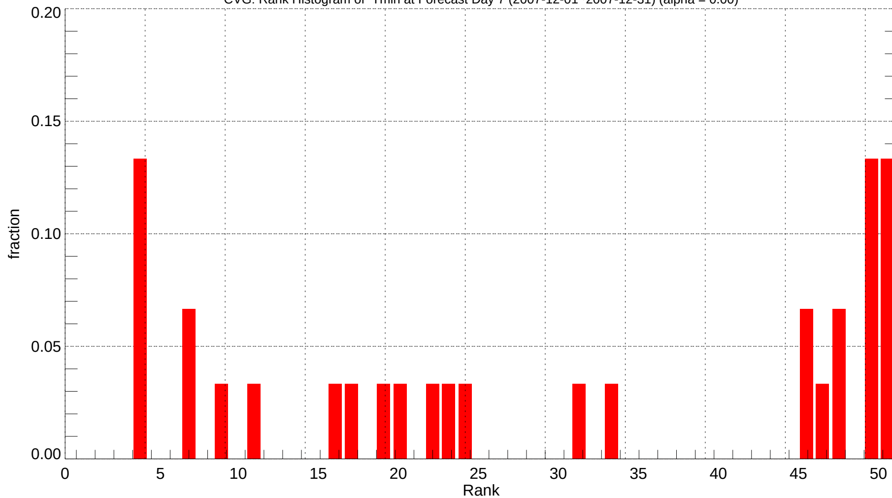
CVG: Rank Histogram of Tmin at Forecast Day 7 (2007-12-01~2007-12-31) (alpha = 0.00)
