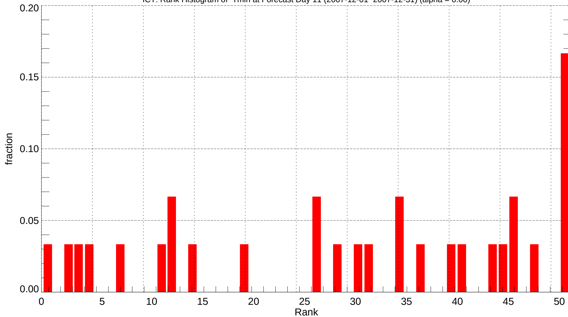
ICT: Rank Histogram of Tmin at Forecast Day 11 (2007-12-01~2007-12-31) (alpha = 0.00)
