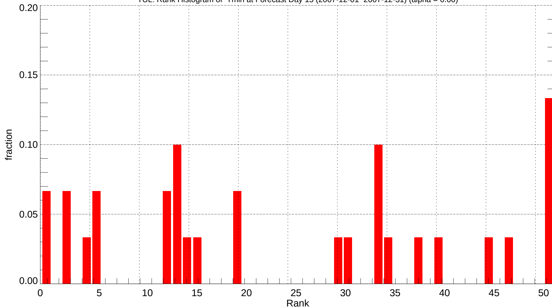
TUL: Rank Histogram of Tmin at Forecast Day 15 (2007-12-01~2007-12-31) (alpha = 0.00)
