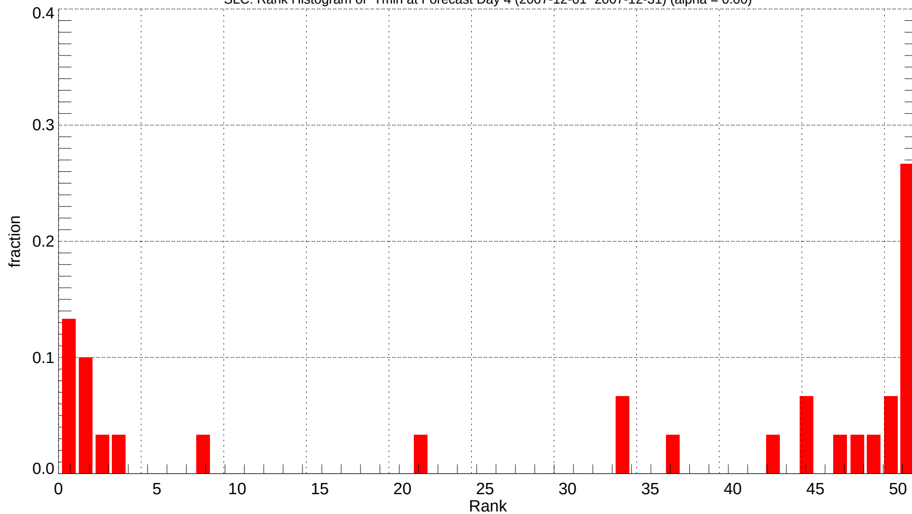
SLC: Rank Histogram of Tmin at Forecast Day 4 (2007-12-01~2007-12-31) (alpha = 0.00)
