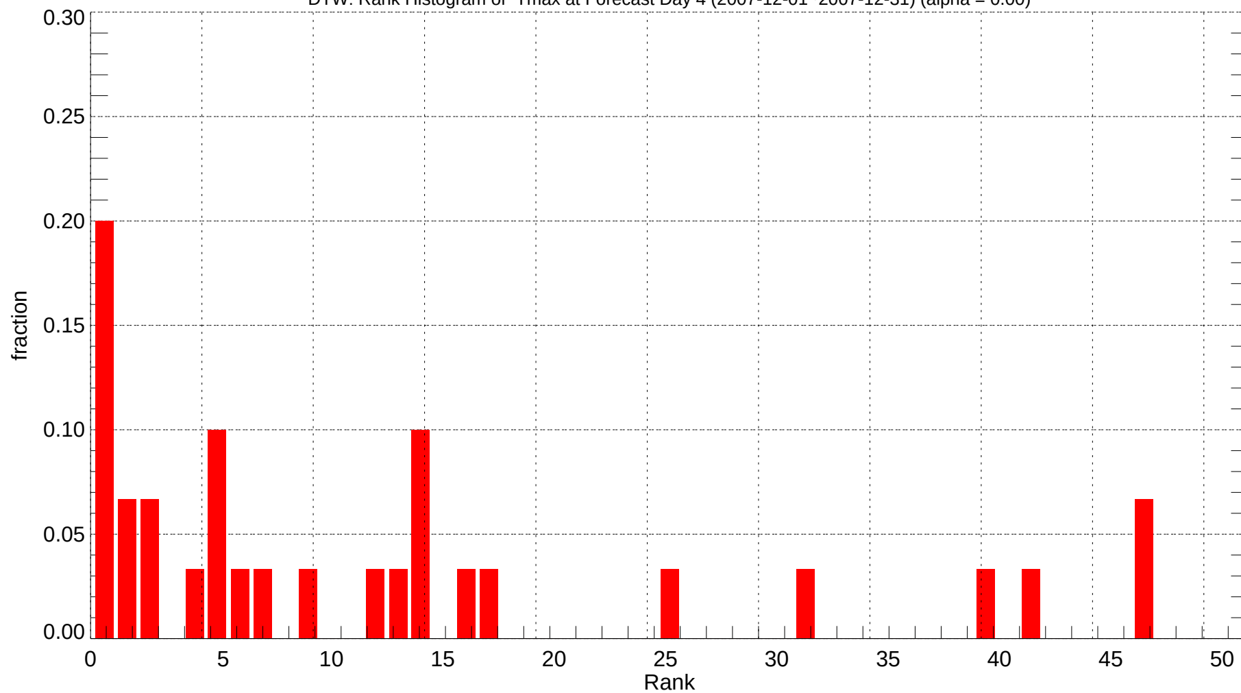
DTW: Rank Histogram of Tmax at Forecast Day 4 (2007-12-01~2007-12-31) (alpha = 0.00)
