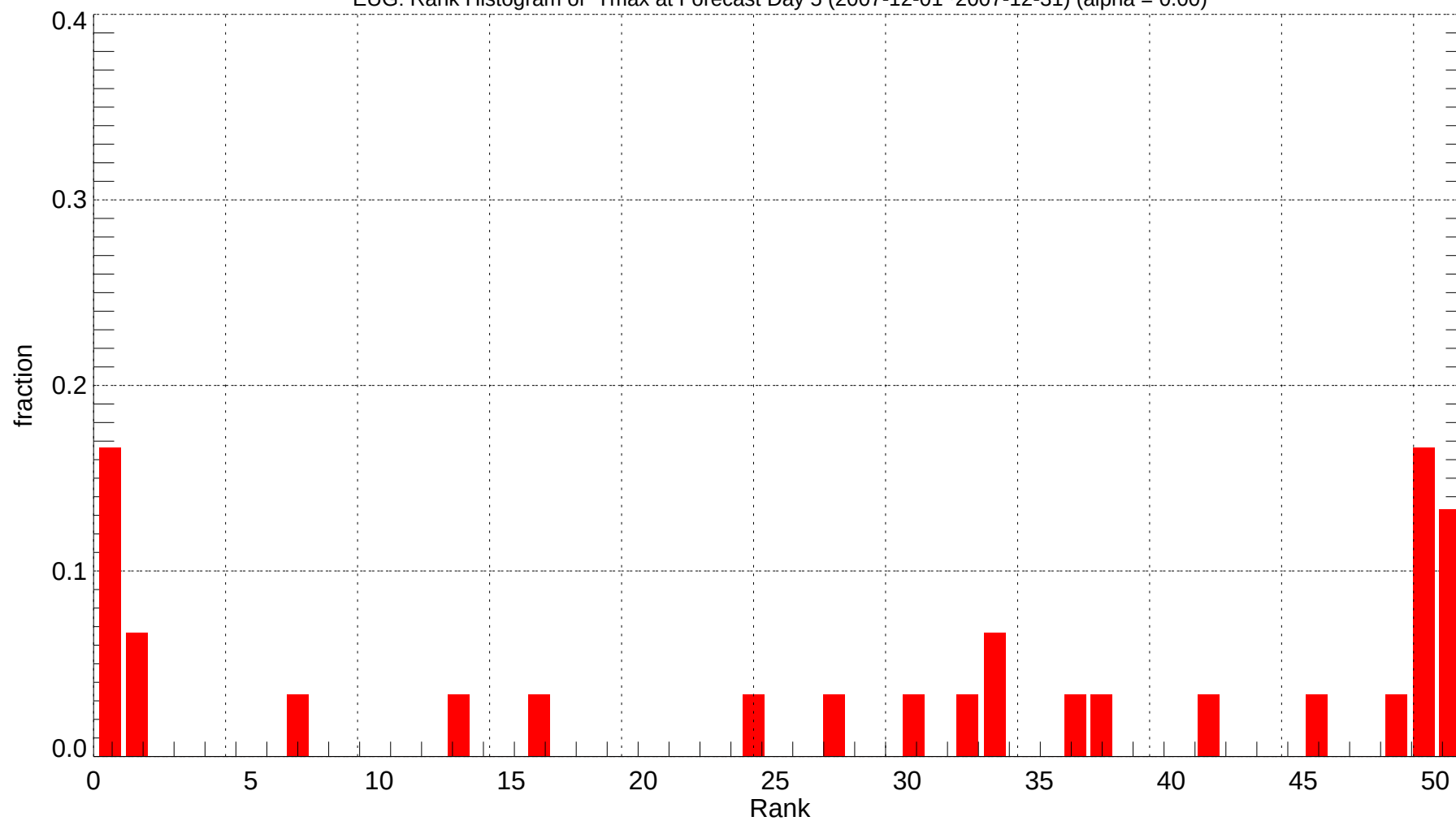
EUG: Rank Histogram of Tmax at Forecast Day 5 (2007-12-01~2007-12-31) (alpha = 0.00)
