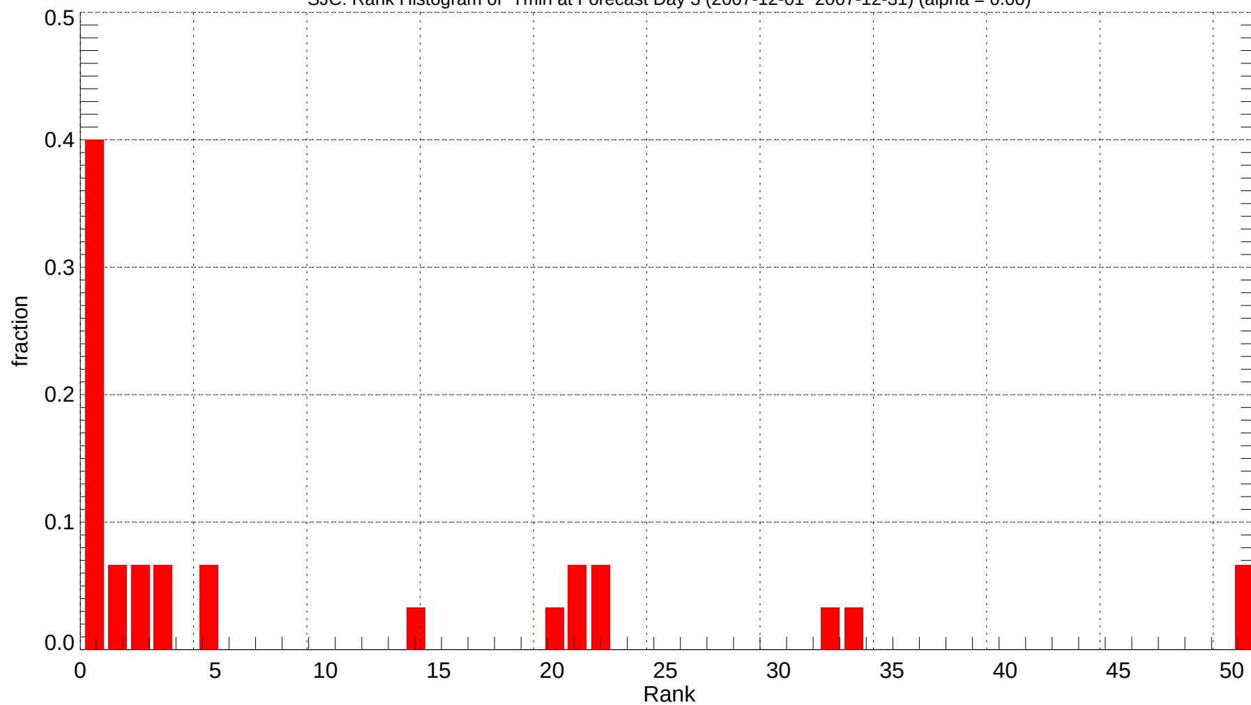
SJC: Rank Histogram of Tmin at Forecast Day 3 (2007-12-01~2007-12-31) (alpha = 0.00)
