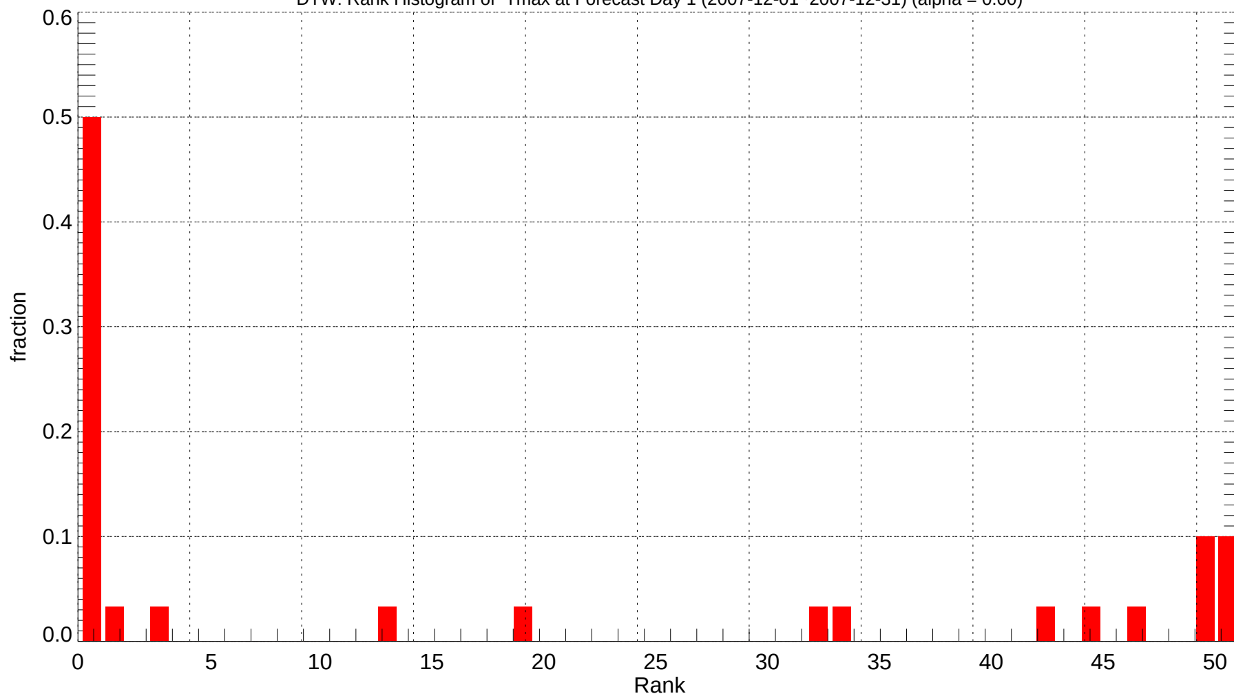
DTW: Rank Histogram of Tmax at Forecast Day 1 (2007-12-01~2007-12-31) (alpha = 0.00)
