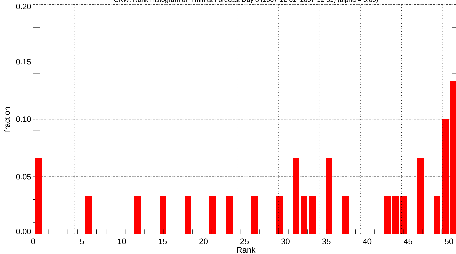
CRW: Rank Histogram of Tmin at Forecast Day 8 (2007-12-01~2007-12-31) (alpha = 0.00)
