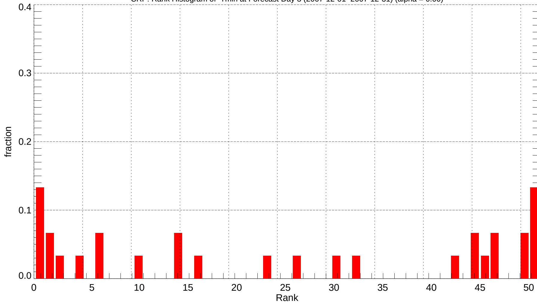
CRP: Rank Histogram of Tmin at Forecast Day 3 (2007-12-01~2007-12-31) (alpha = 0.00)
