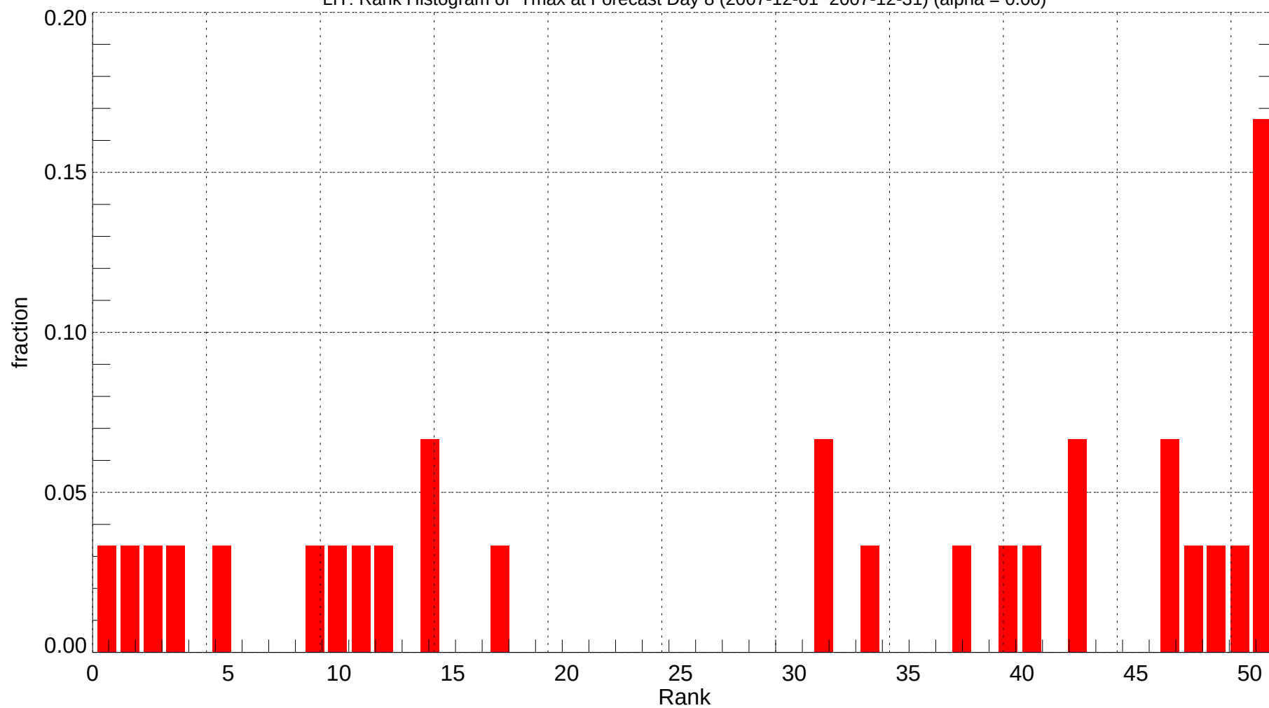
LIT: Rank Histogram of Tmax at Forecast Day 8 (2007-12-01~2007-12-31) (alpha = 0.00)
