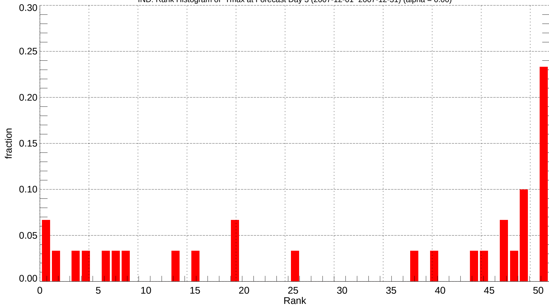
IND: Rank Histogram of Tmax at Forecast Day 3 (2007-12-01~2007-12-31) (alpha = 0.00)
