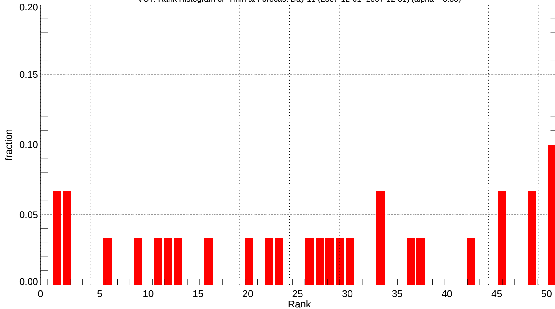
VCT: Rank Histogram of Tmin at Forecast Day 11 (2007-12-01~2007-12-31) (alpha = 0.00)
