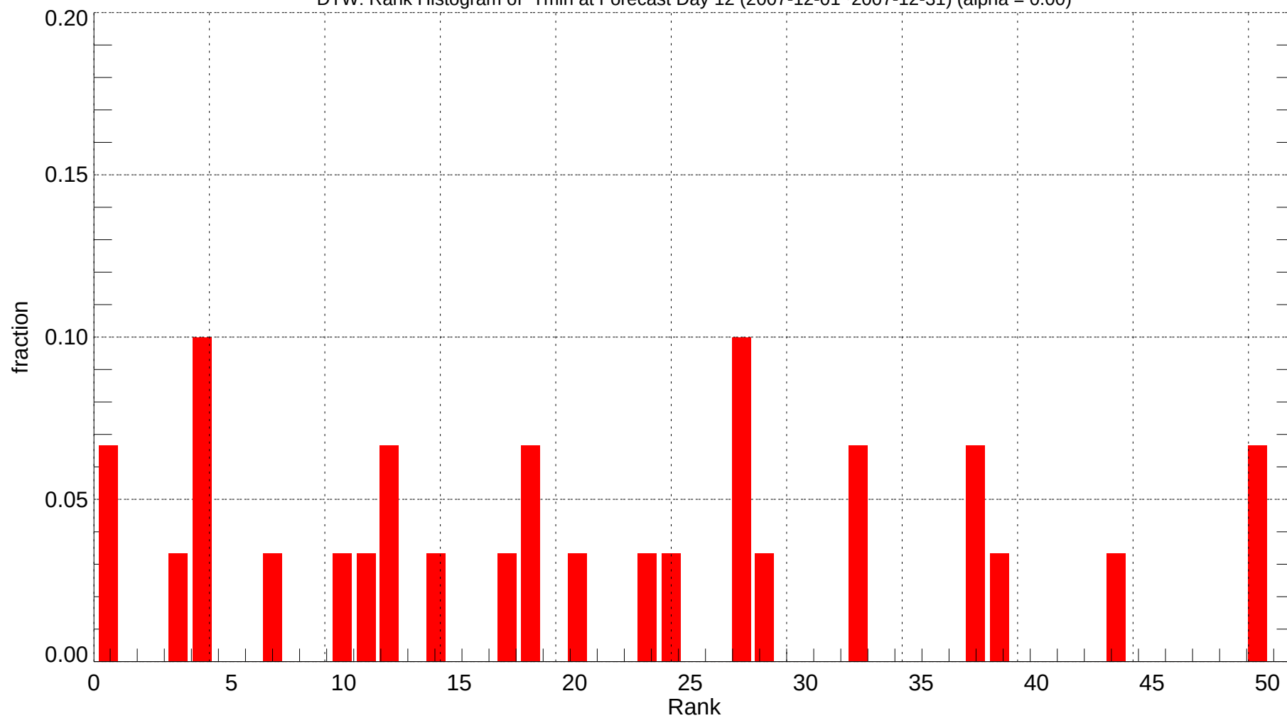
DTW: Rank Histogram of Tmin at Forecast Day 12 (2007-12-01~2007-12-31) (alpha = 0.00)
