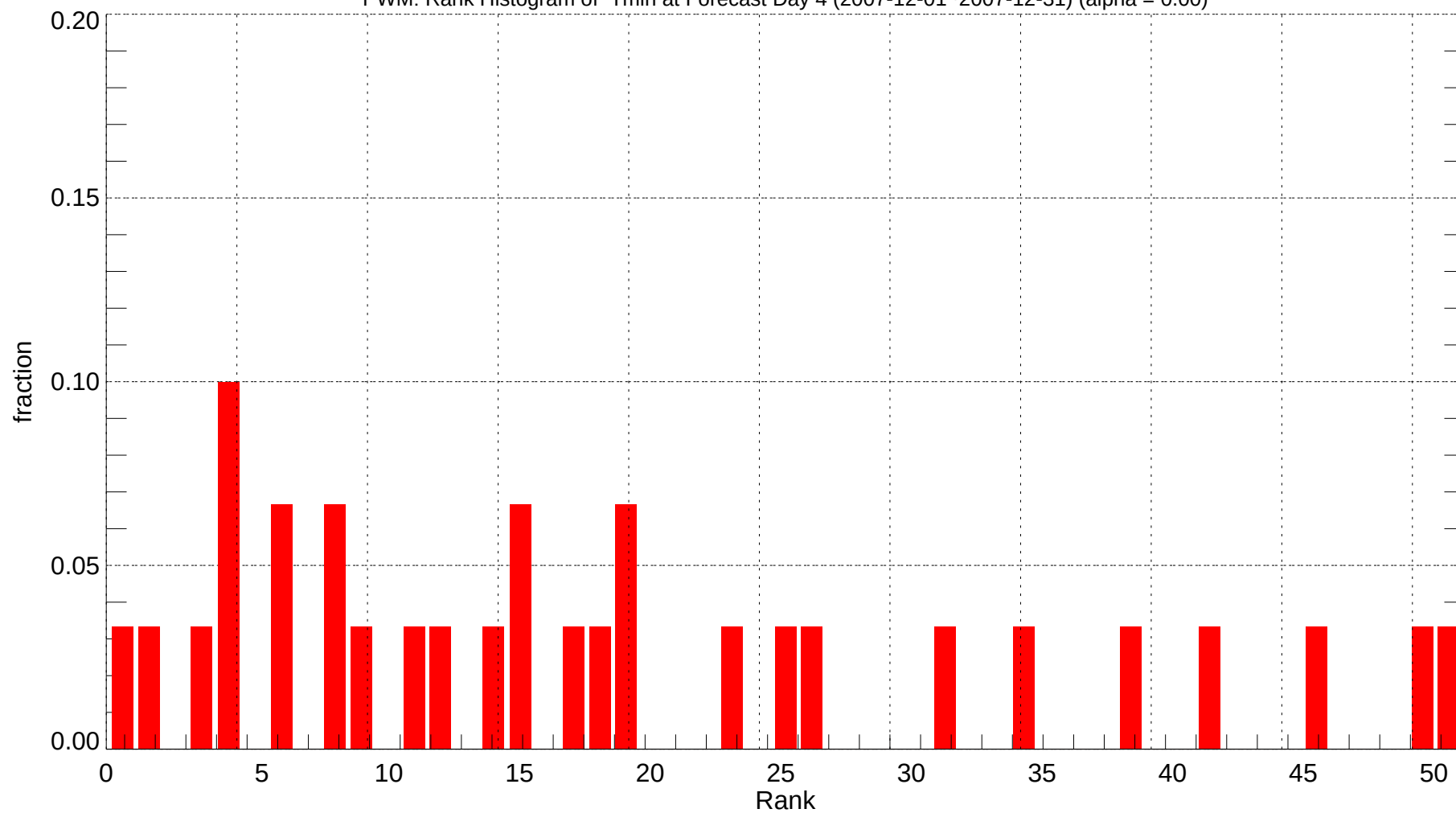
PWM: Rank Histogram of Tmin at Forecast Day 4 (2007-12-01~2007-12-31) (alpha = 0.00)
