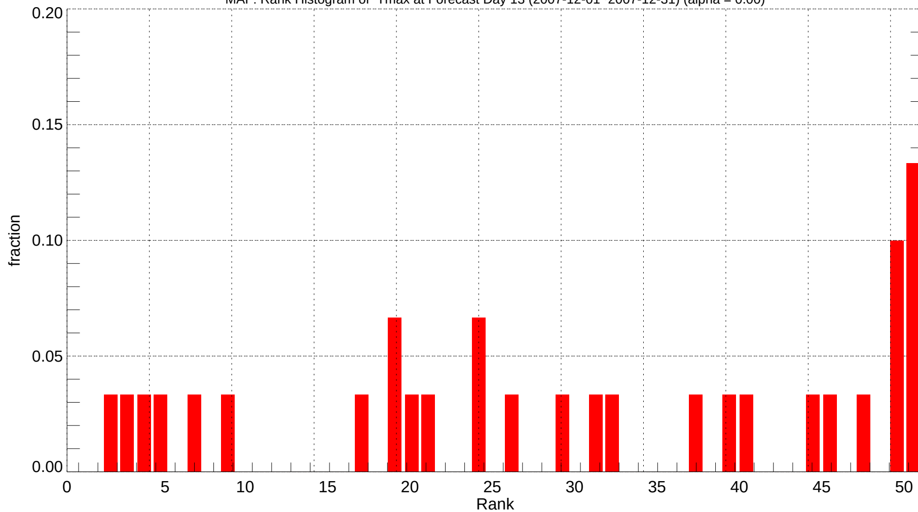
MAF: Rank Histogram of Tmax at Forecast Day 13 (2007-12-01~2007-12-31) (alpha = 0.00)
