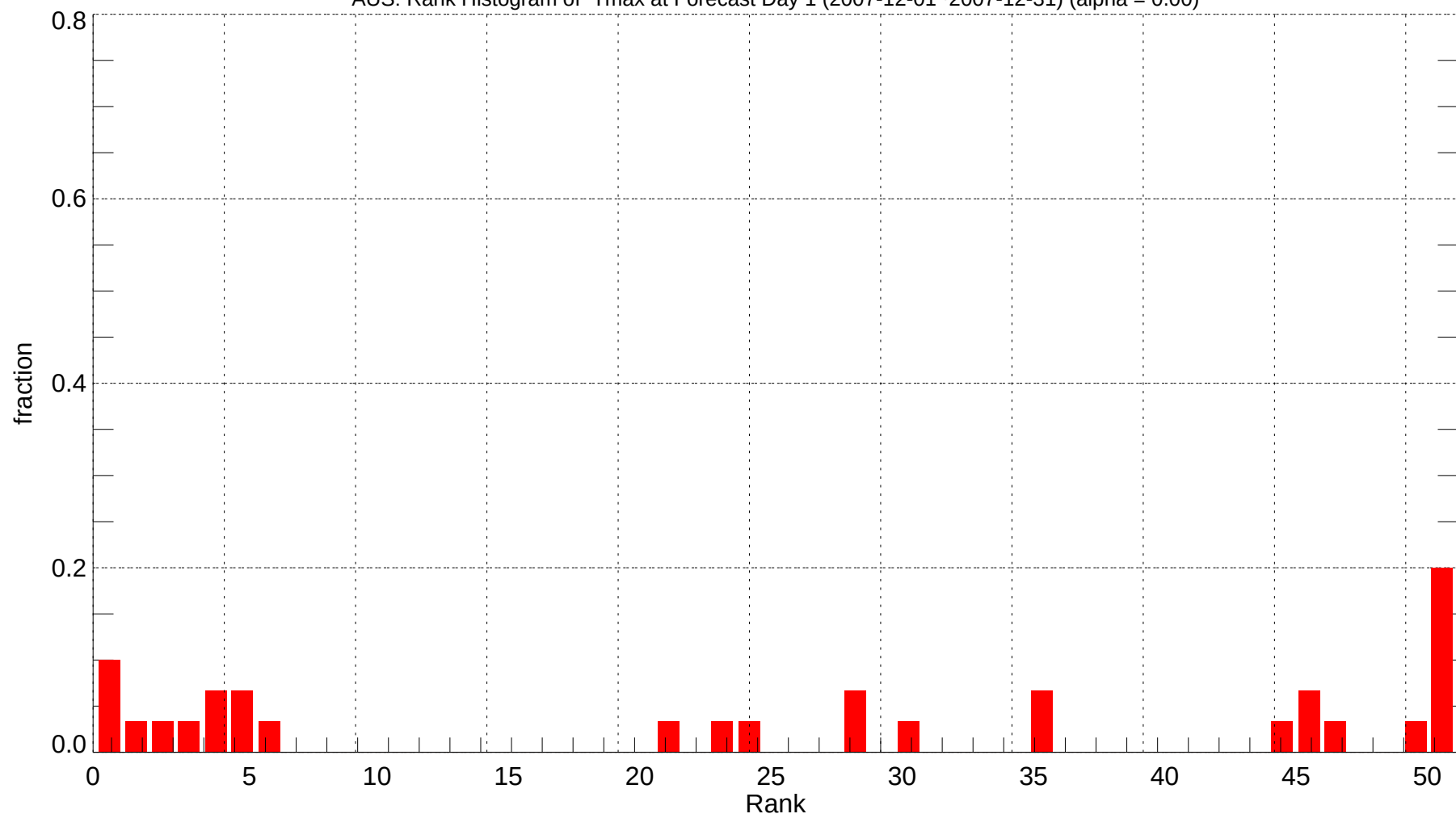
AUS: Rank Histogram of Tmax at Forecast Day 1 (2007-12-01~2007-12-31) (alpha = 0.00)
