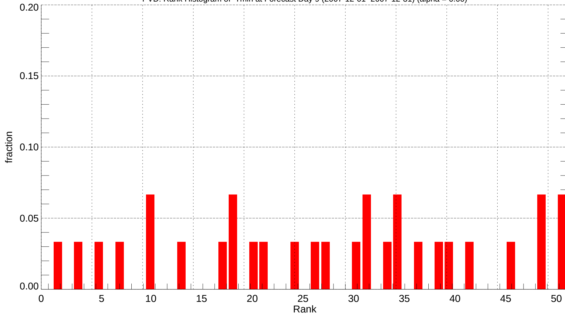
PVD: Rank Histogram of Tmin at Forecast Day 9 (2007-12-01~2007-12-31) (alpha = 0.00)
