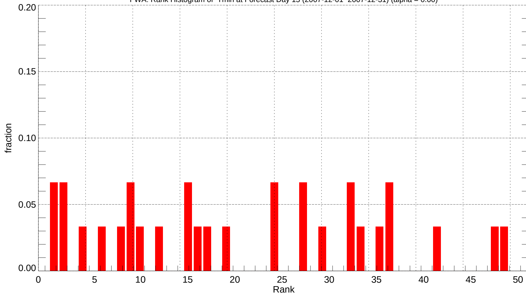
FWA: Rank Histogram of Tmin at Forecast Day 15 (2007-12-01~2007-12-31) (alpha = 0.00)
