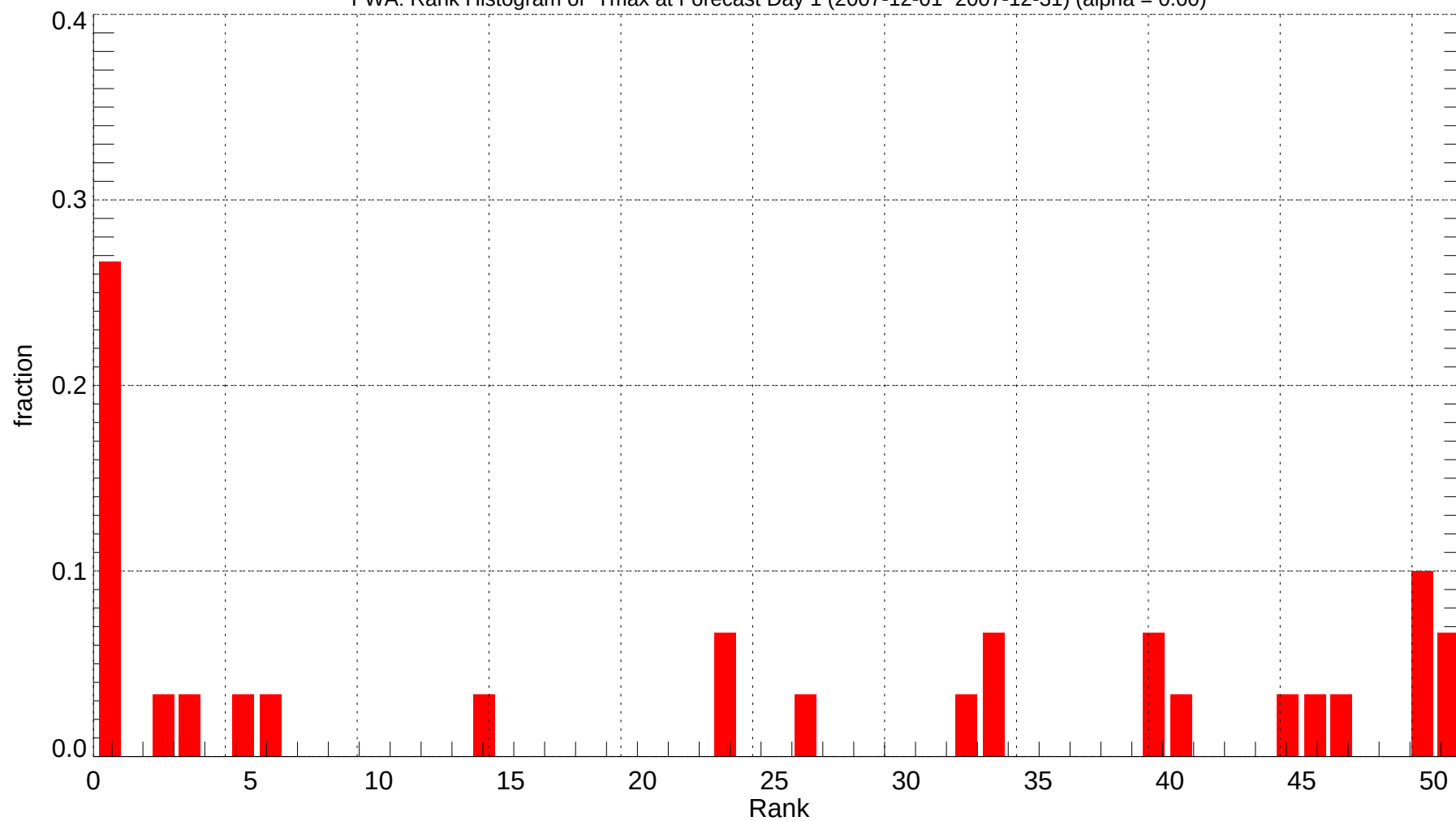
FWA: Rank Histogram of Tmax at Forecast Day 1 (2007-12-01~2007-12-31) (alpha = 0.00)
