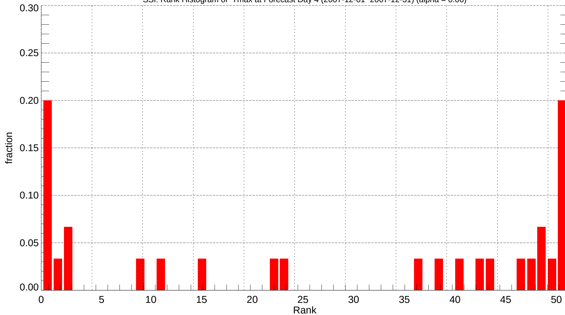
SSI: Rank Histogram of Tmax at Forecast Day 4 (2007-12-01~2007-12-31) (alpha = 0.00)
