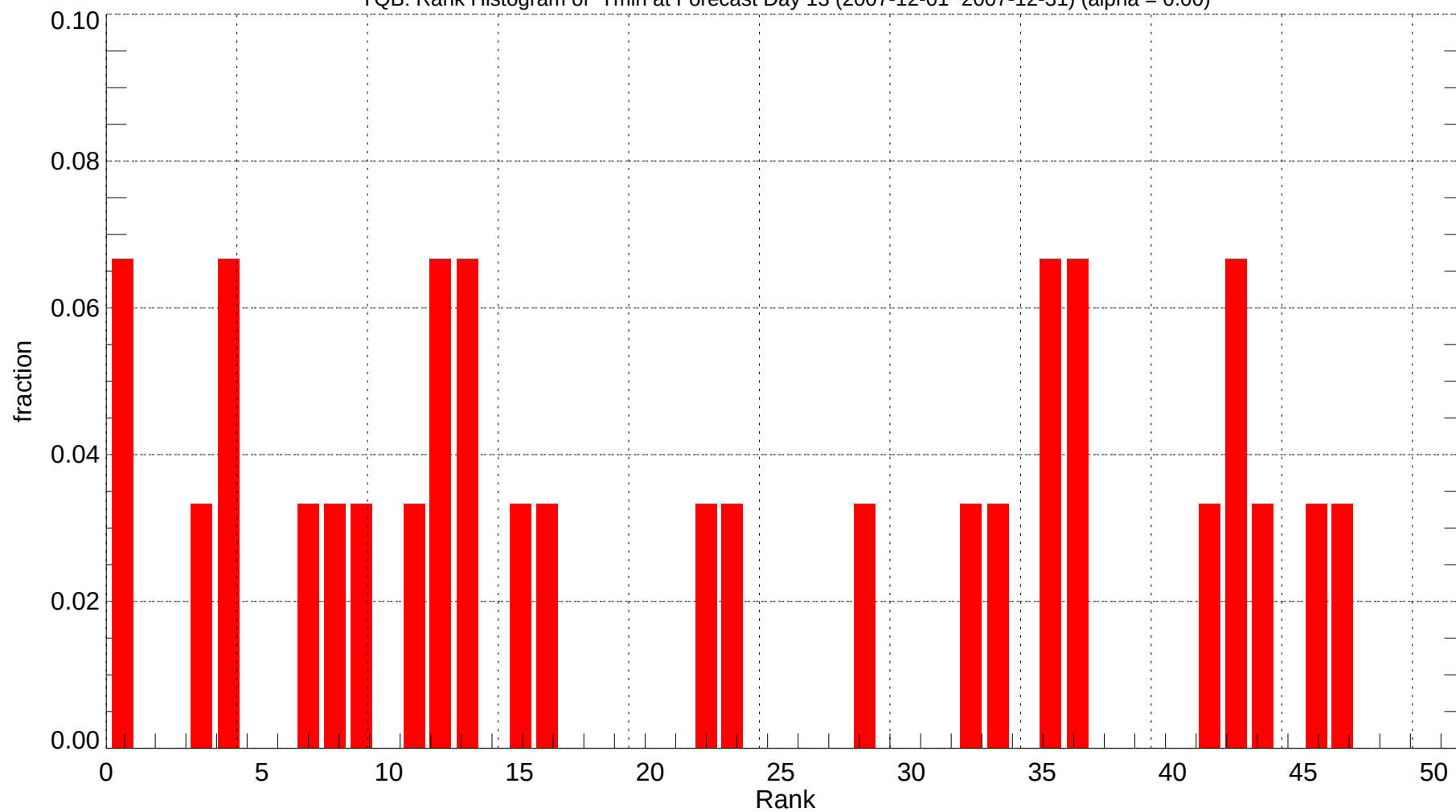
YQB: Rank Histogram of Tmin at Forecast Day 13 (2007-12-01~2007-12-31) (alpha = 0.00)
