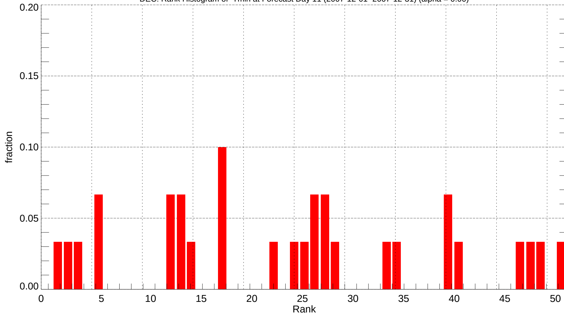
DEC: Rank Histogram of Tmin at Forecast Day 11 (2007-12-01~2007-12-31) (alpha = 0.00)
