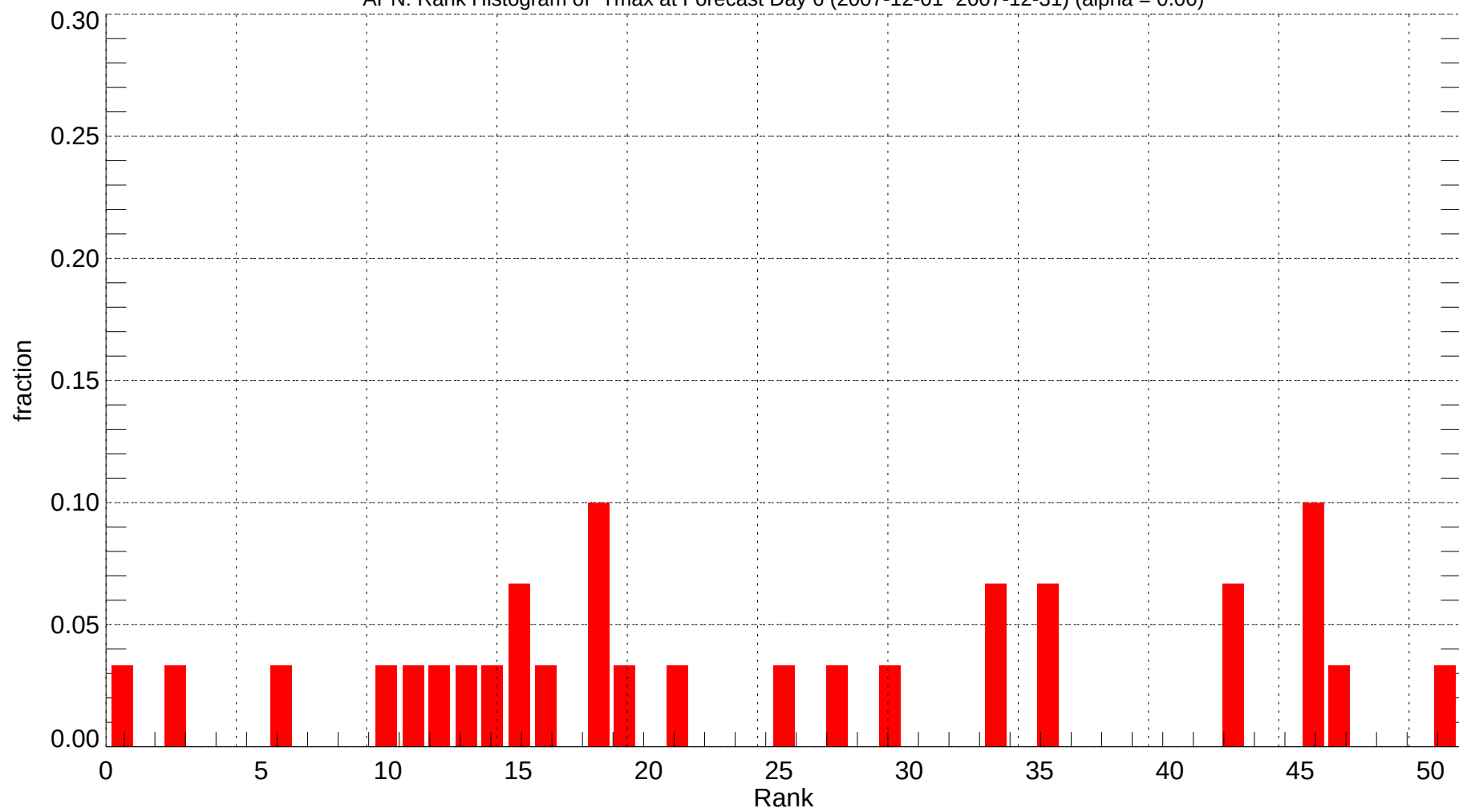
APN: Rank Histogram of Tmax at Forecast Day 6 (2007-12-01~2007-12-31) (alpha = 0.00)
