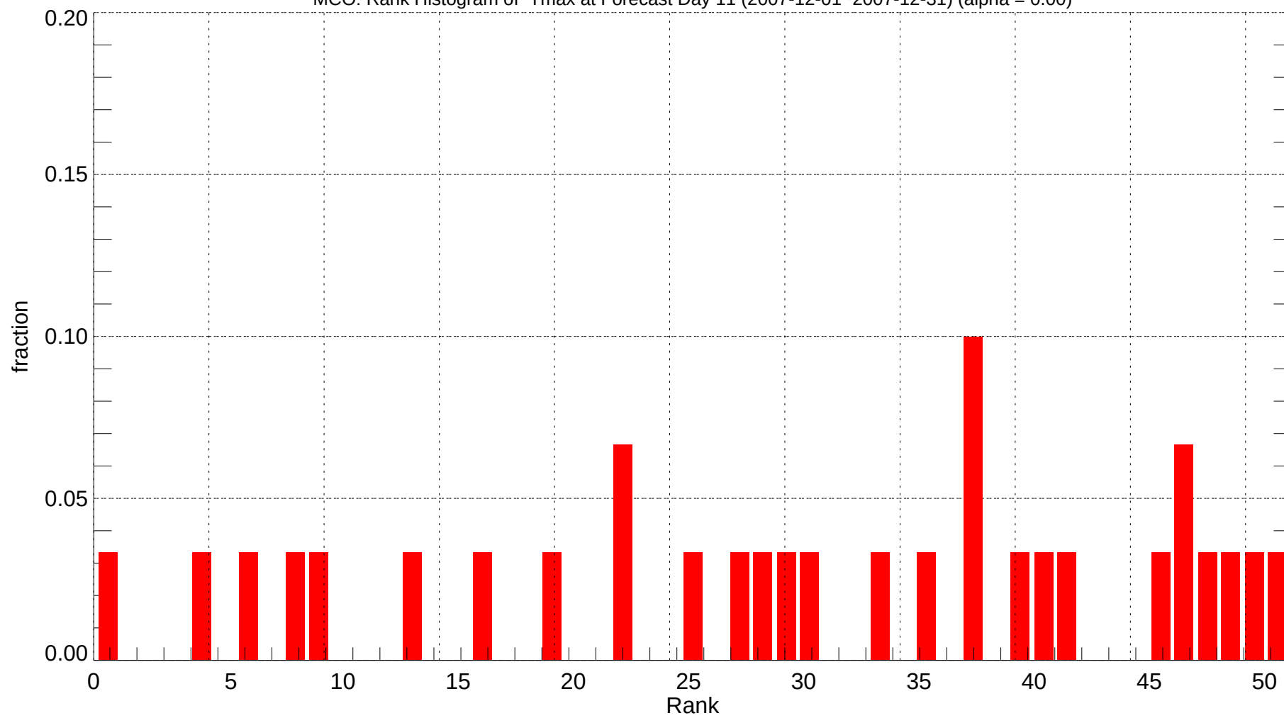
MCO: Rank Histogram of Tmax at Forecast Day 11 (2007-12-01~2007-12-31) (alpha = 0.00)
