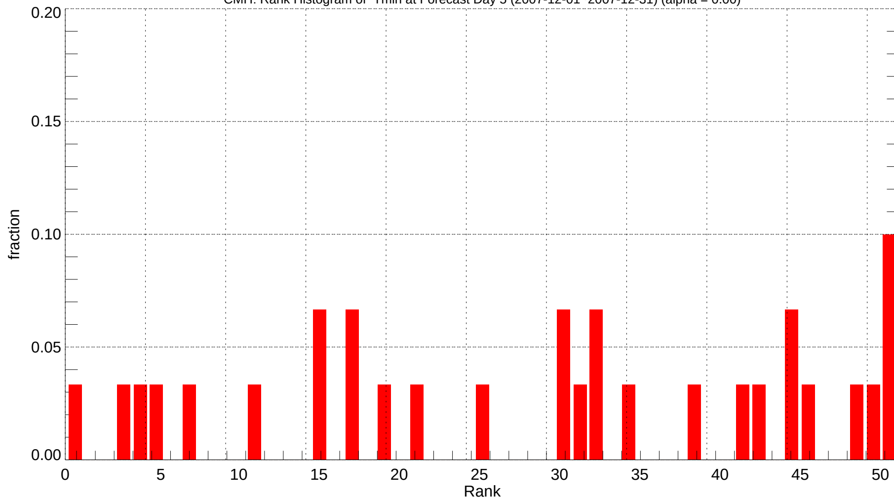
CMH: Rank Histogram of Tmin at Forecast Day 5 (2007-12-01~2007-12-31) (alpha = 0.00)
