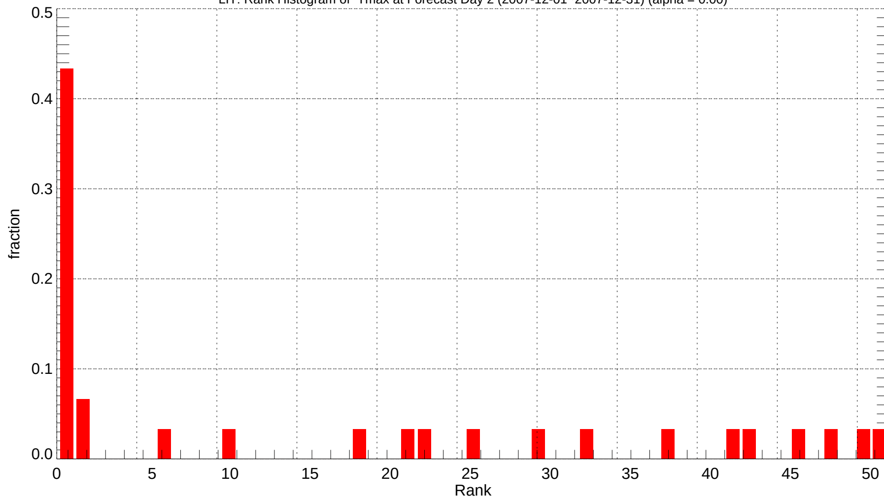
LIT: Rank Histogram of Tmax at Forecast Day 2 (2007-12-01~2007-12-31) (alpha = 0.00)
