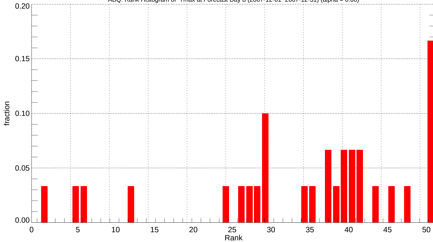
ABQ: Rank Histogram of Tmax at Forecast Day 8 (2007-12-01~2007-12-31) (alpha = 0.00)
