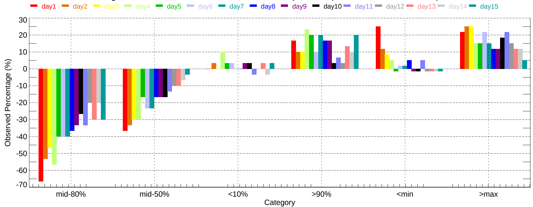
Observed Percentage Deviation of Ensembles - ABI: Max Temperature (2007-12-01~2007-12-31)
