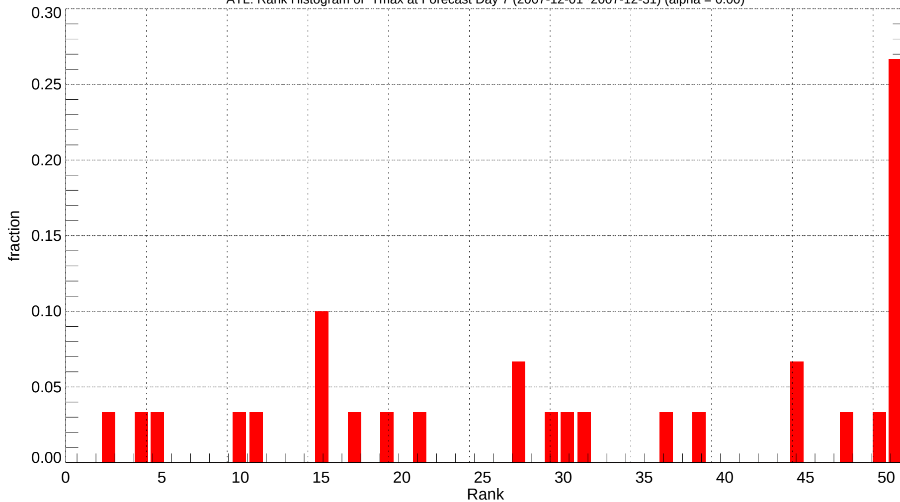
ATL: Rank Histogram of Tmax at Forecast Day 7 (2007-12-01~2007-12-31) (alpha = 0.00)
