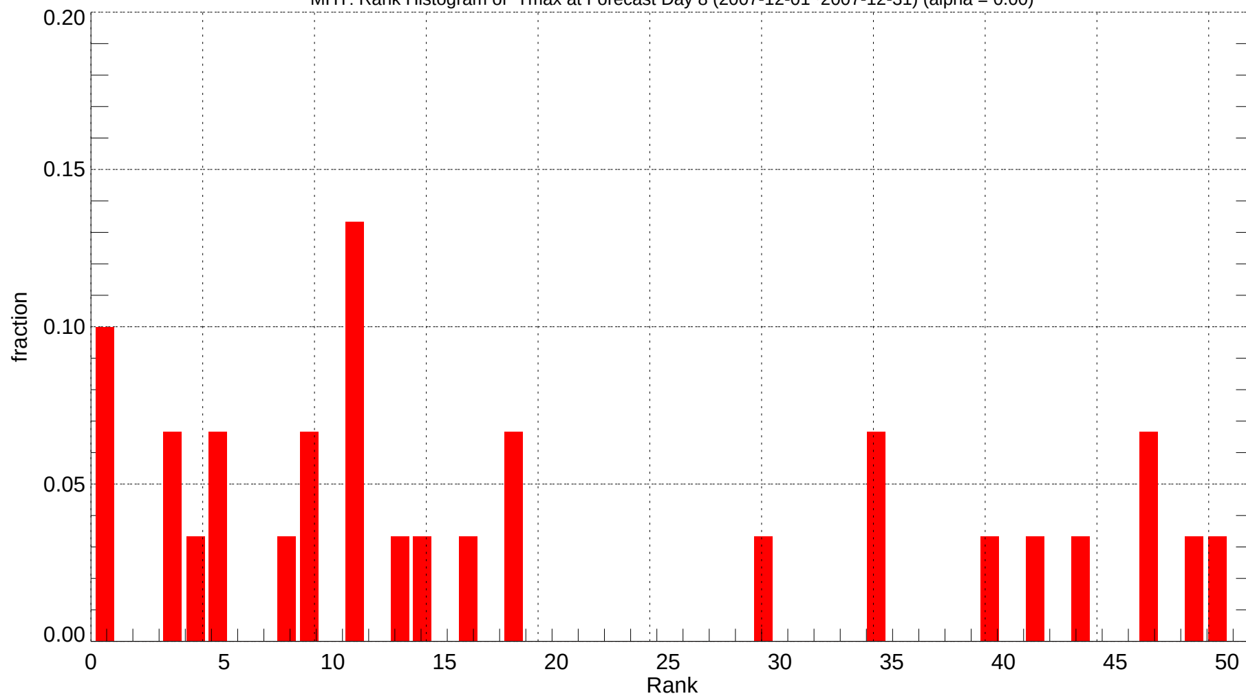
MHT: Rank Histogram of Tmax at Forecast Day 8 (2007-12-01~2007-12-31) (alpha = 0.00)
