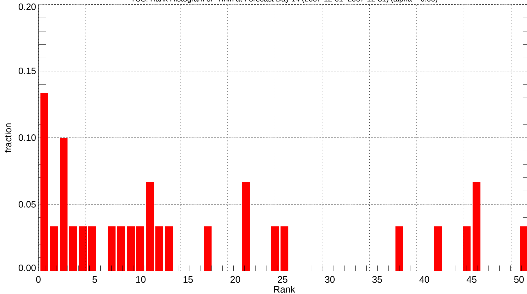
TUS: Rank Histogram of Tmin at Forecast Day 14 (2007-12-01~2007-12-31) (alpha = 0.00)
