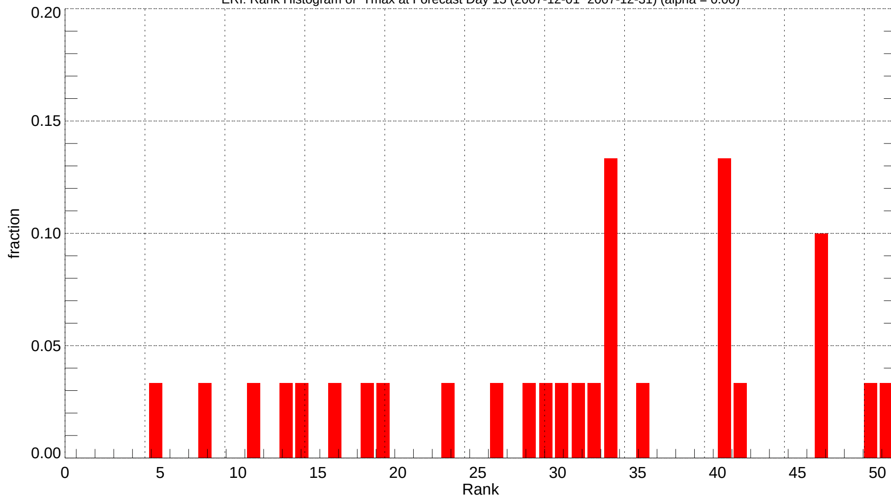
ERI: Rank Histogram of Tmax at Forecast Day 15 (2007-12-01~2007-12-31) (alpha = 0.00)
