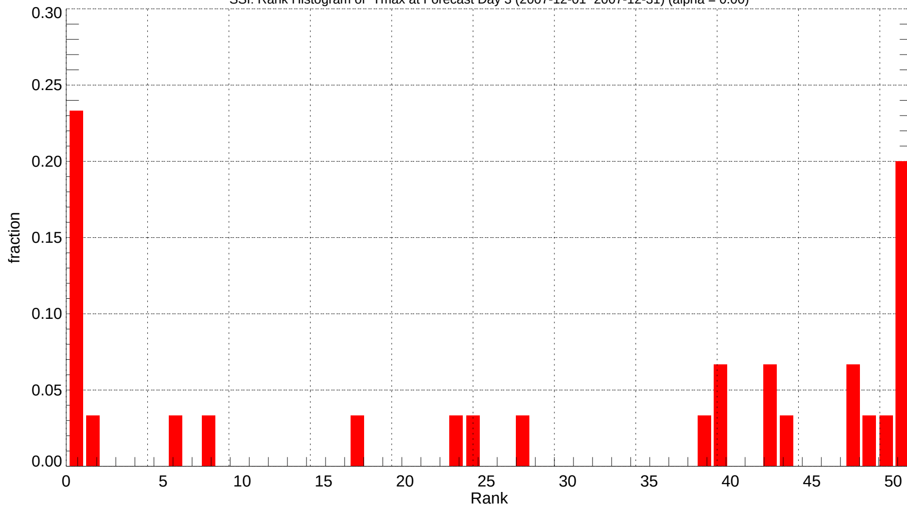
SSI: Rank Histogram of Tmax at Forecast Day 3 (2007-12-01~2007-12-31) (alpha = 0.00)
