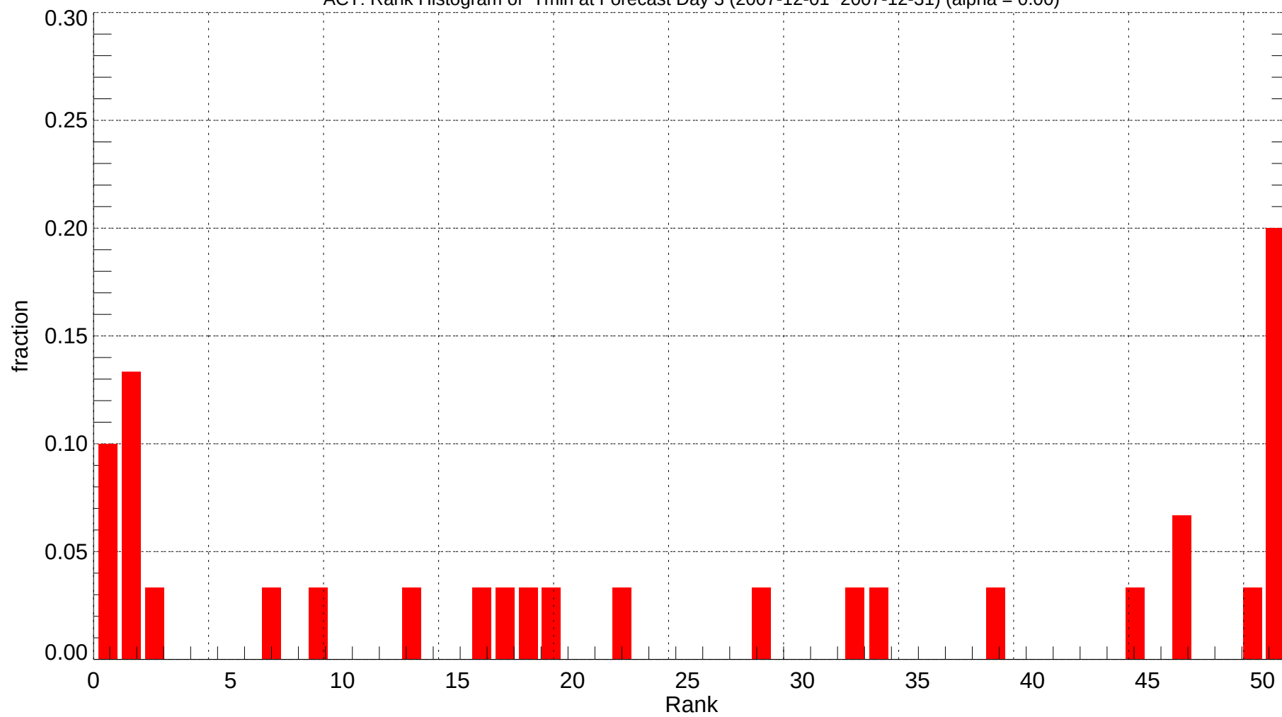
ACT: Rank Histogram of Tmin at Forecast Day 3 (2007-12-01~2007-12-31) (alpha = 0.00)
