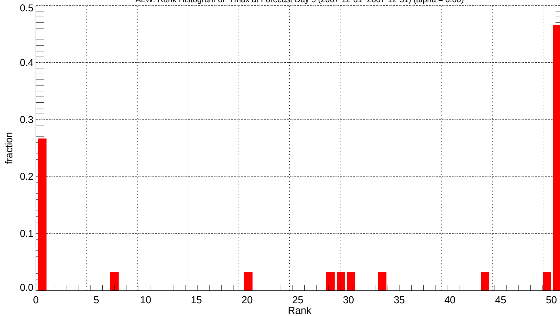
ALW: Rank Histogram of Tmax at Forecast Day 3 (2007-12-01~2007-12-31) (alpha = 0.00)
