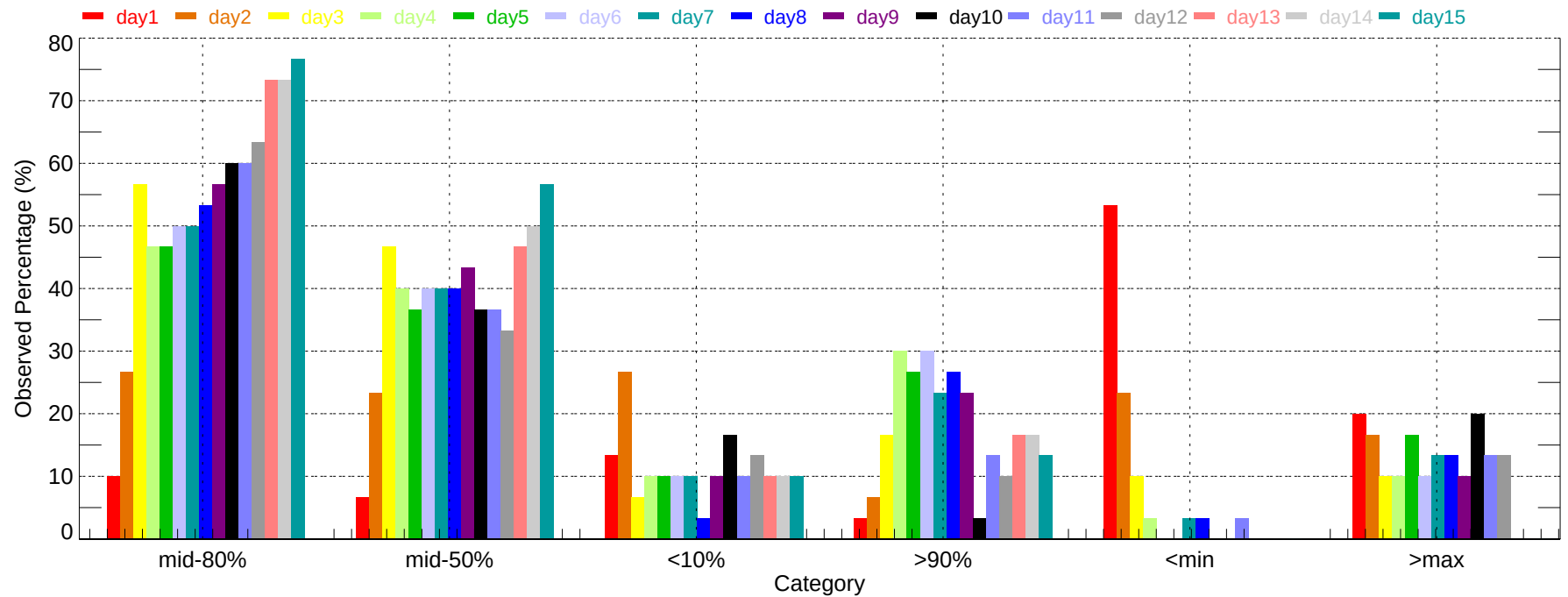
Observed Percentage of Ensembles - OMA: Max Temperature (2007-12-01~2007-12-31)
