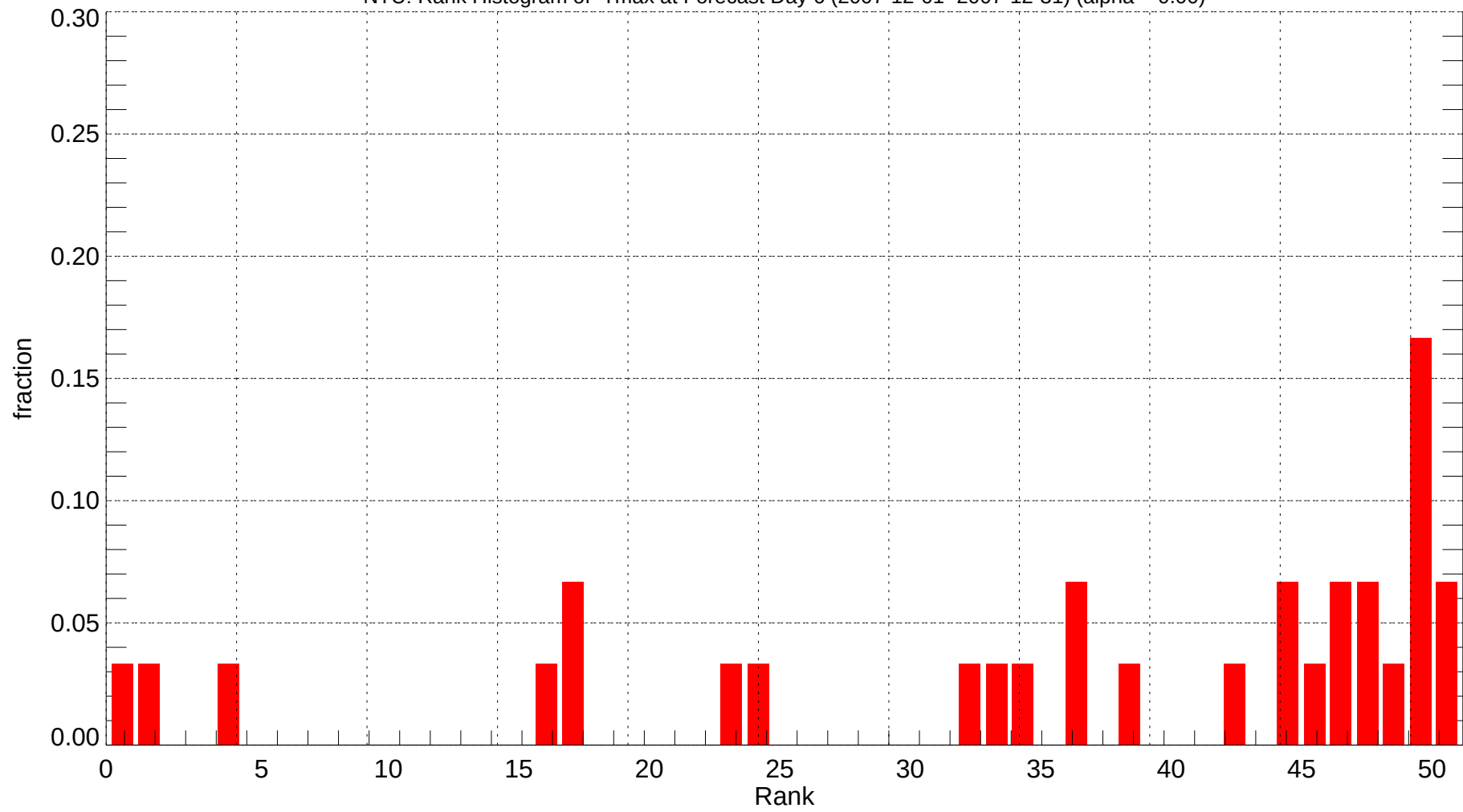
NTU: Rank Histogram of Tmax at Forecast Day 6 (2007-12-01~2007-12-31) (alpha = 0.00)
