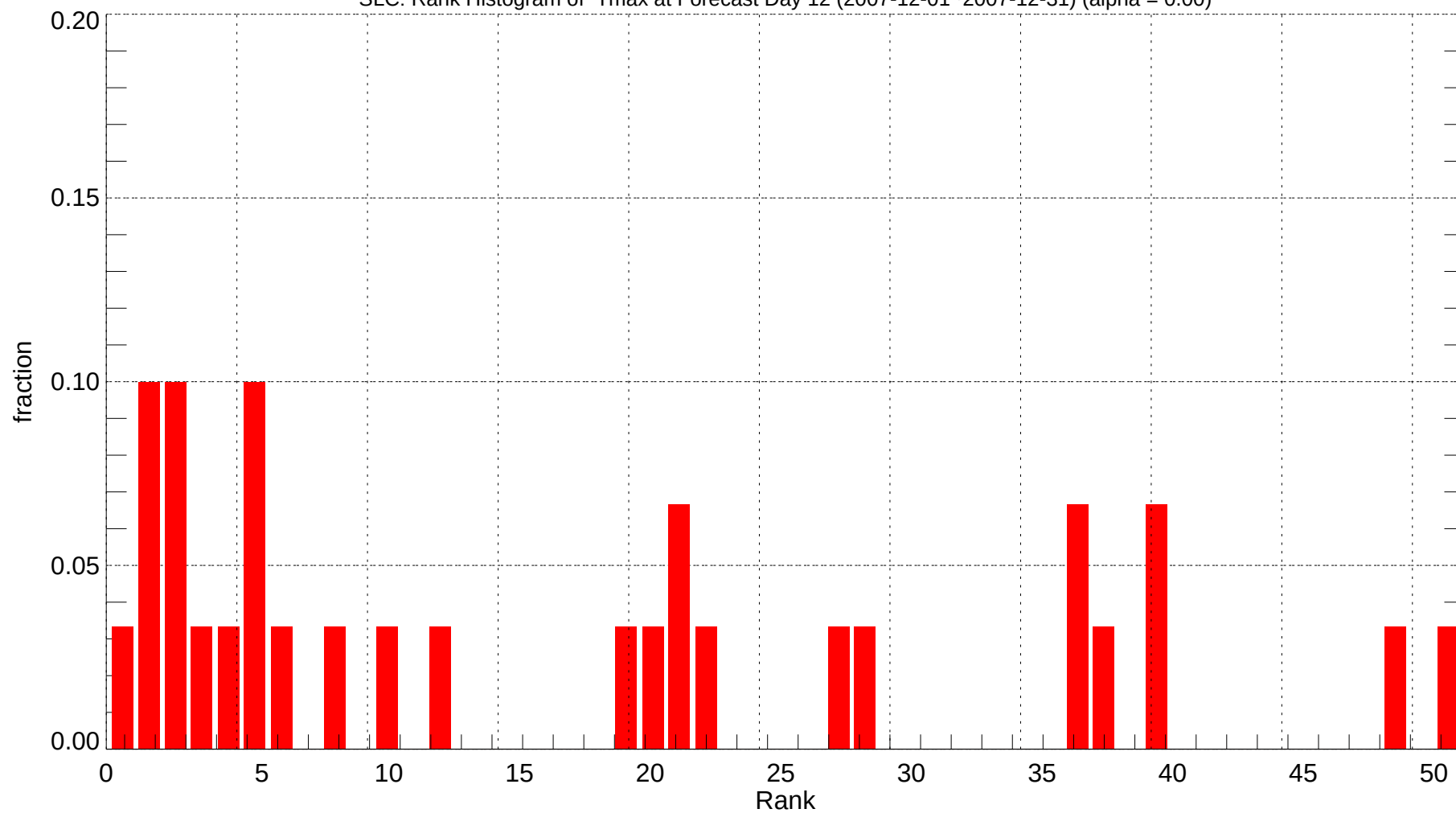
SLC: Rank Histogram of Tmax at Forecast Day 12 (2007-12-01~2007-12-31) (alpha = 0.00)
