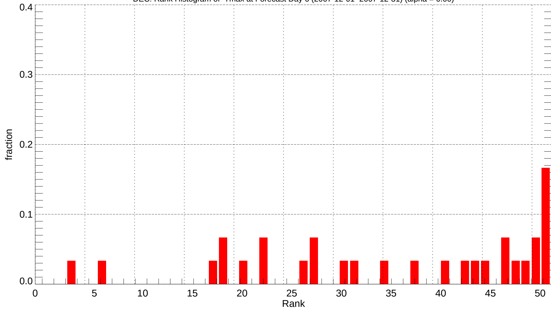
DEC: Rank Histogram of Tmax at Forecast Day 6 (2007-12-01~2007-12-31) (alpha = 0.00)
