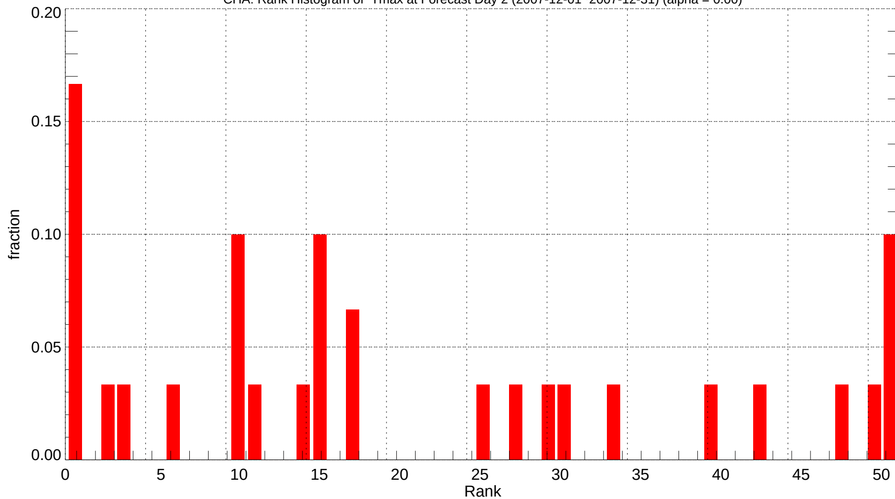
CHA: Rank Histogram of Tmax at Forecast Day 2 (2007-12-01~2007-12-31) (alpha = 0.00)
