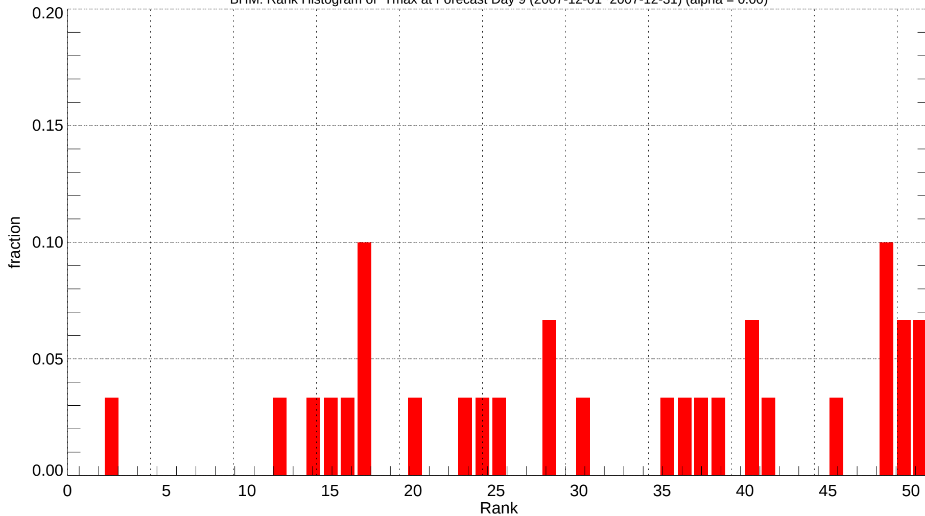
BHM: Rank Histogram of Tmax at Forecast Day 9 (2007-12-01~2007-12-31) (alpha = 0.00)
