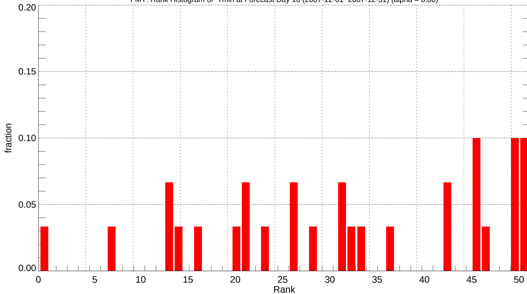
FMY: Rank Histogram of Tmin at Forecast Day 10 (2007-12-01~2007-12-31) (alpha = 0.00)
