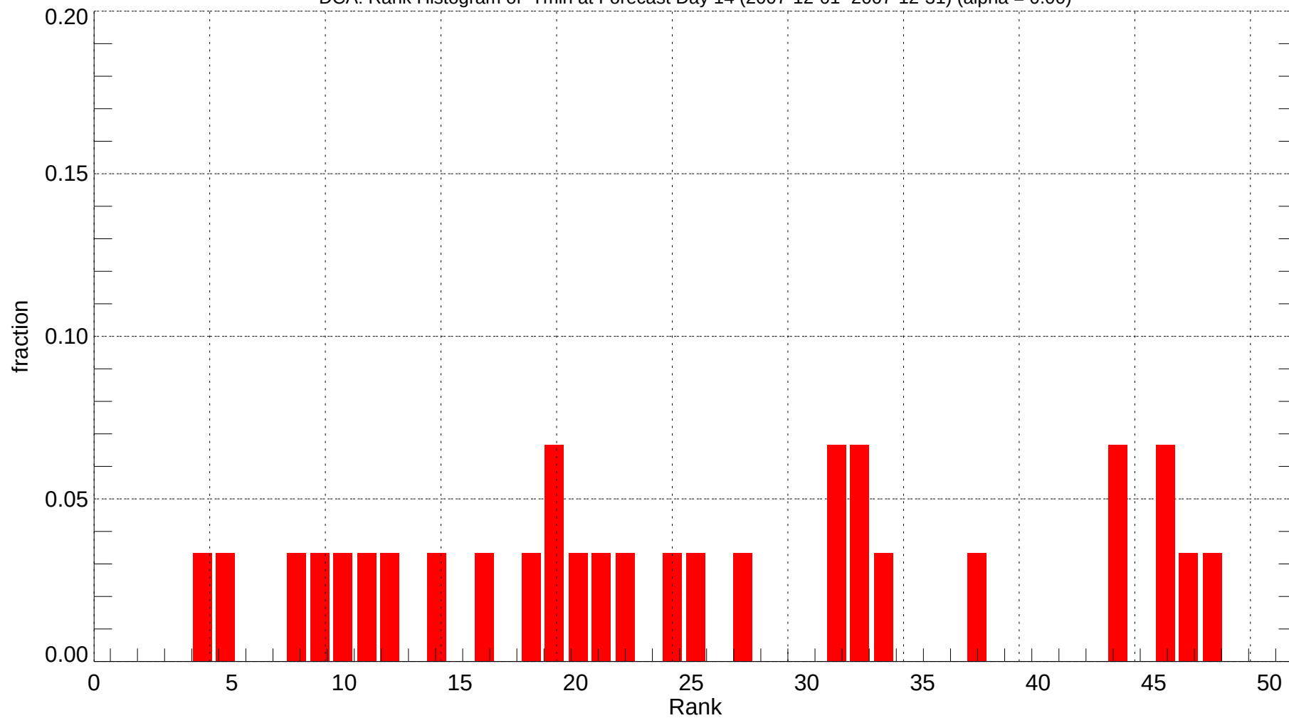
DCA: Rank Histogram of Tmin at Forecast Day 14 (2007-12-01~2007-12-31) (alpha = 0.00)
