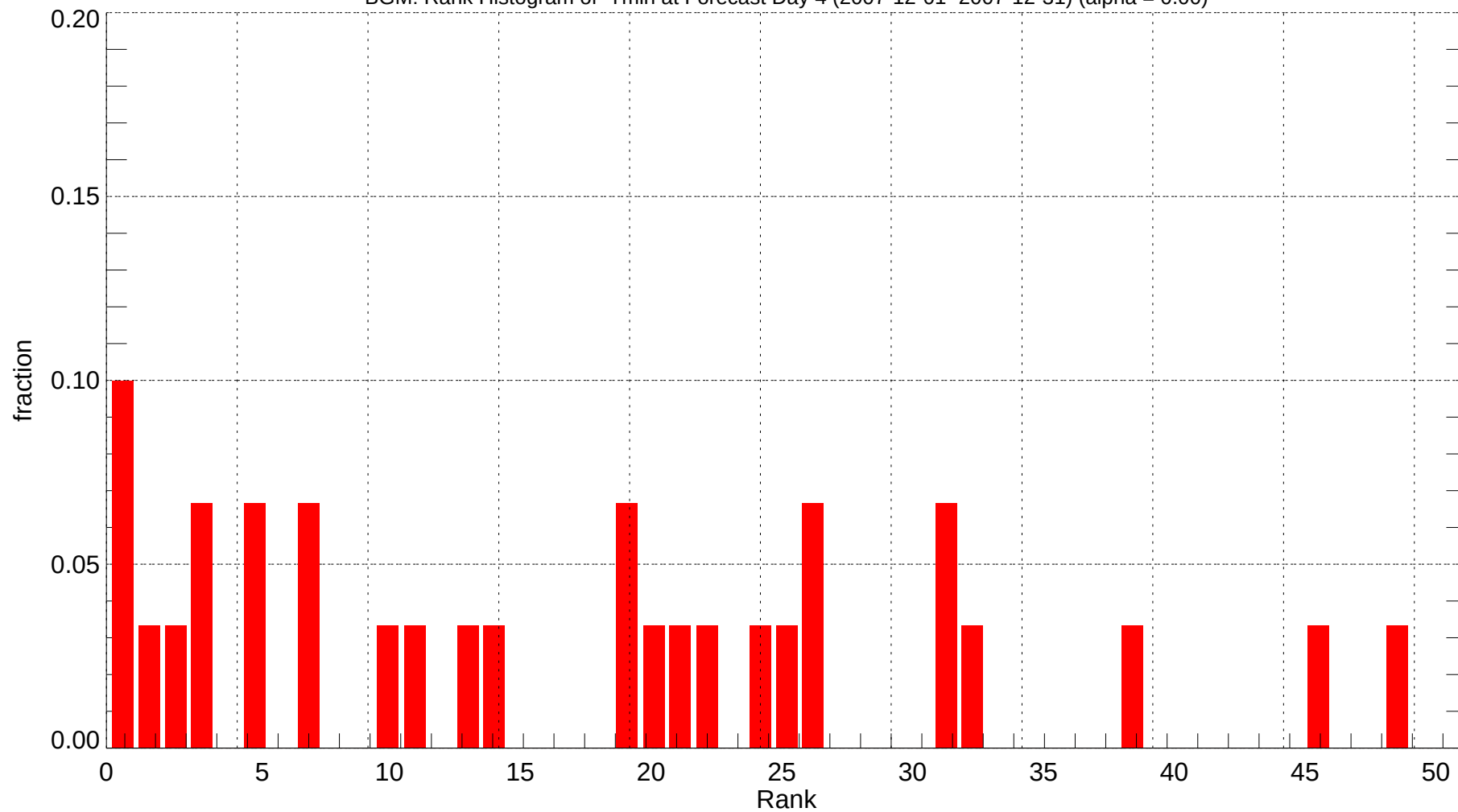
BGM: Rank Histogram of Tmin at Forecast Day 4 (2007-12-01~2007-12-31) (alpha = 0.00)
