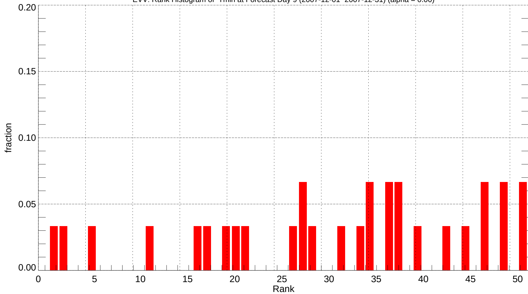
EVV: Rank Histogram of Tmin at Forecast Day 9 (2007-12-01~2007-12-31) (alpha = 0.00)
