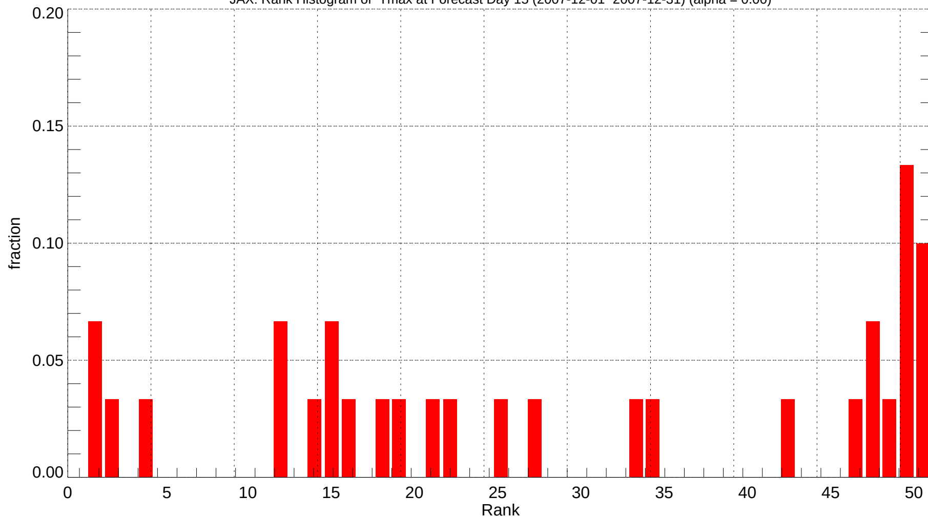
JAX: Rank Histogram of Tmax at Forecast Day 15 (2007-12-01~2007-12-31) (alpha = 0.00)
