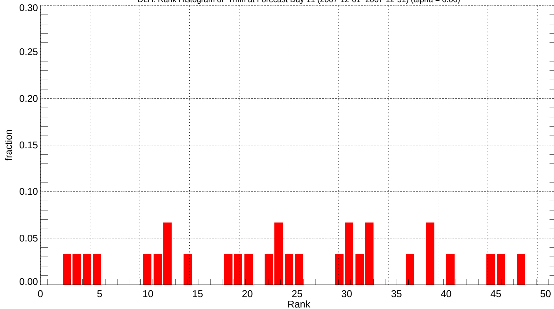
DLH: Rank Histogram of Tmin at Forecast Day 11 (2007-12-01~2007-12-31) (alpha = 0.00)
