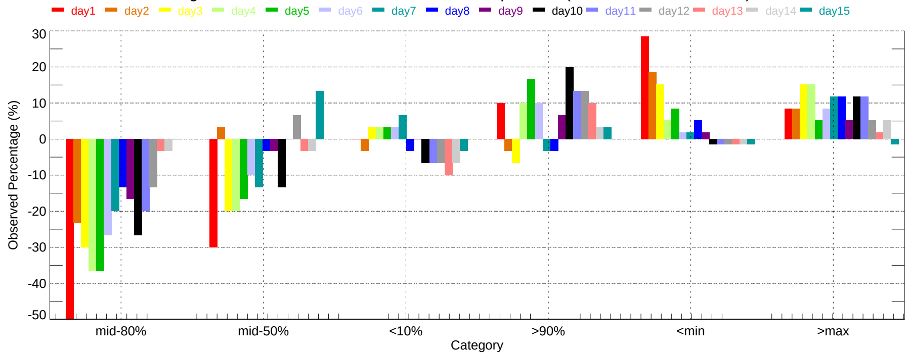
Observed Percentage Deviation of Ensembles - SEA: Min Temperature (2007-12-01~2007-12-31)
