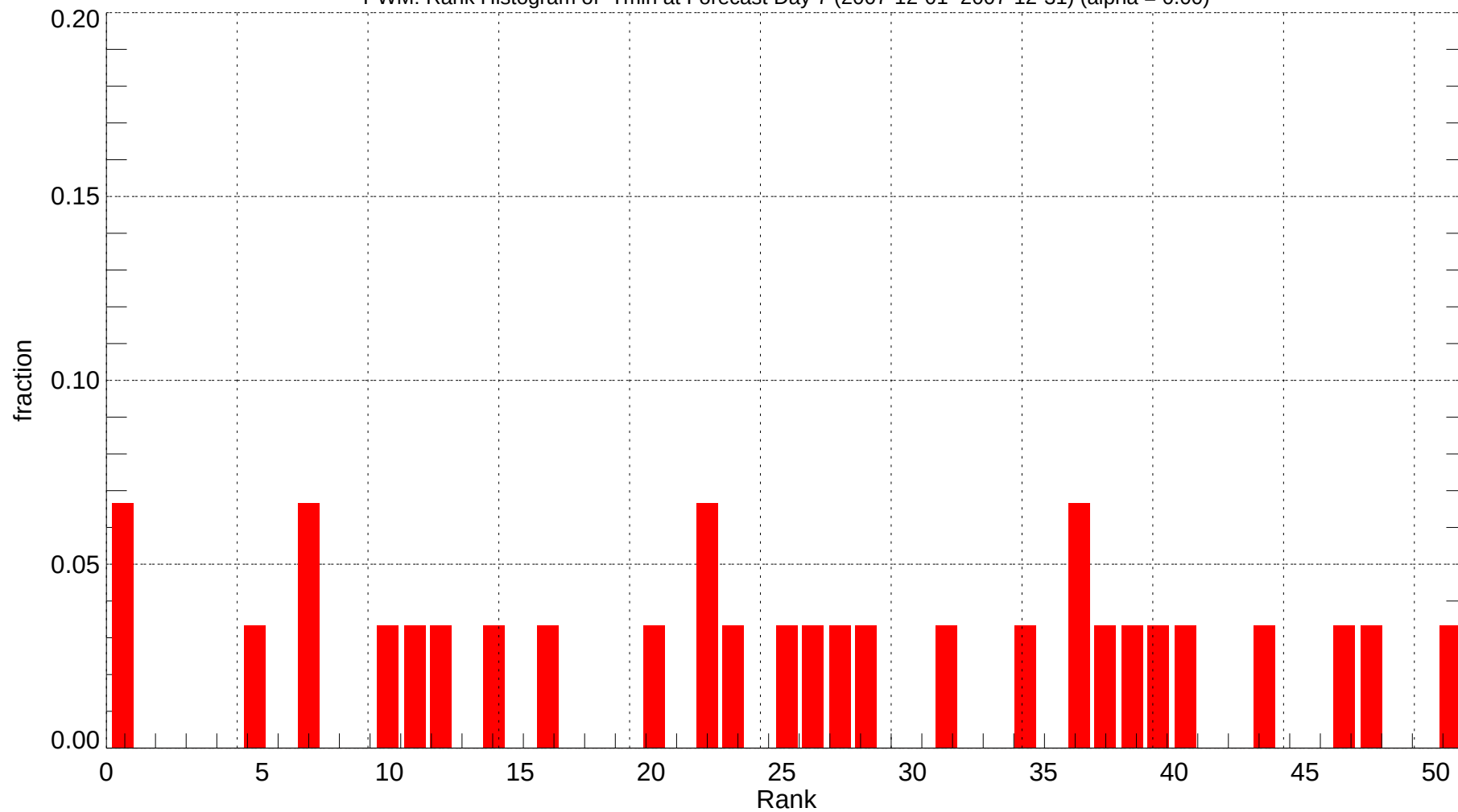
PWM: Rank Histogram of Tmin at Forecast Day 7 (2007-12-01~2007-12-31) (alpha = 0.00)
