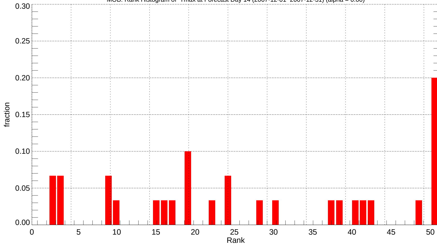
MOB: Rank Histogram of Tmax at Forecast Day 14 (2007-12-01~2007-12-31) (alpha = 0.00)
