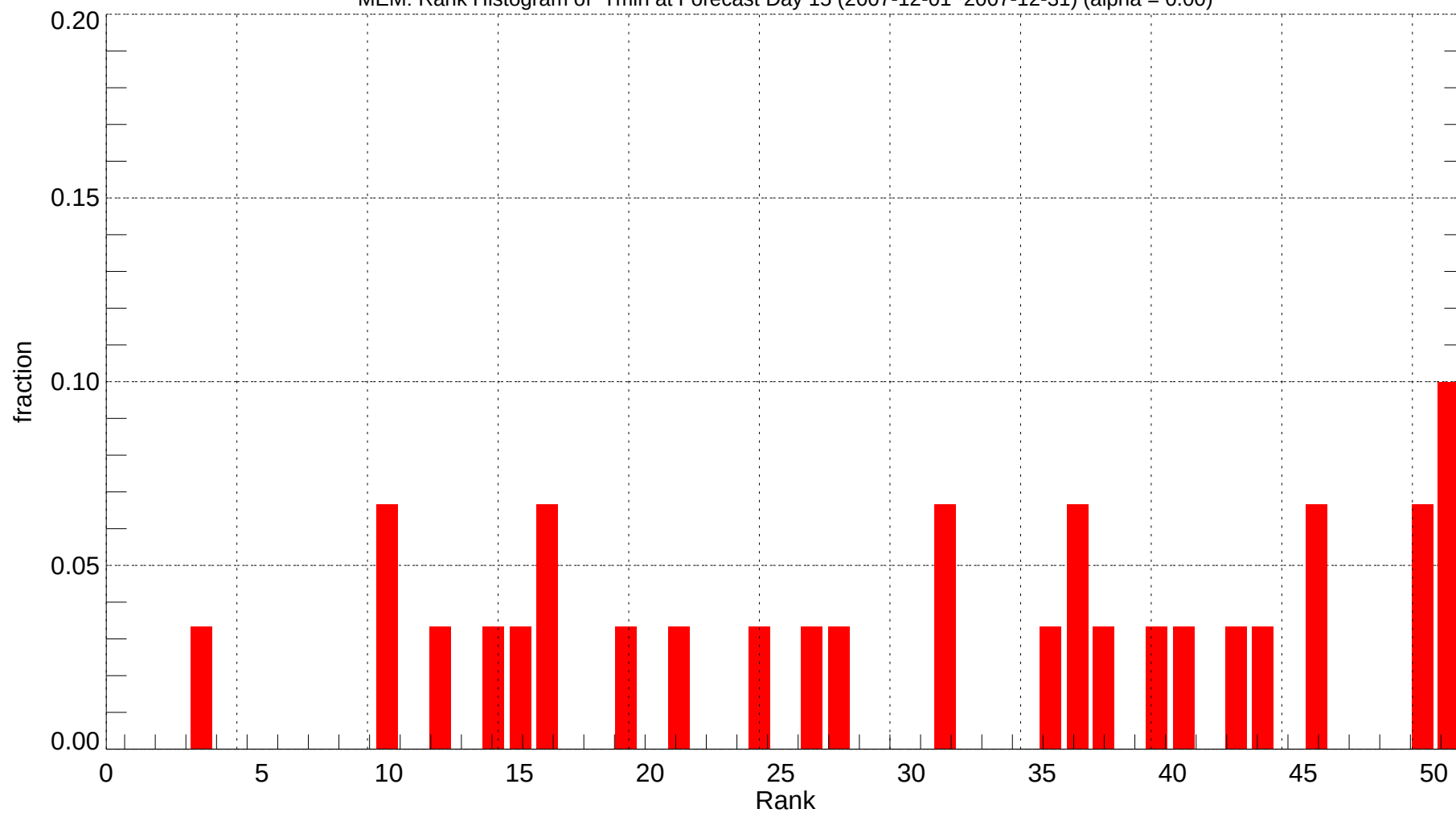
MEM: Rank Histogram of Tmin at Forecast Day 15 (2007-12-01~2007-12-31) (alpha = 0.00)
