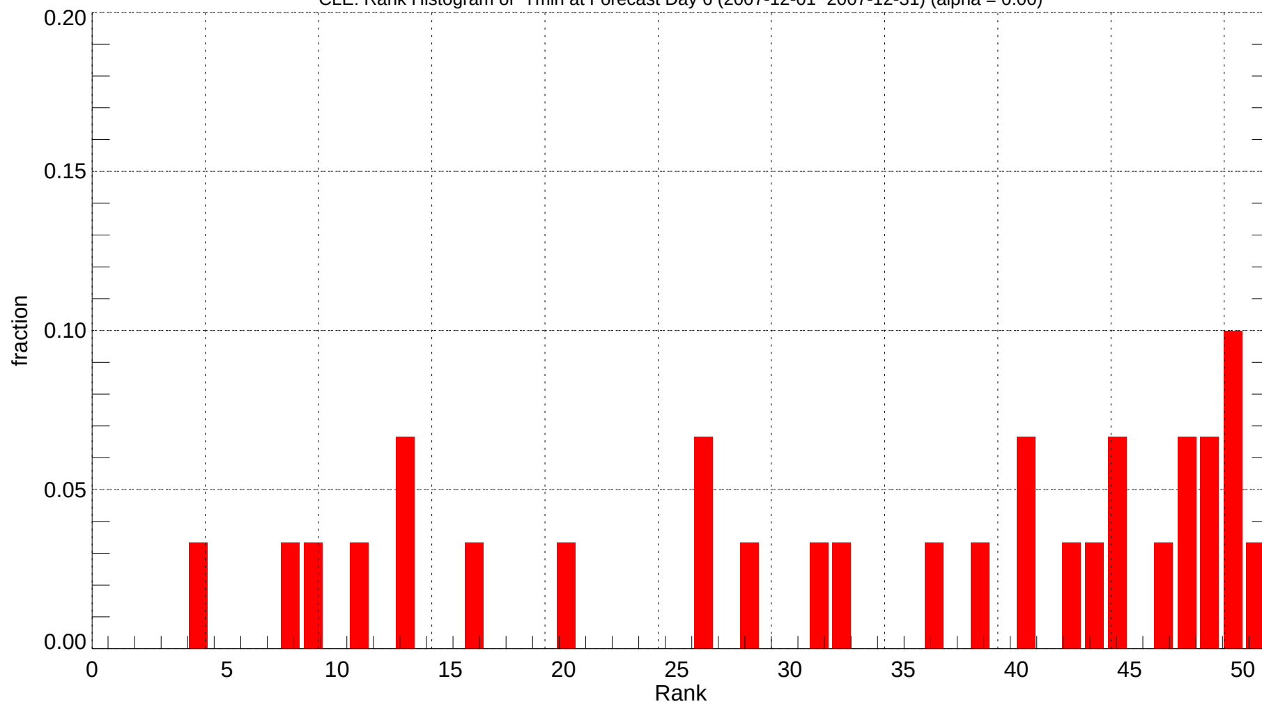
CLE: Rank Histogram of Tmin at Forecast Day 6 (2007-12-01~2007-12-31) (alpha = 0.00)
