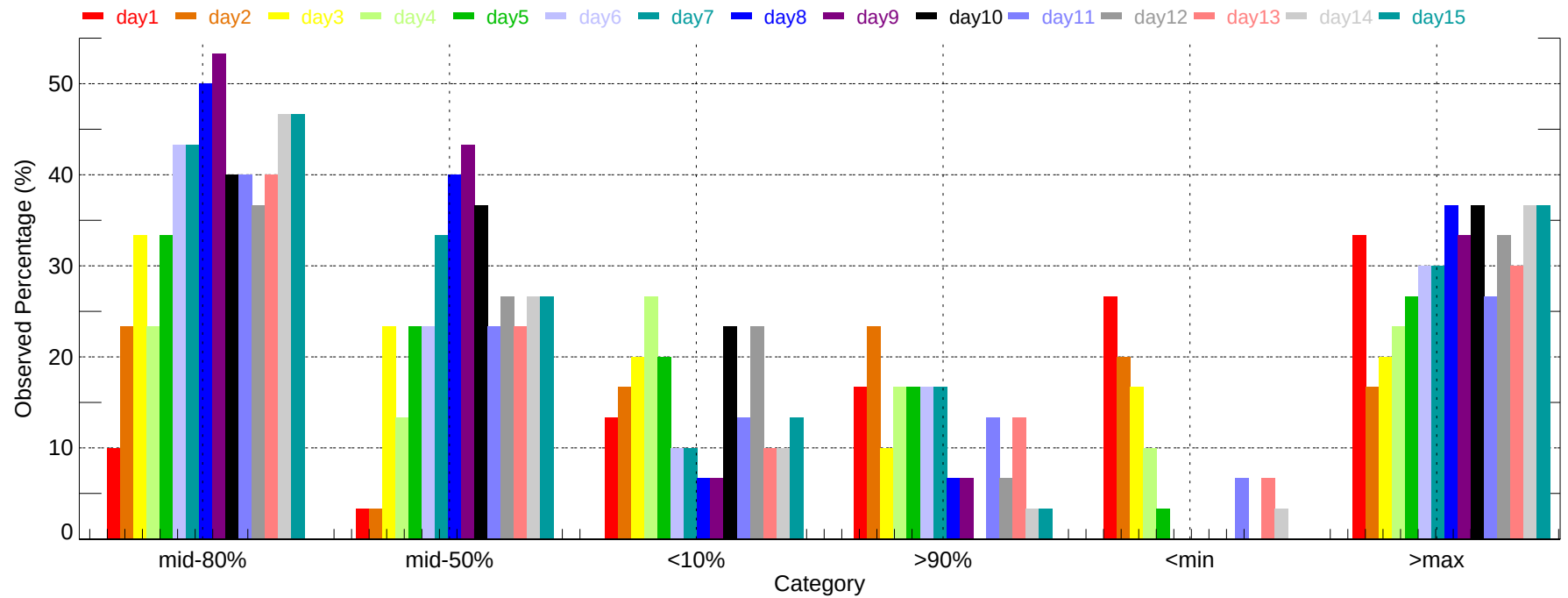
Observed Percentage of Ensembles - MSY: Max Temperature (2007-12-01~2007-12-31)
