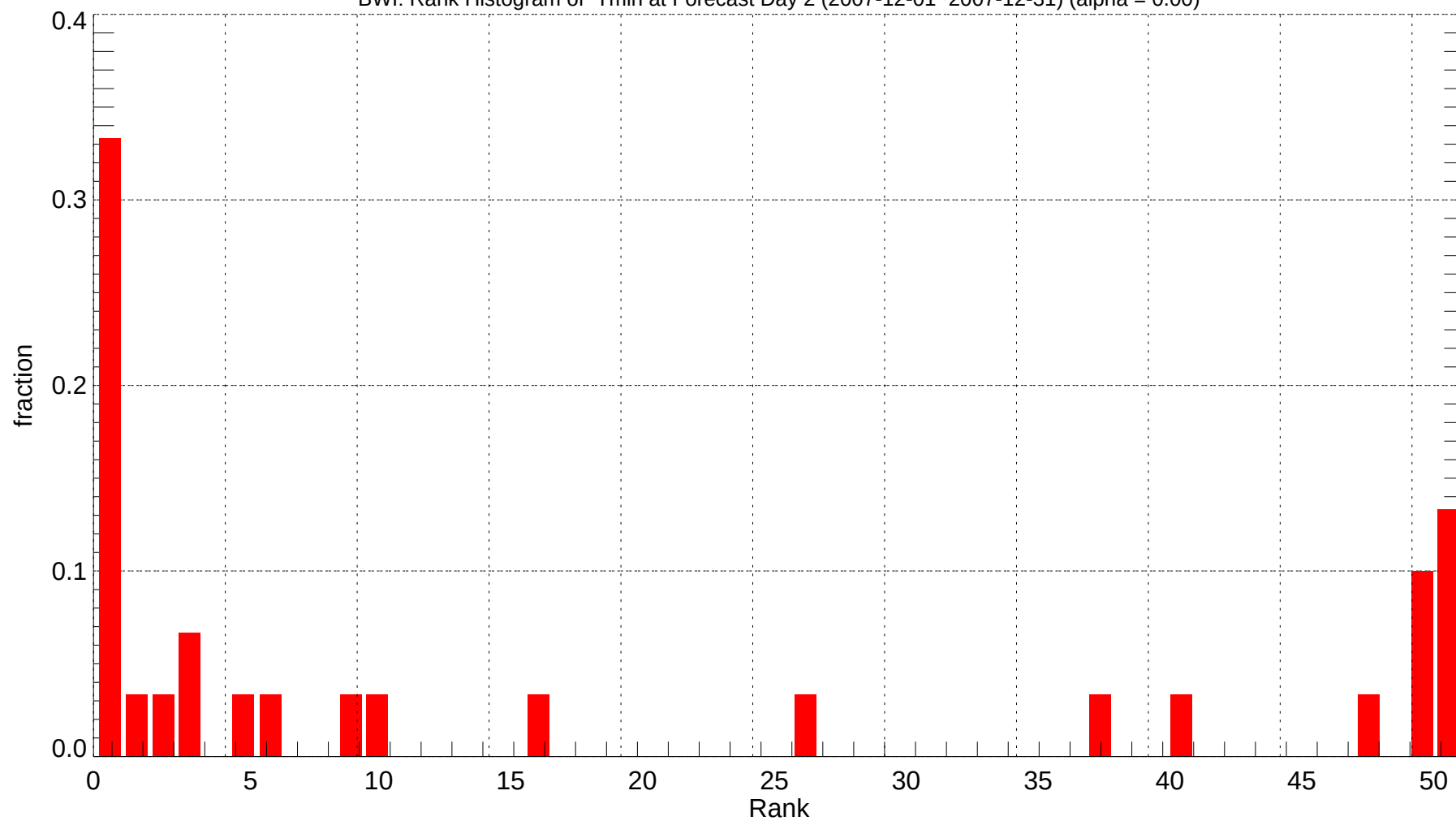
BWI: Rank Histogram of Tmin at Forecast Day 2 (2007-12-01~2007-12-31) (alpha = 0.00)
