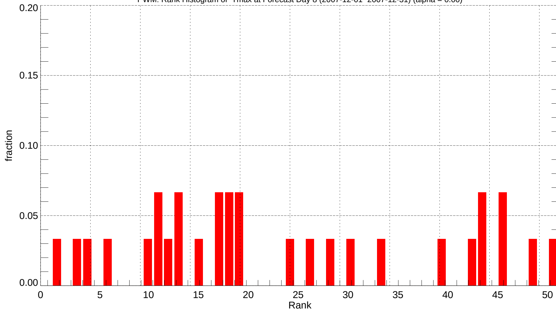
PWM: Rank Histogram of Tmax at Forecast Day 8 (2007-12-01~2007-12-31) (alpha = 0.00)
