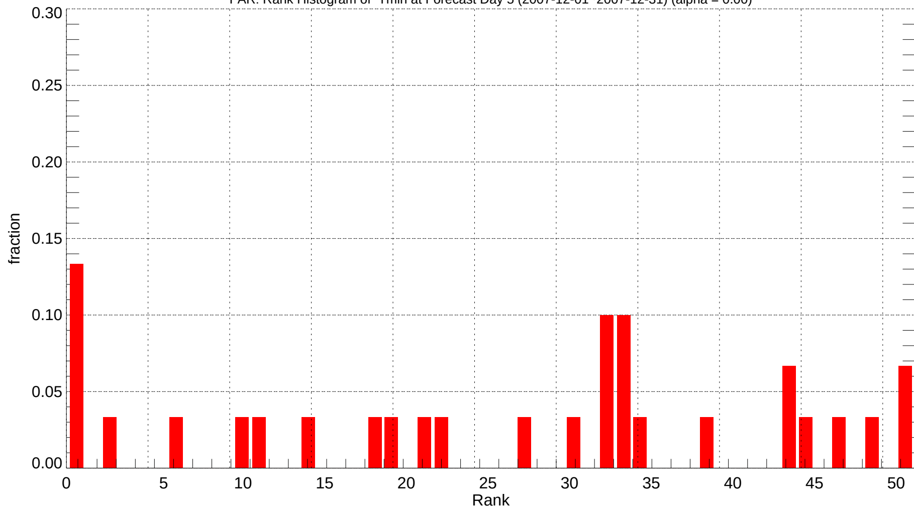
FAR: Rank Histogram of Tmin at Forecast Day 5 (2007-12-01~2007-12-31) (alpha = 0.00)
