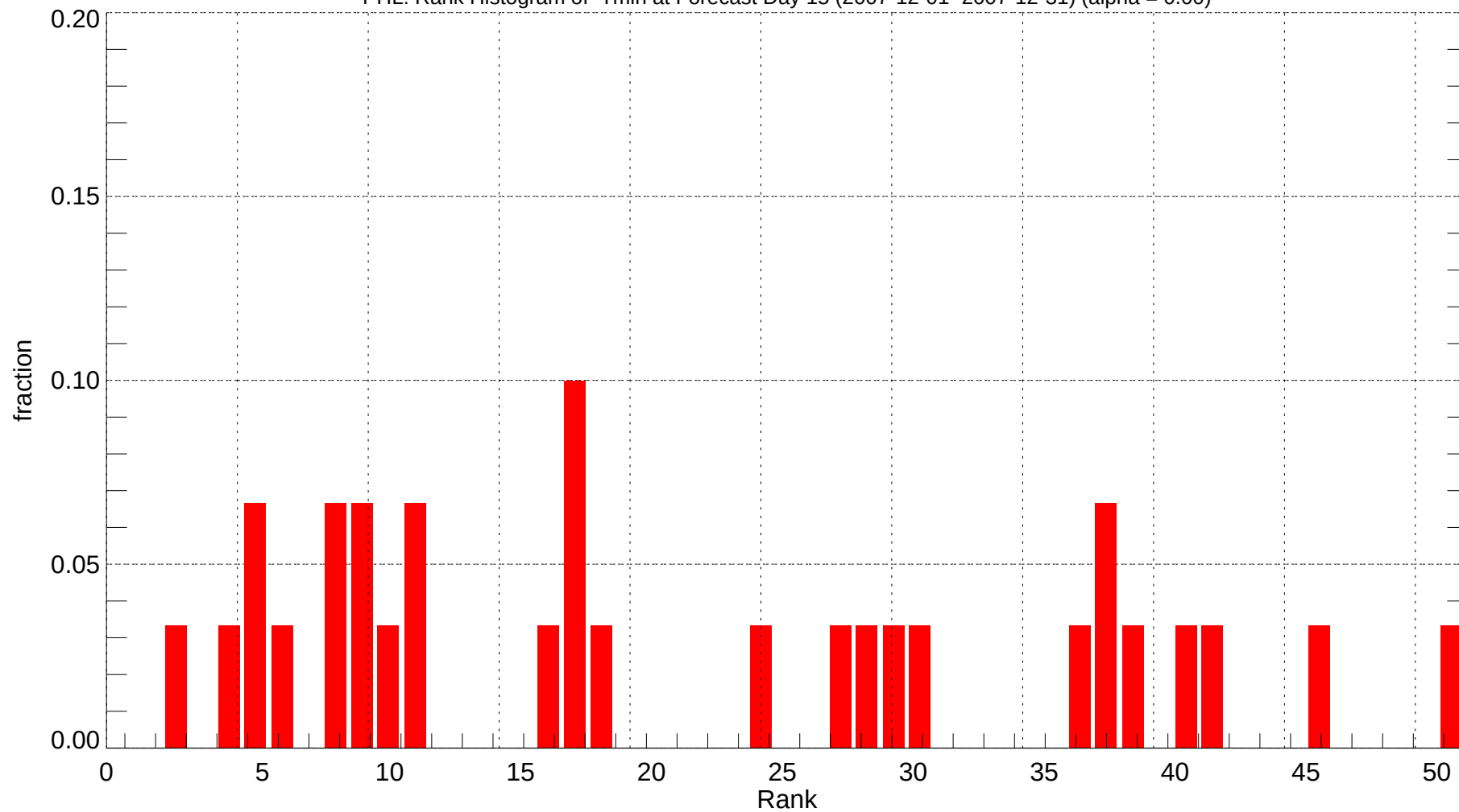
PHL: Rank Histogram of Tmin at Forecast Day 15 (2007-12-01~2007-12-31) (alpha = 0.00)
