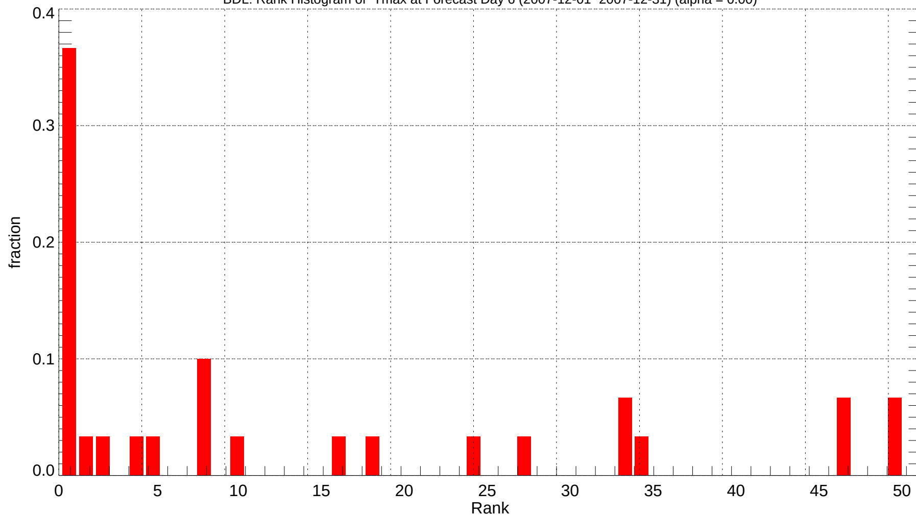
BDL: Rank Histogram of Tmax at Forecast Day 6 (2007-12-01~2007-12-31) (alpha = 0.00)
