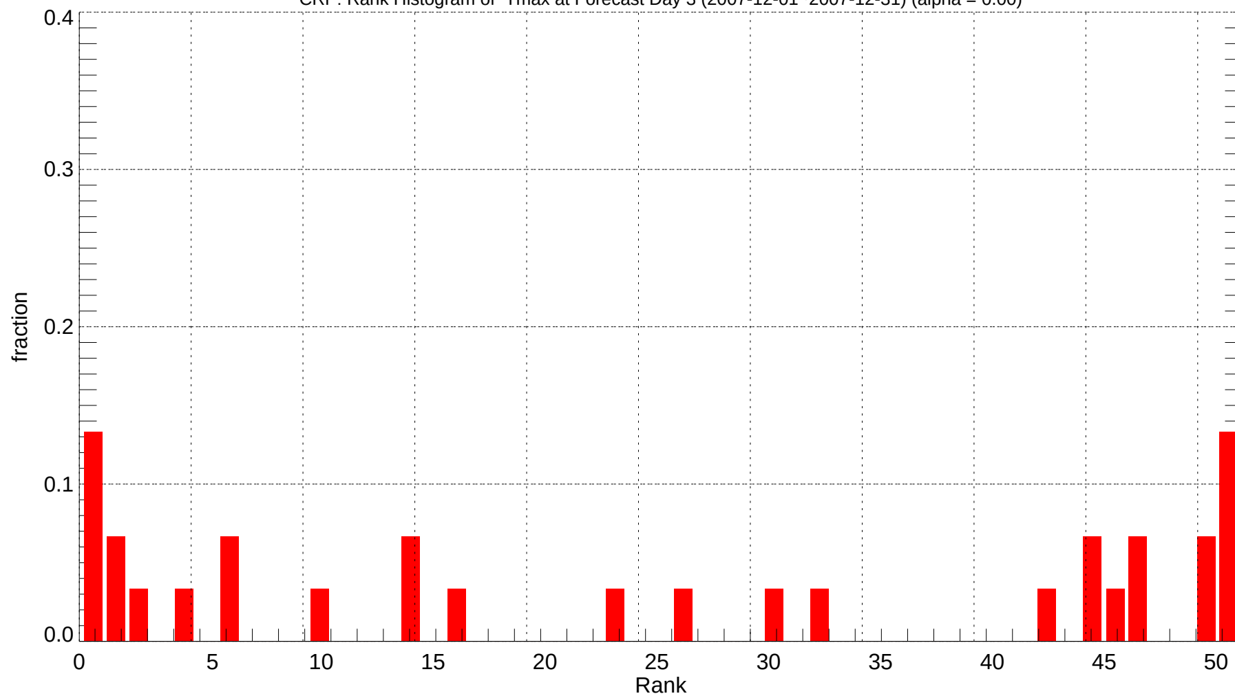
CRP: Rank Histogram of Tmax at Forecast Day 3 (2007-12-01~2007-12-31) (alpha = 0.00)
