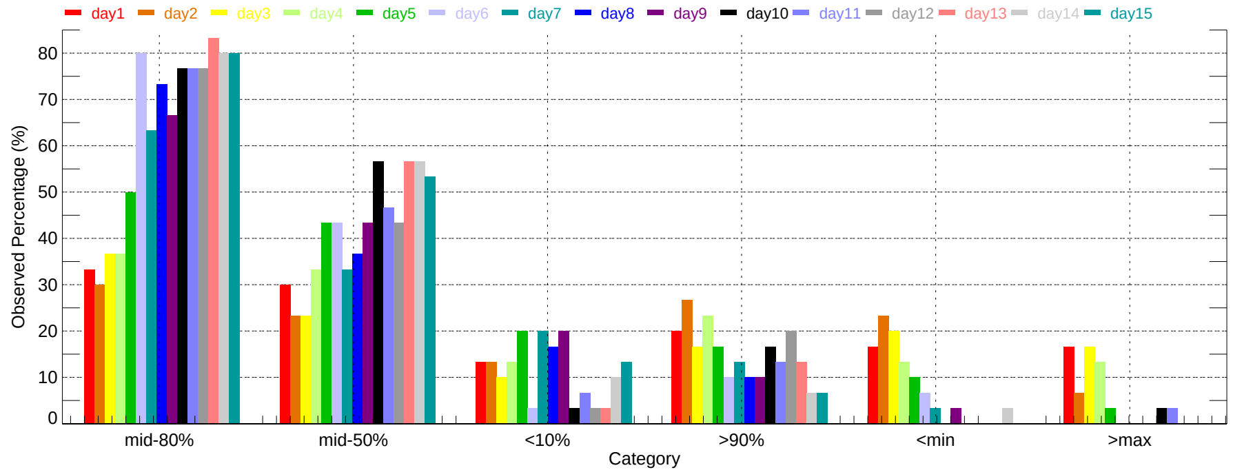
Observed Percentage of Ensembles - WJF: Min Temperature (2007-12-01~2007-12-31)
