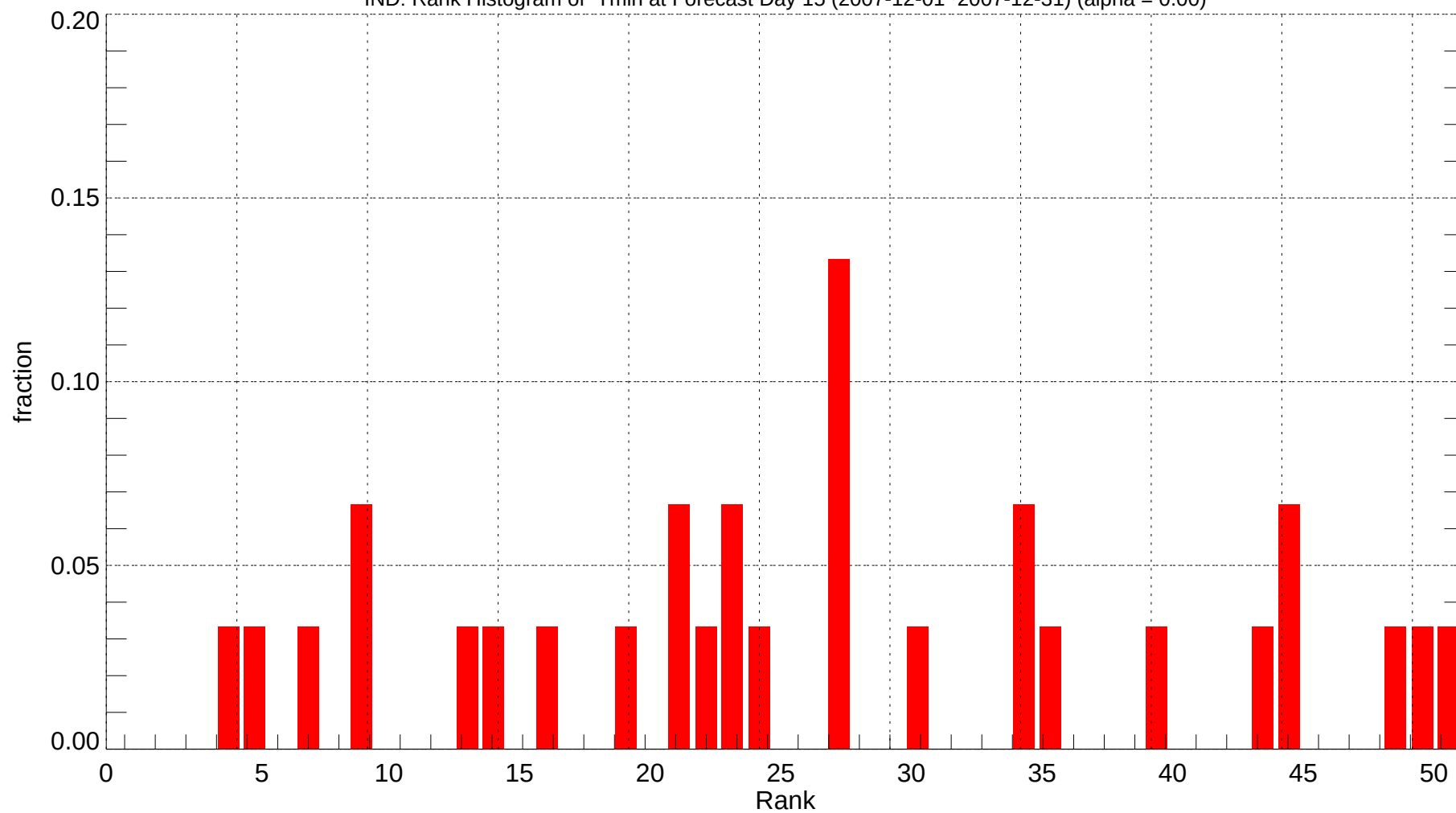
IND: Rank Histogram of Tmin at Forecast Day 15 (2007-12-01~2007-12-31) (alpha = 0.00)
