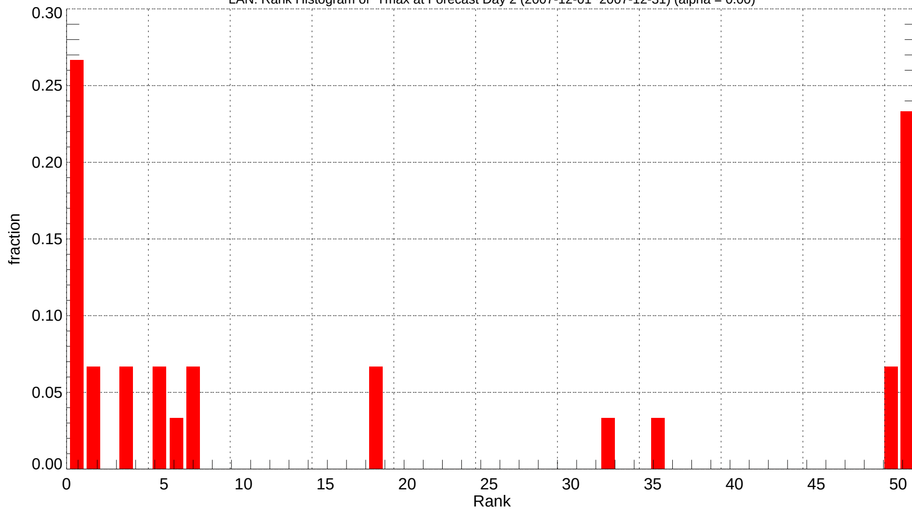
LAN: Rank Histogram of Tmax at Forecast Day 2 (2007-12-01~2007-12-31) (alpha = 0.00)
