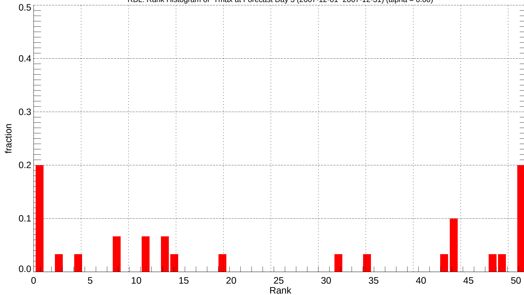
RBL: Rank Histogram of Tmax at Forecast Day 3 (2007-12-01~2007-12-31) (alpha = 0.00)
