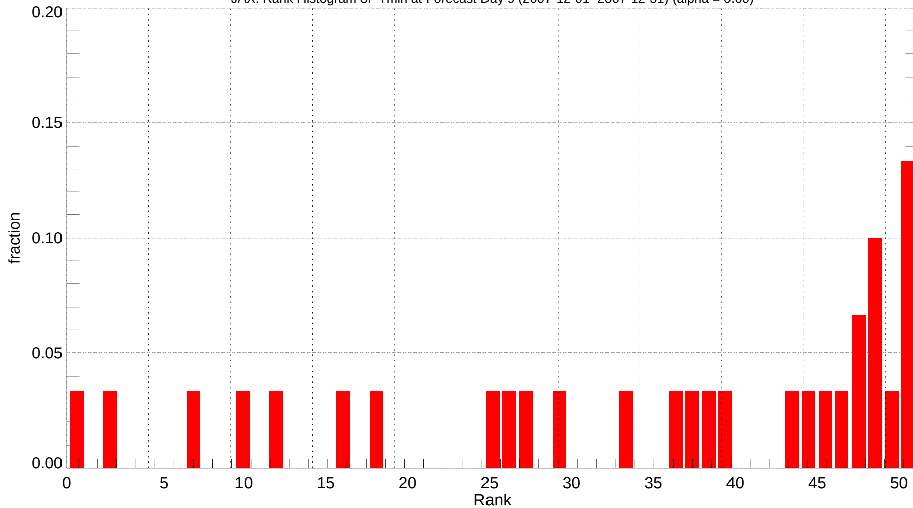
JAX: Rank Histogram of Tmin at Forecast Day 9 (2007-12-01~2007-12-31) (alpha = 0.00)
