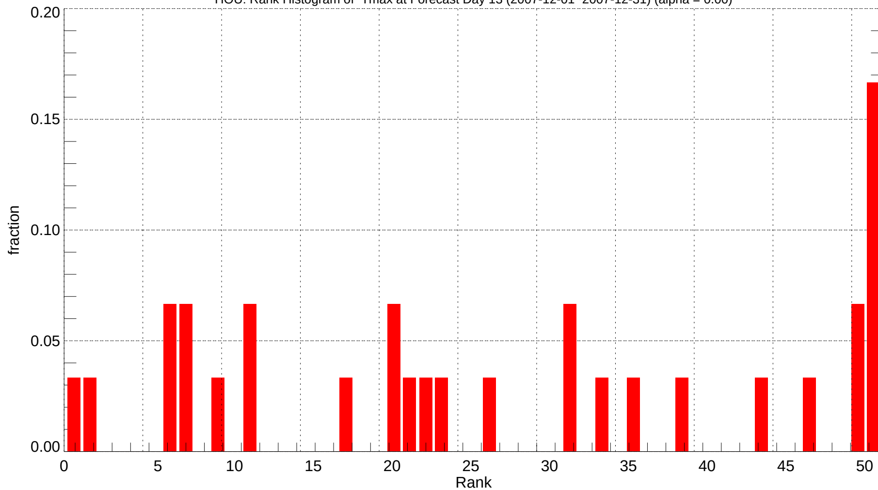
HOU: Rank Histogram of Tmax at Forecast Day 13 (2007-12-01~2007-12-31) (alpha = 0.00)
