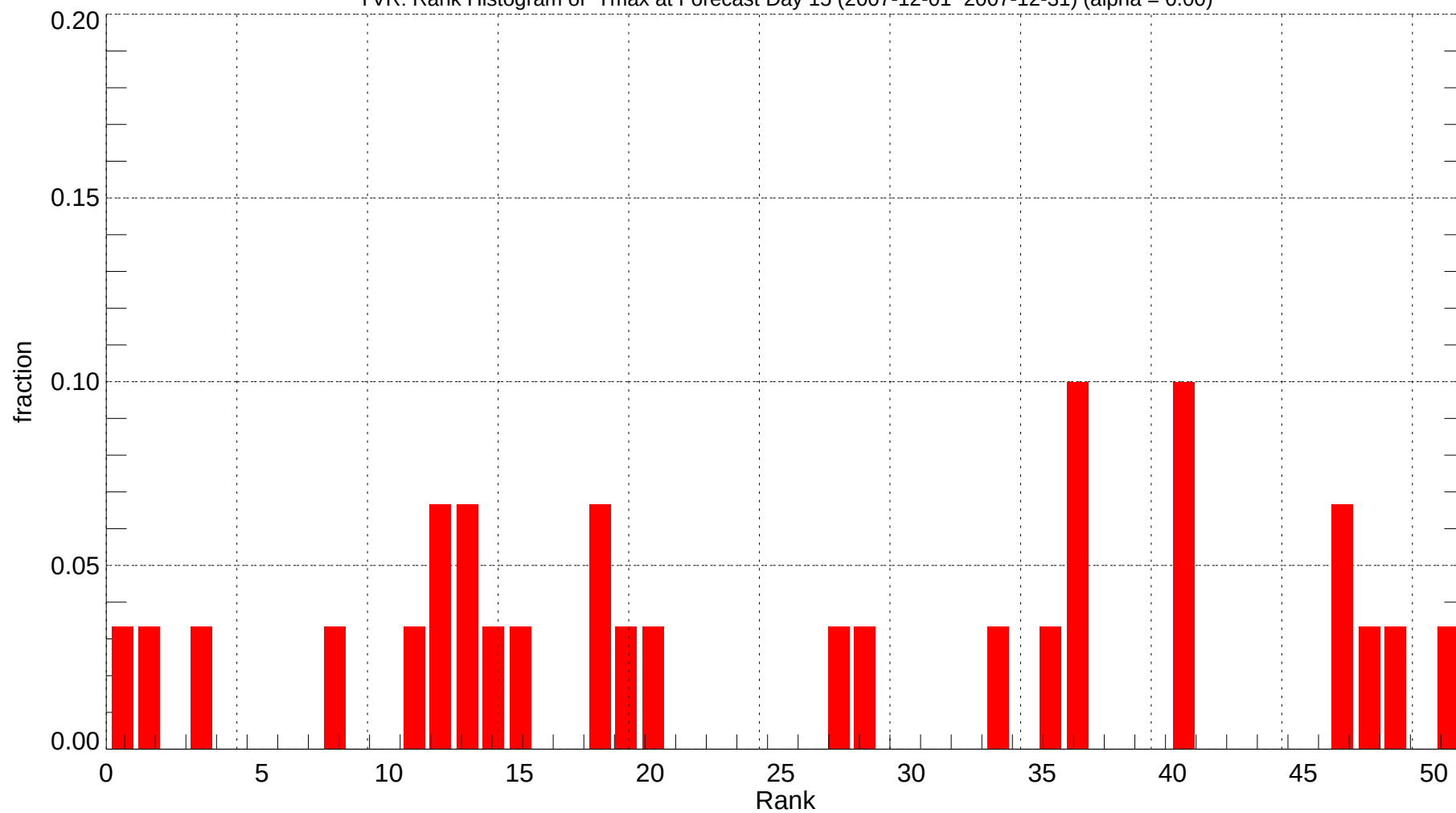
YVR: Rank Histogram of Tmax at Forecast Day 15 (2007-12-01~2007-12-31) (alpha = 0.00)
