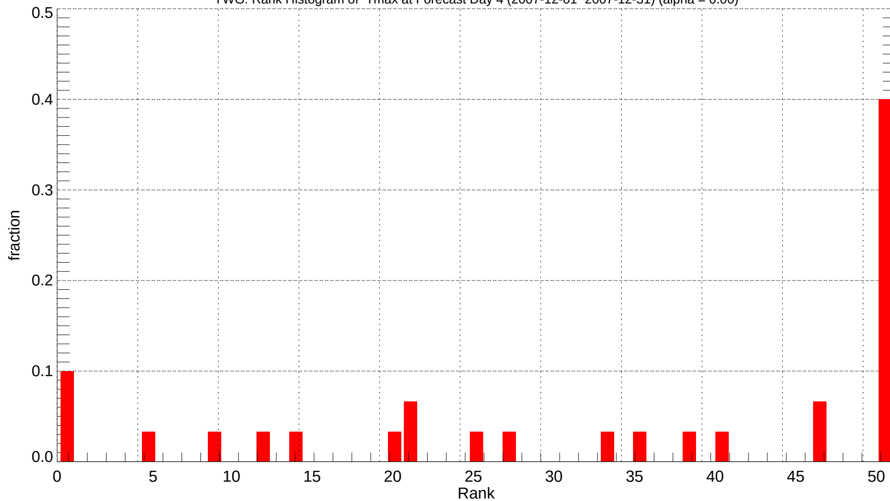
YWG: Rank Histogram of Tmax at Forecast Day 4 (2007-12-01~2007-12-31) (alpha = 0.00)
