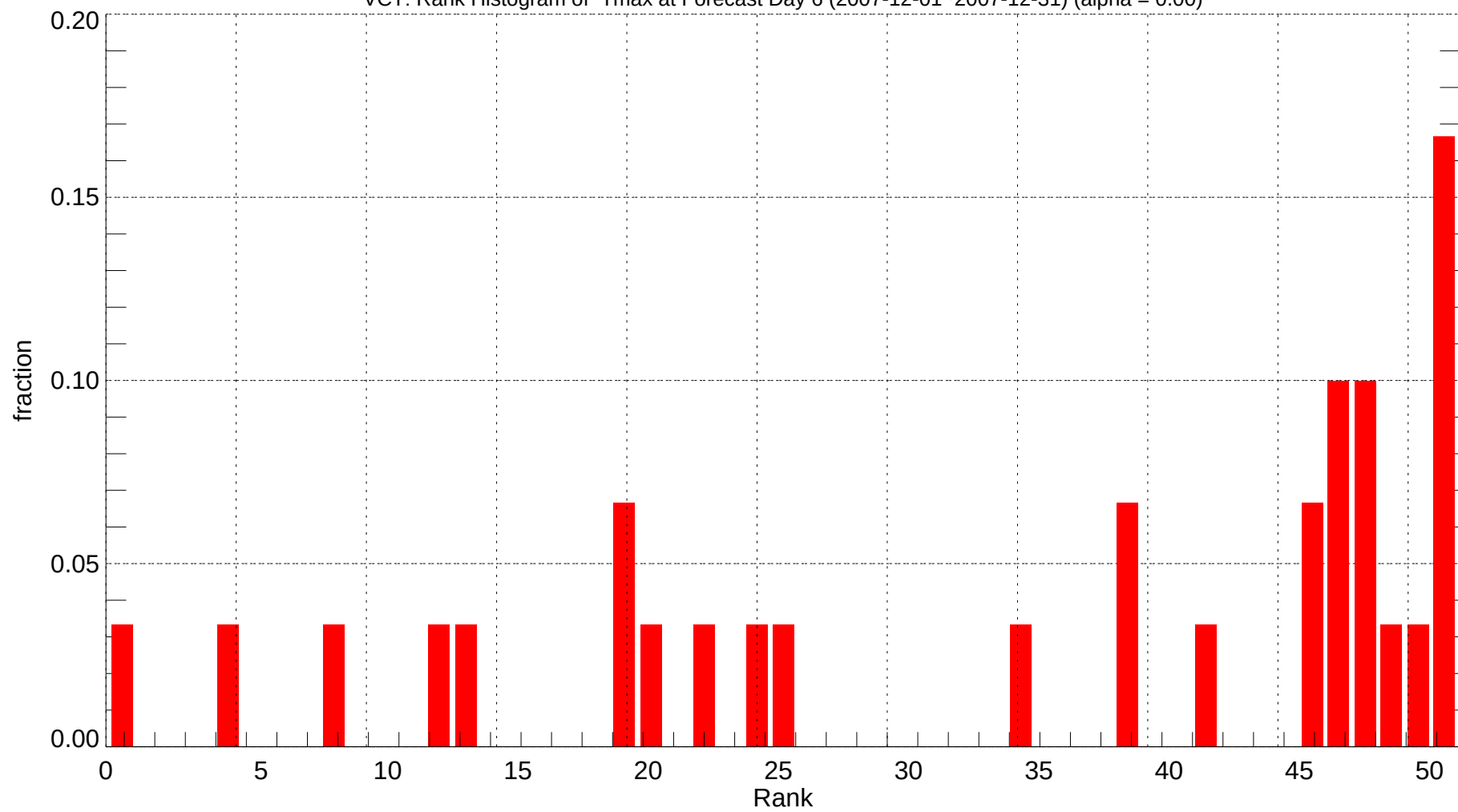
VCT: Rank Histogram of Tmax at Forecast Day 6 (2007-12-01~2007-12-31) (alpha = 0.00)
