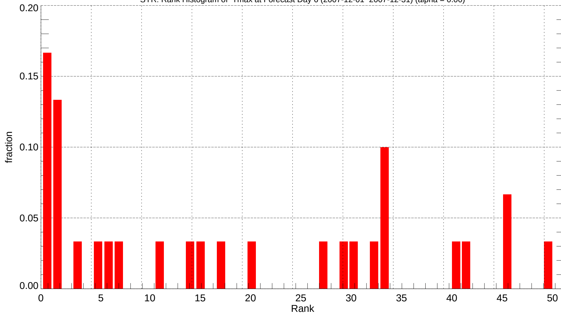
SYR: Rank Histogram of Tmax at Forecast Day 6 (2007-12-01~2007-12-31) (alpha = 0.00)
