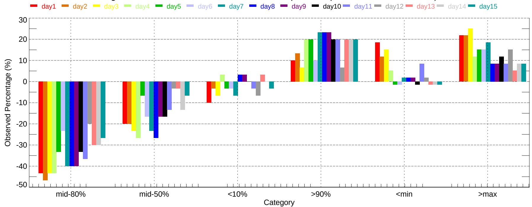
Observed Percentage Deviation of Ensembles - SJT: Min Temperature (2007-12-01~2007-12-31)
