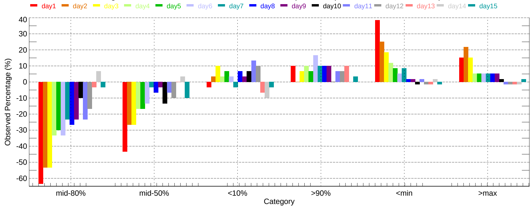
Observed Percentage Deviation of Ensembles - LNS: Max Temperature (2007-12-01~2007-12-31)
