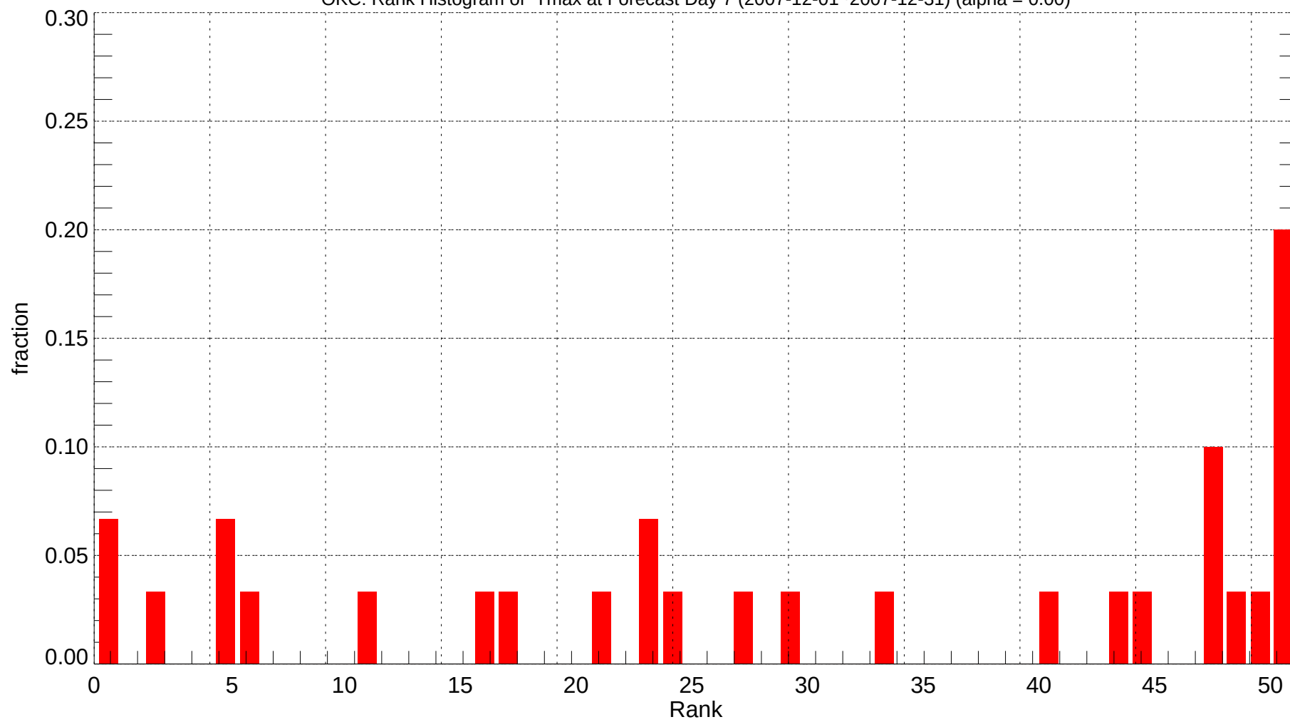
OKC: Rank Histogram of Tmax at Forecast Day 7 (2007-12-01~2007-12-31) (alpha = 0.00)
