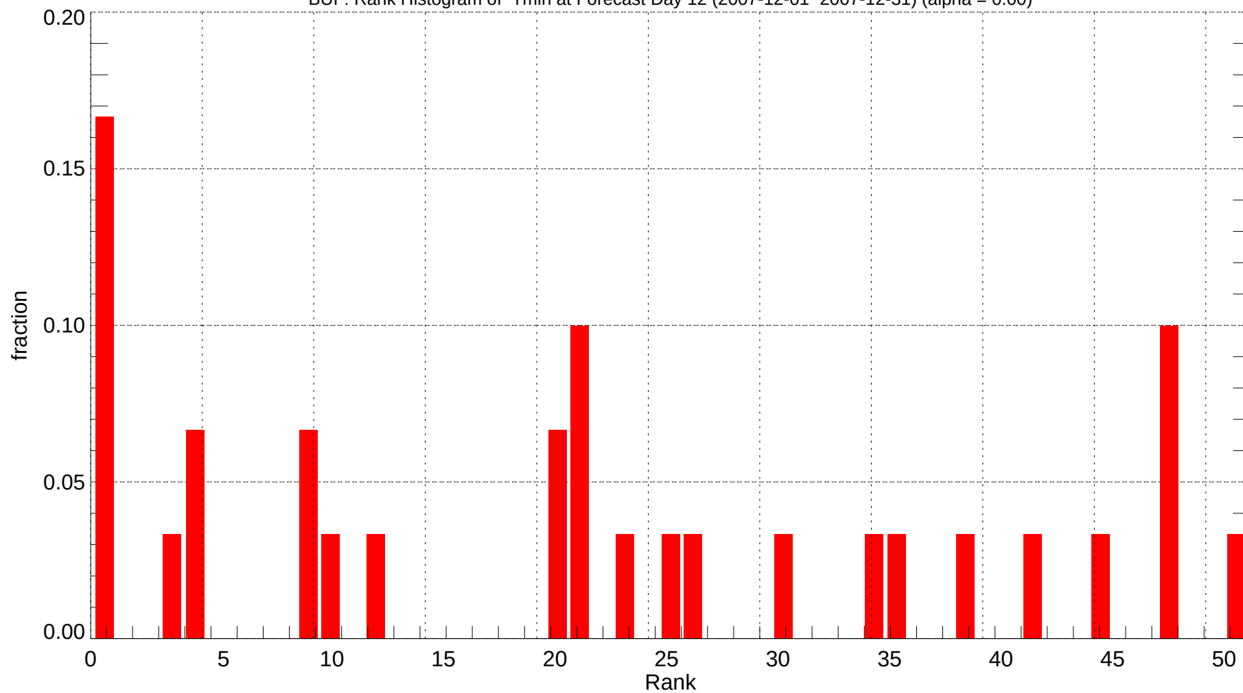
BUF: Rank Histogram of Tmin at Forecast Day 12 (2007-12-01~2007-12-31) (alpha = 0.00)
