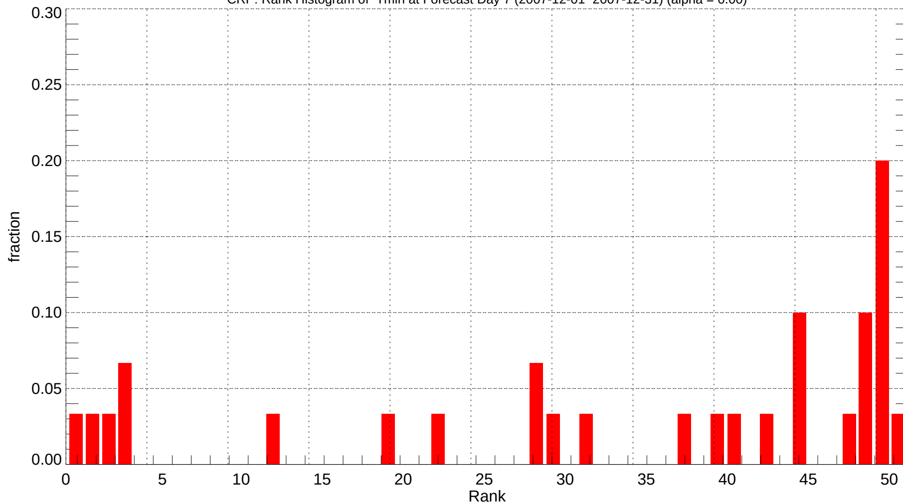
CRP: Rank Histogram of Tmin at Forecast Day 7 (2007-12-01~2007-12-31) (alpha = 0.00)
