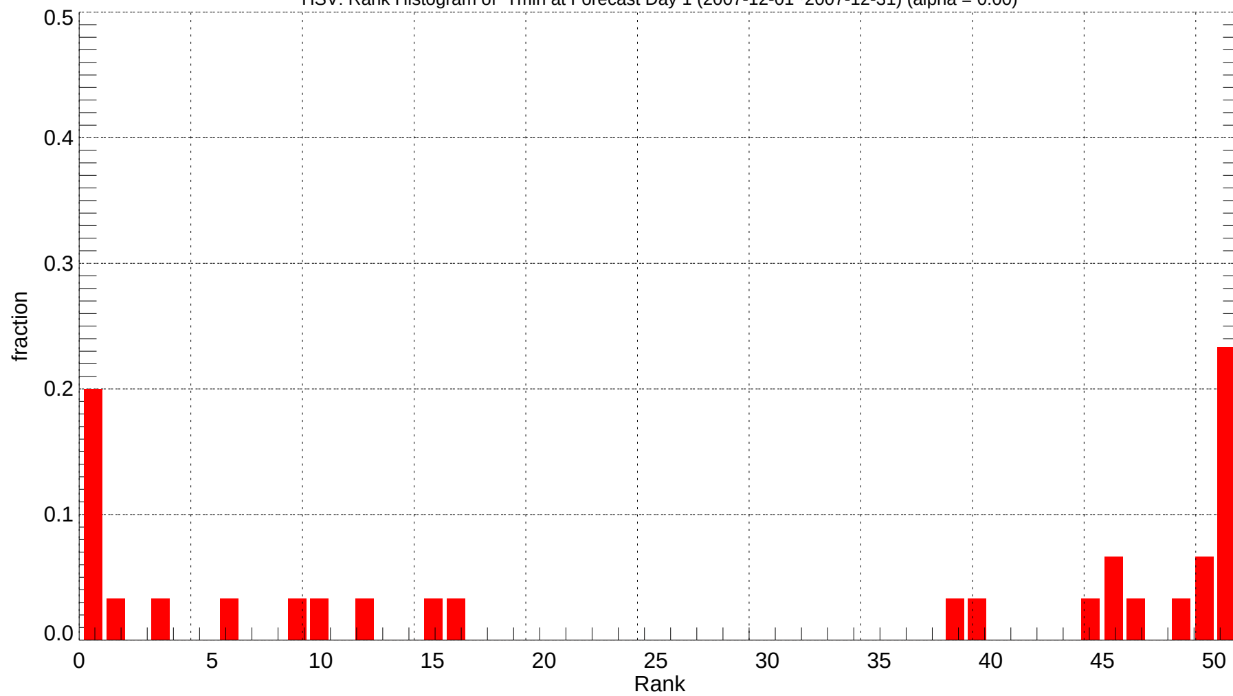
HSV: Rank Histogram of Tmin at Forecast Day 1 (2007-12-01~2007-12-31) (alpha = 0.00)
