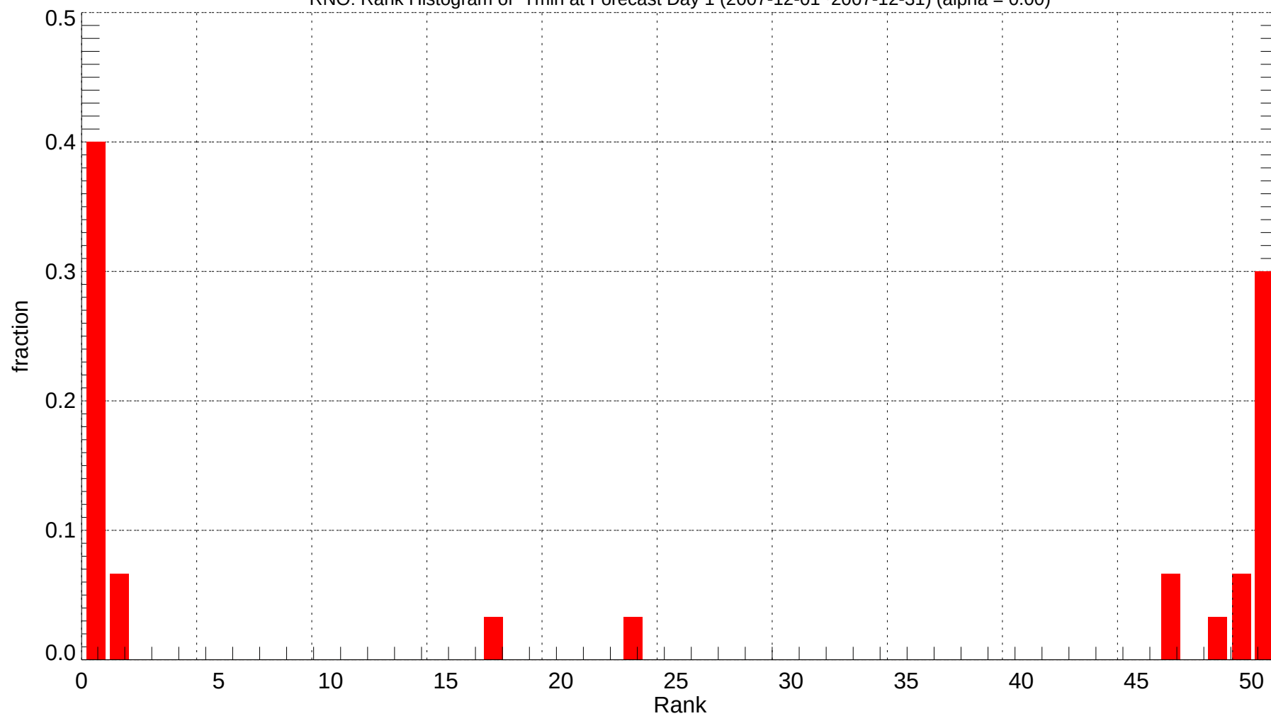
RNO: Rank Histogram of Tmin at Forecast Day 1 (2007-12-01~2007-12-31) (alpha = 0.00)
