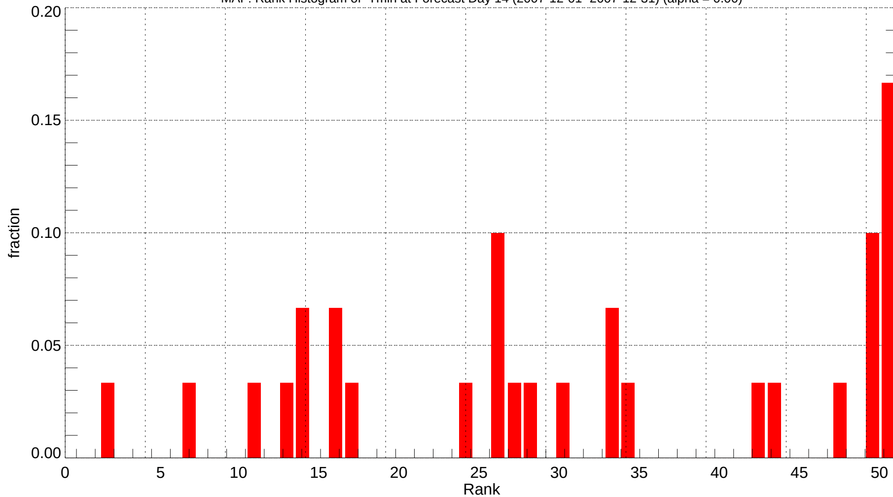
MAF: Rank Histogram of Tmin at Forecast Day 14 (2007-12-01~2007-12-31) (alpha = 0.00)
