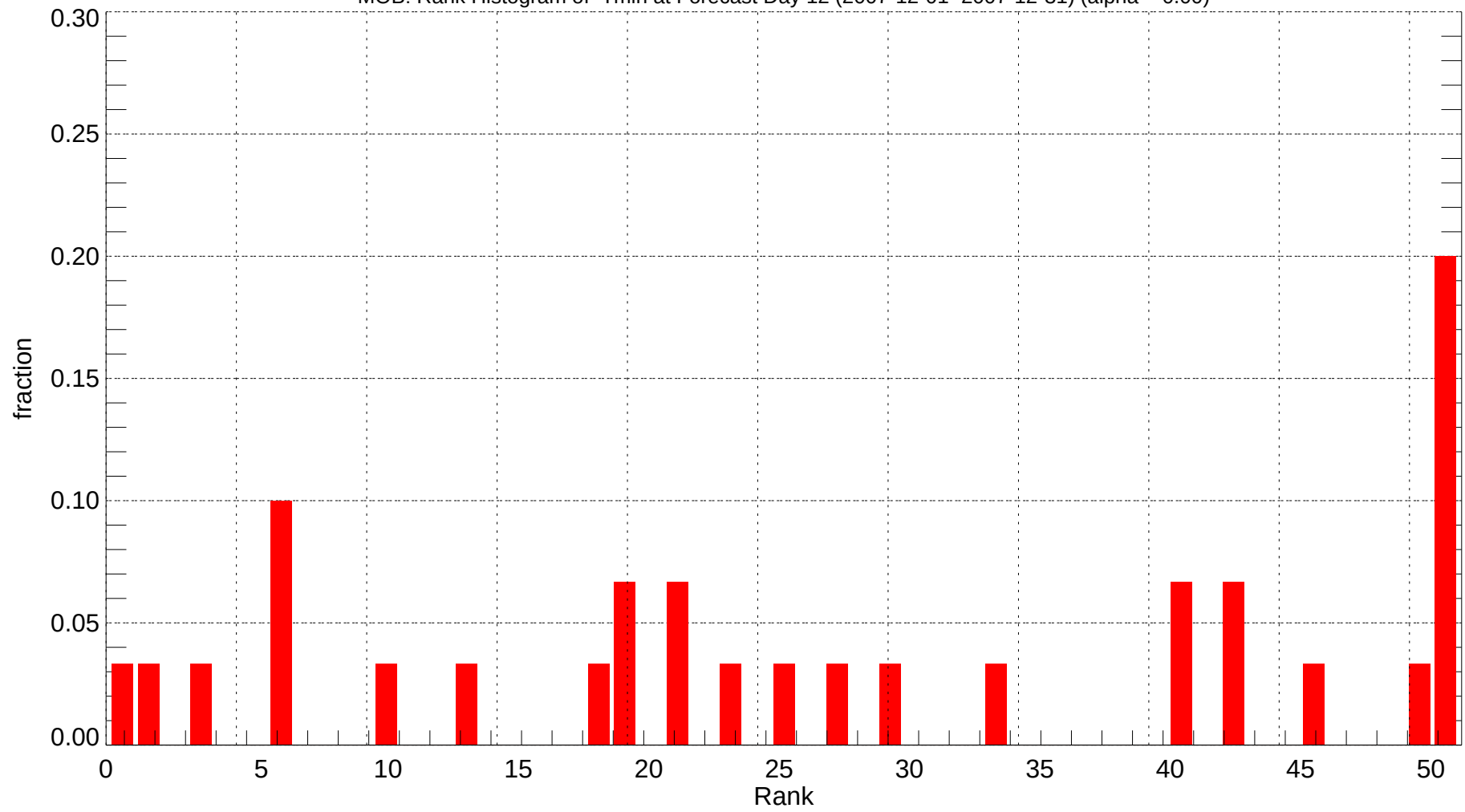
MOB: Rank Histogram of Tmin at Forecast Day 12 (2007-12-01~2007-12-31) (alpha = 0.00)
