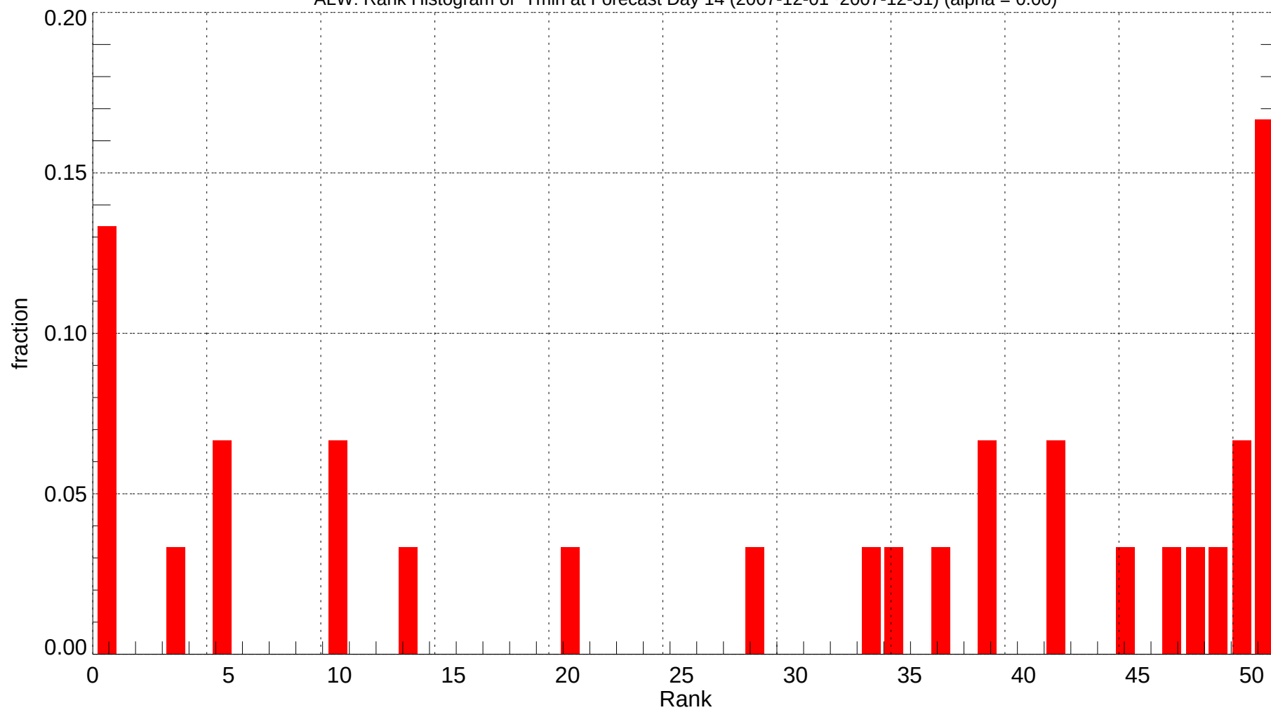
ALW: Rank Histogram of Tmin at Forecast Day 14 (2007-12-01~2007-12-31) (alpha = 0.00)
