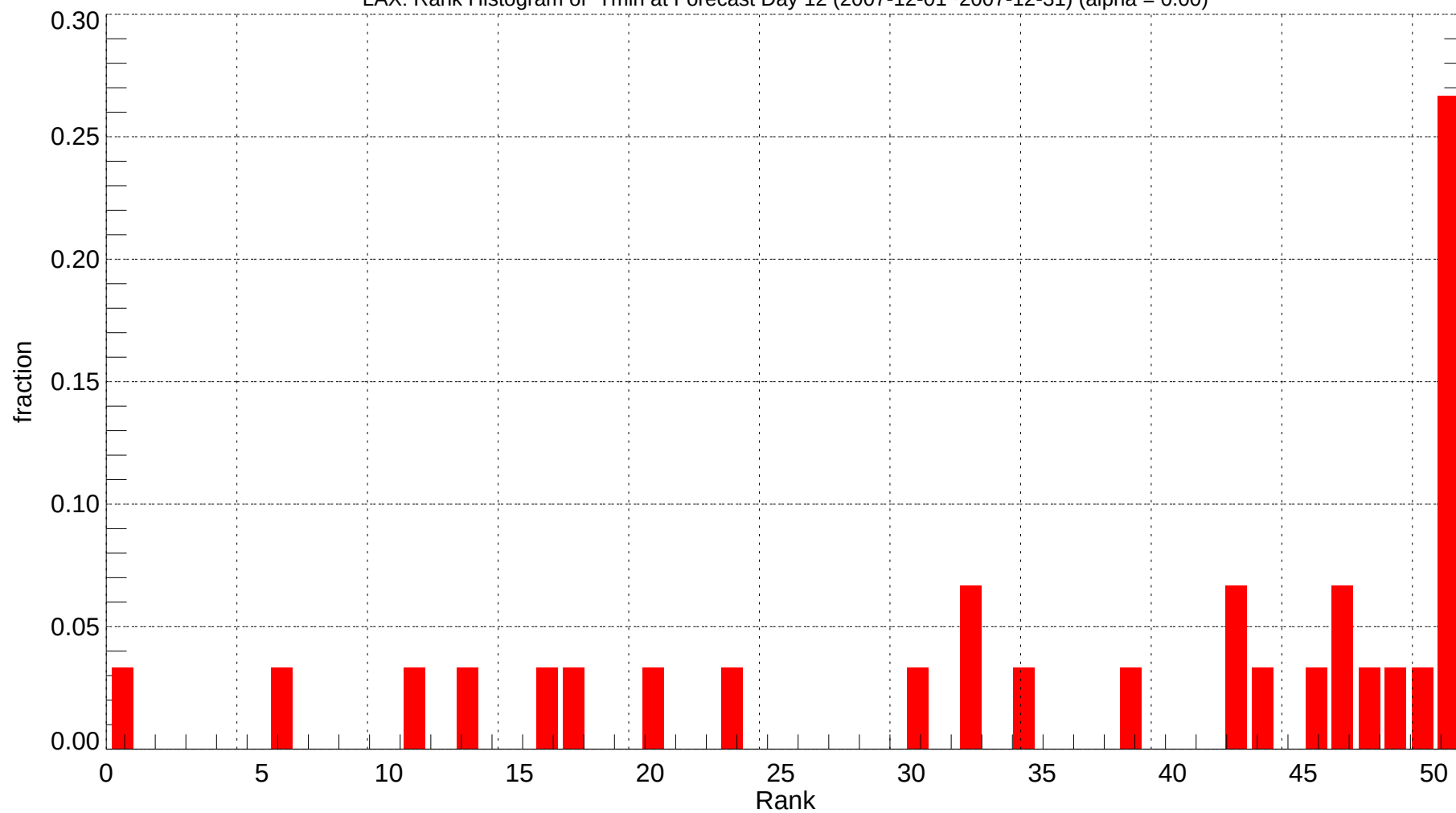
LAX: Rank Histogram of Tmin at Forecast Day 12 (2007-12-01~2007-12-31) (alpha = 0.00)
