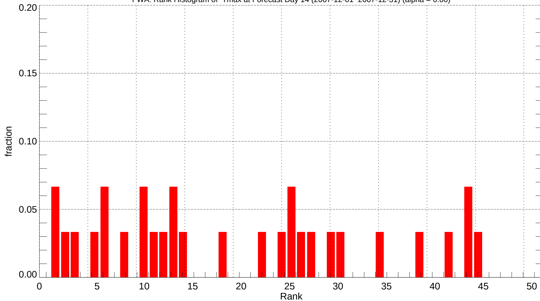
FWA: Rank Histogram of Tmax at Forecast Day 14 (2007-12-01~2007-12-31) (alpha = 0.00)
