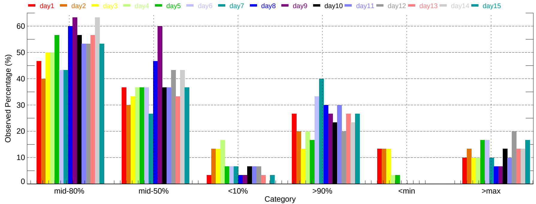
Observed Percentage of Ensembles - BHM: Min Temperature (2007-12-01~2007-12-31)
