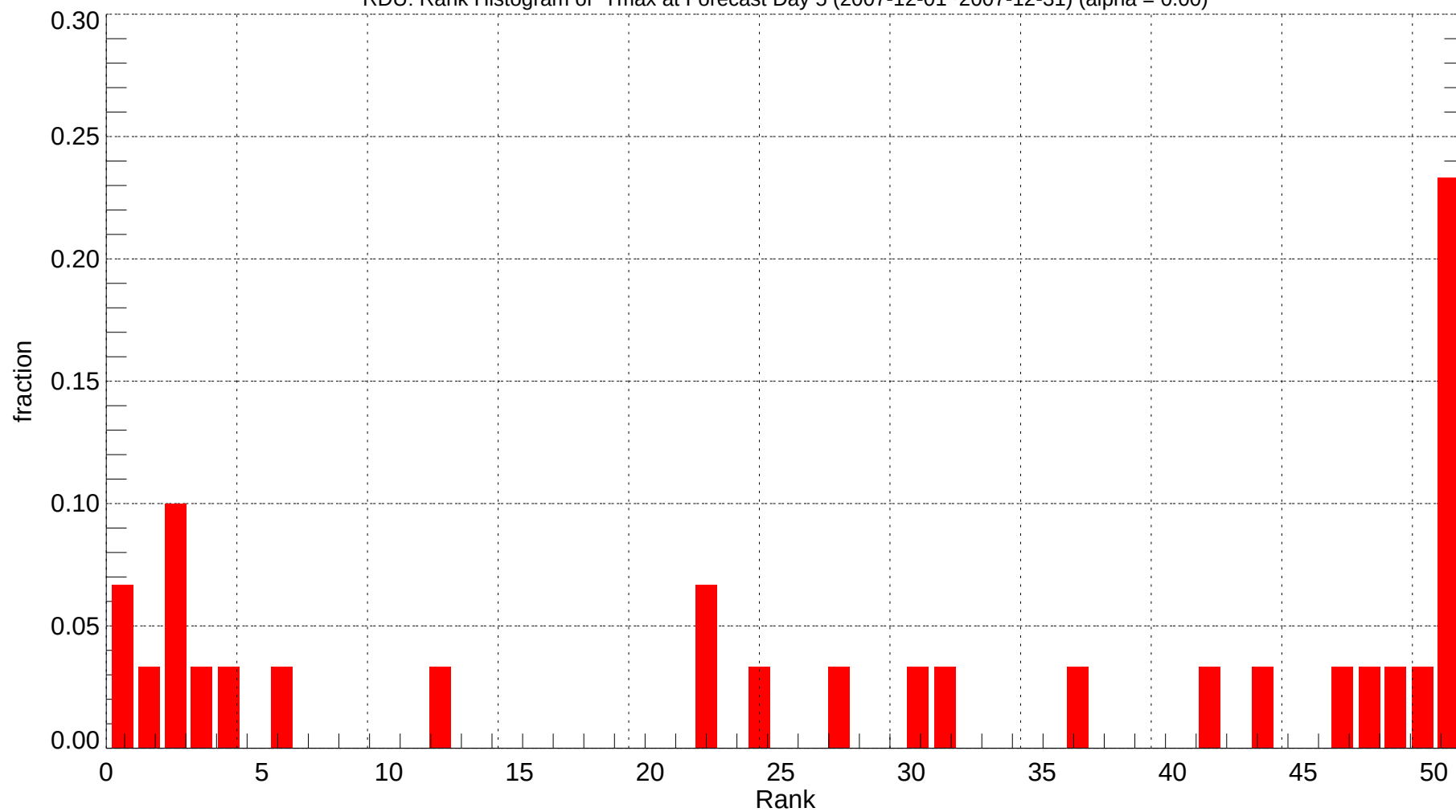
RDU: Rank Histogram of Tmax at Forecast Day 5 (2007-12-01~2007-12-31) (alpha = 0.00)
