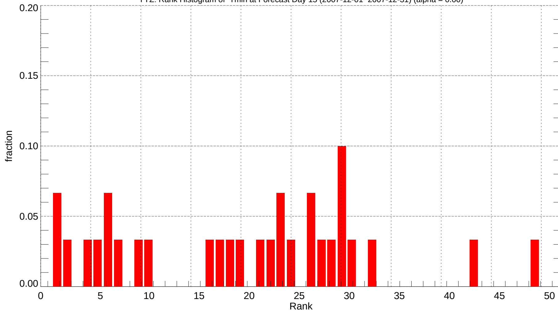
YYZ: Rank Histogram of Tmin at Forecast Day 15 (2007-12-01~2007-12-31) (alpha = 0.00)
