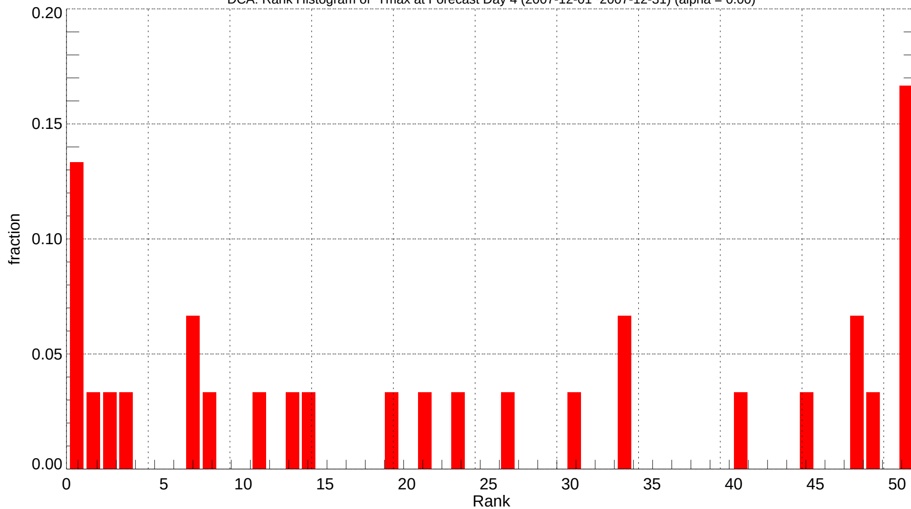
DCA: Rank Histogram of Tmax at Forecast Day 4 (2007-12-01~2007-12-31) (alpha = 0.00)
