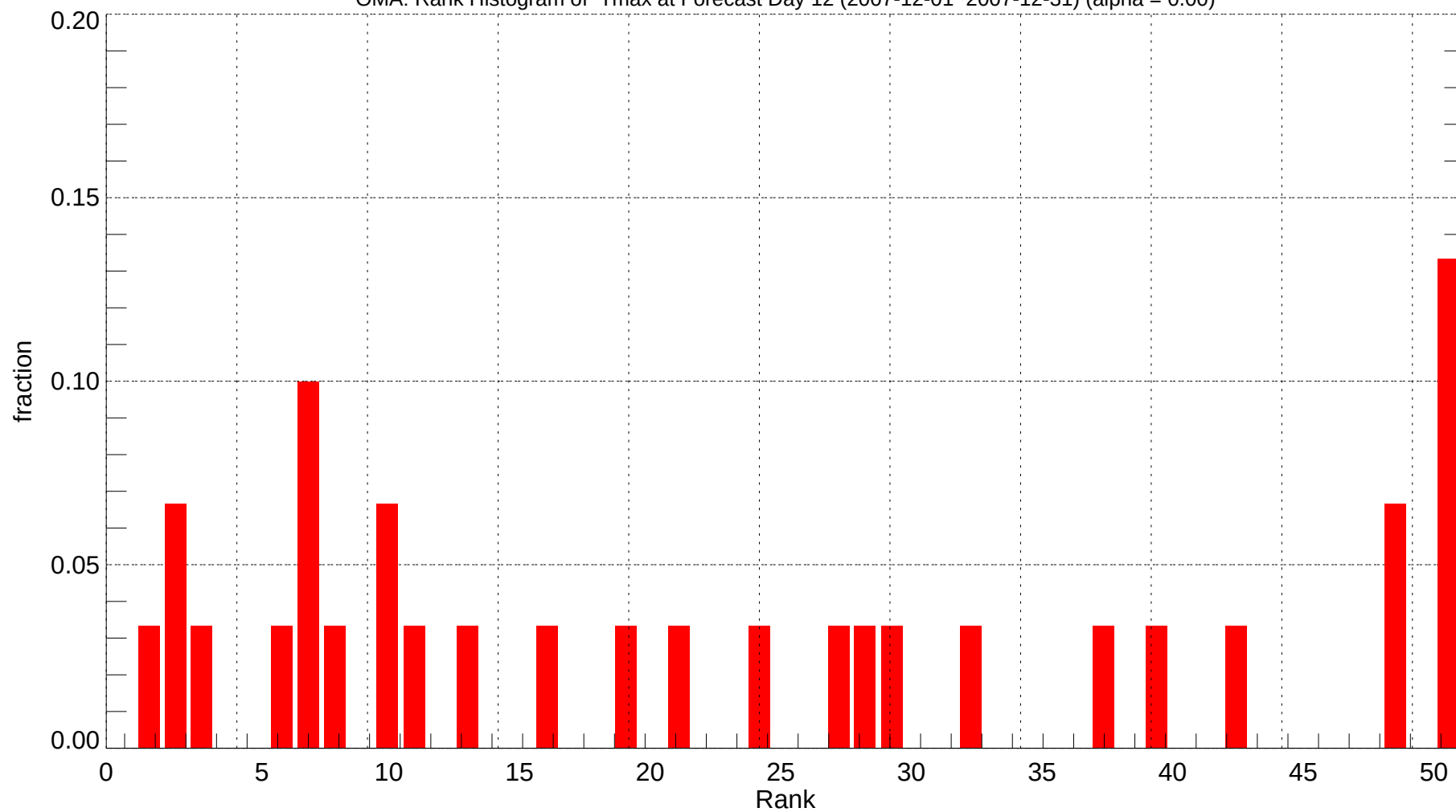
OMA: Rank Histogram of Tmax at Forecast Day 12 (2007-12-01~2007-12-31) (alpha = 0.00)
