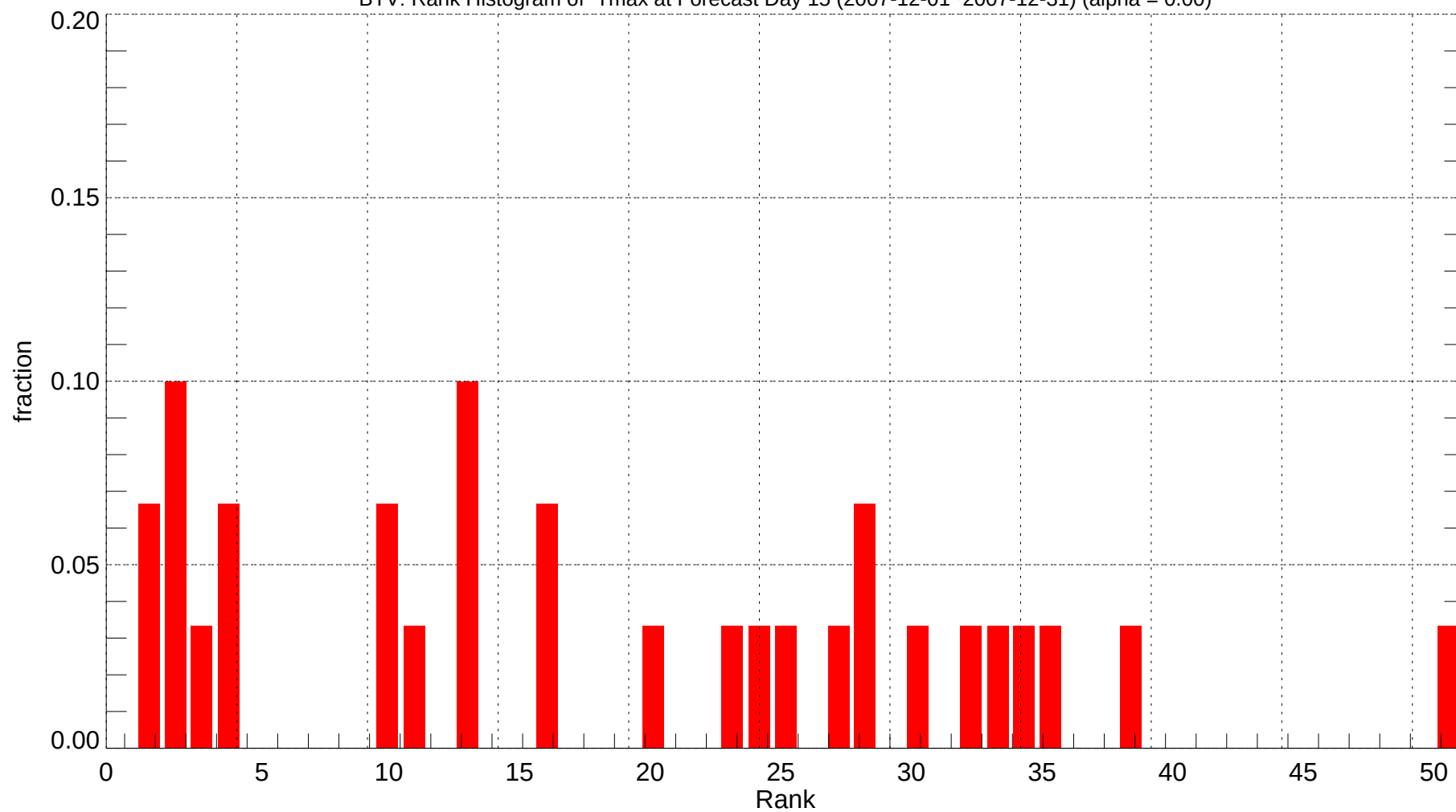
BTV: Rank Histogram of Tmax at Forecast Day 15 (2007-12-01~2007-12-31) (alpha = 0.00)
