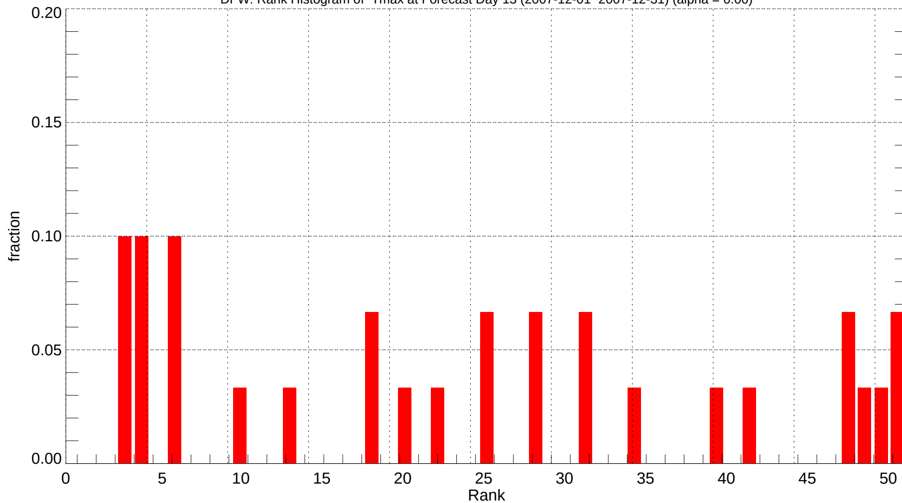
DFW: Rank Histogram of Tmax at Forecast Day 13 (2007-12-01~2007-12-31) (alpha = 0.00)
