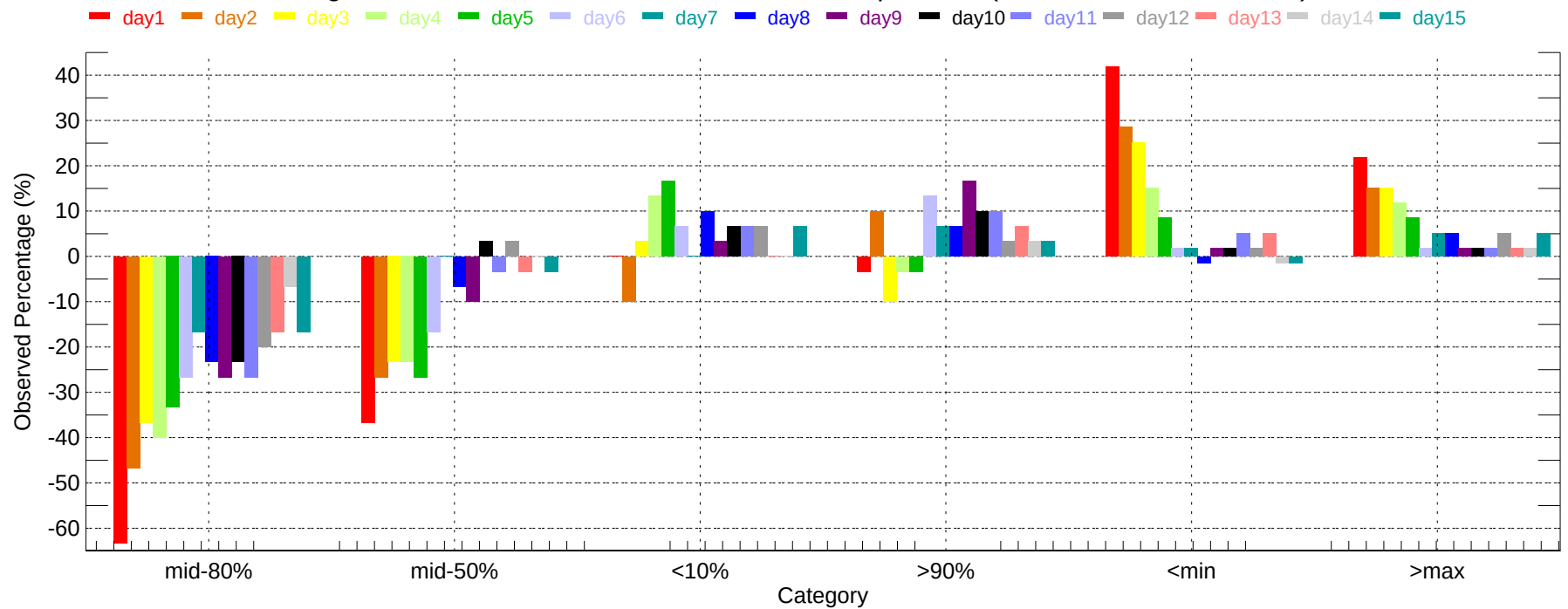
Observed Percentage Deviation of Ensembles - AOO: Max Temperature (2007-12-01~2007-12-31)
