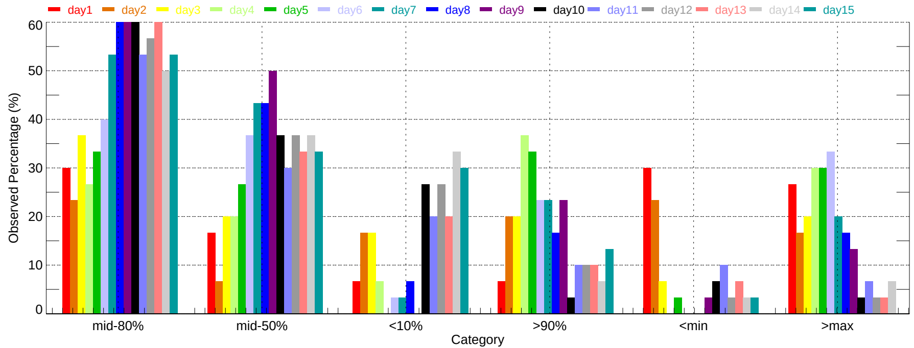
Observed Percentage of Ensembles - ABQ: Max Temperature (2007-12-01~2007-12-31)
