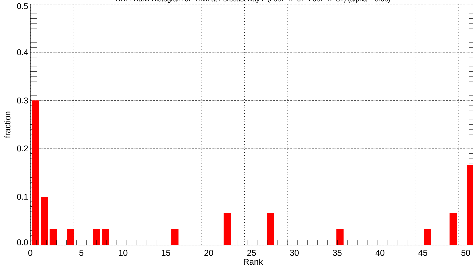
RAP: Rank Histogram of Tmin at Forecast Day 2 (2007-12-01~2007-12-31) (alpha = 0.00)
