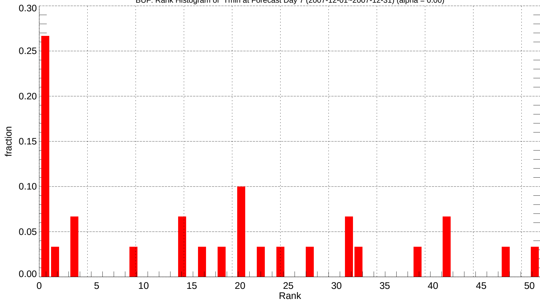
BUF: Rank Histogram of Tmin at Forecast Day 7 (2007-12-01~2007-12-31) (alpha = 0.00)
