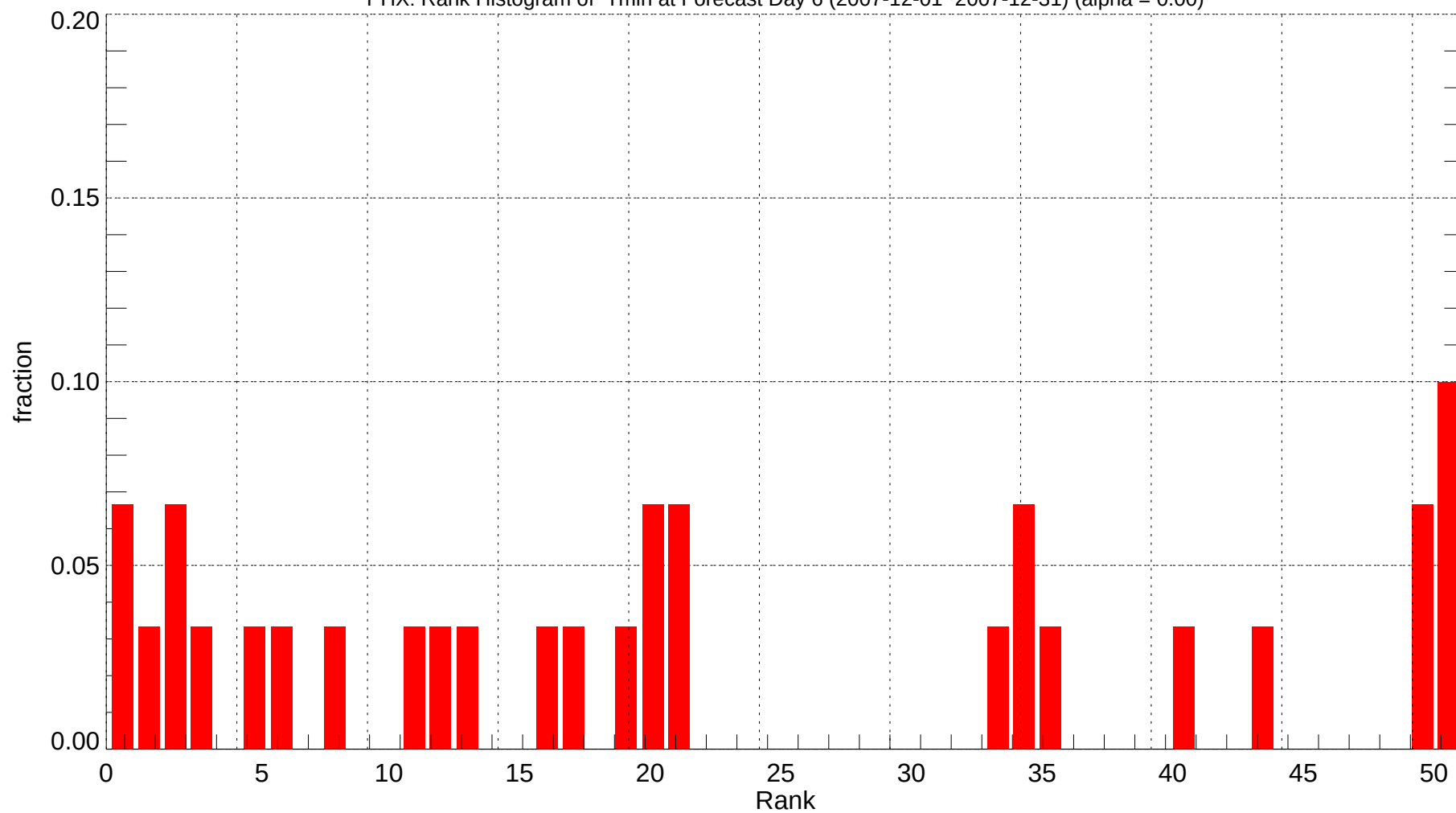
PHX: Rank Histogram of Tmin at Forecast Day 6 (2007-12-01~2007-12-31) (alpha = 0.00)
