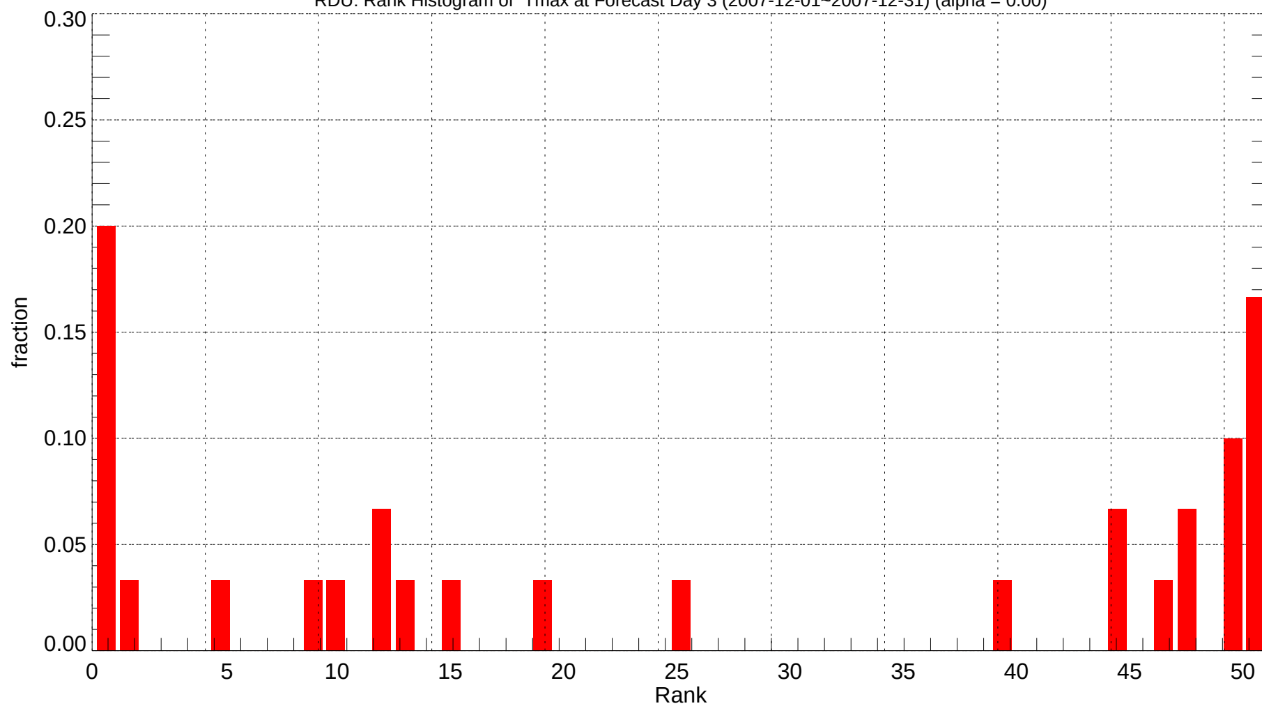
RDU: Rank Histogram of Tmax at Forecast Day 3 (2007-12-01~2007-12-31) (alpha = 0.00)
