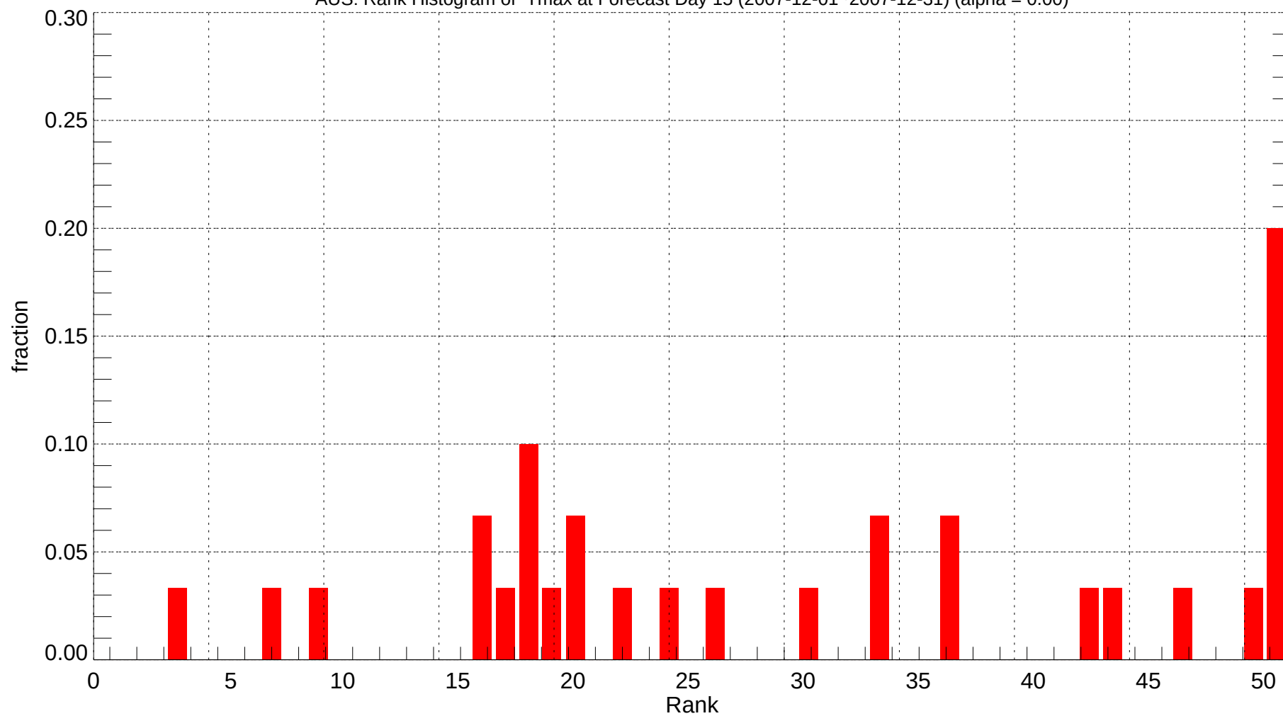
AUS: Rank Histogram of Tmax at Forecast Day 15 (2007-12-01~2007-12-31) (alpha = 0.00)
