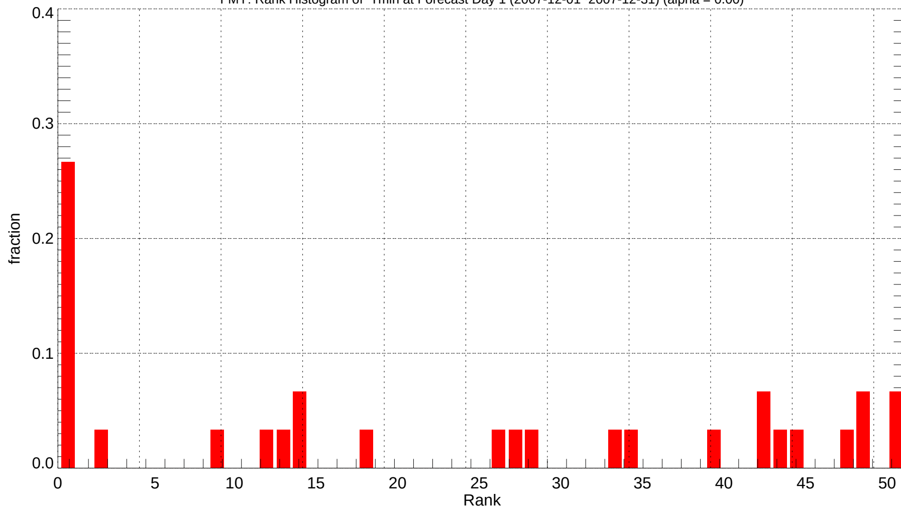
FMY: Rank Histogram of Tmin at Forecast Day 1 (2007-12-01~2007-12-31) (alpha = 0.00)
