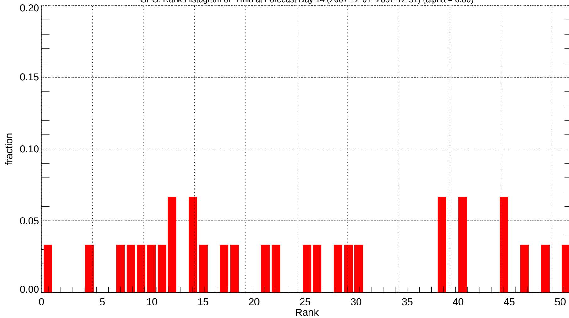
GEG: Rank Histogram of Tmin at Forecast Day 14 (2007-12-01~2007-12-31) (alpha = 0.00)
