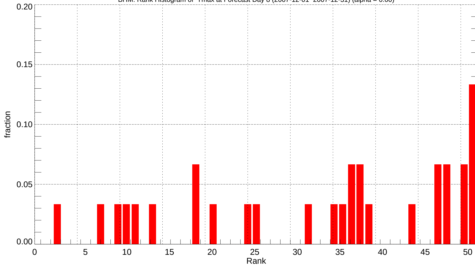
BHM: Rank Histogram of Tmax at Forecast Day 8 (2007-12-01~2007-12-31) (alpha = 0.00)
