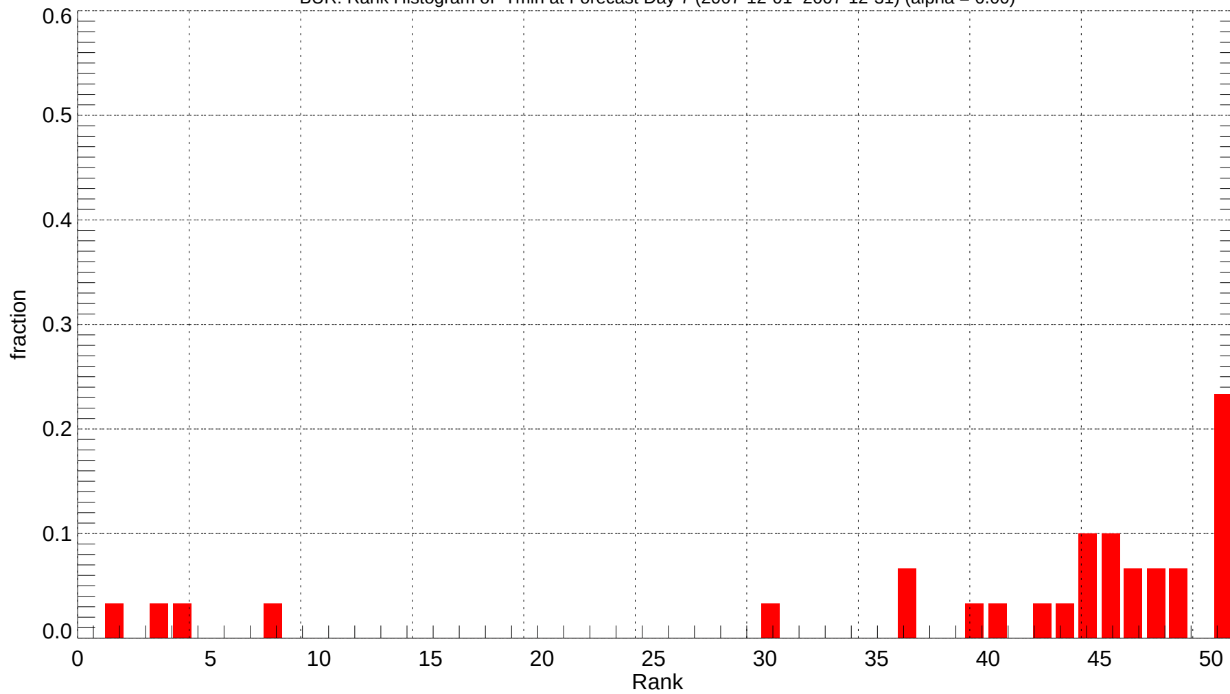
BUR: Rank Histogram of Tmin at Forecast Day 7 (2007-12-01~2007-12-31) (alpha = 0.00)
