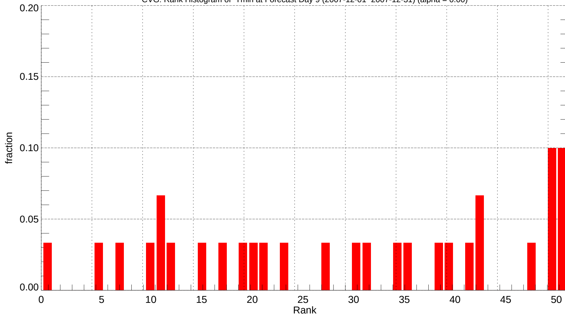
CVG: Rank Histogram of Tmin at Forecast Day 9 (2007-12-01~2007-12-31) (alpha = 0.00)
