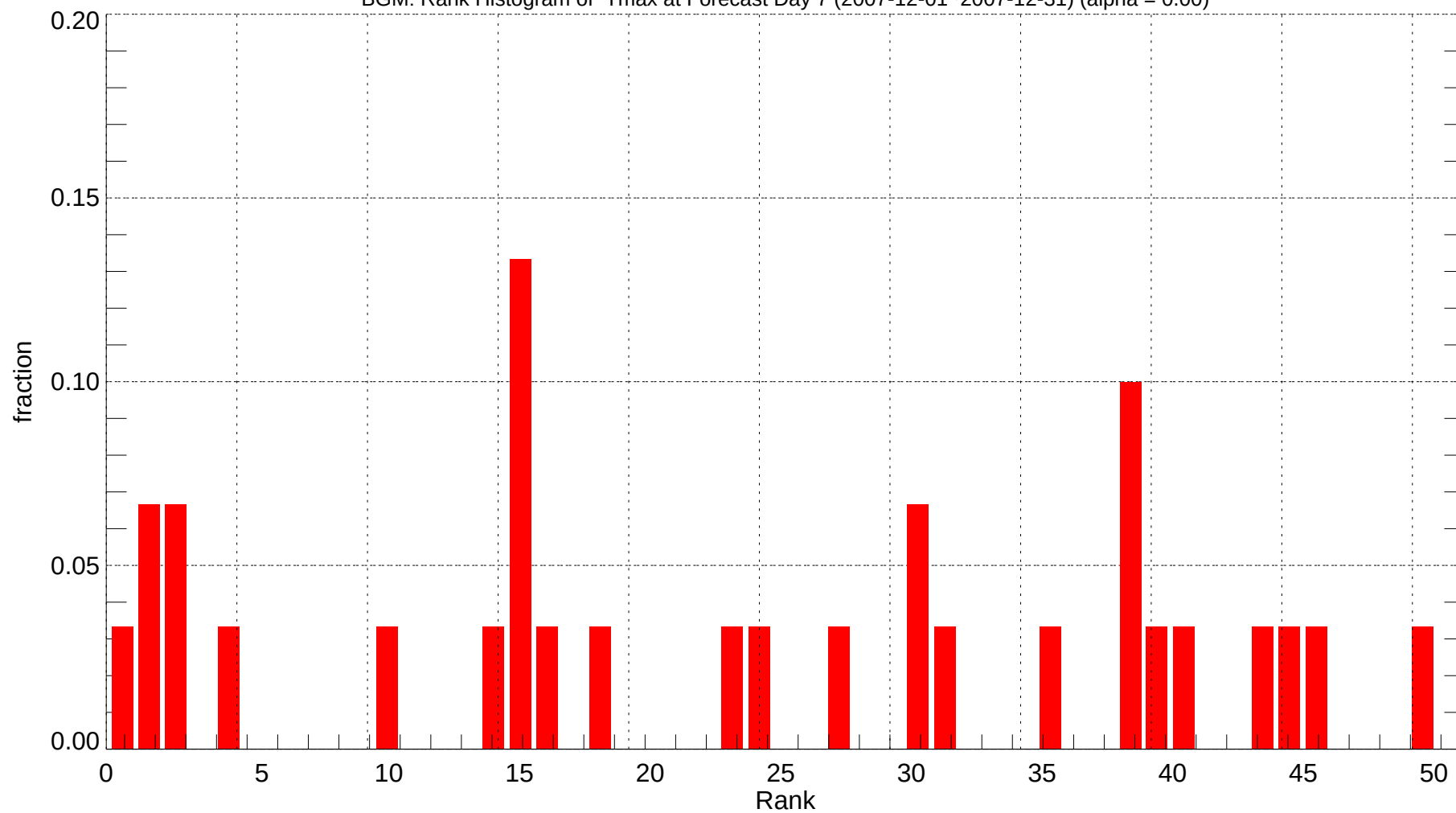
BGM: Rank Histogram of Tmax at Forecast Day 7 (2007-12-01~2007-12-31) (alpha = 0.00)
