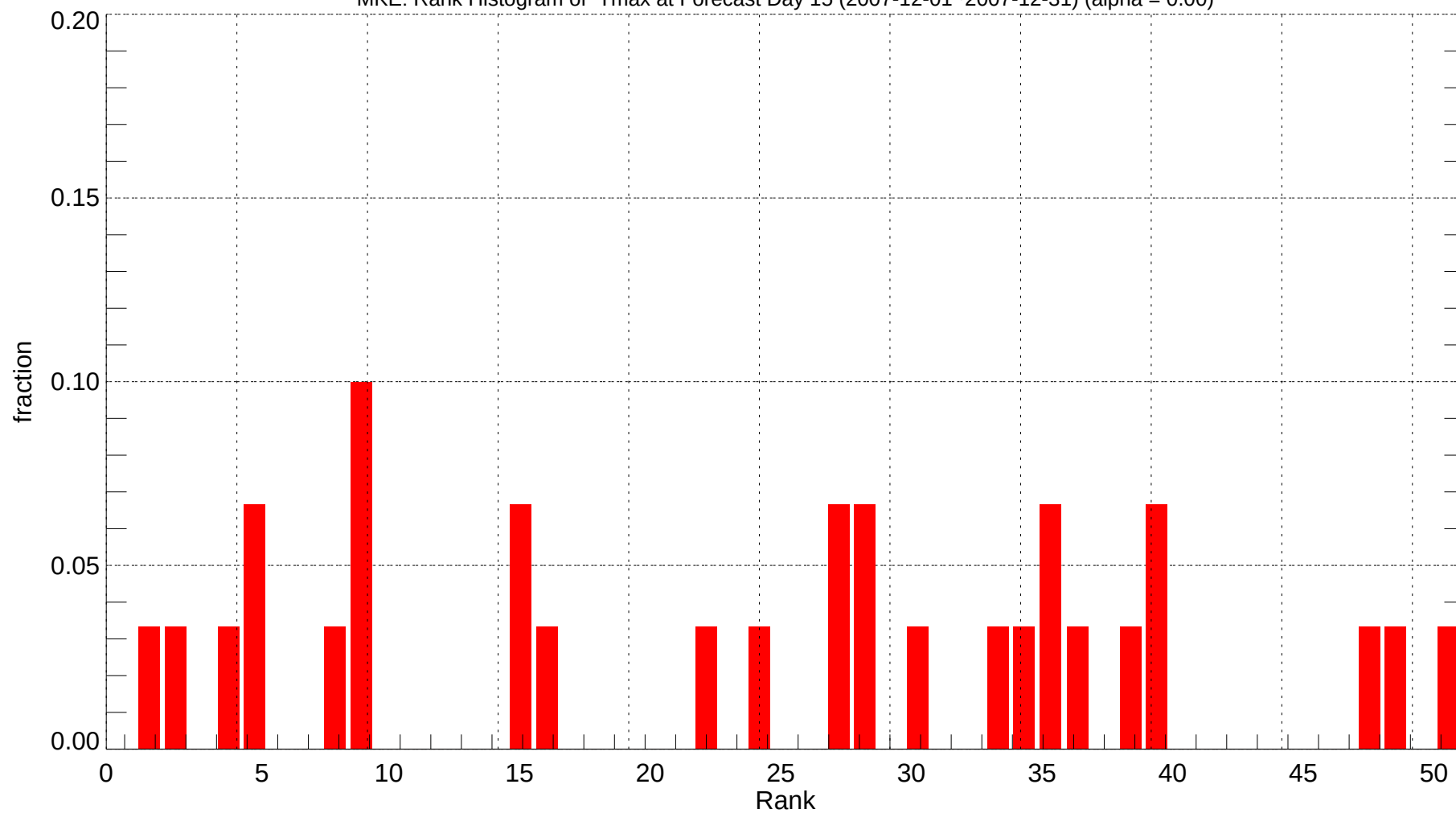
MKE: Rank Histogram of Tmax at Forecast Day 15 (2007-12-01~2007-12-31) (alpha = 0.00)
