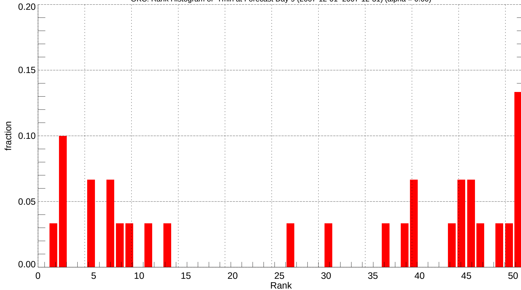
OKC: Rank Histogram of Tmin at Forecast Day 9 (2007-12-01~2007-12-31) (alpha = 0.00)
