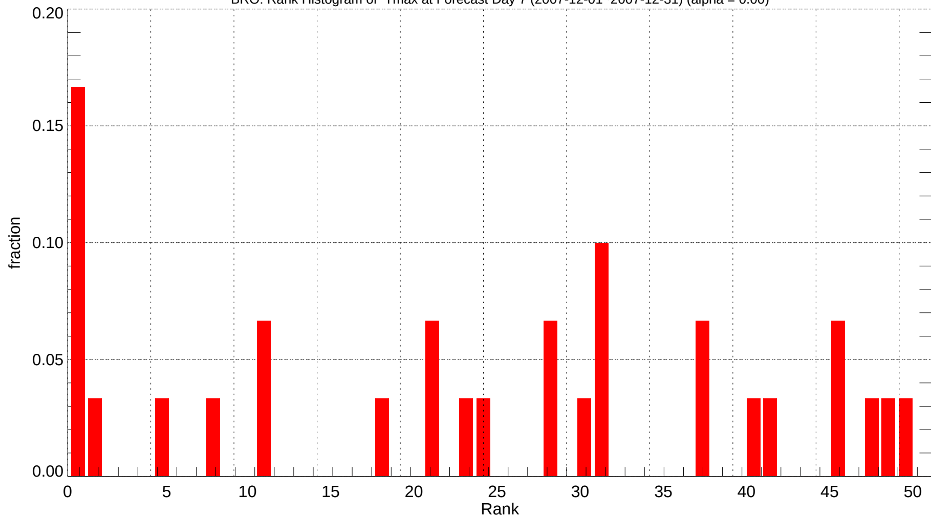
BRO: Rank Histogram of Tmax at Forecast Day 7 (2007-12-01~2007-12-31) (alpha = 0.00)
