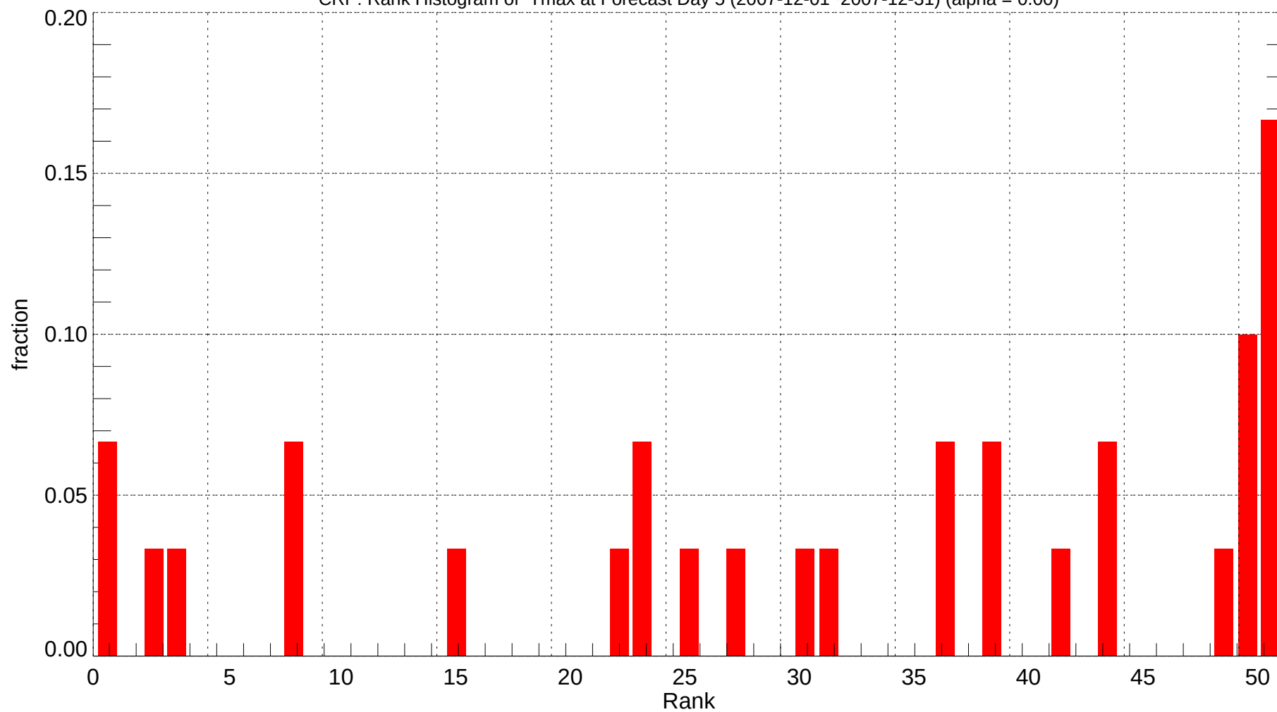
CRP: Rank Histogram of Tmax at Forecast Day 5 (2007-12-01~2007-12-31) (alpha = 0.00)
