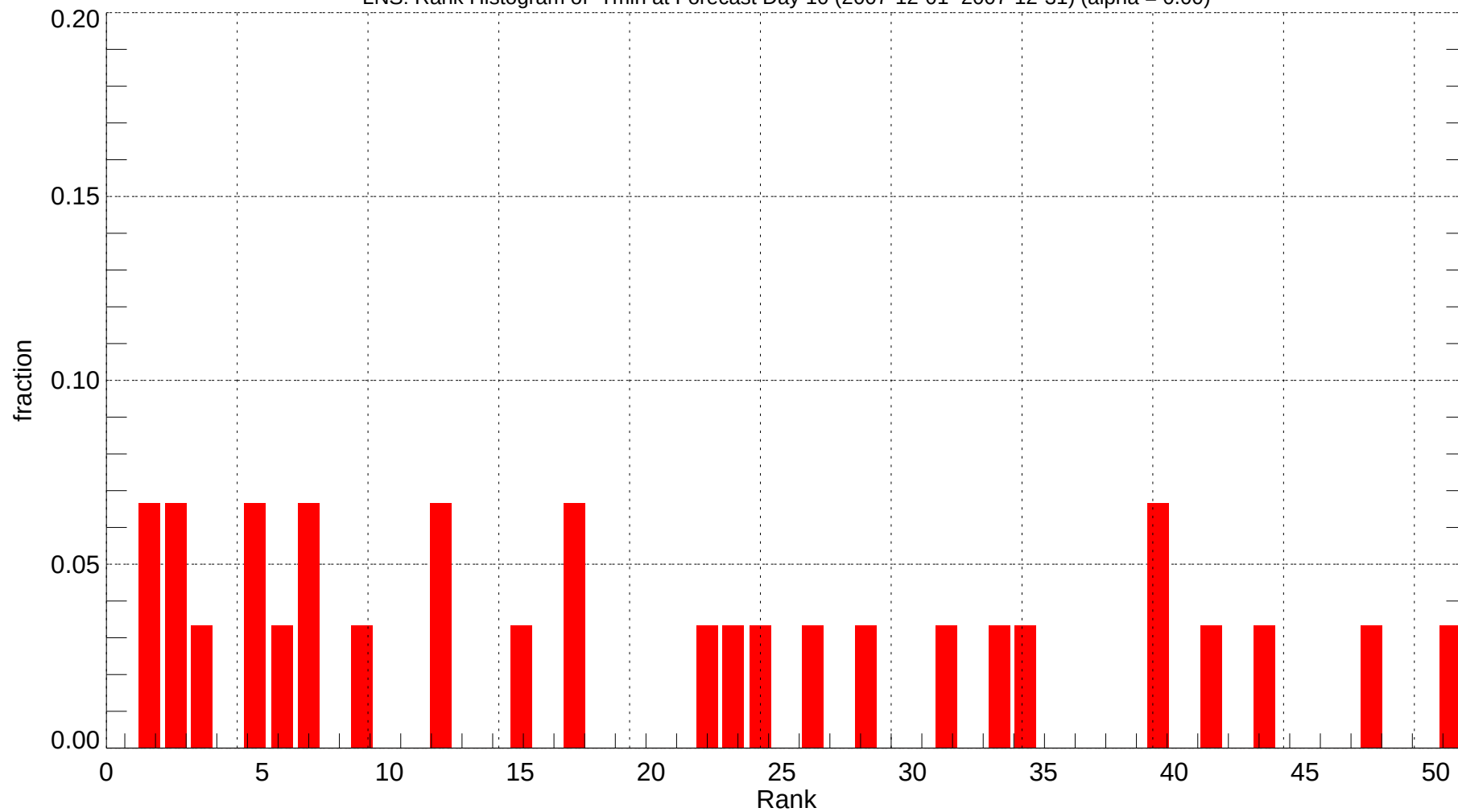
LNS: Rank Histogram of Tmin at Forecast Day 10 (2007-12-01~2007-12-31) (alpha = 0.00)
