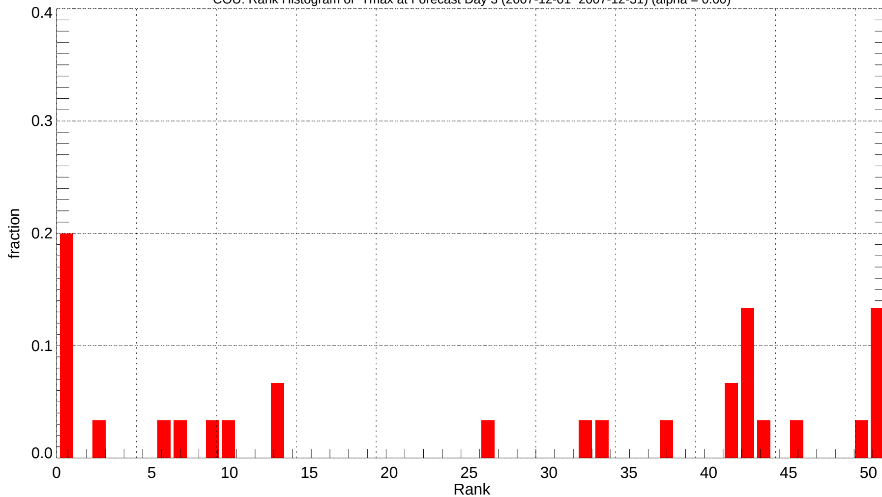
COU: Rank Histogram of Tmax at Forecast Day 3 (2007-12-01~2007-12-31) (alpha = 0.00)
