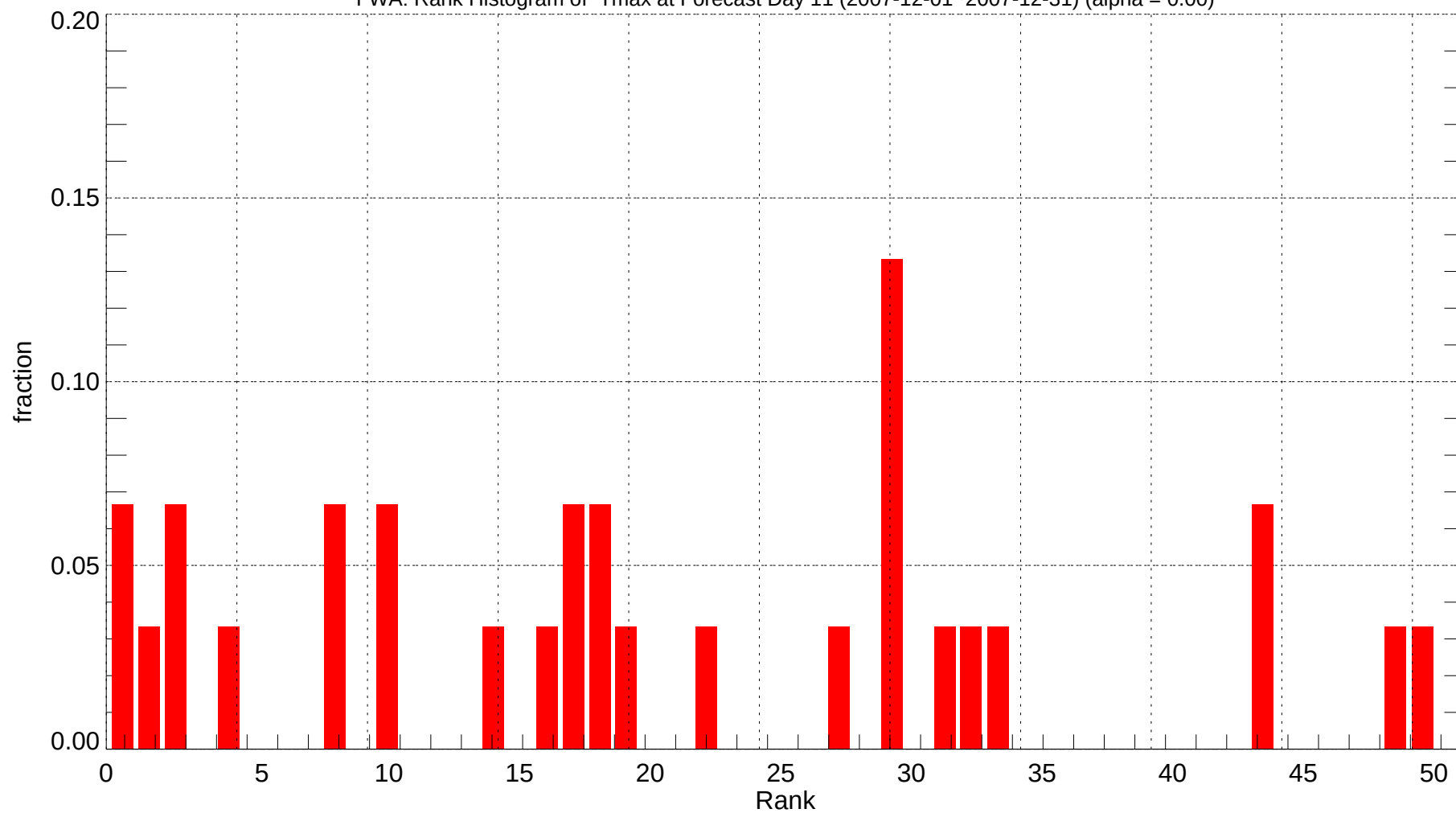
FWA: Rank Histogram of Tmax at Forecast Day 11 (2007-12-01~2007-12-31) (alpha = 0.00)
