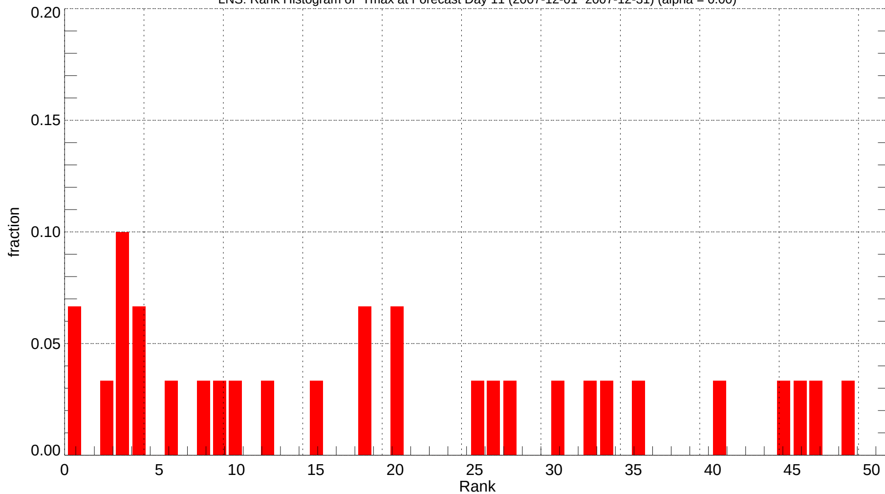
LNS: Rank Histogram of Tmax at Forecast Day 11 (2007-12-01~2007-12-31) (alpha = 0.00)
