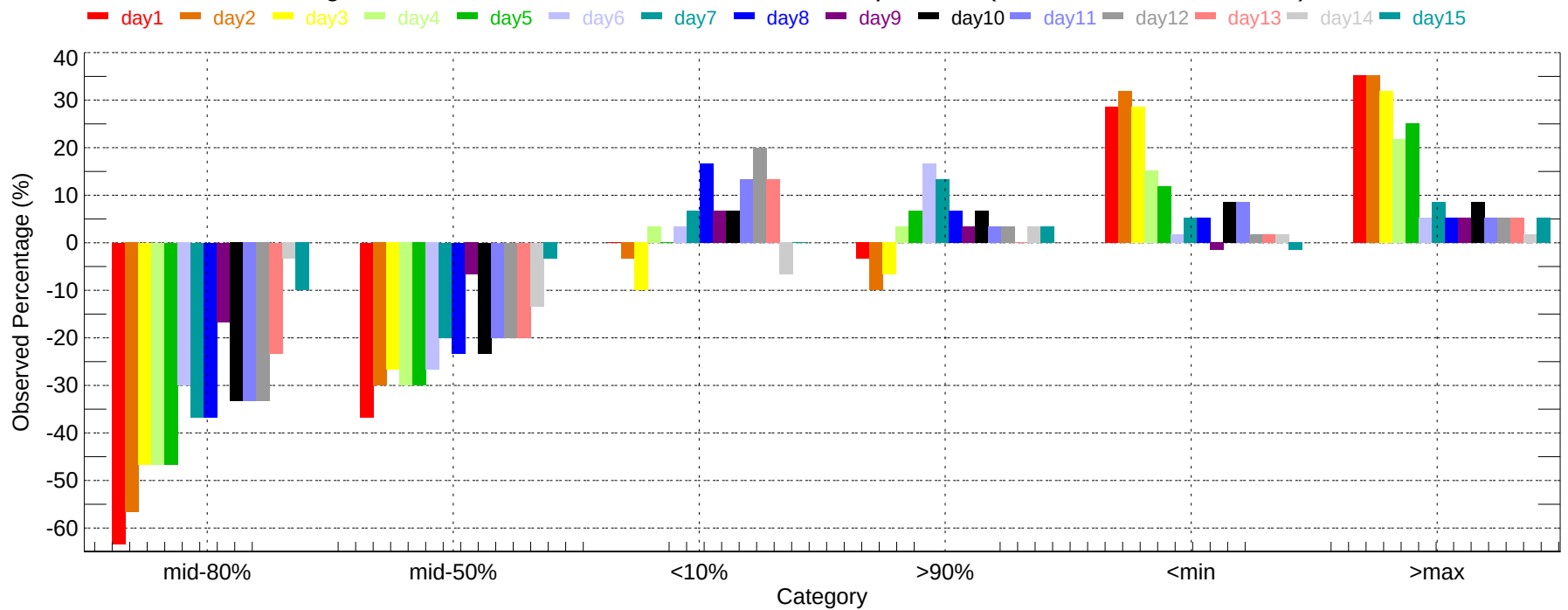
Observed Percentage Deviation of Ensembles - YKM: Max Temperature (2007-12-01~2007-12-31)
