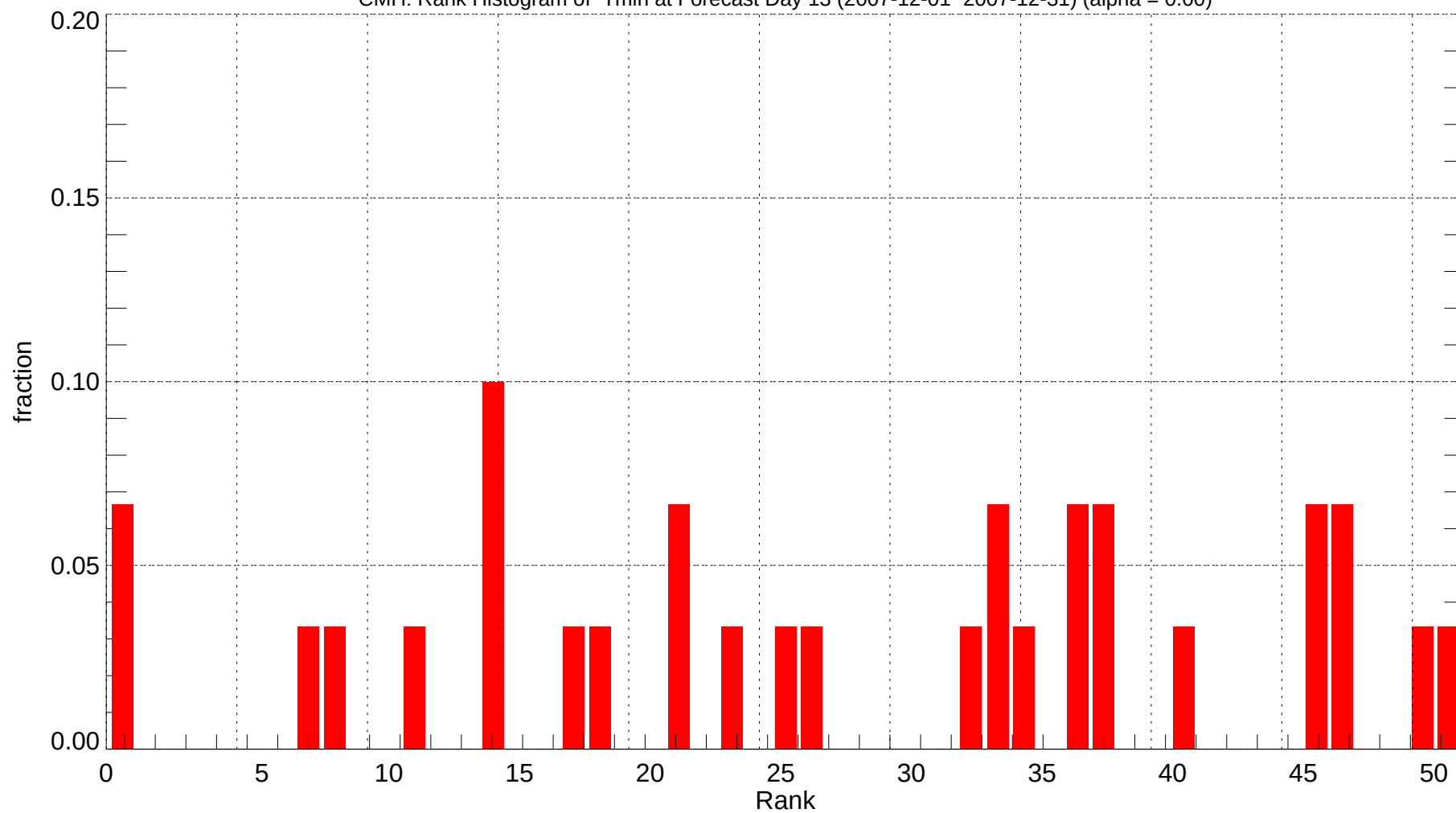
CMH: Rank Histogram of Tmin at Forecast Day 13 (2007-12-01~2007-12-31) (alpha = 0.00)
