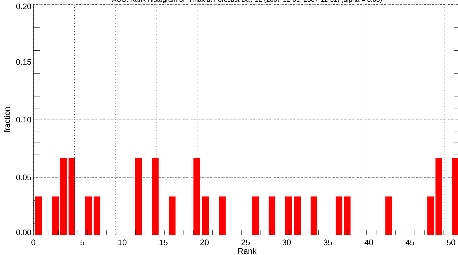
AOO: Rank Histogram of Tmax at Forecast Day 12 (2007-12-01~2007-12-31) (alpha = 0.00)
