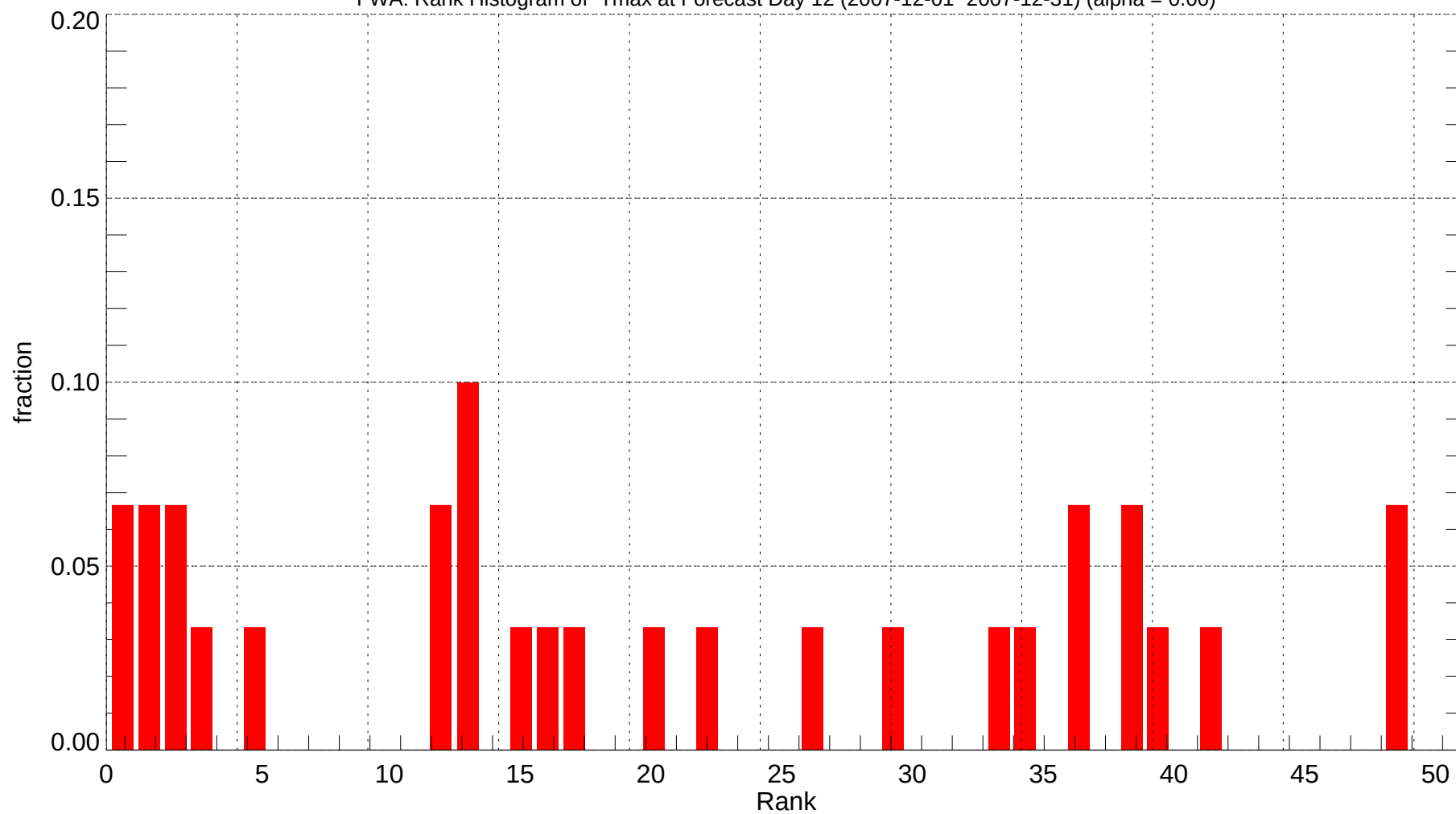
FWA: Rank Histogram of Tmax at Forecast Day 12 (2007-12-01~2007-12-31) (alpha = 0.00)
