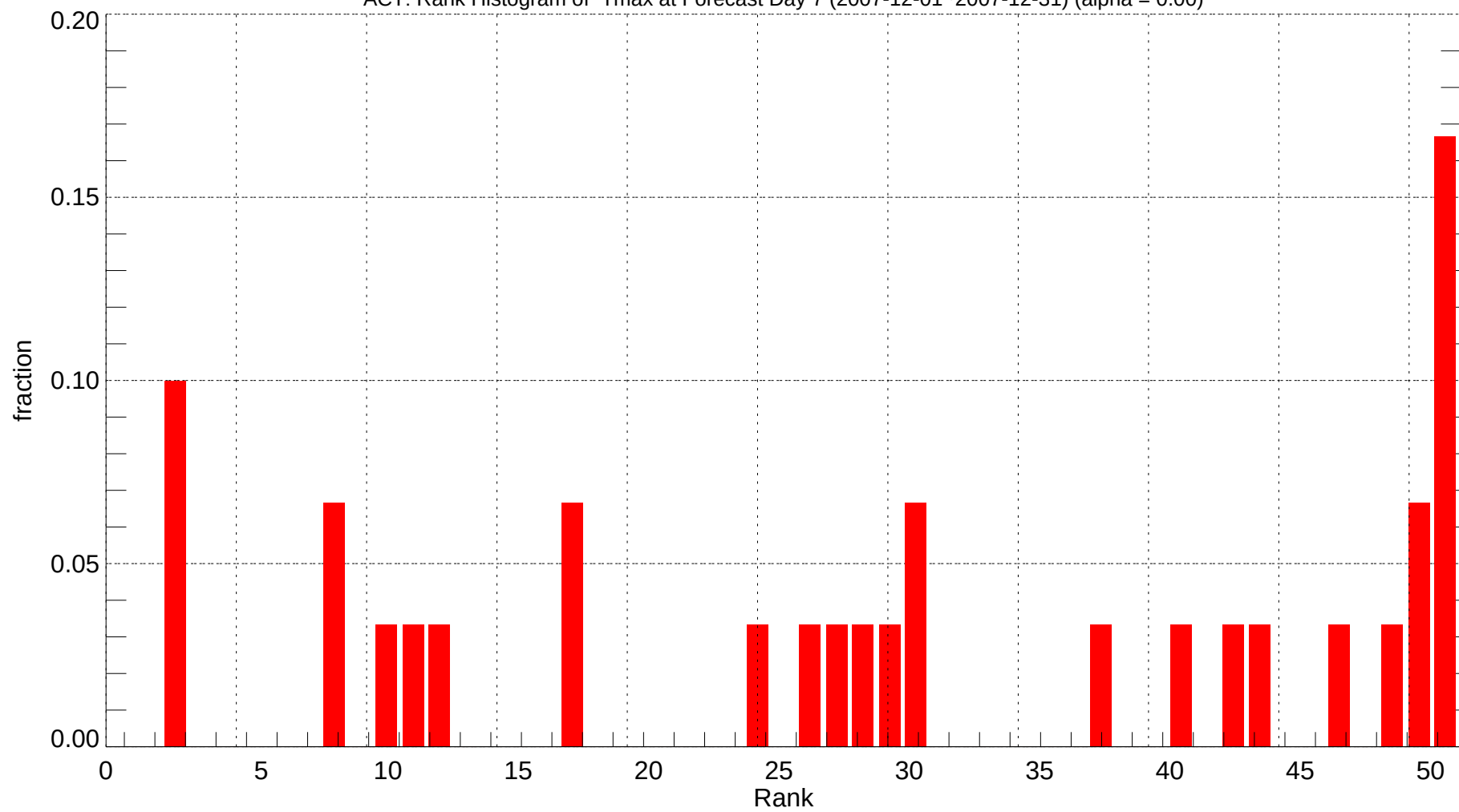
ACT: Rank Histogram of Tmax at Forecast Day 7 (2007-12-01~2007-12-31) (alpha = 0.00)
