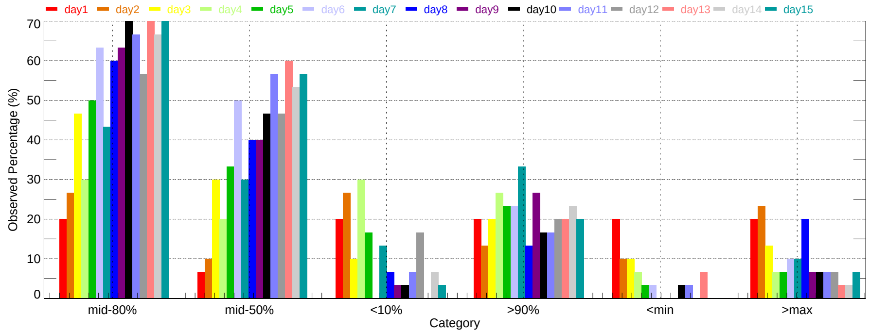
Observed Percentage of Ensembles - CVG: Max Temperature (2007-12-01~2007-12-31)
