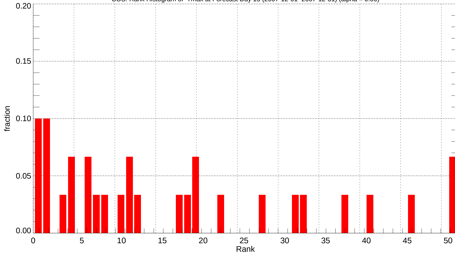
COS: Rank Histogram of Tmax at Forecast Day 15 (2007-12-01~2007-12-31) (alpha = 0.00)
