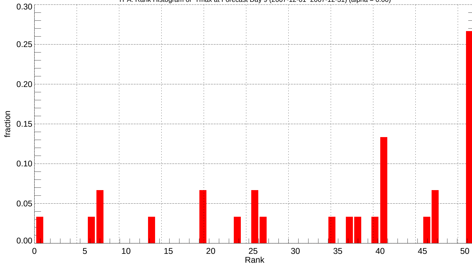
TPA: Rank Histogram of Tmax at Forecast Day 9 (2007-12-01~2007-12-31) (alpha = 0.00)
