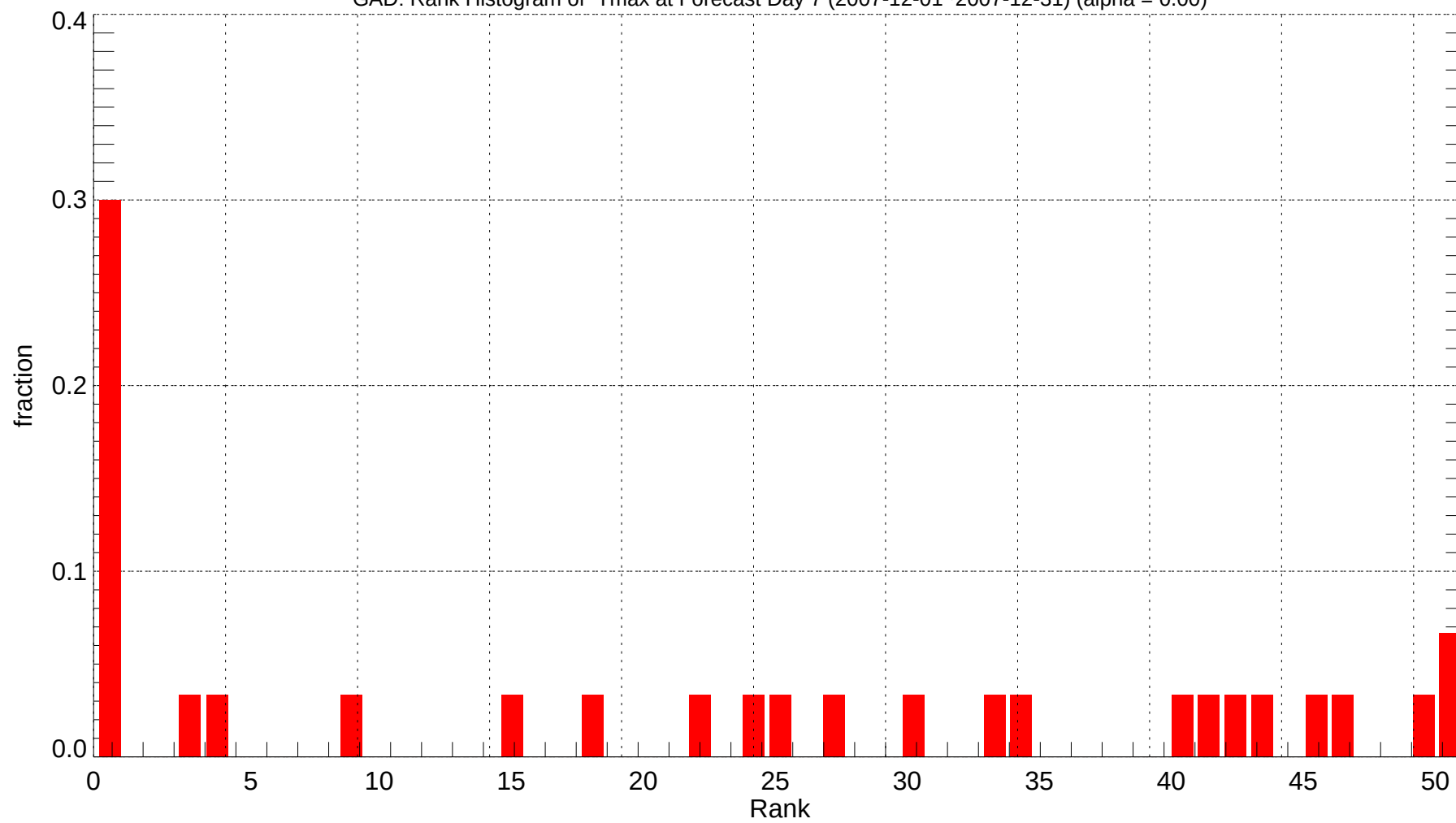
GAD: Rank Histogram of Tmax at Forecast Day 7 (2007-12-01~2007-12-31) (alpha = 0.00)
