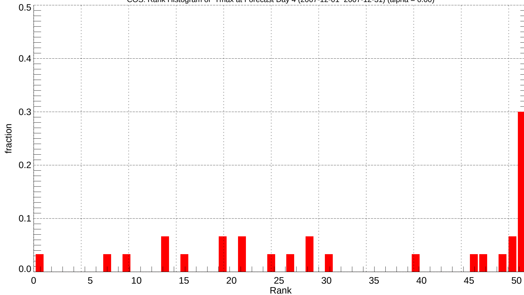
COS: Rank Histogram of Tmax at Forecast Day 4 (2007-12-01~2007-12-31) (alpha = 0.00)
