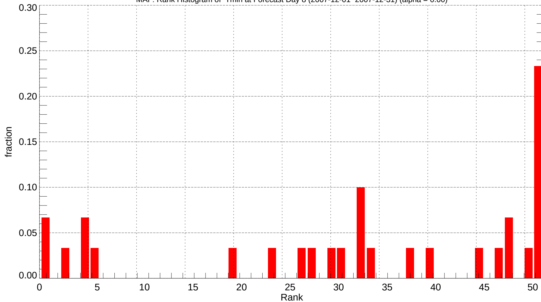
MAF: Rank Histogram of Tmin at Forecast Day 8 (2007-12-01~2007-12-31) (alpha = 0.00)
