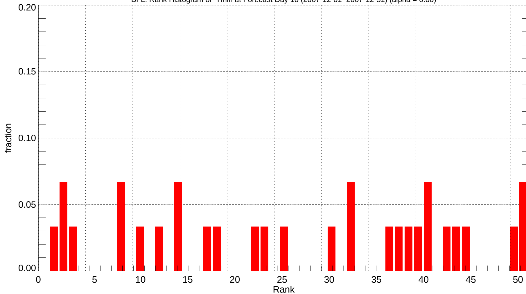
BFL: Rank Histogram of Tmin at Forecast Day 10 (2007-12-01~2007-12-31) (alpha = 0.00)
