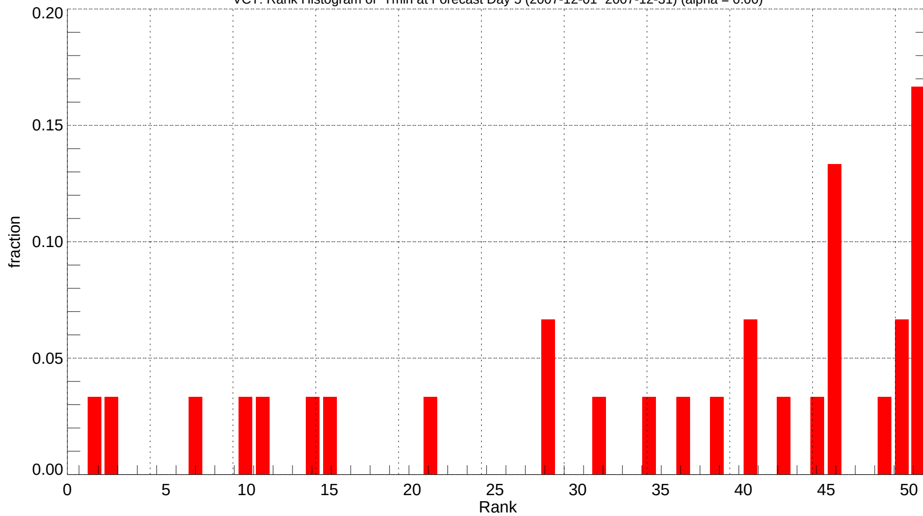
VCT: Rank Histogram of Tmin at Forecast Day 5 (2007-12-01~2007-12-31) (alpha = 0.00)
