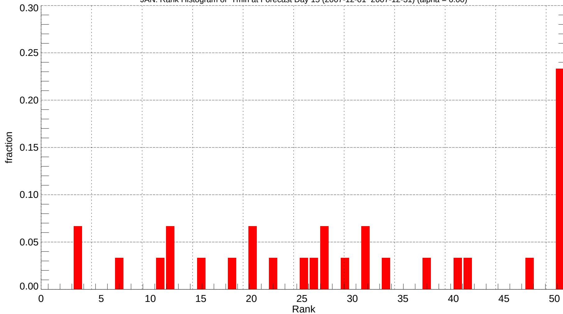
JAN: Rank Histogram of Tmin at Forecast Day 15 (2007-12-01~2007-12-31) (alpha = 0.00)
