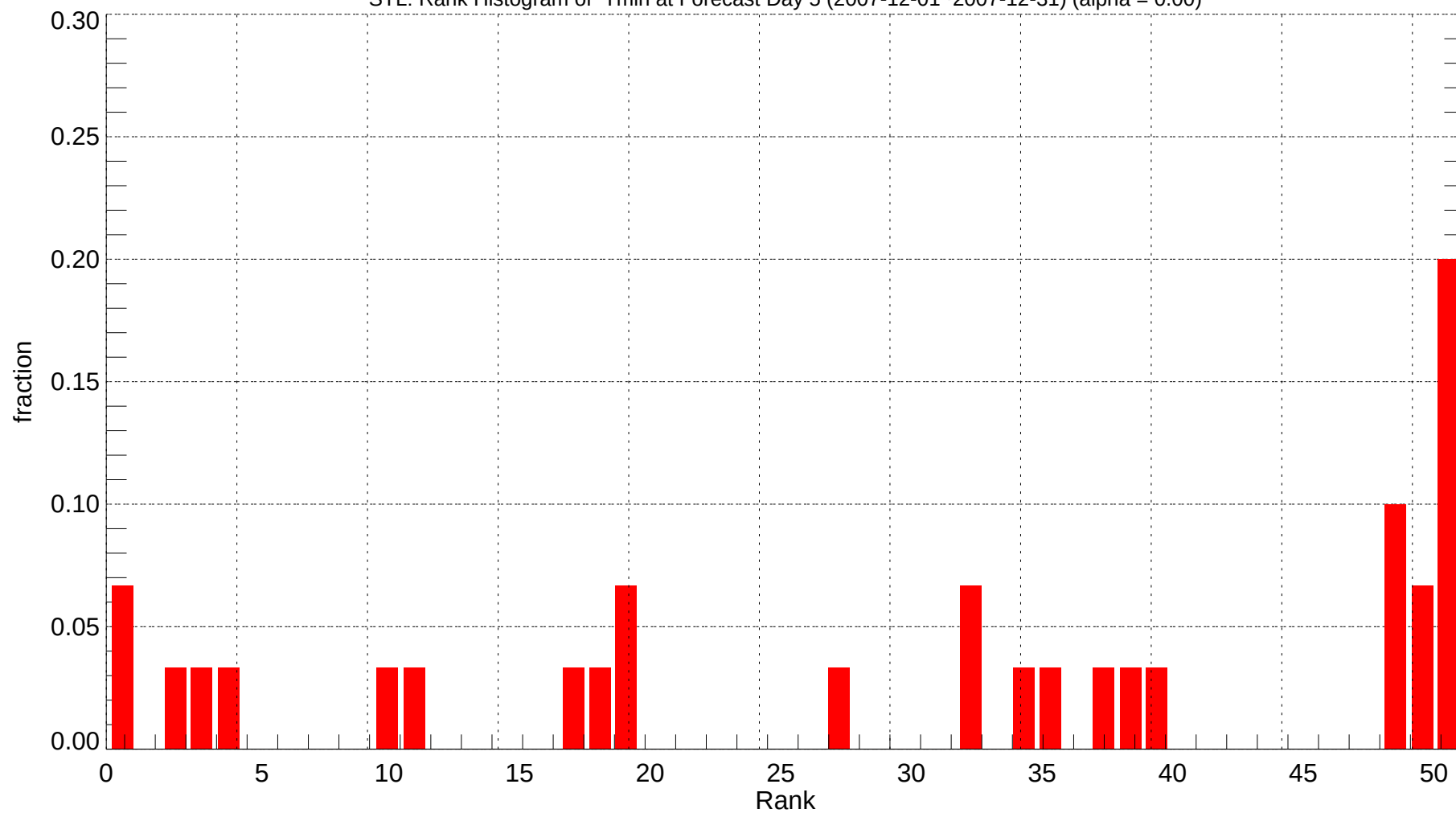
STL: Rank Histogram of Tmin at Forecast Day 5 (2007-12-01~2007-12-31) (alpha = 0.00)
