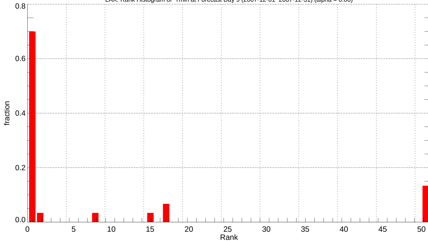
LAX: Rank Histogram of Tmin at Forecast Day 9 (2007-12-01~2007-12-31) (alpha = 0.00)
