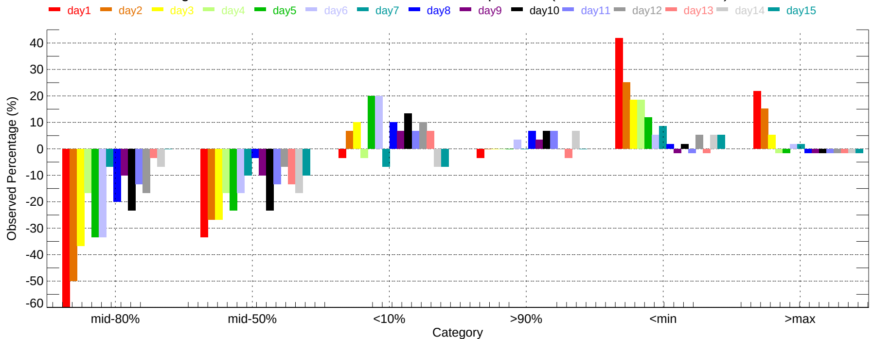
Observed Percentage Deviation of Ensembles - CON: Max Temperature (2007-12-01~2007-12-31)
