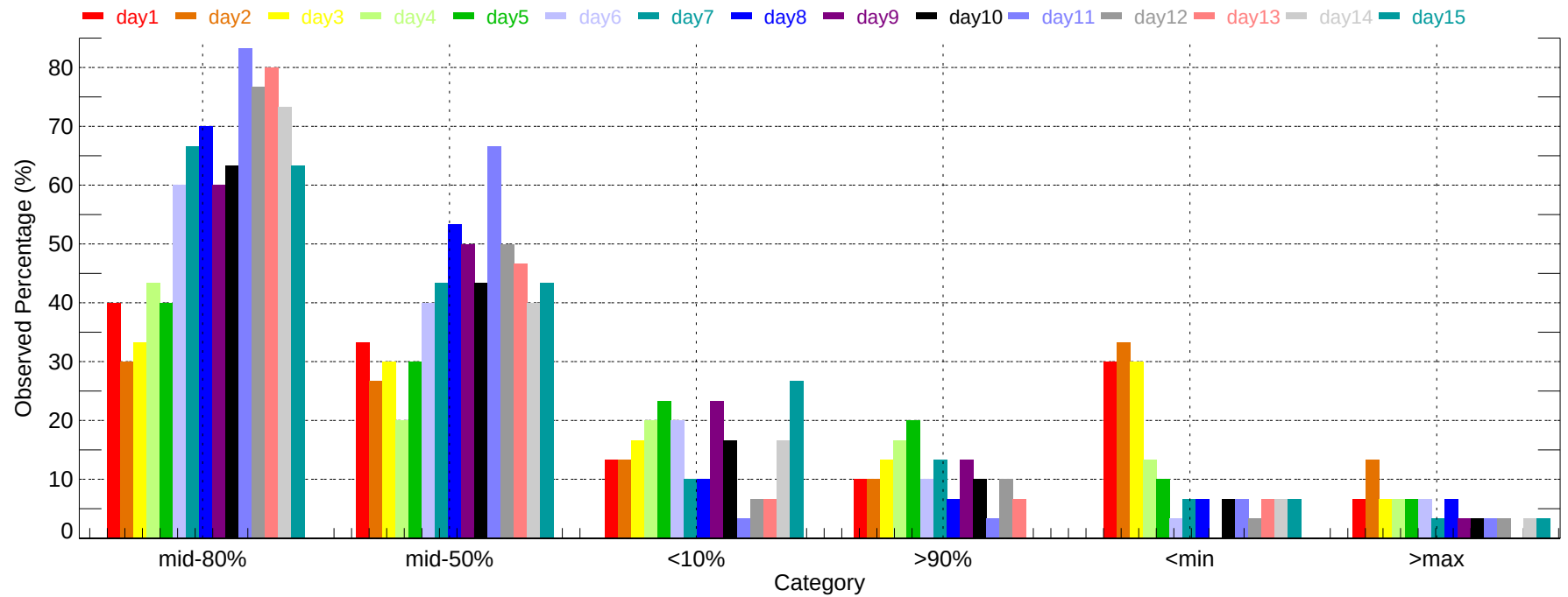
Observed Percentage of Ensembles - SFO: Max Temperature (2007-12-01~2007-12-31)
