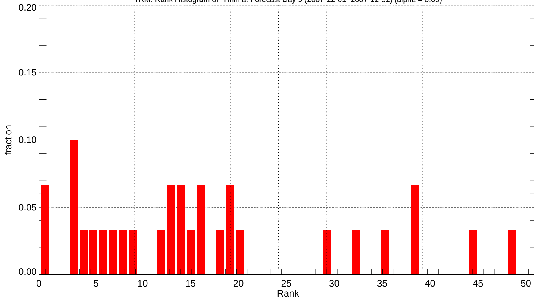
TRM: Rank Histogram of Tmin at Forecast Day 9 (2007-12-01~2007-12-31) (alpha = 0.00)
