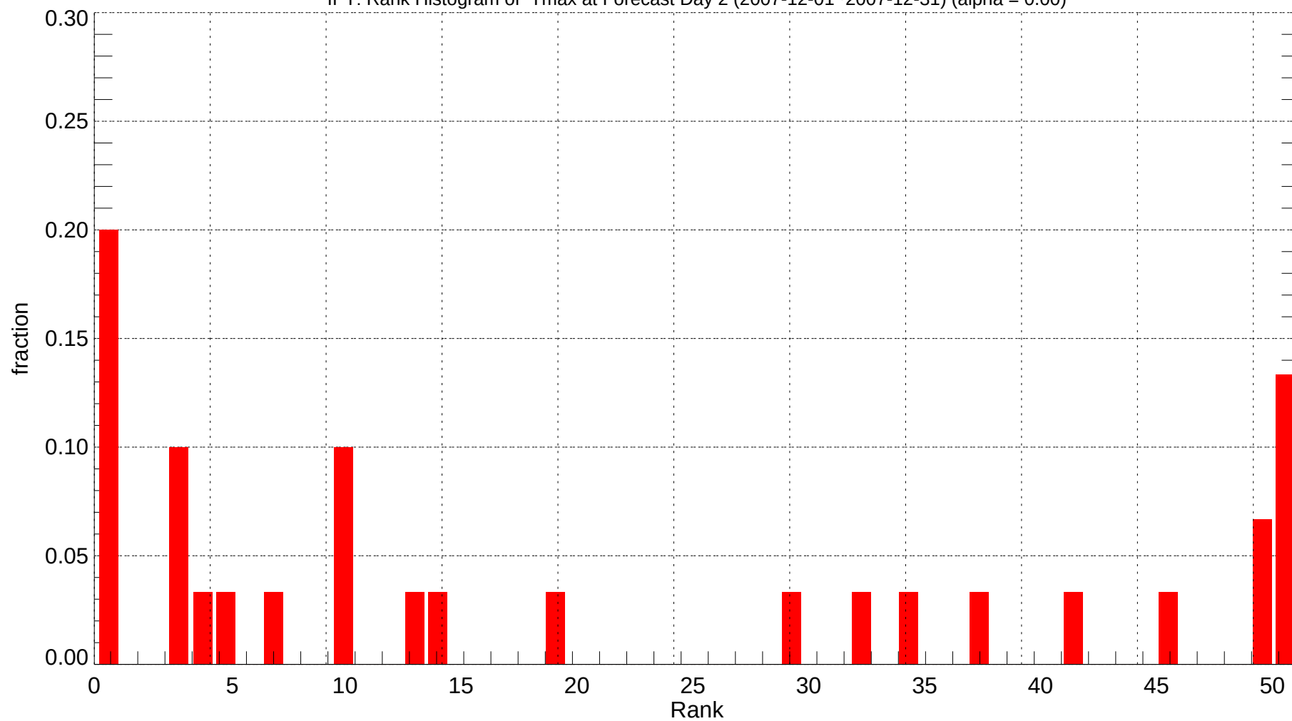
IPT: Rank Histogram of Tmax at Forecast Day 2 (2007-12-01~2007-12-31) (alpha = 0.00)
