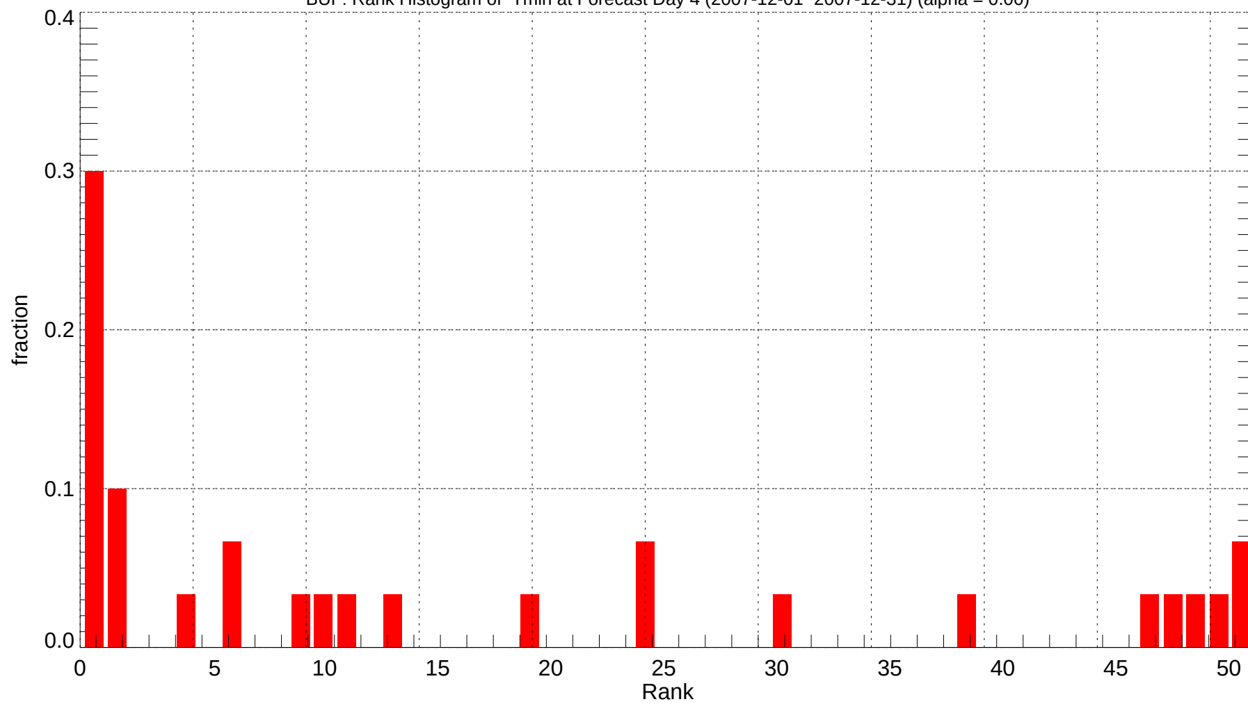
BUF: Rank Histogram of Tmin at Forecast Day 4 (2007-12-01~2007-12-31) (alpha = 0.00)
