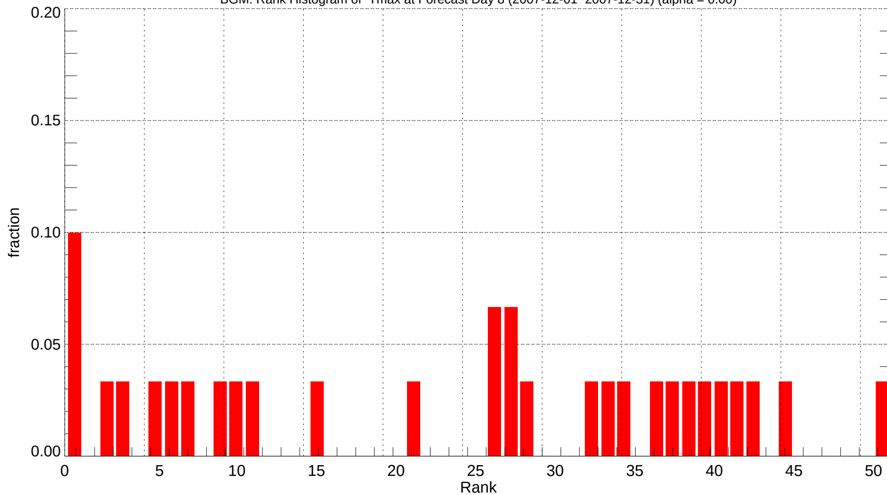
BGM: Rank Histogram of Tmax at Forecast Day 8 (2007-12-01~2007-12-31) (alpha = 0.00)
