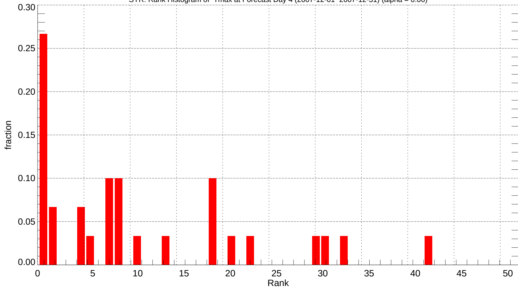
SYR: Rank Histogram of Tmax at Forecast Day 4 (2007-12-01~2007-12-31) (alpha = 0.00)
