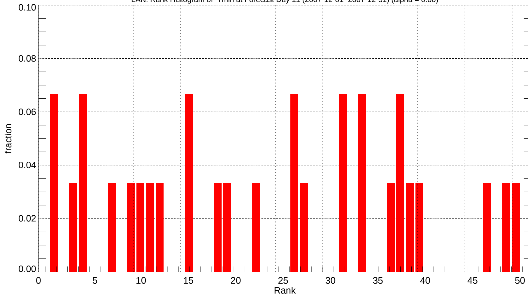
LAN: Rank Histogram of Tmin at Forecast Day 11 (2007-12-01~2007-12-31) (alpha = 0.00)
