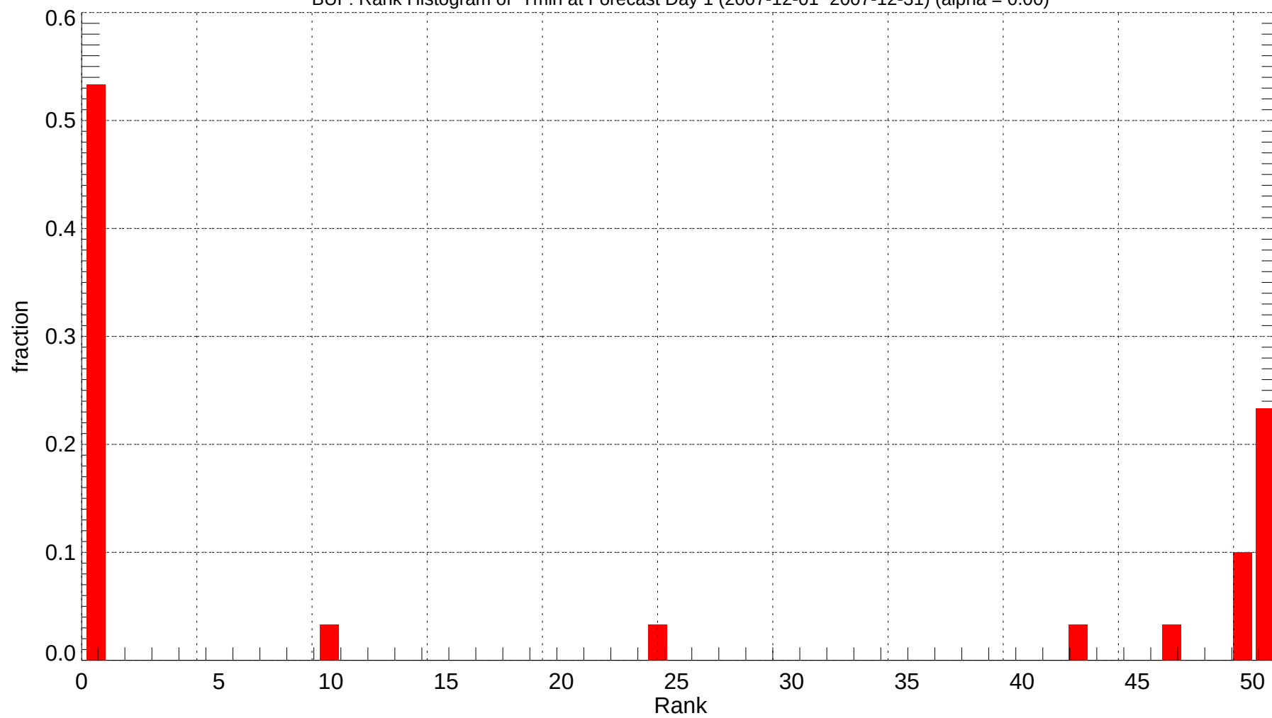
BUF: Rank Histogram of Tmin at Forecast Day 1 (2007-12-01~2007-12-31) (alpha = 0.00)
