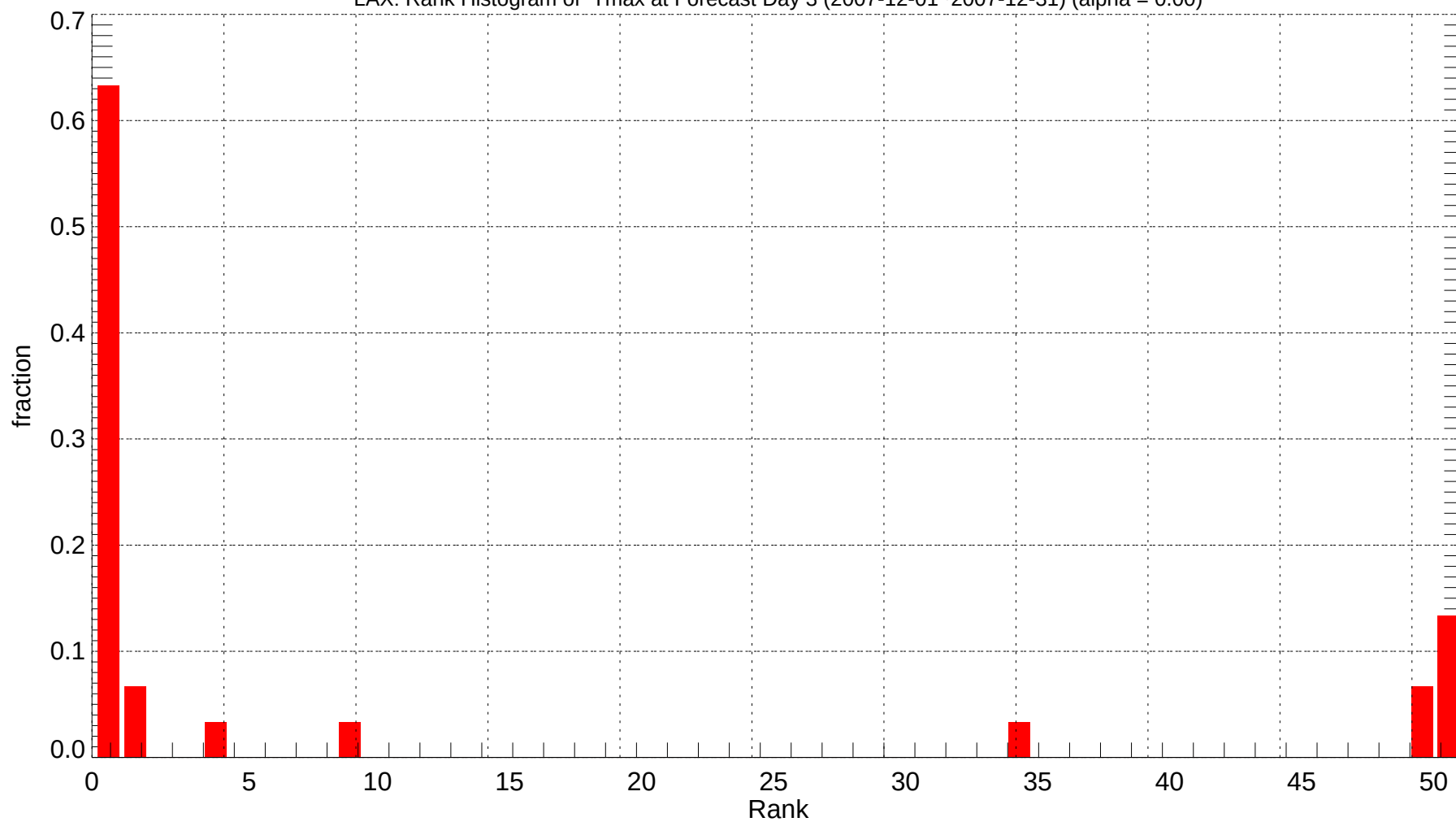
LAX: Rank Histogram of Tmax at Forecast Day 3 (2007-12-01~2007-12-31) (alpha = 0.00)
