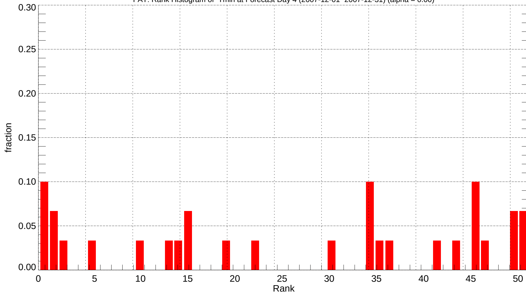
FAT: Rank Histogram of Tmin at Forecast Day 4 (2007-12-01~2007-12-31) (alpha = 0.00)
