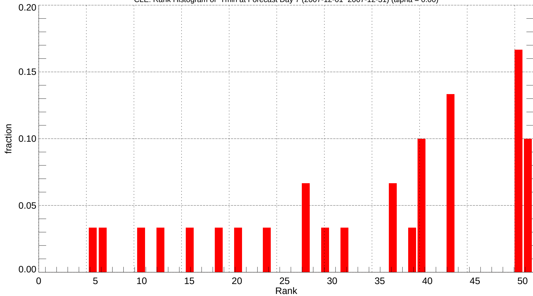
CLE: Rank Histogram of Tmin at Forecast Day 7 (2007-12-01~2007-12-31) (alpha = 0.00)
