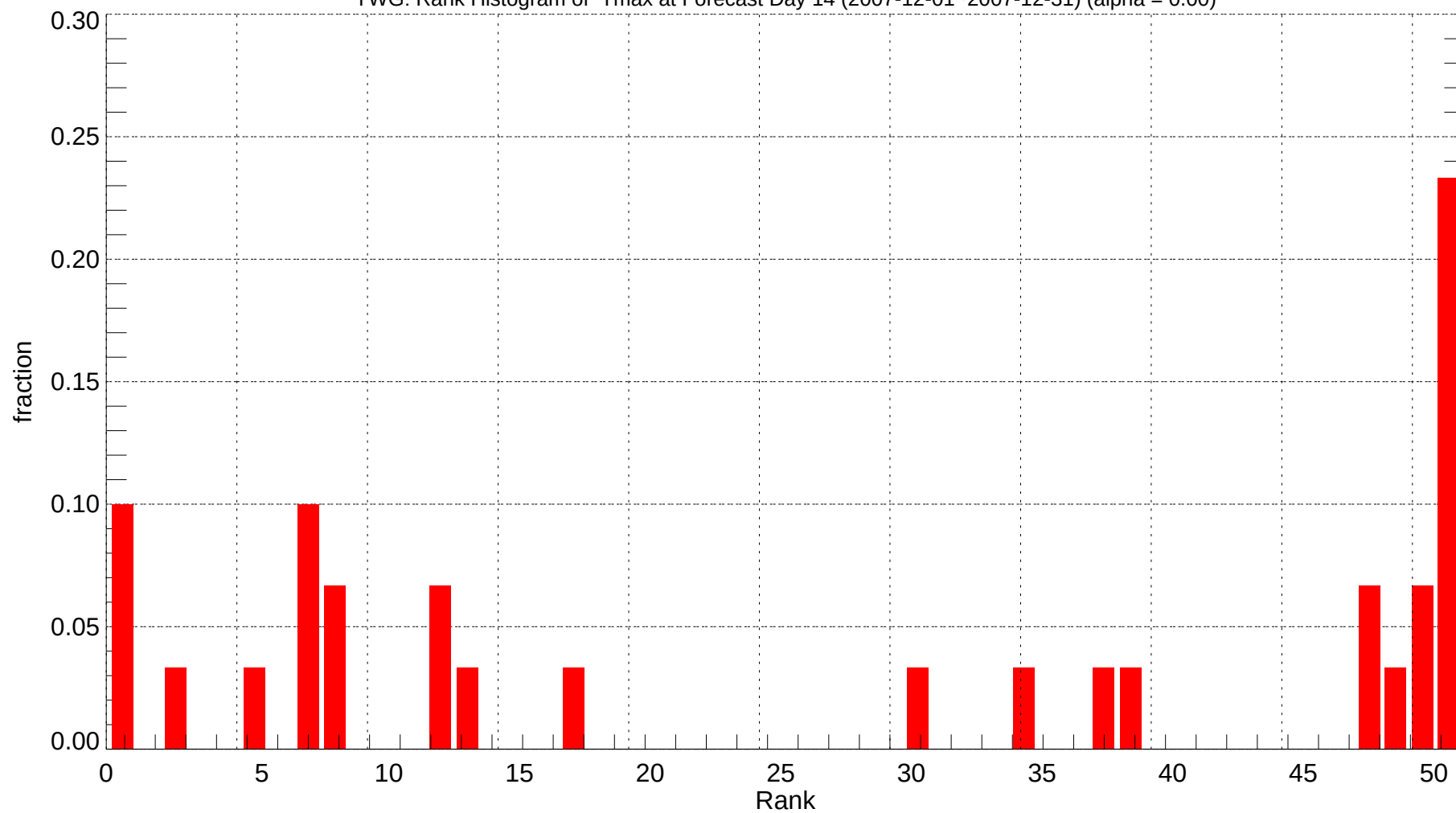
YWG: Rank Histogram of Tmax at Forecast Day 14 (2007-12-01~2007-12-31) (alpha = 0.00)
