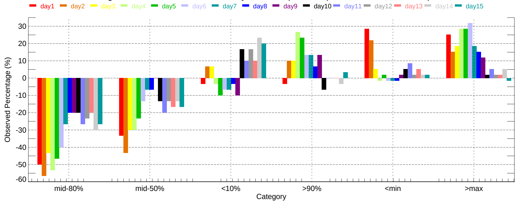
Observed Percentage Deviation of Ensembles - ABQ: Max Temperature (2007-12-01~2007-12-31)
