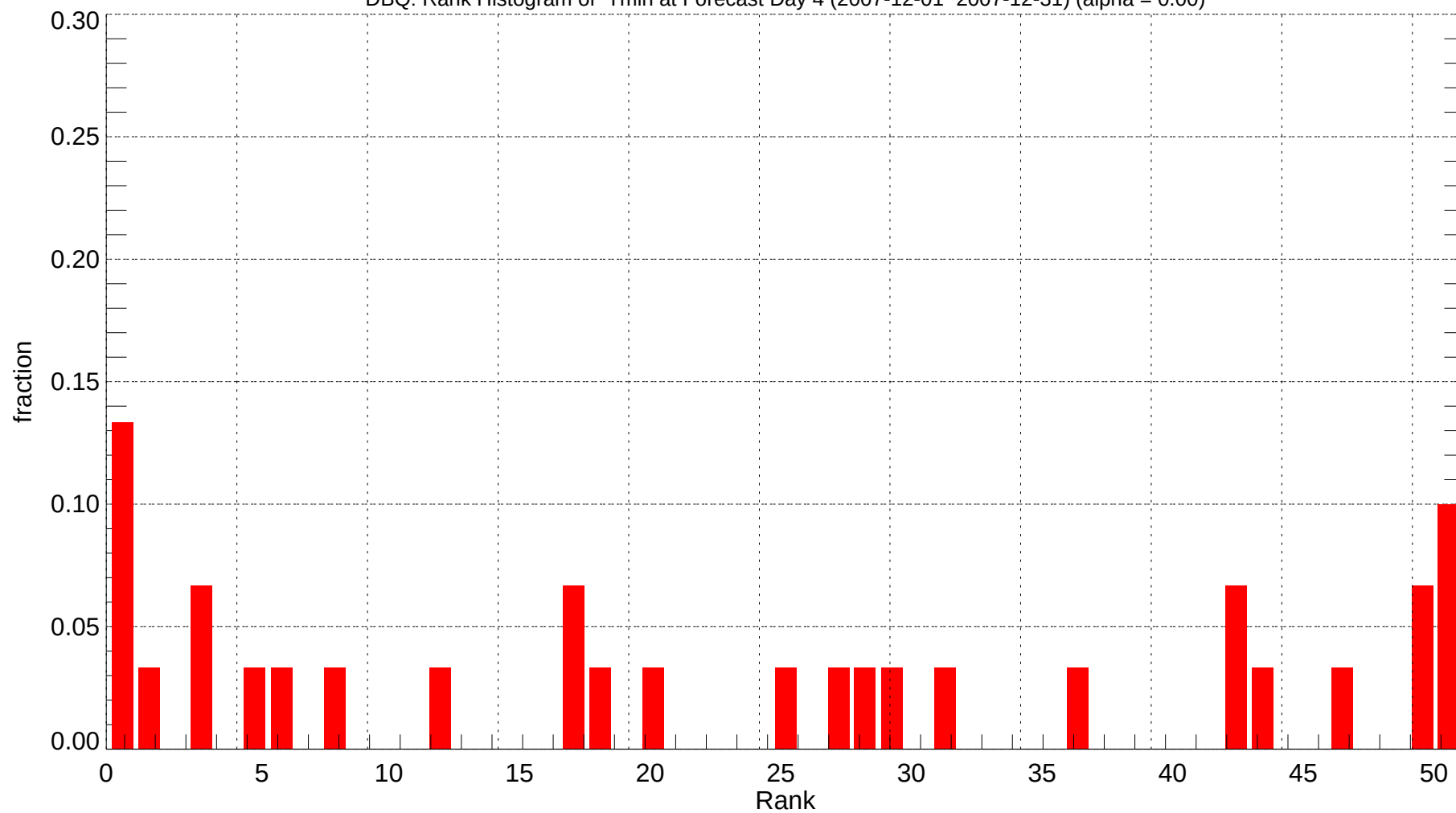
DBQ: Rank Histogram of Tmin at Forecast Day 4 (2007-12-01~2007-12-31) (alpha = 0.00)
