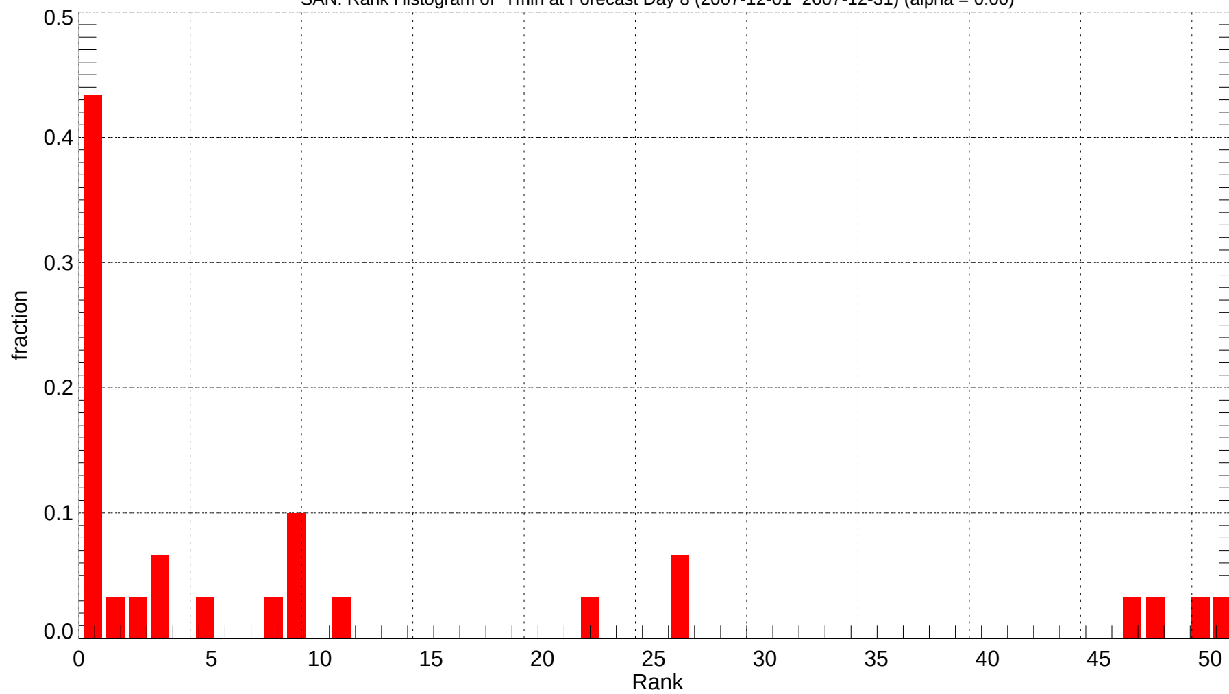
SAN: Rank Histogram of Tmin at Forecast Day 8 (2007-12-01~2007-12-31) (alpha = 0.00)
