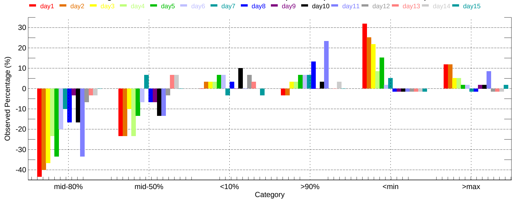
Observed Percentage Deviation of Ensembles - ABE: Max Temperature (2007-12-01~2007-12-31)
