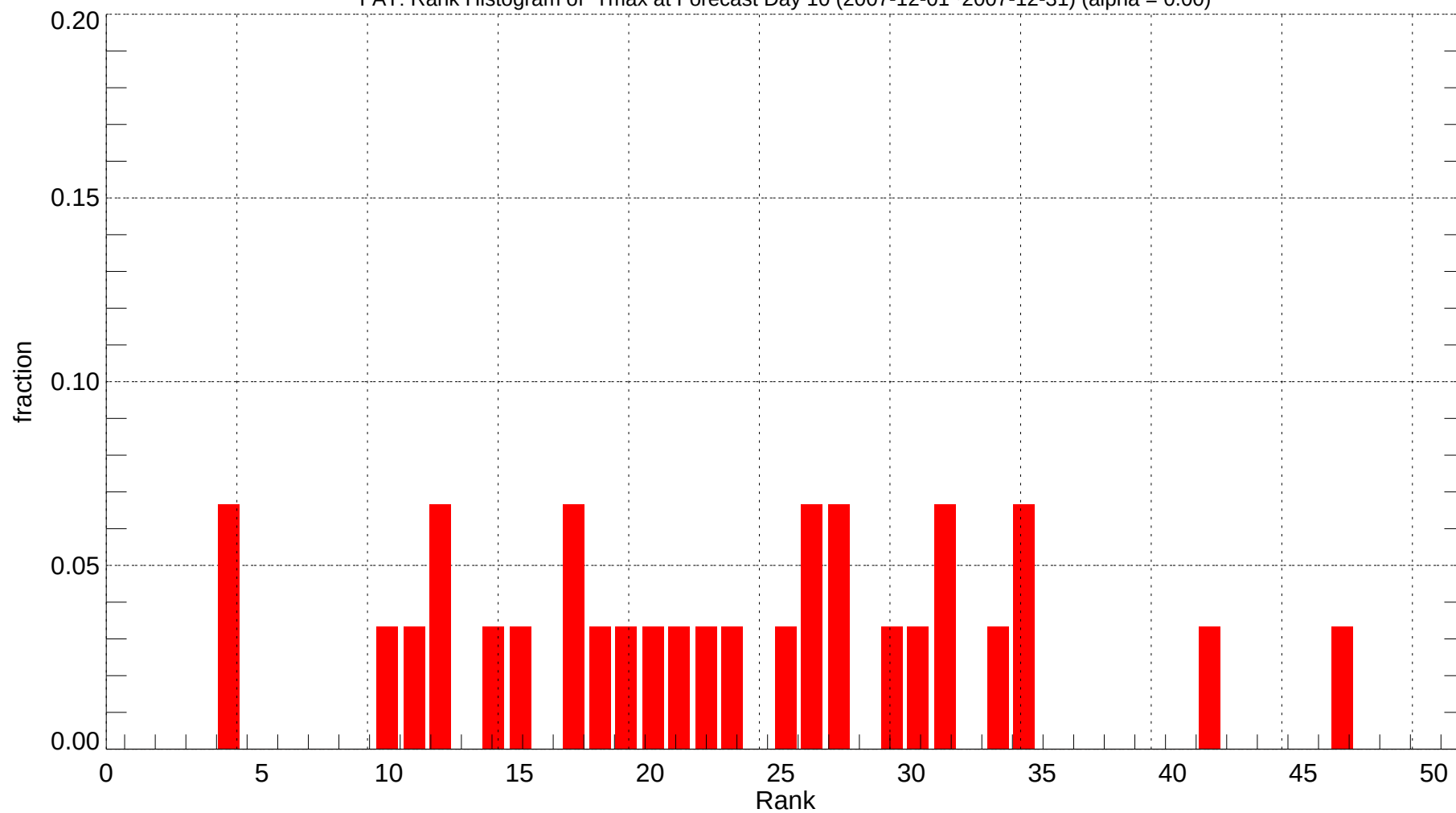
FAT: Rank Histogram of Tmax at Forecast Day 10 (2007-12-01~2007-12-31) (alpha = 0.00)
