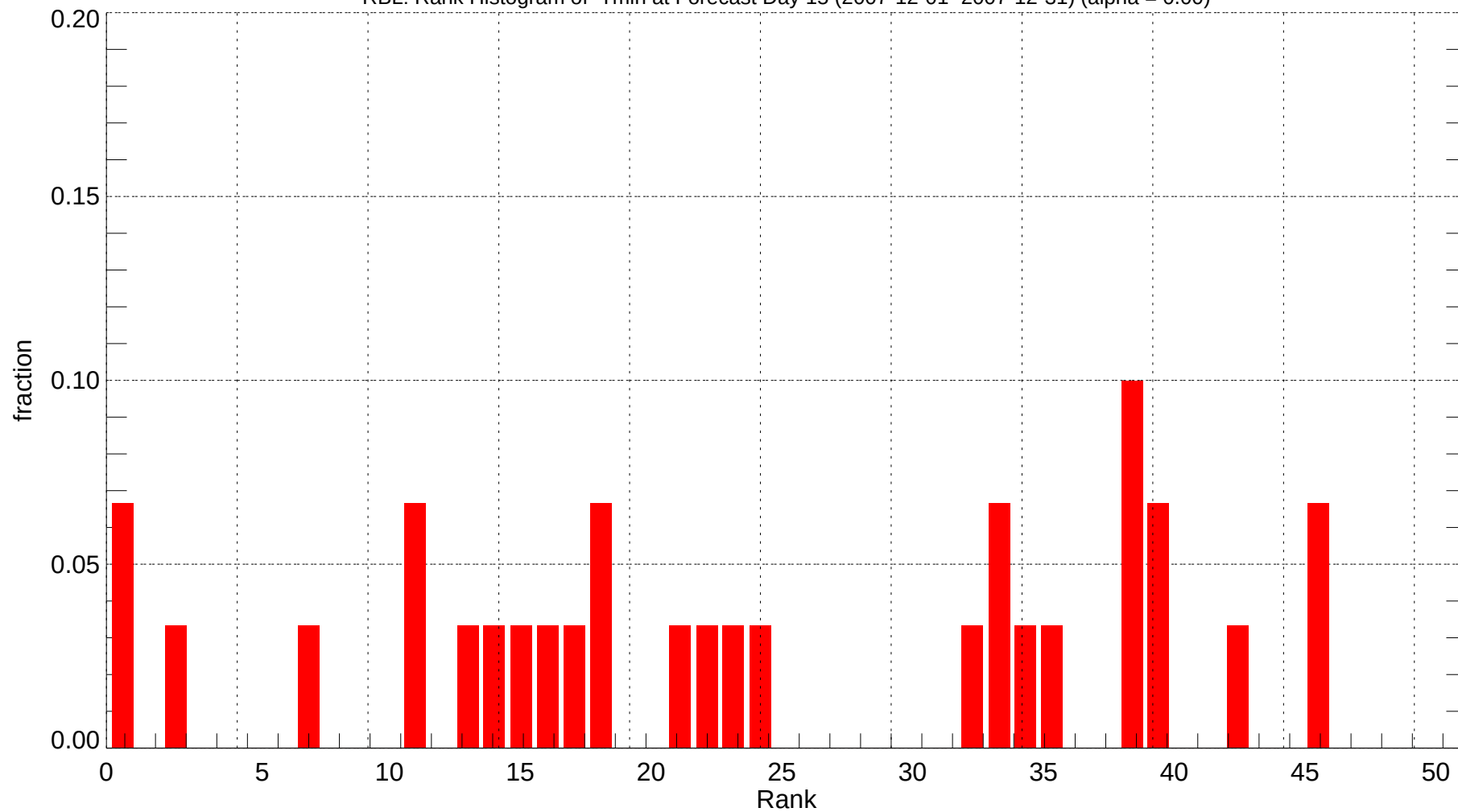
RBL: Rank Histogram of Tmin at Forecast Day 15 (2007-12-01~2007-12-31) (alpha = 0.00)
