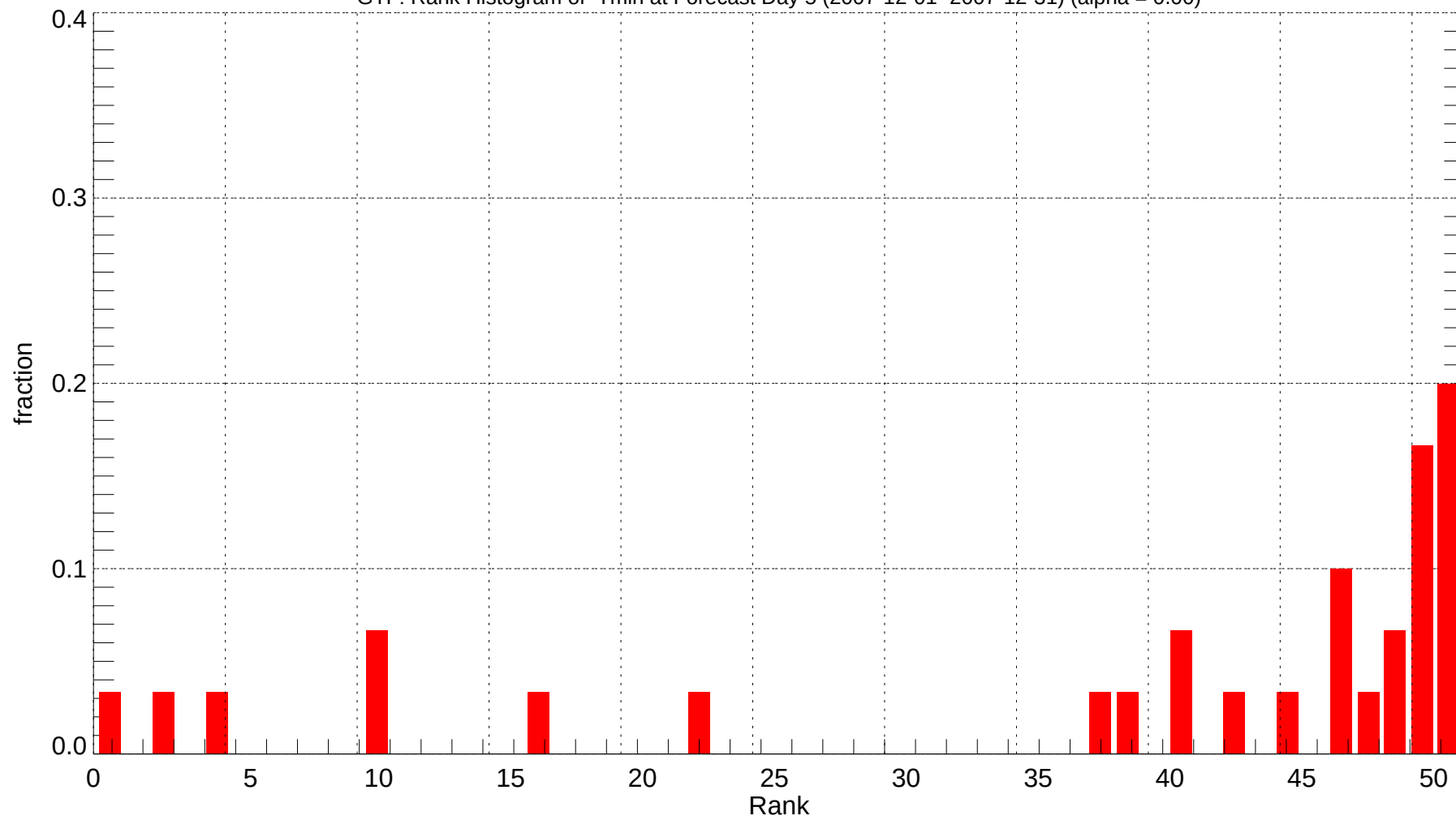
GTF: Rank Histogram of Tmin at Forecast Day 5 (2007-12-01~2007-12-31) (alpha = 0.00)
