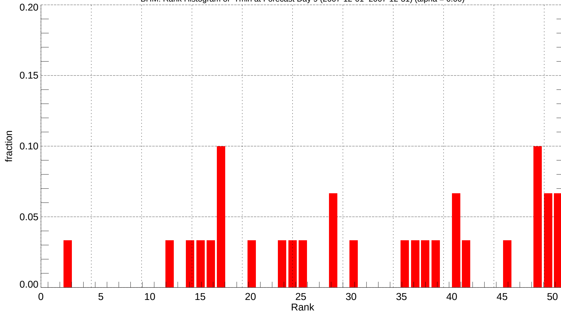
BHM: Rank Histogram of Tmin at Forecast Day 9 (2007-12-01~2007-12-31) (alpha = 0.00)
