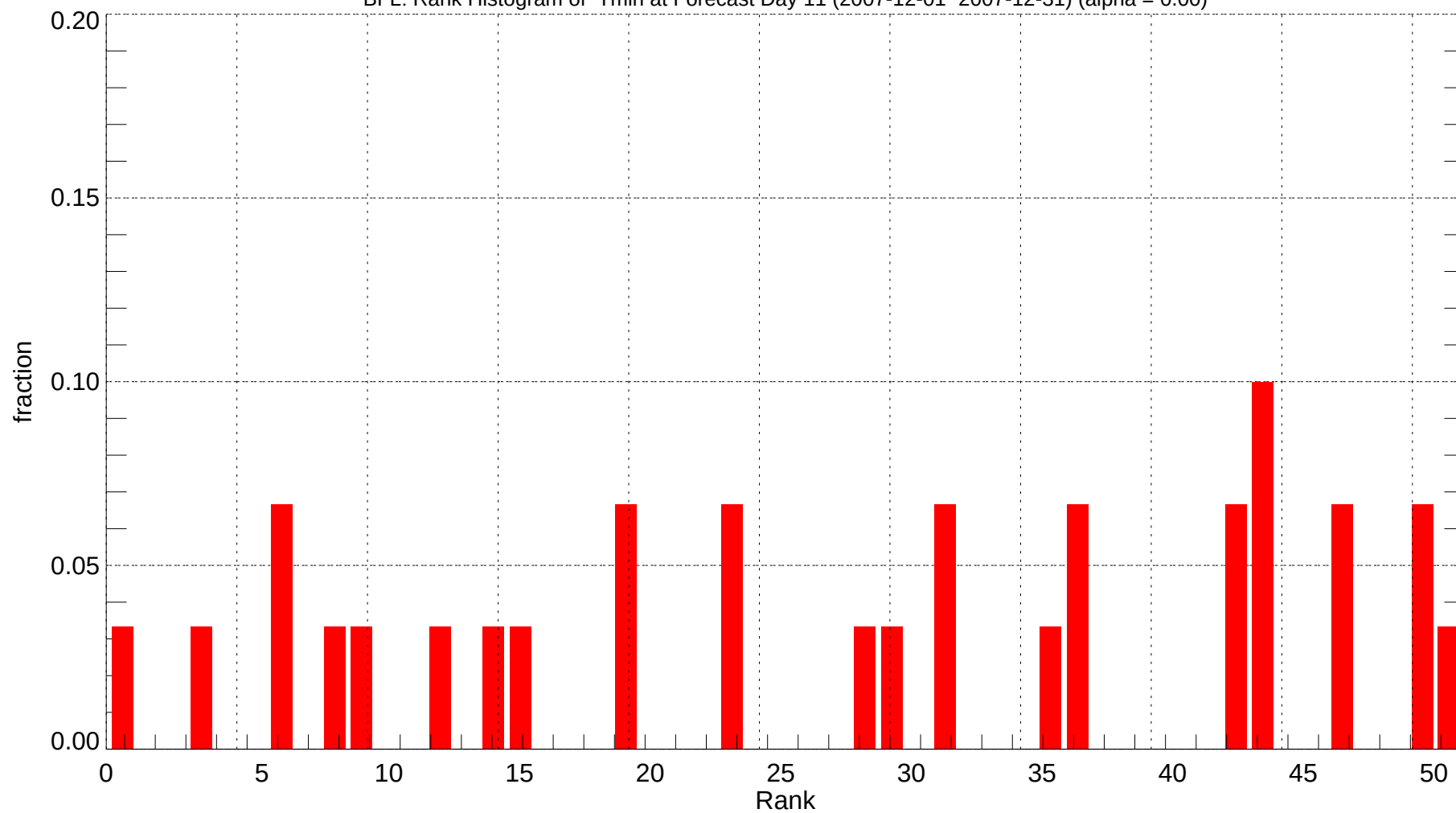
BFL: Rank Histogram of Tmin at Forecast Day 11 (2007-12-01~2007-12-31) (alpha = 0.00)
