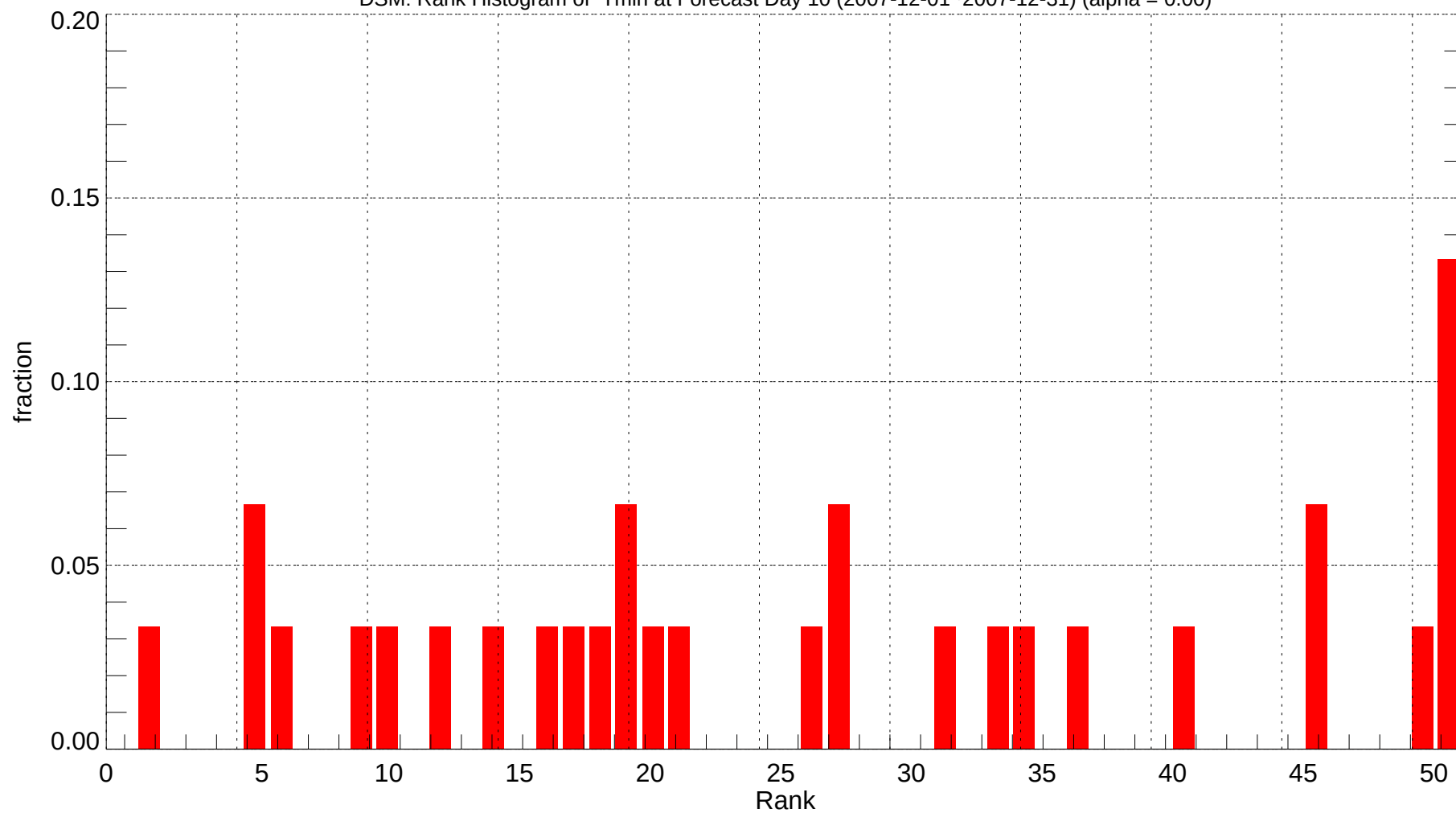
DSM: Rank Histogram of Tmin at Forecast Day 10 (2007-12-01~2007-12-31) (alpha = 0.00)
