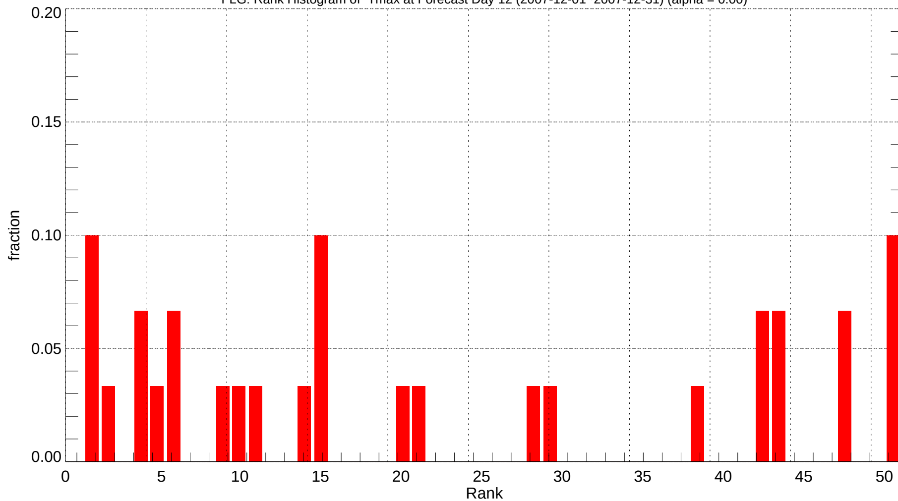
FLG: Rank Histogram of Tmax at Forecast Day 12 (2007-12-01~2007-12-31) (alpha = 0.00)
