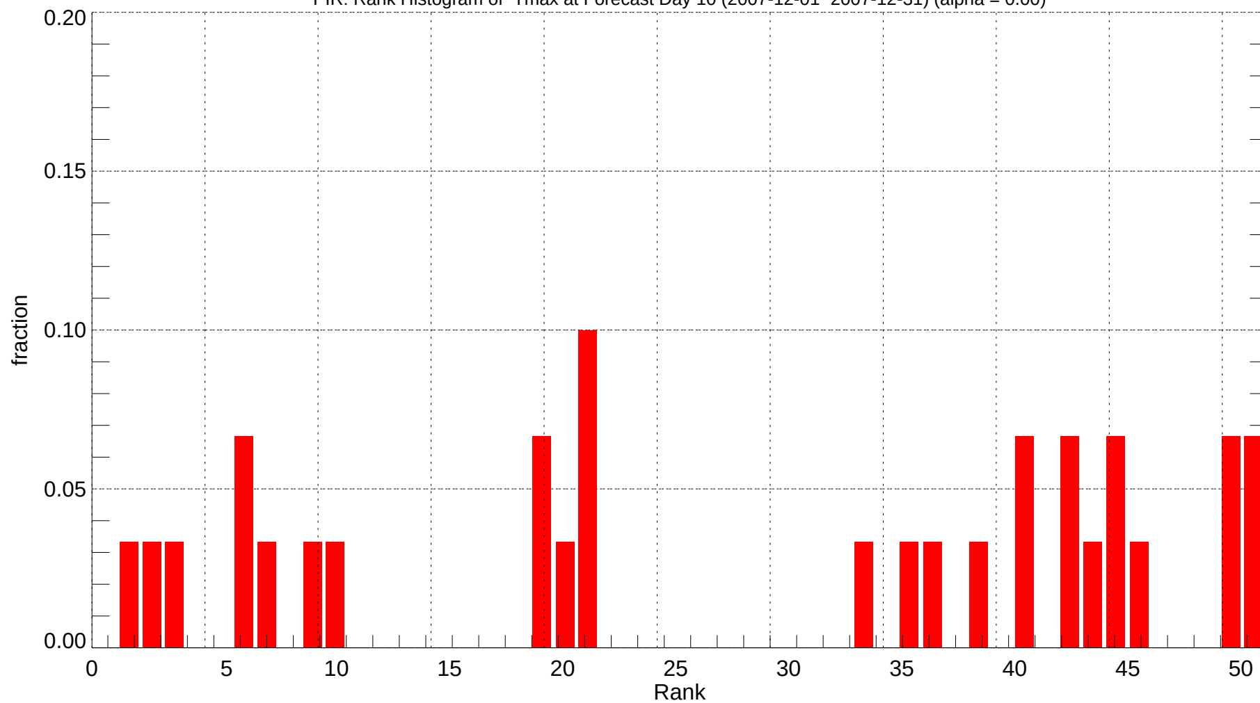
PIR: Rank Histogram of Tmax at Forecast Day 10 (2007-12-01~2007-12-31) (alpha = 0.00)
