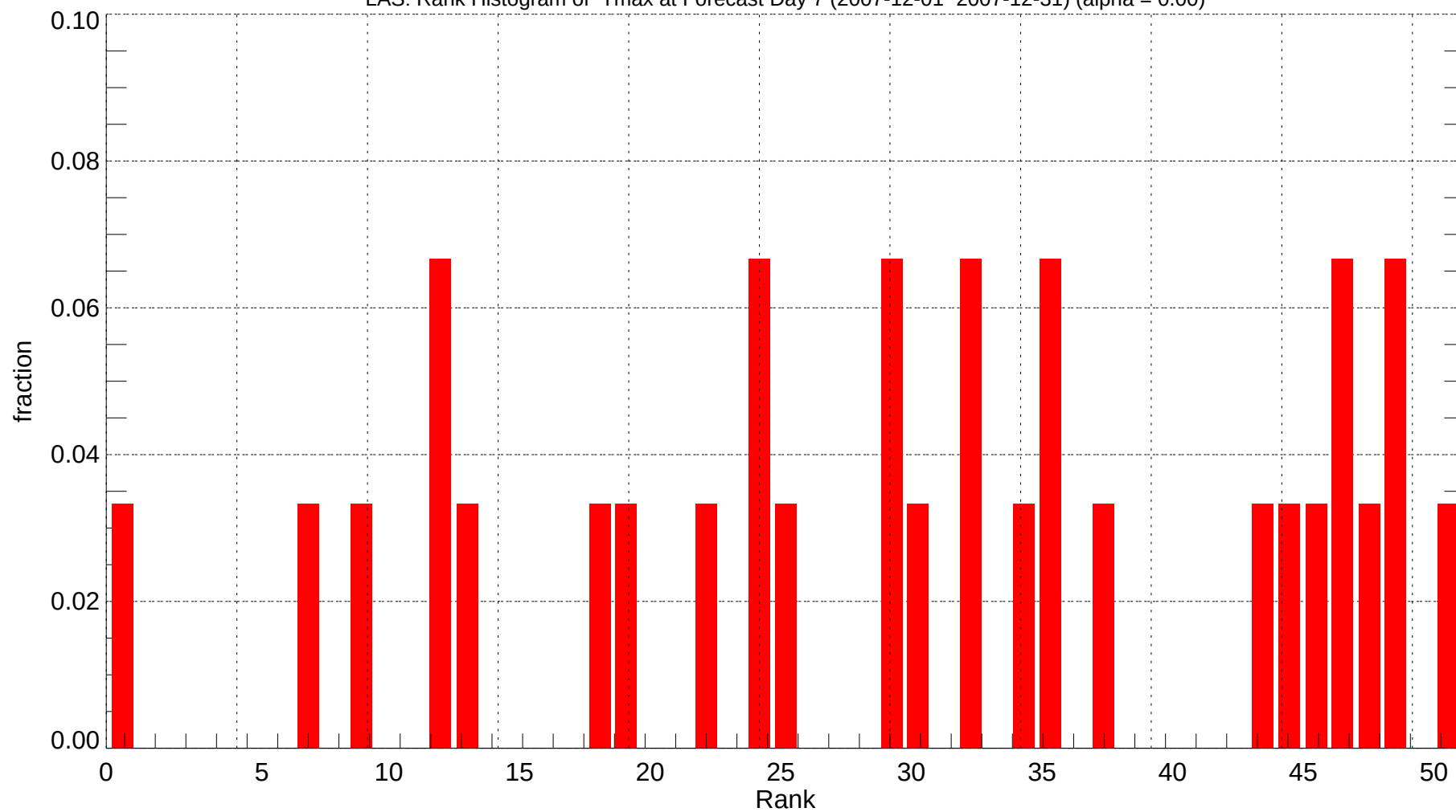
LAS: Rank Histogram of Tmax at Forecast Day 7 (2007-12-01~2007-12-31) (alpha = 0.00)
