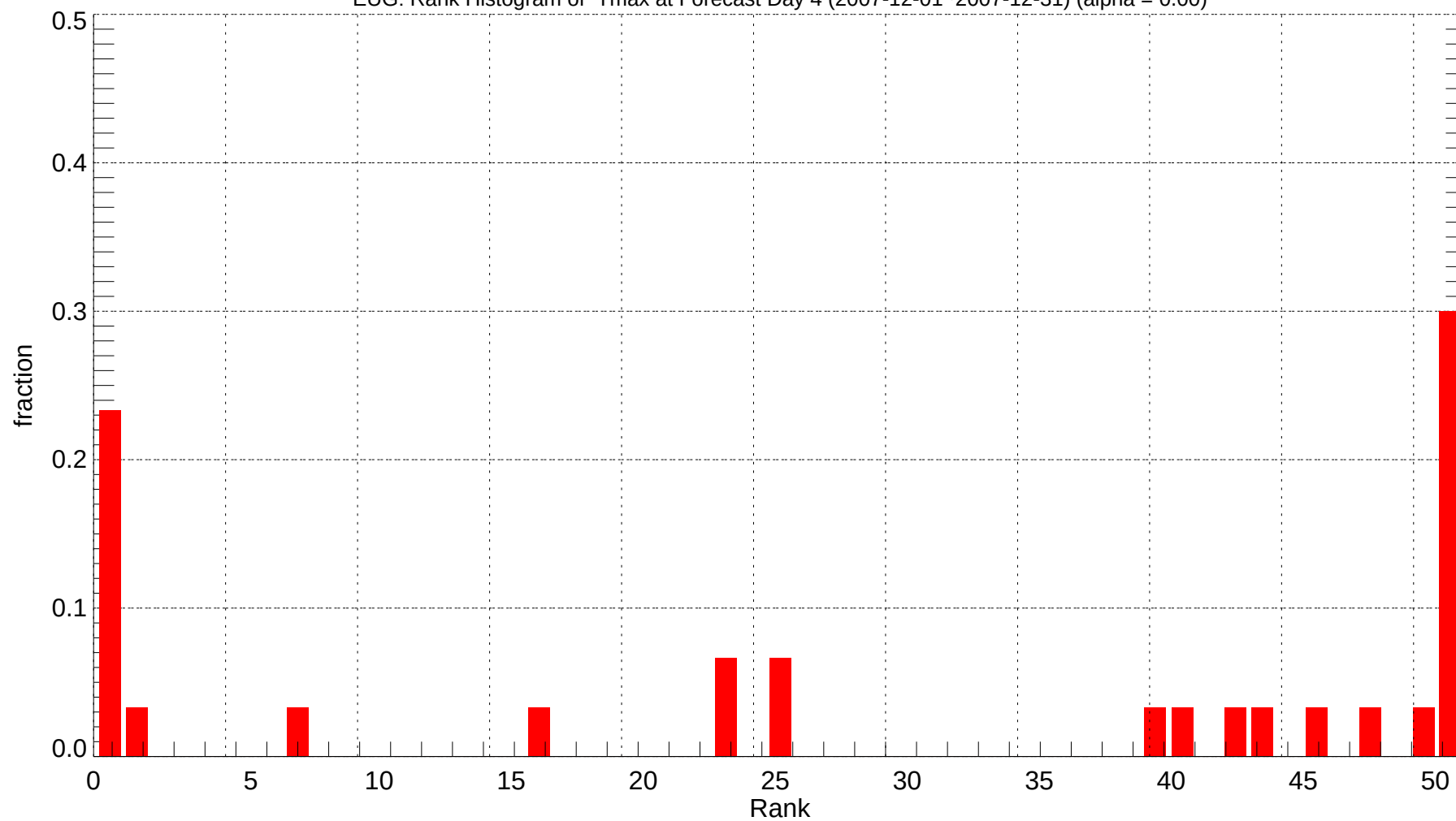
EUG: Rank Histogram of Tmax at Forecast Day 4 (2007-12-01~2007-12-31) (alpha = 0.00)
