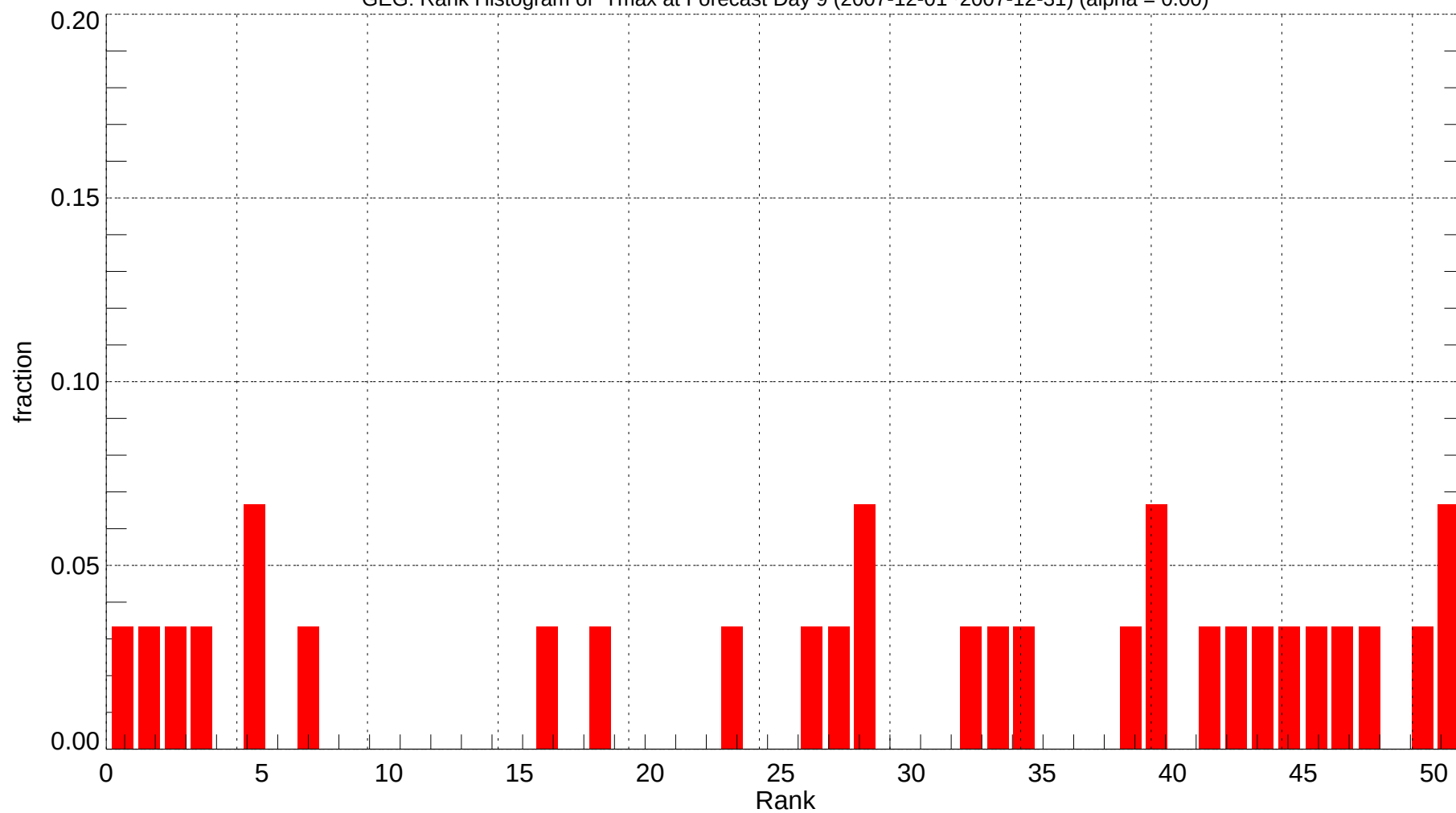
GEG: Rank Histogram of Tmax at Forecast Day 9 (2007-12-01~2007-12-31) (alpha = 0.00)
