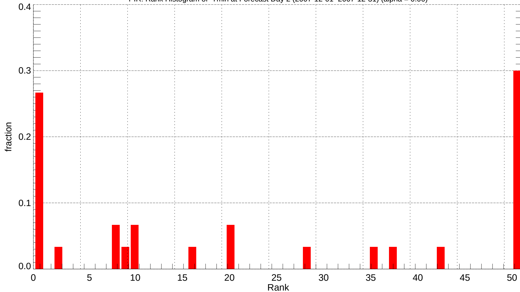
PIR: Rank Histogram of Tmin at Forecast Day 2 (2007-12-01~2007-12-31) (alpha = 0.00)
