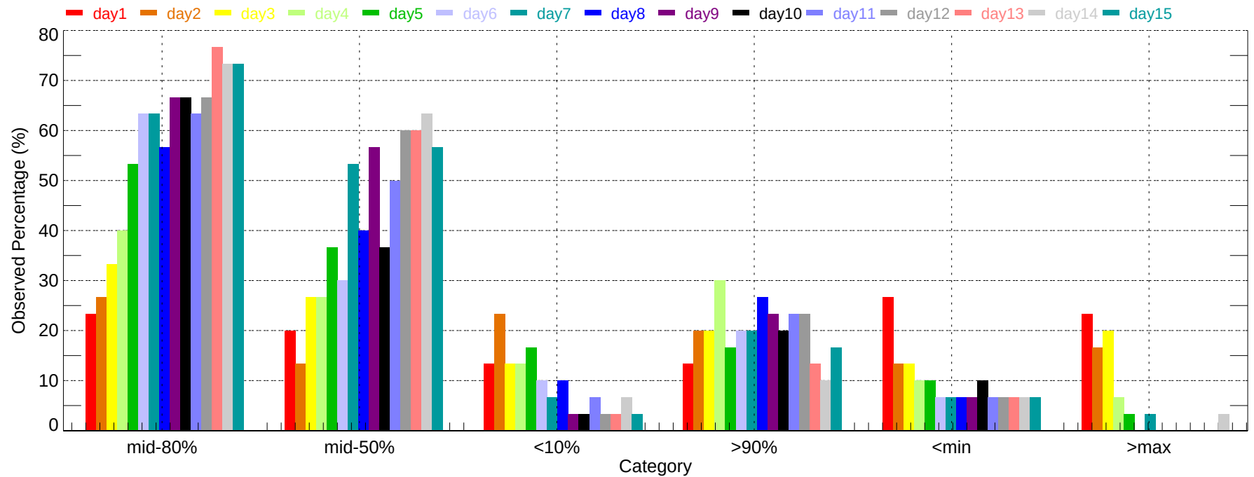
Observed Percentage of Ensembles - RBL: Min Temperature (2007-12-01~2007-12-31)
