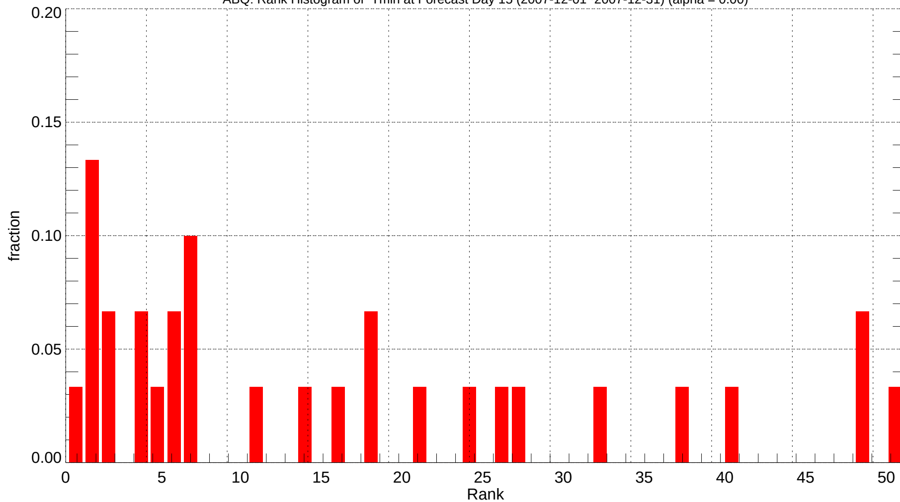
ABQ: Rank Histogram of Tmin at Forecast Day 15 (2007-12-01~2007-12-31) (alpha = 0.00)
