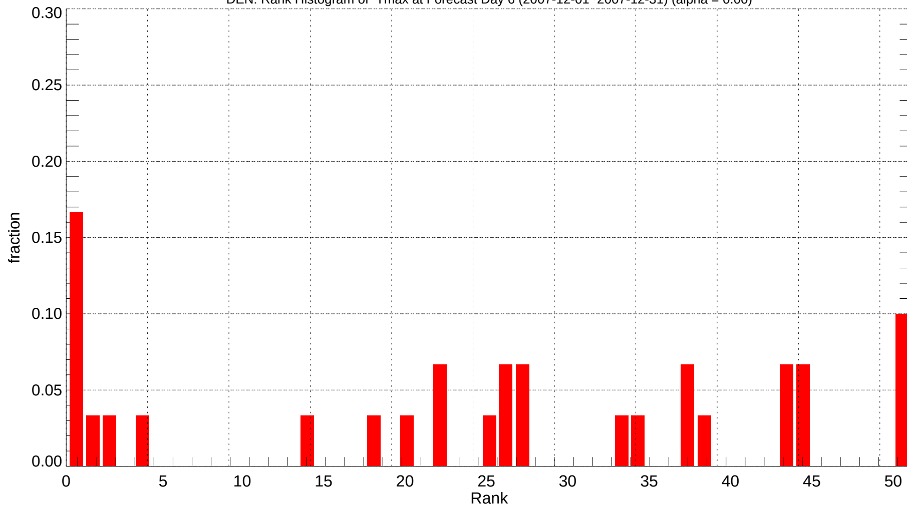
DEN: Rank Histogram of Tmax at Forecast Day 6 (2007-12-01~2007-12-31) (alpha = 0.00)
