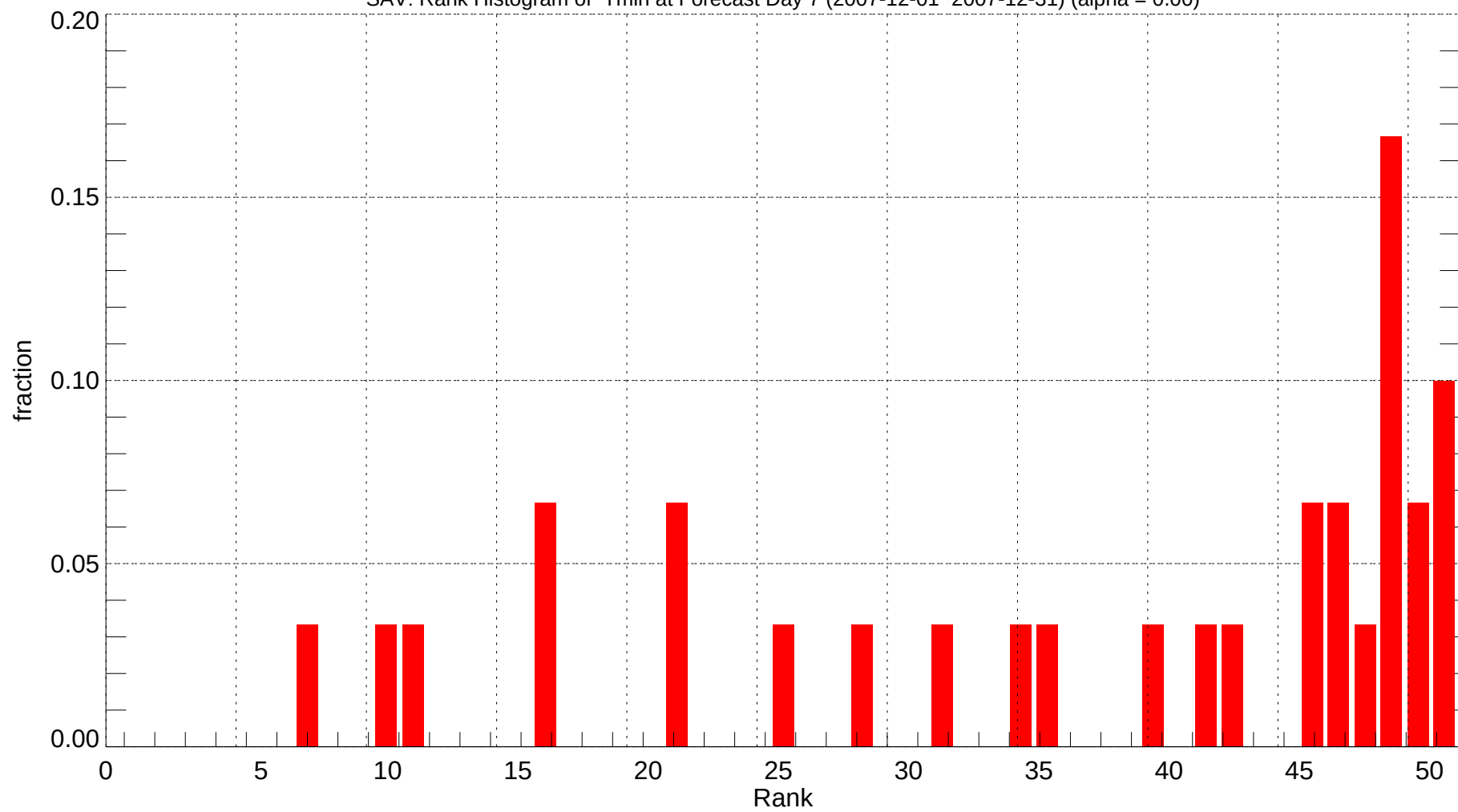
SAV: Rank Histogram of Tmin at Forecast Day 7 (2007-12-01~2007-12-31) (alpha = 0.00)
