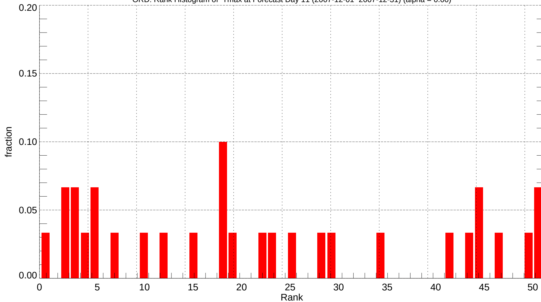
ORD: Rank Histogram of Tmax at Forecast Day 11 (2007-12-01~2007-12-31) (alpha = 0.00)
