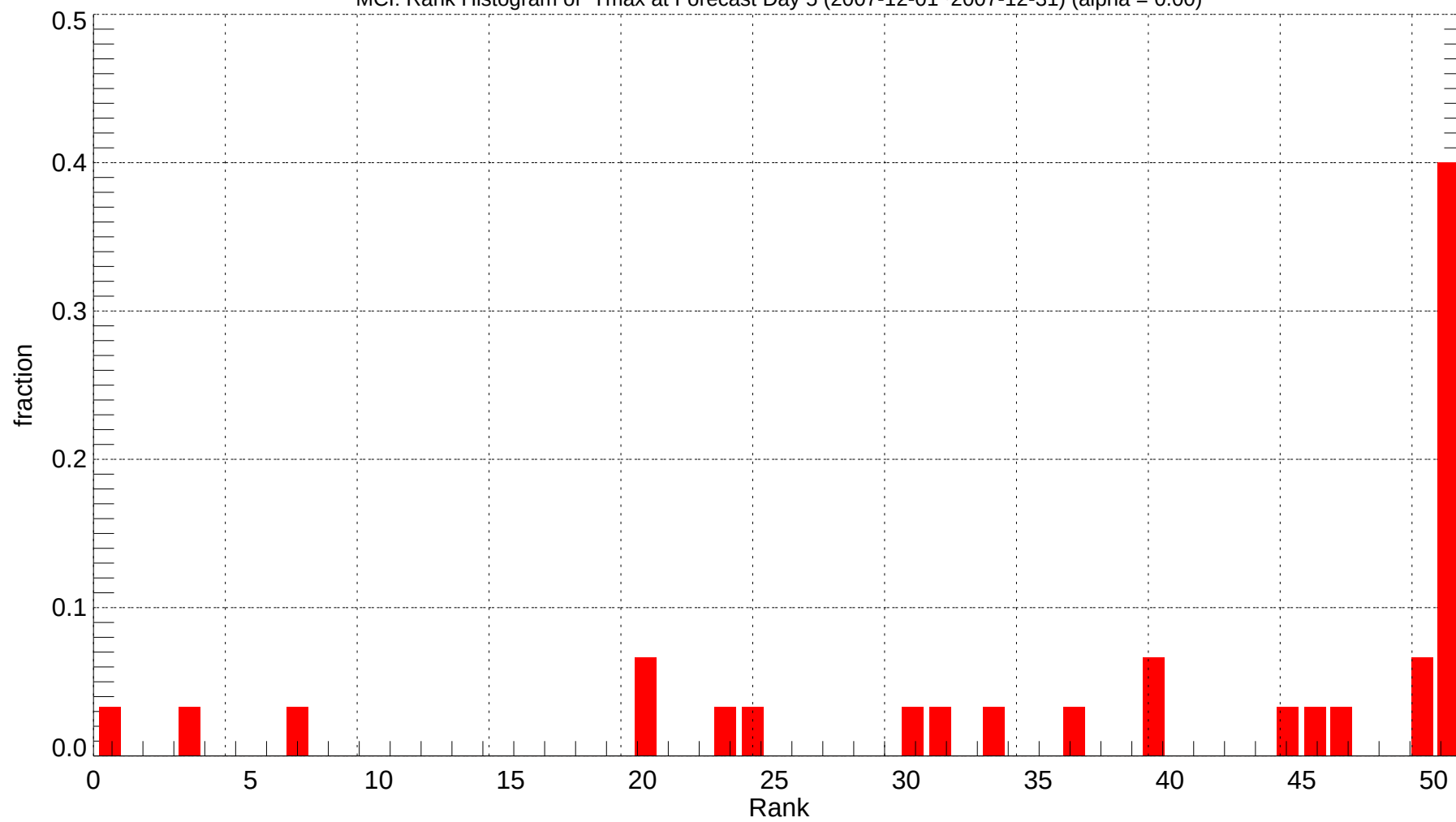
MCI: Rank Histogram of Tmax at Forecast Day 5 (2007-12-01~2007-12-31) (alpha = 0.00)
