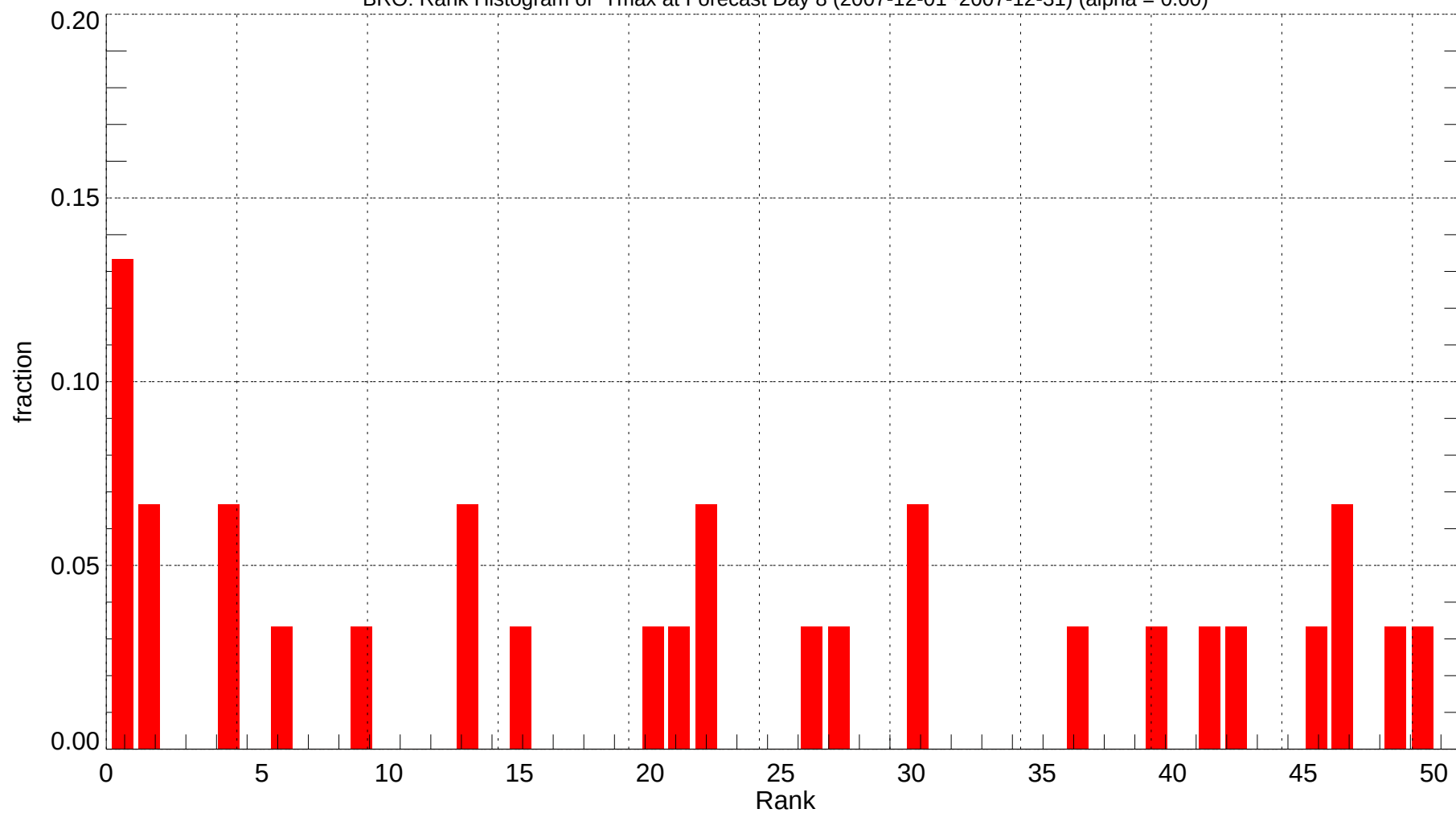
BRO: Rank Histogram of Tmax at Forecast Day 8 (2007-12-01~2007-12-31) (alpha = 0.00)
