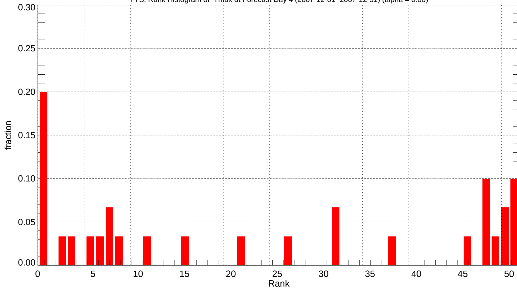
TYS: Rank Histogram of Tmax at Forecast Day 4 (2007-12-01~2007-12-31) (alpha = 0.00)
