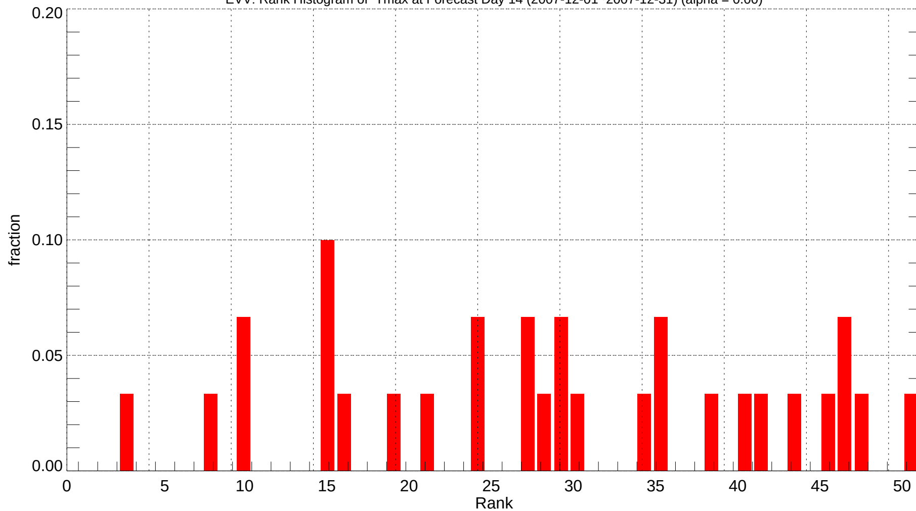
EVV: Rank Histogram of Tmax at Forecast Day 14 (2007-12-01~2007-12-31) (alpha = 0.00)
