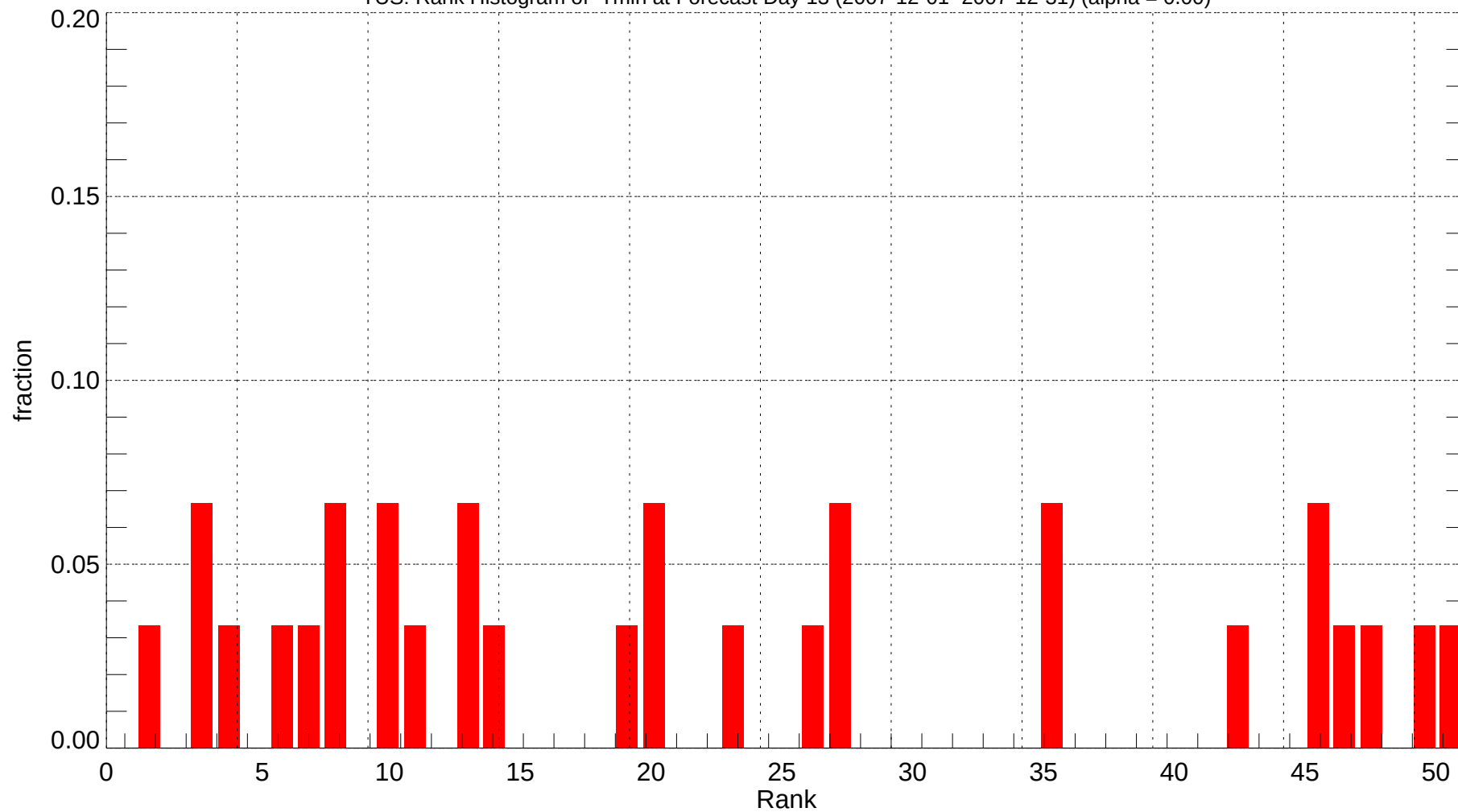
TUS: Rank Histogram of Tmin at Forecast Day 13 (2007-12-01~2007-12-31) (alpha = 0.00)
