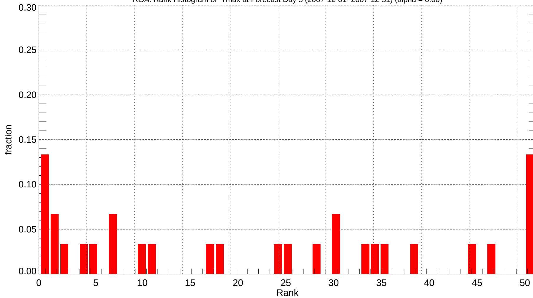
ROA: Rank Histogram of Tmax at Forecast Day 3 (2007-12-01~2007-12-31) (alpha = 0.00)
