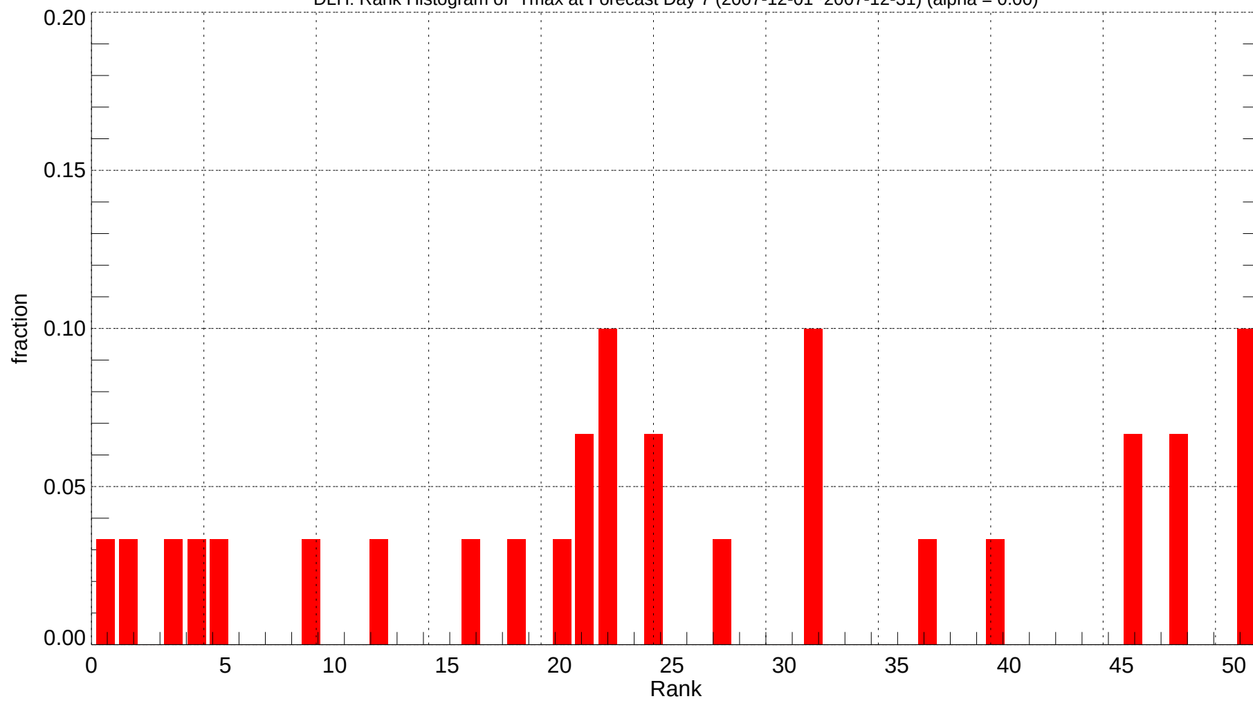
DLH: Rank Histogram of Tmax at Forecast Day 7 (2007-12-01~2007-12-31) (alpha = 0.00)
