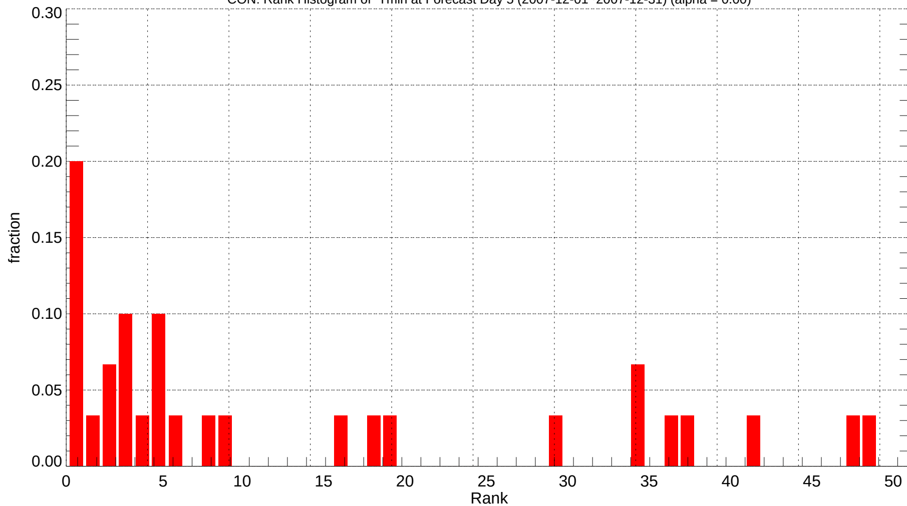
CON: Rank Histogram of Tmin at Forecast Day 5 (2007-12-01~2007-12-31) (alpha = 0.00)
