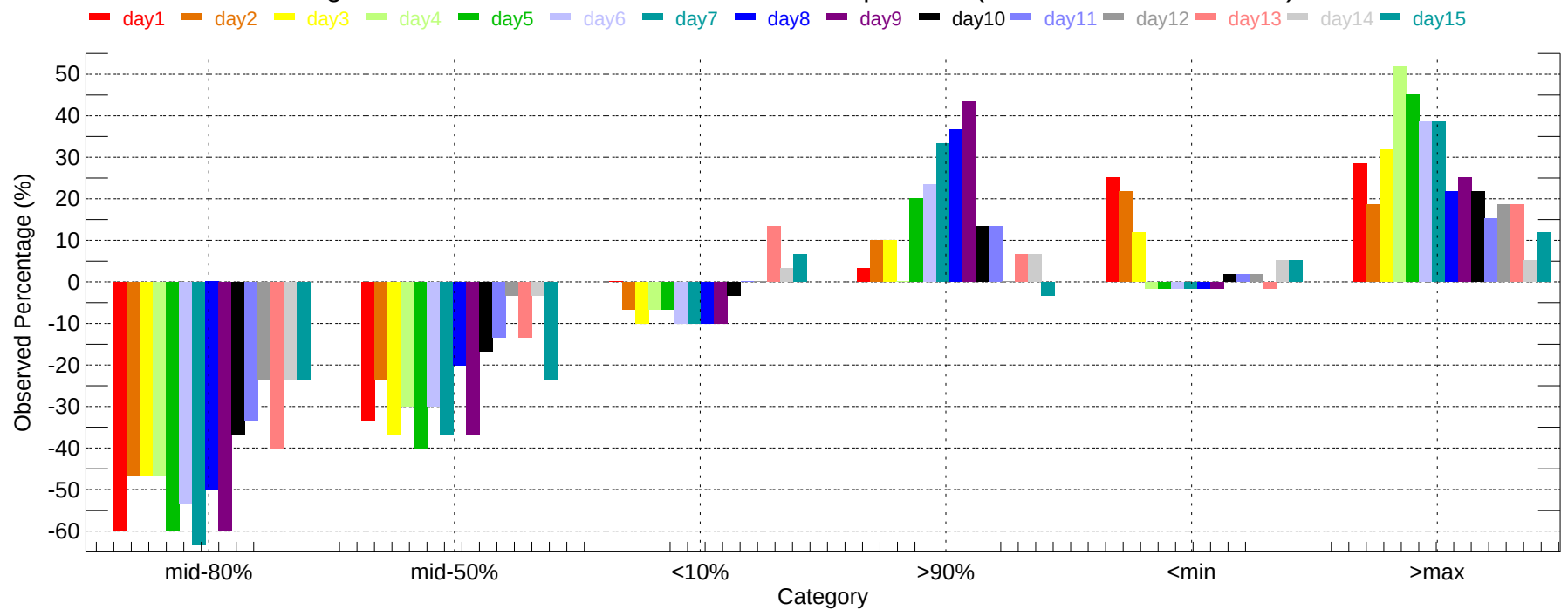
Observed Percentage Deviation of Ensembles - LGB: Min Temperature (2007-12-01~2007-12-31)
