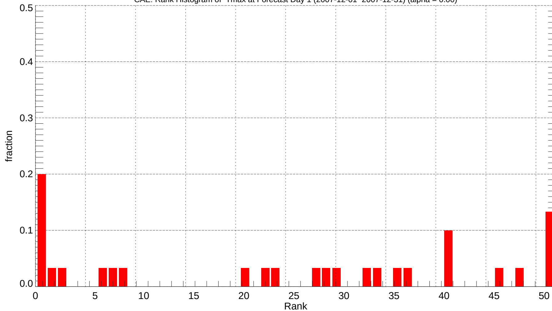
CAE: Rank Histogram of Tmax at Forecast Day 1 (2007-12-01~2007-12-31) (alpha = 0.00)
