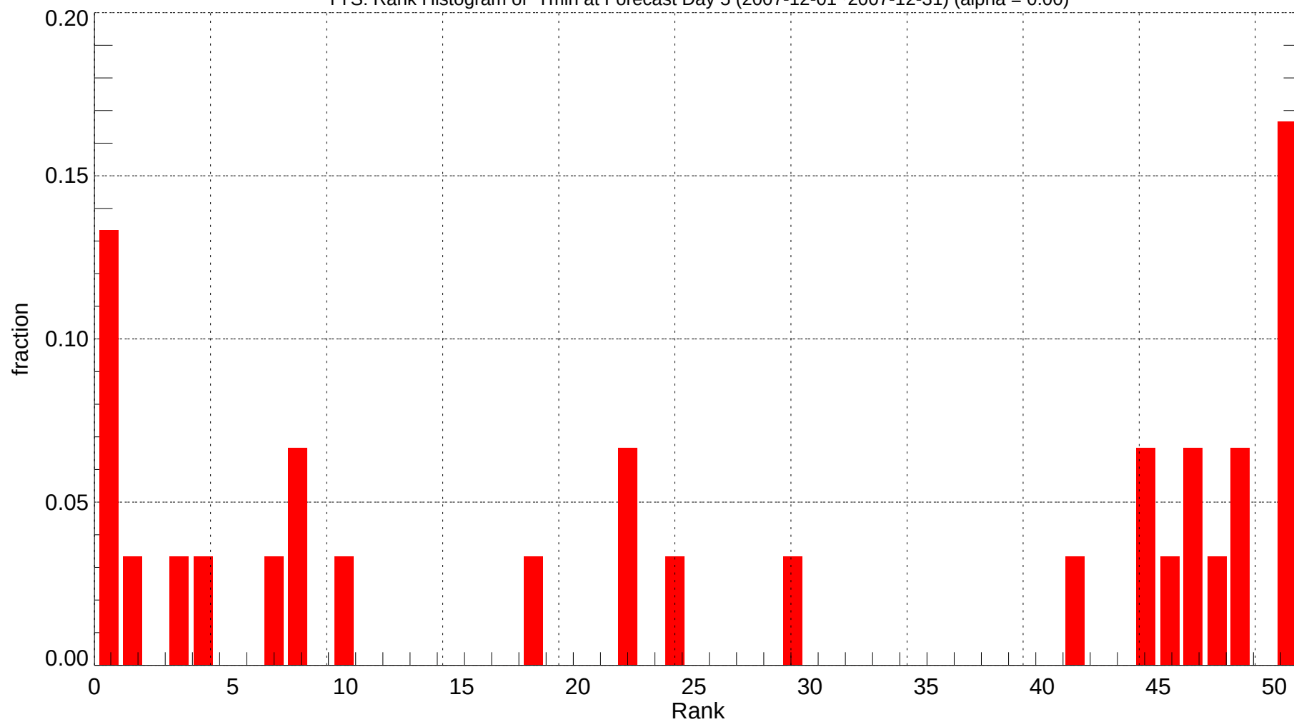
TYS: Rank Histogram of Tmin at Forecast Day 5 (2007-12-01~2007-12-31) (alpha = 0.00)
