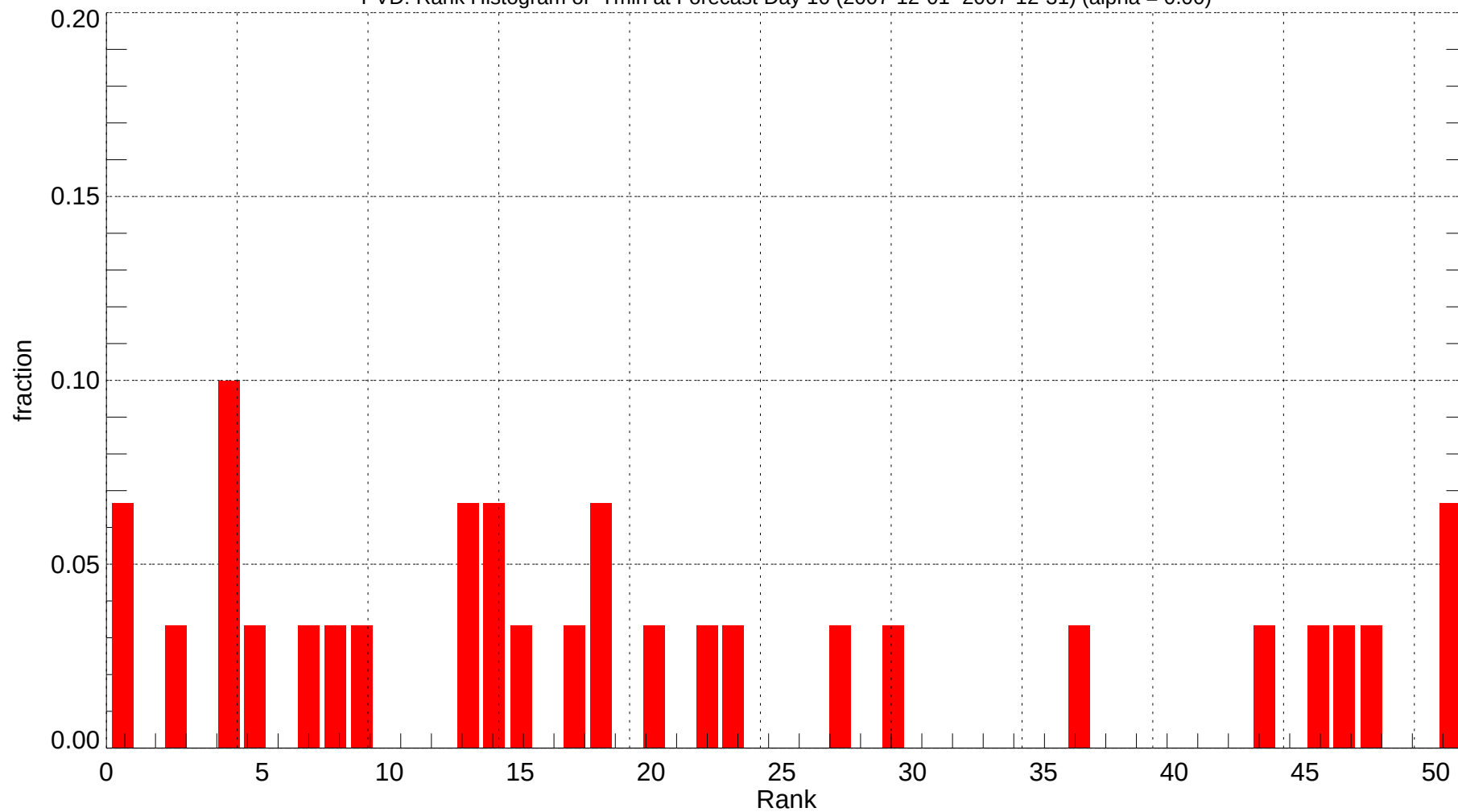
PVD: Rank Histogram of Tmin at Forecast Day 10 (2007-12-01~2007-12-31) (alpha = 0.00)
