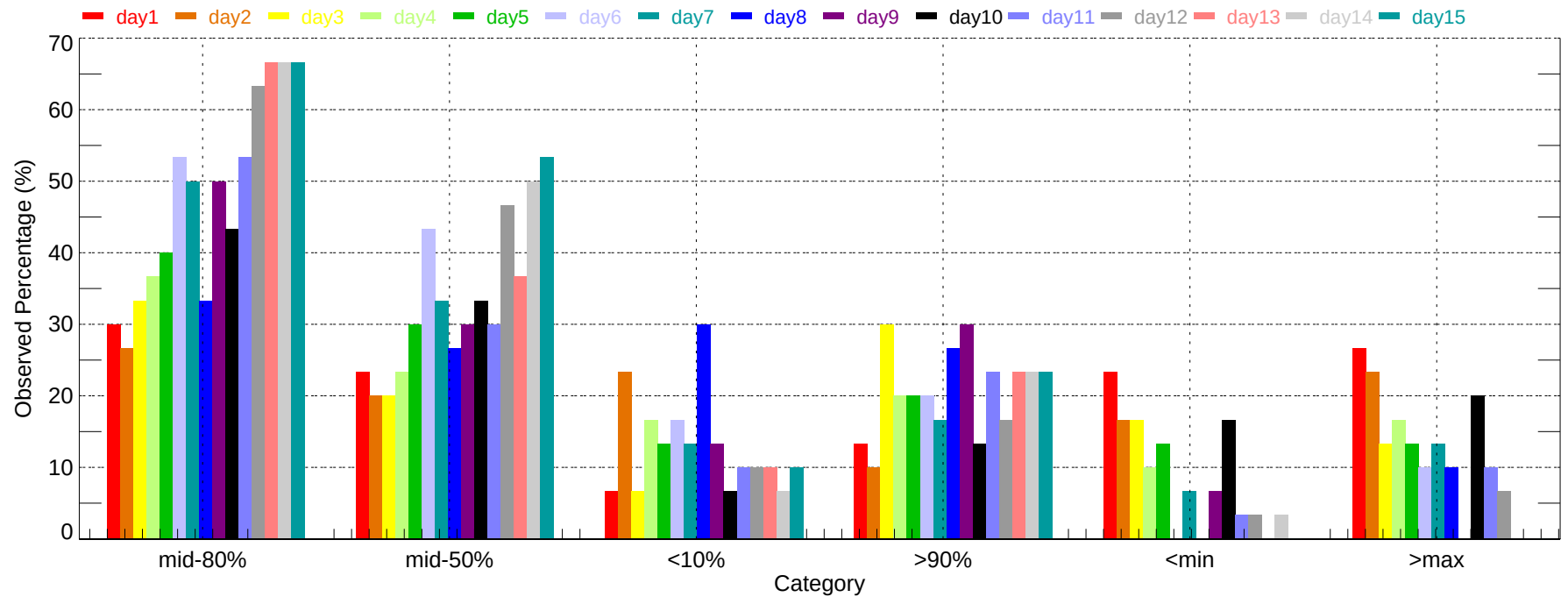
Observed Percentage of Ensembles - COU: Min Temperature (2007-12-01~2007-12-31)
