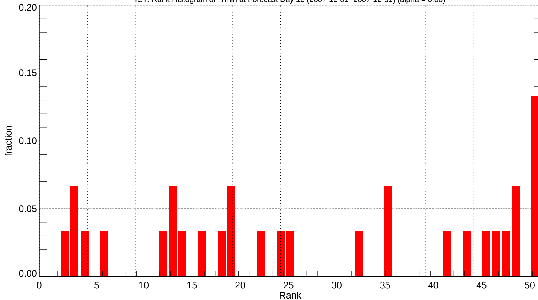
ICT: Rank Histogram of Tmin at Forecast Day 12 (2007-12-01~2007-12-31) (alpha = 0.00)
