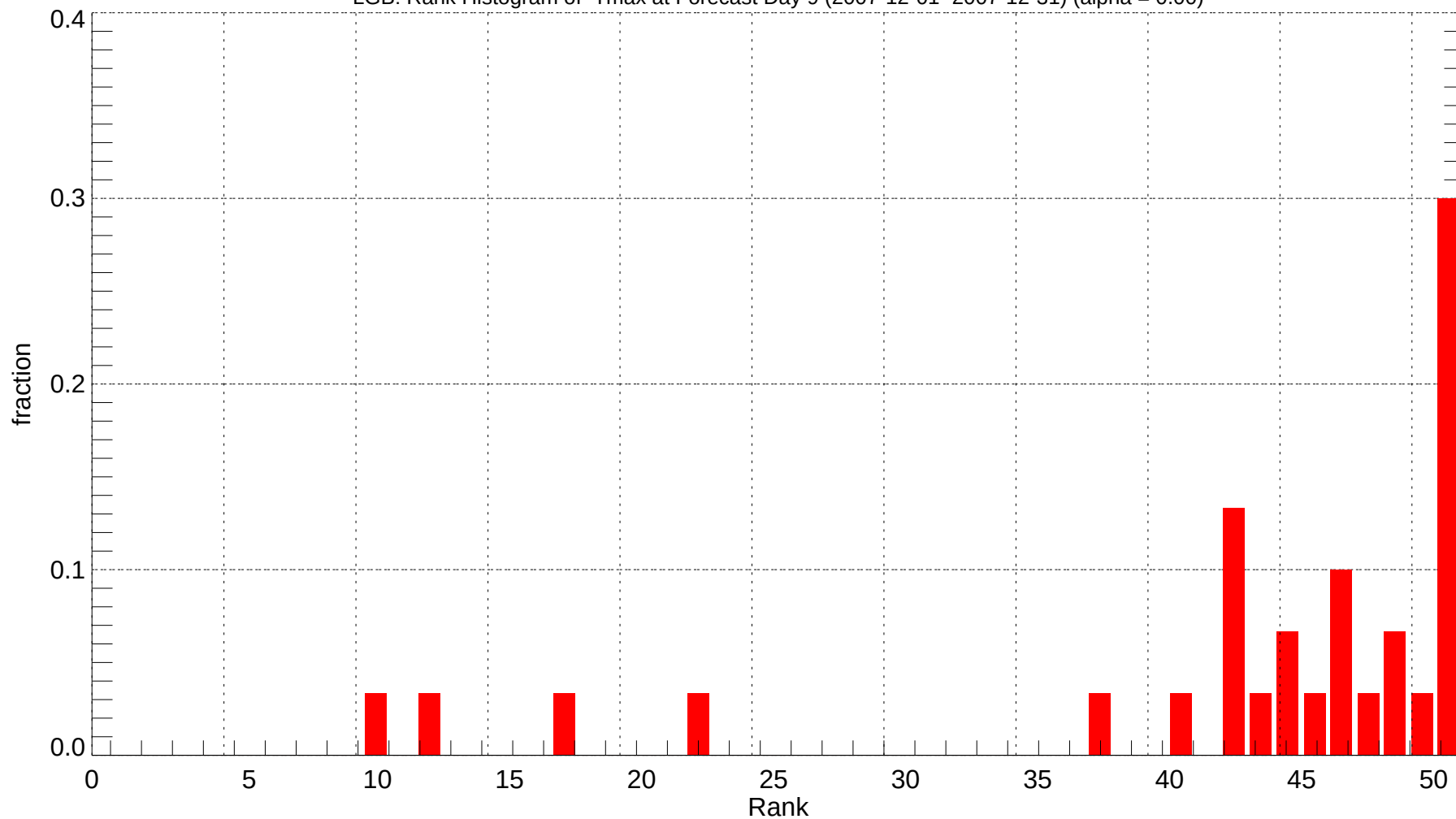
LGB: Rank Histogram of Tmax at Forecast Day 9 (2007-12-01~2007-12-31) (alpha = 0.00)
