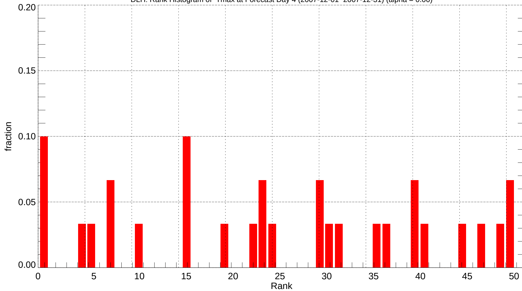
DLH: Rank Histogram of Tmax at Forecast Day 4 (2007-12-01~2007-12-31) (alpha = 0.00)
