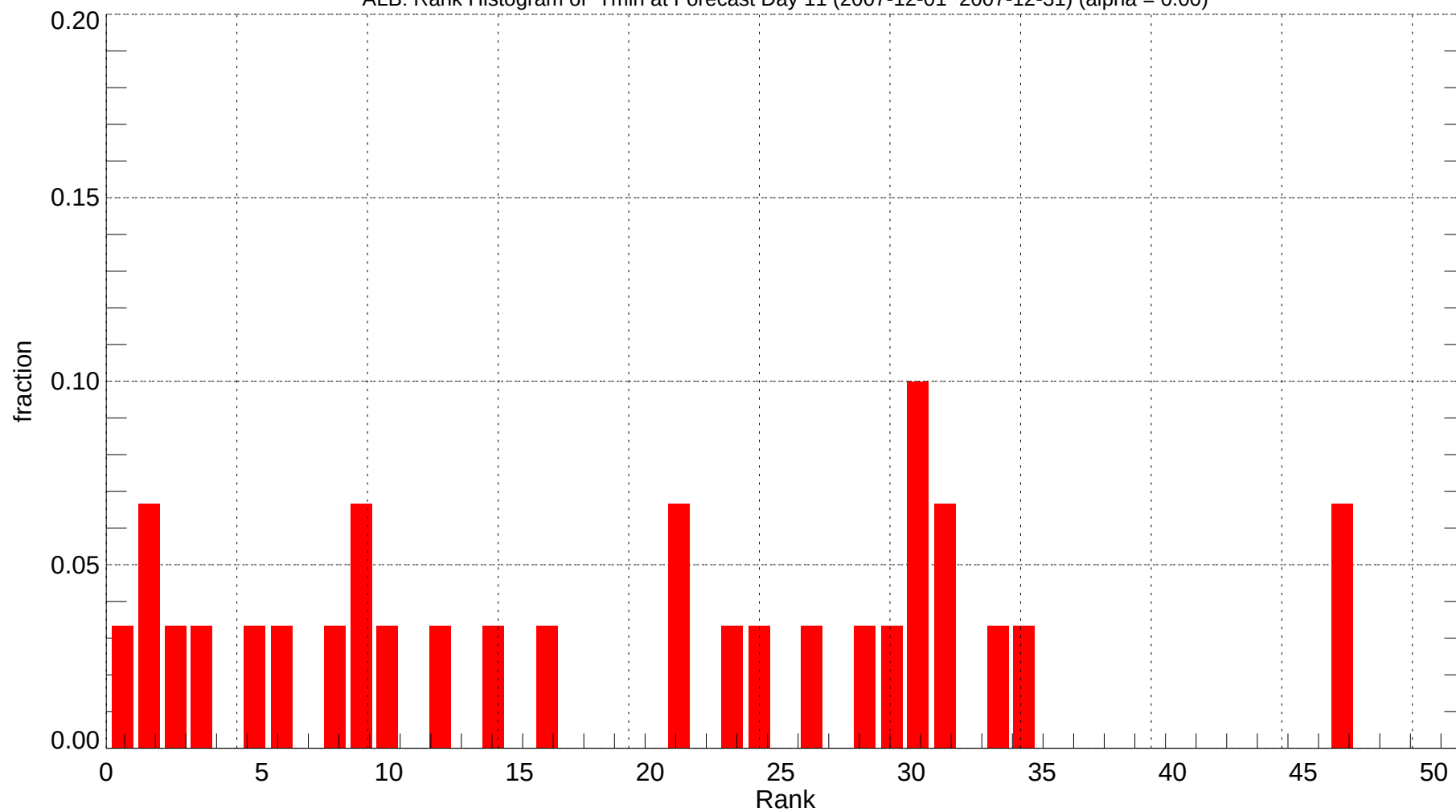
ALB: Rank Histogram of Tmin at Forecast Day 11 (2007-12-01~2007-12-31) (alpha = 0.00)
