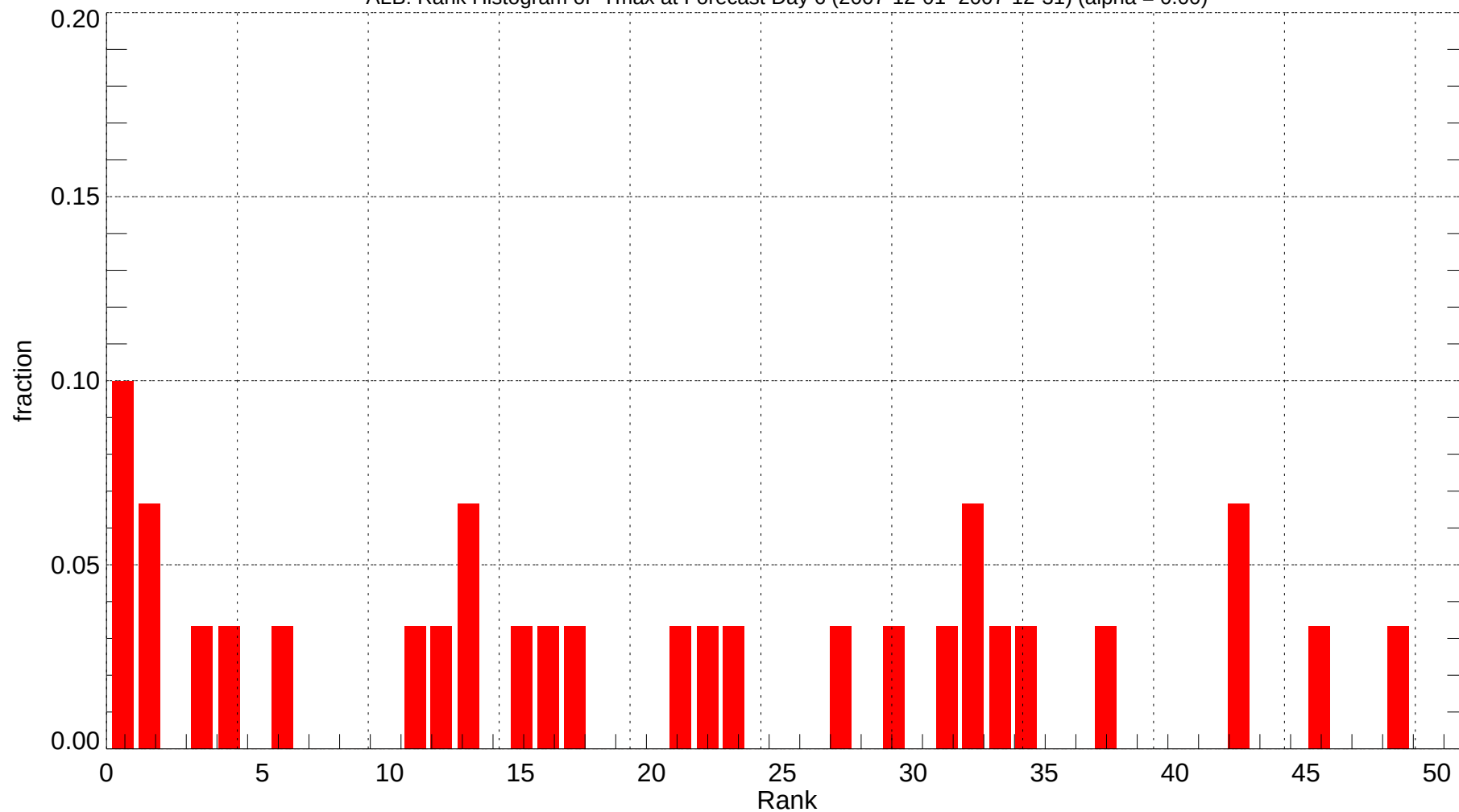
ALB: Rank Histogram of Tmax at Forecast Day 6 (2007-12-01~2007-12-31) (alpha = 0.00)
