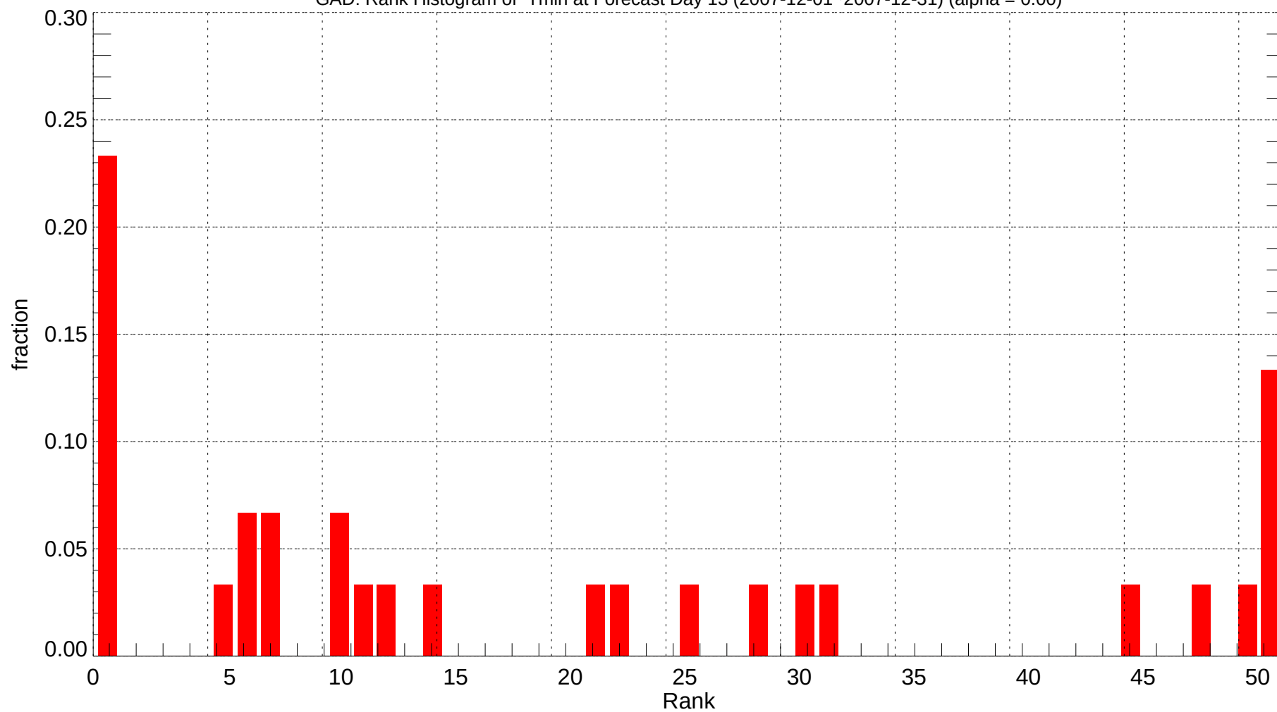
GAD: Rank Histogram of Tmin at Forecast Day 13 (2007-12-01~2007-12-31) (alpha = 0.00)
