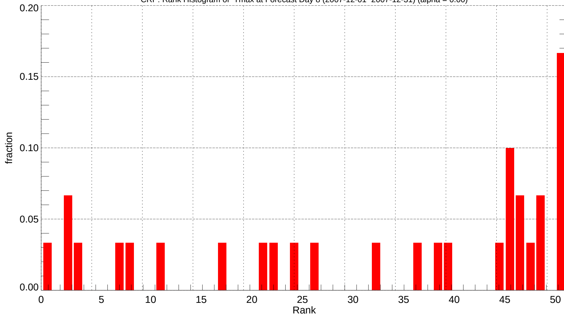
CRP: Rank Histogram of Tmax at Forecast Day 8 (2007-12-01~2007-12-31) (alpha = 0.00)
