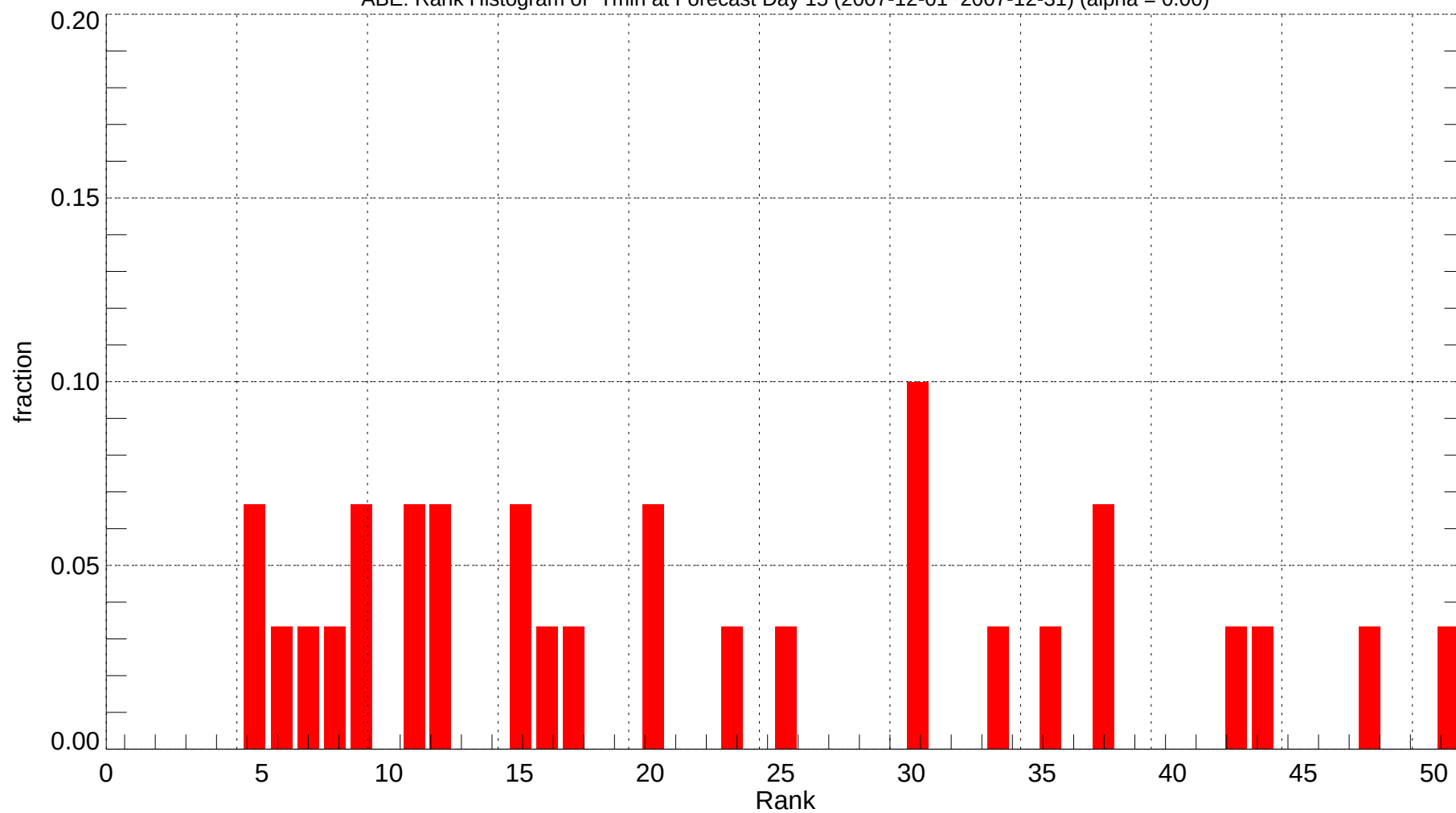
ABE: Rank Histogram of Tmin at Forecast Day 15 (2007-12-01~2007-12-31) (alpha = 0.00)
