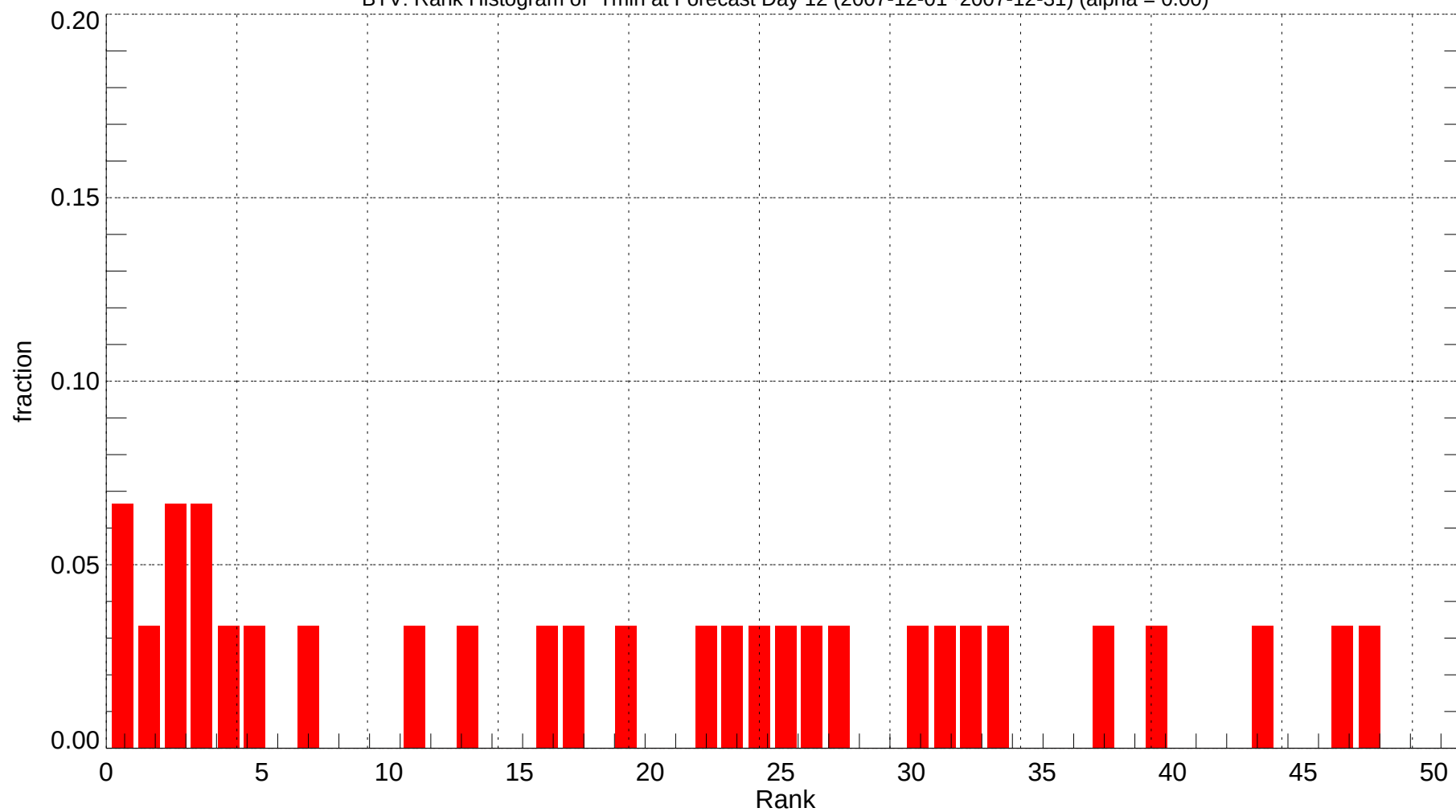
BTV: Rank Histogram of Tmin at Forecast Day 12 (2007-12-01~2007-12-31) (alpha = 0.00)
