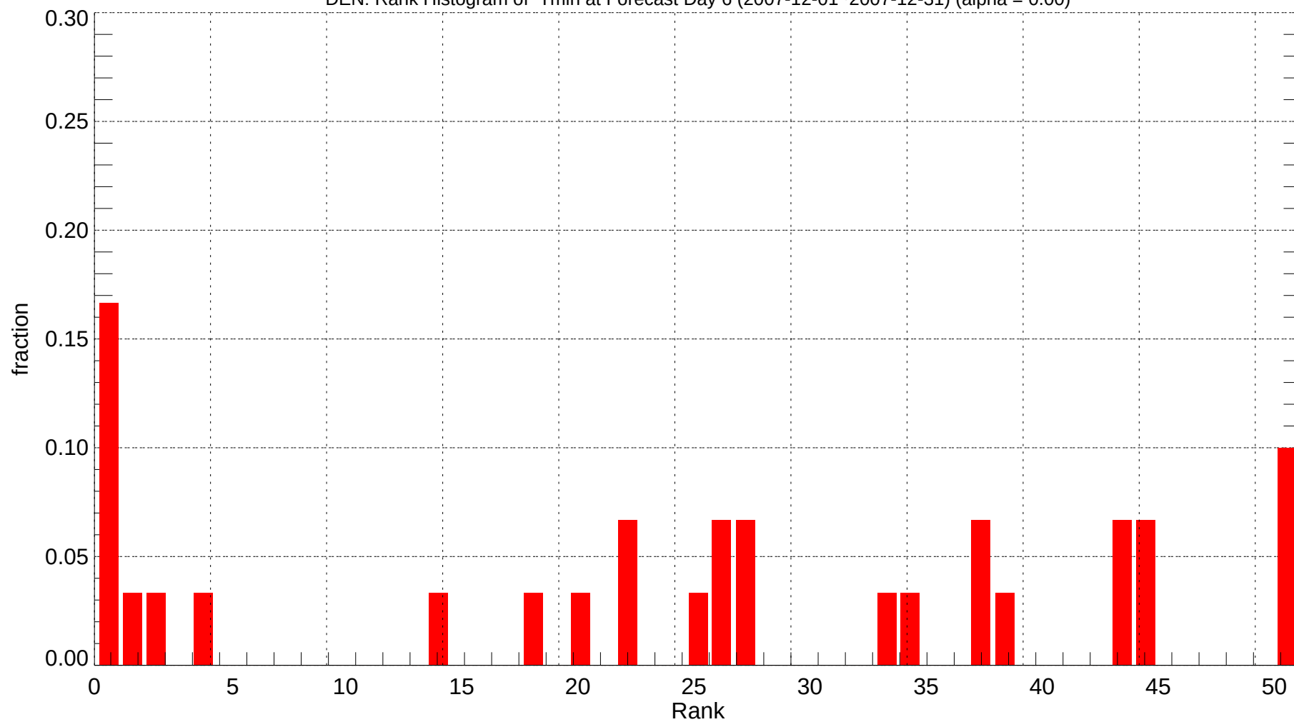
DEN: Rank Histogram of Tmin at Forecast Day 6 (2007-12-01~2007-12-31) (alpha = 0.00)
