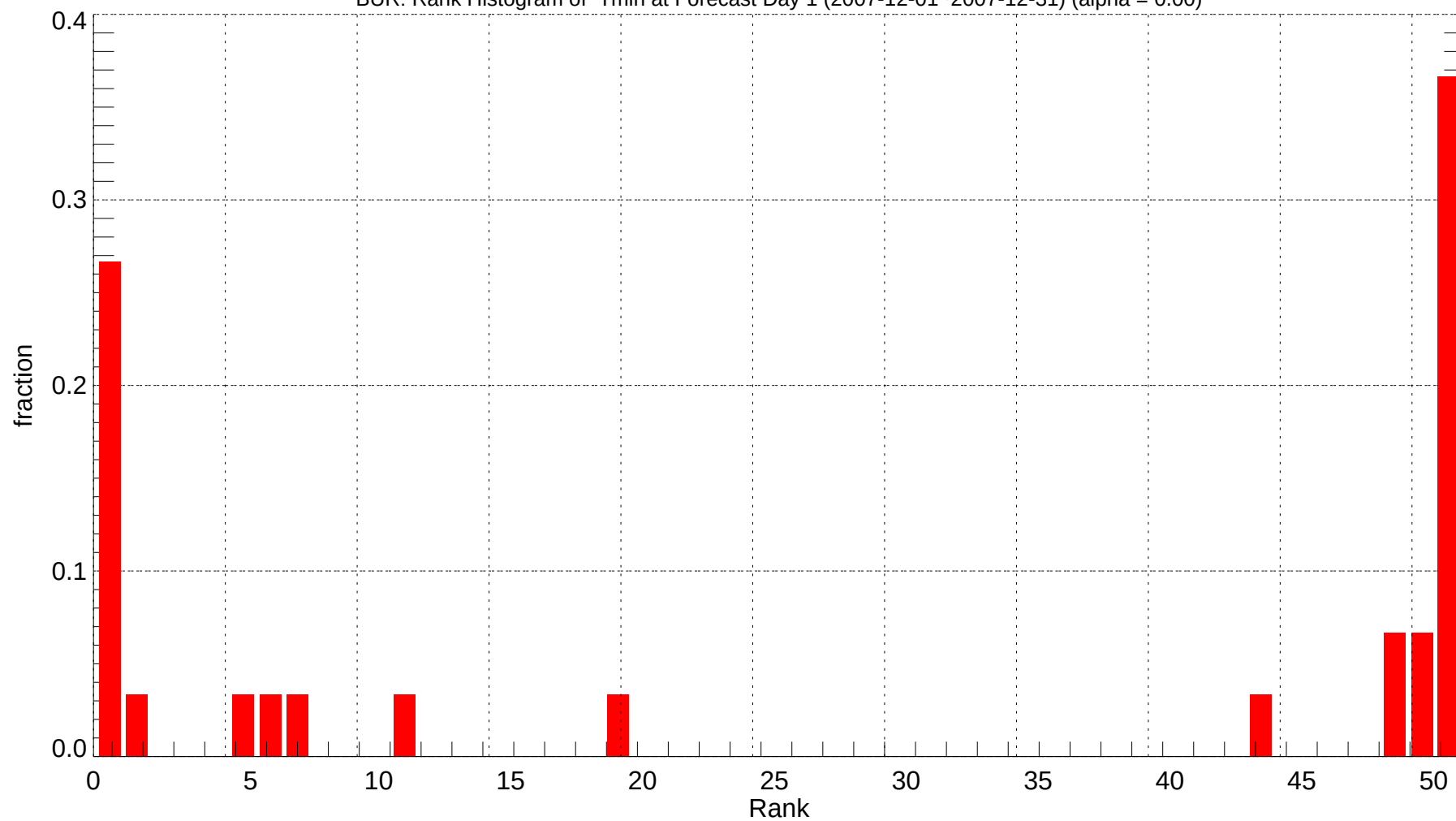
BUR: Rank Histogram of Tmin at Forecast Day 1 (2007-12-01~2007-12-31) (alpha = 0.00)
