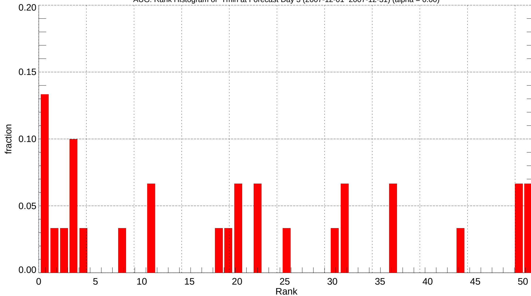
AUG: Rank Histogram of Tmin at Forecast Day 3 (2007-12-01~2007-12-31) (alpha = 0.00)
