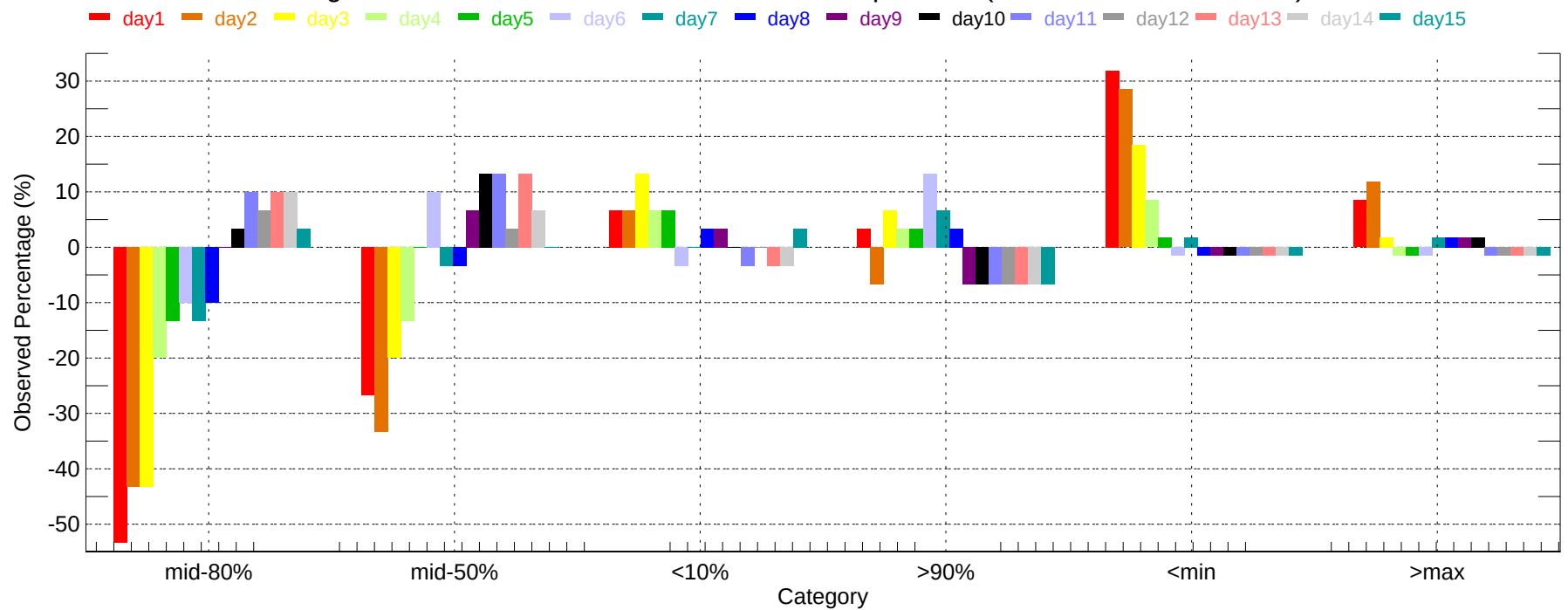
Observed Percentage Deviation of Ensembles - APN: Max Temperature (2007-12-01~2007-12-31)
