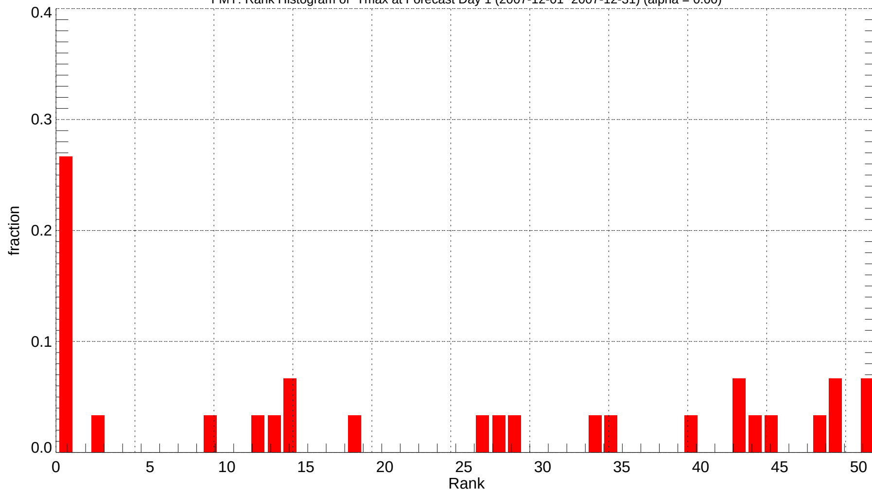
FMY: Rank Histogram of Tmax at Forecast Day 1 (2007-12-01~2007-12-31) (alpha = 0.00)
