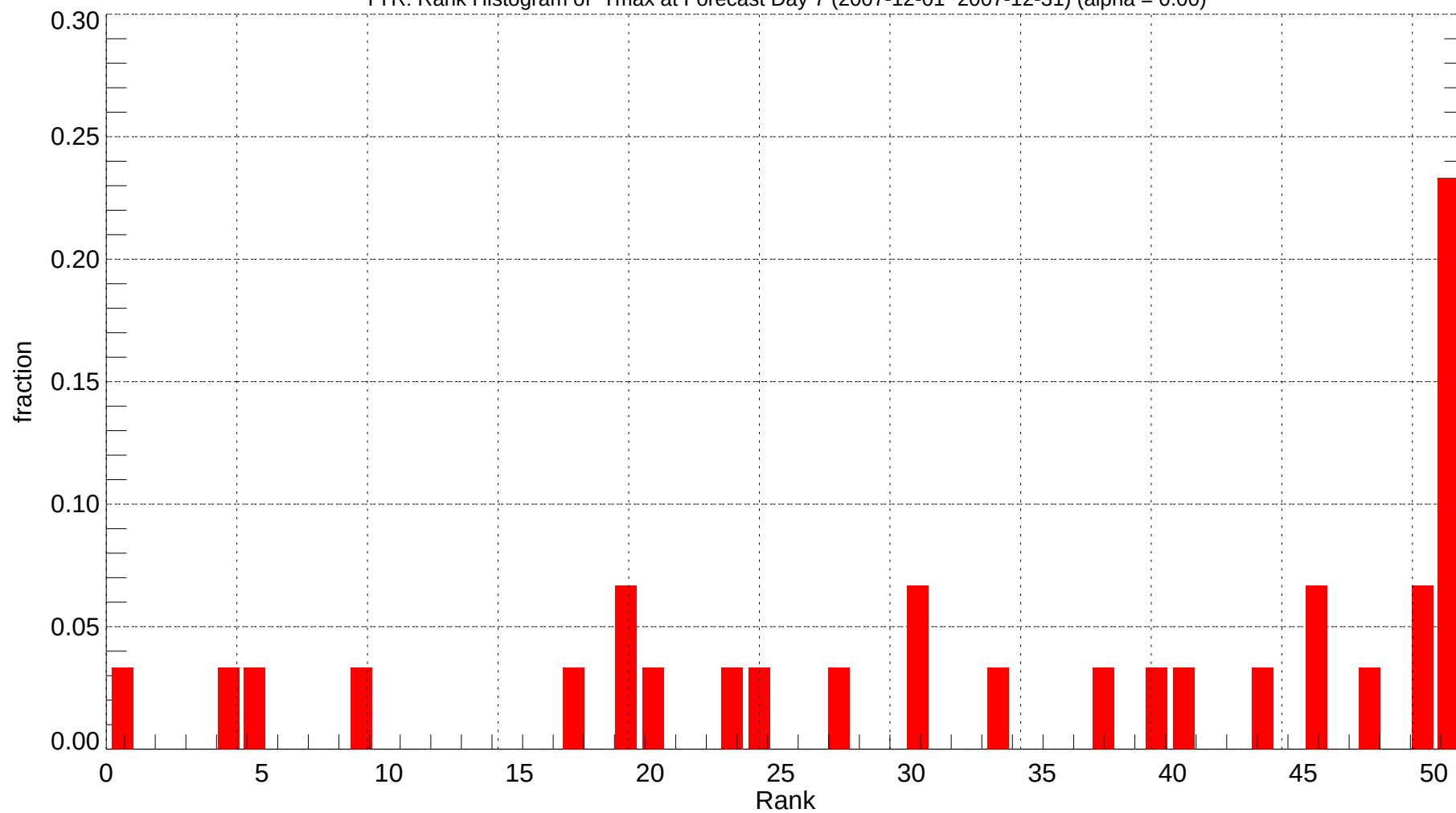
TYR: Rank Histogram of Tmax at Forecast Day 7 (2007-12-01~2007-12-31) (alpha = 0.00)
