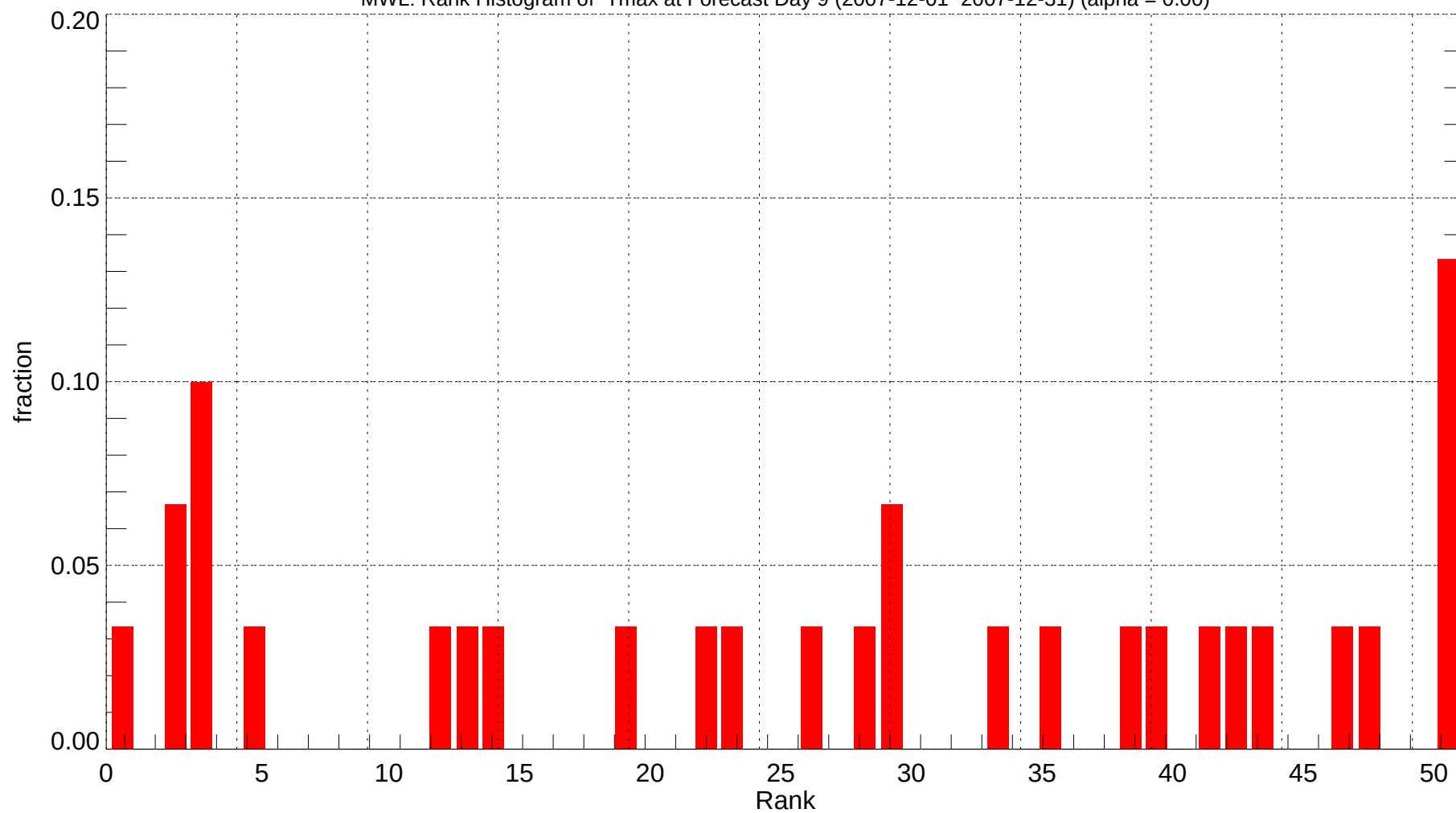
MWL: Rank Histogram of Tmax at Forecast Day 9 (2007-12-01~2007-12-31) (alpha = 0.00)
