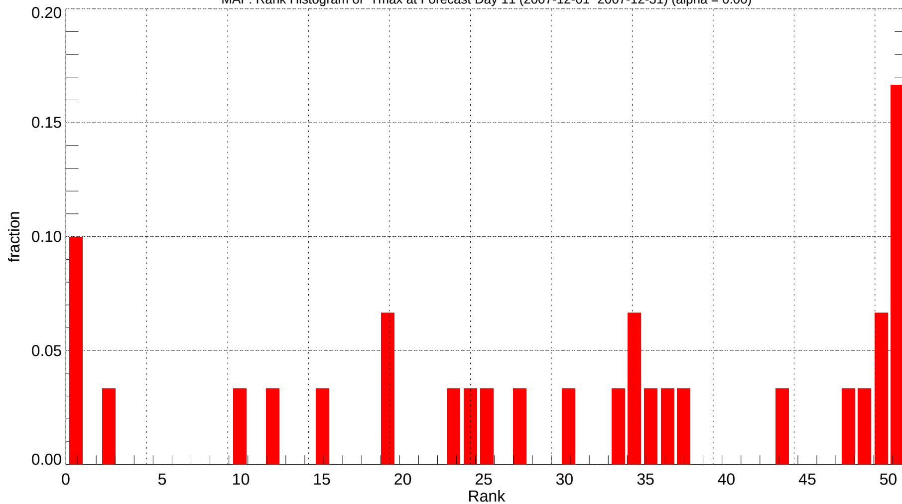
MAF: Rank Histogram of Tmax at Forecast Day 11 (2007-12-01~2007-12-31) (alpha = 0.00)
