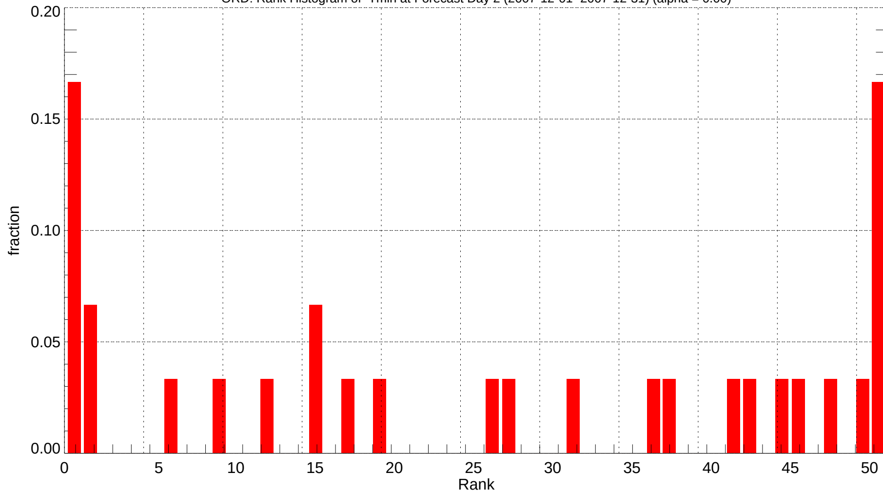
ORD: Rank Histogram of Tmin at Forecast Day 2 (2007-12-01~2007-12-31) (alpha = 0.00)
