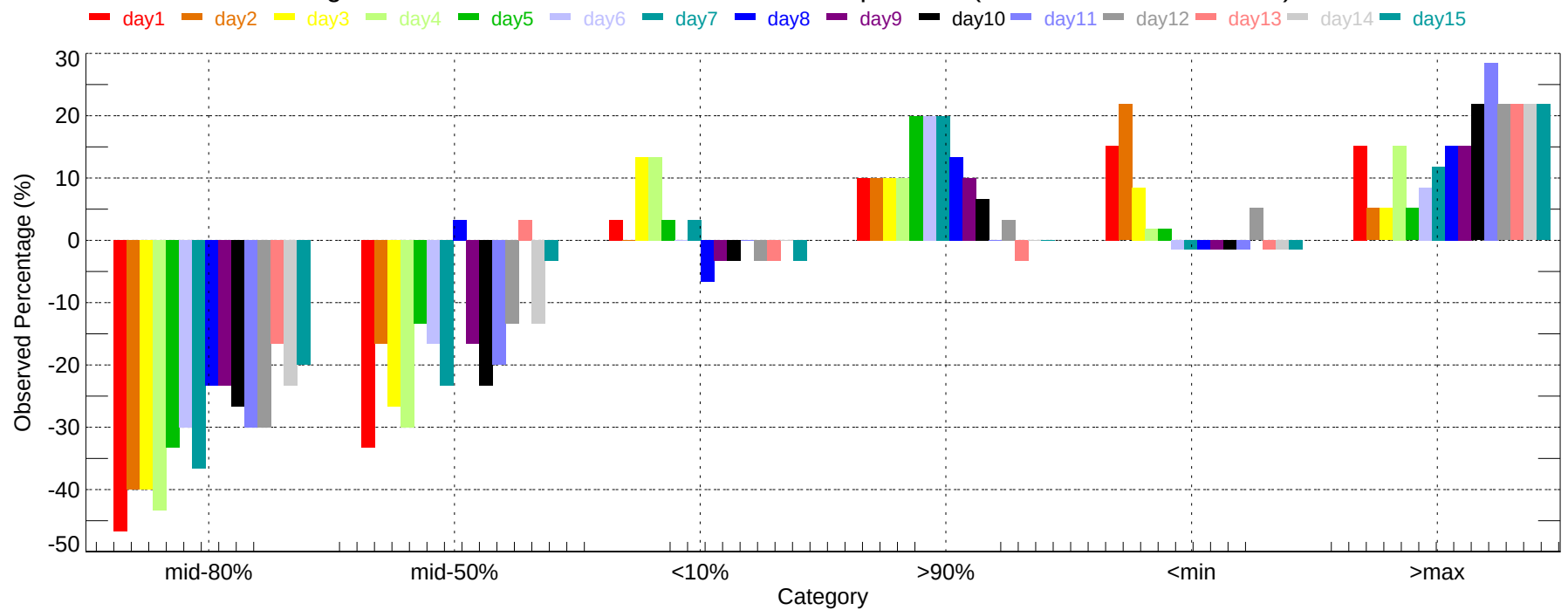
Observed Percentage Deviation of Ensembles - JAN: Min Temperature (2007-12-01~2007-12-31)
