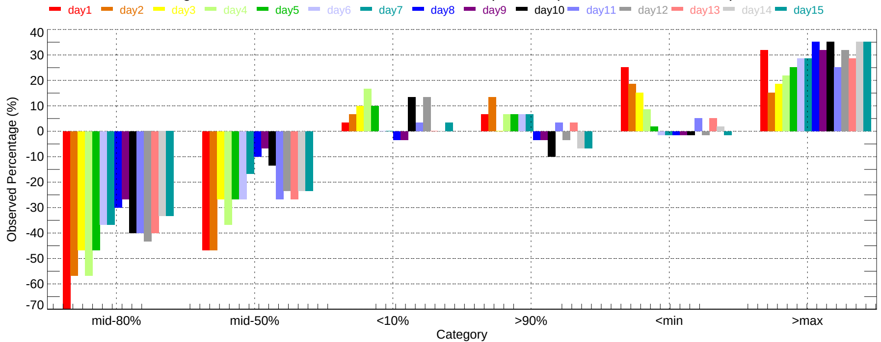
Observed Percentage Deviation of Ensembles - MSY: Max Temperature (2007-12-01~2007-12-31)
