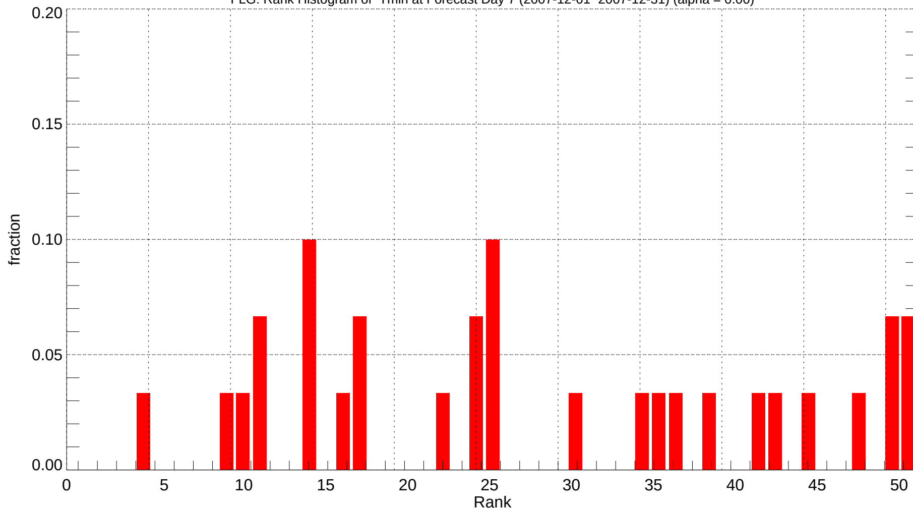
FLG: Rank Histogram of Tmin at Forecast Day 7 (2007-12-01~2007-12-31) (alpha = 0.00)
