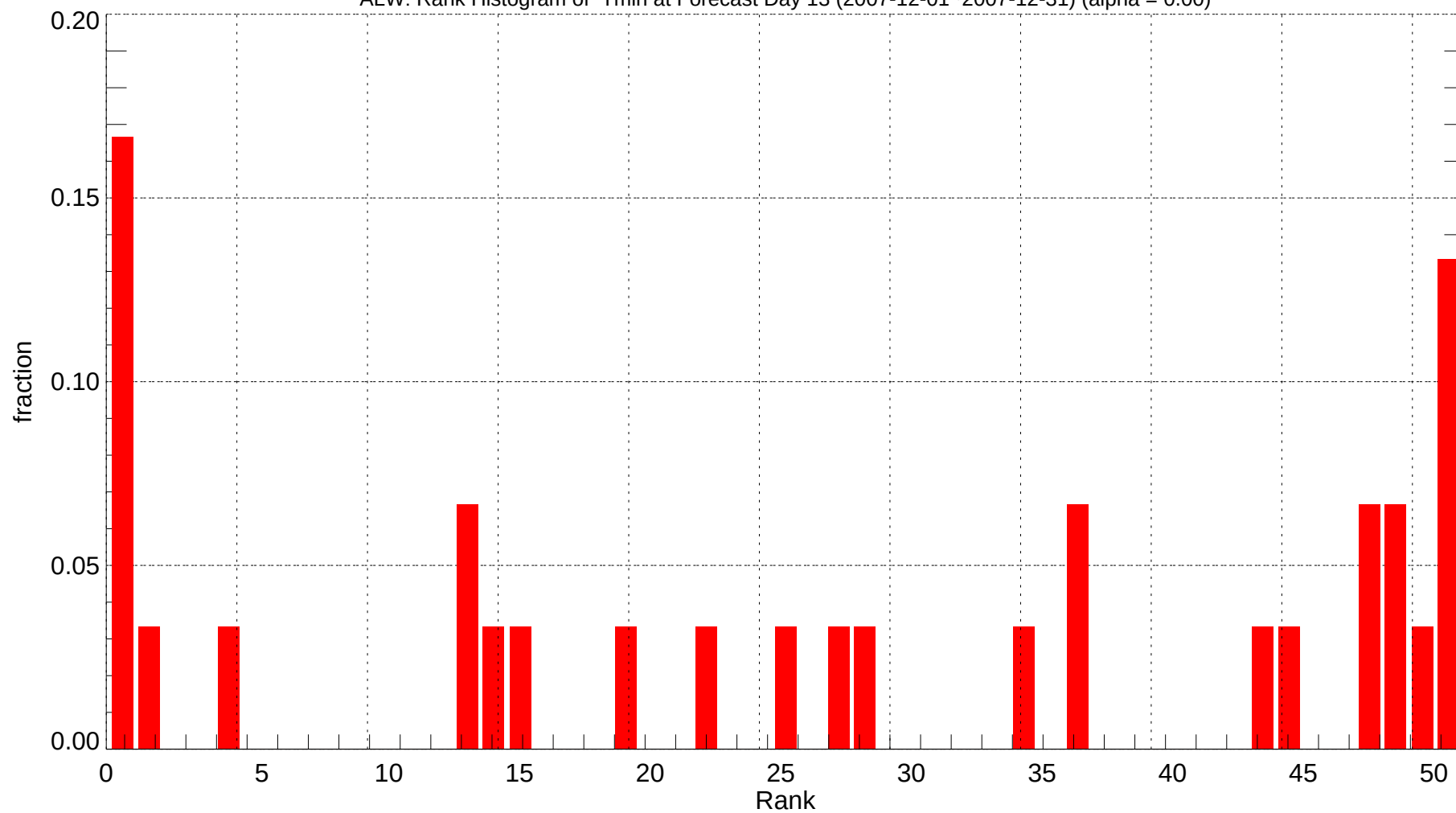
ALW: Rank Histogram of Tmin at Forecast Day 13 (2007-12-01~2007-12-31) (alpha = 0.00)
