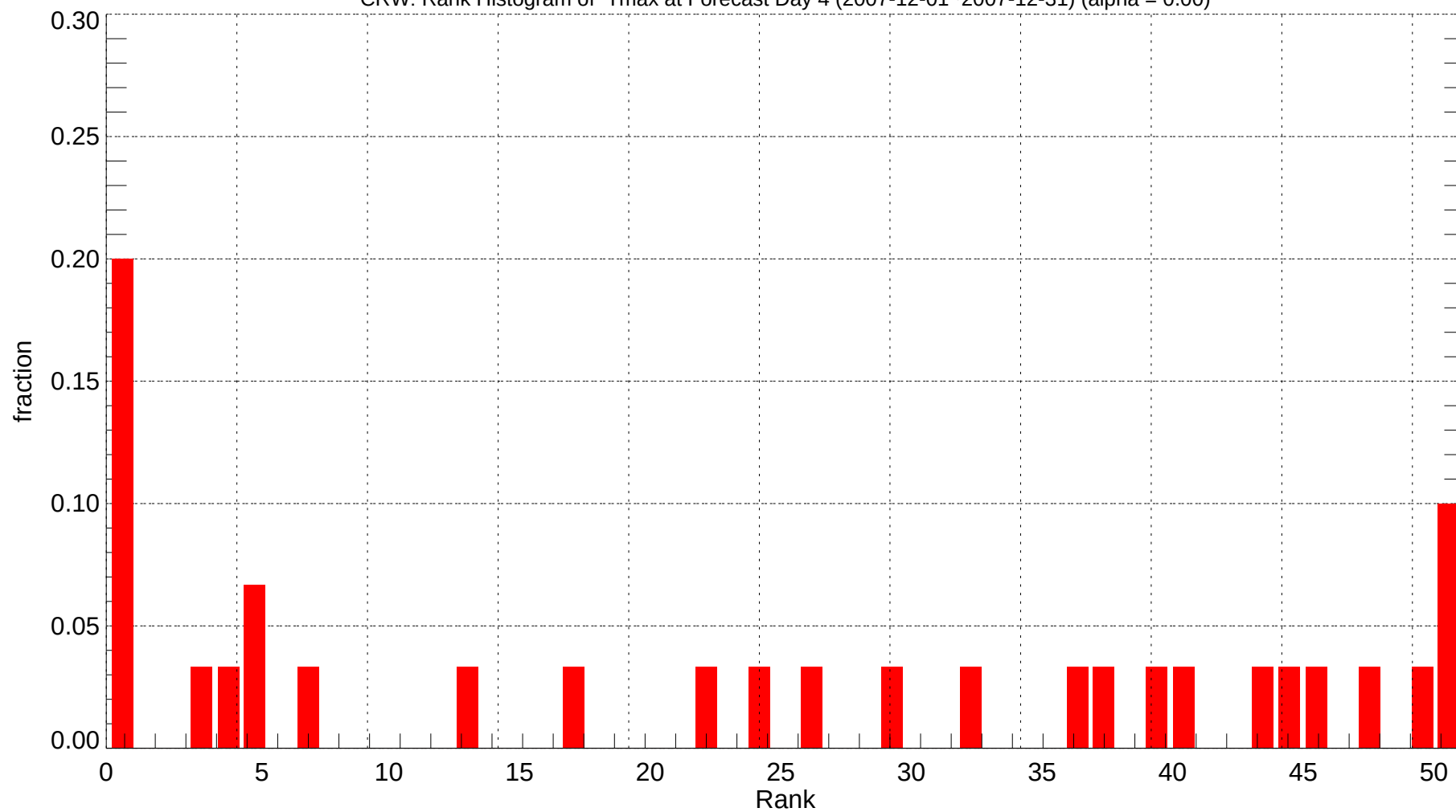
CRW: Rank Histogram of Tmax at Forecast Day 4 (2007-12-01~2007-12-31) (alpha = 0.00)
