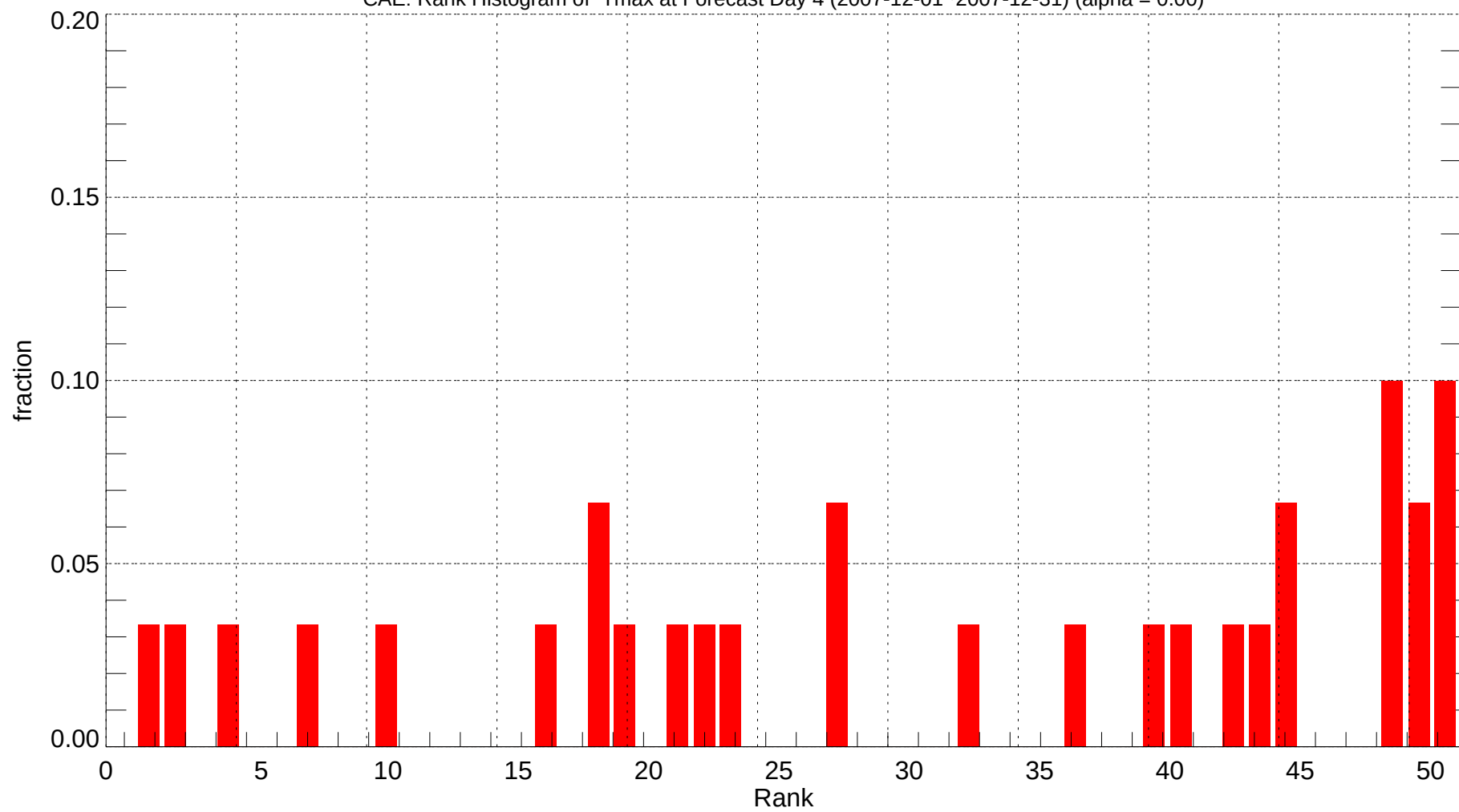
CAE: Rank Histogram of Tmax at Forecast Day 4 (2007-12-01~2007-12-31) (alpha = 0.00)
