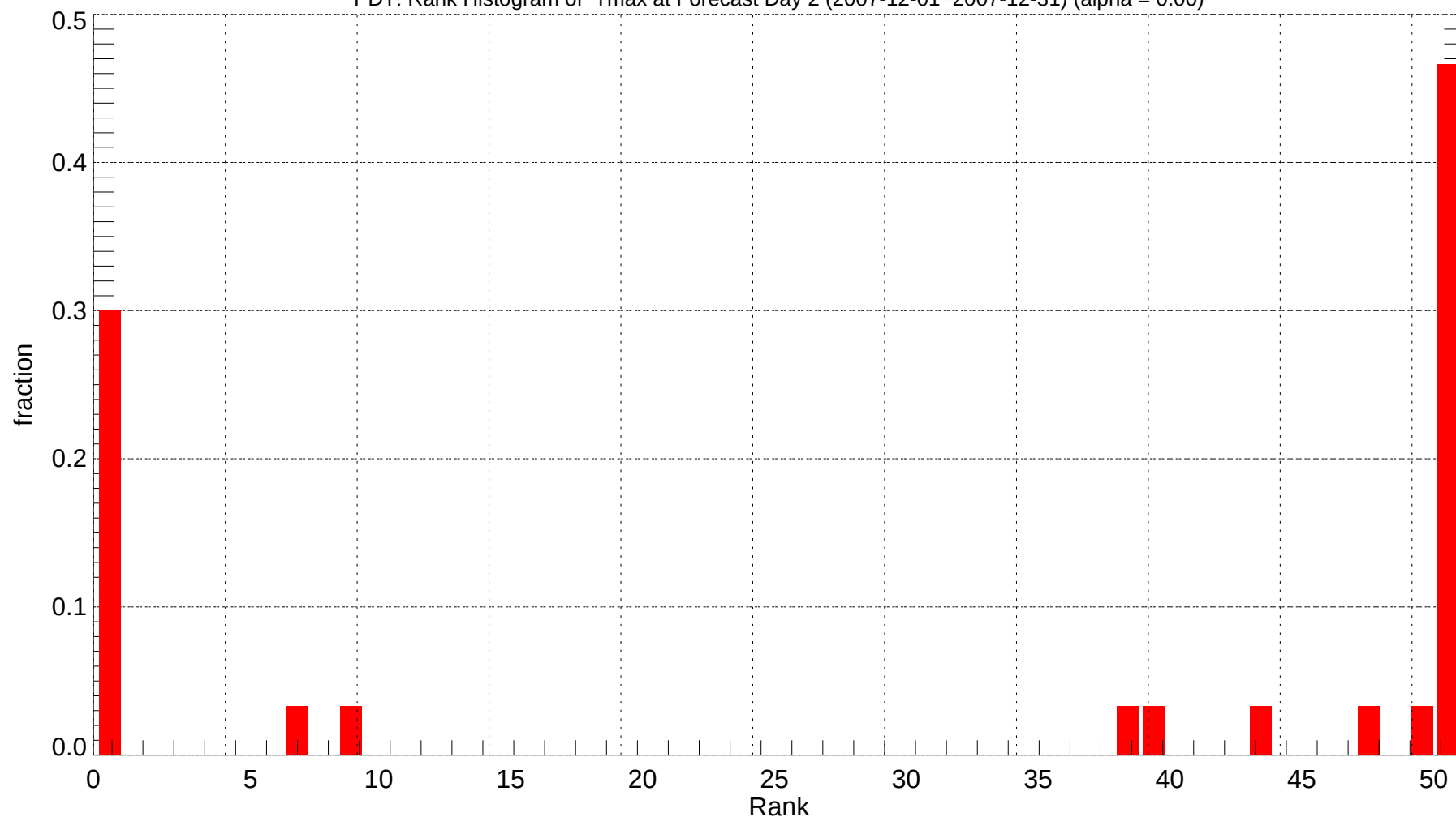
PDT: Rank Histogram of Tmax at Forecast Day 2 (2007-12-01~2007-12-31) (alpha = 0.00)
