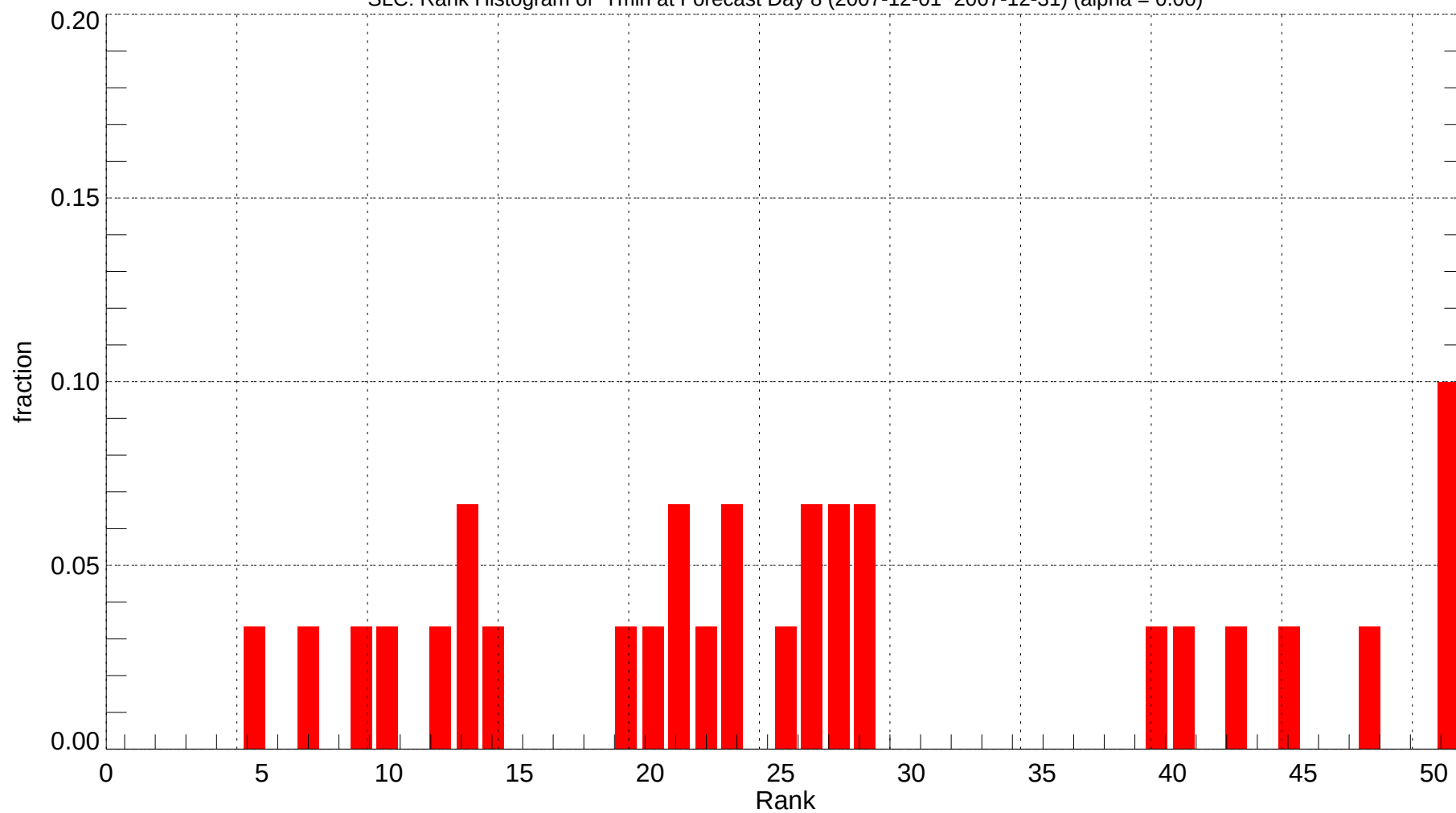
SLC: Rank Histogram of Tmin at Forecast Day 8 (2007-12-01~2007-12-31) (alpha = 0.00)
