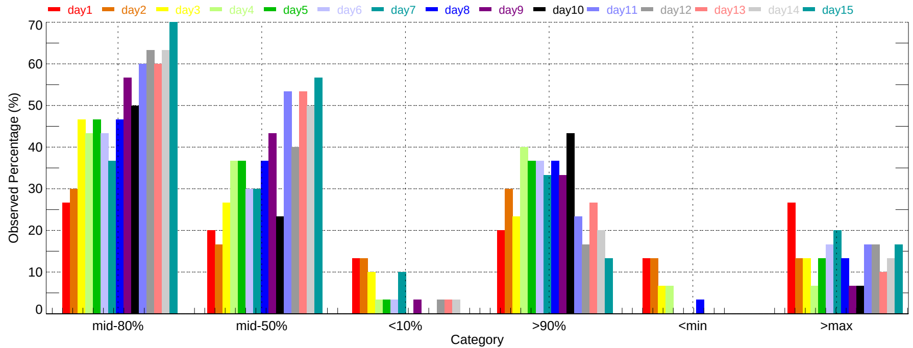
Observed Percentage of Ensembles - BNA: Min Temperature (2007-12-01~2007-12-31)
