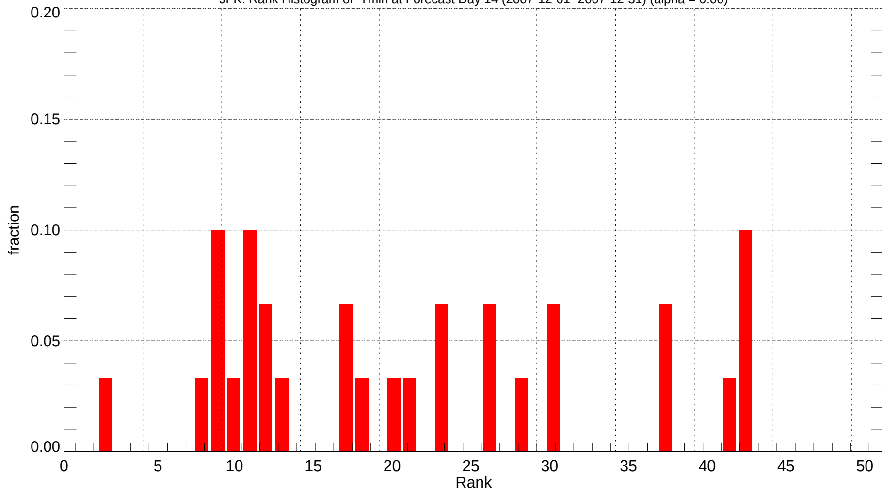
JFK: Rank Histogram of Tmin at Forecast Day 14 (2007-12-01~2007-12-31) (alpha = 0.00)
