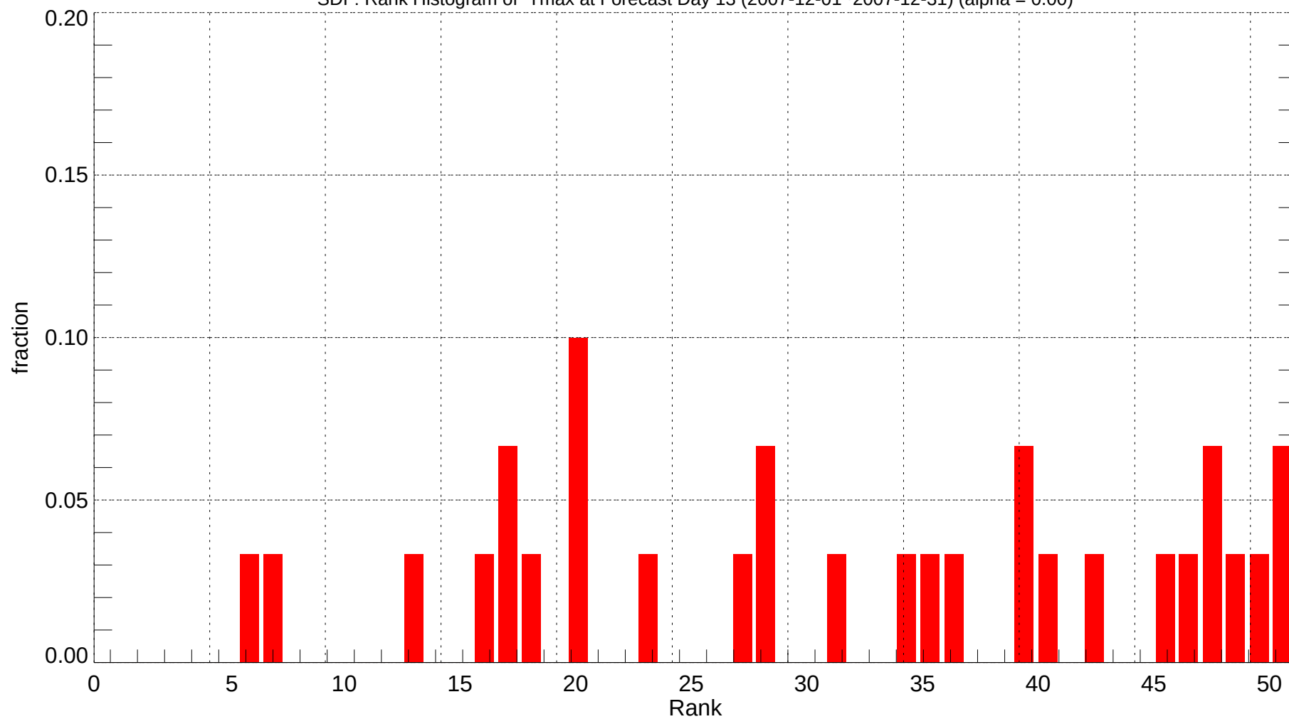
SDF: Rank Histogram of Tmax at Forecast Day 13 (2007-12-01~2007-12-31) (alpha = 0.00)
