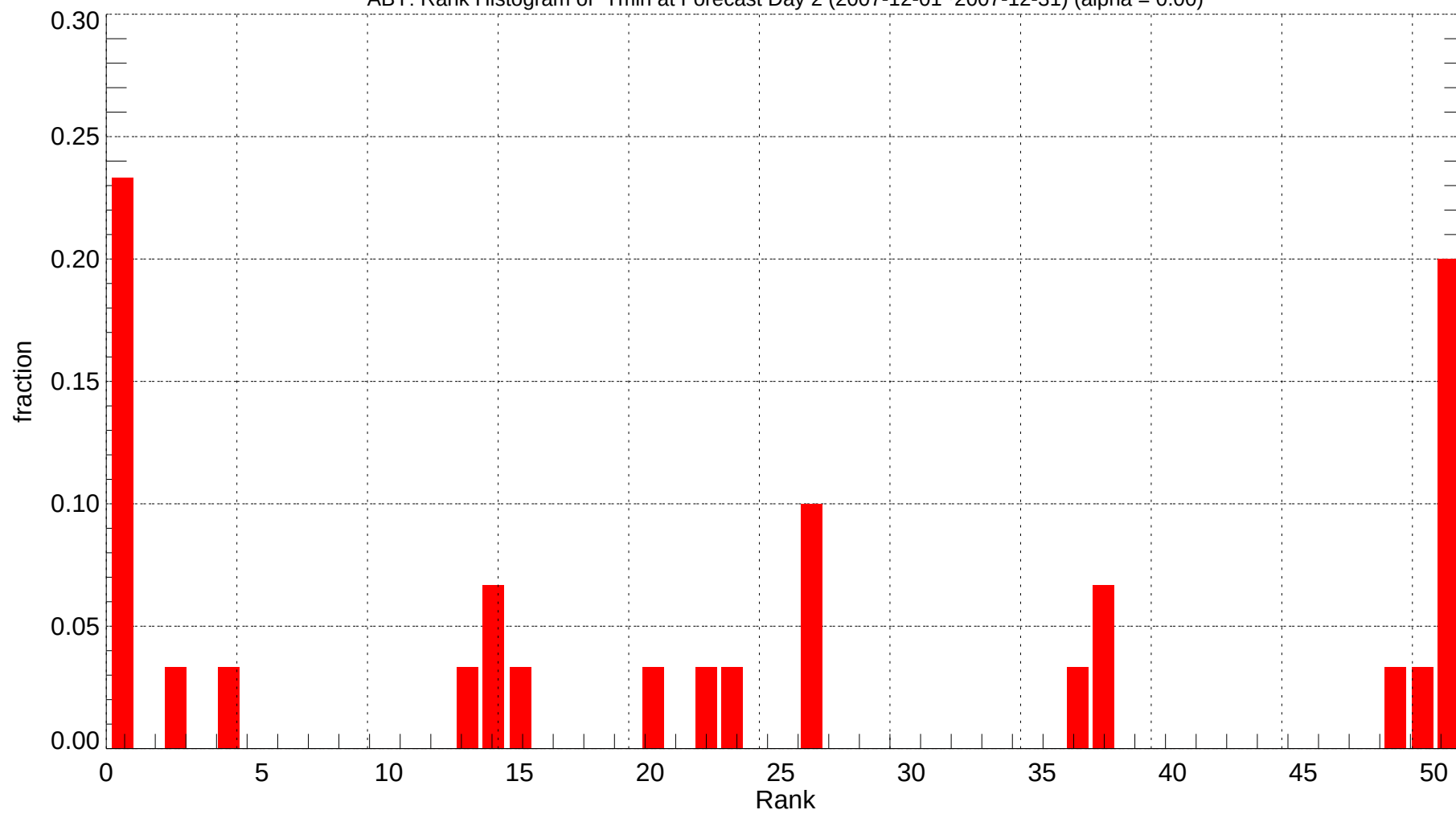
ABY: Rank Histogram of Tmin at Forecast Day 2 (2007-12-01~2007-12-31) (alpha = 0.00)
