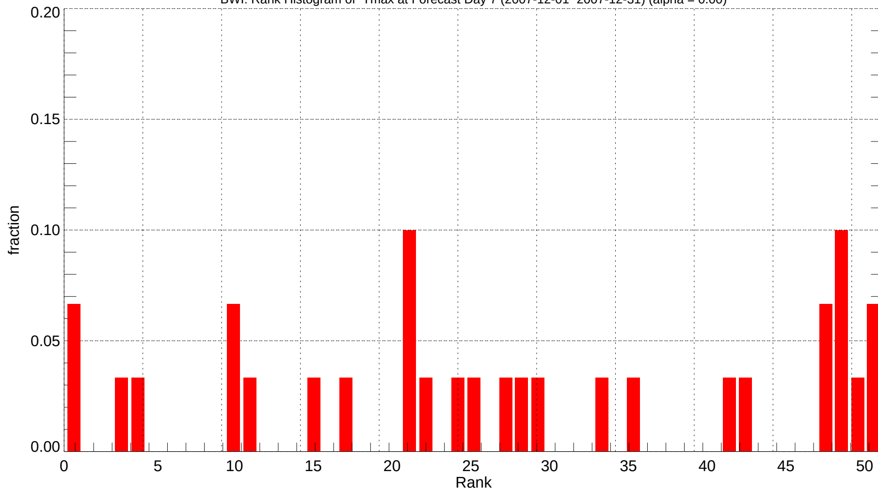
BWI: Rank Histogram of Tmax at Forecast Day 7 (2007-12-01~2007-12-31) (alpha = 0.00)
