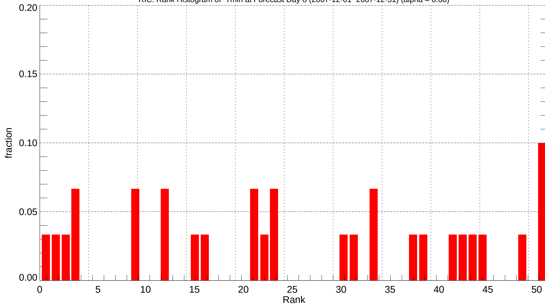
RIC: Rank Histogram of Tmin at Forecast Day 8 (2007-12-01~2007-12-31) (alpha = 0.00)
