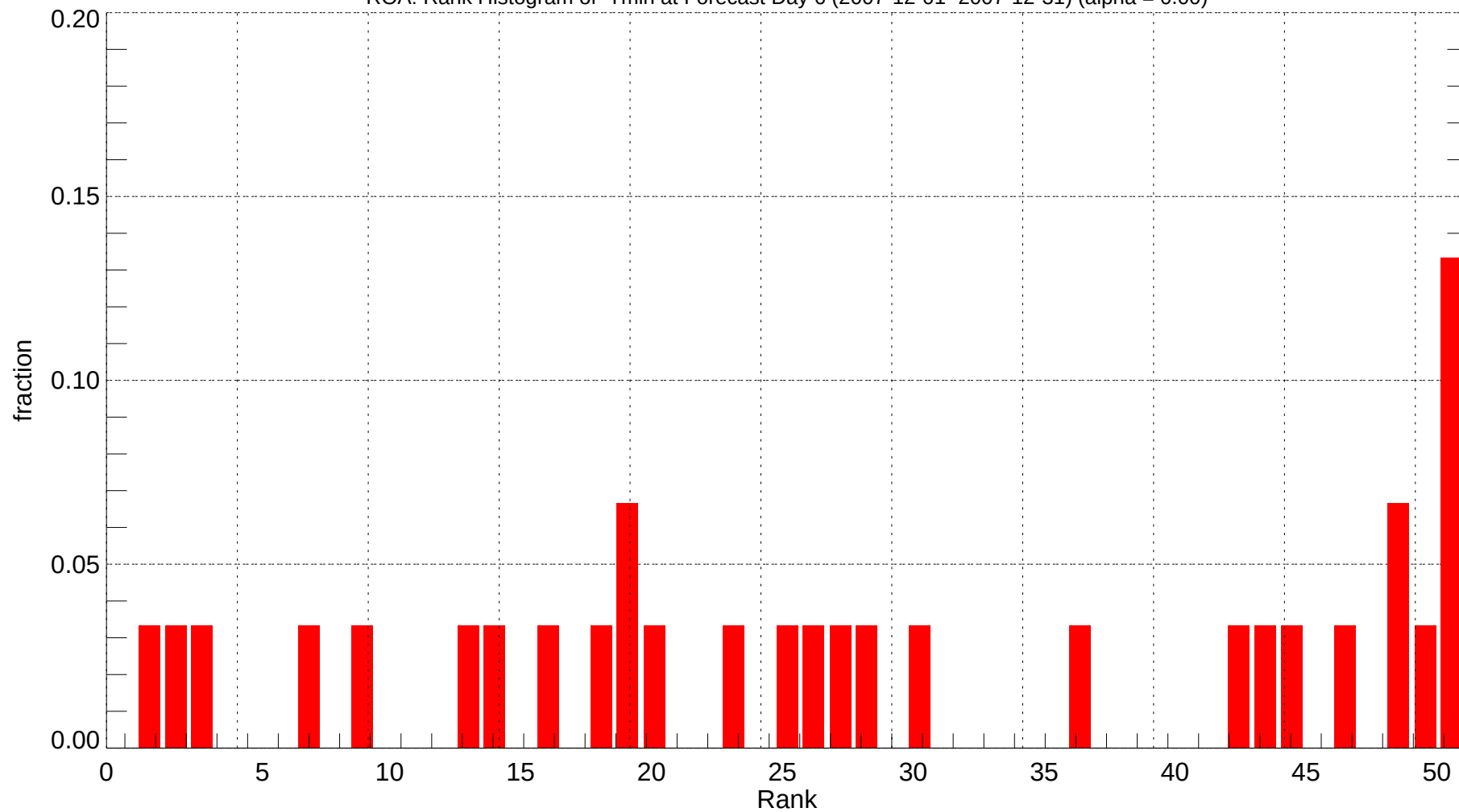
ROA: Rank Histogram of Tmin at Forecast Day 6 (2007-12-01~2007-12-31) (alpha = 0.00)
