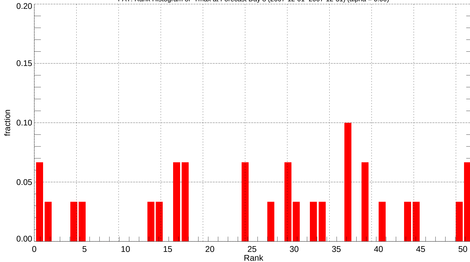
FAT: Rank Histogram of Tmax at Forecast Day 8 (2007-12-01~2007-12-31) (alpha = 0.00)
