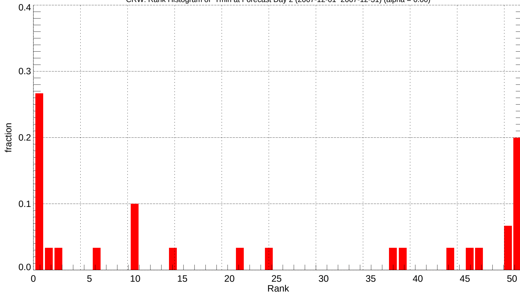
CRW: Rank Histogram of Tmin at Forecast Day 2 (2007-12-01~2007-12-31) (alpha = 0.00)
