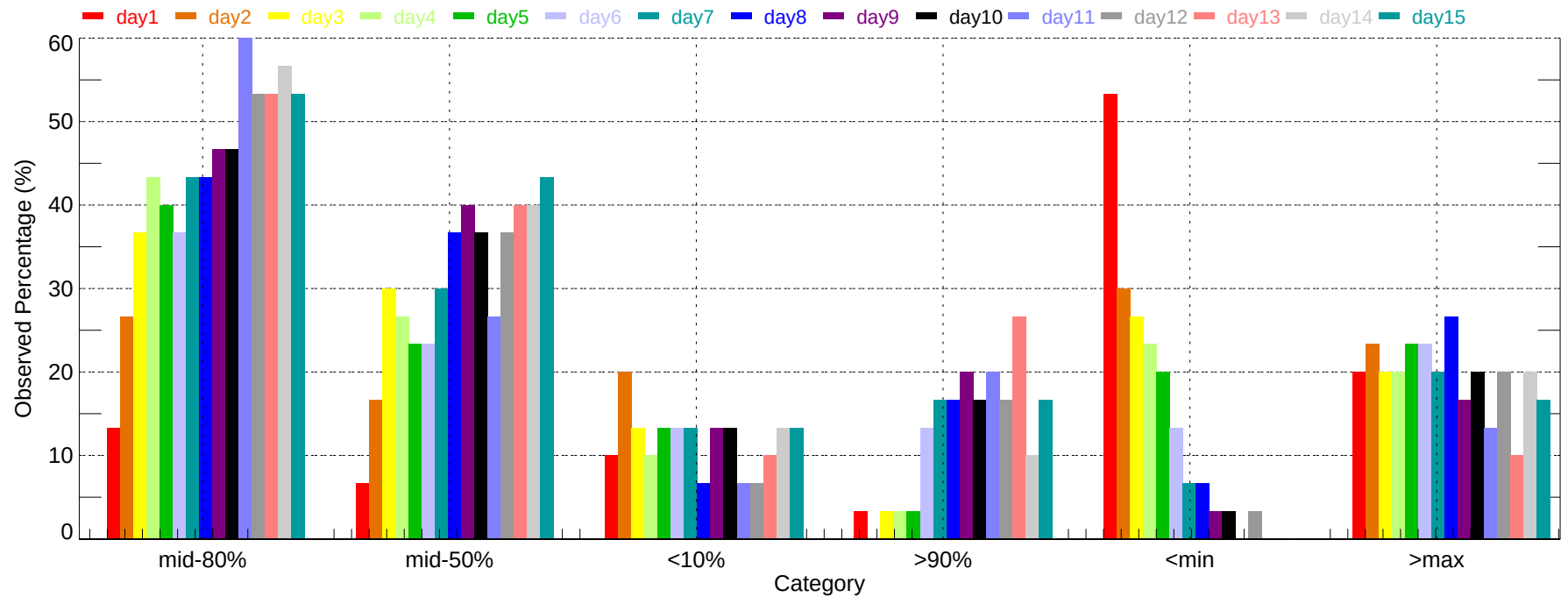
Observed Percentage of Ensembles - MOB: Min Temperature (2007-12-01~2007-12-31)
