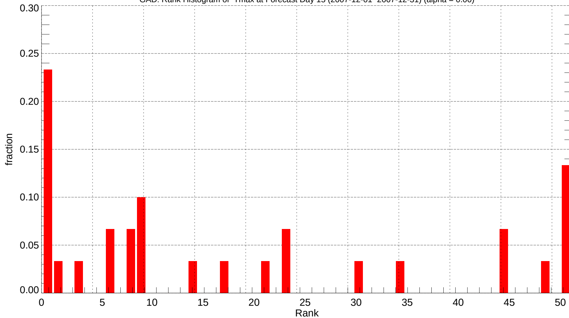
GAD: Rank Histogram of Tmax at Forecast Day 15 (2007-12-01~2007-12-31) (alpha = 0.00)
