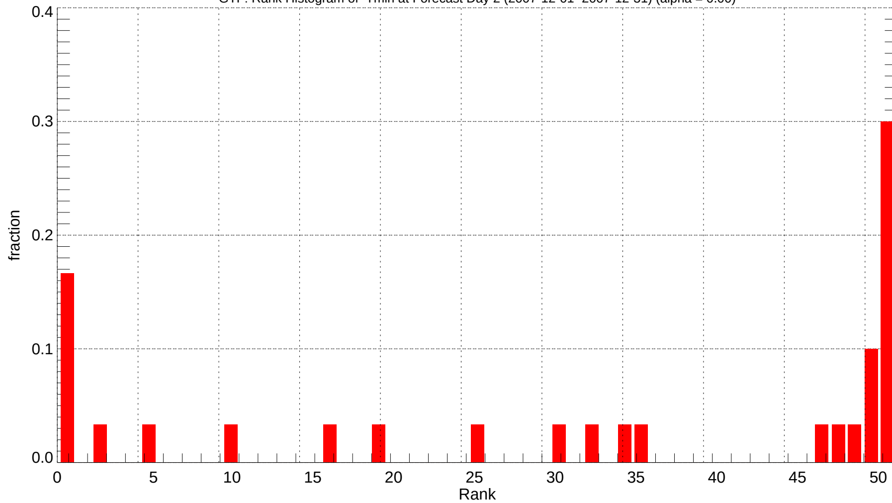
GTF: Rank Histogram of Tmin at Forecast Day 2 (2007-12-01~2007-12-31) (alpha = 0.00)
