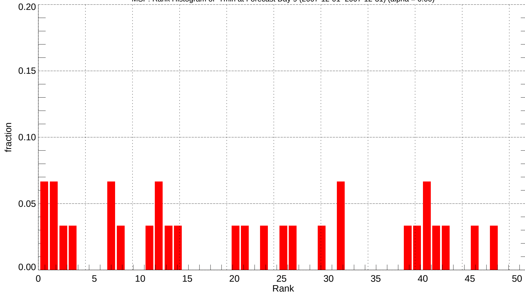
MSP: Rank Histogram of Tmin at Forecast Day 9 (2007-12-01~2007-12-31) (alpha = 0.00)
