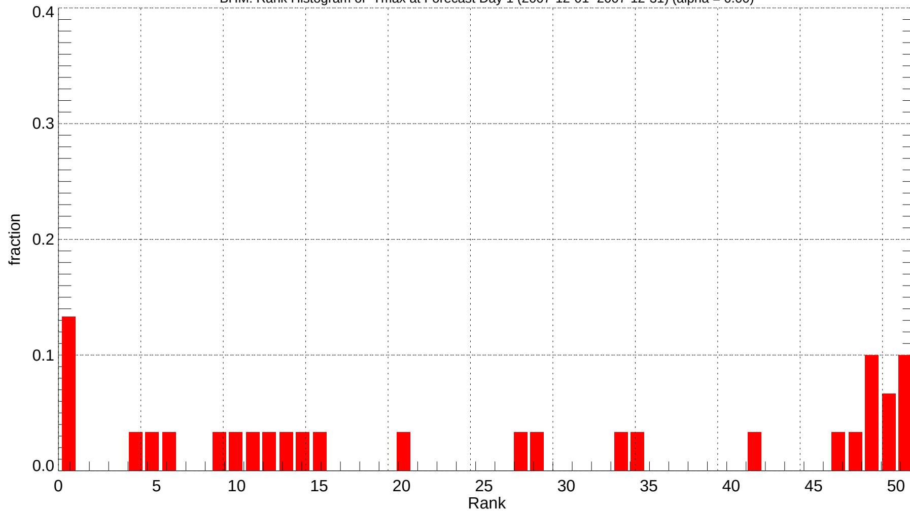
BHM: Rank Histogram of Tmax at Forecast Day 1 (2007-12-01~2007-12-31) (alpha = 0.00)
