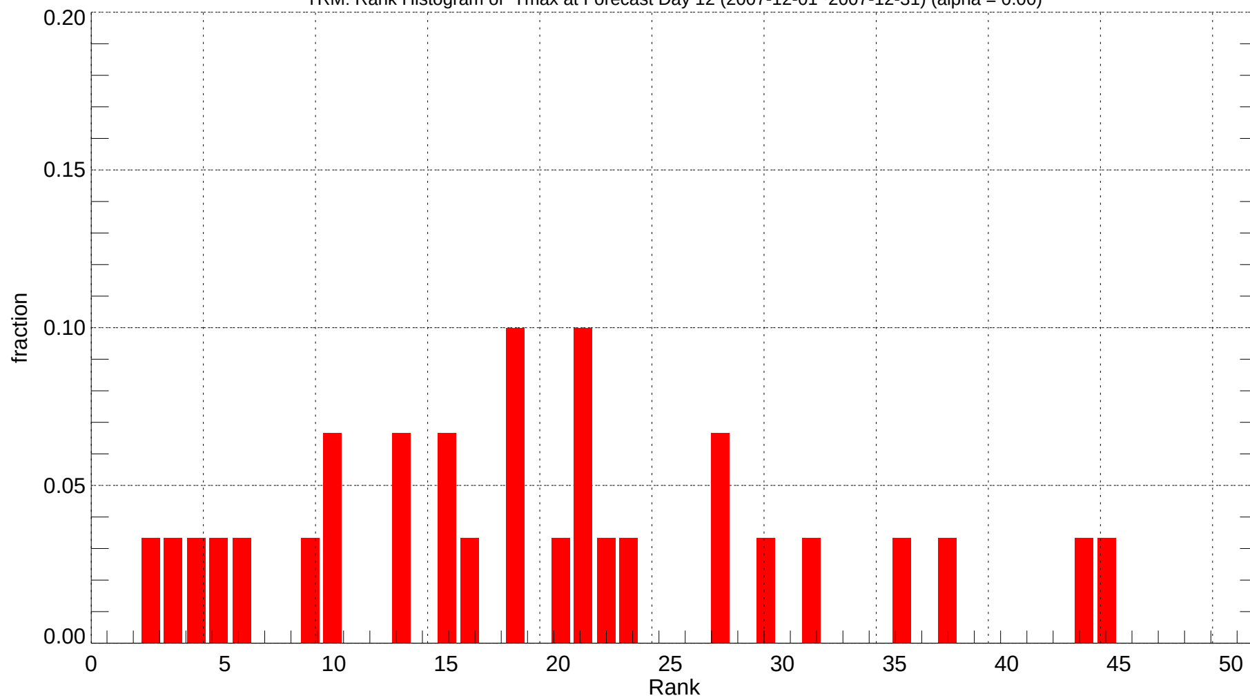
TRM: Rank Histogram of Tmax at Forecast Day 12 (2007-12-01~2007-12-31) (alpha = 0.00)
