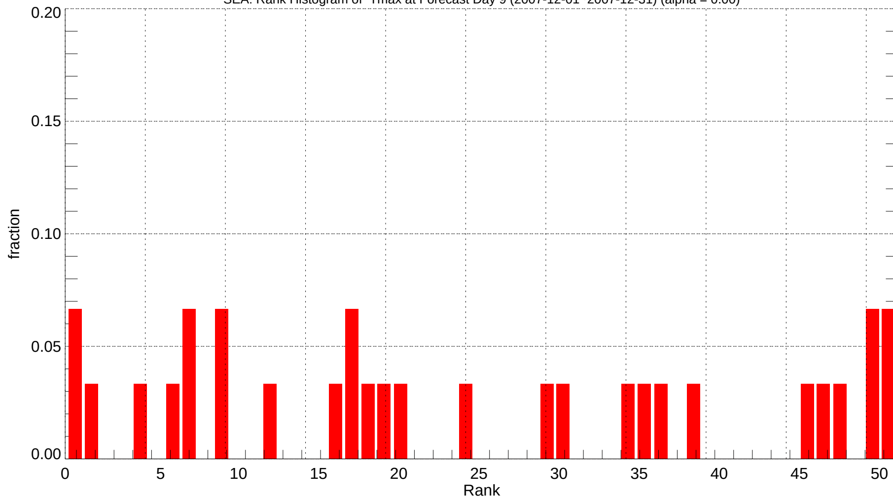
SEA: Rank Histogram of Tmax at Forecast Day 9 (2007-12-01~2007-12-31) (alpha = 0.00)
