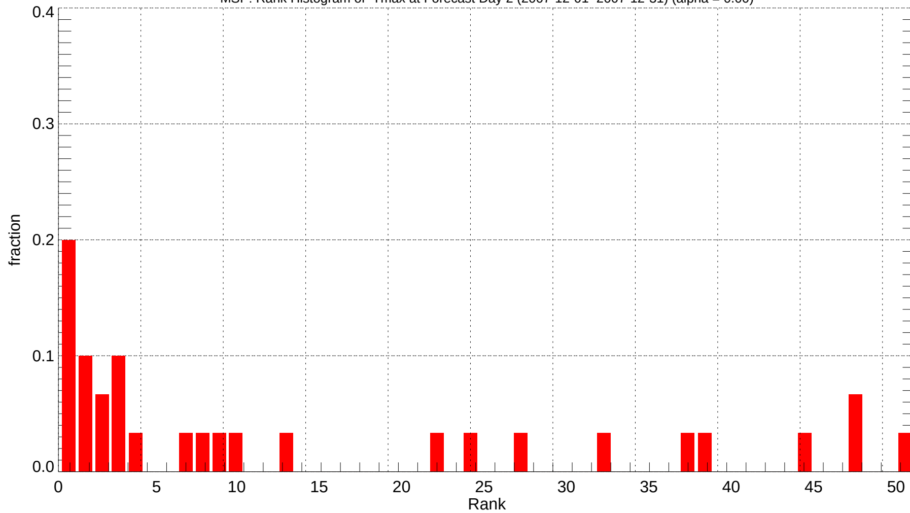
MSP: Rank Histogram of Tmax at Forecast Day 2 (2007-12-01~2007-12-31) (alpha = 0.00)
