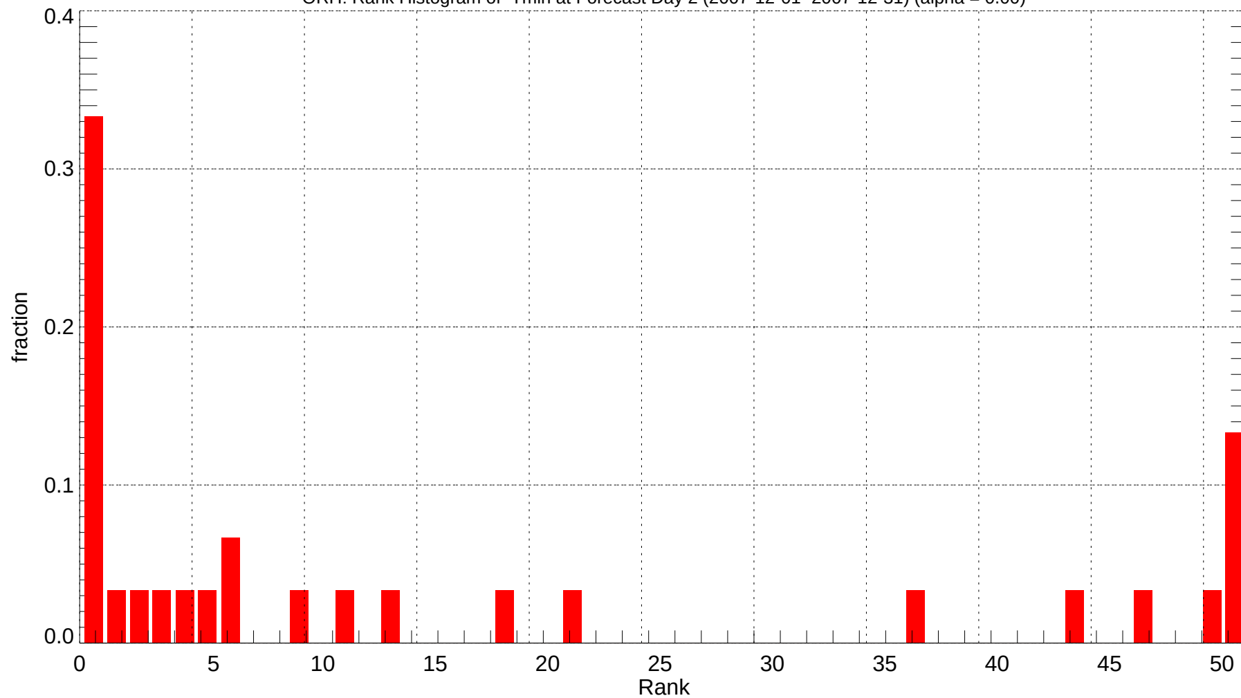
ORH: Rank Histogram of Tmin at Forecast Day 2 (2007-12-01~2007-12-31) (alpha = 0.00)
