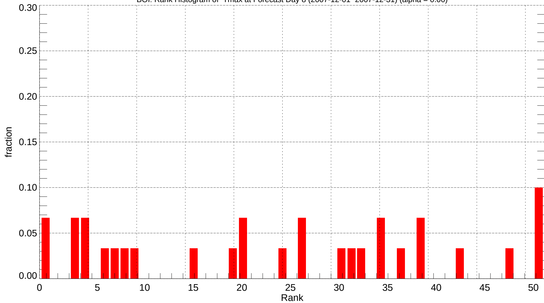
BOI: Rank Histogram of Tmax at Forecast Day 8 (2007-12-01~2007-12-31) (alpha = 0.00)
