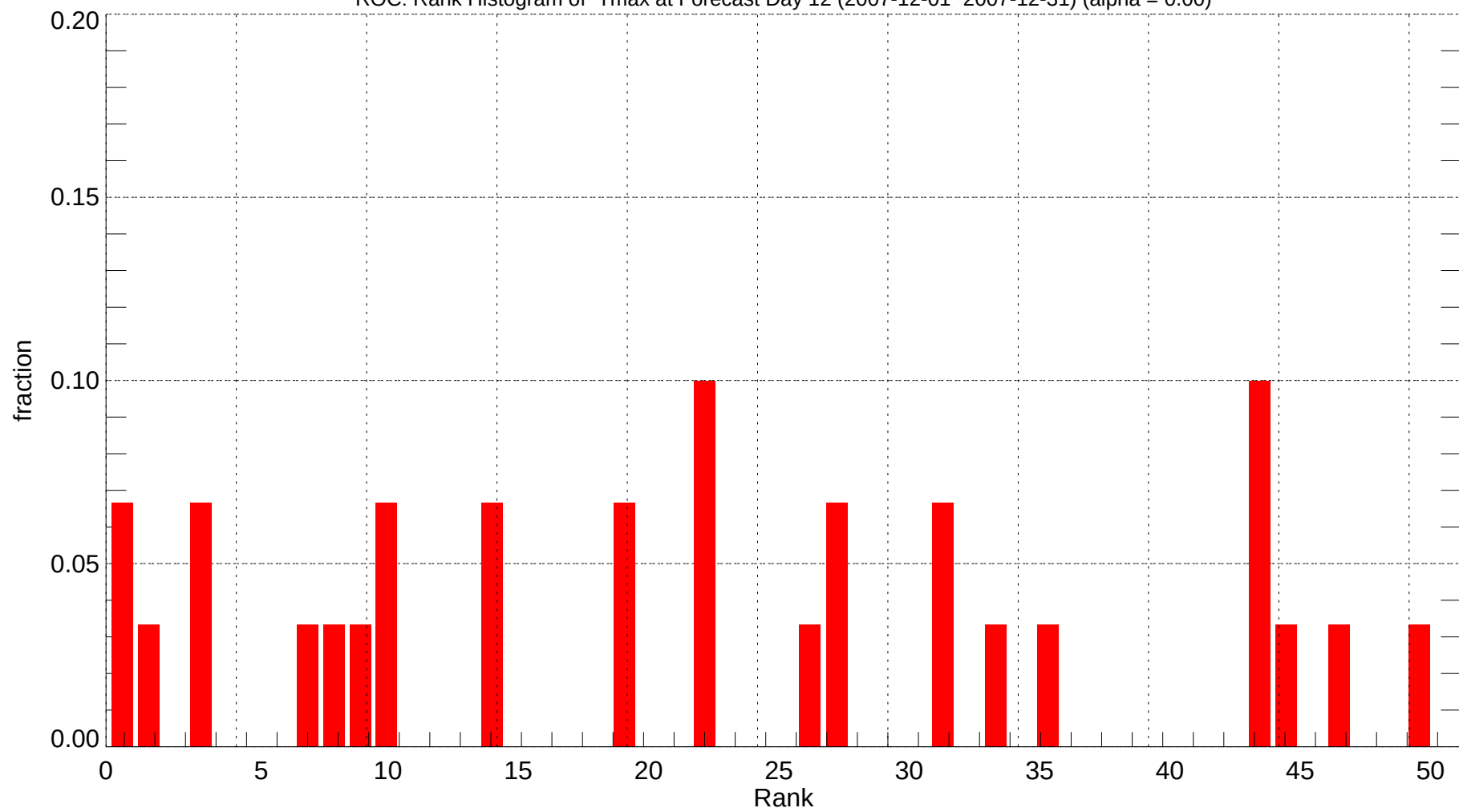
ROC: Rank Histogram of Tmax at Forecast Day 12 (2007-12-01~2007-12-31) (alpha = 0.00)
