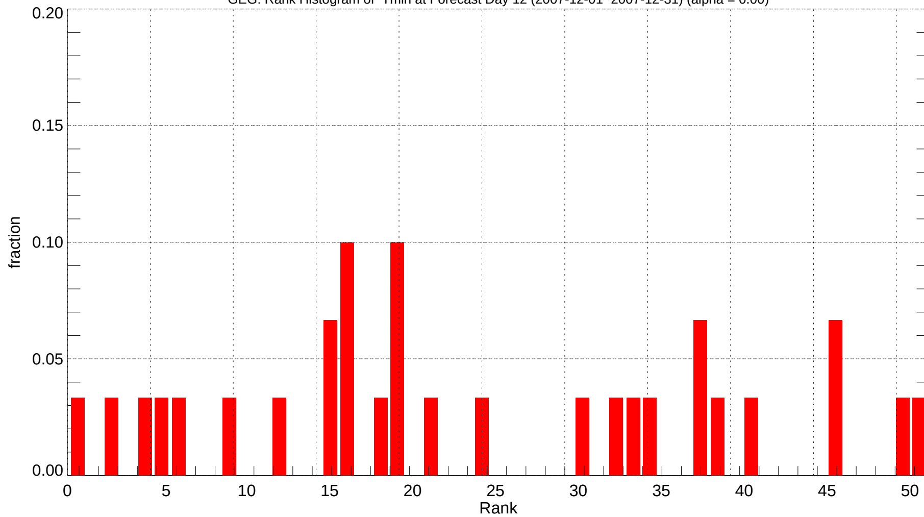
GEG: Rank Histogram of Tmin at Forecast Day 12 (2007-12-01~2007-12-31) (alpha = 0.00)
