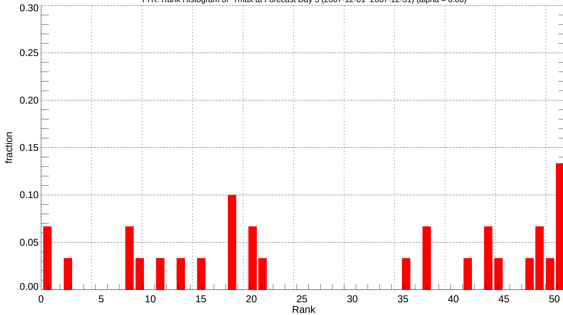
TYR: Rank Histogram of Tmax at Forecast Day 3 (2007-12-01~2007-12-31) (alpha = 0.00)
