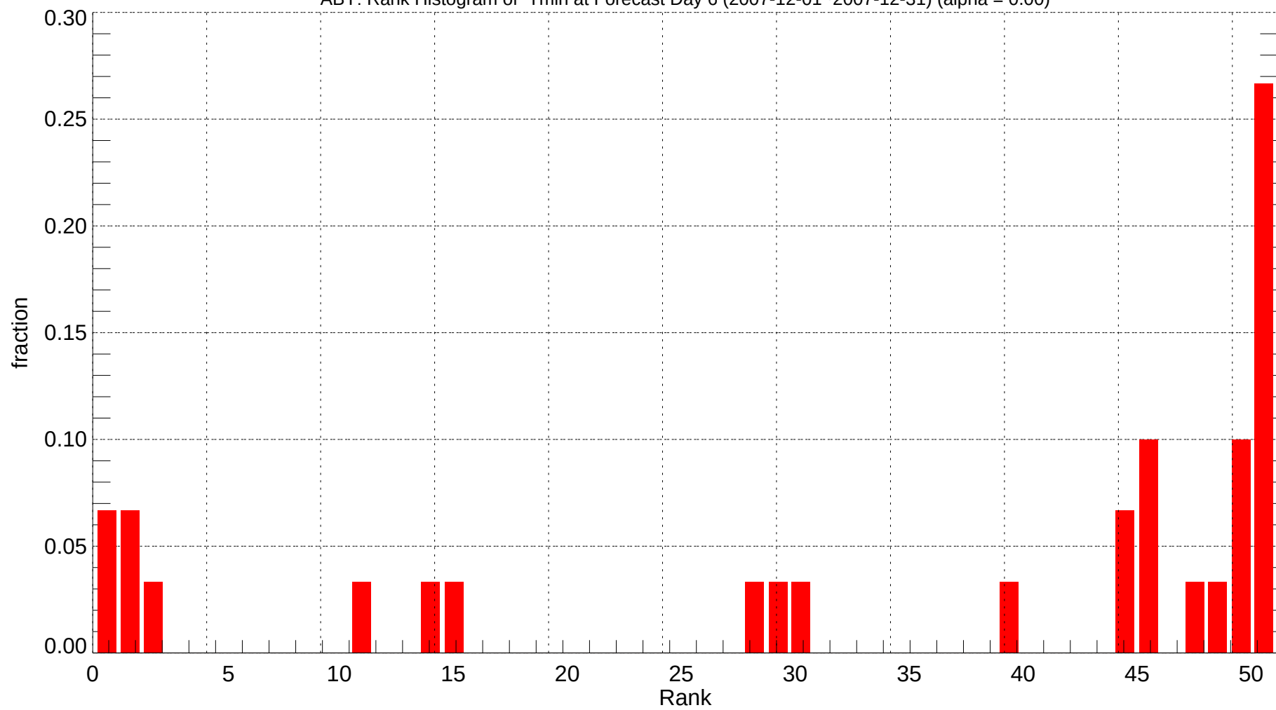
ABY: Rank Histogram of Tmin at Forecast Day 6 (2007-12-01~2007-12-31) (alpha = 0.00)
