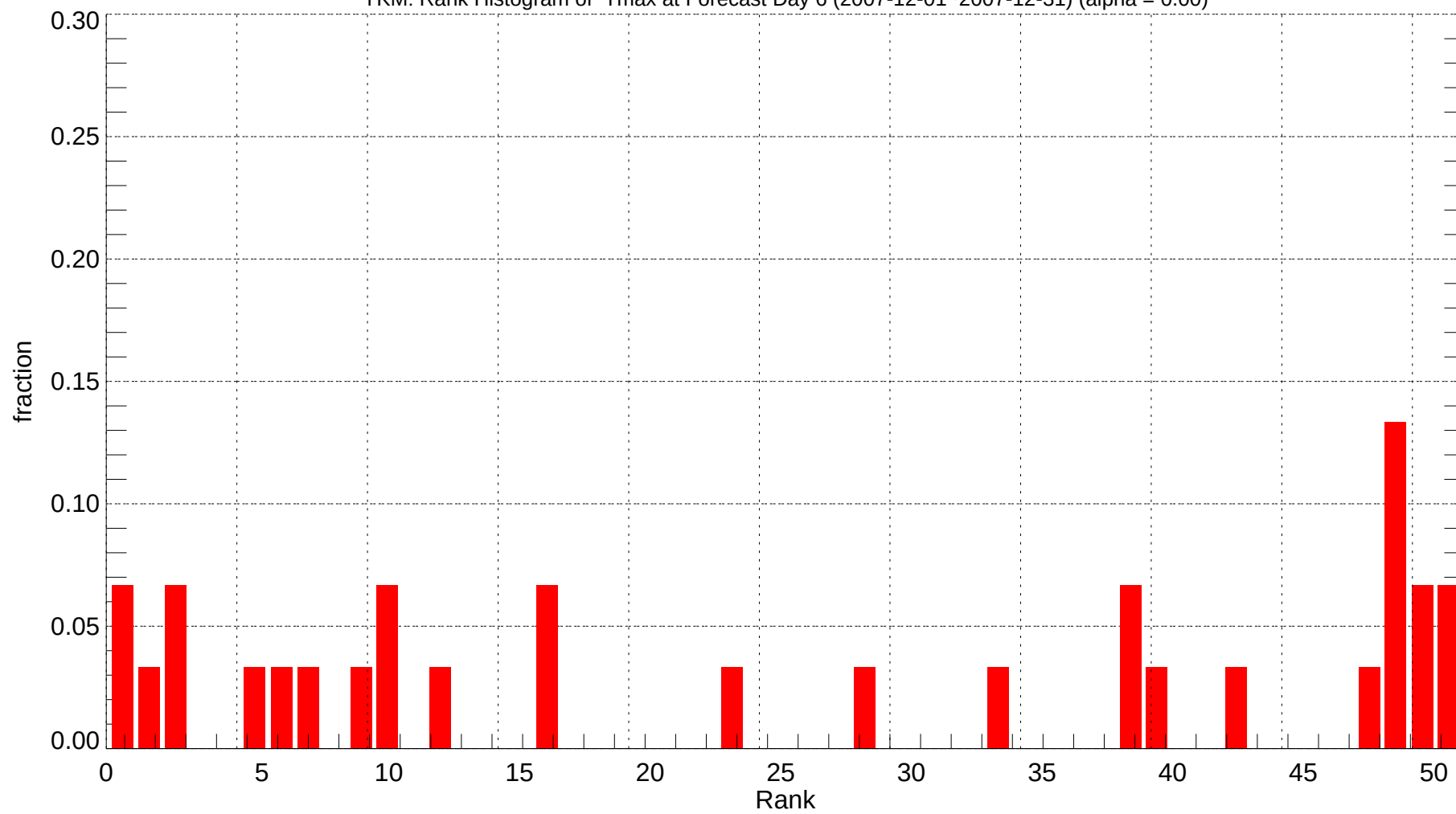
YKM: Rank Histogram of Tmax at Forecast Day 6 (2007-12-01~2007-12-31) (alpha = 0.00)
