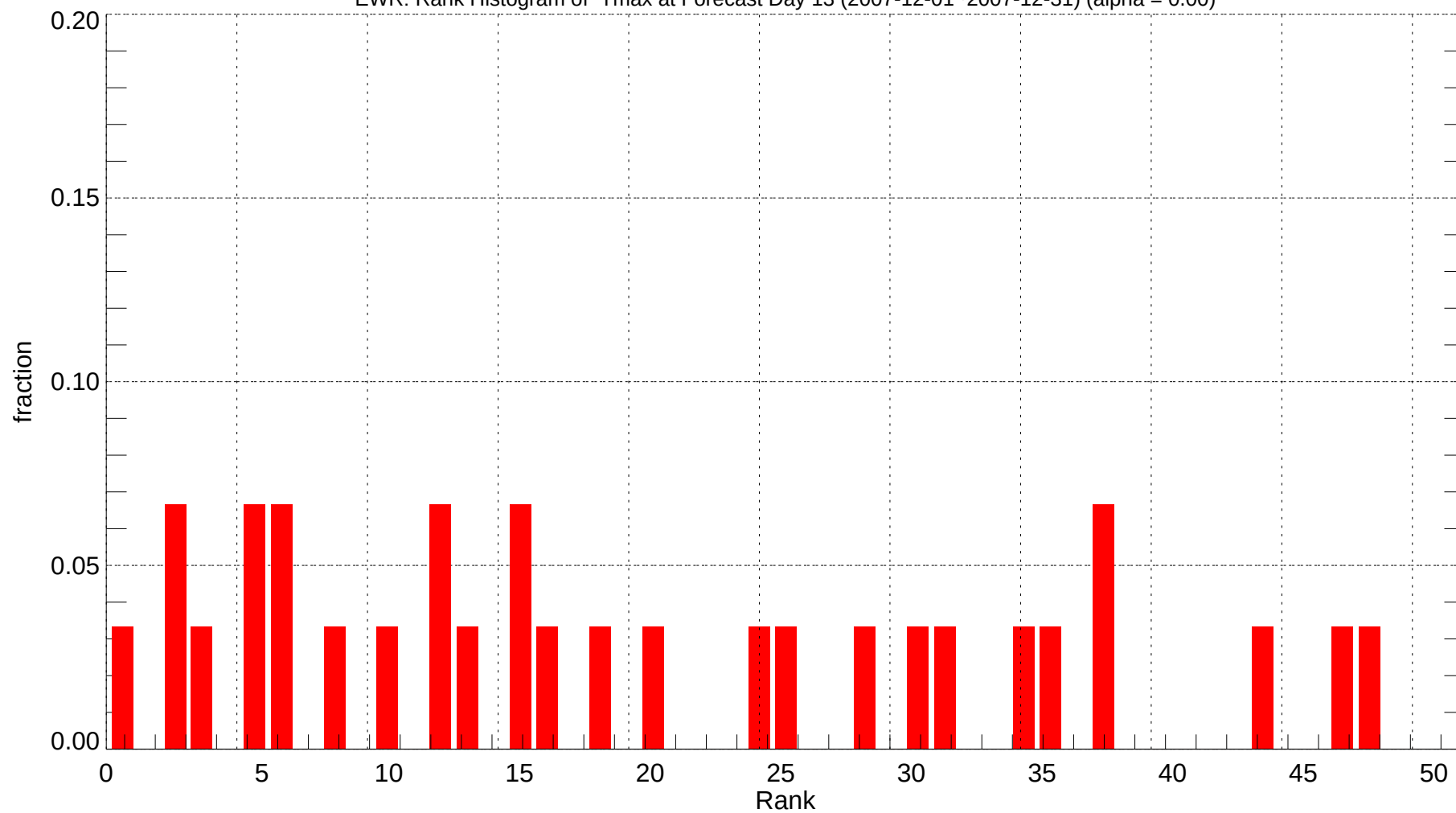
EWR: Rank Histogram of Tmax at Forecast Day 13 (2007-12-01~2007-12-31) (alpha = 0.00)
