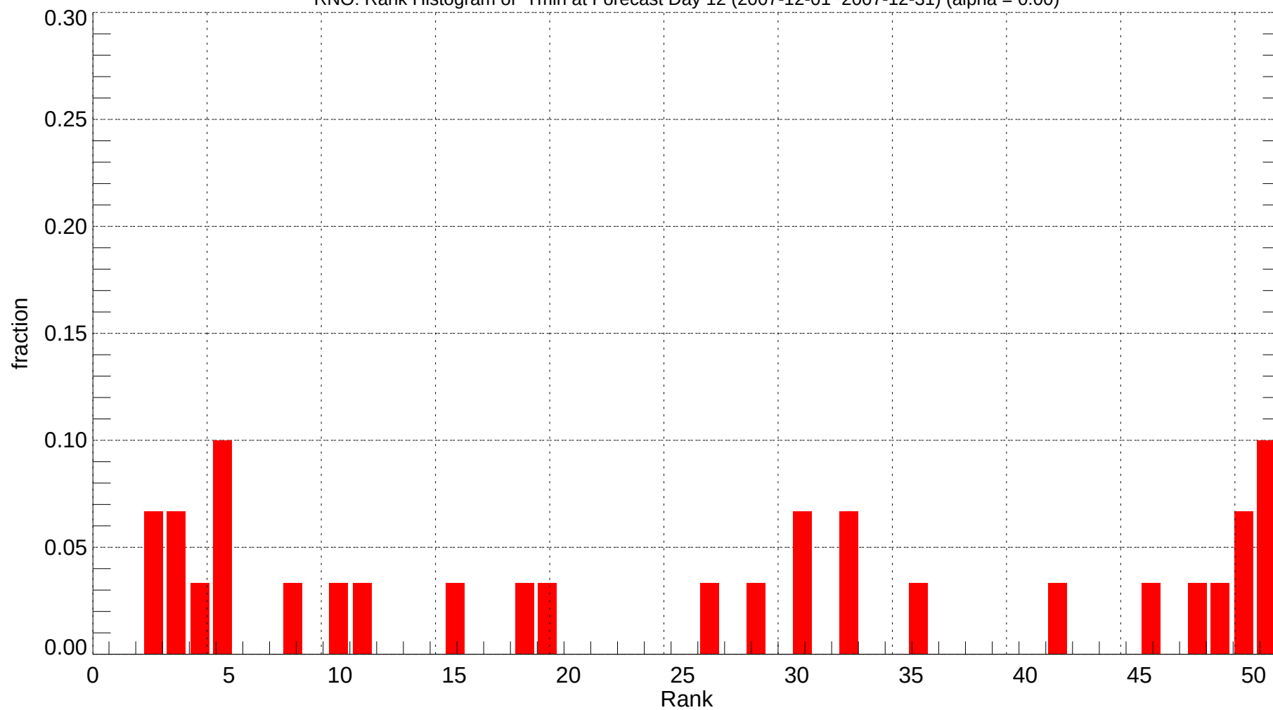
RNO: Rank Histogram of Tmin at Forecast Day 12 (2007-12-01~2007-12-31) (alpha = 0.00)
