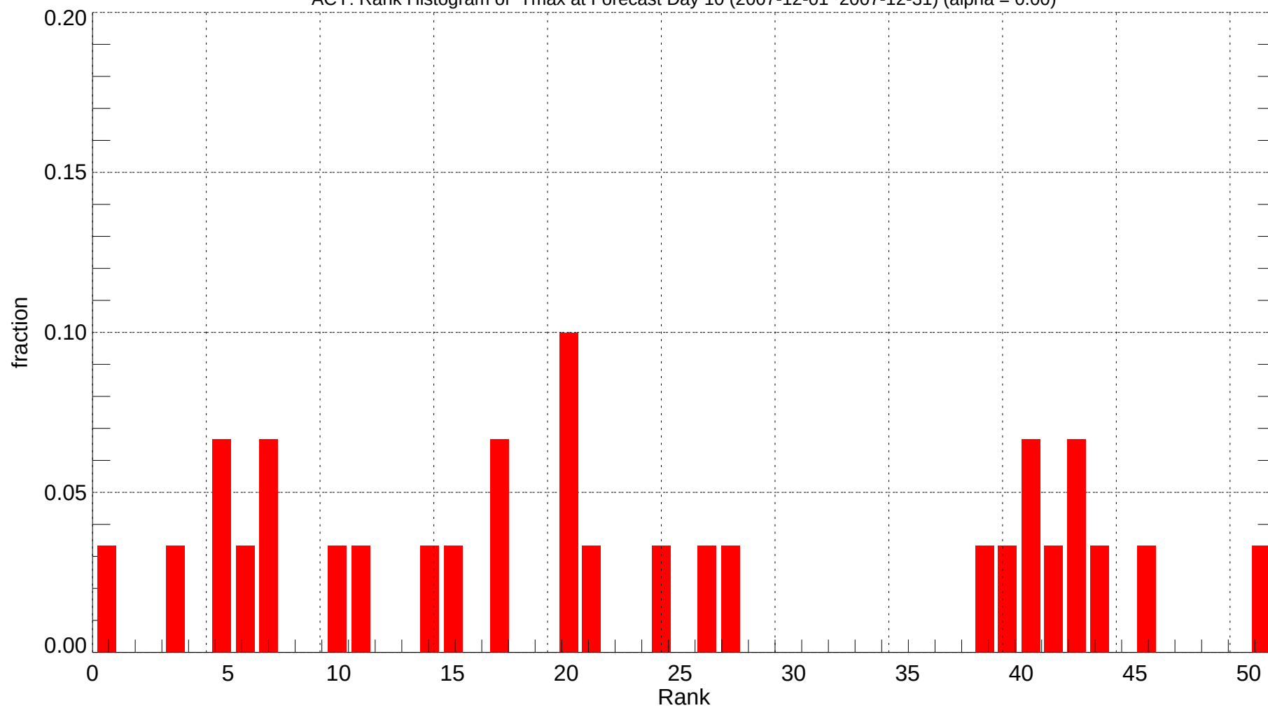
ACY: Rank Histogram of Tmax at Forecast Day 10 (2007-12-01~2007-12-31) (alpha = 0.00)
