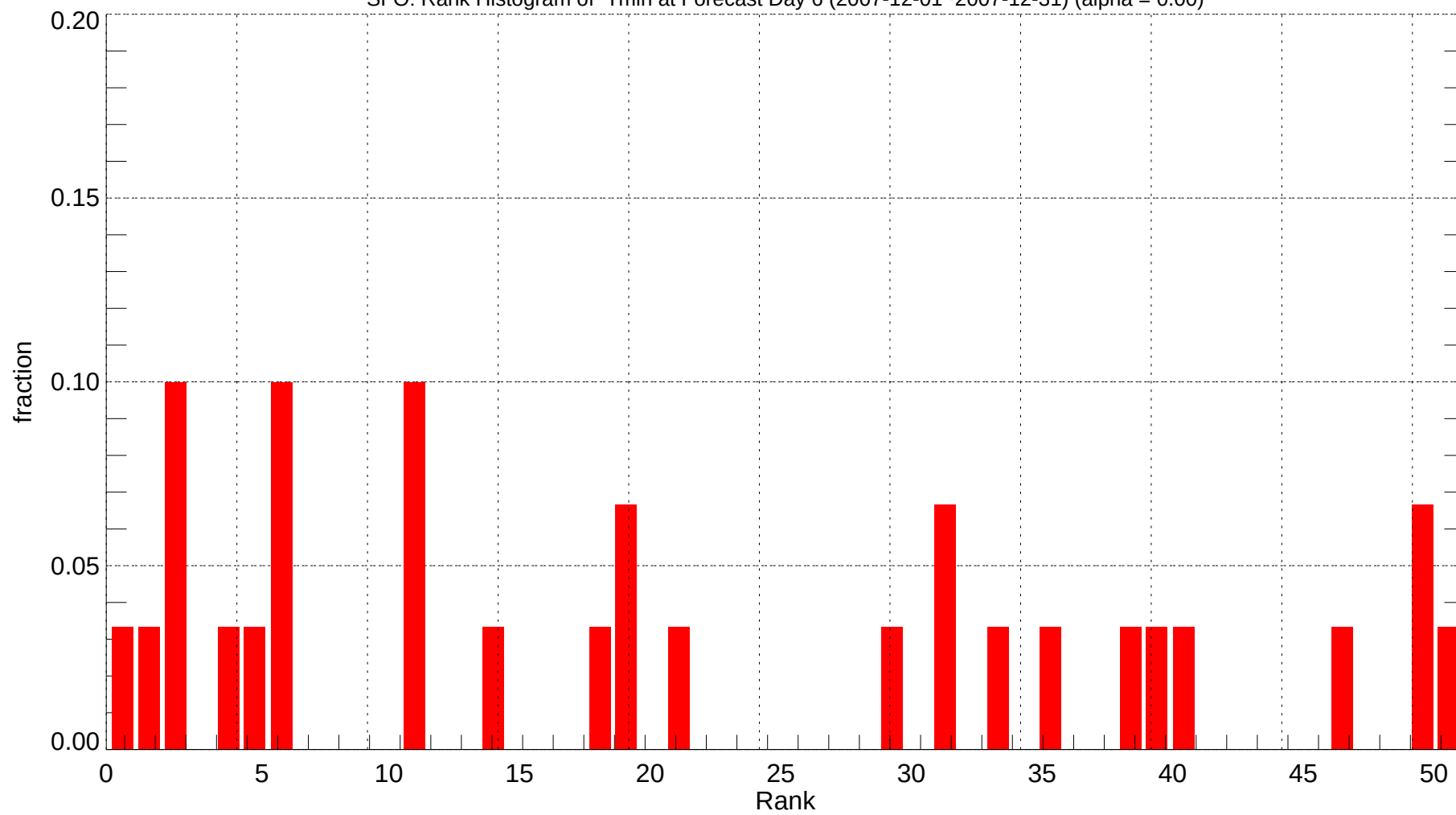
SFO: Rank Histogram of Tmin at Forecast Day 6 (2007-12-01~2007-12-31) (alpha = 0.00)
