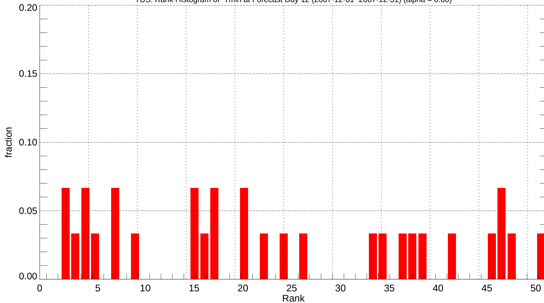
TUS: Rank Histogram of Tmin at Forecast Day 12 (2007-12-01~2007-12-31) (alpha = 0.00)
