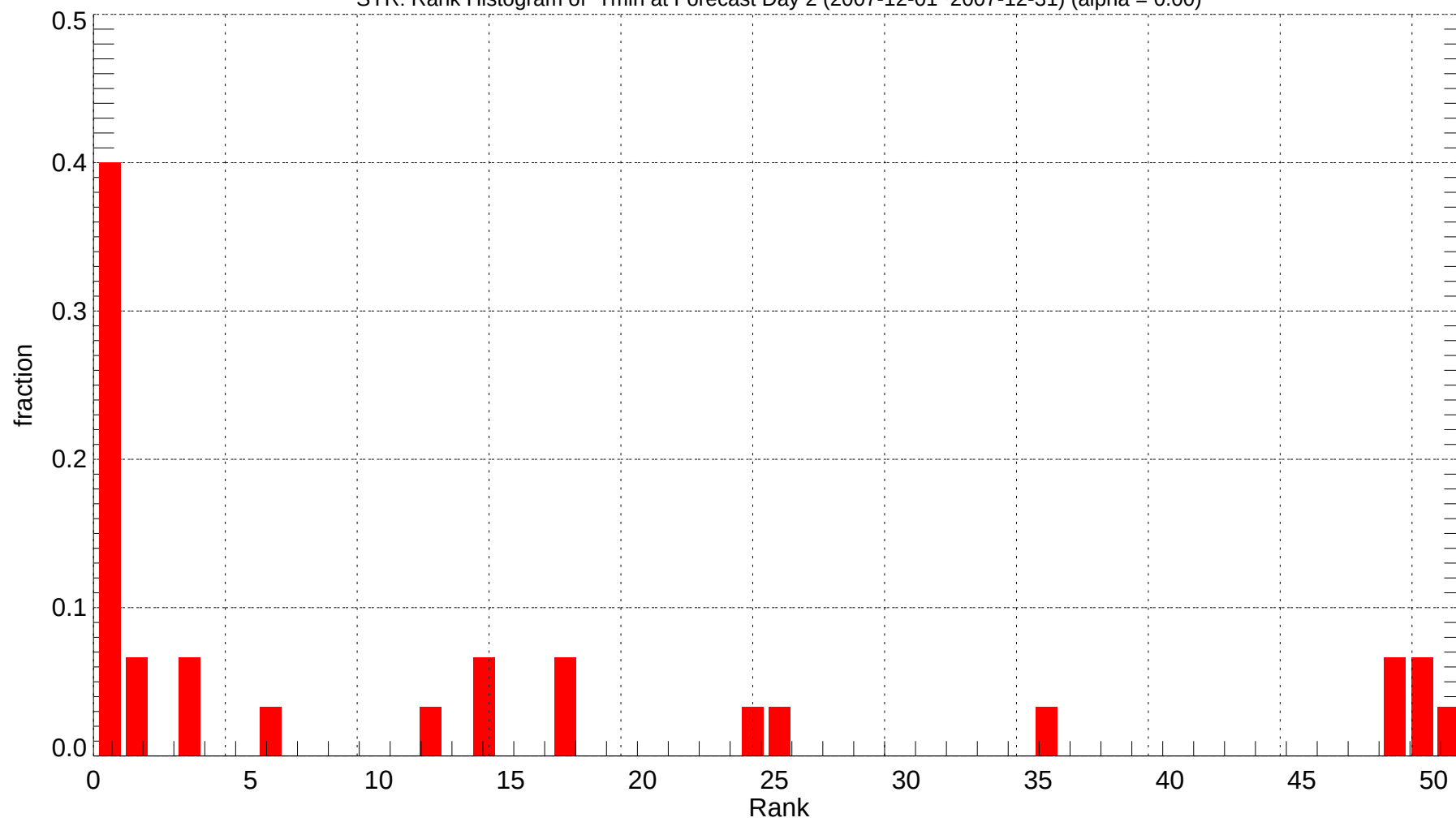
SYR: Rank Histogram of Tmin at Forecast Day 2 (2007-12-01~2007-12-31) (alpha = 0.00)
