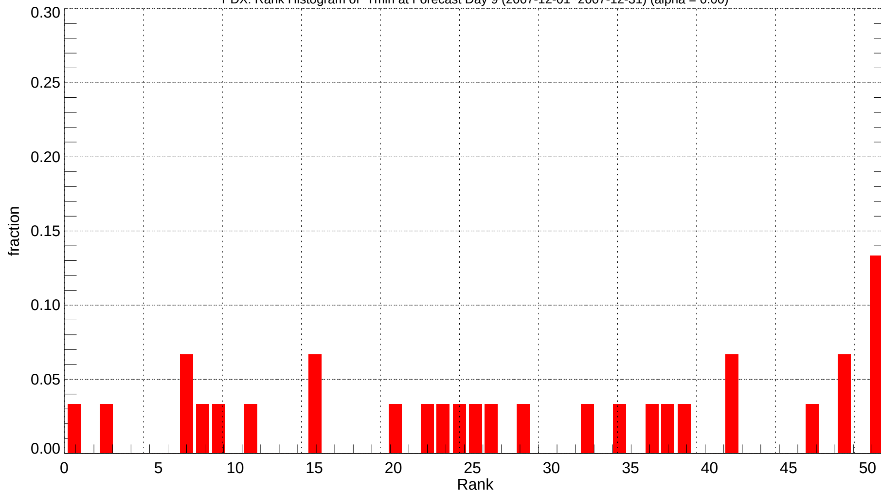
PDX: Rank Histogram of Tmin at Forecast Day 9 (2007-12-01~2007-12-31) (alpha = 0.00)
