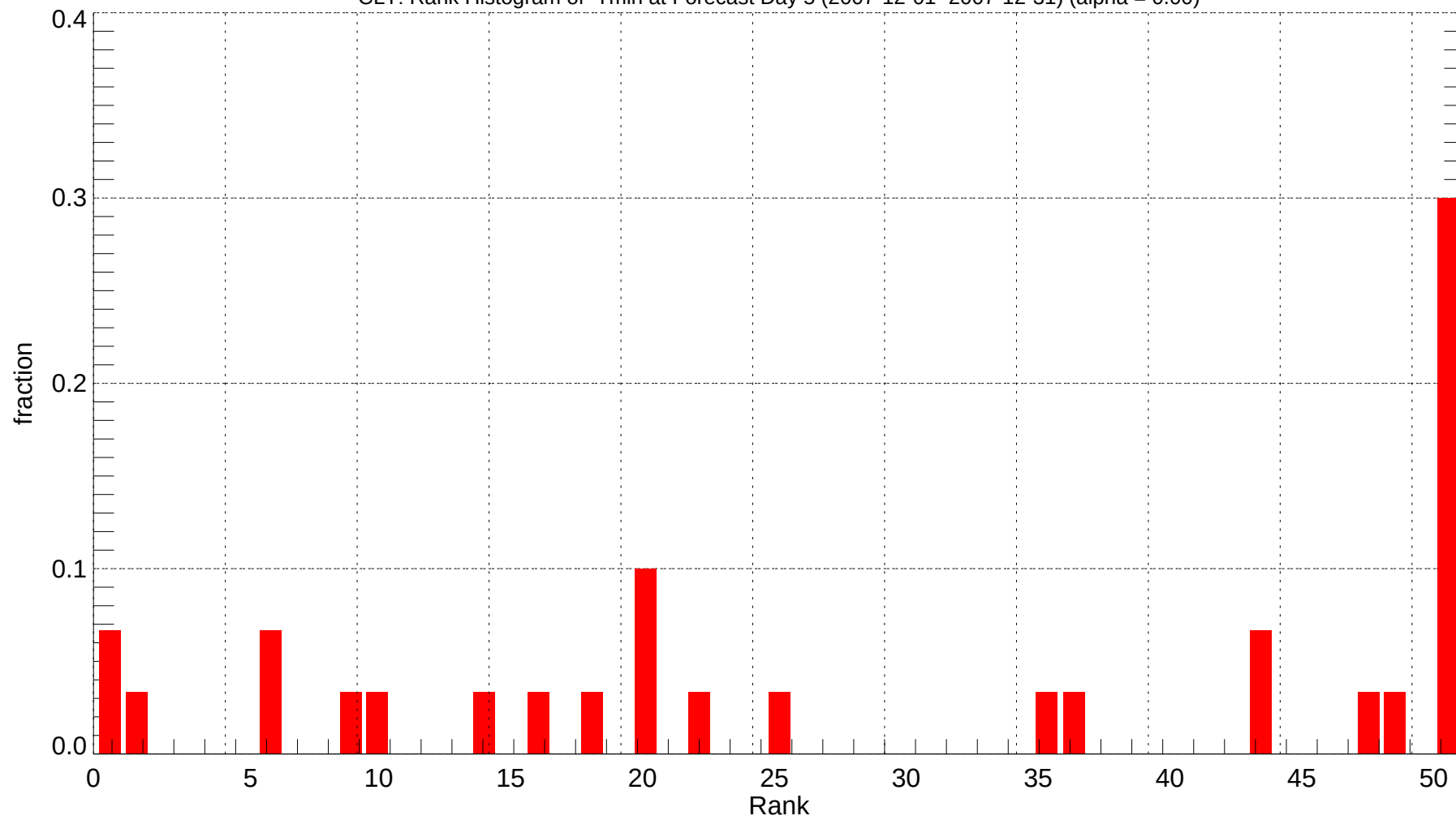
CLT: Rank Histogram of Tmin at Forecast Day 5 (2007-12-01~2007-12-31) (alpha = 0.00)
