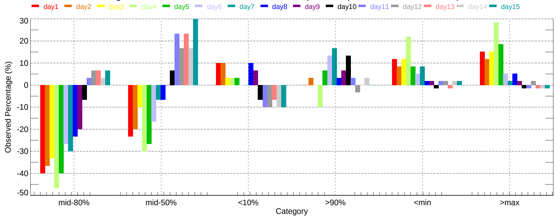
Observed Percentage Deviation of Ensembles - SAC: Min Temperature (2007-12-01~2007-12-31)
