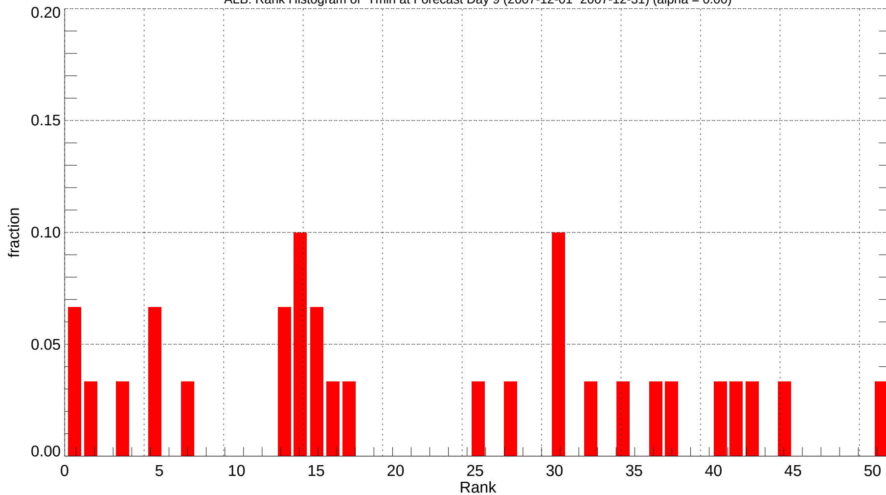
ALB: Rank Histogram of Tmin at Forecast Day 9 (2007-12-01~2007-12-31) (alpha = 0.00)
