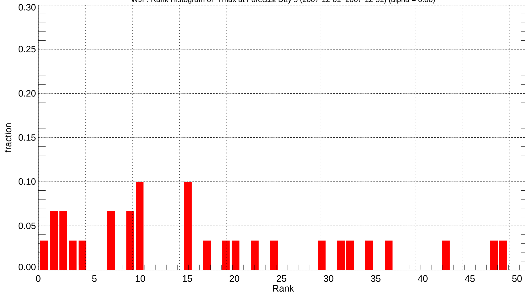
WJF: Rank Histogram of Tmax at Forecast Day 9 (2007-12-01~2007-12-31) (alpha = 0.00)
