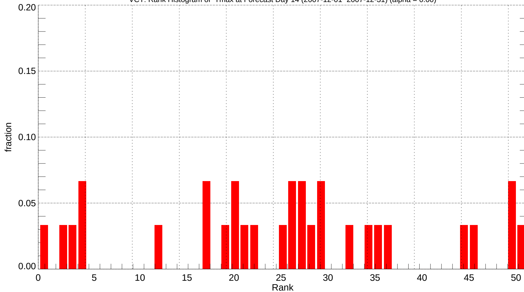
VCT: Rank Histogram of Tmax at Forecast Day 14 (2007-12-01~2007-12-31) (alpha = 0.00)
