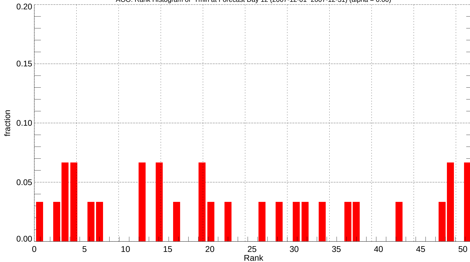
AOO: Rank Histogram of Tmin at Forecast Day 12 (2007-12-01~2007-12-31) (alpha = 0.00)
