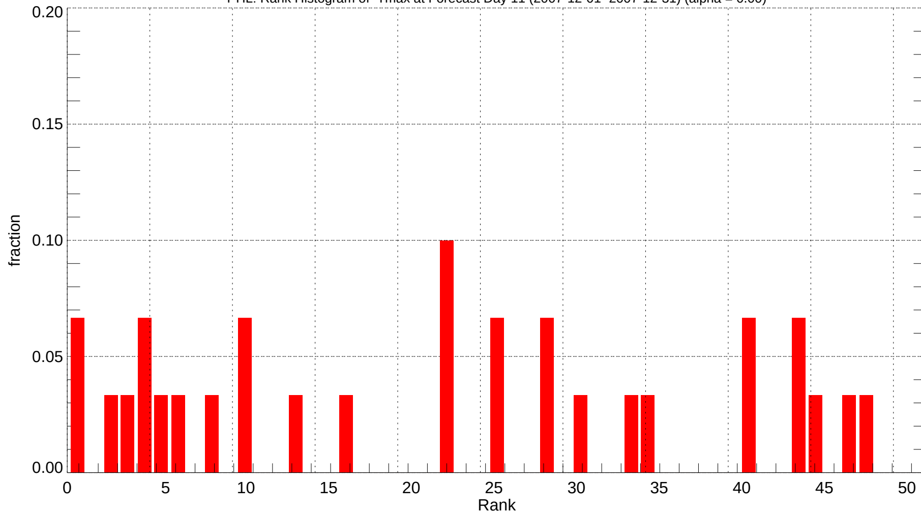
PHL: Rank Histogram of Tmax at Forecast Day 11 (2007-12-01~2007-12-31) (alpha = 0.00)
