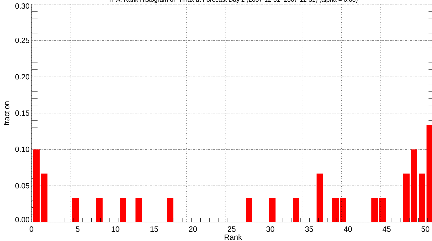
TPA: Rank Histogram of Tmax at Forecast Day 2 (2007-12-01~2007-12-31) (alpha = 0.00)
