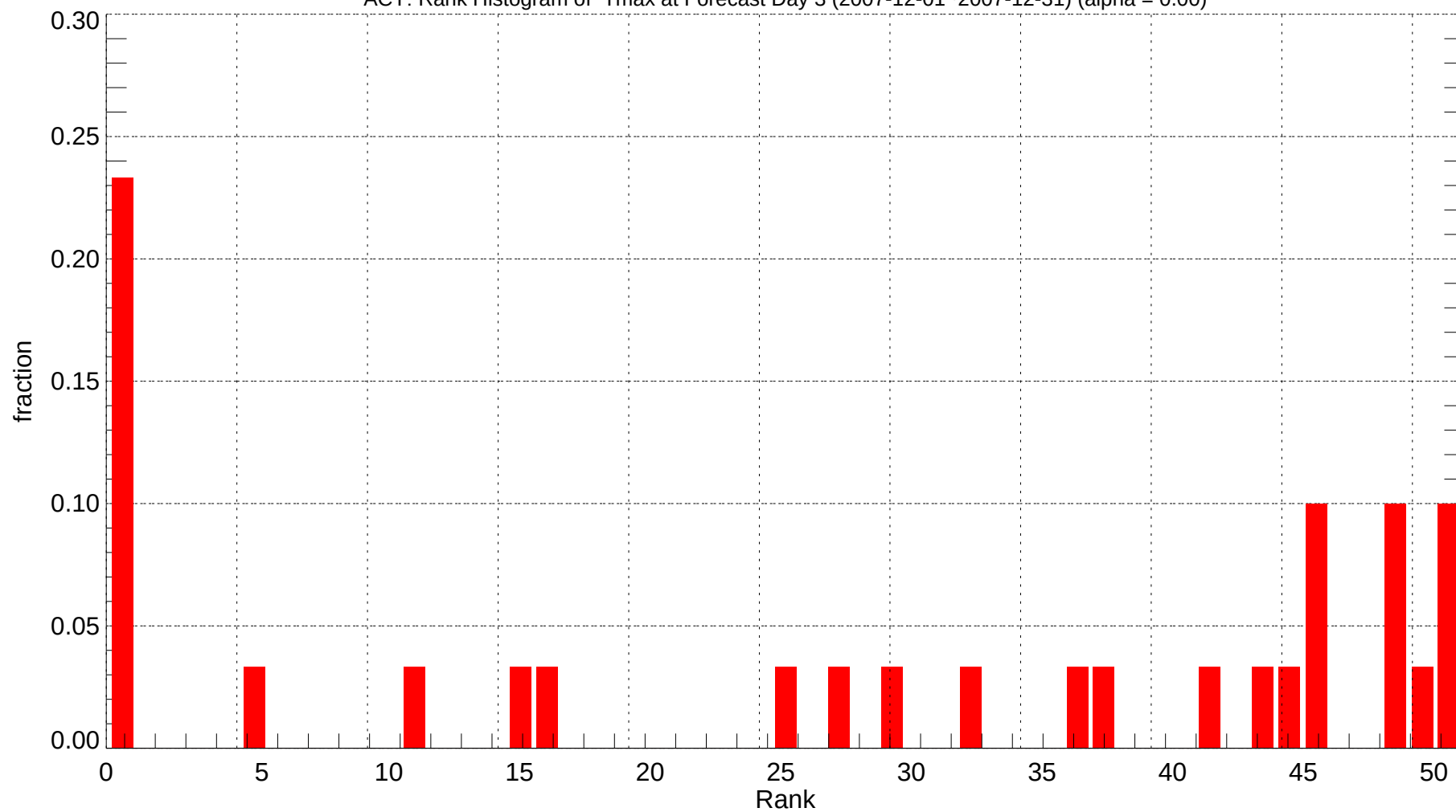
ACY: Rank Histogram of Tmax at Forecast Day 3 (2007-12-01~2007-12-31) (alpha = 0.00)
