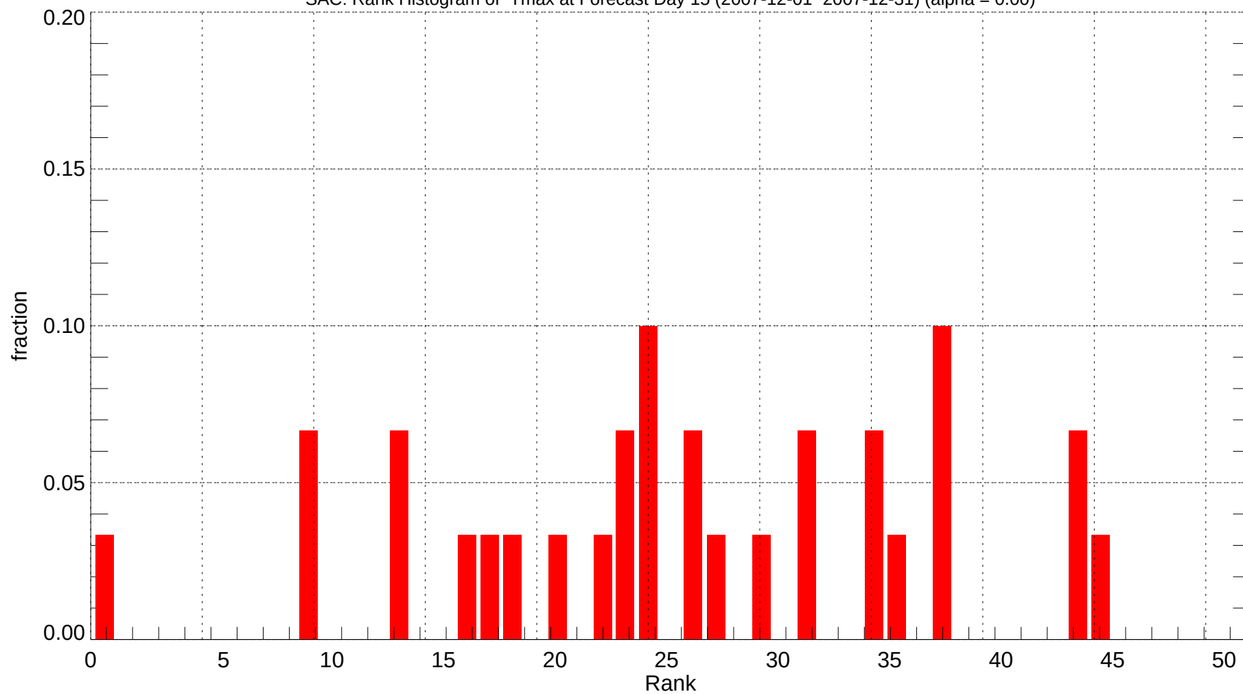
SAC: Rank Histogram of Tmax at Forecast Day 15 (2007-12-01~2007-12-31) (alpha = 0.00)
