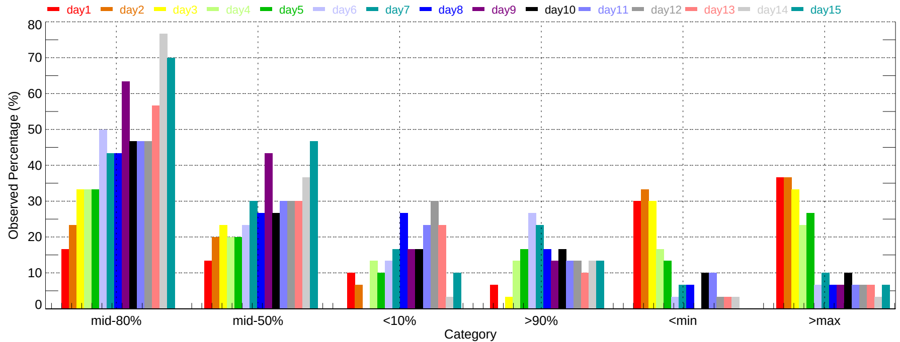
Observed Percentage of Ensembles - YKM: Max Temperature (2007-12-01~2007-12-31)
