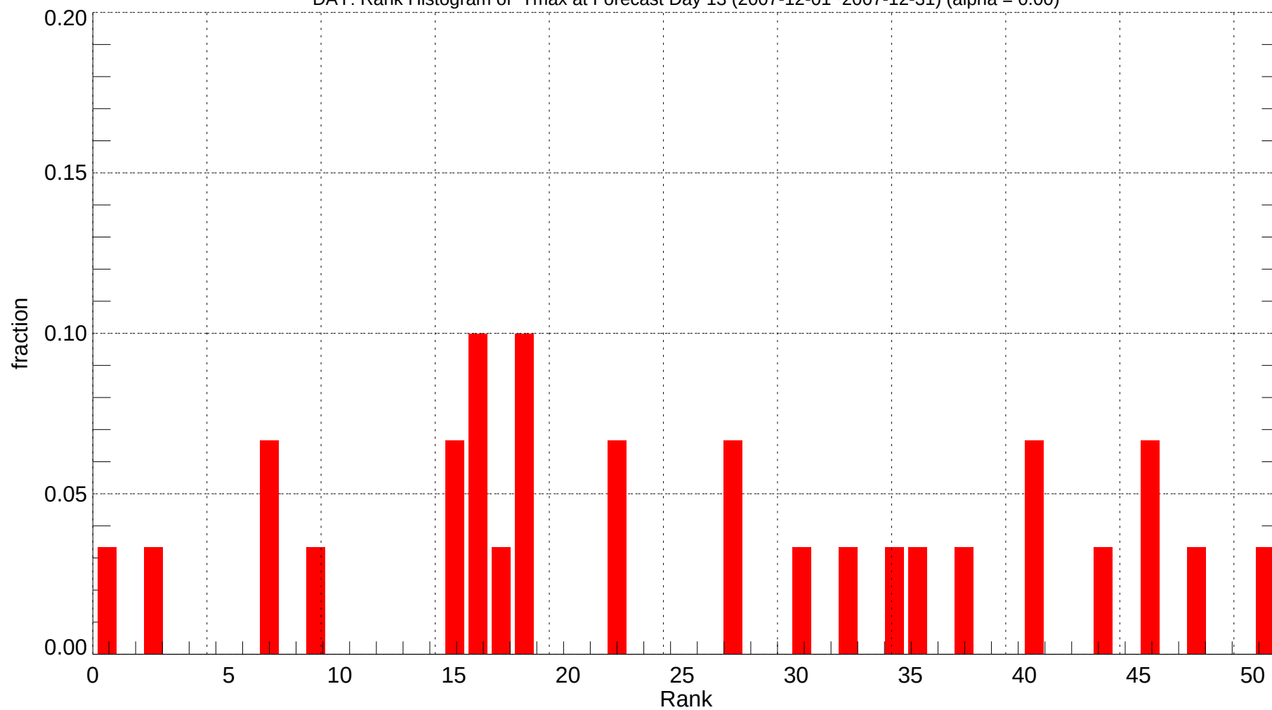
DAY: Rank Histogram of Tmax at Forecast Day 13 (2007-12-01~2007-12-31) (alpha = 0.00)
