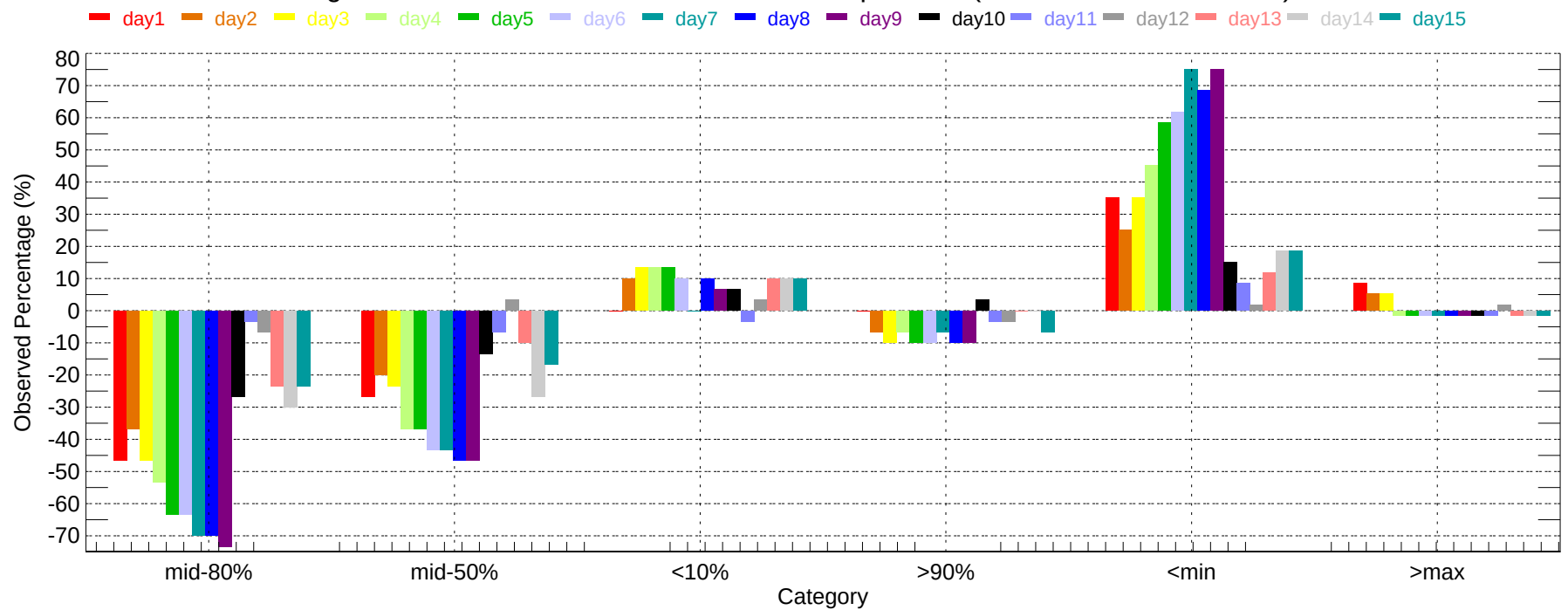
Observed Percentage Deviation of Ensembles - SJC: Min Temperature (2007-12-01~2007-12-31)
