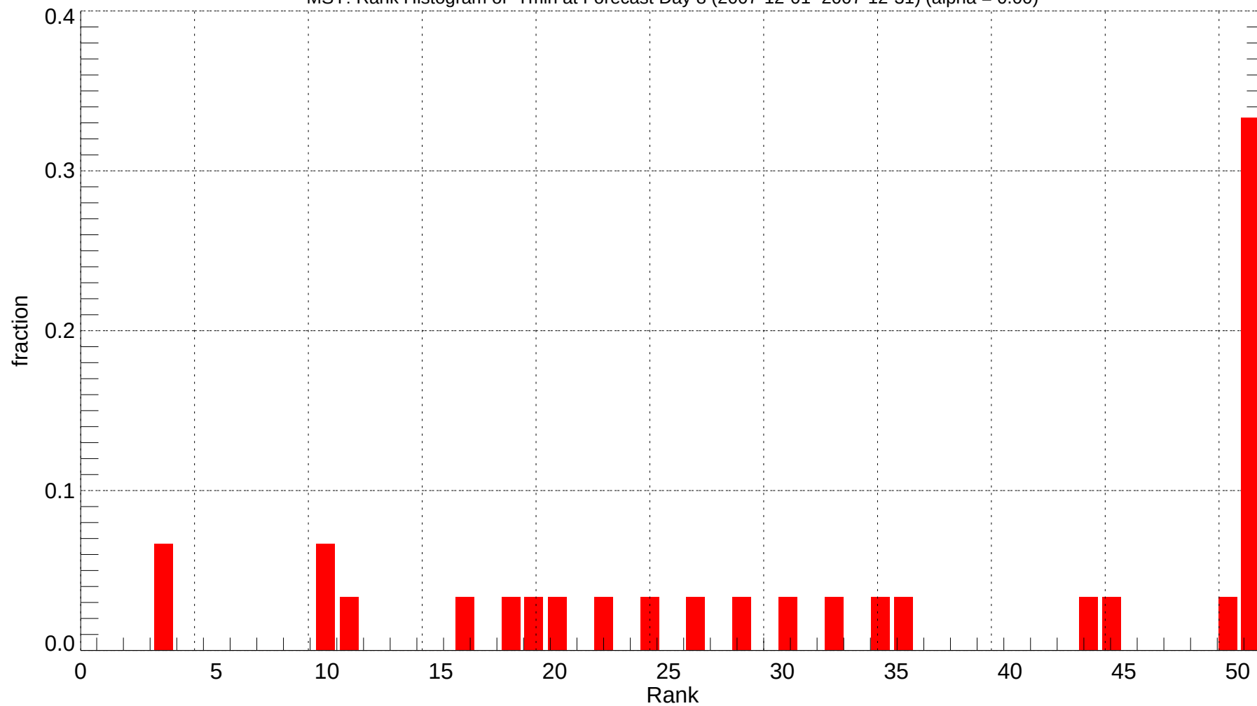
MSY: Rank Histogram of Tmin at Forecast Day 8 (2007-12-01~2007-12-31) (alpha = 0.00)
