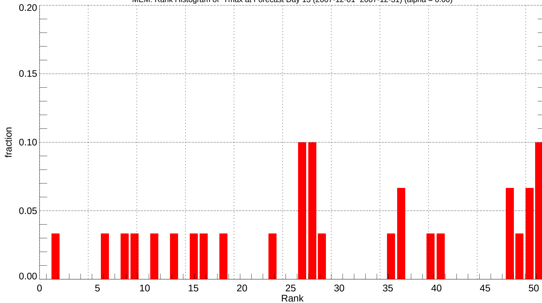
MEM: Rank Histogram of Tmax at Forecast Day 13 (2007-12-01~2007-12-31) (alpha = 0.00)
