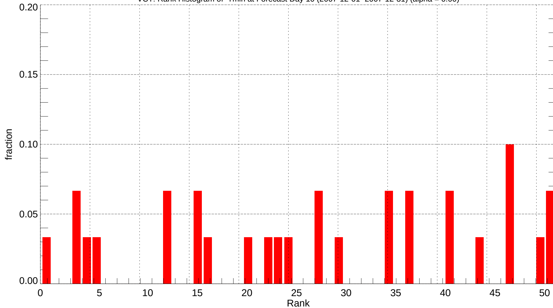
VCT: Rank Histogram of Tmin at Forecast Day 10 (2007-12-01~2007-12-31) (alpha = 0.00)
