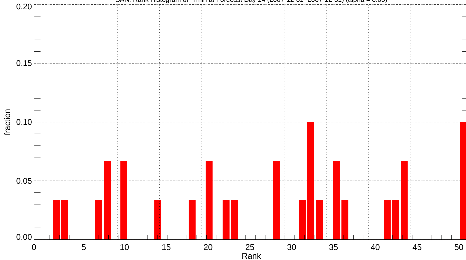
SAN: Rank Histogram of Tmin at Forecast Day 14 (2007-12-01~2007-12-31) (alpha = 0.00)
