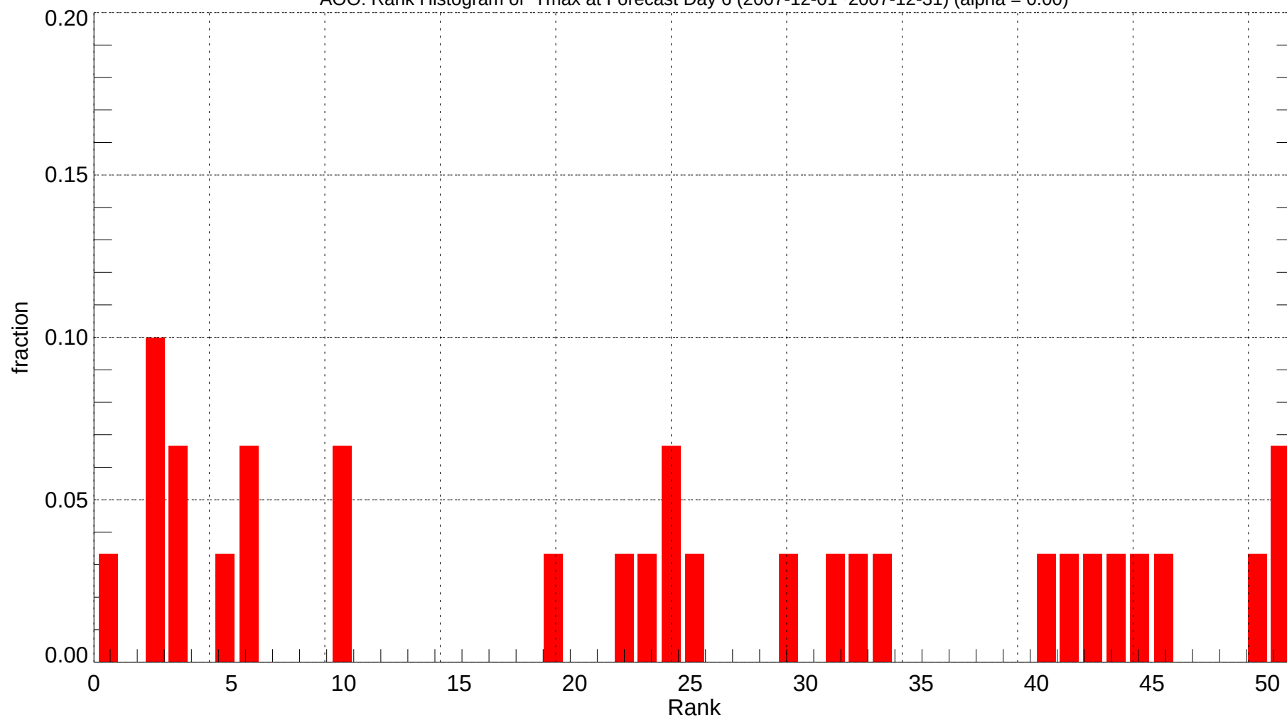
AOO: Rank Histogram of Tmax at Forecast Day 6 (2007-12-01~2007-12-31) (alpha = 0.00)
