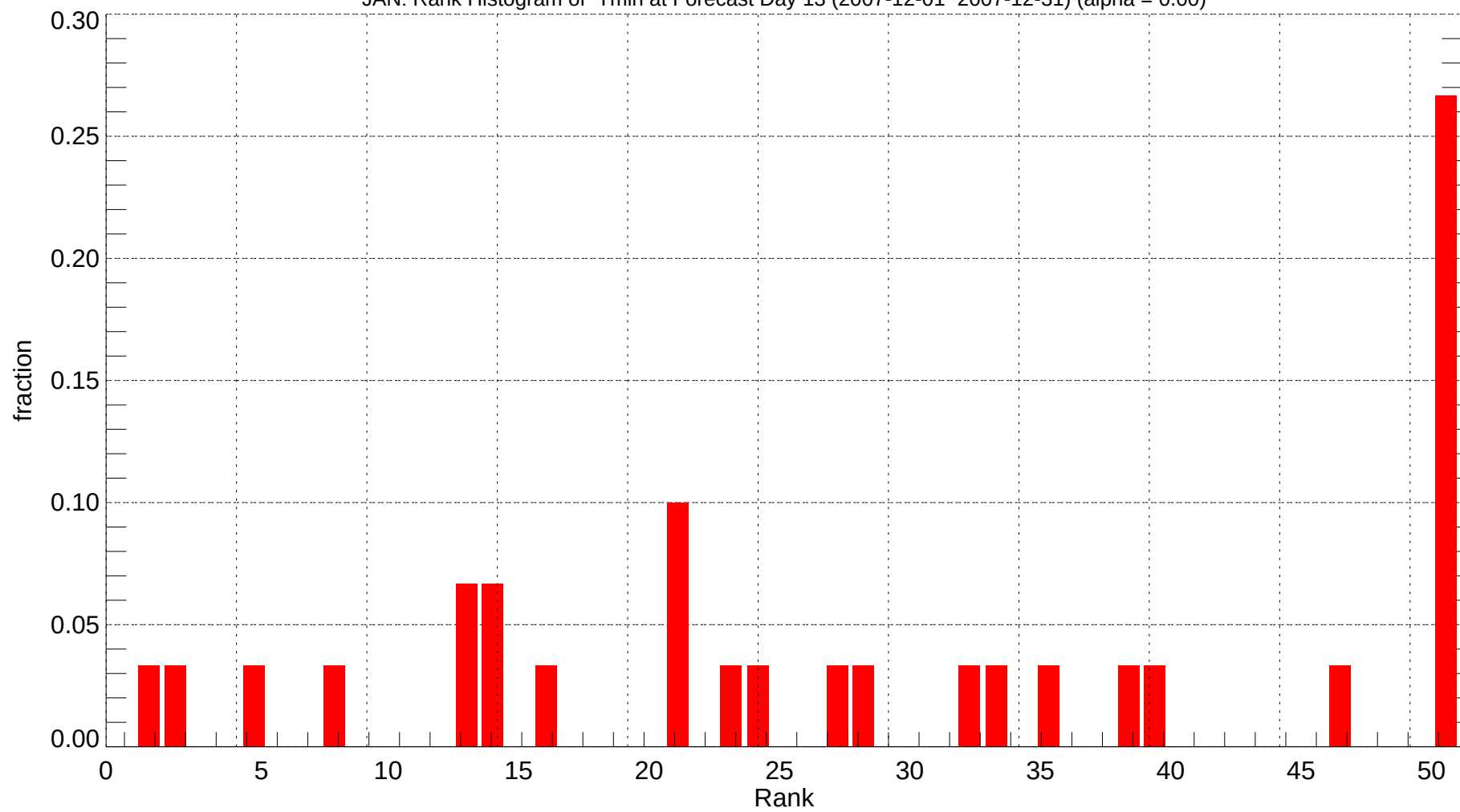
JAN: Rank Histogram of Tmin at Forecast Day 13 (2007-12-01~2007-12-31) (alpha = 0.00)
