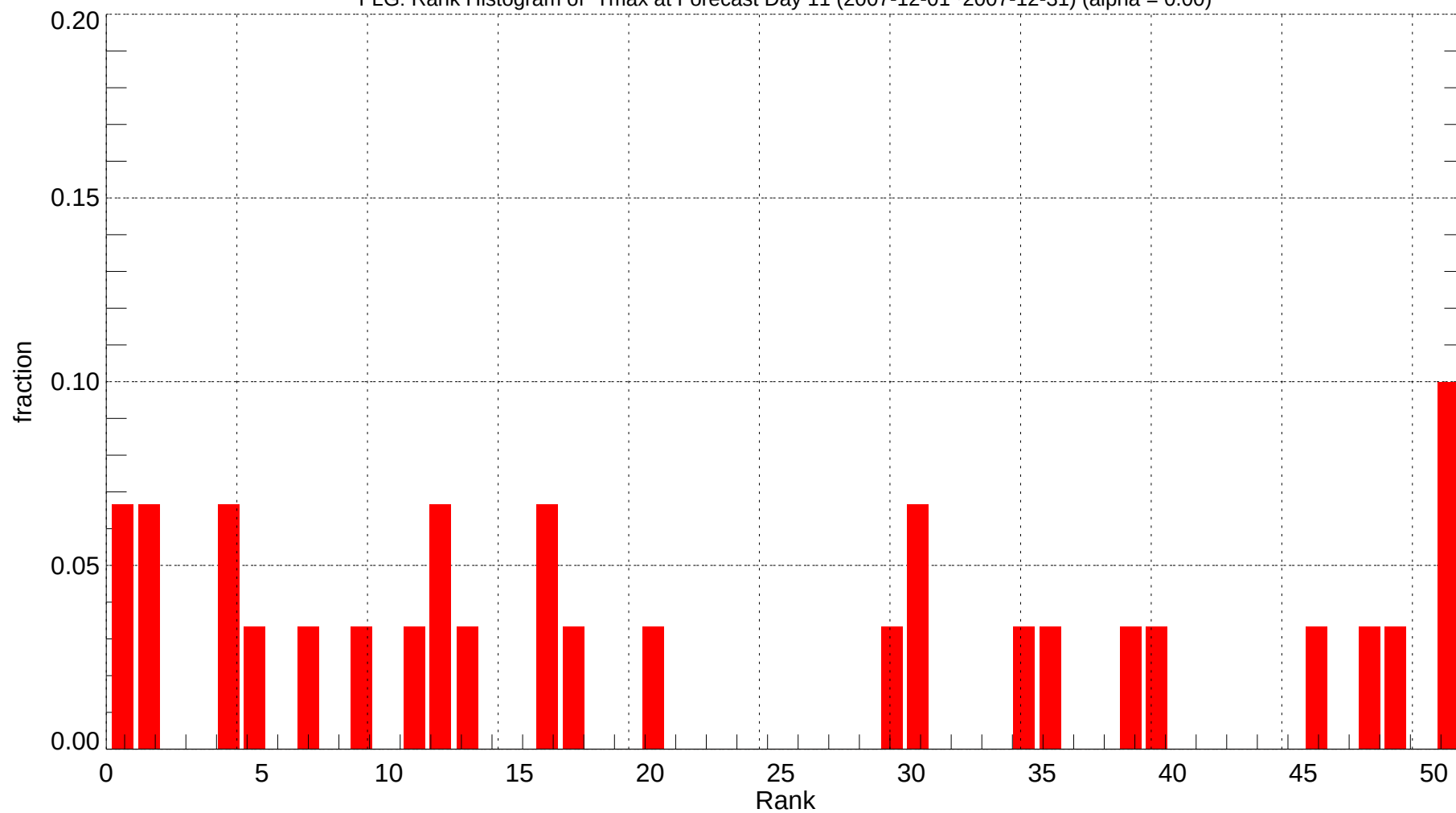
FLG: Rank Histogram of Tmax at Forecast Day 11 (2007-12-01~2007-12-31) (alpha = 0.00)
