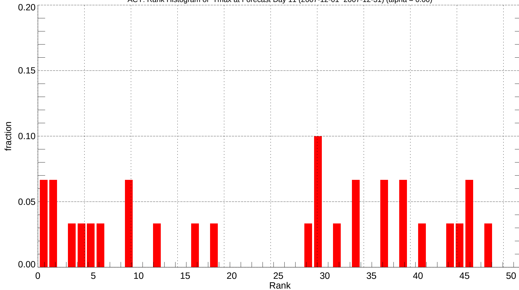
ACY: Rank Histogram of Tmax at Forecast Day 11 (2007-12-01~2007-12-31) (alpha = 0.00)
