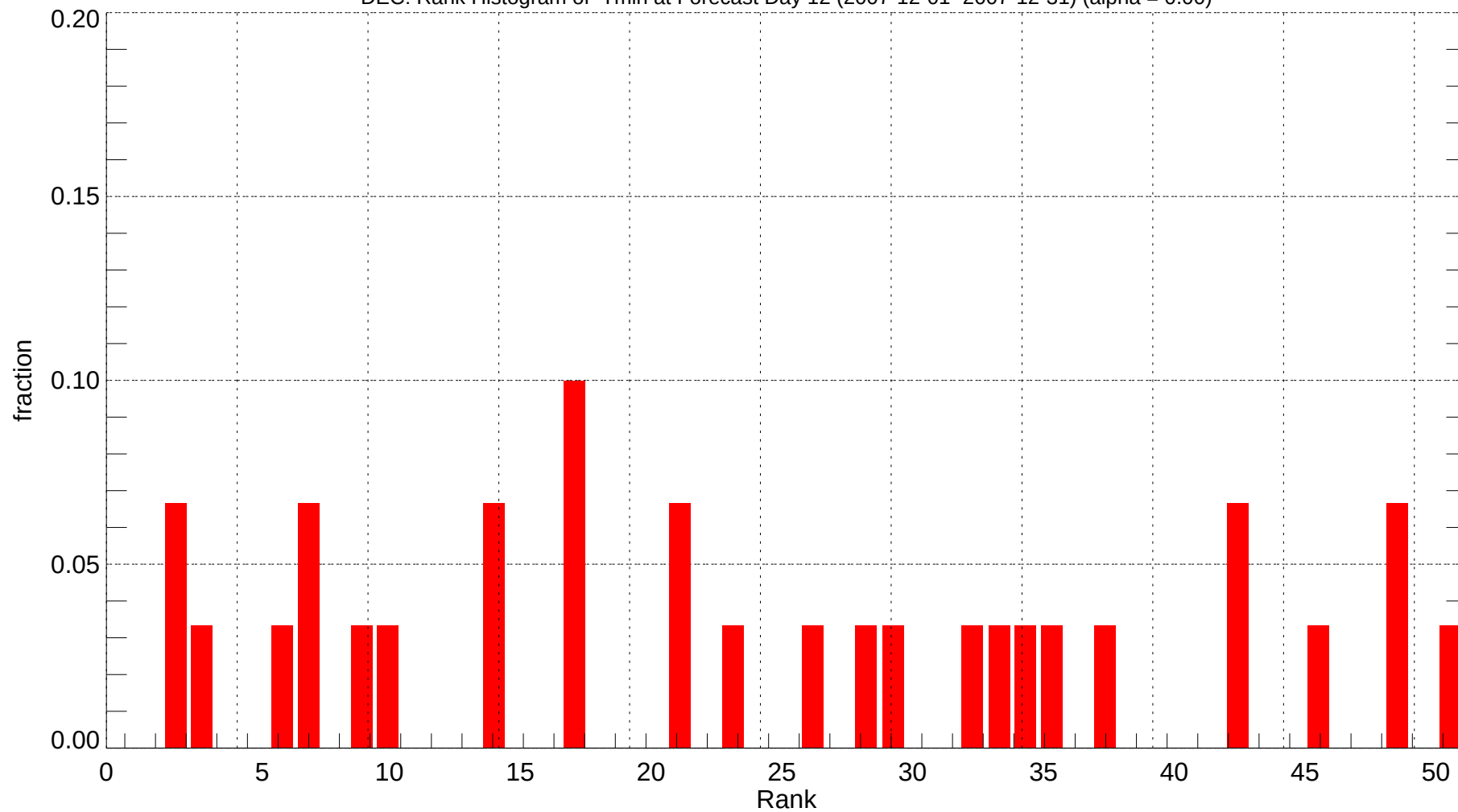
DEC: Rank Histogram of Tmin at Forecast Day 12 (2007-12-01~2007-12-31) (alpha = 0.00)
