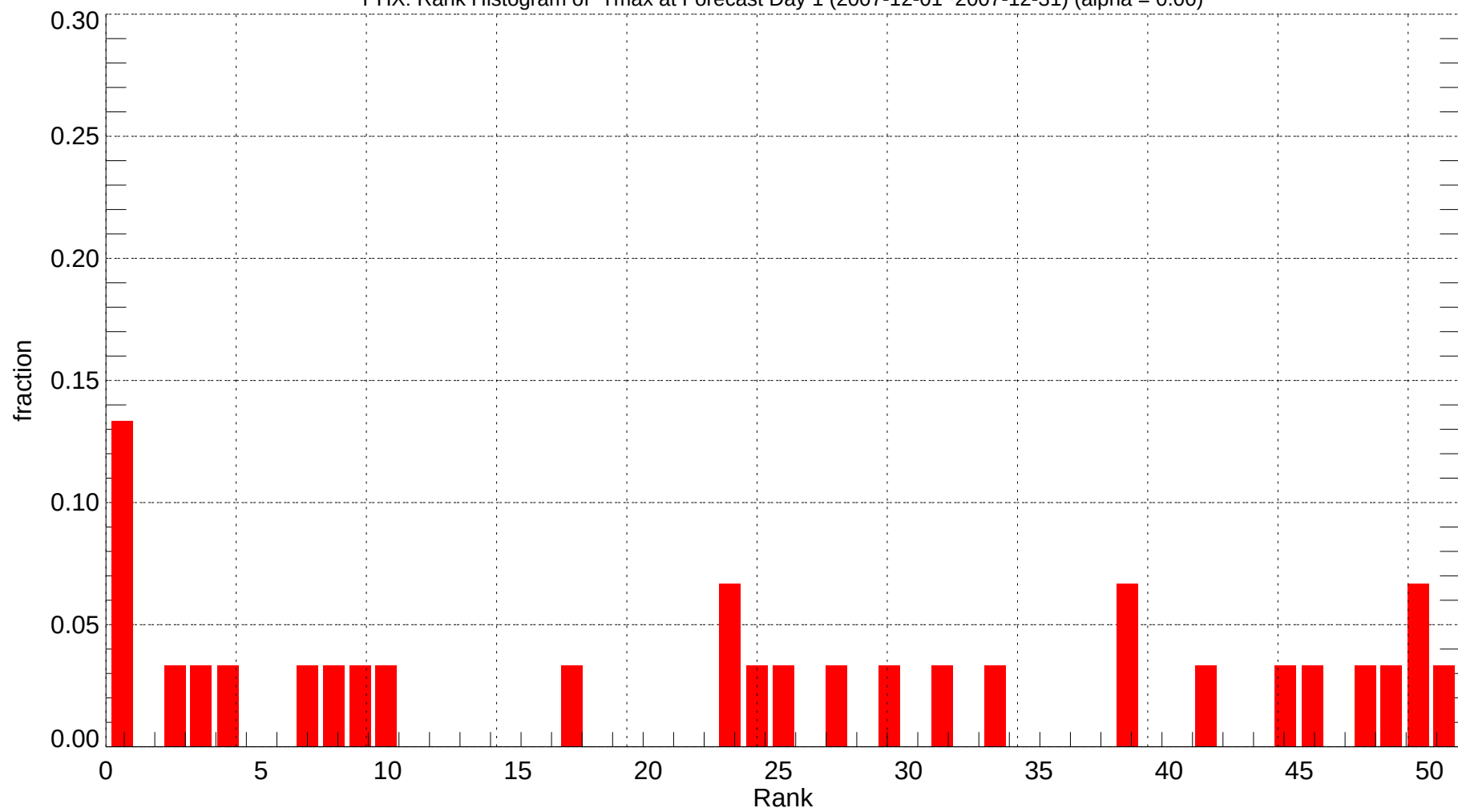
PHX: Rank Histogram of Tmax at Forecast Day 1 (2007-12-01~2007-12-31) (alpha = 0.00)
