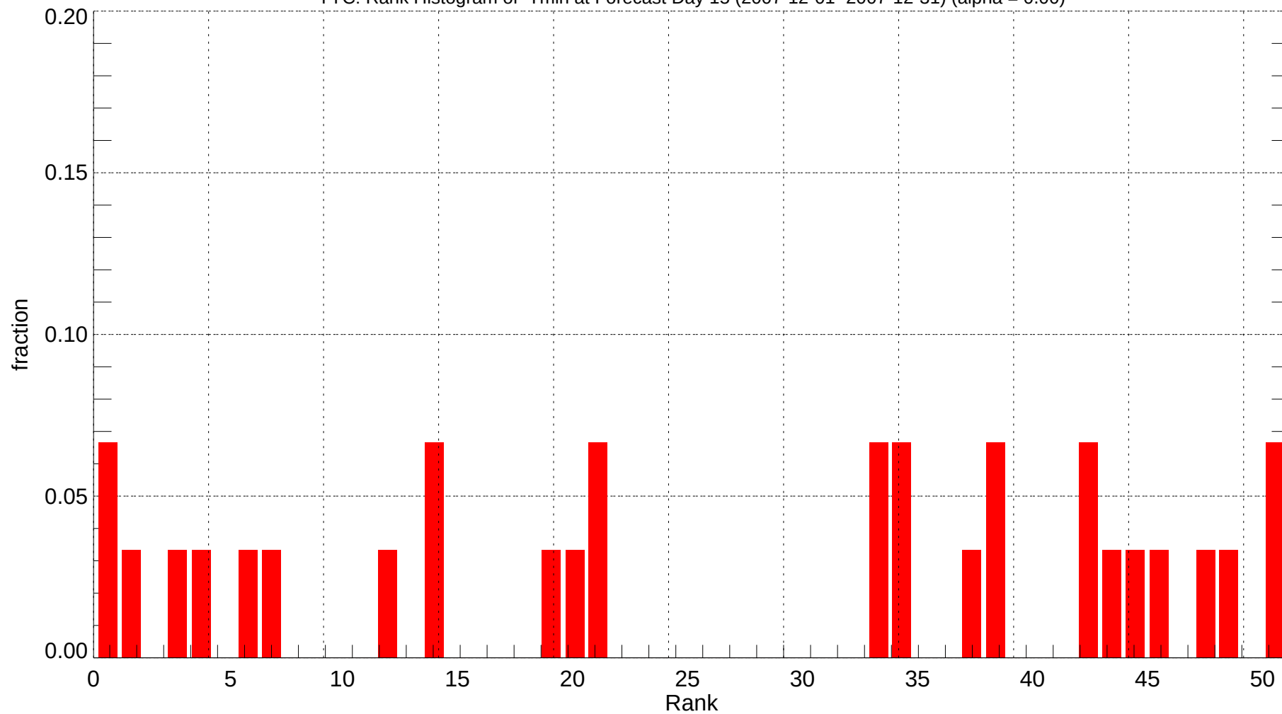
YYC: Rank Histogram of Tmin at Forecast Day 15 (2007-12-01~2007-12-31) (alpha = 0.00)
