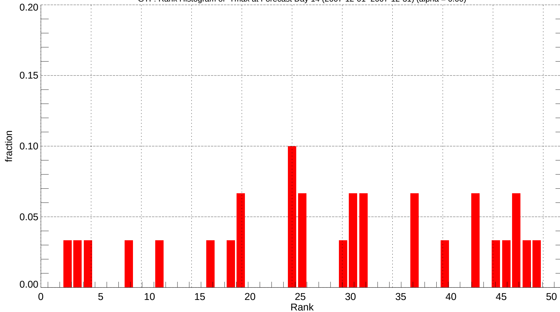
GTF: Rank Histogram of Tmax at Forecast Day 14 (2007-12-01~2007-12-31) (alpha = 0.00)
