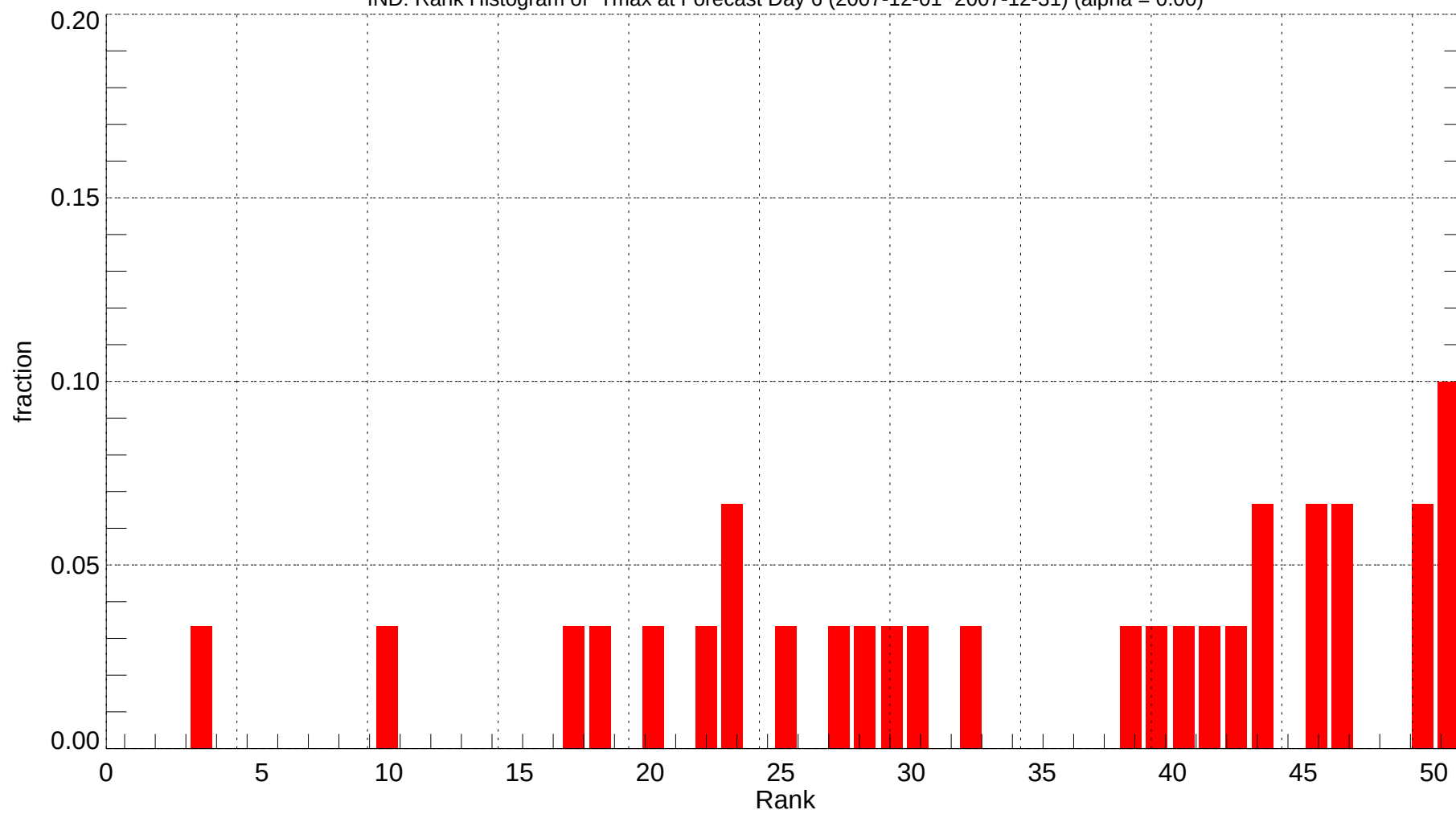
IND: Rank Histogram of Tmax at Forecast Day 6 (2007-12-01~2007-12-31) (alpha = 0.00)
