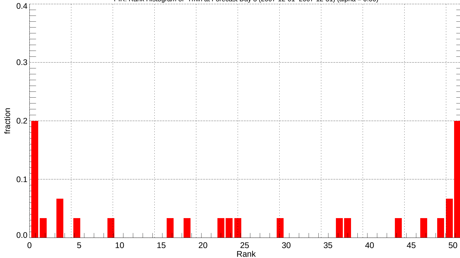
PIR: Rank Histogram of Tmin at Forecast Day 3 (2007-12-01~2007-12-31) (alpha = 0.00)
