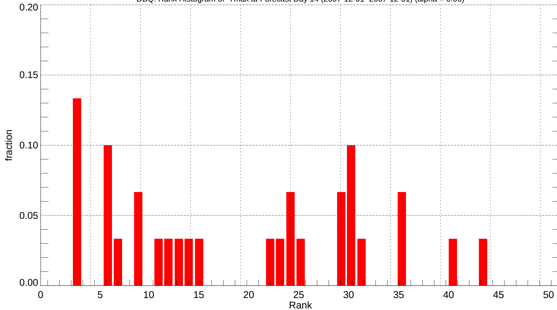
DBQ: Rank Histogram of Tmax at Forecast Day 14 (2007-12-01~2007-12-31) (alpha = 0.00)
