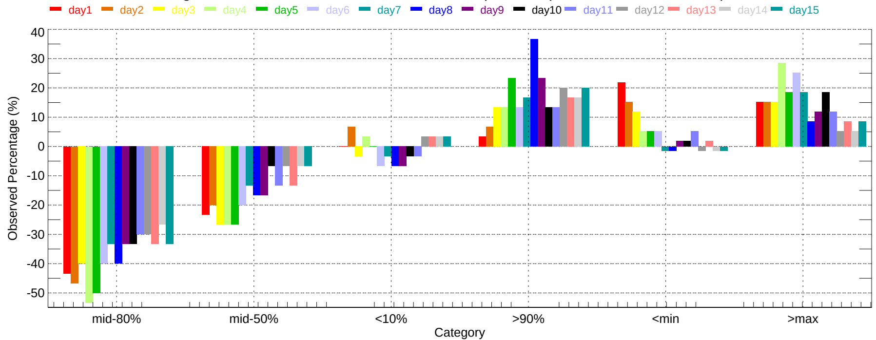
Observed Percentage Deviation of Ensembles - JAX: Max Temperature (2007-12-01~2007-12-31)
