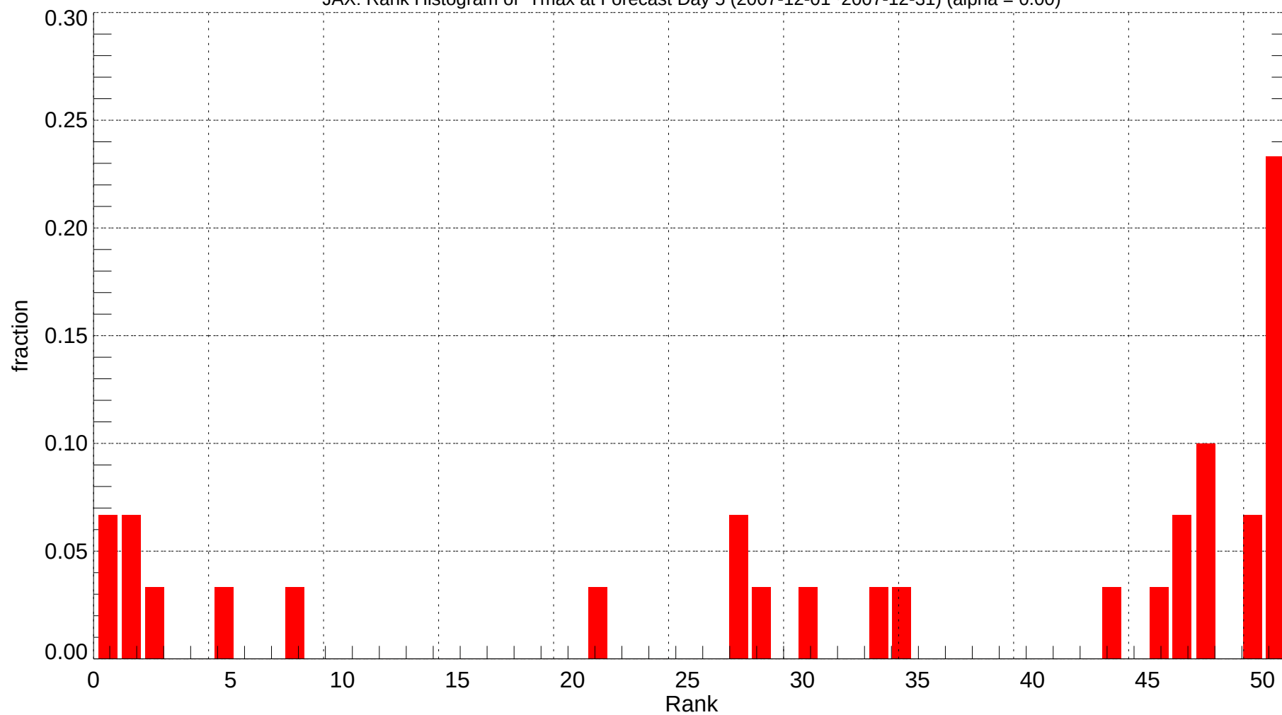
JAX: Rank Histogram of Tmax at Forecast Day 5 (2007-12-01~2007-12-31) (alpha = 0.00)
