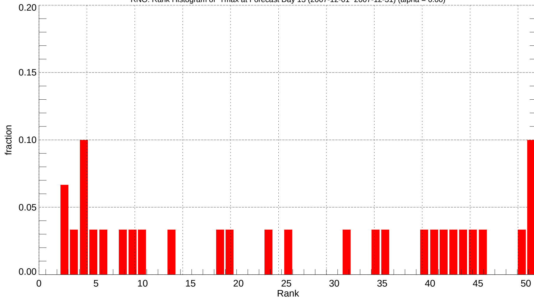
RNO: Rank Histogram of Tmax at Forecast Day 13 (2007-12-01~2007-12-31) (alpha = 0.00)
