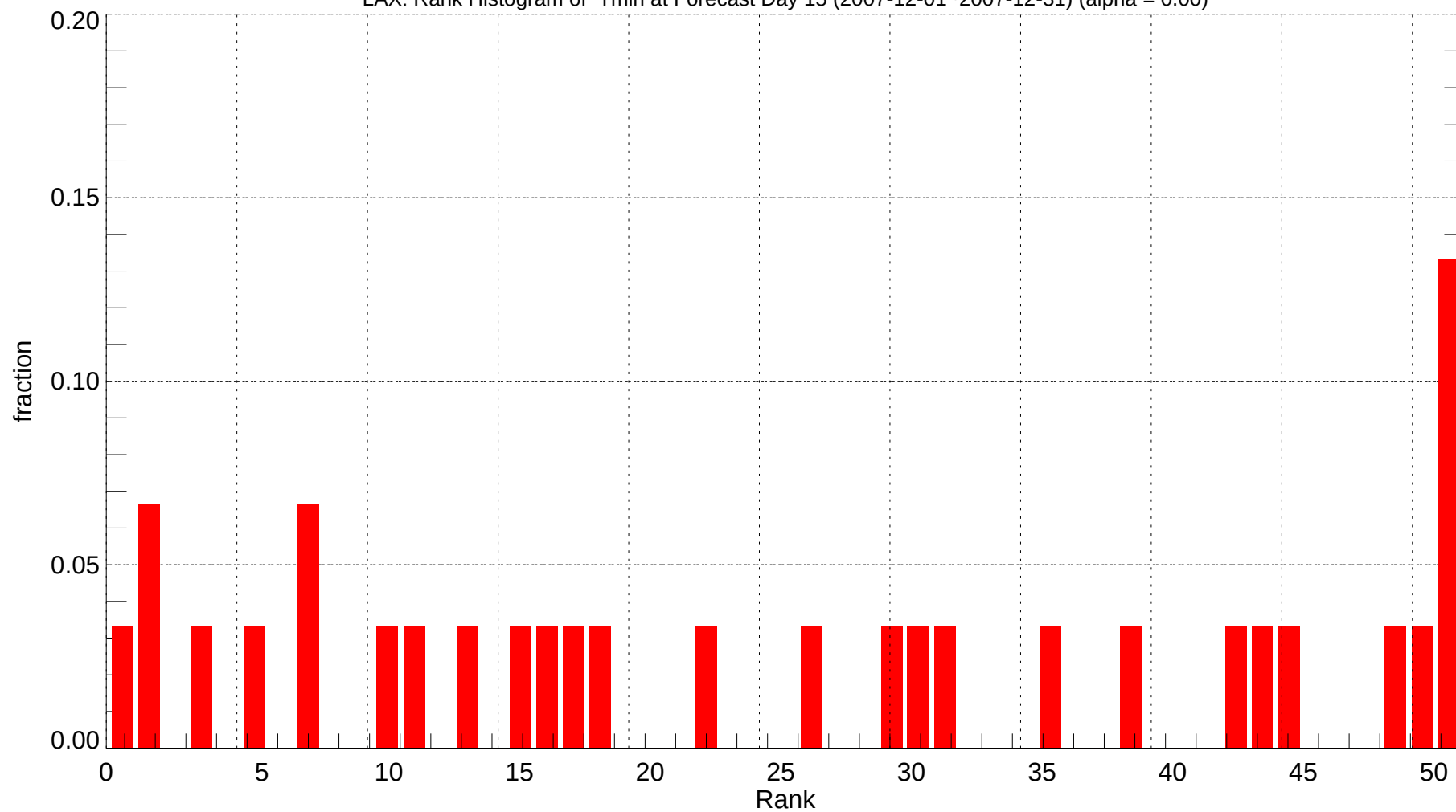
LAX: Rank Histogram of Tmin at Forecast Day 15 (2007-12-01~2007-12-31) (alpha = 0.00)
