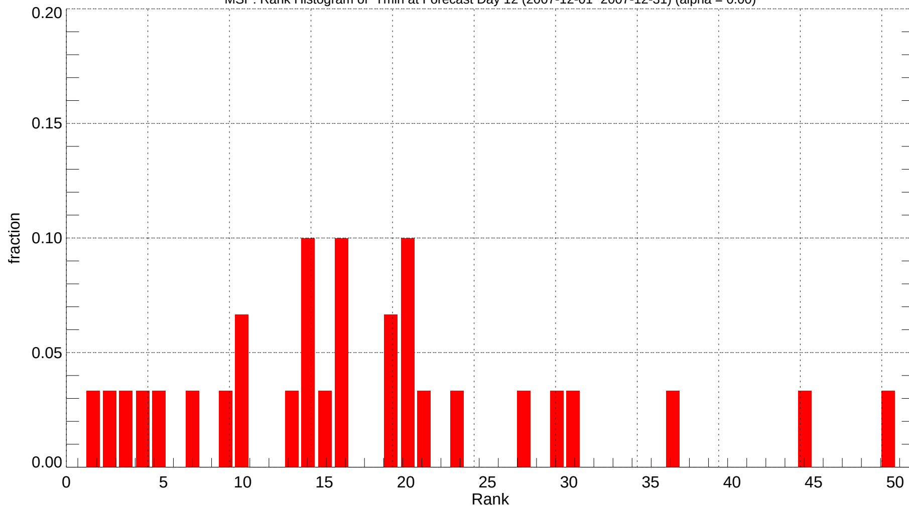
MSP: Rank Histogram of Tmin at Forecast Day 12 (2007-12-01~2007-12-31) (alpha = 0.00)
