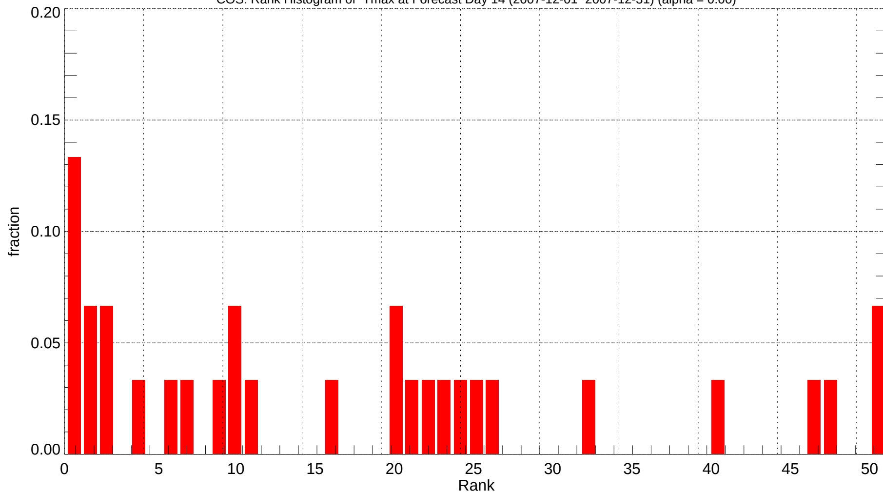
COS: Rank Histogram of Tmax at Forecast Day 14 (2007-12-01~2007-12-31) (alpha = 0.00)
