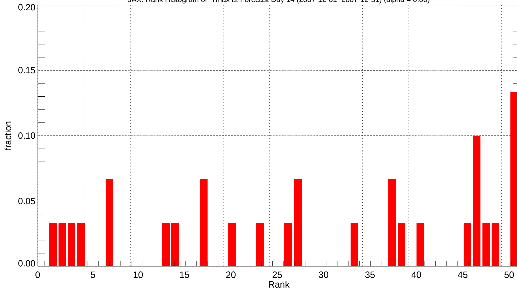
JAX: Rank Histogram of Tmax at Forecast Day 14 (2007-12-01~2007-12-31) (alpha = 0.00)
