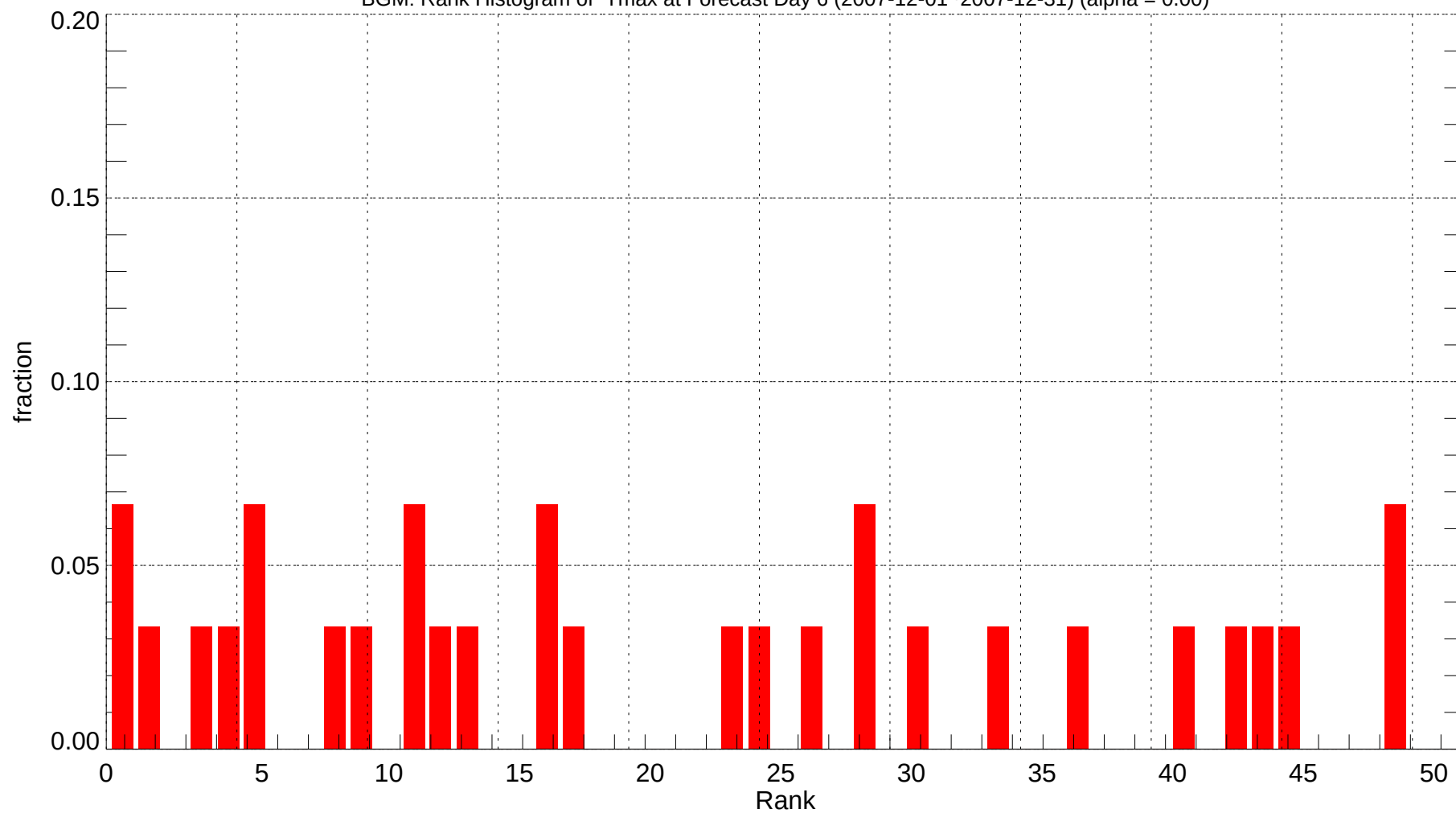
BGM: Rank Histogram of Tmax at Forecast Day 6 (2007-12-01~2007-12-31) (alpha = 0.00)
