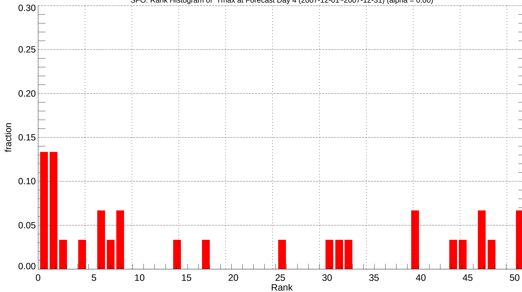
SFO: Rank Histogram of Tmax at Forecast Day 4 (2007-12-01~2007-12-31) (alpha = 0.00)
