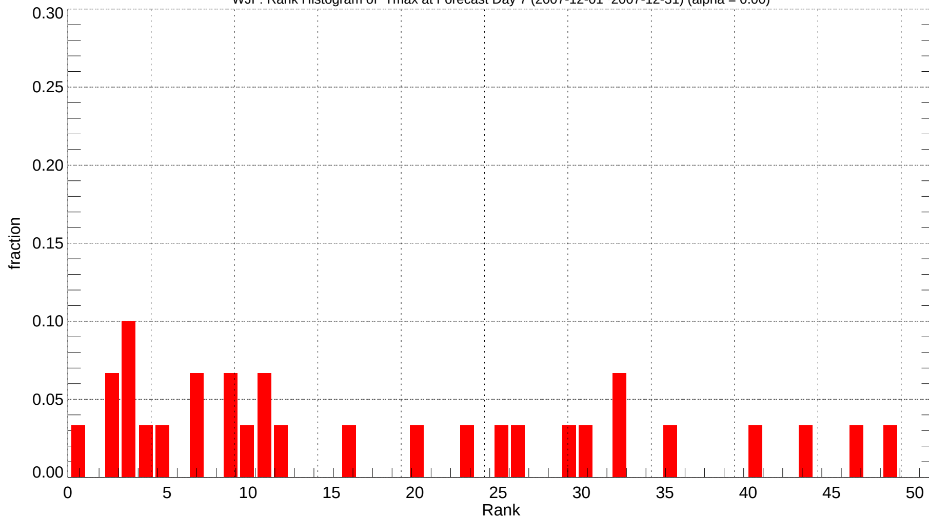
WJF: Rank Histogram of Tmax at Forecast Day 7 (2007-12-01~2007-12-31) (alpha = 0.00)
