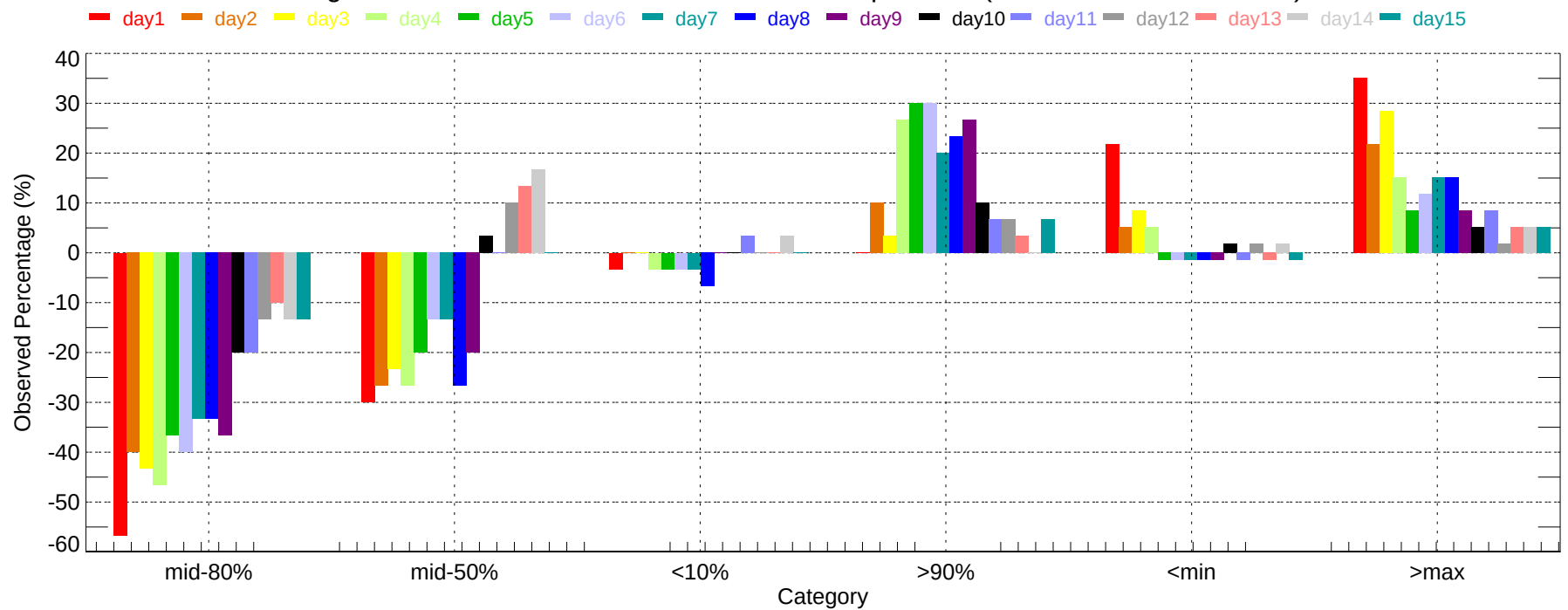
Observed Percentage Deviation of Ensembles - VCT: Max Temperature (2007-12-01~2007-12-31)
