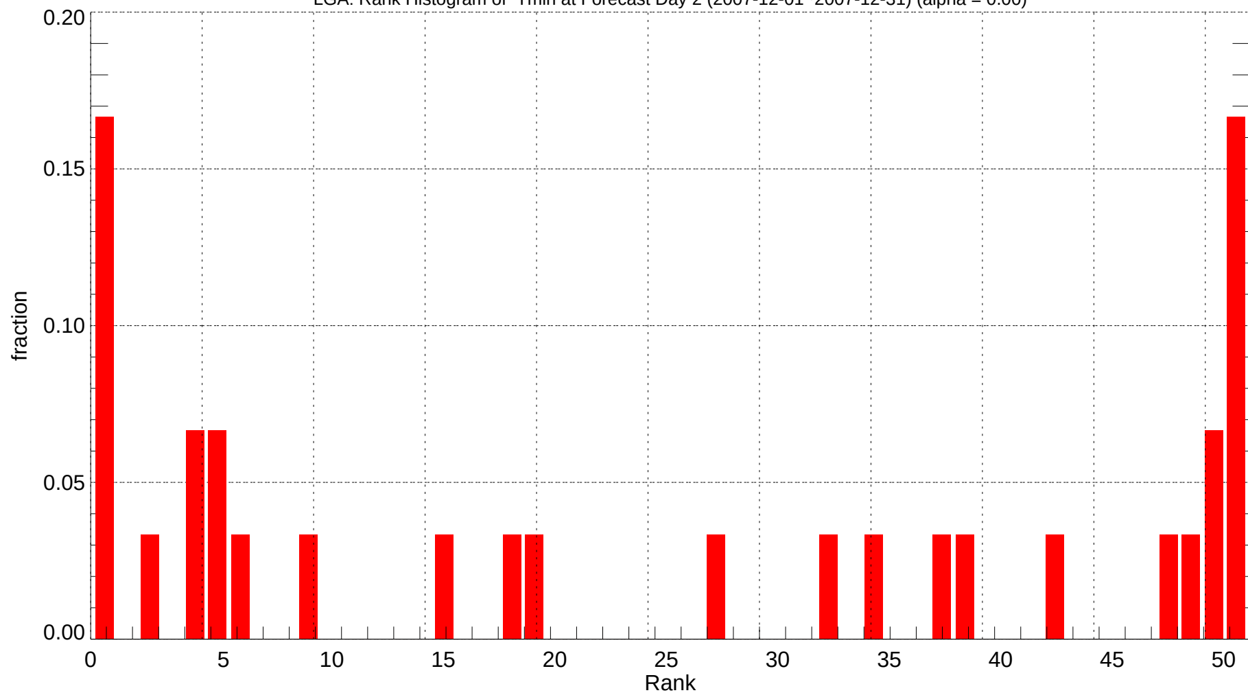
LGA: Rank Histogram of Tmin at Forecast Day 2 (2007-12-01~2007-12-31) (alpha = 0.00)
