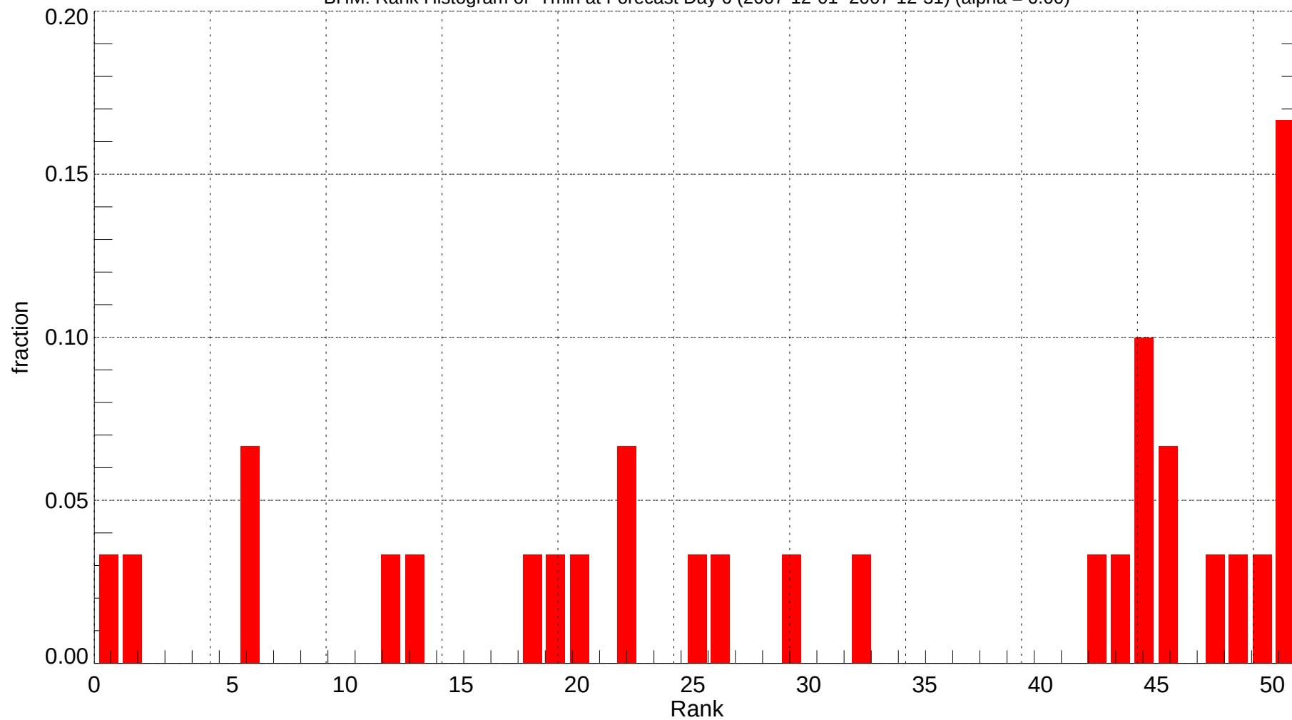
BHM: Rank Histogram of Tmin at Forecast Day 6 (2007-12-01~2007-12-31) (alpha = 0.00)
