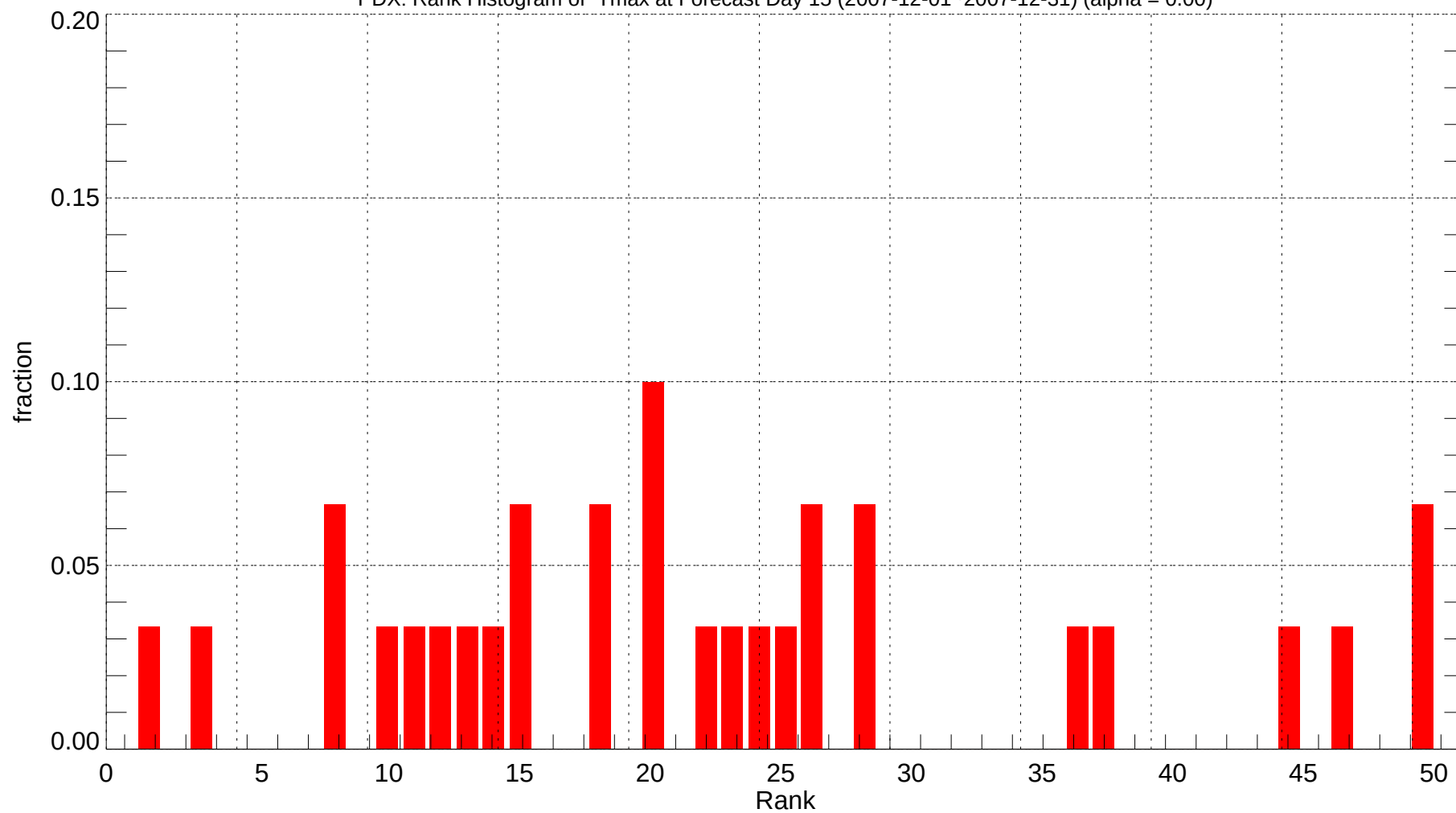
PDX: Rank Histogram of Tmax at Forecast Day 15 (2007-12-01~2007-12-31) (alpha = 0.00)
