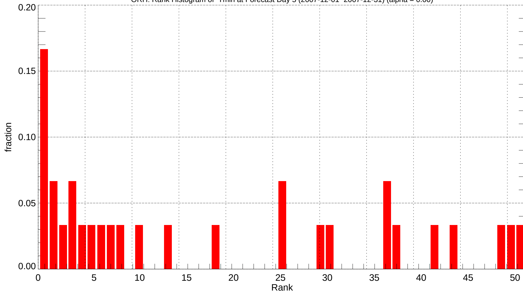
ORH: Rank Histogram of Tmin at Forecast Day 5 (2007-12-01~2007-12-31) (alpha = 0.00)
