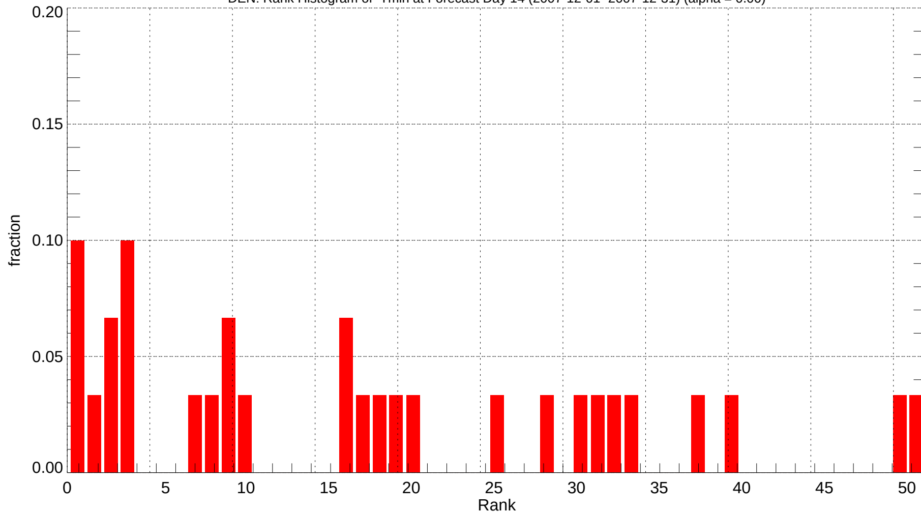
DEN: Rank Histogram of Tmin at Forecast Day 14 (2007-12-01~2007-12-31) (alpha = 0.00)
