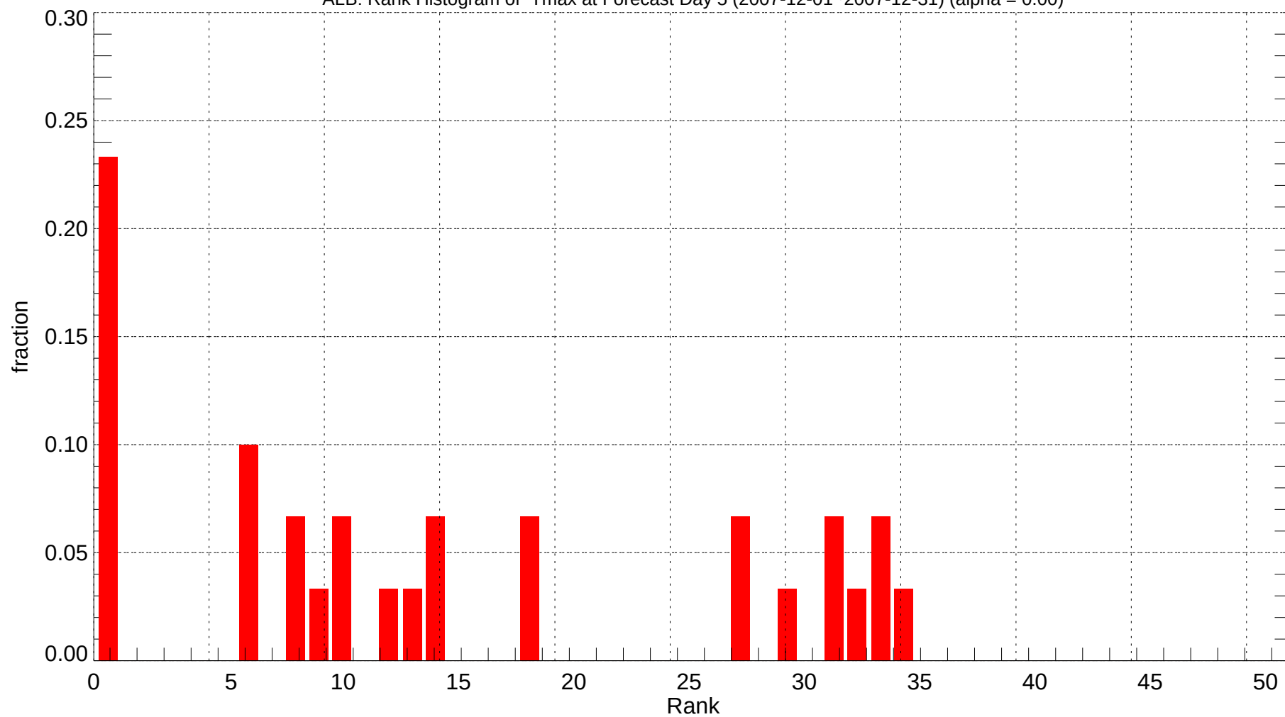
ALB: Rank Histogram of Tmax at Forecast Day 5 (2007-12-01~2007-12-31) (alpha = 0.00)
