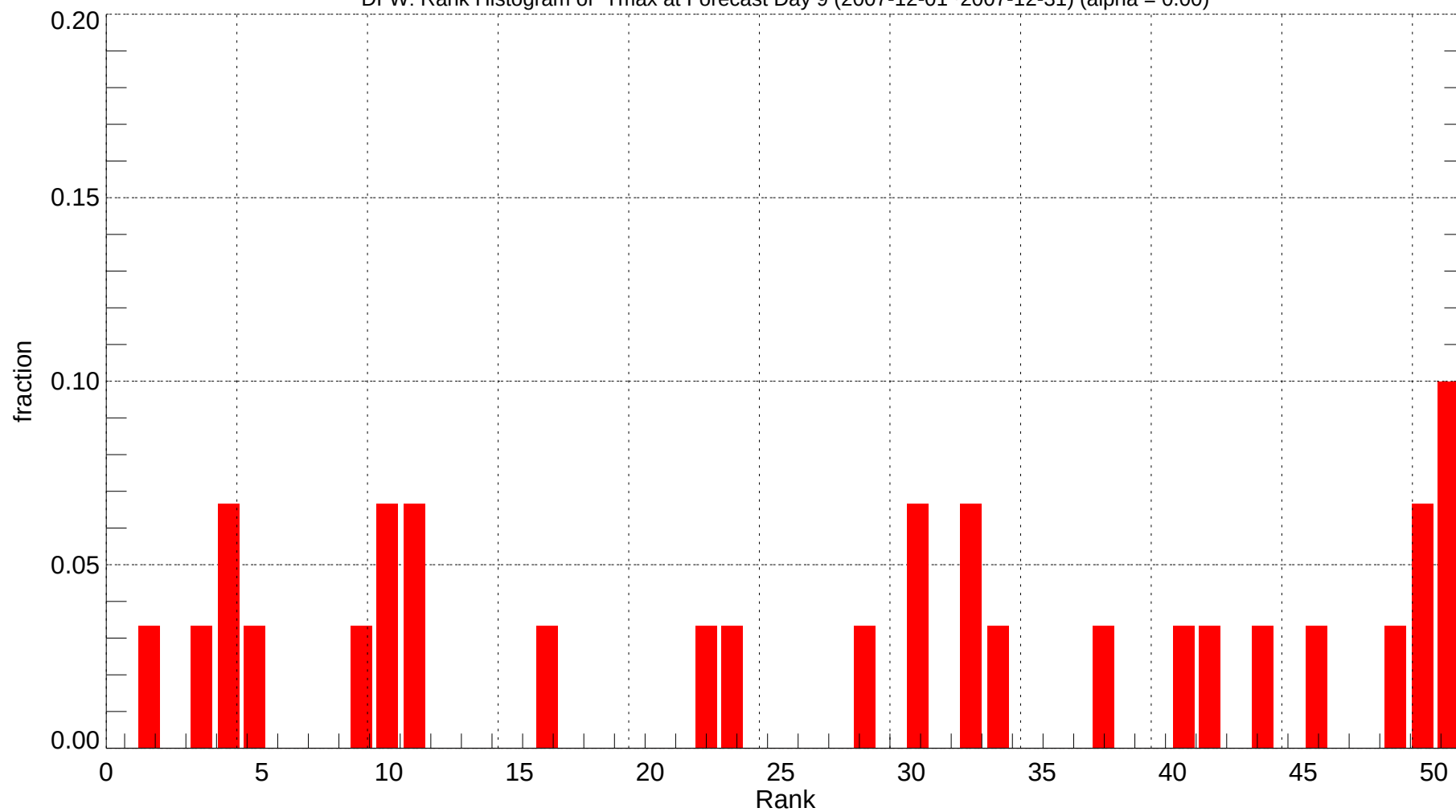
DFW: Rank Histogram of Tmax at Forecast Day 9 (2007-12-01~2007-12-31) (alpha = 0.00)
