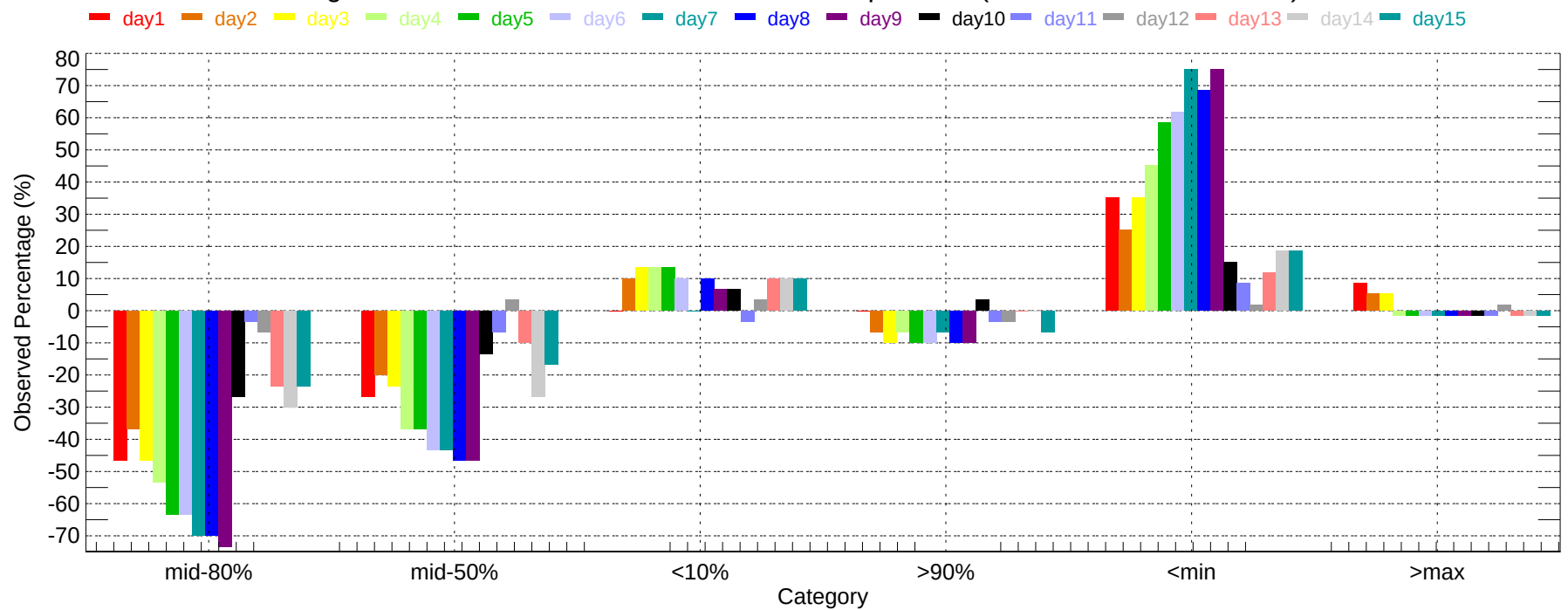
Observed Percentage Deviation of Ensembles - SJC: Max Temperature (2007-12-01~2007-12-31)
