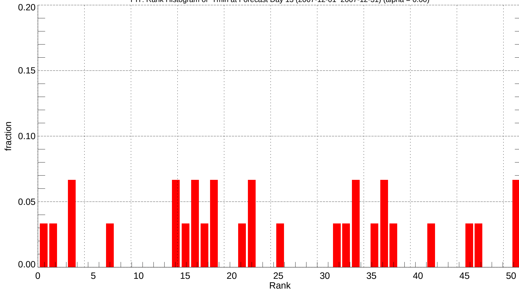
PIT: Rank Histogram of Tmin at Forecast Day 13 (2007-12-01~2007-12-31) (alpha = 0.00)
