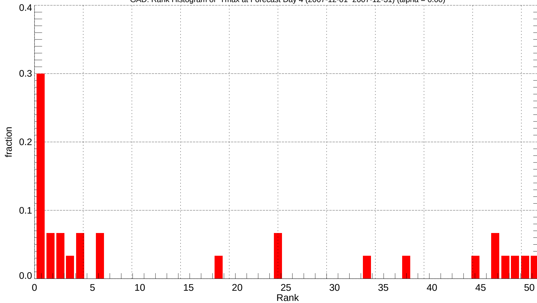
GAD: Rank Histogram of Tmax at Forecast Day 4 (2007-12-01~2007-12-31) (alpha = 0.00)
