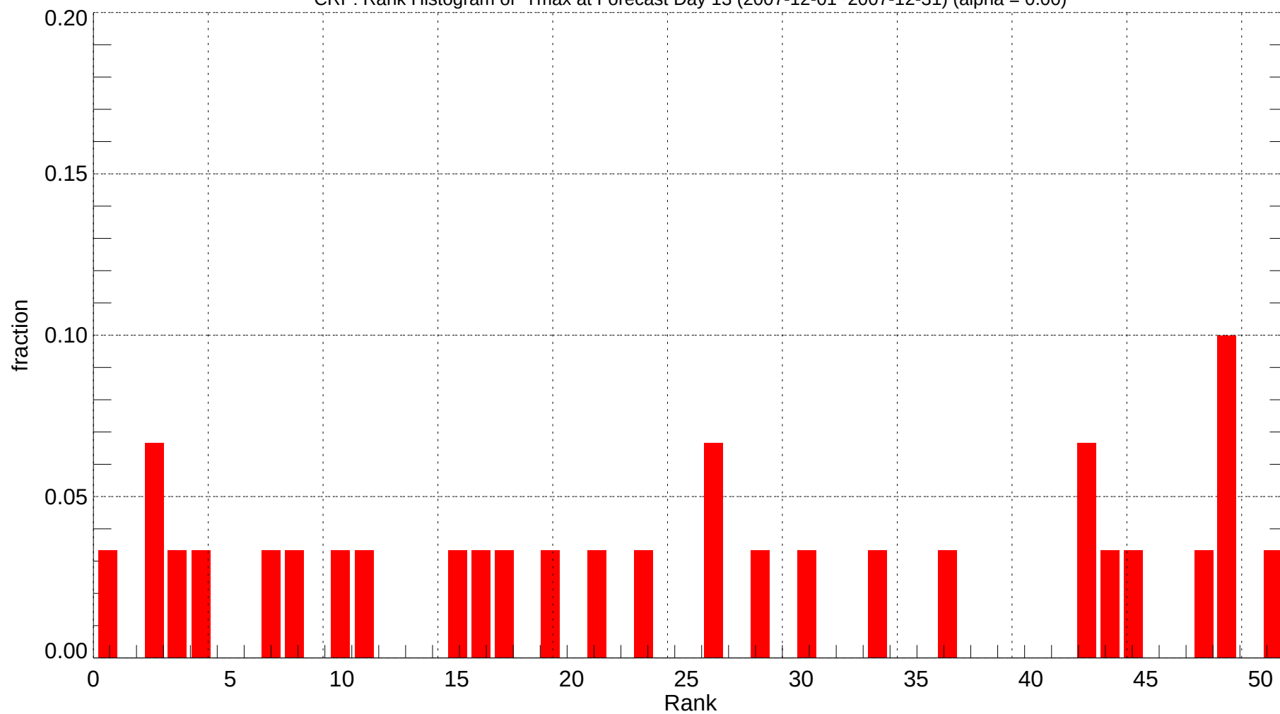
CRP: Rank Histogram of Tmax at Forecast Day 13 (2007-12-01~2007-12-31) (alpha = 0.00)
