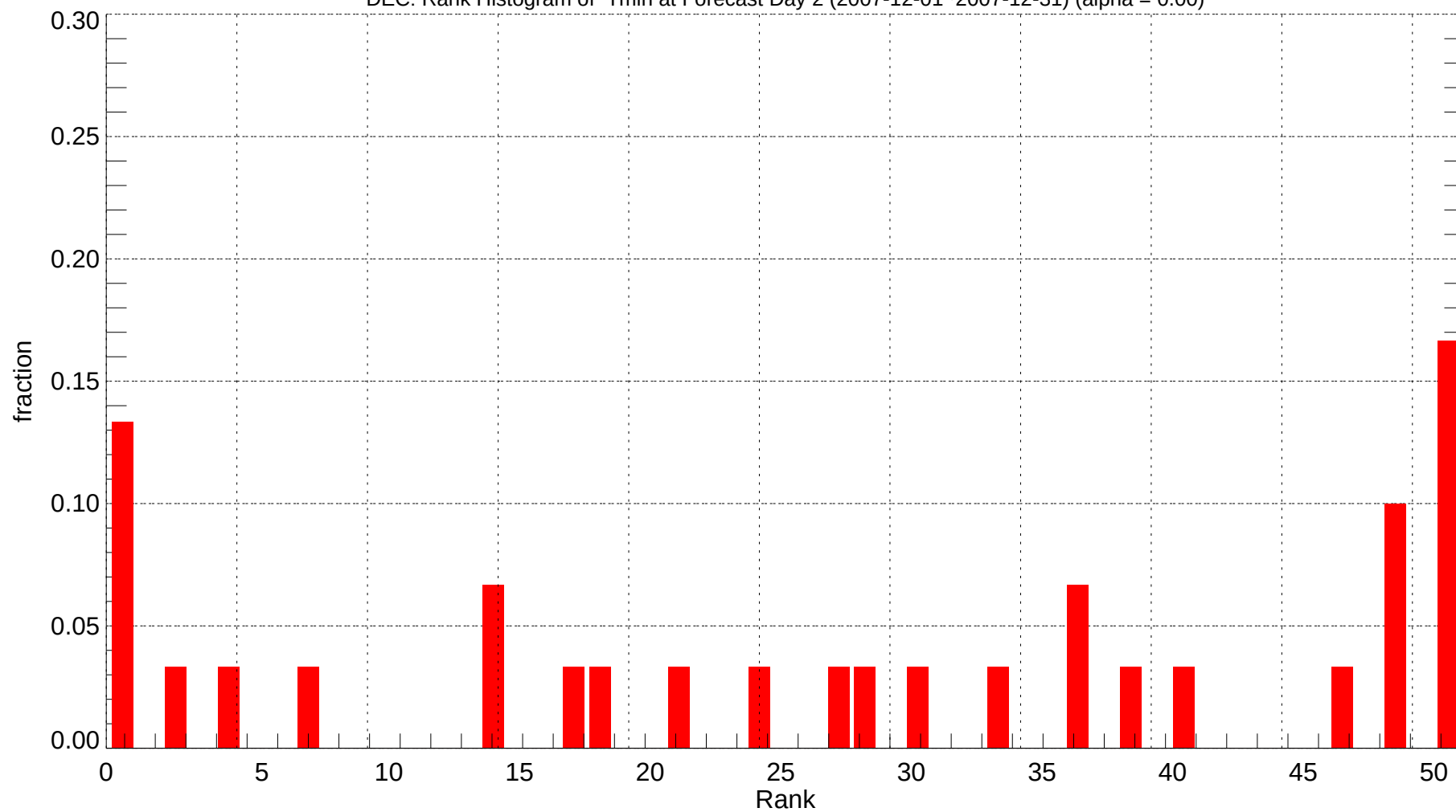
DEC: Rank Histogram of Tmin at Forecast Day 2 (2007-12-01~2007-12-31) (alpha = 0.00)
