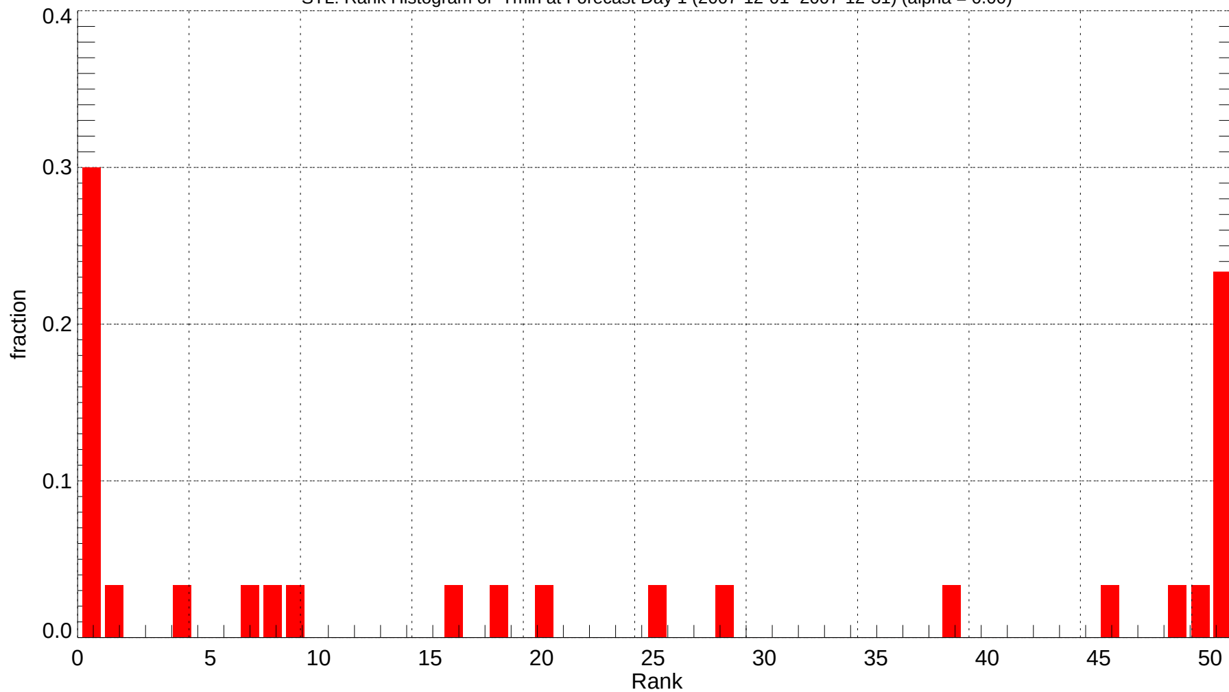
STL: Rank Histogram of Tmin at Forecast Day 1 (2007-12-01~2007-12-31) (alpha = 0.00)
