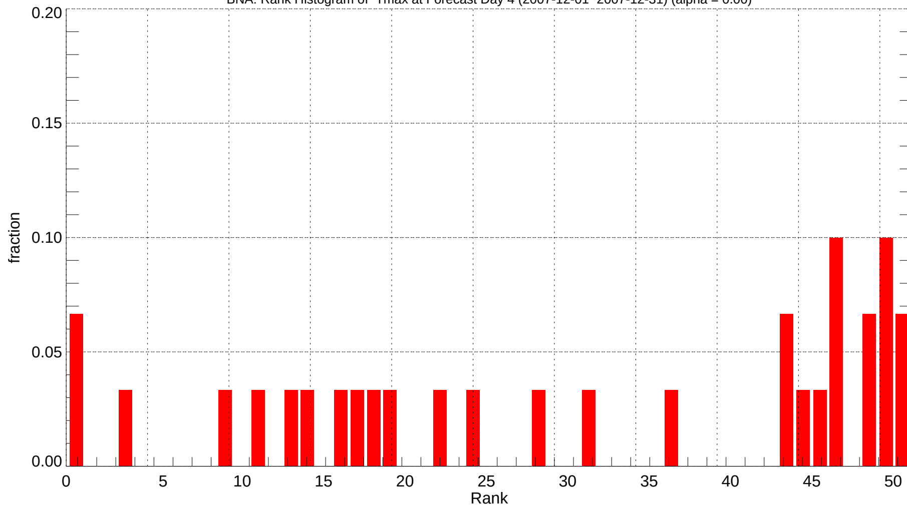
BNA: Rank Histogram of Tmax at Forecast Day 4 (2007-12-01~2007-12-31) (alpha = 0.00)
