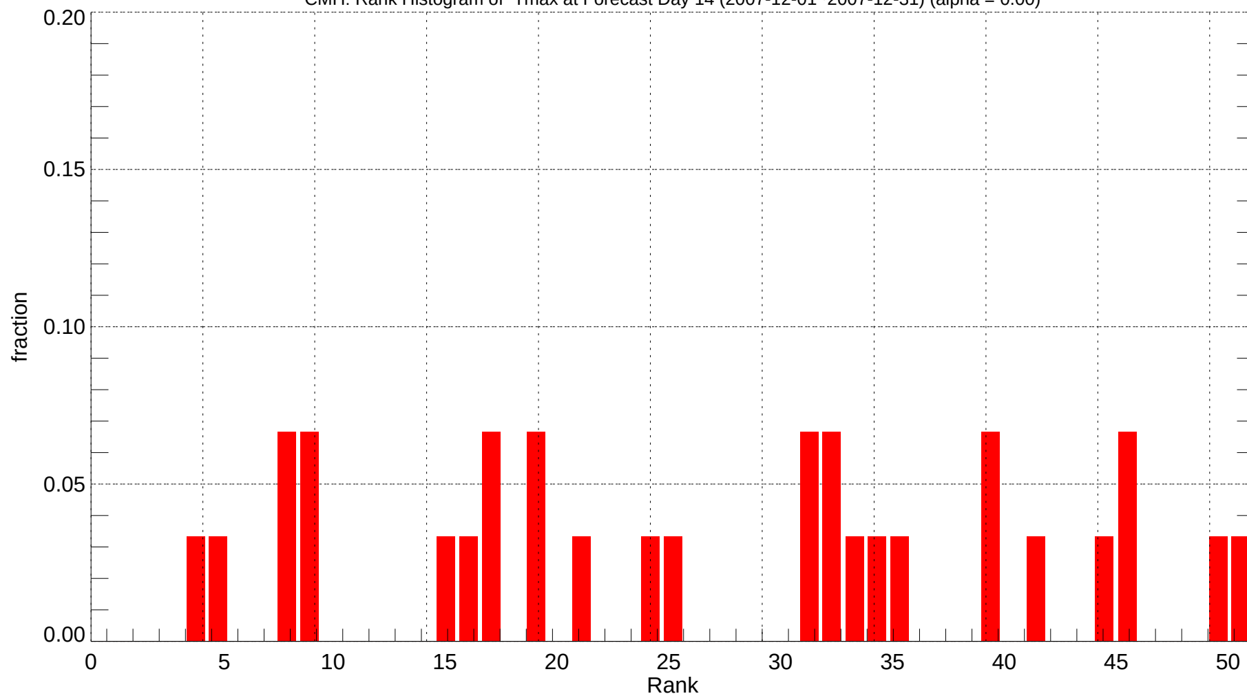
CMH: Rank Histogram of Tmax at Forecast Day 14 (2007-12-01~2007-12-31) (alpha = 0.00)
