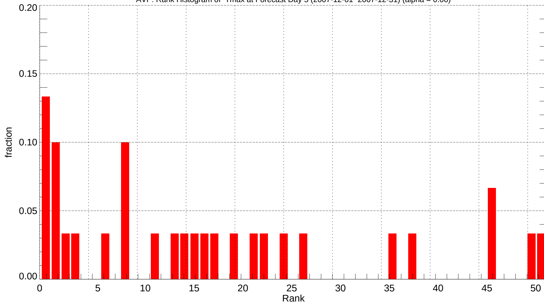
AVP: Rank Histogram of Tmax at Forecast Day 5 (2007-12-01~2007-12-31) (alpha = 0.00)
