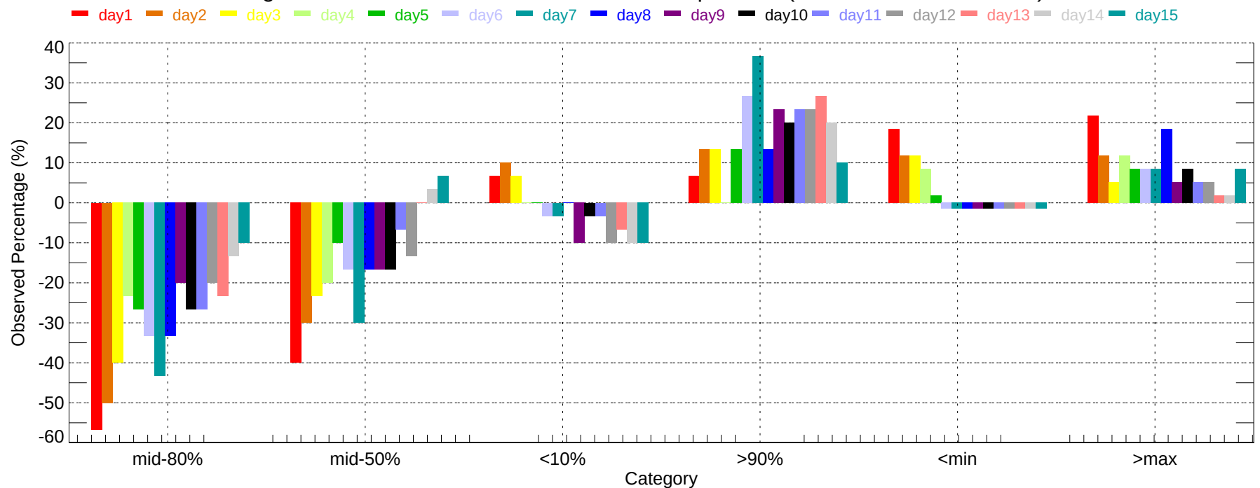
Observed Percentage Deviation of Ensembles - LEX: Max Temperature (2007-12-01~2007-12-31)
