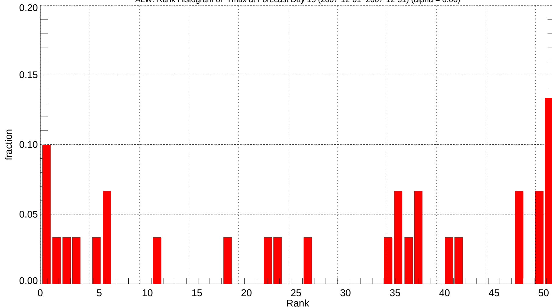
ALW: Rank Histogram of Tmax at Forecast Day 15 (2007-12-01~2007-12-31) (alpha = 0.00)
