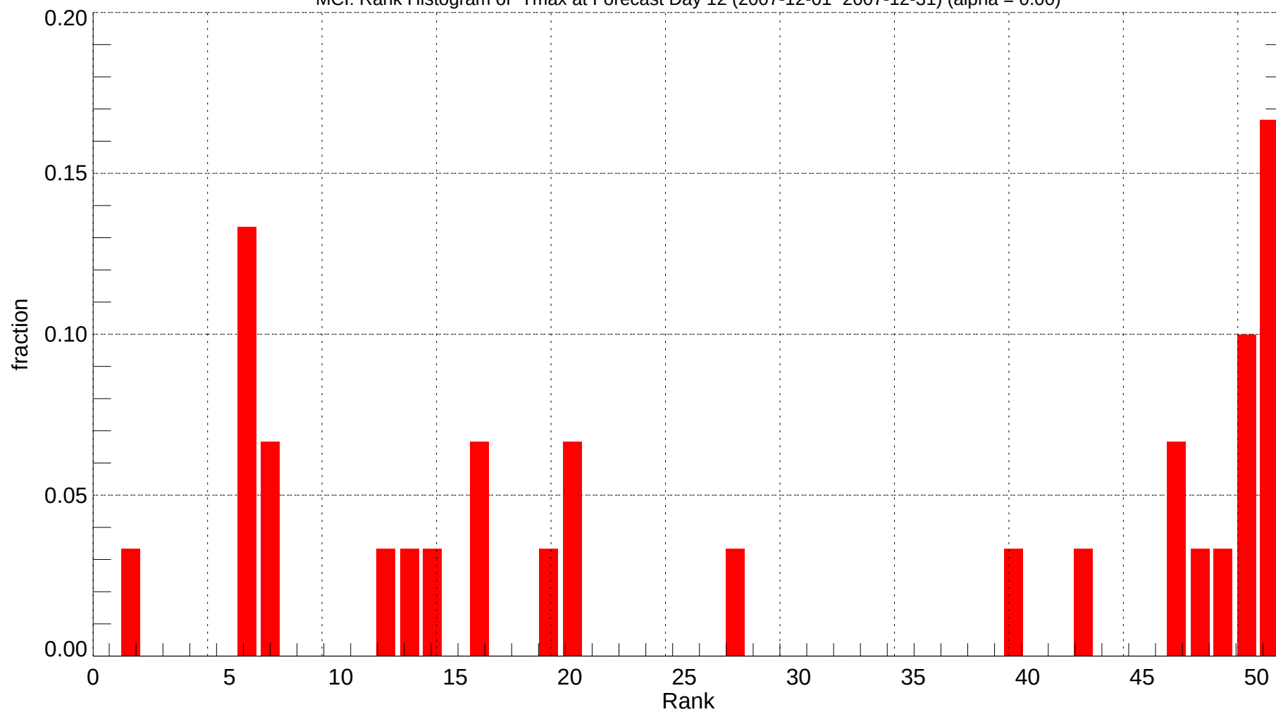
MCI: Rank Histogram of Tmax at Forecast Day 12 (2007-12-01~2007-12-31) (alpha = 0.00)
