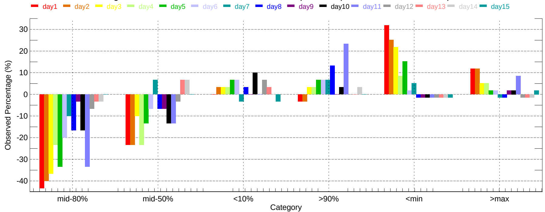
Observed Percentage Deviation of Ensembles - ABE: Min Temperature (2007-12-01~2007-12-31)
