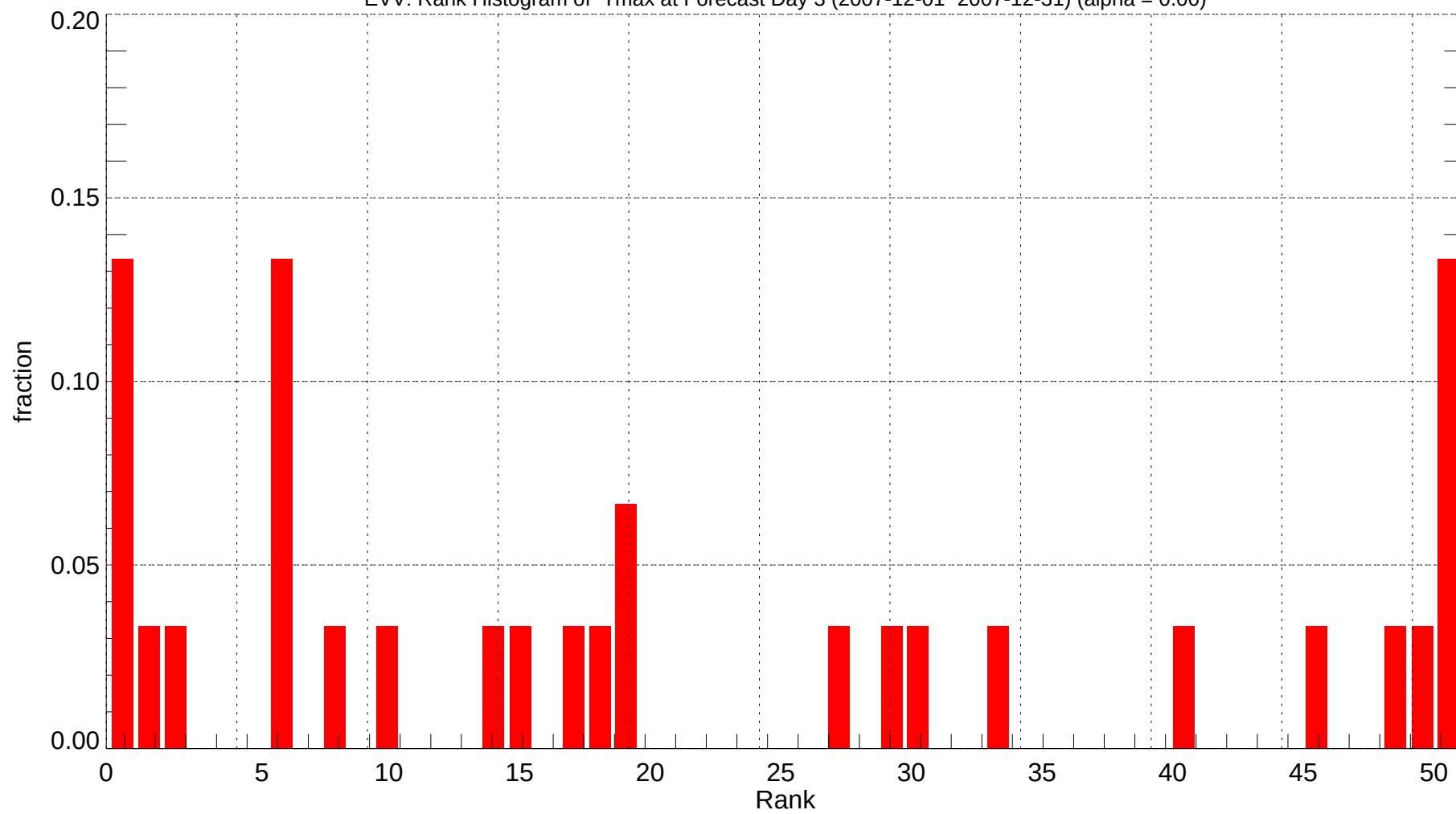
EVV: Rank Histogram of Tmax at Forecast Day 3 (2007-12-01~2007-12-31) (alpha = 0.00)
