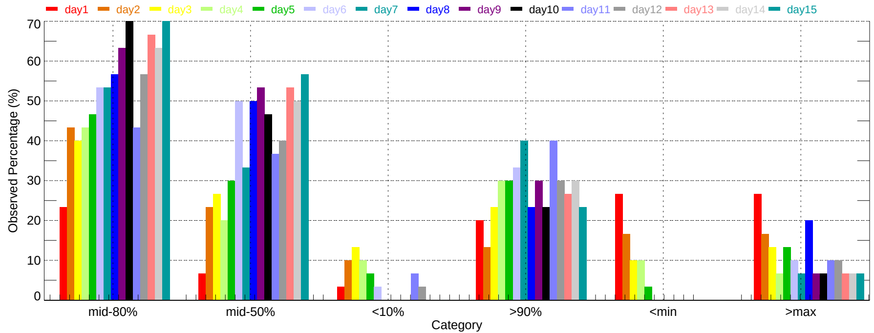
Observed Percentage of Ensembles - SDF: Max Temperature (2007-12-01~2007-12-31)
