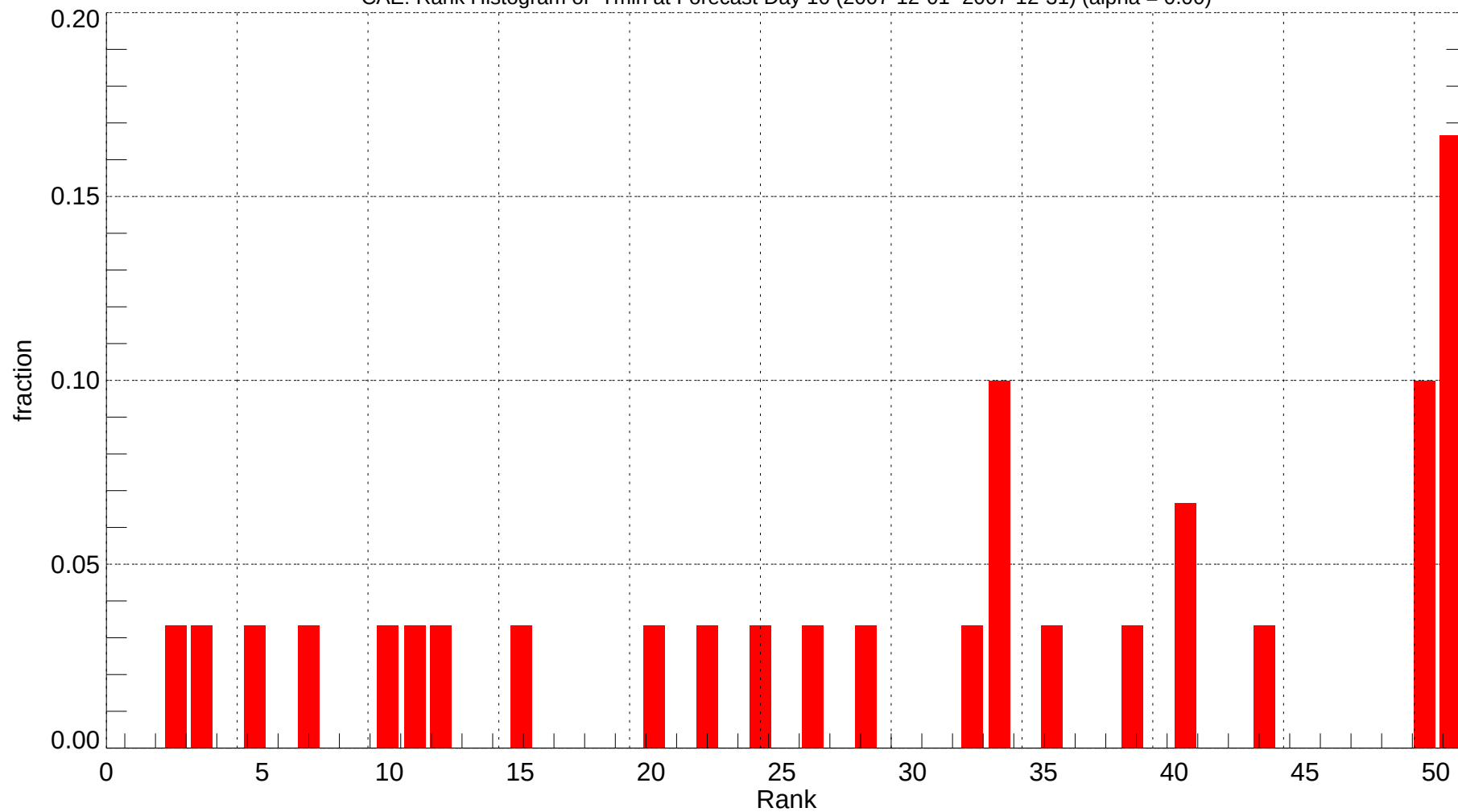
CAE: Rank Histogram of Tmin at Forecast Day 10 (2007-12-01~2007-12-31) (alpha = 0.00)
