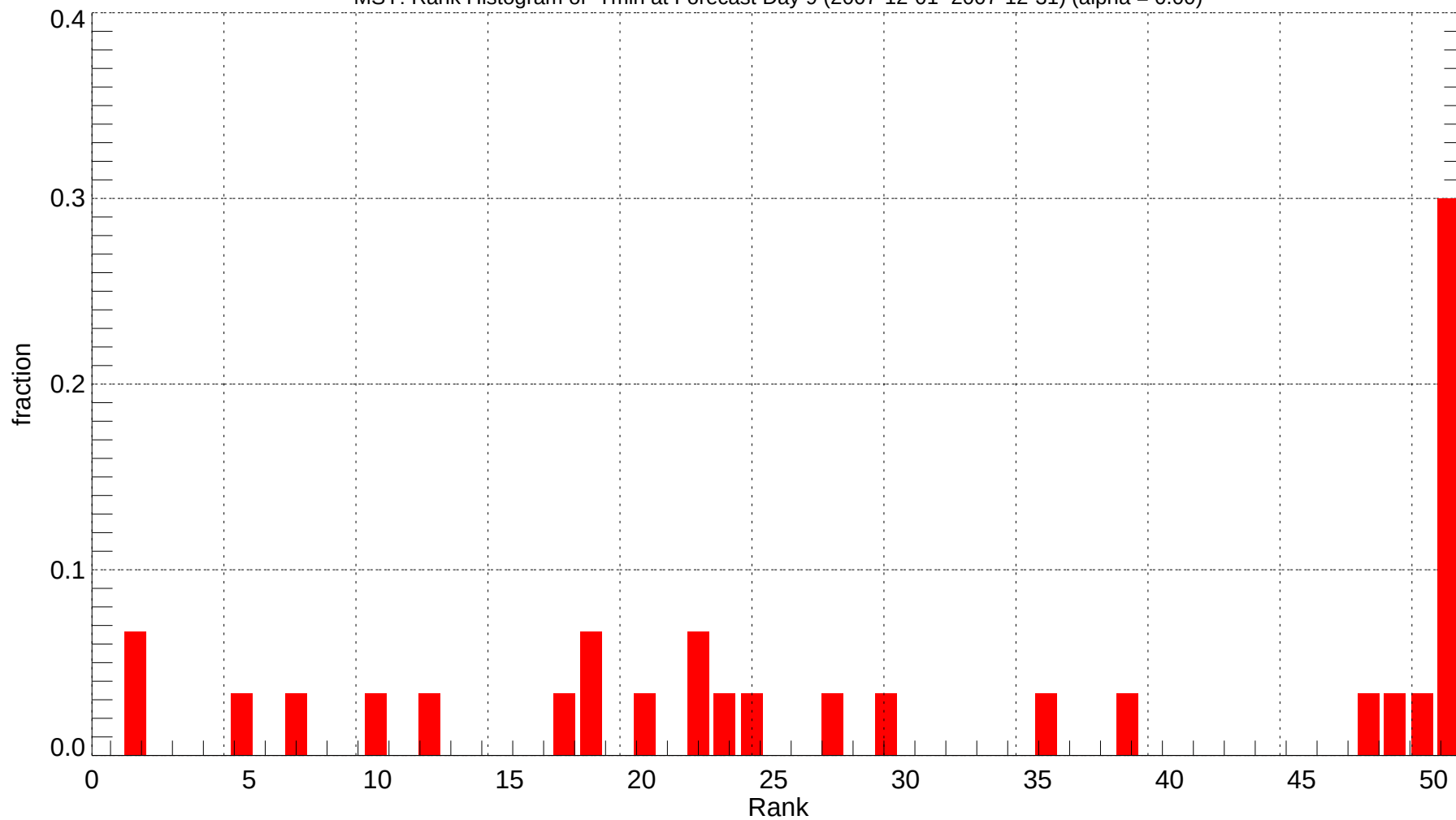
MSY: Rank Histogram of Tmin at Forecast Day 9 (2007-12-01~2007-12-31) (alpha = 0.00)
