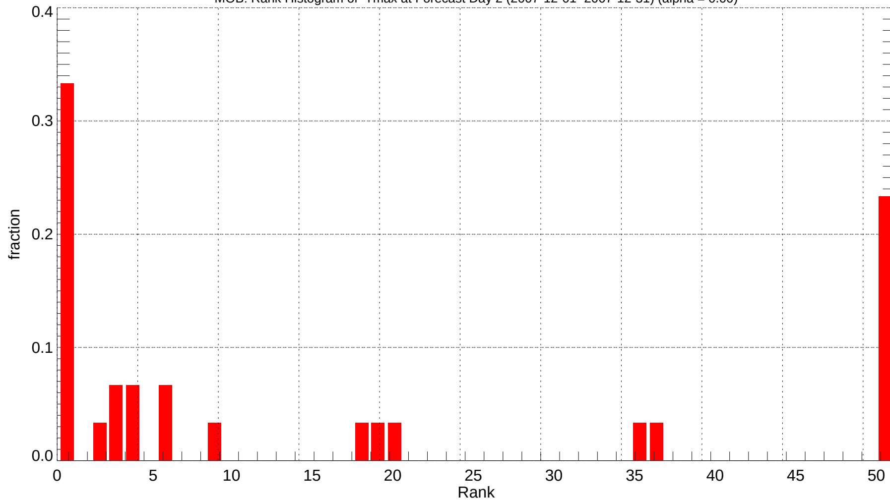
MOB: Rank Histogram of Tmax at Forecast Day 2 (2007-12-01~2007-12-31) (alpha = 0.00)
