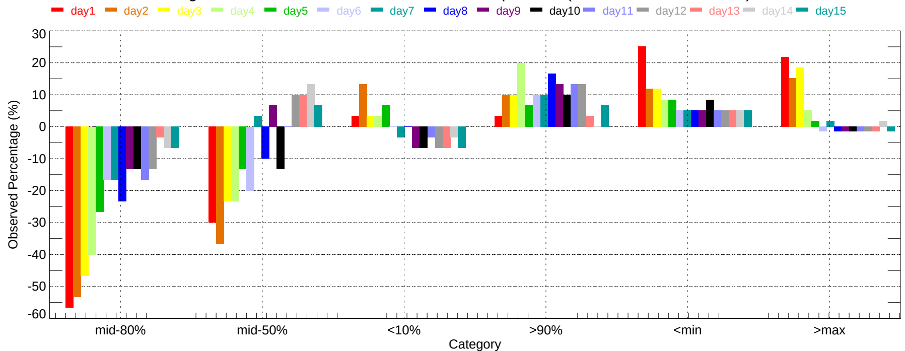
Observed Percentage Deviation of Ensembles - RBL: Max Temperature (2007-12-01~2007-12-31)
