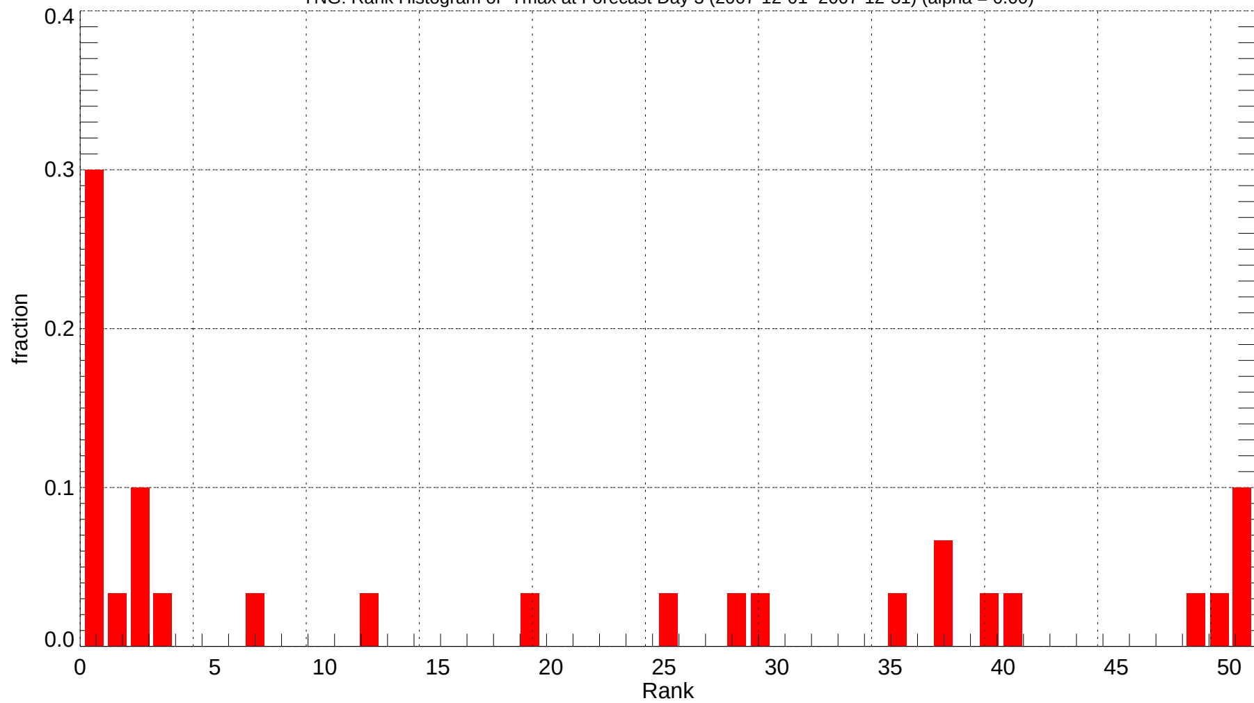
YNG: Rank Histogram of Tmax at Forecast Day 3 (2007-12-01~2007-12-31) (alpha = 0.00)
