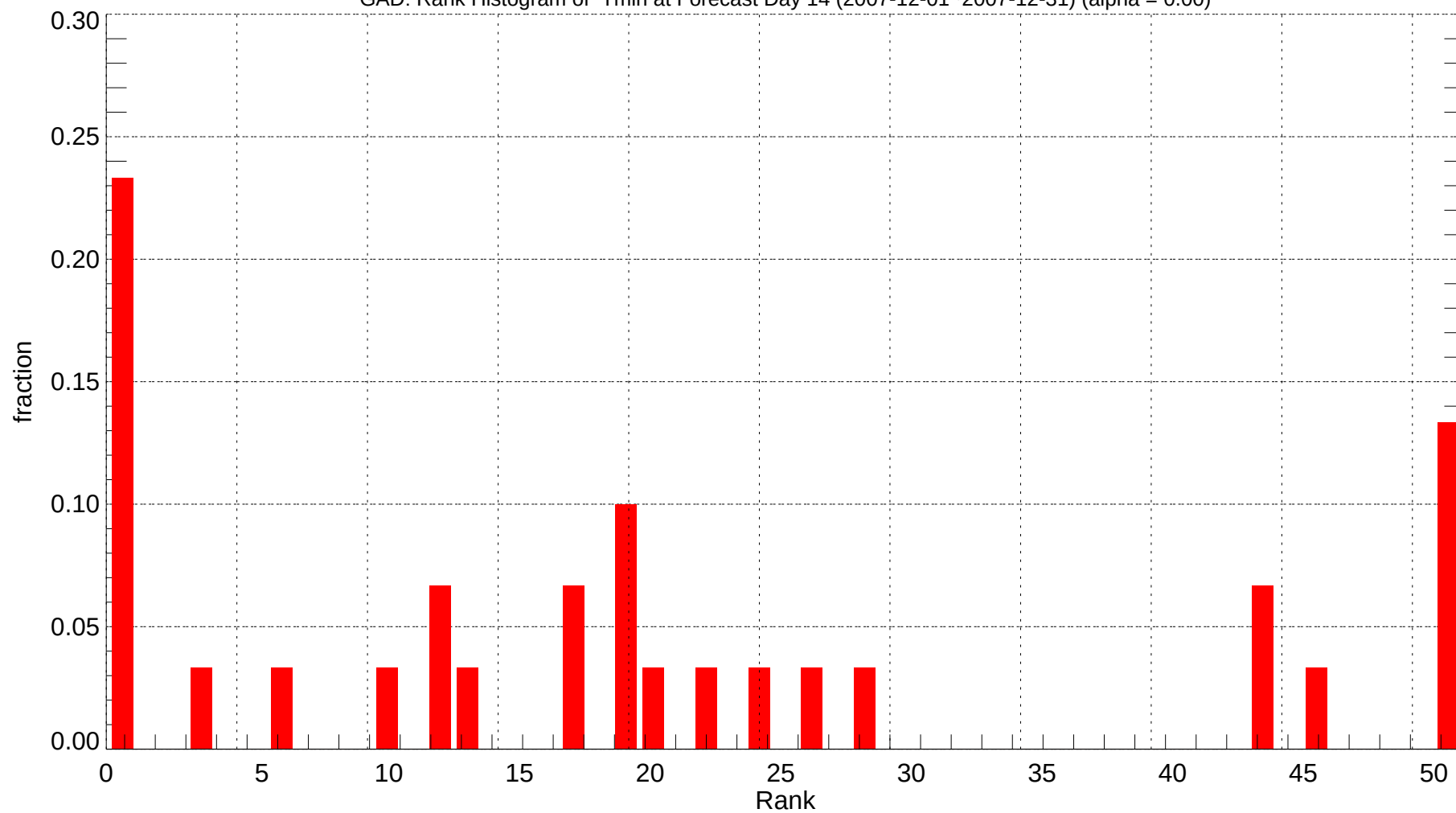
GAD: Rank Histogram of Tmin at Forecast Day 14 (2007-12-01~2007-12-31) (alpha = 0.00)
