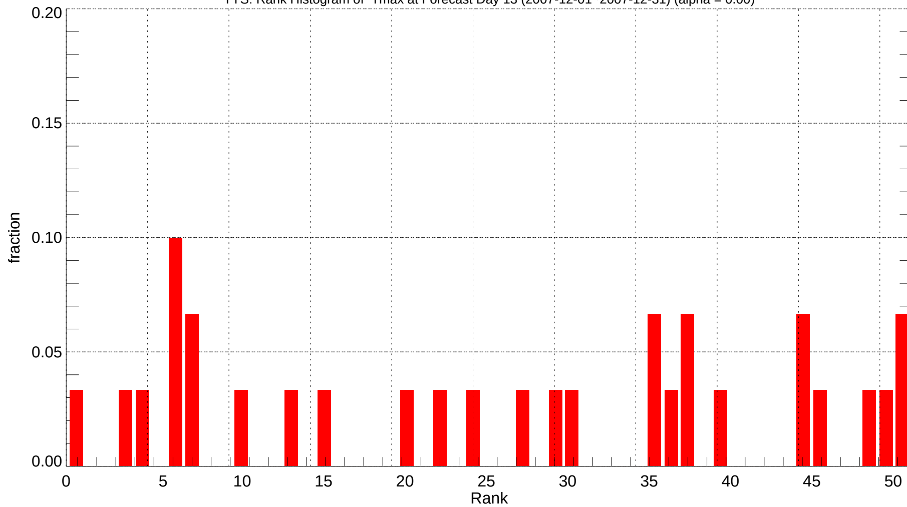
TYS: Rank Histogram of Tmax at Forecast Day 13 (2007-12-01~2007-12-31) (alpha = 0.00)
