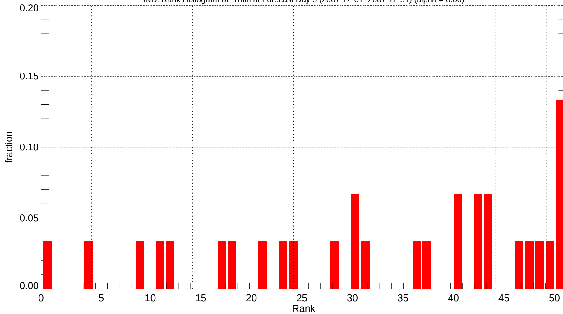
IND: Rank Histogram of Tmin at Forecast Day 5 (2007-12-01~2007-12-31) (alpha = 0.00)
