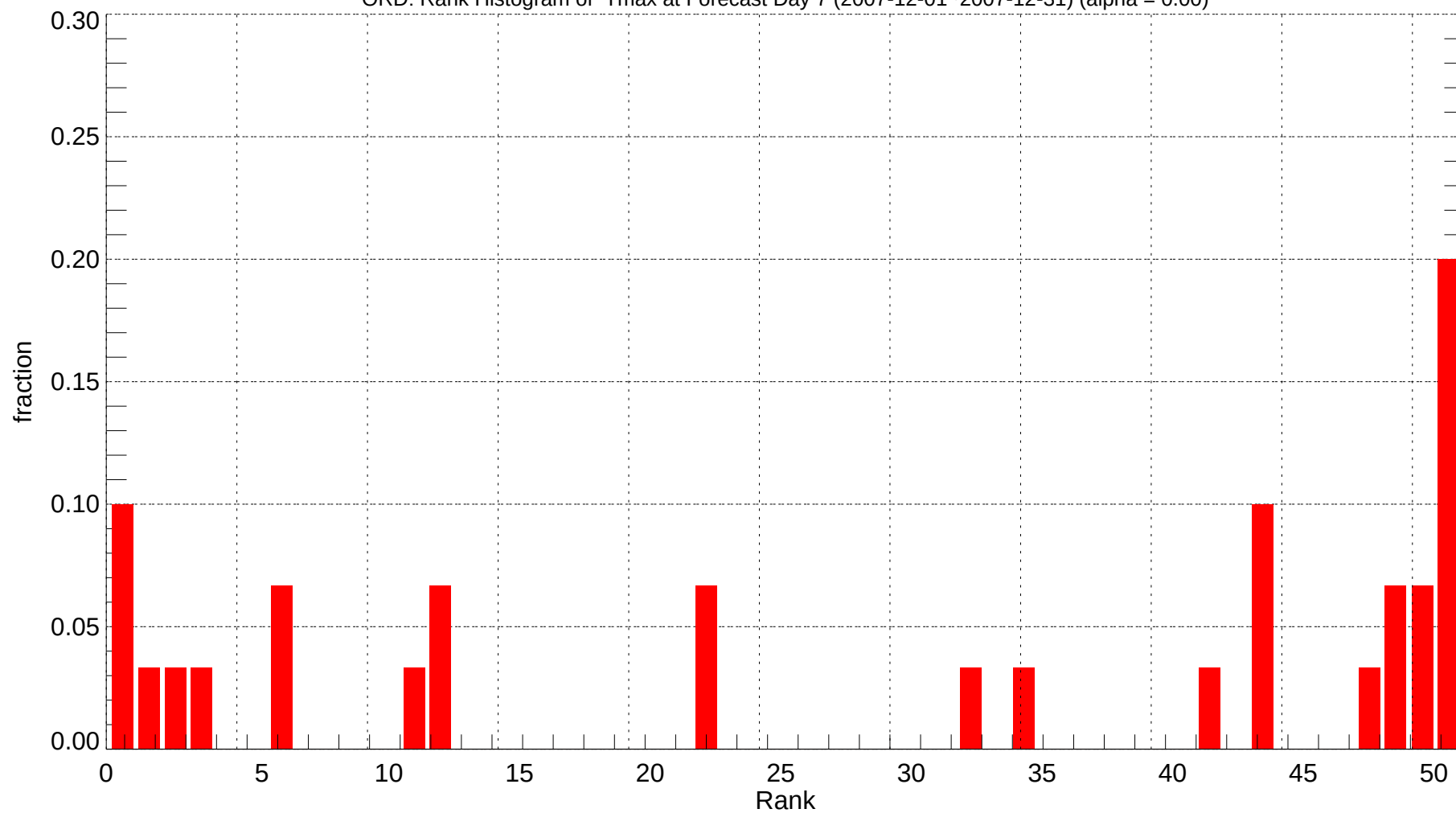
ORD: Rank Histogram of Tmax at Forecast Day 7 (2007-12-01~2007-12-31) (alpha = 0.00)
