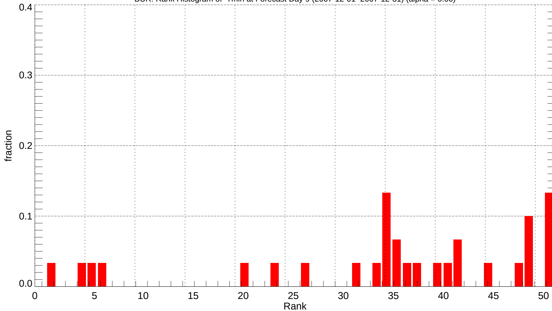
BUR: Rank Histogram of Tmin at Forecast Day 9 (2007-12-01~2007-12-31) (alpha = 0.00)
