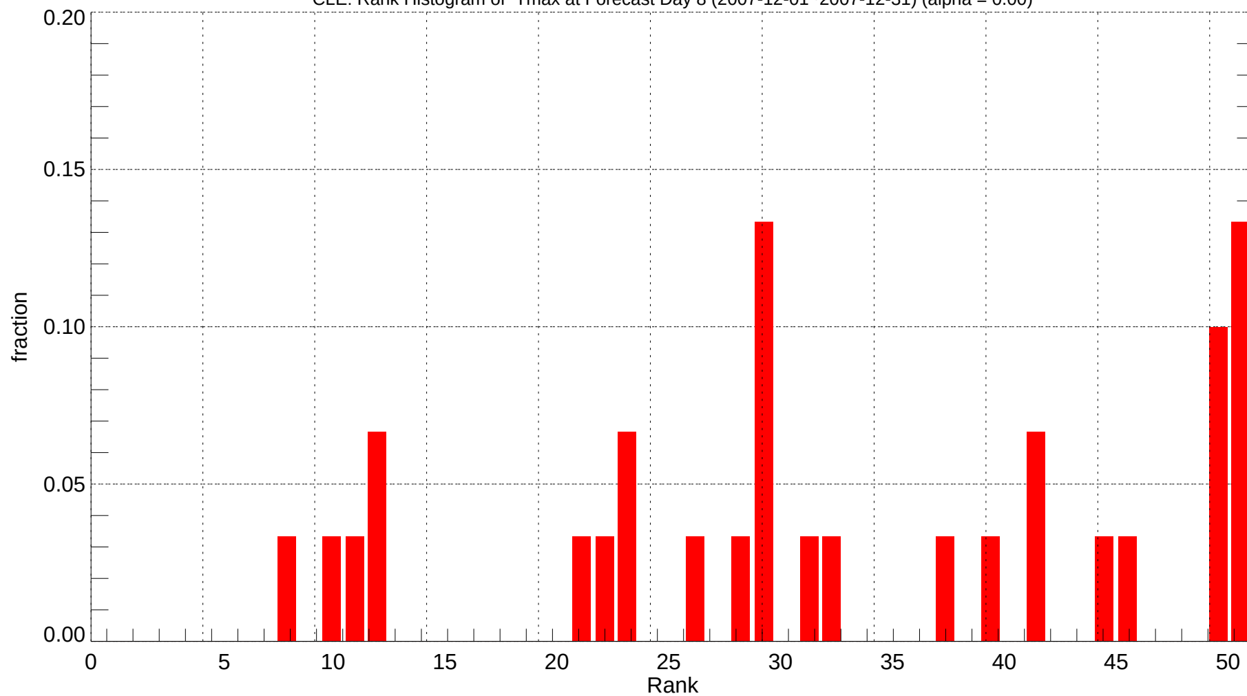
CLE: Rank Histogram of Tmax at Forecast Day 8 (2007-12-01~2007-12-31) (alpha = 0.00)
