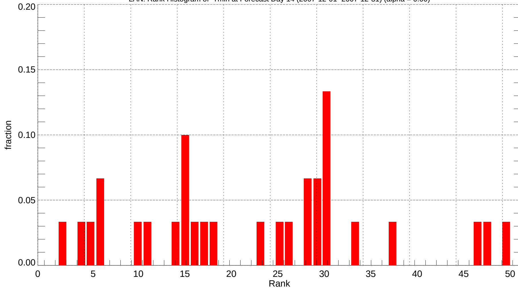
LAN: Rank Histogram of Tmin at Forecast Day 14 (2007-12-01~2007-12-31) (alpha = 0.00)
