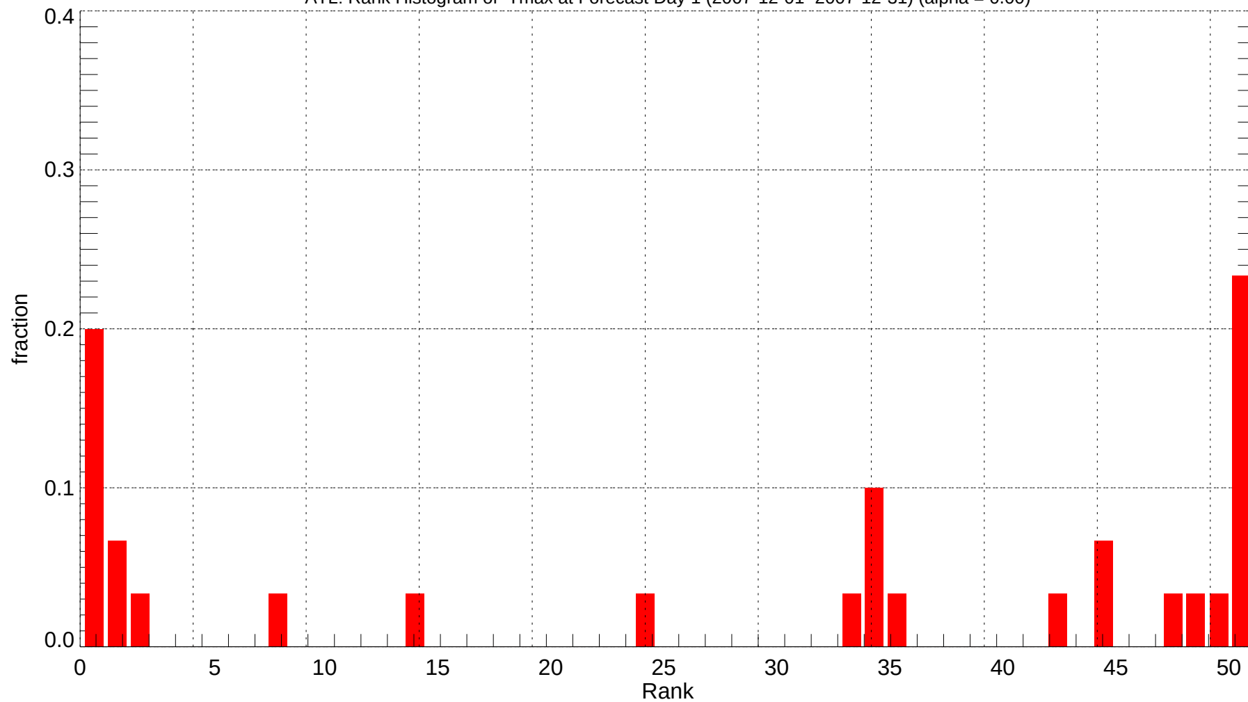
ATL: Rank Histogram of Tmax at Forecast Day 1 (2007-12-01~2007-12-31) (alpha = 0.00)
