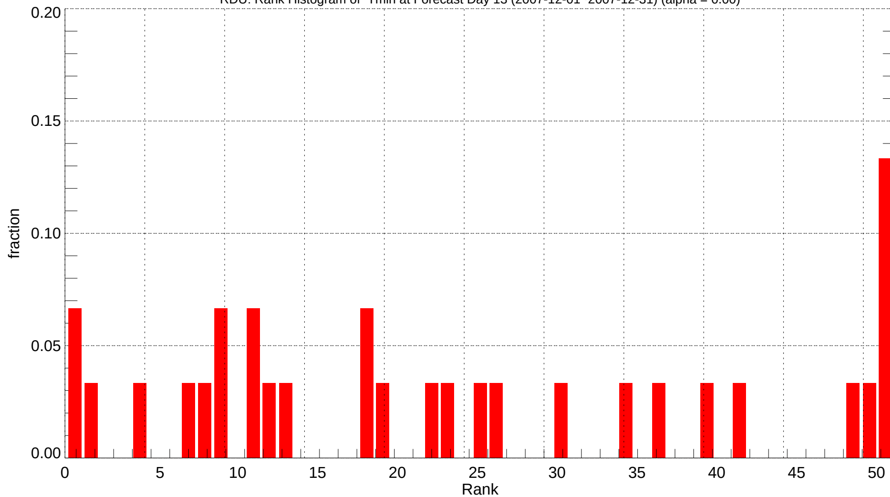
RDU: Rank Histogram of Tmin at Forecast Day 13 (2007-12-01~2007-12-31) (alpha = 0.00)
