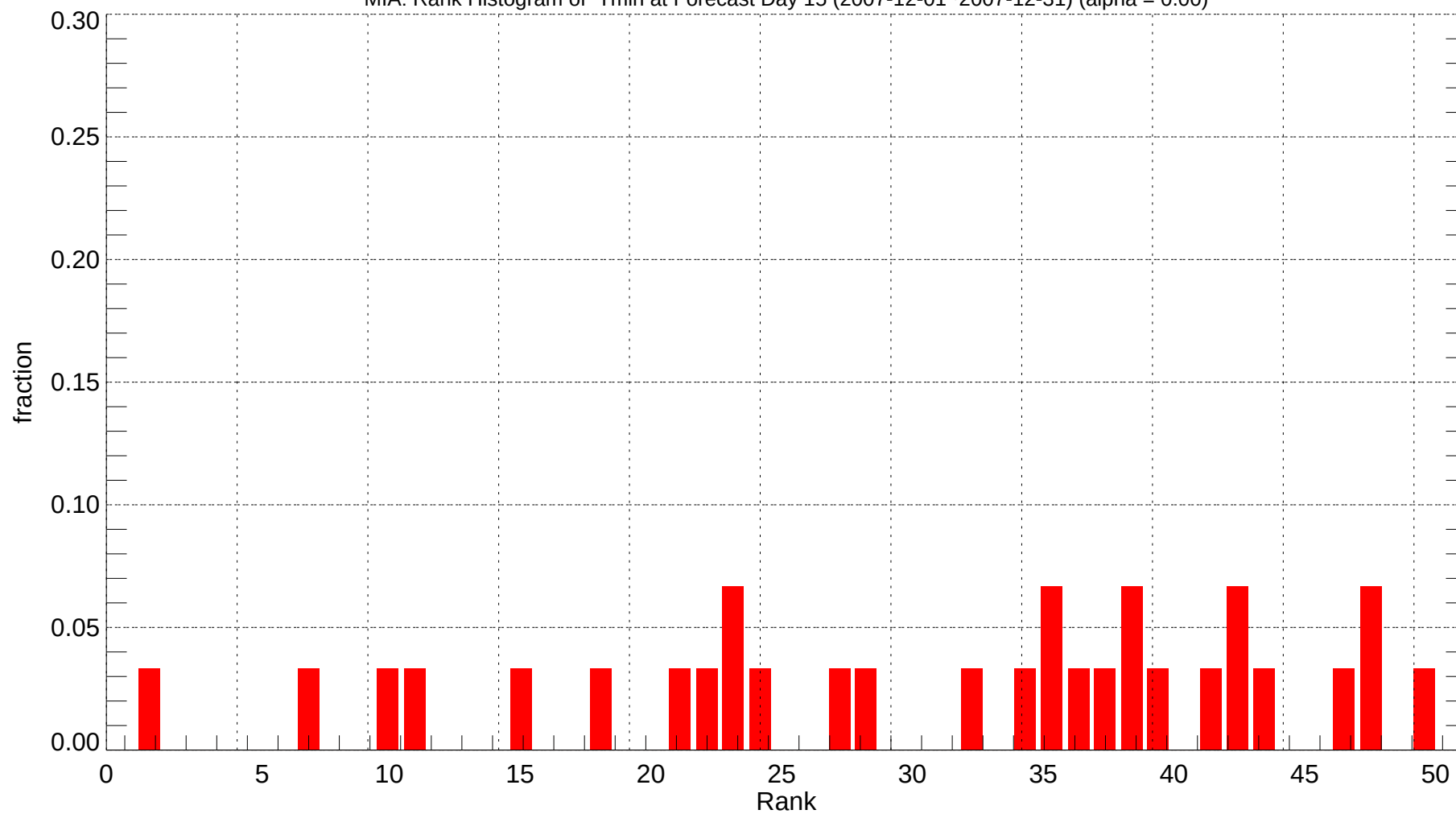
MIA: Rank Histogram of Tmin at Forecast Day 15 (2007-12-01~2007-12-31) (alpha = 0.00)
