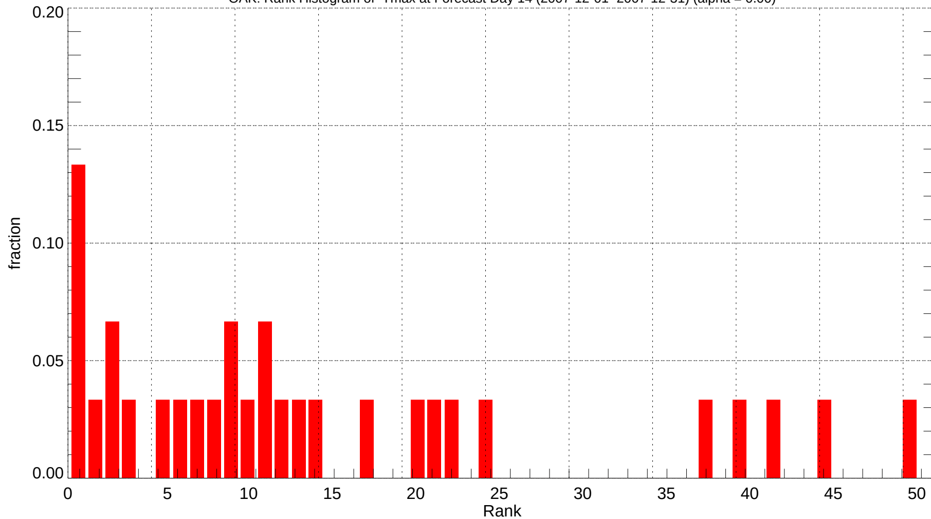
OAK: Rank Histogram of Tmax at Forecast Day 14 (2007-12-01~2007-12-31) (alpha = 0.00)
