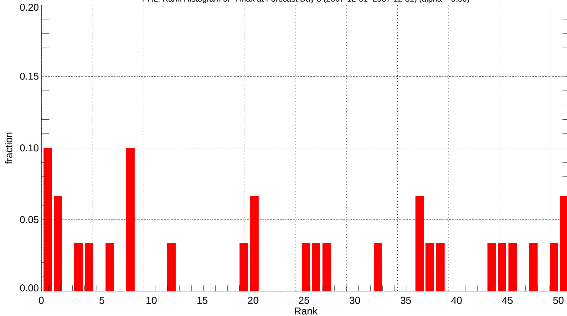
PHL: Rank Histogram of Tmax at Forecast Day 5 (2007-12-01~2007-12-31) (alpha = 0.00)
