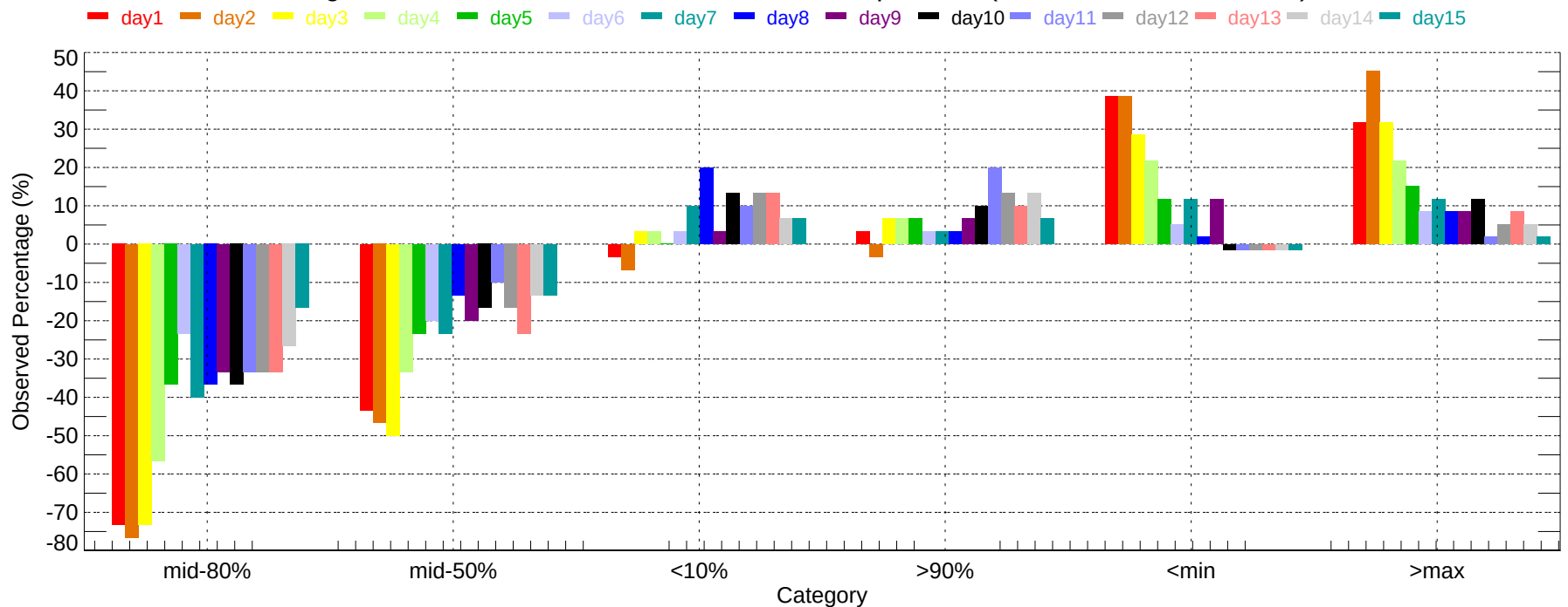
Observed Percentage Deviation of Ensembles - RNO: Max Temperature (2007-12-01~2007-12-31)
