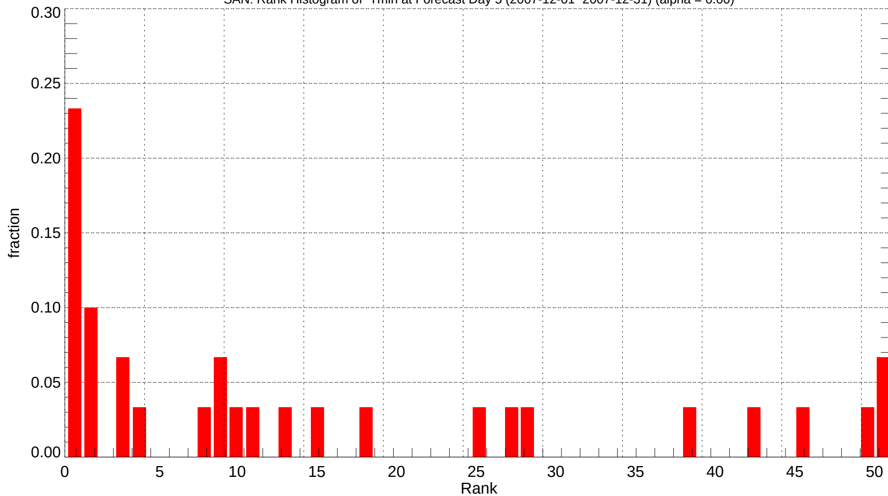
SAN: Rank Histogram of Tmin at Forecast Day 5 (2007-12-01~2007-12-31) (alpha = 0.00)
