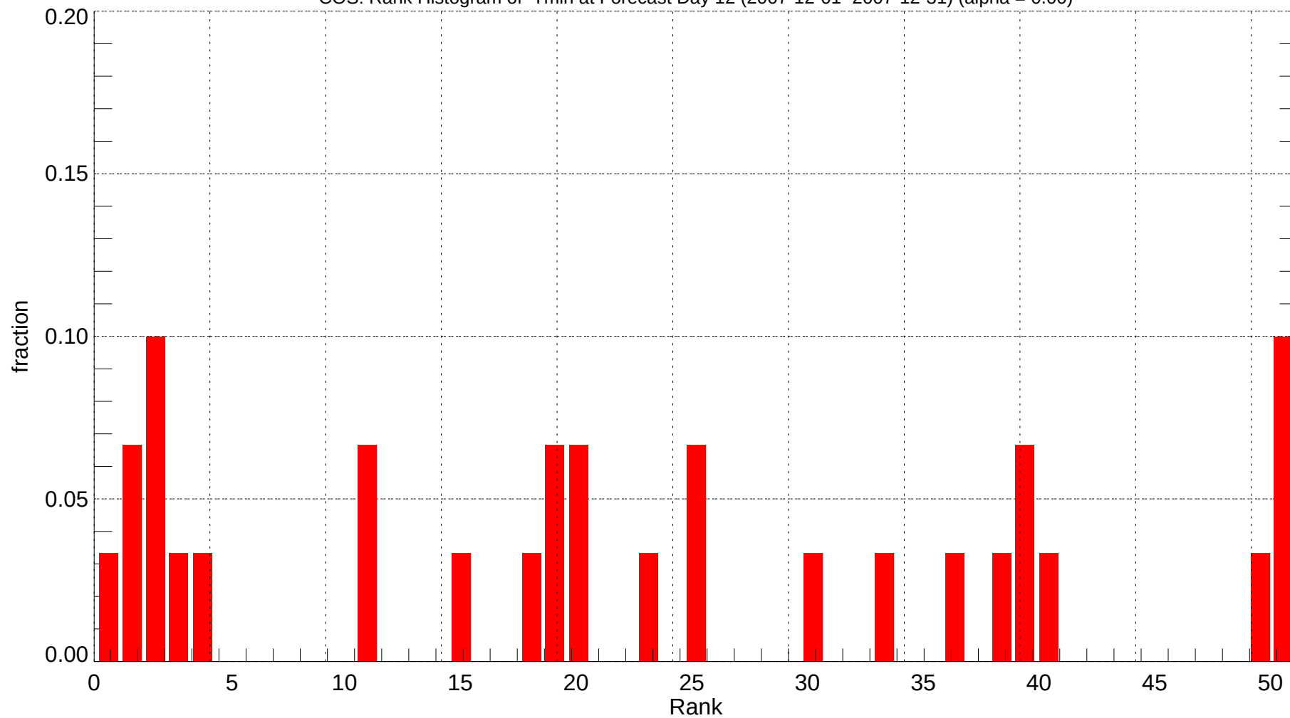
COS: Rank Histogram of Tmin at Forecast Day 12 (2007-12-01~2007-12-31) (alpha = 0.00)
