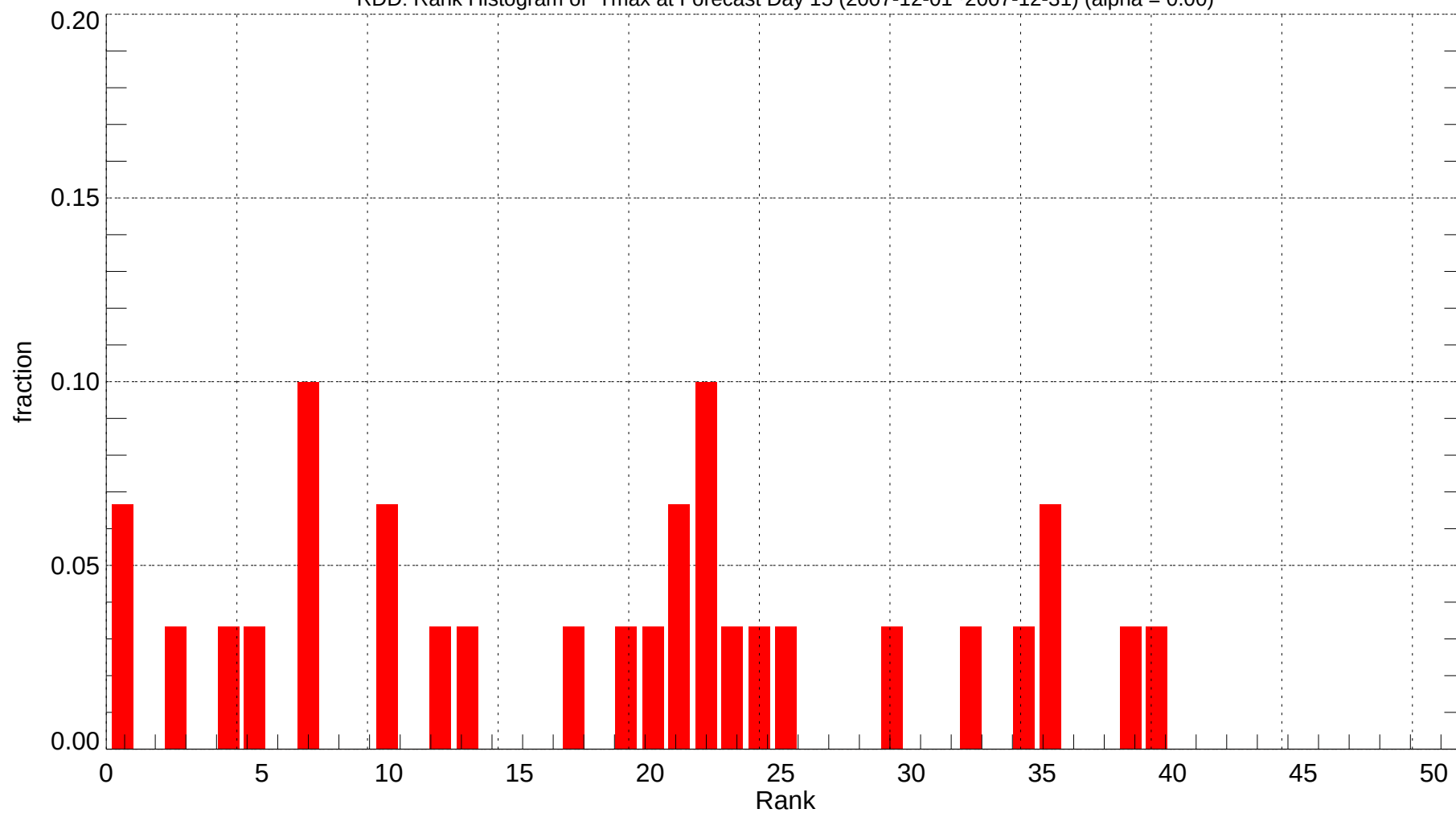
RDD: Rank Histogram of Tmax at Forecast Day 15 (2007-12-01~2007-12-31) (alpha = 0.00)
