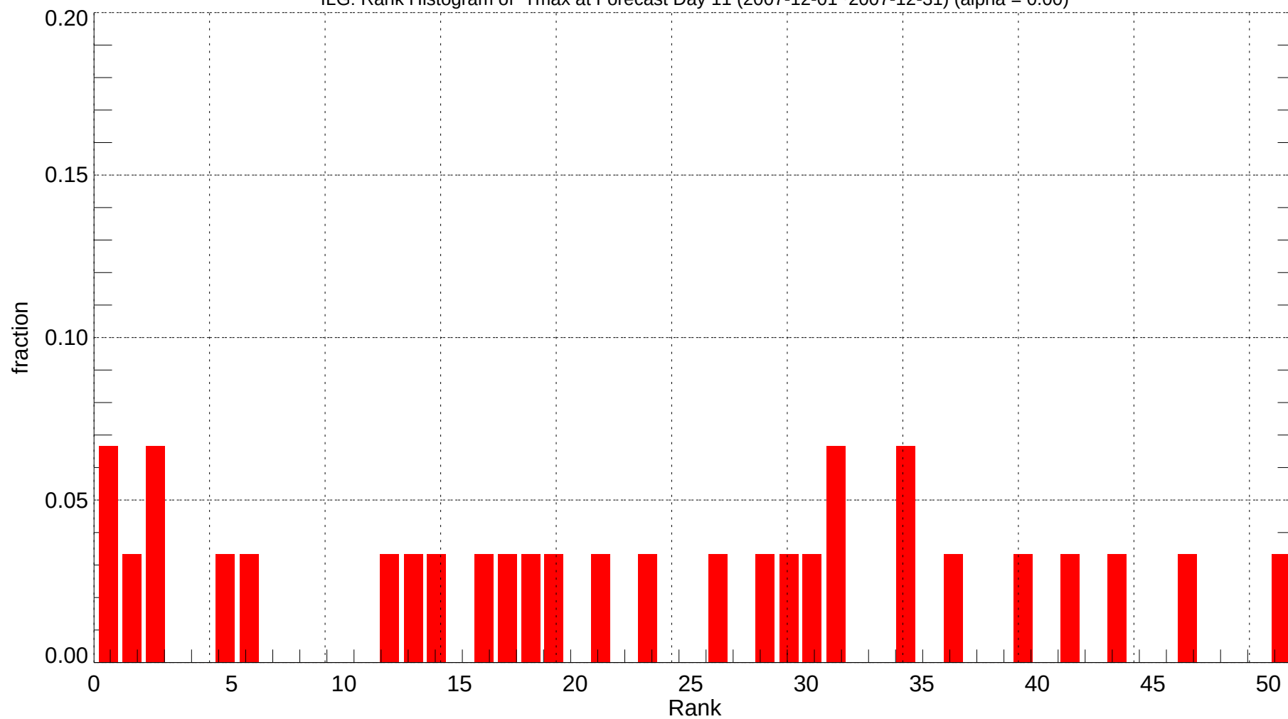
ILG: Rank Histogram of Tmax at Forecast Day 11 (2007-12-01~2007-12-31) (alpha = 0.00)
