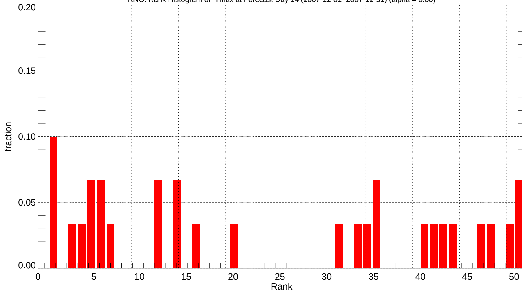
RNO: Rank Histogram of Tmax at Forecast Day 14 (2007-12-01~2007-12-31) (alpha = 0.00)
