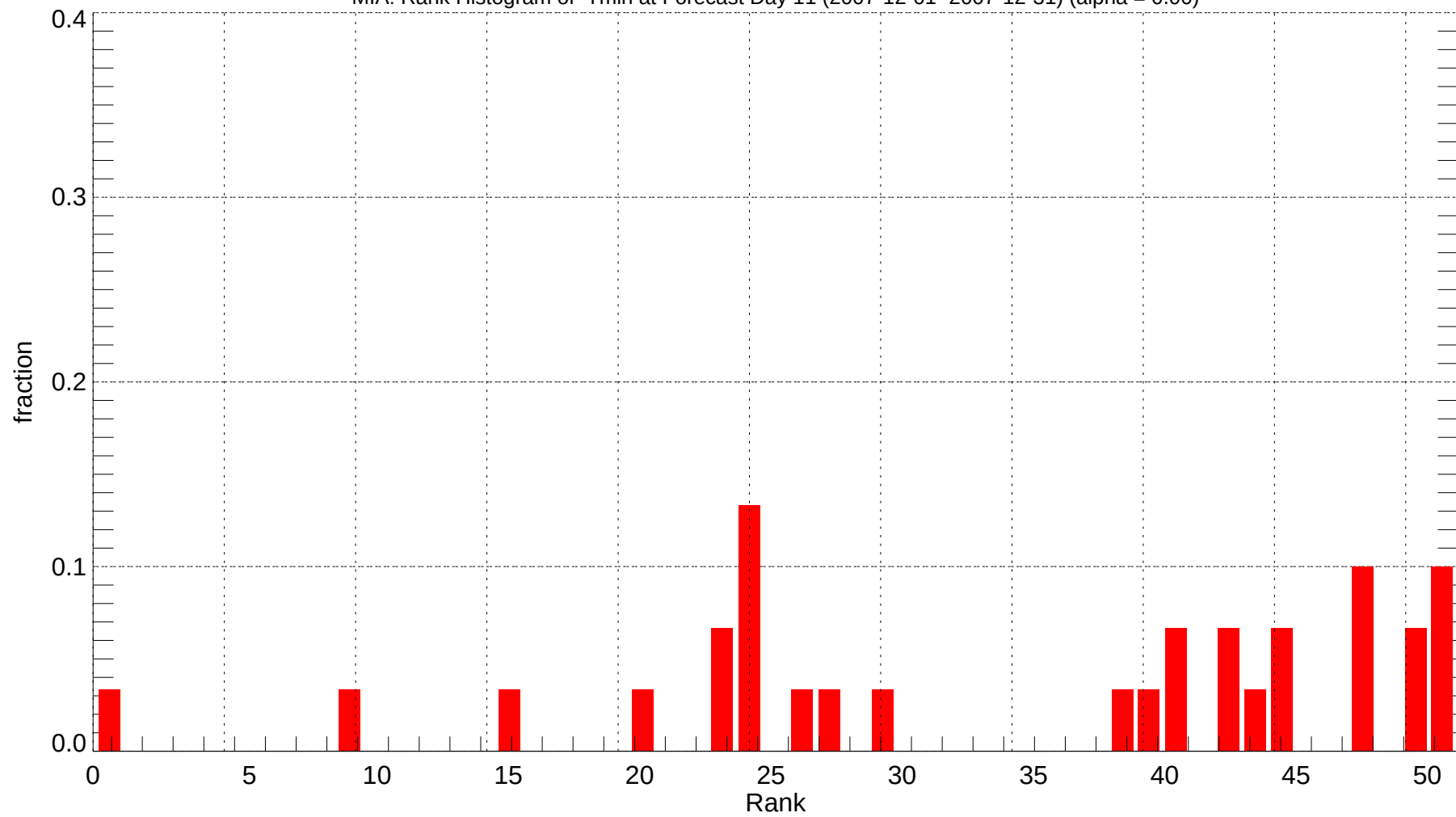
MIA: Rank Histogram of Tmin at Forecast Day 11 (2007-12-01~2007-12-31) (alpha = 0.00)
