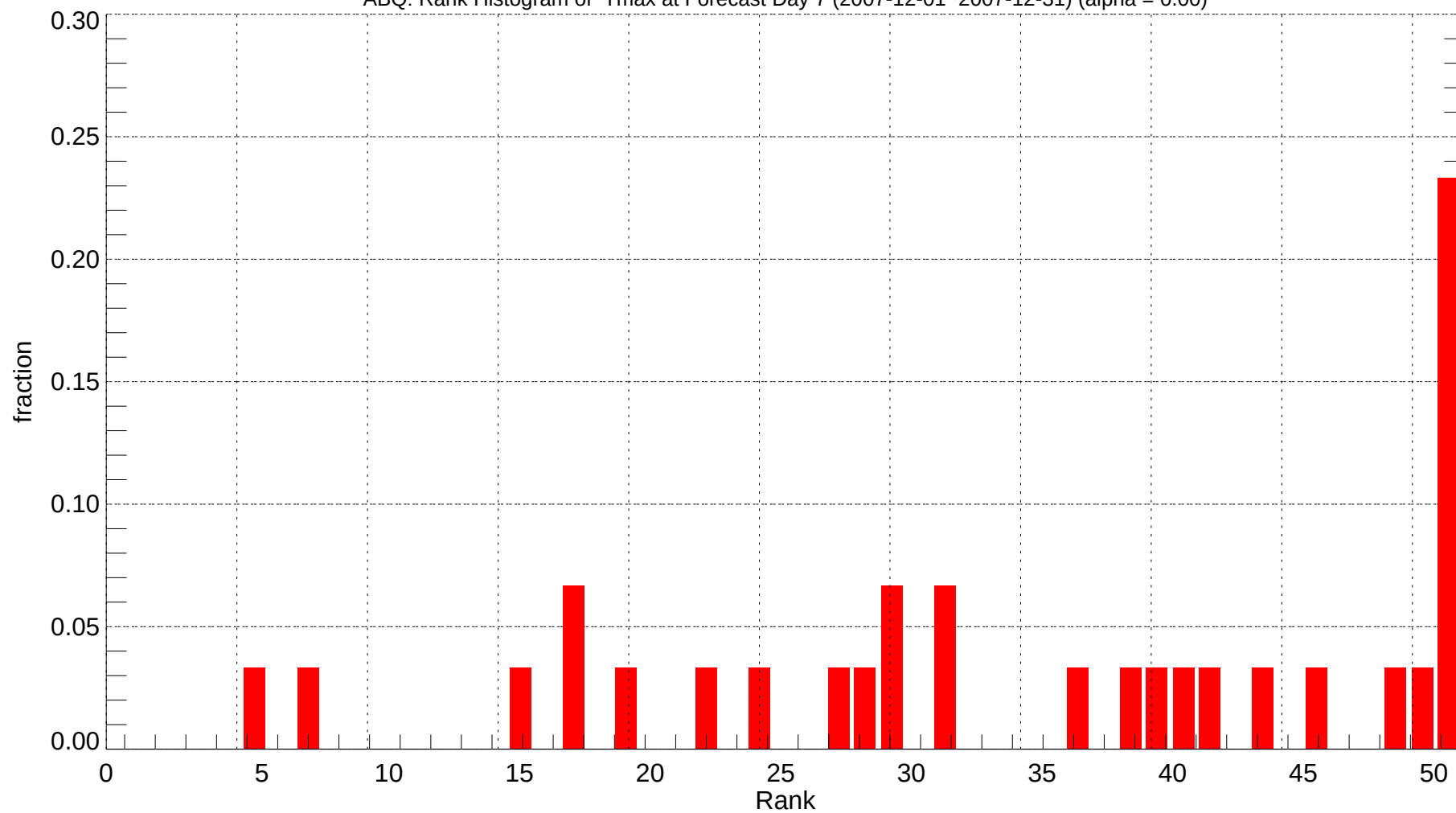
ABQ: Rank Histogram of Tmax at Forecast Day 7 (2007-12-01~2007-12-31) (alpha = 0.00)
