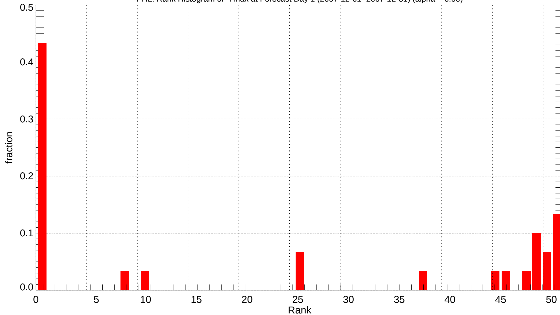
PHL: Rank Histogram of Tmax at Forecast Day 1 (2007-12-01~2007-12-31) (alpha = 0.00)
