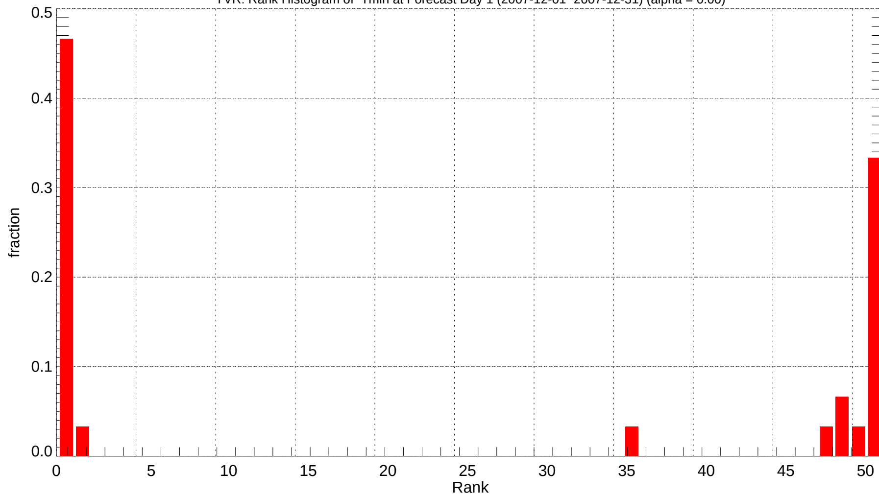
YVR: Rank Histogram of Tmin at Forecast Day 1 (2007-12-01~2007-12-31) (alpha = 0.00)
