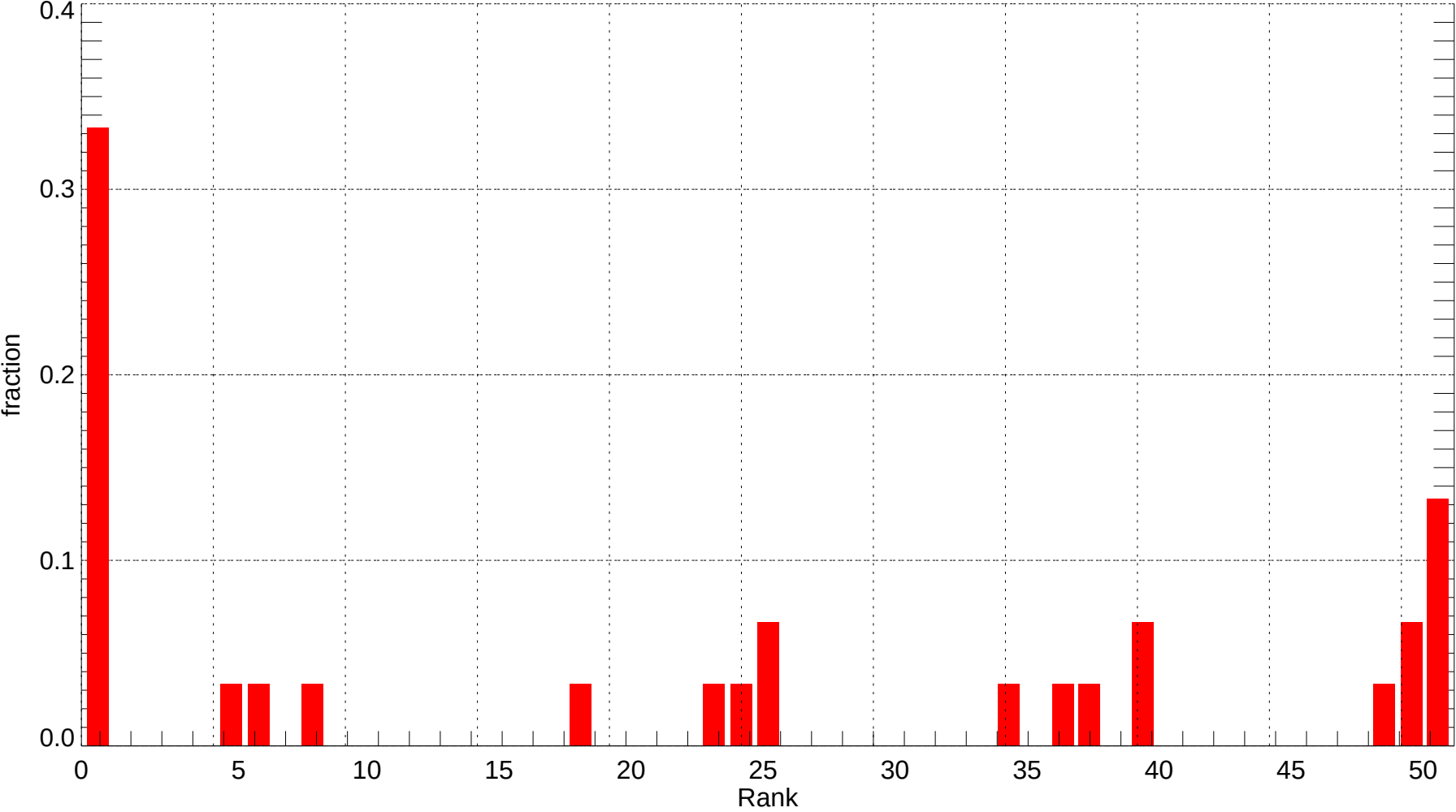
PIT: Rank Histogram of Tmax at Forecast Day 3 (2007-12-01~2007-12-31) (alpha = 0.00)
