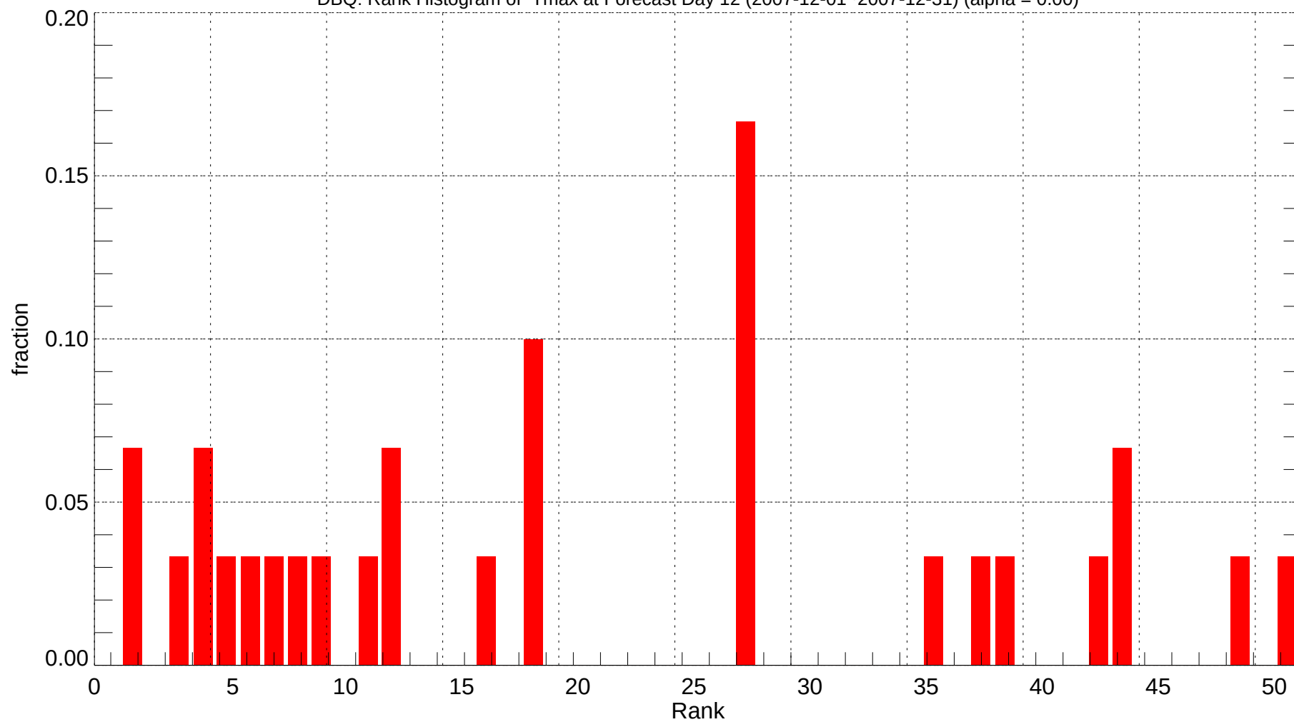
DBQ: Rank Histogram of Tmax at Forecast Day 12 (2007-12-01~2007-12-31) (alpha = 0.00)
