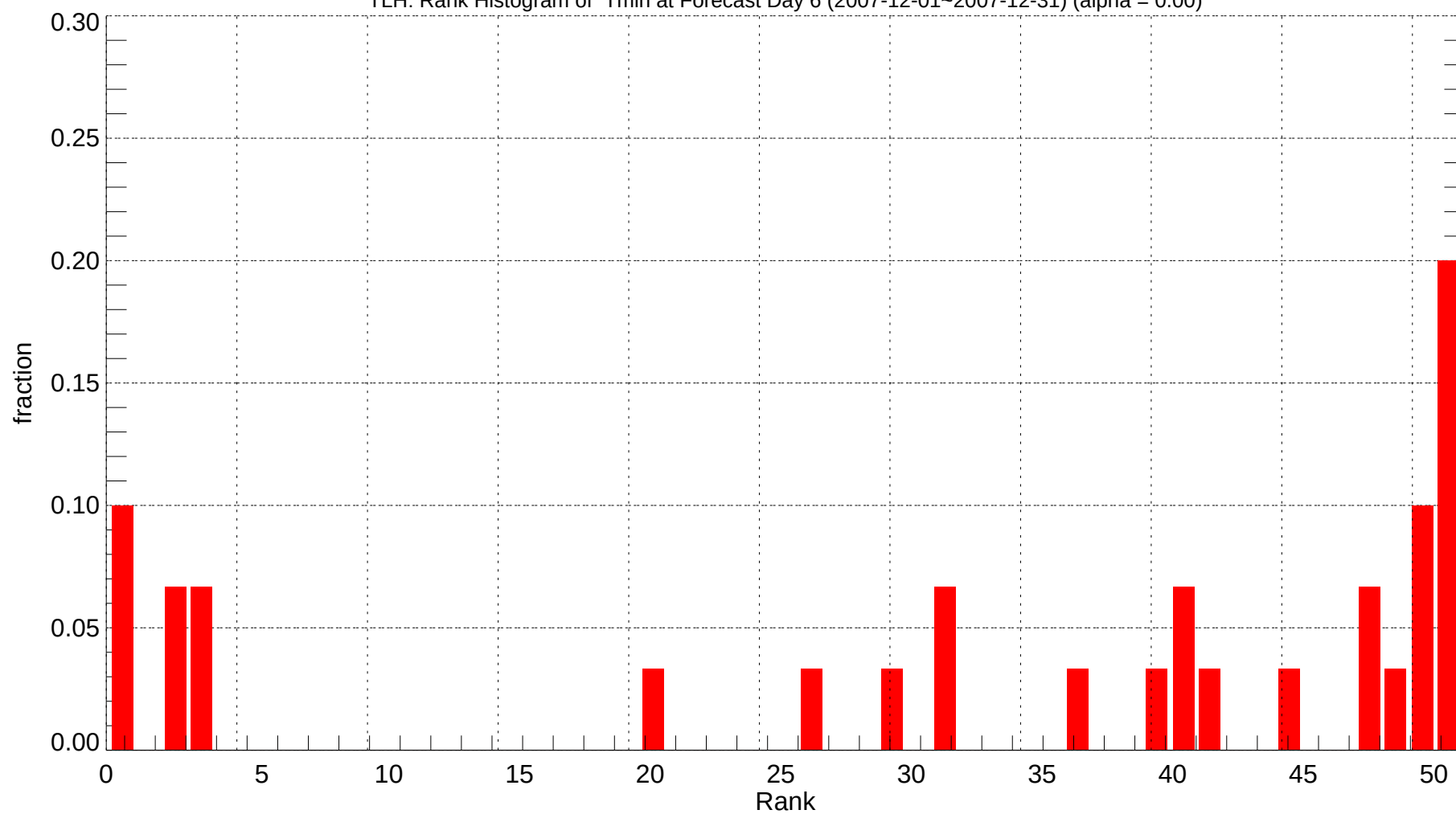
TLH: Rank Histogram of Tmin at Forecast Day 6 (2007-12-01~2007-12-31) (alpha = 0.00)
