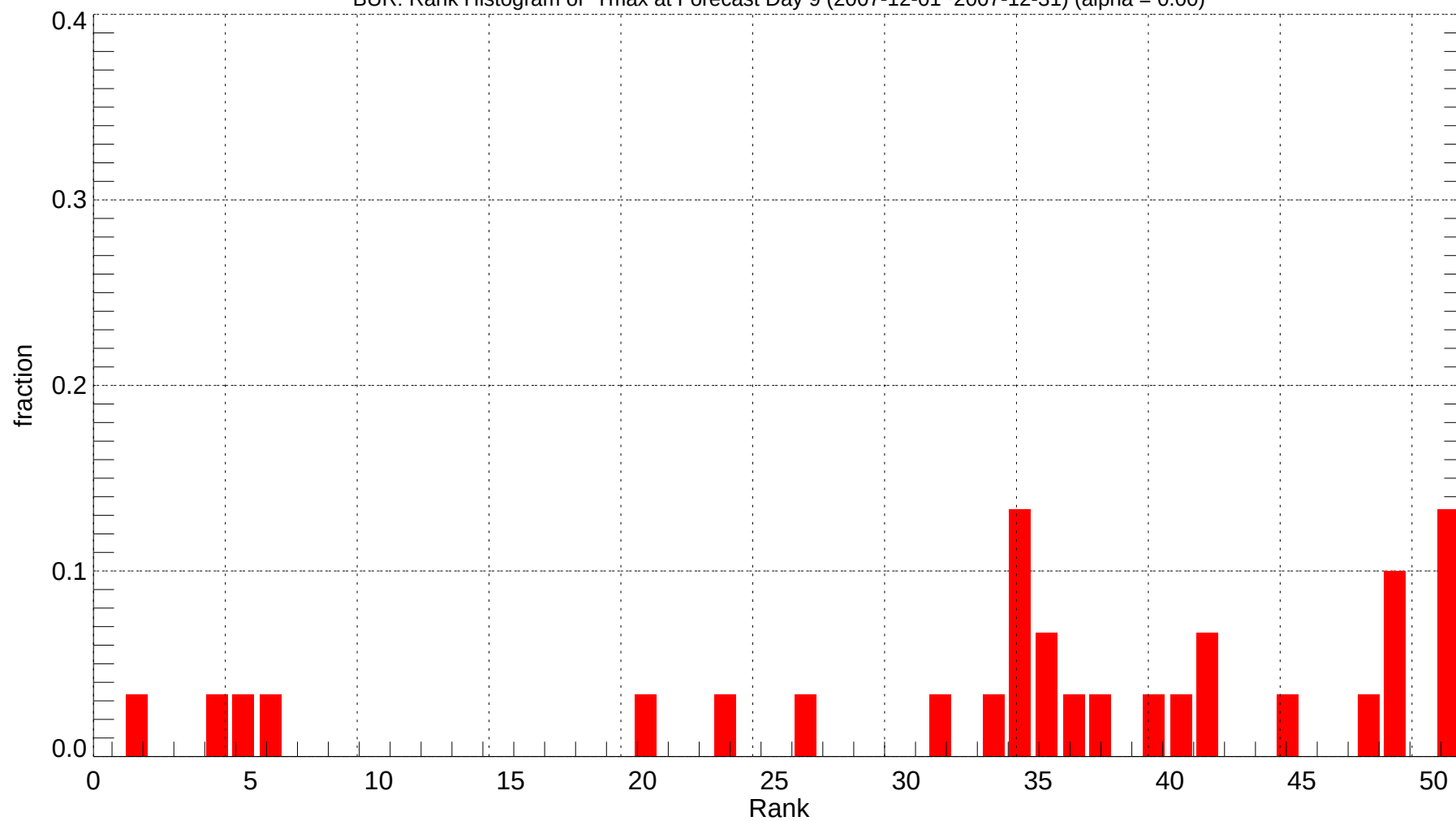
BUR: Rank Histogram of Tmax at Forecast Day 9 (2007-12-01~2007-12-31) (alpha = 0.00)
