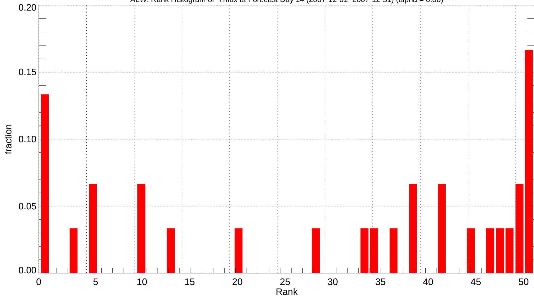
ALW: Rank Histogram of Tmax at Forecast Day 14 (2007-12-01~2007-12-31) (alpha = 0.00)
