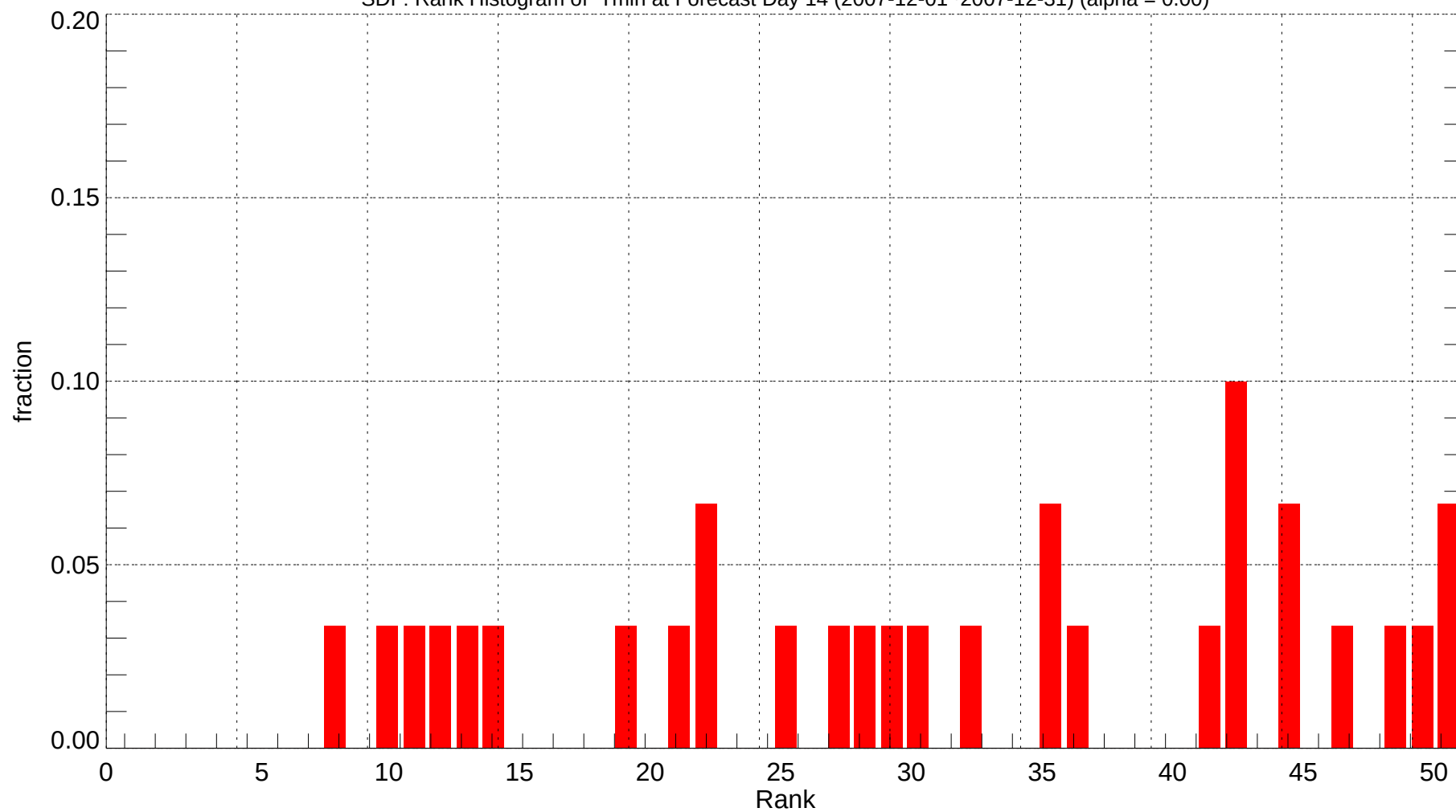
SDF: Rank Histogram of Tmin at Forecast Day 14 (2007-12-01~2007-12-31) (alpha = 0.00)
