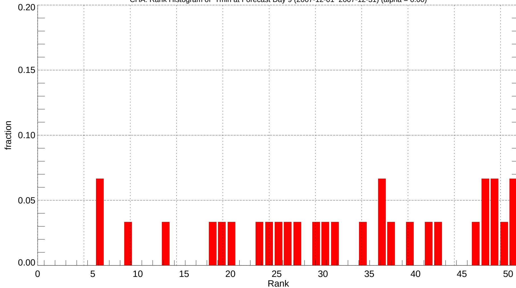
CHA: Rank Histogram of Tmin at Forecast Day 9 (2007-12-01~2007-12-31) (alpha = 0.00)
