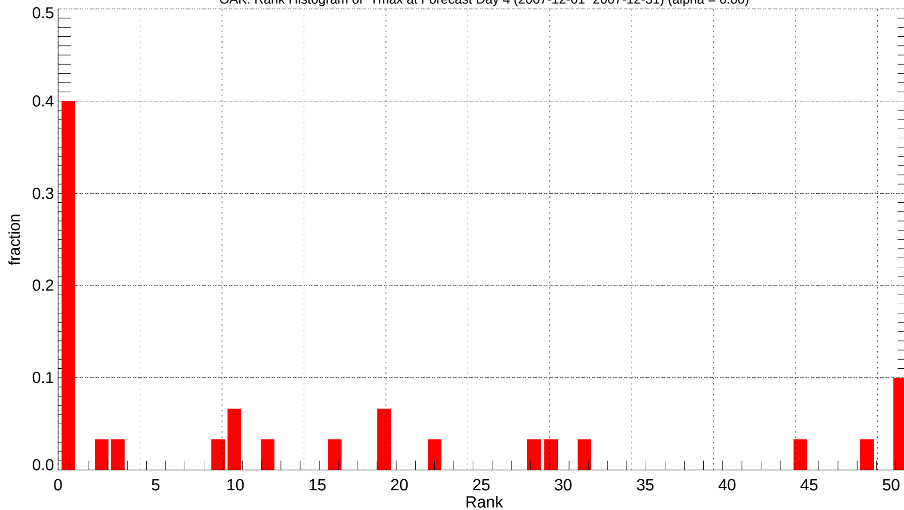
OAK: Rank Histogram of Tmax at Forecast Day 4 (2007-12-01~2007-12-31) (alpha = 0.00)
