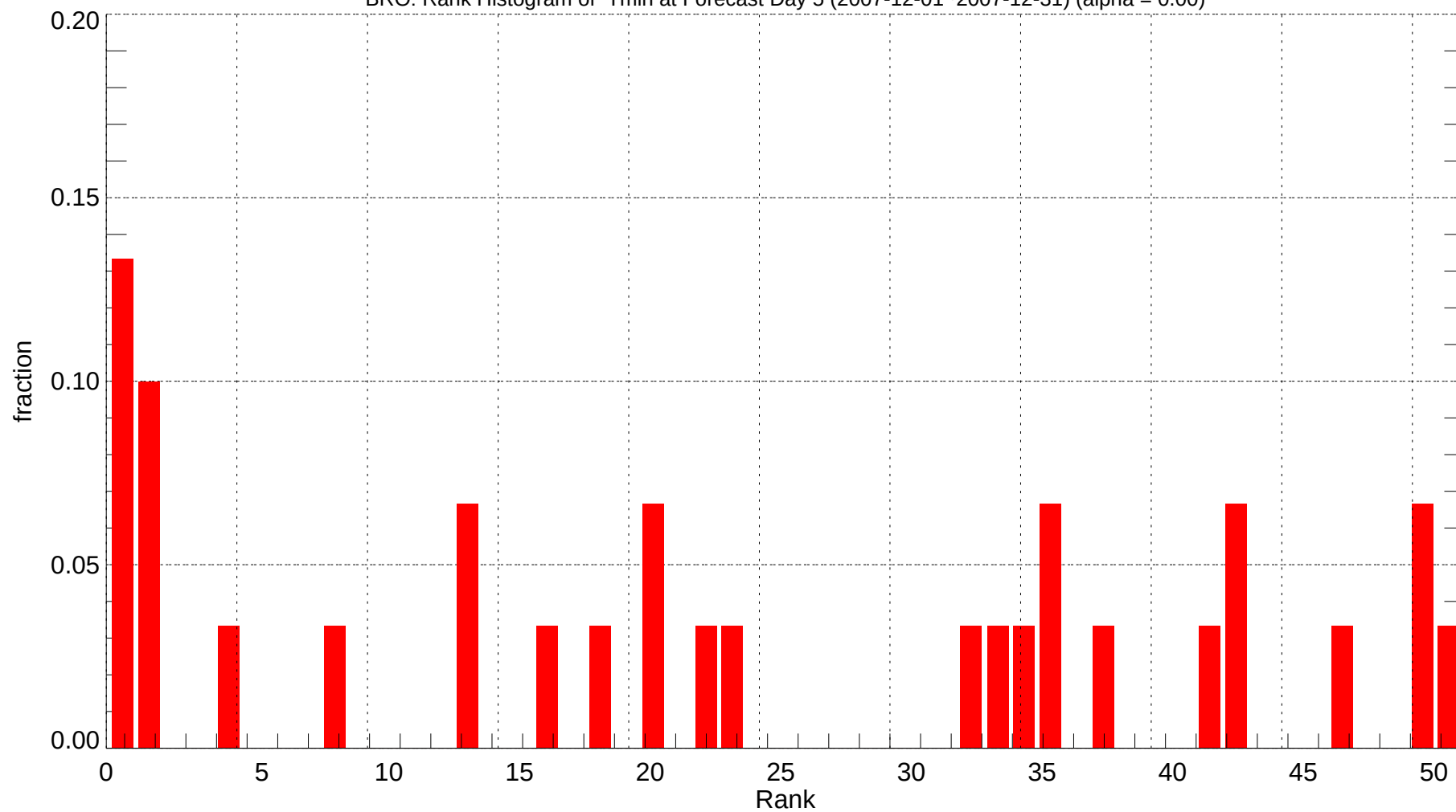
BRO: Rank Histogram of Tmin at Forecast Day 5 (2007-12-01~2007-12-31) (alpha = 0.00)
