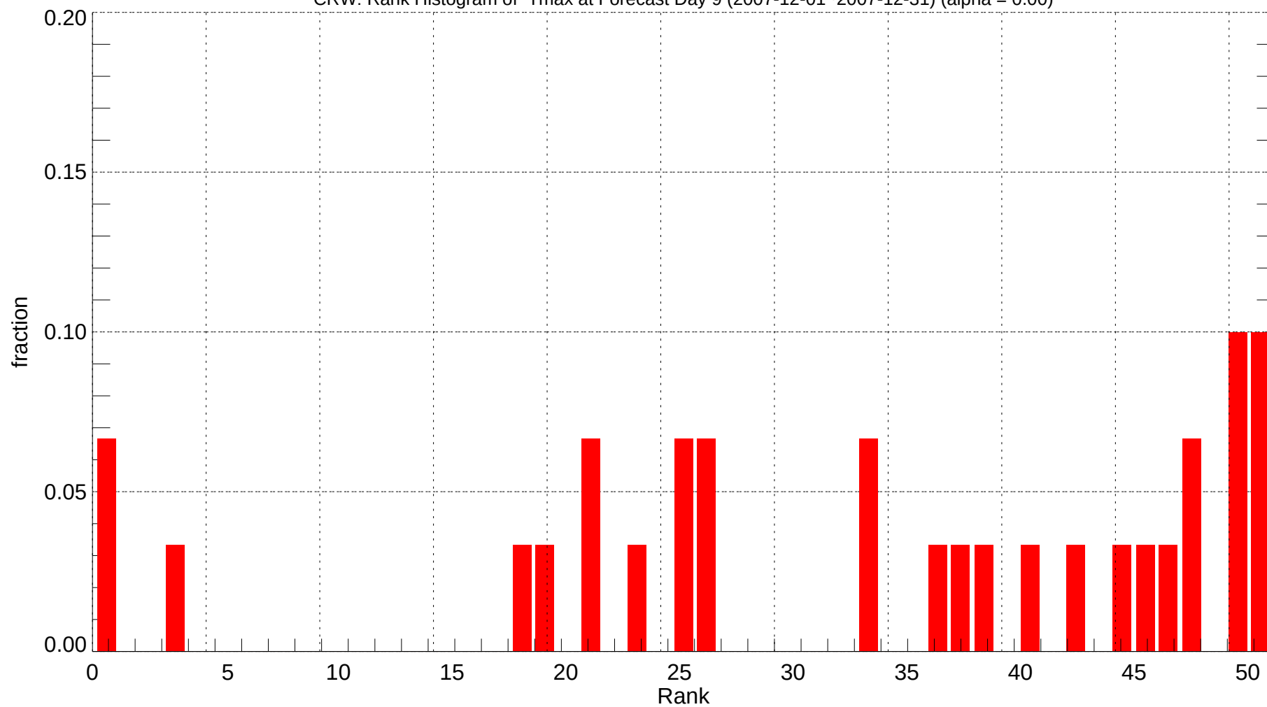
CRW: Rank Histogram of Tmax at Forecast Day 9 (2007-12-01~2007-12-31) (alpha = 0.00)
