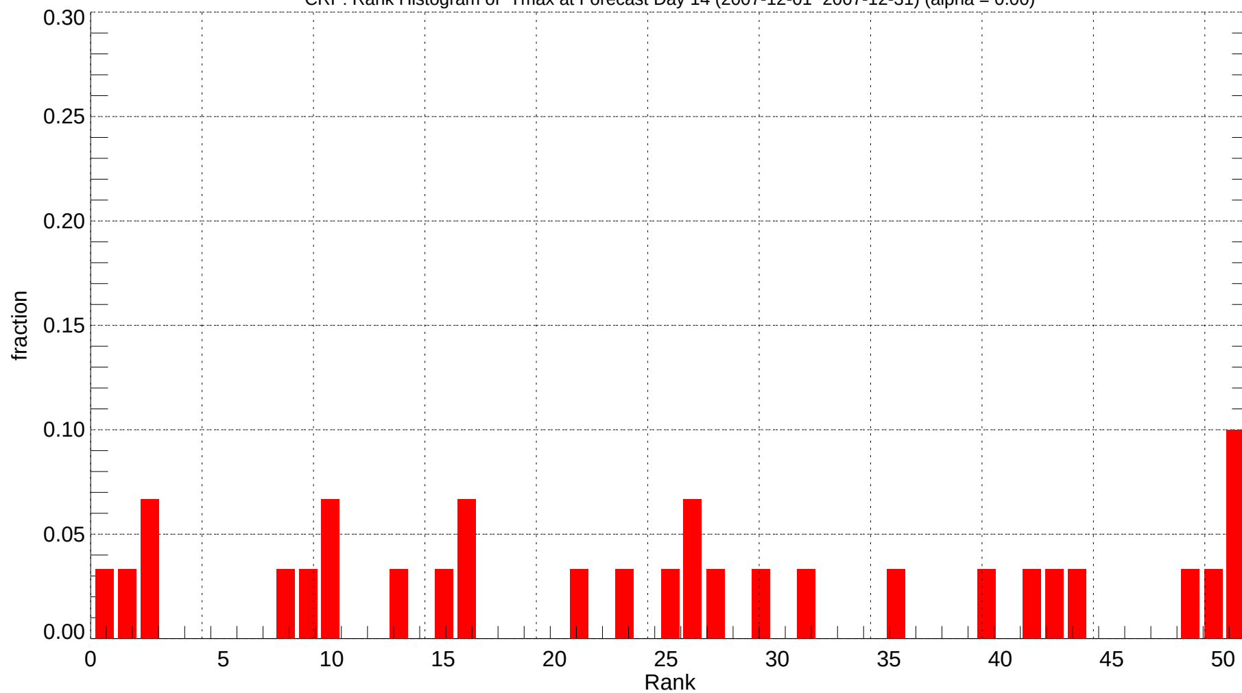
CRP: Rank Histogram of Tmax at Forecast Day 14 (2007-12-01~2007-12-31) (alpha = 0.00)
