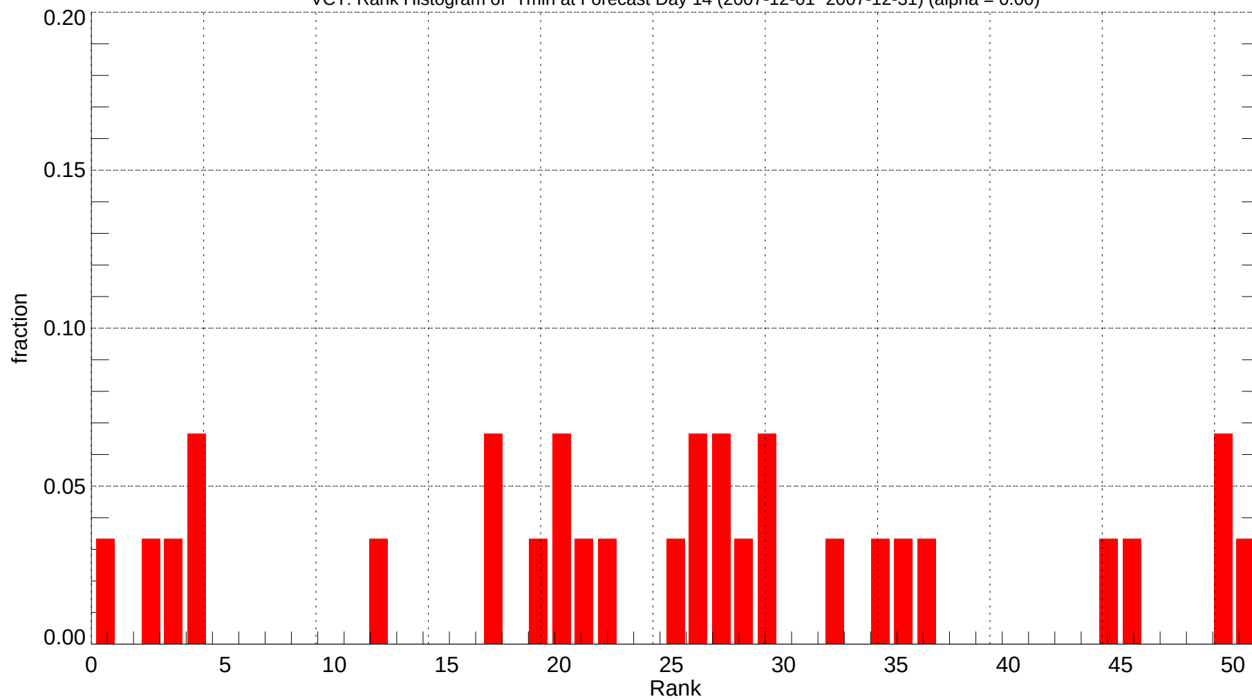
VCT: Rank Histogram of Tmin at Forecast Day 14 (2007-12-01~2007-12-31) (alpha = 0.00)
