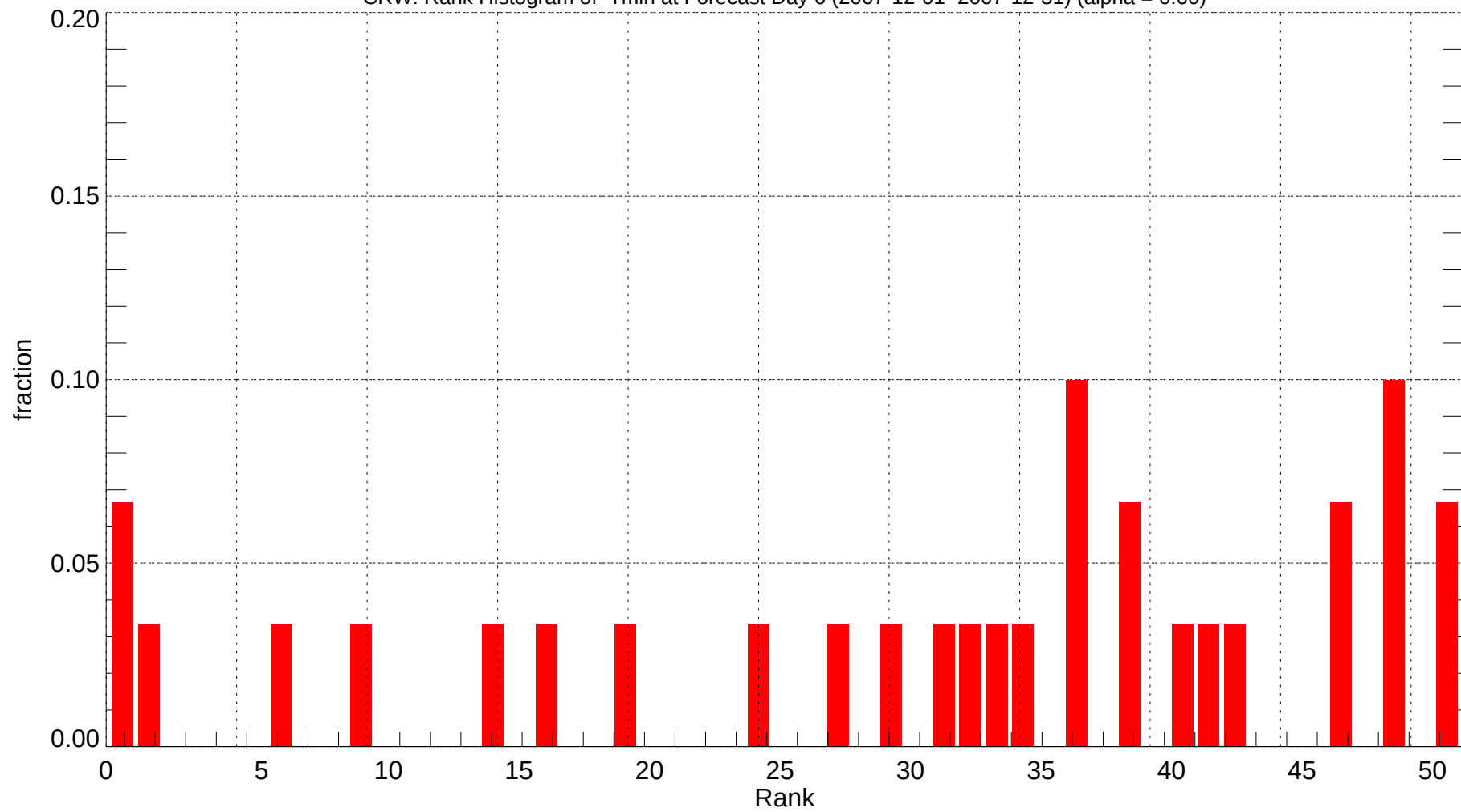
CRW: Rank Histogram of Tmin at Forecast Day 6 (2007-12-01~2007-12-31) (alpha = 0.00)
