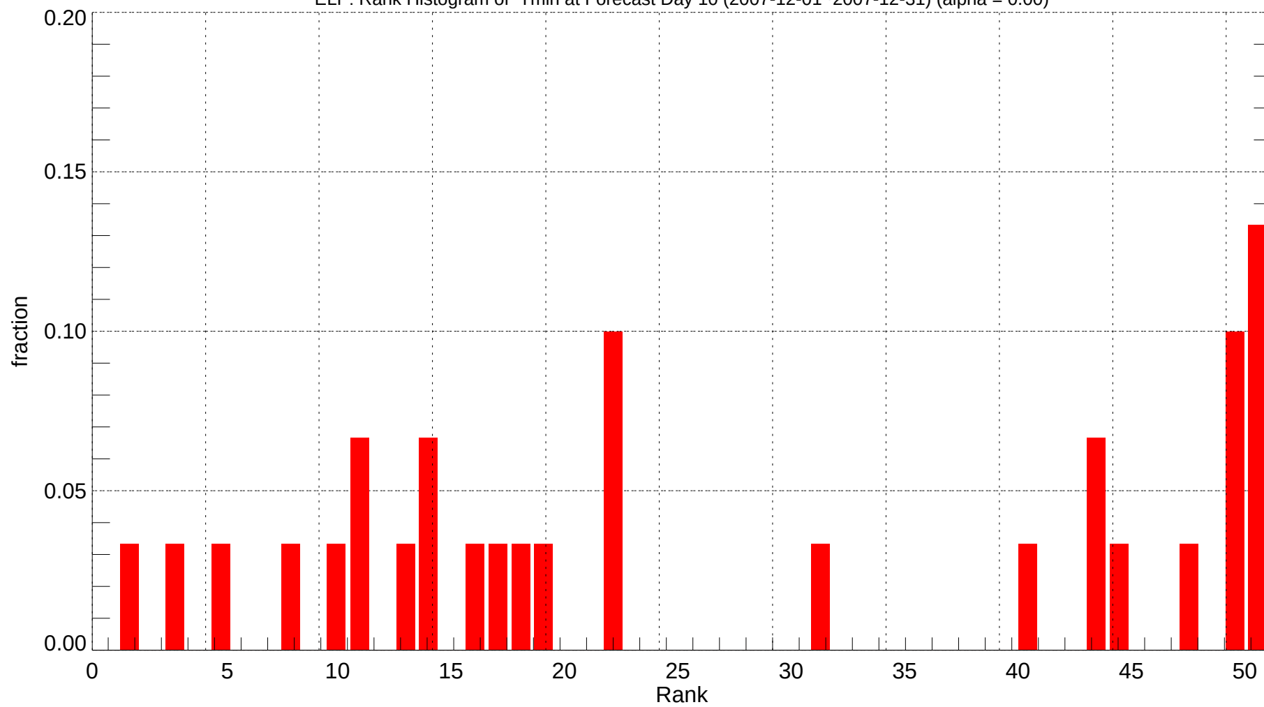
ELP: Rank Histogram of Tmin at Forecast Day 10 (2007-12-01~2007-12-31) (alpha = 0.00)
