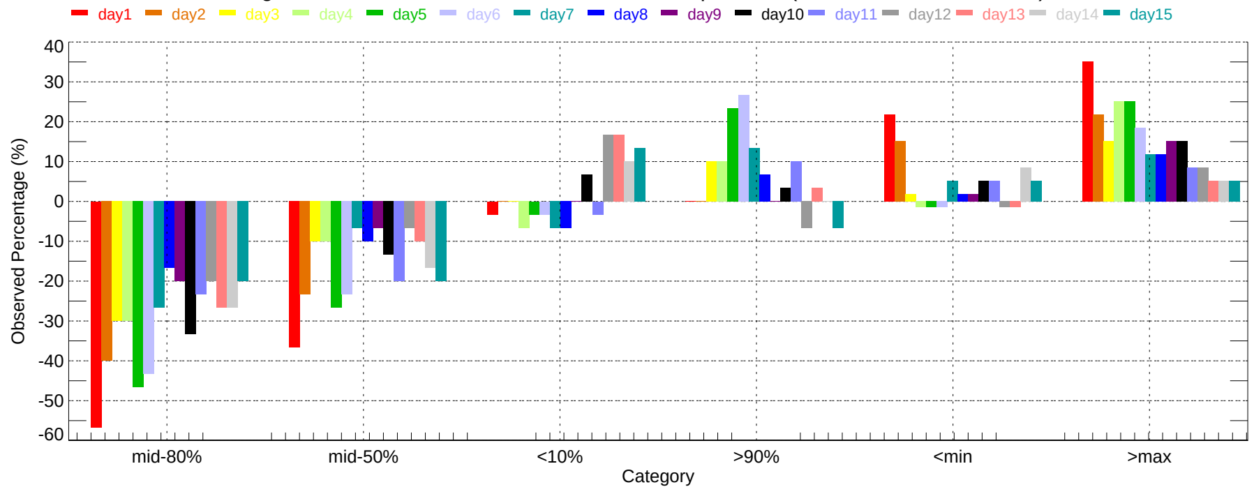
Observed Percentage Deviation of Ensembles - COS: Max Temperature (2007-12-01~2007-12-31)
