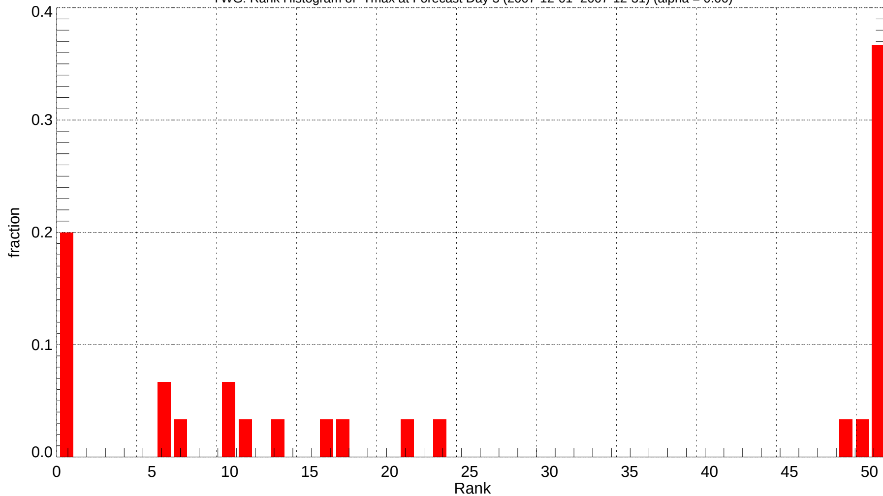
YWG: Rank Histogram of Tmax at Forecast Day 3 (2007-12-01~2007-12-31) (alpha = 0.00)
