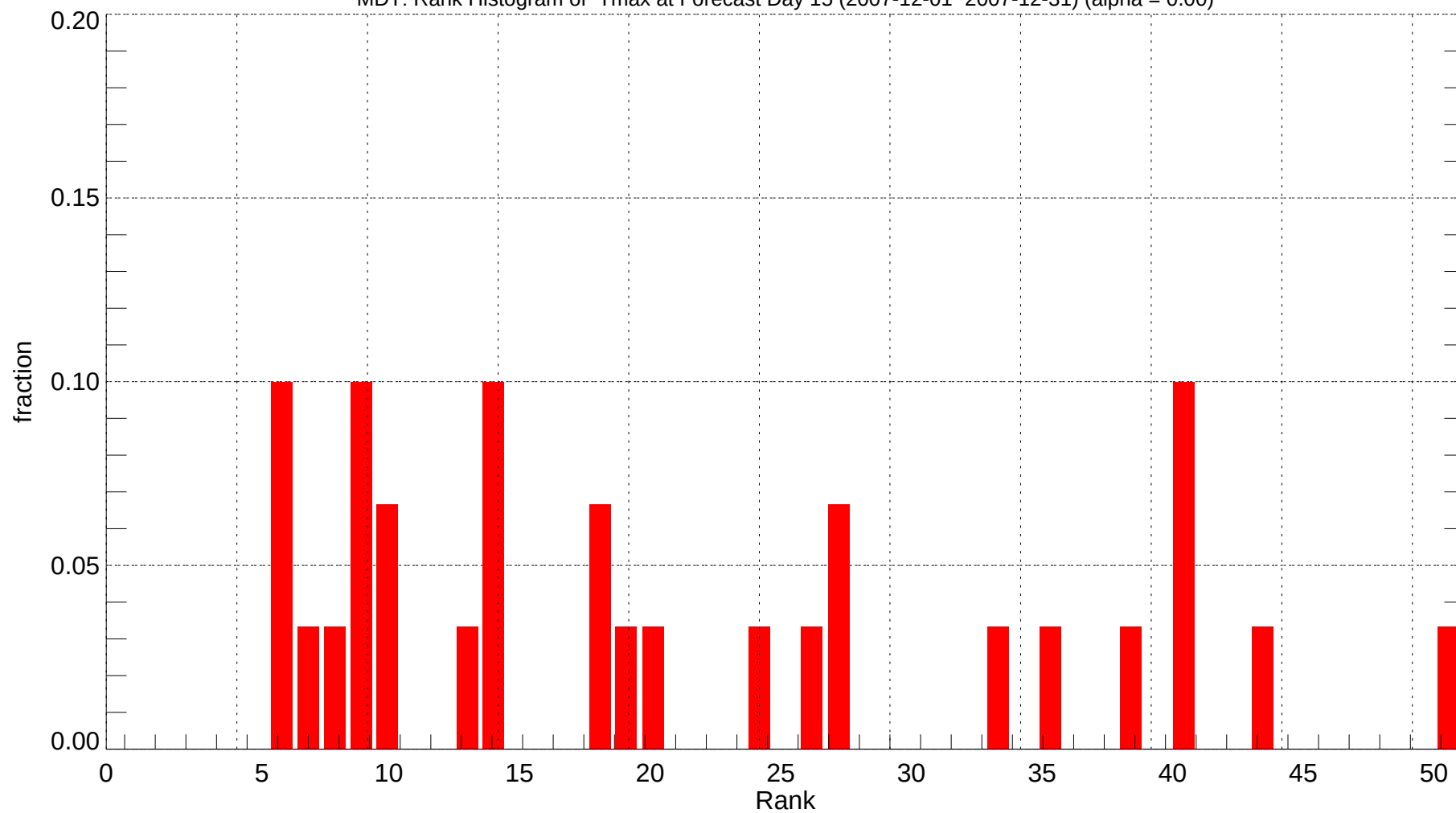
MDT: Rank Histogram of Tmax at Forecast Day 15 (2007-12-01~2007-12-31) (alpha = 0.00)
