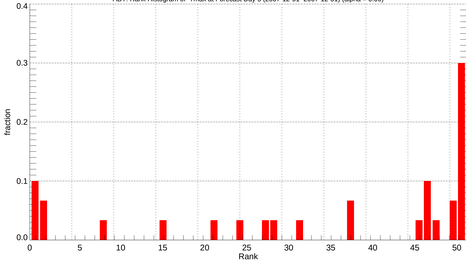
ABY: Rank Histogram of Tmax at Forecast Day 5 (2007-12-01~2007-12-31) (alpha = 0.00)
