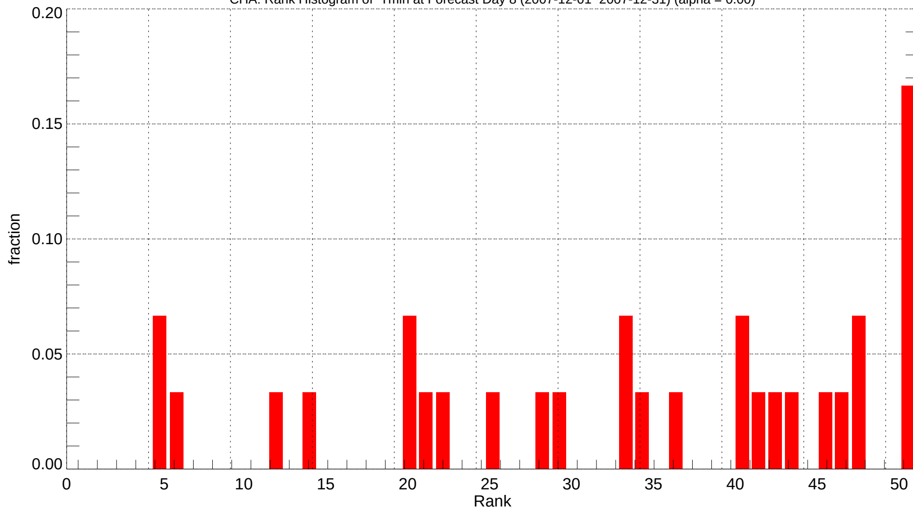
CHA: Rank Histogram of Tmin at Forecast Day 8 (2007-12-01~2007-12-31) (alpha = 0.00)
