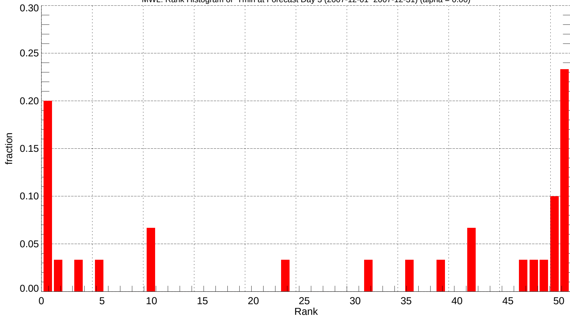
MWL: Rank Histogram of Tmin at Forecast Day 3 (2007-12-01~2007-12-31) (alpha = 0.00)
