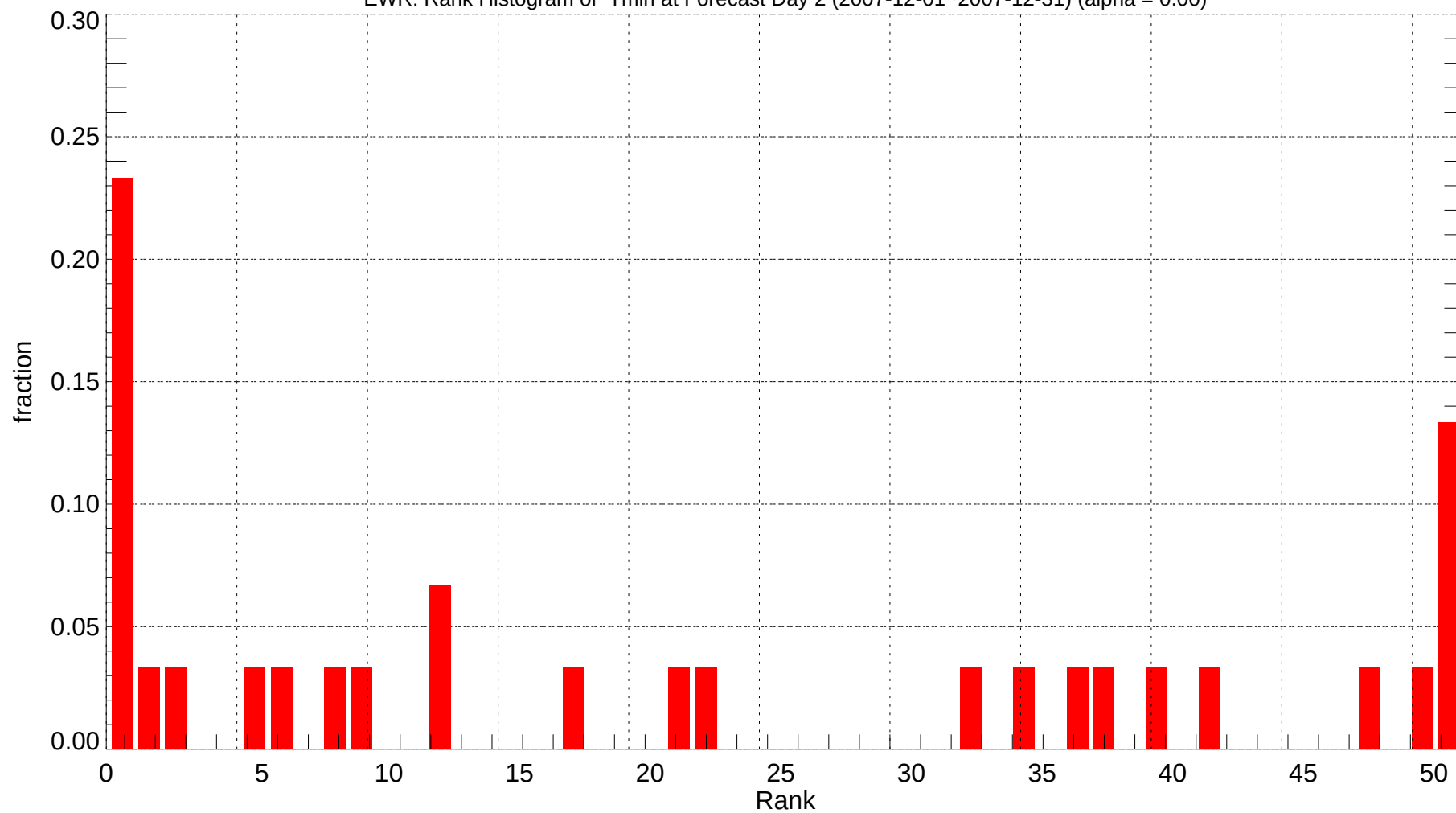
EWR: Rank Histogram of Tmin at Forecast Day 2 (2007-12-01~2007-12-31) (alpha = 0.00)
