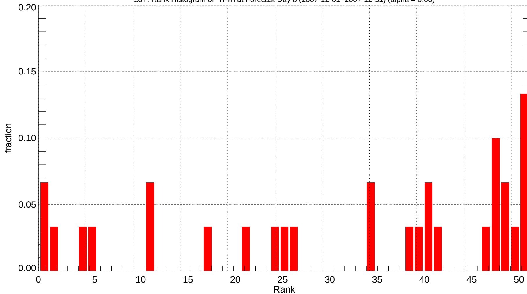
SJT: Rank Histogram of Tmin at Forecast Day 8 (2007-12-01~2007-12-31) (alpha = 0.00)
