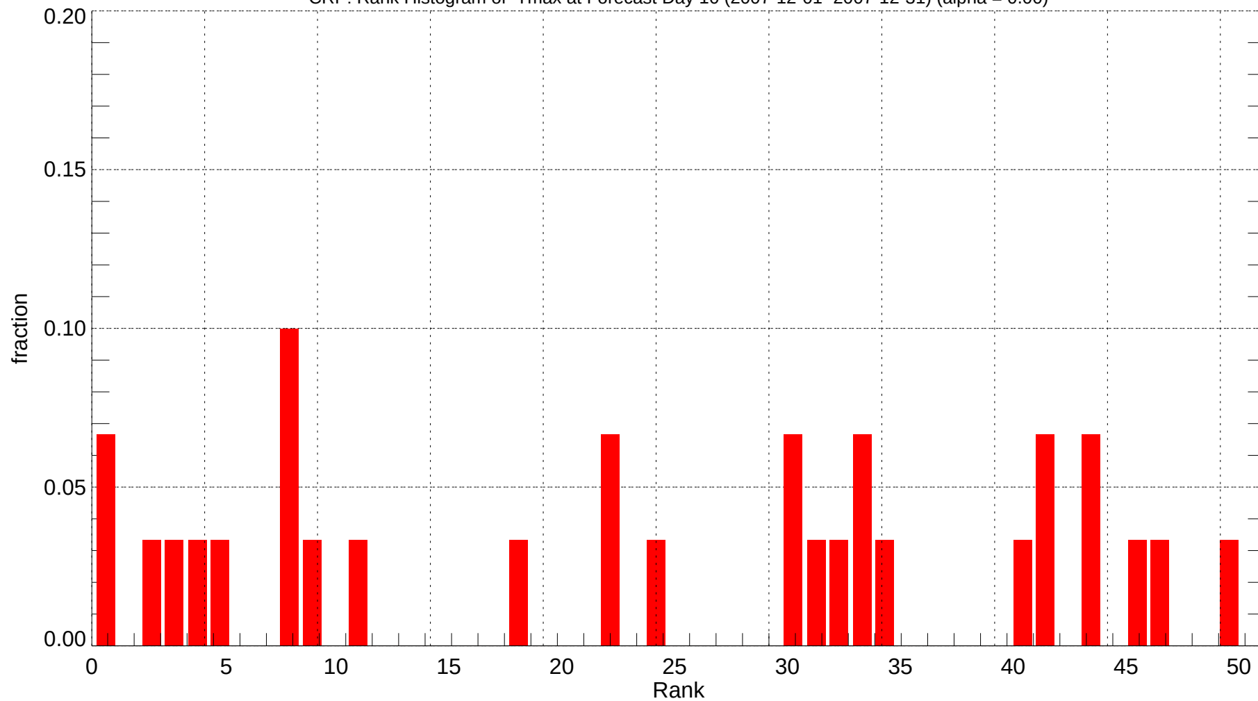
CRP: Rank Histogram of Tmax at Forecast Day 10 (2007-12-01~2007-12-31) (alpha = 0.00)
