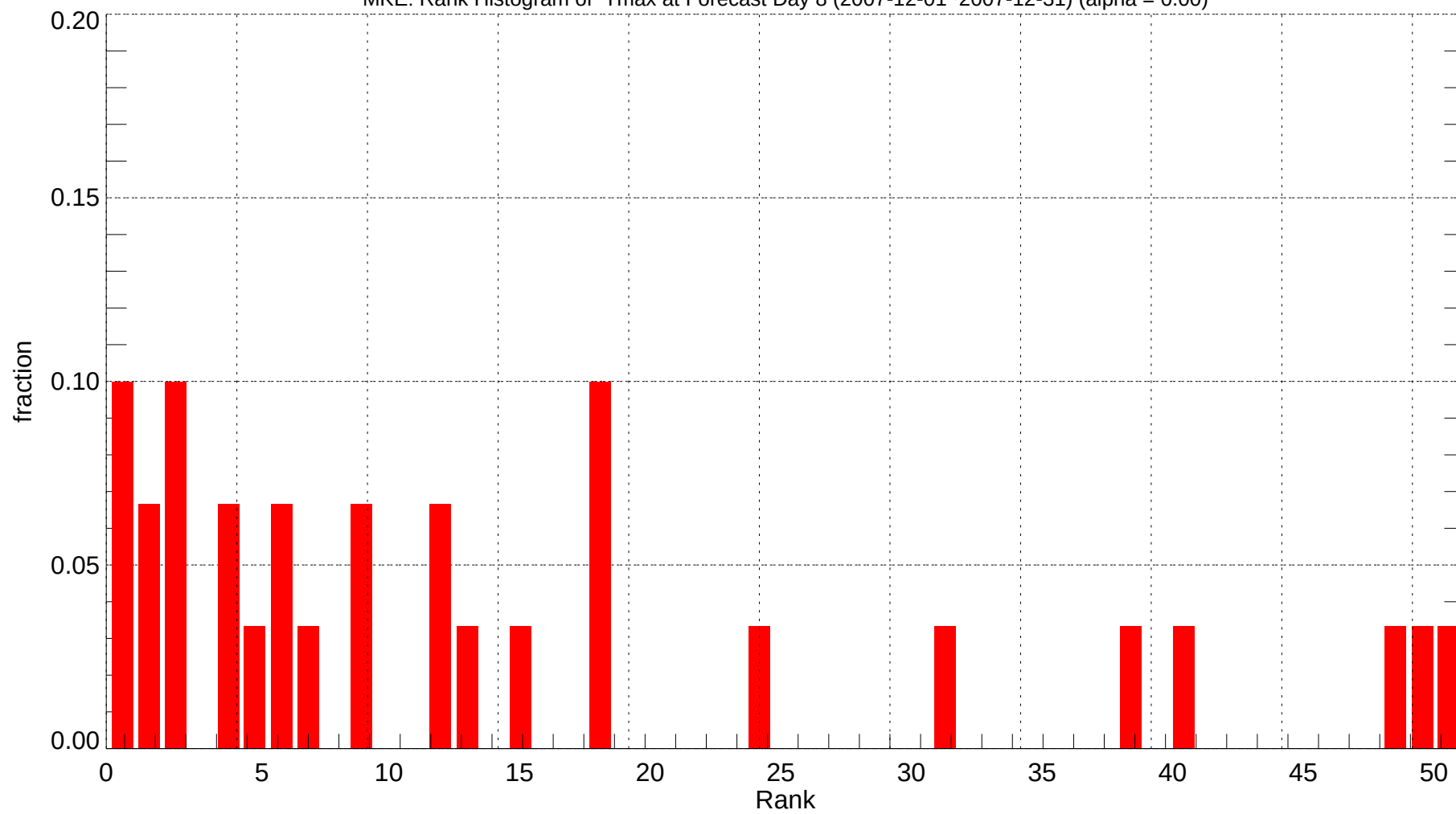
MKE: Rank Histogram of Tmax at Forecast Day 8 (2007-12-01~2007-12-31) (alpha = 0.00)
