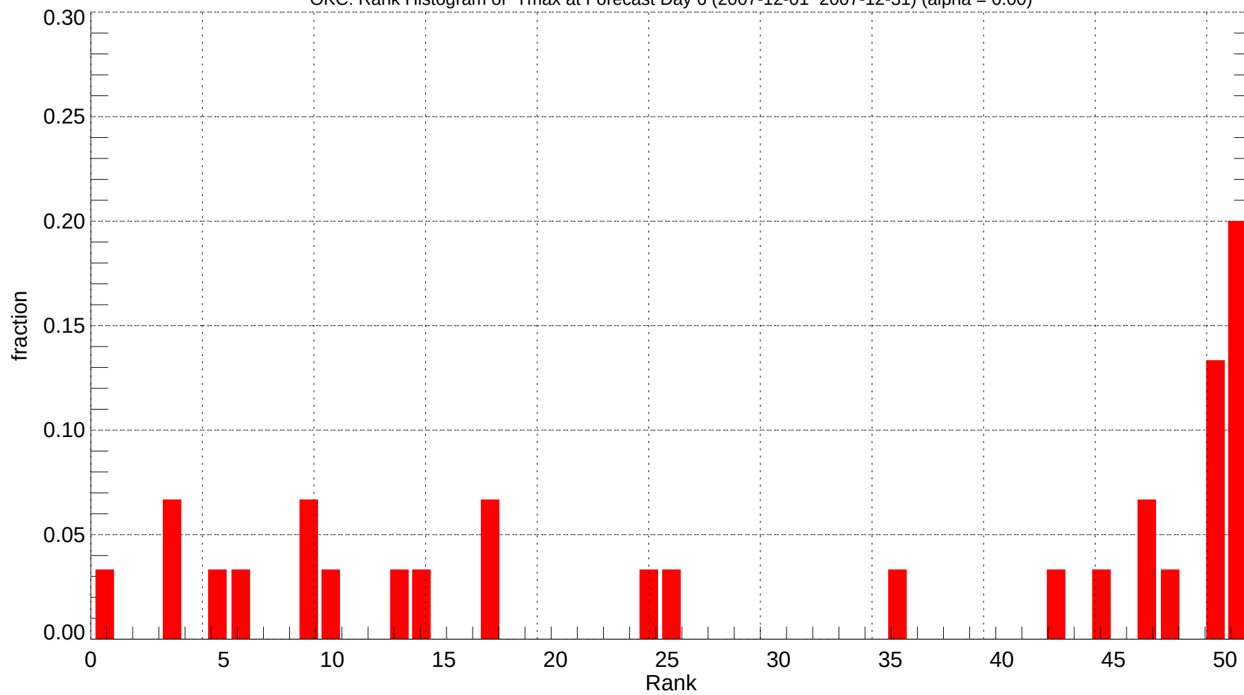
OKC: Rank Histogram of Tmax at Forecast Day 6 (2007-12-01~2007-12-31) (alpha = 0.00)
