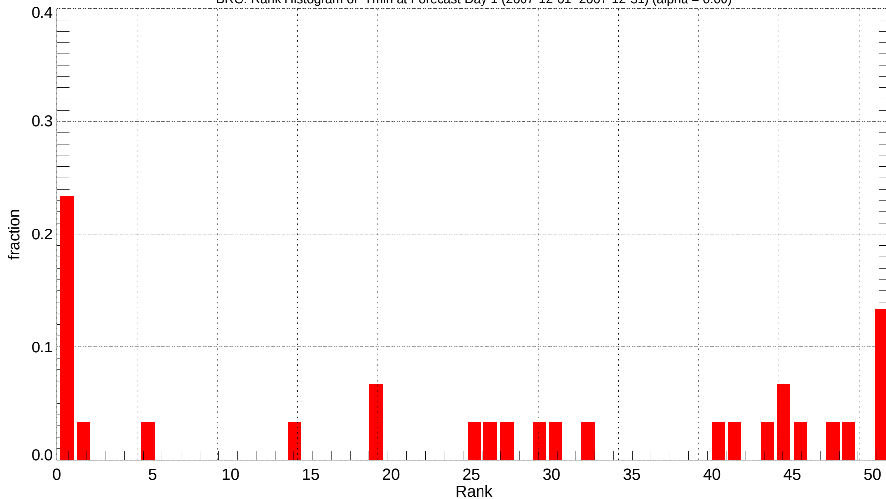
BRO: Rank Histogram of Tmin at Forecast Day 1 (2007-12-01~2007-12-31) (alpha = 0.00)
