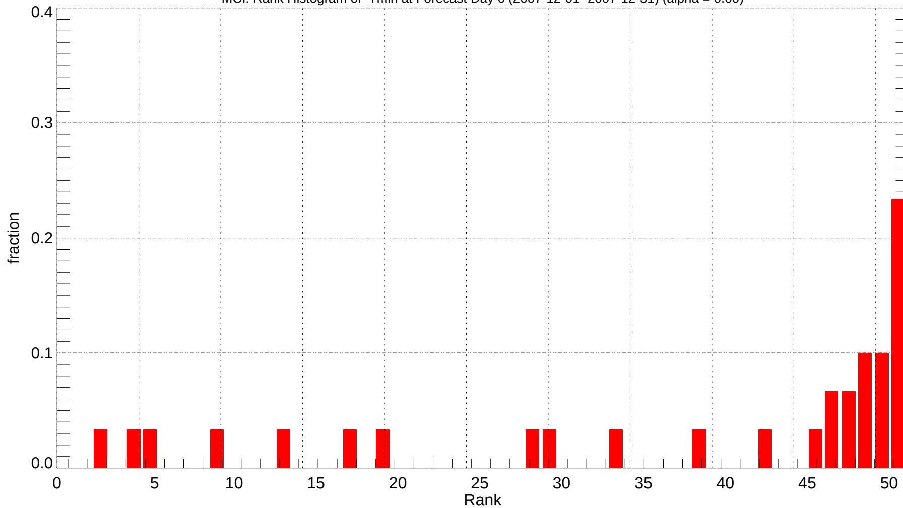
MCI: Rank Histogram of Tmin at Forecast Day 6 (2007-12-01~2007-12-31) (alpha = 0.00)
