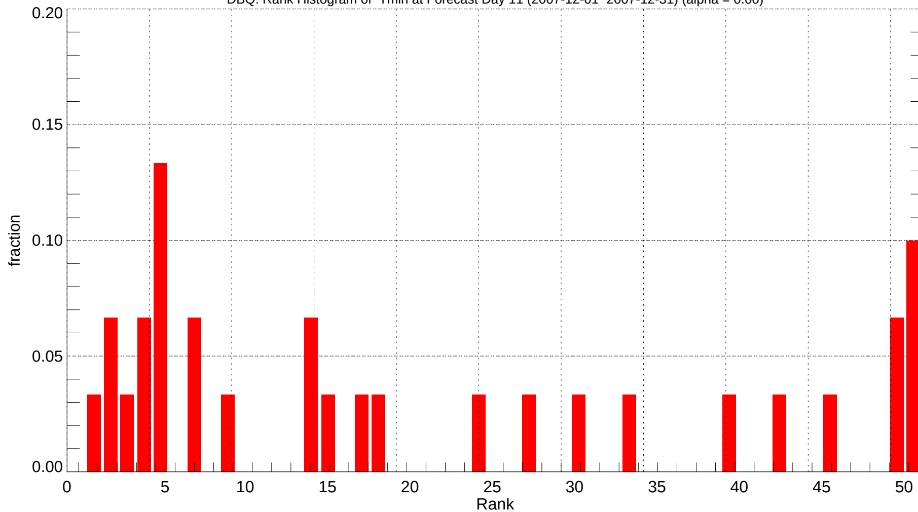
DBQ: Rank Histogram of Tmin at Forecast Day 11 (2007-12-01~2007-12-31) (alpha = 0.00)
