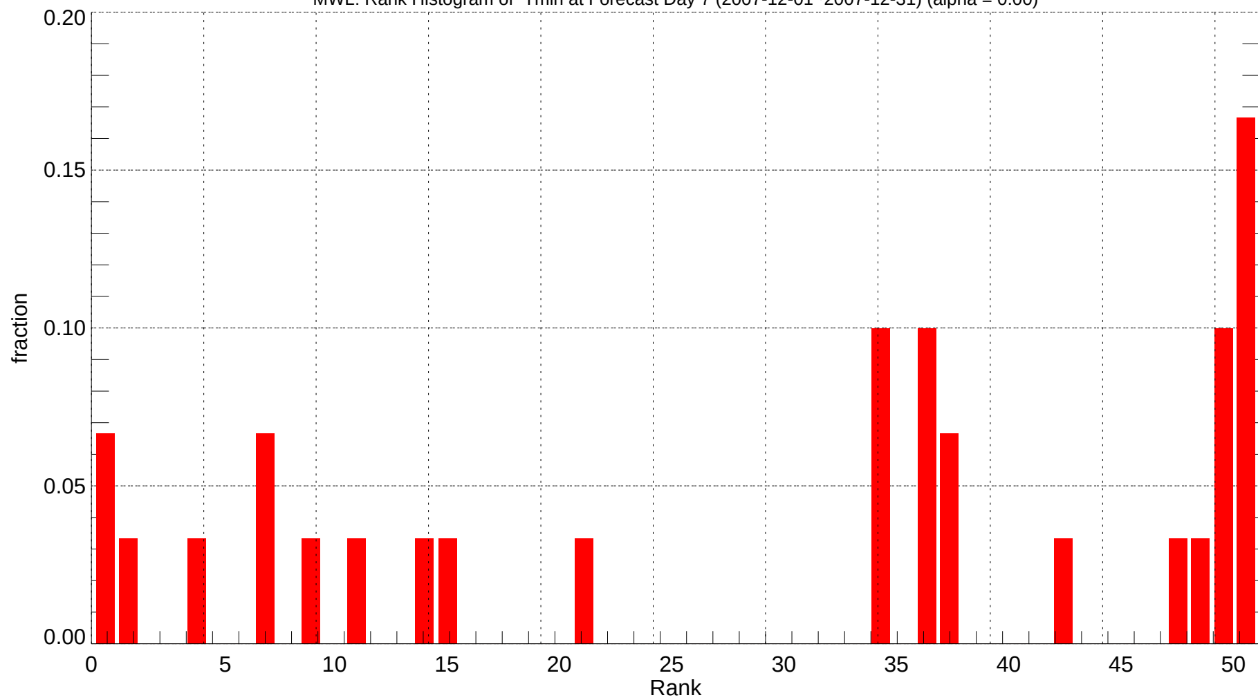
MWL: Rank Histogram of Tmin at Forecast Day 7 (2007-12-01~2007-12-31) (alpha = 0.00)
