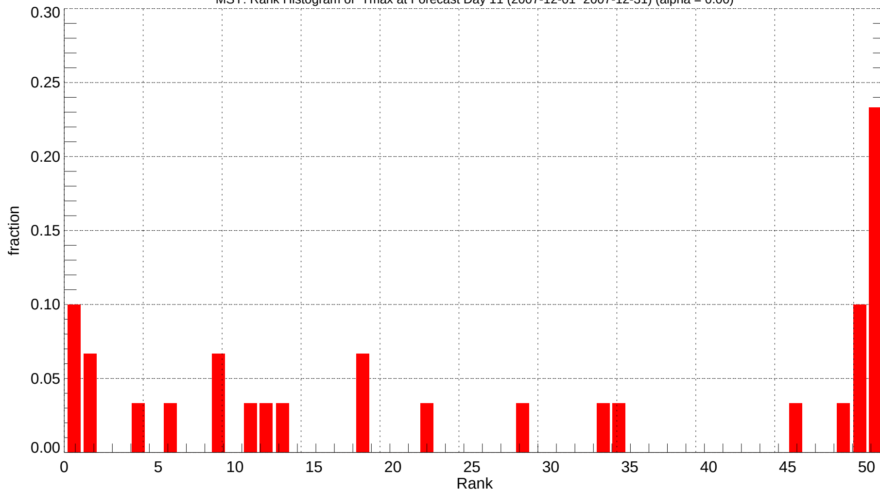
MSY: Rank Histogram of Tmax at Forecast Day 11 (2007-12-01~2007-12-31) (alpha = 0.00)
