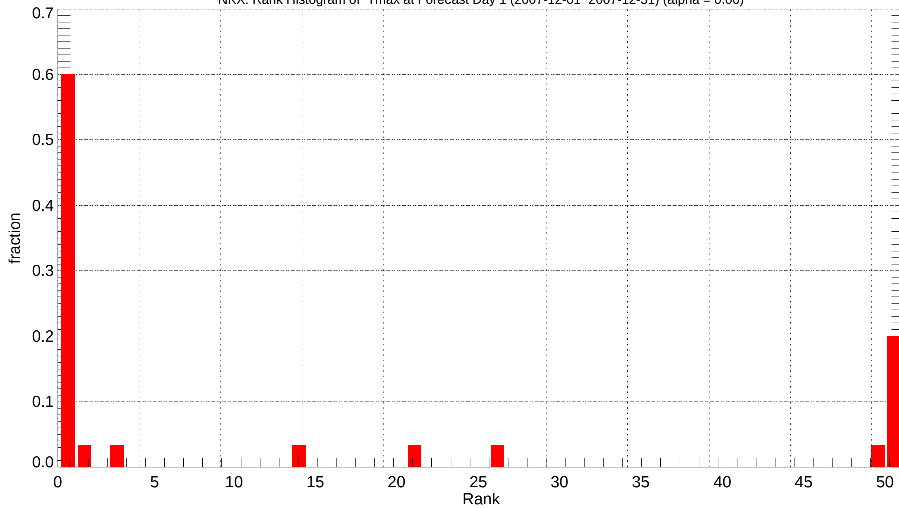
NKX: Rank Histogram of Tmax at Forecast Day 1 (2007-12-01~2007-12-31) (alpha = 0.00)
