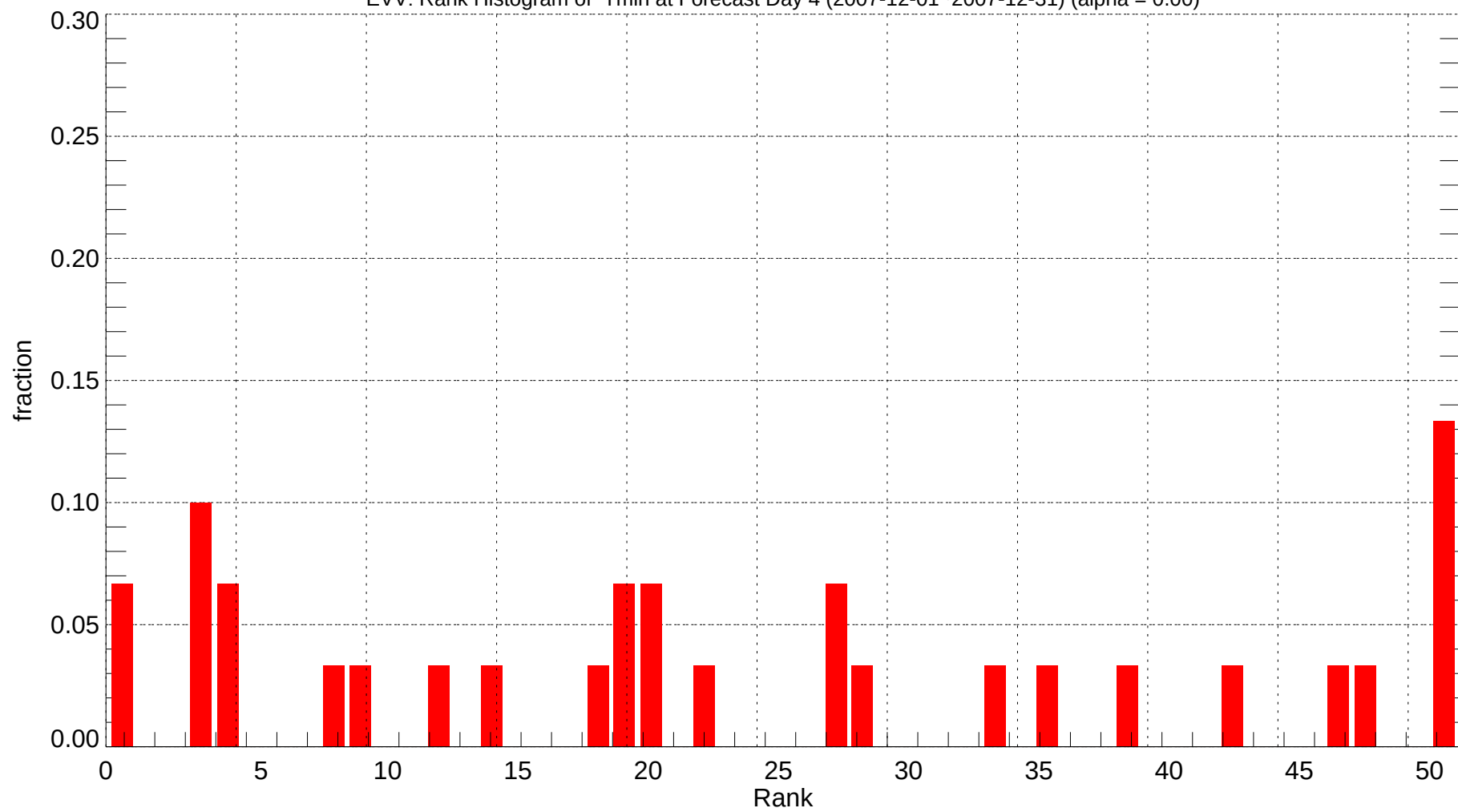
EVV: Rank Histogram of Tmin at Forecast Day 4 (2007-12-01~2007-12-31) (alpha = 0.00)
