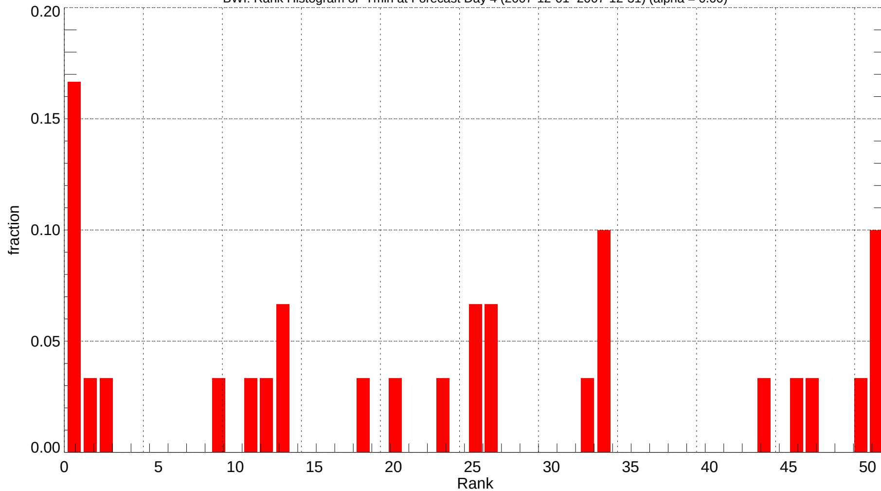
BWI: Rank Histogram of Tmin at Forecast Day 4 (2007-12-01~2007-12-31) (alpha = 0.00)
