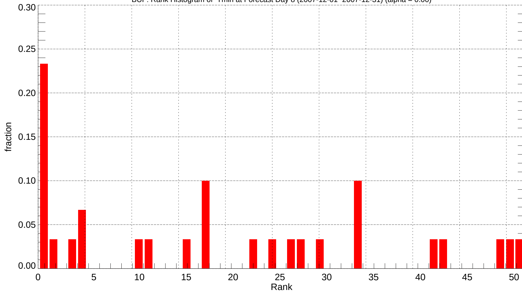
BUF: Rank Histogram of Tmin at Forecast Day 8 (2007-12-01~2007-12-31) (alpha = 0.00)
