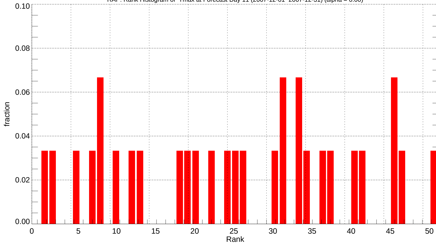
RAP: Rank Histogram of Tmax at Forecast Day 11 (2007-12-01~2007-12-31) (alpha = 0.00)
