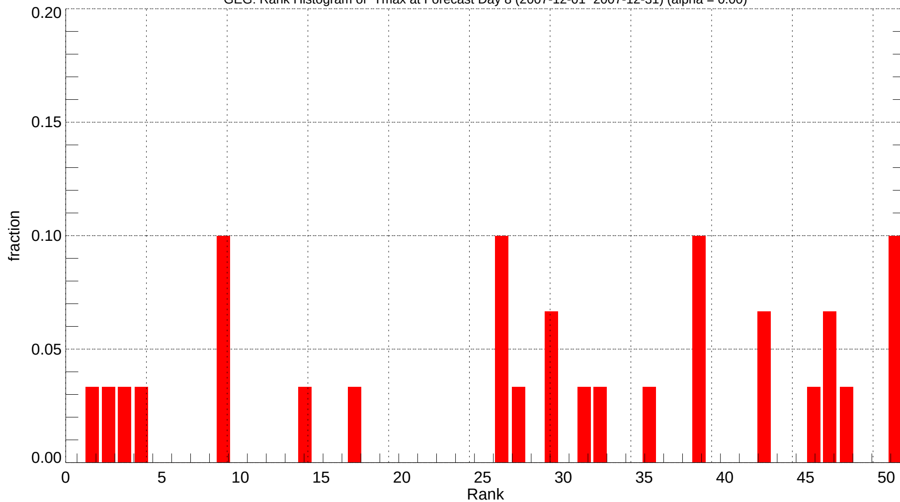
GEG: Rank Histogram of Tmax at Forecast Day 8 (2007-12-01~2007-12-31) (alpha = 0.00)
