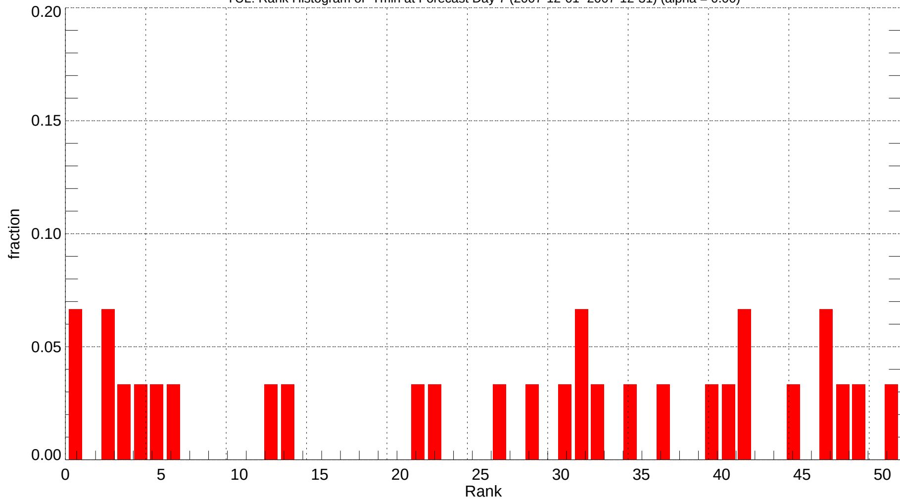
YUL: Rank Histogram of Tmin at Forecast Day 7 (2007-12-01~2007-12-31) (alpha = 0.00)
