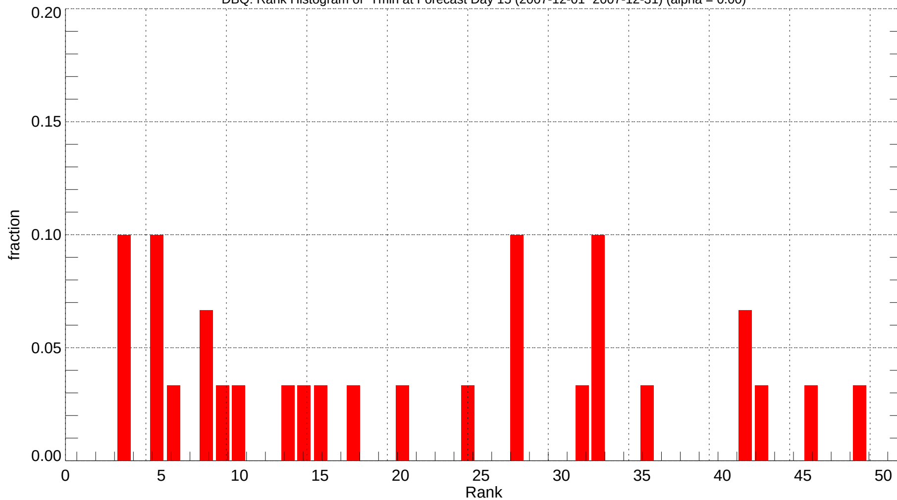
DBQ: Rank Histogram of Tmin at Forecast Day 15 (2007-12-01~2007-12-31) (alpha = 0.00)
