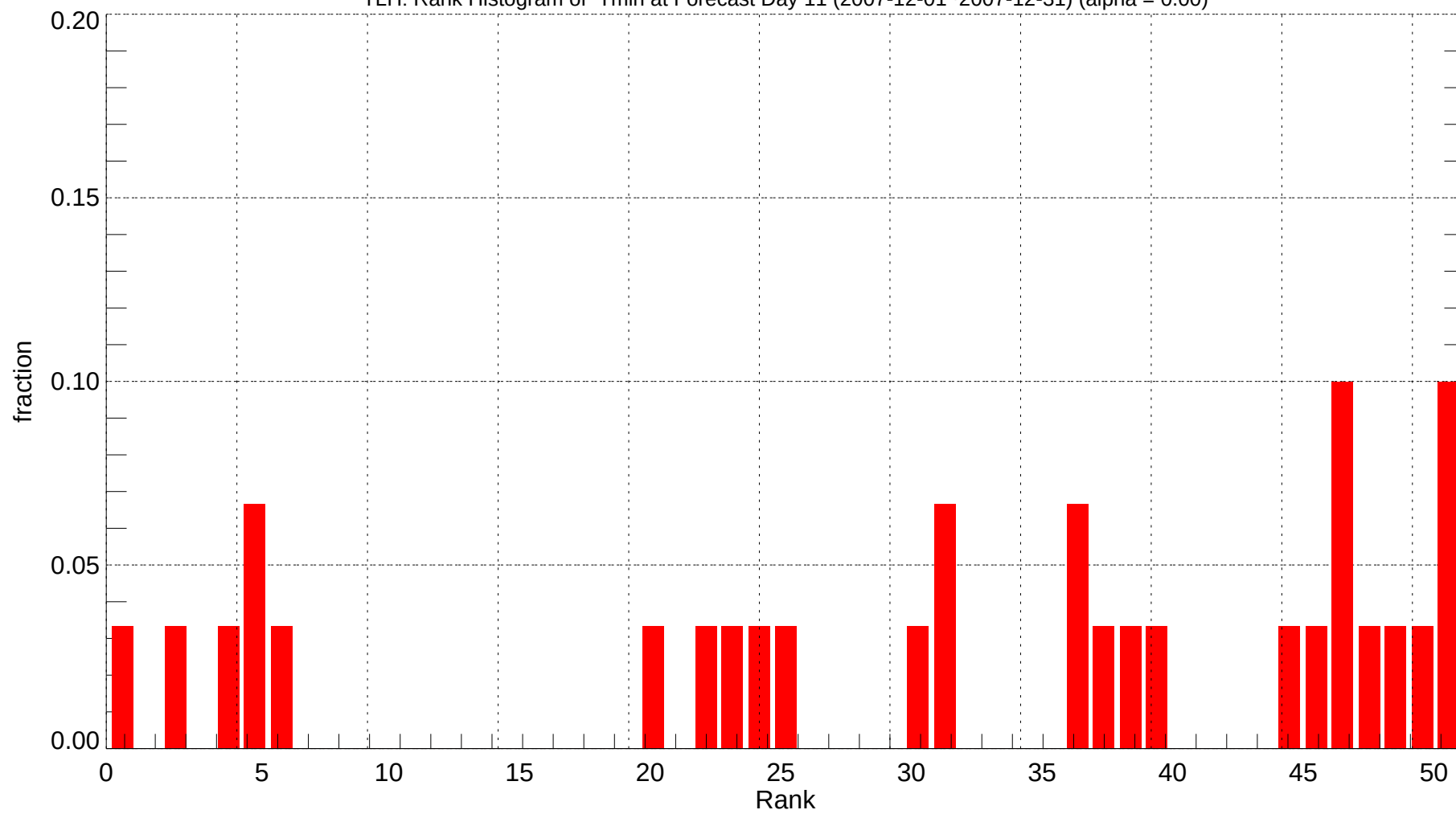
TLH: Rank Histogram of Tmin at Forecast Day 11 (2007-12-01~2007-12-31) (alpha = 0.00)
