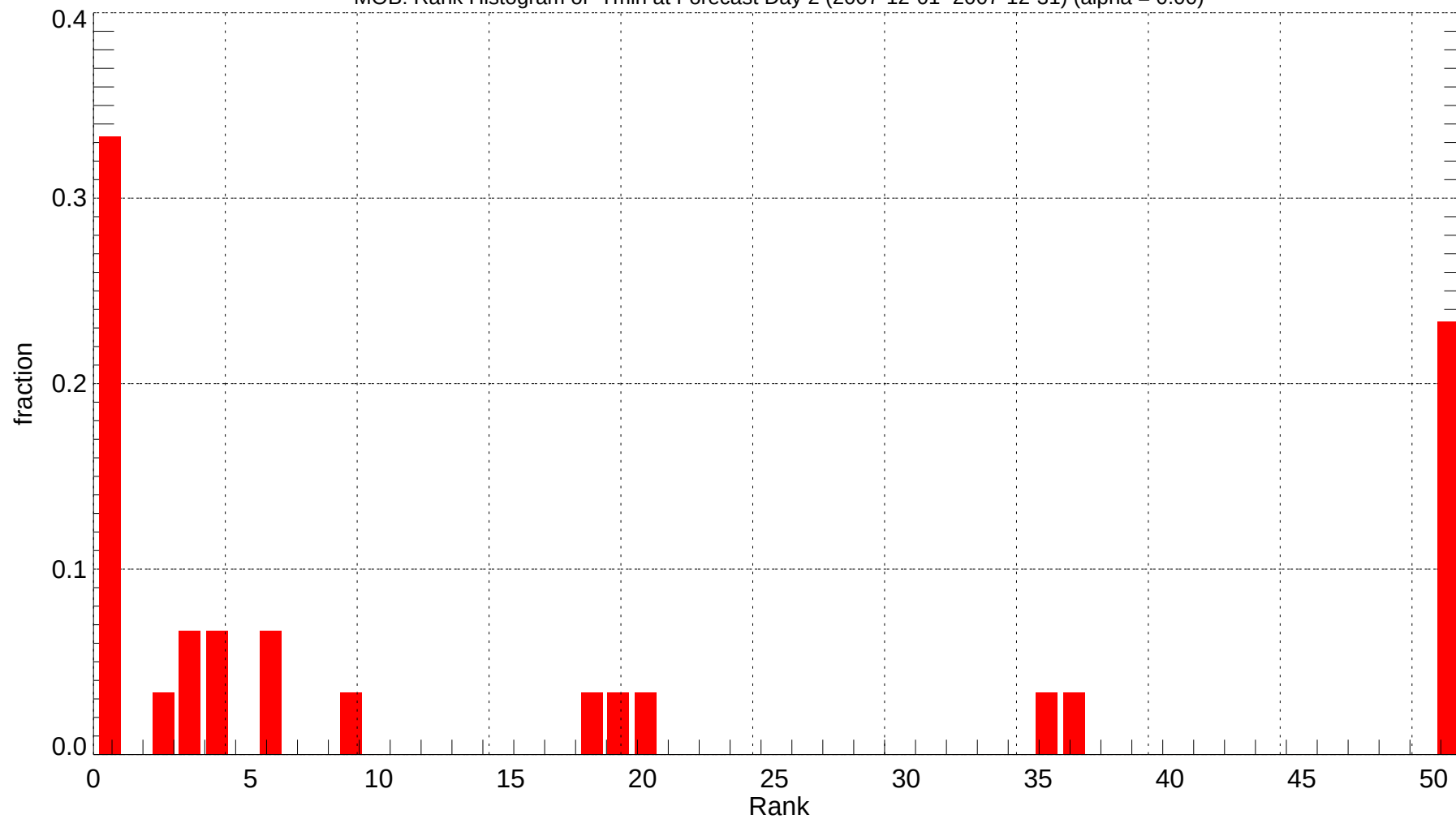
MOB: Rank Histogram of Tmin at Forecast Day 2 (2007-12-01~2007-12-31) (alpha = 0.00)
