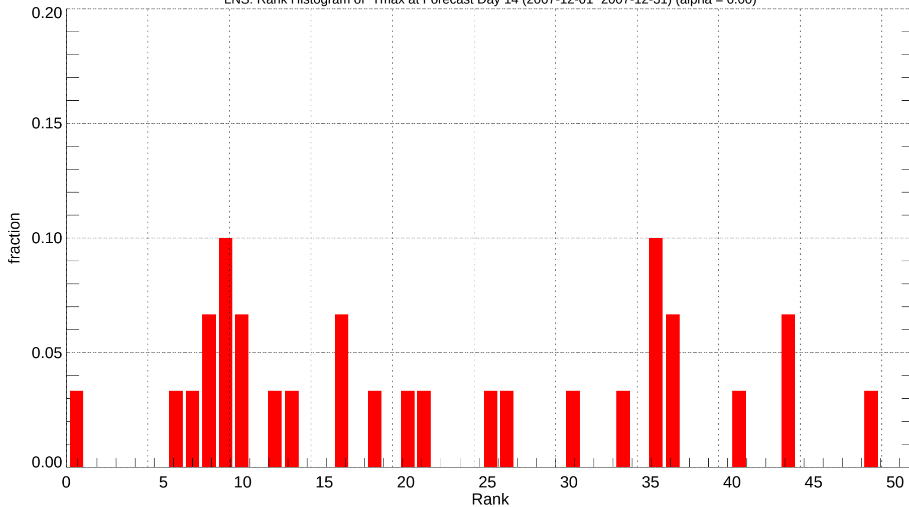
LNS: Rank Histogram of Tmax at Forecast Day 14 (2007-12-01~2007-12-31) (alpha = 0.00)
