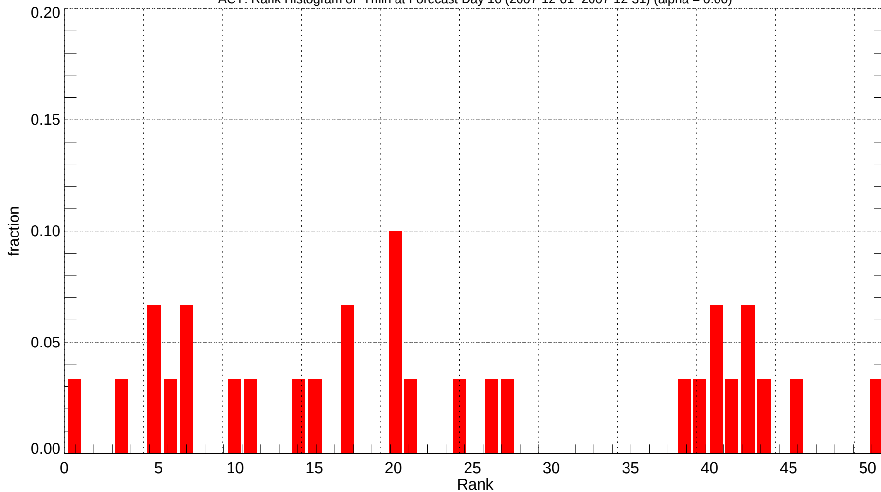
ACY: Rank Histogram of Tmin at Forecast Day 10 (2007-12-01~2007-12-31) (alpha = 0.00)
