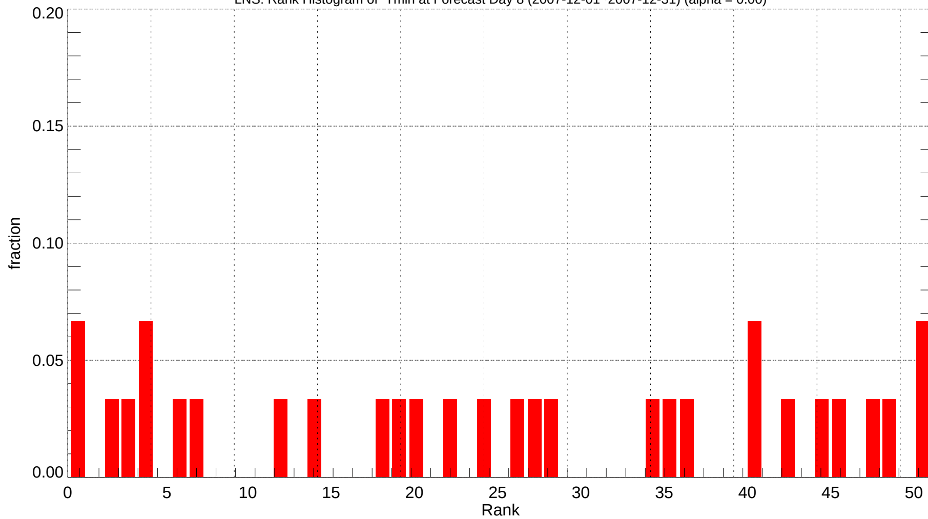
LNS: Rank Histogram of Tmin at Forecast Day 8 (2007-12-01~2007-12-31) (alpha = 0.00)
