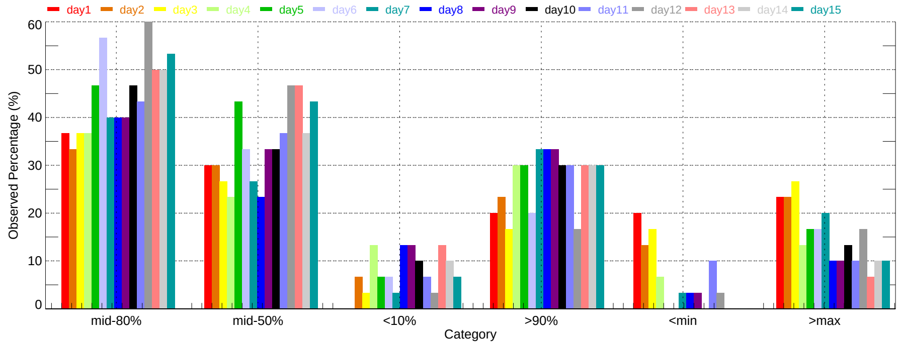
Observed Percentage of Ensembles - SJT: Max Temperature (2007-12-01~2007-12-31)
