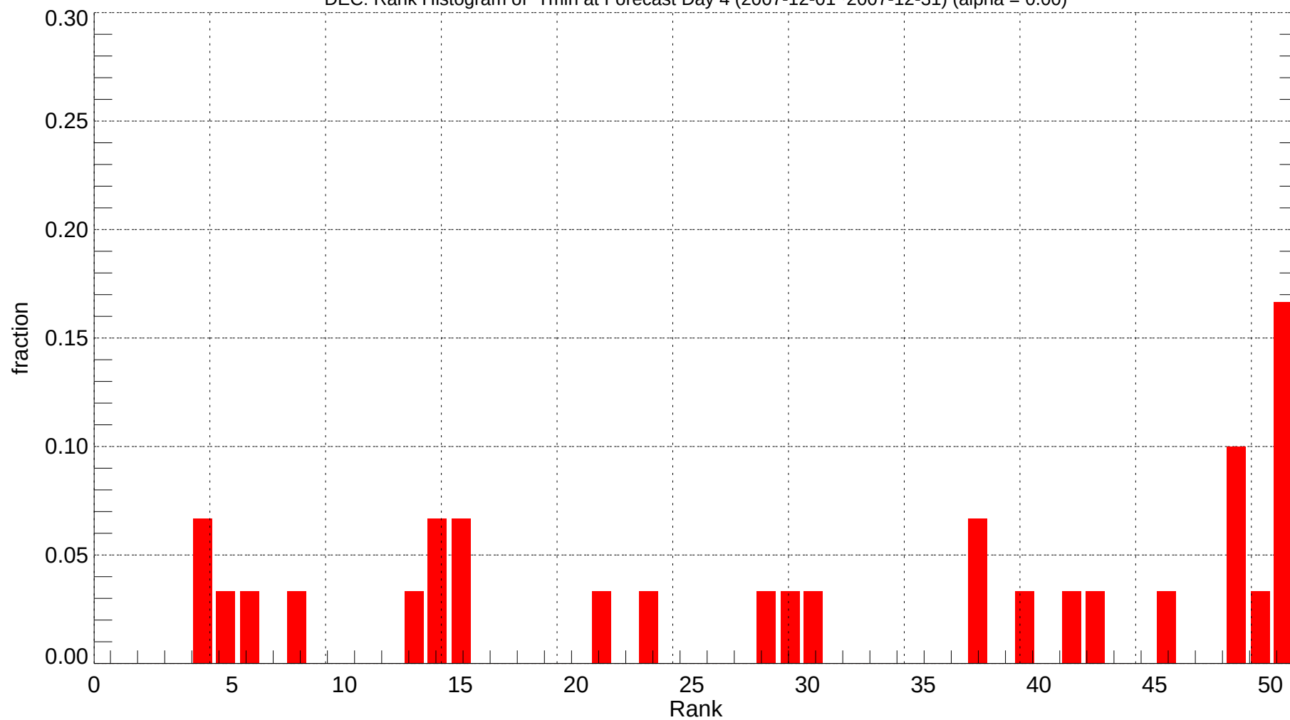
DEC: Rank Histogram of Tmin at Forecast Day 4 (2007-12-01~2007-12-31) (alpha = 0.00)
