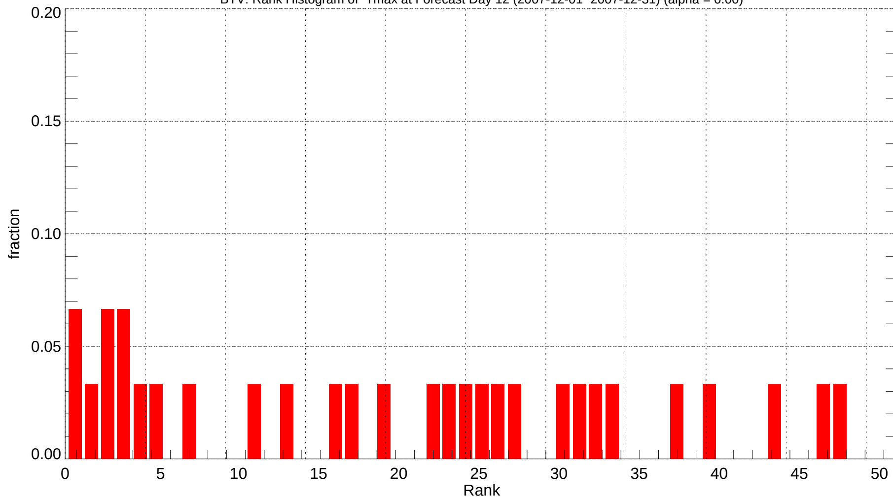
BTV: Rank Histogram of Tmax at Forecast Day 12 (2007-12-01~2007-12-31) (alpha = 0.00)
