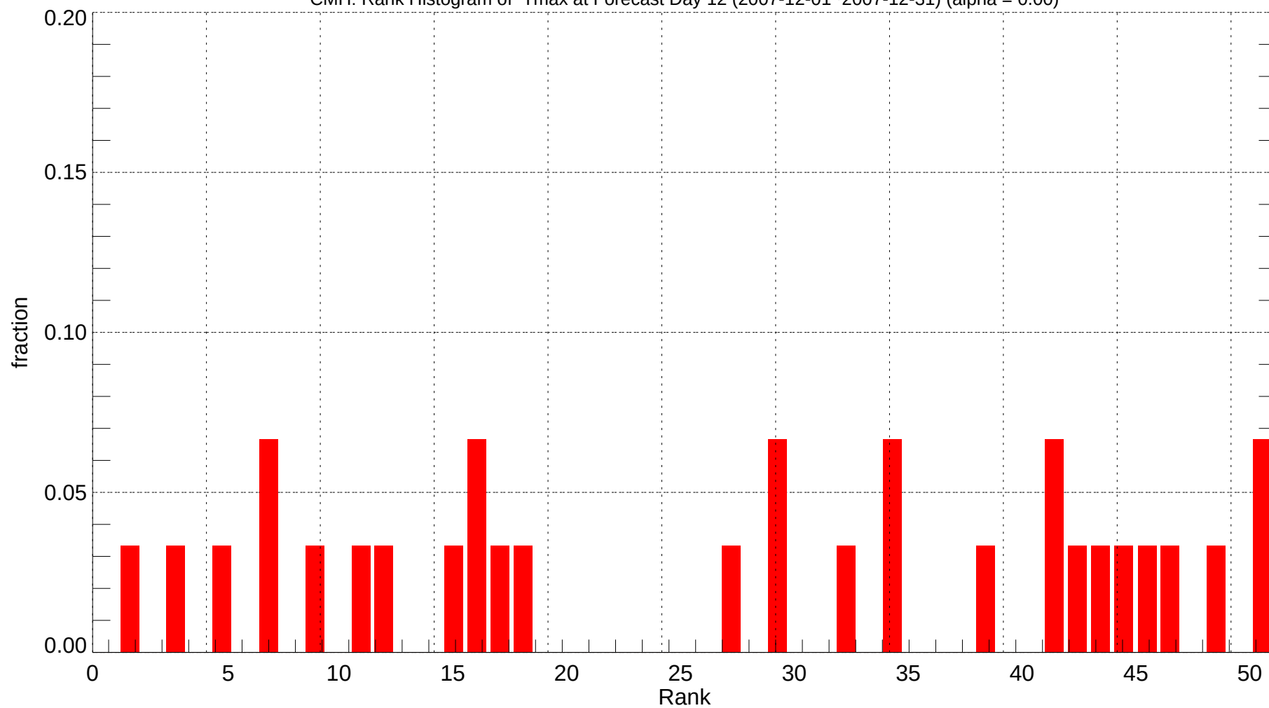
CMH: Rank Histogram of Tmax at Forecast Day 12 (2007-12-01~2007-12-31) (alpha = 0.00)
