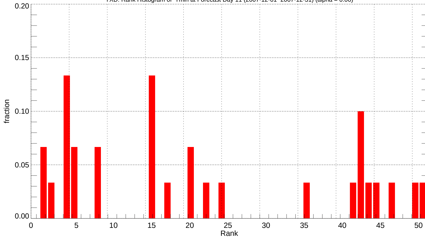
YXD: Rank Histogram of Tmin at Forecast Day 11 (2007-12-01~2007-12-31) (alpha = 0.00)
