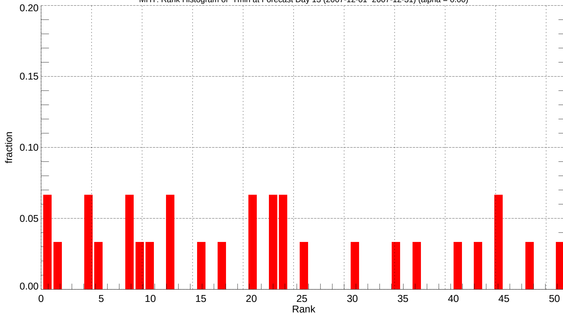
MHT: Rank Histogram of Tmin at Forecast Day 13 (2007-12-01~2007-12-31) (alpha = 0.00)
