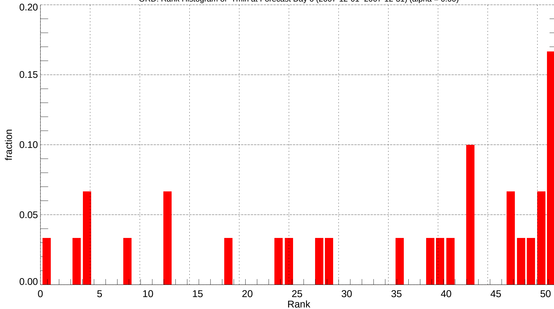
ORD: Rank Histogram of Tmin at Forecast Day 6 (2007-12-01~2007-12-31) (alpha = 0.00)
