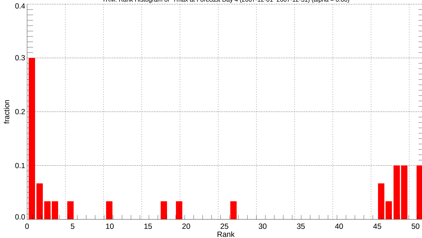
TRM: Rank Histogram of Tmax at Forecast Day 4 (2007-12-01~2007-12-31) (alpha = 0.00)
