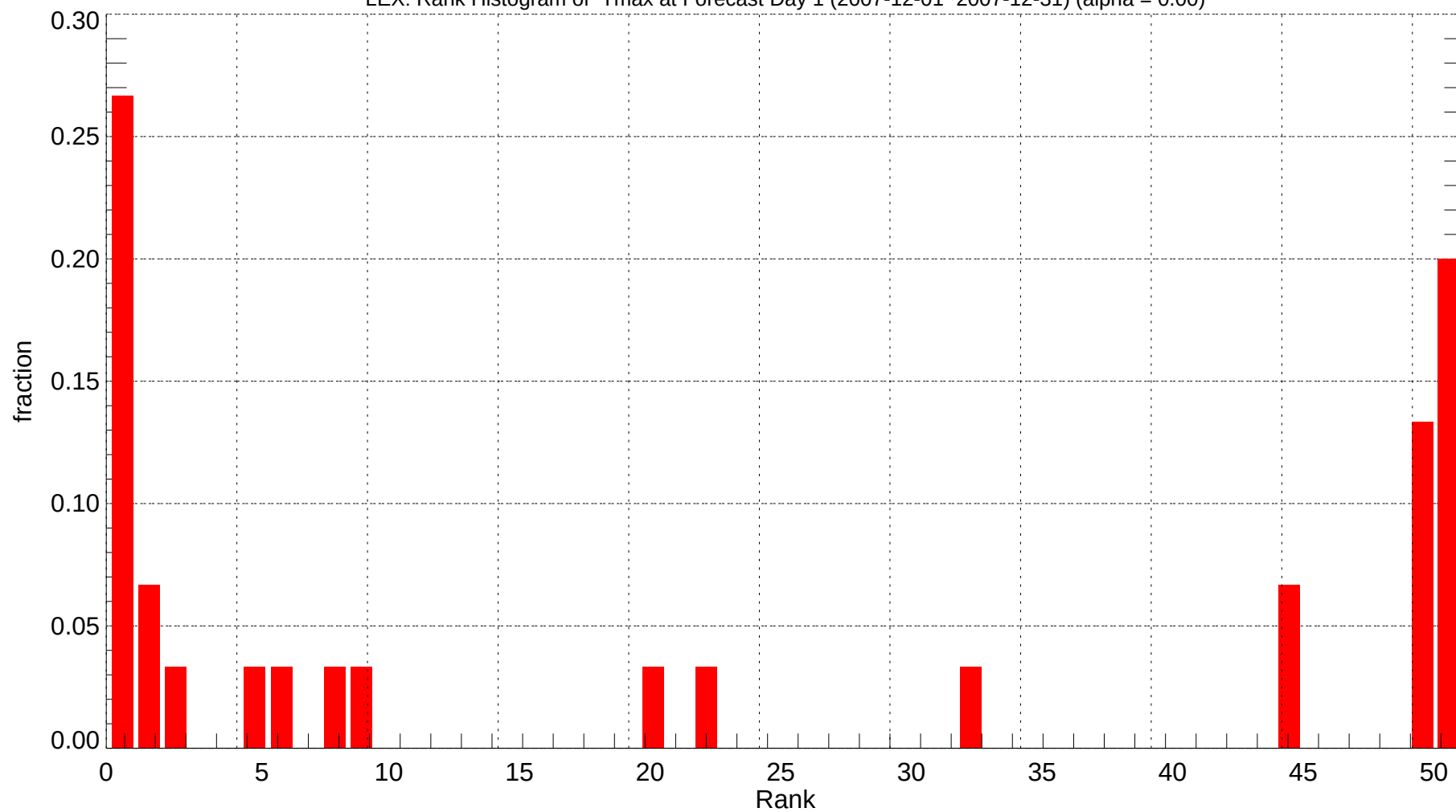
LEX: Rank Histogram of Tmax at Forecast Day 1 (2007-12-01~2007-12-31) (alpha = 0.00)
