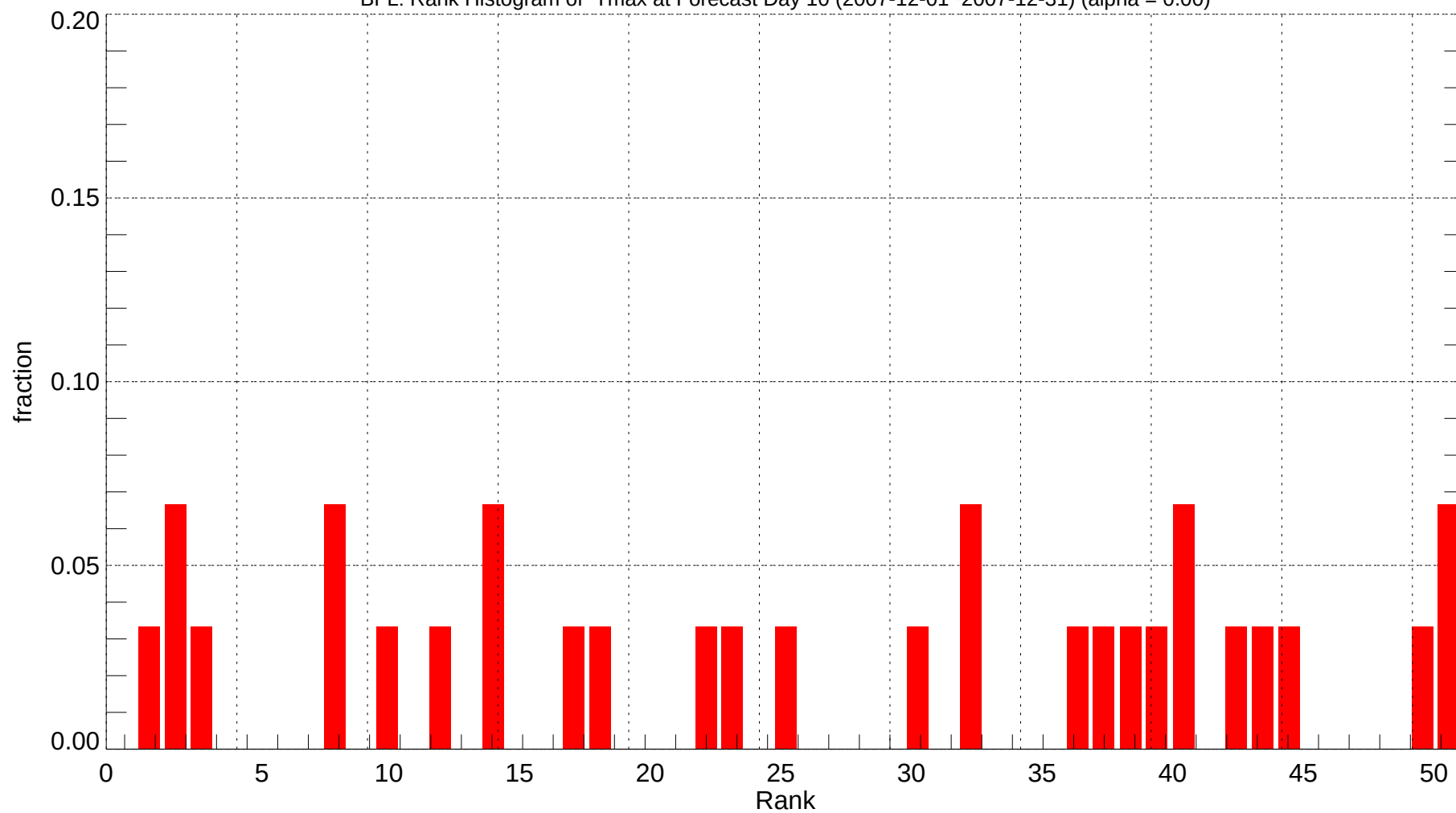
BFL: Rank Histogram of Tmax at Forecast Day 10 (2007-12-01~2007-12-31) (alpha = 0.00)
