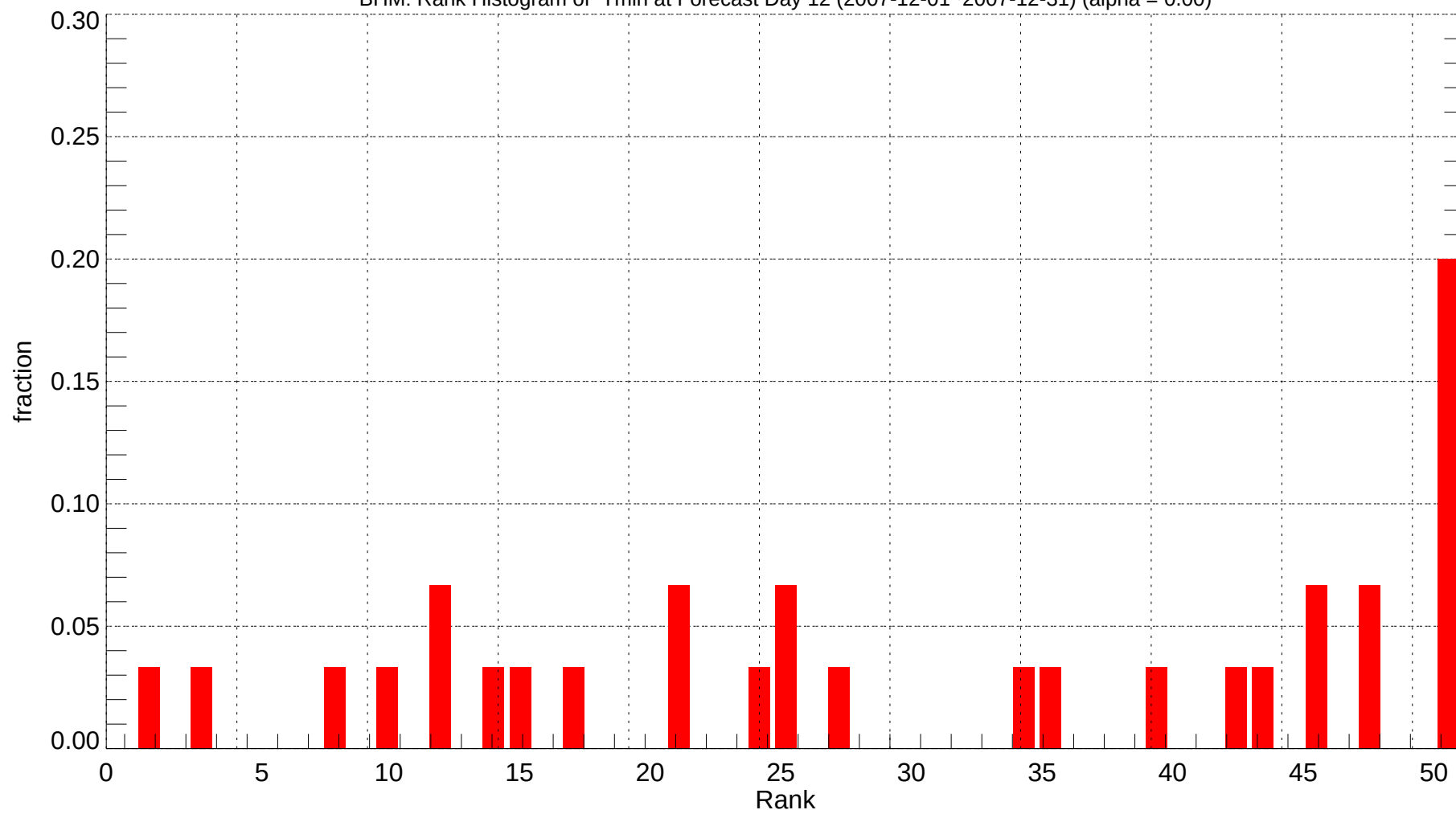
BHM: Rank Histogram of Tmin at Forecast Day 12 (2007-12-01~2007-12-31) (alpha = 0.00)
