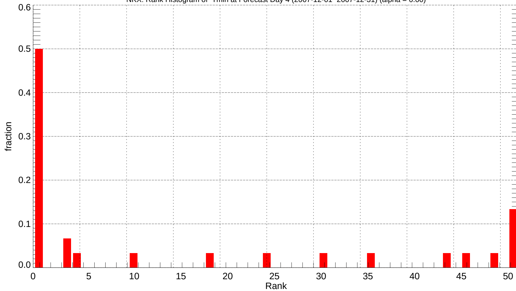
NKX: Rank Histogram of Tmin at Forecast Day 4 (2007-12-01~2007-12-31) (alpha = 0.00)
