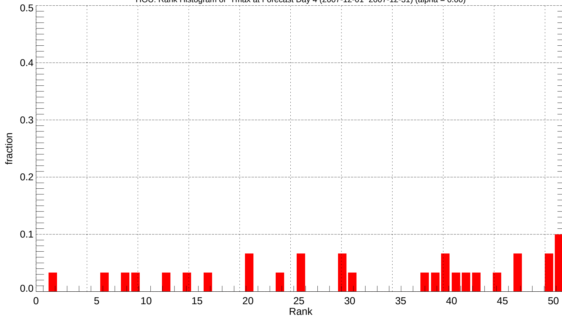
HOU: Rank Histogram of Tmax at Forecast Day 4 (2007-12-01~2007-12-31) (alpha = 0.00)
