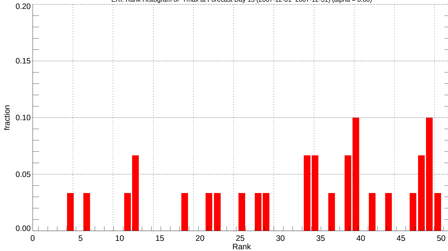
ERI: Rank Histogram of Tmax at Forecast Day 13 (2007-12-01~2007-12-31) (alpha = 0.00)
