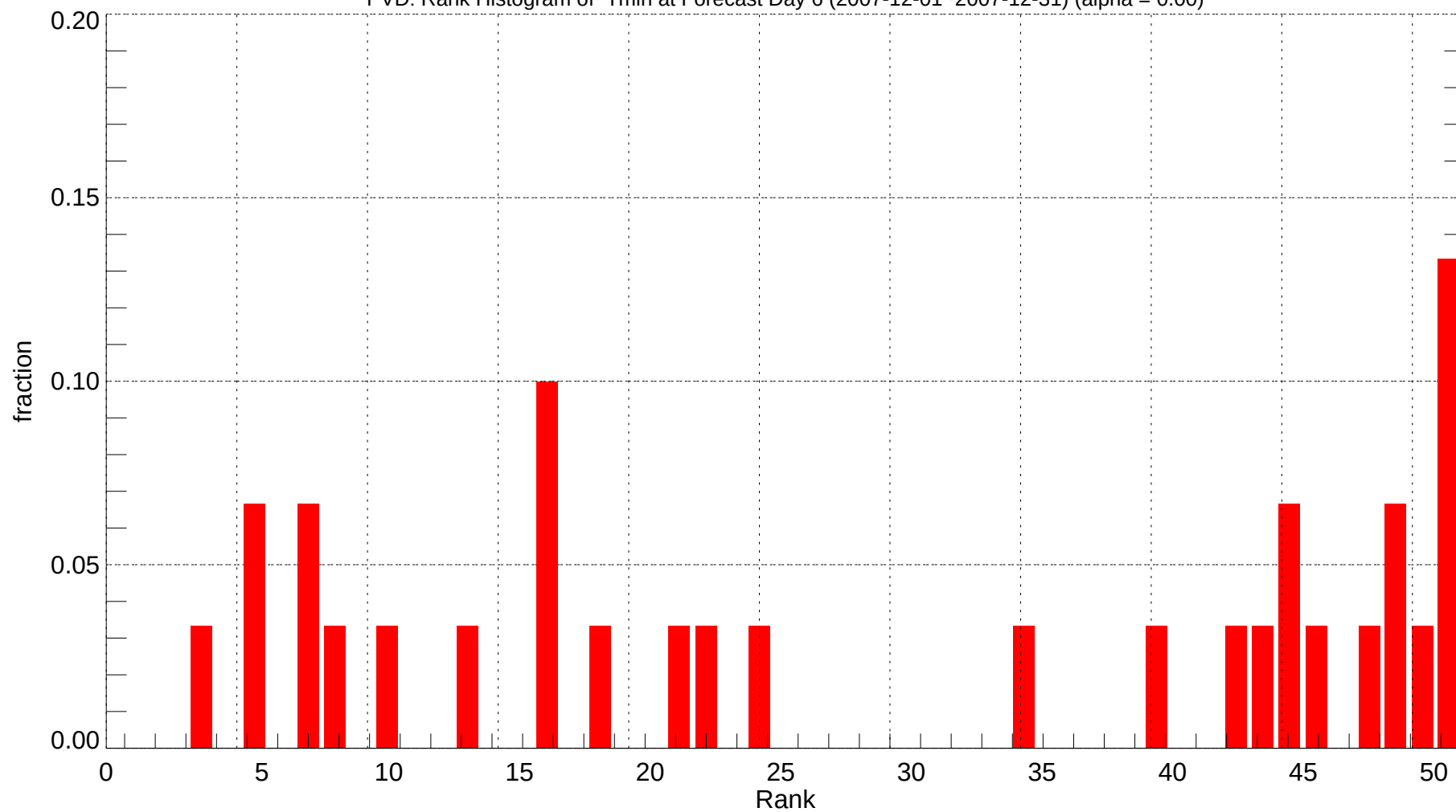
PVD: Rank Histogram of Tmin at Forecast Day 6 (2007-12-01~2007-12-31) (alpha = 0.00)
