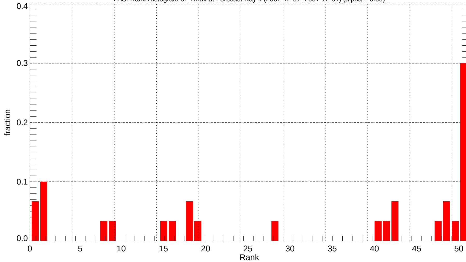
LAS: Rank Histogram of Tmax at Forecast Day 4 (2007-12-01~2007-12-31) (alpha = 0.00)
