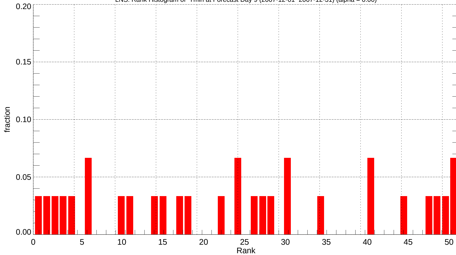
LNS: Rank Histogram of Tmin at Forecast Day 9 (2007-12-01~2007-12-31) (alpha = 0.00)
