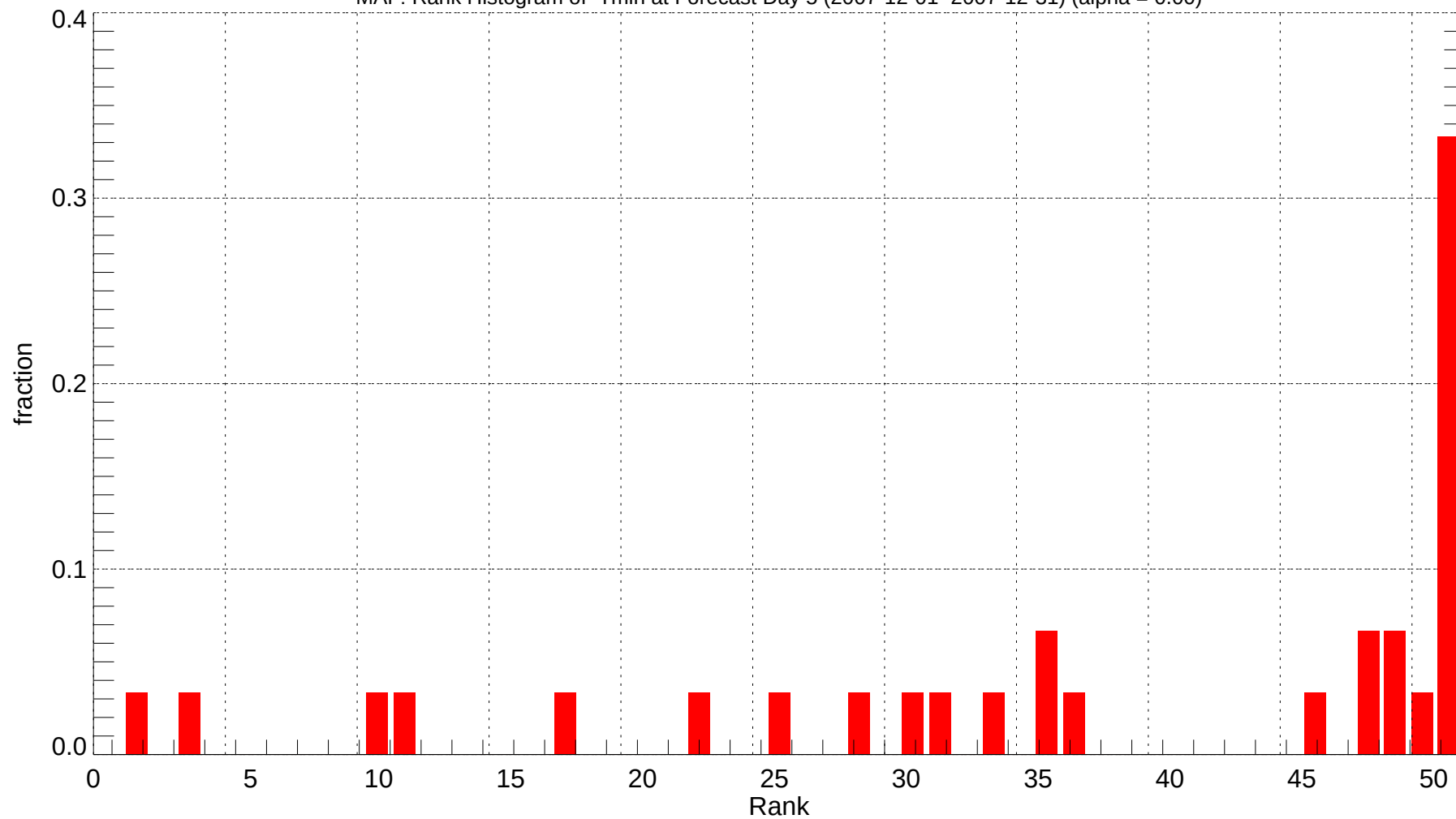
MAF: Rank Histogram of Tmin at Forecast Day 5 (2007-12-01~2007-12-31) (alpha = 0.00)
