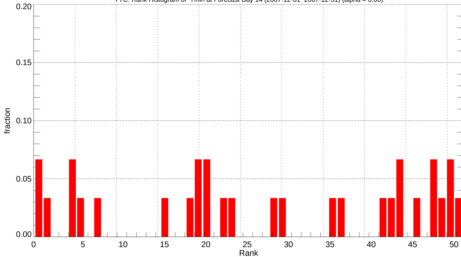
YYC: Rank Histogram of Tmin at Forecast Day 14 (2007-12-01~2007-12-31) (alpha = 0.00)
