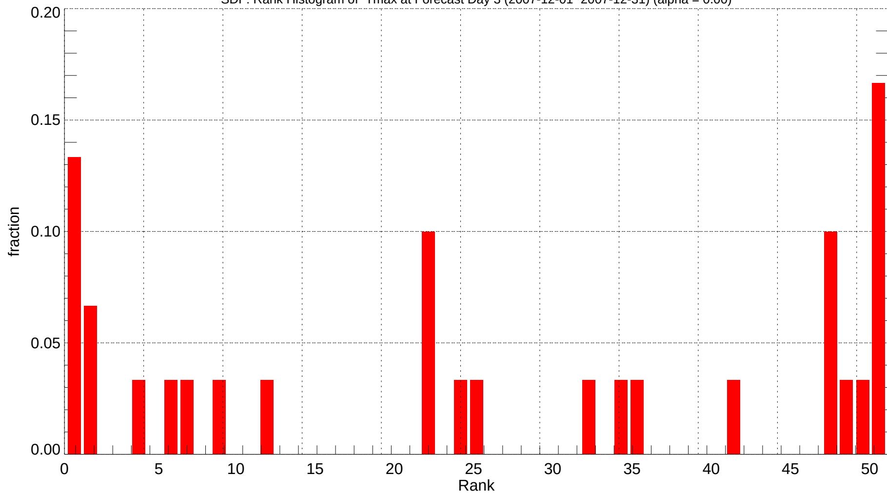
SDF: Rank Histogram of Tmax at Forecast Day 3 (2007-12-01~2007-12-31) (alpha = 0.00)
