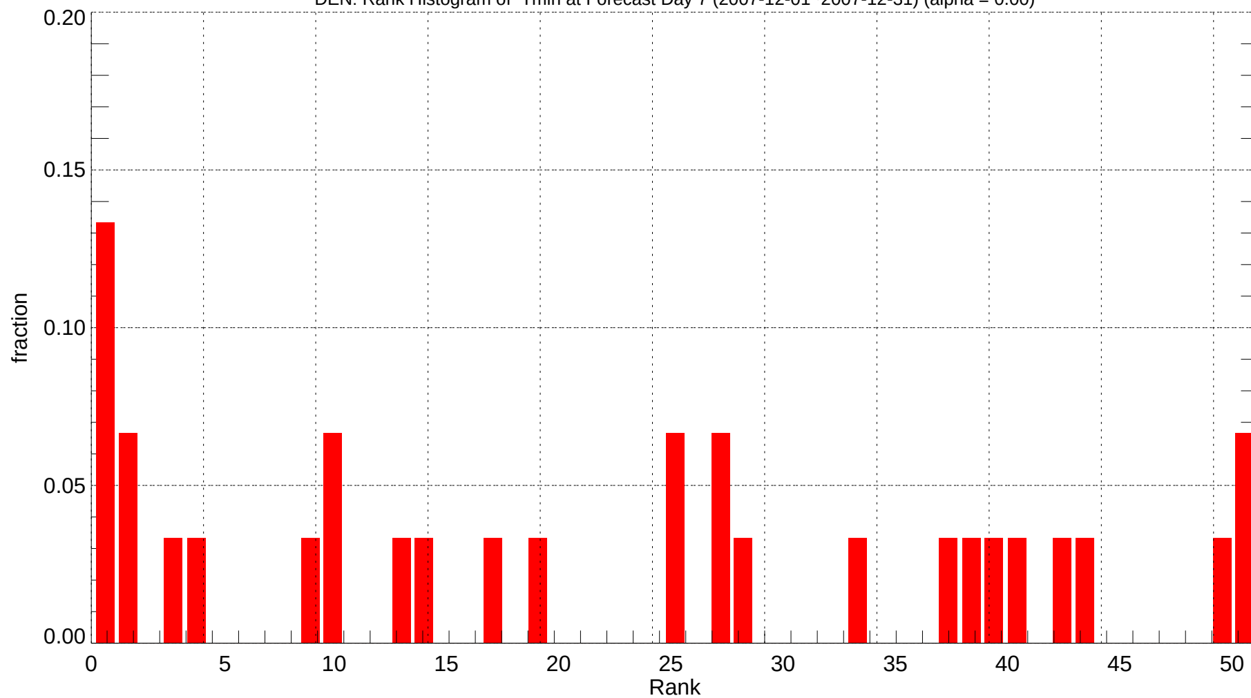
DEN: Rank Histogram of Tmin at Forecast Day 7 (2007-12-01~2007-12-31) (alpha = 0.00)
