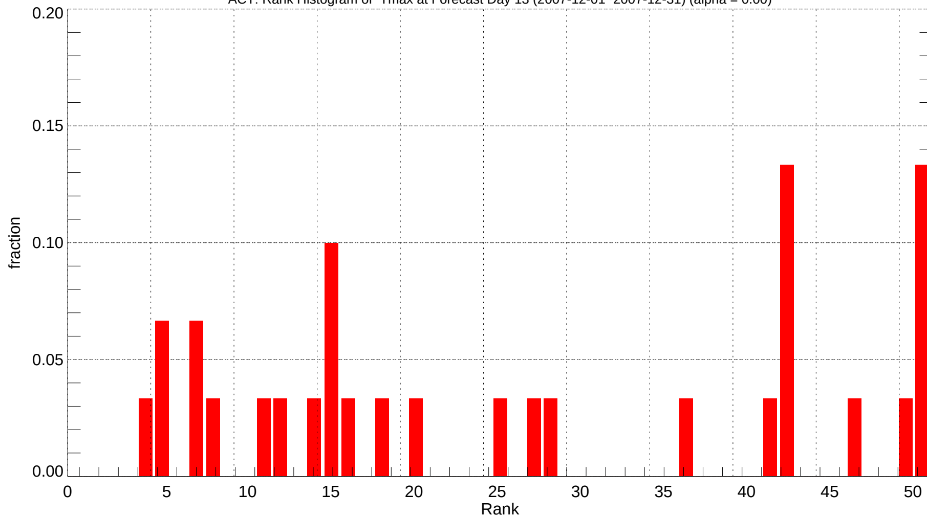
ACT: Rank Histogram of Tmax at Forecast Day 13 (2007-12-01~2007-12-31) (alpha = 0.00)
