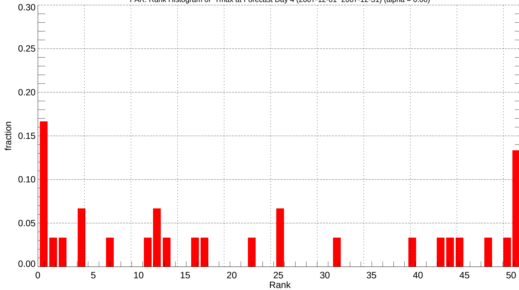
FAR: Rank Histogram of Tmax at Forecast Day 4 (2007-12-01~2007-12-31) (alpha = 0.00)
