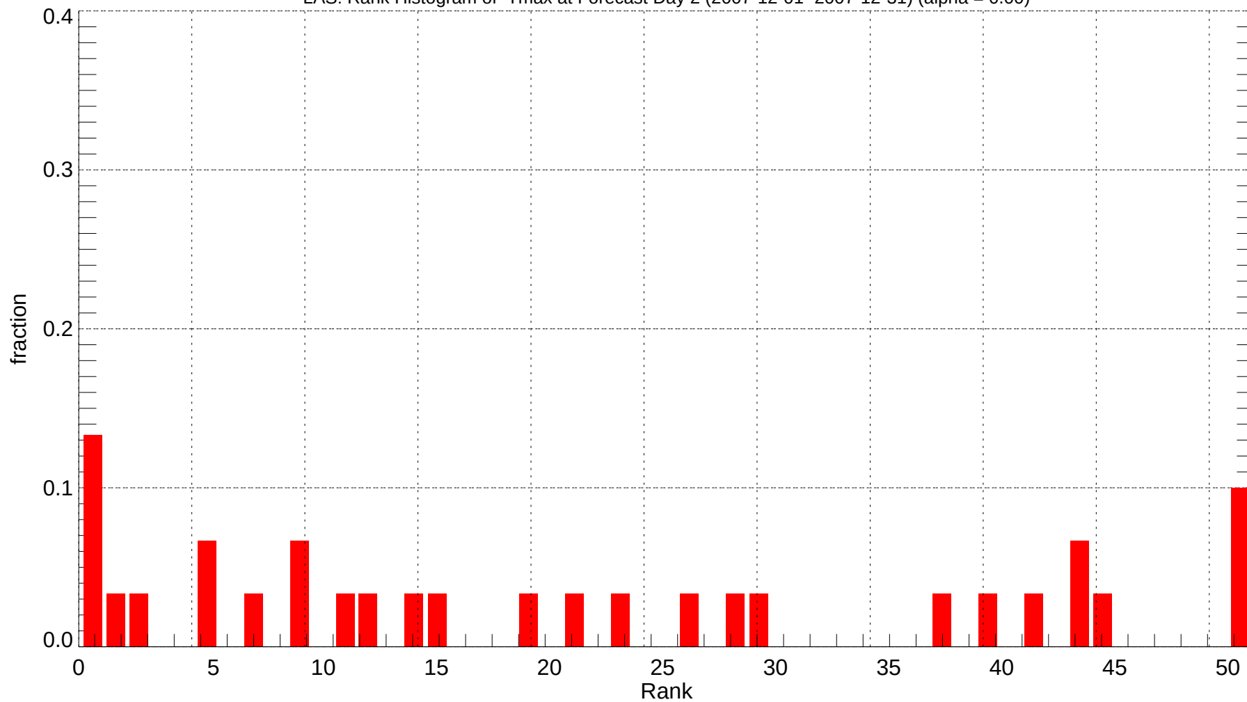
LAS: Rank Histogram of Tmax at Forecast Day 2 (2007-12-01~2007-12-31) (alpha = 0.00)
