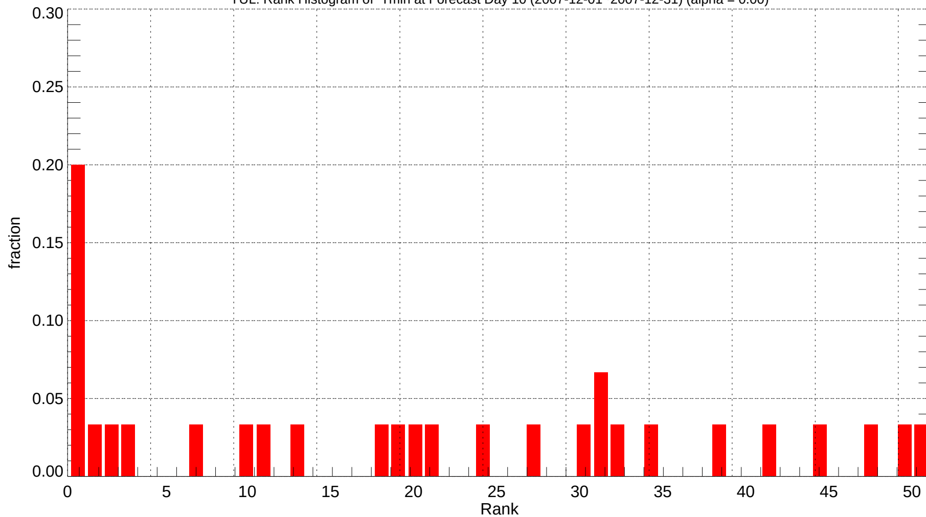
YUL: Rank Histogram of Tmin at Forecast Day 10 (2007-12-01~2007-12-31) (alpha = 0.00)
