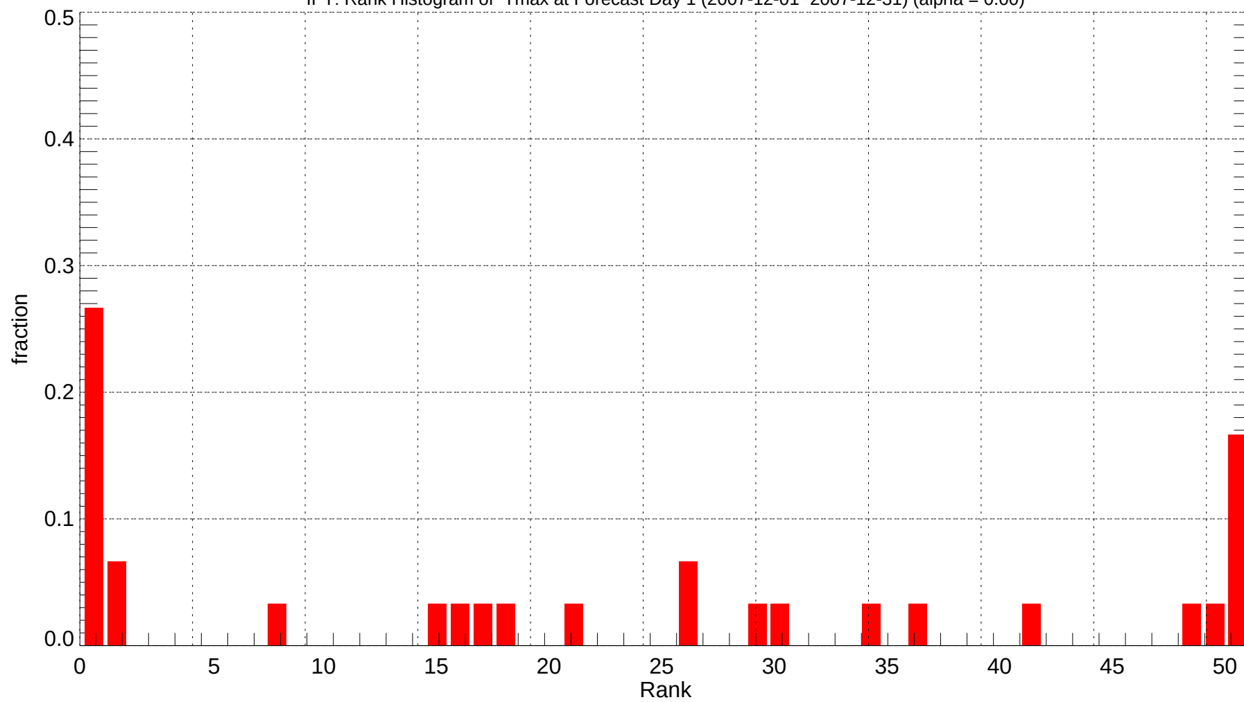
IPT: Rank Histogram of Tmax at Forecast Day 1 (2007-12-01~2007-12-31) (alpha = 0.00)
