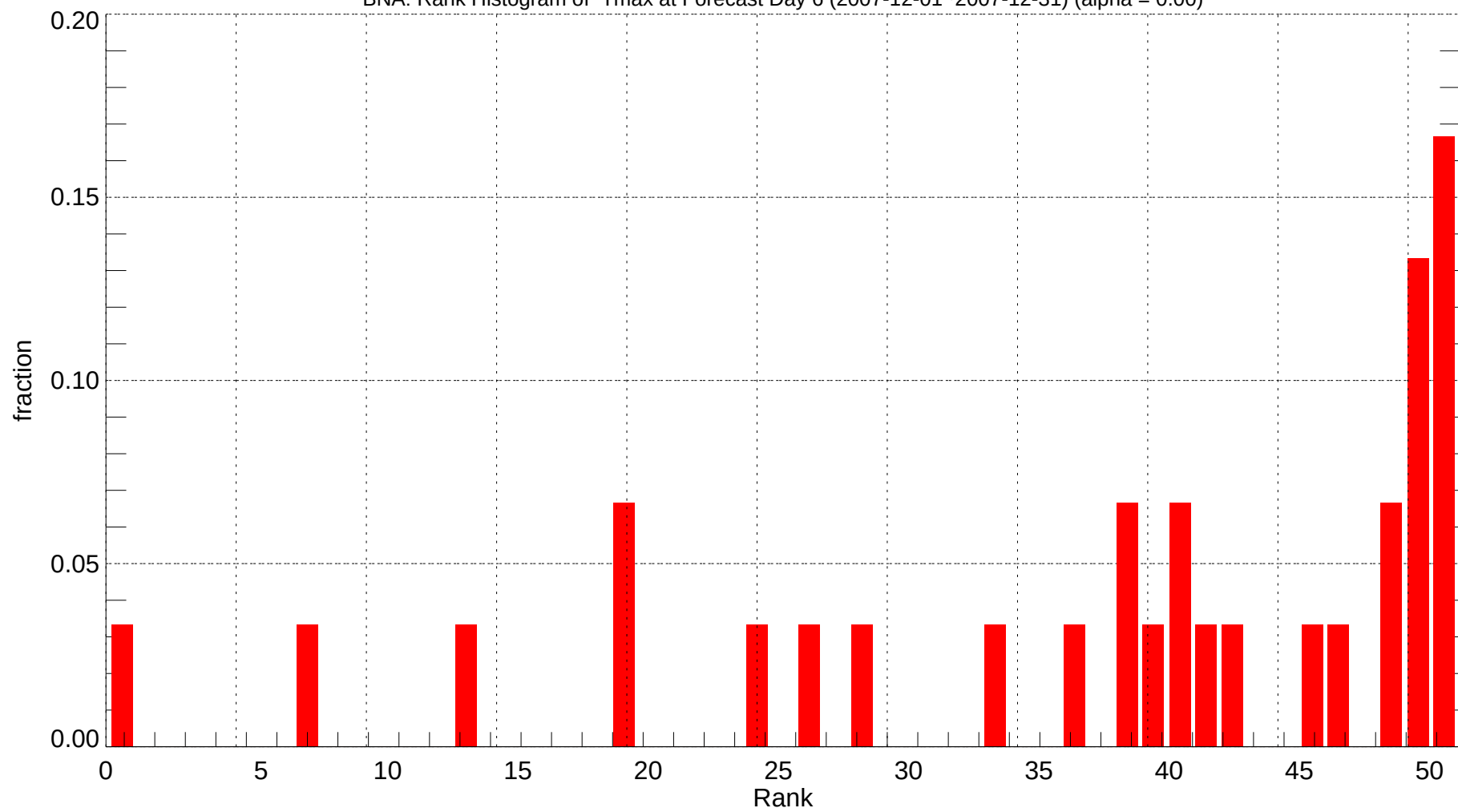
BNA: Rank Histogram of Tmax at Forecast Day 6 (2007-12-01~2007-12-31) (alpha = 0.00)
