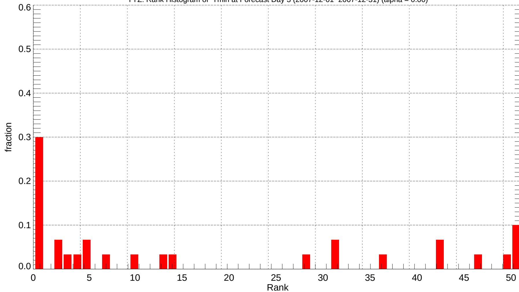
YYZ: Rank Histogram of Tmin at Forecast Day 3 (2007-12-01~2007-12-31) (alpha = 0.00)
