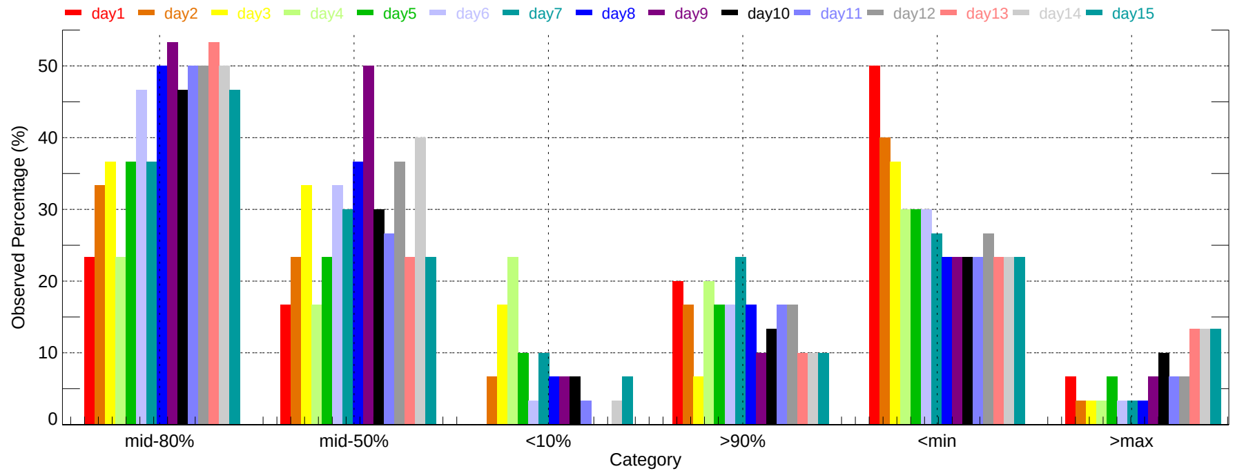
Observed Percentage of Ensembles - GAD: Min Temperature (2007-12-01~2007-12-31)
