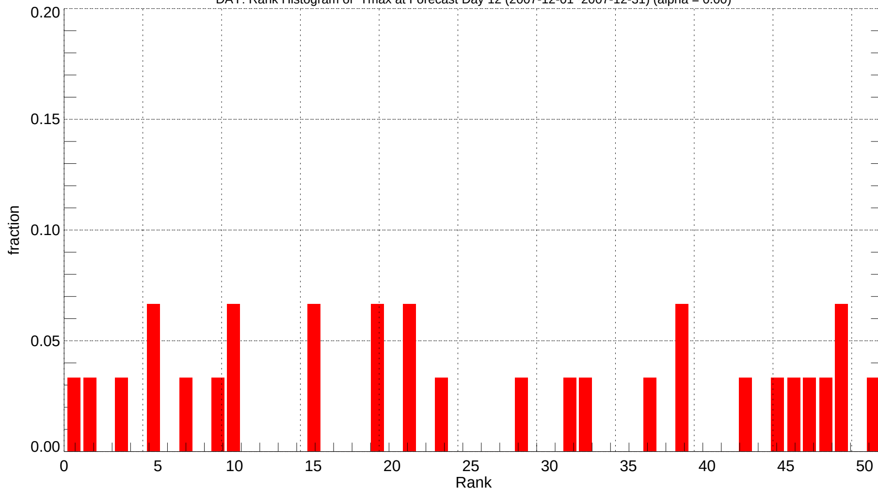
DAY: Rank Histogram of Tmax at Forecast Day 12 (2007-12-01~2007-12-31) (alpha = 0.00)
