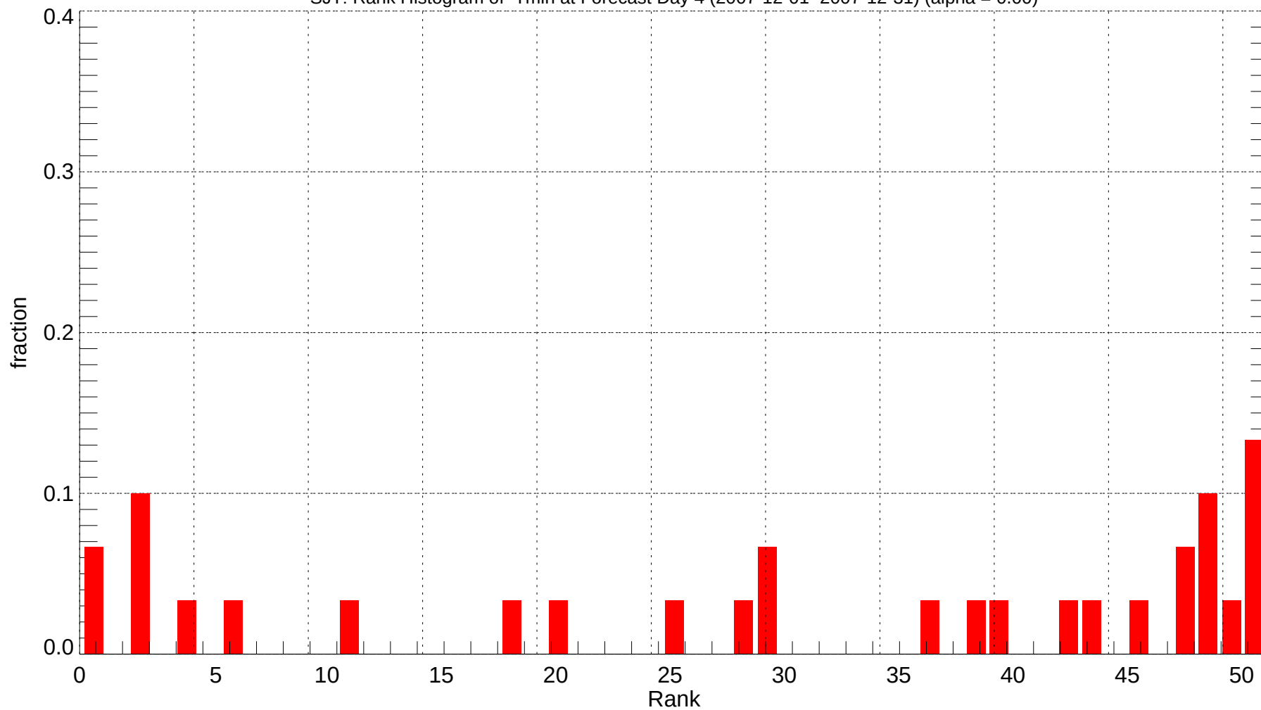
SJT: Rank Histogram of Tmin at Forecast Day 4 (2007-12-01~2007-12-31) (alpha = 0.00)
