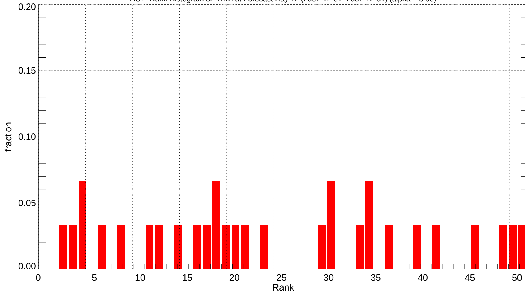
ACY: Rank Histogram of Tmin at Forecast Day 12 (2007-12-01~2007-12-31) (alpha = 0.00)
