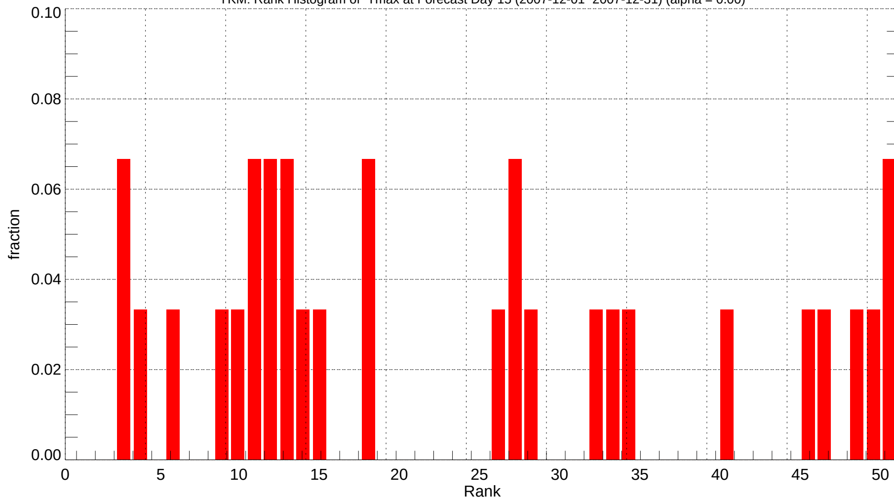
YKM: Rank Histogram of Tmax at Forecast Day 15 (2007-12-01~2007-12-31) (alpha = 0.00)
