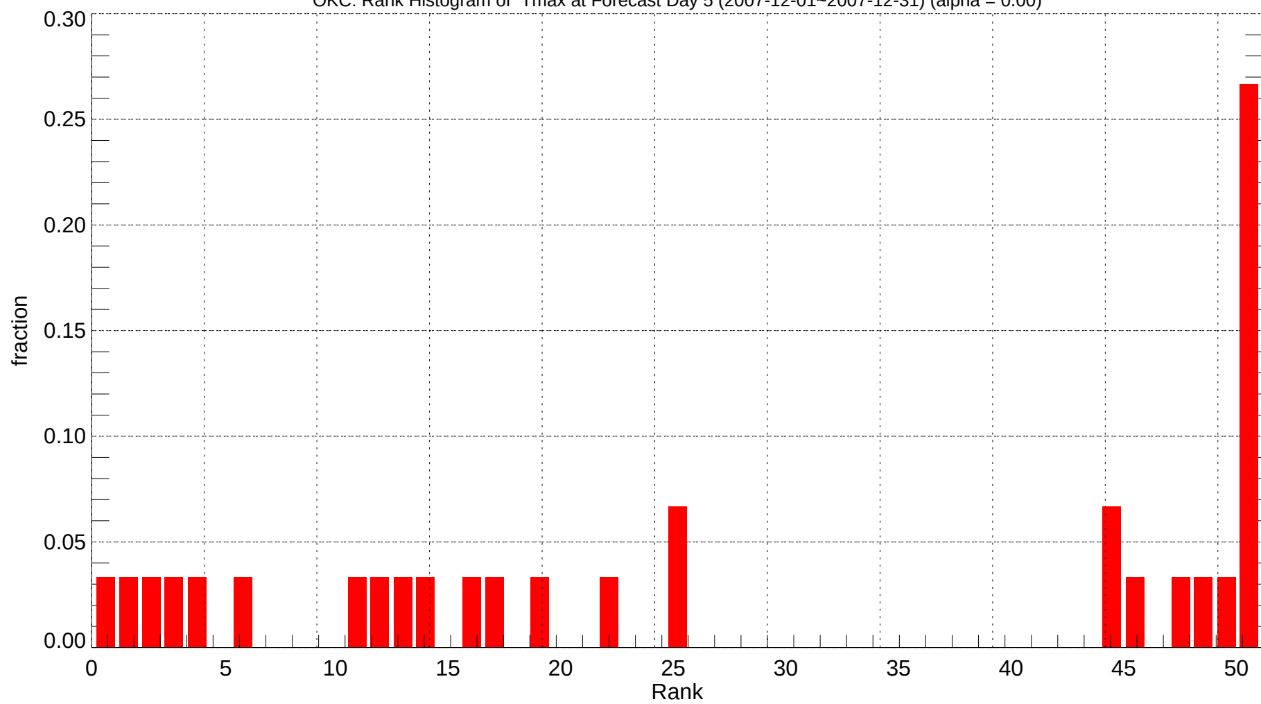
OKC: Rank Histogram of Tmax at Forecast Day 5 (2007-12-01~2007-12-31) (alpha = 0.00)
