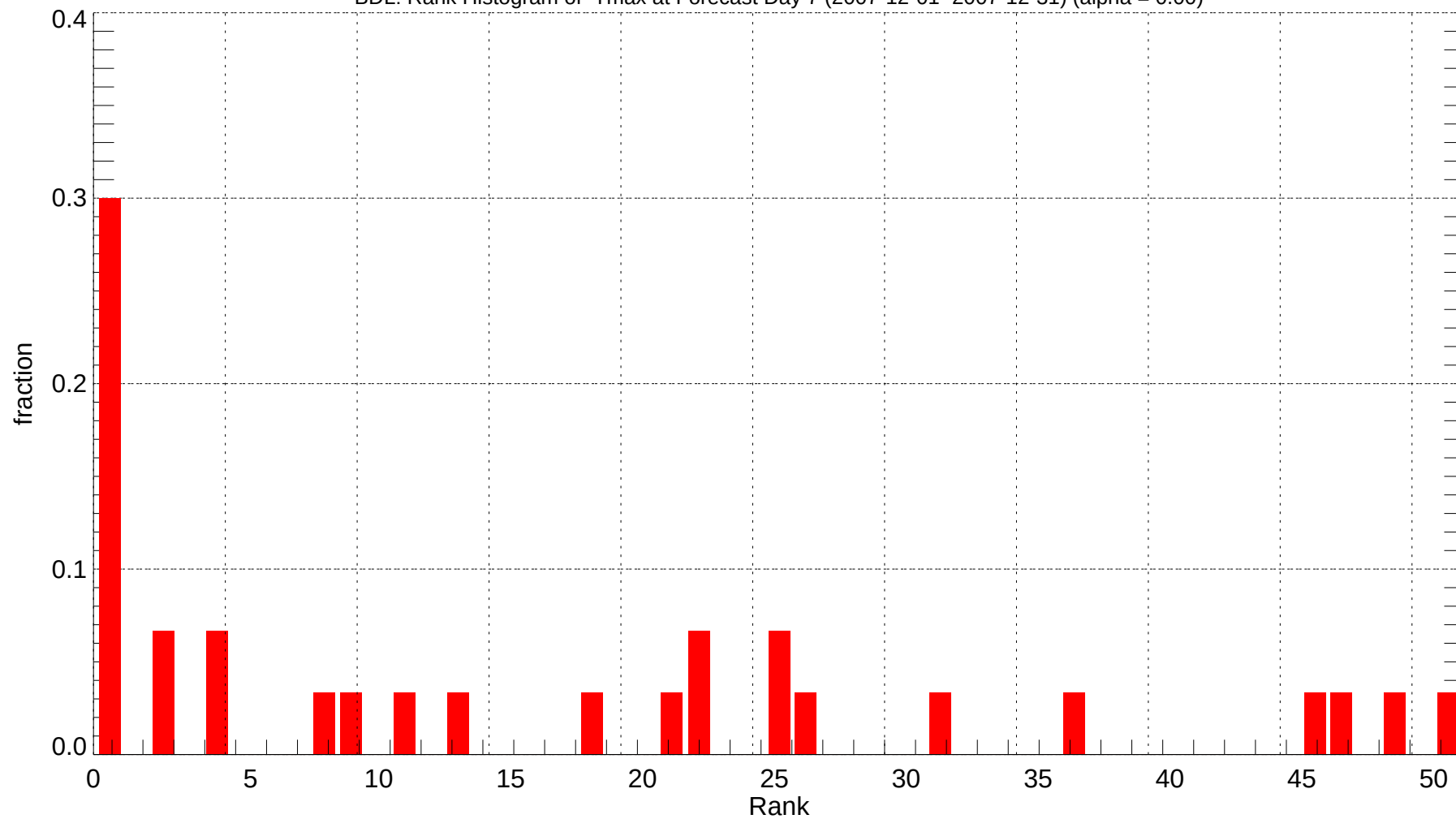
BDL: Rank Histogram of Tmax at Forecast Day 7 (2007-12-01~2007-12-31) (alpha = 0.00)
