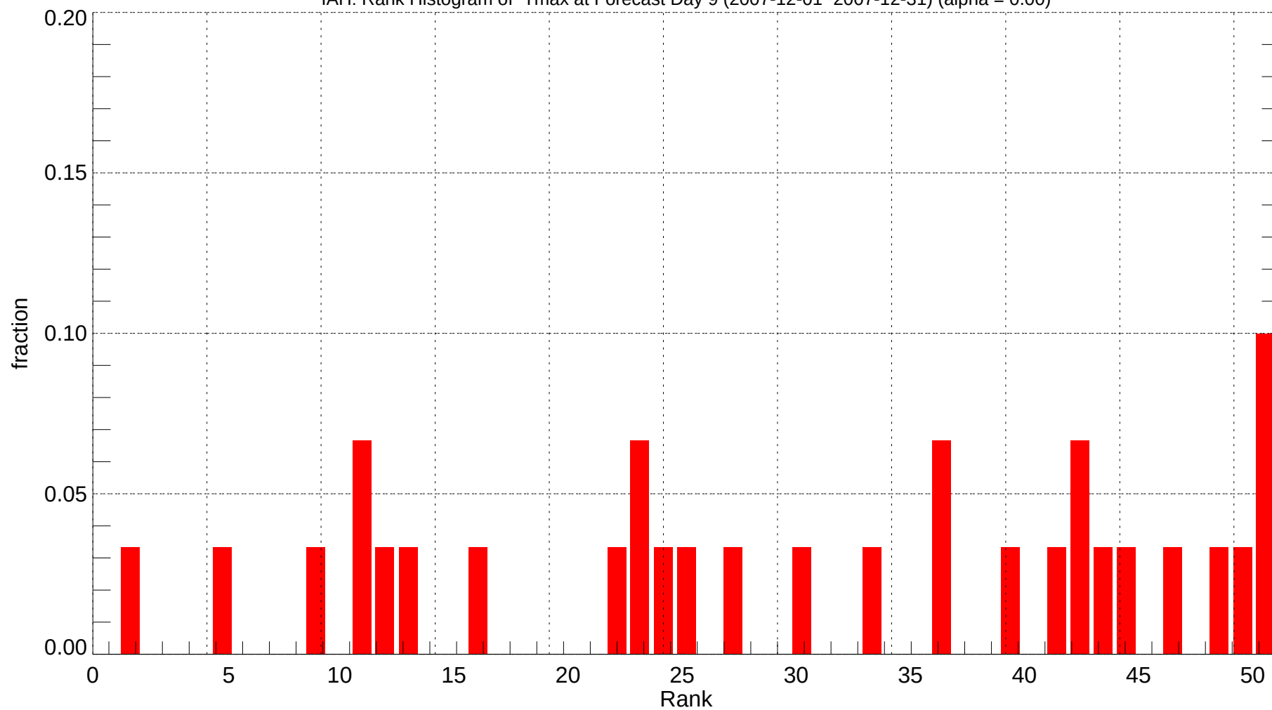
IAH: Rank Histogram of Tmax at Forecast Day 9 (2007-12-01~2007-12-31) (alpha = 0.00)
