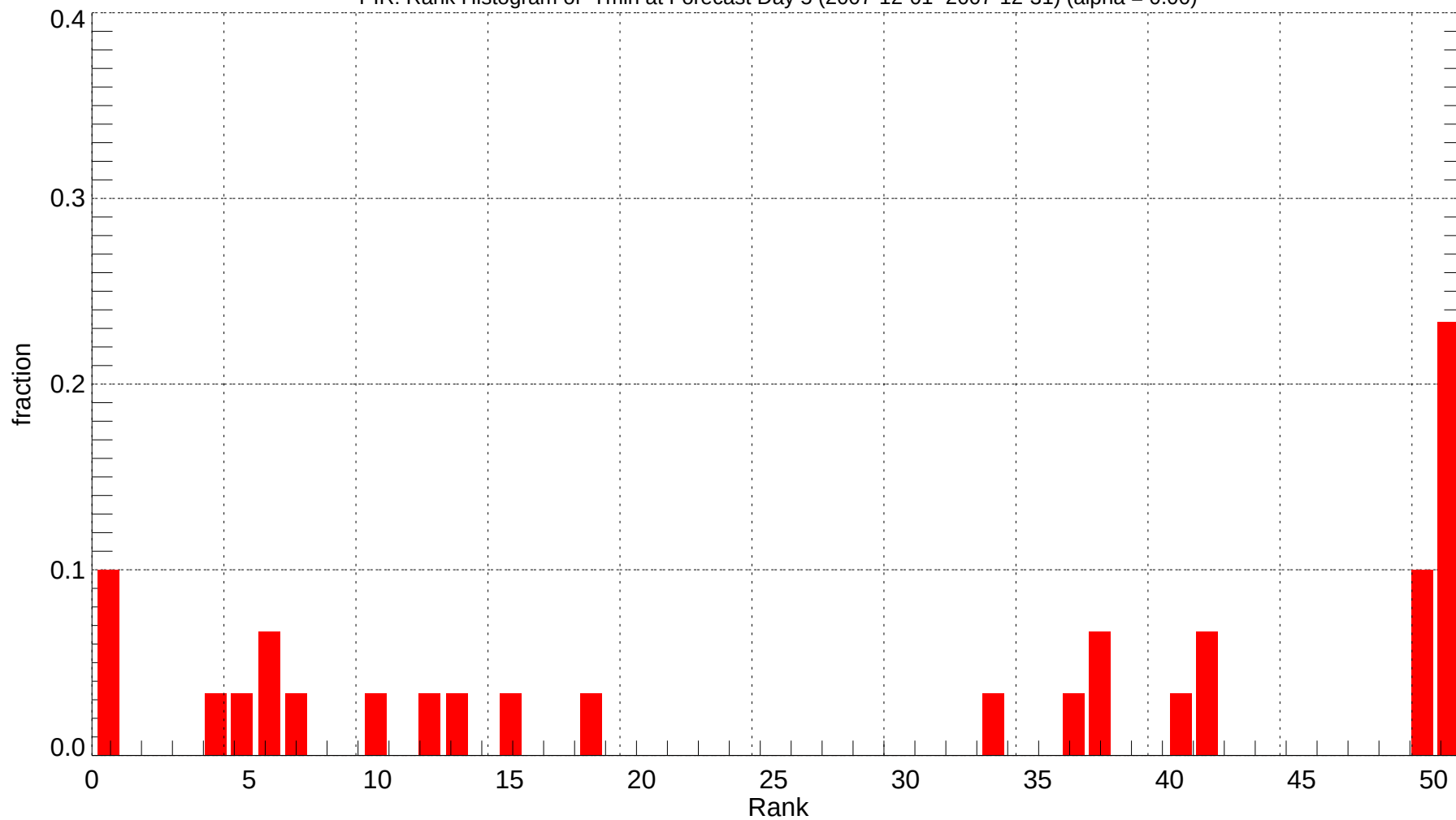
PIR: Rank Histogram of Tmin at Forecast Day 5 (2007-12-01~2007-12-31) (alpha = 0.00)
