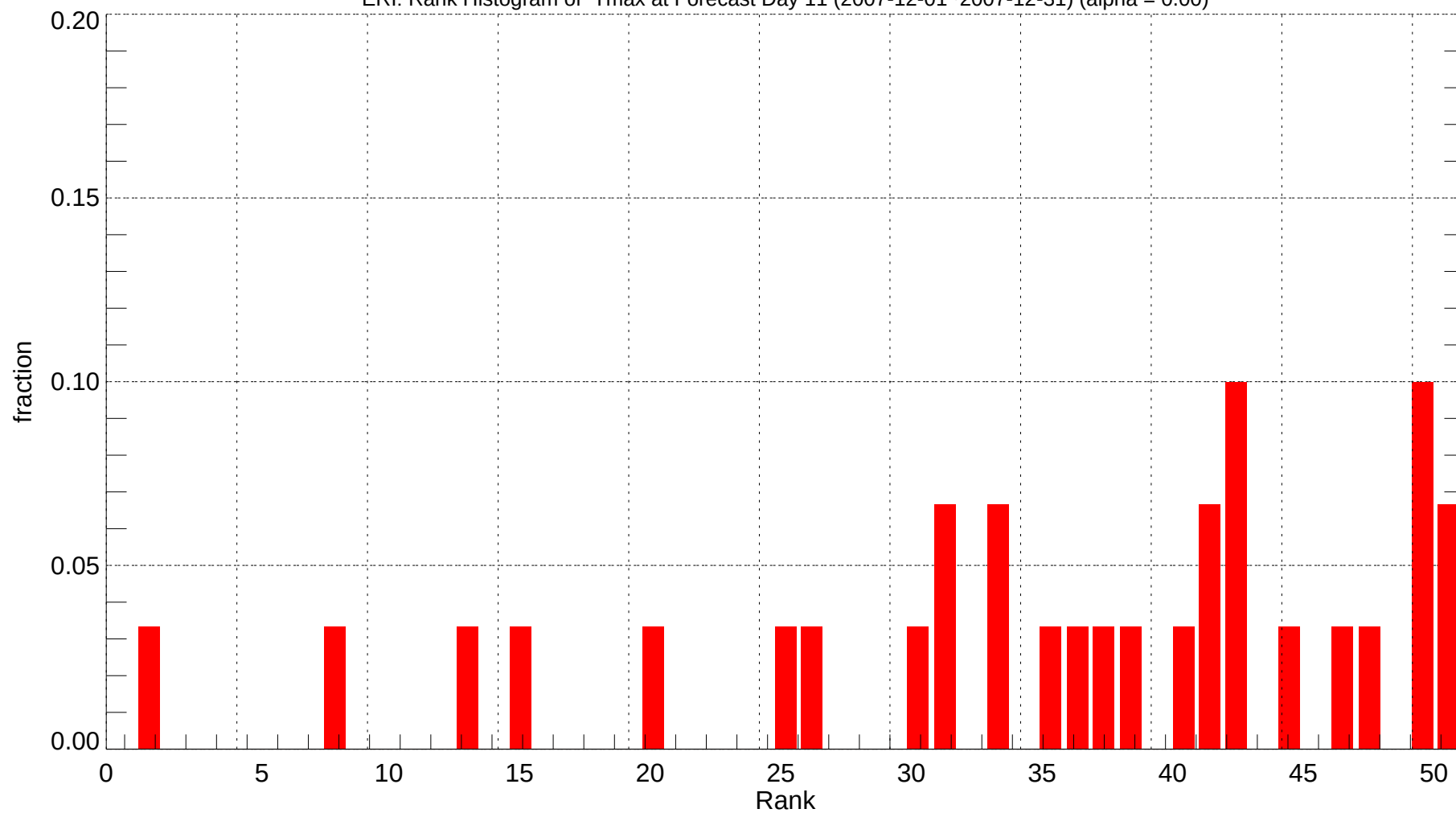
ERI: Rank Histogram of Tmax at Forecast Day 11 (2007-12-01~2007-12-31) (alpha = 0.00)
