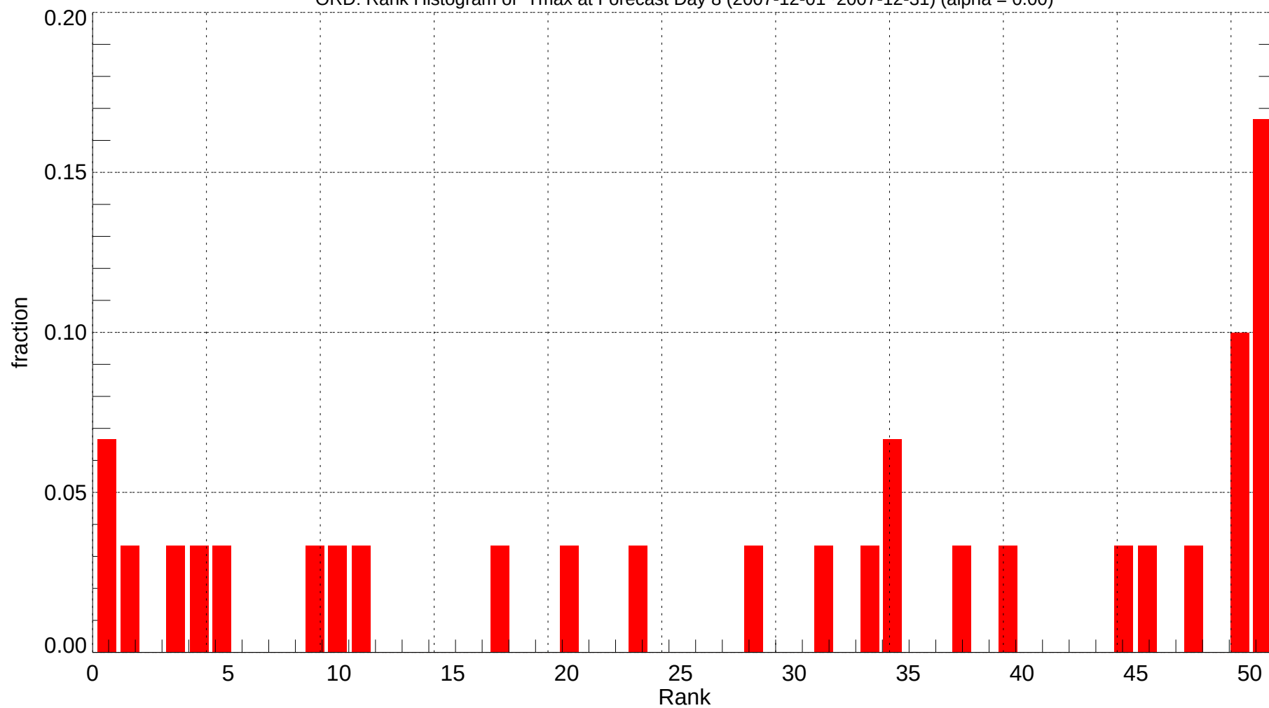
ORD: Rank Histogram of Tmax at Forecast Day 8 (2007-12-01~2007-12-31) (alpha = 0.00)
