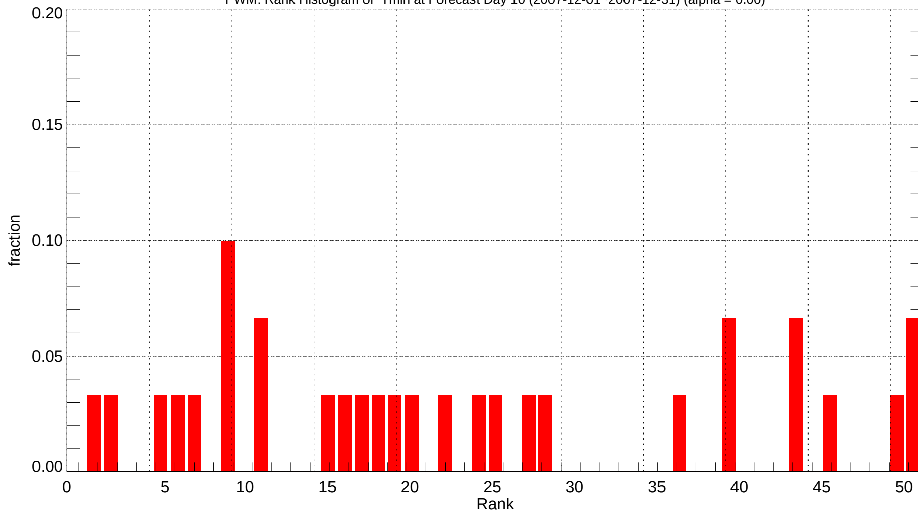
PWM: Rank Histogram of Tmin at Forecast Day 10 (2007-12-01~2007-12-31) (alpha = 0.00)
