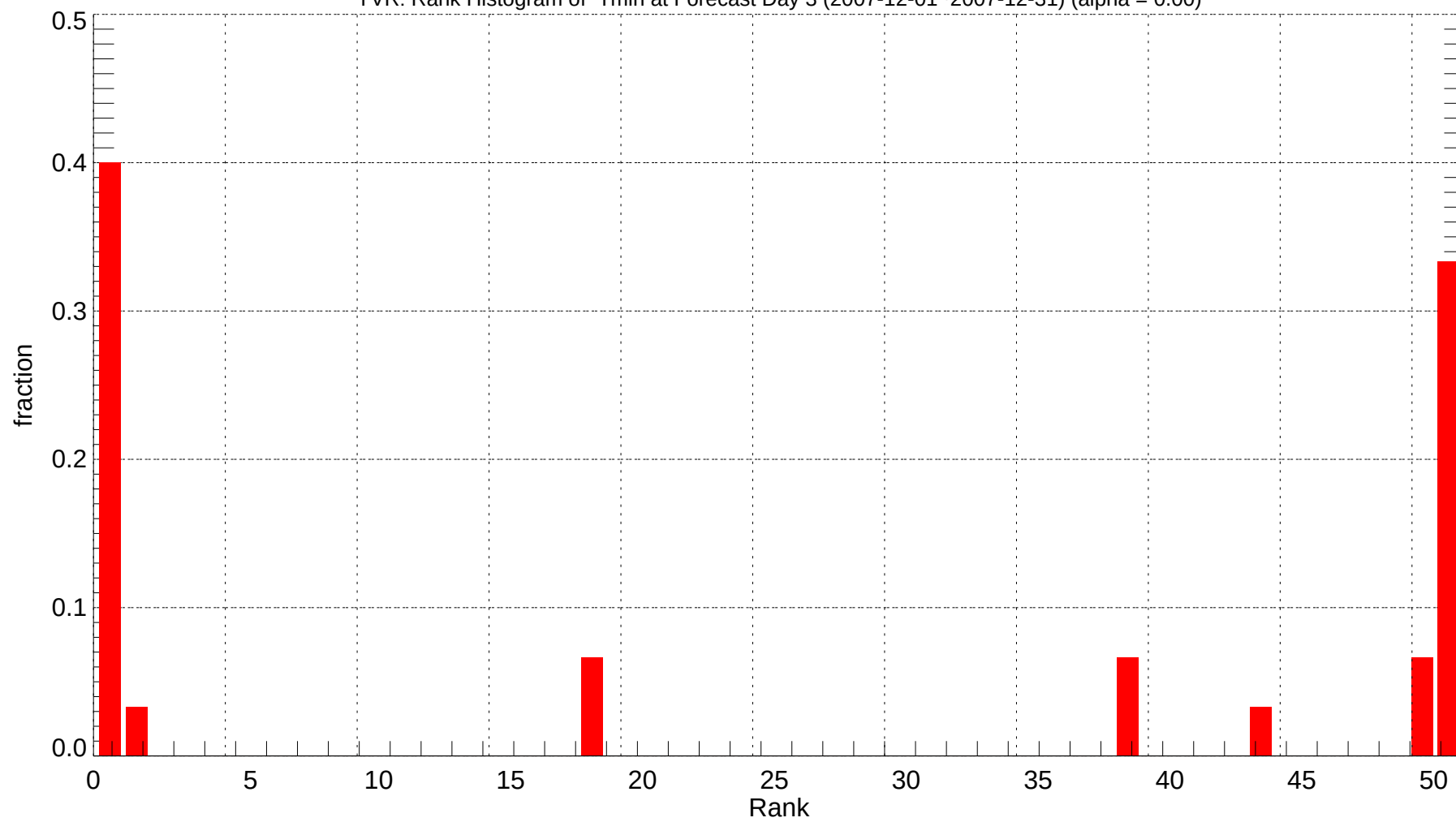
YVR: Rank Histogram of Tmin at Forecast Day 3 (2007-12-01~2007-12-31) (alpha = 0.00)
