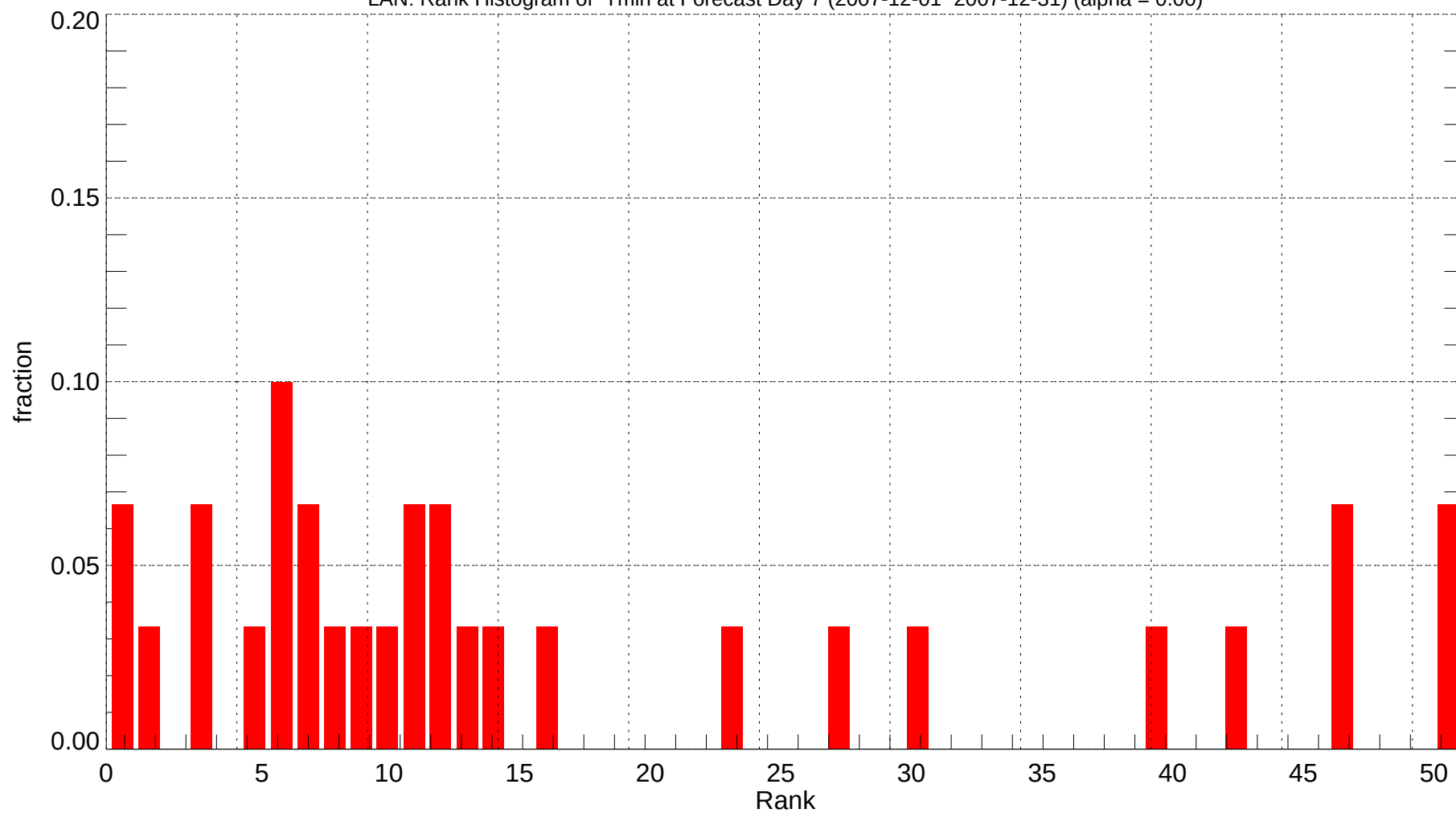
LAN: Rank Histogram of Tmin at Forecast Day 7 (2007-12-01~2007-12-31) (alpha = 0.00)
