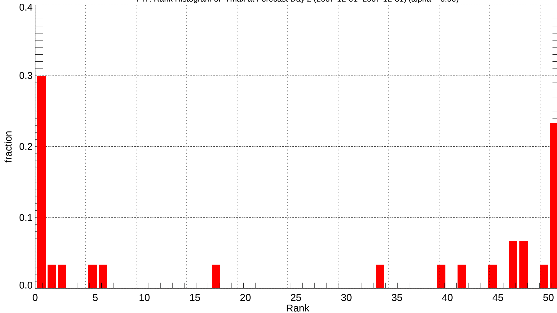
PIT: Rank Histogram of Tmax at Forecast Day 2 (2007-12-01~2007-12-31) (alpha = 0.00)
