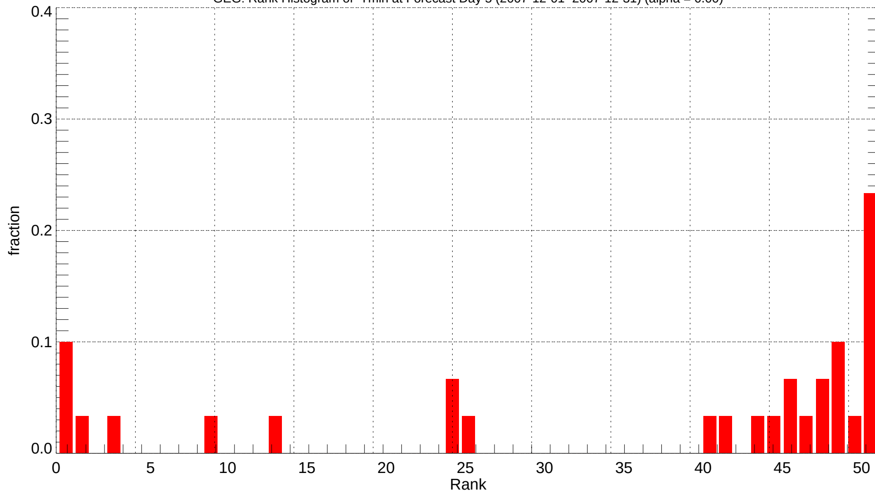
GEG: Rank Histogram of Tmin at Forecast Day 5 (2007-12-01~2007-12-31) (alpha = 0.00)
