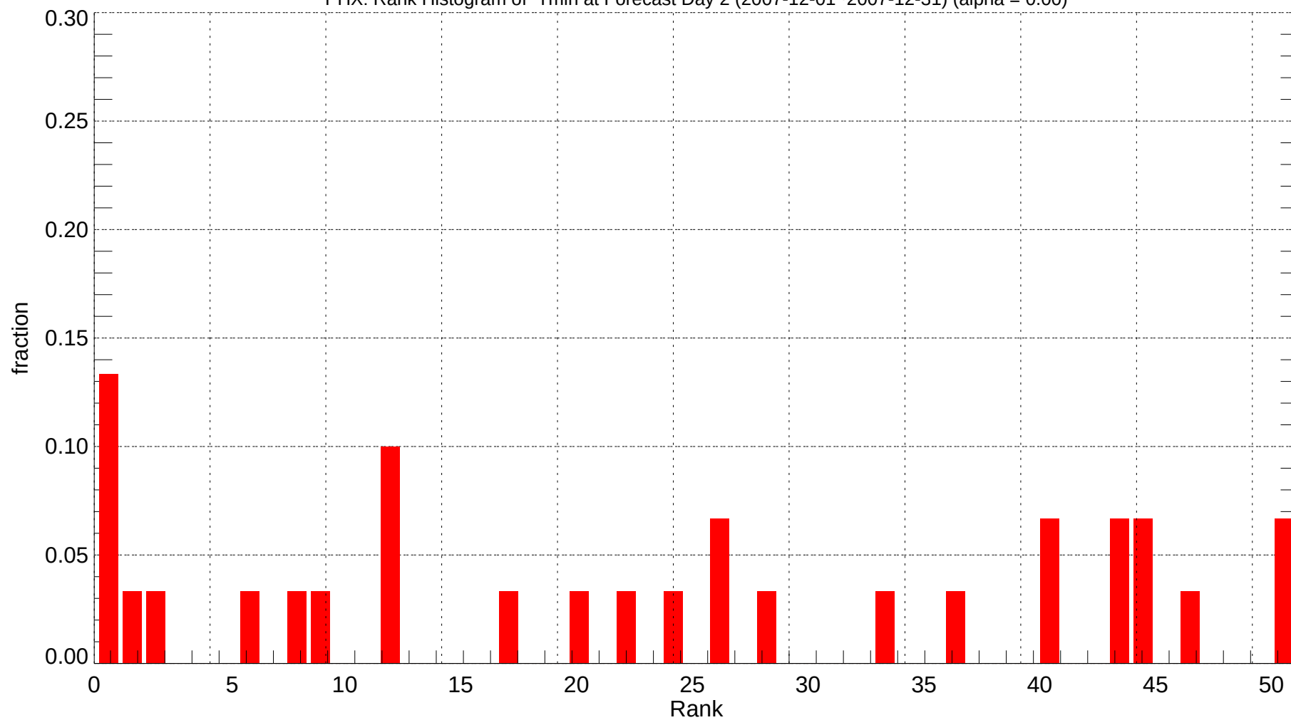
PHX: Rank Histogram of Tmin at Forecast Day 2 (2007-12-01~2007-12-31) (alpha = 0.00)
