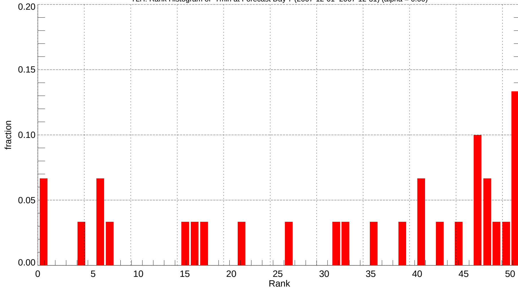
TLH: Rank Histogram of Tmin at Forecast Day 7 (2007-12-01~2007-12-31) (alpha = 0.00)
