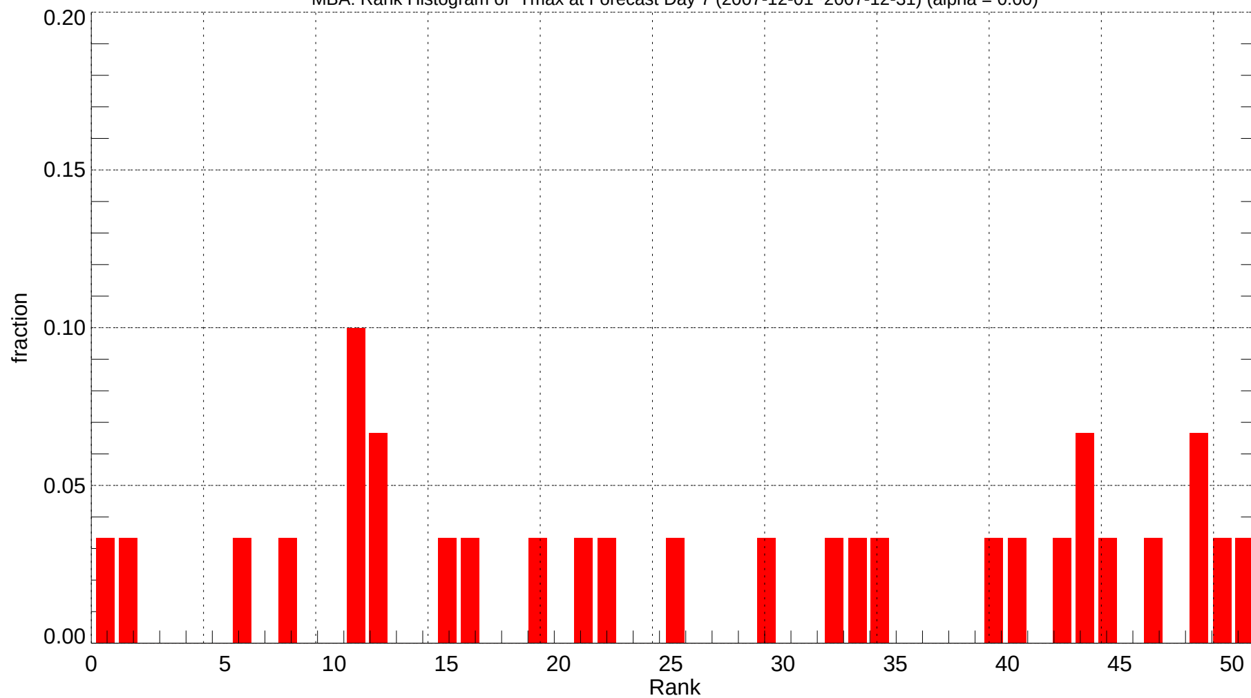
MBA: Rank Histogram of Tmax at Forecast Day 7 (2007-12-01~2007-12-31) (alpha = 0.00)
