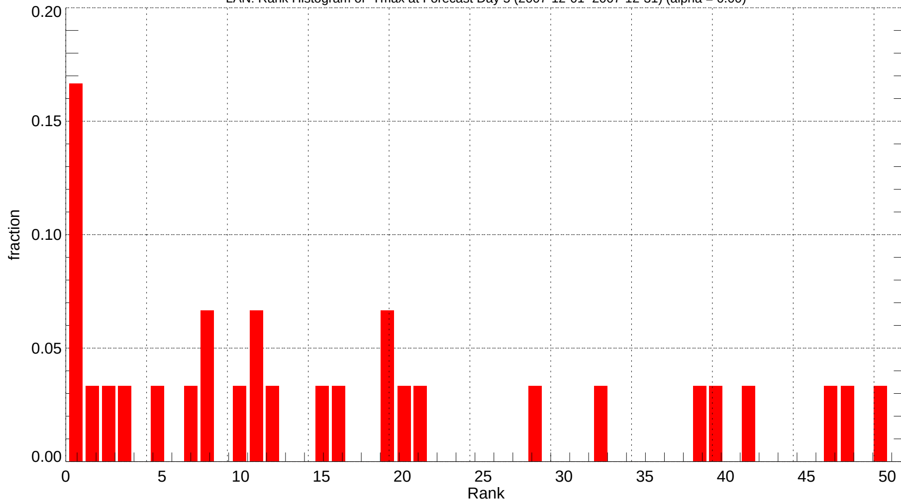
LAN: Rank Histogram of Tmax at Forecast Day 5 (2007-12-01~2007-12-31) (alpha = 0.00)
