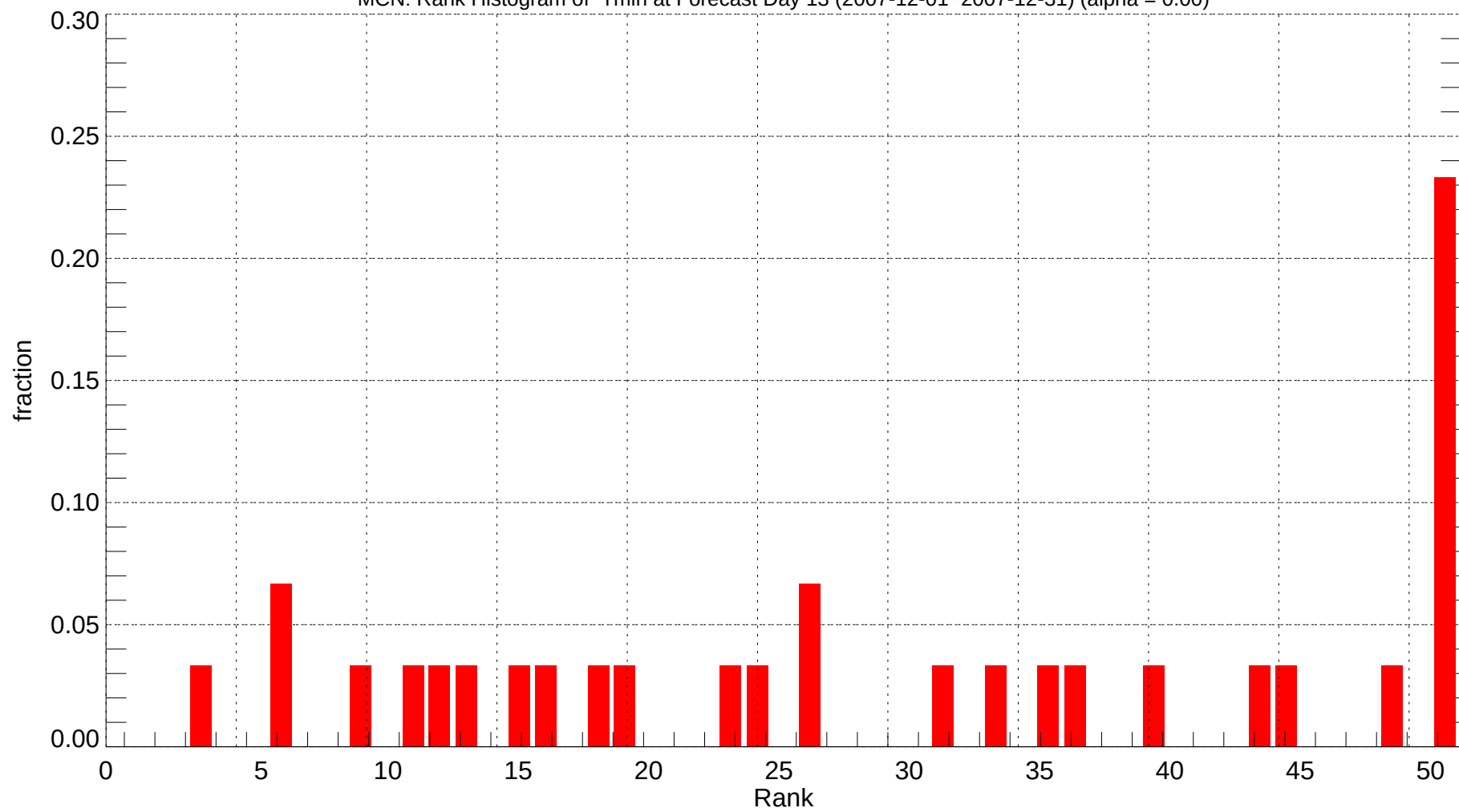
MCN: Rank Histogram of Tmin at Forecast Day 13 (2007-12-01~2007-12-31) (alpha = 0.00)
