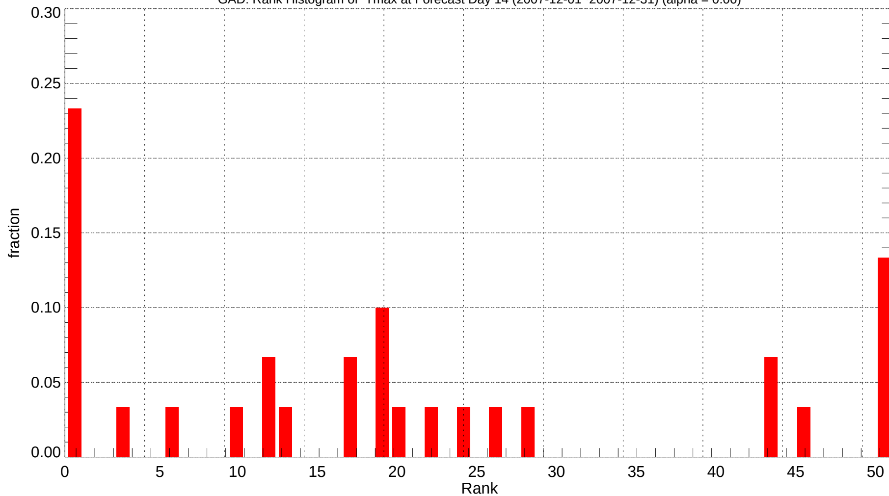
GAD: Rank Histogram of Tmax at Forecast Day 14 (2007-12-01~2007-12-31) (alpha = 0.00)
