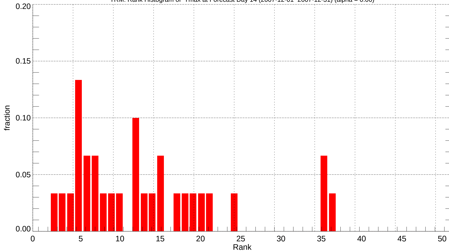
TRM: Rank Histogram of Tmax at Forecast Day 14 (2007-12-01~2007-12-31) (alpha = 0.00)
