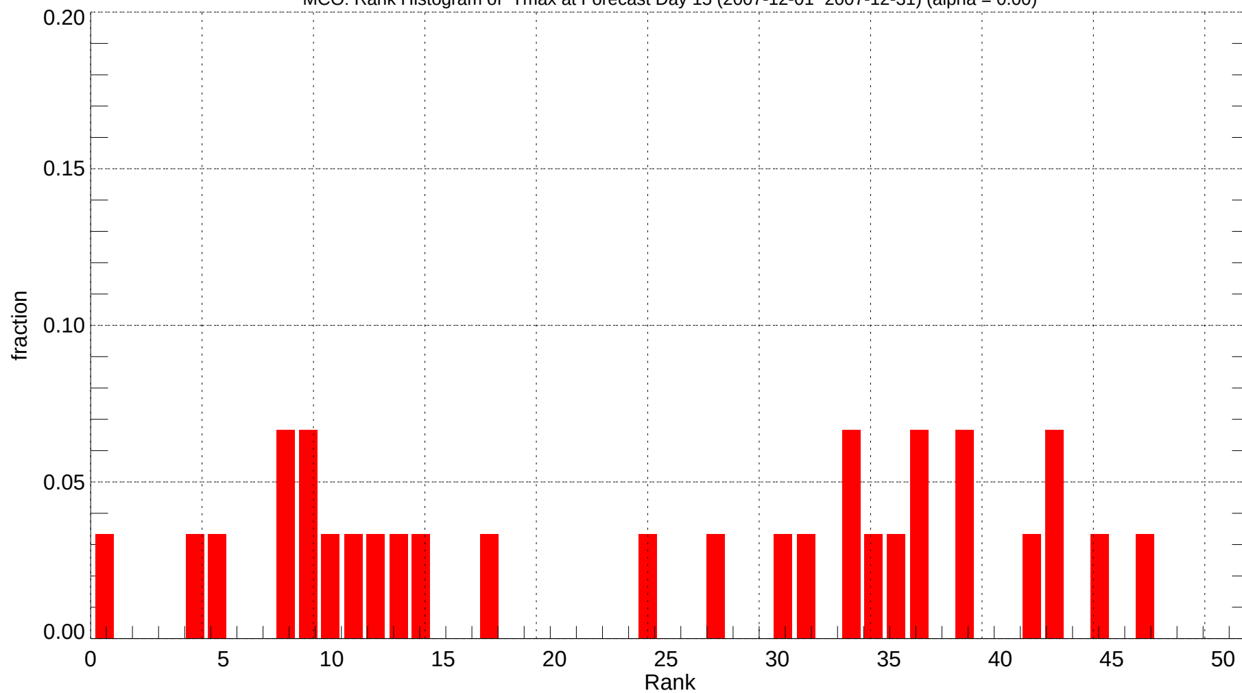
MCO: Rank Histogram of Tmax at Forecast Day 15 (2007-12-01~2007-12-31) (alpha = 0.00)
