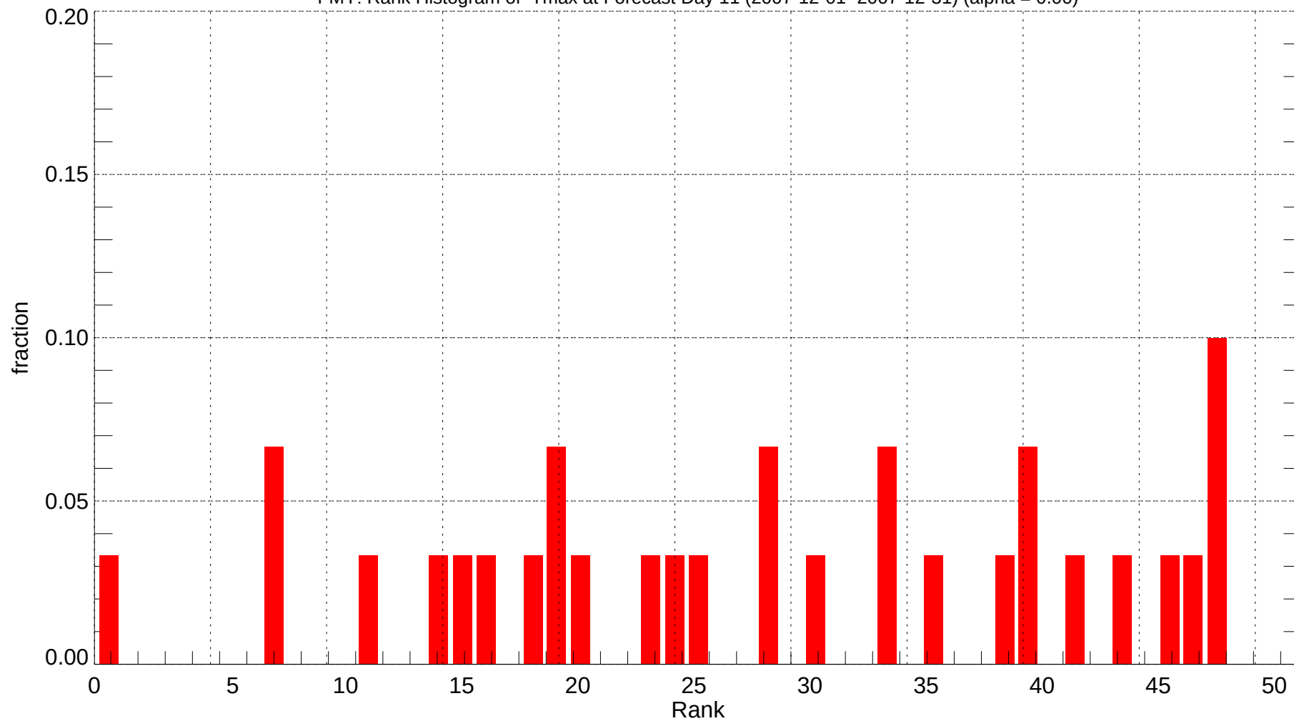
FMY: Rank Histogram of Tmax at Forecast Day 11 (2007-12-01~2007-12-31) (alpha = 0.00)
