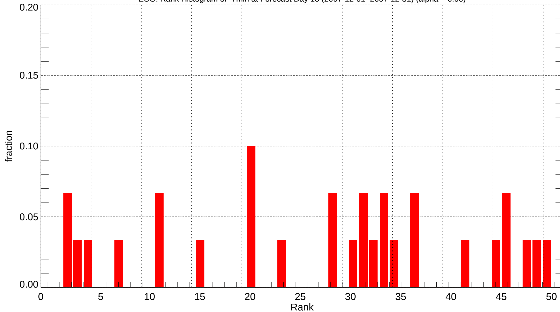
EUG: Rank Histogram of Tmin at Forecast Day 15 (2007-12-01~2007-12-31) (alpha = 0.00)
