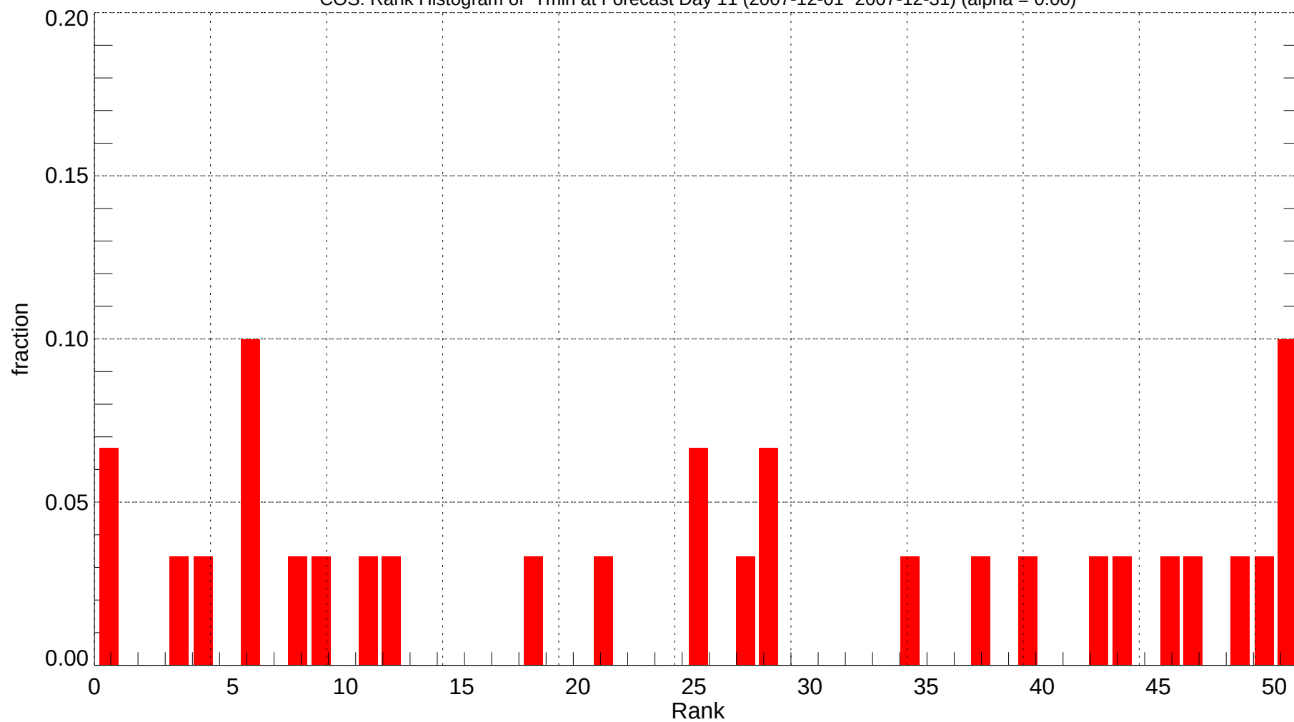
COS: Rank Histogram of Tmin at Forecast Day 11 (2007-12-01~2007-12-31) (alpha = 0.00)
