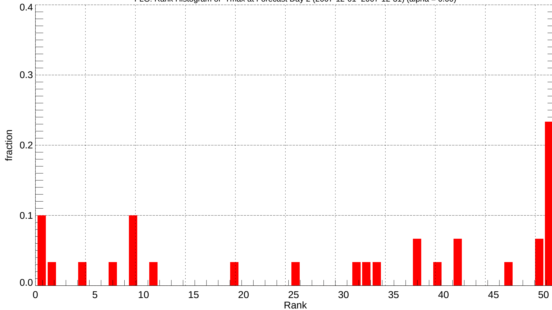
FLG: Rank Histogram of Tmax at Forecast Day 2 (2007-12-01~2007-12-31) (alpha = 0.00)
