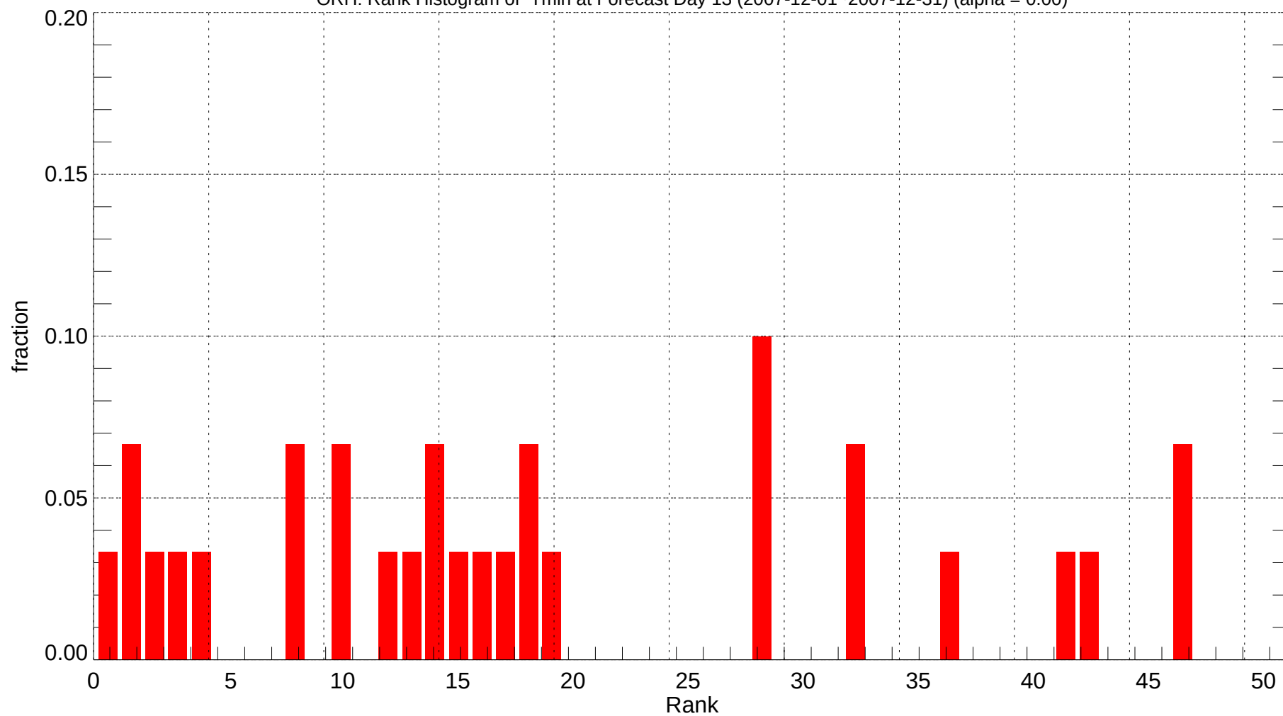
ORH: Rank Histogram of Tmin at Forecast Day 13 (2007-12-01~2007-12-31) (alpha = 0.00)
