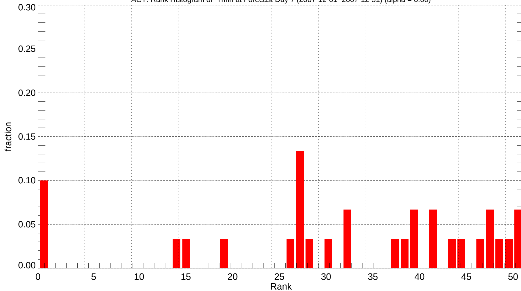
ACY: Rank Histogram of Tmin at Forecast Day 7 (2007-12-01~2007-12-31) (alpha = 0.00)
