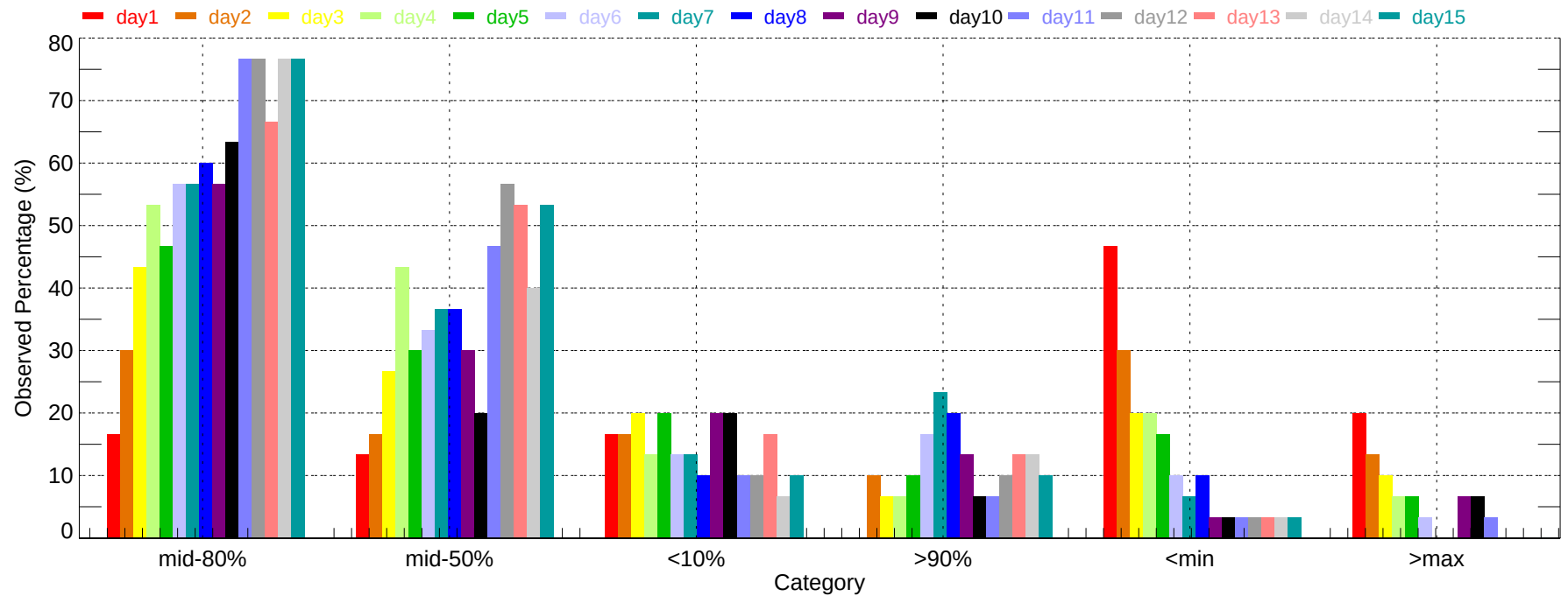
Observed Percentage of Ensembles - ORH: Min Temperature (2007-12-01~2007-12-31)
