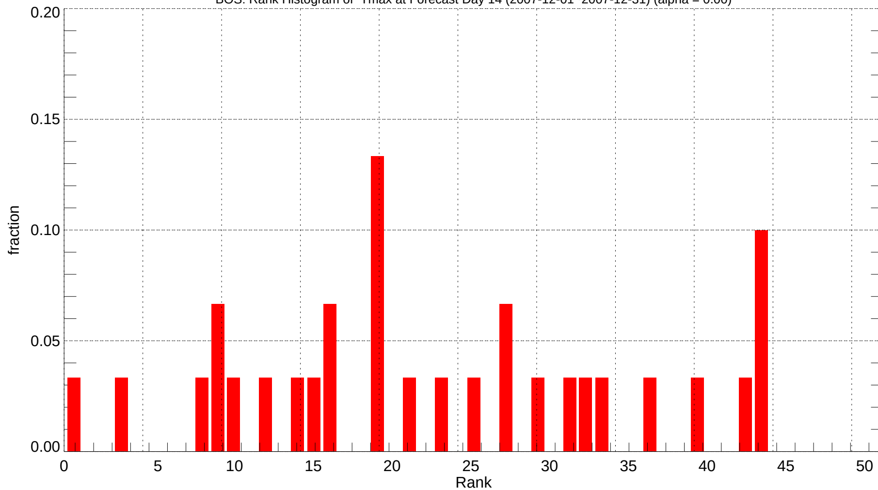
BOS: Rank Histogram of Tmax at Forecast Day 14 (2007-12-01~2007-12-31) (alpha = 0.00)
