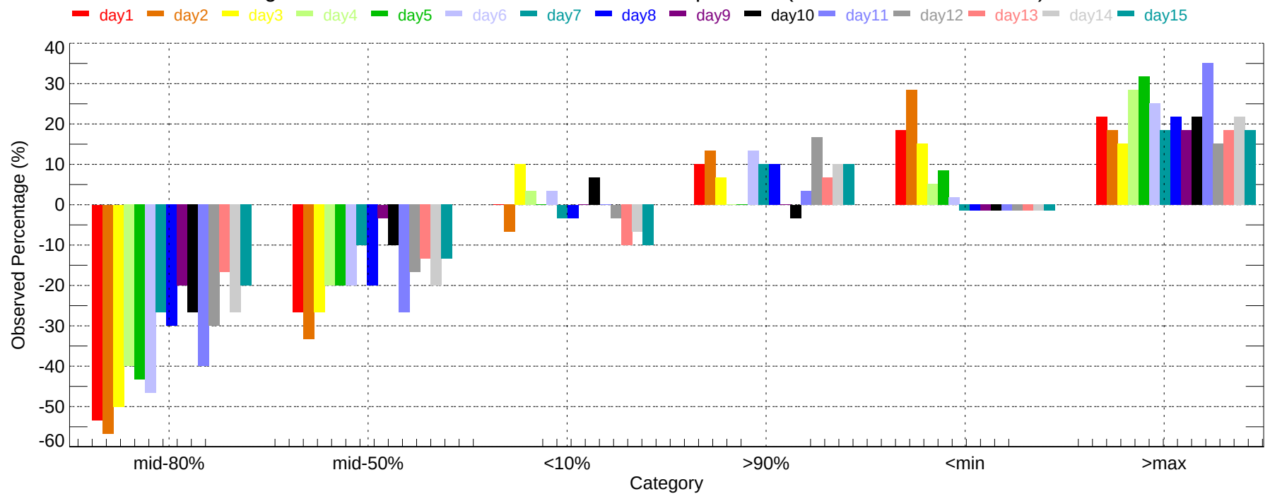
Observed Percentage Deviation of Ensembles - ATL: Min Temperature (2007-12-01~2007-12-31)
