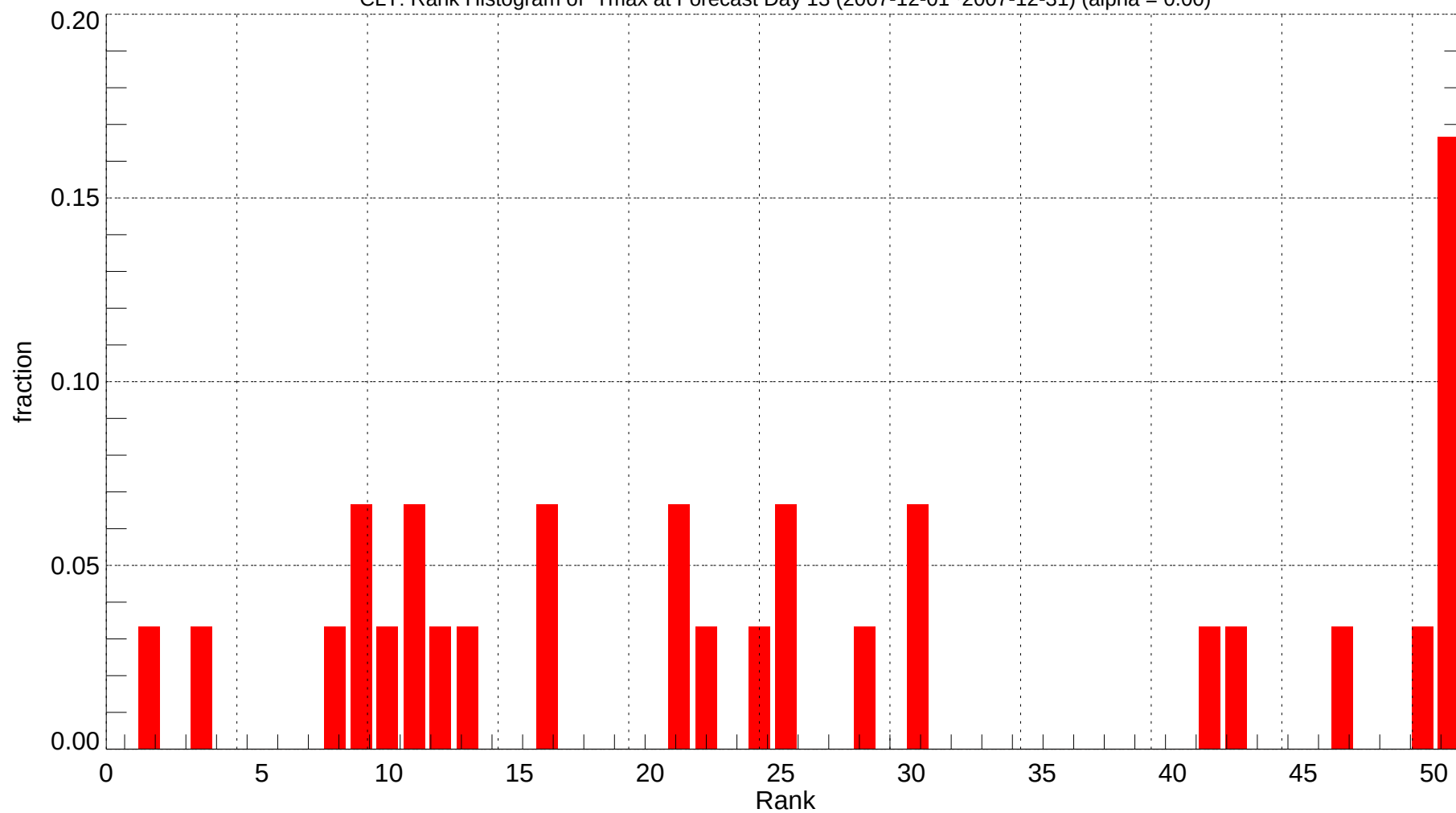
CLT: Rank Histogram of Tmax at Forecast Day 13 (2007-12-01~2007-12-31) (alpha = 0.00)
