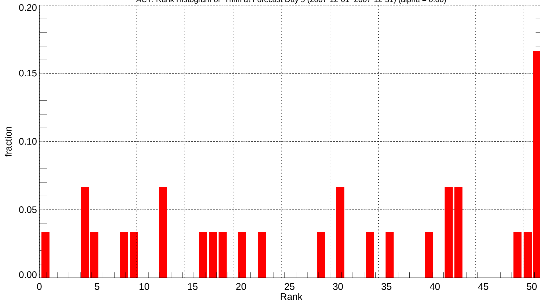
ACT: Rank Histogram of Tmin at Forecast Day 9 (2007-12-01~2007-12-31) (alpha = 0.00)
