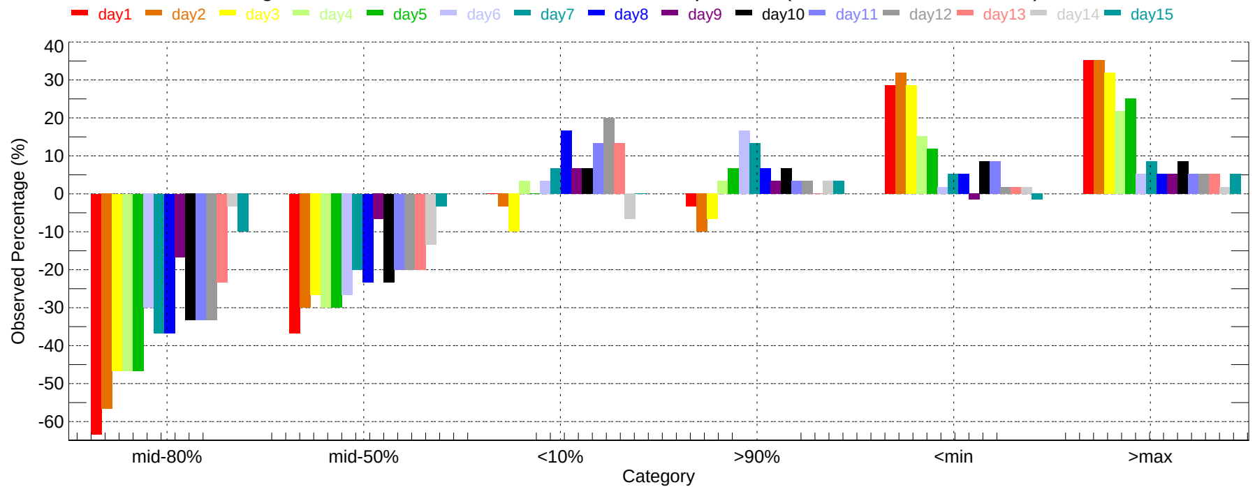
Observed Percentage Deviation of Ensembles - YKM: Min Temperature (2007-12-01~2007-12-31)
