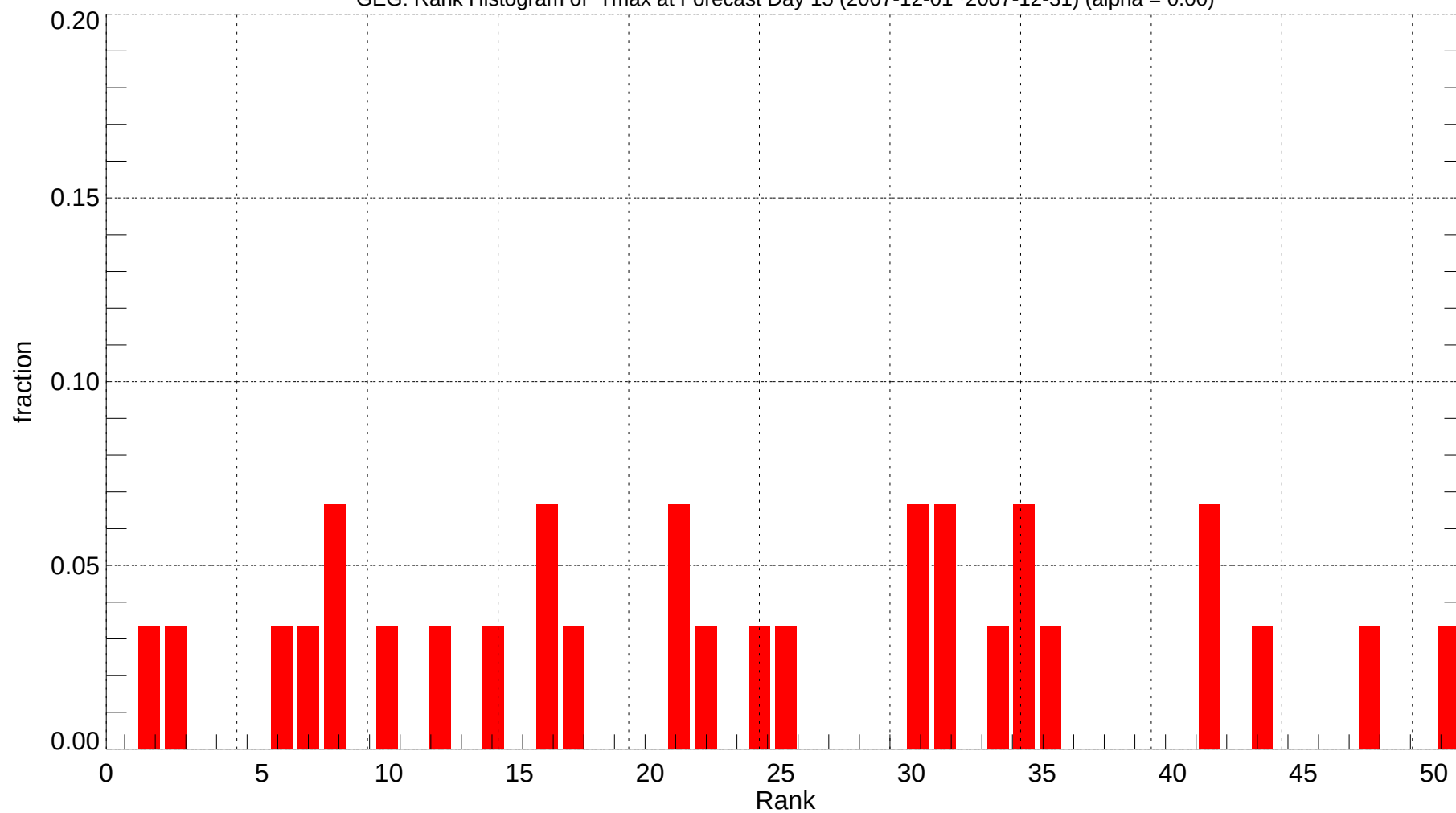
GEG: Rank Histogram of Tmax at Forecast Day 15 (2007-12-01~2007-12-31) (alpha = 0.00)
