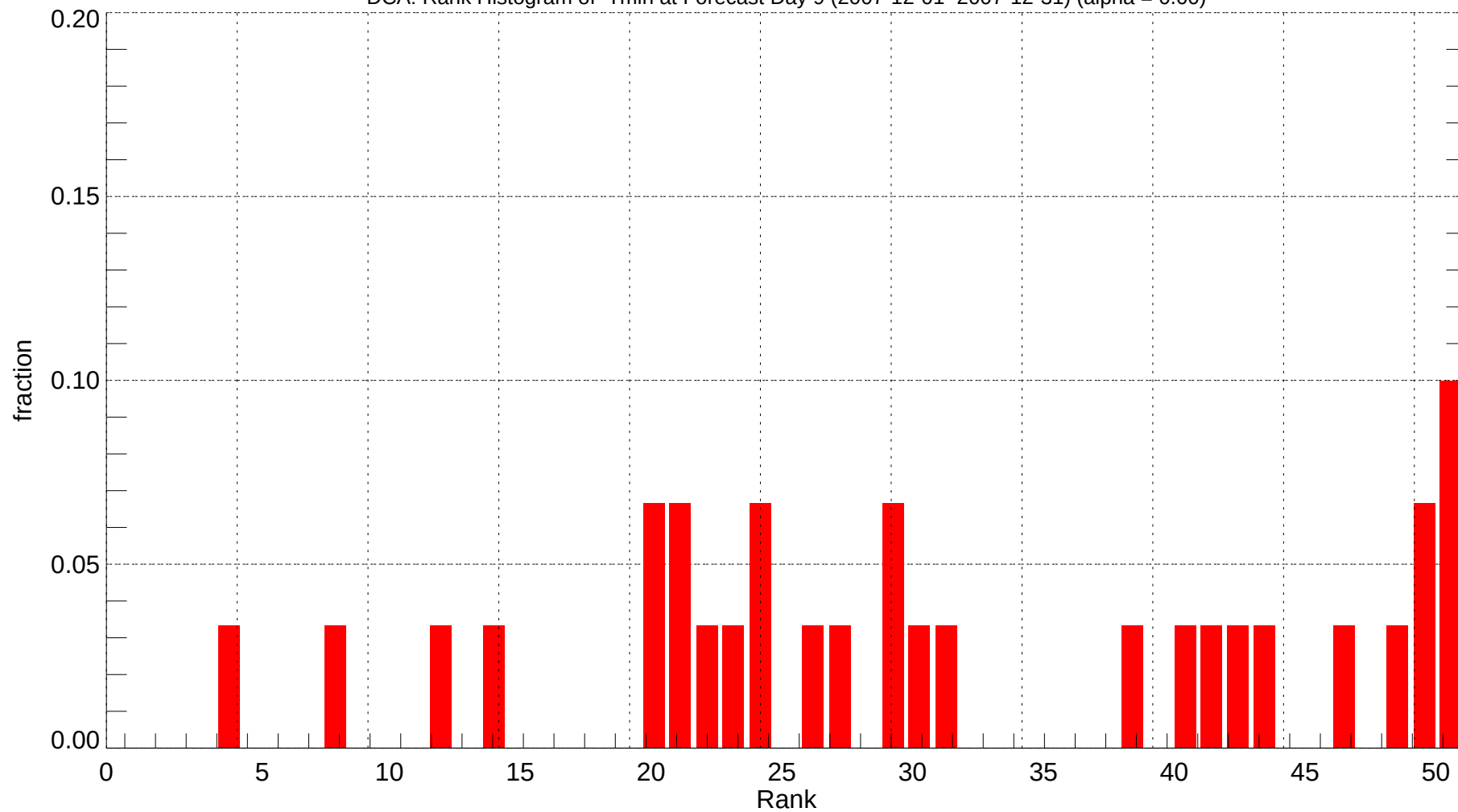
DCA: Rank Histogram of Tmin at Forecast Day 9 (2007-12-01~2007-12-31) (alpha = 0.00)
