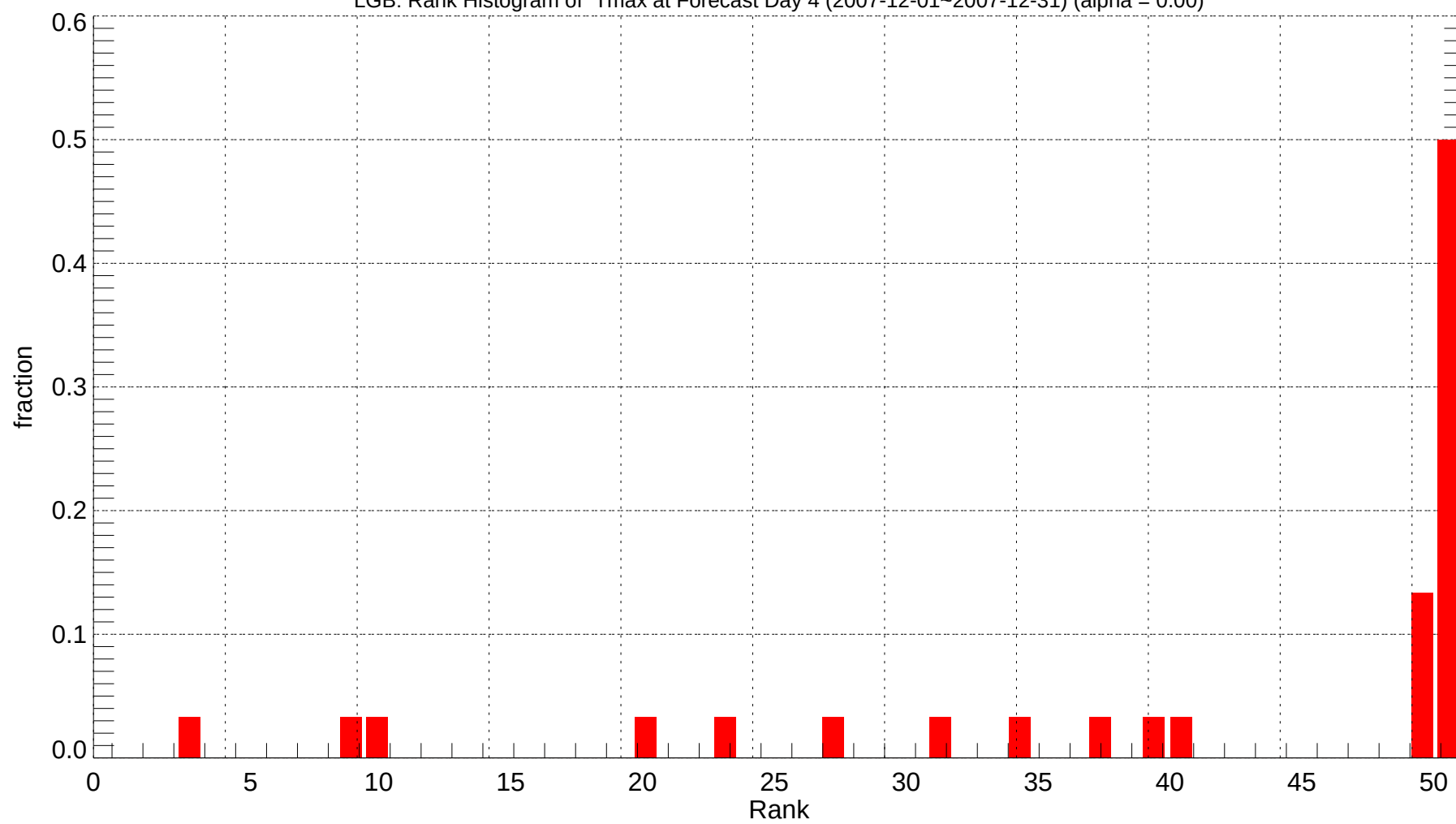
LGB: Rank Histogram of Tmax at Forecast Day 4 (2007-12-01~2007-12-31) (alpha = 0.00)
