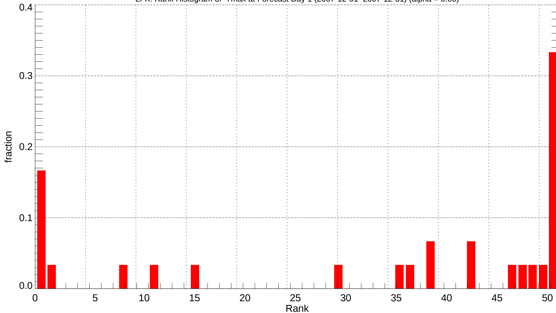
LFK: Rank Histogram of Tmax at Forecast Day 1 (2007-12-01~2007-12-31) (alpha = 0.00)
