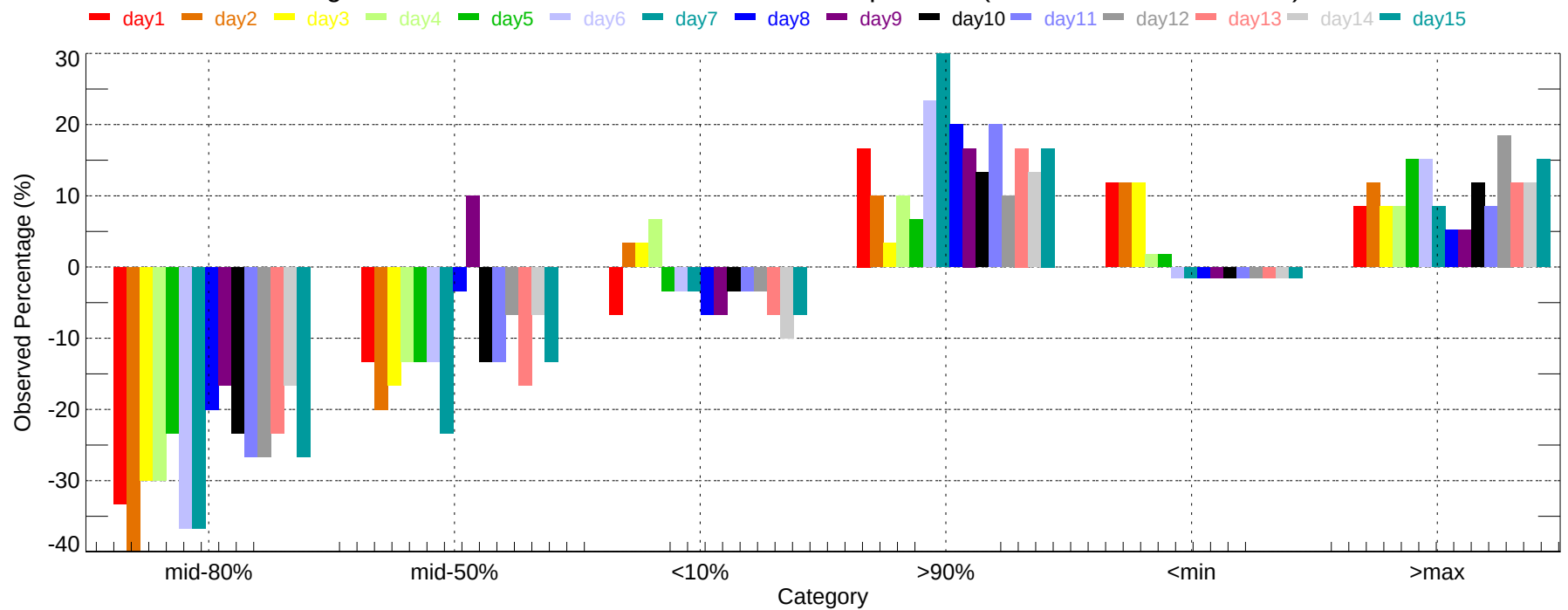
Observed Percentage Deviation of Ensembles - BHM: Min Temperature (2007-12-01~2007-12-31)
