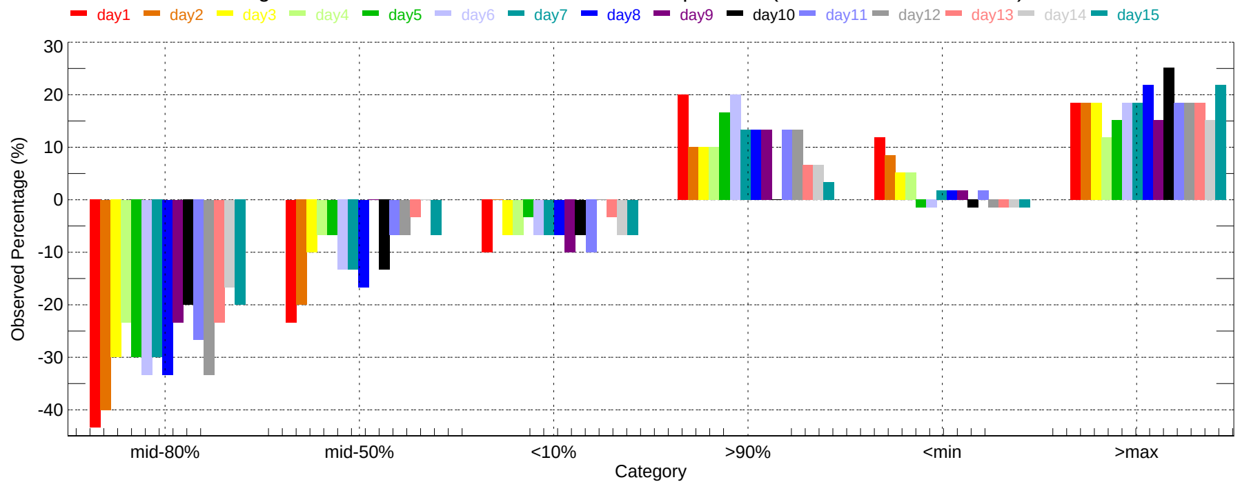
Observed Percentage Deviation of Ensembles - TYR: Min Temperature (2007-12-01~2007-12-31)
