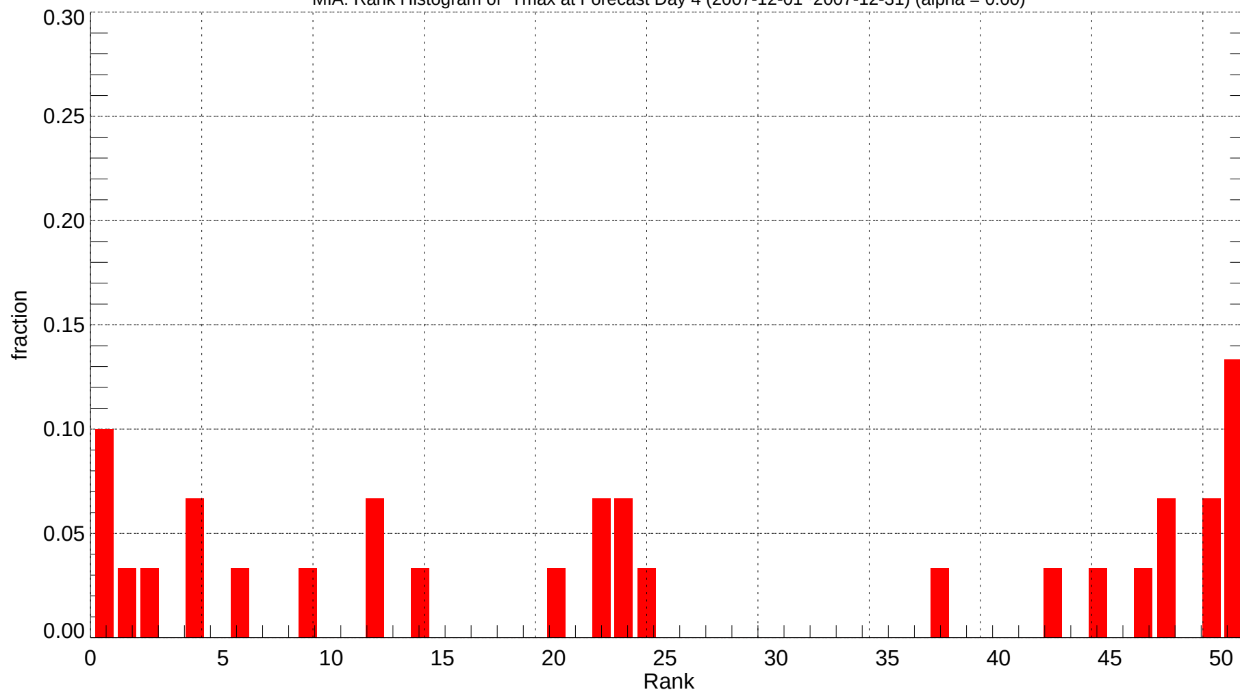
MIA: Rank Histogram of Tmax at Forecast Day 4 (2007-12-01~2007-12-31) (alpha = 0.00)
