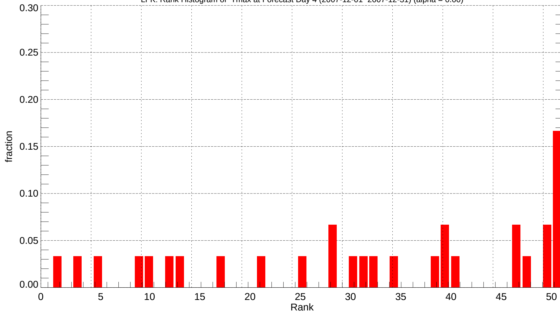
LFK: Rank Histogram of Tmax at Forecast Day 4 (2007-12-01~2007-12-31) (alpha = 0.00)
