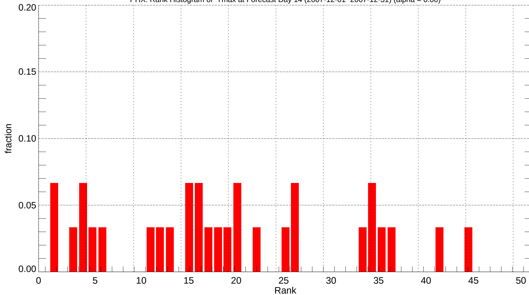
PHX: Rank Histogram of Tmax at Forecast Day 14 (2007-12-01~2007-12-31) (alpha = 0.00)
