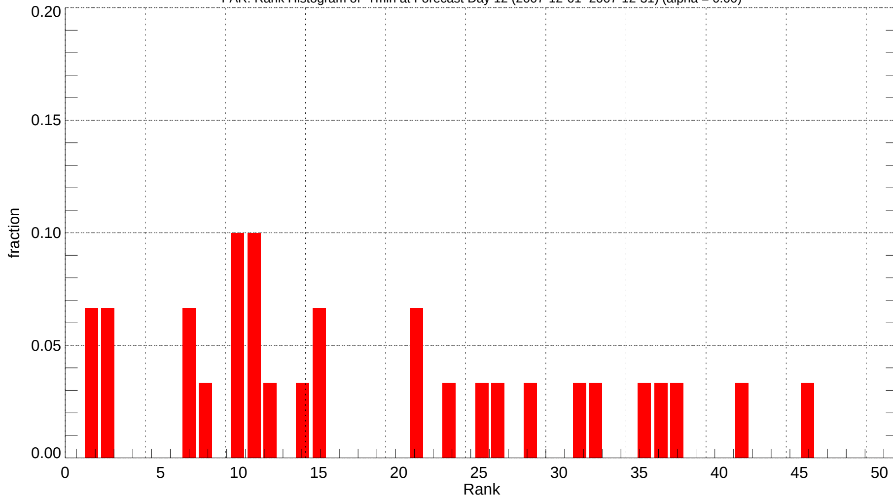
FAR: Rank Histogram of Tmin at Forecast Day 12 (2007-12-01~2007-12-31) (alpha = 0.00)
