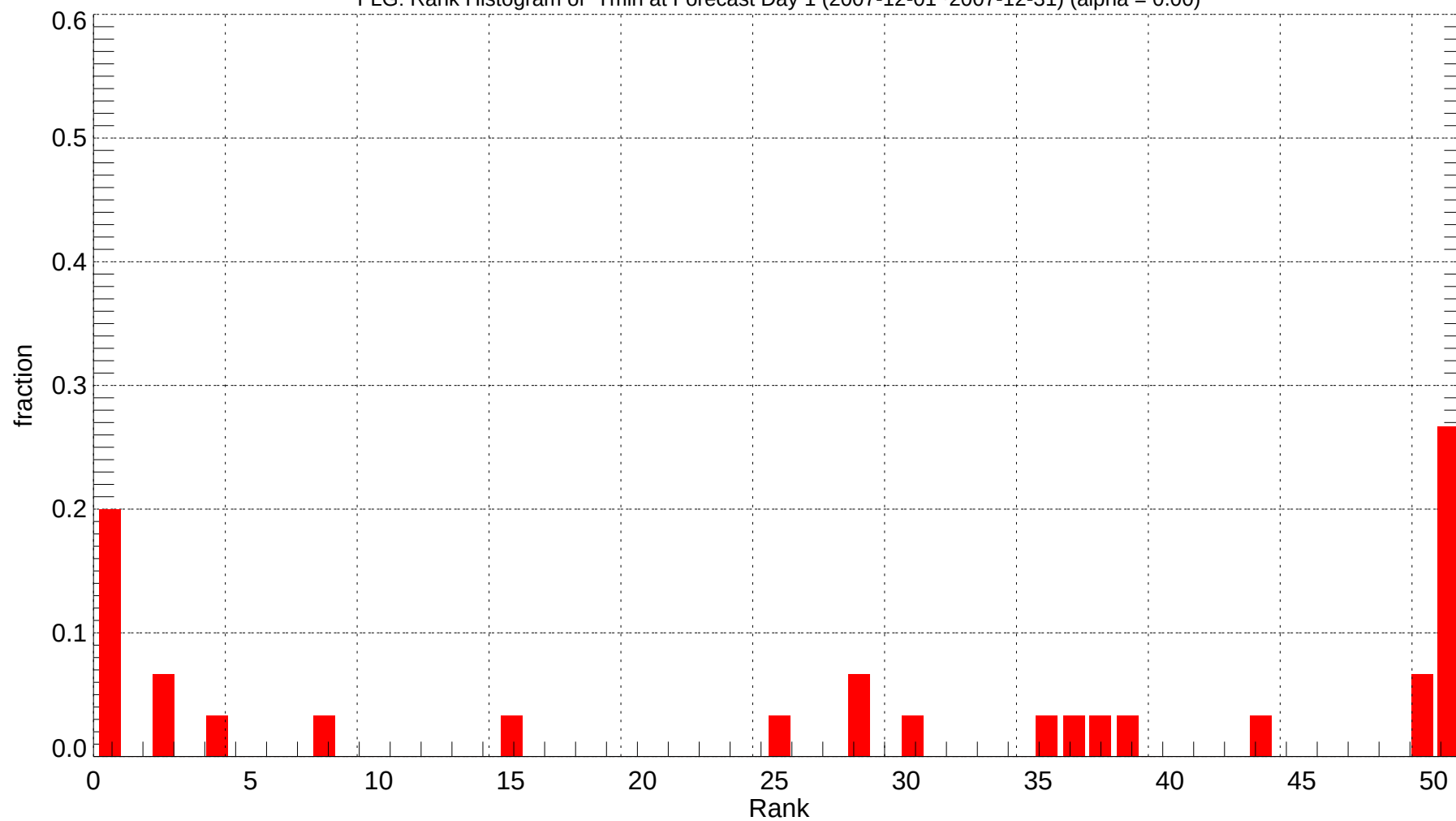
FLG: Rank Histogram of Tmin at Forecast Day 1 (2007-12-01~2007-12-31) (alpha = 0.00)
