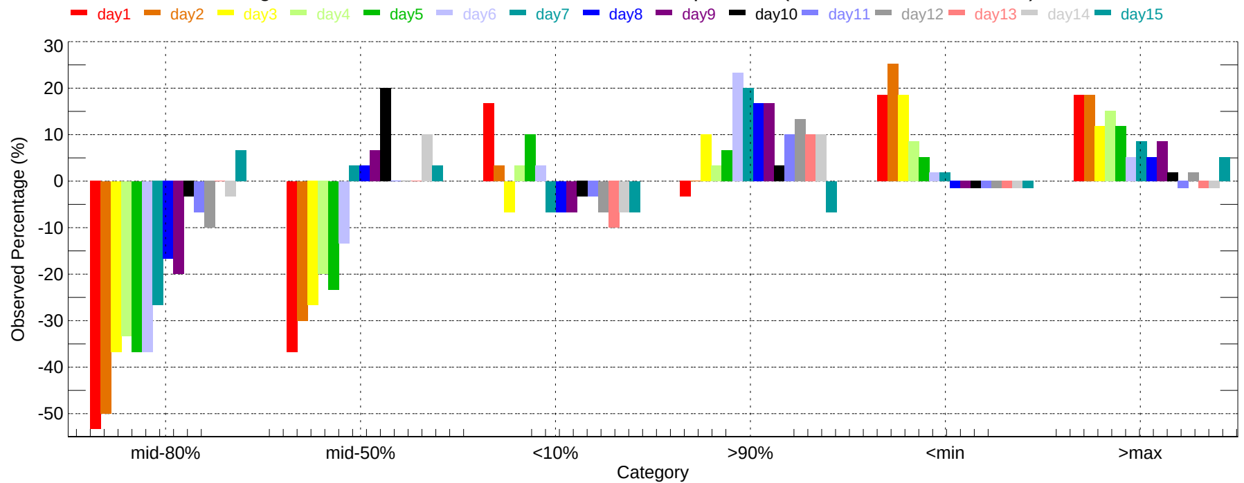
Observed Percentage Deviation of Ensembles - DCA: Max Temperature (2007-12-01~2007-12-31)
