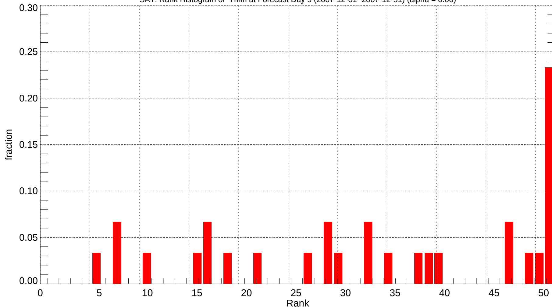
SAT: Rank Histogram of Tmin at Forecast Day 9 (2007-12-01~2007-12-31) (alpha = 0.00)
