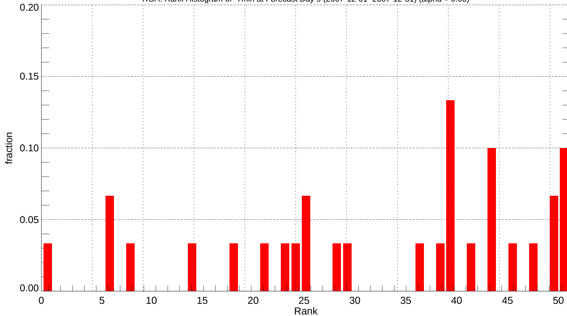
ROA: Rank Histogram of Tmin at Forecast Day 9 (2007-12-01~2007-12-31) (alpha = 0.00)
