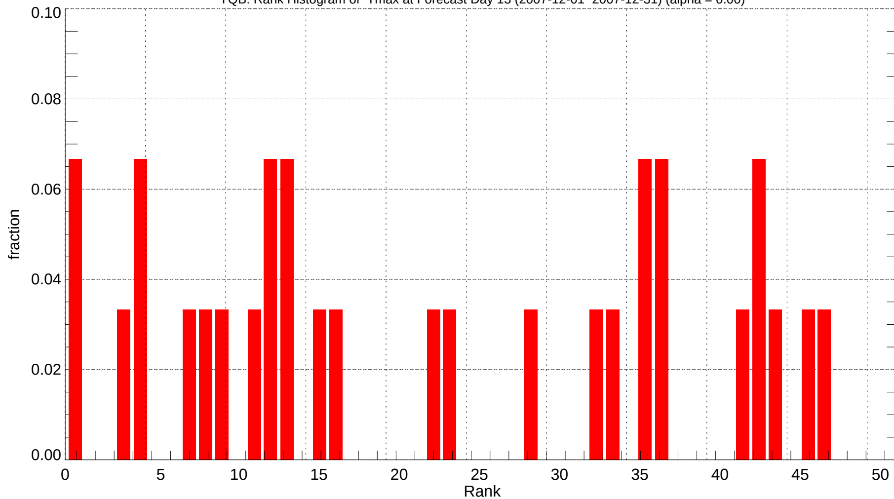
YQB: Rank Histogram of Tmax at Forecast Day 13 (2007-12-01~2007-12-31) (alpha = 0.00)
