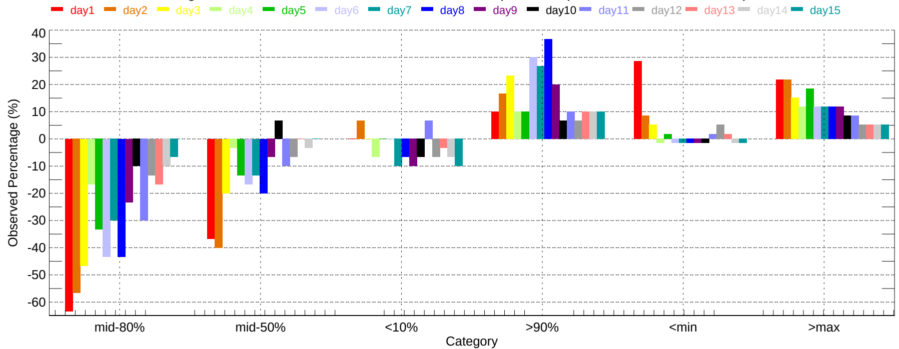
Observed Percentage Deviation of Ensembles - NTU: Max Temperature (2007-12-01~2007-12-31)
