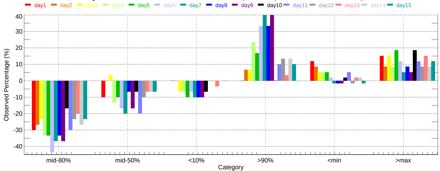
Observed Percentage Deviation of Ensembles - SAV: Min Temperature (2007-12-01~2007-12-31)
