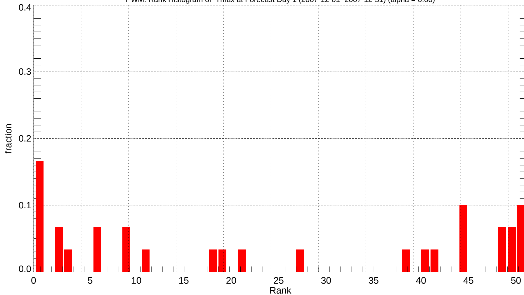
PWM: Rank Histogram of Tmax at Forecast Day 1 (2007-12-01~2007-12-31) (alpha = 0.00)
