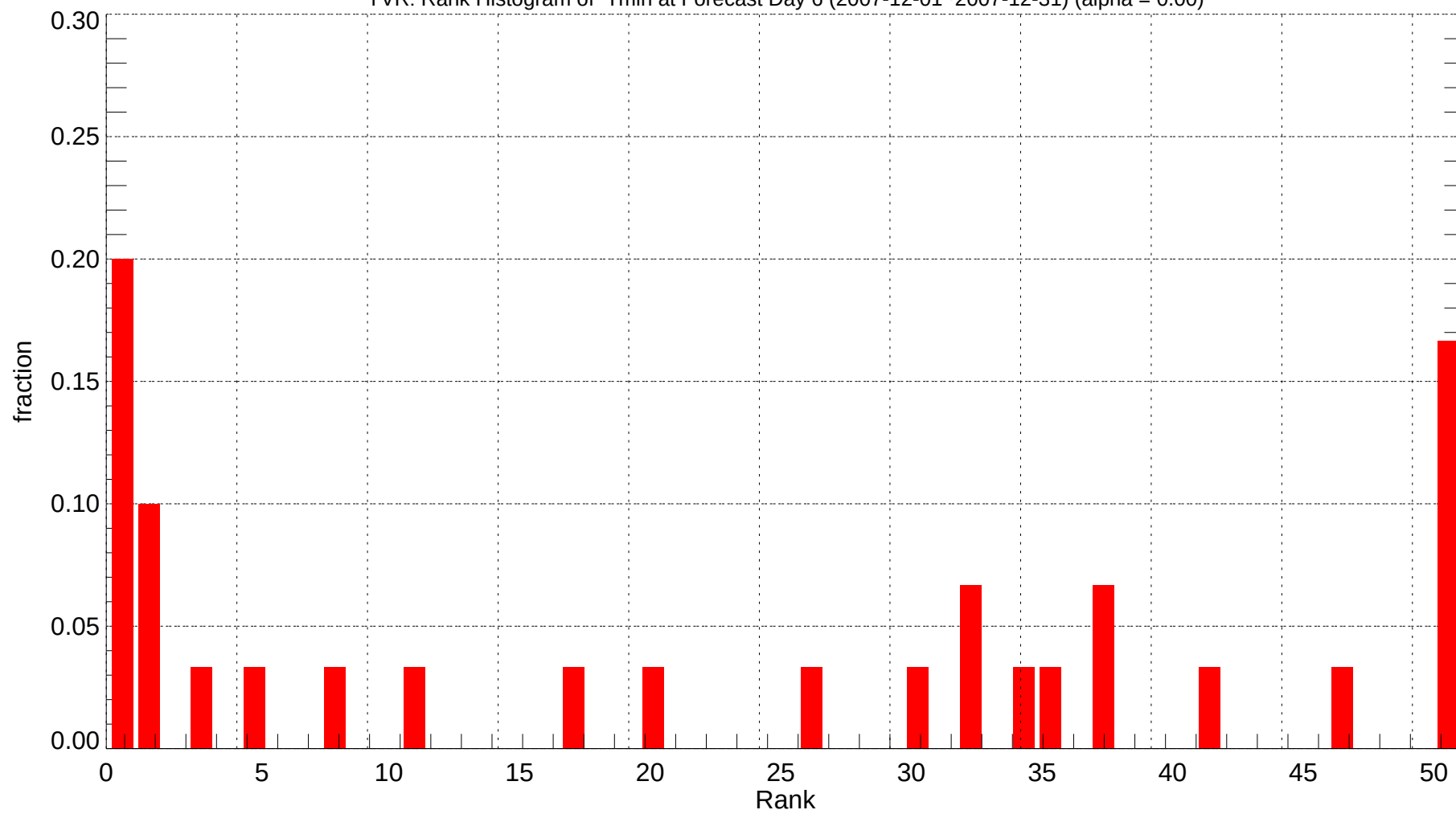
YVR: Rank Histogram of Tmin at Forecast Day 6 (2007-12-01~2007-12-31) (alpha = 0.00)
