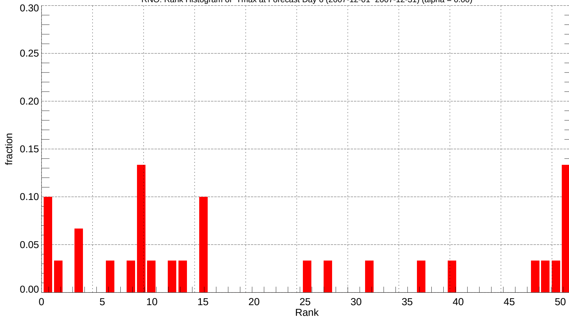
RNO: Rank Histogram of Tmax at Forecast Day 6 (2007-12-01~2007-12-31) (alpha = 0.00)
