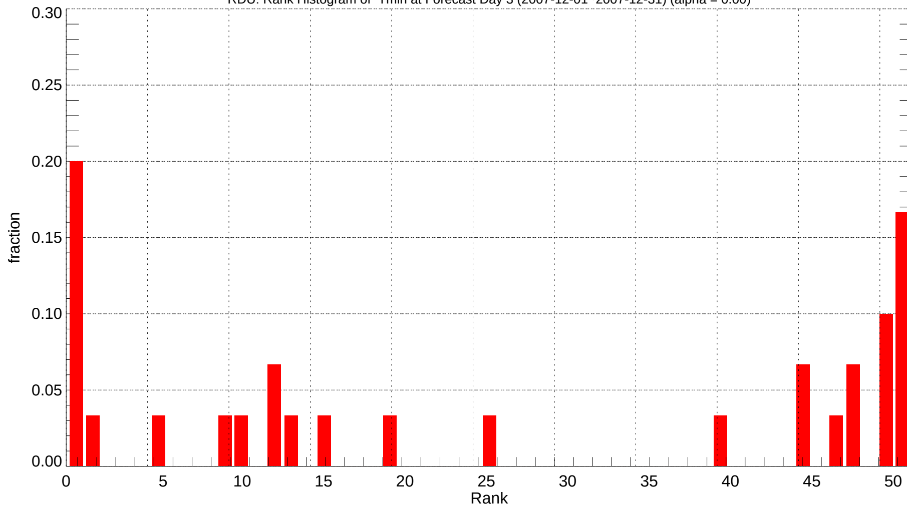
RDU: Rank Histogram of Tmin at Forecast Day 3 (2007-12-01~2007-12-31) (alpha = 0.00)
