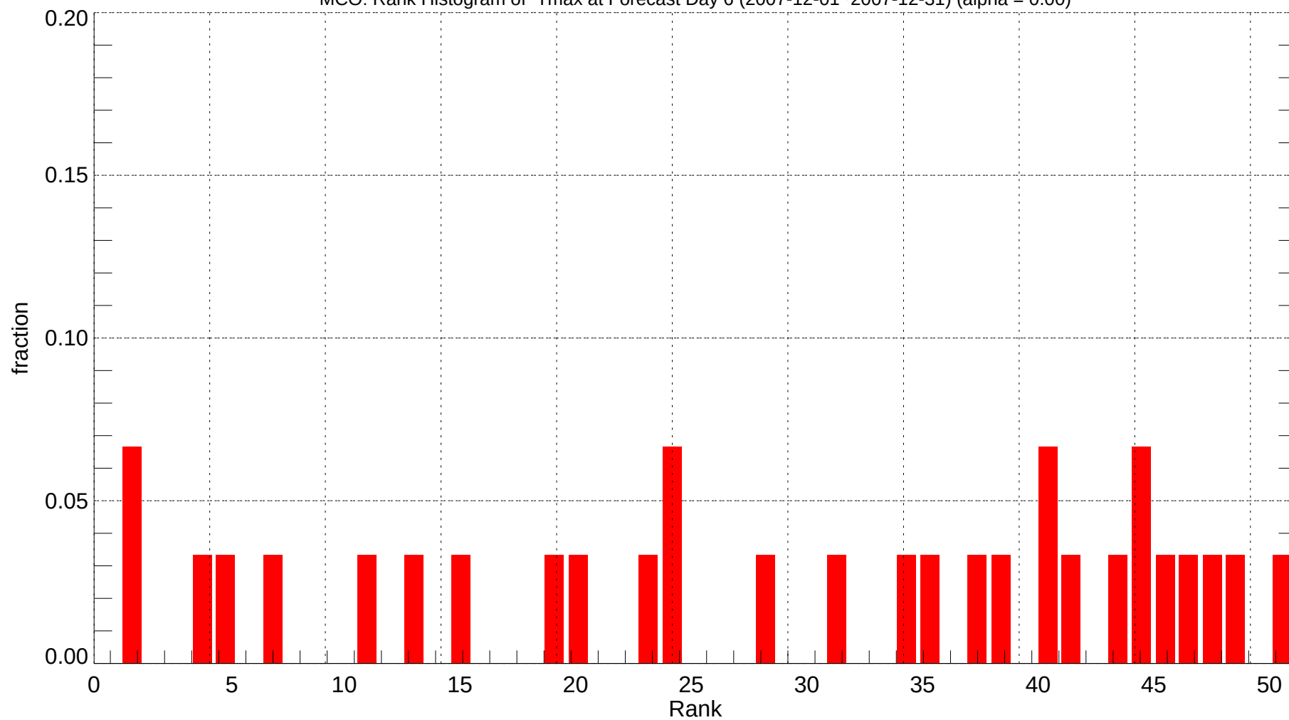
MCO: Rank Histogram of Tmax at Forecast Day 6 (2007-12-01~2007-12-31) (alpha = 0.00)
