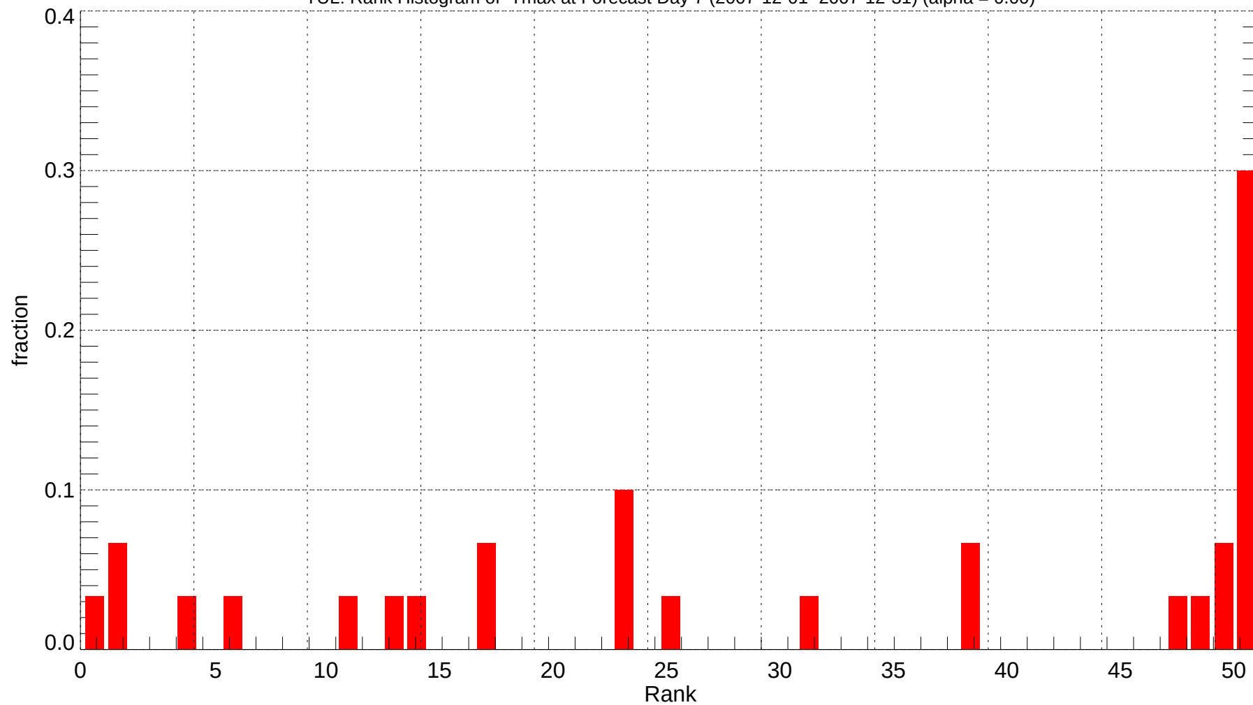
TUL: Rank Histogram of Tmax at Forecast Day 7 (2007-12-01~2007-12-31) (alpha = 0.00)
