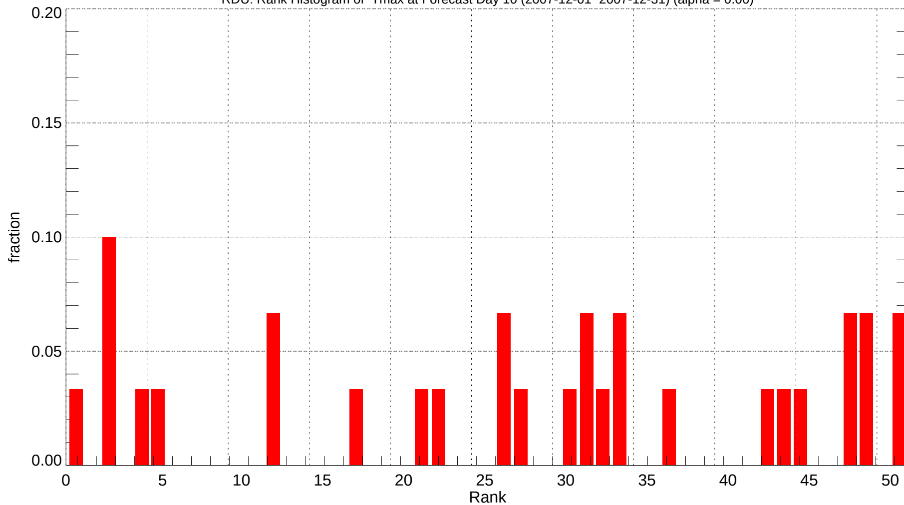
RDU: Rank Histogram of Tmax at Forecast Day 10 (2007-12-01~2007-12-31) (alpha = 0.00)
