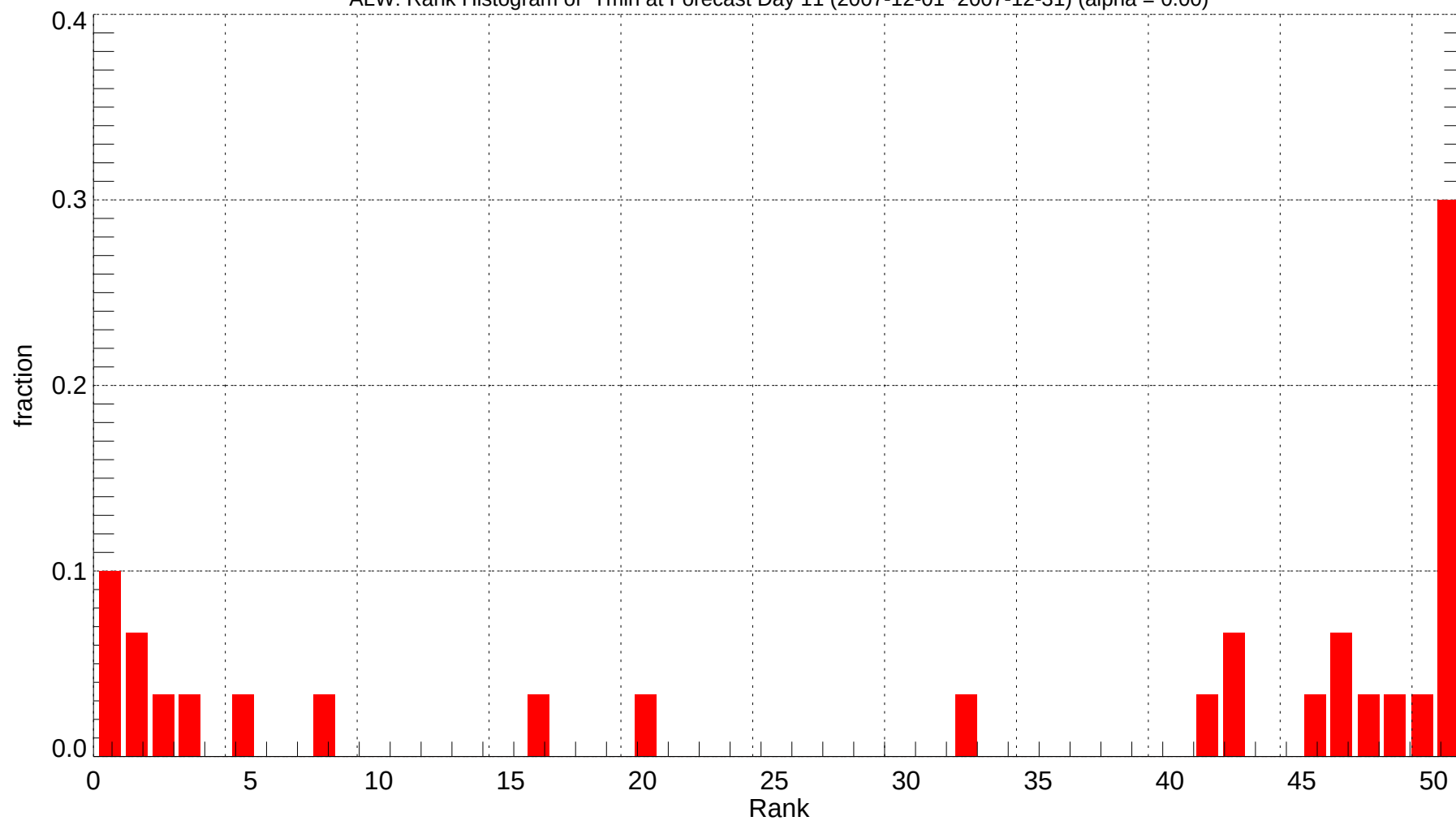
ALW: Rank Histogram of Tmin at Forecast Day 11 (2007-12-01~2007-12-31) (alpha = 0.00)
