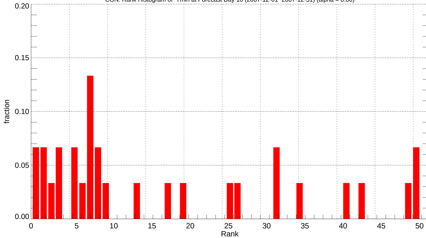
CON: Rank Histogram of Tmin at Forecast Day 10 (2007-12-01~2007-12-31) (alpha = 0.00)
