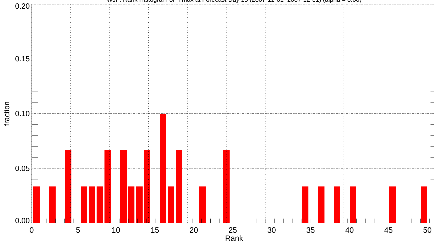
WJF: Rank Histogram of Tmax at Forecast Day 15 (2007-12-01~2007-12-31) (alpha = 0.00)
