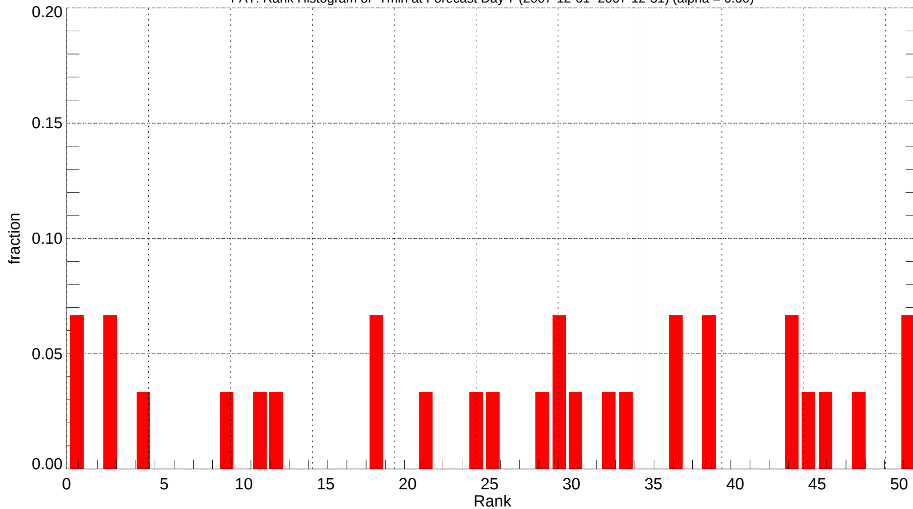
FAT: Rank Histogram of Tmin at Forecast Day 7 (2007-12-01~2007-12-31) (alpha = 0.00)
