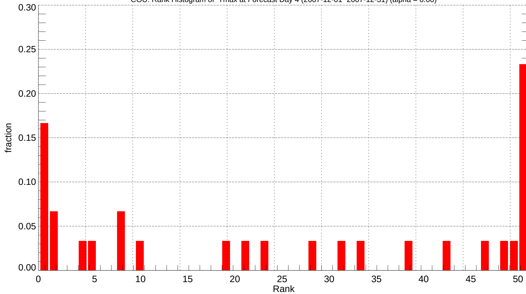
COU: Rank Histogram of Tmax at Forecast Day 4 (2007-12-01~2007-12-31) (alpha = 0.00)
