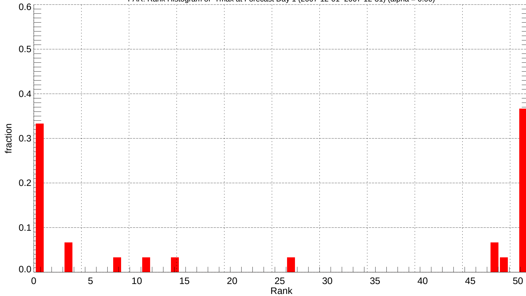
FAR: Rank Histogram of Tmax at Forecast Day 1 (2007-12-01~2007-12-31) (alpha = 0.00)
