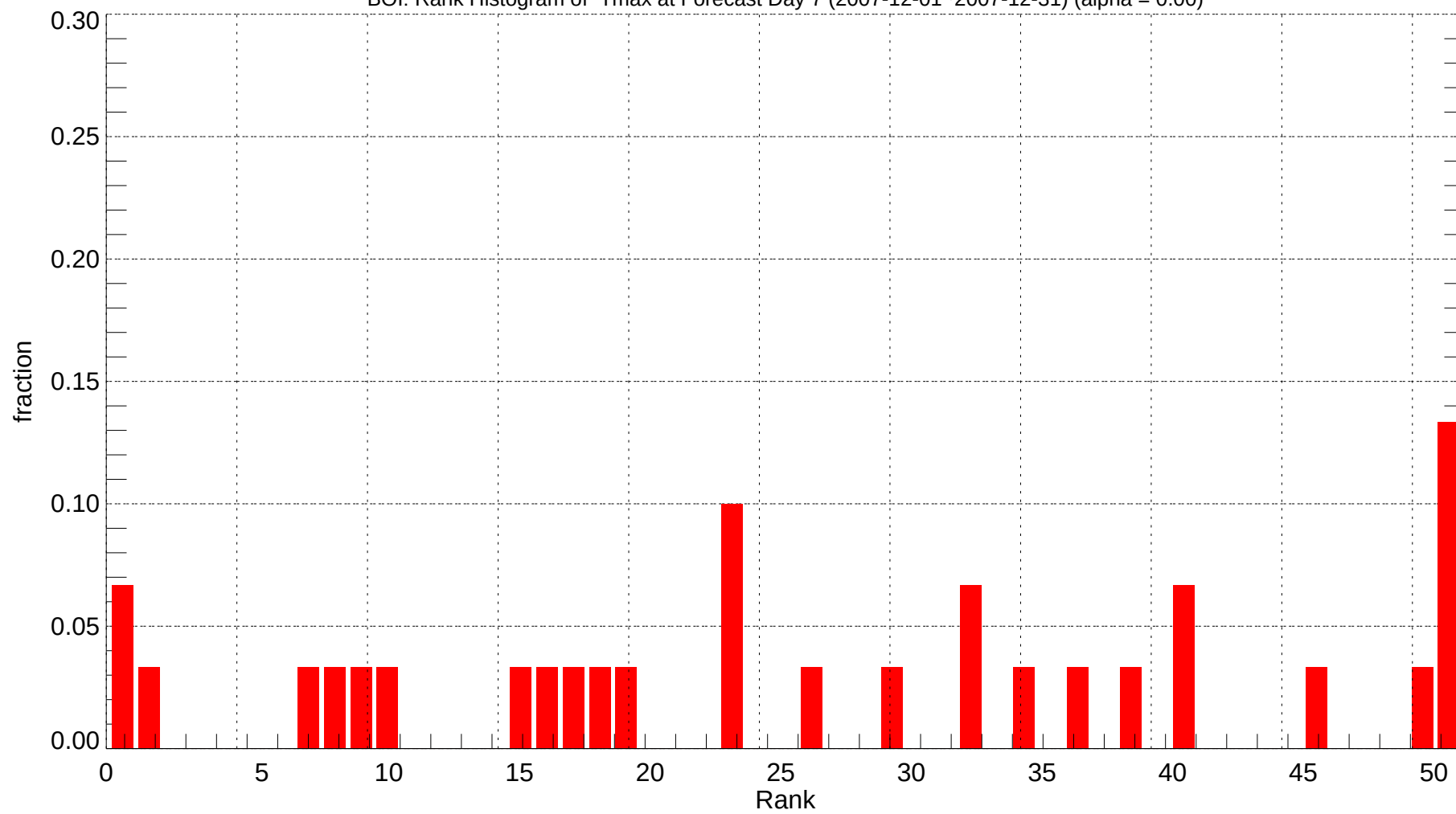
BOI: Rank Histogram of Tmax at Forecast Day 7 (2007-12-01~2007-12-31) (alpha = 0.00)
