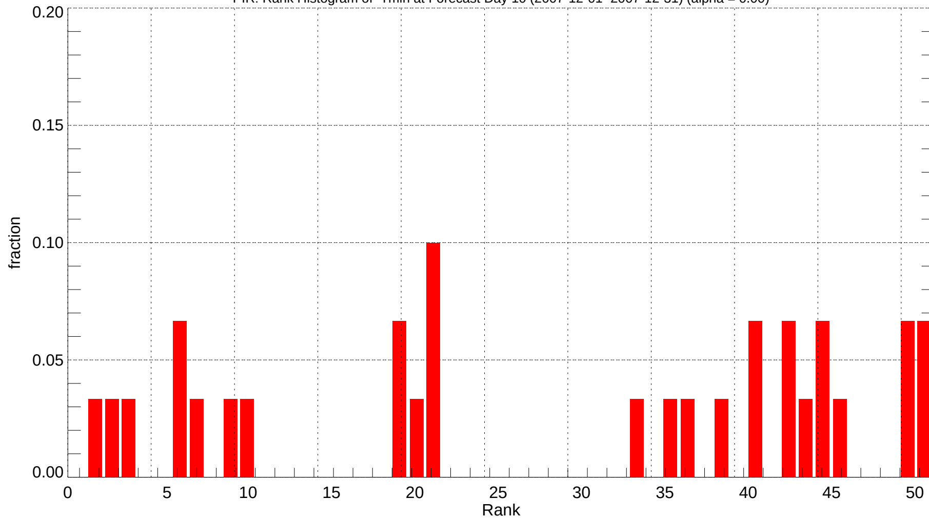
PIR: Rank Histogram of Tmin at Forecast Day 10 (2007-12-01~2007-12-31) (alpha = 0.00)
