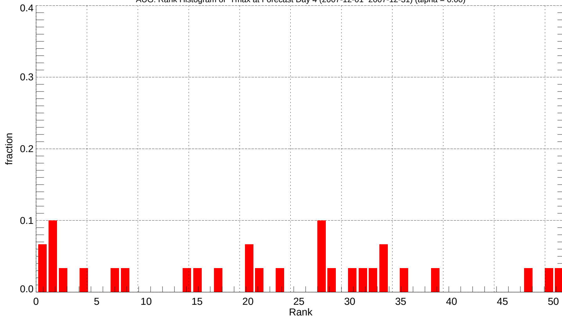
AUG: Rank Histogram of Tmax at Forecast Day 4 (2007-12-01~2007-12-31) (alpha = 0.00)
