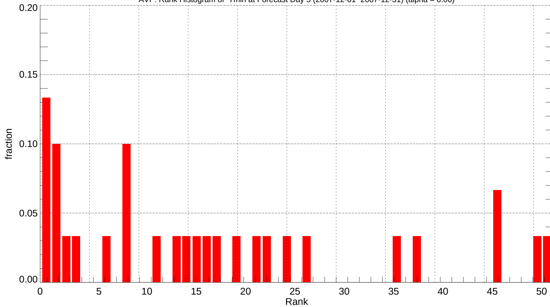
AVP: Rank Histogram of Tmin at Forecast Day 5 (2007-12-01~2007-12-31) (alpha = 0.00)
