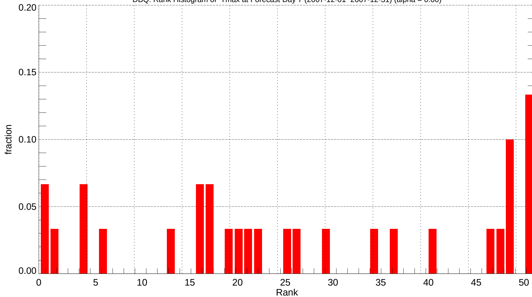
DBQ: Rank Histogram of Tmax at Forecast Day 7 (2007-12-01~2007-12-31) (alpha = 0.00)
