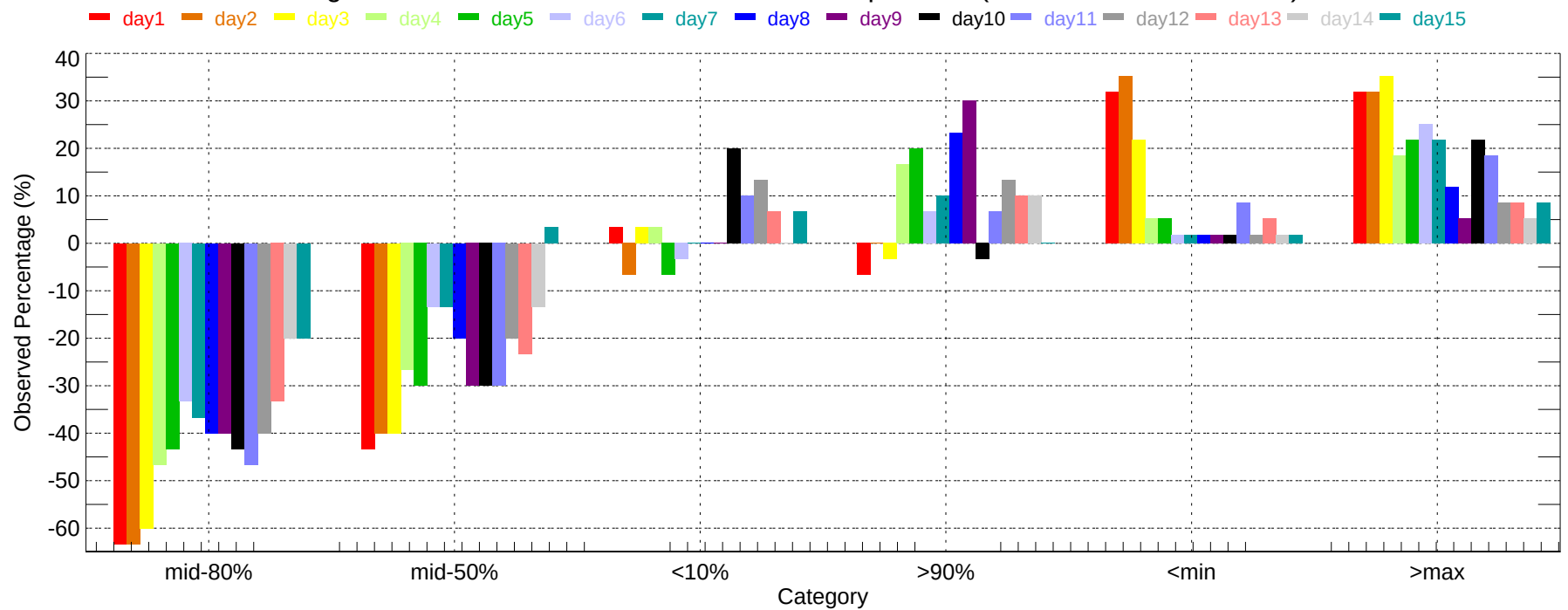
Observed Percentage Deviation of Ensembles - TUL: Max Temperature (2007-12-01~2007-12-31)
