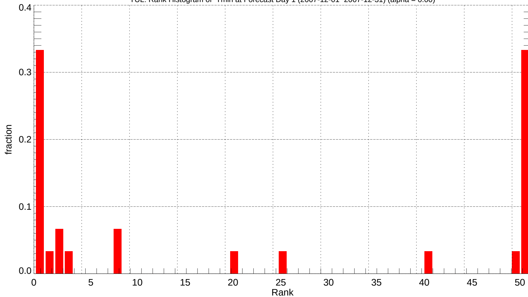
TUL: Rank Histogram of Tmin at Forecast Day 1 (2007-12-01~2007-12-31) (alpha = 0.00)
