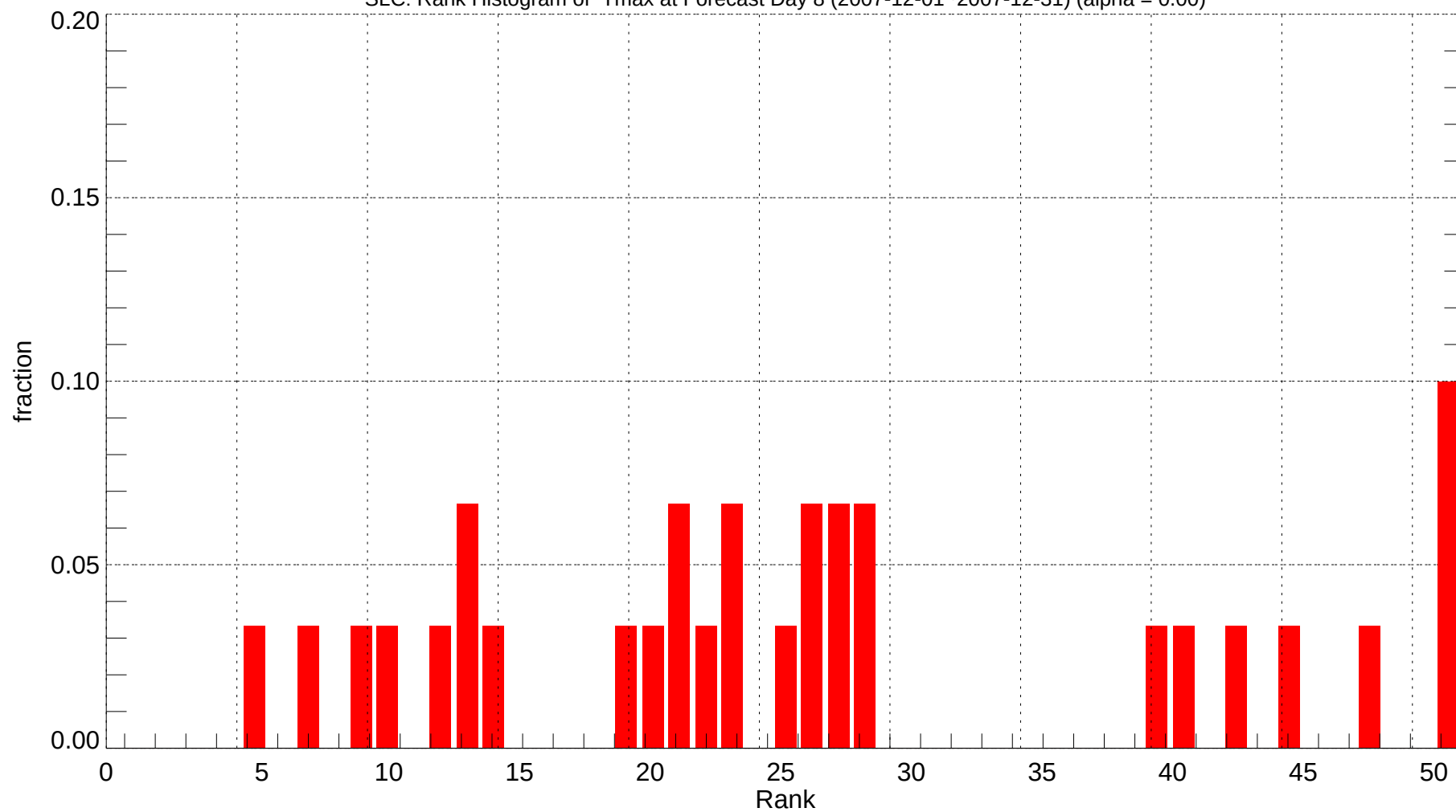
SLC: Rank Histogram of Tmax at Forecast Day 8 (2007-12-01~2007-12-31) (alpha = 0.00)
