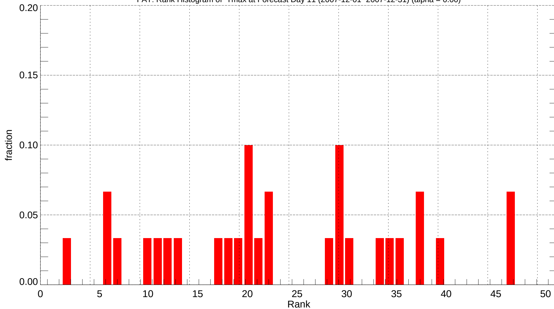
FAT: Rank Histogram of Tmax at Forecast Day 11 (2007-12-01~2007-12-31) (alpha = 0.00)
