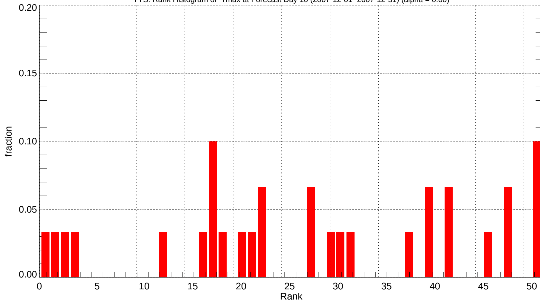
TYS: Rank Histogram of Tmax at Forecast Day 10 (2007-12-01~2007-12-31) (alpha = 0.00)
