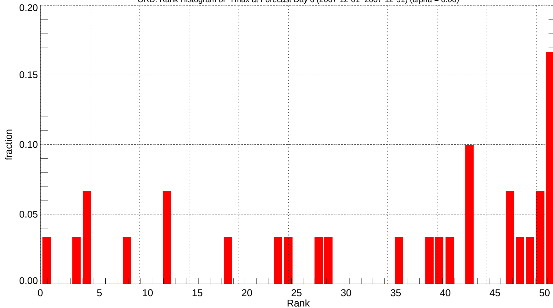
ORD: Rank Histogram of Tmax at Forecast Day 6 (2007-12-01~2007-12-31) (alpha = 0.00)
