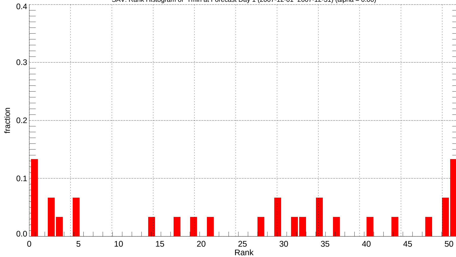
SAV: Rank Histogram of Tmin at Forecast Day 1 (2007-12-01~2007-12-31) (alpha = 0.00)
