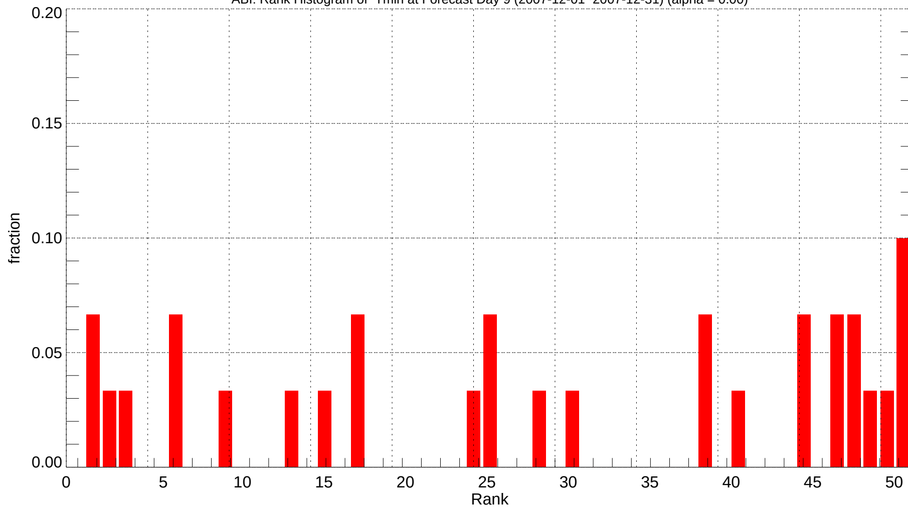
ABI: Rank Histogram of Tmin at Forecast Day 9 (2007-12-01~2007-12-31) (alpha = 0.00)
