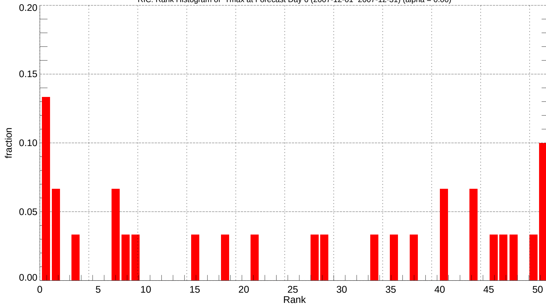
RIC: Rank Histogram of Tmax at Forecast Day 6 (2007-12-01~2007-12-31) (alpha = 0.00)
