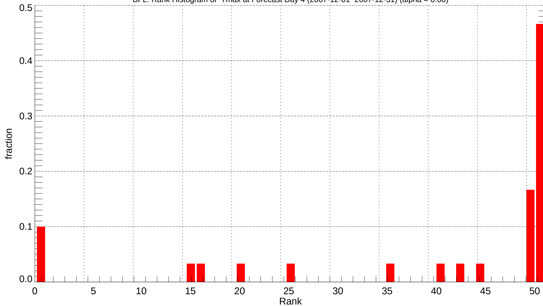
BFL: Rank Histogram of Tmax at Forecast Day 4 (2007-12-01~2007-12-31) (alpha = 0.00)
