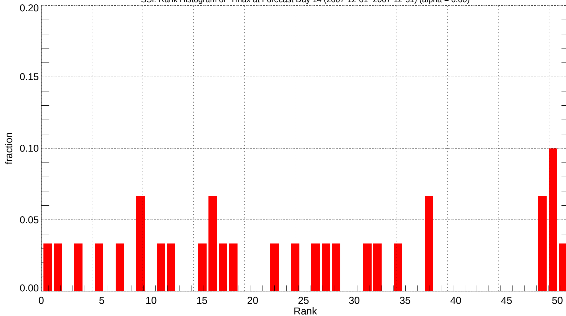
SSI: Rank Histogram of Tmax at Forecast Day 14 (2007-12-01~2007-12-31) (alpha = 0.00)
