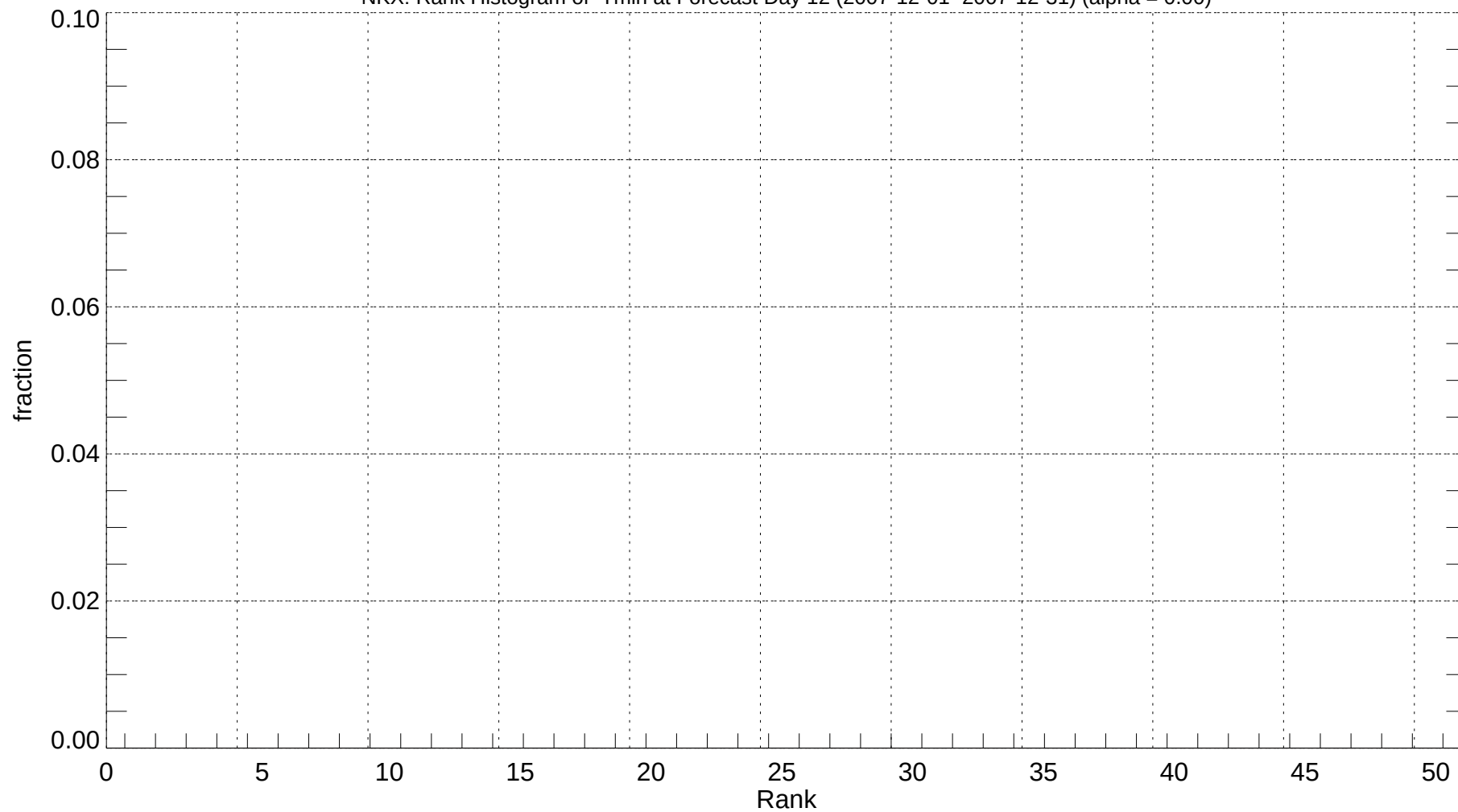
NKX: Rank Histogram of Tmin at Forecast Day 12 (2007-12-01~2007-12-31) (alpha = 0.00)
