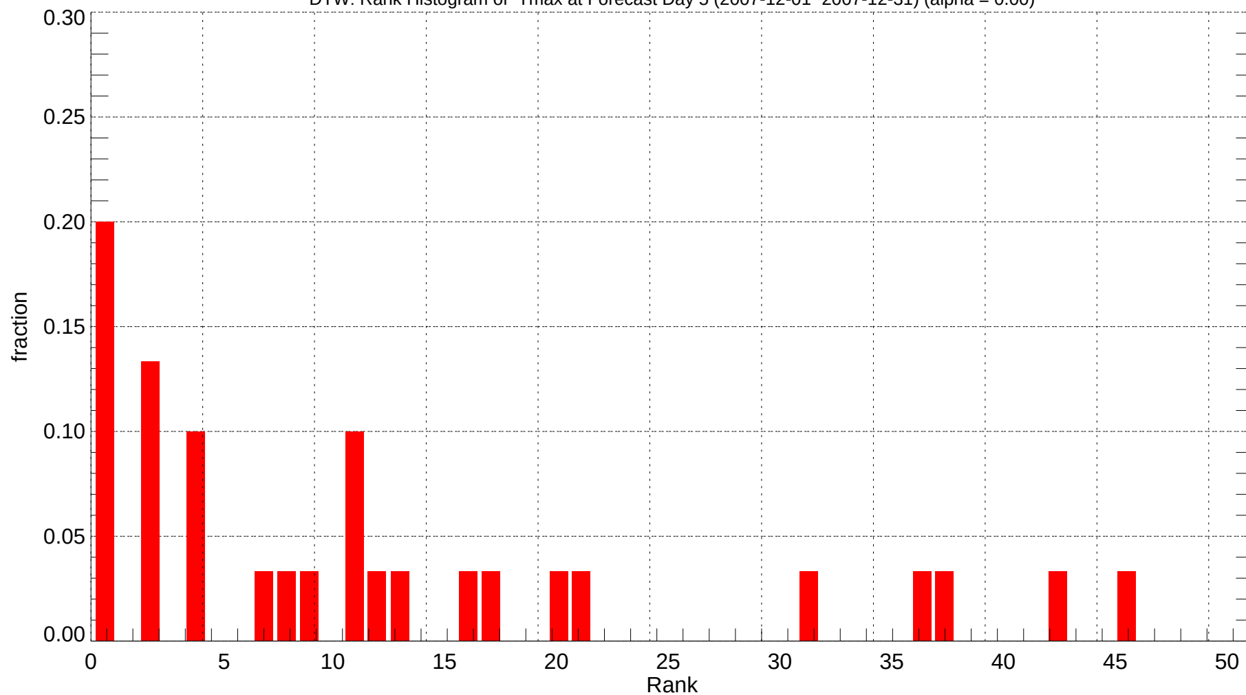
DTW: Rank Histogram of Tmax at Forecast Day 5 (2007-12-01~2007-12-31) (alpha = 0.00)
