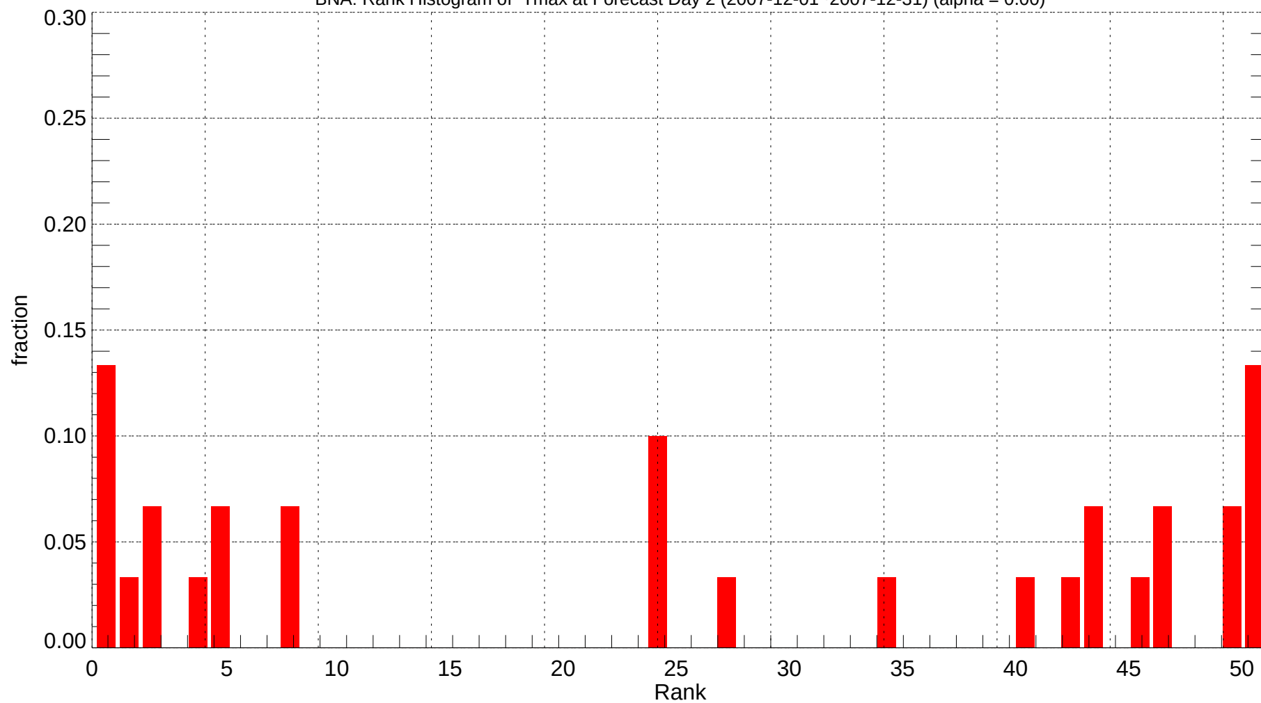
BNA: Rank Histogram of Tmax at Forecast Day 2 (2007-12-01~2007-12-31) (alpha = 0.00)
