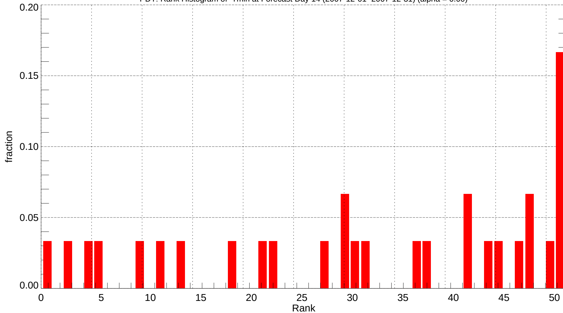
PDT: Rank Histogram of Tmin at Forecast Day 14 (2007-12-01~2007-12-31) (alpha = 0.00)
