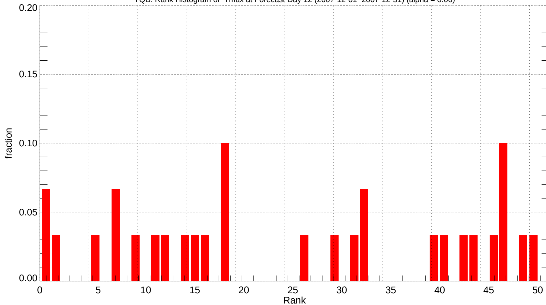
YQB: Rank Histogram of Tmax at Forecast Day 12 (2007-12-01~2007-12-31) (alpha = 0.00)
