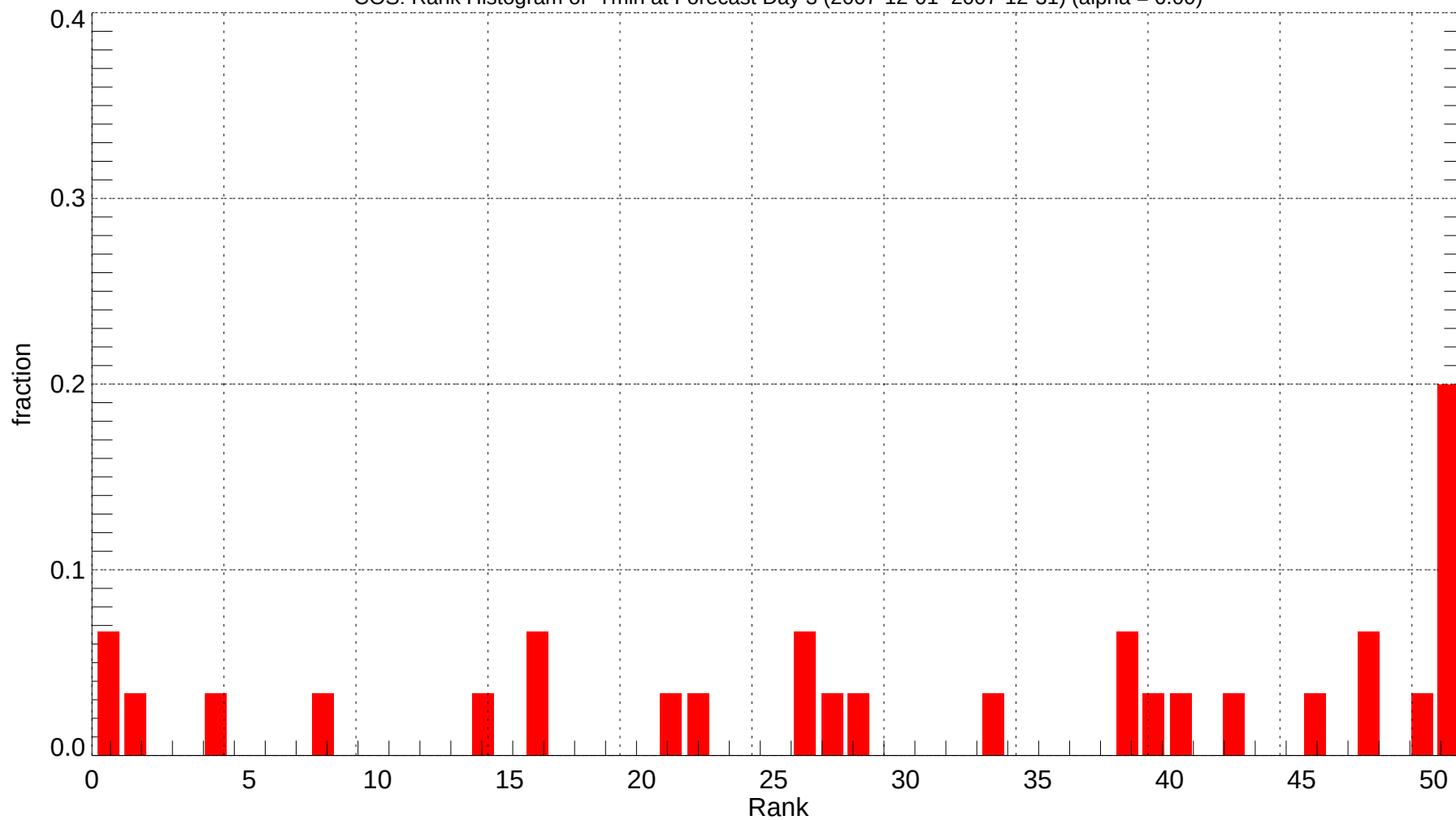
COS: Rank Histogram of Tmin at Forecast Day 3 (2007-12-01~2007-12-31) (alpha = 0.00)
