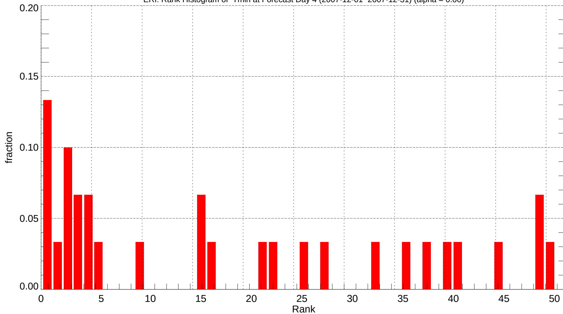
ERI: Rank Histogram of Tmin at Forecast Day 4 (2007-12-01~2007-12-31) (alpha = 0.00)
