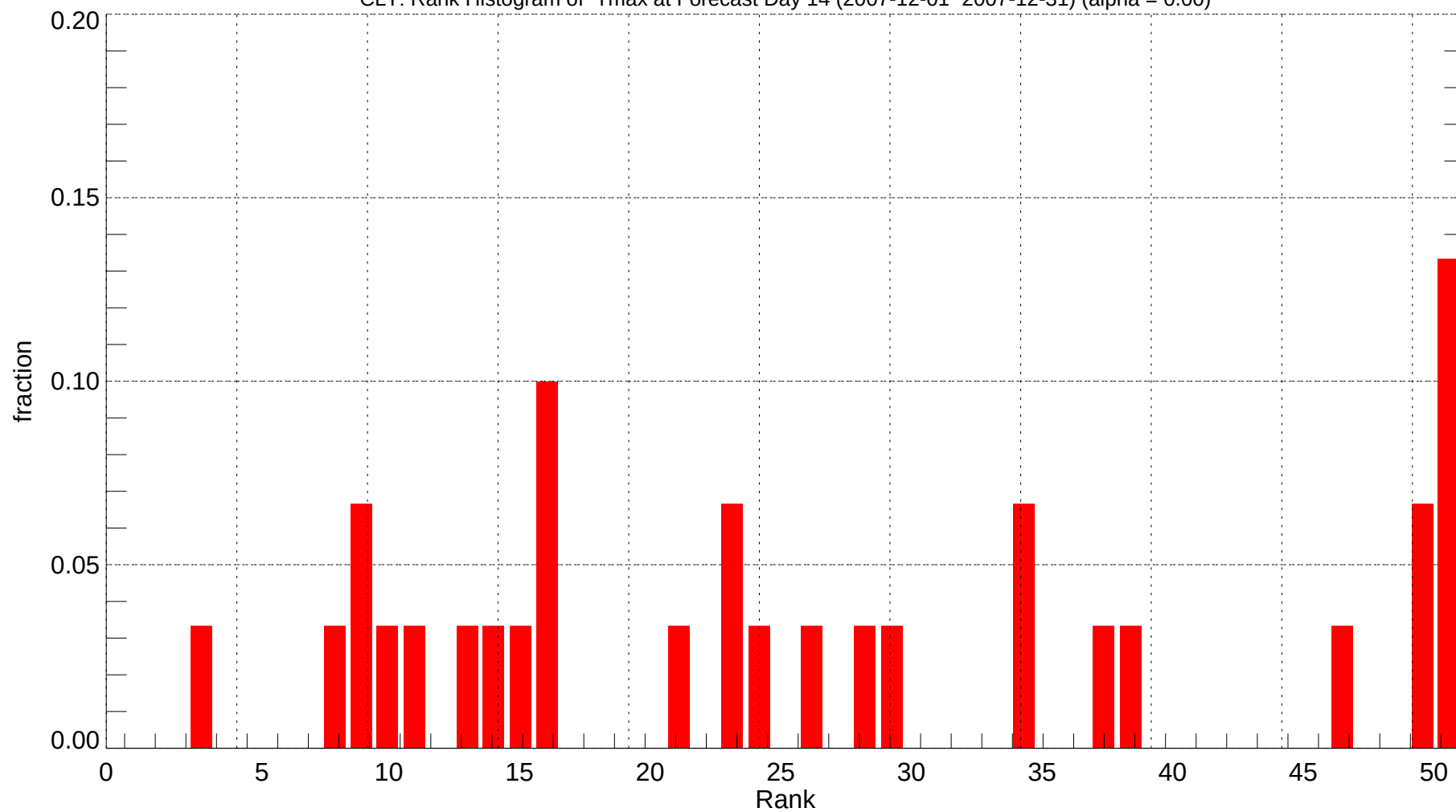
CLT: Rank Histogram of Tmax at Forecast Day 14 (2007-12-01~2007-12-31) (alpha = 0.00)
