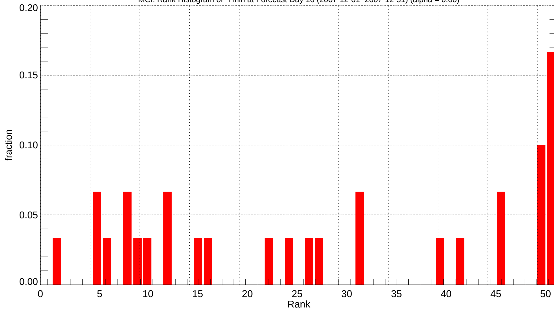
MCI: Rank Histogram of Tmin at Forecast Day 10 (2007-12-01~2007-12-31) (alpha = 0.00)
