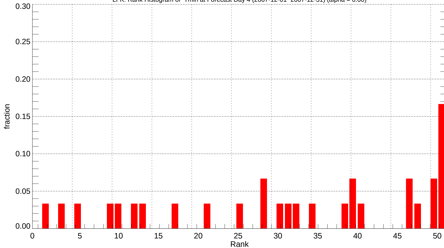
LFK: Rank Histogram of Tmin at Forecast Day 4 (2007-12-01~2007-12-31) (alpha = 0.00)
