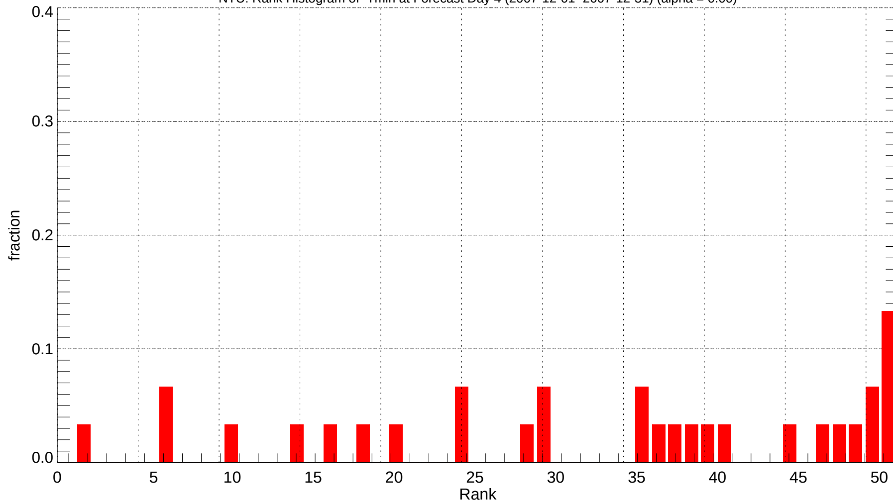
NTU: Rank Histogram of Tmin at Forecast Day 4 (2007-12-01~2007-12-31) (alpha = 0.00)
