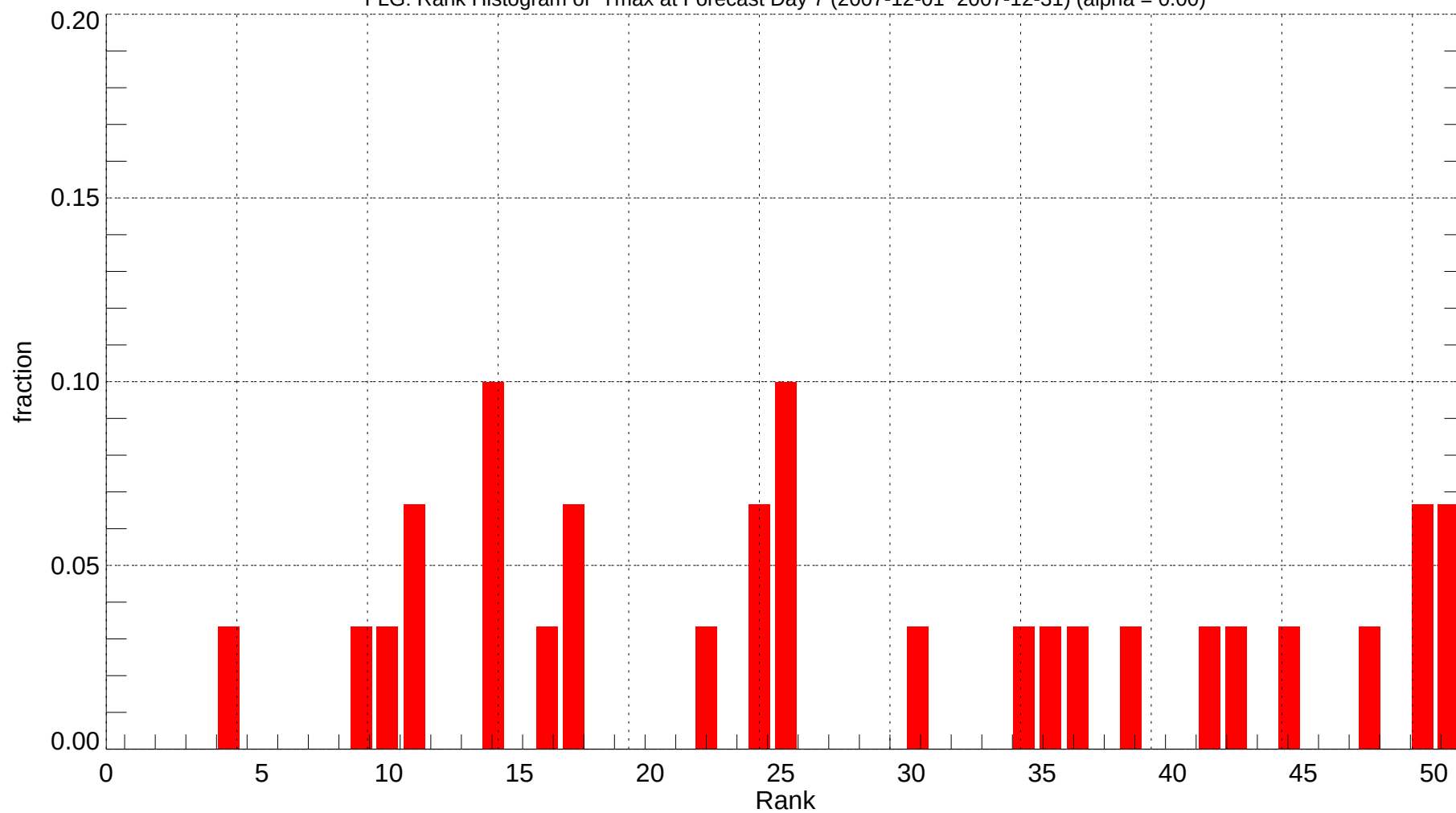
FLG: Rank Histogram of Tmax at Forecast Day 7 (2007-12-01~2007-12-31) (alpha = 0.00)
