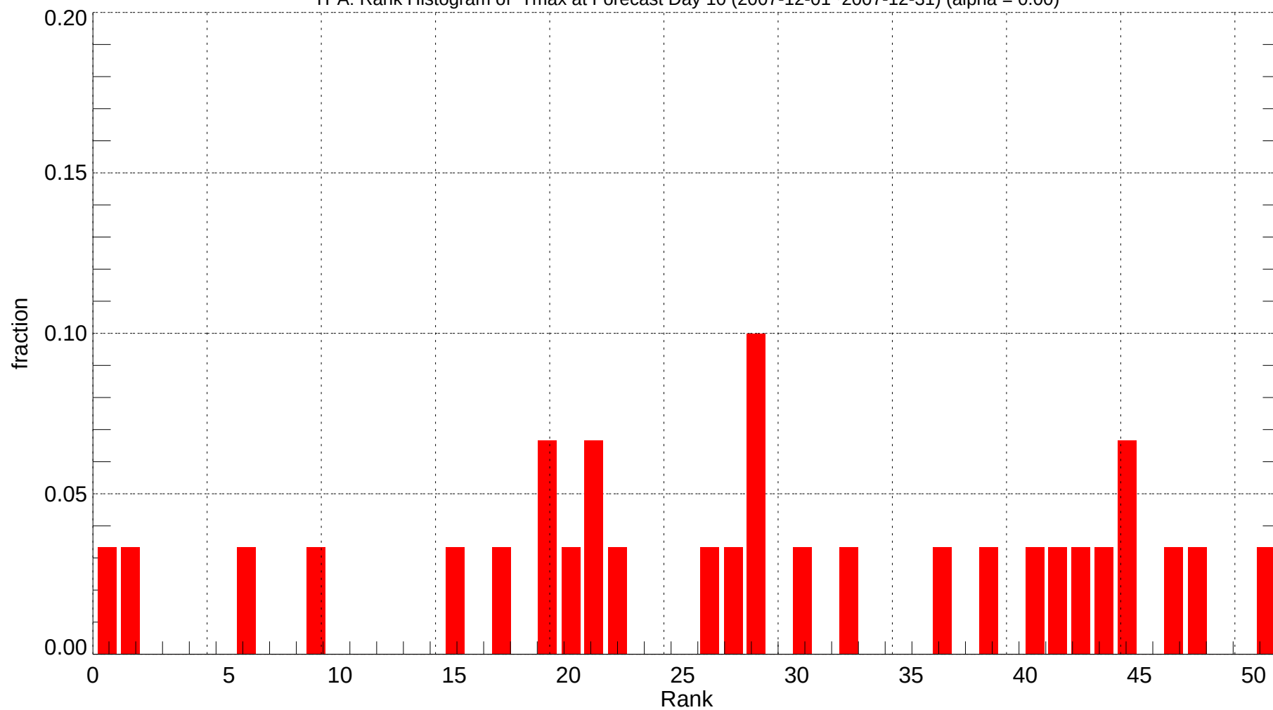
TPA: Rank Histogram of Tmax at Forecast Day 10 (2007-12-01~2007-12-31) (alpha = 0.00)
