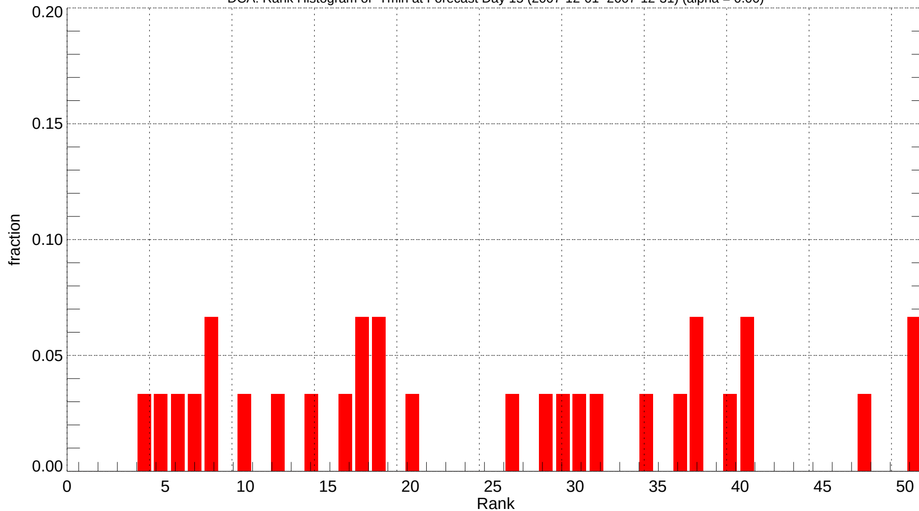
DCA: Rank Histogram of Tmin at Forecast Day 15 (2007-12-01~2007-12-31) (alpha = 0.00)
