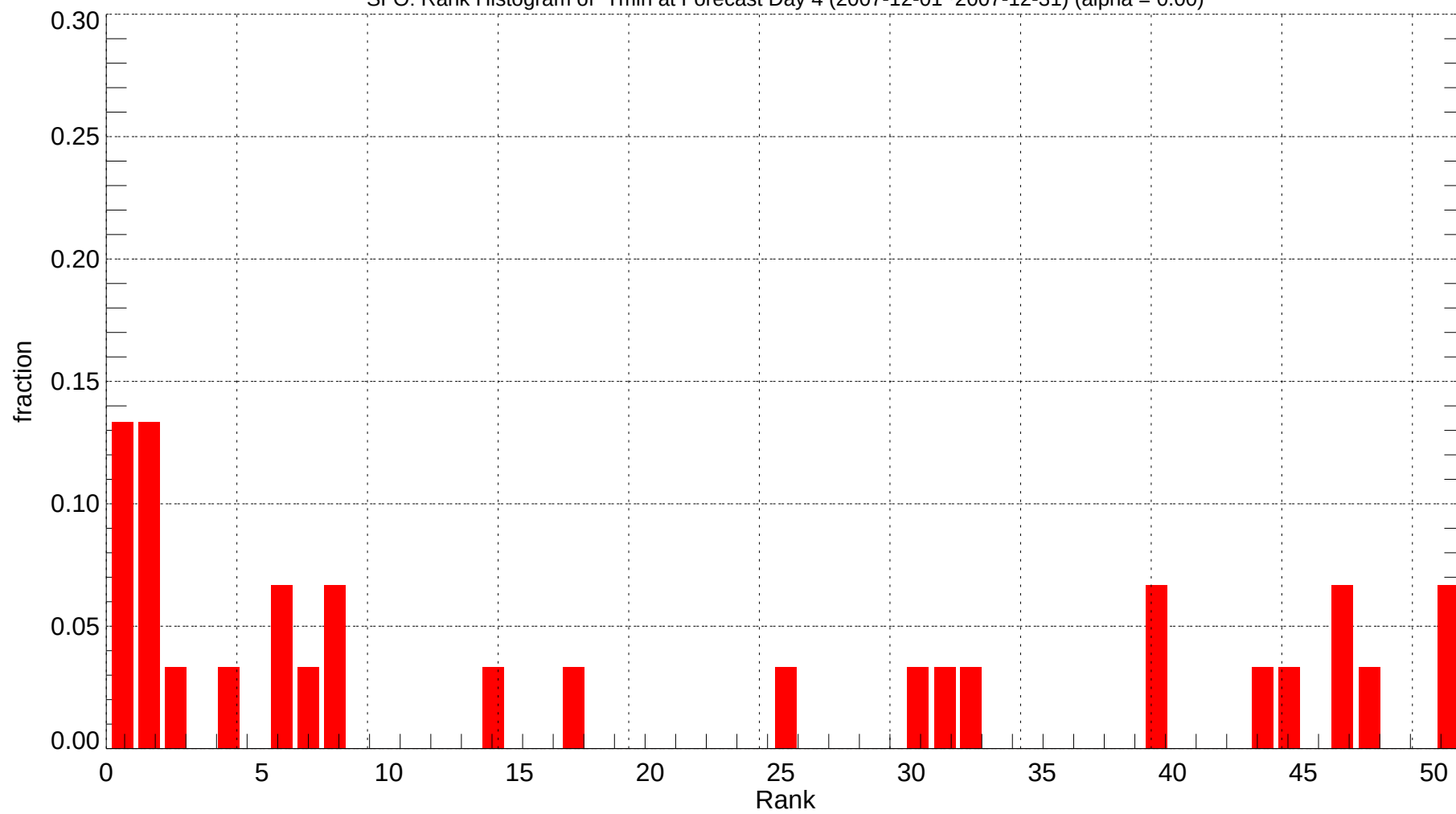
SFO: Rank Histogram of Tmin at Forecast Day 4 (2007-12-01~2007-12-31) (alpha = 0.00)
