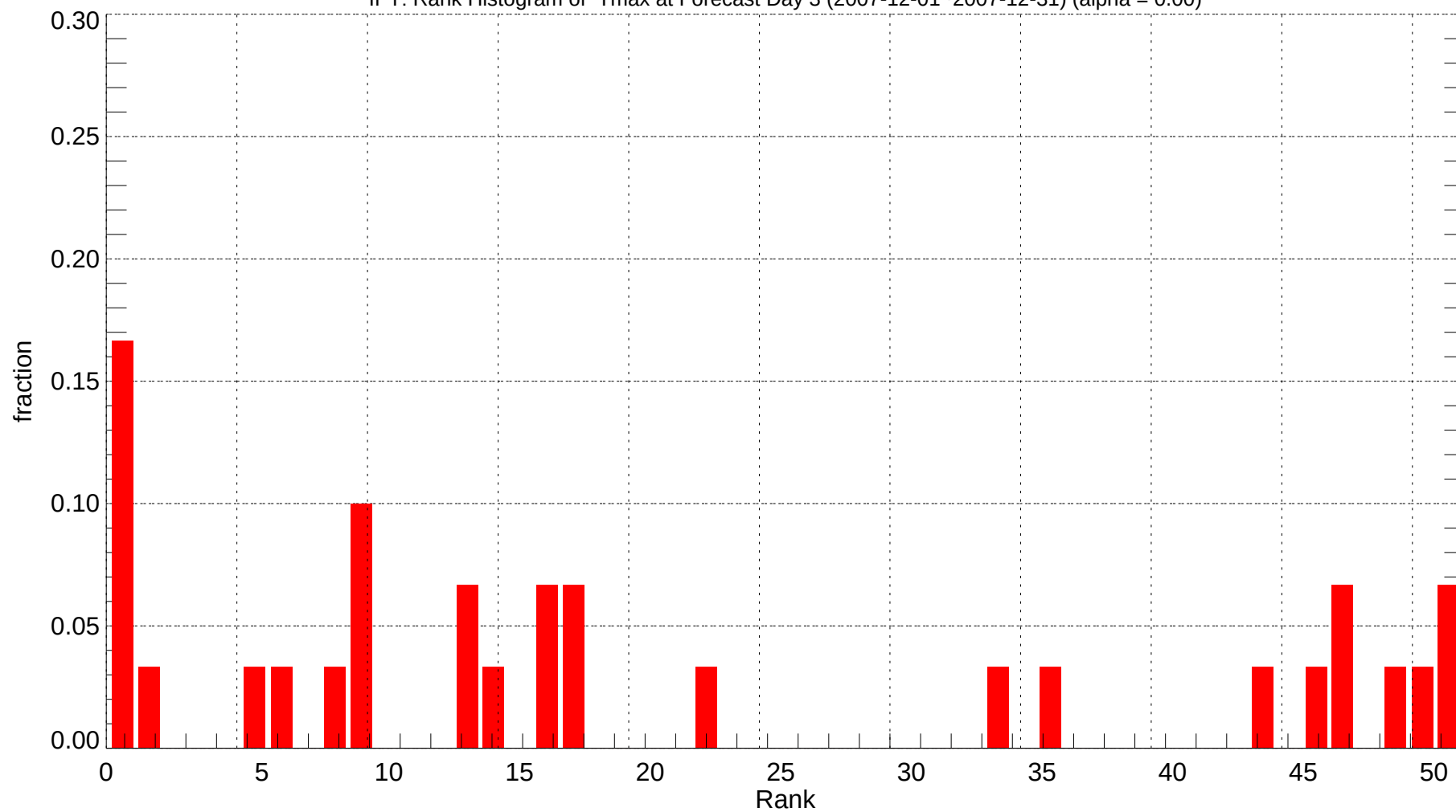
IPT: Rank Histogram of Tmax at Forecast Day 3 (2007-12-01~2007-12-31) (alpha = 0.00)
