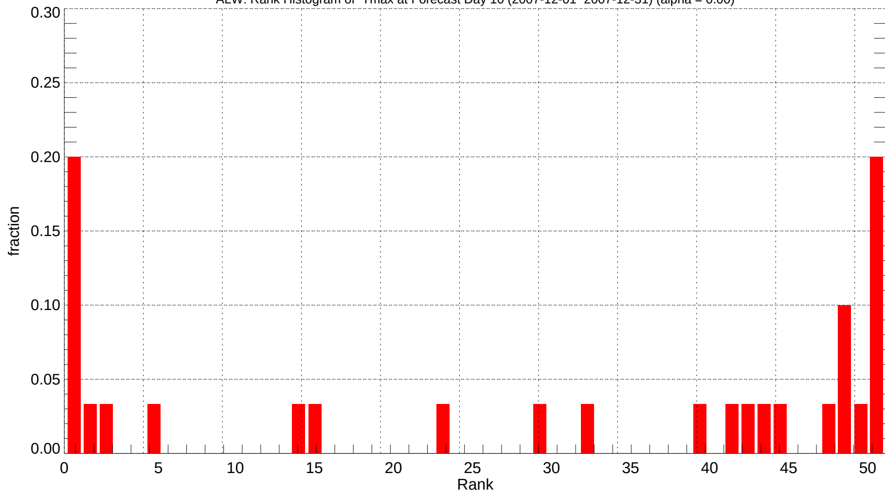
ALW: Rank Histogram of Tmax at Forecast Day 10 (2007-12-01~2007-12-31) (alpha = 0.00)
