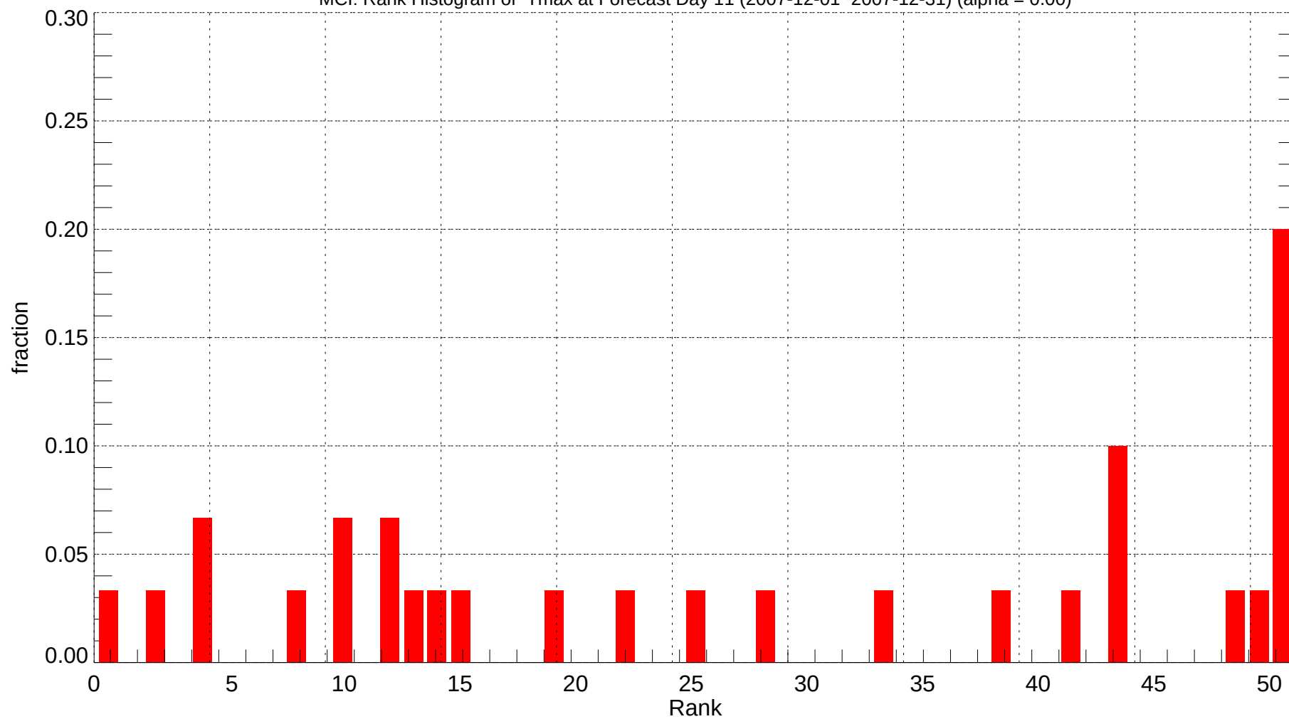
MCI: Rank Histogram of Tmax at Forecast Day 11 (2007-12-01~2007-12-31) (alpha = 0.00)
