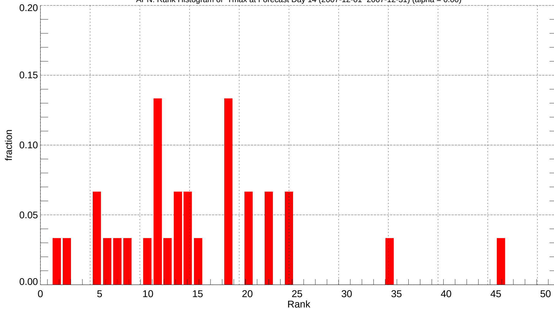
APN: Rank Histogram of Tmax at Forecast Day 14 (2007-12-01~2007-12-31) (alpha = 0.00)
