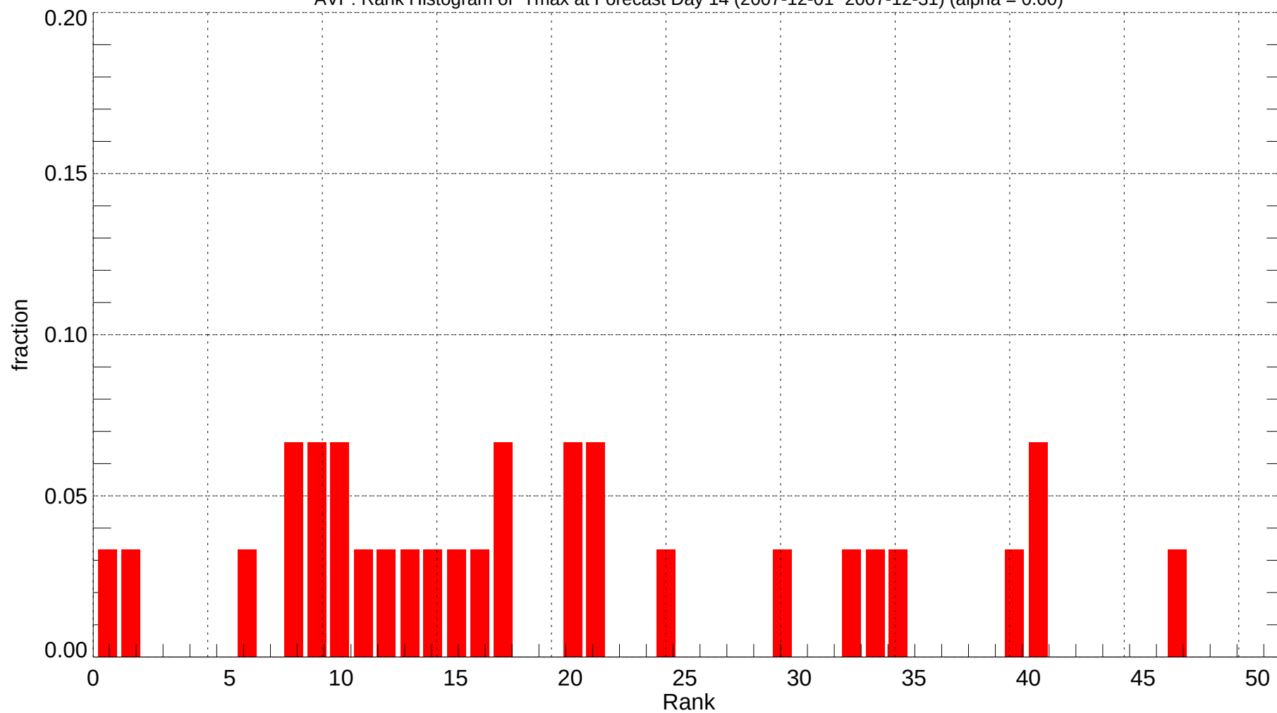
AVP: Rank Histogram of Tmax at Forecast Day 14 (2007-12-01~2007-12-31) (alpha = 0.00)
