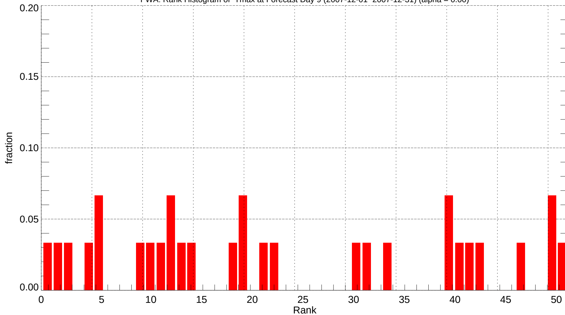
FWA: Rank Histogram of Tmax at Forecast Day 9 (2007-12-01~2007-12-31) (alpha = 0.00)
