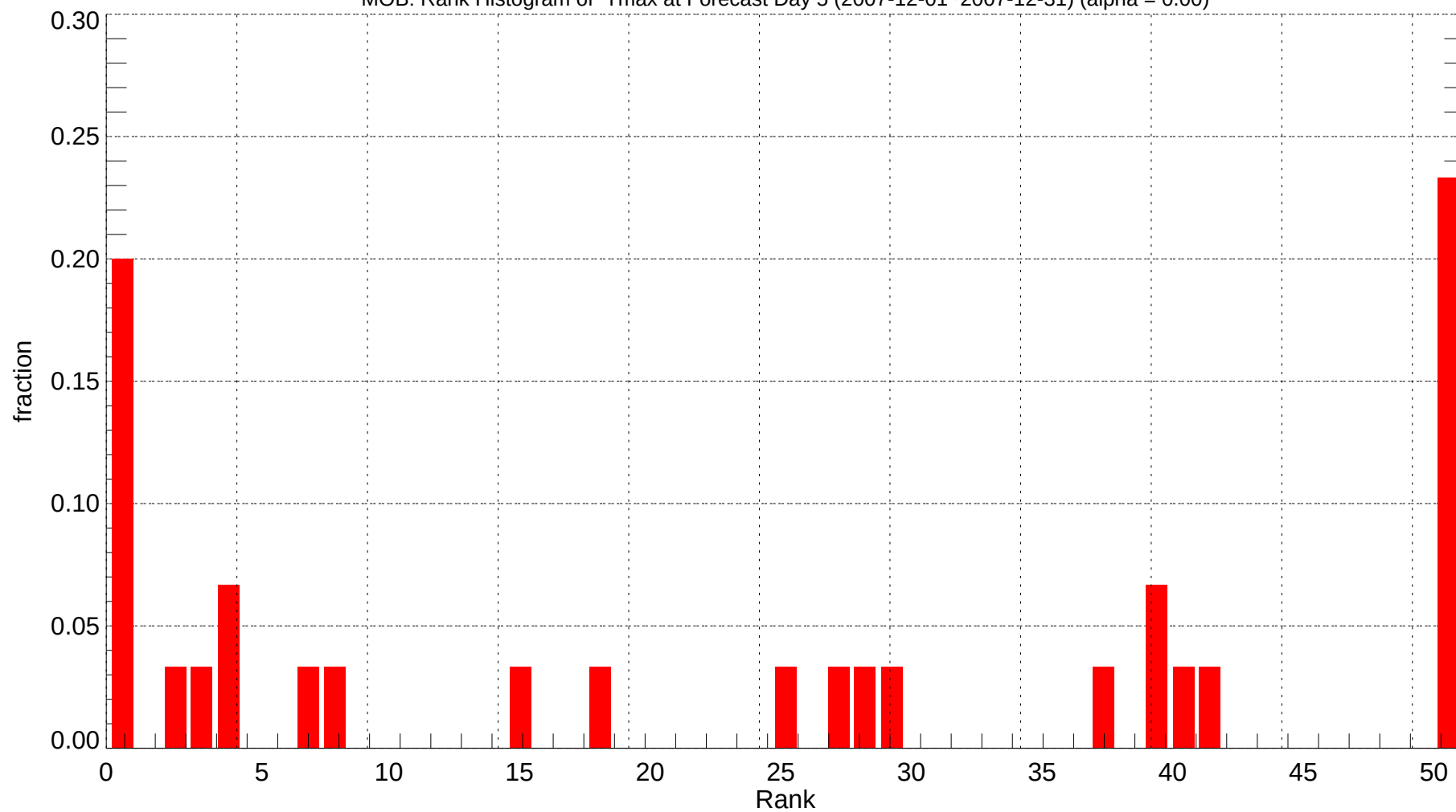
MOB: Rank Histogram of Tmax at Forecast Day 5 (2007-12-01~2007-12-31) (alpha = 0.00)
