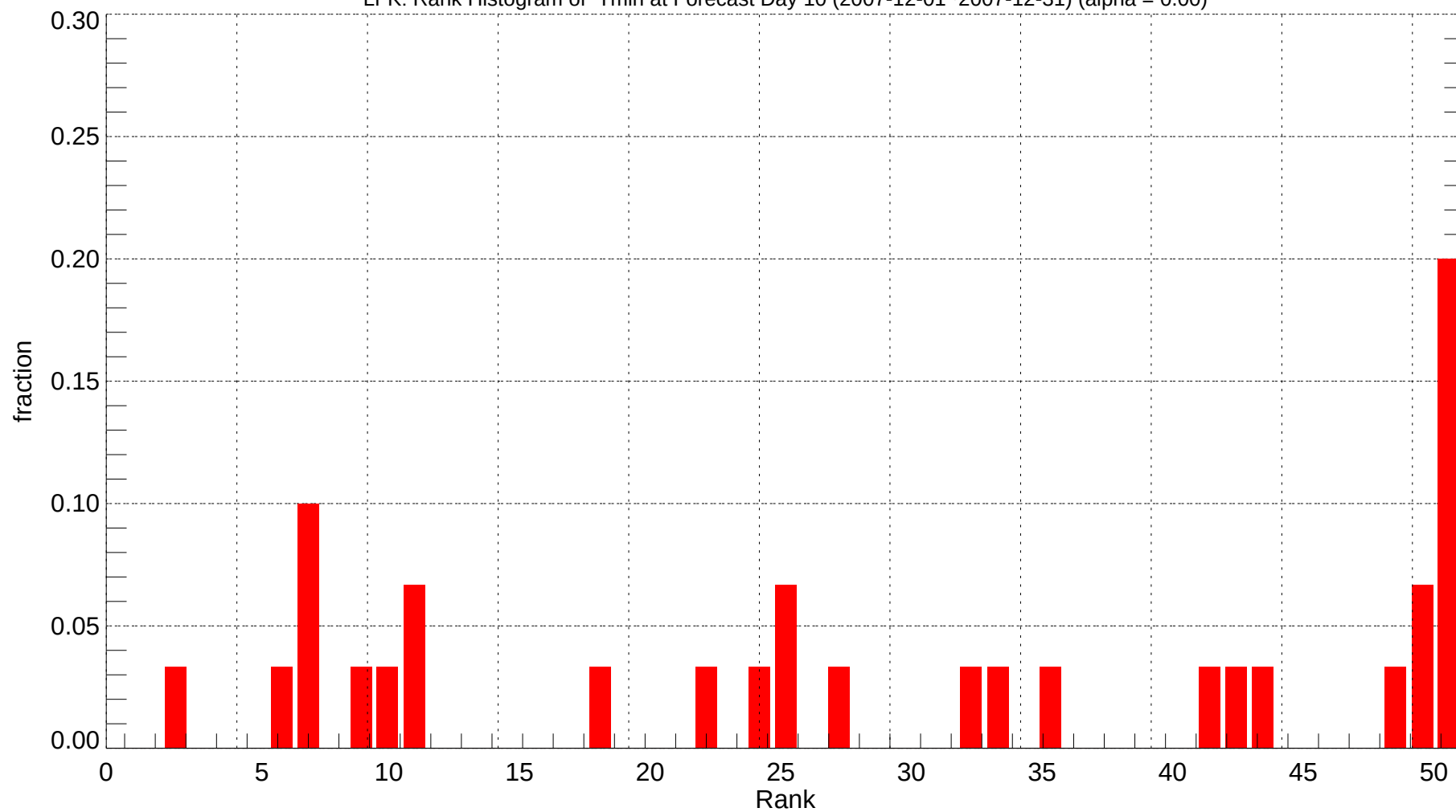
LFK: Rank Histogram of Tmin at Forecast Day 10 (2007-12-01~2007-12-31) (alpha = 0.00)
