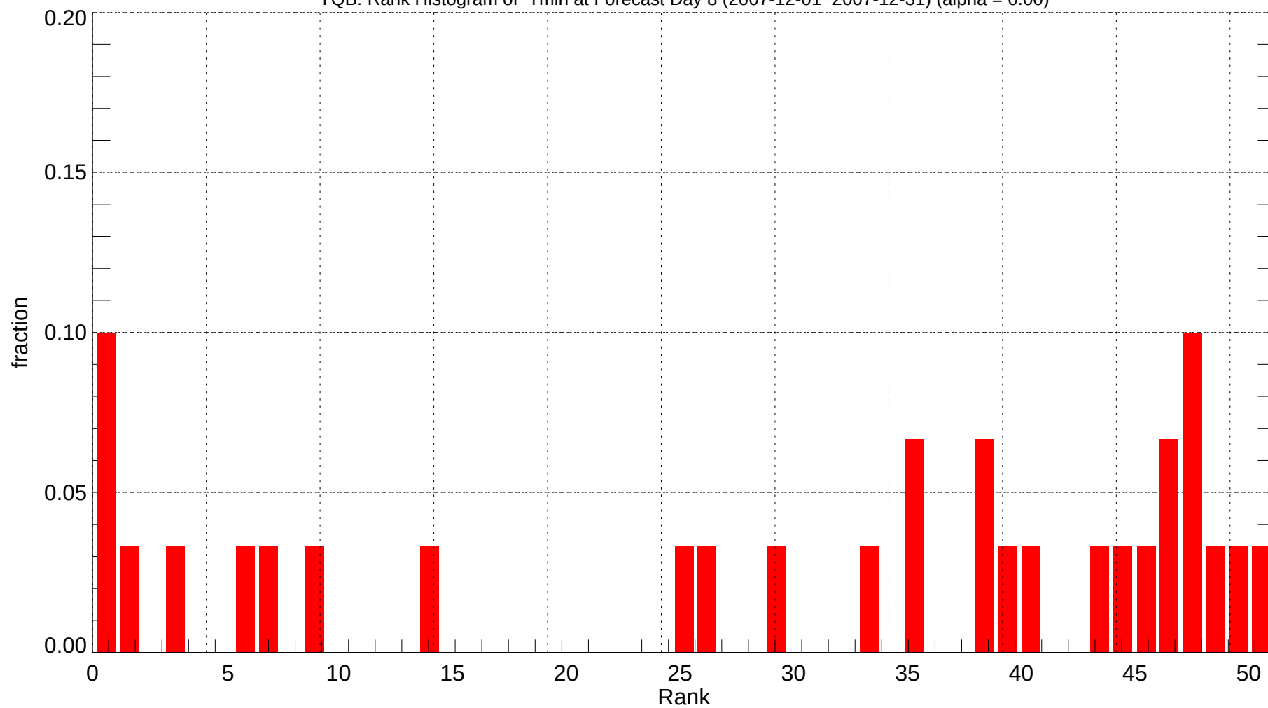
YQB: Rank Histogram of Tmin at Forecast Day 8 (2007-12-01~2007-12-31) (alpha = 0.00)
