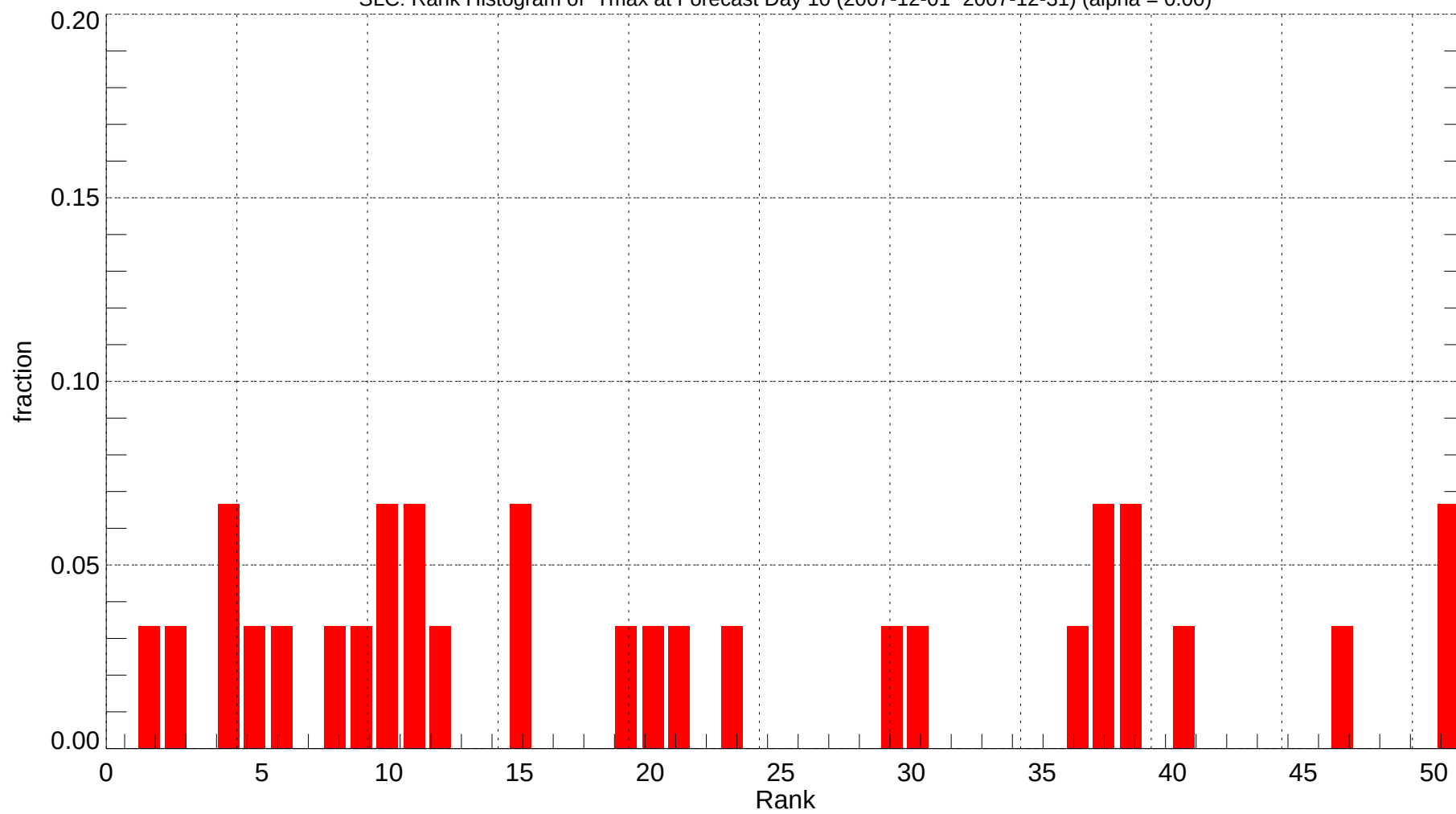
SLC: Rank Histogram of Tmax at Forecast Day 10 (2007-12-01~2007-12-31) (alpha = 0.00)
