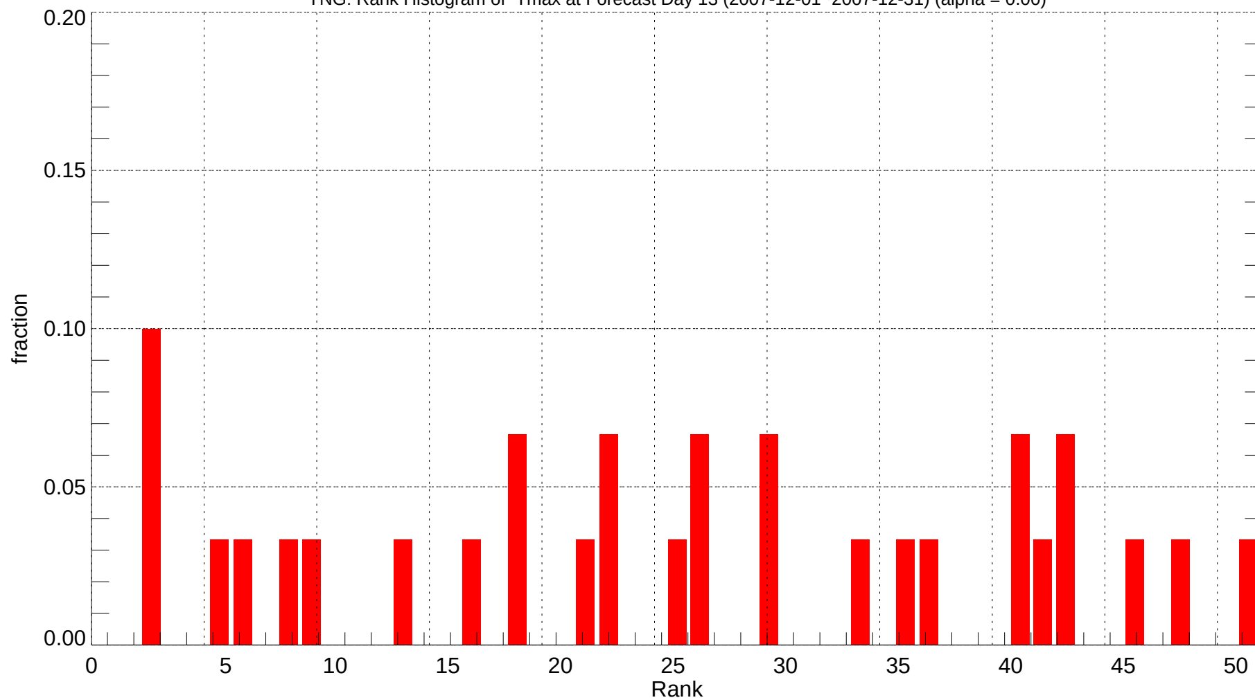
YNG: Rank Histogram of Tmax at Forecast Day 13 (2007-12-01~2007-12-31) (alpha = 0.00)
