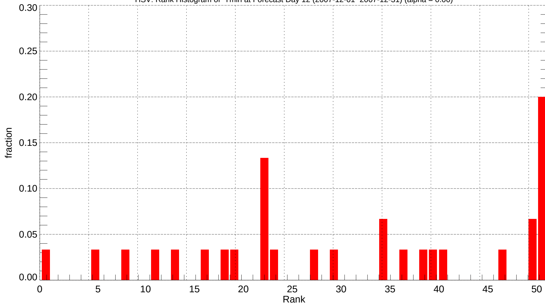
HSV: Rank Histogram of Tmin at Forecast Day 12 (2007-12-01~2007-12-31) (alpha = 0.00)
