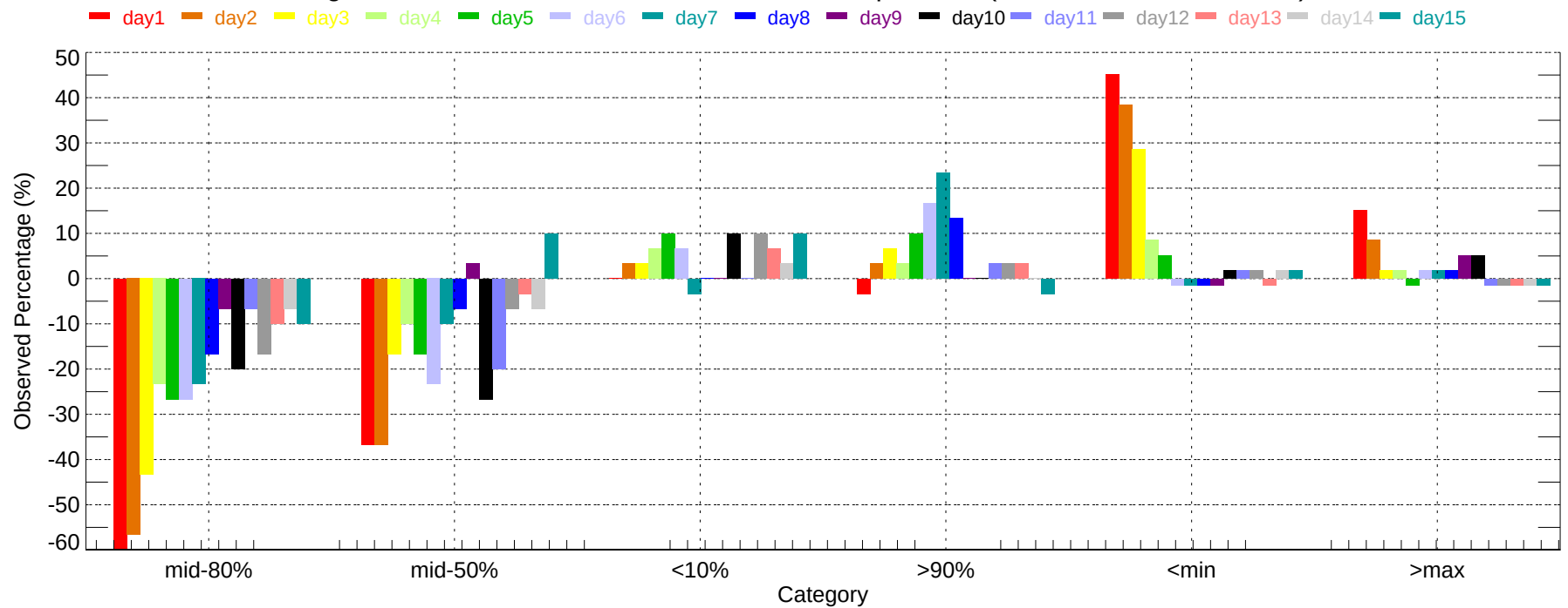
Observed Percentage Deviation of Ensembles - MBA: Max Temperature (2007-12-01~2007-12-31)
