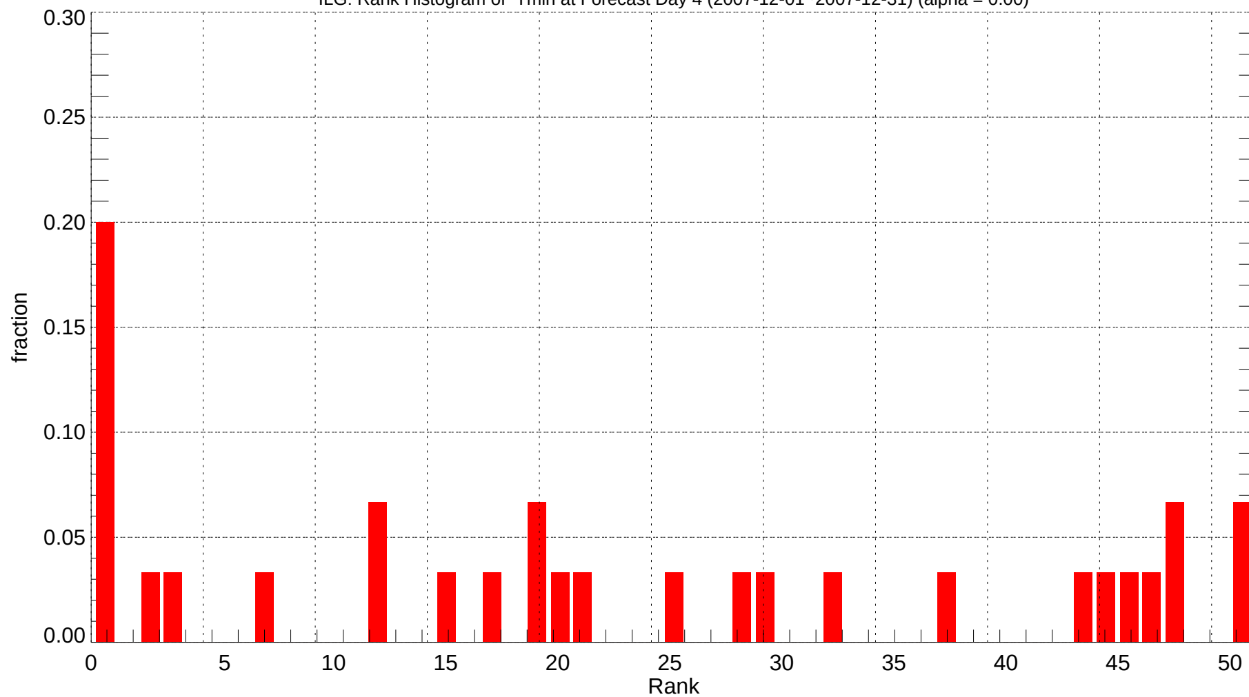
ILG: Rank Histogram of Tmin at Forecast Day 4 (2007-12-01~2007-12-31) (alpha = 0.00)
