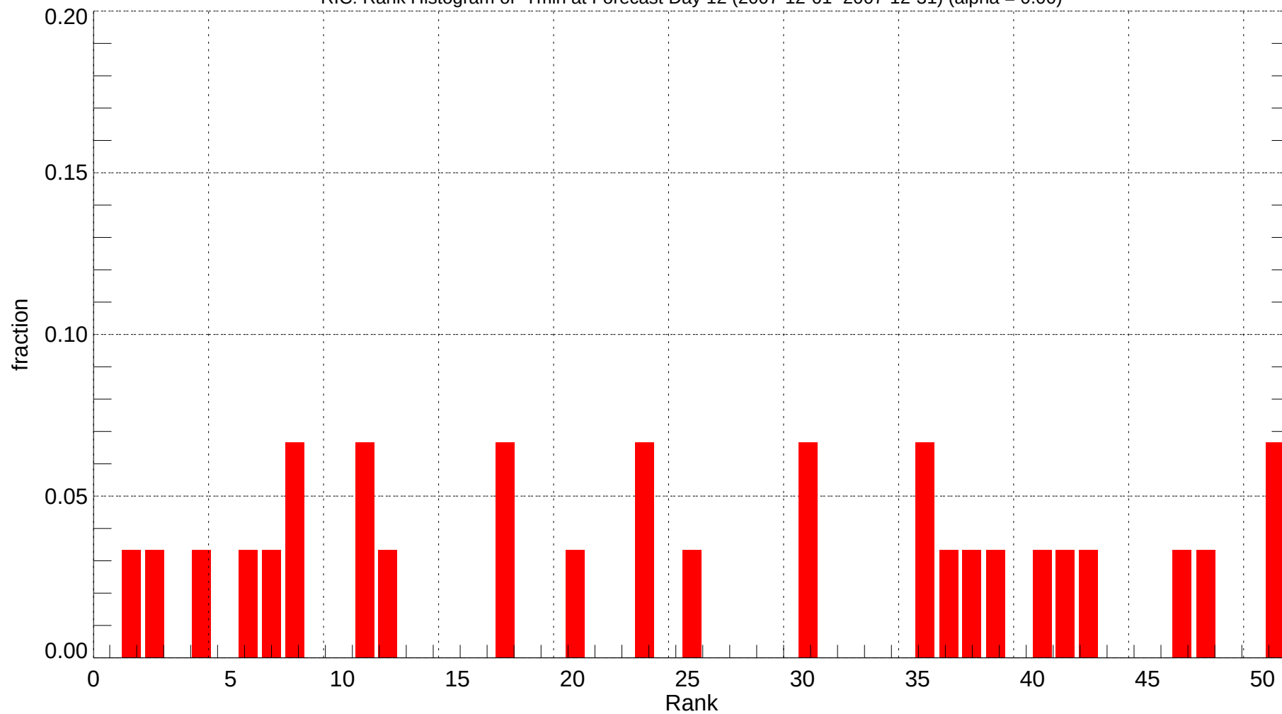
RIC: Rank Histogram of Tmin at Forecast Day 12 (2007-12-01~2007-12-31) (alpha = 0.00)
