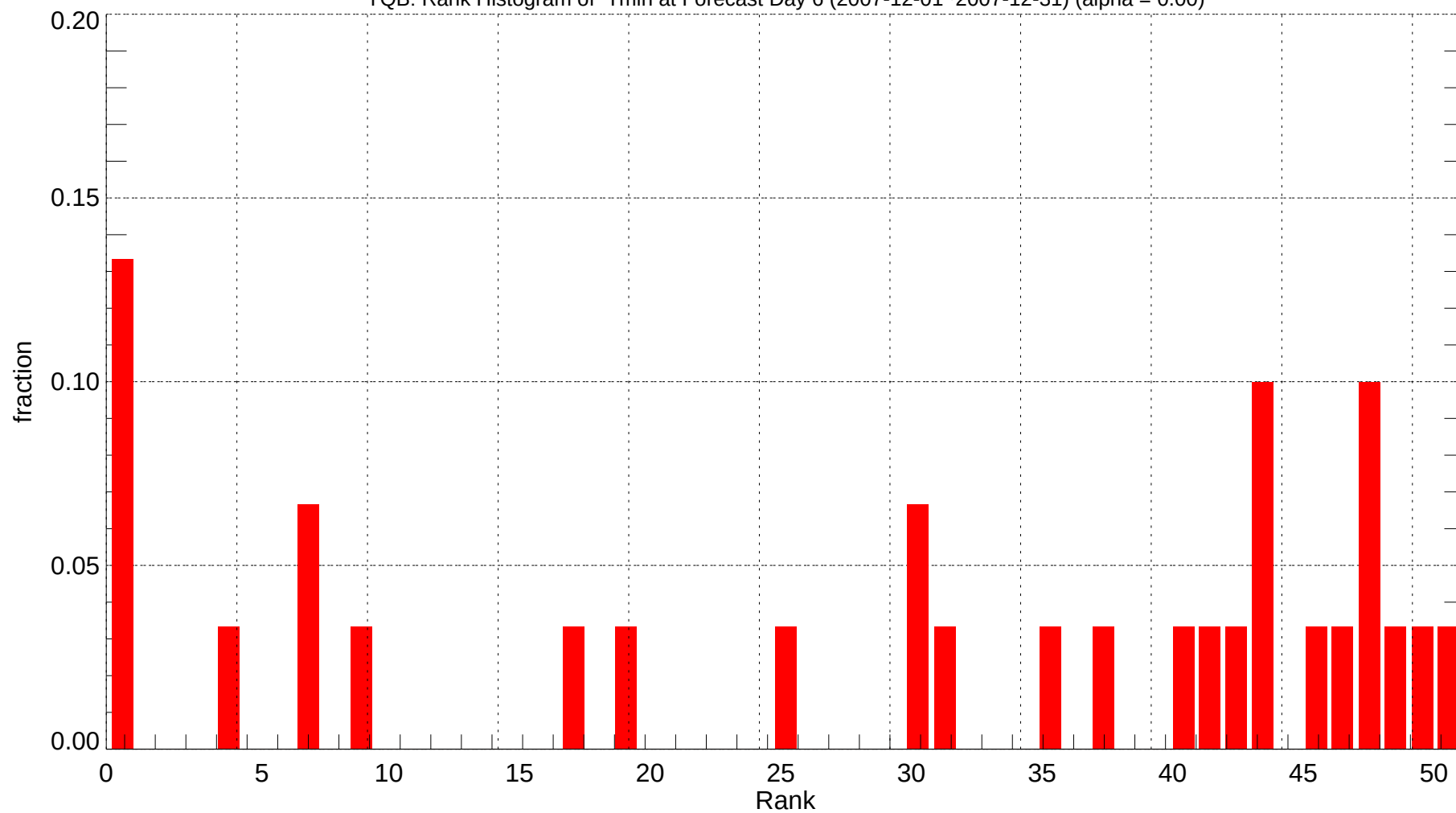
YQB: Rank Histogram of Tmin at Forecast Day 6 (2007-12-01~2007-12-31) (alpha = 0.00)
