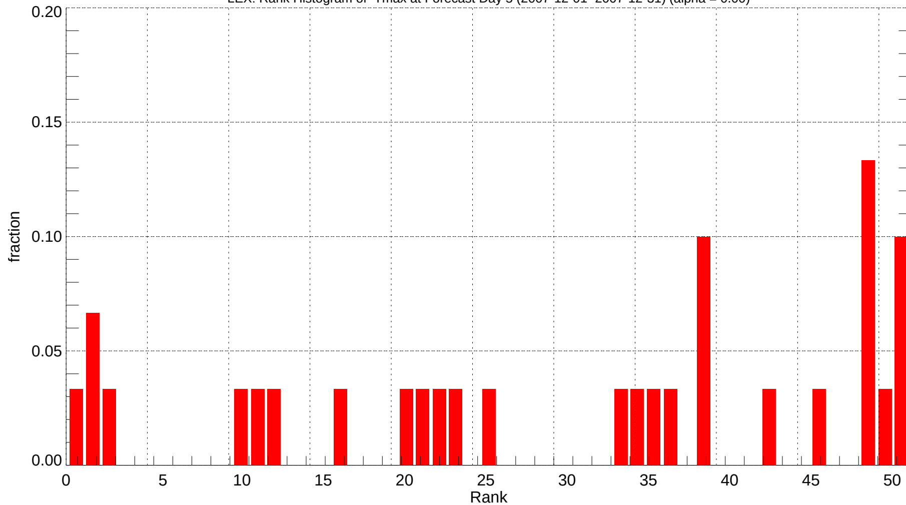
LEX: Rank Histogram of Tmax at Forecast Day 5 (2007-12-01~2007-12-31) (alpha = 0.00)
