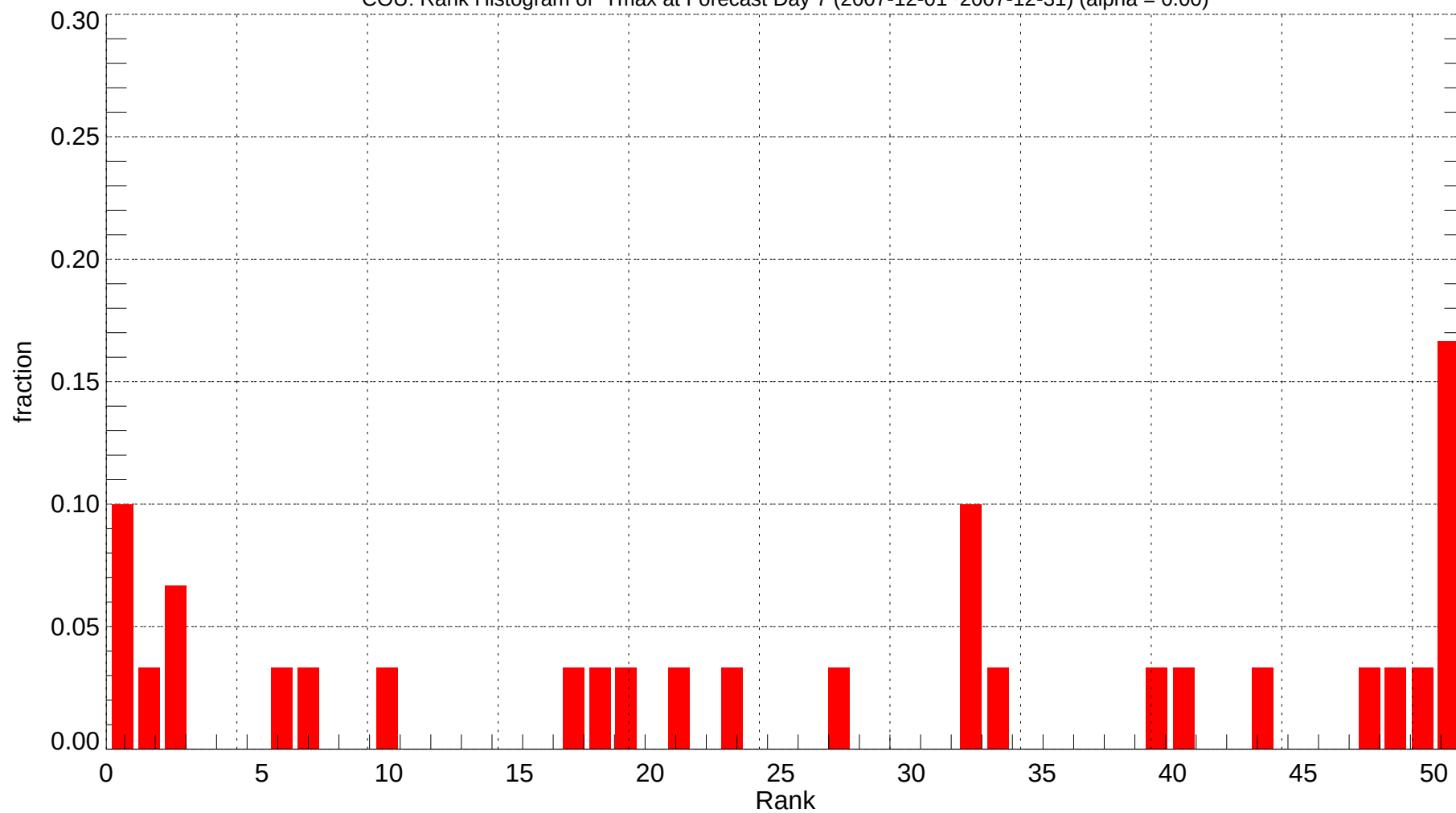
COU: Rank Histogram of Tmax at Forecast Day 7 (2007-12-01~2007-12-31) (alpha = 0.00)
