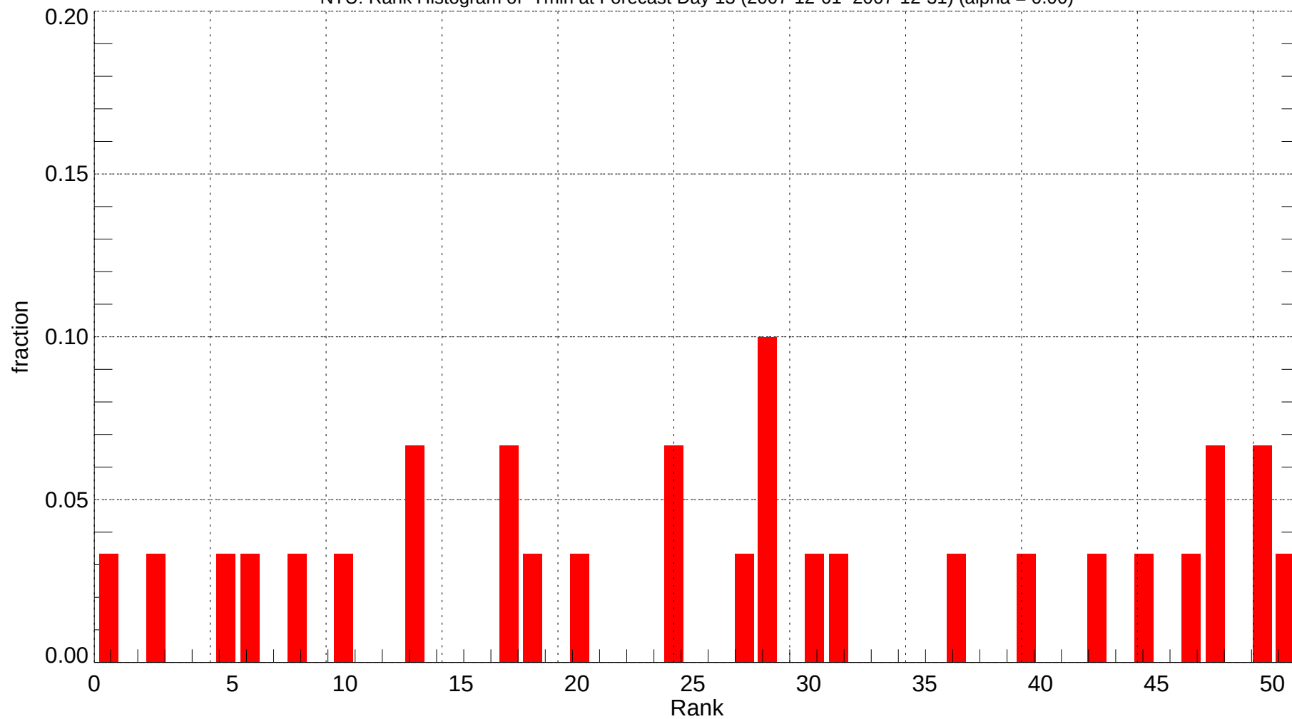
NTU: Rank Histogram of Tmin at Forecast Day 13 (2007-12-01~2007-12-31) (alpha = 0.00)
