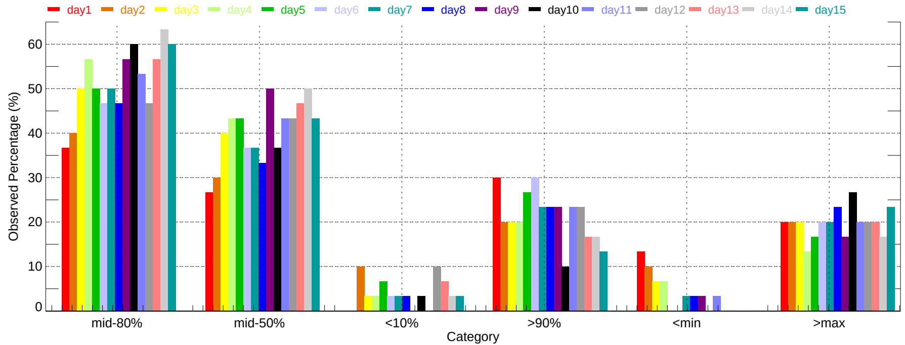
Observed Percentage of Ensembles - TYR: Min Temperature (2007-12-01~2007-12-31)
