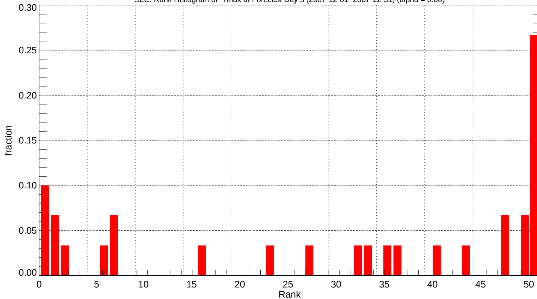
SLC: Rank Histogram of Tmax at Forecast Day 5 (2007-12-01~2007-12-31) (alpha = 0.00)
