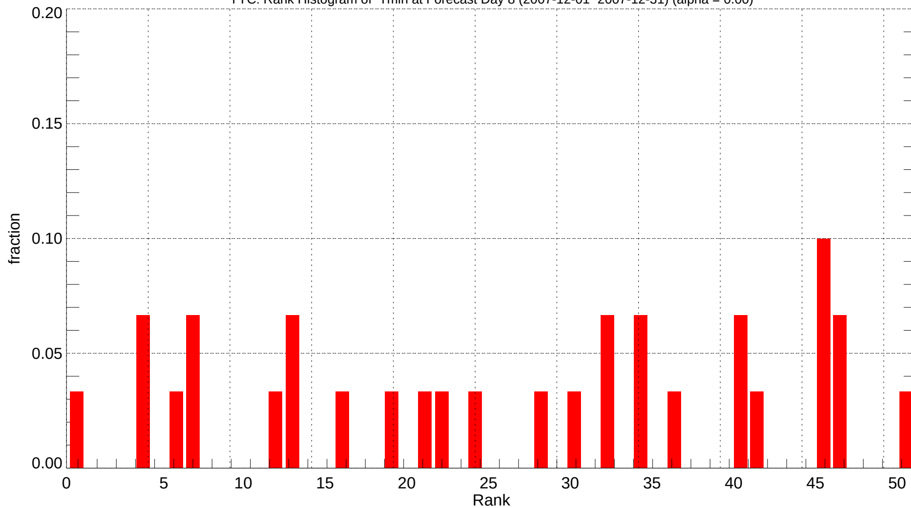
YYC: Rank Histogram of Tmin at Forecast Day 8 (2007-12-01~2007-12-31) (alpha = 0.00)
