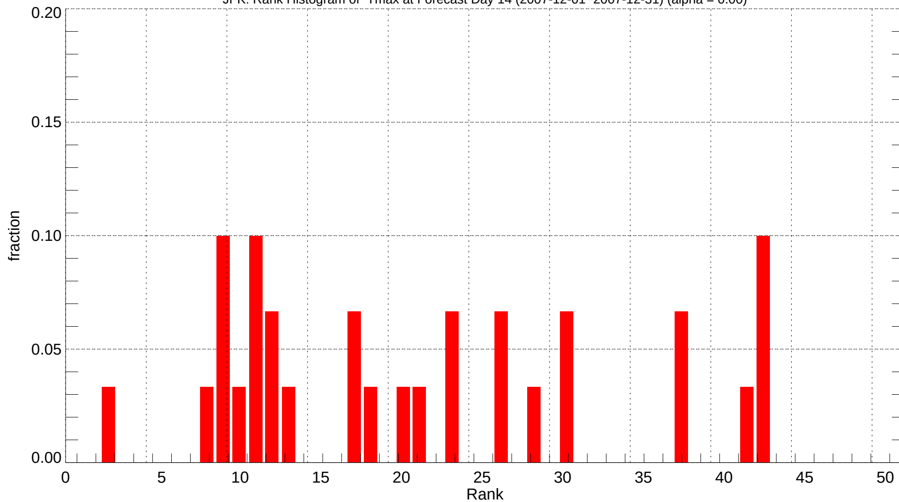
JFK: Rank Histogram of Tmax at Forecast Day 14 (2007-12-01~2007-12-31) (alpha = 0.00)
