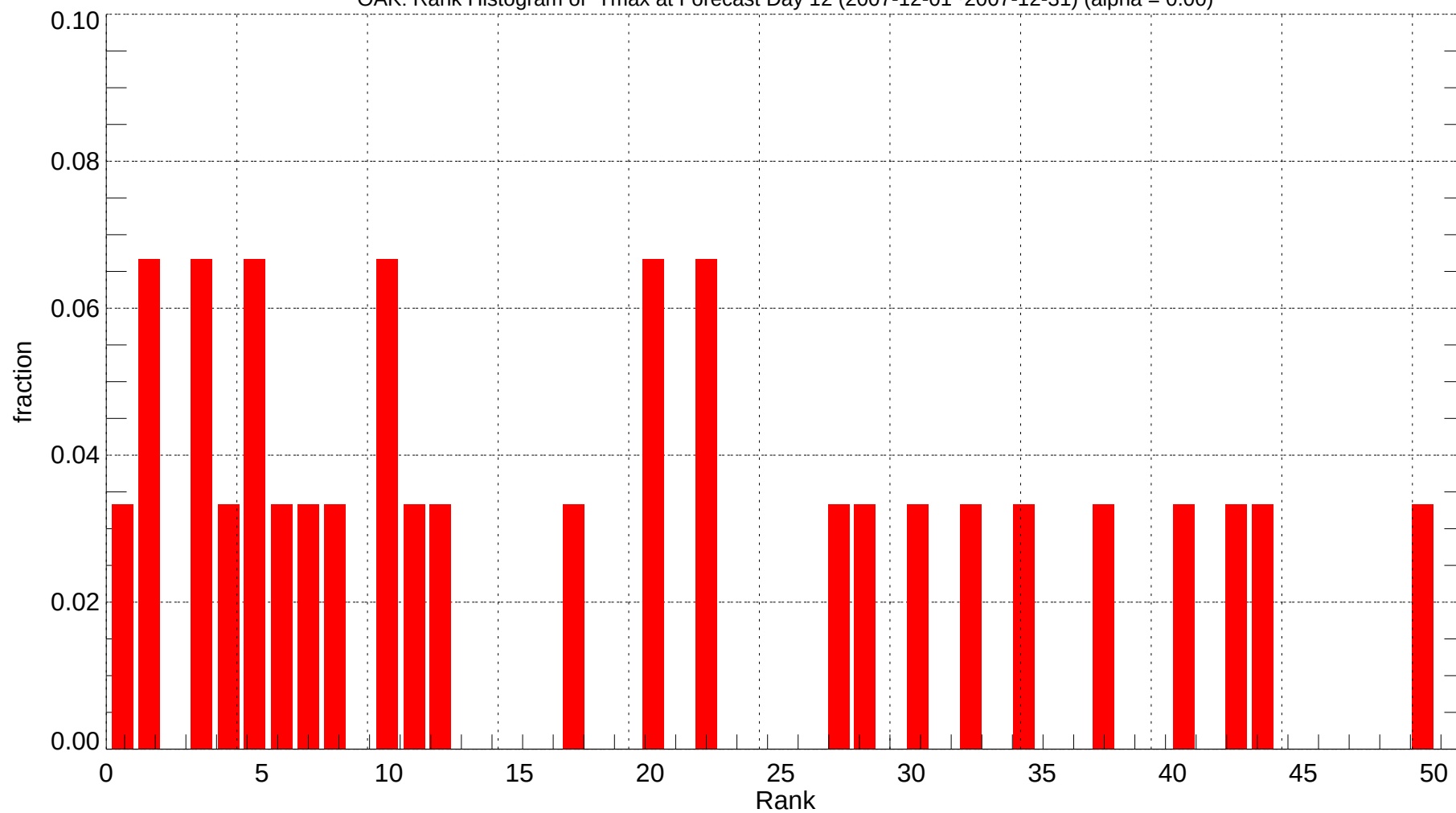
OAK: Rank Histogram of Tmax at Forecast Day 12 (2007-12-01~2007-12-31) (alpha = 0.00)
