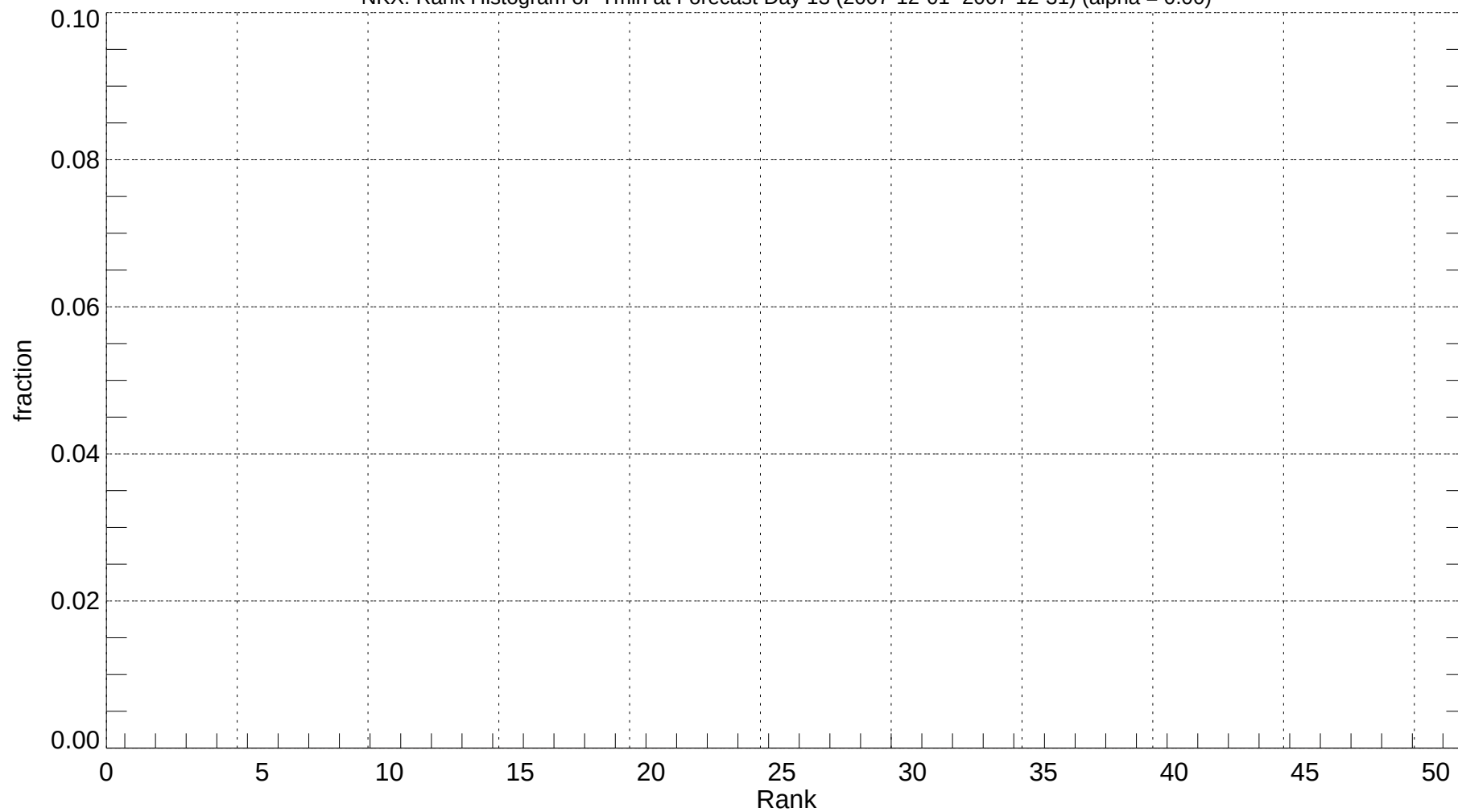
NKX: Rank Histogram of Tmin at Forecast Day 13 (2007-12-01~2007-12-31) (alpha = 0.00)
