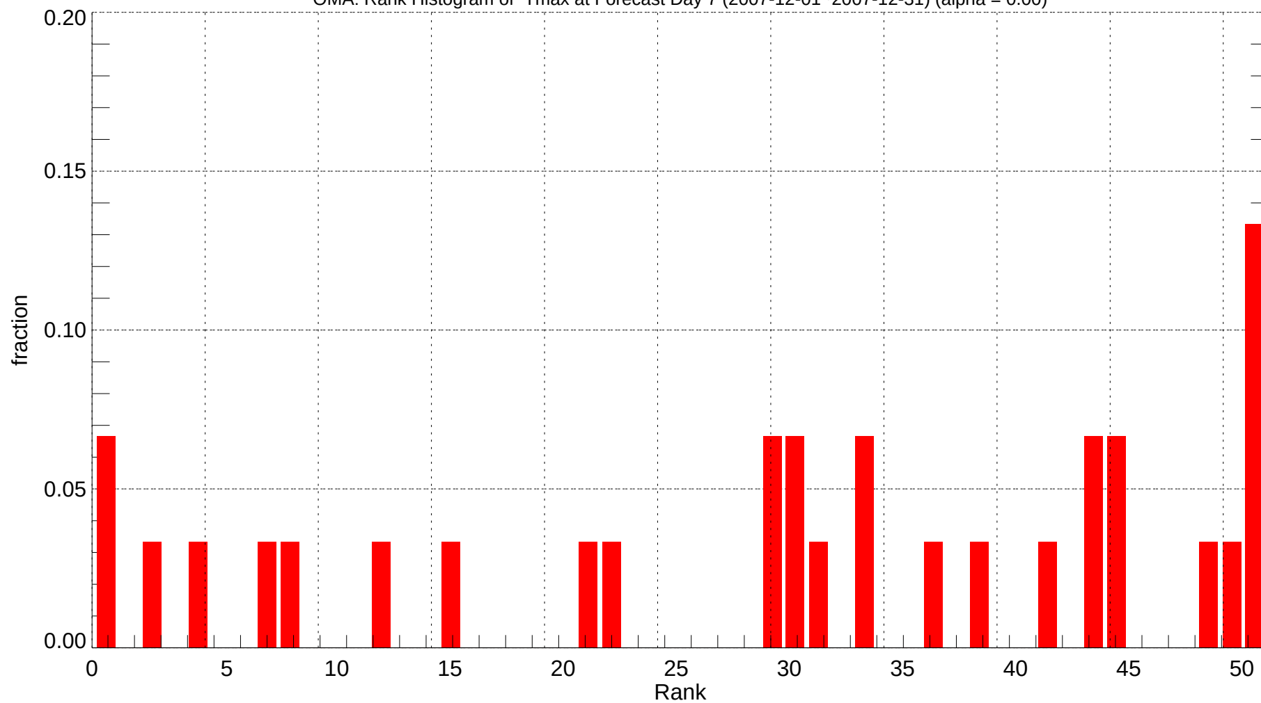
OMA: Rank Histogram of Tmax at Forecast Day 7 (2007-12-01~2007-12-31) (alpha = 0.00)
