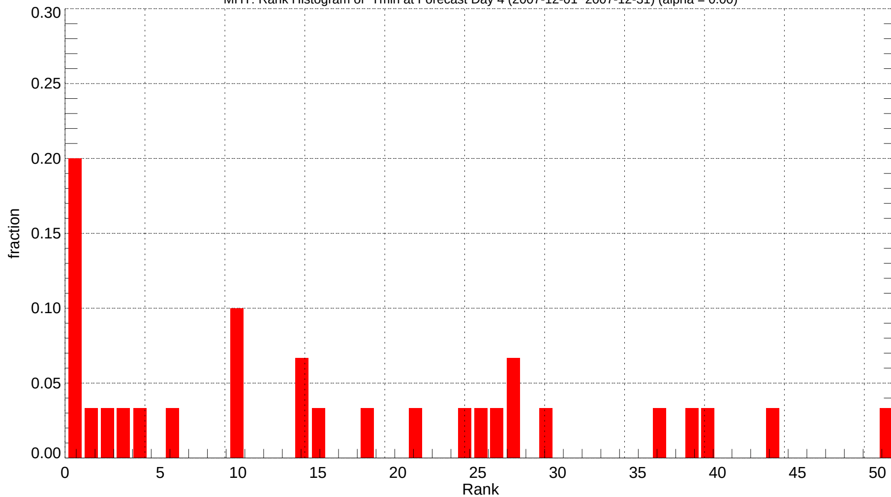
MHT: Rank Histogram of Tmin at Forecast Day 4 (2007-12-01~2007-12-31) (alpha = 0.00)
