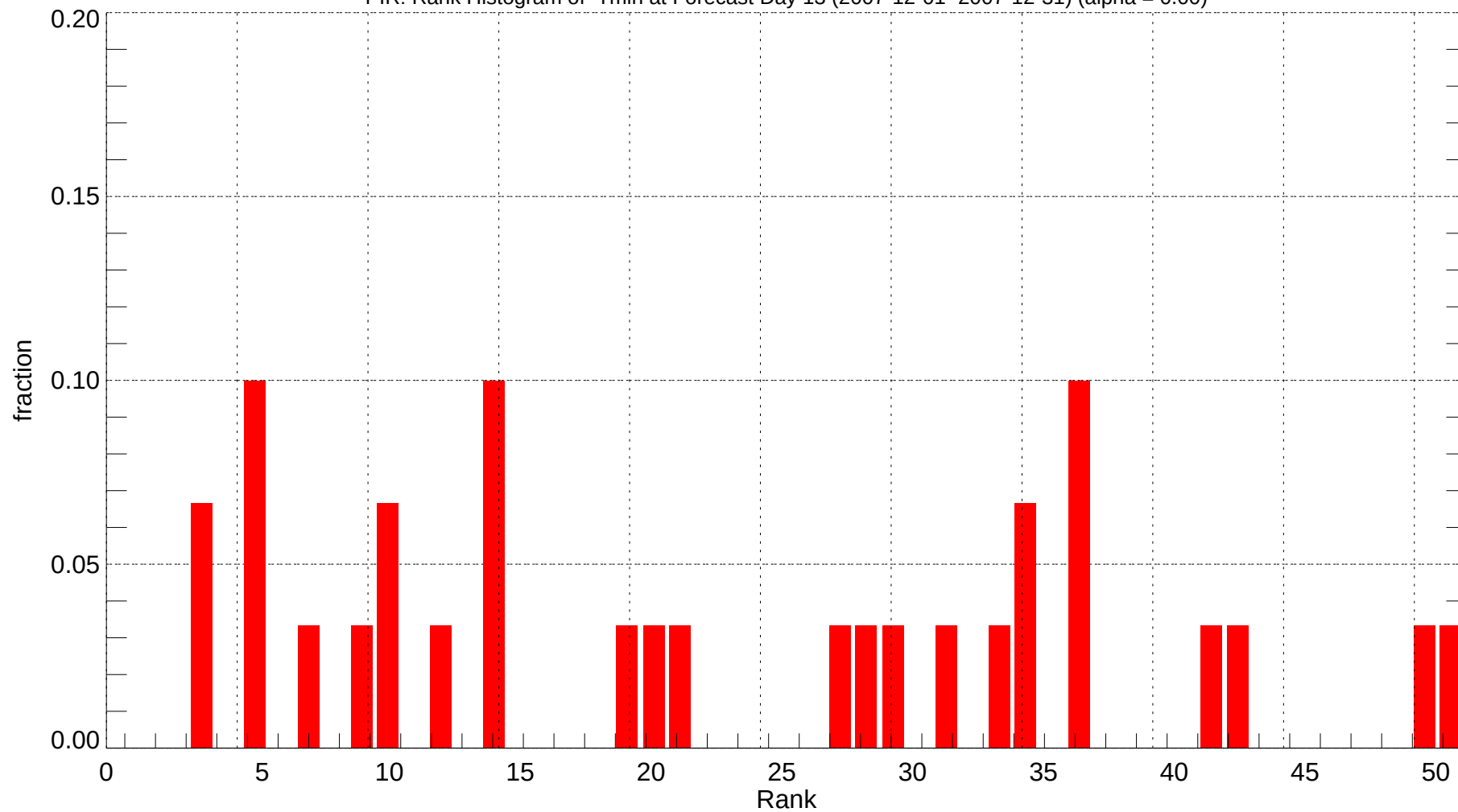
PIR: Rank Histogram of Tmin at Forecast Day 13 (2007-12-01~2007-12-31) (alpha = 0.00)
