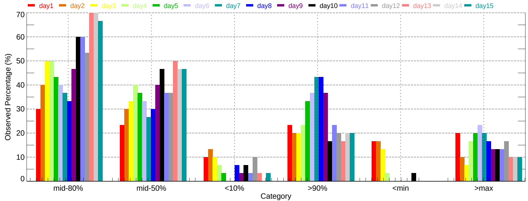
Observed Percentage of Ensembles - MEM: Max Temperature (2007-12-01~2007-12-31)
