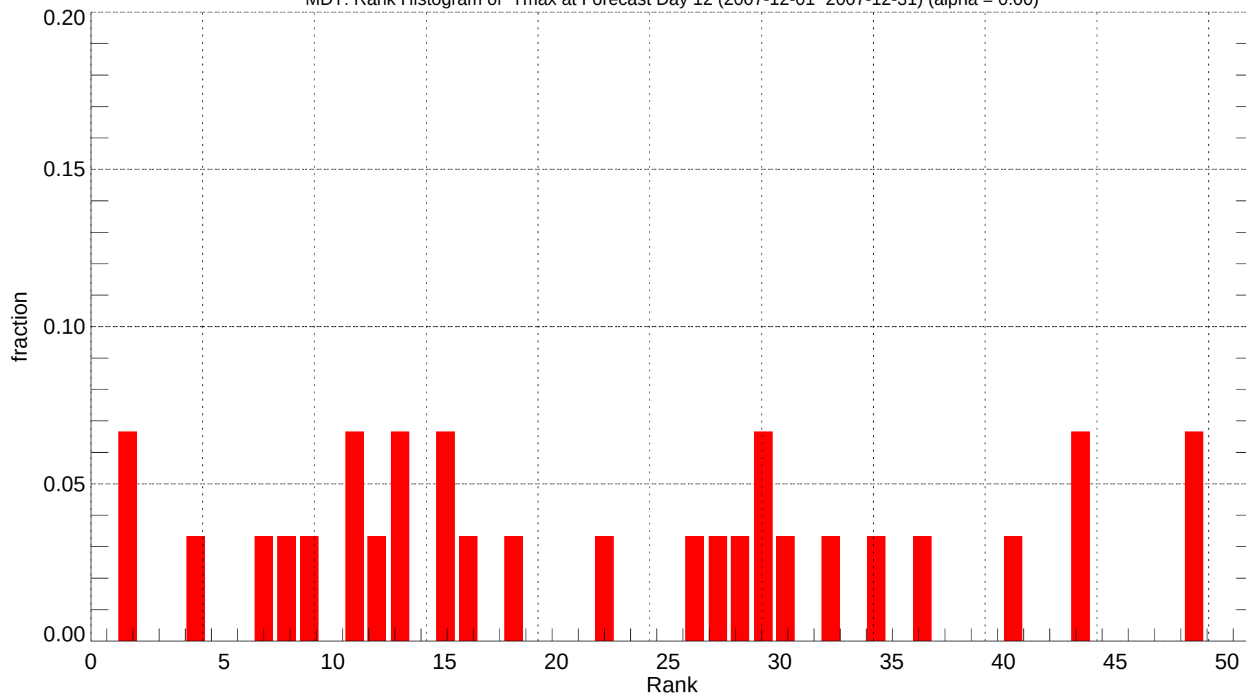
MDT: Rank Histogram of Tmax at Forecast Day 12 (2007-12-01~2007-12-31) (alpha = 0.00)
