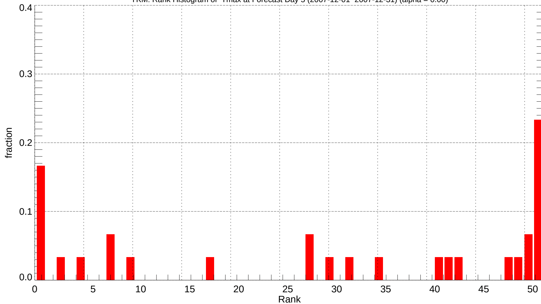
YKM: Rank Histogram of Tmax at Forecast Day 5 (2007-12-01~2007-12-31) (alpha = 0.00)
