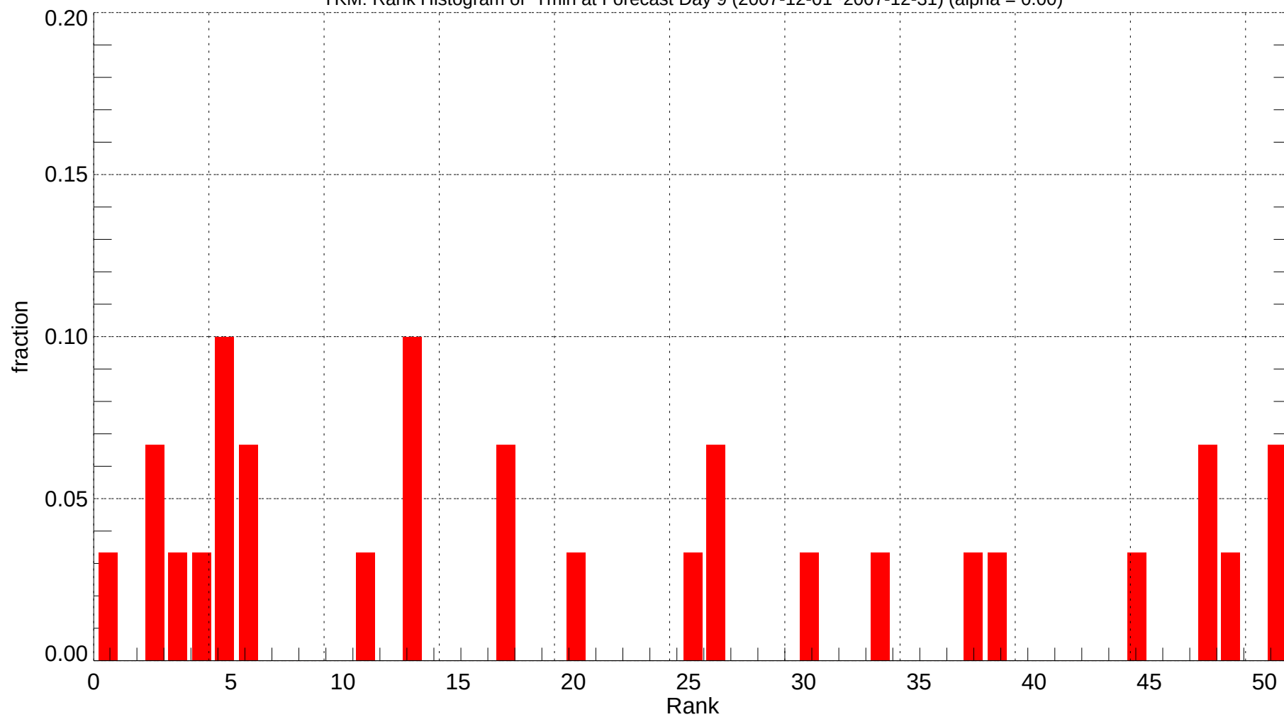
YKM: Rank Histogram of Tmin at Forecast Day 9 (2007-12-01~2007-12-31) (alpha = 0.00)
