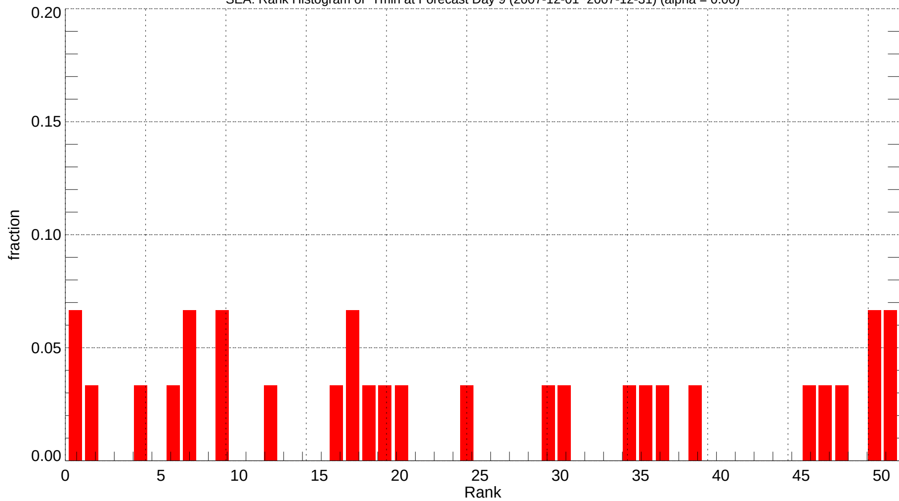
SEA: Rank Histogram of Tmin at Forecast Day 9 (2007-12-01~2007-12-31) (alpha = 0.00)
