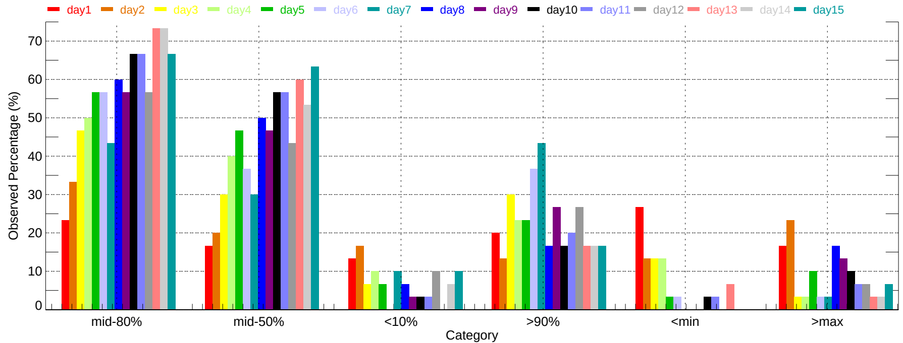
Observed Percentage of Ensembles - CMH: Max Temperature (2007-12-01~2007-12-31)
