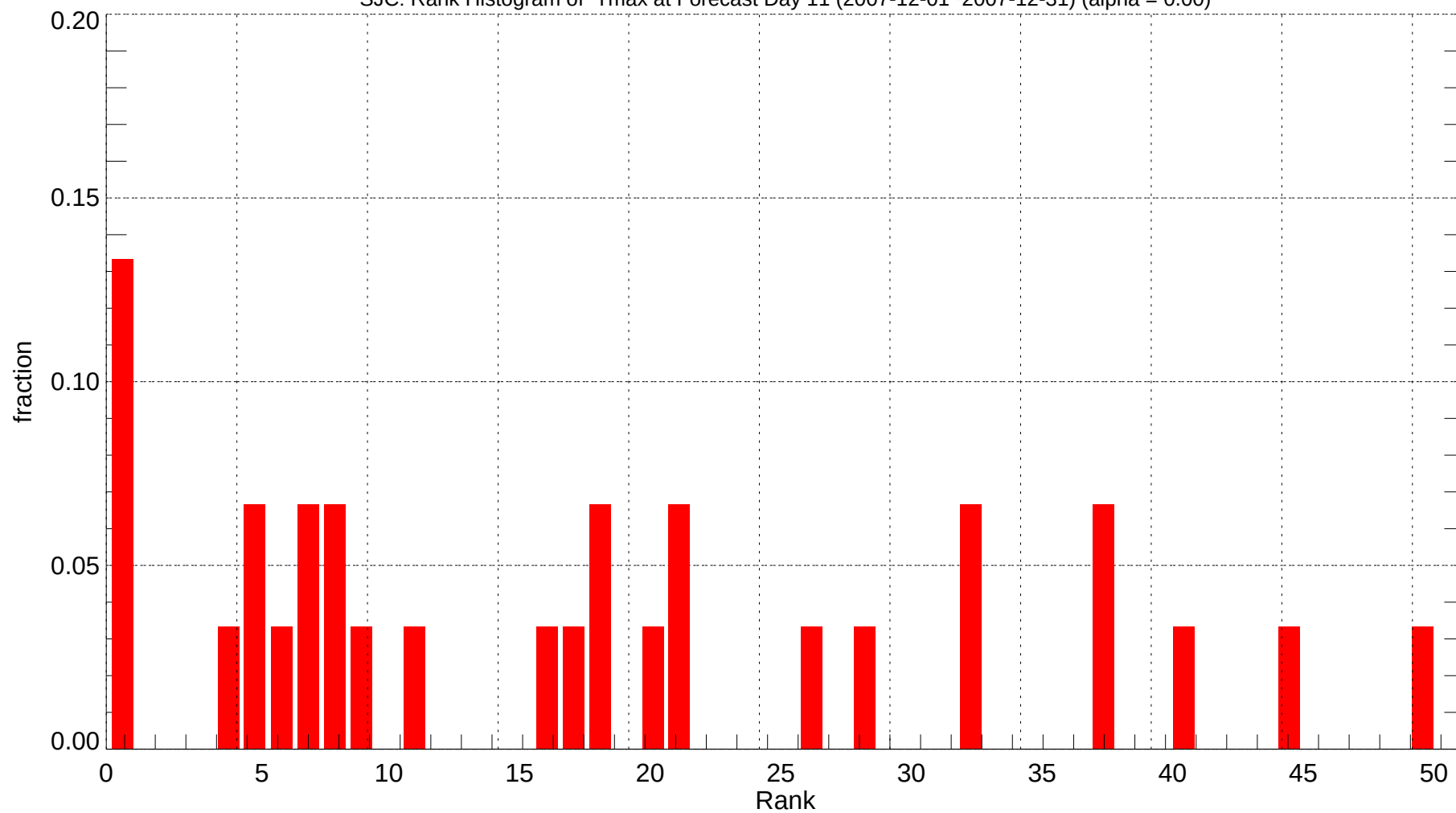
SJC: Rank Histogram of Tmax at Forecast Day 11 (2007-12-01~2007-12-31) (alpha = 0.00)
