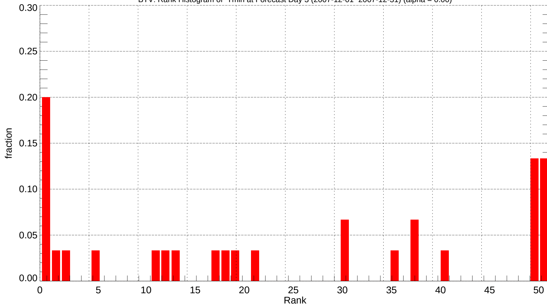
BTV: Rank Histogram of Tmin at Forecast Day 3 (2007-12-01~2007-12-31) (alpha = 0.00)
