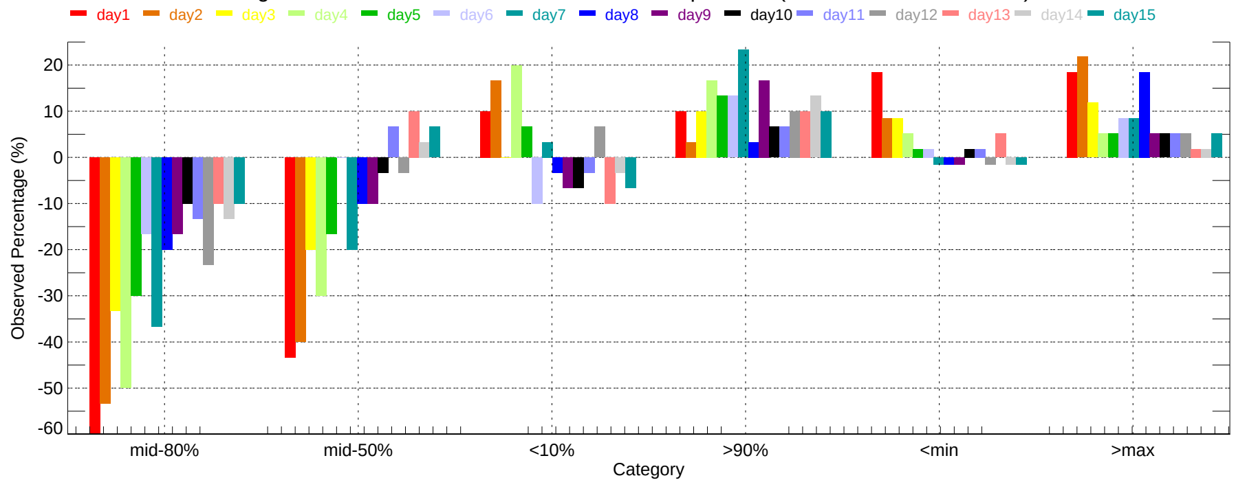
Observed Percentage Deviation of Ensembles - CVG: Max Temperature (2007-12-01~2007-12-31)
