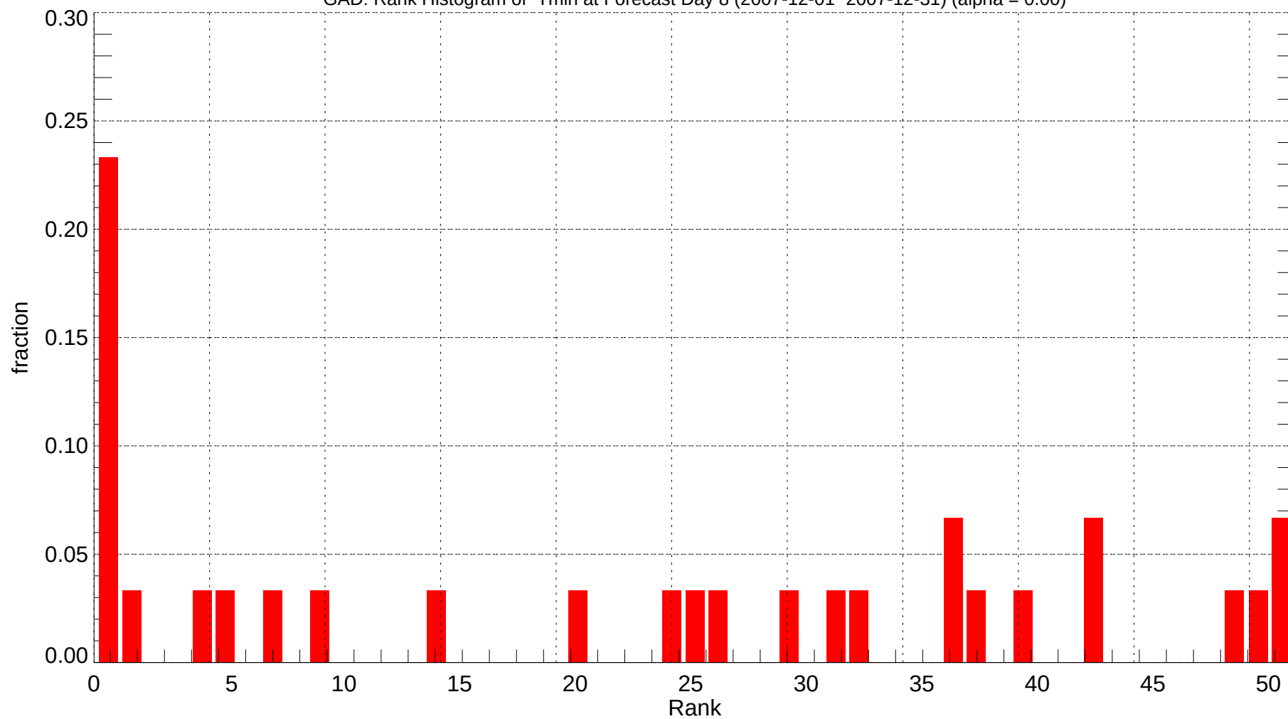
GAD: Rank Histogram of Tmin at Forecast Day 8 (2007-12-01~2007-12-31) (alpha = 0.00)
