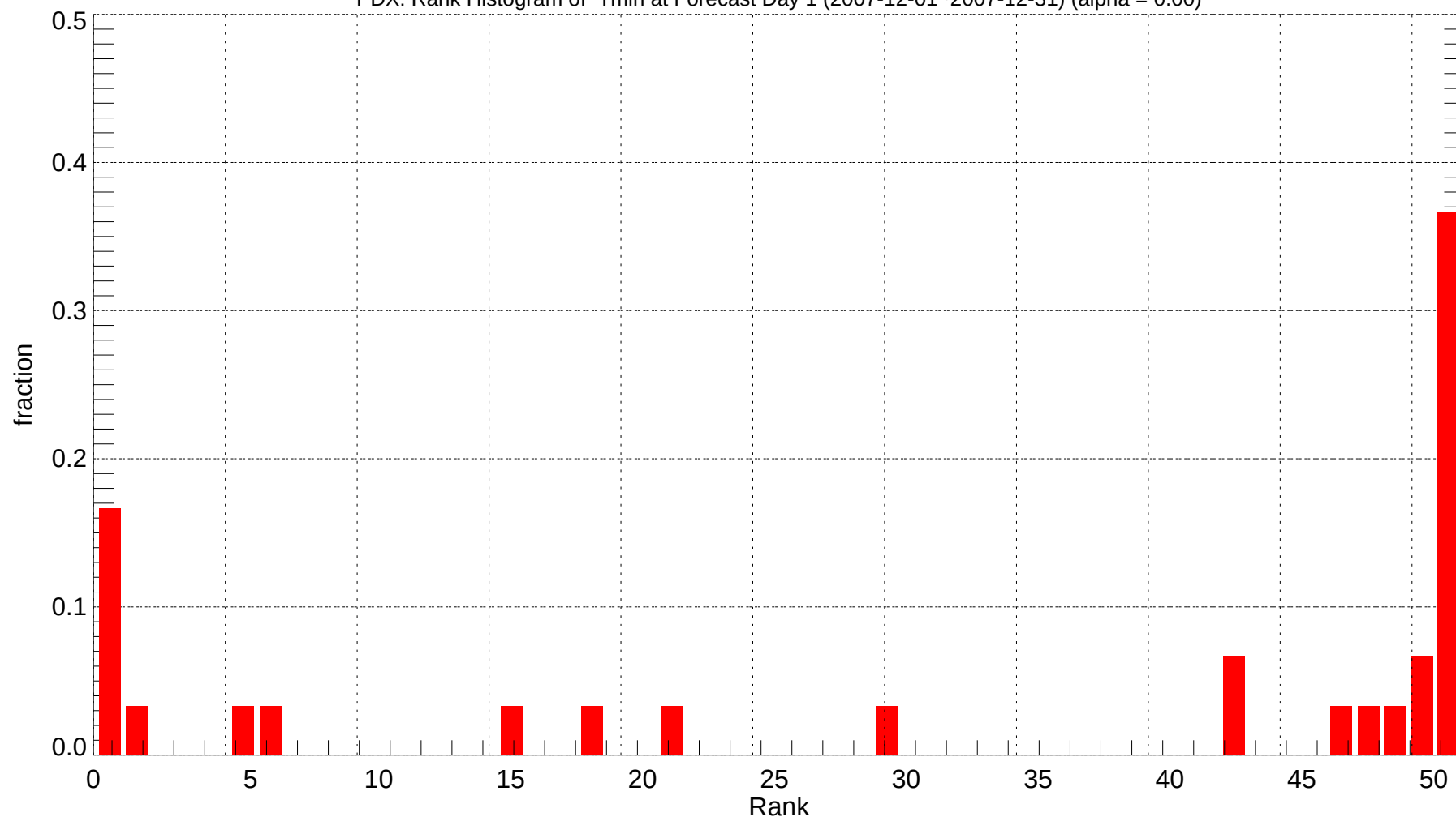
PDX: Rank Histogram of Tmin at Forecast Day 1 (2007-12-01~2007-12-31) (alpha = 0.00)
