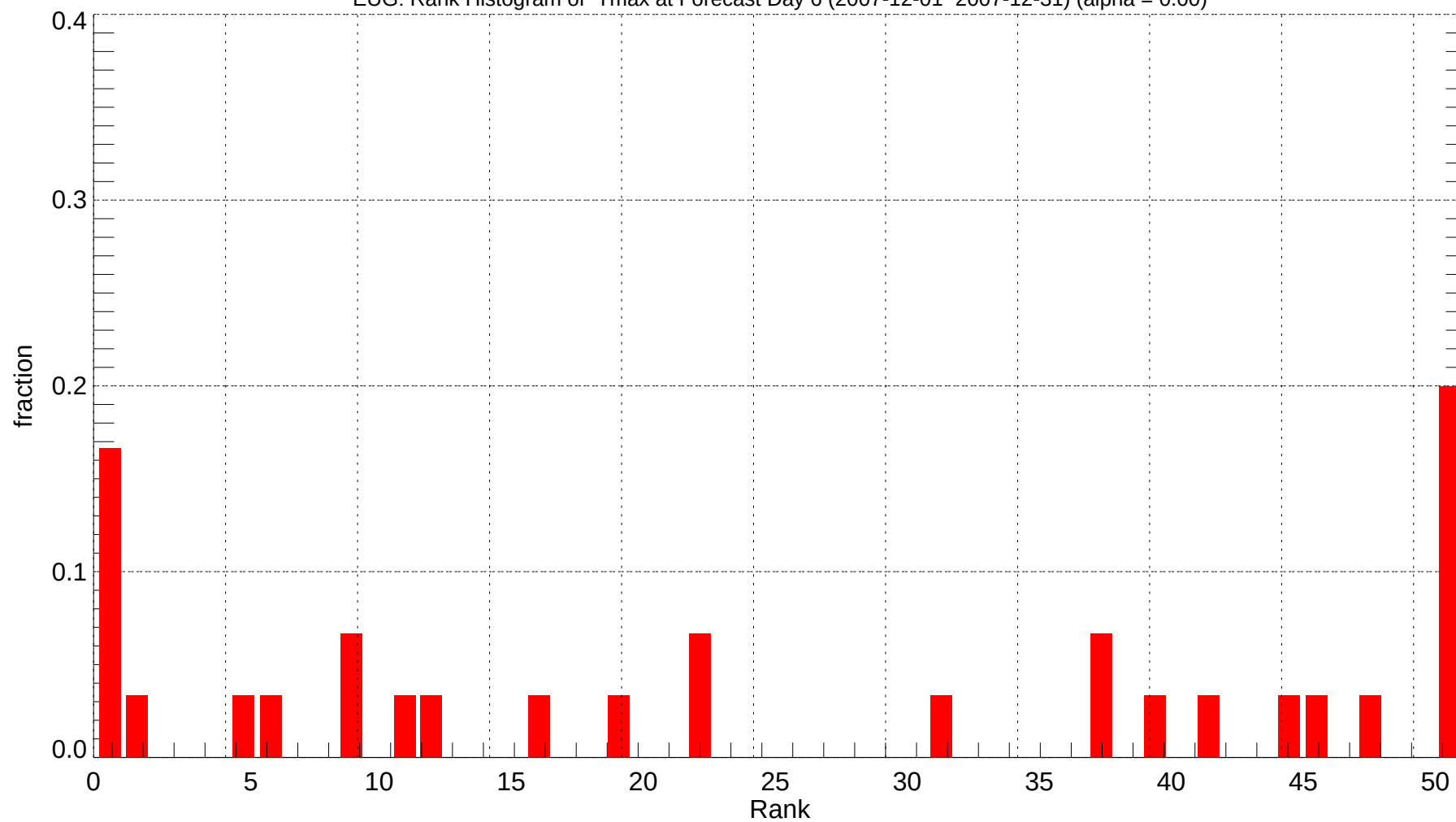
EUG: Rank Histogram of Tmax at Forecast Day 6 (2007-12-01~2007-12-31) (alpha = 0.00)
