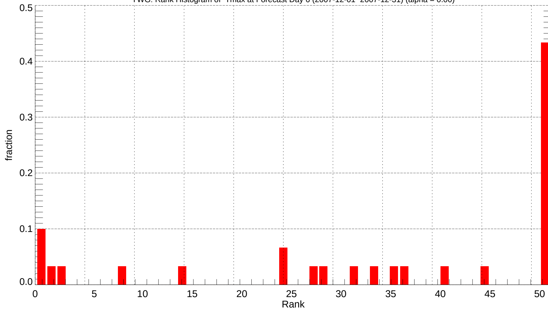
YWG: Rank Histogram of Tmax at Forecast Day 6 (2007-12-01~2007-12-31) (alpha = 0.00)
