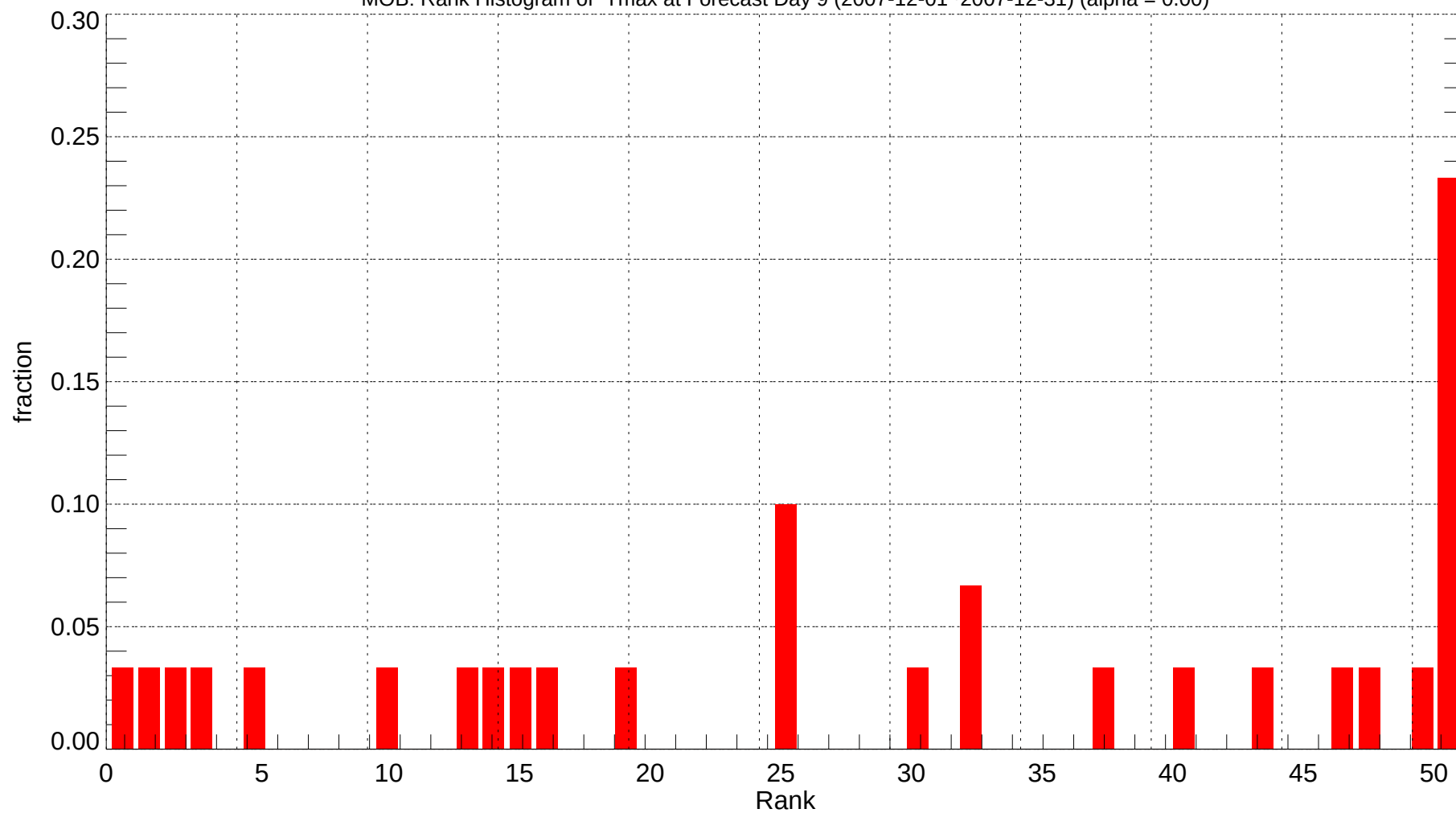
MOB: Rank Histogram of Tmax at Forecast Day 9 (2007-12-01~2007-12-31) (alpha = 0.00)
