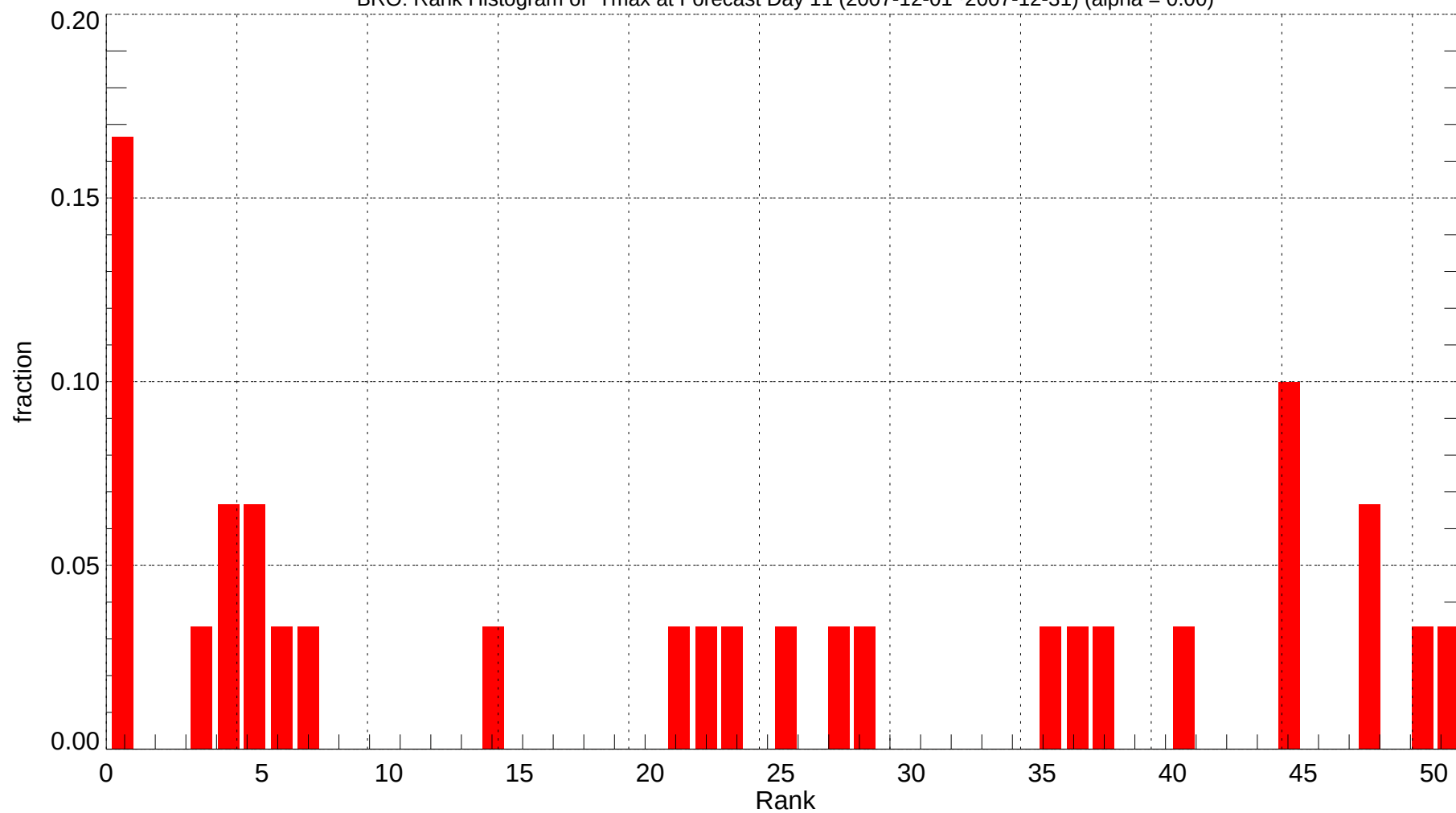
BRO: Rank Histogram of Tmax at Forecast Day 11 (2007-12-01~2007-12-31) (alpha = 0.00)
