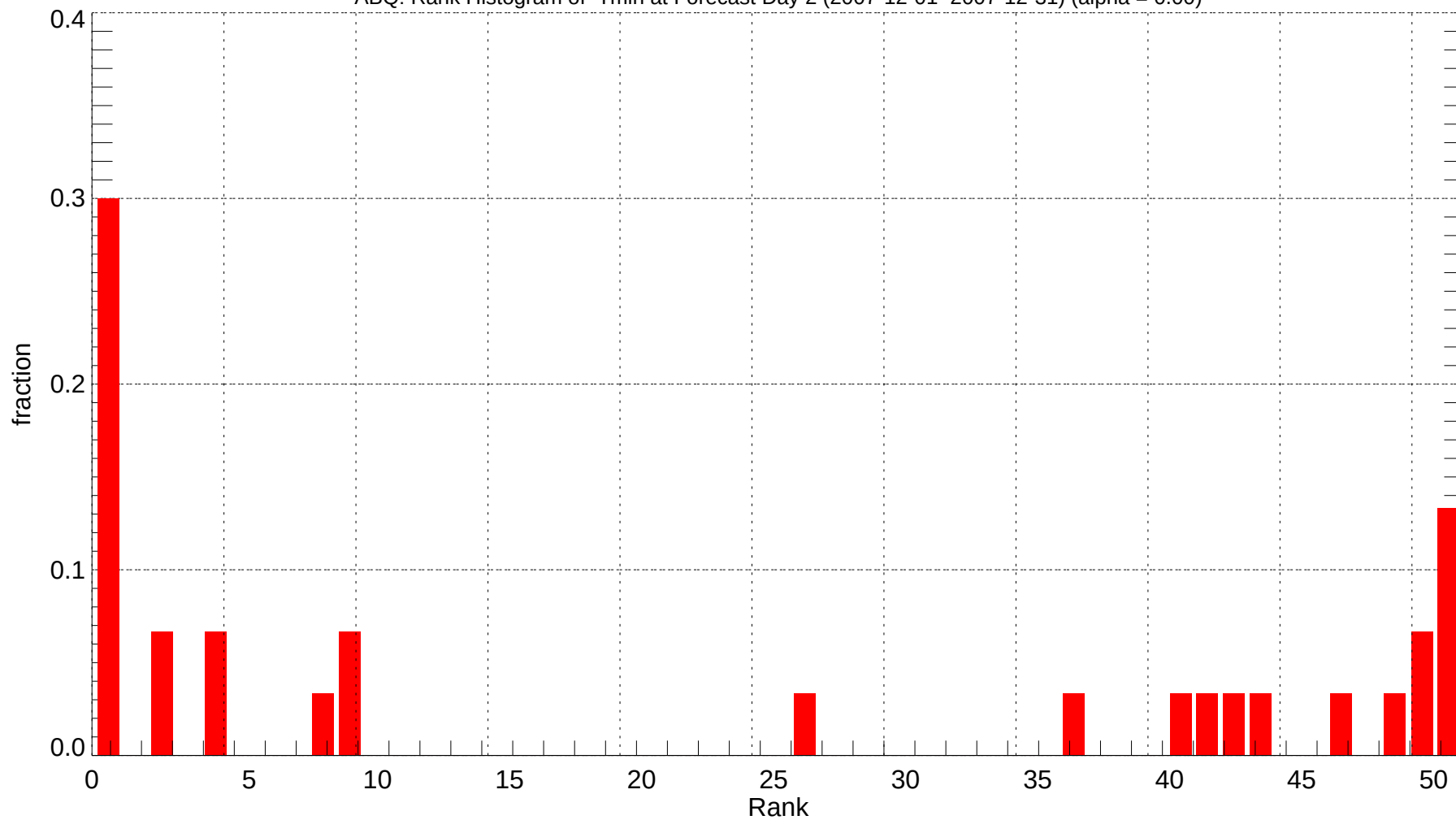
ABQ: Rank Histogram of Tmin at Forecast Day 2 (2007-12-01~2007-12-31) (alpha = 0.00)
