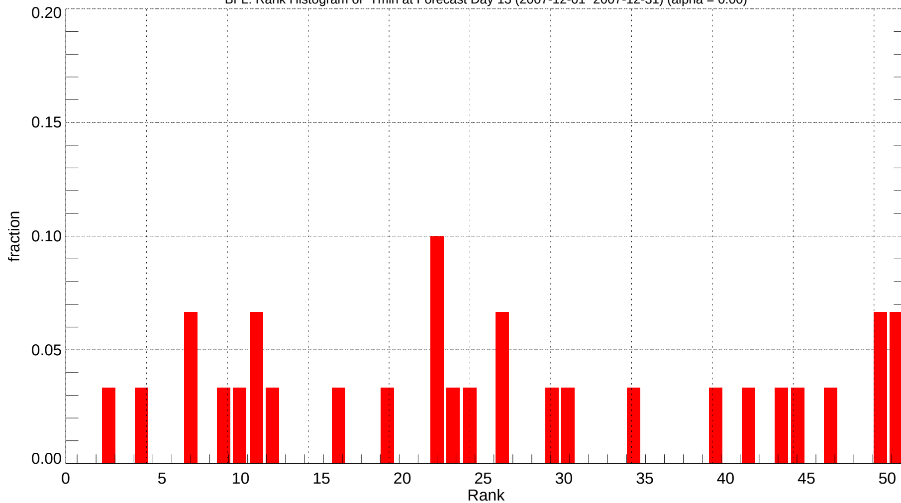
BFL: Rank Histogram of Tmin at Forecast Day 13 (2007-12-01~2007-12-31) (alpha = 0.00)
