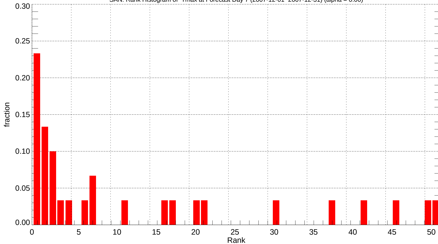
SAN: Rank Histogram of Tmax at Forecast Day 7 (2007-12-01~2007-12-31) (alpha = 0.00)
