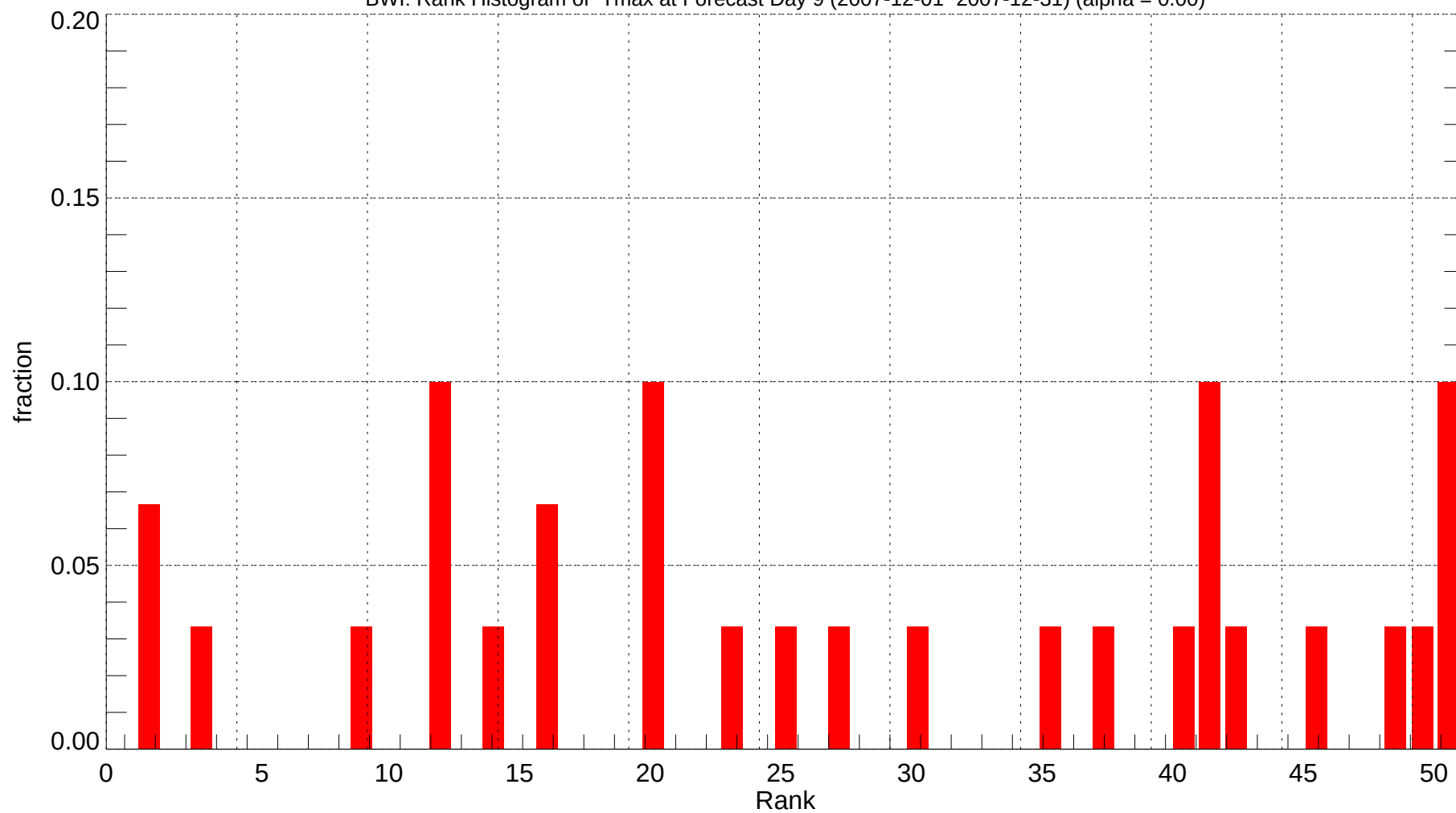
BWI: Rank Histogram of Tmax at Forecast Day 9 (2007-12-01~2007-12-31) (alpha = 0.00)
