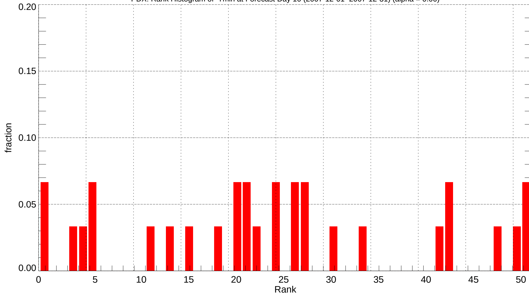
PDX: Rank Histogram of Tmin at Forecast Day 10 (2007-12-01~2007-12-31) (alpha = 0.00)
