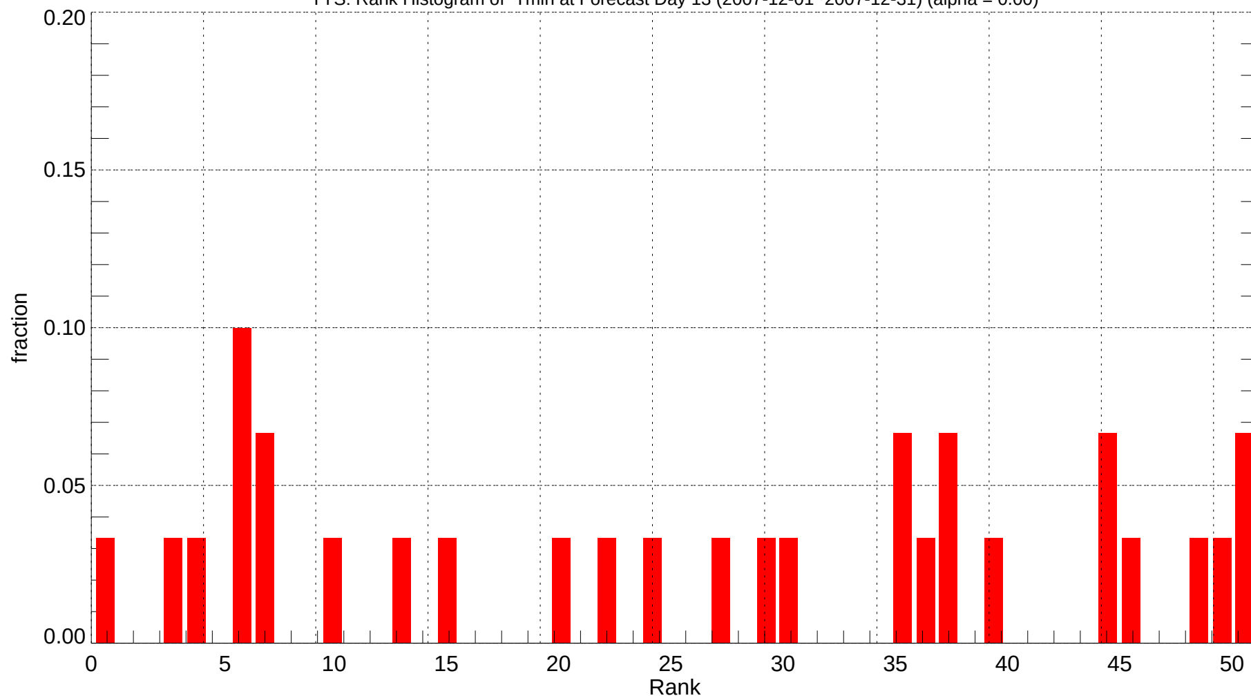
TYS: Rank Histogram of Tmin at Forecast Day 13 (2007-12-01~2007-12-31) (alpha = 0.00)
