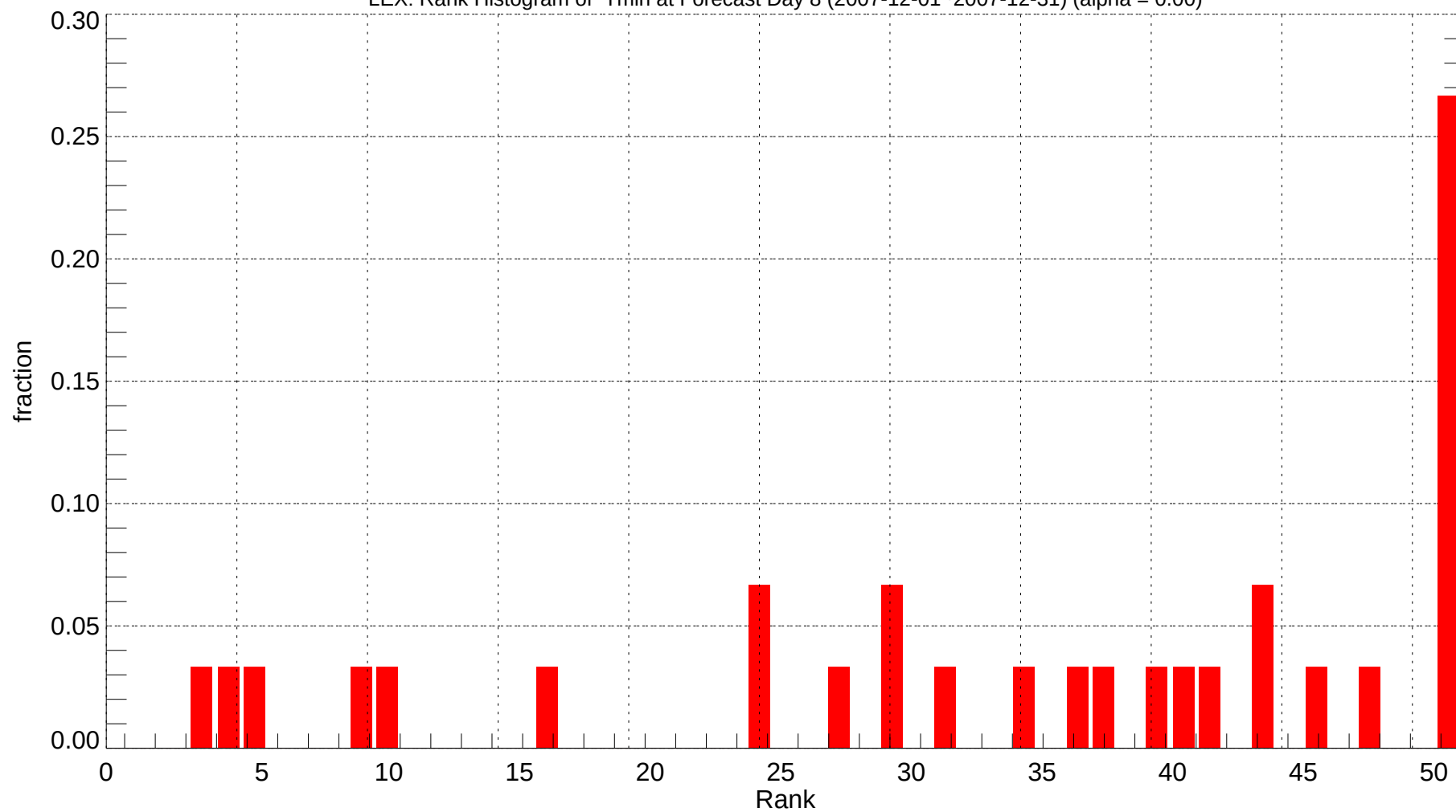
LEX: Rank Histogram of Tmin at Forecast Day 8 (2007-12-01~2007-12-31) (alpha = 0.00)
