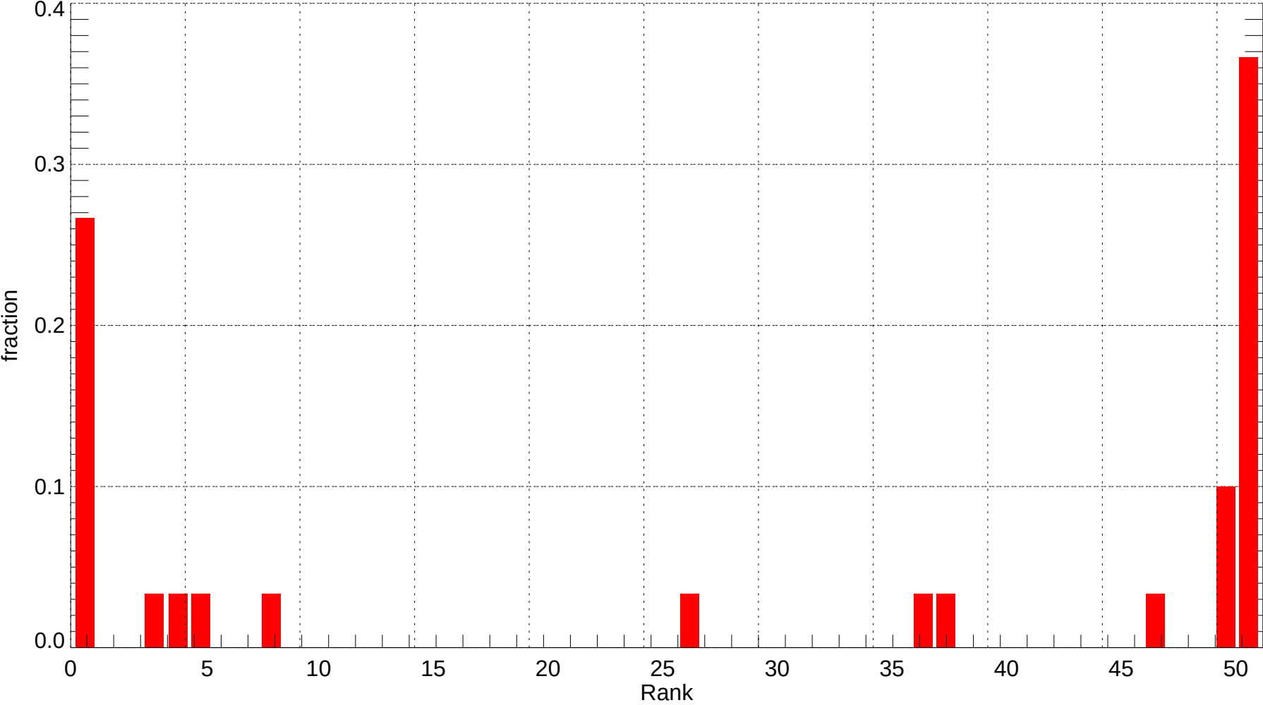
BFL: Rank Histogram of Tmin at Forecast Day 1 (2007-12-01~2007-12-31) (alpha = 0.00)
