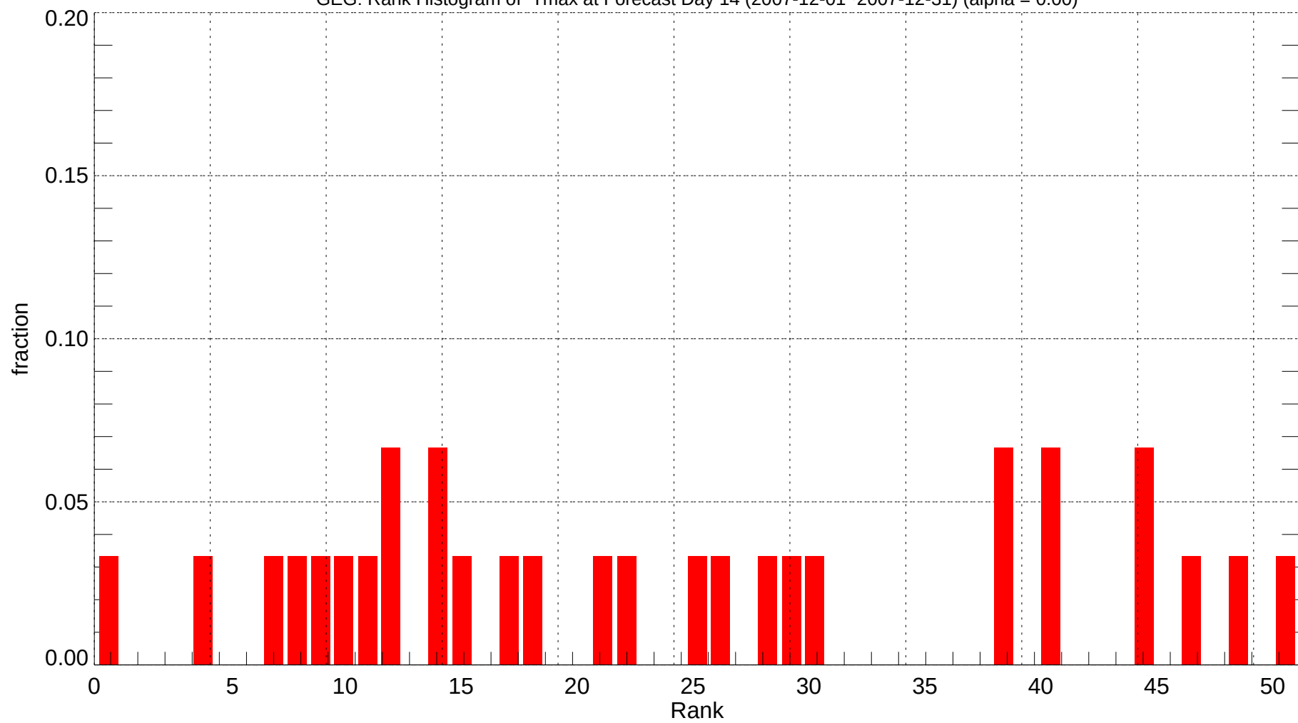
GEG: Rank Histogram of Tmax at Forecast Day 14 (2007-12-01~2007-12-31) (alpha = 0.00)
