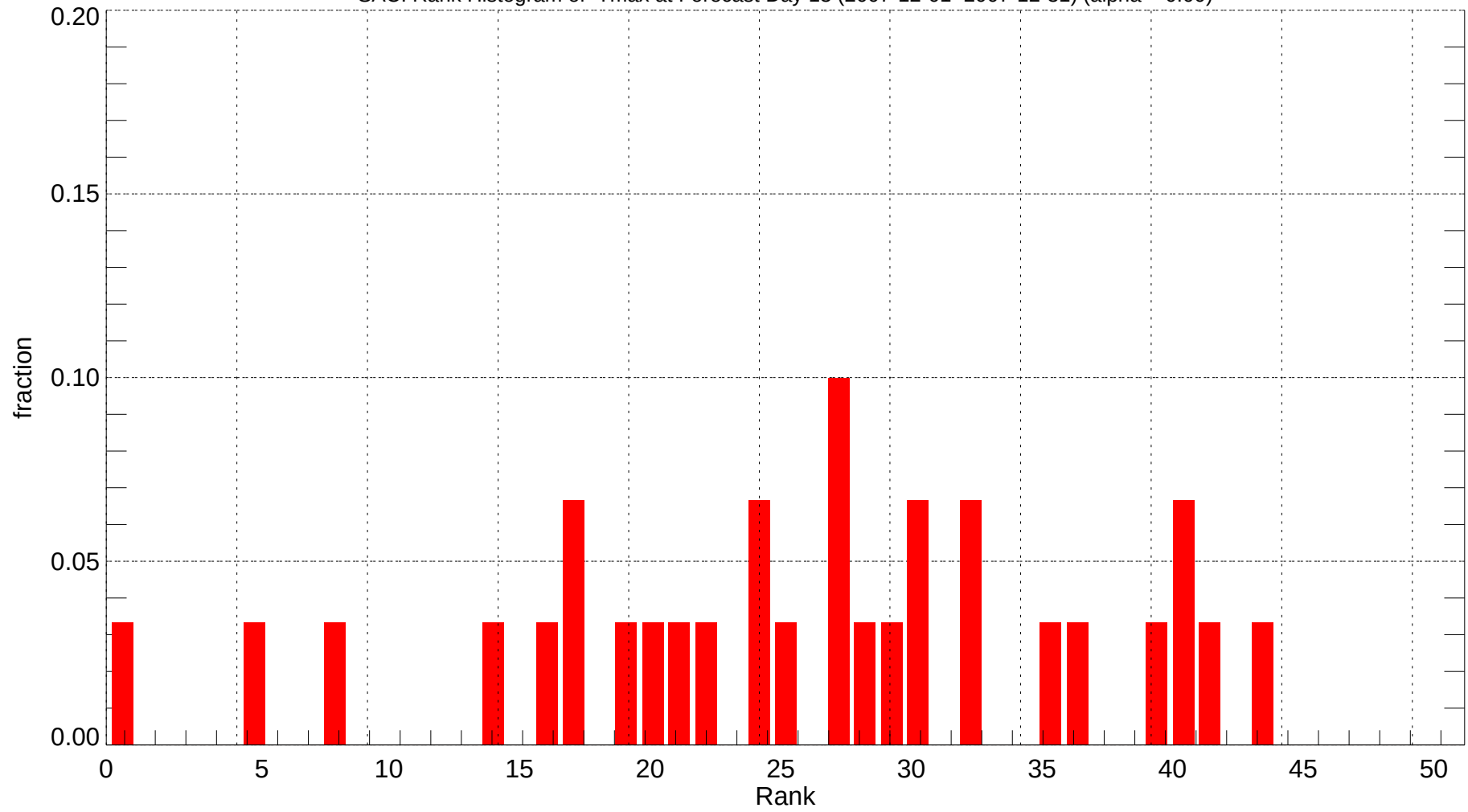
SAC: Rank Histogram of Tmax at Forecast Day 13 (2007-12-01~2007-12-31) (alpha = 0.00)
