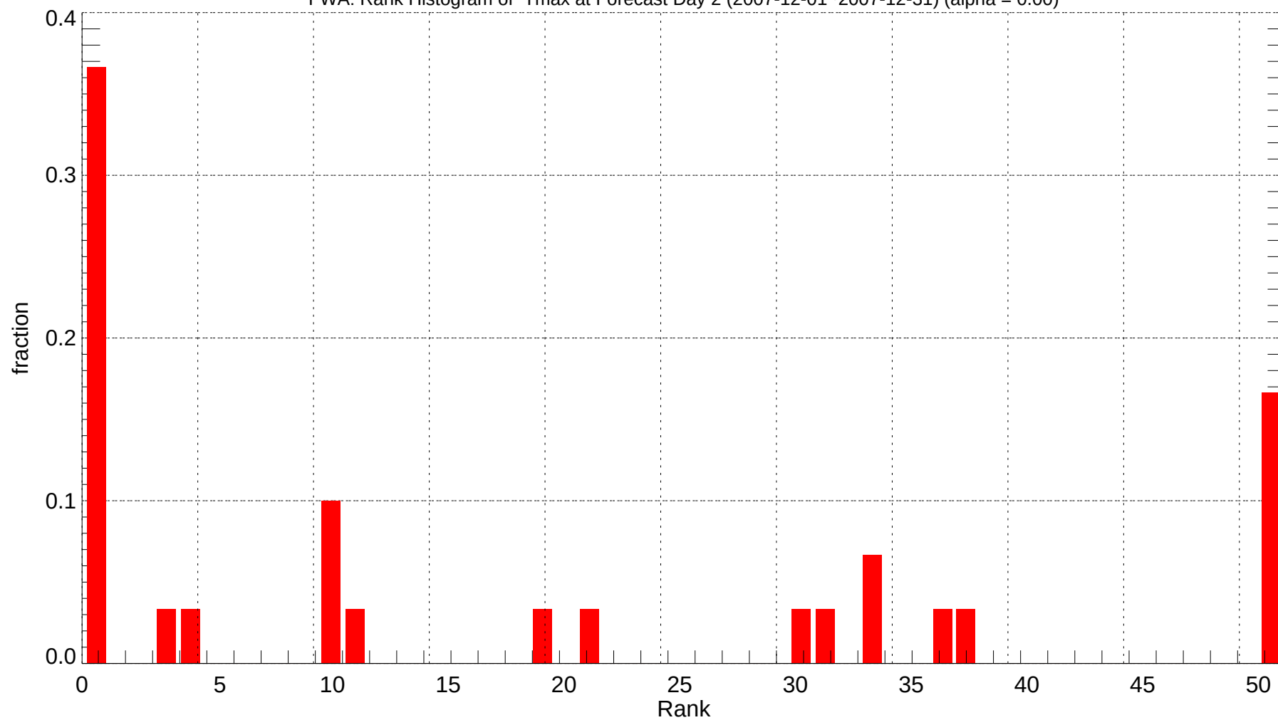
FWA: Rank Histogram of Tmax at Forecast Day 2 (2007-12-01~2007-12-31) (alpha = 0.00)
