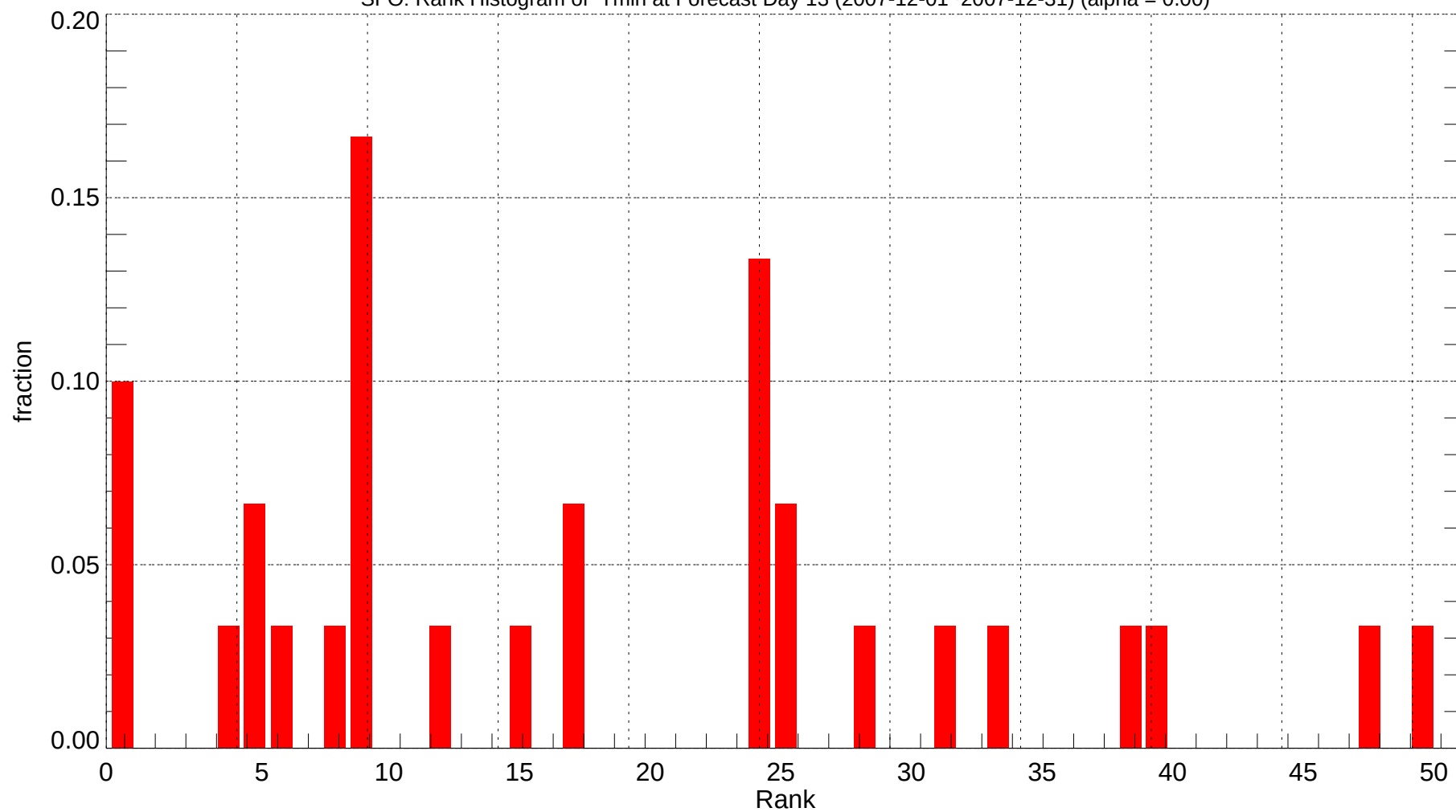
SFO: Rank Histogram of Tmin at Forecast Day 13 (2007-12-01~2007-12-31) (alpha = 0.00)
