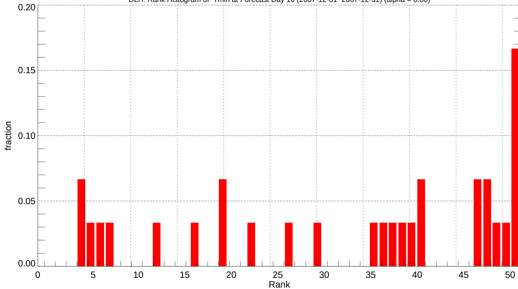
DLH: Rank Histogram of Tmin at Forecast Day 10 (2007-12-01~2007-12-31) (alpha = 0.00)
