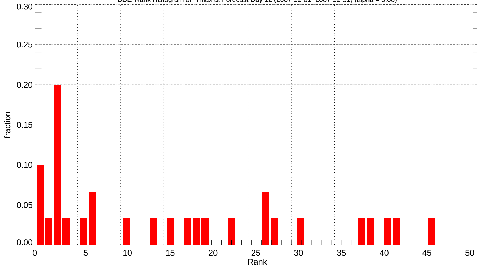
BDL: Rank Histogram of Tmax at Forecast Day 12 (2007-12-01~2007-12-31) (alpha = 0.00)
