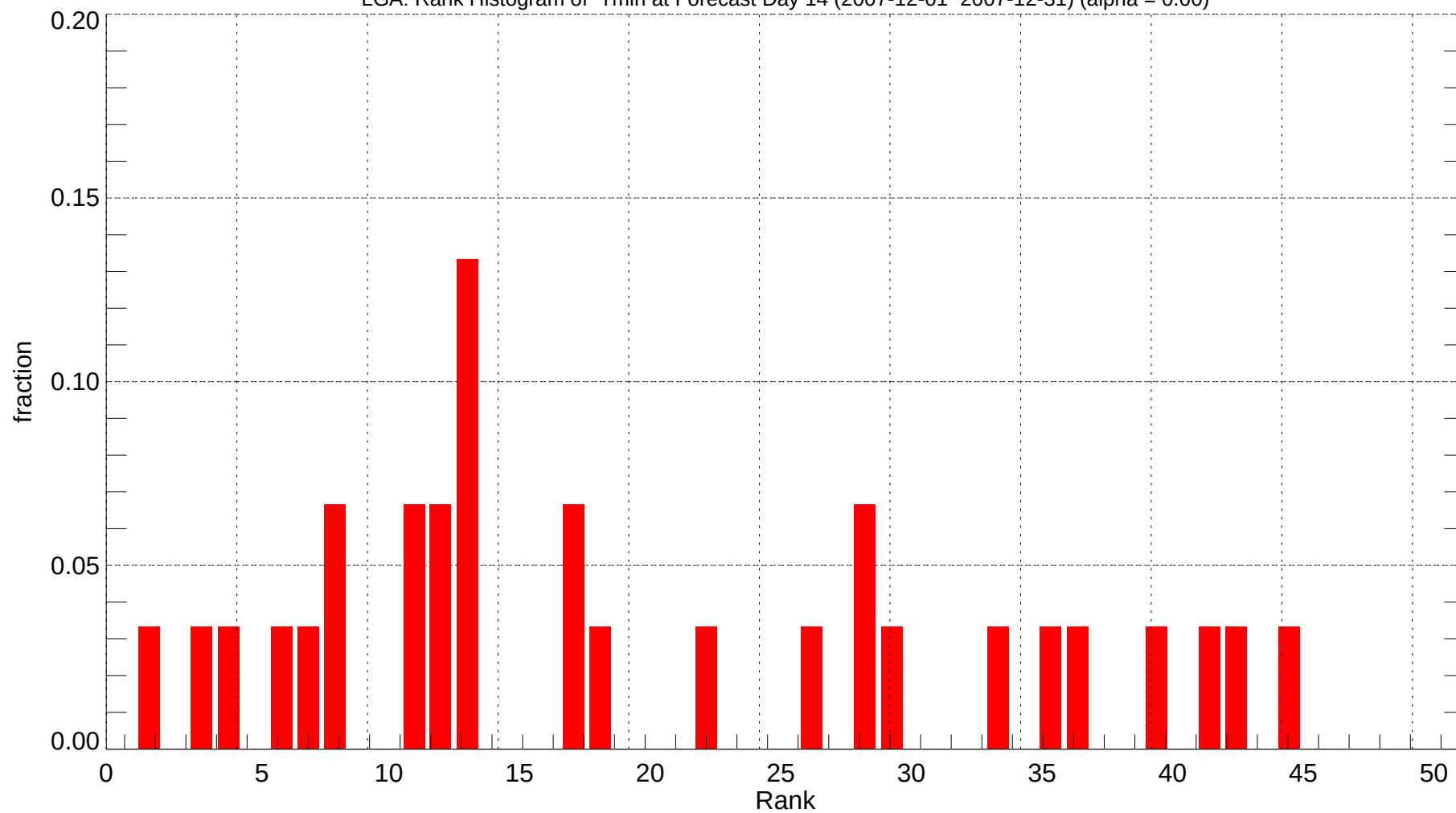
LGA: Rank Histogram of Tmin at Forecast Day 14 (2007-12-01~2007-12-31) (alpha = 0.00)
