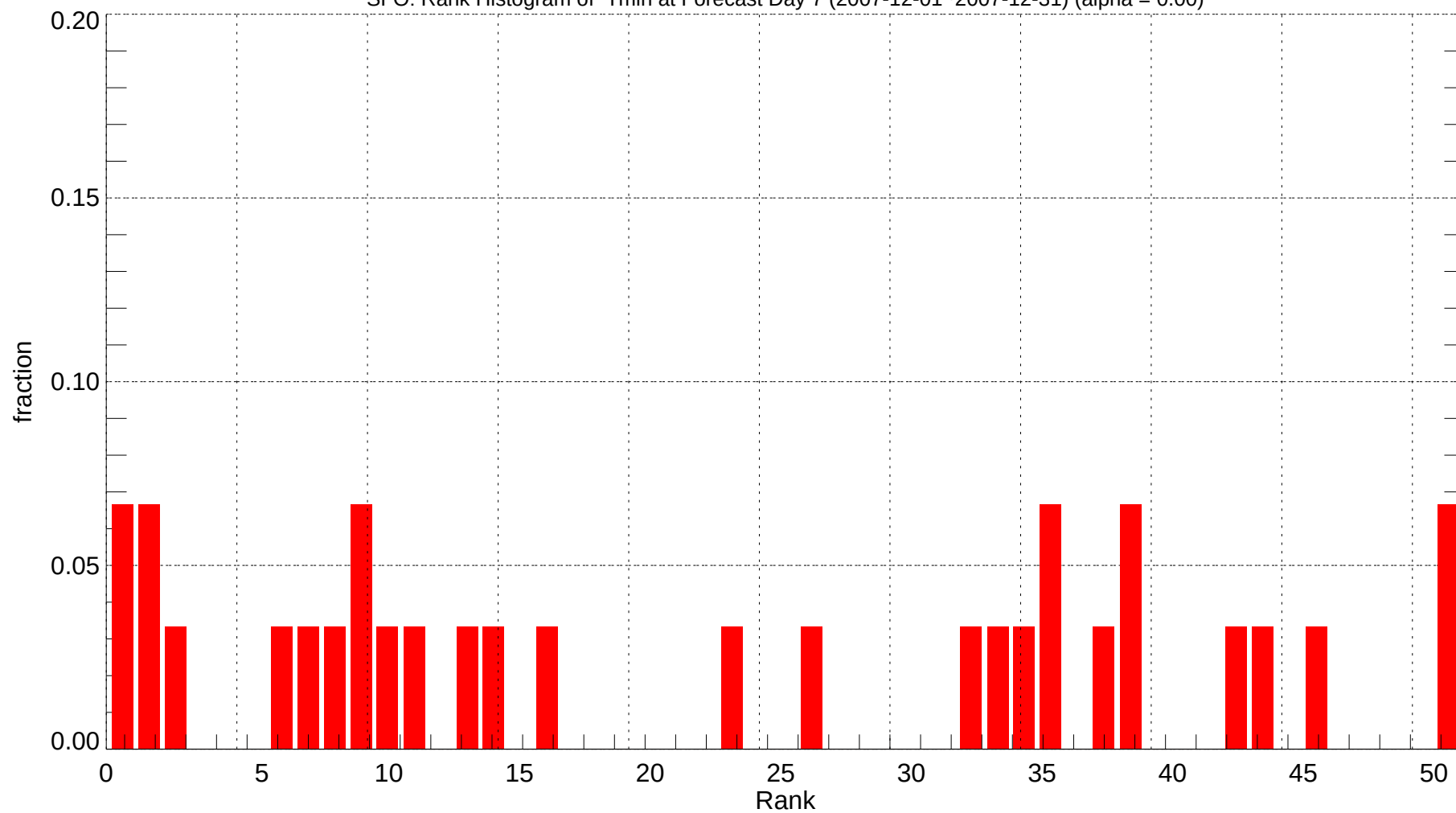
SFO: Rank Histogram of Tmin at Forecast Day 7 (2007-12-01~2007-12-31) (alpha = 0.00)
