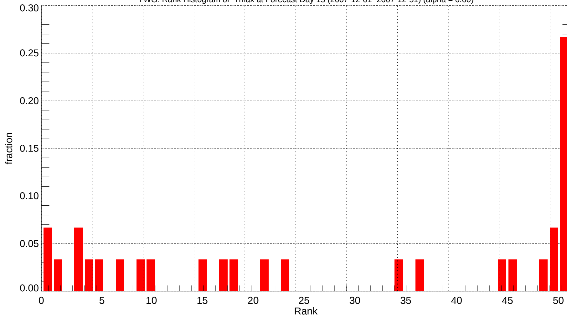
YWG: Rank Histogram of Tmax at Forecast Day 15 (2007-12-01~2007-12-31) (alpha = 0.00)
