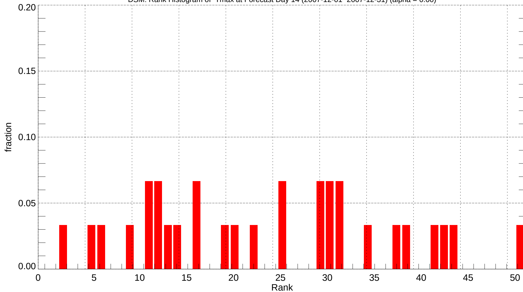
DSM: Rank Histogram of Tmax at Forecast Day 14 (2007-12-01~2007-12-31) (alpha = 0.00)
