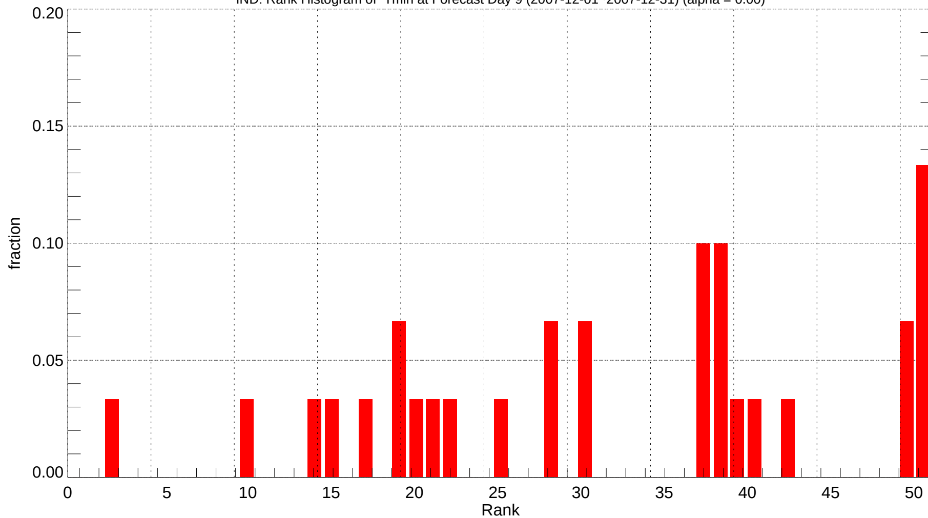
IND: Rank Histogram of Tmin at Forecast Day 9 (2007-12-01~2007-12-31) (alpha = 0.00)
