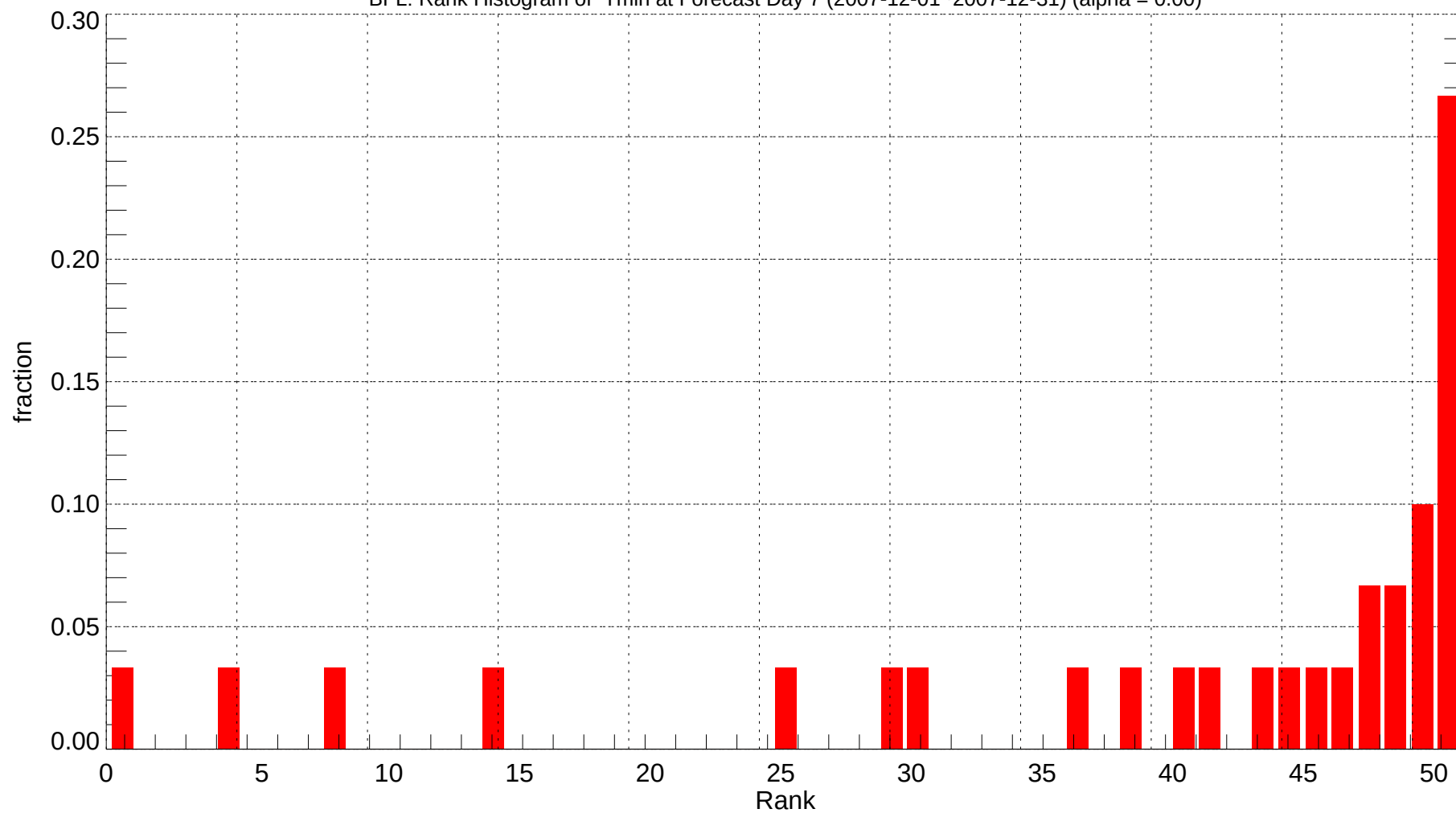
BFL: Rank Histogram of Tmin at Forecast Day 7 (2007-12-01~2007-12-31) (alpha = 0.00)
