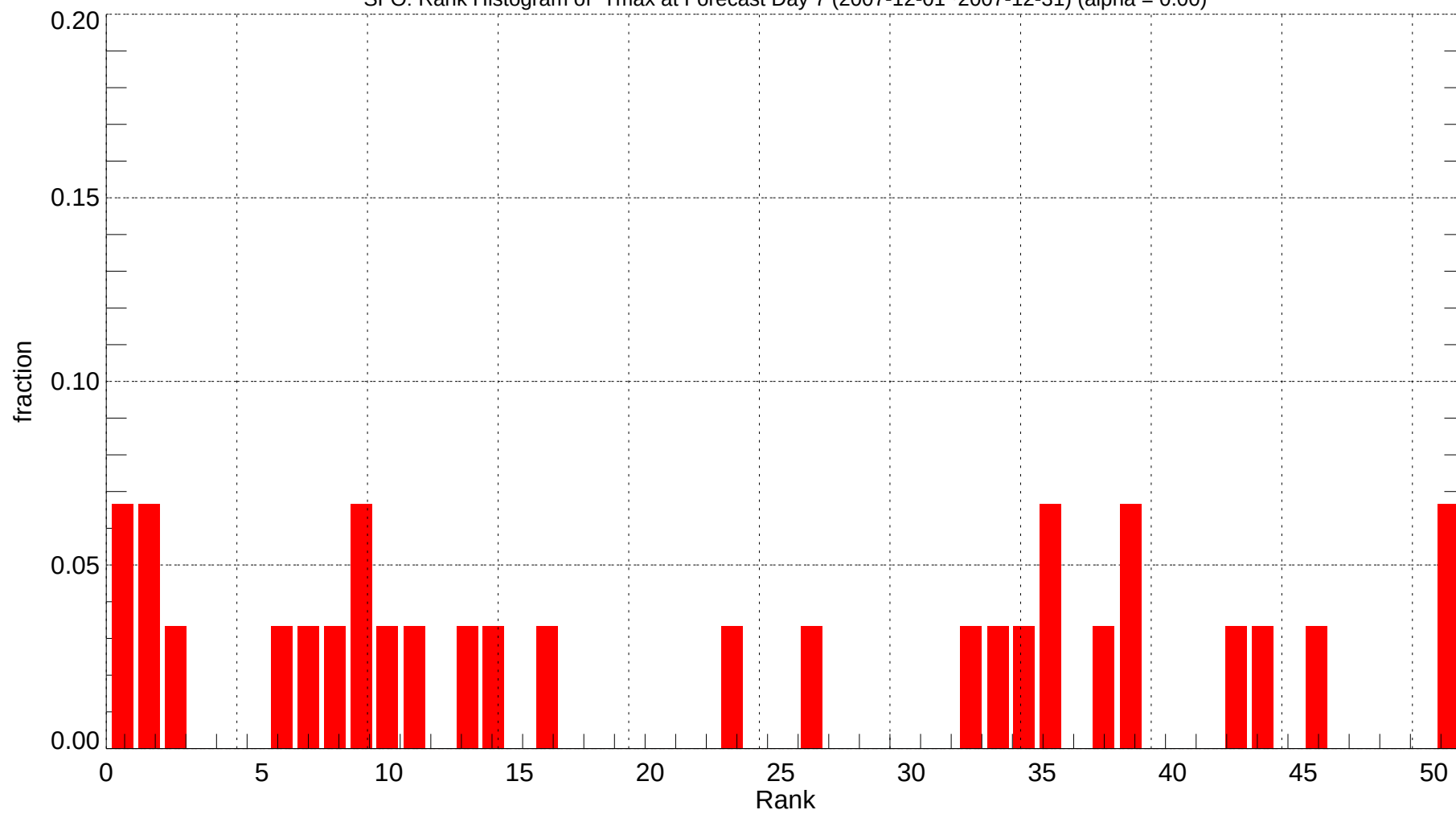
SFO: Rank Histogram of Tmax at Forecast Day 7 (2007-12-01~2007-12-31) (alpha = 0.00)
