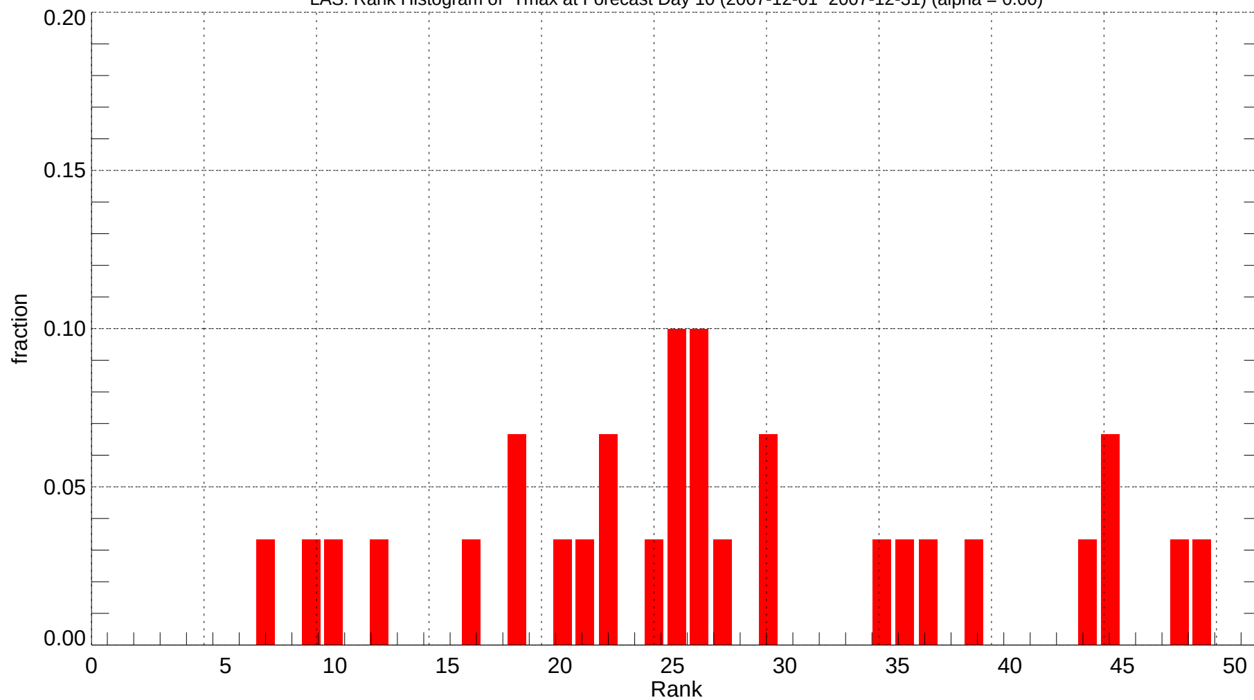
LAS: Rank Histogram of Tmax at Forecast Day 10 (2007-12-01~2007-12-31) (alpha = 0.00)
