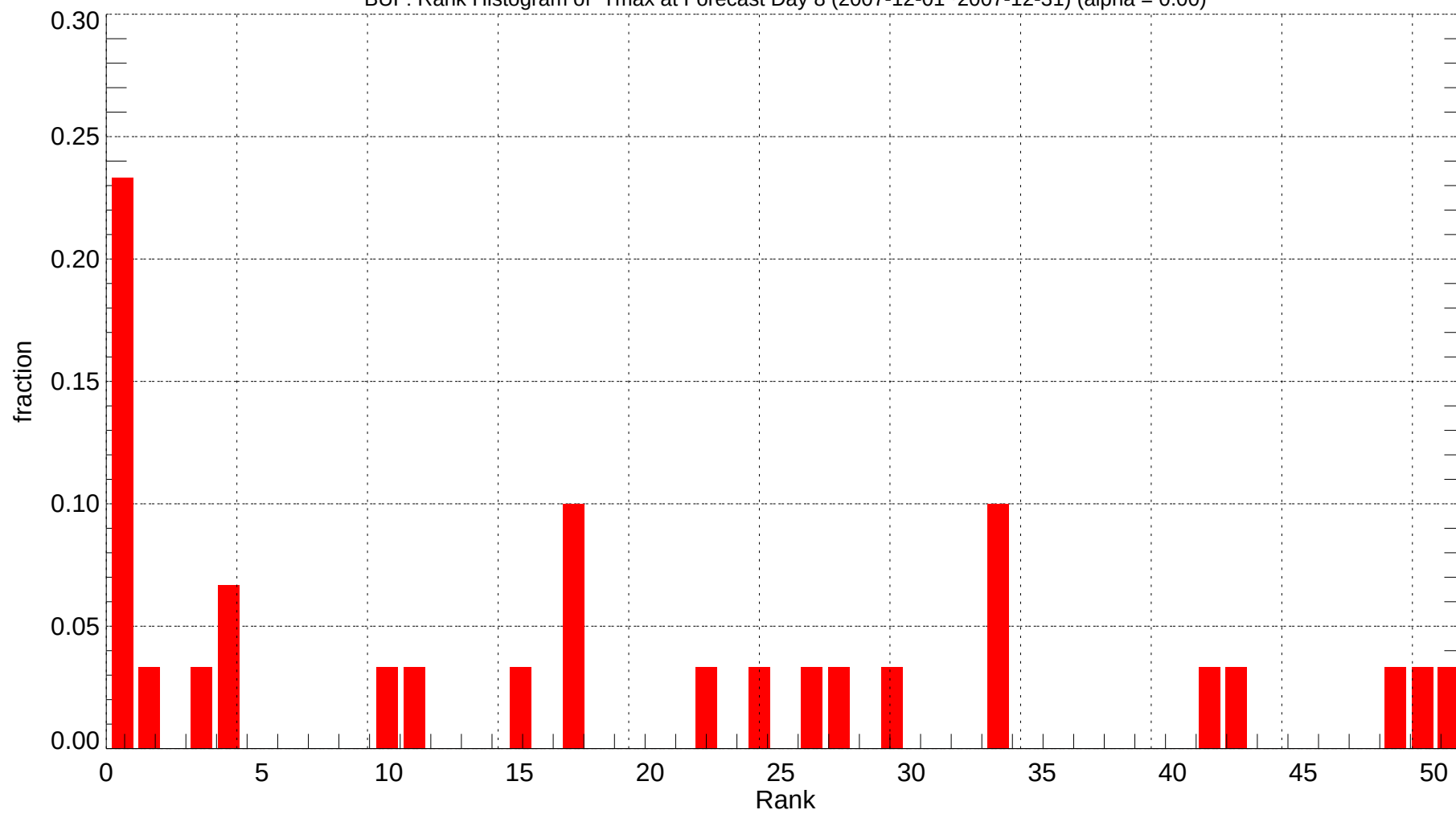
BUF: Rank Histogram of Tmax at Forecast Day 8 (2007-12-01~2007-12-31) (alpha = 0.00)
