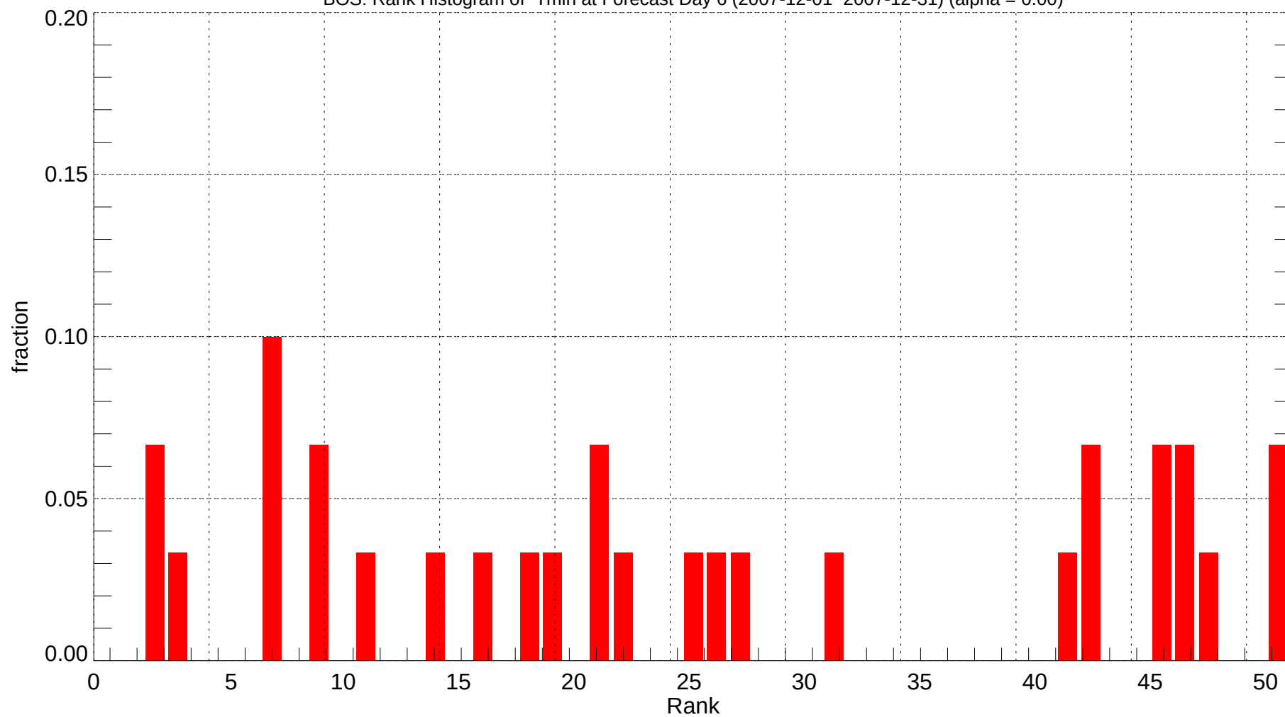
BOS: Rank Histogram of Tmin at Forecast Day 6 (2007-12-01~2007-12-31) (alpha = 0.00)
