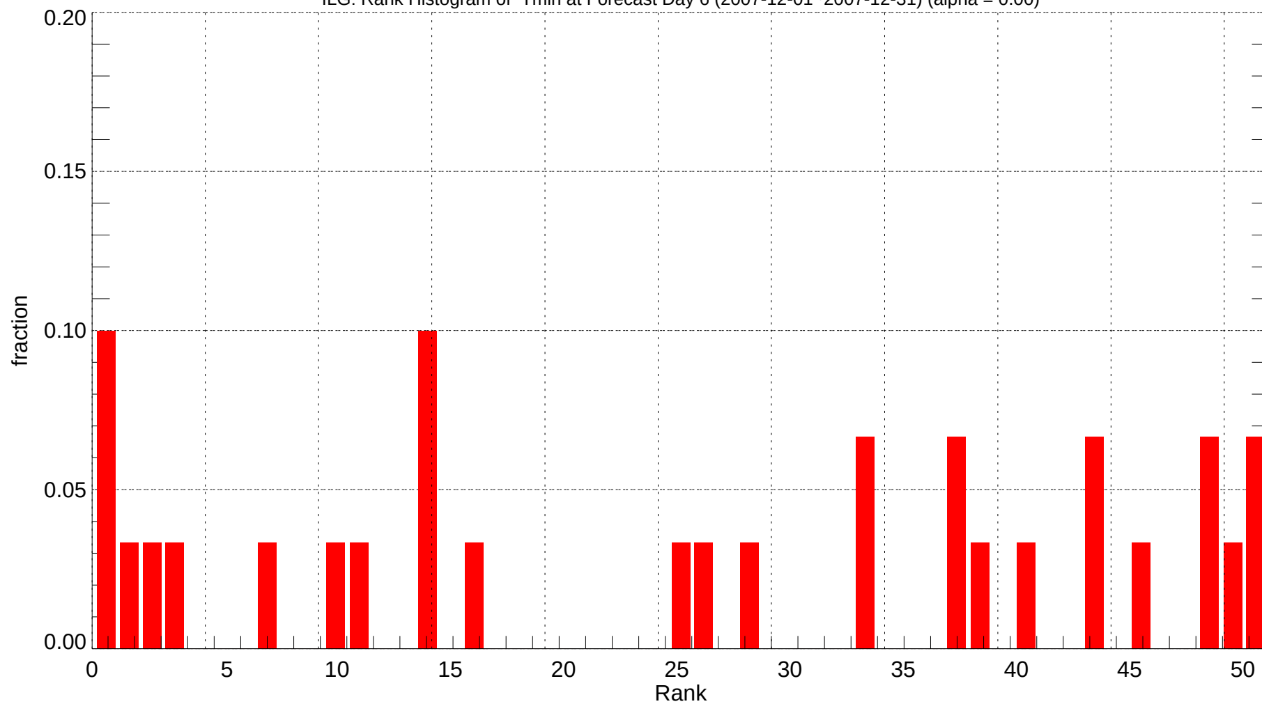
ILG: Rank Histogram of Tmin at Forecast Day 6 (2007-12-01~2007-12-31) (alpha = 0.00)
