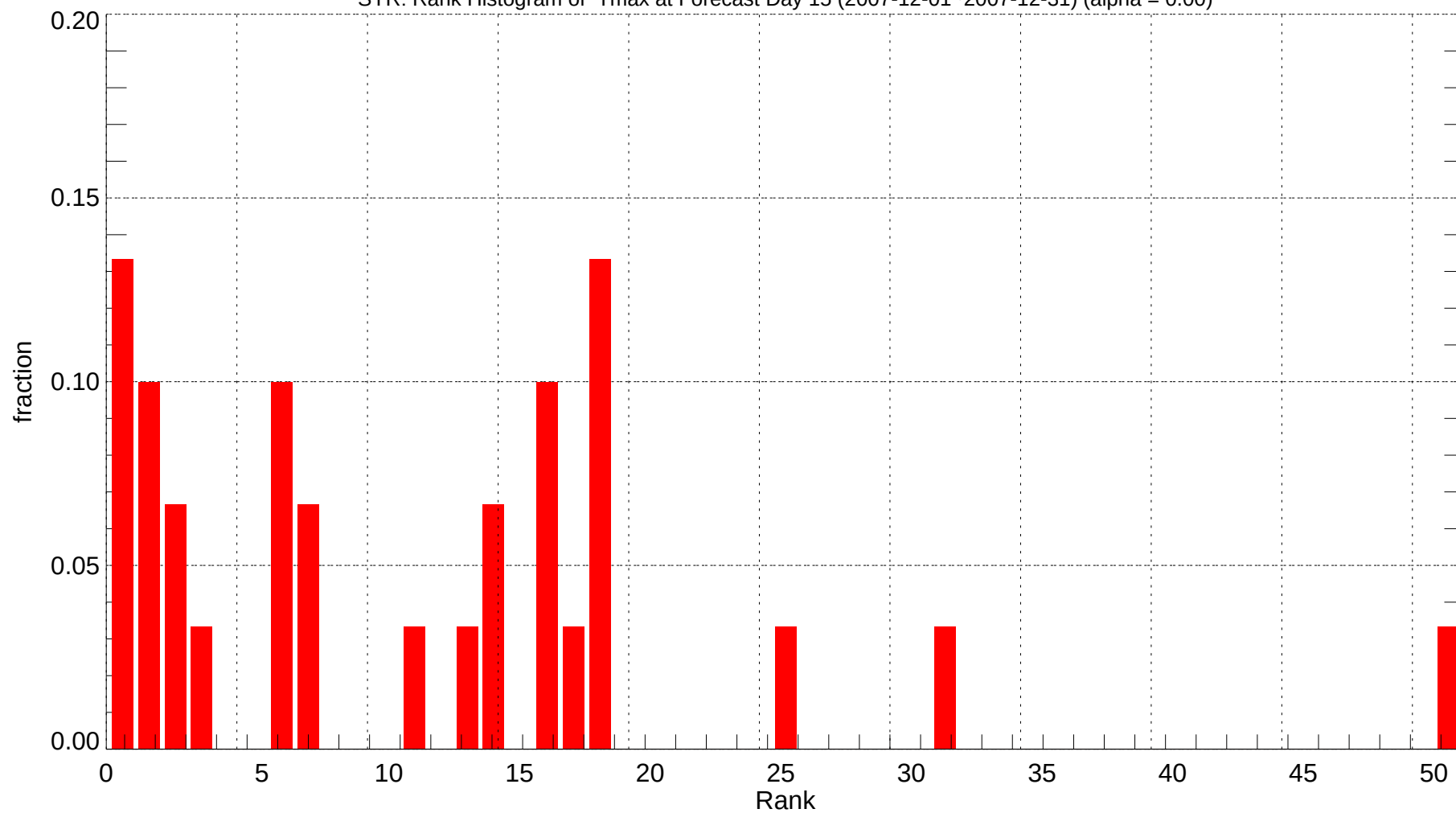
SYR: Rank Histogram of Tmax at Forecast Day 15 (2007-12-01~2007-12-31) (alpha = 0.00)
