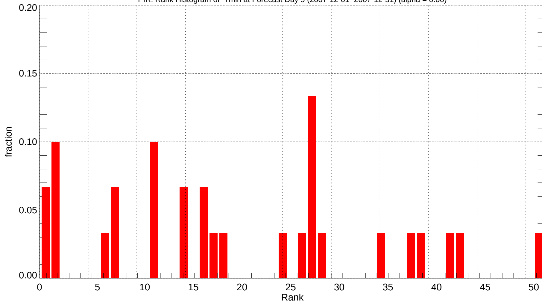
PIR: Rank Histogram of Tmin at Forecast Day 9 (2007-12-01~2007-12-31) (alpha = 0.00)
