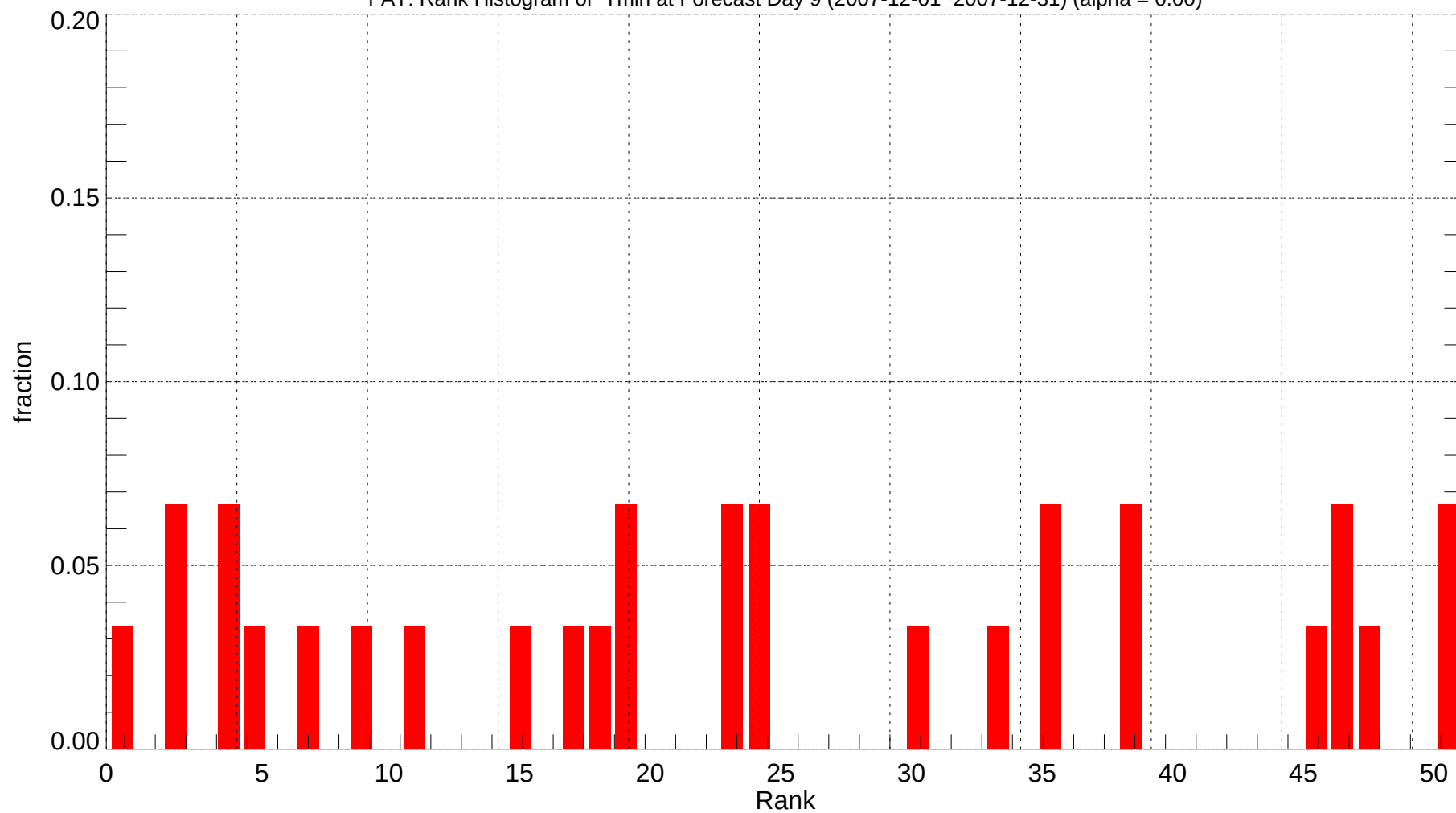
FAT: Rank Histogram of Tmin at Forecast Day 9 (2007-12-01~2007-12-31) (alpha = 0.00)
