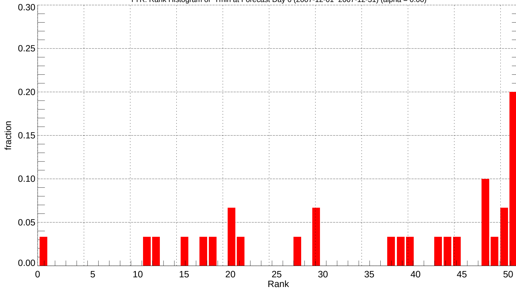
TYR: Rank Histogram of Tmin at Forecast Day 6 (2007-12-01~2007-12-31) (alpha = 0.00)
