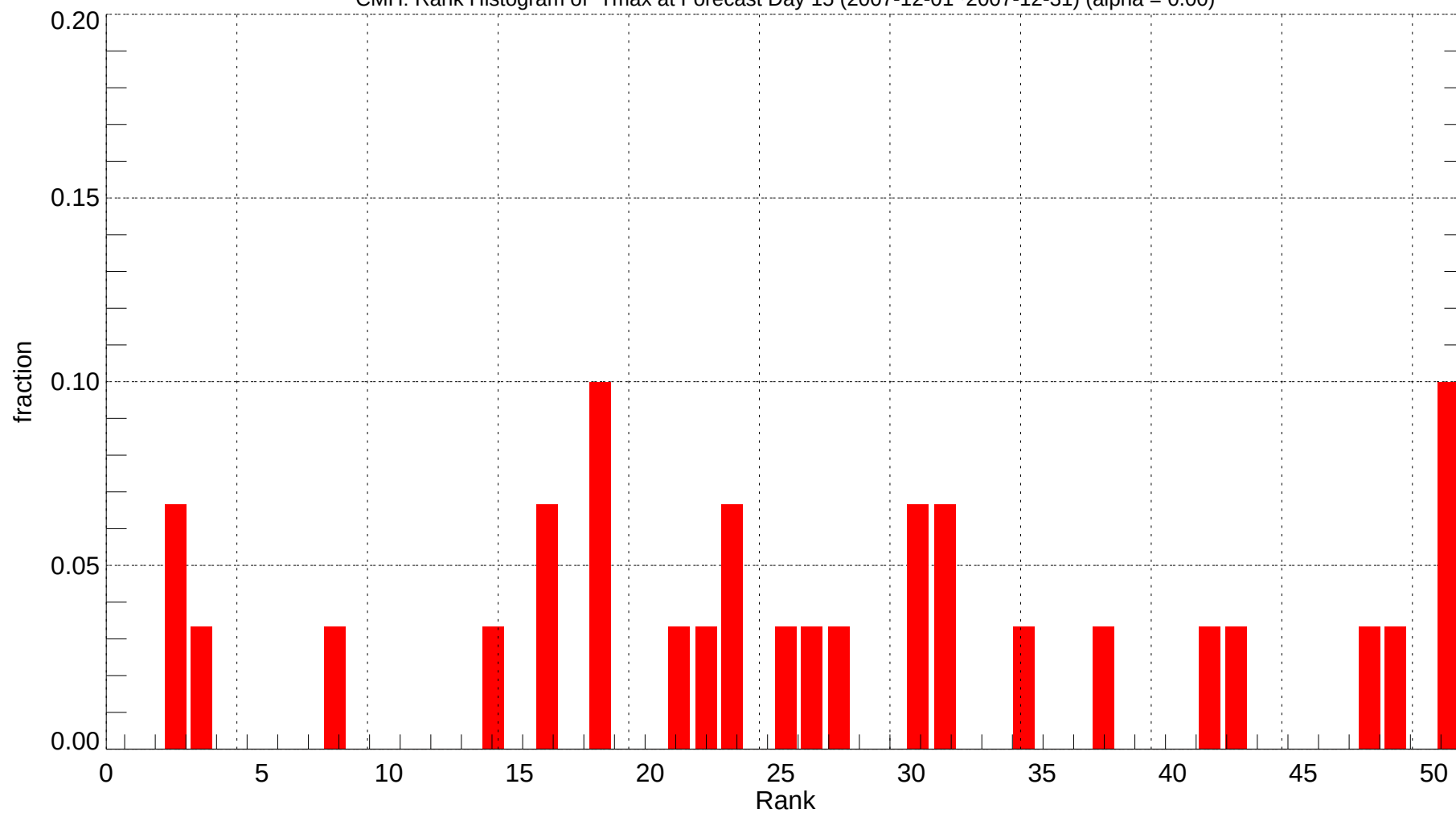
CMH: Rank Histogram of Tmax at Forecast Day 15 (2007-12-01~2007-12-31) (alpha = 0.00)
