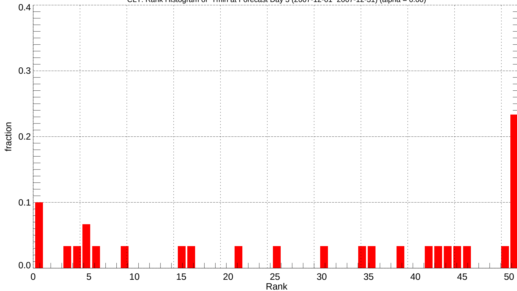
CLT: Rank Histogram of Tmin at Forecast Day 3 (2007-12-01~2007-12-31) (alpha = 0.00)
