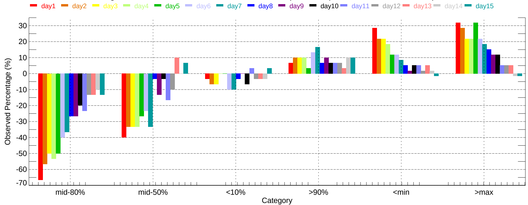
Observed Percentage Deviation of Ensembles - SSI: Max Temperature (2007-12-01~2007-12-31)
