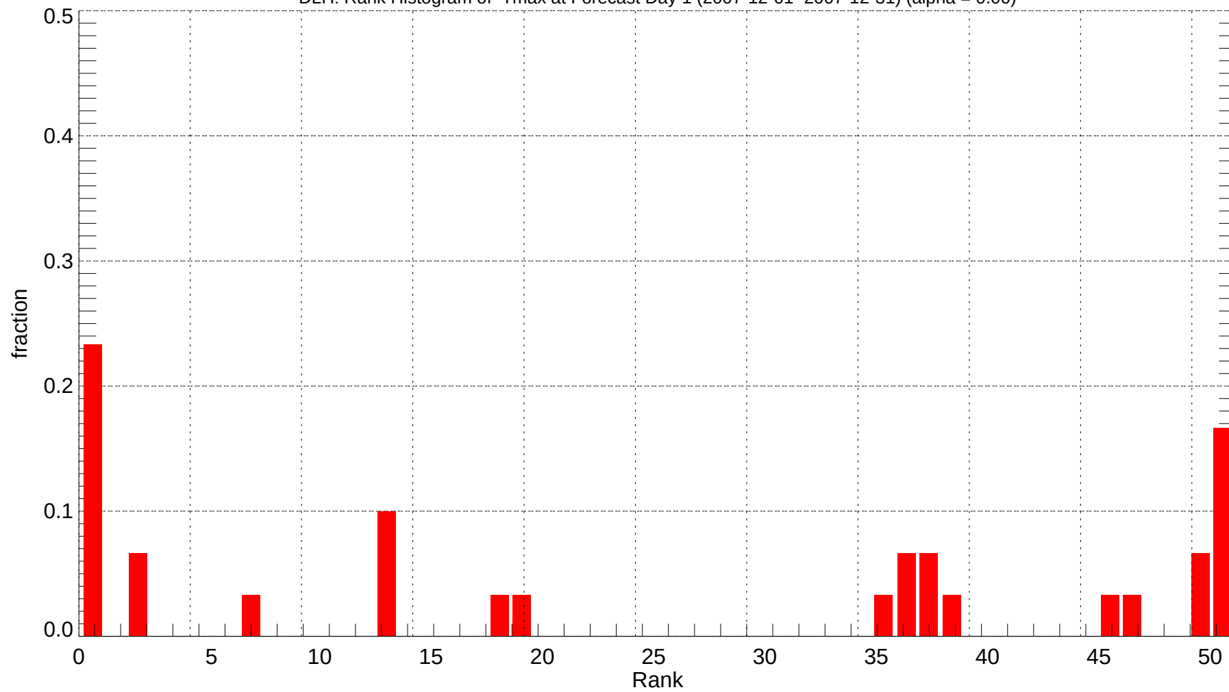
DLH: Rank Histogram of Tmax at Forecast Day 1 (2007-12-01~2007-12-31) (alpha = 0.00)
