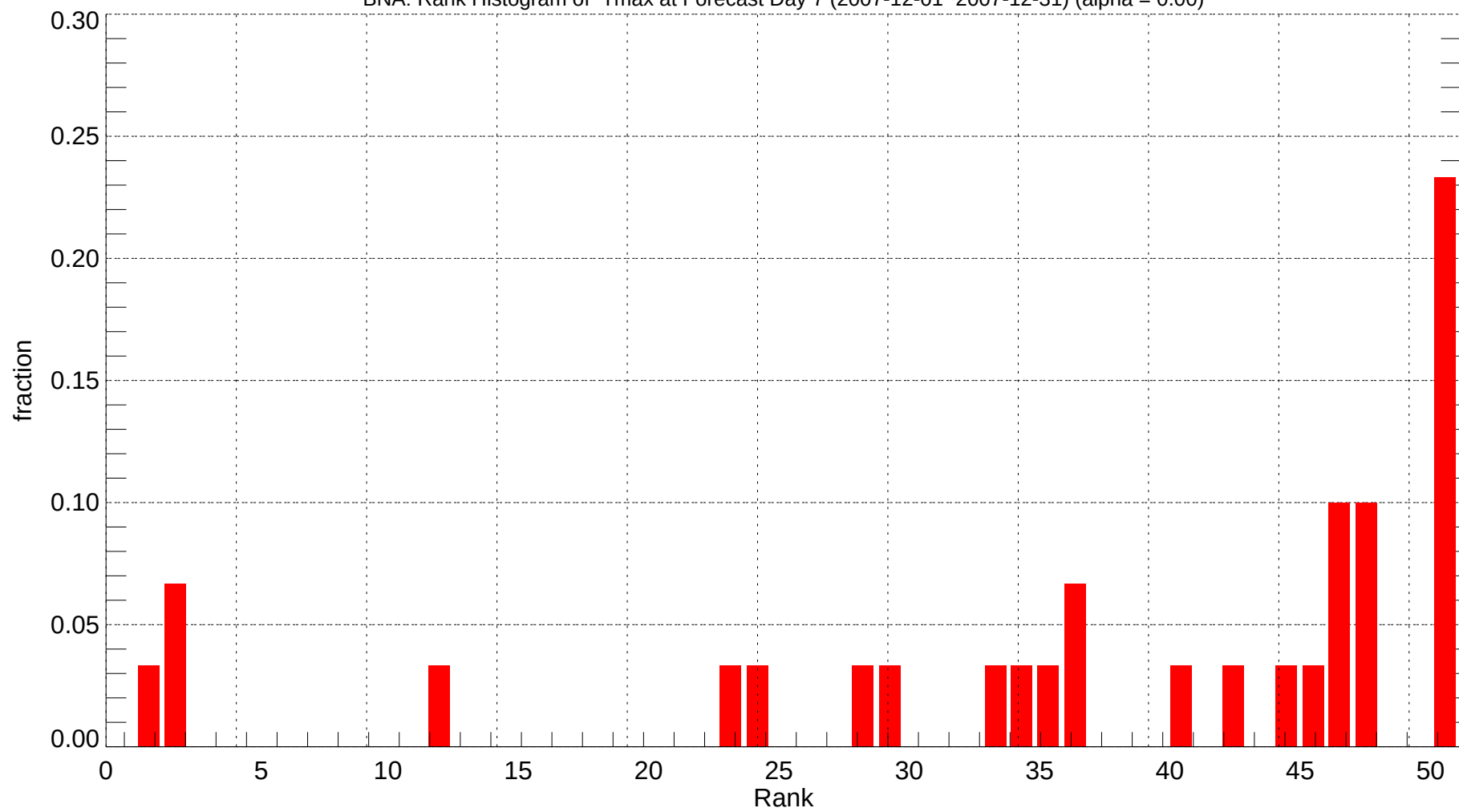
BNA: Rank Histogram of Tmax at Forecast Day 7 (2007-12-01~2007-12-31) (alpha = 0.00)
