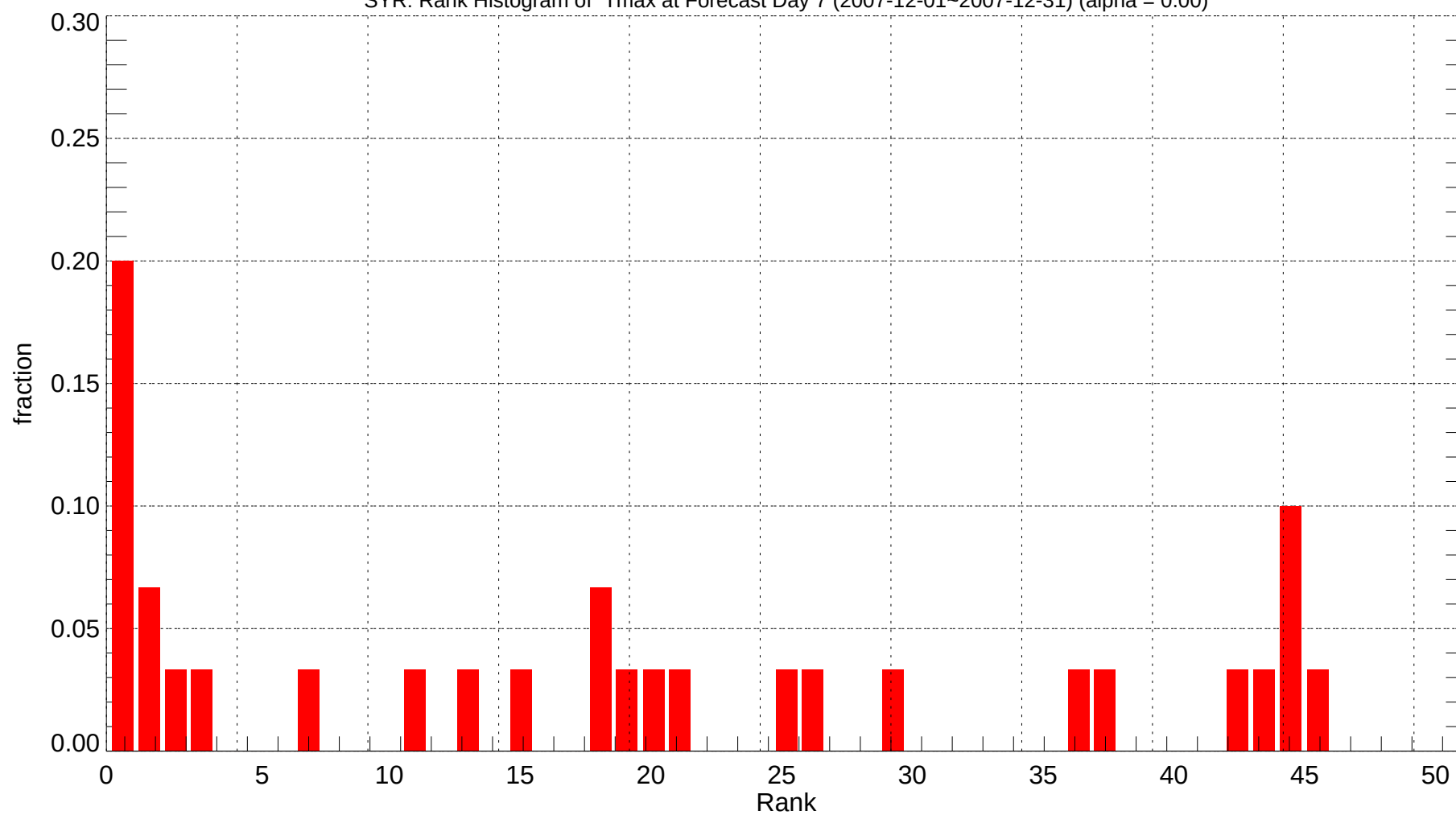
SYR: Rank Histogram of Tmax at Forecast Day 7 (2007-12-01~2007-12-31) (alpha = 0.00)
