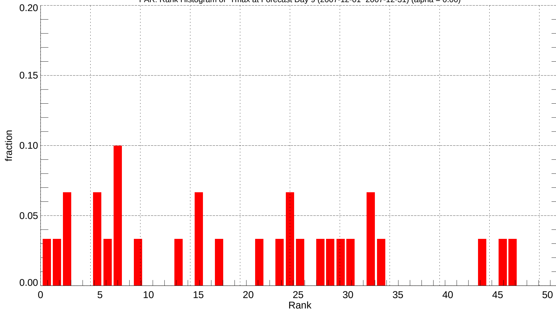
FAR: Rank Histogram of Tmax at Forecast Day 9 (2007-12-01~2007-12-31) (alpha = 0.00)
