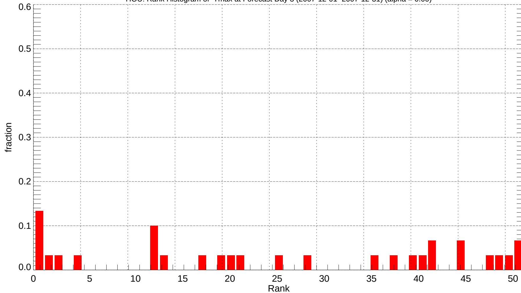
HOU: Rank Histogram of Tmax at Forecast Day 3 (2007-12-01~2007-12-31) (alpha = 0.00)
