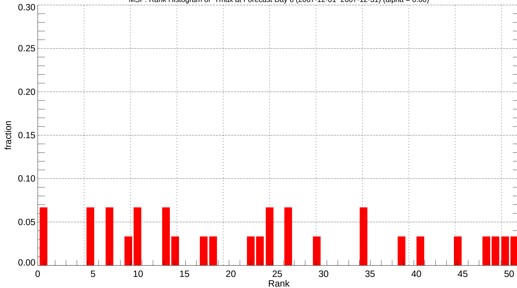
MSP: Rank Histogram of Tmax at Forecast Day 6 (2007-12-01~2007-12-31) (alpha = 0.00)
