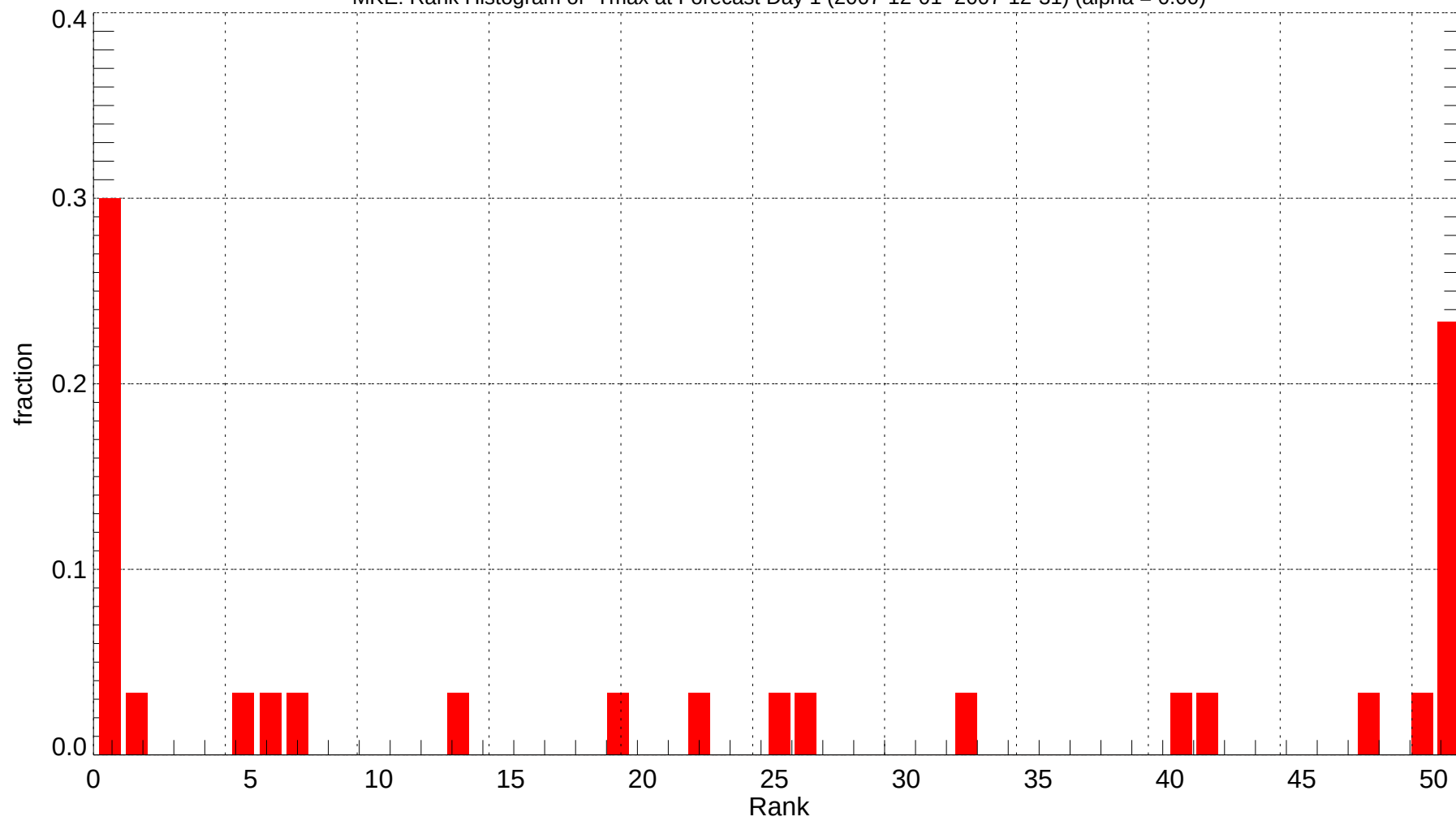
MKE: Rank Histogram of Tmax at Forecast Day 1 (2007-12-01~2007-12-31) (alpha = 0.00)
