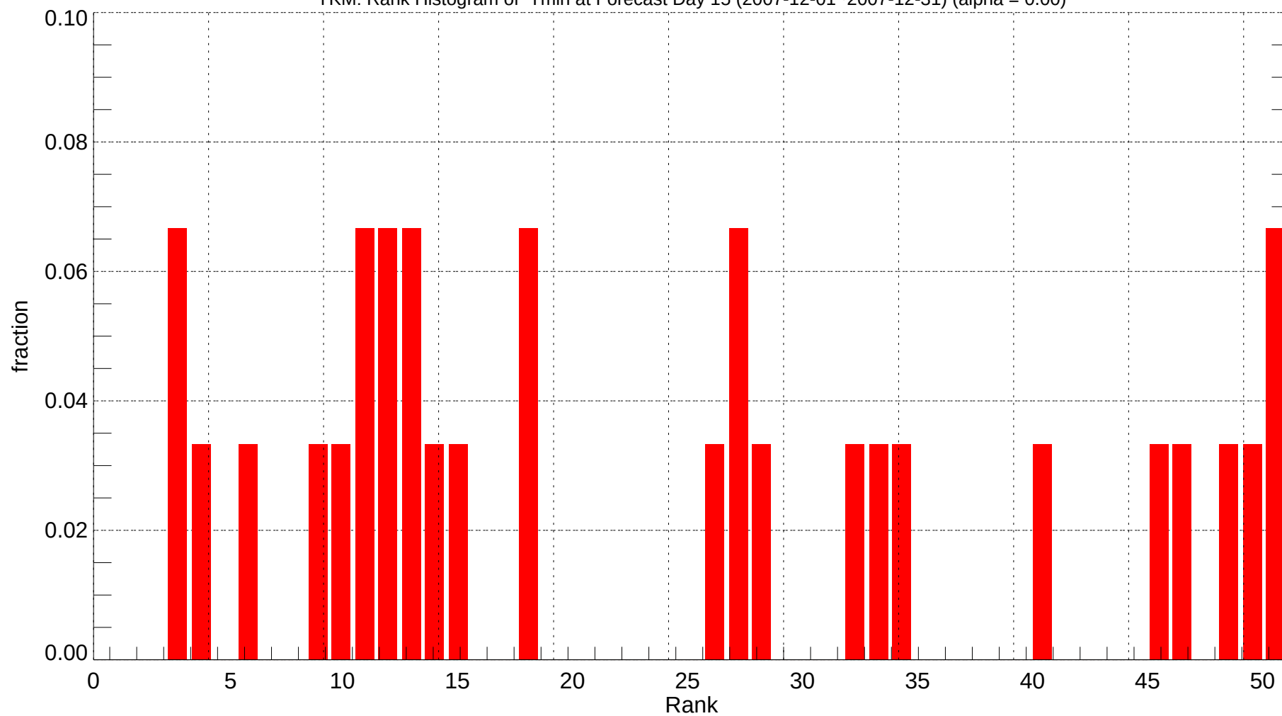
YKM: Rank Histogram of Tmin at Forecast Day 15 (2007-12-01~2007-12-31) (alpha = 0.00)
