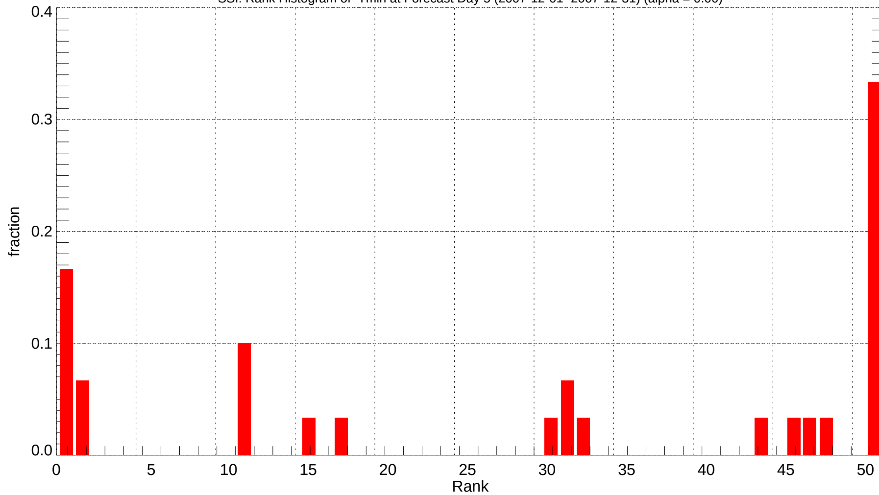
SSI: Rank Histogram of Tmin at Forecast Day 5 (2007-12-01~2007-12-31) (alpha = 0.00)
