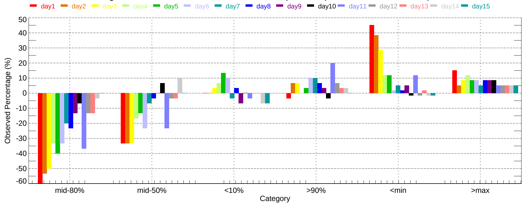
Observed Percentage Deviation of Ensembles - RIC: Min Temperature (2007-12-01~2007-12-31)
