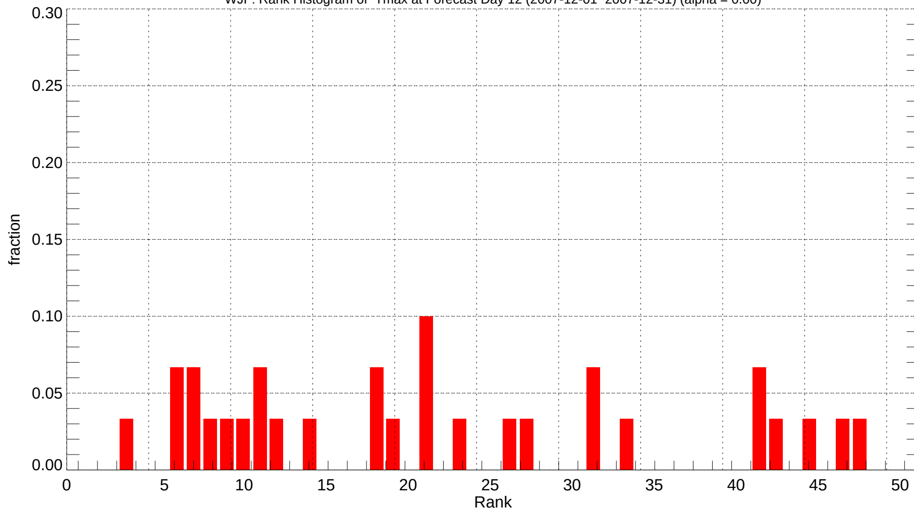
WJF: Rank Histogram of Tmax at Forecast Day 12 (2007-12-01~2007-12-31) (alpha = 0.00)
