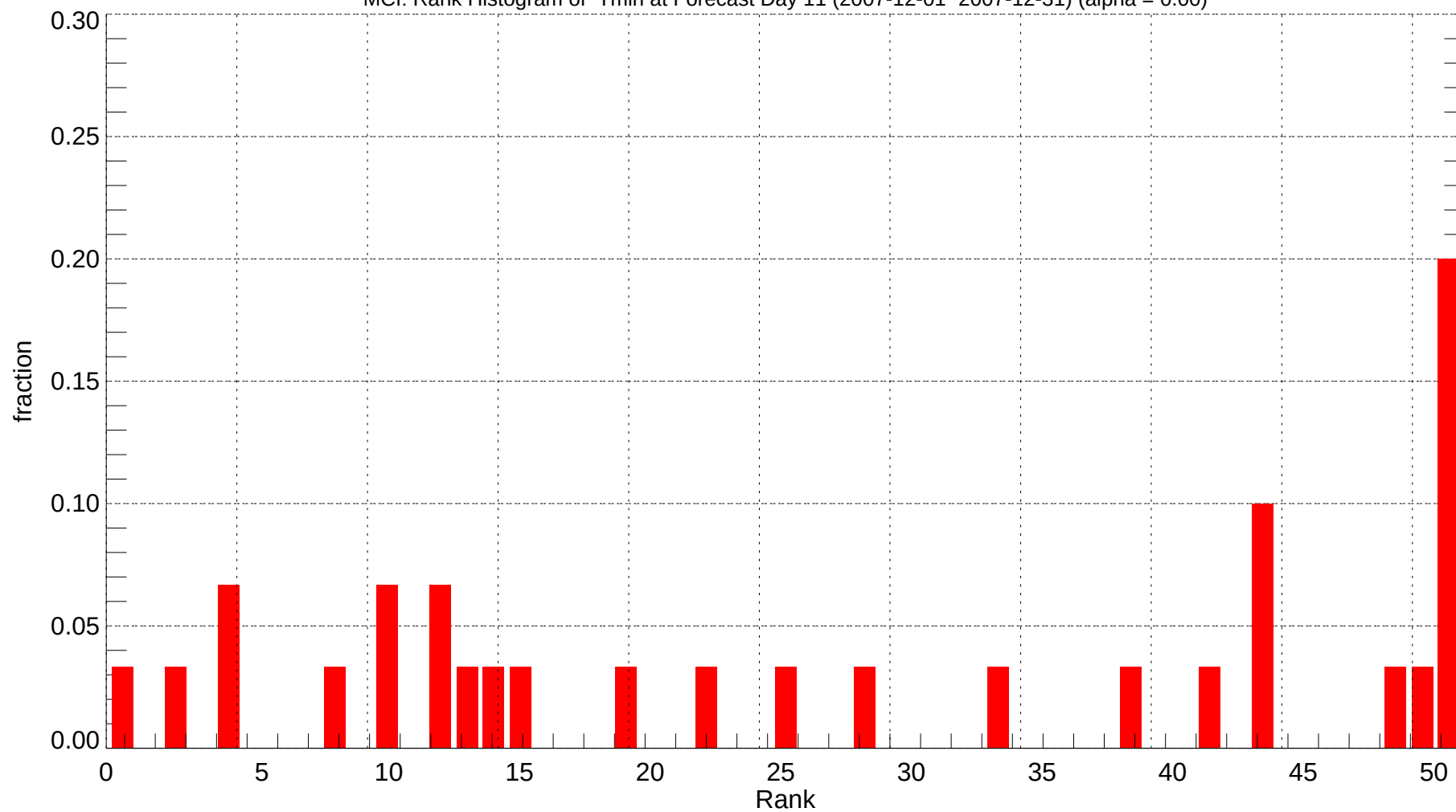
MCI: Rank Histogram of Tmin at Forecast Day 11 (2007-12-01~2007-12-31) (alpha = 0.00)
