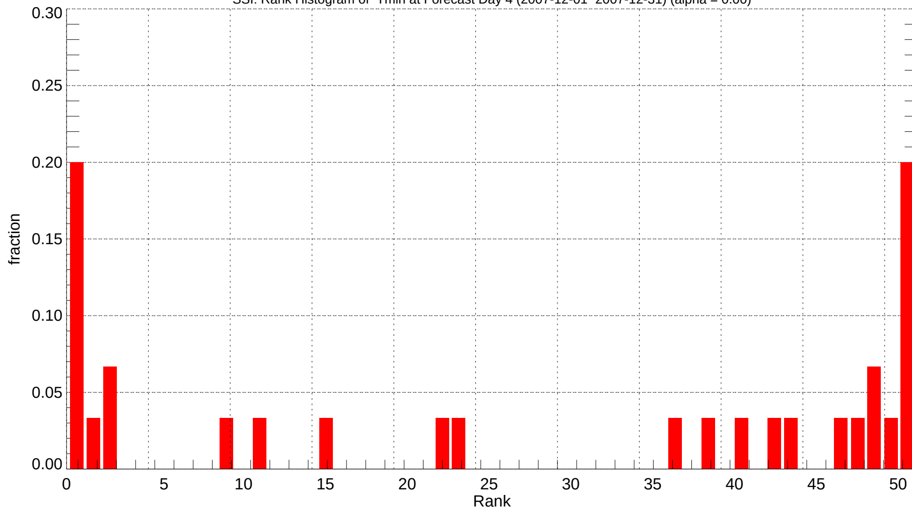
SSI: Rank Histogram of Tmin at Forecast Day 4 (2007-12-01~2007-12-31) (alpha = 0.00)
