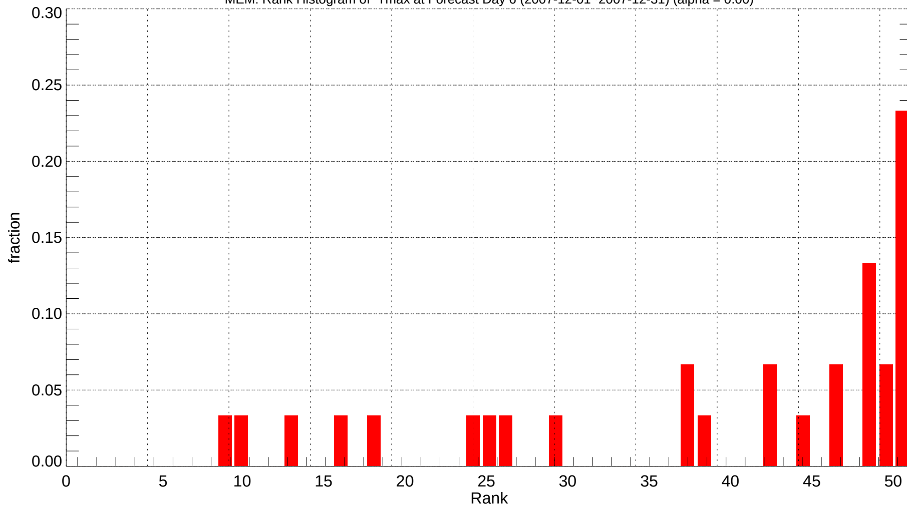
MEM: Rank Histogram of Tmax at Forecast Day 6 (2007-12-01~2007-12-31) (alpha = 0.00)
