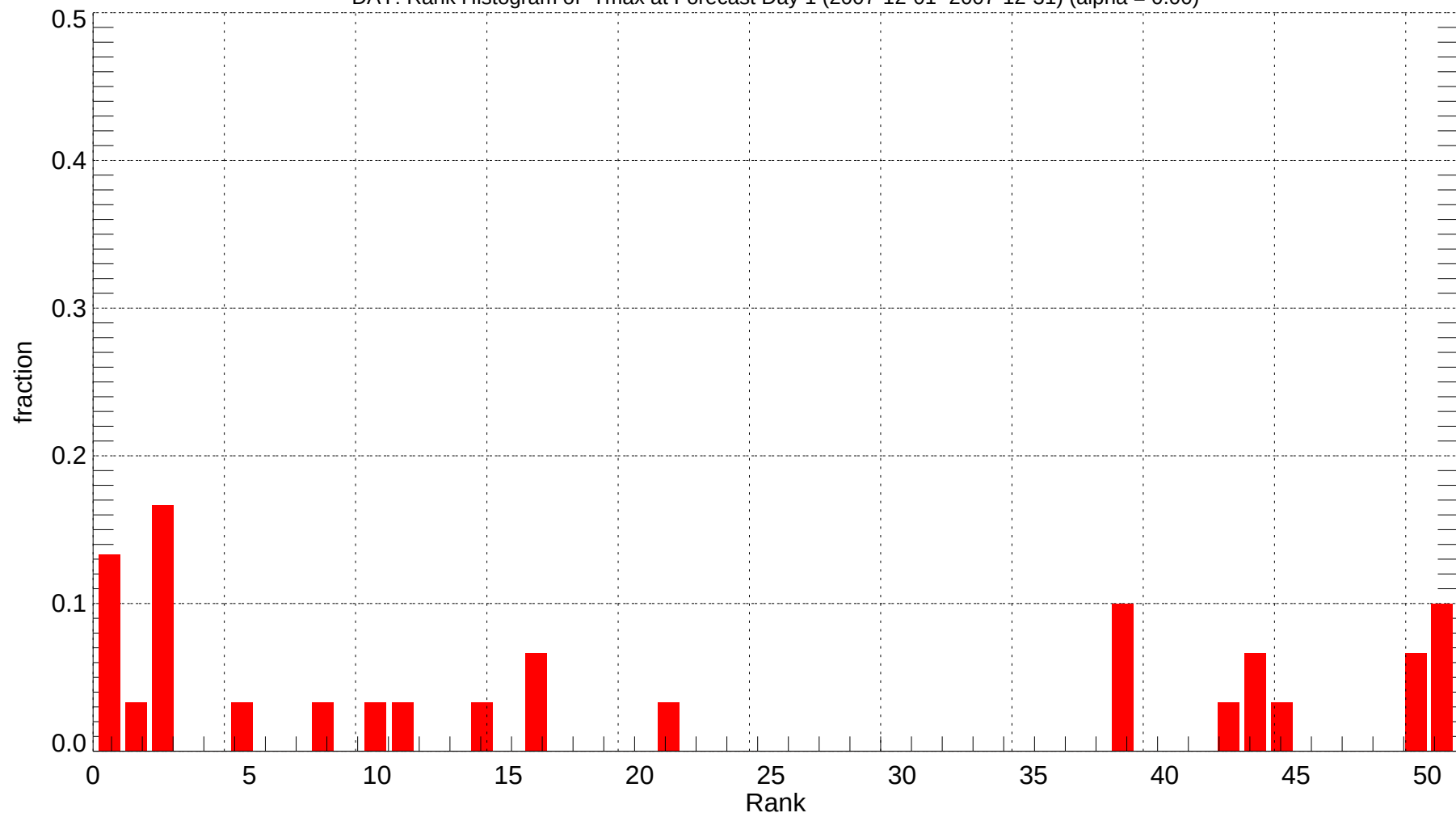
DAY: Rank Histogram of Tmax at Forecast Day 1 (2007-12-01~2007-12-31) (alpha = 0.00)
