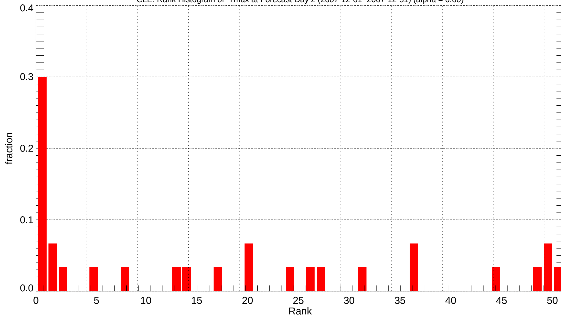
CLE: Rank Histogram of Tmax at Forecast Day 2 (2007-12-01~2007-12-31) (alpha = 0.00)
