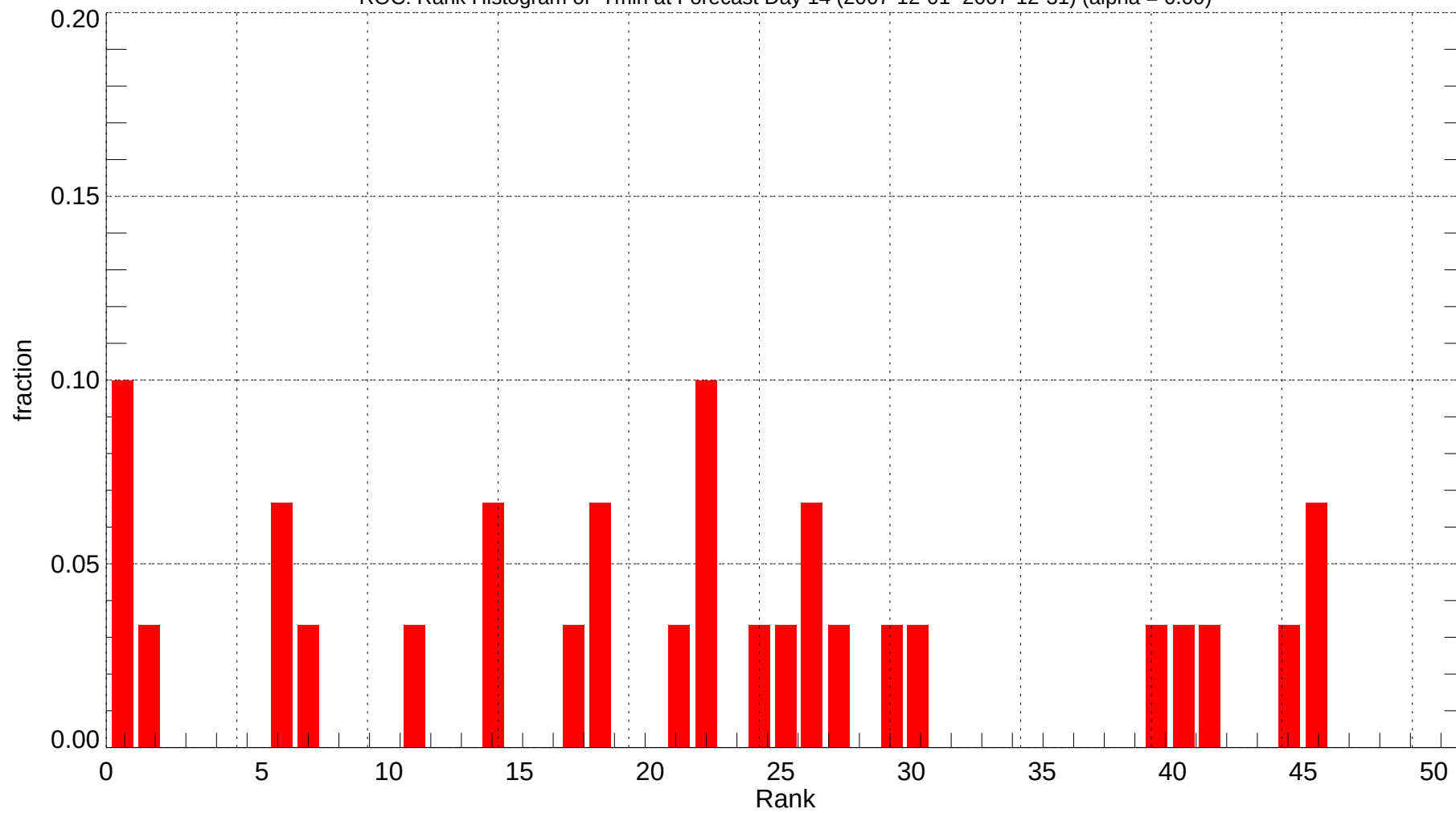
ROC: Rank Histogram of Tmin at Forecast Day 14 (2007-12-01~2007-12-31) (alpha = 0.00)
