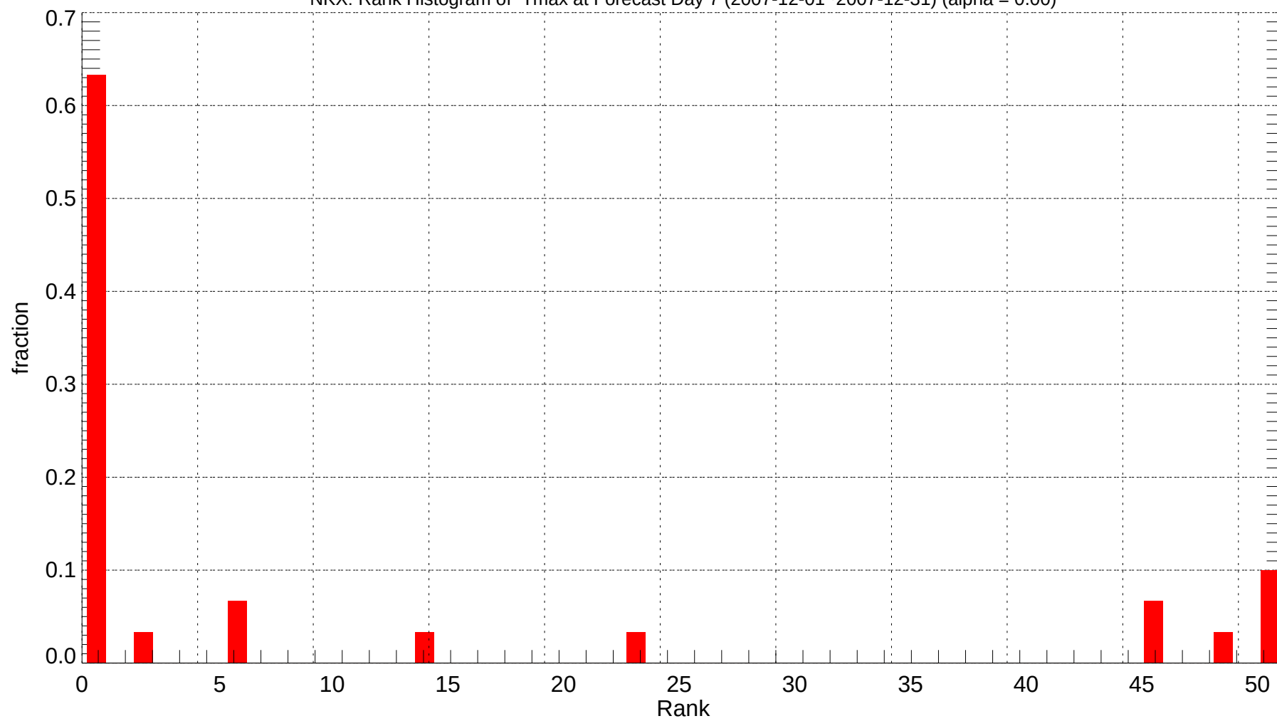
NKX: Rank Histogram of Tmax at Forecast Day 7 (2007-12-01~2007-12-31) (alpha = 0.00)
