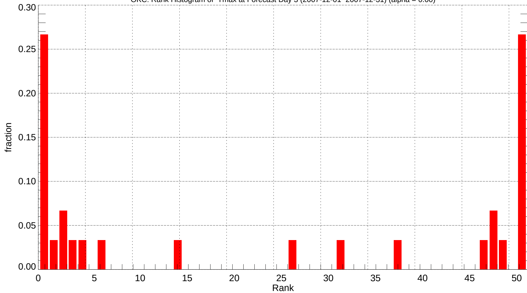
OKC: Rank Histogram of Tmax at Forecast Day 3 (2007-12-01~2007-12-31) (alpha = 0.00)
