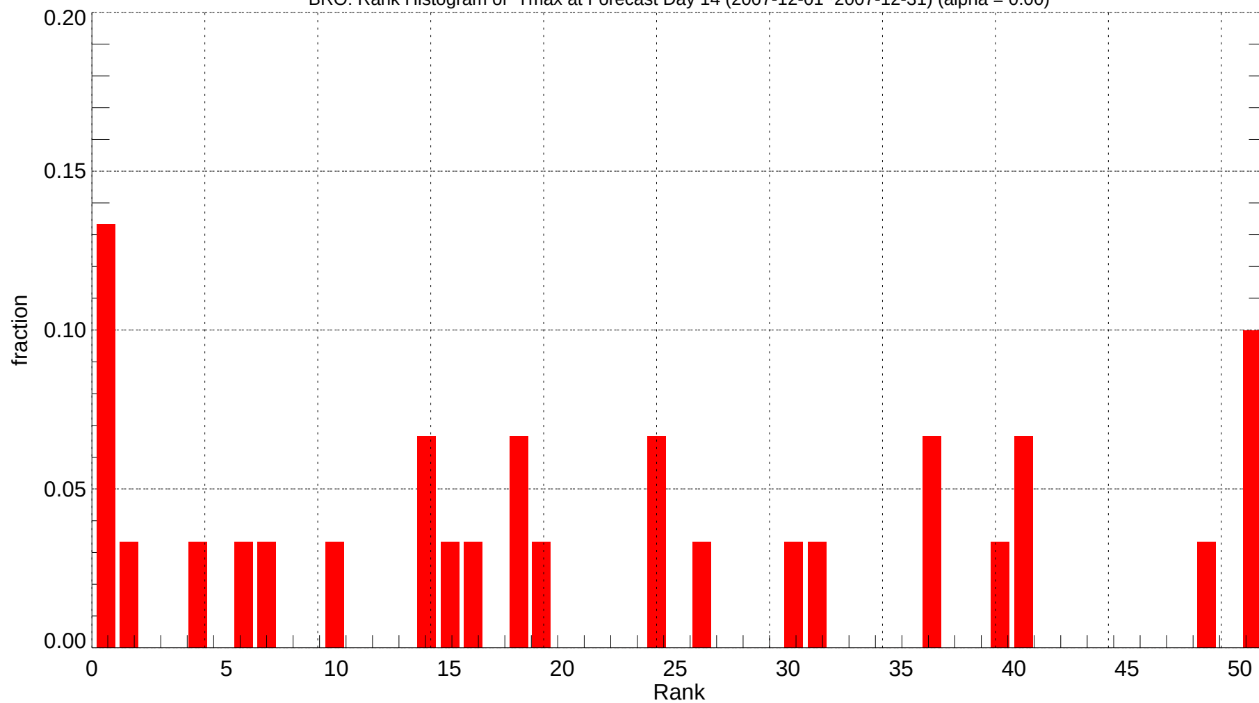
BRO: Rank Histogram of Tmax at Forecast Day 14 (2007-12-01~2007-12-31) (alpha = 0.00)
