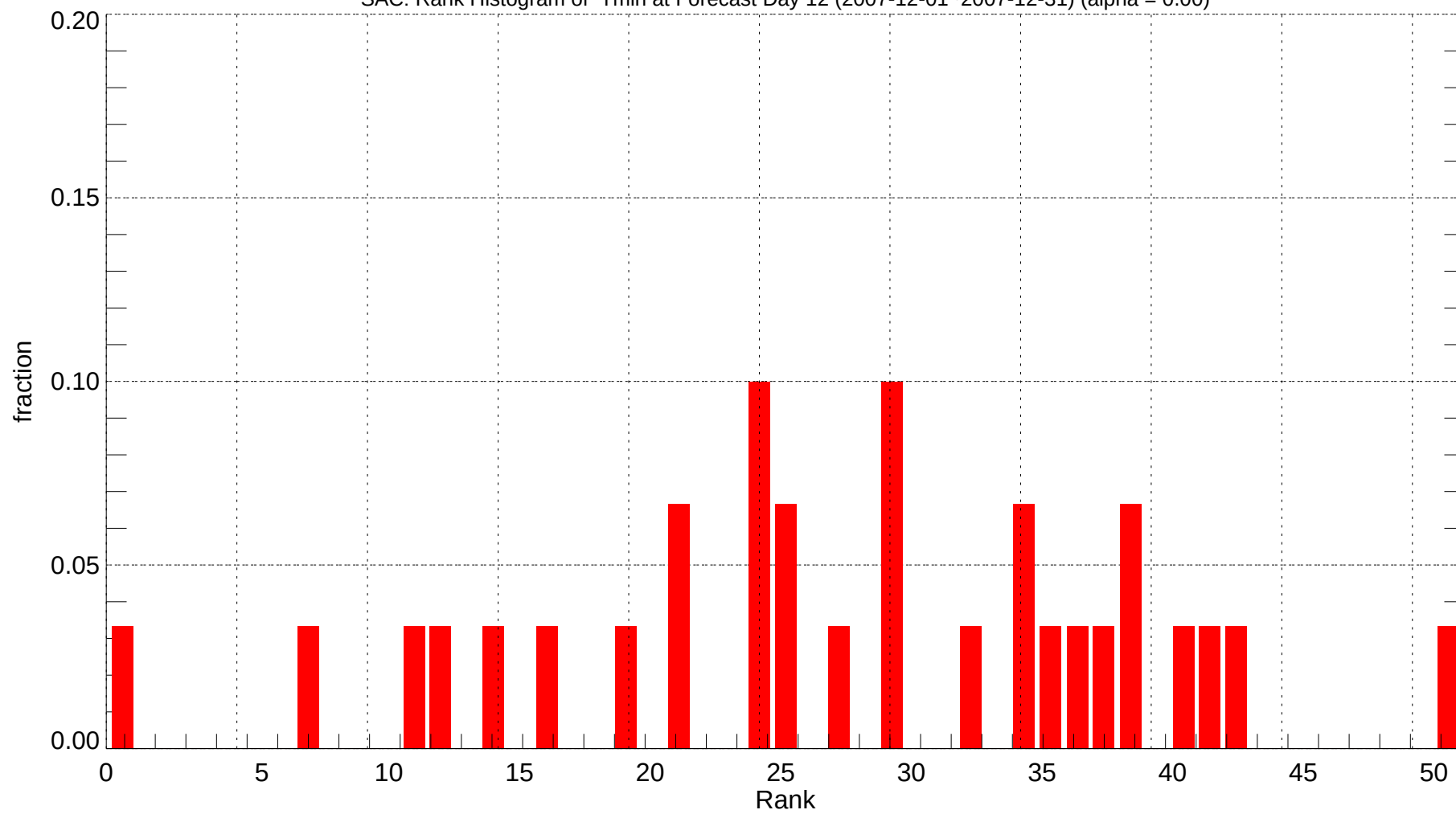
SAC: Rank Histogram of Tmin at Forecast Day 12 (2007-12-01~2007-12-31) (alpha = 0.00)
