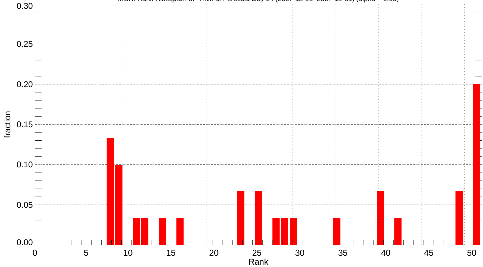
MCN: Rank Histogram of Tmin at Forecast Day 14 (2007-12-01~2007-12-31) (alpha = 0.00)
