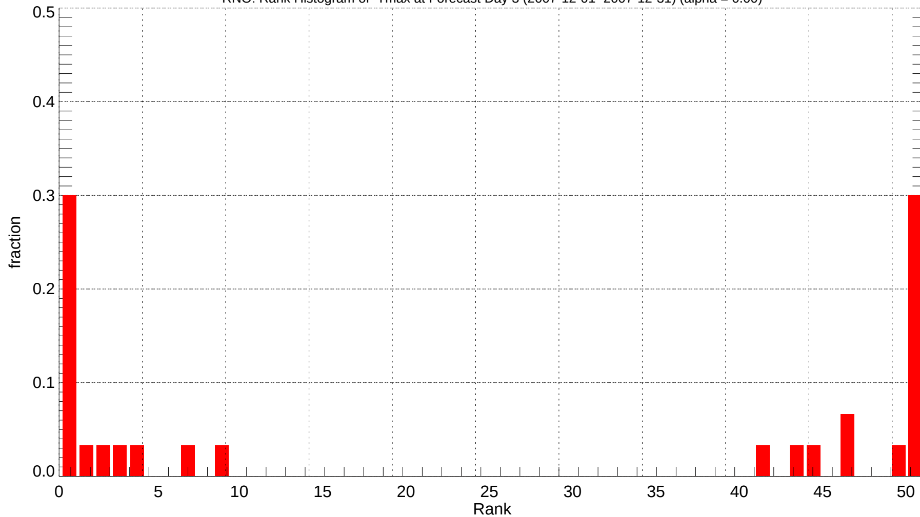
RNO: Rank Histogram of Tmax at Forecast Day 3 (2007-12-01~2007-12-31) (alpha = 0.00)
