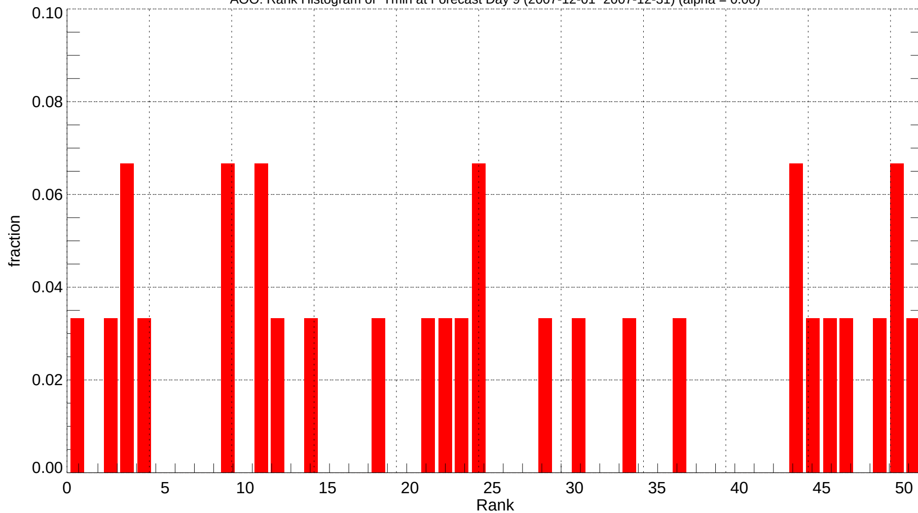
AOO: Rank Histogram of Tmin at Forecast Day 9 (2007-12-01~2007-12-31) (alpha = 0.00)
