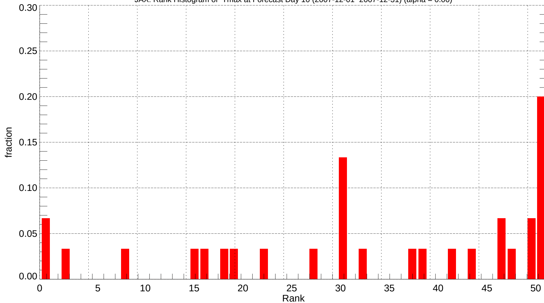
JAX: Rank Histogram of Tmax at Forecast Day 10 (2007-12-01~2007-12-31) (alpha = 0.00)
