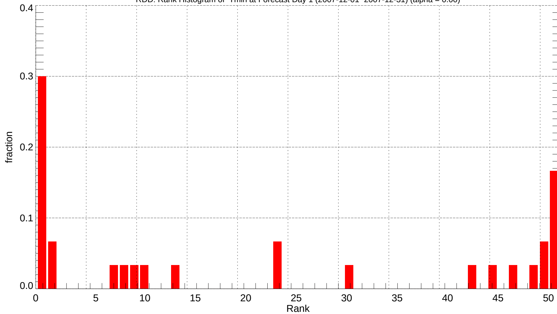
RDD: Rank Histogram of Tmin at Forecast Day 1 (2007-12-01~2007-12-31) (alpha = 0.00)
