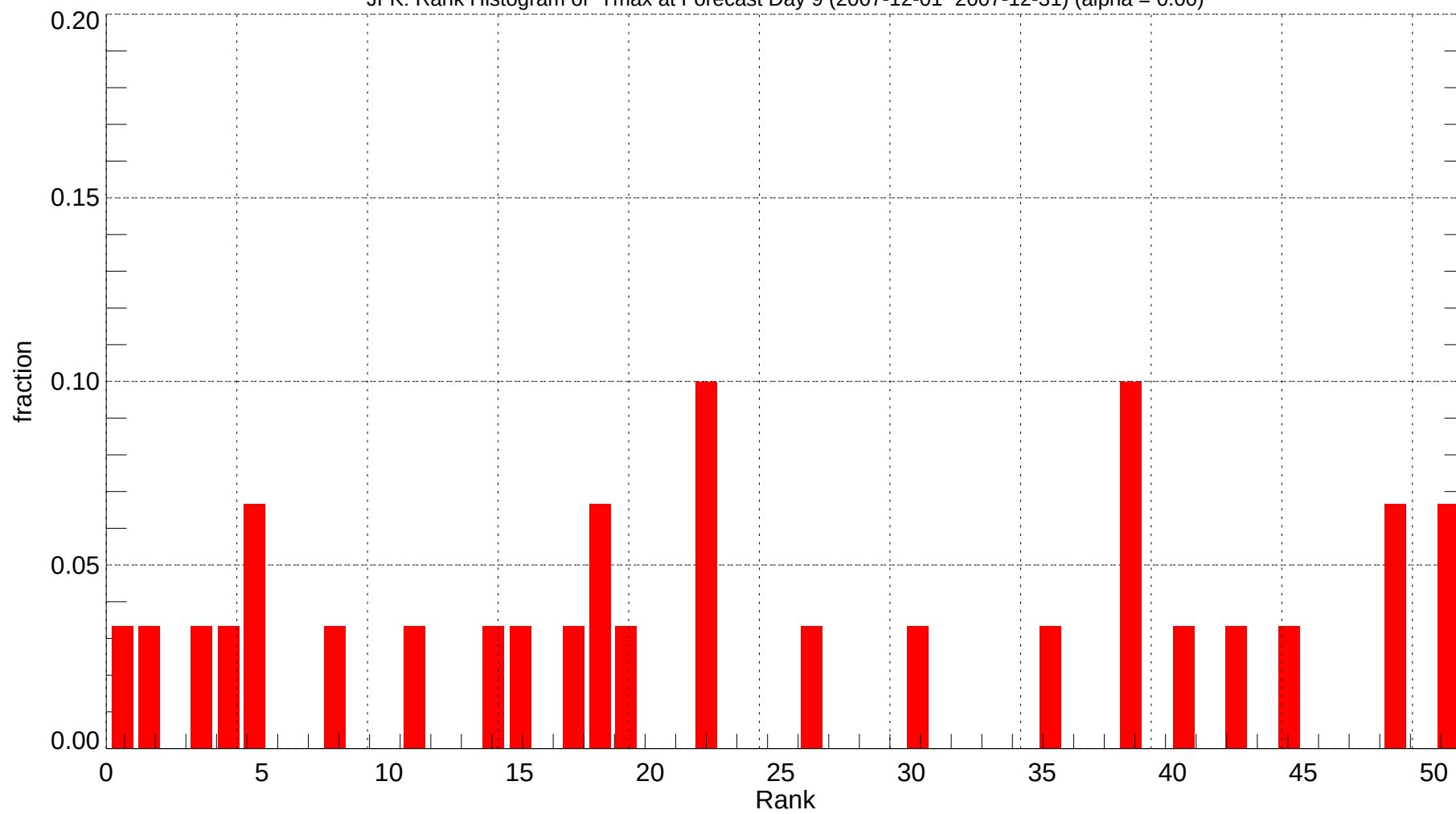
JFK: Rank Histogram of Tmax at Forecast Day 9 (2007-12-01~2007-12-31) (alpha = 0.00)
