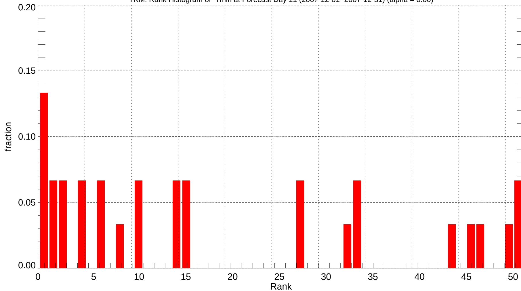
YKM: Rank Histogram of Tmin at Forecast Day 11 (2007-12-01~2007-12-31) (alpha = 0.00)
