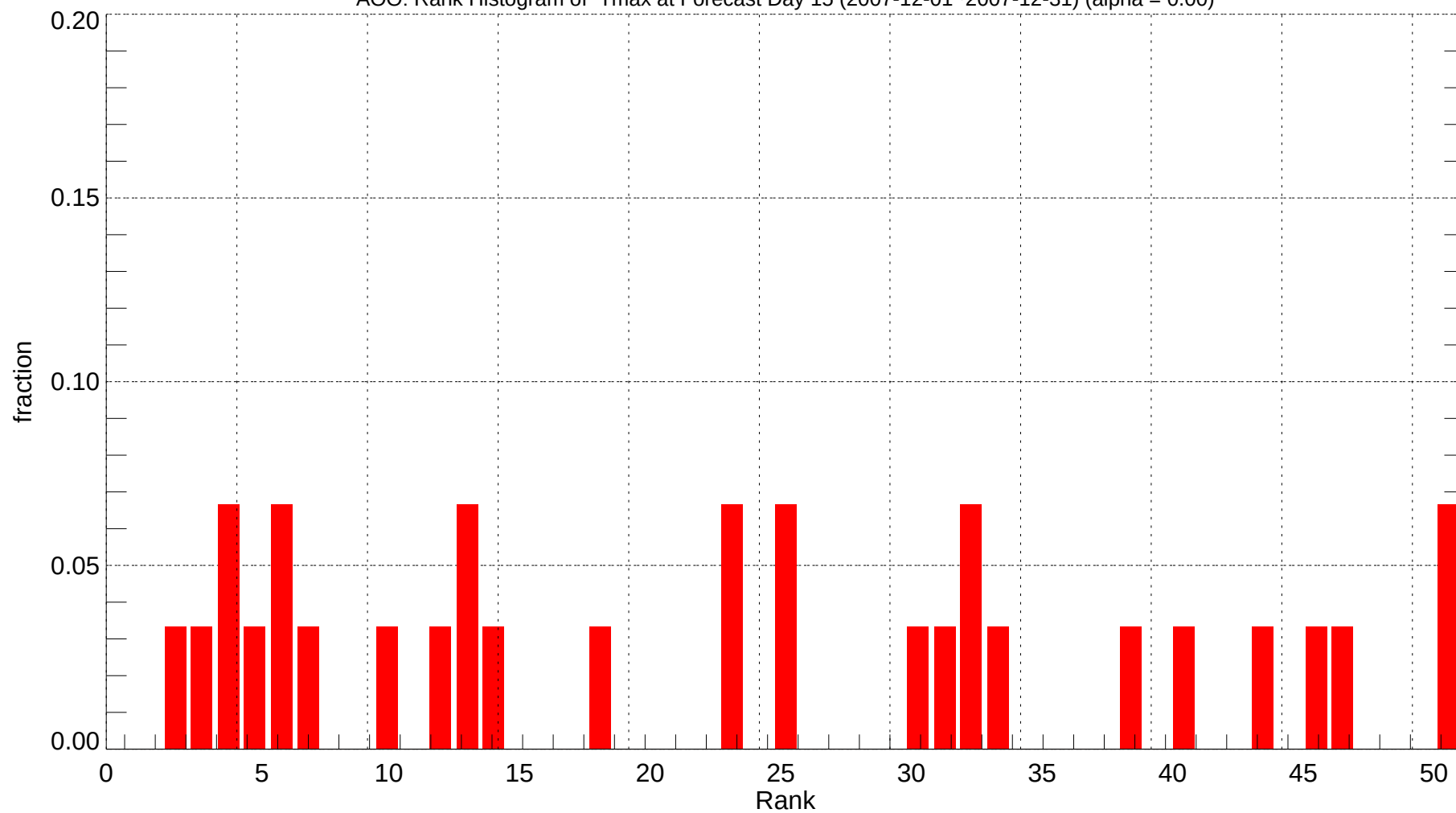
AOO: Rank Histogram of Tmax at Forecast Day 15 (2007-12-01~2007-12-31) (alpha = 0.00)
