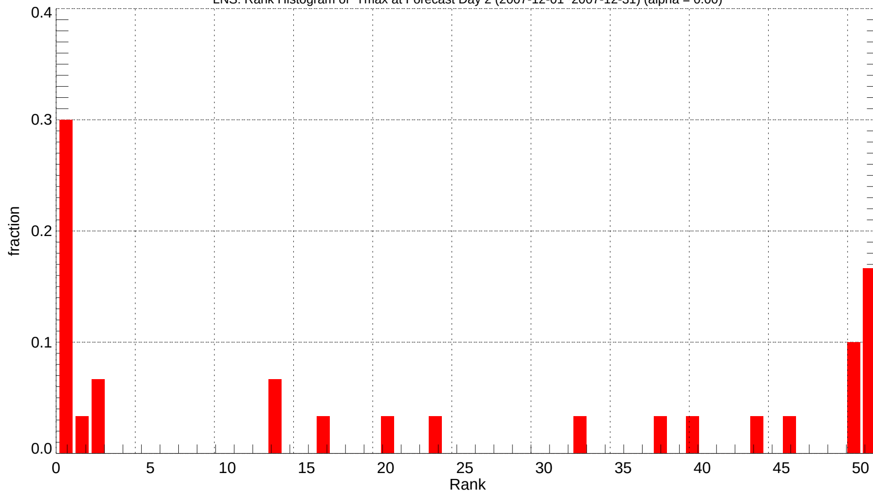
LNS: Rank Histogram of Tmax at Forecast Day 2 (2007-12-01~2007-12-31) (alpha = 0.00)
