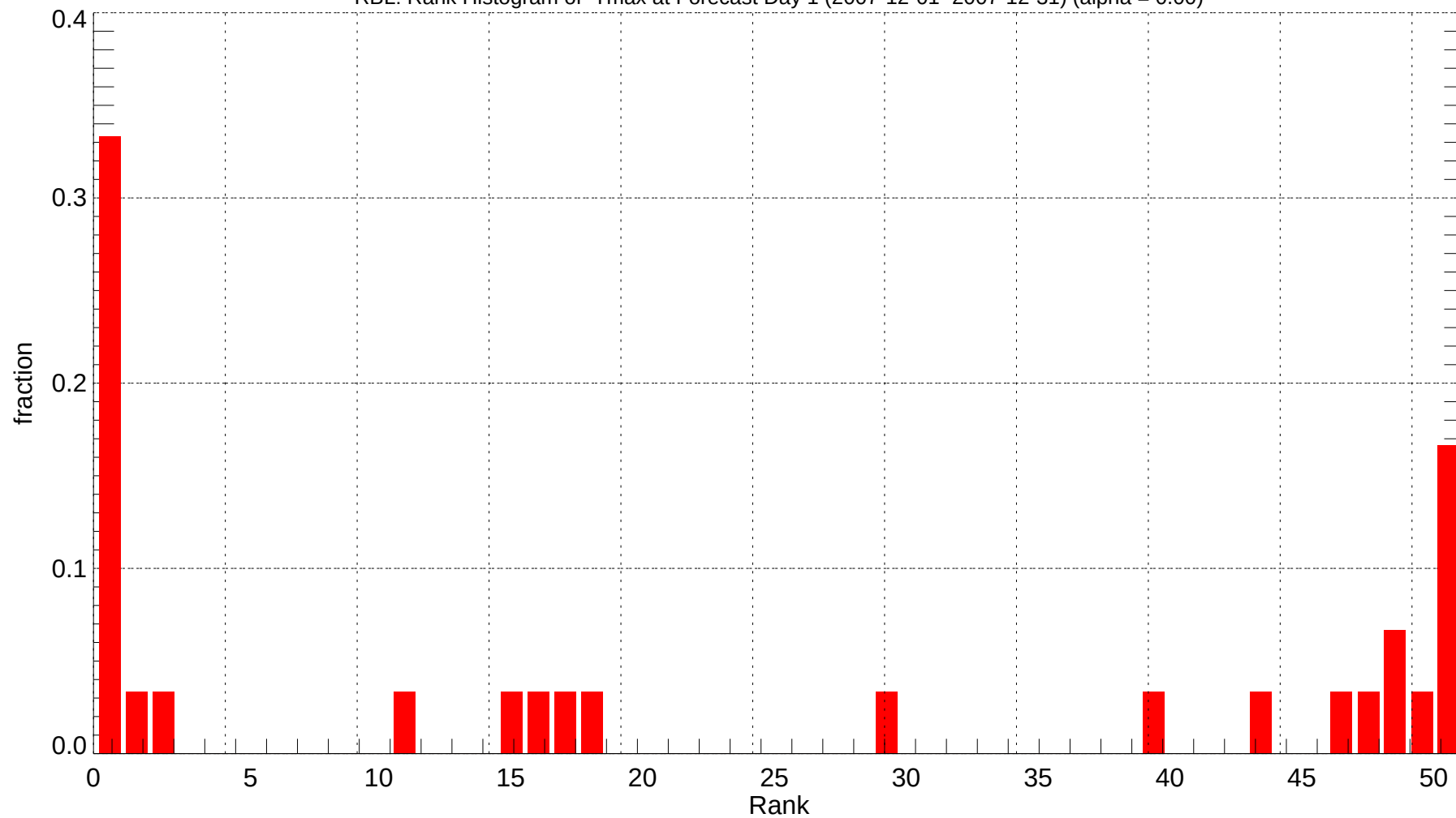
RBL: Rank Histogram of Tmax at Forecast Day 1 (2007-12-01~2007-12-31) (alpha = 0.00)
