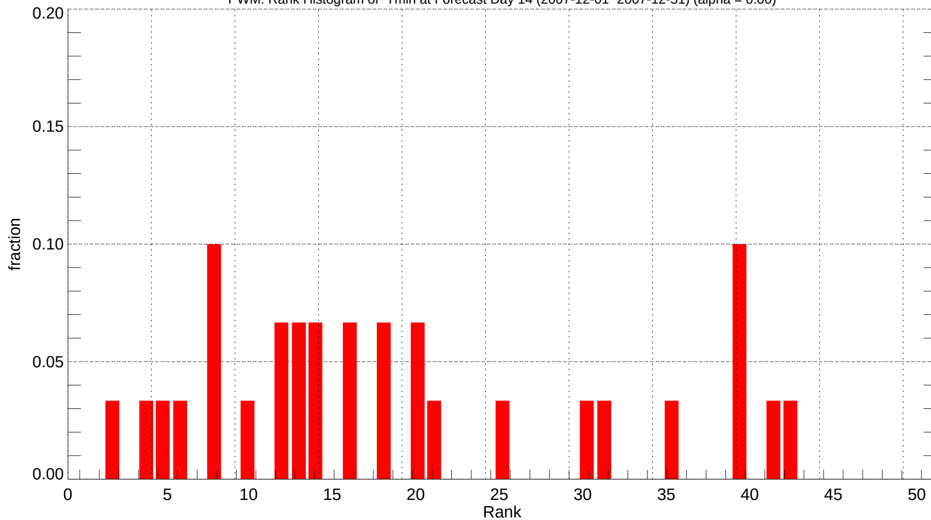
PWM: Rank Histogram of Tmin at Forecast Day 14 (2007-12-01~2007-12-31) (alpha = 0.00)
