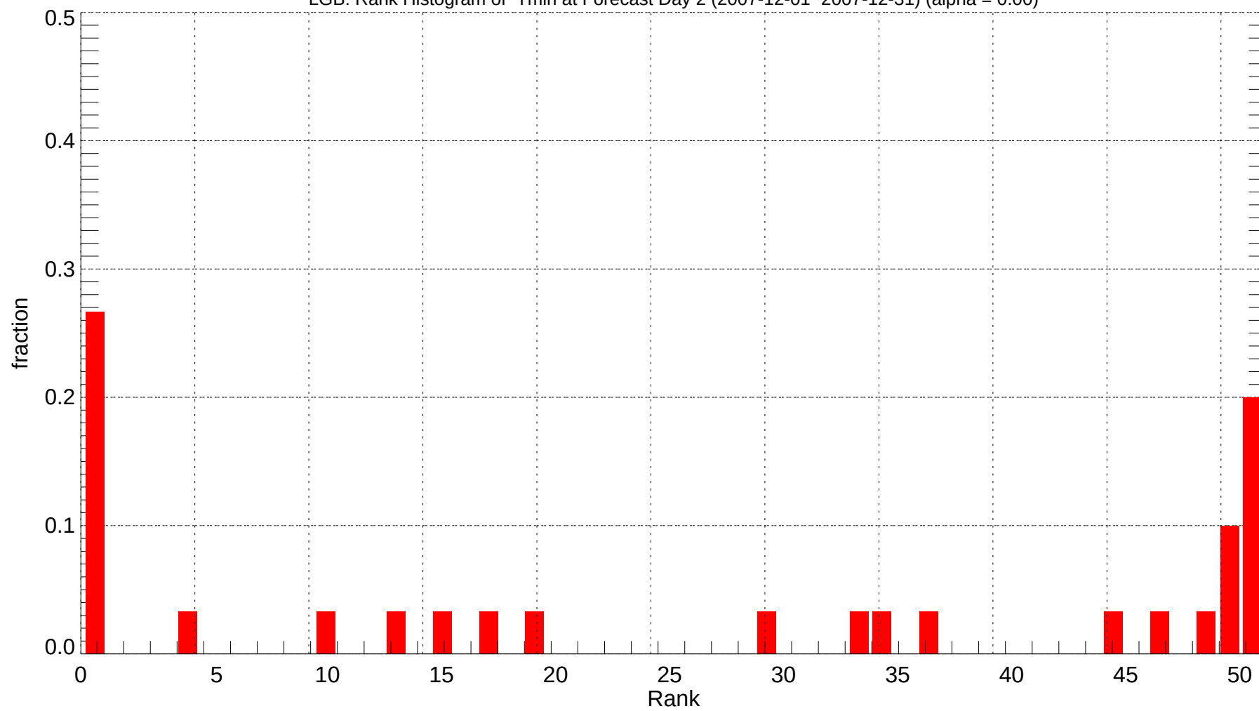
LGB: Rank Histogram of Tmin at Forecast Day 2 (2007-12-01~2007-12-31) (alpha = 0.00)
