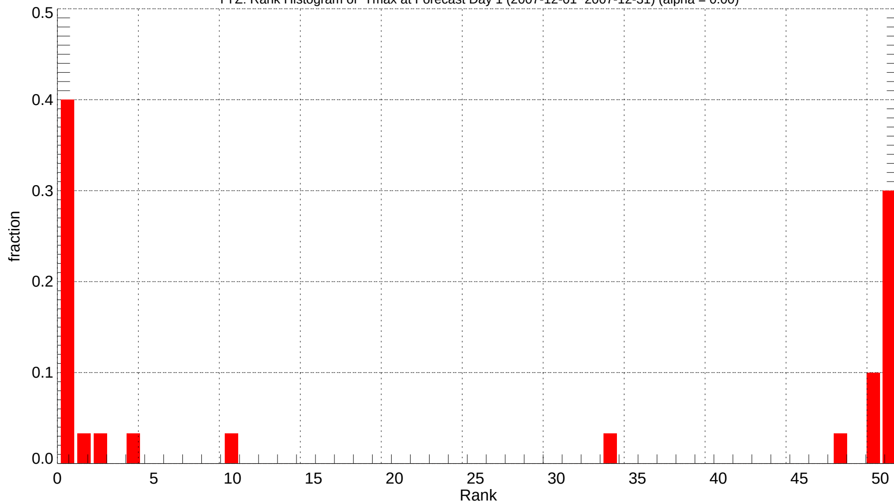
YYZ: Rank Histogram of Tmax at Forecast Day 1 (2007-12-01~2007-12-31) (alpha = 0.00)
