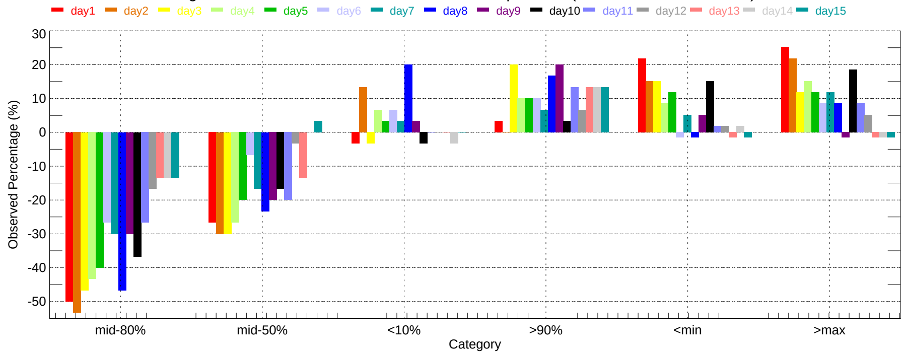
Observed Percentage Deviation of Ensembles - COU: Max Temperature (2007-12-01~2007-12-31)
