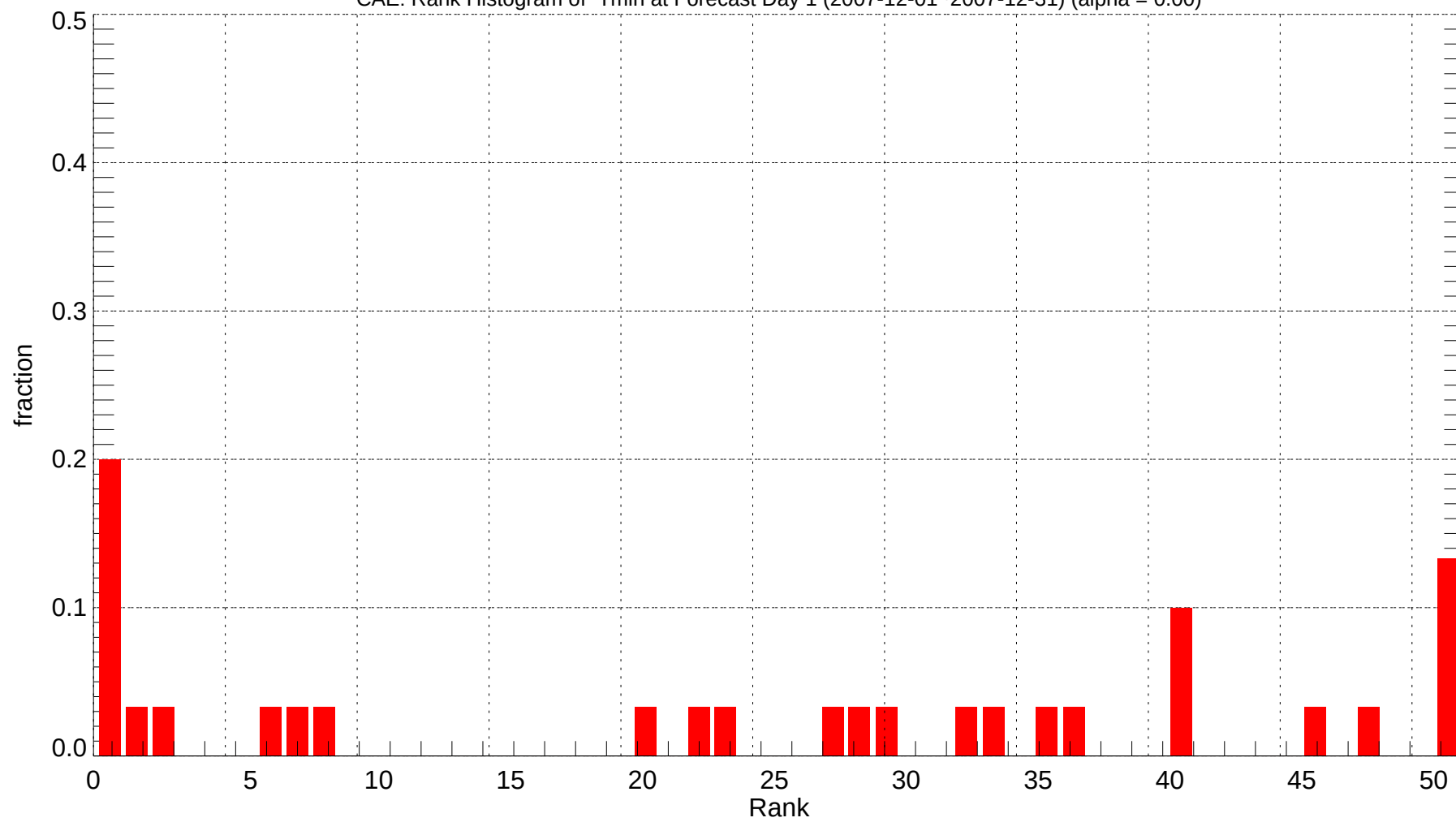
CAE: Rank Histogram of Tmin at Forecast Day 1 (2007-12-01~2007-12-31) (alpha = 0.00)
