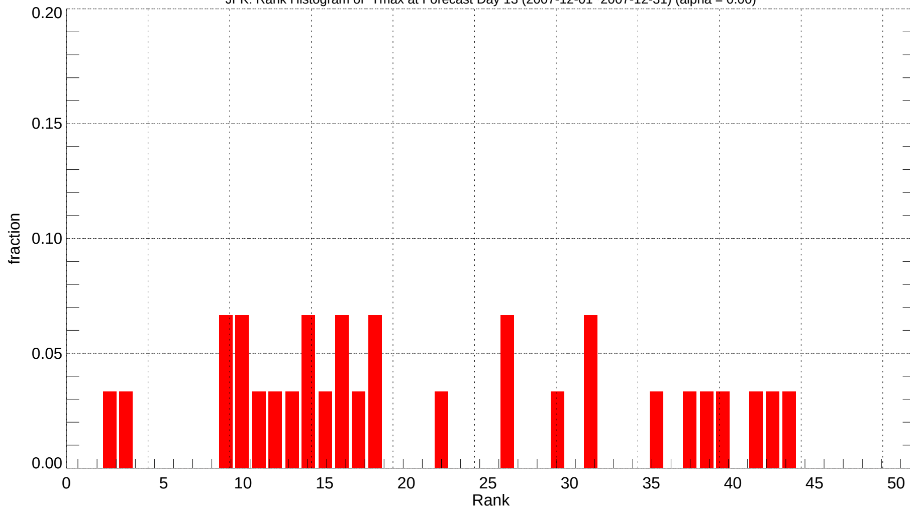
JFK: Rank Histogram of Tmax at Forecast Day 13 (2007-12-01~2007-12-31) (alpha = 0.00)
