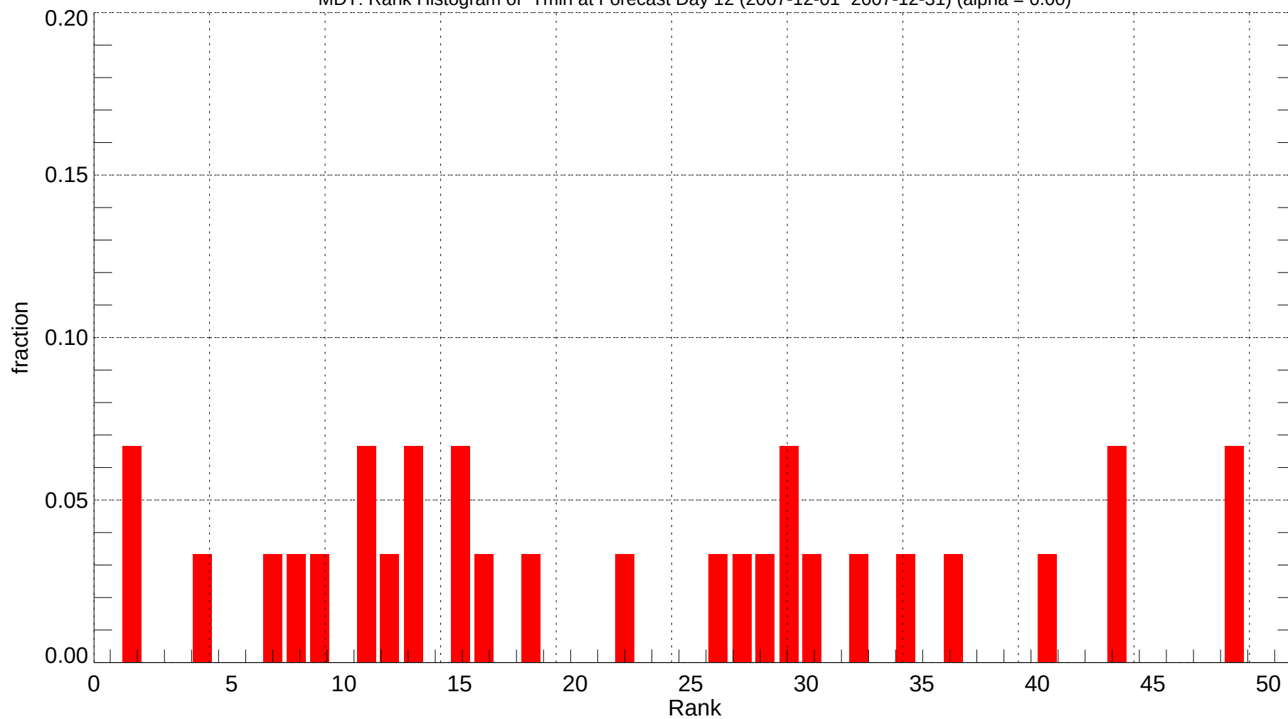
MDT: Rank Histogram of Tmin at Forecast Day 12 (2007-12-01~2007-12-31) (alpha = 0.00)
