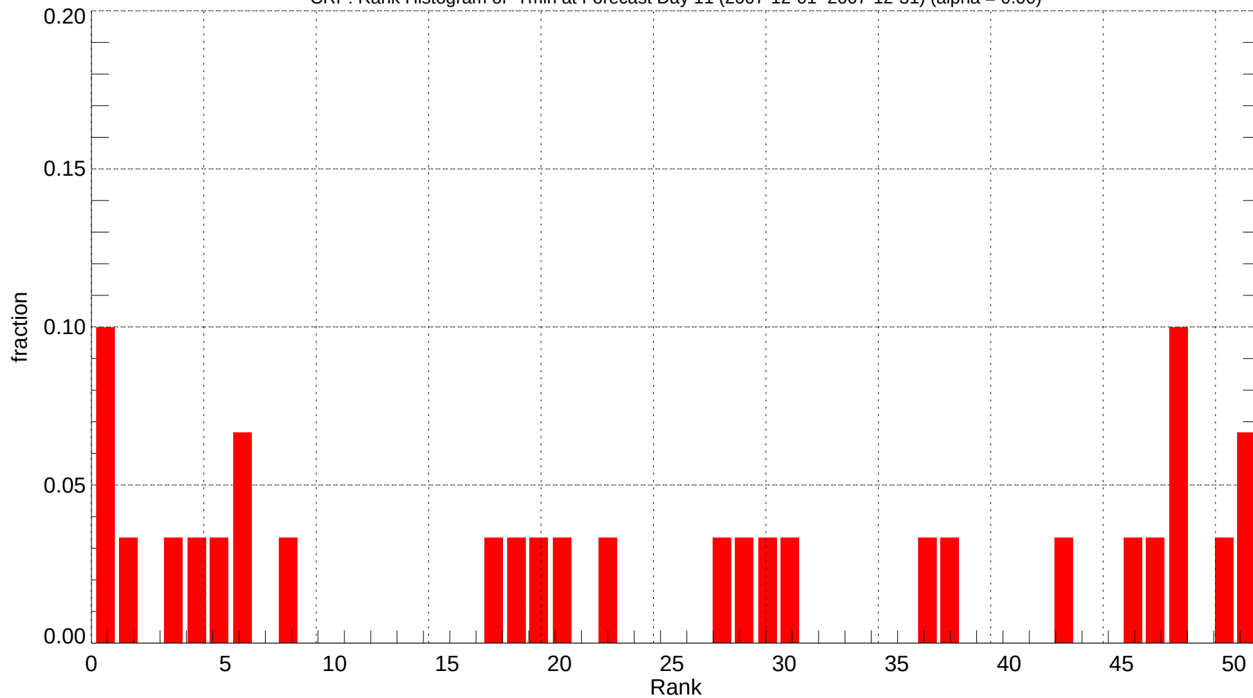
CRP: Rank Histogram of Tmin at Forecast Day 11 (2007-12-01~2007-12-31) (alpha = 0.00)
