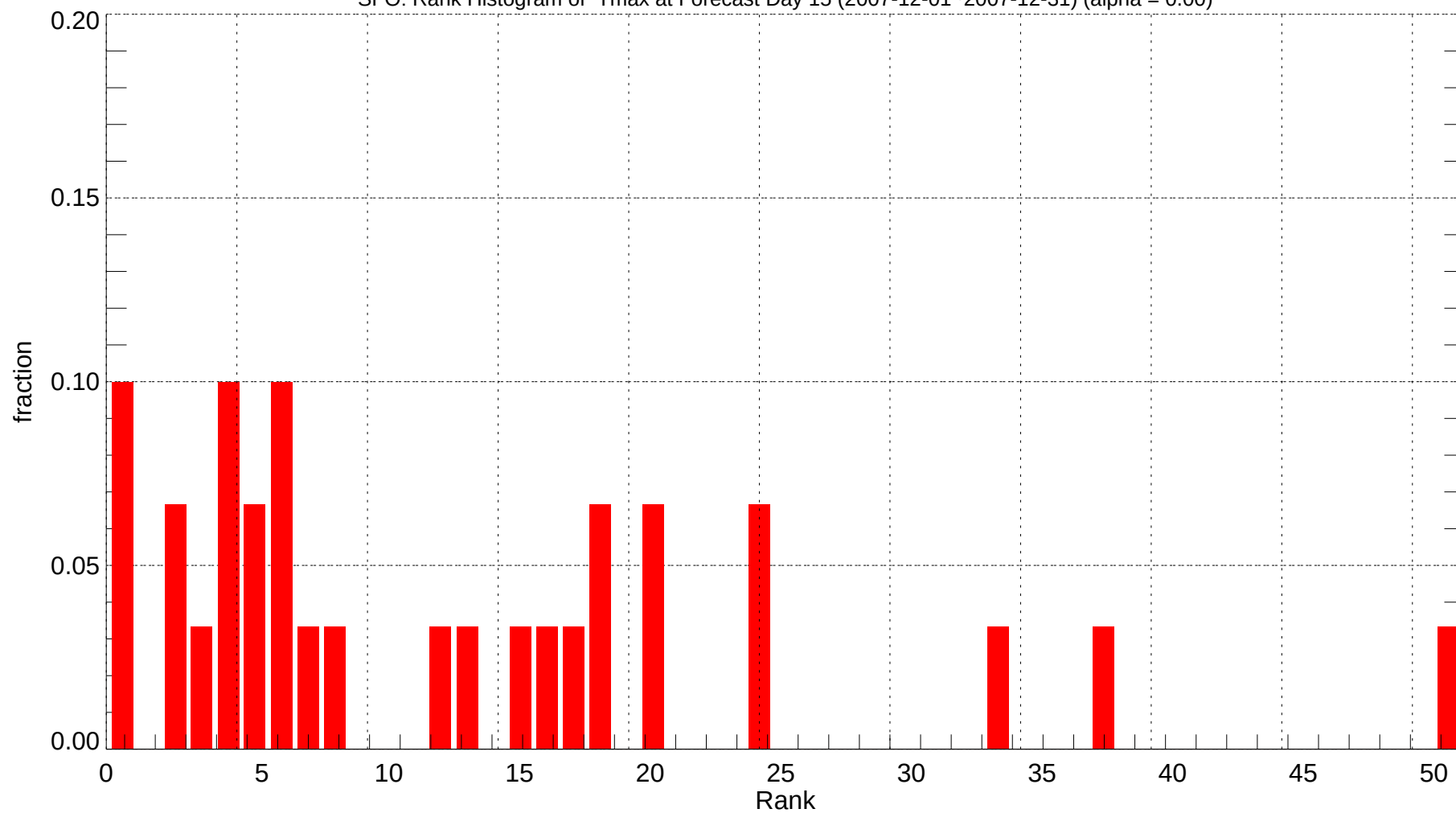
SFO: Rank Histogram of Tmax at Forecast Day 15 (2007-12-01~2007-12-31) (alpha = 0.00)
