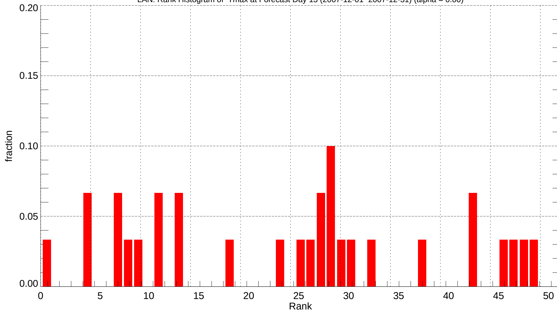
LAN: Rank Histogram of Tmax at Forecast Day 13 (2007-12-01~2007-12-31) (alpha = 0.00)
