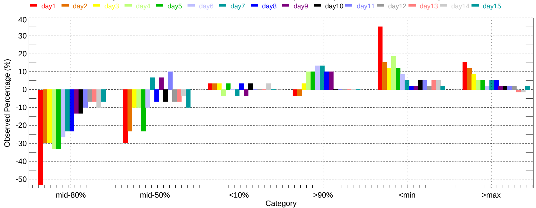
Observed Percentage Deviation of Ensembles - ILG: Max Temperature (2007-12-01~2007-12-31)
