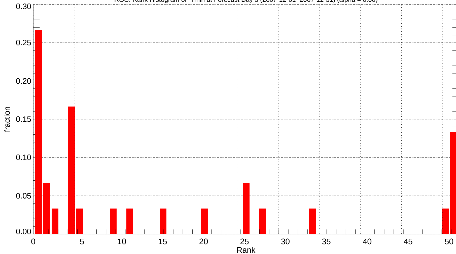
ROC: Rank Histogram of Tmin at Forecast Day 3 (2007-12-01~2007-12-31) (alpha = 0.00)
