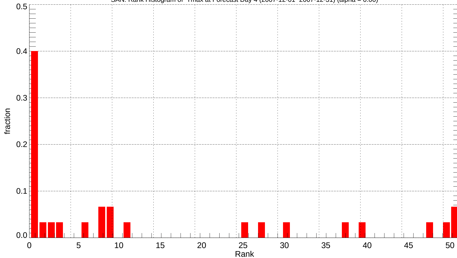
SAN: Rank Histogram of Tmax at Forecast Day 4 (2007-12-01~2007-12-31) (alpha = 0.00)
