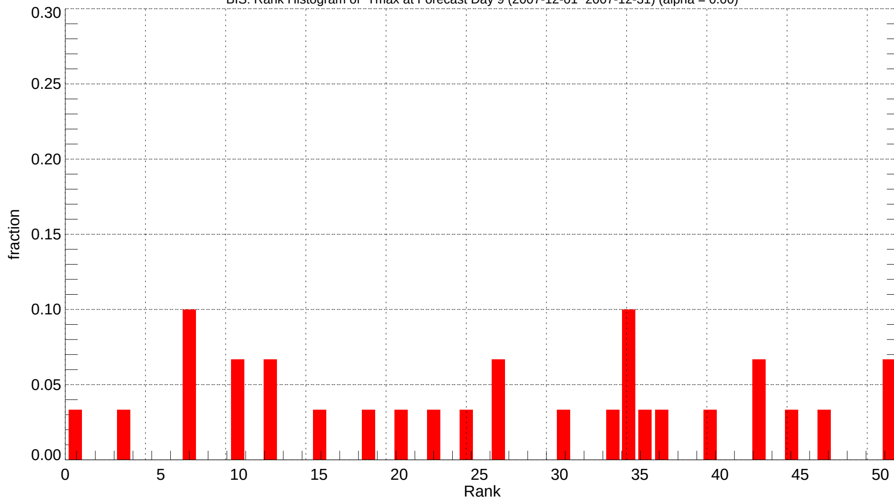
BIS: Rank Histogram of Tmax at Forecast Day 9 (2007-12-01~2007-12-31) (alpha = 0.00)
