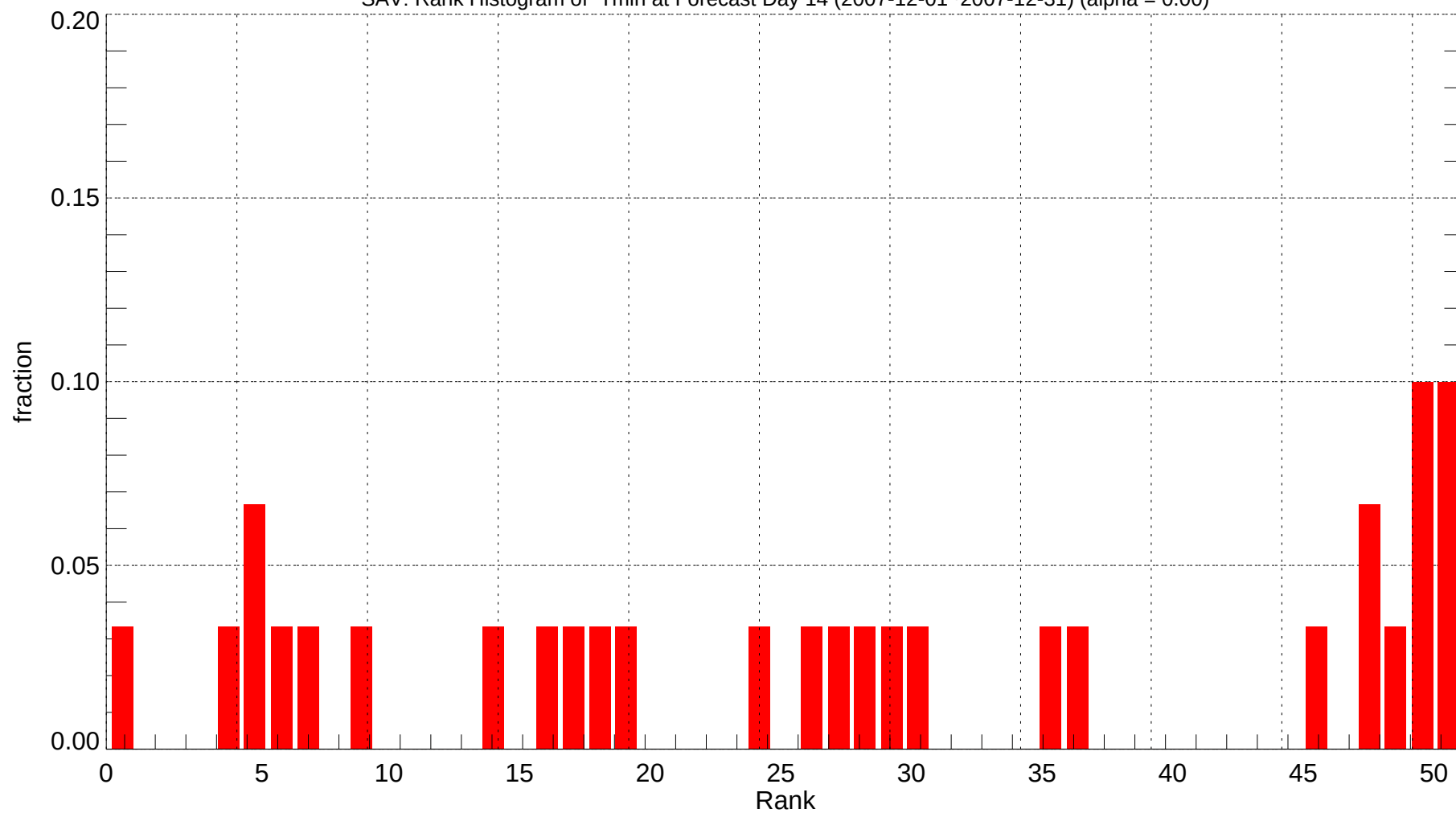
SAV: Rank Histogram of Tmin at Forecast Day 14 (2007-12-01~2007-12-31) (alpha = 0.00)
