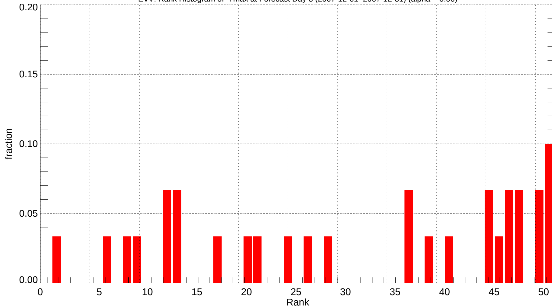
EVV: Rank Histogram of Tmax at Forecast Day 8 (2007-12-01~2007-12-31) (alpha = 0.00)
