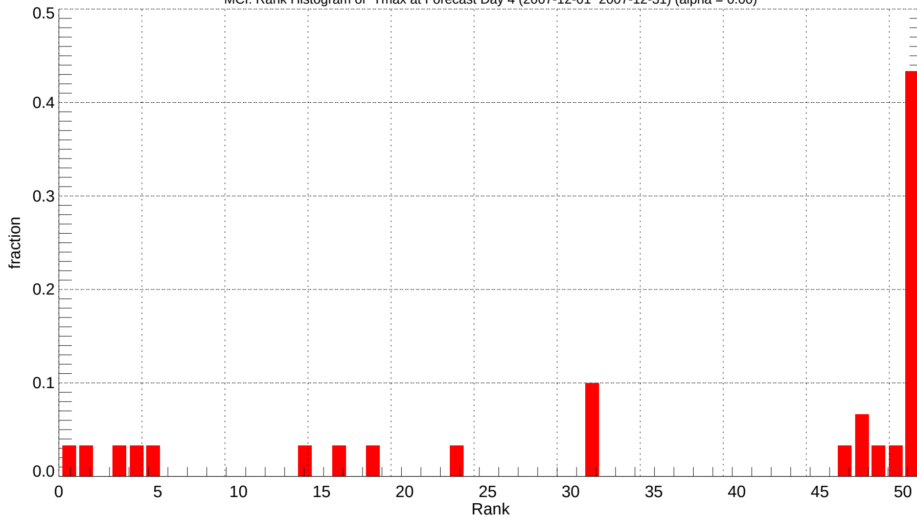
MCI: Rank Histogram of Tmax at Forecast Day 4 (2007-12-01~2007-12-31) (alpha = 0.00)
