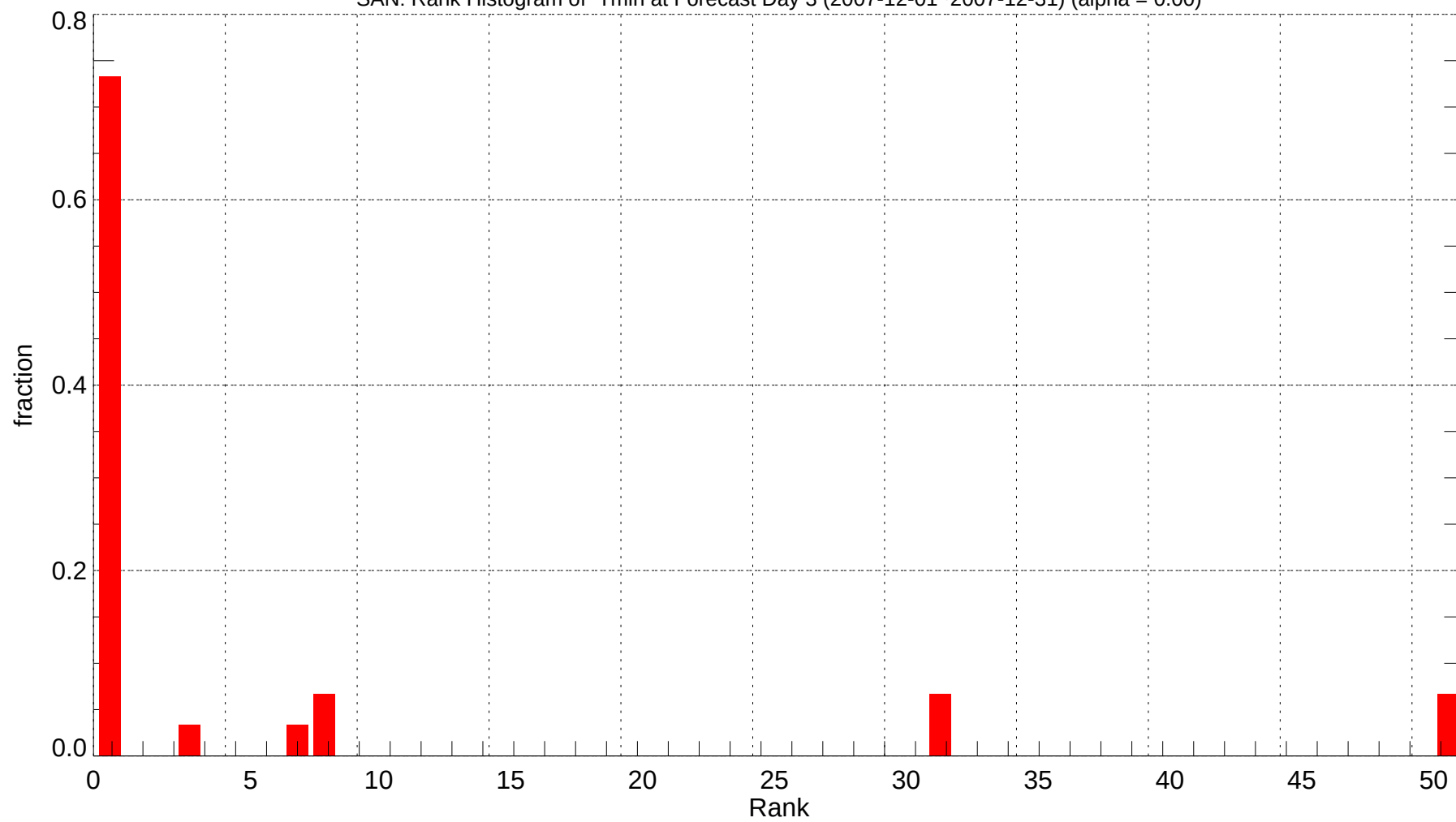
SAN: Rank Histogram of Tmin at Forecast Day 3 (2007-12-01~2007-12-31) (alpha = 0.00)
