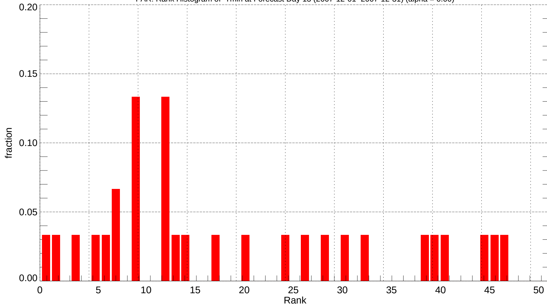
FAR: Rank Histogram of Tmin at Forecast Day 13 (2007-12-01~2007-12-31) (alpha = 0.00)
