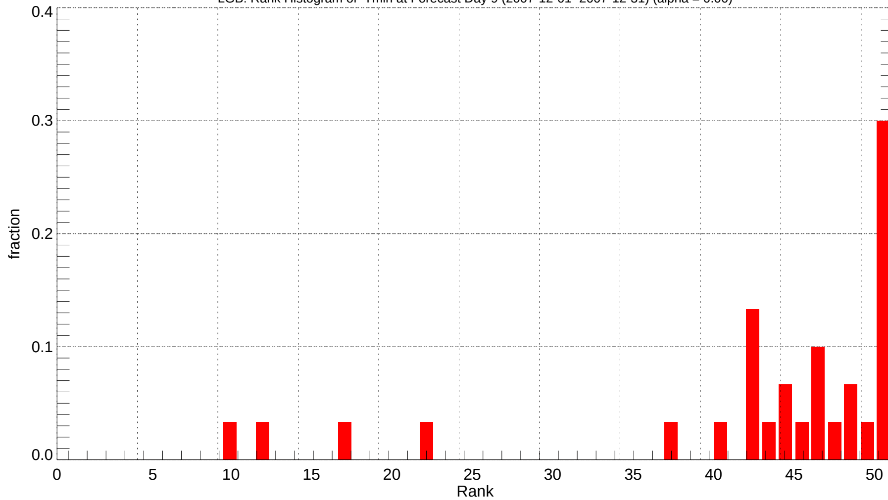
LGB: Rank Histogram of Tmin at Forecast Day 9 (2007-12-01~2007-12-31) (alpha = 0.00)
