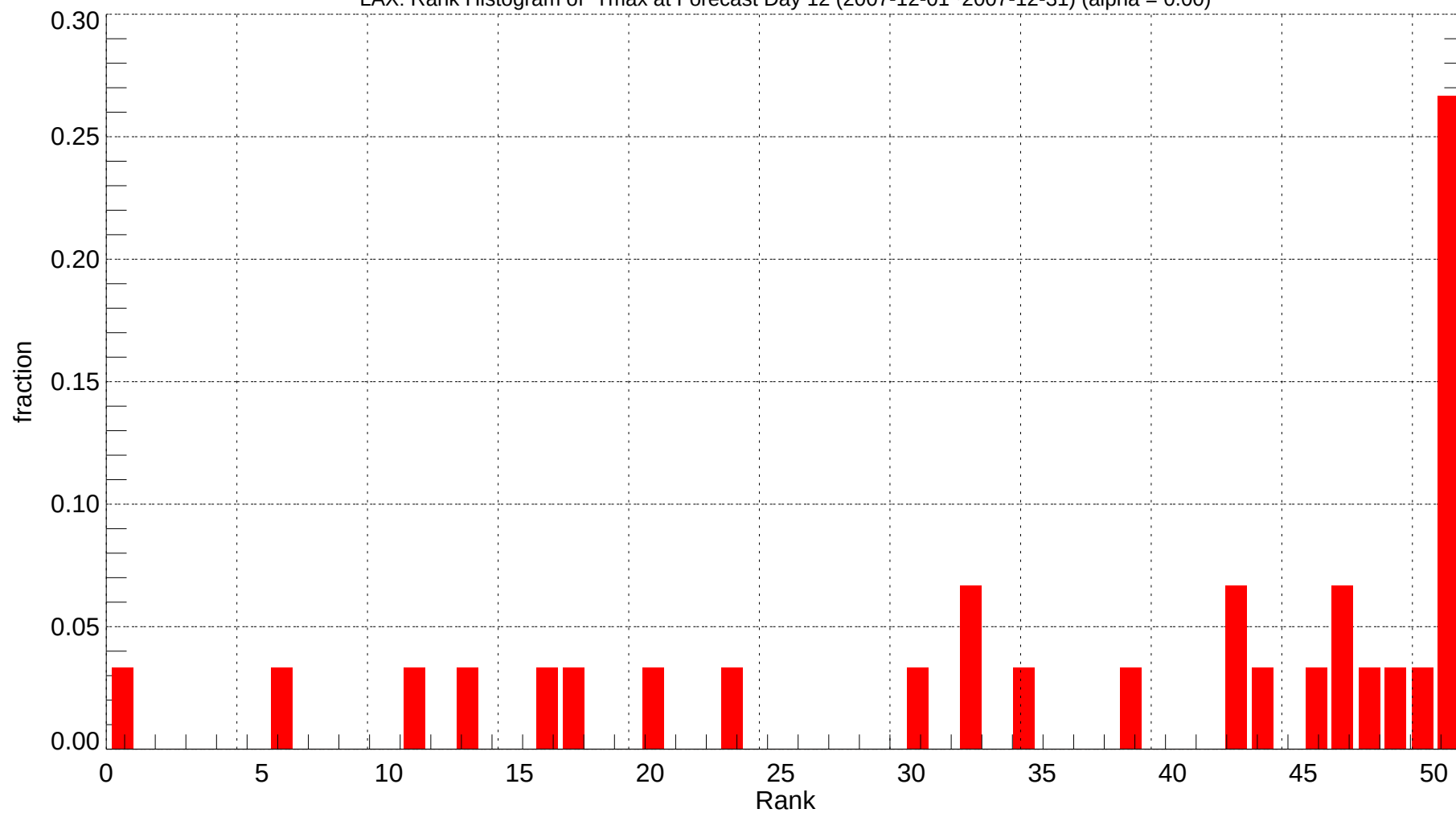
LAX: Rank Histogram of Tmax at Forecast Day 12 (2007-12-01~2007-12-31) (alpha = 0.00)
