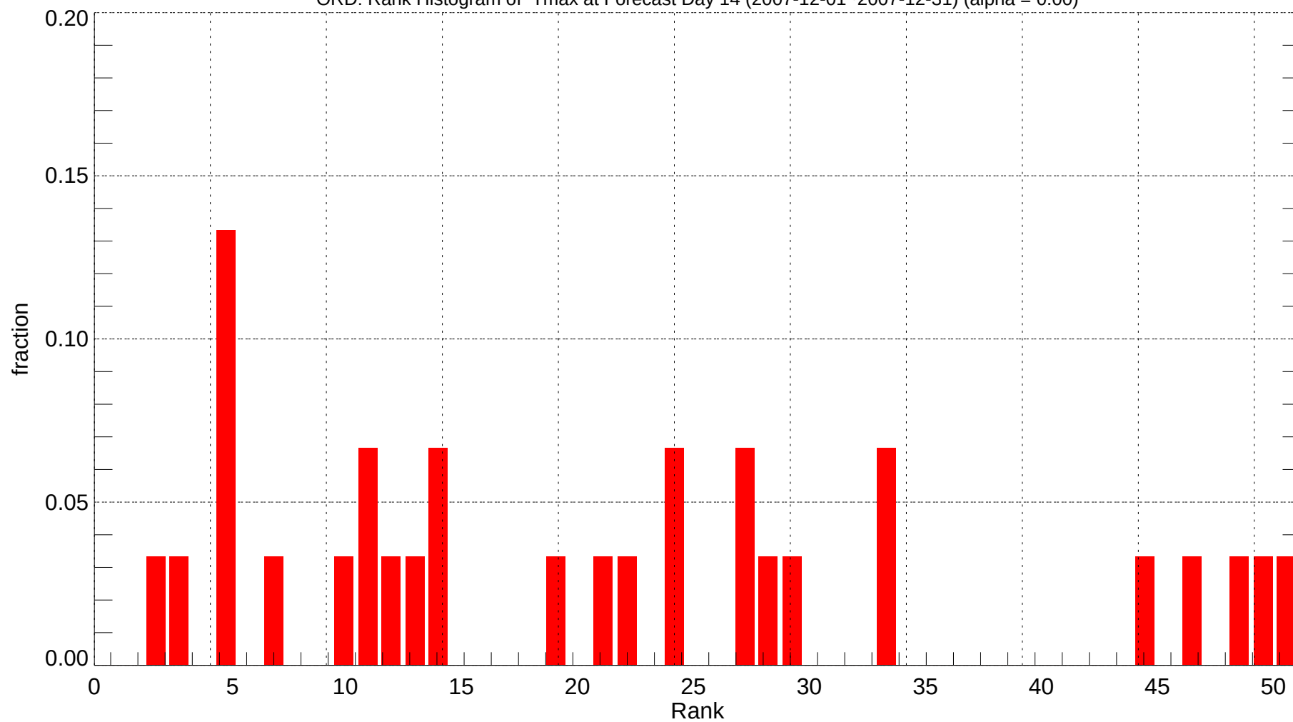
ORD: Rank Histogram of Tmax at Forecast Day 14 (2007-12-01~2007-12-31) (alpha = 0.00)
