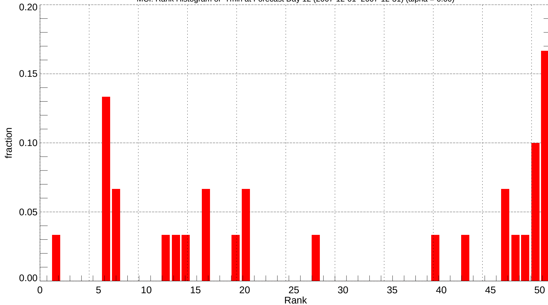
MCI: Rank Histogram of Tmin at Forecast Day 12 (2007-12-01~2007-12-31) (alpha = 0.00)
