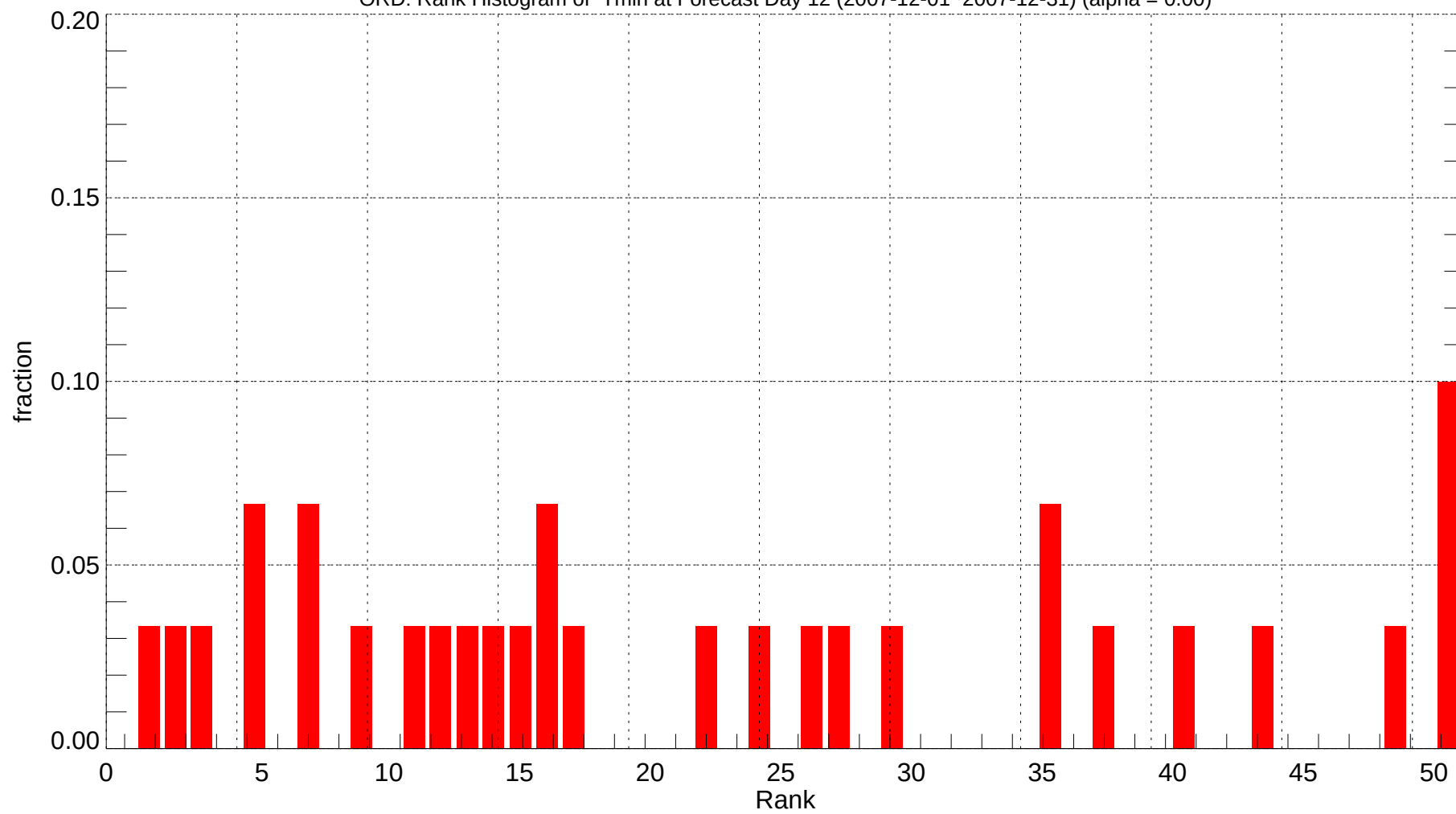
ORD: Rank Histogram of Tmin at Forecast Day 12 (2007-12-01~2007-12-31) (alpha = 0.00)
