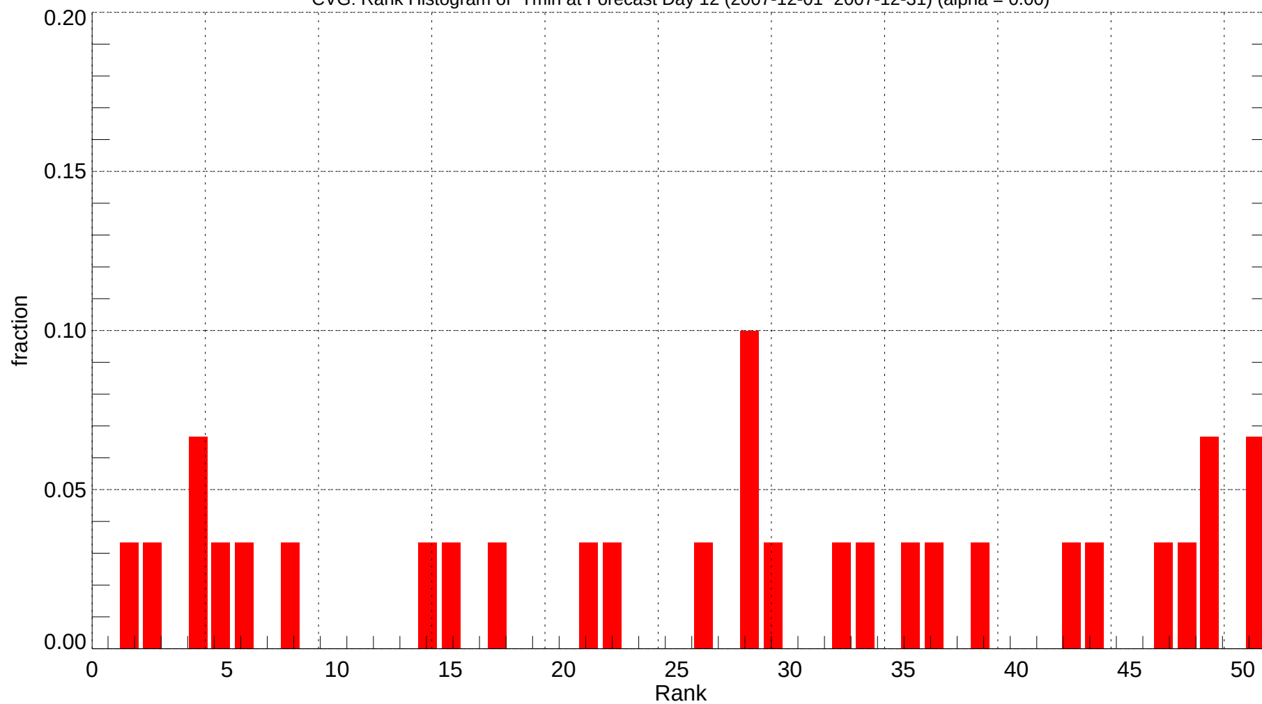
CVG: Rank Histogram of Tmin at Forecast Day 12 (2007-12-01~2007-12-31) (alpha = 0.00)
