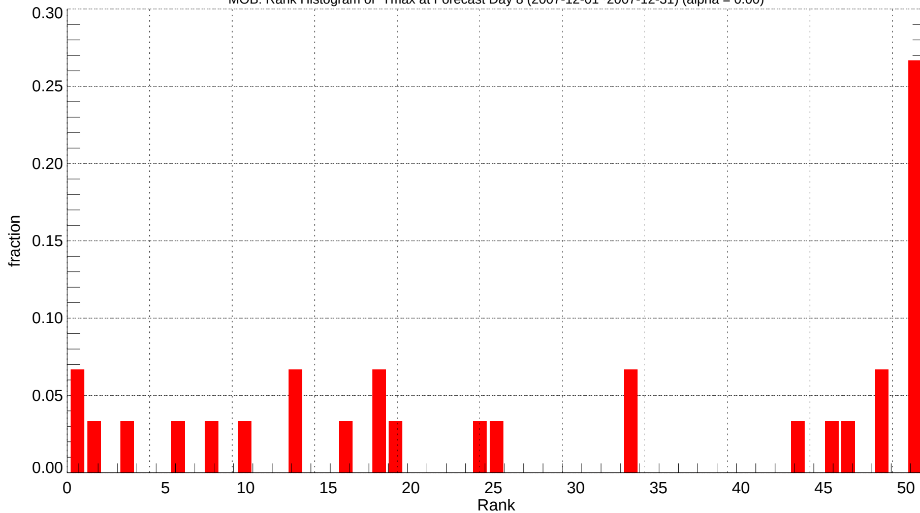
MOB: Rank Histogram of Tmax at Forecast Day 8 (2007-12-01~2007-12-31) (alpha = 0.00)
