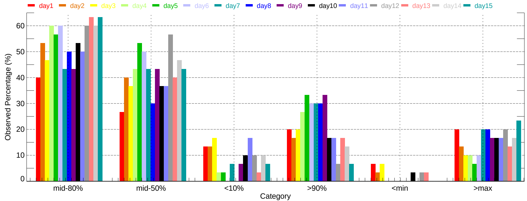
Observed Percentage of Ensembles - HOU: Max Temperature (2007-12-01~2007-12-31)
