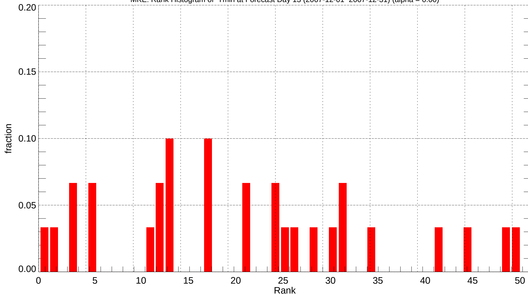
MKE: Rank Histogram of Tmin at Forecast Day 13 (2007-12-01~2007-12-31) (alpha = 0.00)
