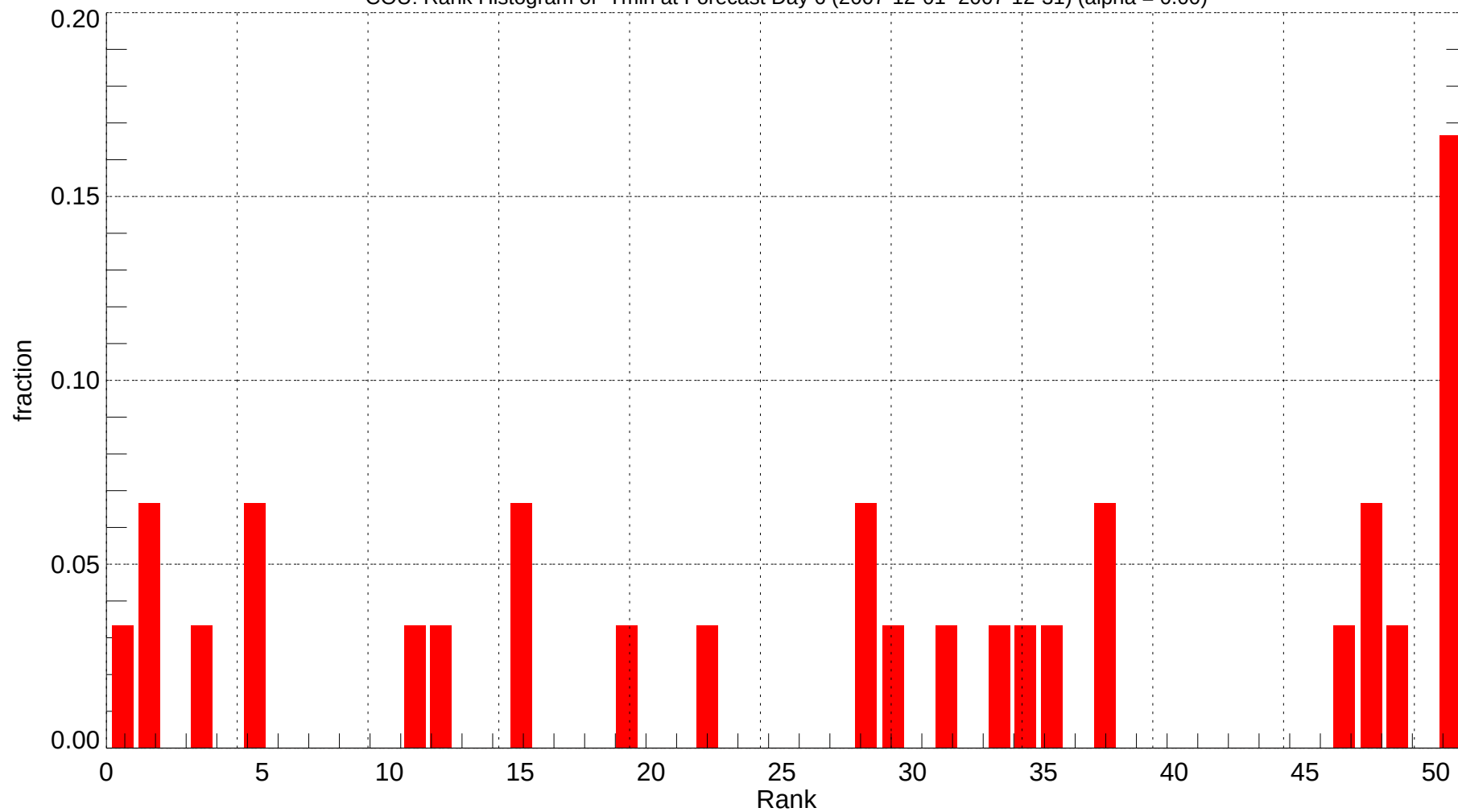
COU: Rank Histogram of Tmin at Forecast Day 6 (2007-12-01~2007-12-31) (alpha = 0.00)
