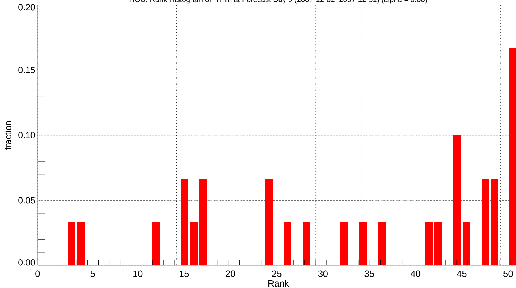
HOU: Rank Histogram of Tmin at Forecast Day 9 (2007-12-01~2007-12-31) (alpha = 0.00)
