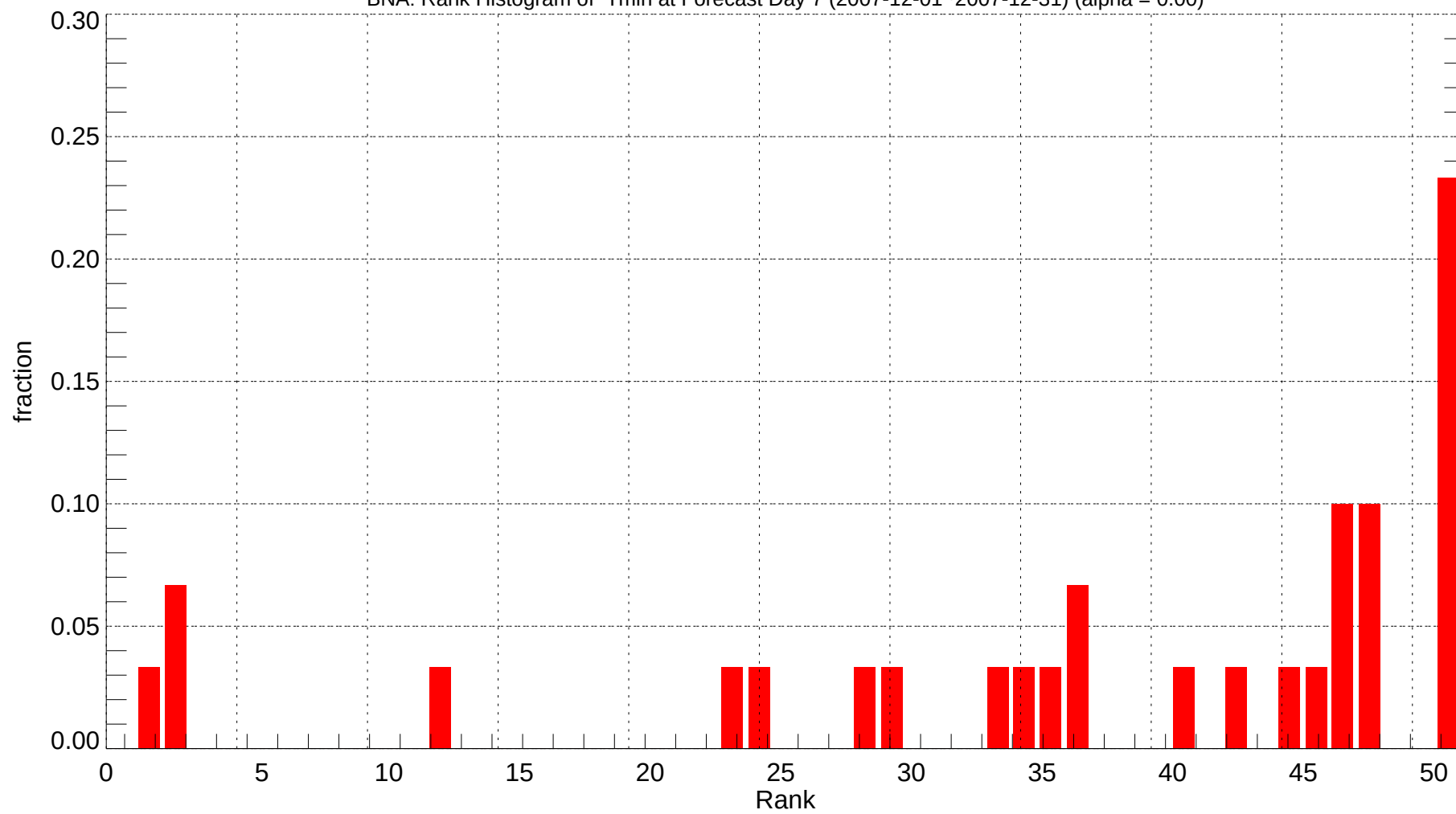
BNA: Rank Histogram of Tmin at Forecast Day 7 (2007-12-01~2007-12-31) (alpha = 0.00)
