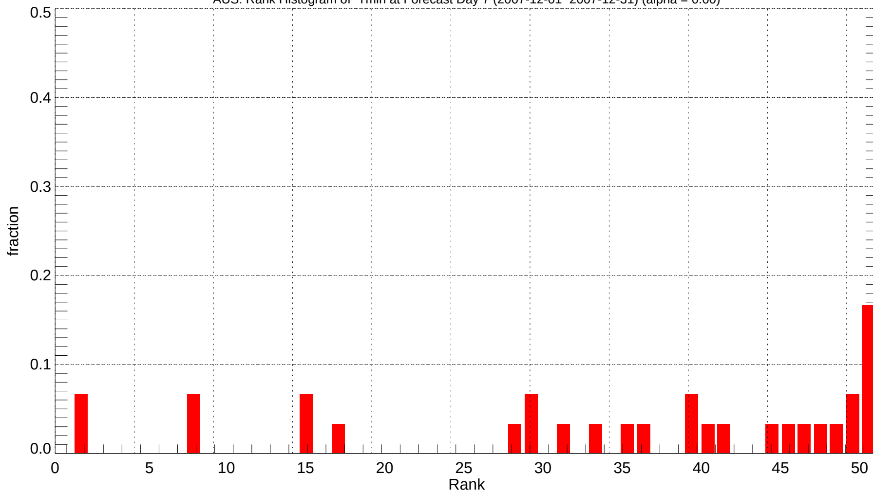
AUS: Rank Histogram of Tmin at Forecast Day 7 (2007-12-01~2007-12-31) (alpha = 0.00)
