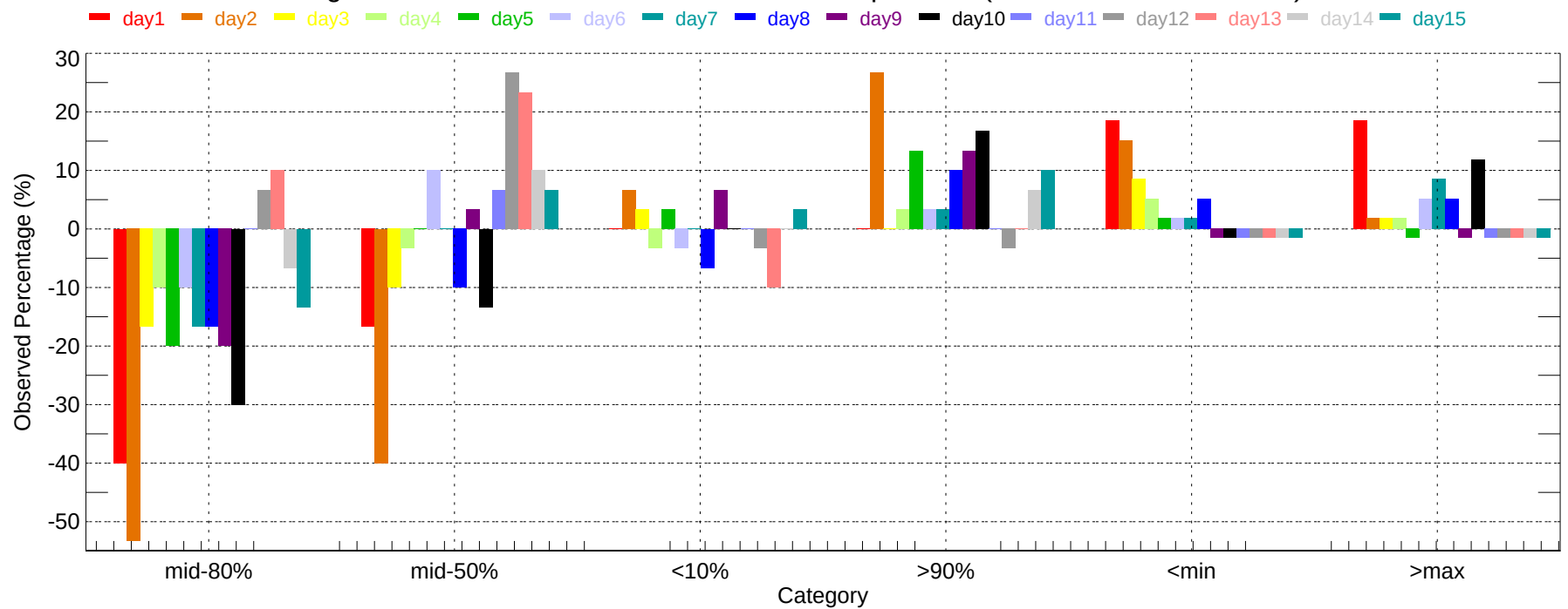
Observed Percentage Deviation of Ensembles - DLH: Max Temperature (2007-12-01~2007-12-31)
