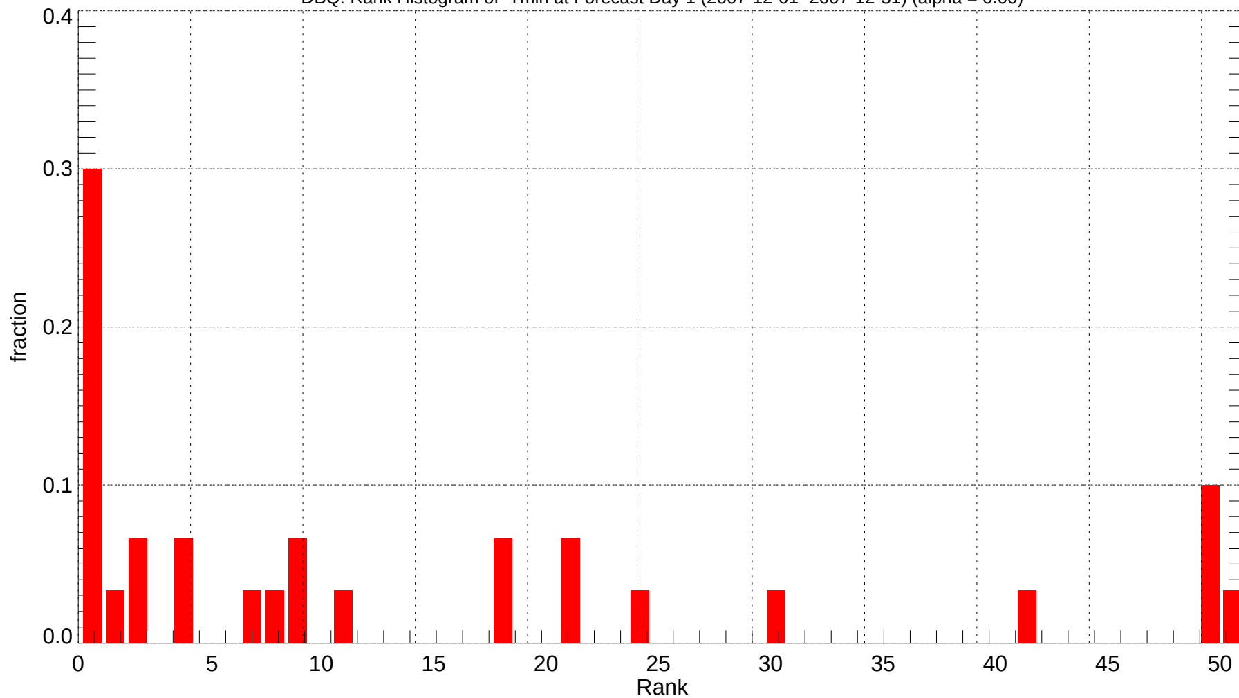
DBQ: Rank Histogram of Tmin at Forecast Day 1 (2007-12-01~2007-12-31) (alpha = 0.00)
