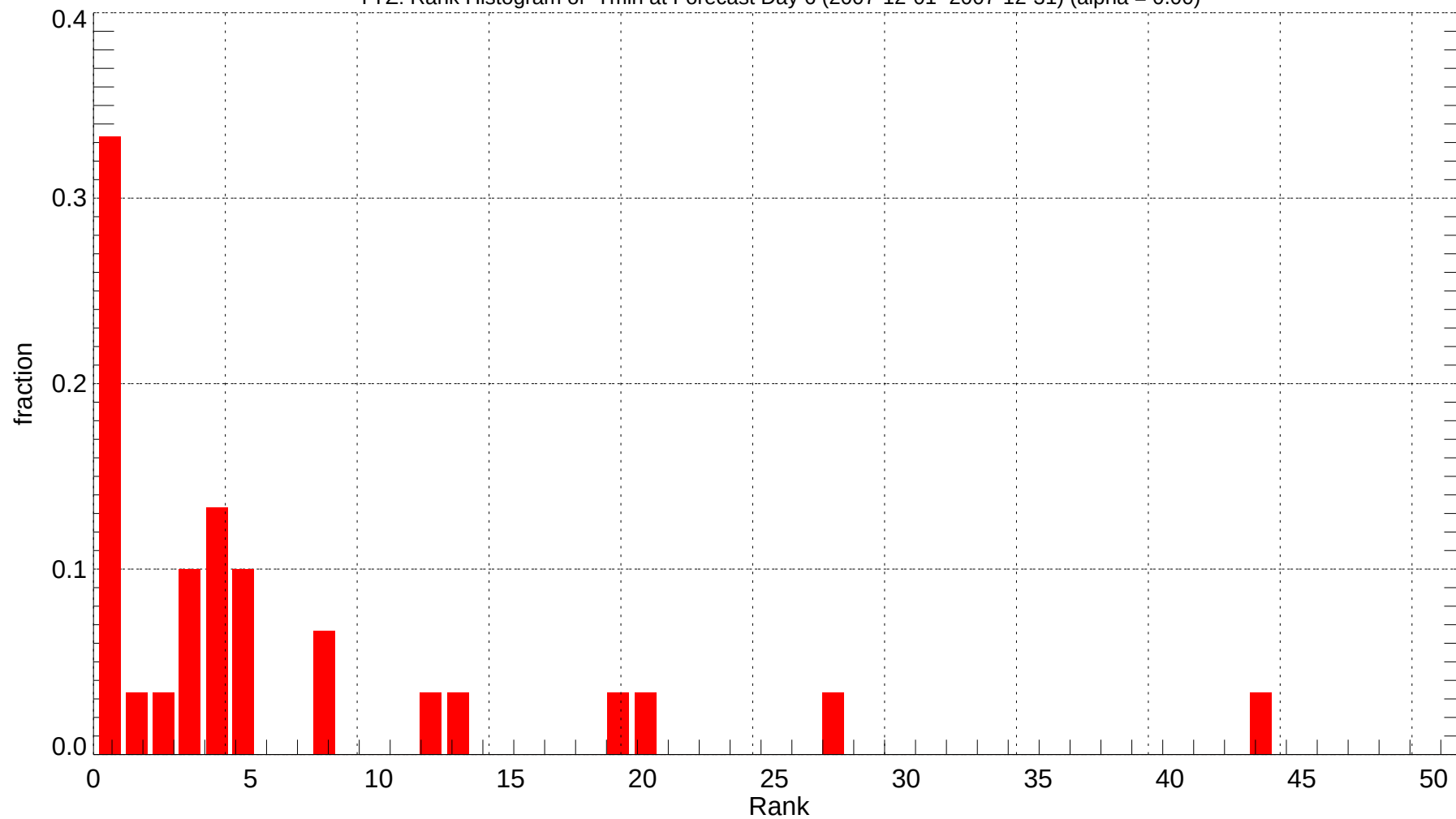
YYZ: Rank Histogram of Tmin at Forecast Day 6 (2007-12-01~2007-12-31) (alpha = 0.00)
