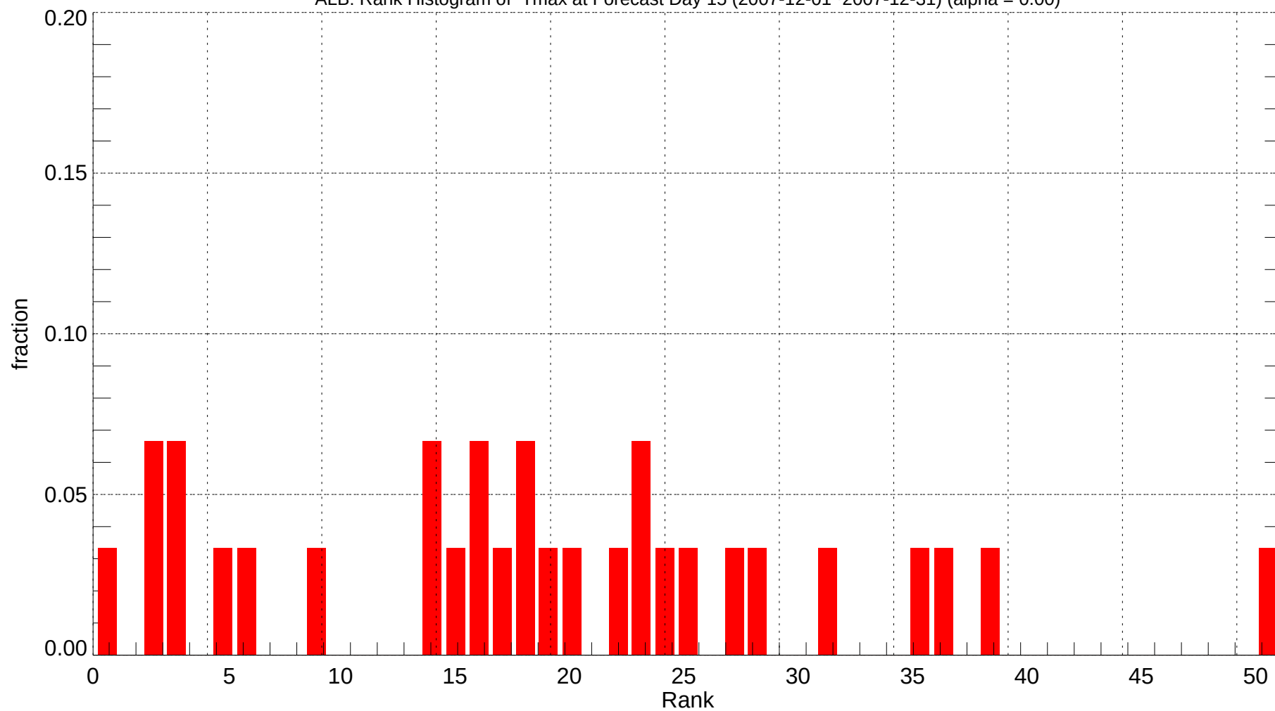
ALB: Rank Histogram of Tmax at Forecast Day 15 (2007-12-01~2007-12-31) (alpha = 0.00)
