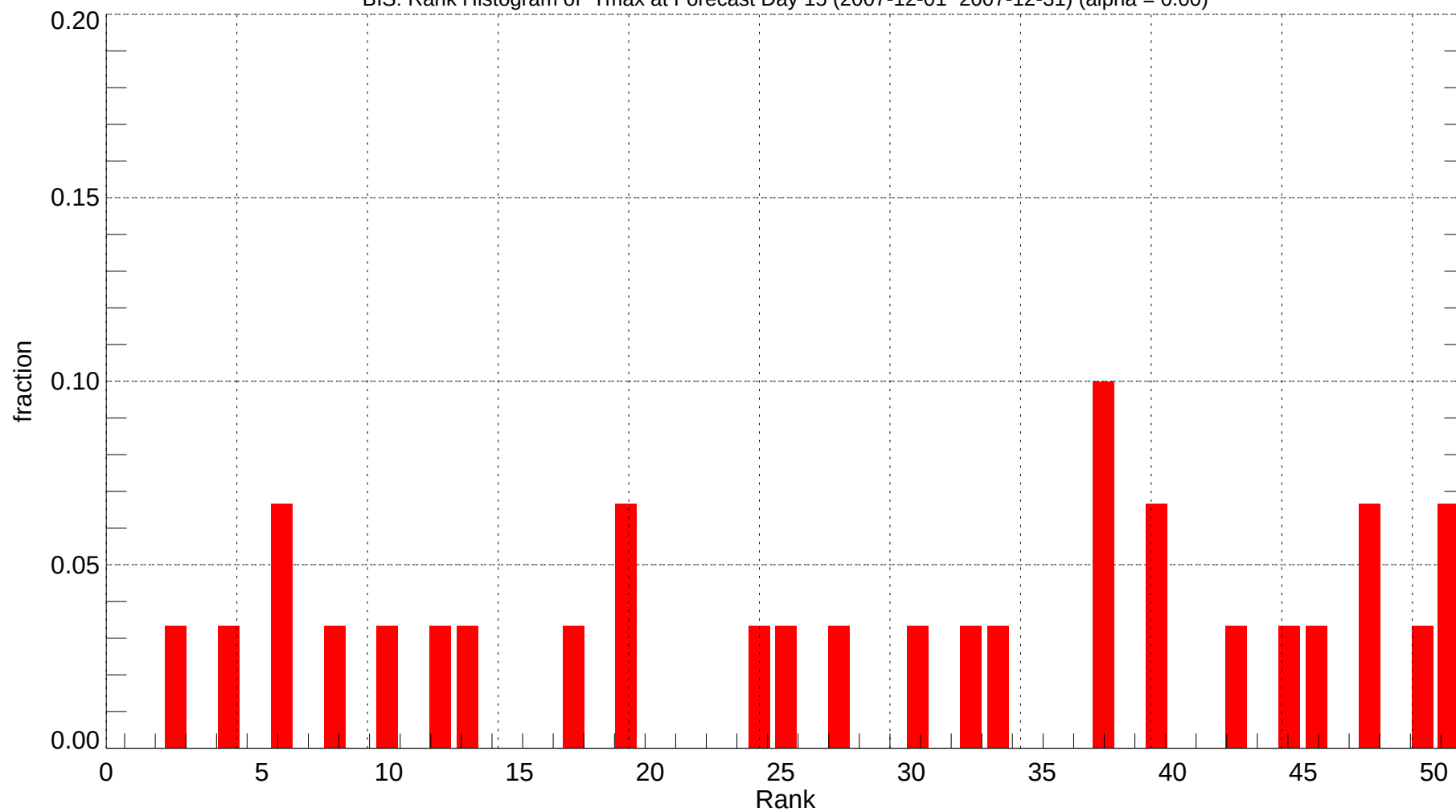
BIS: Rank Histogram of Tmax at Forecast Day 15 (2007-12-01~2007-12-31) (alpha = 0.00)
