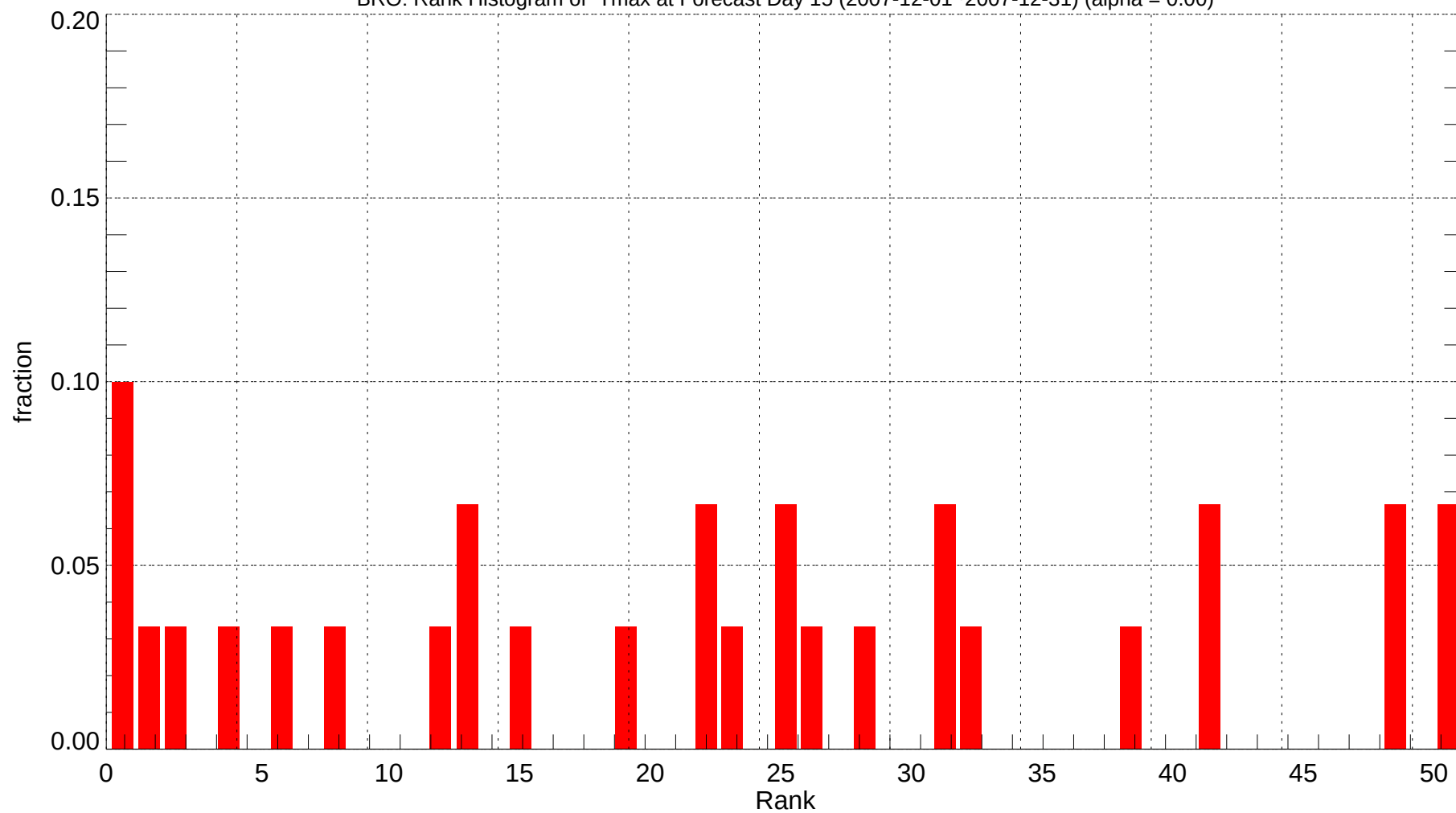
BRO: Rank Histogram of Tmax at Forecast Day 15 (2007-12-01~2007-12-31) (alpha = 0.00)
