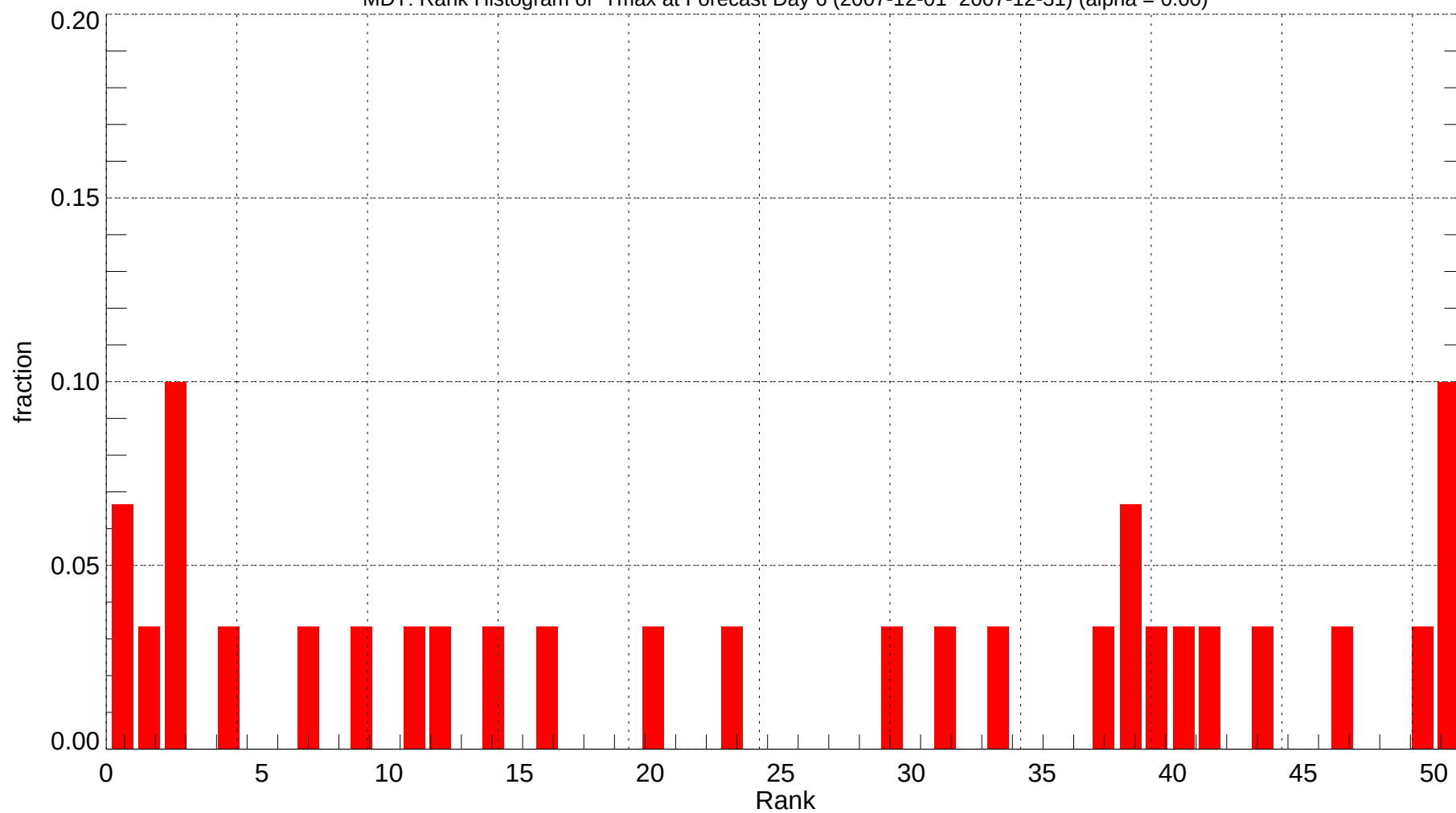
MDT: Rank Histogram of Tmax at Forecast Day 6 (2007-12-01~2007-12-31) (alpha = 0.00)
