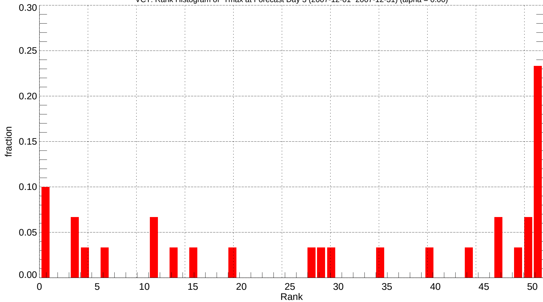
VCT: Rank Histogram of Tmax at Forecast Day 3 (2007-12-01~2007-12-31) (alpha = 0.00)
