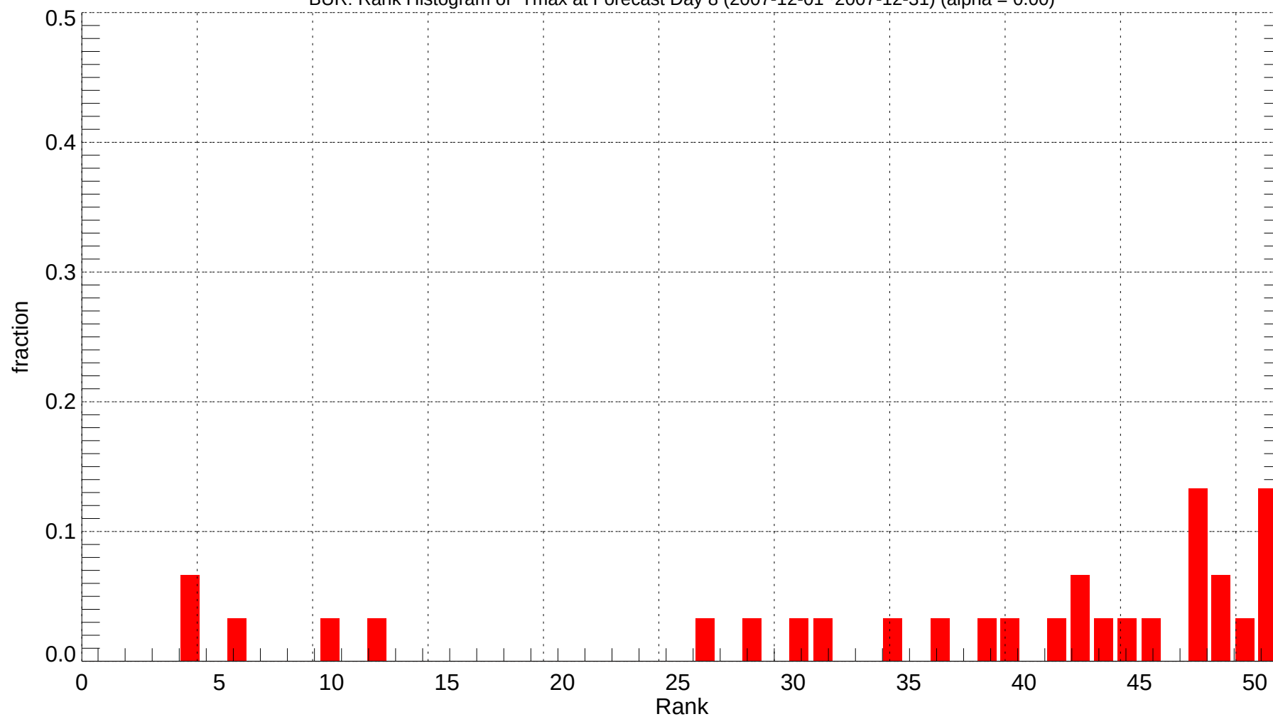
BUR: Rank Histogram of Tmax at Forecast Day 8 (2007-12-01~2007-12-31) (alpha = 0.00)
