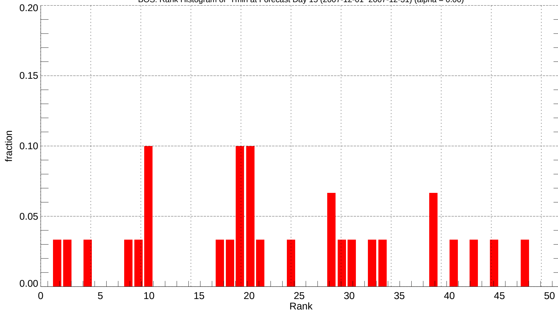
BOS: Rank Histogram of Tmin at Forecast Day 15 (2007-12-01~2007-12-31) (alpha = 0.00)
