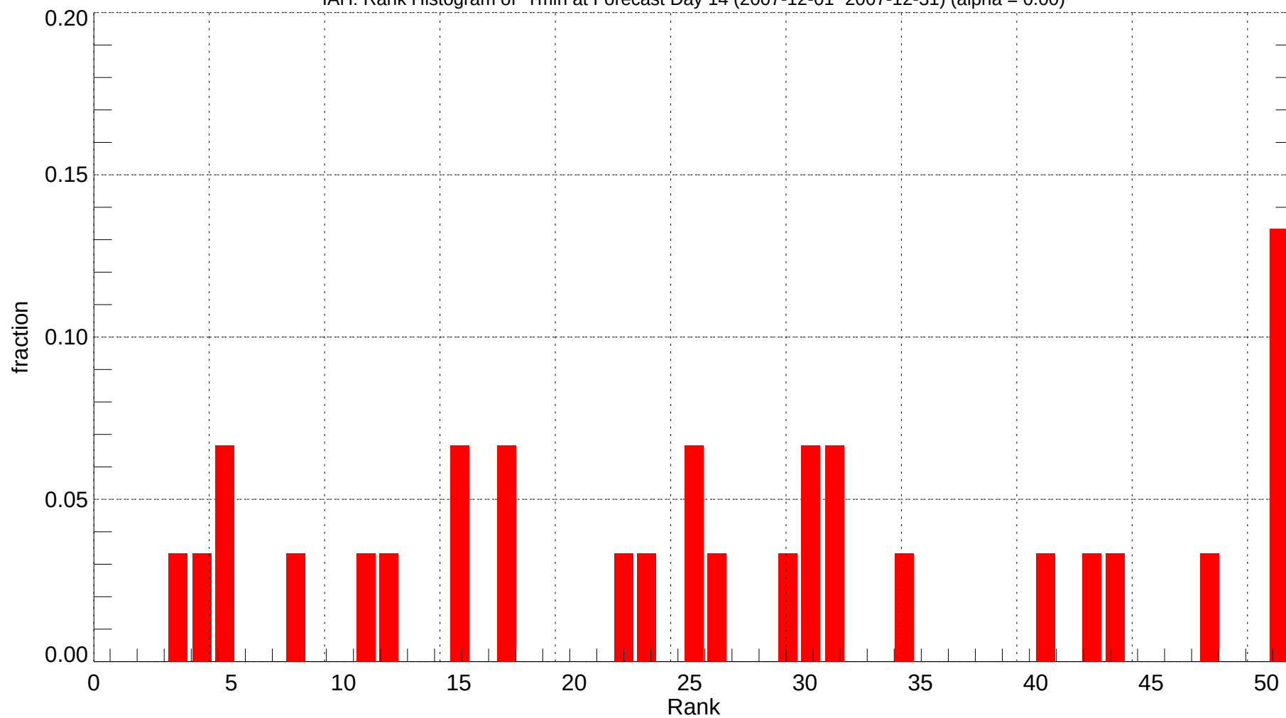
IAH: Rank Histogram of Tmin at Forecast Day 14 (2007-12-01~2007-12-31) (alpha = 0.00)
