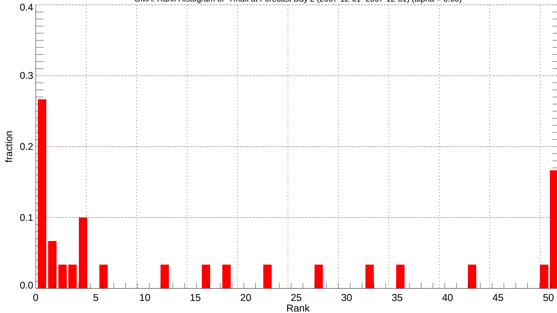
OMA: Rank Histogram of Tmax at Forecast Day 2 (2007-12-01~2007-12-31) (alpha = 0.00)
