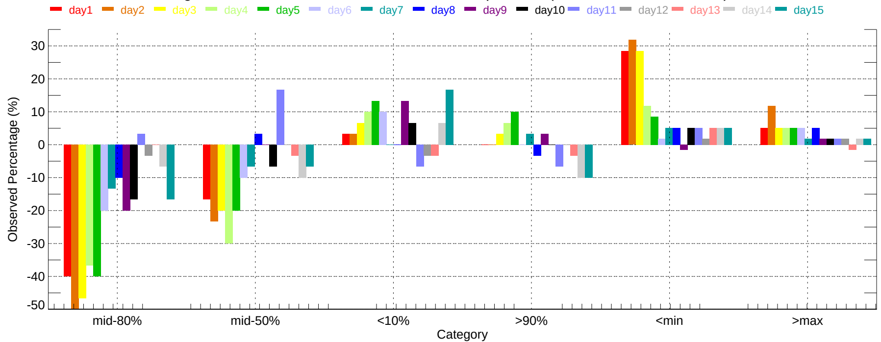
Observed Percentage Deviation of Ensembles - SFO: Min Temperature (2007-12-01~2007-12-31)
