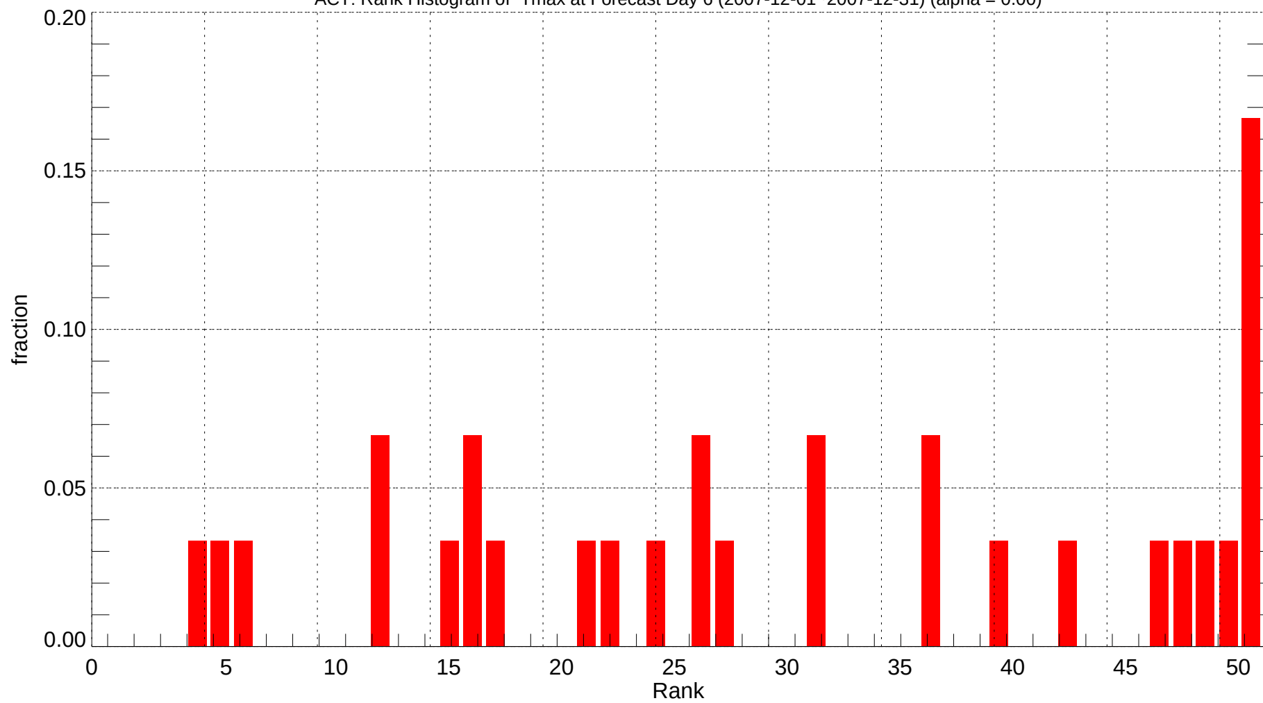
ACT: Rank Histogram of Tmax at Forecast Day 6 (2007-12-01~2007-12-31) (alpha = 0.00)
