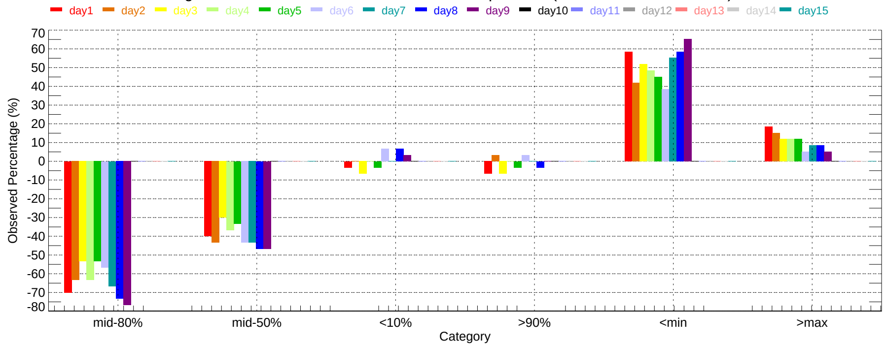
Observed Percentage Deviation of Ensembles - NKX: Min Temperature (2007-12-01~2007-12-31)
