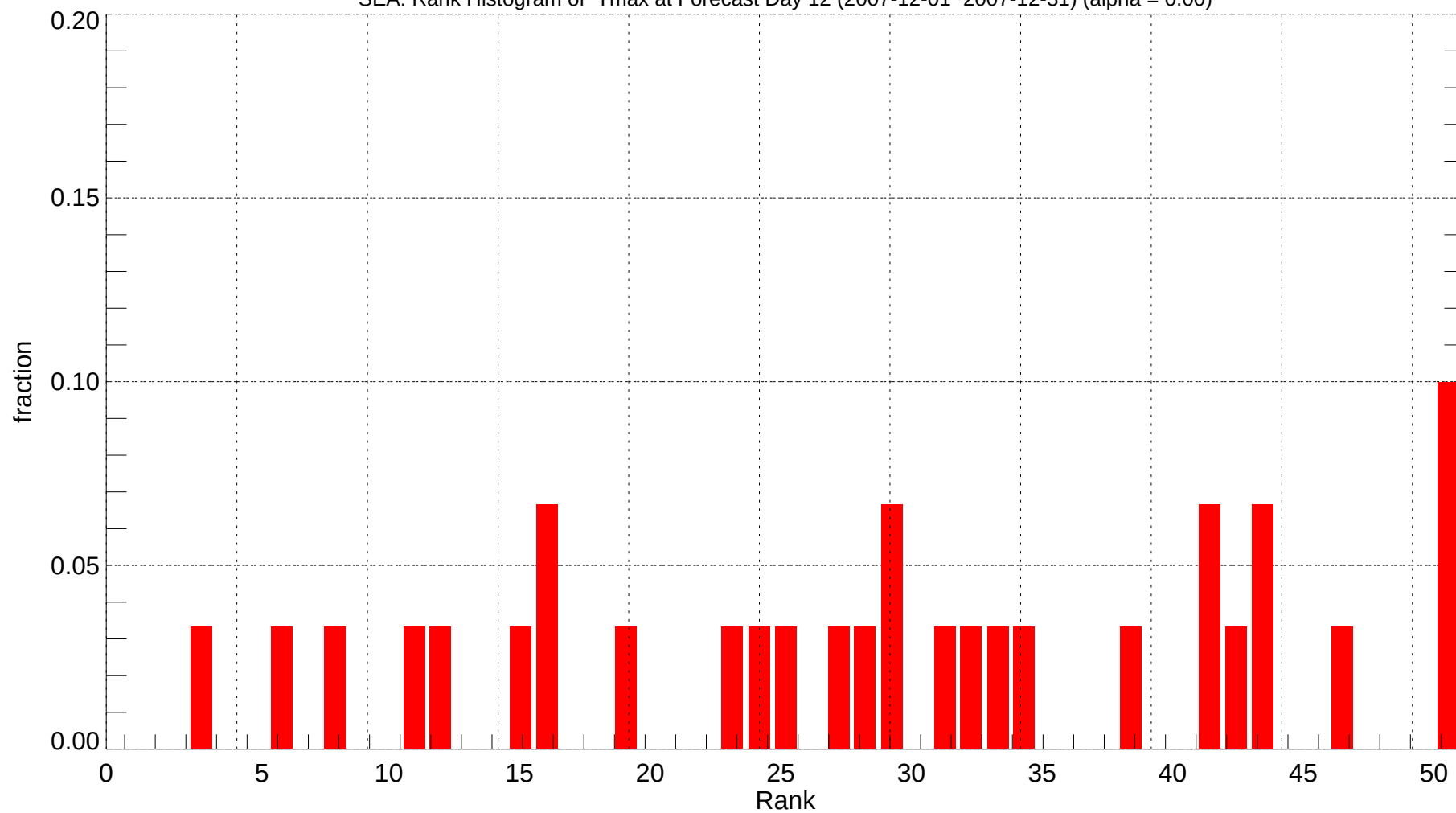
SEA: Rank Histogram of Tmax at Forecast Day 12 (2007-12-01~2007-12-31) (alpha = 0.00)
