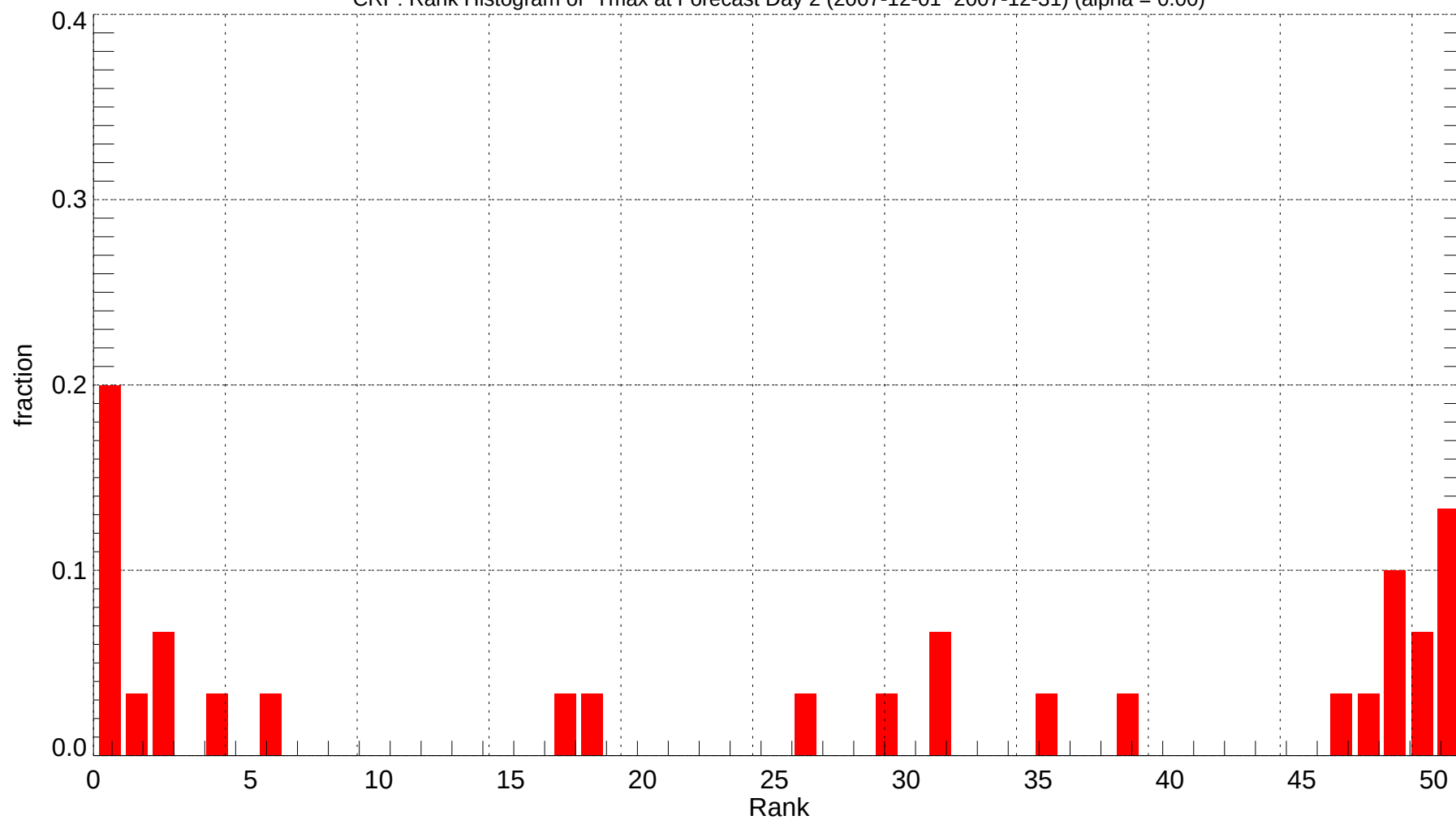
CRP: Rank Histogram of Tmax at Forecast Day 2 (2007-12-01~2007-12-31) (alpha = 0.00)
