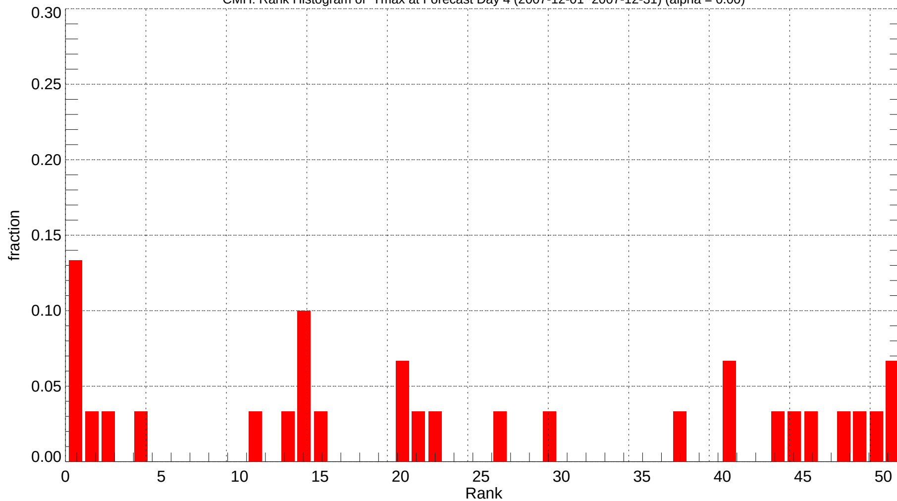
CMH: Rank Histogram of Tmax at Forecast Day 4 (2007-12-01~2007-12-31) (alpha = 0.00)
