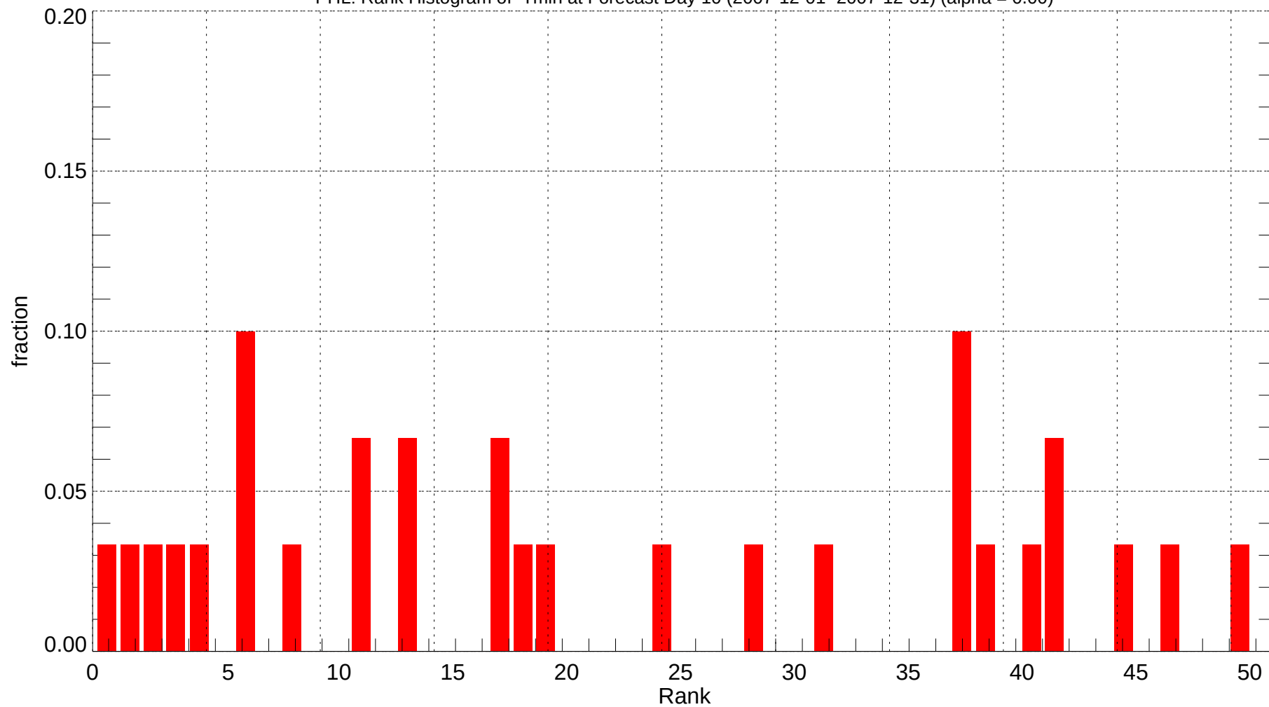
PHL: Rank Histogram of Tmin at Forecast Day 10 (2007-12-01~2007-12-31) (alpha = 0.00)
