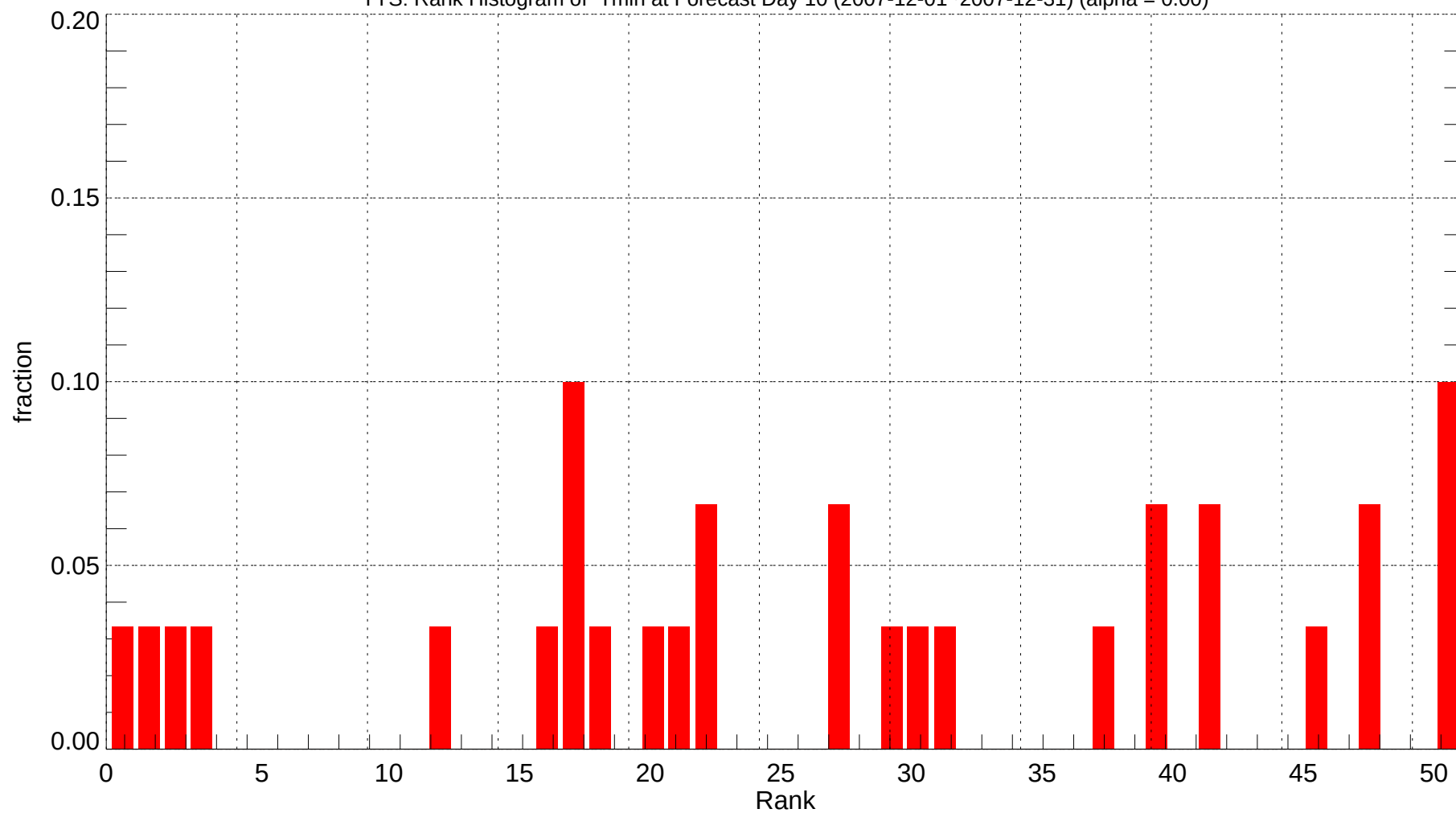
TYS: Rank Histogram of Tmin at Forecast Day 10 (2007-12-01~2007-12-31) (alpha = 0.00)
