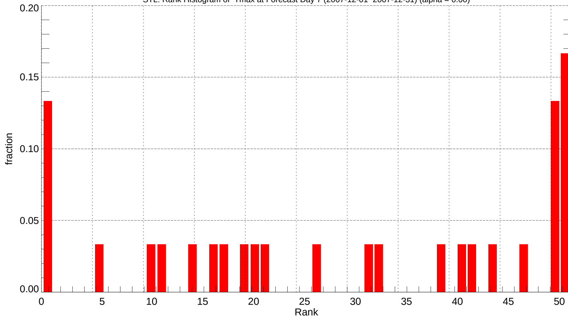
STL: Rank Histogram of Tmax at Forecast Day 7 (2007-12-01~2007-12-31) (alpha = 0.00)
