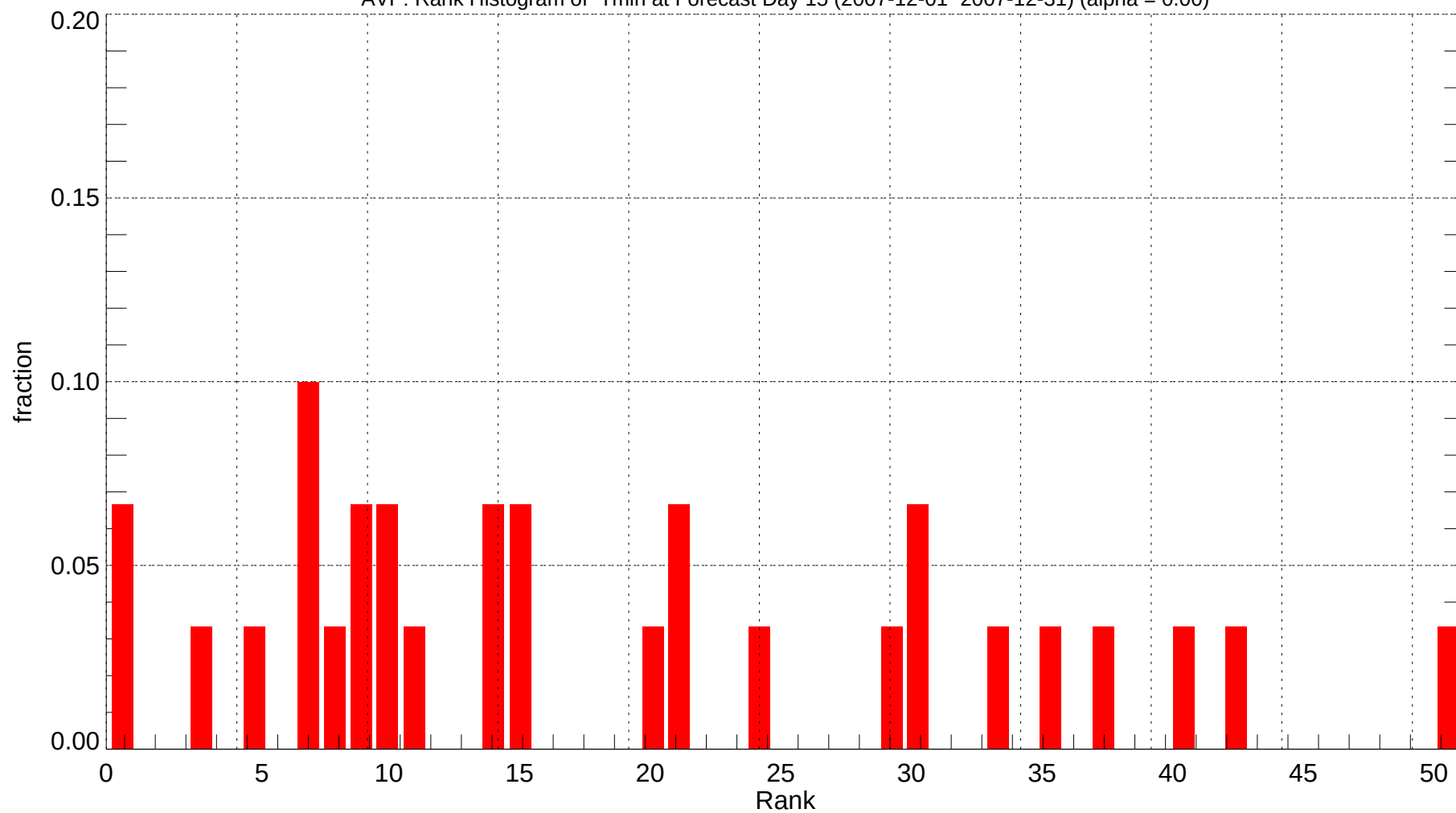
AVP: Rank Histogram of Tmin at Forecast Day 15 (2007-12-01~2007-12-31) (alpha = 0.00)
