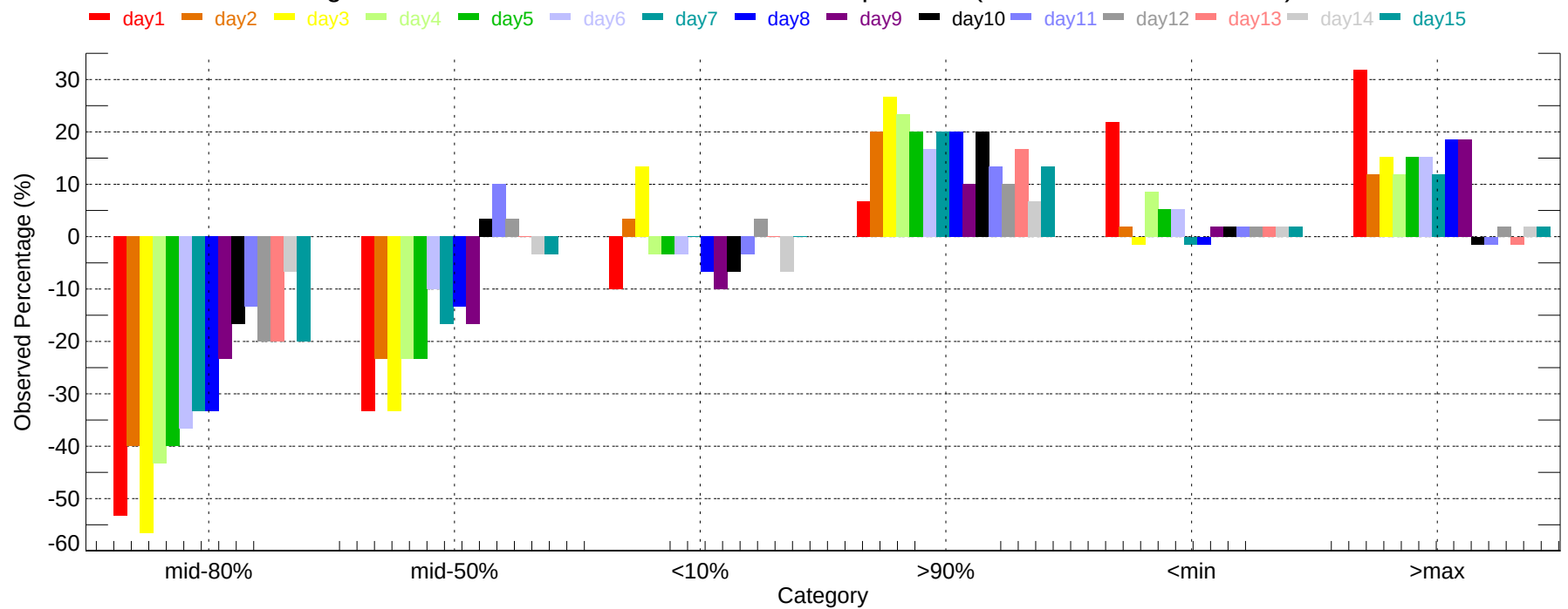
Observed Percentage Deviation of Ensembles - TPA: Min Temperature (2007-12-01~2007-12-31)
