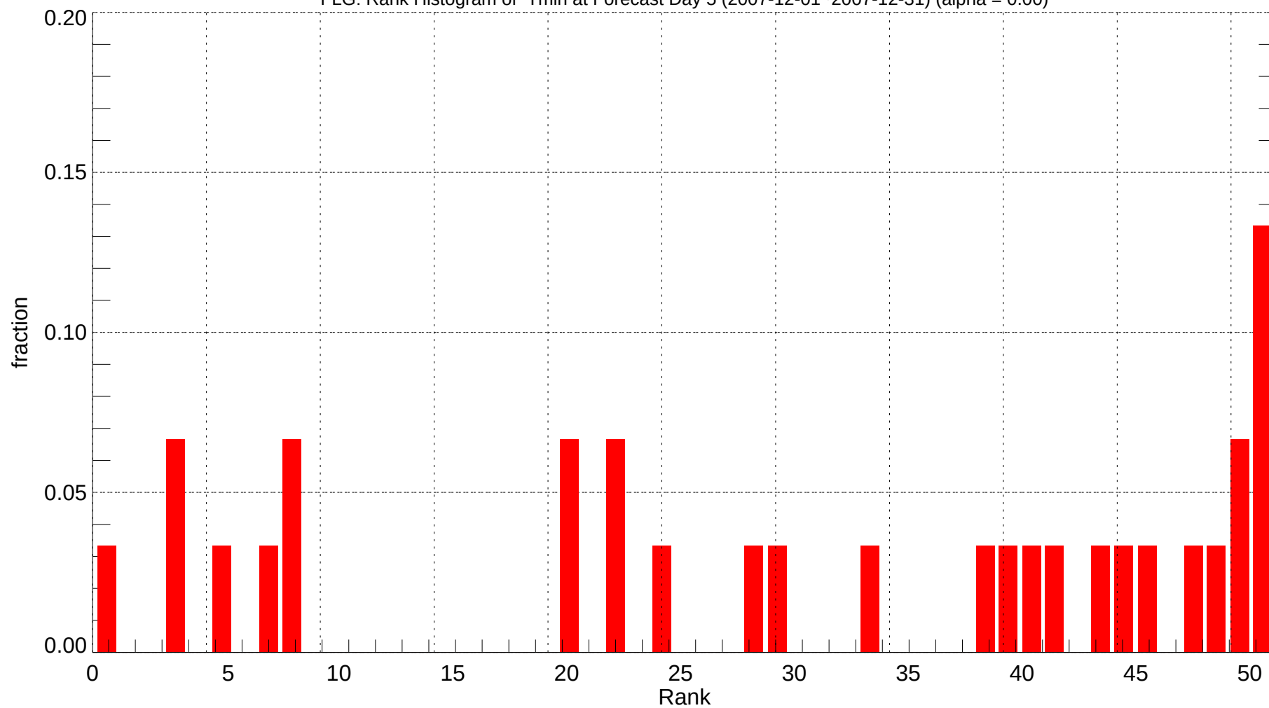
FLG: Rank Histogram of Tmin at Forecast Day 5 (2007-12-01~2007-12-31) (alpha = 0.00)
