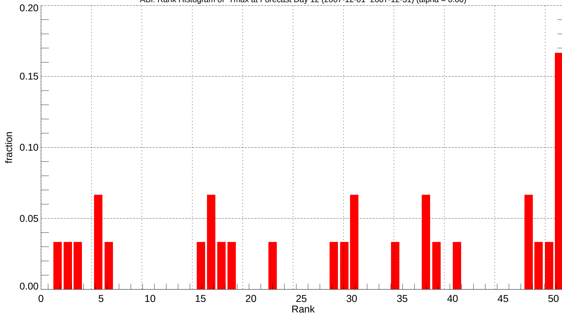
ABI: Rank Histogram of Tmax at Forecast Day 12 (2007-12-01~2007-12-31) (alpha = 0.00)
