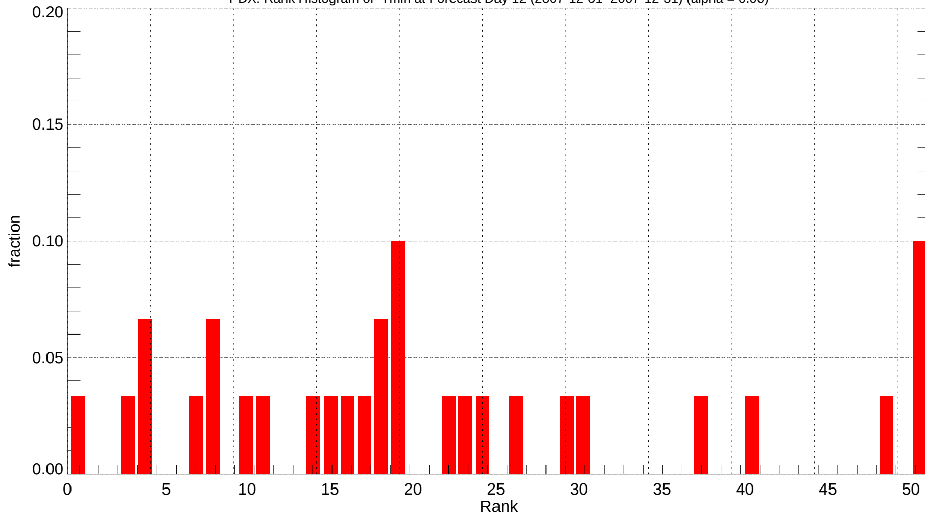
PDX: Rank Histogram of Tmin at Forecast Day 12 (2007-12-01~2007-12-31) (alpha = 0.00)
