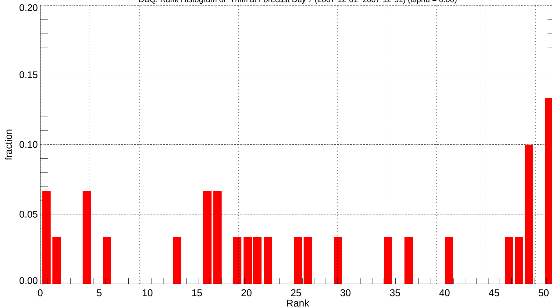
DBQ: Rank Histogram of Tmin at Forecast Day 7 (2007-12-01~2007-12-31) (alpha = 0.00)
