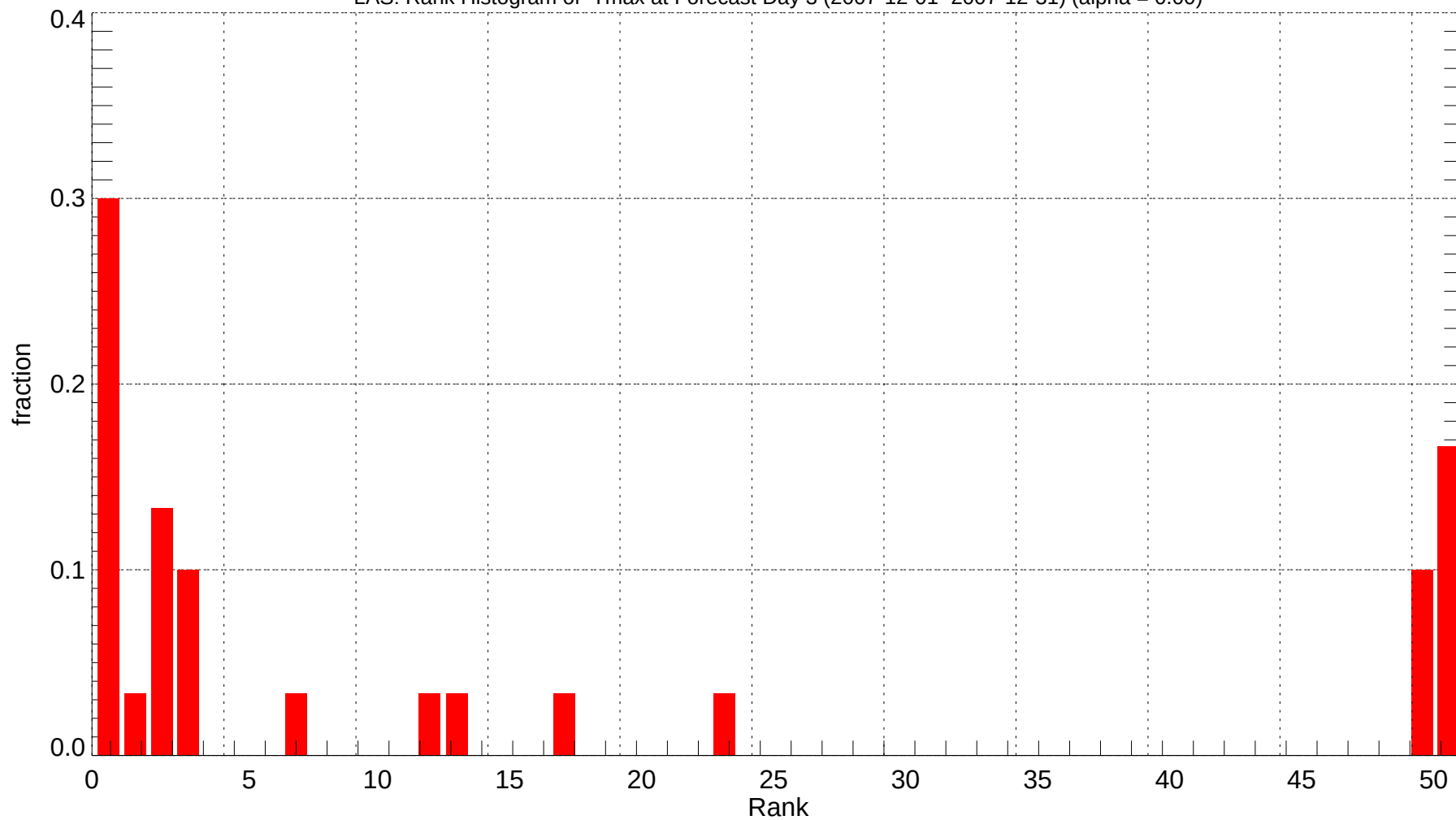
LAS: Rank Histogram of Tmax at Forecast Day 3 (2007-12-01~2007-12-31) (alpha = 0.00)
