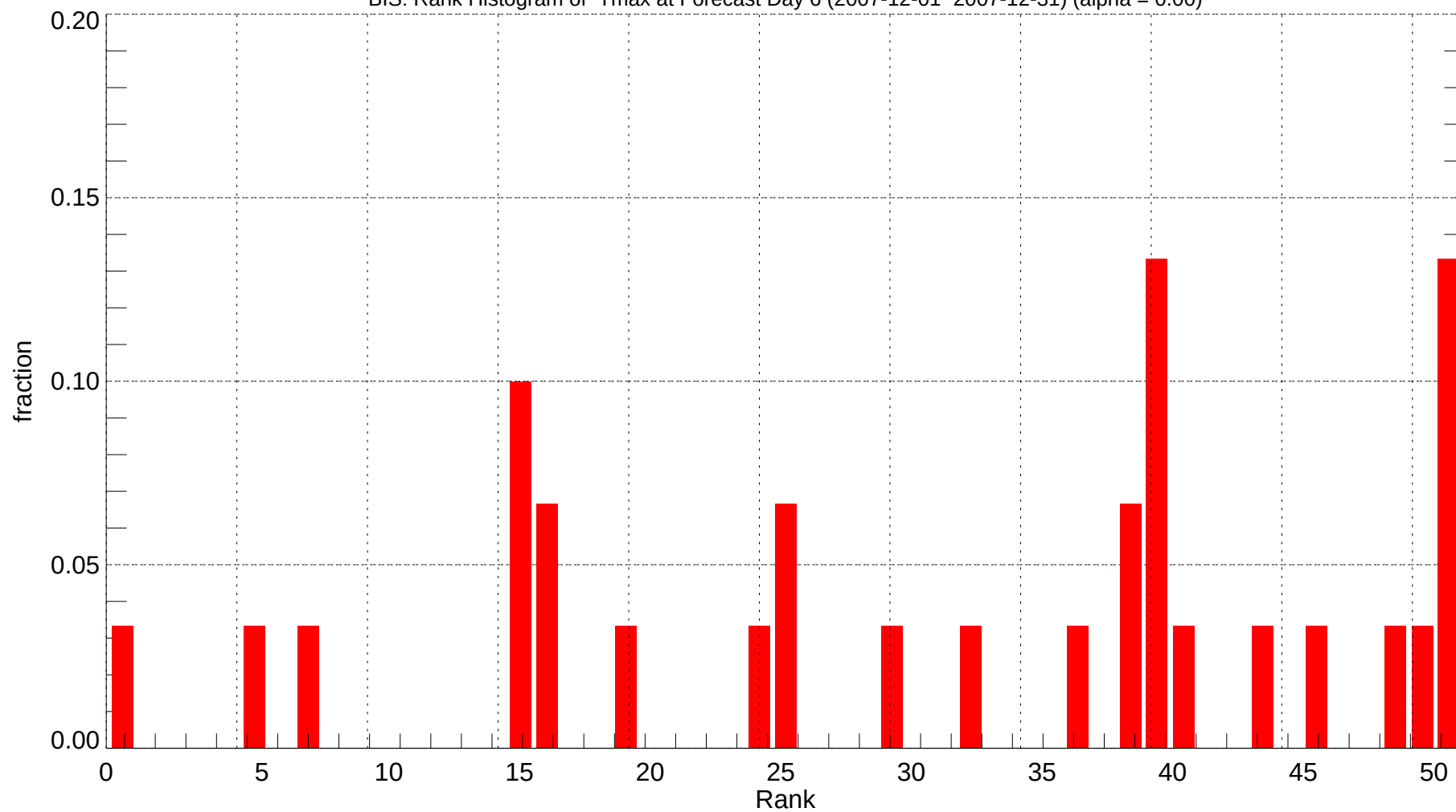
BIS: Rank Histogram of Tmax at Forecast Day 6 (2007-12-01~2007-12-31) (alpha = 0.00)
