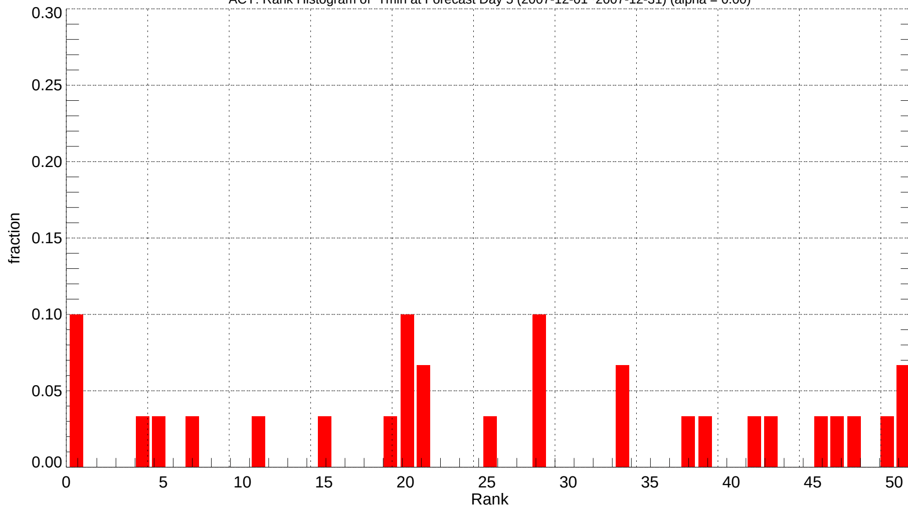
ACY: Rank Histogram of Tmin at Forecast Day 5 (2007-12-01~2007-12-31) (alpha = 0.00)
