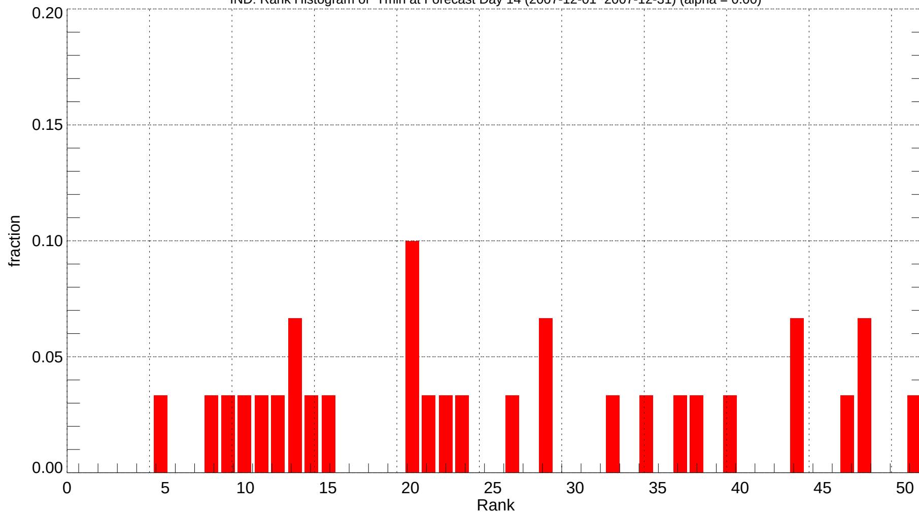
IND: Rank Histogram of Tmin at Forecast Day 14 (2007-12-01~2007-12-31) (alpha = 0.00)
