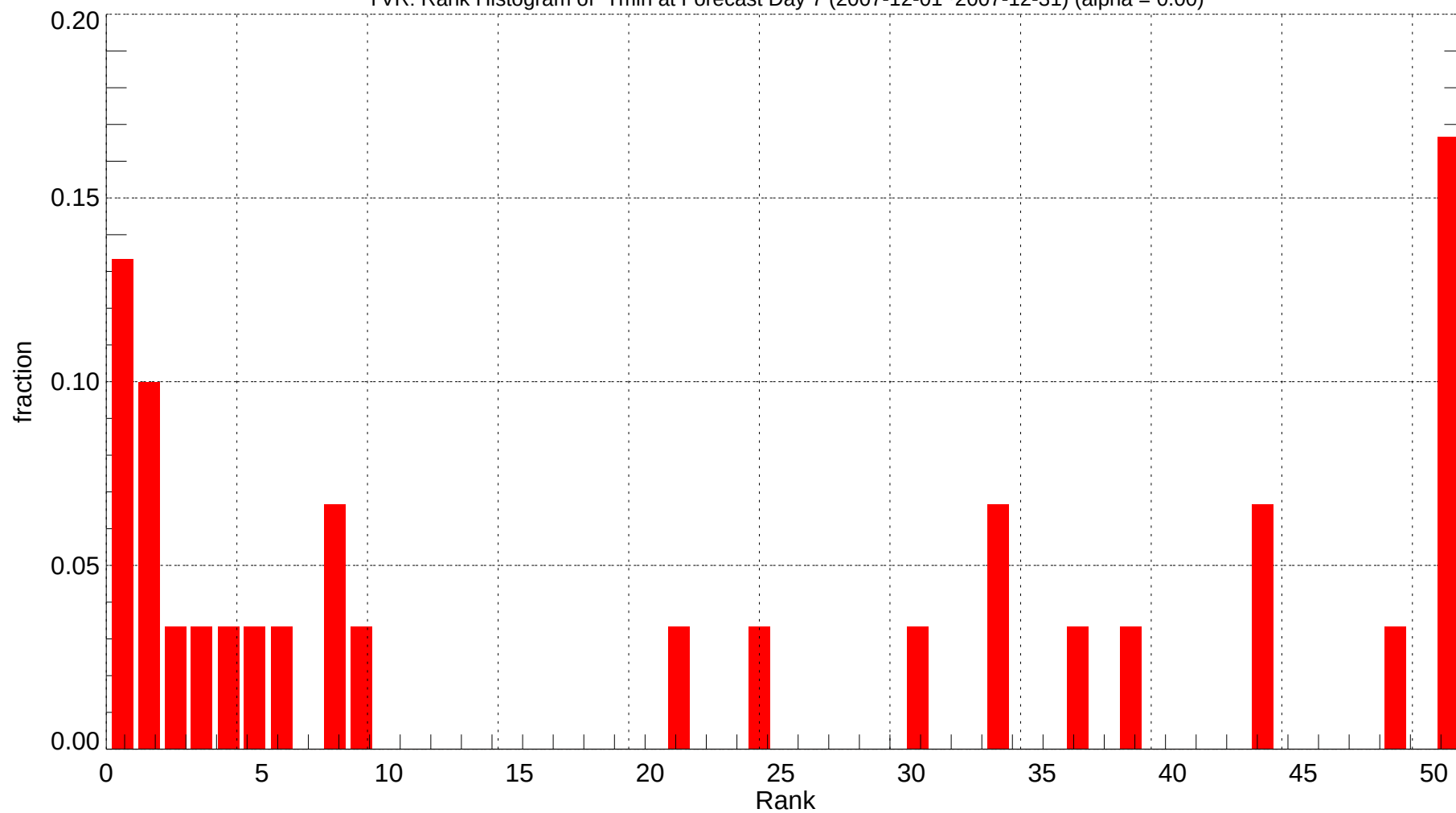
YVR: Rank Histogram of Tmin at Forecast Day 7 (2007-12-01~2007-12-31) (alpha = 0.00)
