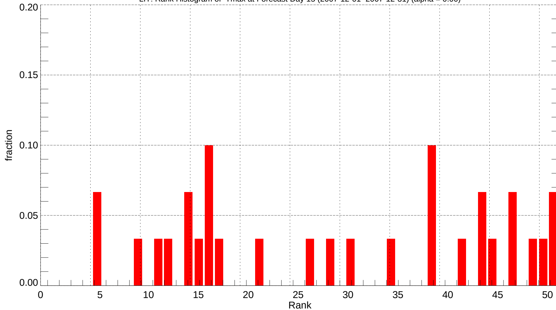
LIT: Rank Histogram of Tmax at Forecast Day 15 (2007-12-01~2007-12-31) (alpha = 0.00)
