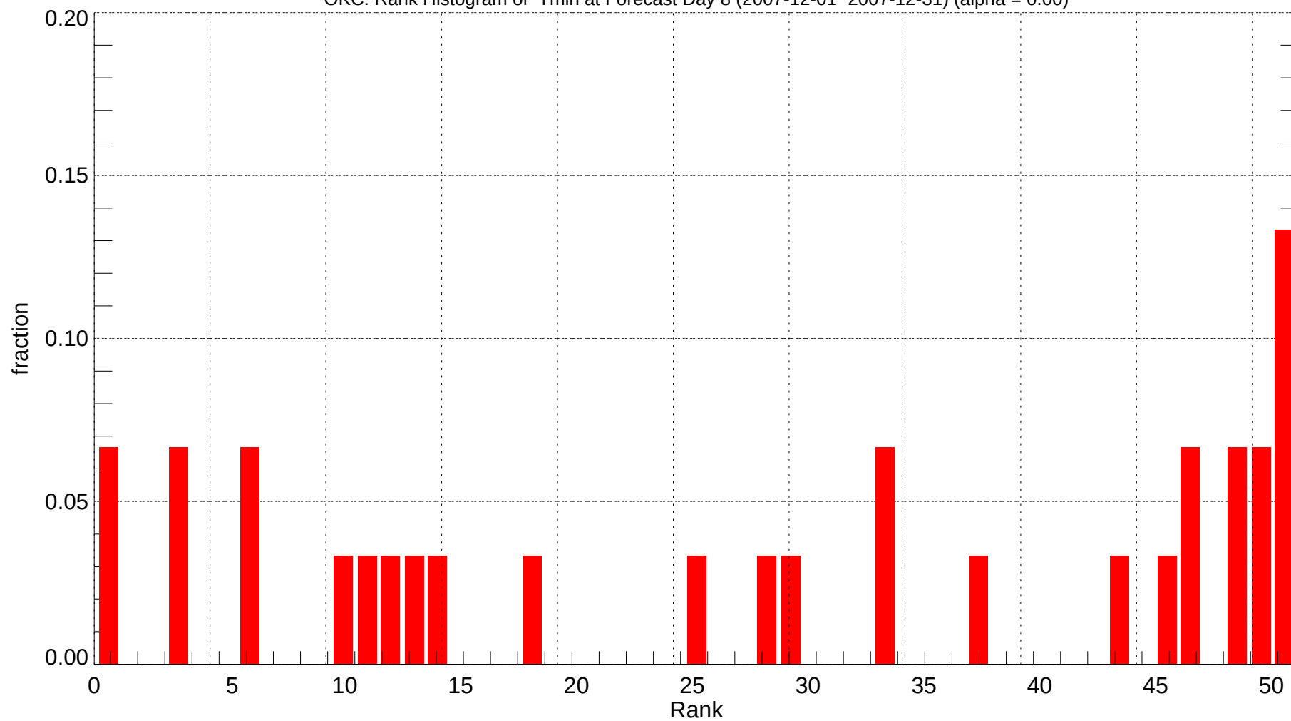
OKC: Rank Histogram of Tmin at Forecast Day 8 (2007-12-01~2007-12-31) (alpha = 0.00)
