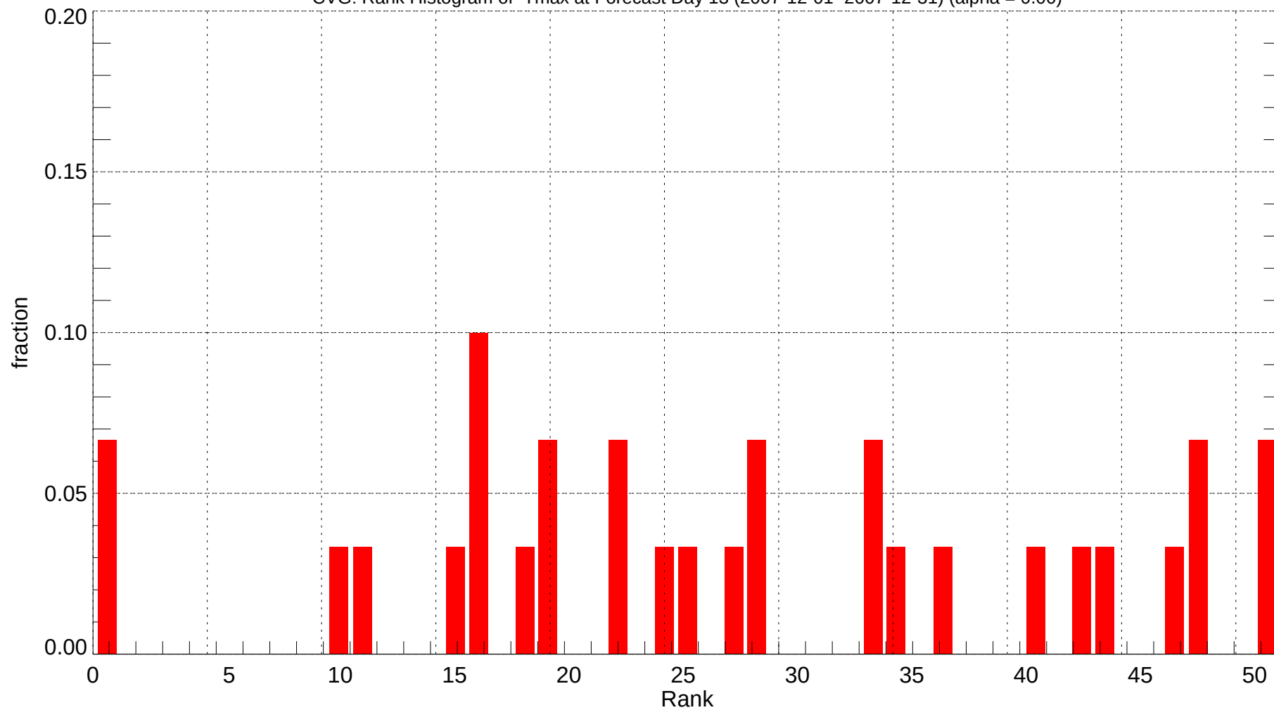
CVG: Rank Histogram of Tmax at Forecast Day 13 (2007-12-01~2007-12-31) (alpha = 0.00)
