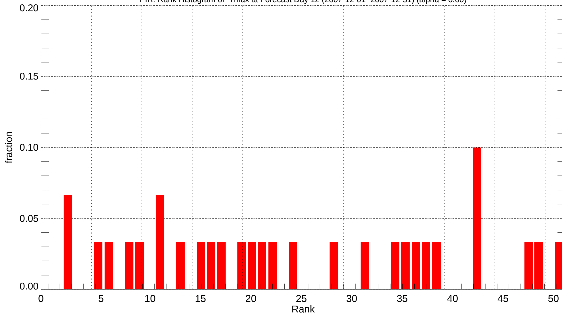
PIR: Rank Histogram of Tmax at Forecast Day 12 (2007-12-01~2007-12-31) (alpha = 0.00)
