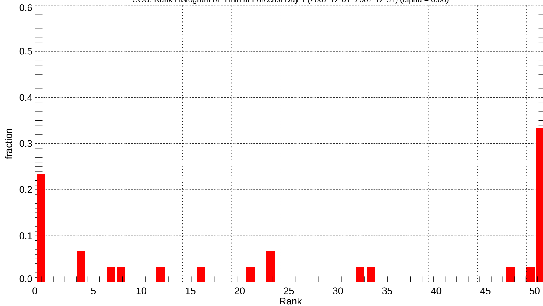
COU: Rank Histogram of Tmin at Forecast Day 1 (2007-12-01~2007-12-31) (alpha = 0.00)
