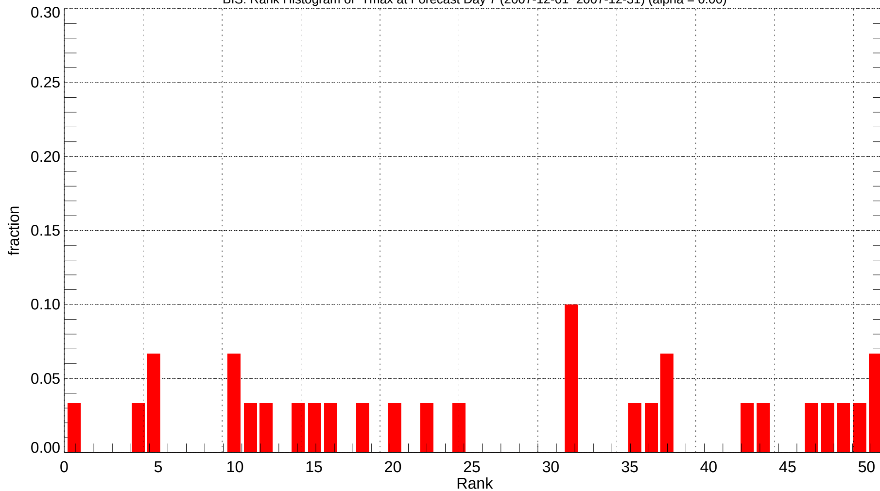
BIS: Rank Histogram of Tmax at Forecast Day 7 (2007-12-01~2007-12-31) (alpha = 0.00)
