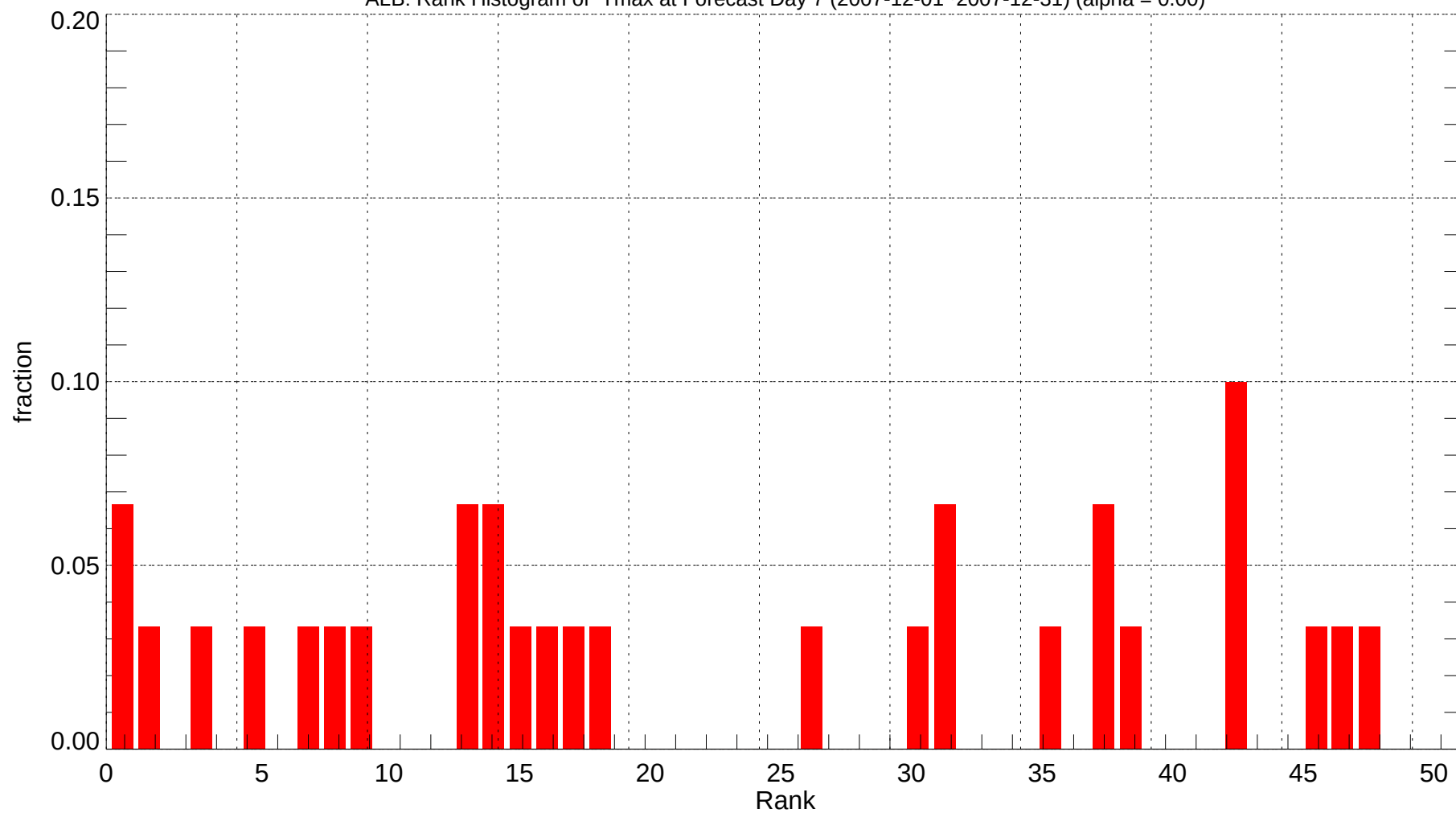
ALB: Rank Histogram of Tmax at Forecast Day 7 (2007-12-01~2007-12-31) (alpha = 0.00)
