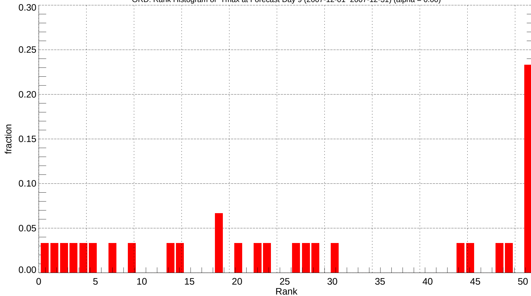
ORD: Rank Histogram of Tmax at Forecast Day 9 (2007-12-01~2007-12-31) (alpha = 0.00)
