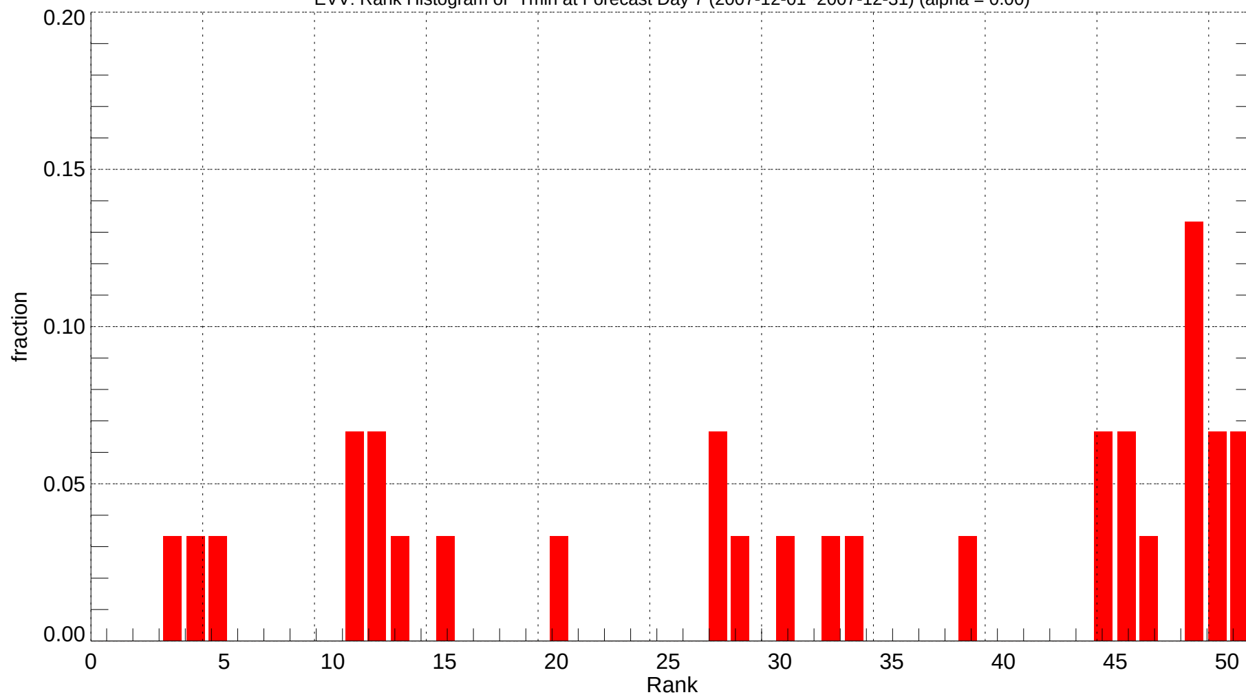
EVV: Rank Histogram of Tmin at Forecast Day 7 (2007-12-01~2007-12-31) (alpha = 0.00)
