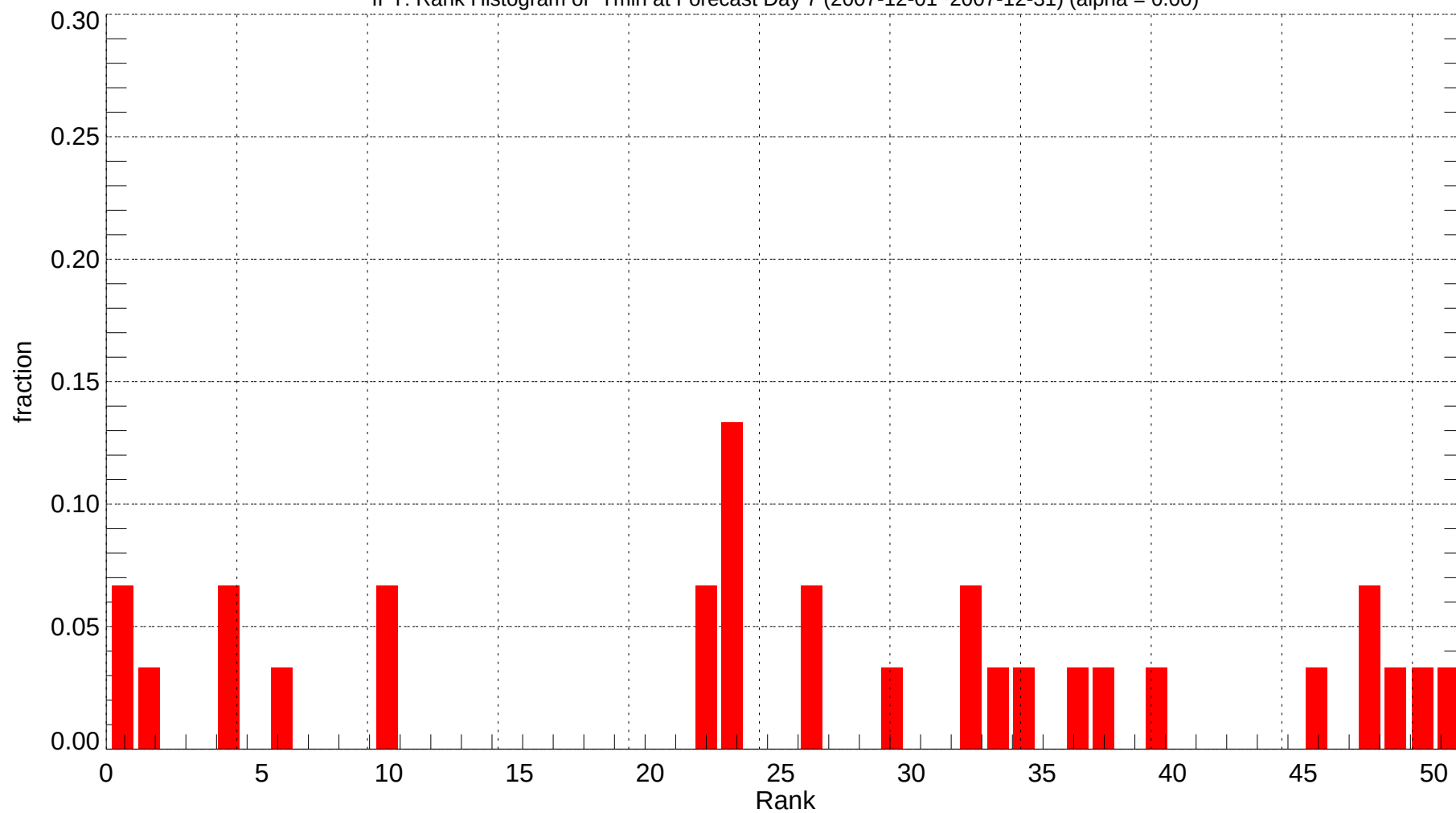
IPT: Rank Histogram of Tmin at Forecast Day 7 (2007-12-01~2007-12-31) (alpha = 0.00)
