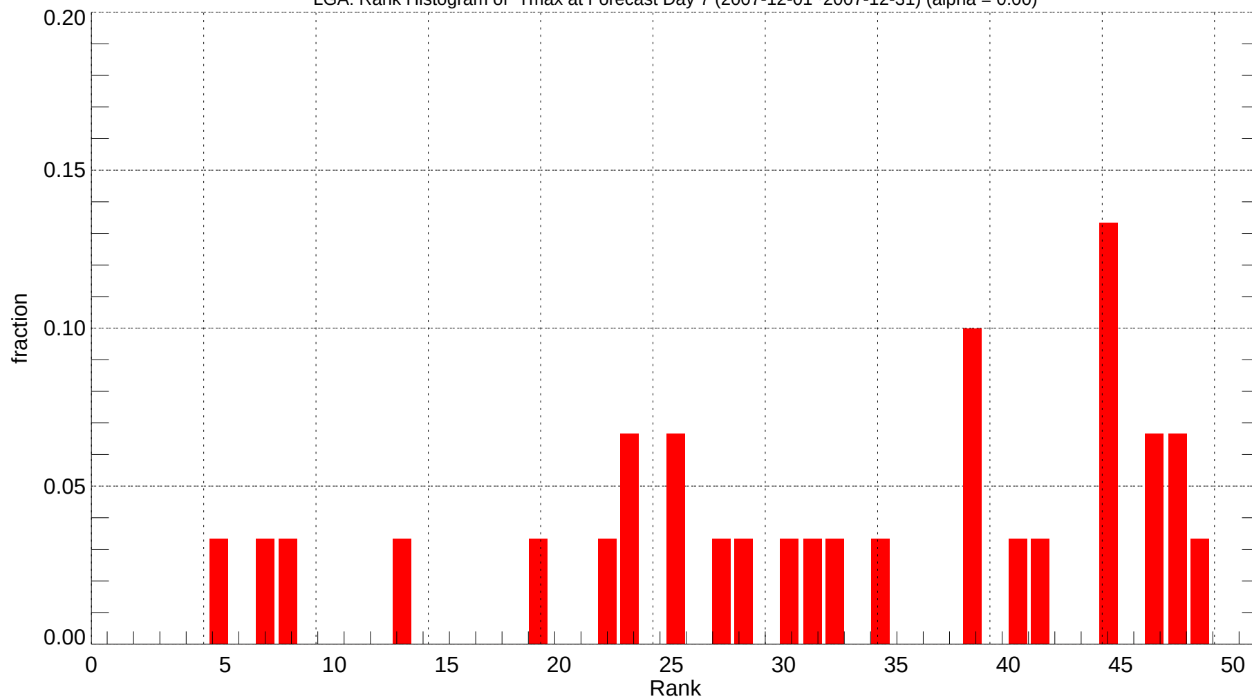
LGA: Rank Histogram of Tmax at Forecast Day 7 (2007-12-01~2007-12-31) (alpha = 0.00)
