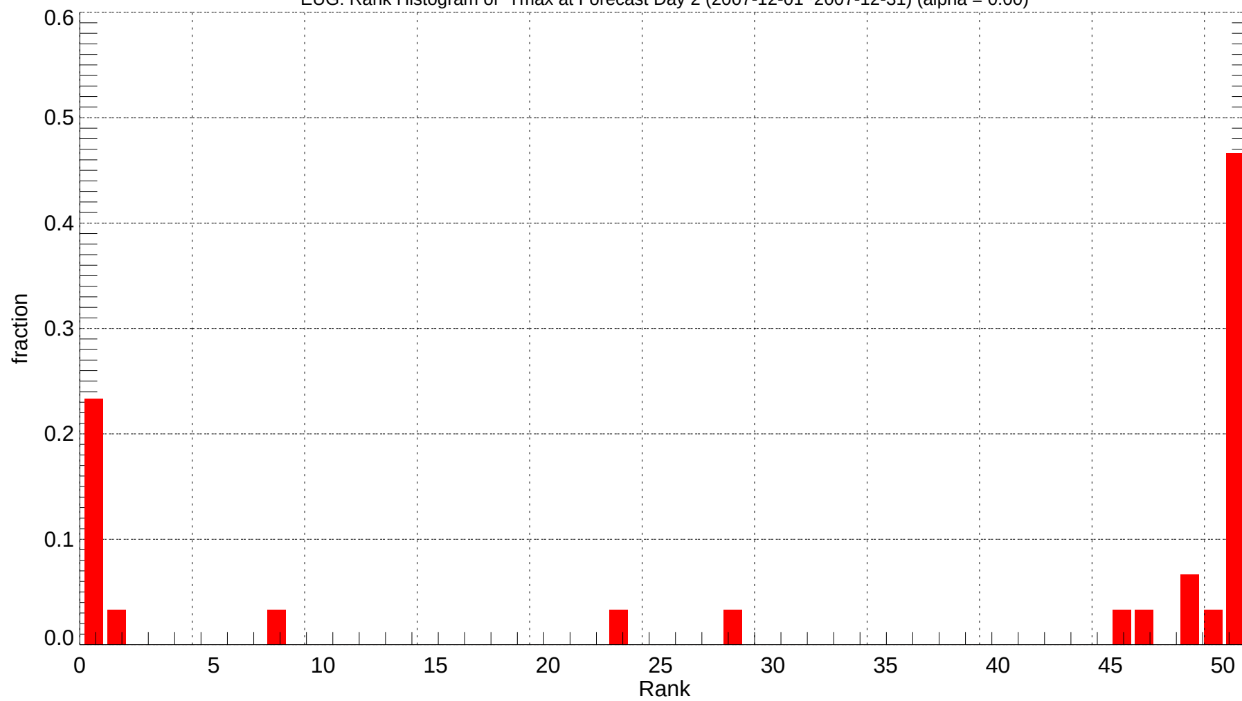
EUG: Rank Histogram of Tmax at Forecast Day 2 (2007-12-01~2007-12-31) (alpha = 0.00)
