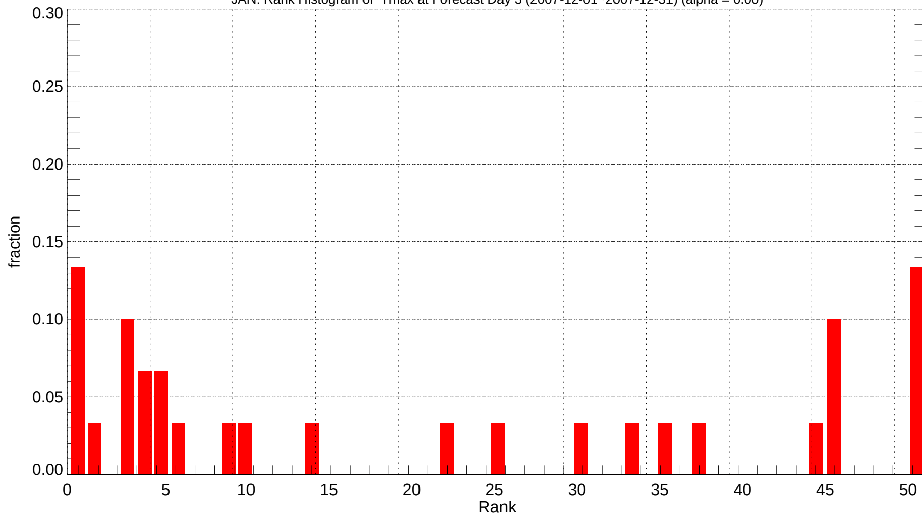
JAN: Rank Histogram of Tmax at Forecast Day 3 (2007-12-01~2007-12-31) (alpha = 0.00)
