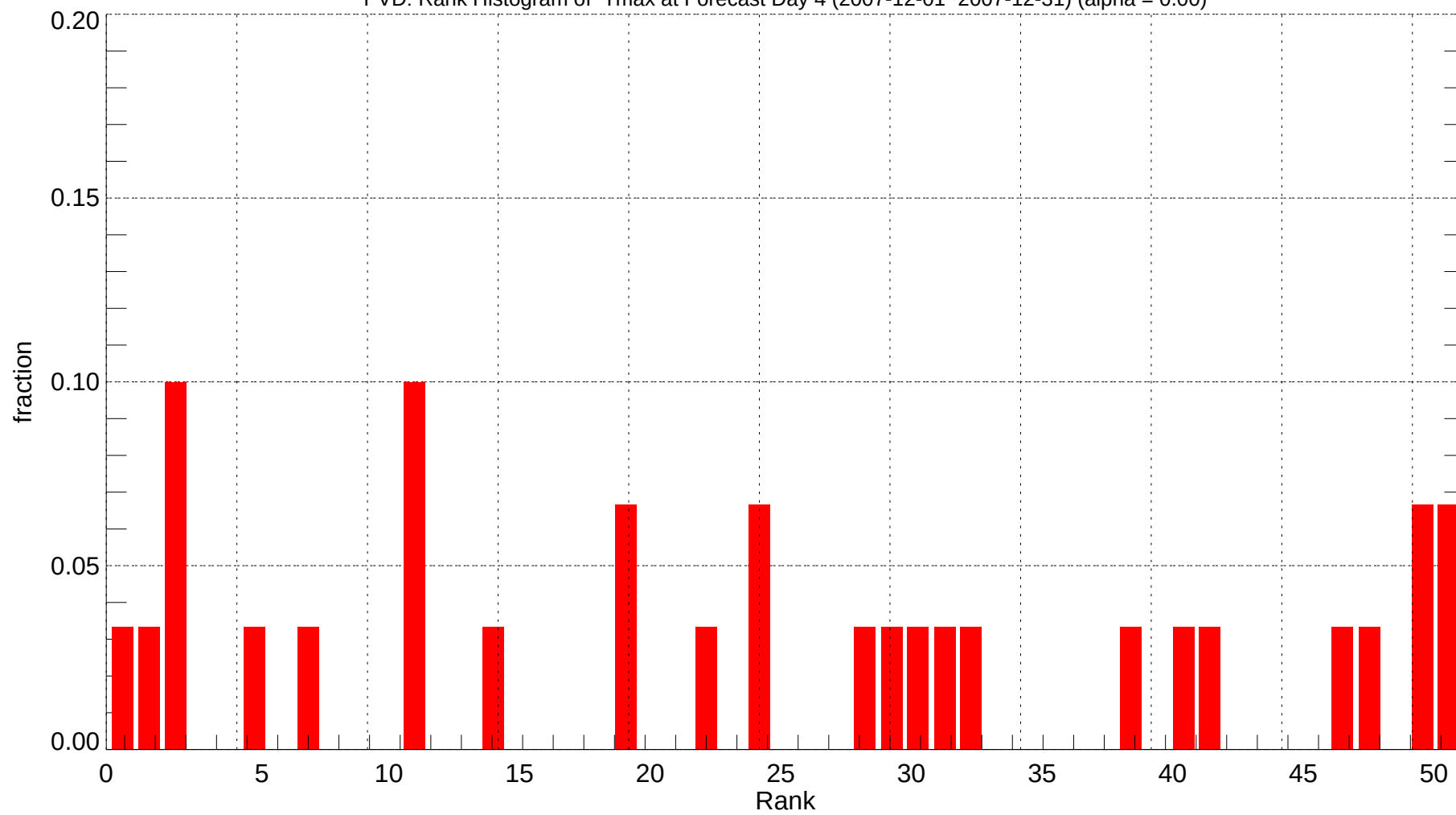
PVD: Rank Histogram of Tmax at Forecast Day 4 (2007-12-01~2007-12-31) (alpha = 0.00)
