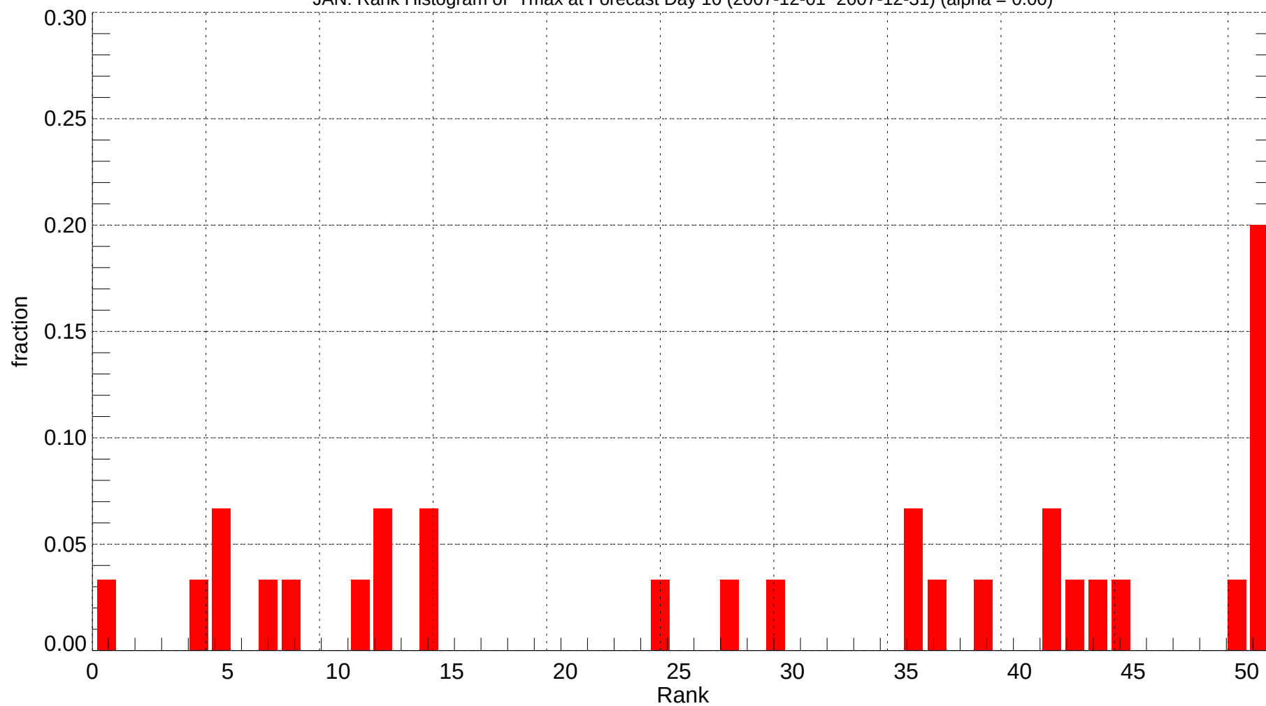
JAN: Rank Histogram of Tmax at Forecast Day 10 (2007-12-01~2007-12-31) (alpha = 0.00)
