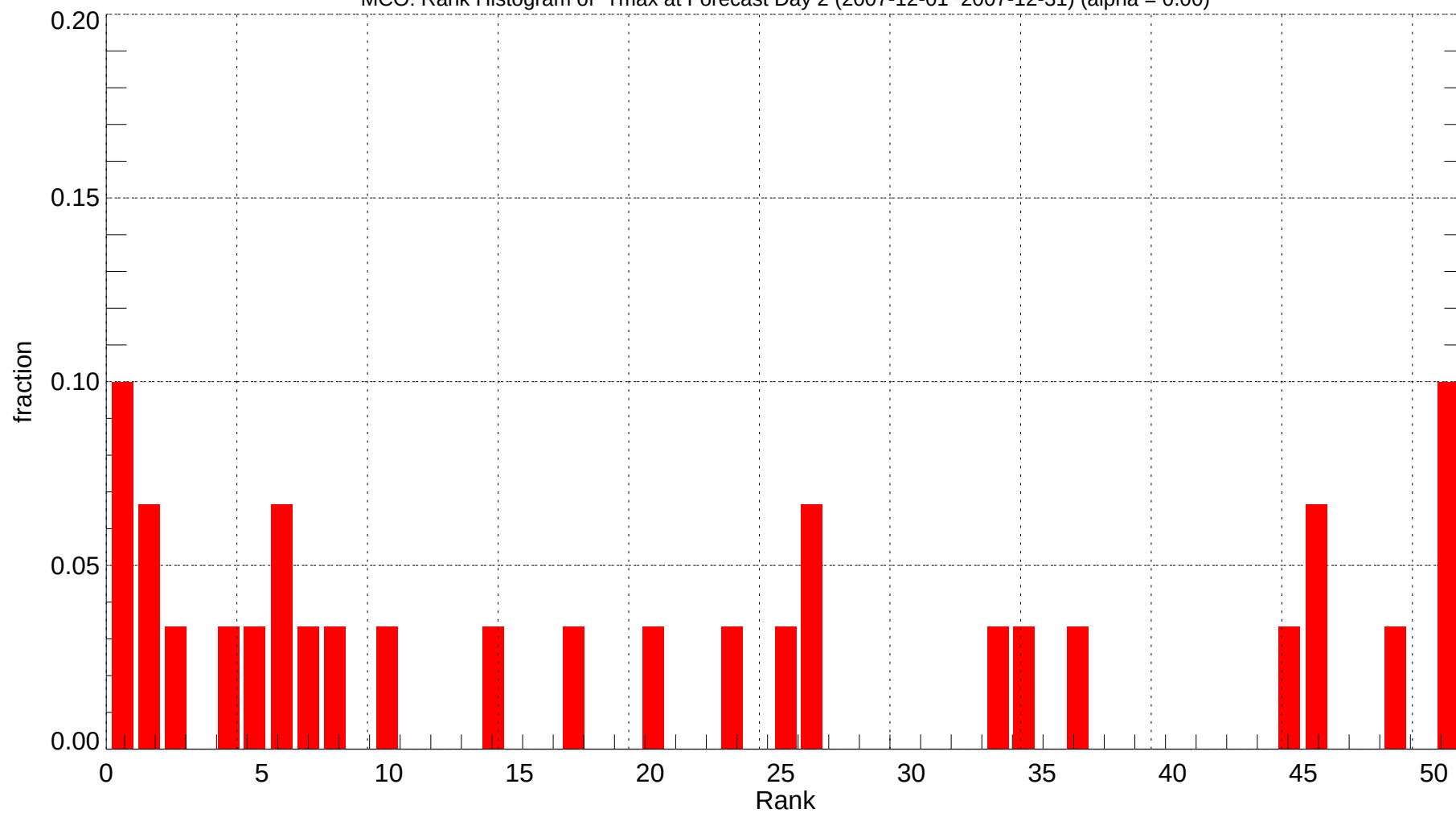
MCO: Rank Histogram of Tmax at Forecast Day 2 (2007-12-01~2007-12-31) (alpha = 0.00)
