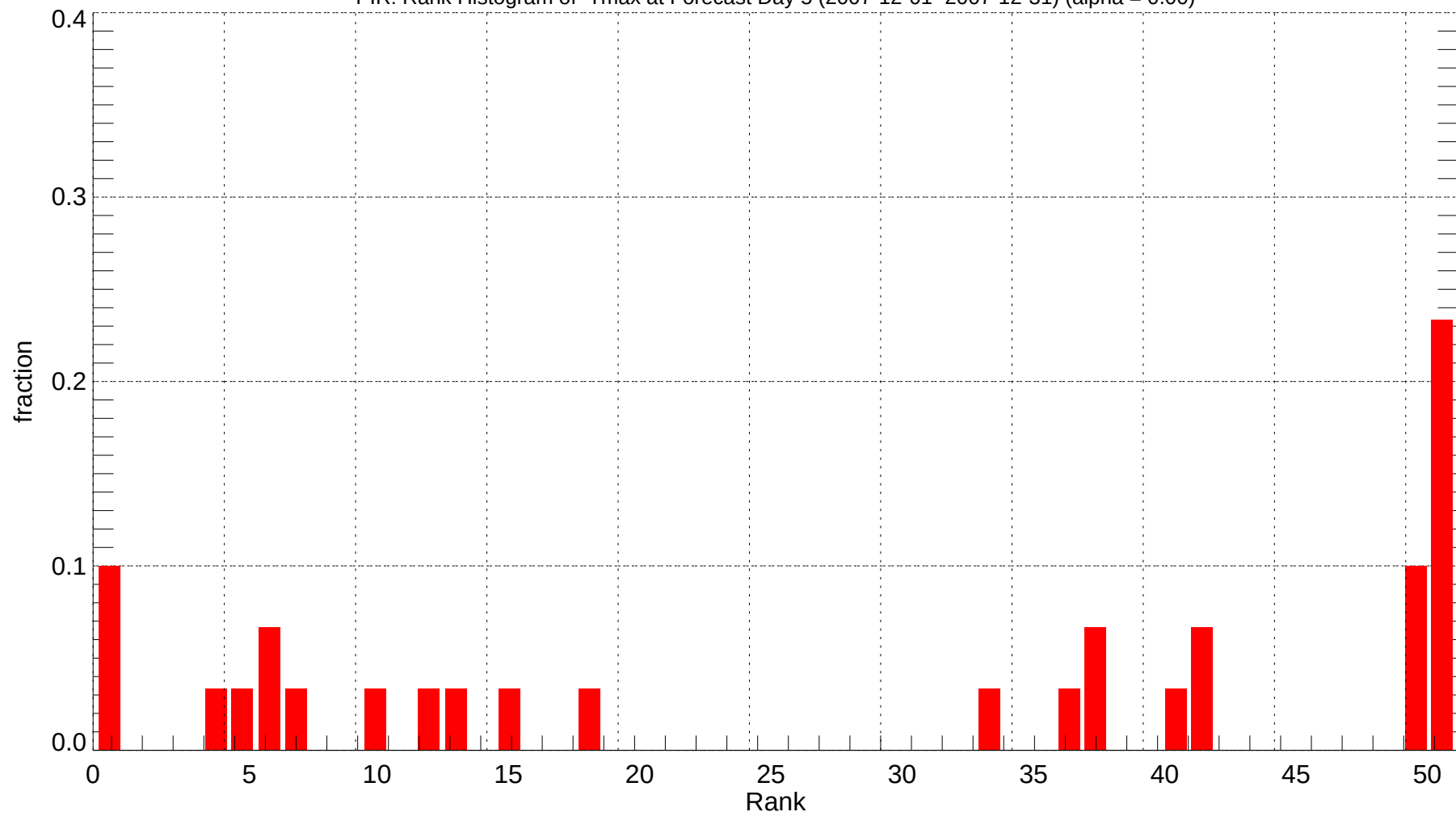
PIR: Rank Histogram of Tmax at Forecast Day 5 (2007-12-01~2007-12-31) (alpha = 0.00)
