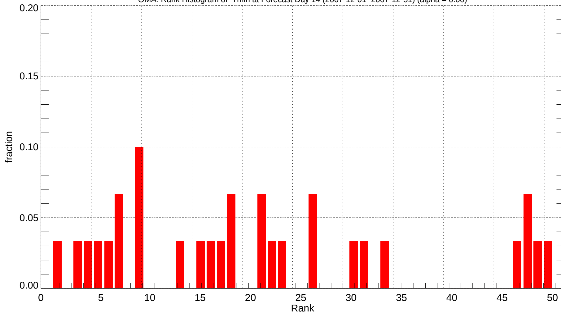
OMA: Rank Histogram of Tmin at Forecast Day 14 (2007-12-01~2007-12-31) (alpha = 0.00)
