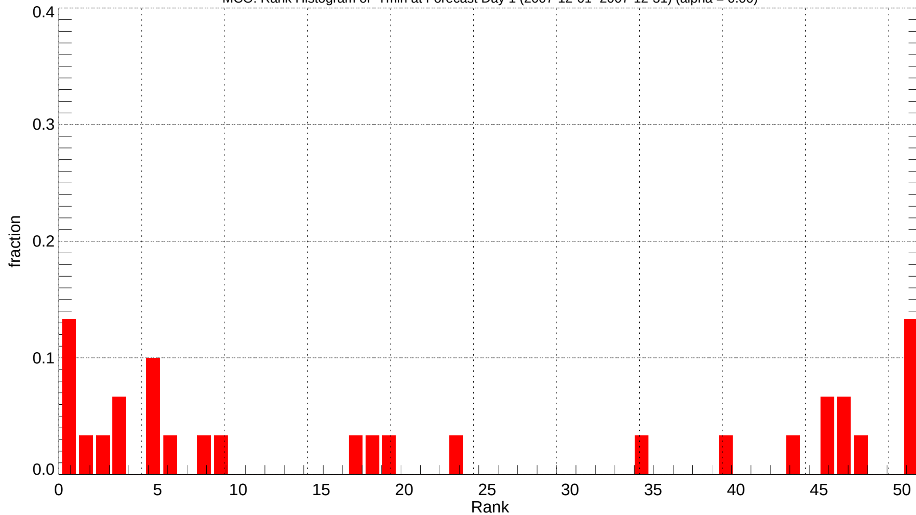
MCO: Rank Histogram of Tmin at Forecast Day 1 (2007-12-01~2007-12-31) (alpha = 0.00)
