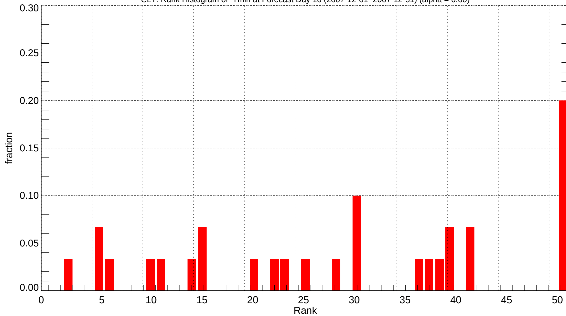
CLT: Rank Histogram of Tmin at Forecast Day 10 (2007-12-01~2007-12-31) (alpha = 0.00)
