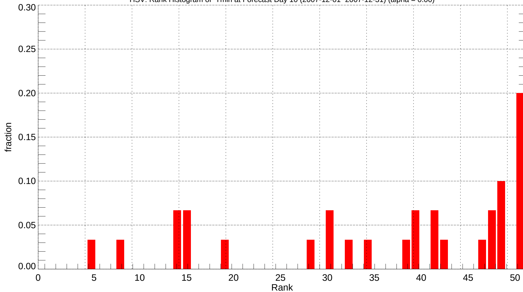
HSV: Rank Histogram of Tmin at Forecast Day 10 (2007-12-01~2007-12-31) (alpha = 0.00)
