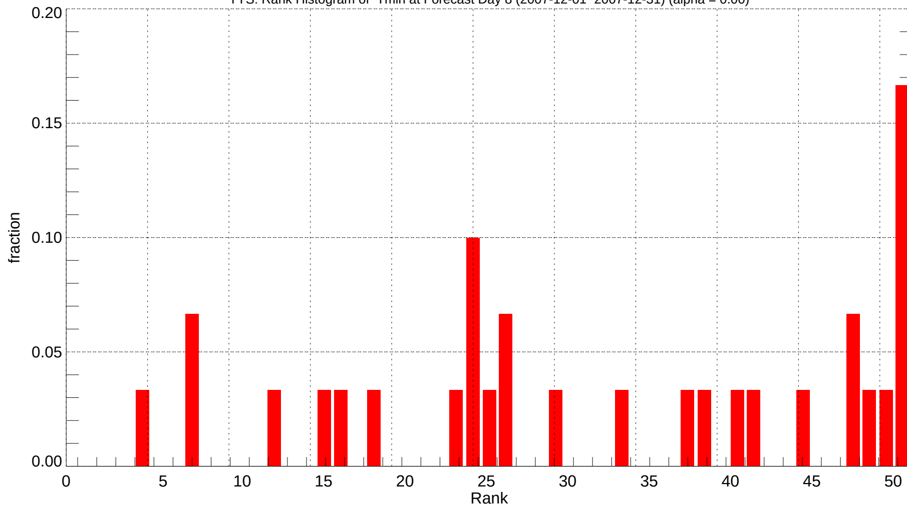
TYS: Rank Histogram of Tmin at Forecast Day 8 (2007-12-01~2007-12-31) (alpha = 0.00)
