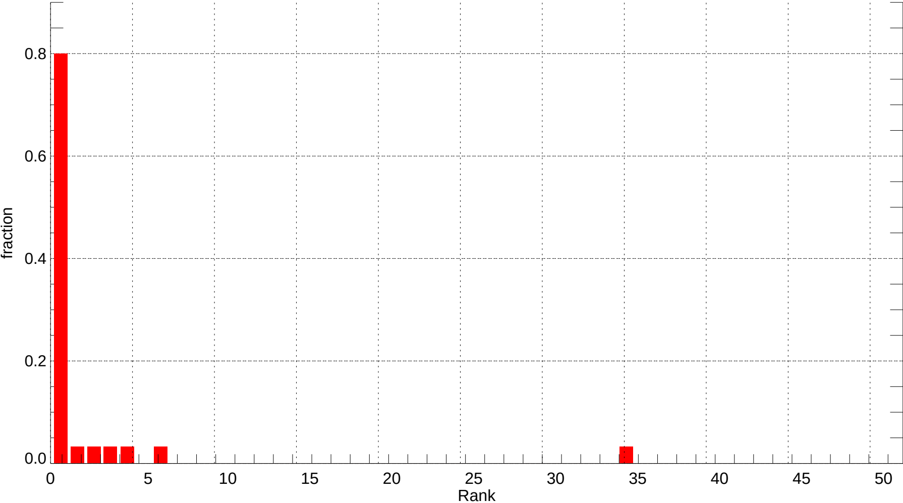
SJC: Rank Histogram of Tmin at Forecast Day 9 (2007-12-01~2007-12-31) (alpha = 0.00)
