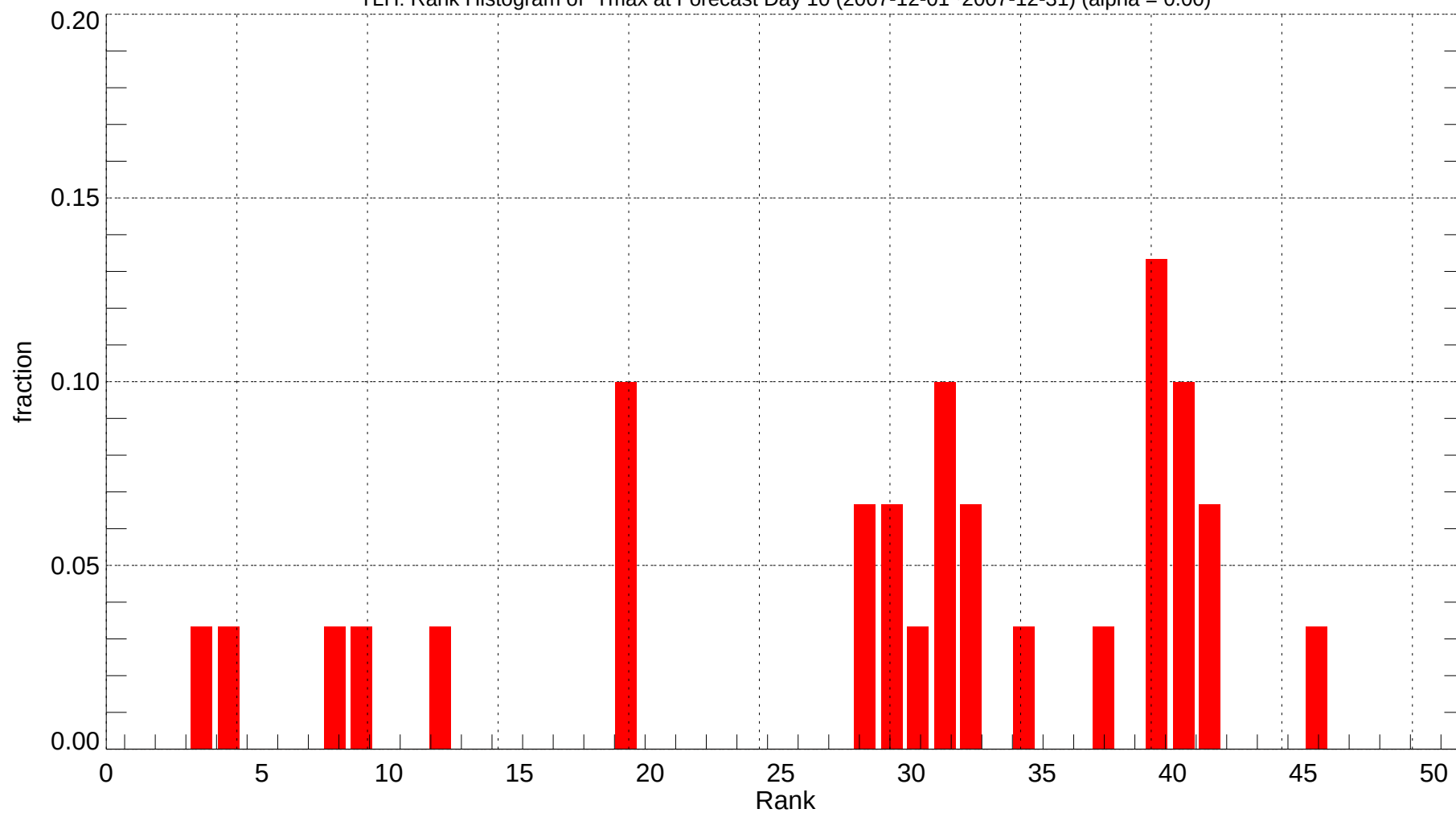
TLH: Rank Histogram of Tmax at Forecast Day 10 (2007-12-01~2007-12-31) (alpha = 0.00)
