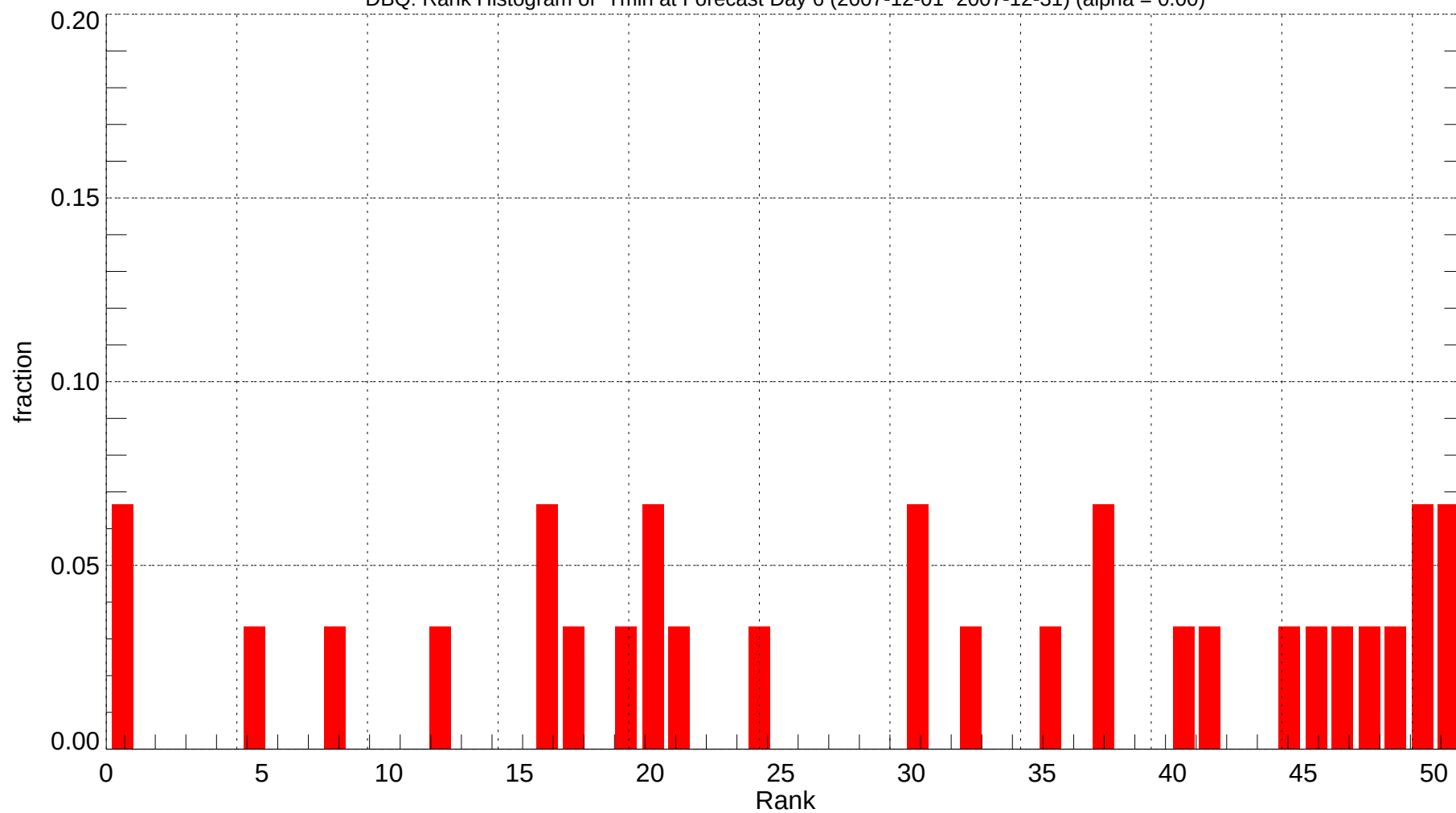
DBQ: Rank Histogram of Tmin at Forecast Day 6 (2007-12-01~2007-12-31) (alpha = 0.00)
