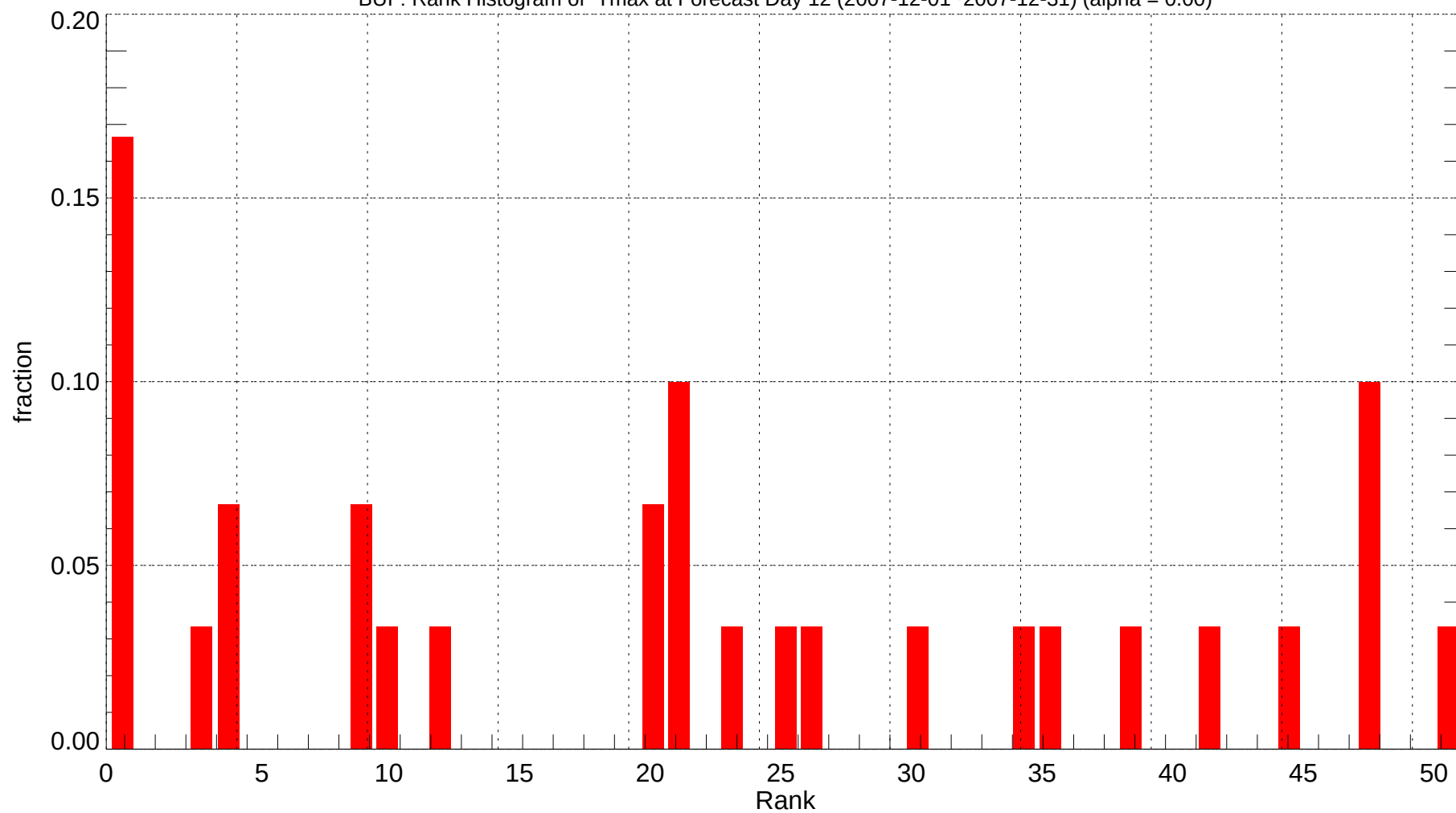
BUF: Rank Histogram of Tmax at Forecast Day 12 (2007-12-01~2007-12-31) (alpha = 0.00)
