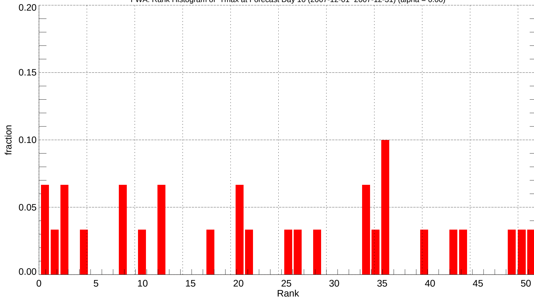
FWA: Rank Histogram of Tmax at Forecast Day 10 (2007-12-01~2007-12-31) (alpha = 0.00)
