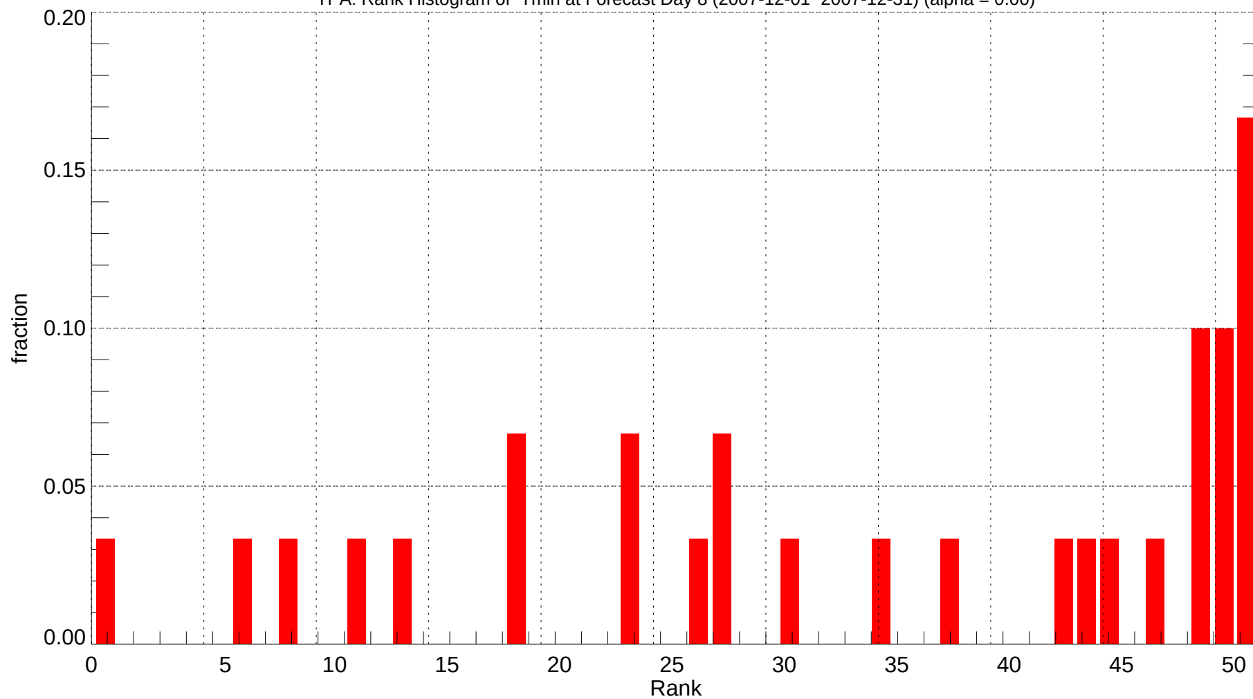
TPA: Rank Histogram of Tmin at Forecast Day 8 (2007-12-01~2007-12-31) (alpha = 0.00)
