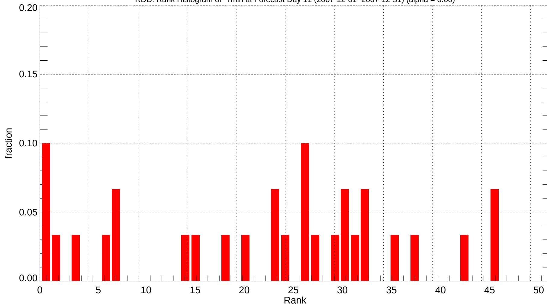
RDD: Rank Histogram of Tmin at Forecast Day 11 (2007-12-01~2007-12-31) (alpha = 0.00)
