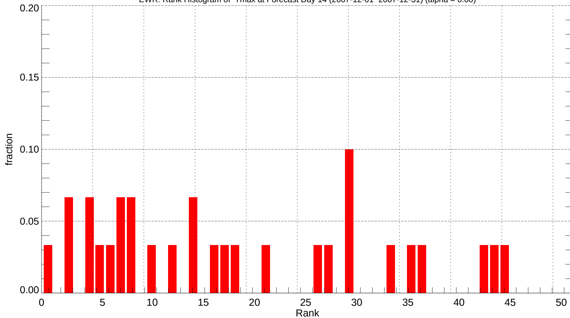
EWR: Rank Histogram of Tmax at Forecast Day 14 (2007-12-01~2007-12-31) (alpha = 0.00)
