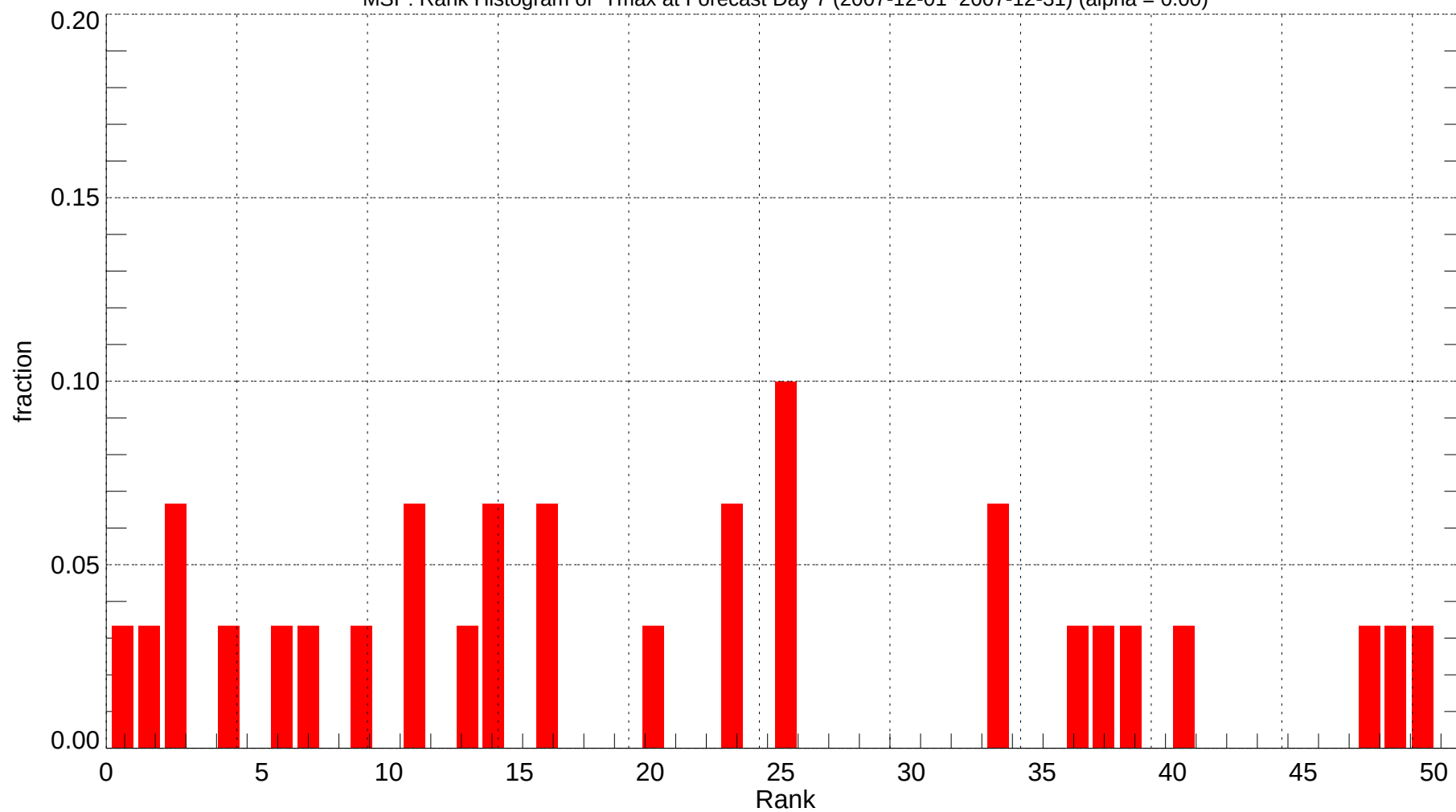
MSP: Rank Histogram of Tmax at Forecast Day 7 (2007-12-01~2007-12-31) (alpha = 0.00)
