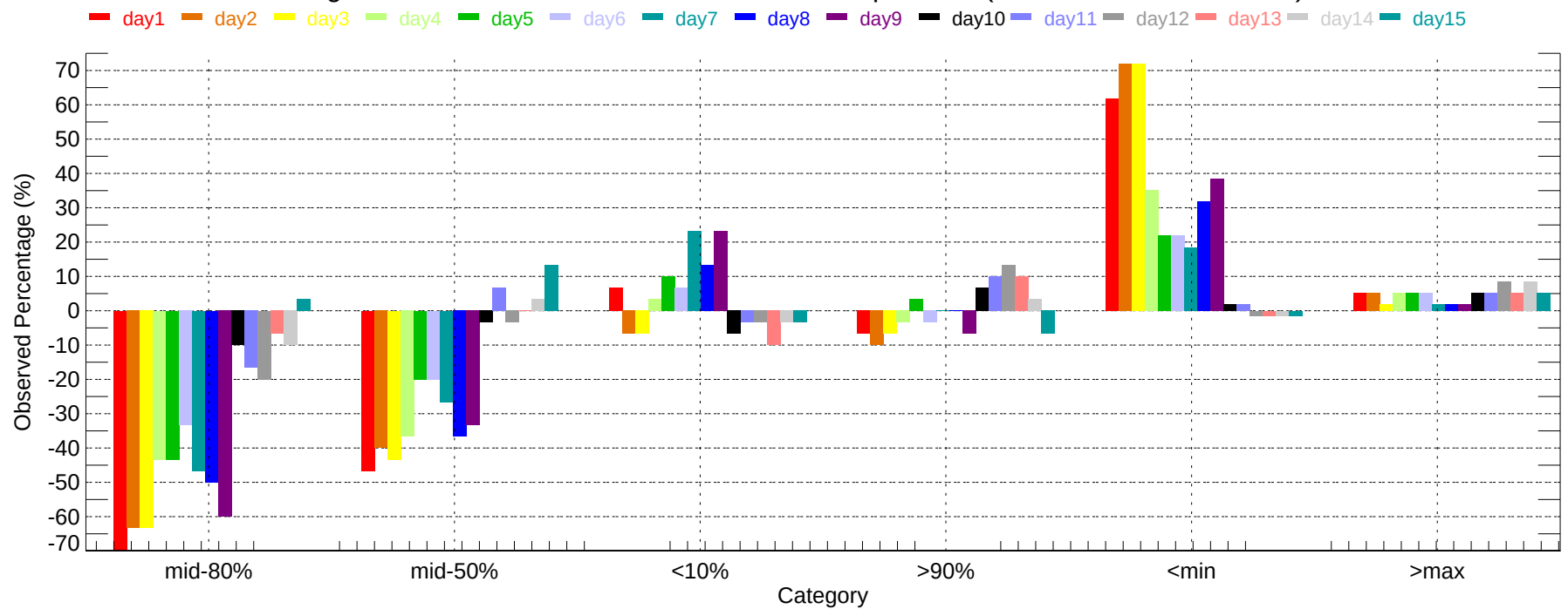
Observed Percentage Deviation of Ensembles - SAN: Max Temperature (2007-12-01~2007-12-31)
