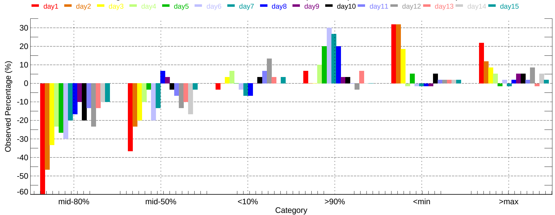
Observed Percentage Deviation of Ensembles - PVD: Min Temperature (2007-12-01~2007-12-31)
