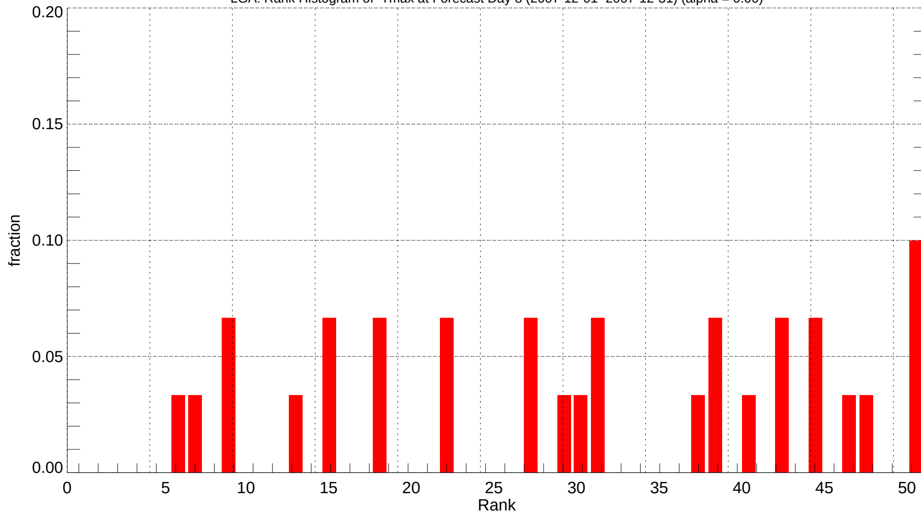
LGA: Rank Histogram of Tmax at Forecast Day 8 (2007-12-01~2007-12-31) (alpha = 0.00)
