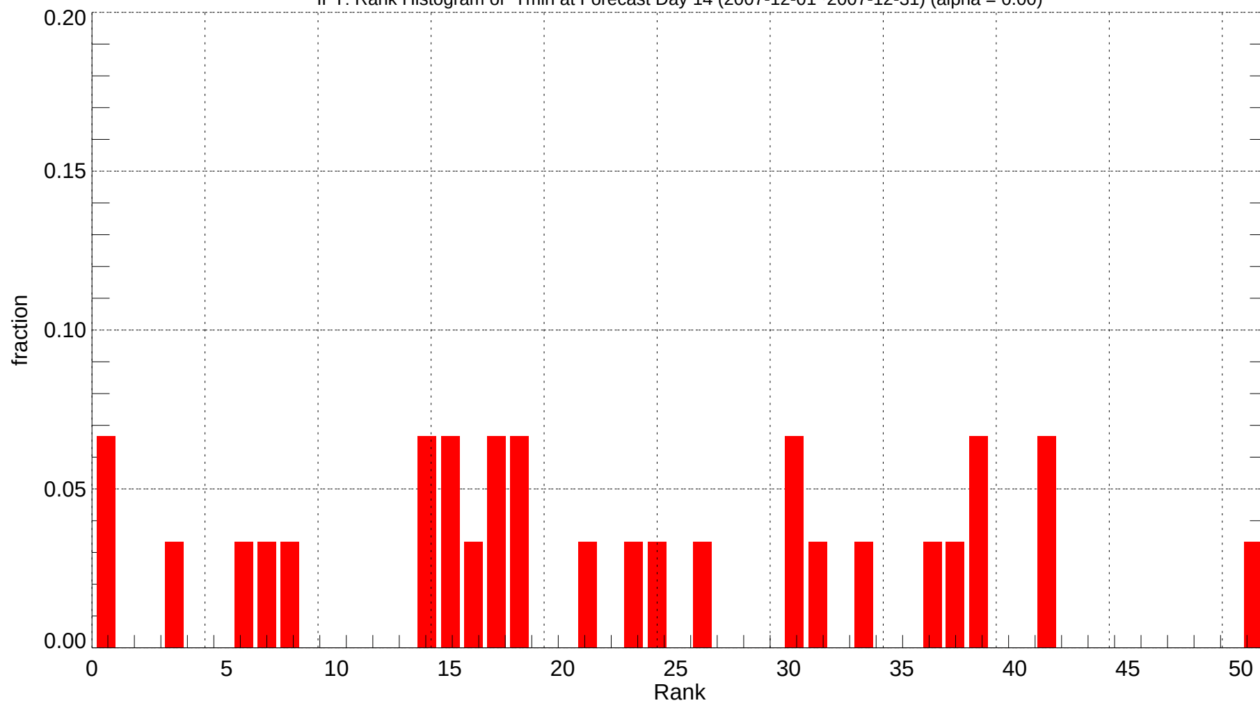
IPT: Rank Histogram of Tmin at Forecast Day 14 (2007-12-01~2007-12-31) (alpha = 0.00)
