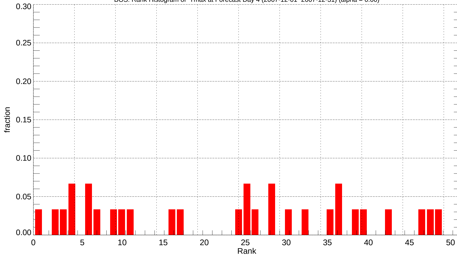
BOS: Rank Histogram of Tmax at Forecast Day 4 (2007-12-01~2007-12-31) (alpha = 0.00)
