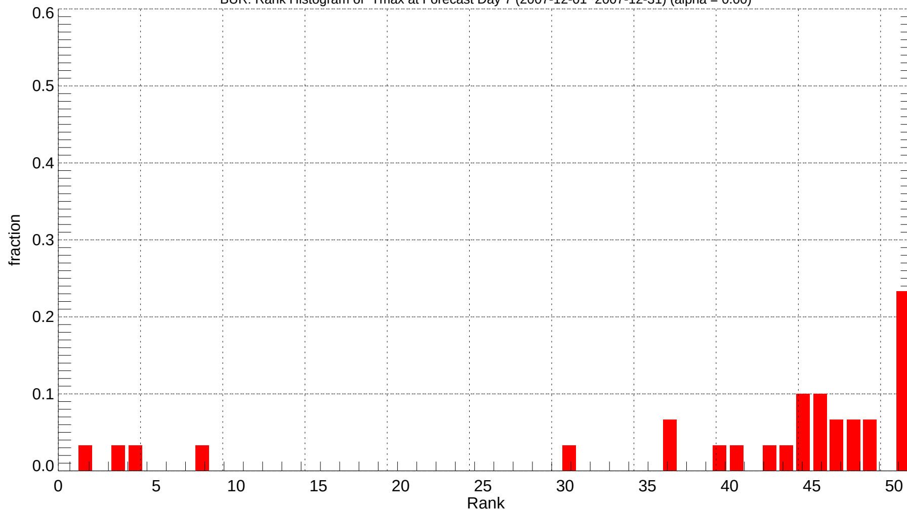
BUR: Rank Histogram of Tmax at Forecast Day 7 (2007-12-01~2007-12-31) (alpha = 0.00)
