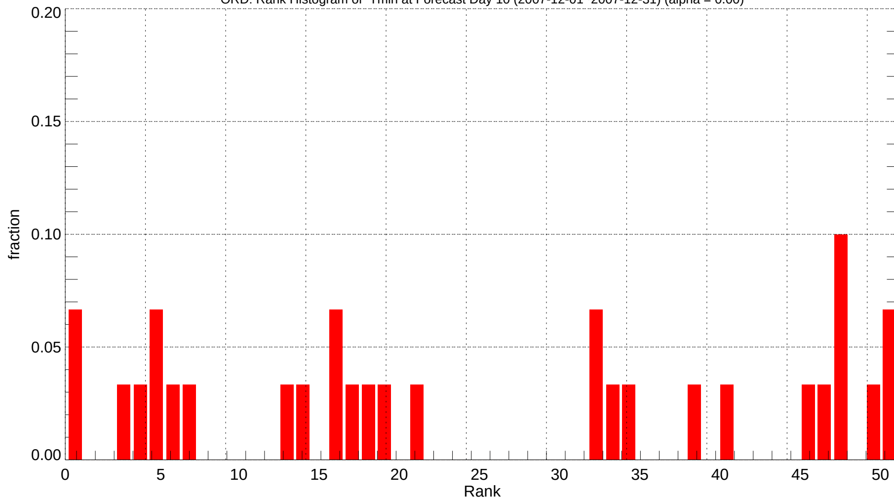
ORD: Rank Histogram of Tmin at Forecast Day 10 (2007-12-01~2007-12-31) (alpha = 0.00)
