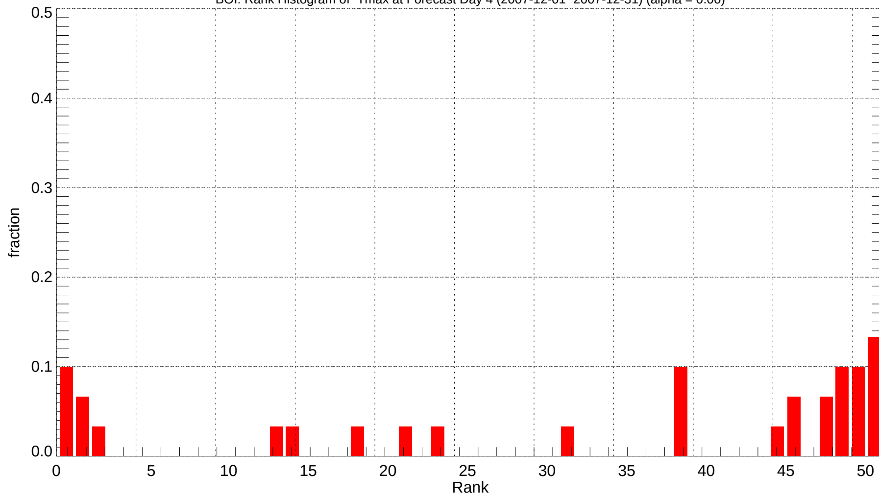
BOI: Rank Histogram of Tmax at Forecast Day 4 (2007-12-01~2007-12-31) (alpha = 0.00)
