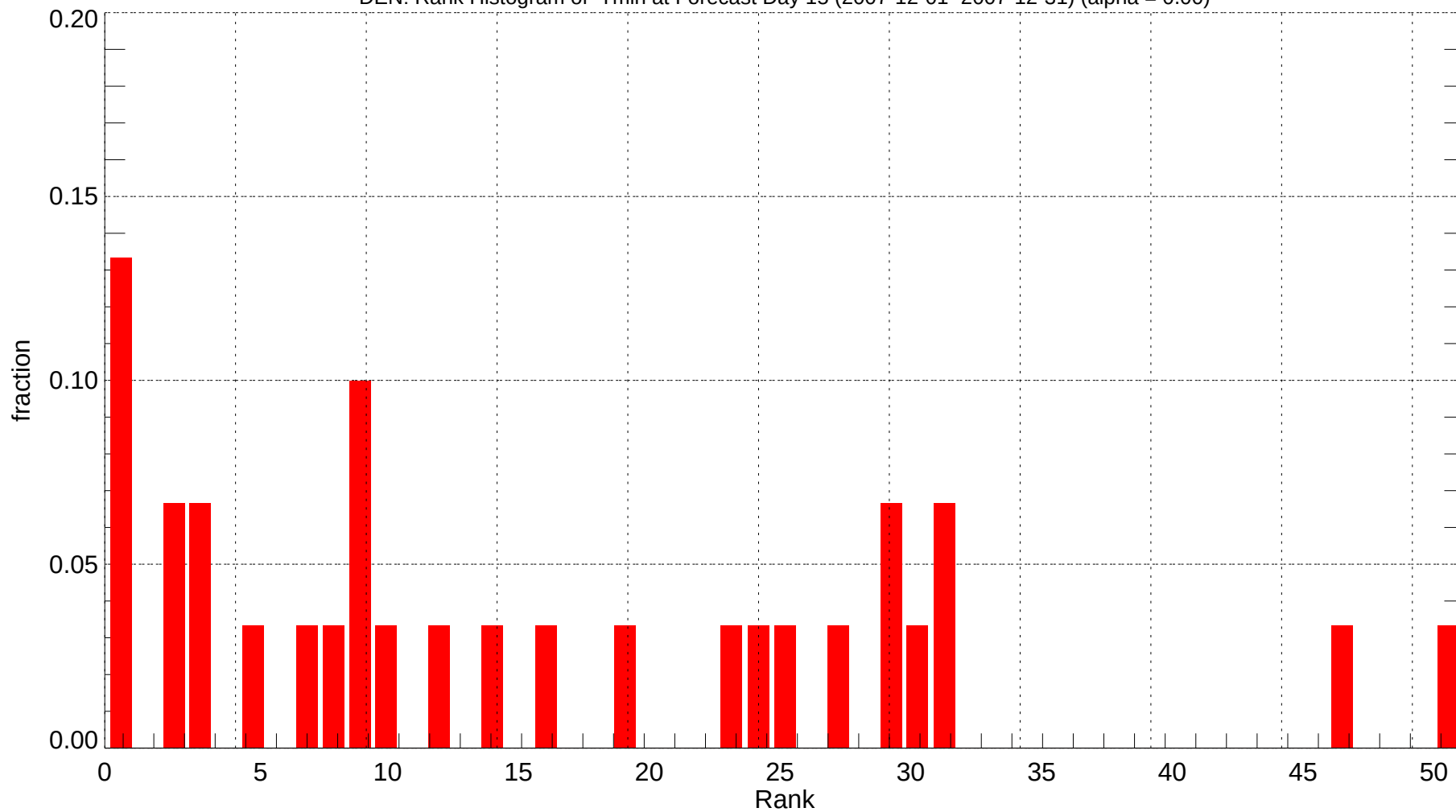
DEN: Rank Histogram of Tmin at Forecast Day 15 (2007-12-01~2007-12-31) (alpha = 0.00)
