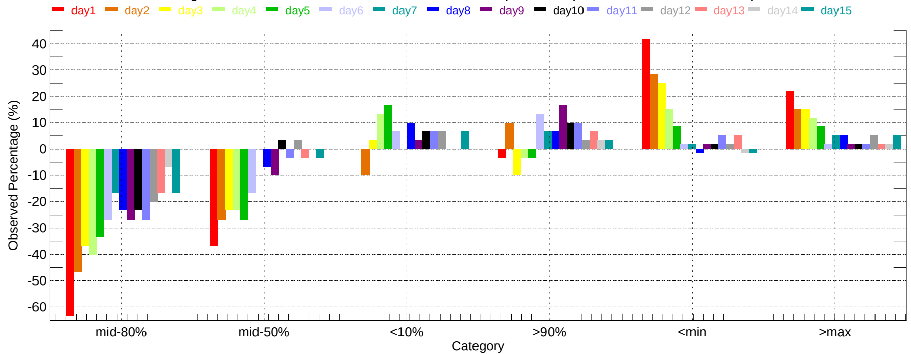
Observed Percentage Deviation of Ensembles - AOO: Min Temperature (2007-12-01~2007-12-31)
