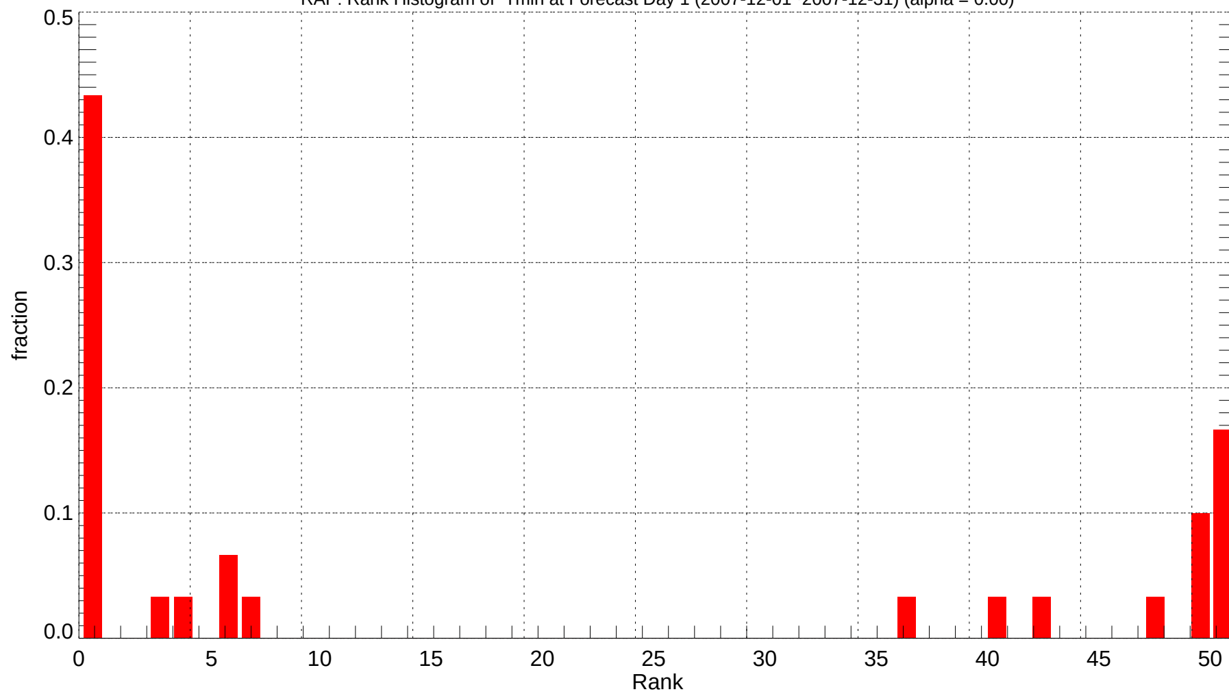
RAP: Rank Histogram of Tmin at Forecast Day 1 (2007-12-01~2007-12-31) (alpha = 0.00)
