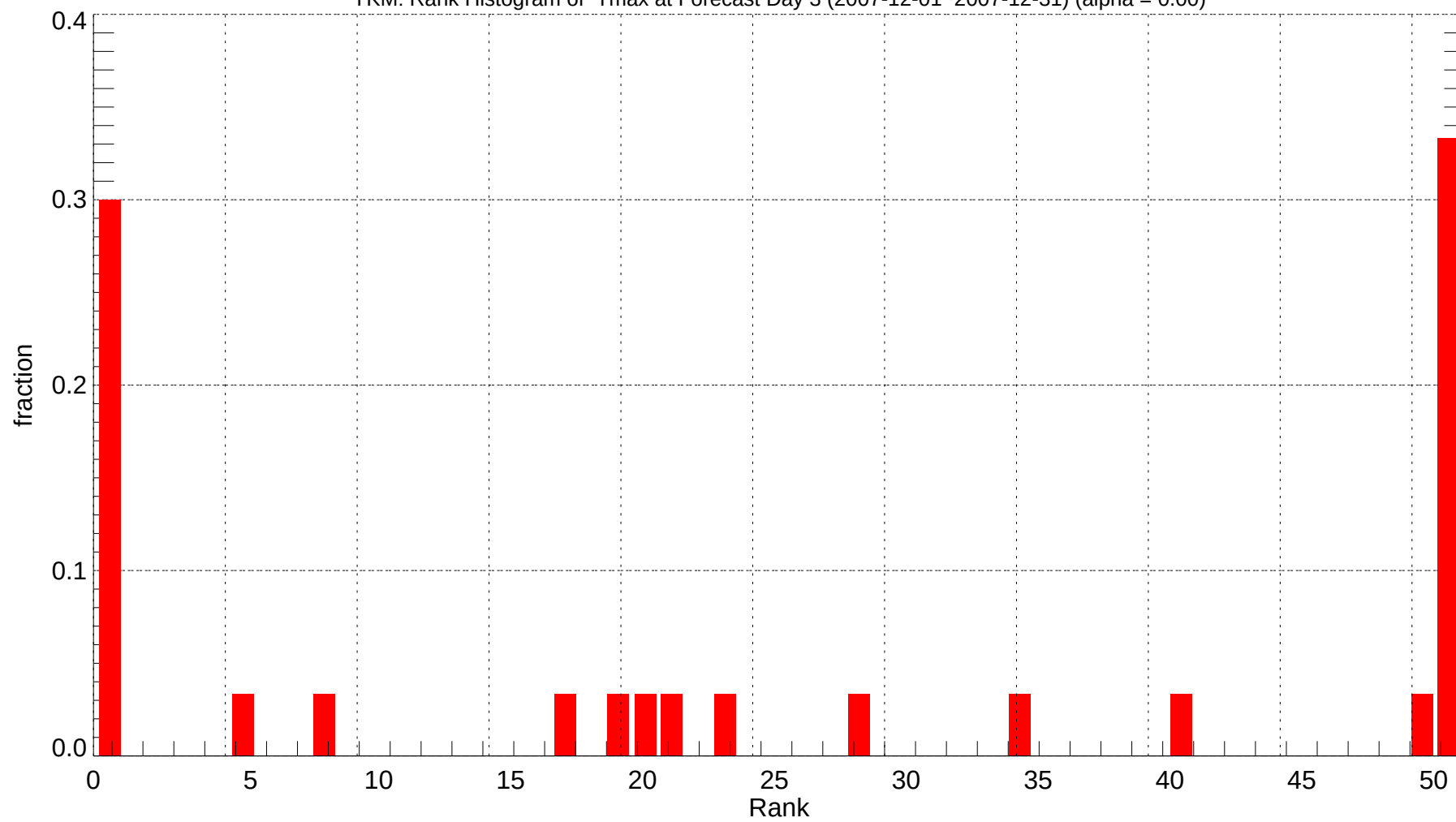
YKM: Rank Histogram of Tmax at Forecast Day 3 (2007-12-01~2007-12-31) (alpha = 0.00)
