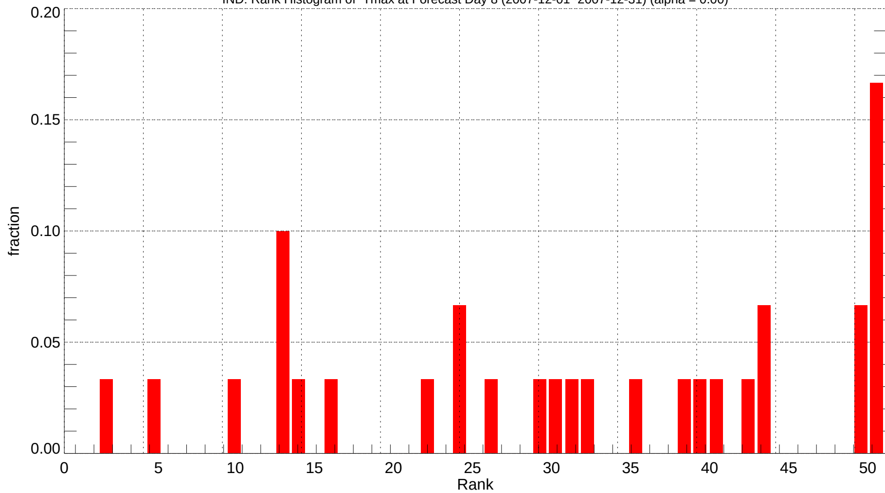
IND: Rank Histogram of Tmax at Forecast Day 8 (2007-12-01~2007-12-31) (alpha = 0.00)
