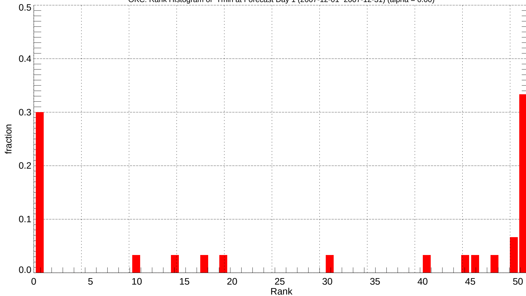
OKC: Rank Histogram of Tmin at Forecast Day 1 (2007-12-01~2007-12-31) (alpha = 0.00)
