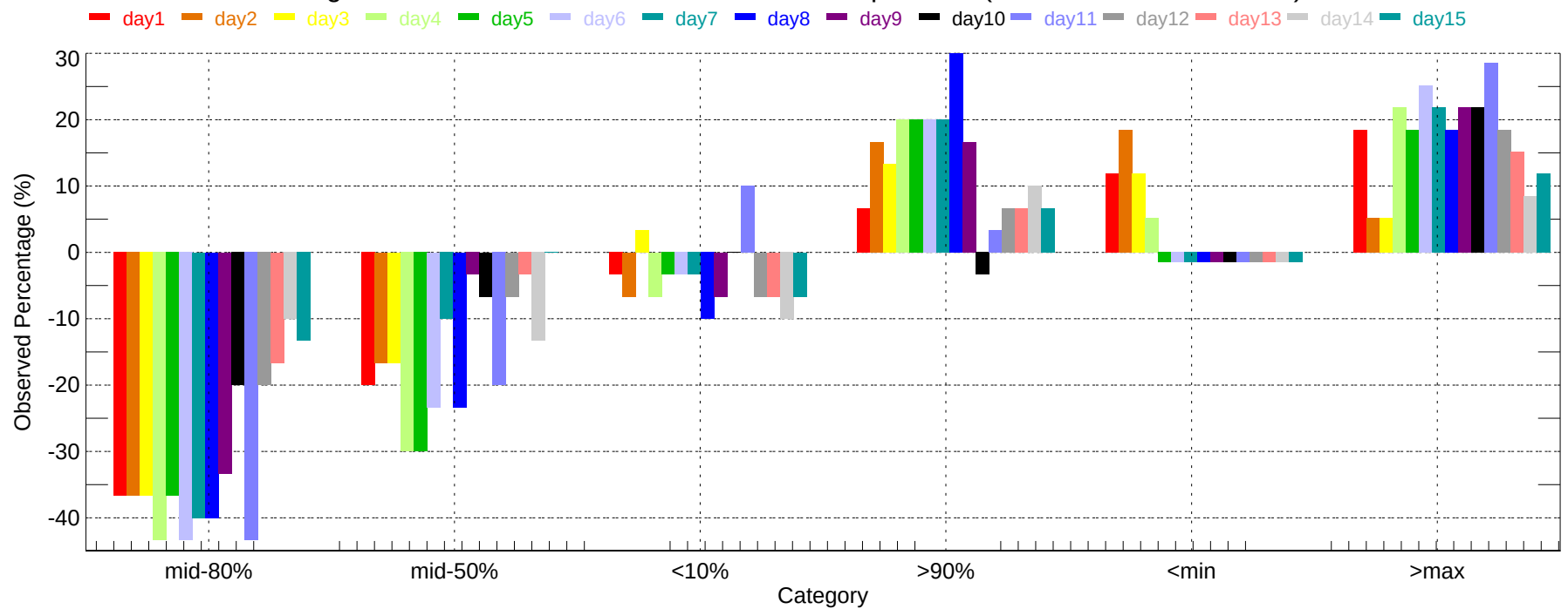
Observed Percentage Deviation of Ensembles - MCN: Min Temperature (2007-12-01~2007-12-31)
