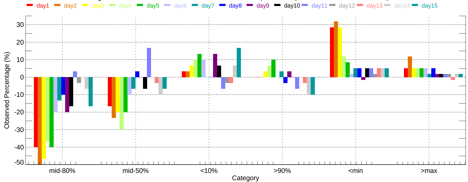
Observed Percentage Deviation of Ensembles - SFO: Max Temperature (2007-12-01~2007-12-31)
