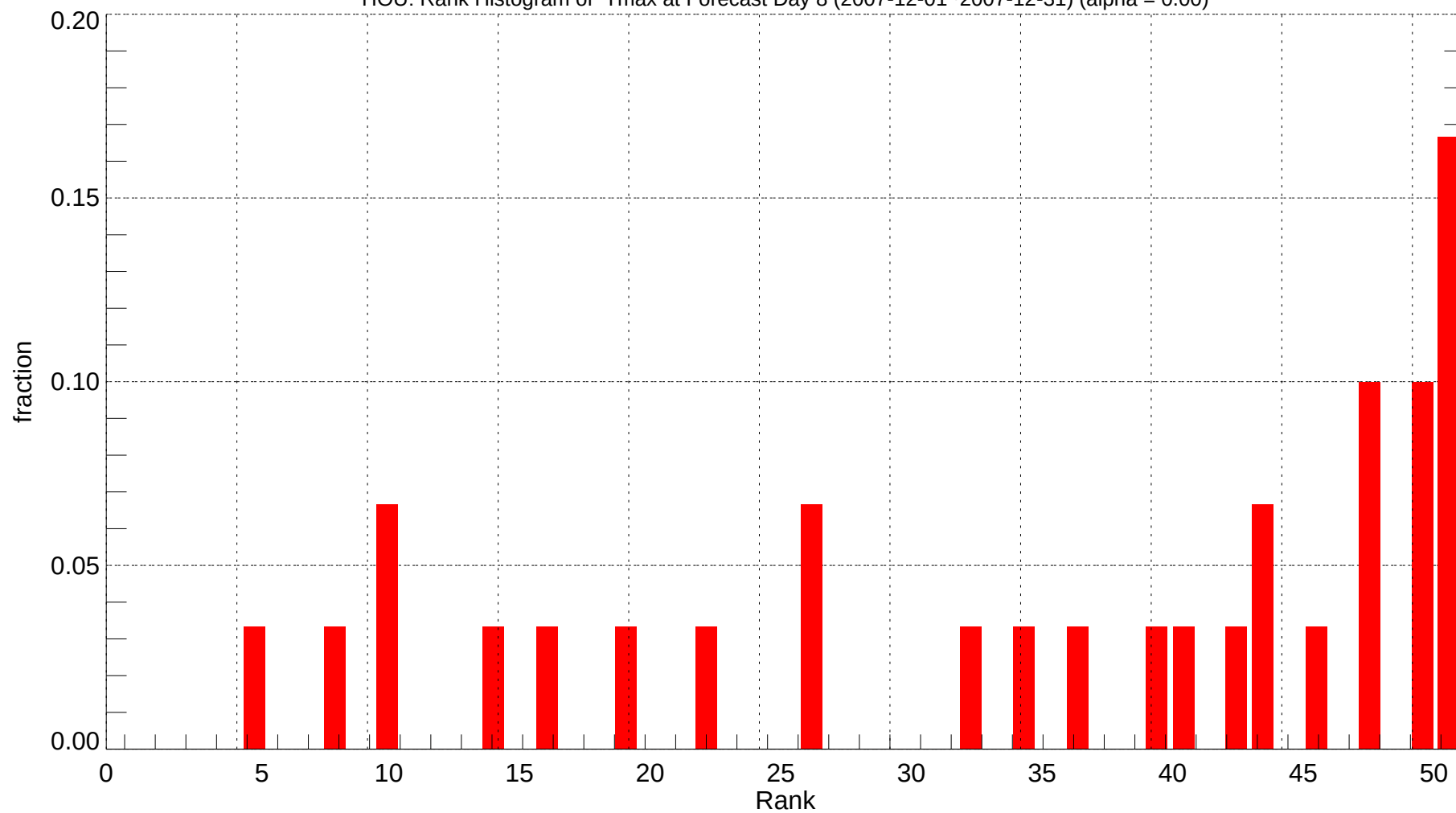
HOU: Rank Histogram of Tmax at Forecast Day 8 (2007-12-01~2007-12-31) (alpha = 0.00)
