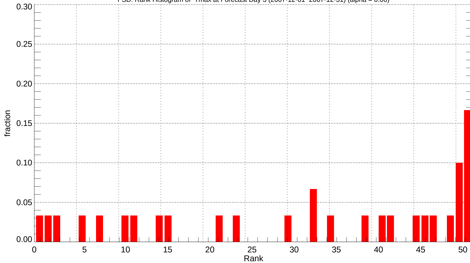
FSD: Rank Histogram of Tmax at Forecast Day 3 (2007-12-01~2007-12-31) (alpha = 0.00)
