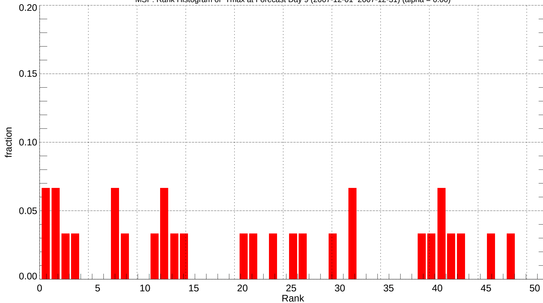
MSP: Rank Histogram of Tmax at Forecast Day 9 (2007-12-01~2007-12-31) (alpha = 0.00)
