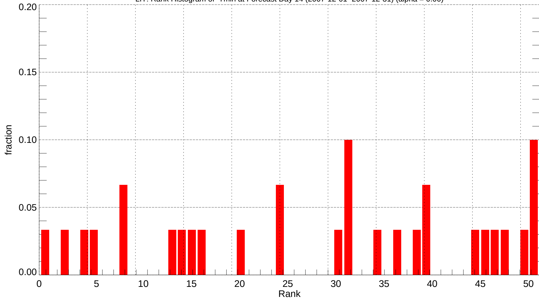
LIT: Rank Histogram of Tmin at Forecast Day 14 (2007-12-01~2007-12-31) (alpha = 0.00)
