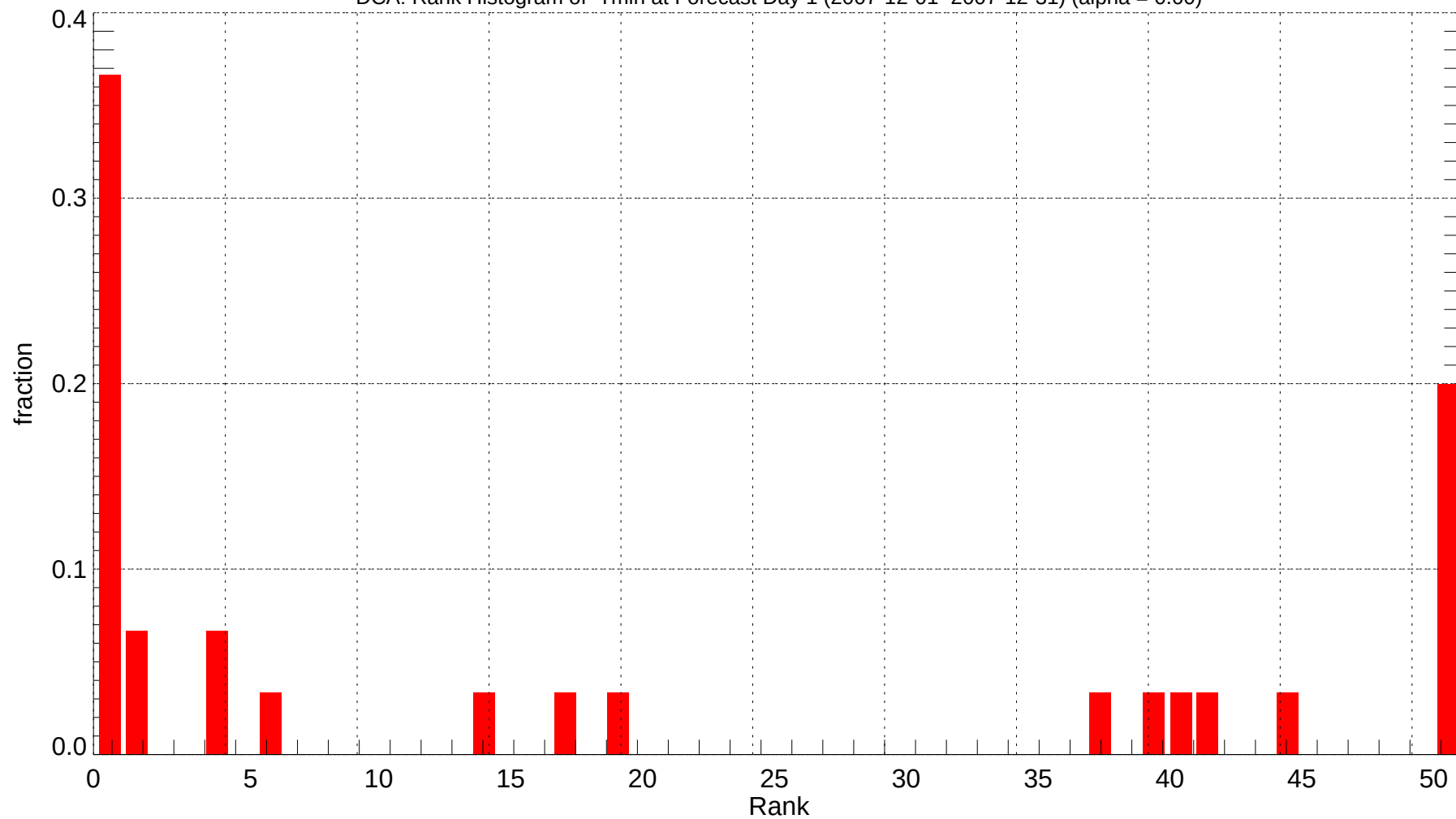
DCA: Rank Histogram of Tmin at Forecast Day 1 (2007-12-01~2007-12-31) (alpha = 0.00)
