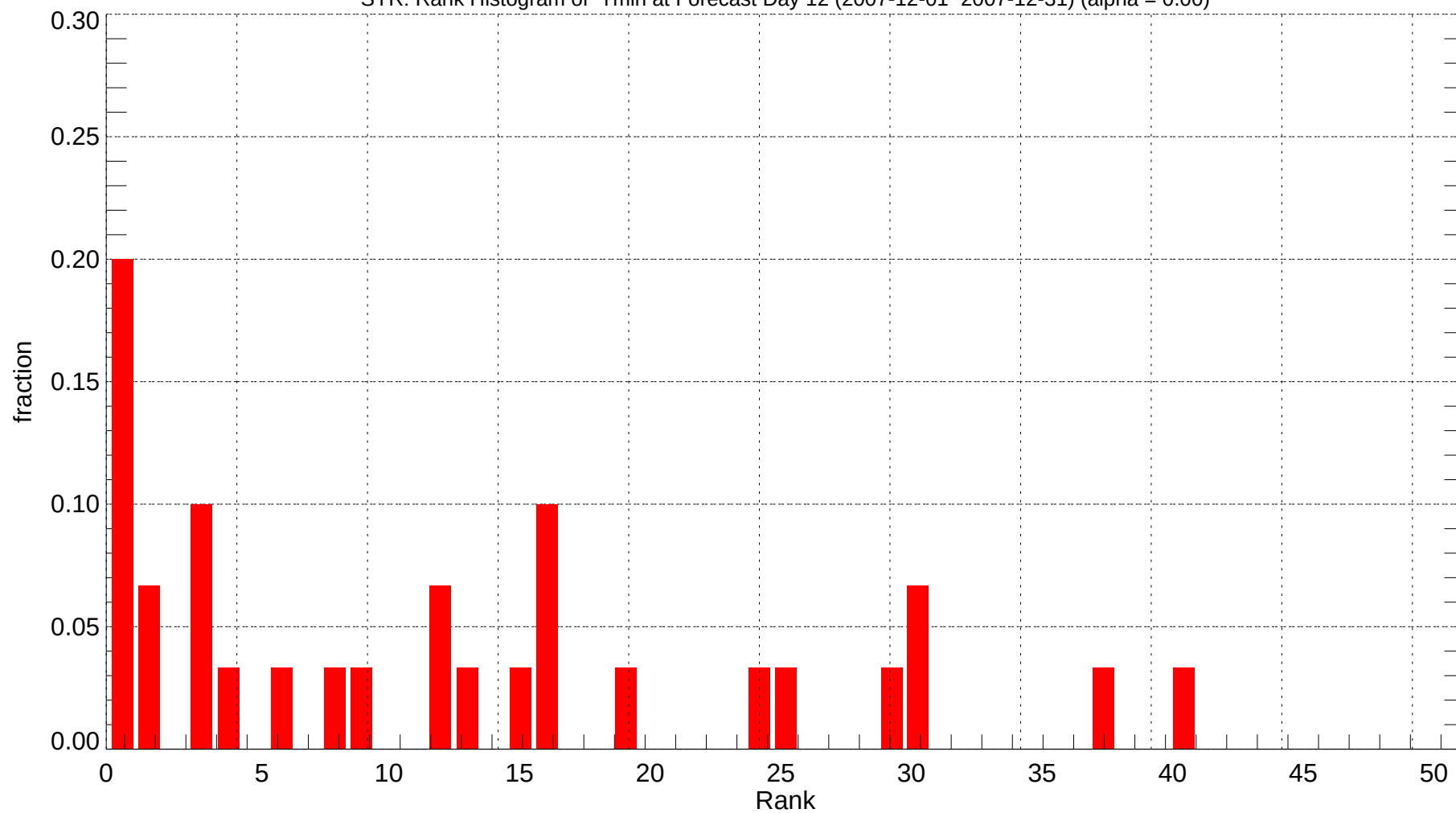
SYR: Rank Histogram of Tmin at Forecast Day 12 (2007-12-01~2007-12-31) (alpha = 0.00)
