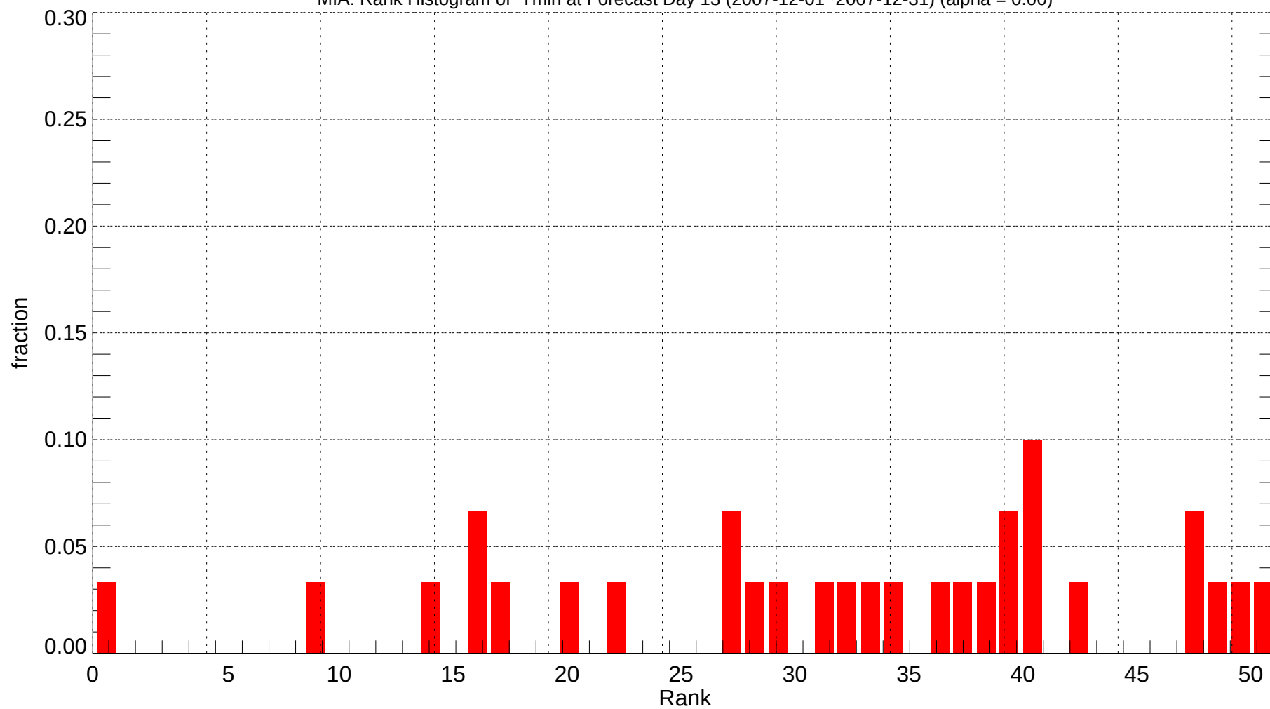
MIA: Rank Histogram of Tmin at Forecast Day 13 (2007-12-01~2007-12-31) (alpha = 0.00)
