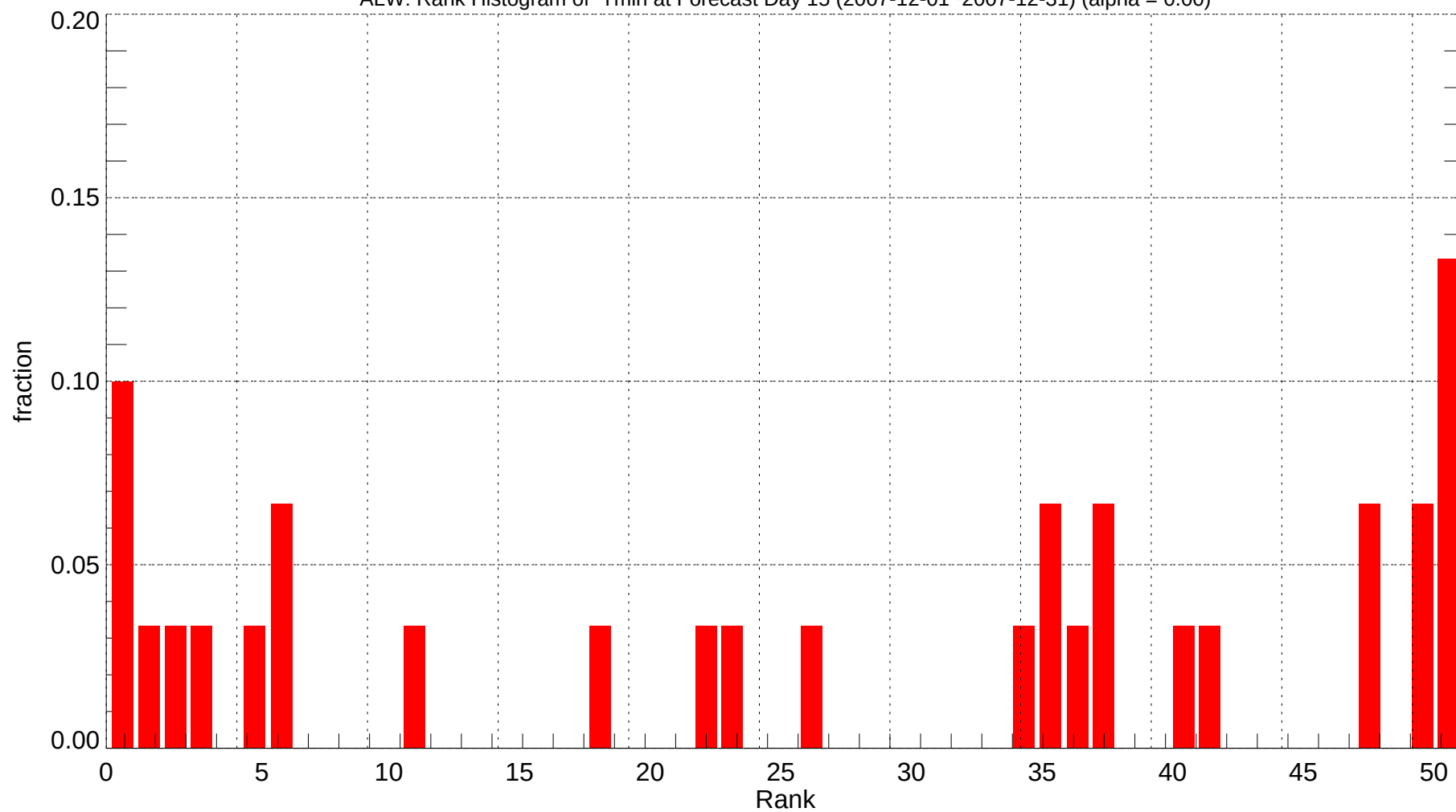
ALW: Rank Histogram of Tmin at Forecast Day 15 (2007-12-01~2007-12-31) (alpha = 0.00)
