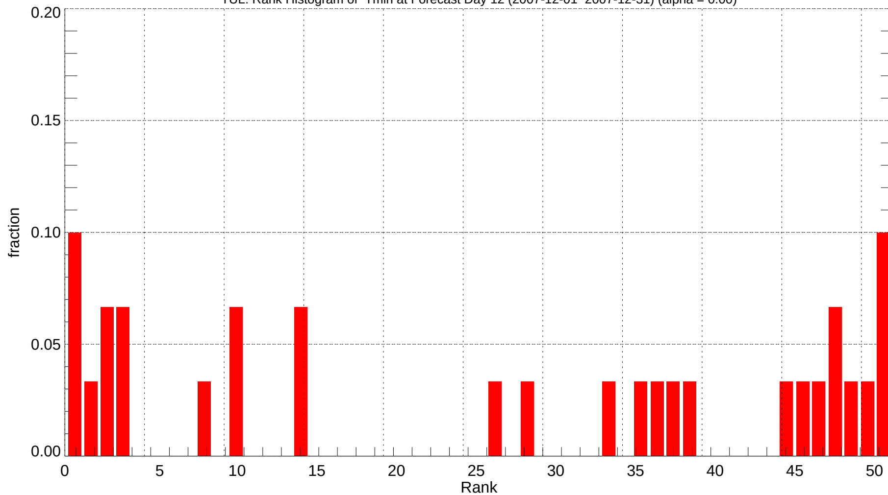
TUL: Rank Histogram of Tmin at Forecast Day 12 (2007-12-01~2007-12-31) (alpha = 0.00)
