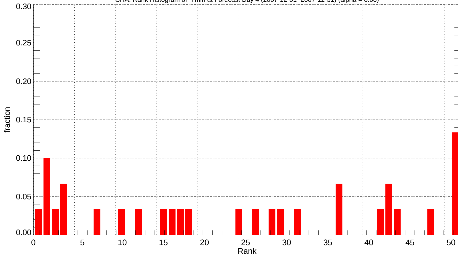
CHA: Rank Histogram of Tmin at Forecast Day 4 (2007-12-01~2007-12-31) (alpha = 0.00)
