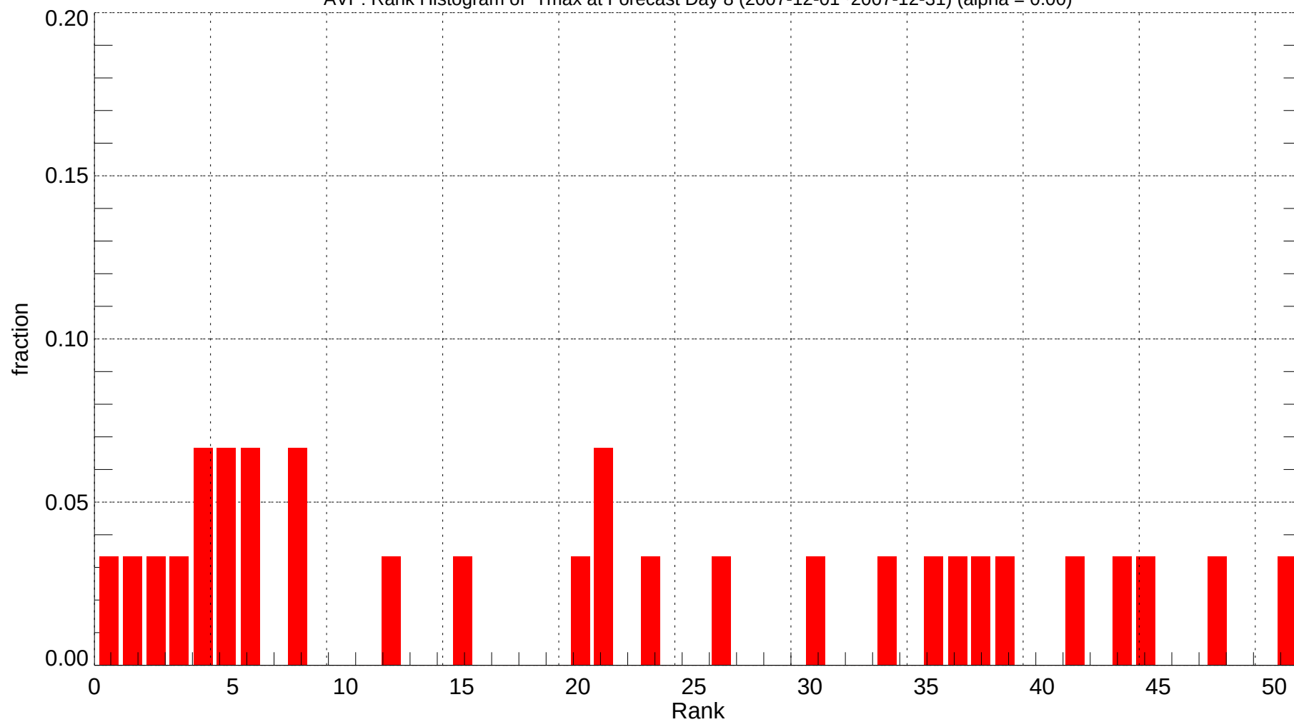
AVP: Rank Histogram of Tmax at Forecast Day 8 (2007-12-01~2007-12-31) (alpha = 0.00)
