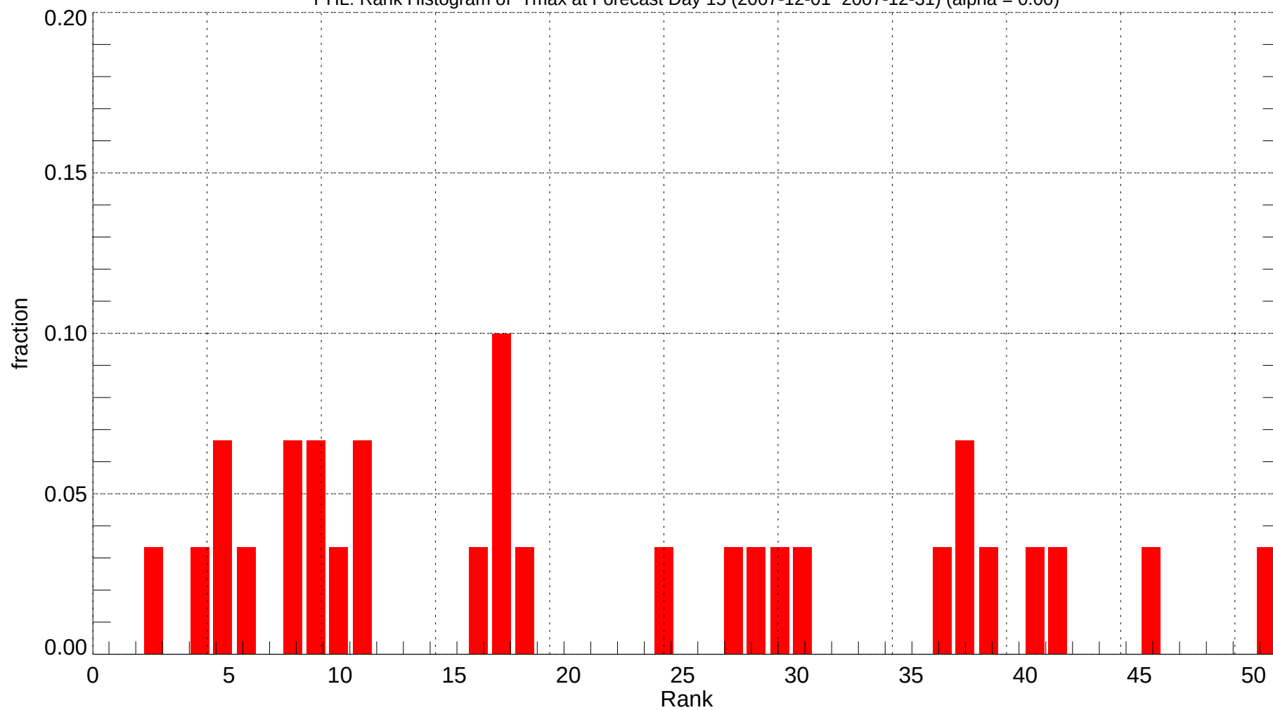
PHL: Rank Histogram of Tmax at Forecast Day 15 (2007-12-01~2007-12-31) (alpha = 0.00)
