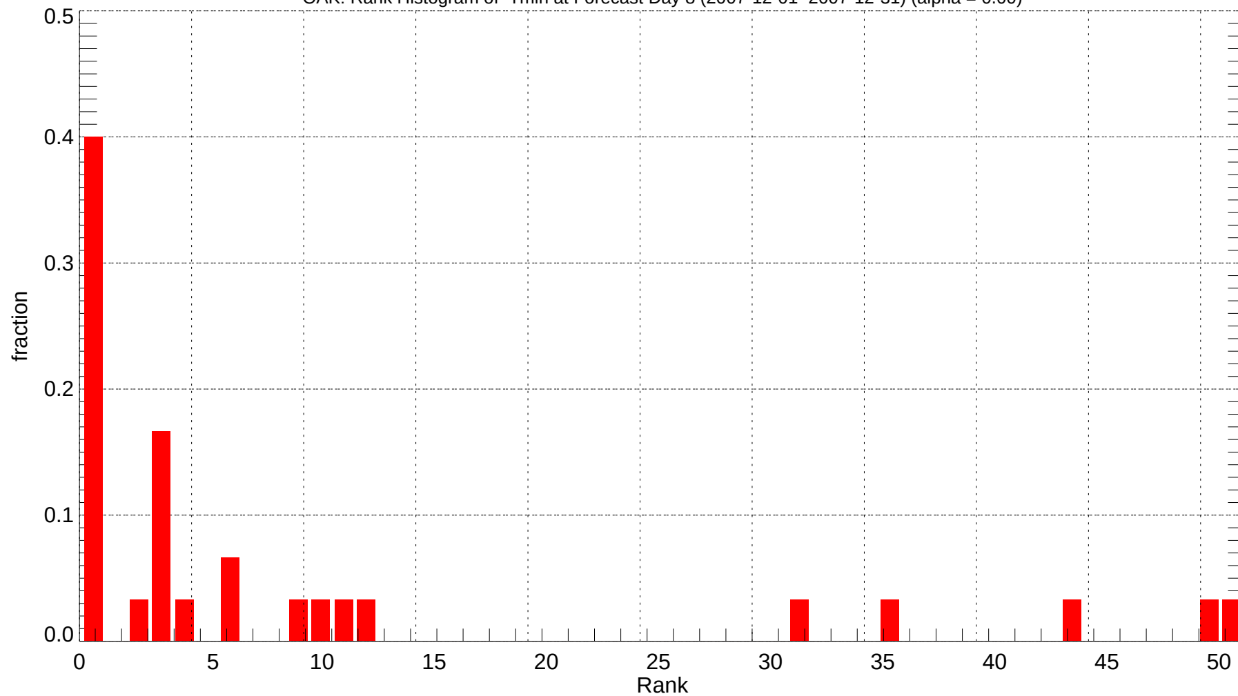
OAK: Rank Histogram of Tmin at Forecast Day 8 (2007-12-01~2007-12-31) (alpha = 0.00)
