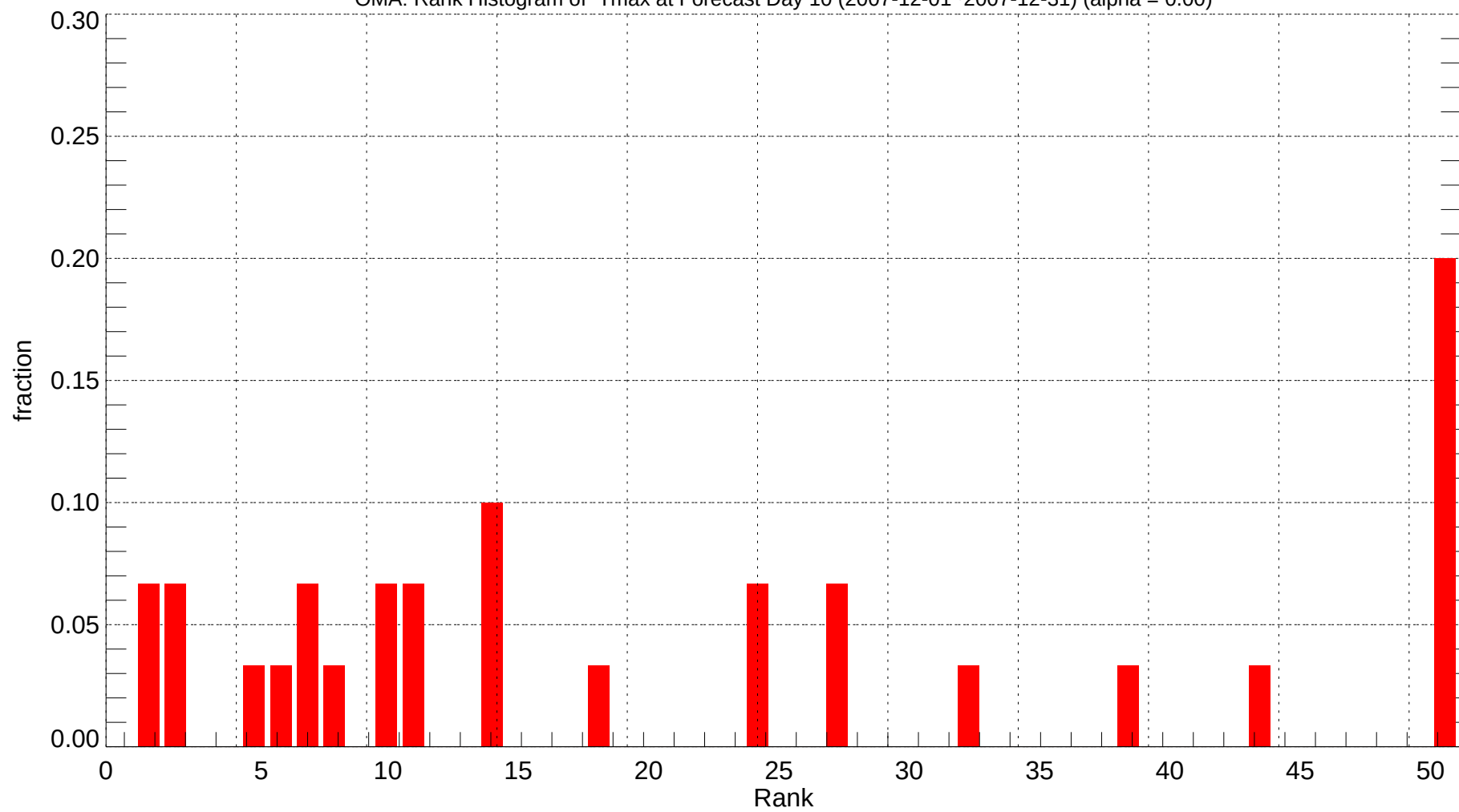
OMA: Rank Histogram of Tmax at Forecast Day 10 (2007-12-01~2007-12-31) (alpha = 0.00)
