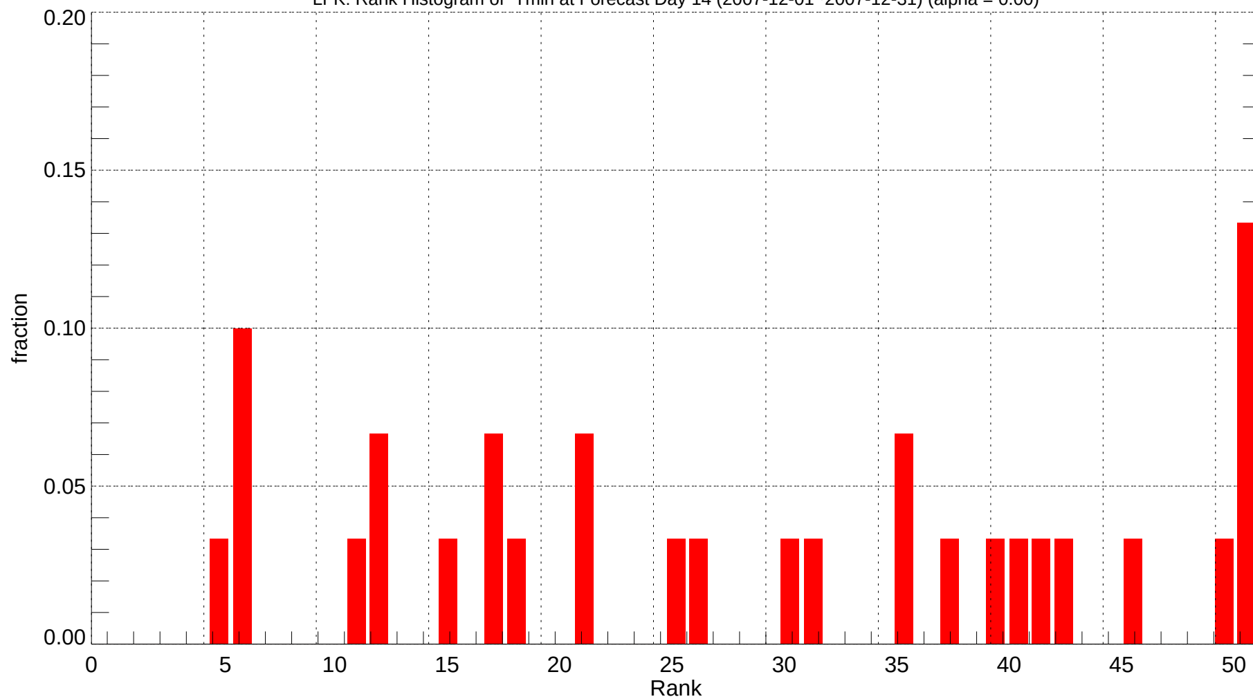
LFK: Rank Histogram of Tmin at Forecast Day 14 (2007-12-01~2007-12-31) (alpha = 0.00)
