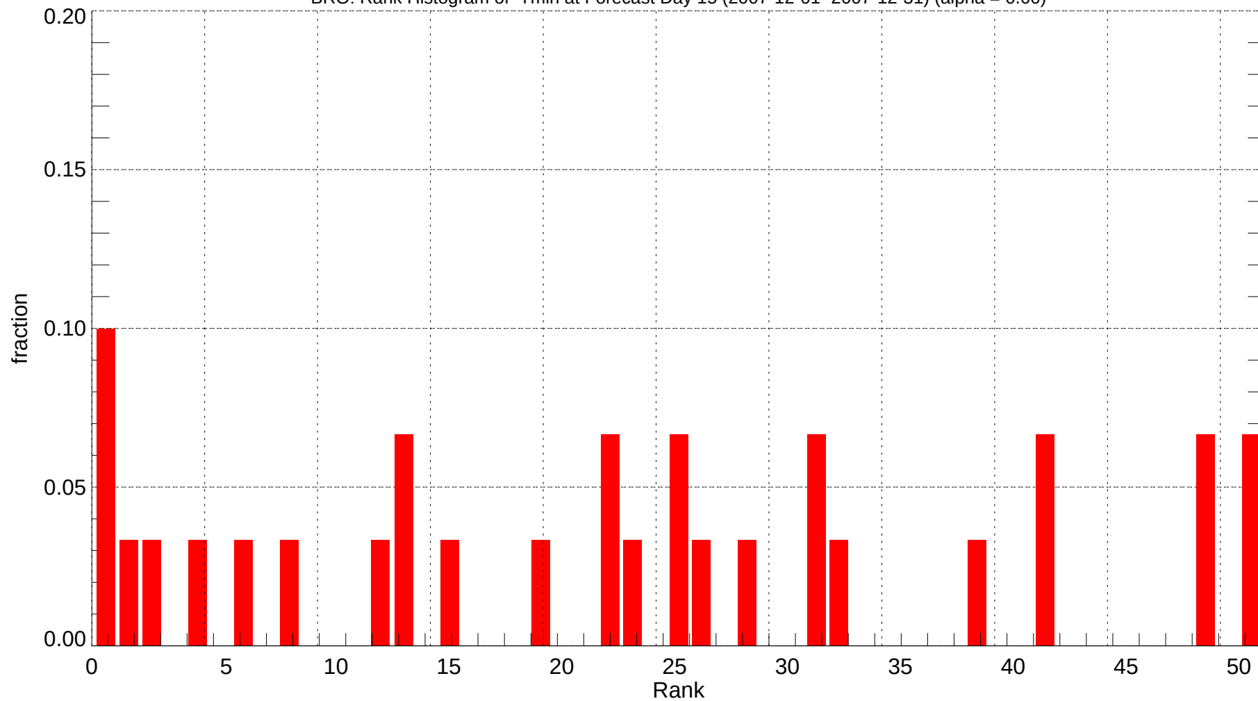
BRO: Rank Histogram of Tmin at Forecast Day 15 (2007-12-01~2007-12-31) (alpha = 0.00)
