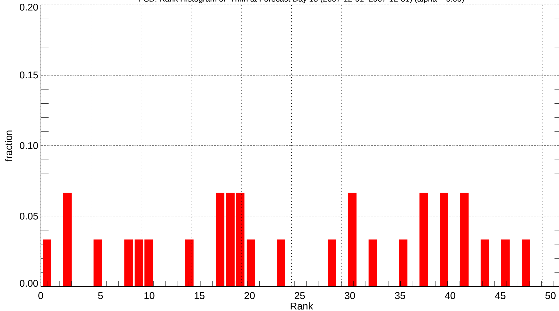
FSD: Rank Histogram of Tmin at Forecast Day 15 (2007-12-01~2007-12-31) (alpha = 0.00)
