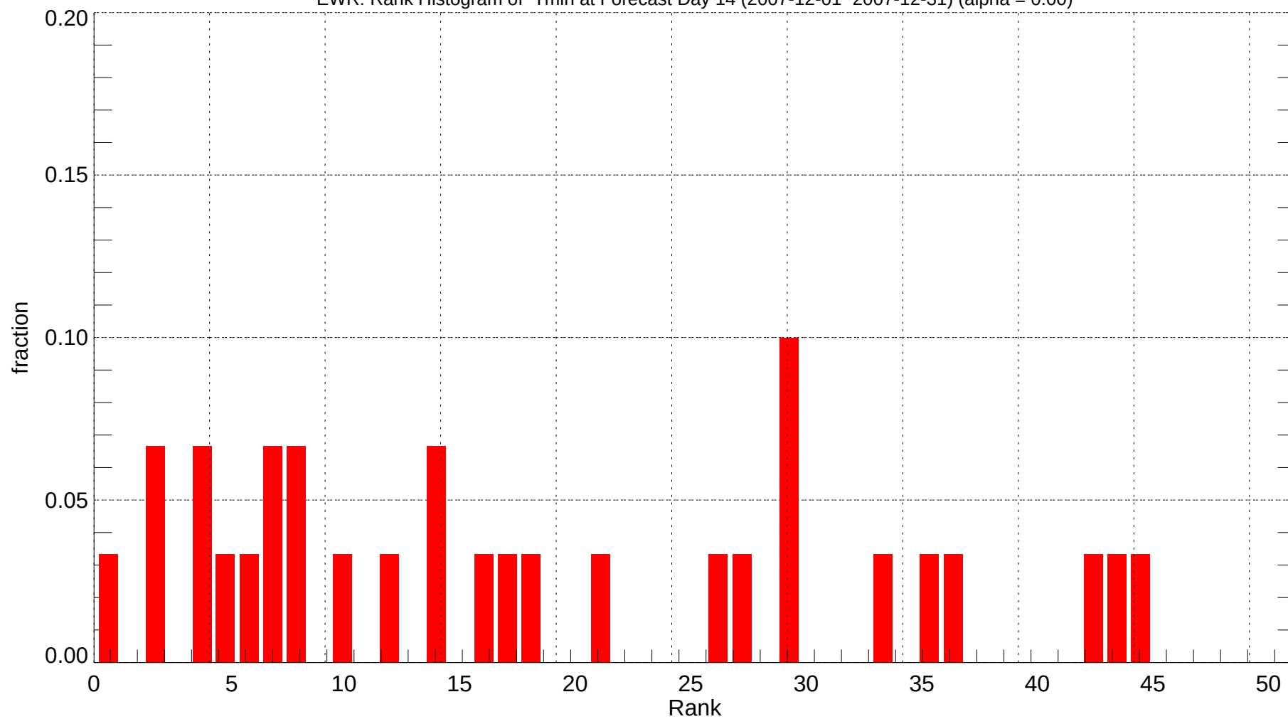
EWR: Rank Histogram of Tmin at Forecast Day 14 (2007-12-01~2007-12-31) (alpha = 0.00)
