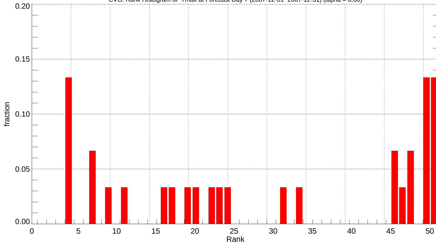
CVG: Rank Histogram of Tmax at Forecast Day 7 (2007-12-01~2007-12-31) (alpha = 0.00)
