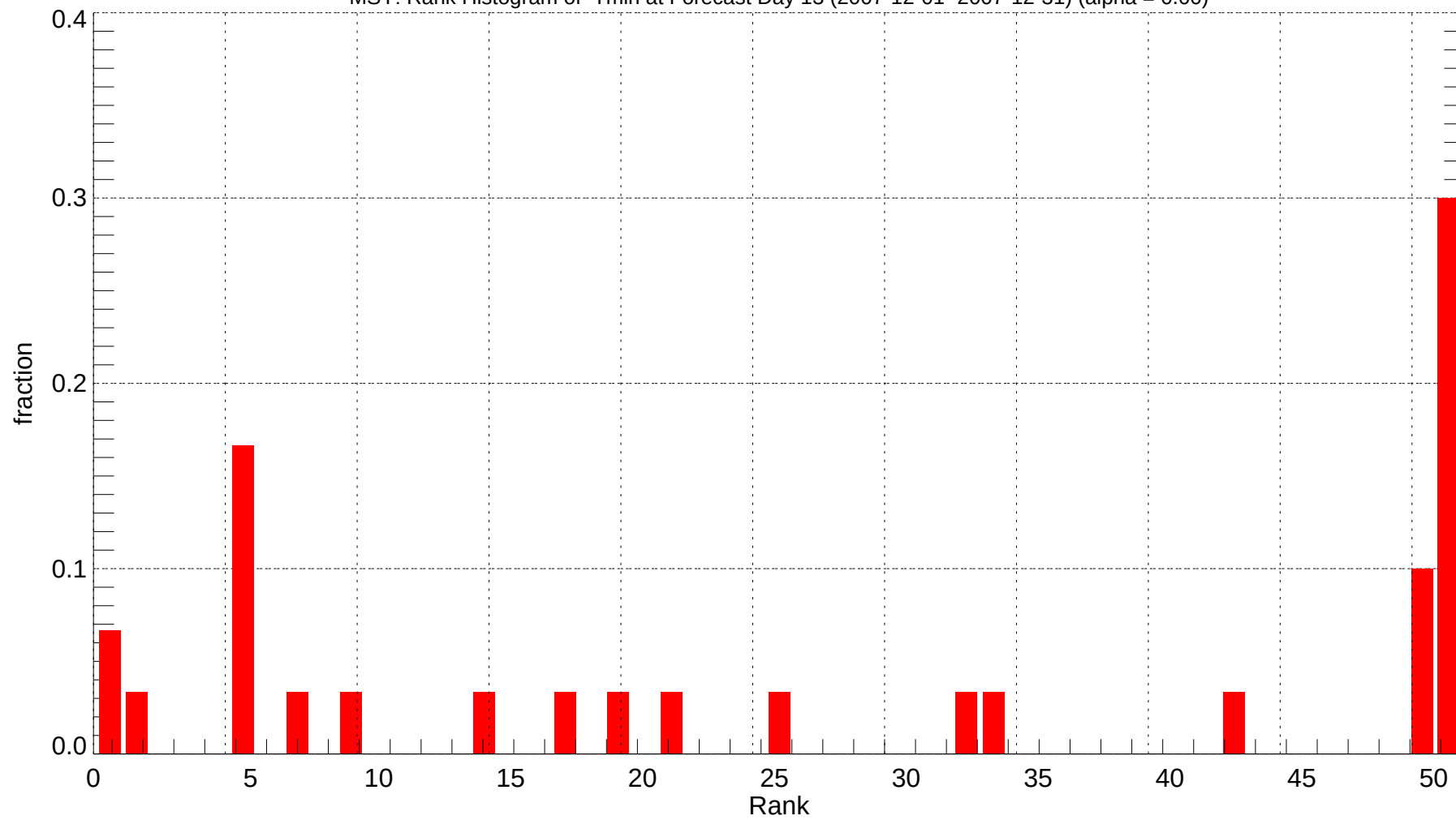
MSY: Rank Histogram of Tmin at Forecast Day 13 (2007-12-01~2007-12-31) (alpha = 0.00)
