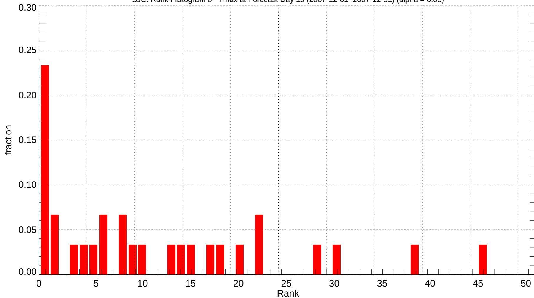
SJC: Rank Histogram of Tmax at Forecast Day 15 (2007-12-01~2007-12-31) (alpha = 0.00)
