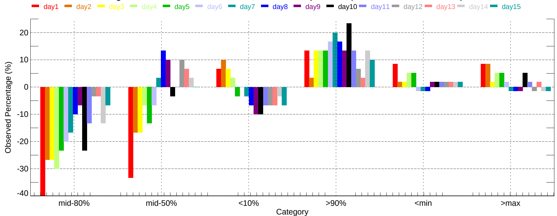
Observed Percentage Deviation of Ensembles - MCO: Min Temperature (2007-12-01~2007-12-31)
