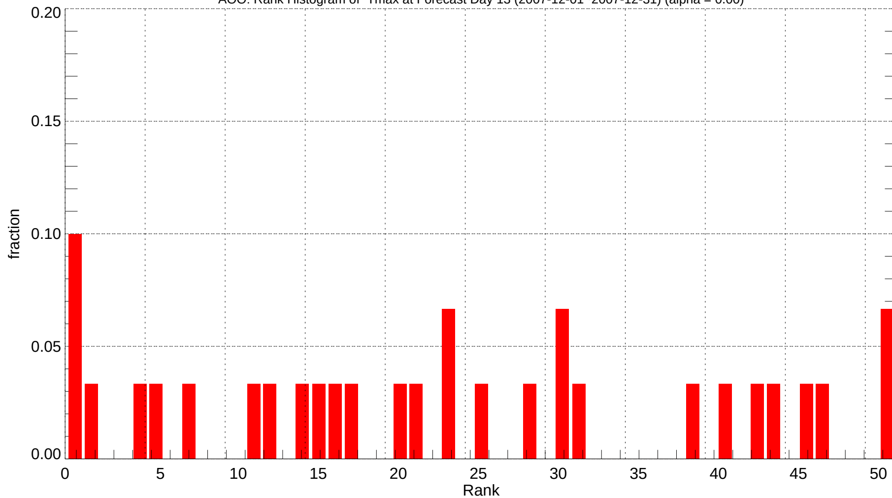
AOO: Rank Histogram of Tmax at Forecast Day 13 (2007-12-01~2007-12-31) (alpha = 0.00)
