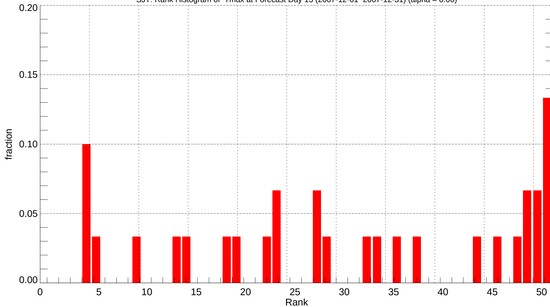
SJT: Rank Histogram of Tmax at Forecast Day 13 (2007-12-01~2007-12-31) (alpha = 0.00)
