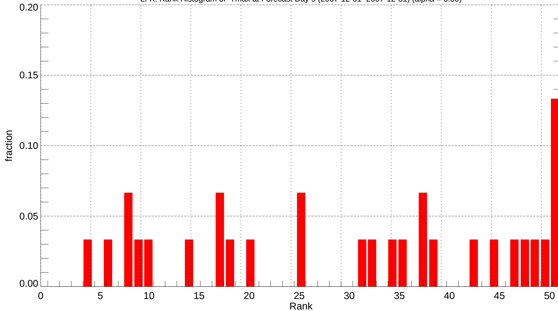
LFK: Rank Histogram of Tmax at Forecast Day 9 (2007-12-01~2007-12-31) (alpha = 0.00)
