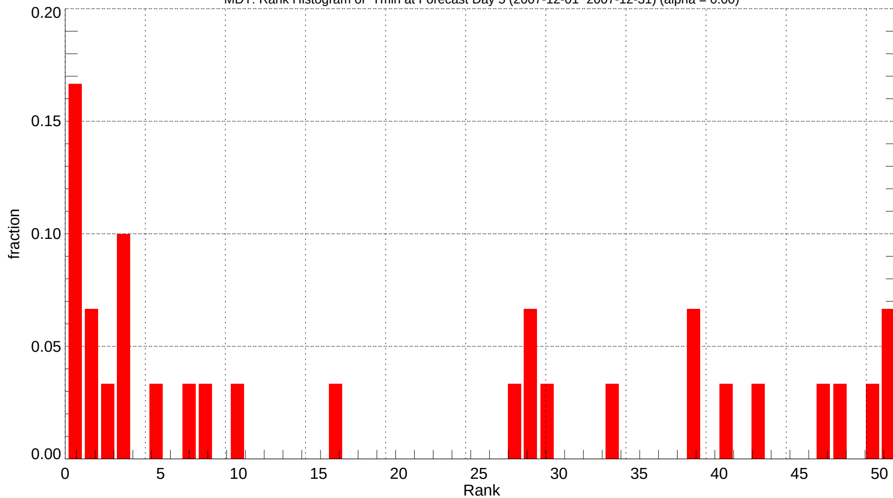
MDT: Rank Histogram of Tmin at Forecast Day 5 (2007-12-01~2007-12-31) (alpha = 0.00)
