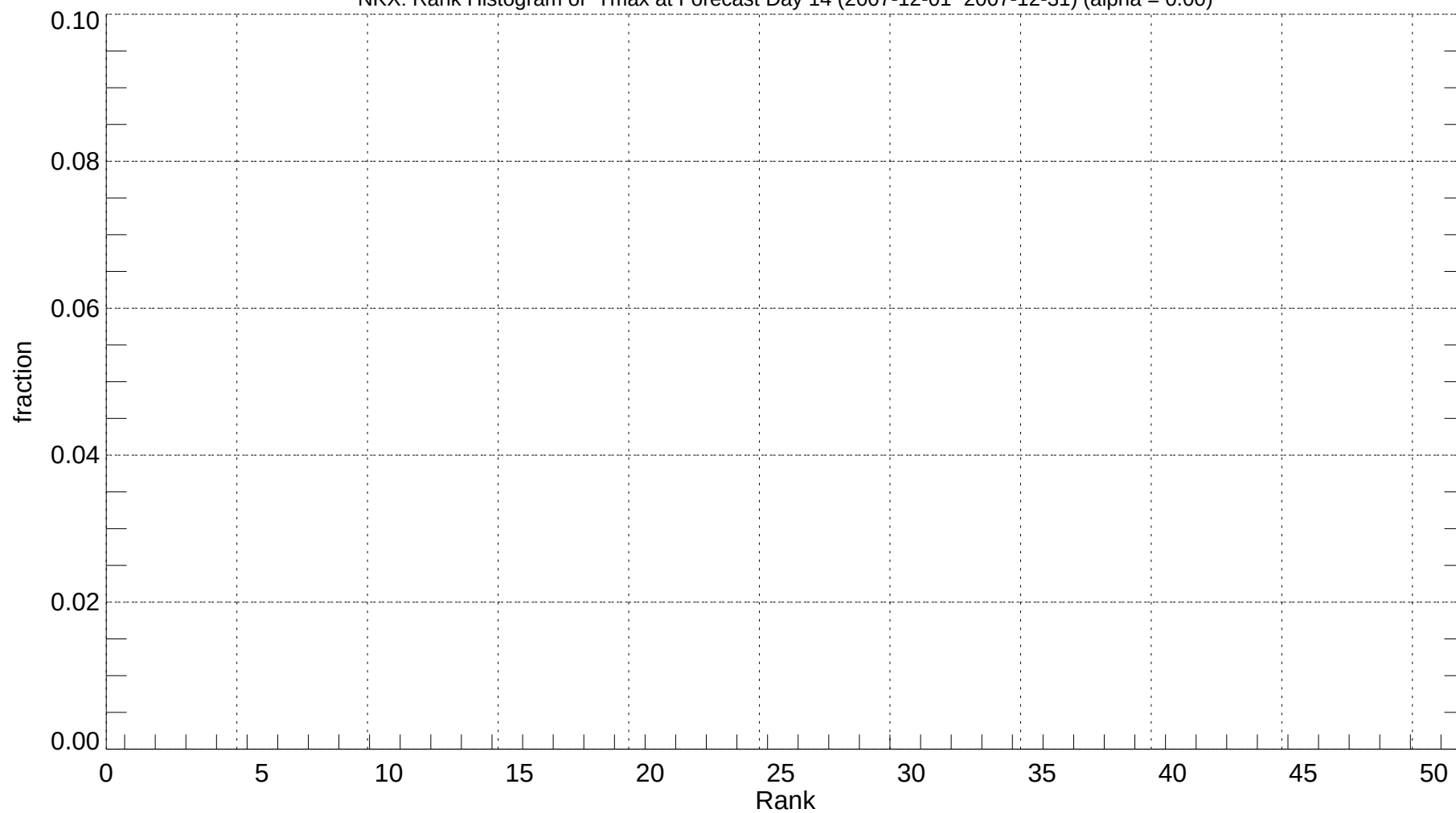
NKX: Rank Histogram of Tmax at Forecast Day 14 (2007-12-01~2007-12-31) (alpha = 0.00)
