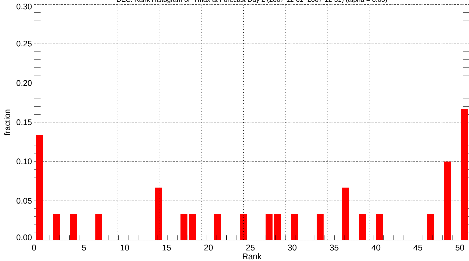
DEC: Rank Histogram of Tmax at Forecast Day 2 (2007-12-01~2007-12-31) (alpha = 0.00)
