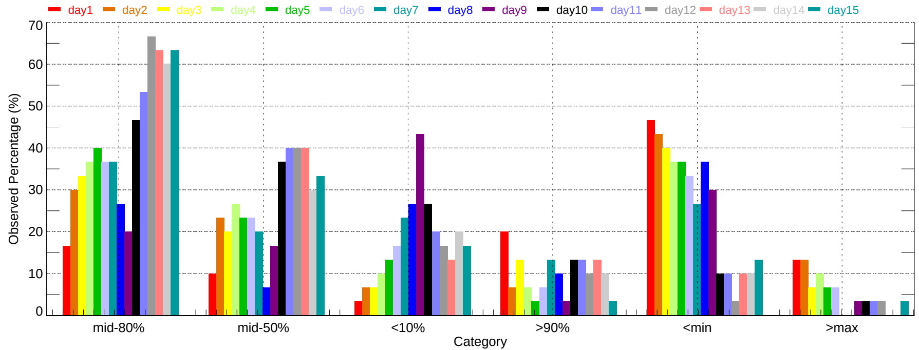
Observed Percentage of Ensembles - OAK: Min Temperature (2007-12-01~2007-12-31)
