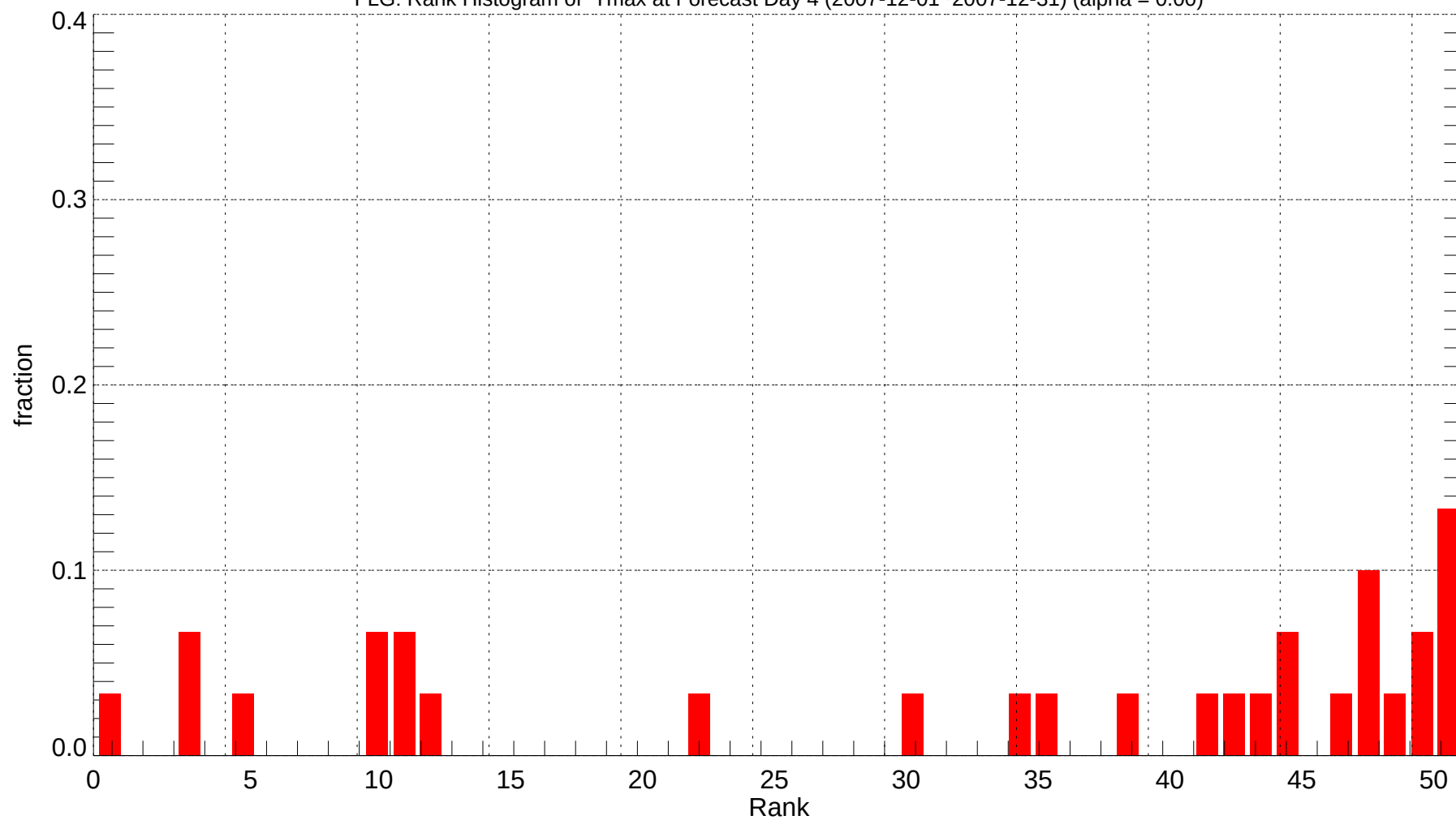
FLG: Rank Histogram of Tmax at Forecast Day 4 (2007-12-01~2007-12-31) (alpha = 0.00)
