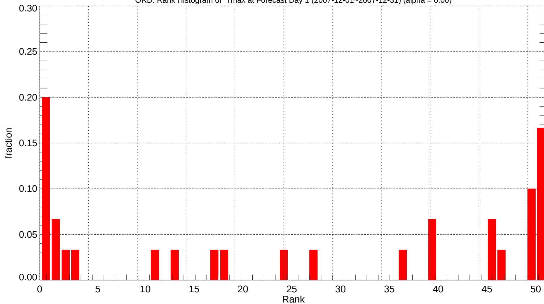
ORD: Rank Histogram of Tmax at Forecast Day 1 (2007-12-01~2007-12-31) (alpha = 0.00)
