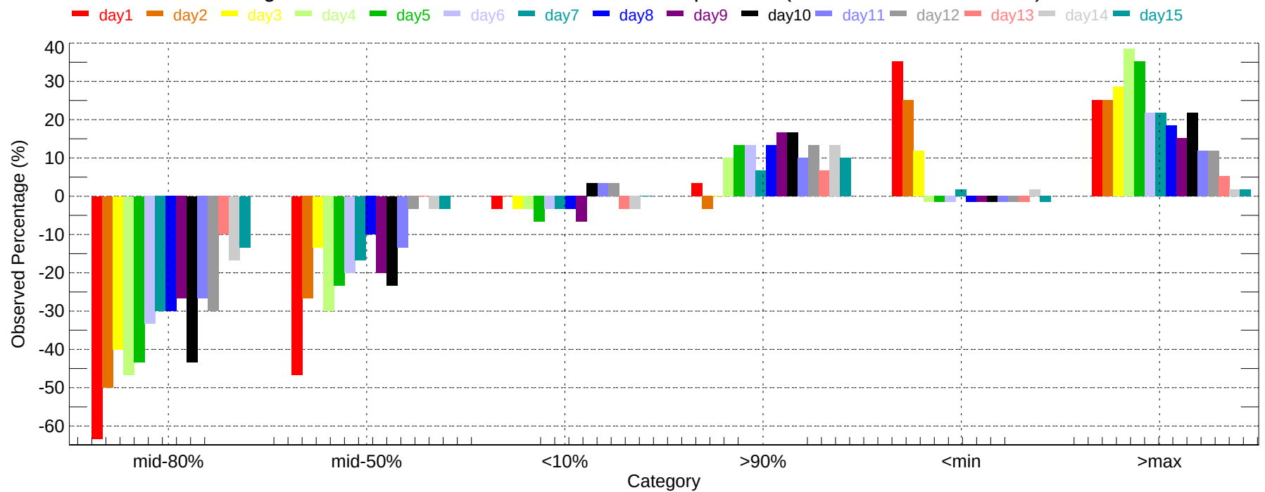
Observed Percentage Deviation of Ensembles - ICT: Max Temperature (2007-12-01~2007-12-31)
