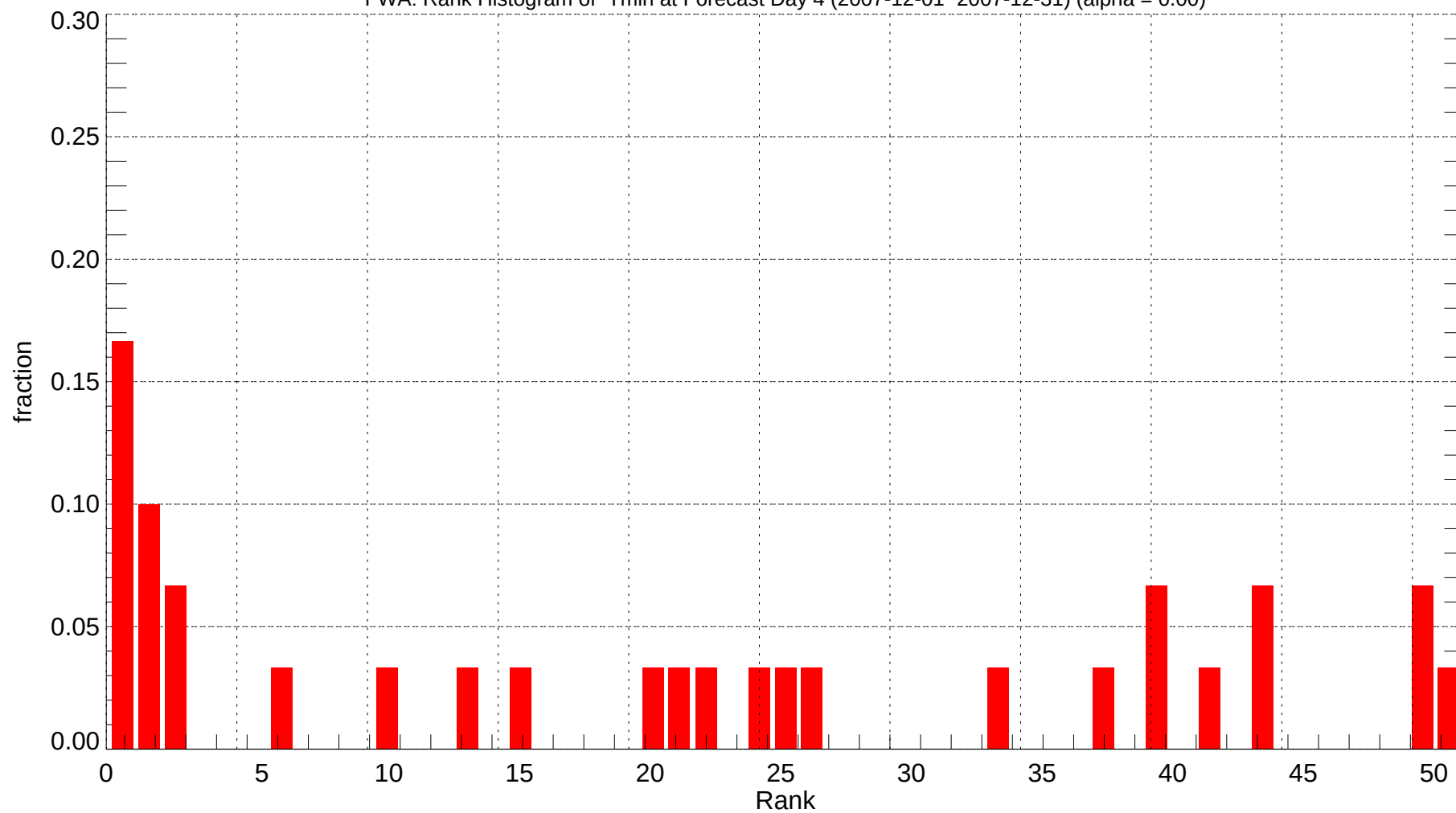
FWA: Rank Histogram of Tmin at Forecast Day 4 (2007-12-01~2007-12-31) (alpha = 0.00)
