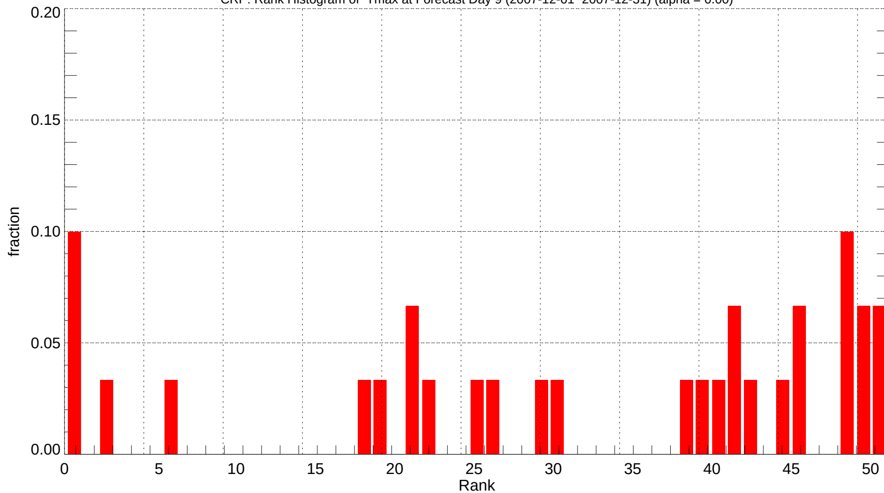
CRP: Rank Histogram of Tmax at Forecast Day 9 (2007-12-01~2007-12-31) (alpha = 0.00)
