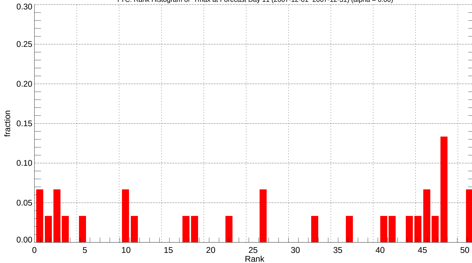
YYC: Rank Histogram of Tmax at Forecast Day 11 (2007-12-01~2007-12-31) (alpha = 0.00)
