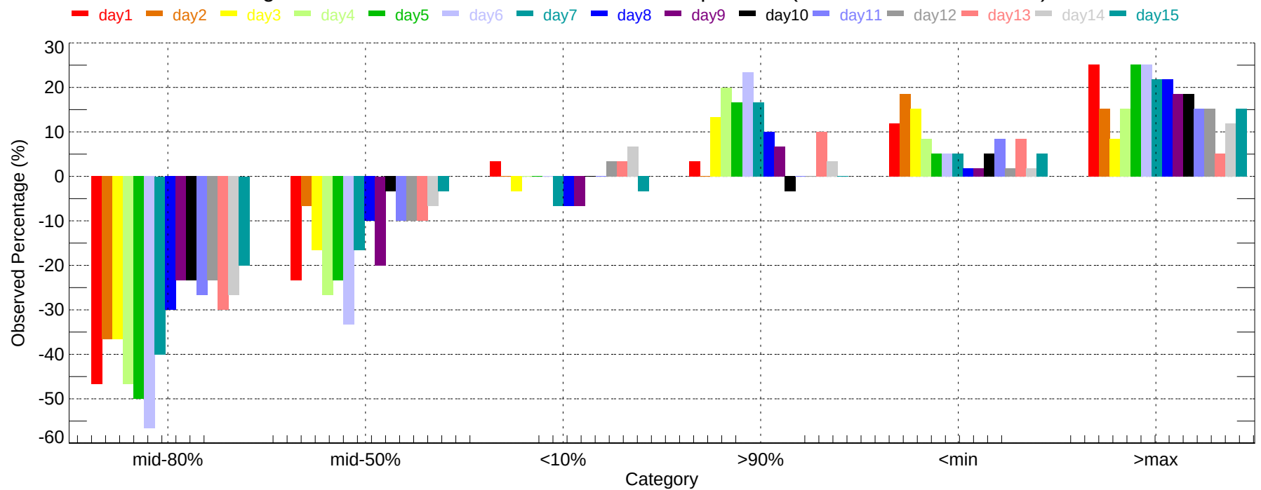
Observed Percentage Deviation of Ensembles - ABY: Max Temperature (2007-12-01~2007-12-31)
