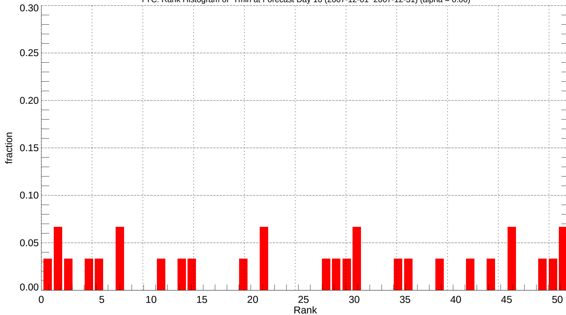
YYC: Rank Histogram of Tmin at Forecast Day 10 (2007-12-01~2007-12-31) (alpha = 0.00)
