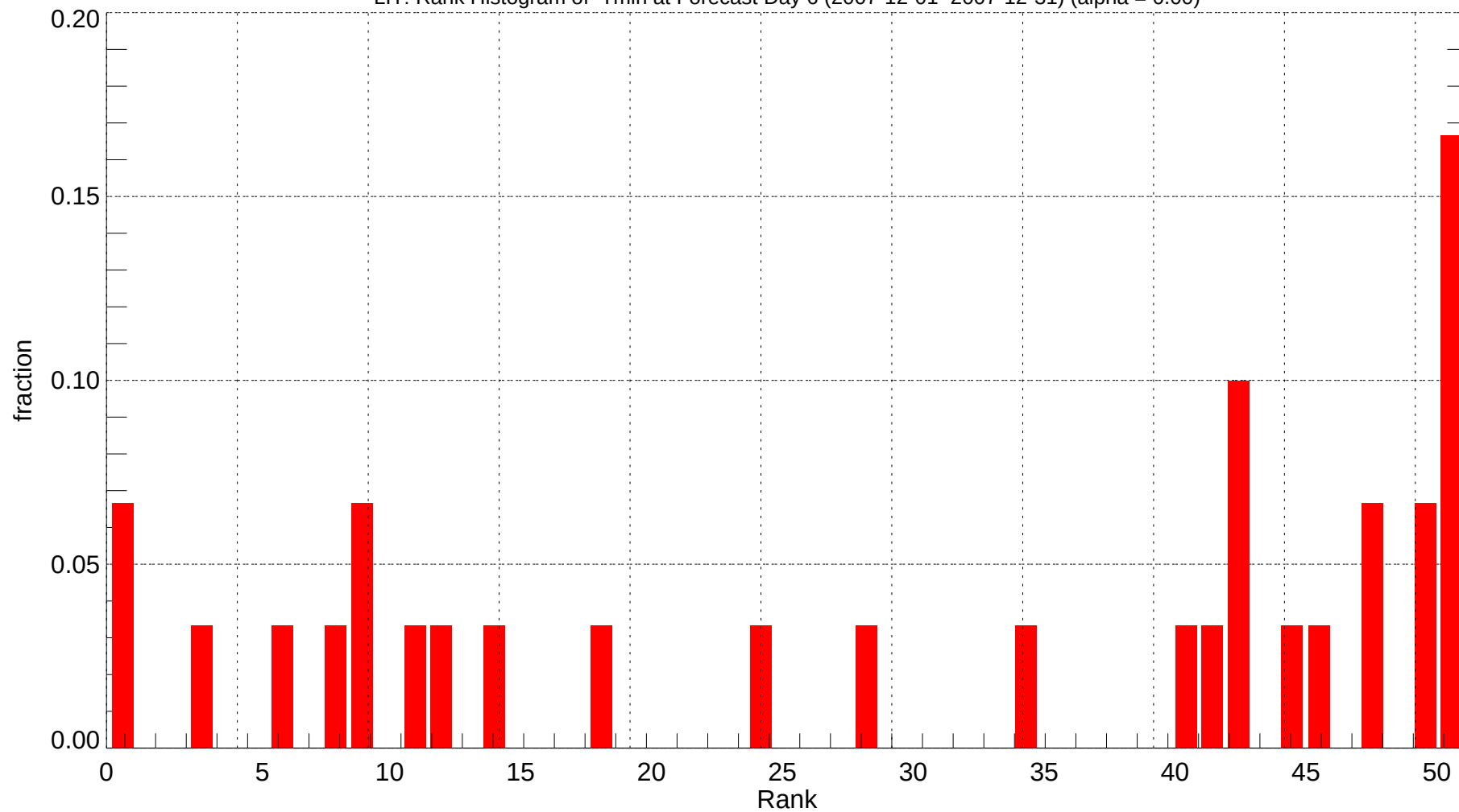
LIT: Rank Histogram of Tmin at Forecast Day 6 (2007-12-01~2007-12-31) (alpha = 0.00)
