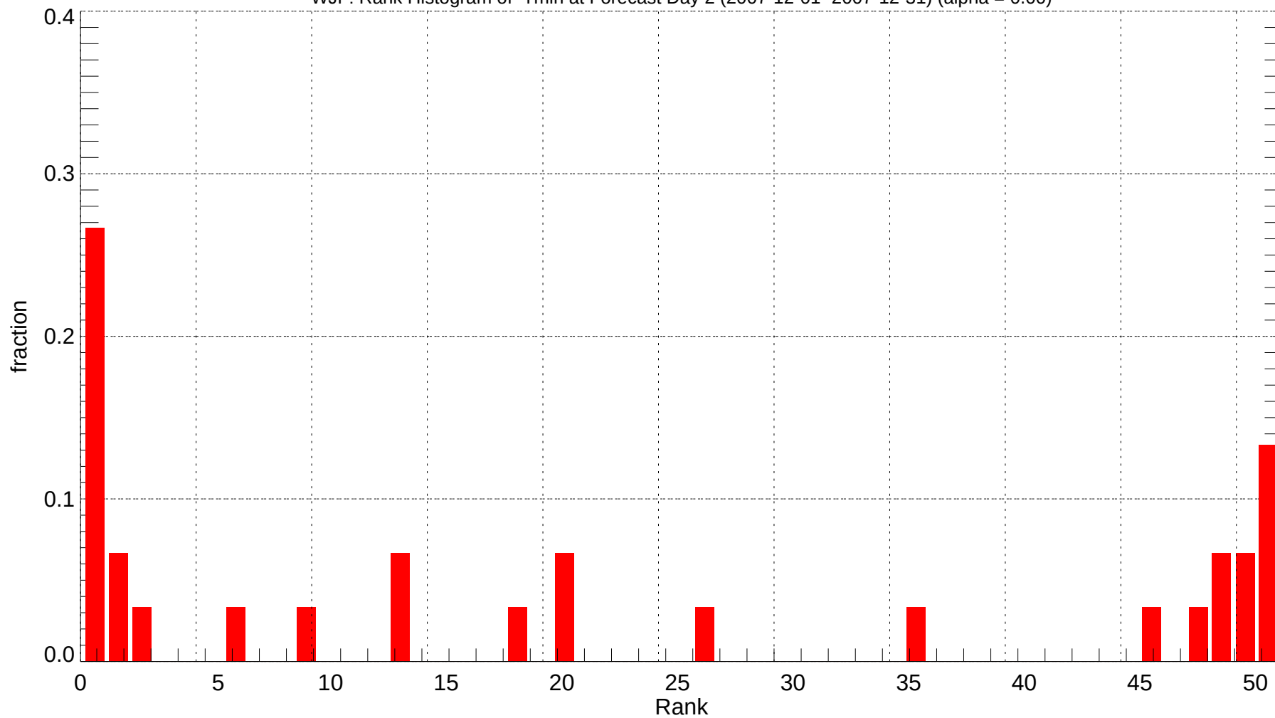
WJF: Rank Histogram of Tmin at Forecast Day 2 (2007-12-01~2007-12-31) (alpha = 0.00)
