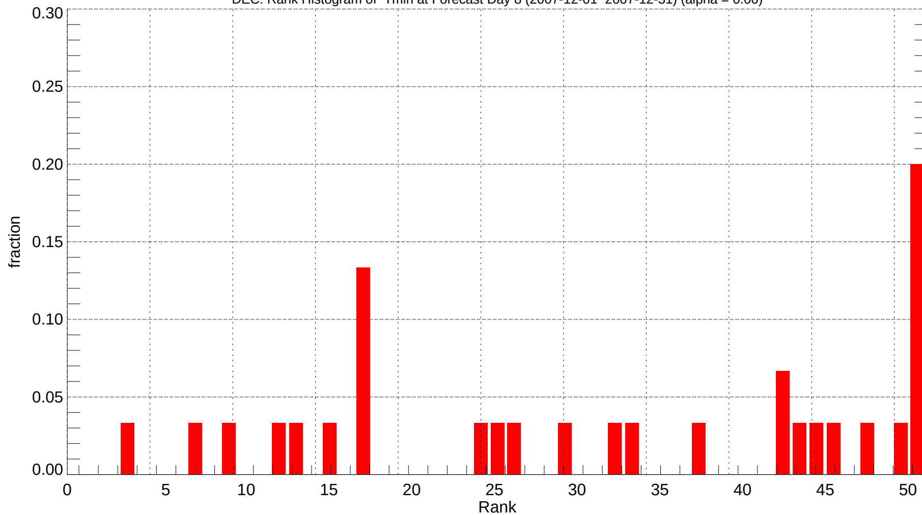
DEC: Rank Histogram of Tmin at Forecast Day 8 (2007-12-01~2007-12-31) (alpha = 0.00)
