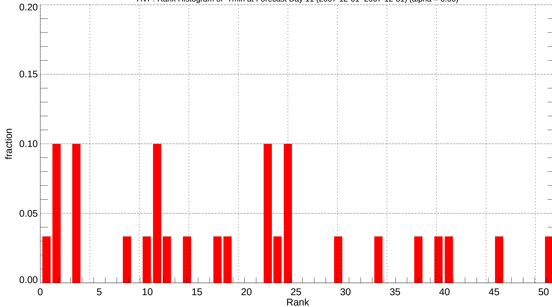
AVP: Rank Histogram of Tmin at Forecast Day 11 (2007-12-01~2007-12-31) (alpha = 0.00)
