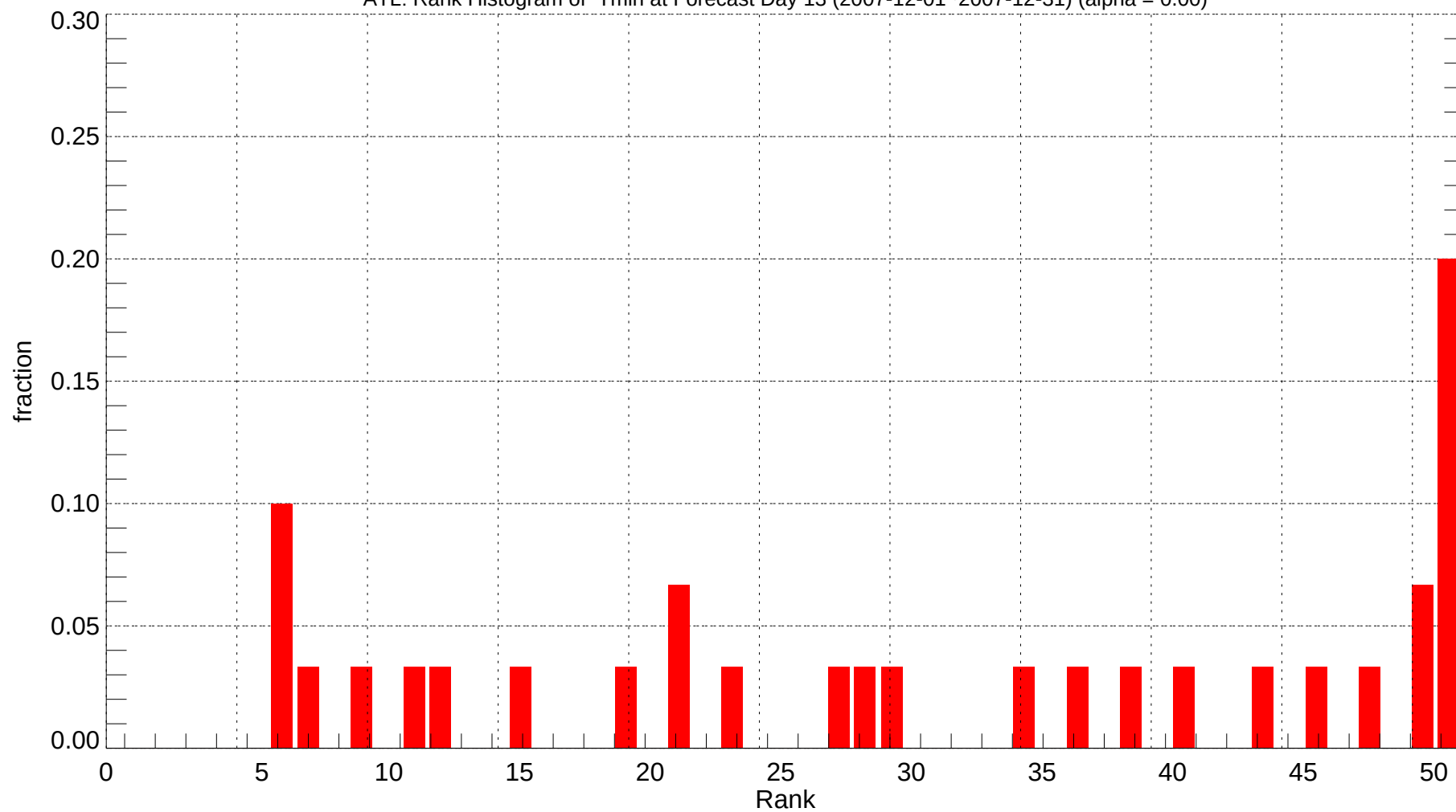
ATL: Rank Histogram of Tmin at Forecast Day 13 (2007-12-01~2007-12-31) (alpha = 0.00)
