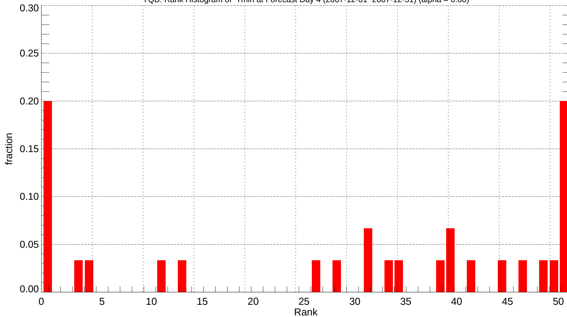
YQB: Rank Histogram of Tmin at Forecast Day 4 (2007-12-01~2007-12-31) (alpha = 0.00)
