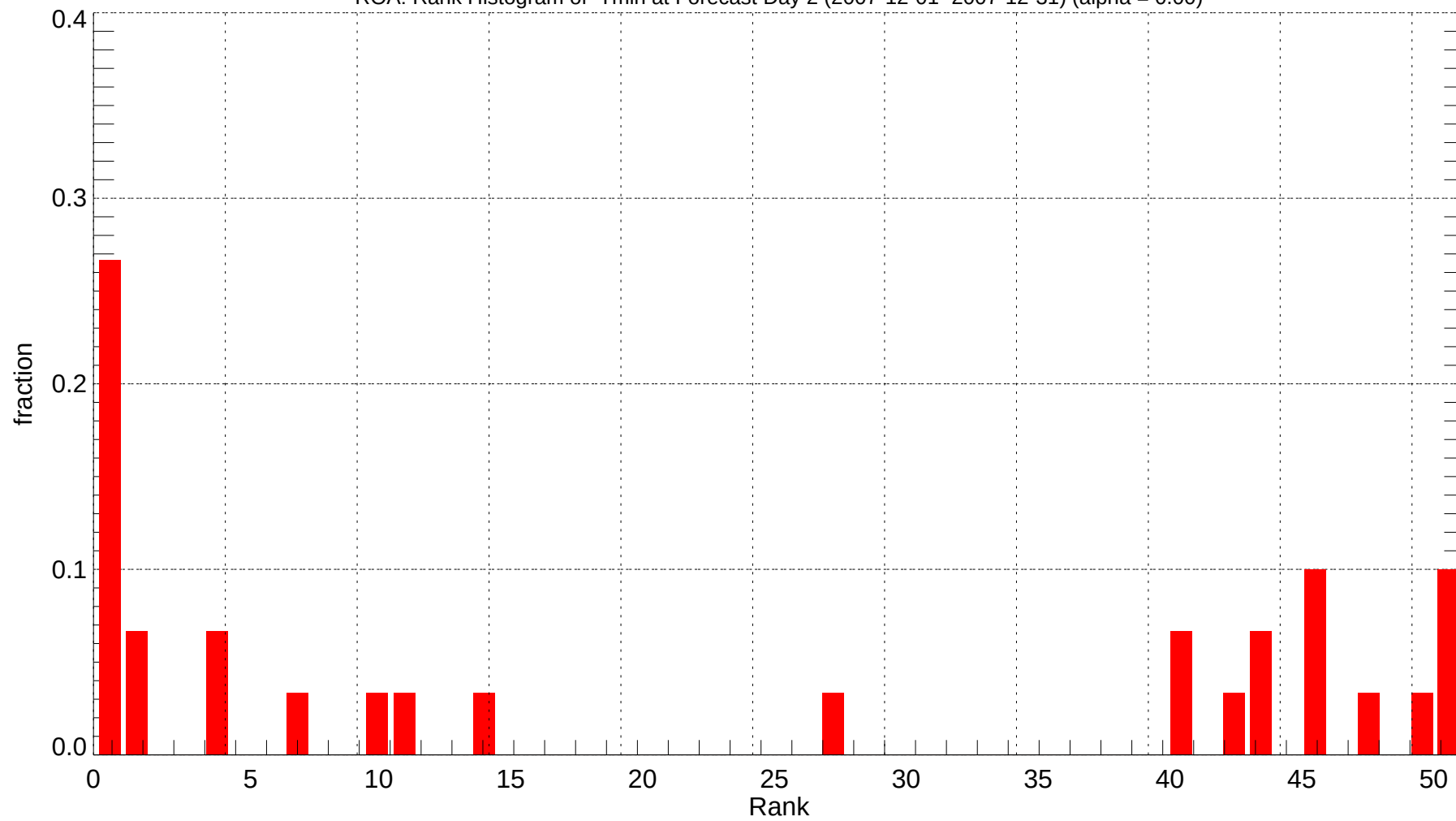
ROA: Rank Histogram of Tmin at Forecast Day 2 (2007-12-01~2007-12-31) (alpha = 0.00)
