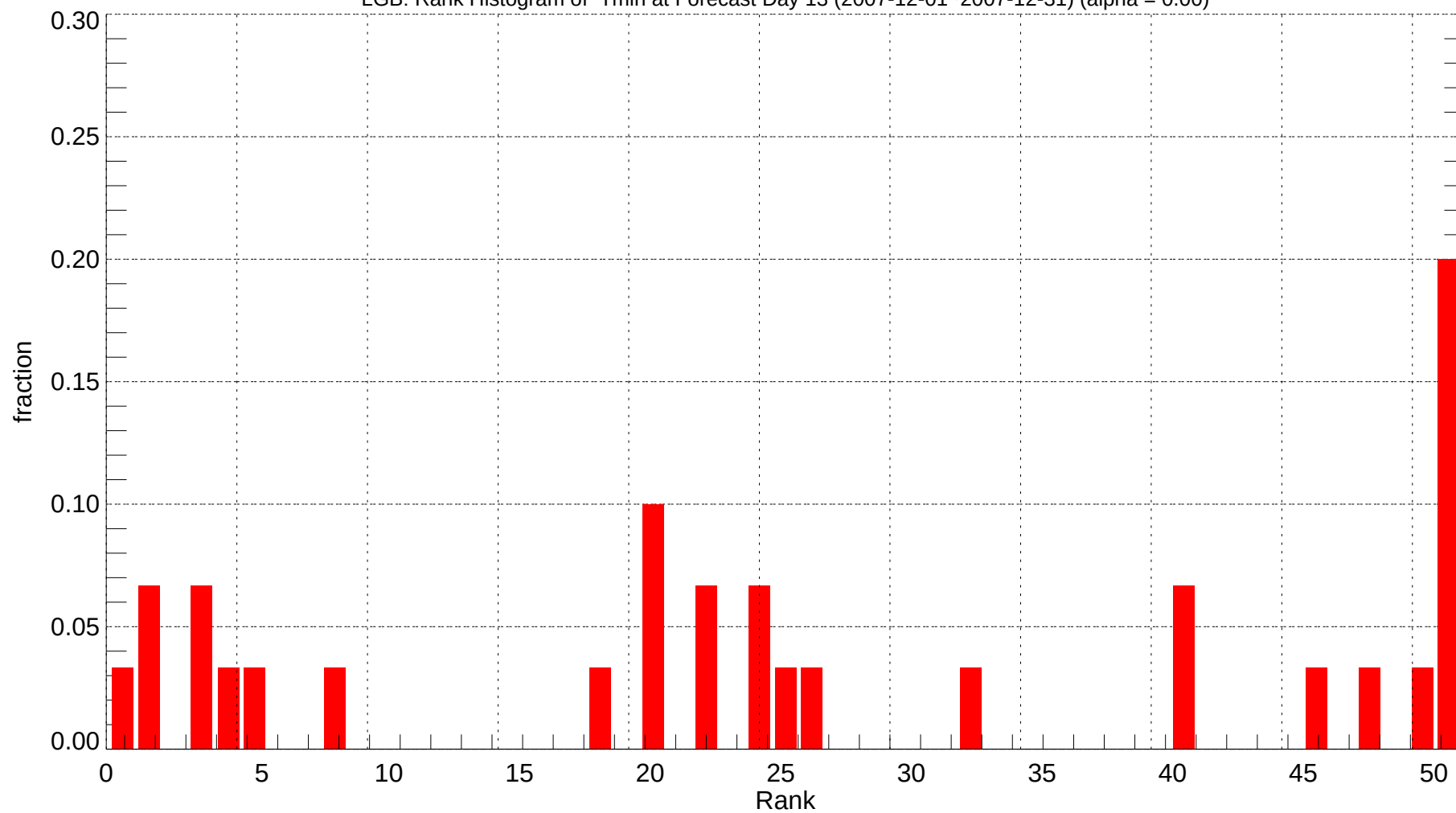
LGB: Rank Histogram of Tmin at Forecast Day 13 (2007-12-01~2007-12-31) (alpha = 0.00)
