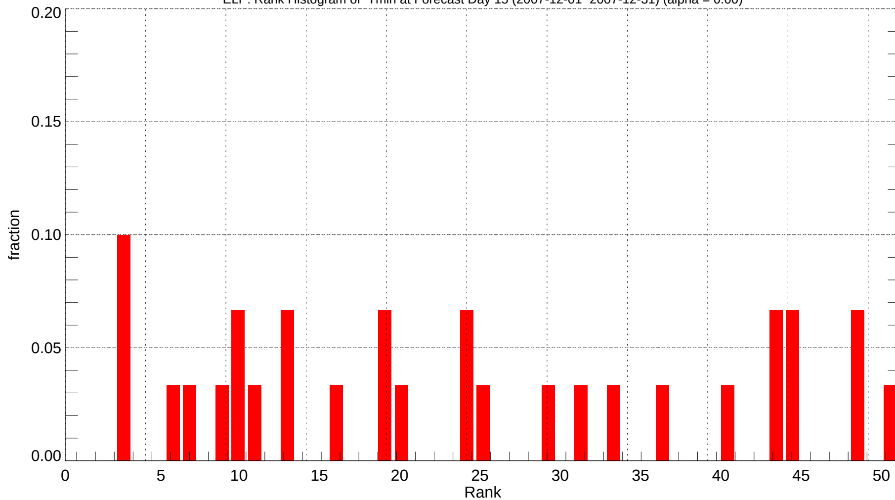
ELP: Rank Histogram of Tmin at Forecast Day 15 (2007-12-01~2007-12-31) (alpha = 0.00)
