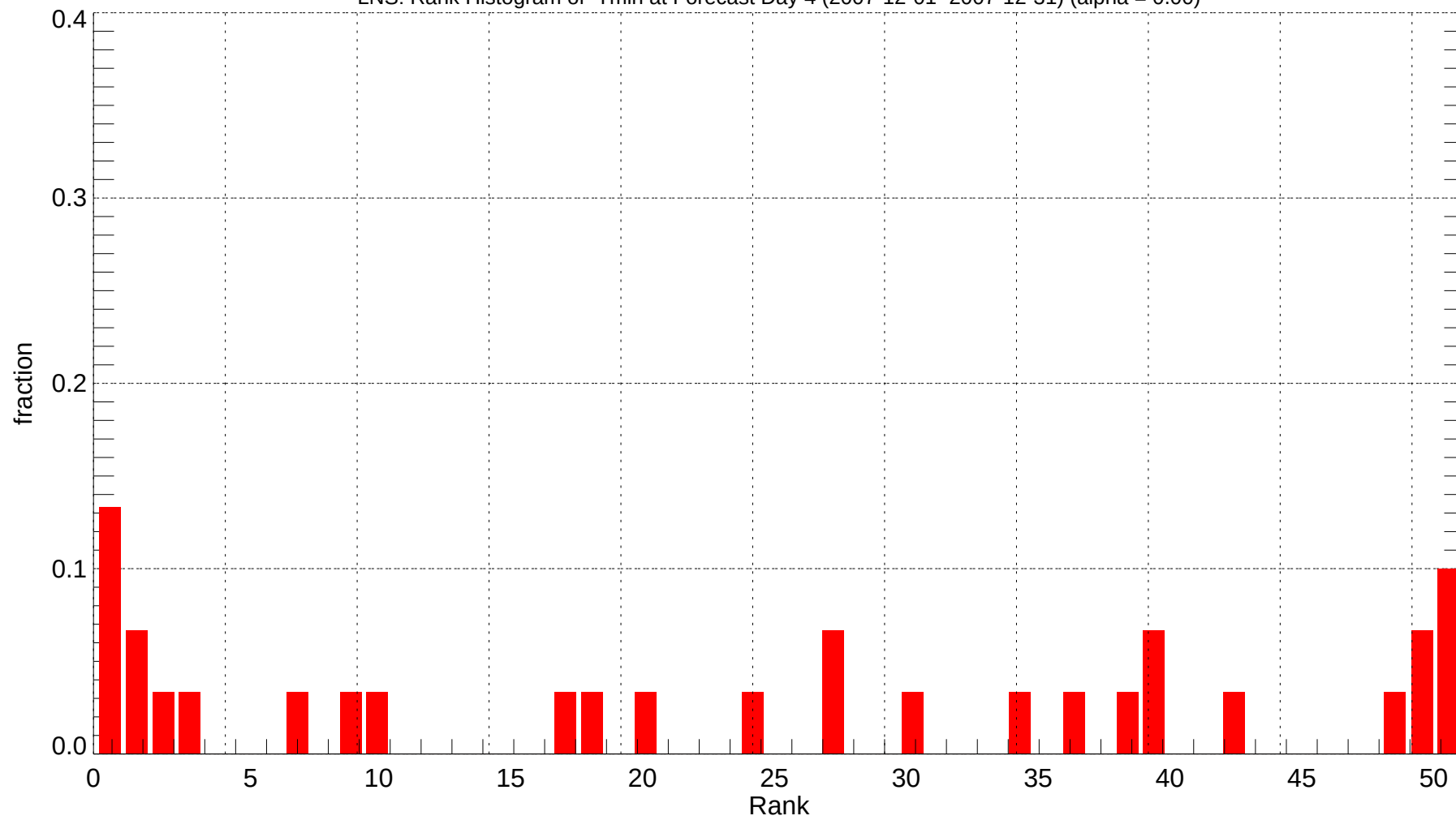
LNS: Rank Histogram of Tmin at Forecast Day 4 (2007-12-01~2007-12-31) (alpha = 0.00)
