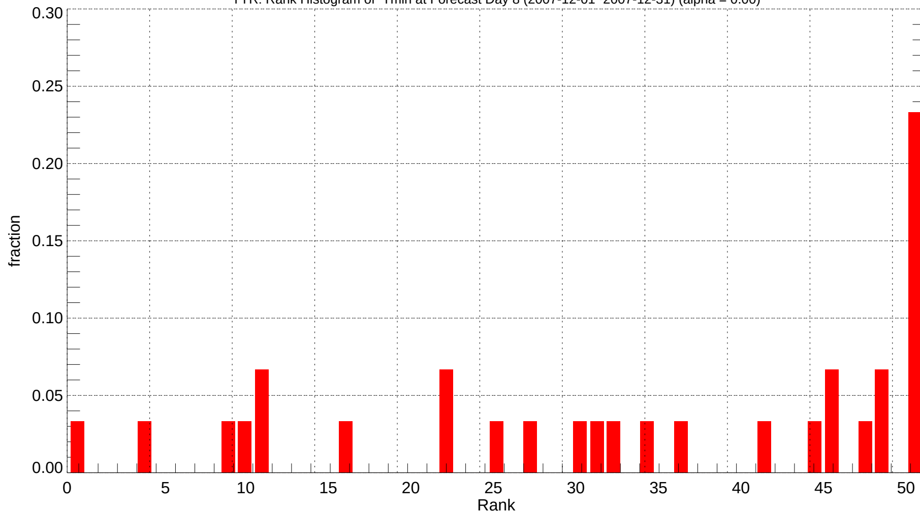
TYR: Rank Histogram of Tmin at Forecast Day 8 (2007-12-01~2007-12-31) (alpha = 0.00)
