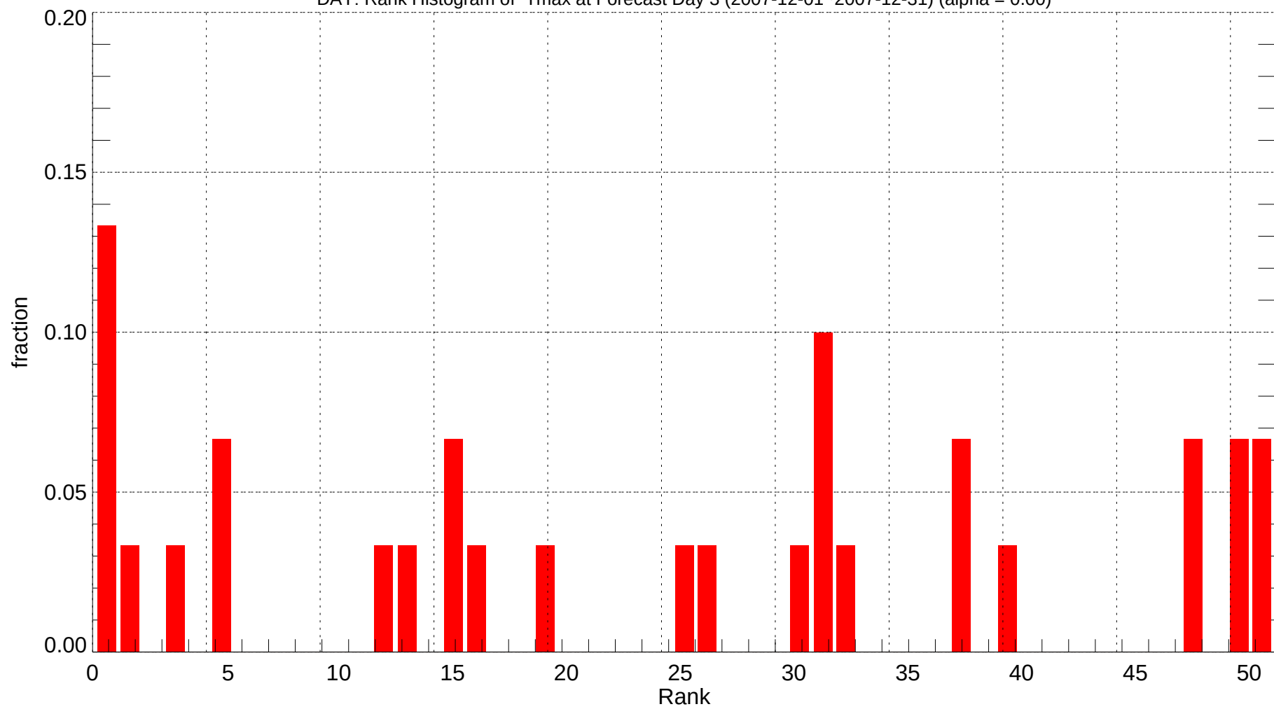
DAY: Rank Histogram of Tmax at Forecast Day 3 (2007-12-01~2007-12-31) (alpha = 0.00)
