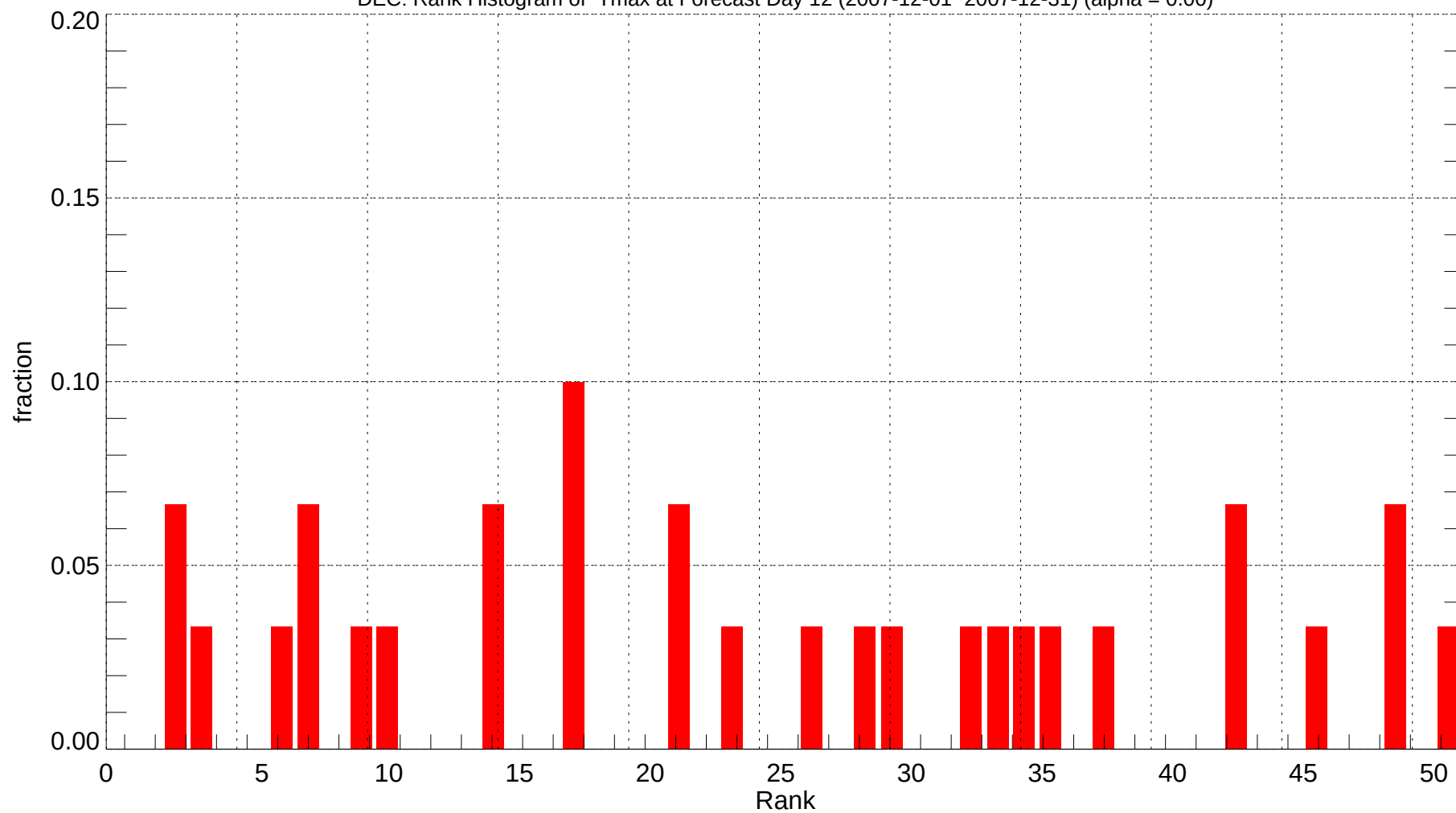
DEC: Rank Histogram of Tmax at Forecast Day 12 (2007-12-01~2007-12-31) (alpha = 0.00)
