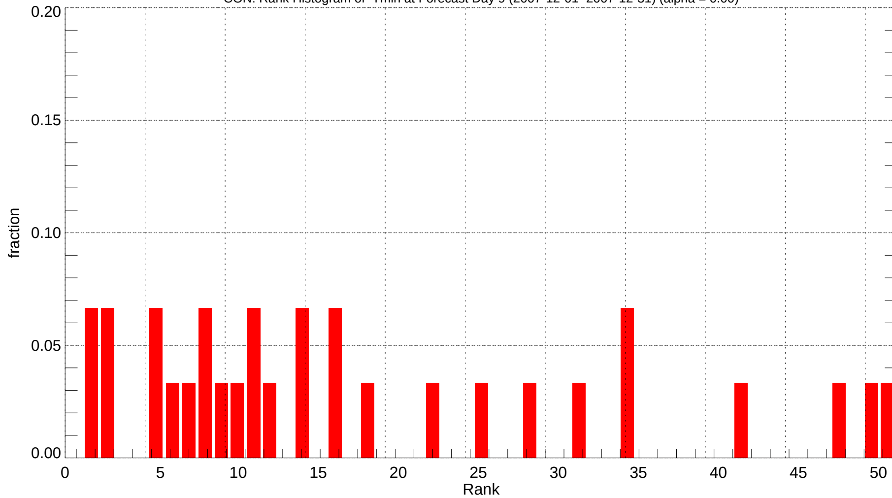
CON: Rank Histogram of Tmin at Forecast Day 9 (2007-12-01~2007-12-31) (alpha = 0.00)
