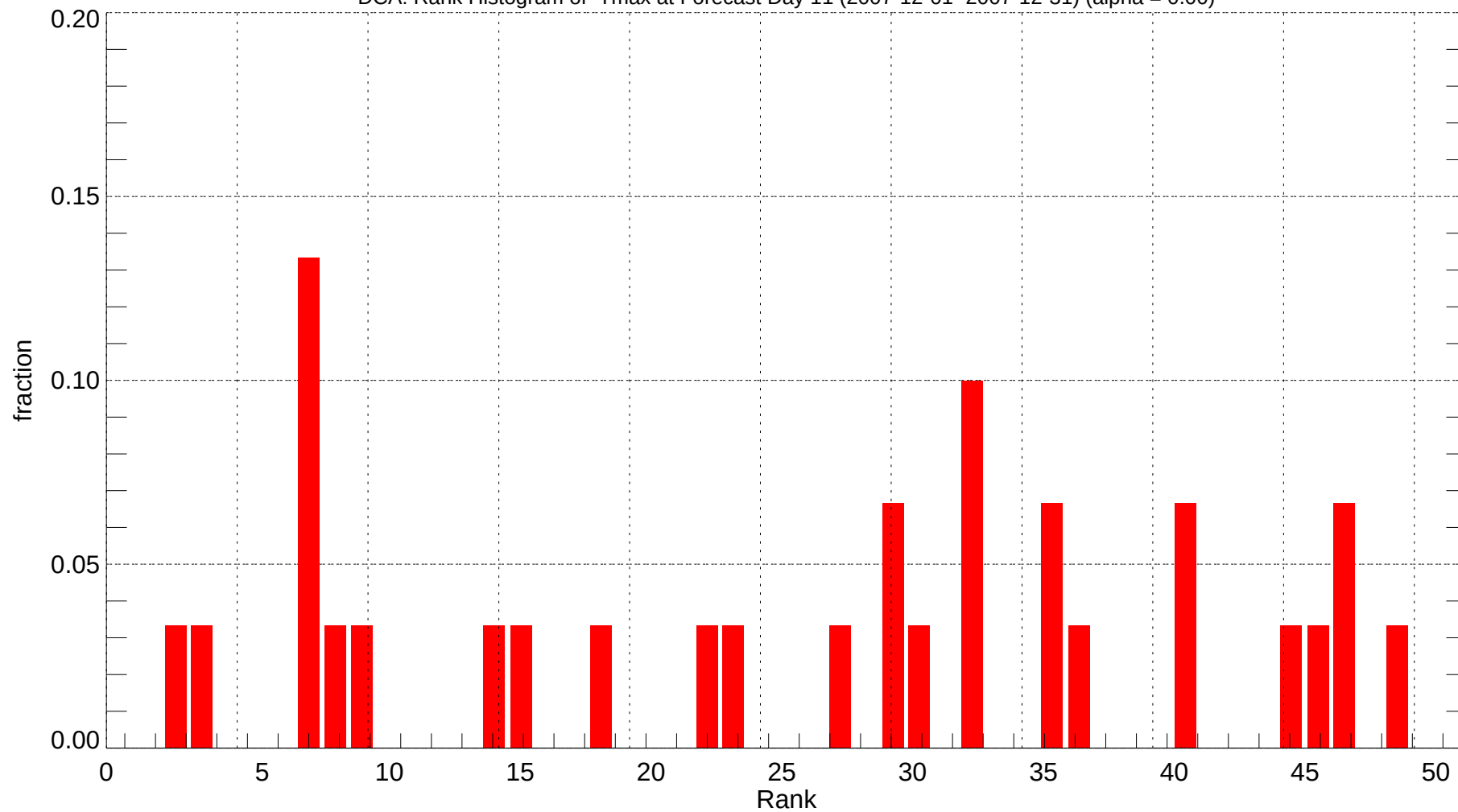
DCA: Rank Histogram of Tmax at Forecast Day 11 (2007-12-01~2007-12-31) (alpha = 0.00)
