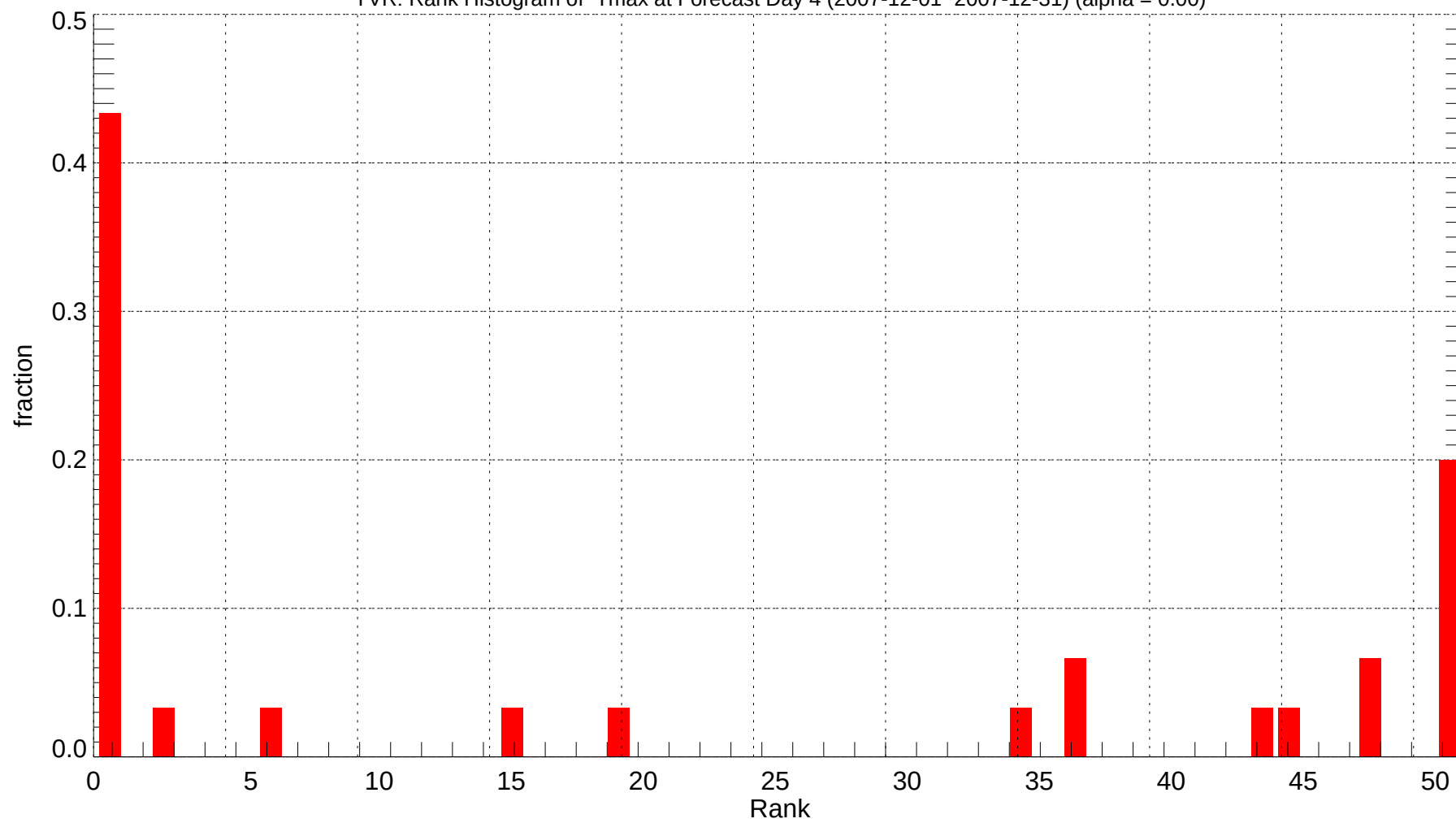
YVR: Rank Histogram of Tmax at Forecast Day 4 (2007-12-01~2007-12-31) (alpha = 0.00)
