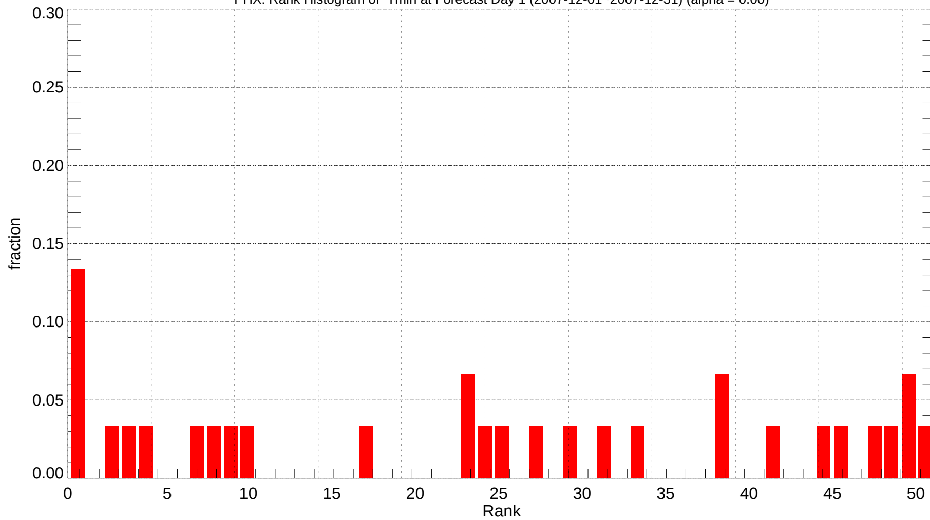
PHX: Rank Histogram of Tmin at Forecast Day 1 (2007-12-01~2007-12-31) (alpha = 0.00)
