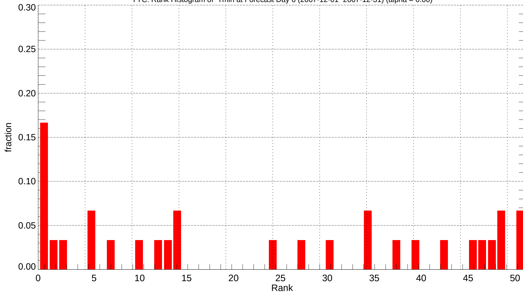
YYC: Rank Histogram of Tmin at Forecast Day 6 (2007-12-01~2007-12-31) (alpha = 0.00)
