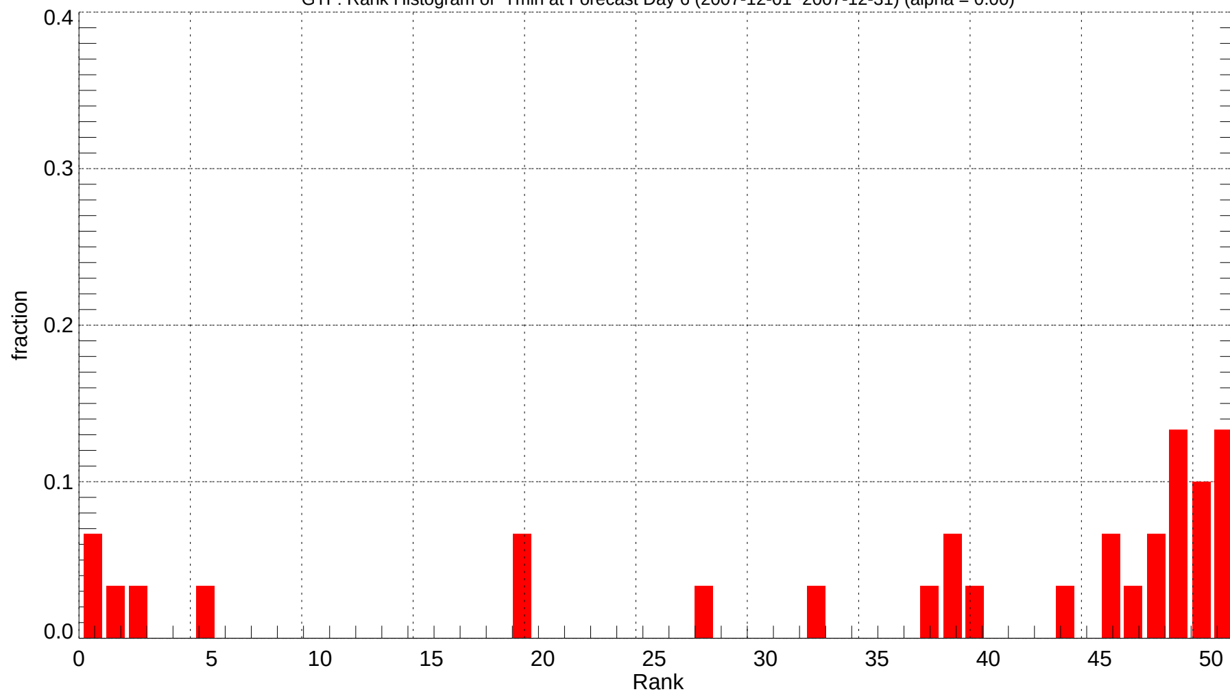
GTF: Rank Histogram of Tmin at Forecast Day 6 (2007-12-01~2007-12-31) (alpha = 0.00)
