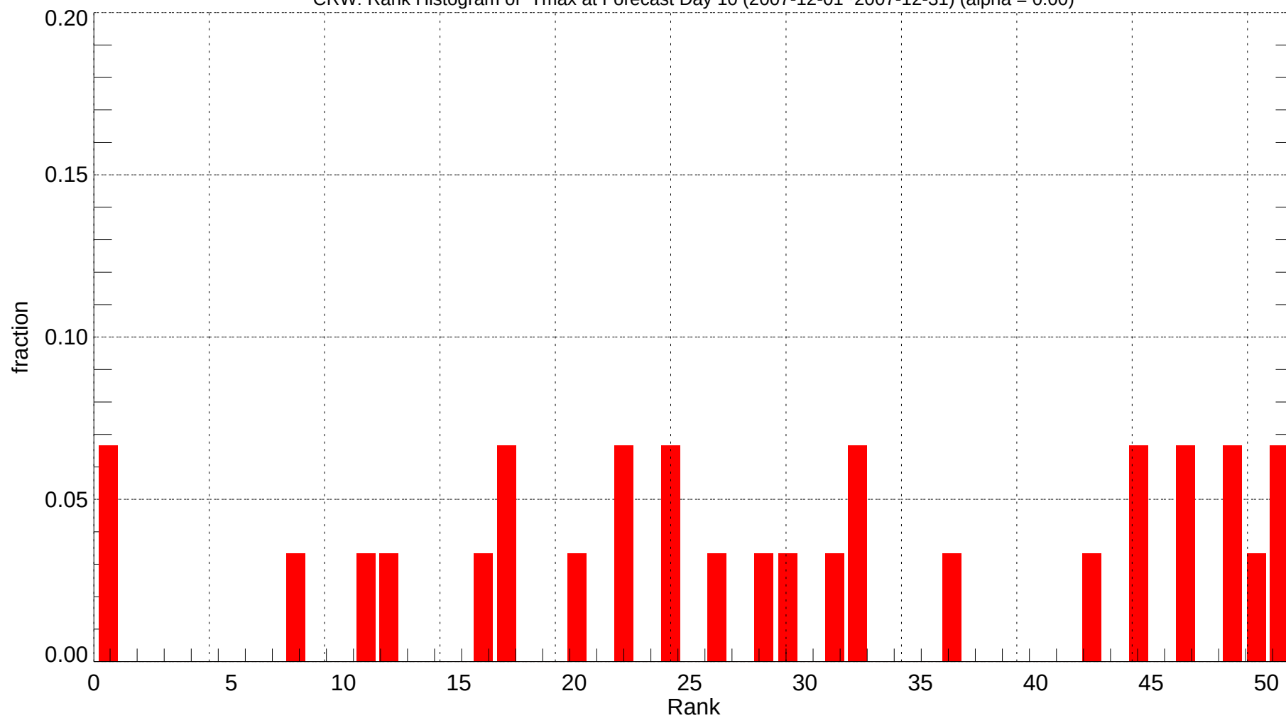
CRW: Rank Histogram of Tmax at Forecast Day 10 (2007-12-01~2007-12-31) (alpha = 0.00)
