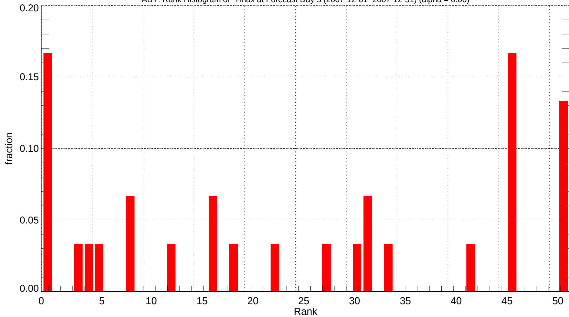
ABY: Rank Histogram of Tmax at Forecast Day 3 (2007-12-01~2007-12-31) (alpha = 0.00)
