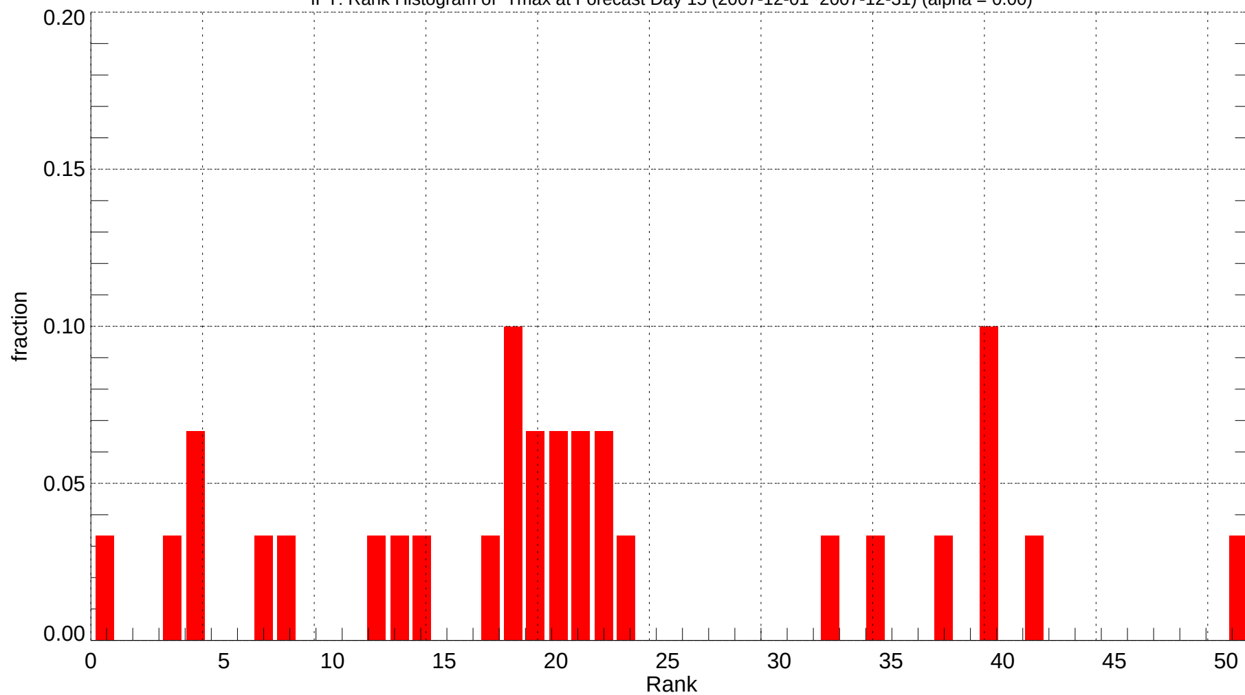
IPT: Rank Histogram of Tmax at Forecast Day 15 (2007-12-01~2007-12-31) (alpha = 0.00)
