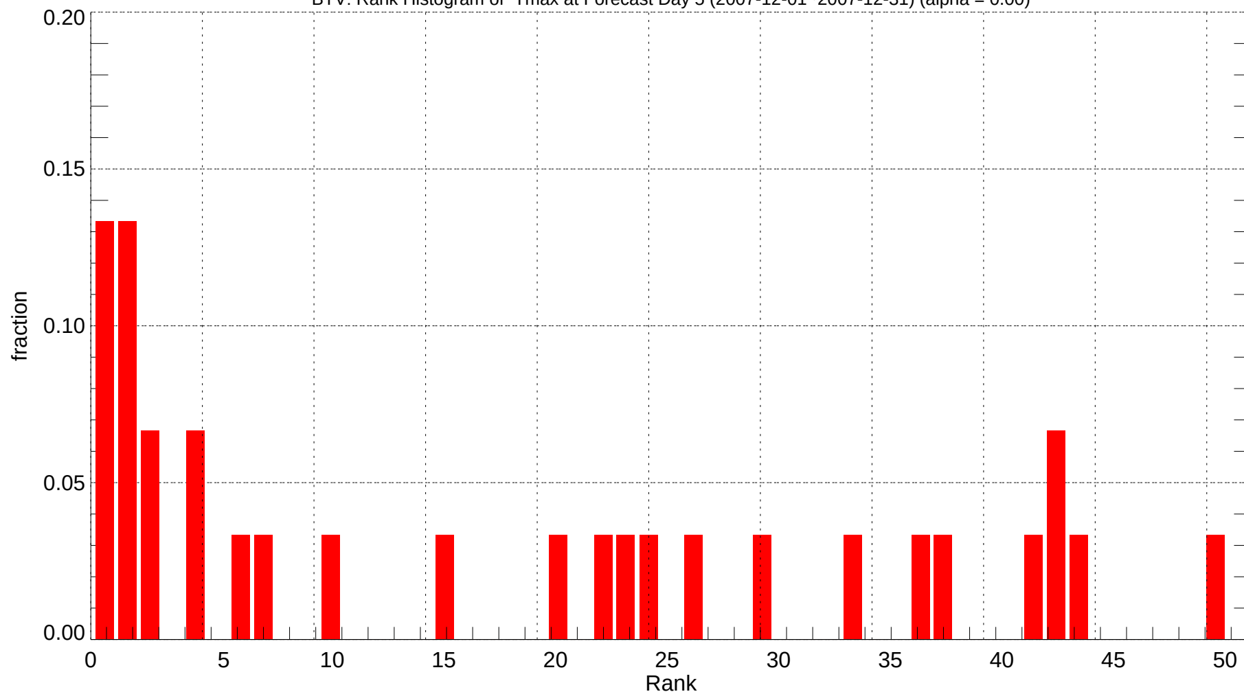
BTV: Rank Histogram of Tmax at Forecast Day 5 (2007-12-01~2007-12-31) (alpha = 0.00)
