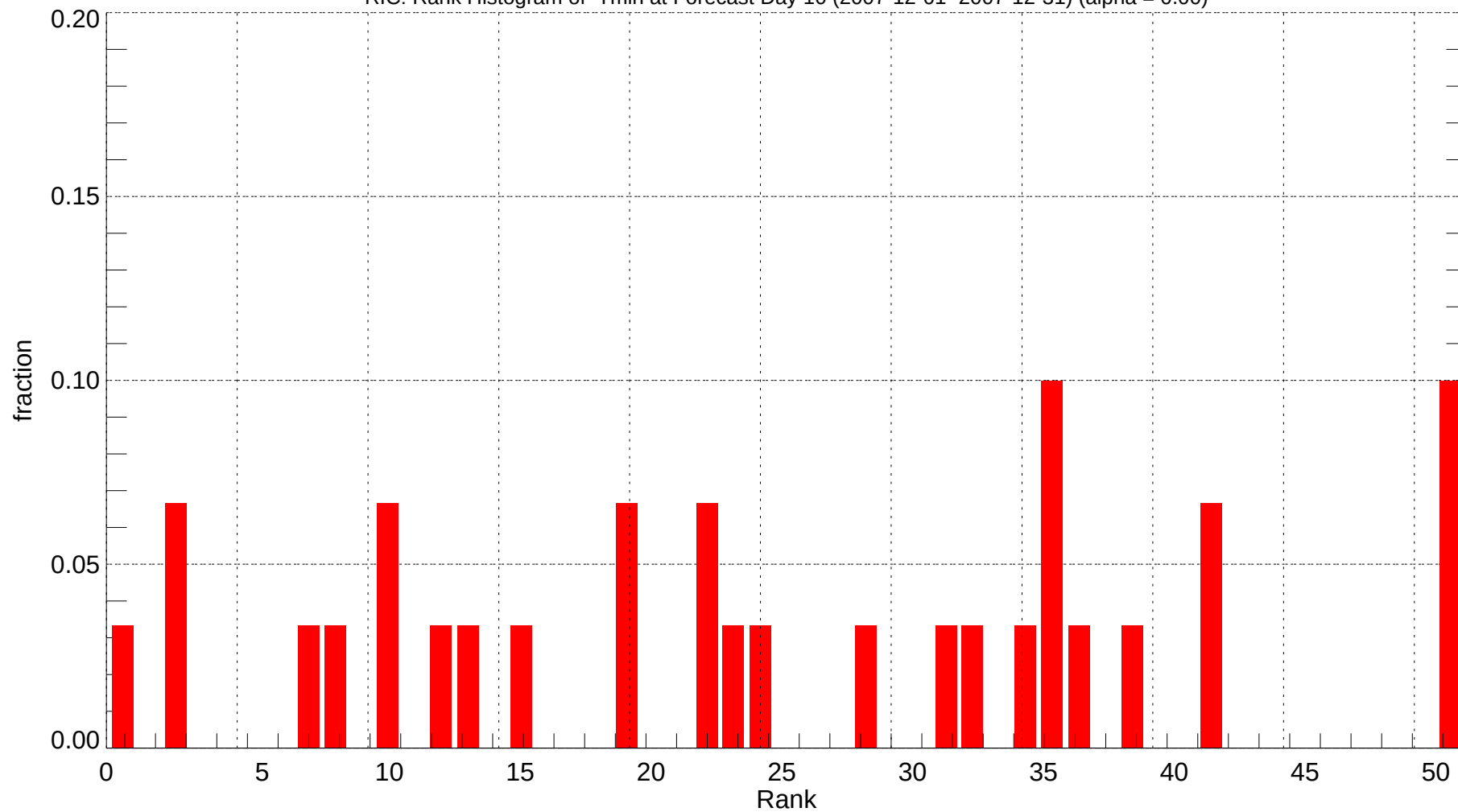
RIC: Rank Histogram of Tmin at Forecast Day 10 (2007-12-01~2007-12-31) (alpha = 0.00)
