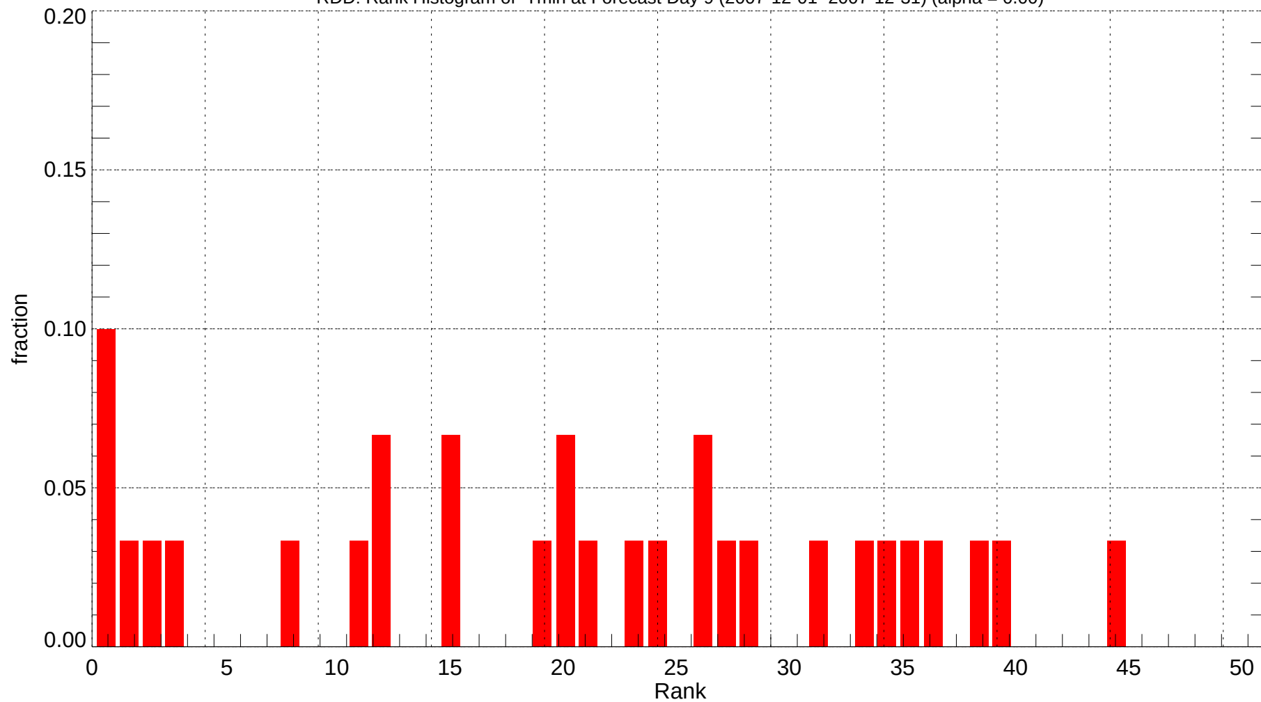
RDD: Rank Histogram of Tmin at Forecast Day 9 (2007-12-01~2007-12-31) (alpha = 0.00)
