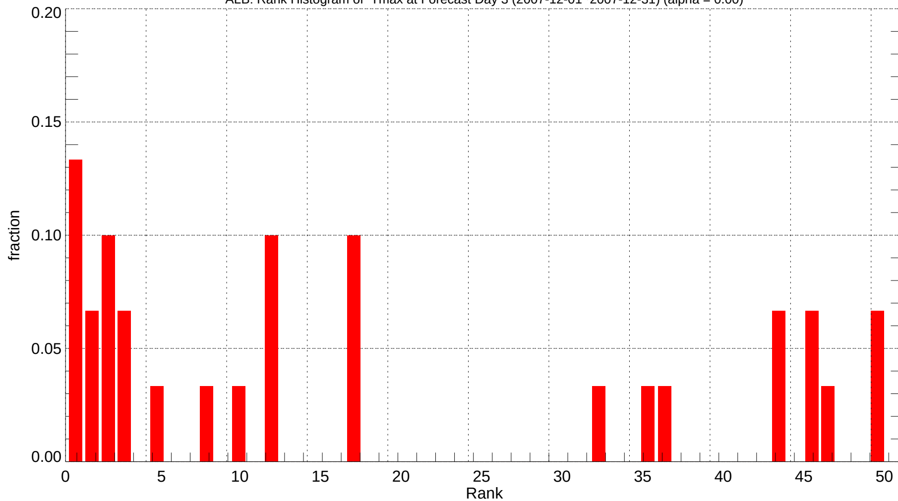
ALB: Rank Histogram of Tmax at Forecast Day 3 (2007-12-01~2007-12-31) (alpha = 0.00)
