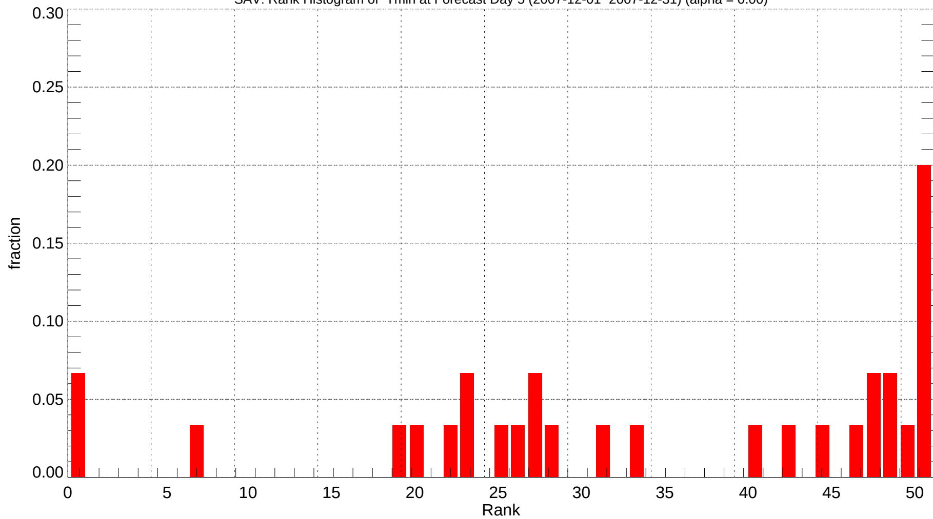
SAV: Rank Histogram of Tmin at Forecast Day 5 (2007-12-01~2007-12-31) (alpha = 0.00)
