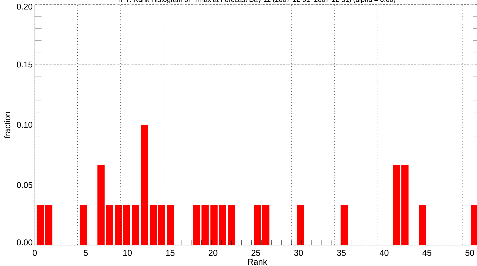
IPT: Rank Histogram of Tmax at Forecast Day 12 (2007-12-01~2007-12-31) (alpha = 0.00)
