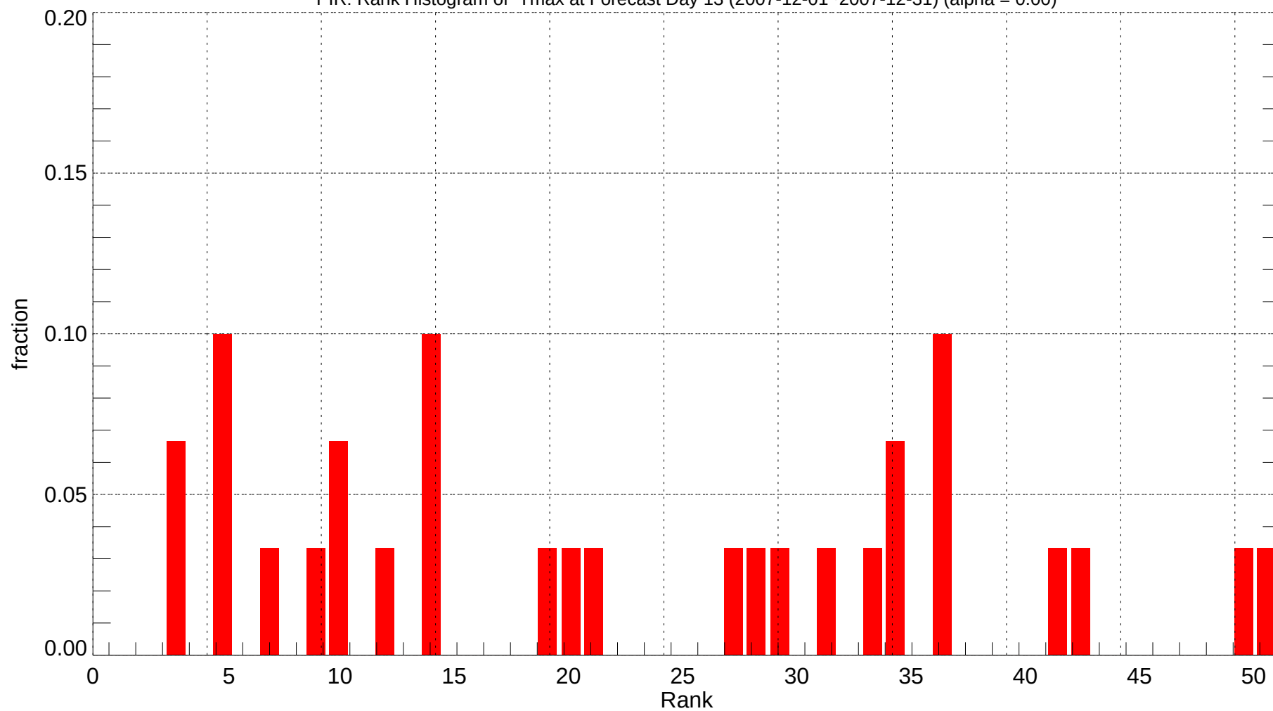
PIR: Rank Histogram of Tmax at Forecast Day 13 (2007-12-01~2007-12-31) (alpha = 0.00)
