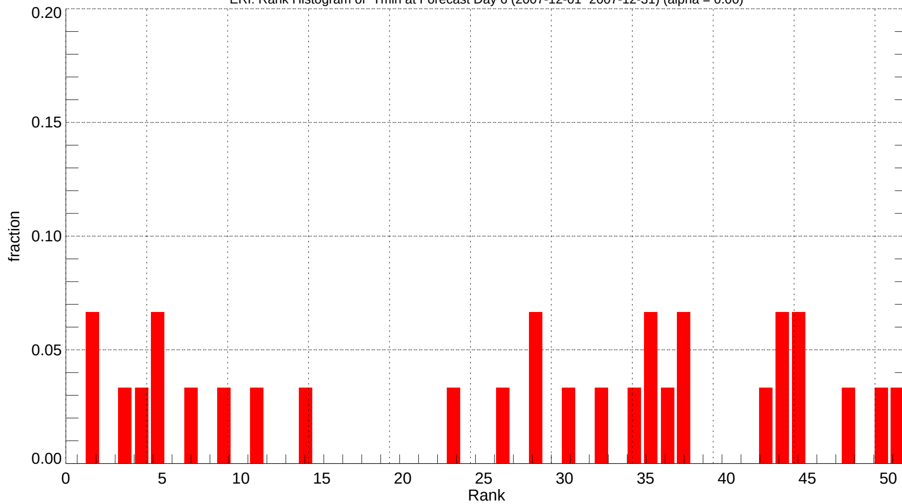
ERI: Rank Histogram of Tmin at Forecast Day 6 (2007-12-01~2007-12-31) (alpha = 0.00)
