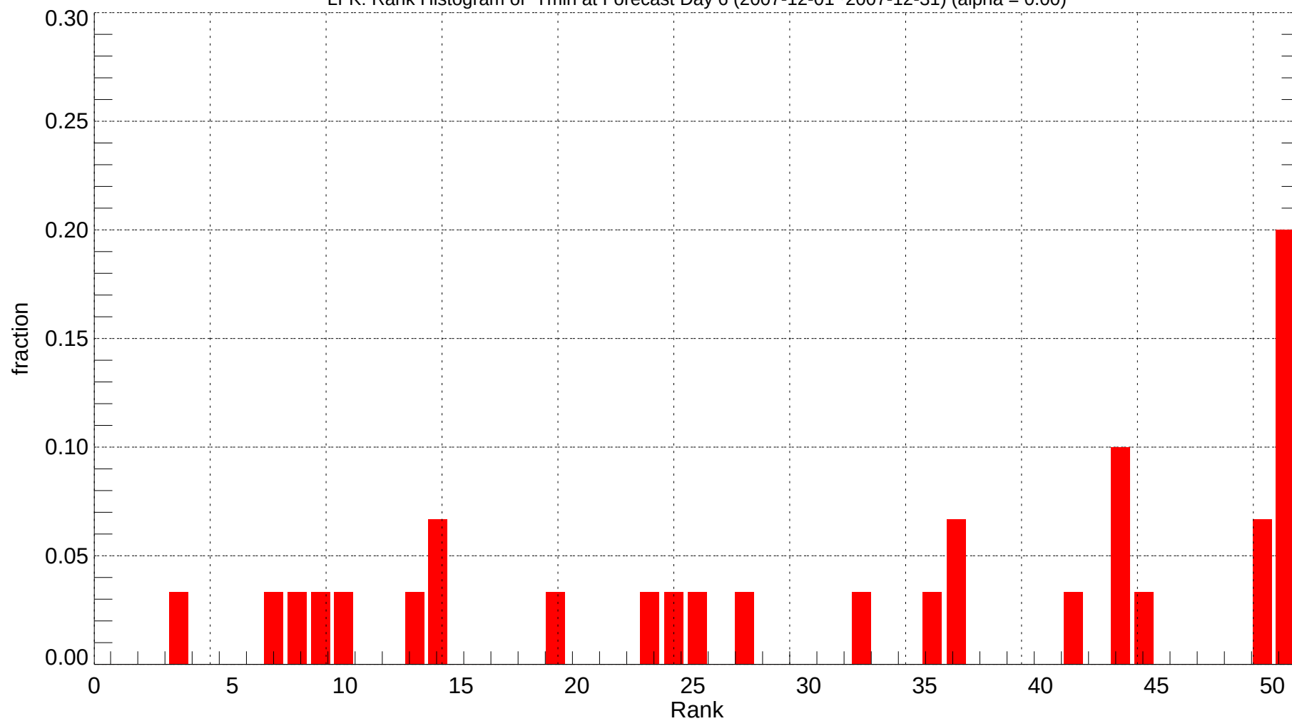
LFK: Rank Histogram of Tmin at Forecast Day 6 (2007-12-01~2007-12-31) (alpha = 0.00)
