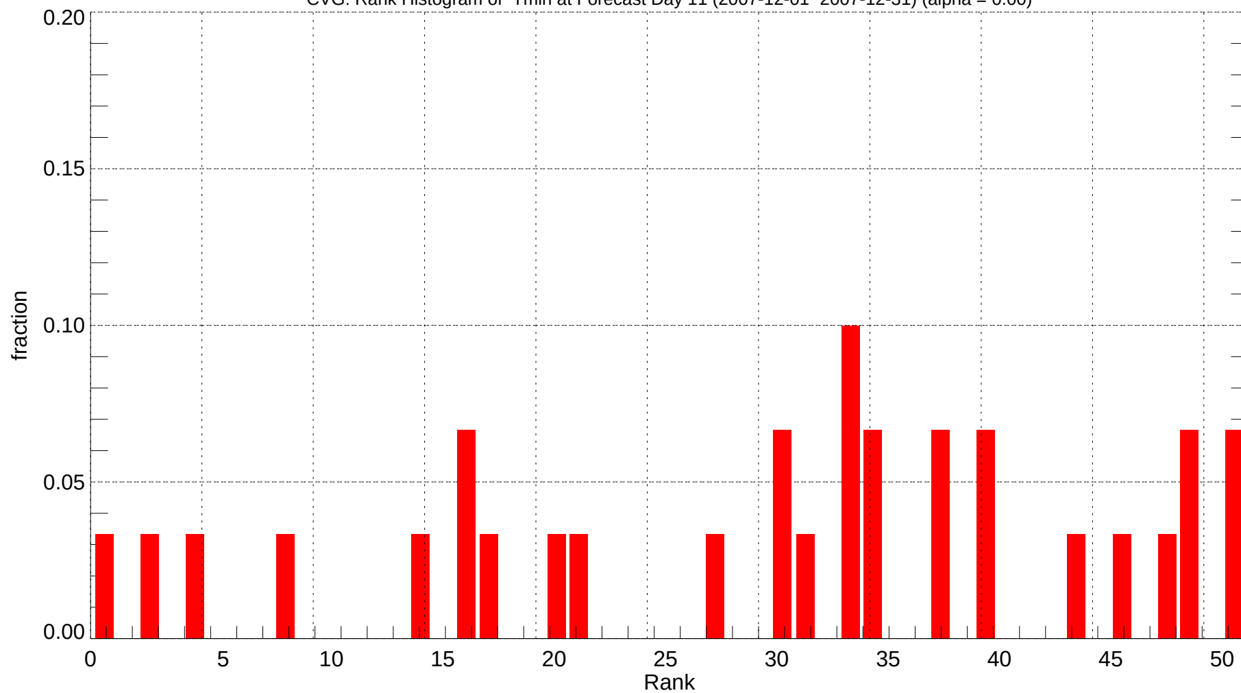
CVG: Rank Histogram of Tmin at Forecast Day 11 (2007-12-01~2007-12-31) (alpha = 0.00)
