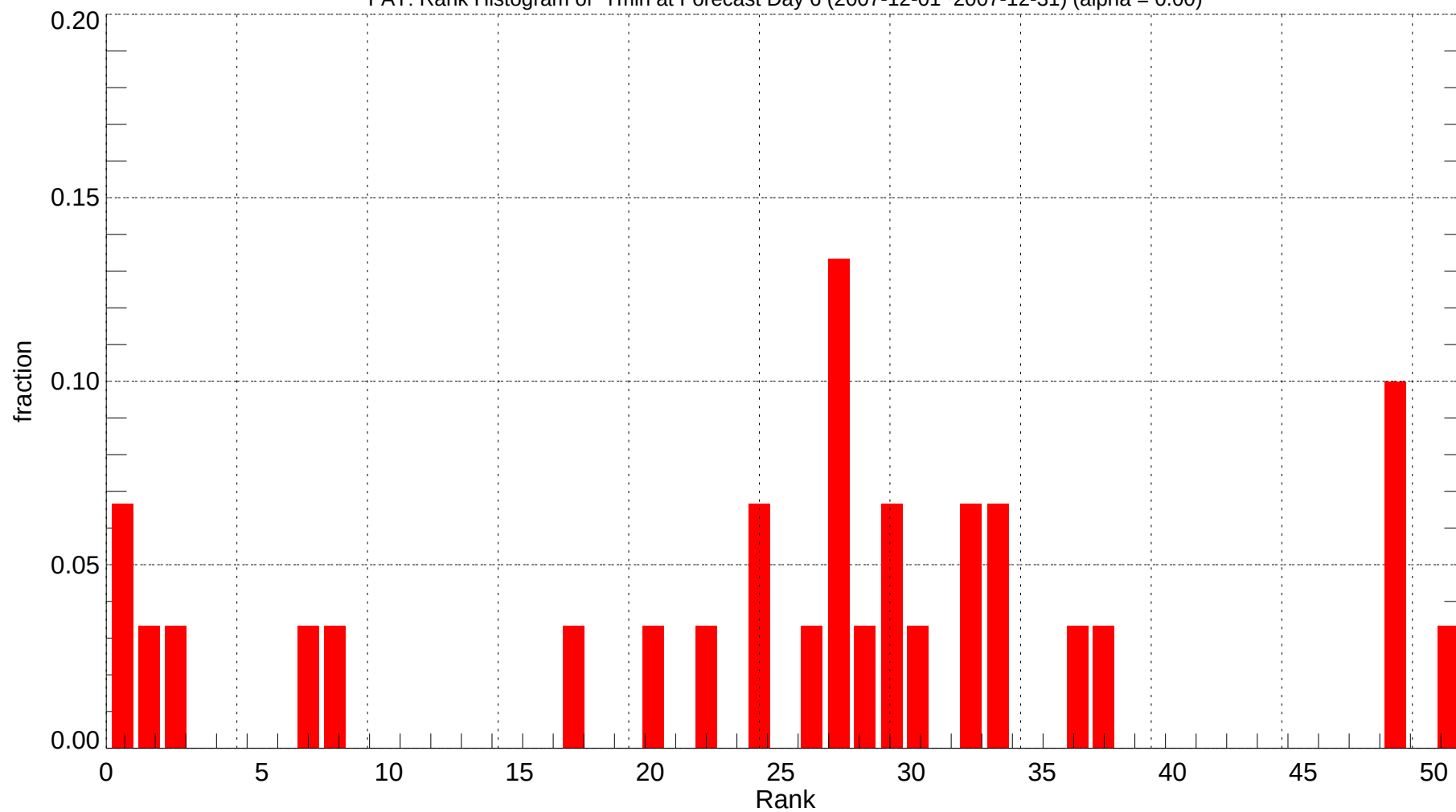
FAT: Rank Histogram of Tmin at Forecast Day 6 (2007-12-01~2007-12-31) (alpha = 0.00)
