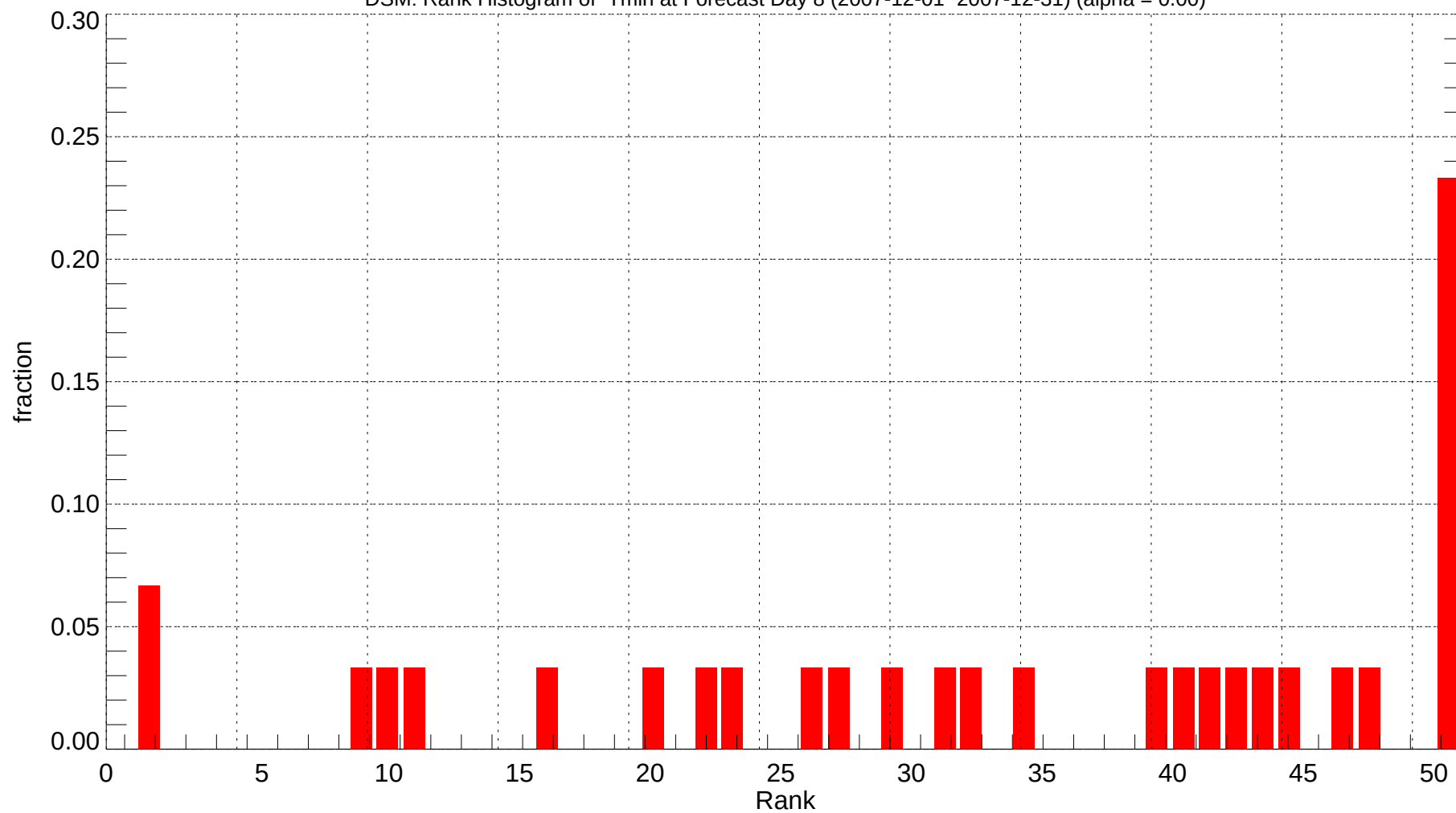
DSM: Rank Histogram of Tmin at Forecast Day 8 (2007-12-01~2007-12-31) (alpha = 0.00)
