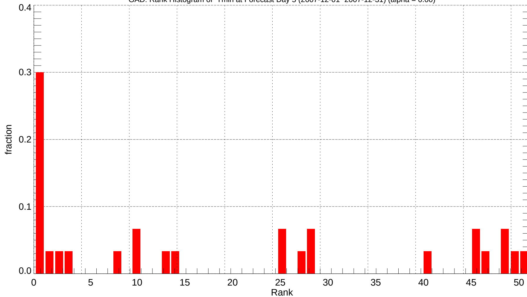
GAD: Rank Histogram of Tmin at Forecast Day 5 (2007-12-01~2007-12-31) (alpha = 0.00)
