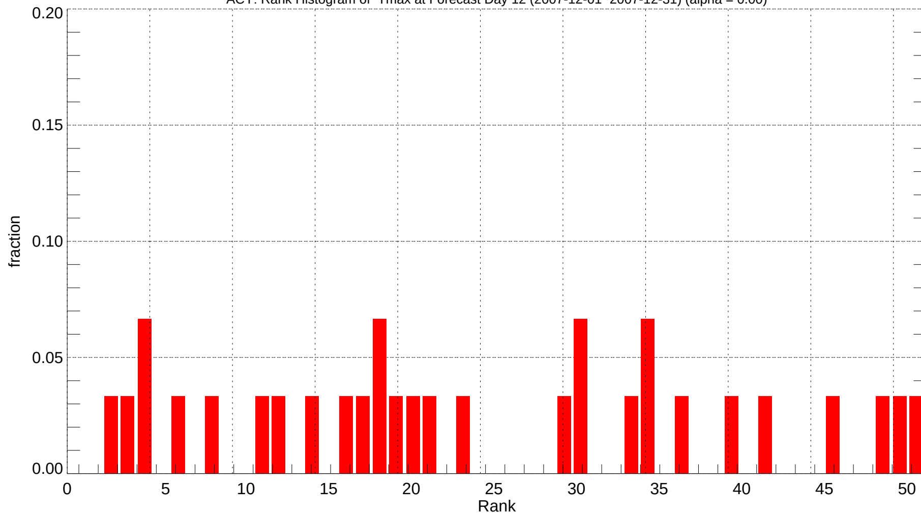
ACY: Rank Histogram of Tmax at Forecast Day 12 (2007-12-01~2007-12-31) (alpha = 0.00)
