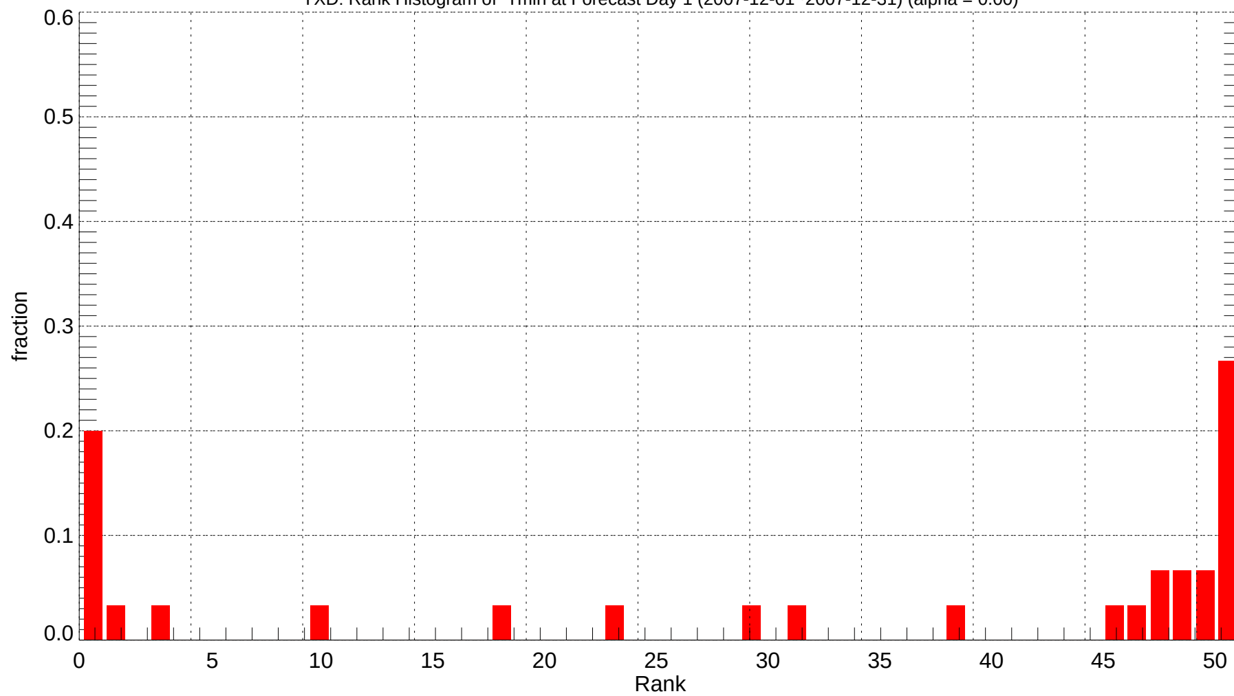
YXD: Rank Histogram of Tmin at Forecast Day 1 (2007-12-01~2007-12-31) (alpha = 0.00)
