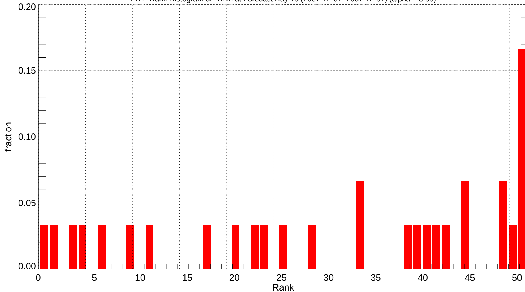
PDT: Rank Histogram of Tmin at Forecast Day 15 (2007-12-01~2007-12-31) (alpha = 0.00)
