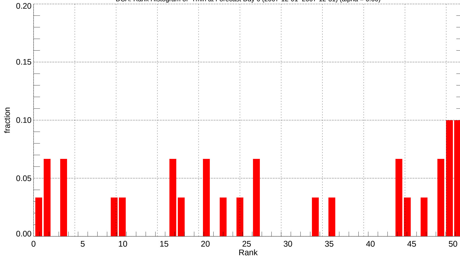
DCA: Rank Histogram of Tmin at Forecast Day 6 (2007-12-01~2007-12-31) (alpha = 0.00)
