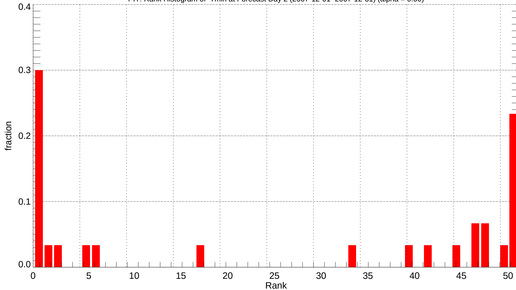
PIT: Rank Histogram of Tmin at Forecast Day 2 (2007-12-01~2007-12-31) (alpha = 0.00)
