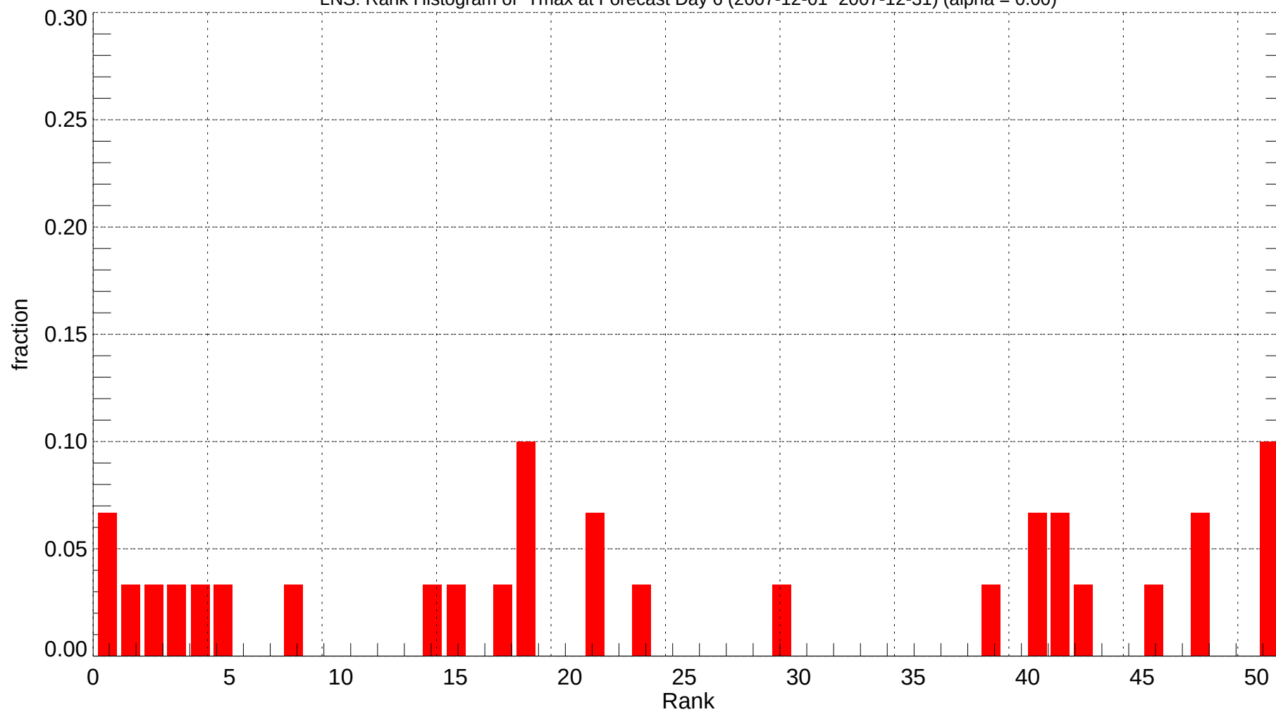
LNS: Rank Histogram of Tmax at Forecast Day 6 (2007-12-01~2007-12-31) (alpha = 0.00)
