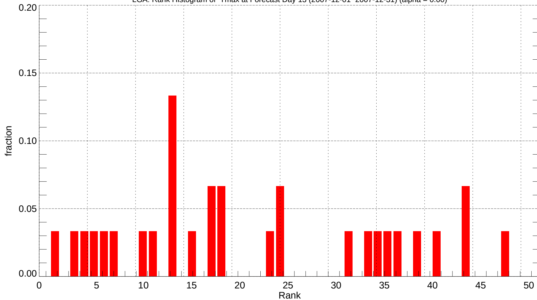
LGA: Rank Histogram of Tmax at Forecast Day 13 (2007-12-01~2007-12-31) (alpha = 0.00)
