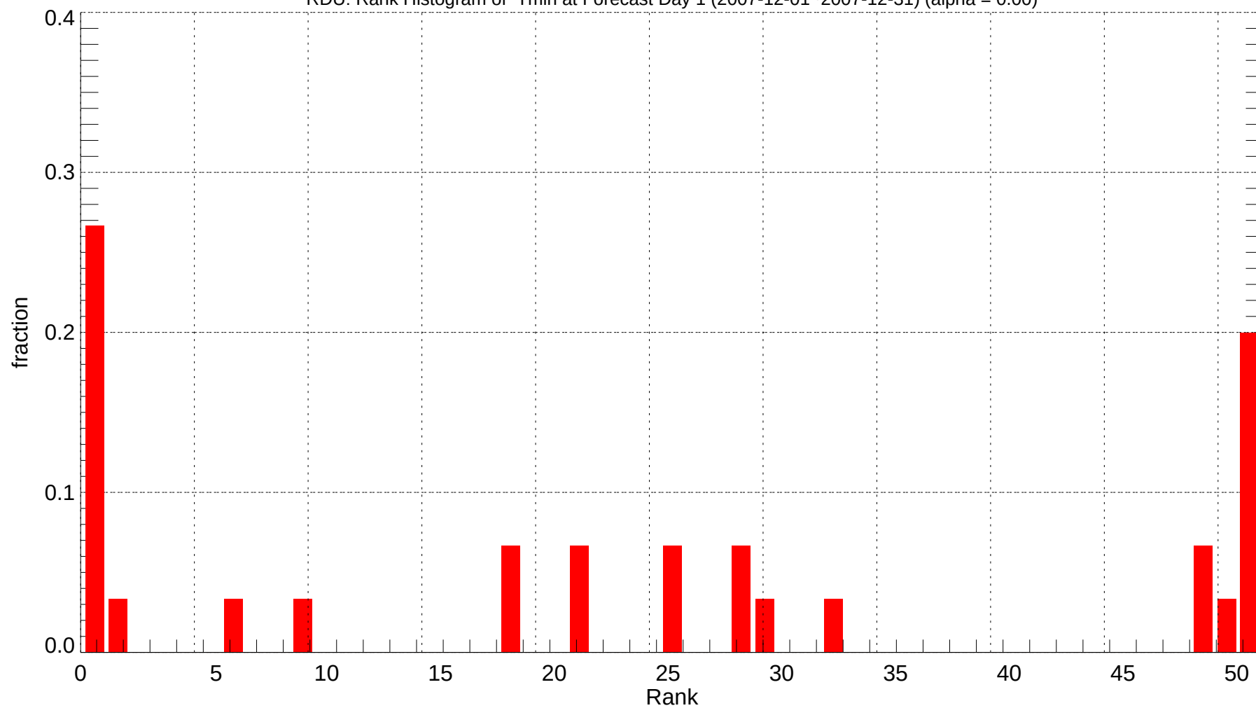
RDU: Rank Histogram of Tmin at Forecast Day 1 (2007-12-01~2007-12-31) (alpha = 0.00)
