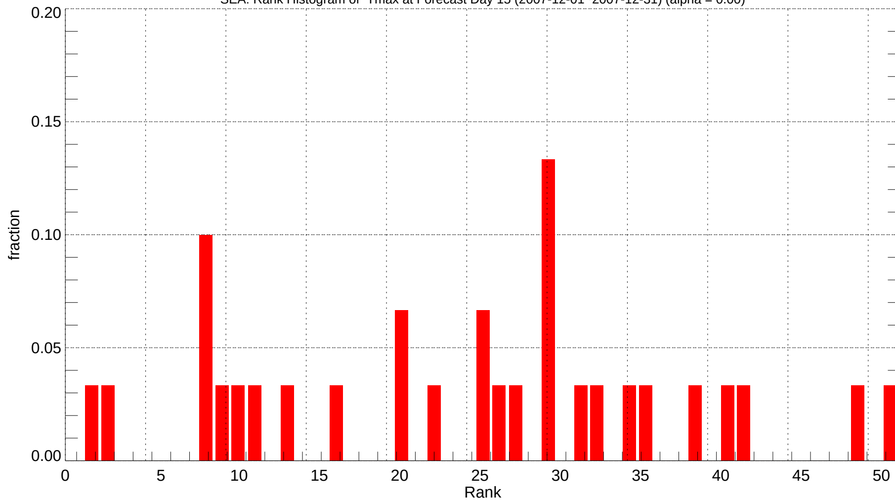
SEA: Rank Histogram of Tmax at Forecast Day 15 (2007-12-01~2007-12-31) (alpha = 0.00)
