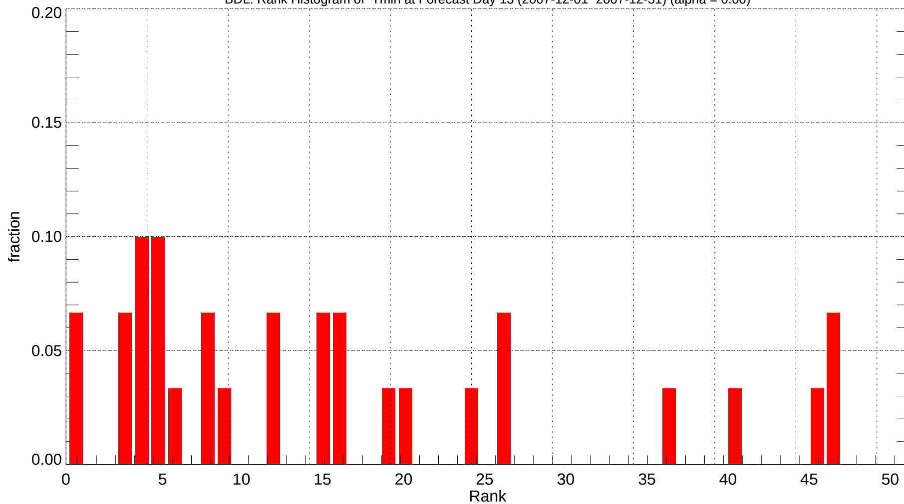
BDL: Rank Histogram of Tmin at Forecast Day 13 (2007-12-01~2007-12-31) (alpha = 0.00)
