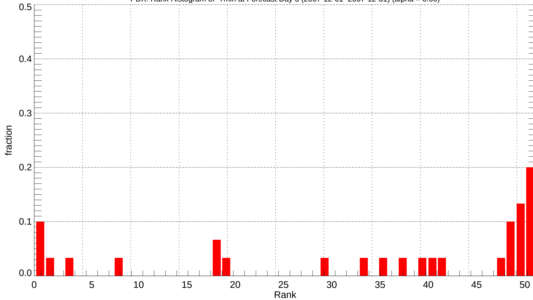
PDX: Rank Histogram of Tmin at Forecast Day 3 (2007-12-01~2007-12-31) (alpha = 0.00)
