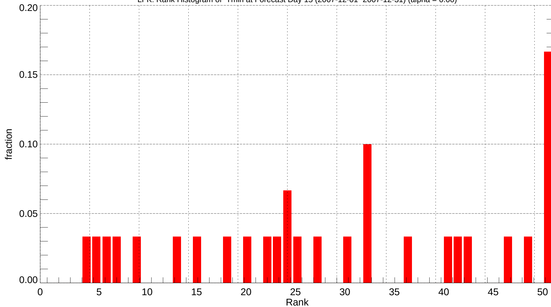
LFK: Rank Histogram of Tmin at Forecast Day 15 (2007-12-01~2007-12-31) (alpha = 0.00)
