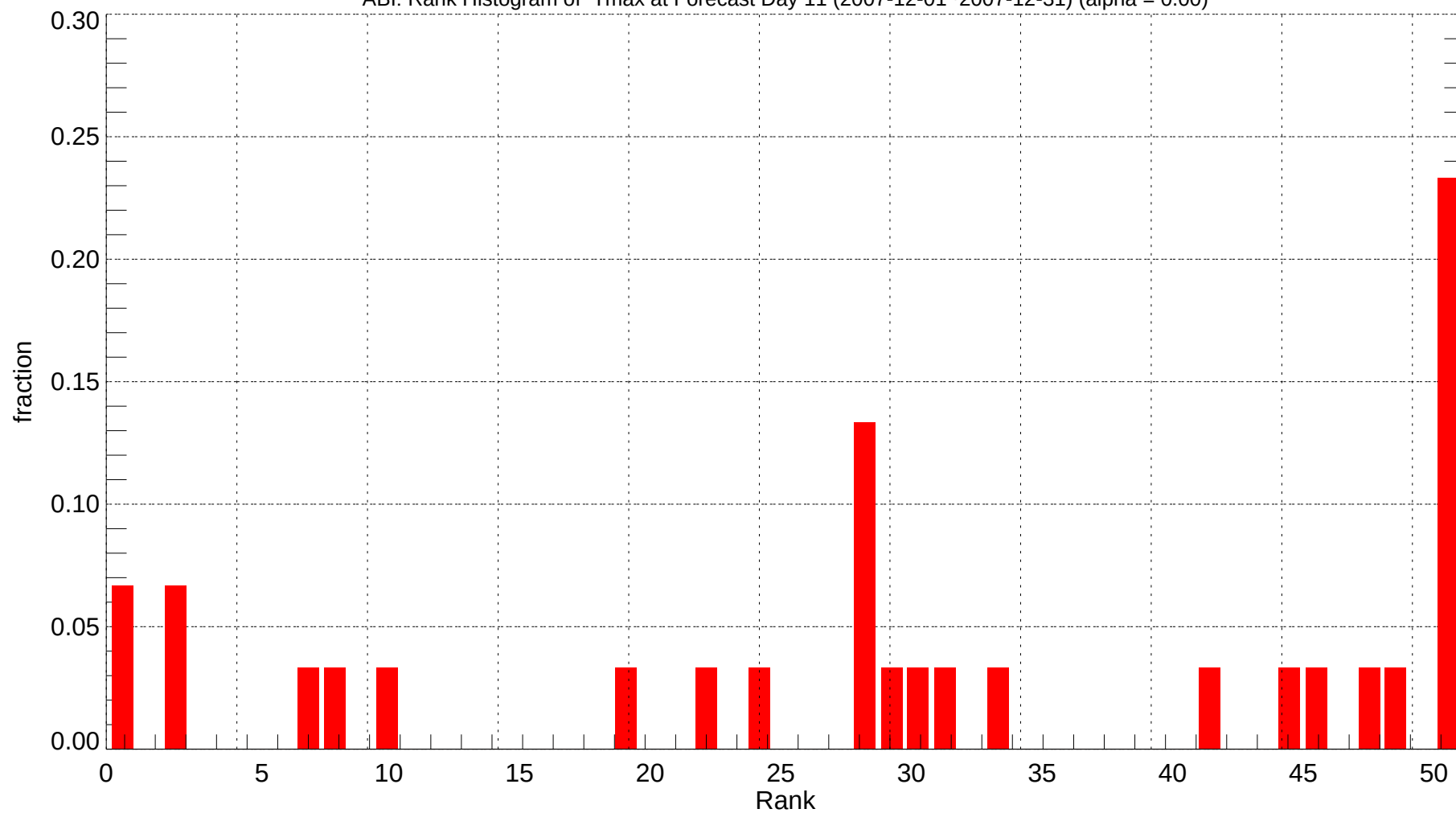
ABI: Rank Histogram of Tmax at Forecast Day 11 (2007-12-01~2007-12-31) (alpha = 0.00)
