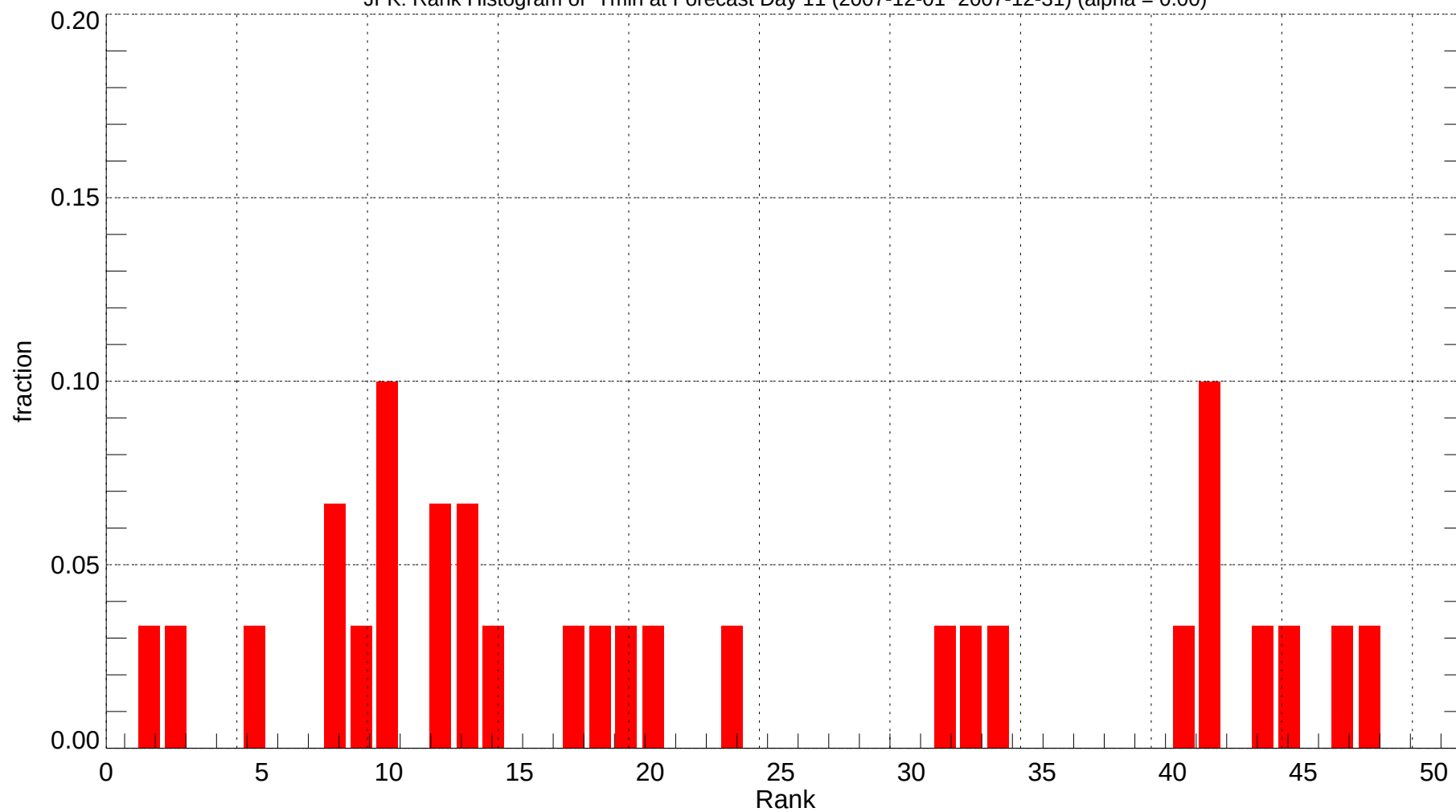
JFK: Rank Histogram of Tmin at Forecast Day 11 (2007-12-01~2007-12-31) (alpha = 0.00)
