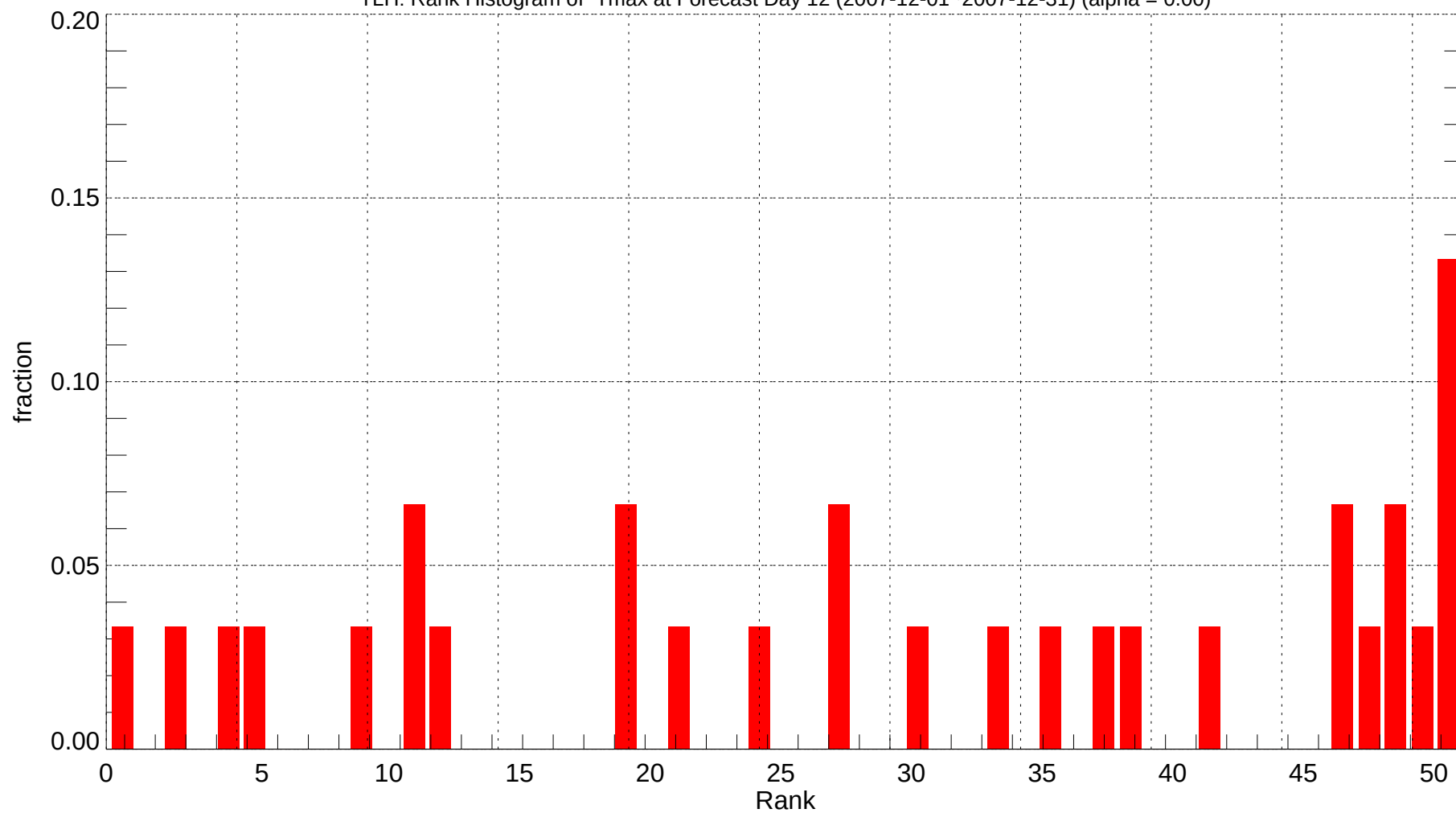
TLH: Rank Histogram of Tmax at Forecast Day 12 (2007-12-01~2007-12-31) (alpha = 0.00)
