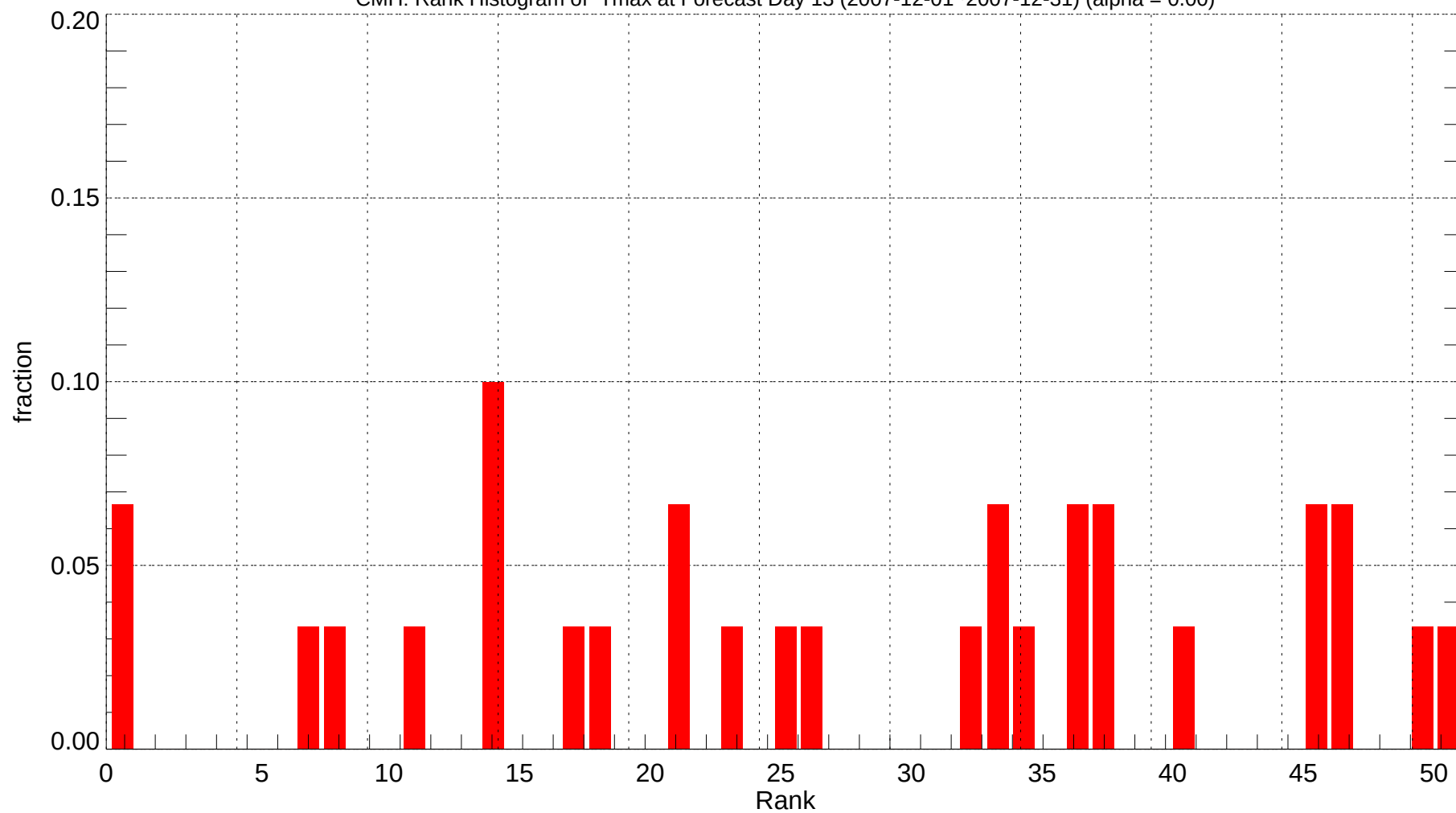
CMH: Rank Histogram of Tmax at Forecast Day 13 (2007-12-01~2007-12-31) (alpha = 0.00)
