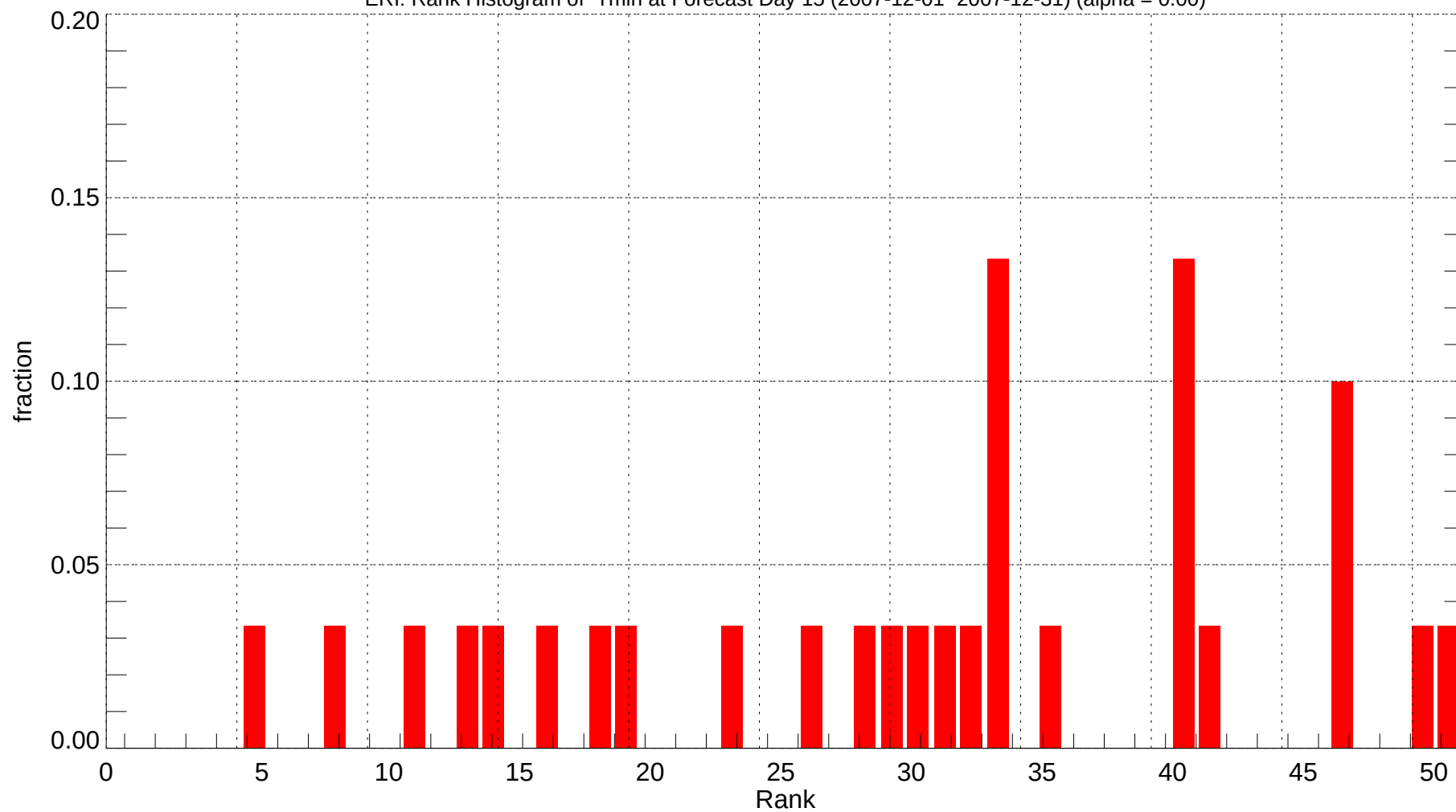
ERI: Rank Histogram of Tmin at Forecast Day 15 (2007-12-01~2007-12-31) (alpha = 0.00)
