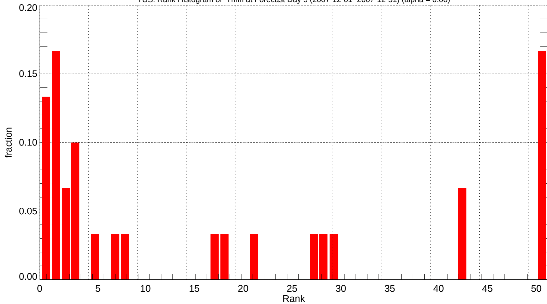
TUS: Rank Histogram of Tmin at Forecast Day 3 (2007-12-01~2007-12-31) (alpha = 0.00)
