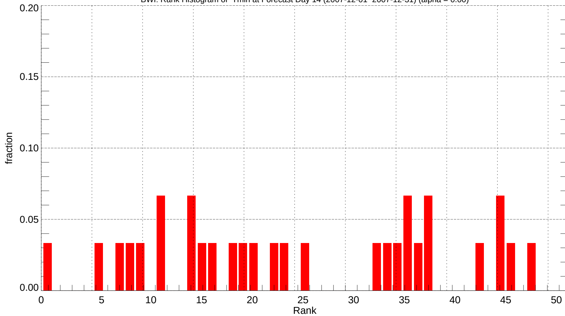
BWl: Rank Histogram of Tmin at Forecast Day 14 (2007-12-01~2007-12-31) (alpha = 0.00)
