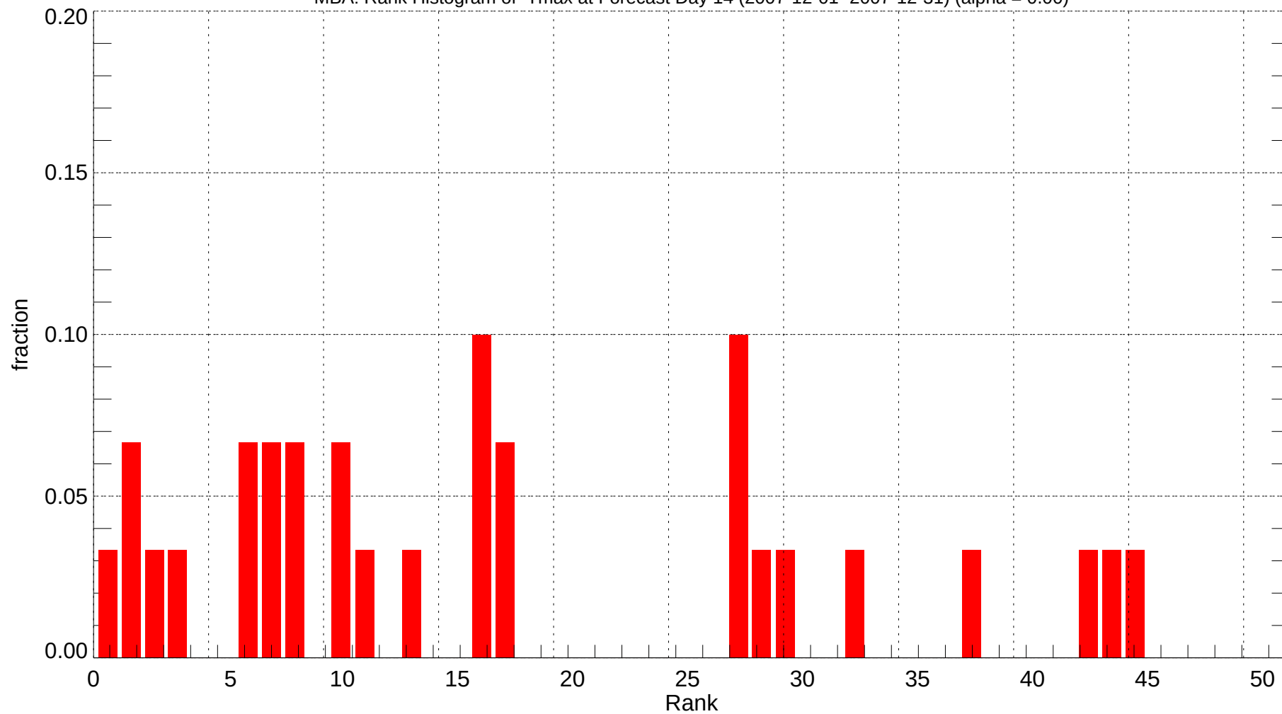
MBA: Rank Histogram of Tmax at Forecast Day 14 (2007-12-01~2007-12-31) (alpha = 0.00)
