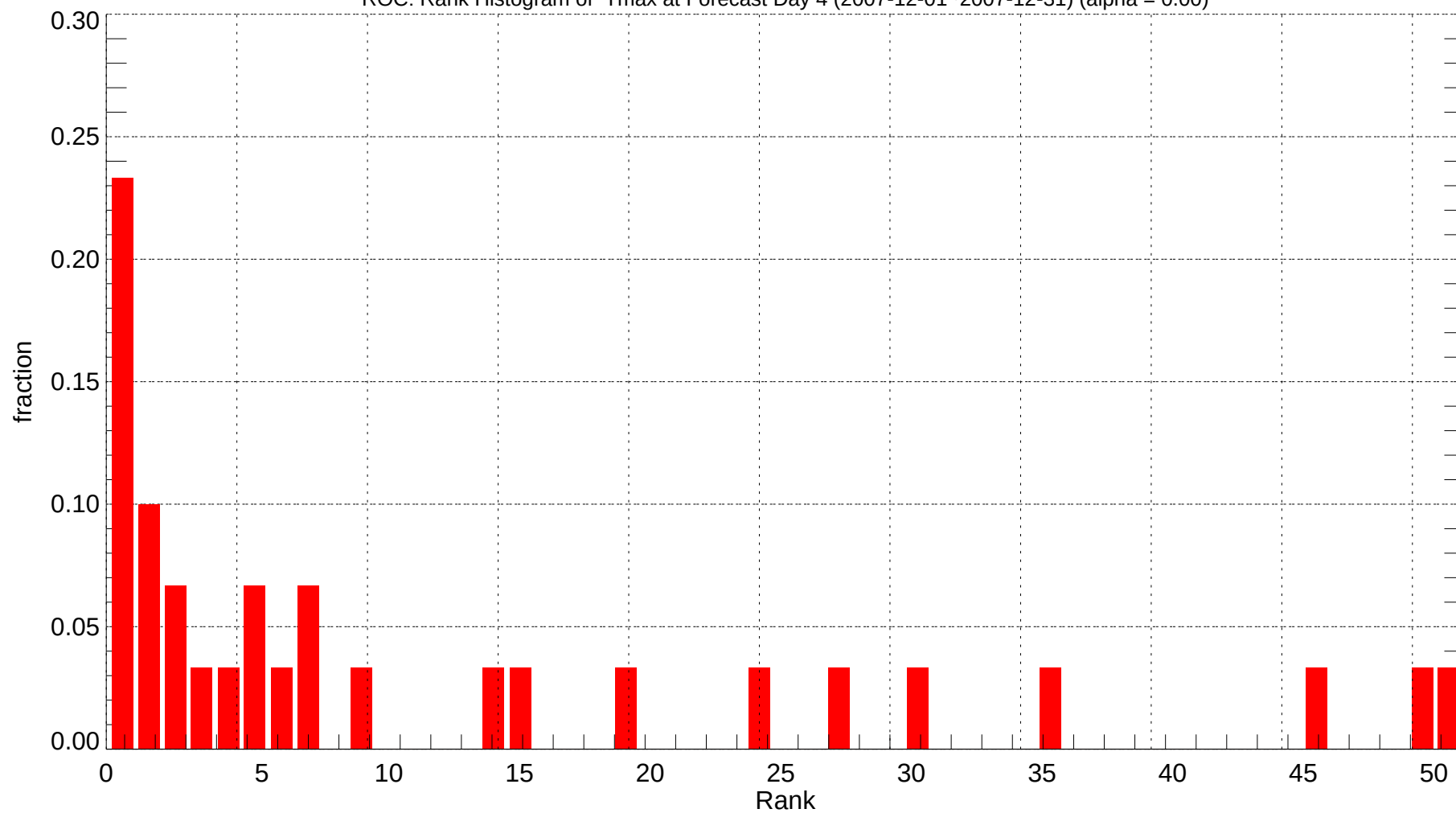
ROC: Rank Histogram of Tmax at Forecast Day 4 (2007-12-01~2007-12-31) (alpha = 0.00)
