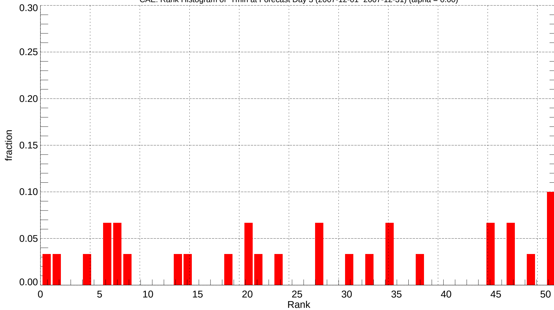
CAE: Rank Histogram of Tmin at Forecast Day 3 (2007-12-01~2007-12-31) (alpha = 0.00)
