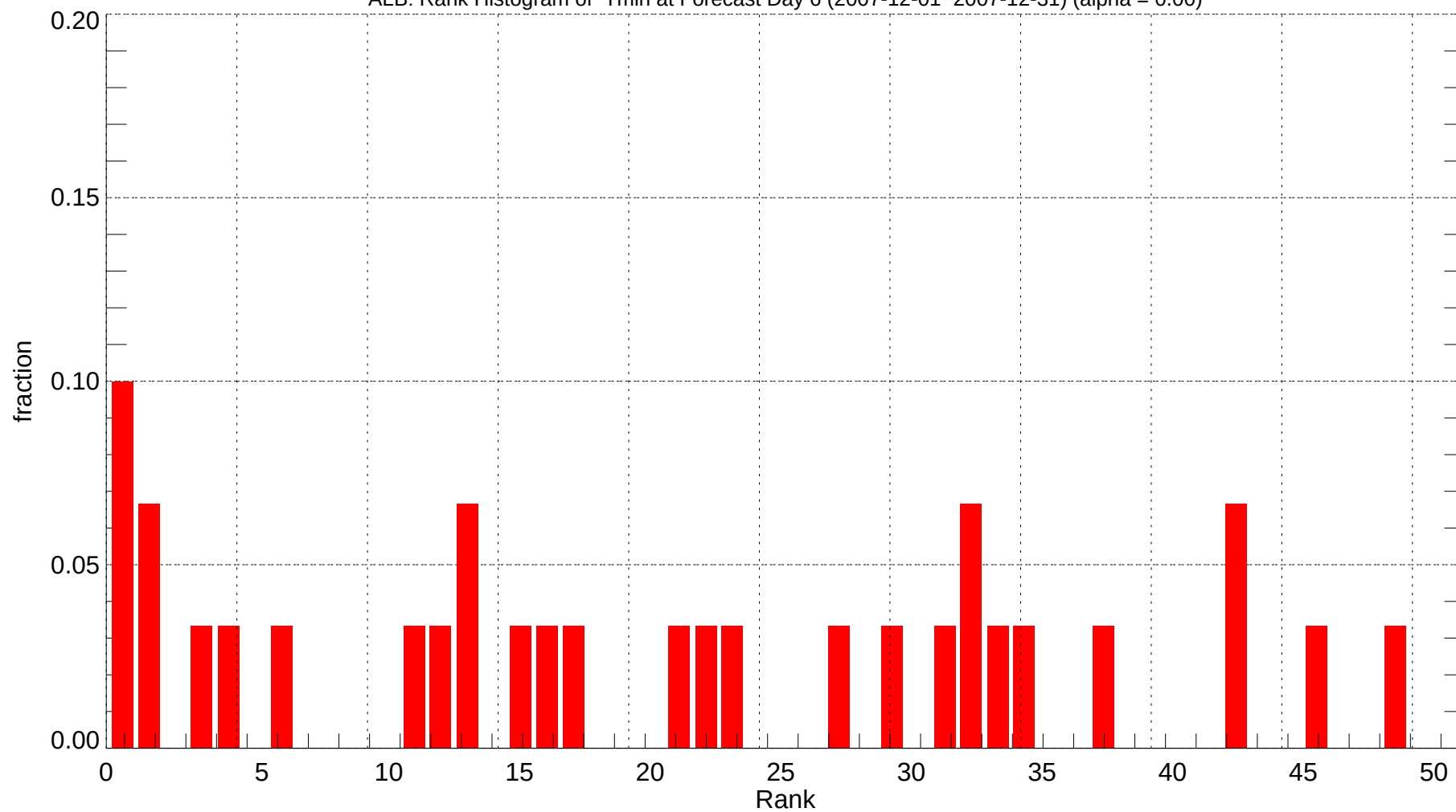
ALB: Rank Histogram of Tmin at Forecast Day 6 (2007-12-01~2007-12-31) (alpha = 0.00)
