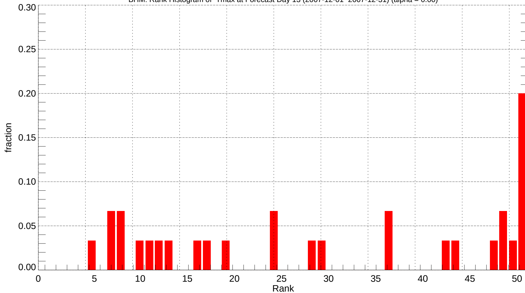
BHM: Rank Histogram of Tmax at Forecast Day 13 (2007-12-01~2007-12-31) (alpha = 0.00)
