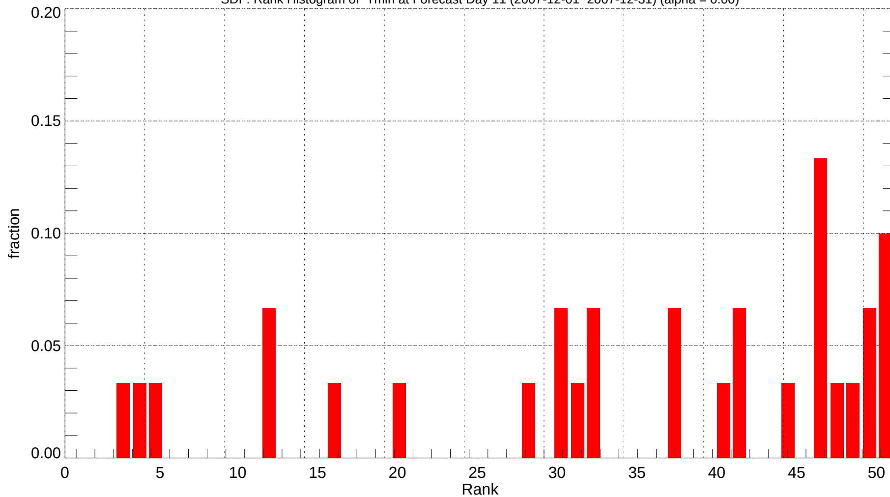
SDF: Rank Histogram of Tmin at Forecast Day 11 (2007-12-01~2007-12-31) (alpha = 0.00)
