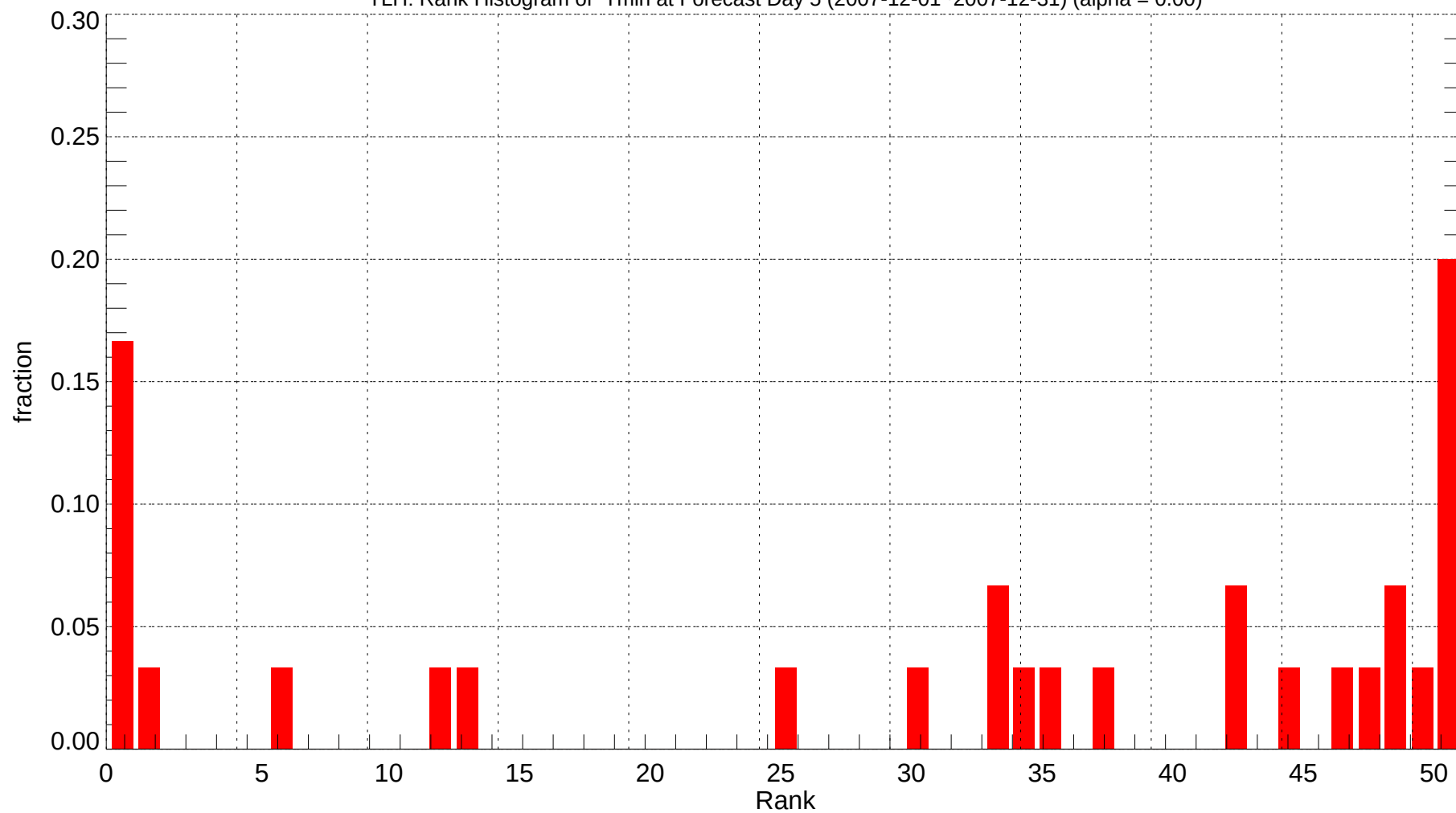
TLH: Rank Histogram of Tmin at Forecast Day 5 (2007-12-01~2007-12-31) (alpha = 0.00)
