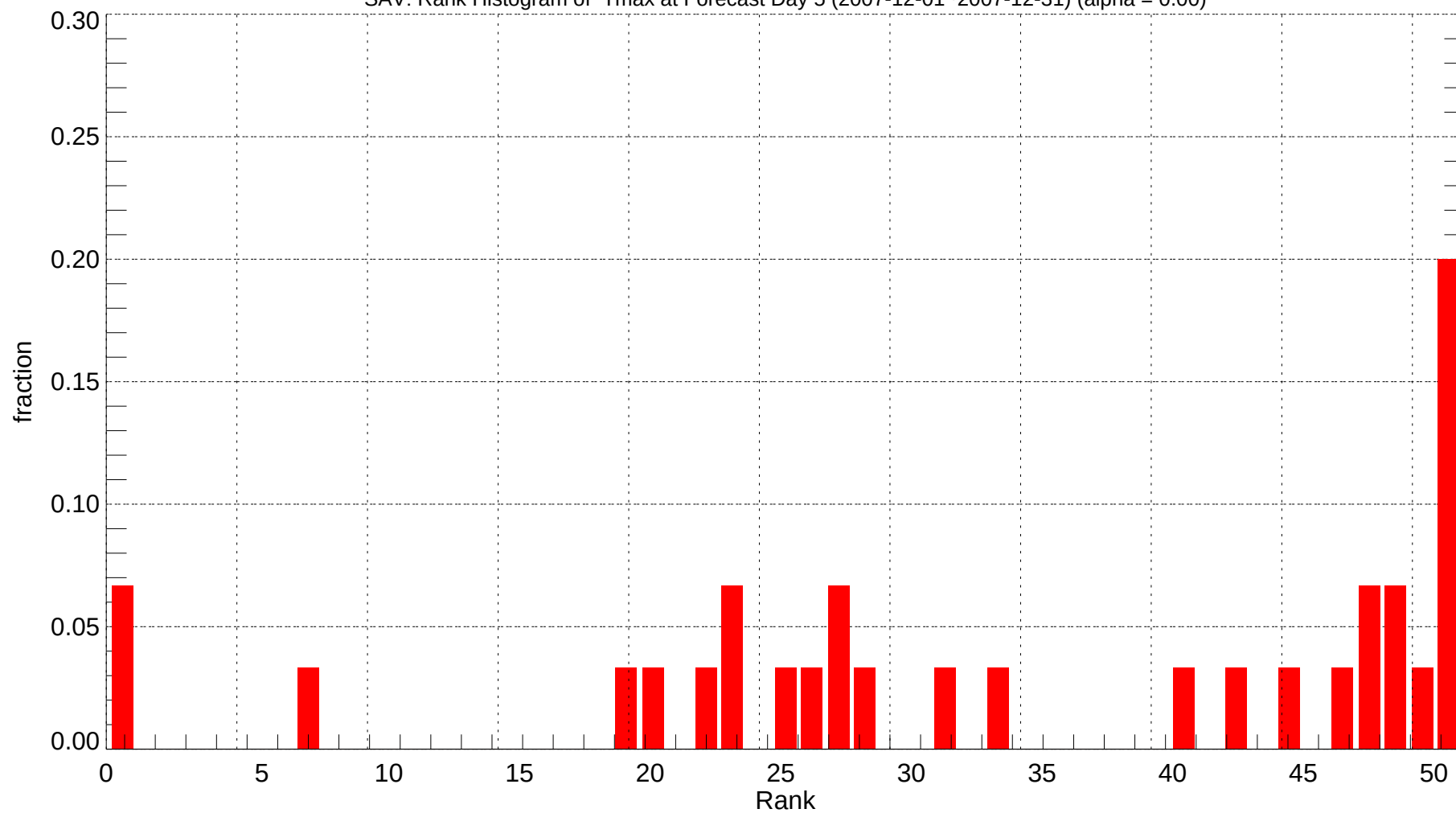
SAV: Rank Histogram of Tmax at Forecast Day 5 (2007-12-01~2007-12-31) (alpha = 0.00)
