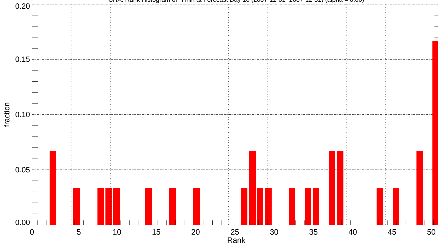
CHA: Rank Histogram of Tmin at Forecast Day 10 (2007-12-01~2007-12-31) (alpha = 0.00)
