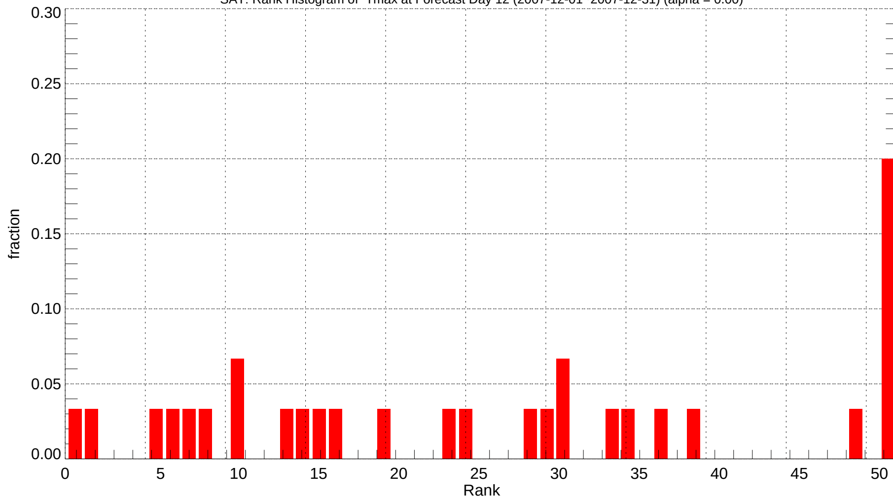
SAT: Rank Histogram of Tmax at Forecast Day 12 (2007-12-01~2007-12-31) (alpha = 0.00)
