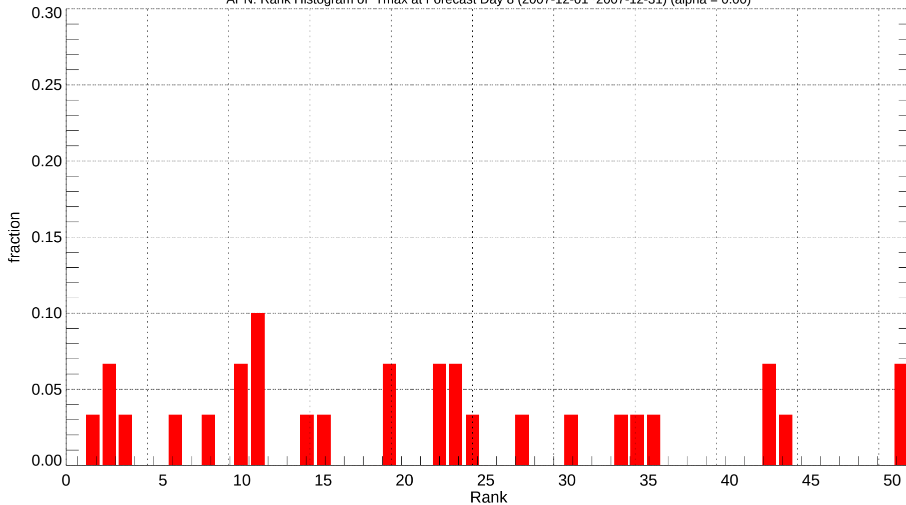
APN: Rank Histogram of Tmax at Forecast Day 8 (2007-12-01~2007-12-31) (alpha = 0.00)
