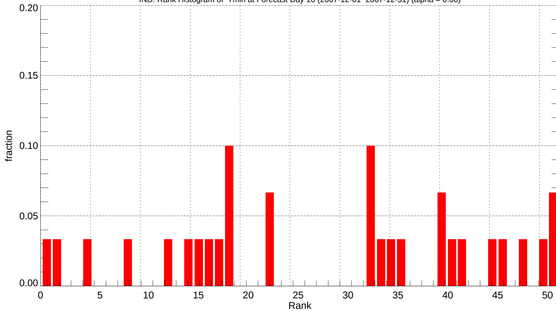
IND: Rank Histogram of Tmin at Forecast Day 10 (2007-12-01~2007-12-31) (alpha = 0.00)
