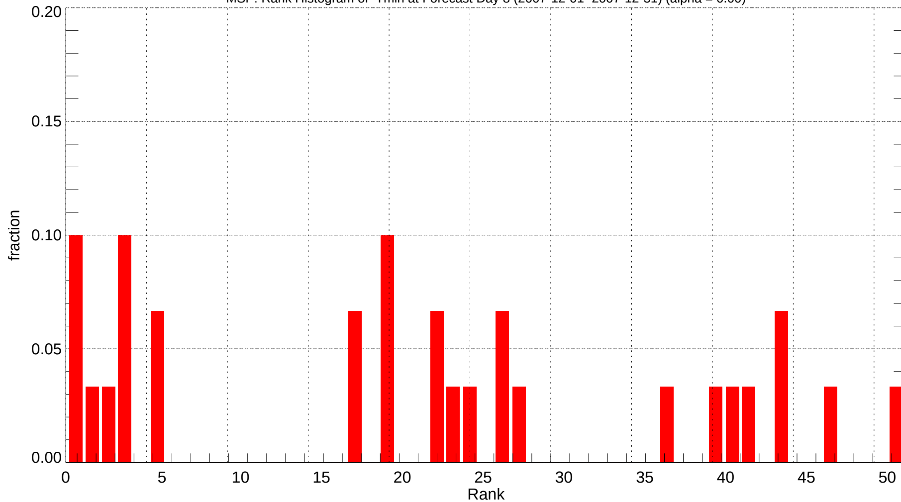
MSP: Rank Histogram of Tmin at Forecast Day 8 (2007-12-01~2007-12-31) (alpha = 0.00)
