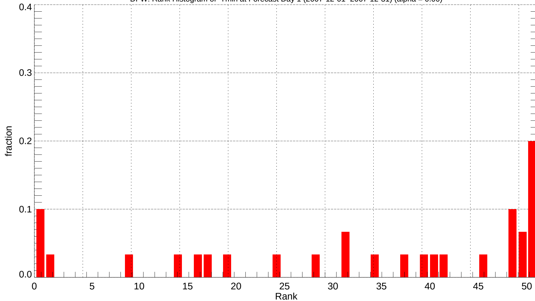
DFW: Rank Histogram of Tmin at Forecast Day 1 (2007-12-01~2007-12-31) (alpha = 0.00)
