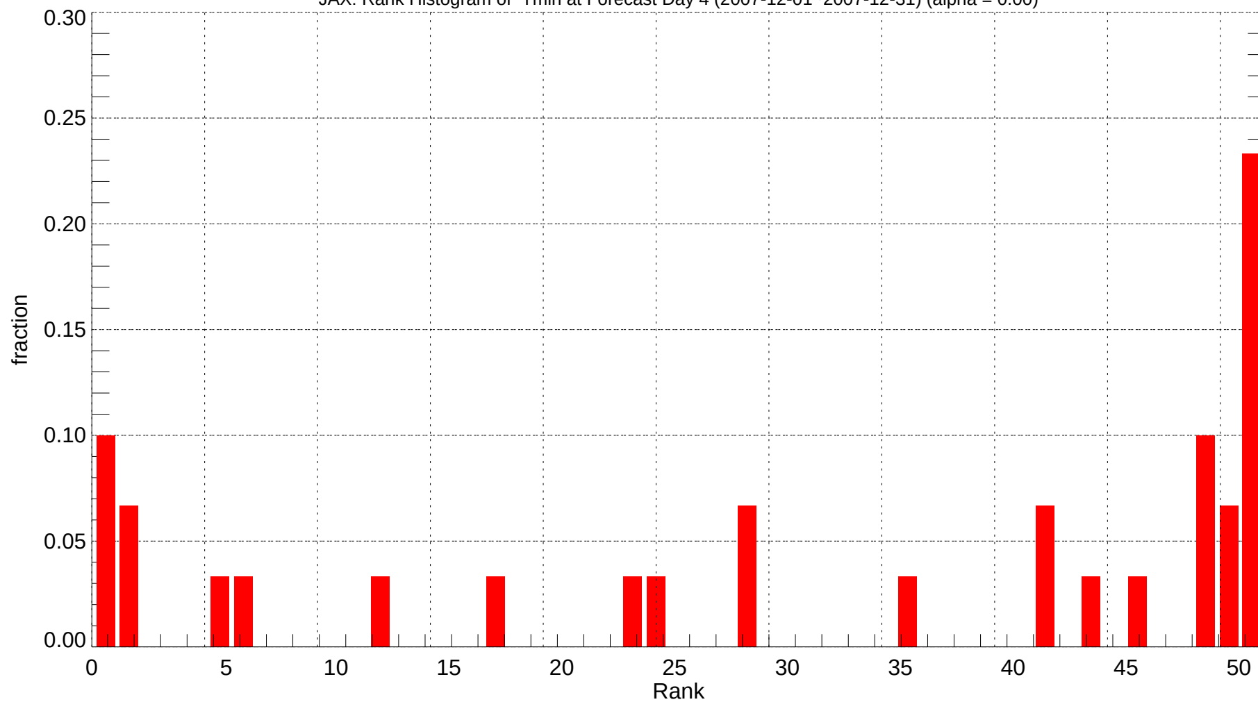
JAX: Rank Histogram of Tmin at Forecast Day 4 (2007-12-01~2007-12-31) (alpha = 0.00)
