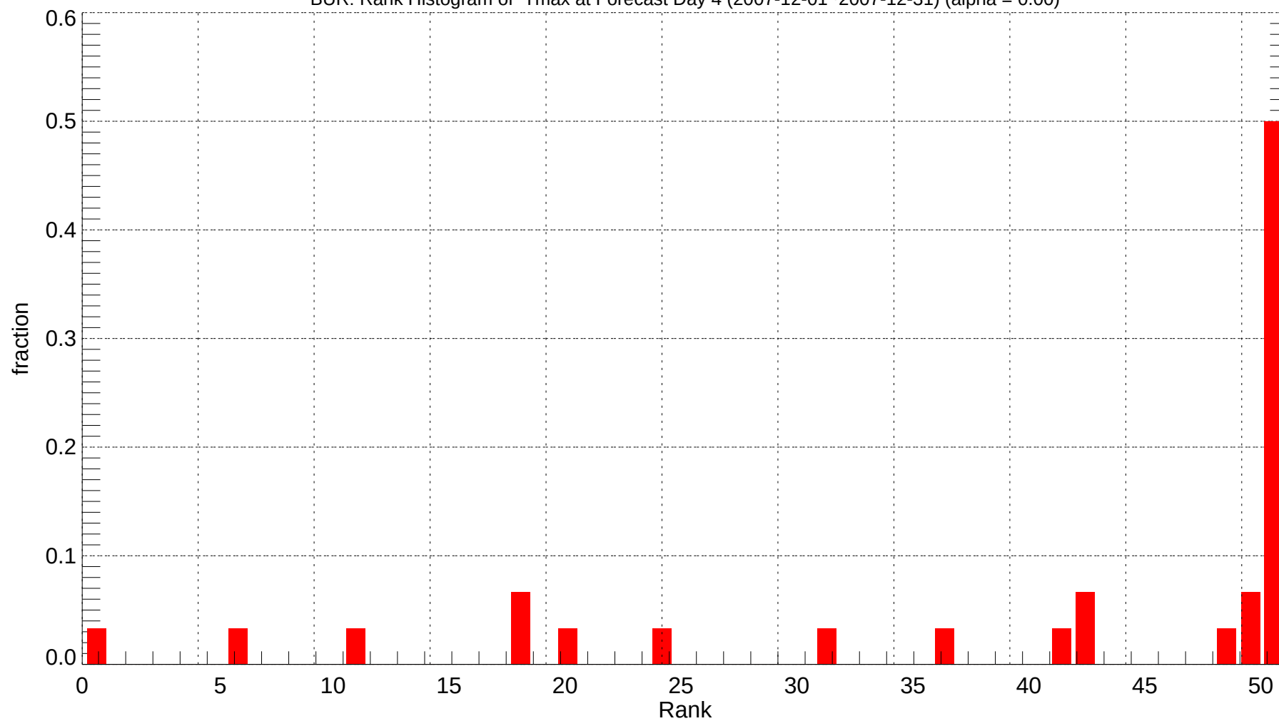
BUR: Rank Histogram of Tmax at Forecast Day 4 (2007-12-01~2007-12-31) (alpha = 0.00)
