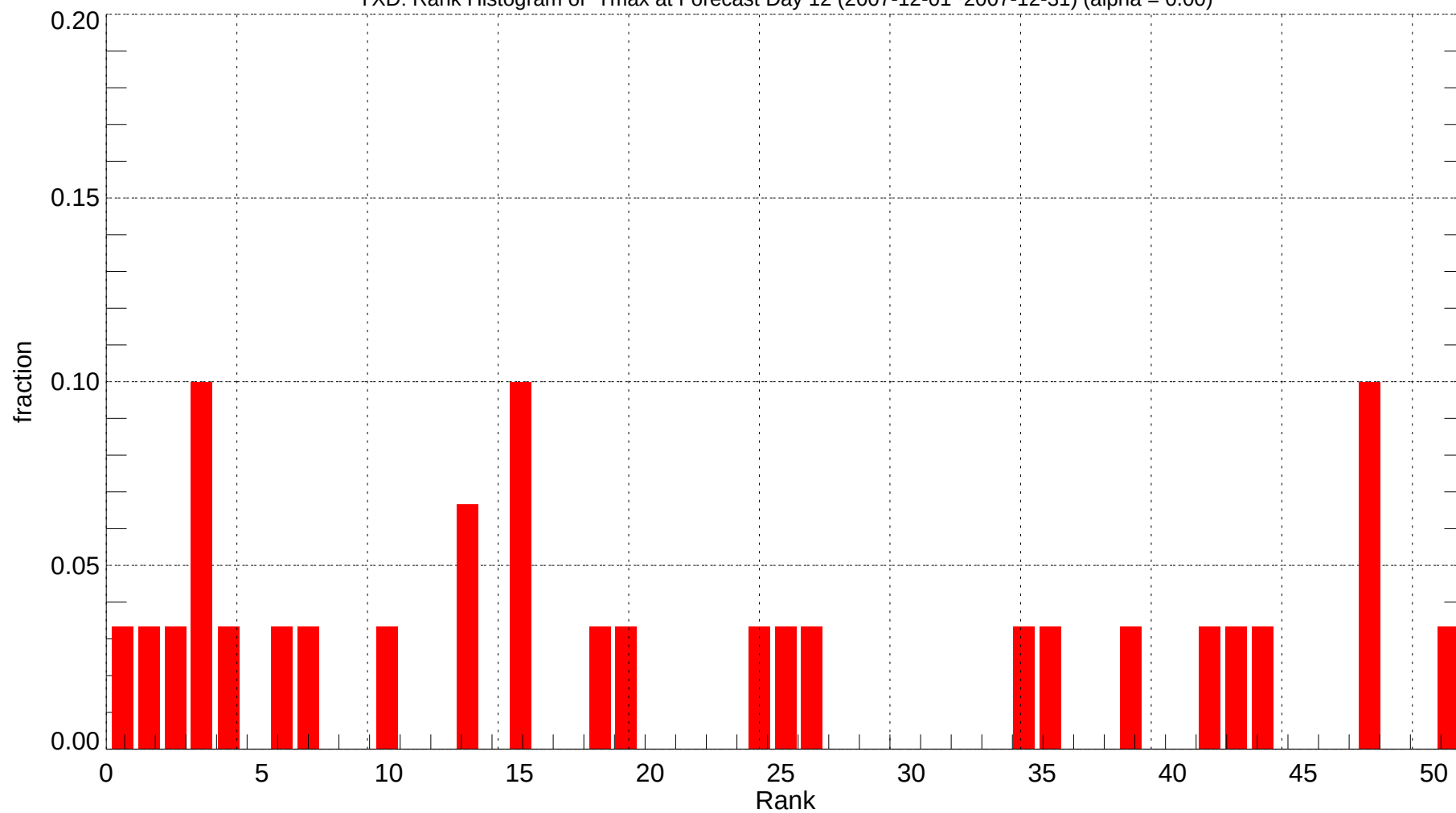
YXD: Rank Histogram of Tmax at Forecast Day 12 (2007-12-01~2007-12-31) (alpha = 0.00)
