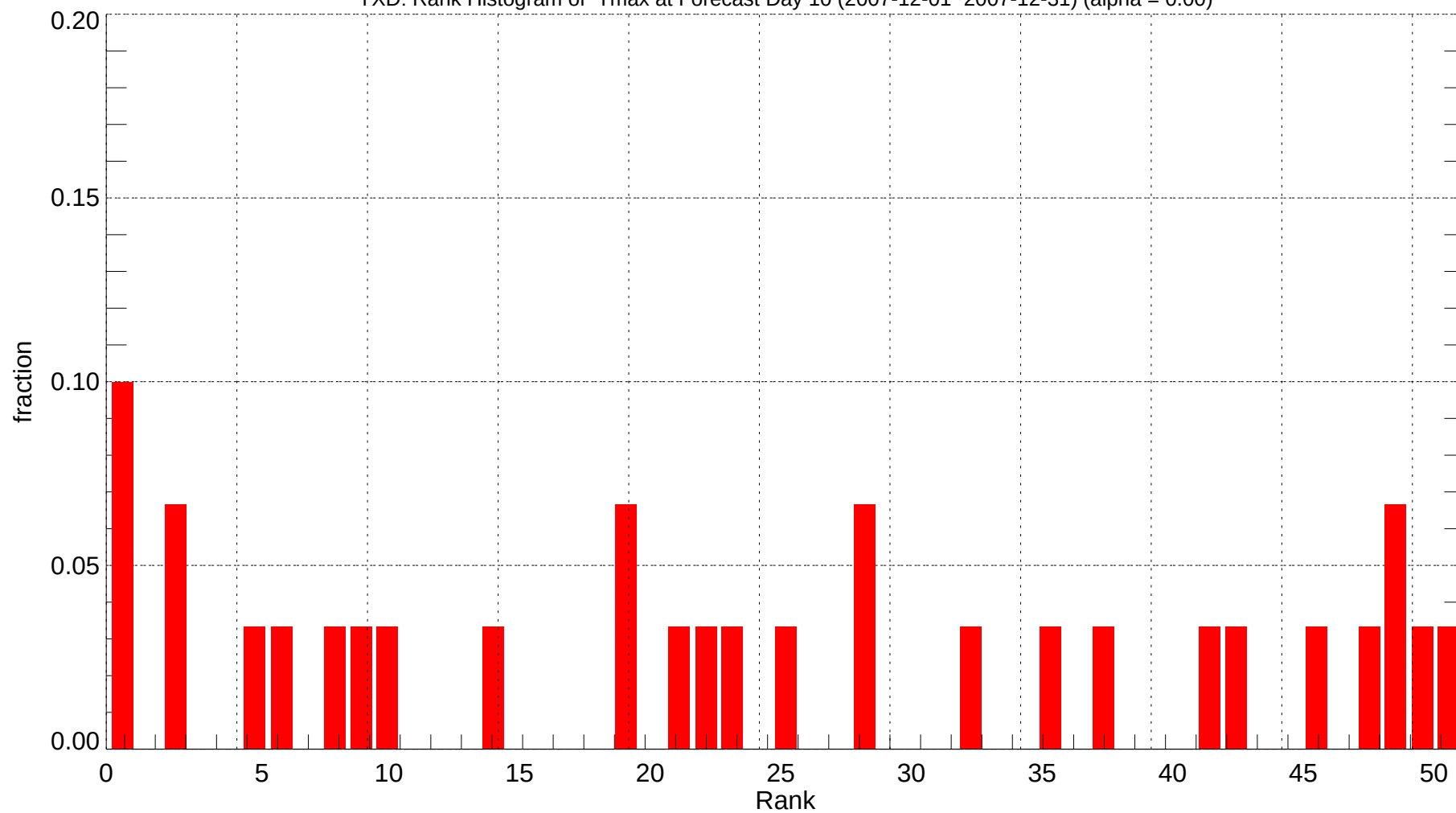
YXD: Rank Histogram of Tmax at Forecast Day 10 (2007-12-01~2007-12-31) (alpha = 0.00)
