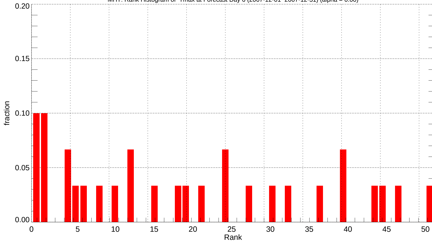
MHT: Rank Histogram of Tmax at Forecast Day 6 (2007-12-01~2007-12-31) (alpha = 0.00)
