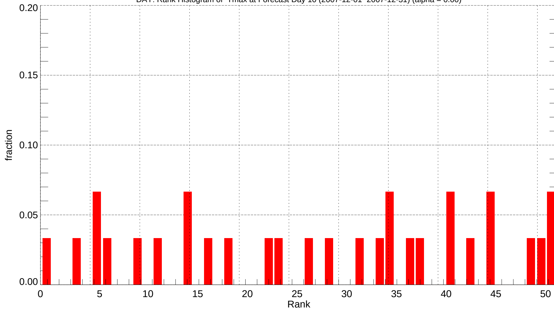
DAY: Rank Histogram of Tmax at Forecast Day 10 (2007-12-01~2007-12-31) (alpha = 0.00)
