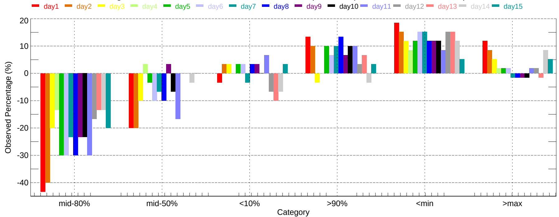
Observed Percentage Deviation of Ensembles - BRO: Max Temperature (2007-12-01~2007-12-31)
