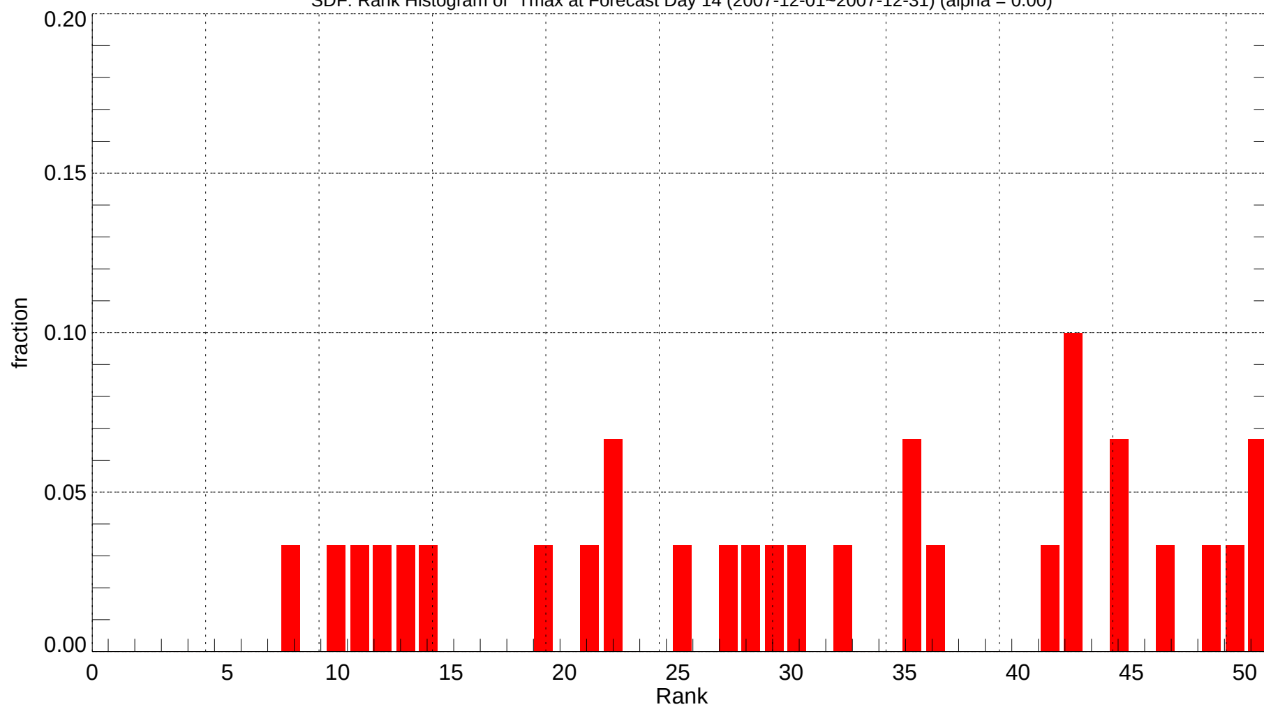
SDF: Rank Histogram of Tmax at Forecast Day 14 (2007-12-01~2007-12-31) (alpha = 0.00)
