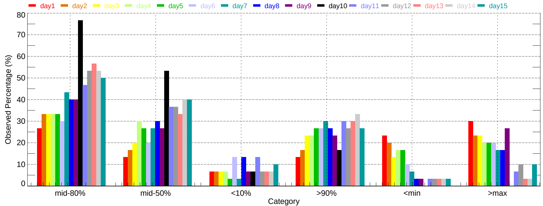
Observed Percentage of Ensembles - TLH: Min Temperature (2007-12-01~2007-12-31)
