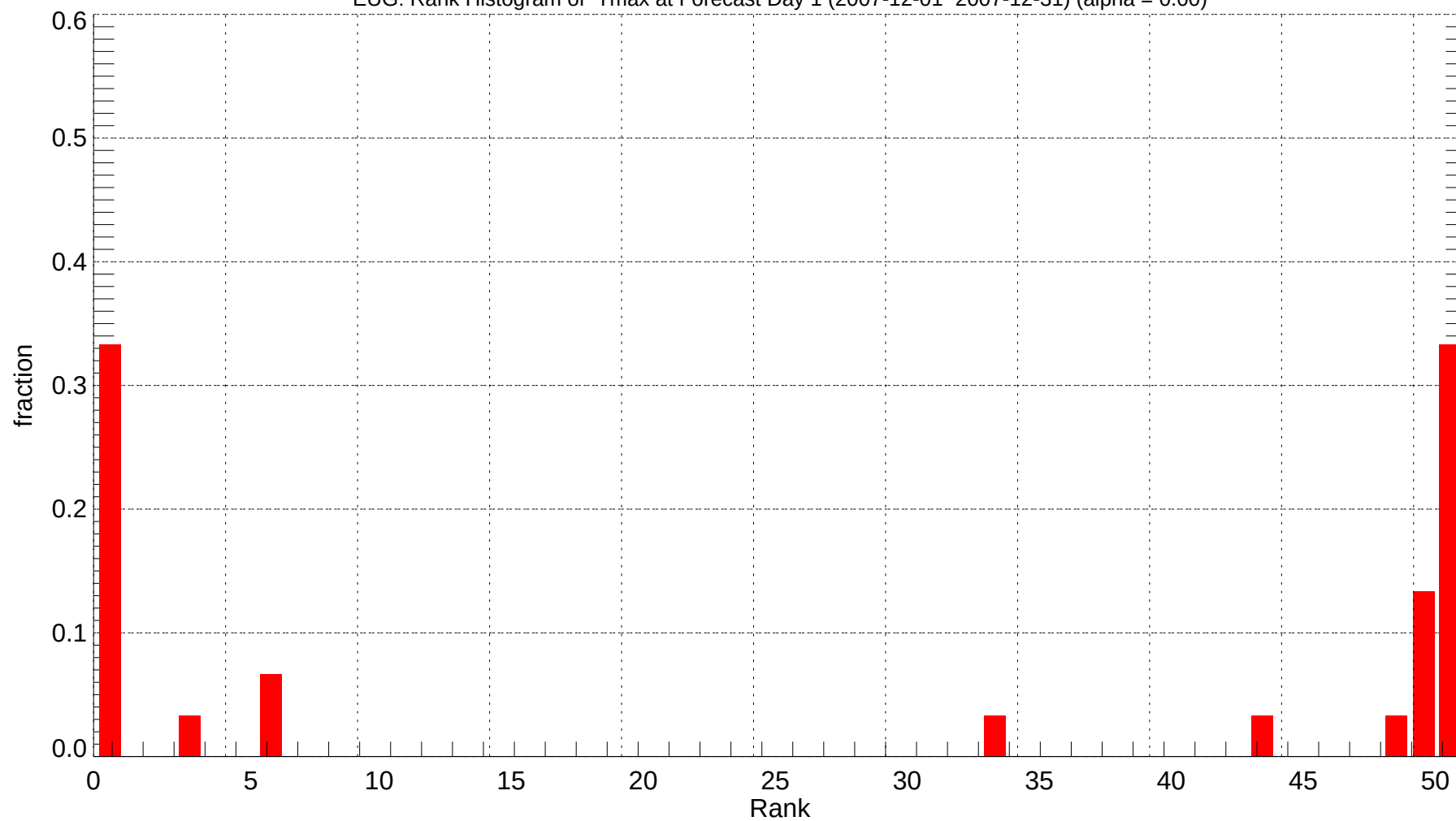
EUG: Rank Histogram of Tmax at Forecast Day 1 (2007-12-01~2007-12-31) (alpha = 0.00)
