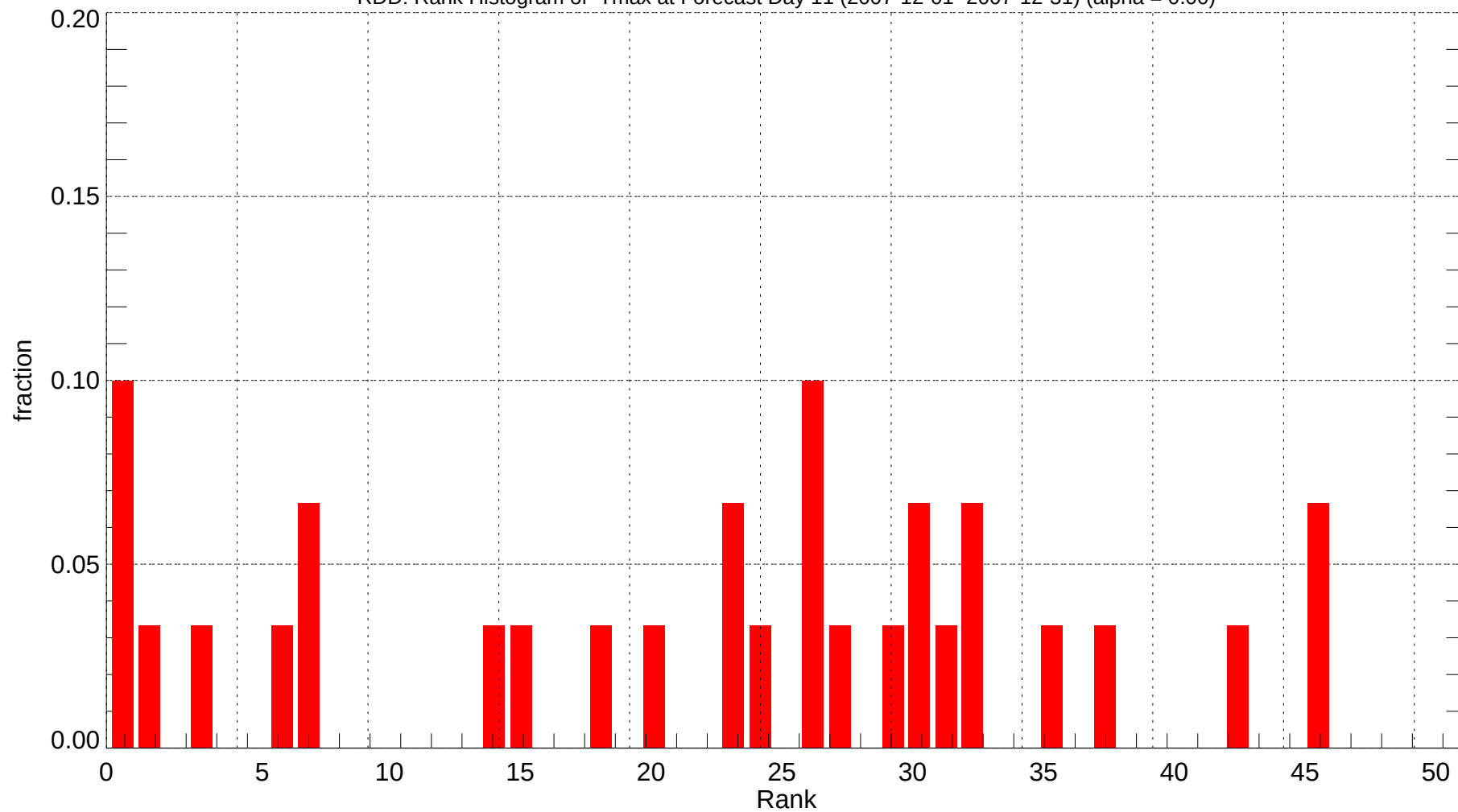
RDD: Rank Histogram of Tmax at Forecast Day 11 (2007-12-01~2007-12-31) (alpha = 0.00)
