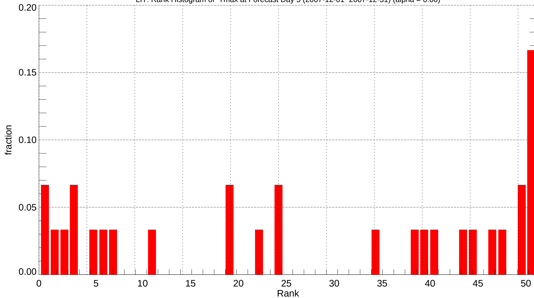
LIT: Rank Histogram of Tmax at Forecast Day 5 (2007-12-01~2007-12-31) (alpha = 0.00)
