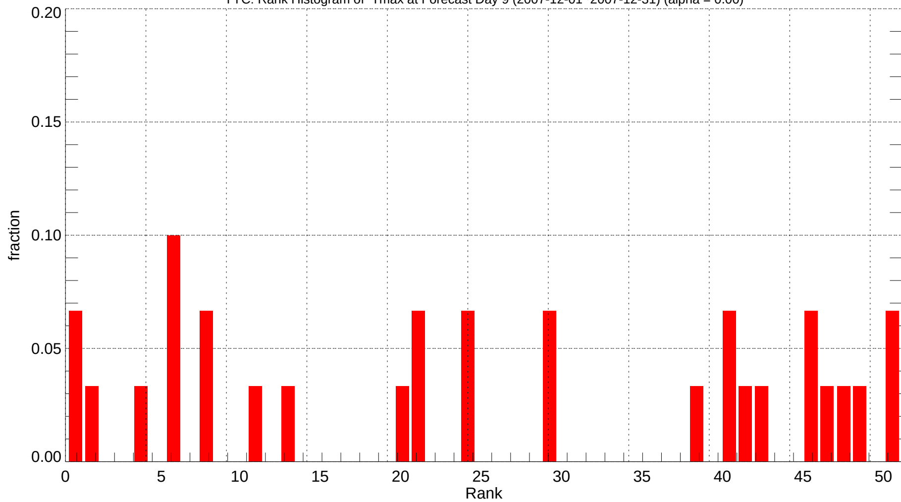
YYC: Rank Histogram of Tmax at Forecast Day 9 (2007-12-01~2007-12-31) (alpha = 0.00)
