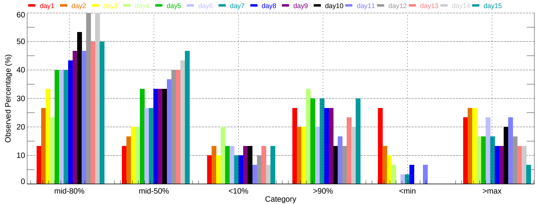
Observed Percentage of Ensembles - ABI: Max Temperature (2007-12-01~2007-12-31)
