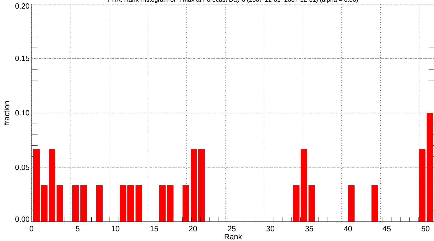
PHX: Rank Histogram of Tmax at Forecast Day 6 (2007-12-01~2007-12-31) (alpha = 0.00)
