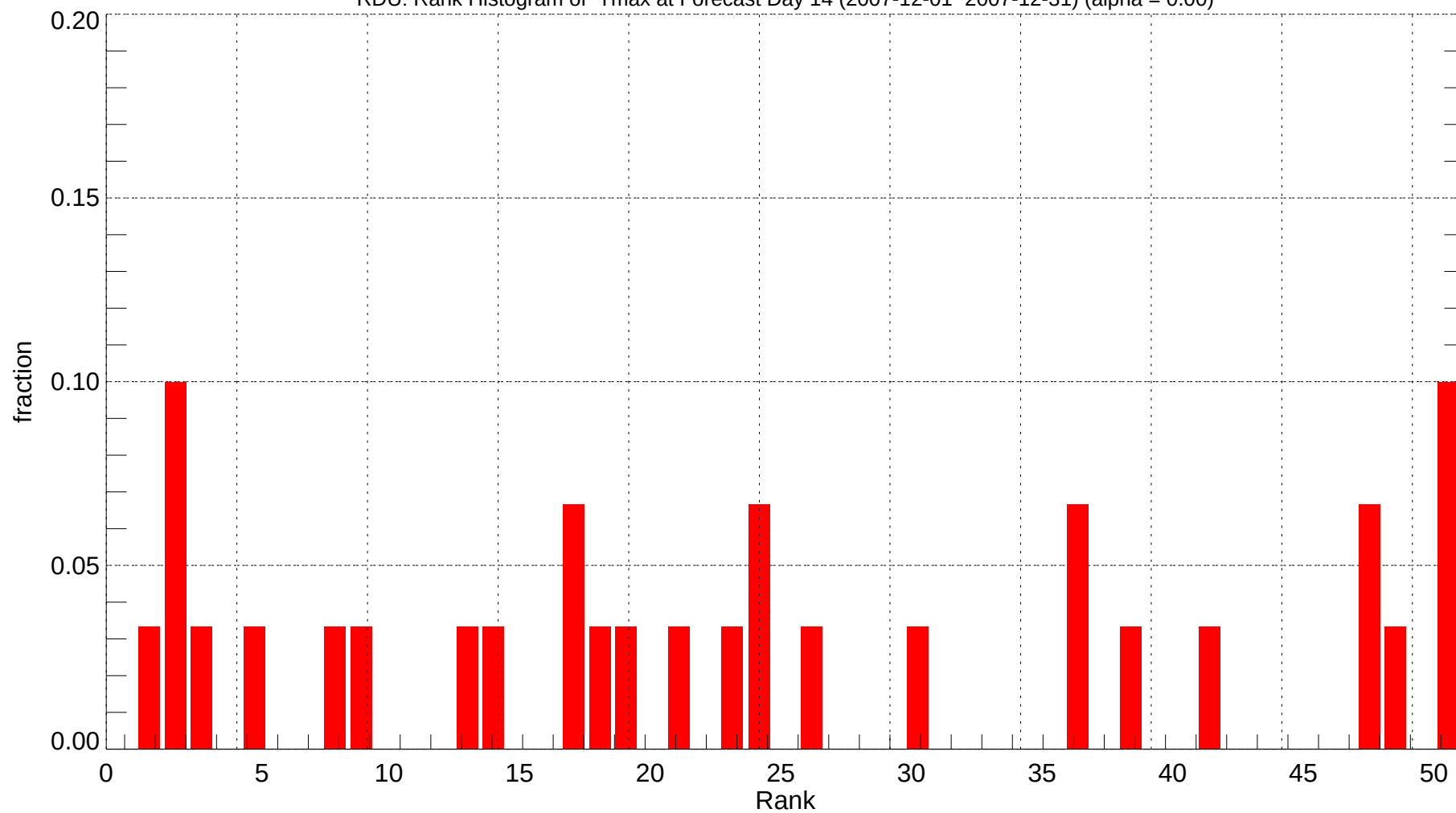
RDU: Rank Histogram of Tmax at Forecast Day 14 (2007-12-01~2007-12-31) (alpha = 0.00)
