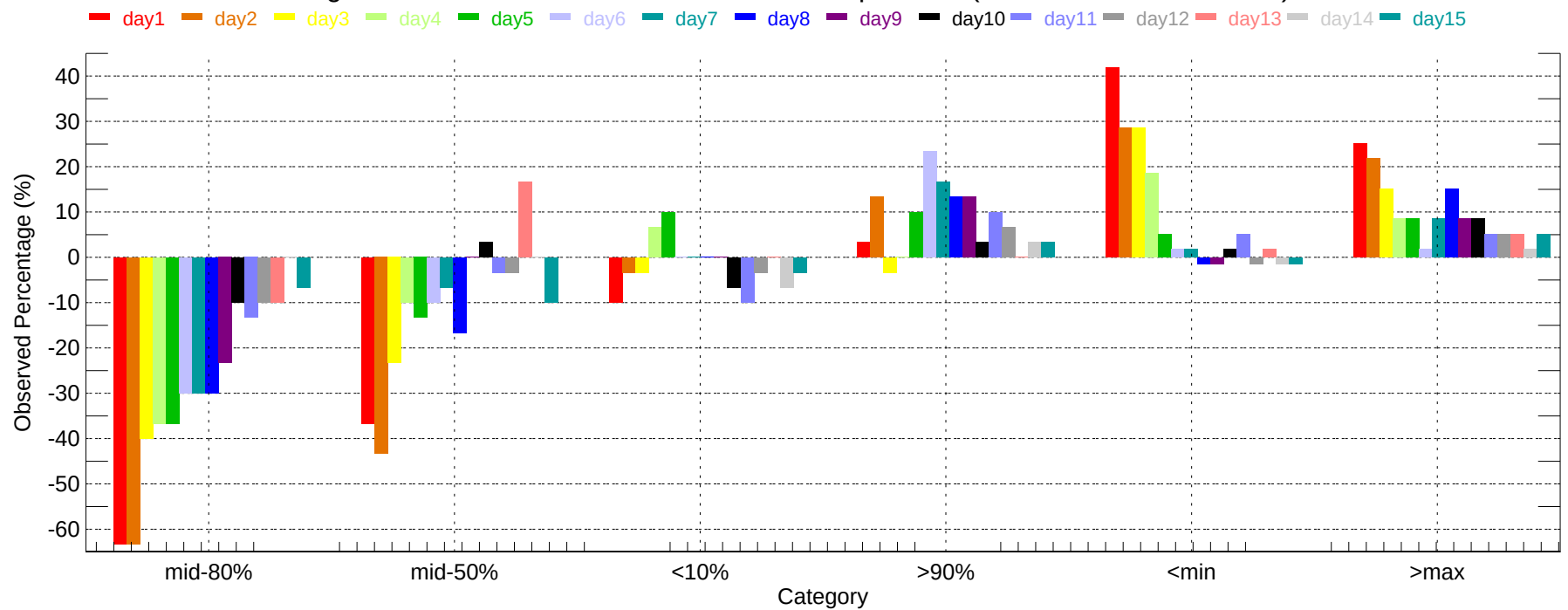
Observed Percentage Deviation of Ensembles - PIT: Max Temperature (2007-12-01~2007-12-31)
