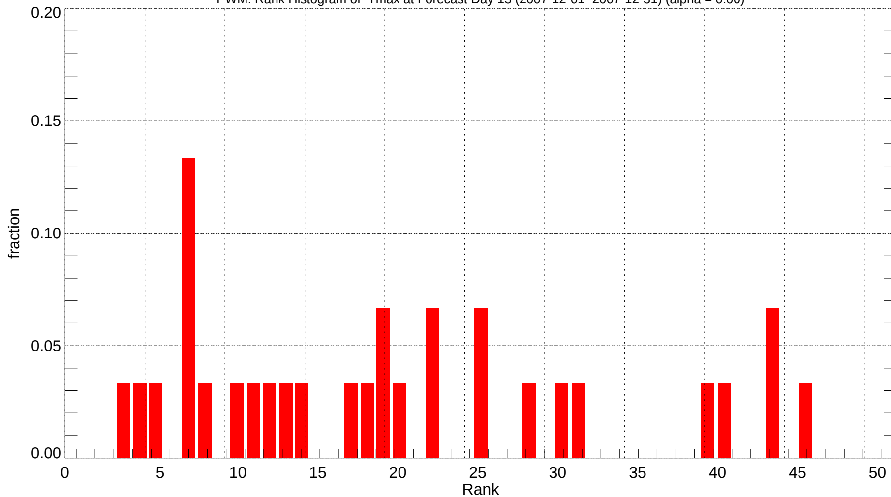
PWM: Rank Histogram of Tmax at Forecast Day 13 (2007-12-01~2007-12-31) (alpha = 0.00)
