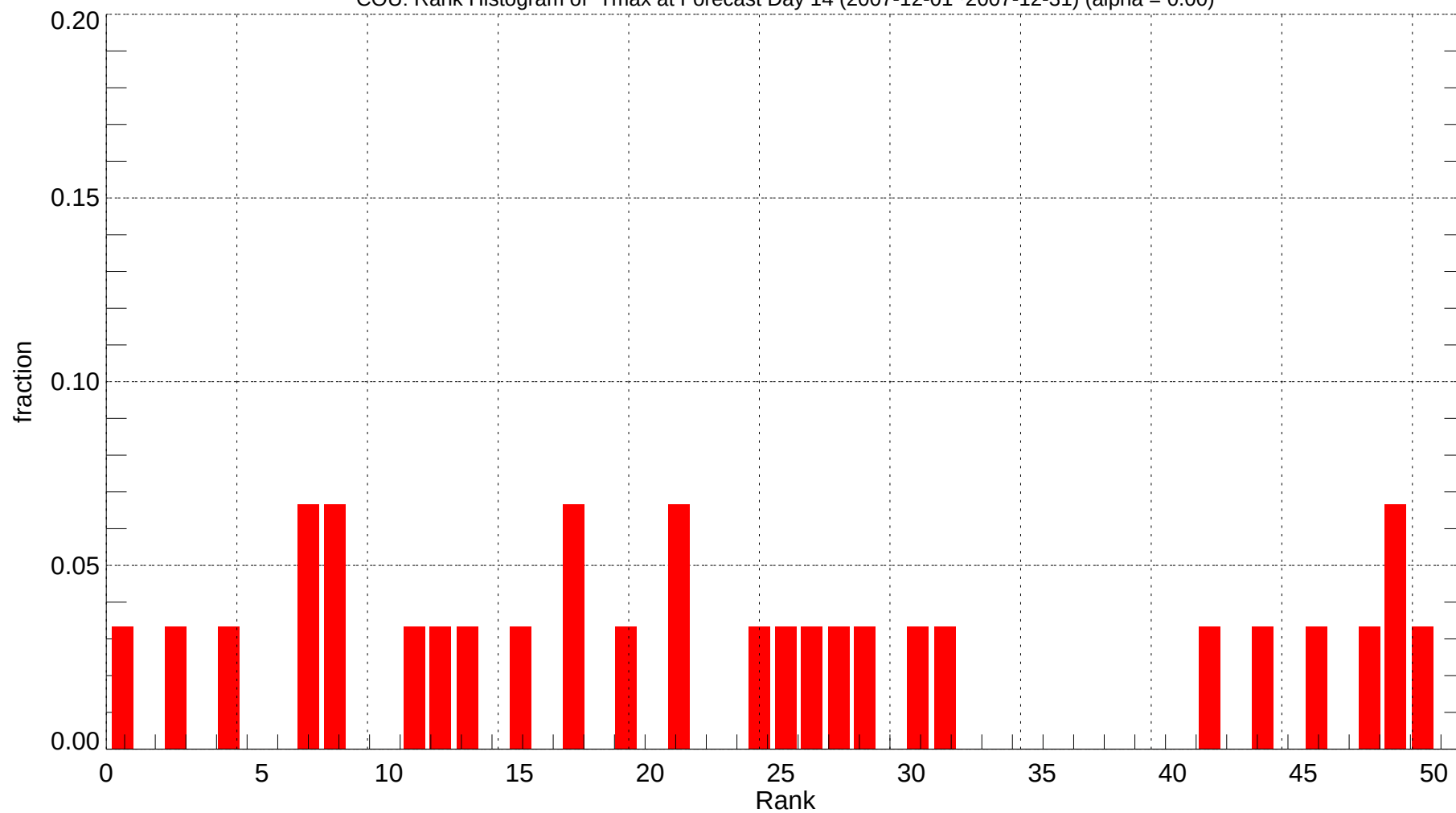
COU: Rank Histogram of Tmax at Forecast Day 14 (2007-12-01~2007-12-31) (alpha = 0.00)
