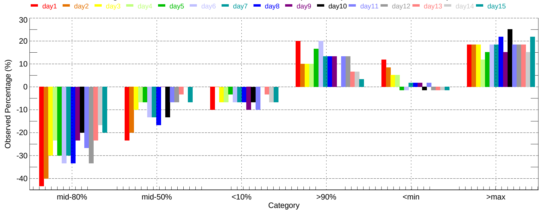
Observed Percentage Deviation of Ensembles - TYR: Max Temperature (2007-12-01~2007-12-31)
