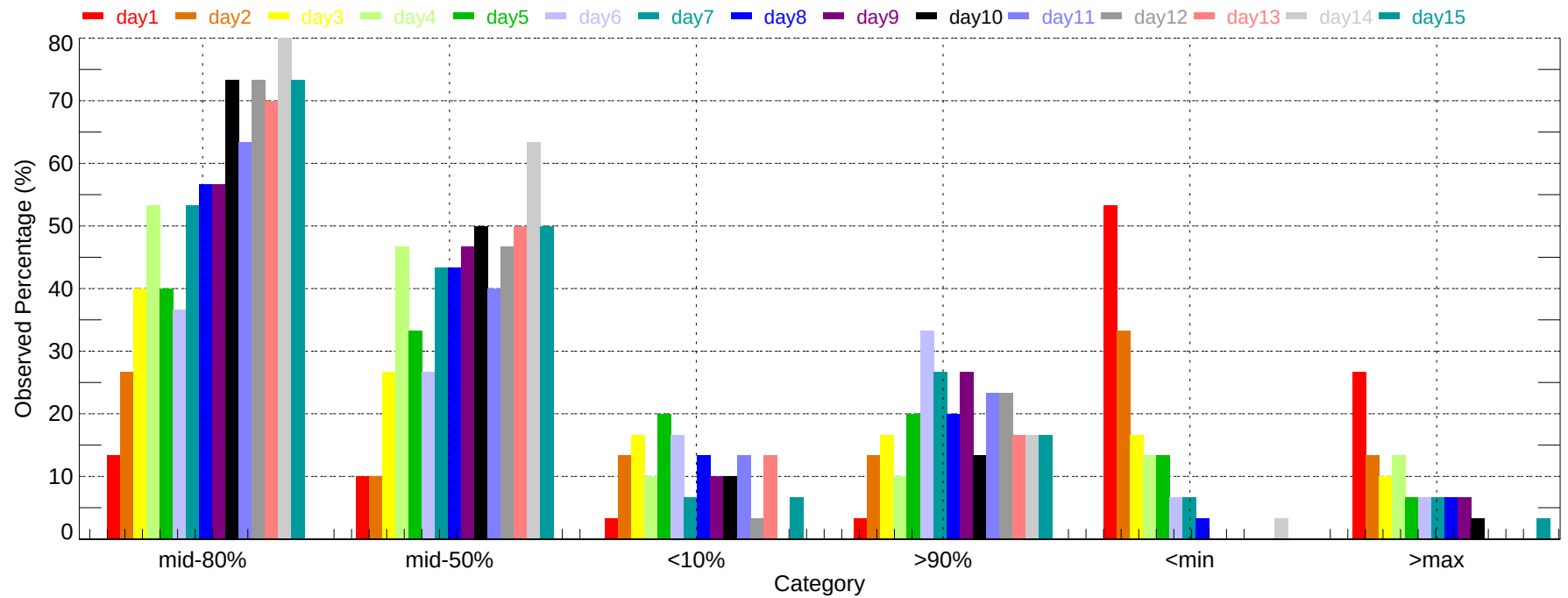
Observed Percentage of Ensembles - BWI: Min Temperature (2007-12-01~2007-12-31)
