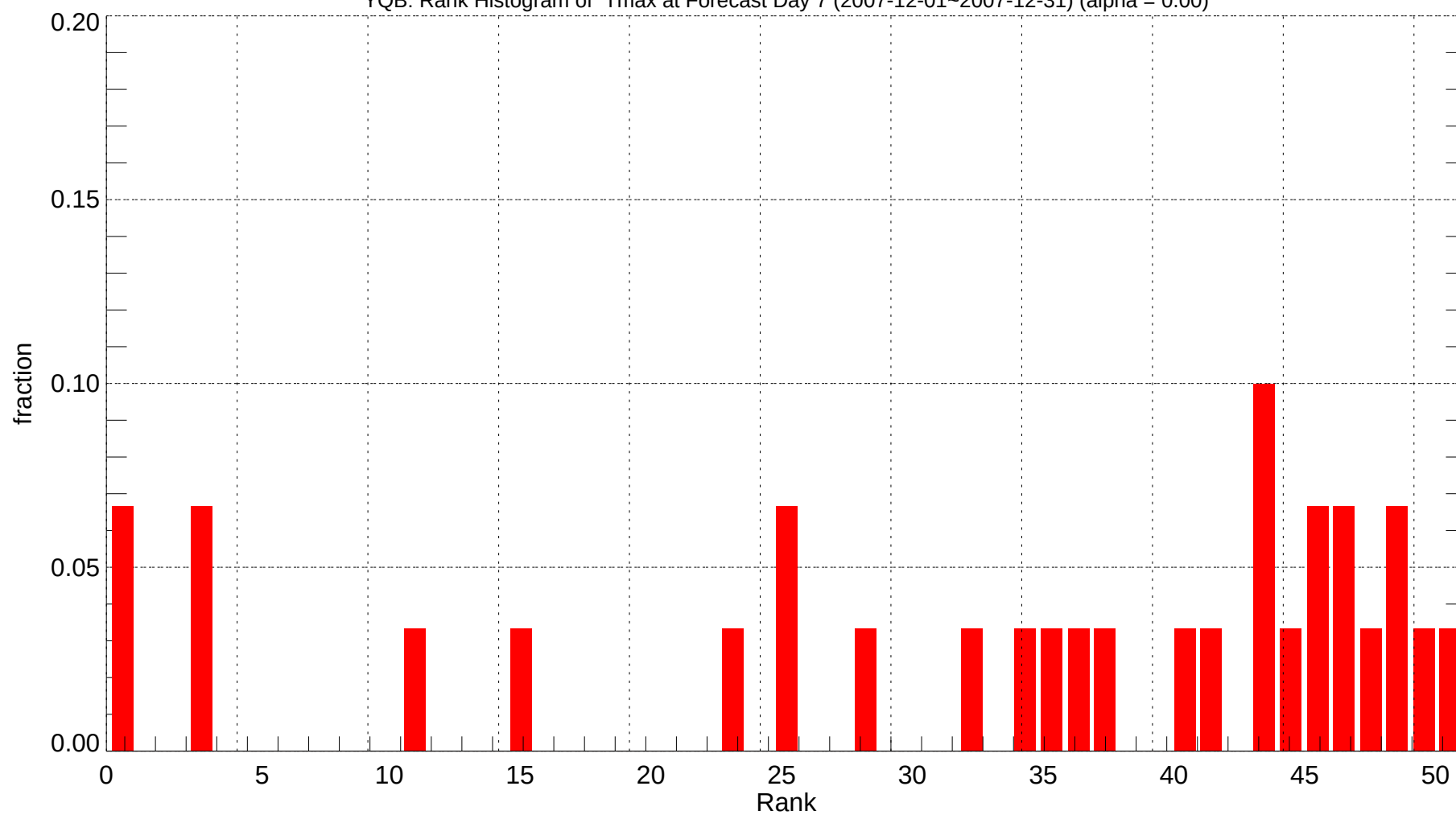
YQB: Rank Histogram of Tmax at Forecast Day 7 (2007-12-01~2007-12-31) (alpha = 0.00)
