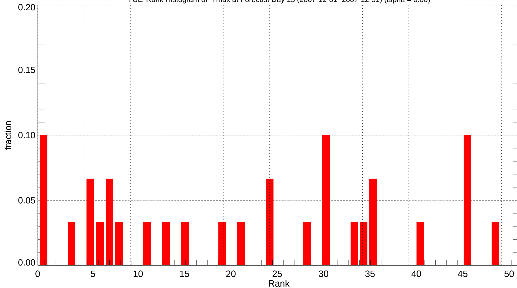
YUL: Rank Histogram of Tmax at Forecast Day 13 (2007-12-01~2007-12-31) (alpha = 0.00)
