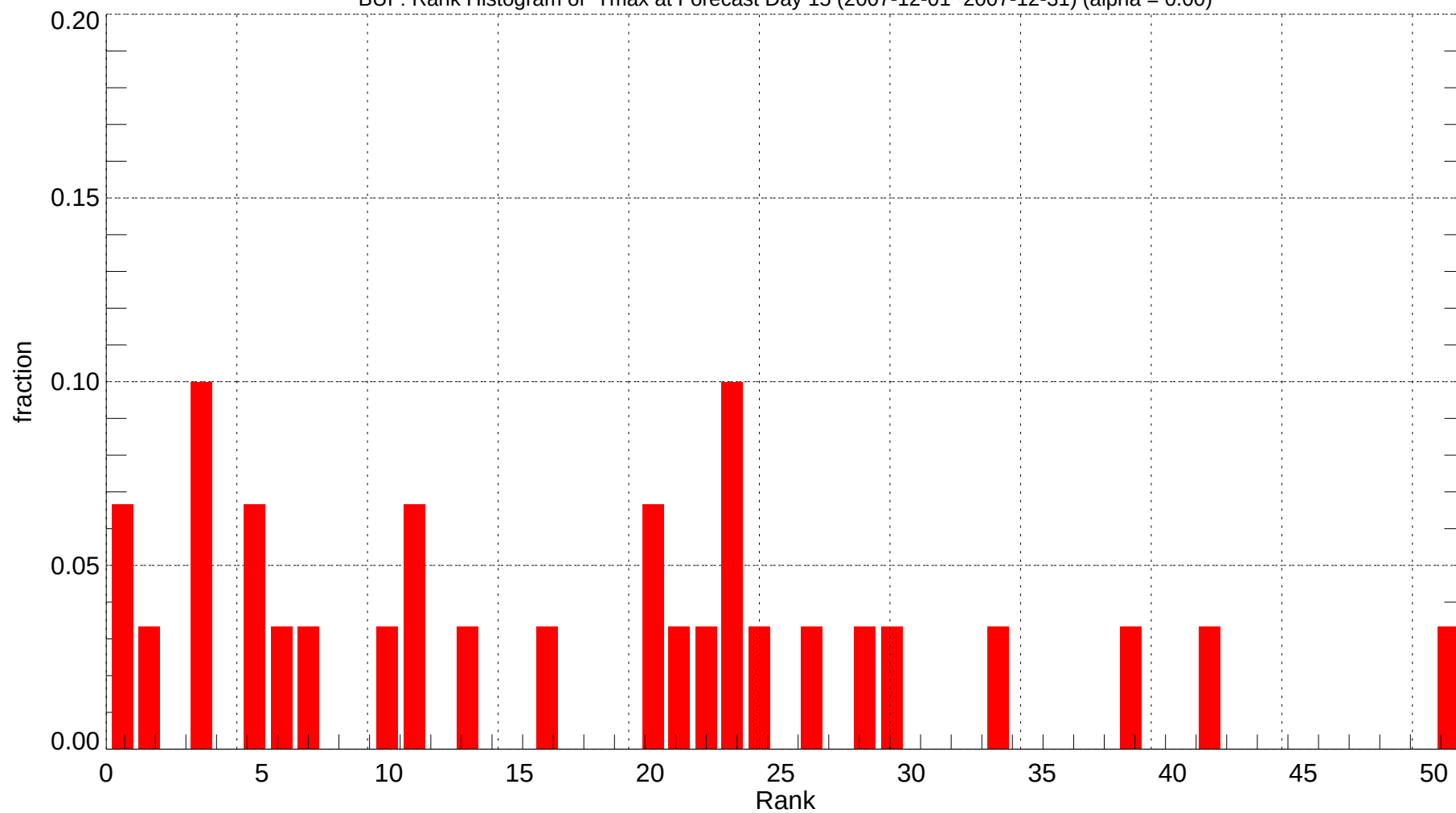
BUF: Rank Histogram of Tmax at Forecast Day 15 (2007-12-01~2007-12-31) (alpha = 0.00)
