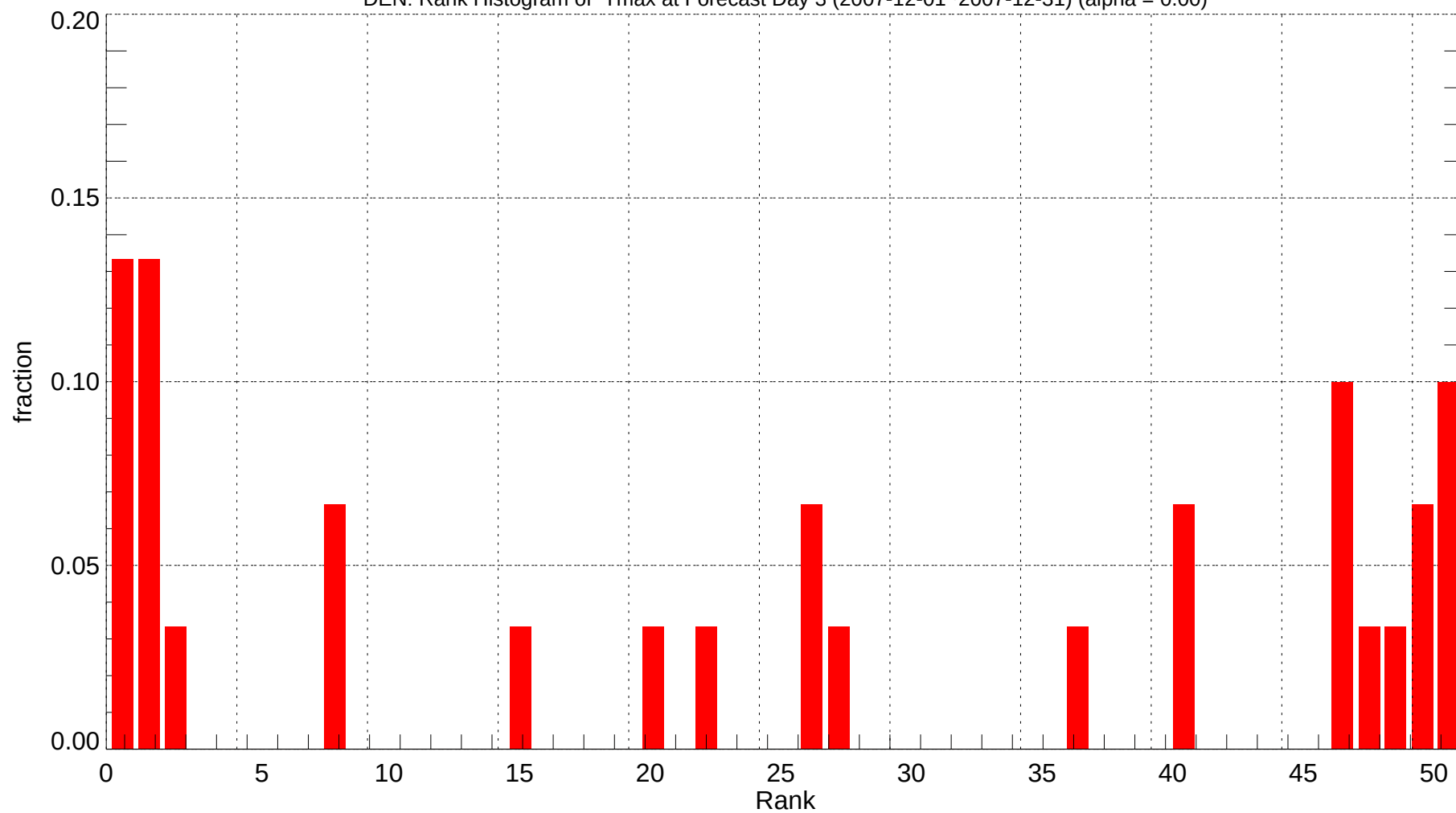
DEN: Rank Histogram of Tmax at Forecast Day 3 (2007-12-01~2007-12-31) (alpha = 0.00)
