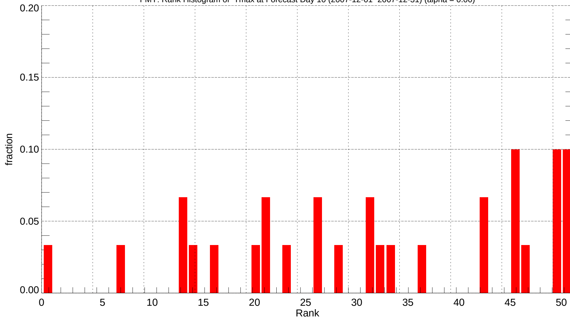
FMY: Rank Histogram of Tmax at Forecast Day 10 (2007-12-01~2007-12-31) (alpha = 0.00)
