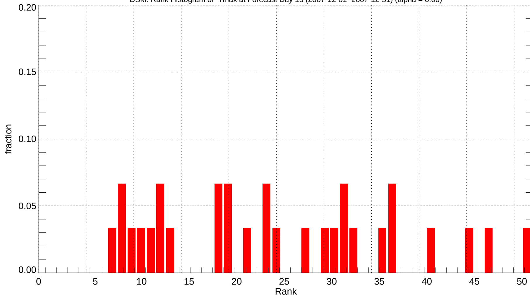
DSM: Rank Histogram of Tmax at Forecast Day 13 (2007-12-01~2007-12-31) (alpha = 0.00)
