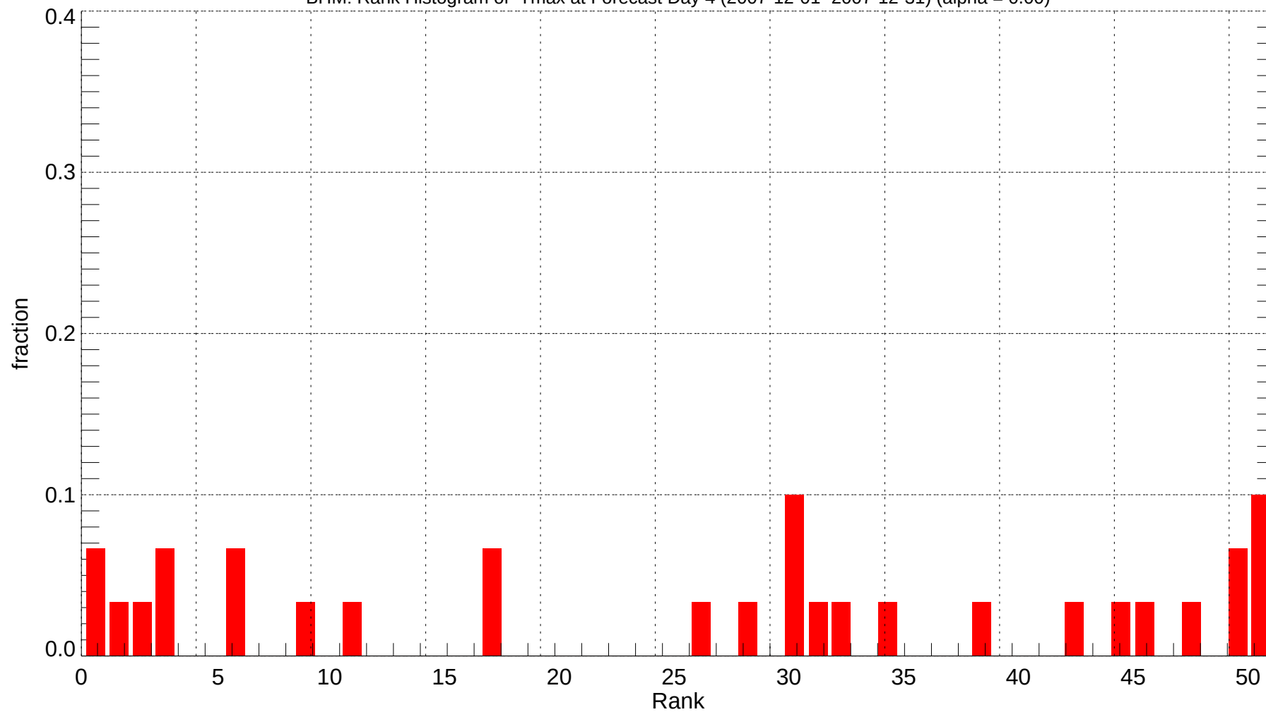
BHM: Rank Histogram of Tmax at Forecast Day 4 (2007-12-01~2007-12-31) (alpha = 0.00)
