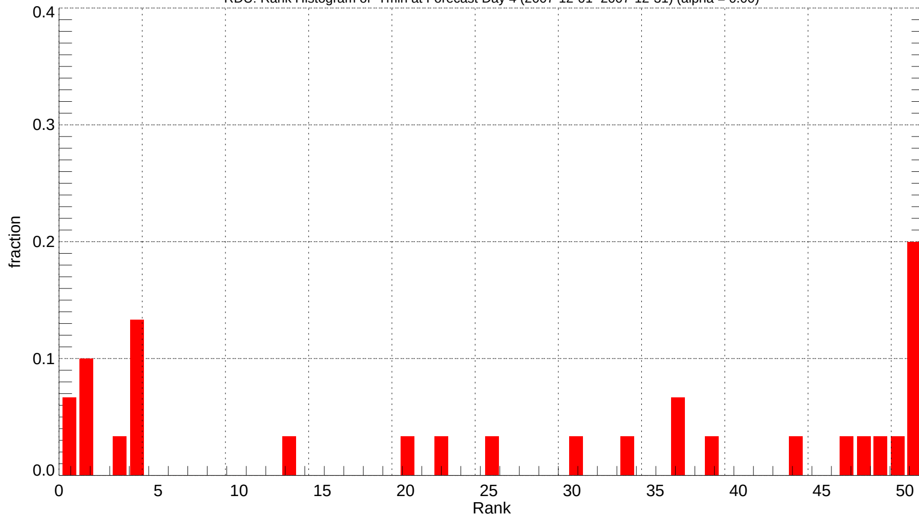
RDU: Rank Histogram of Tmin at Forecast Day 4 (2007-12-01~2007-12-31) (alpha = 0.00)
