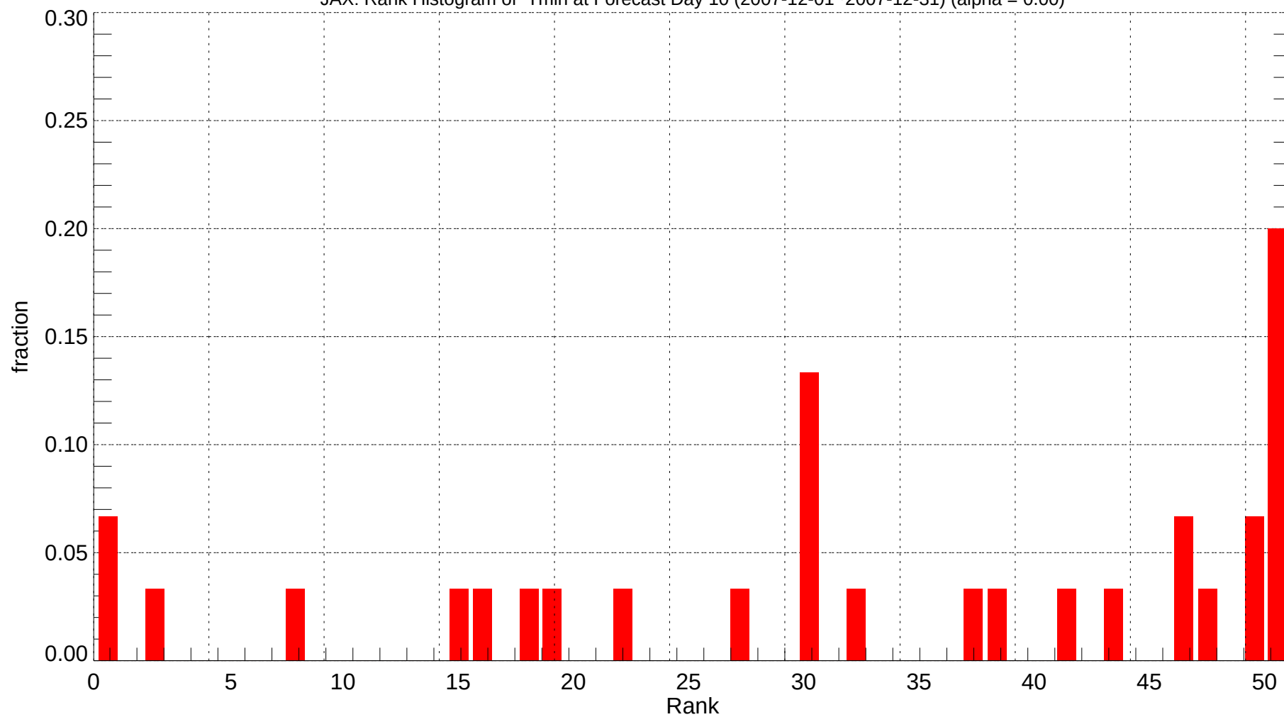
JAX: Rank Histogram of Tmin at Forecast Day 10 (2007-12-01~2007-12-31) (alpha = 0.00)
