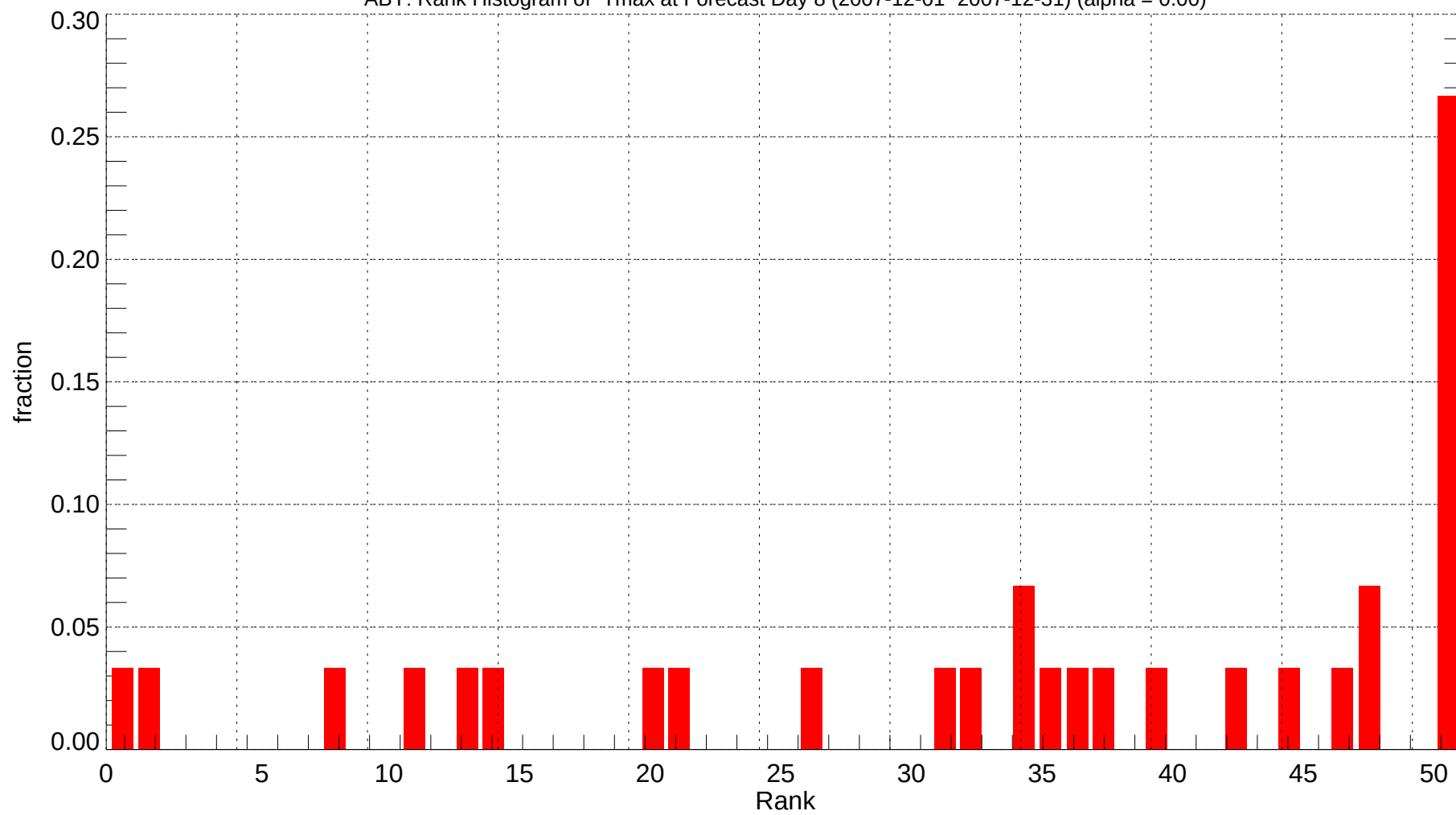
ABY: Rank Histogram of Tmax at Forecast Day 8 (2007-12-01~2007-12-31) (alpha = 0.00)
