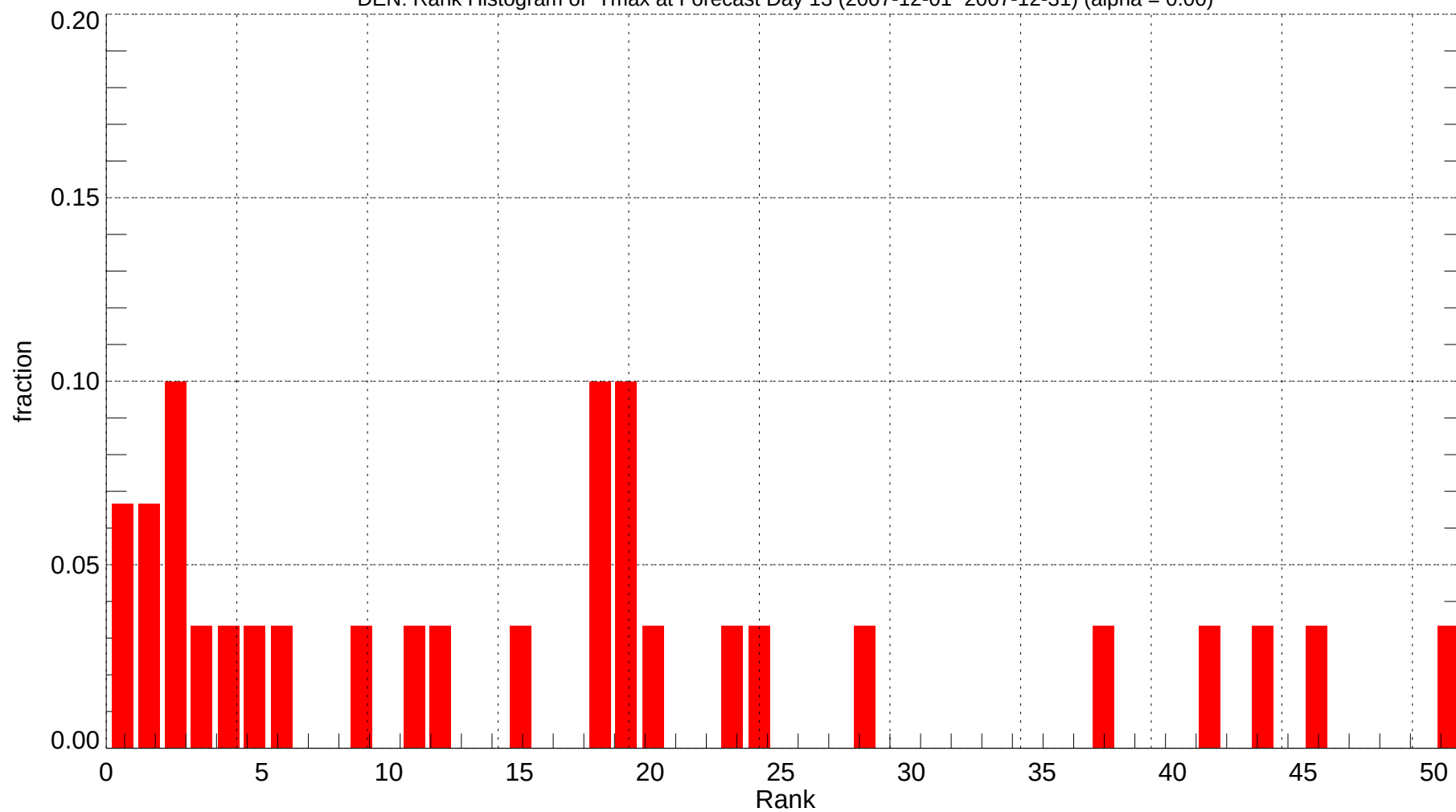
DEN: Rank Histogram of Tmax at Forecast Day 13 (2007-12-01~2007-12-31) (alpha = 0.00)
