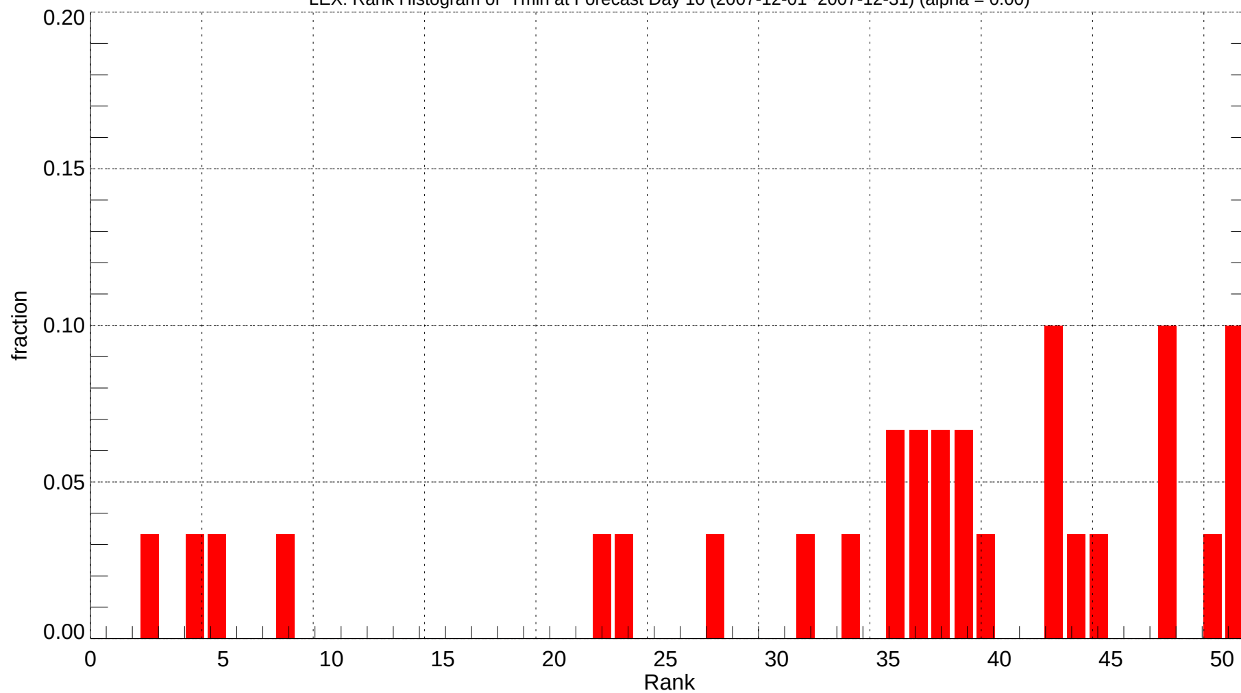
LEX: Rank Histogram of Tmin at Forecast Day 10 (2007-12-01~2007-12-31) (alpha = 0.00)
