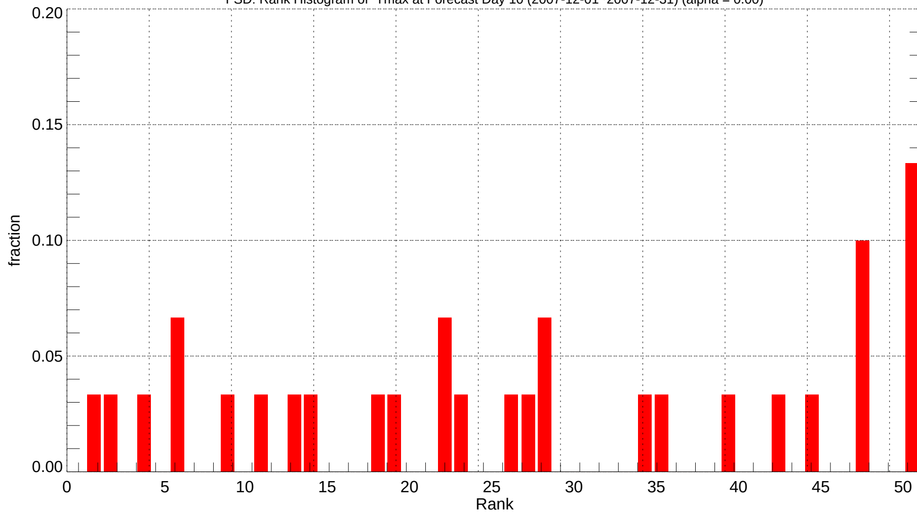
FSD: Rank Histogram of Tmax at Forecast Day 10 (2007-12-01~2007-12-31) (alpha = 0.00)
