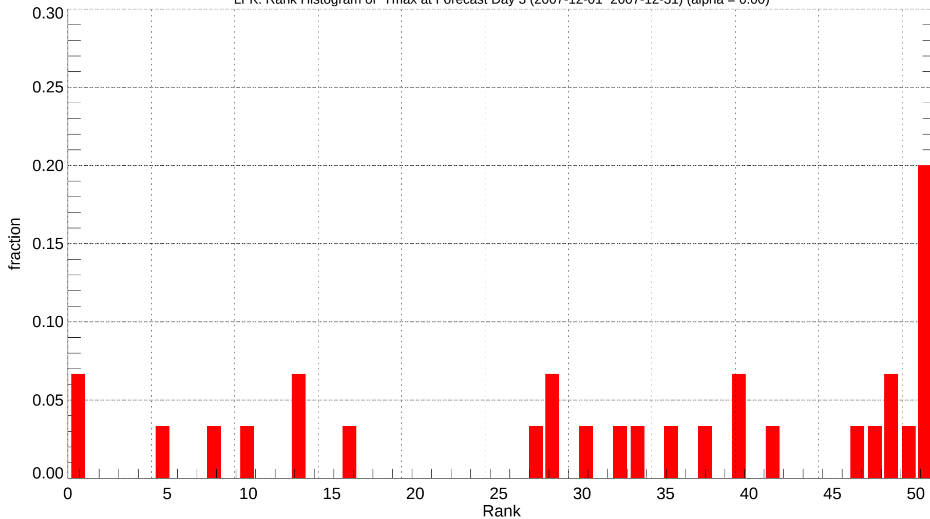
LFK: Rank Histogram of Tmax at Forecast Day 3 (2007-12-01~2007-12-31) (alpha = 0.00)
