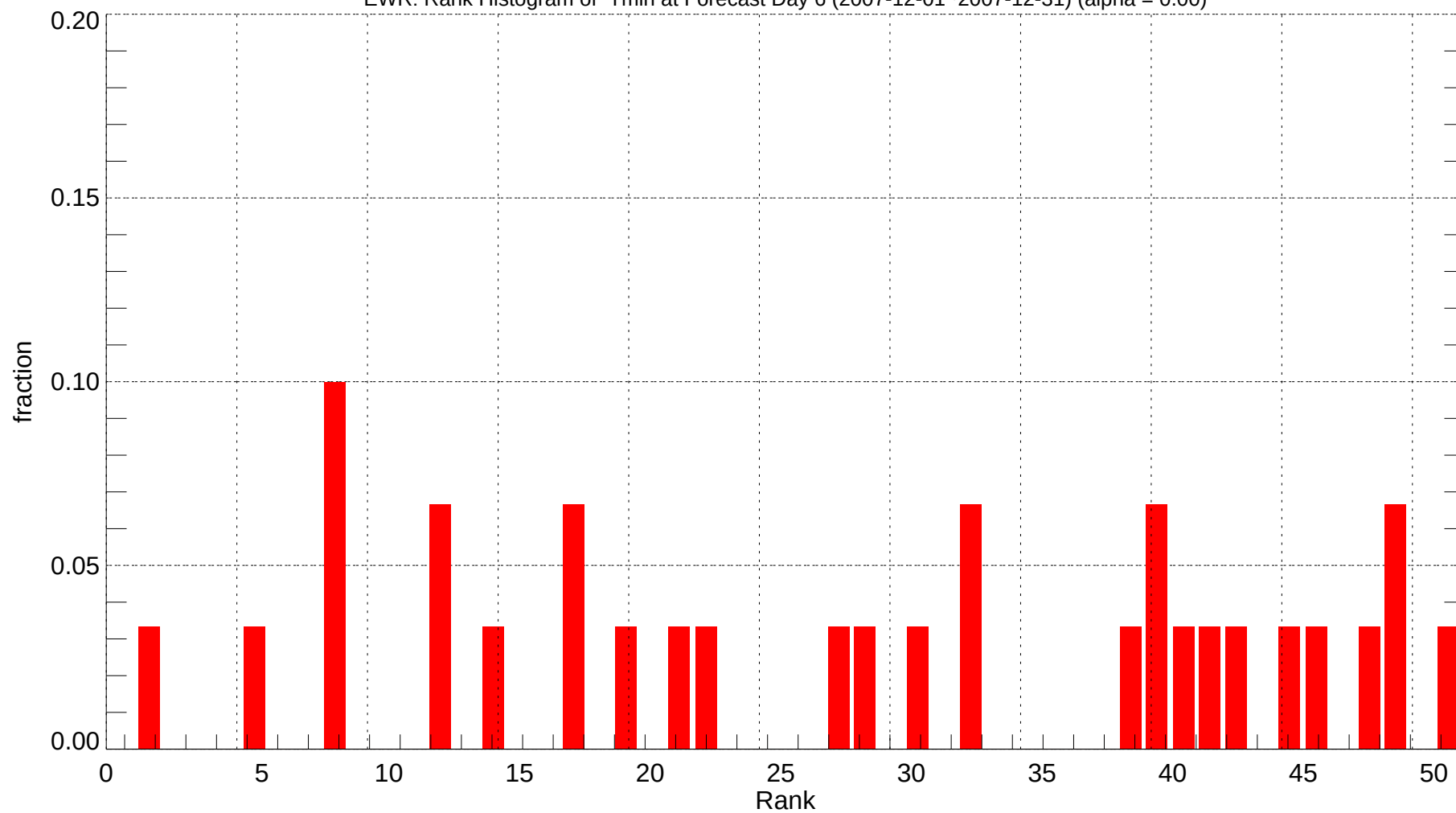
EWR: Rank Histogram of Tmin at Forecast Day 6 (2007-12-01~2007-12-31) (alpha = 0.00)
