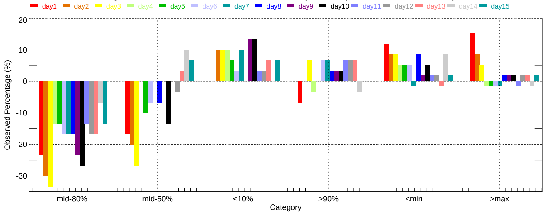
Observed Percentage Deviation of Ensembles - BGM: Max Temperature (2007-12-01~2007-12-31)
