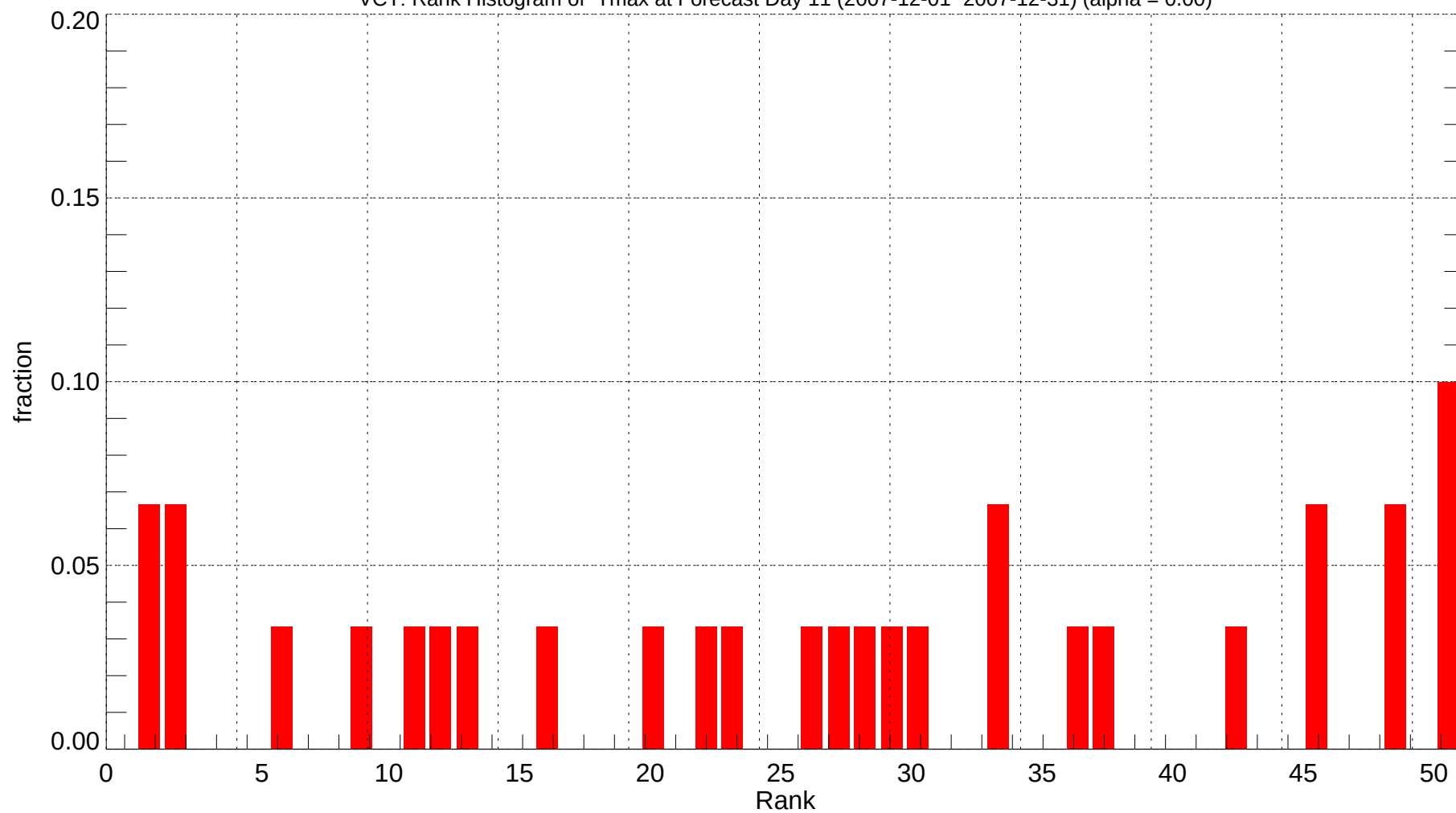
VCT: Rank Histogram of Tmax at Forecast Day 11 (2007-12-01~2007-12-31) (alpha = 0.00)
