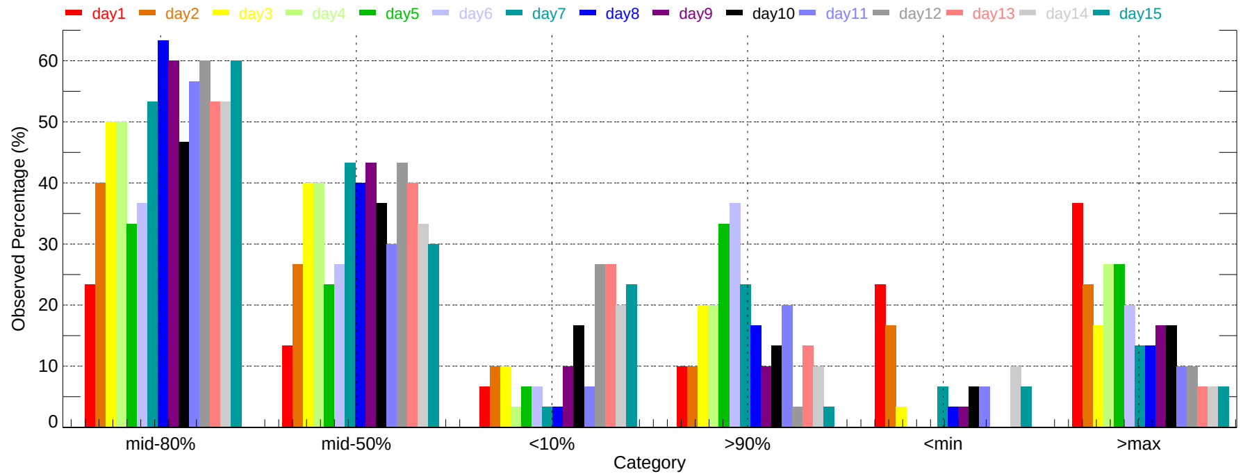
Observed Percentage of Ensembles - COS: Max Temperature (2007-12-01~2007-12-31)
