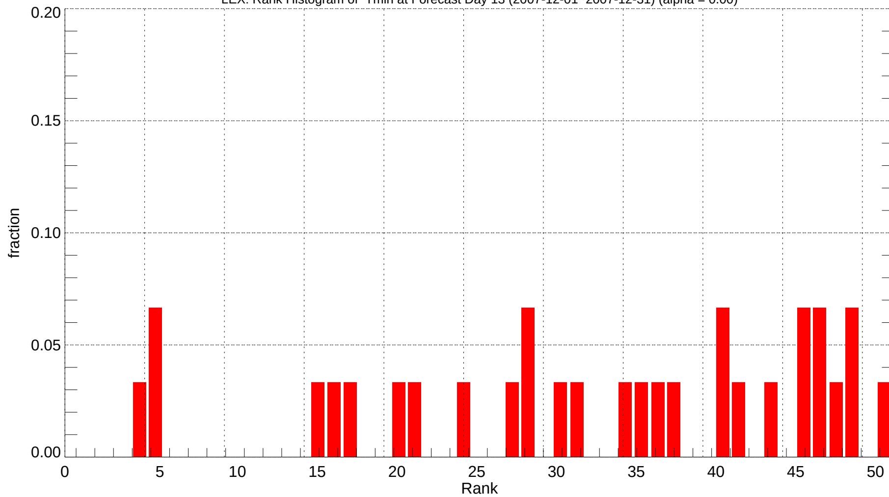
LEX: Rank Histogram of Tmin at Forecast Day 13 (2007-12-01~2007-12-31) (alpha = 0.00)
