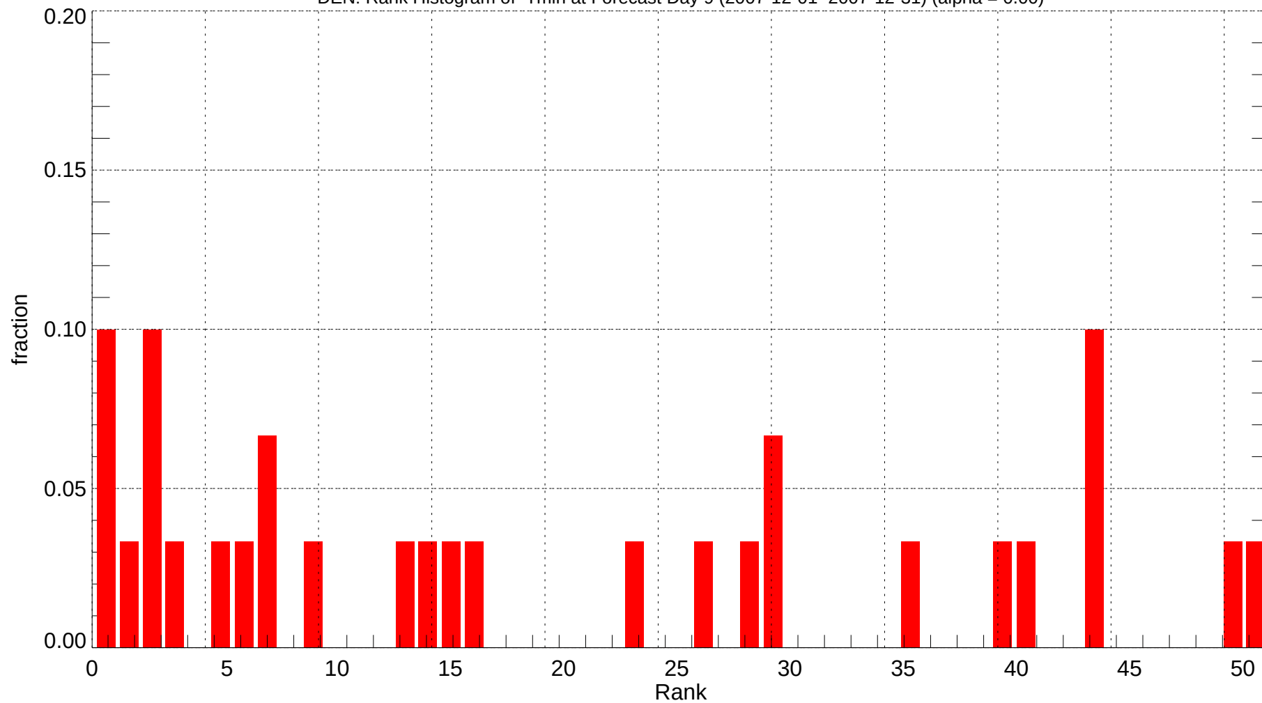
DEN: Rank Histogram of Tmin at Forecast Day 9 (2007-12-01~2007-12-31) (alpha = 0.00)
