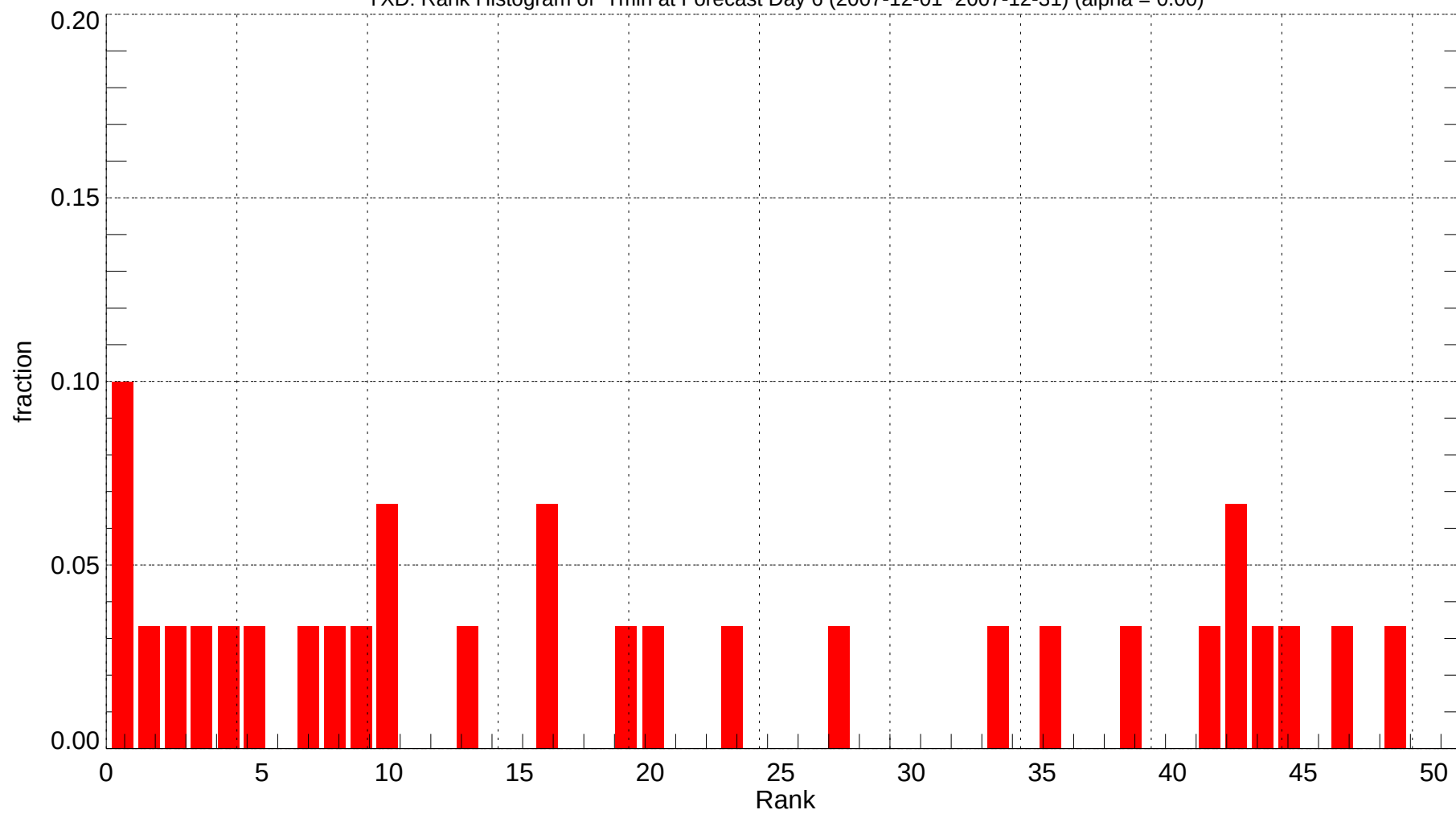
YXD: Rank Histogram of Tmin at Forecast Day 6 (2007-12-01~2007-12-31) (alpha = 0.00)
