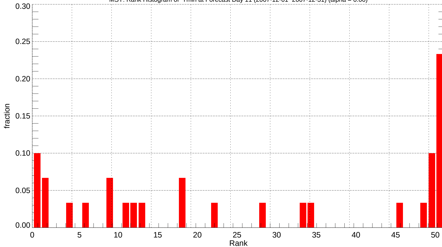
MSY: Rank Histogram of Tmin at Forecast Day 11 (2007-12-01~2007-12-31) (alpha = 0.00)
