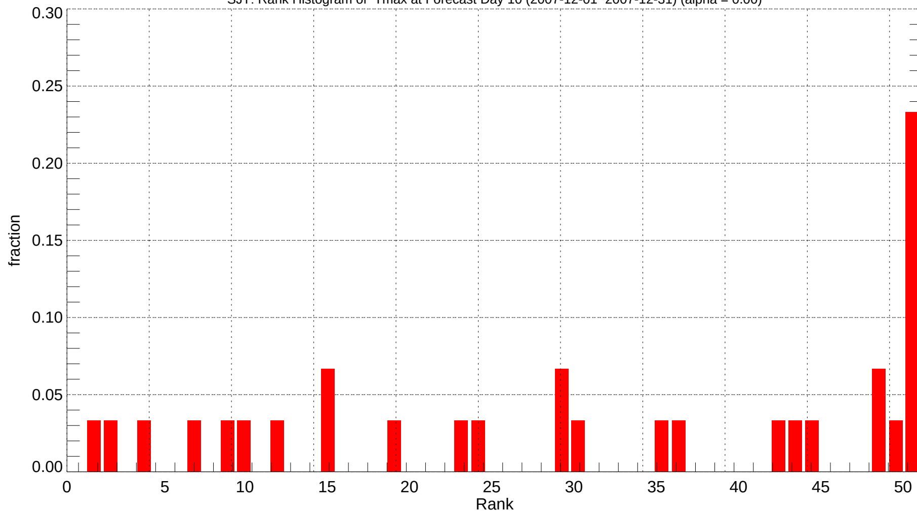
SJT: Rank Histogram of Tmax at Forecast Day 10 (2007-12-01~2007-12-31) (alpha = 0.00)
