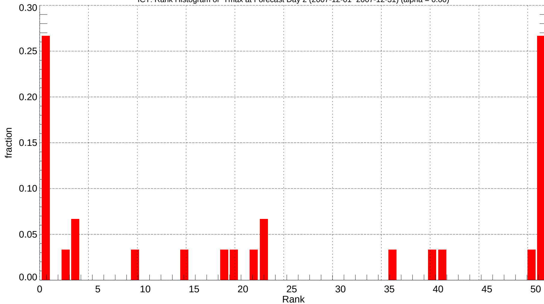
ICT: Rank Histogram of Tmax at Forecast Day 2 (2007-12-01~2007-12-31) (alpha = 0.00)
