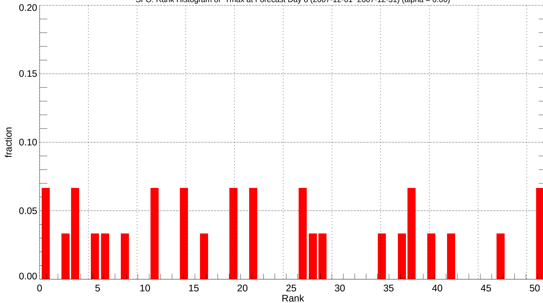
SFO: Rank Histogram of Tmax at Forecast Day 8 (2007-12-01~2007-12-31) (alpha = 0.00)
