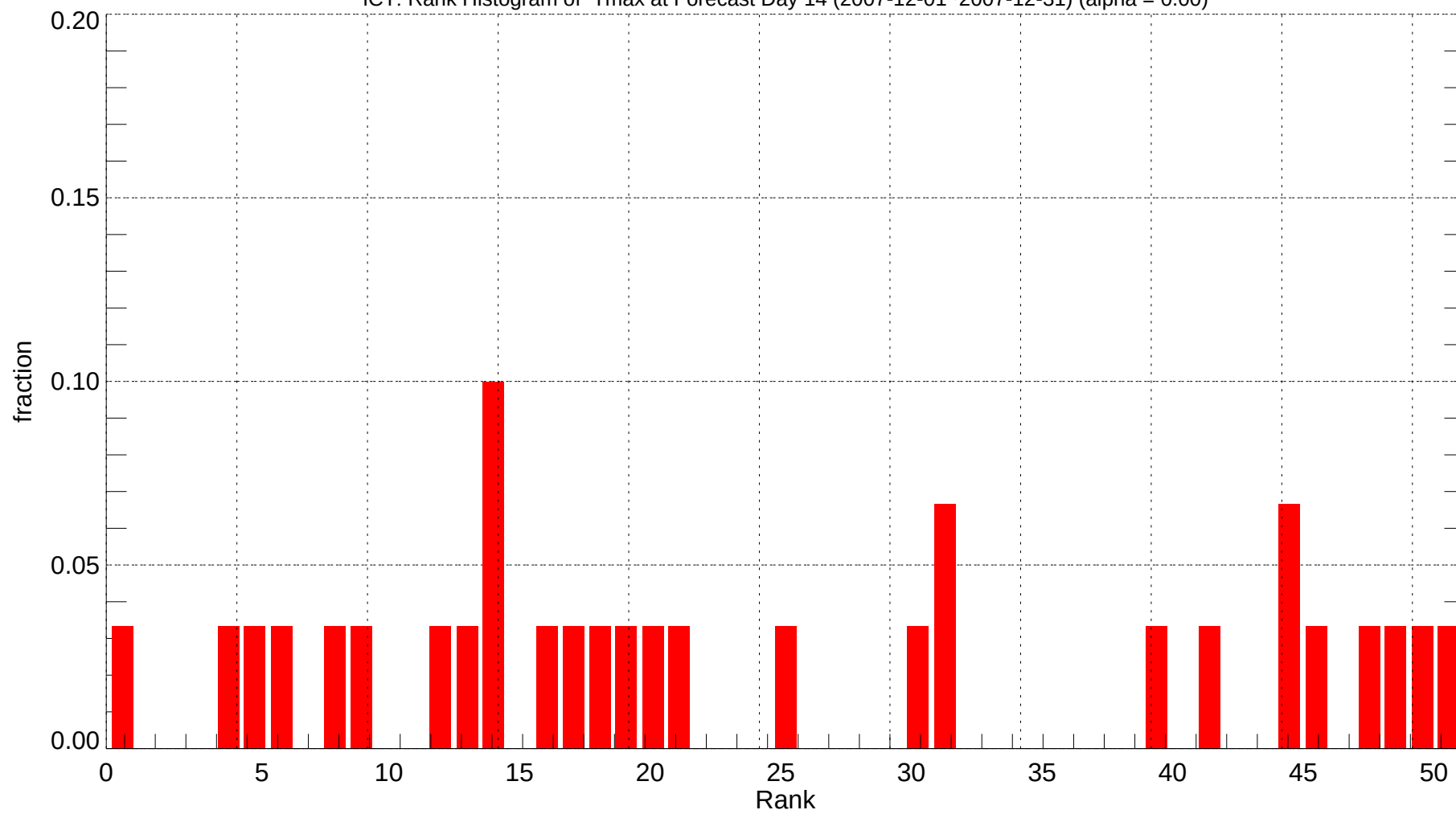
ICT: Rank Histogram of Tmax at Forecast Day 14 (2007-12-01~2007-12-31) (alpha = 0.00)
