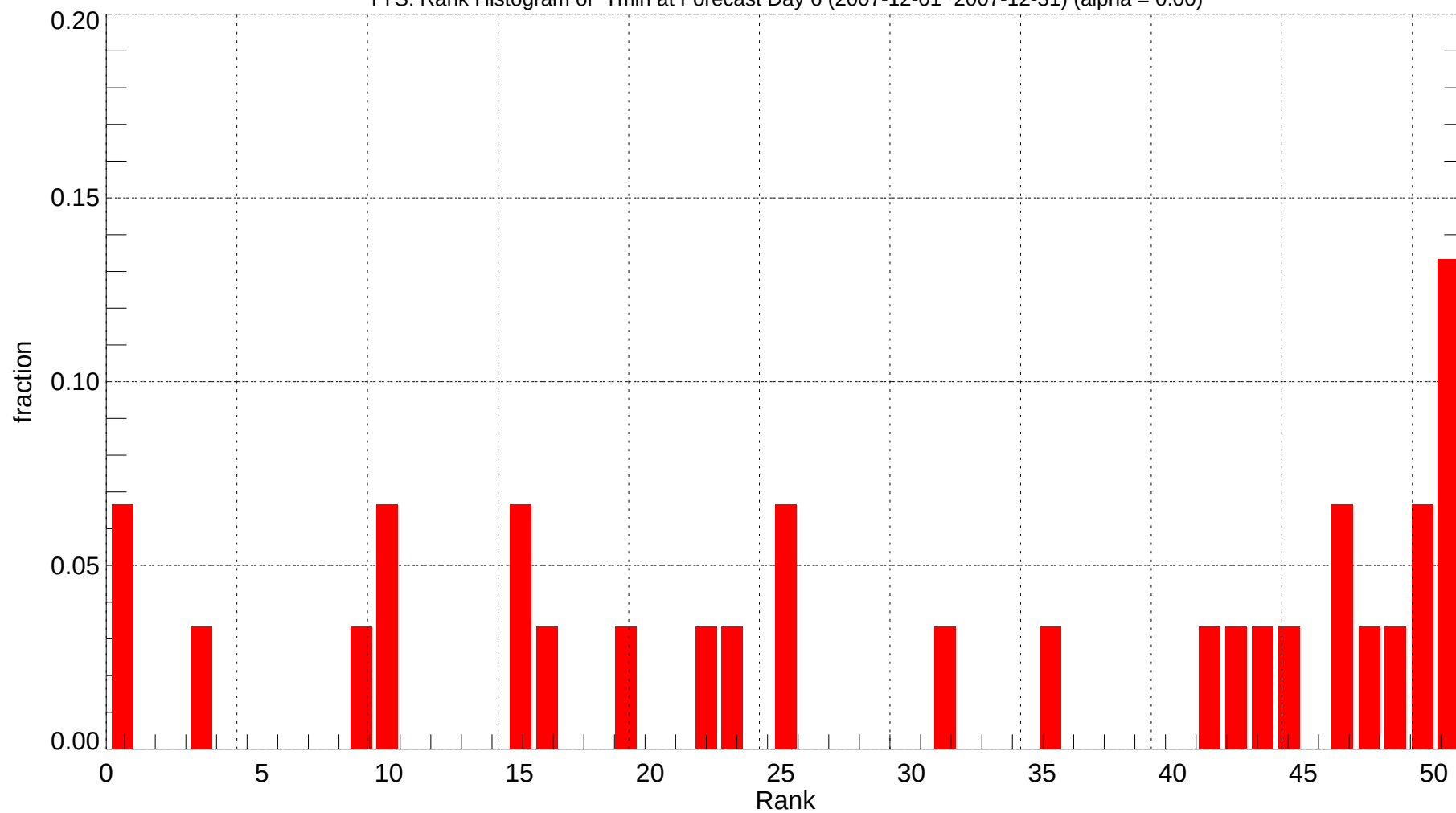
TYS: Rank Histogram of Tmin at Forecast Day 6 (2007-12-01~2007-12-31) (alpha = 0.00)
