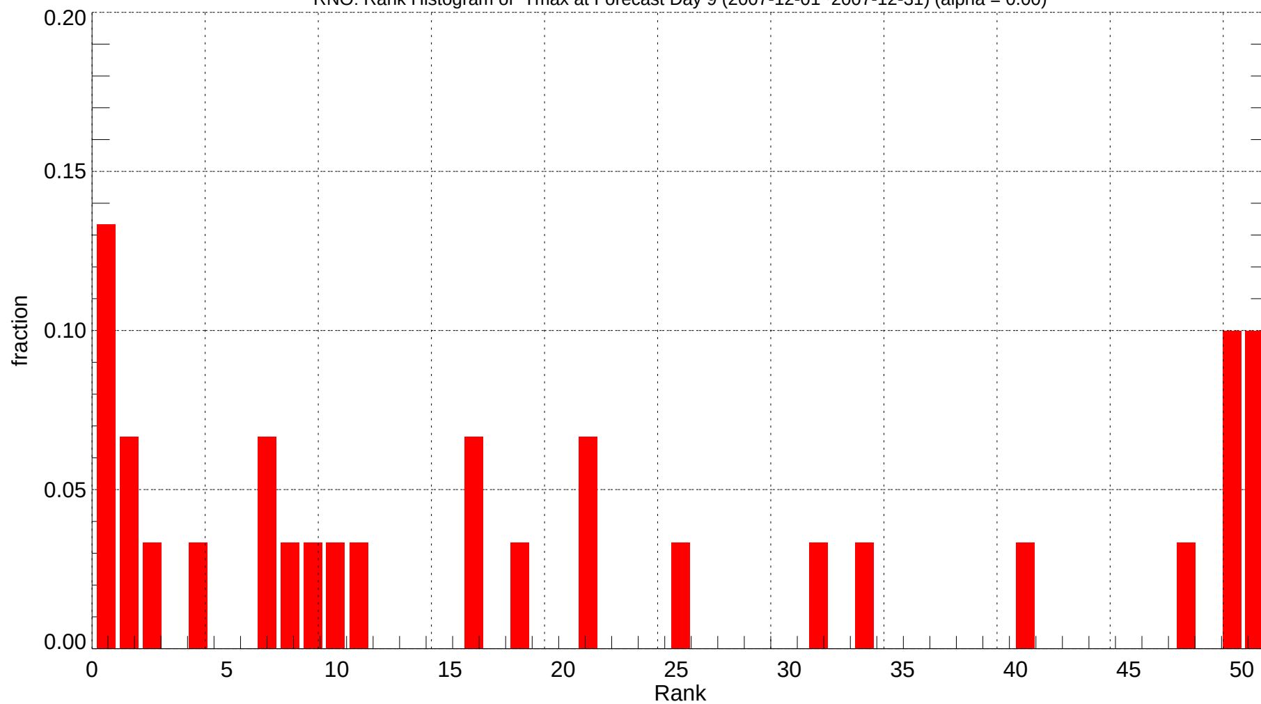
RNO: Rank Histogram of Tmax at Forecast Day 9 (2007-12-01~2007-12-31) (alpha = 0.00)
