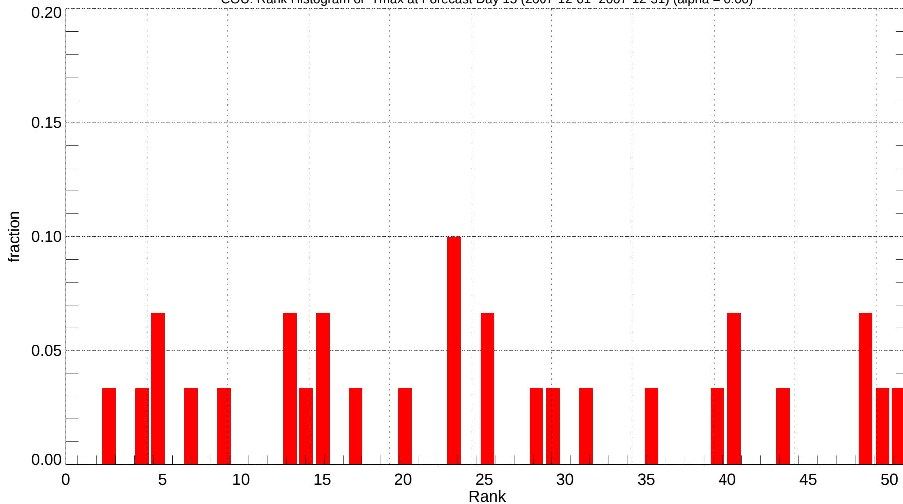
COU: Rank Histogram of Tmax at Forecast Day 15 (2007-12-01~2007-12-31) (alpha = 0.00)
