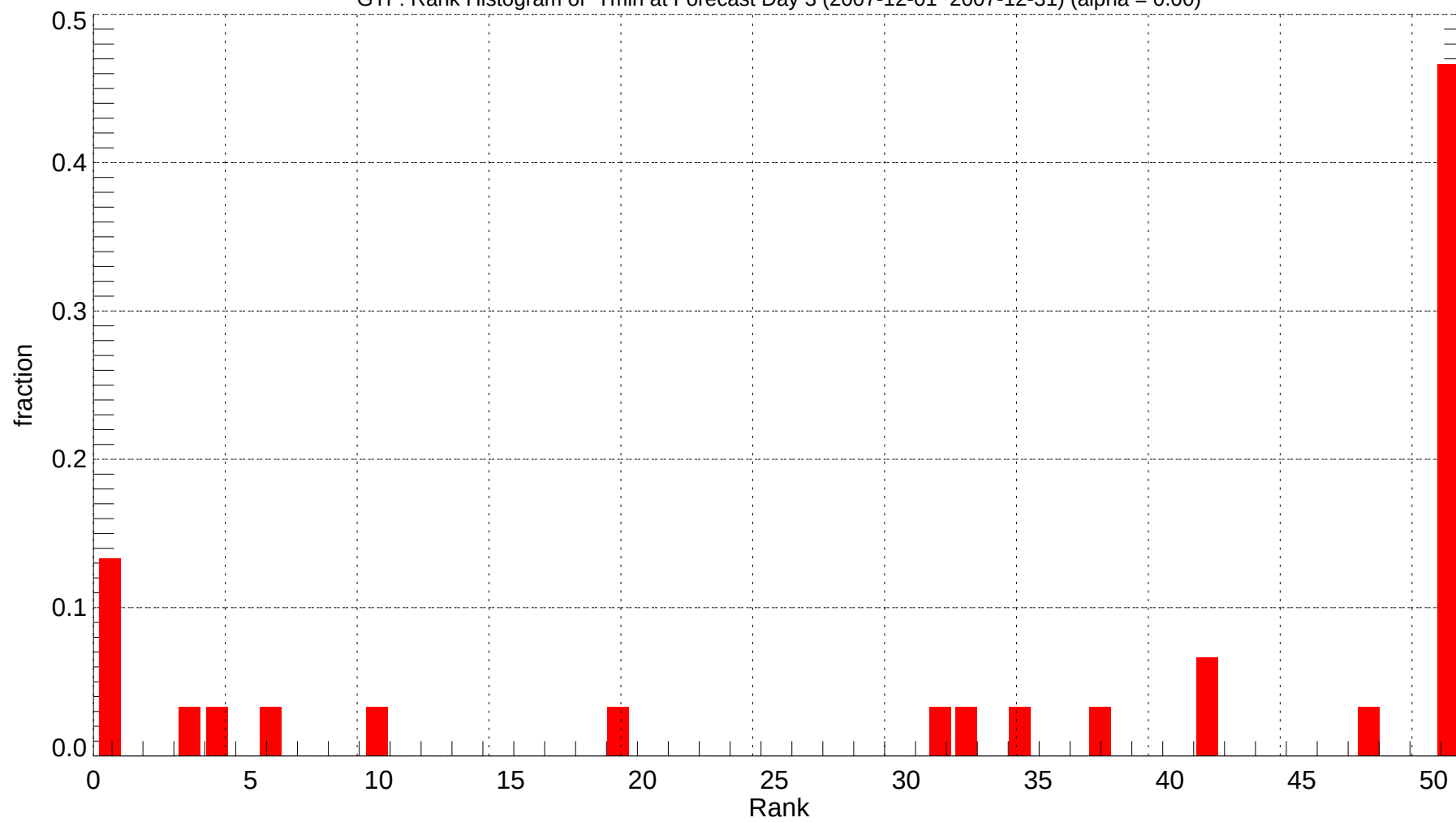
GTF: Rank Histogram of Tmin at Forecast Day 3 (2007-12-01~2007-12-31) (alpha = 0.00)
