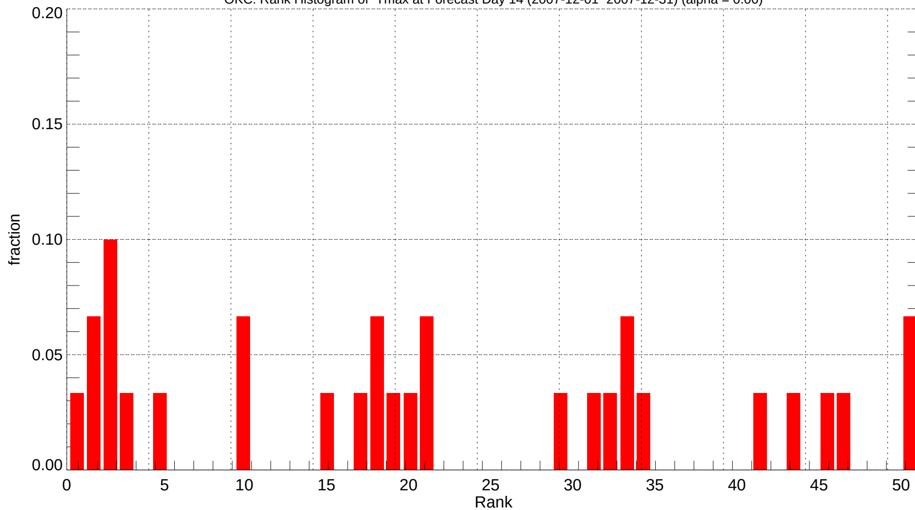
OKC: Rank Histogram of Tmax at Forecast Day 14 (2007-12-01~2007-12-31) (alpha = 0.00)
