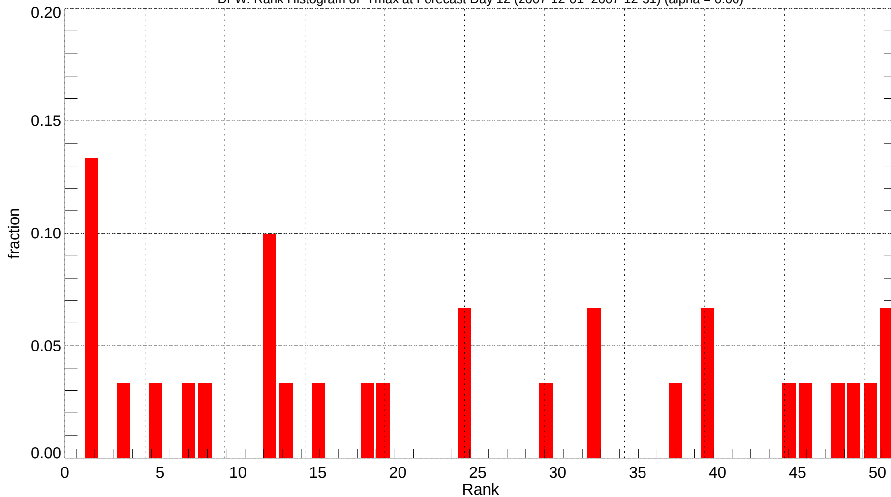
DFW: Rank Histogram of Tmax at Forecast Day 12 (2007-12-01~2007-12-31) (alpha = 0.00)
