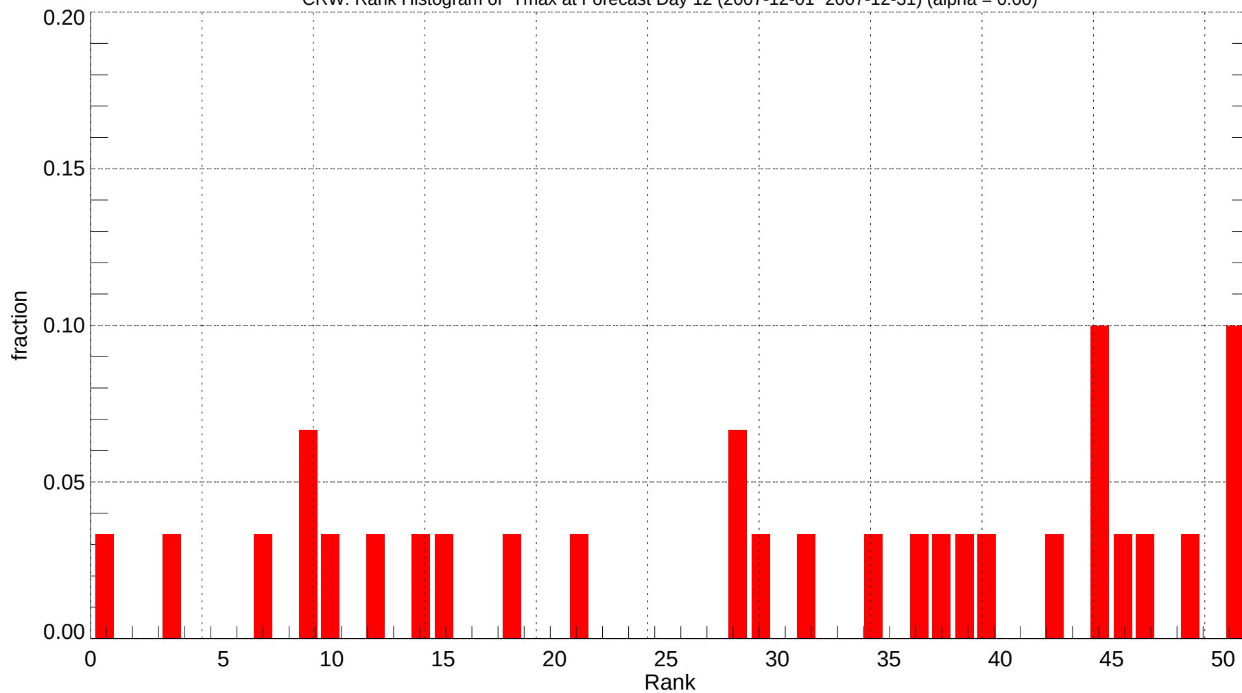
CRW: Rank Histogram of Tmax at Forecast Day 12 (2007-12-01~2007-12-31) (alpha = 0.00)
