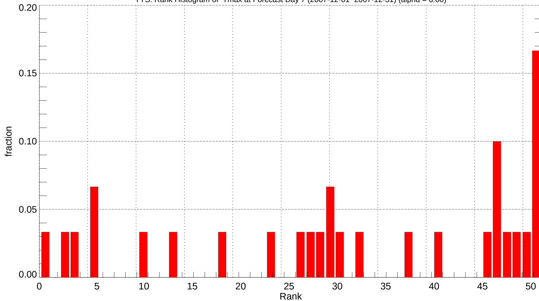
TYS: Rank Histogram of Tmax at Forecast Day 7 (2007-12-01~2007-12-31) (alpha = 0.00)
