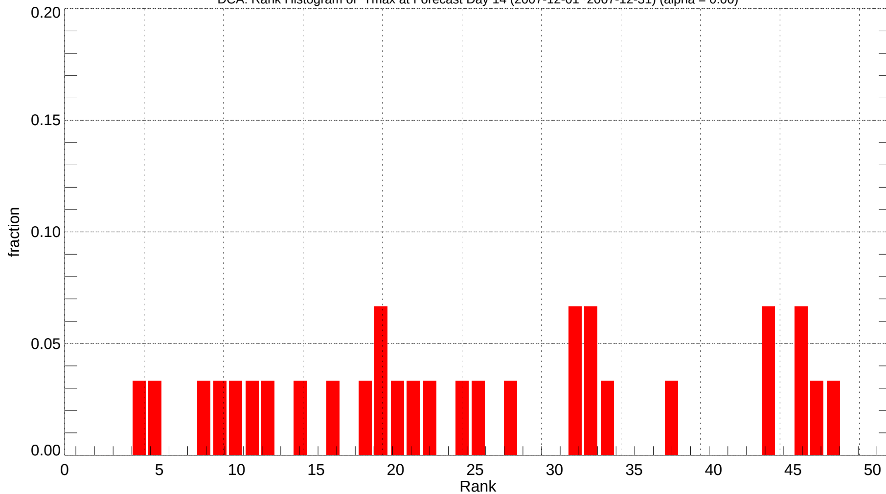
DCA: Rank Histogram of Tmax at Forecast Day 14 (2007-12-01~2007-12-31) (alpha = 0.00)
