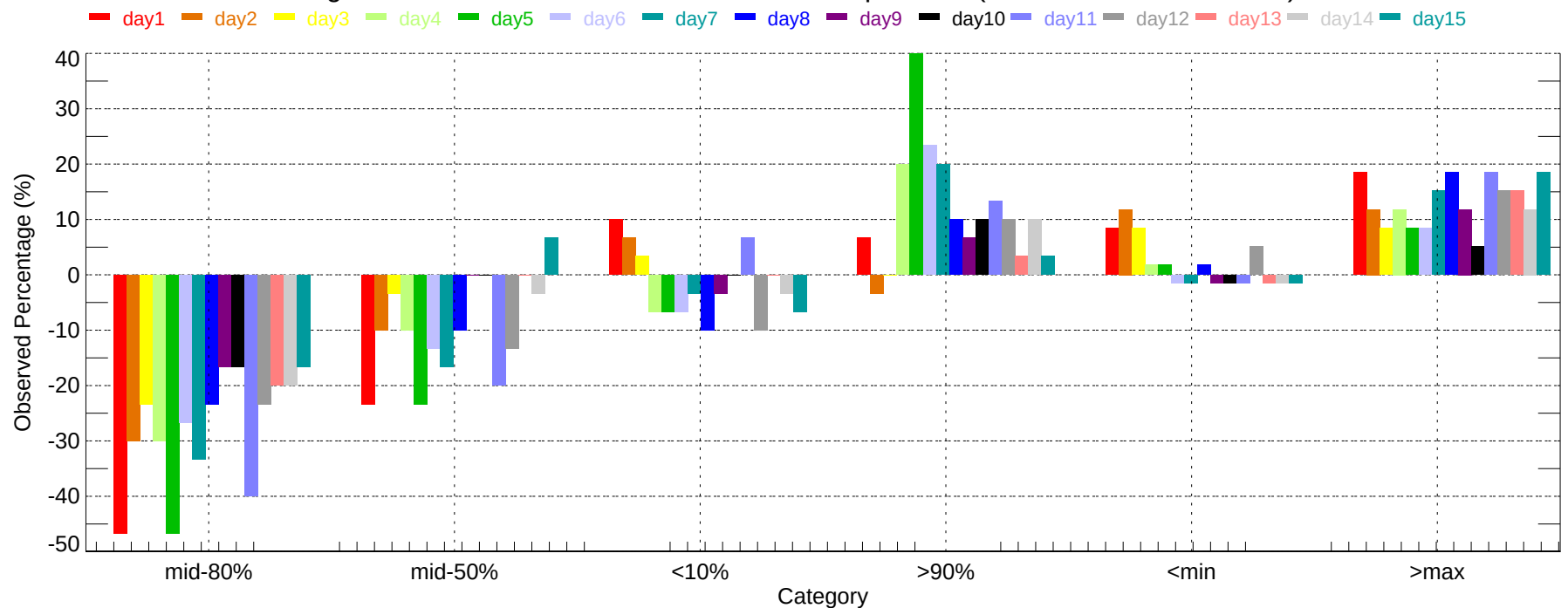
Observed Percentage Deviation of Ensembles - AUS: Min Temperature (2007-12-01~2007-12-31)
