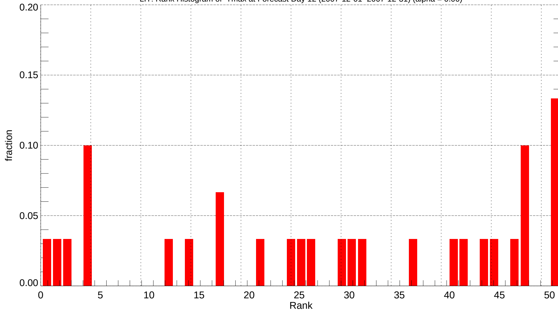
LIT: Rank Histogram of Tmax at Forecast Day 12 (2007-12-01~2007-12-31) (alpha = 0.00)
