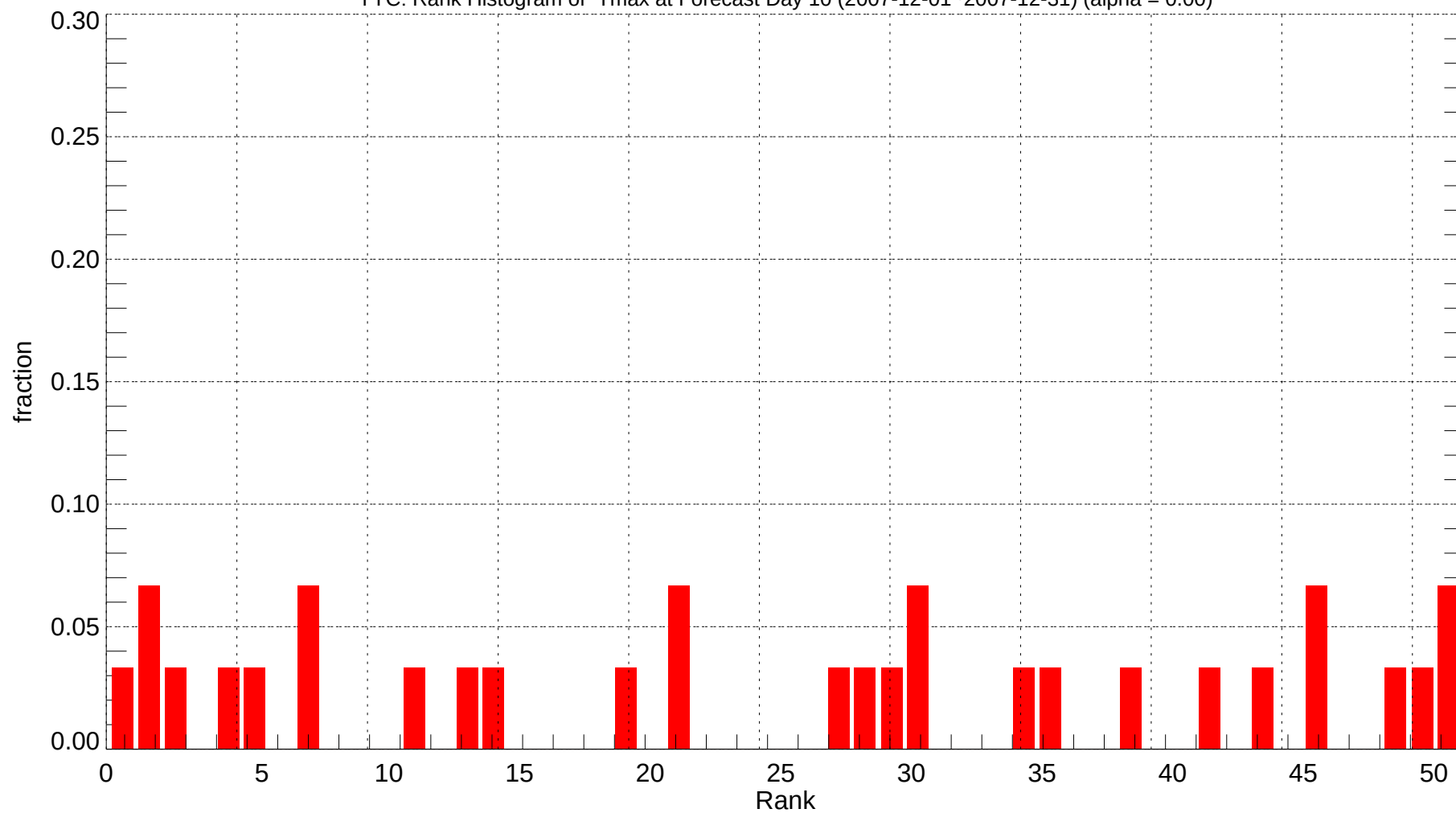
YYC: Rank Histogram of Tmax at Forecast Day 10 (2007-12-01~2007-12-31) (alpha = 0.00)
