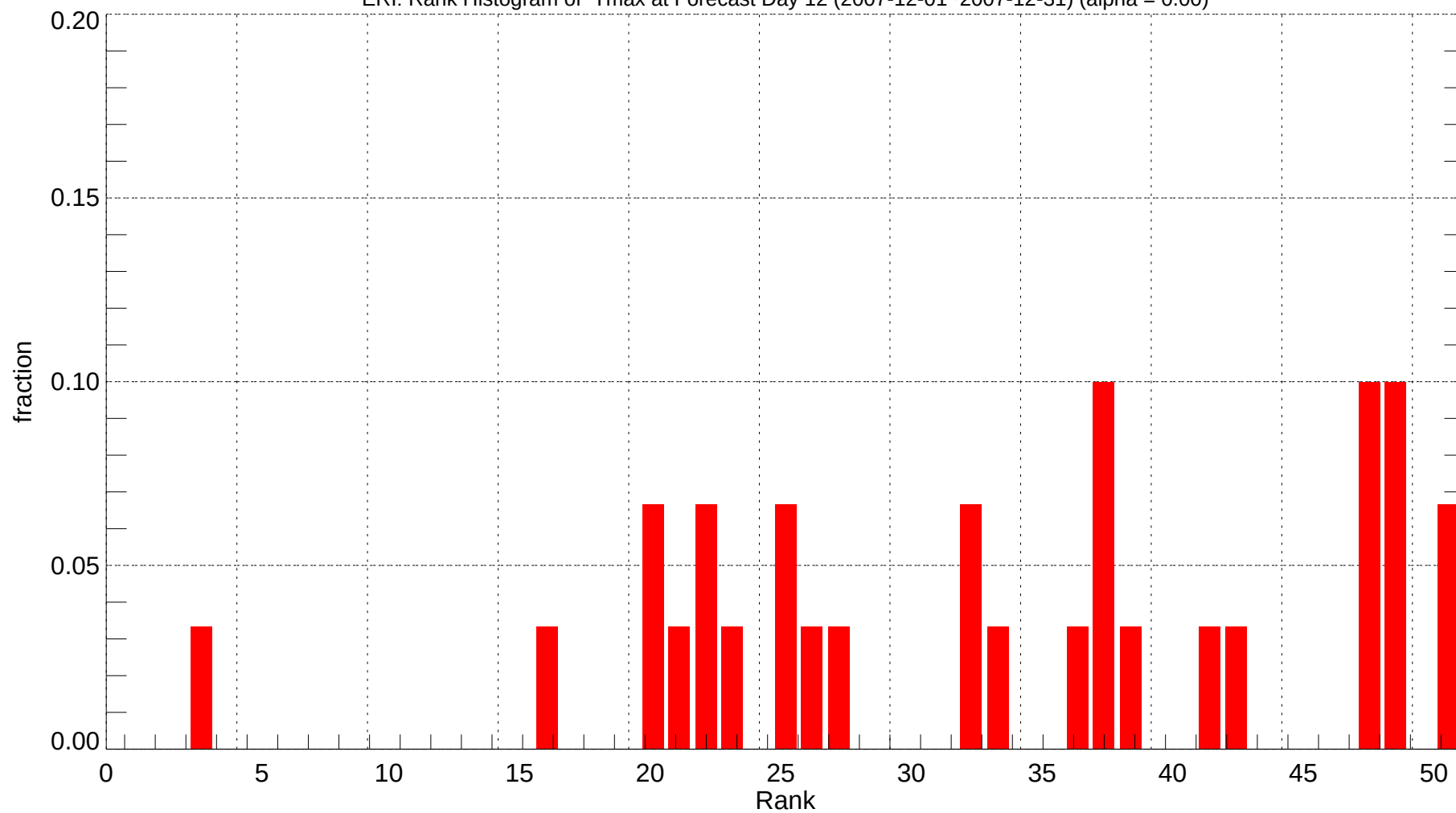
ERI: Rank Histogram of Tmax at Forecast Day 12 (2007-12-01~2007-12-31) (alpha = 0.00)
