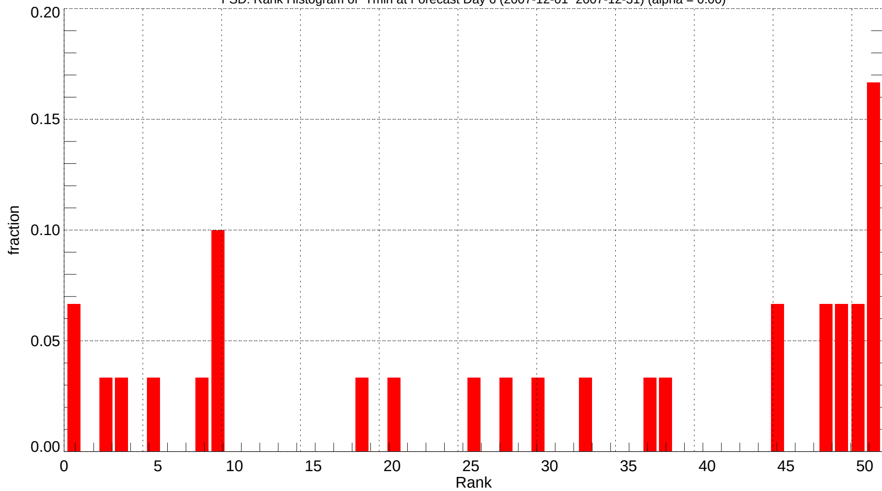
FSD: Rank Histogram of Tmin at Forecast Day 6 (2007-12-01~2007-12-31) (alpha = 0.00)
