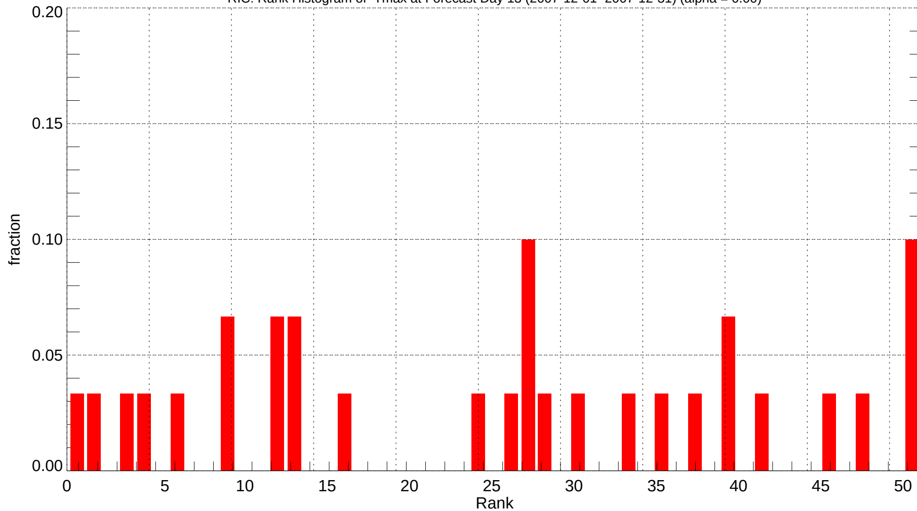
RIC: Rank Histogram of Tmax at Forecast Day 13 (2007-12-01~2007-12-31) (alpha = 0.00)
