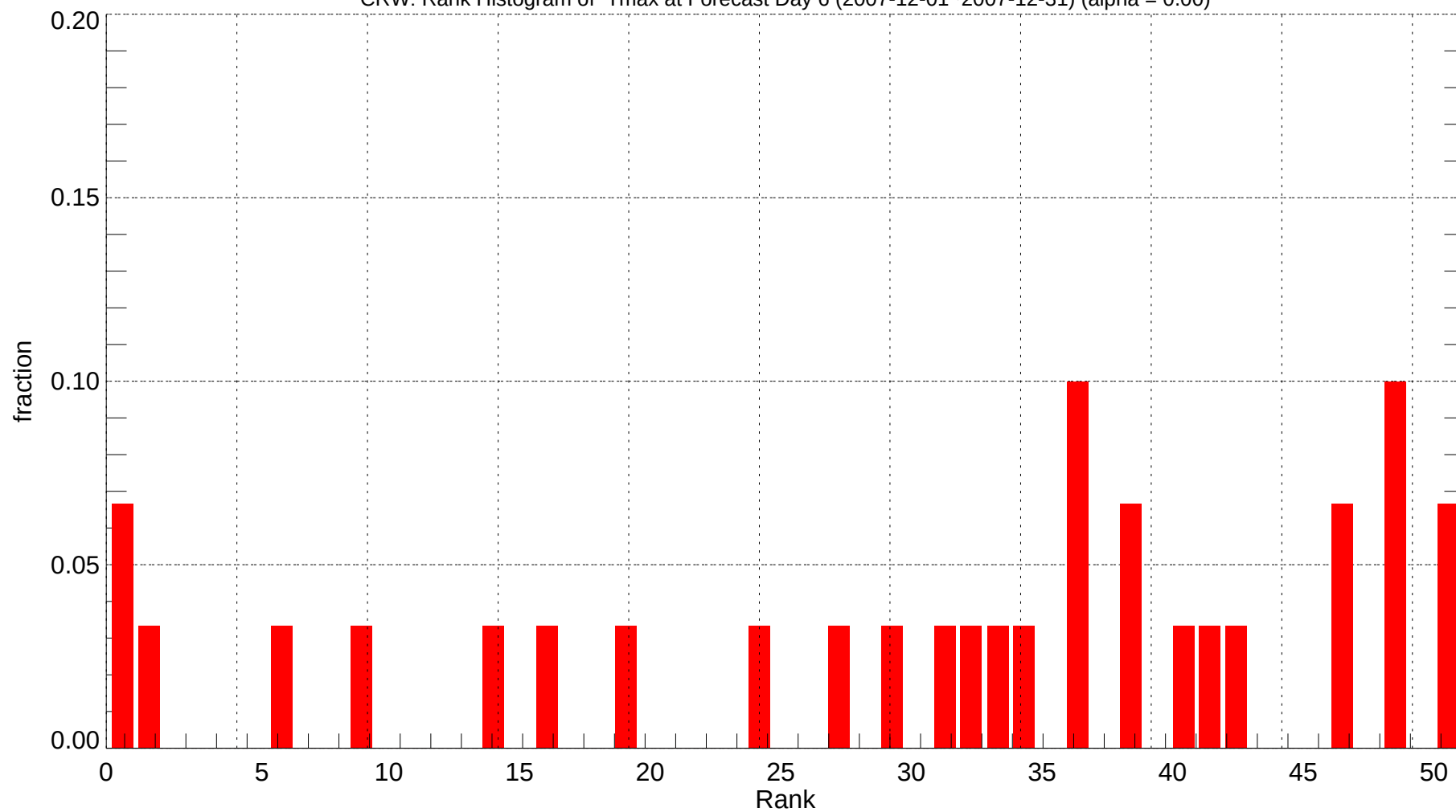
CRW: Rank Histogram of Tmax at Forecast Day 6 (2007-12-01~2007-12-31) (alpha = 0.00)
