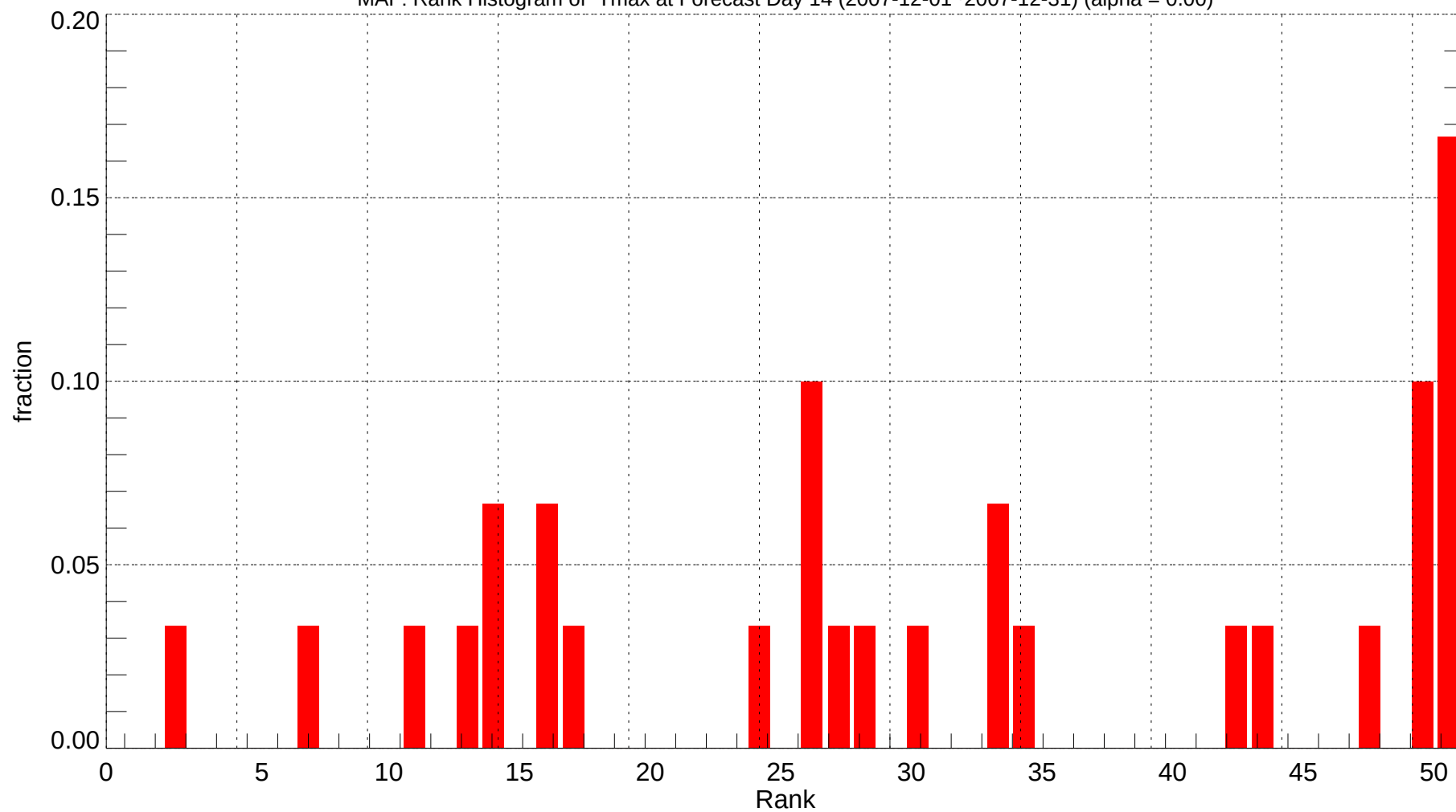
MAF: Rank Histogram of Tmax at Forecast Day 14 (2007-12-01~2007-12-31) (alpha = 0.00)
