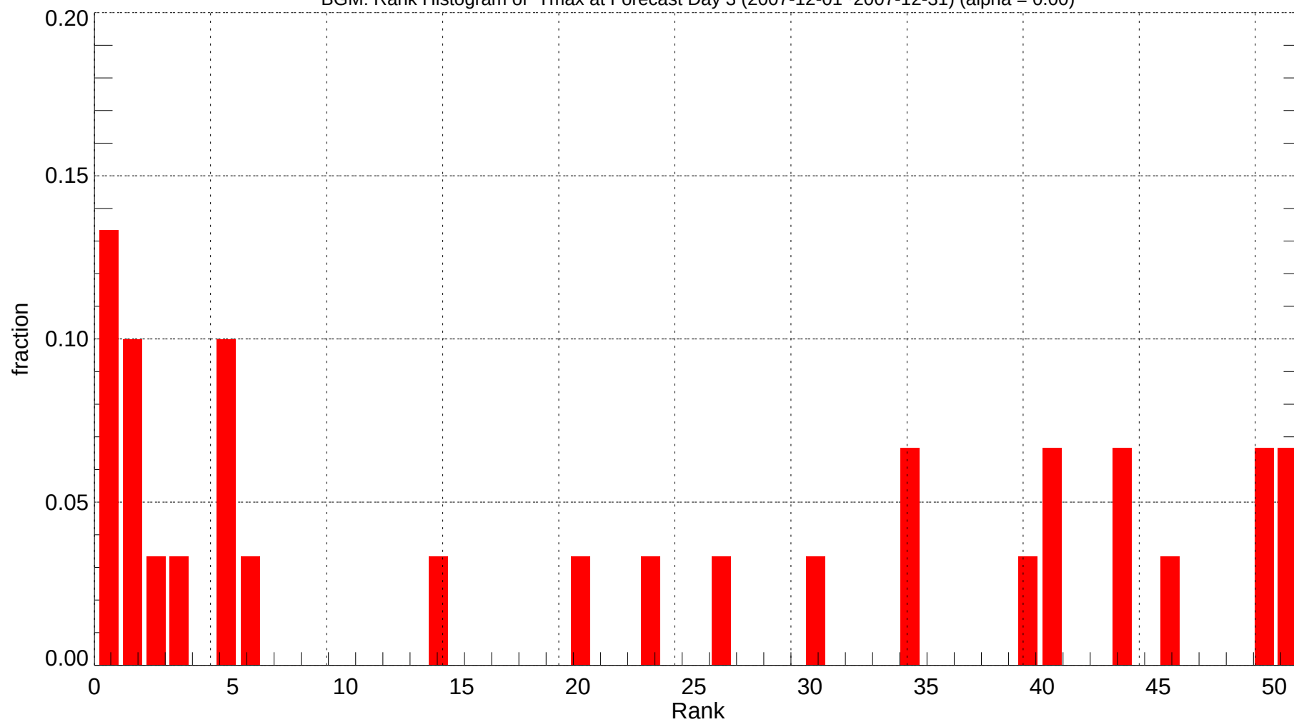
BGM: Rank Histogram of Tmax at Forecast Day 3 (2007-12-01~2007-12-31) (alpha = 0.00)
