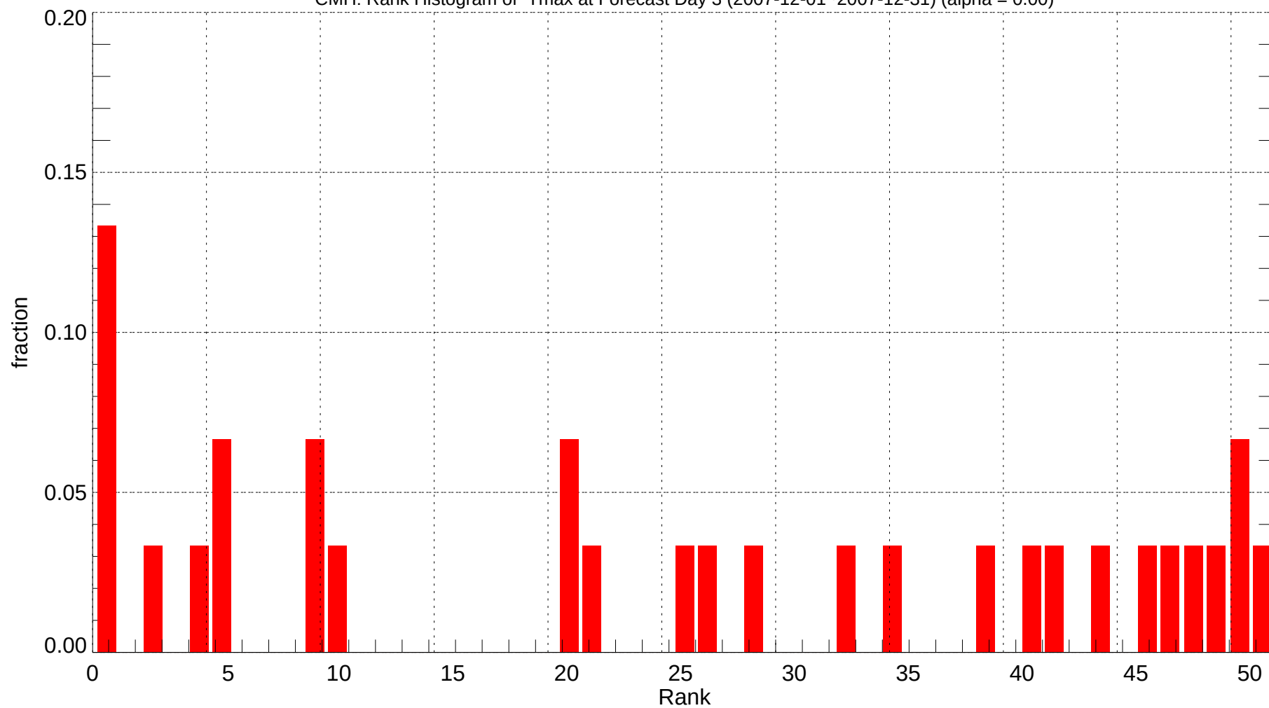
CMH: Rank Histogram of Tmax at Forecast Day 3 (2007-12-01~2007-12-31) (alpha = 0.00)
