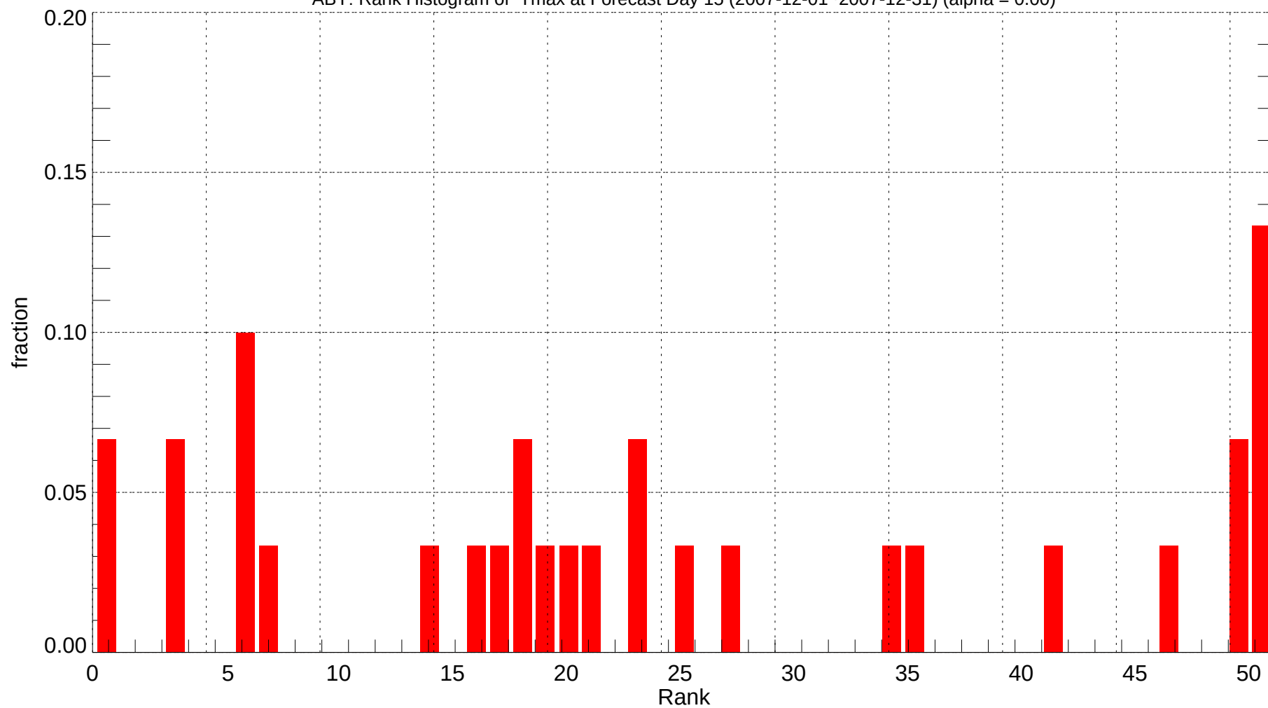
ABY: Rank Histogram of Tmax at Forecast Day 15 (2007-12-01~2007-12-31) (alpha = 0.00)
