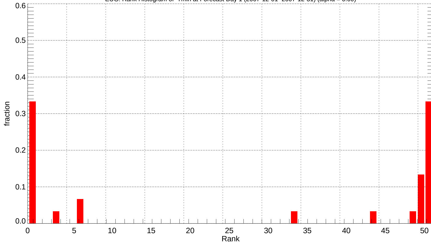
EUG: Rank Histogram of Tmin at Forecast Day 1 (2007-12-01~2007-12-31) (alpha = 0.00)
