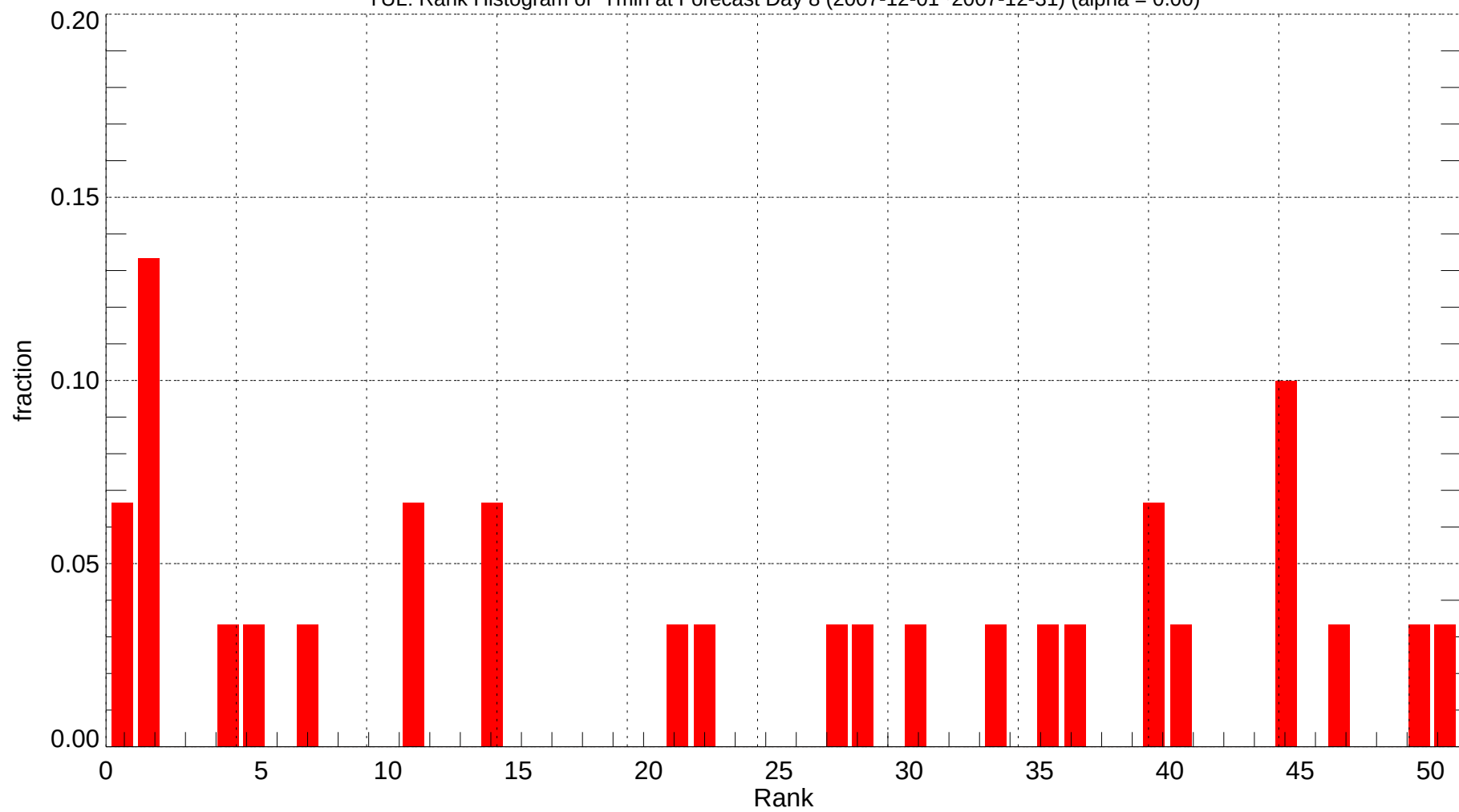
YUL: Rank Histogram of Tmin at Forecast Day 8 (2007-12-01~2007-12-31) (alpha = 0.00)
