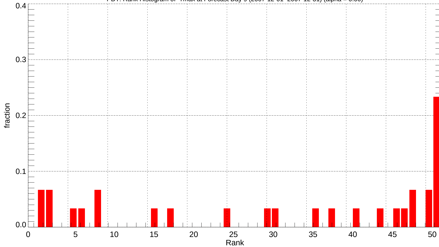
PDT: Rank Histogram of Tmax at Forecast Day 9 (2007-12-01~2007-12-31) (alpha = 0.00)
