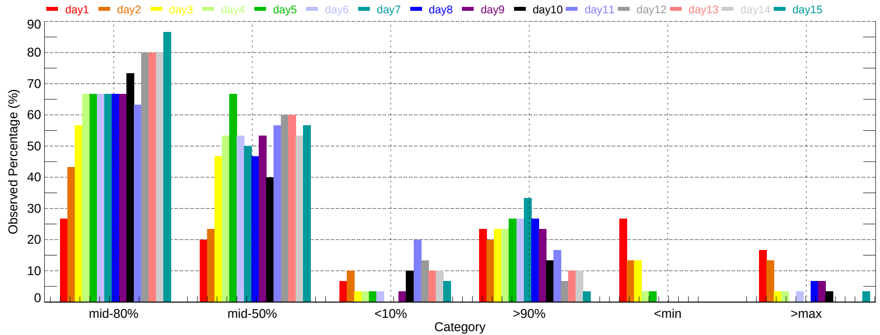
Observed Percentage of Ensembles - LGA: Min Temperature (2007-12-01~2007-12-31)
