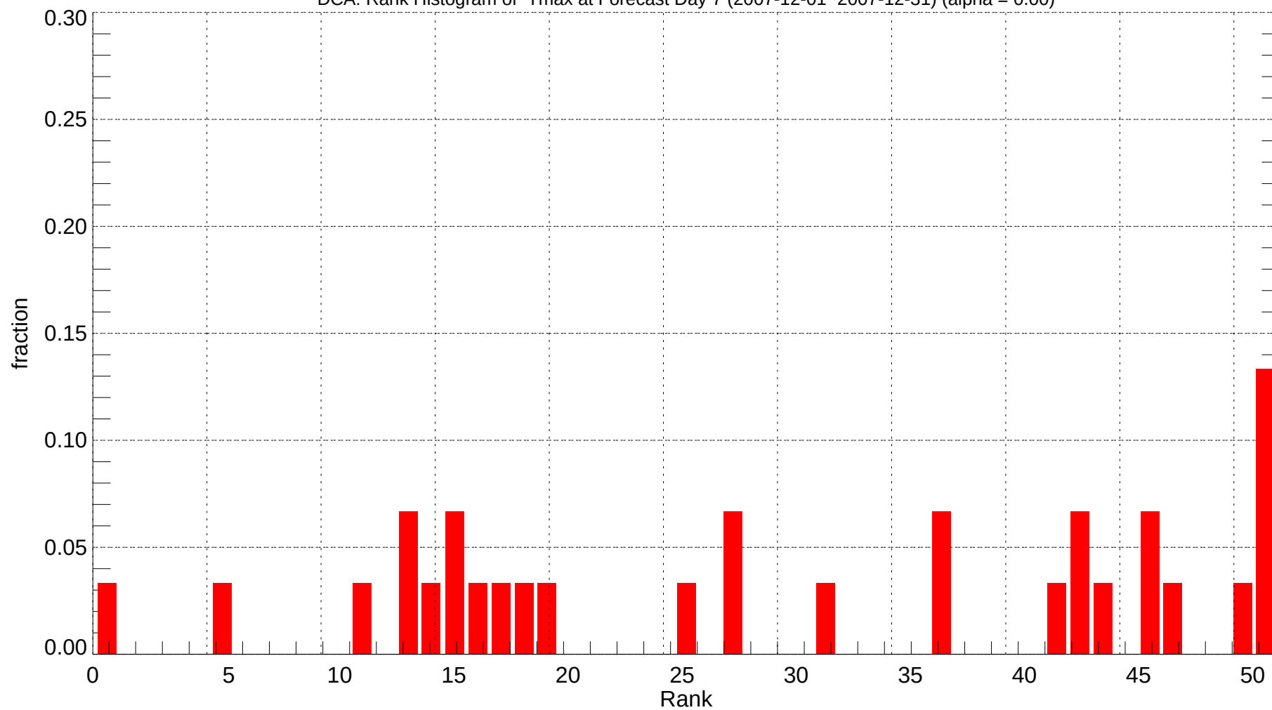
DCA: Rank Histogram of Tmax at Forecast Day 7 (2007-12-01~2007-12-31) (alpha = 0.00)
