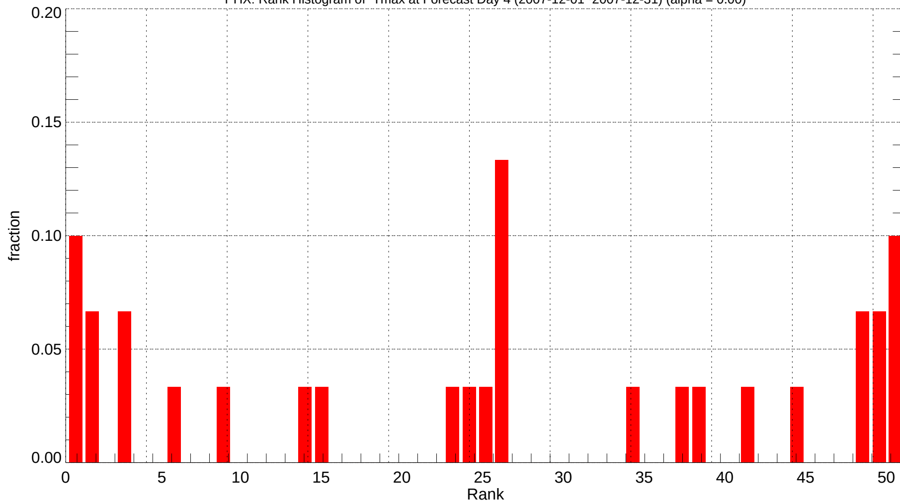
PHX: Rank Histogram of Tmax at Forecast Day 4 (2007-12-01~2007-12-31) (alpha = 0.00)
