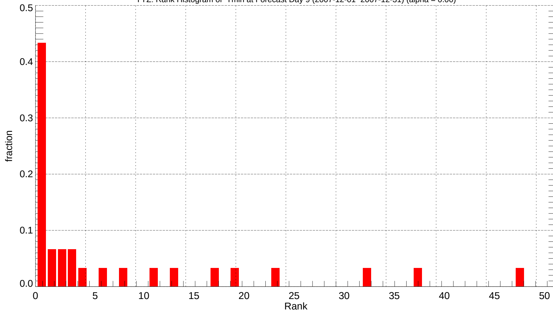
YYZ: Rank Histogram of Tmin at Forecast Day 9 (2007-12-01~2007-12-31) (alpha = 0.00)
