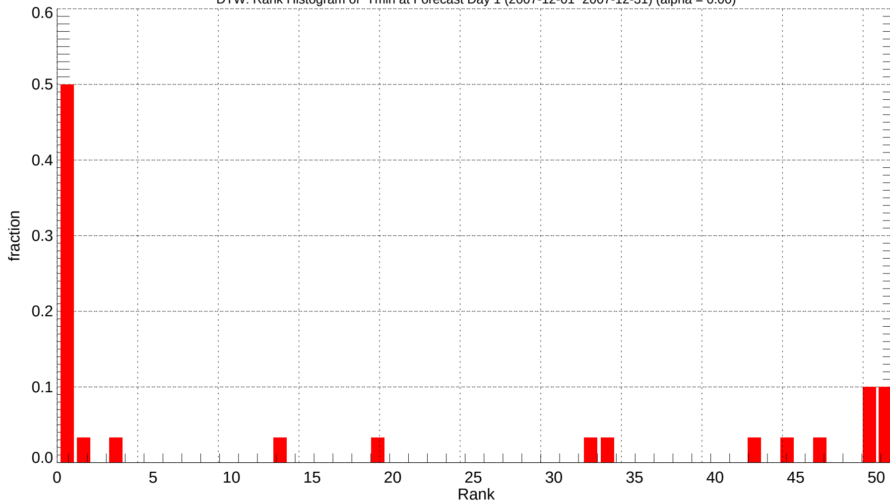
DTW: Rank Histogram of Tmin at Forecast Day 1 (2007-12-01~2007-12-31) (alpha = 0.00)
