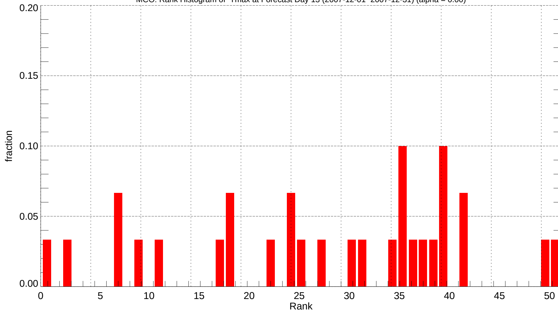
MCO: Rank Histogram of Tmax at Forecast Day 13 (2007-12-01~2007-12-31) (alpha = 0.00)
