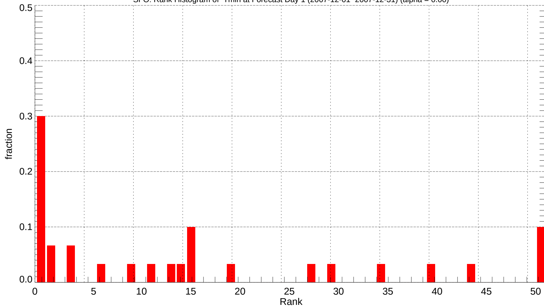
SFO: Rank Histogram of Tmin at Forecast Day 1 (2007-12-01~2007-12-31) (alpha = 0.00)
