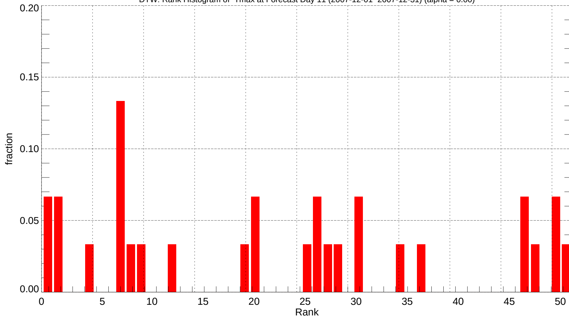
DTW: Rank Histogram of Tmax at Forecast Day 11 (2007-12-01~2007-12-31) (alpha = 0.00)
