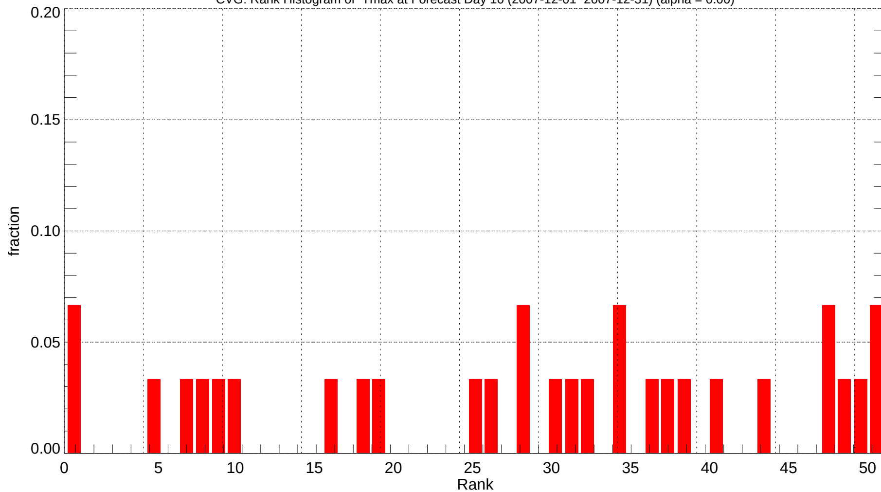
CVG: Rank Histogram of Tmax at Forecast Day 10 (2007-12-01~2007-12-31) (alpha = 0.00)
