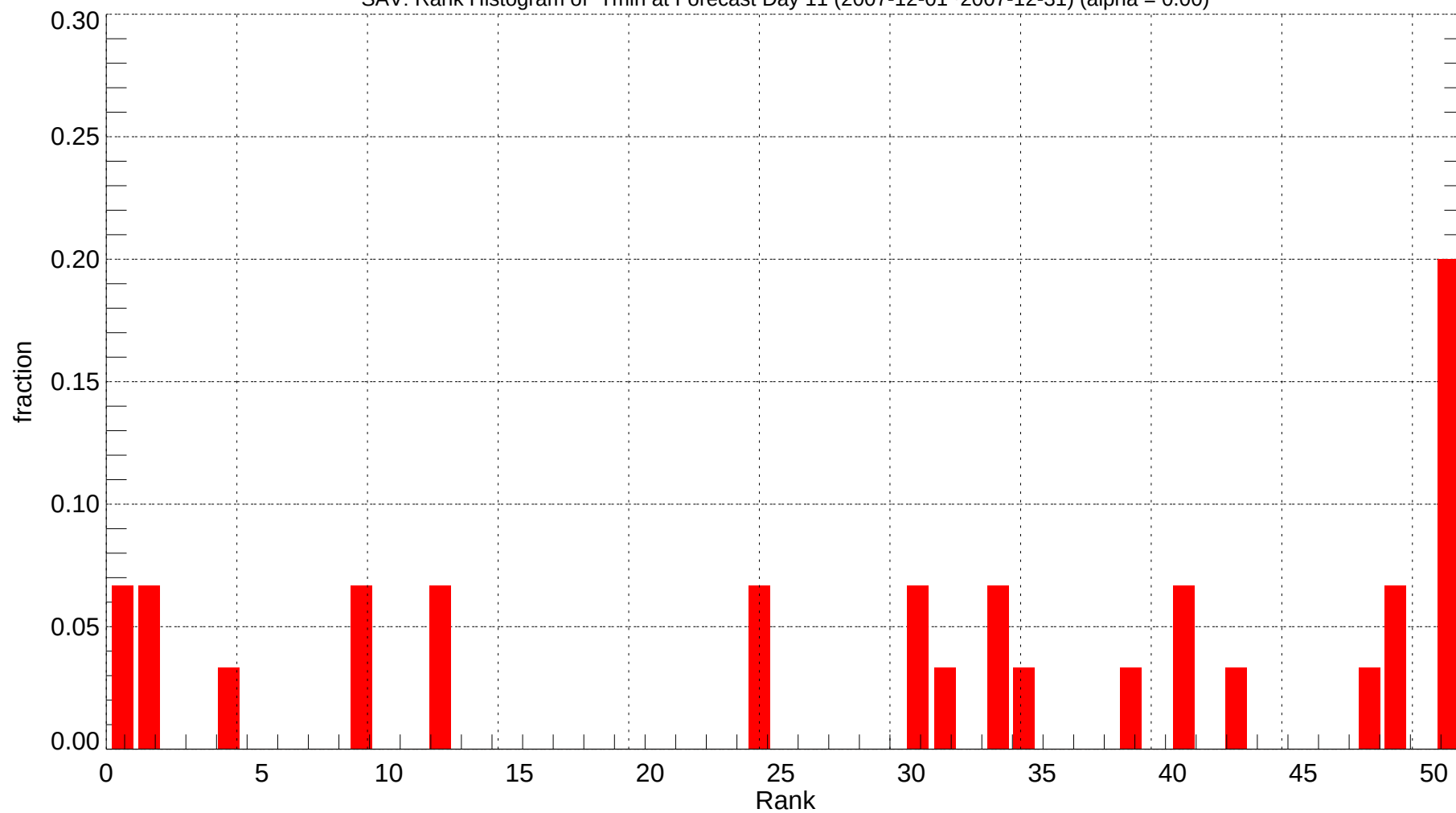
SAV: Rank Histogram of Tmin at Forecast Day 11 (2007-12-01~2007-12-31) (alpha = 0.00)
