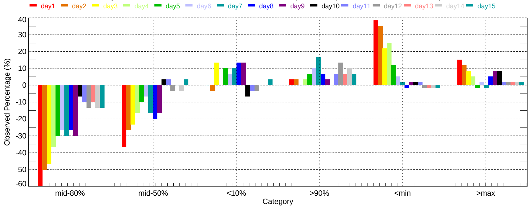
Observed Percentage Deviation of Ensembles - YNG: Max Temperature (2007-12-01~2007-12-31)
