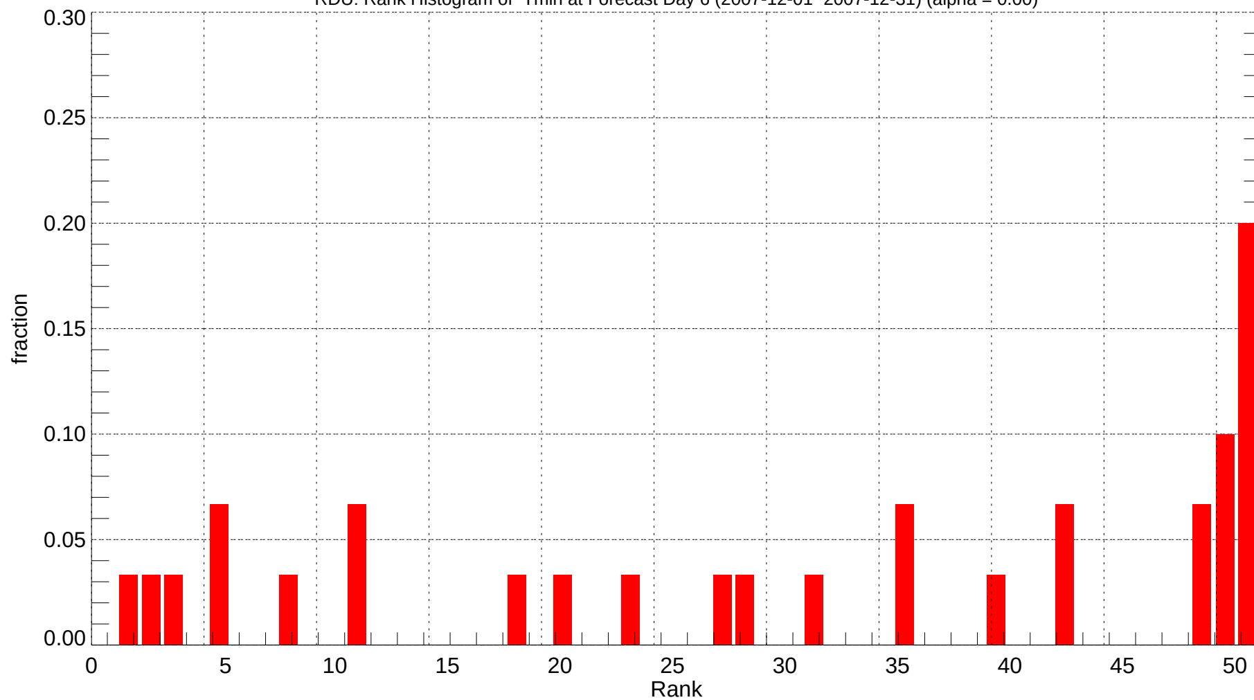
RDU: Rank Histogram of Tmin at Forecast Day 6 (2007-12-01~2007-12-31) (alpha = 0.00)
