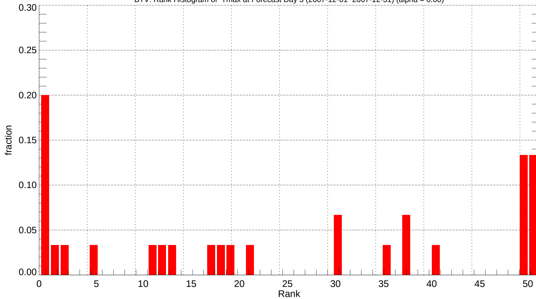
BTV: Rank Histogram of Tmax at Forecast Day 3 (2007-12-01~2007-12-31) (alpha = 0.00)
