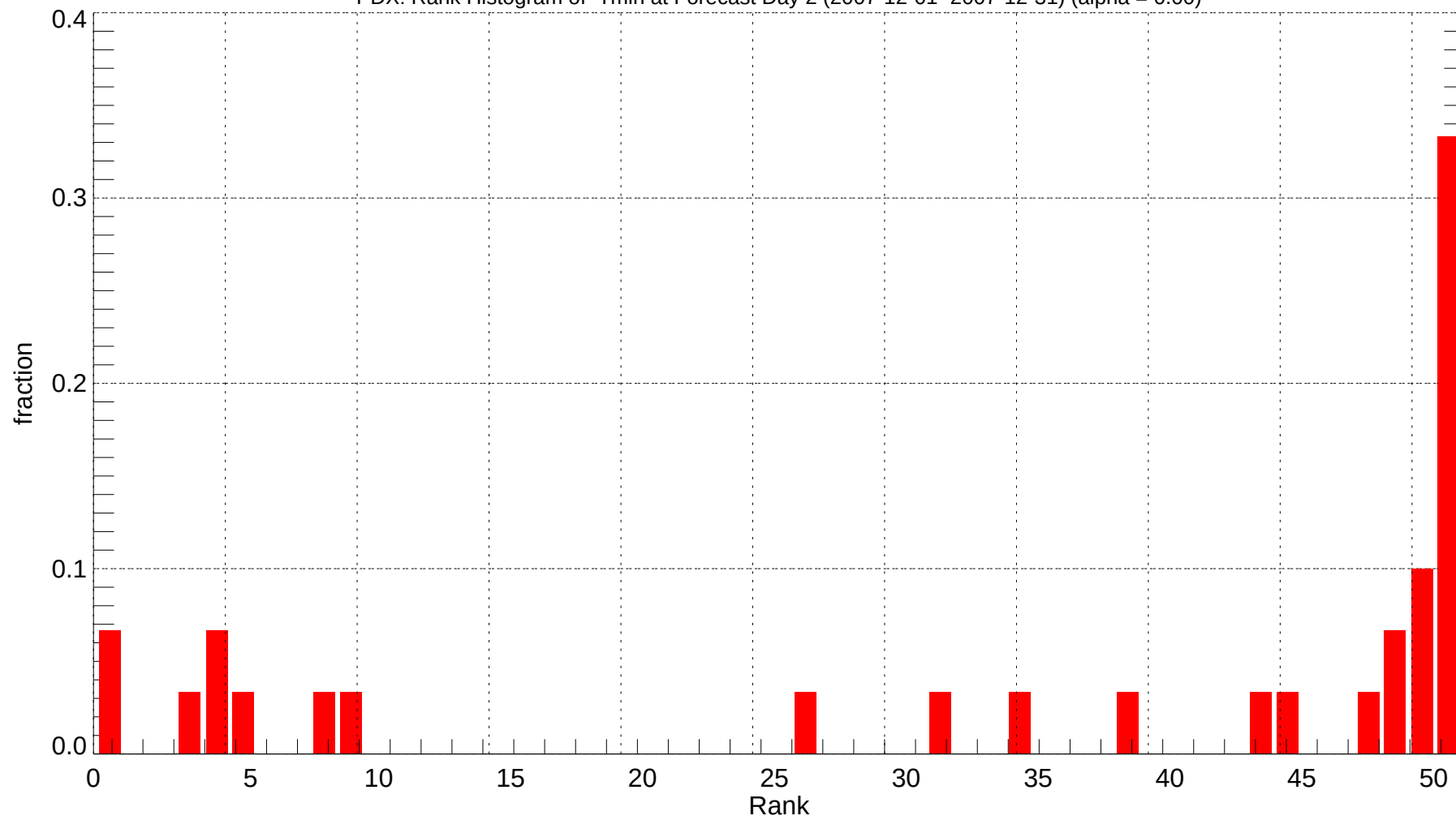
PDX: Rank Histogram of Tmin at Forecast Day 2 (2007-12-01~2007-12-31) (alpha = 0.00)
