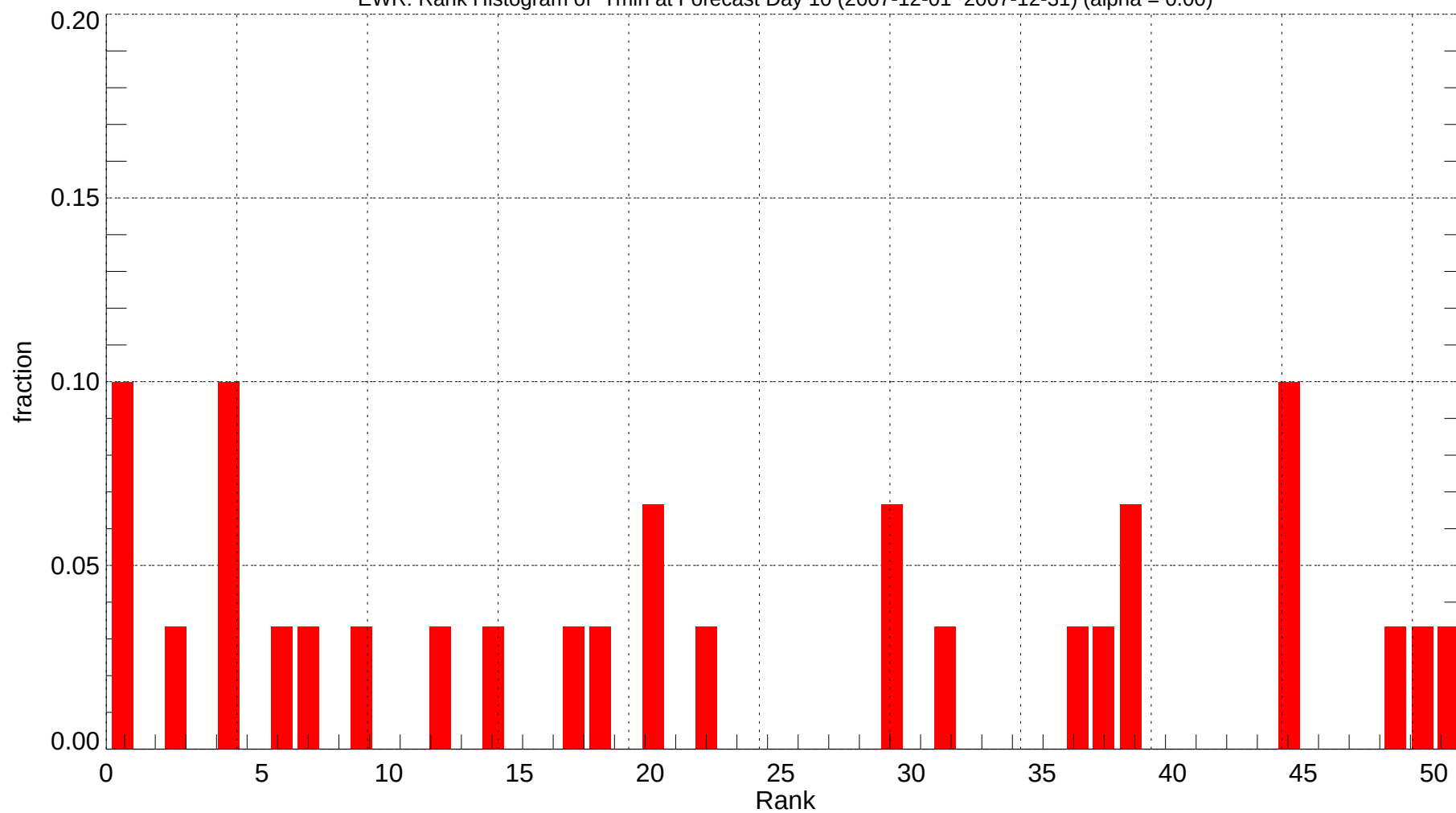
EWR: Rank Histogram of Tmin at Forecast Day 10 (2007-12-01~2007-12-31) (alpha = 0.00)
