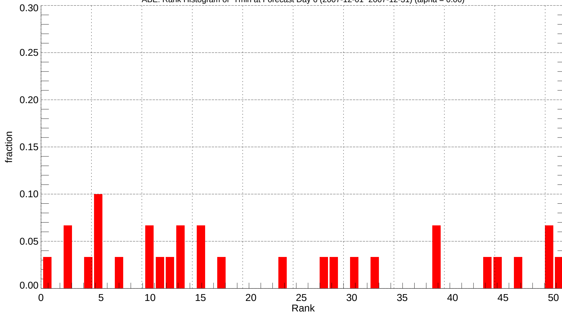
ABE: Rank Histogram of Tmin at Forecast Day 6 (2007-12-01~2007-12-31) (alpha = 0.00)
