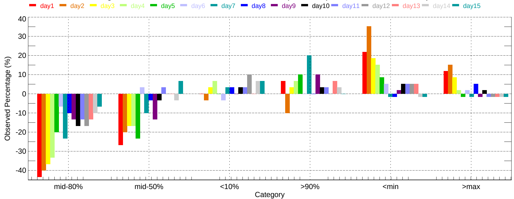
Observed Percentage Deviation of Ensembles - FWA: Max Temperature (2007-12-01~2007-12-31)
