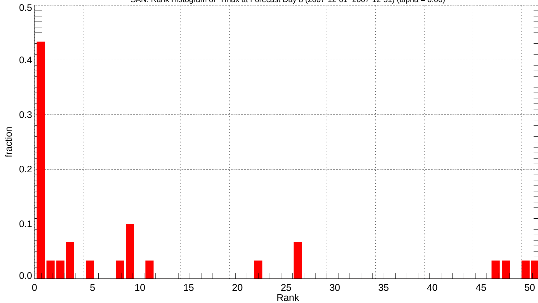
SAN: Rank Histogram of Tmax at Forecast Day 8 (2007-12-01~2007-12-31) (alpha = 0.00)
