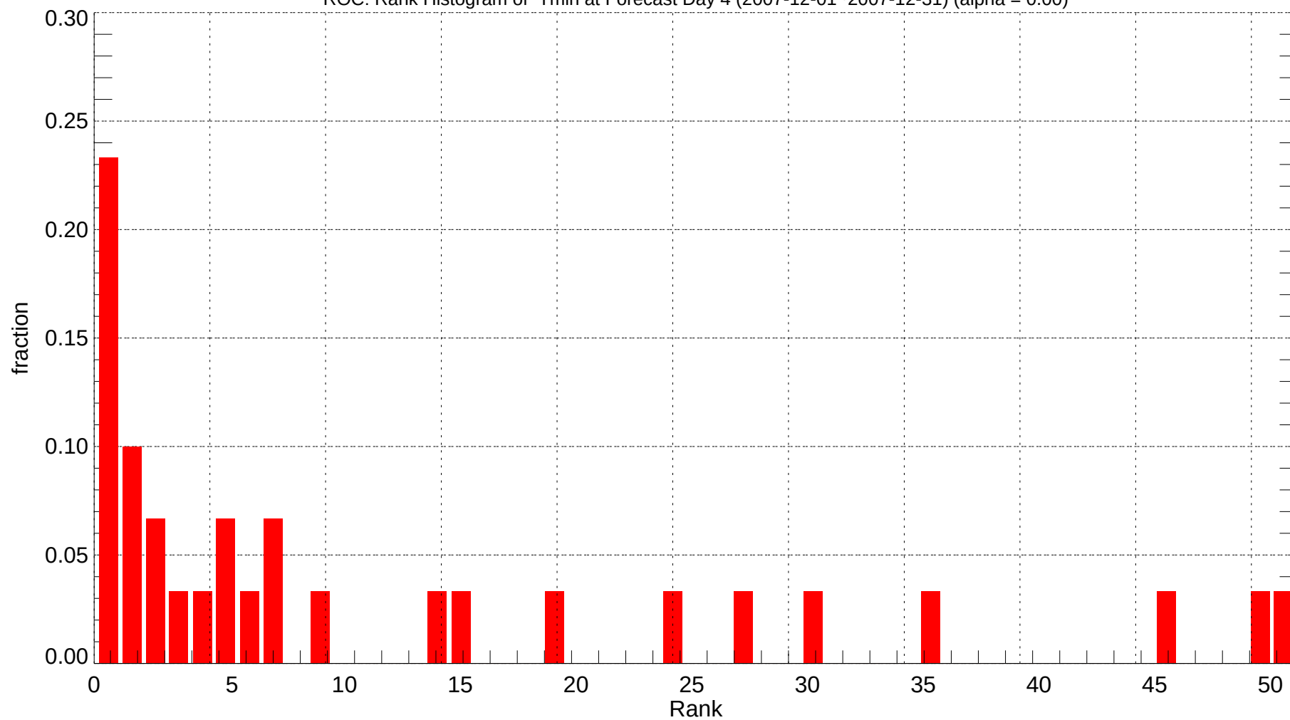
ROC: Rank Histogram of Tmin at Forecast Day 4 (2007-12-01~2007-12-31) (alpha = 0.00)
