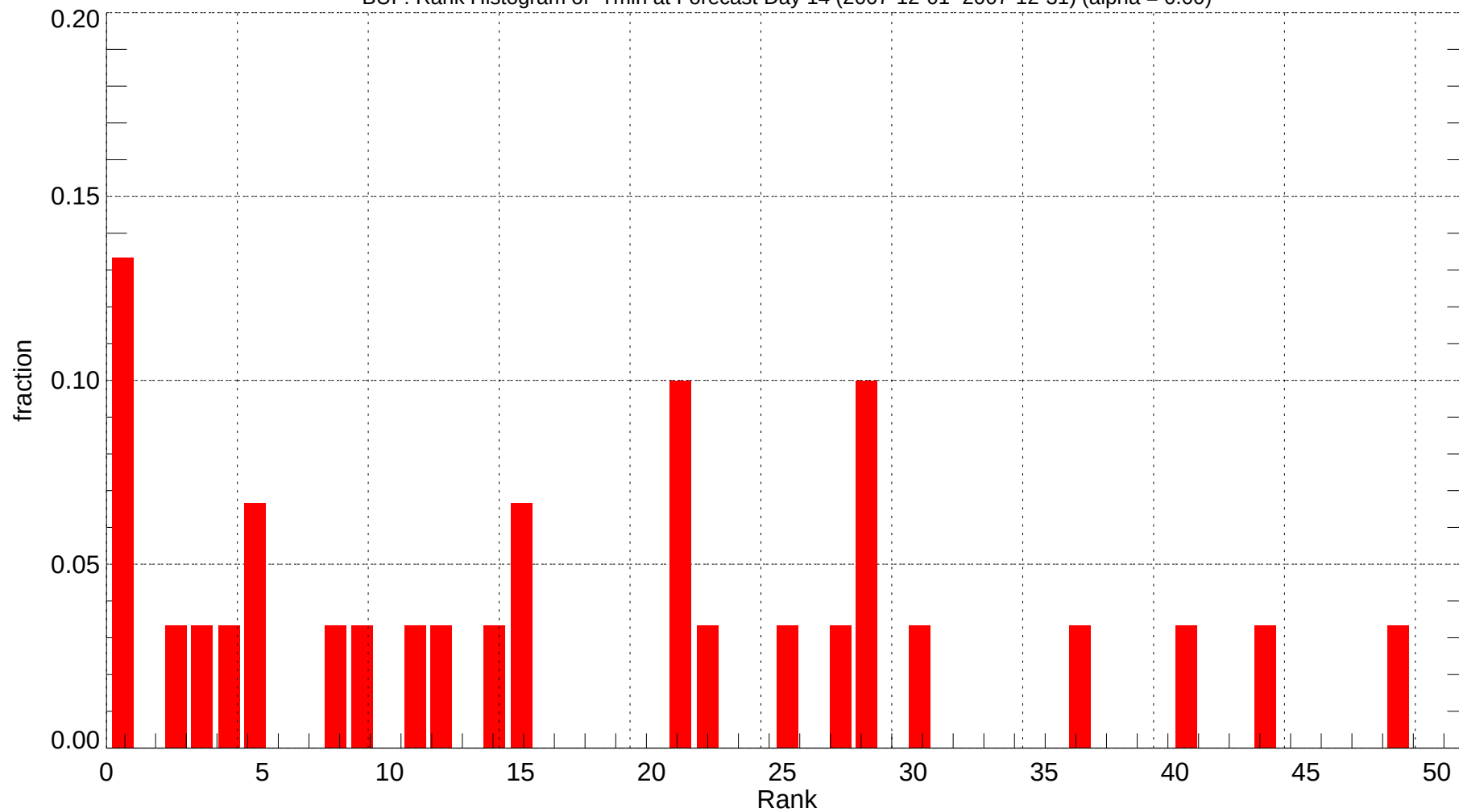
BUF: Rank Histogram of Tmin at Forecast Day 14 (2007-12-01~2007-12-31) (alpha = 0.00)
