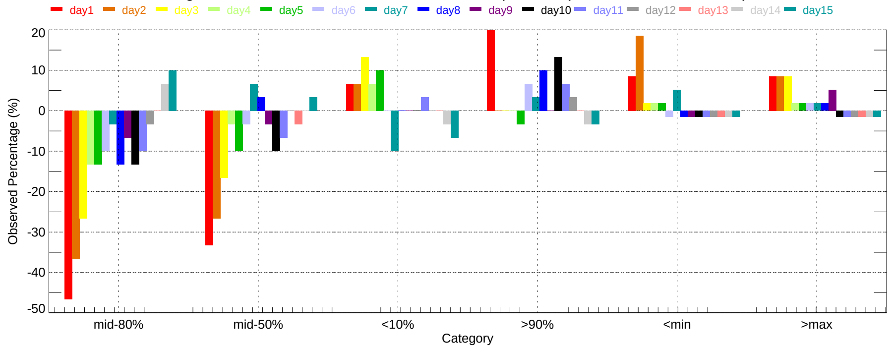
Observed Percentage Deviation of Ensembles - PWM: Max Temperature (2007-12-01~2007-12-31)
