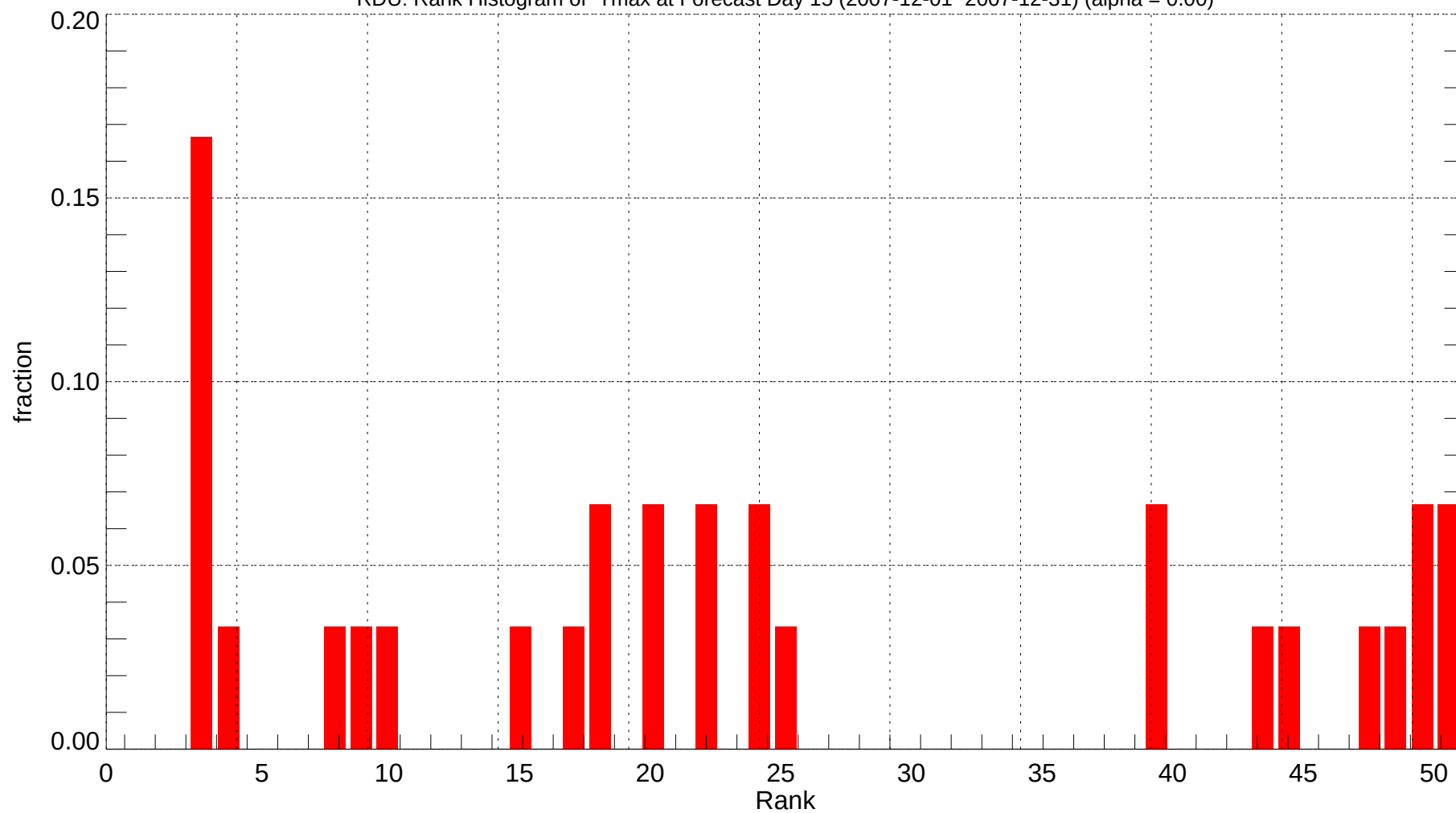
RDU: Rank Histogram of Tmax at Forecast Day 15 (2007-12-01~2007-12-31) (alpha = 0.00)
