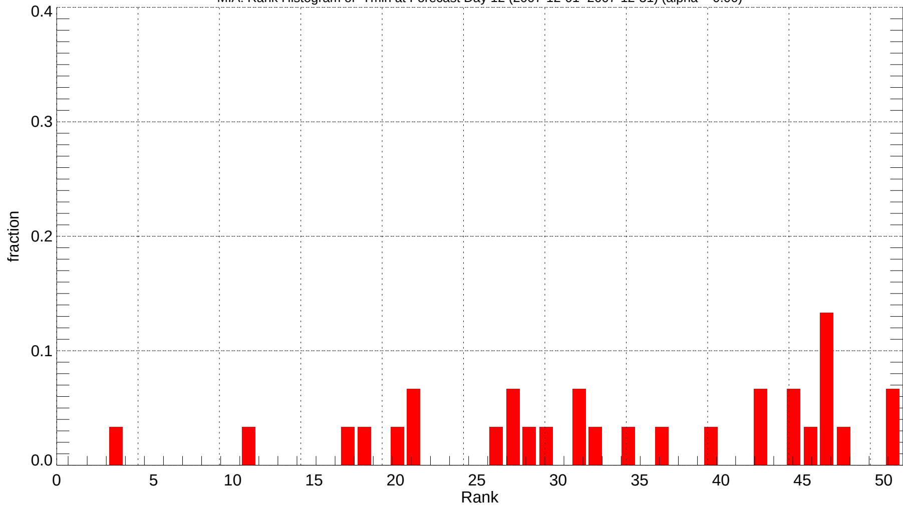
MIA: Rank Histogram of Tmin at Forecast Day 12 (2007-12-01~2007-12-31) (alpha = 0.00)
