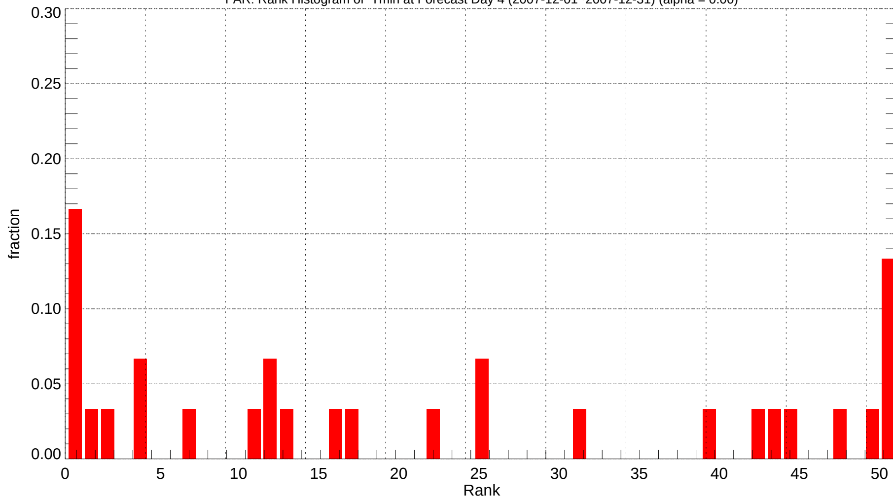
FAR: Rank Histogram of Tmin at Forecast Day 4 (2007-12-01~2007-12-31) (alpha = 0.00)
