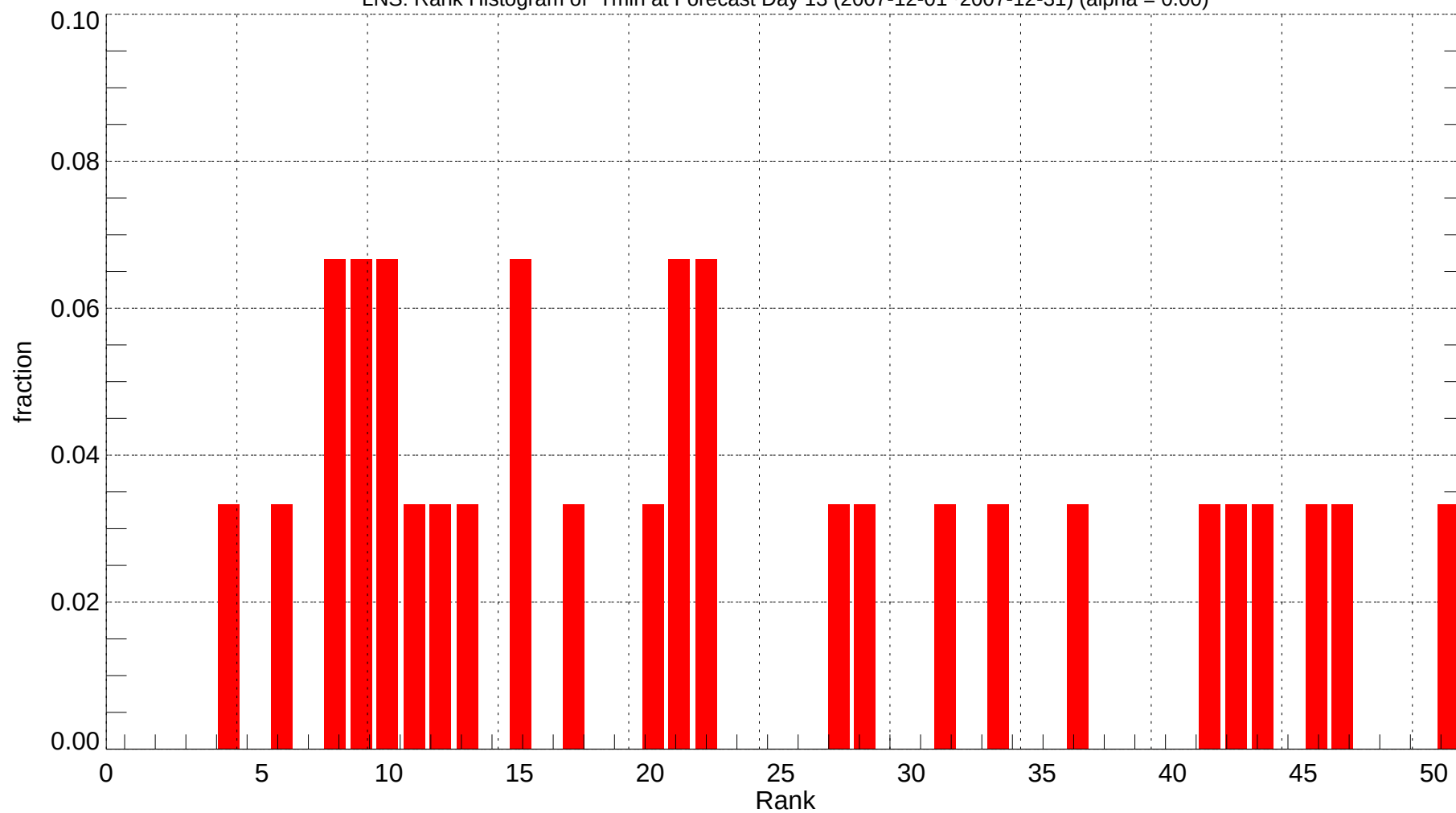
LNS: Rank Histogram of Tmin at Forecast Day 13 (2007-12-01~2007-12-31) (alpha = 0.00)
