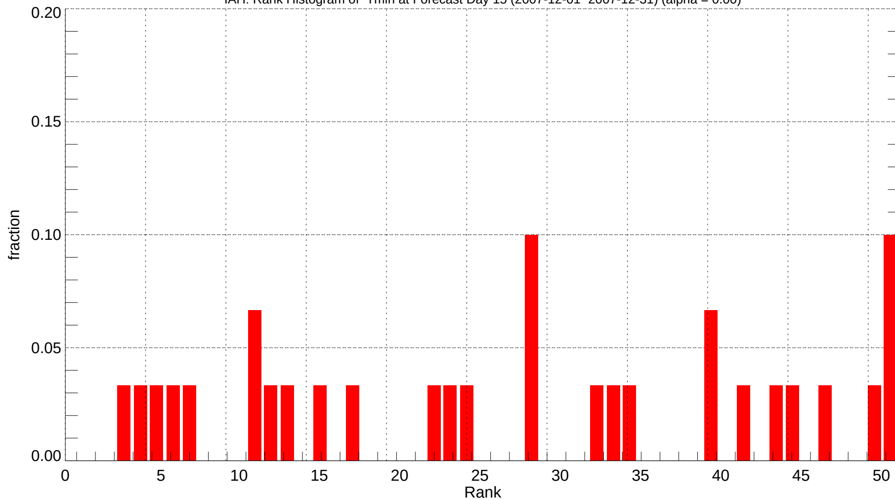
IAH: Rank Histogram of Tmin at Forecast Day 15 (2007-12-01~2007-12-31) (alpha = 0.00)
