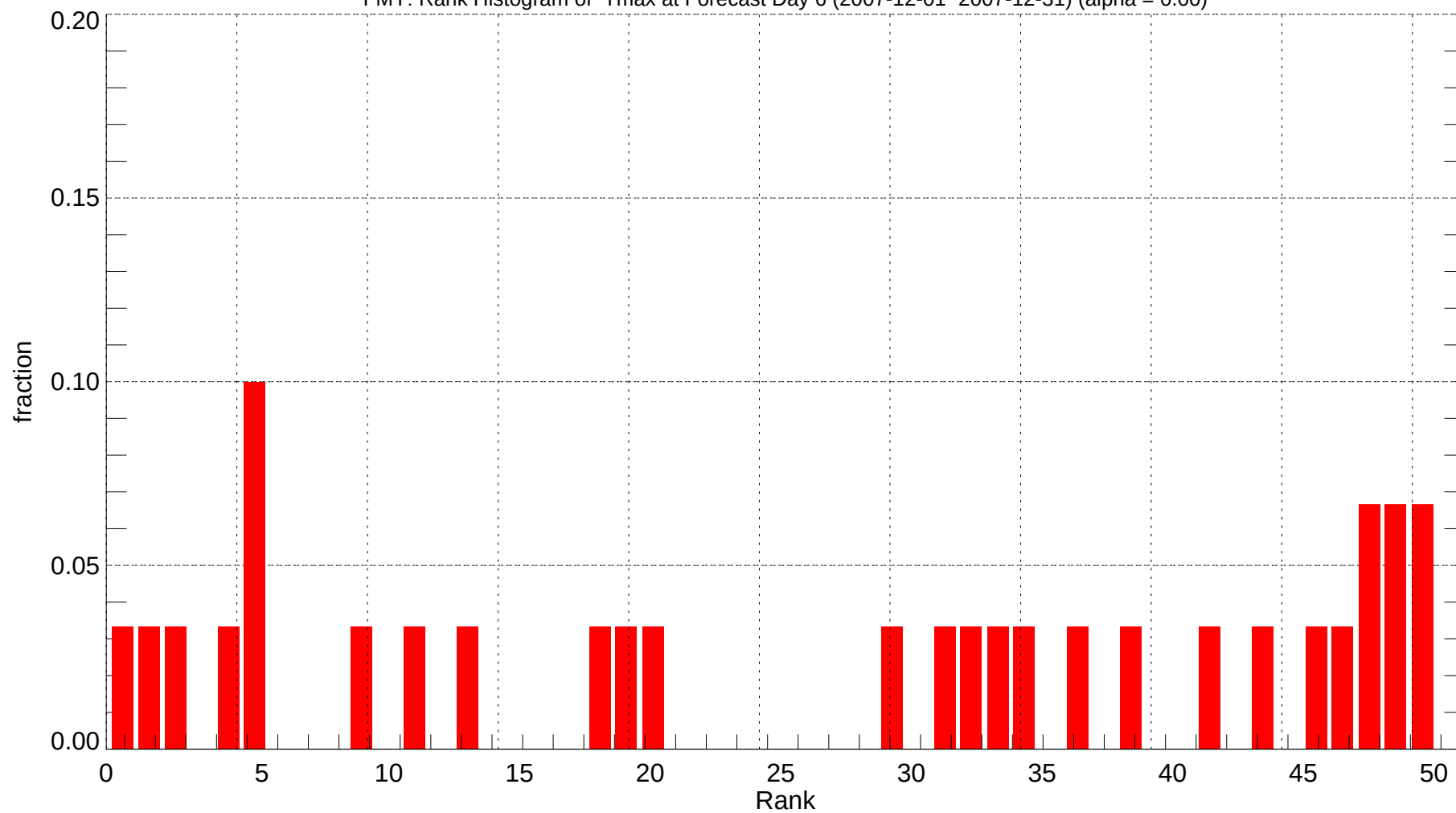
FMY: Rank Histogram of Tmax at Forecast Day 6 (2007-12-01~2007-12-31) (alpha = 0.00)
