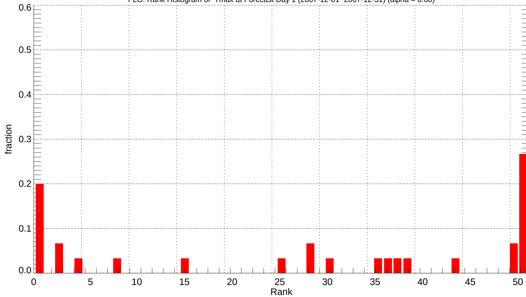
FLG: Rank Histogram of Tmax at Forecast Day 1 (2007-12-01~2007-12-31) (alpha = 0.00)
