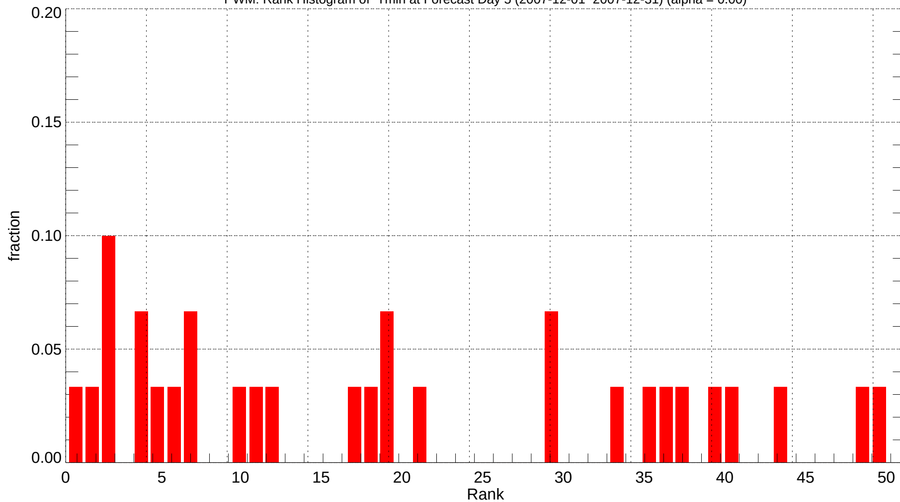
PWM: Rank Histogram of Tmin at Forecast Day 5 (2007-12-01~2007-12-31) (alpha = 0.00)
