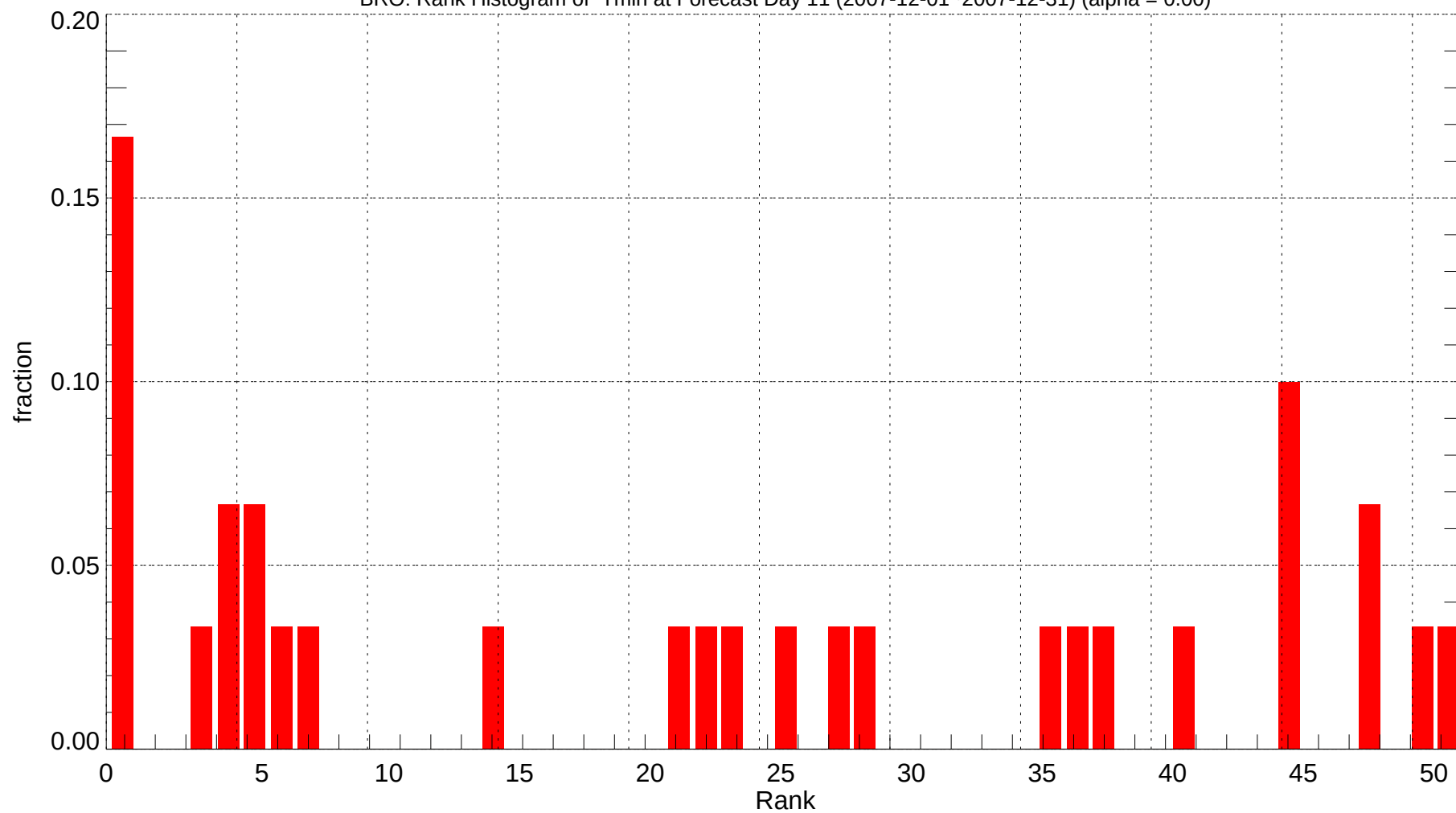
BRO: Rank Histogram of Tmin at Forecast Day 11 (2007-12-01~2007-12-31) (alpha = 0.00)
