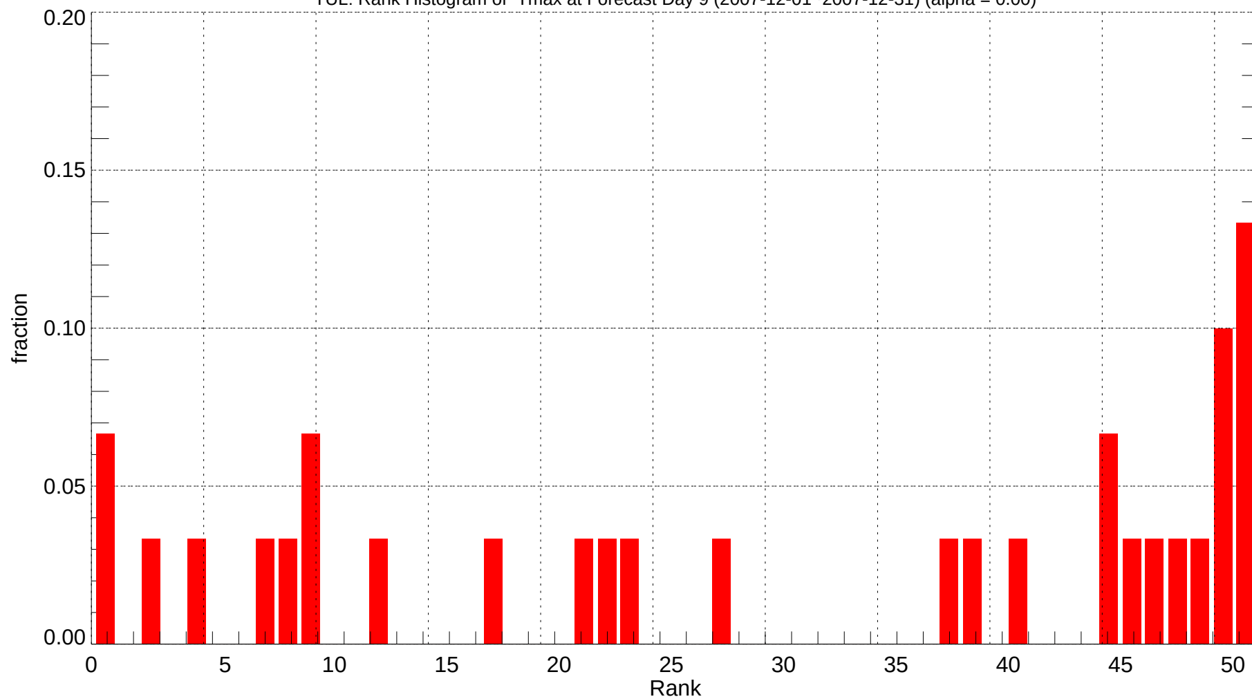
TUL: Rank Histogram of Tmax at Forecast Day 9 (2007-12-01~2007-12-31) (alpha = 0.00)
