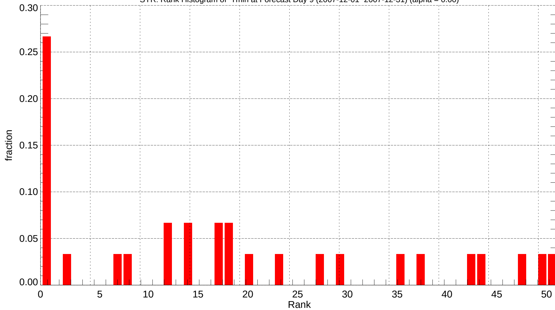
SYR: Rank Histogram of Tmin at Forecast Day 9 (2007-12-01~2007-12-31) (alpha = 0.00)
