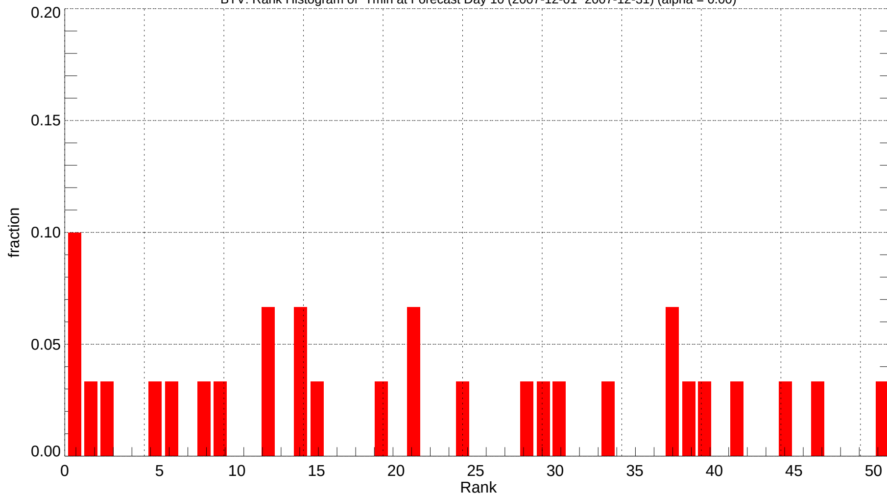
BTV: Rank Histogram of Tmin at Forecast Day 10 (2007-12-01~2007-12-31) (alpha = 0.00)
