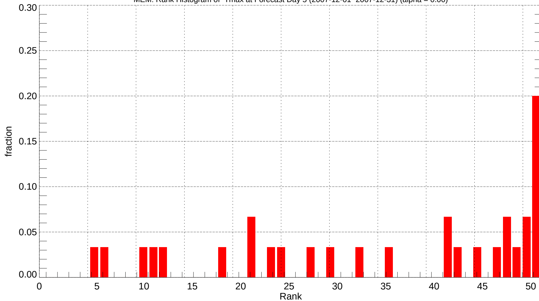
MEM: Rank Histogram of Tmax at Forecast Day 5 (2007-12-01~2007-12-31) (alpha = 0.00)
