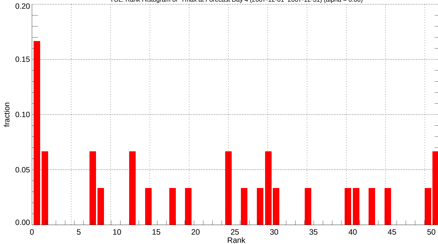
YUL: Rank Histogram of Tmax at Forecast Day 4 (2007-12-01~2007-12-31) (alpha = 0.00)
