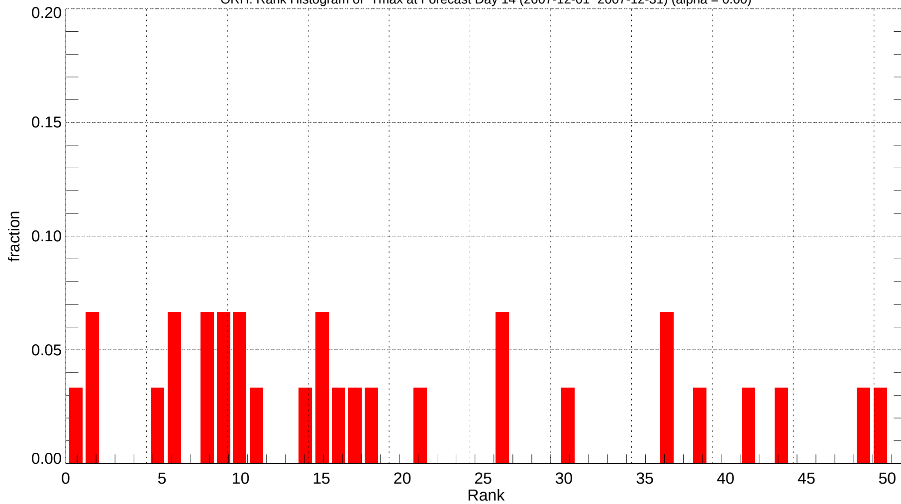
ORH: Rank Histogram of Tmax at Forecast Day 14 (2007-12-01~2007-12-31) (alpha = 0.00)
