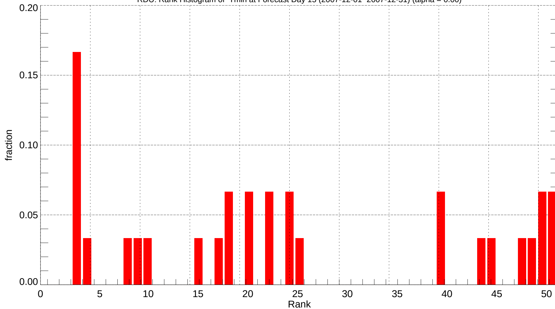
RDU: Rank Histogram of Tmin at Forecast Day 15 (2007-12-01~2007-12-31) (alpha = 0.00)
