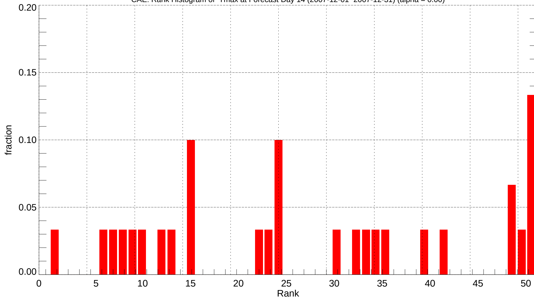
CAE: Rank Histogram of Tmax at Forecast Day 14 (2007-12-01~2007-12-31) (alpha = 0.00)
