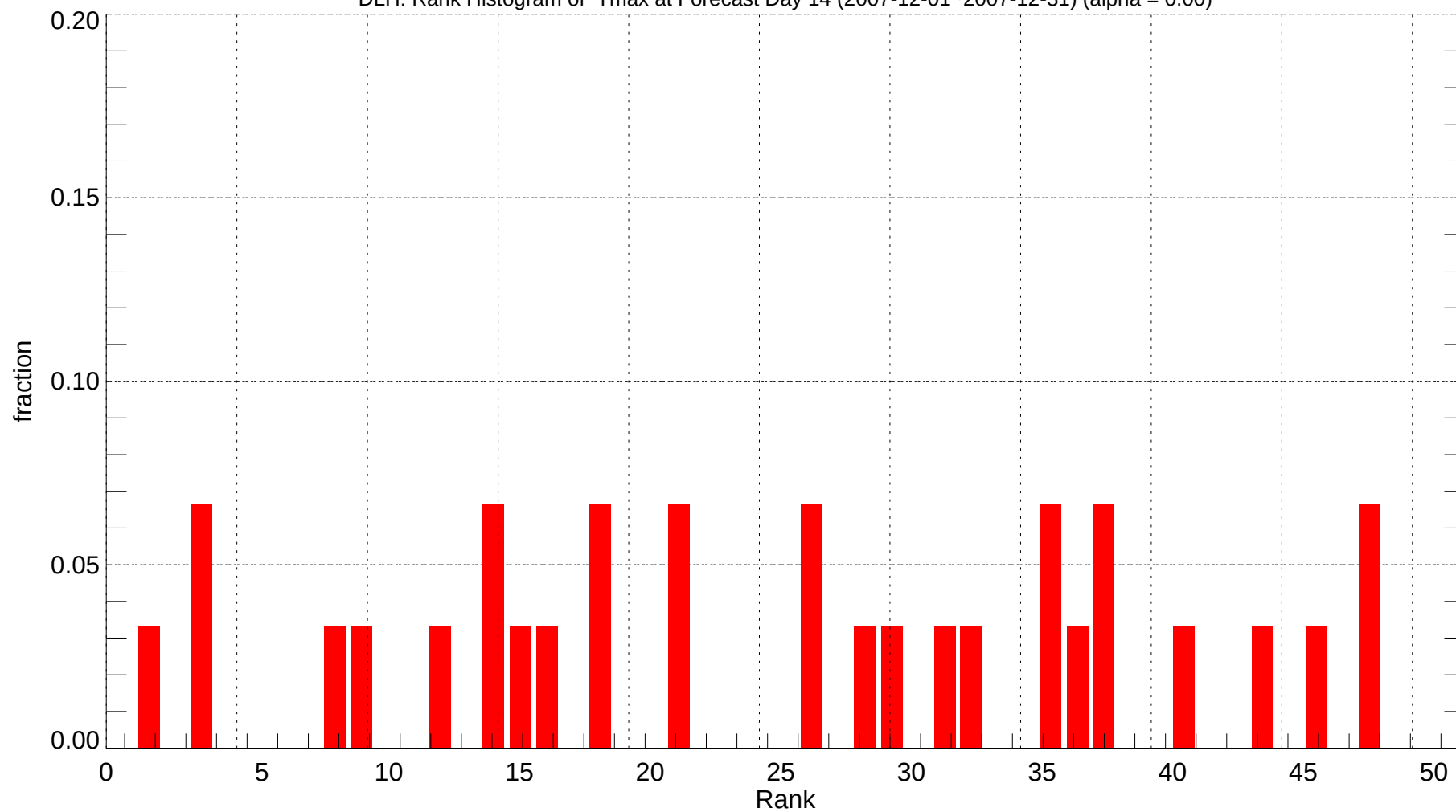
DLH: Rank Histogram of Tmax at Forecast Day 14 (2007-12-01~2007-12-31) (alpha = 0.00)
