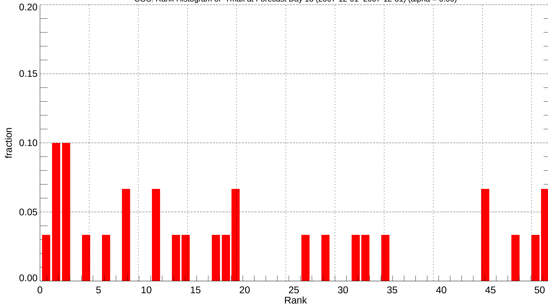
COS: Rank Histogram of Tmax at Forecast Day 13 (2007-12-01~2007-12-31) (alpha = 0.00)
