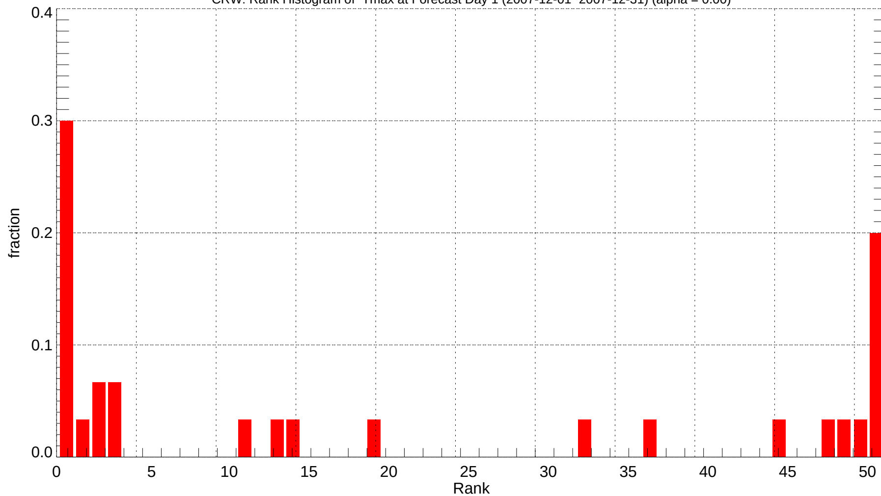
CRW: Rank Histogram of Tmax at Forecast Day 1 (2007-12-01~2007-12-31) (alpha = 0.00)
