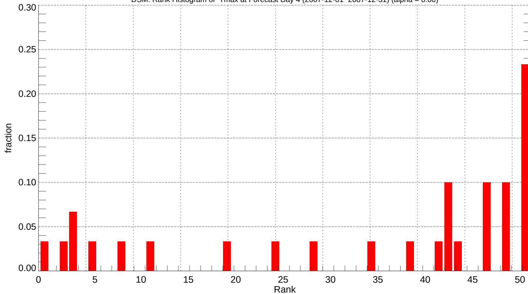
DSM: Rank Histogram of Tmax at Forecast Day 4 (2007-12-01~2007-12-31) (alpha = 0.00)
