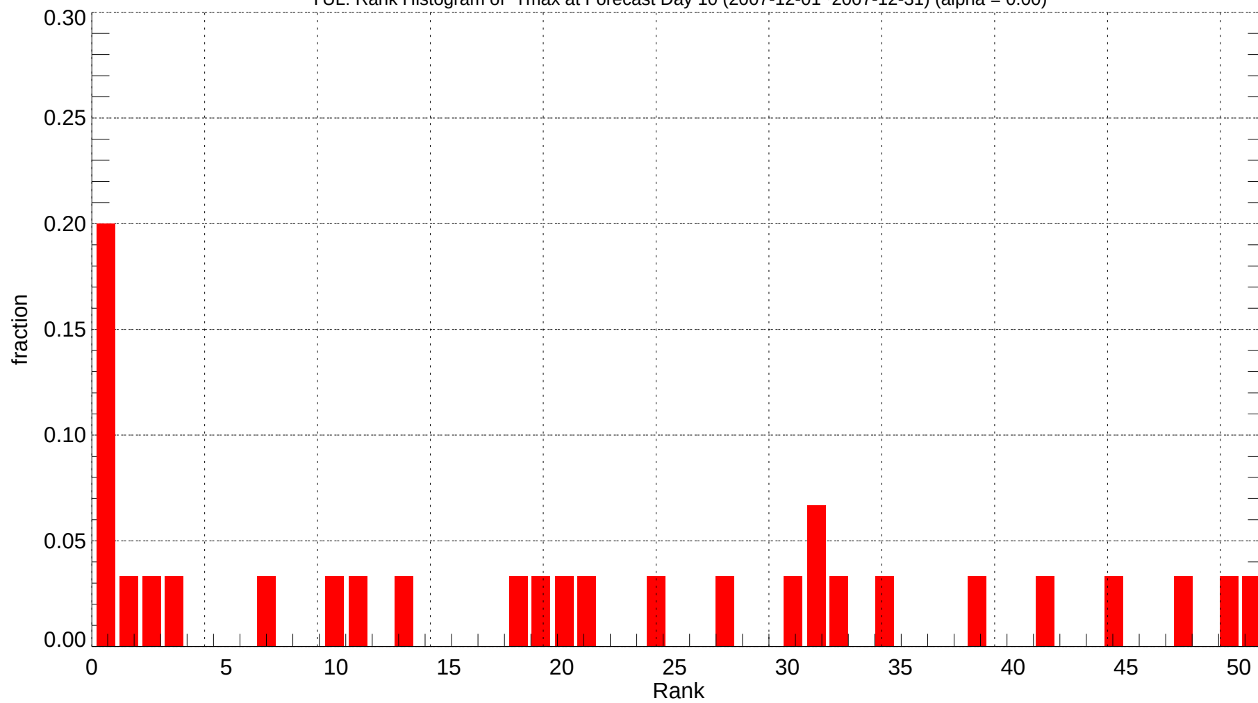
YUL: Rank Histogram of Tmax at Forecast Day 10 (2007-12-01~2007-12-31) (alpha = 0.00)
