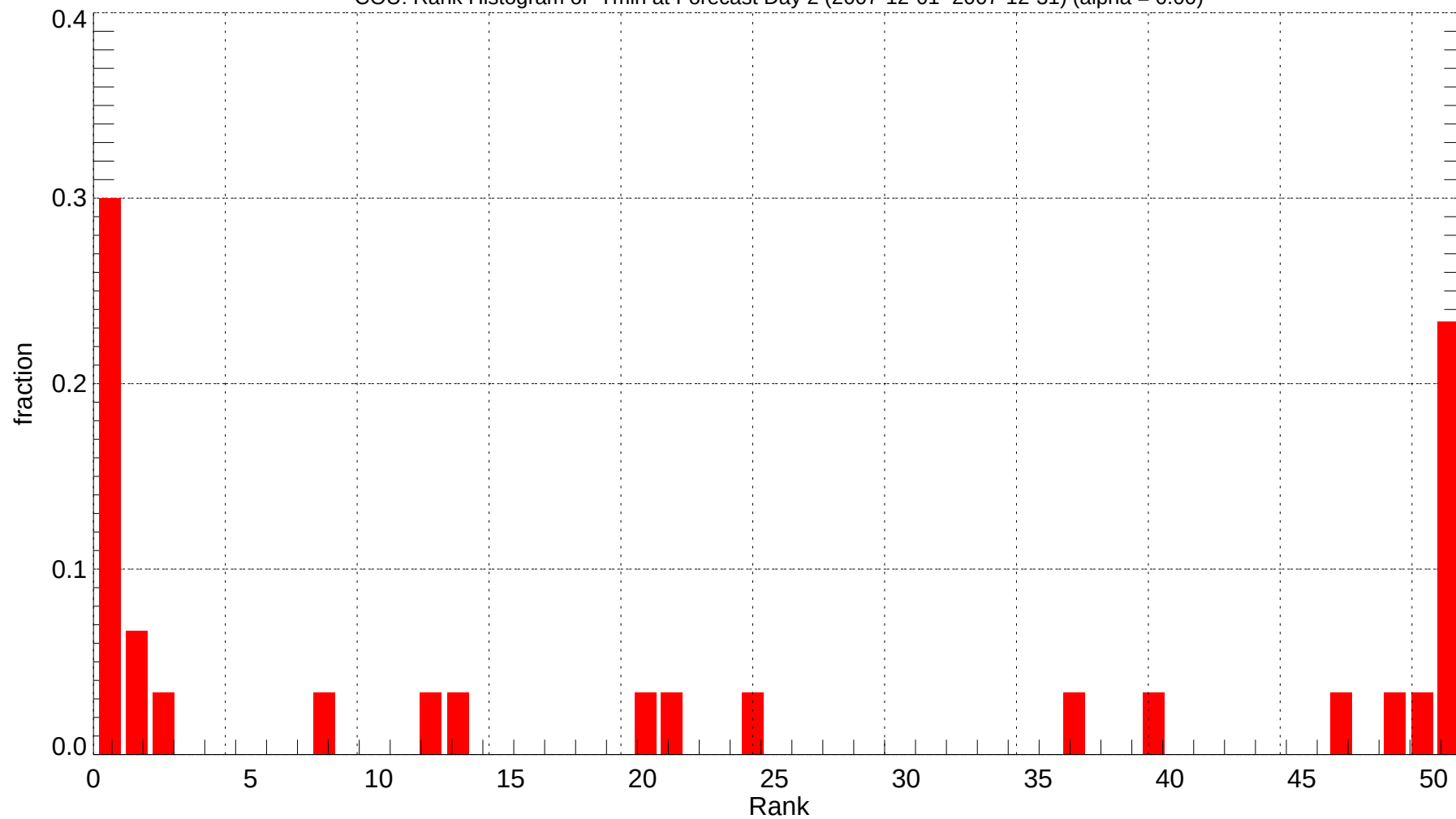
COU: Rank Histogram of Tmin at Forecast Day 2 (2007-12-01~2007-12-31) (alpha = 0.00)
