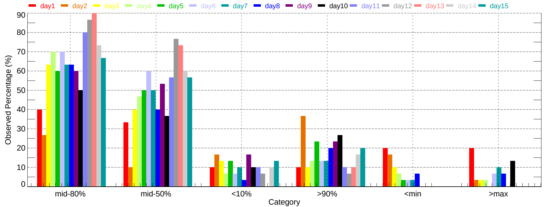
Observed Percentage of Ensembles - DLH: Max Temperature (2007-12-01~2007-12-31)
