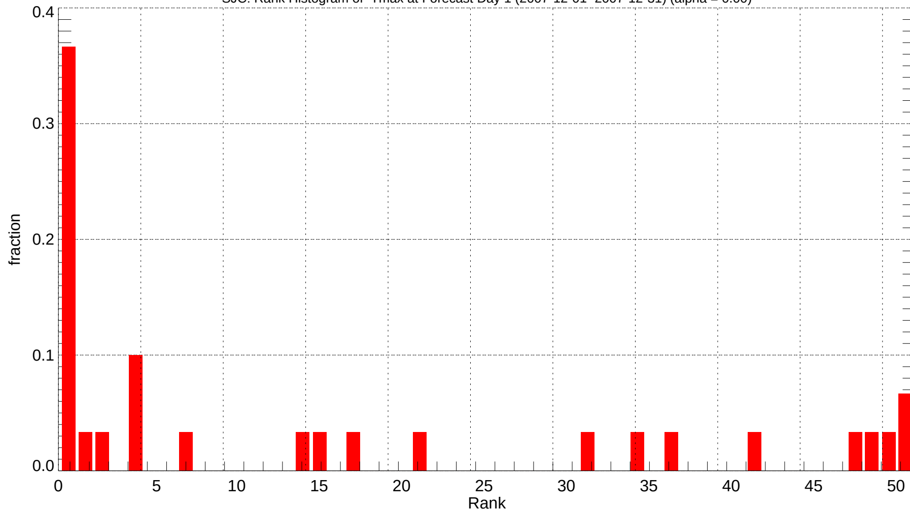
SJC: Rank Histogram of Tmax at Forecast Day 1 (2007-12-01~2007-12-31) (alpha = 0.00)
