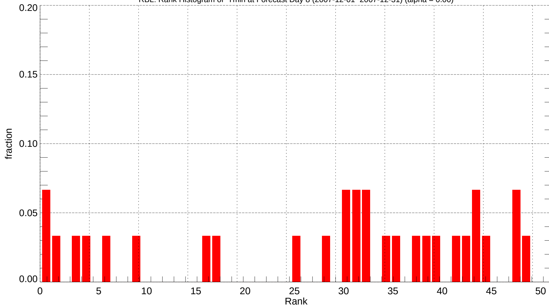
RBL: Rank Histogram of Tmin at Forecast Day 8 (2007-12-01~2007-12-31) (alpha = 0.00)
