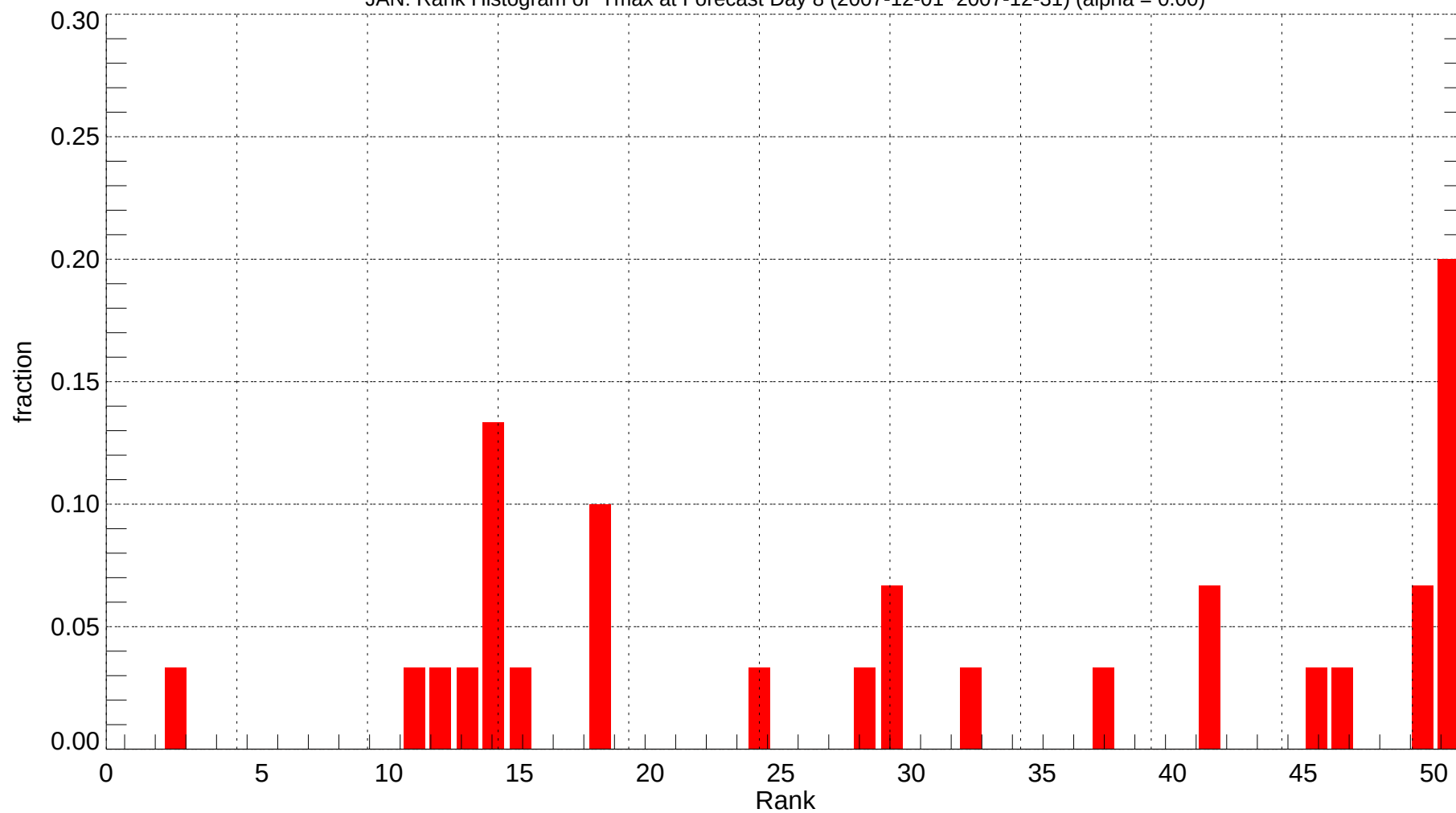
JAN: Rank Histogram of Tmax at Forecast Day 8 (2007-12-01~2007-12-31) (alpha = 0.00)
