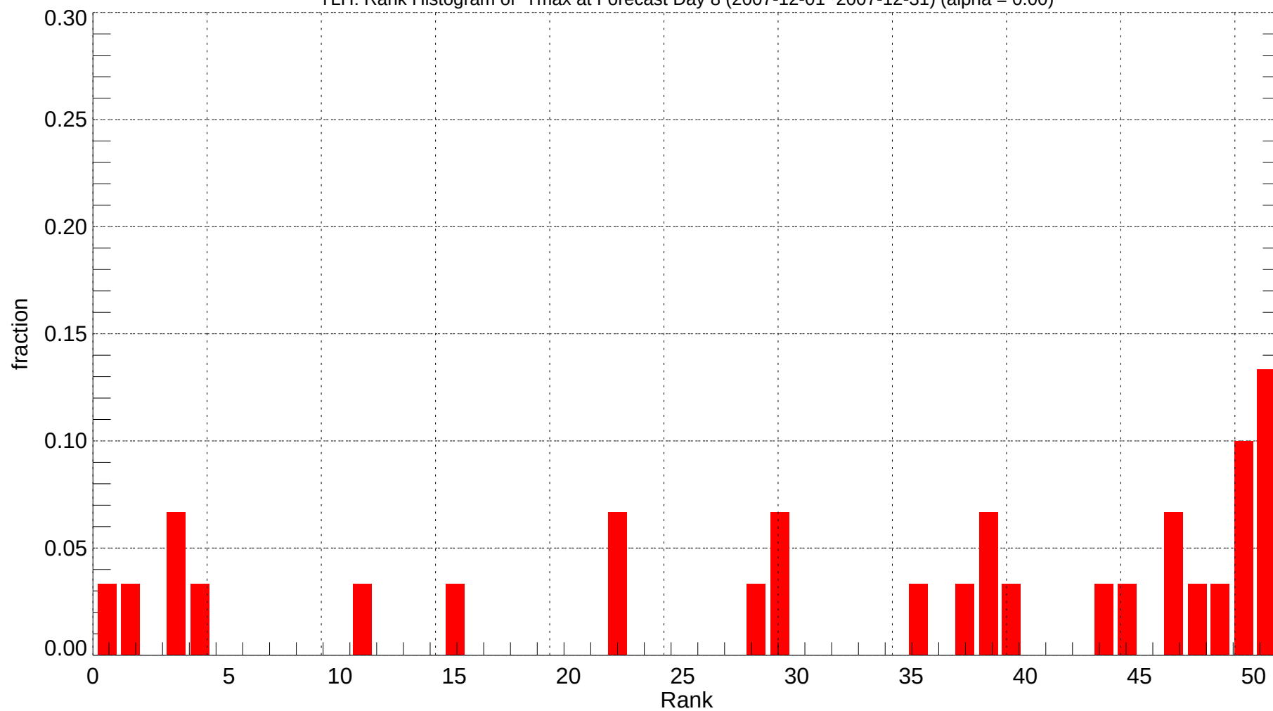
TLH: Rank Histogram of Tmax at Forecast Day 8 (2007-12-01~2007-12-31) (alpha = 0.00)
