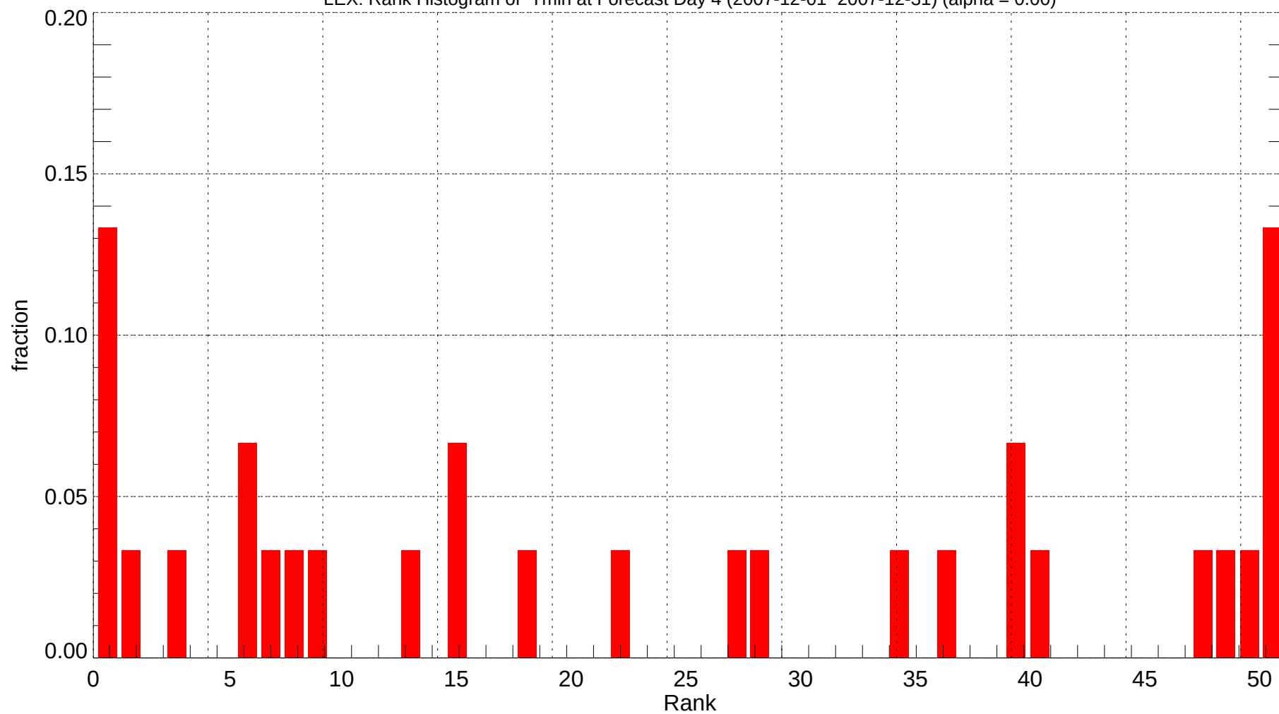
LEX: Rank Histogram of Tmin at Forecast Day 4 (2007-12-01~2007-12-31) (alpha = 0.00)
