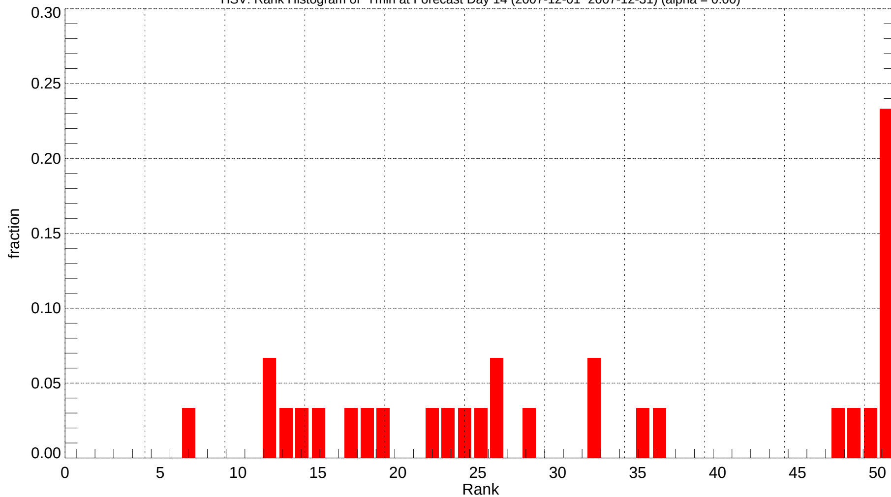
HSV: Rank Histogram of Tmin at Forecast Day 14 (2007-12-01~2007-12-31) (alpha = 0.00)
