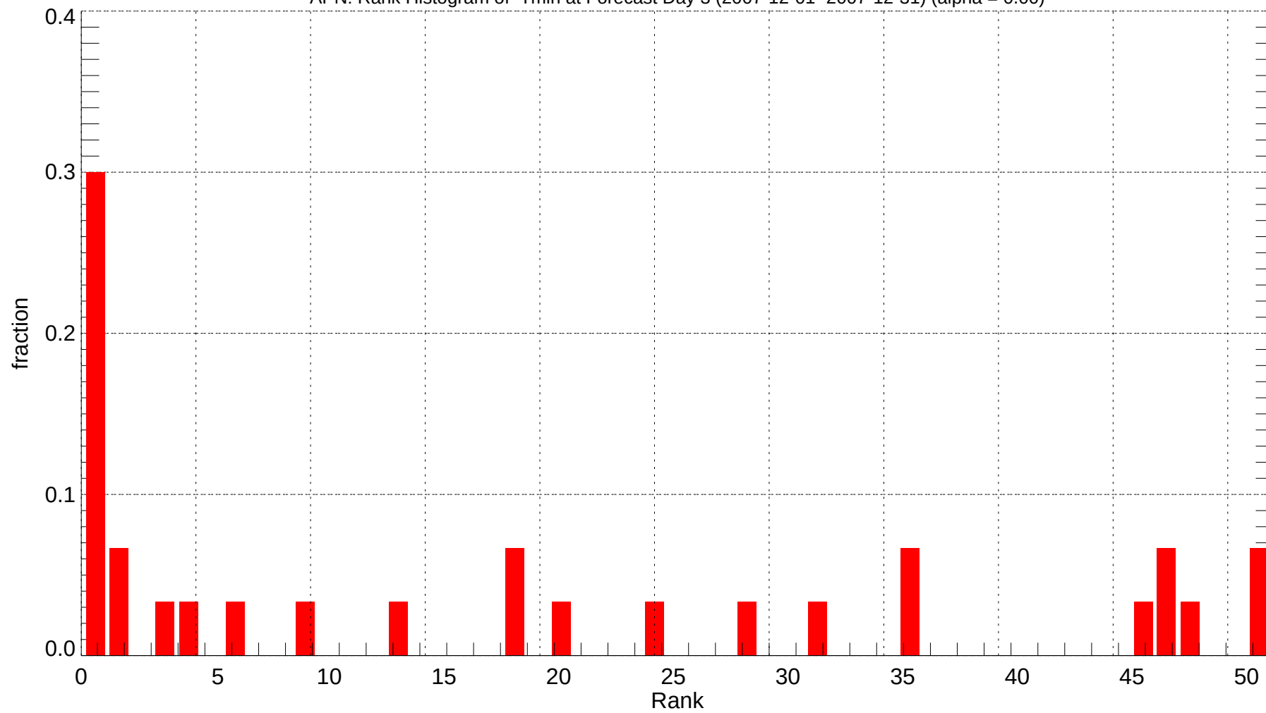
APN: Rank Histogram of Tmin at Forecast Day 3 (2007-12-01~2007-12-31) (alpha = 0.00)
