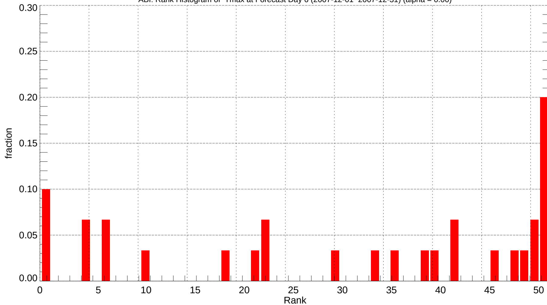
ABI: Rank Histogram of Tmax at Forecast Day 6 (2007-12-01~2007-12-31) (alpha = 0.00)
