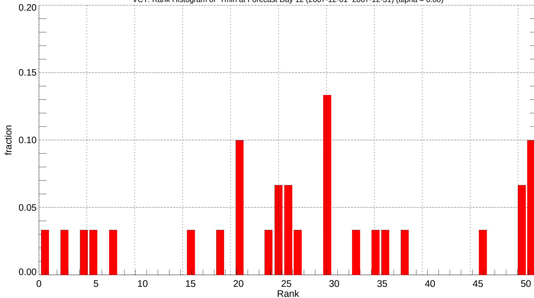
VCT: Rank Histogram of Tmin at Forecast Day 12 (2007-12-01~2007-12-31) (alpha = 0.00)
