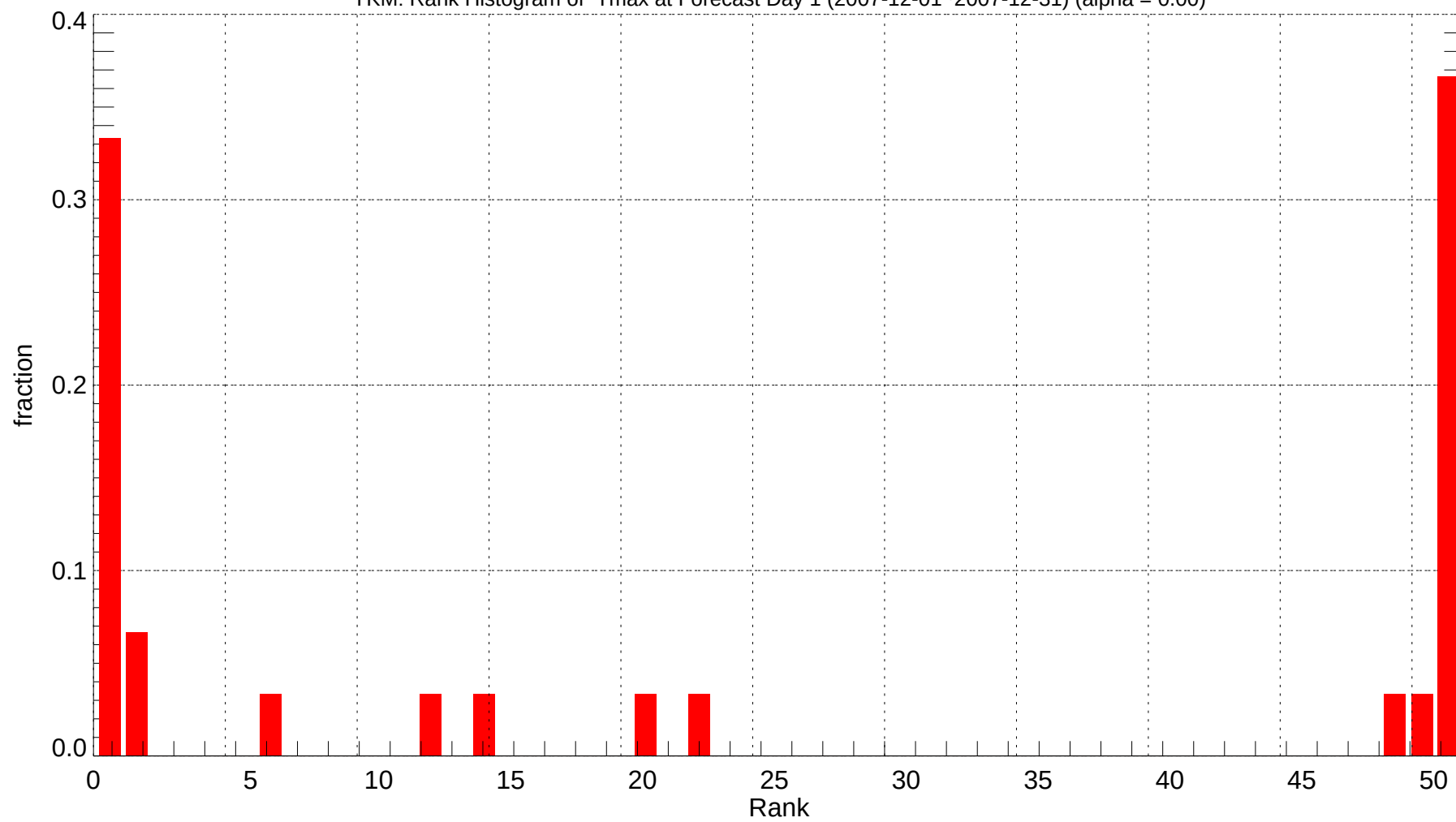
YKM: Rank Histogram of Tmax at Forecast Day 1 (2007-12-01~2007-12-31) (alpha = 0.00)
