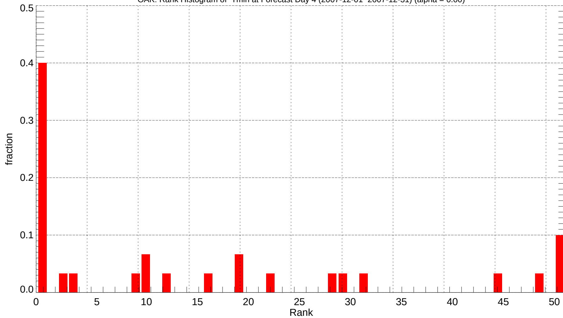
OAK: Rank Histogram of Tmin at Forecast Day 4 (2007-12-01~2007-12-31) (alpha = 0.00)
