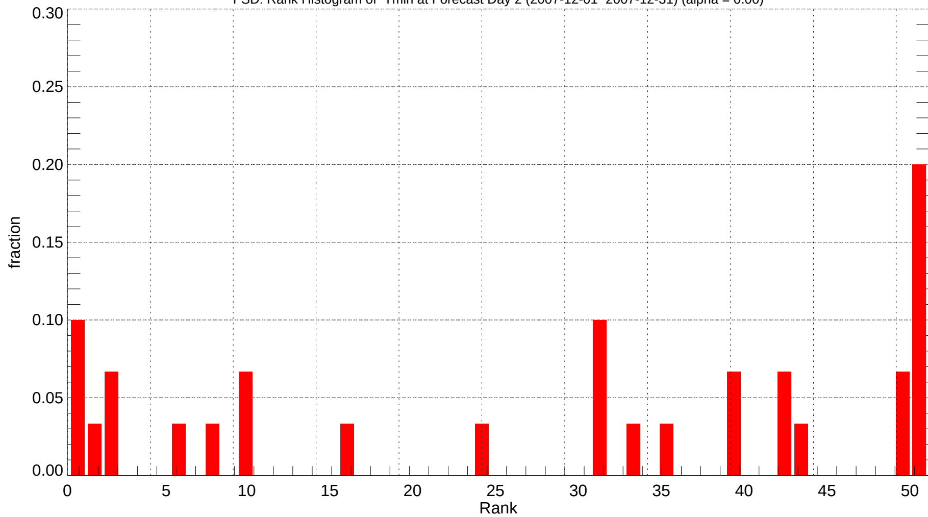
FSD: Rank Histogram of Tmin at Forecast Day 2 (2007-12-01~2007-12-31) (alpha = 0.00)
