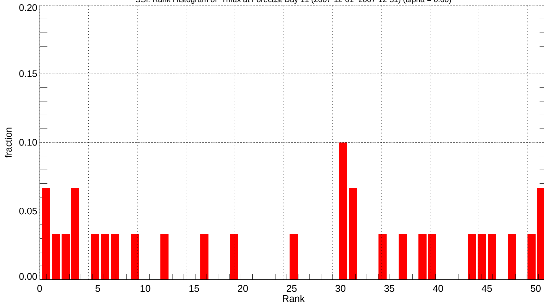
SSI: Rank Histogram of Tmax at Forecast Day 11 (2007-12-01~2007-12-31) (alpha = 0.00)
