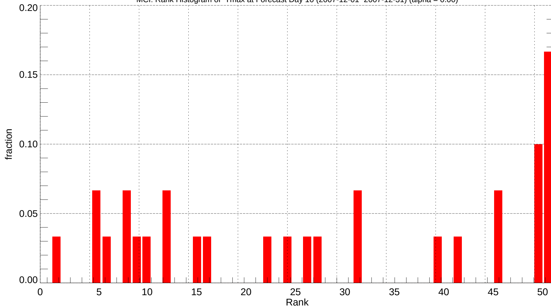
MCI: Rank Histogram of Tmax at Forecast Day 10 (2007-12-01~2007-12-31) (alpha = 0.00)
