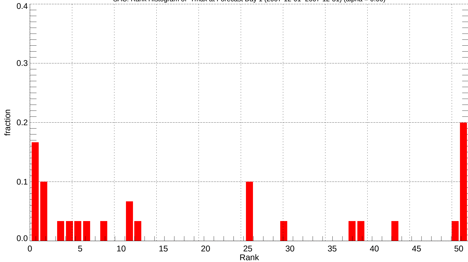
SAC: Rank Histogram of Tmax at Forecast Day 1 (2007-12-01~2007-12-31) (alpha = 0.00)
