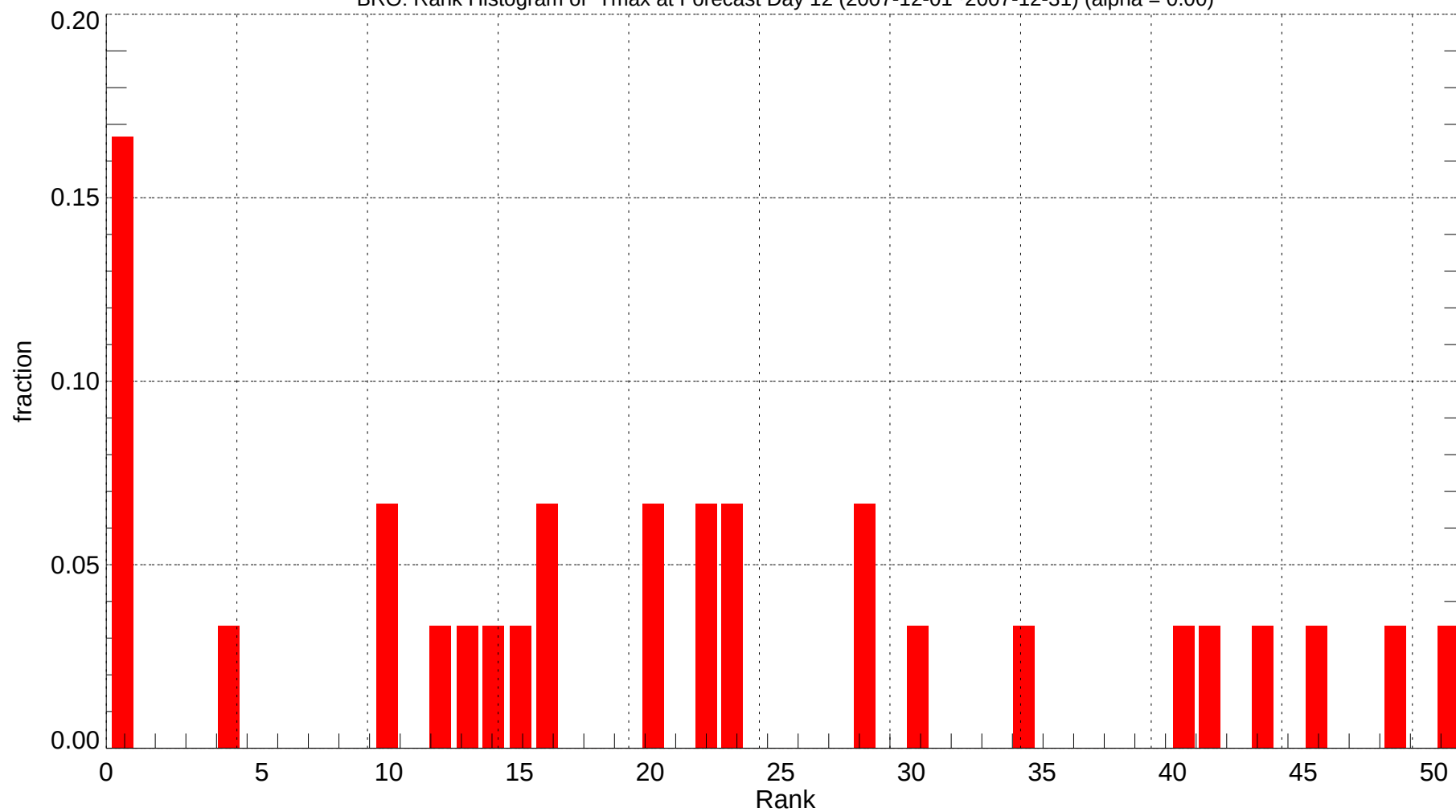
BRO: Rank Histogram of Tmax at Forecast Day 12 (2007-12-01~2007-12-31) (alpha = 0.00)
