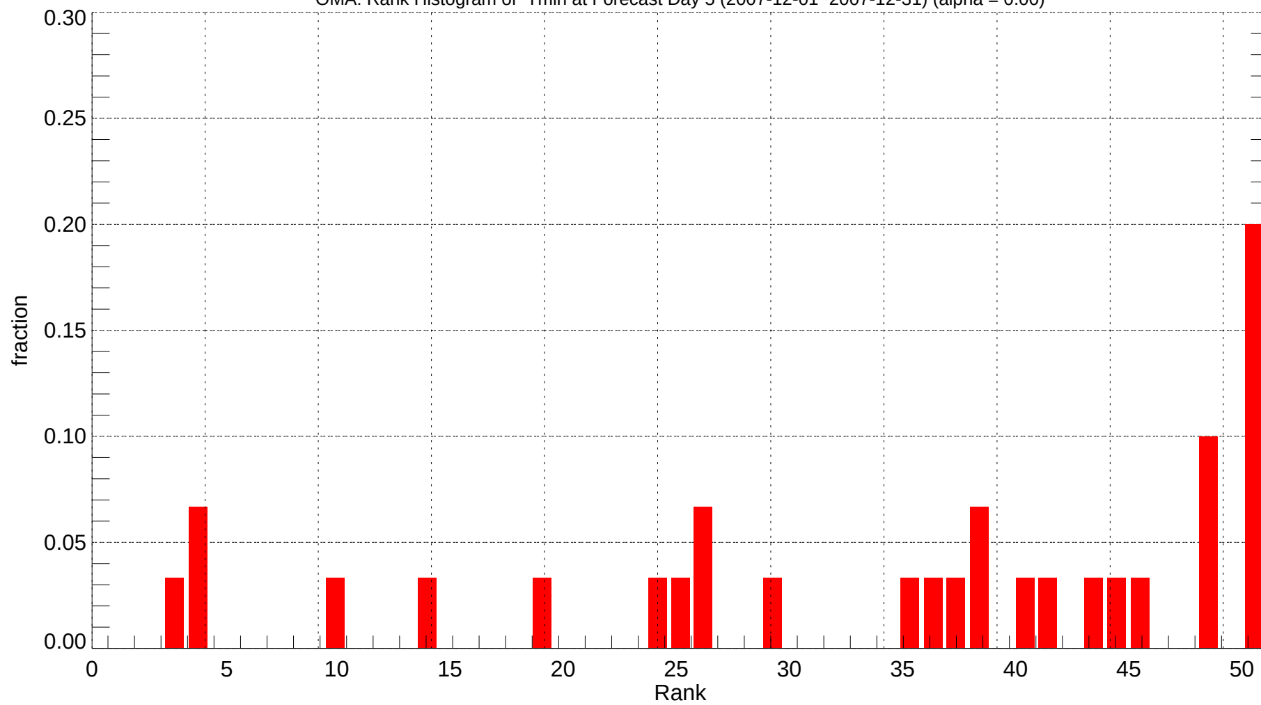
OMA: Rank Histogram of Tmin at Forecast Day 5 (2007-12-01~2007-12-31) (alpha = 0.00)
