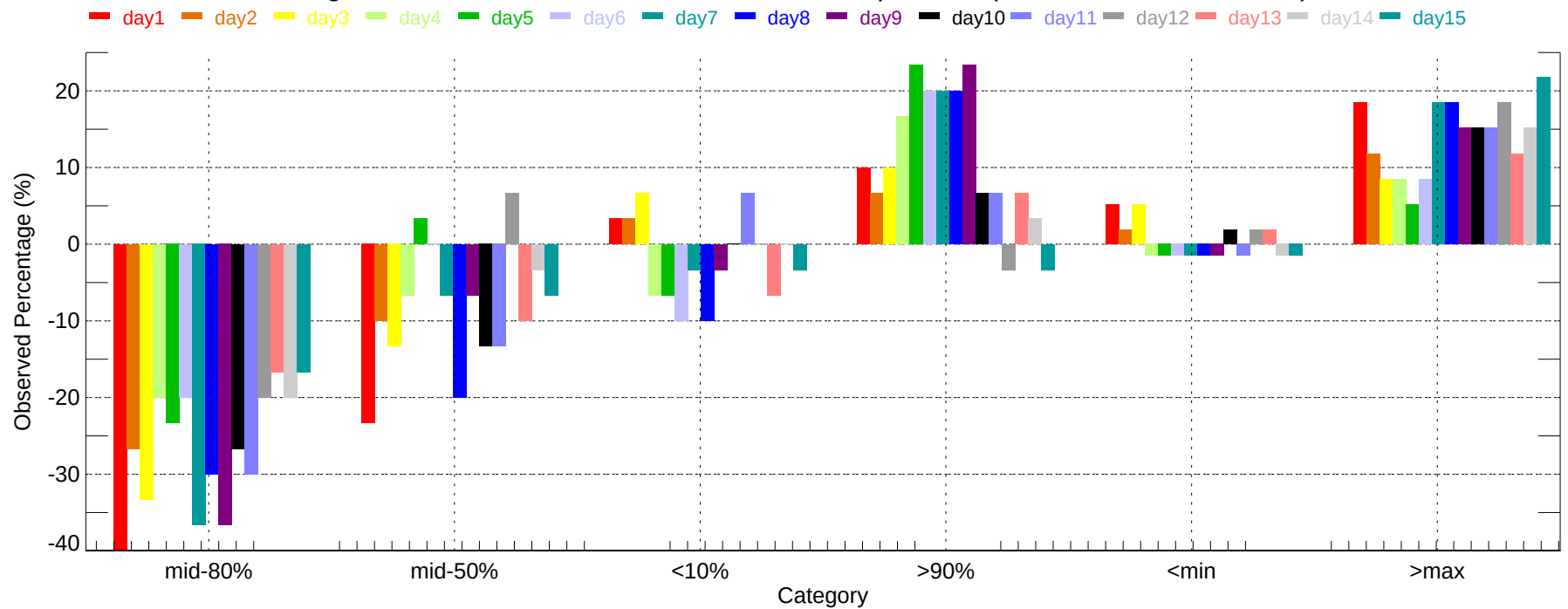
Observed Percentage Deviation of Ensembles - HOU: Max Temperature (2007-12-01~2007-12-31)
