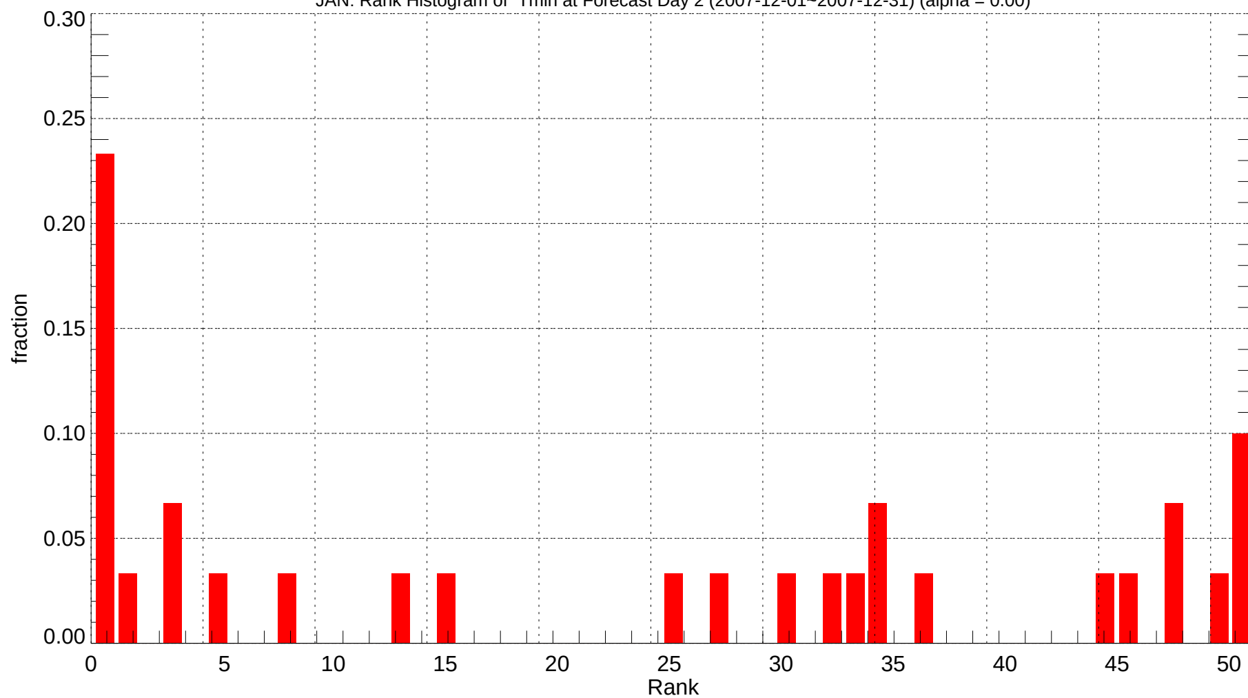
JAN: Rank Histogram of Tmin at Forecast Day 2 (2007-12-01~2007-12-31) (alpha = 0.00)
