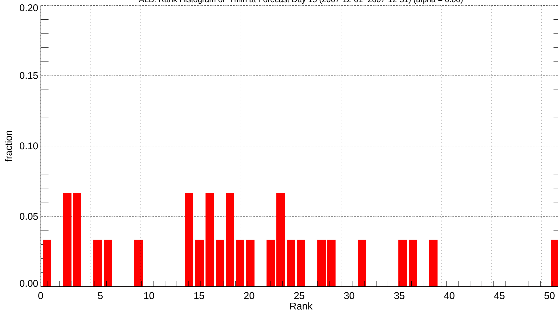
ALB: Rank Histogram of Tmin at Forecast Day 15 (2007-12-01~2007-12-31) (alpha = 0.00)
