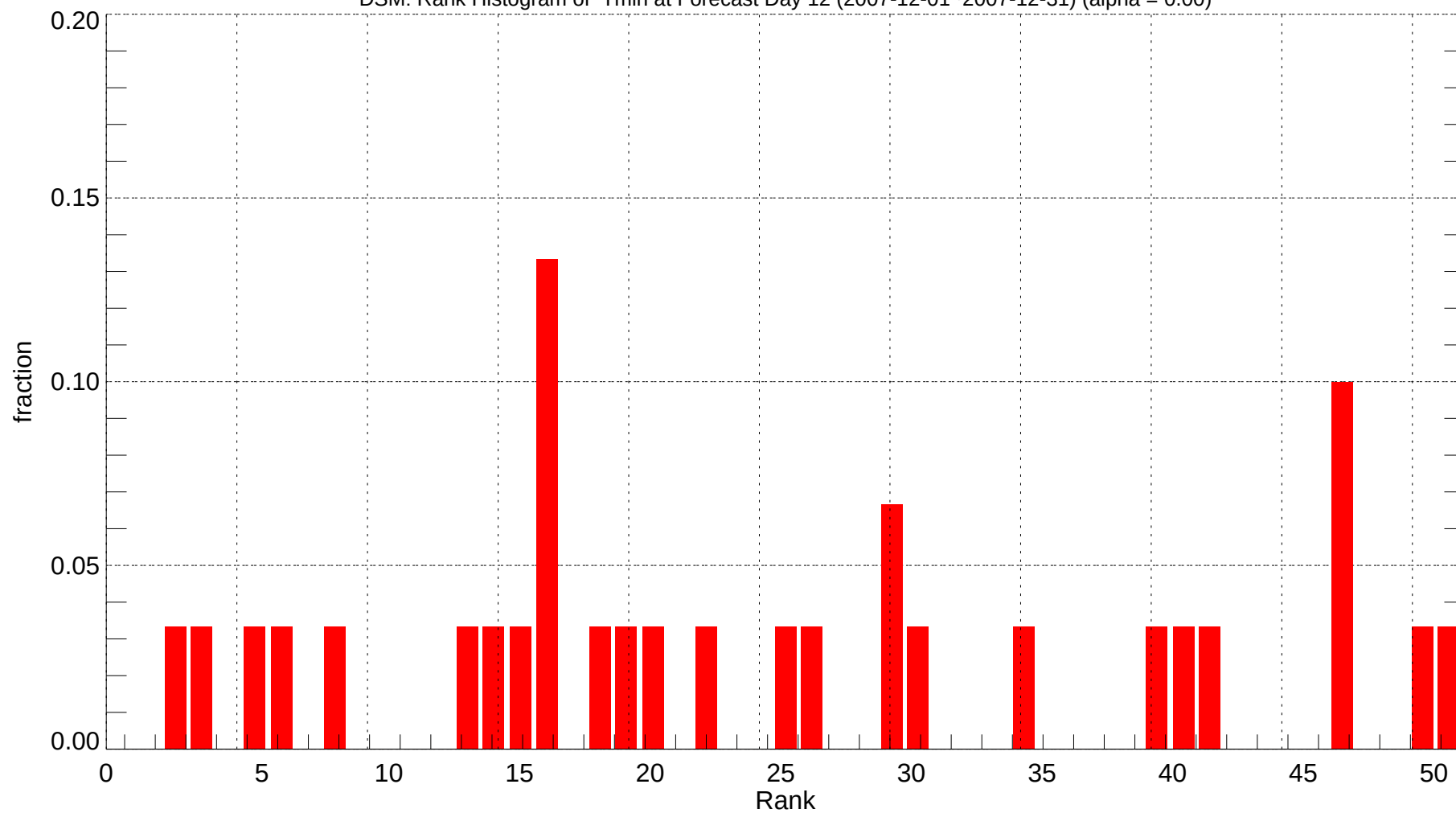
DSM: Rank Histogram of Tmin at Forecast Day 12 (2007-12-01~2007-12-31) (alpha = 0.00)
