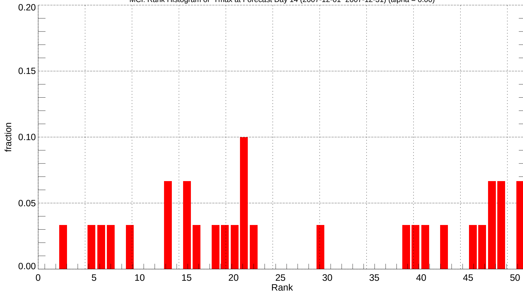
MCI: Rank Histogram of Tmax at Forecast Day 14 (2007-12-01~2007-12-31) (alpha = 0.00)
