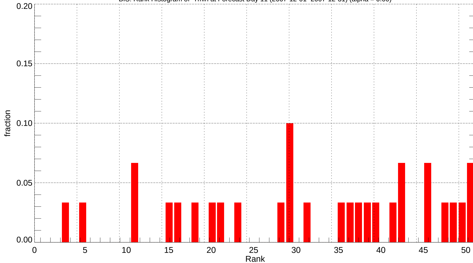
BIS: Rank Histogram of Tmin at Forecast Day 11 (2007-12-01~2007-12-31) (alpha = 0.00)
