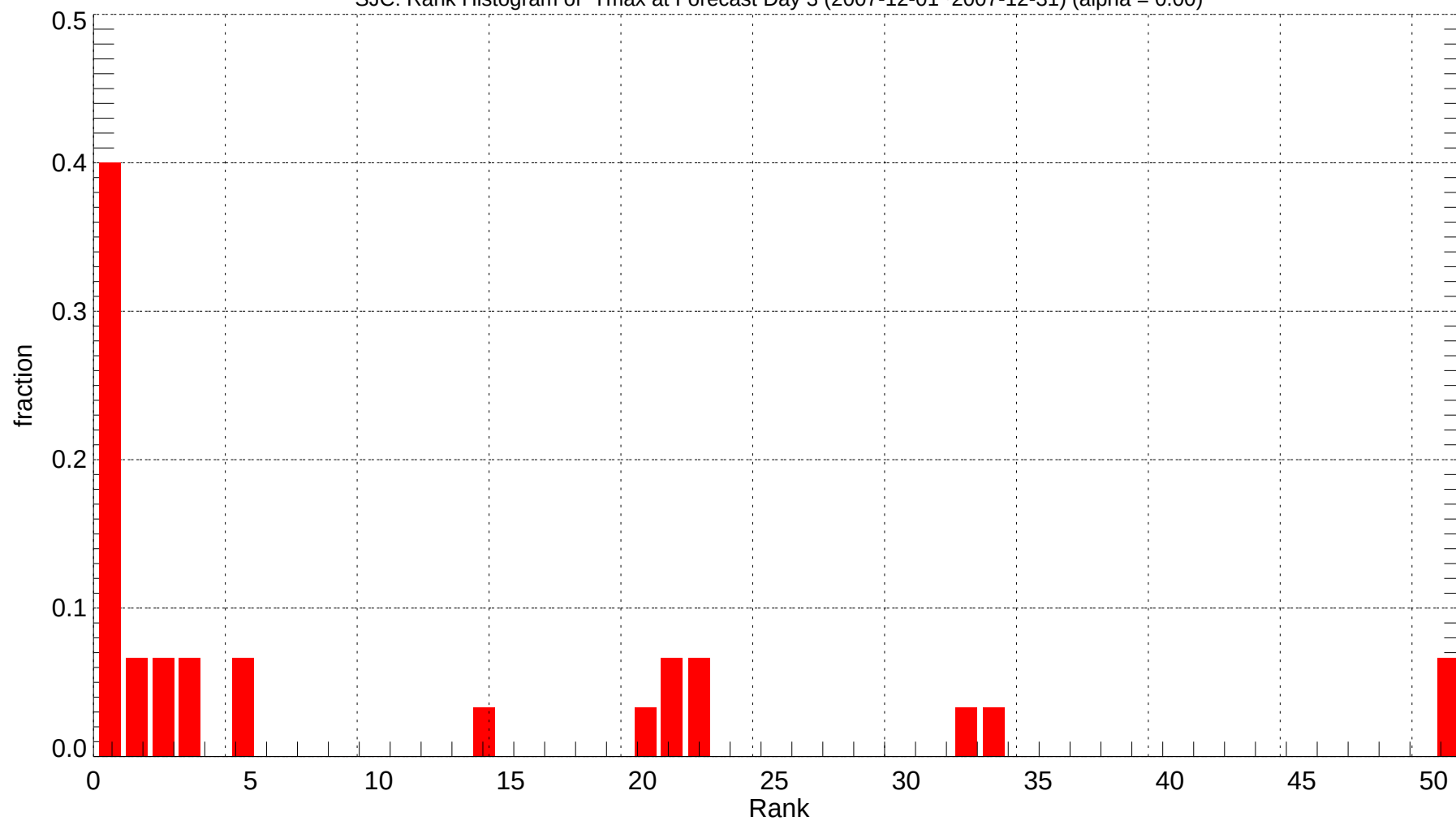
SJC: Rank Histogram of Tmax at Forecast Day 3 (2007-12-01~2007-12-31) (alpha = 0.00)
