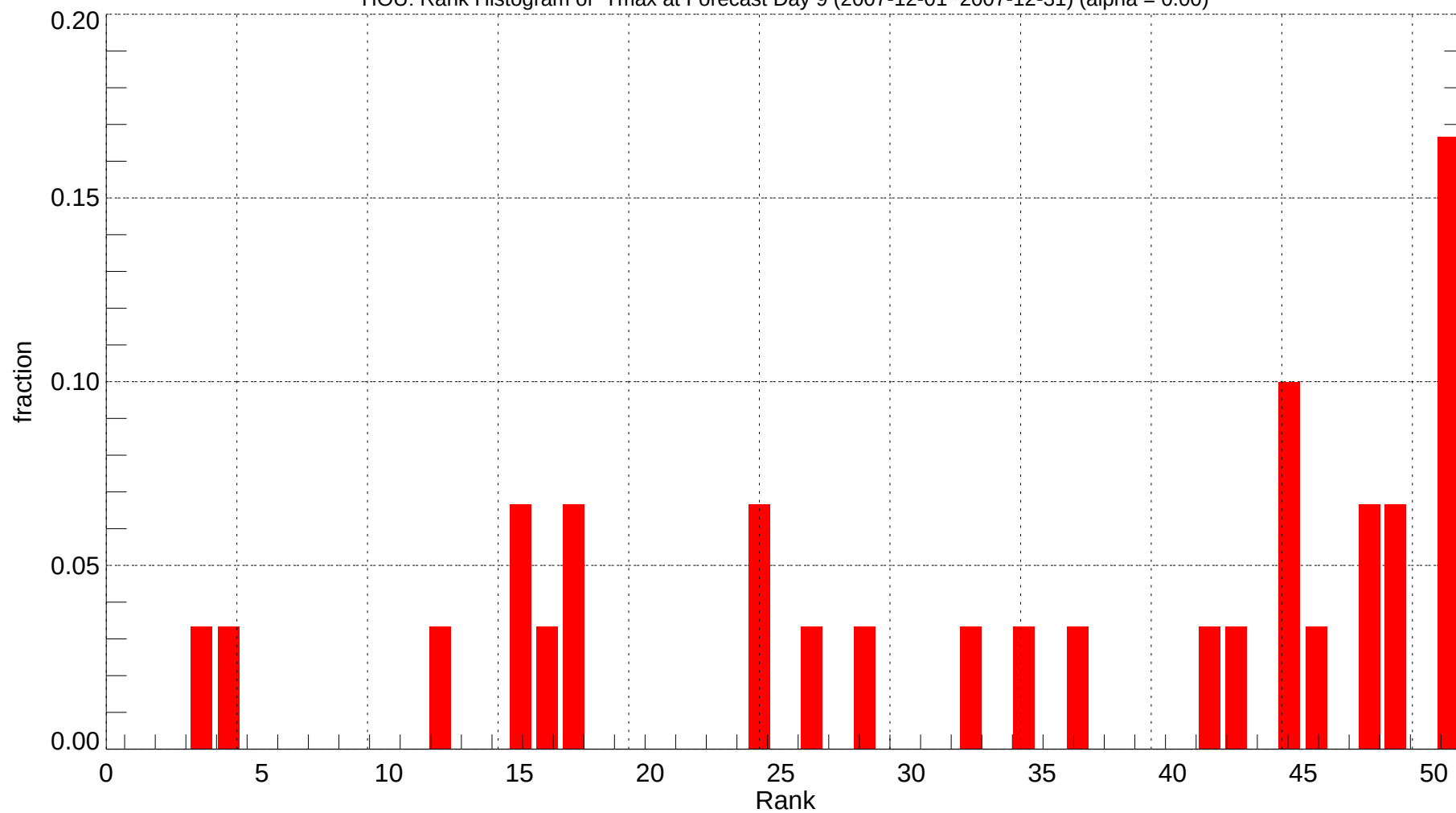
HOU: Rank Histogram of Tmax at Forecast Day 9 (2007-12-01~2007-12-31) (alpha = 0.00)
