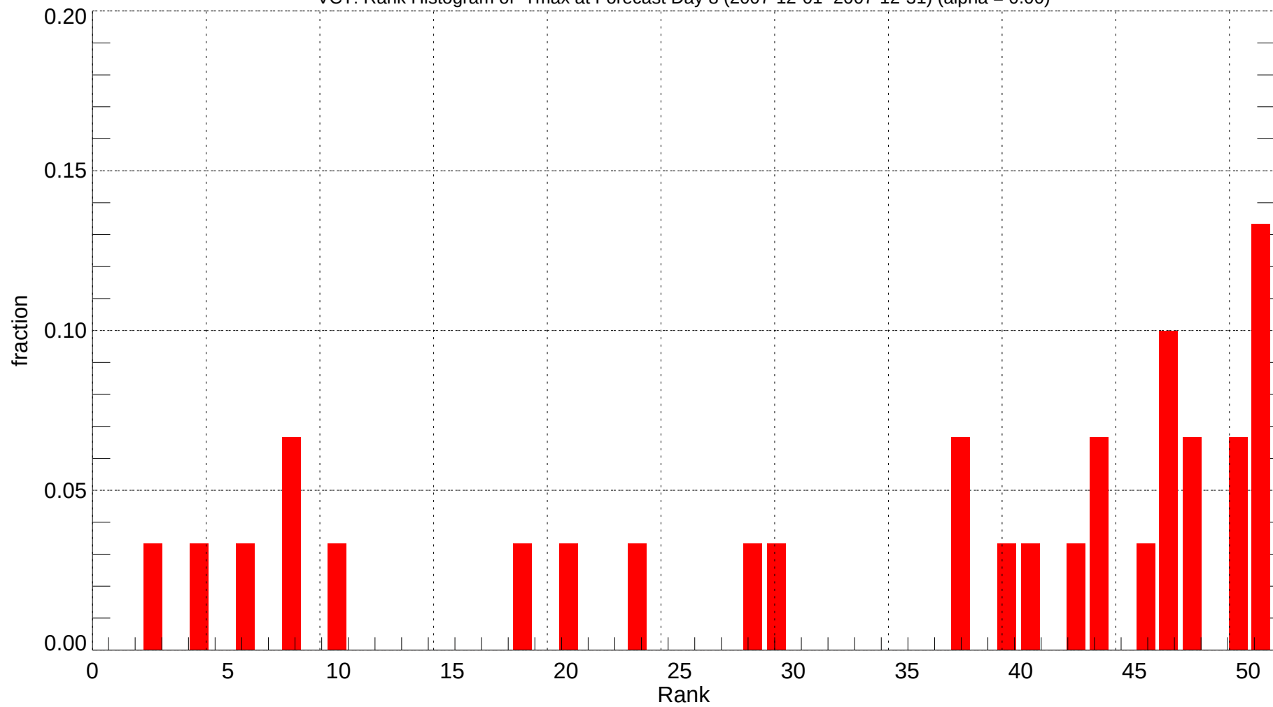
VCT: Rank Histogram of Tmax at Forecast Day 8 (2007-12-01~2007-12-31) (alpha = 0.00)
