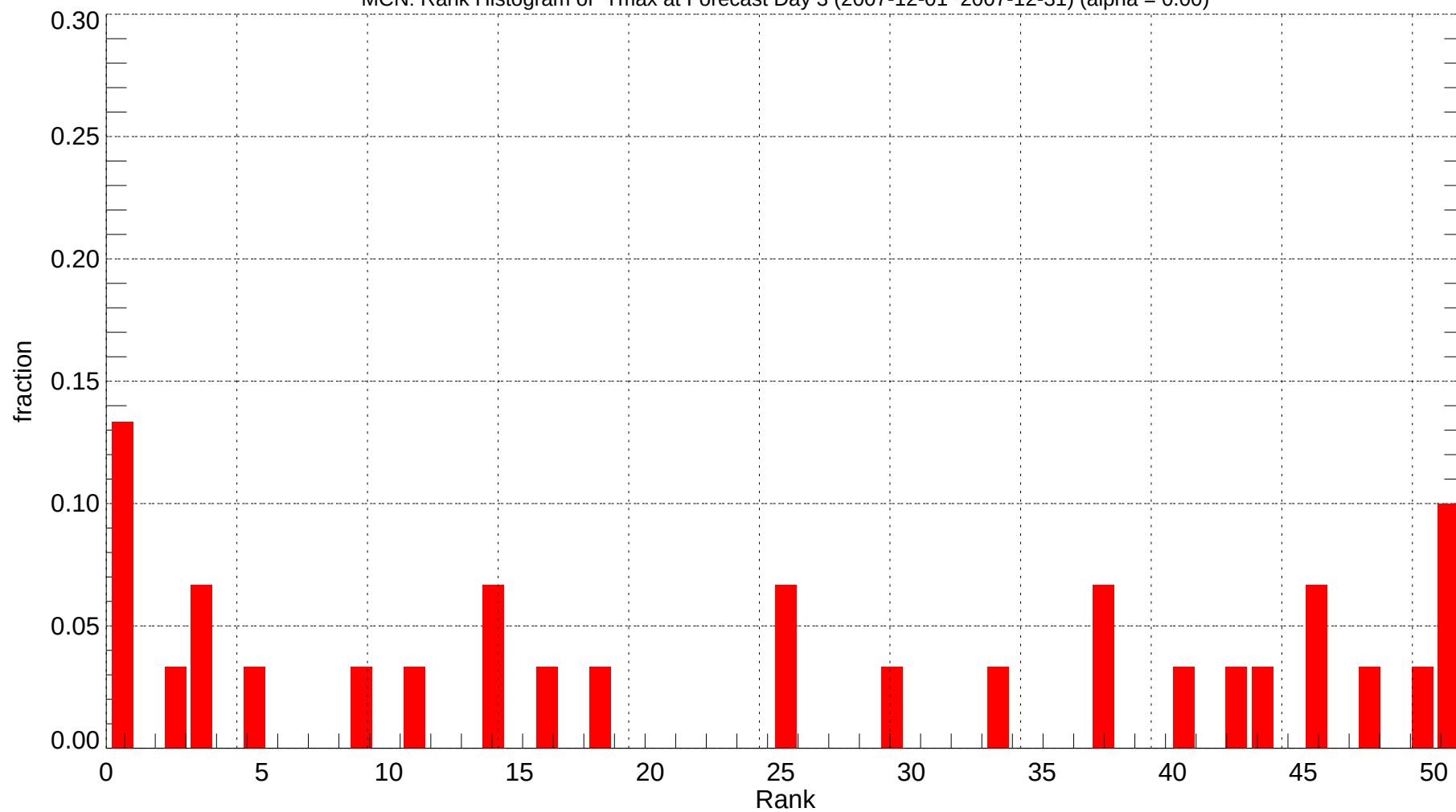
MCN: Rank Histogram of Tmax at Forecast Day 3 (2007-12-01~2007-12-31) (alpha = 0.00)
