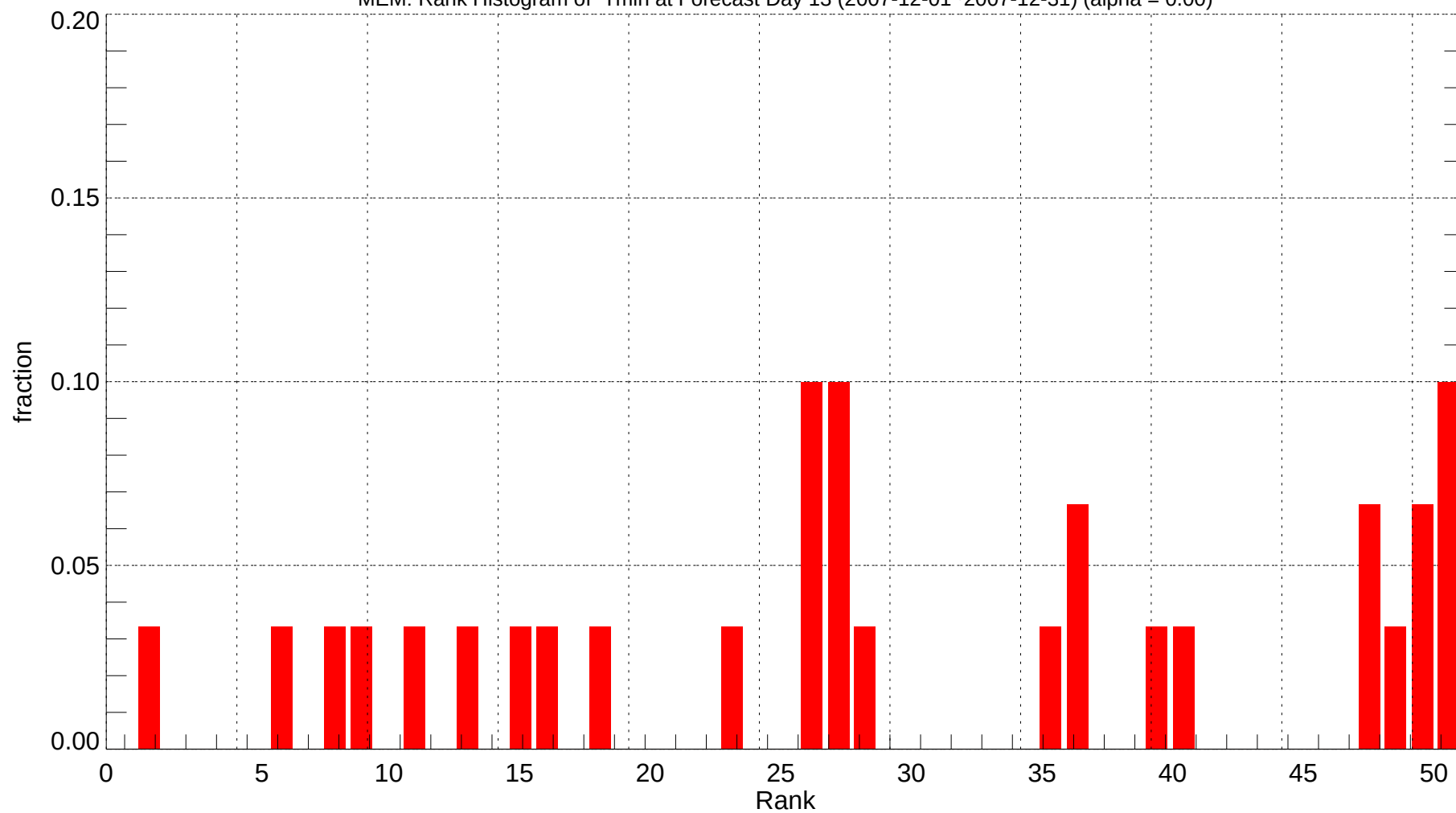
MEM: Rank Histogram of Tmin at Forecast Day 13 (2007-12-01~2007-12-31) (alpha = 0.00)
