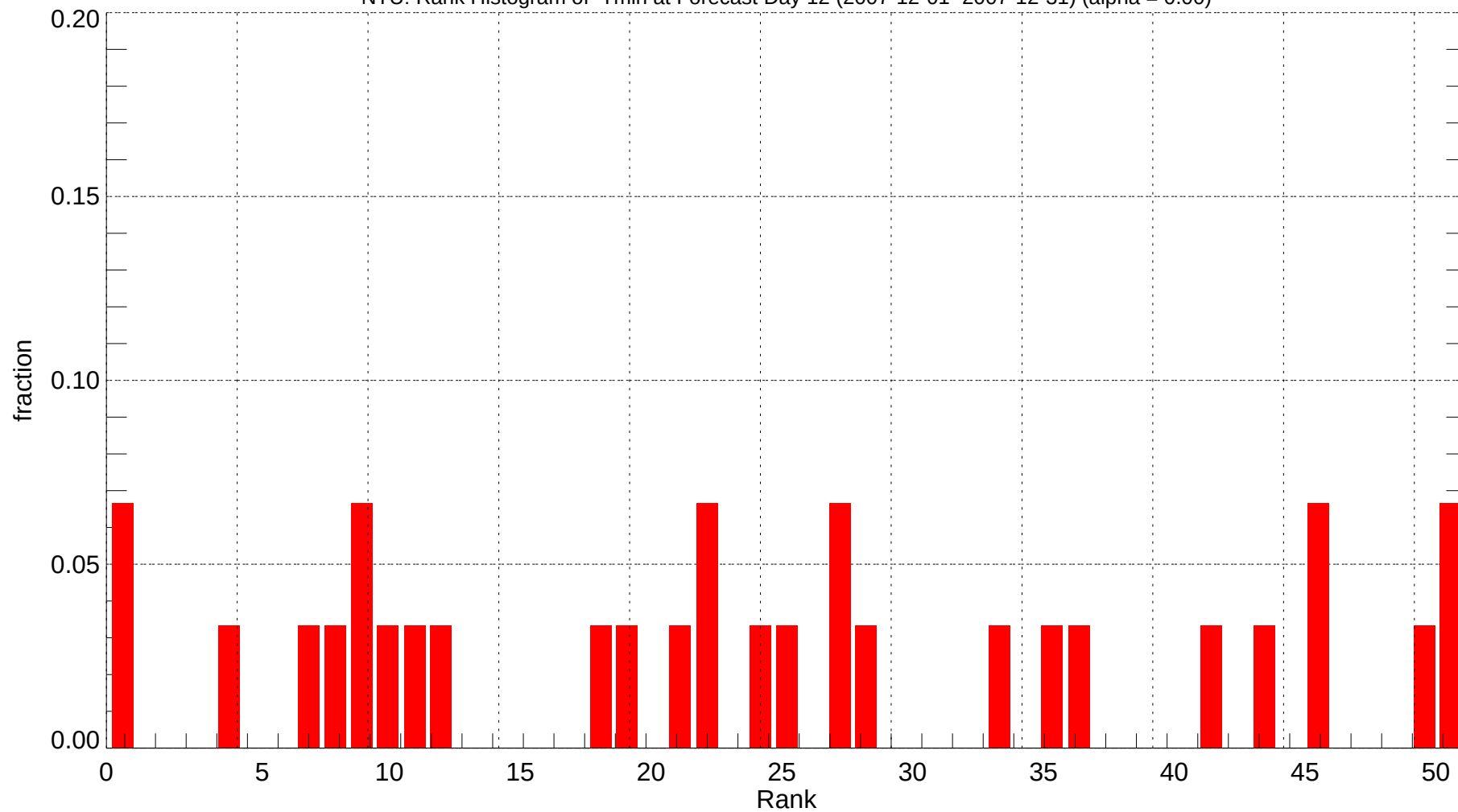
NTU: Rank Histogram of Tmin at Forecast Day 12 (2007-12-01~2007-12-31) (alpha = 0.00)
