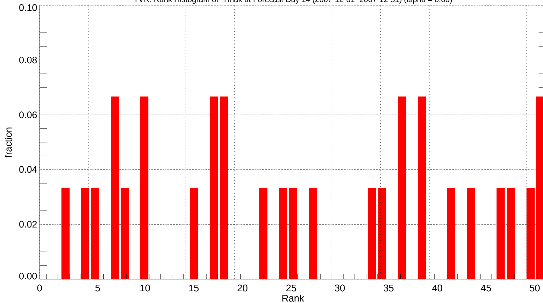
YVR: Rank Histogram of Tmax at Forecast Day 14 (2007-12-01~2007-12-31) (alpha = 0.00)
