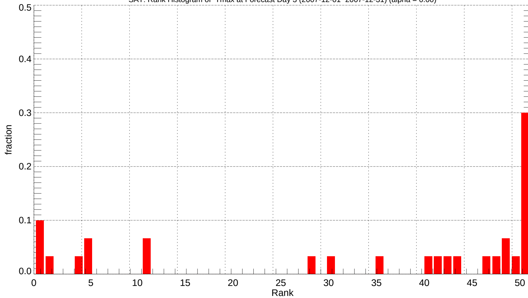
SAT: Rank Histogram of Tmax at Forecast Day 3 (2007-12-01~2007-12-31) (alpha = 0.00)
