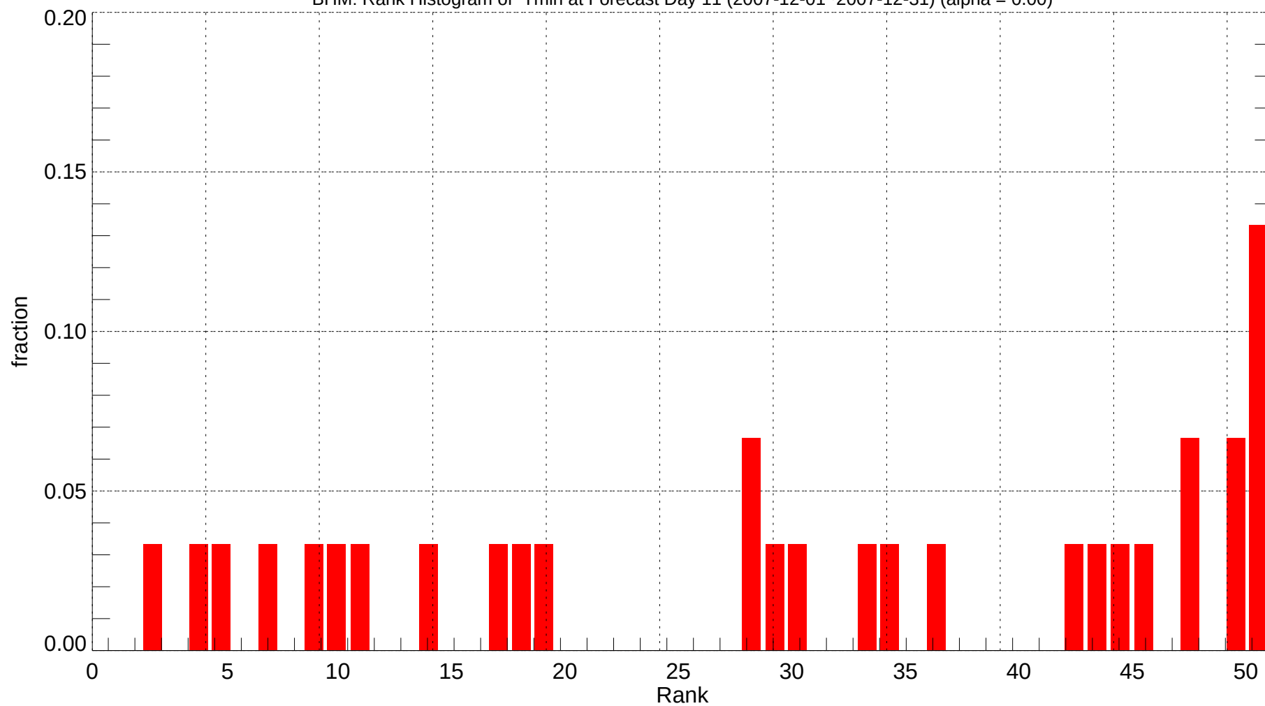
BHM: Rank Histogram of Tmin at Forecast Day 11 (2007-12-01~2007-12-31) (alpha = 0.00)
