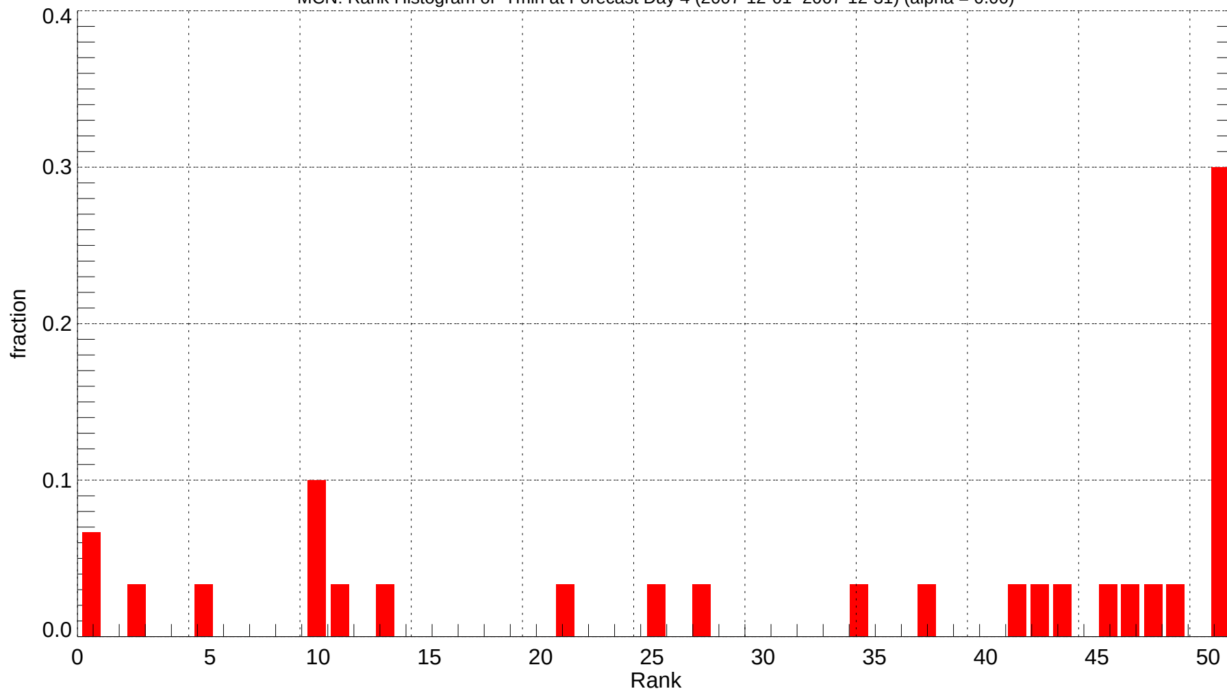
MCN: Rank Histogram of Tmin at Forecast Day 4 (2007-12-01~2007-12-31) (alpha = 0.00)
