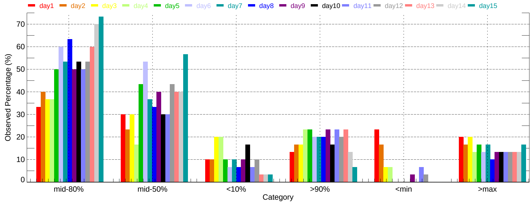
Observed Percentage of Ensembles - ACT: Max Temperature (2007-12-01~2007-12-31)
