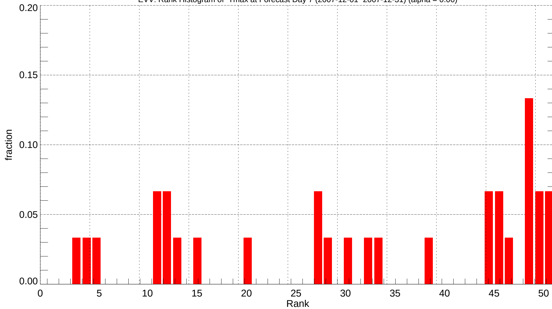
EVV: Rank Histogram of Tmax at Forecast Day 7 (2007-12-01~2007-12-31) (alpha = 0.00)
