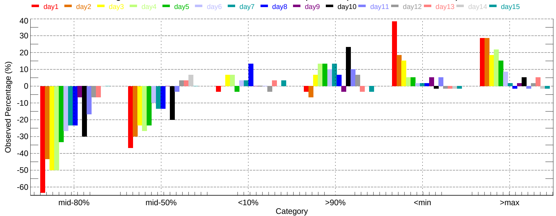
Observed Percentage Deviation of Ensembles - PIR: Max Temperature (2007-12-01~2007-12-31)
