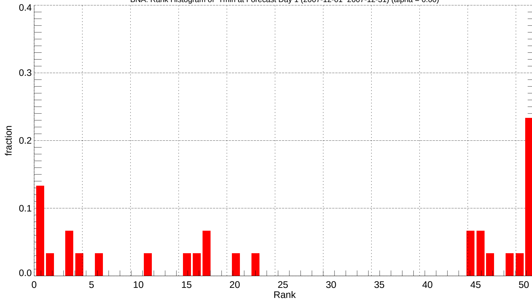
BNA: Rank Histogram of Tmin at Forecast Day 1 (2007-12-01~2007-12-31) (alpha = 0.00)
