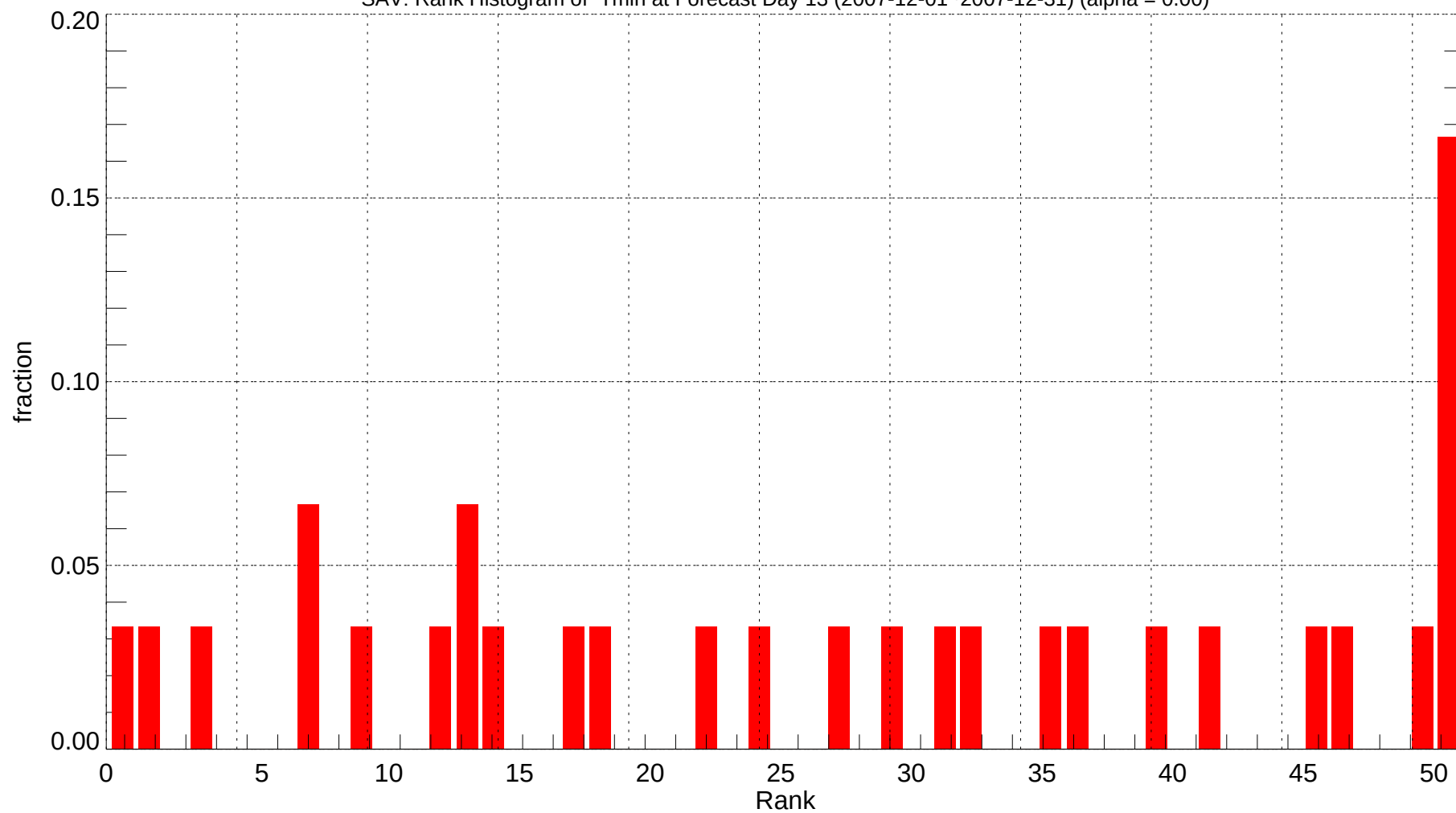
SAV: Rank Histogram of Tmin at Forecast Day 13 (2007-12-01~2007-12-31) (alpha = 0.00)
