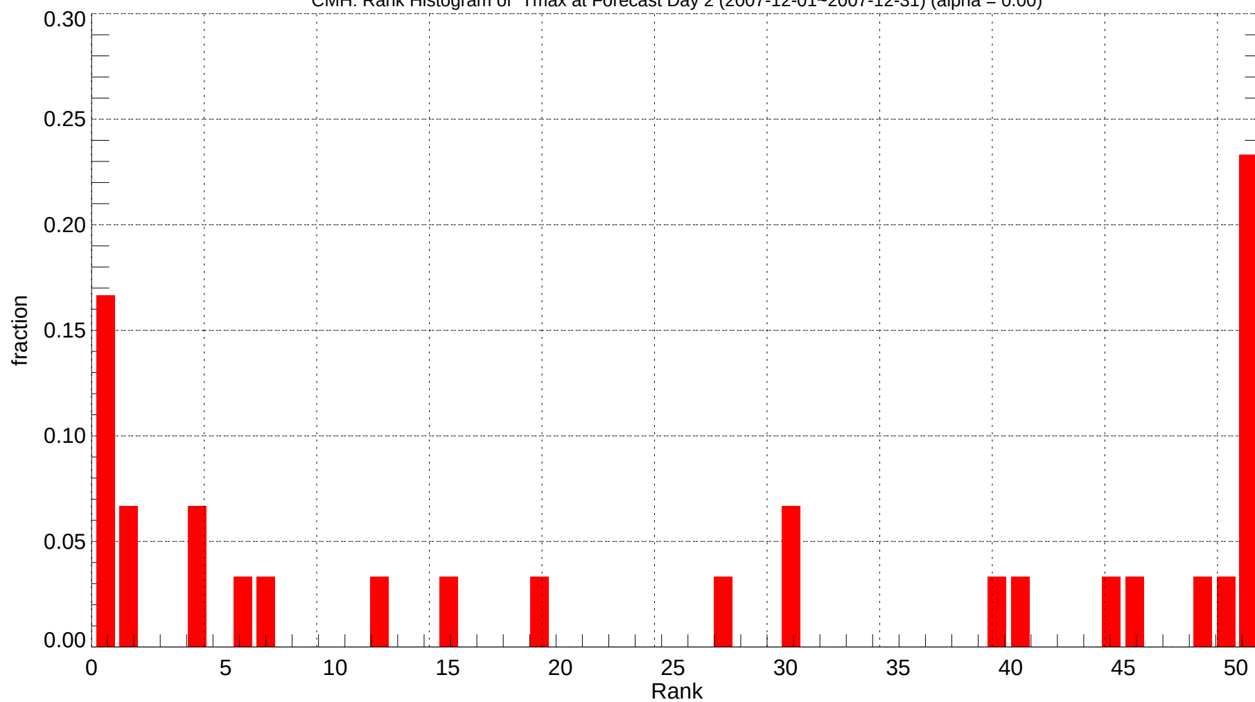
CMH: Rank Histogram of Tmax at Forecast Day 2 (2007-12-01~2007-12-31) (alpha = 0.00)
