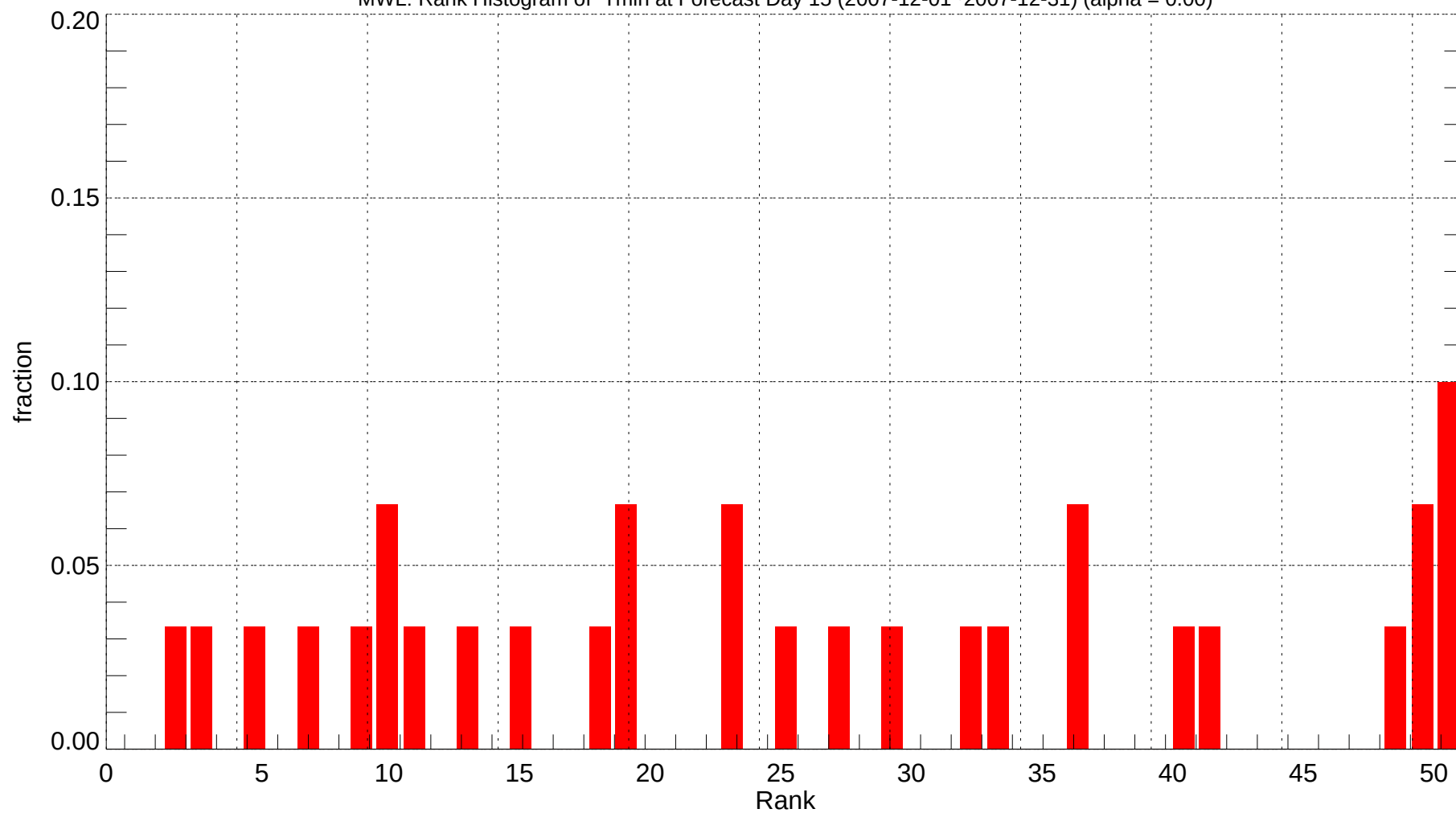
MWL: Rank Histogram of Tmin at Forecast Day 15 (2007-12-01~2007-12-31) (alpha = 0.00)
