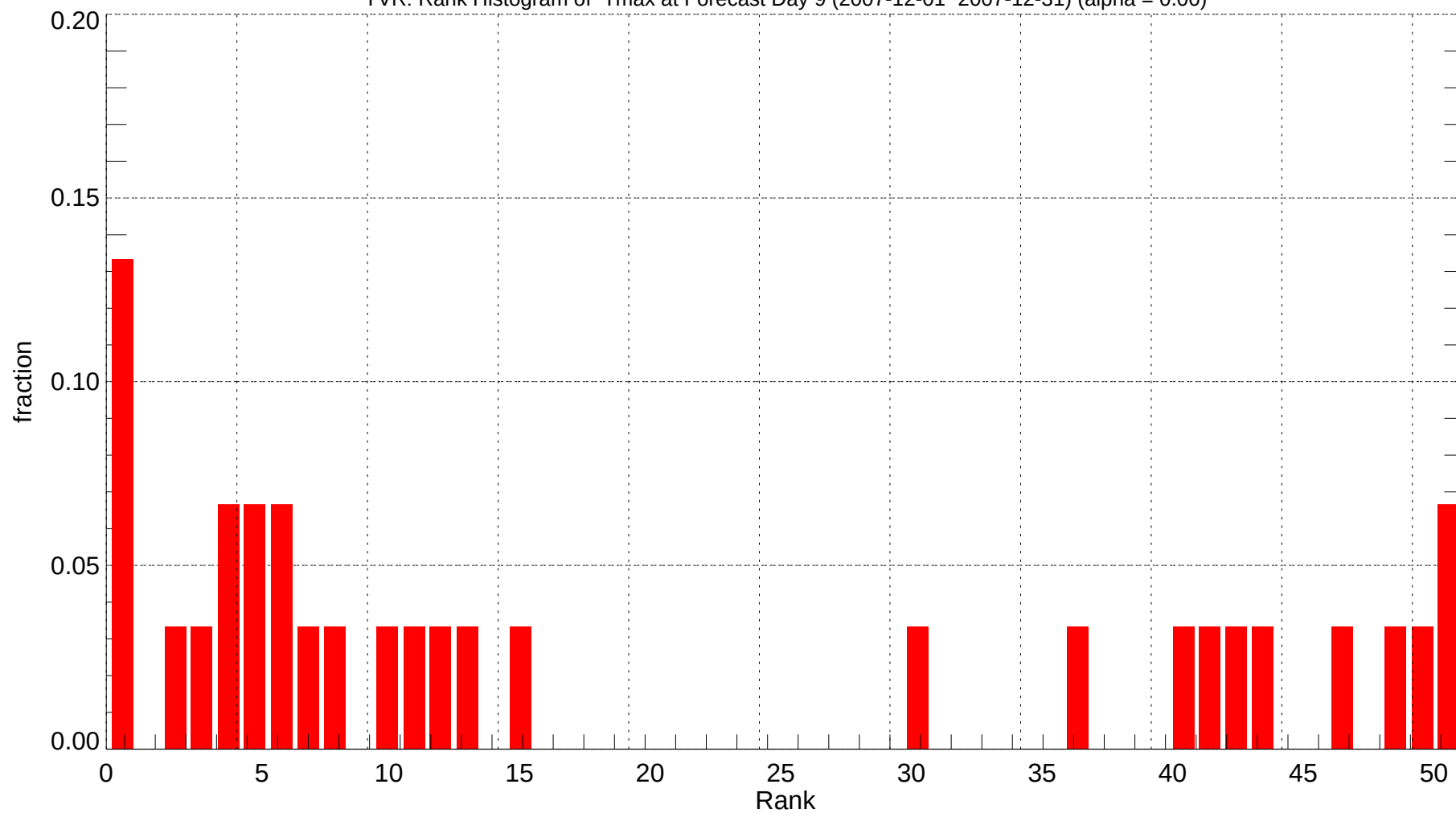
YVR: Rank Histogram of Tmax at Forecast Day 9 (2007-12-01~2007-12-31) (alpha = 0.00)
