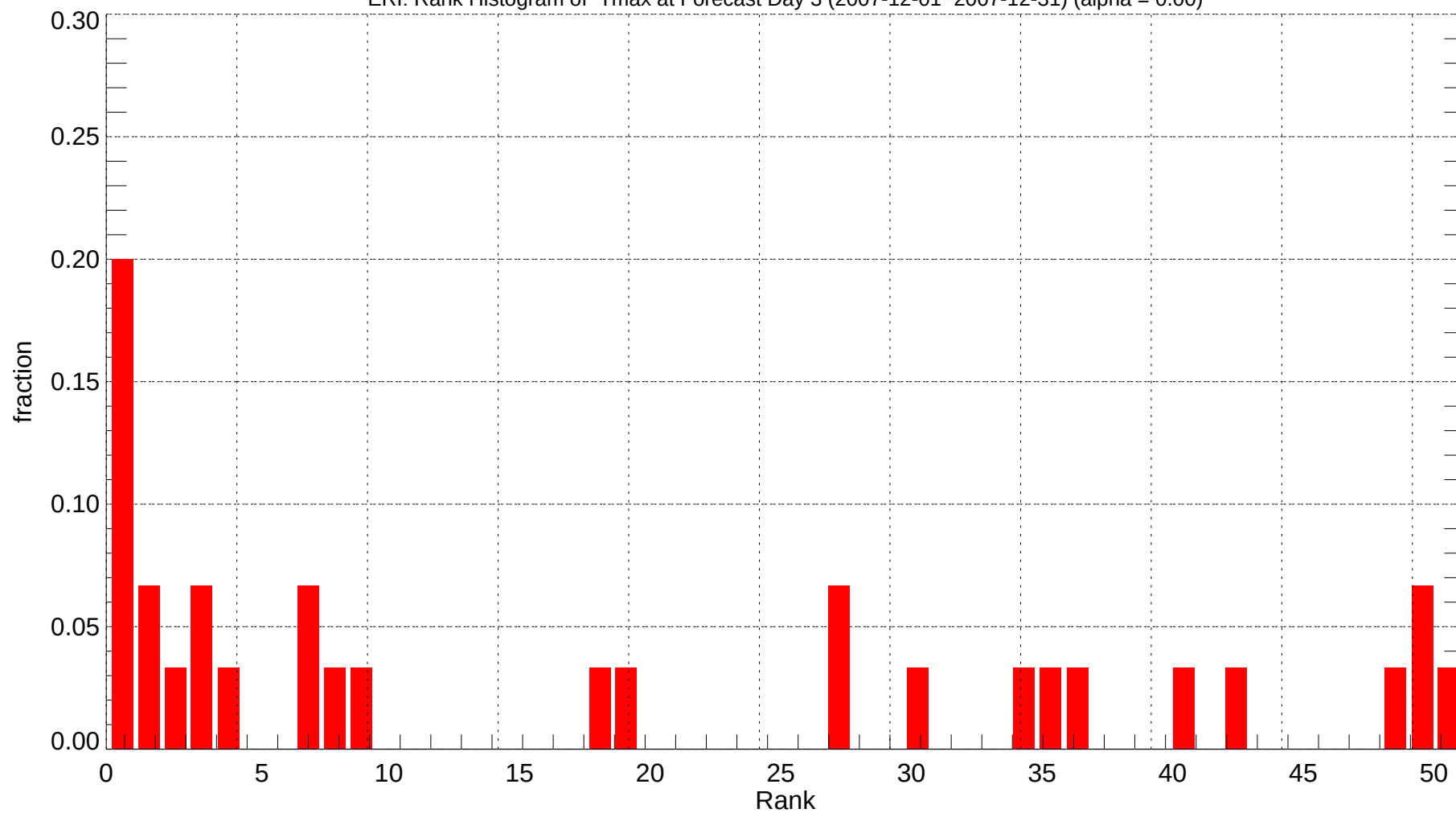
ERI: Rank Histogram of Tmax at Forecast Day 3 (2007-12-01~2007-12-31) (alpha = 0.00)
