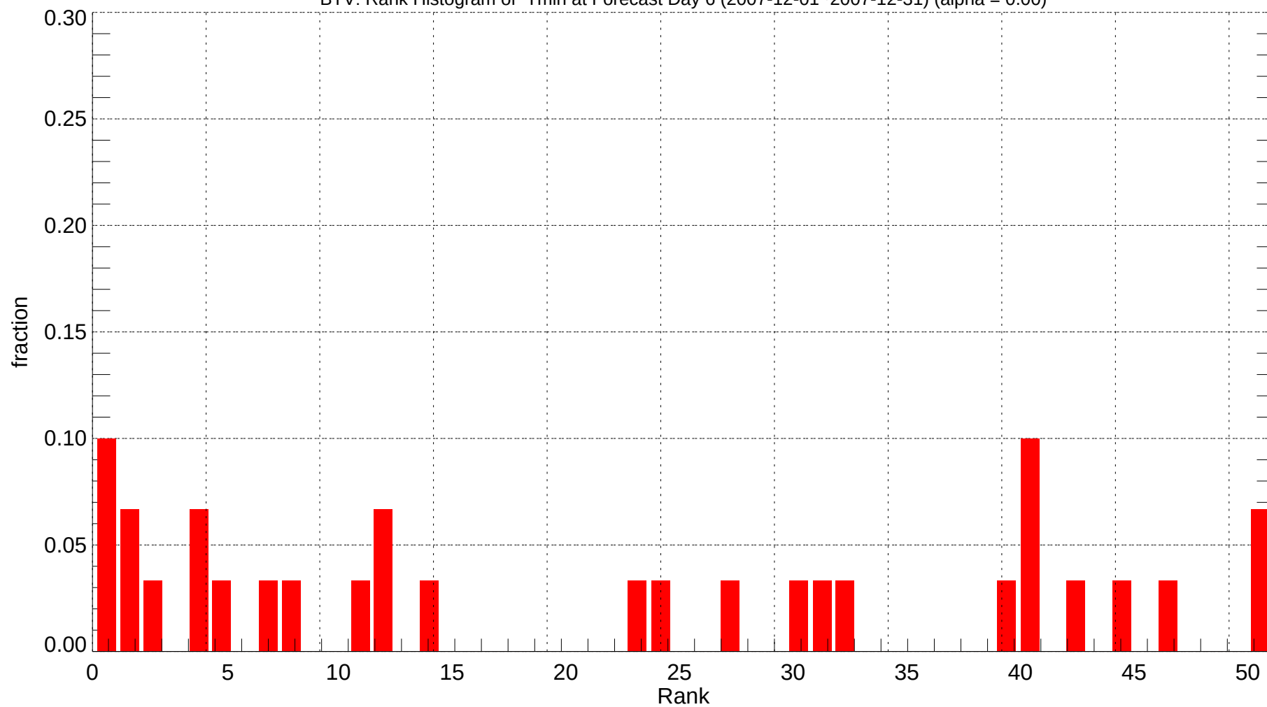
BTV: Rank Histogram of Tmin at Forecast Day 6 (2007-12-01~2007-12-31) (alpha = 0.00)
