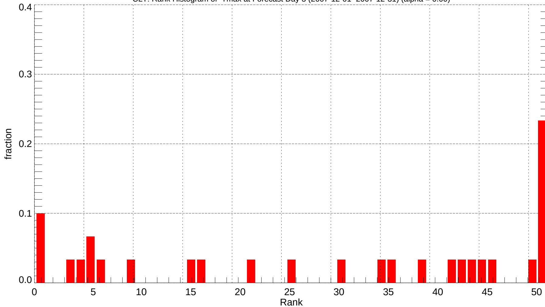
CLT: Rank Histogram of Tmax at Forecast Day 3 (2007-12-01~2007-12-31) (alpha = 0.00)
