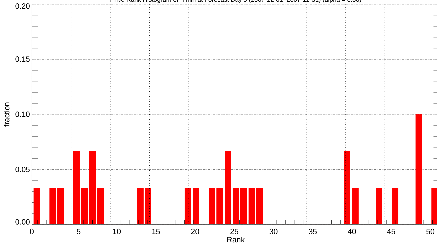
PHX: Rank Histogram of Tmin at Forecast Day 9 (2007-12-01~2007-12-31) (alpha = 0.00)
