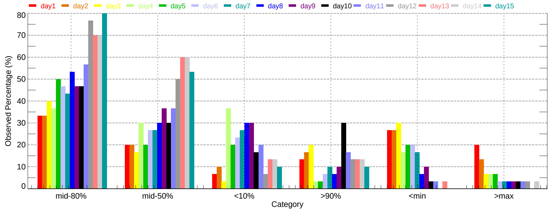
Observed Percentage of Ensembles - MKE: Min Temperature (2007-12-01~2007-12-31)
