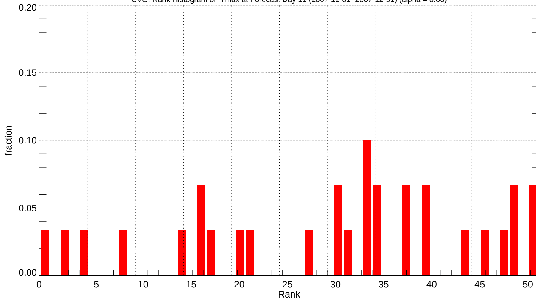
CVG: Rank Histogram of Tmax at Forecast Day 11 (2007-12-01~2007-12-31) (alpha = 0.00)
