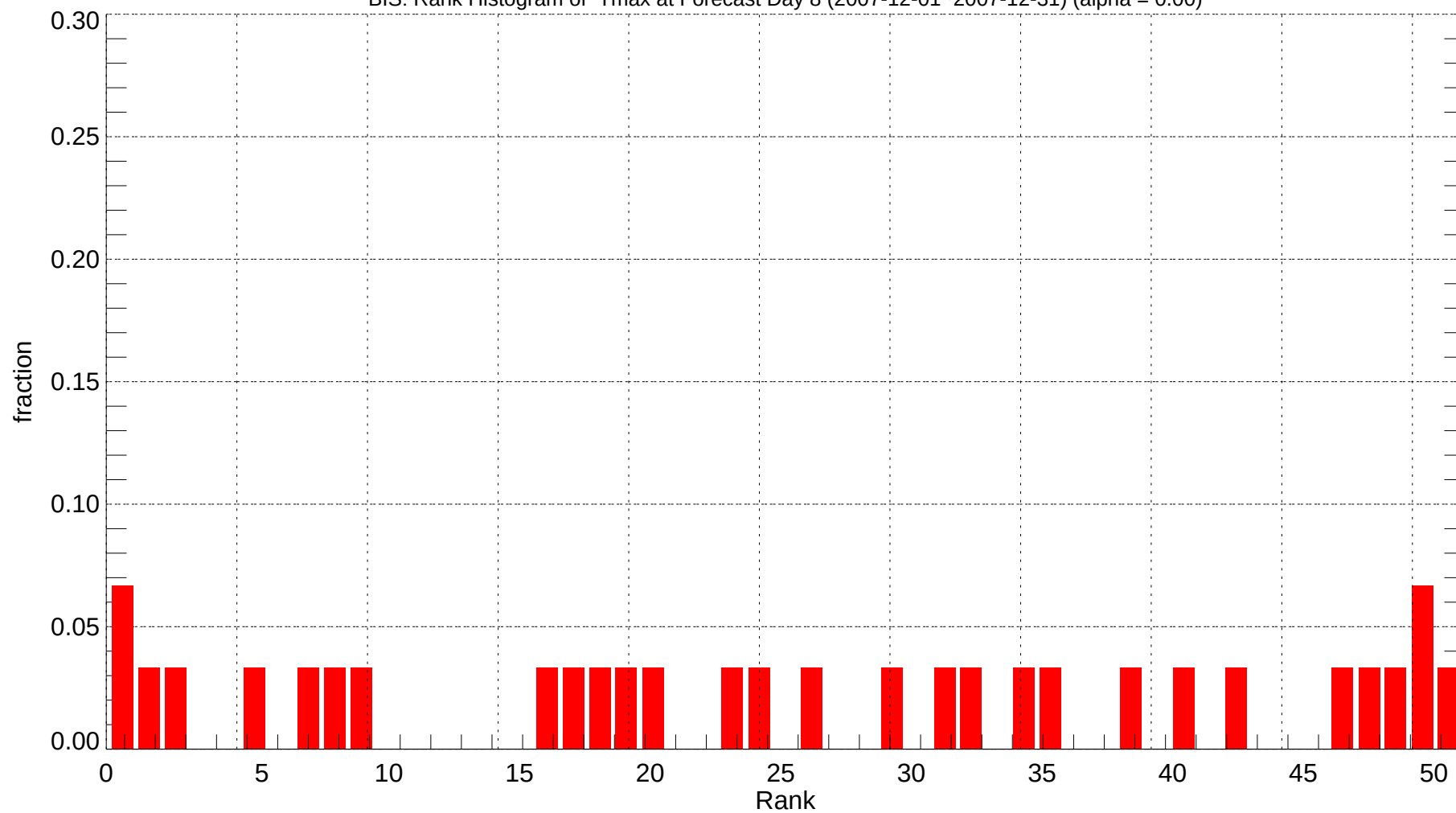
BIS: Rank Histogram of Tmax at Forecast Day 8 (2007-12-01~2007-12-31) (alpha = 0.00)
