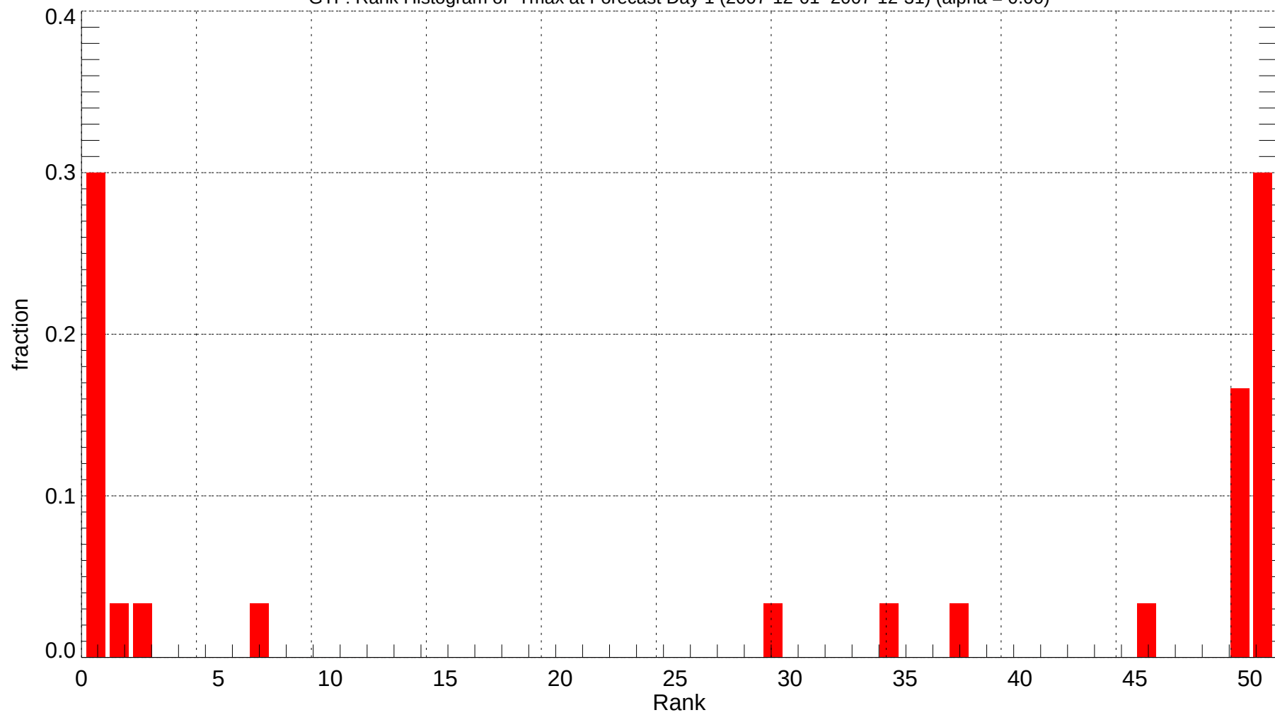
GTF: Rank Histogram of Tmax at Forecast Day 1 (2007-12-01~2007-12-31) (alpha = 0.00)
