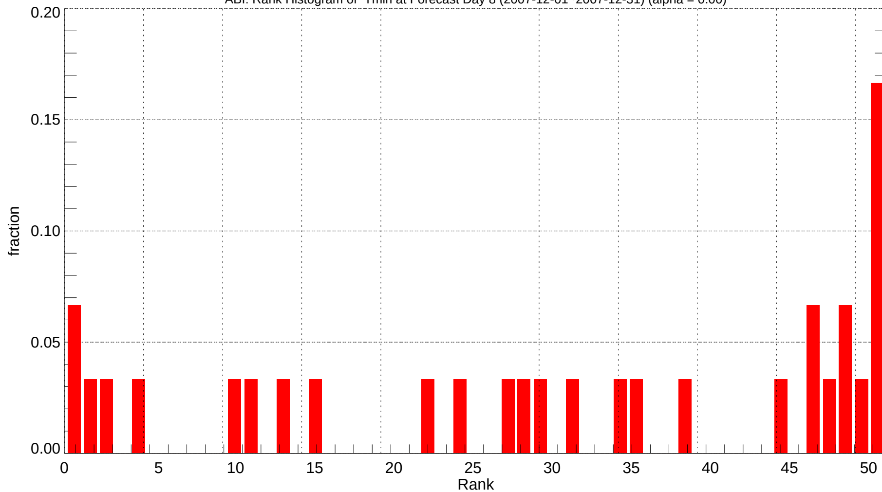
ABI: Rank Histogram of Tmin at Forecast Day 8 (2007-12-01~2007-12-31) (alpha = 0.00)
