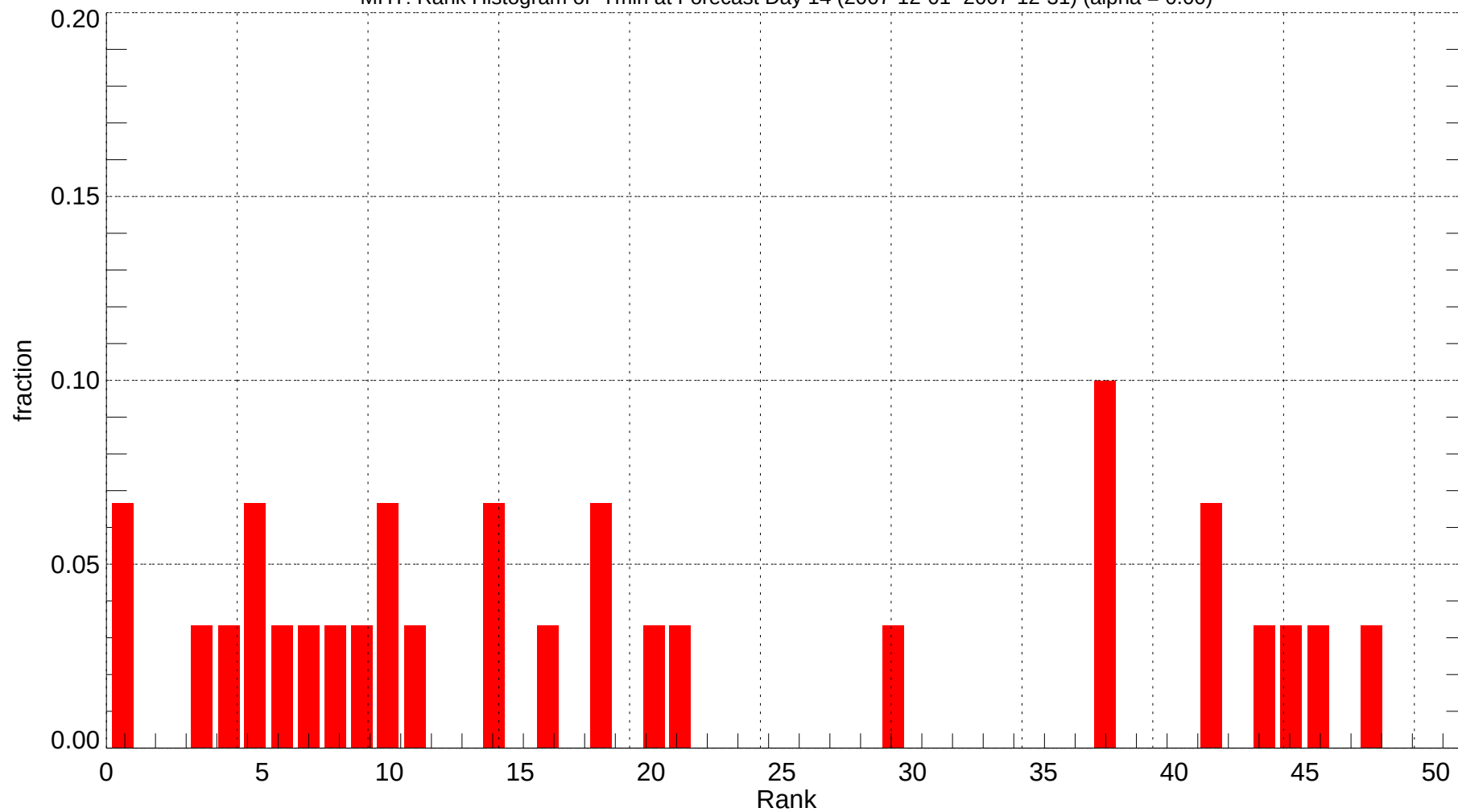
MHT: Rank Histogram of Tmin at Forecast Day 14 (2007-12-01~2007-12-31) (alpha = 0.00)
