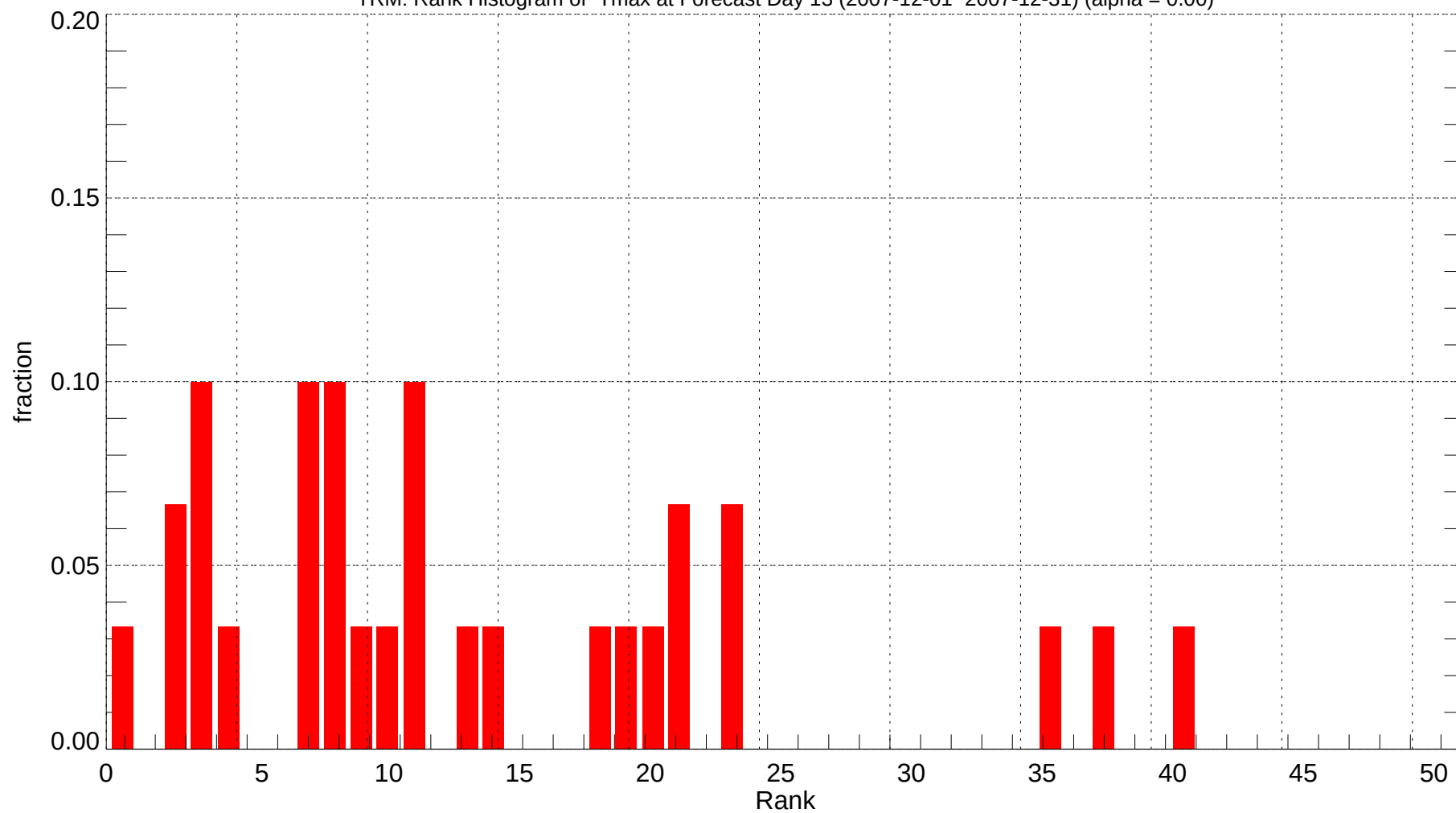
TRM: Rank Histogram of Tmax at Forecast Day 13 (2007-12-01~2007-12-31) (alpha = 0.00)
