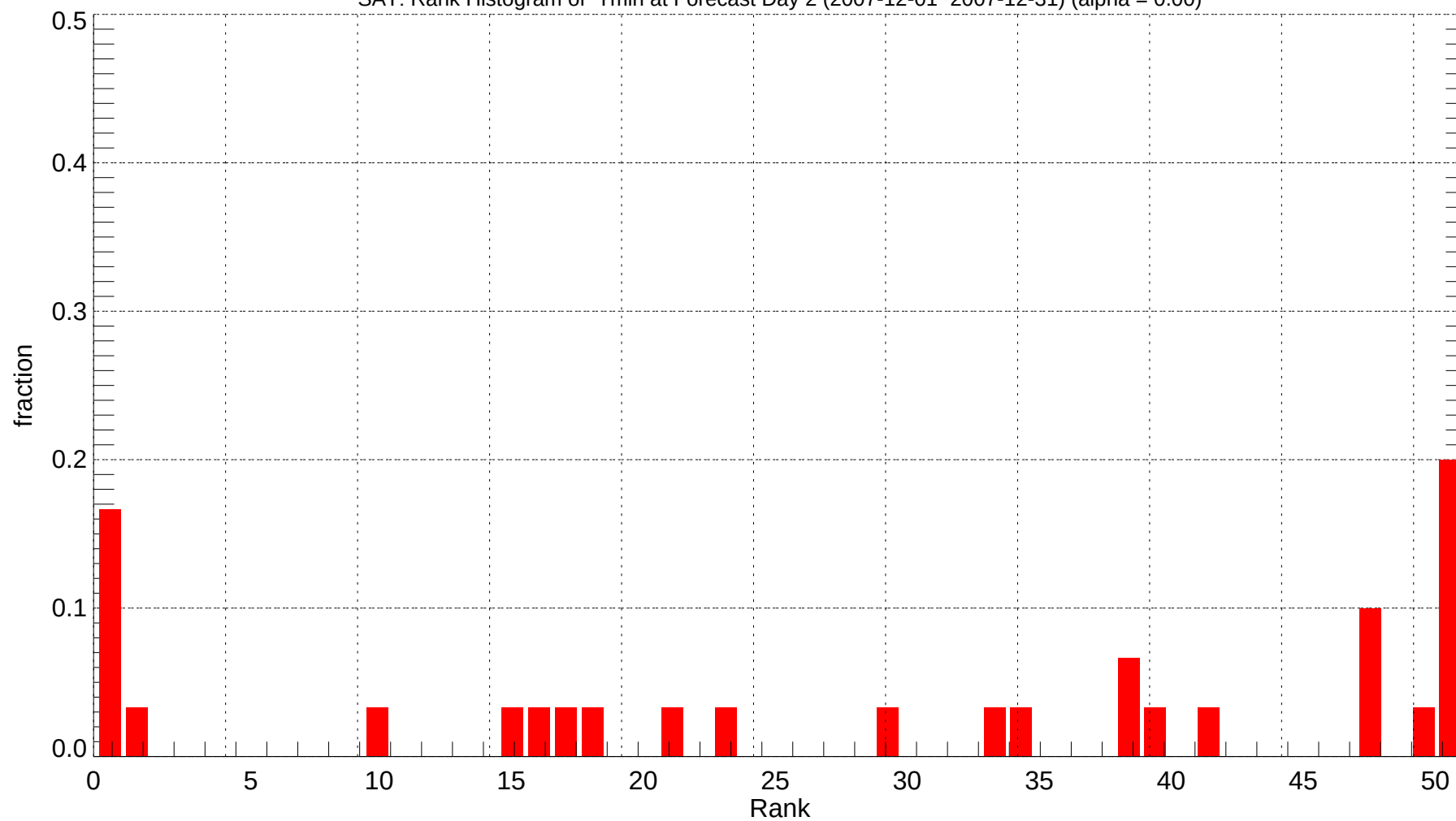
SAT: Rank Histogram of Tmin at Forecast Day 2 (2007-12-01~2007-12-31) (alpha = 0.00)
