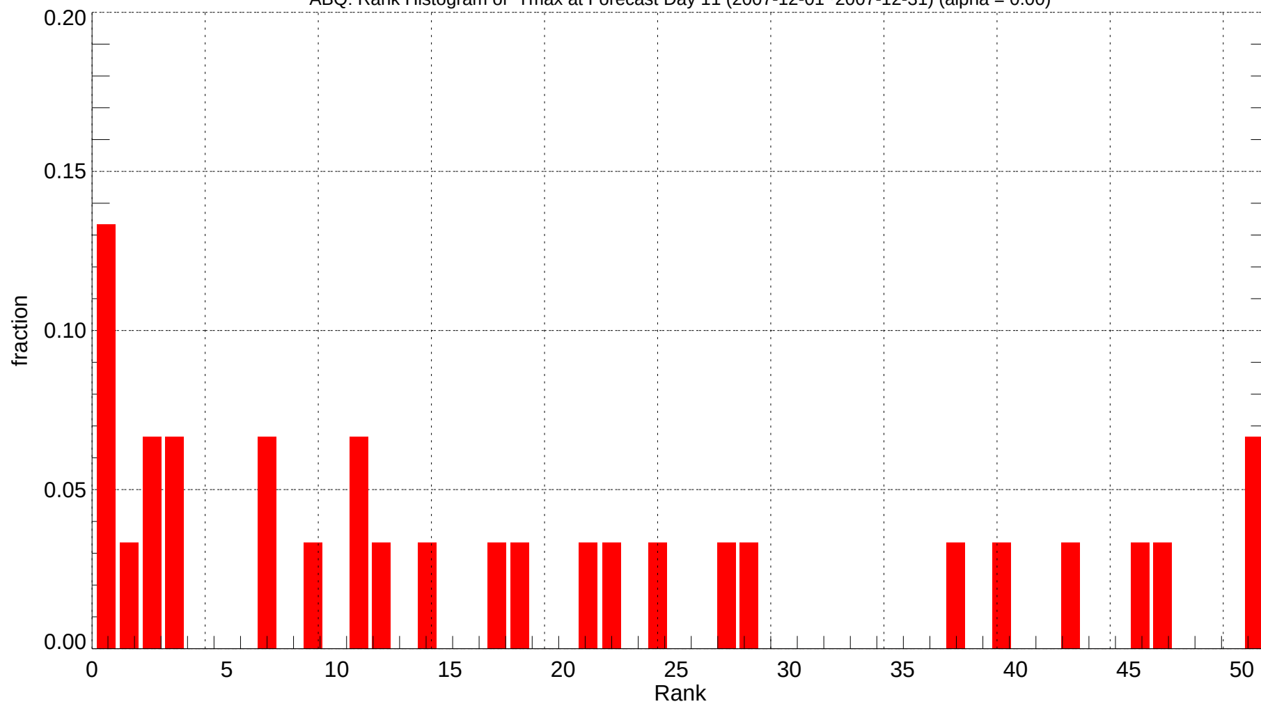
ABQ: Rank Histogram of Tmax at Forecast Day 11 (2007-12-01~2007-12-31) (alpha = 0.00)
