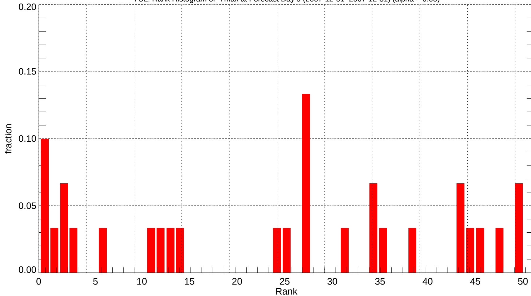
YUL: Rank Histogram of Tmax at Forecast Day 9 (2007-12-01~2007-12-31) (alpha = 0.00)
