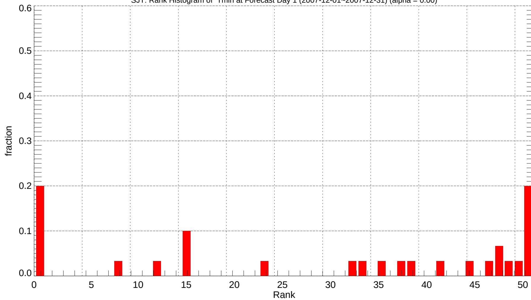
SJT: Rank Histogram of Tmin at Forecast Day 1 (2007-12-01~2007-12-31) (alpha = 0.00)
