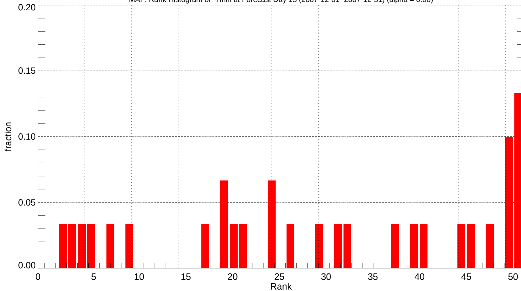
MAF: Rank Histogram of Tmin at Forecast Day 13 (2007-12-01~2007-12-31) (alpha = 0.00)
