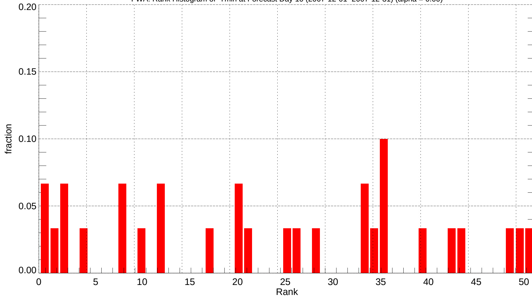
FWA: Rank Histogram of Tmin at Forecast Day 10 (2007-12-01~2007-12-31) (alpha = 0.00)
