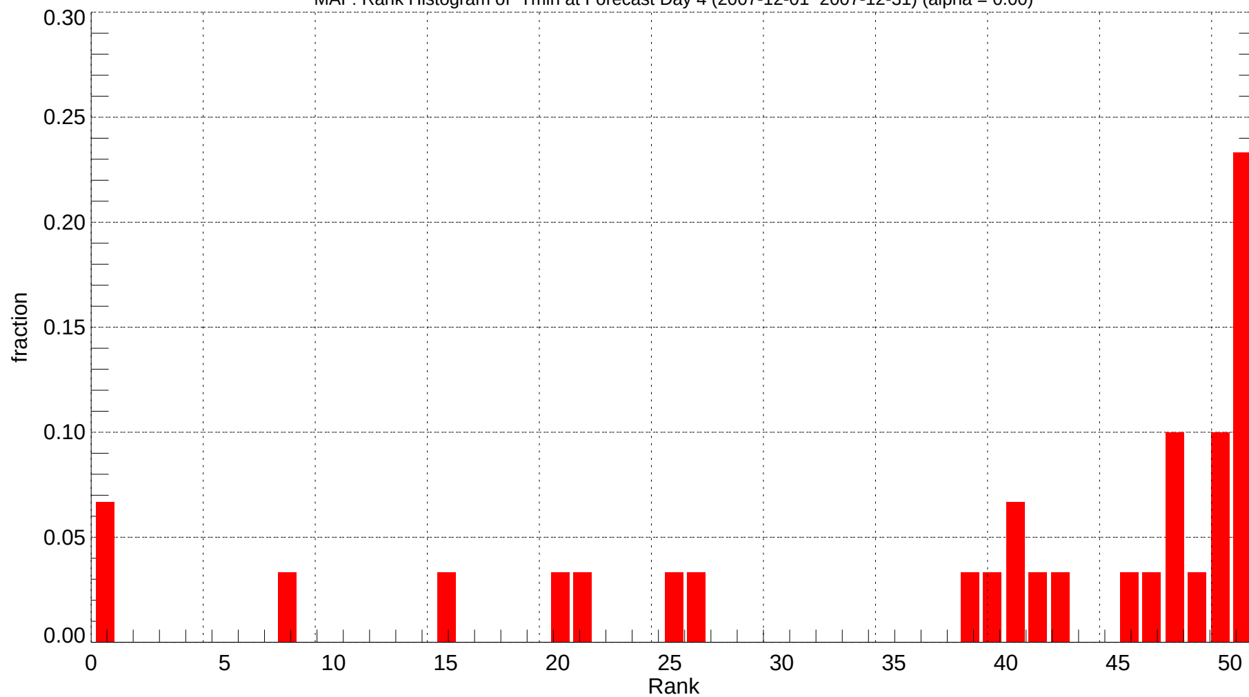
MAF: Rank Histogram of Tmin at Forecast Day 4 (2007-12-01~2007-12-31) (alpha = 0.00)
