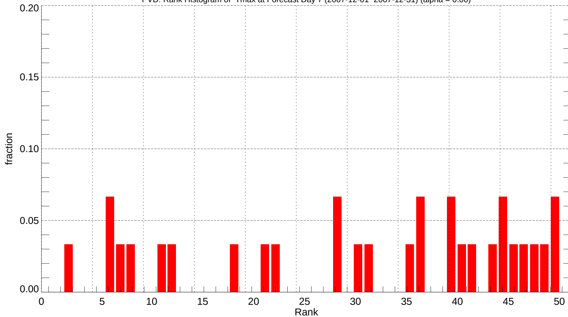
PVD: Rank Histogram of Tmax at Forecast Day 7 (2007-12-01~2007-12-31) (alpha = 0.00)
