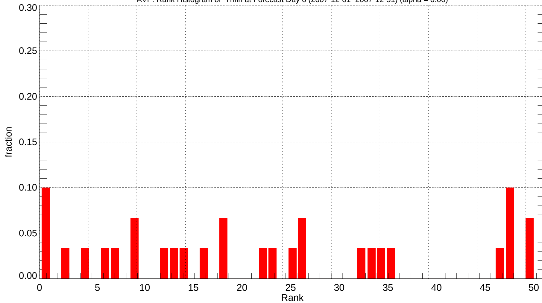
AVP: Rank Histogram of Tmin at Forecast Day 6 (2007-12-01~2007-12-31) (alpha = 0.00)
