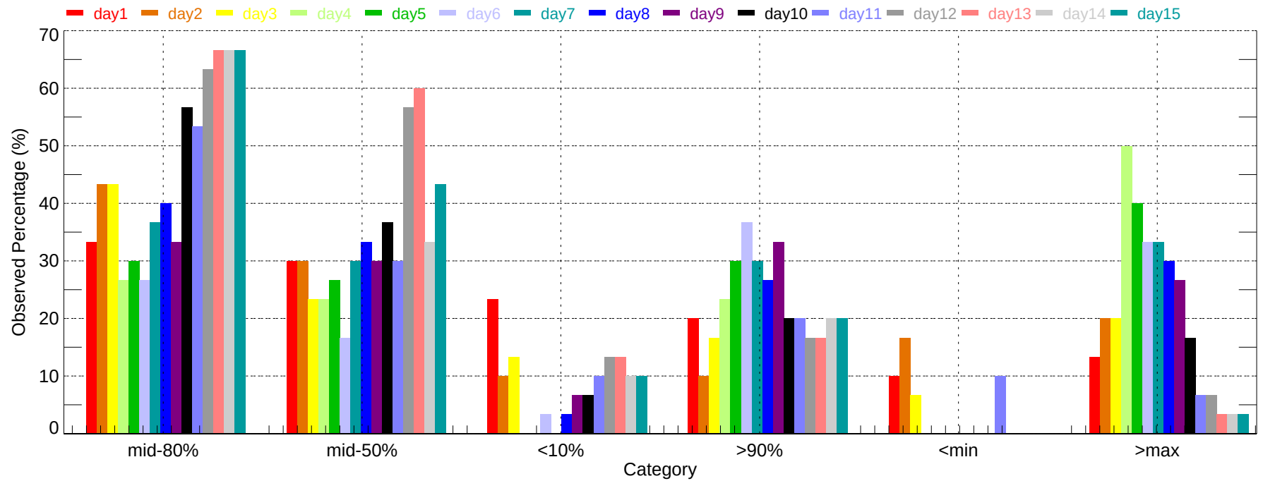
Observed Percentage of Ensembles - ELP: Min Temperature (2007-12-01~2007-12-31)
