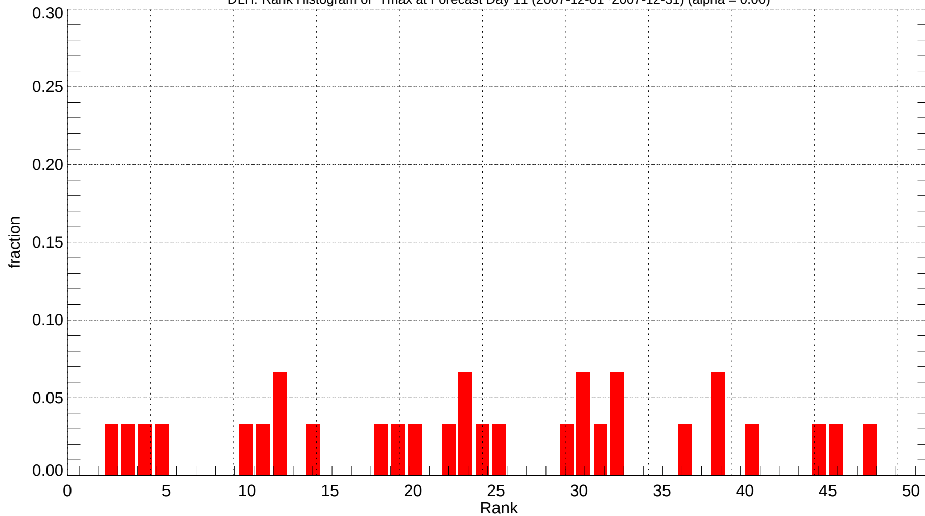
DLH: Rank Histogram of Tmax at Forecast Day 11 (2007-12-01~2007-12-31) (alpha = 0.00)
