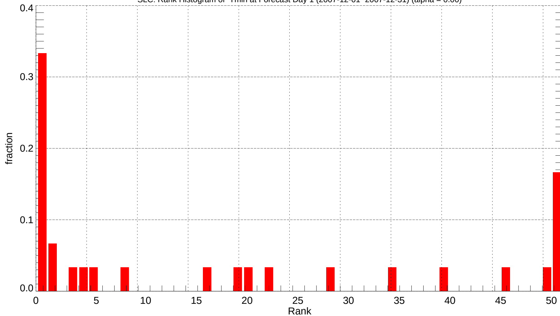
SLC: Rank Histogram of Tmin at Forecast Day 1 (2007-12-01~2007-12-31) (alpha = 0.00)
