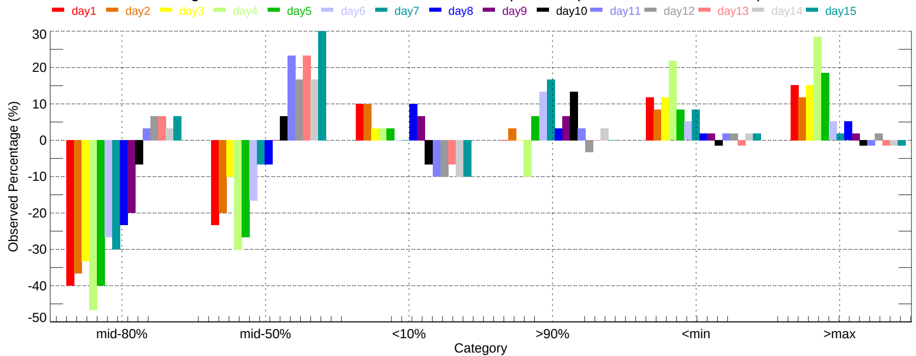
Observed Percentage Deviation of Ensembles - SAC: Max Temperature (2007-12-01~2007-12-31)
