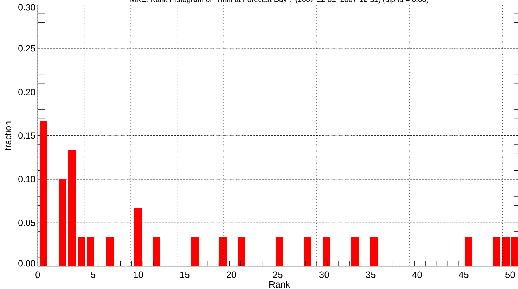
MKE: Rank Histogram of Tmin at Forecast Day 7 (2007-12-01~2007-12-31) (alpha = 0.00)
