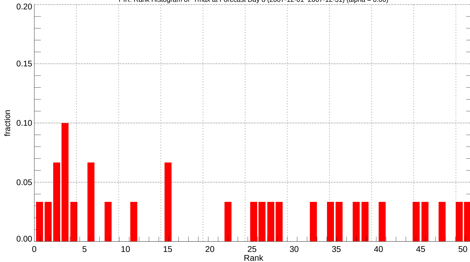
PIR: Rank Histogram of Tmax at Forecast Day 8 (2007-12-01~2007-12-31) (alpha = 0.00)
