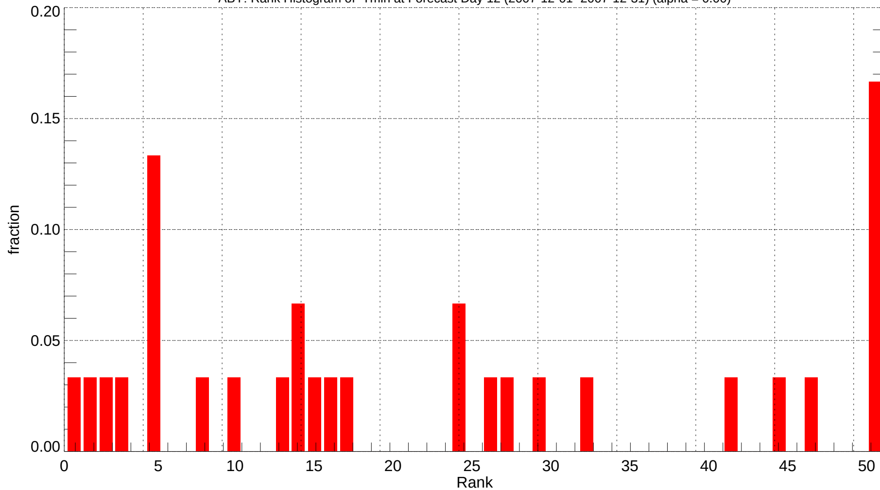
ABY: Rank Histogram of Tmin at Forecast Day 12 (2007-12-01~2007-12-31) (alpha = 0.00)
