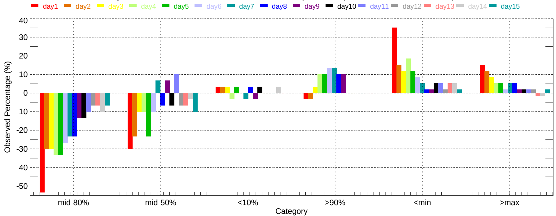
Observed Percentage Deviation of Ensembles - ILG: Min Temperature (2007-12-01~2007-12-31)
