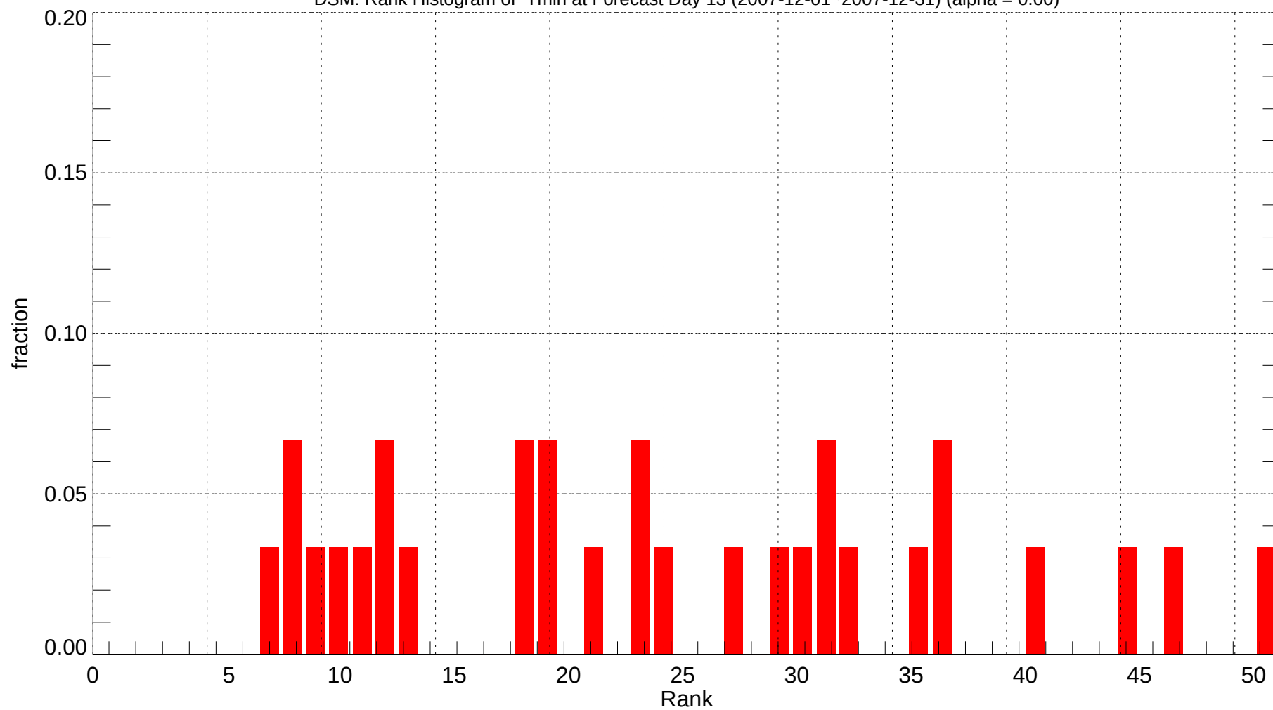
DSM: Rank Histogram of Tmin at Forecast Day 13 (2007-12-01~2007-12-31) (alpha = 0.00)
