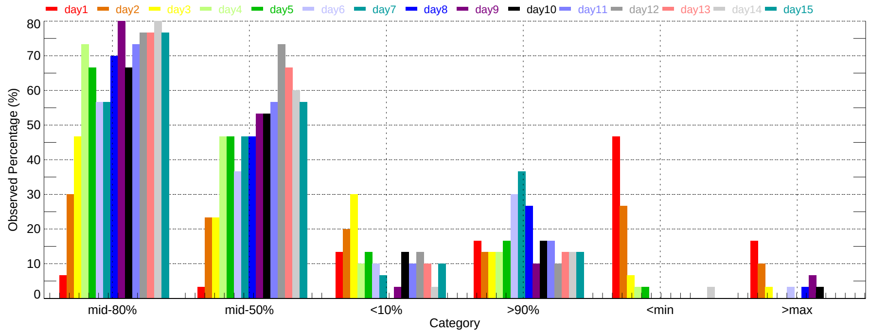
Observed Percentage of Ensembles - BOS: Min Temperature (2007-12-01~2007-12-31)
