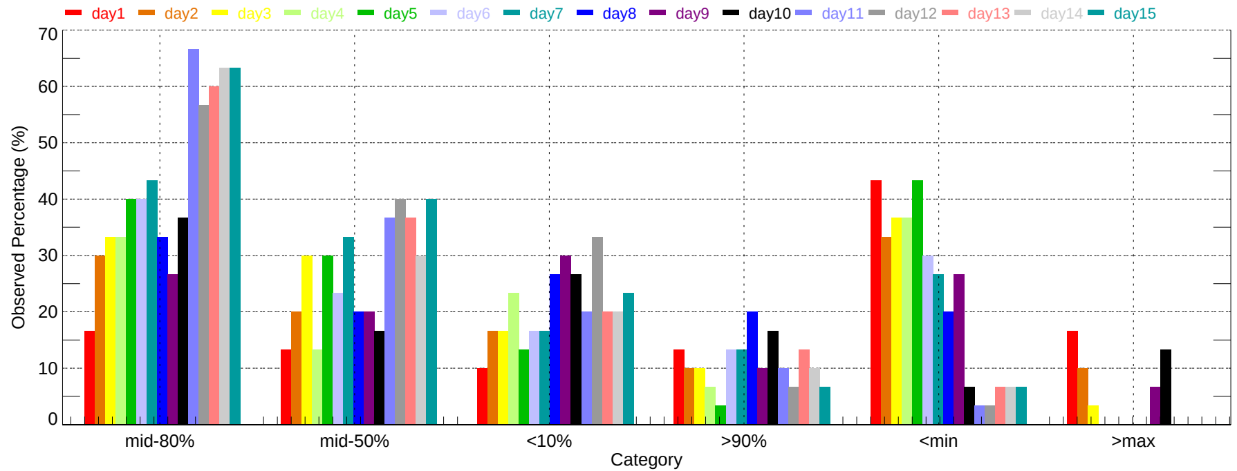
Observed Percentage of Ensembles - BDL: Max Temperature (2007-12-01~2007-12-31)
