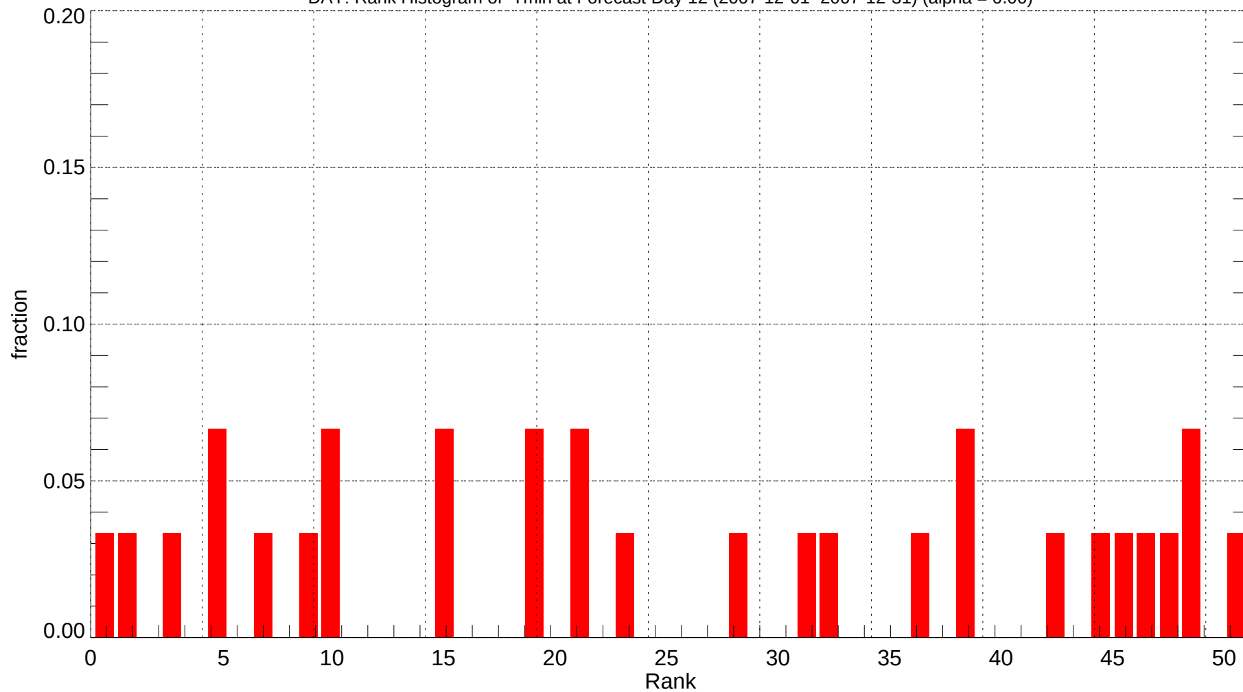
DAY: Rank Histogram of Tmin at Forecast Day 12 (2007-12-01~2007-12-31) (alpha = 0.00)
