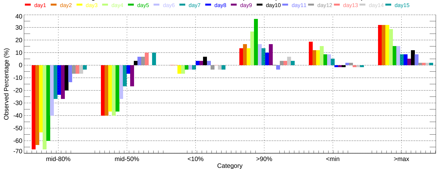
Observed Percentage Deviation of Ensembles - GEG: Min Temperature (2007-12-01~2007-12-31)
