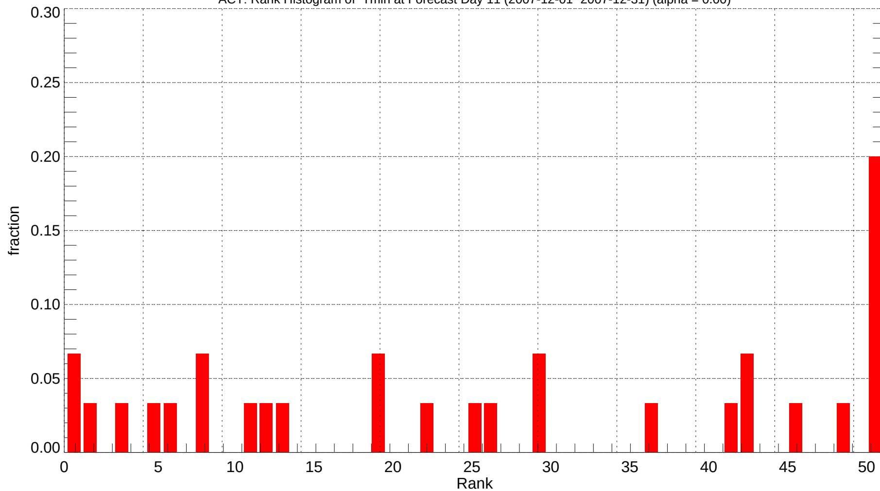
ACT: Rank Histogram of Tmin at Forecast Day 11 (2007-12-01~2007-12-31) (alpha = 0.00)
