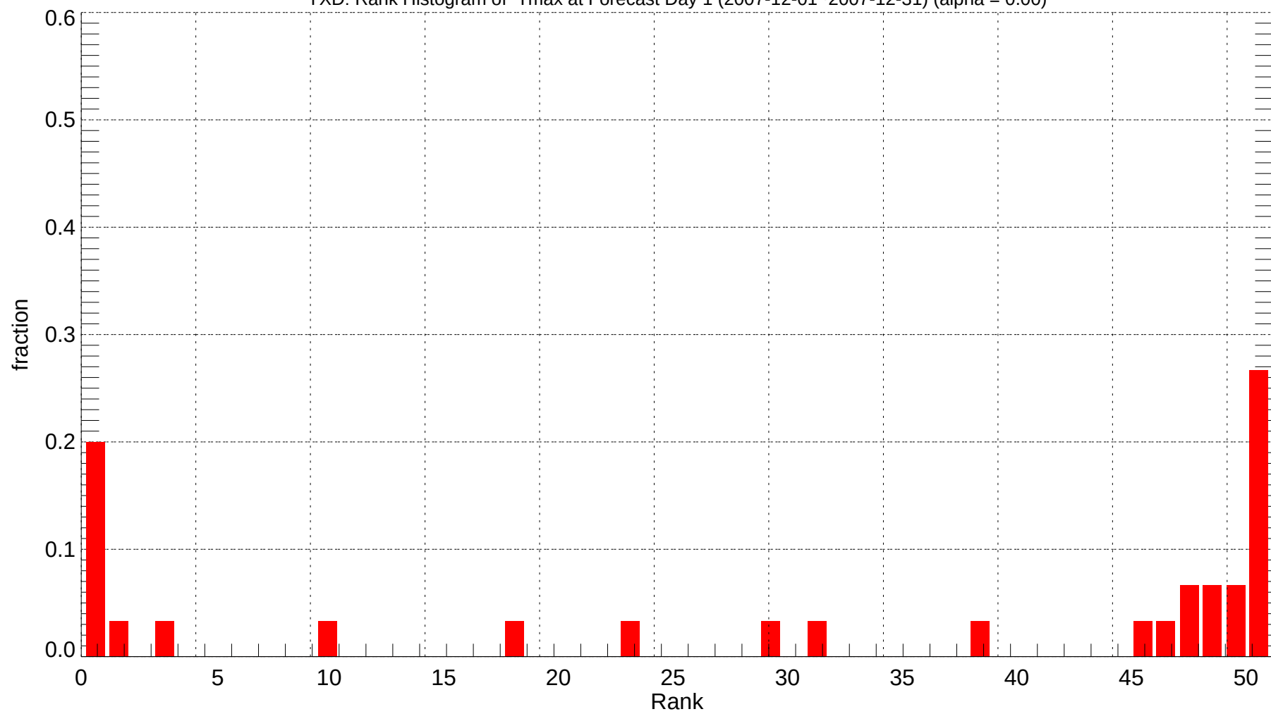
YXD: Rank Histogram of Tmax at Forecast Day 1 (2007-12-01~2007-12-31) (alpha = 0.00)
