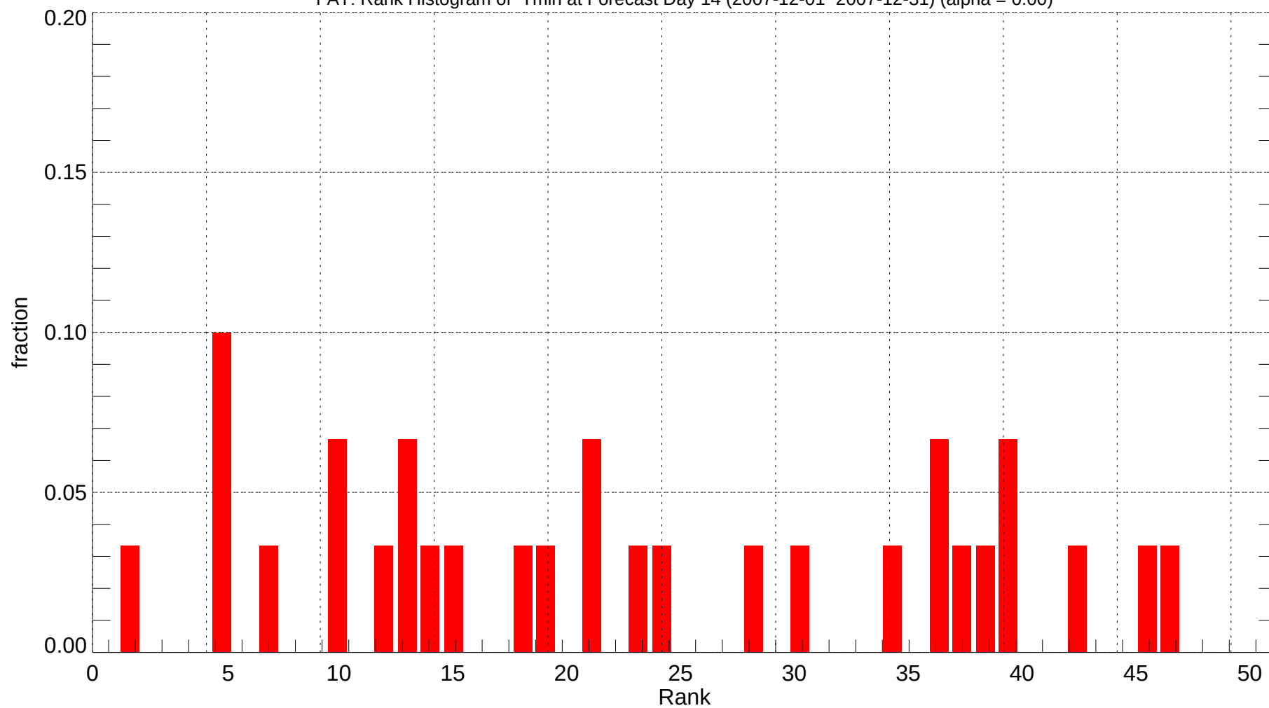
FAT: Rank Histogram of Tmin at Forecast Day 14 (2007-12-01~2007-12-31) (alpha = 0.00)
