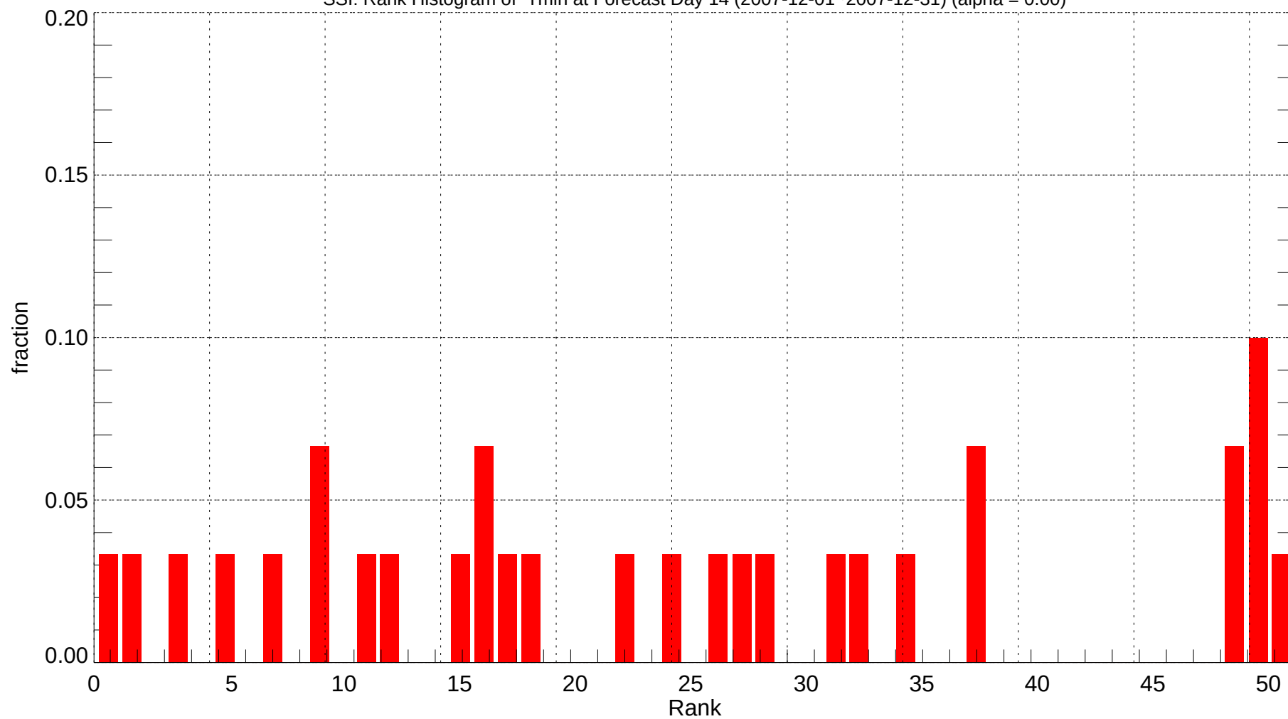
SSI: Rank Histogram of Tmin at Forecast Day 14 (2007-12-01~2007-12-31) (alpha = 0.00)
