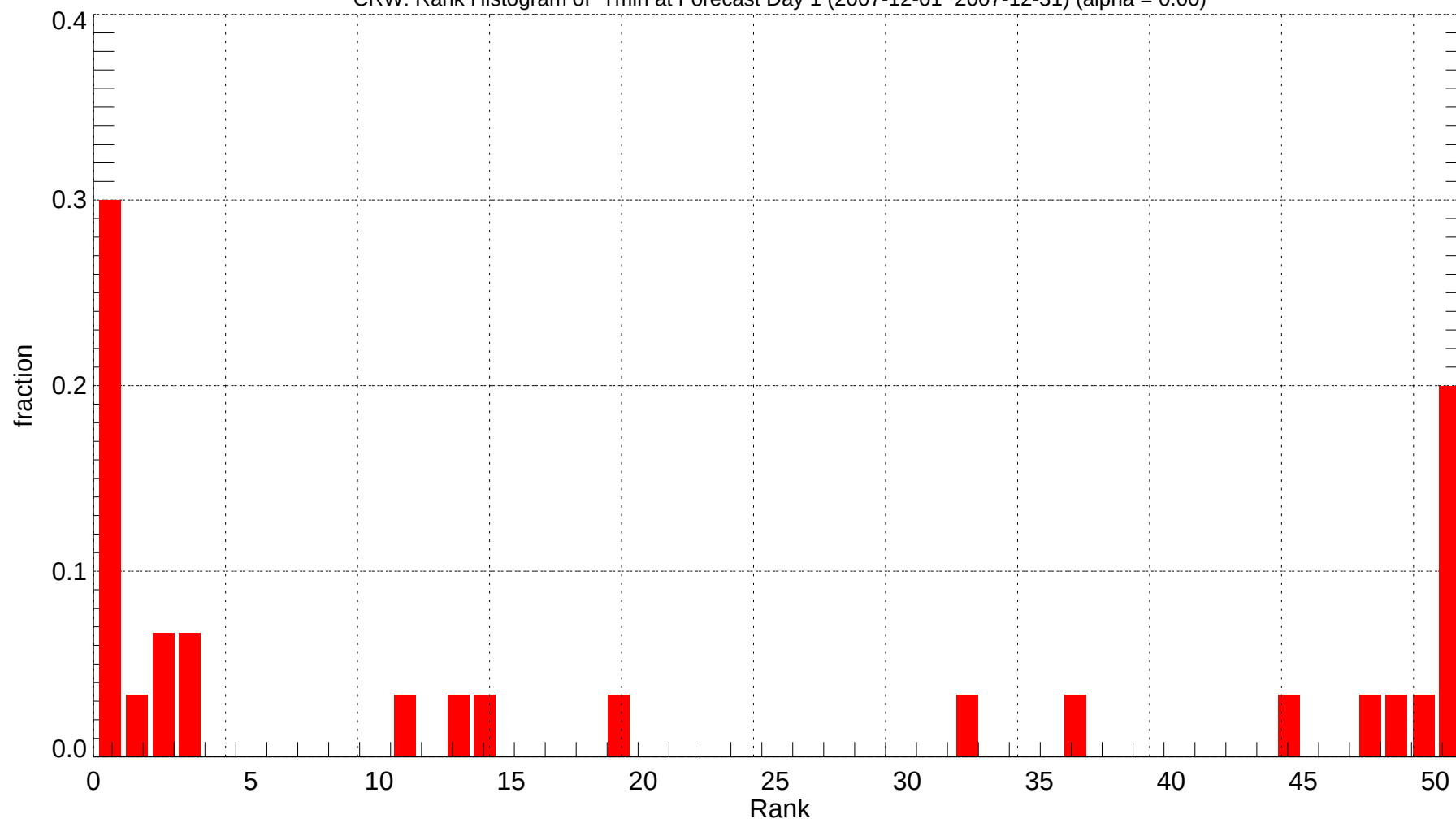
CRW: Rank Histogram of Tmin at Forecast Day 1 (2007-12-01~2007-12-31) (alpha = 0.00)
