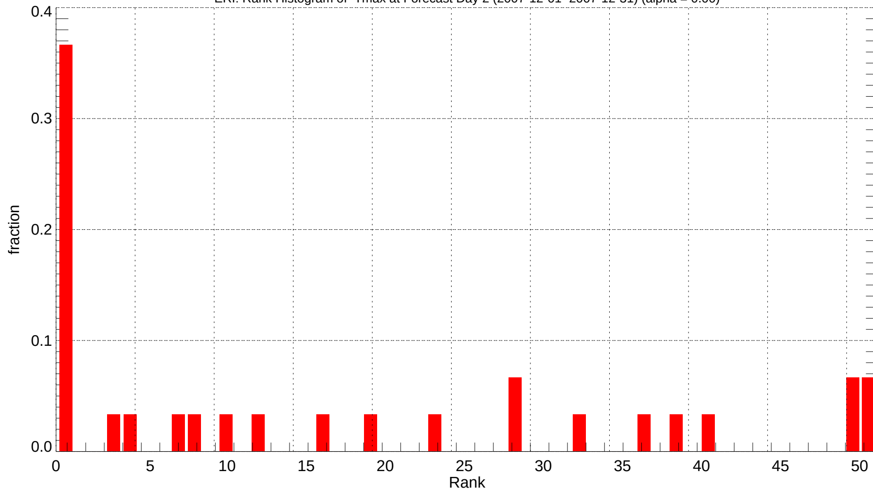
ERI: Rank Histogram of Tmax at Forecast Day 2 (2007-12-01~2007-12-31) (alpha = 0.00)
