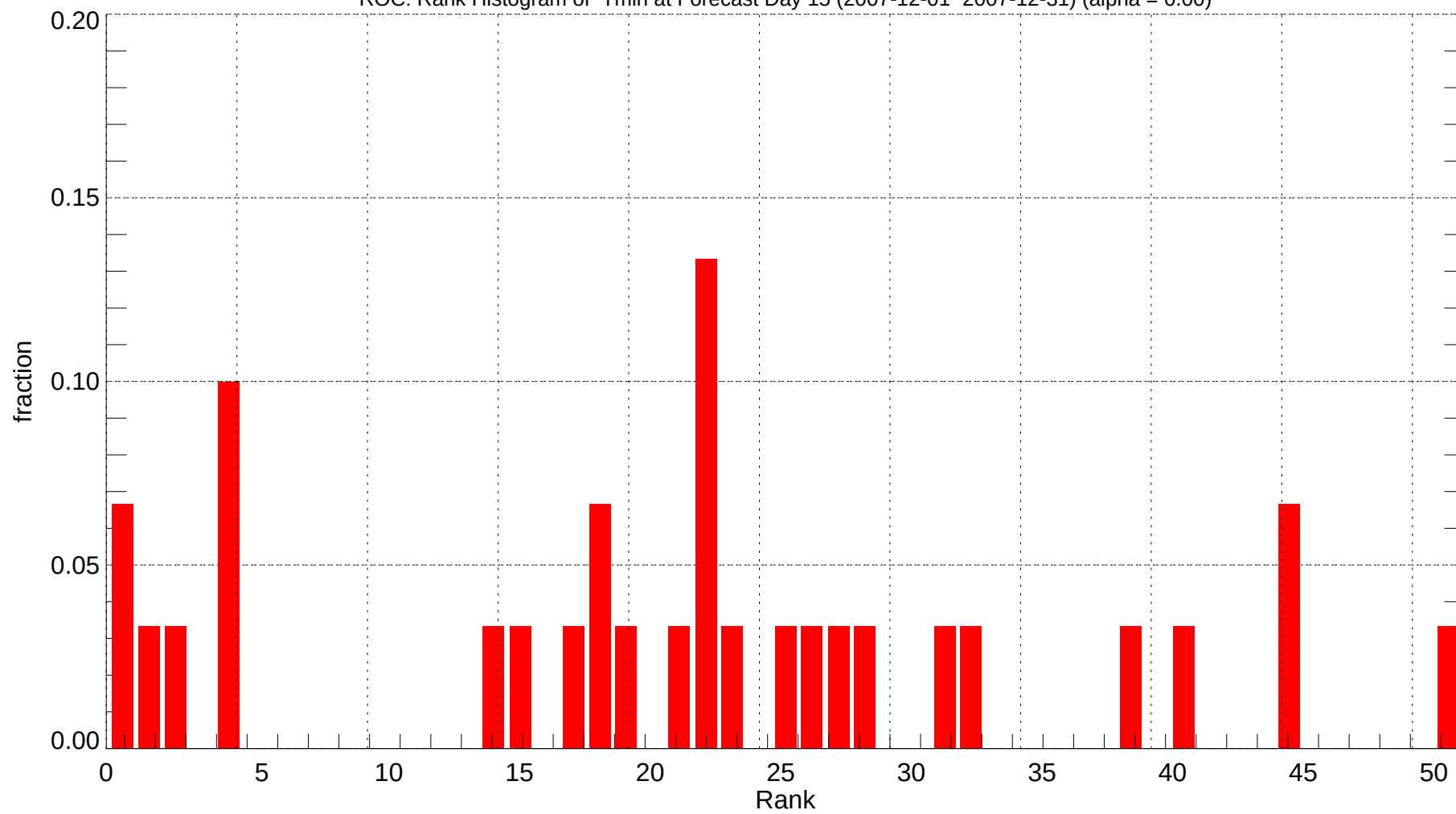
ROC: Rank Histogram of Tmin at Forecast Day 15 (2007-12-01~2007-12-31) (alpha = 0.00)
