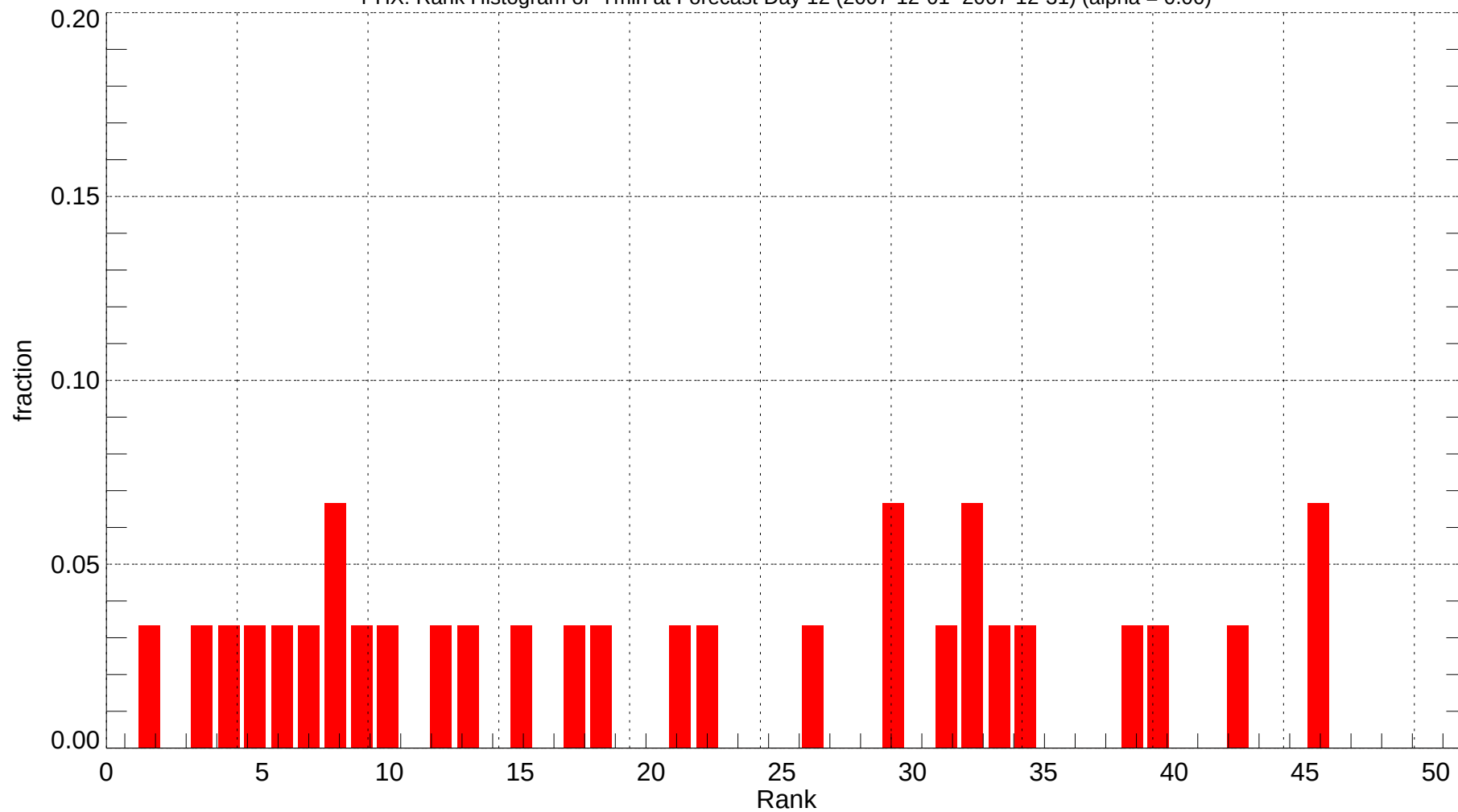
PHX: Rank Histogram of Tmin at Forecast Day 12 (2007-12-01~2007-12-31) (alpha = 0.00)
