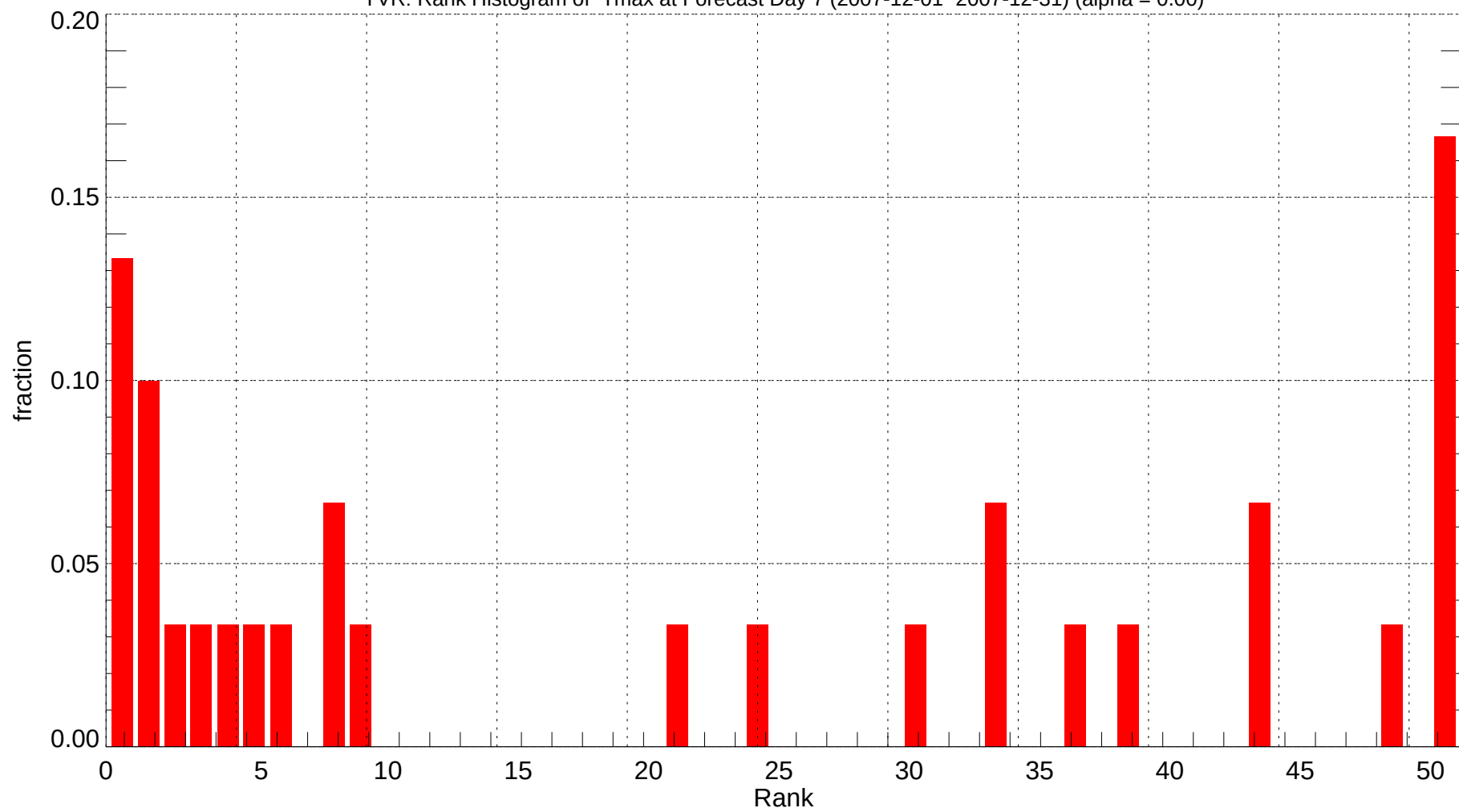
YVR: Rank Histogram of Tmax at Forecast Day 7 (2007-12-01~2007-12-31) (alpha = 0.00)
