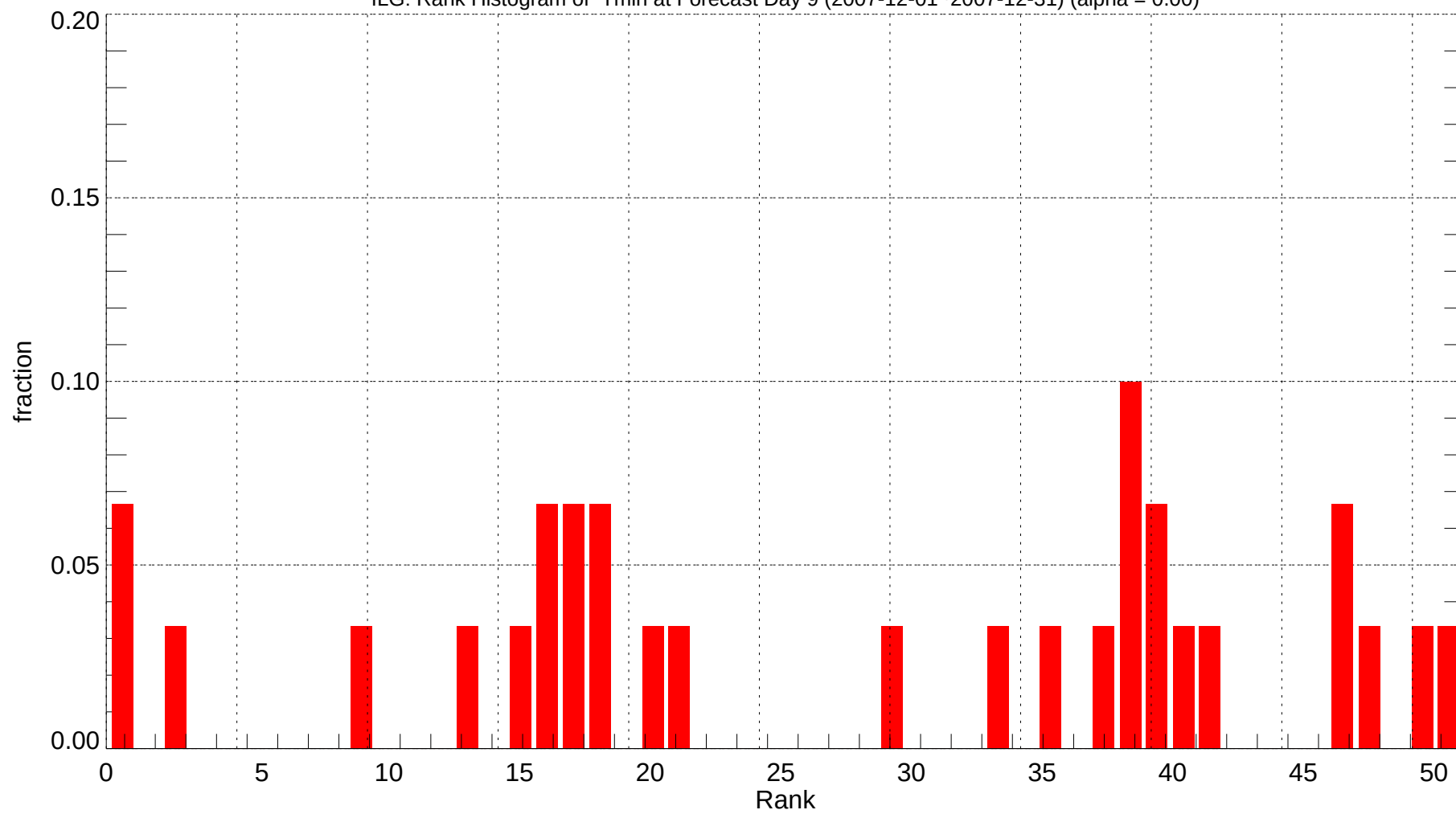
ILG: Rank Histogram of Tmin at Forecast Day 9 (2007-12-01~2007-12-31) (alpha = 0.00)
