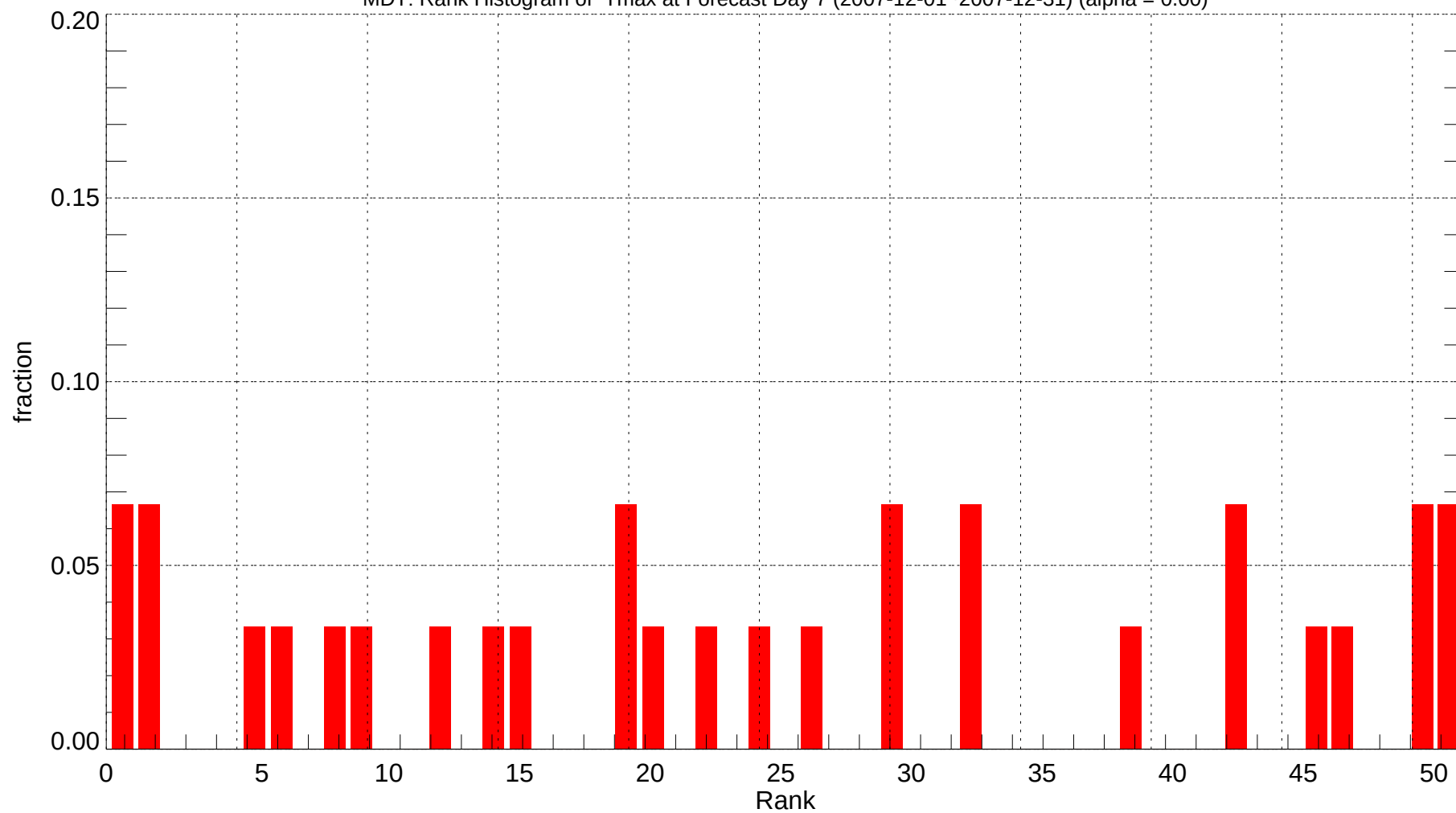
MDT: Rank Histogram of Tmax at Forecast Day 7 (2007-12-01~2007-12-31) (alpha = 0.00)
