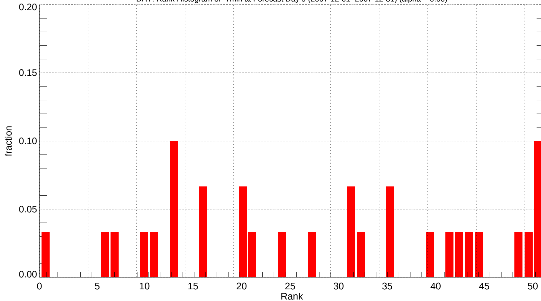
DAY: Rank Histogram of Tmin at Forecast Day 9 (2007-12-01~2007-12-31) (alpha = 0.00)
