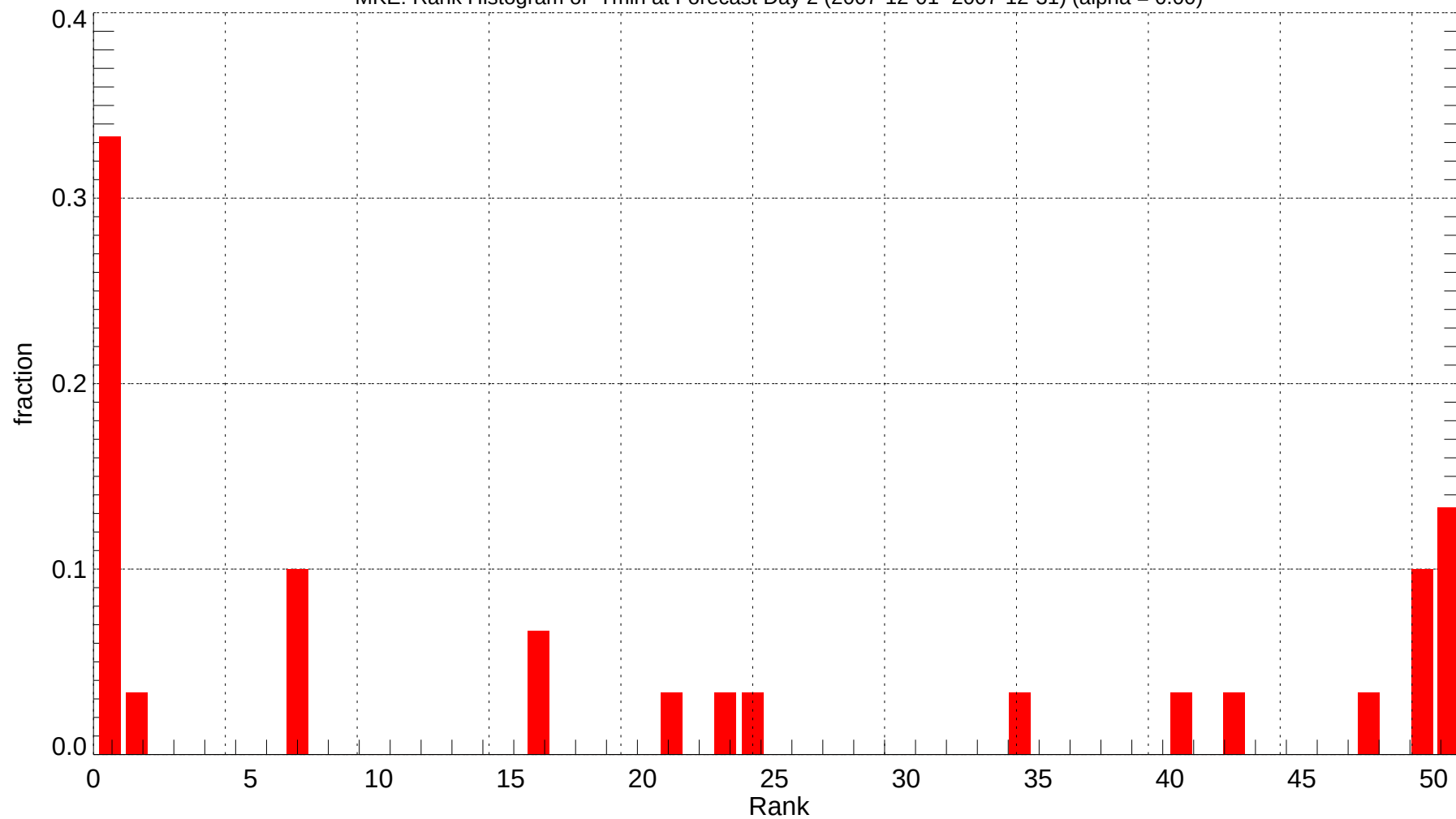
MKE: Rank Histogram of Tmin at Forecast Day 2 (2007-12-01~2007-12-31) (alpha = 0.00)
