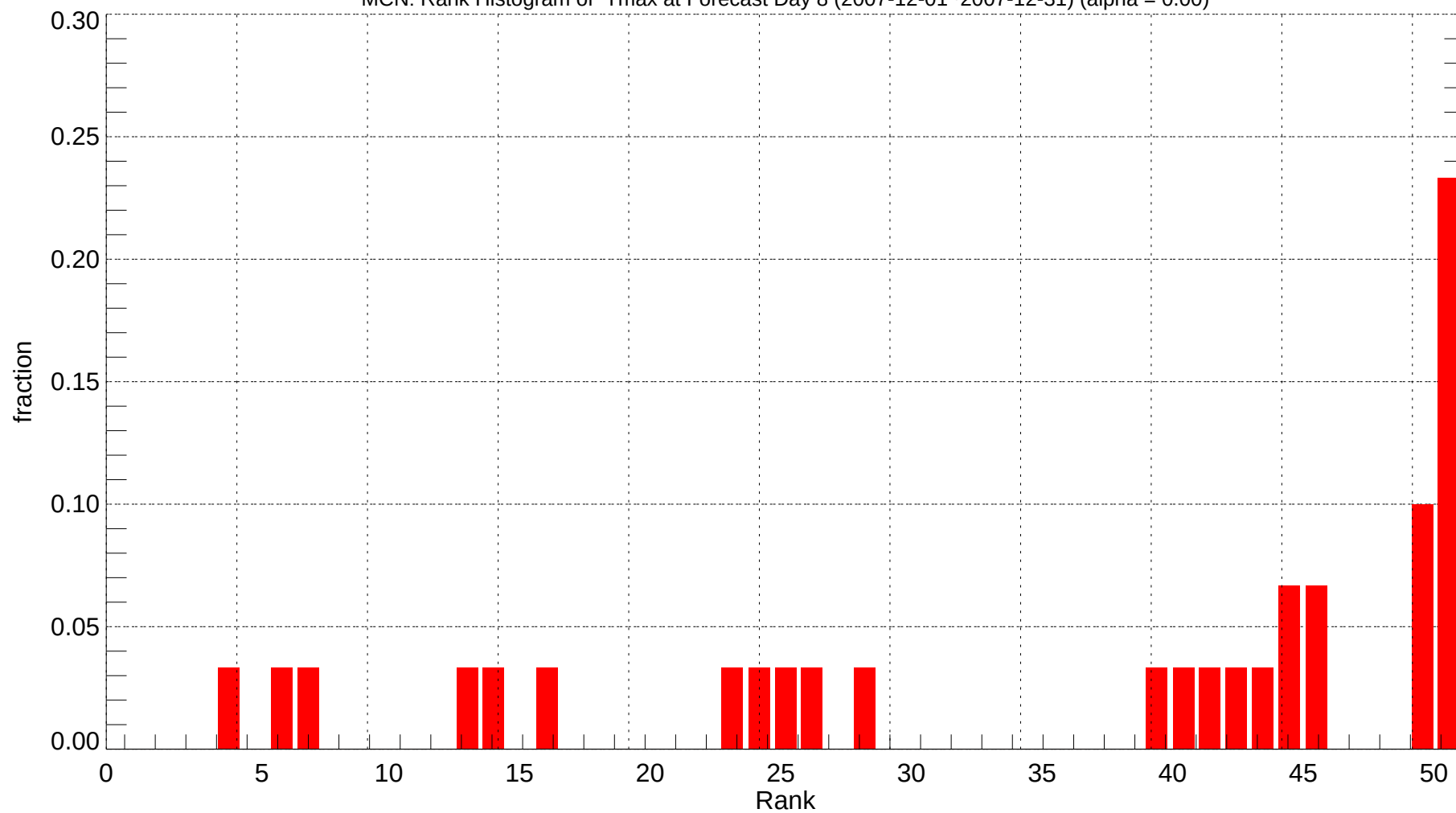
MCN: Rank Histogram of Tmax at Forecast Day 8 (2007-12-01~2007-12-31) (alpha = 0.00)
