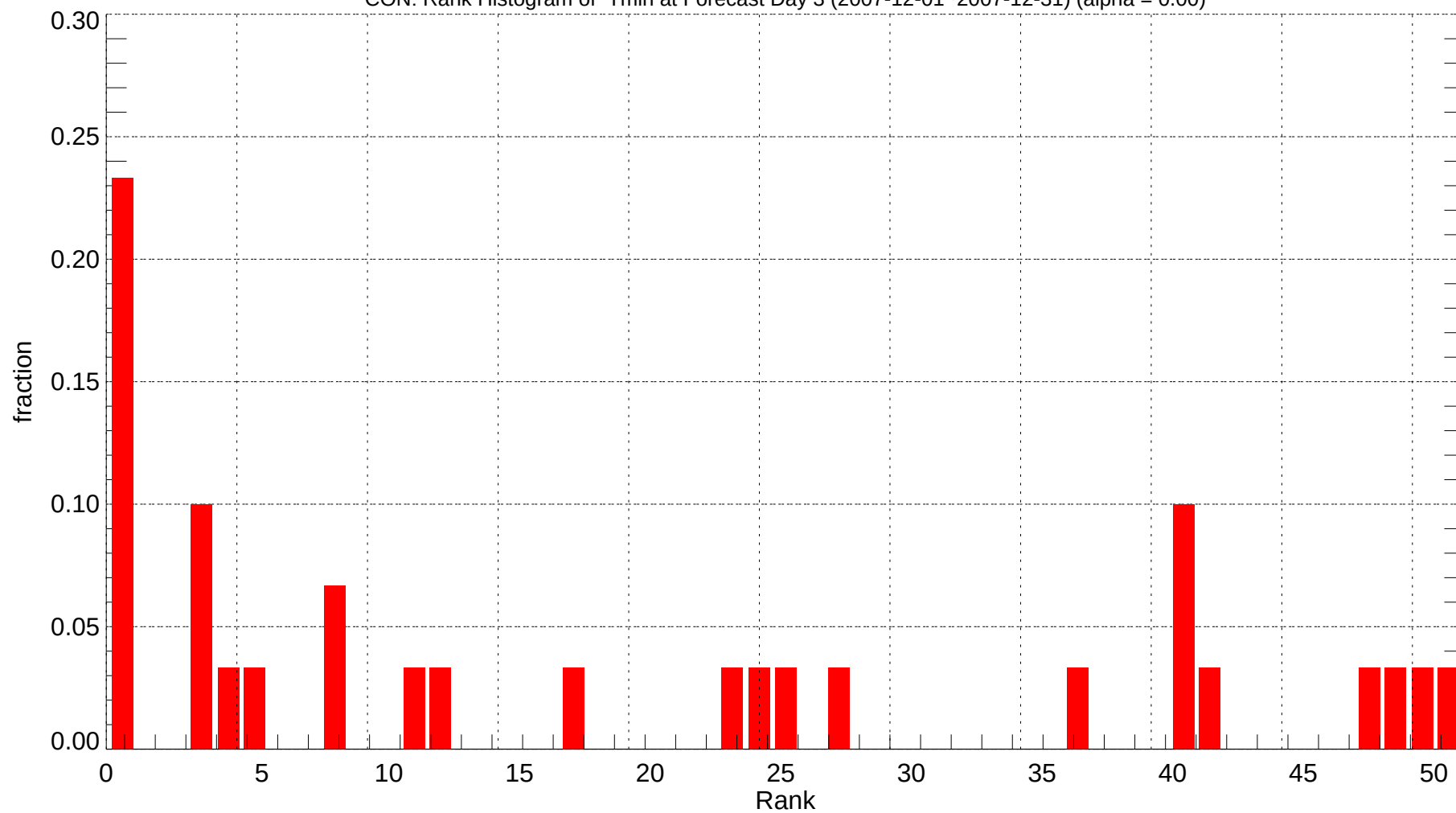
CON: Rank Histogram of Tmin at Forecast Day 3 (2007-12-01~2007-12-31) (alpha = 0.00)
