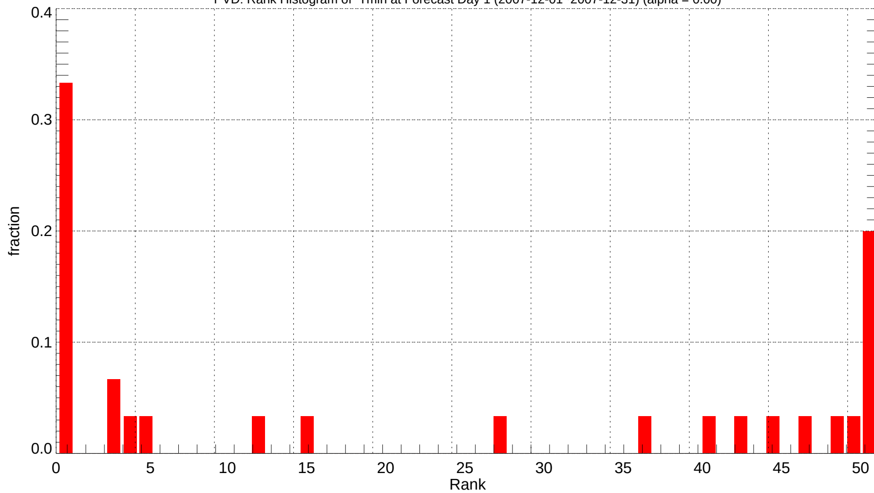
PVD: Rank Histogram of Tmin at Forecast Day 1 (2007-12-01~2007-12-31) (alpha = 0.00)
