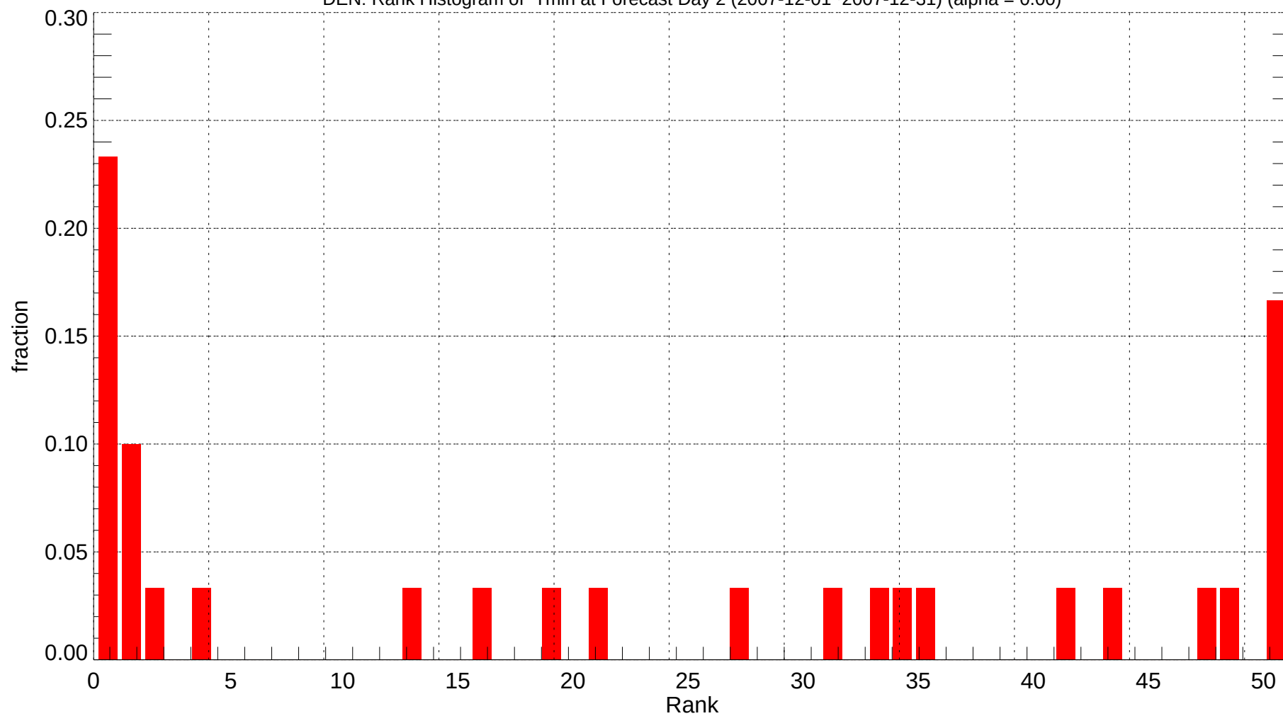
DEN: Rank Histogram of Tmin at Forecast Day 2 (2007-12-01~2007-12-31) (alpha = 0.00)
