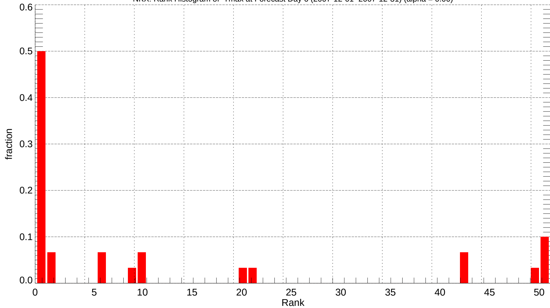
NKX: Rank Histogram of Tmax at Forecast Day 6 (2007-12-01~2007-12-31) (alpha = 0.00)
