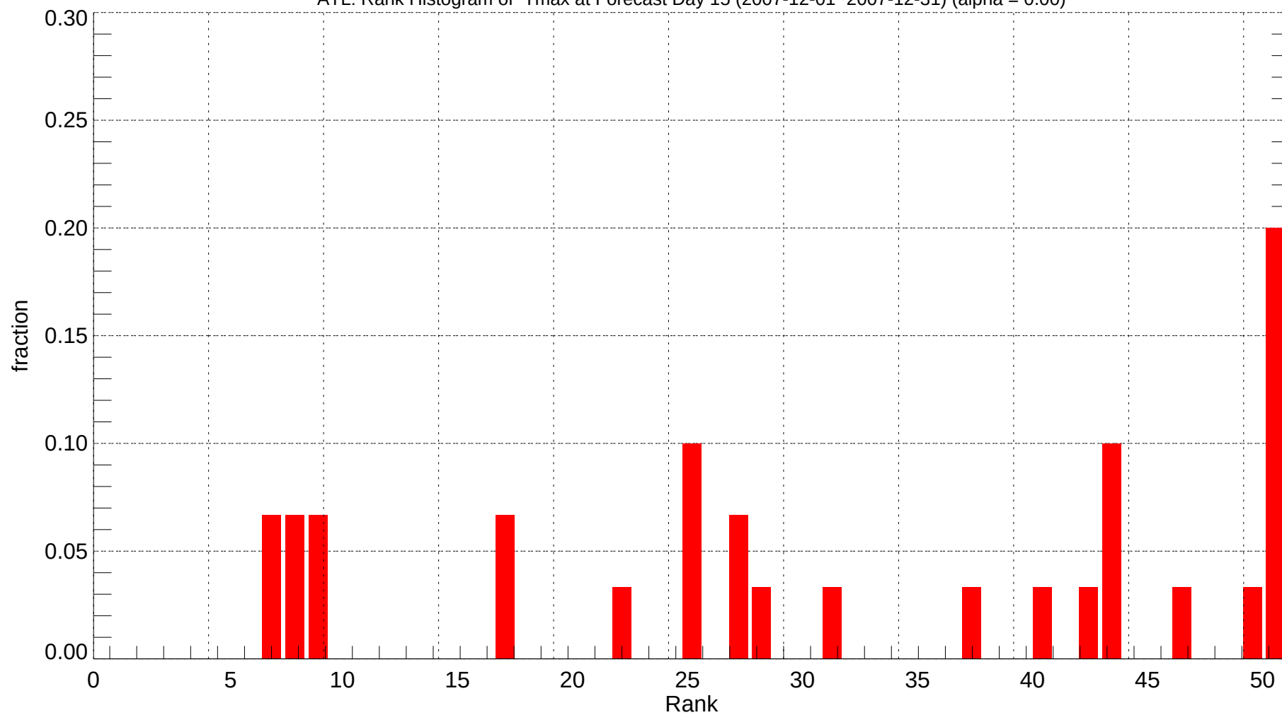
ATL: Rank Histogram of Tmax at Forecast Day 15 (2007-12-01~2007-12-31) (alpha = 0.00)
