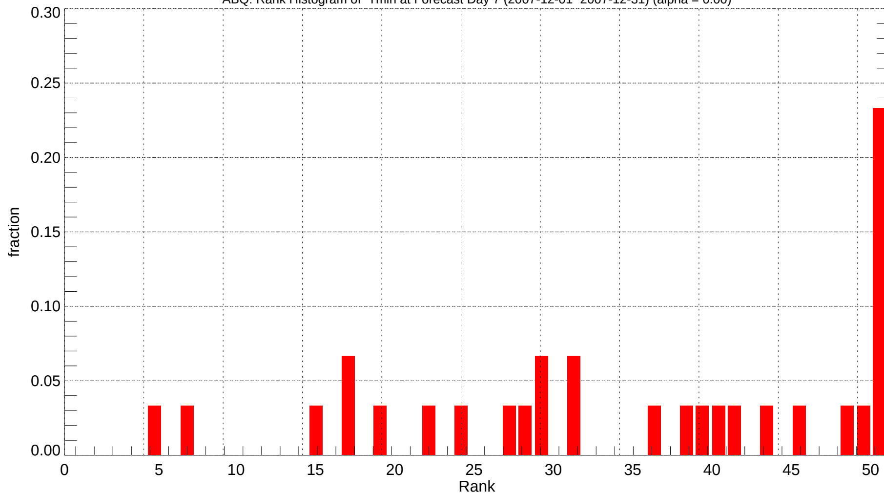
ABQ: Rank Histogram of Tmin at Forecast Day 7 (2007-12-01~2007-12-31) (alpha = 0.00)
