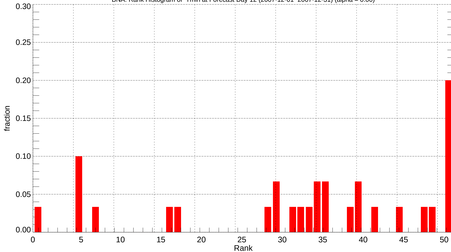
BNA: Rank Histogram of Tmin at Forecast Day 12 (2007-12-01~2007-12-31) (alpha = 0.00)
