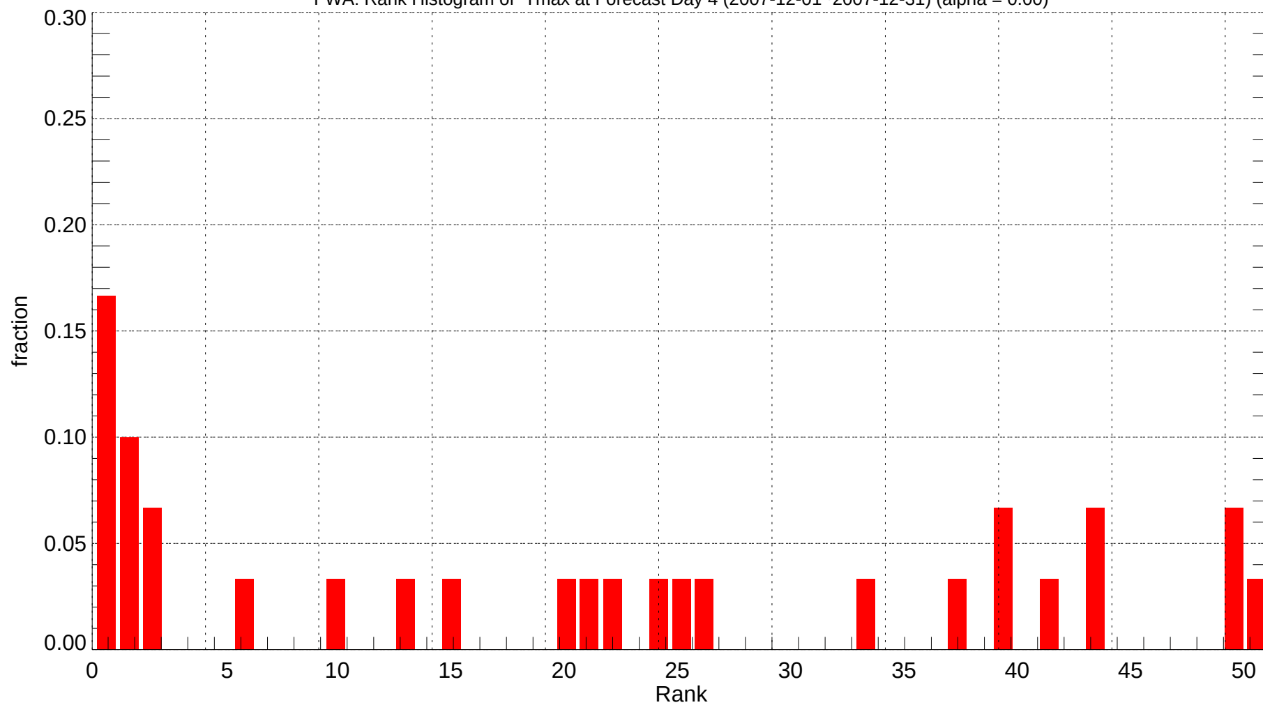
FWA: Rank Histogram of Tmax at Forecast Day 4 (2007-12-01~2007-12-31) (alpha = 0.00)
