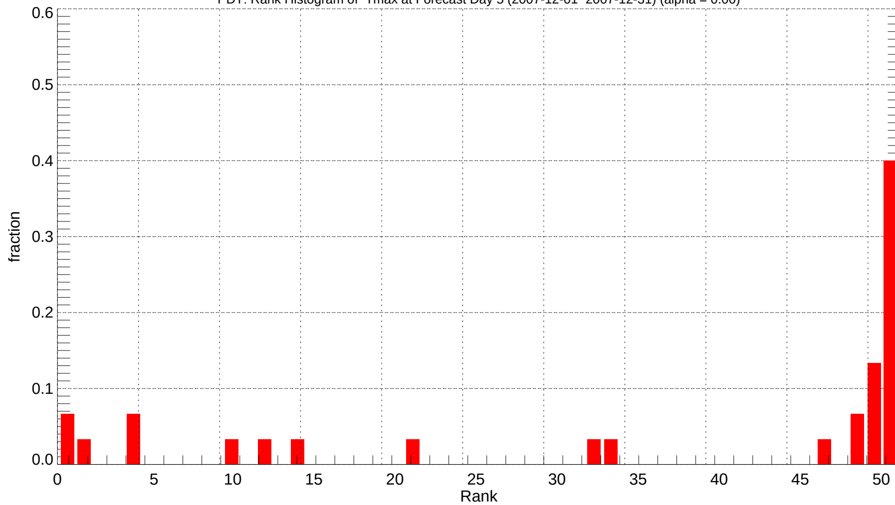
PDT: Rank Histogram of Tmax at Forecast Day 5 (2007-12-01~2007-12-31) (alpha = 0.00)
