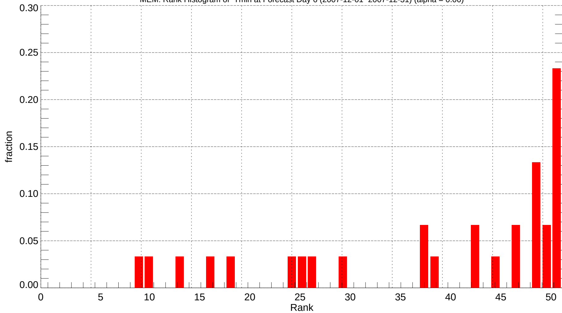
MEM: Rank Histogram of Tmin at Forecast Day 6 (2007-12-01~2007-12-31) (alpha = 0.00)
