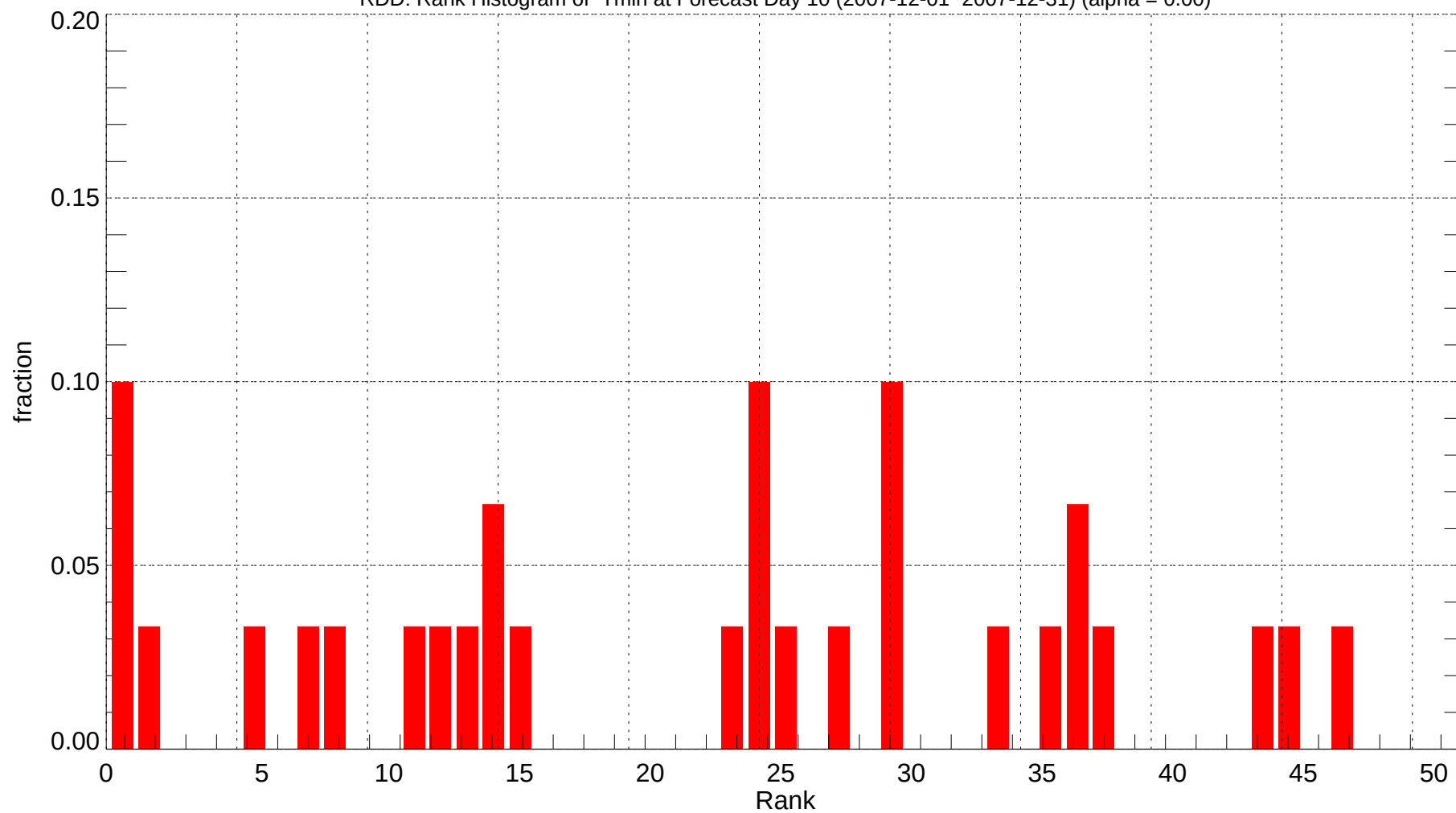
RDD: Rank Histogram of Tmin at Forecast Day 10 (2007-12-01~2007-12-31) (alpha = 0.00)
