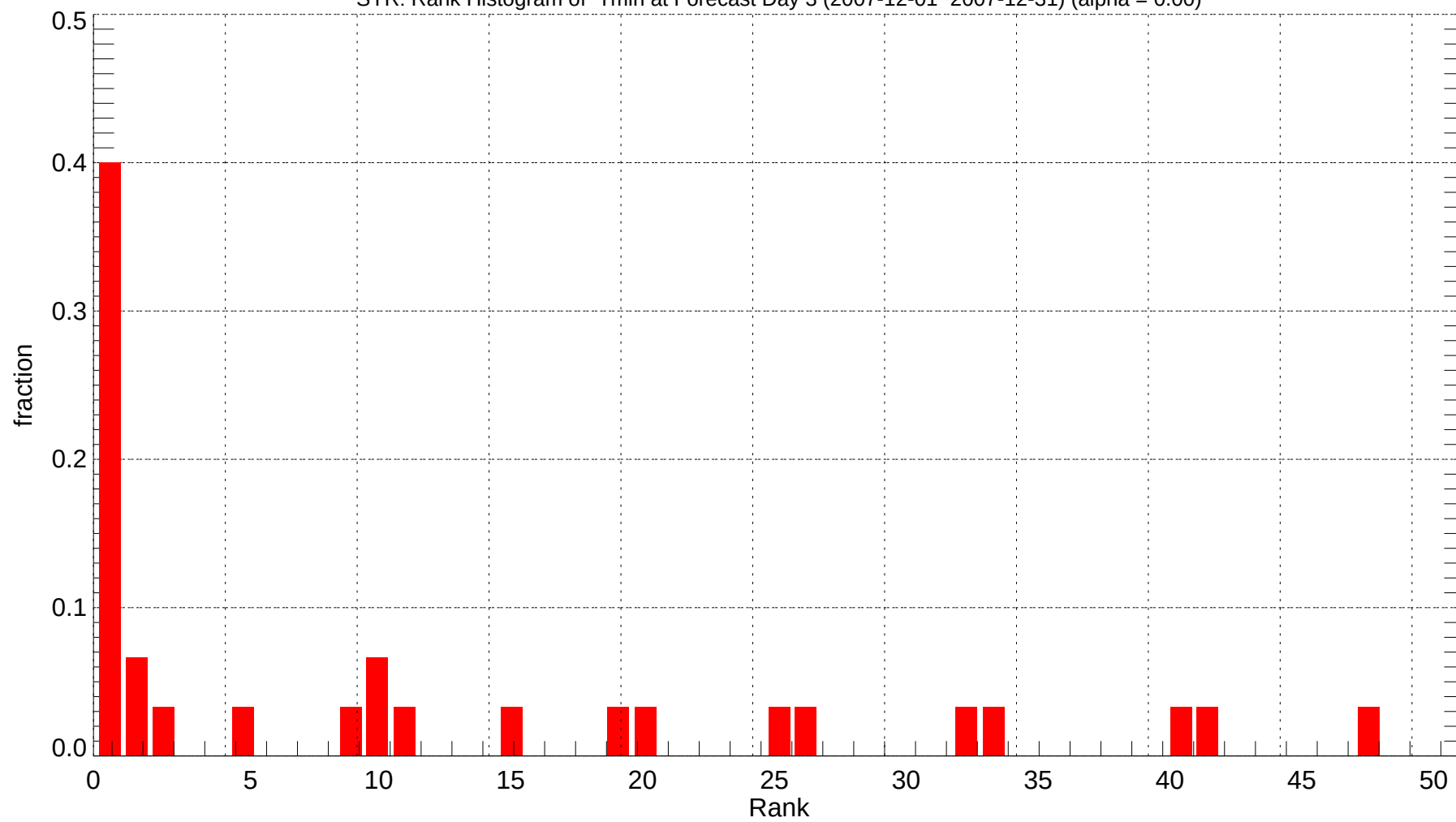
SYR: Rank Histogram of Tmin at Forecast Day 3 (2007-12-01~2007-12-31) (alpha = 0.00)
