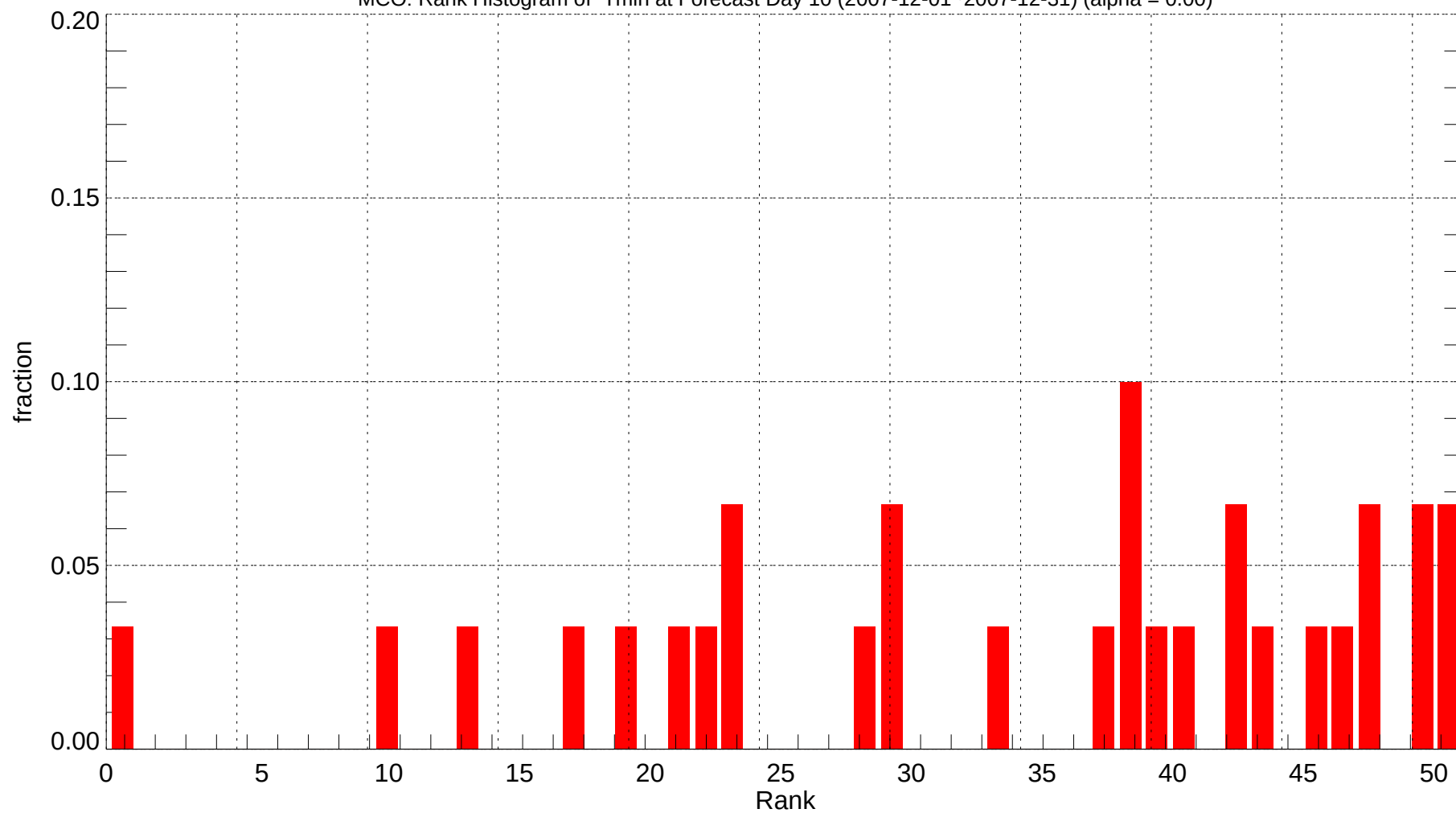
MCO: Rank Histogram of Tmin at Forecast Day 10 (2007-12-01~2007-12-31) (alpha = 0.00)
