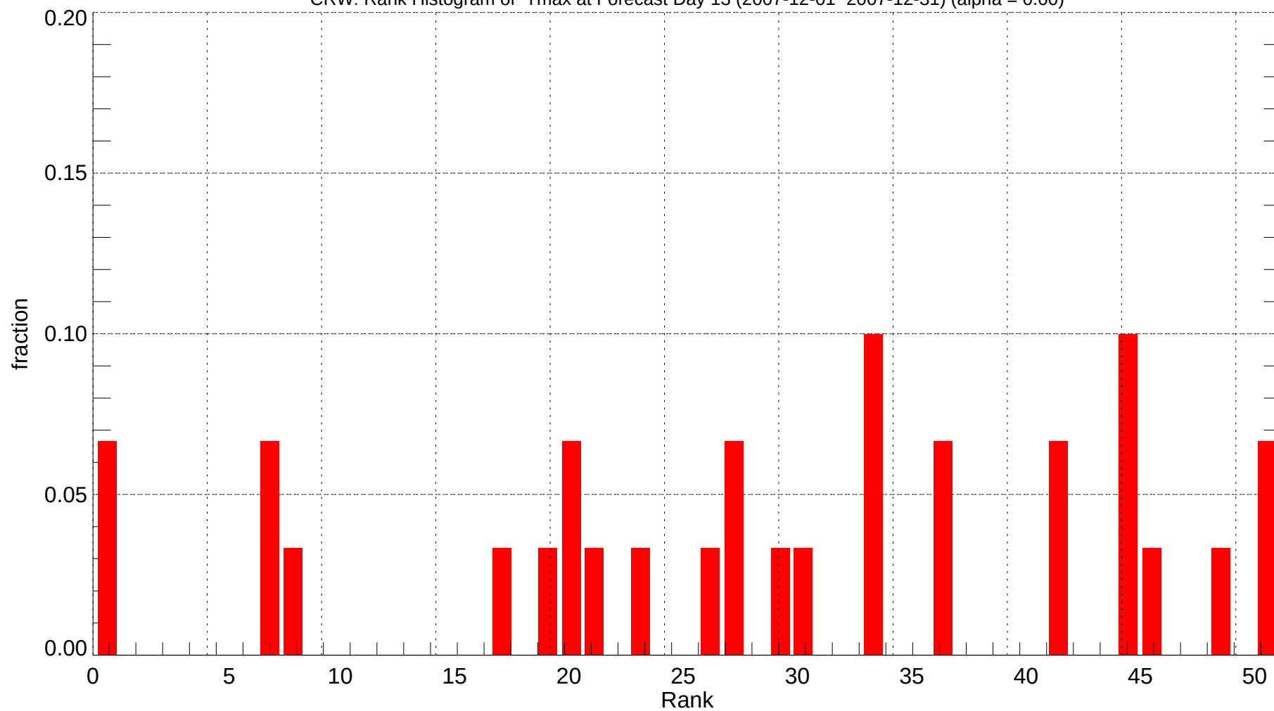
CRW: Rank Histogram of Tmax at Forecast Day 13 (2007-12-01~2007-12-31) (alpha = 0.00)
