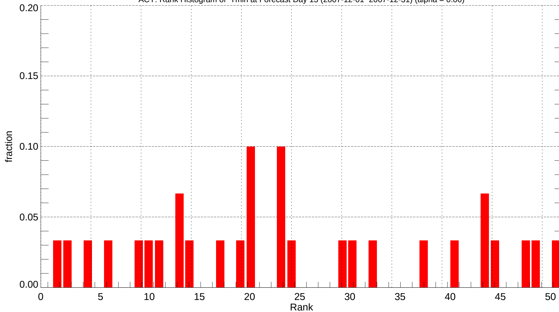
ACY: Rank Histogram of Tmin at Forecast Day 13 (2007-12-01~2007-12-31) (alpha = 0.00)
