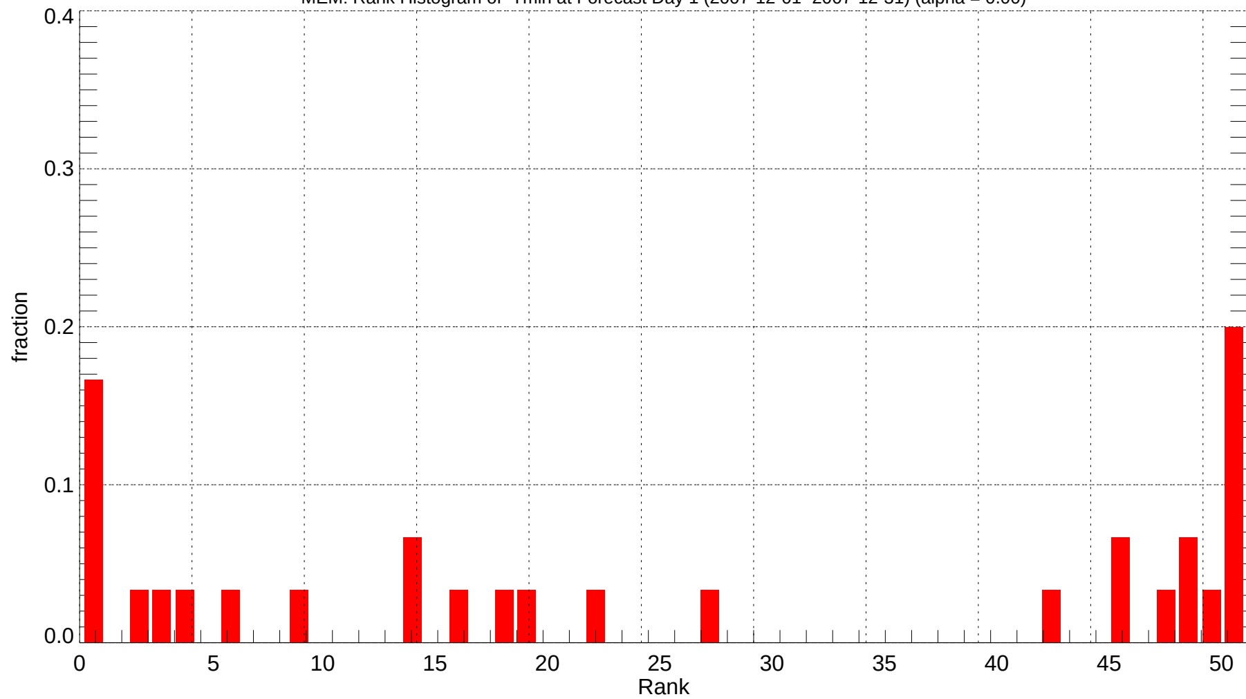
MEM: Rank Histogram of Tmin at Forecast Day 1 (2007-12-01~2007-12-31) (alpha = 0.00)
