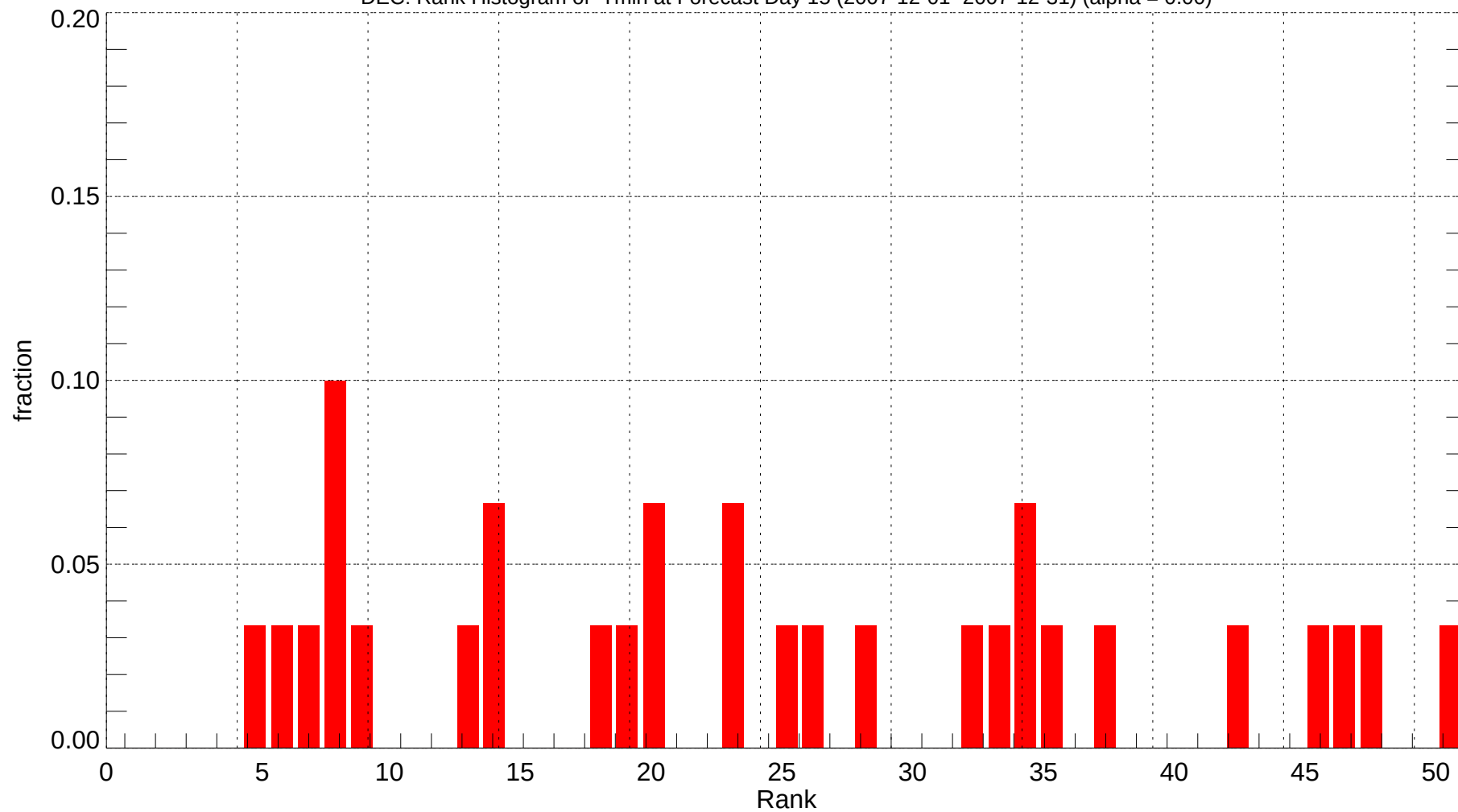
DEC: Rank Histogram of Tmin at Forecast Day 15 (2007-12-01~2007-12-31) (alpha = 0.00)
