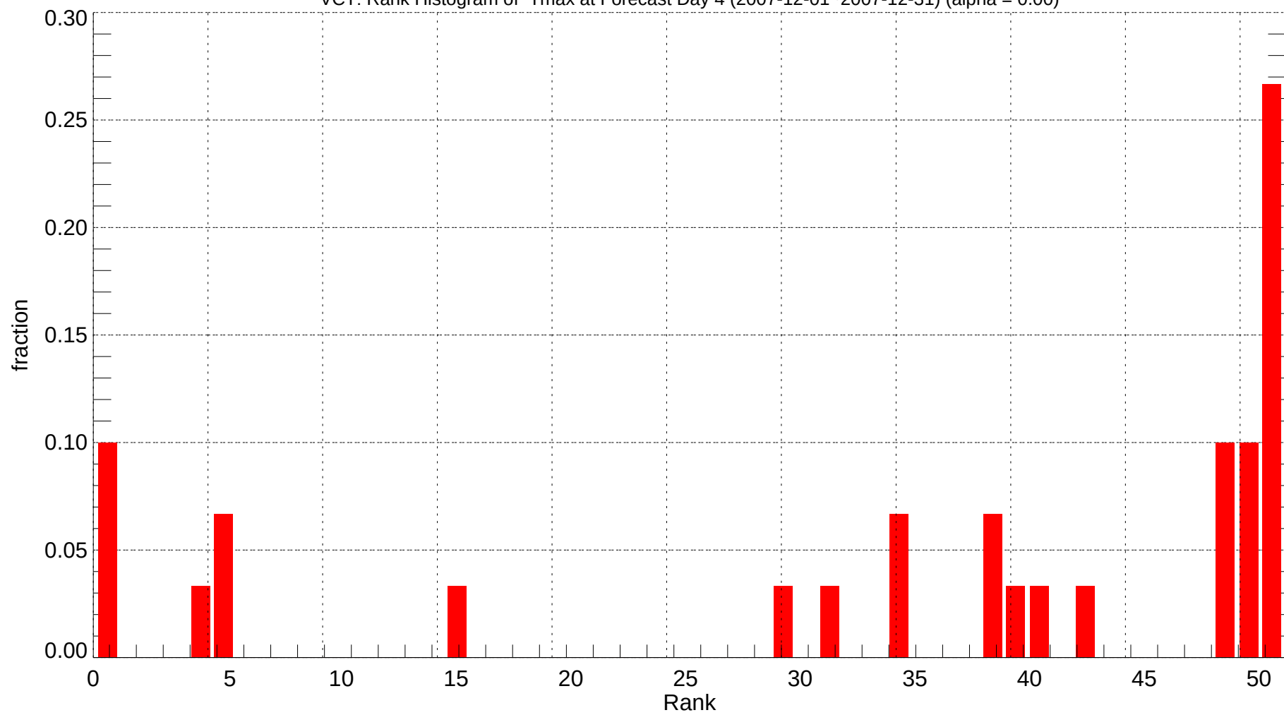
VCT: Rank Histogram of Tmax at Forecast Day 4 (2007-12-01~2007-12-31) (alpha = 0.00)
