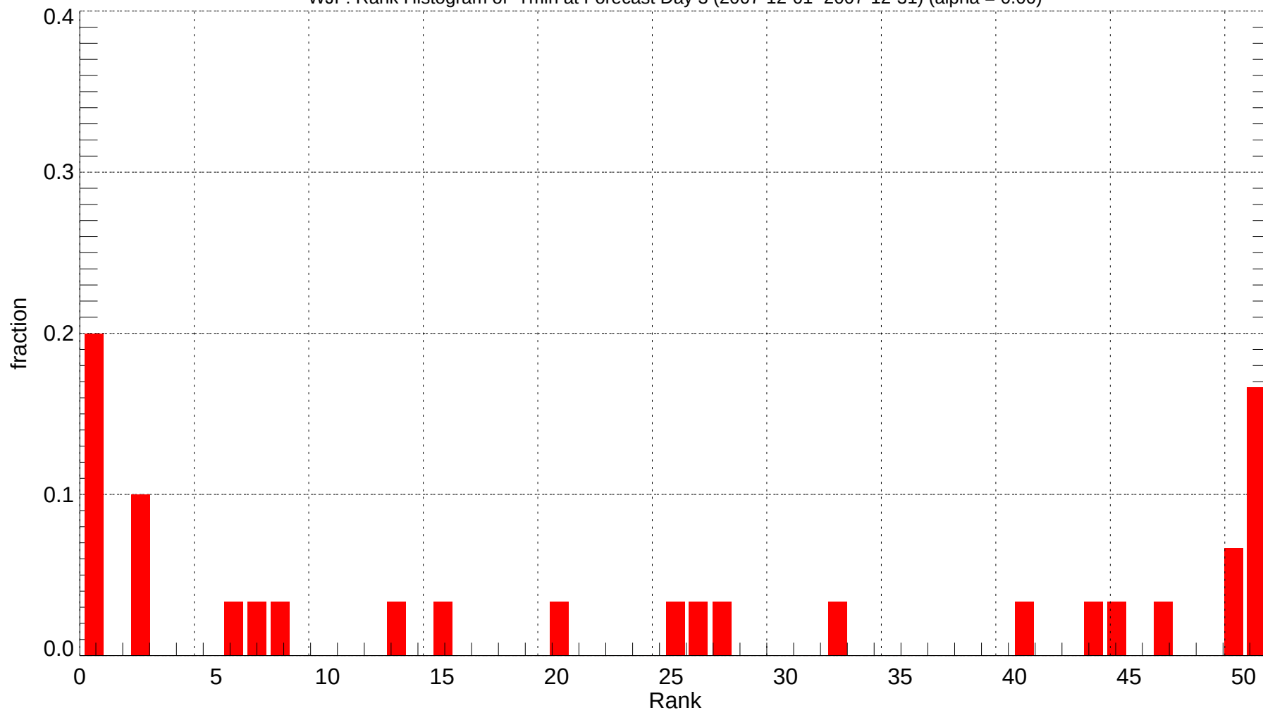
WJF: Rank Histogram of Tmin at Forecast Day 3 (2007-12-01~2007-12-31) (alpha = 0.00)
