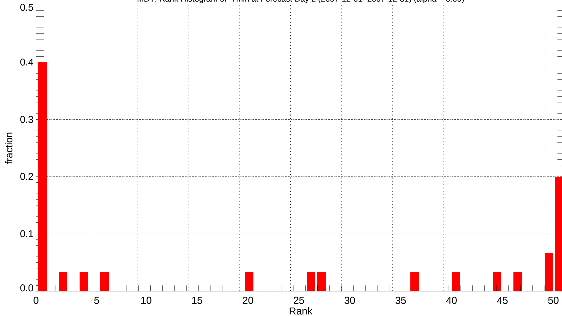
MDT: Rank Histogram of Tmin at Forecast Day 2 (2007-12-01~2007-12-31) (alpha = 0.00)
