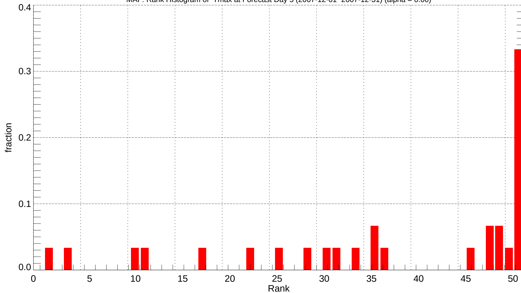
MAF: Rank Histogram of Tmax at Forecast Day 5 (2007-12-01~2007-12-31) (alpha = 0.00)
