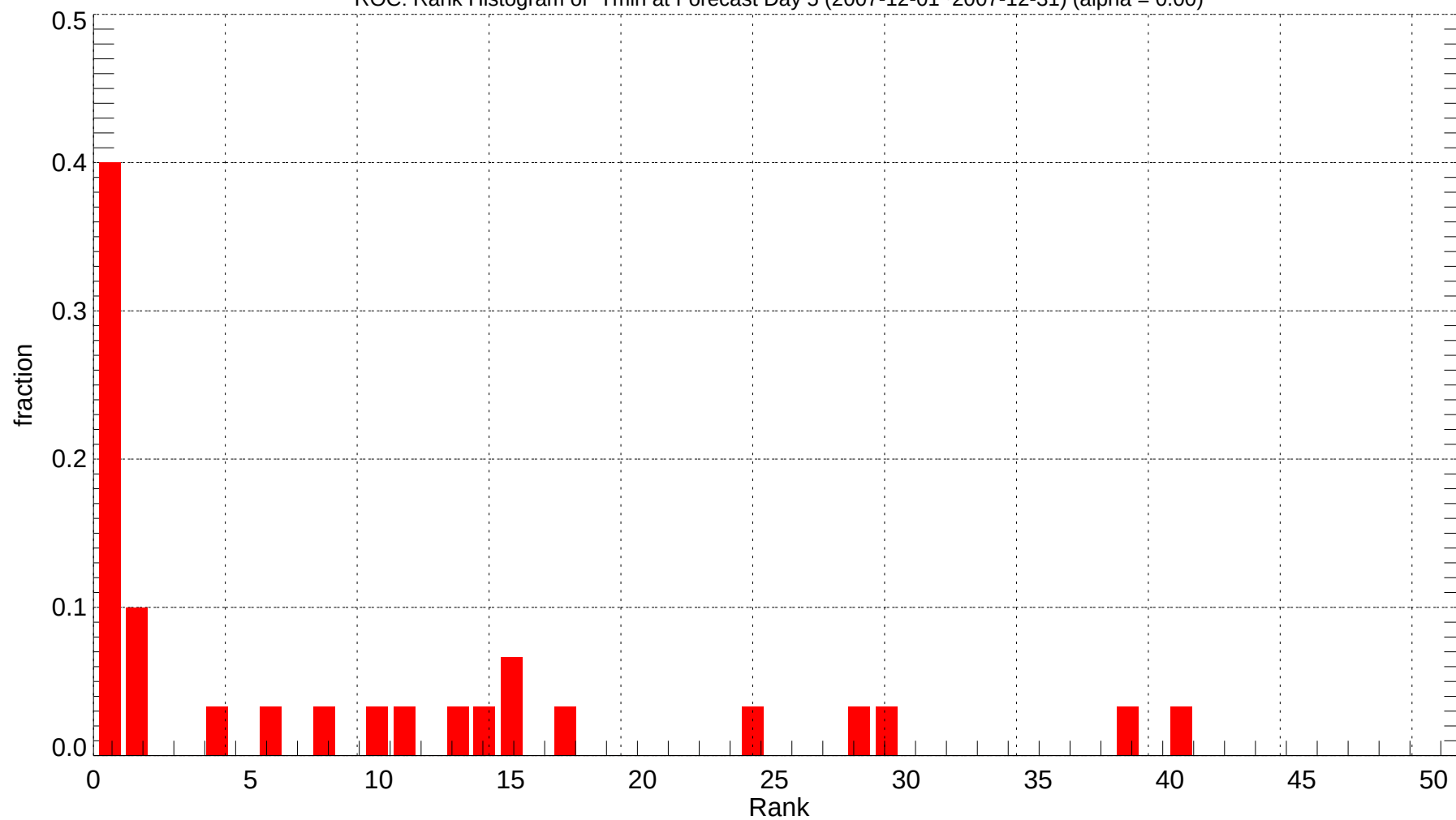
ROC: Rank Histogram of Tmin at Forecast Day 5 (2007-12-01~2007-12-31) (alpha = 0.00)
