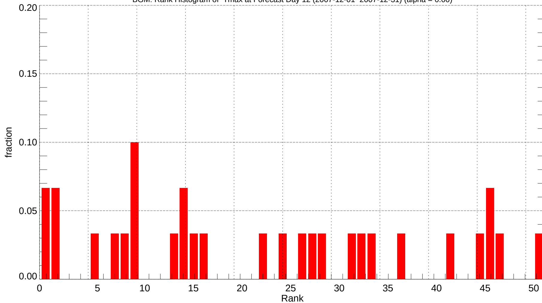
BGM: Rank Histogram of Tmax at Forecast Day 12 (2007-12-01~2007-12-31) (alpha = 0.00)
