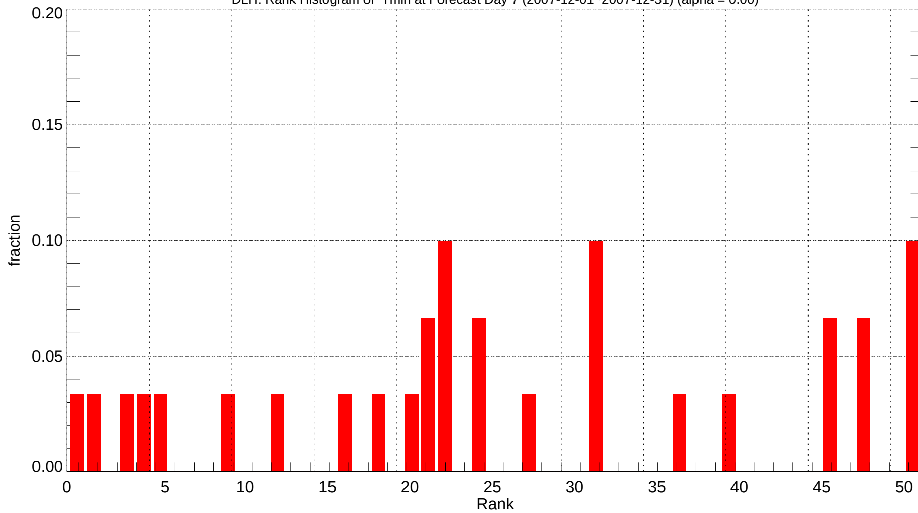
DLH: Rank Histogram of Tmin at Forecast Day 7 (2007-12-01~2007-12-31) (alpha = 0.00)
