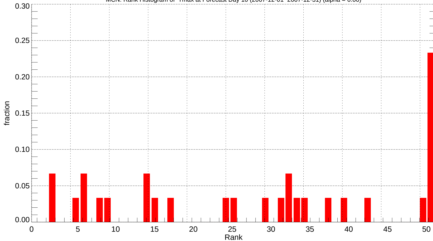
MCN: Rank Histogram of Tmax at Forecast Day 10 (2007-12-01~2007-12-31) (alpha = 0.00)
