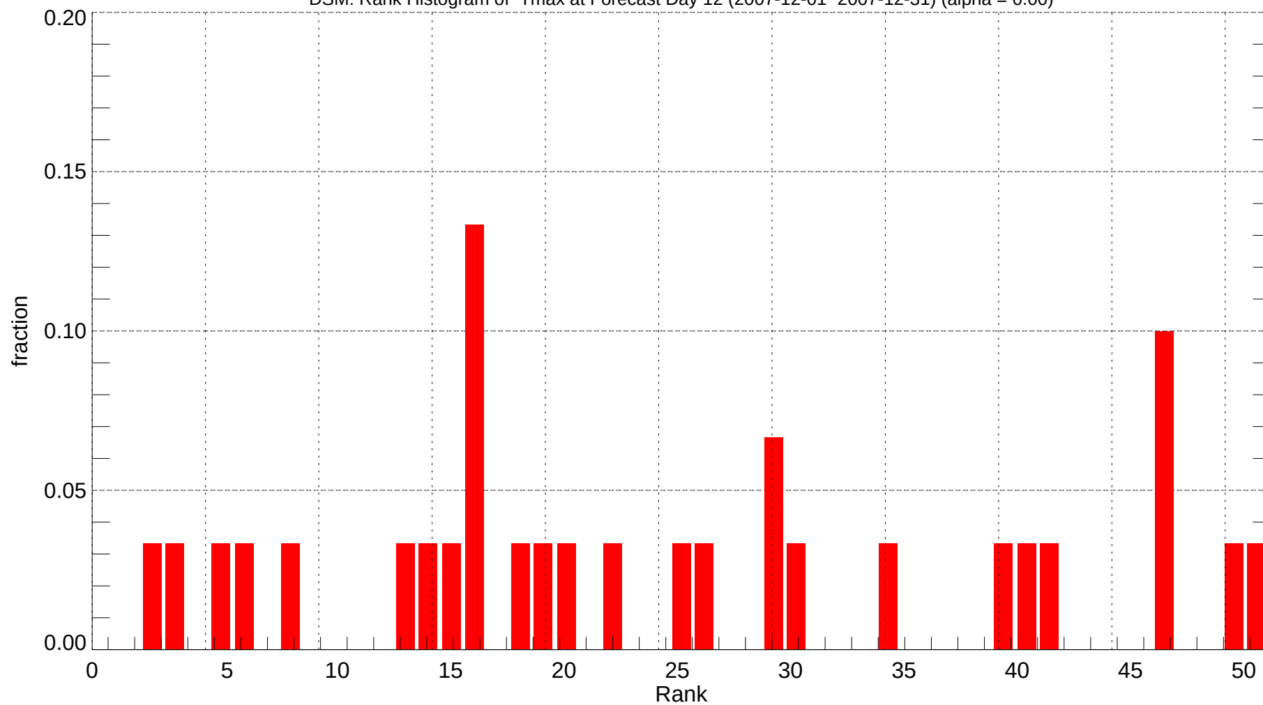
DSM: Rank Histogram of Tmax at Forecast Day 12 (2007-12-01~2007-12-31) (alpha = 0.00)
