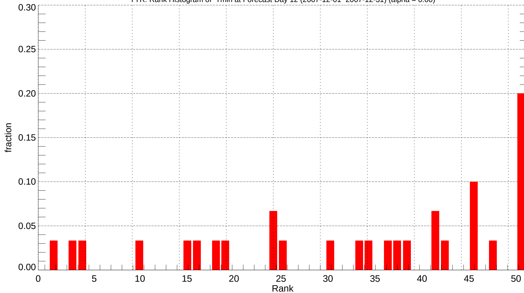
TYR: Rank Histogram of Tmin at Forecast Day 12 (2007-12-01~2007-12-31) (alpha = 0.00)
