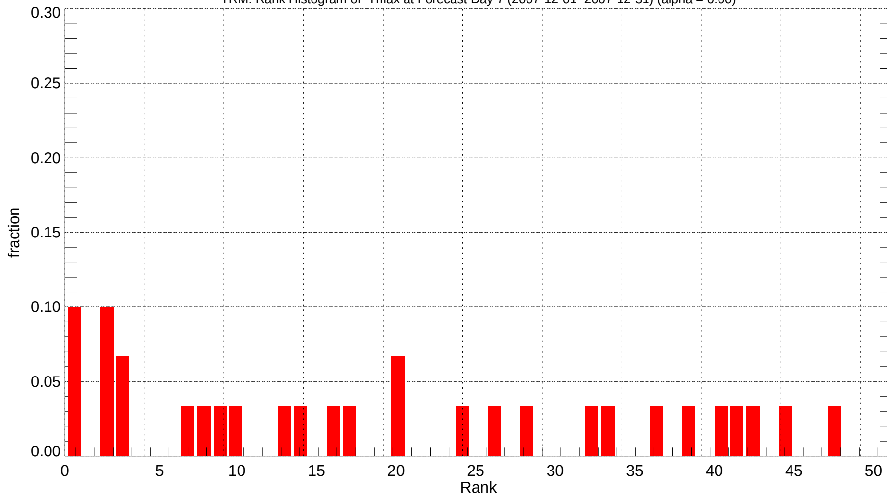
TRM: Rank Histogram of Tmax at Forecast Day 7 (2007-12-01~2007-12-31) (alpha = 0.00)
