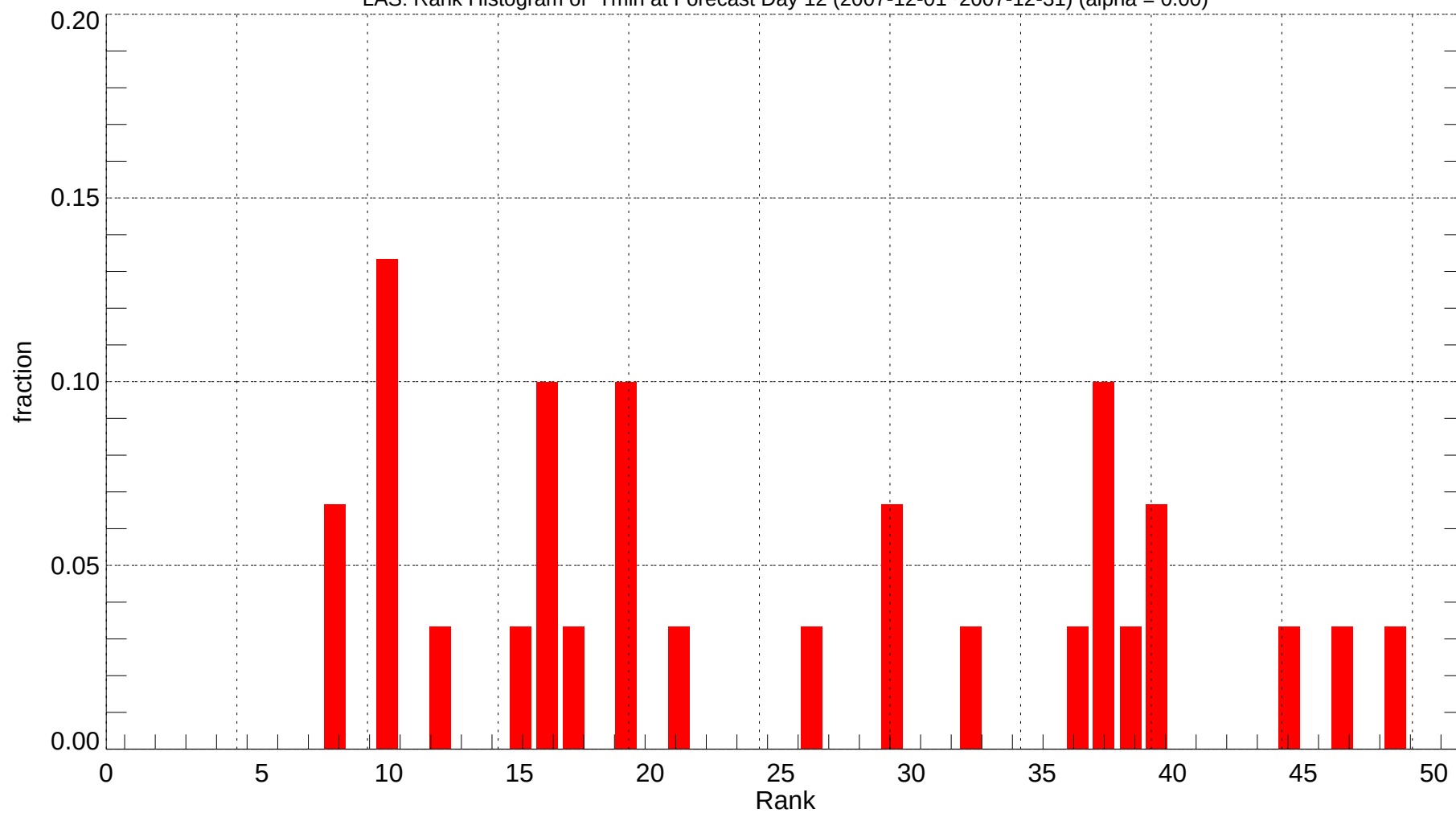
LAS: Rank Histogram of Tmin at Forecast Day 12 (2007-12-01~2007-12-31) (alpha = 0.00)
