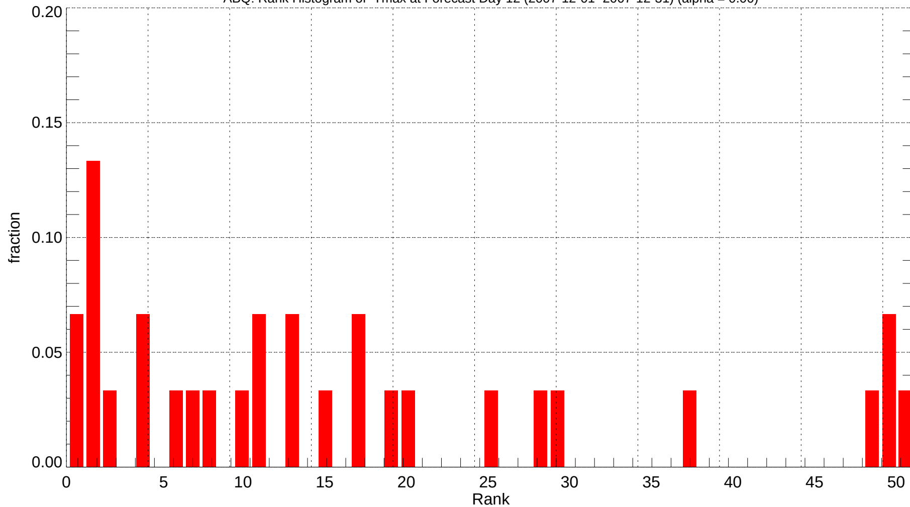
ABQ: Rank Histogram of Tmax at Forecast Day 12 (2007-12-01~2007-12-31) (alpha = 0.00)
