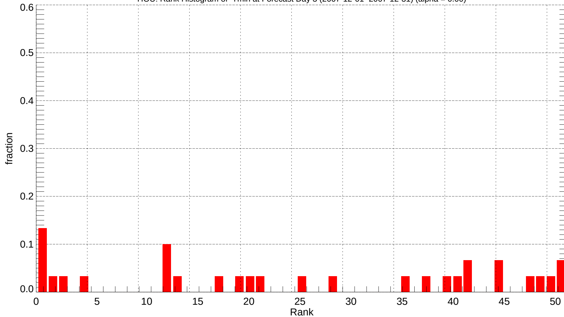
HOU: Rank Histogram of Tmin at Forecast Day 3 (2007-12-01~2007-12-31) (alpha = 0.00)
