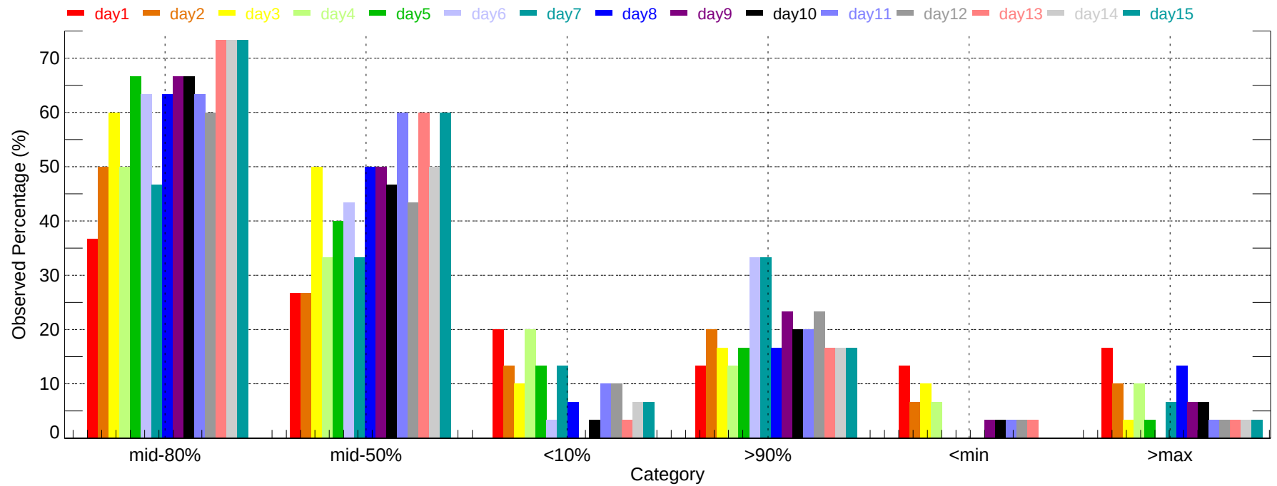
Observed Percentage of Ensembles - DAY: Min Temperature (2007-12-01~2007-12-31)
