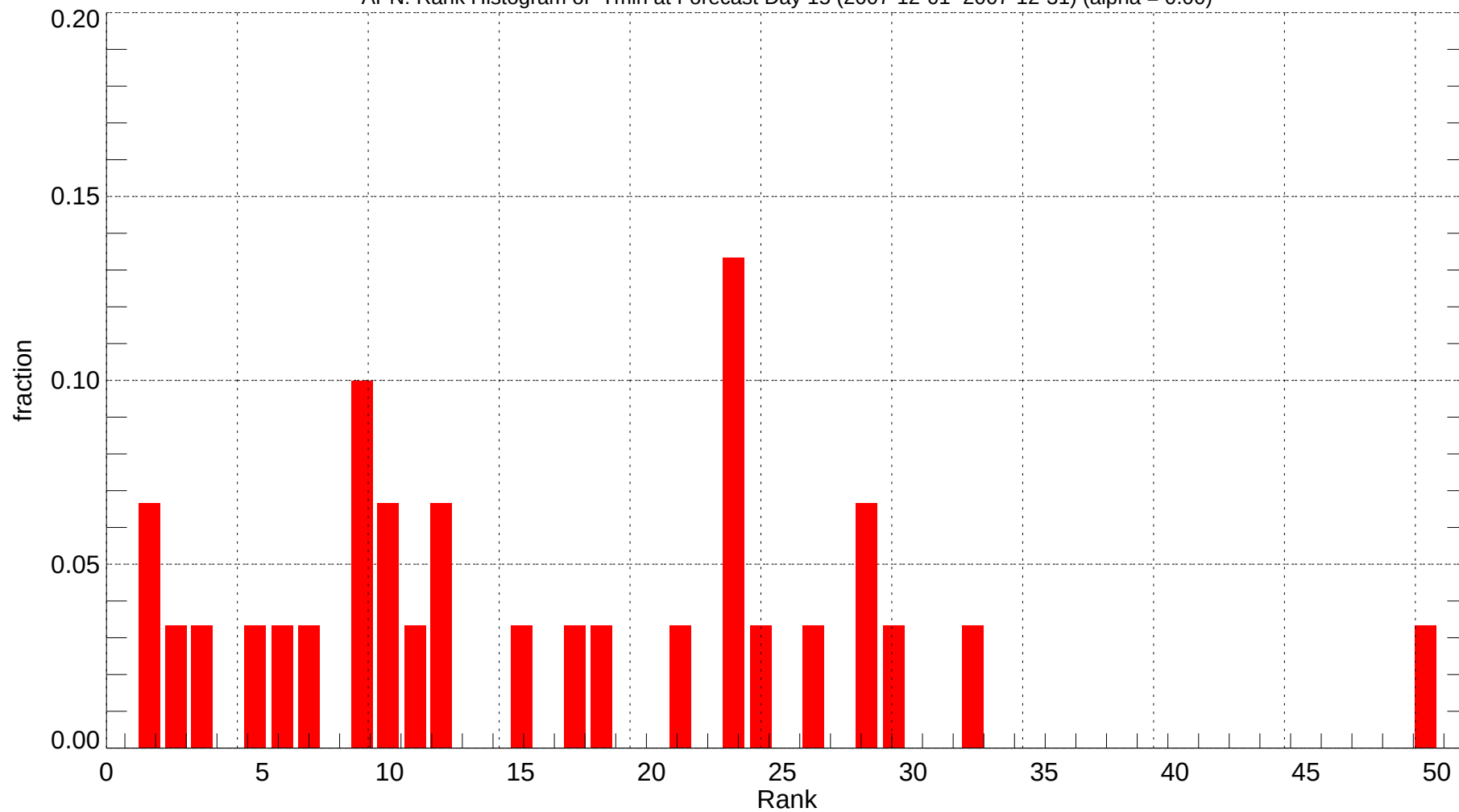
APN: Rank Histogram of Tmin at Forecast Day 15 (2007-12-01~2007-12-31) (alpha = 0.00)
