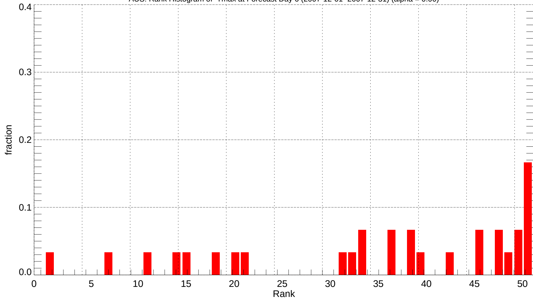
AUS: Rank Histogram of Tmax at Forecast Day 6 (2007-12-01~2007-12-31) (alpha = 0.00)
