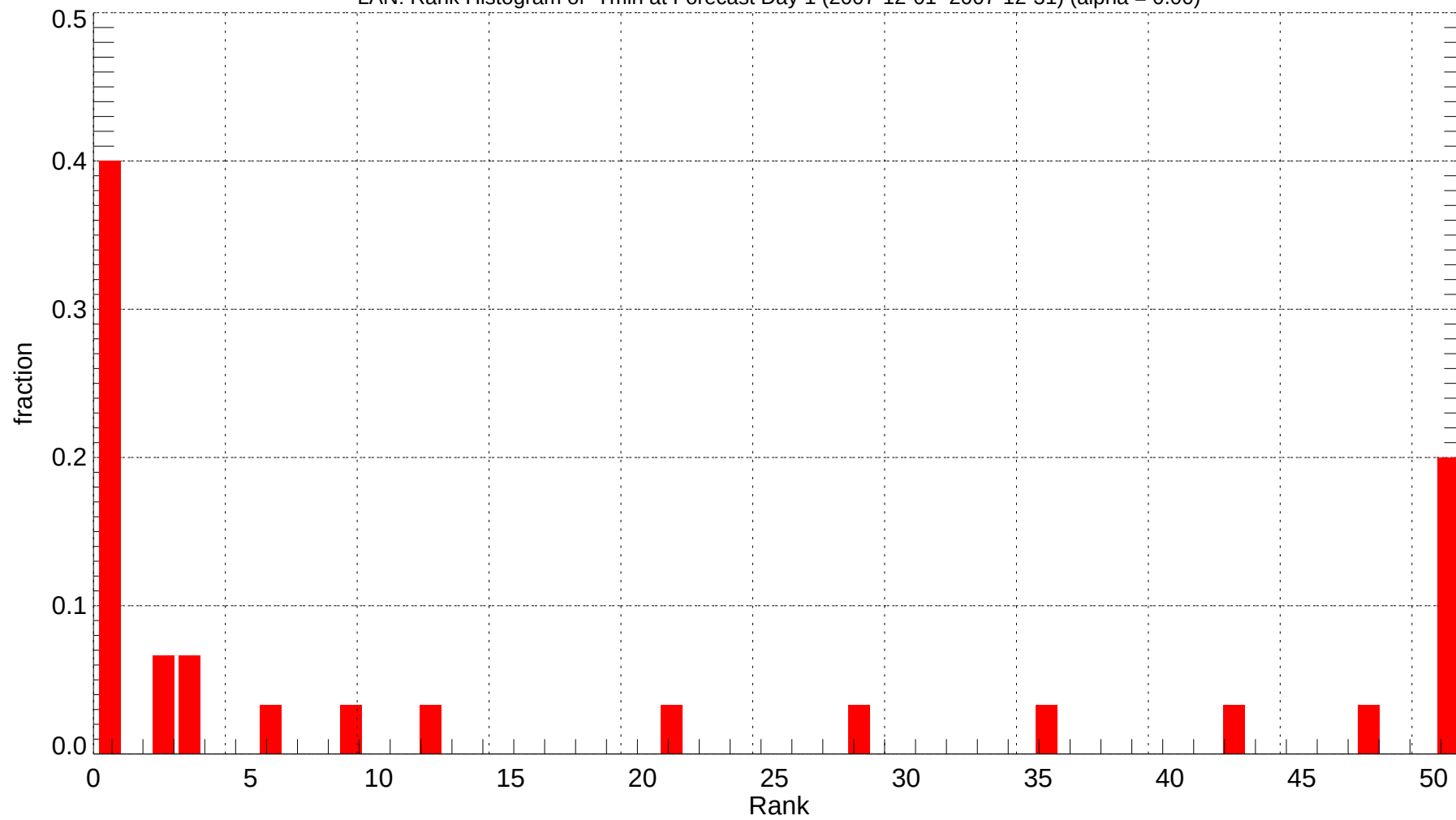
LAN: Rank Histogram of Tmin at Forecast Day 1 (2007-12-01~2007-12-31) (alpha = 0.00)
