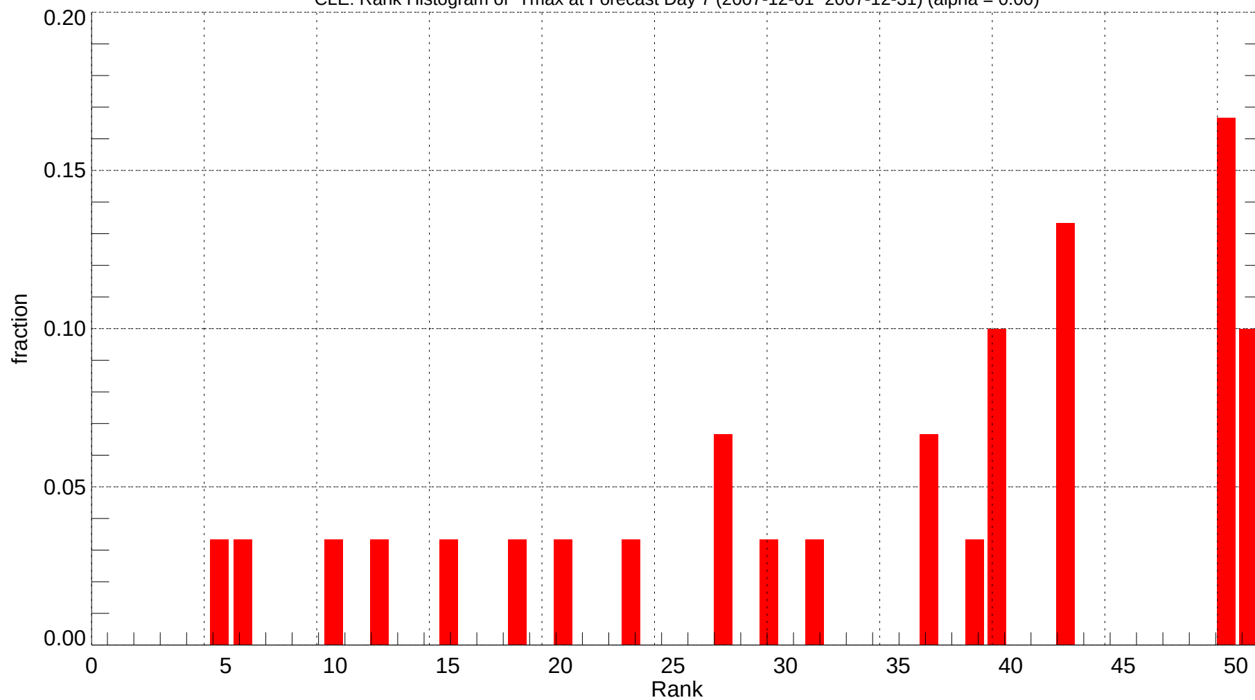
CLE: Rank Histogram of Tmax at Forecast Day 7 (2007-12-01~2007-12-31) (alpha = 0.00)
