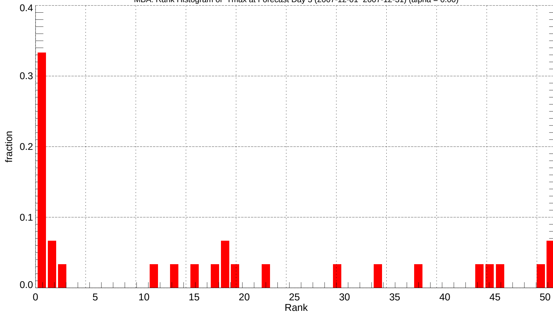
MBA: Rank Histogram of Tmax at Forecast Day 3 (2007-12-01~2007-12-31) (alpha = 0.00)
