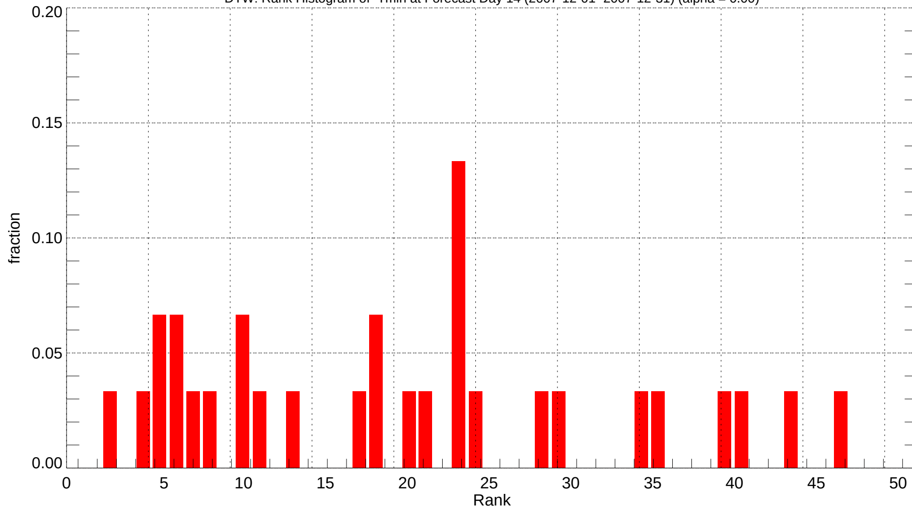
DTW: Rank Histogram of Tmin at Forecast Day 14 (2007-12-01~2007-12-31) (alpha = 0.00)
