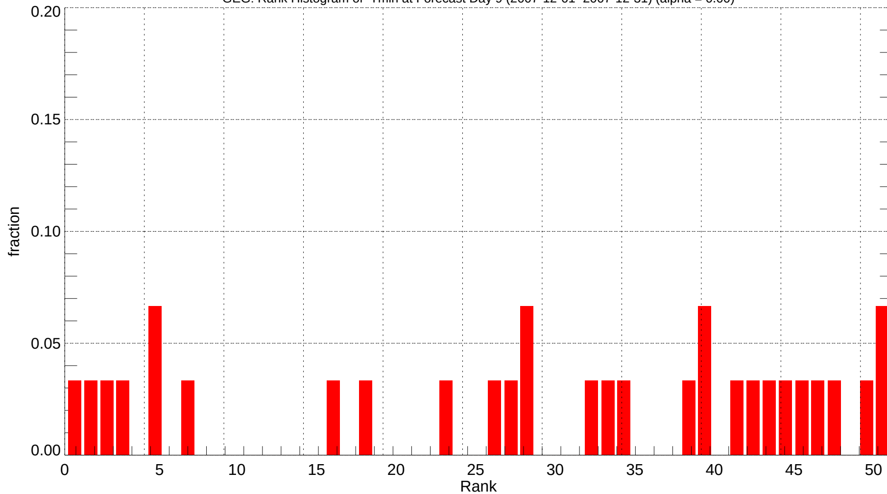
GEG: Rank Histogram of Tmin at Forecast Day 9 (2007-12-01~2007-12-31) (alpha = 0.00)
