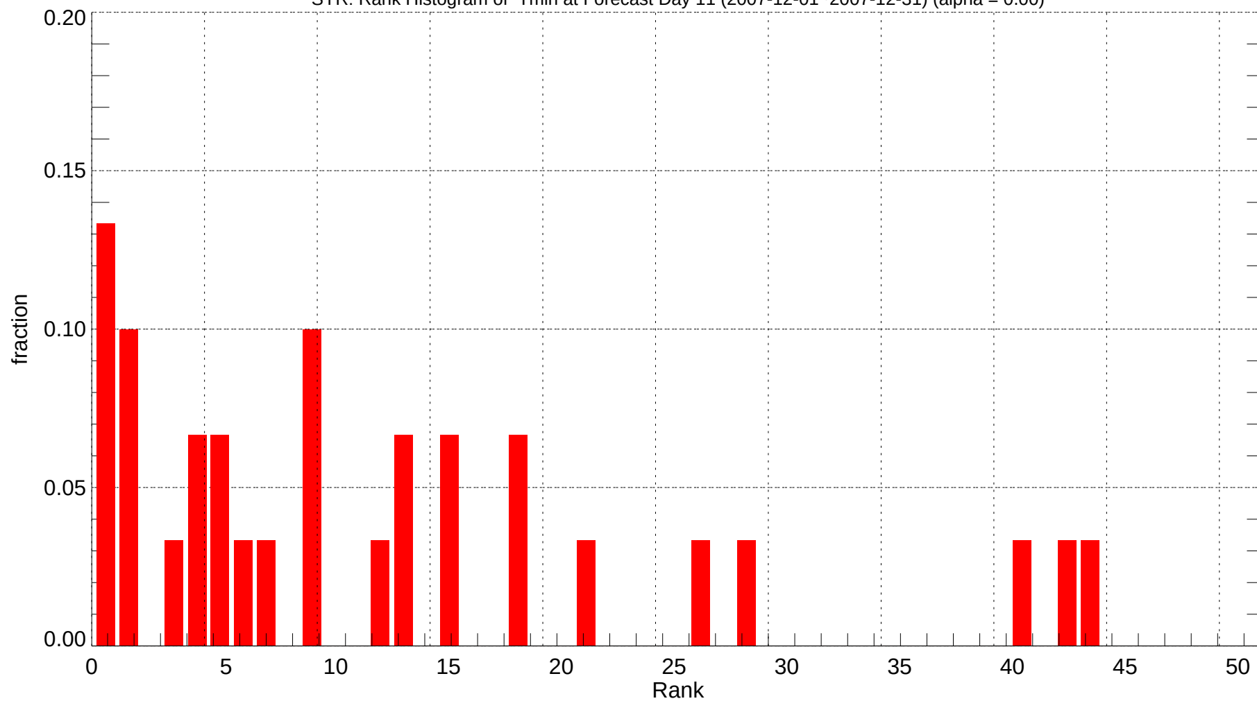
SYR: Rank Histogram of Tmin at Forecast Day 11 (2007-12-01~2007-12-31) (alpha = 0.00)
