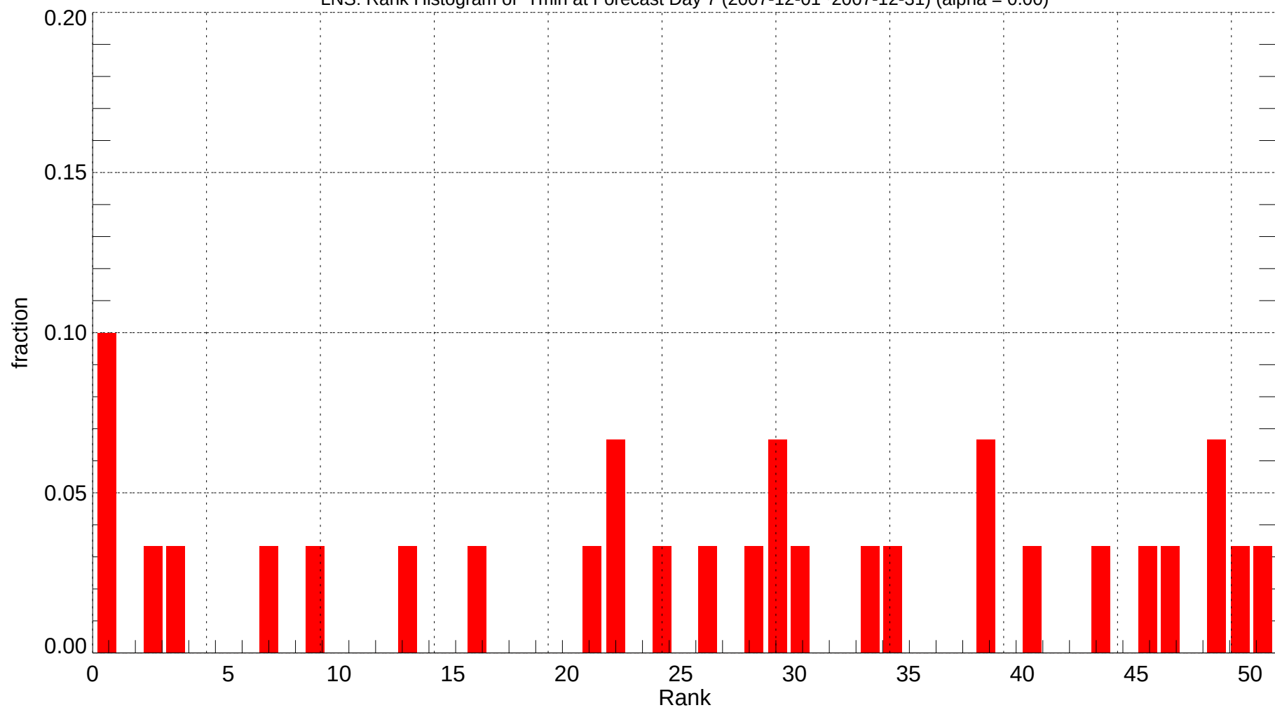
LNS: Rank Histogram of Tmin at Forecast Day 7 (2007-12-01~2007-12-31) (alpha = 0.00)
