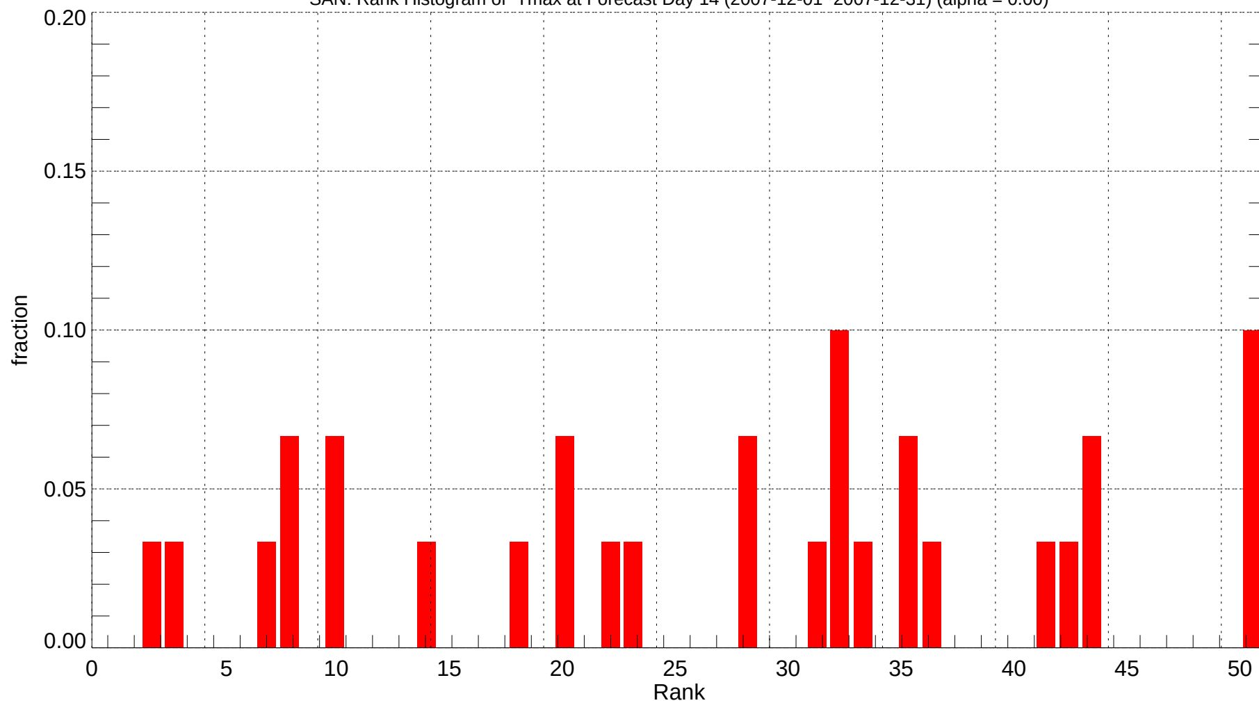
SAN: Rank Histogram of Tmax at Forecast Day 14 (2007-12-01~2007-12-31) (alpha = 0.00)
