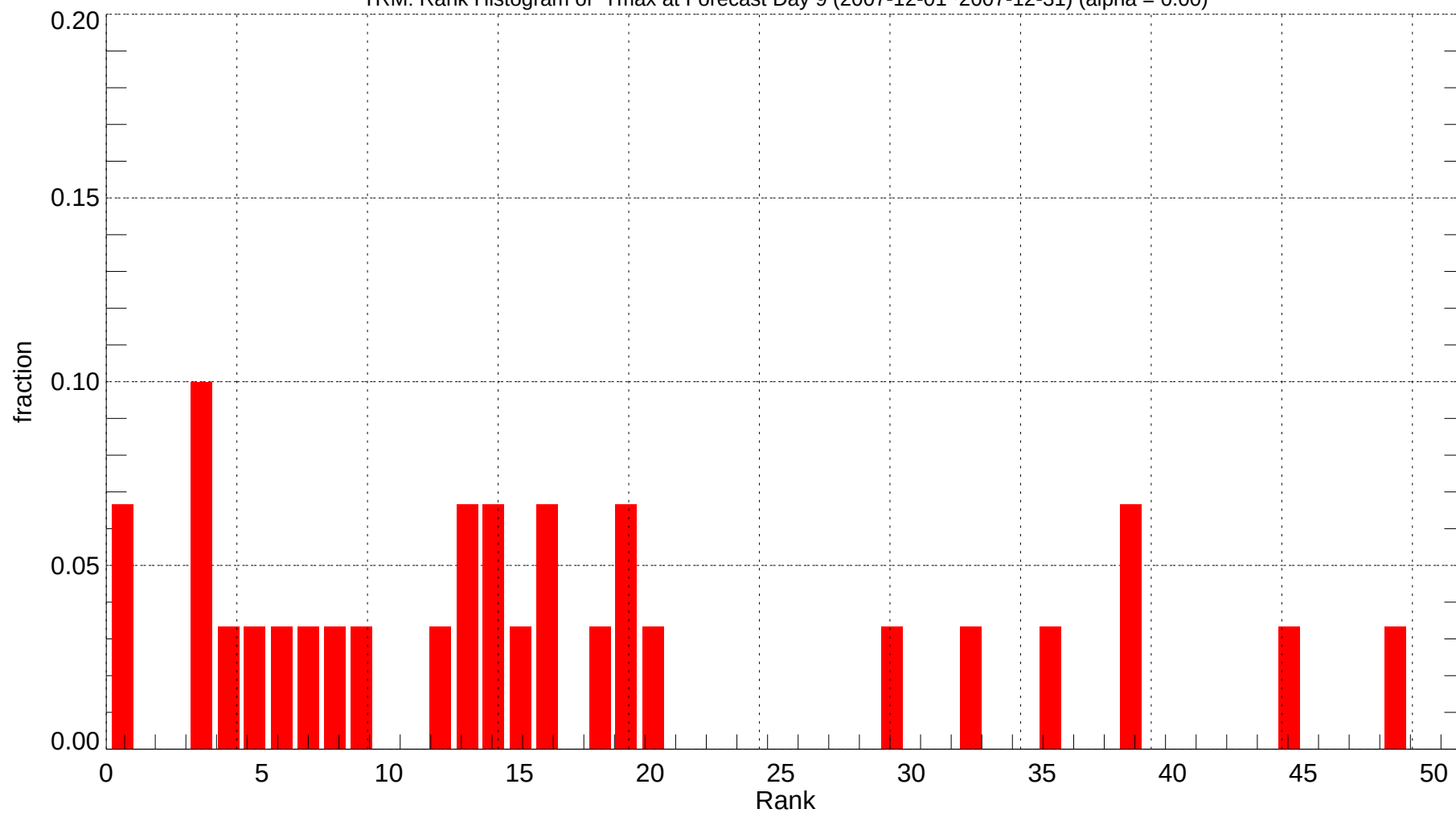
TRM: Rank Histogram of Tmax at Forecast Day 9 (2007-12-01~2007-12-31) (alpha = 0.00)
