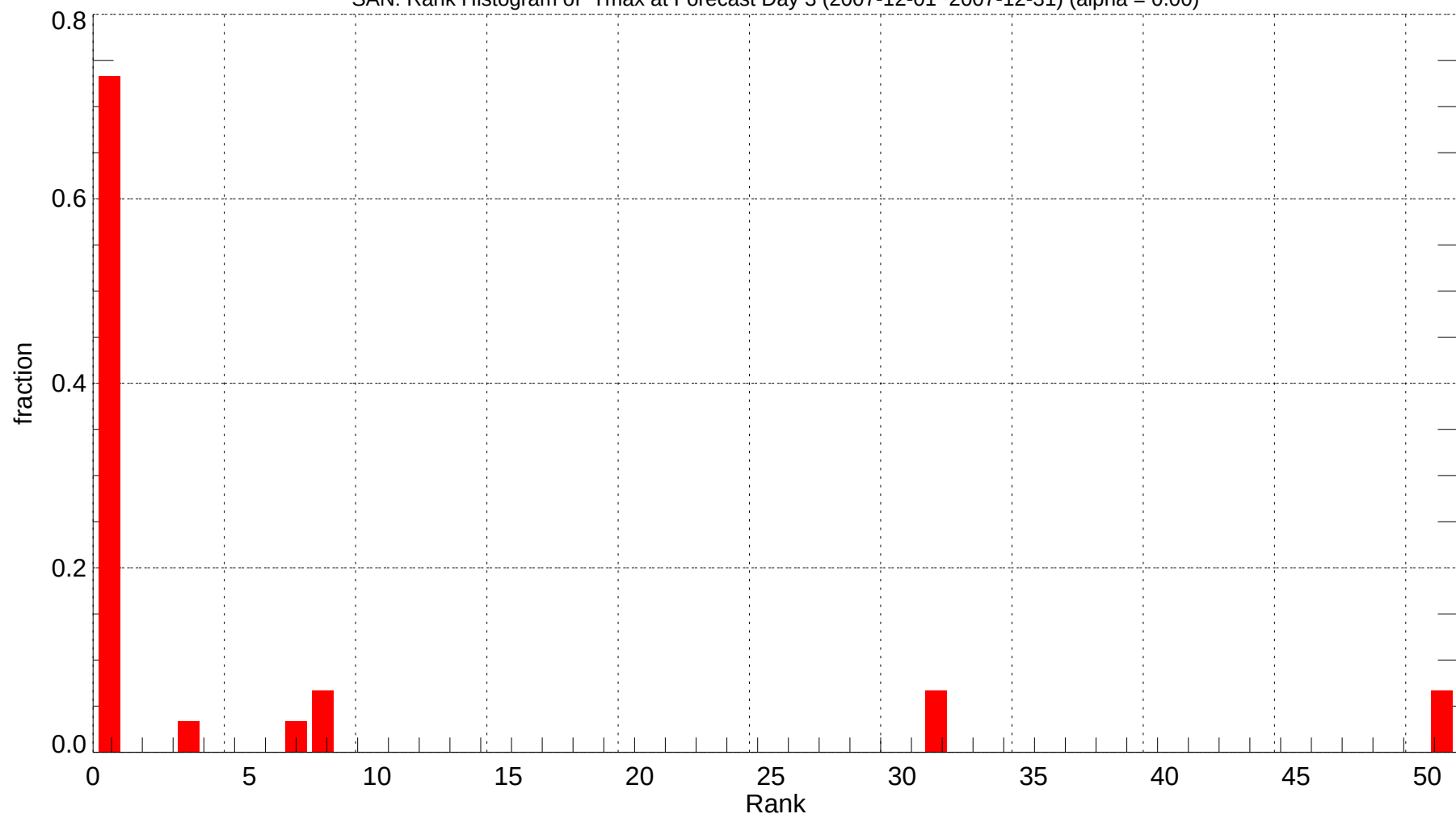
SAN: Rank Histogram of Tmax at Forecast Day 3 (2007-12-01~2007-12-31) (alpha = 0.00)
