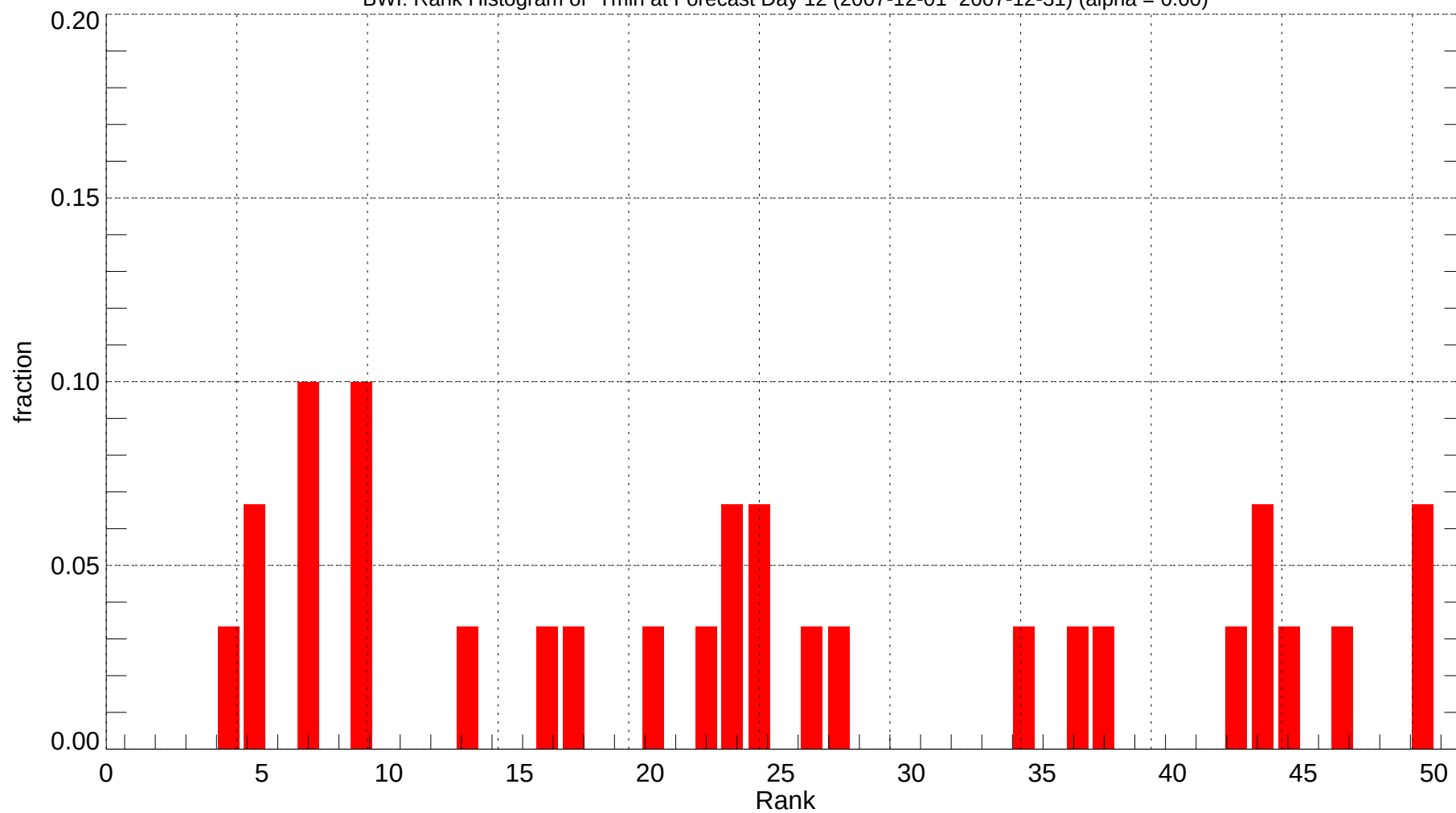
BWl: Rank Histogram of Tmin at Forecast Day 12 (2007-12-01~2007-12-31) (alpha = 0.00)
