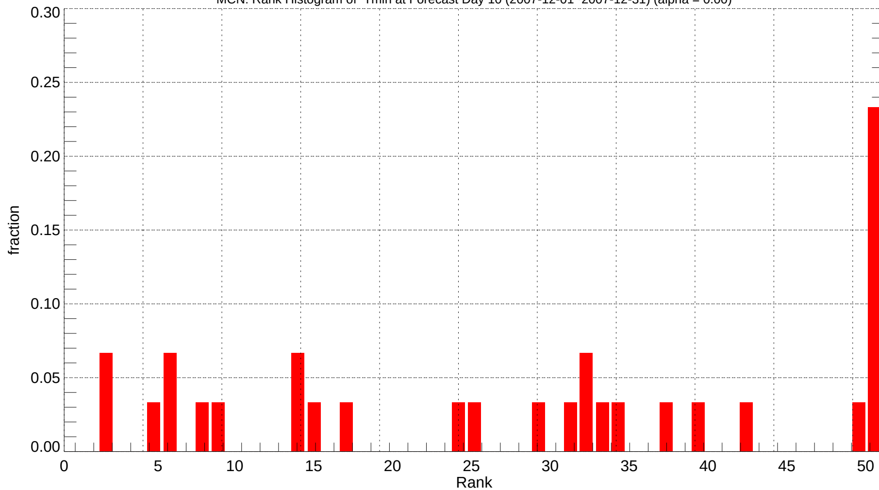
MCN: Rank Histogram of Tmin at Forecast Day 10 (2007-12-01~2007-12-31) (alpha = 0.00)
