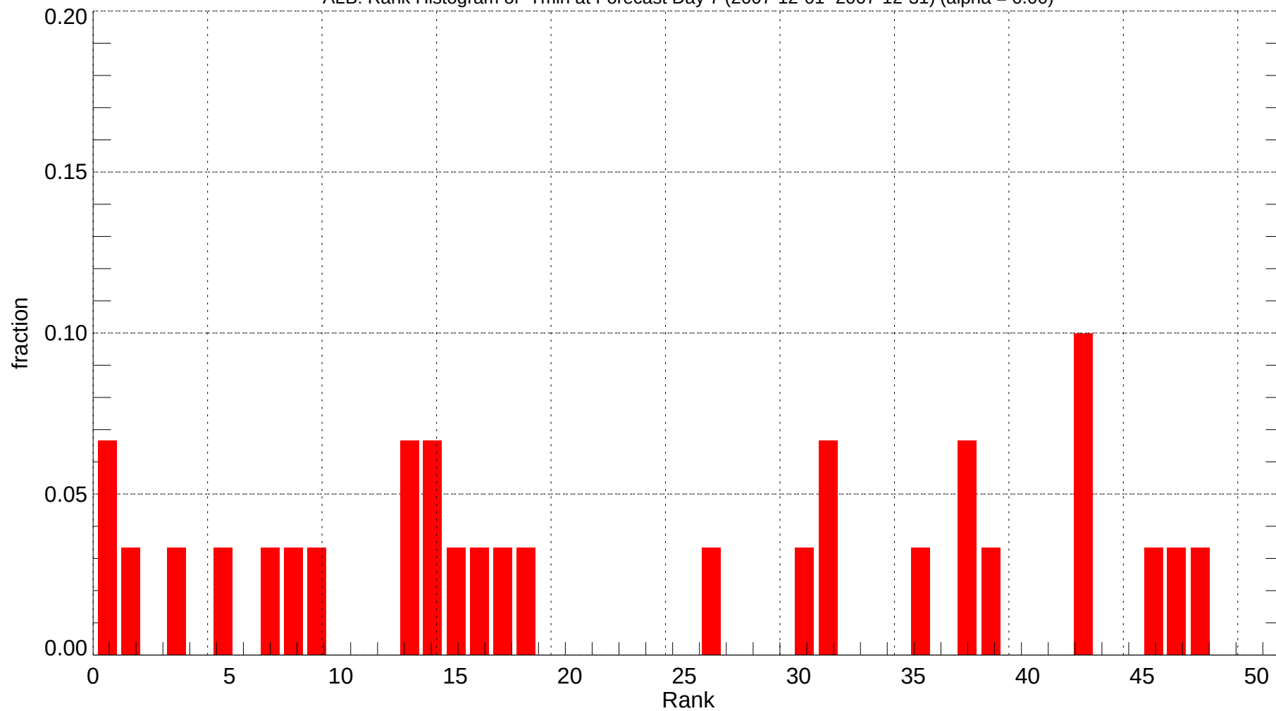
ALB: Rank Histogram of Tmin at Forecast Day 7 (2007-12-01~2007-12-31) (alpha = 0.00)
