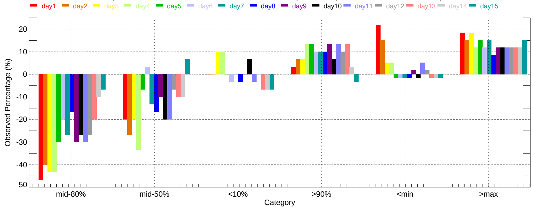
Observed Percentage Deviation of Ensembles - ACT: Max Temperature (2007-12-01~2007-12-31)
