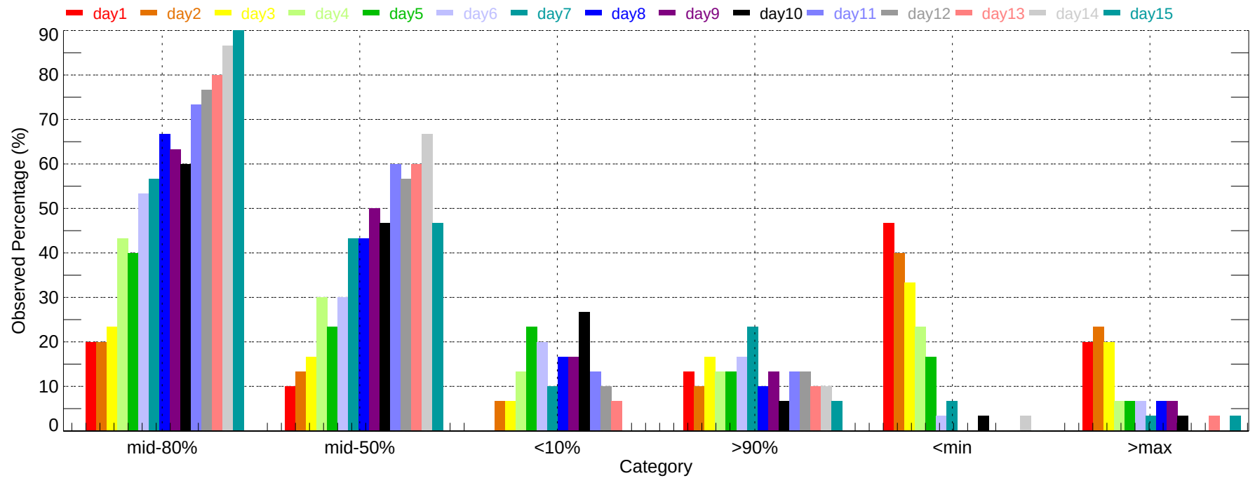
Observed Percentage of Ensembles - MDT: Max Temperature (2007-12-01~2007-12-31)
