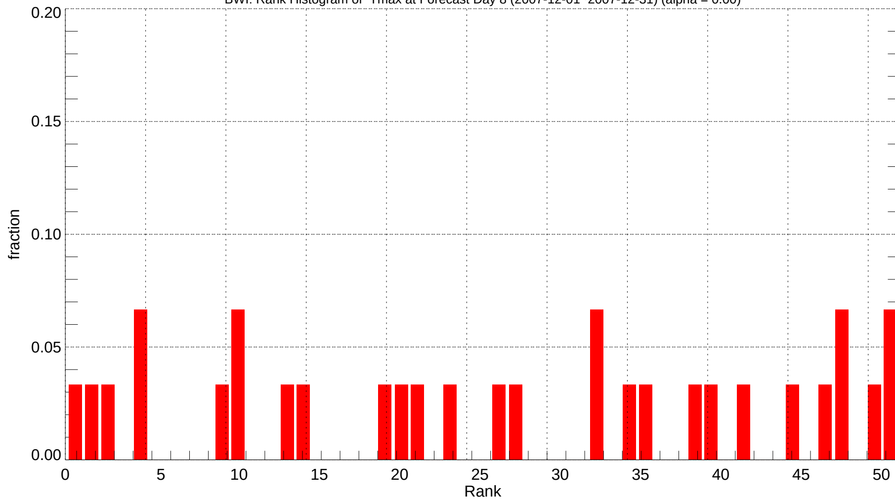
BWI: Rank Histogram of Tmax at Forecast Day 8 (2007-12-01~2007-12-31) (alpha = 0.00)
