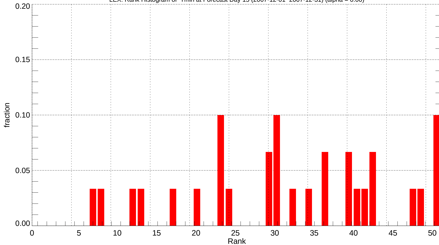
LEX: Rank Histogram of Tmin at Forecast Day 15 (2007-12-01~2007-12-31) (alpha = 0.00)
