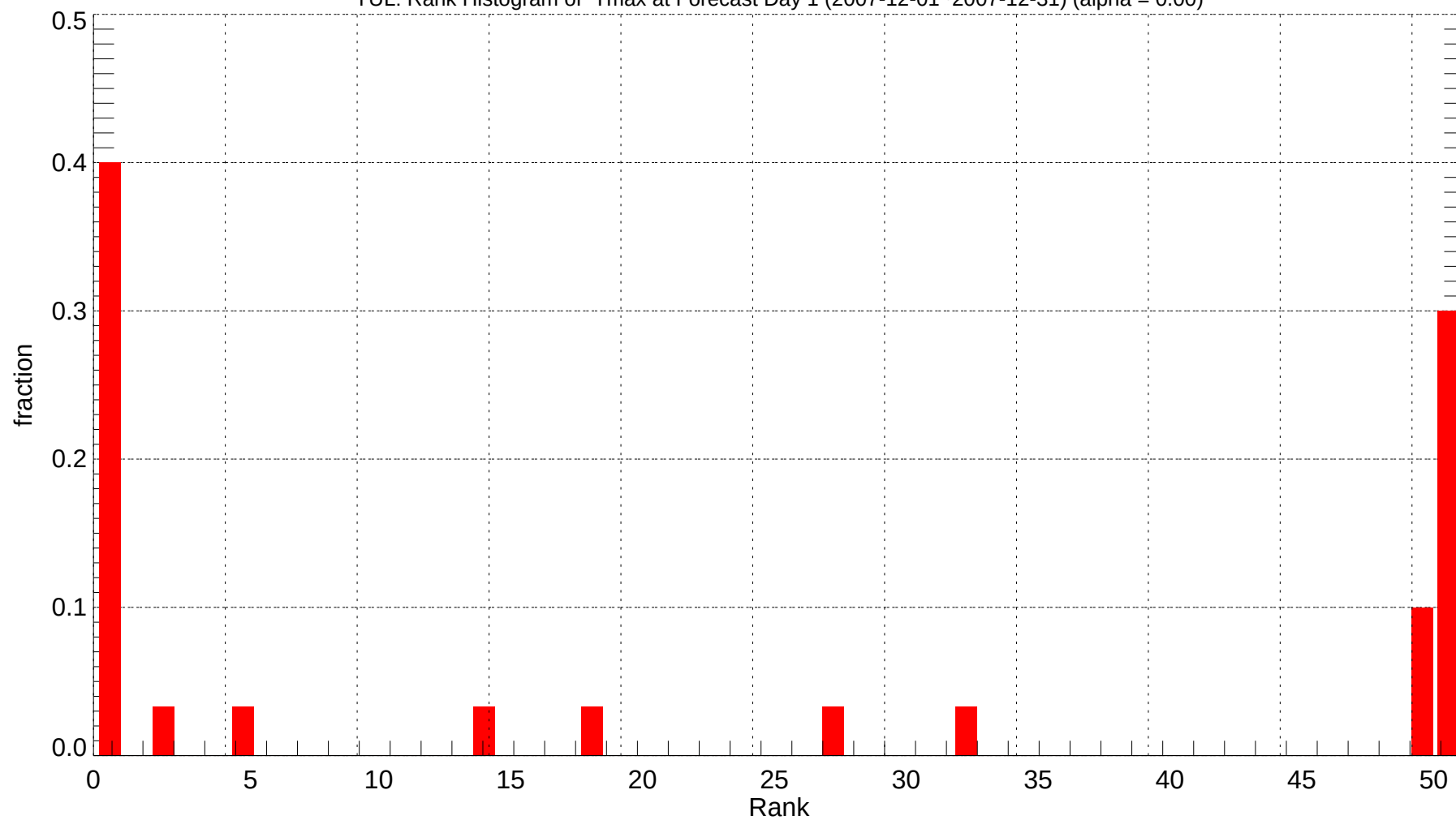
YUL: Rank Histogram of Tmax at Forecast Day 1 (2007-12-01~2007-12-31) (alpha = 0.00)
