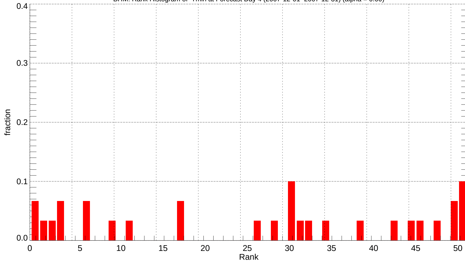
BHM: Rank Histogram of Tmin at Forecast Day 4 (2007-12-01~2007-12-31) (alpha = 0.00)
