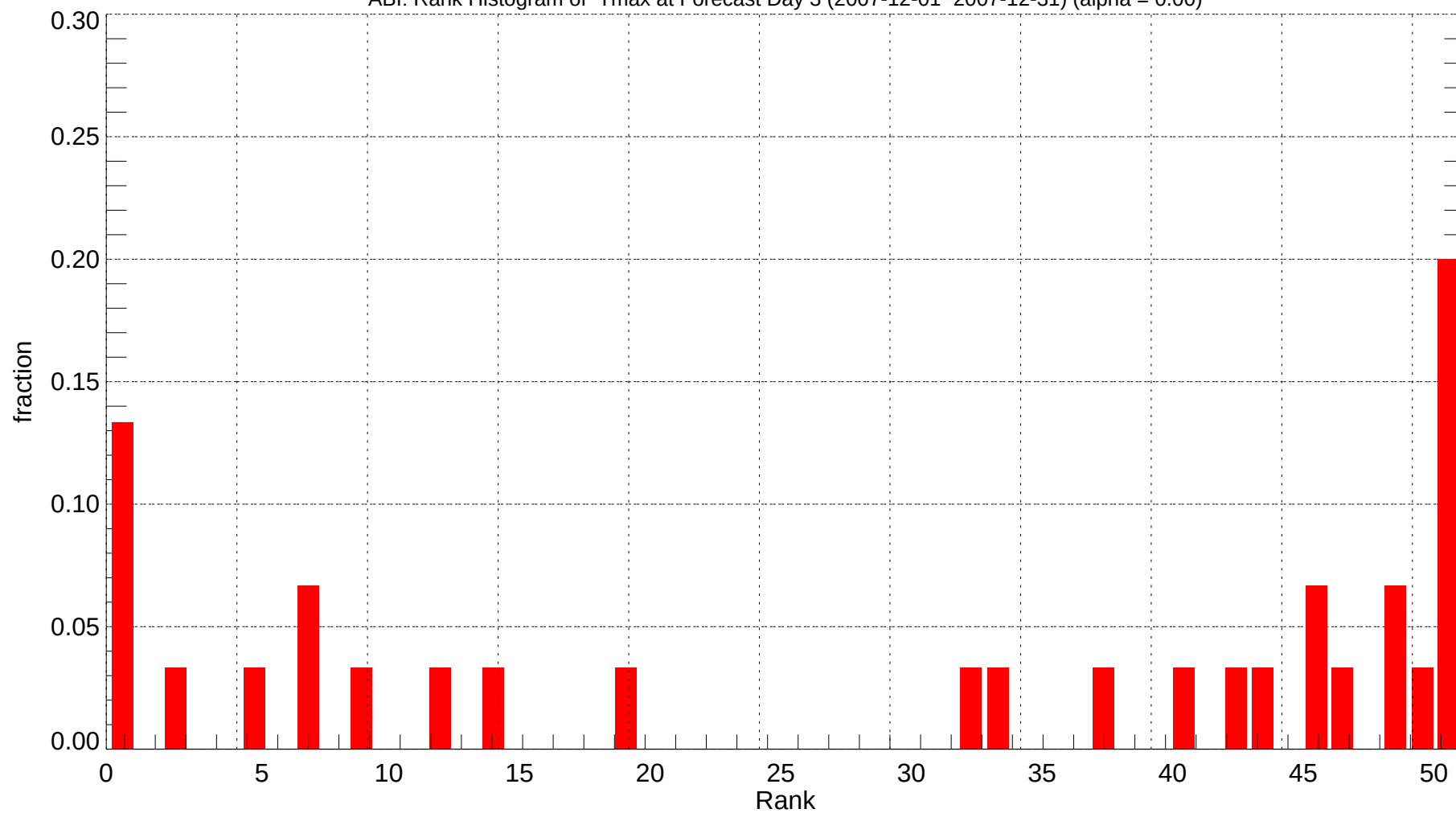
ABI: Rank Histogram of Tmax at Forecast Day 3 (2007-12-01~2007-12-31) (alpha = 0.00)
