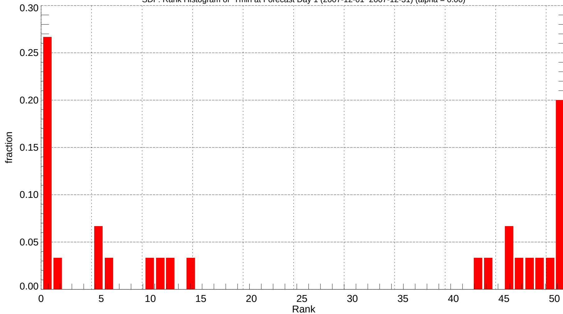
SDF: Rank Histogram of Tmin at Forecast Day 1 (2007-12-01~2007-12-31) (alpha = 0.00)
