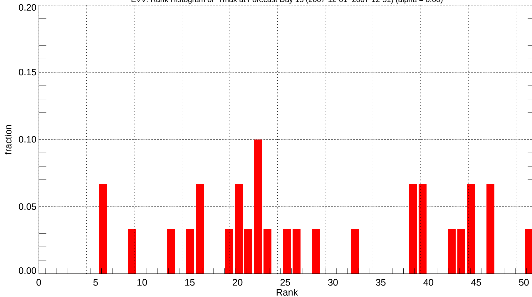
EVV: Rank Histogram of Tmax at Forecast Day 13 (2007-12-01~2007-12-31) (alpha = 0.00)
