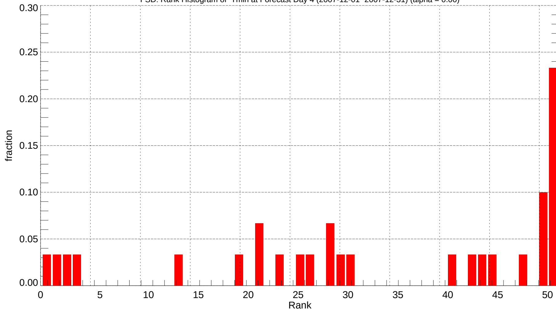
FSD: Rank Histogram of Tmin at Forecast Day 4 (2007-12-01~2007-12-31) (alpha = 0.00)
