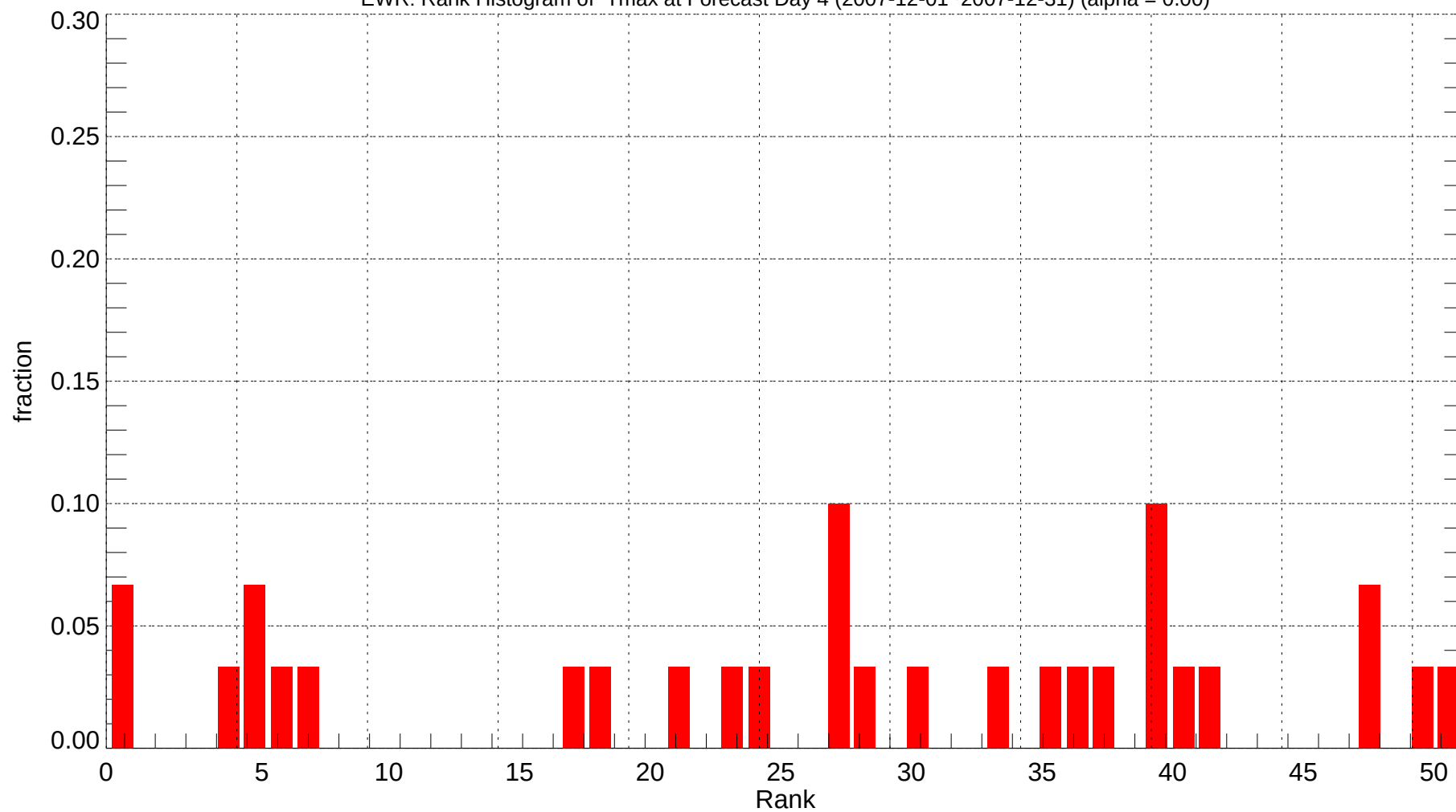
EWR: Rank Histogram of Tmax at Forecast Day 4 (2007-12-01~2007-12-31) (alpha = 0.00)
