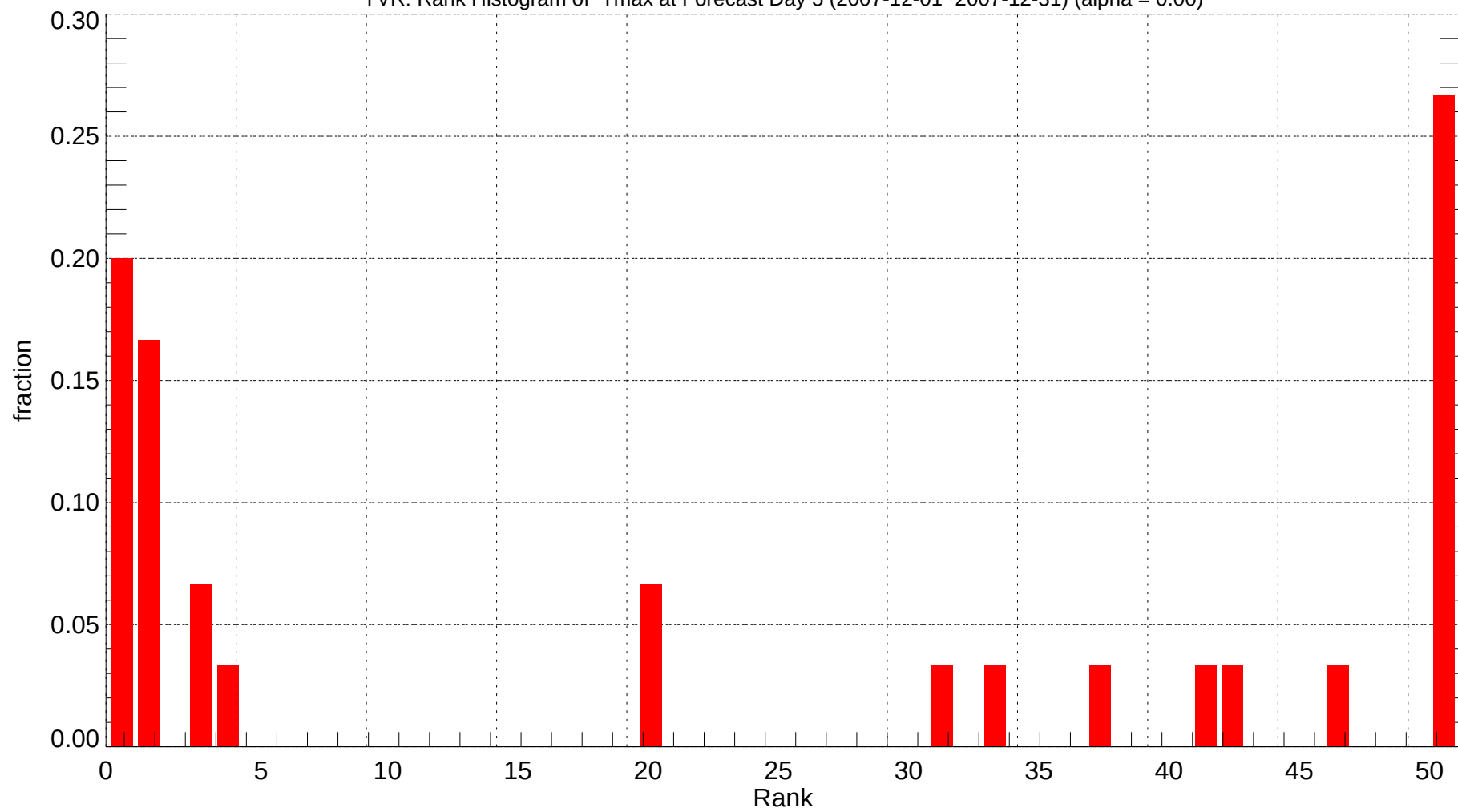
YVR: Rank Histogram of Tmax at Forecast Day 5 (2007-12-01~2007-12-31) (alpha = 0.00)
