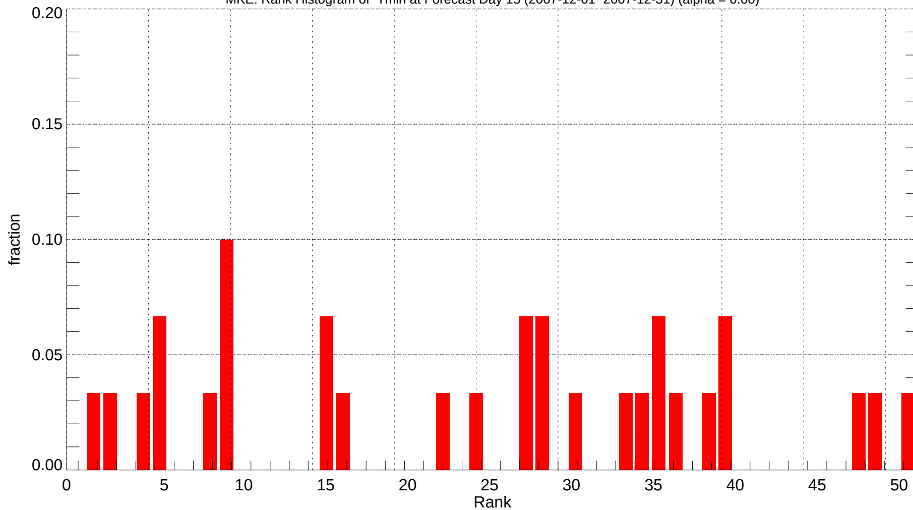
MKE: Rank Histogram of Tmin at Forecast Day 15 (2007-12-01~2007-12-31) (alpha = 0.00)
