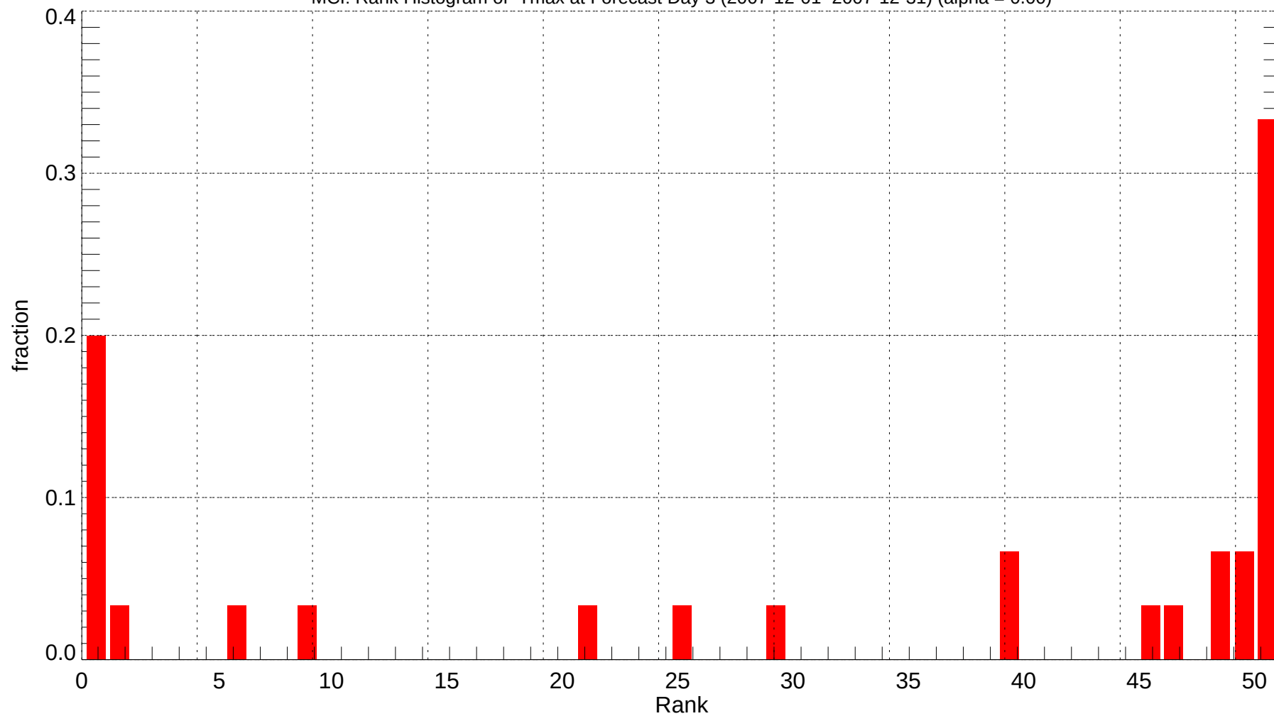
MCI: Rank Histogram of Tmax at Forecast Day 3 (2007-12-01~2007-12-31) (alpha = 0.00)
