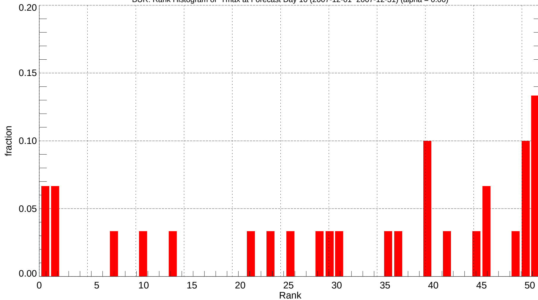
BUR: Rank Histogram of Tmax at Forecast Day 10 (2007-12-01~2007-12-31) (alpha = 0.00)
