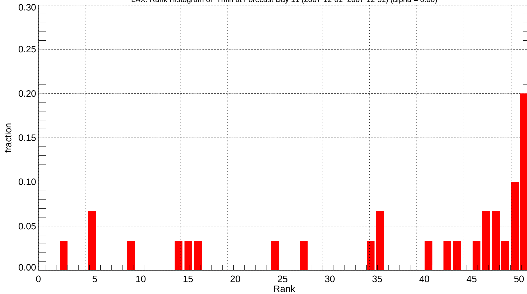
LAX: Rank Histogram of Tmin at Forecast Day 11 (2007-12-01~2007-12-31) (alpha = 0.00)
