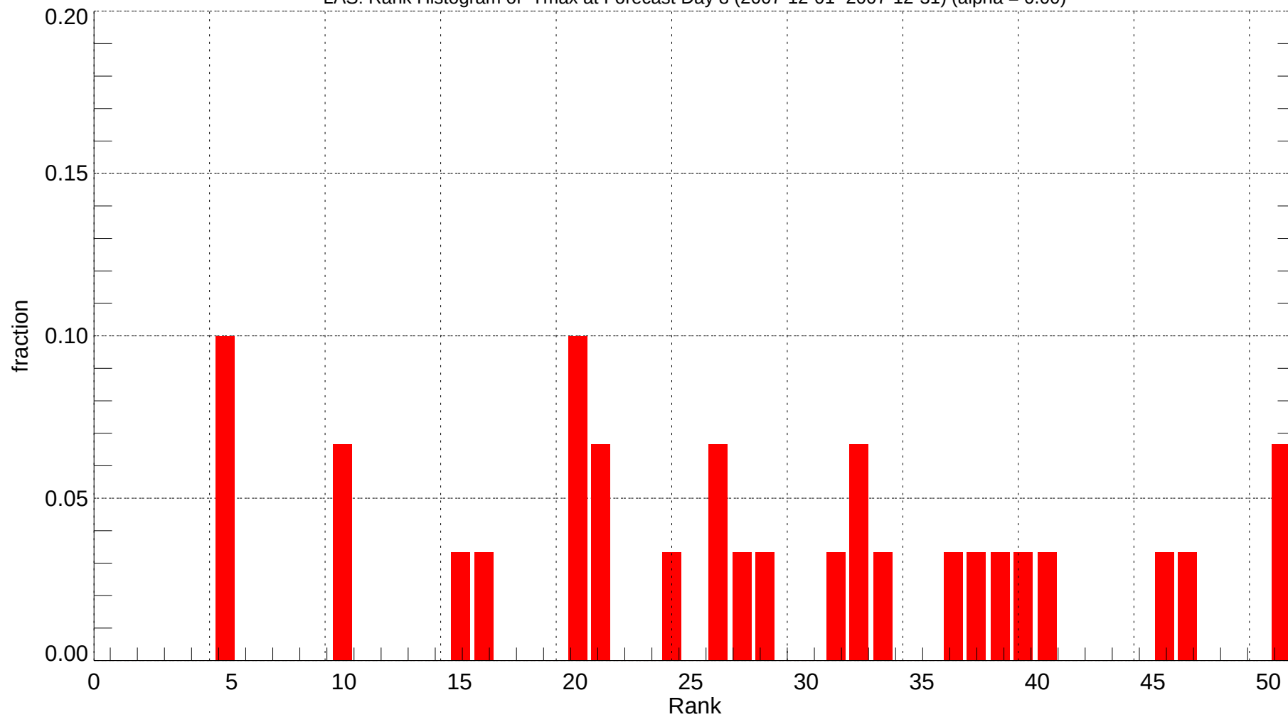
LAS: Rank Histogram of Tmax at Forecast Day 8 (2007-12-01~2007-12-31) (alpha = 0.00)
