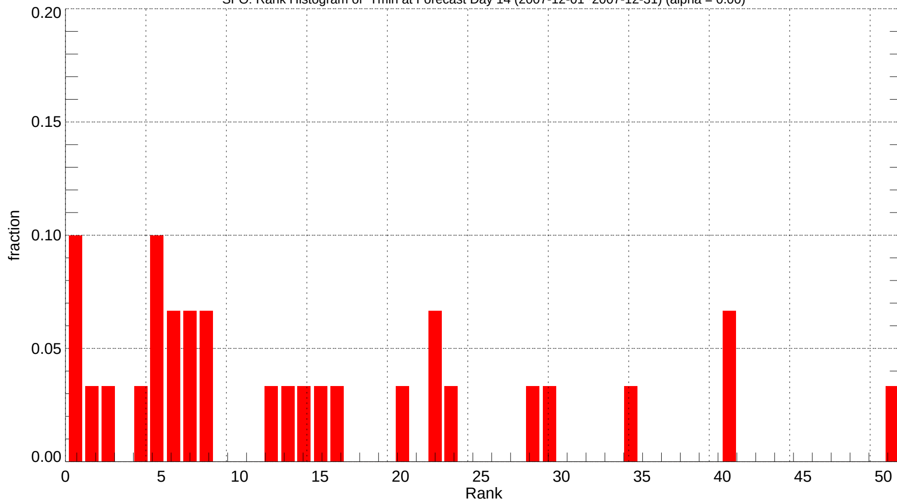
SFO: Rank Histogram of Tmin at Forecast Day 14 (2007-12-01~2007-12-31) (alpha = 0.00)
