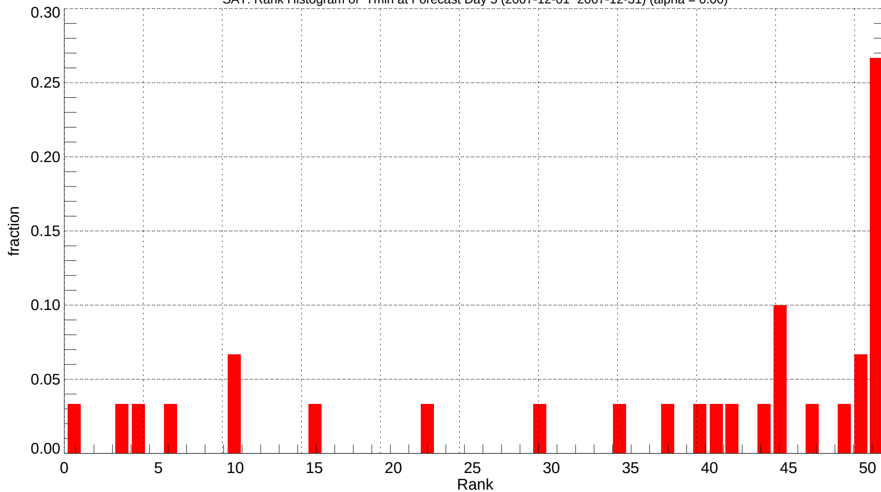
SAT: Rank Histogram of Tmin at Forecast Day 5 (2007-12-01~2007-12-31) (alpha = 0.00)
