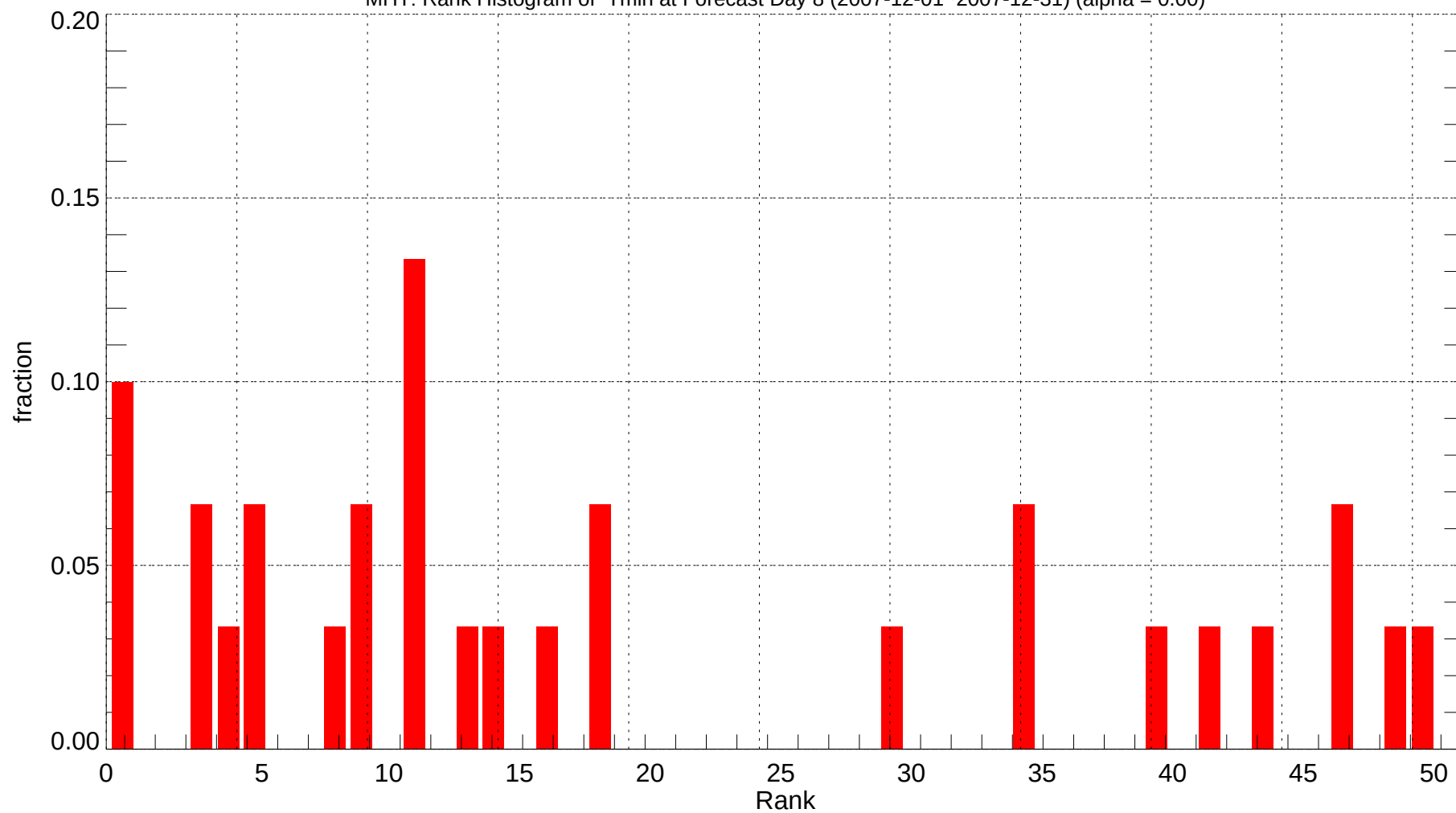
MHT: Rank Histogram of Tmin at Forecast Day 8 (2007-12-01~2007-12-31) (alpha = 0.00)
