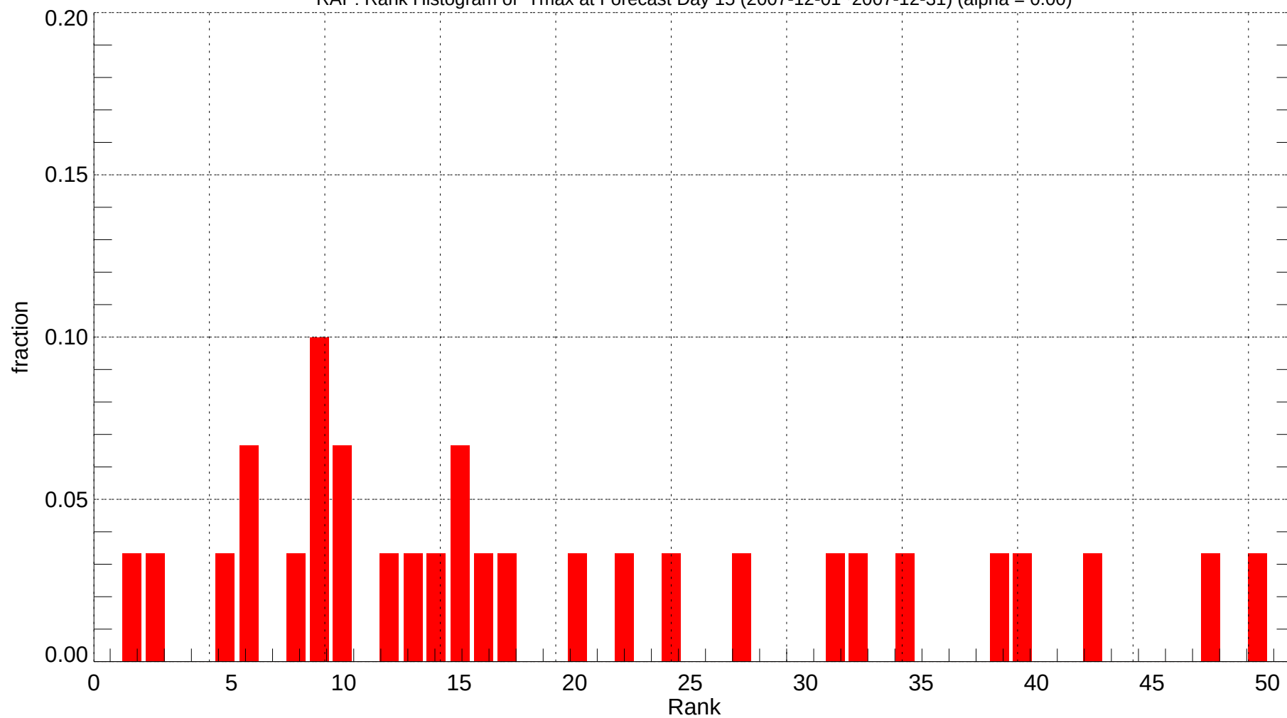
RAP: Rank Histogram of Tmax at Forecast Day 15 (2007-12-01~2007-12-31) (alpha = 0.00)
