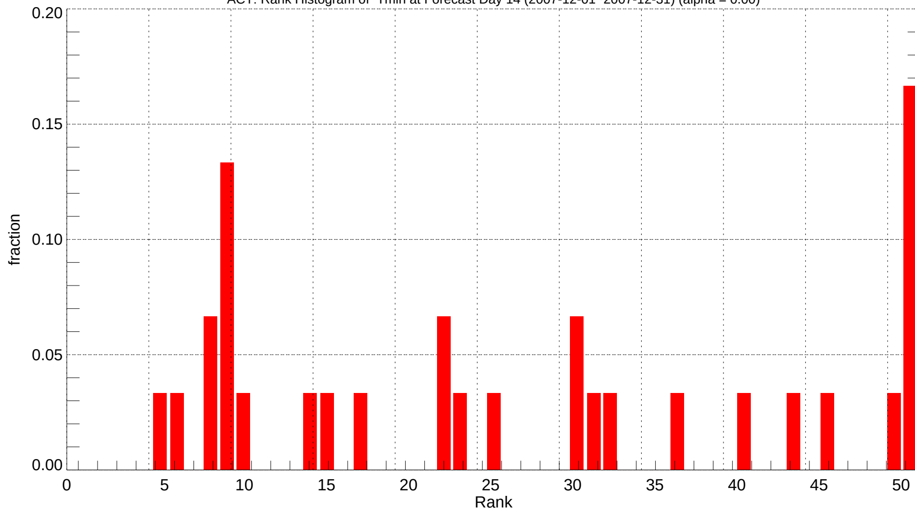
ACT: Rank Histogram of Tmin at Forecast Day 14 (2007-12-01~2007-12-31) (alpha = 0.00)
