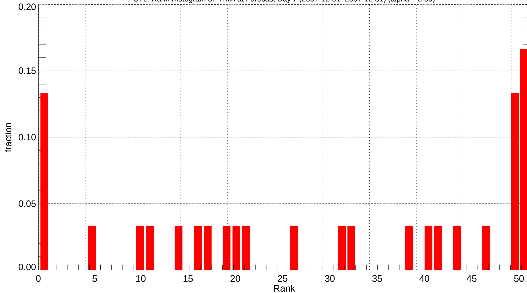
STL: Rank Histogram of Tmin at Forecast Day 7 (2007-12-01~2007-12-31) (alpha = 0.00)
