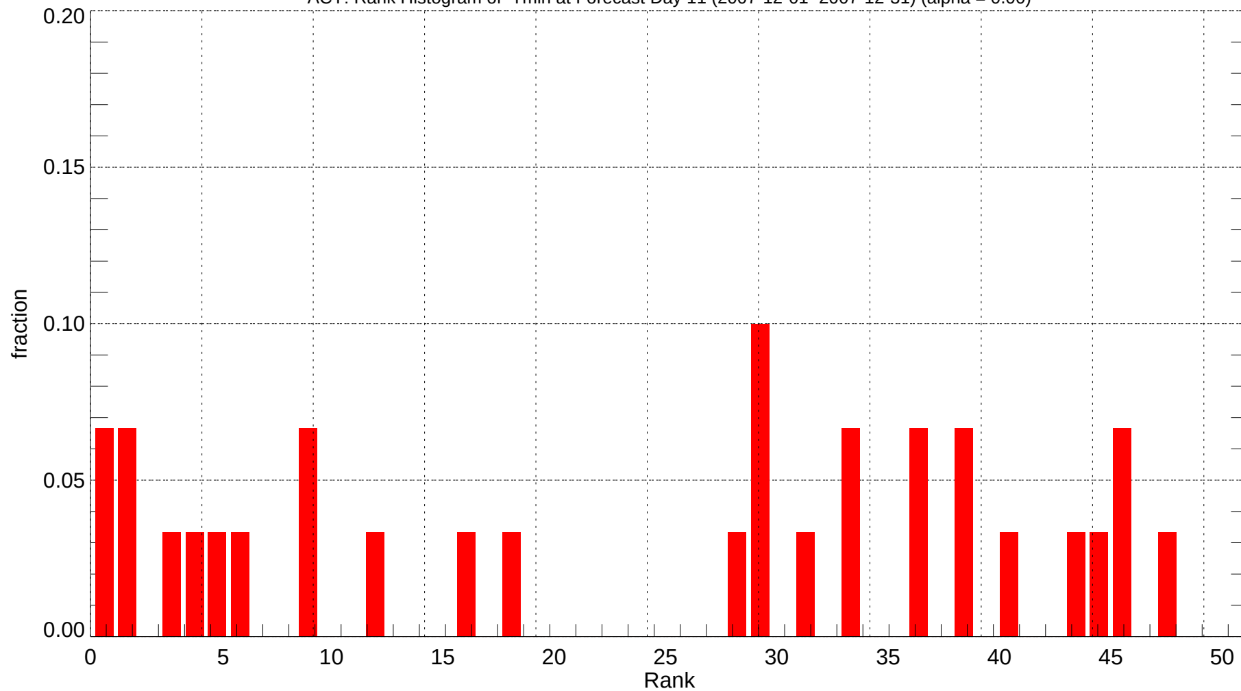
ACY: Rank Histogram of Tmin at Forecast Day 11 (2007-12-01~2007-12-31) (alpha = 0.00)
