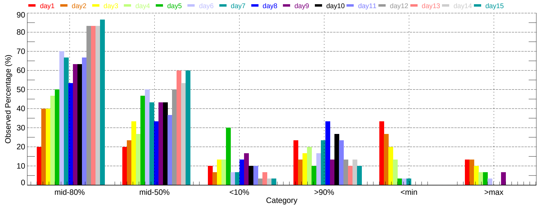
Observed Percentage of Ensembles - JFK: Max Temperature (2007-12-01~2007-12-31)
