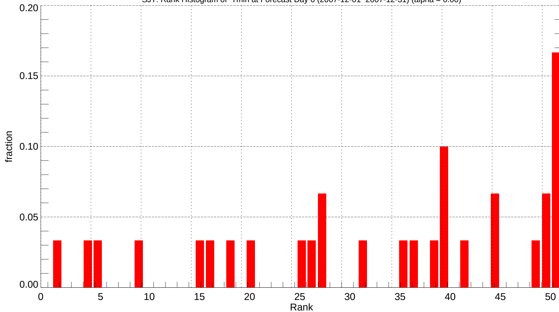
SJT: Rank Histogram of Tmin at Forecast Day 6 (2007-12-01~2007-12-31) (alpha = 0.00)
