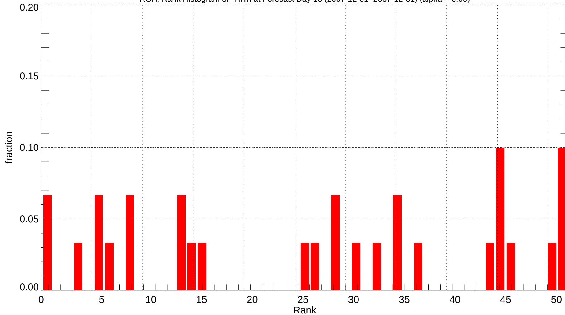
ROA: Rank Histogram of Tmin at Forecast Day 13 (2007-12-01~2007-12-31) (alpha = 0.00)
