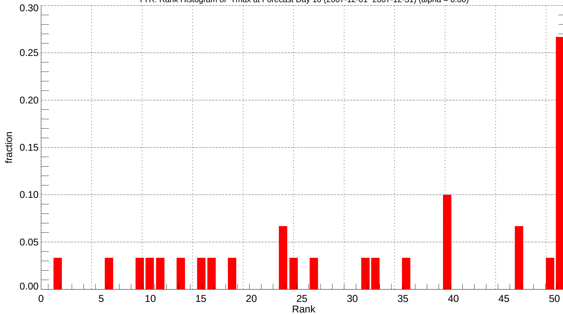
TYR: Rank Histogram of Tmax at Forecast Day 10 (2007-12-01~2007-12-31) (alpha = 0.00)
