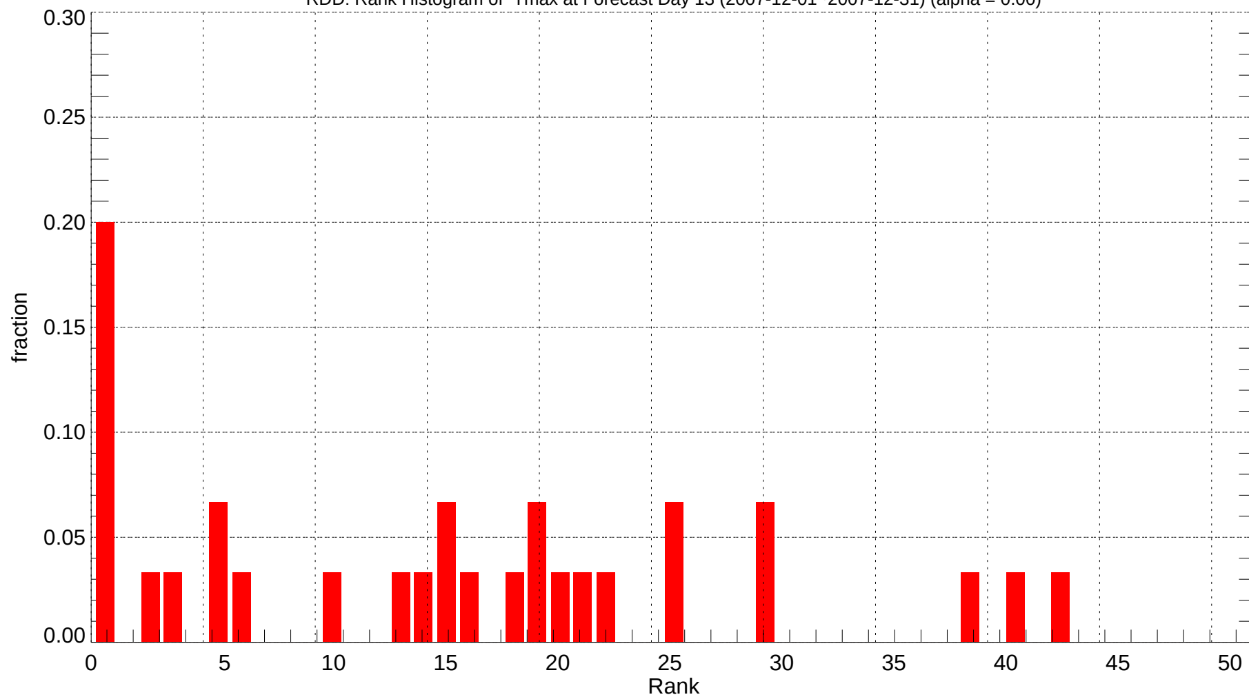
RDD: Rank Histogram of Tmax at Forecast Day 13 (2007-12-01~2007-12-31) (alpha = 0.00)
