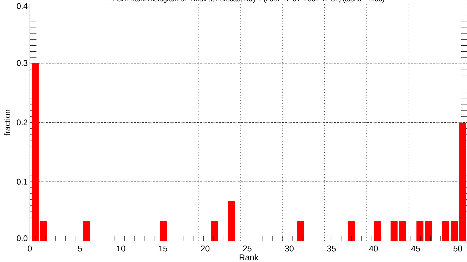
LGA: Rank Histogram of Tmax at Forecast Day 1 (2007-12-01~2007-12-31) (alpha = 0.00)
