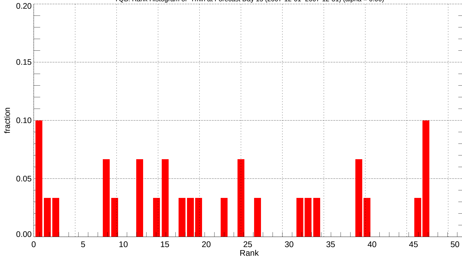
YQB: Rank Histogram of Tmin at Forecast Day 15 (2007-12-01~2007-12-31) (alpha = 0.00)
