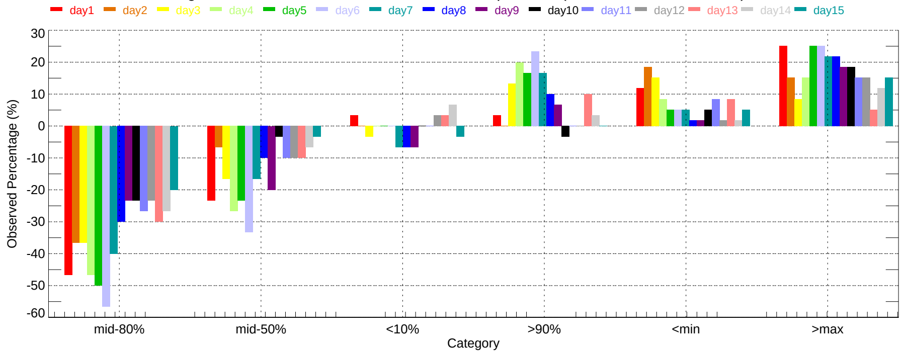
Observed Percentage Deviation of Ensembles - ABY: Min Temperature (2007-12-01~2007-12-31)
