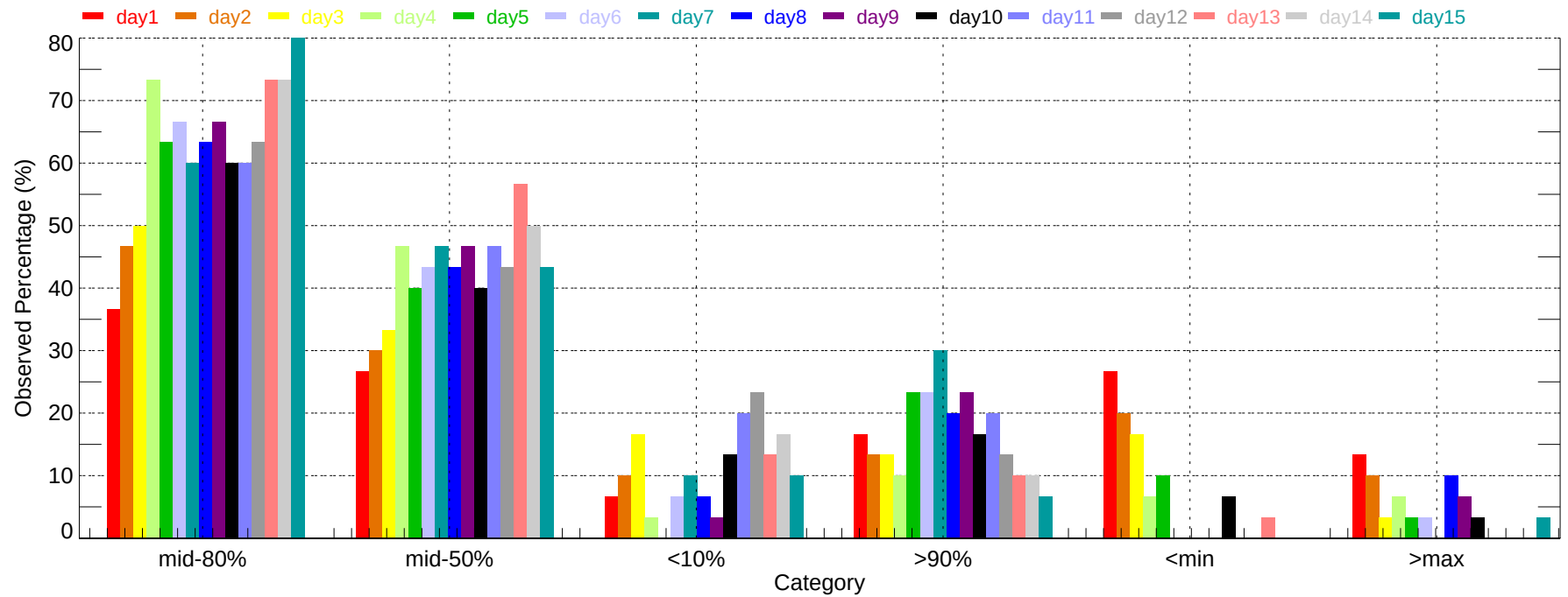
Observed Percentage of Ensembles - EWR: Min Temperature (2007-12-01~2007-12-31)
