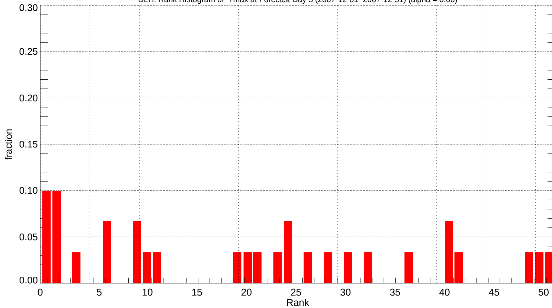
DLH: Rank Histogram of Tmax at Forecast Day 3 (2007-12-01~2007-12-31) (alpha = 0.00)
