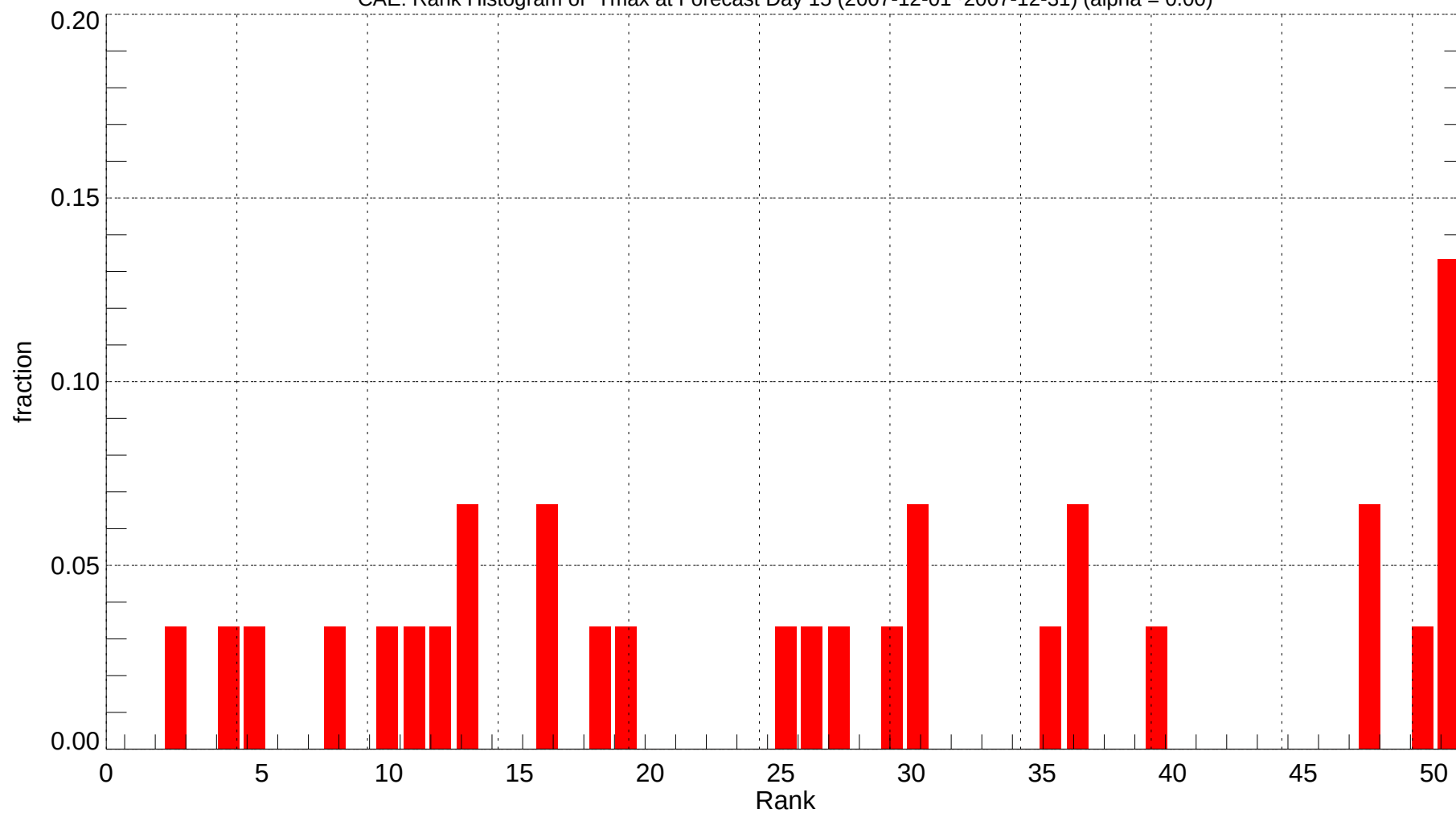
CAE: Rank Histogram of Tmax at Forecast Day 15 (2007-12-01~2007-12-31) (alpha = 0.00)
