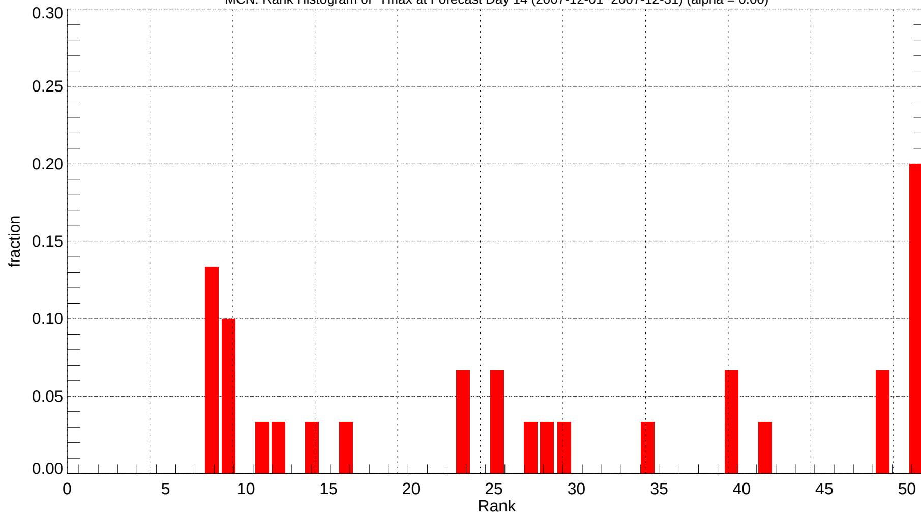
MCN: Rank Histogram of Tmax at Forecast Day 14 (2007-12-01~2007-12-31) (alpha = 0.00)
