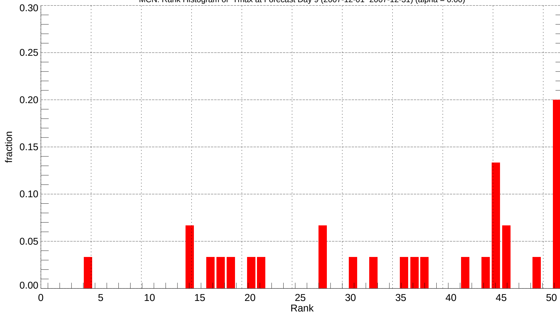
MCN: Rank Histogram of Tmax at Forecast Day 9 (2007-12-01~2007-12-31) (alpha = 0.00)
