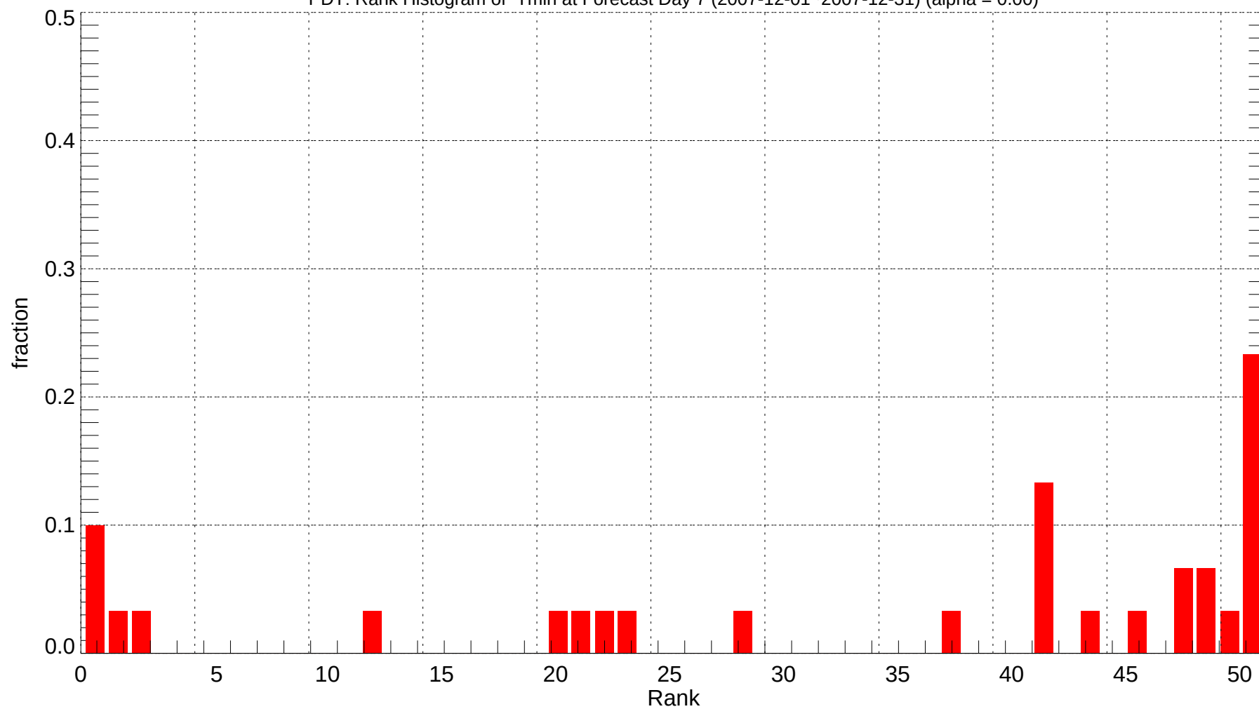
PDT: Rank Histogram of Tmin at Forecast Day 7 (2007-12-01~2007-12-31) (alpha = 0.00)
