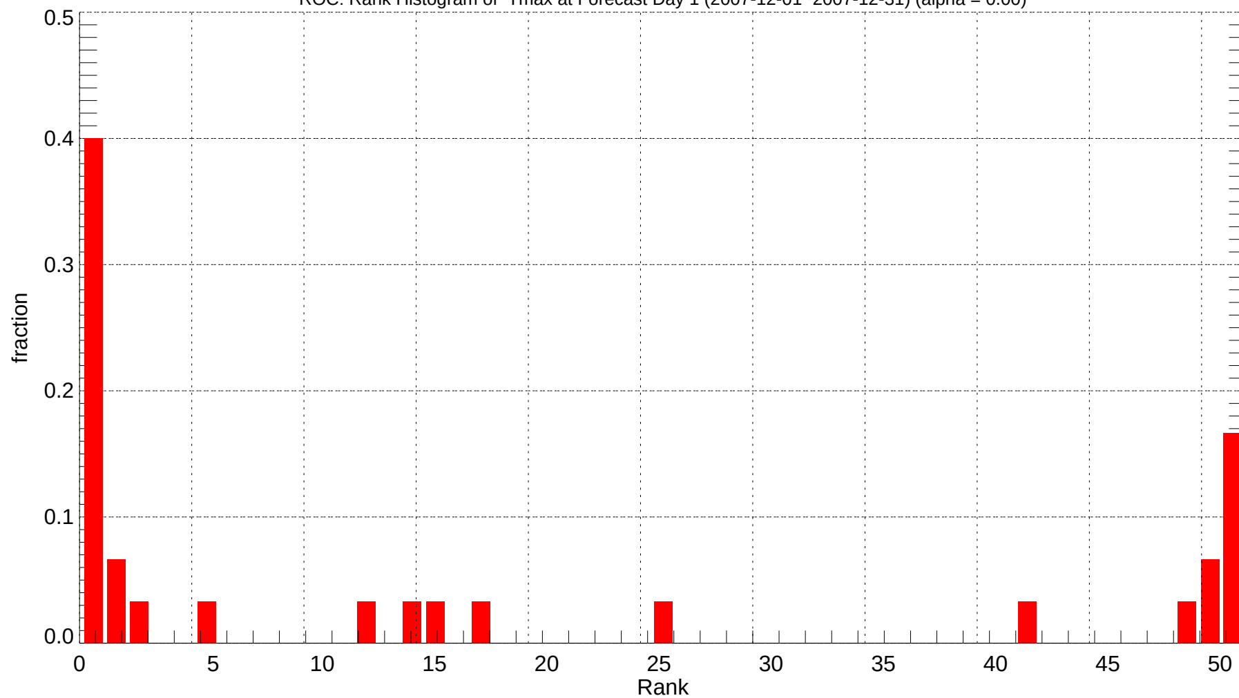
ROC: Rank Histogram of Tmax at Forecast Day 1 (2007-12-01~2007-12-31) (alpha = 0.00)
