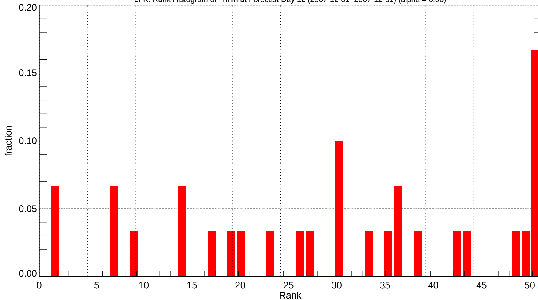
LFK: Rank Histogram of Tmin at Forecast Day 12 (2007-12-01~2007-12-31) (alpha = 0.00)
