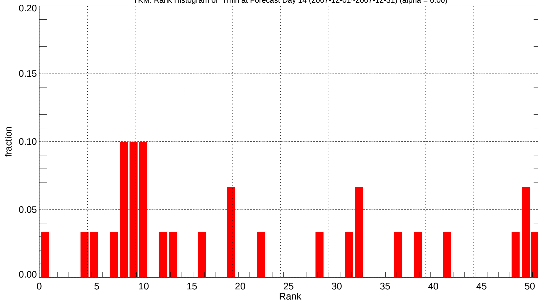
YKM: Rank Histogram of Tmin at Forecast Day 14 (2007-12-01~2007-12-31) (alpha = 0.00)
