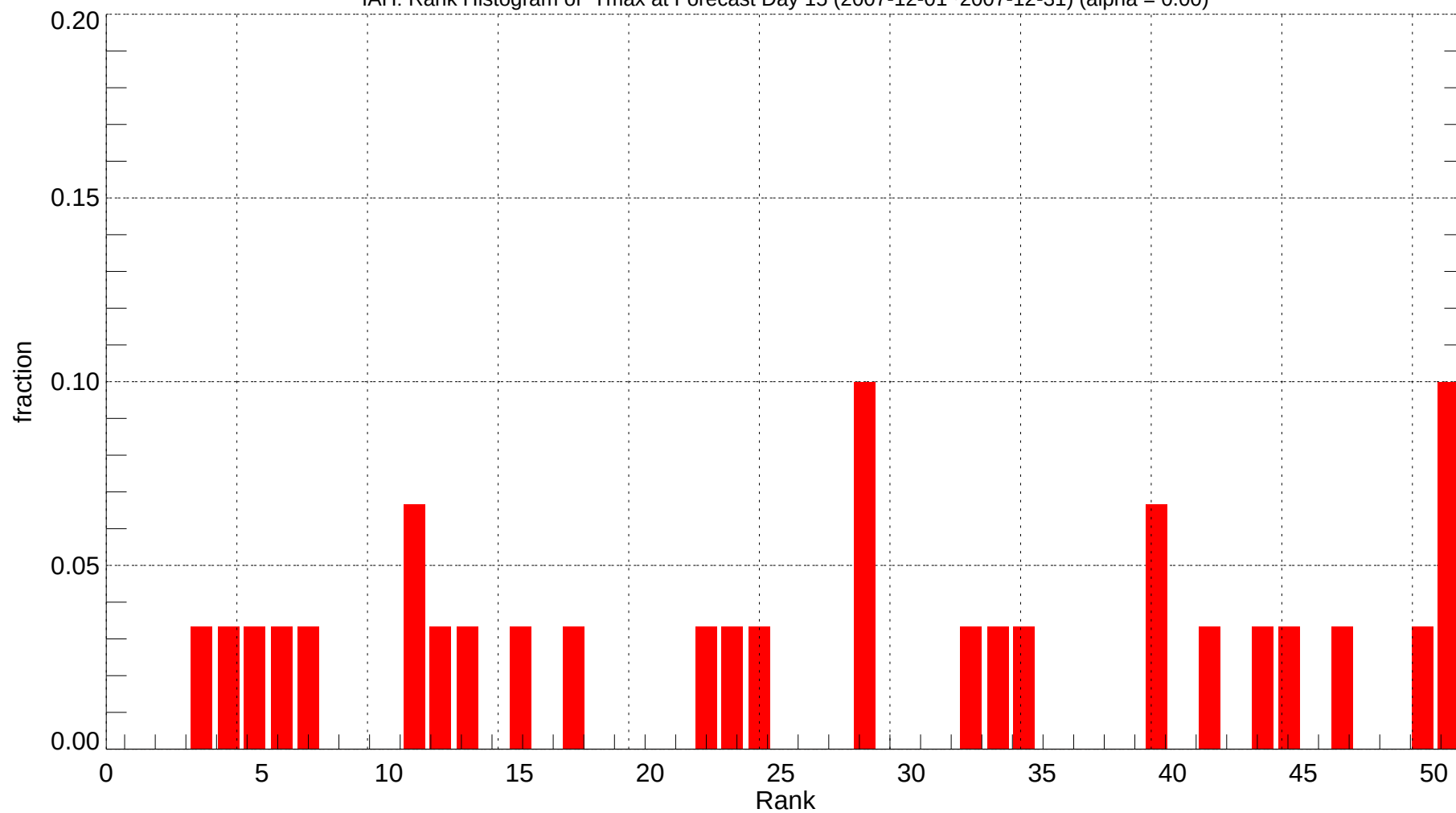
IAH: Rank Histogram of Tmax at Forecast Day 15 (2007-12-01~2007-12-31) (alpha = 0.00)
