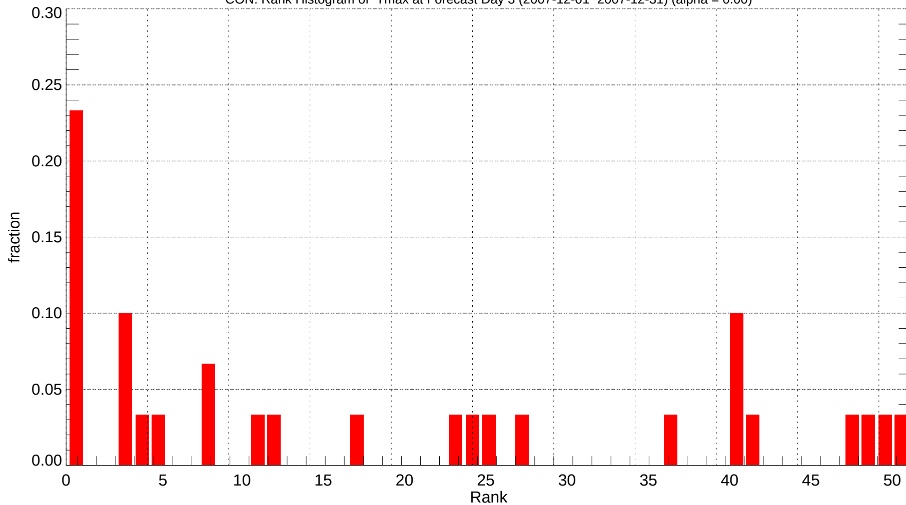
CON: Rank Histogram of Tmax at Forecast Day 3 (2007-12-01~2007-12-31) (alpha = 0.00)
