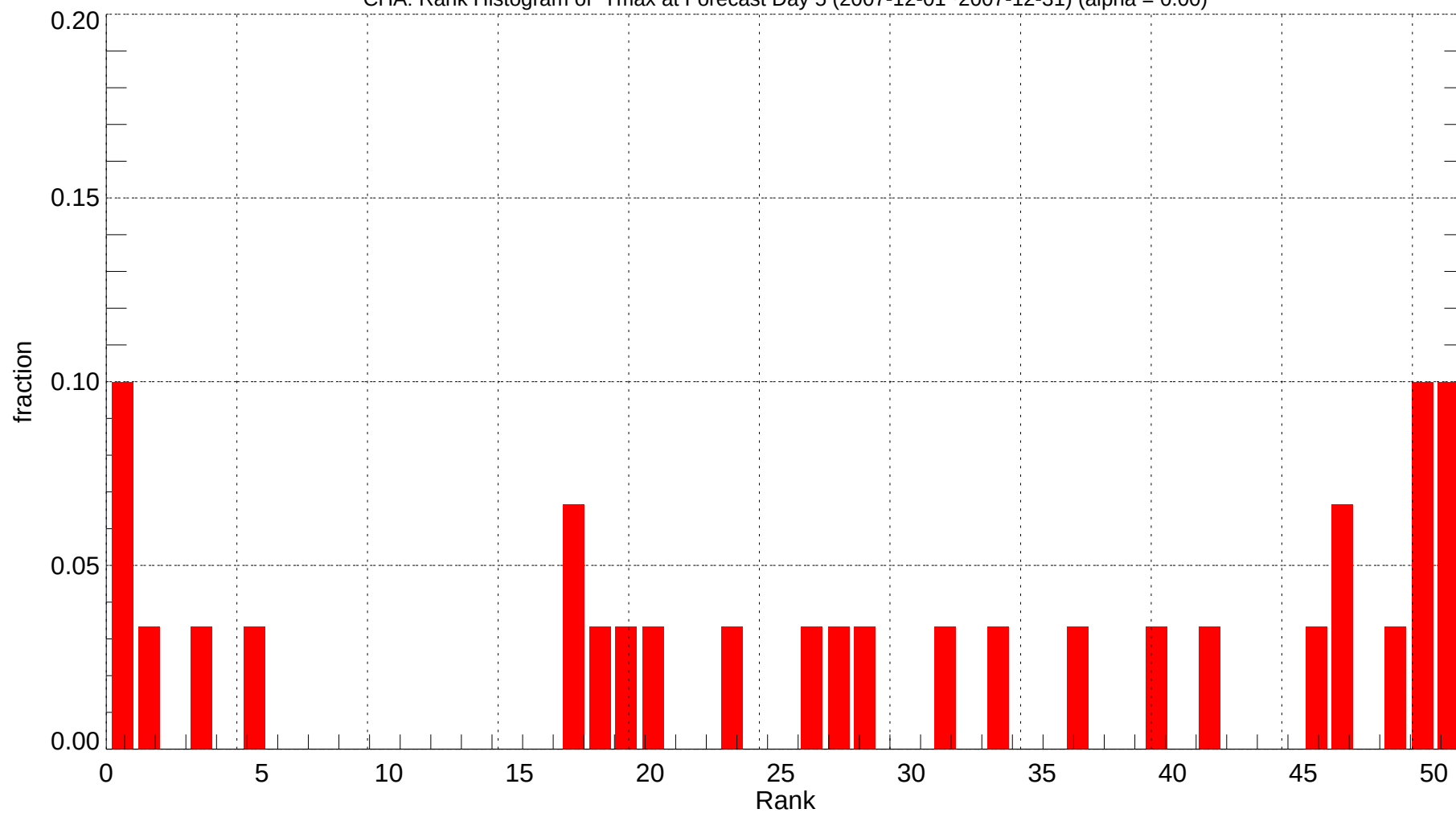
CHA: Rank Histogram of Tmax at Forecast Day 5 (2007-12-01~2007-12-31) (alpha = 0.00)
