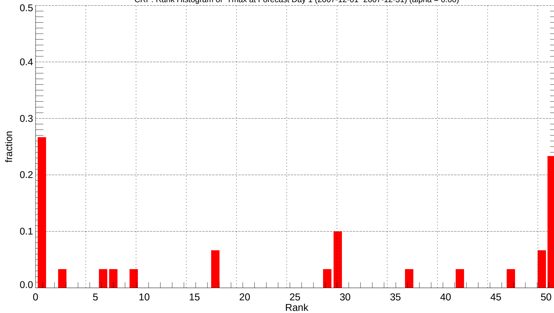
CRP: Rank Histogram of Tmax at Forecast Day 1 (2007-12-01~2007-12-31) (alpha = 0.00)
