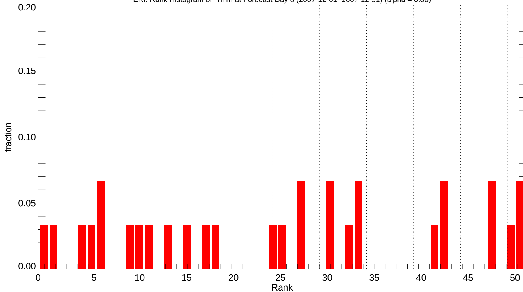
ERI: Rank Histogram of Tmin at Forecast Day 8 (2007-12-01~2007-12-31) (alpha = 0.00)
