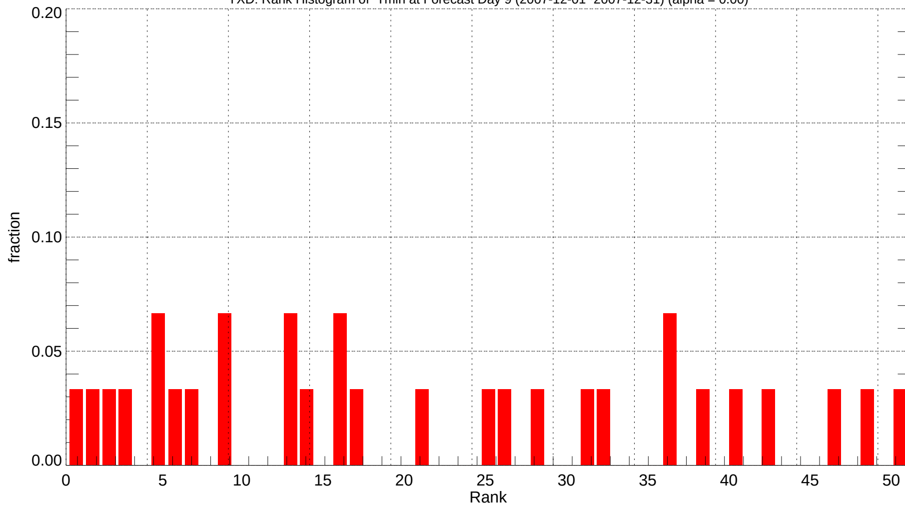
YXD: Rank Histogram of Tmin at Forecast Day 9 (2007-12-01~2007-12-31) (alpha = 0.00)
