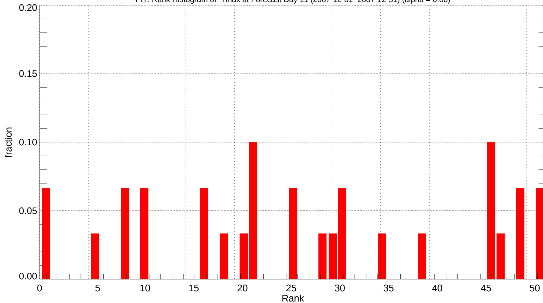
PIT: Rank Histogram of Tmax at Forecast Day 11 (2007-12-01~2007-12-31) (alpha = 0.00)
