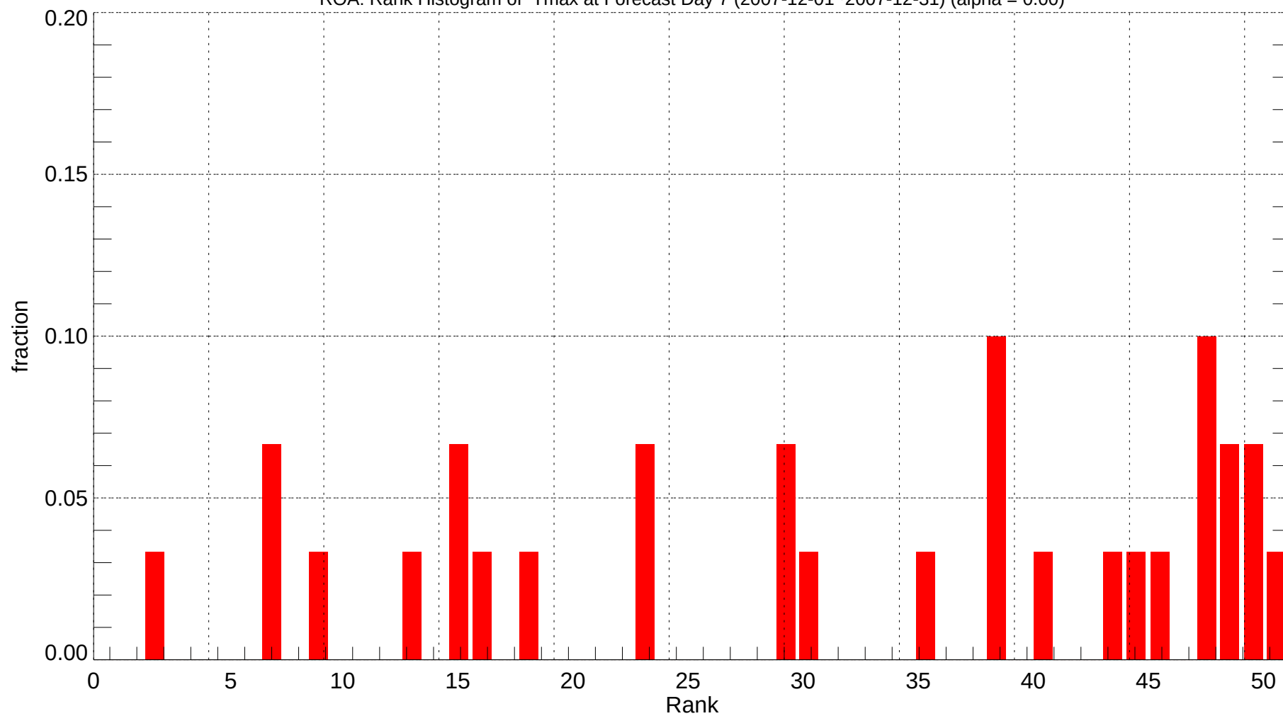
ROA: Rank Histogram of Tmax at Forecast Day 7 (2007-12-01~2007-12-31) (alpha = 0.00)
