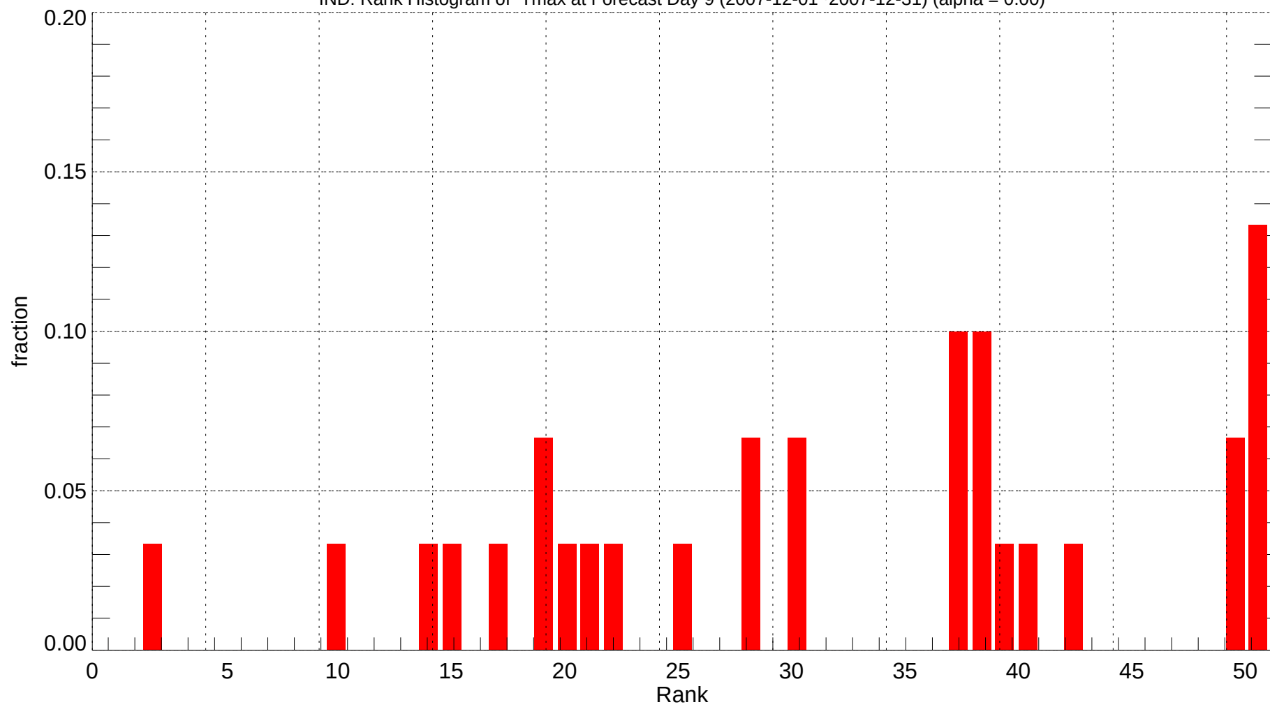
IND: Rank Histogram of Tmax at Forecast Day 9 (2007-12-01~2007-12-31) (alpha = 0.00)
