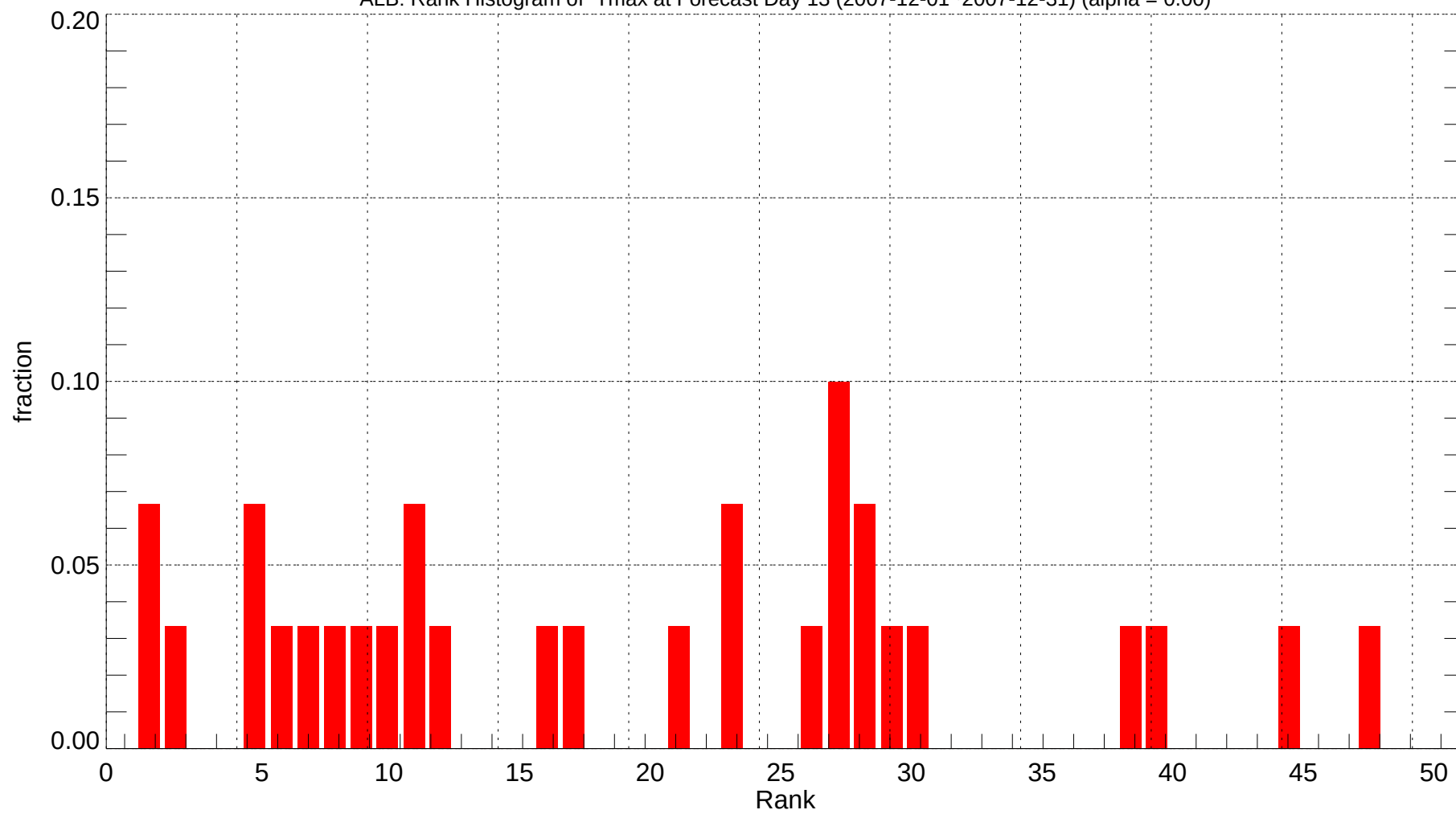
ALB: Rank Histogram of Tmax at Forecast Day 13 (2007-12-01~2007-12-31) (alpha = 0.00)
