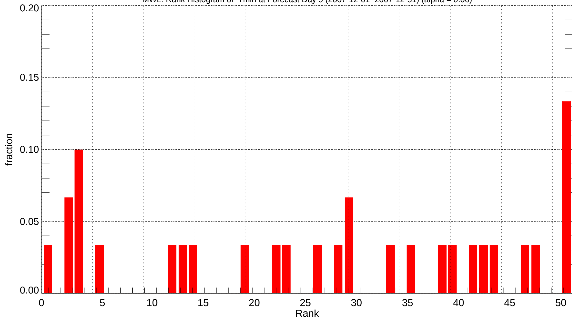
MWL: Rank Histogram of Tmin at Forecast Day 9 (2007-12-01~2007-12-31) (alpha = 0.00)
