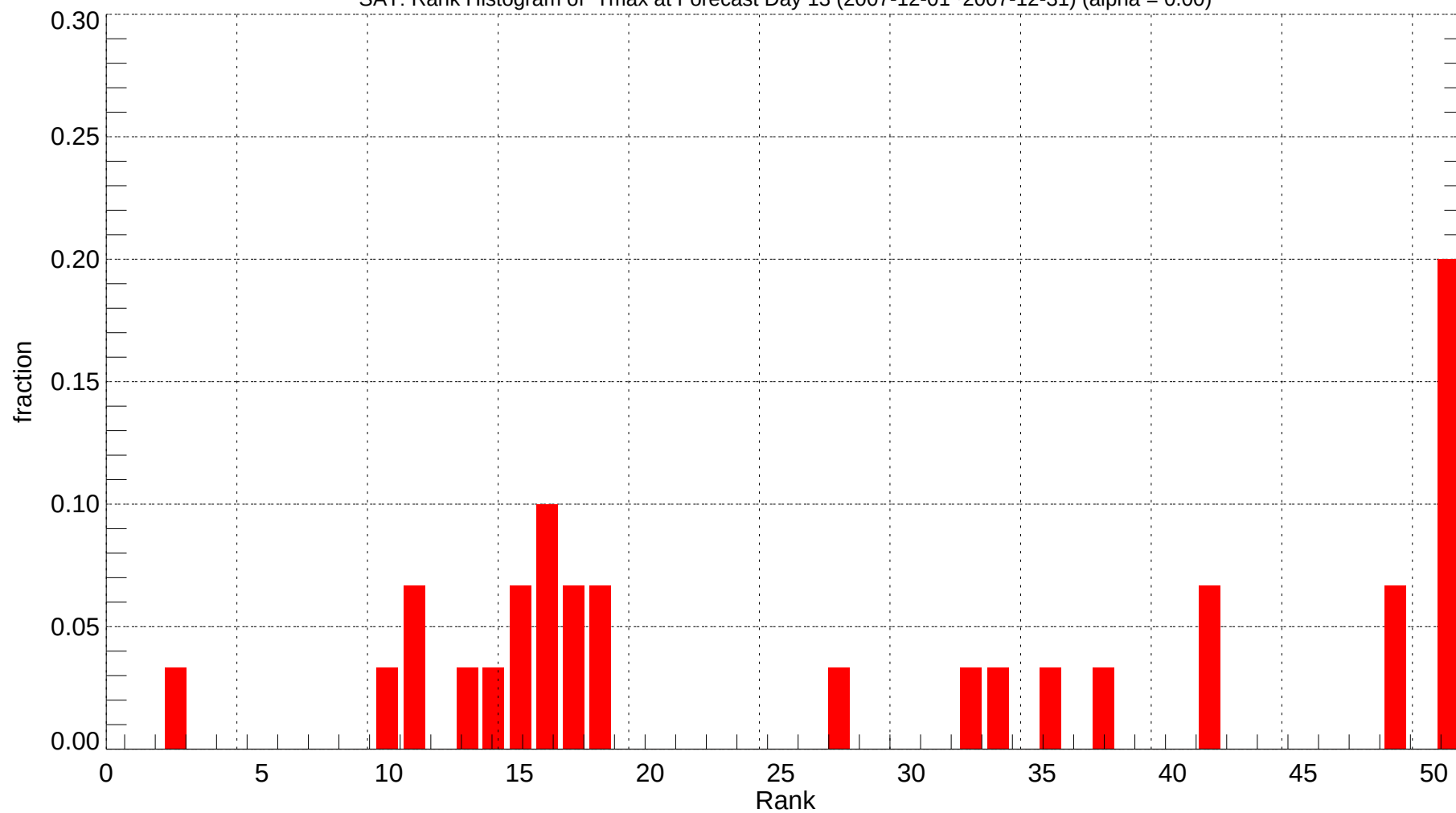
SAT: Rank Histogram of Tmax at Forecast Day 13 (2007-12-01~2007-12-31) (alpha = 0.00)
