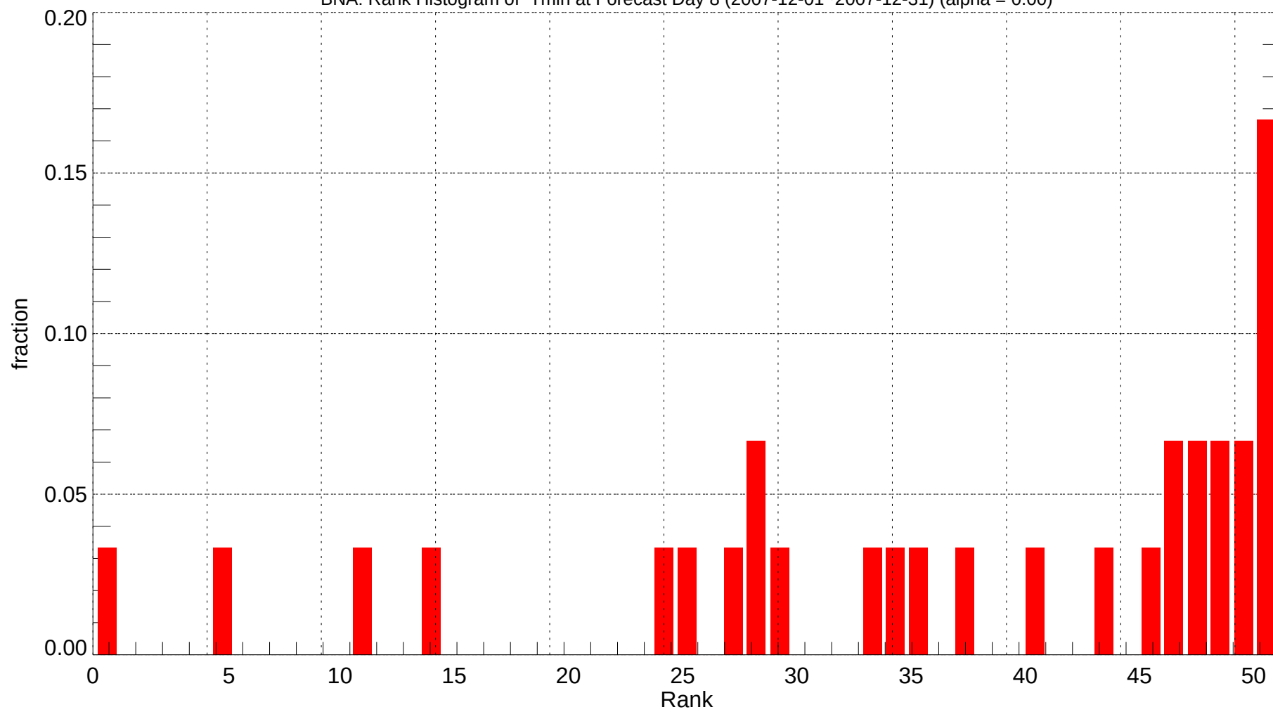
BNA: Rank Histogram of Tmin at Forecast Day 8 (2007-12-01~2007-12-31) (alpha = 0.00)
