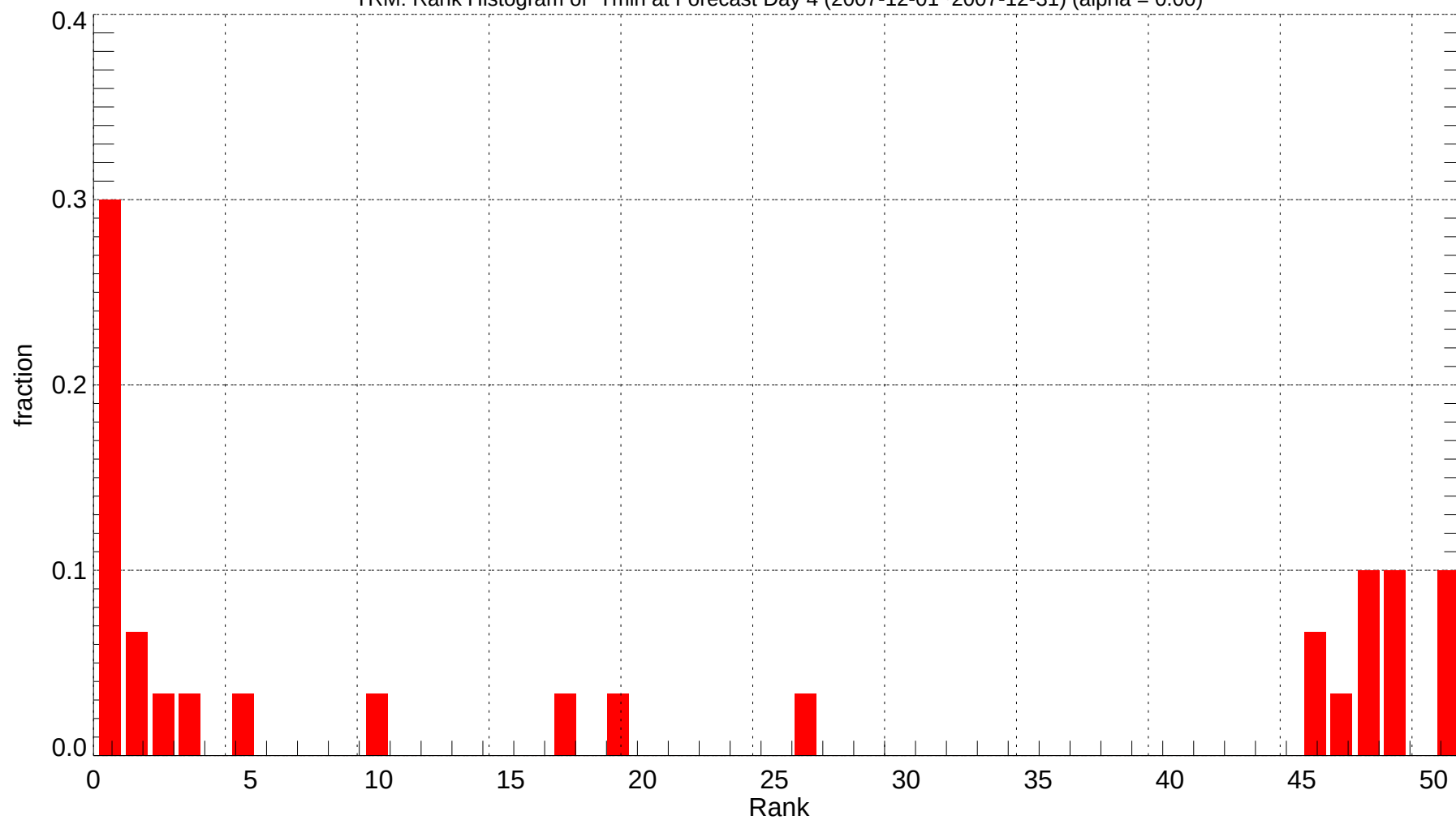
TRM: Rank Histogram of Tmin at Forecast Day 4 (2007-12-01~2007-12-31) (alpha = 0.00)
