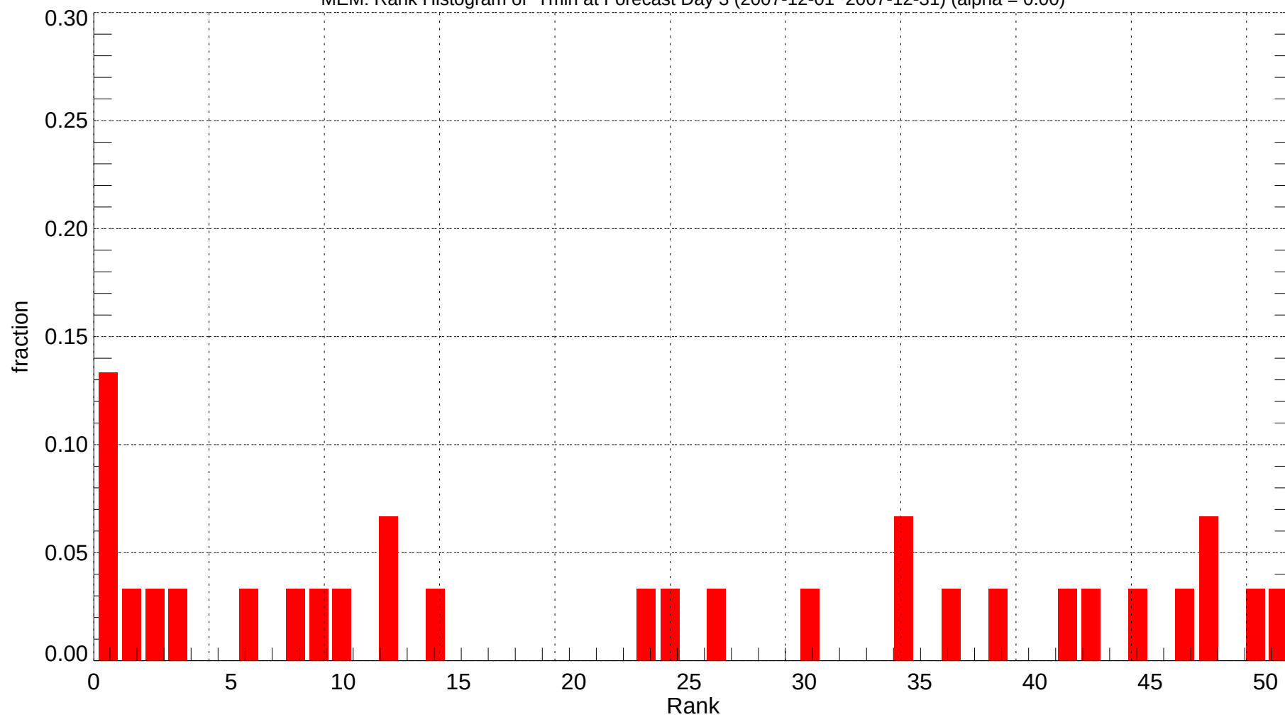
MEM: Rank Histogram of Tmin at Forecast Day 3 (2007-12-01~2007-12-31) (alpha = 0.00)
