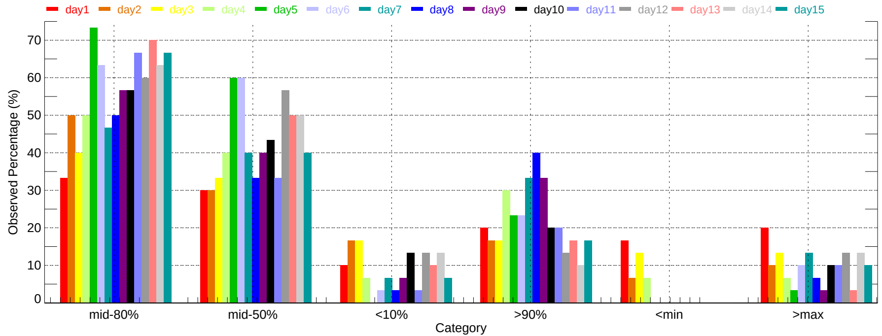
Observed Percentage of Ensembles - IAH: Max Temperature (2007-12-01~2007-12-31)
