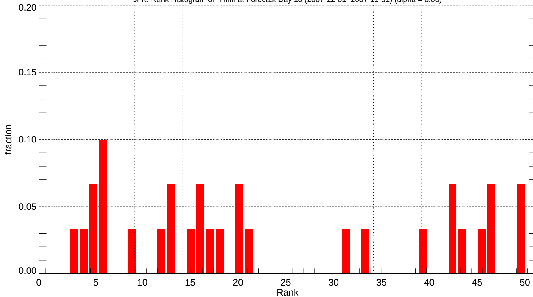
JFK: Rank Histogram of Tmin at Forecast Day 10 (2007-12-01~2007-12-31) (alpha = 0.00)
