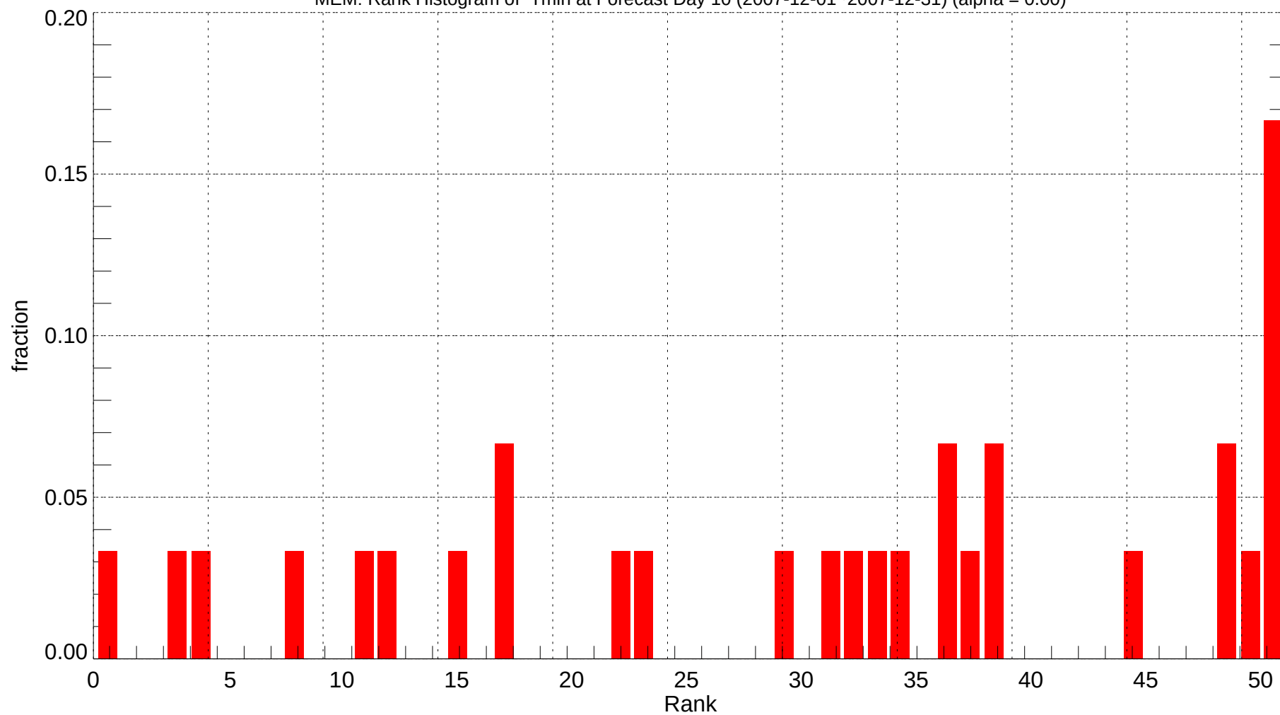
MEM: Rank Histogram of Tmin at Forecast Day 10 (2007-12-01~2007-12-31) (alpha = 0.00)
