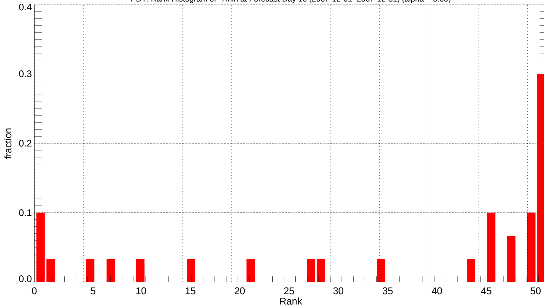
PDT: Rank Histogram of Tmin at Forecast Day 10 (2007-12-01~2007-12-31) (alpha = 0.00)
