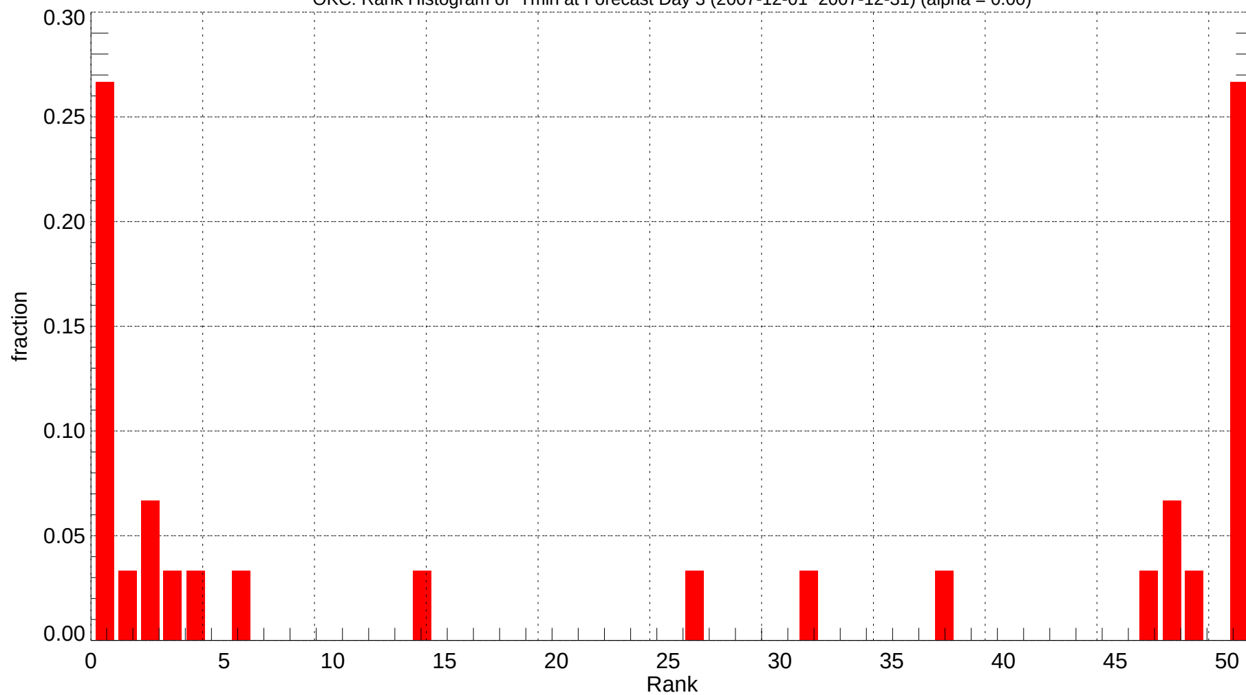
OKC: Rank Histogram of Tmin at Forecast Day 3 (2007-12-01~2007-12-31) (alpha = 0.00)
