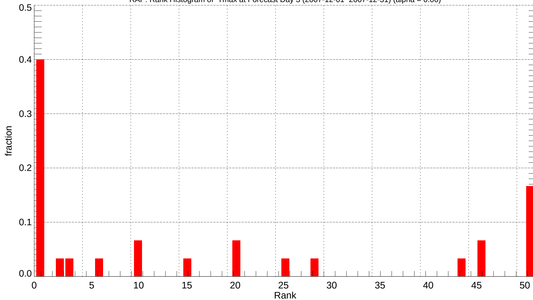
RAP: Rank Histogram of Tmax at Forecast Day 3 (2007-12-01~2007-12-31) (alpha = 0.00)
