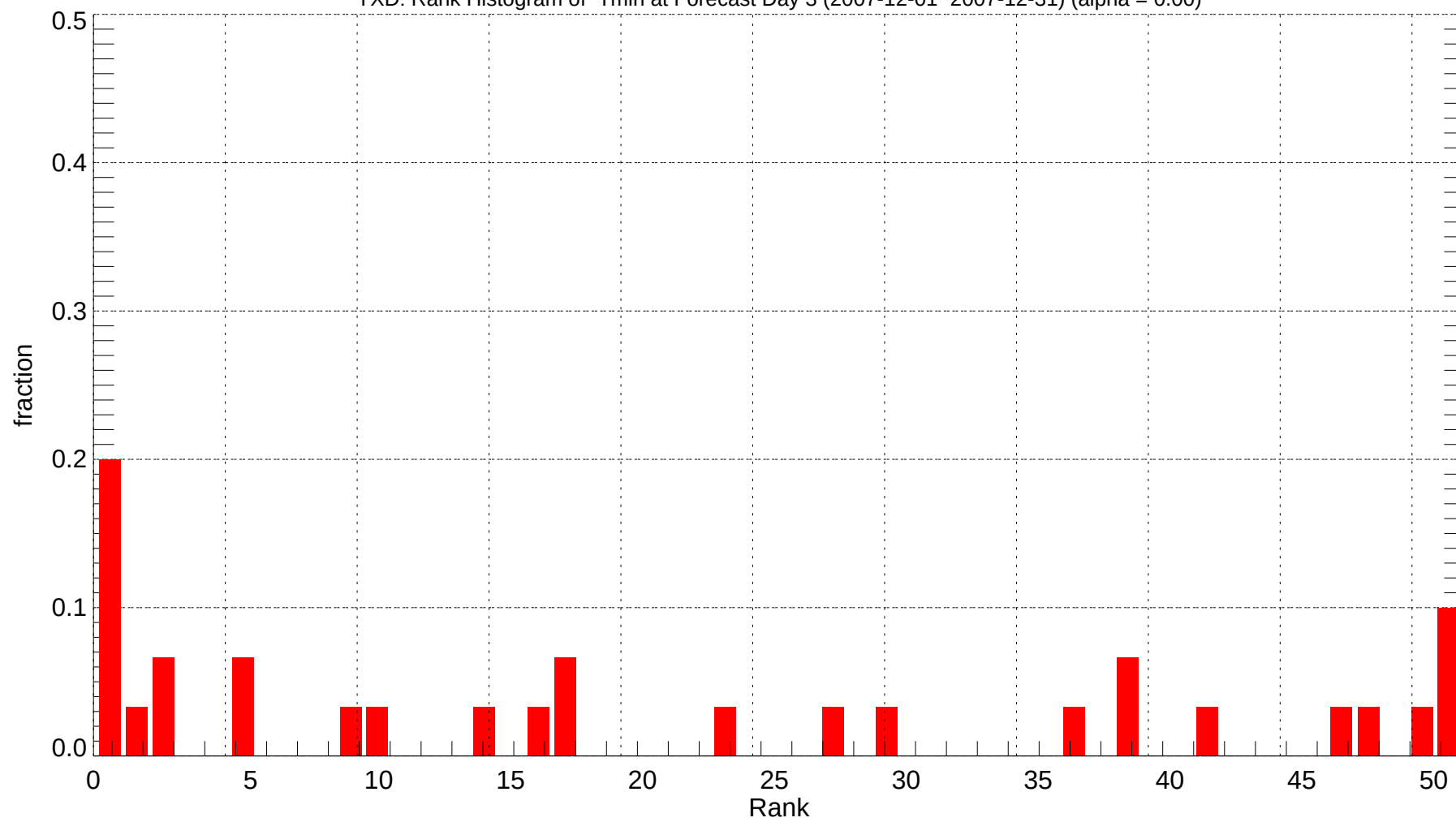
YXD: Rank Histogram of Tmin at Forecast Day 3 (2007-12-01~2007-12-31) (alpha = 0.00)
