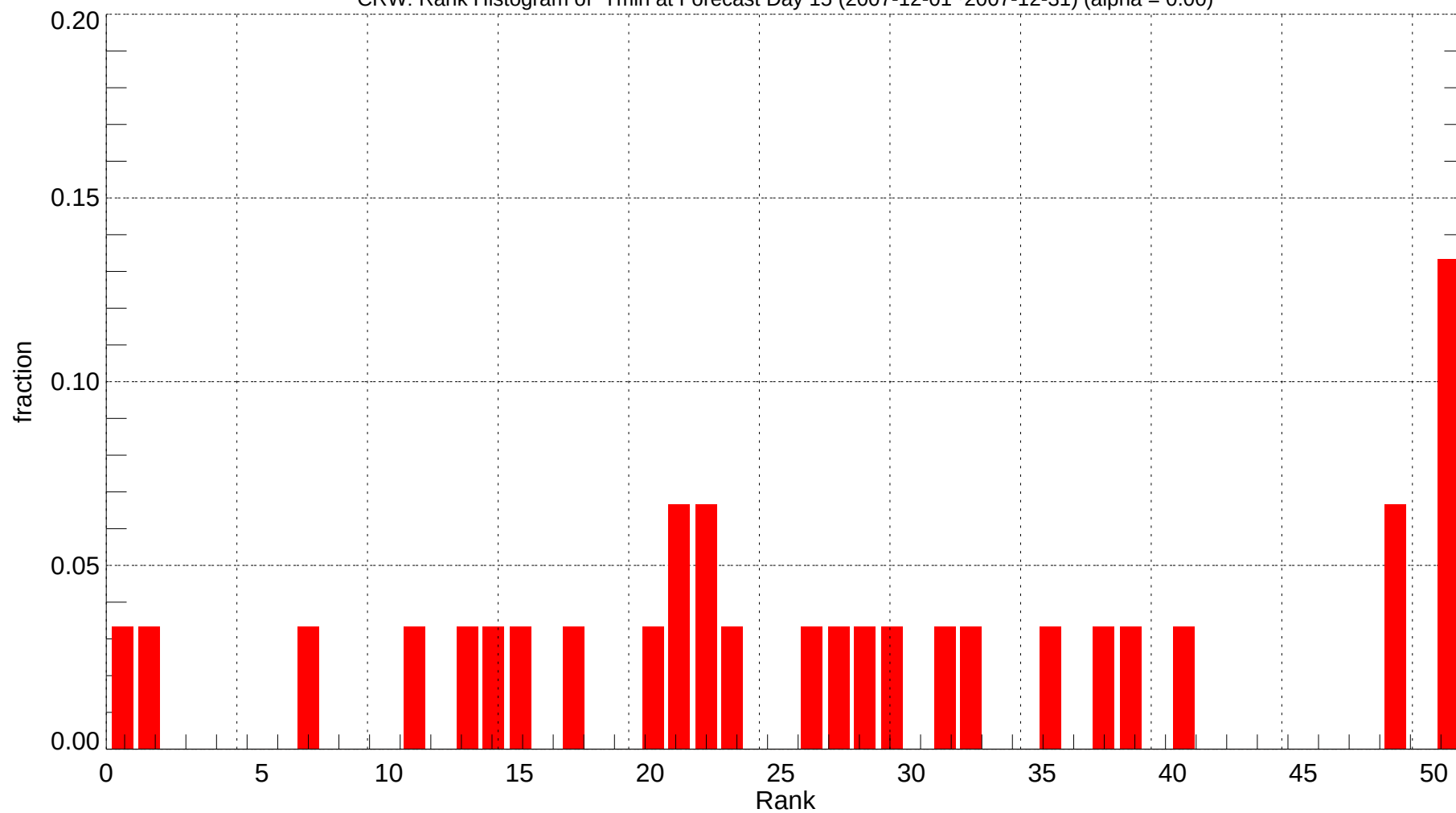
CRW: Rank Histogram of Tmin at Forecast Day 15 (2007-12-01~2007-12-31) (alpha = 0.00)
