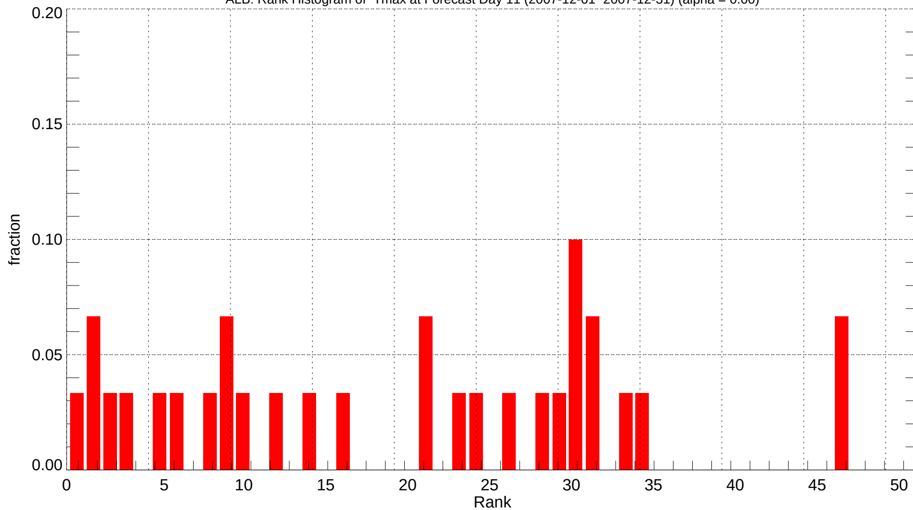
ALB: Rank Histogram of Tmax at Forecast Day 11 (2007-12-01~2007-12-31) (alpha = 0.00)
