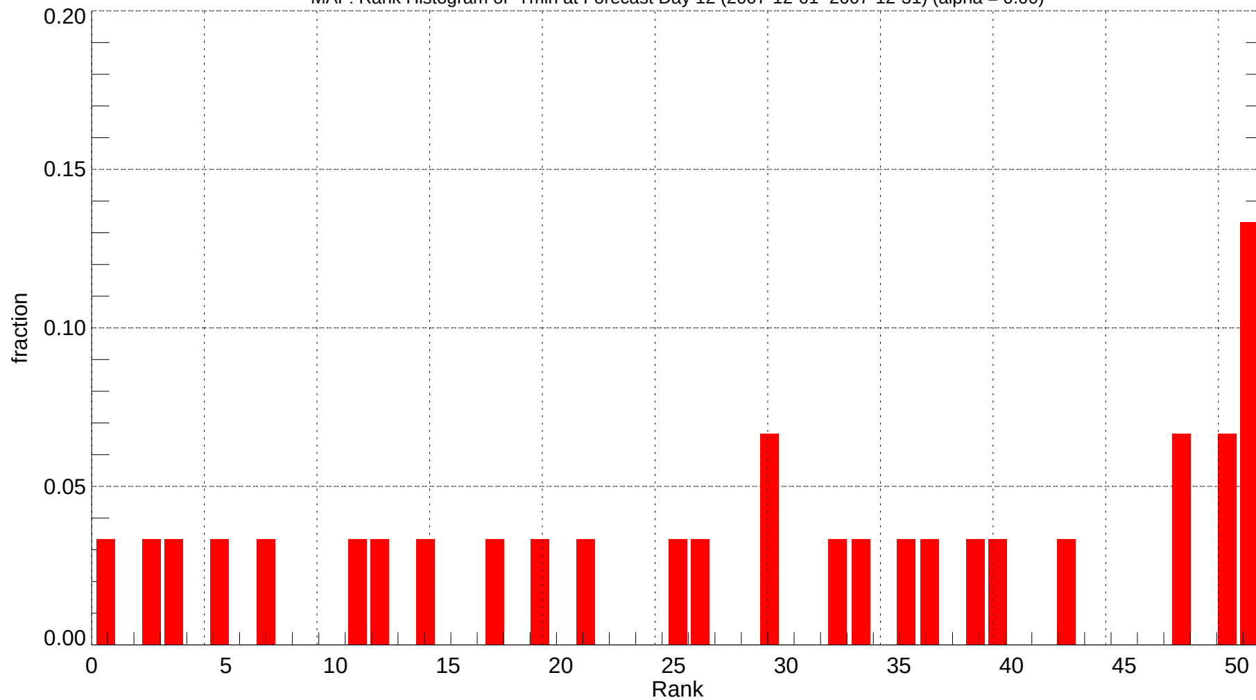
MAF: Rank Histogram of Tmin at Forecast Day 12 (2007-12-01~2007-12-31) (alpha = 0.00)
