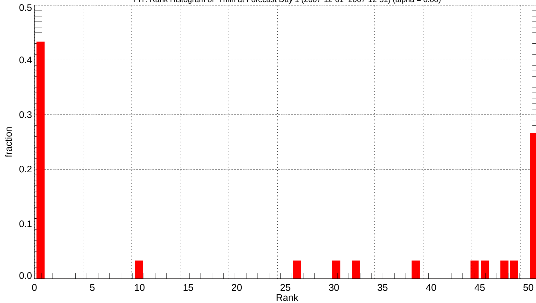
PIT: Rank Histogram of Tmin at Forecast Day 1 (2007-12-01~2007-12-31) (alpha = 0.00)
