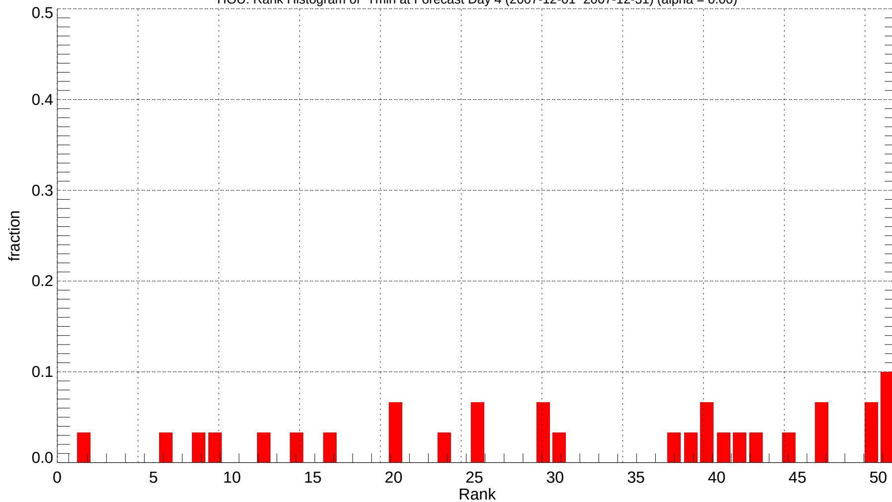
HOU: Rank Histogram of Tmin at Forecast Day 4 (2007-12-01~2007-12-31) (alpha = 0.00)
