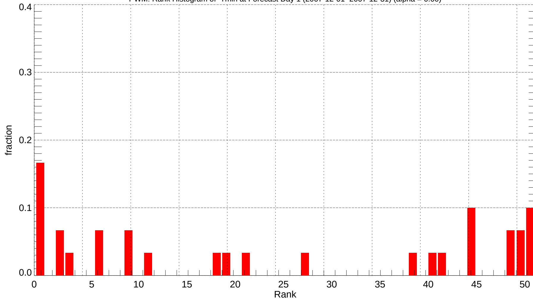
PWM: Rank Histogram of Tmin at Forecast Day 1 (2007-12-01~2007-12-31) (alpha = 0.00)
