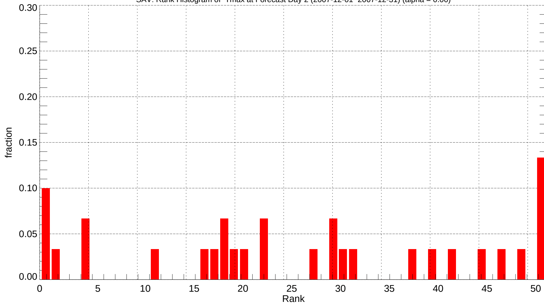
SAV: Rank Histogram of Tmax at Forecast Day 2 (2007-12-01~2007-12-31) (alpha = 0.00)
