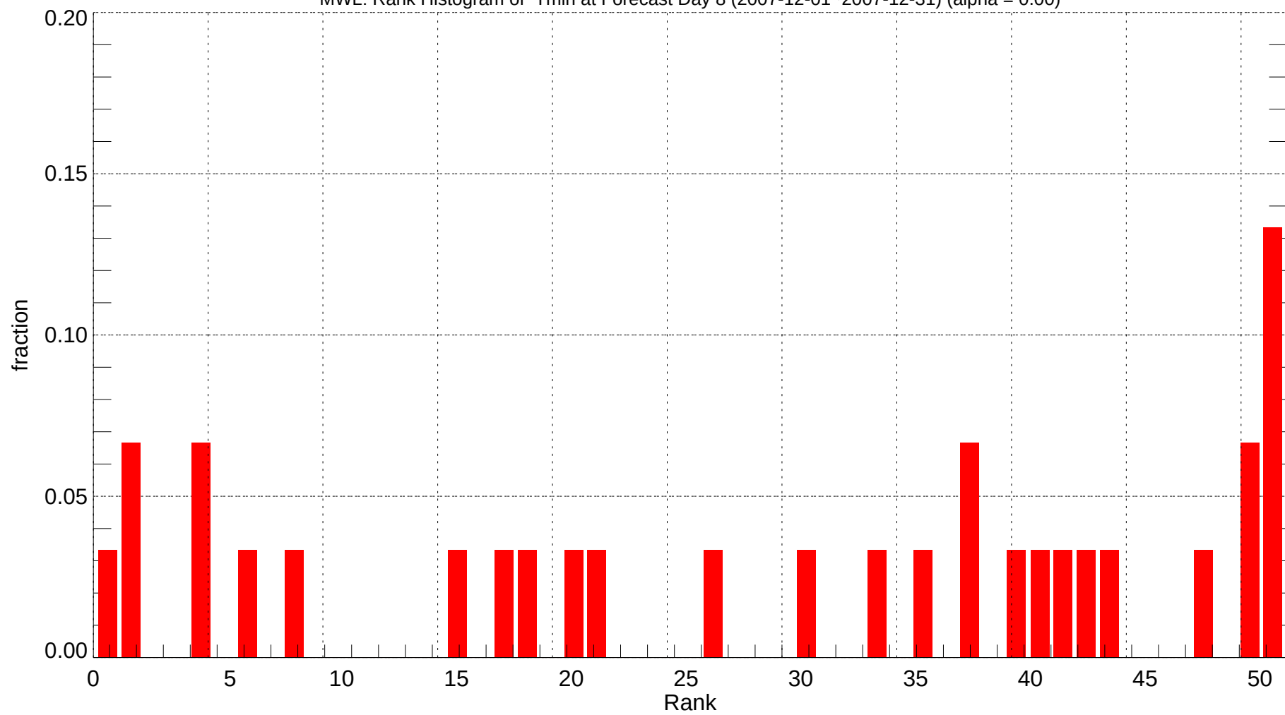
MWL: Rank Histogram of Tmin at Forecast Day 8 (2007-12-01~2007-12-31) (alpha = 0.00)
