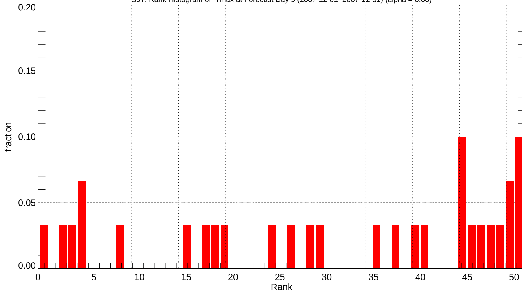
SJT: Rank Histogram of Tmax at Forecast Day 9 (2007-12-01~2007-12-31) (alpha = 0.00)
