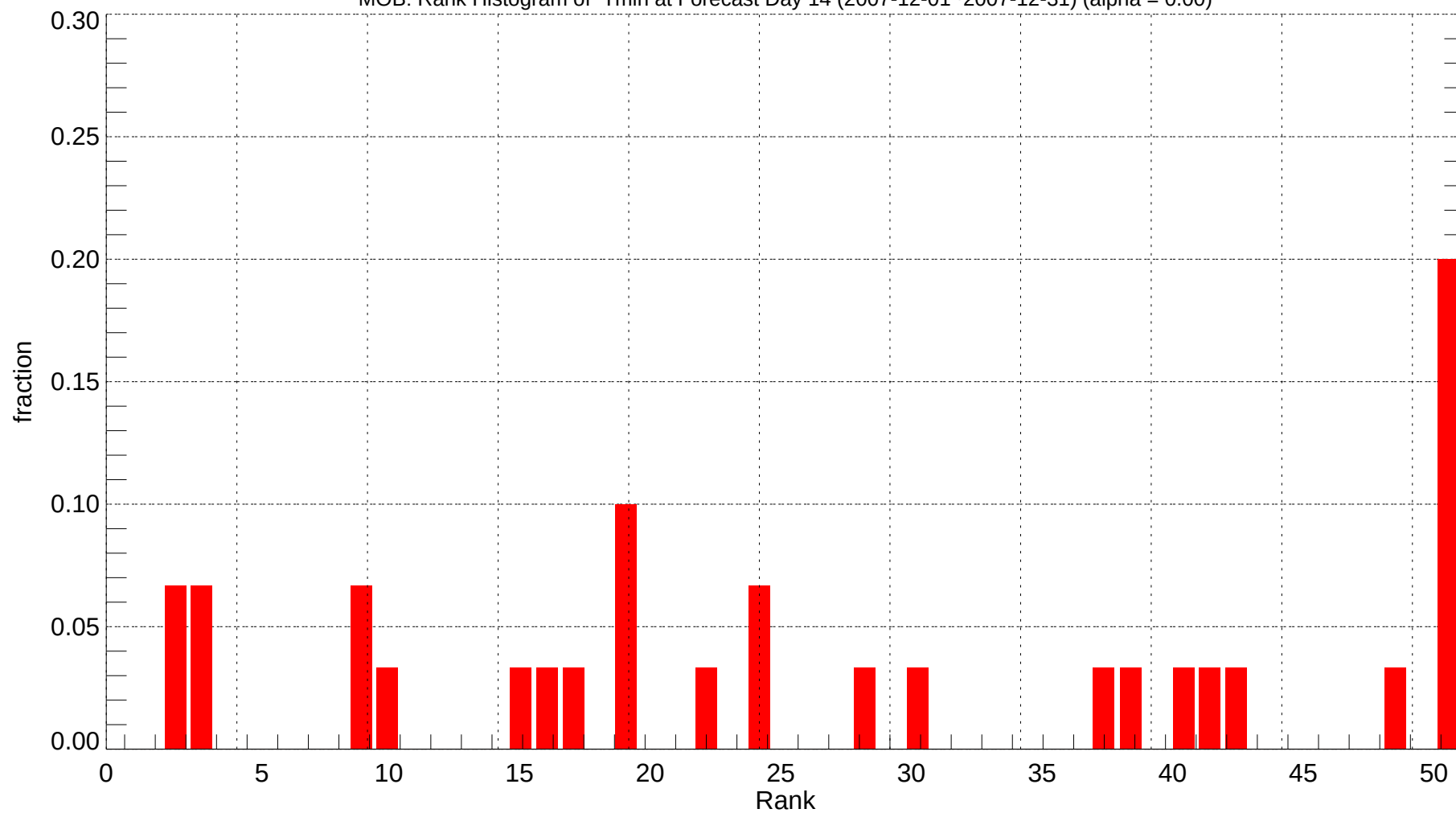
MOB: Rank Histogram of Tmin at Forecast Day 14 (2007-12-01~2007-12-31) (alpha = 0.00)
