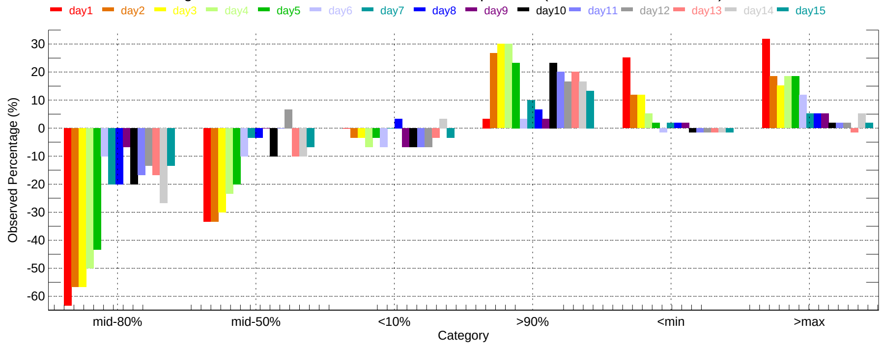
Observed Percentage Deviation of Ensembles - BIS: Min Temperature (2007-12-01~2007-12-31)
