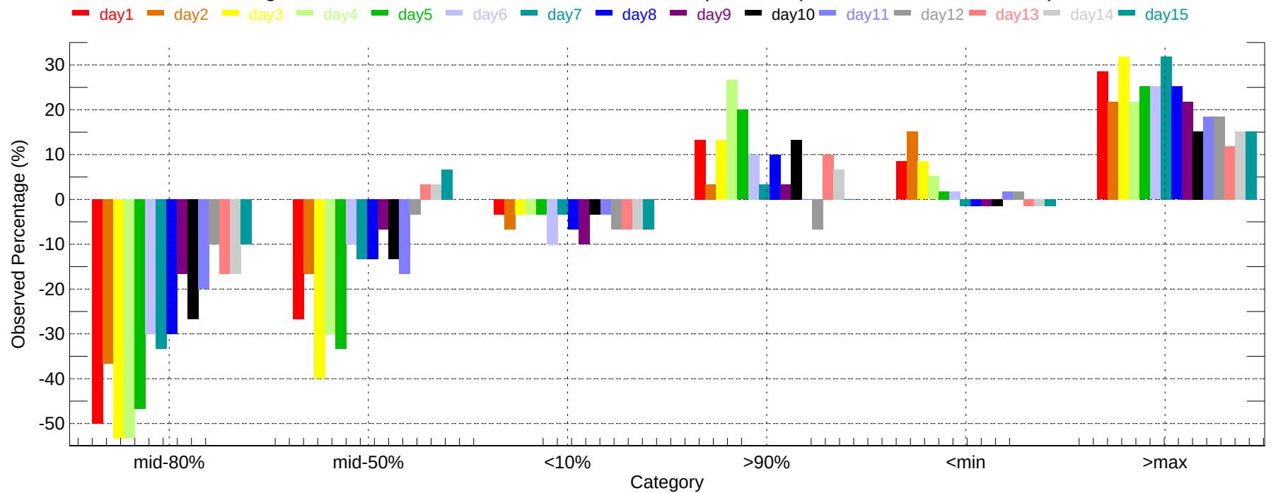
Observed Percentage Deviation of Ensembles - SAT: Max Temperature (2007-12-01~2007-12-31)
