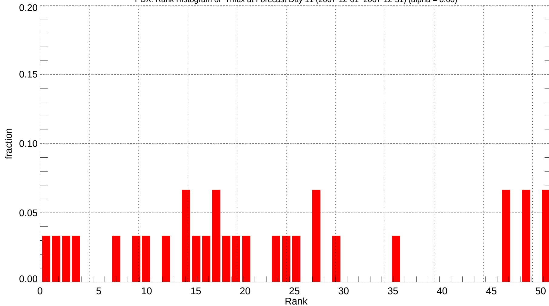
PDX: Rank Histogram of Tmax at Forecast Day 11 (2007-12-01~2007-12-31) (alpha = 0.00)
