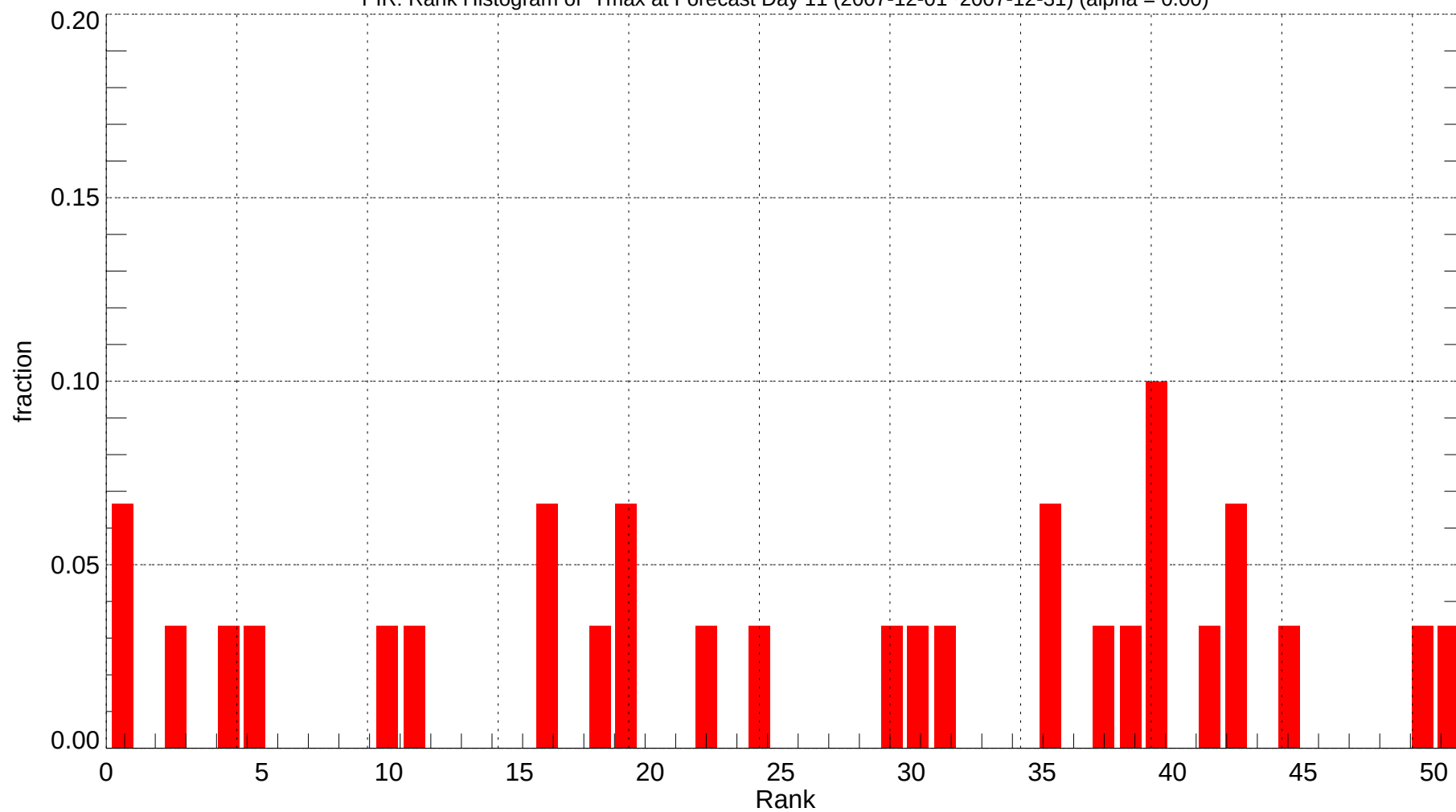
PIR: Rank Histogram of Tmax at Forecast Day 11 (2007-12-01~2007-12-31) (alpha = 0.00)
