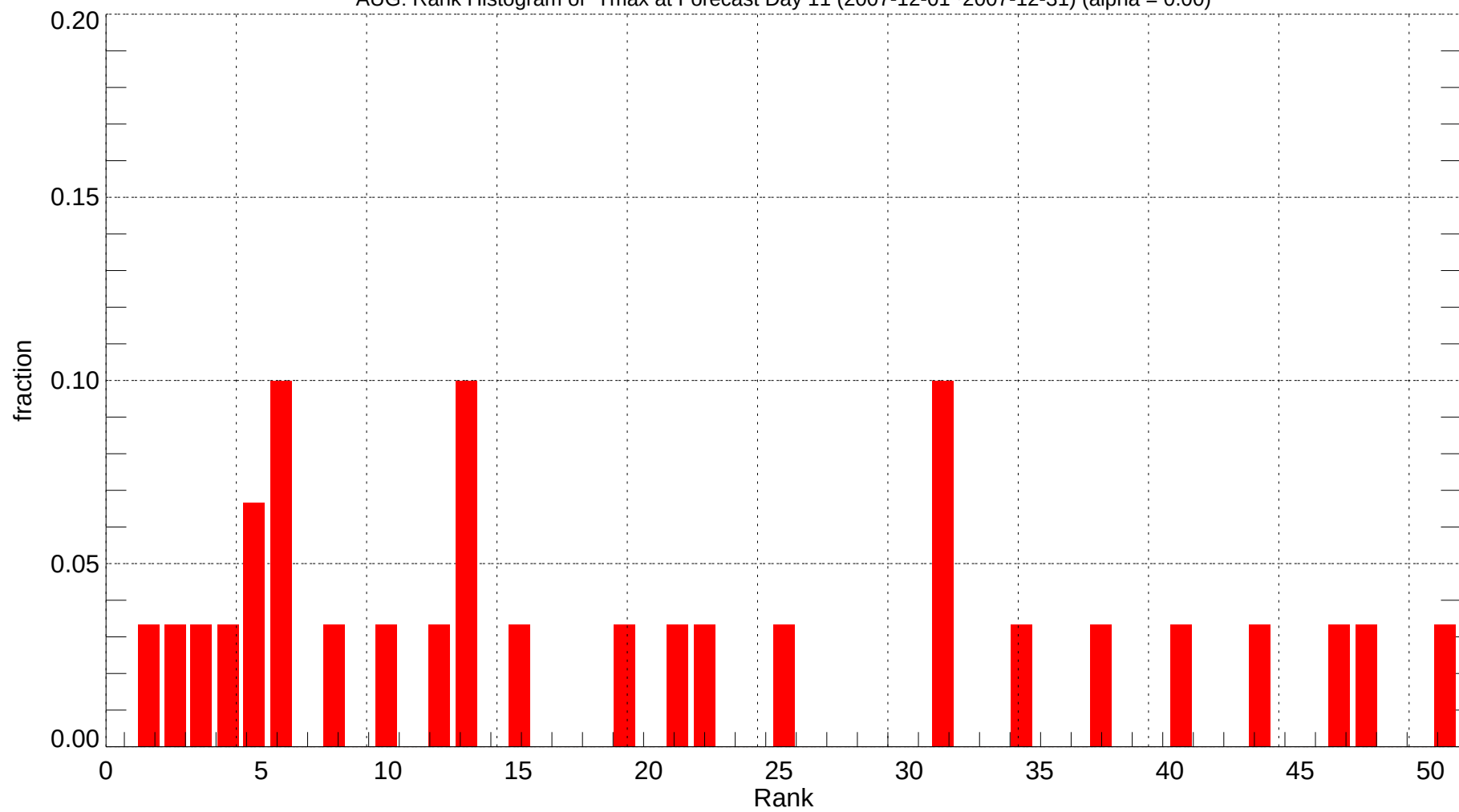
AUG: Rank Histogram of Tmax at Forecast Day 11 (2007-12-01~2007-12-31) (alpha = 0.00)
