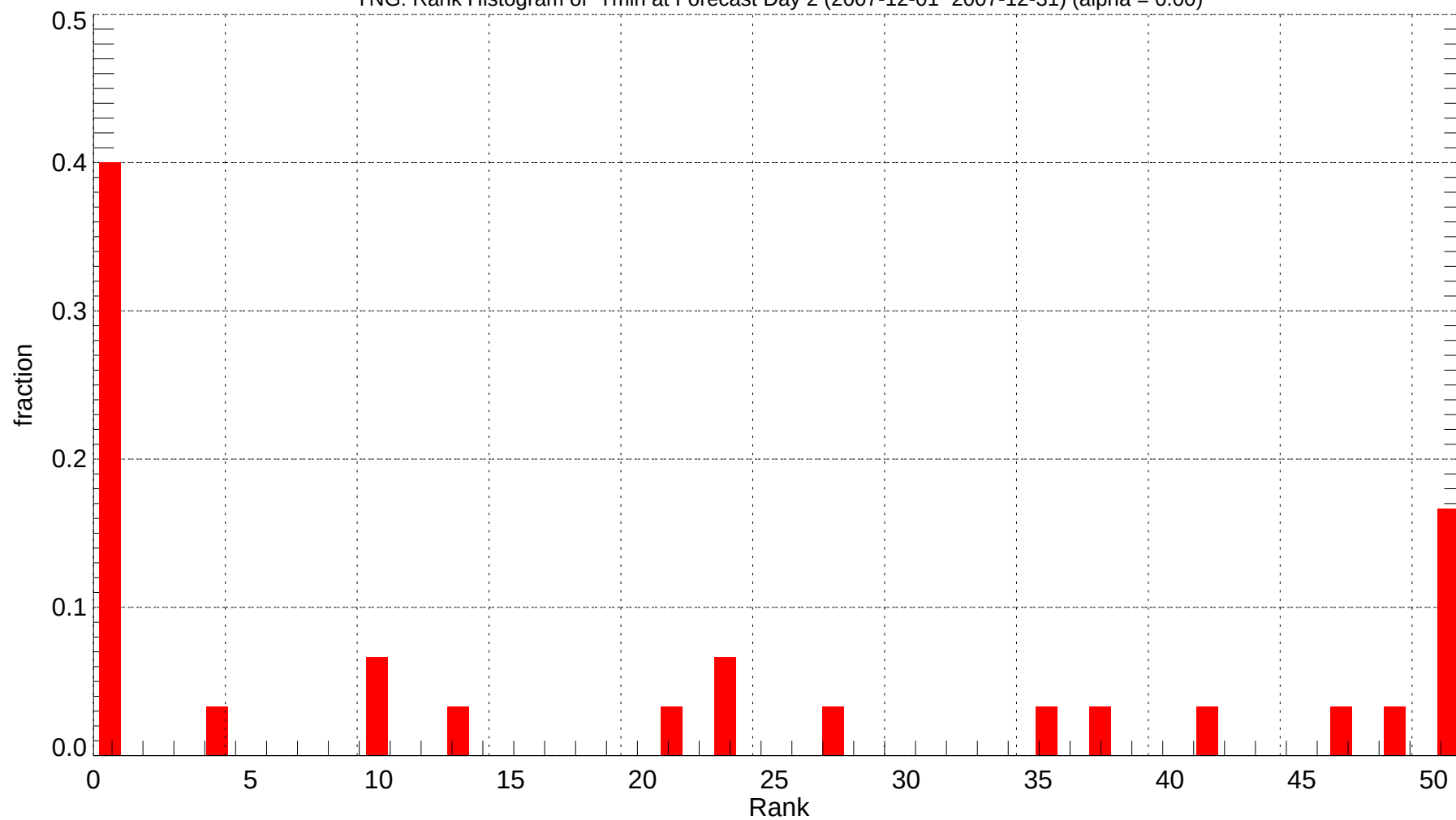
YNG: Rank Histogram of Tmin at Forecast Day 2 (2007-12-01~2007-12-31) (alpha = 0.00)
