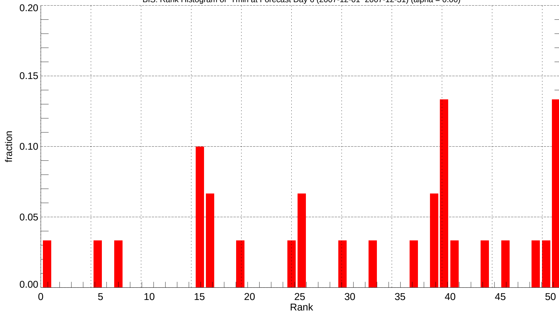
BIS: Rank Histogram of Tmin at Forecast Day 6 (2007-12-01~2007-12-31) (alpha = 0.00)
