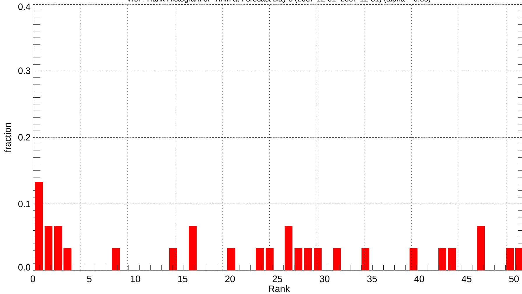
WJF: Rank Histogram of Tmin at Forecast Day 5 (2007-12-01~2007-12-31) (alpha = 0.00)
