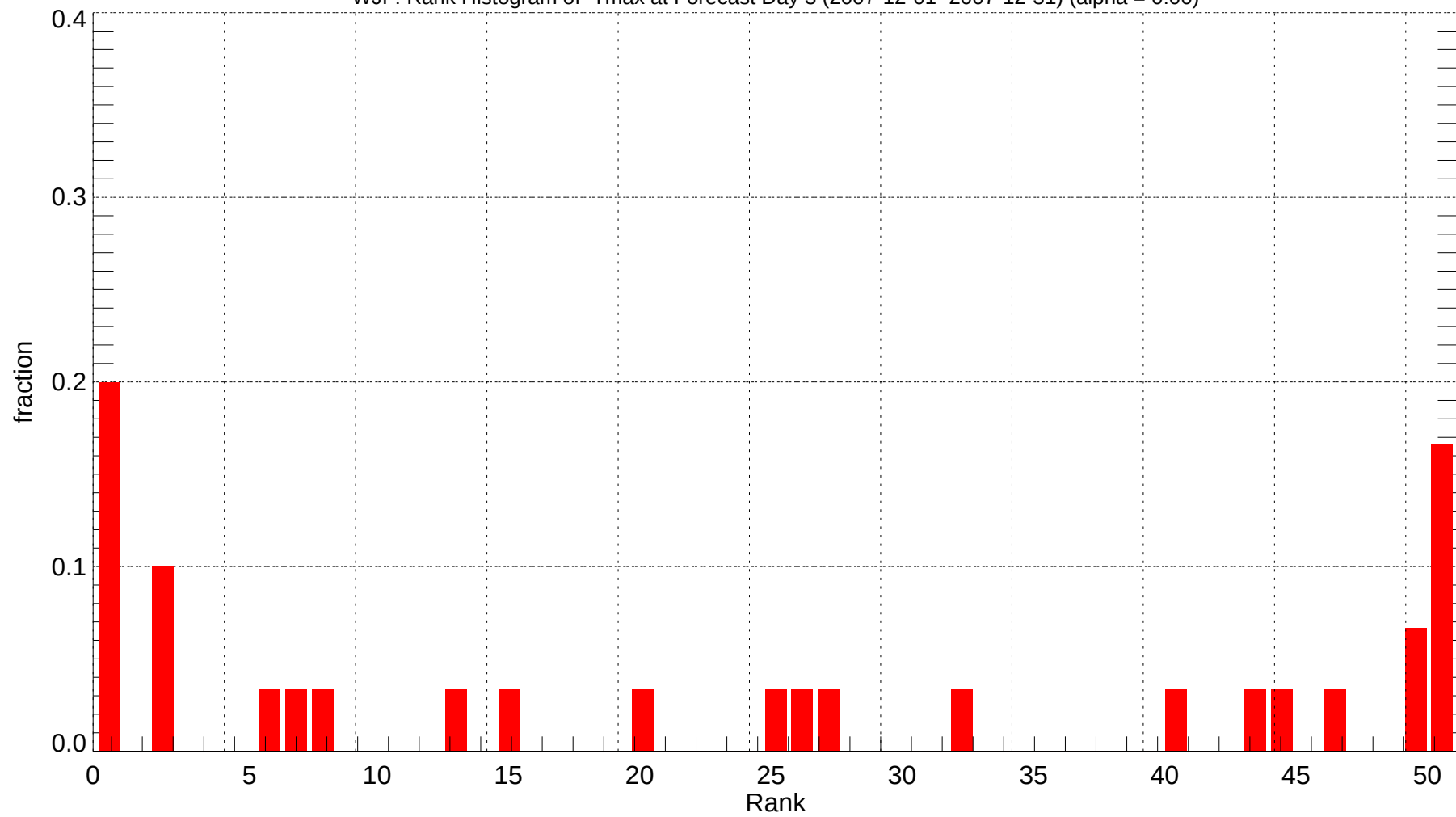
WJF: Rank Histogram of Tmax at Forecast Day 3 (2007-12-01~2007-12-31) (alpha = 0.00)
