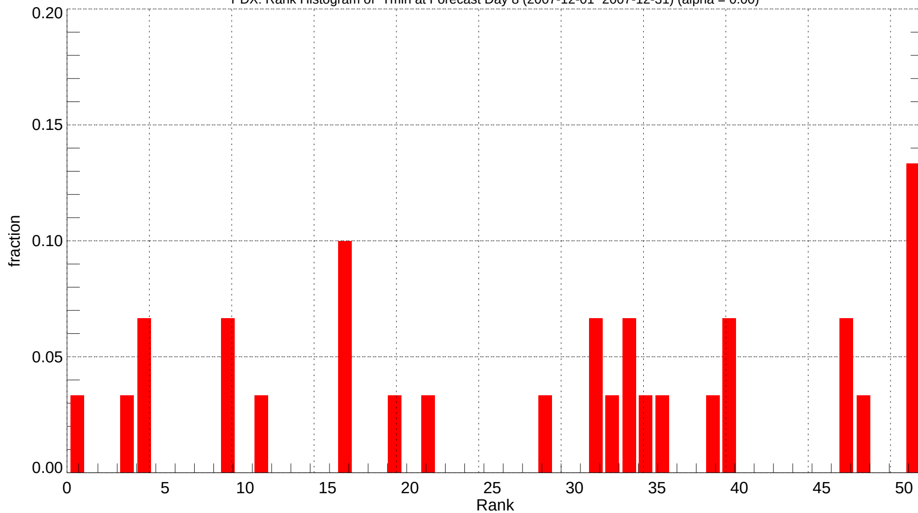
PDX: Rank Histogram of Tmin at Forecast Day 8 (2007-12-01~2007-12-31) (alpha = 0.00)
