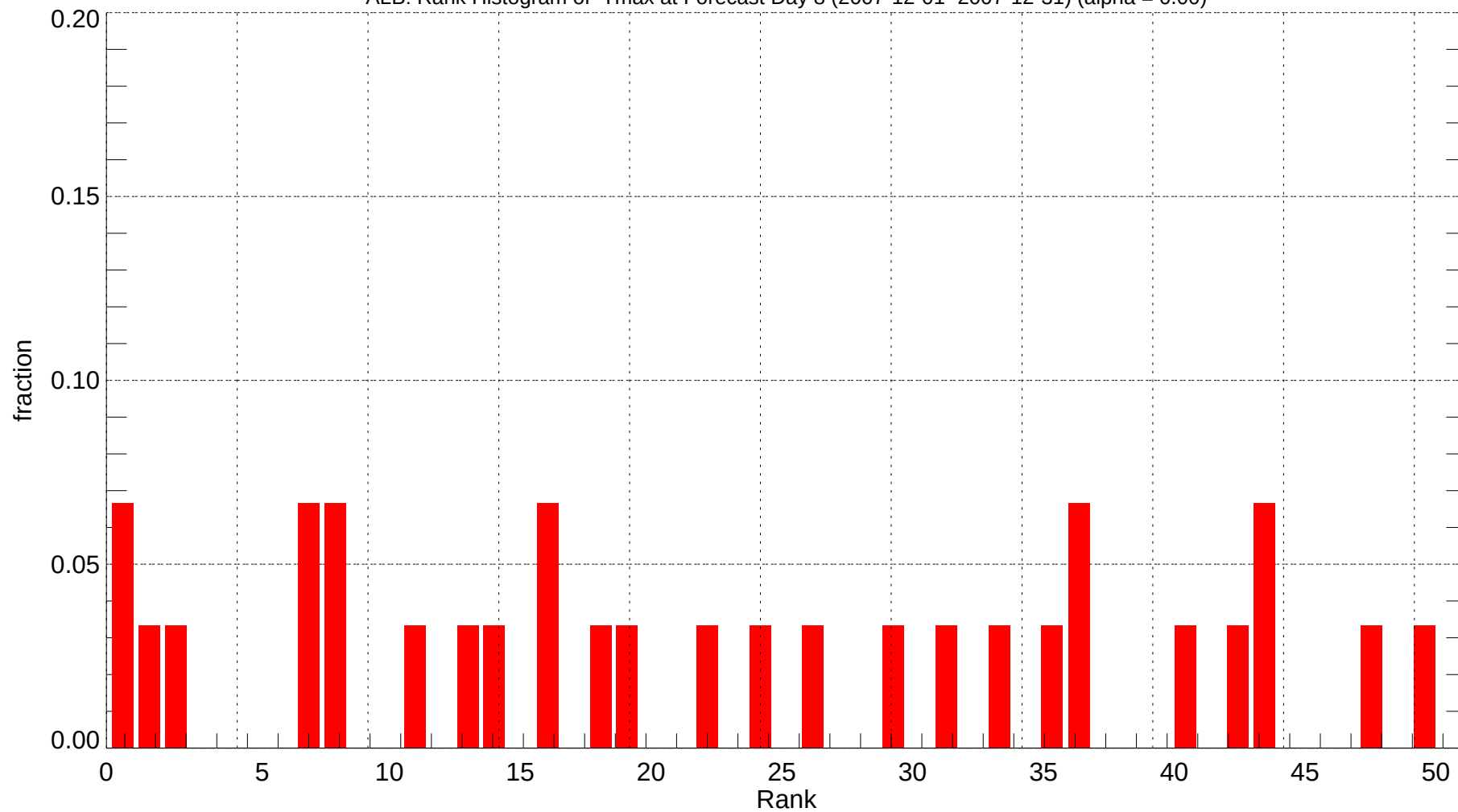
ALB: Rank Histogram of Tmax at Forecast Day 8 (2007-12-01~2007-12-31) (alpha = 0.00)
