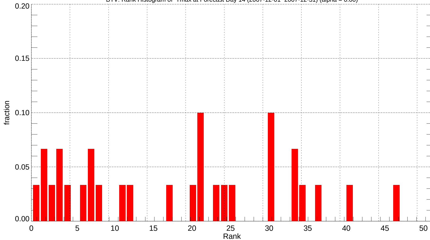
BTV: Rank Histogram of Tmax at Forecast Day 14 (2007-12-01~2007-12-31) (alpha = 0.00)
