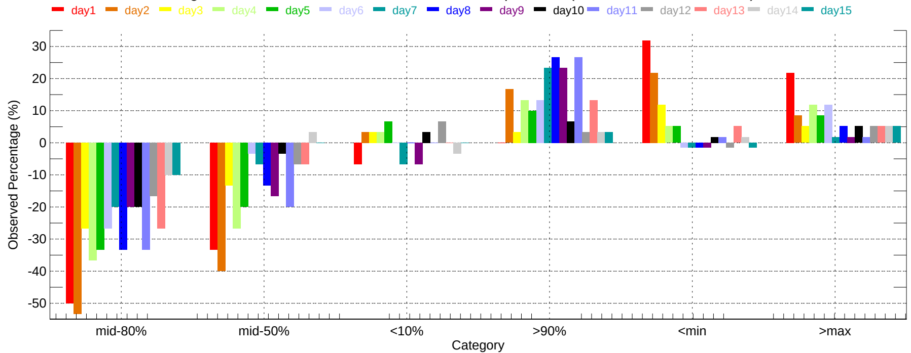
Observed Percentage Deviation of Ensembles - ROA: Min Temperature (2007-12-01~2007-12-31)
