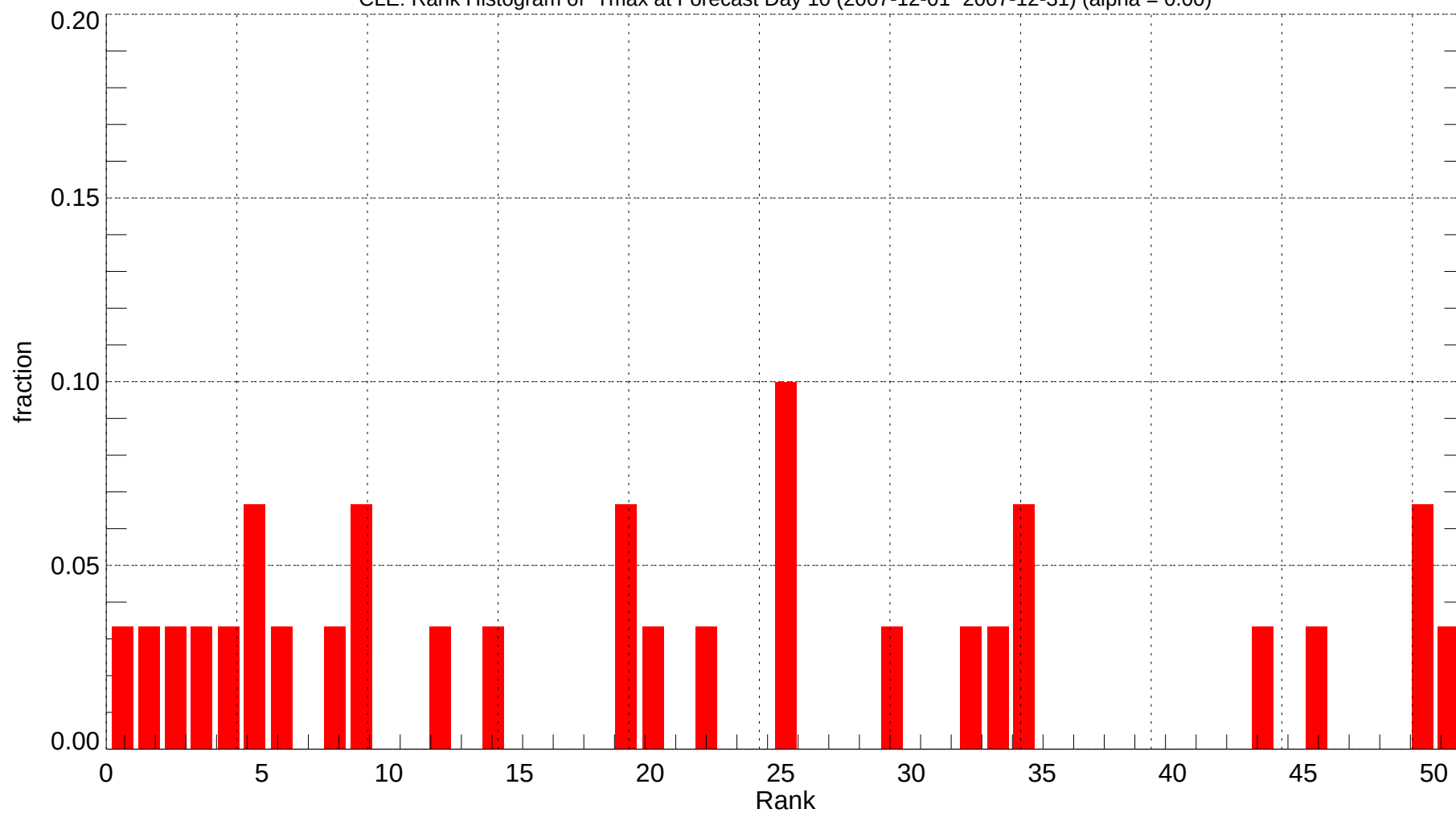
CLE: Rank Histogram of Tmax at Forecast Day 10 (2007-12-01~2007-12-31) (alpha = 0.00)
