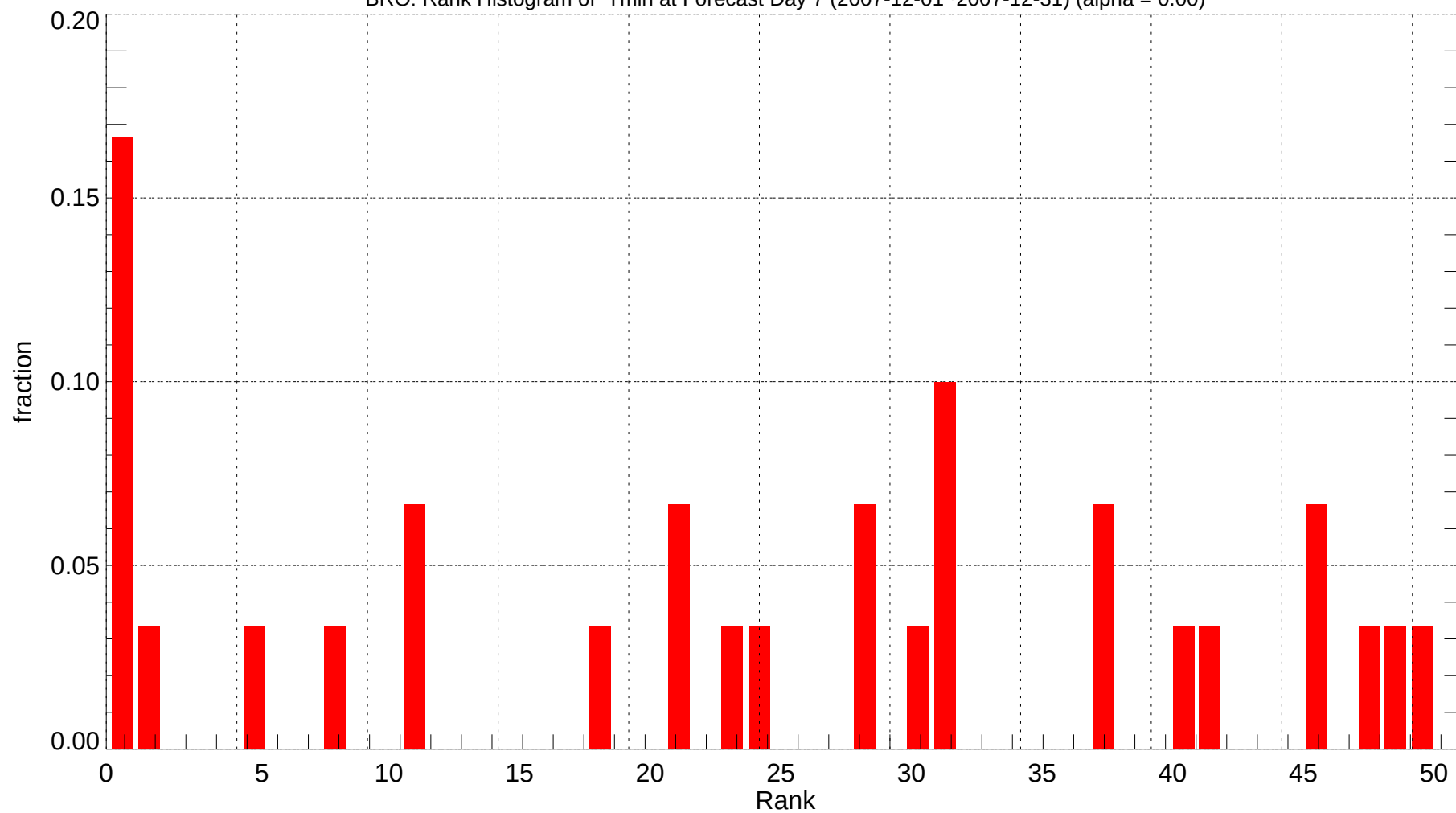
BRO: Rank Histogram of Tmin at Forecast Day 7 (2007-12-01~2007-12-31) (alpha = 0.00)
