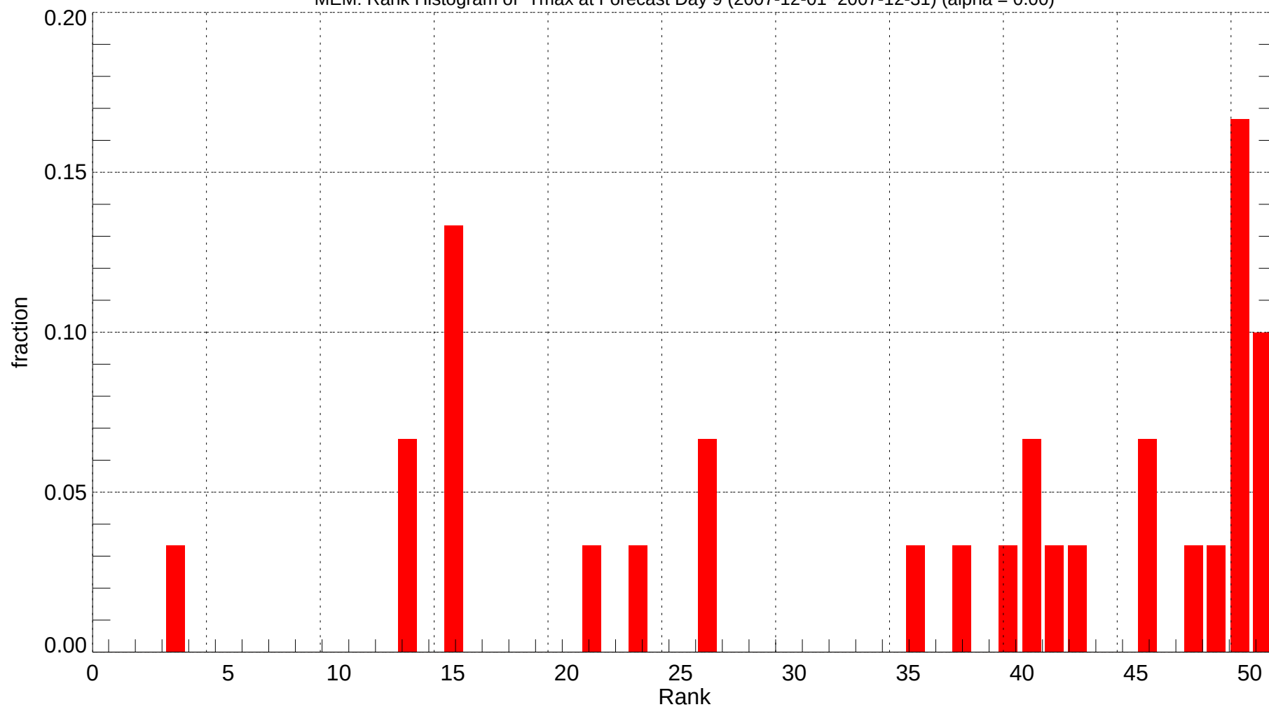
MEM: Rank Histogram of Tmax at Forecast Day 9 (2007-12-01~2007-12-31) (alpha = 0.00)
