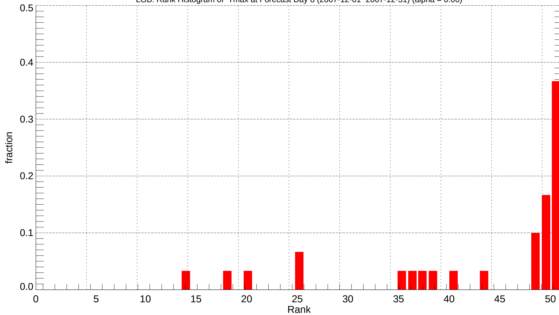
LGB: Rank Histogram of Tmax at Forecast Day 8 (2007-12-01~2007-12-31) (alpha = 0.00)
