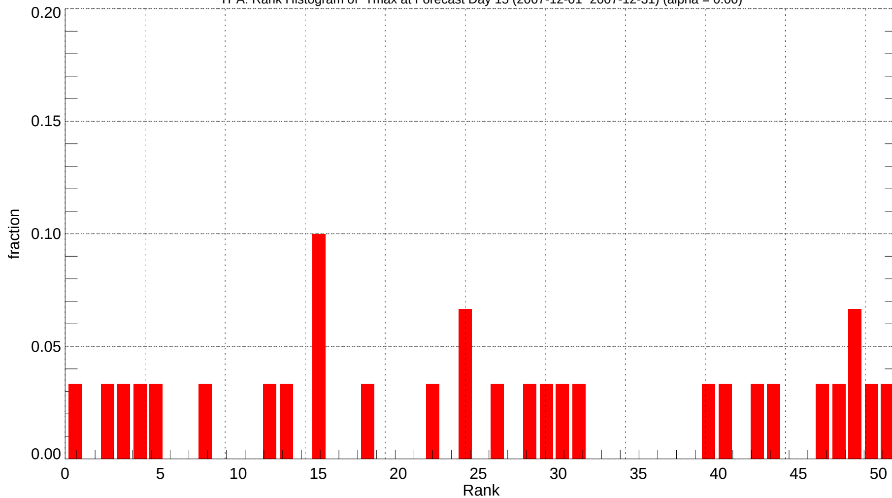
TPA: Rank Histogram of Tmax at Forecast Day 15 (2007-12-01~2007-12-31) (alpha = 0.00)
