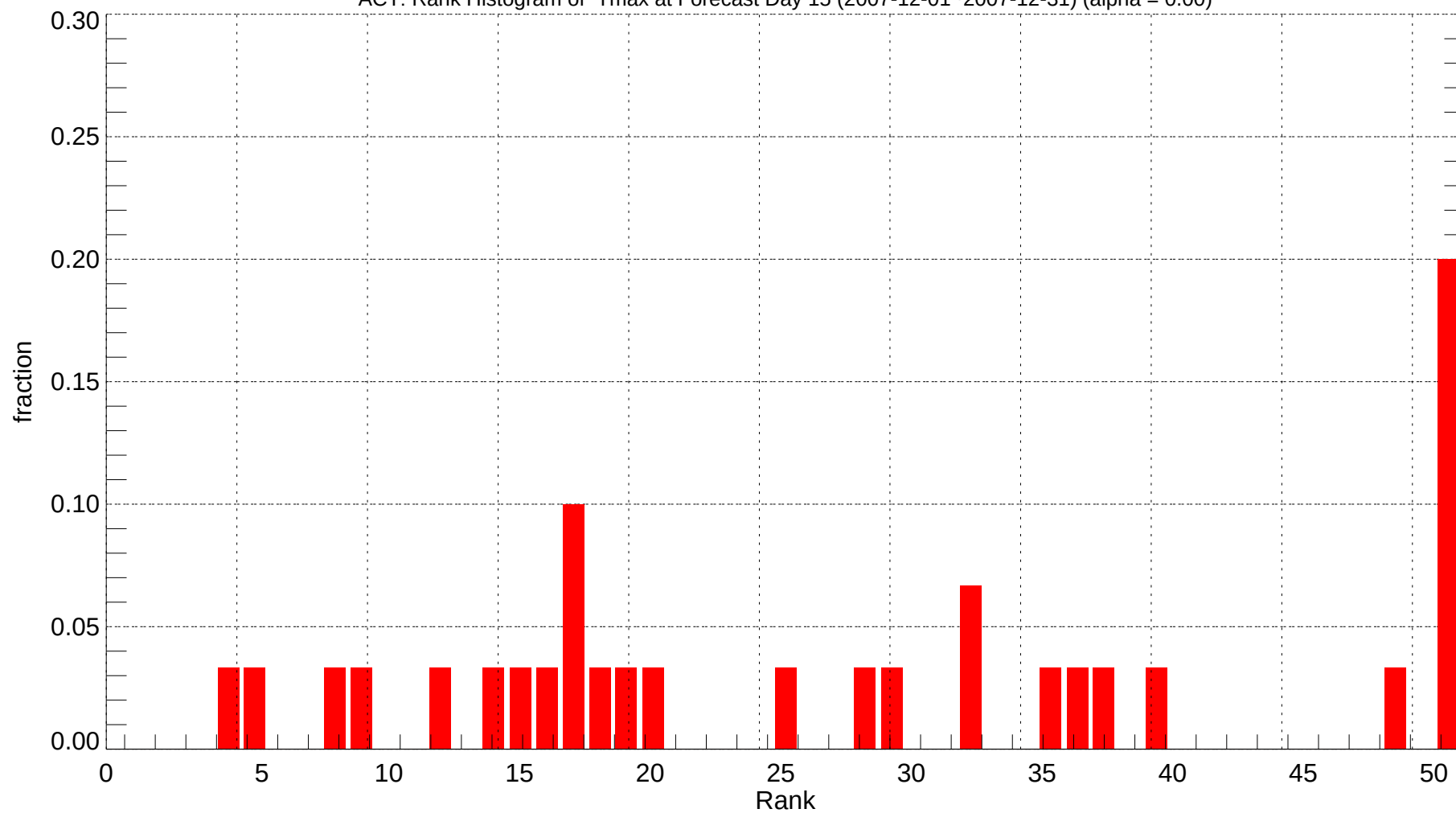
ACT: Rank Histogram of Tmax at Forecast Day 15 (2007-12-01~2007-12-31) (alpha = 0.00)
