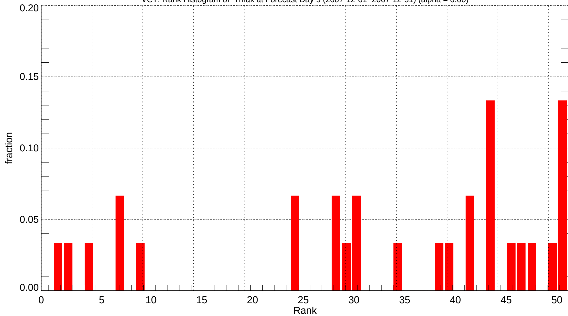
VCT: Rank Histogram of Tmax at Forecast Day 9 (2007-12-01~2007-12-31) (alpha = 0.00)
