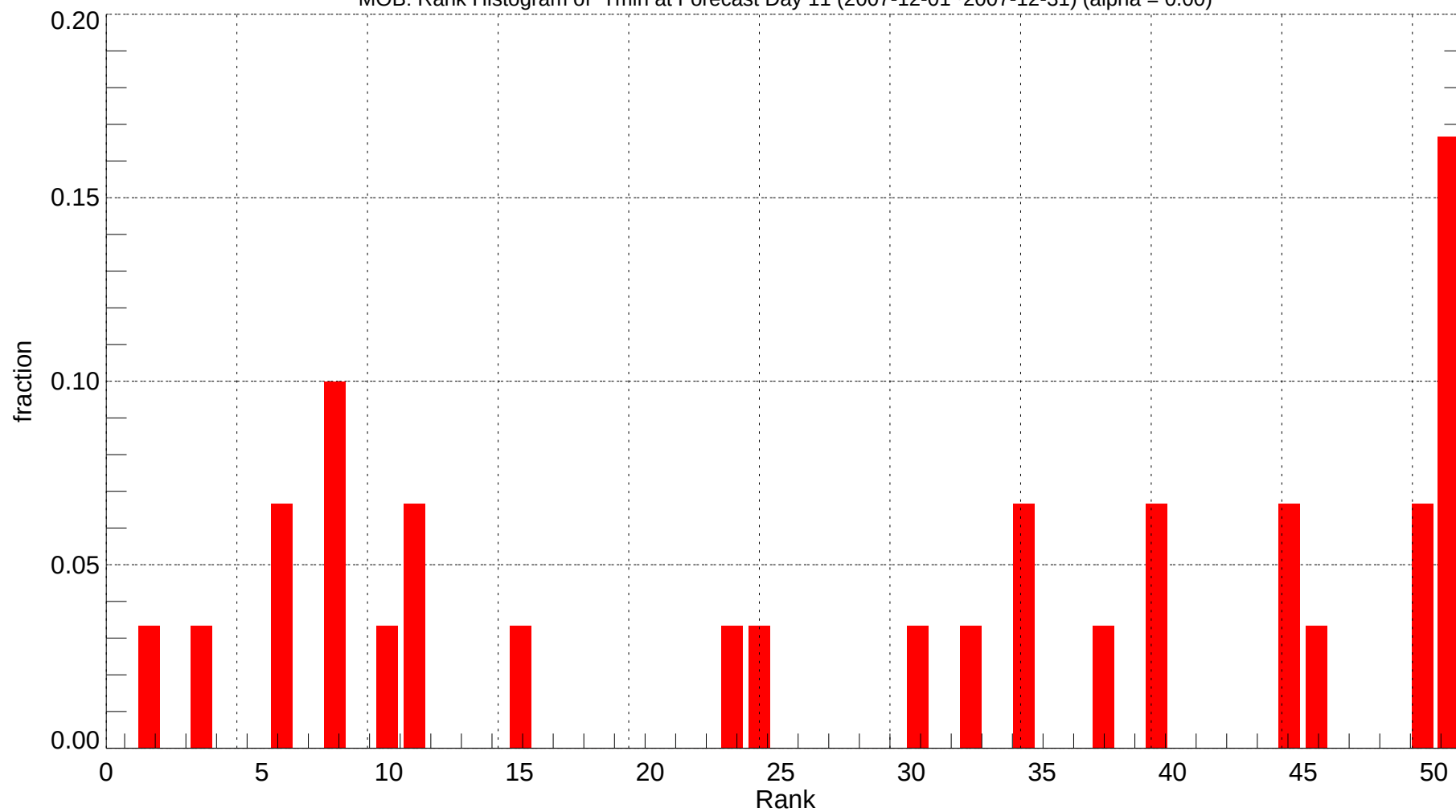
MOB: Rank Histogram of Tmin at Forecast Day 11 (2007-12-01~2007-12-31) (alpha = 0.00)
