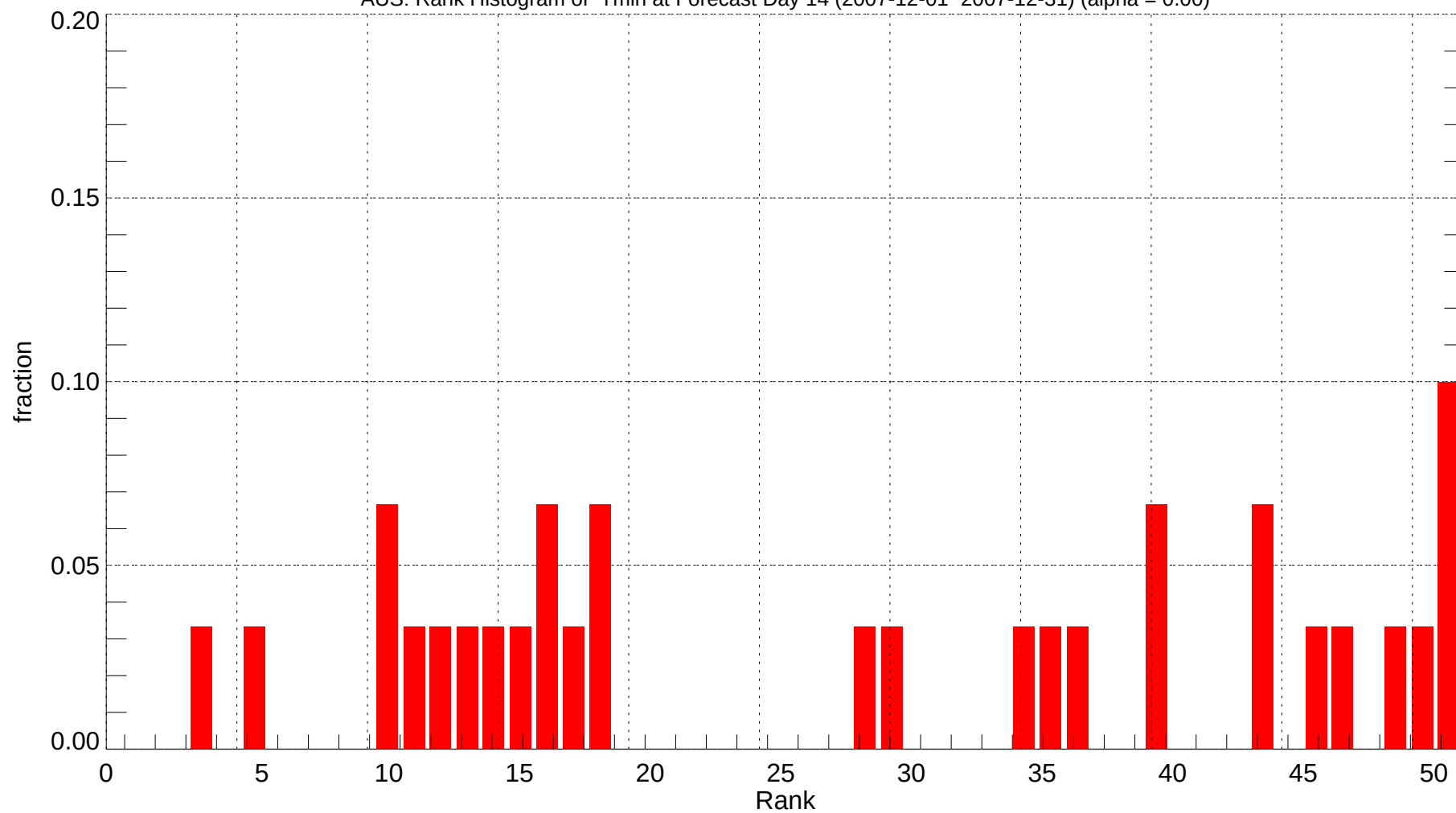
AUS: Rank Histogram of Tmin at Forecast Day 14 (2007-12-01~2007-12-31) (alpha = 0.00)
