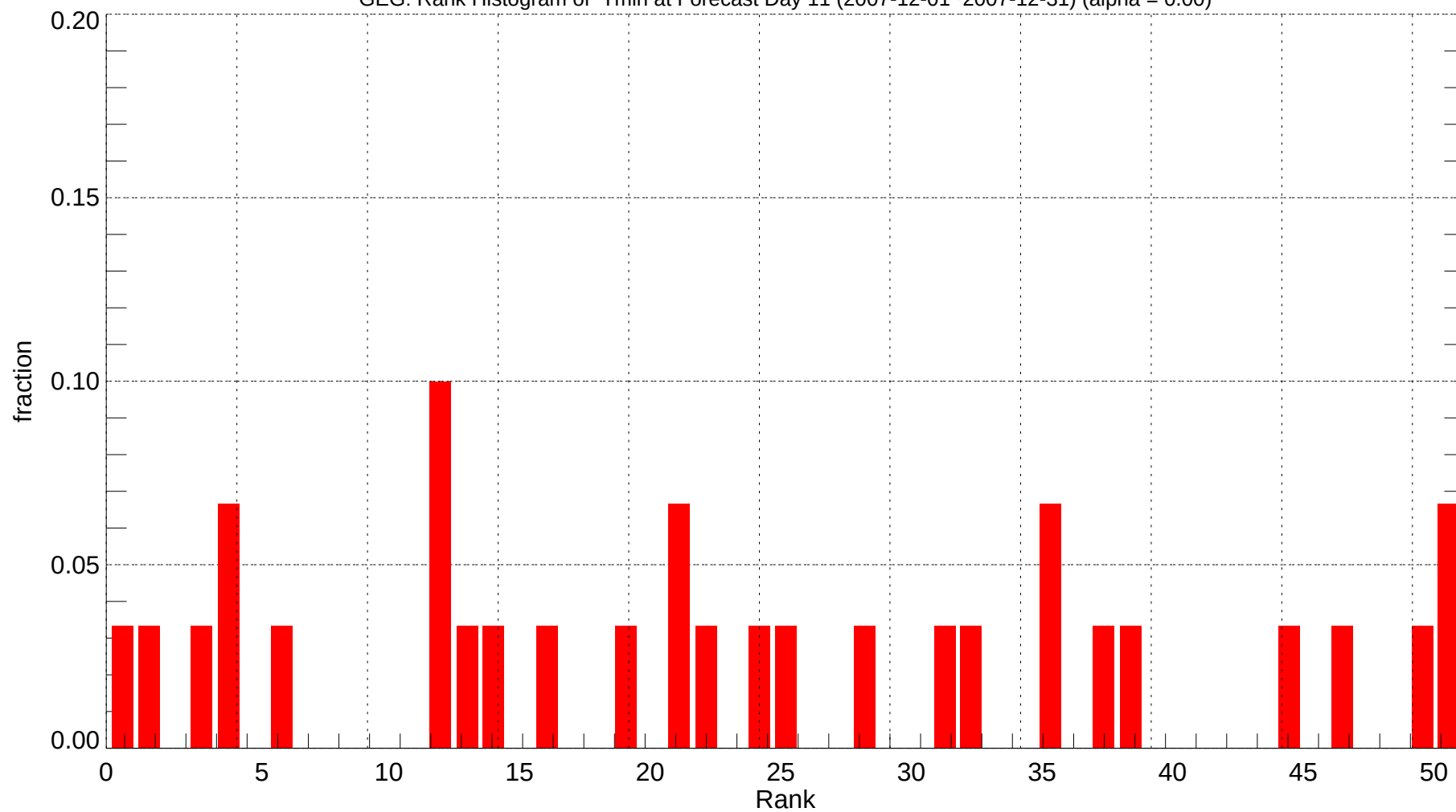
GEG: Rank Histogram of Tmin at Forecast Day 11 (2007-12-01~2007-12-31) (alpha = 0.00)
