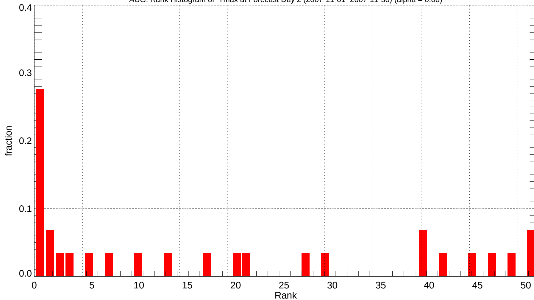
AUG: Rank Histogram of Tmax at Forecast Day 2 (2007-11-01~2007-11-30) (alpha = 0.00)
