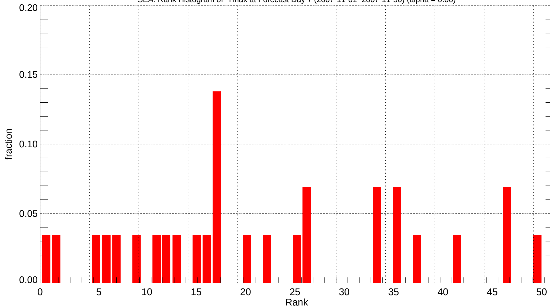
SEA: Rank Histogram of Tmax at Forecast Day 7 (2007-11-01~2007-11-30) (alpha = 0.00)
