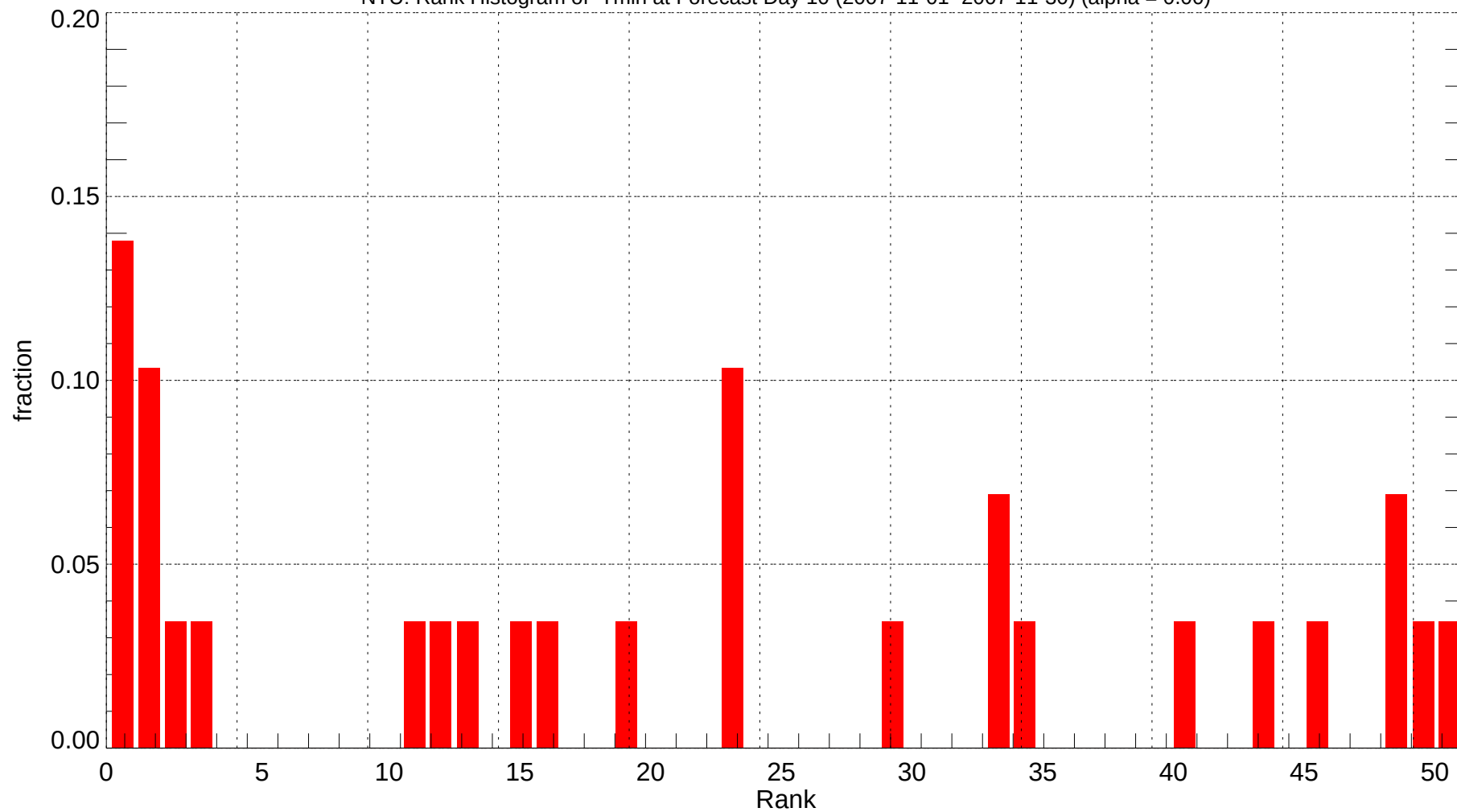
NTU: Rank Histogram of Tmin at Forecast Day 10 (2007-11-01~2007-11-30) (alpha = 0.00)
