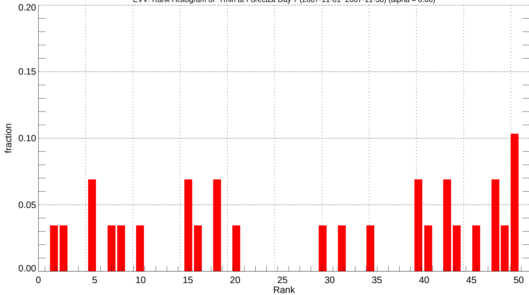
EVV: Rank Histogram of Tmin at Forecast Day 7 (2007-11-01~2007-11-30) (alpha = 0.00)
