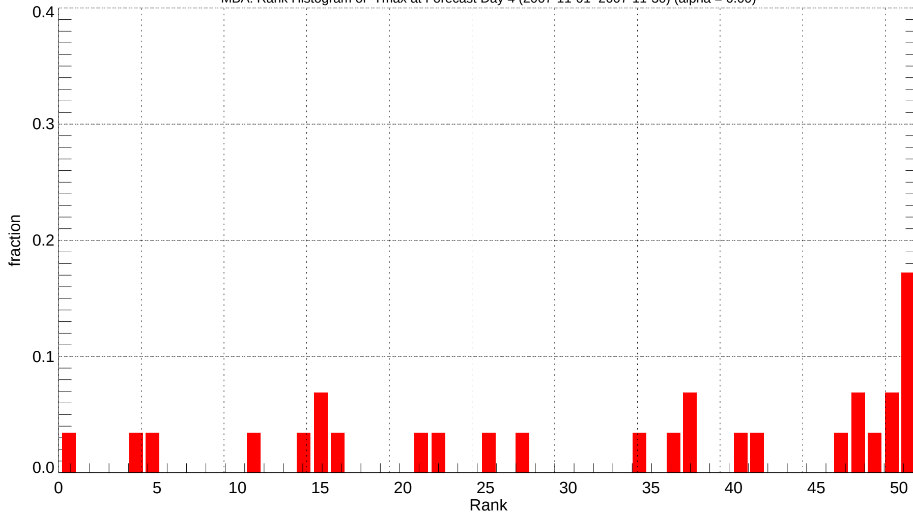
MBA: Rank Histogram of Tmax at Forecast Day 4 (2007-11-01~2007-11-30) (alpha = 0.00)
