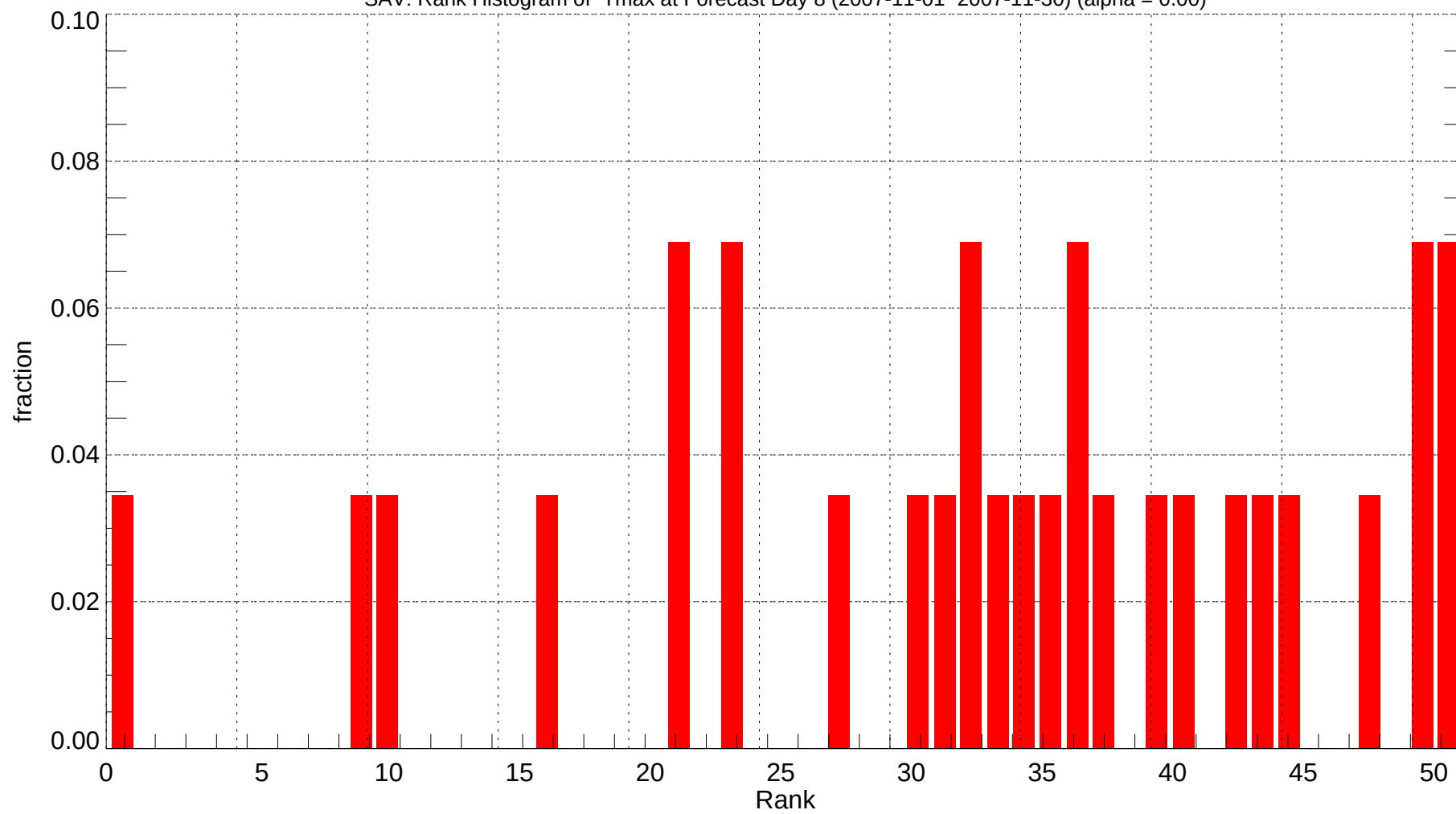
SAV: Rank Histogram of Tmax at Forecast Day 8 (2007-11-01~2007-11-30) (alpha = 0.00)
