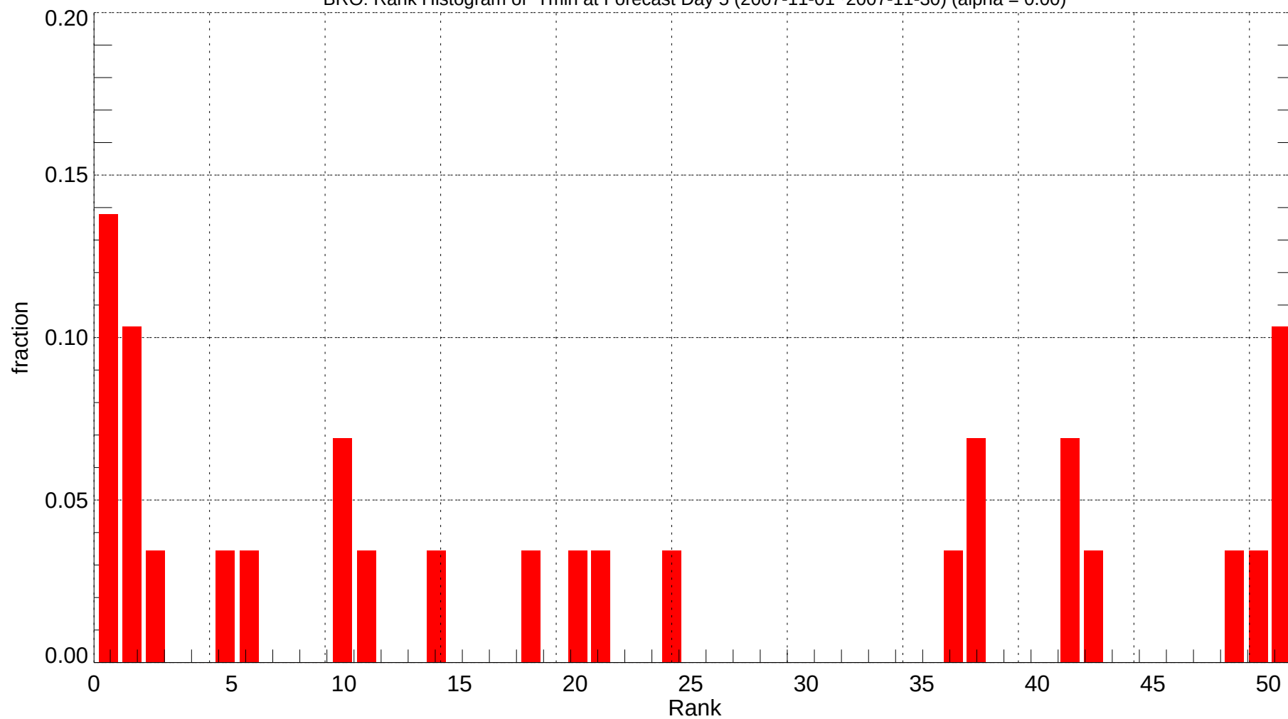
BRO: Rank Histogram of Tmin at Forecast Day 5 (2007-11-01~2007-11-30) (alpha = 0.00)
