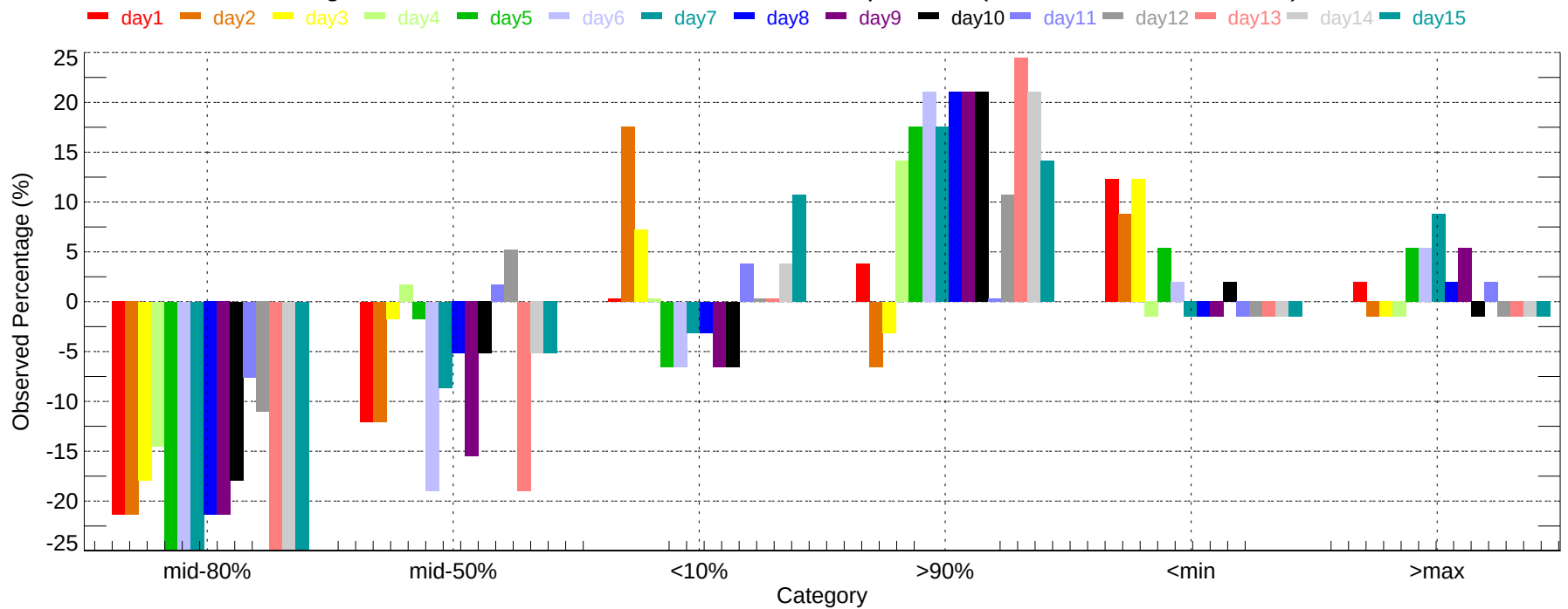
Observed Percentage Deviation of Ensembles - ELP: Max Temperature (2007-11-01~2007-11-30)
