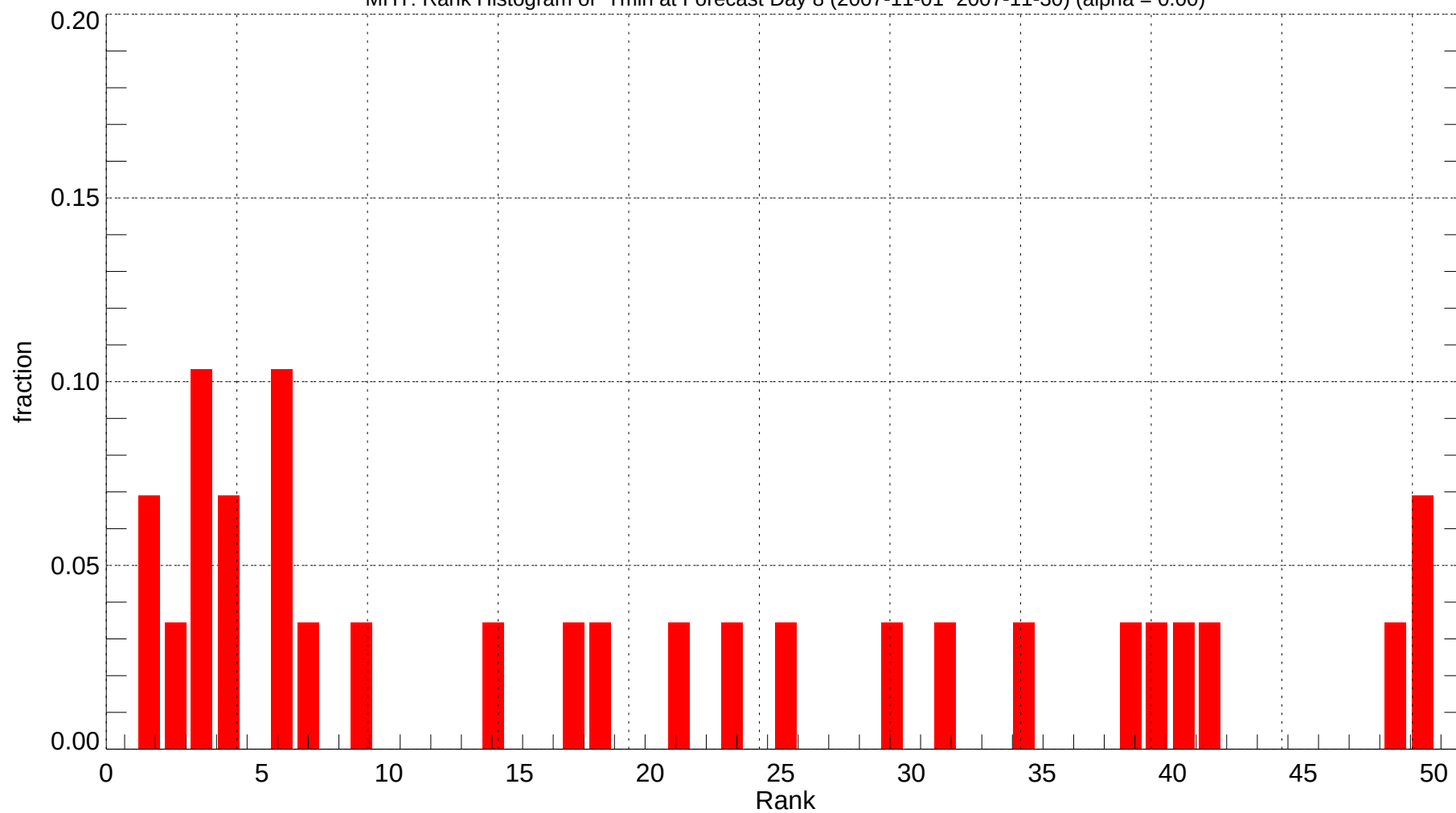
MHT: Rank Histogram of Tmin at Forecast Day 8 (2007-11-01~2007-11-30) (alpha = 0.00)
