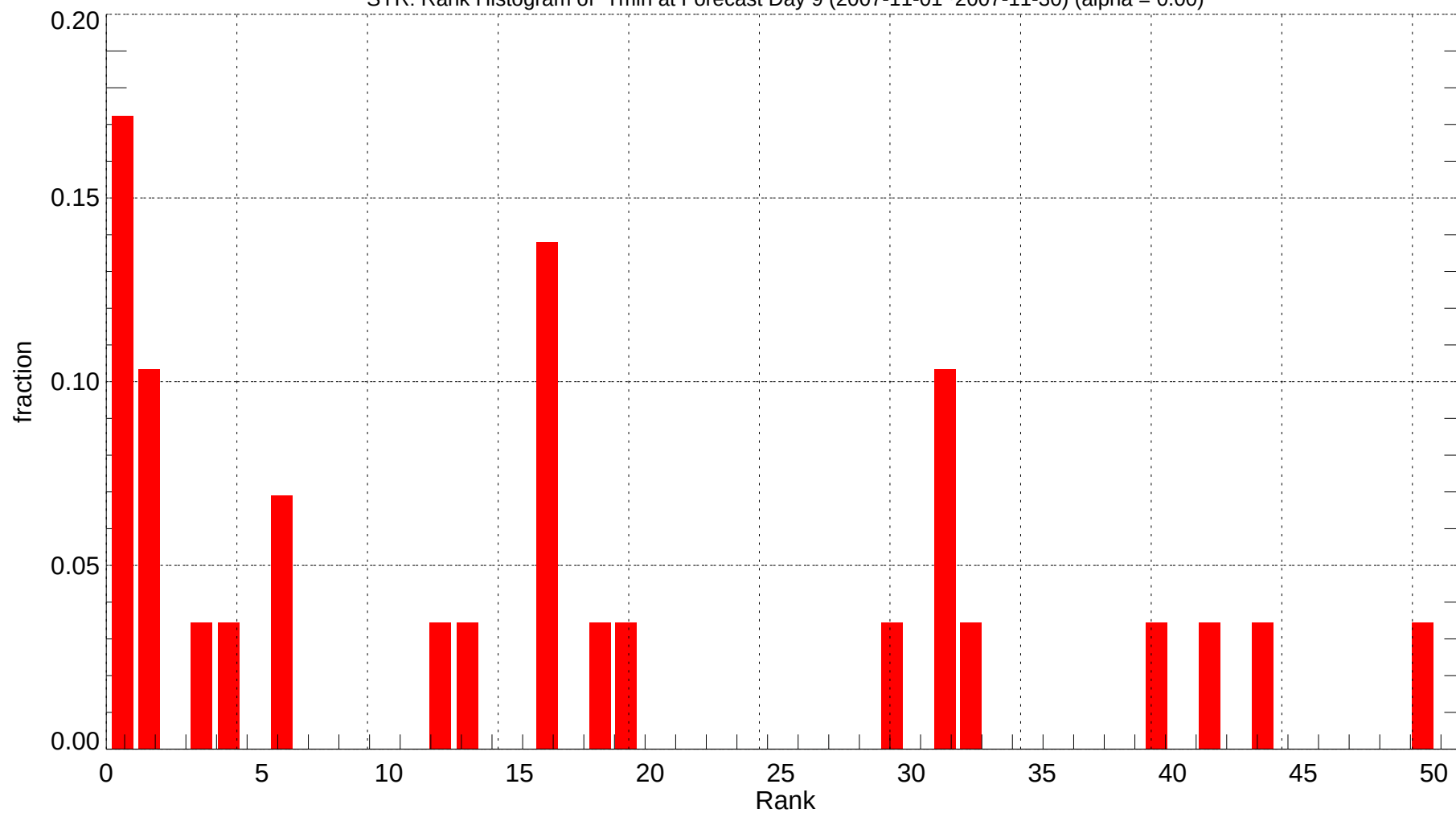
SYR: Rank Histogram of Tmin at Forecast Day 9 (2007-11-01~2007-11-30) (alpha = 0.00)
