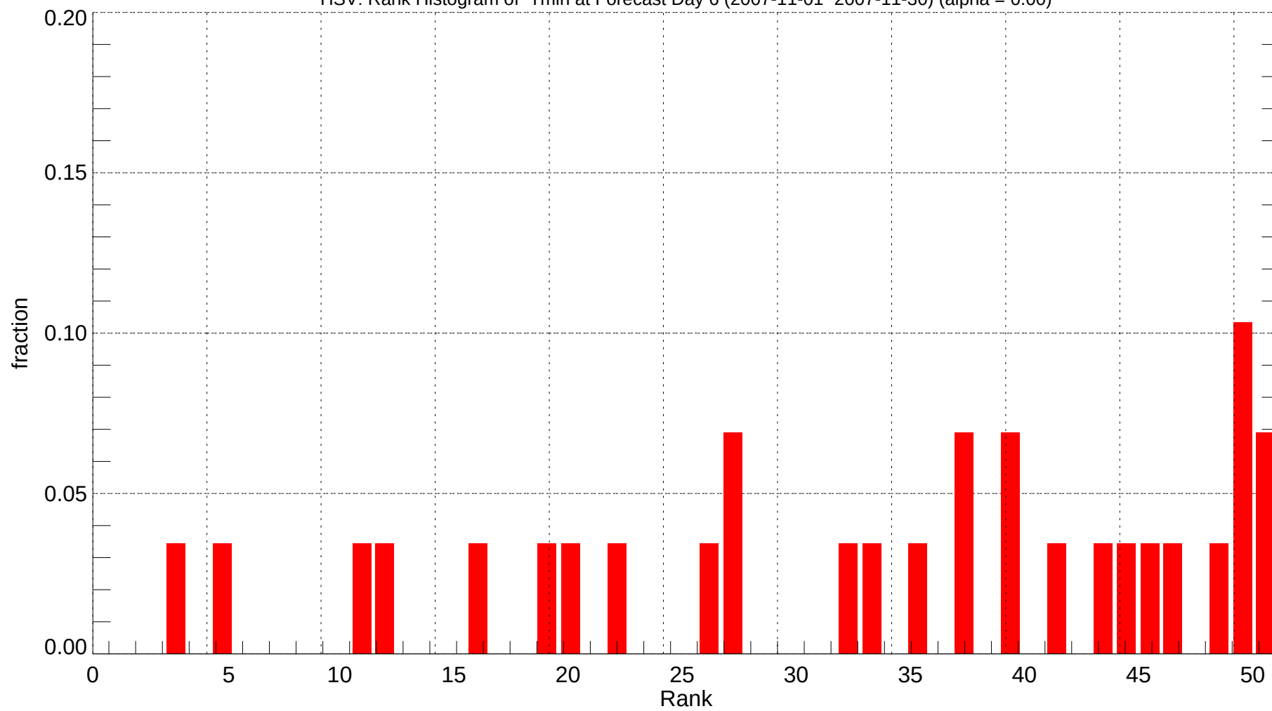
HSV: Rank Histogram of Tmin at Forecast Day 6 (2007-11-01~2007-11-30) (alpha = 0.00)
