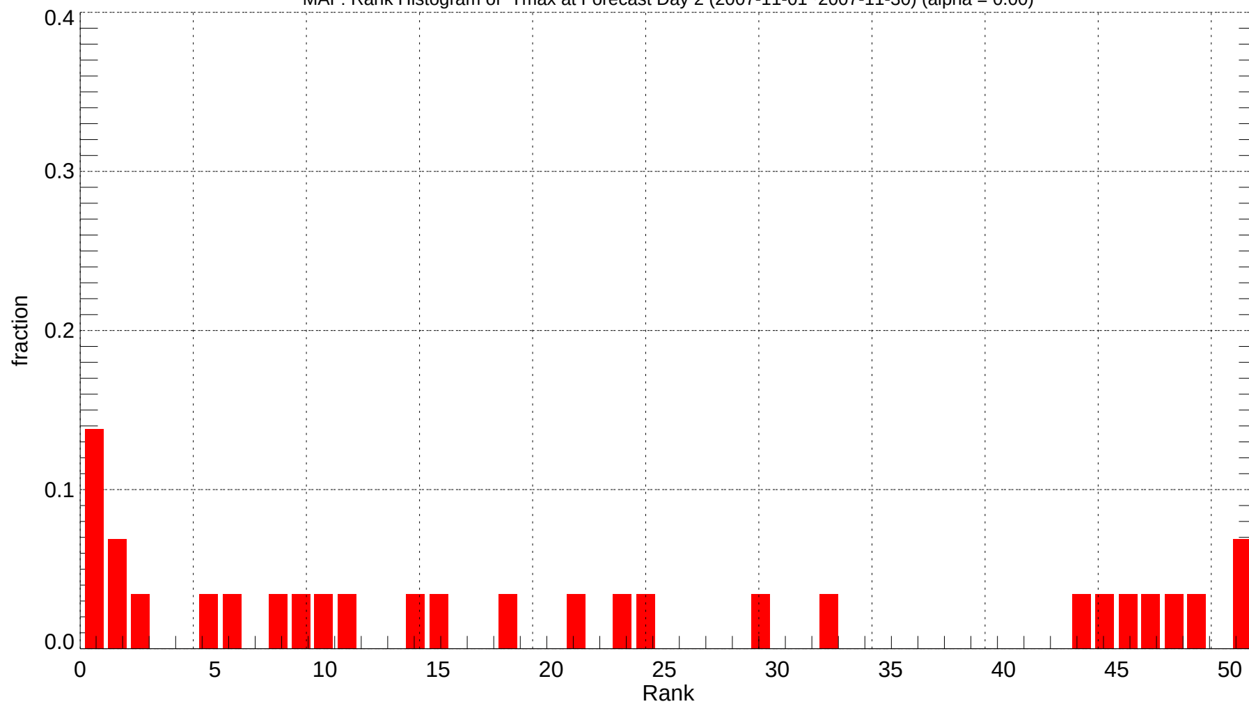
MAF: Rank Histogram of Tmax at Forecast Day 2 (2007-11-01~2007-11-30) (alpha = 0.00)
