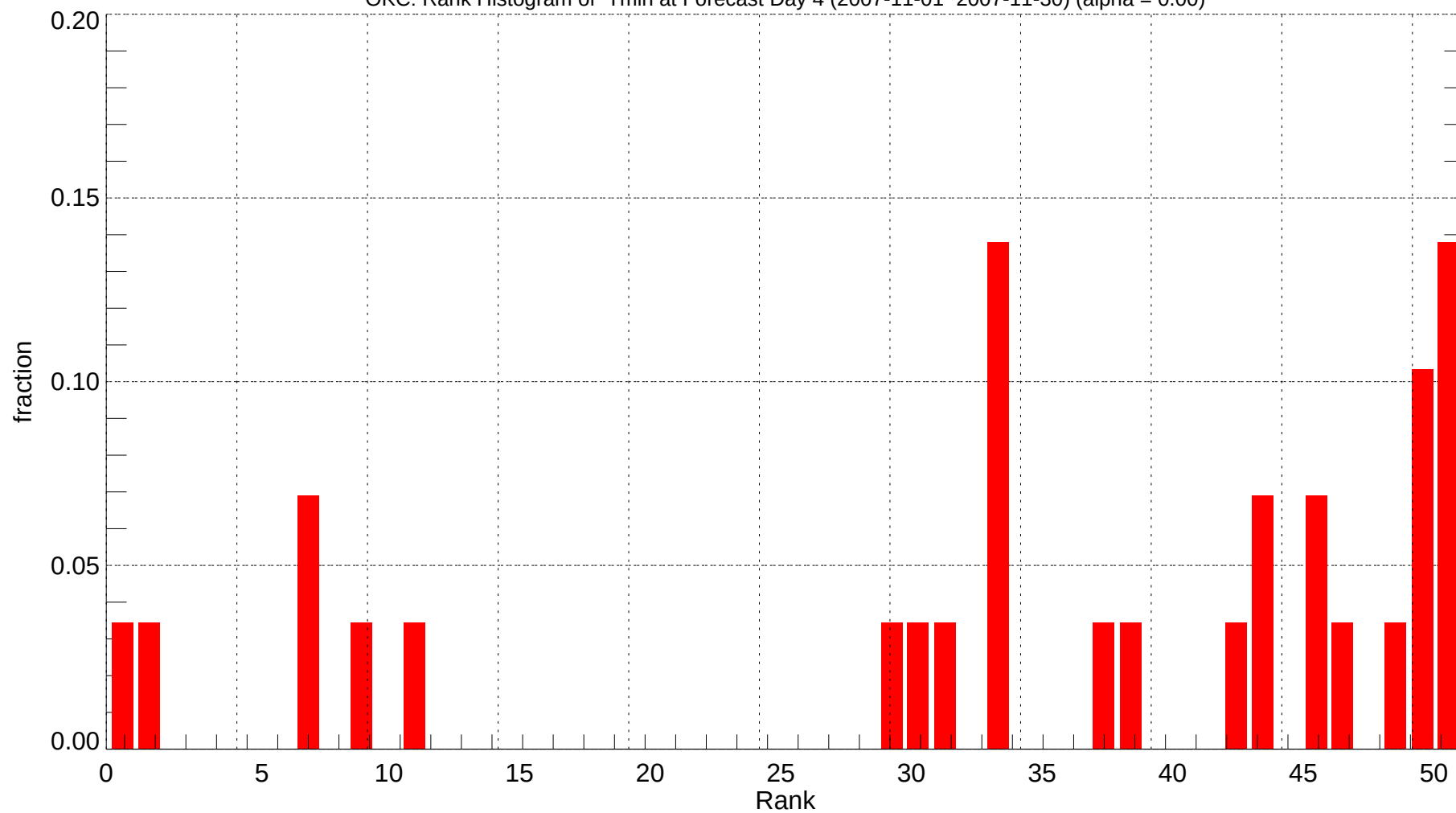
OKC: Rank Histogram of Tmin at Forecast Day 4 (2007-11-01~2007-11-30) (alpha = 0.00)
