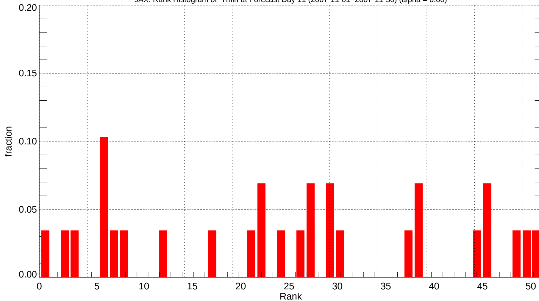
JAX: Rank Histogram of Tmin at Forecast Day 11 (2007-11-01~2007-11-30) (alpha = 0.00)
