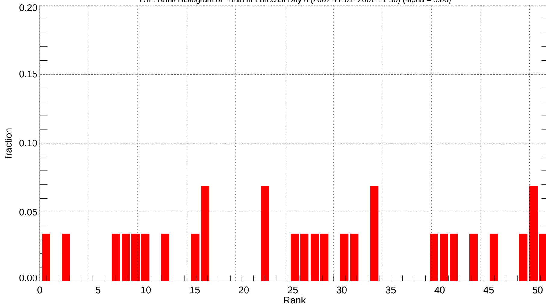
YUL: Rank Histogram of Tmin at Forecast Day 8 (2007-11-01~2007-11-30) (alpha = 0.00)
