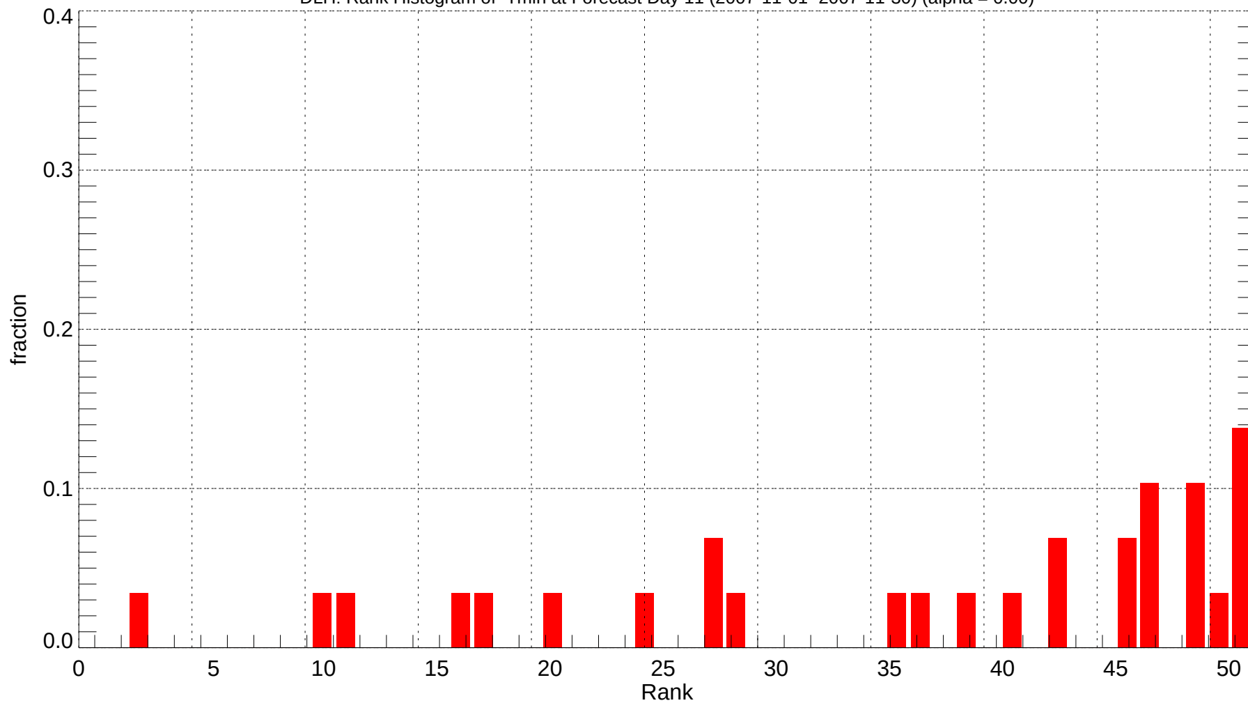
DLH: Rank Histogram of Tmin at Forecast Day 11 (2007-11-01~2007-11-30) (alpha = 0.00)
