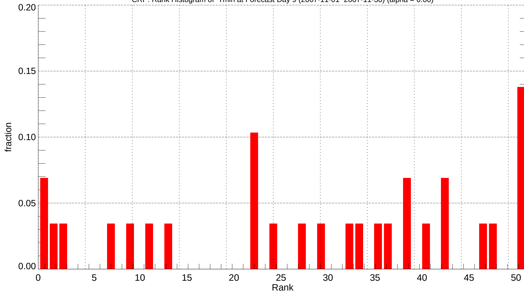
CRP: Rank Histogram of Tmin at Forecast Day 9 (2007-11-01~2007-11-30) (alpha = 0.00)
