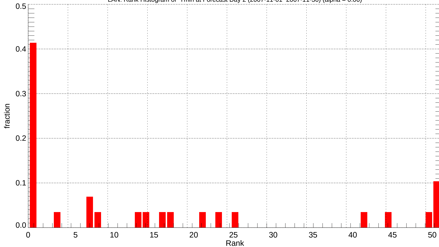
LAN: Rank Histogram of Tmin at Forecast Day 2 (2007-11-01~2007-11-30) (alpha = 0.00)
