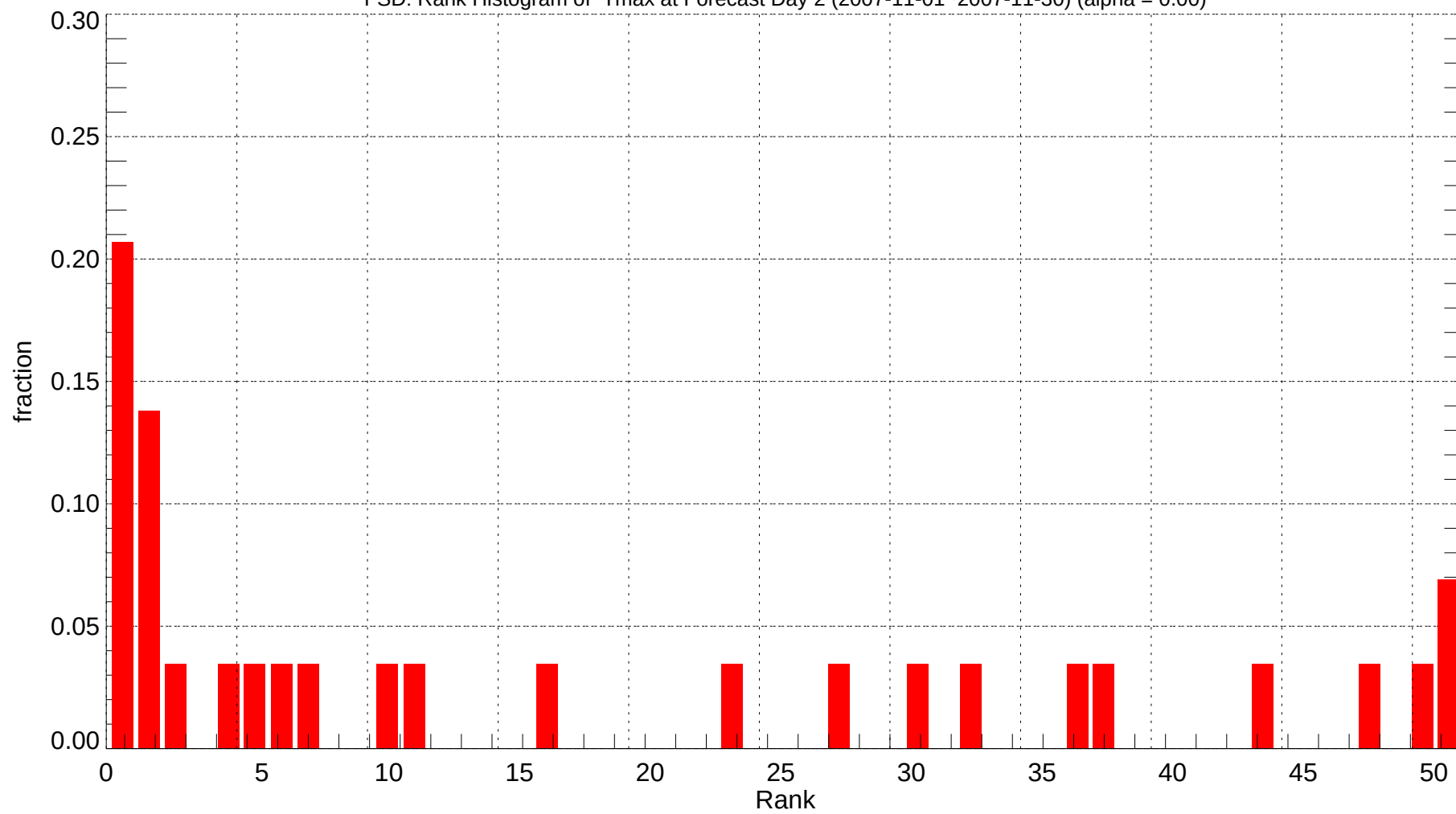
FSD: Rank Histogram of Tmax at Forecast Day 2 (2007-11-01~2007-11-30) (alpha = 0.00)
