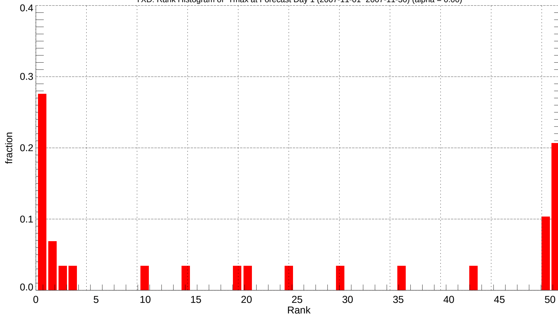
YXD: Rank Histogram of Tmax at Forecast Day 1 (2007-11-01~2007-11-30) (alpha = 0.00)
