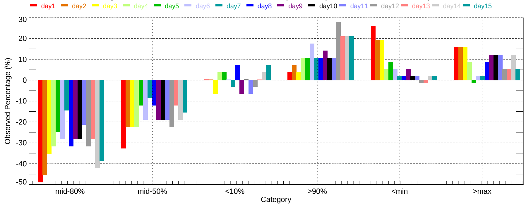
Observed Percentage Deviation of Ensembles - ABI: Min Temperature (2007-11-01~2007-11-30)
