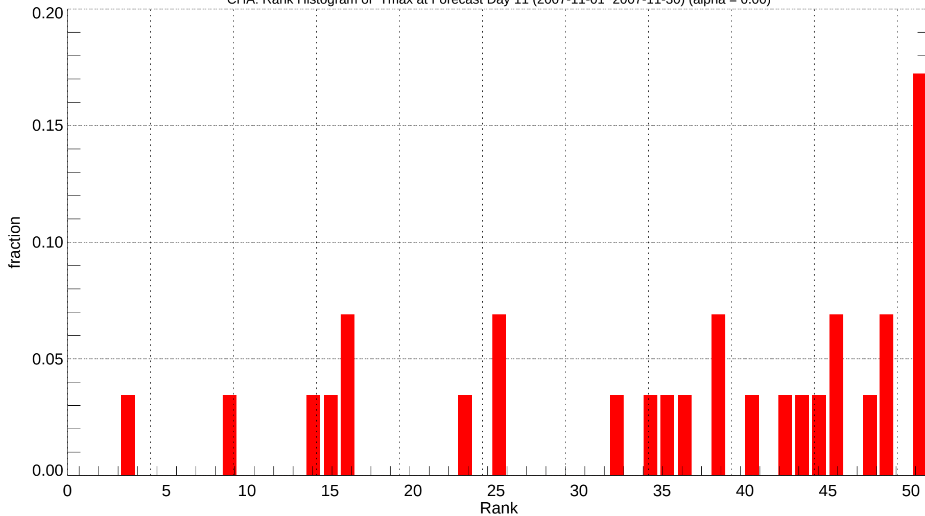
CHA: Rank Histogram of Tmax at Forecast Day 11 (2007-11-01~2007-11-30) (alpha = 0.00)
