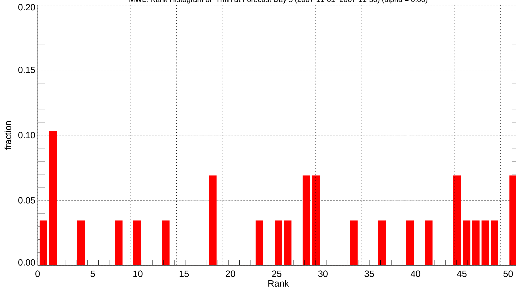
MWL: Rank Histogram of Tmin at Forecast Day 5 (2007-11-01~2007-11-30) (alpha = 0.00)
