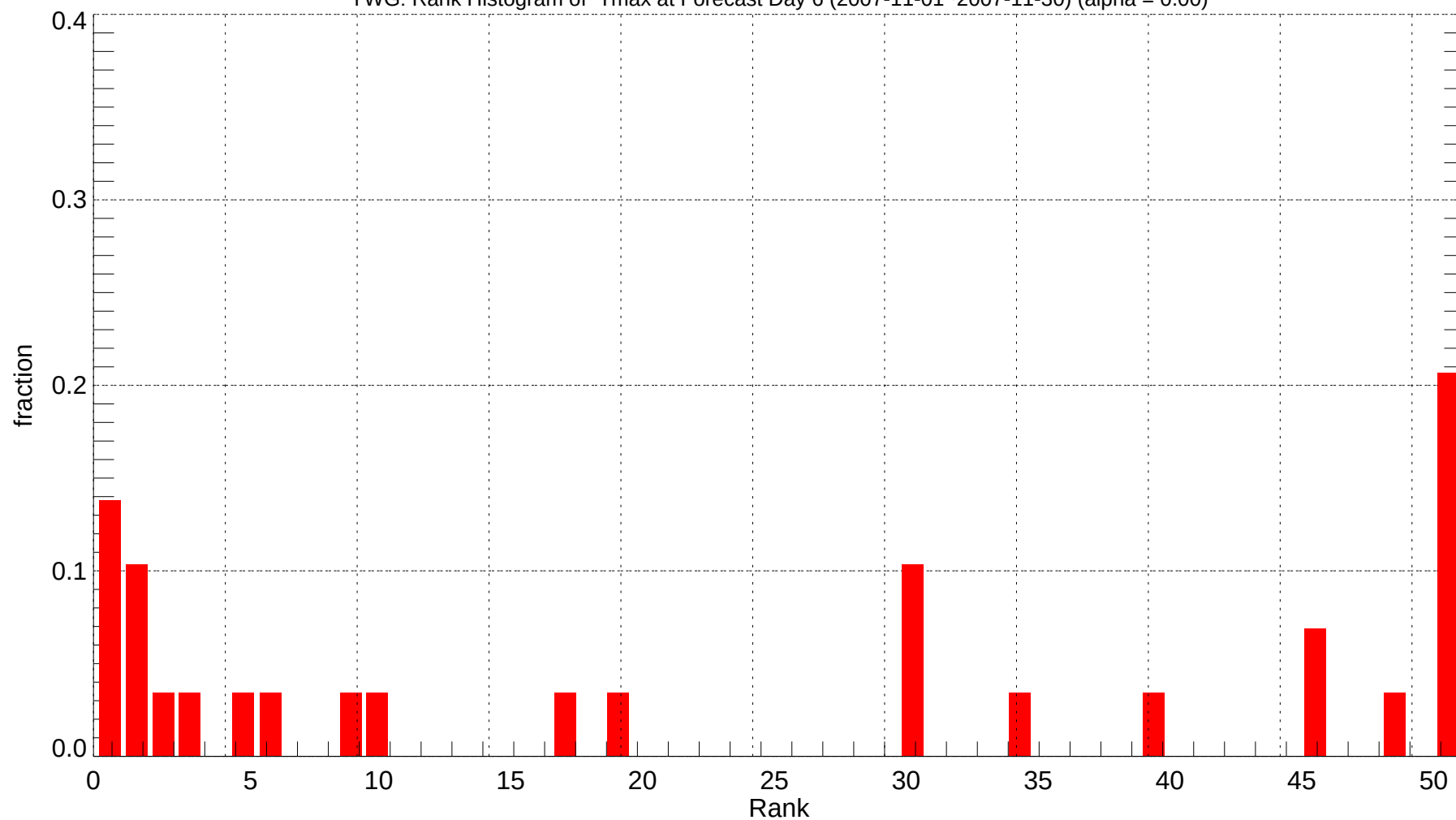
YWG: Rank Histogram of Tmax at Forecast Day 6 (2007-11-01~2007-11-30) (alpha = 0.00)
