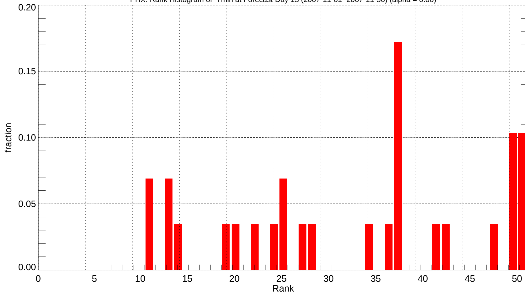
PHX: Rank Histogram of Tmin at Forecast Day 13 (2007-11-01~2007-11-30) (alpha = 0.00)
