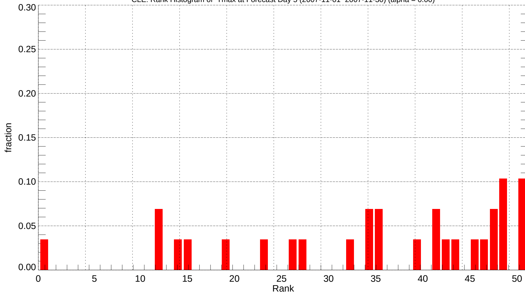
CLE: Rank Histogram of Tmax at Forecast Day 5 (2007-11-01~2007-11-30) (alpha = 0.00)
