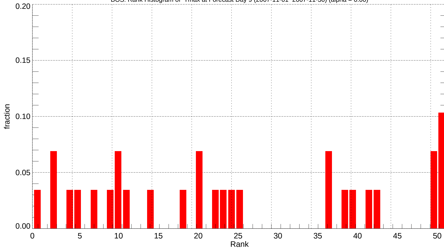
BOS: Rank Histogram of Tmax at Forecast Day 9 (2007-11-01~2007-11-30) (alpha = 0.00)
