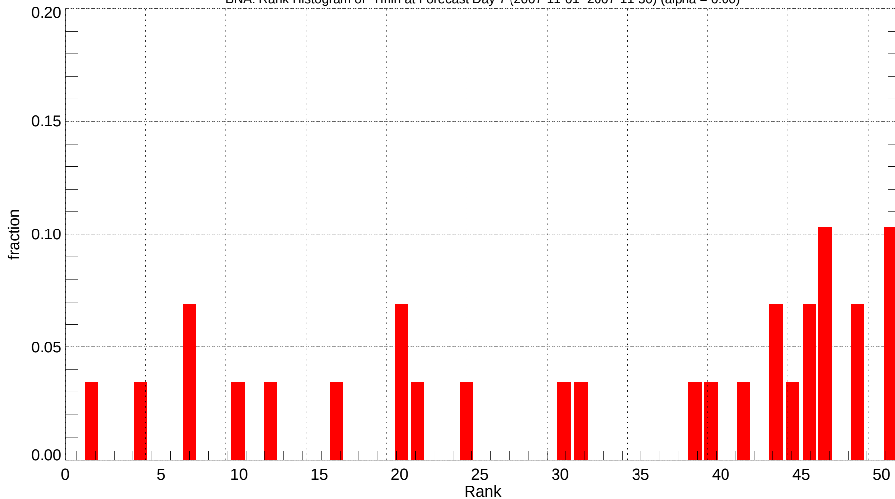
BNA: Rank Histogram of Tmin at Forecast Day 7 (2007-11-01~2007-11-30) (alpha = 0.00)
