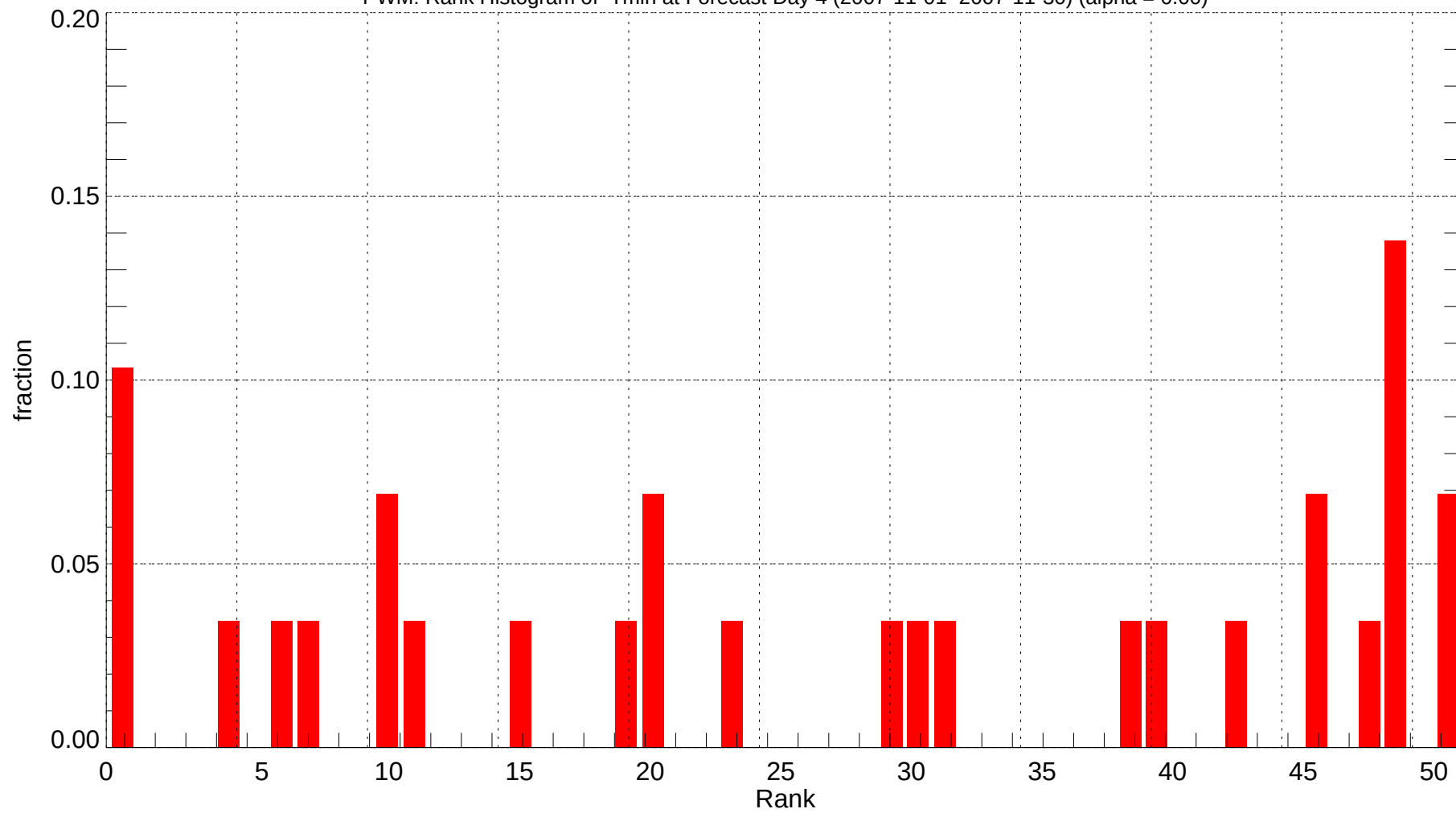
PWM: Rank Histogram of Tmin at Forecast Day 4 (2007-11-01~2007-11-30) (alpha = 0.00)
