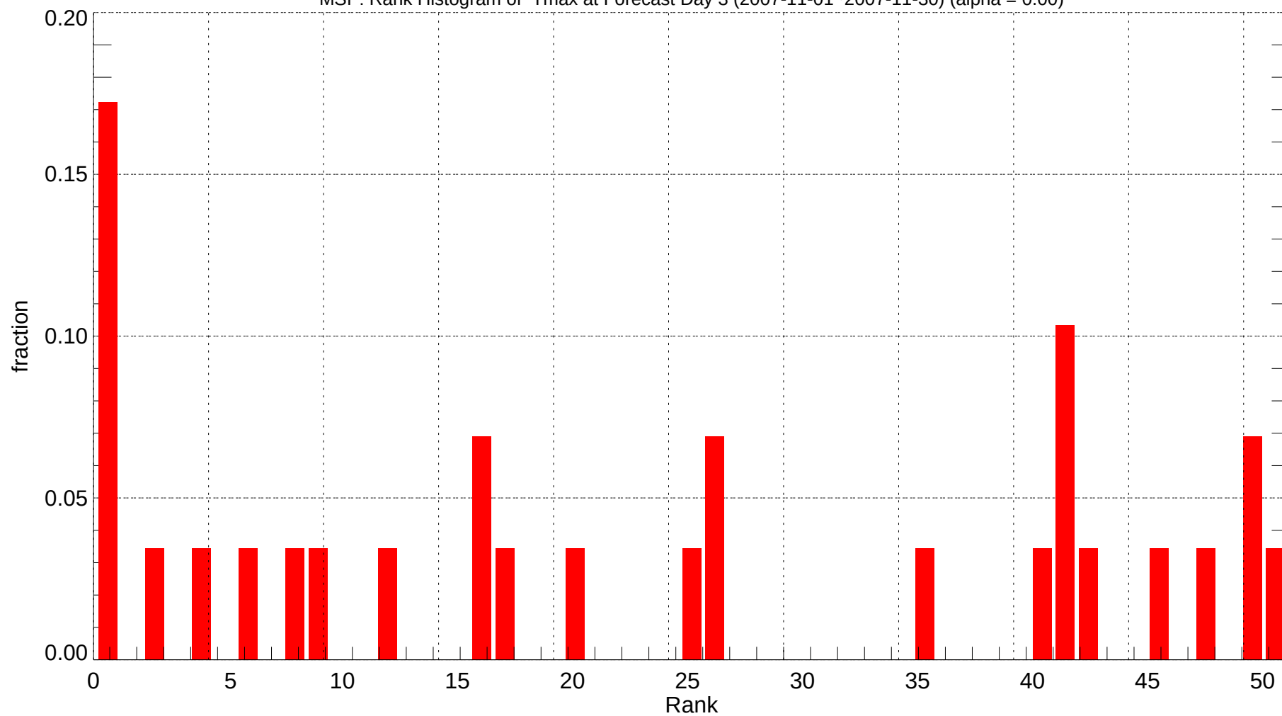
MSP: Rank Histogram of Tmax at Forecast Day 3 (2007-11-01~2007-11-30) (alpha = 0.00)
