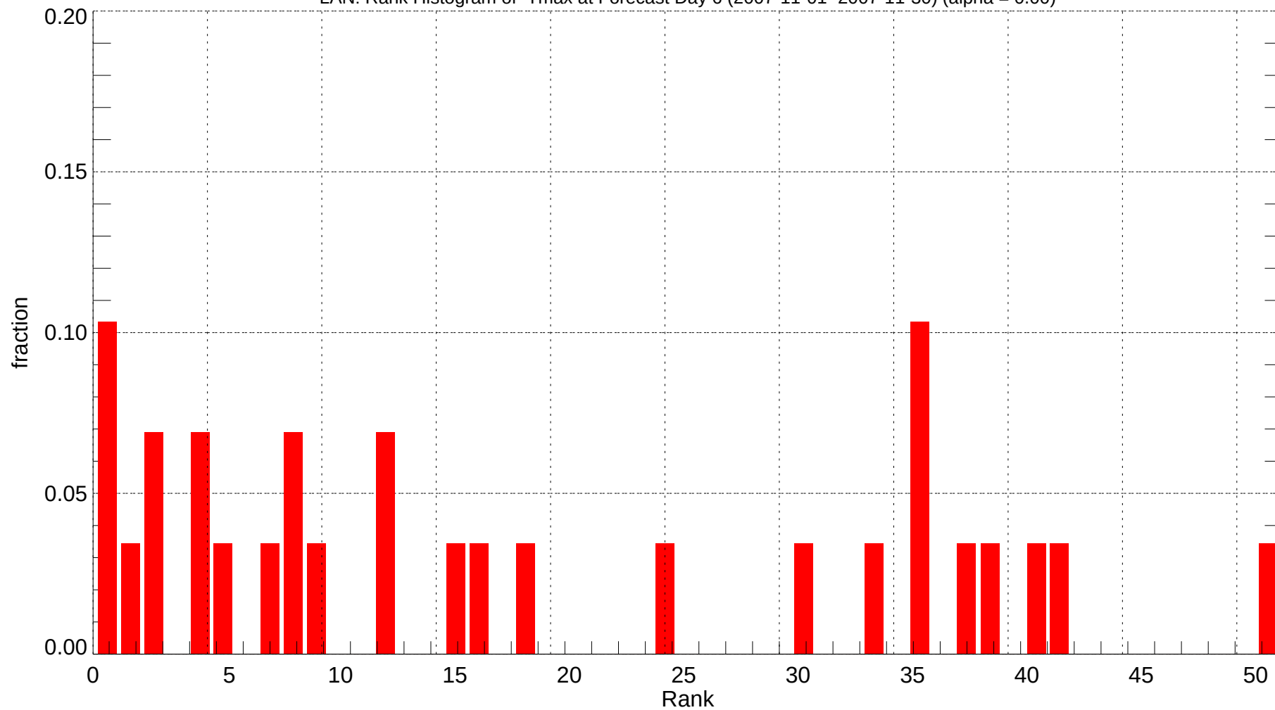
LAN: Rank Histogram of Tmax at Forecast Day 6 (2007-11-01~2007-11-30) (alpha = 0.00)
