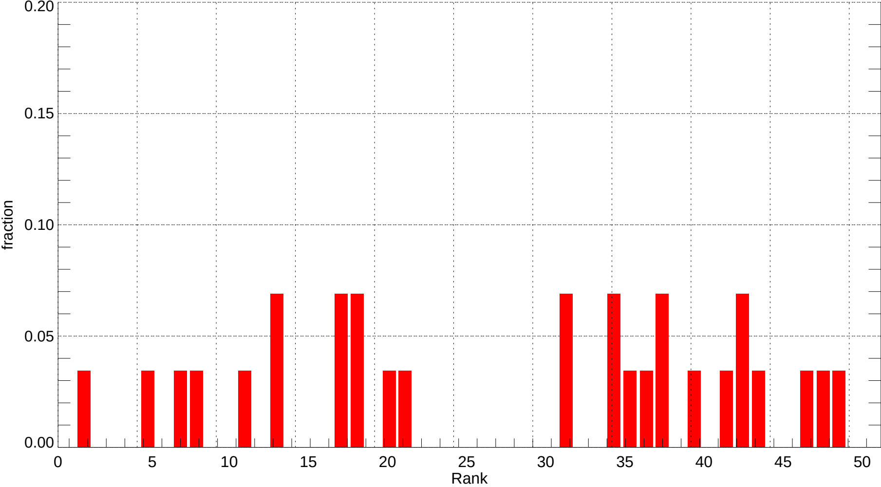
BFL: Rank Histogram of Tmin at Forecast Day 7 (2007-11-01~2007-11-30) (alpha = 0.00)
