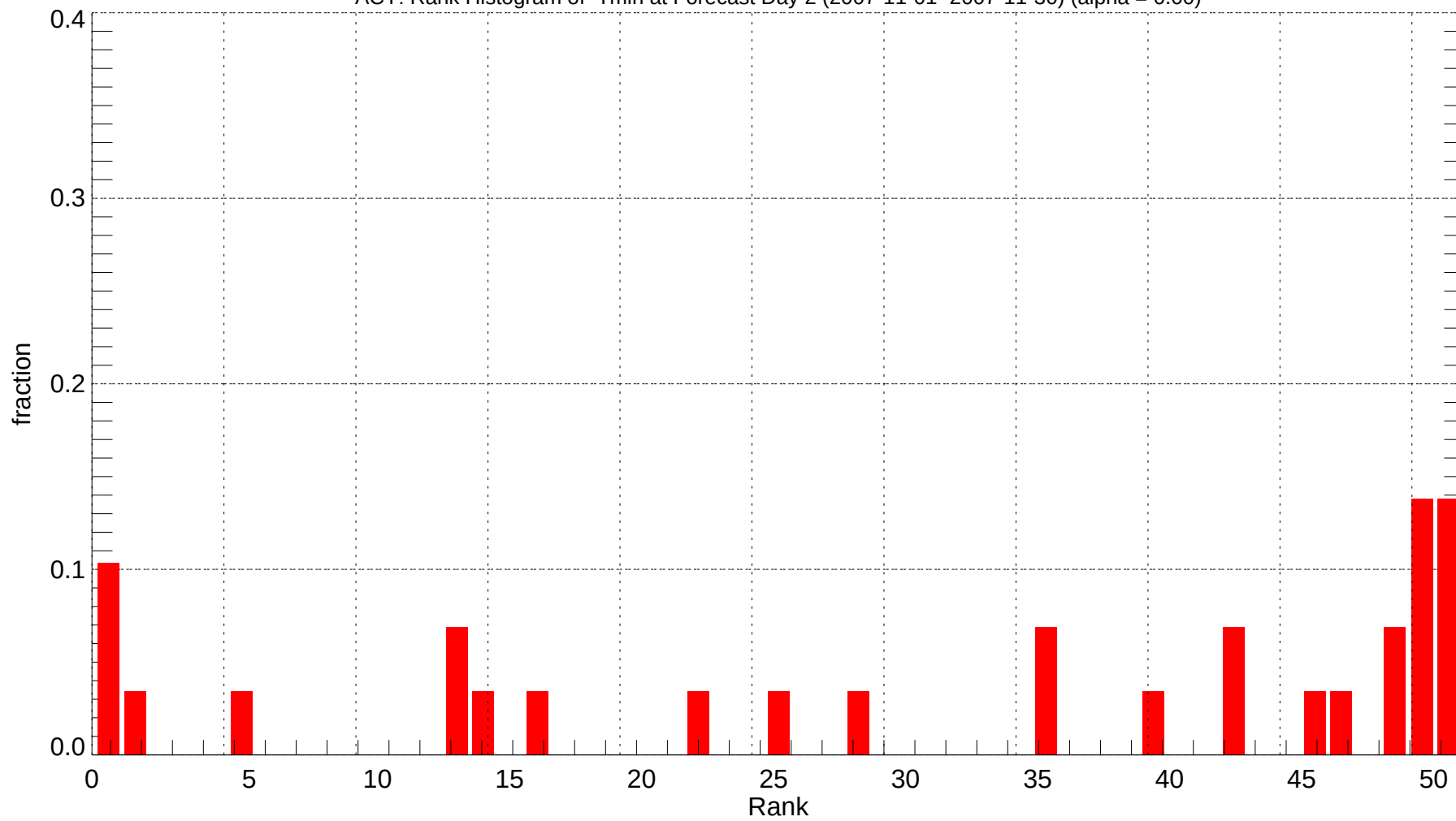
ACY: Rank Histogram of Tmin at Forecast Day 2 (2007-11-01~2007-11-30) (alpha = 0.00)
