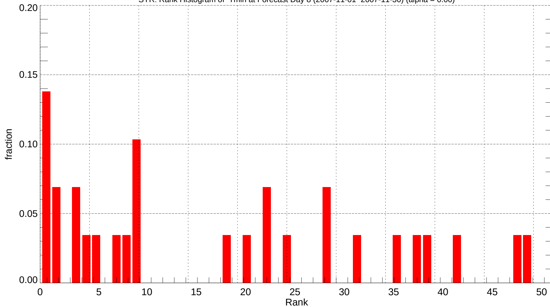
SYR: Rank Histogram of Tmin at Forecast Day 8 (2007-11-01~2007-11-30) (alpha = 0.00)
