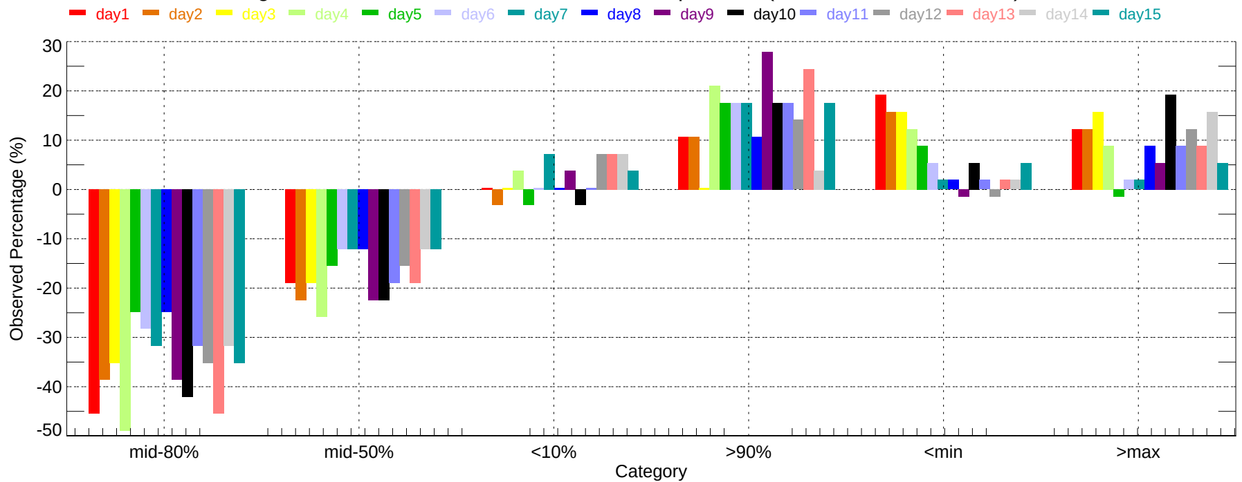
Observed Percentage Deviation of Ensembles - SJT: Min Temperature (2007-11-01~2007-11-30)
