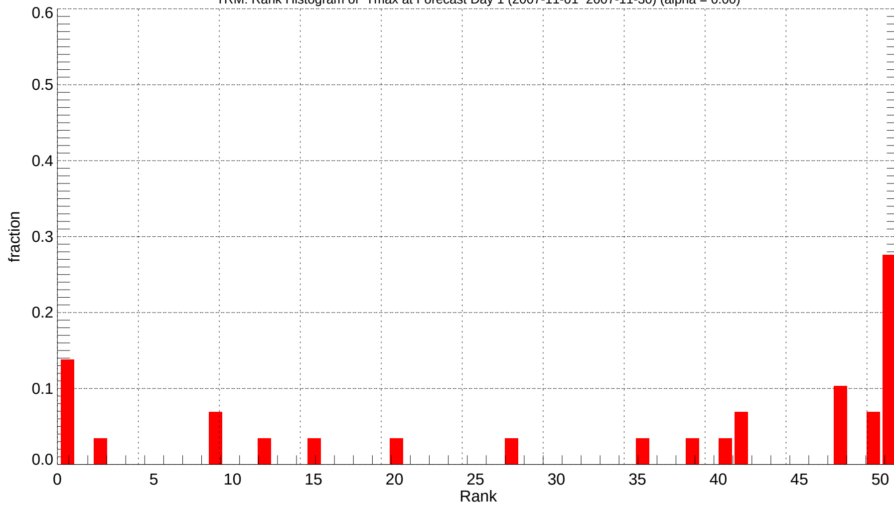
TRM: Rank Histogram of Tmax at Forecast Day 1 (2007-11-01~2007-11-30) (alpha = 0.00)
