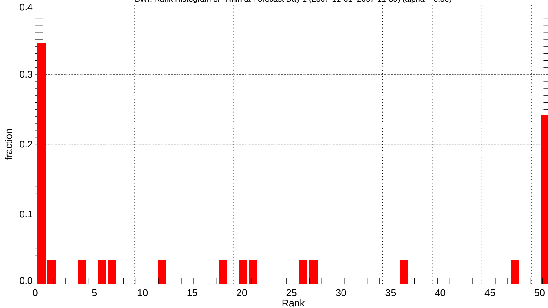
BWI: Rank Histogram of Tmin at Forecast Day 1 (2007-11-01~2007-11-30) (alpha = 0.00)
