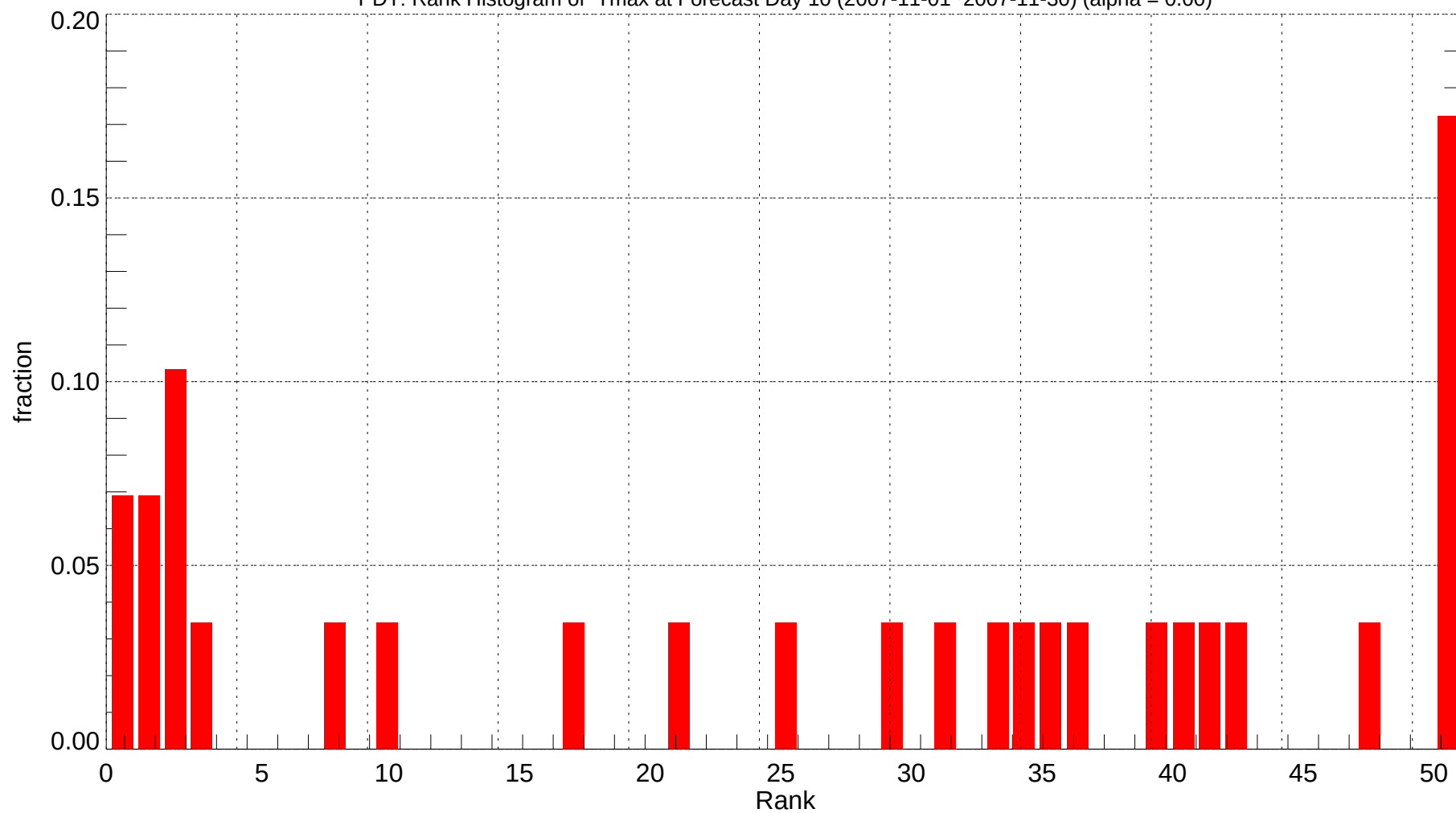
PDT: Rank Histogram of Tmax at Forecast Day 10 (2007-11-01~2007-11-30) (alpha = 0.00)
