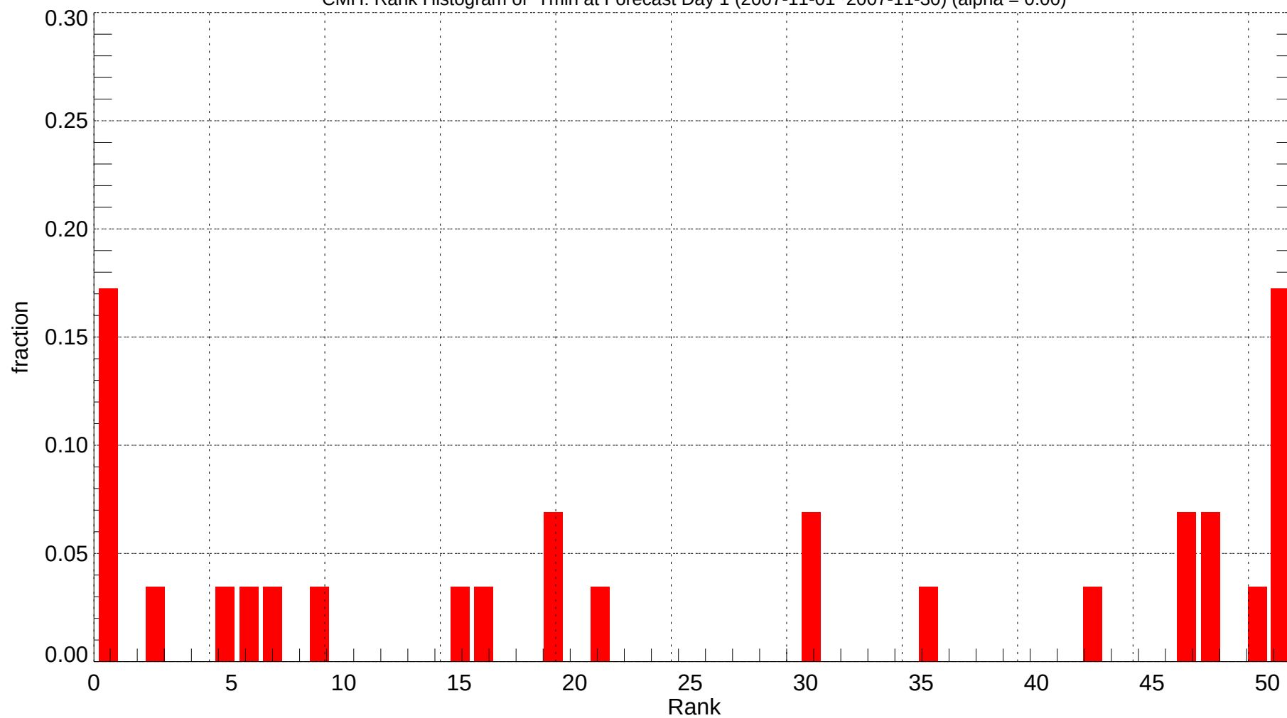
CMH: Rank Histogram of Tmin at Forecast Day 1 (2007-11-01~2007-11-30) (alpha = 0.00)
