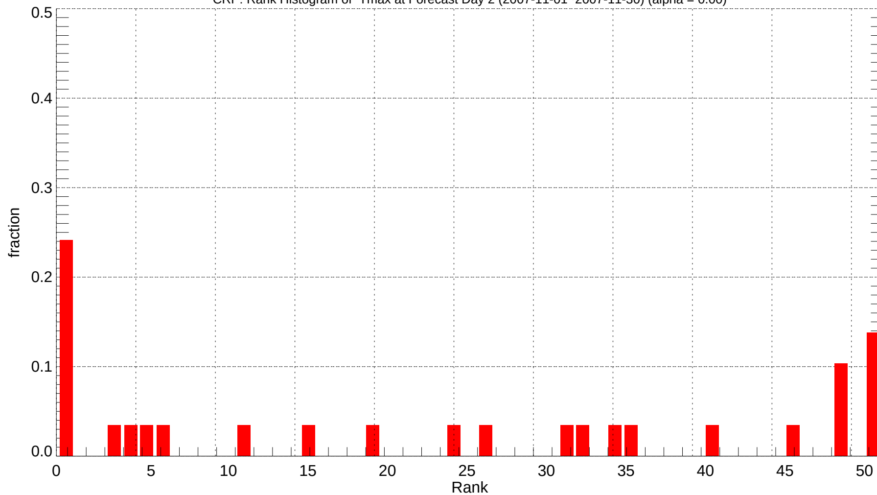
CRP: Rank Histogram of Tmax at Forecast Day 2 (2007-11-01~2007-11-30) (alpha = 0.00)
