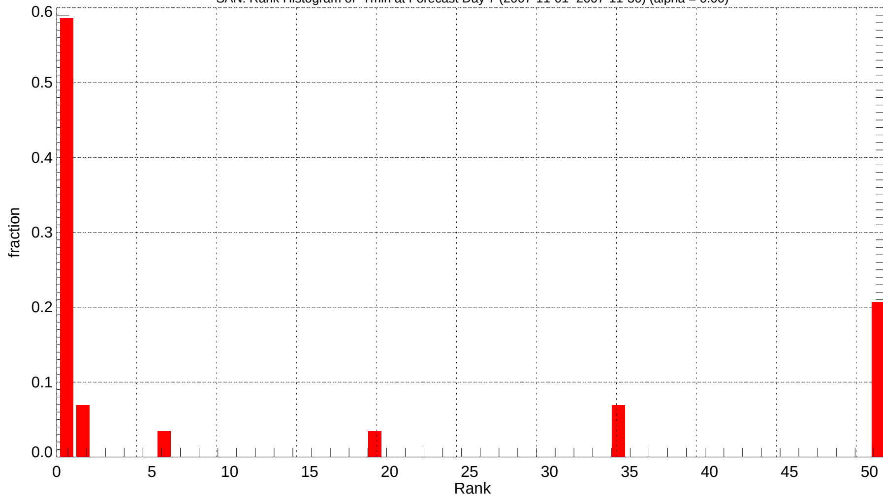
SAN: Rank Histogram of Tmin at Forecast Day 7 (2007-11-01~2007-11-30) (alpha = 0.00)
