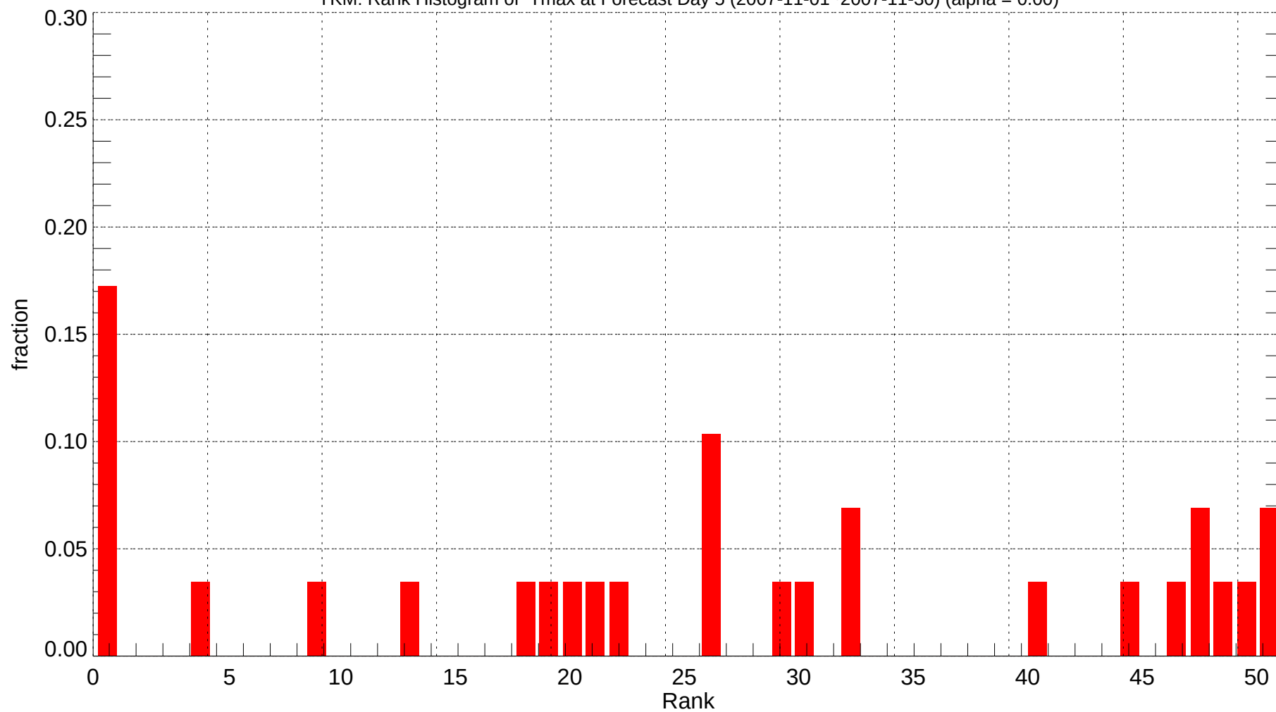
YKM: Rank Histogram of Tmax at Forecast Day 5 (2007-11-01~2007-11-30) (alpha = 0.00)
