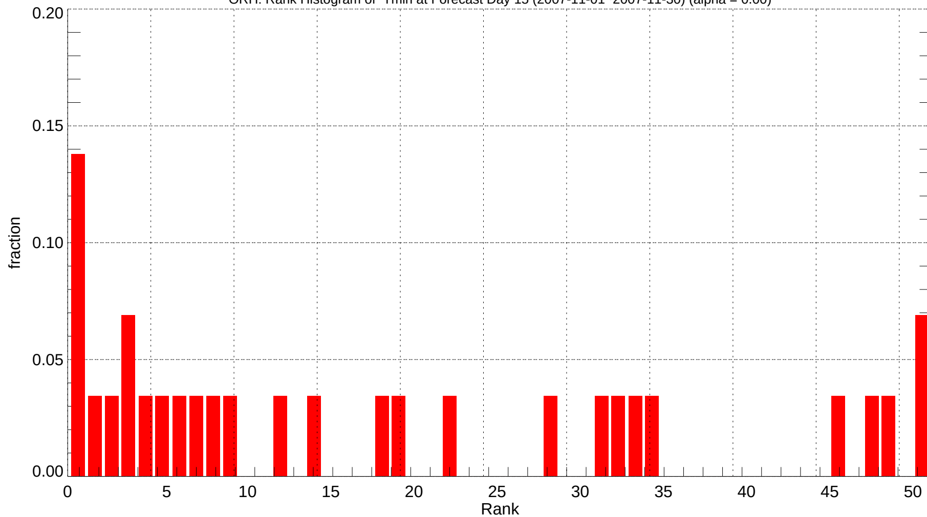
ORH: Rank Histogram of Tmin at Forecast Day 15 (2007-11-01~2007-11-30) (alpha = 0.00)
