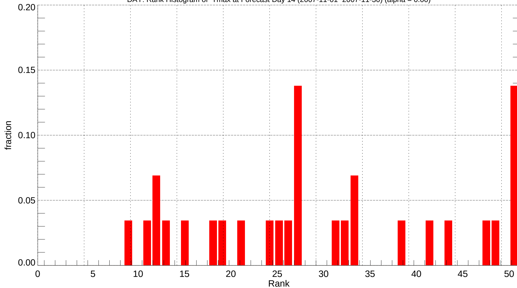
DAY: Rank Histogram of Tmax at Forecast Day 14 (2007-11-01~2007-11-30) (alpha = 0.00)
