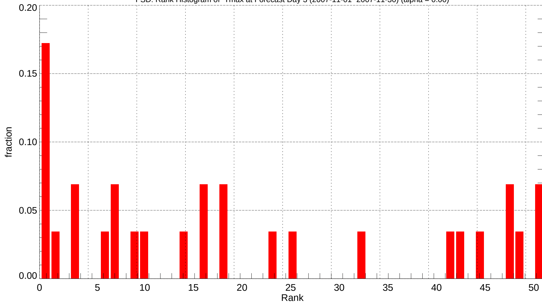
FSD: Rank Histogram of Tmax at Forecast Day 3 (2007-11-01~2007-11-30) (alpha = 0.00)
