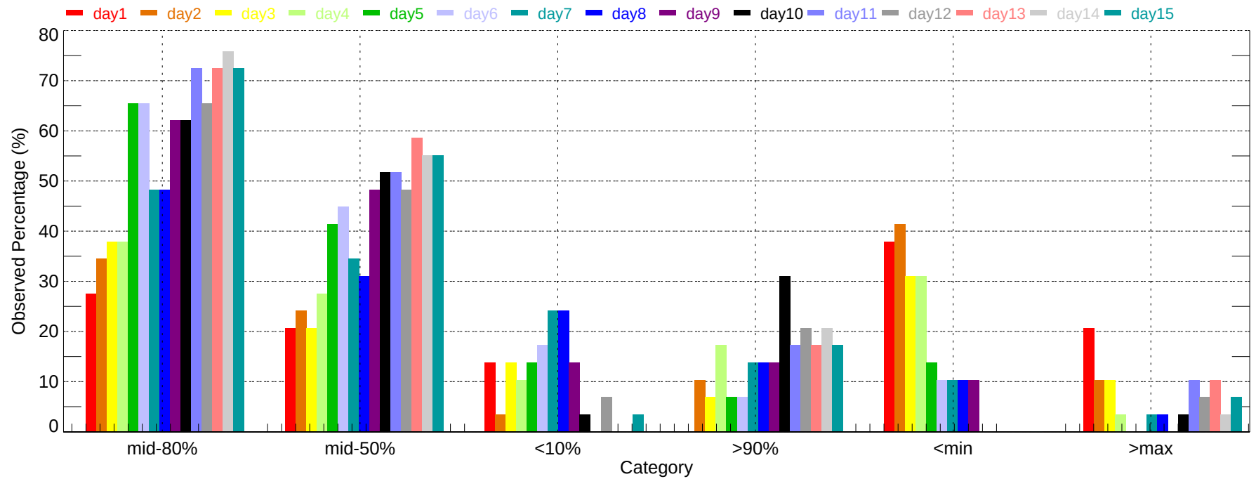
Observed Percentage of Ensembles - LAN: Max Temperature (2007-11-01~2007-11-30)
