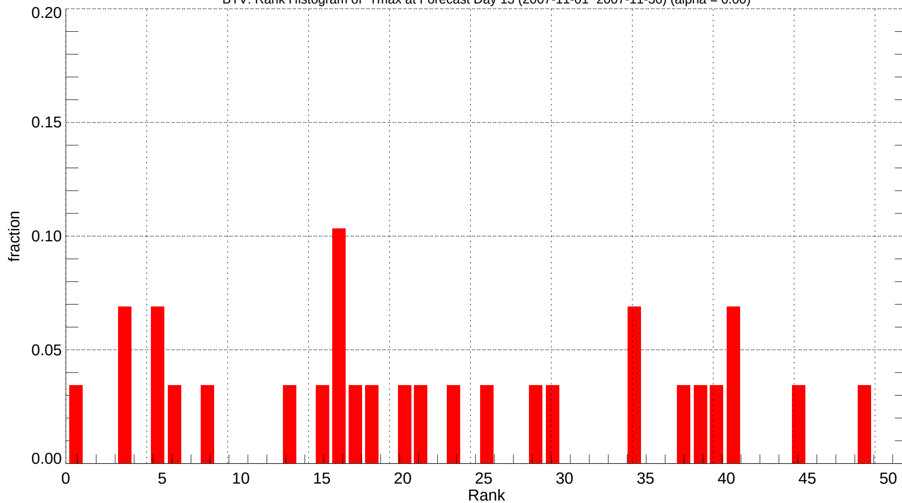
BTV: Rank Histogram of Tmax at Forecast Day 13 (2007-11-01~2007-11-30) (alpha = 0.00)
