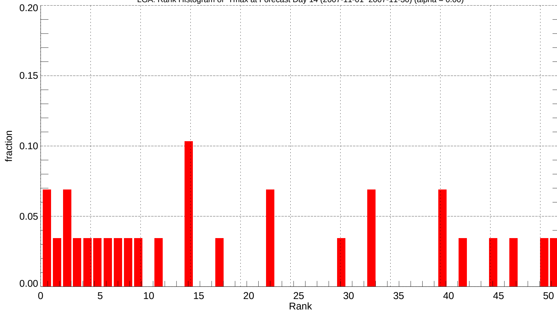
LGA: Rank Histogram of Tmax at Forecast Day 14 (2007-11-01~2007-11-30) (alpha = 0.00)
