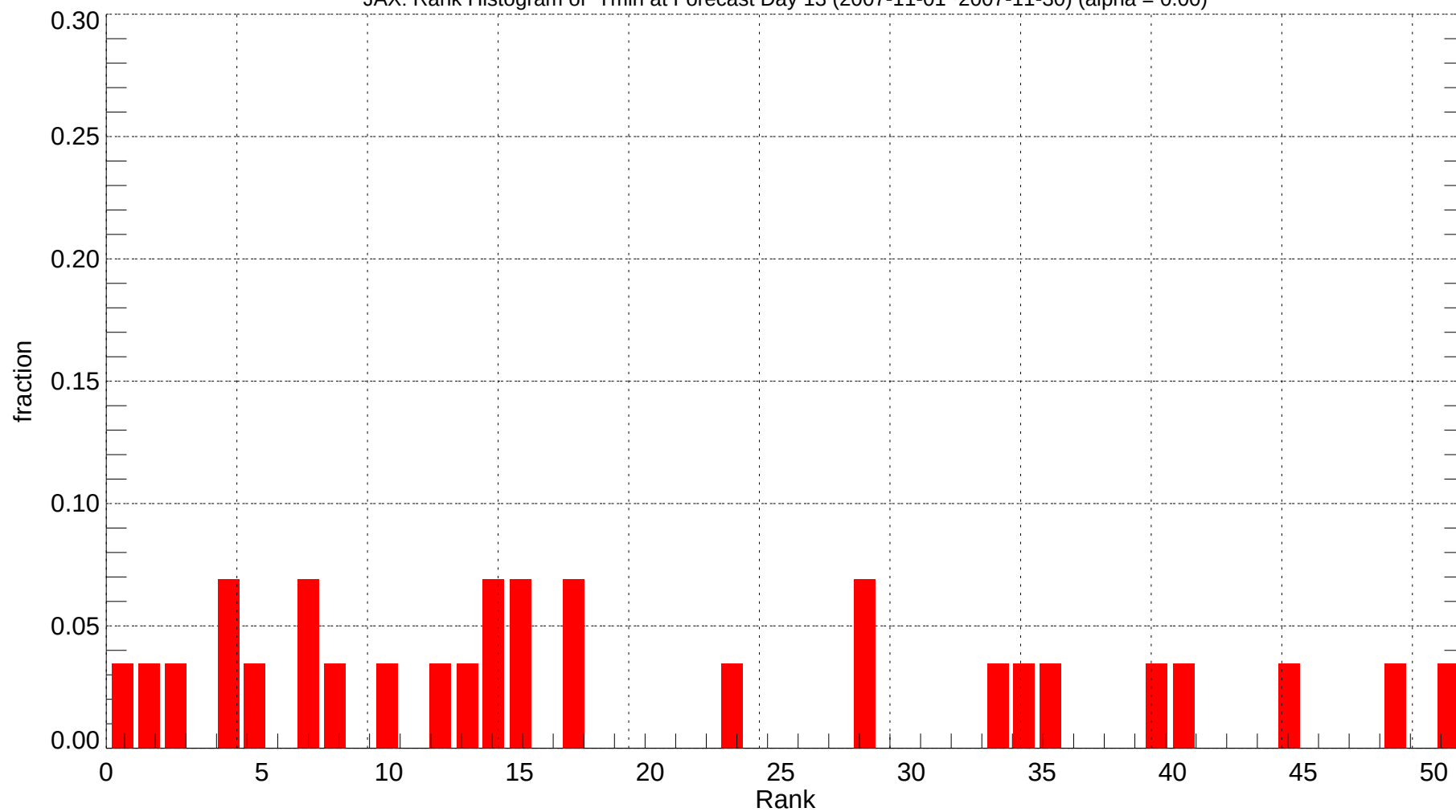
JAX: Rank Histogram of Tmin at Forecast Day 13 (2007-11-01~2007-11-30) (alpha = 0.00)
