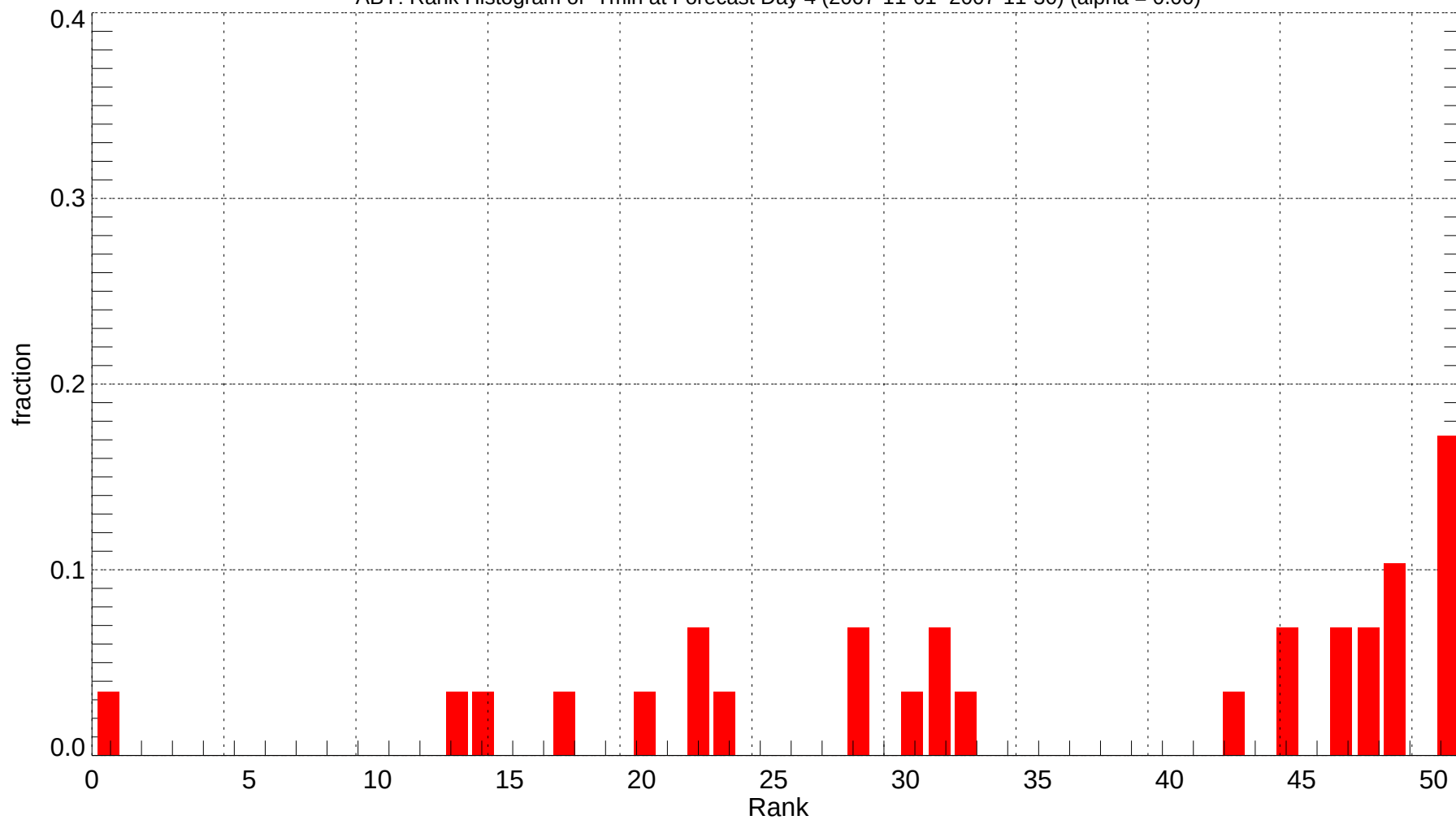
ABY: Rank Histogram of Tmin at Forecast Day 4 (2007-11-01~2007-11-30) (alpha = 0.00)
