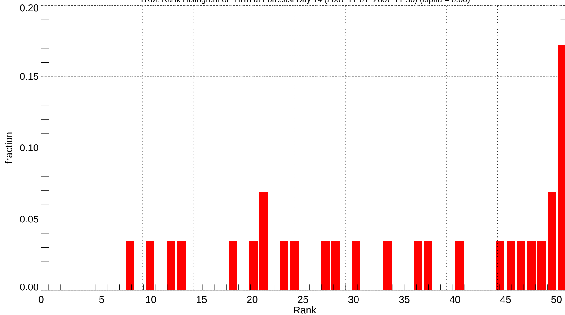
TRM: Rank Histogram of Tmin at Forecast Day 14 (2007-11-01~2007-11-30) (alpha = 0.00)
