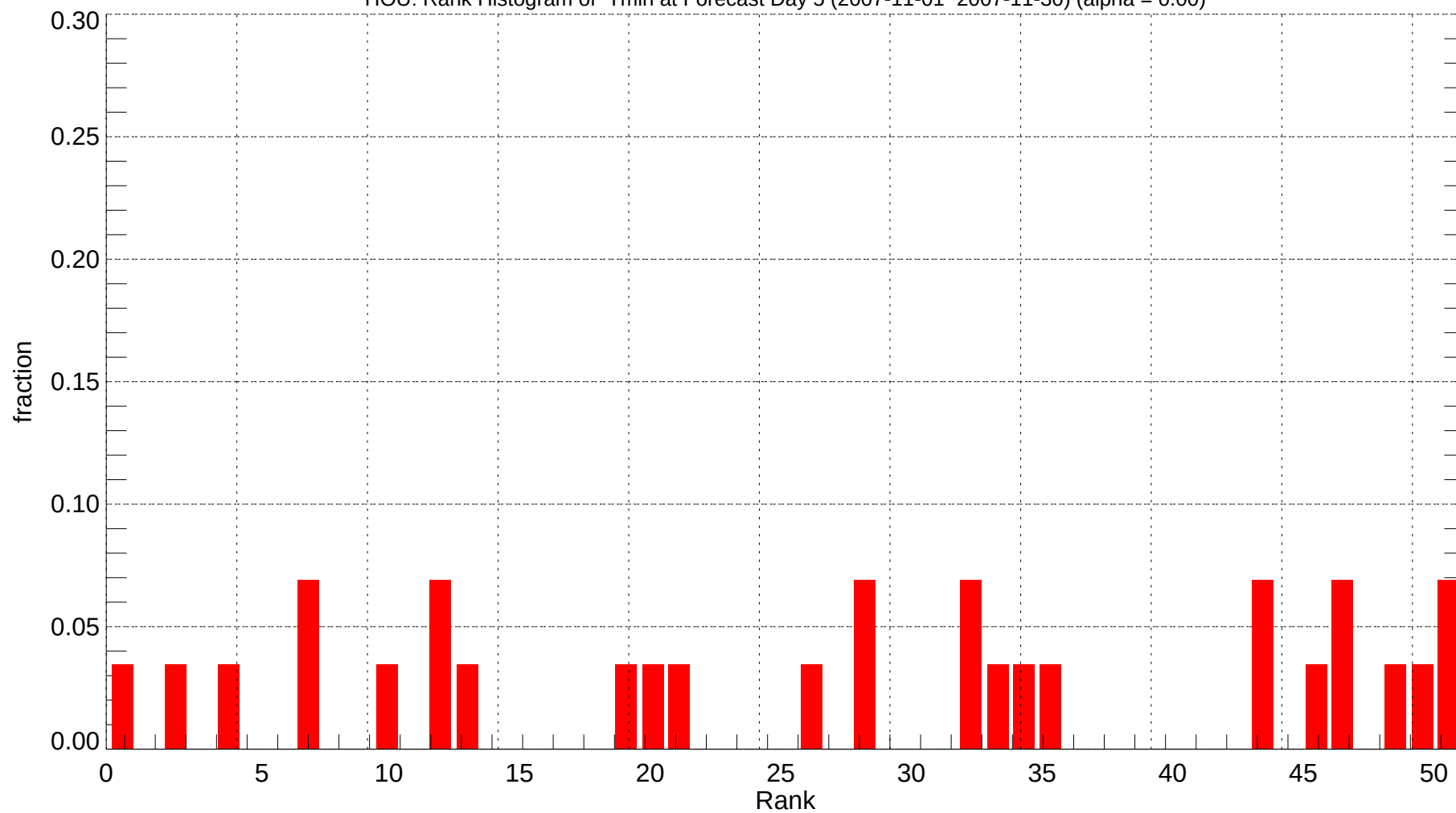
HOU: Rank Histogram of Tmin at Forecast Day 5 (2007-11-01~2007-11-30) (alpha = 0.00)
