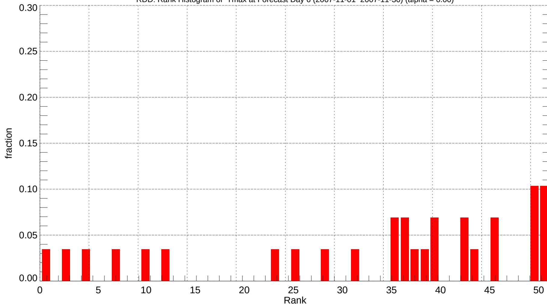
RDD: Rank Histogram of Tmax at Forecast Day 6 (2007-11-01~2007-11-30) (alpha = 0.00)
