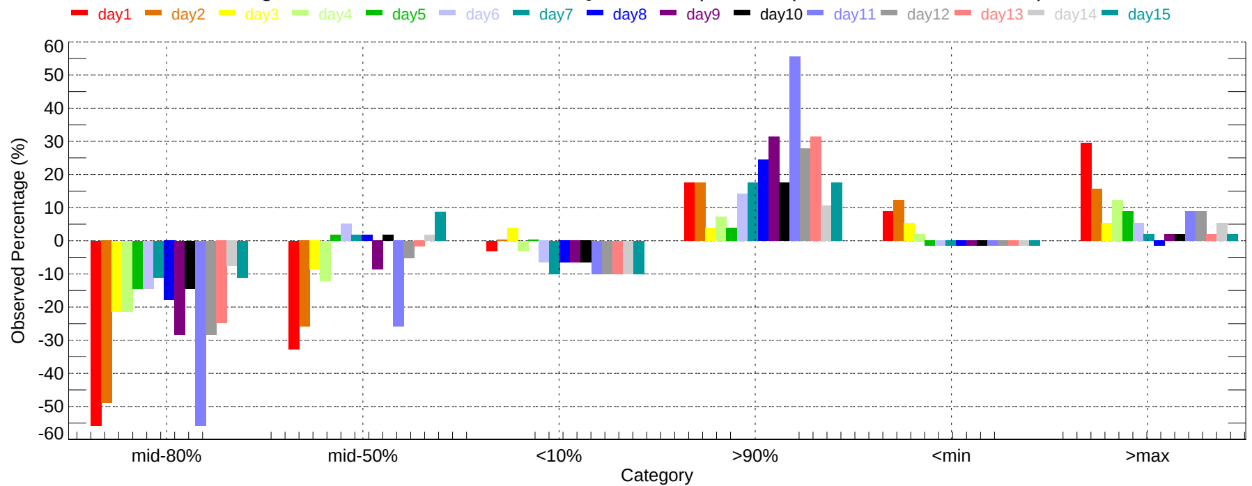
Observed Percentage Deviation of Ensembles - DBQ: Max Temperature (2007-11-01~2007-11-30)
