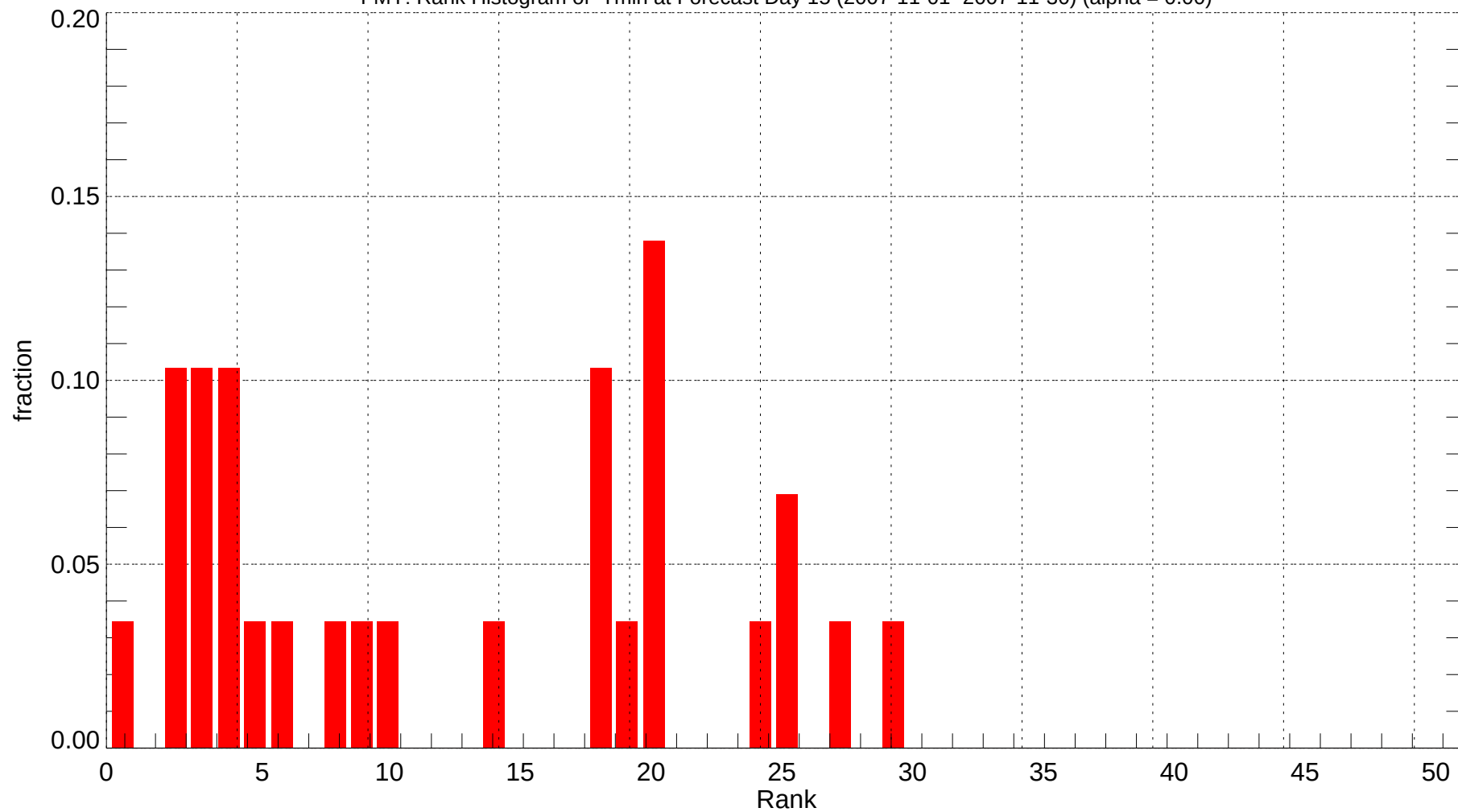
FMY: Rank Histogram of Tmin at Forecast Day 15 (2007-11-01~2007-11-30) (alpha = 0.00)
