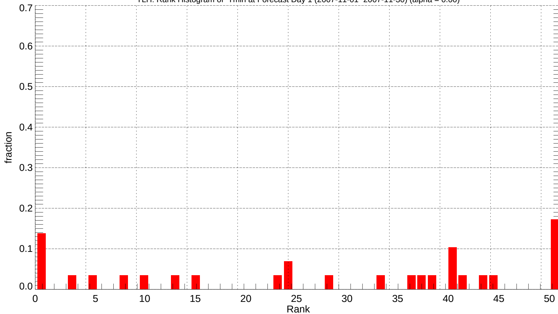
TLH: Rank Histogram of Tmin at Forecast Day 1 (2007-11-01~2007-11-30) (alpha = 0.00)
