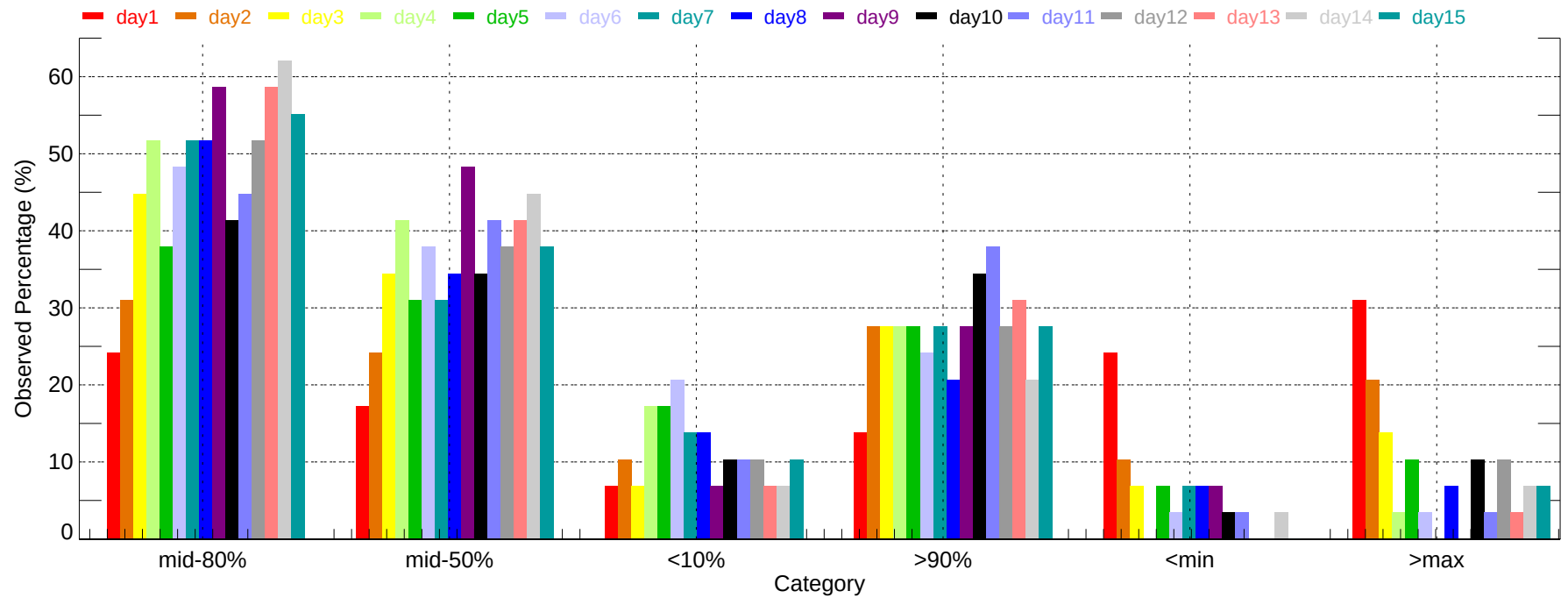
Observed Percentage of Ensembles - BIS: Min Temperature (2007-11-01~2007-11-30)
