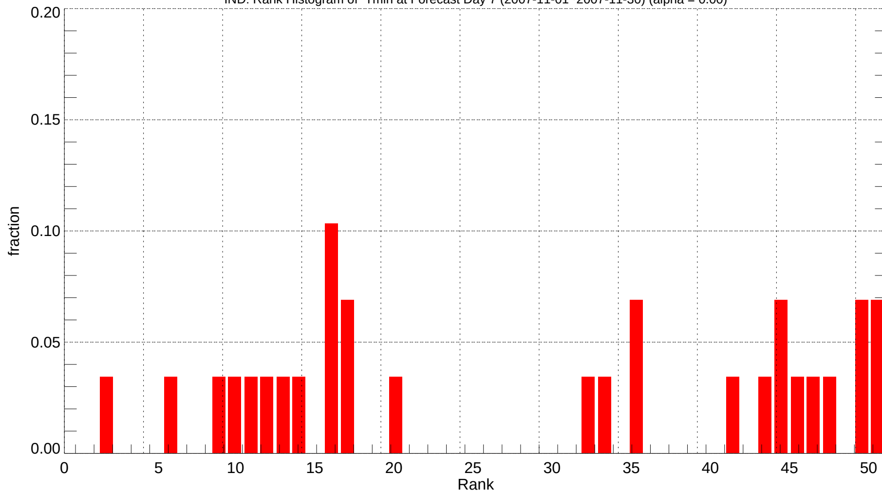
IND: Rank Histogram of Tmin at Forecast Day 7 (2007-11-01~2007-11-30) (alpha = 0.00)
