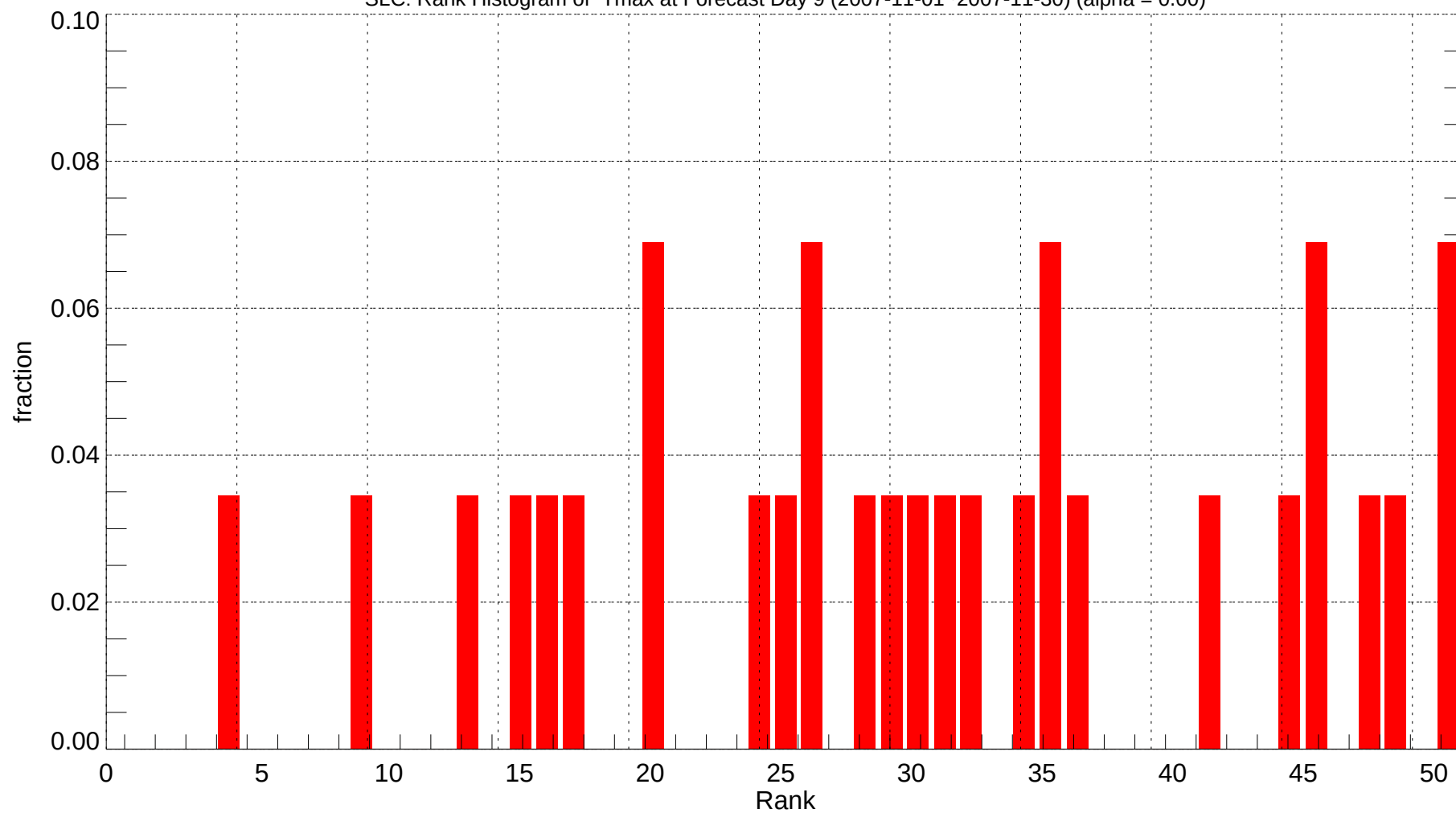
SLC: Rank Histogram of Tmax at Forecast Day 9 (2007-11-01~2007-11-30) (alpha = 0.00)
