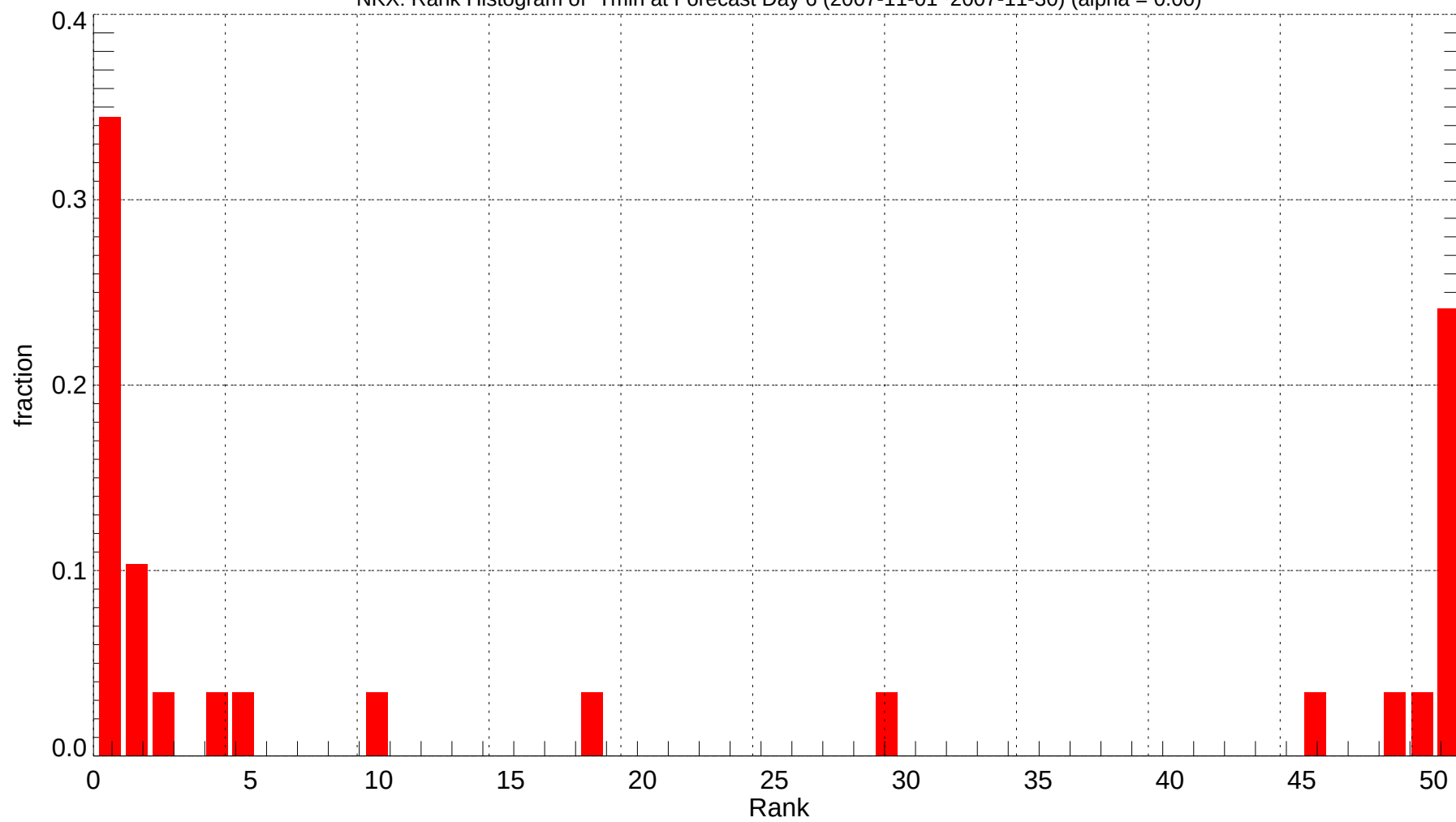
NKX: Rank Histogram of Tmin at Forecast Day 6 (2007-11-01~2007-11-30) (alpha = 0.00)
