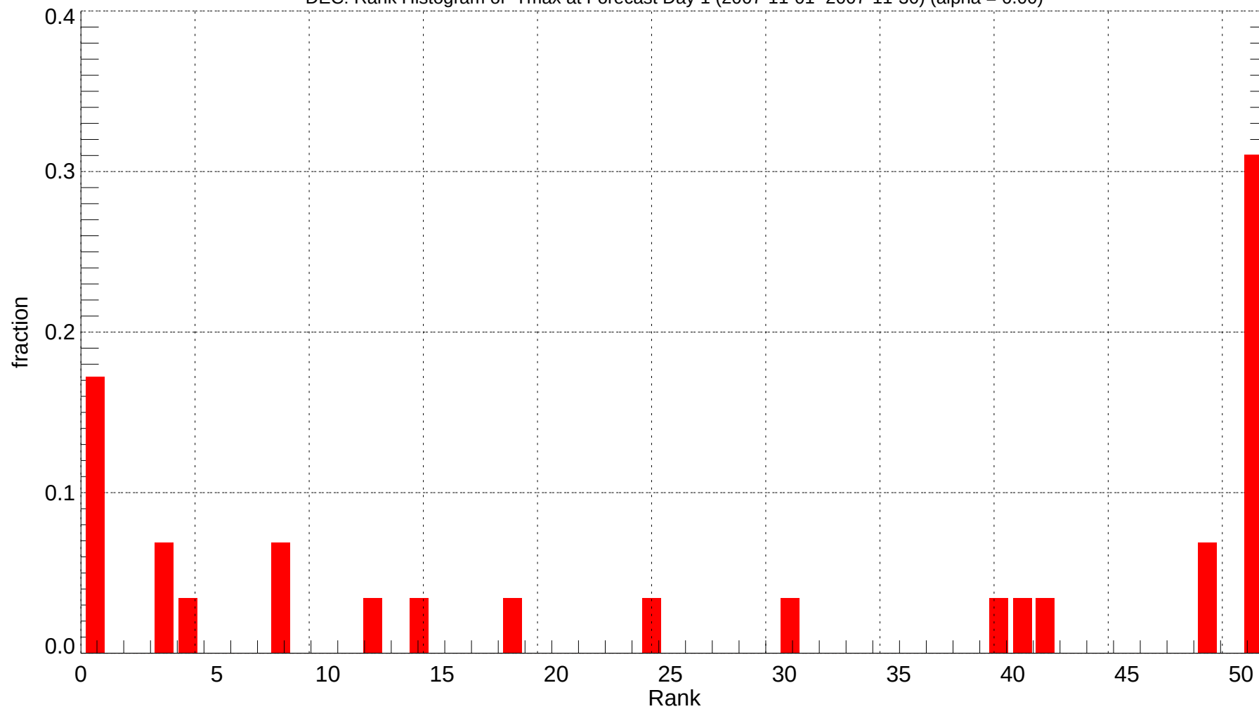
DEC: Rank Histogram of Tmax at Forecast Day 1 (2007-11-01~2007-11-30) (alpha = 0.00)
