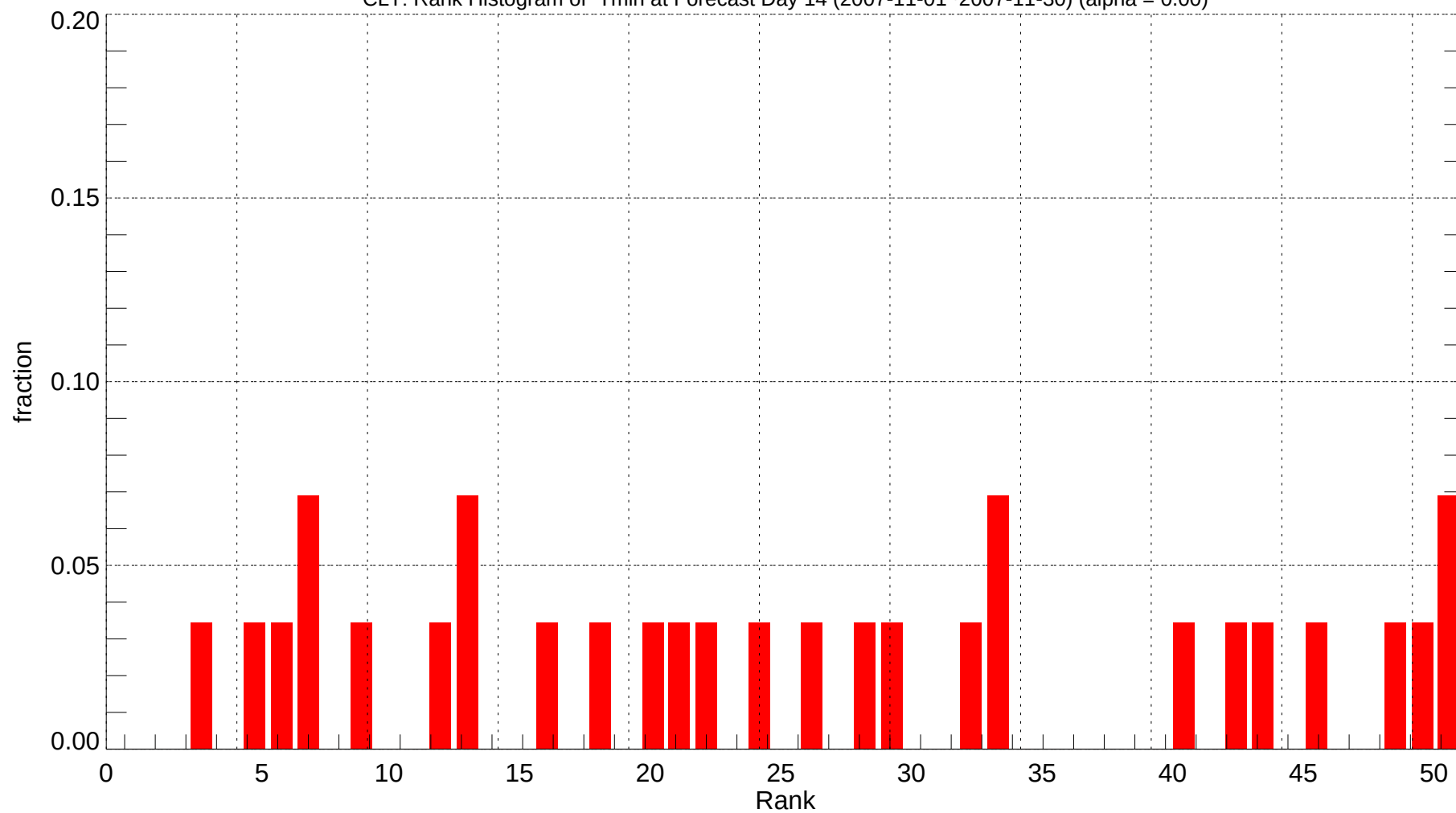
CLT: Rank Histogram of Tmin at Forecast Day 14 (2007-11-01~2007-11-30) (alpha = 0.00)
