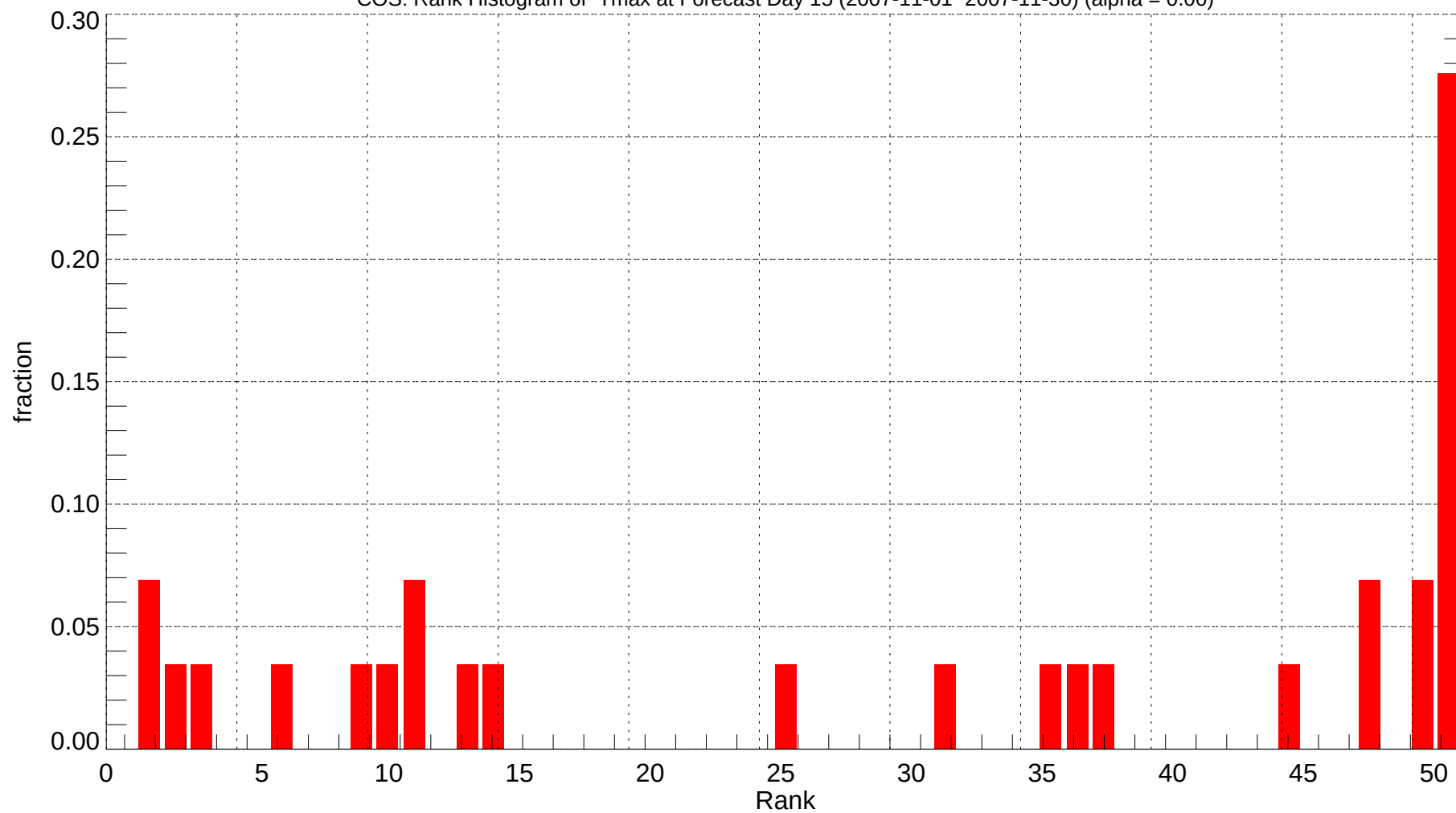
COS: Rank Histogram of Tmax at Forecast Day 15 (2007-11-01~2007-11-30) (alpha = 0.00)
