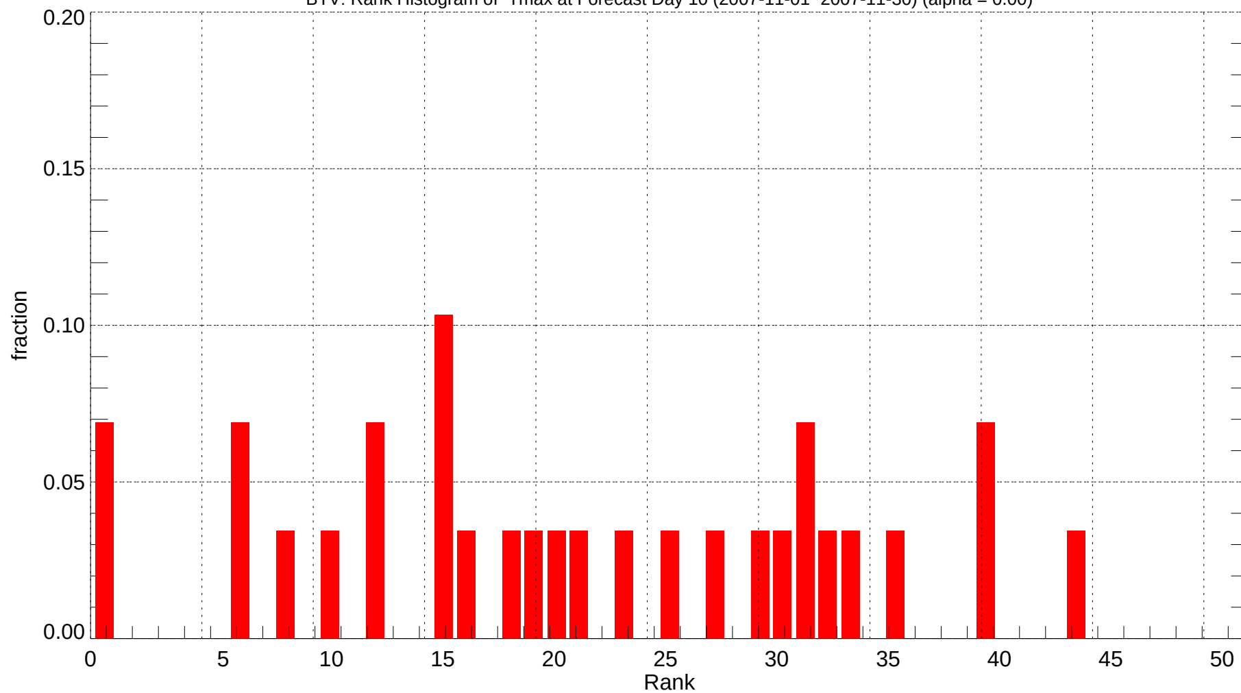
BTV: Rank Histogram of Tmax at Forecast Day 10 (2007-11-01~2007-11-30) (alpha = 0.00)
