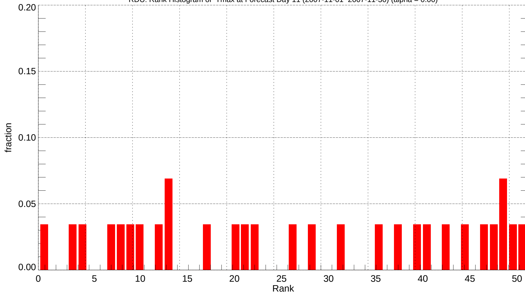
RDU: Rank Histogram of Tmax at Forecast Day 11 (2007-11-01~2007-11-30) (alpha = 0.00)
