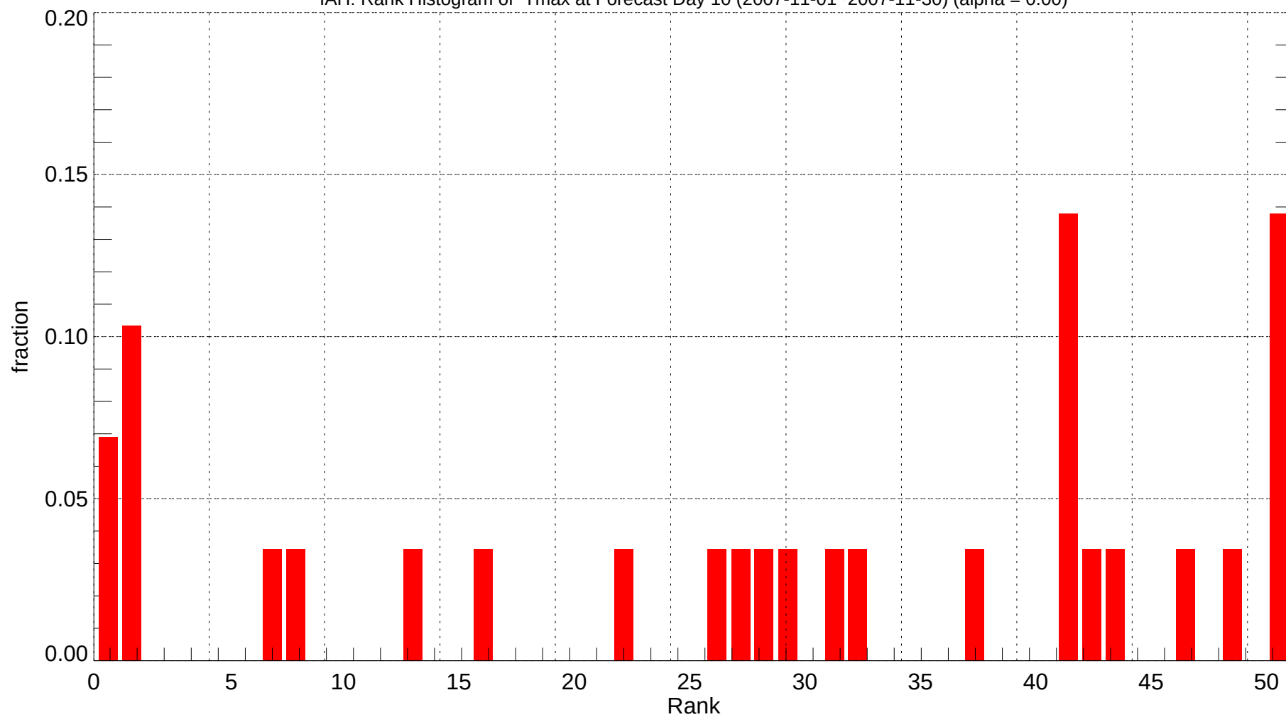
IAH: Rank Histogram of Tmax at Forecast Day 10 (2007-11-01~2007-11-30) (alpha = 0.00)
