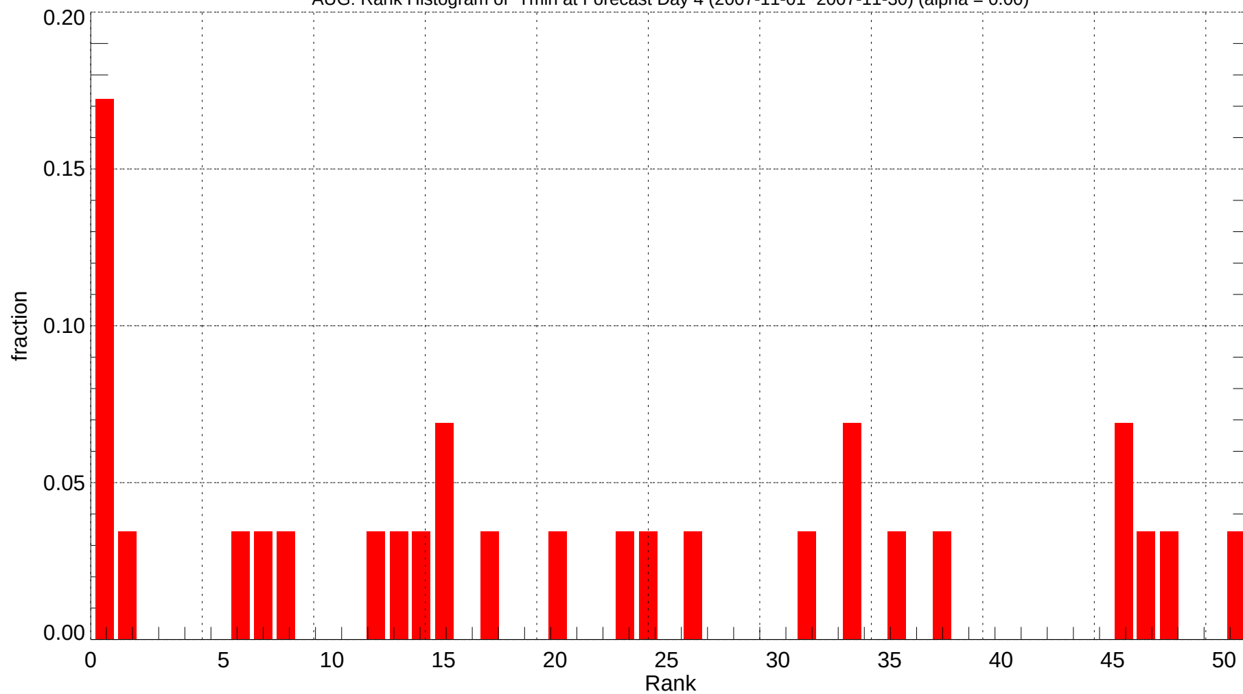
AUG: Rank Histogram of Tmin at Forecast Day 4 (2007-11-01~2007-11-30) (alpha = 0.00)
