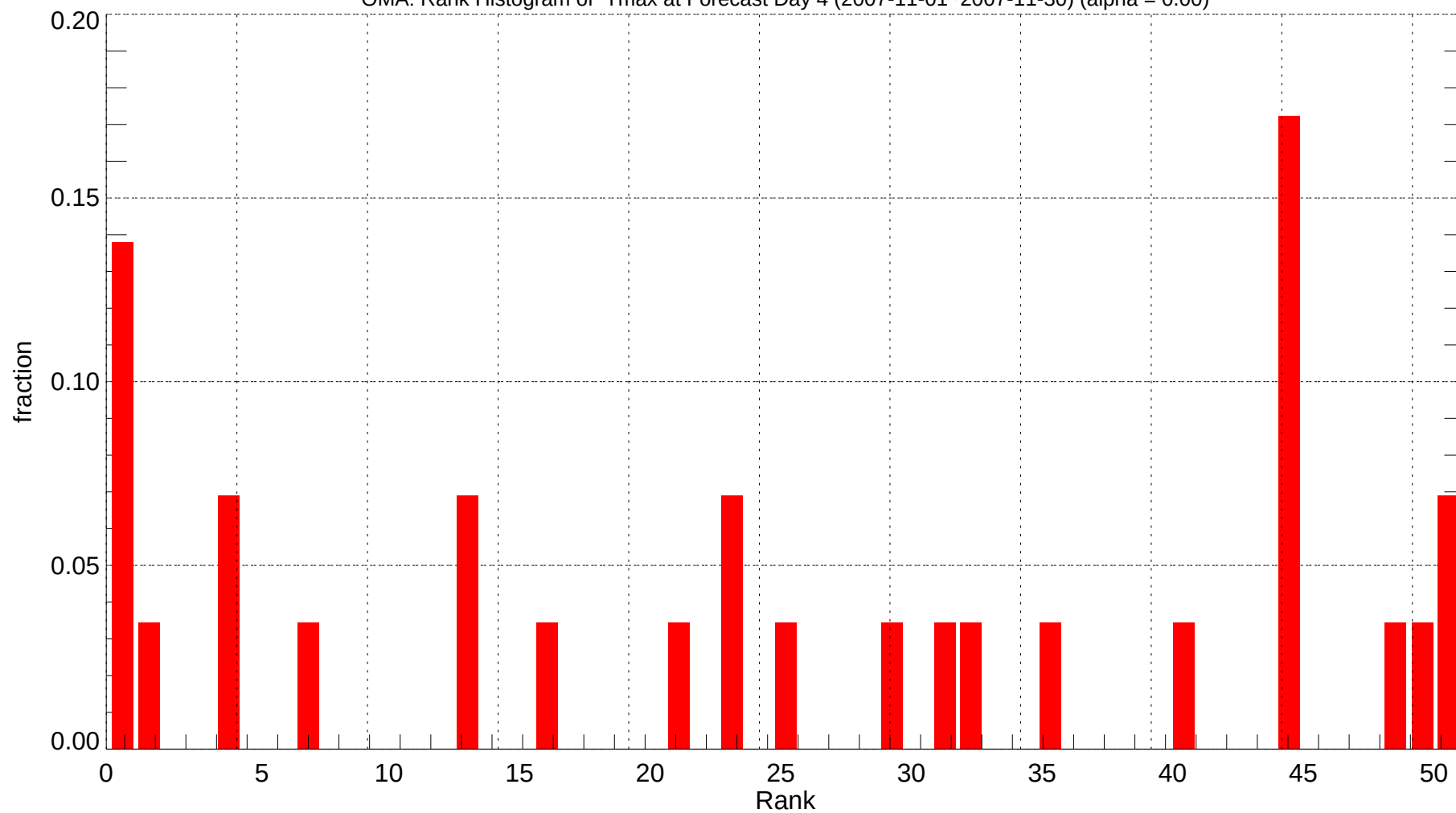
OMA: Rank Histogram of Tmax at Forecast Day 4 (2007-11-01~2007-11-30) (alpha = 0.00)
