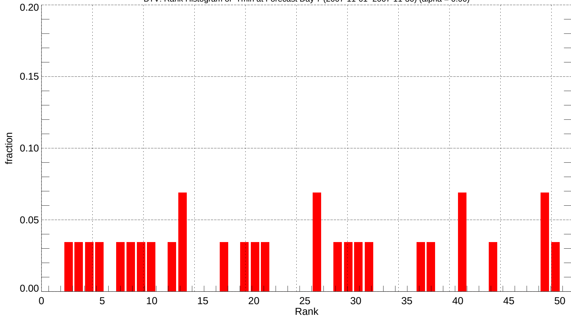
BTV: Rank Histogram of Tmin at Forecast Day 7 (2007-11-01~2007-11-30) (alpha = 0.00)
