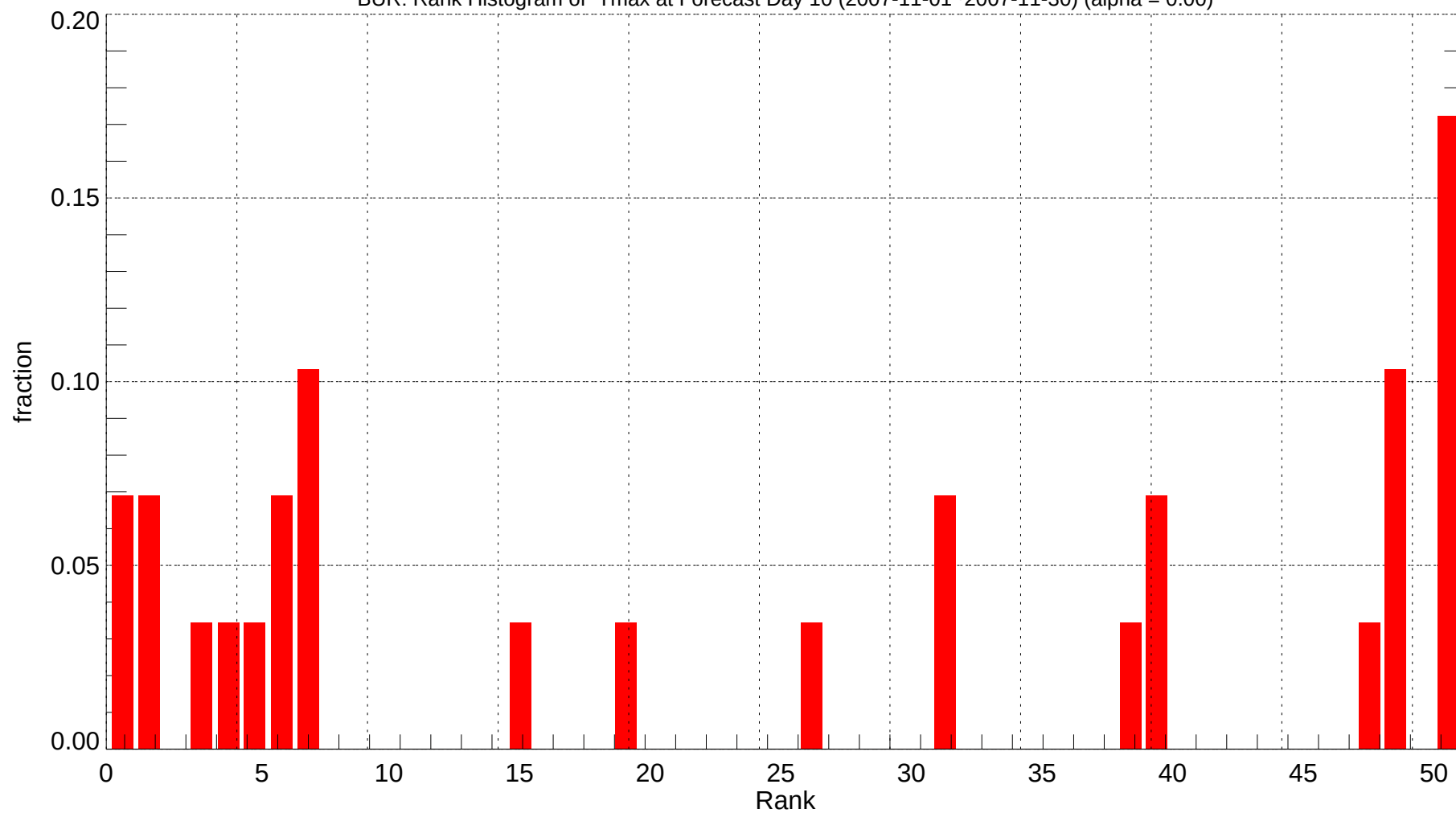
BUR: Rank Histogram of Tmax at Forecast Day 10 (2007-11-01~2007-11-30) (alpha = 0.00)
