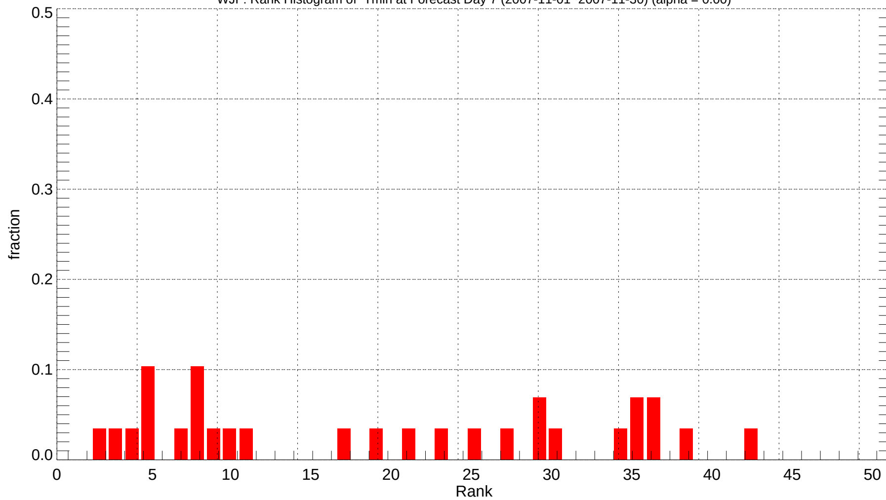
WJF: Rank Histogram of Tmin at Forecast Day 7 (2007-11-01~2007-11-30) (alpha = 0.00)
