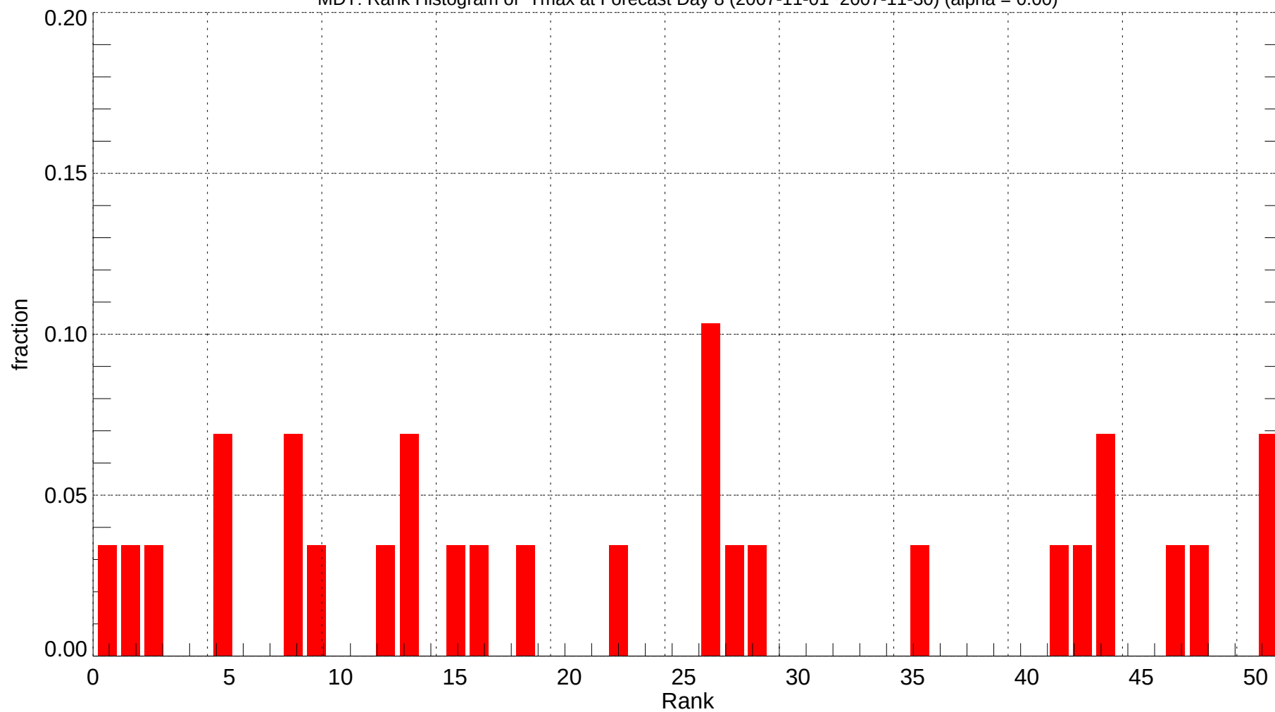
MDT: Rank Histogram of Tmax at Forecast Day 8 (2007-11-01~2007-11-30) (alpha = 0.00)
