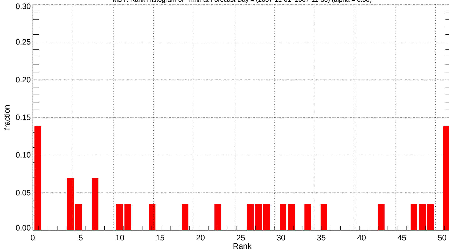
MDT: Rank Histogram of Tmin at Forecast Day 4 (2007-11-01~2007-11-30) (alpha = 0.00)
