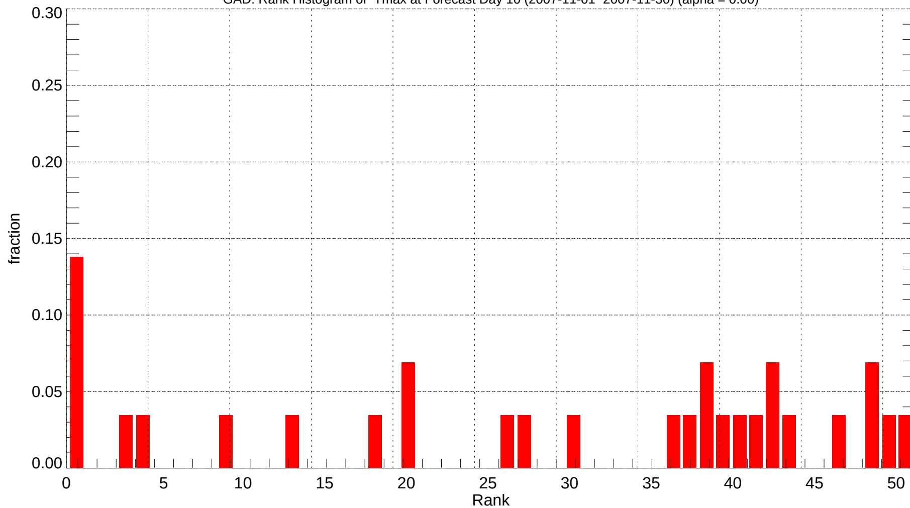
GAD: Rank Histogram of Tmax at Forecast Day 10 (2007-11-01~2007-11-30) (alpha = 0.00)
