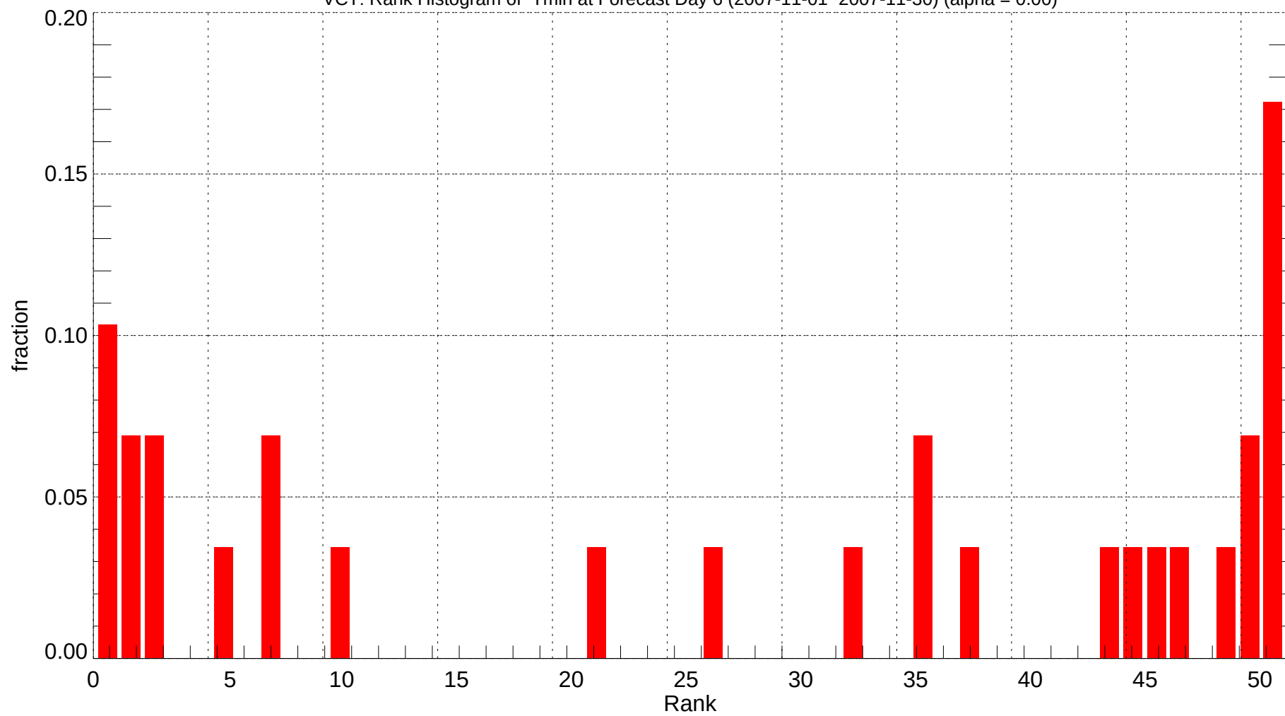
VCT: Rank Histogram of Tmin at Forecast Day 6 (2007-11-01~2007-11-30) (alpha = 0.00)
