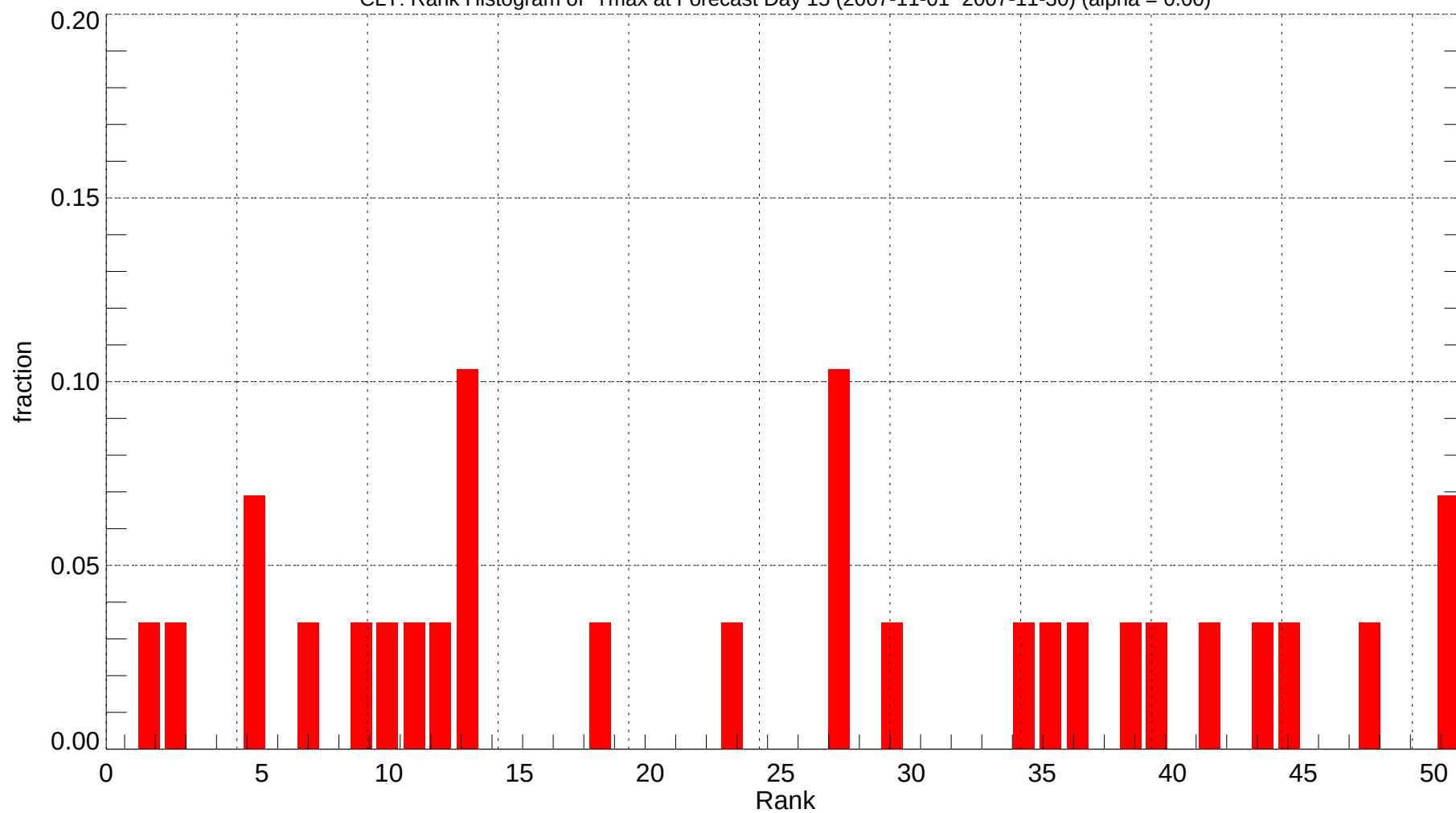
CLT: Rank Histogram of Tmax at Forecast Day 15 (2007-11-01~2007-11-30) (alpha = 0.00)
