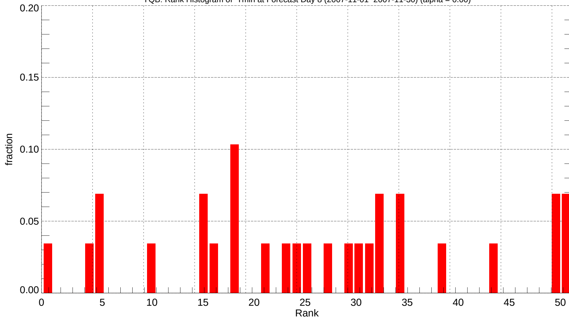
YQB: Rank Histogram of Tmin at Forecast Day 8 (2007-11-01~2007-11-30) (alpha = 0.00)
