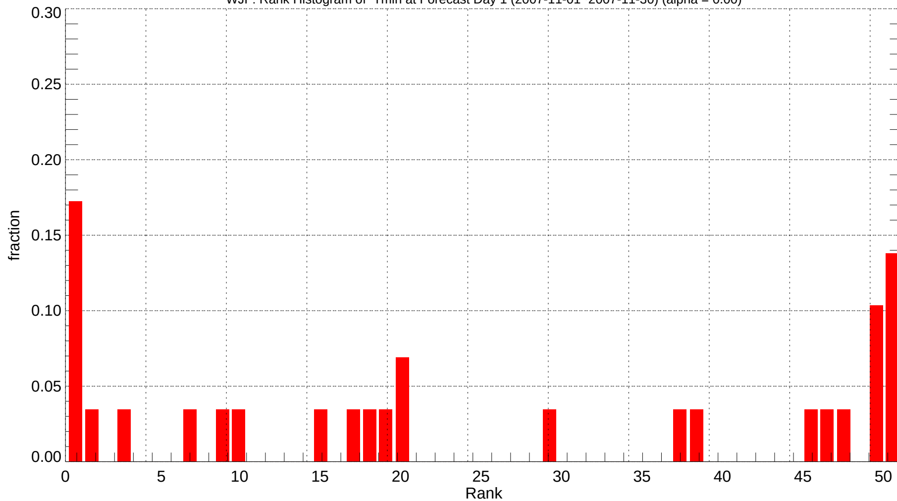
WJF: Rank Histogram of Tmin at Forecast Day 1 (2007-11-01~2007-11-30) (alpha = 0.00)
