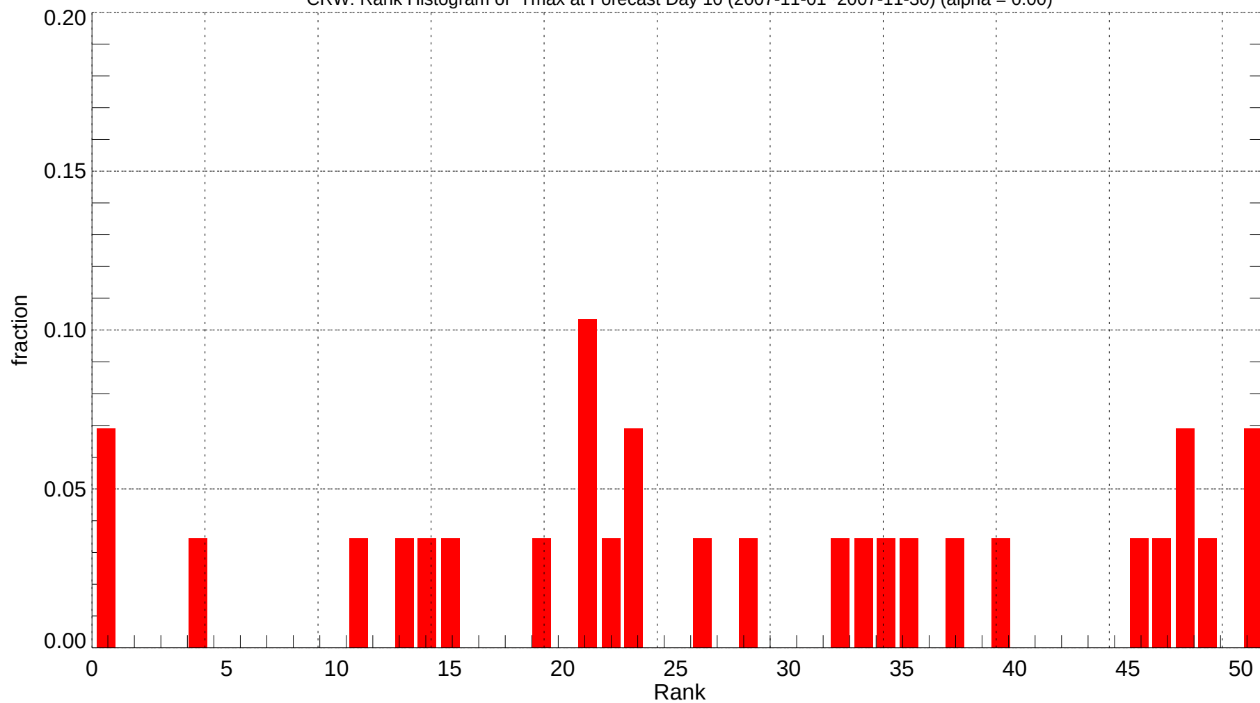
CRW: Rank Histogram of Tmax at Forecast Day 10 (2007-11-01~2007-11-30) (alpha = 0.00)
