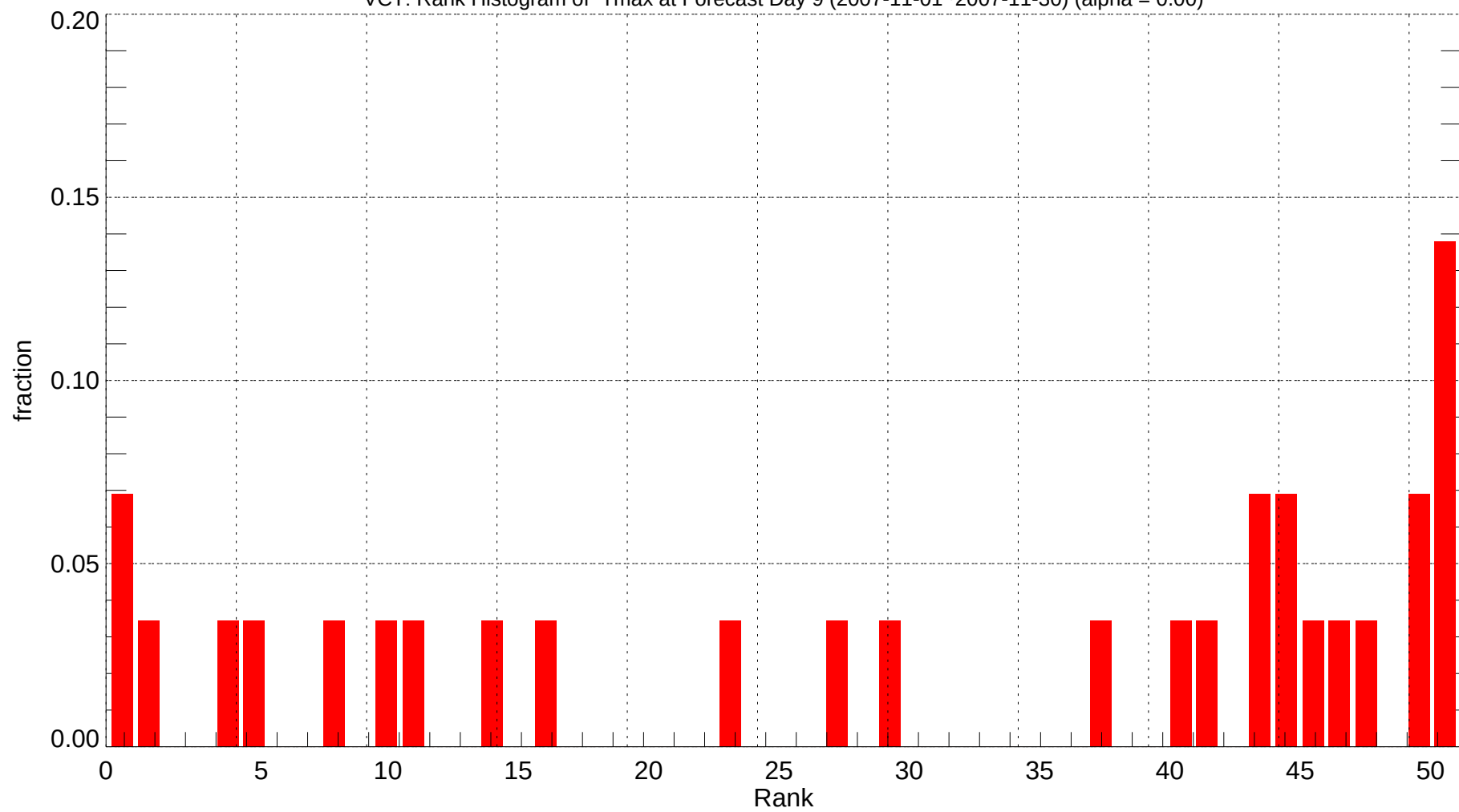
VCT: Rank Histogram of Tmax at Forecast Day 9 (2007-11-01~2007-11-30) (alpha = 0.00)
