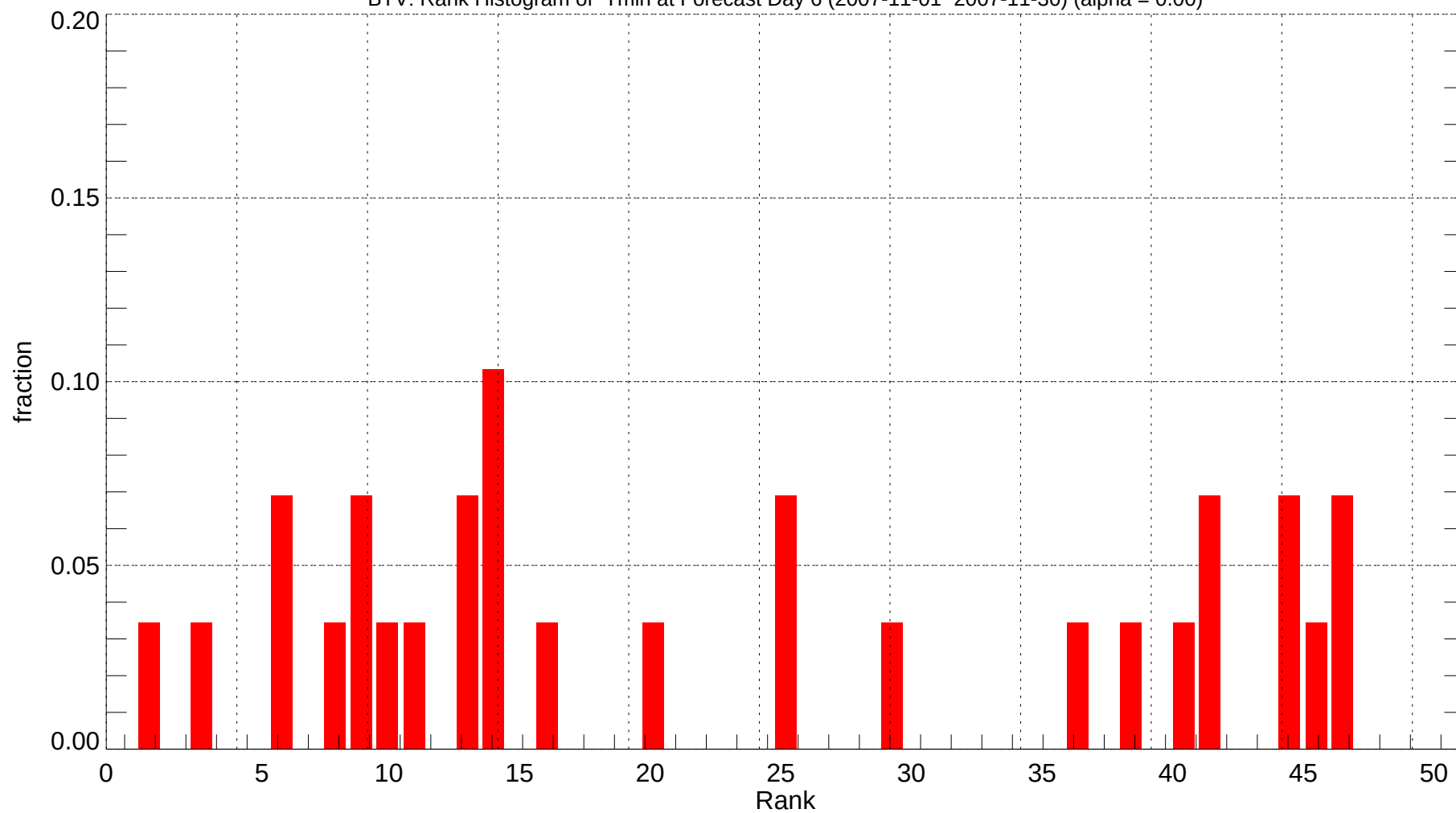
BTV: Rank Histogram of Tmin at Forecast Day 6 (2007-11-01~2007-11-30) (alpha = 0.00)
