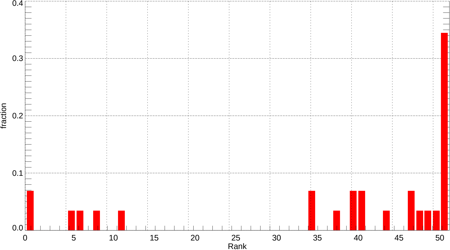
TUL: Rank Histogram of Tmin at Forecast Day 4 (2007-11-01~2007-11-30) (alpha = 0.00)
