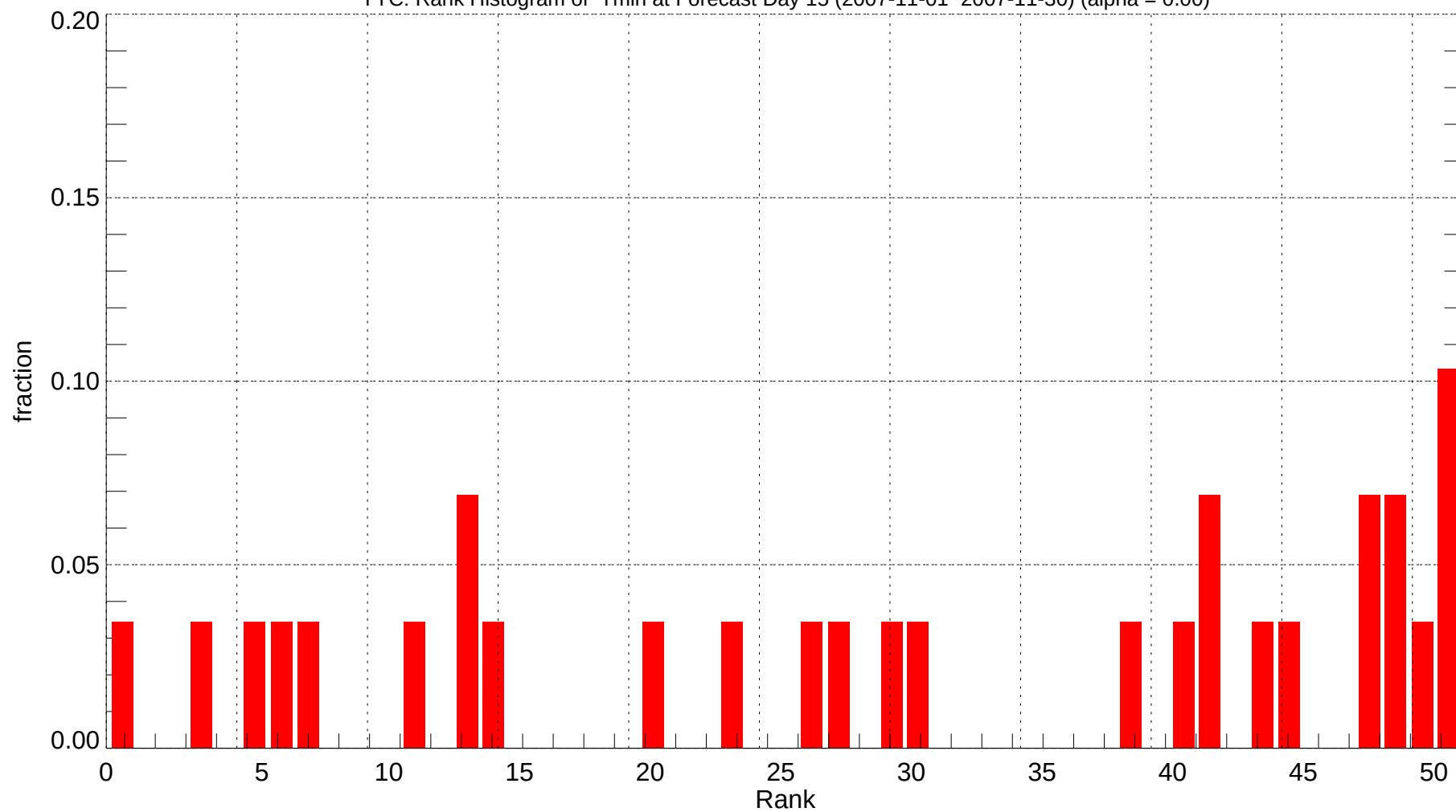
YYC: Rank Histogram of Tmin at Forecast Day 15 (2007-11-01~2007-11-30) (alpha = 0.00)
