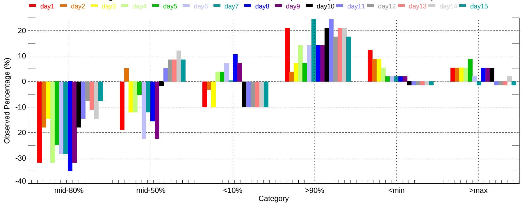
Observed Percentage Deviation of Ensembles - SAC: Max Temperature (2007-11-01~2007-11-30)
