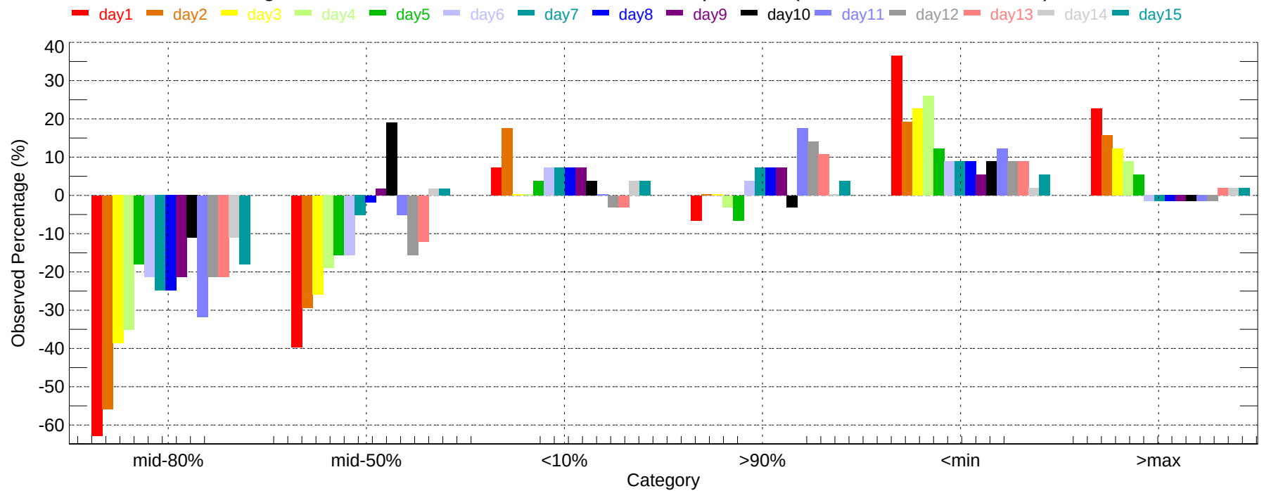
Observed Percentage Deviation of Ensembles - BUF: Max Temperature (2007-11-01~2007-11-30)
