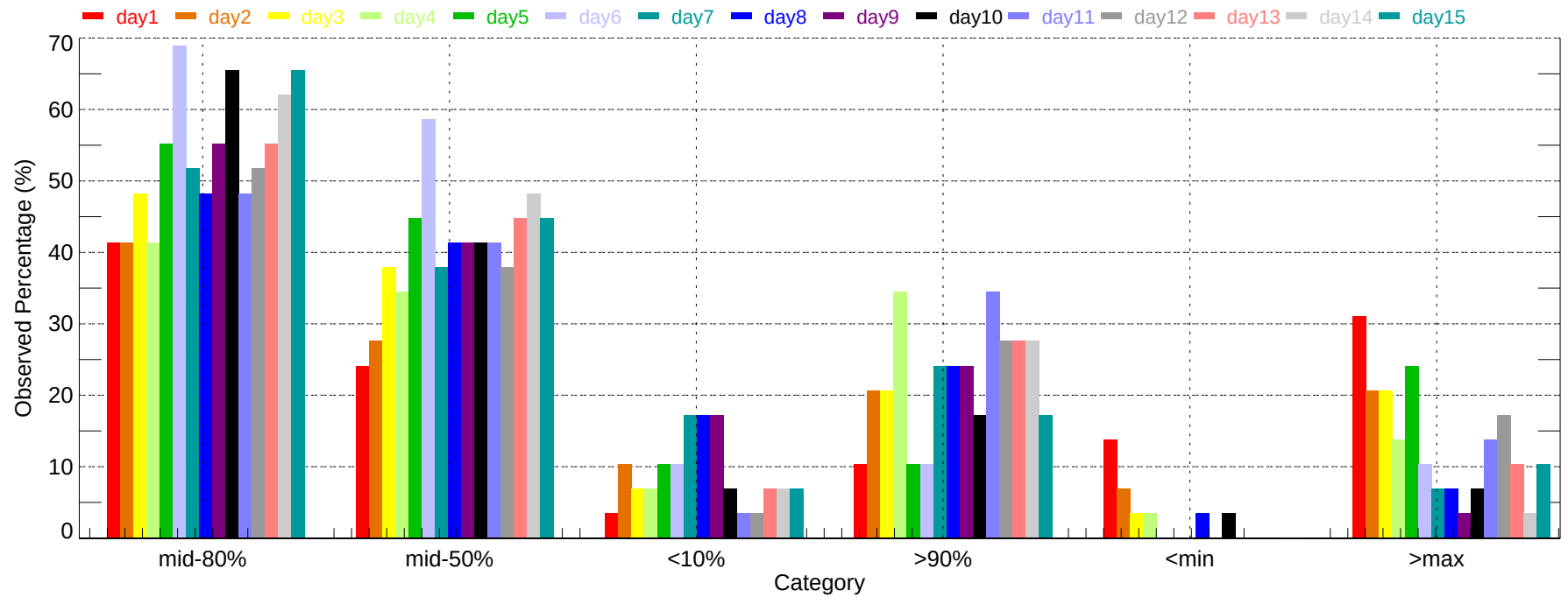
Observed Percentage of Ensembles - RIC: Max Temperature (2007-11-01~2007-11-30)
