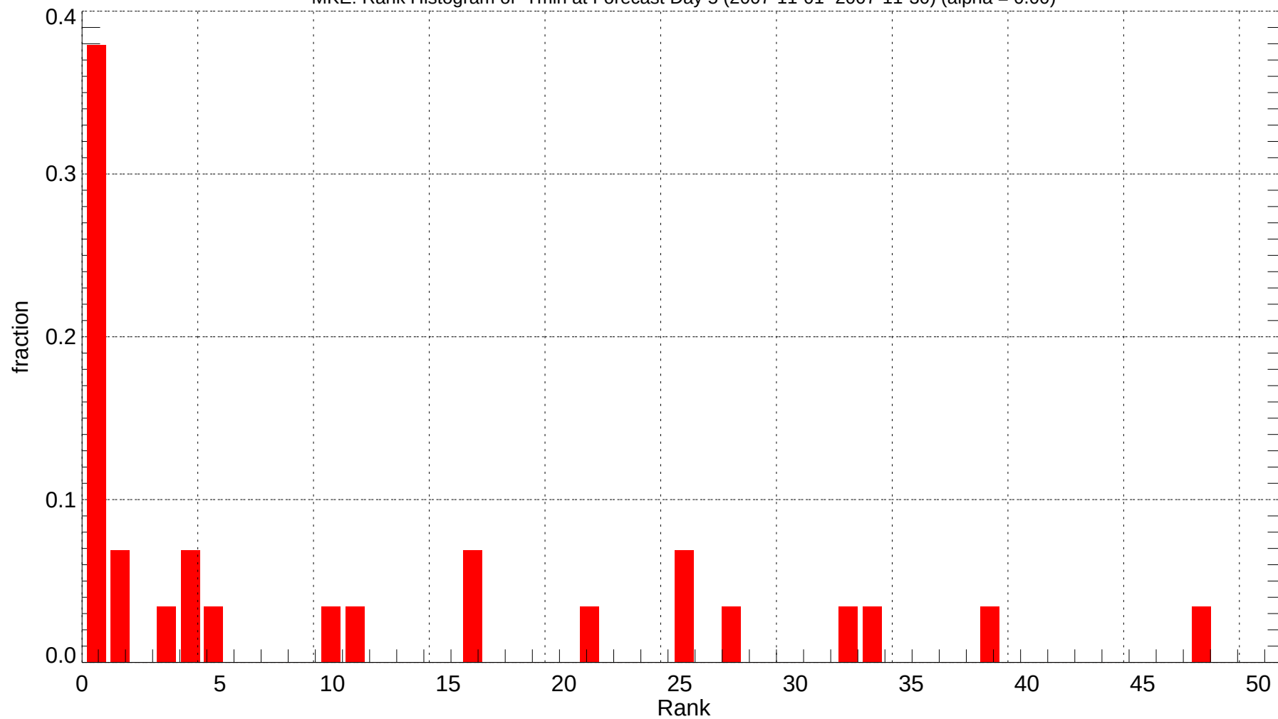
MKE: Rank Histogram of Tmin at Forecast Day 5 (2007-11-01~2007-11-30) (alpha = 0.00)
