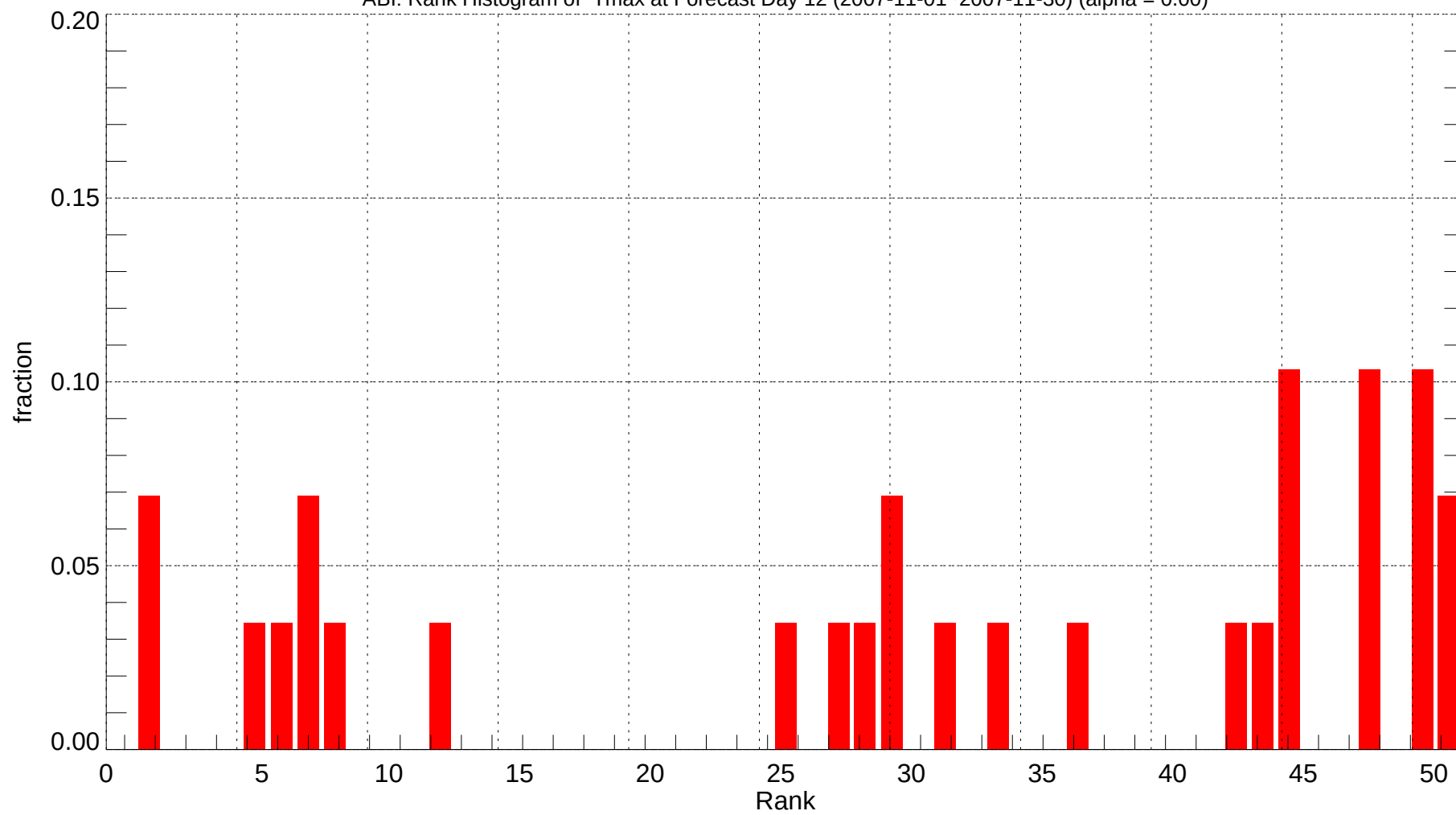
ABI: Rank Histogram of Tmax at Forecast Day 12 (2007-11-01~2007-11-30) (alpha = 0.00)
