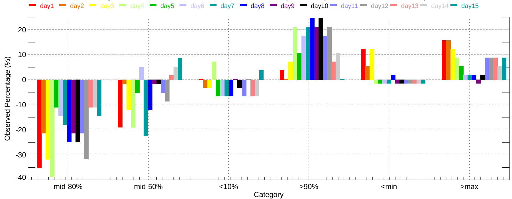
Observed Percentage Deviation of Ensembles - CVG: Max Temperature (2007-11-01~2007-11-30)
