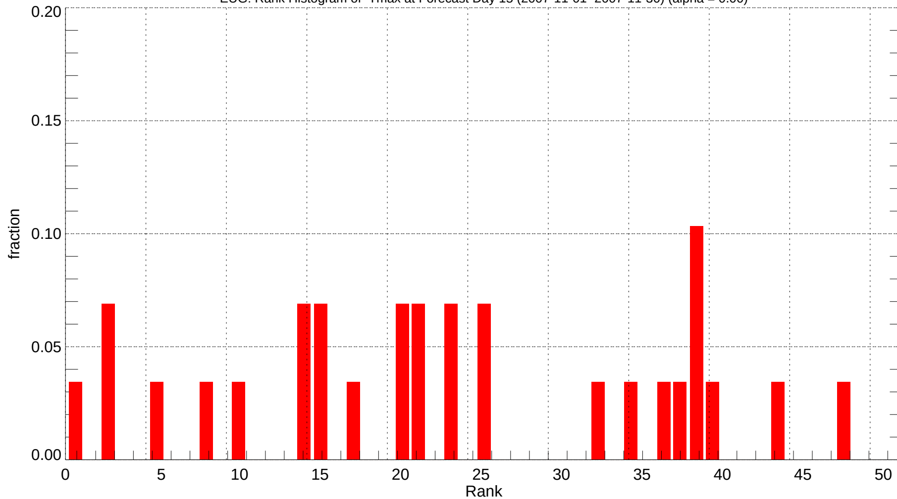
EUG: Rank Histogram of Tmax at Forecast Day 15 (2007-11-01~2007-11-30) (alpha = 0.00)
