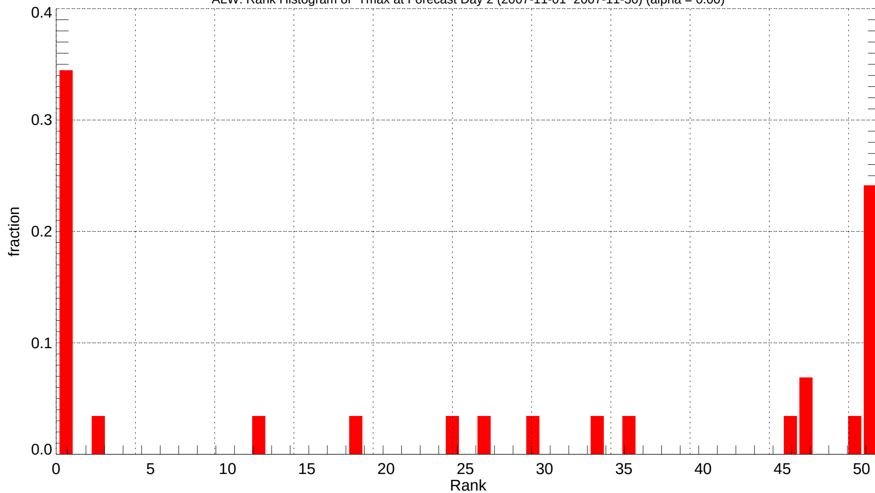
ALW: Rank Histogram of Tmax at Forecast Day 2 (2007-11-01~2007-11-30) (alpha = 0.00)
