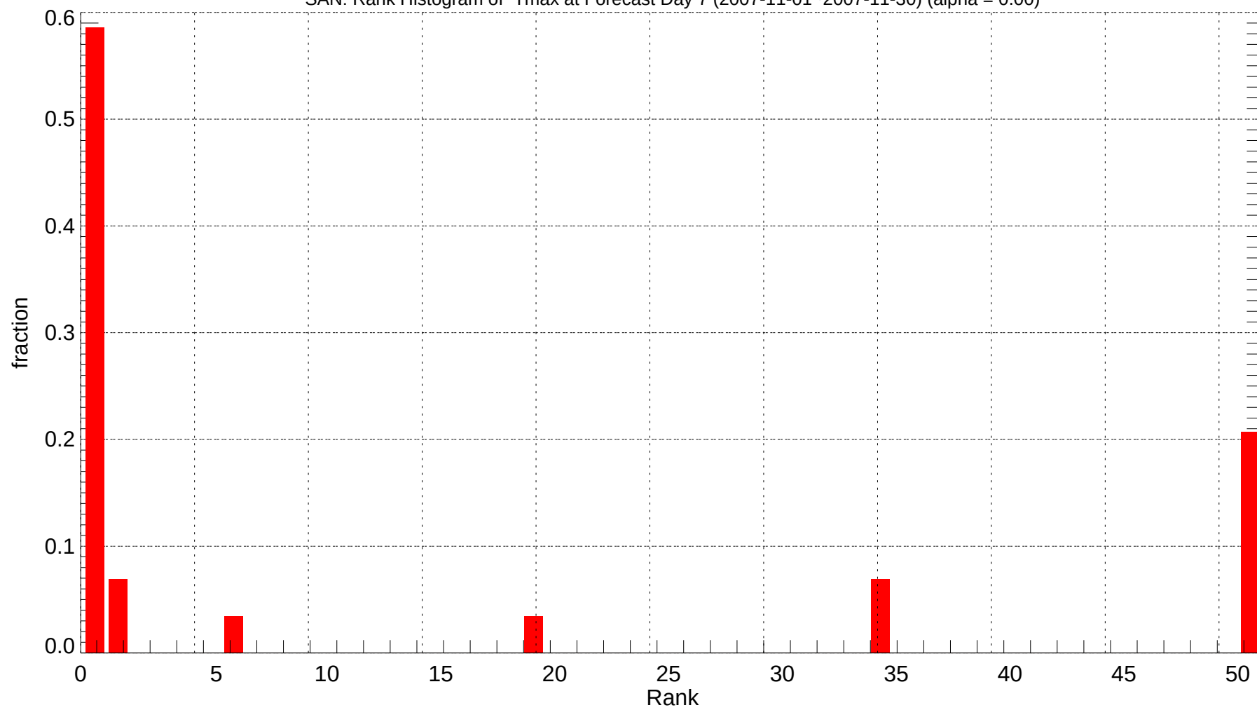
SAN: Rank Histogram of Tmax at Forecast Day 7 (2007-11-01~2007-11-30) (alpha = 0.00)
