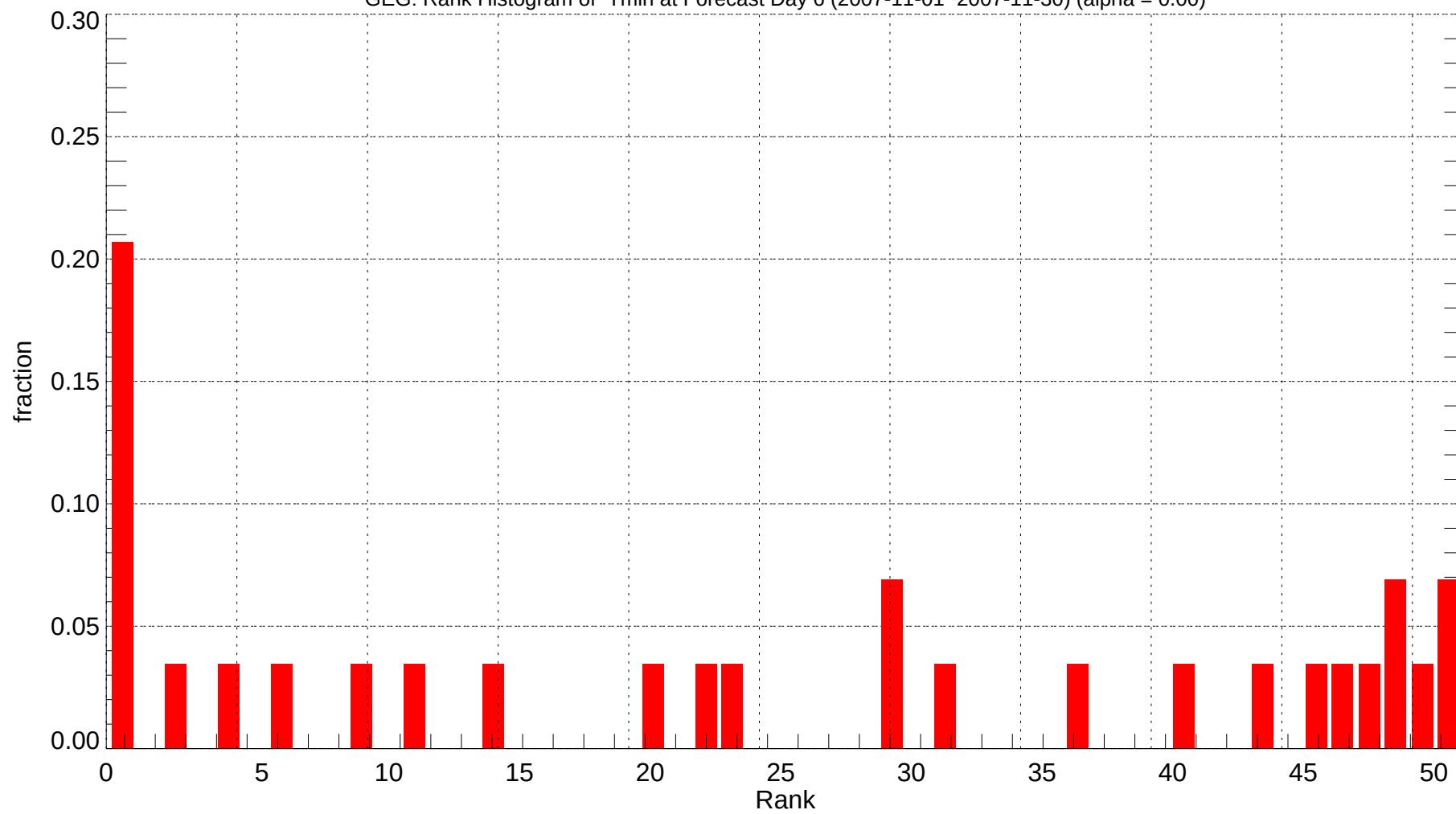
GEG: Rank Histogram of Tmin at Forecast Day 6 (2007-11-01~2007-11-30) (alpha = 0.00)
