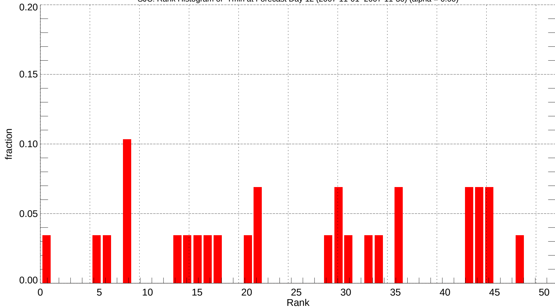
SJC: Rank Histogram of Tmin at Forecast Day 12 (2007-11-01~2007-11-30) (alpha = 0.00)
