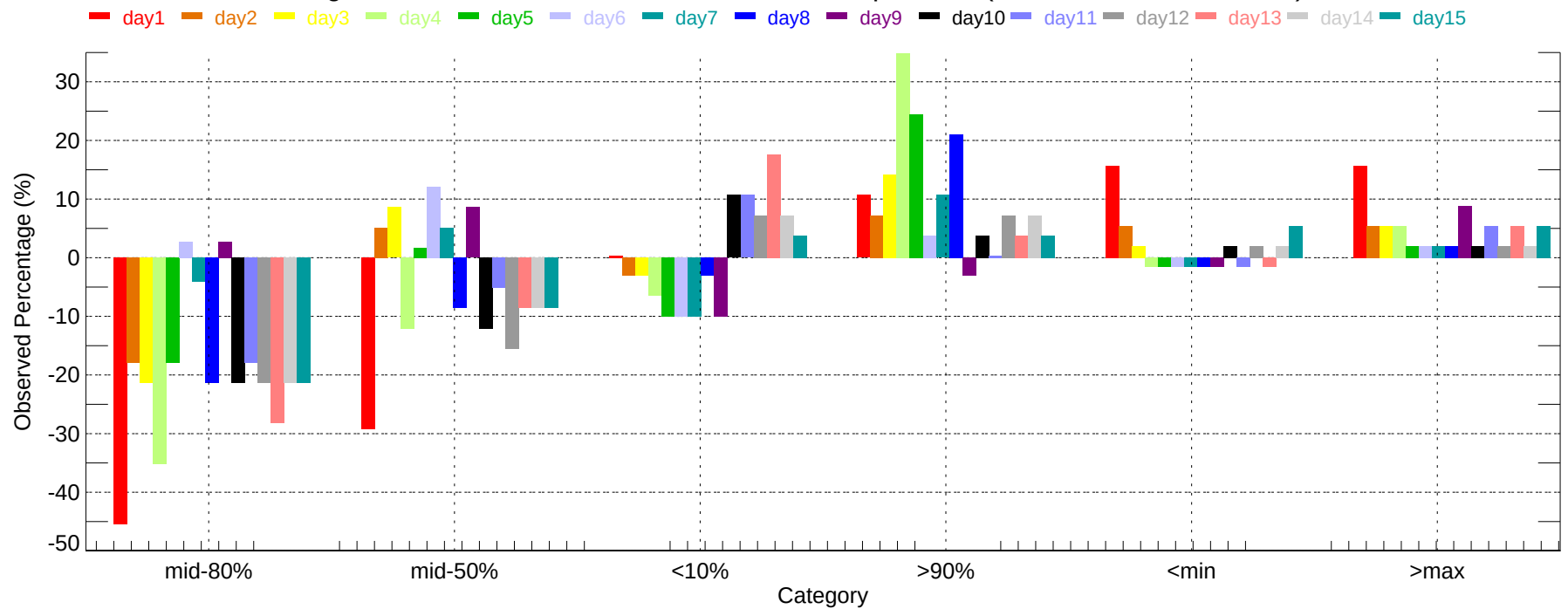
Observed Percentage Deviation of Ensembles - EWR: Min Temperature (2007-11-01~2007-11-30)
