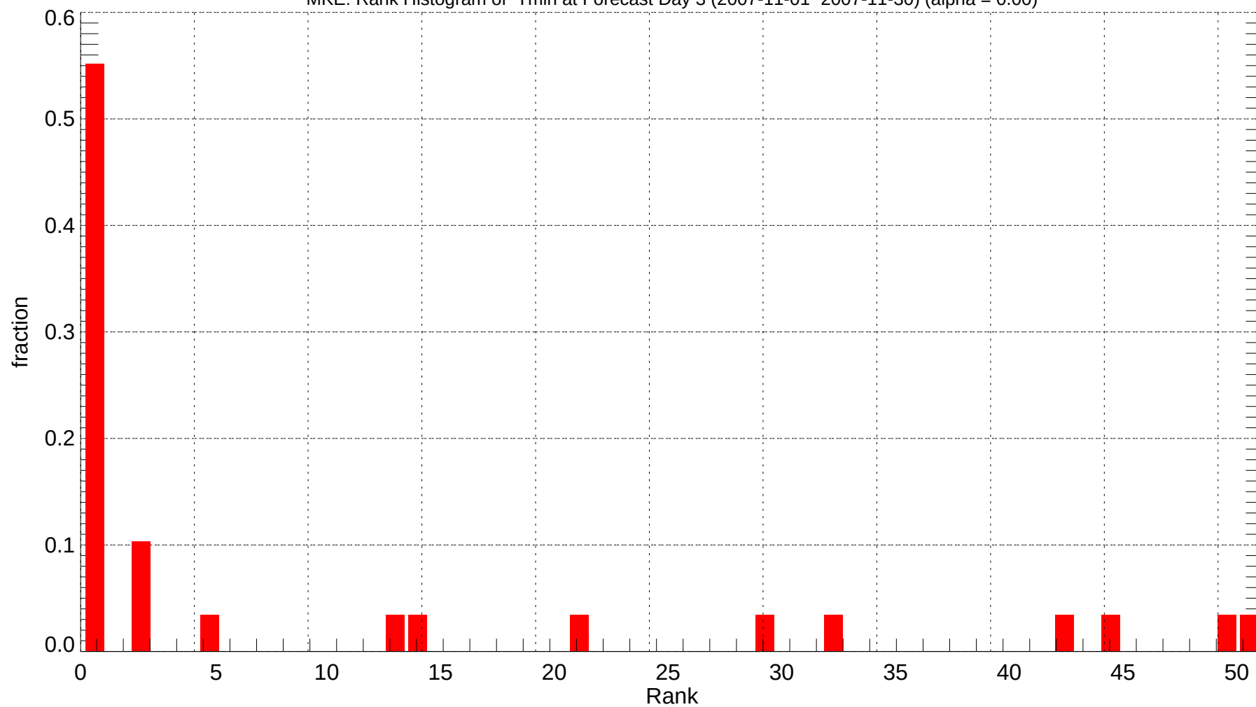
MKE: Rank Histogram of Tmin at Forecast Day 3 (2007-11-01~2007-11-30) (alpha = 0.00)
