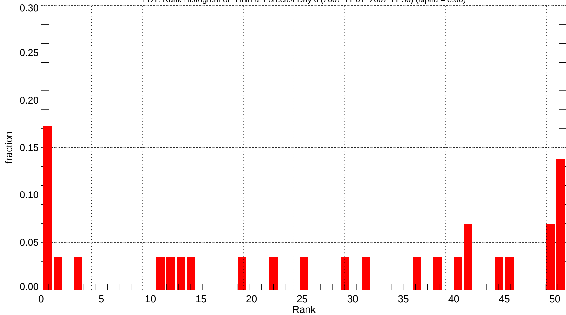
PDT: Rank Histogram of Tmin at Forecast Day 6 (2007-11-01~2007-11-30) (alpha = 0.00)
