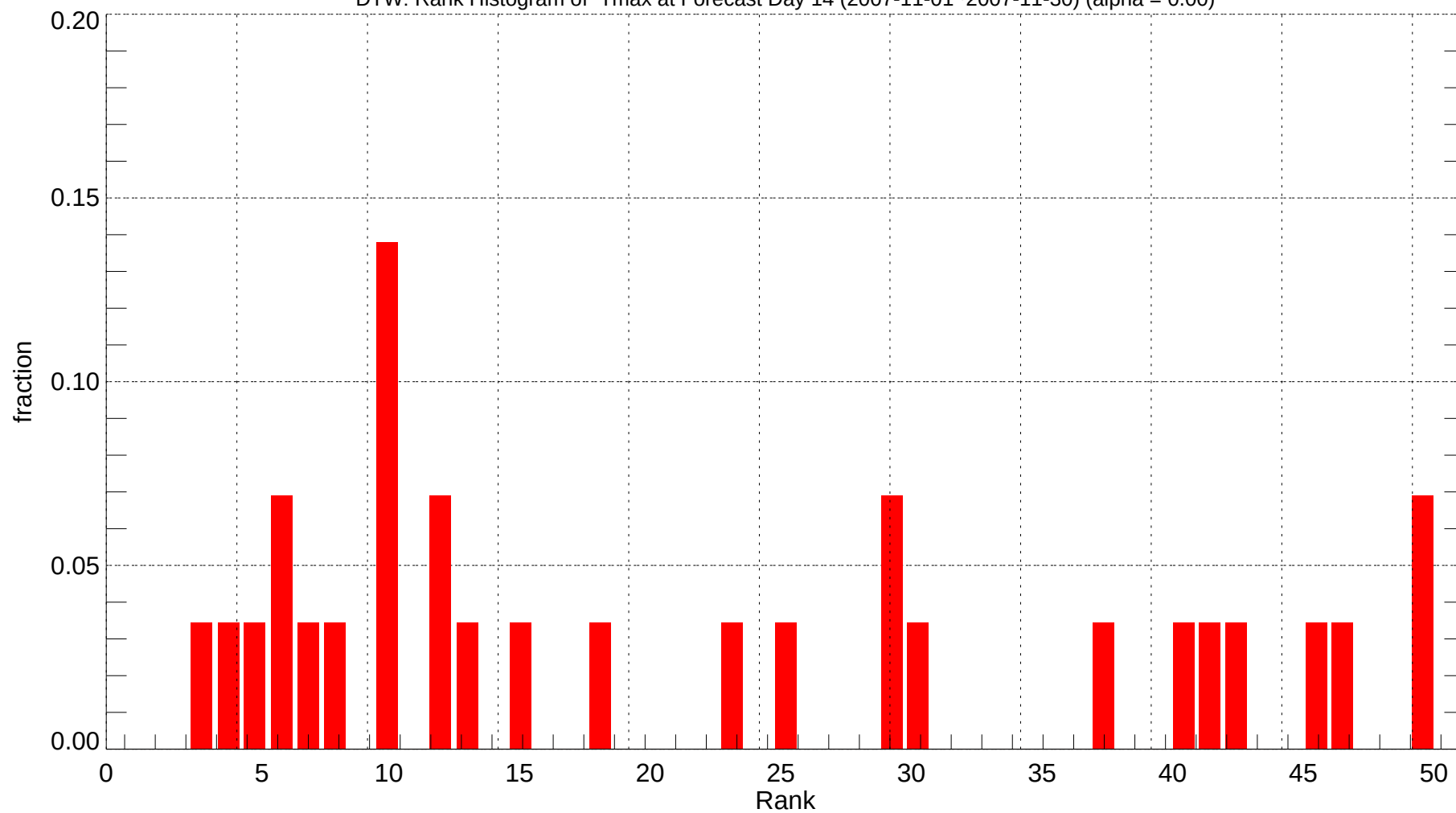
DTW: Rank Histogram of Tmax at Forecast Day 14 (2007-11-01~2007-11-30) (alpha = 0.00)
