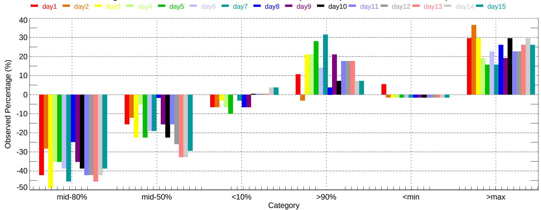
Observed Percentage Deviation of Ensembles - COS: Min Temperature (2007-11-01~2007-11-30)
