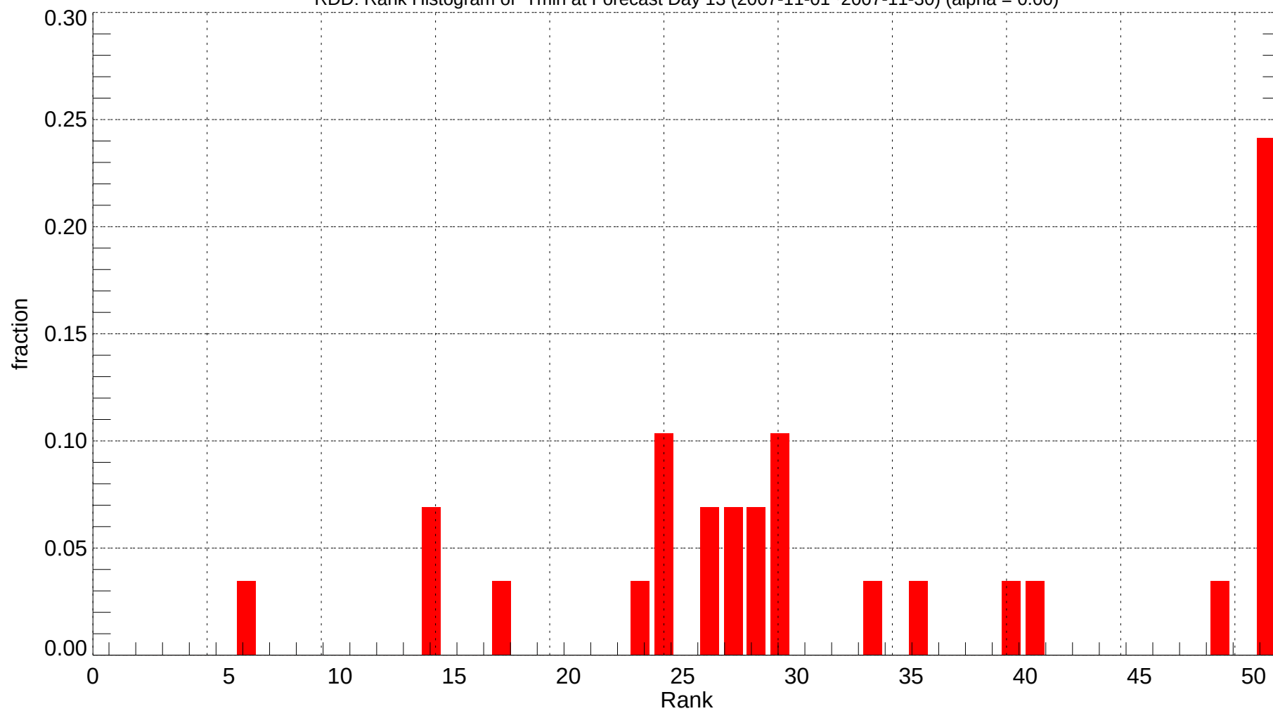
RDD: Rank Histogram of Tmin at Forecast Day 13 (2007-11-01~2007-11-30) (alpha = 0.00)
