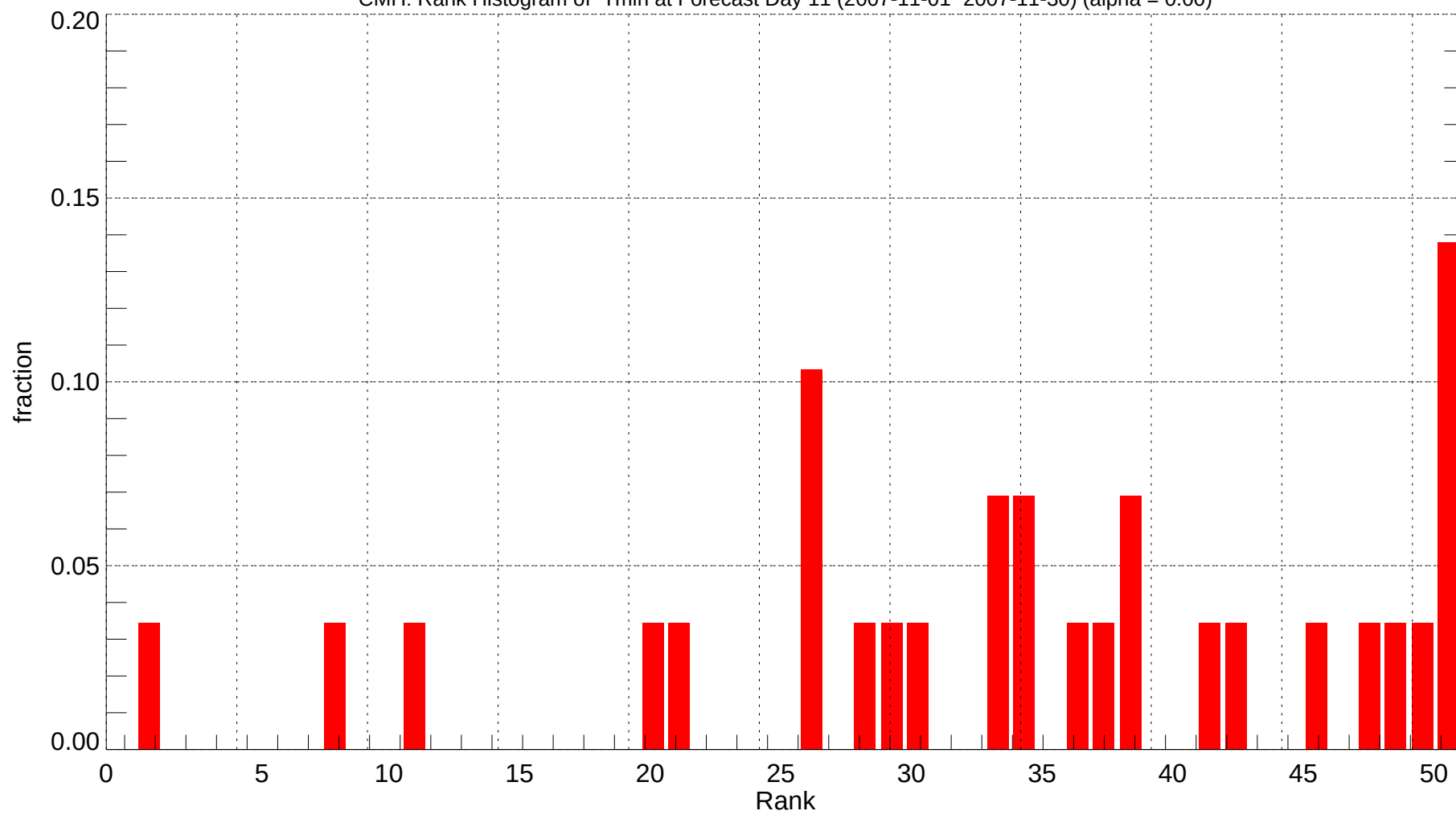
CMH: Rank Histogram of Tmin at Forecast Day 11 (2007-11-01~2007-11-30) (alpha = 0.00)
