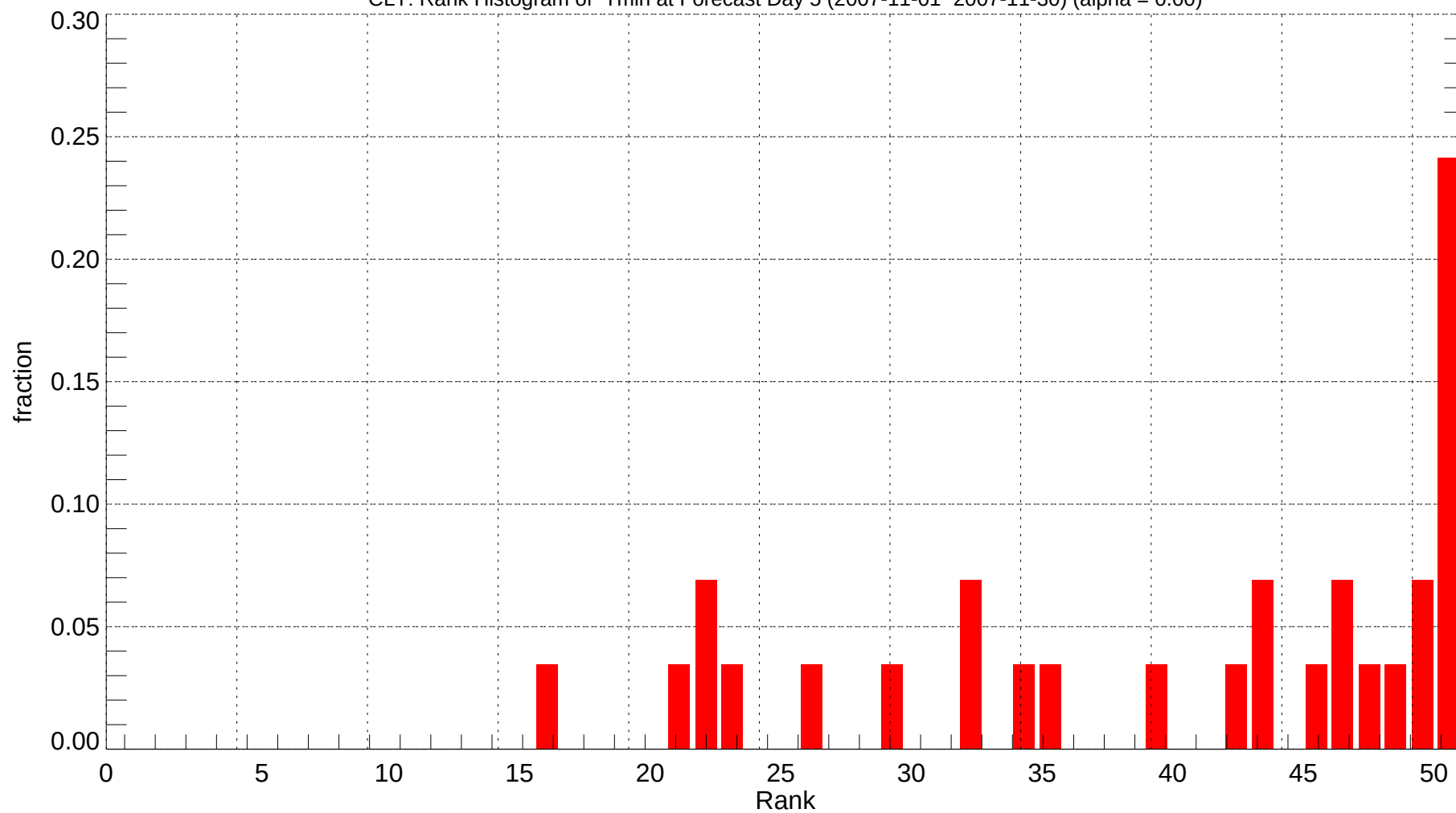
CLT: Rank Histogram of Tmin at Forecast Day 5 (2007-11-01~2007-11-30) (alpha = 0.00)
