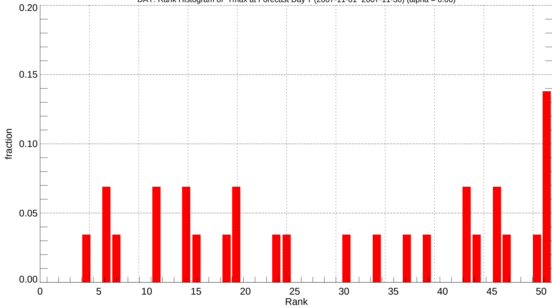
DAY: Rank Histogram of Tmax at Forecast Day 7 (2007-11-01~2007-11-30) (alpha = 0.00)
