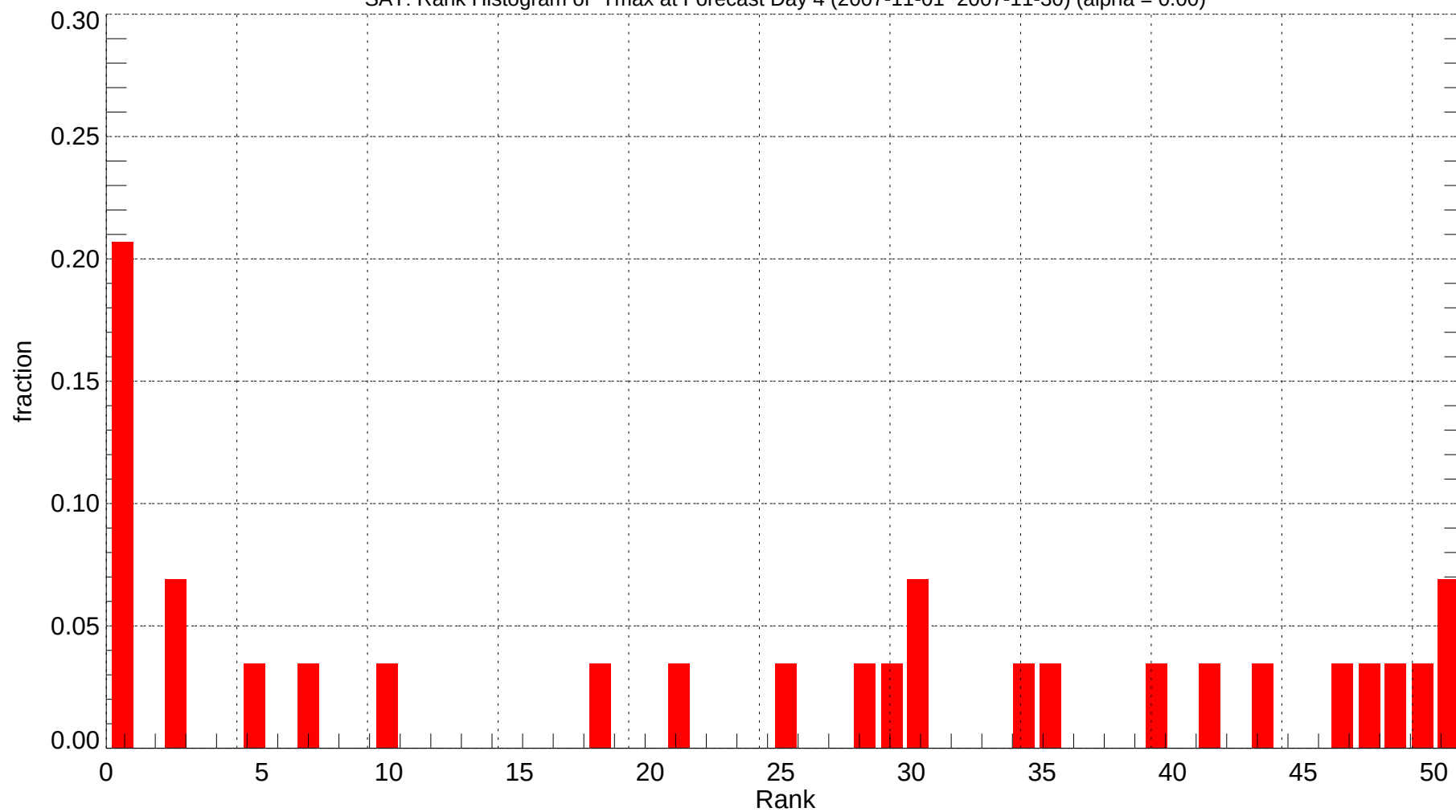
SAT: Rank Histogram of Tmax at Forecast Day 4 (2007-11-01~2007-11-30) (alpha = 0.00)
