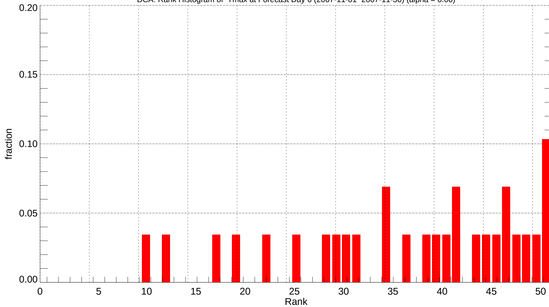
DCA: Rank Histogram of Tmax at Forecast Day 6 (2007-11-01~2007-11-30) (alpha = 0.00)
