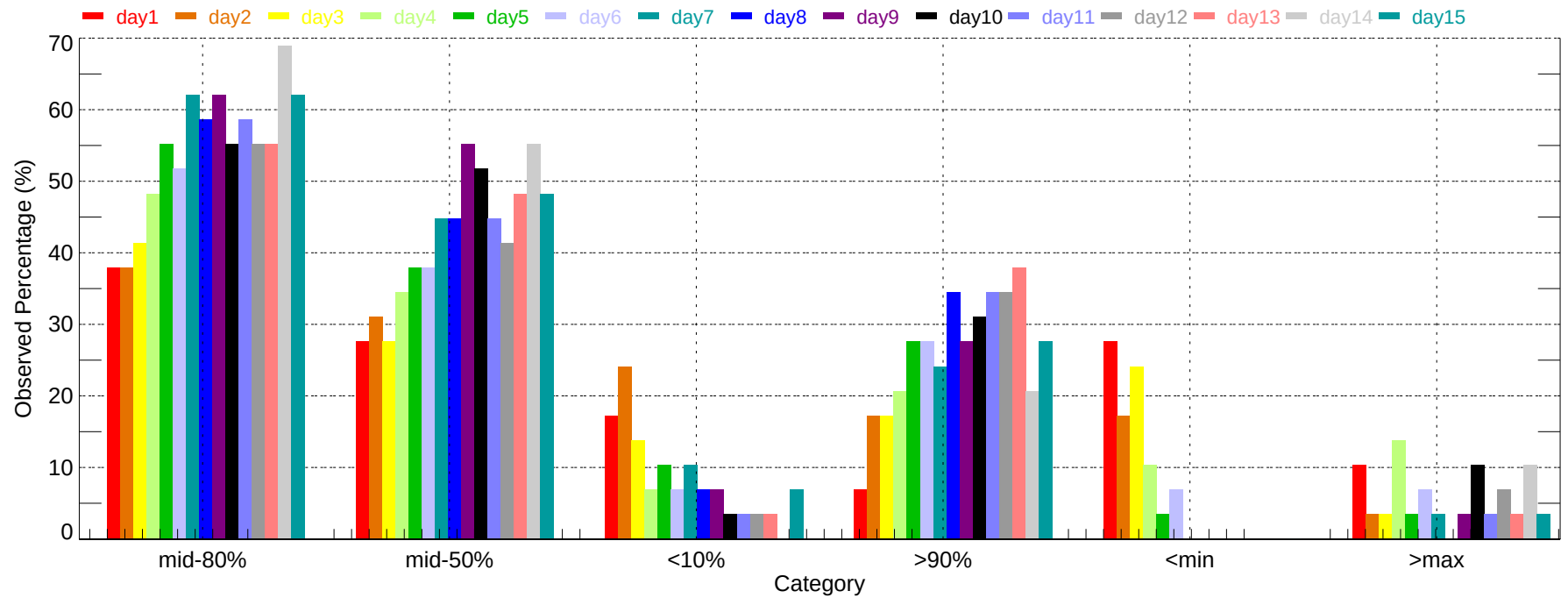
Observed Percentage of Ensembles - DSM: Max Temperature (2007-11-01~2007-11-30)
