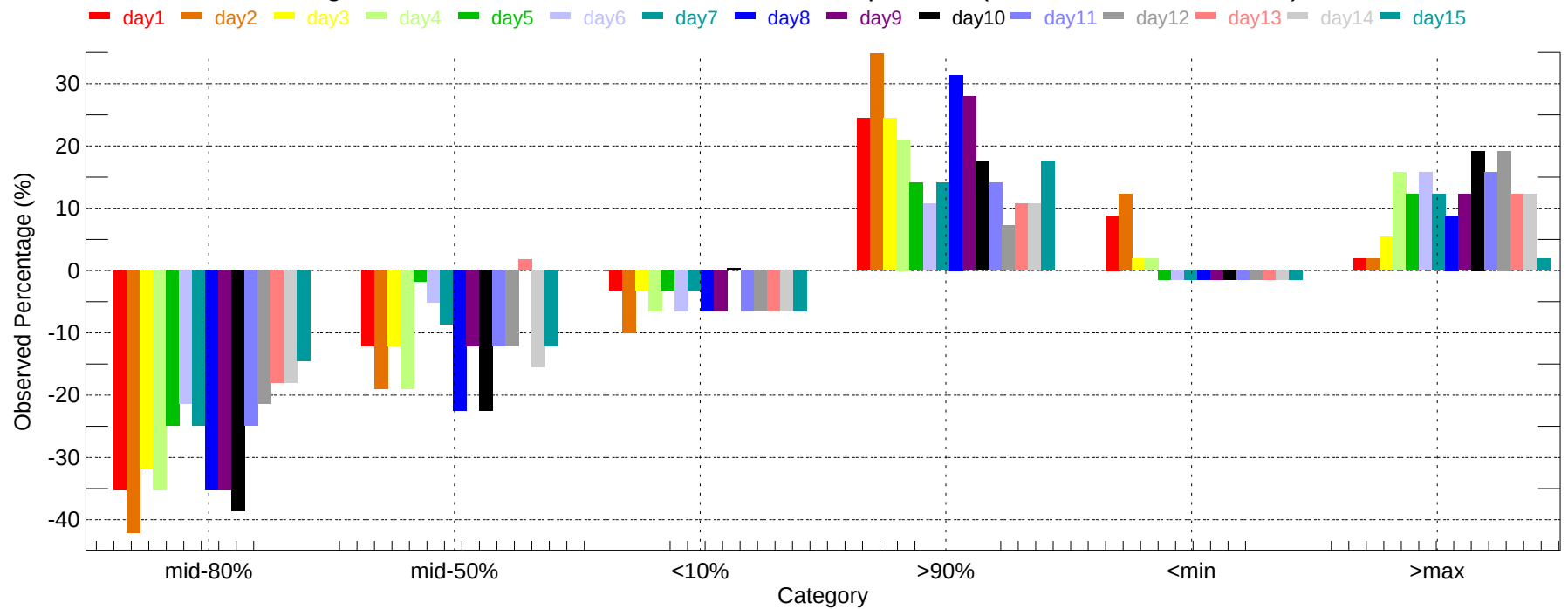
Observed Percentage Deviation of Ensembles - OKC: Min Temperature (2007-11-01~2007-11-30)
