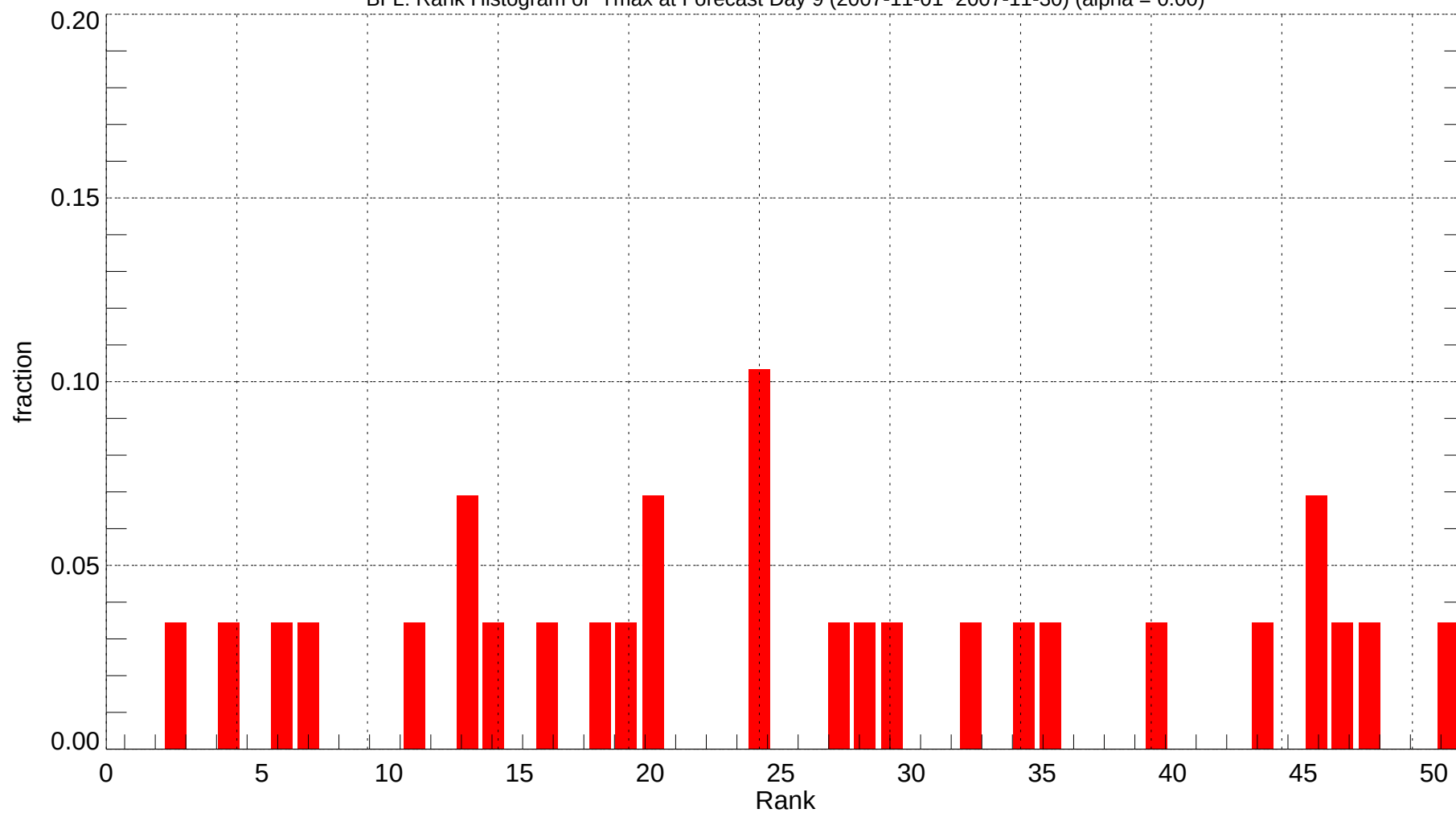
BFL: Rank Histogram of Tmax at Forecast Day 9 (2007-11-01~2007-11-30) (alpha = 0.00)
