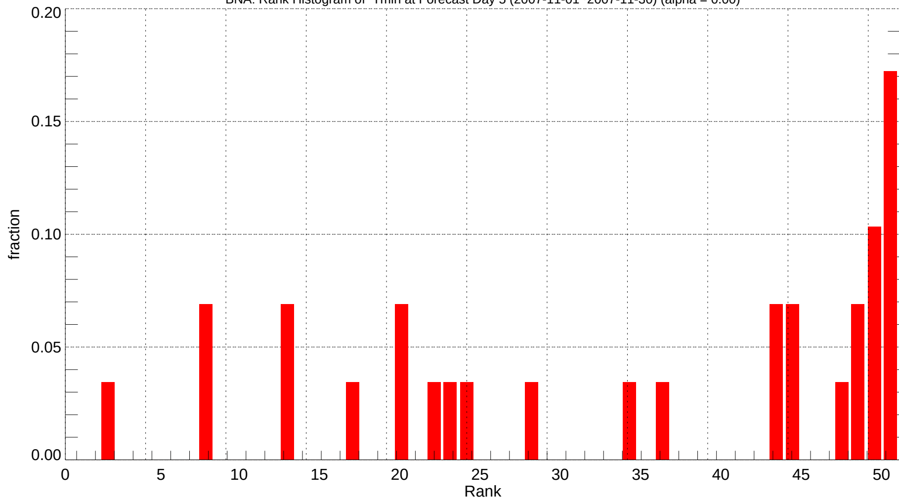
BNA: Rank Histogram of Tmin at Forecast Day 5 (2007-11-01~2007-11-30) (alpha = 0.00)
