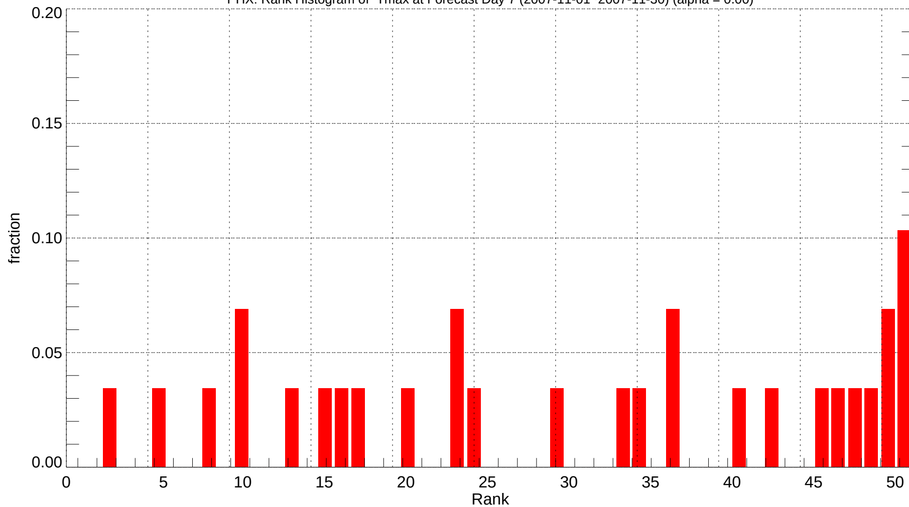
PHX: Rank Histogram of Tmax at Forecast Day 7 (2007-11-01~2007-11-30) (alpha = 0.00)
