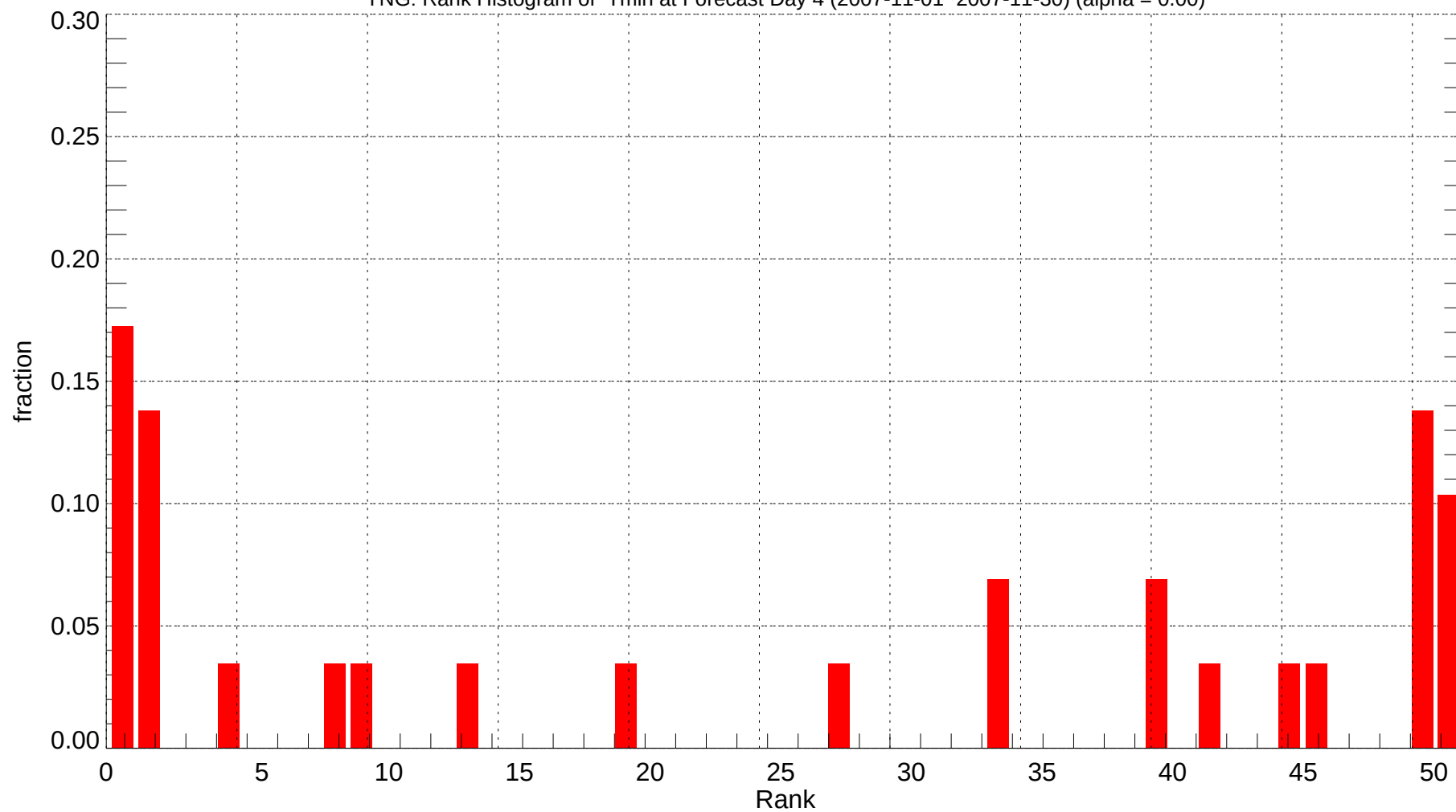
YNG: Rank Histogram of Tmin at Forecast Day 4 (2007-11-01~2007-11-30) (alpha = 0.00)
