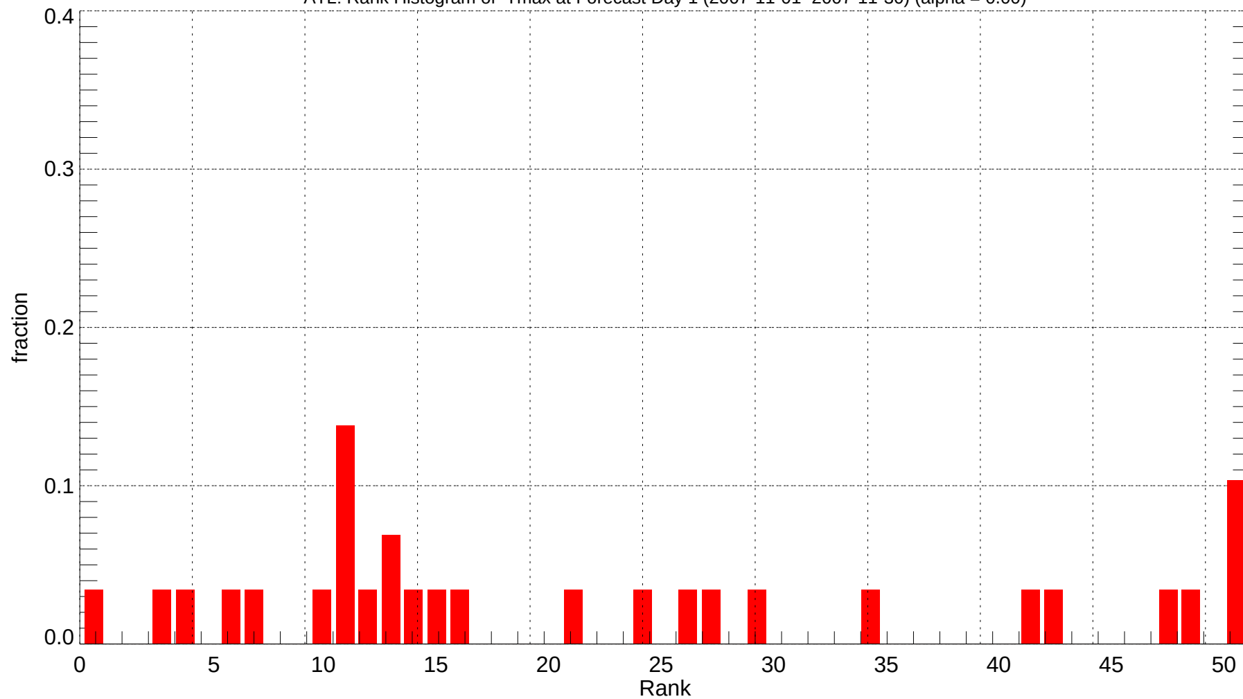
ATL: Rank Histogram of Tmax at Forecast Day 1 (2007-11-01~2007-11-30) (alpha = 0.00)
