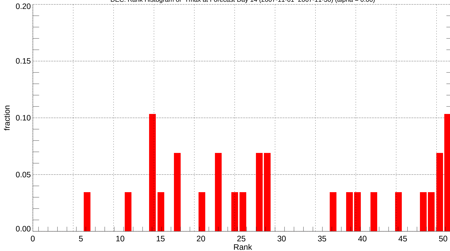
DEC: Rank Histogram of Tmax at Forecast Day 14 (2007-11-01~2007-11-30) (alpha = 0.00)
