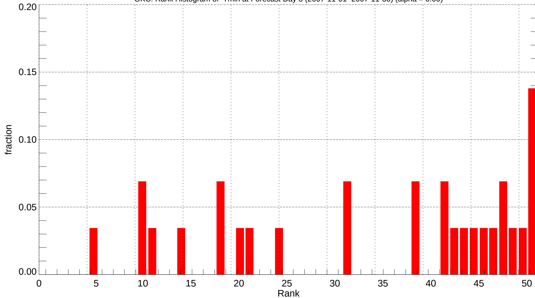
OKC: Rank Histogram of Tmin at Forecast Day 8 (2007-11-01~2007-11-30) (alpha = 0.00)
