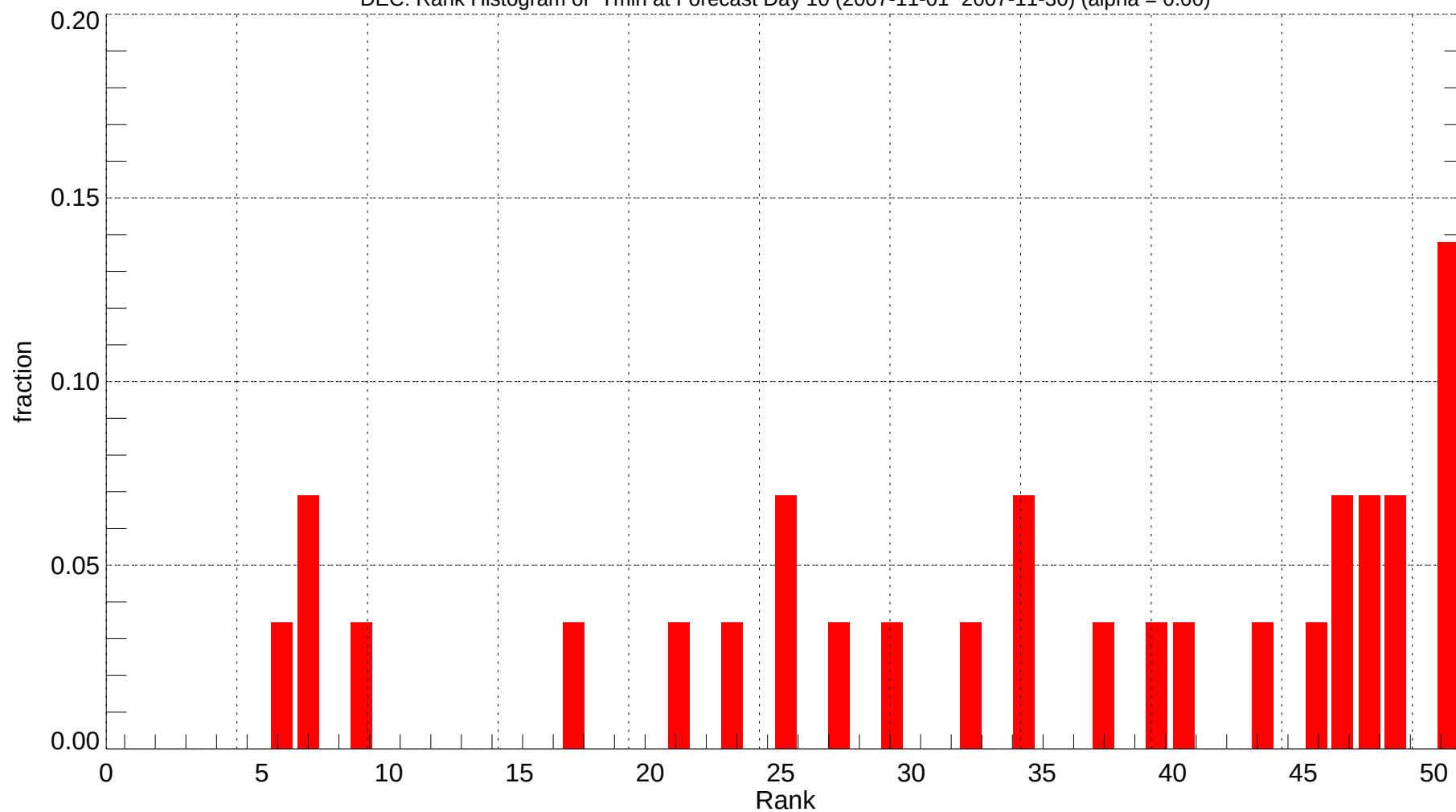
DEC: Rank Histogram of Tmin at Forecast Day 10 (2007-11-01~2007-11-30) (alpha = 0.00)
