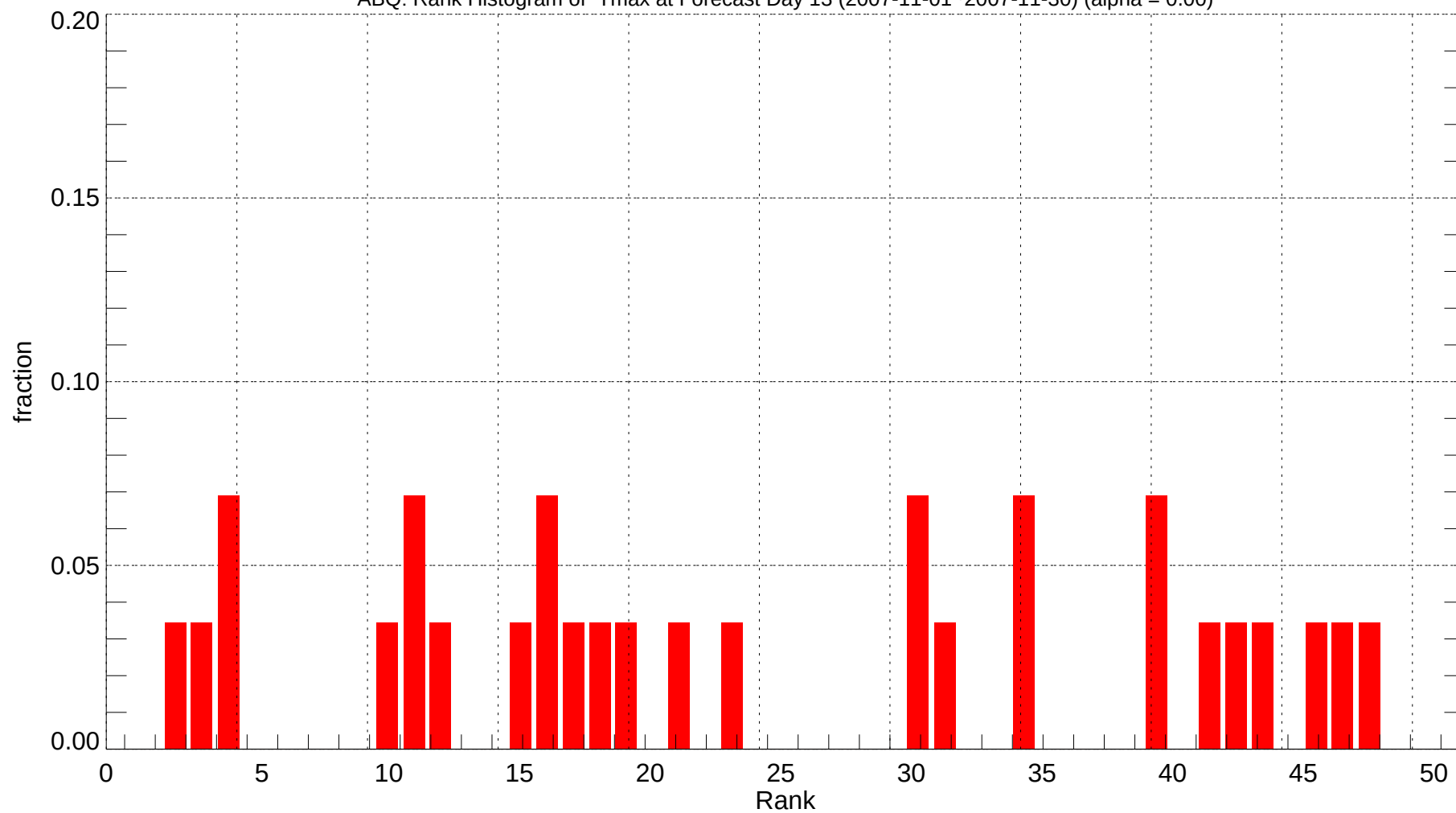
ABQ: Rank Histogram of Tmax at Forecast Day 13 (2007-11-01~2007-11-30) (alpha = 0.00)
