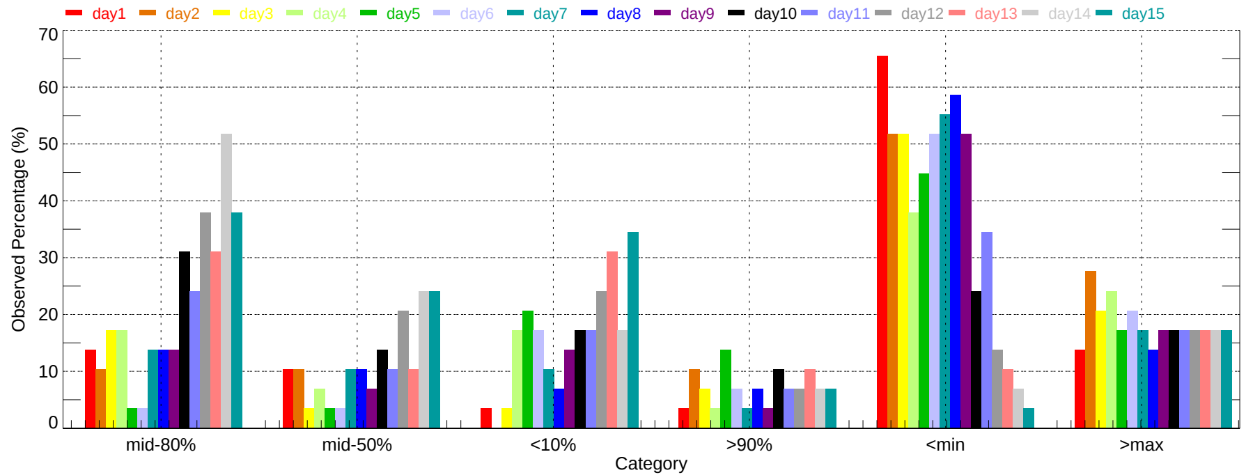
Observed Percentage of Ensembles - SAN: Min Temperature (2007-11-01~2007-11-30)
