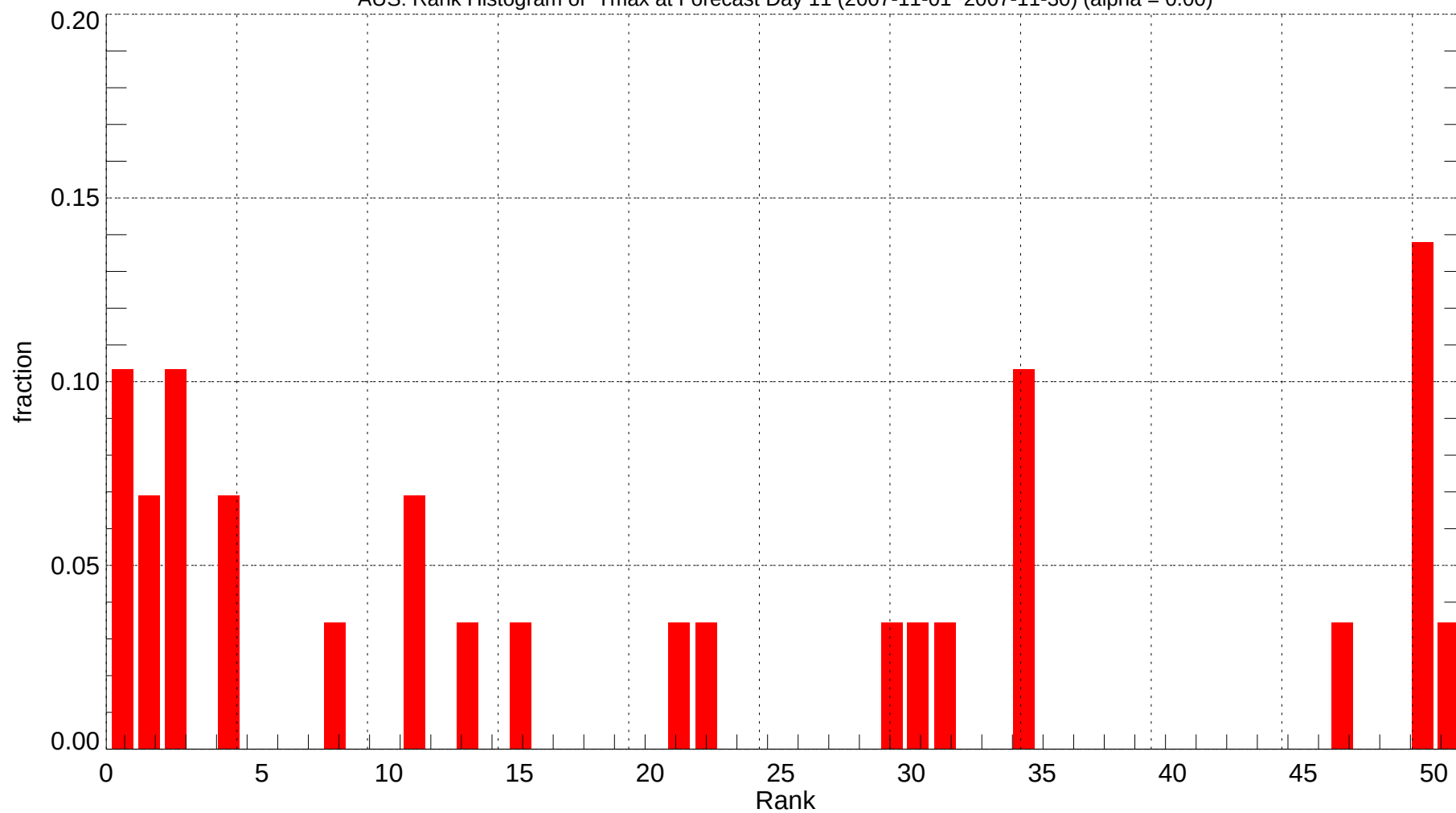
AUS: Rank Histogram of Tmax at Forecast Day 11 (2007-11-01~2007-11-30) (alpha = 0.00)
