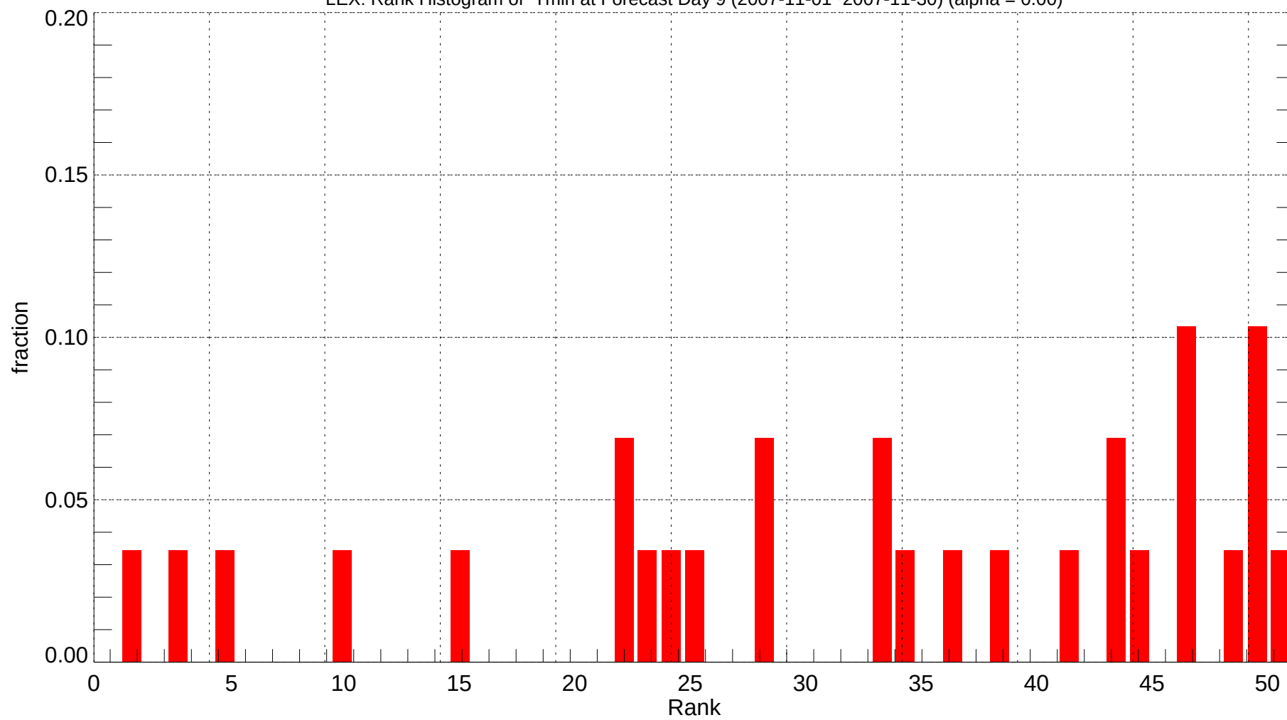
LEX: Rank Histogram of Tmin at Forecast Day 9 (2007-11-01~2007-11-30) (alpha = 0.00)
