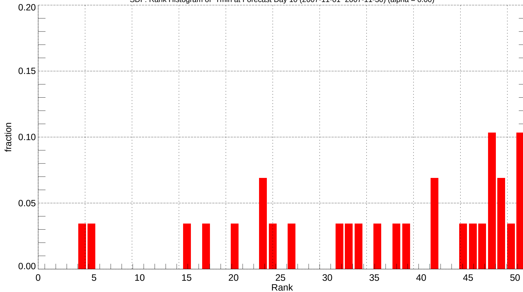
SDF: Rank Histogram of Tmin at Forecast Day 10 (2007-11-01~2007-11-30) (alpha = 0.00)
