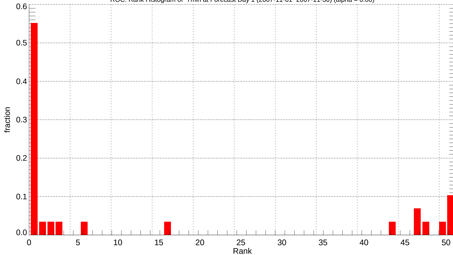
ROC: Rank Histogram of Tmin at Forecast Day 1 (2007-11-01~2007-11-30) (alpha = 0.00)
