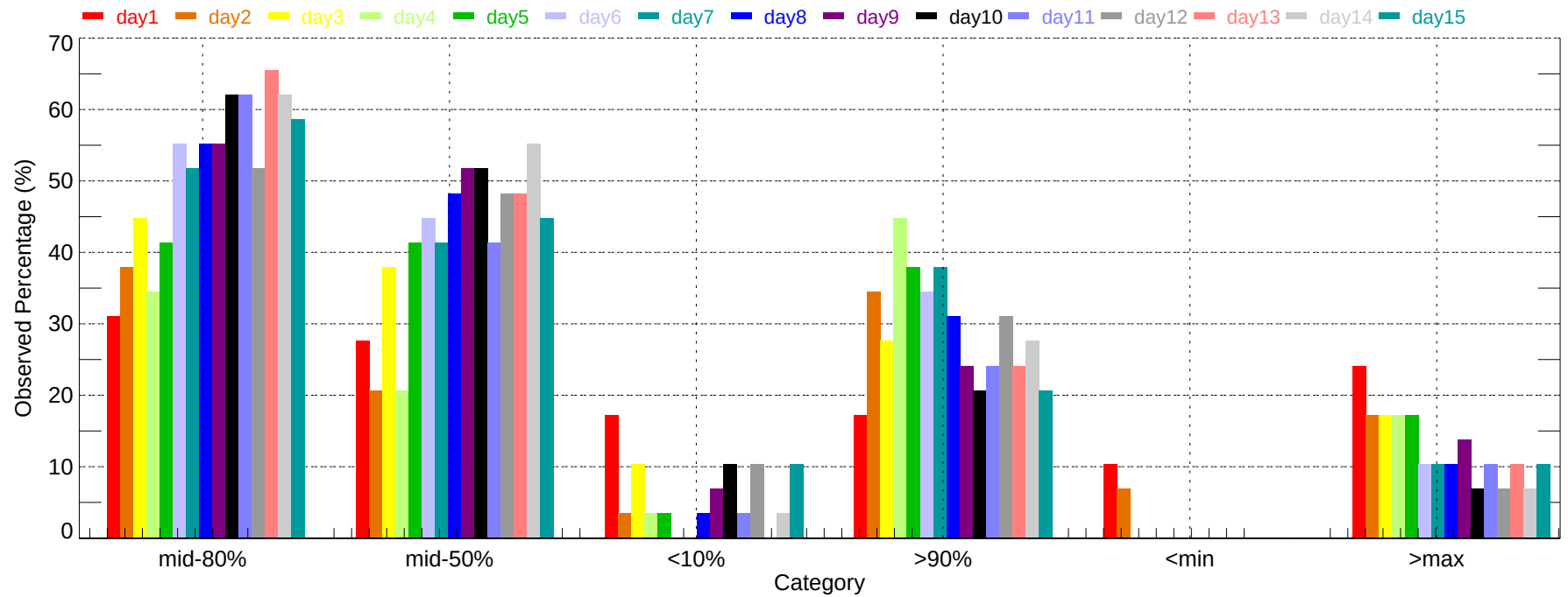
Observed Percentage of Ensembles - DCA: Max Temperature (2007-11-01~2007-11-30)
