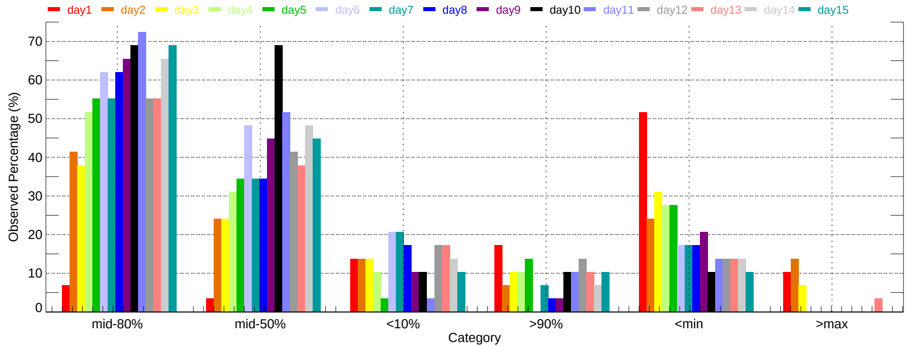
Observed Percentage of Ensembles - ROC: Min Temperature (2007-11-01~2007-11-30)
