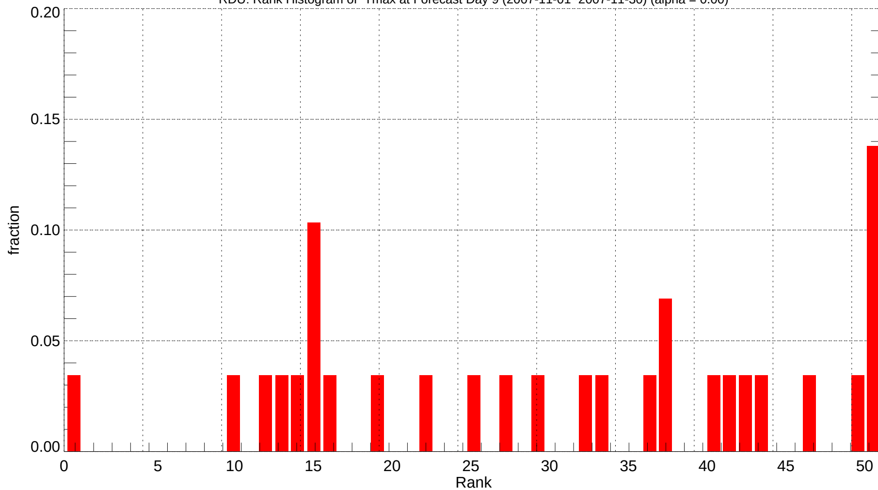
RDU: Rank Histogram of Tmax at Forecast Day 9 (2007-11-01~2007-11-30) (alpha = 0.00)
