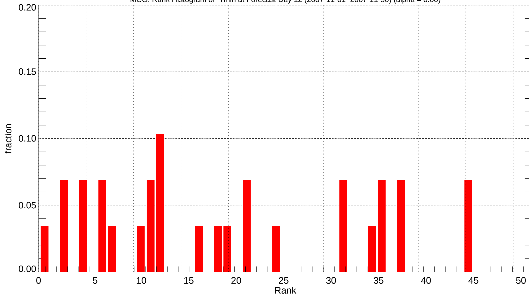
MCO: Rank Histogram of Tmin at Forecast Day 12 (2007-11-01~2007-11-30) (alpha = 0.00)
