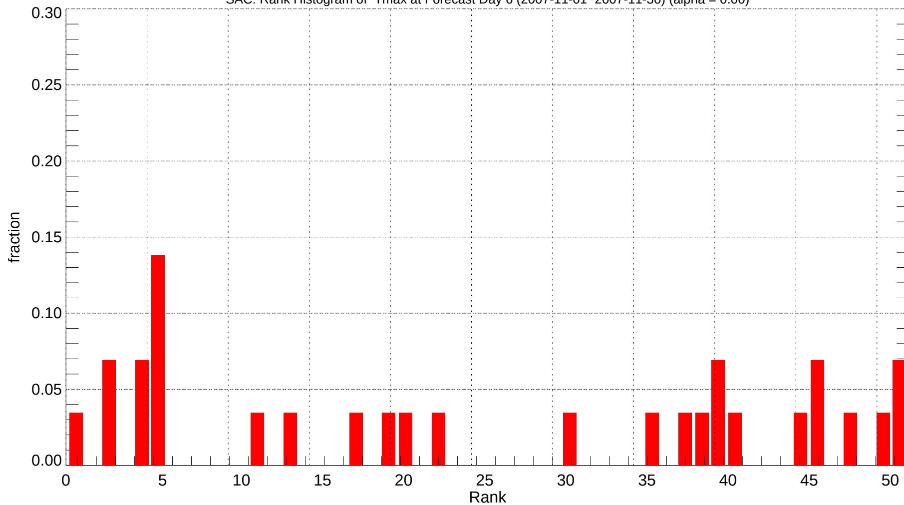
SAC: Rank Histogram of Tmax at Forecast Day 6 (2007-11-01~2007-11-30) (alpha = 0.00)
