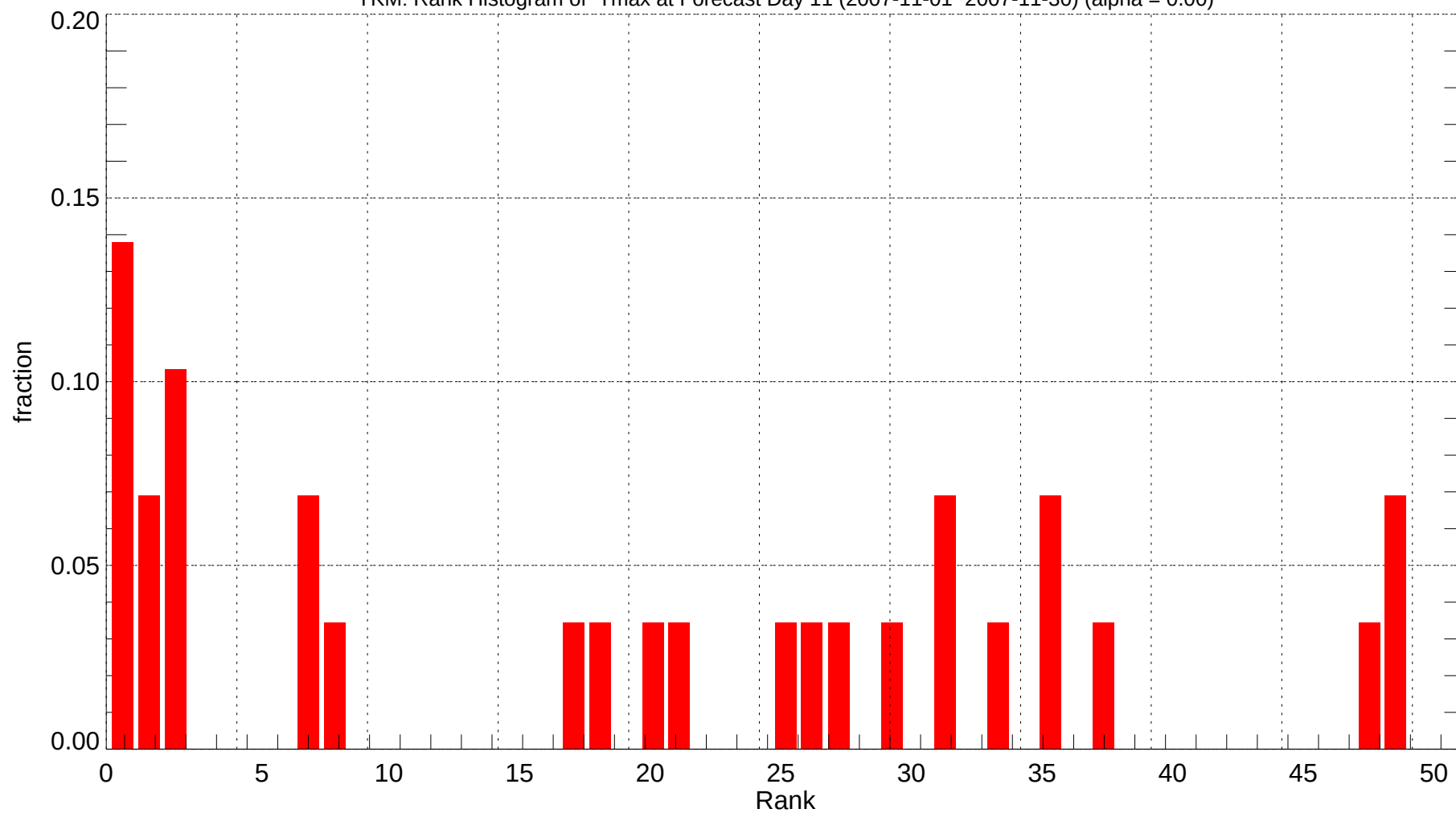
YKM: Rank Histogram of Tmax at Forecast Day 11 (2007-11-01~2007-11-30) (alpha = 0.00)
