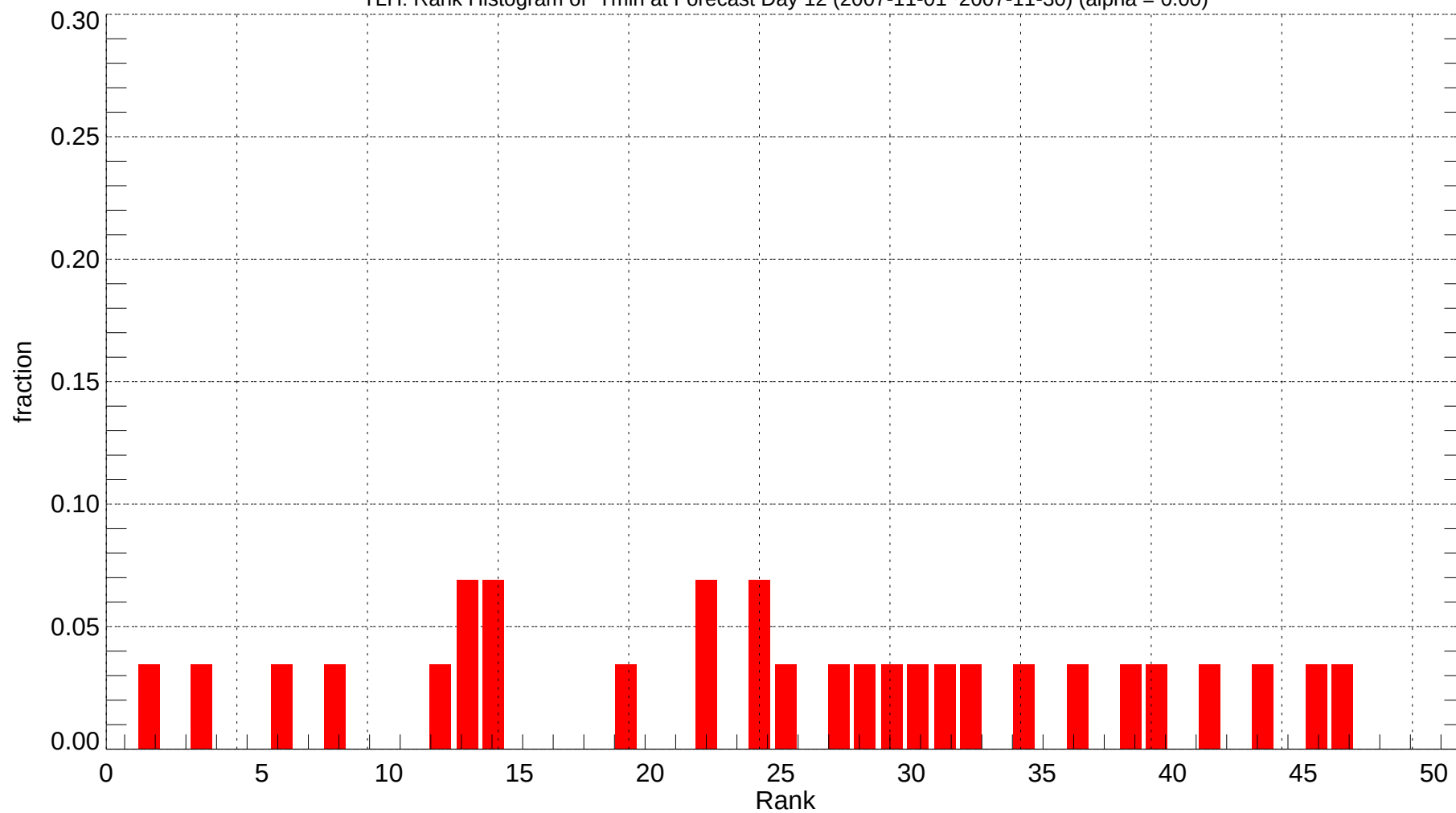
TLH: Rank Histogram of Tmin at Forecast Day 12 (2007-11-01~2007-11-30) (alpha = 0.00)
