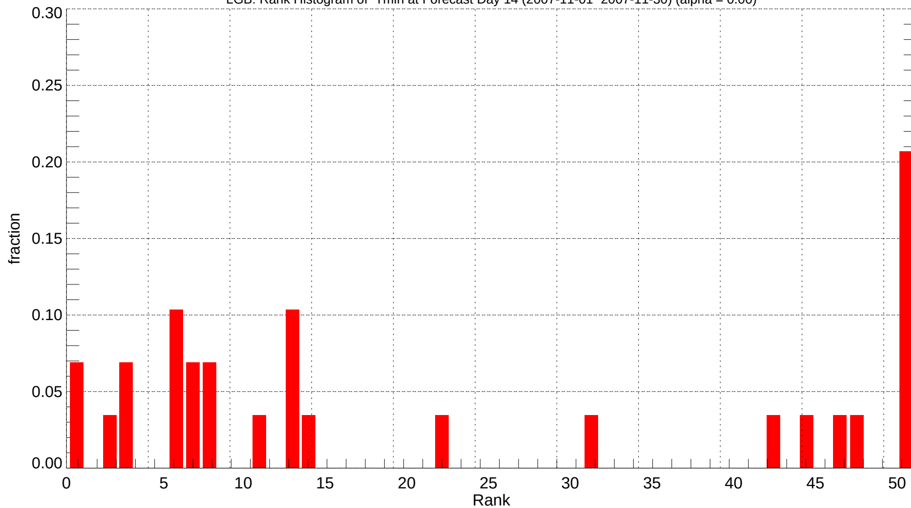
LGB: Rank Histogram of Tmin at Forecast Day 14 (2007-11-01~2007-11-30) (alpha = 0.00)
