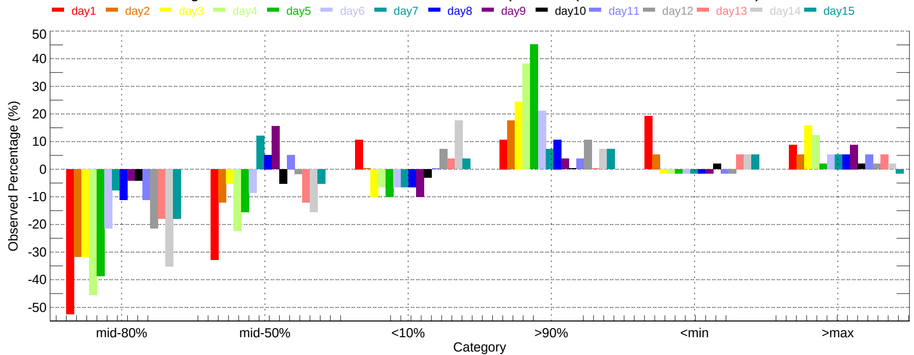
Observed Percentage Deviation of Ensembles - PVD: Max Temperature (2007-11-01~2007-11-30)
