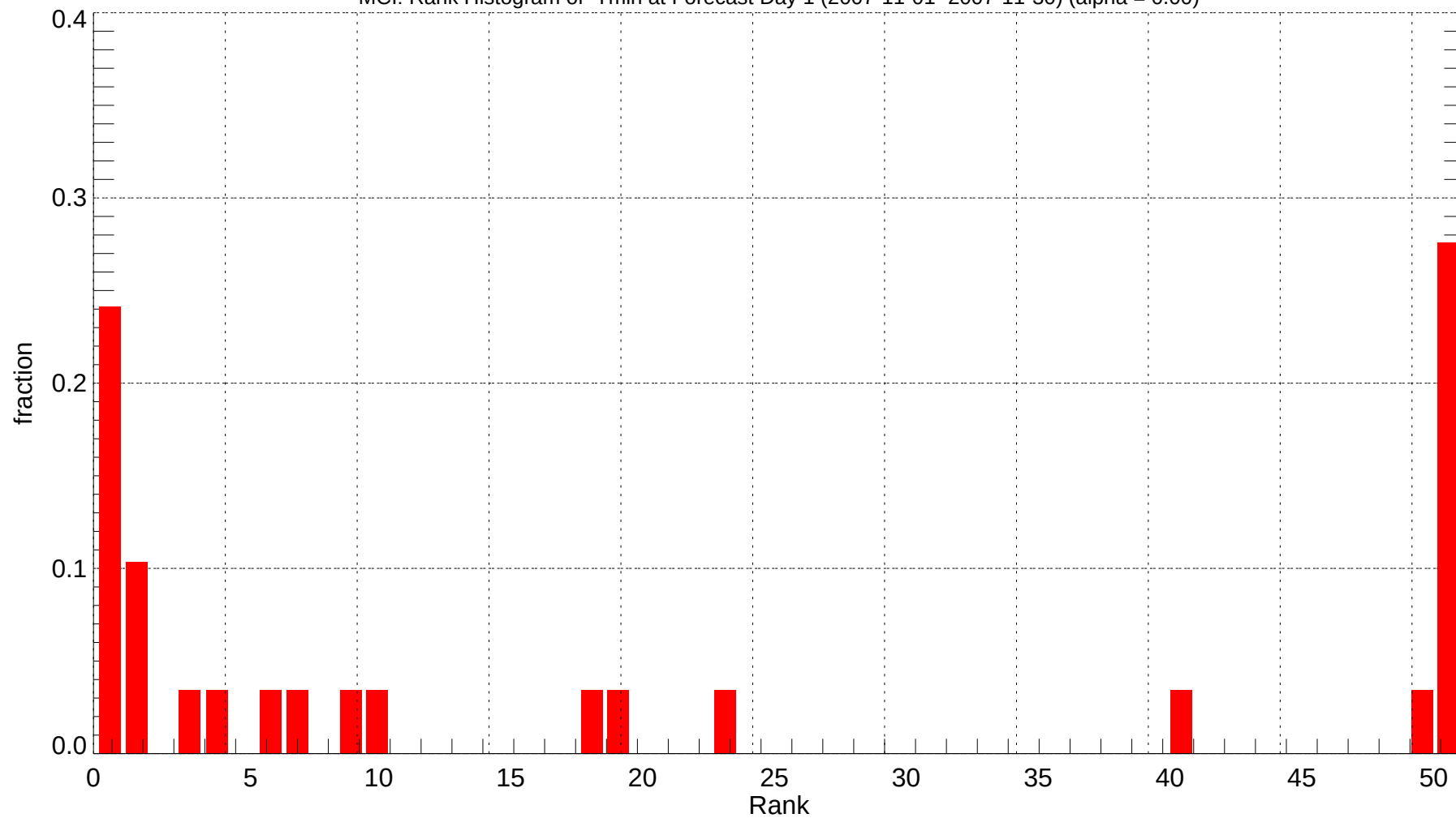
MCI: Rank Histogram of Tmin at Forecast Day 1 (2007-11-01~2007-11-30) (alpha = 0.00)
