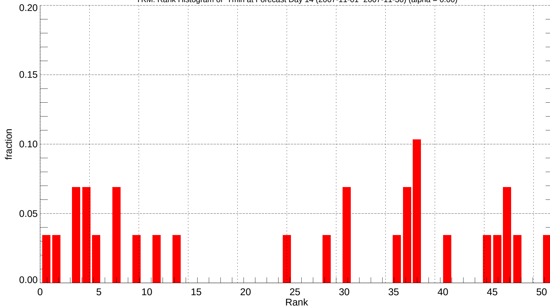
YKM: Rank Histogram of Tmin at Forecast Day 14 (2007-11-01~2007-11-30) (alpha = 0.00)
