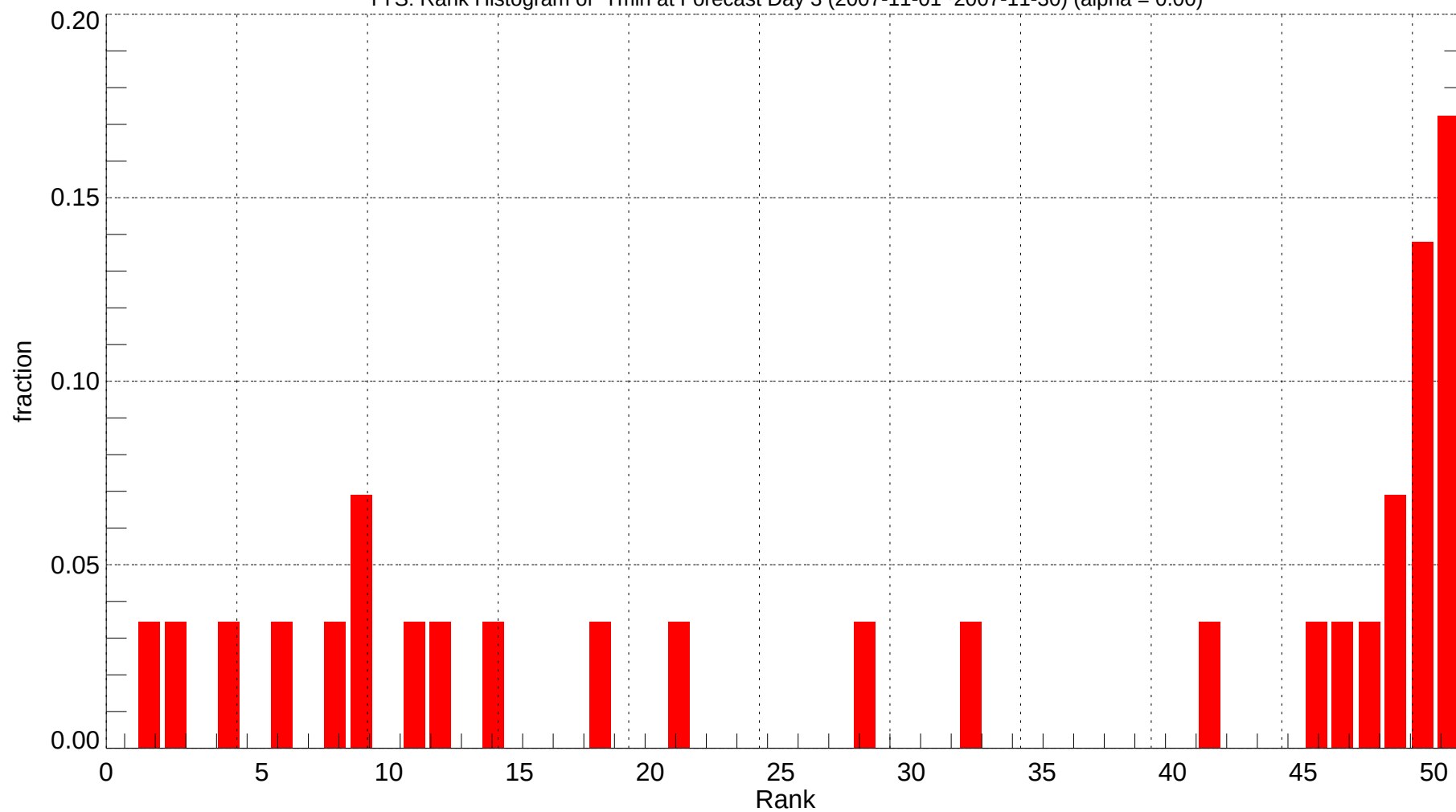
TYS: Rank Histogram of Tmin at Forecast Day 3 (2007-11-01~2007-11-30) (alpha = 0.00)
