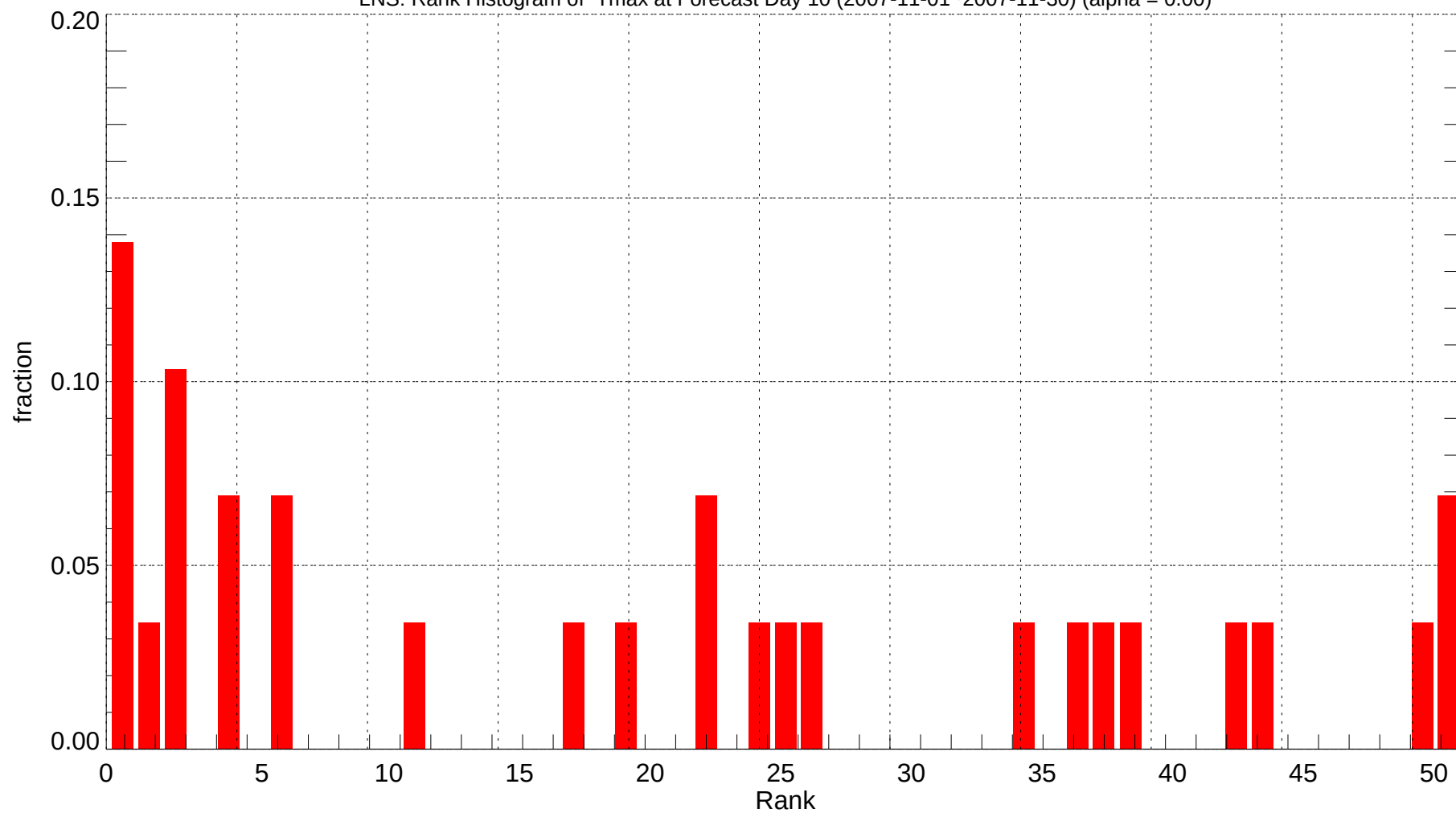
LNS: Rank Histogram of Tmax at Forecast Day 10 (2007-11-01~2007-11-30) (alpha = 0.00)
