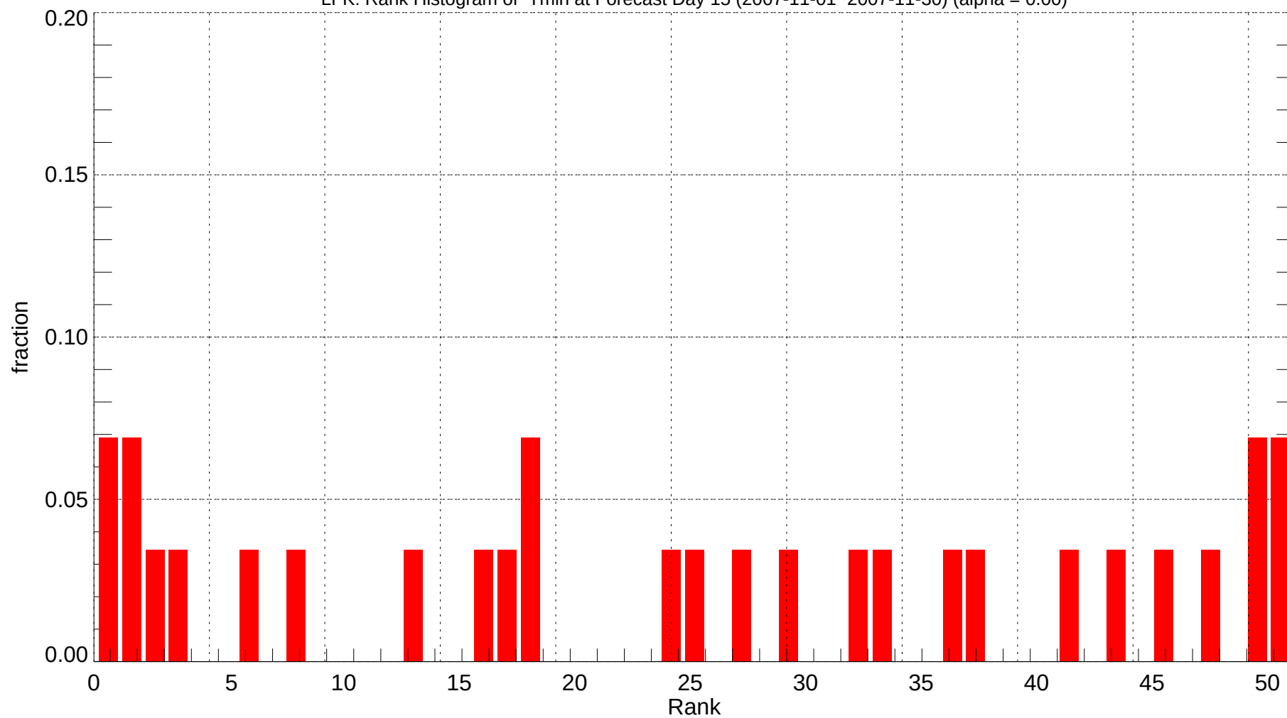
LFK: Rank Histogram of Tmin at Forecast Day 15 (2007-11-01~2007-11-30) (alpha = 0.00)
