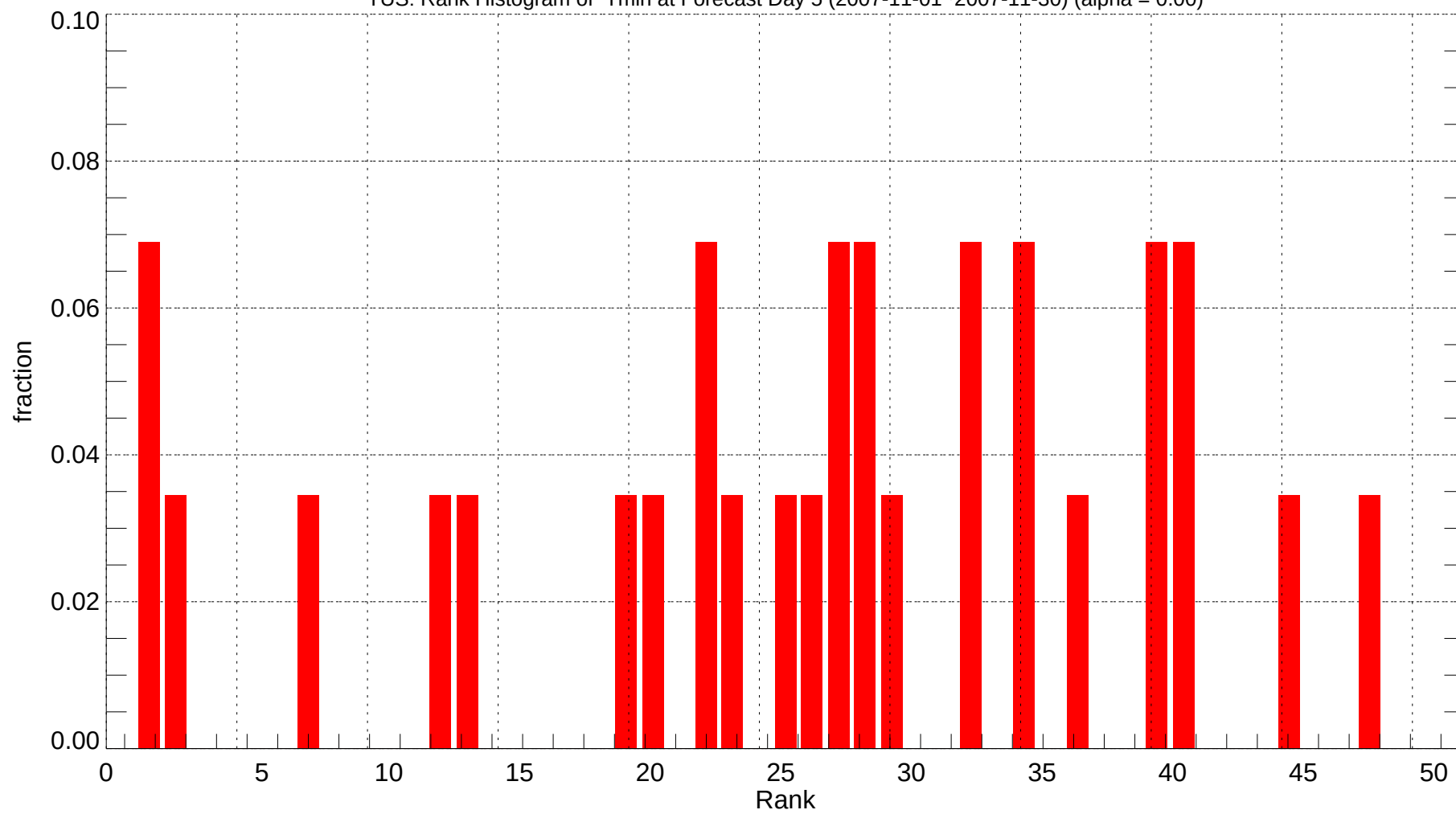
TUS: Rank Histogram of Tmin at Forecast Day 5 (2007-11-01~2007-11-30) (alpha = 0.00)
