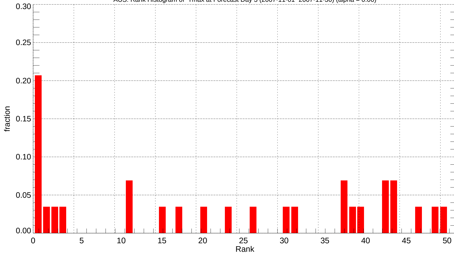
AUS: Rank Histogram of Tmax at Forecast Day 3 (2007-11-01~2007-11-30) (alpha = 0.00)
