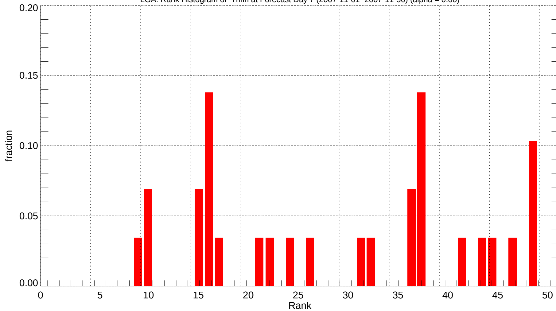
LGA: Rank Histogram of Tmin at Forecast Day 7 (2007-11-01~2007-11-30) (alpha = 0.00)
