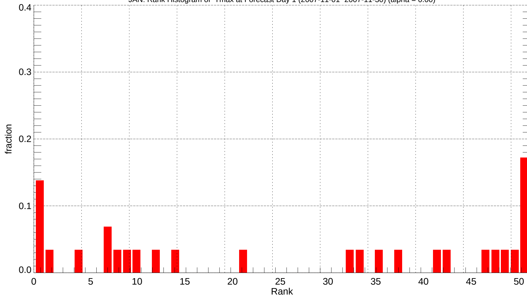
JAN: Rank Histogram of Tmax at Forecast Day 1 (2007-11-01~2007-11-30) (alpha = 0.00)
