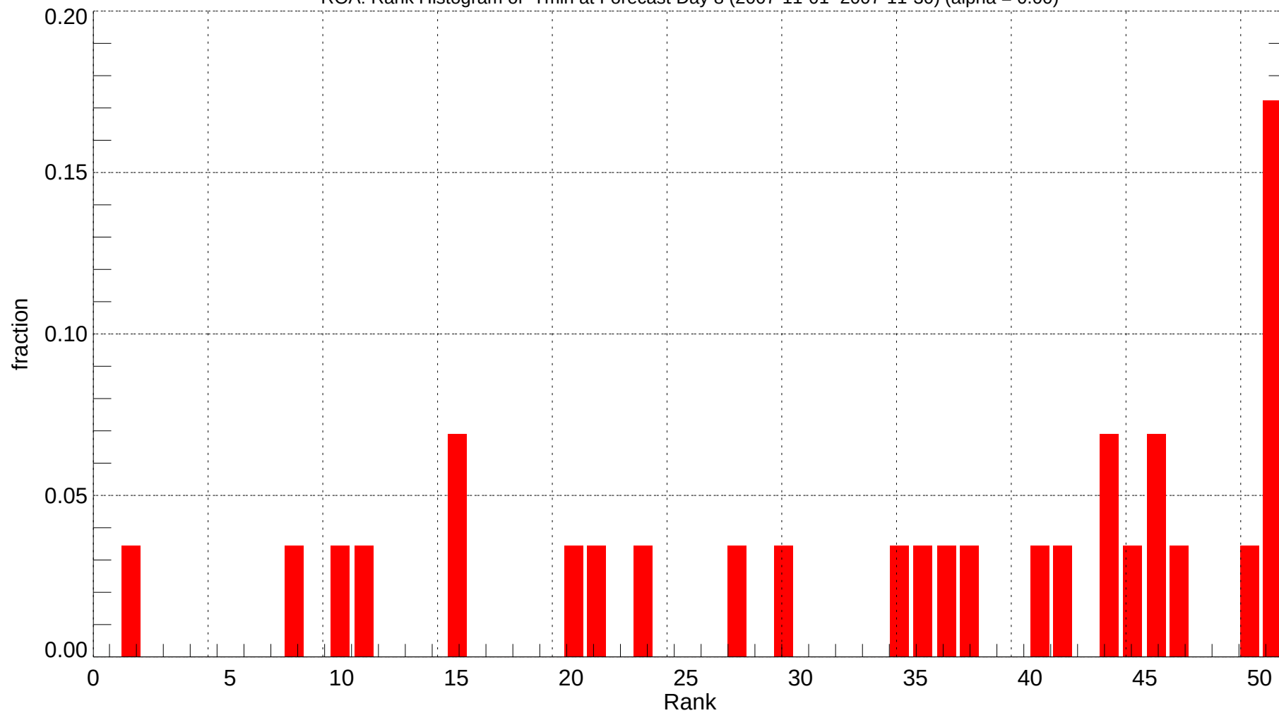
ROA: Rank Histogram of Tmin at Forecast Day 8 (2007-11-01~2007-11-30) (alpha = 0.00)
