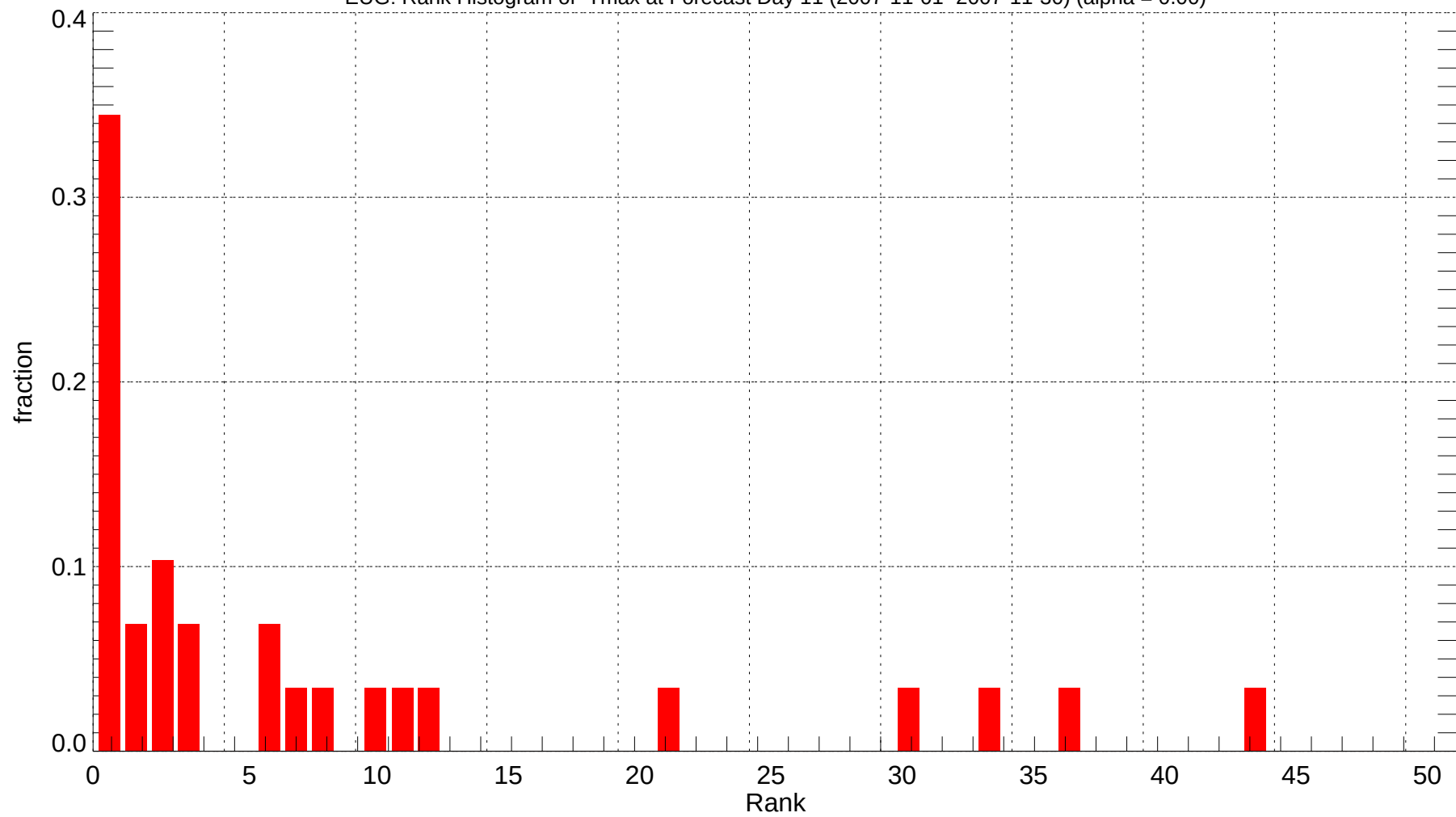
EUG: Rank Histogram of Tmax at Forecast Day 11 (2007-11-01~2007-11-30) (alpha = 0.00)
