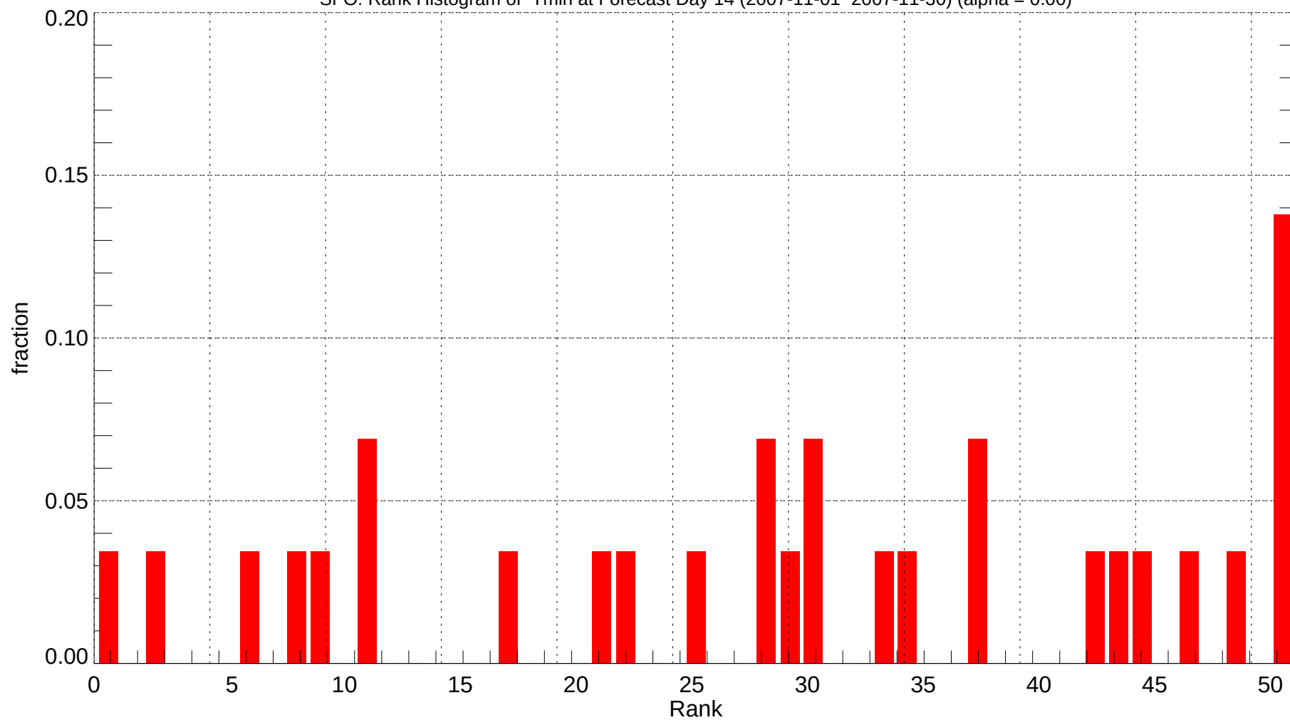
SFO: Rank Histogram of Tmin at Forecast Day 14 (2007-11-01~2007-11-30) (alpha = 0.00)
