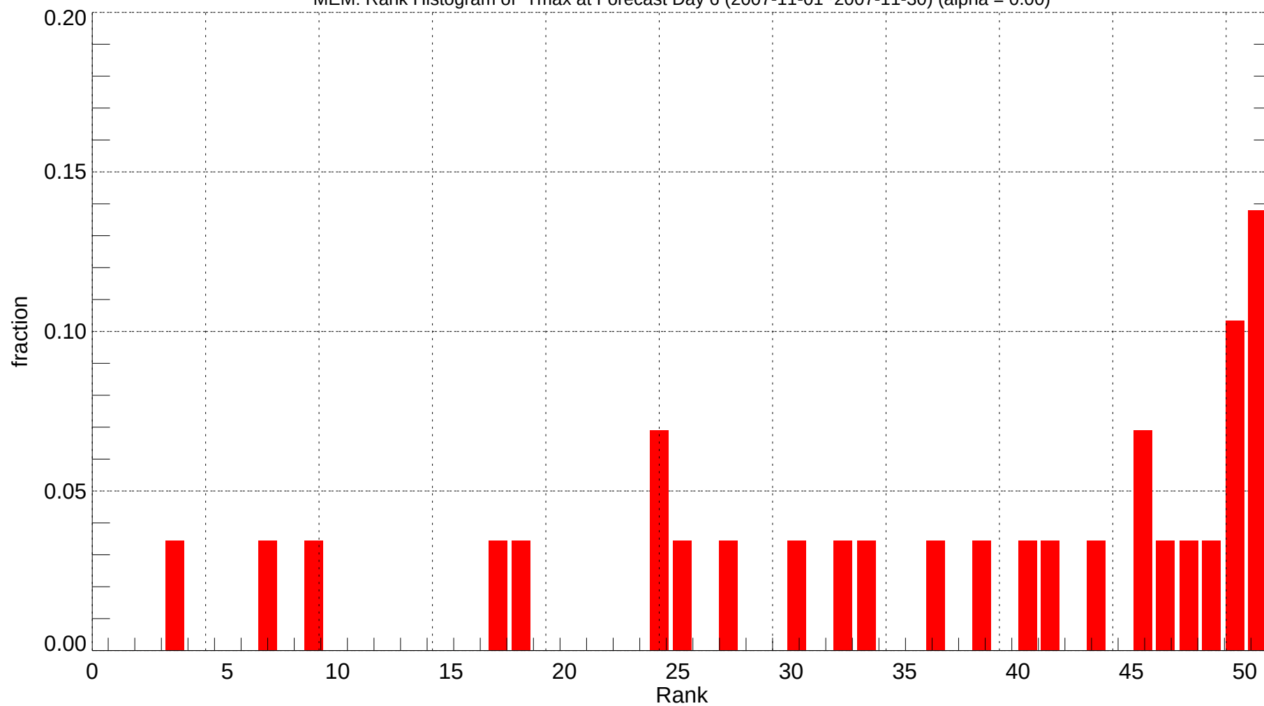
MEM: Rank Histogram of Tmax at Forecast Day 6 (2007-11-01~2007-11-30) (alpha = 0.00)
