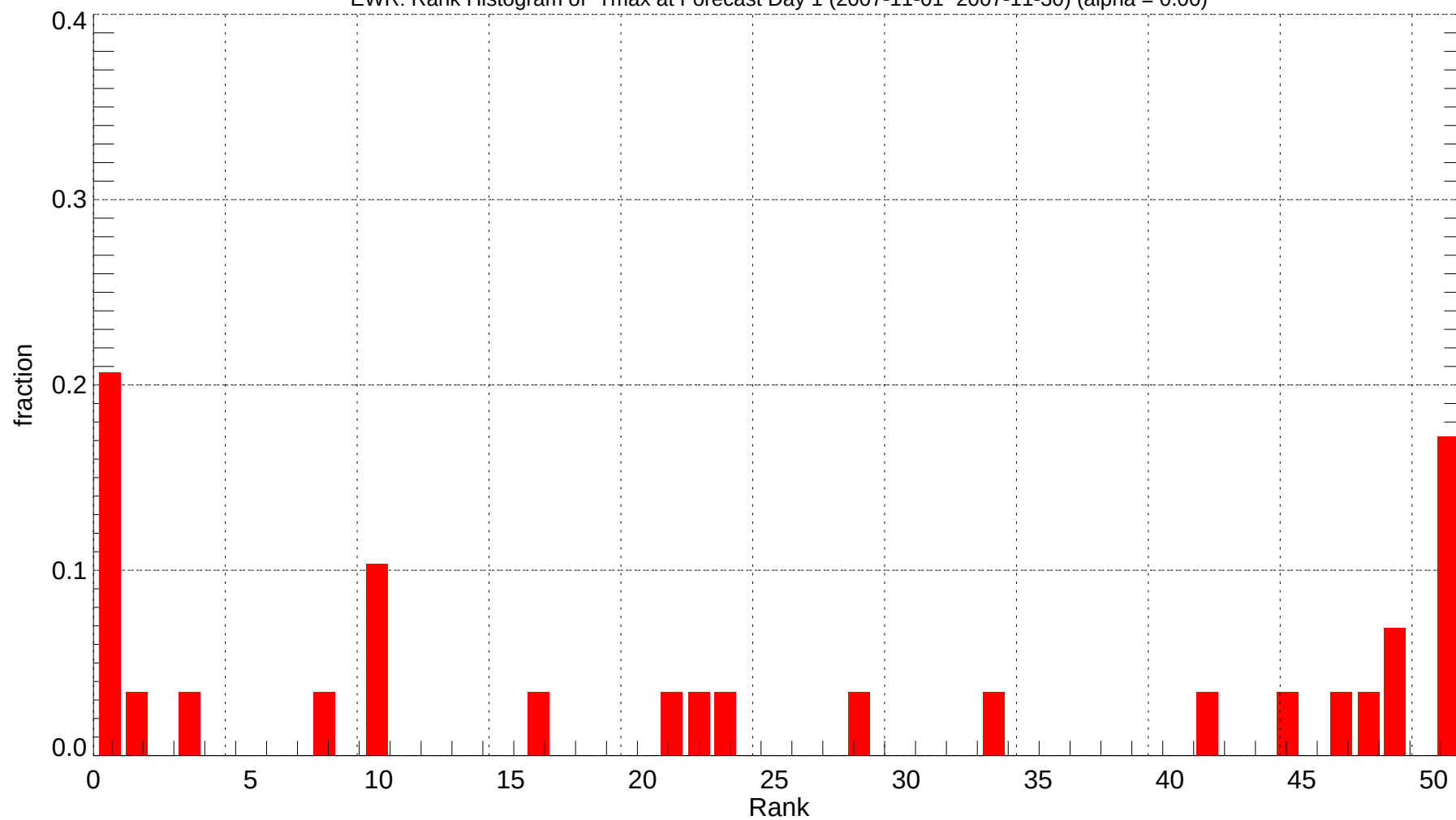
EWR: Rank Histogram of Tmax at Forecast Day 1 (2007-11-01~2007-11-30) (alpha = 0.00)
