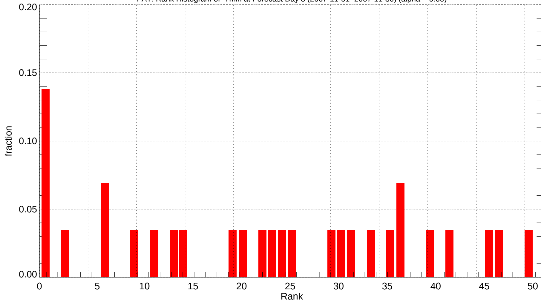
FAT: Rank Histogram of Tmin at Forecast Day 3 (2007-11-01~2007-11-30) (alpha = 0.00)
