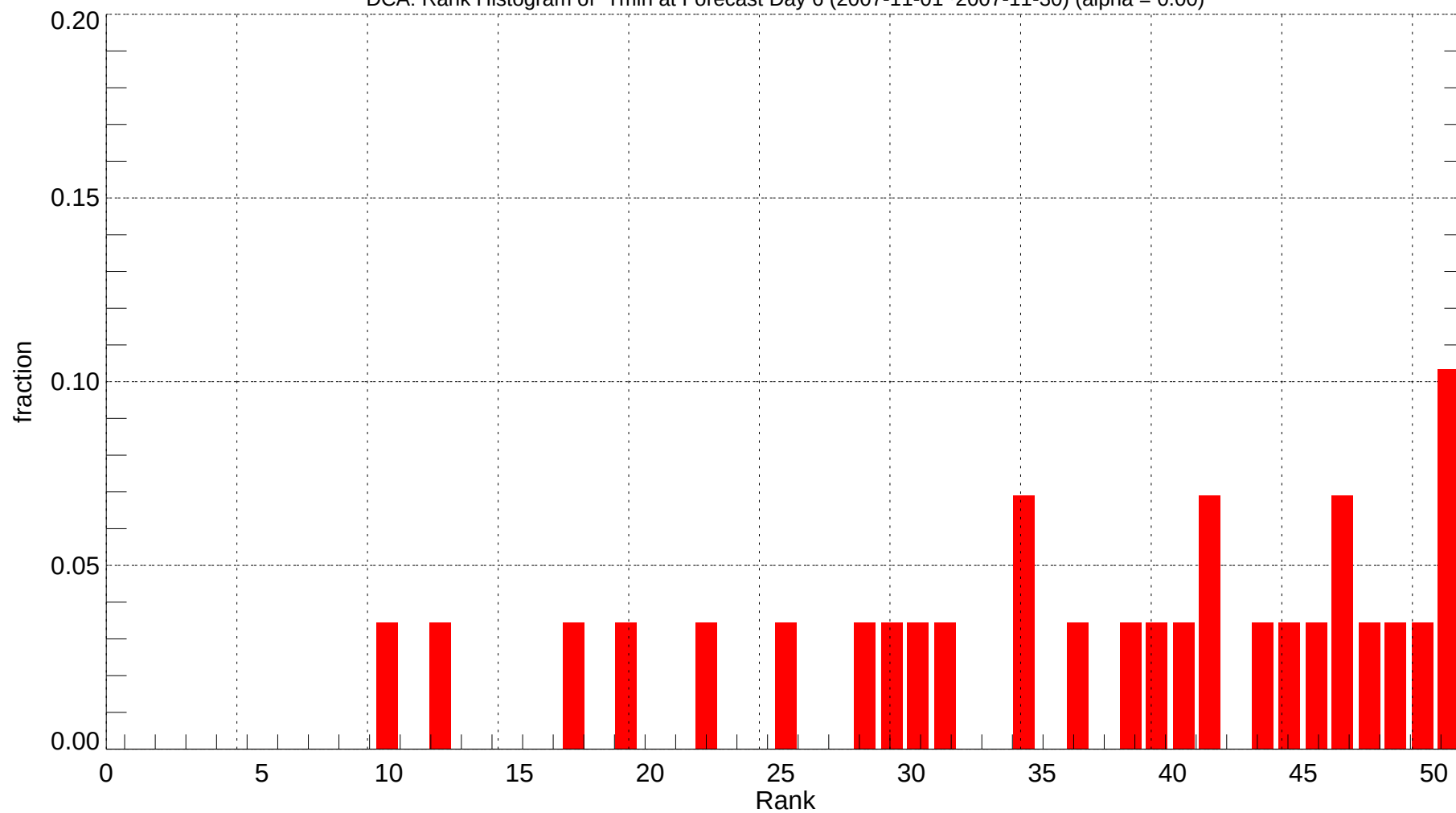
DCA: Rank Histogram of Tmin at Forecast Day 6 (2007-11-01~2007-11-30) (alpha = 0.00)
