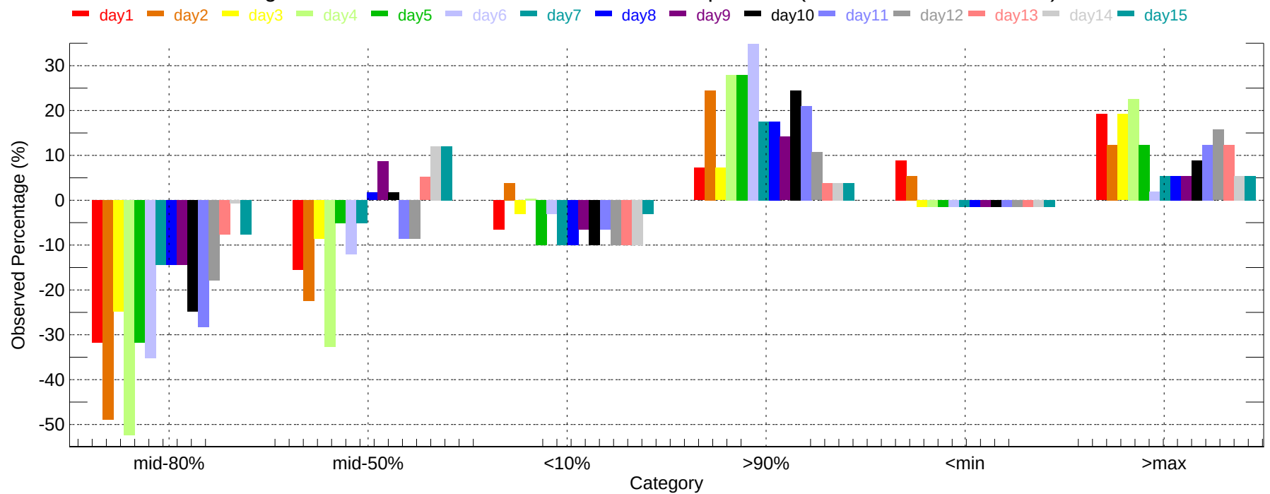
Observed Percentage Deviation of Ensembles - CHA: Max Temperature (2007-11-01~2007-11-30)
