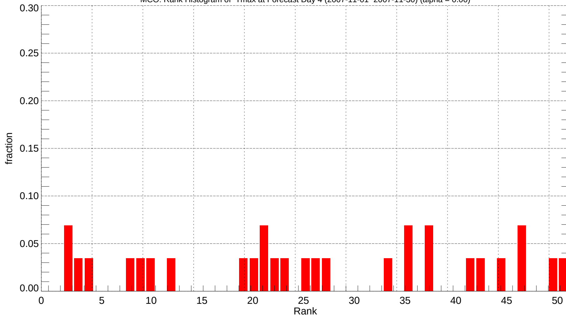
MCO: Rank Histogram of Tmax at Forecast Day 4 (2007-11-01~2007-11-30) (alpha = 0.00)
