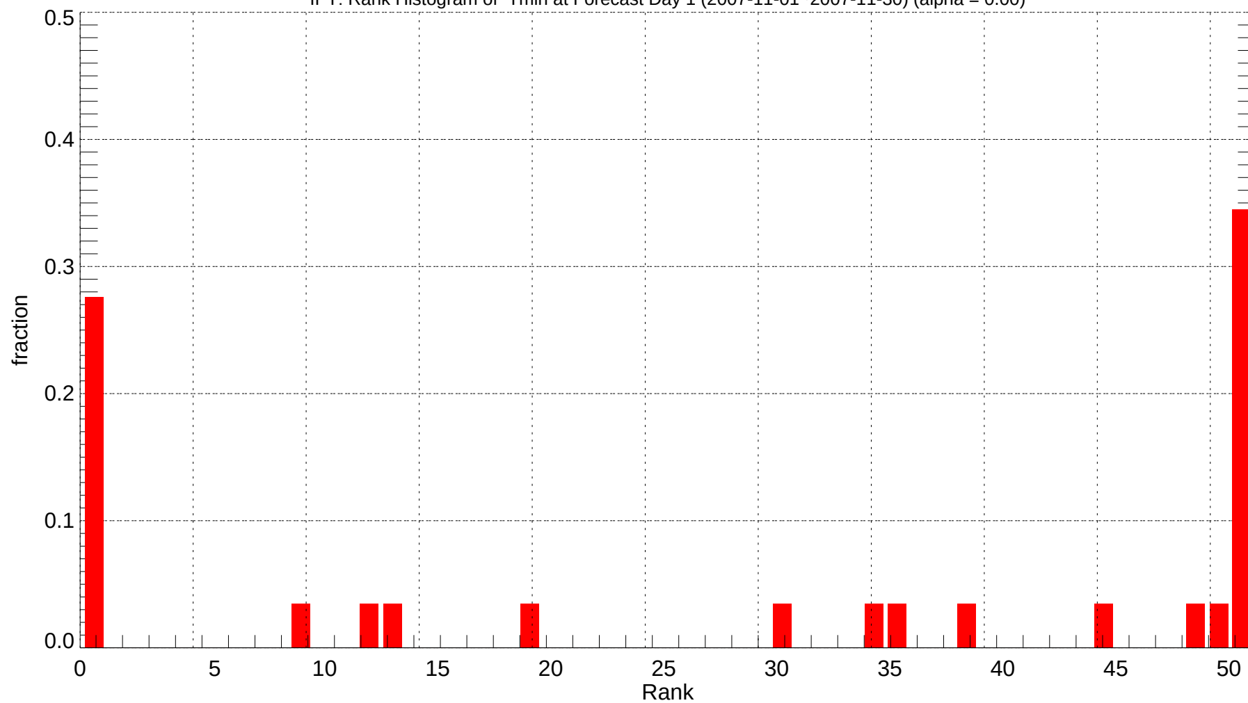
IPT: Rank Histogram of Tmin at Forecast Day 1 (2007-11-01~2007-11-30) (alpha = 0.00)
