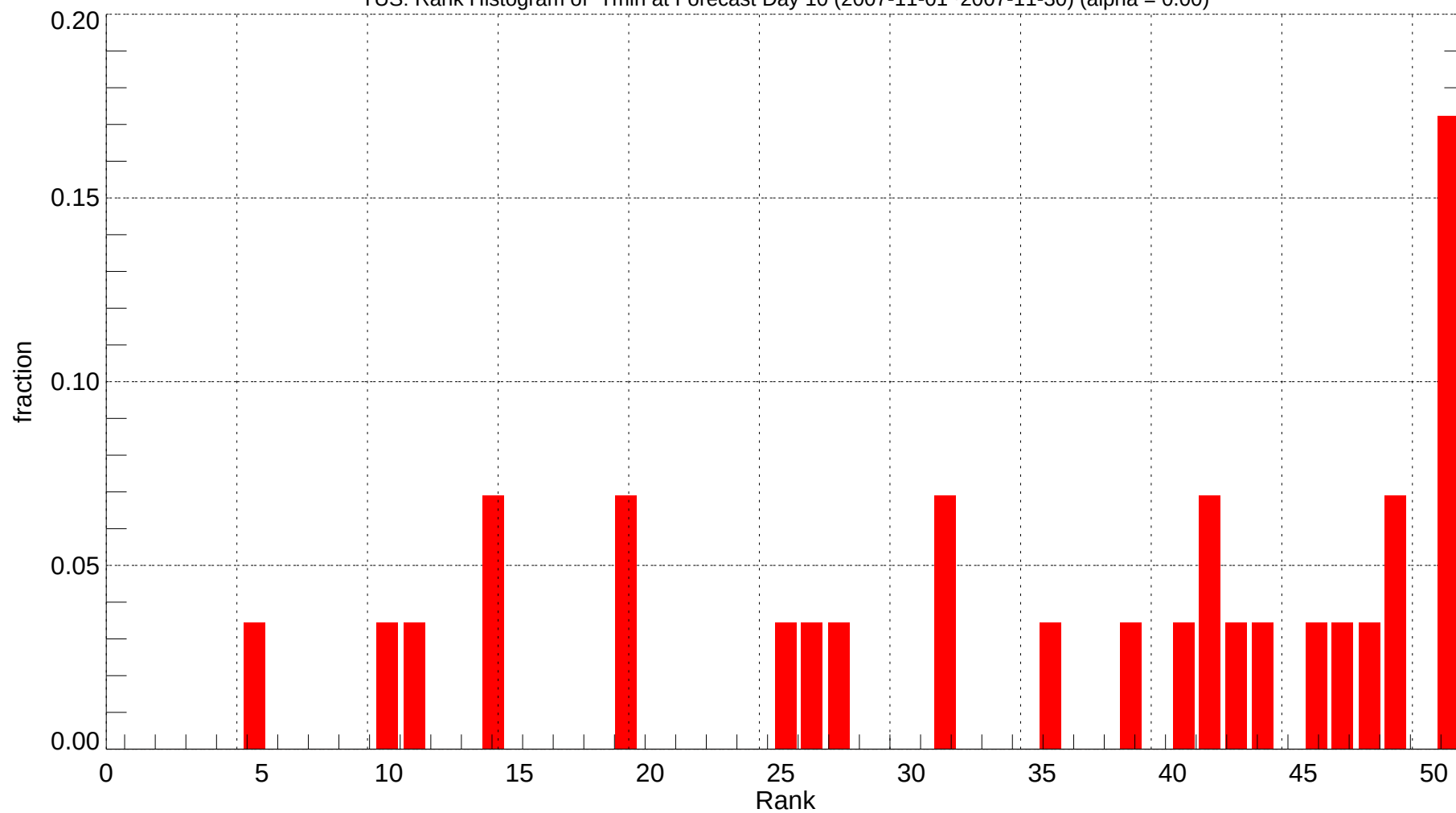
TUS: Rank Histogram of Tmin at Forecast Day 10 (2007-11-01~2007-11-30) (alpha = 0.00)
