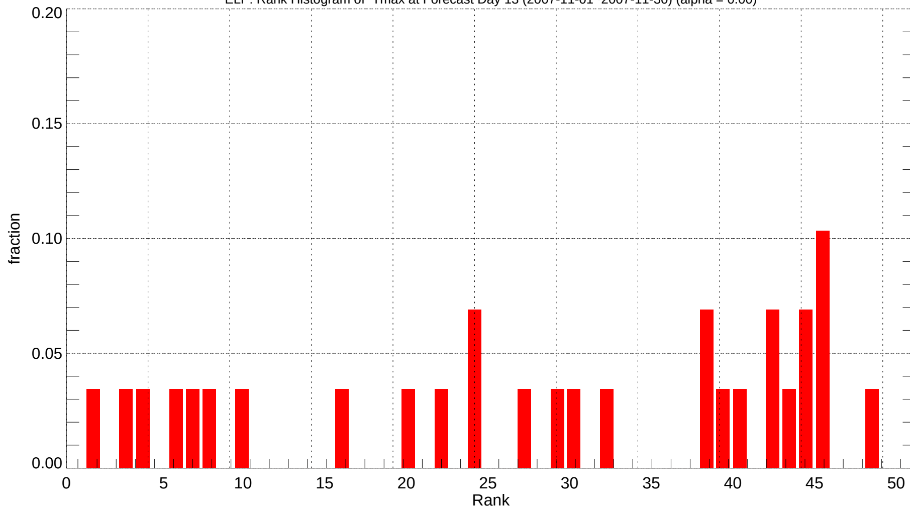
ELP: Rank Histogram of Tmax at Forecast Day 13 (2007-11-01~2007-11-30) (alpha = 0.00)
