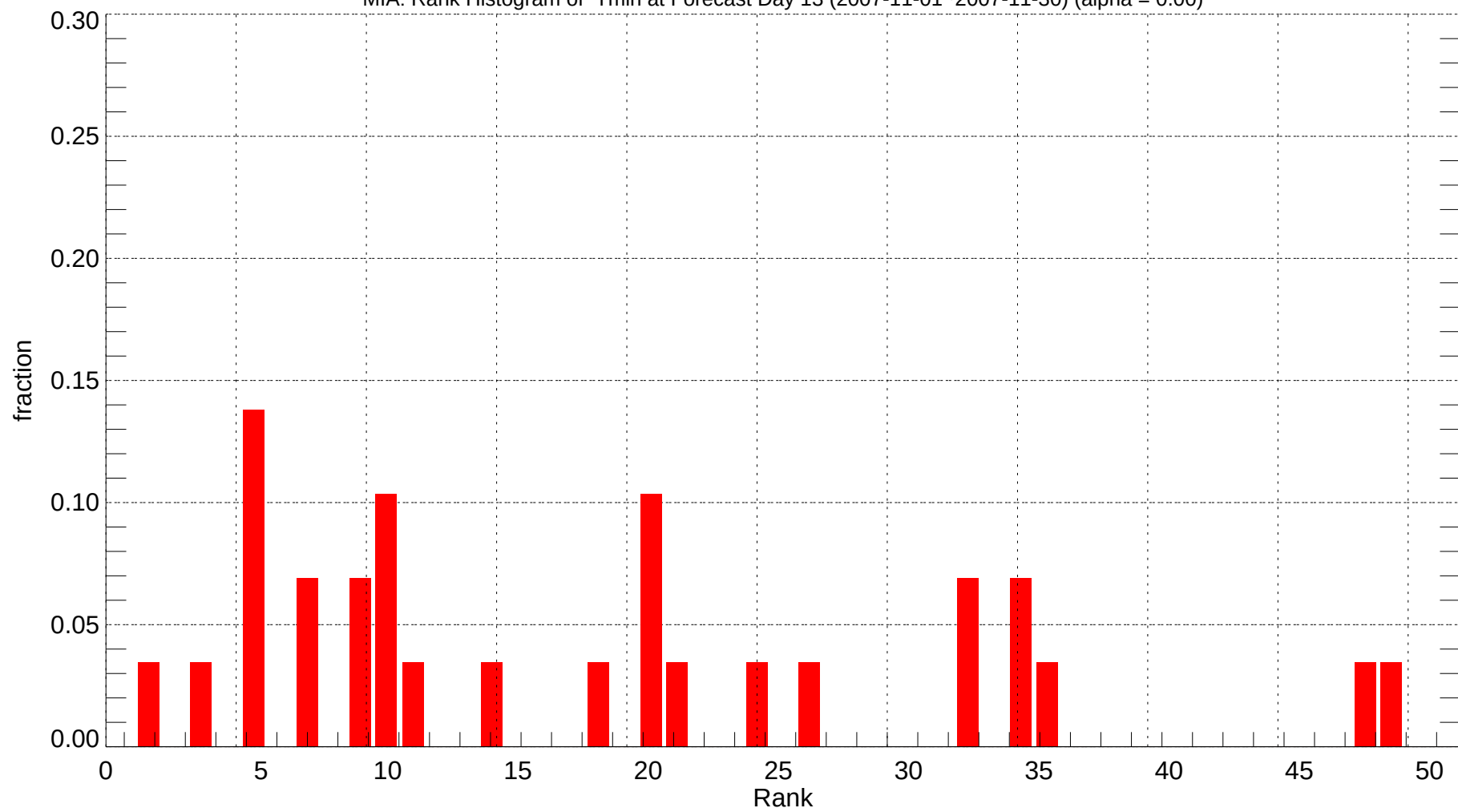
MIA: Rank Histogram of Tmin at Forecast Day 13 (2007-11-01~2007-11-30) (alpha = 0.00)
