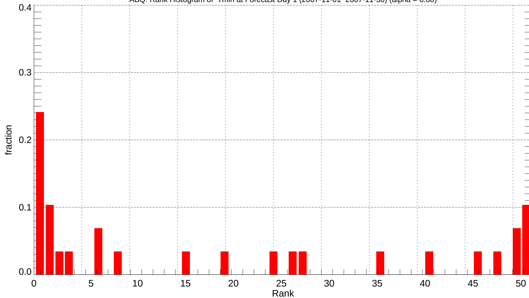
ABQ: Rank Histogram of Tmin at Forecast Day 1 (2007-11-01~2007-11-30) (alpha = 0.00)
