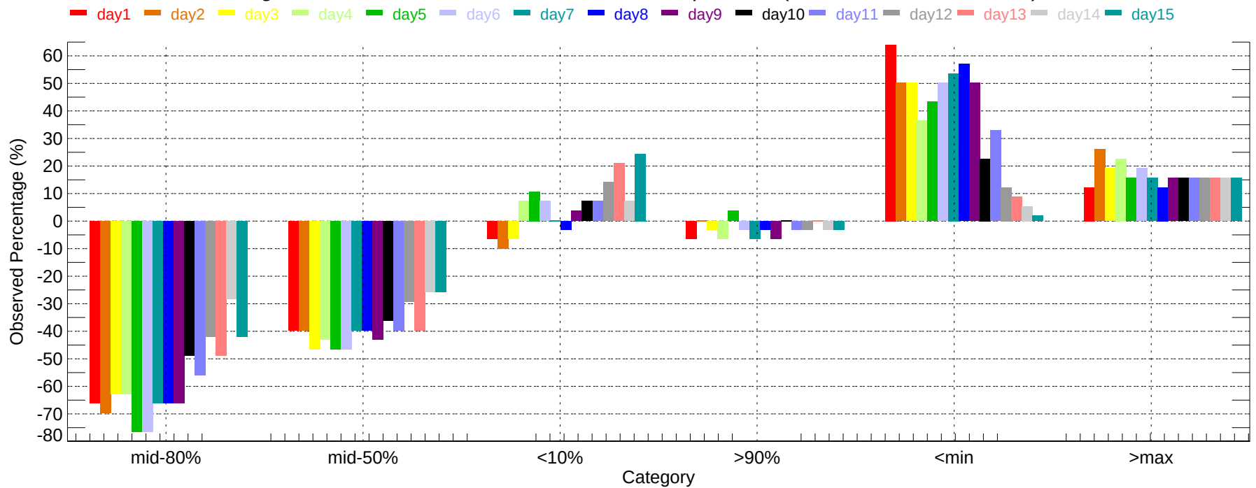
Observed Percentage Deviation of Ensembles - SAN: Min Temperature (2007-11-01~2007-11-30)
