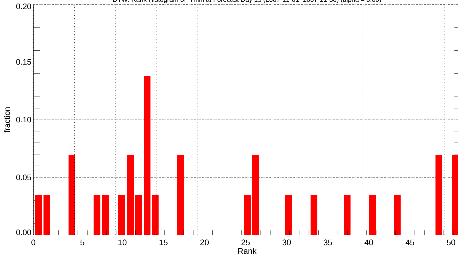
DTW: Rank Histogram of Tmin at Forecast Day 15 (2007-11-01~2007-11-30) (alpha = 0.00)
