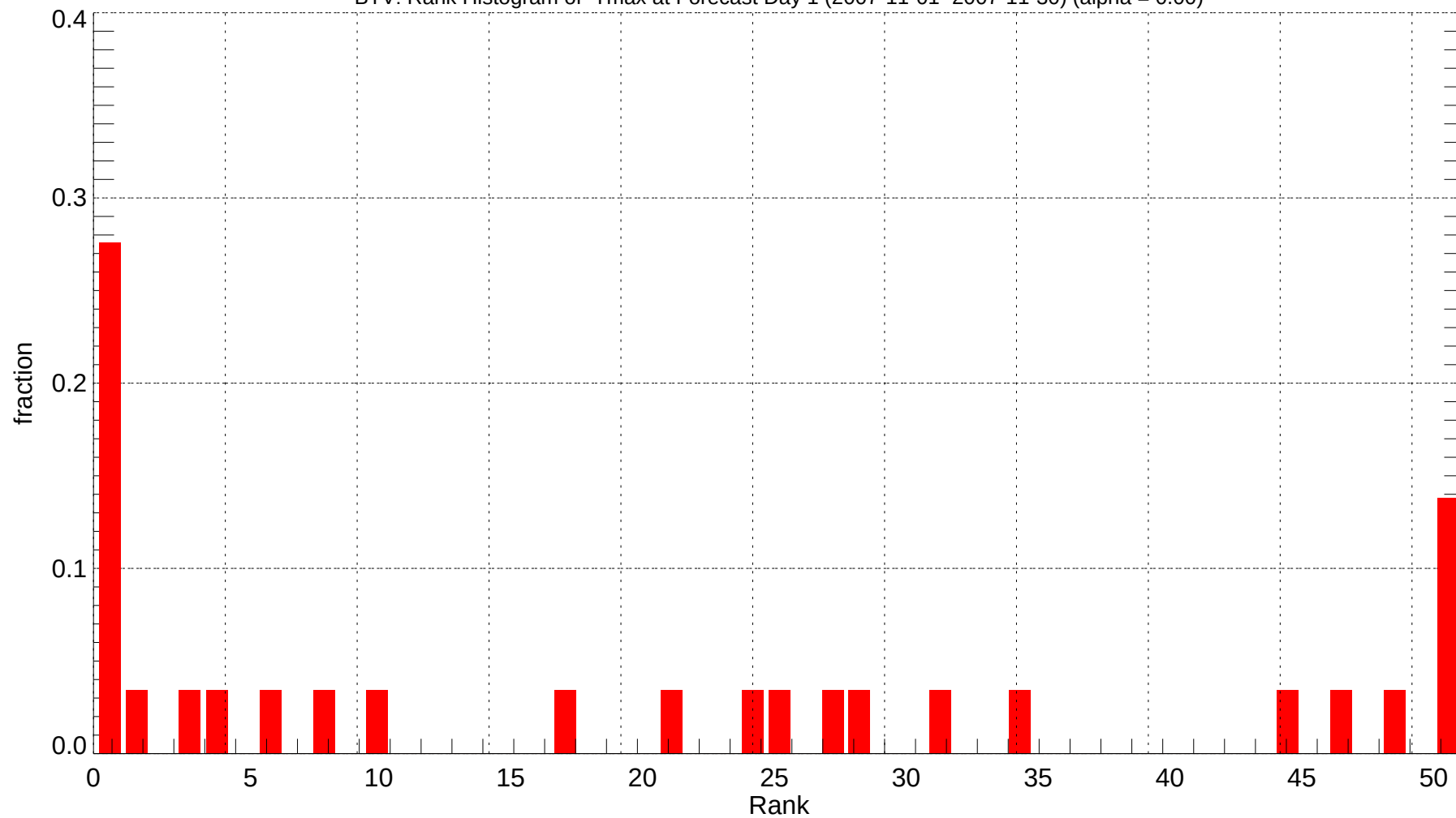
BTV: Rank Histogram of Tmax at Forecast Day 1 (2007-11-01~2007-11-30) (alpha = 0.00)
