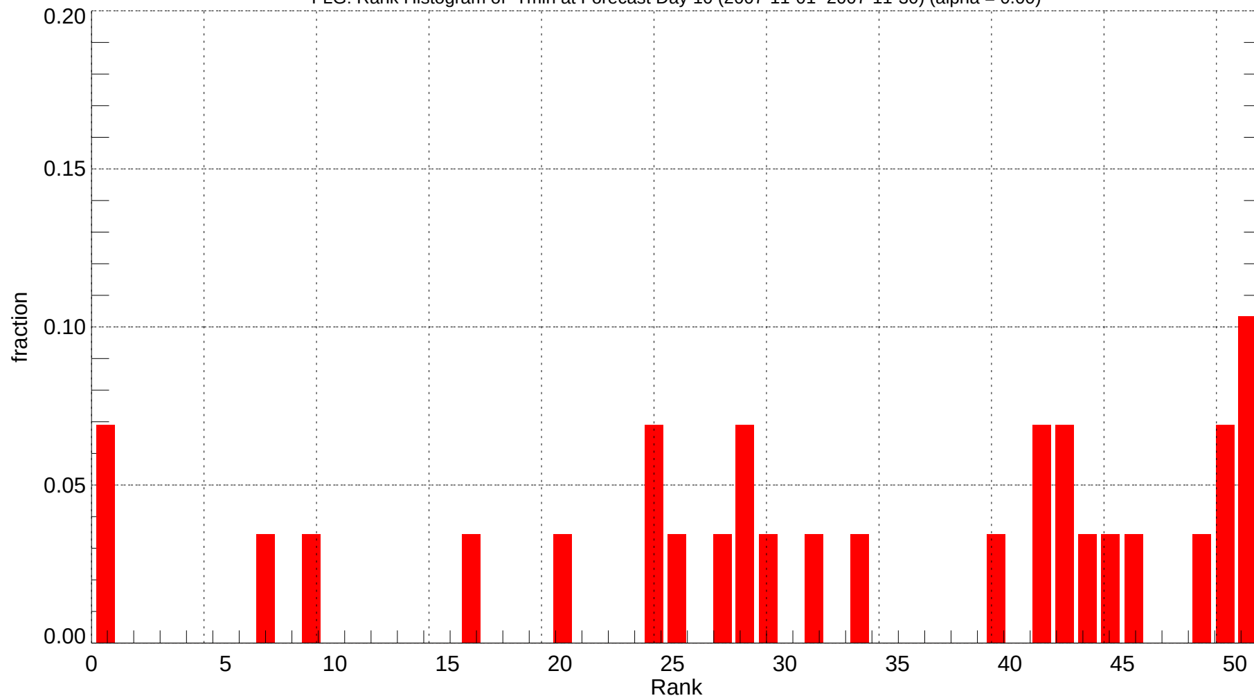
FLG: Rank Histogram of Tmin at Forecast Day 10 (2007-11-01~2007-11-30) (alpha = 0.00)
