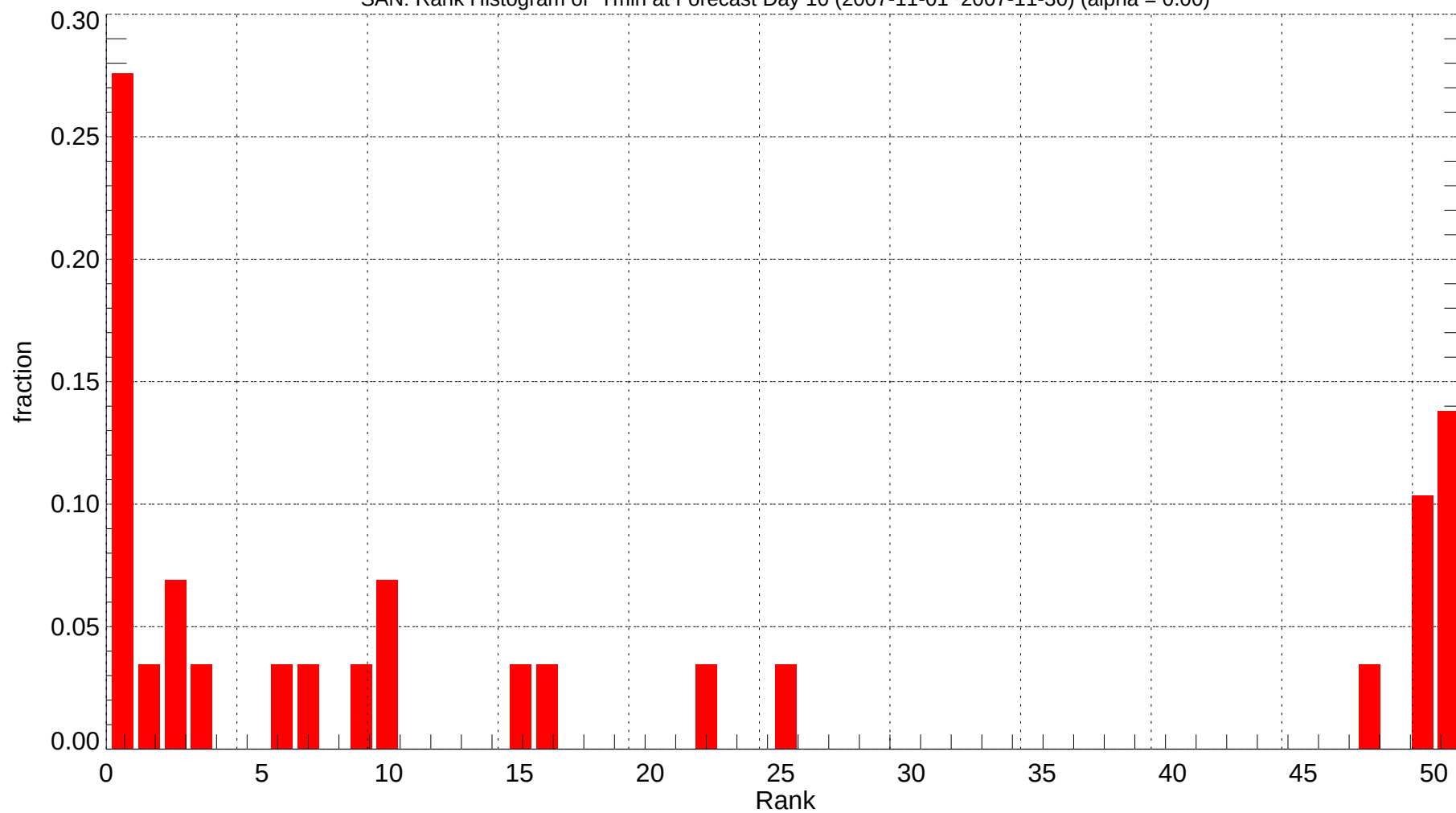
SAN: Rank Histogram of Tmin at Forecast Day 10 (2007-11-01~2007-11-30) (alpha = 0.00)
