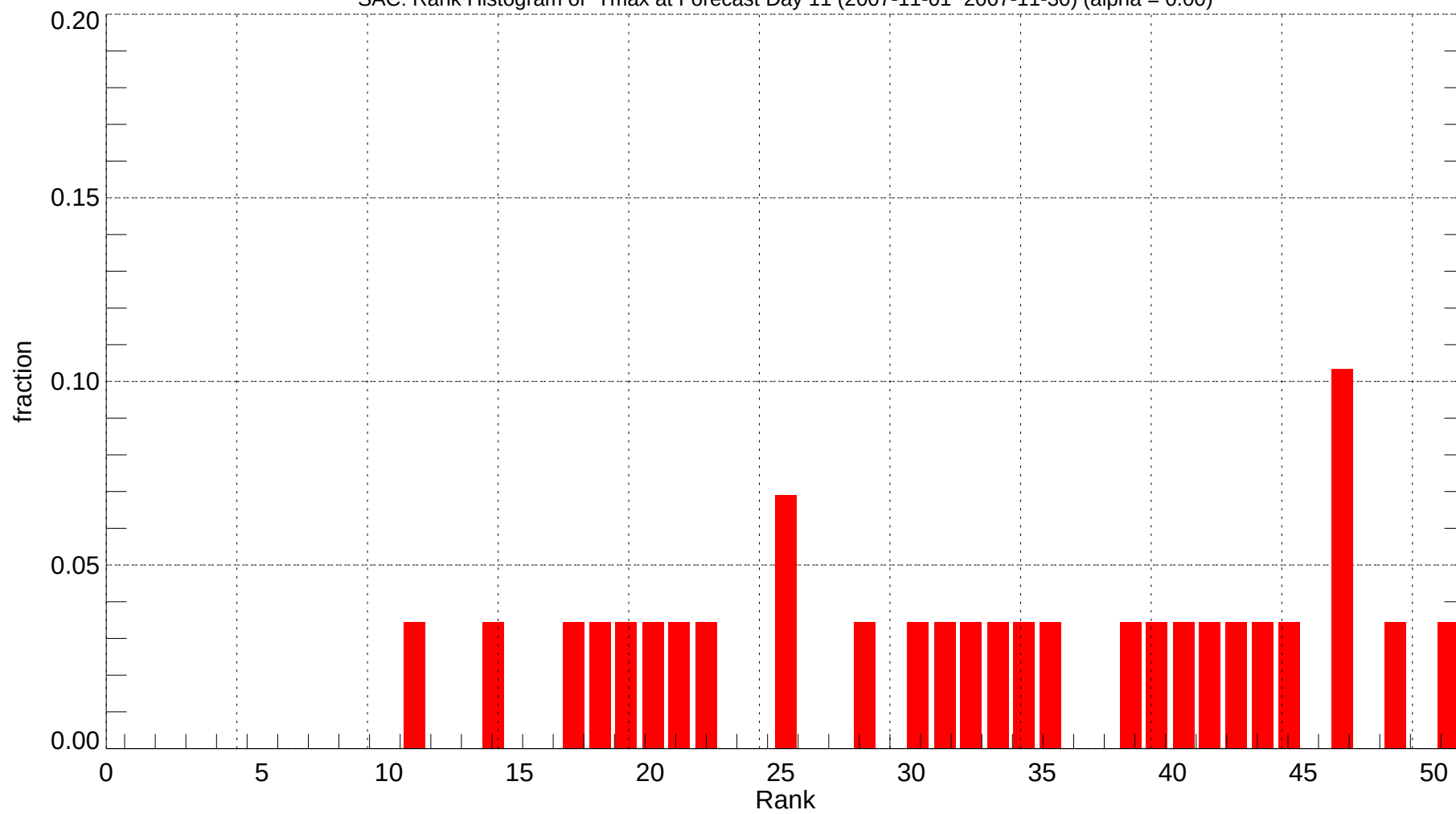
SAC: Rank Histogram of Tmax at Forecast Day 11 (2007-11-01~2007-11-30) (alpha = 0.00)
