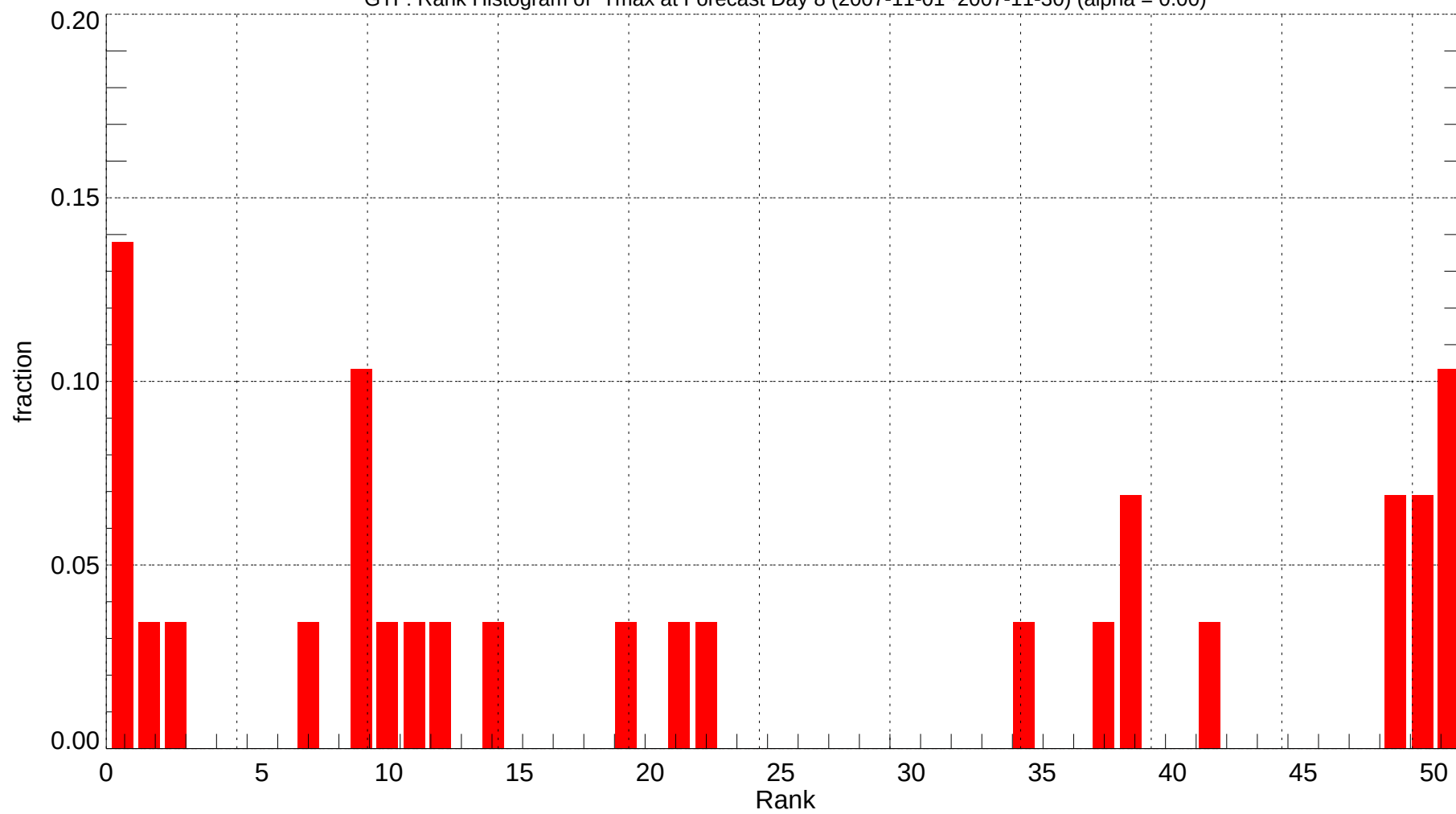
GTF: Rank Histogram of Tmax at Forecast Day 8 (2007-11-01~2007-11-30) (alpha = 0.00)
