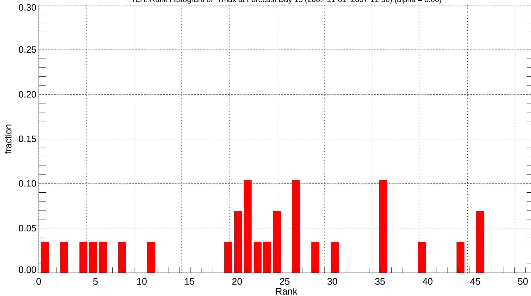
TLH: Rank Histogram of Tmax at Forecast Day 13 (2007-11-01~2007-11-30) (alpha = 0.00)
