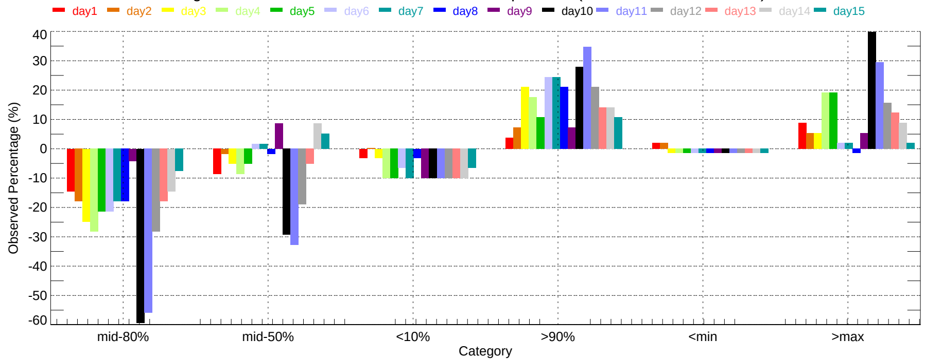
Observed Percentage Deviation of Ensembles - ATL: Max Temperature (2007-11-01~2007-11-30)
