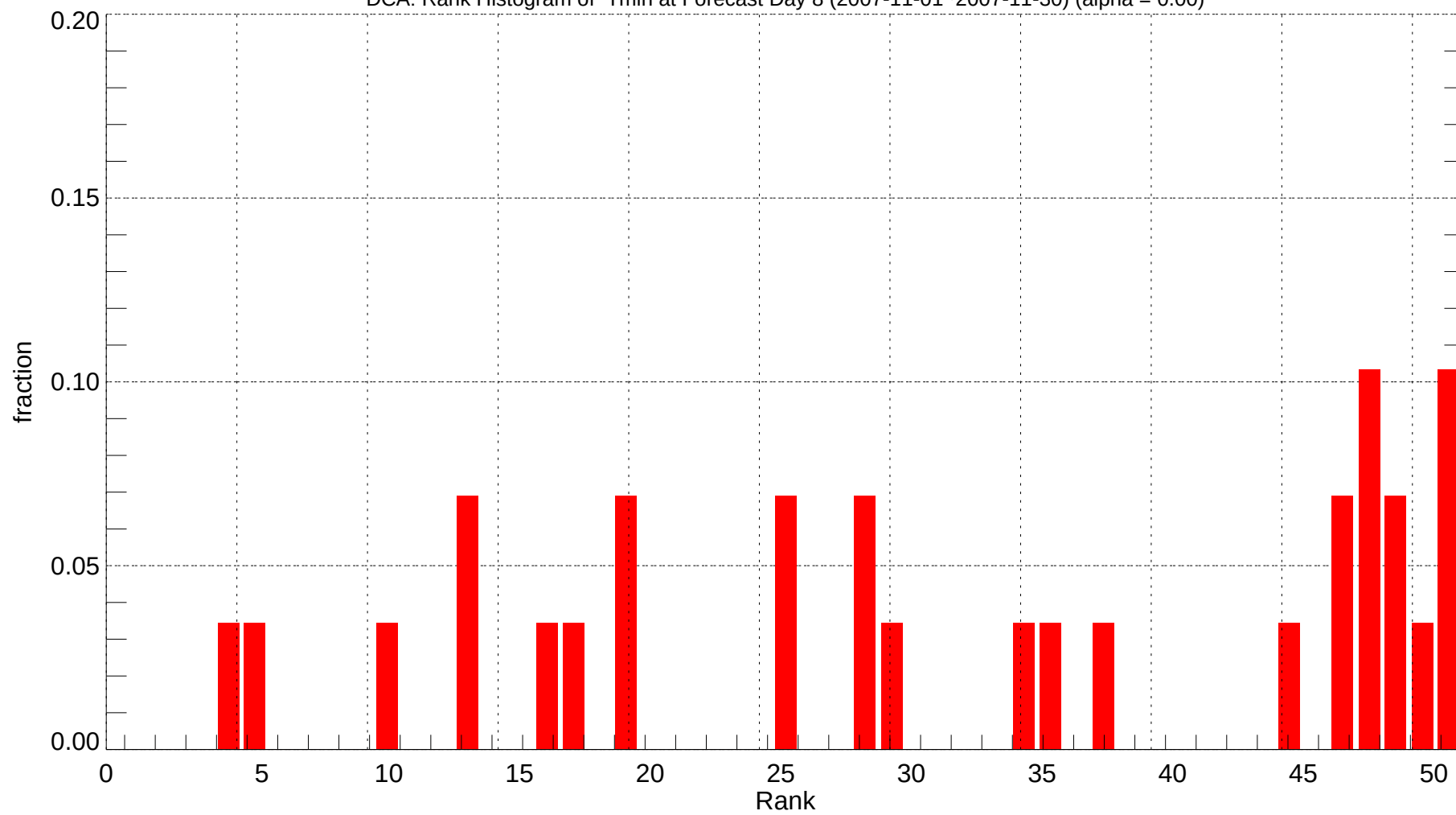
DCA: Rank Histogram of Tmin at Forecast Day 8 (2007-11-01~2007-11-30) (alpha = 0.00)
