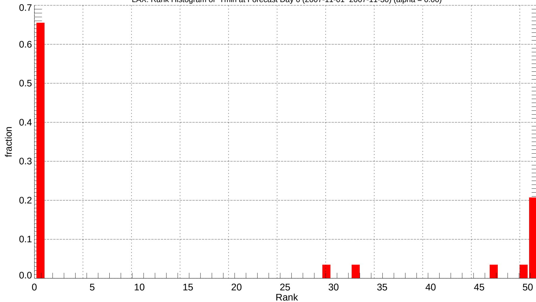
LAX: Rank Histogram of Tmin at Forecast Day 6 (2007-11-01~2007-11-30) (alpha = 0.00)
