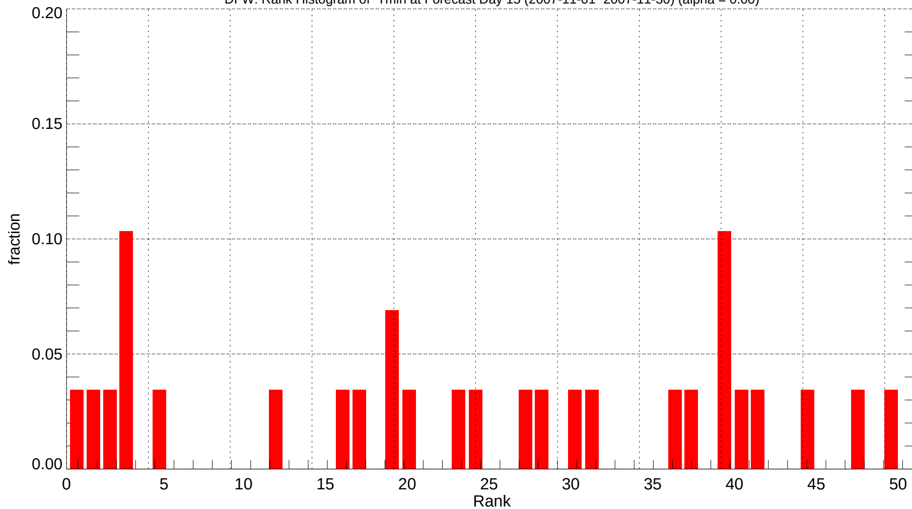
DFW: Rank Histogram of Tmin at Forecast Day 15 (2007-11-01~2007-11-30) (alpha = 0.00)
