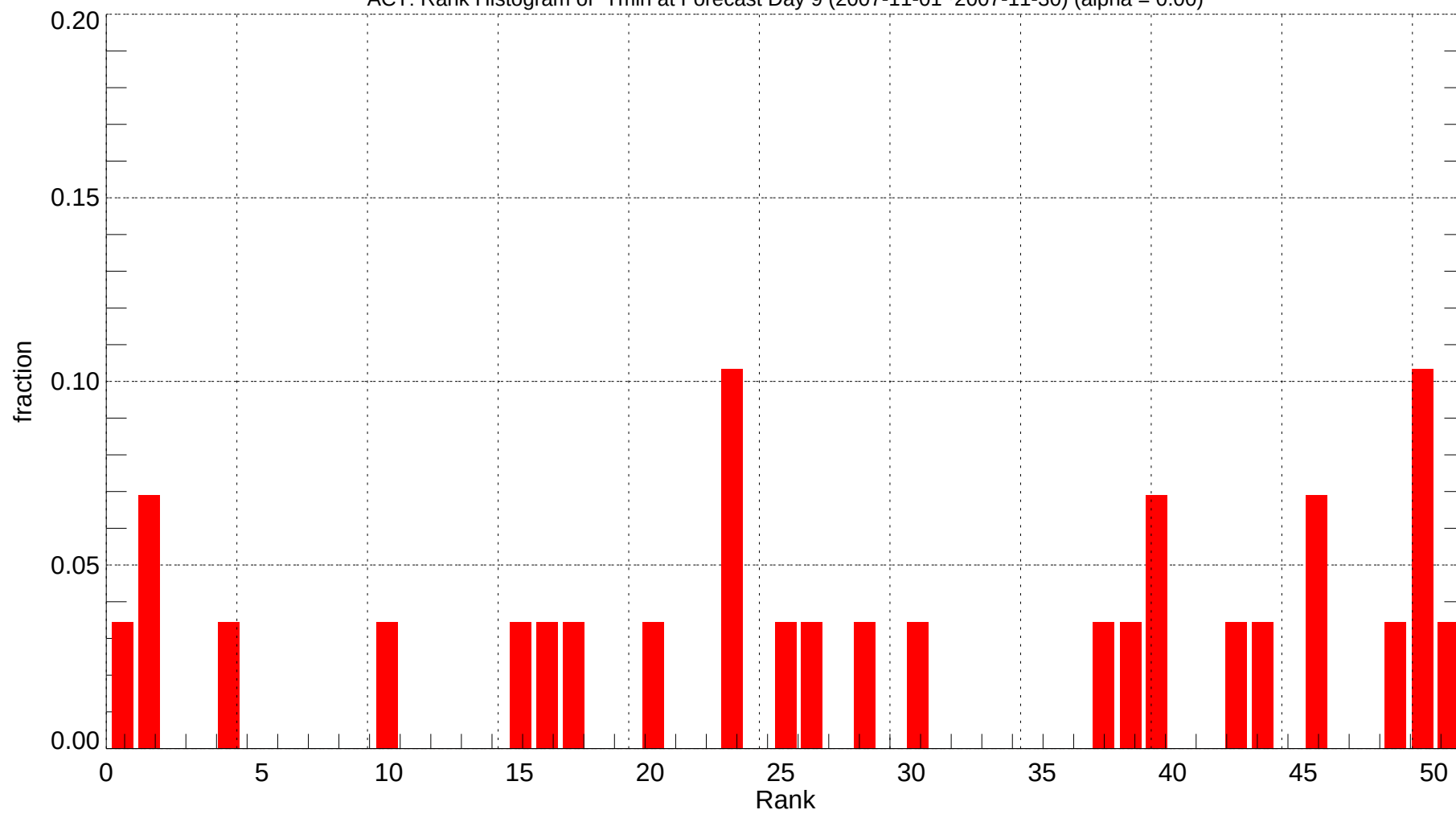
ACT: Rank Histogram of Tmin at Forecast Day 9 (2007-11-01~2007-11-30) (alpha = 0.00)
