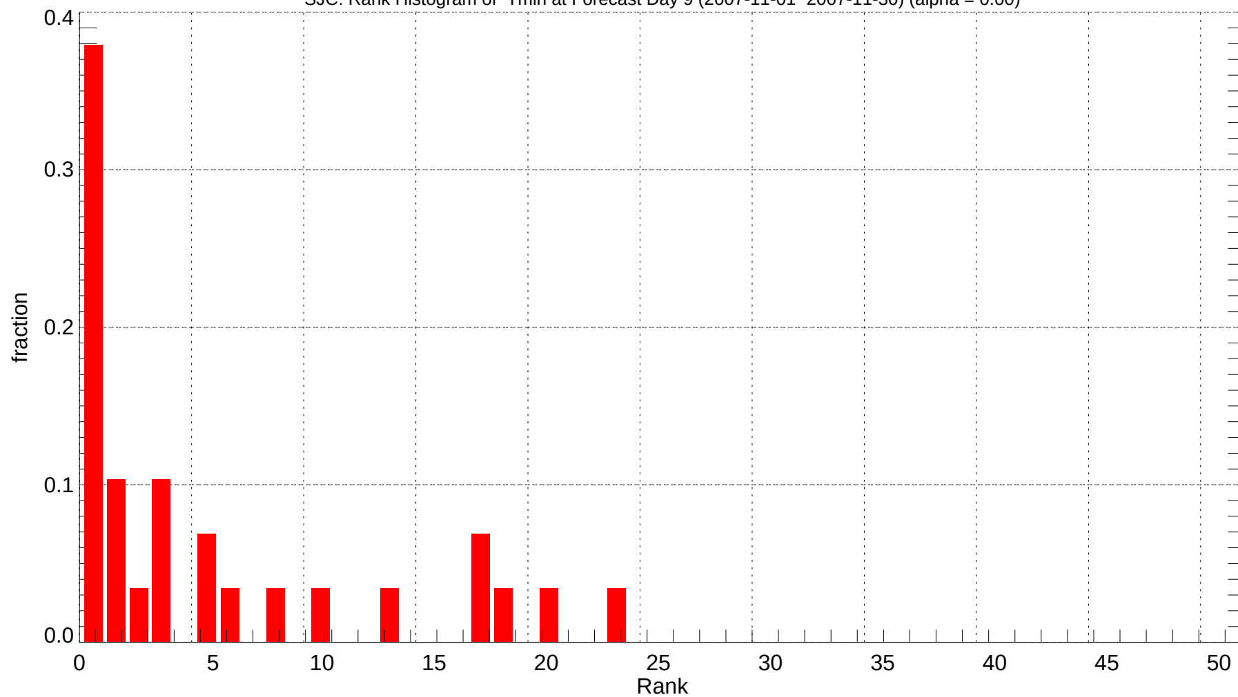
SJC: Rank Histogram of Tmin at Forecast Day 9 (2007-11-01~2007-11-30) (alpha = 0.00)
