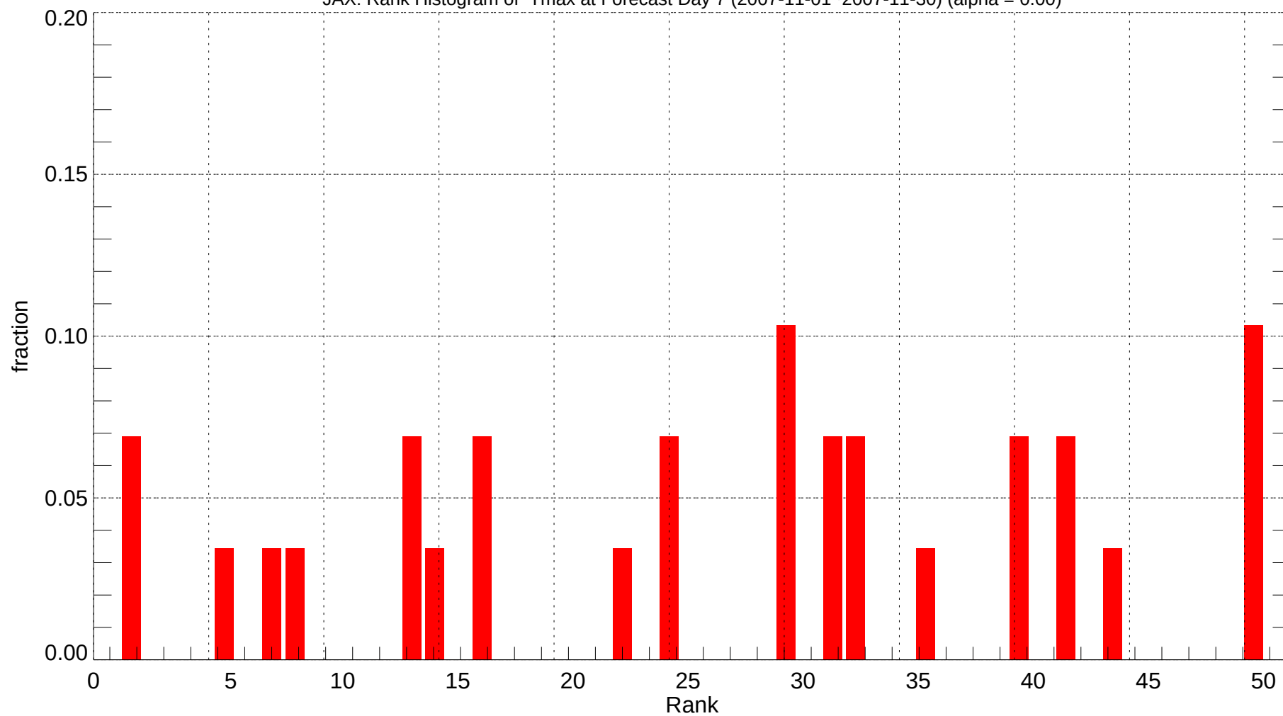
JAX: Rank Histogram of Tmax at Forecast Day 7 (2007-11-01~2007-11-30) (alpha = 0.00)
