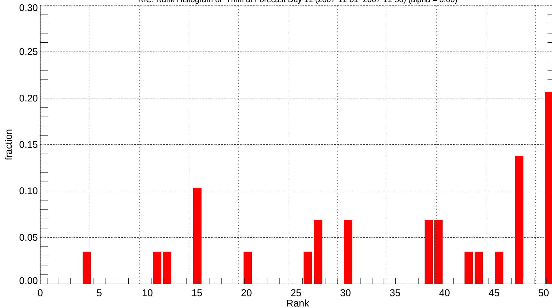
RIC: Rank Histogram of Tmin at Forecast Day 11 (2007-11-01~2007-11-30) (alpha = 0.00)
