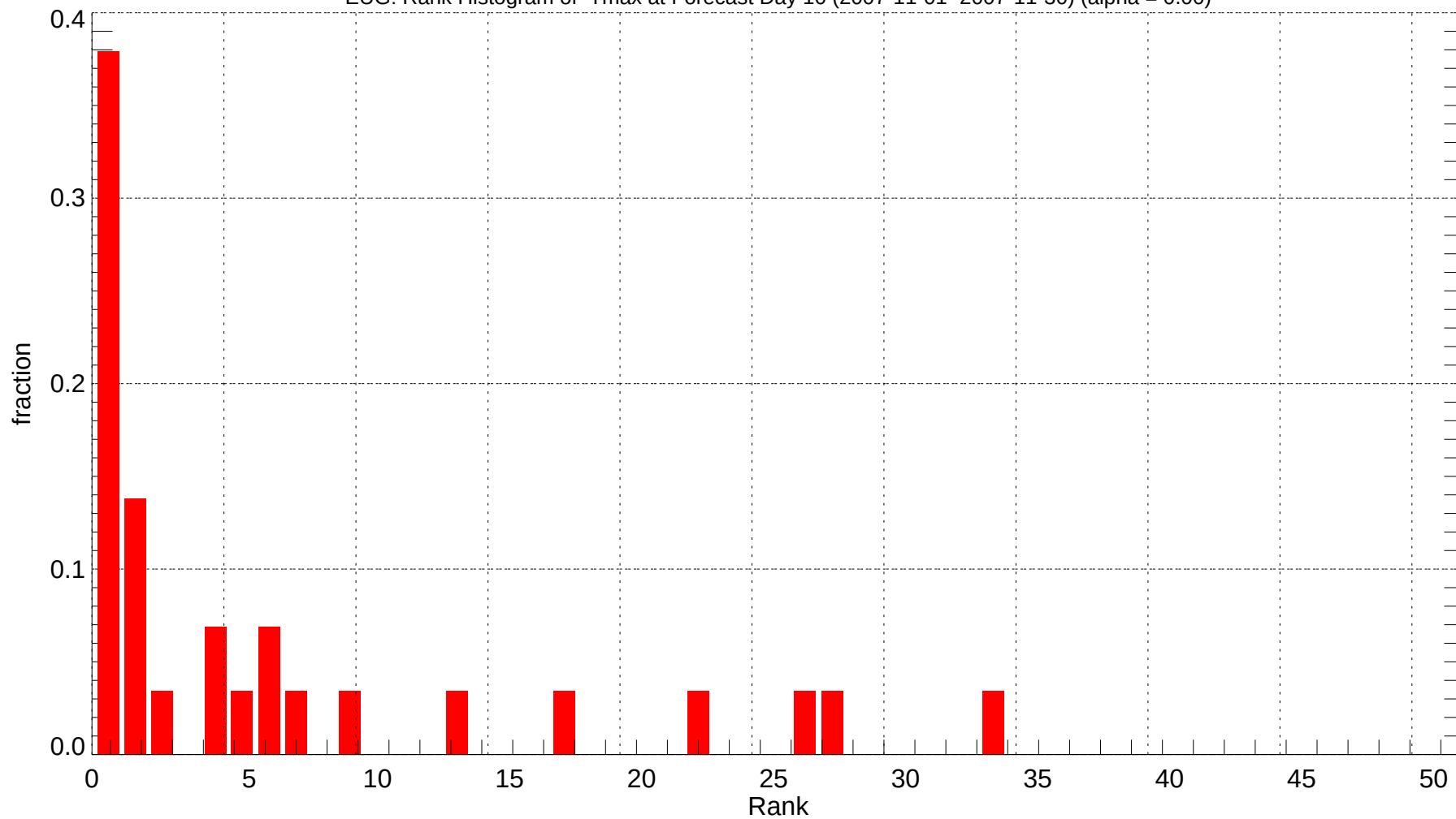
EUG: Rank Histogram of Tmax at Forecast Day 10 (2007-11-01~2007-11-30) (alpha = 0.00)
