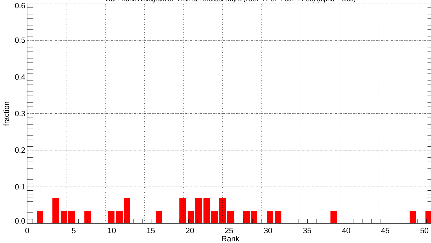
WJF: Rank Histogram of Tmin at Forecast Day 5 (2007-11-01~2007-11-30) (alpha = 0.00)
