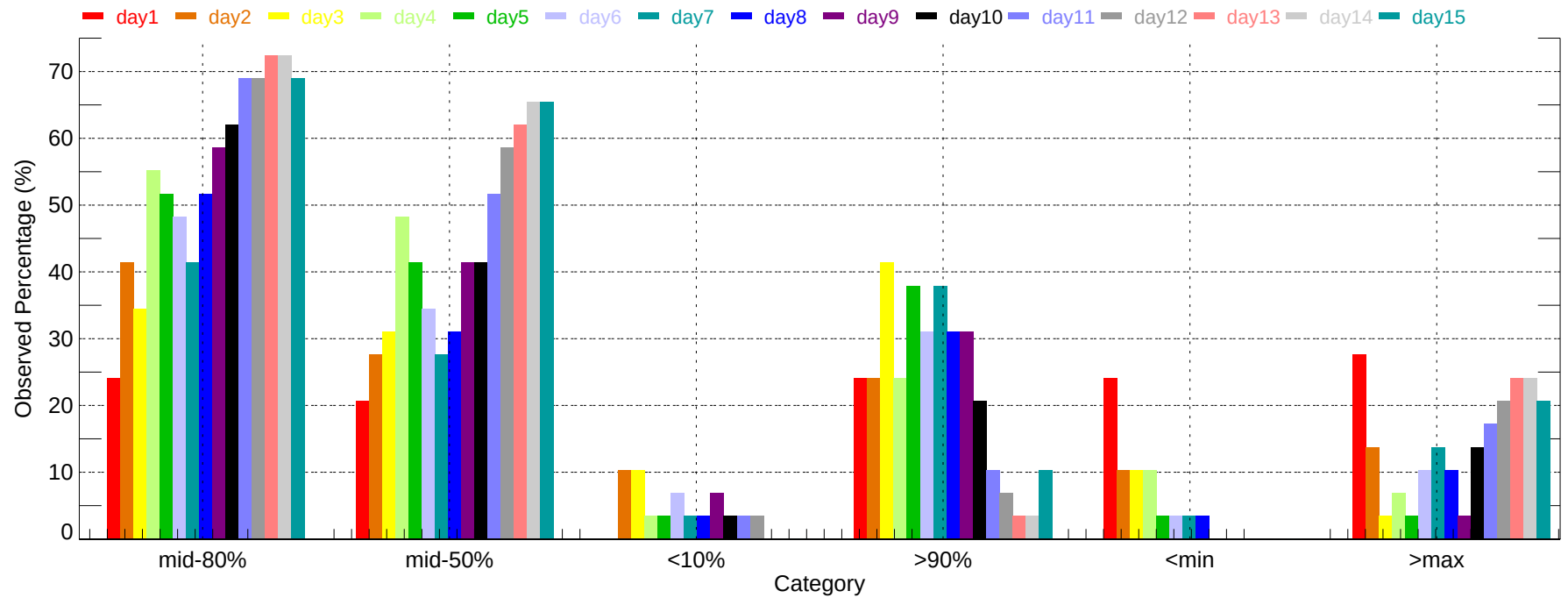
Observed Percentage of Ensembles - RDD: Max Temperature (2007-11-01~2007-11-30)
