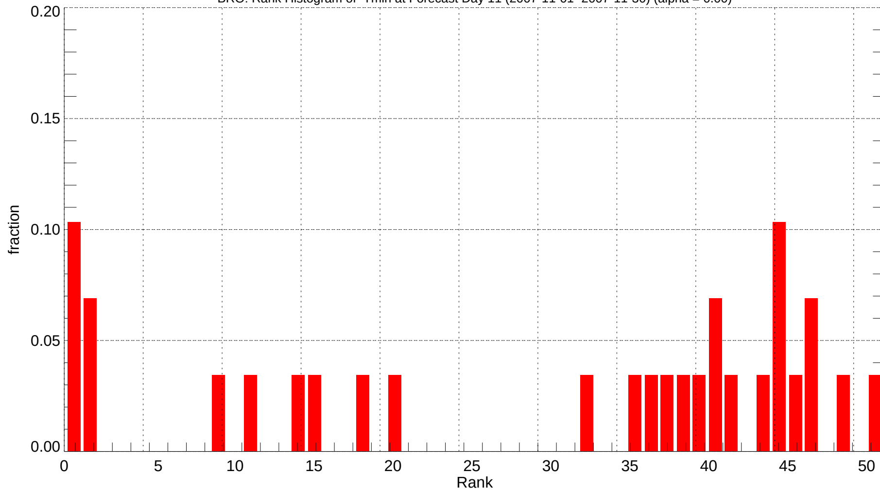
BRO: Rank Histogram of Tmin at Forecast Day 11 (2007-11-01~2007-11-30) (alpha = 0.00)
