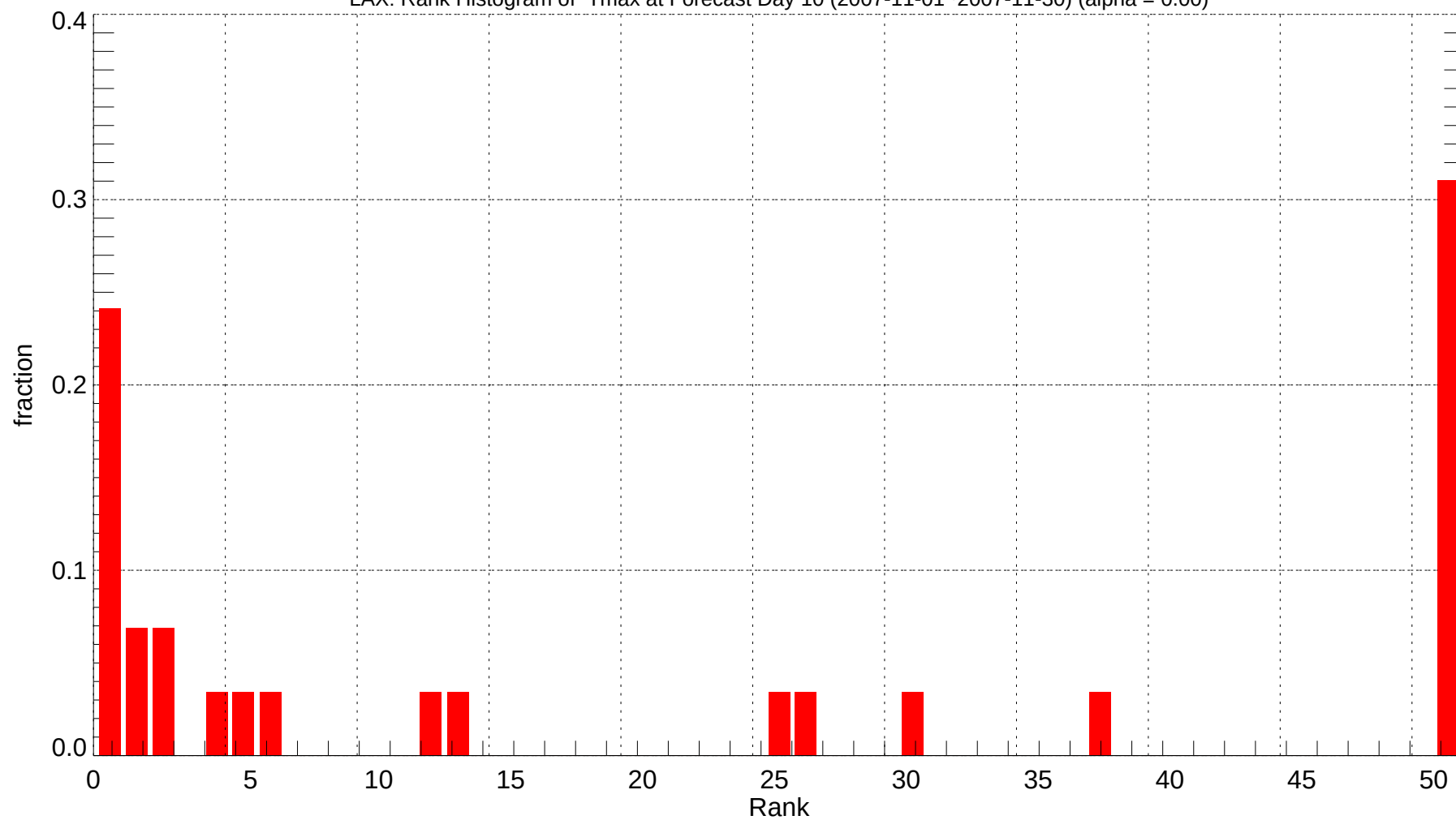
LAX: Rank Histogram of Tmax at Forecast Day 10 (2007-11-01~2007-11-30) (alpha = 0.00)
