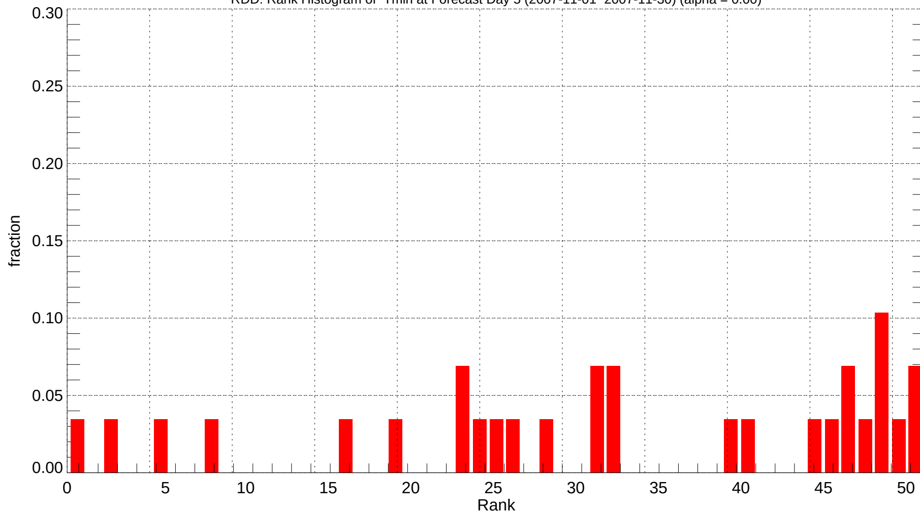
RDD: Rank Histogram of Tmin at Forecast Day 5 (2007-11-01~2007-11-30) (alpha = 0.00)
