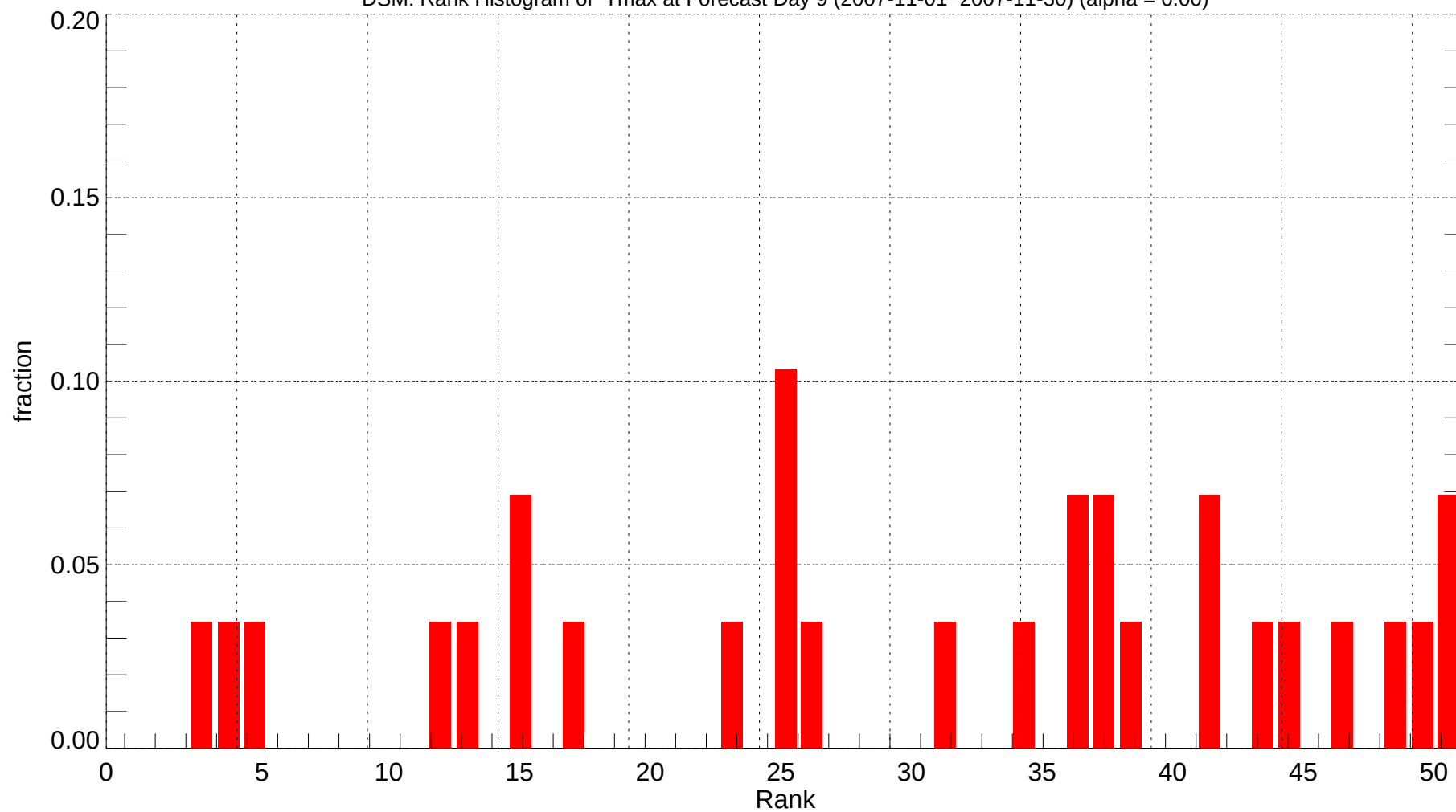
DSM: Rank Histogram of Tmax at Forecast Day 9 (2007-11-01~2007-11-30) (alpha = 0.00)
