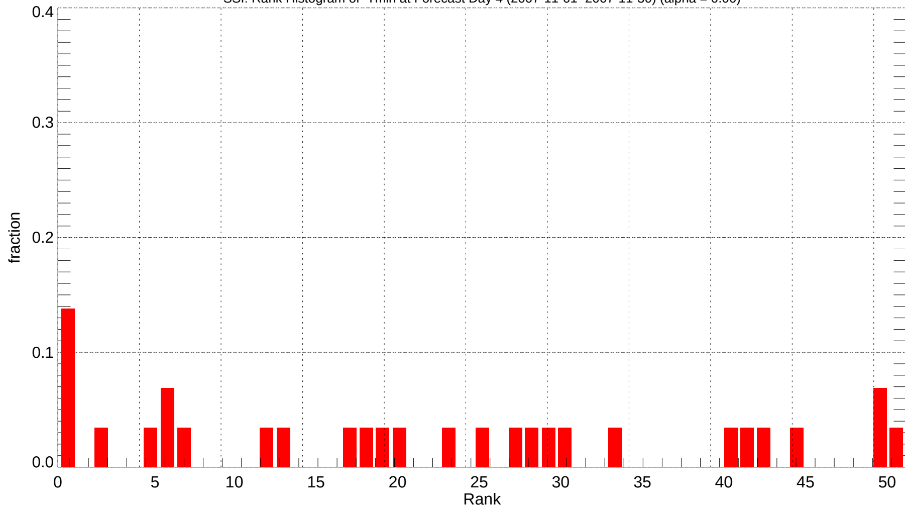
SSI: Rank Histogram of Tmin at Forecast Day 4 (2007-11-01~2007-11-30) (alpha = 0.00)
