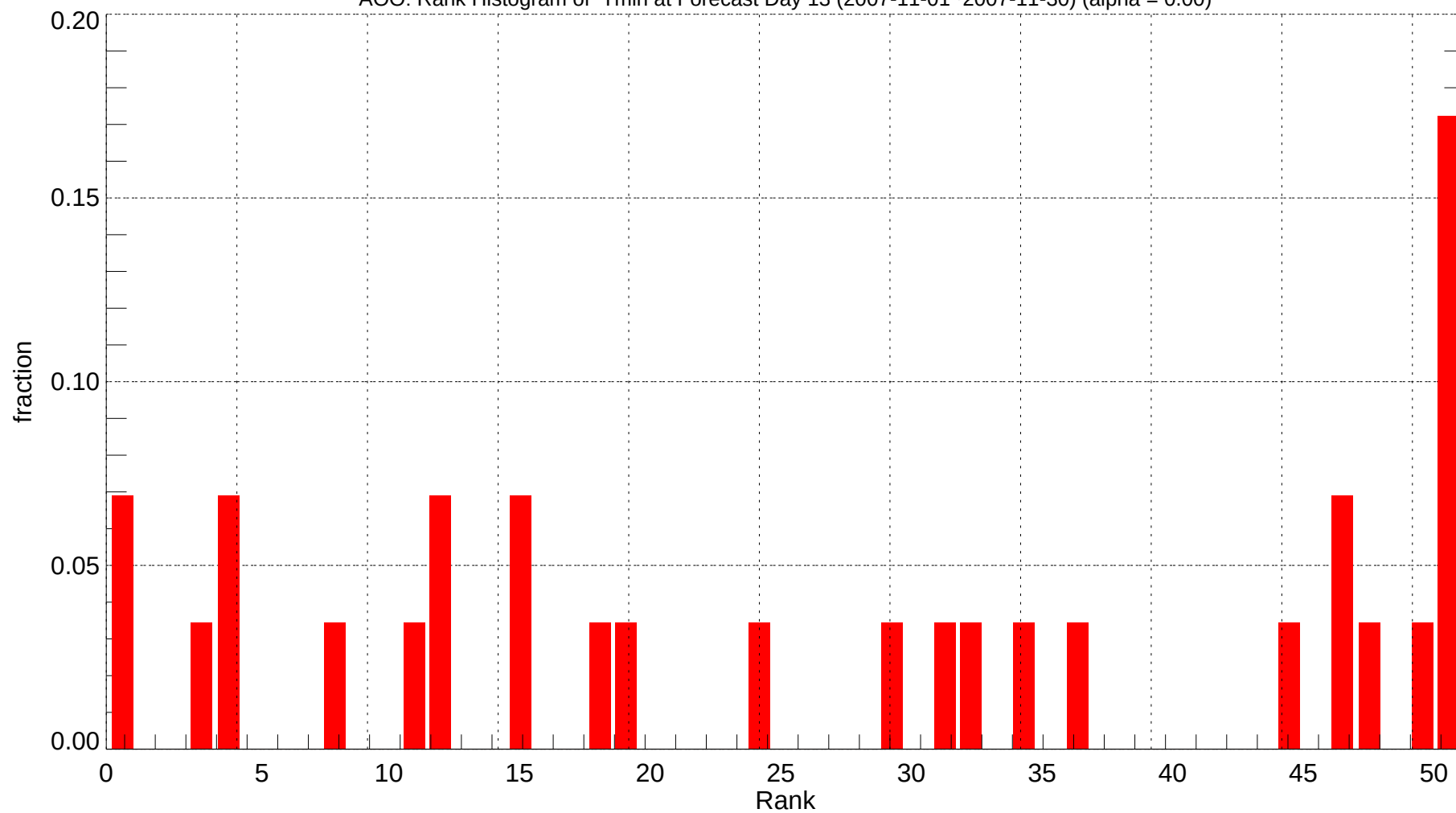
AOO: Rank Histogram of Tmin at Forecast Day 13 (2007-11-01~2007-11-30) (alpha = 0.00)
