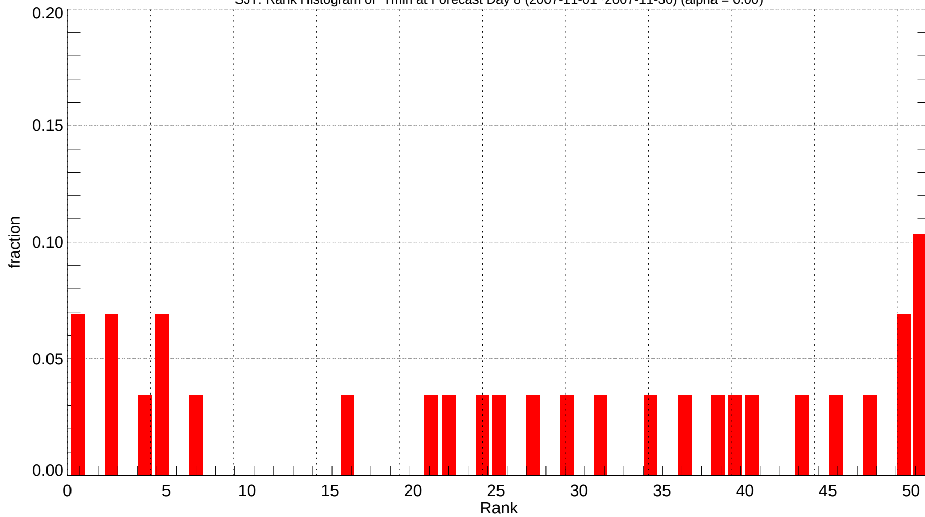
SJT: Rank Histogram of Tmin at Forecast Day 8 (2007-11-01~2007-11-30) (alpha = 0.00)
