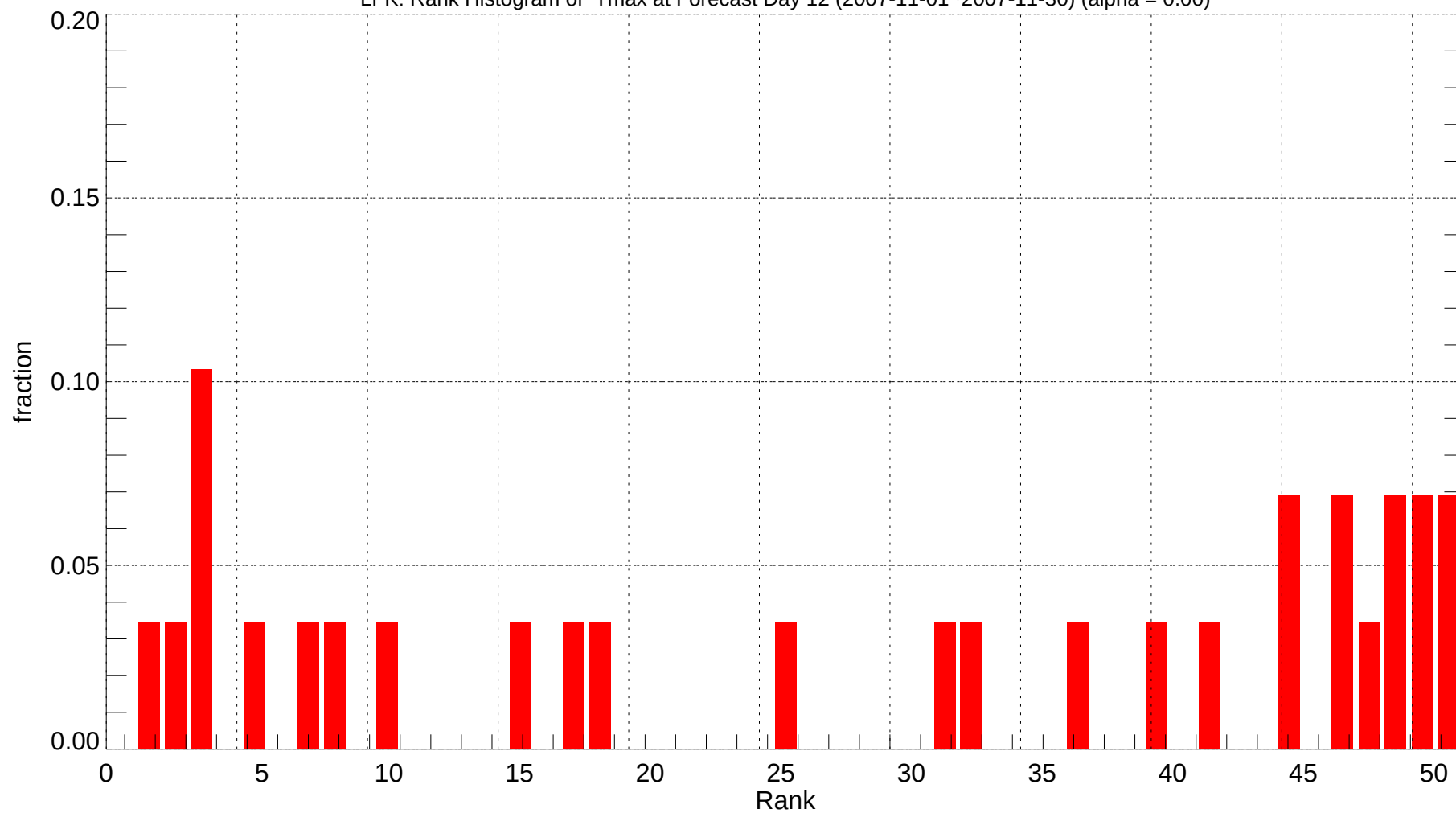
LFK: Rank Histogram of Tmax at Forecast Day 12 (2007-11-01~2007-11-30) (alpha = 0.00)
