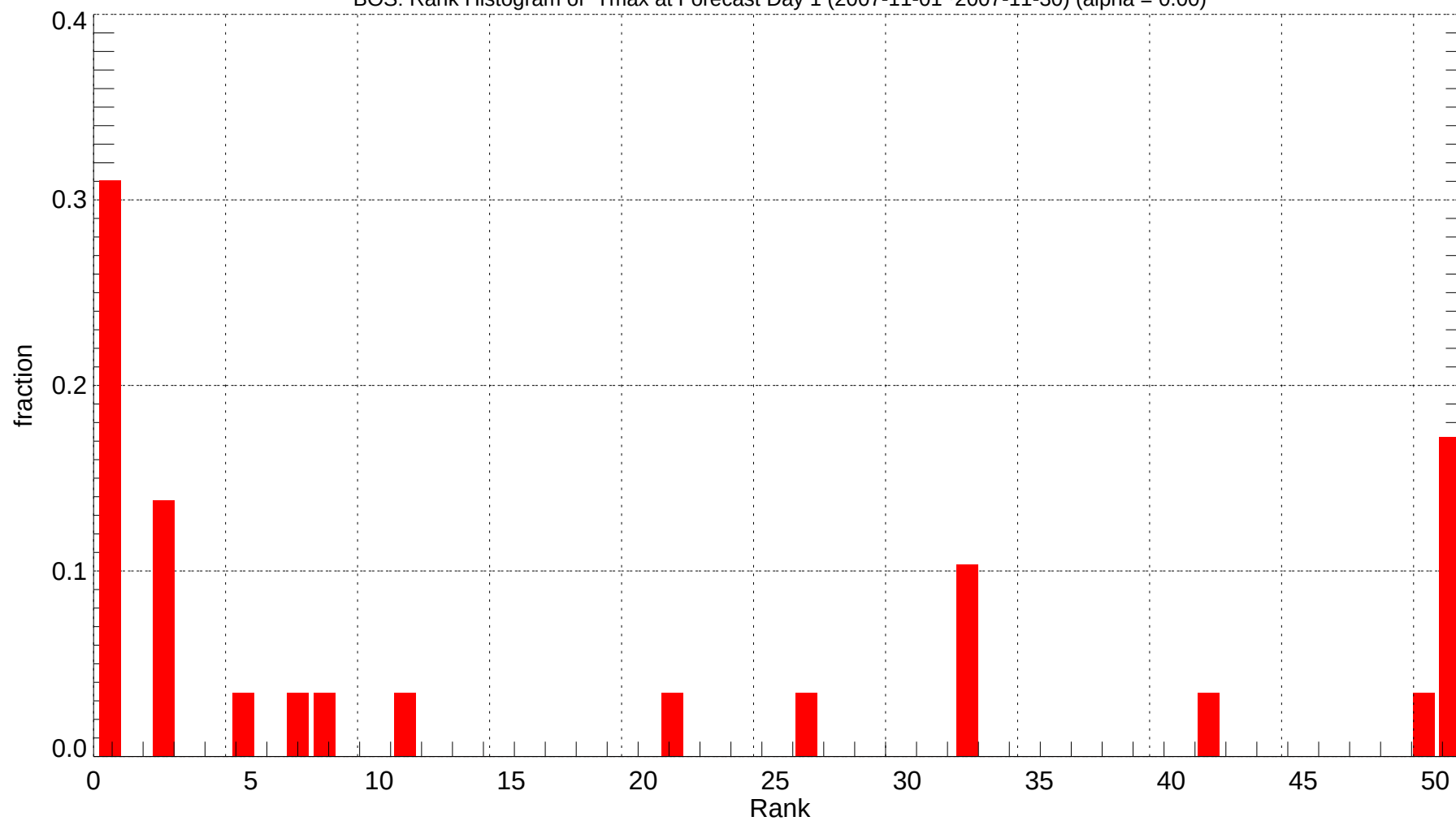
BOS: Rank Histogram of Tmax at Forecast Day 1 (2007-11-01~2007-11-30) (alpha = 0.00)
