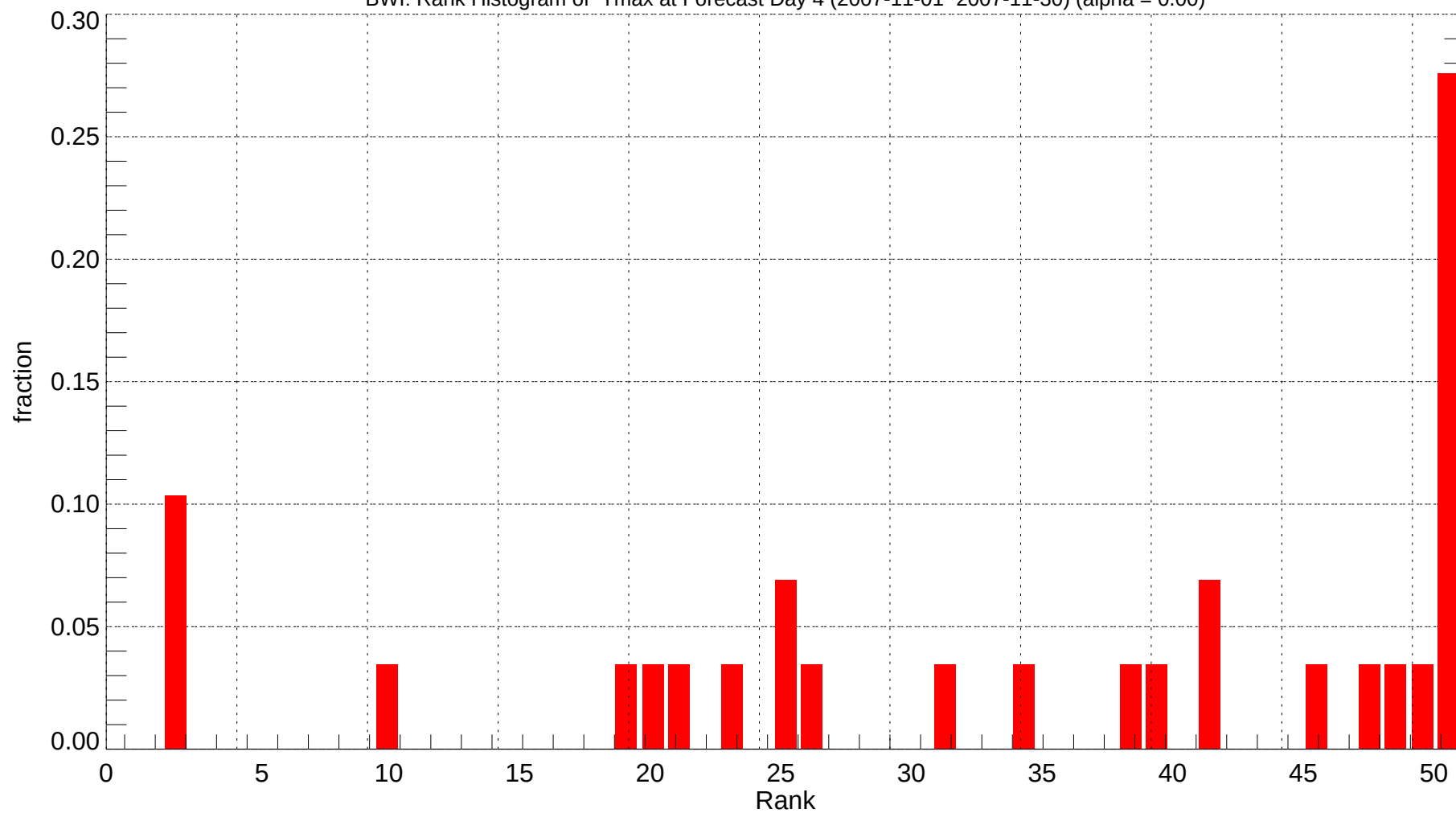
BWI: Rank Histogram of Tmax at Forecast Day 4 (2007-11-01~2007-11-30) (alpha = 0.00)
