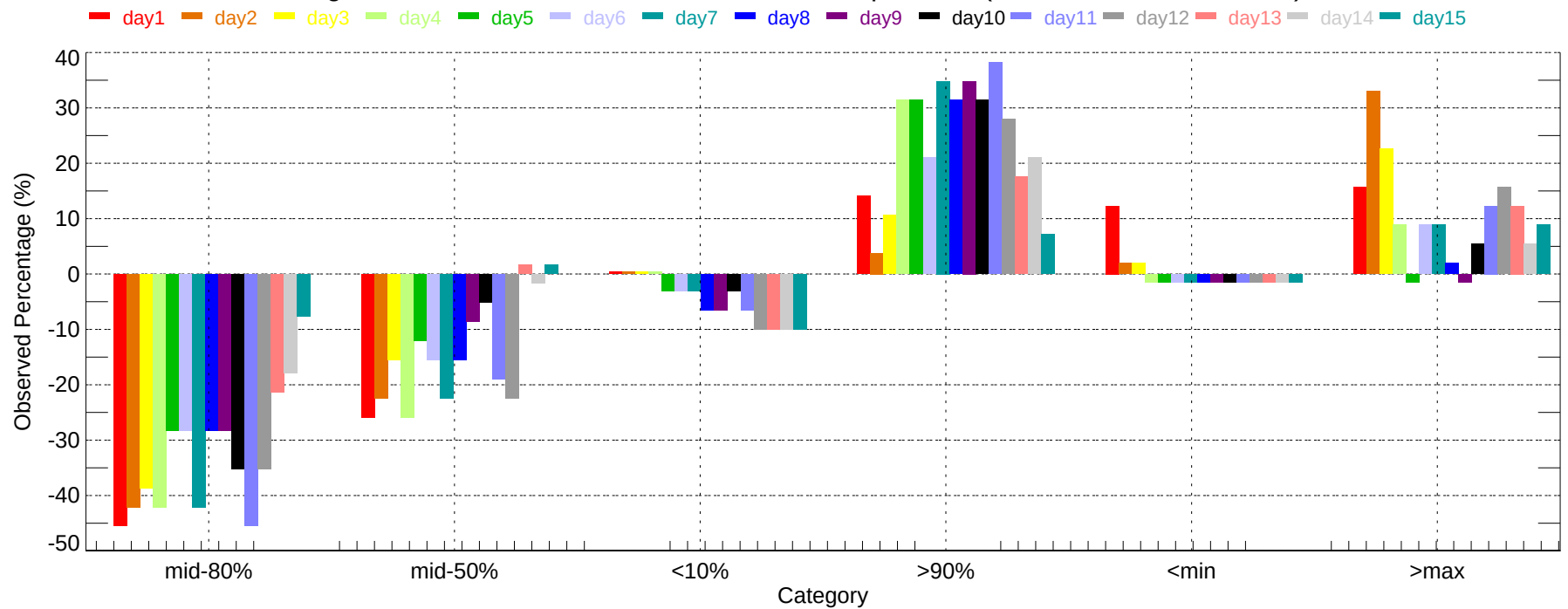
Observed Percentage Deviation of Ensembles - SDF: Max Temperature (2007-11-01~2007-11-30)
