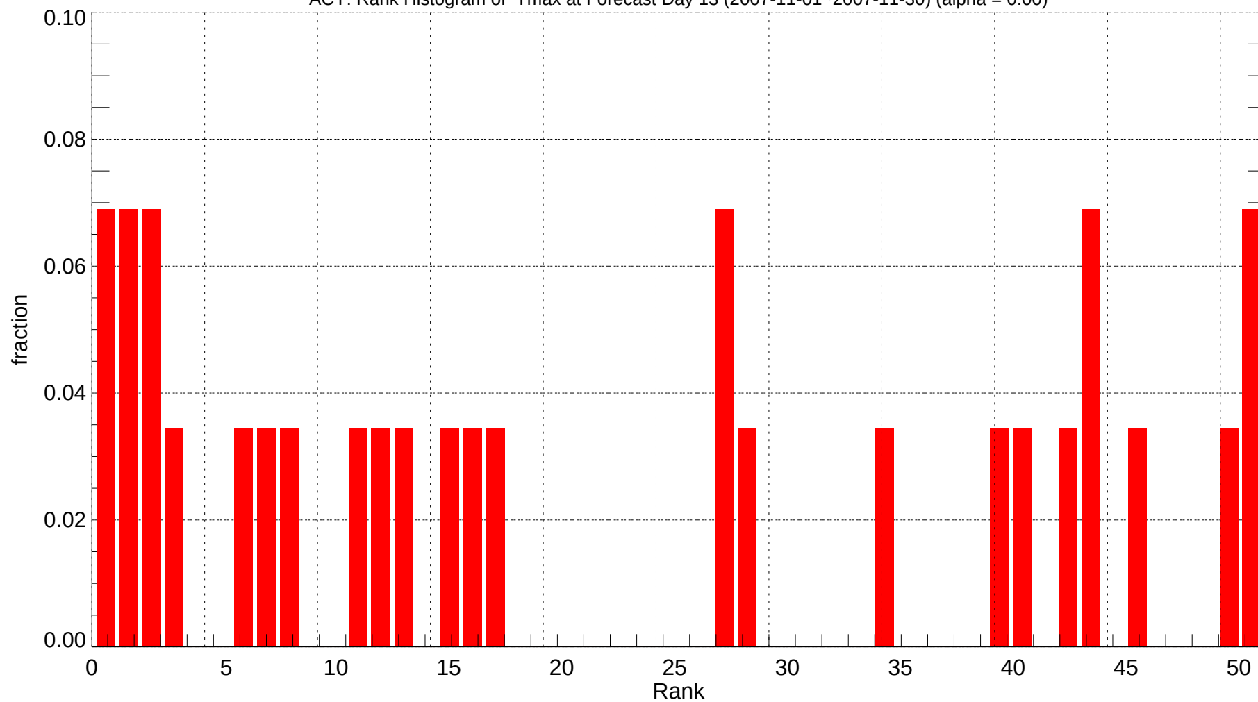
ACY: Rank Histogram of Tmax at Forecast Day 13 (2007-11-01~2007-11-30) (alpha = 0.00)
