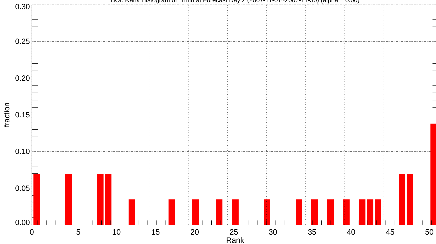
BOI: Rank Histogram of Tmin at Forecast Day 2 (2007-11-01~2007-11-30) (alpha = 0.00)
