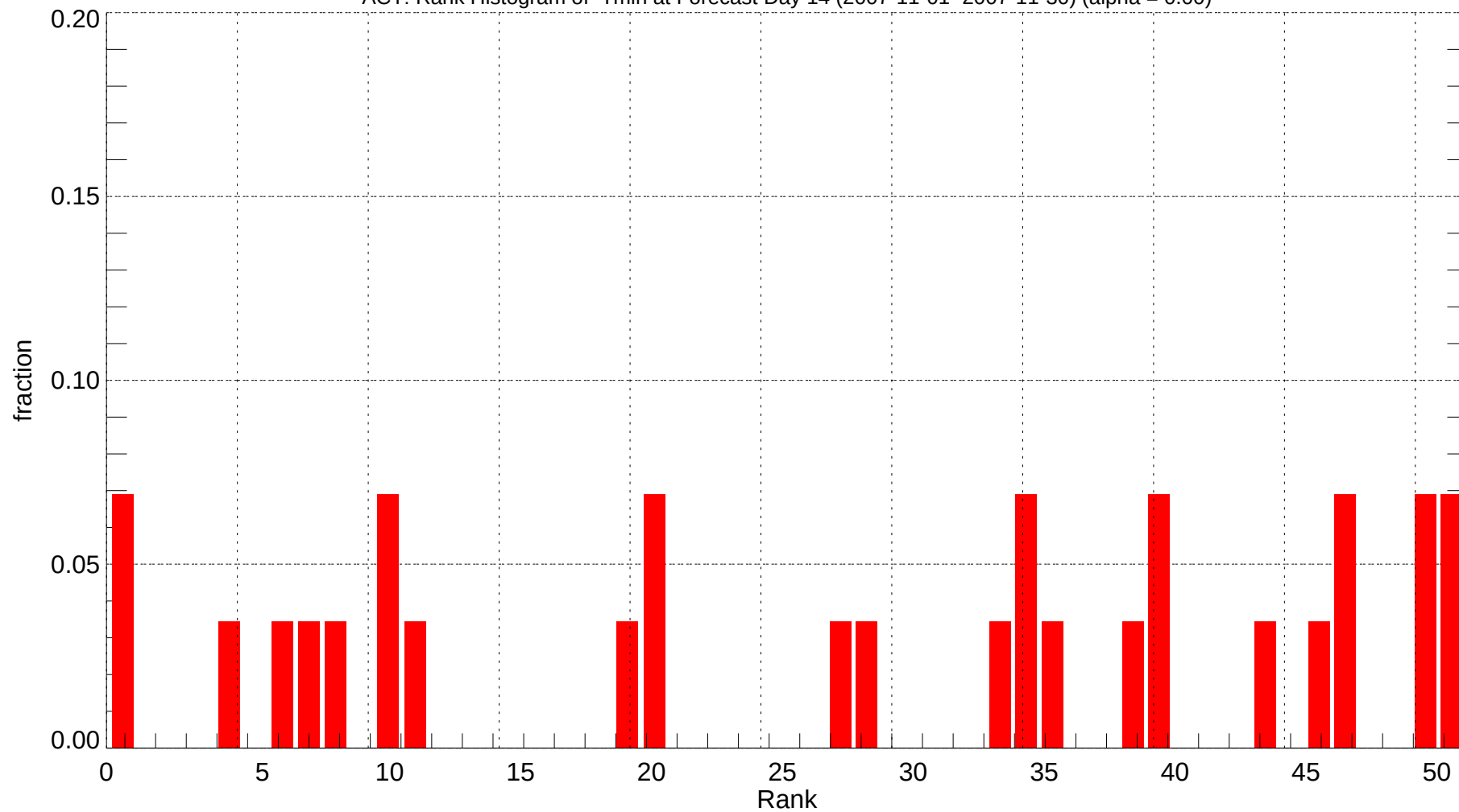
ACT: Rank Histogram of Tmin at Forecast Day 14 (2007-11-01~2007-11-30) (alpha = 0.00)
