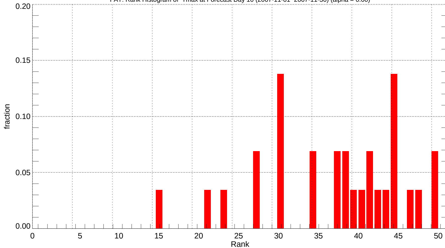
FAT: Rank Histogram of Tmax at Forecast Day 10 (2007-11-01~2007-11-30) (alpha = 0.00)
