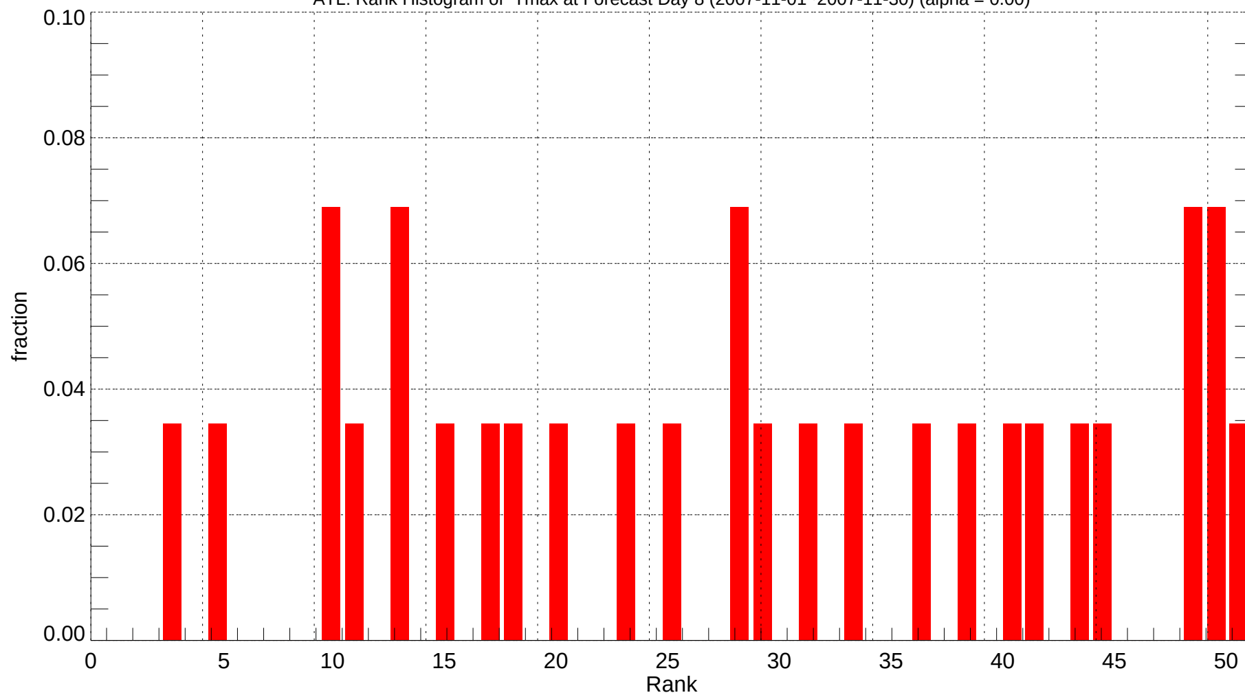
ATL: Rank Histogram of Tmax at Forecast Day 8 (2007-11-01~2007-11-30) (alpha = 0.00)
