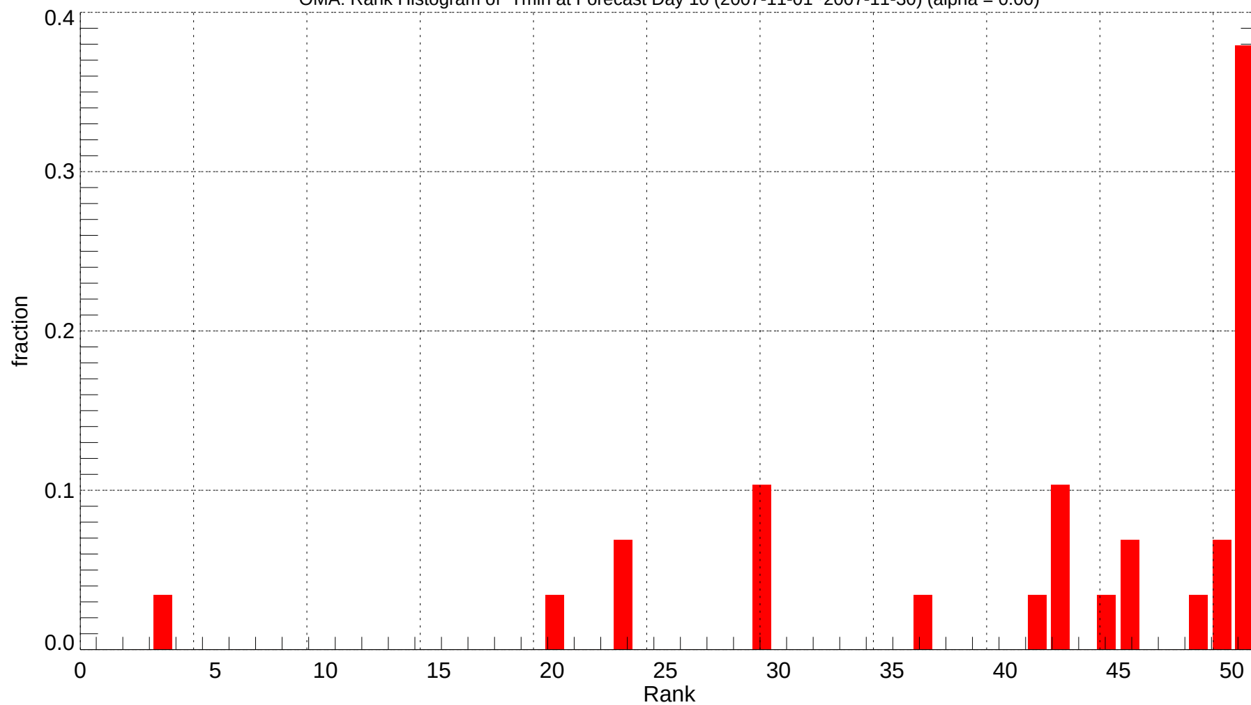
OMA: Rank Histogram of Tmin at Forecast Day 10 (2007-11-01~2007-11-30) (alpha = 0.00)
