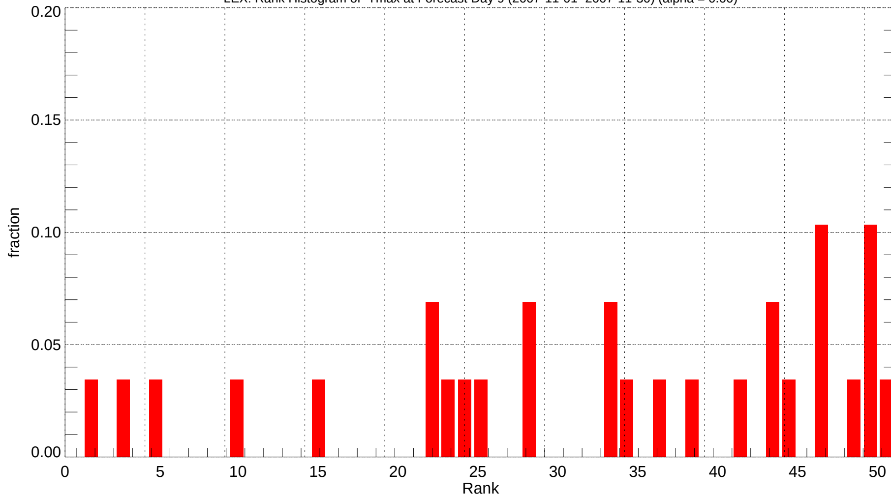
LEX: Rank Histogram of Tmax at Forecast Day 9 (2007-11-01~2007-11-30) (alpha = 0.00)
