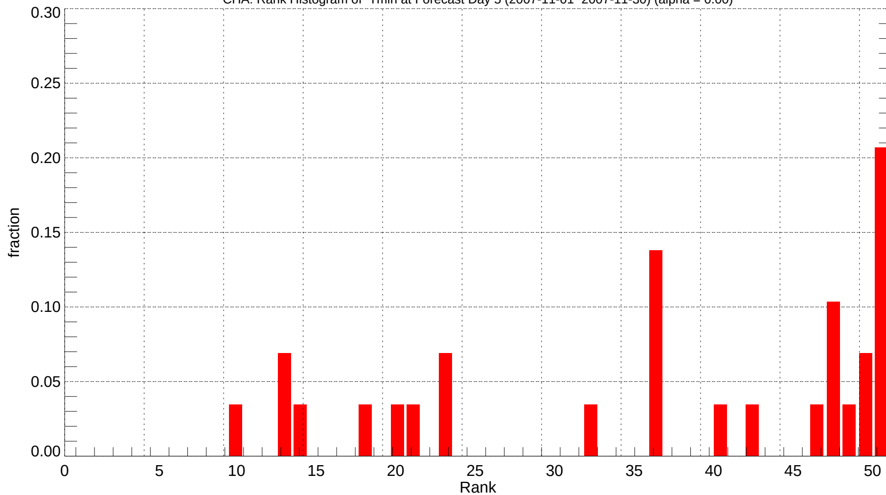
CHA: Rank Histogram of Tmin at Forecast Day 5 (2007-11-01~2007-11-30) (alpha = 0.00)
