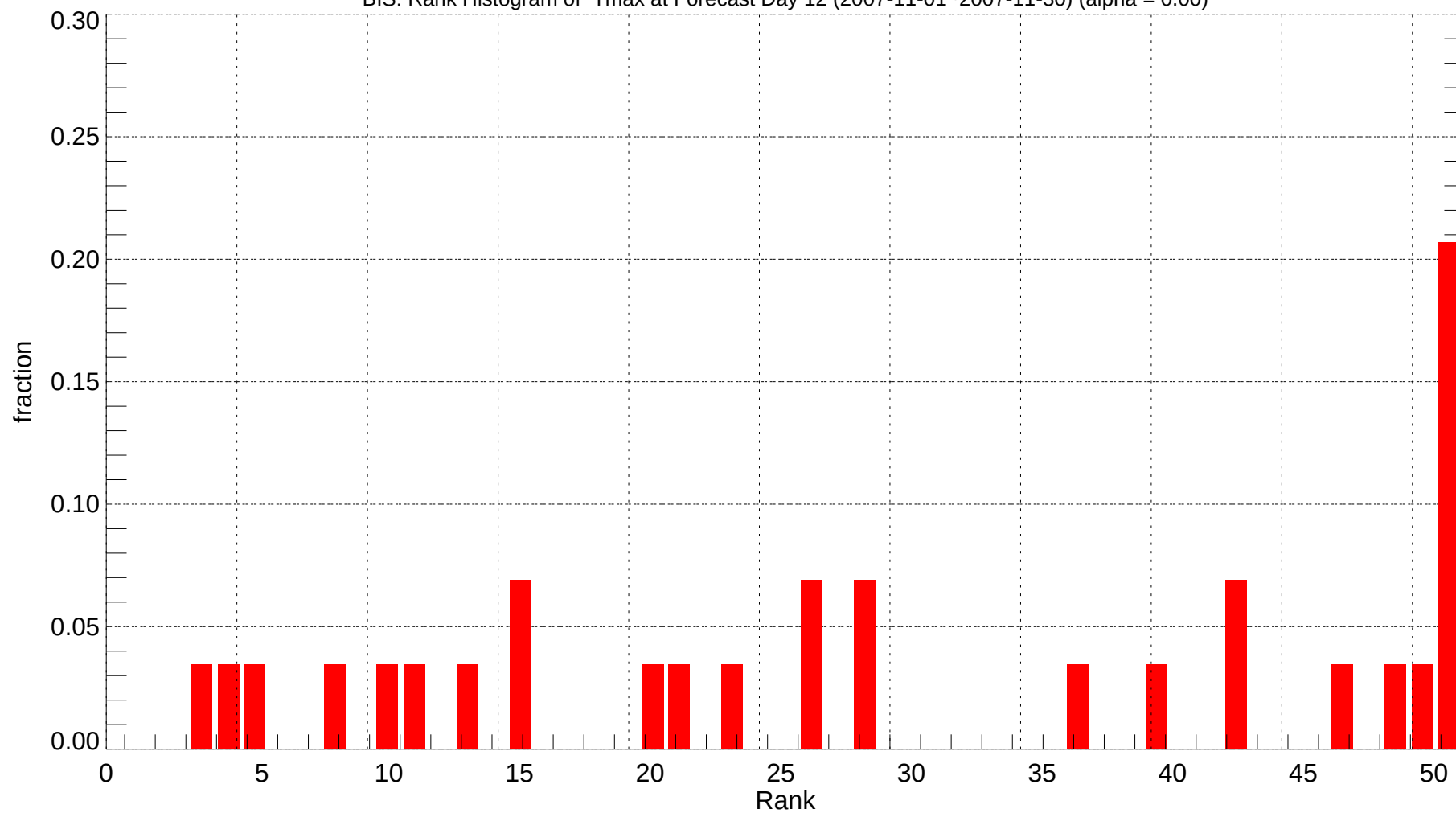
BIS: Rank Histogram of Tmax at Forecast Day 12 (2007-11-01~2007-11-30) (alpha = 0.00)
