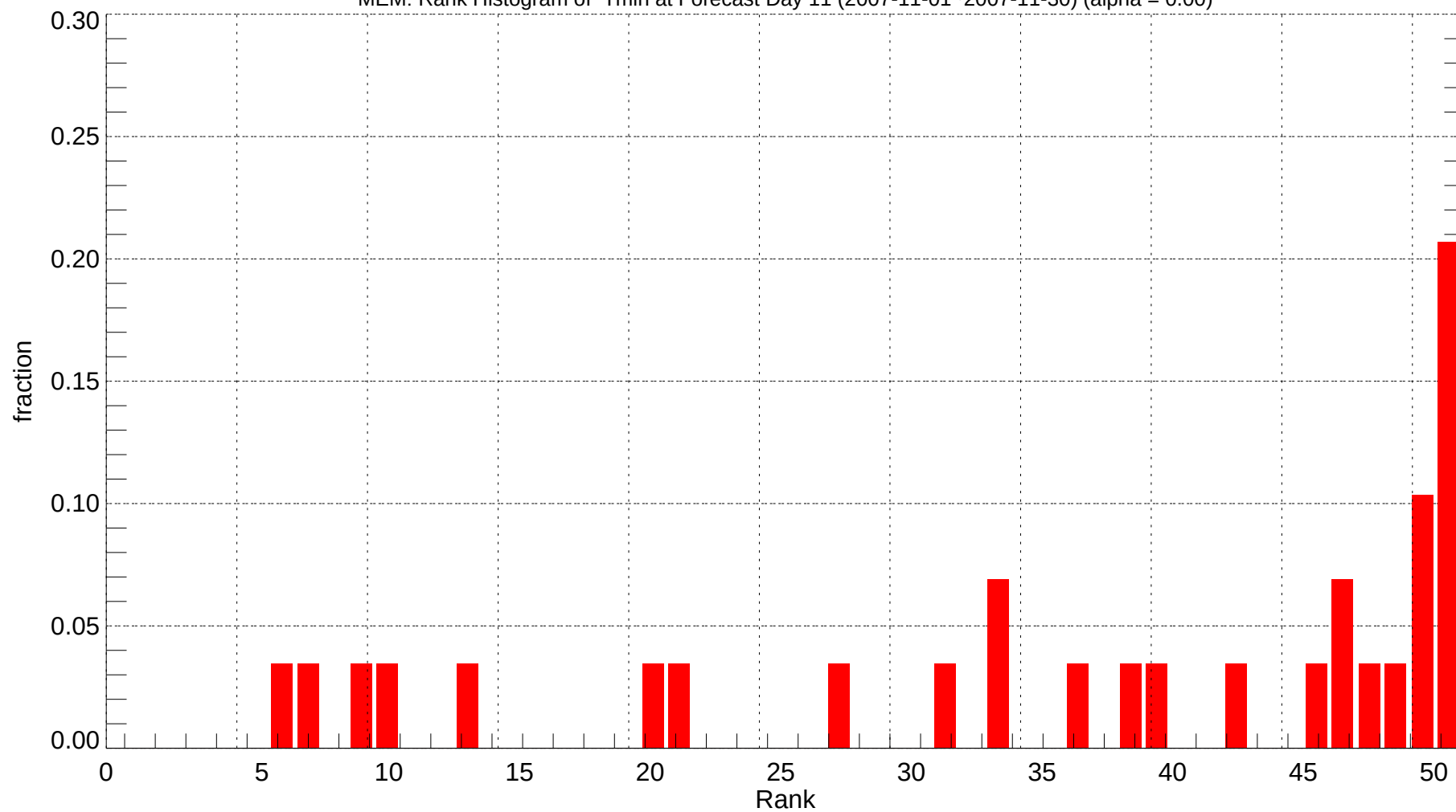
MEM: Rank Histogram of Tmin at Forecast Day 11 (2007-11-01~2007-11-30) (alpha = 0.00)
