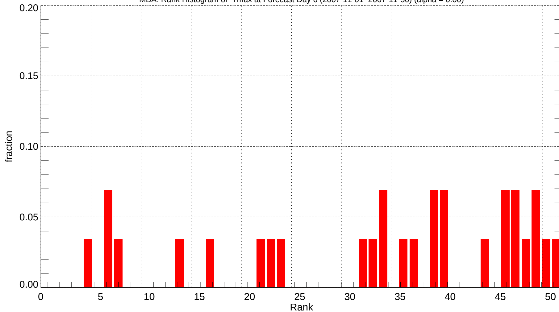
MBA: Rank Histogram of Tmax at Forecast Day 6 (2007-11-01~2007-11-30) (alpha = 0.00)
