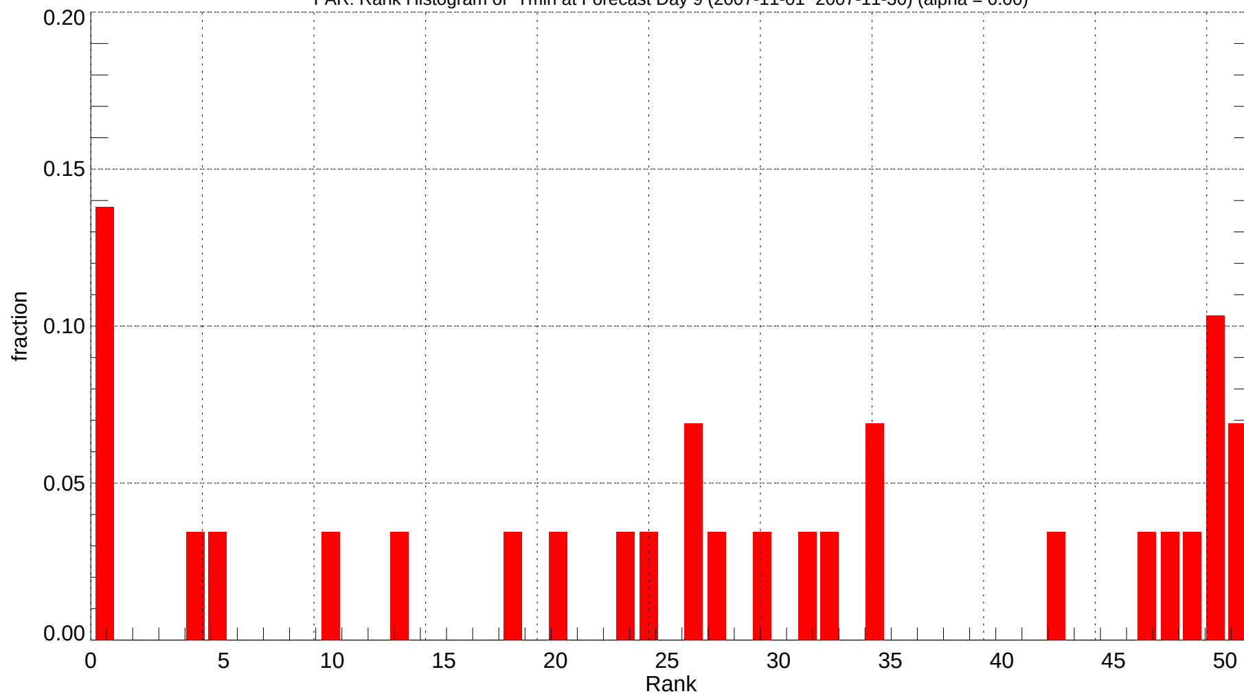
FAR: Rank Histogram of Tmin at Forecast Day 9 (2007-11-01~2007-11-30) (alpha = 0.00)
