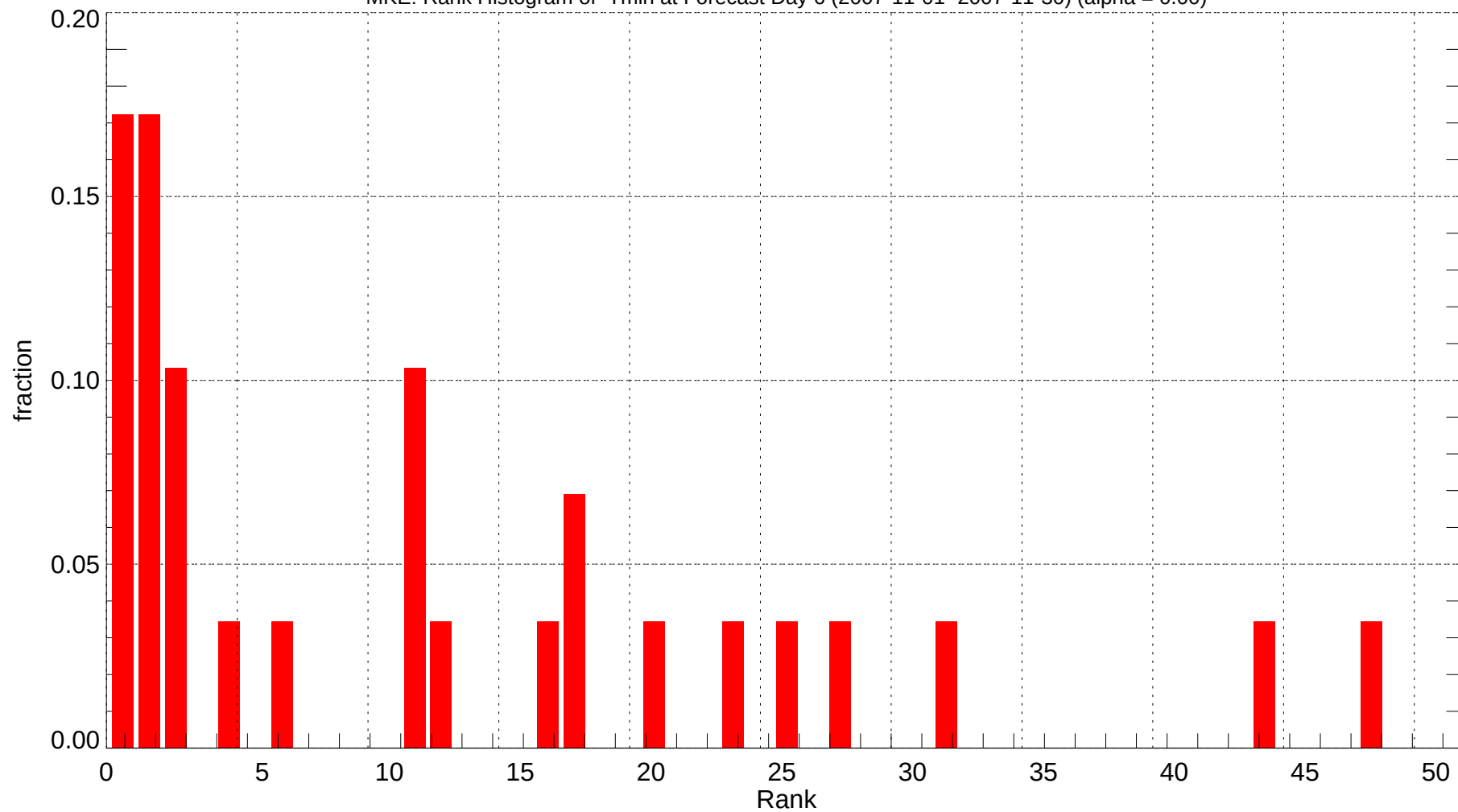
MKE: Rank Histogram of Tmin at Forecast Day 6 (2007-11-01~2007-11-30) (alpha = 0.00)
