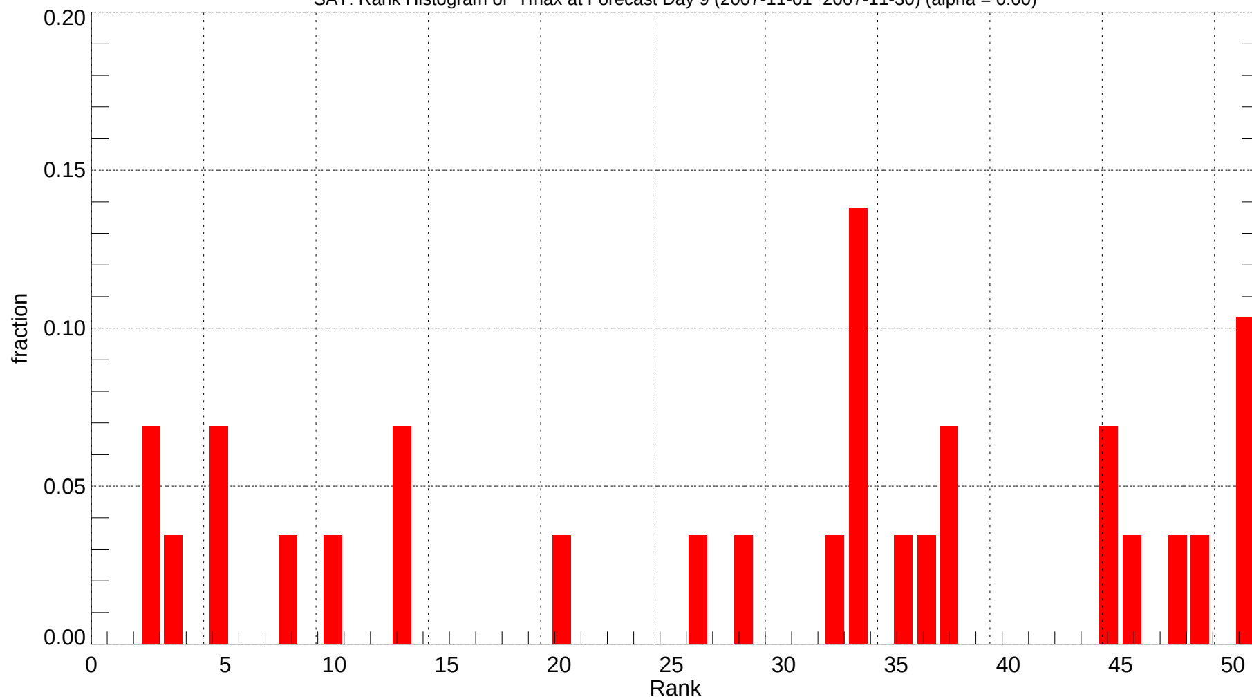
SAT: Rank Histogram of Tmax at Forecast Day 9 (2007-11-01~2007-11-30) (alpha = 0.00)
