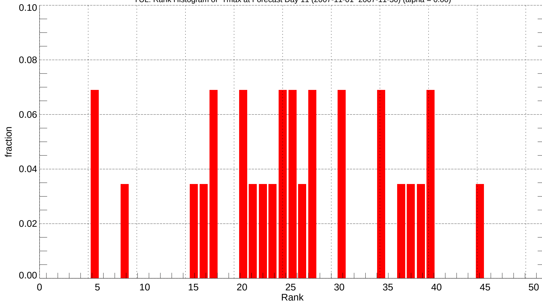
YUL: Rank Histogram of Tmax at Forecast Day 11 (2007-11-01~2007-11-30) (alpha = 0.00)
