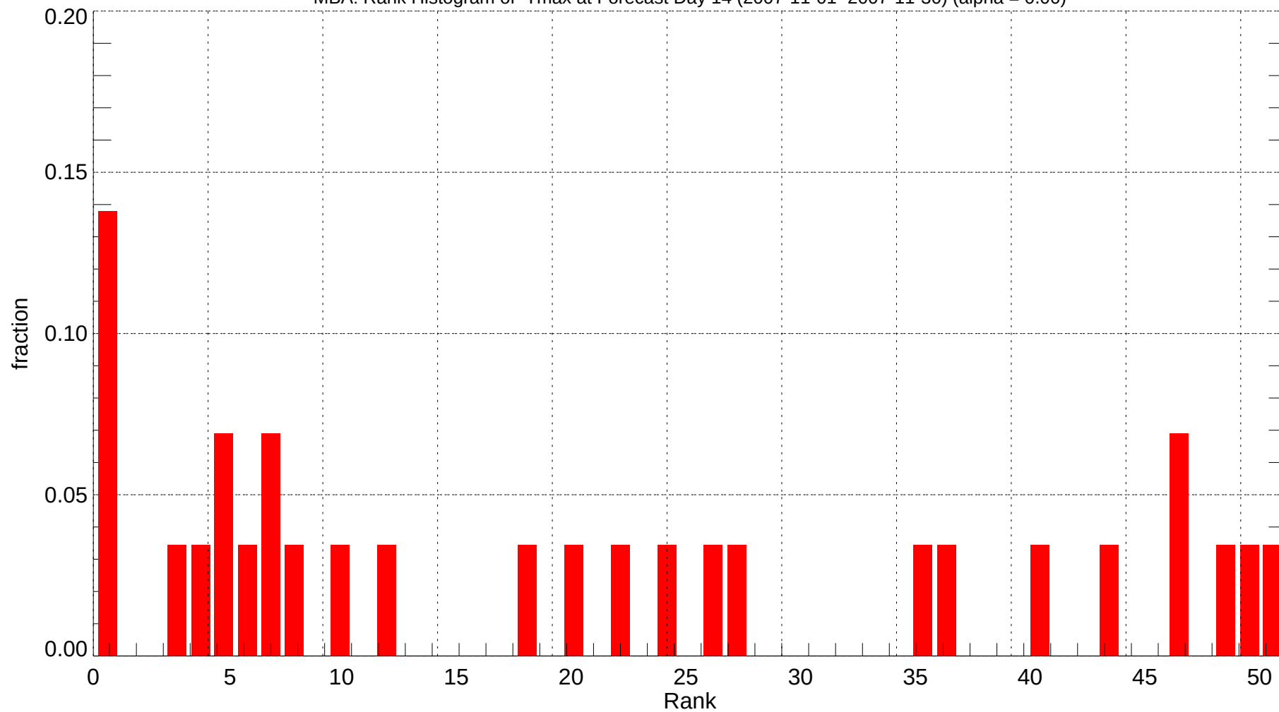
MBA: Rank Histogram of Tmax at Forecast Day 14 (2007-11-01~2007-11-30) (alpha = 0.00)
