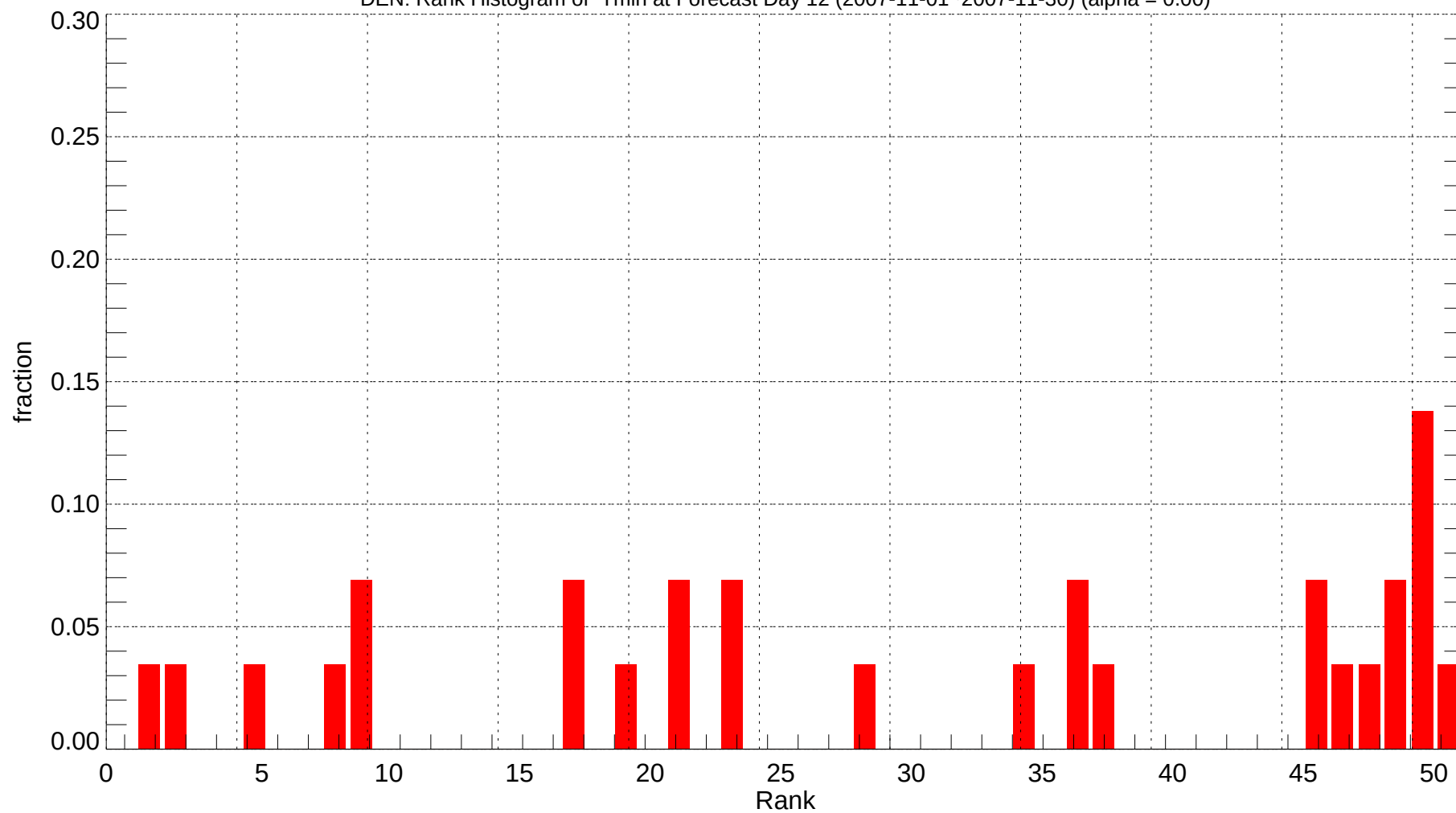
DEN: Rank Histogram of Tmin at Forecast Day 12 (2007-11-01~2007-11-30) (alpha = 0.00)
