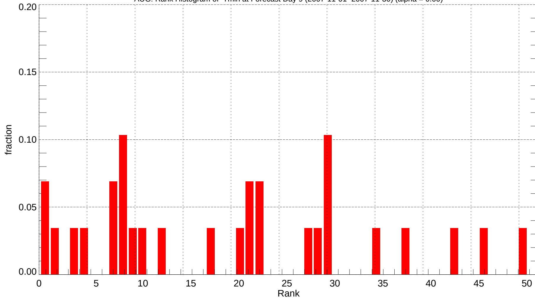
AUG: Rank Histogram of Tmin at Forecast Day 9 (2007-11-01~2007-11-30) (alpha = 0.00)
