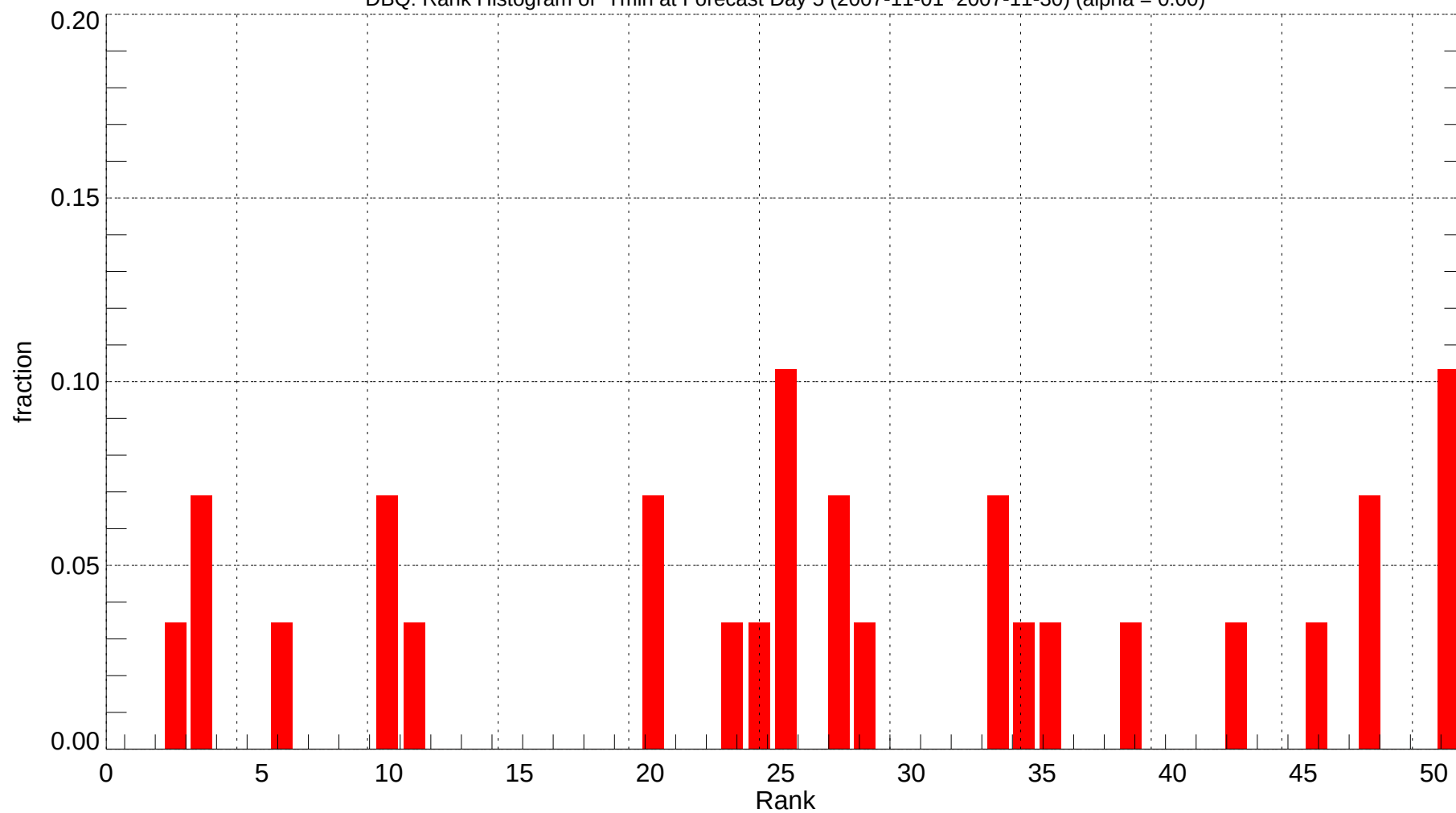
DBQ: Rank Histogram of Tmin at Forecast Day 5 (2007-11-01~2007-11-30) (alpha = 0.00)
