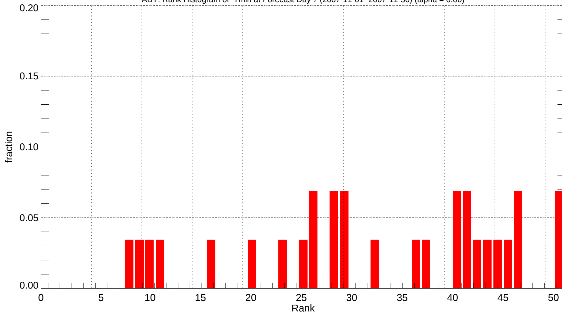
ABY: Rank Histogram of Tmin at Forecast Day 7 (2007-11-01~2007-11-30) (alpha = 0.00)
