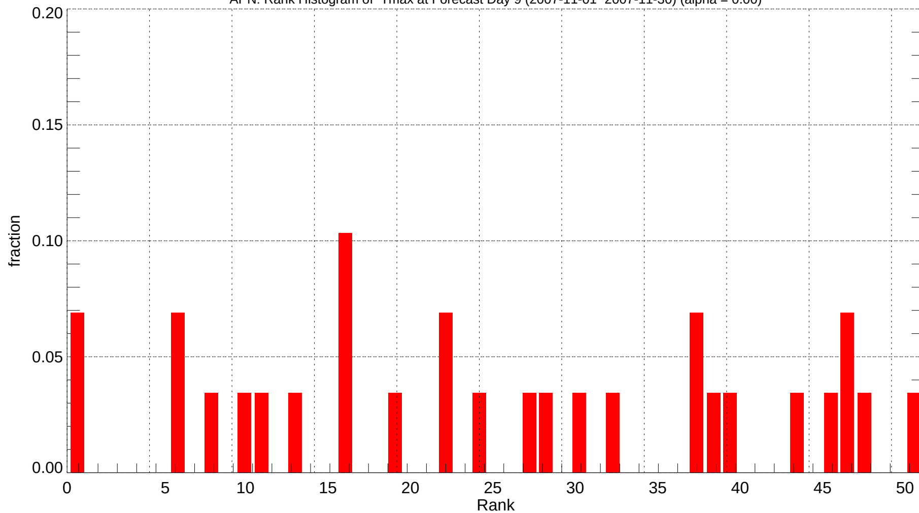
APN: Rank Histogram of Tmax at Forecast Day 9 (2007-11-01~2007-11-30) (alpha = 0.00)
