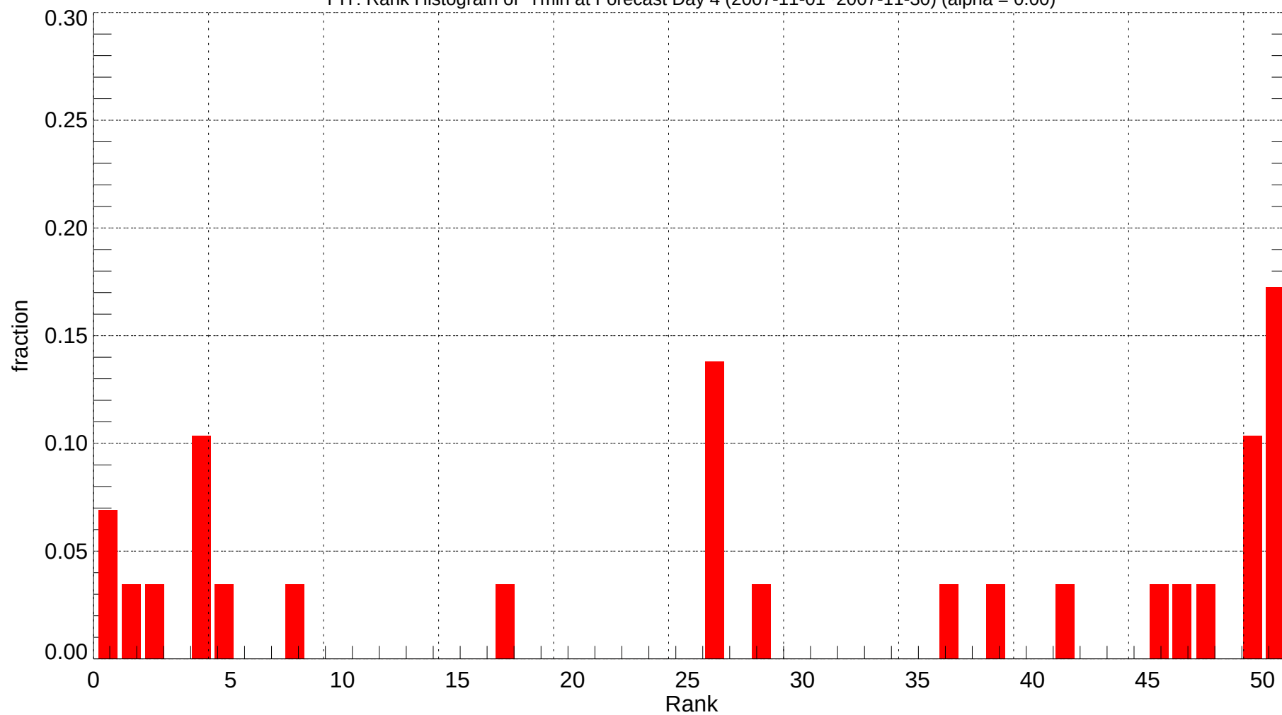
PIT: Rank Histogram of Tmin at Forecast Day 4 (2007-11-01~2007-11-30) (alpha = 0.00)
