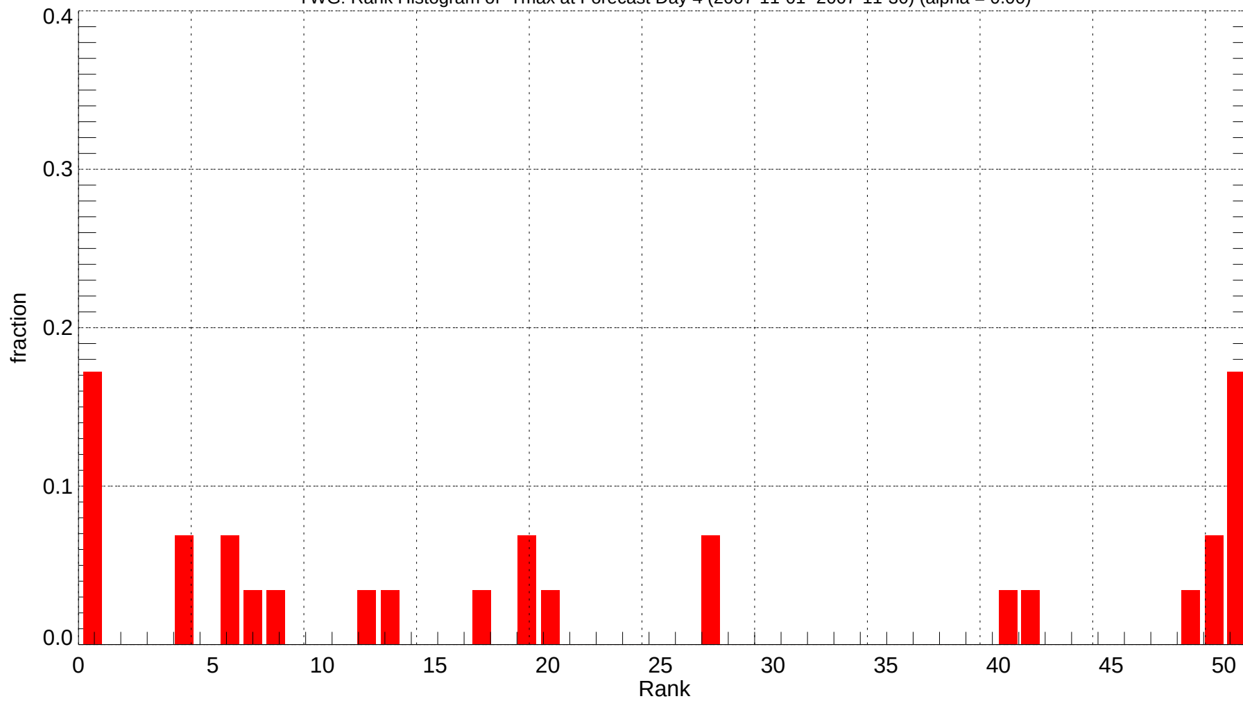
YWG: Rank Histogram of Tmax at Forecast Day 4 (2007-11-01~2007-11-30) (alpha = 0.00)
