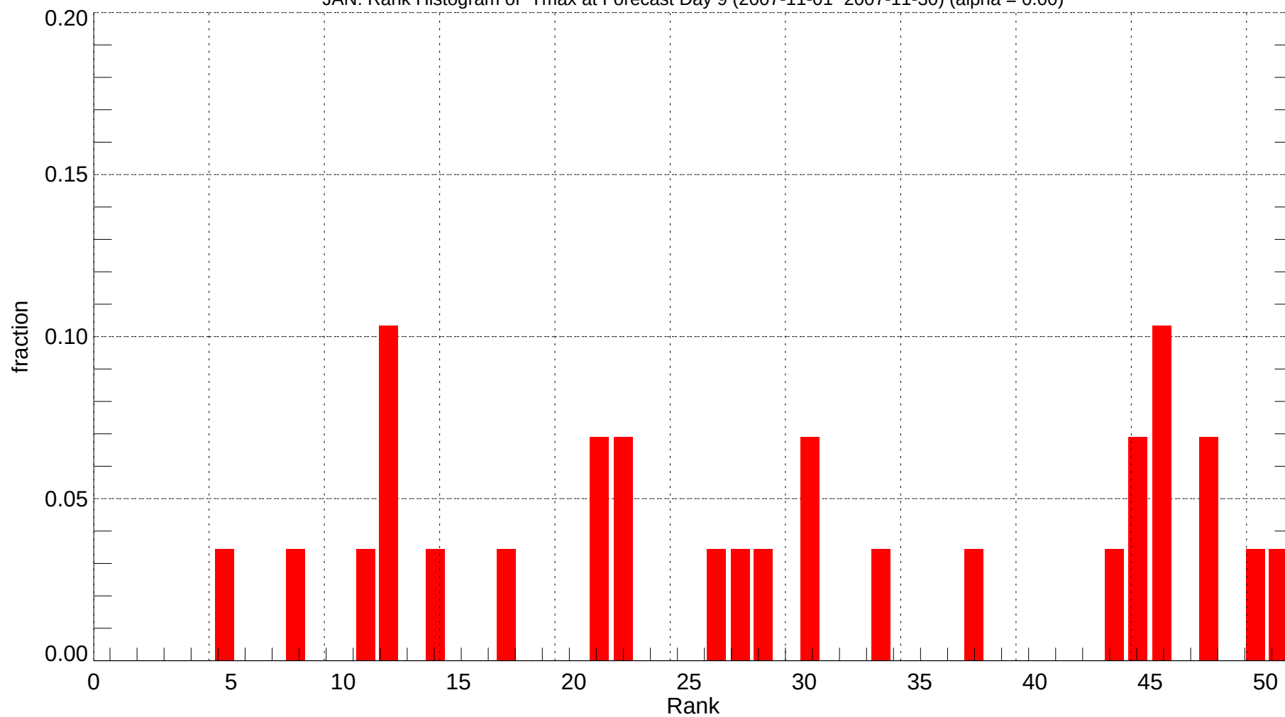
JAN: Rank Histogram of Tmax at Forecast Day 9 (2007-11-01~2007-11-30) (alpha = 0.00)
