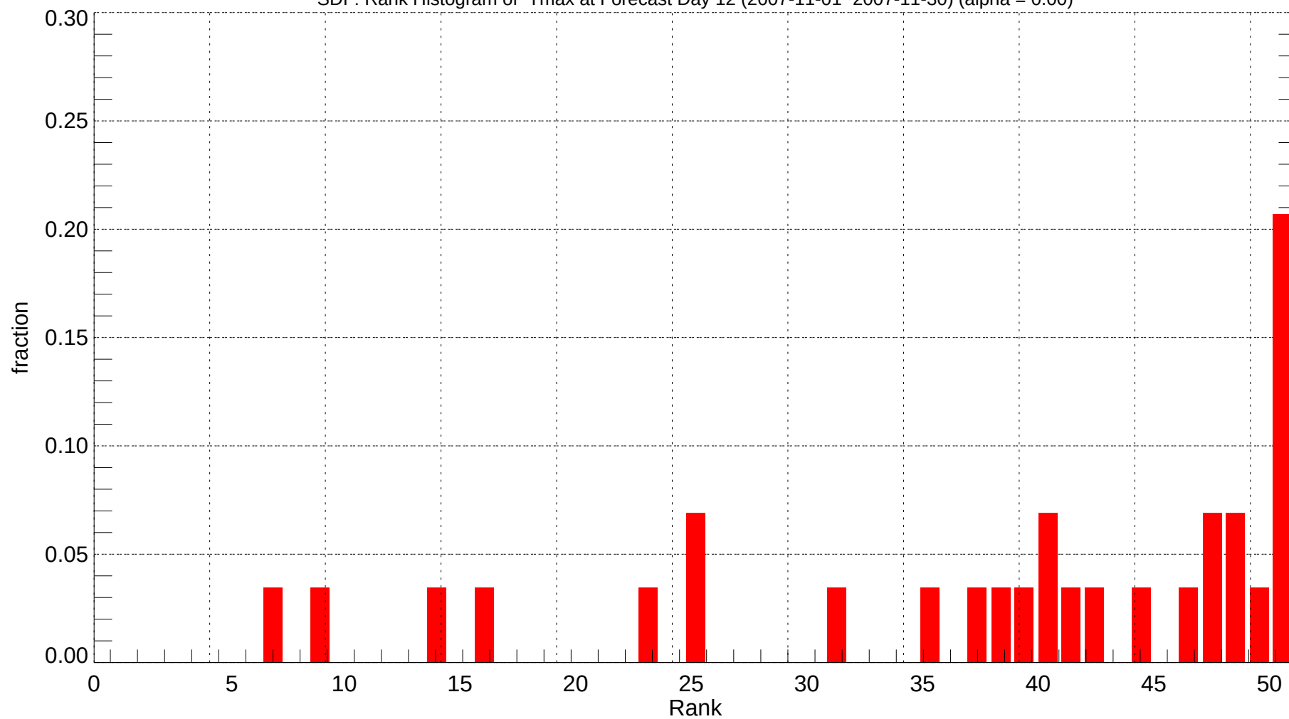
SDF: Rank Histogram of Tmax at Forecast Day 12 (2007-11-01~2007-11-30) (alpha = 0.00)
