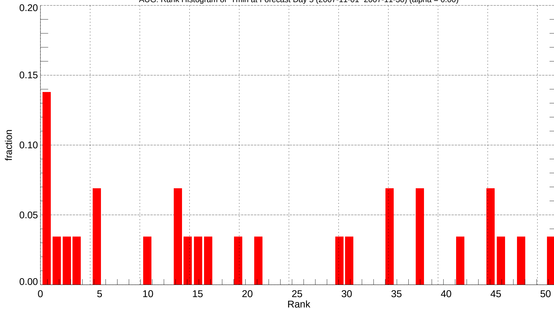
AUG: Rank Histogram of Tmin at Forecast Day 5 (2007-11-01~2007-11-30) (alpha = 0.00)
