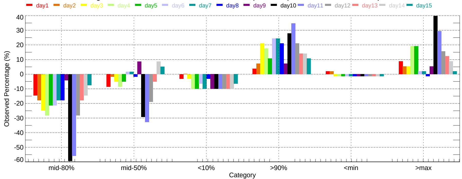
Observed Percentage Deviation of Ensembles - ATL: Min Temperature (2007-11-01~2007-11-30)
