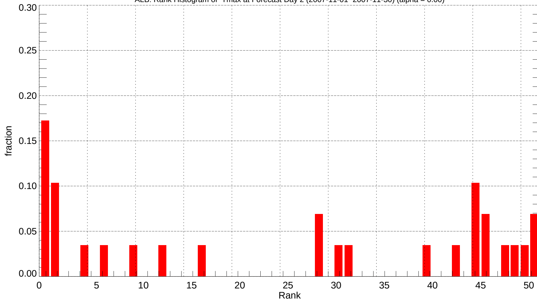
ALB: Rank Histogram of Tmax at Forecast Day 2 (2007-11-01~2007-11-30) (alpha = 0.00)
