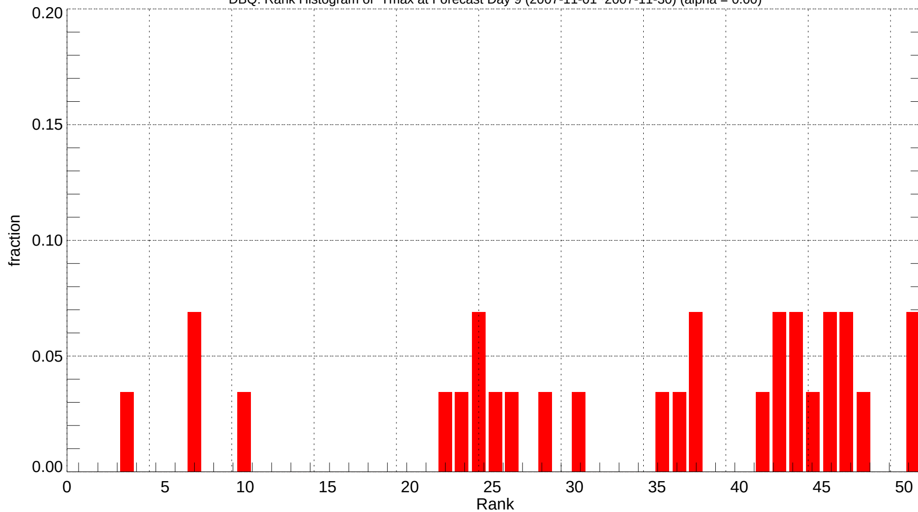
DBQ: Rank Histogram of Tmax at Forecast Day 9 (2007-11-01~2007-11-30) (alpha = 0.00)
