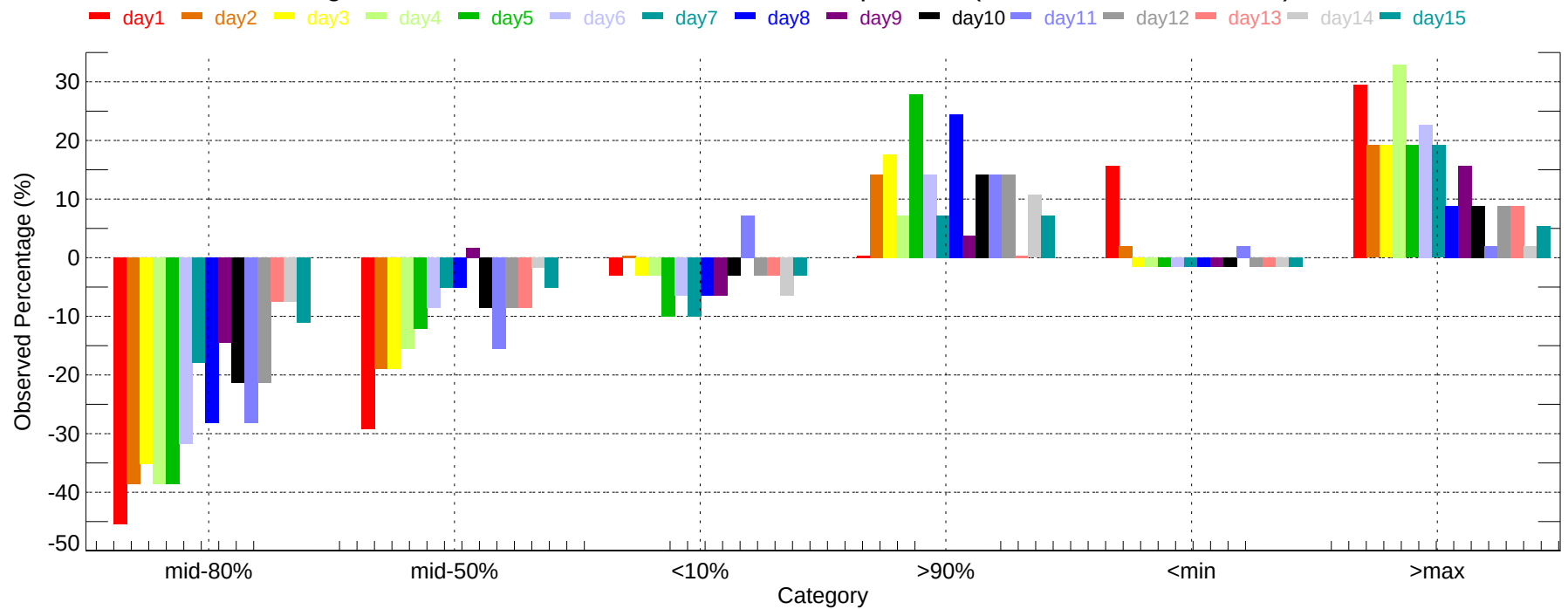
Observed Percentage Deviation of Ensembles - CLT: Min Temperature (2007-11-01~2007-11-30)
