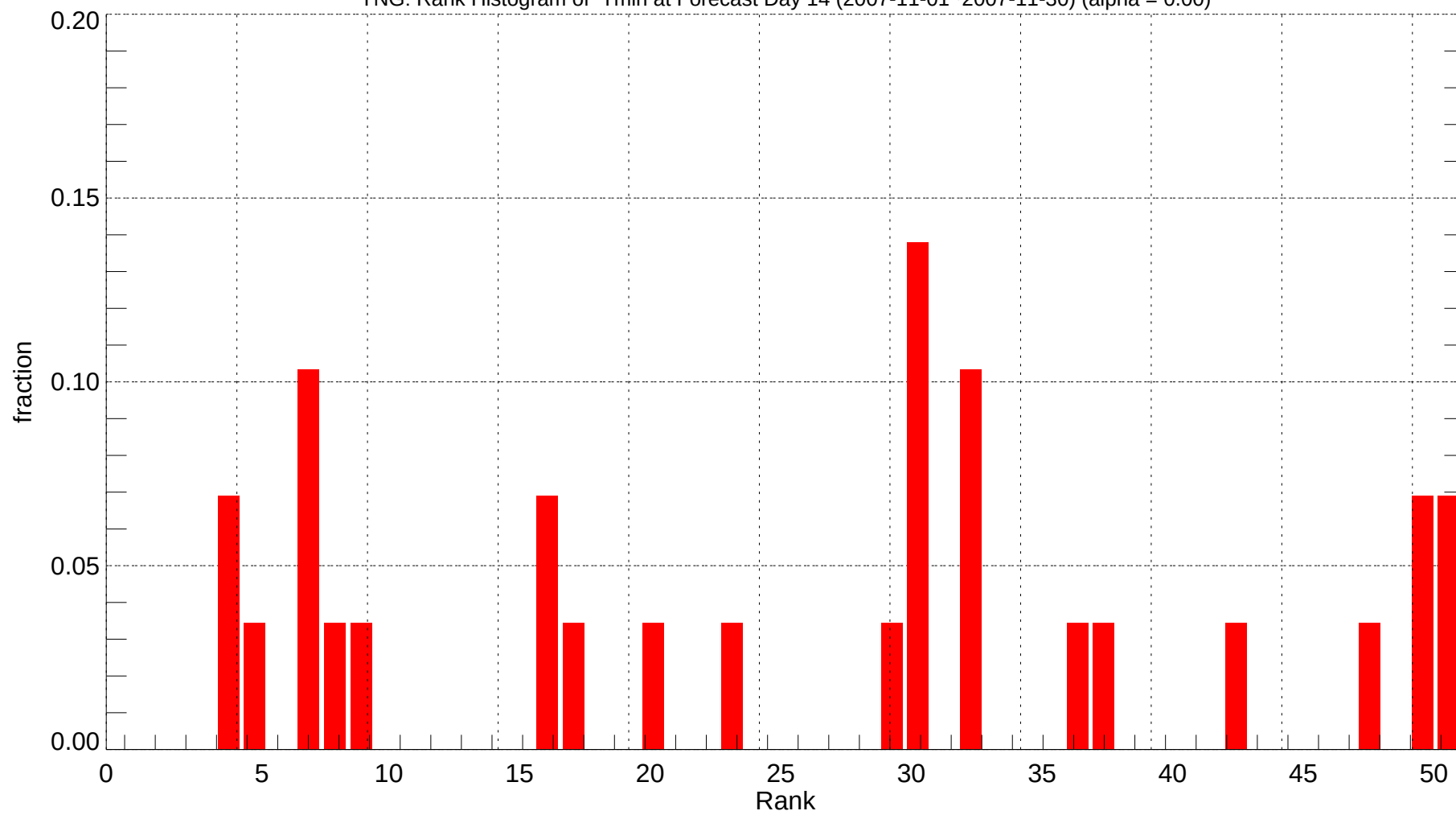
YNG: Rank Histogram of Tmin at Forecast Day 14 (2007-11-01~2007-11-30) (alpha = 0.00)
