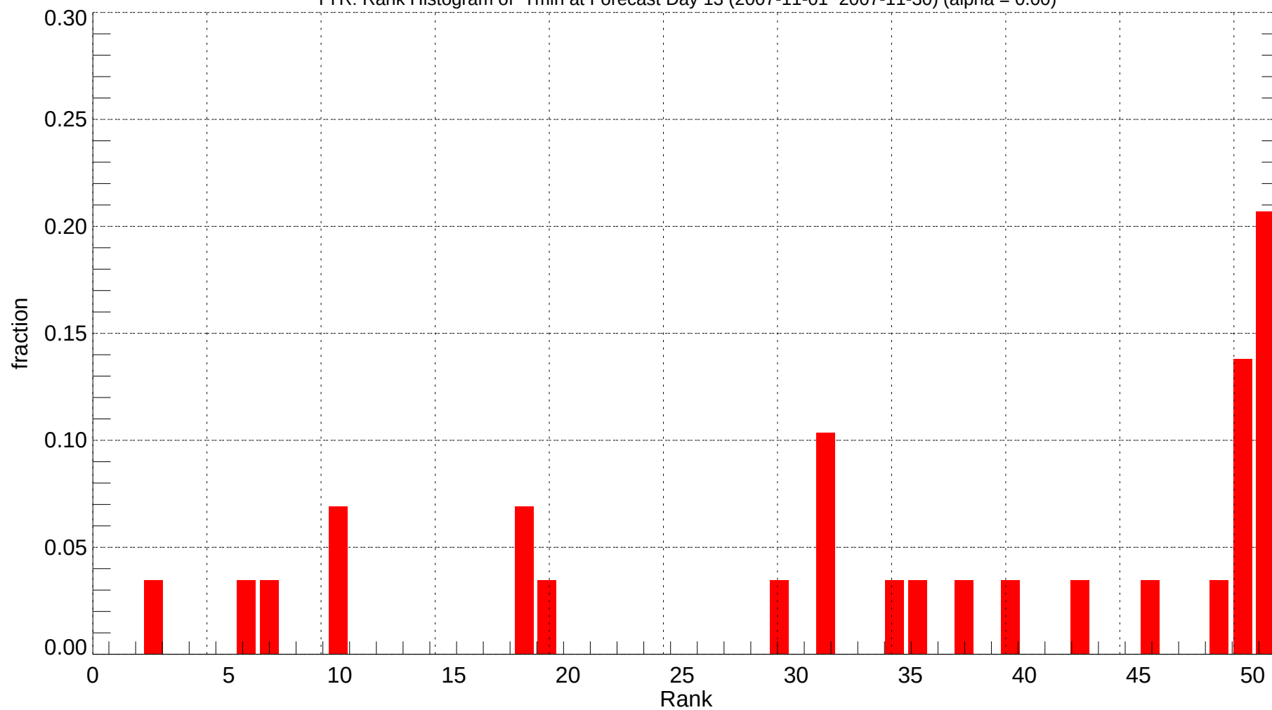
TYR: Rank Histogram of Tmin at Forecast Day 13 (2007-11-01~2007-11-30) (alpha = 0.00)
