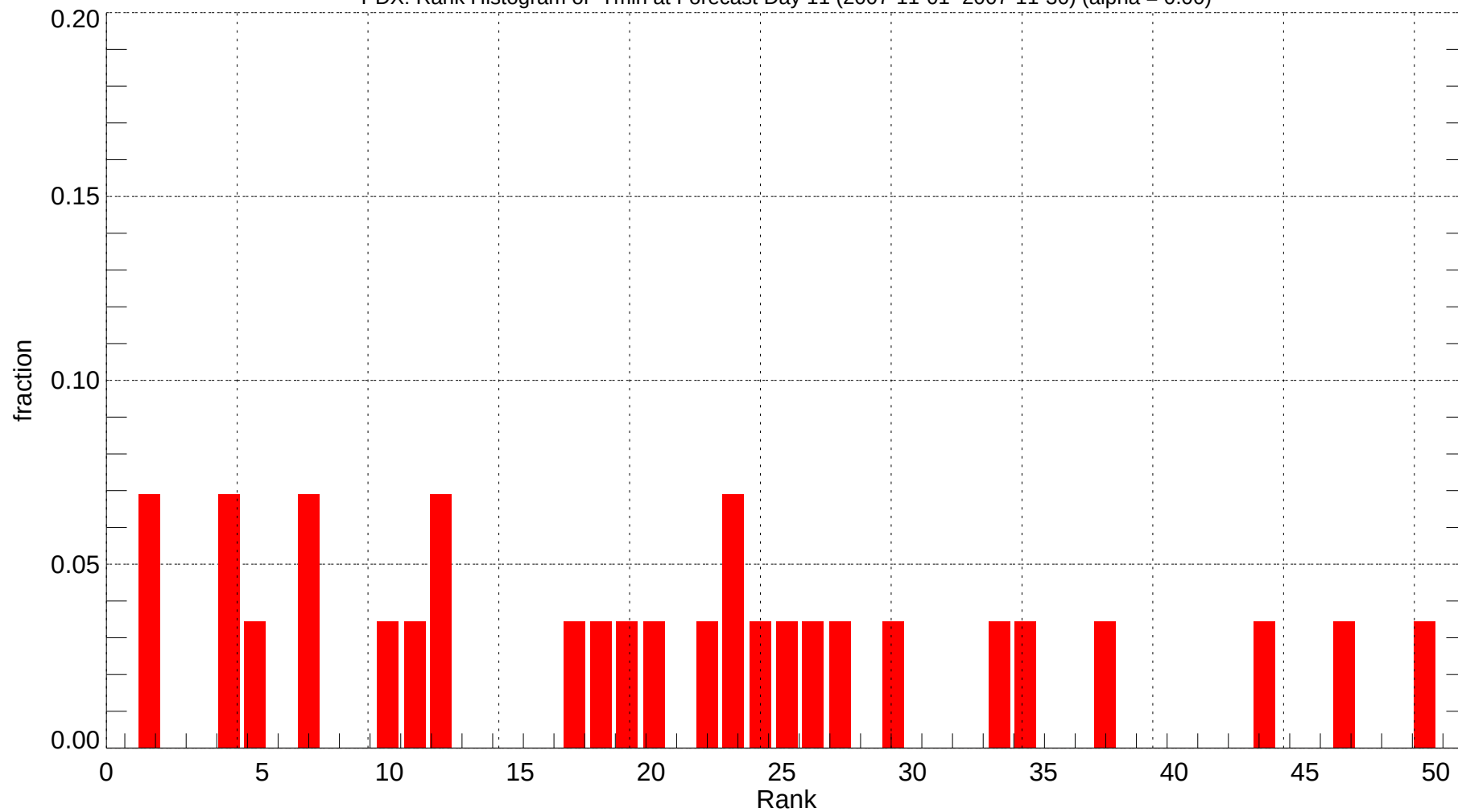
PDX: Rank Histogram of Tmin at Forecast Day 11 (2007-11-01~2007-11-30) (alpha = 0.00)
