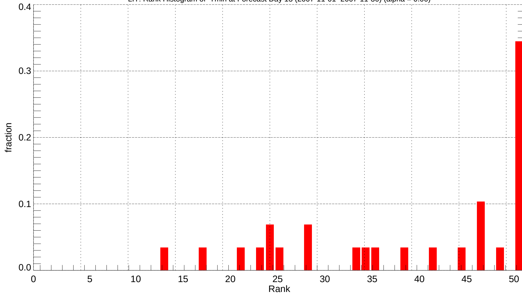
LIT: Rank Histogram of Tmin at Forecast Day 13 (2007-11-01~2007-11-30) (alpha = 0.00)
