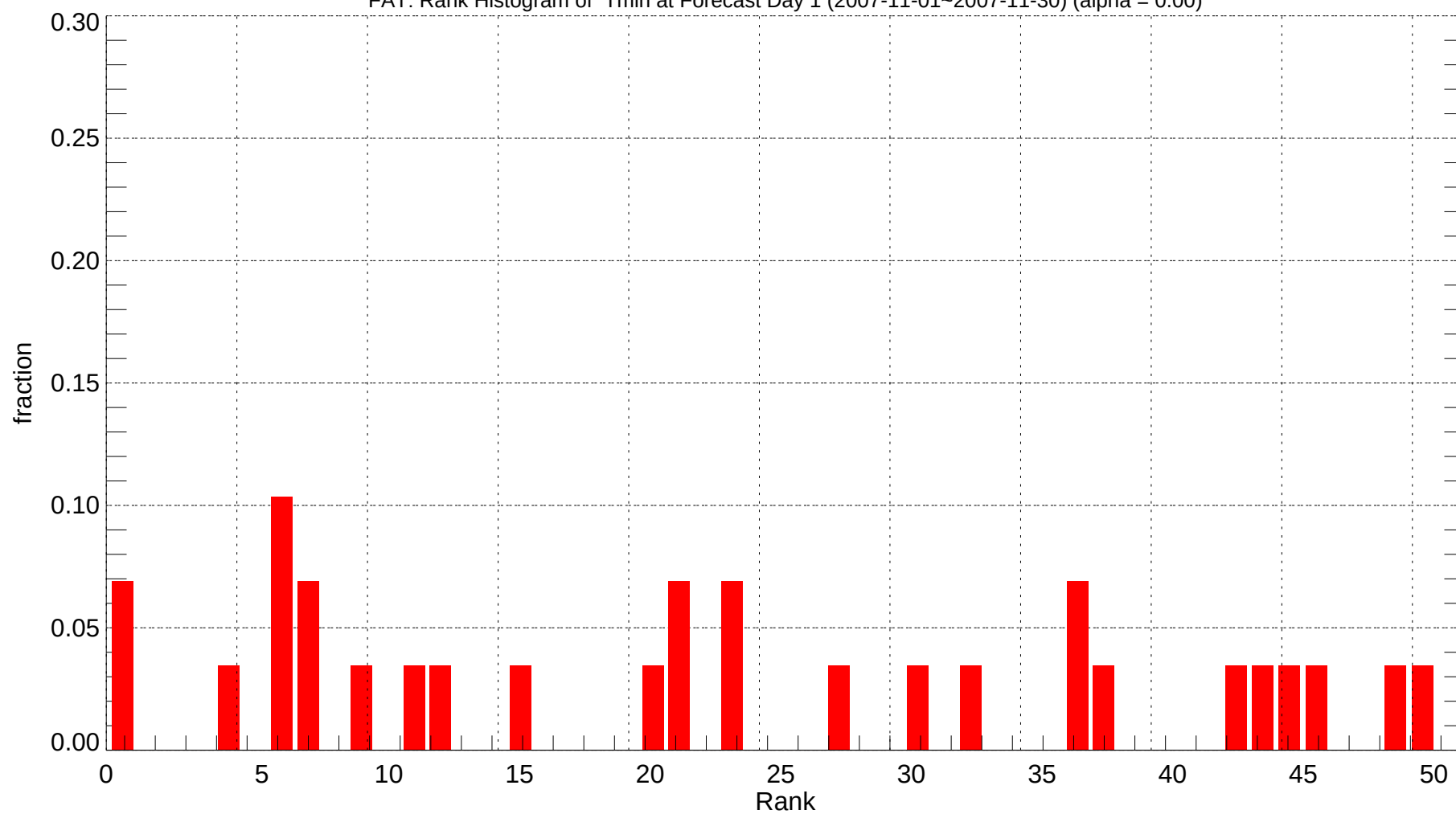
FAT: Rank Histogram of Tmin at Forecast Day 1 (2007-11-01~2007-11-30) (alpha = 0.00)
