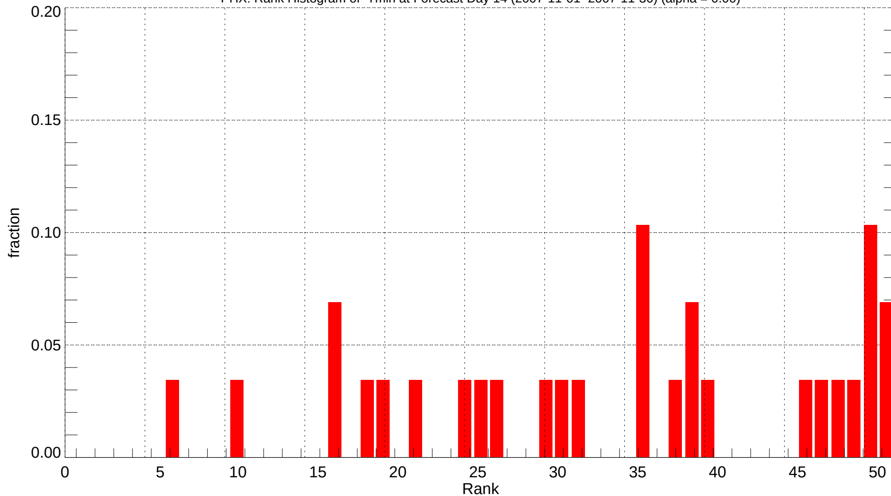
PHX: Rank Histogram of Tmin at Forecast Day 14 (2007-11-01~2007-11-30) (alpha = 0.00)
