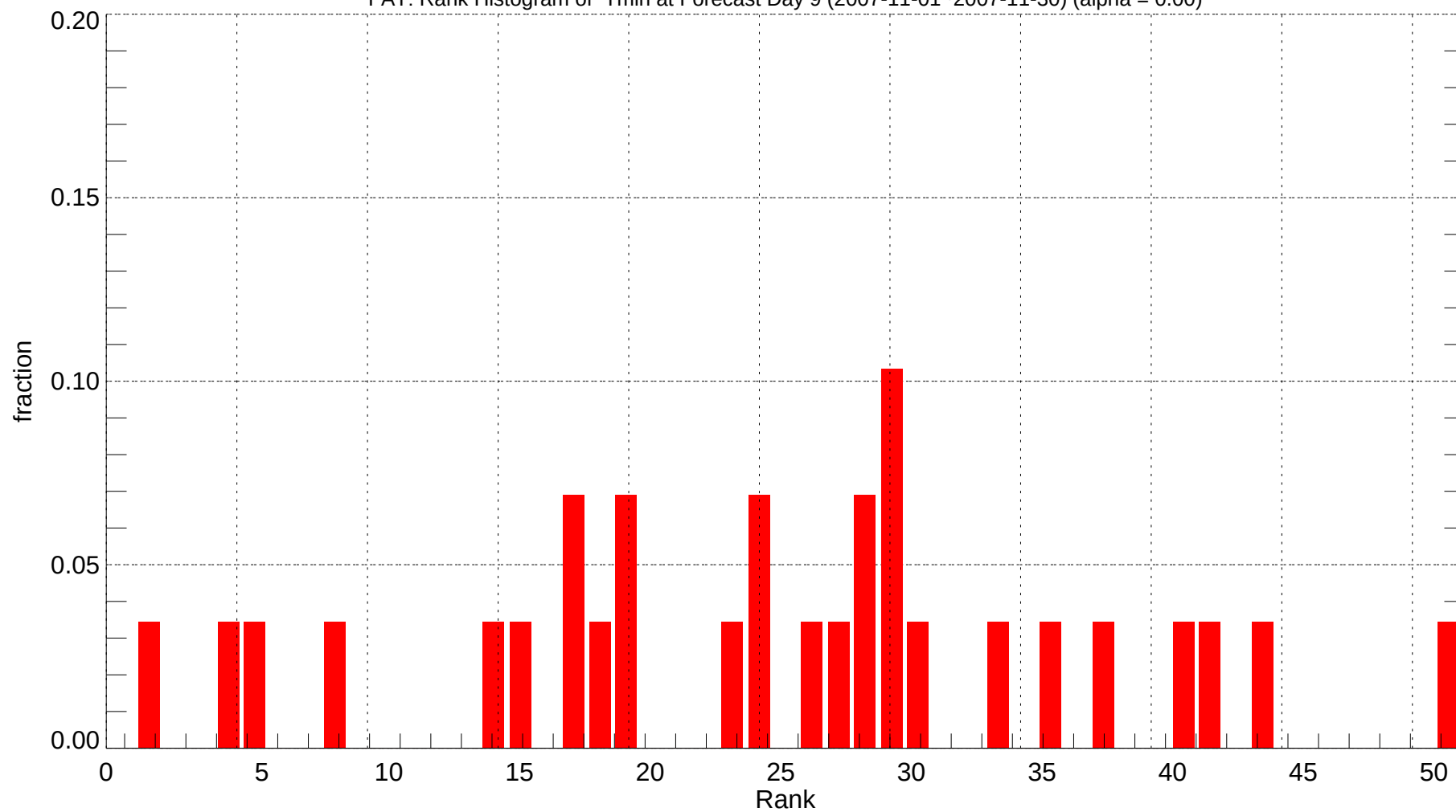
FAT: Rank Histogram of Tmin at Forecast Day 9 (2007-11-01~2007-11-30) (alpha = 0.00)
