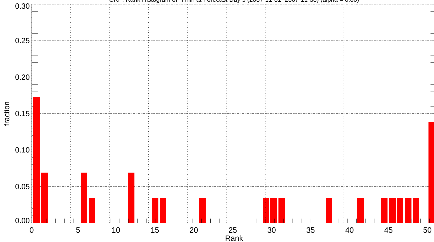
CRP: Rank Histogram of Tmin at Forecast Day 5 (2007-11-01~2007-11-30) (alpha = 0.00)
