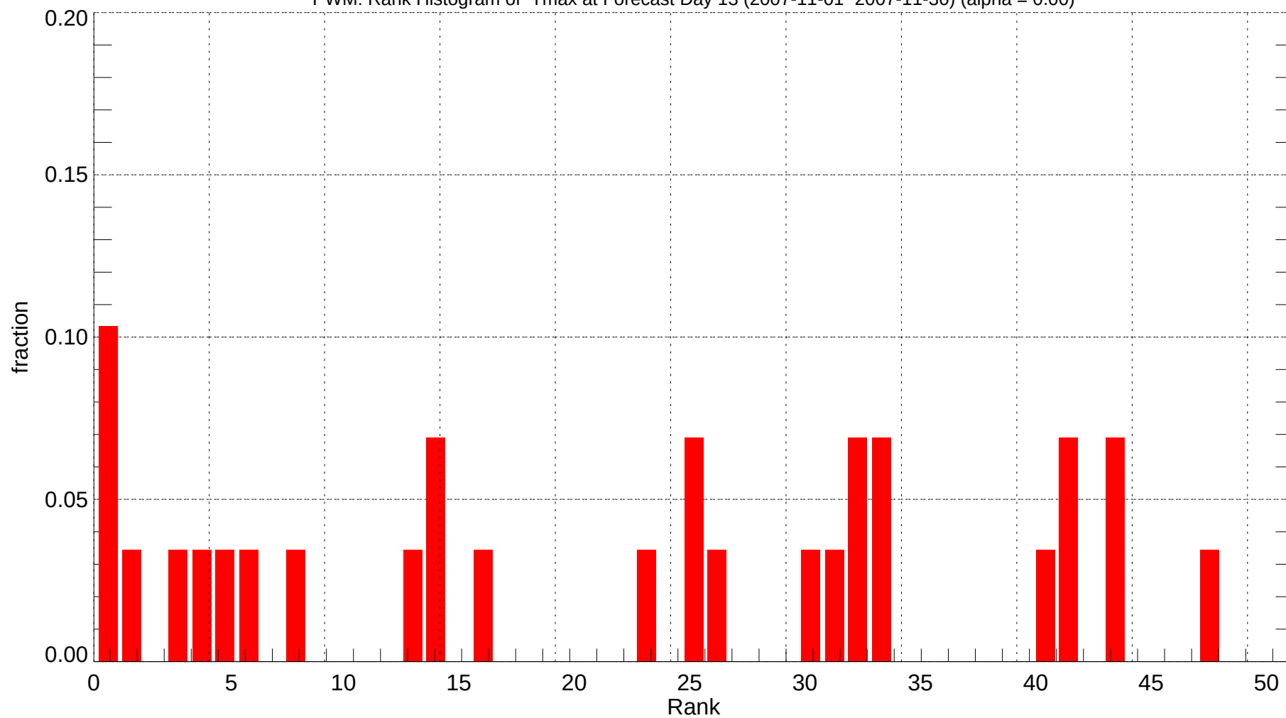
PWM: Rank Histogram of Tmax at Forecast Day 13 (2007-11-01~2007-11-30) (alpha = 0.00)
