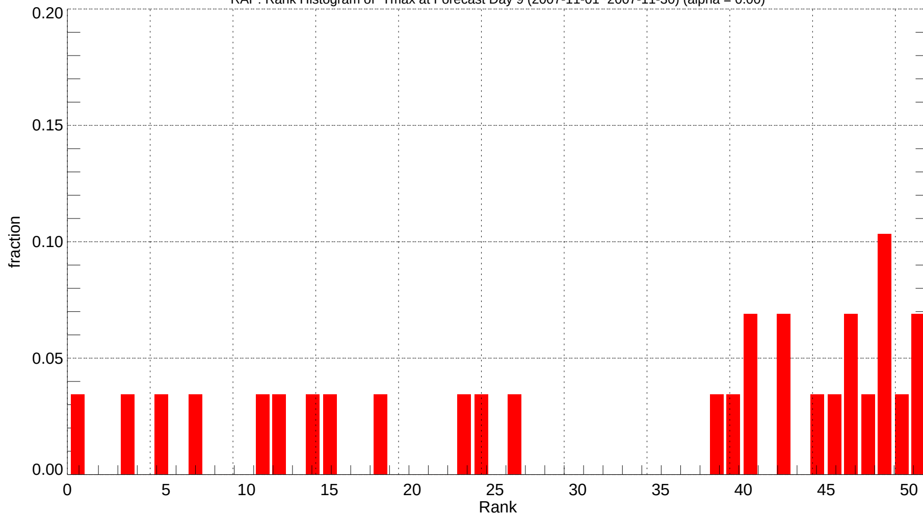
RAP: Rank Histogram of Tmax at Forecast Day 9 (2007-11-01~2007-11-30) (alpha = 0.00)
