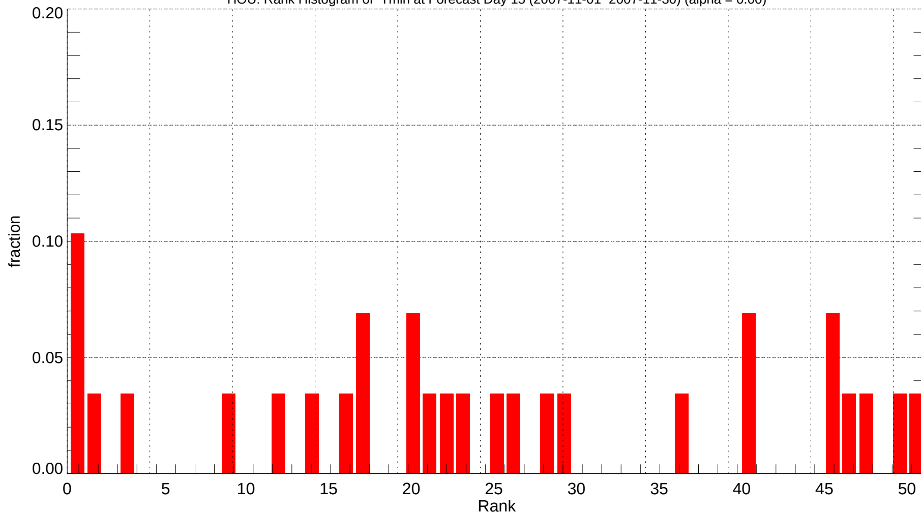
HOU: Rank Histogram of Tmin at Forecast Day 15 (2007-11-01~2007-11-30) (alpha = 0.00)
