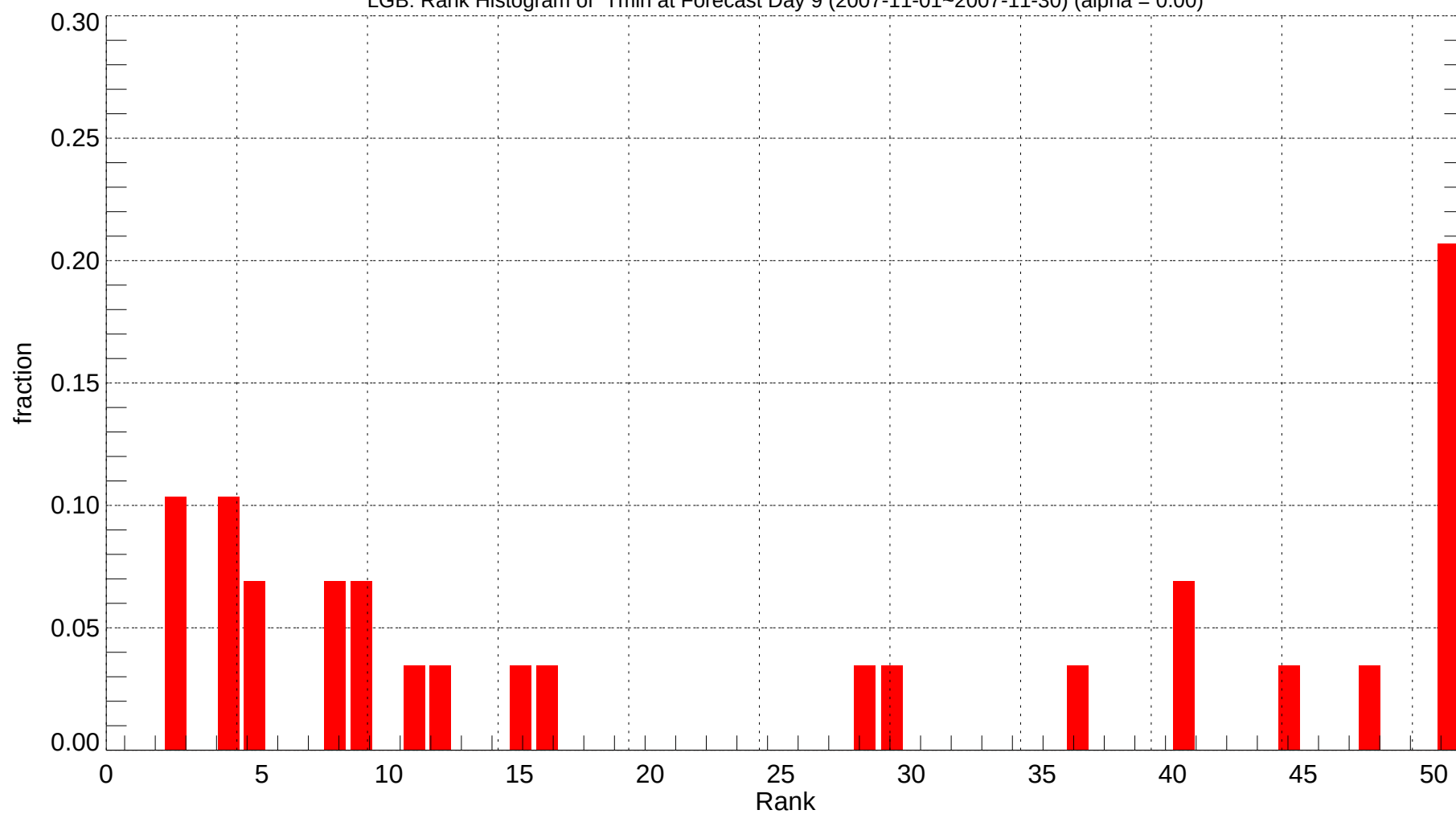
LGB: Rank Histogram of Tmin at Forecast Day 9 (2007-11-01~2007-11-30) (alpha = 0.00)
