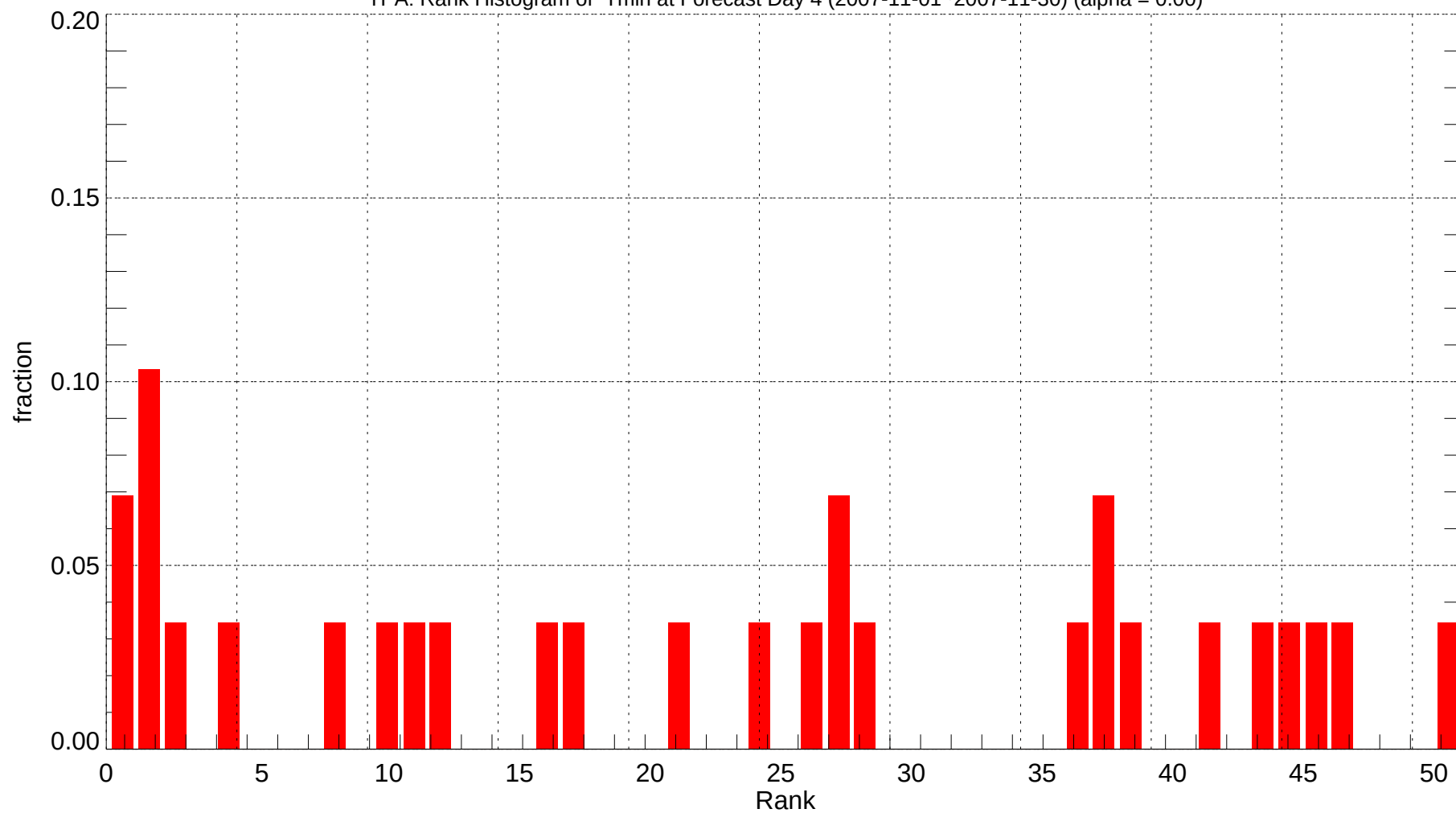
TPA: Rank Histogram of Tmin at Forecast Day 4 (2007-11-01~2007-11-30) (alpha = 0.00)
