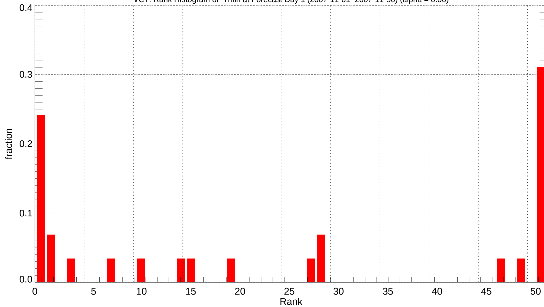
VCT: Rank Histogram of Tmin at Forecast Day 1 (2007-11-01~2007-11-30) (alpha = 0.00)
