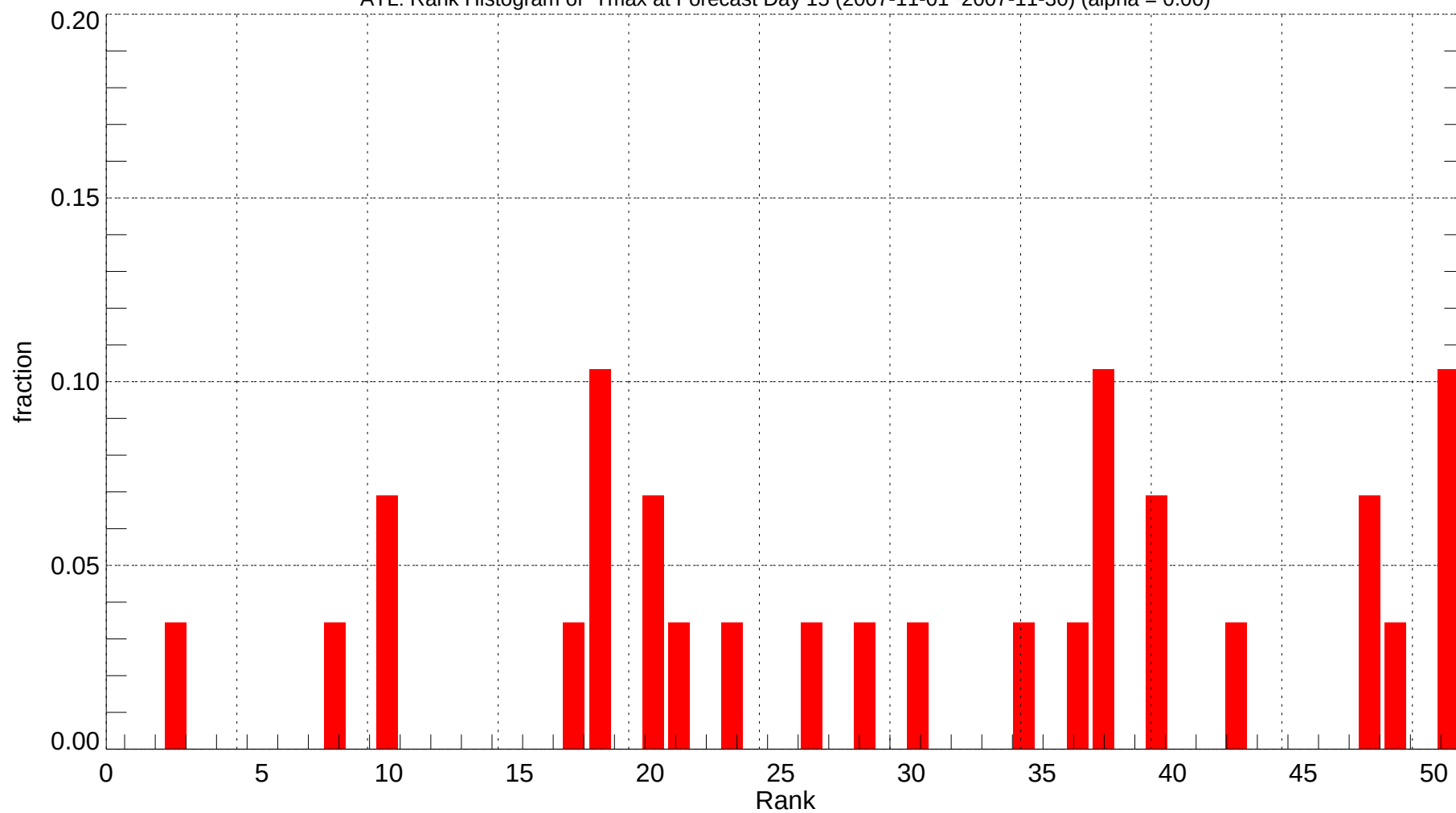
ATL: Rank Histogram of Tmax at Forecast Day 15 (2007-11-01~2007-11-30) (alpha = 0.00)
