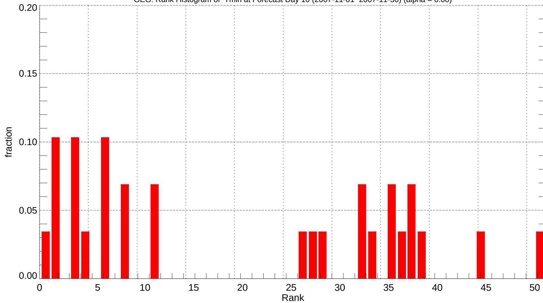
GEG: Rank Histogram of Tmin at Forecast Day 10 (2007-11-01~2007-11-30) (alpha = 0.00)
