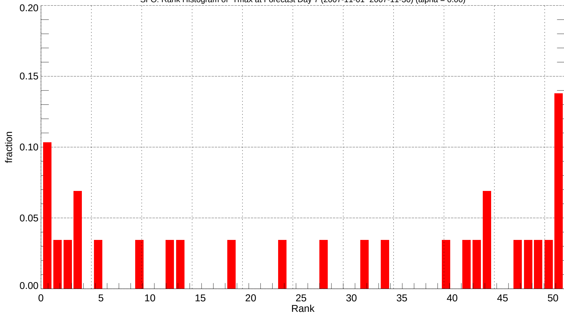
SFO: Rank Histogram of Tmax at Forecast Day 7 (2007-11-01~2007-11-30) (alpha = 0.00)
