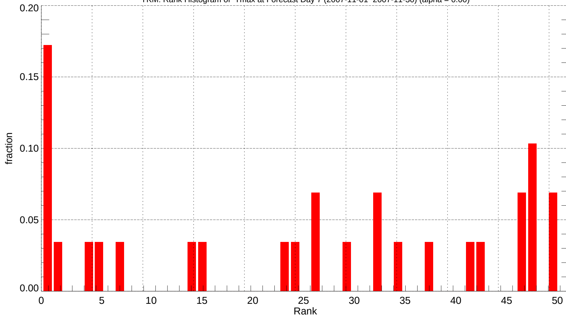
YKM: Rank Histogram of Tmax at Forecast Day 7 (2007-11-01~2007-11-30) (alpha = 0.00)
