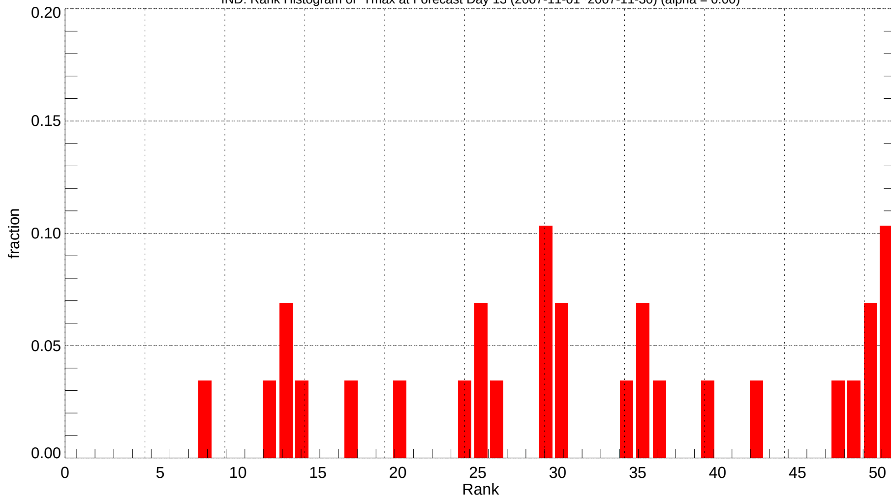
IND: Rank Histogram of Tmax at Forecast Day 13 (2007-11-01~2007-11-30) (alpha = 0.00)
