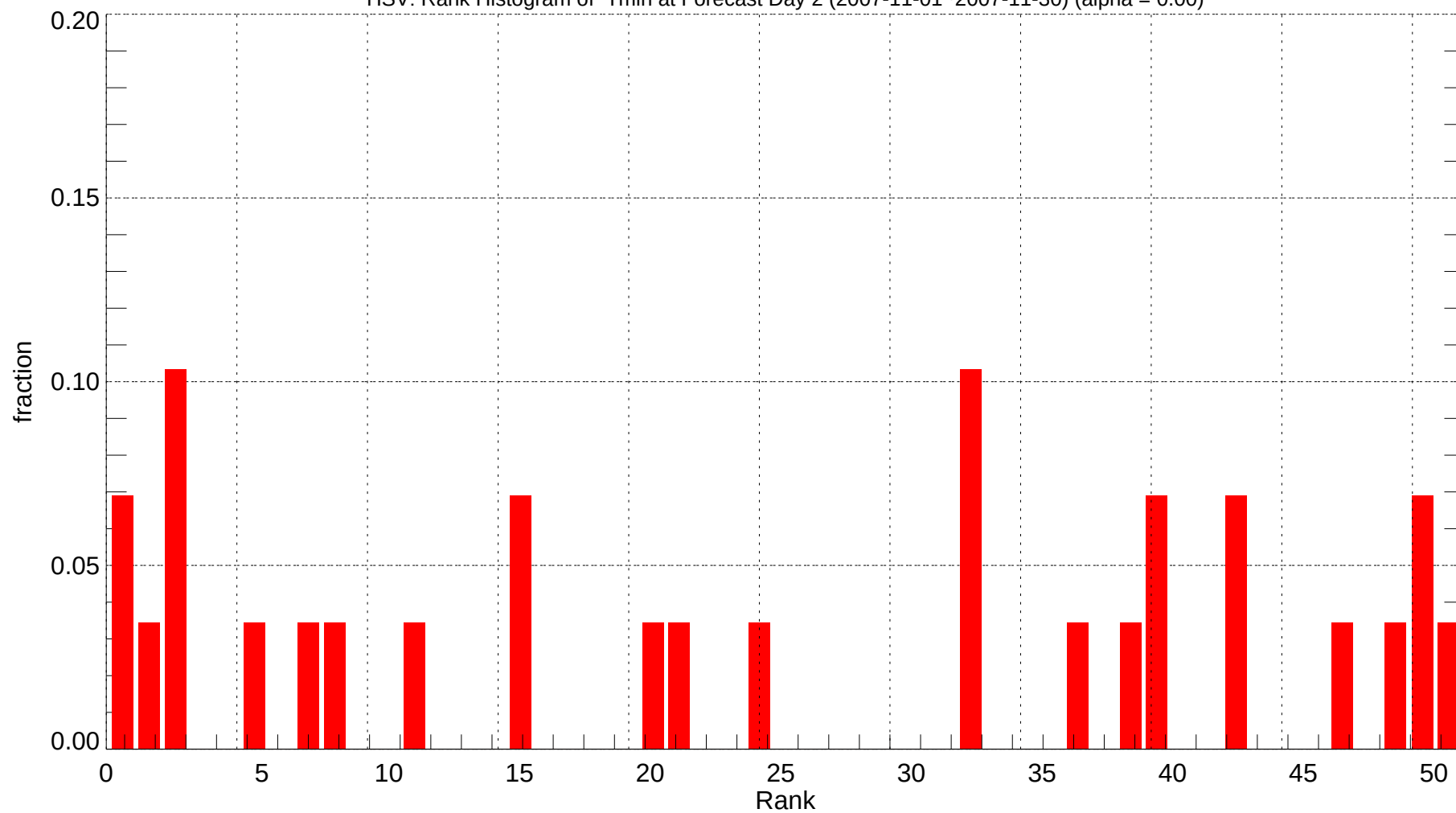
HSV: Rank Histogram of Tmin at Forecast Day 2 (2007-11-01~2007-11-30) (alpha = 0.00)
