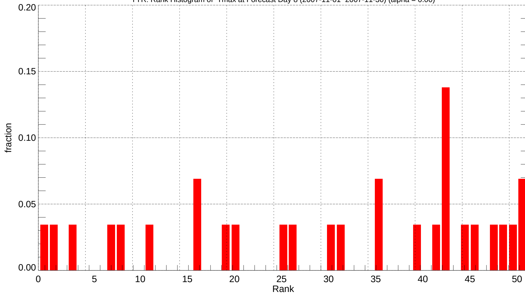
TYR: Rank Histogram of Tmax at Forecast Day 8 (2007-11-01~2007-11-30) (alpha = 0.00)
