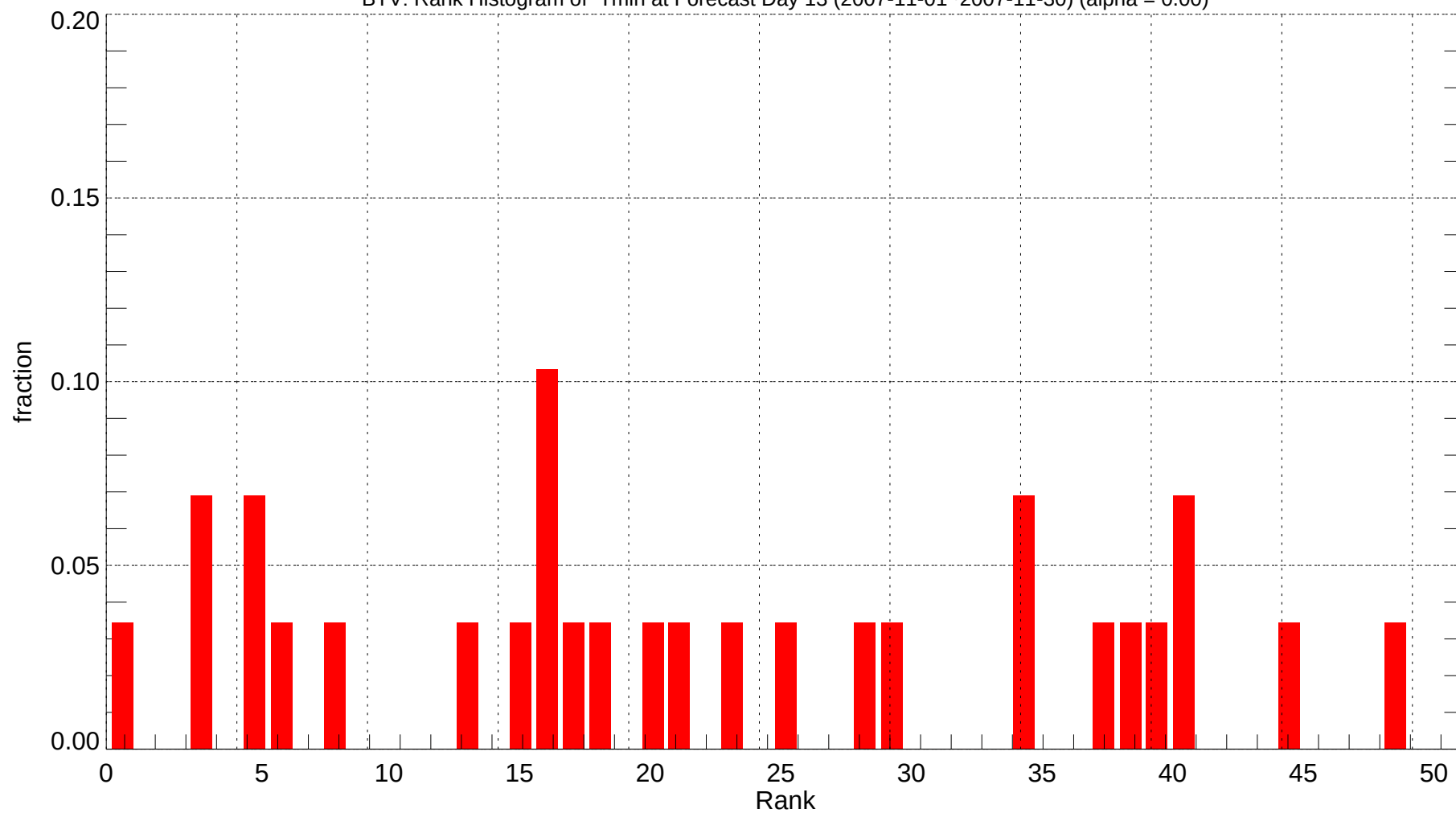
BTV: Rank Histogram of Tmin at Forecast Day 13 (2007-11-01~2007-11-30) (alpha = 0.00)
