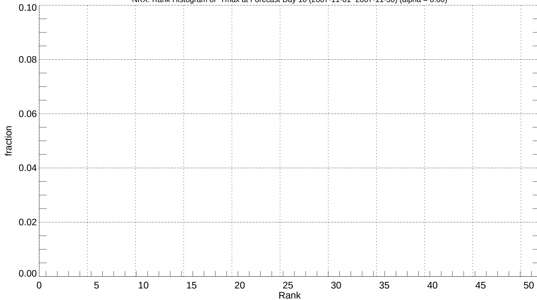
NKX: Rank Histogram of Tmax at Forecast Day 10 (2007-11-01~2007-11-30) (alpha = 0.00)
