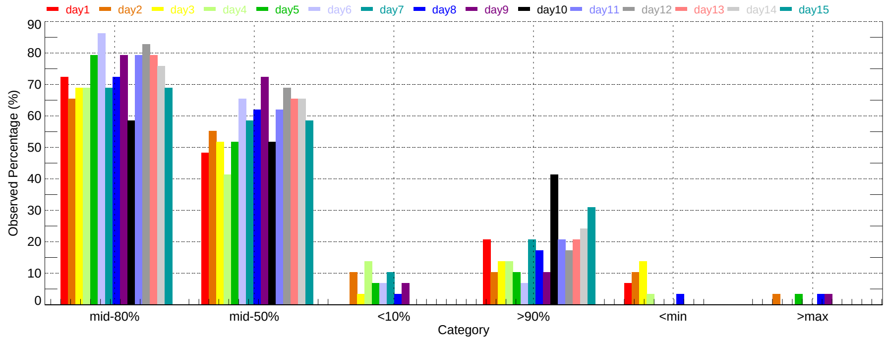
Observed Percentage of Ensembles - FAT: Max Temperature (2007-11-01~2007-11-30)
