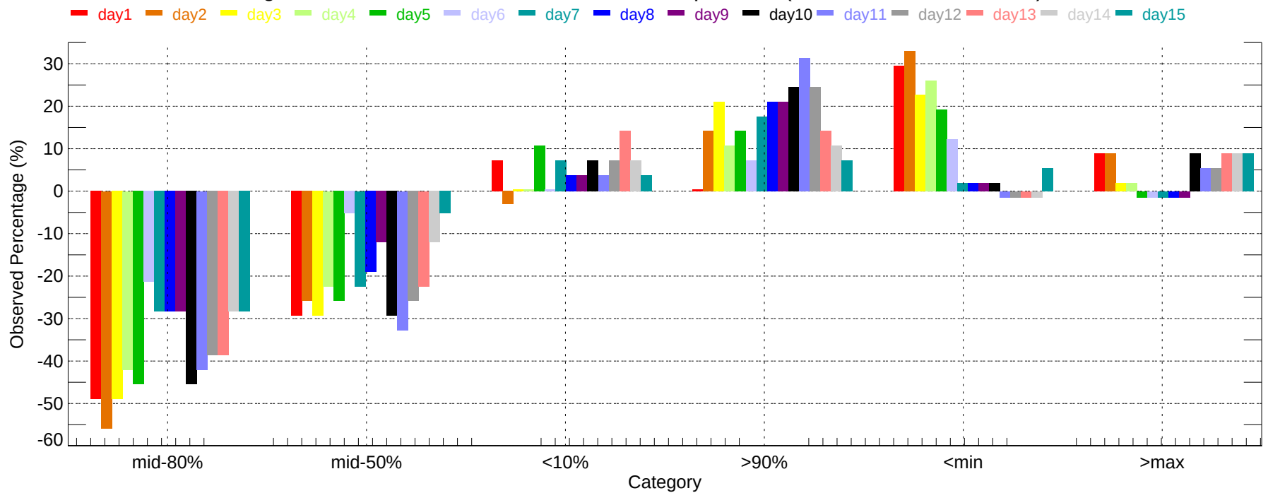
Observed Percentage Deviation of Ensembles - LFK: Min Temperature (2007-11-01~2007-11-30)
