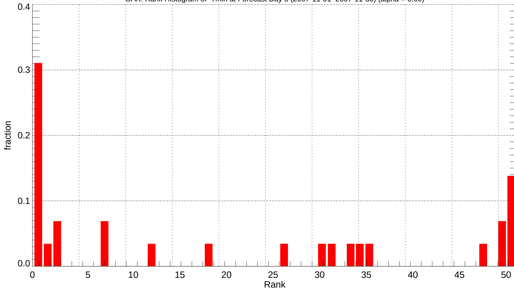
OAK: Rank Histogram of Tmin at Forecast Day 5 (2007-11-01~2007-11-30) (alpha = 0.00)
