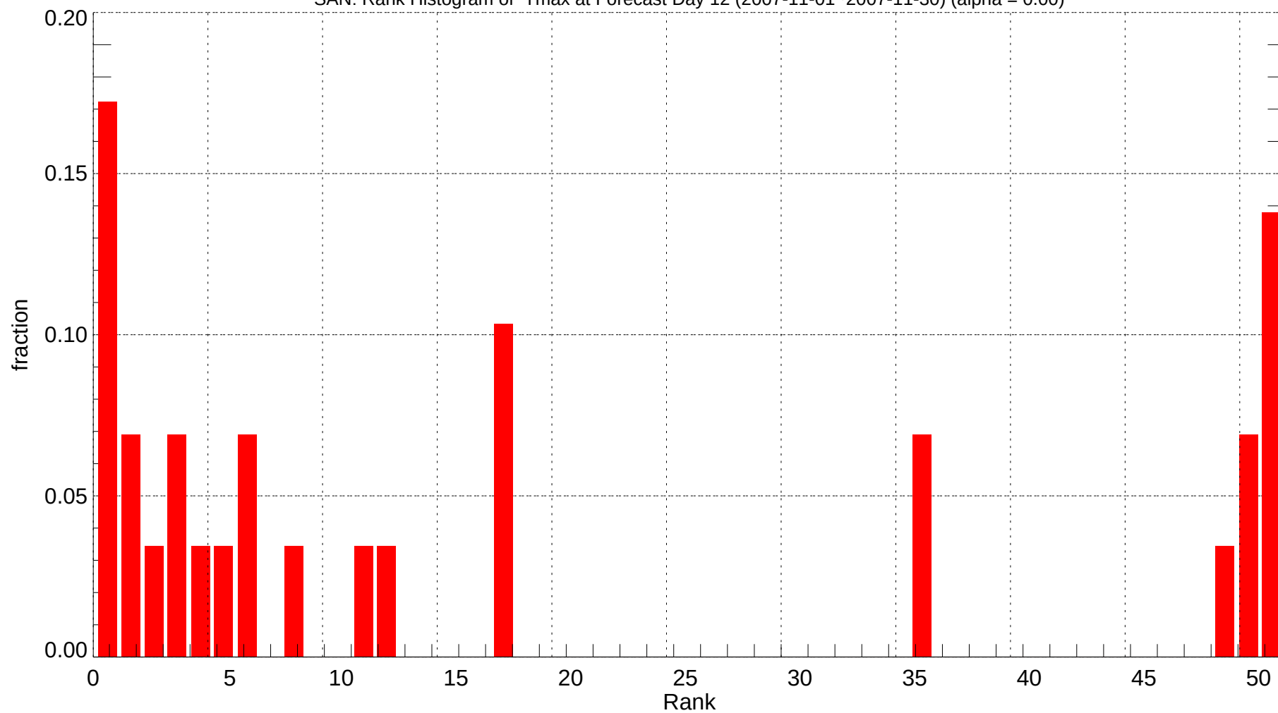
SAN: Rank Histogram of Tmax at Forecast Day 12 (2007-11-01~2007-11-30) (alpha = 0.00)
