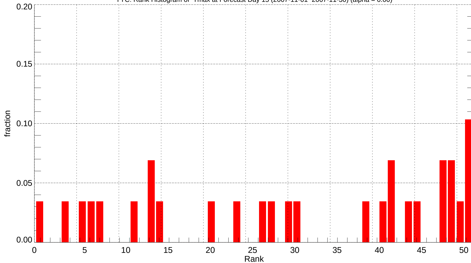
YYC: Rank Histogram of Tmax at Forecast Day 15 (2007-11-01~2007-11-30) (alpha = 0.00)
