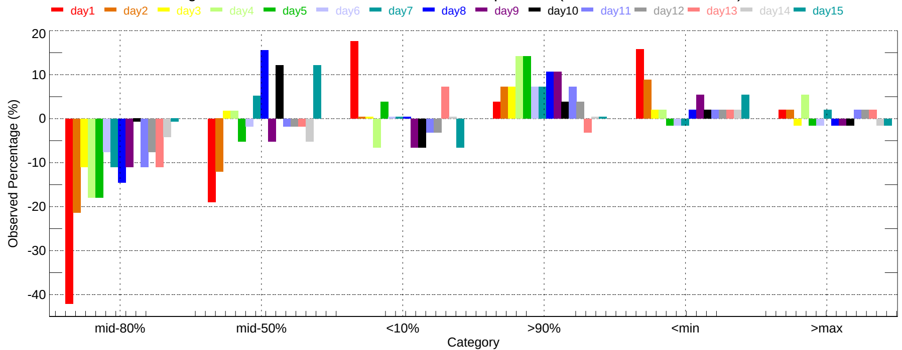
Observed Percentage Deviation of Ensembles - JAX: Min Temperature (2007-11-01~2007-11-30)
