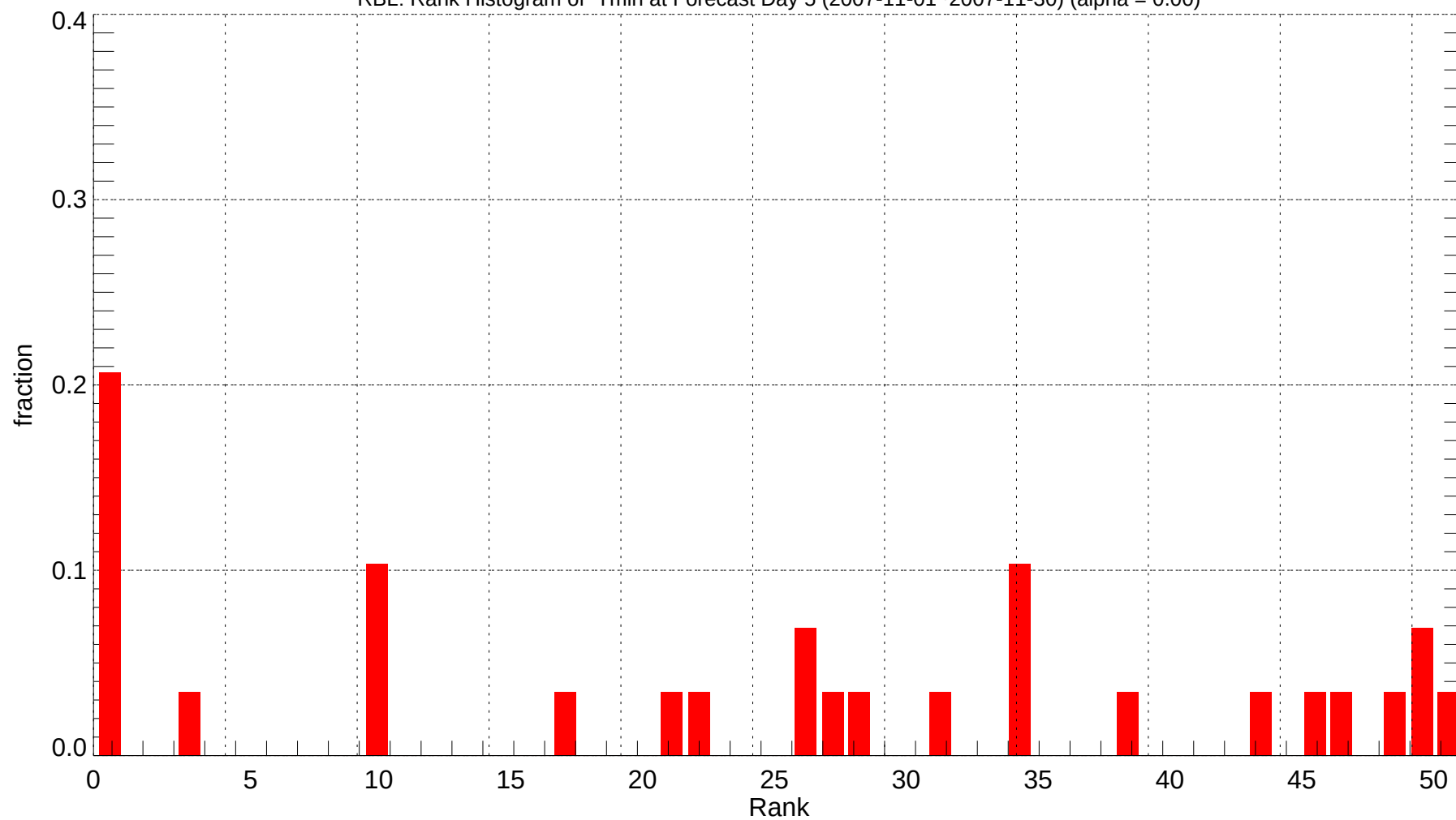
RBL: Rank Histogram of Tmin at Forecast Day 5 (2007-11-01~2007-11-30) (alpha = 0.00)
