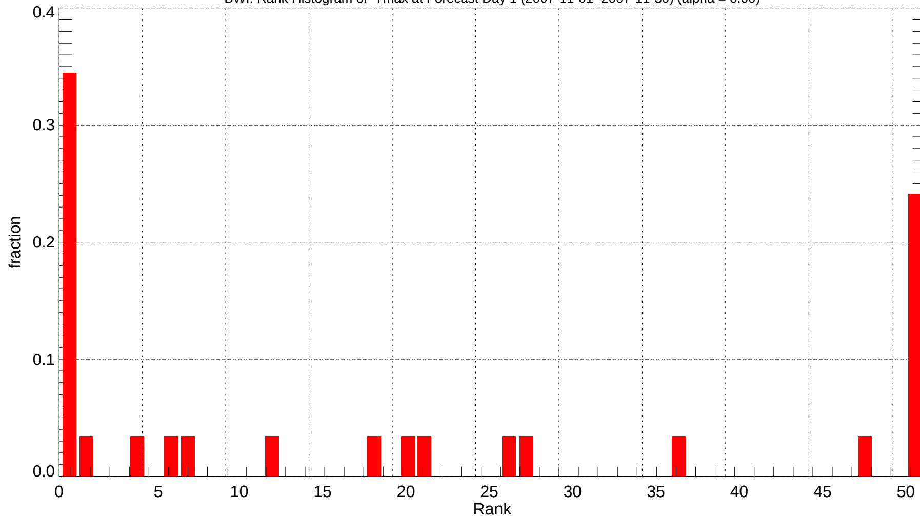
BWI: Rank Histogram of Tmax at Forecast Day 1 (2007-11-01~2007-11-30) (alpha = 0.00)
