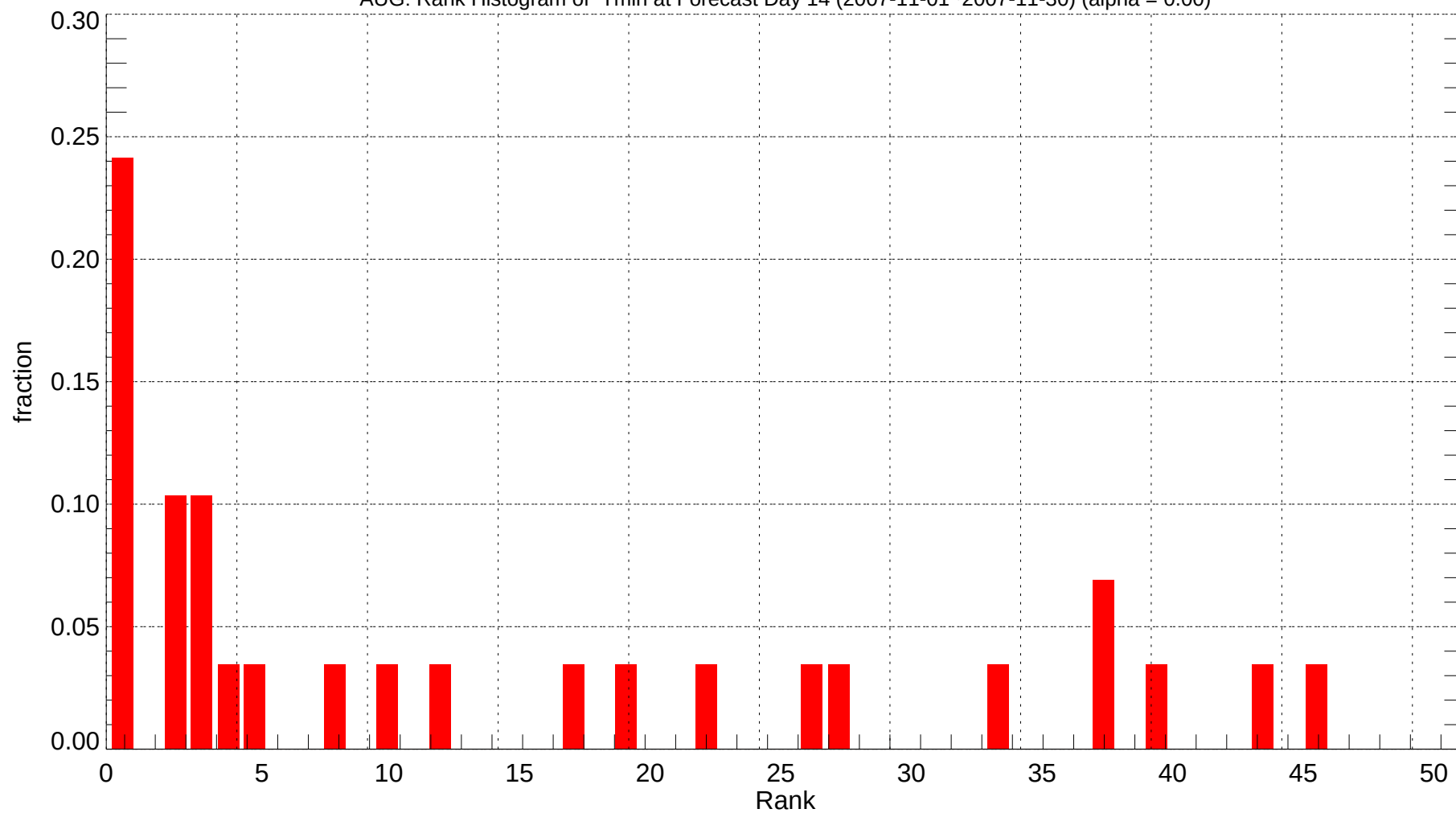
AUG: Rank Histogram of Tmin at Forecast Day 14 (2007-11-01~2007-11-30) (alpha = 0.00)
