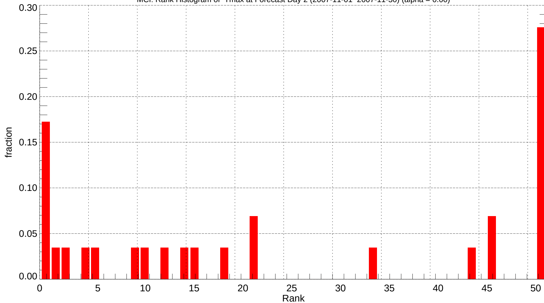
MCI: Rank Histogram of Tmax at Forecast Day 2 (2007-11-01~2007-11-30) (alpha = 0.00)
