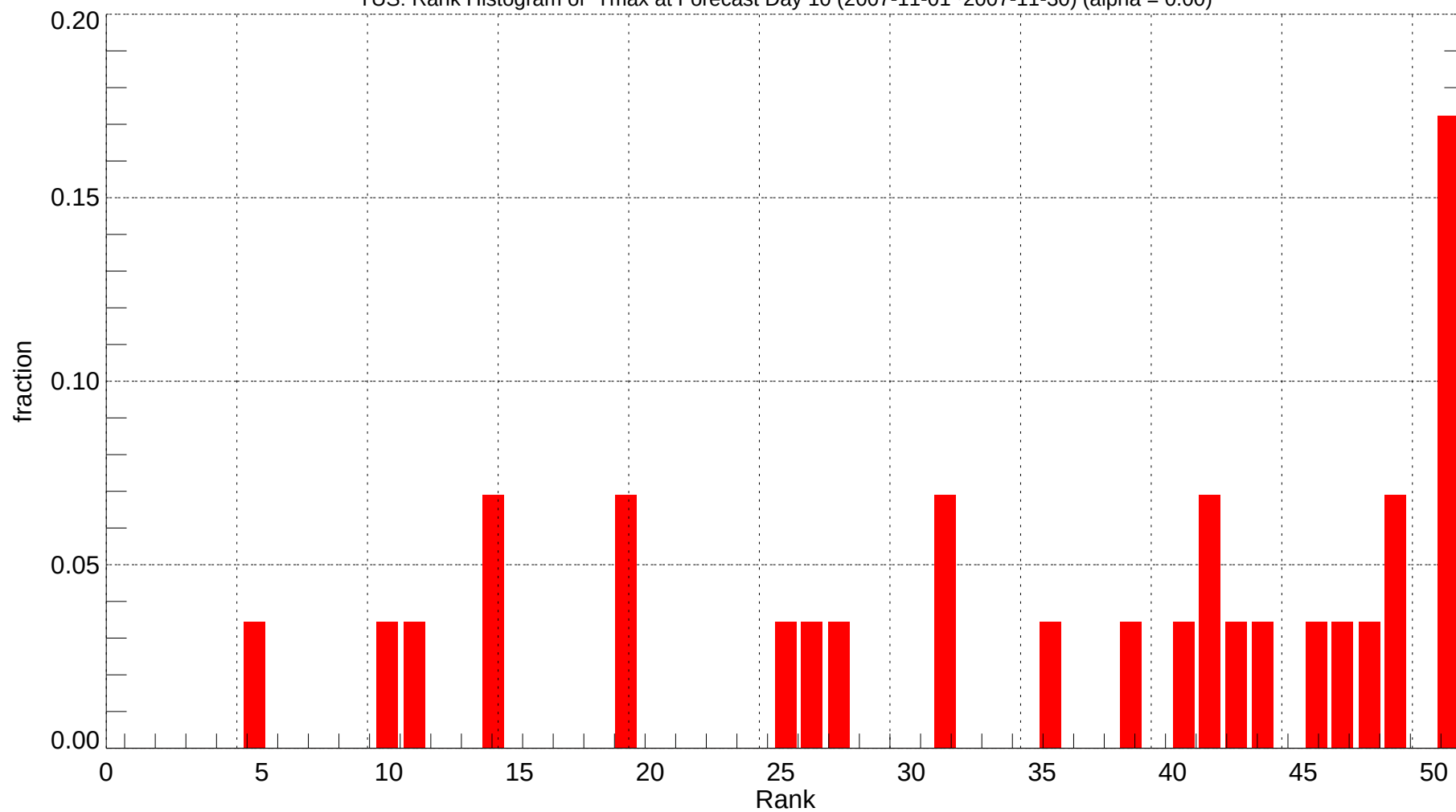
TUS: Rank Histogram of Tmax at Forecast Day 10 (2007-11-01~2007-11-30) (alpha = 0.00)
