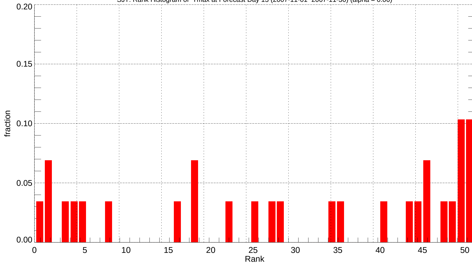
SJT: Rank Histogram of Tmax at Forecast Day 13 (2007-11-01~2007-11-30) (alpha = 0.00)
