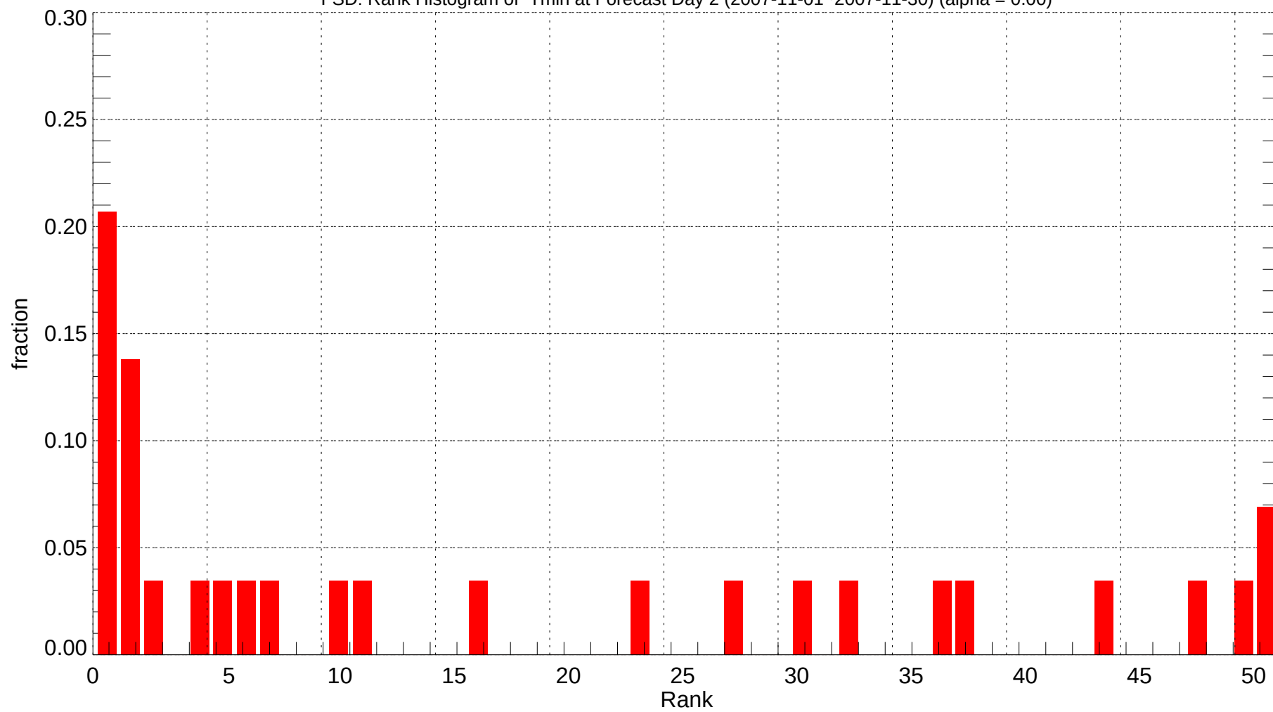
FSD: Rank Histogram of Tmin at Forecast Day 2 (2007-11-01~2007-11-30) (alpha = 0.00)
