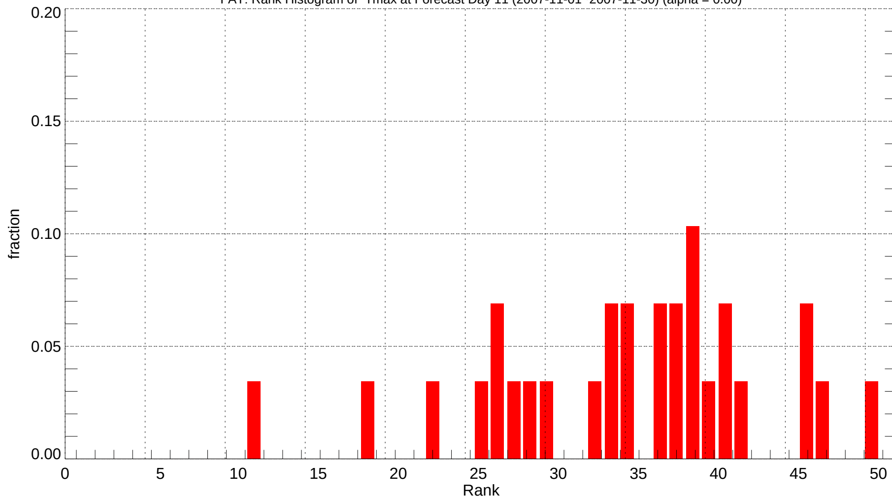
FAT: Rank Histogram of Tmax at Forecast Day 11 (2007-11-01~2007-11-30) (alpha = 0.00)
