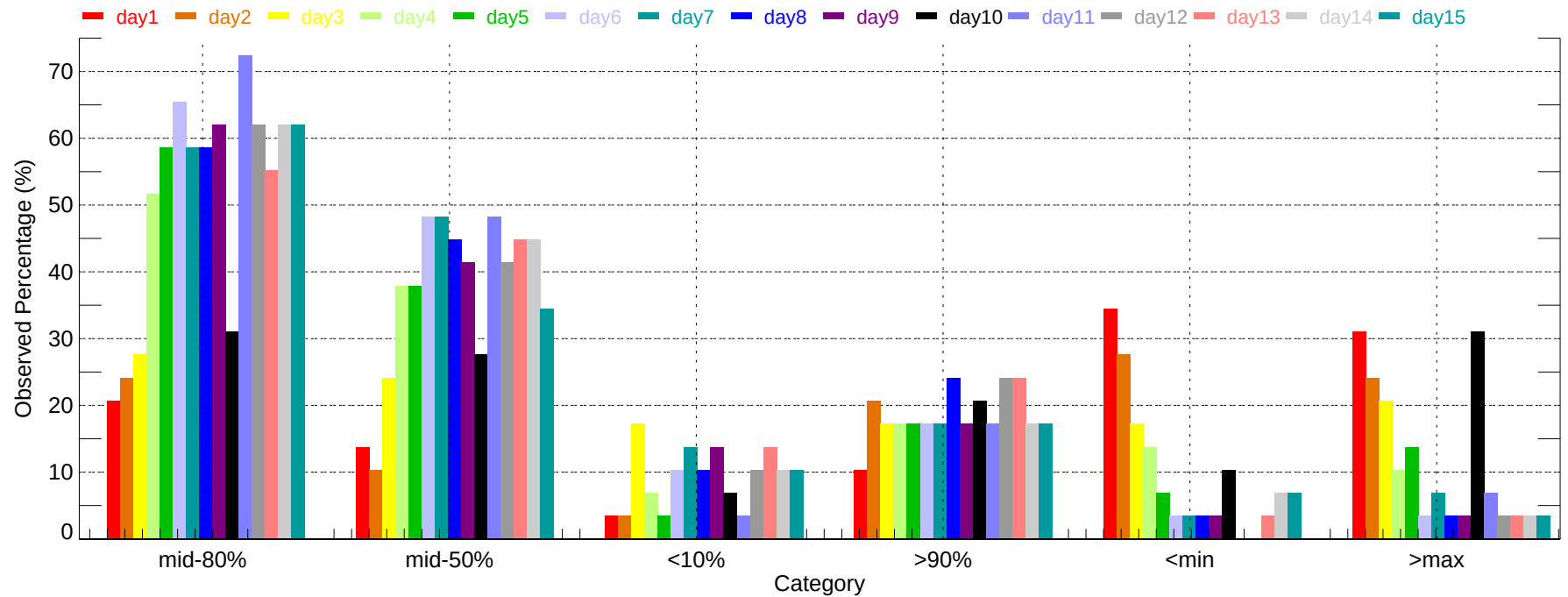
Observed Percentage of Ensembles - MDT: Min Temperature (2007-11-01~2007-11-30)
