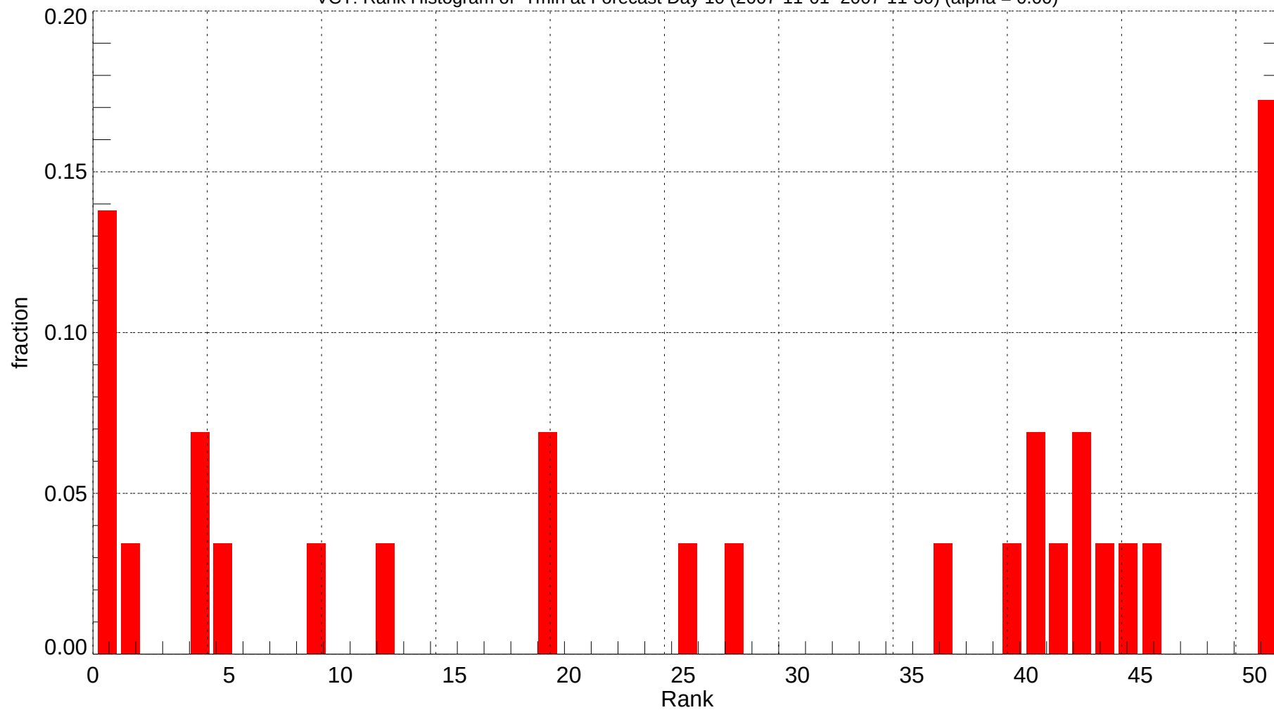
VCT: Rank Histogram of Tmin at Forecast Day 10 (2007-11-01~2007-11-30) (alpha = 0.00)
