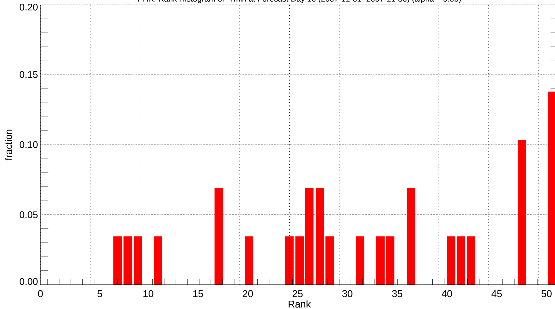
PHX: Rank Histogram of Tmin at Forecast Day 10 (2007-11-01~2007-11-30) (alpha = 0.00)
