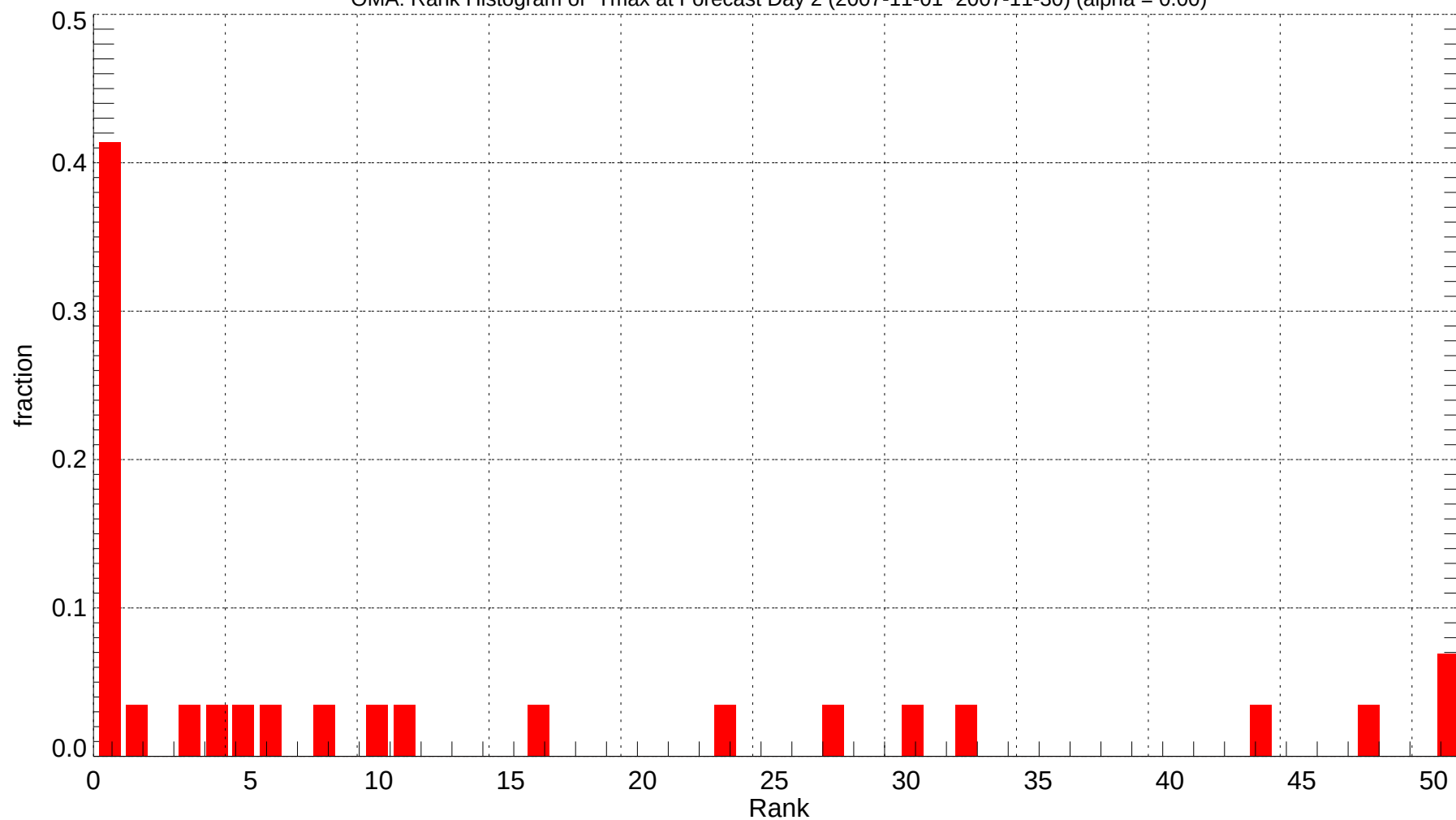
OMA: Rank Histogram of Tmax at Forecast Day 2 (2007-11-01~2007-11-30) (alpha = 0.00)
