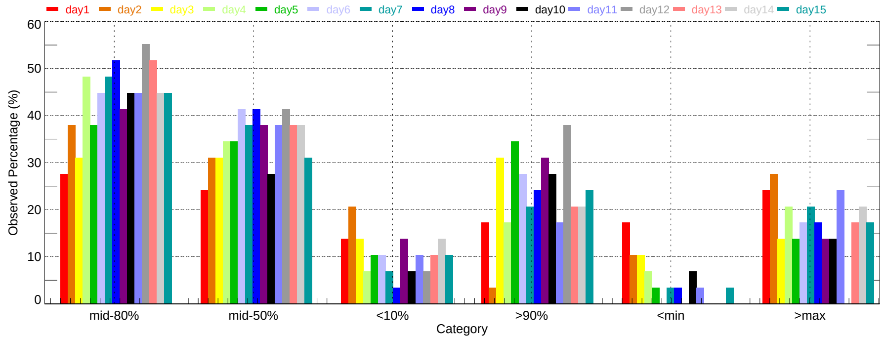
Observed Percentage of Ensembles - DEN: Max Temperature (2007-11-01~2007-11-30)
