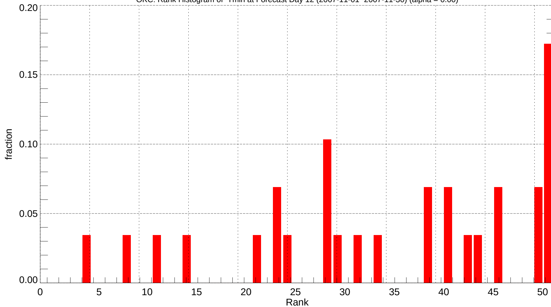
OKC: Rank Histogram of Tmin at Forecast Day 12 (2007-11-01~2007-11-30) (alpha = 0.00)
