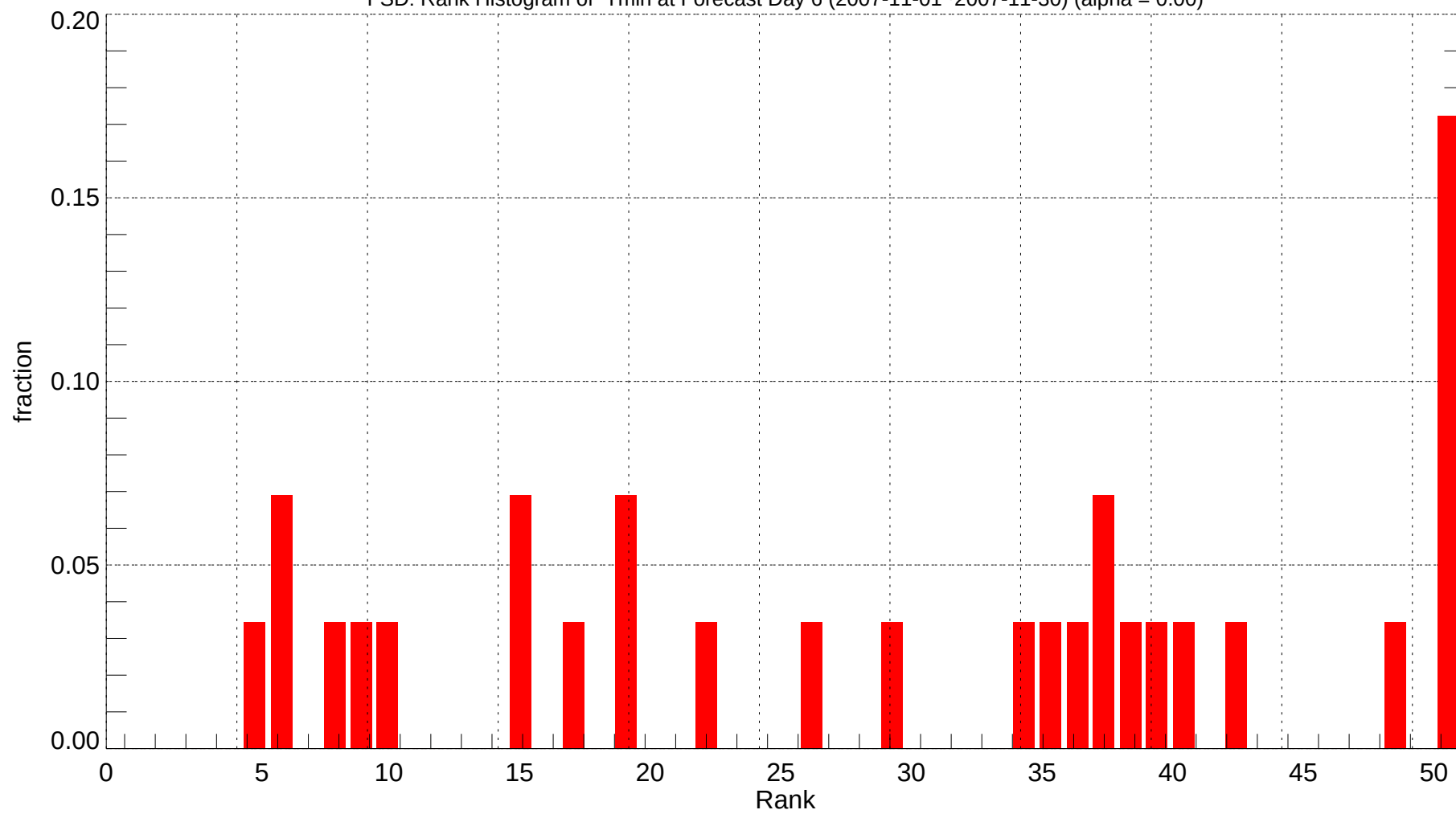
FSD: Rank Histogram of Tmin at Forecast Day 6 (2007-11-01~2007-11-30) (alpha = 0.00)
