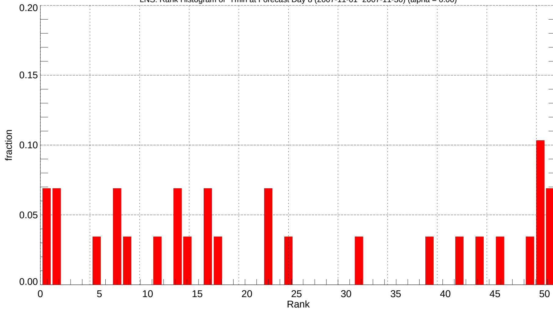
LNS: Rank Histogram of Tmin at Forecast Day 8 (2007-11-01~2007-11-30) (alpha = 0.00)
