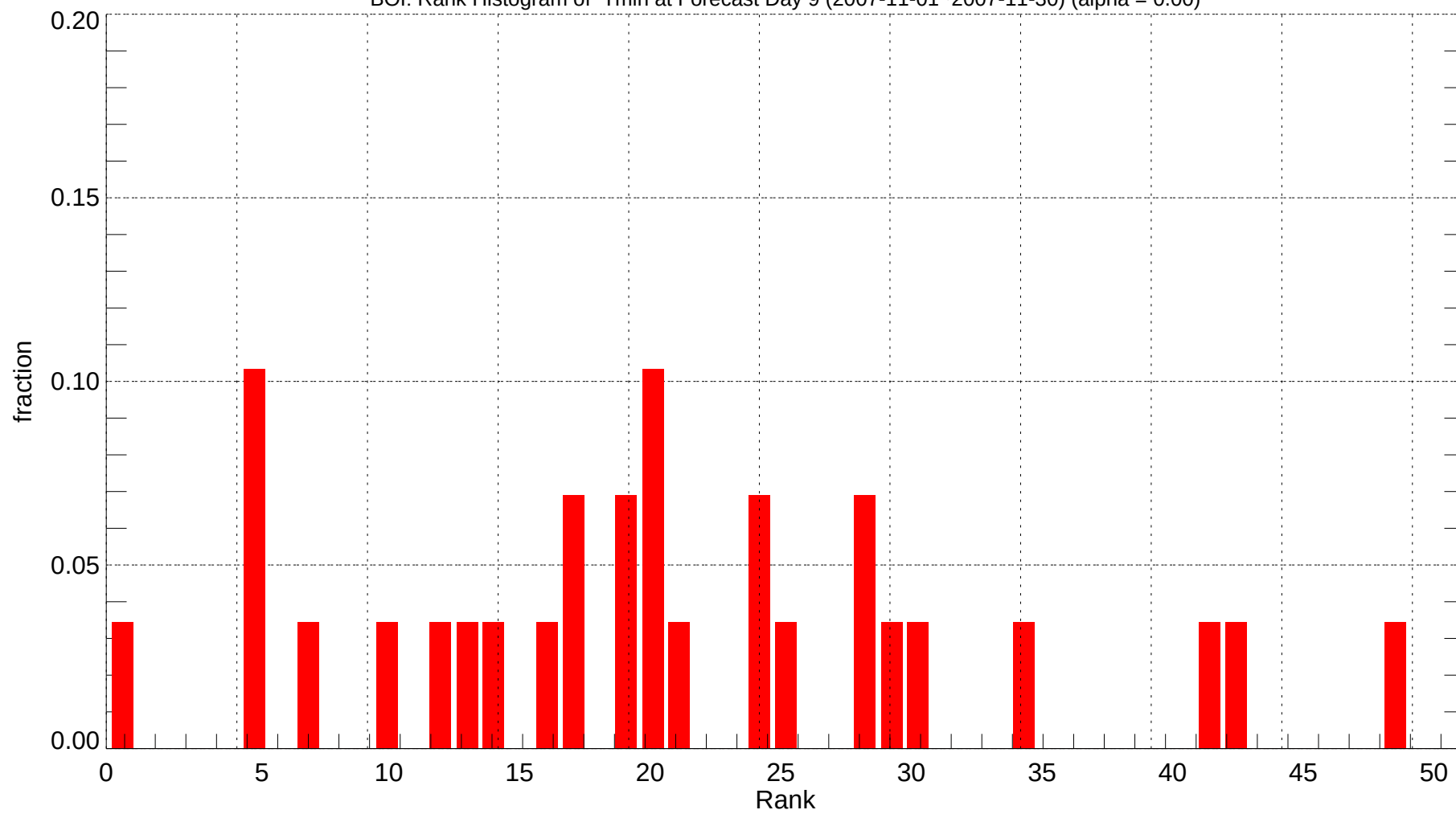
BOI: Rank Histogram of Tmin at Forecast Day 9 (2007-11-01~2007-11-30) (alpha = 0.00)
