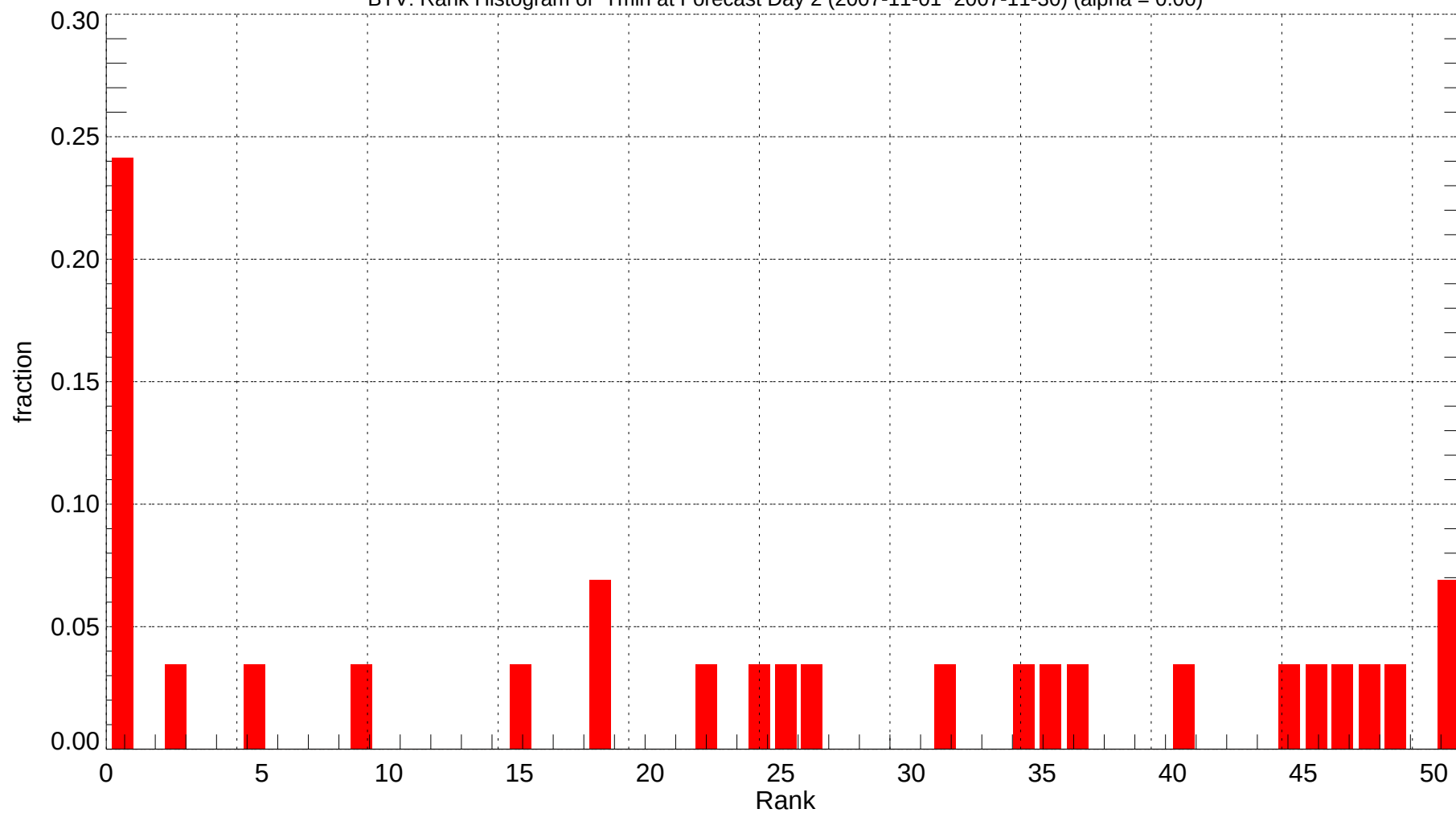
BTV: Rank Histogram of Tmin at Forecast Day 2 (2007-11-01~2007-11-30) (alpha = 0.00)
