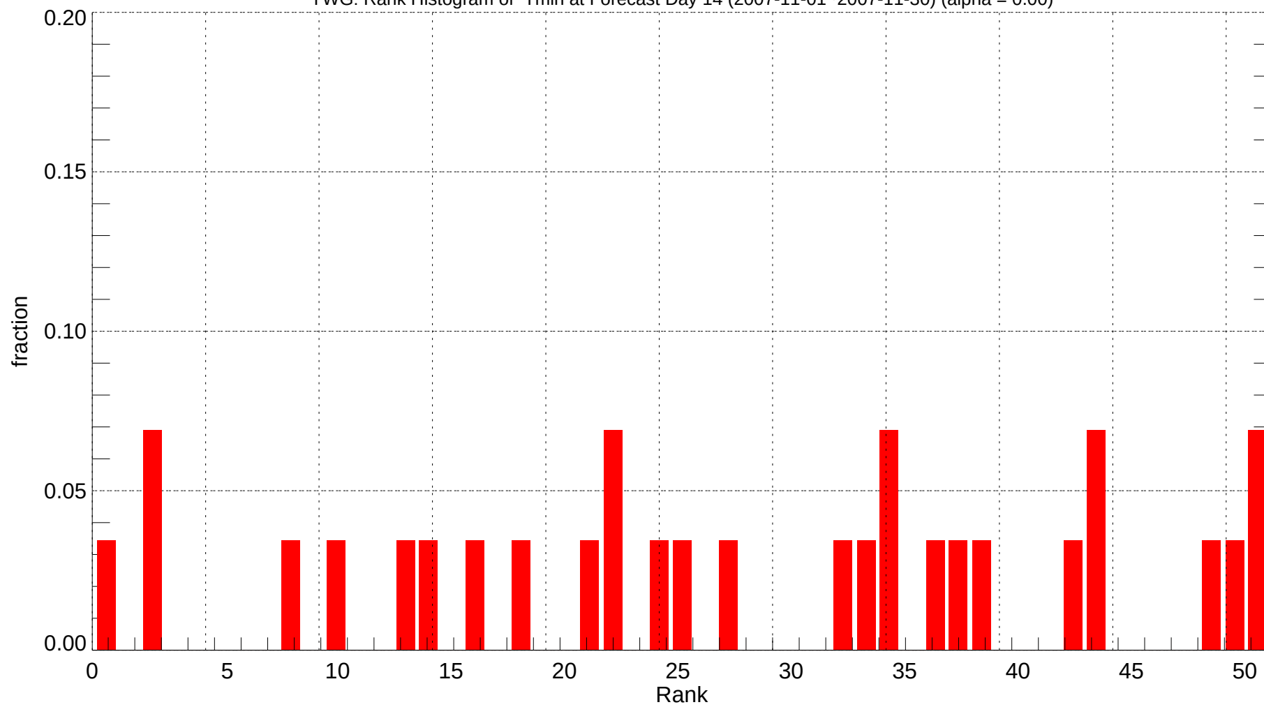
YWG: Rank Histogram of Tmin at Forecast Day 14 (2007-11-01~2007-11-30) (alpha = 0.00)
