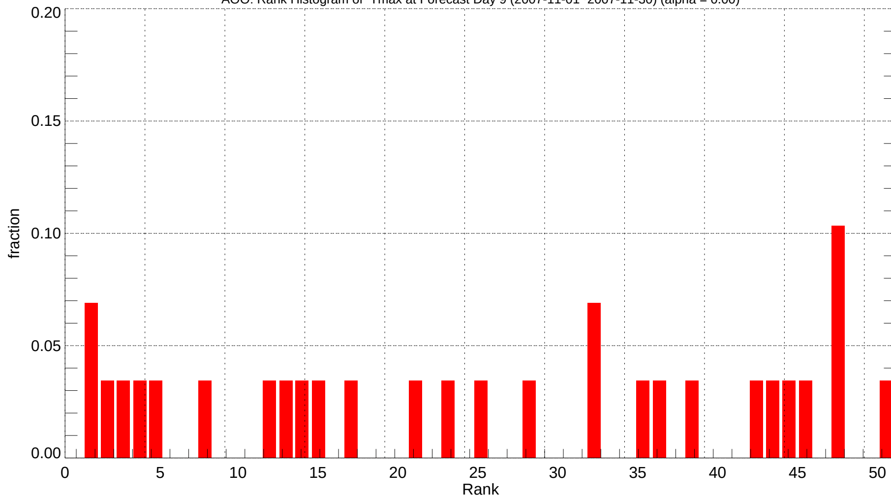
AOO: Rank Histogram of Tmax at Forecast Day 9 (2007-11-01~2007-11-30) (alpha = 0.00)
