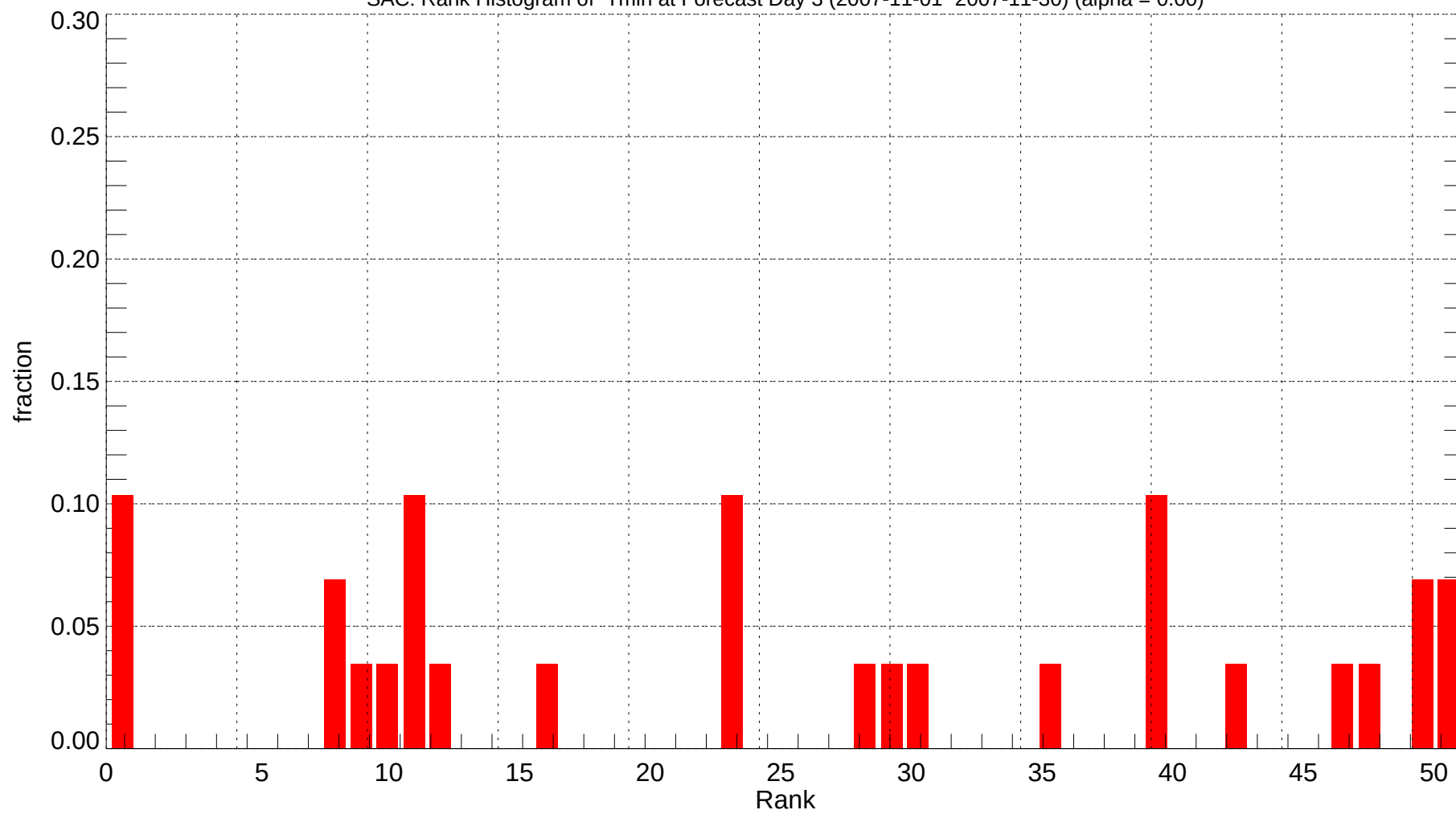
SAC: Rank Histogram of Tmin at Forecast Day 3 (2007-11-01~2007-11-30) (alpha = 0.00)
