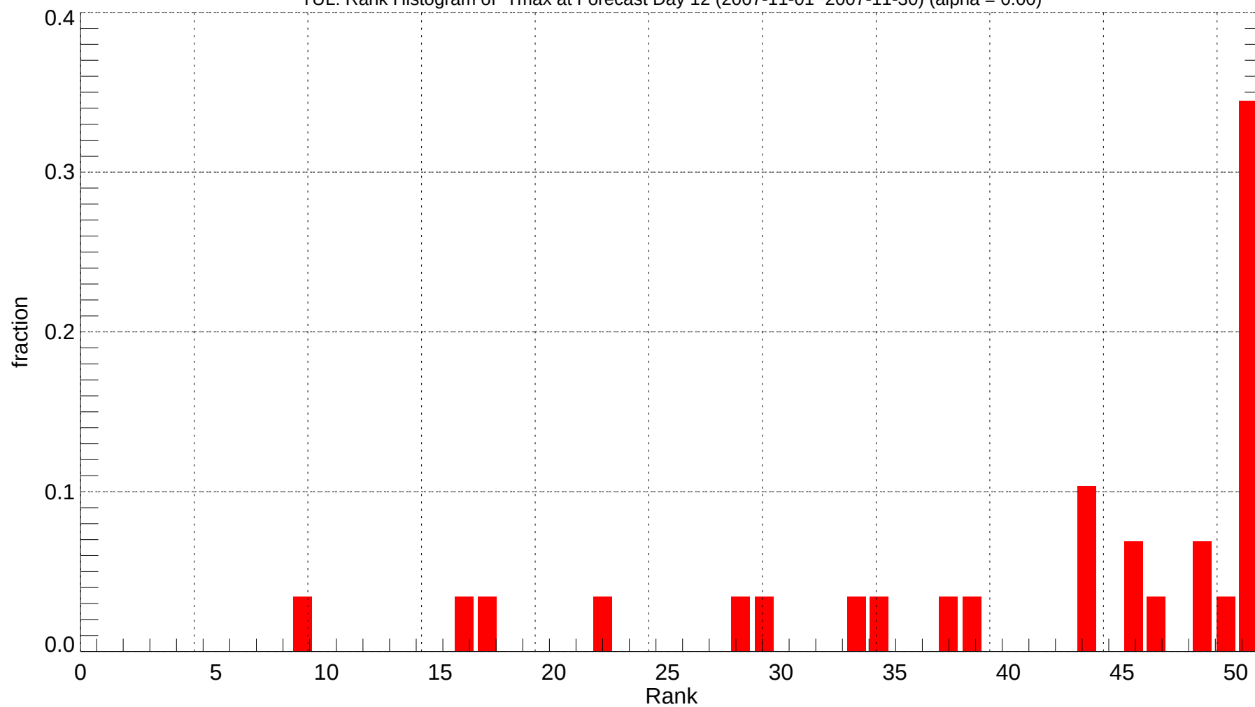
TUL: Rank Histogram of Tmax at Forecast Day 12 (2007-11-01~2007-11-30) (alpha = 0.00)
