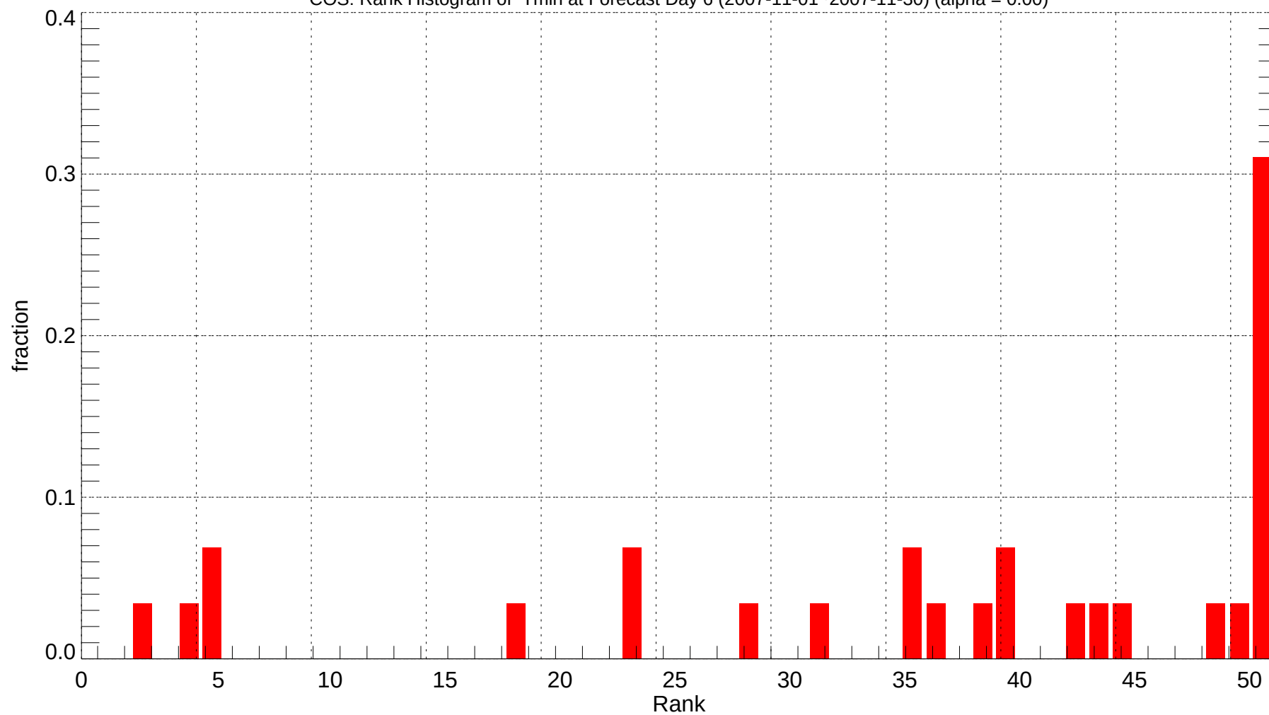
COS: Rank Histogram of Tmin at Forecast Day 6 (2007-11-01~2007-11-30) (alpha = 0.00)
