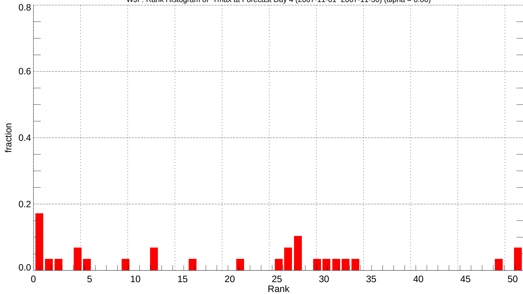
WJF: Rank Histogram of Tmax at Forecast Day 4 (2007-11-01~2007-11-30) (alpha = 0.00)
