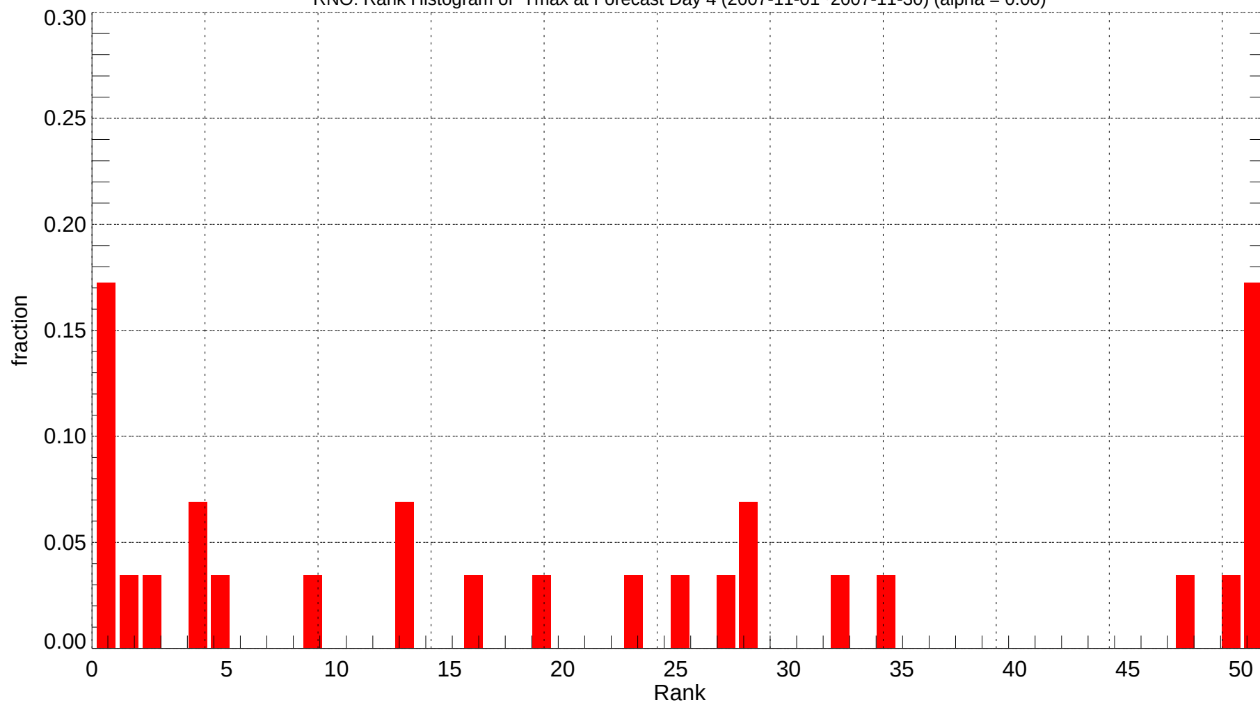
RNO: Rank Histogram of Tmax at Forecast Day 4 (2007-11-01~2007-11-30) (alpha = 0.00)
