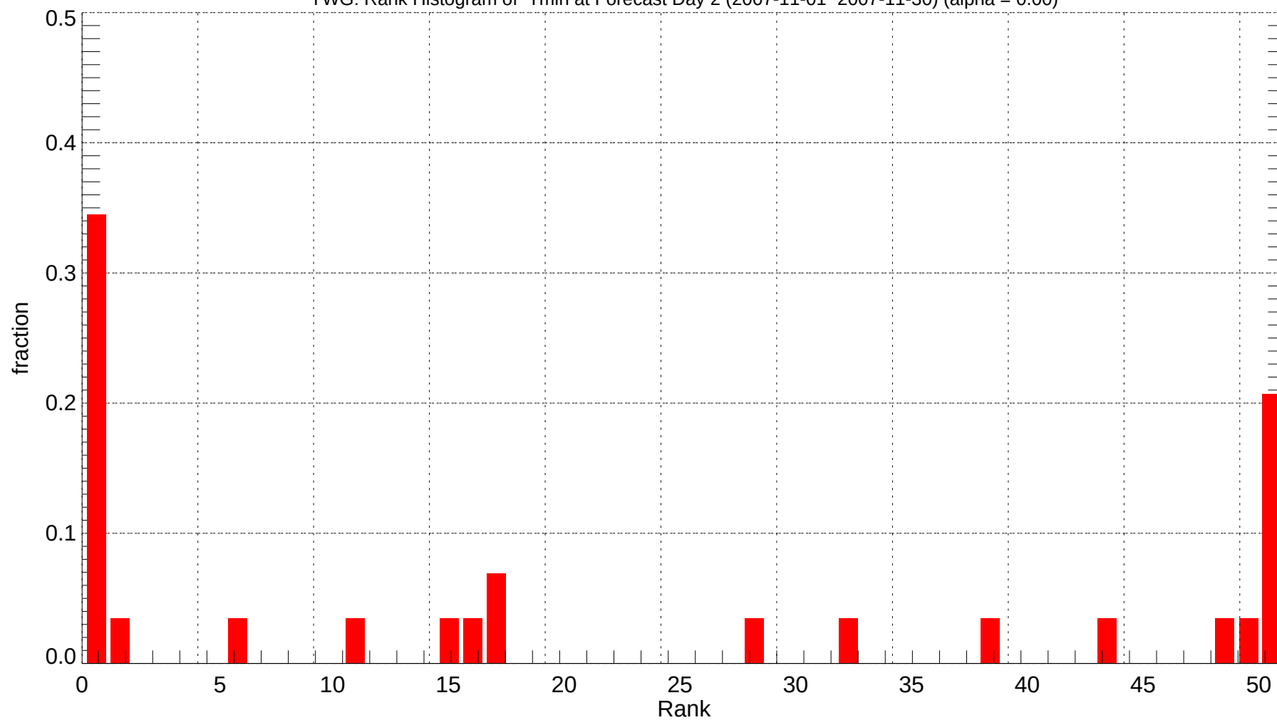
YWG: Rank Histogram of Tmin at Forecast Day 2 (2007-11-01~2007-11-30) (alpha = 0.00)
