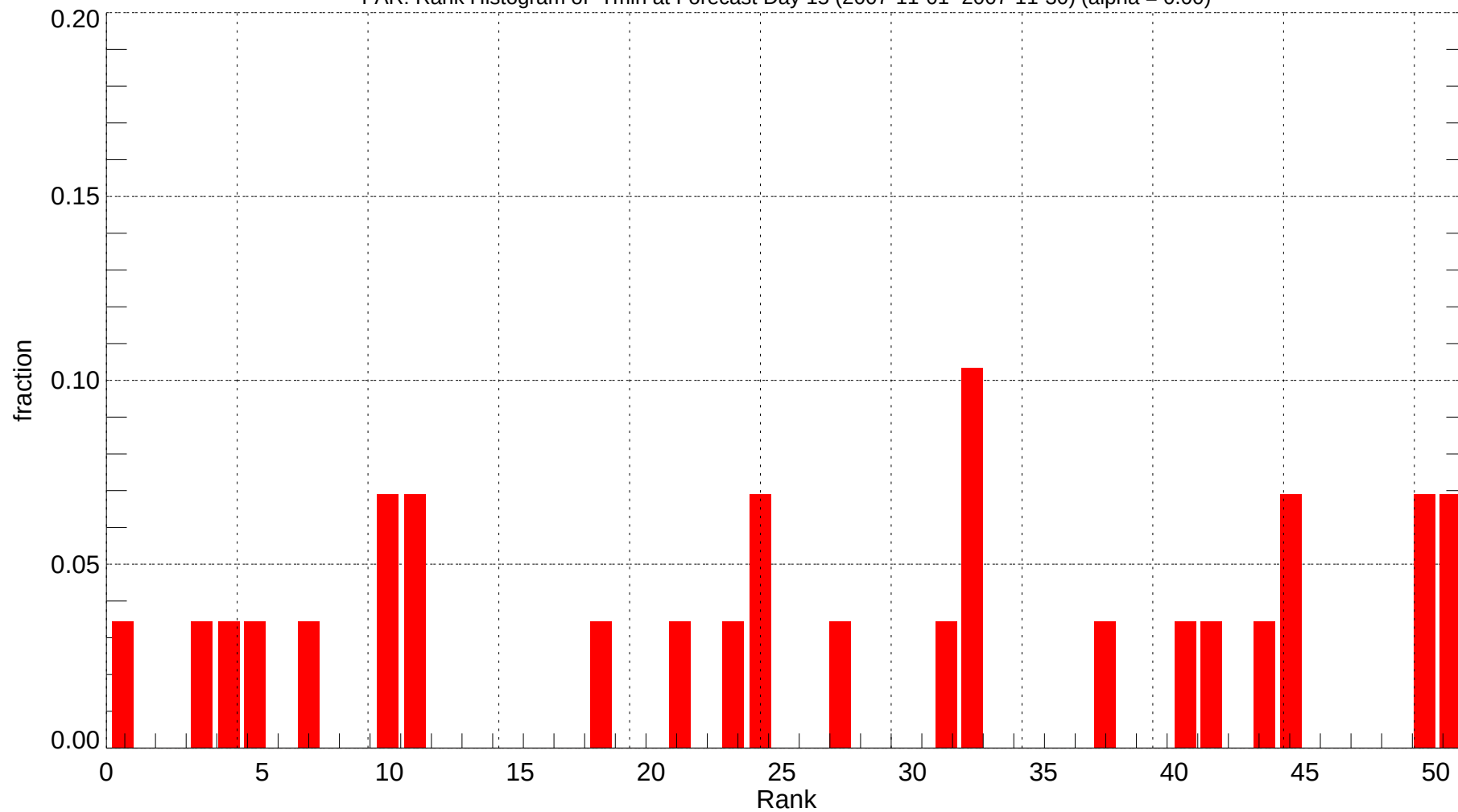
FAR: Rank Histogram of Tmin at Forecast Day 15 (2007-11-01~2007-11-30) (alpha = 0.00)
