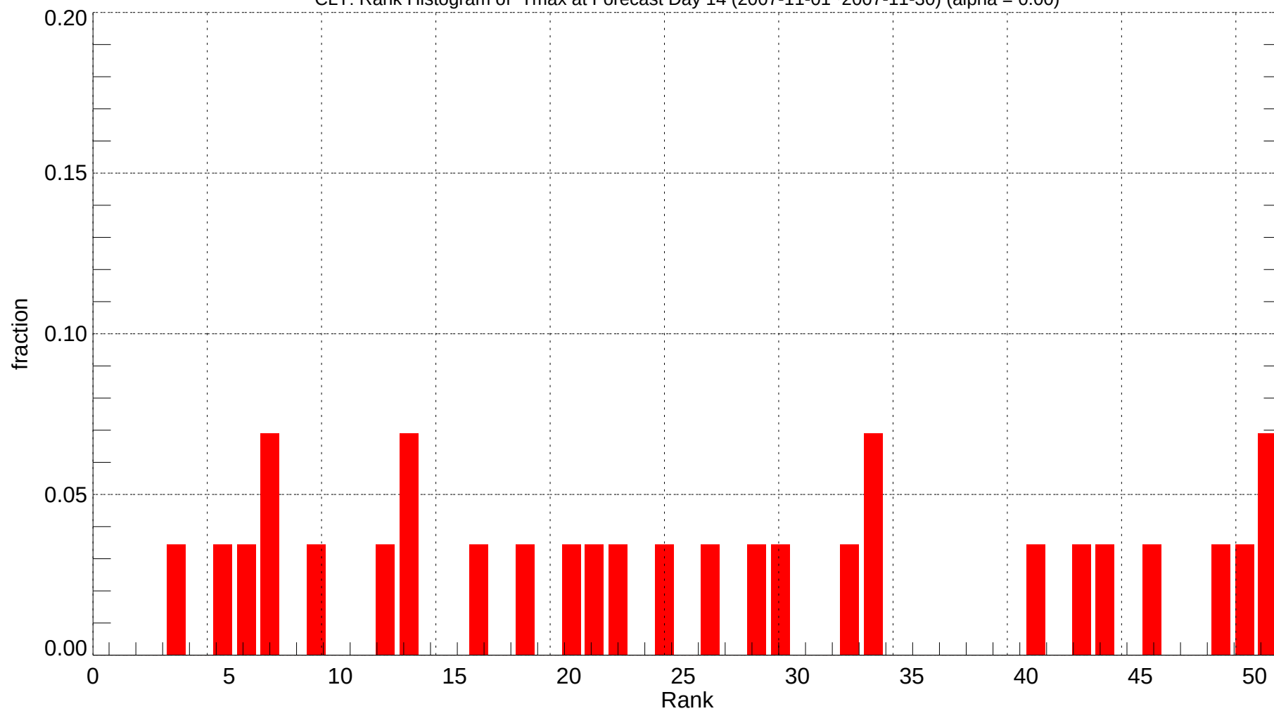
CLT: Rank Histogram of Tmax at Forecast Day 14 (2007-11-01~2007-11-30) (alpha = 0.00)
