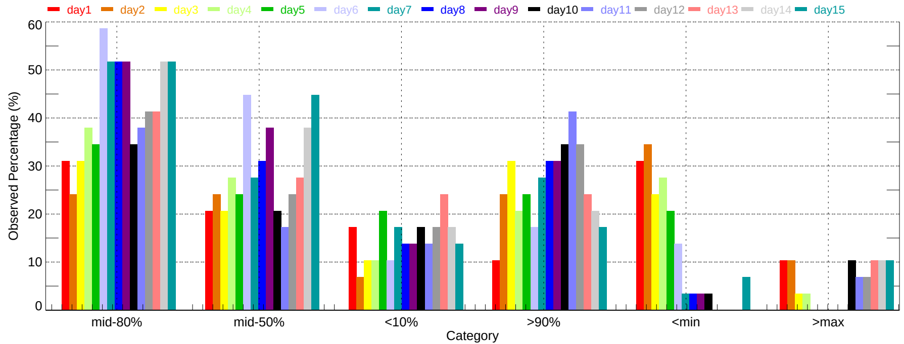
Observed Percentage of Ensembles - LFK: Min Temperature (2007-11-01~2007-11-30)
