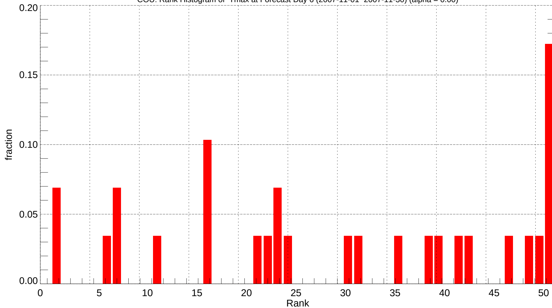
COU: Rank Histogram of Tmax at Forecast Day 6 (2007-11-01~2007-11-30) (alpha = 0.00)
