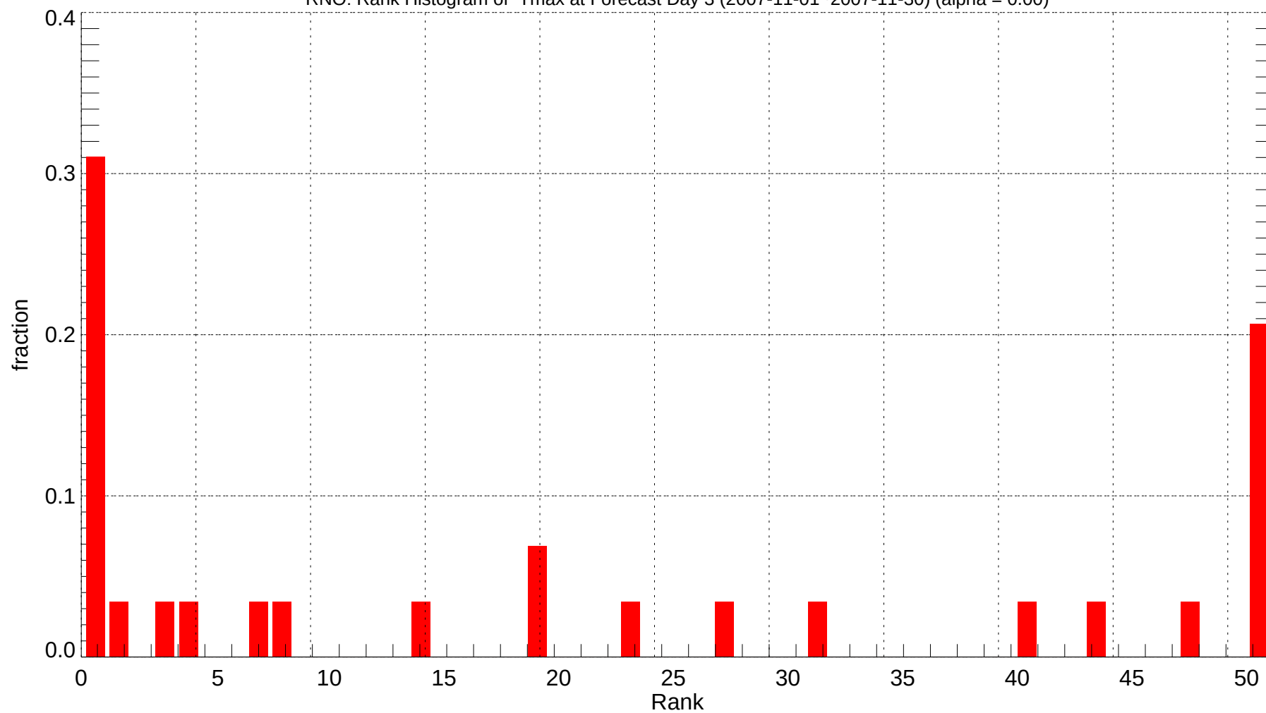
RNO: Rank Histogram of Tmax at Forecast Day 3 (2007-11-01~2007-11-30) (alpha = 0.00)
