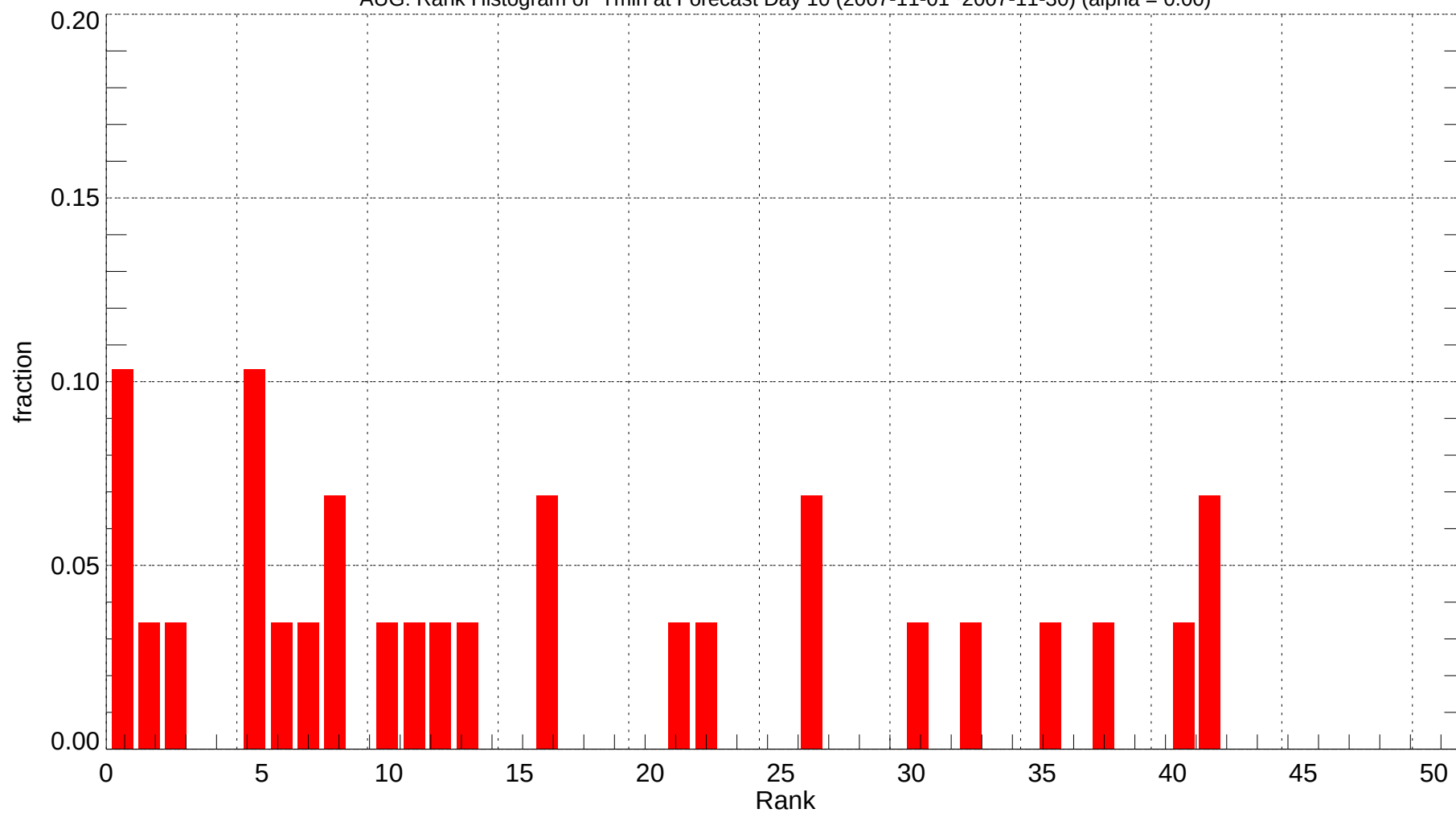
AUG: Rank Histogram of Tmin at Forecast Day 10 (2007-11-01~2007-11-30) (alpha = 0.00)
