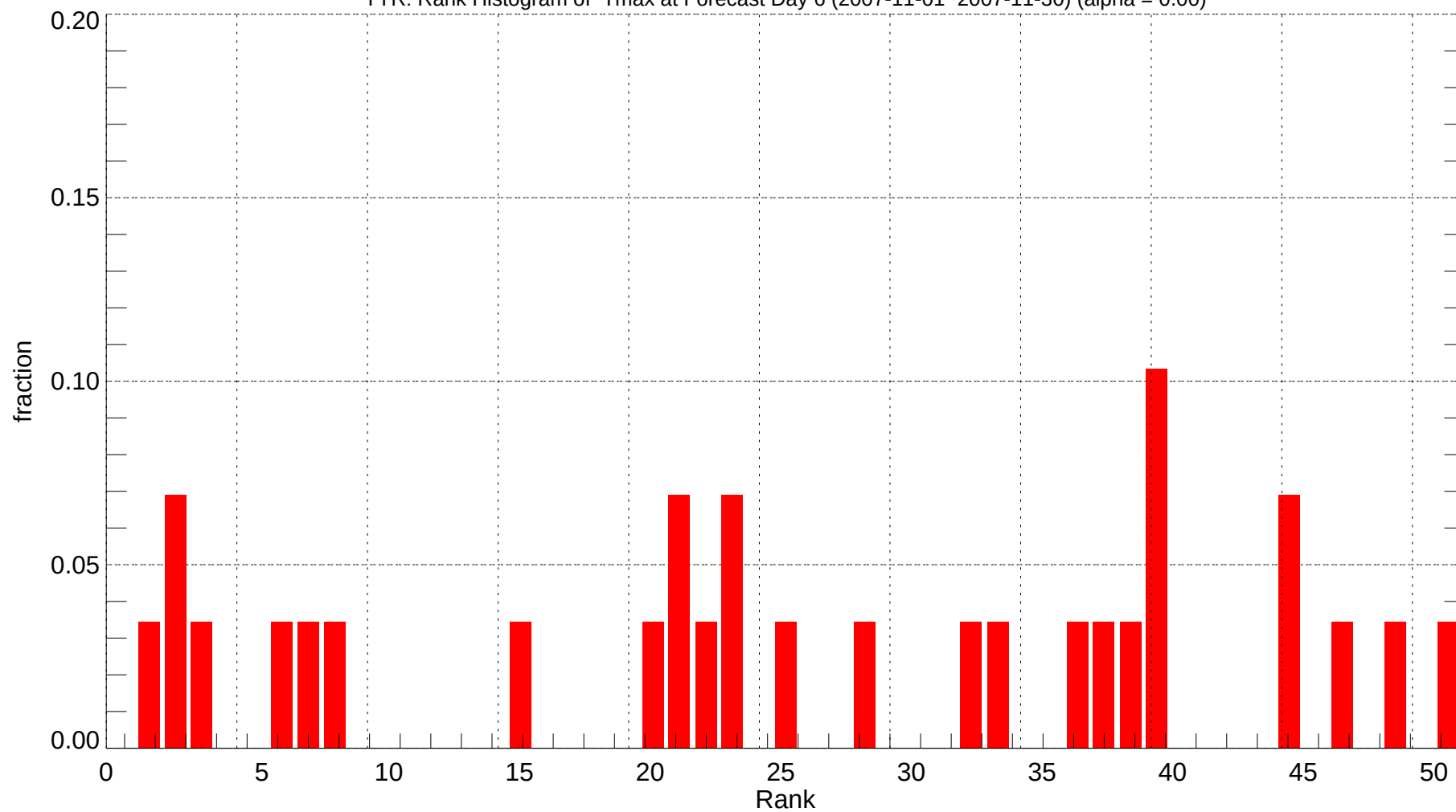
TYR: Rank Histogram of Tmax at Forecast Day 6 (2007-11-01~2007-11-30) (alpha = 0.00)
