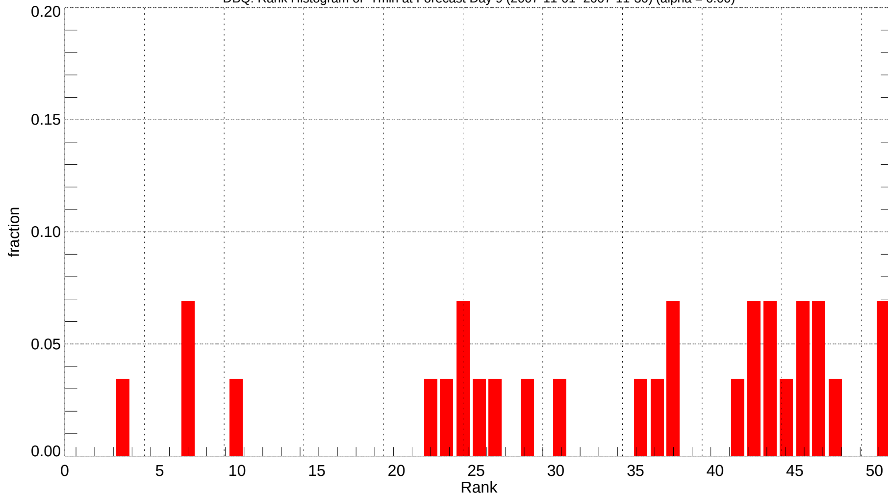
DBQ: Rank Histogram of Tmin at Forecast Day 9 (2007-11-01~2007-11-30) (alpha = 0.00)
