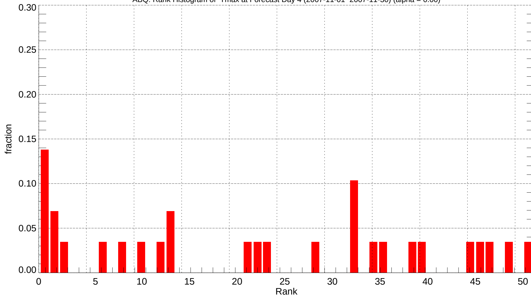
ABQ: Rank Histogram of Tmax at Forecast Day 4 (2007-11-01~2007-11-30) (alpha = 0.00)
