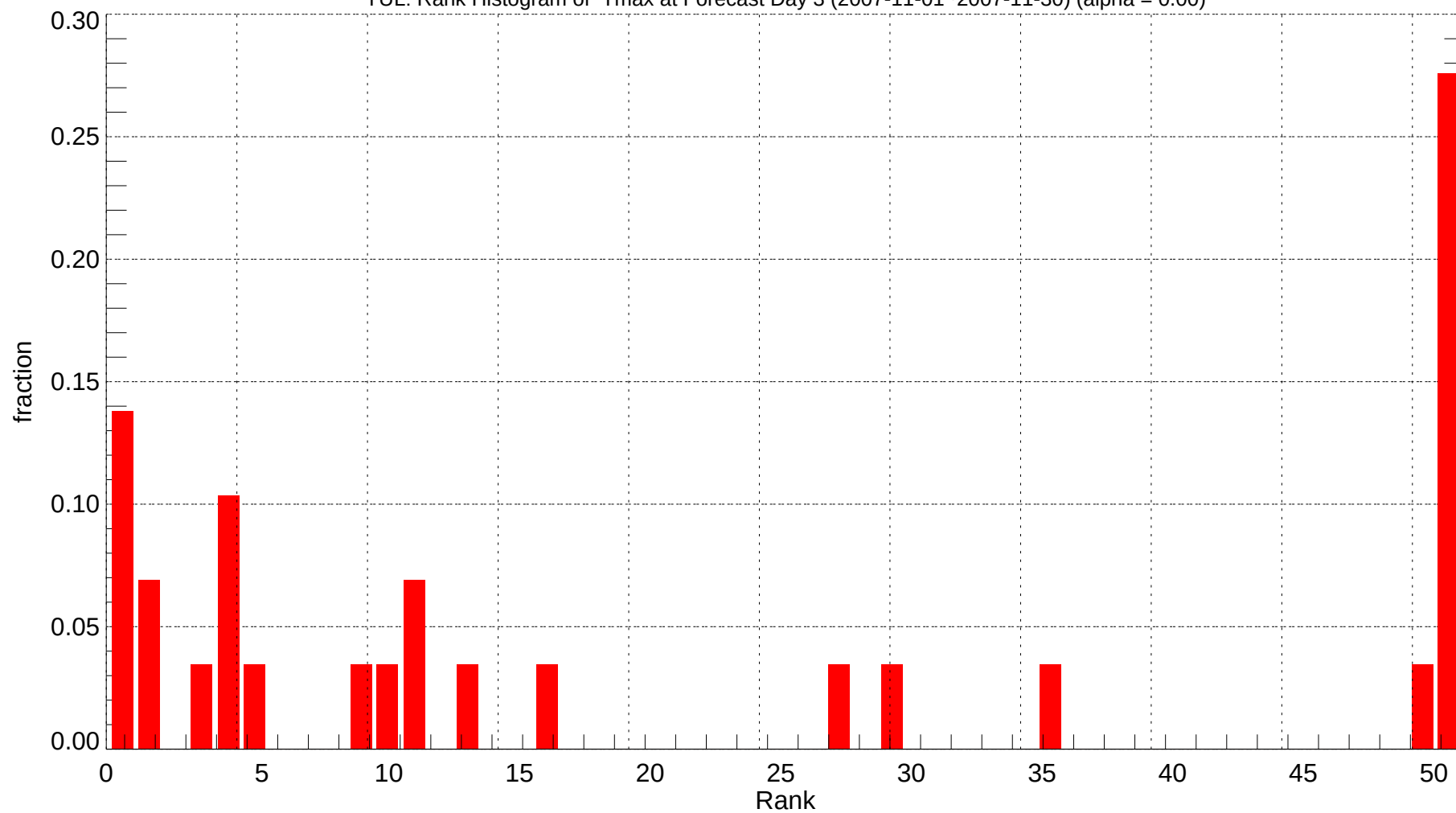
YUL: Rank Histogram of Tmax at Forecast Day 3 (2007-11-01~2007-11-30) (alpha = 0.00)
