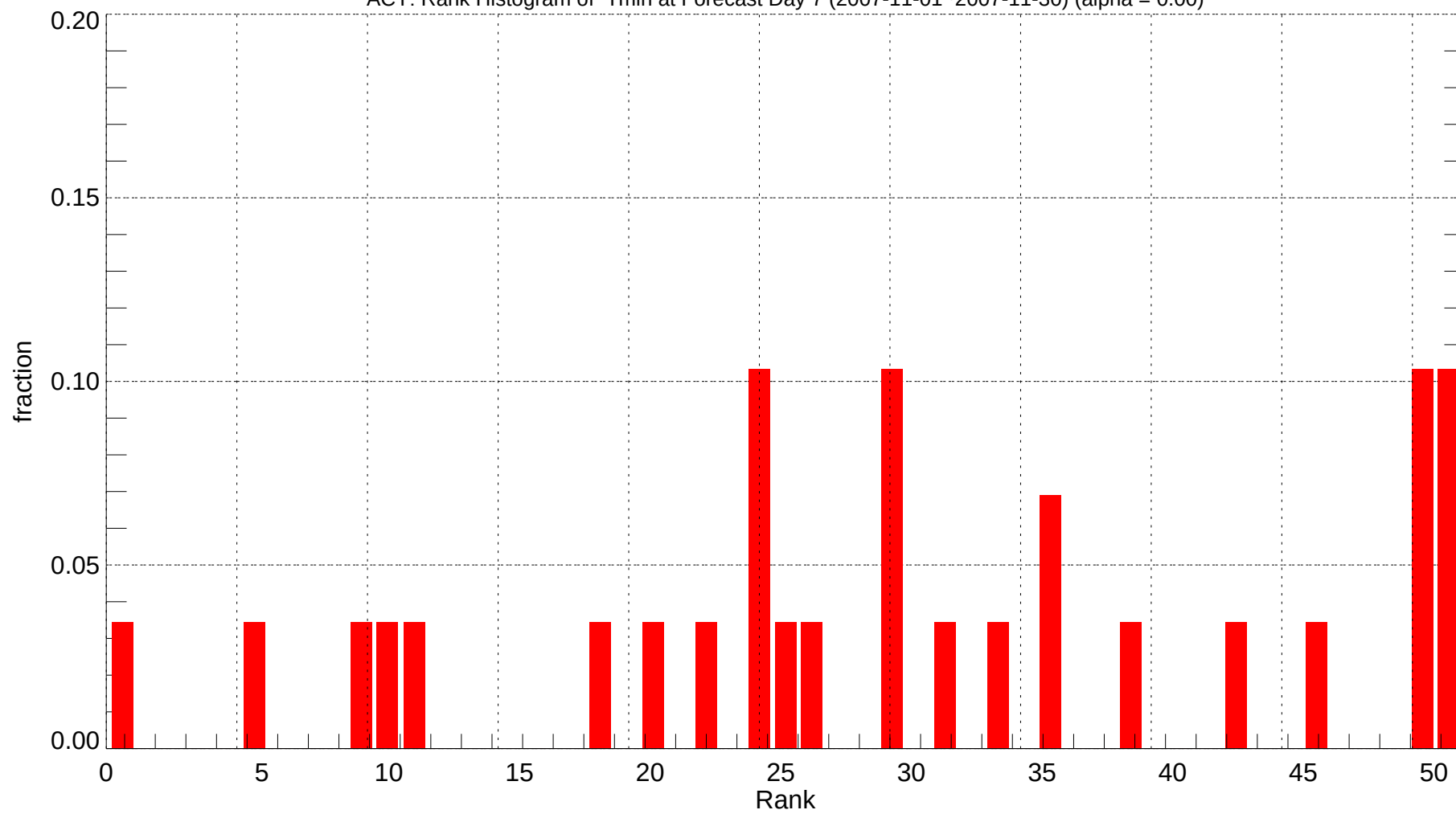
ACY: Rank Histogram of Tmin at Forecast Day 7 (2007-11-01~2007-11-30) (alpha = 0.00)
