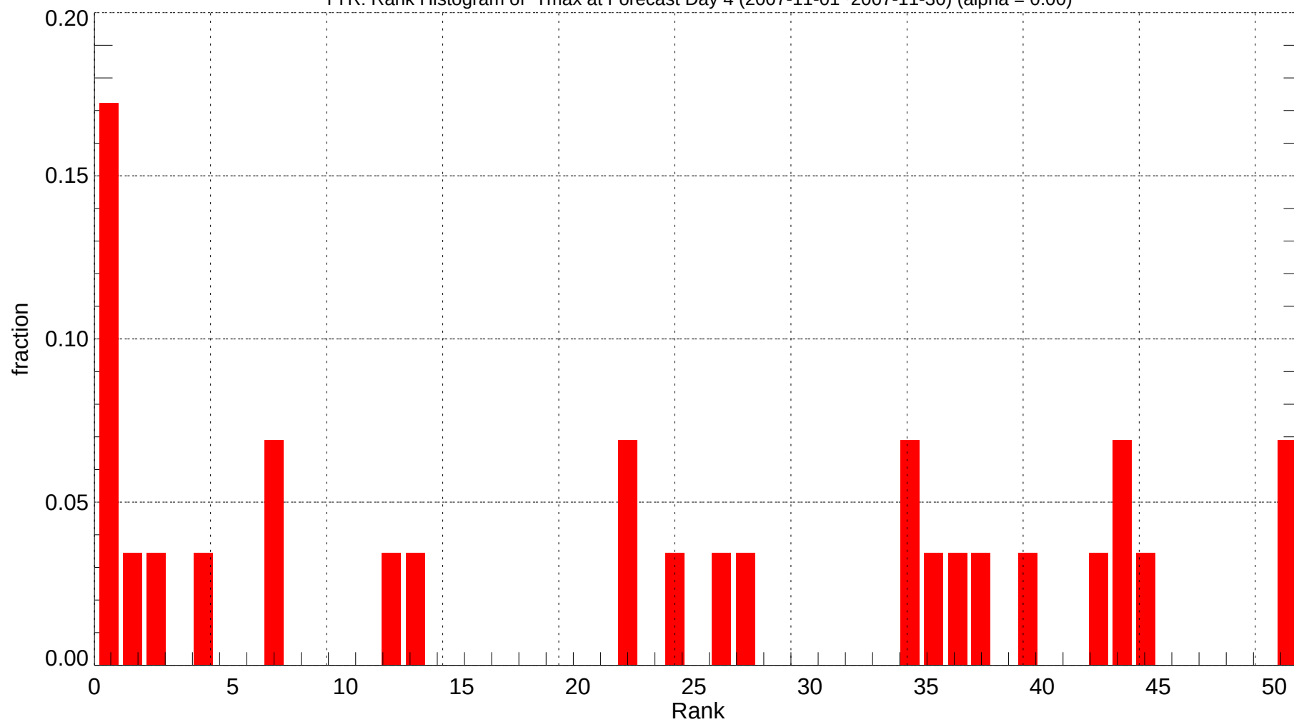
TYR: Rank Histogram of Tmax at Forecast Day 4 (2007-11-01~2007-11-30) (alpha = 0.00)
