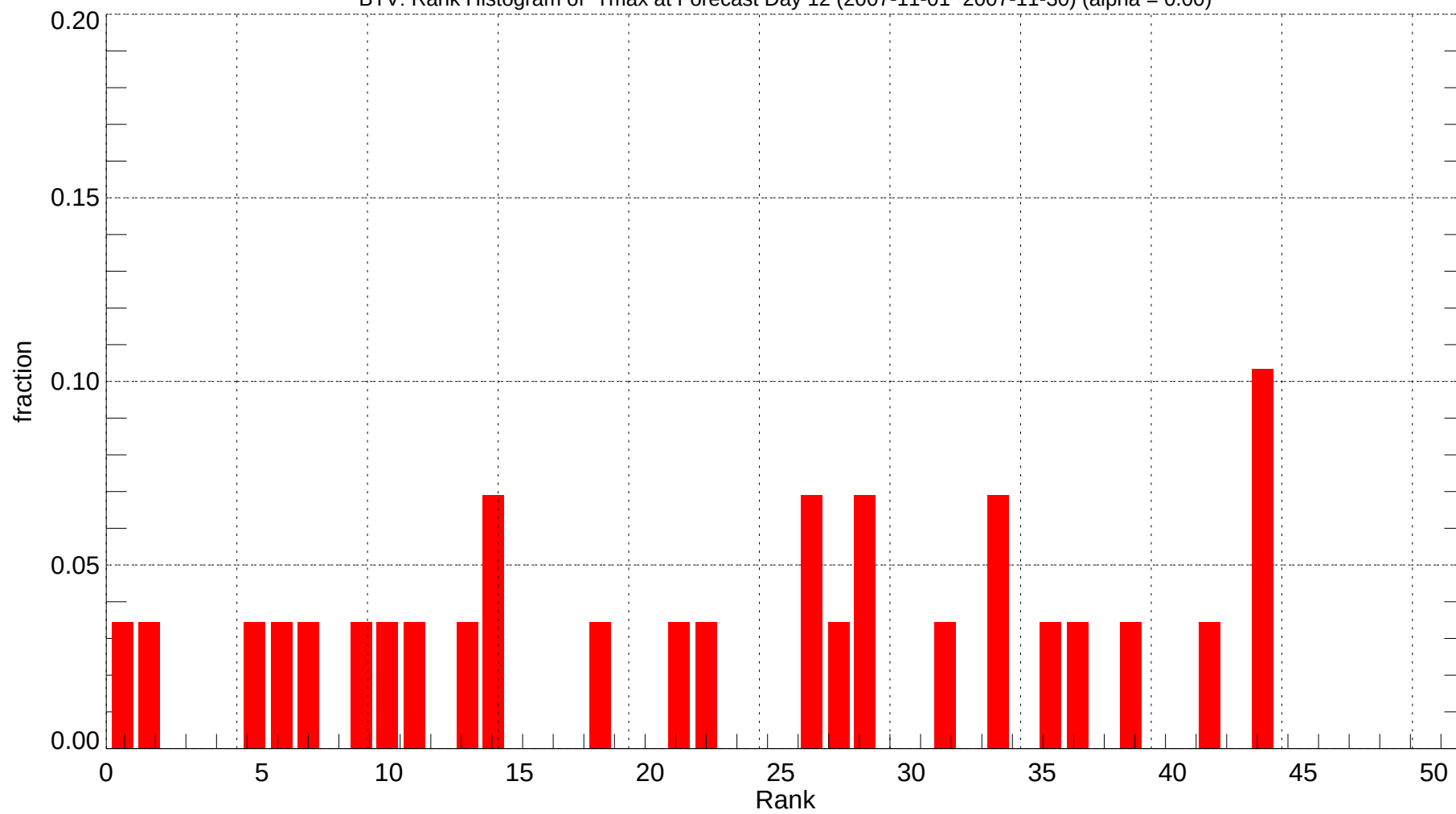
BTV: Rank Histogram of Tmax at Forecast Day 12 (2007-11-01~2007-11-30) (alpha = 0.00)
