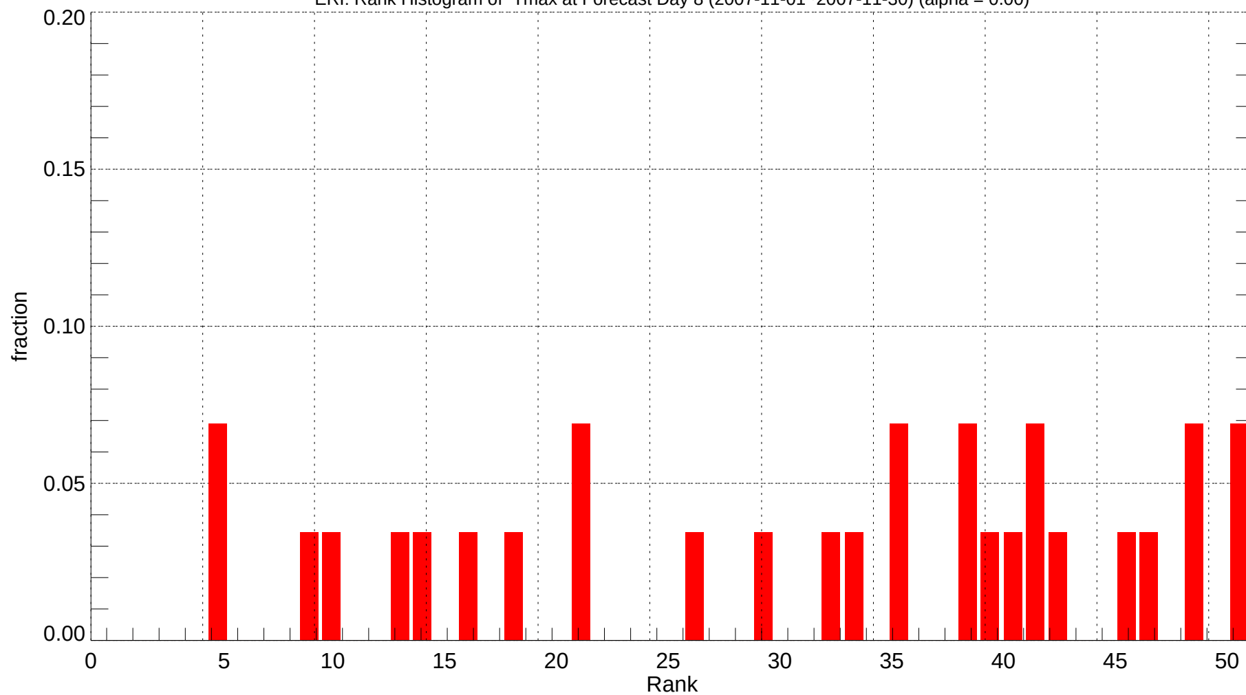
ERI: Rank Histogram of Tmax at Forecast Day 8 (2007-11-01~2007-11-30) (alpha = 0.00)
