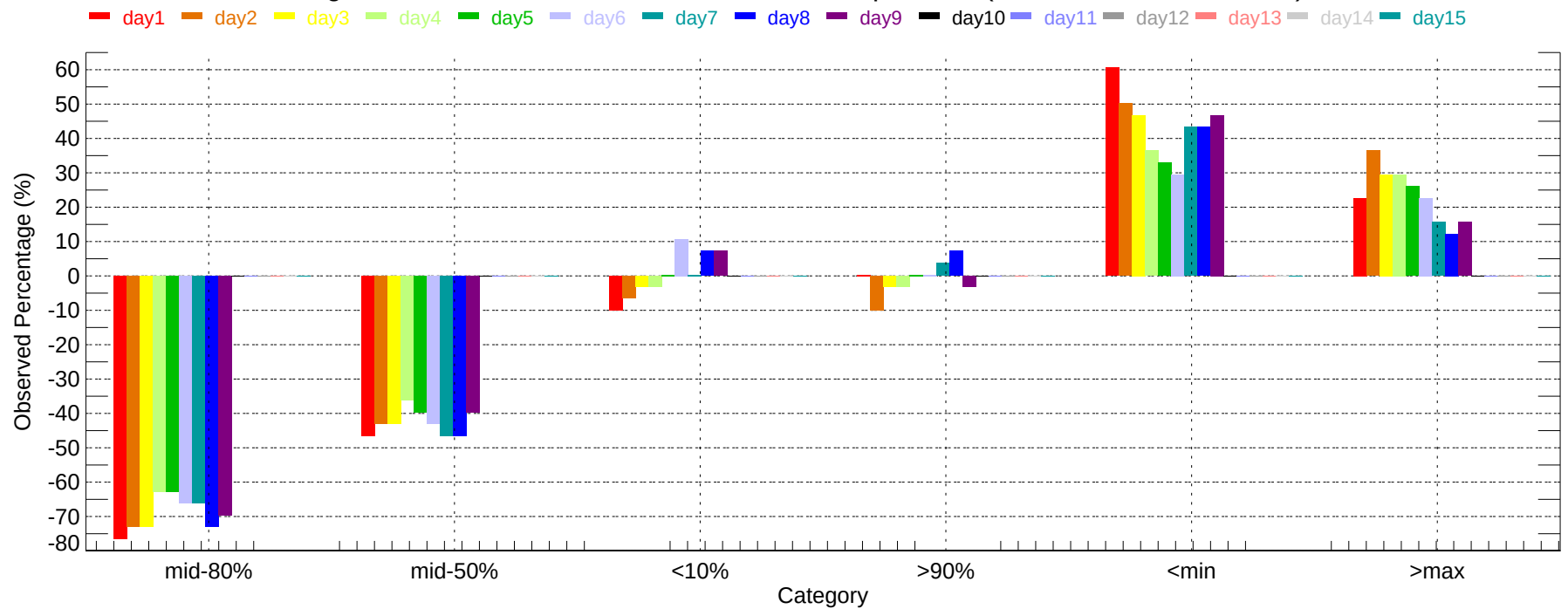
Observed Percentage Deviation of Ensembles - NKX: Max Temperature (2007-11-01~2007-11-30)
