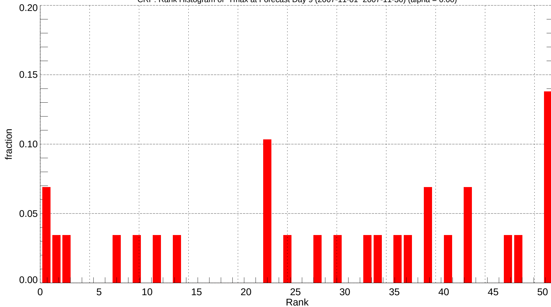
CRP: Rank Histogram of Tmax at Forecast Day 9 (2007-11-01~2007-11-30) (alpha = 0.00)
