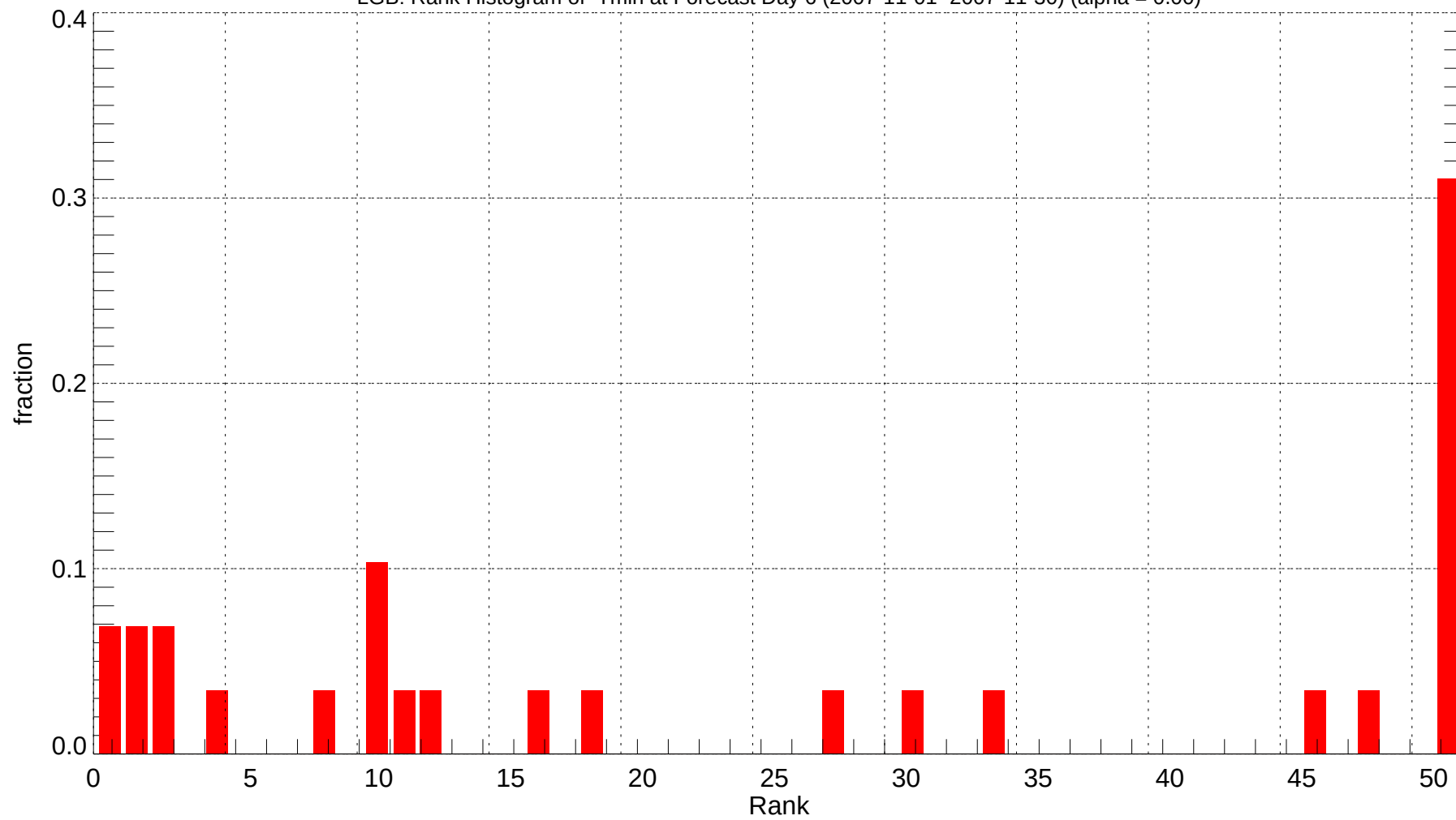
LGB: Rank Histogram of Tmin at Forecast Day 6 (2007-11-01~2007-11-30) (alpha = 0.00)
