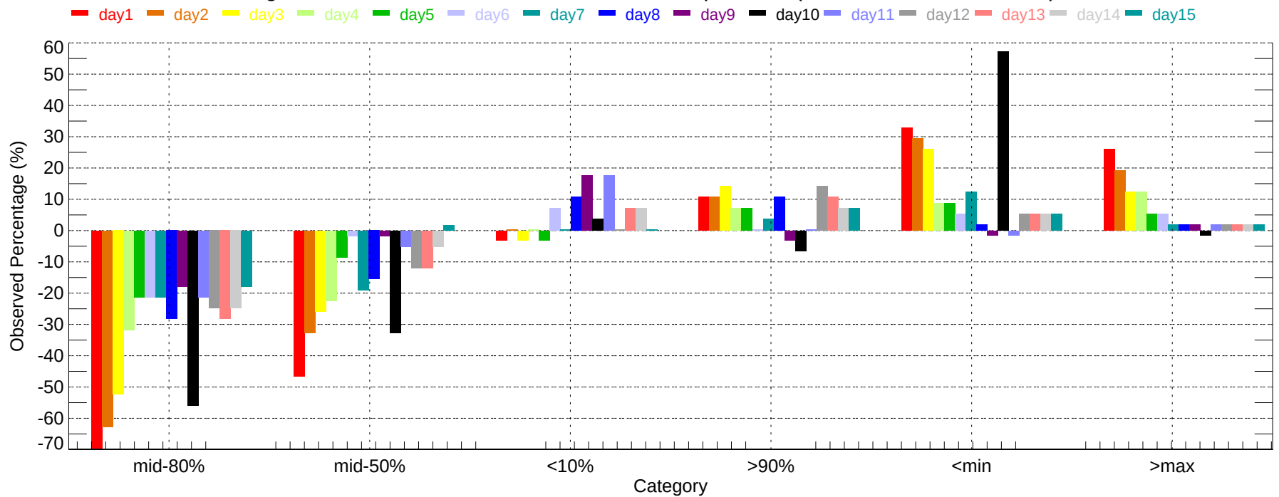
Observed Percentage Deviation of Ensembles - AVP: Min Temperature (2007-11-01~2007-11-30)
