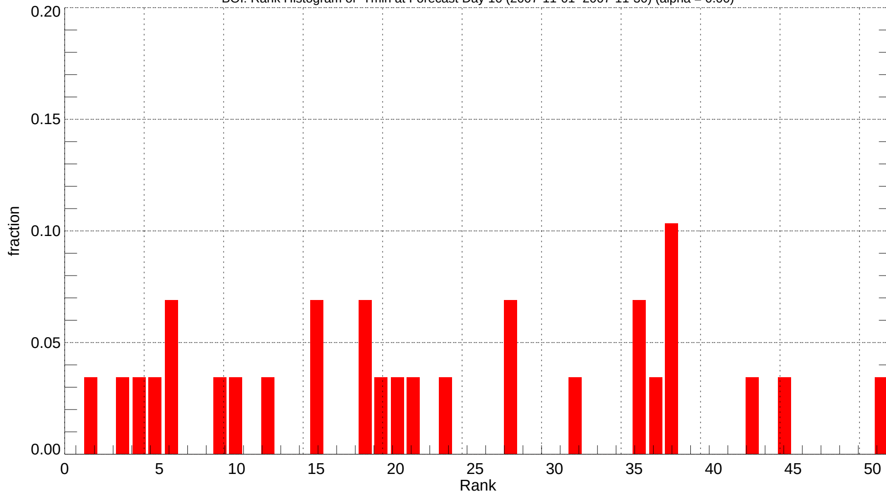
BOI: Rank Histogram of Tmin at Forecast Day 10 (2007-11-01~2007-11-30) (alpha = 0.00)
