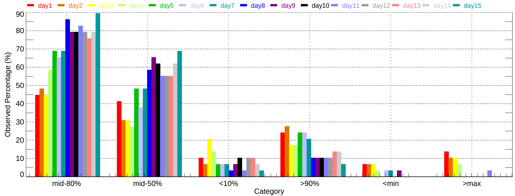
Observed Percentage of Ensembles - BOI: Max Temperature (2007-11-01~2007-11-30)
