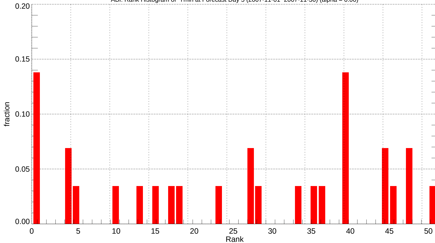
ABI: Rank Histogram of Tmin at Forecast Day 5 (2007-11-01~2007-11-30) (alpha = 0.00)
