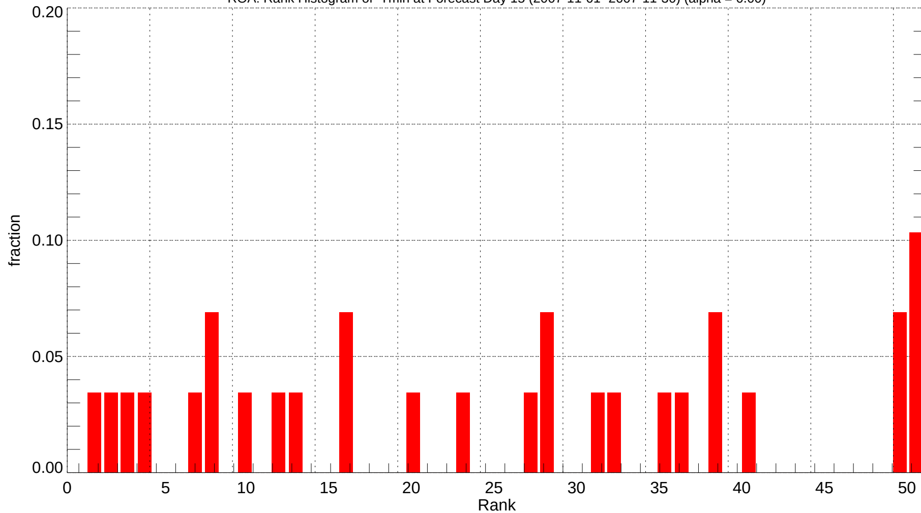
ROA: Rank Histogram of Tmin at Forecast Day 15 (2007-11-01~2007-11-30) (alpha = 0.00)
