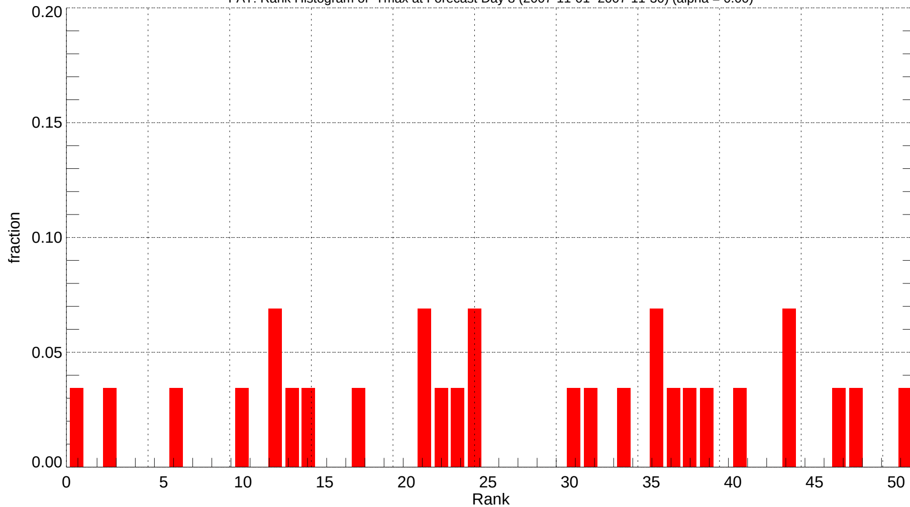
FAT: Rank Histogram of Tmax at Forecast Day 8 (2007-11-01~2007-11-30) (alpha = 0.00)
