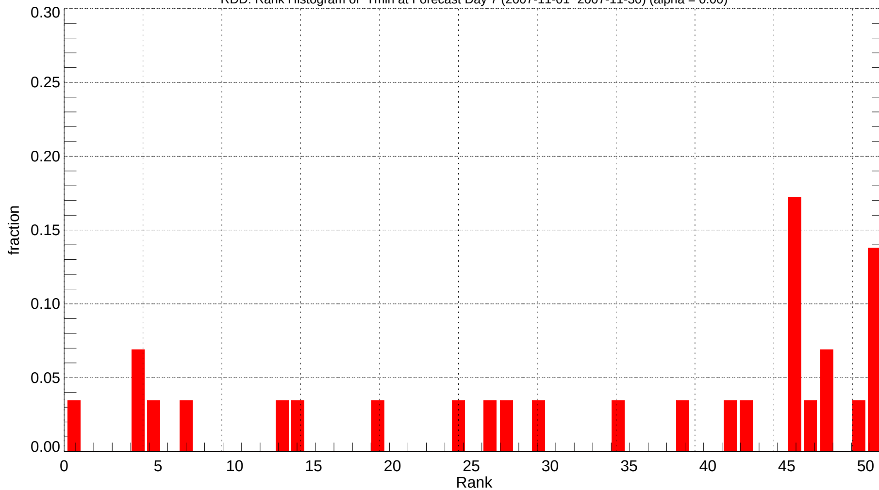
RDD: Rank Histogram of Tmin at Forecast Day 7 (2007-11-01~2007-11-30) (alpha = 0.00)
