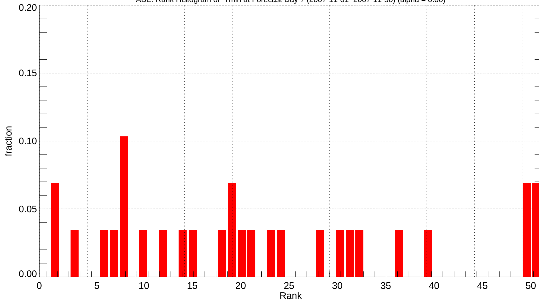
ABE: Rank Histogram of Tmin at Forecast Day 7 (2007-11-01~2007-11-30) (alpha = 0.00)
