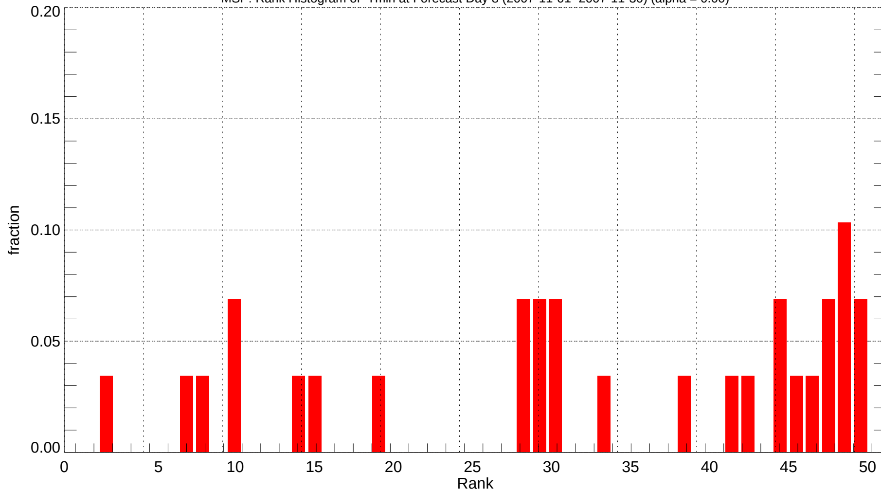
MSP: Rank Histogram of Tmin at Forecast Day 8 (2007-11-01~2007-11-30) (alpha = 0.00)
