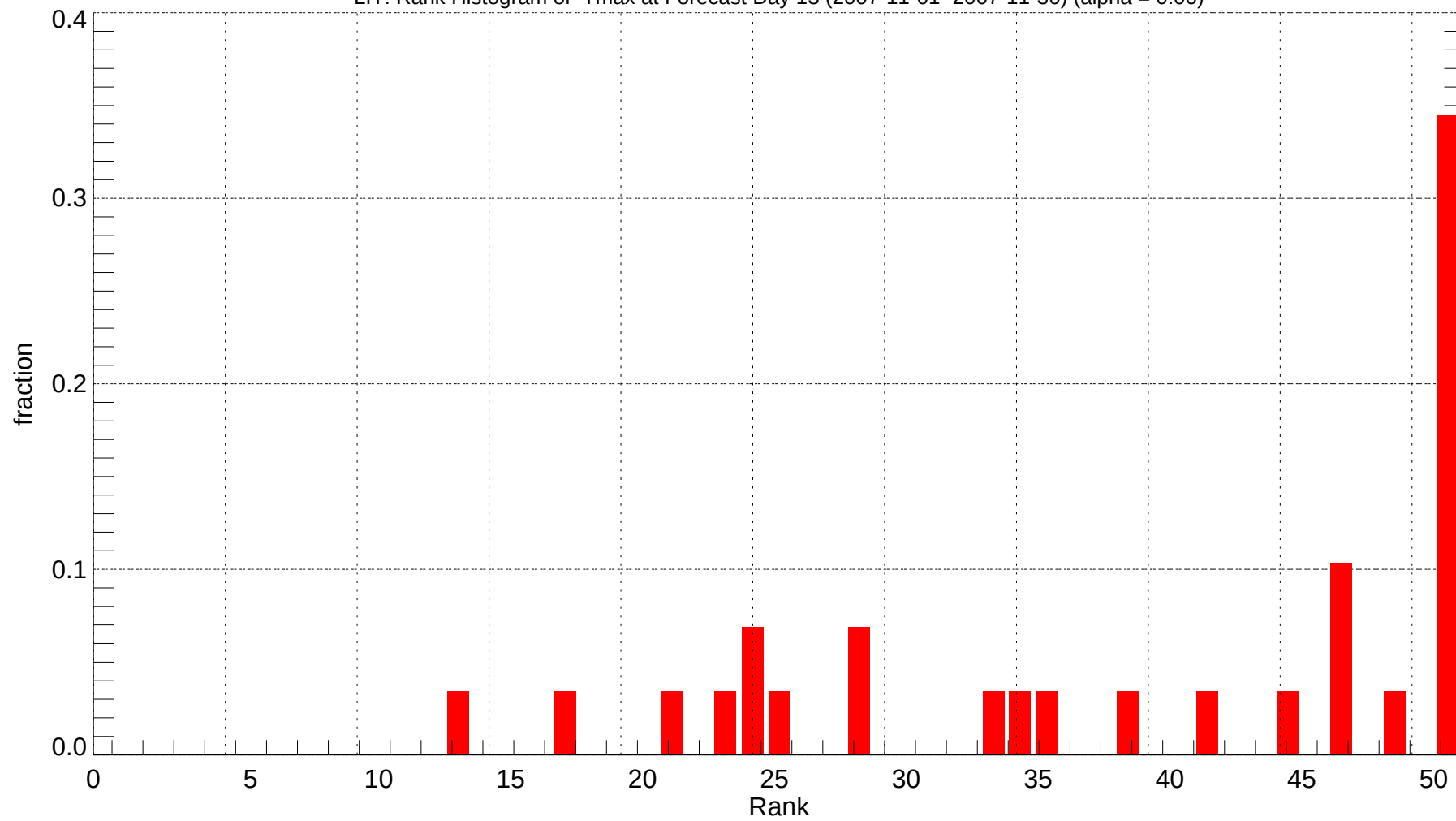
LIT: Rank Histogram of Tmax at Forecast Day 13 (2007-11-01~2007-11-30) (alpha = 0.00)
