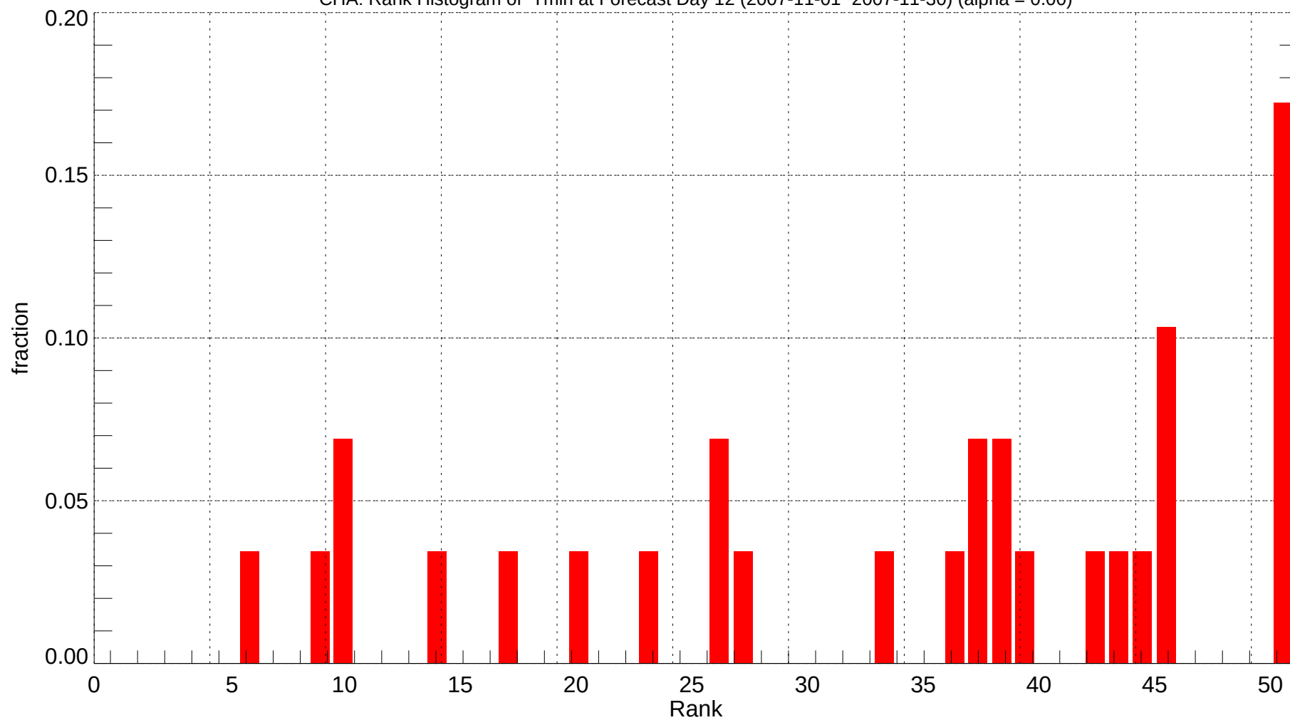
CHA: Rank Histogram of Tmin at Forecast Day 12 (2007-11-01~2007-11-30) (alpha = 0.00)
