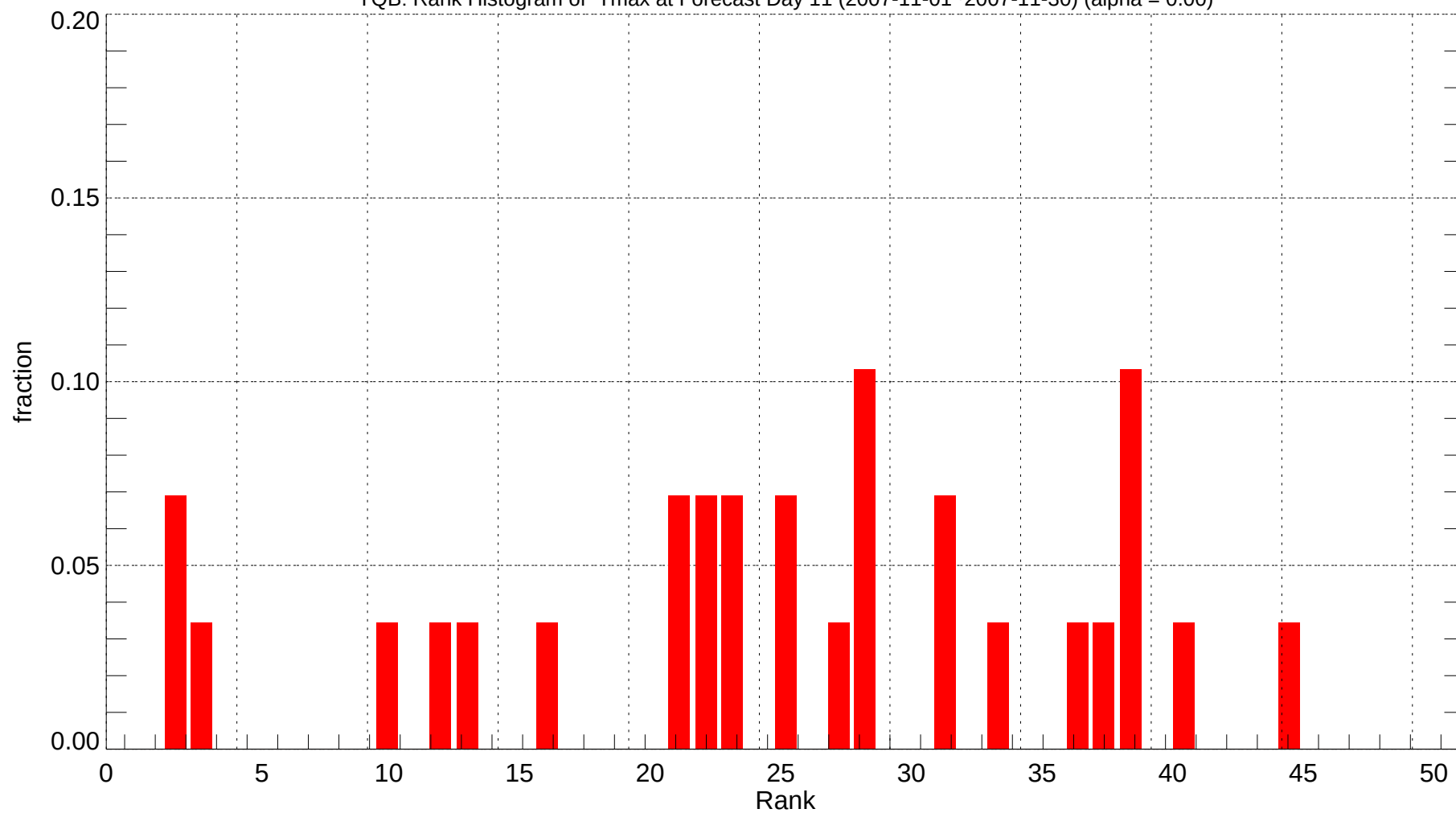
YQB: Rank Histogram of Tmax at Forecast Day 11 (2007-11-01~2007-11-30) (alpha = 0.00)
