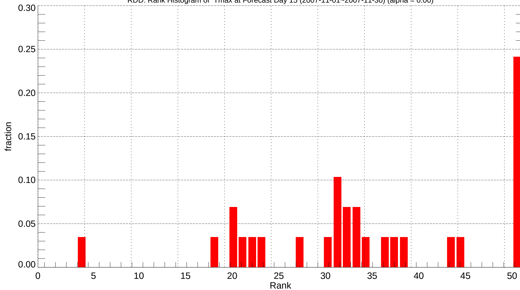
RDD: Rank Histogram of Tmax at Forecast Day 15 (2007-11-01~2007-11-30) (alpha = 0.00)
