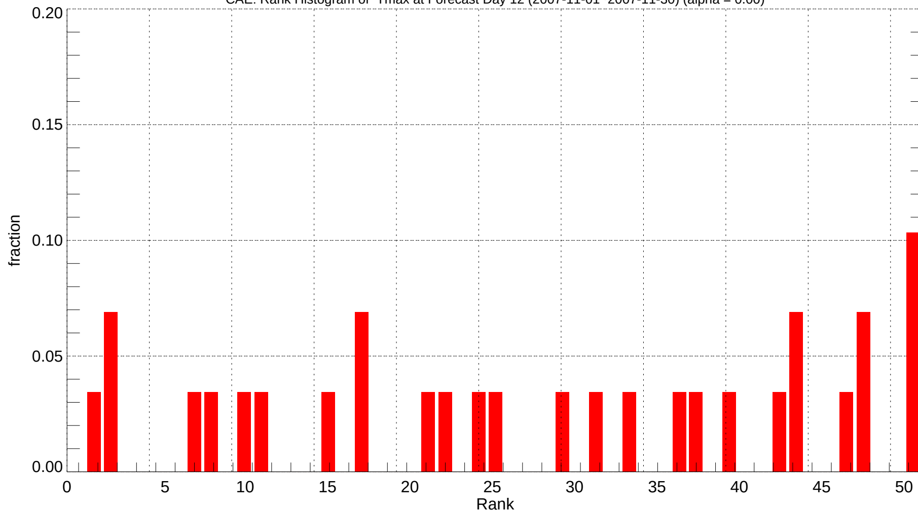
CAE: Rank Histogram of Tmax at Forecast Day 12 (2007-11-01~2007-11-30) (alpha = 0.00)
