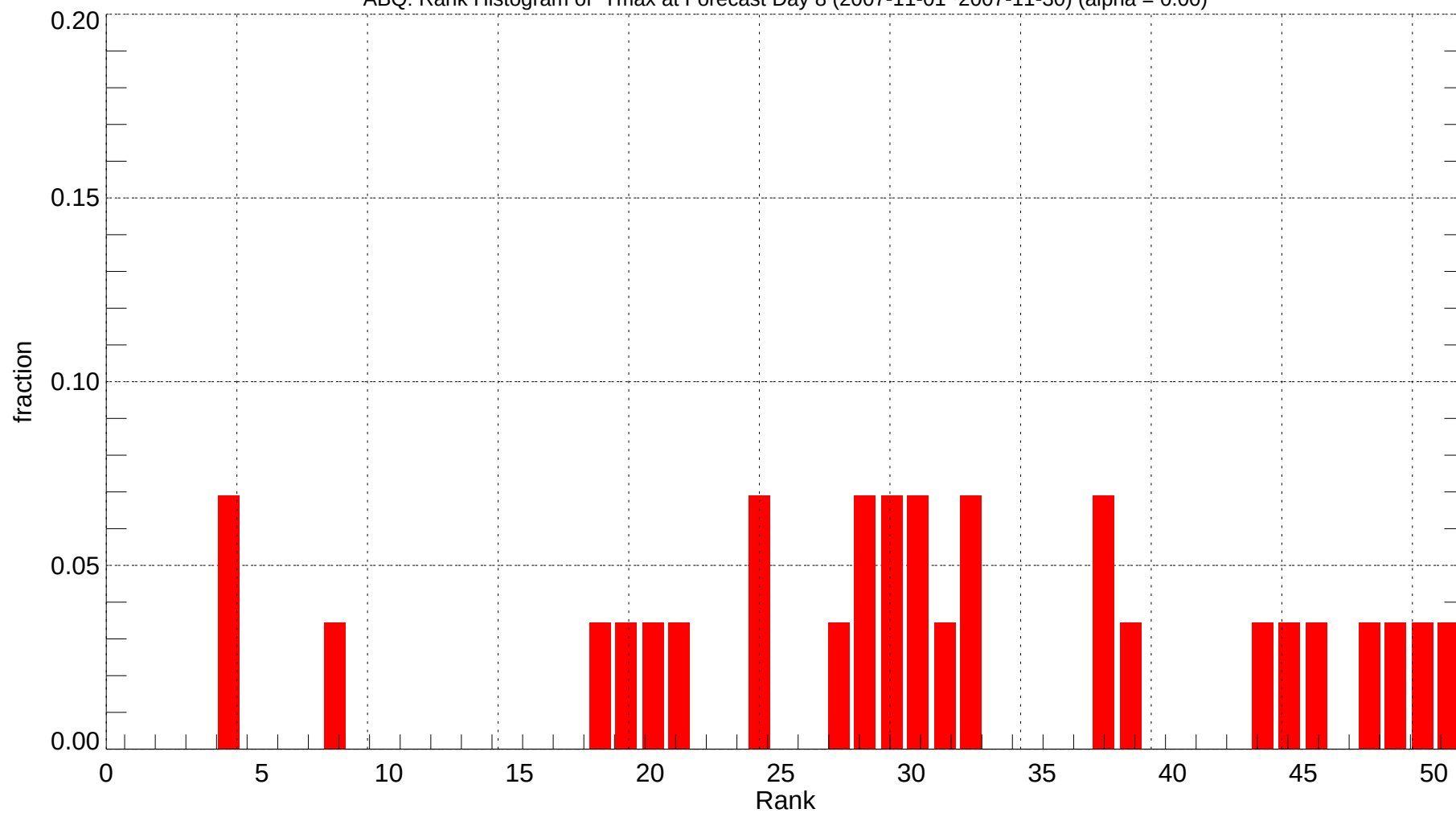
ABQ: Rank Histogram of Tmax at Forecast Day 8 (2007-11-01~2007-11-30) (alpha = 0.00)
