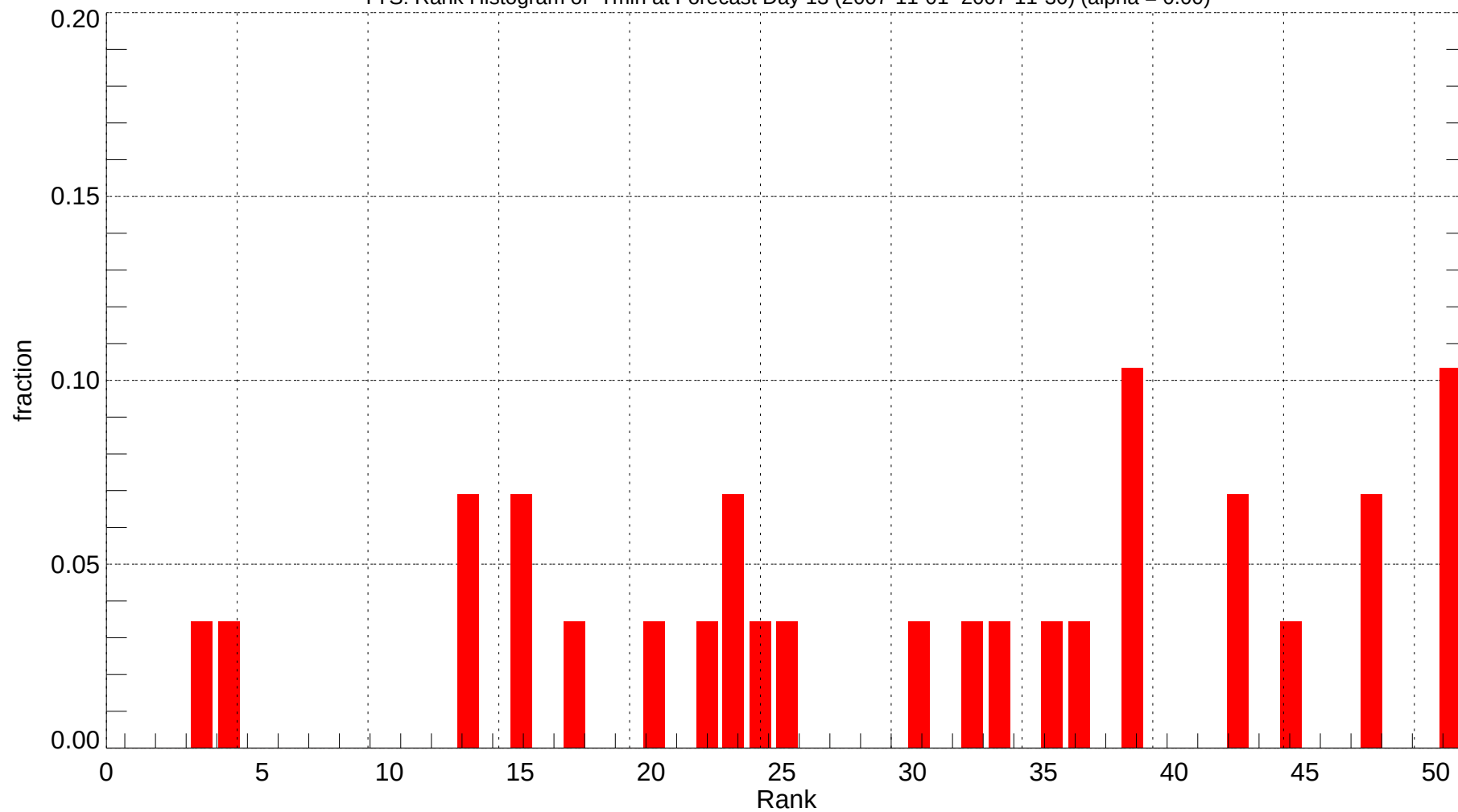
TYS: Rank Histogram of Tmin at Forecast Day 13 (2007-11-01~2007-11-30) (alpha = 0.00)
