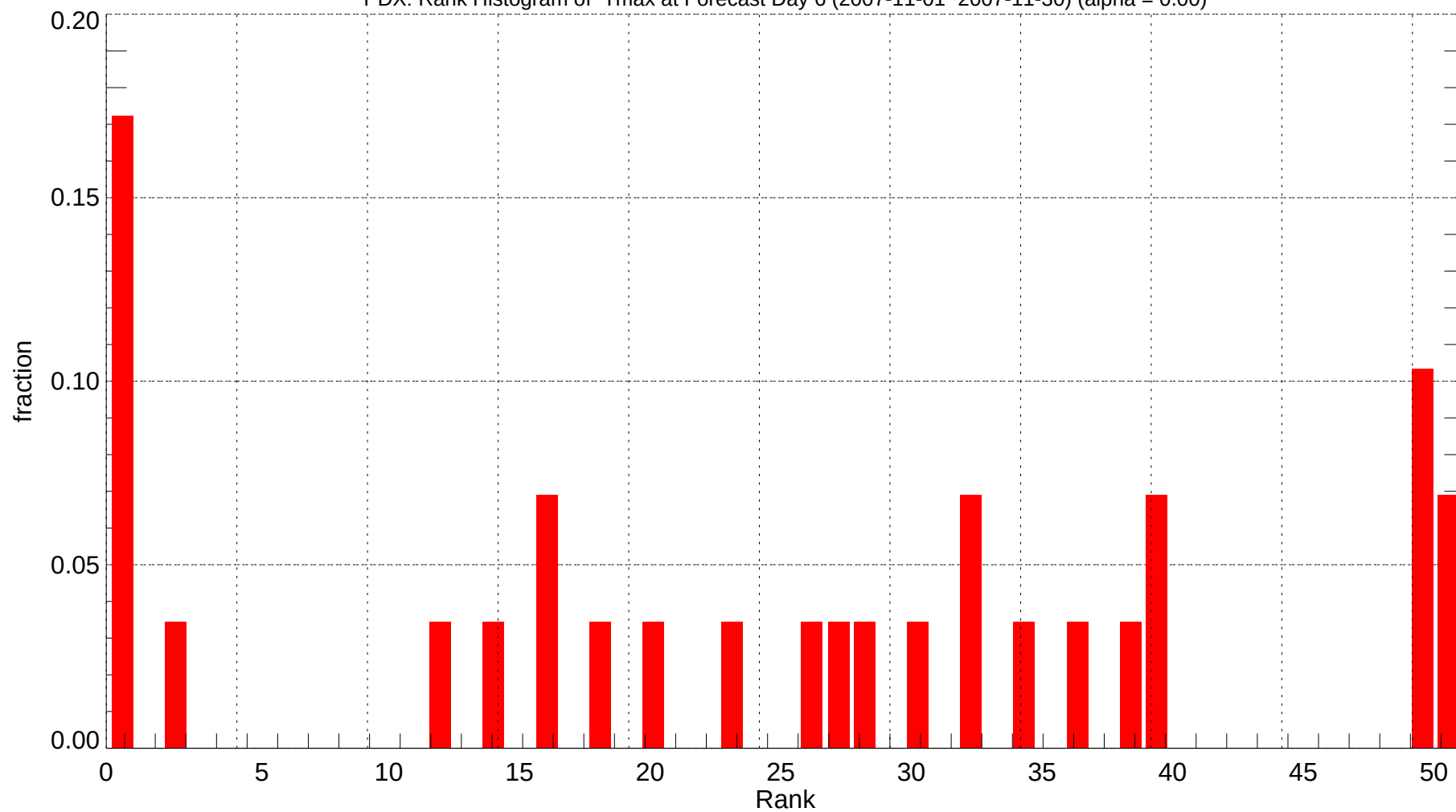
PDX: Rank Histogram of Tmax at Forecast Day 6 (2007-11-01~2007-11-30) (alpha = 0.00)
