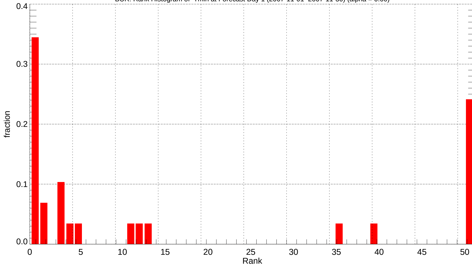
BUR: Rank Histogram of Tmin at Forecast Day 1 (2007-11-01~2007-11-30) (alpha = 0.00)
