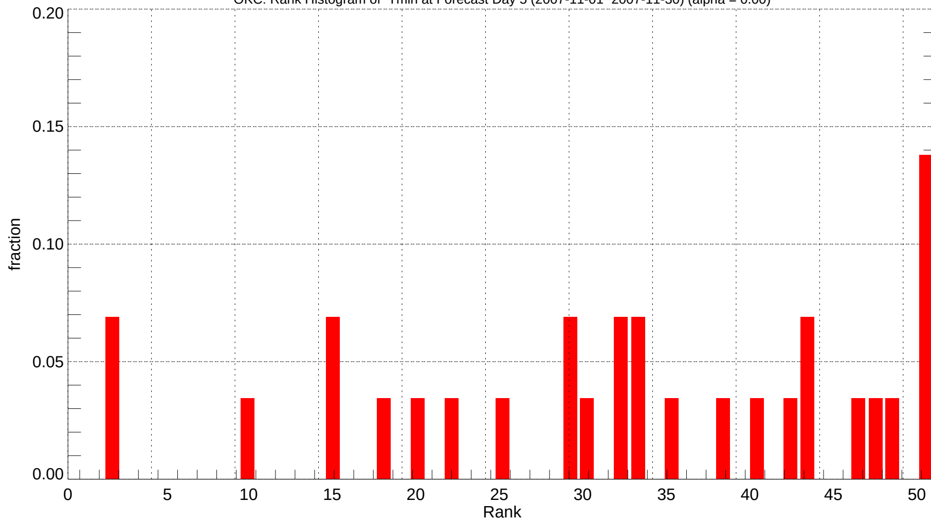
OKC: Rank Histogram of Tmin at Forecast Day 5 (2007-11-01~2007-11-30) (alpha = 0.00)
