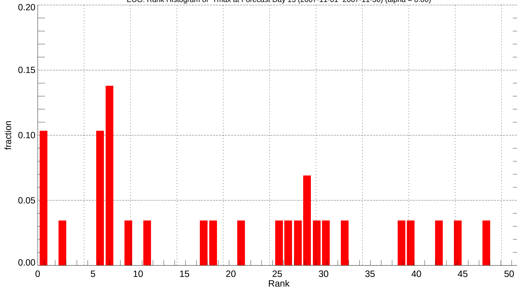
EUG: Rank Histogram of Tmax at Forecast Day 13 (2007-11-01~2007-11-30) (alpha = 0.00)
