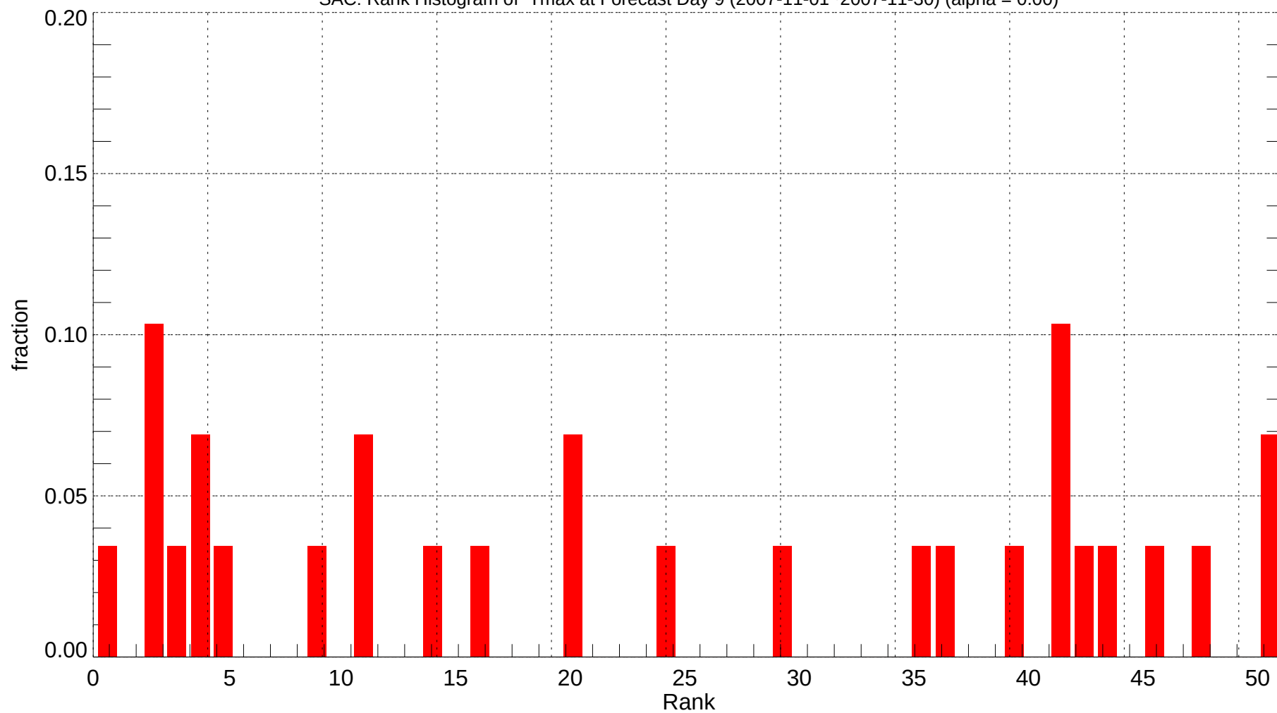
SAC: Rank Histogram of Tmax at Forecast Day 9 (2007-11-01~2007-11-30) (alpha = 0.00)
