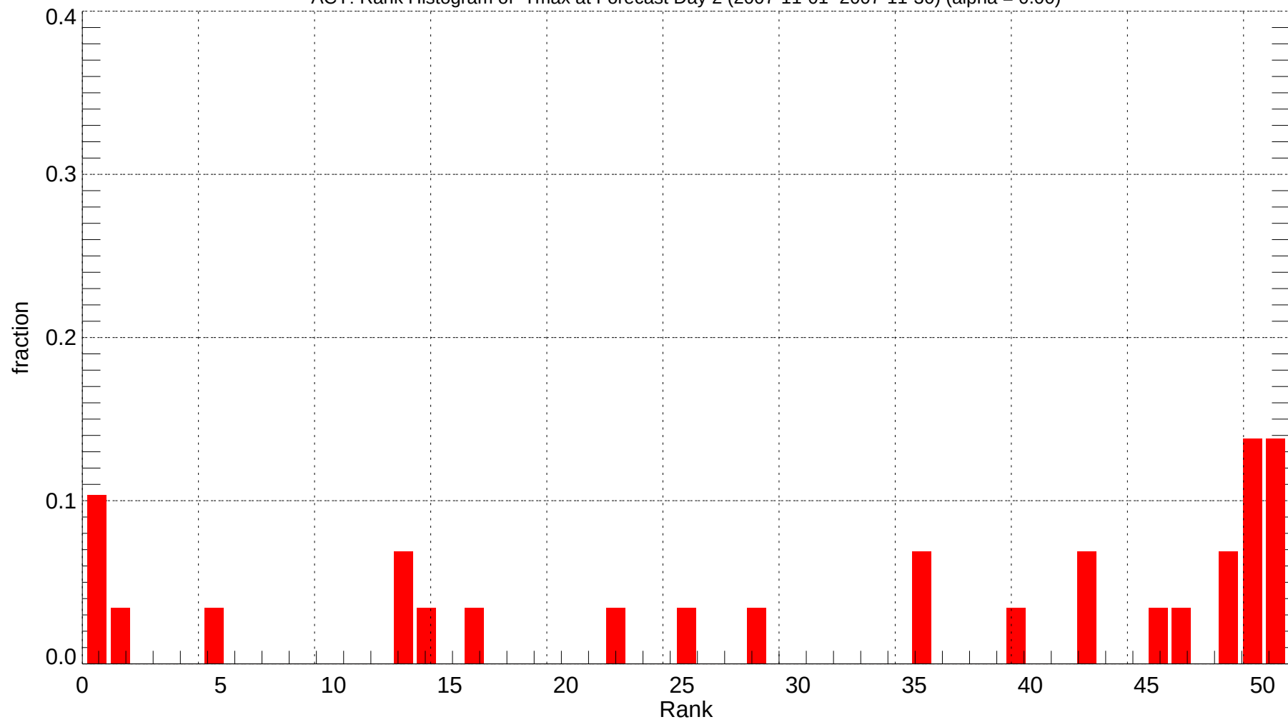
ACY: Rank Histogram of Tmax at Forecast Day 2 (2007-11-01~2007-11-30) (alpha = 0.00)
