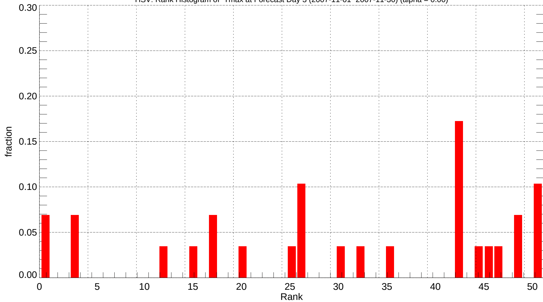
HSV: Rank Histogram of Tmax at Forecast Day 3 (2007-11-01~2007-11-30) (alpha = 0.00)
