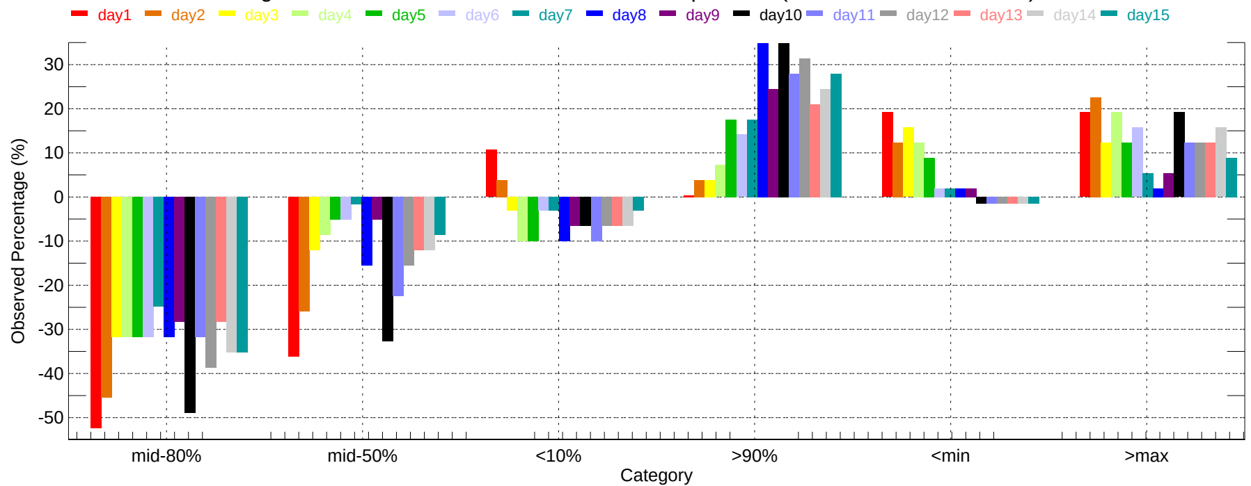
Observed Percentage Deviation of Ensembles - MCI: Max Temperature (2007-11-01~2007-11-30)
