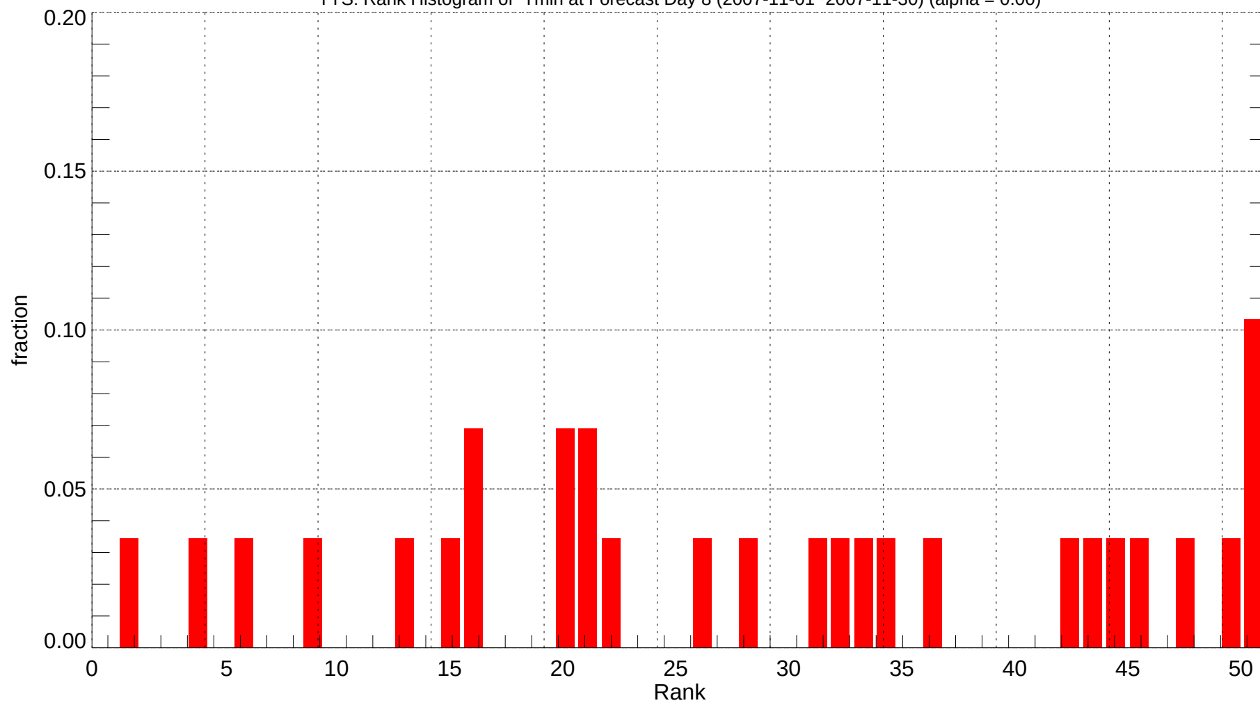
TYS: Rank Histogram of Tmin at Forecast Day 8 (2007-11-01~2007-11-30) (alpha = 0.00)
