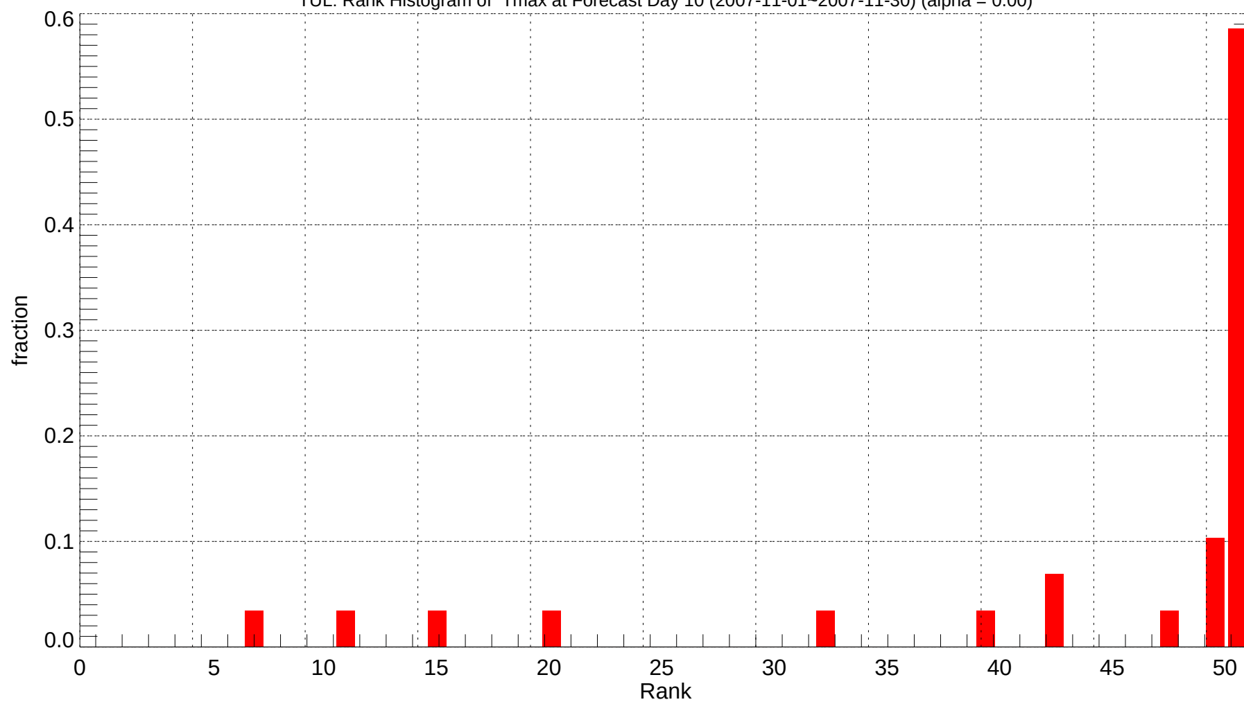
TUL: Rank Histogram of Tmax at Forecast Day 10 (2007-11-01~2007-11-30) (alpha = 0.00)
