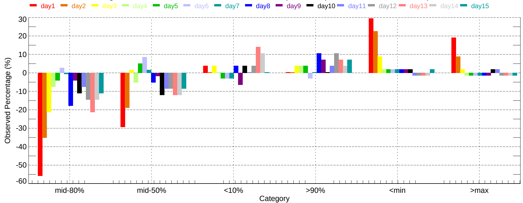
Observed Percentage Deviation of Ensembles - JFK: Min Temperature (2007-11-01~2007-11-30)
