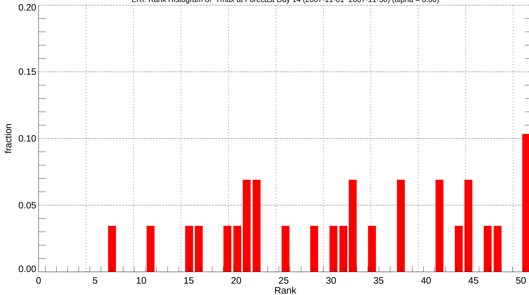
ERI: Rank Histogram of Tmax at Forecast Day 14 (2007-11-01~2007-11-30) (alpha = 0.00)
