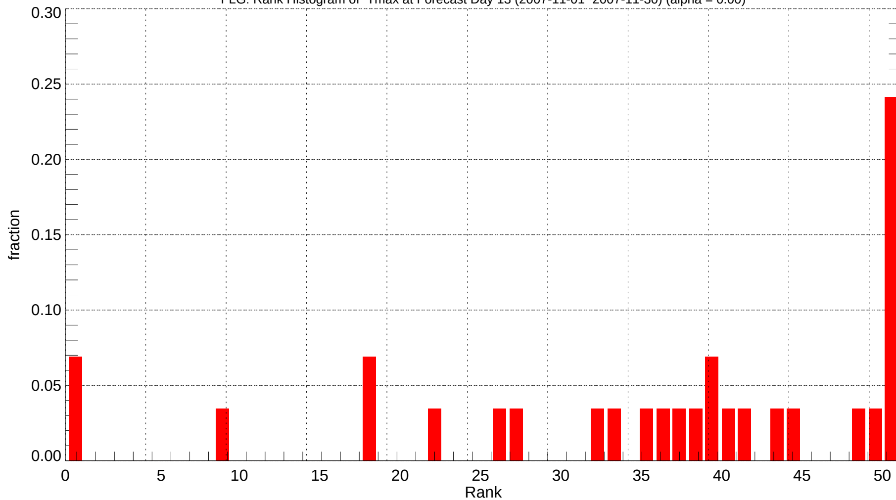
FLG: Rank Histogram of Tmax at Forecast Day 13 (2007-11-01~2007-11-30) (alpha = 0.00)
