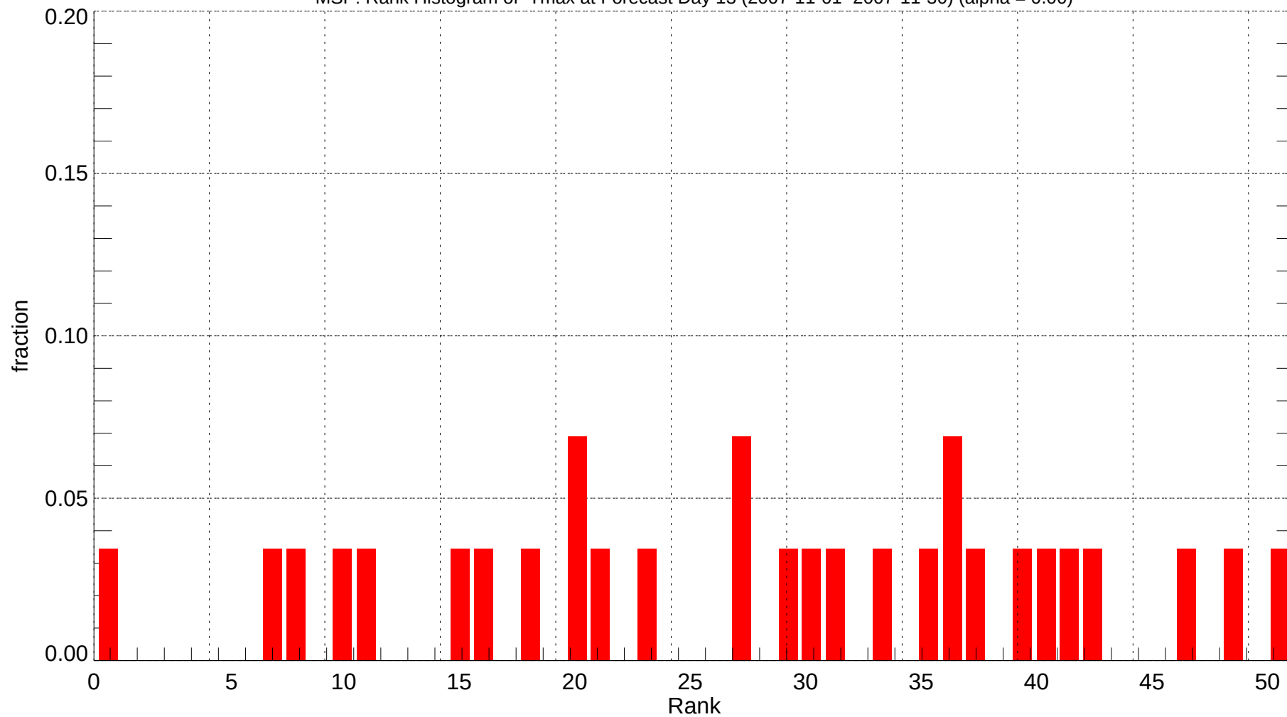
MSP: Rank Histogram of Tmax at Forecast Day 13 (2007-11-01~2007-11-30) (alpha = 0.00)
