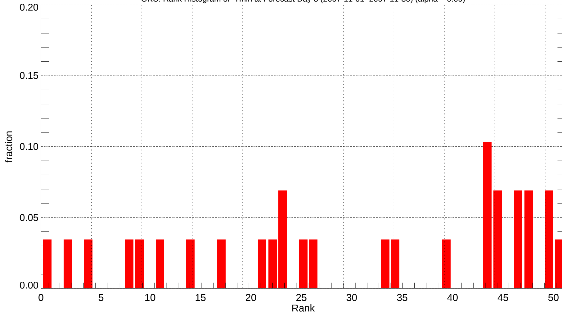
OKC: Rank Histogram of Tmin at Forecast Day 3 (2007-11-01~2007-11-30) (alpha = 0.00)
