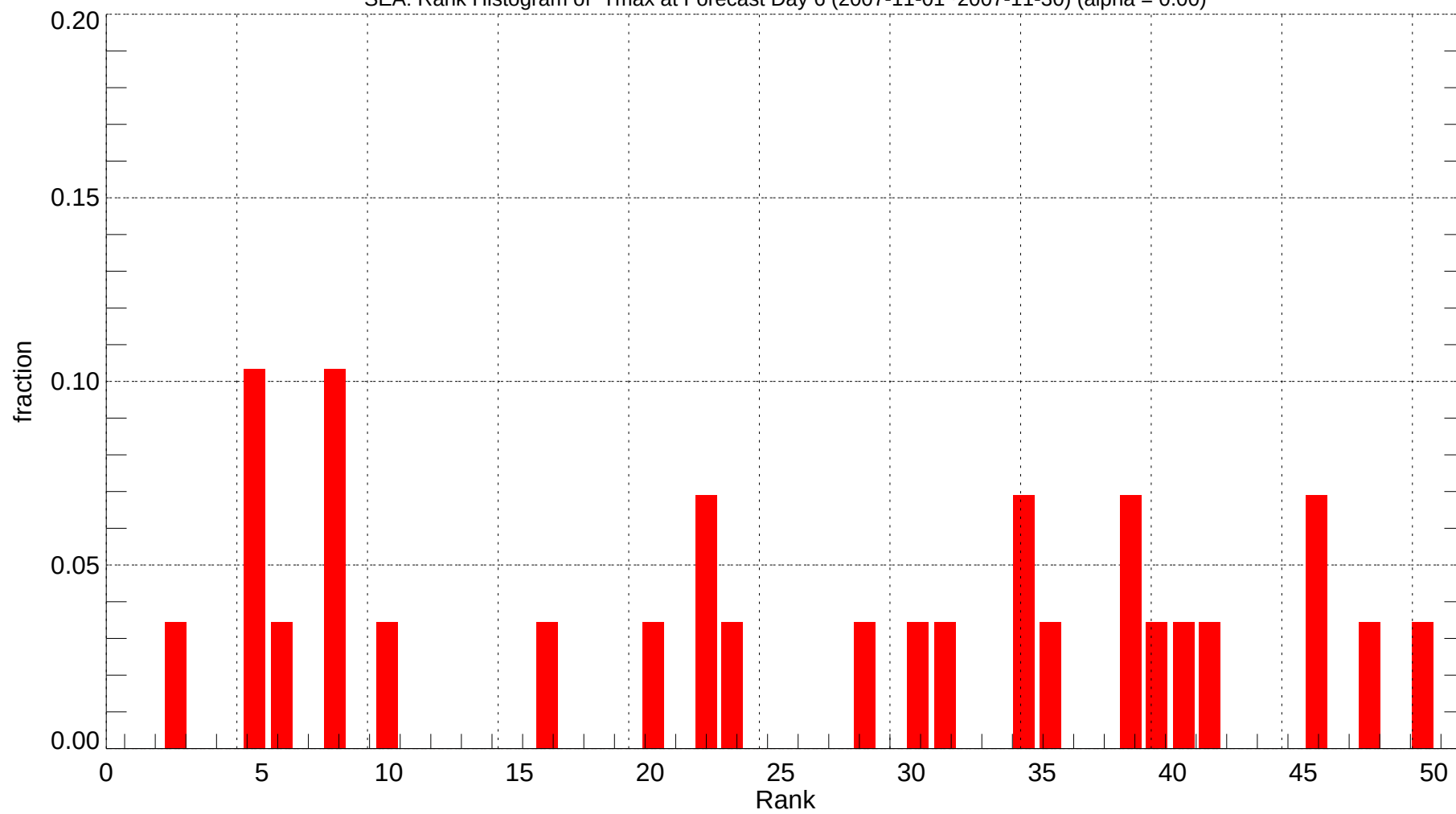
SEA: Rank Histogram of Tmax at Forecast Day 6 (2007-11-01~2007-11-30) (alpha = 0.00)
