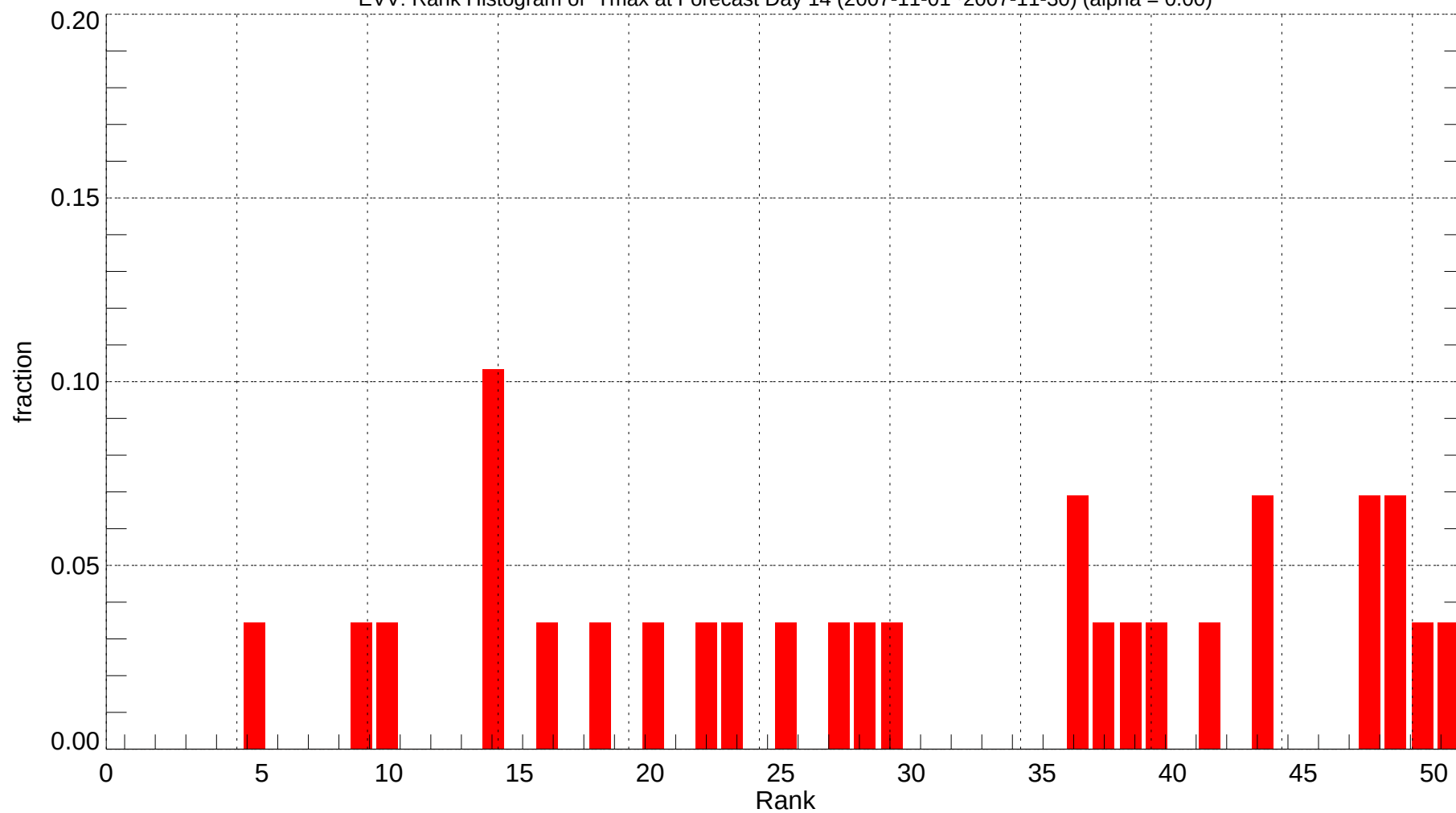
EVV: Rank Histogram of Tmax at Forecast Day 14 (2007-11-01~2007-11-30) (alpha = 0.00)
