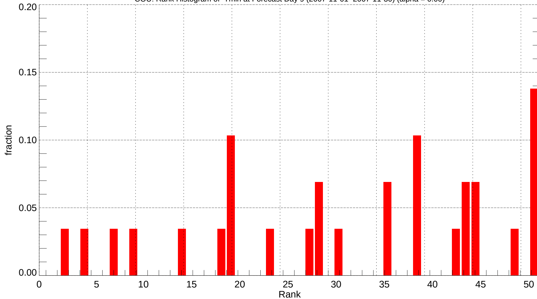
COU: Rank Histogram of Tmin at Forecast Day 9 (2007-11-01~2007-11-30) (alpha = 0.00)
