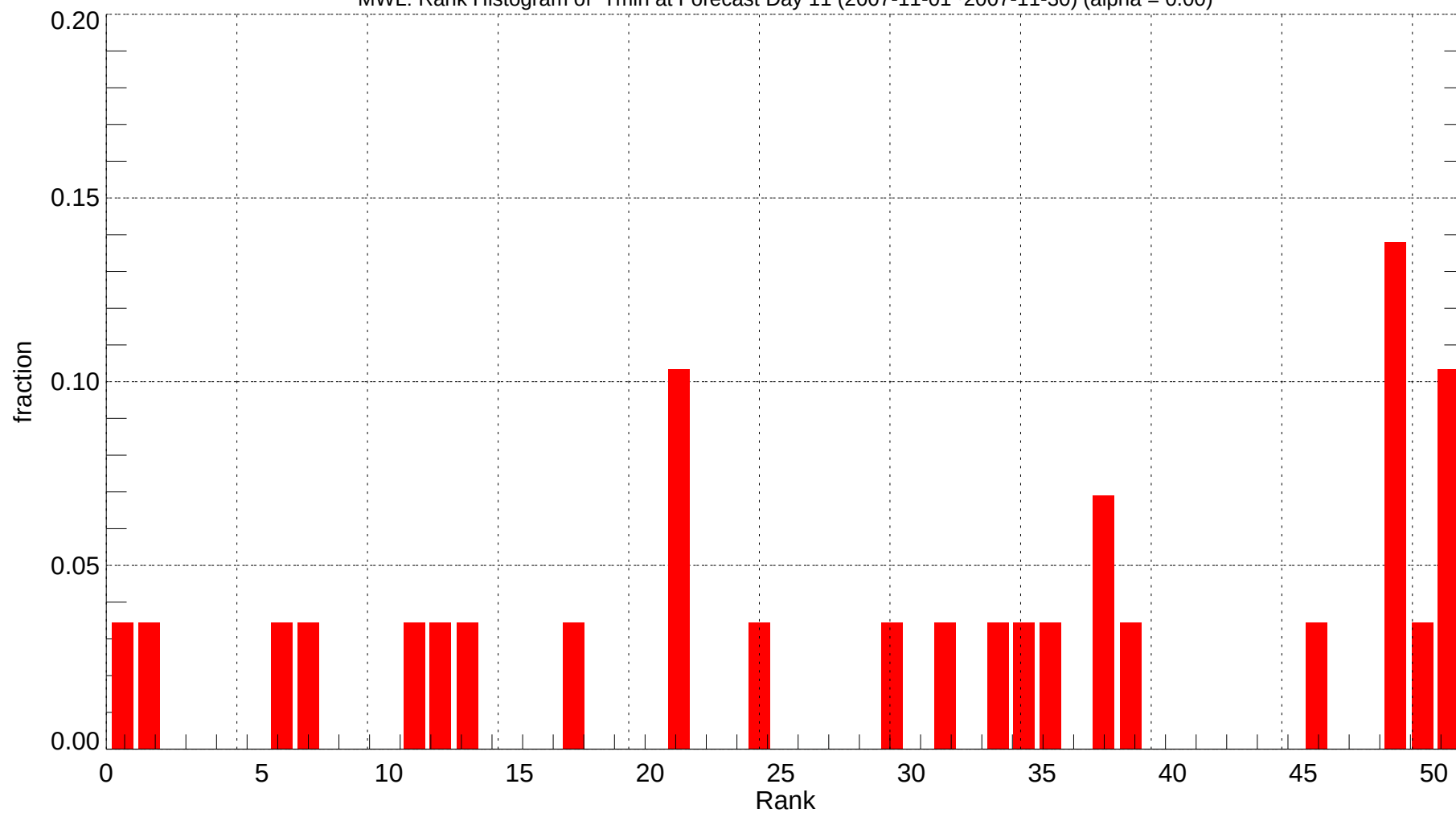
MWL: Rank Histogram of Tmin at Forecast Day 11 (2007-11-01~2007-11-30) (alpha = 0.00)
