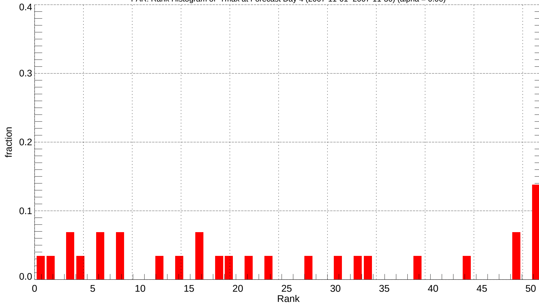
FAR: Rank Histogram of Tmax at Forecast Day 4 (2007-11-01~2007-11-30) (alpha = 0.00)
