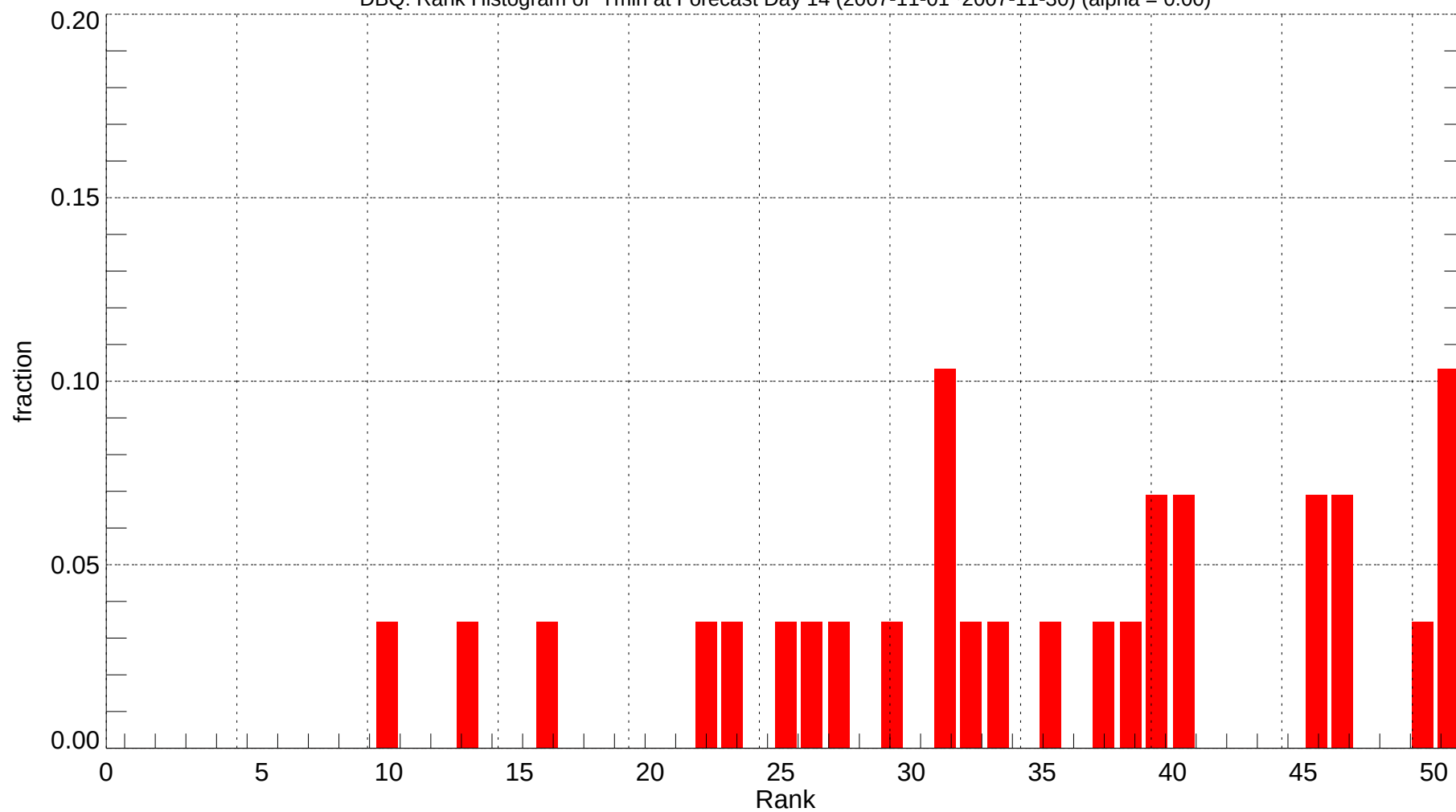
DBQ: Rank Histogram of Tmin at Forecast Day 14 (2007-11-01~2007-11-30) (alpha = 0.00)
