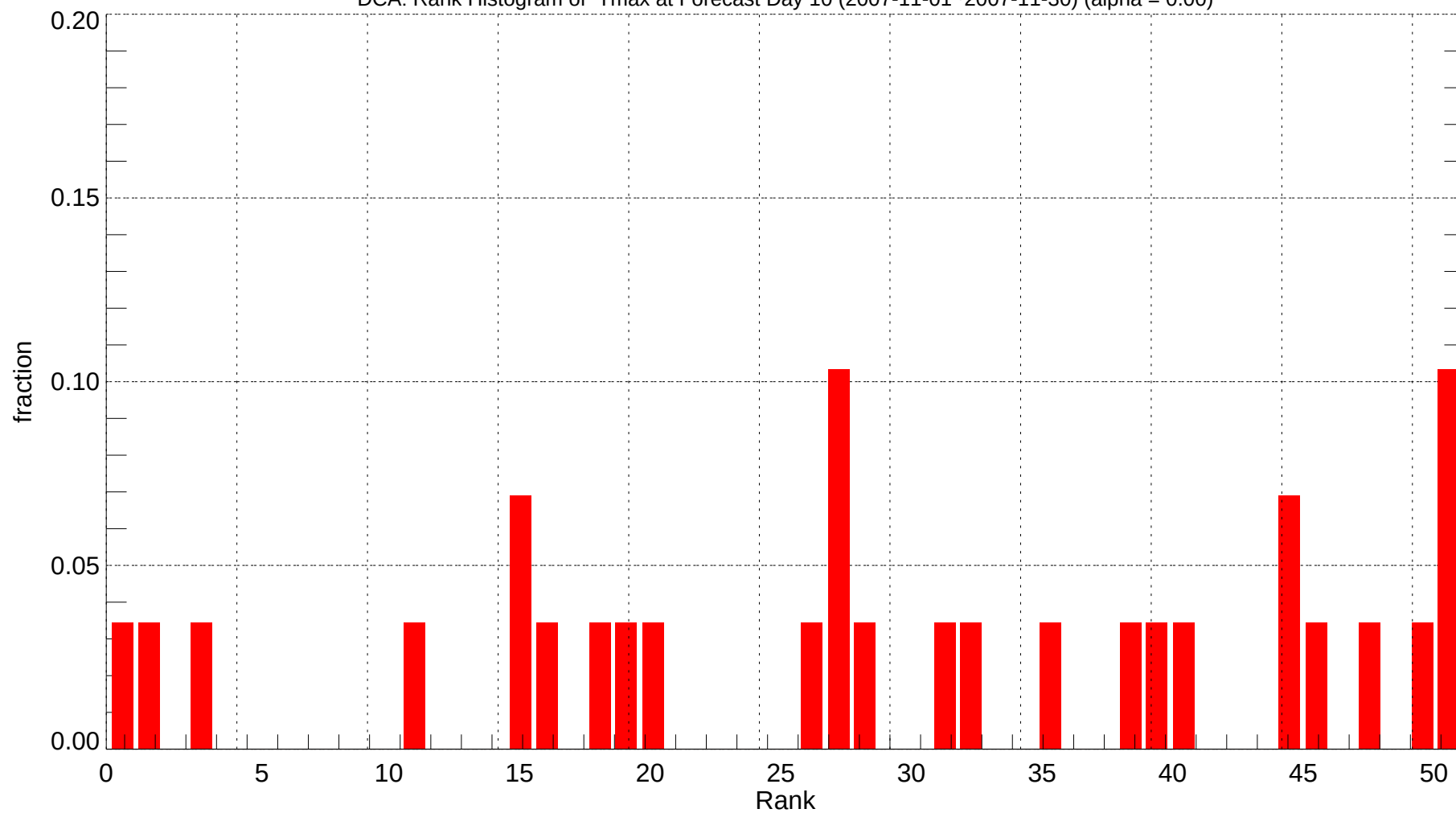
DCA: Rank Histogram of Tmax at Forecast Day 10 (2007-11-01~2007-11-30) (alpha = 0.00)
