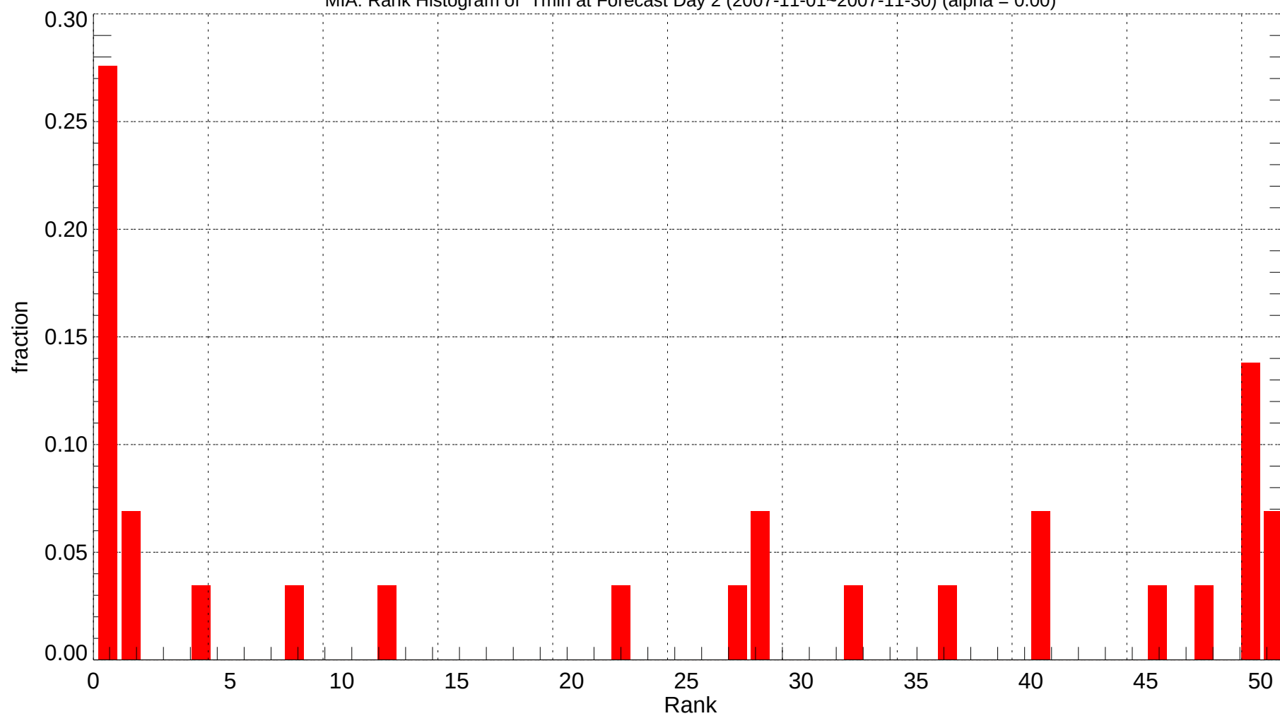
MIA: Rank Histogram of Tmin at Forecast Day 2 (2007-11-01~2007-11-30) (alpha = 0.00)
