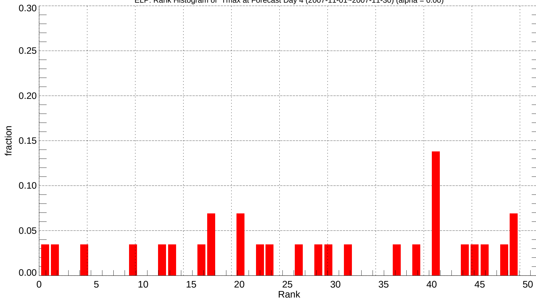
ELP: Rank Histogram of Tmax at Forecast Day 4 (2007-11-01~2007-11-30) (alpha = 0.00)
