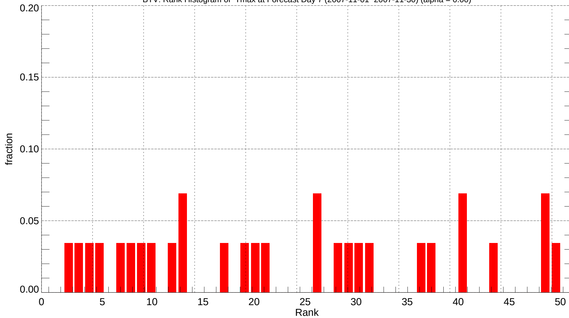
BTV: Rank Histogram of Tmax at Forecast Day 7 (2007-11-01~2007-11-30) (alpha = 0.00)
