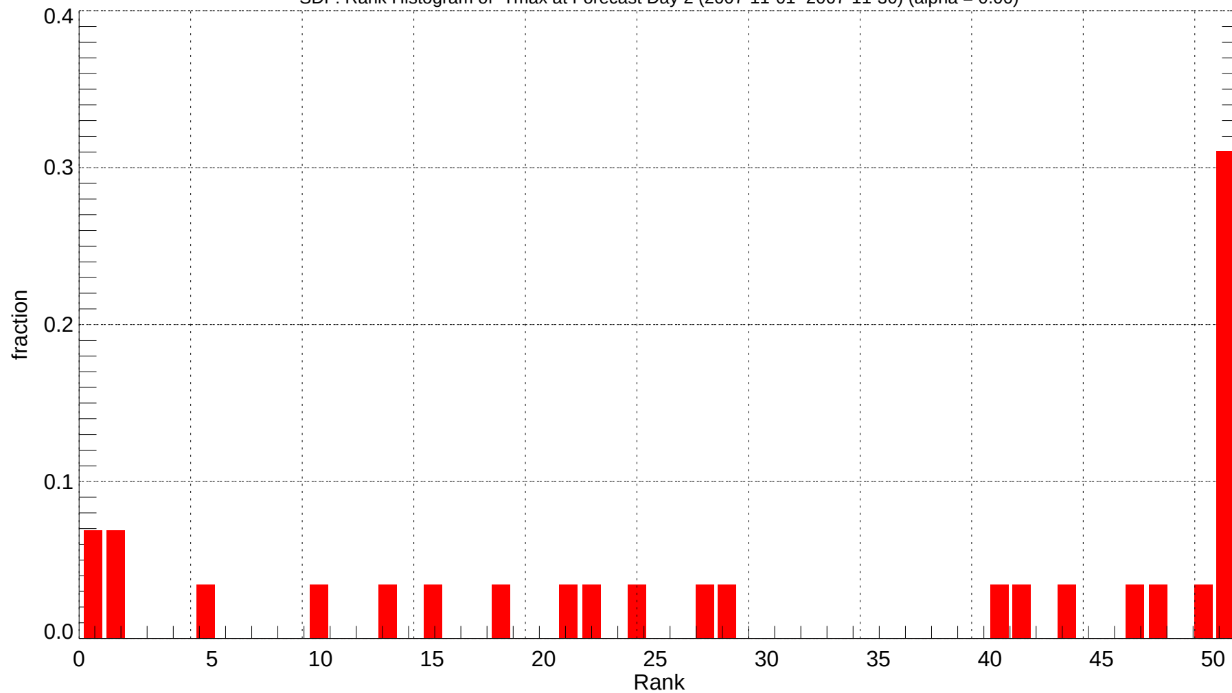
SDF: Rank Histogram of Tmax at Forecast Day 2 (2007-11-01~2007-11-30) (alpha = 0.00)
