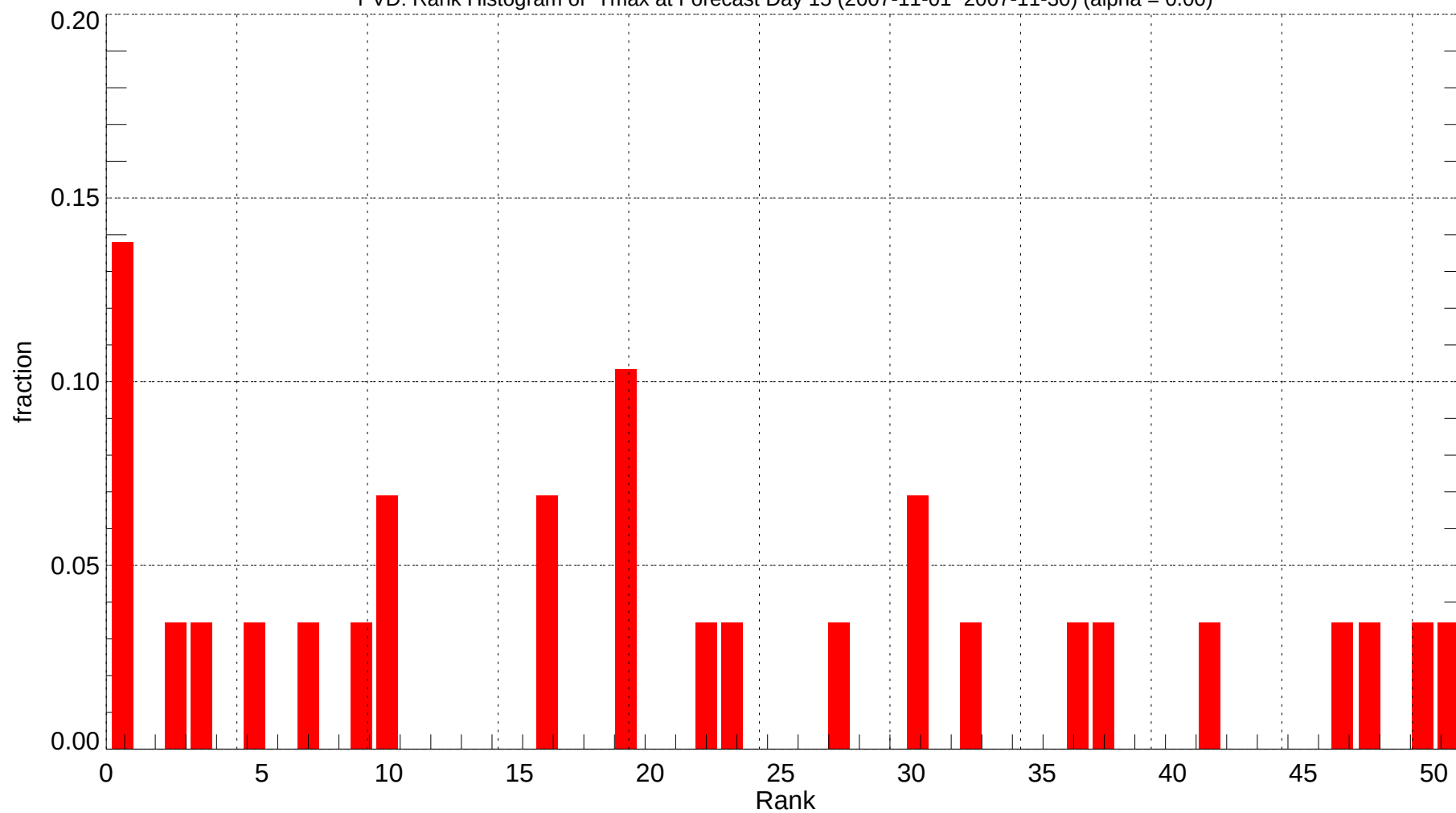
PVD: Rank Histogram of Tmax at Forecast Day 15 (2007-11-01~2007-11-30) (alpha = 0.00)
