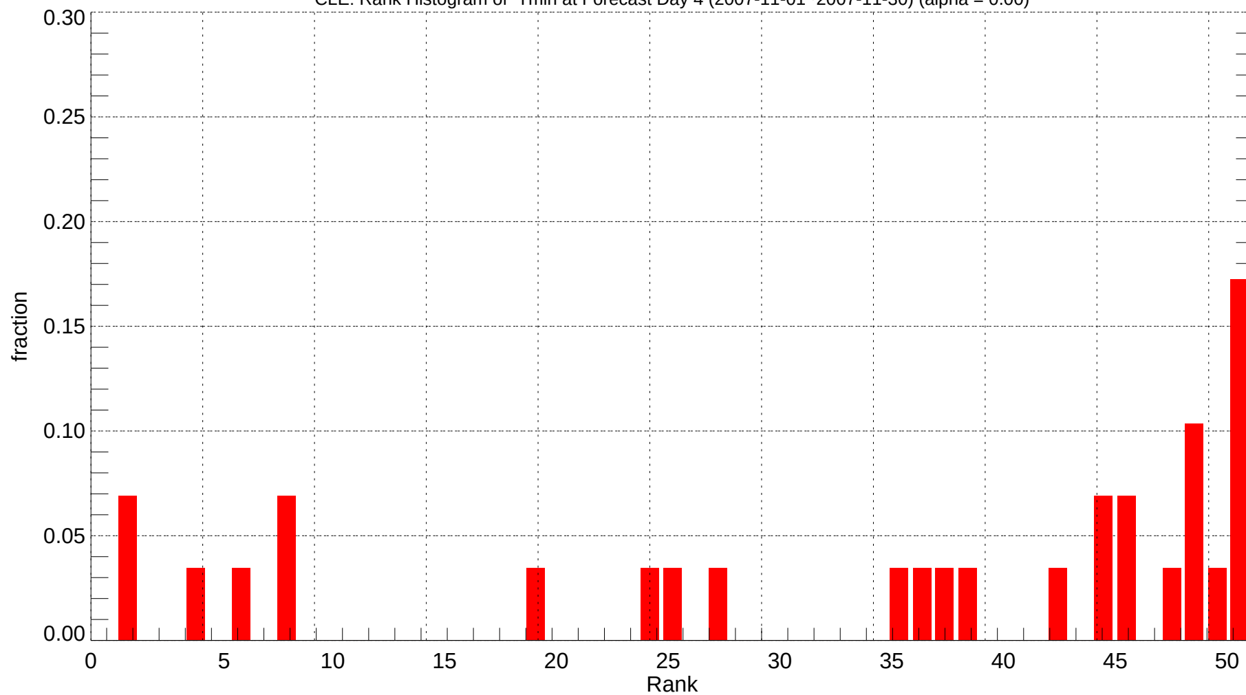
CLE: Rank Histogram of Tmin at Forecast Day 4 (2007-11-01~2007-11-30) (alpha = 0.00)
