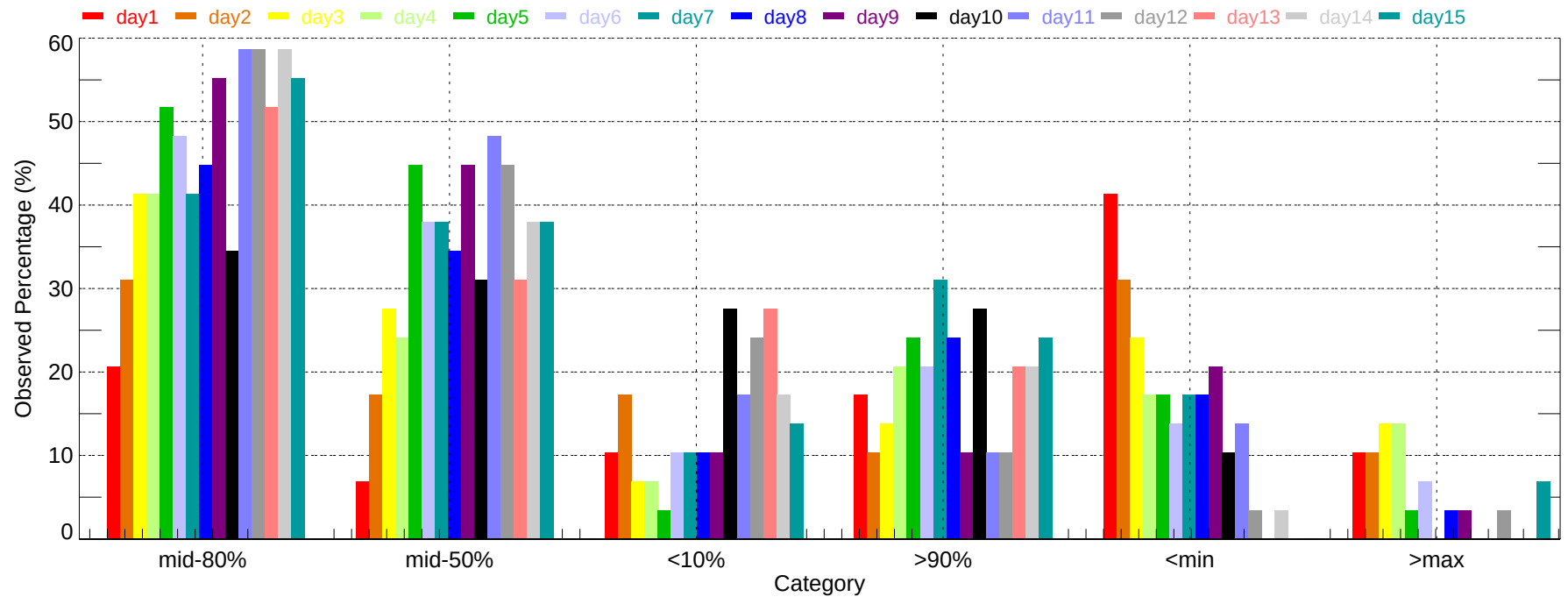
Observed Percentage of Ensembles - YKM: Min Temperature (2007-11-01~2007-11-30)
