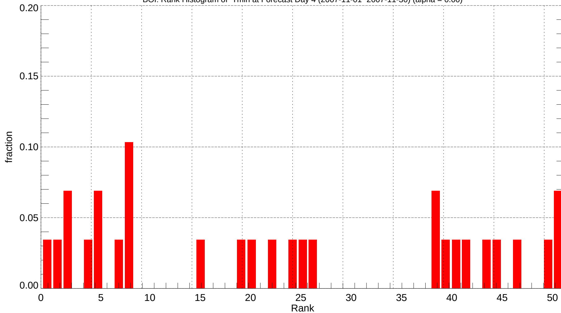
BOI: Rank Histogram of Tmin at Forecast Day 4 (2007-11-01~2007-11-30) (alpha = 0.00)
