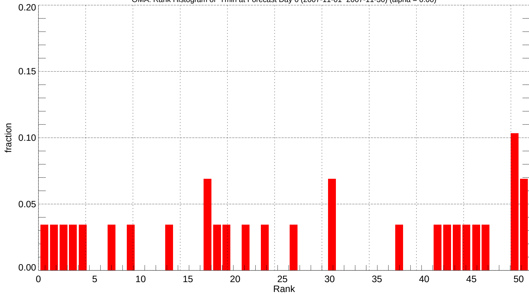
OMA: Rank Histogram of Tmin at Forecast Day 6 (2007-11-01~2007-11-30) (alpha = 0.00)
