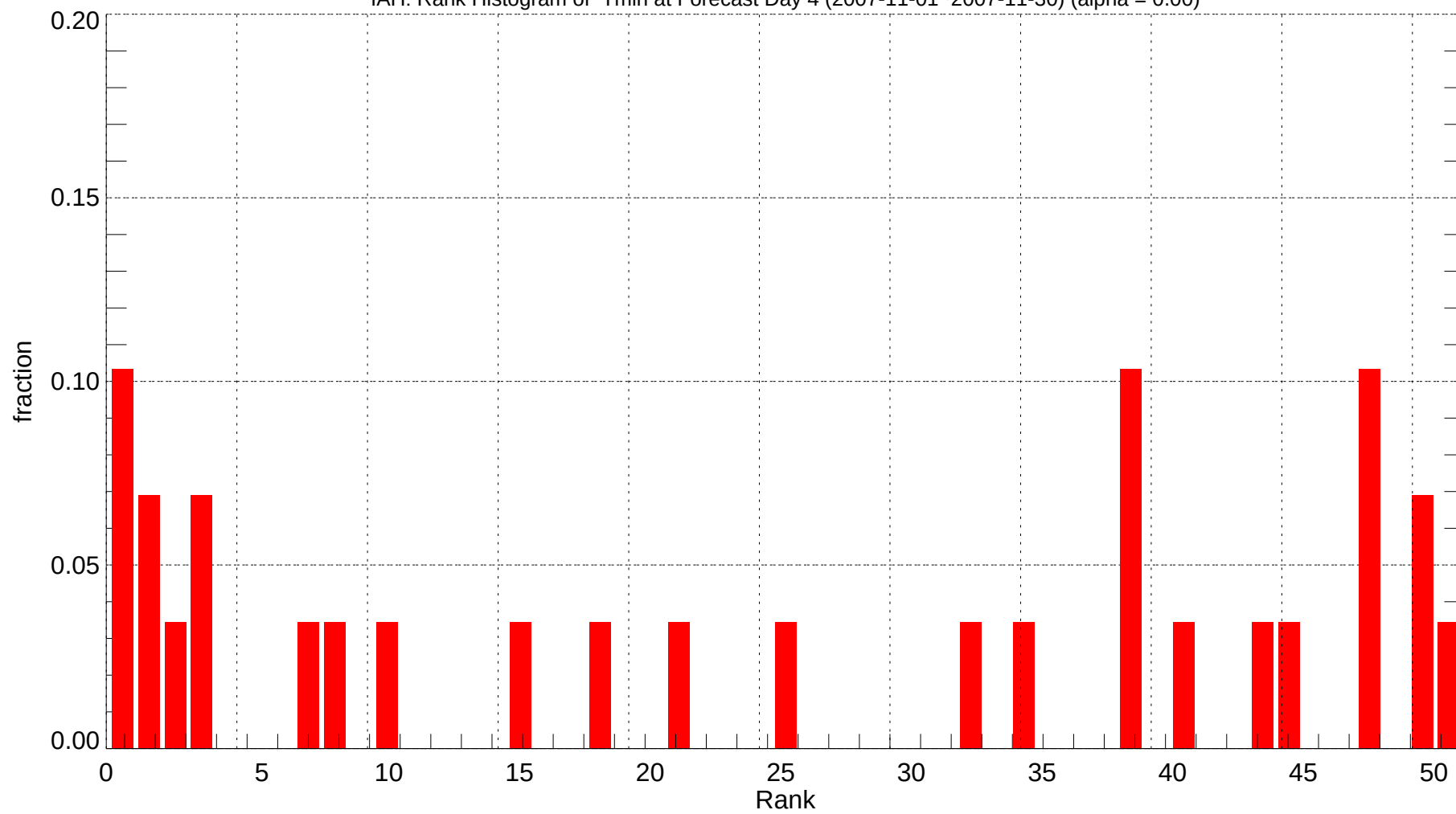
IAH: Rank Histogram of Tmin at Forecast Day 4 (2007-11-01~2007-11-30) (alpha = 0.00)
