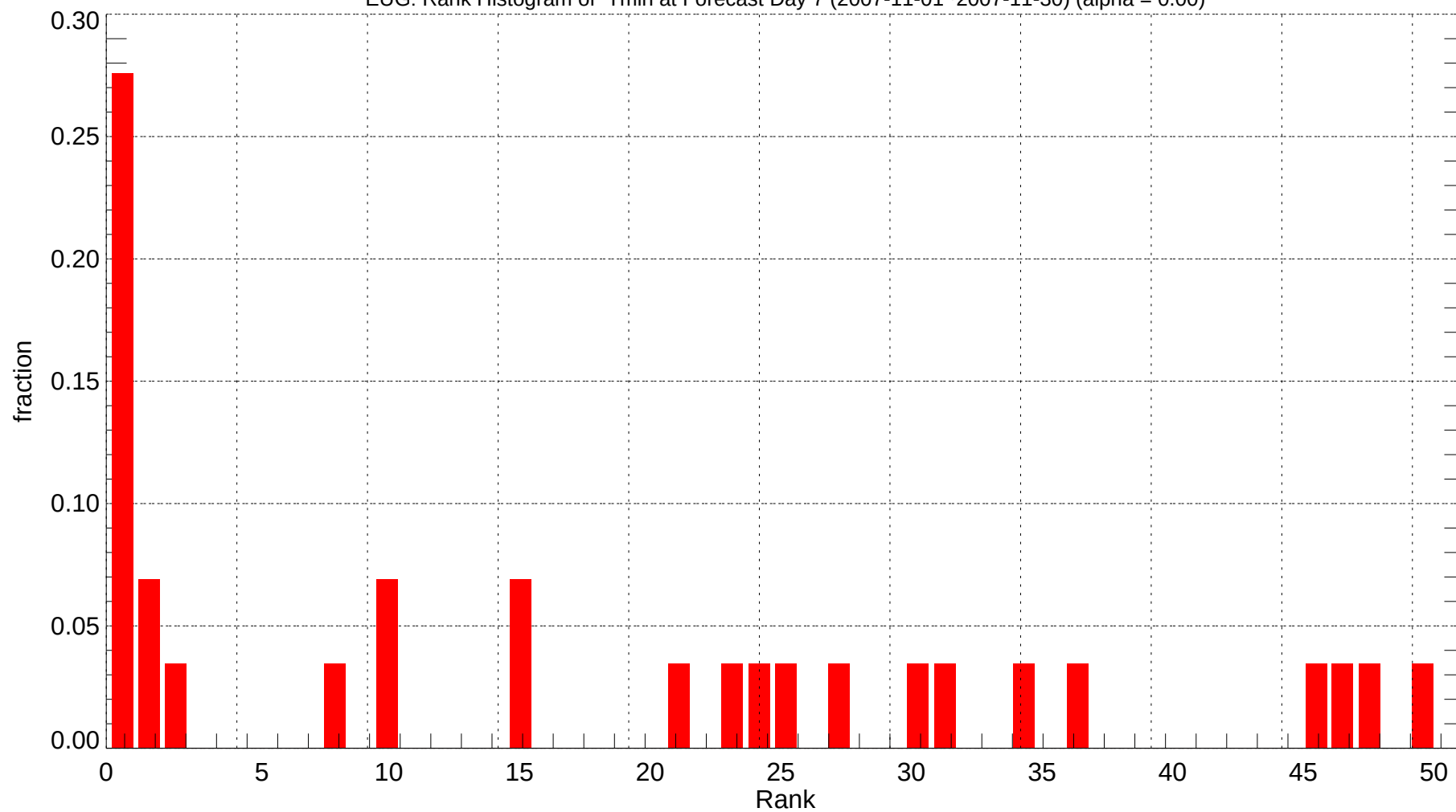
EUG: Rank Histogram of Tmin at Forecast Day 7 (2007-11-01~2007-11-30) (alpha = 0.00)
