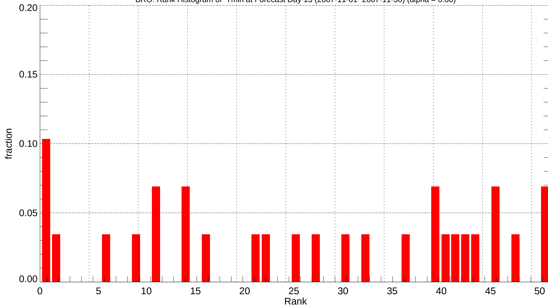
BRO: Rank Histogram of Tmin at Forecast Day 13 (2007-11-01~2007-11-30) (alpha = 0.00)
