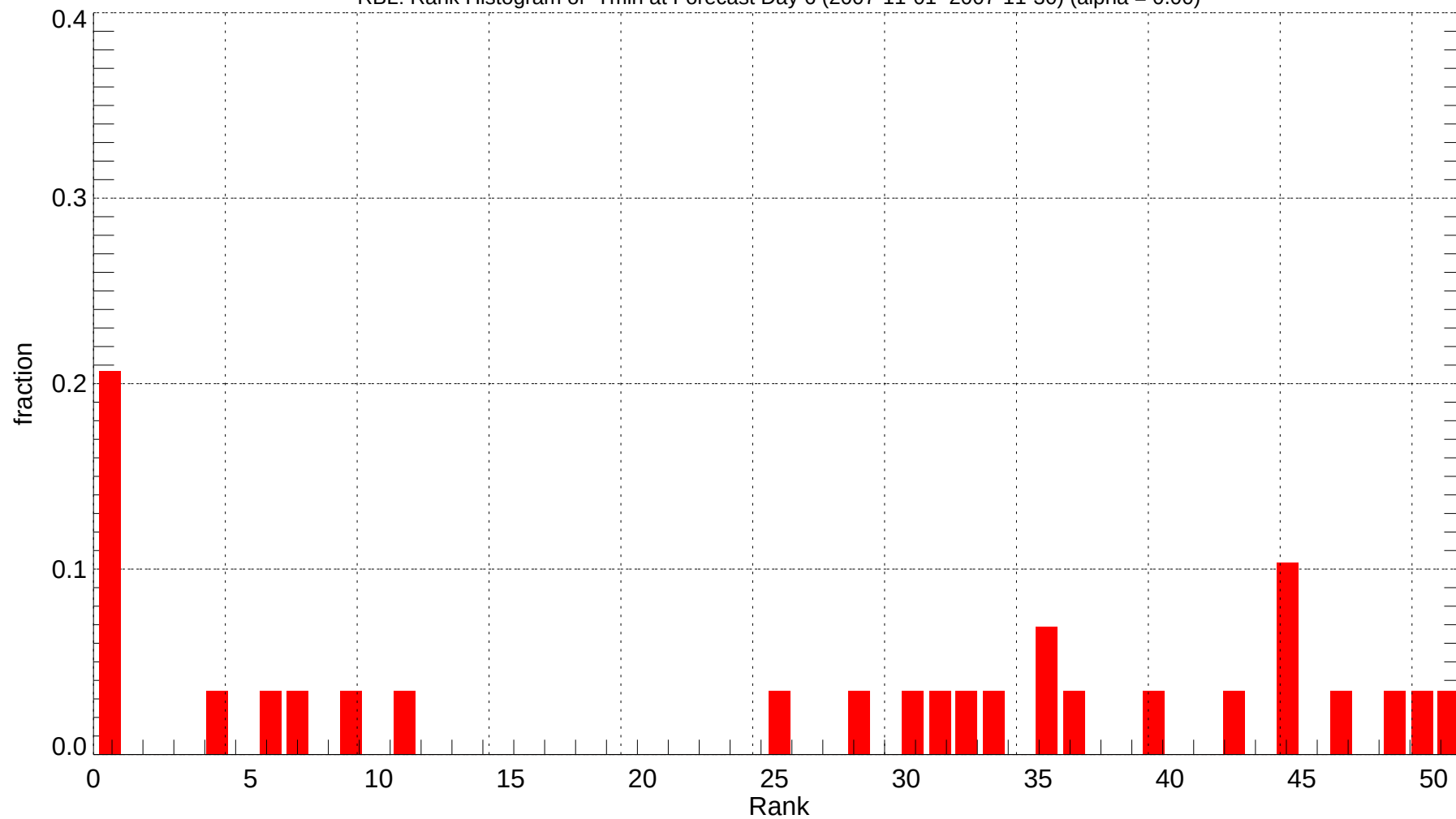
RBL: Rank Histogram of Tmin at Forecast Day 6 (2007-11-01~2007-11-30) (alpha = 0.00)
