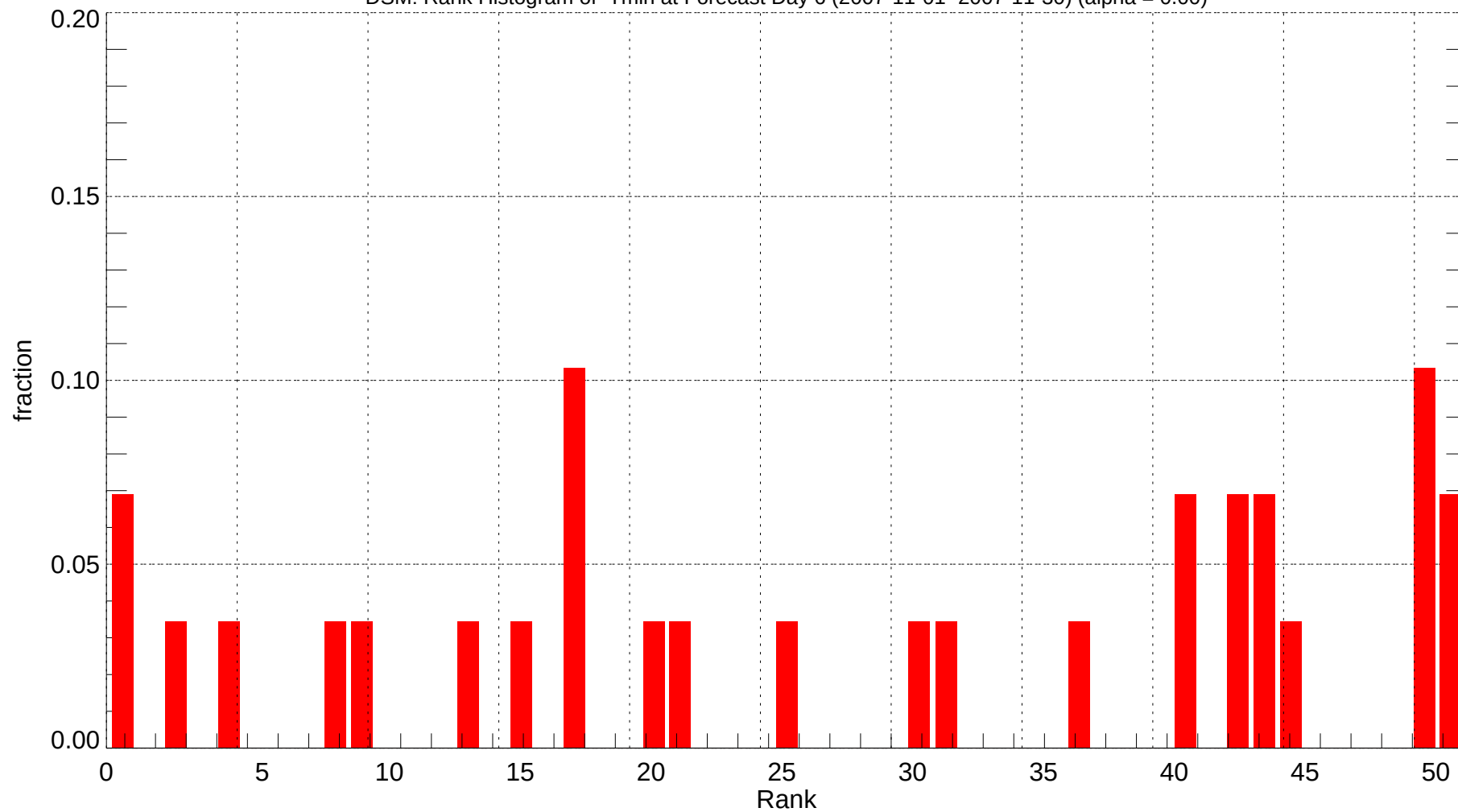
DSM: Rank Histogram of Tmin at Forecast Day 6 (2007-11-01~2007-11-30) (alpha = 0.00)
