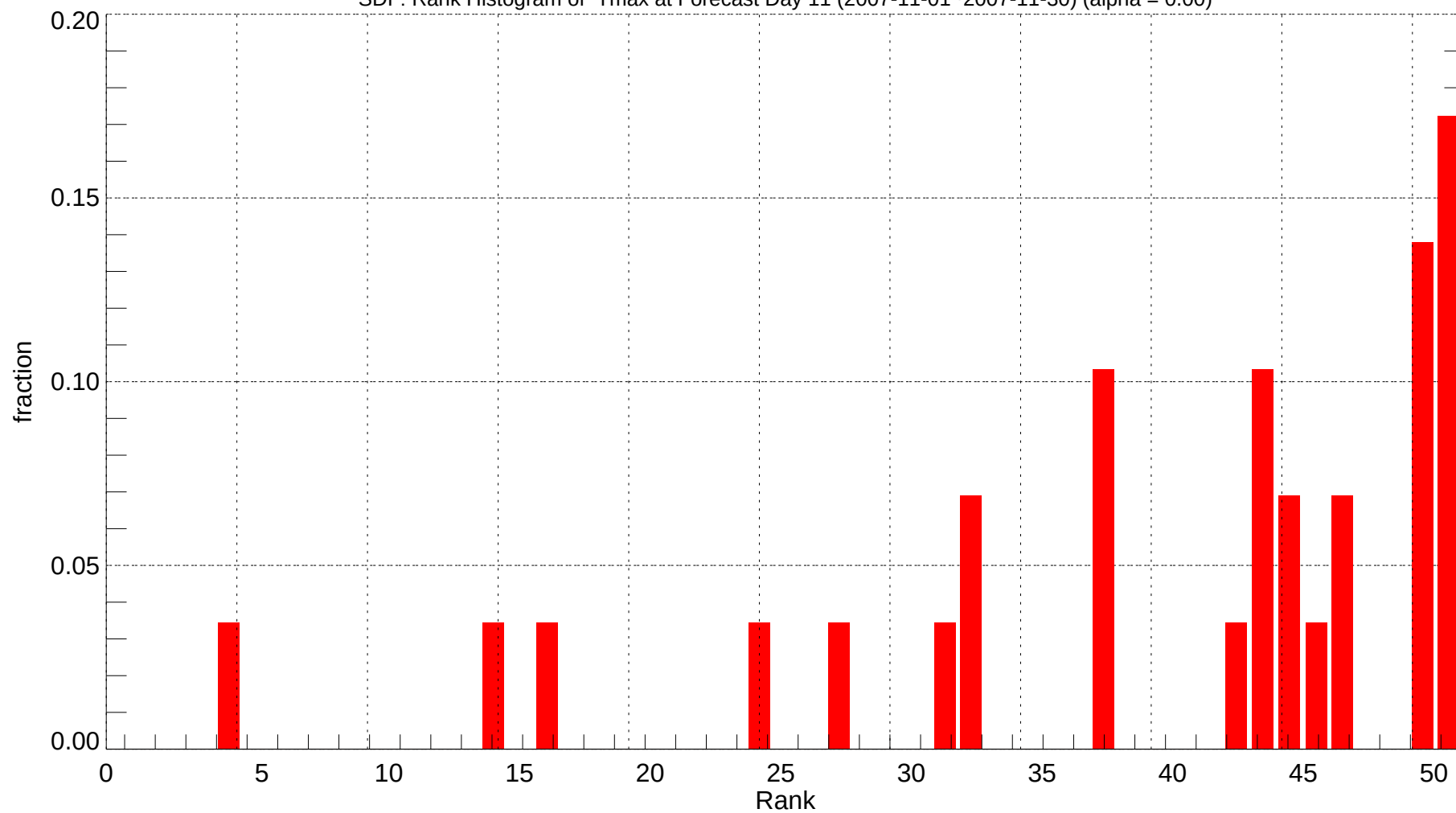
SDF: Rank Histogram of Tmax at Forecast Day 11 (2007-11-01~2007-11-30) (alpha = 0.00)
