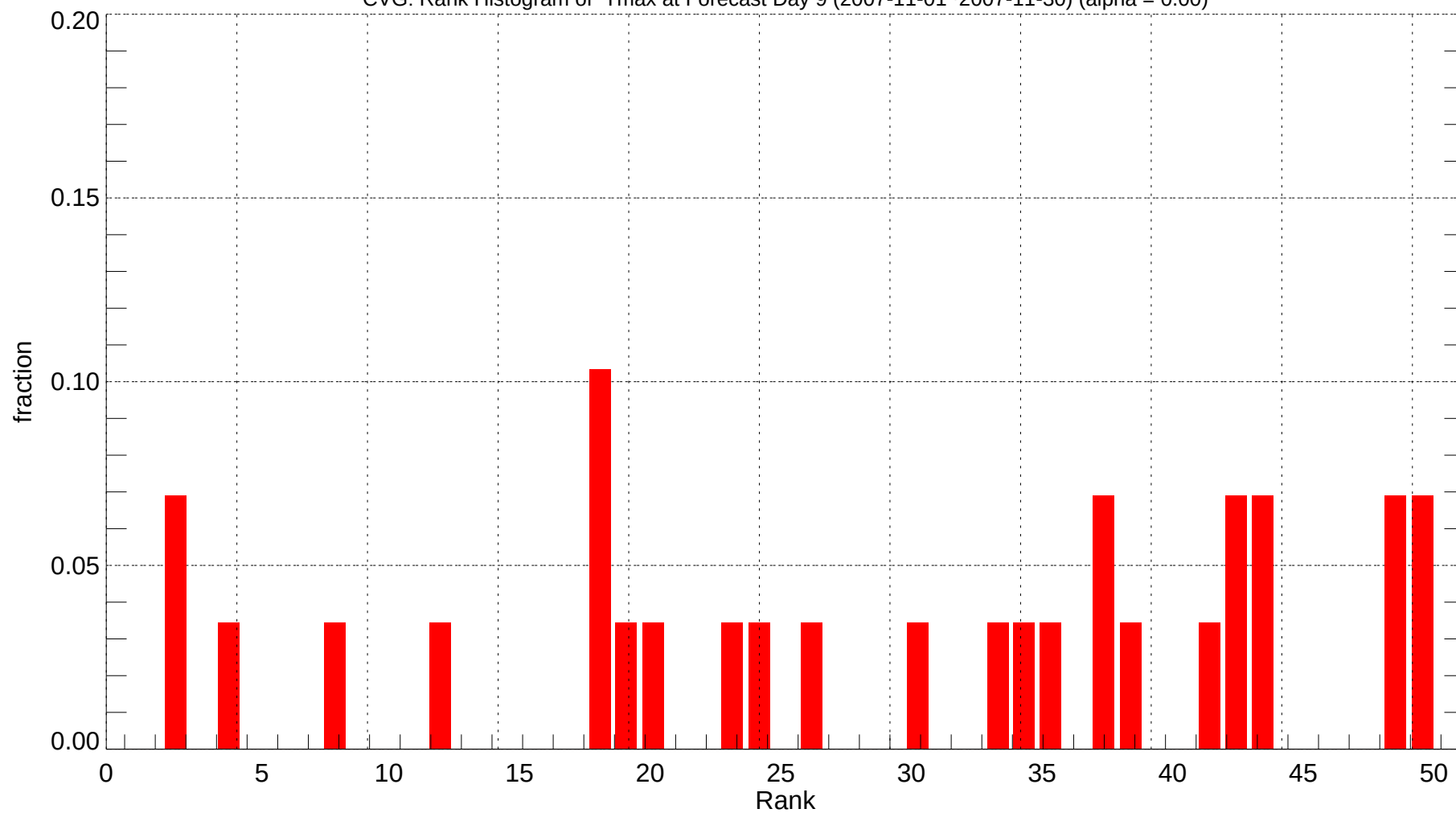
CVG: Rank Histogram of Tmax at Forecast Day 9 (2007-11-01~2007-11-30) (alpha = 0.00)
