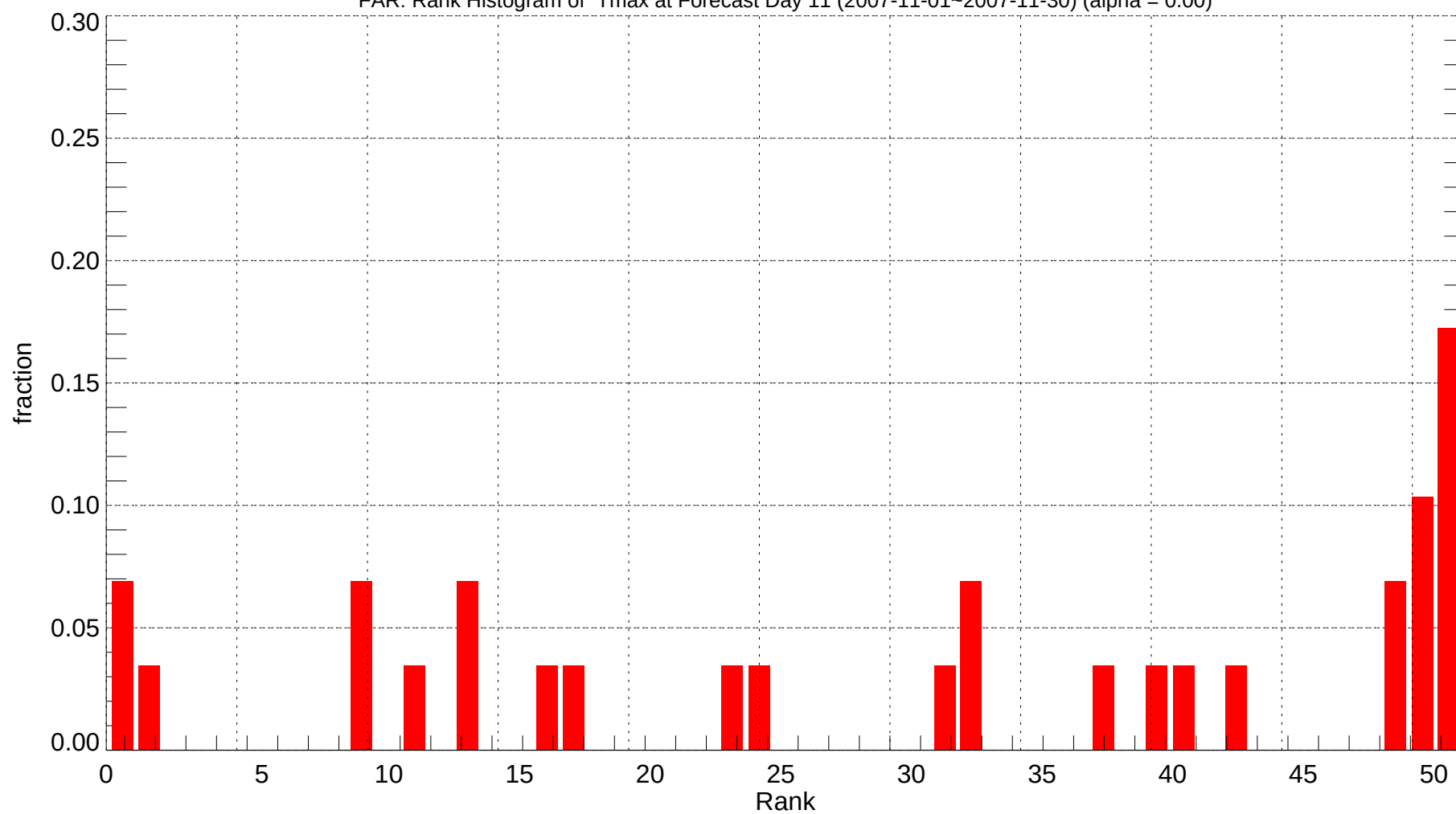
FAR: Rank Histogram of Tmax at Forecast Day 11 (2007-11-01~2007-11-30) (alpha = 0.00)
