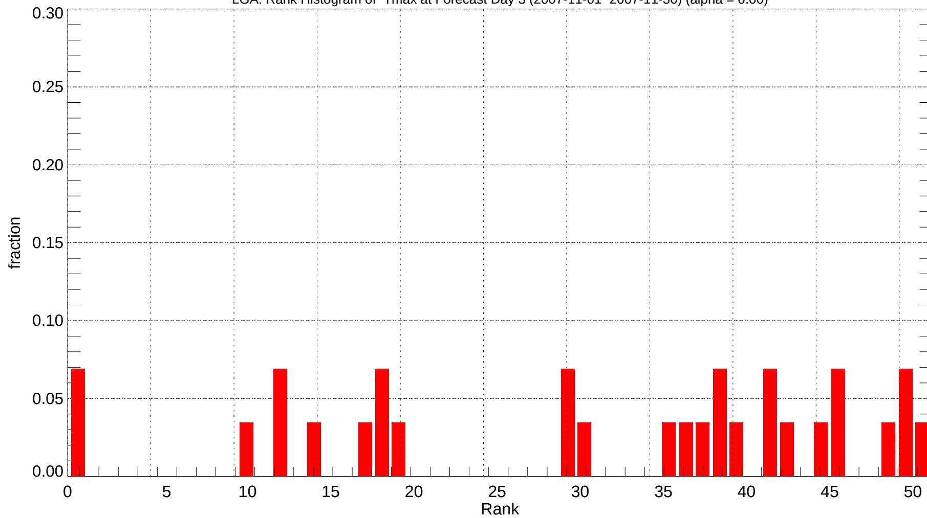
LGA: Rank Histogram of Tmax at Forecast Day 3 (2007-11-01~2007-11-30) (alpha = 0.00)
