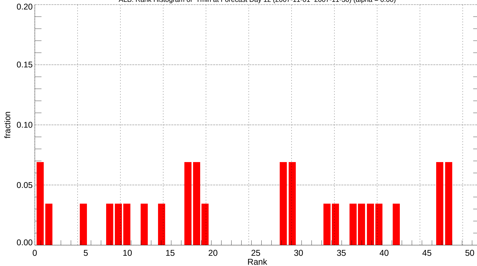
ALB: Rank Histogram of Tmin at Forecast Day 12 (2007-11-01~2007-11-30) (alpha = 0.00)
