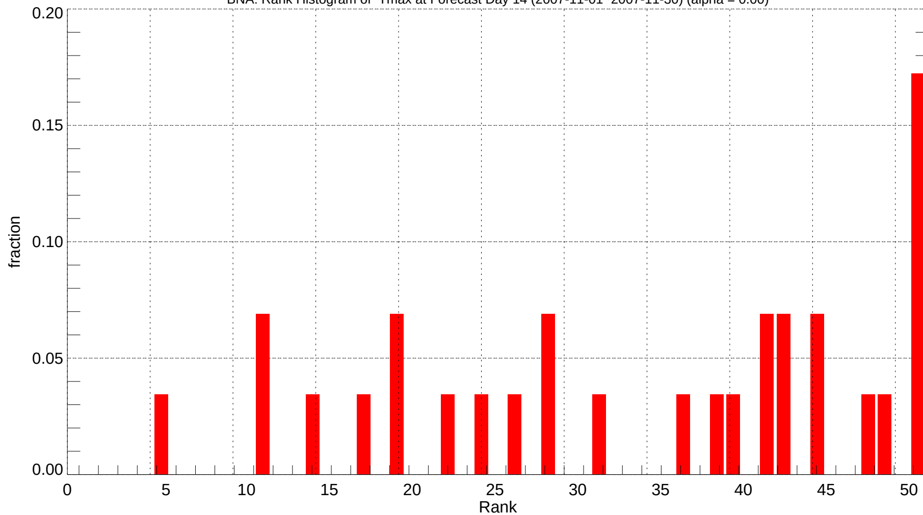
BNA: Rank Histogram of Tmax at Forecast Day 14 (2007-11-01~2007-11-30) (alpha = 0.00)
