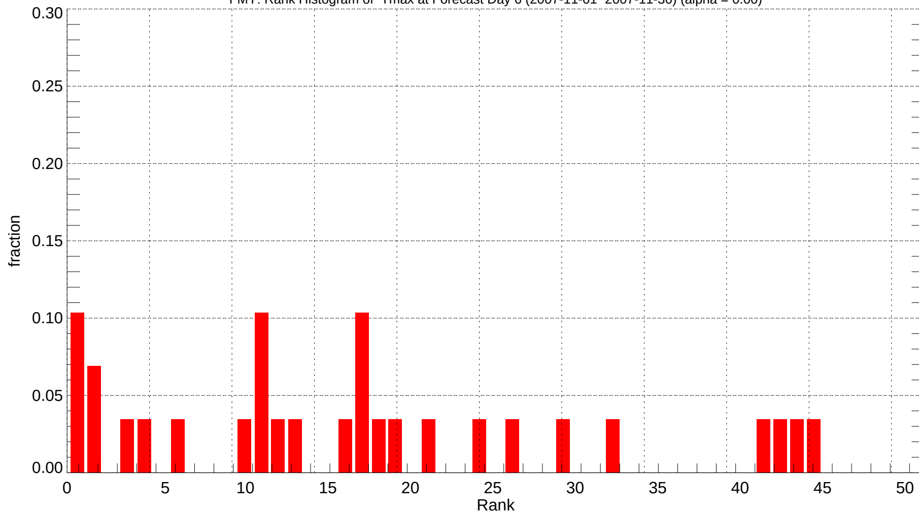
FMY: Rank Histogram of Tmax at Forecast Day 6 (2007-11-01~2007-11-30) (alpha = 0.00)
