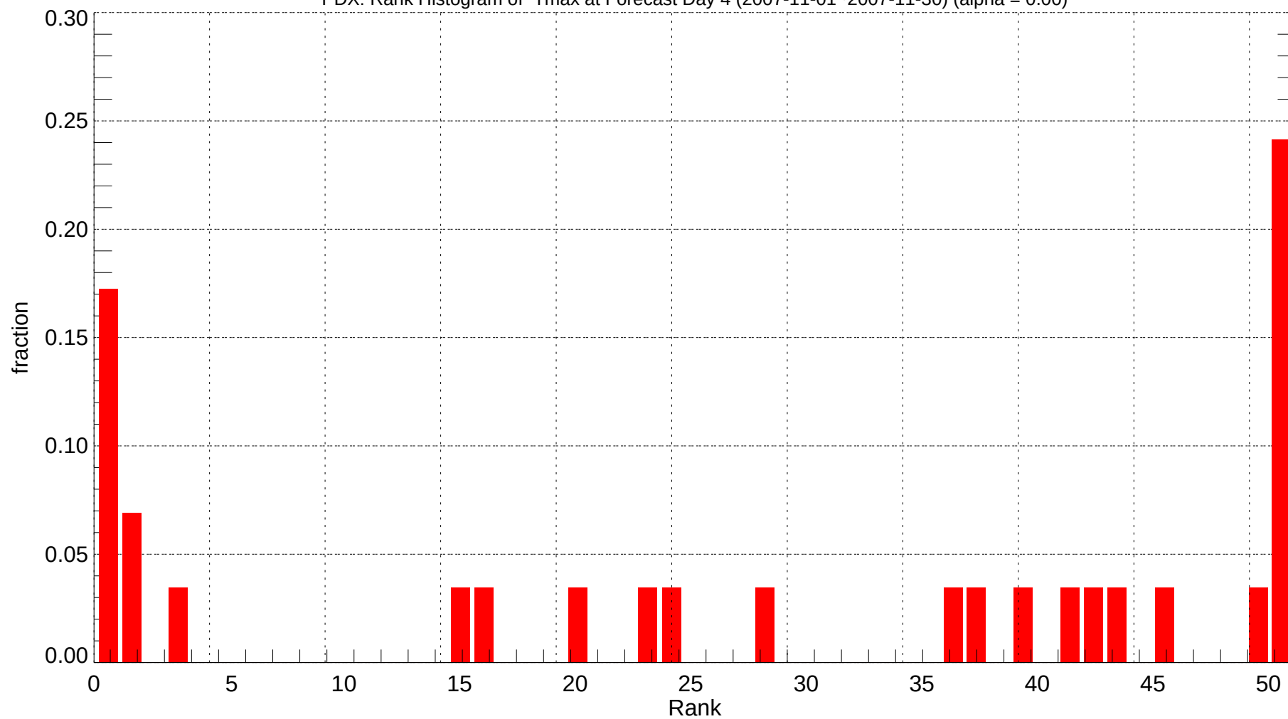
PDX: Rank Histogram of Tmax at Forecast Day 4 (2007-11-01~2007-11-30) (alpha = 0.00)
