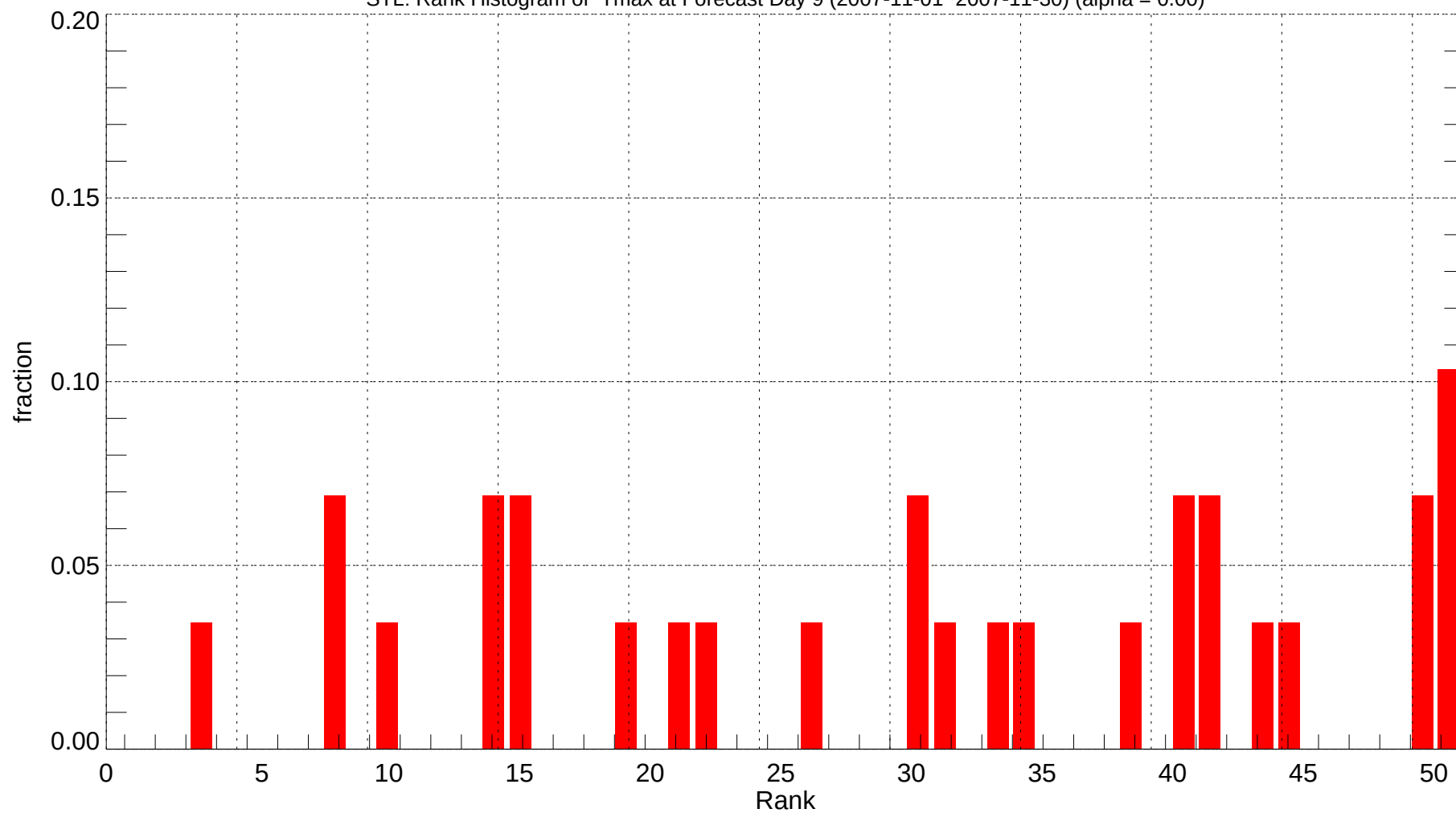
STL: Rank Histogram of Tmax at Forecast Day 9 (2007-11-01~2007-11-30) (alpha = 0.00)
