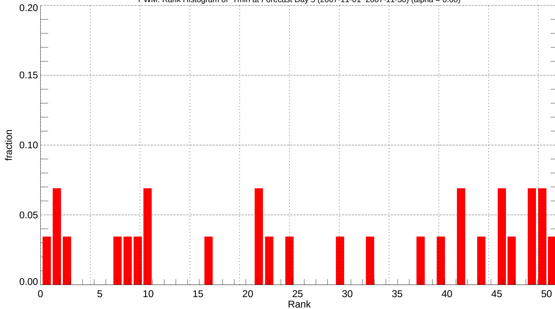
PWM: Rank Histogram of Tmin at Forecast Day 5 (2007-11-01~2007-11-30) (alpha = 0.00)
