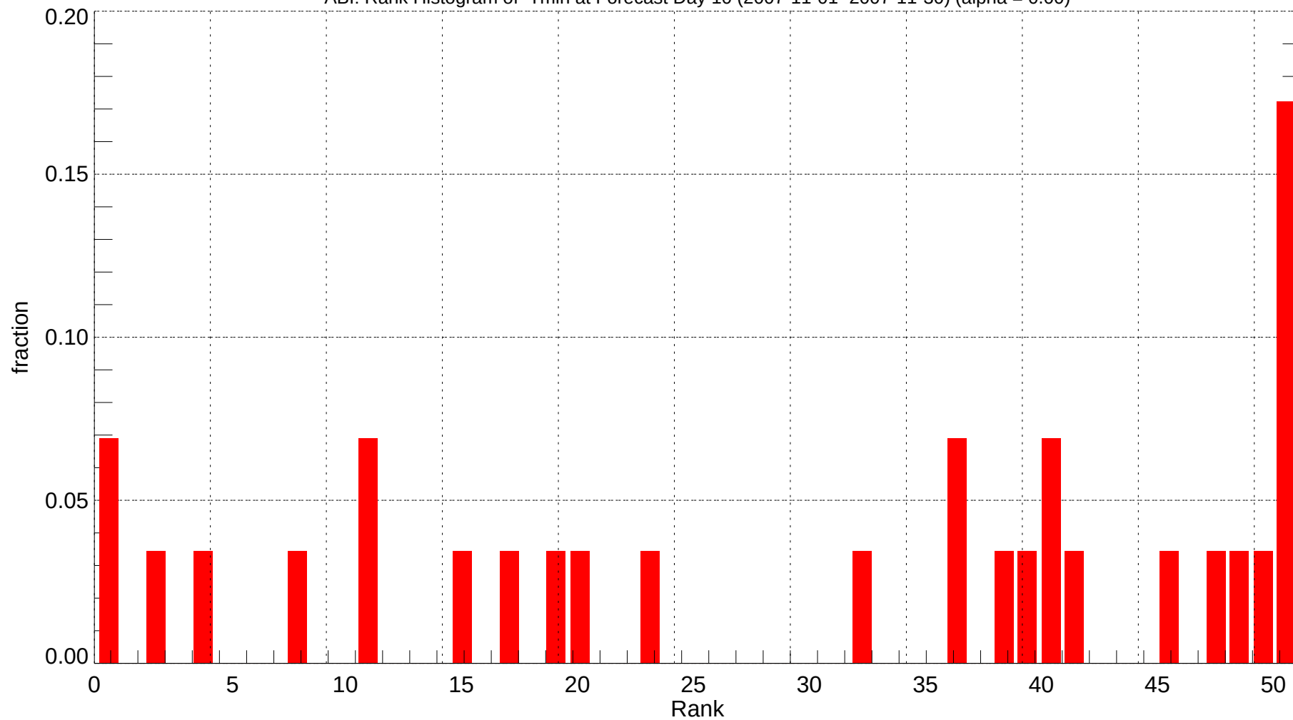
ABI: Rank Histogram of Tmin at Forecast Day 10 (2007-11-01~2007-11-30) (alpha = 0.00)
