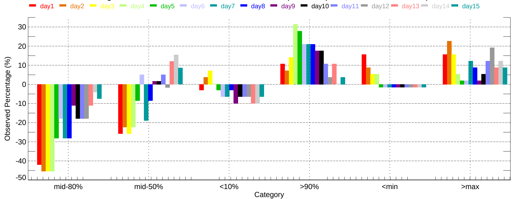
Observed Percentage Deviation of Ensembles - CMH: Max Temperature (2007-11-01~2007-11-30)
