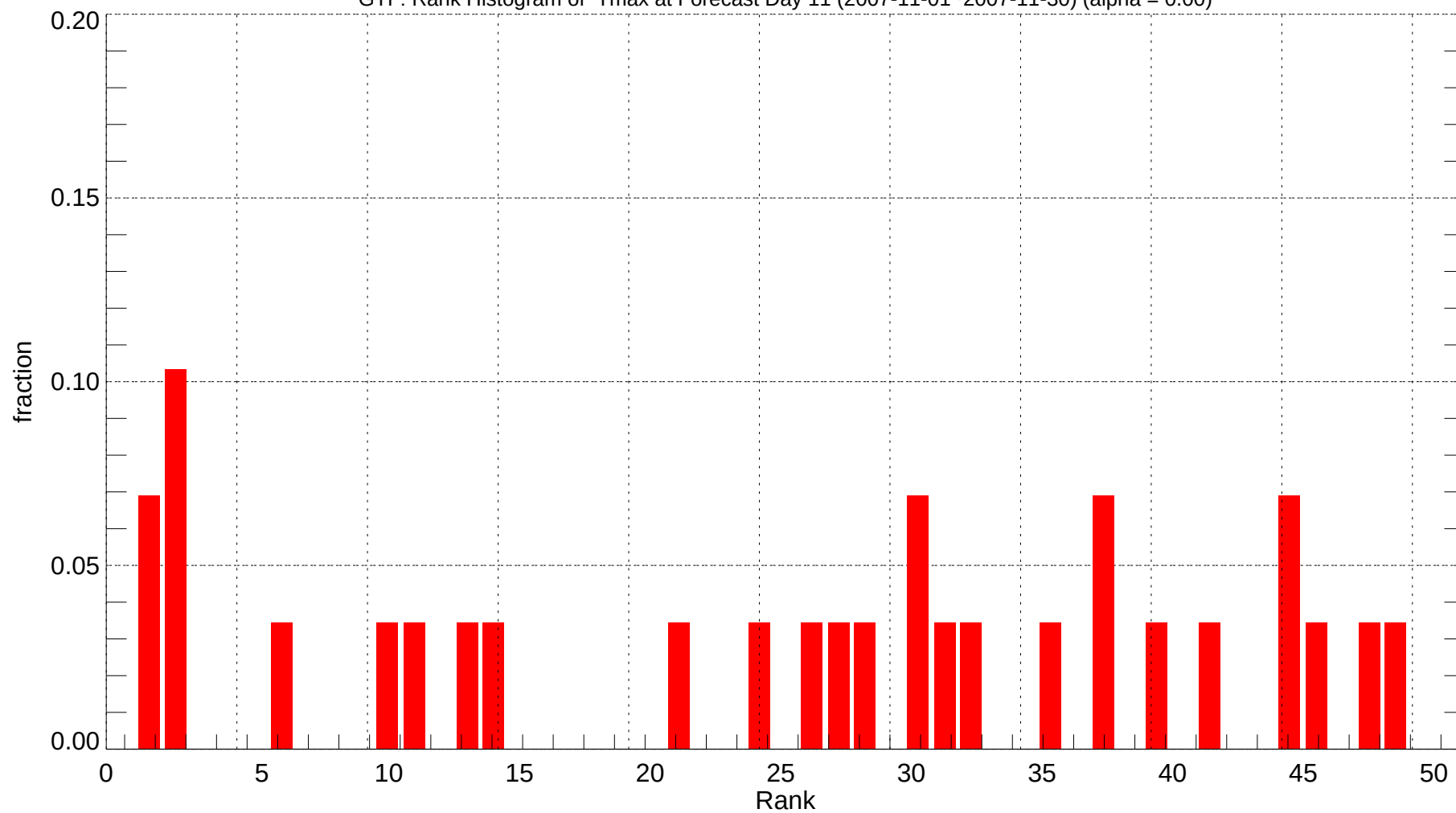
GTF: Rank Histogram of Tmax at Forecast Day 11 (2007-11-01~2007-11-30) (alpha = 0.00)
