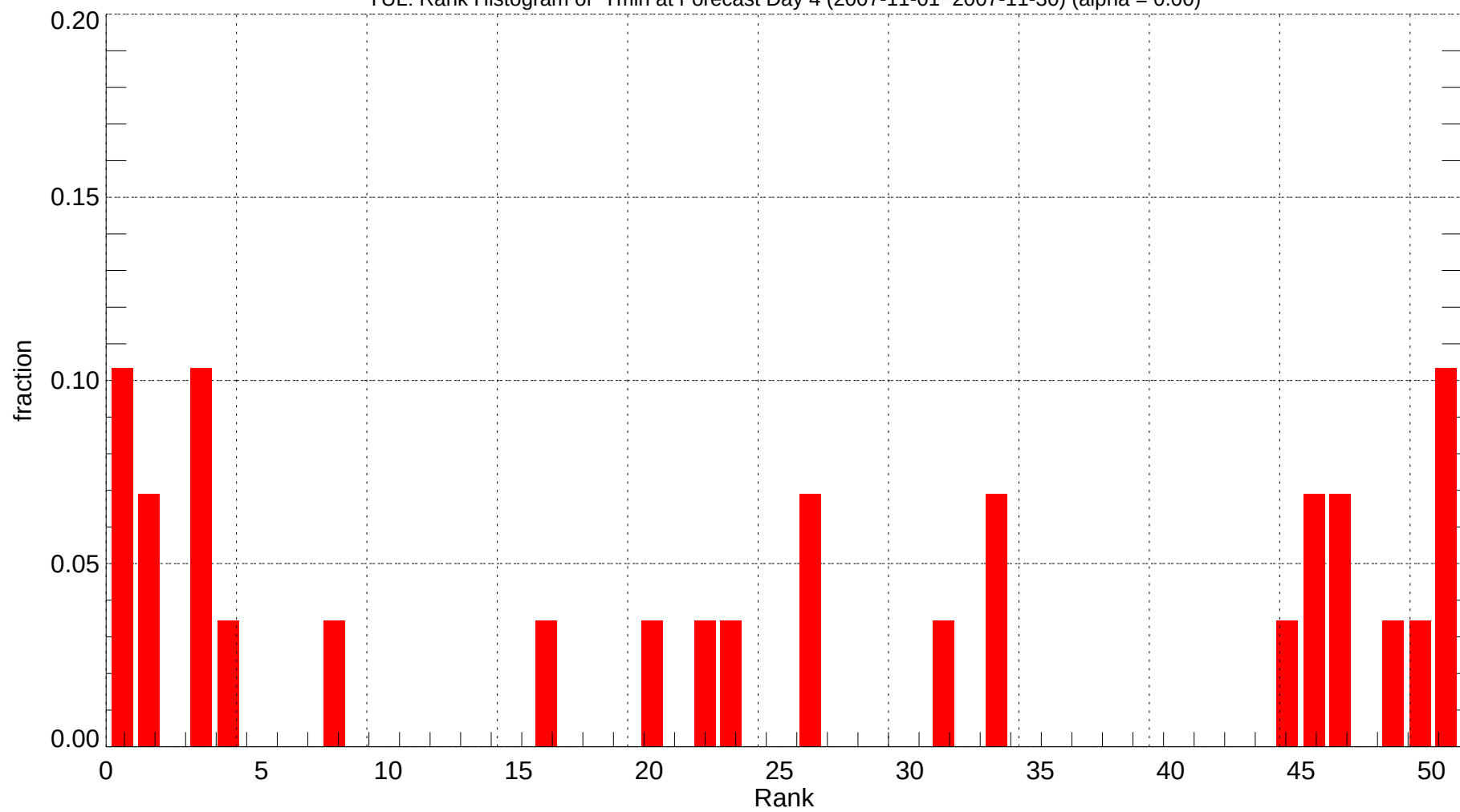
YUL: Rank Histogram of Tmin at Forecast Day 4 (2007-11-01~2007-11-30) (alpha = 0.00)
