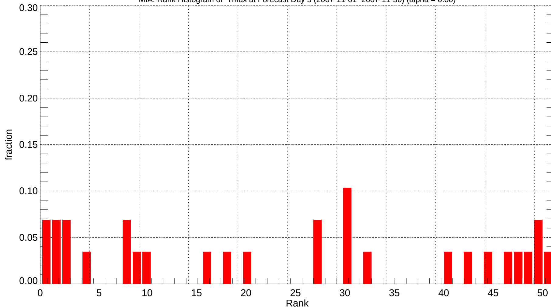
MIA: Rank Histogram of Tmax at Forecast Day 5 (2007-11-01~2007-11-30) (alpha = 0.00)
