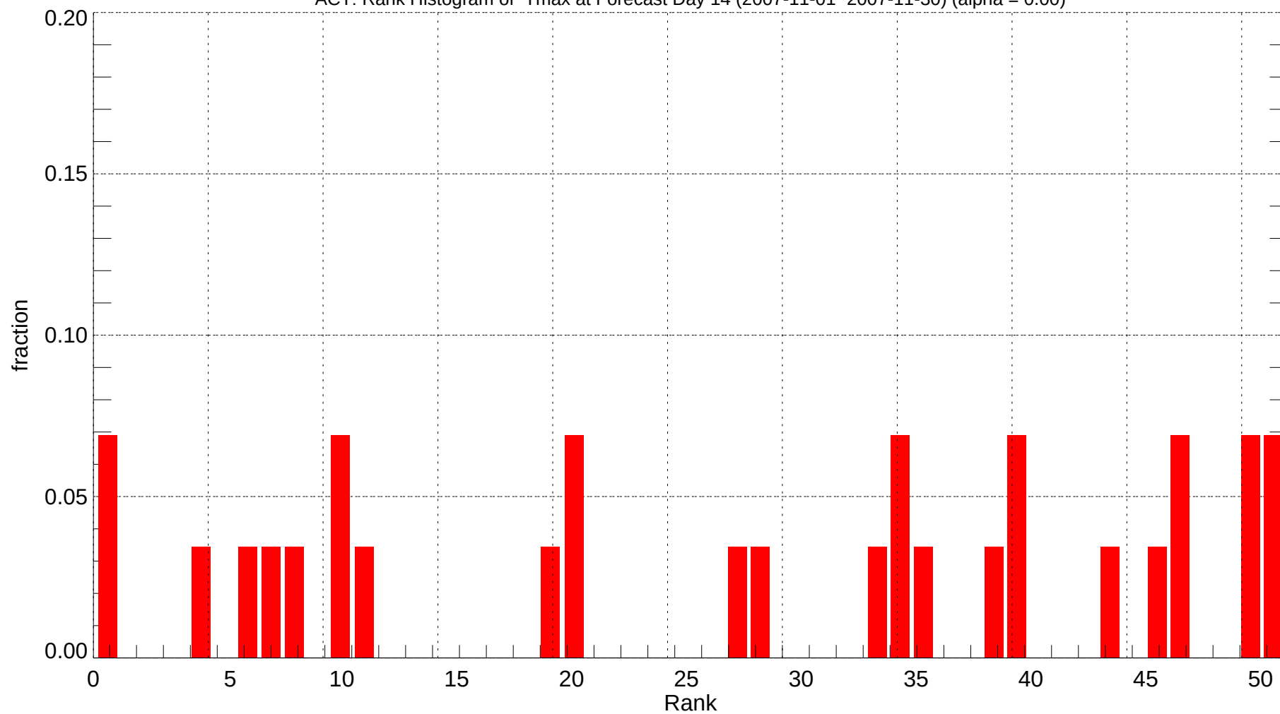
ACT: Rank Histogram of Tmax at Forecast Day 14 (2007-11-01~2007-11-30) (alpha = 0.00)
