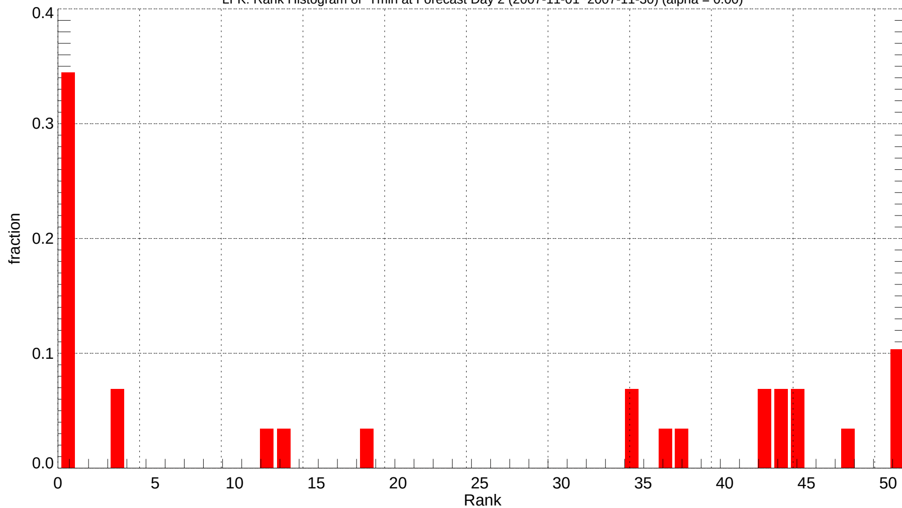
LFK: Rank Histogram of Tmin at Forecast Day 2 (2007-11-01~2007-11-30) (alpha = 0.00)
