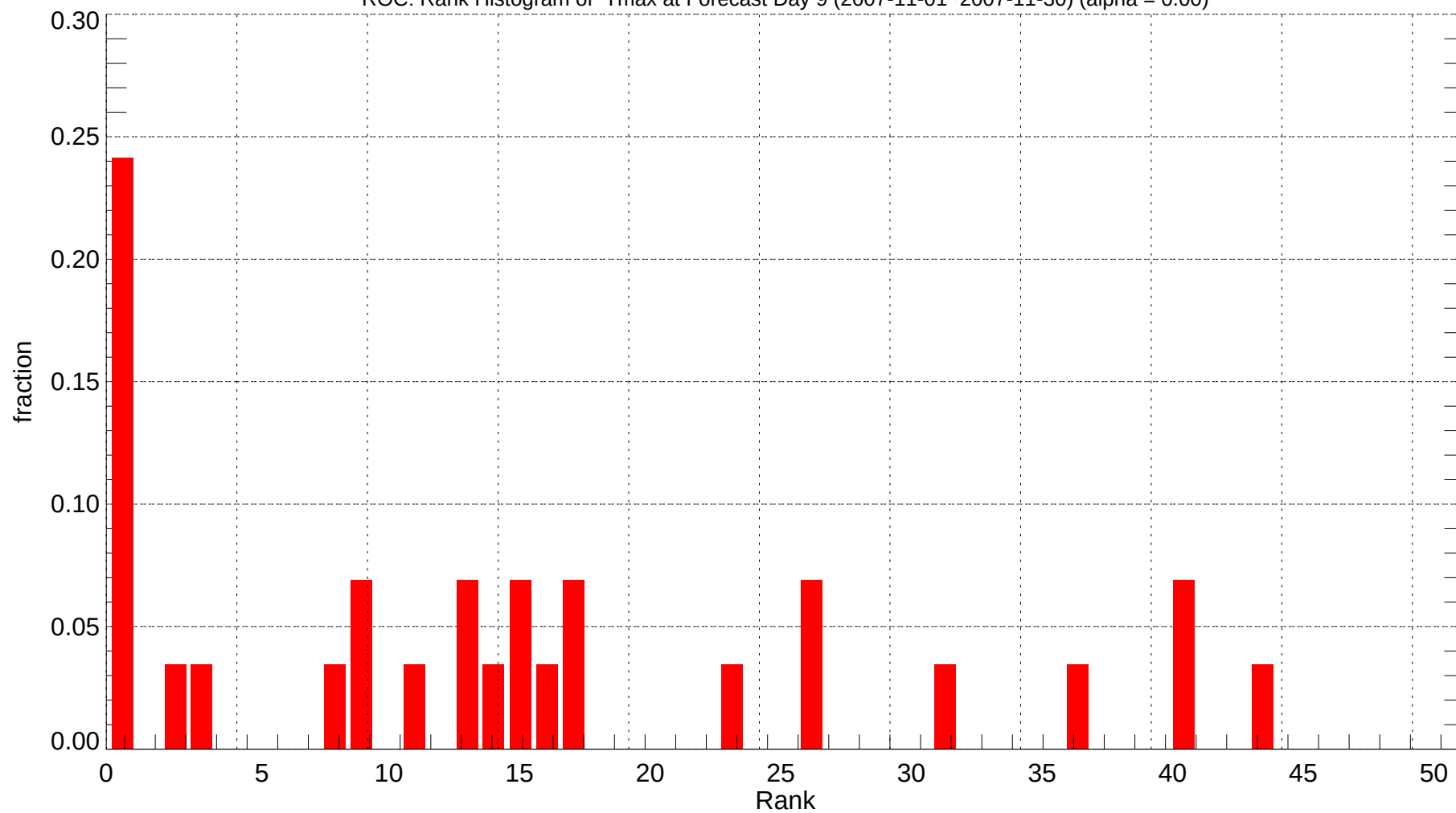
ROC: Rank Histogram of Tmax at Forecast Day 9 (2007-11-01~2007-11-30) (alpha = 0.00)
