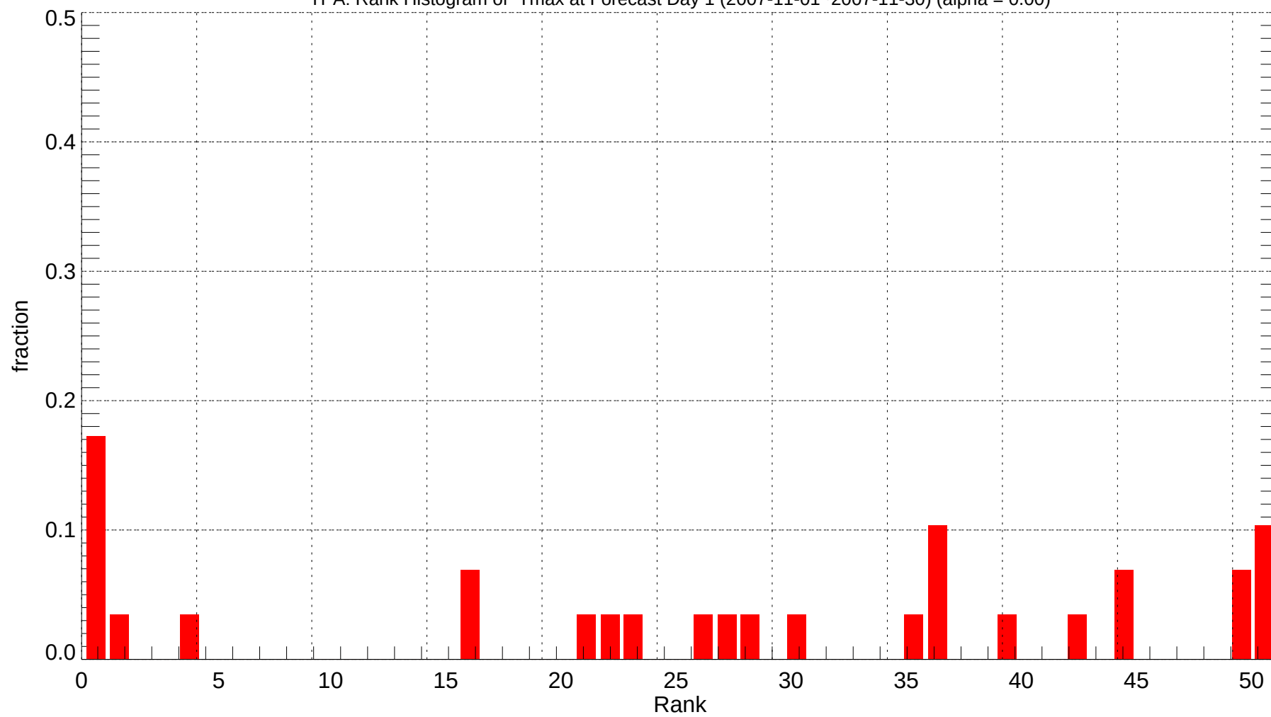
TPA: Rank Histogram of Tmax at Forecast Day 1 (2007-11-01~2007-11-30) (alpha = 0.00)
