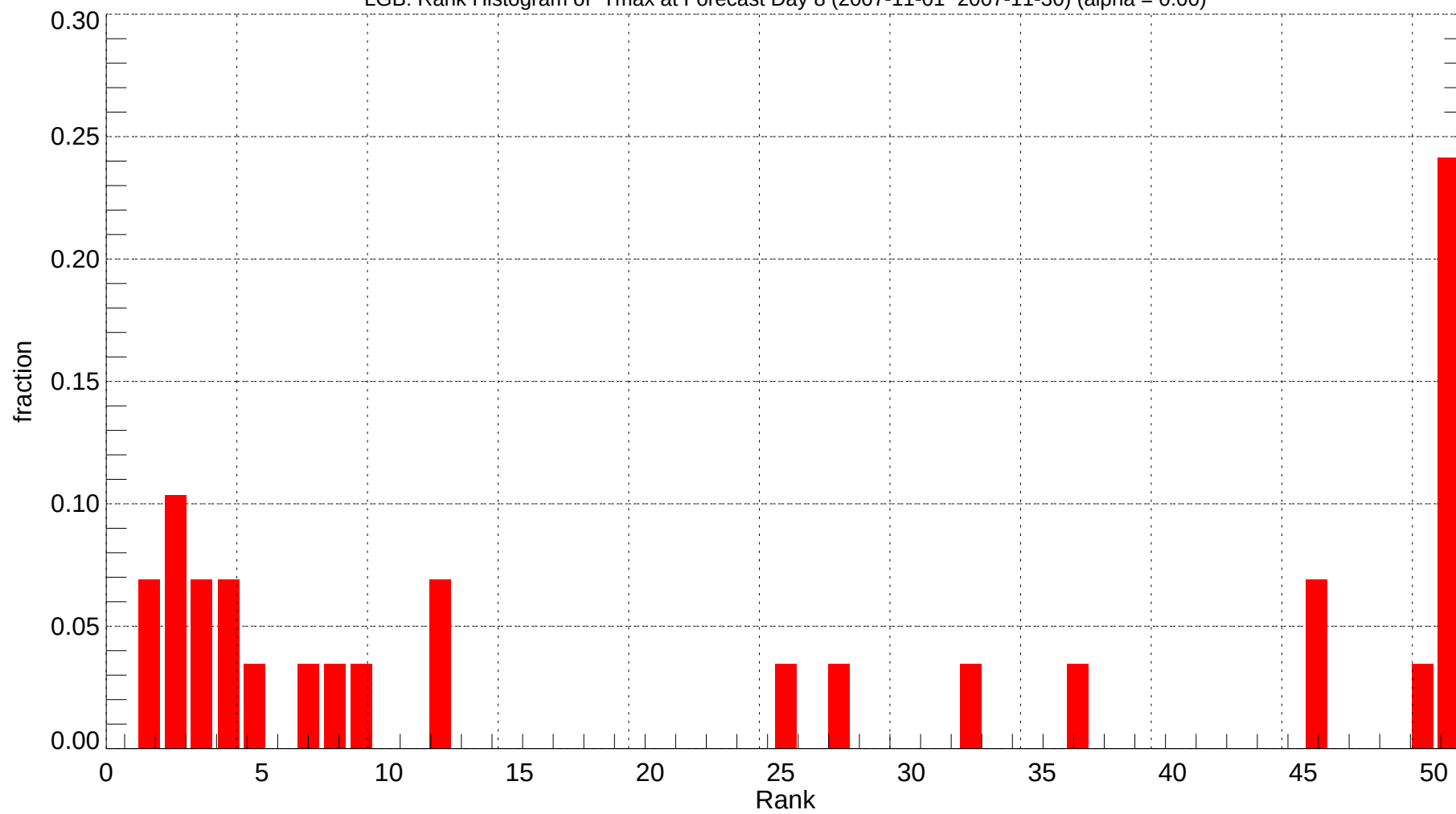
LGB: Rank Histogram of Tmax at Forecast Day 8 (2007-11-01~2007-11-30) (alpha = 0.00)
