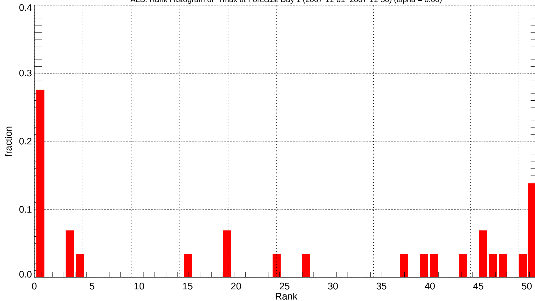
ALB: Rank Histogram of Tmax at Forecast Day 1 (2007-11-01~2007-11-30) (alpha = 0.00)
