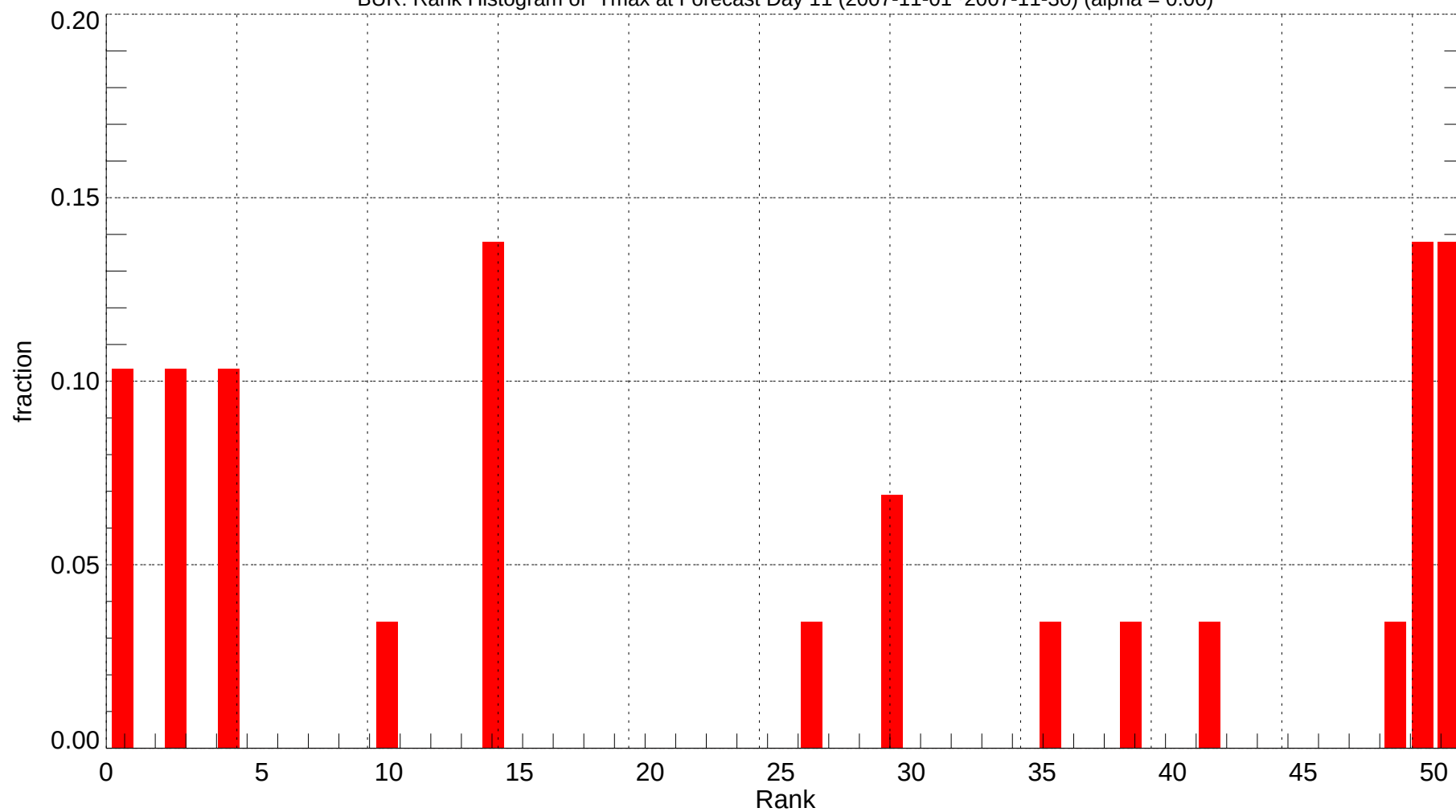
BUR: Rank Histogram of Tmax at Forecast Day 11 (2007-11-01~2007-11-30) (alpha = 0.00)
