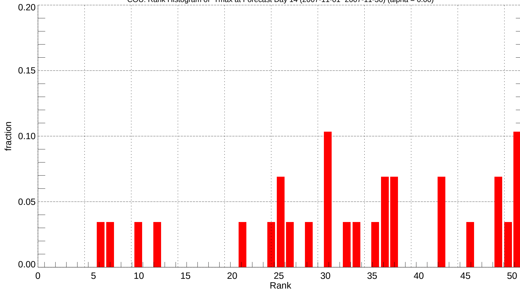
COU: Rank Histogram of Tmax at Forecast Day 14 (2007-11-01~2007-11-30) (alpha = 0.00)
