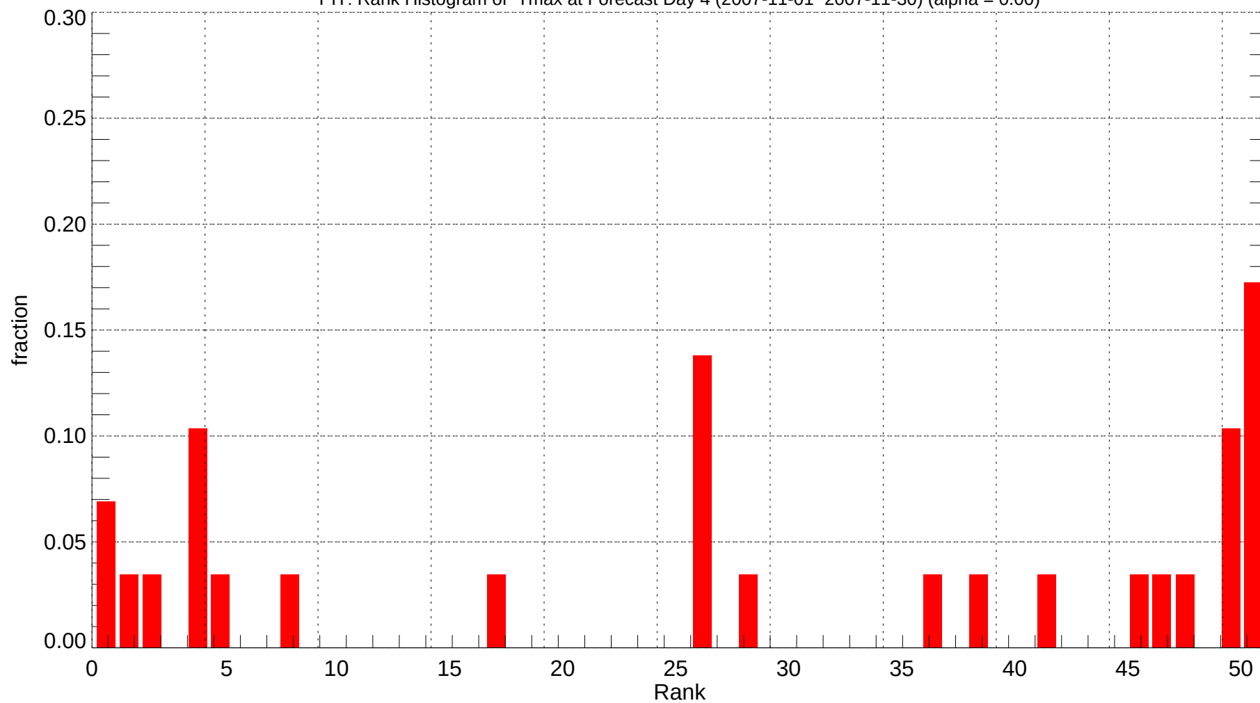
PIT: Rank Histogram of Tmax at Forecast Day 4 (2007-11-01~2007-11-30) (alpha = 0.00)
