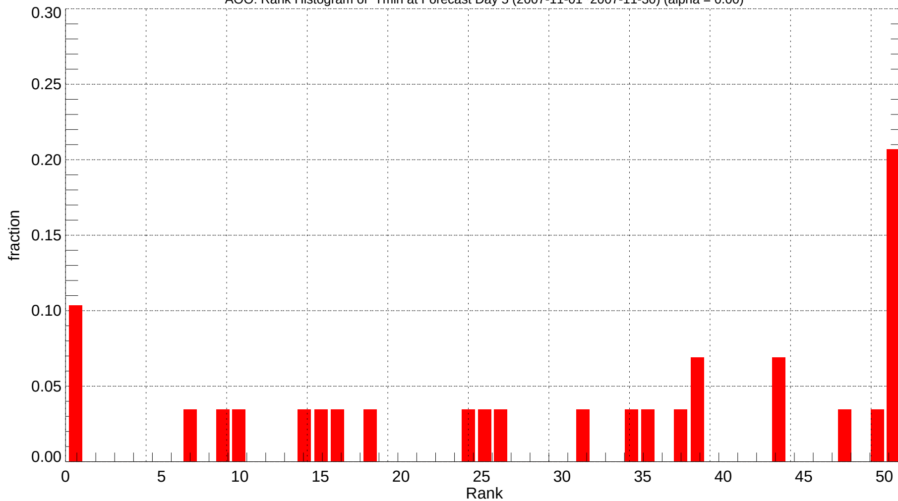
AOO: Rank Histogram of Tmin at Forecast Day 5 (2007-11-01~2007-11-30) (alpha = 0.00)
