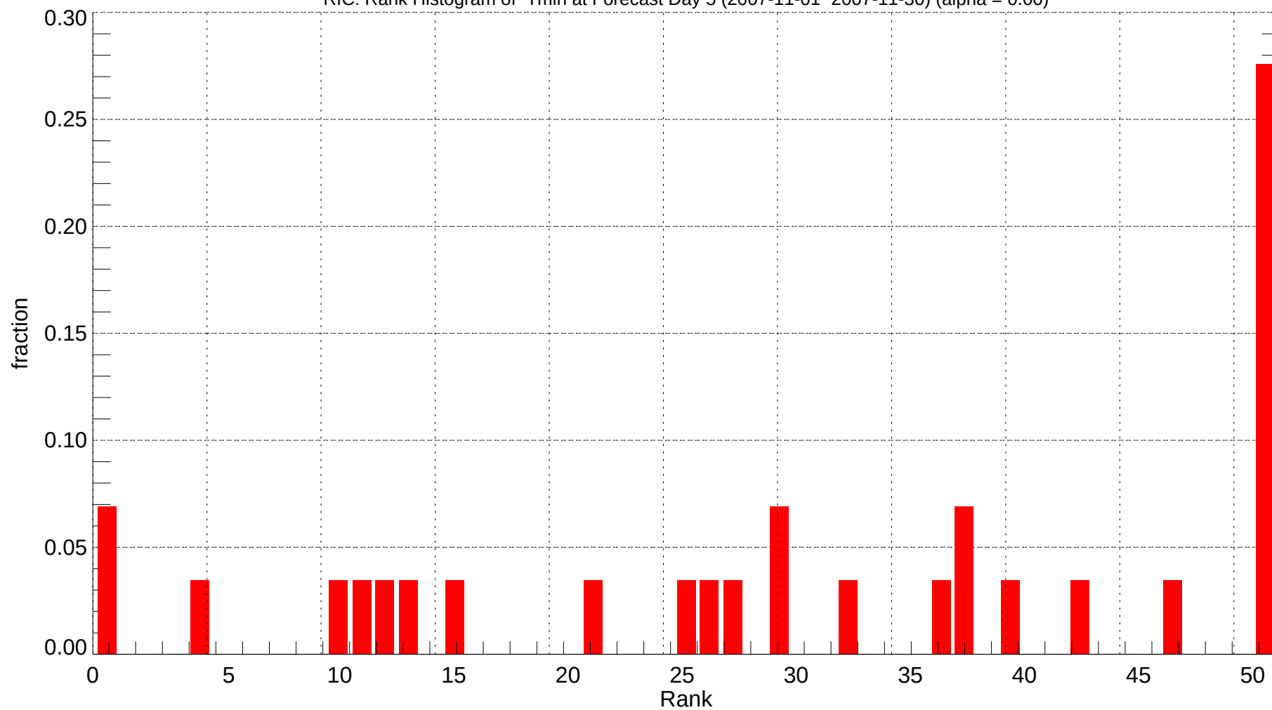
RIC: Rank Histogram of Tmin at Forecast Day 5 (2007-11-01~2007-11-30) (alpha = 0.00)
