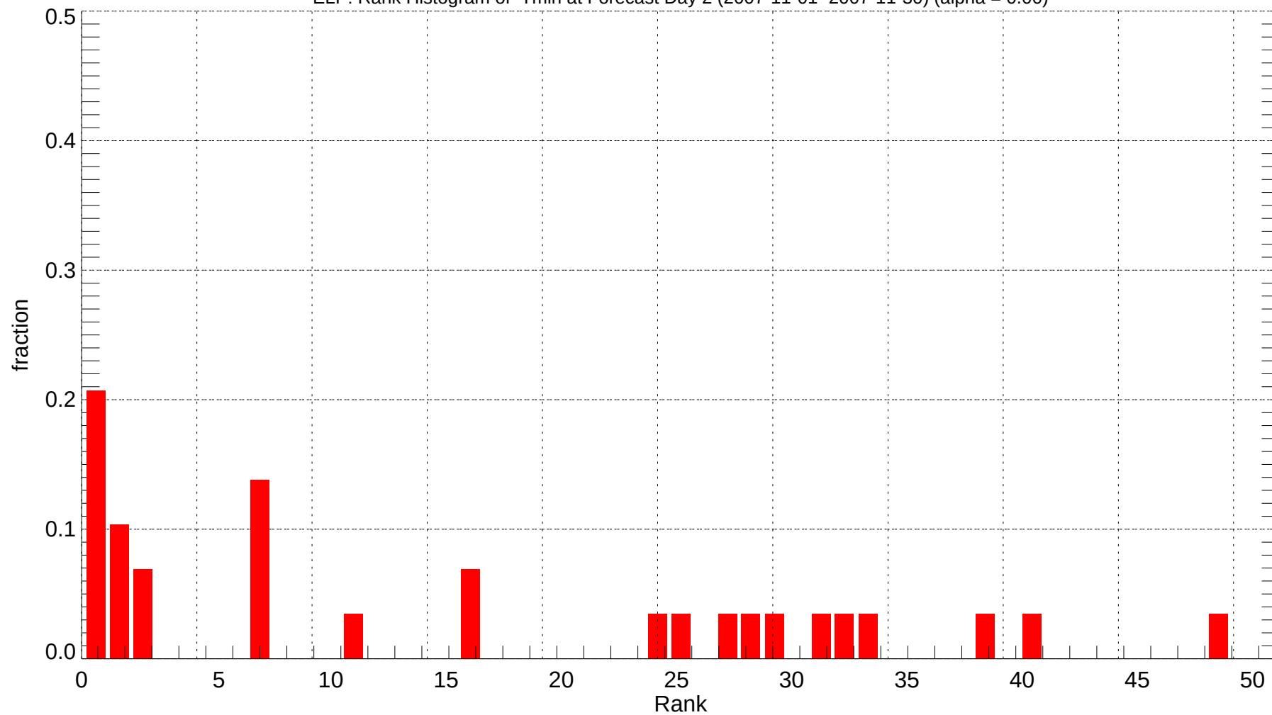
ELP: Rank Histogram of Tmin at Forecast Day 2 (2007-11-01~2007-11-30) (alpha = 0.00)
