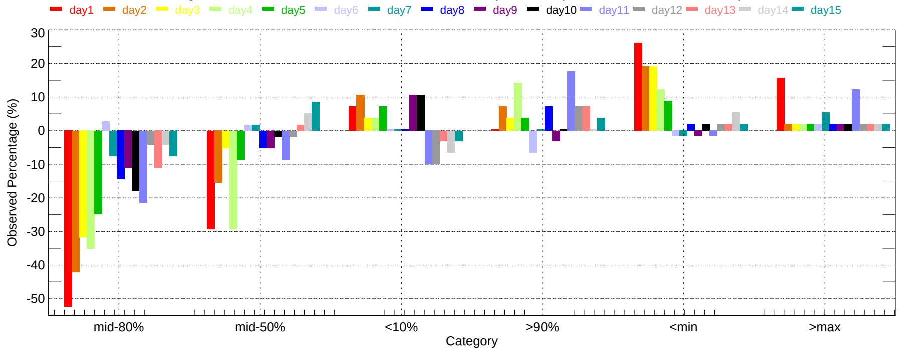
Observed Percentage Deviation of Ensembles - ABE: Min Temperature (2007-11-01~2007-11-30)
