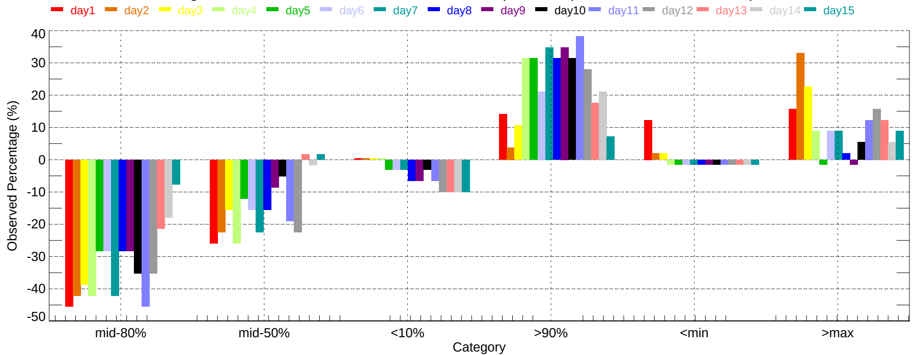
Observed Percentage Deviation of Ensembles - SDF: Min Temperature (2007-11-01~2007-11-30)
