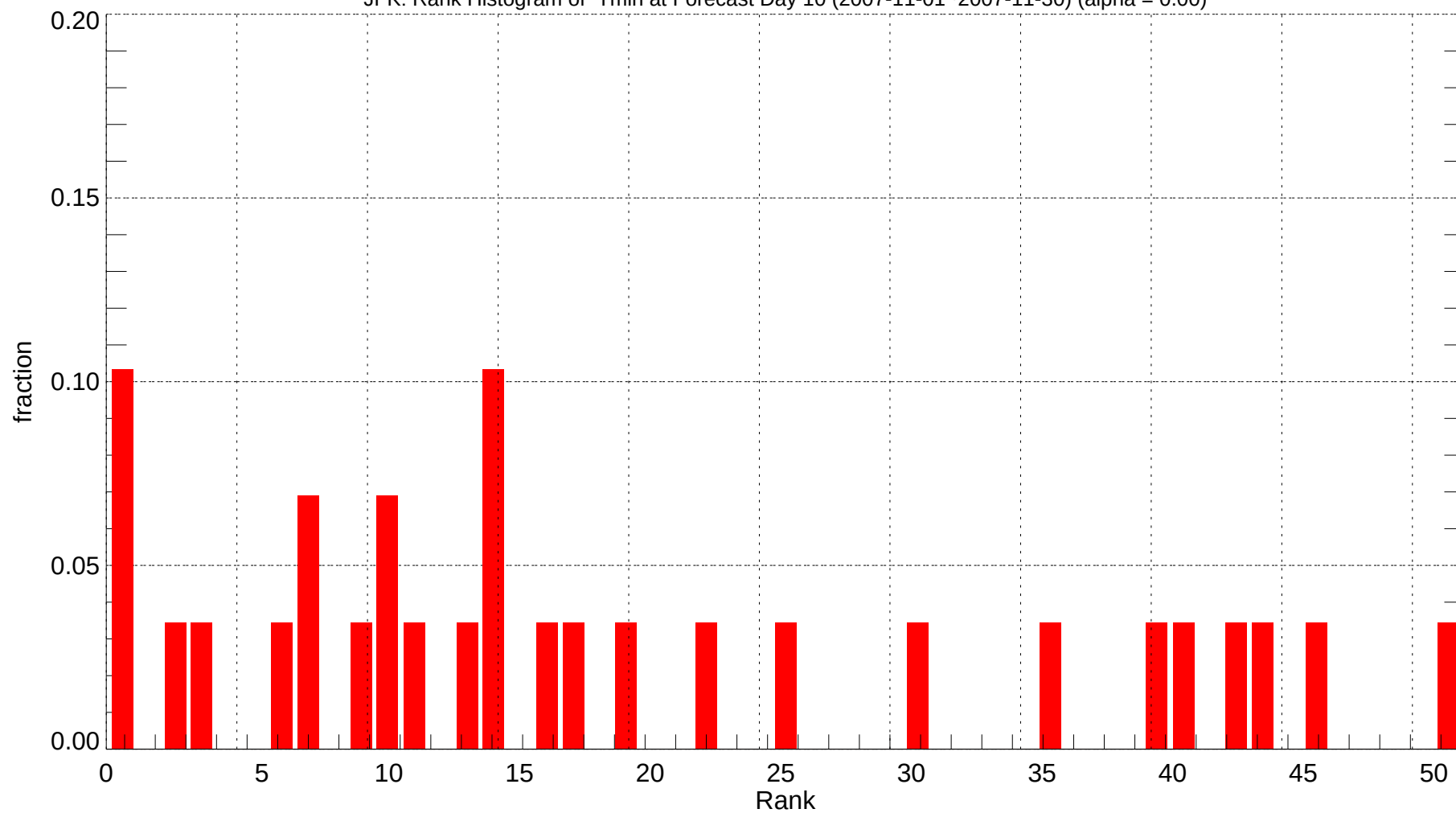
JFK: Rank Histogram of Tmin at Forecast Day 10 (2007-11-01~2007-11-30) (alpha = 0.00)
