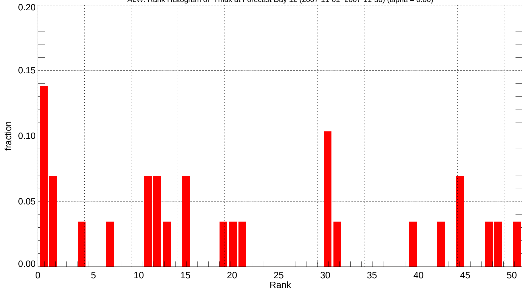
ALW: Rank Histogram of Tmax at Forecast Day 12 (2007-11-01~2007-11-30) (alpha = 0.00)
