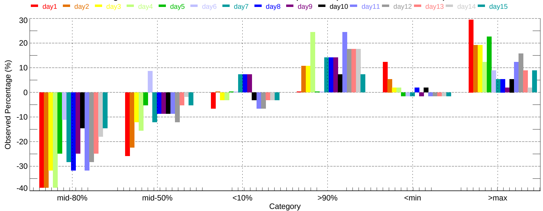
Observed Percentage Deviation of Ensembles - RIC: Min Temperature (2007-11-01~2007-11-30)
