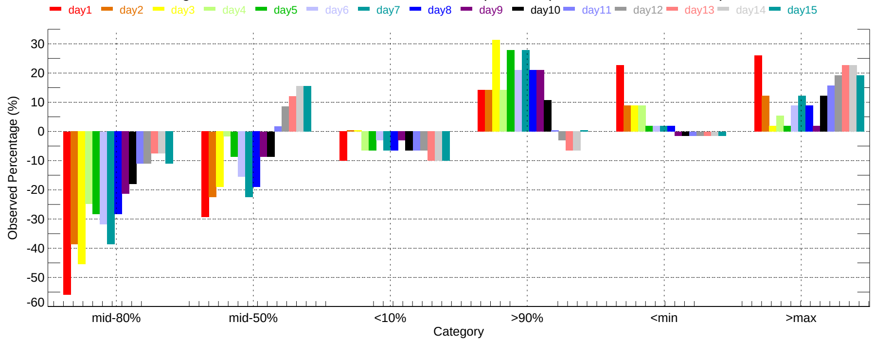
Observed Percentage Deviation of Ensembles - RDD: Min Temperature (2007-11-01~2007-11-30)
