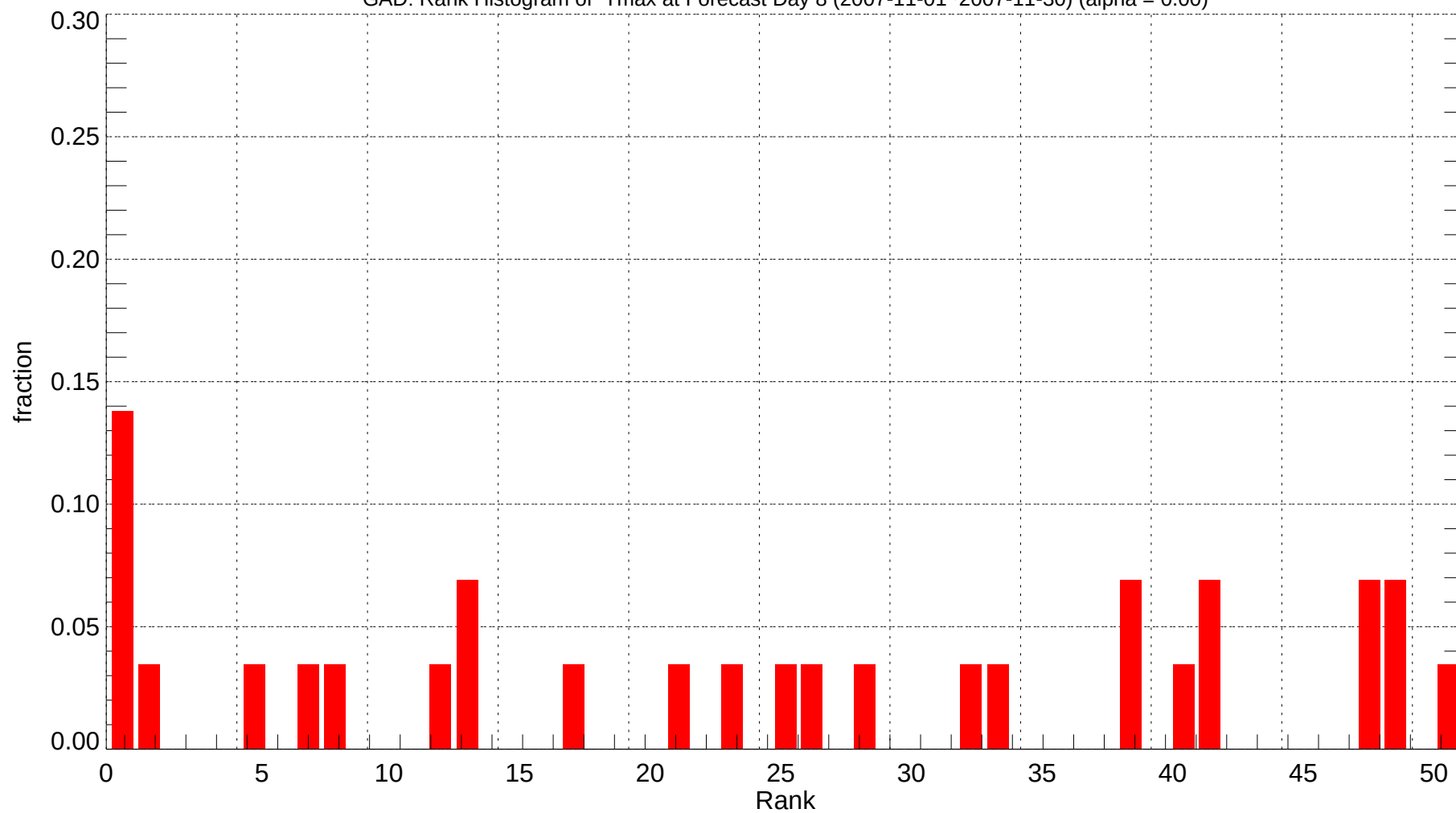
GAD: Rank Histogram of Tmax at Forecast Day 8 (2007-11-01~2007-11-30) (alpha = 0.00)
