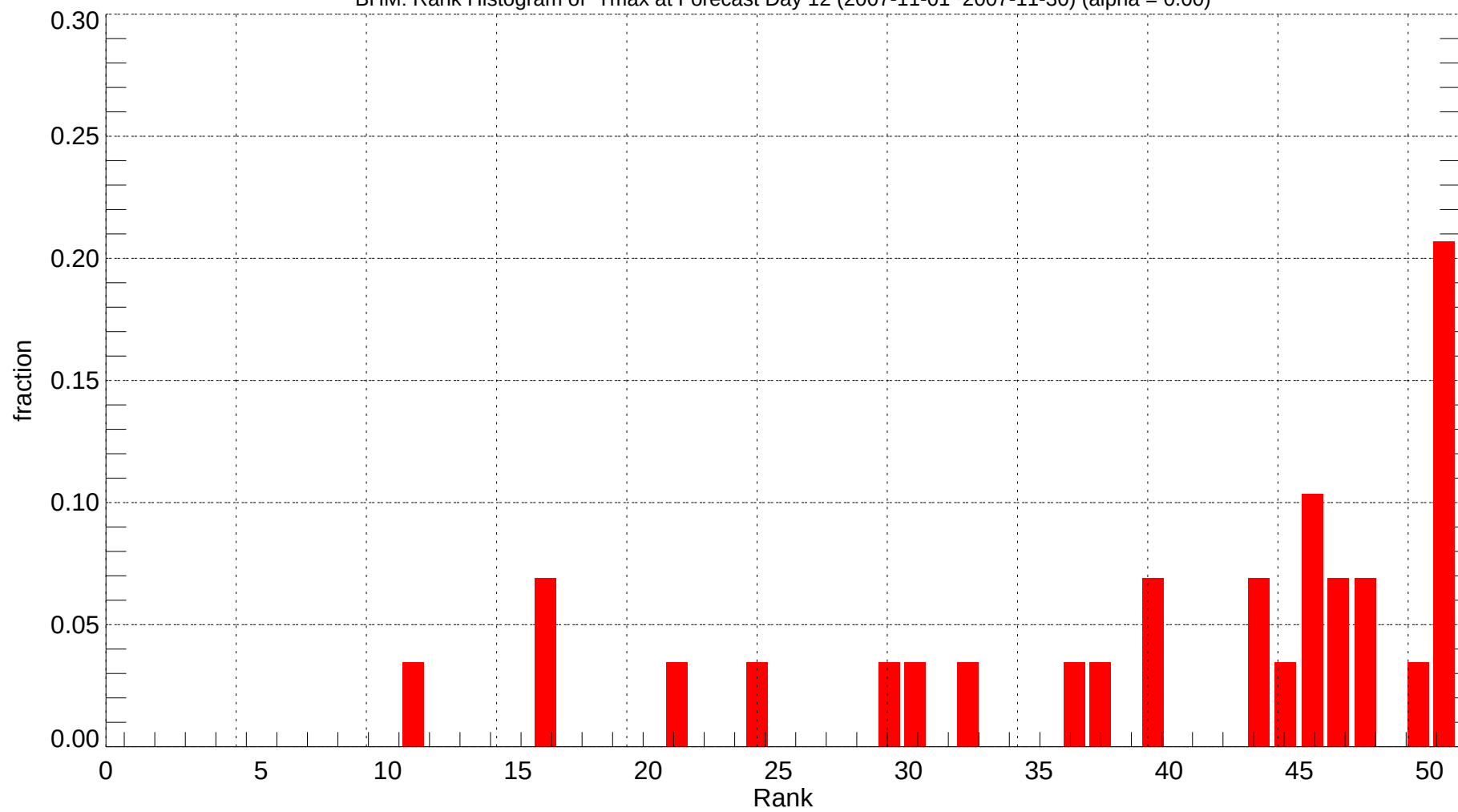
BHM: Rank Histogram of Tmax at Forecast Day 12 (2007-11-01~2007-11-30) (alpha = 0.00)
