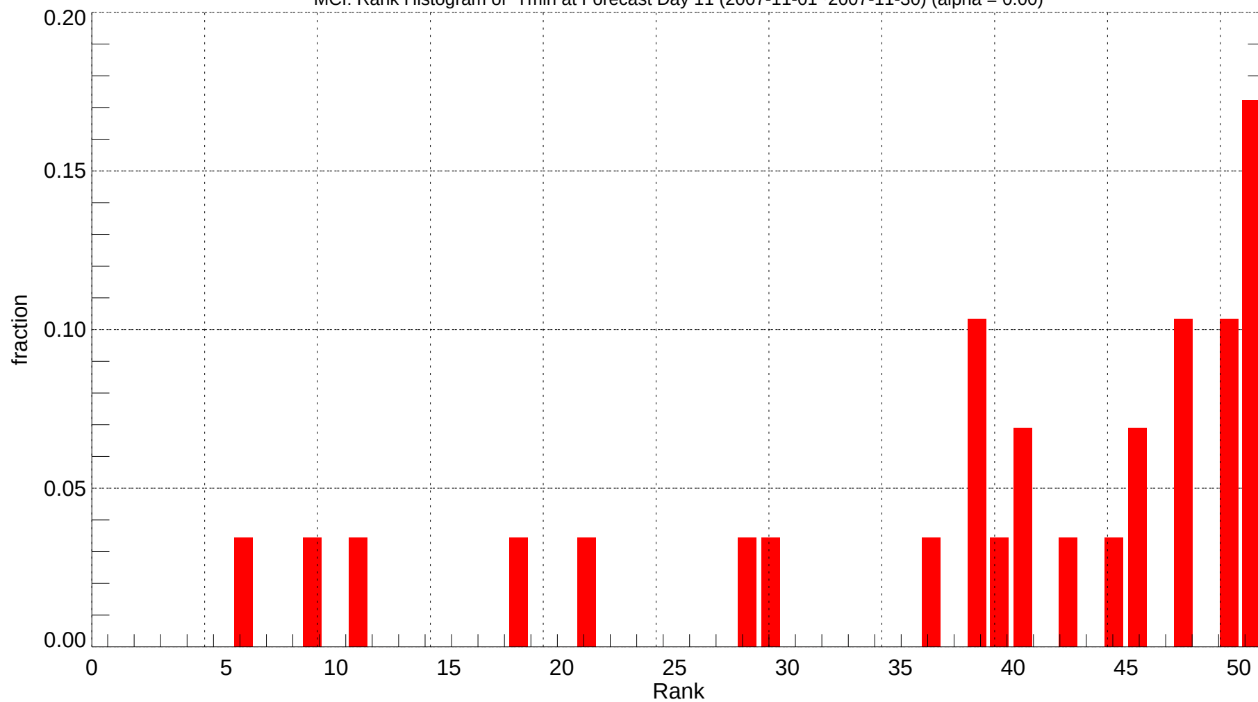
MCI: Rank Histogram of Tmin at Forecast Day 11 (2007-11-01~2007-11-30) (alpha = 0.00)
