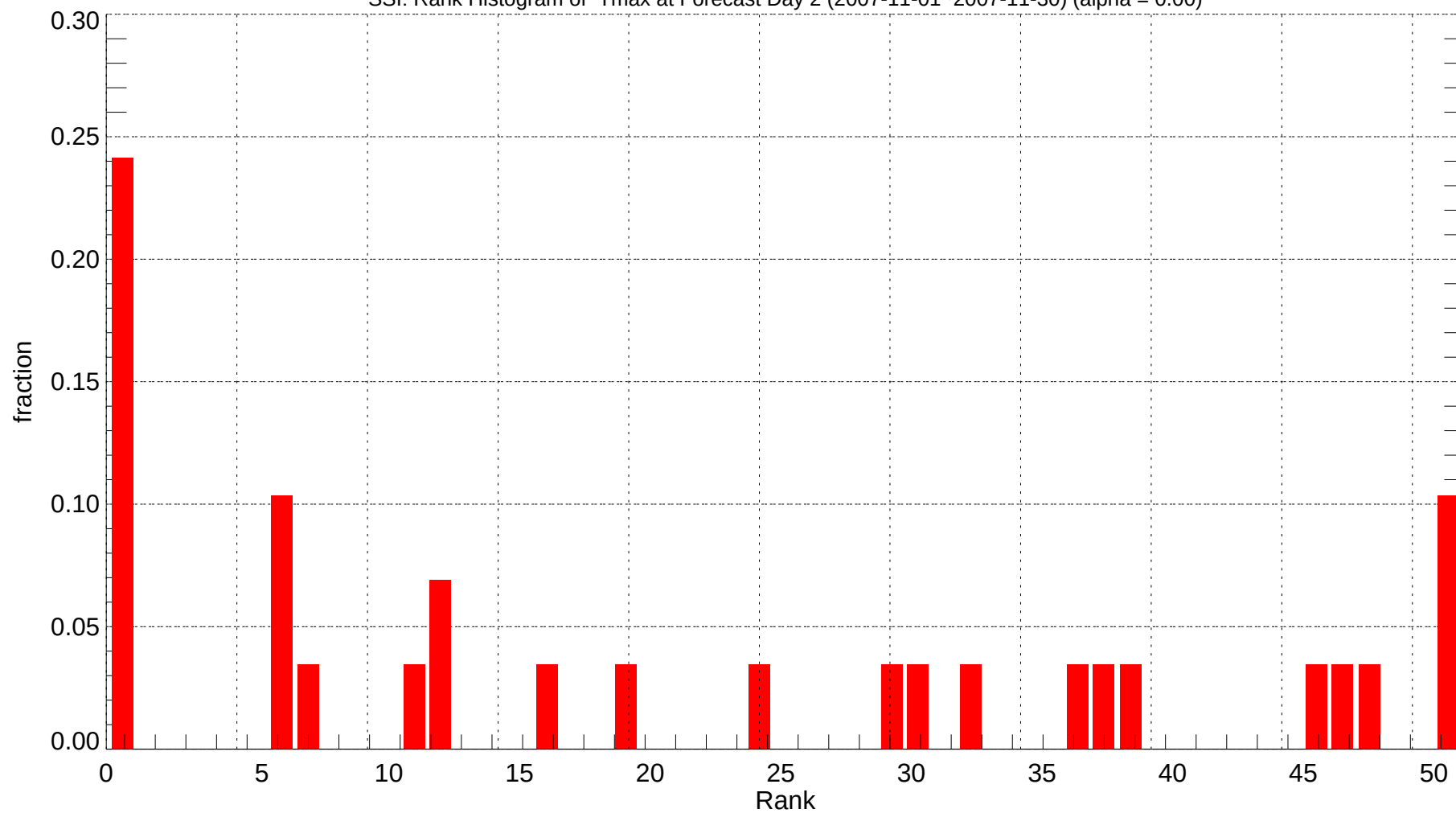
SSI: Rank Histogram of Tmax at Forecast Day 2 (2007-11-01~2007-11-30) (alpha = 0.00)
