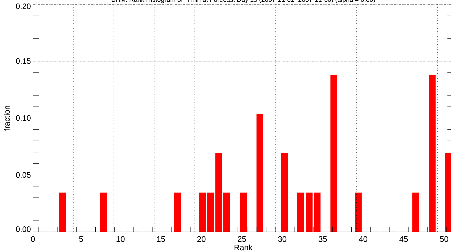
BHM: Rank Histogram of Tmin at Forecast Day 15 (2007-11-01~2007-11-30) (alpha = 0.00)
