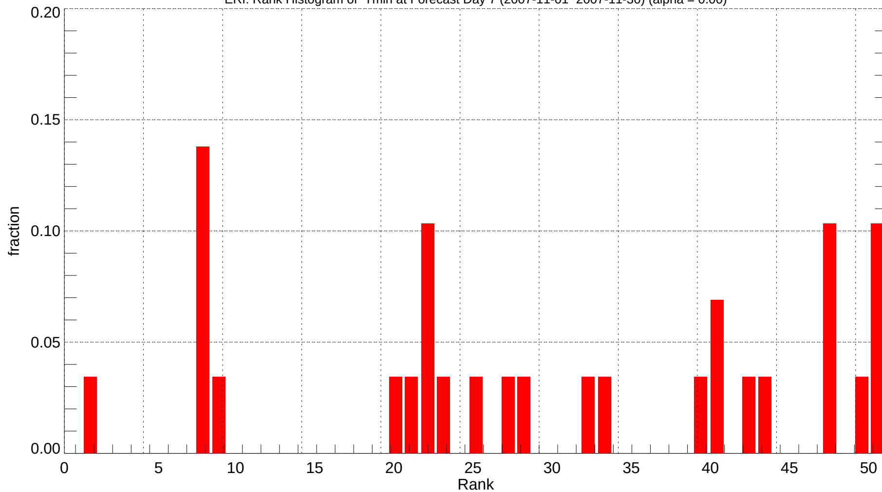
ERI: Rank Histogram of Tmin at Forecast Day 7 (2007-11-01~2007-11-30) (alpha = 0.00)
