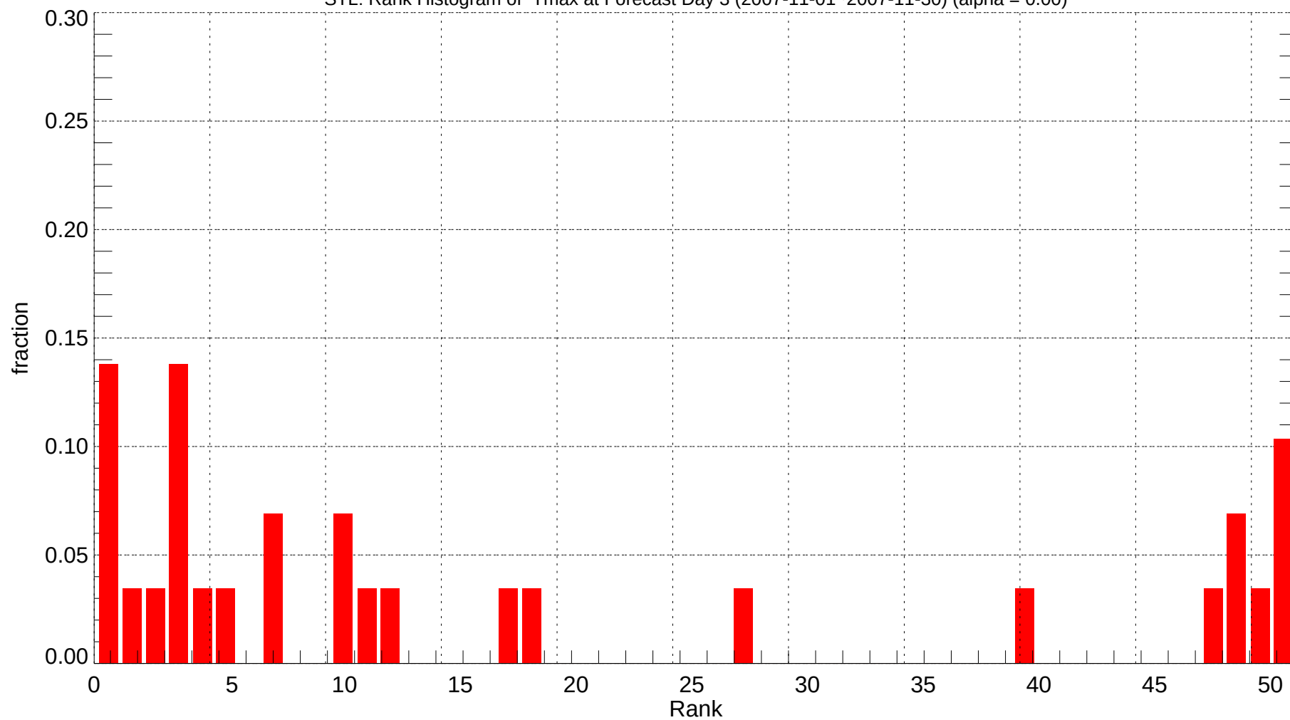
STL: Rank Histogram of Tmax at Forecast Day 3 (2007-11-01~2007-11-30) (alpha = 0.00)
