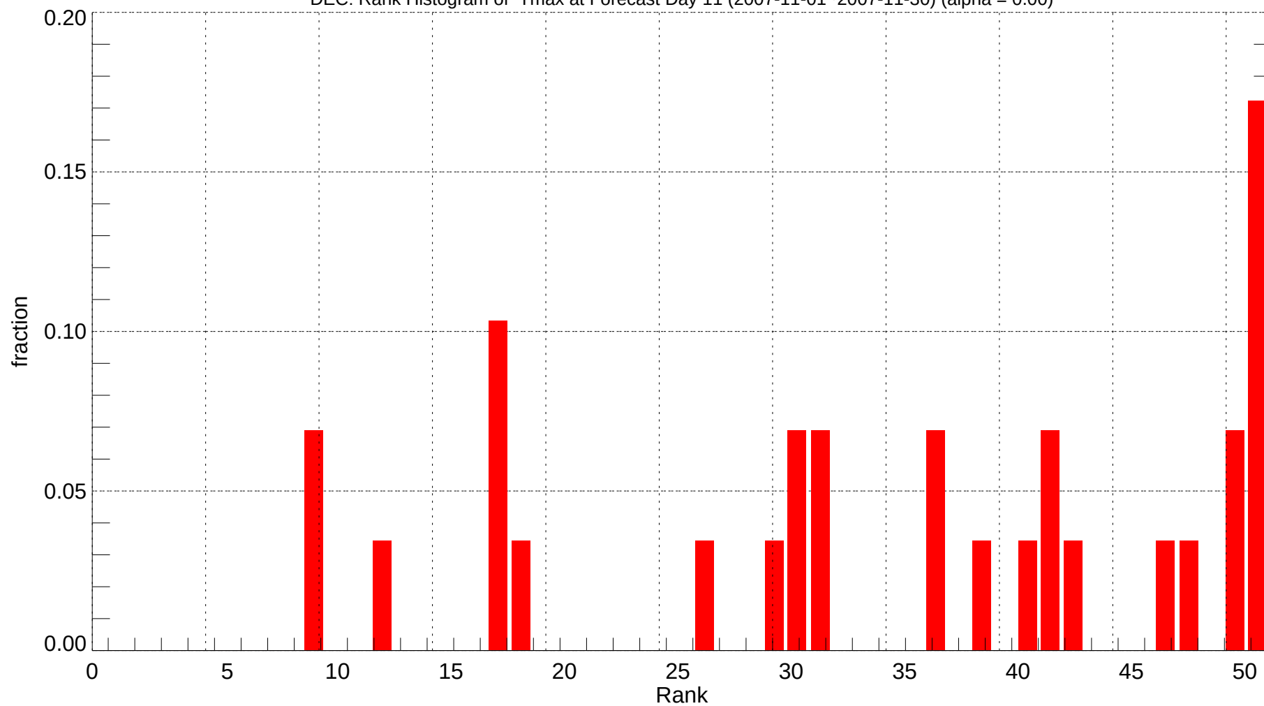
DEC: Rank Histogram of Tmax at Forecast Day 11 (2007-11-01~2007-11-30) (alpha = 0.00)
