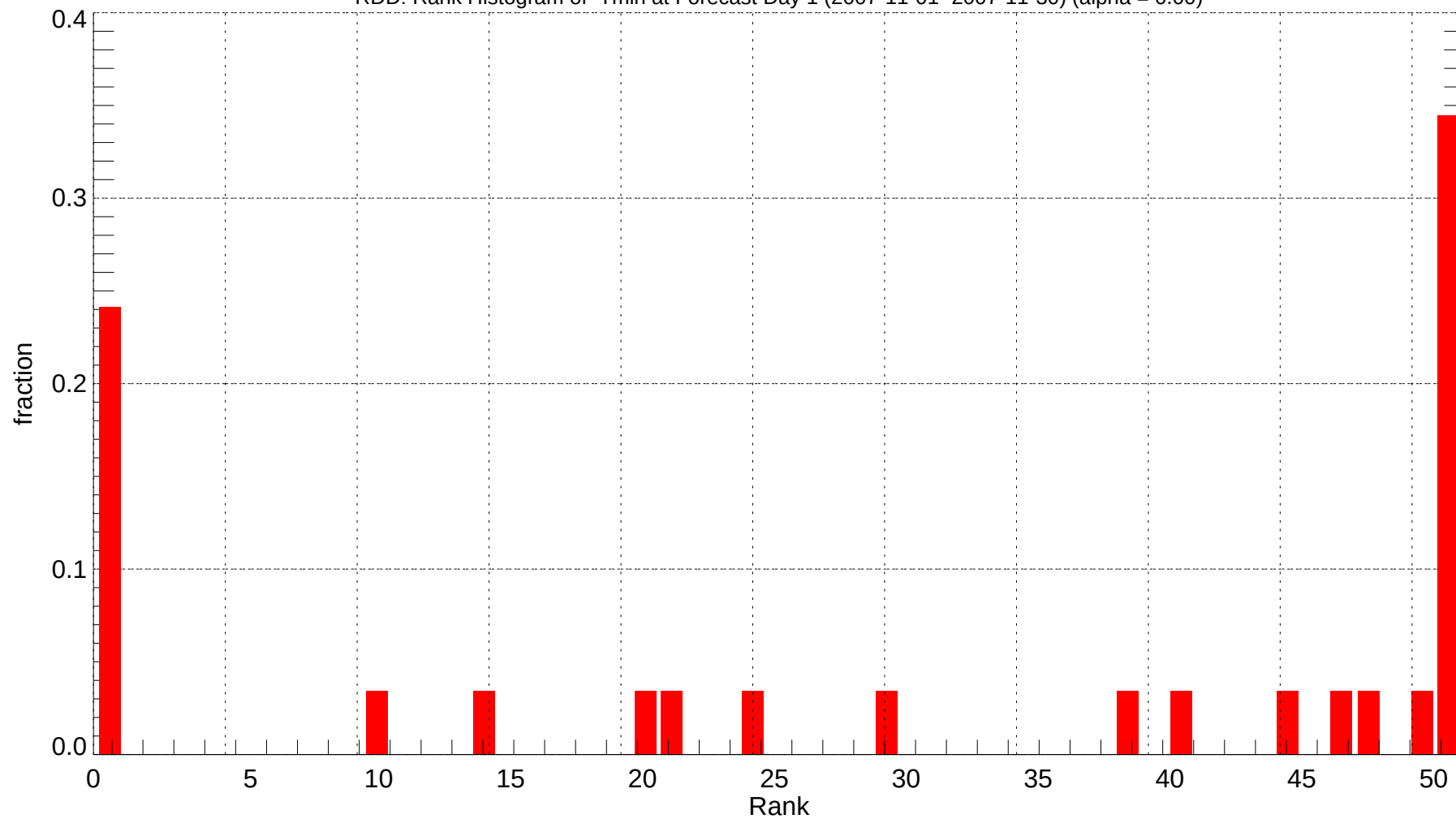
RDD: Rank Histogram of Tmin at Forecast Day 1 (2007-11-01~2007-11-30) (alpha = 0.00)
