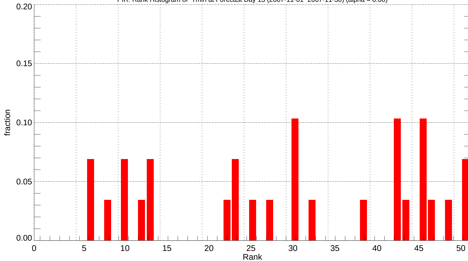
PIR: Rank Histogram of Tmin at Forecast Day 13 (2007-11-01~2007-11-30) (alpha = 0.00)
