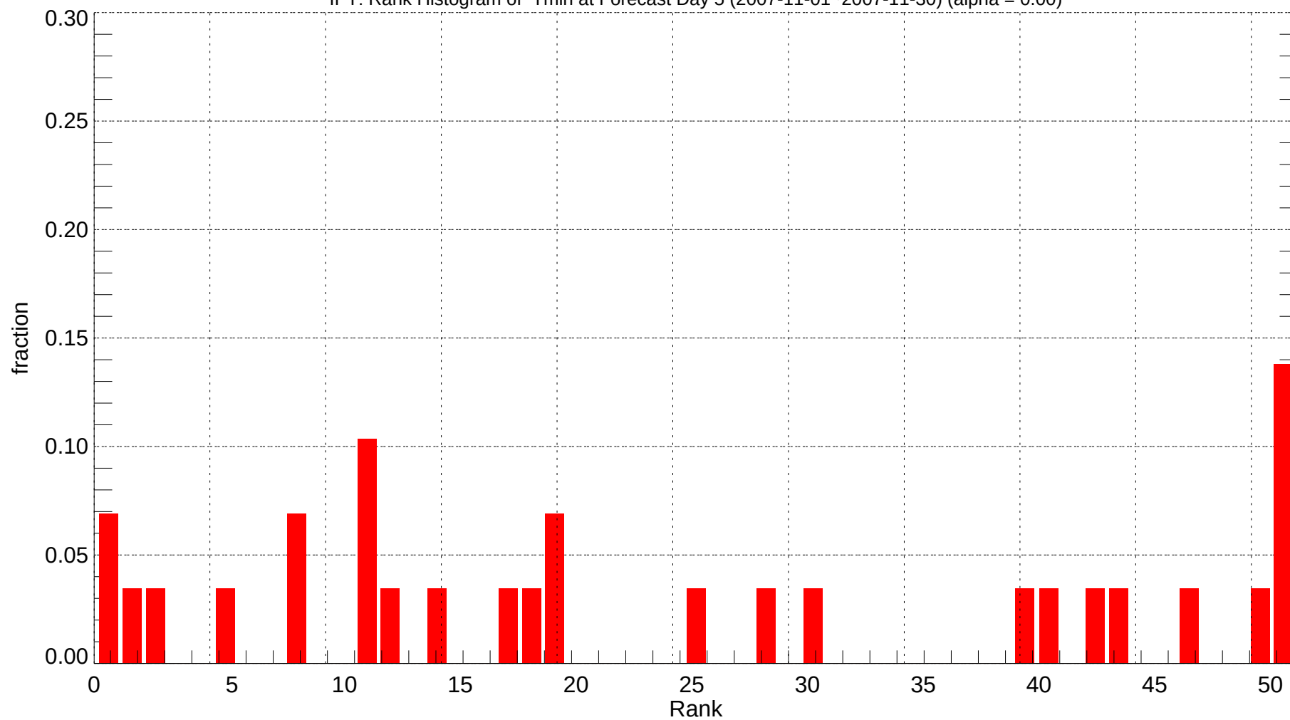
IPT: Rank Histogram of Tmin at Forecast Day 5 (2007-11-01~2007-11-30) (alpha = 0.00)
