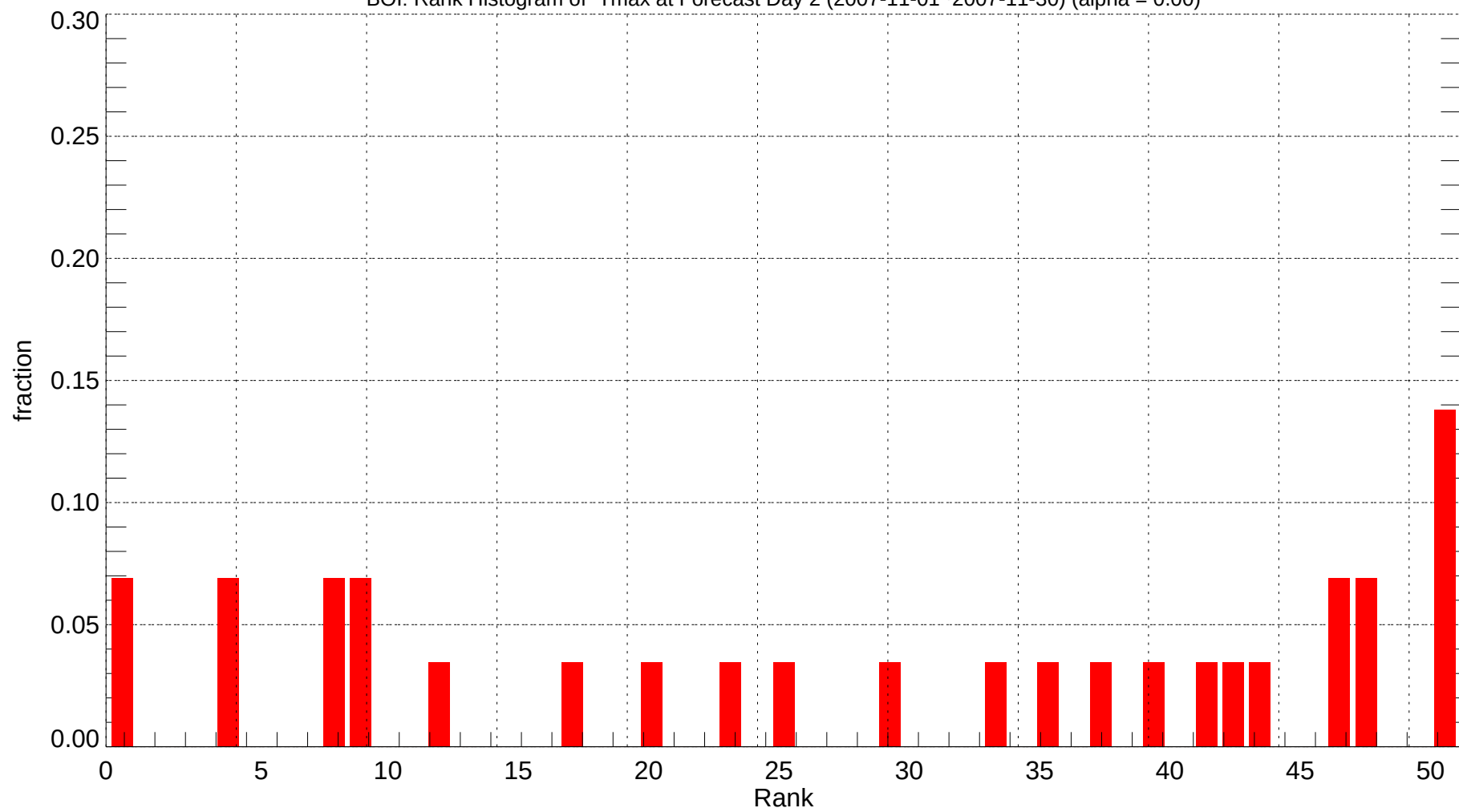
BOI: Rank Histogram of Tmax at Forecast Day 2 (2007-11-01~2007-11-30) (alpha = 0.00)
