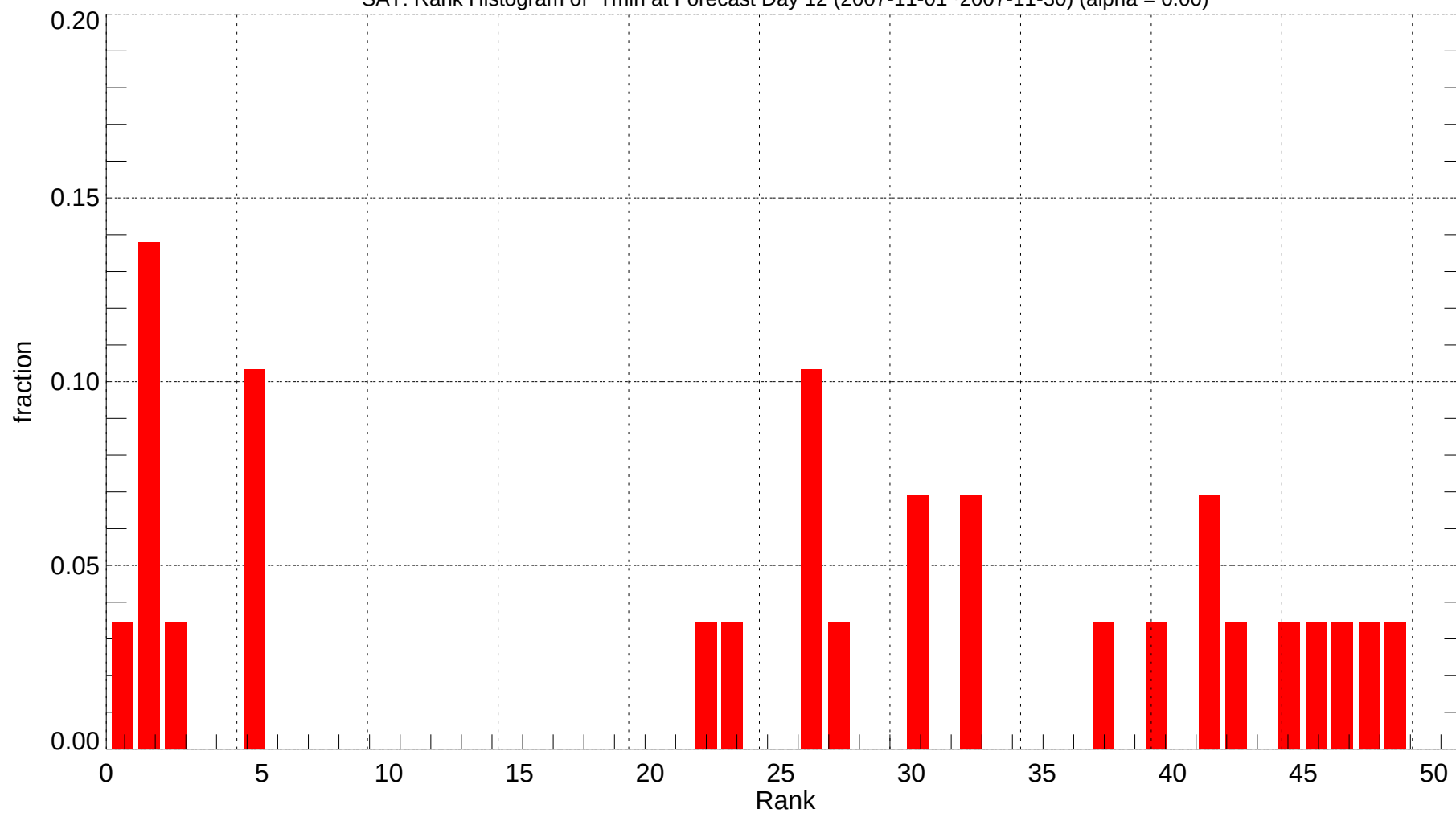
SAT: Rank Histogram of Tmin at Forecast Day 12 (2007-11-01~2007-11-30) (alpha = 0.00)
