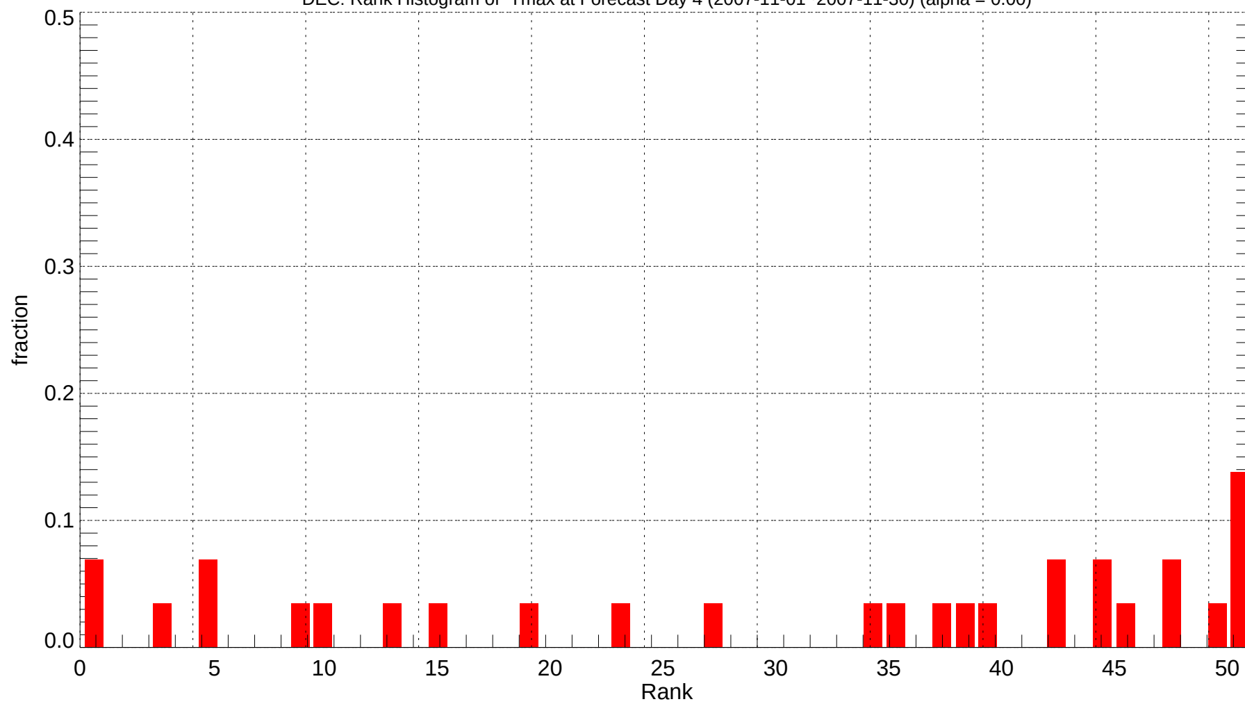
DEC: Rank Histogram of Tmax at Forecast Day 4 (2007-11-01~2007-11-30) (alpha = 0.00)
