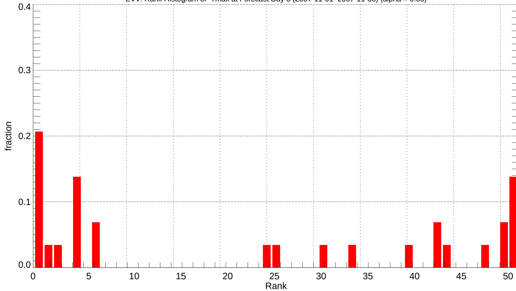
EVV: Rank Histogram of Tmax at Forecast Day 3 (2007-11-01~2007-11-30) (alpha = 0.00)
