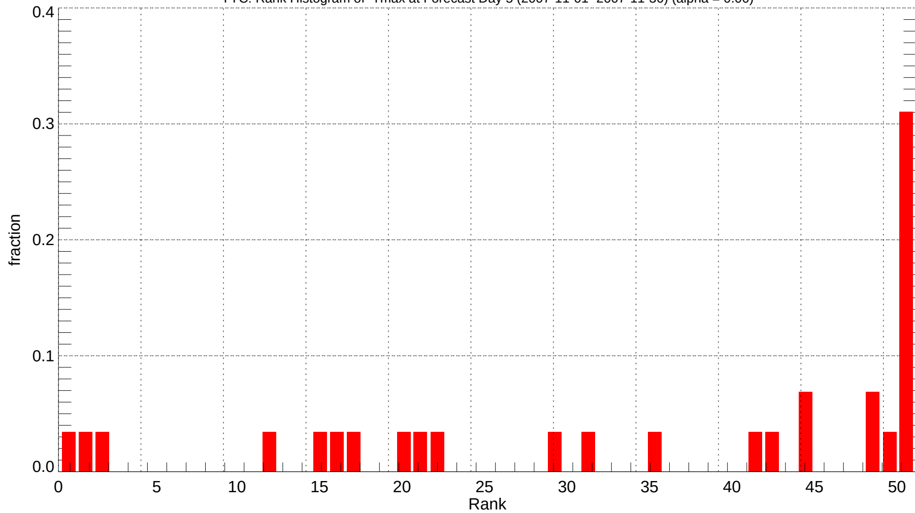
YYC: Rank Histogram of Tmax at Forecast Day 5 (2007-11-01~2007-11-30) (alpha = 0.00)
