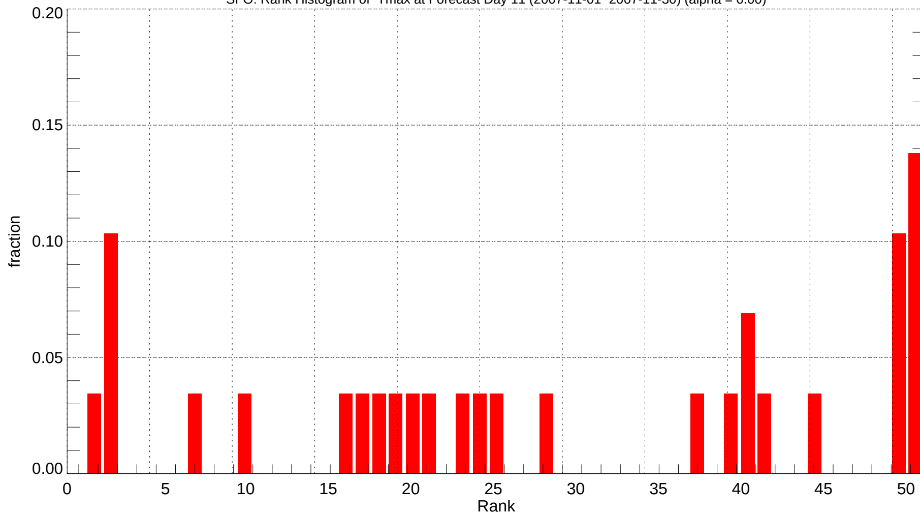
SFO: Rank Histogram of Tmax at Forecast Day 11 (2007-11-01~2007-11-30) (alpha = 0.00)
