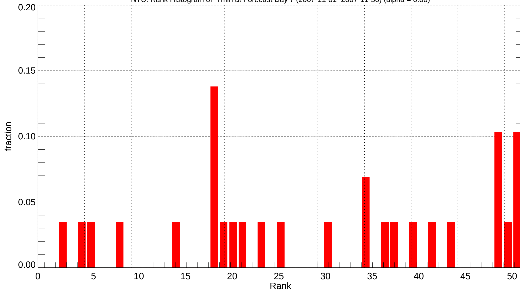
NTU: Rank Histogram of Tmin at Forecast Day 7 (2007-11-01~2007-11-30) (alpha = 0.00)
