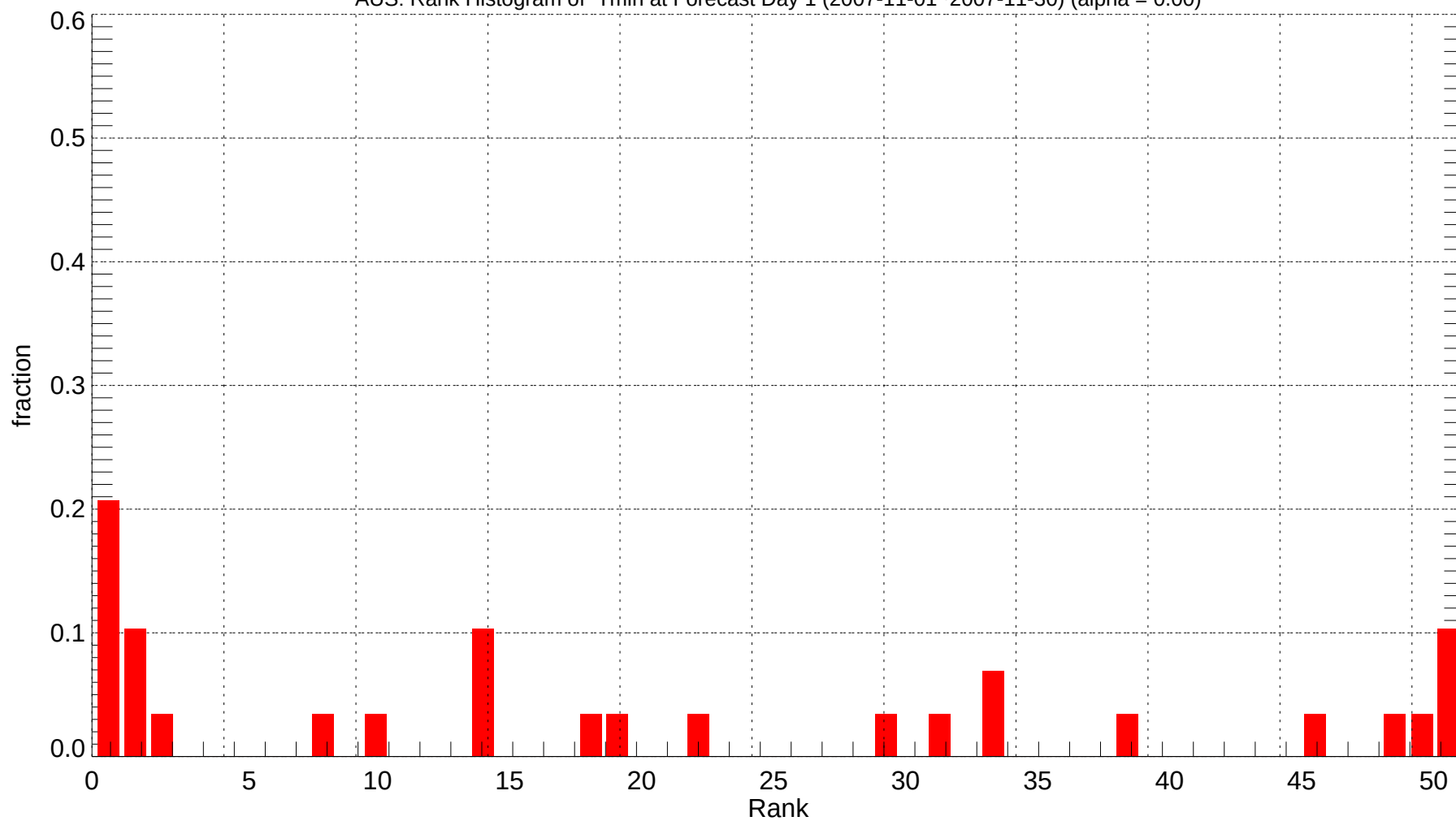
AUS: Rank Histogram of Tmin at Forecast Day 1 (2007-11-01~2007-11-30) (alpha = 0.00)
