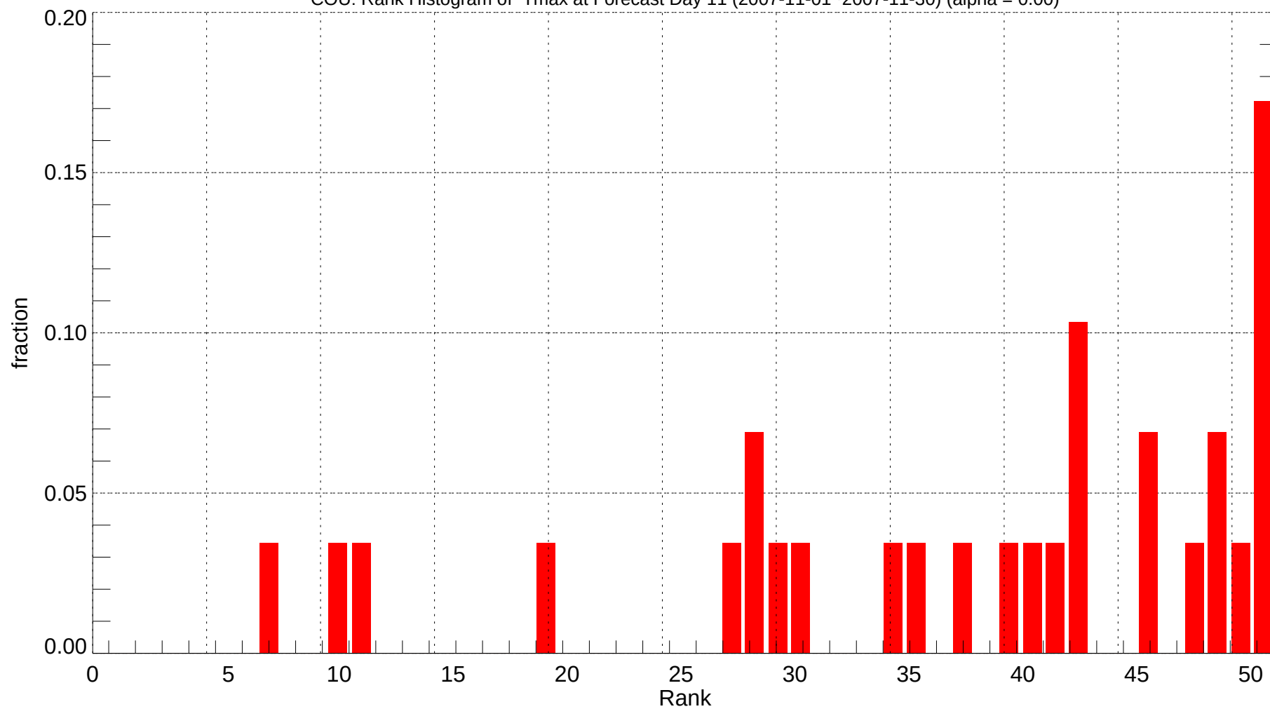
COU: Rank Histogram of Tmax at Forecast Day 11 (2007-11-01~2007-11-30) (alpha = 0.00)
