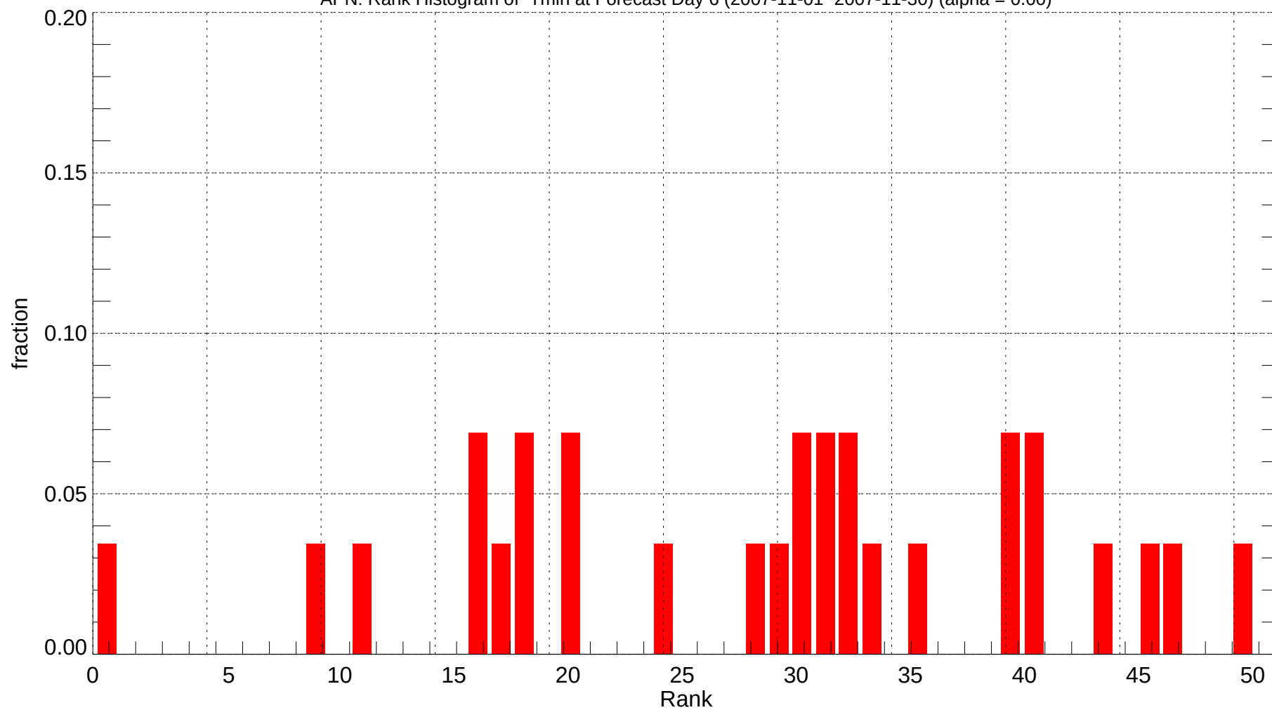
APN: Rank Histogram of Tmin at Forecast Day 6 (2007-11-01~2007-11-30) (alpha = 0.00)
