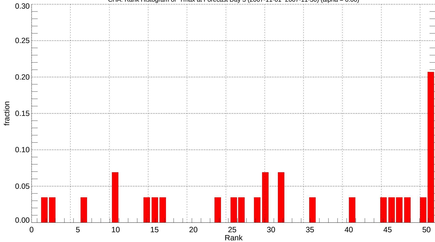
CHA: Rank Histogram of Tmax at Forecast Day 3 (2007-11-01~2007-11-30) (alpha = 0.00)
