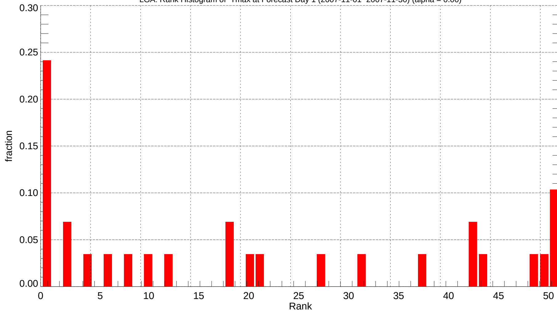
LGA: Rank Histogram of Tmax at Forecast Day 1 (2007-11-01~2007-11-30) (alpha = 0.00)
