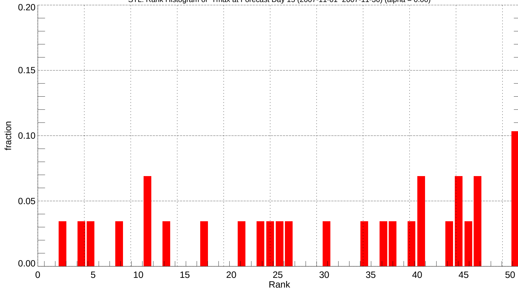
STL: Rank Histogram of Tmax at Forecast Day 15 (2007-11-01~2007-11-30) (alpha = 0.00)
