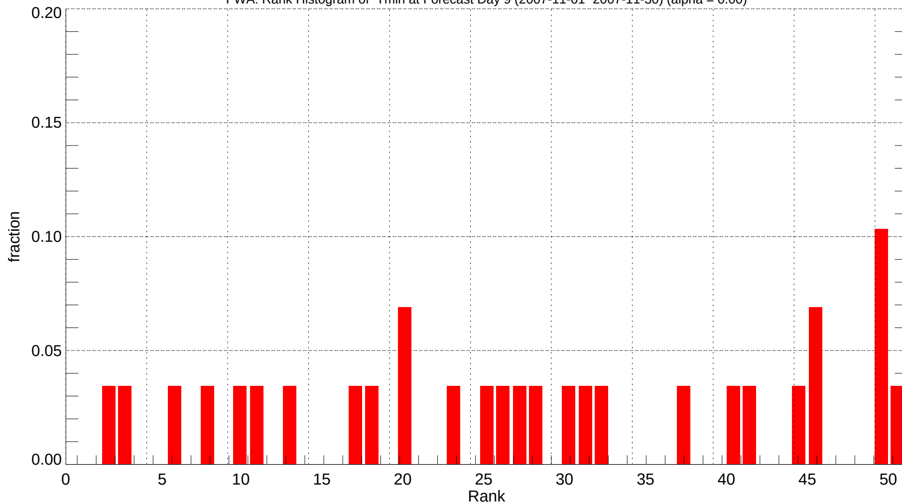
FWA: Rank Histogram of Tmin at Forecast Day 9 (2007-11-01~2007-11-30) (alpha = 0.00)
