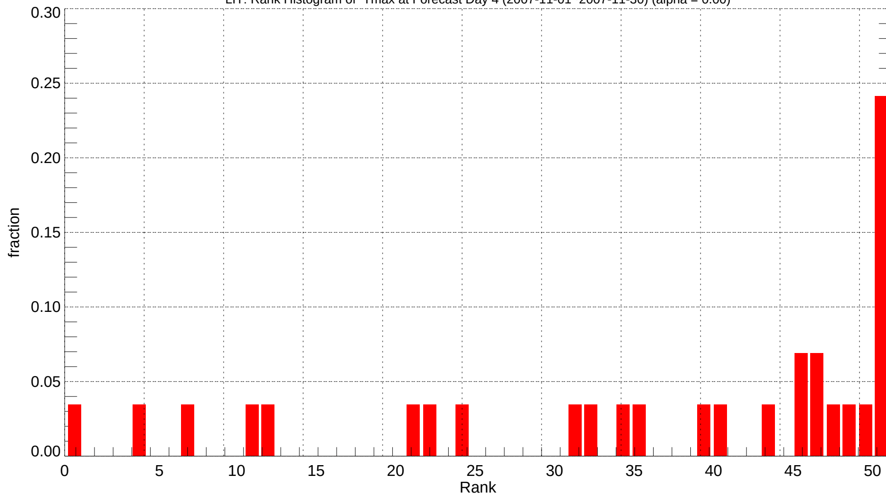
LIT: Rank Histogram of Tmax at Forecast Day 4 (2007-11-01~2007-11-30) (alpha = 0.00)
