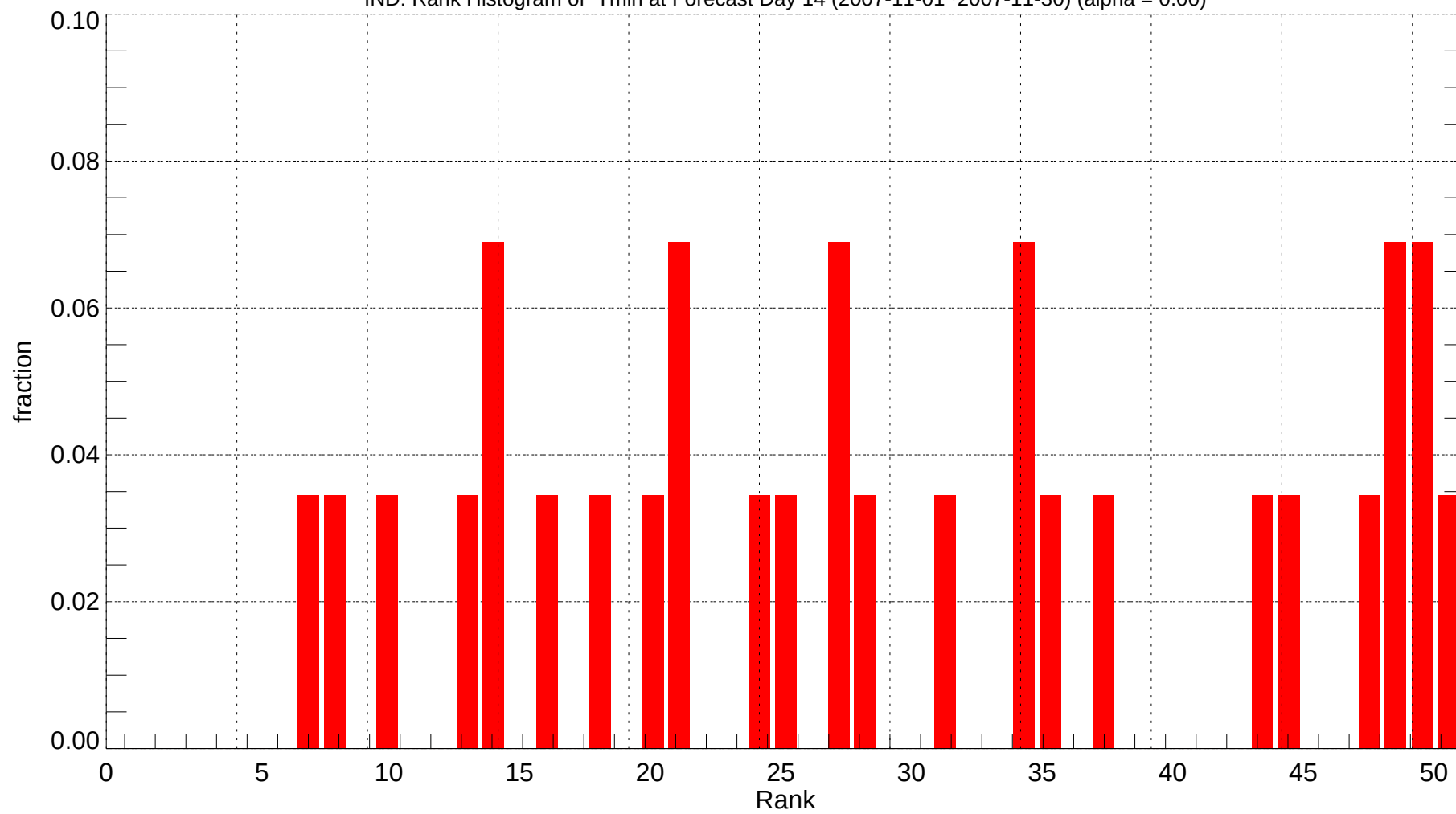
IND: Rank Histogram of Tmin at Forecast Day 14 (2007-11-01~2007-11-30) (alpha = 0.00)
