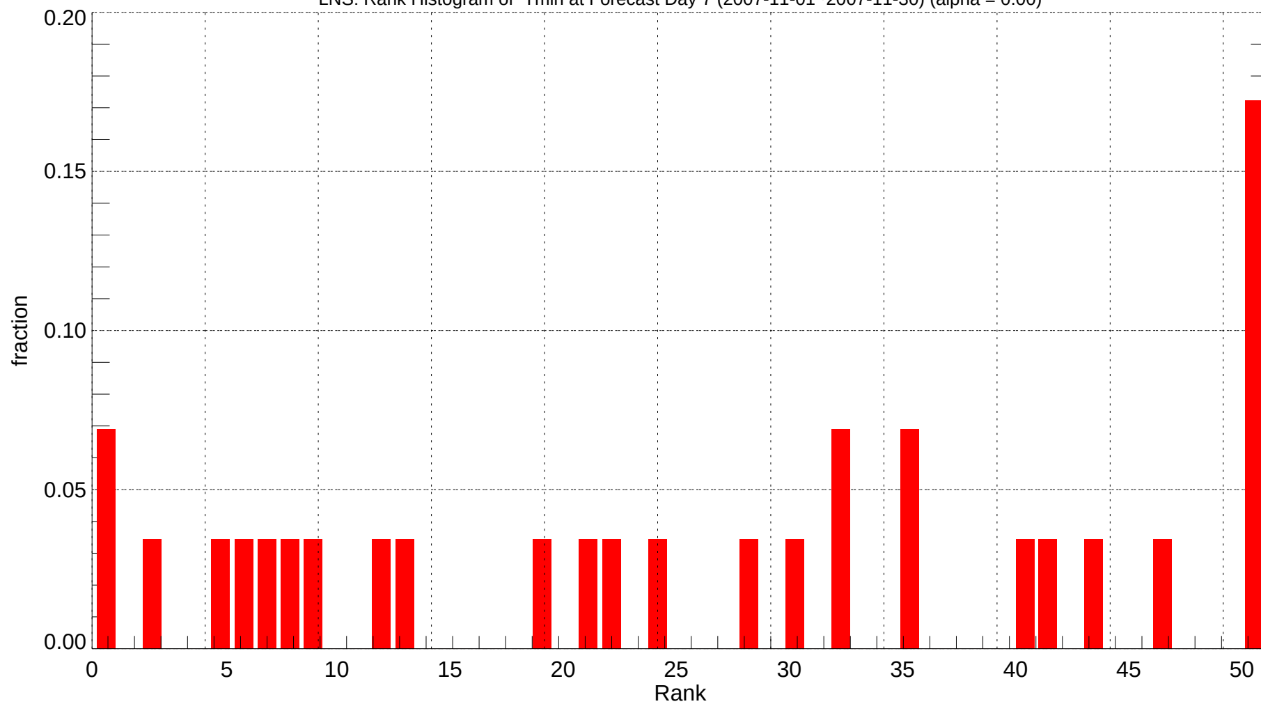
LNS: Rank Histogram of Tmin at Forecast Day 7 (2007-11-01~2007-11-30) (alpha = 0.00)
