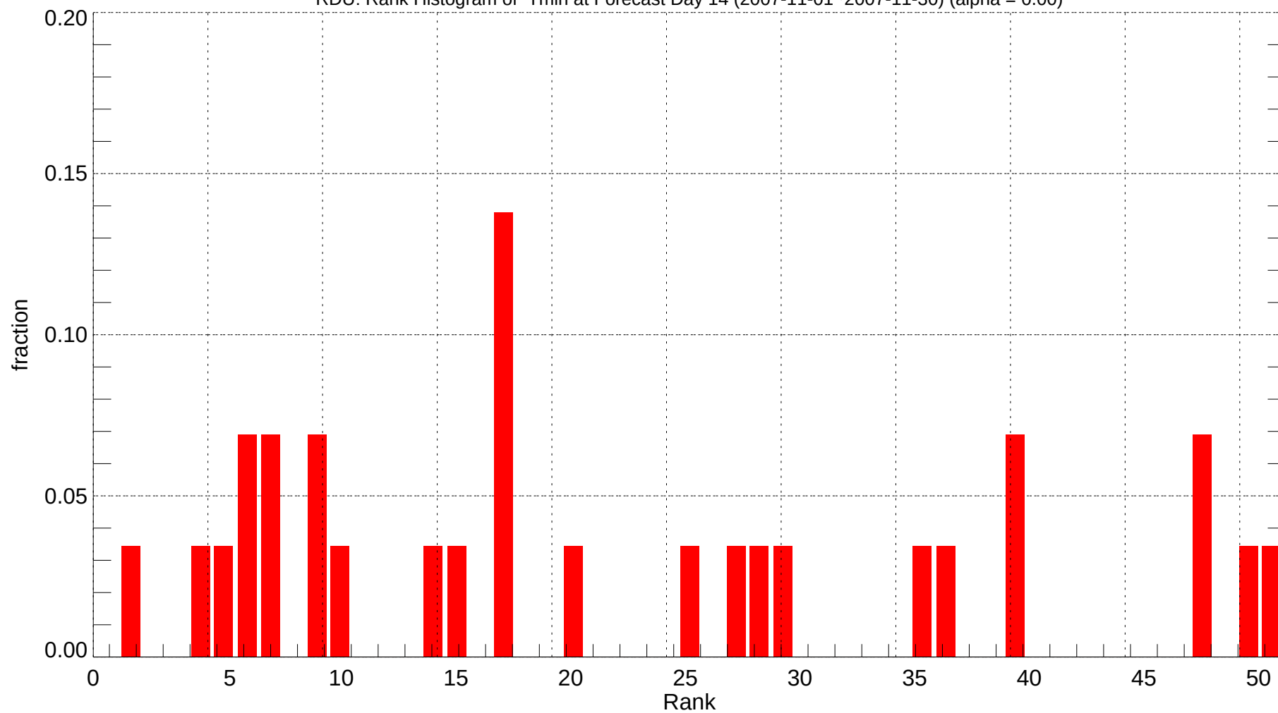
RDU: Rank Histogram of Tmin at Forecast Day 14 (2007-11-01~2007-11-30) (alpha = 0.00)
