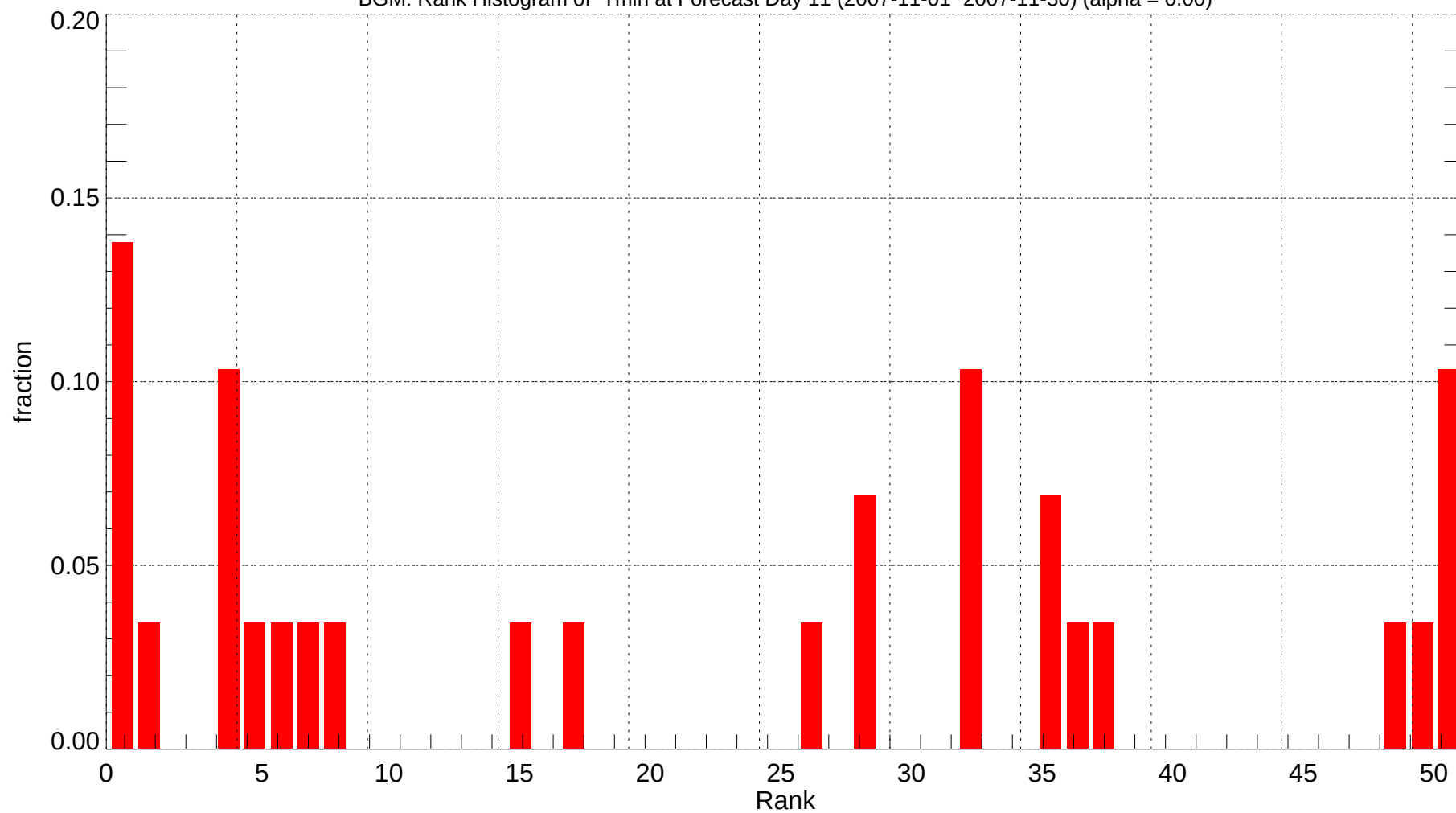
BGM: Rank Histogram of Tmin at Forecast Day 11 (2007-11-01~2007-11-30) (alpha = 0.00)
