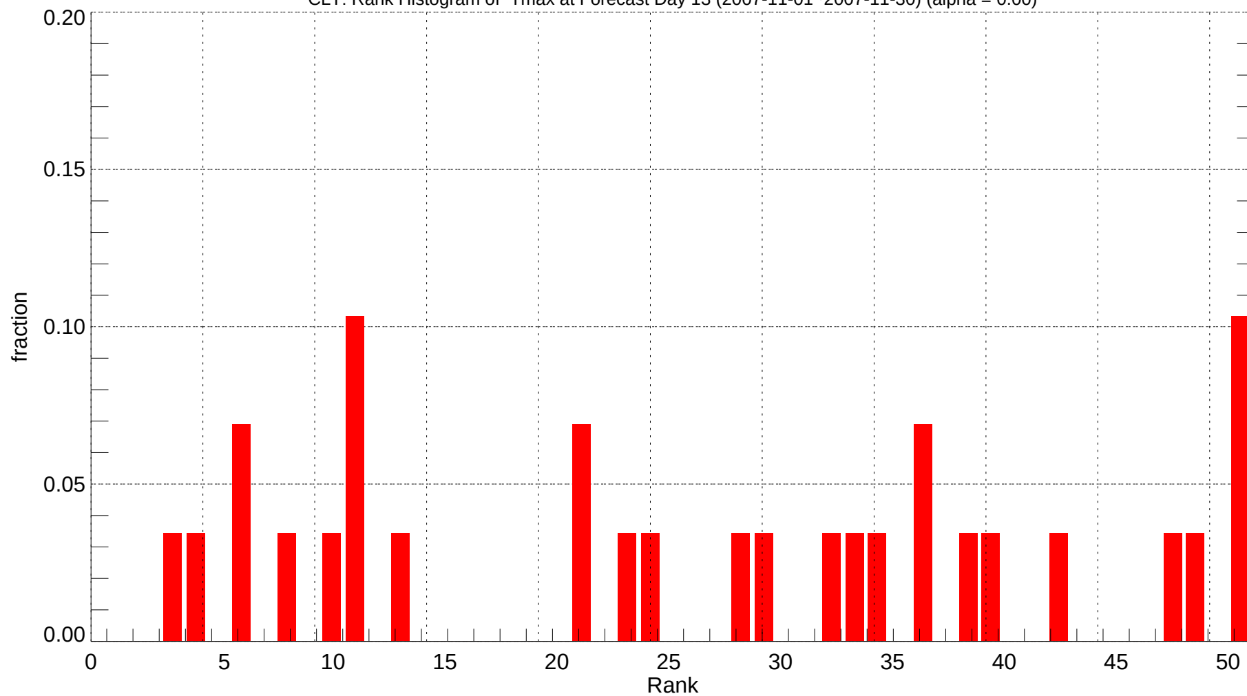
CLT: Rank Histogram of Tmax at Forecast Day 13 (2007-11-01~2007-11-30) (alpha = 0.00)
