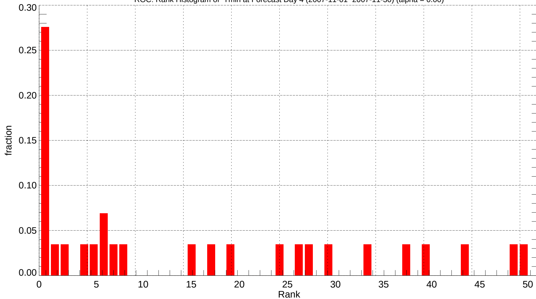
ROC: Rank Histogram of Tmin at Forecast Day 4 (2007-11-01~2007-11-30) (alpha = 0.00)
