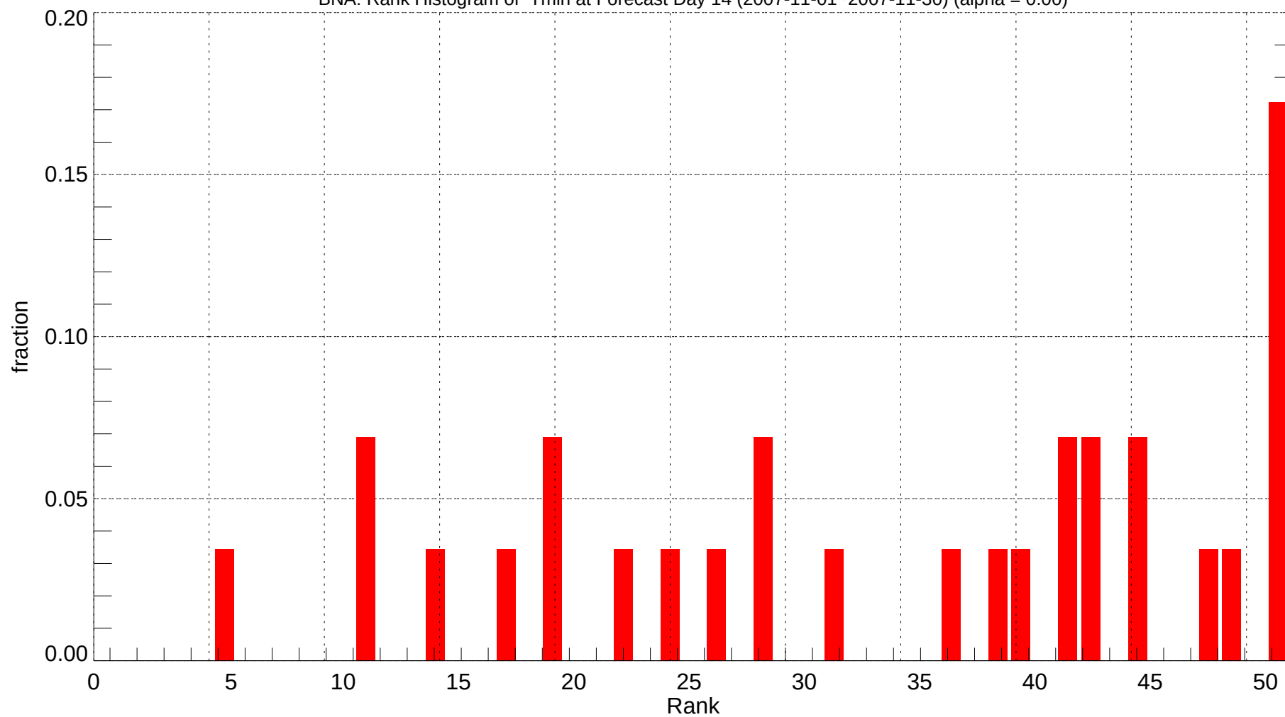
BNA: Rank Histogram of Tmin at Forecast Day 14 (2007-11-01~2007-11-30) (alpha = 0.00)
