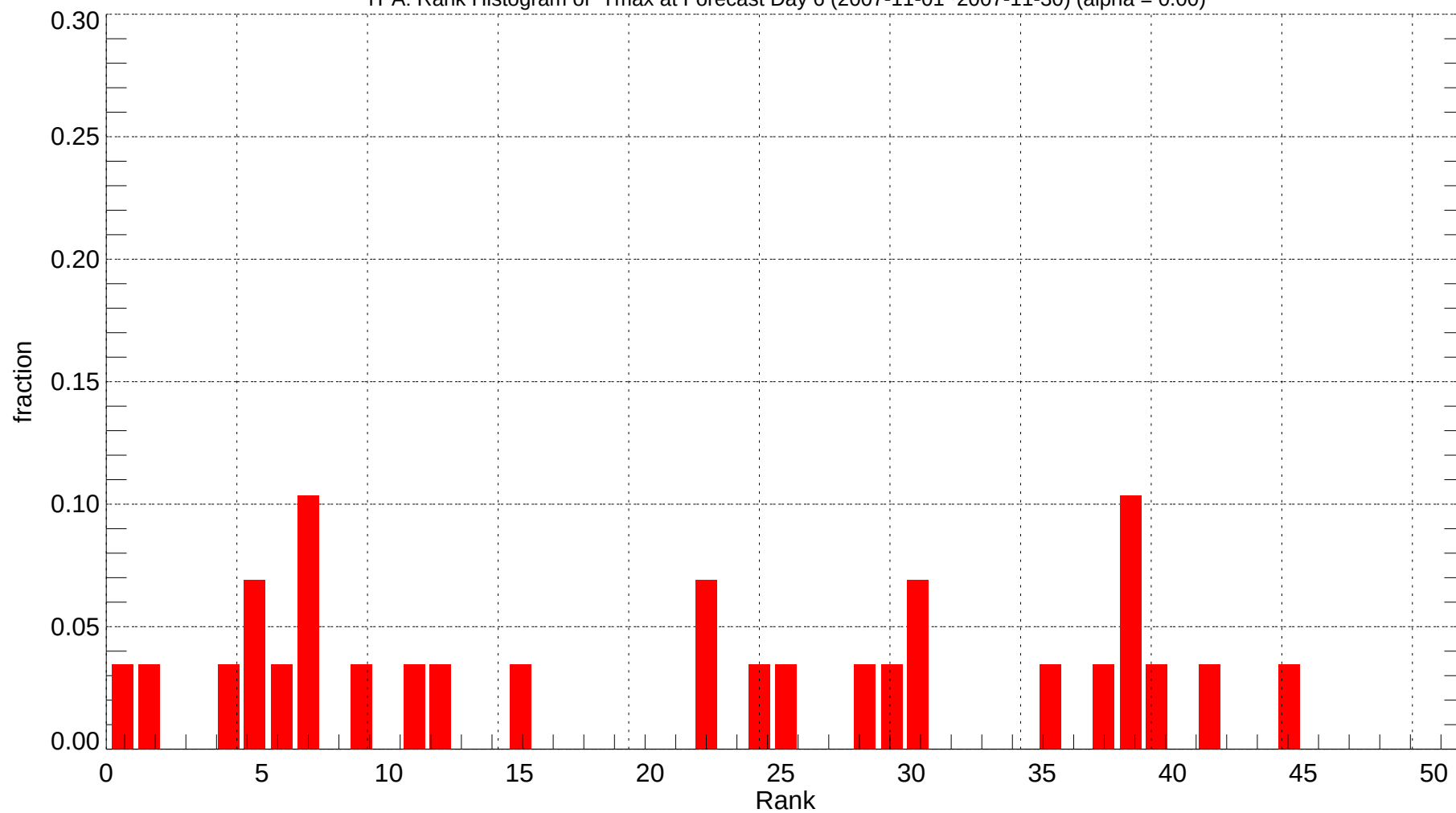
TPA: Rank Histogram of Tmax at Forecast Day 6 (2007-11-01~2007-11-30) (alpha = 0.00)
