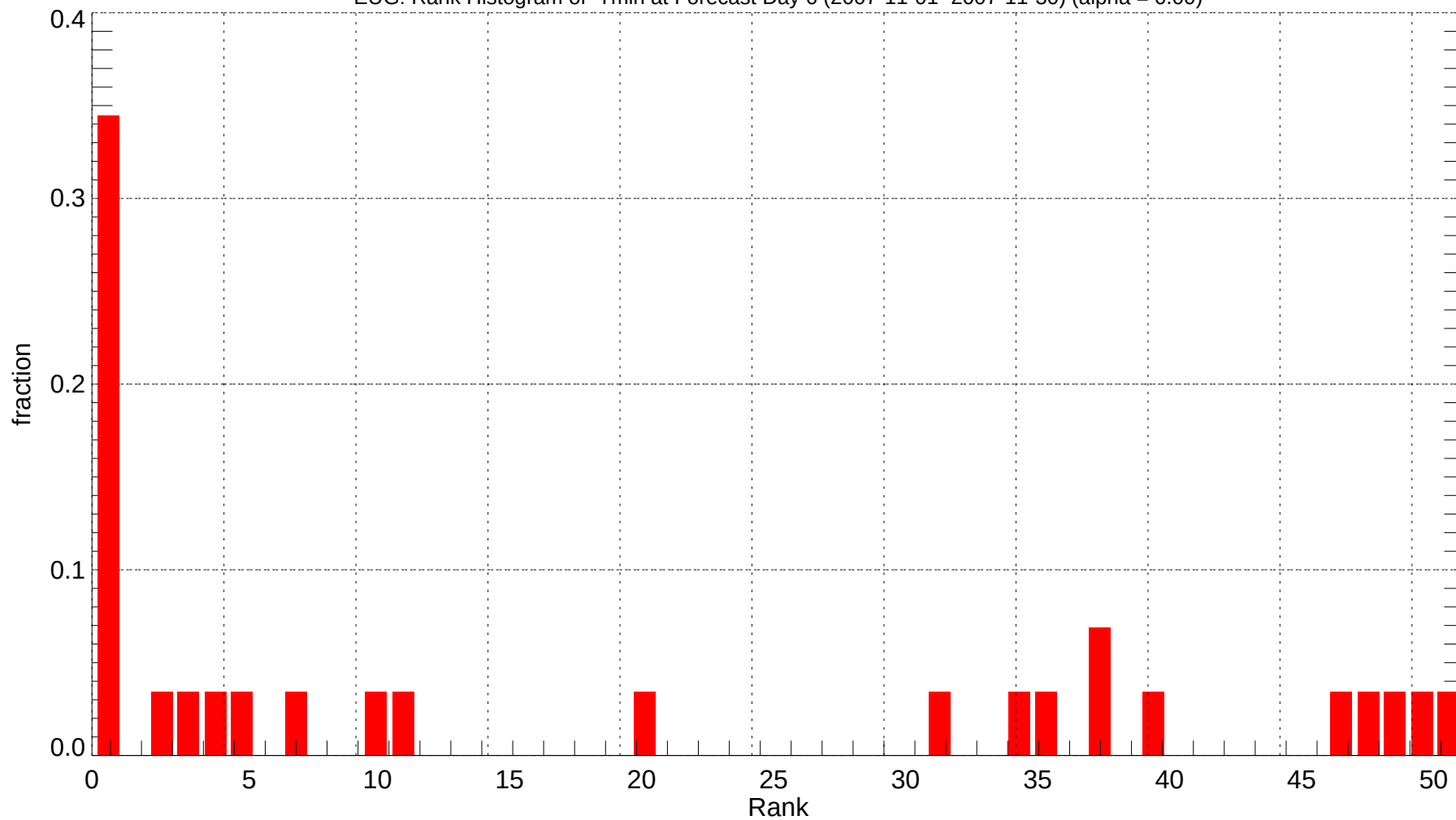
EUG: Rank Histogram of Tmin at Forecast Day 6 (2007-11-01~2007-11-30) (alpha = 0.00)
