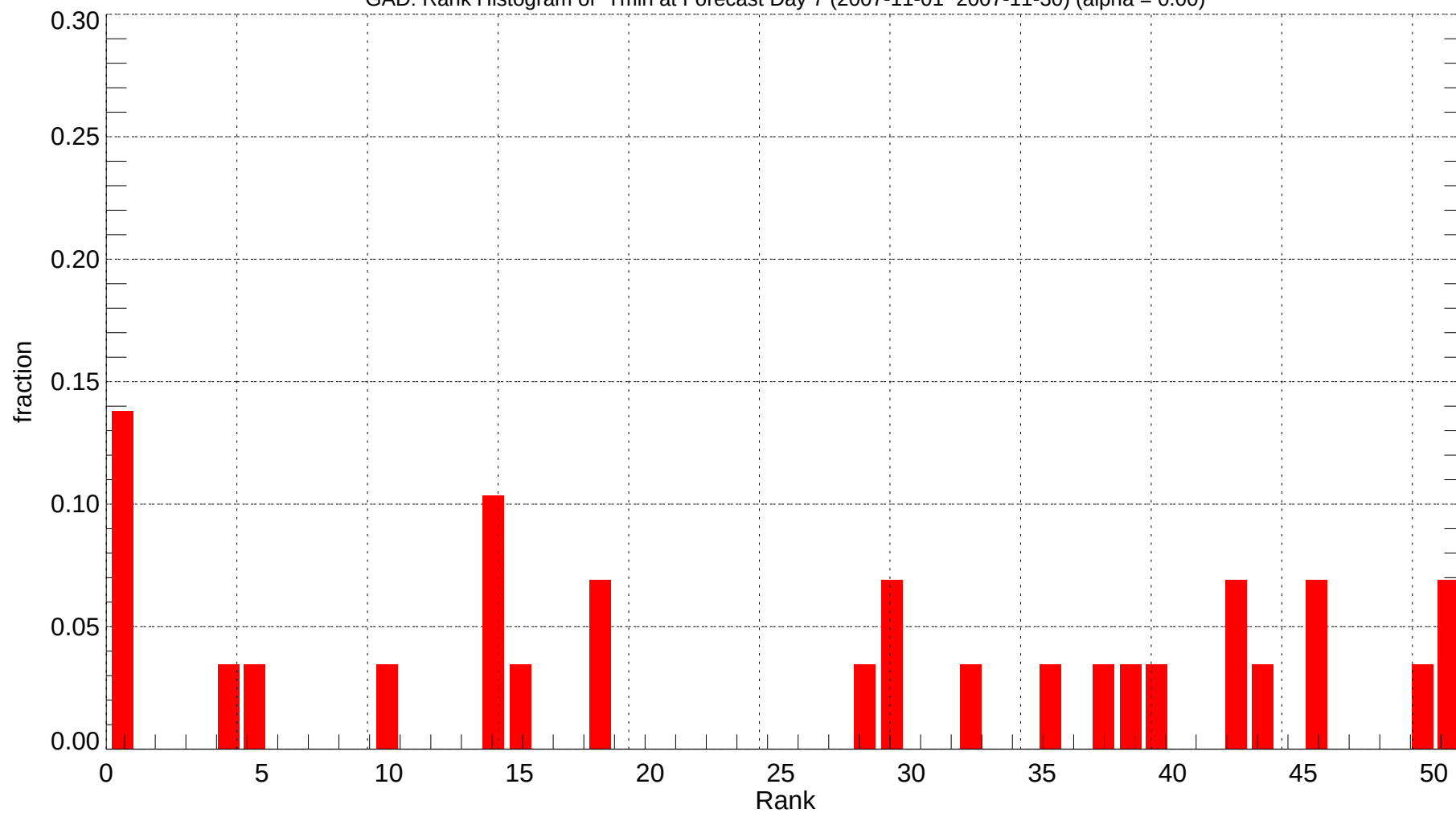
GAD: Rank Histogram of Tmin at Forecast Day 7 (2007-11-01~2007-11-30) (alpha = 0.00)
