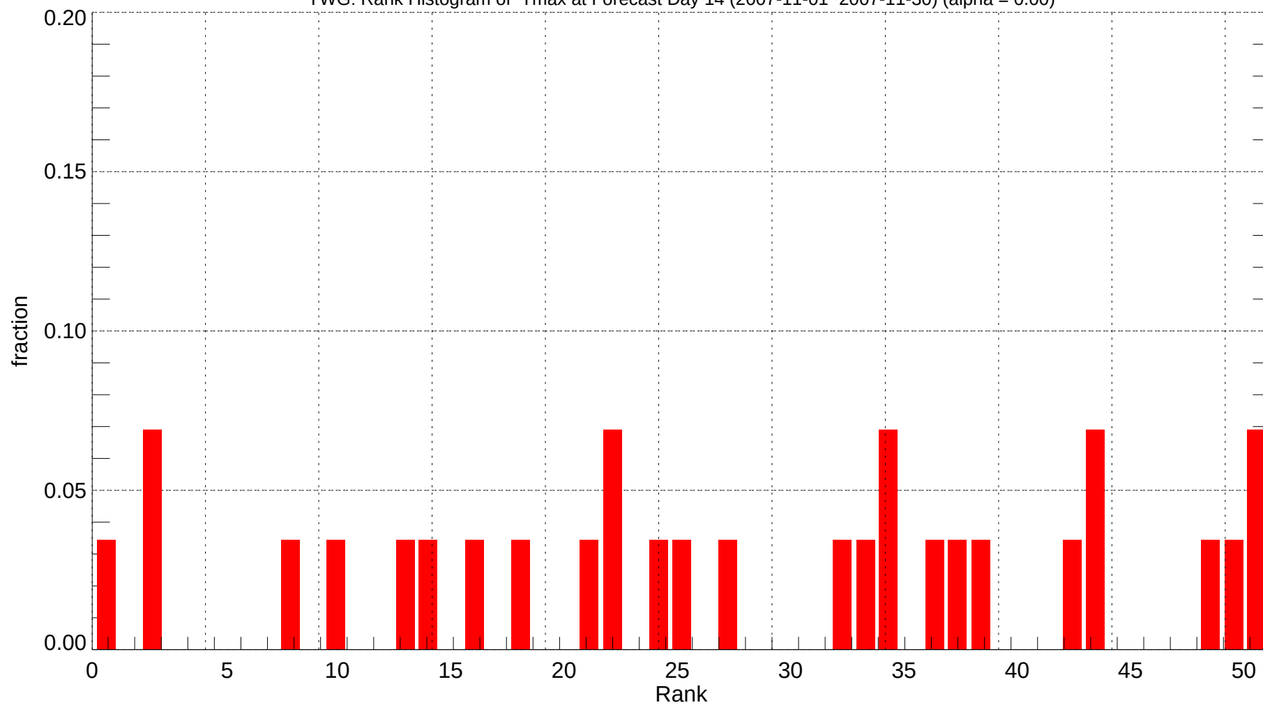
YWG: Rank Histogram of Tmax at Forecast Day 14 (2007-11-01~2007-11-30) (alpha = 0.00)
