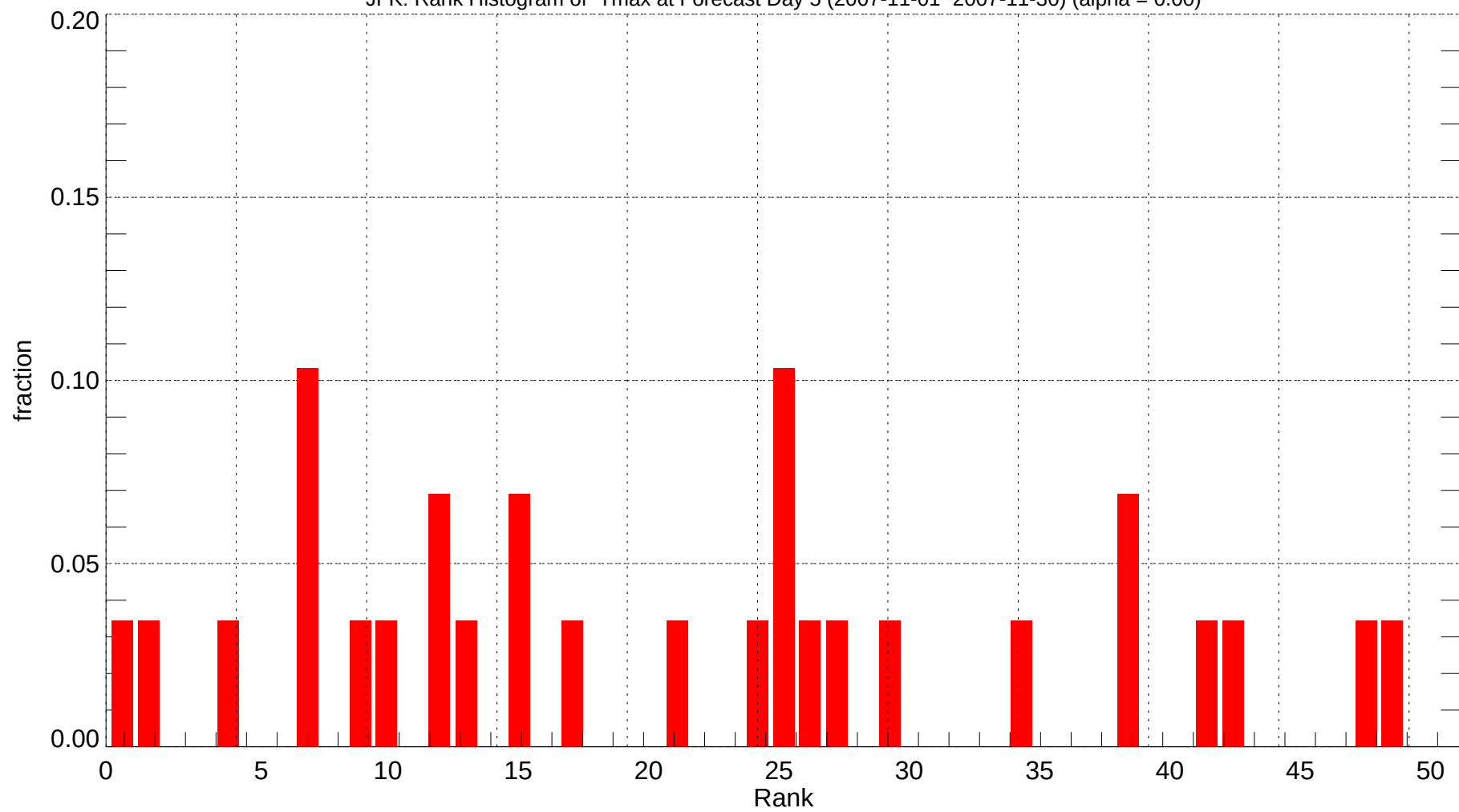
JFK: Rank Histogram of Tmax at Forecast Day 5 (2007-11-01~2007-11-30) (alpha = 0.00)
