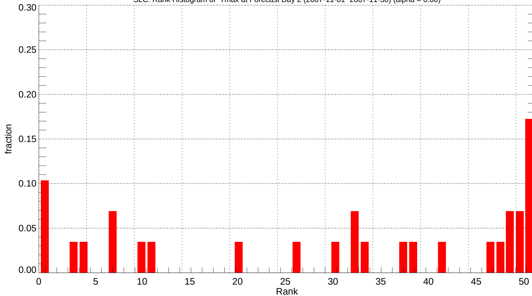
SLC: Rank Histogram of Tmax at Forecast Day 2 (2007-11-01~2007-11-30) (alpha = 0.00)
