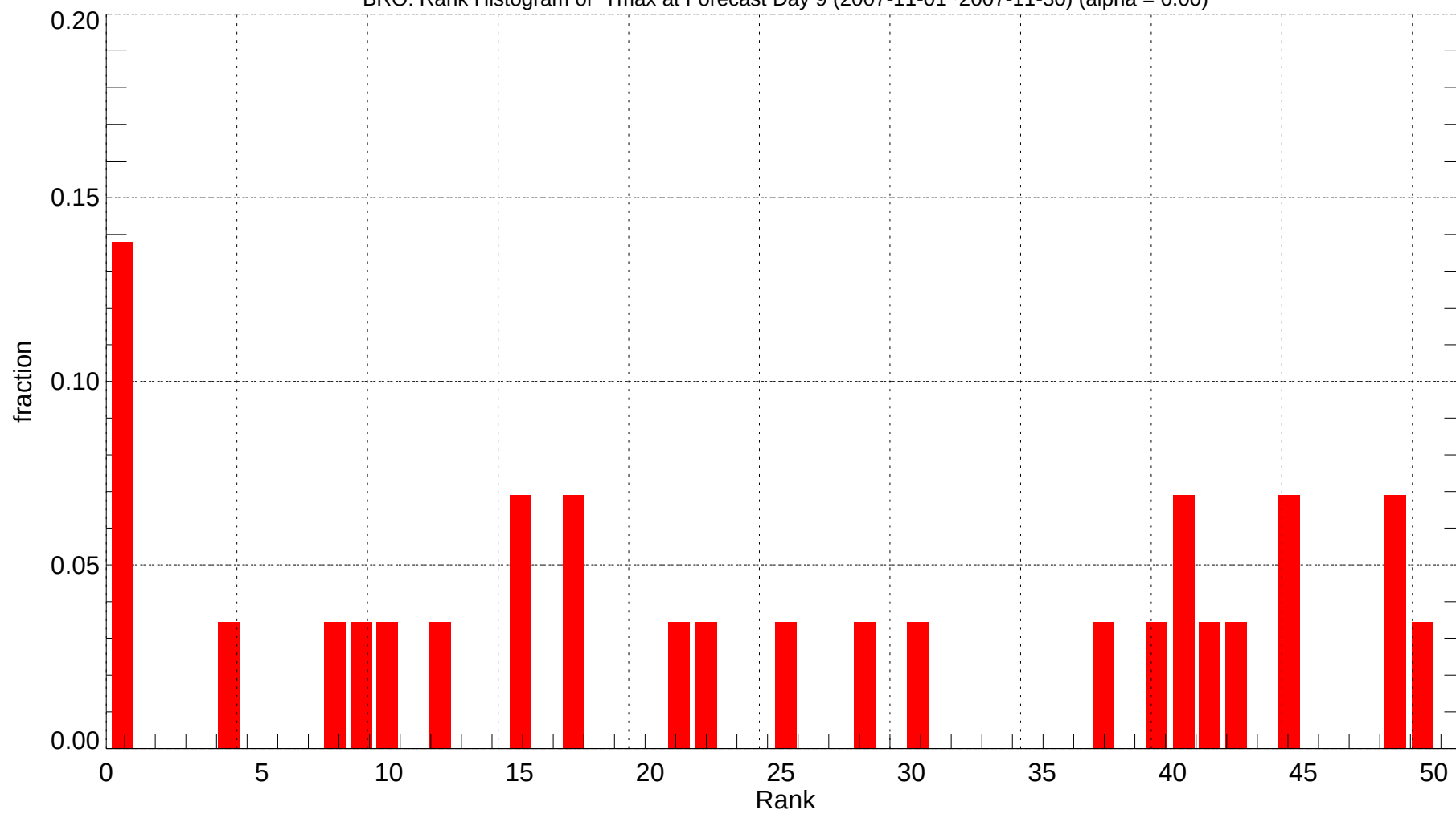
BRO: Rank Histogram of Tmax at Forecast Day 9 (2007-11-01~2007-11-30) (alpha = 0.00)
