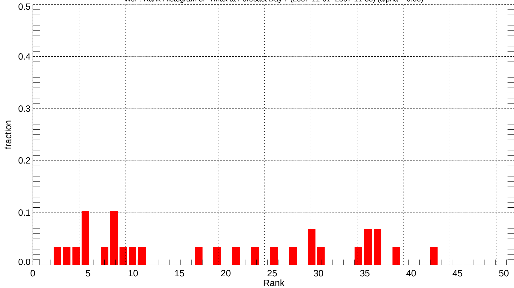
WJF: Rank Histogram of Tmax at Forecast Day 7 (2007-11-01~2007-11-30) (alpha = 0.00)
