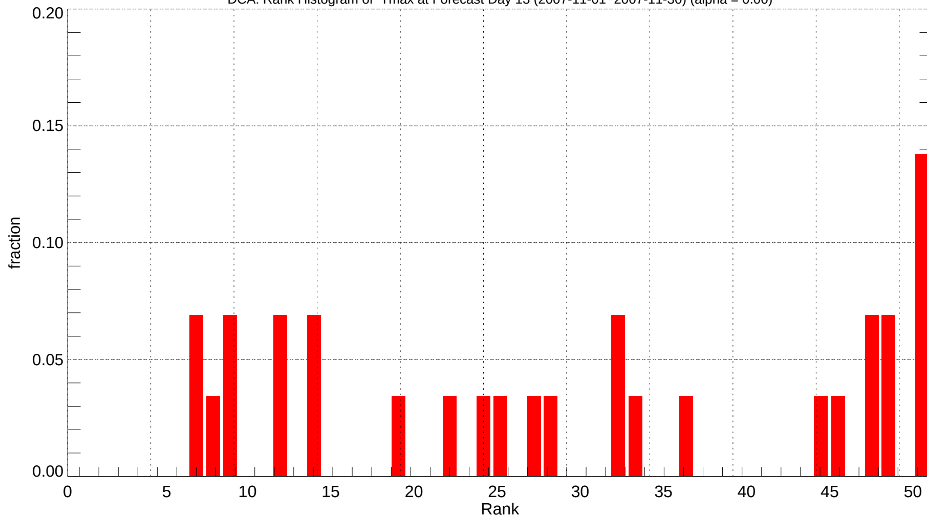
DCA: Rank Histogram of Tmax at Forecast Day 13 (2007-11-01~2007-11-30) (alpha = 0.00)
