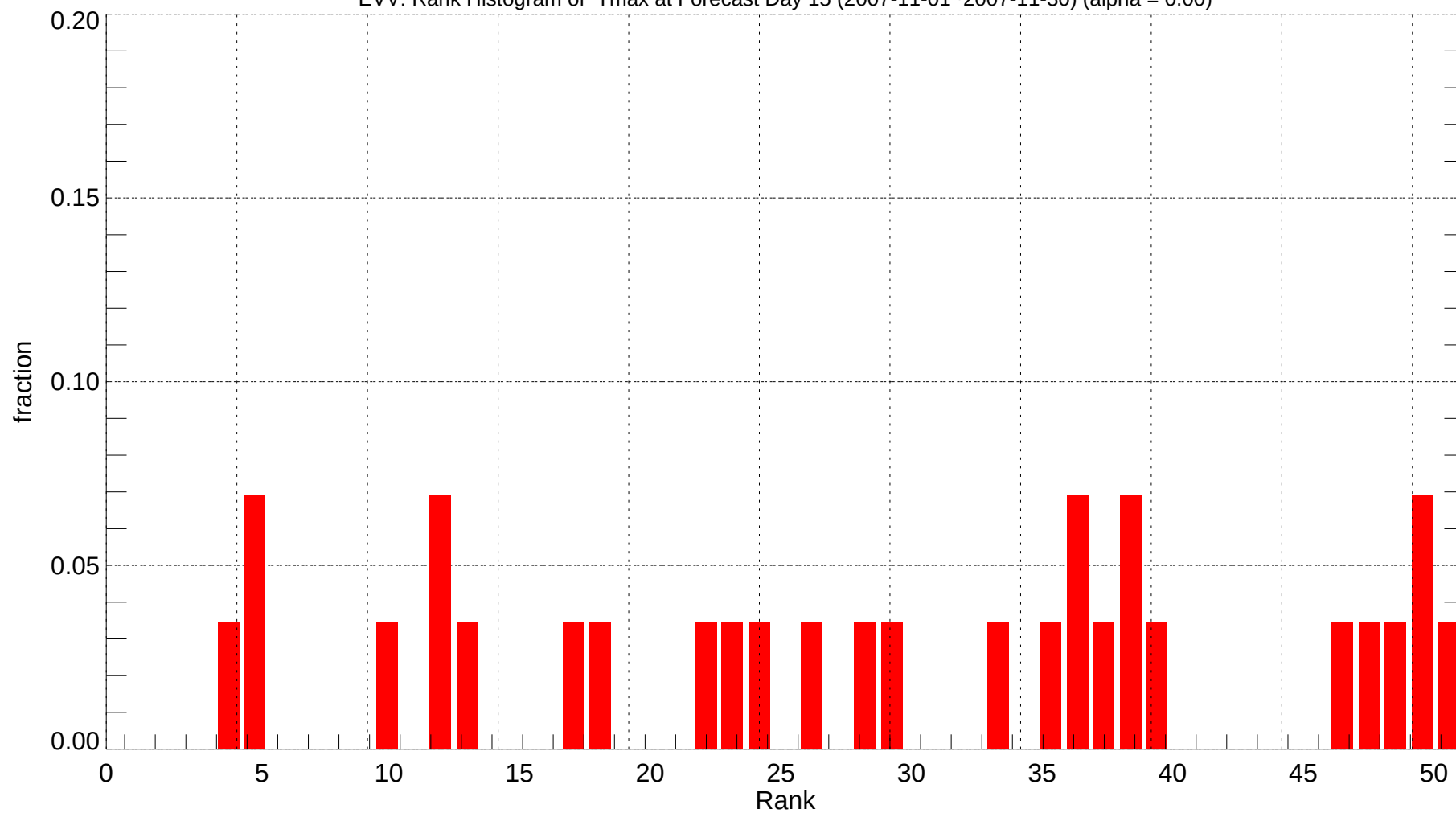
EVV: Rank Histogram of Tmax at Forecast Day 15 (2007-11-01~2007-11-30) (alpha = 0.00)
