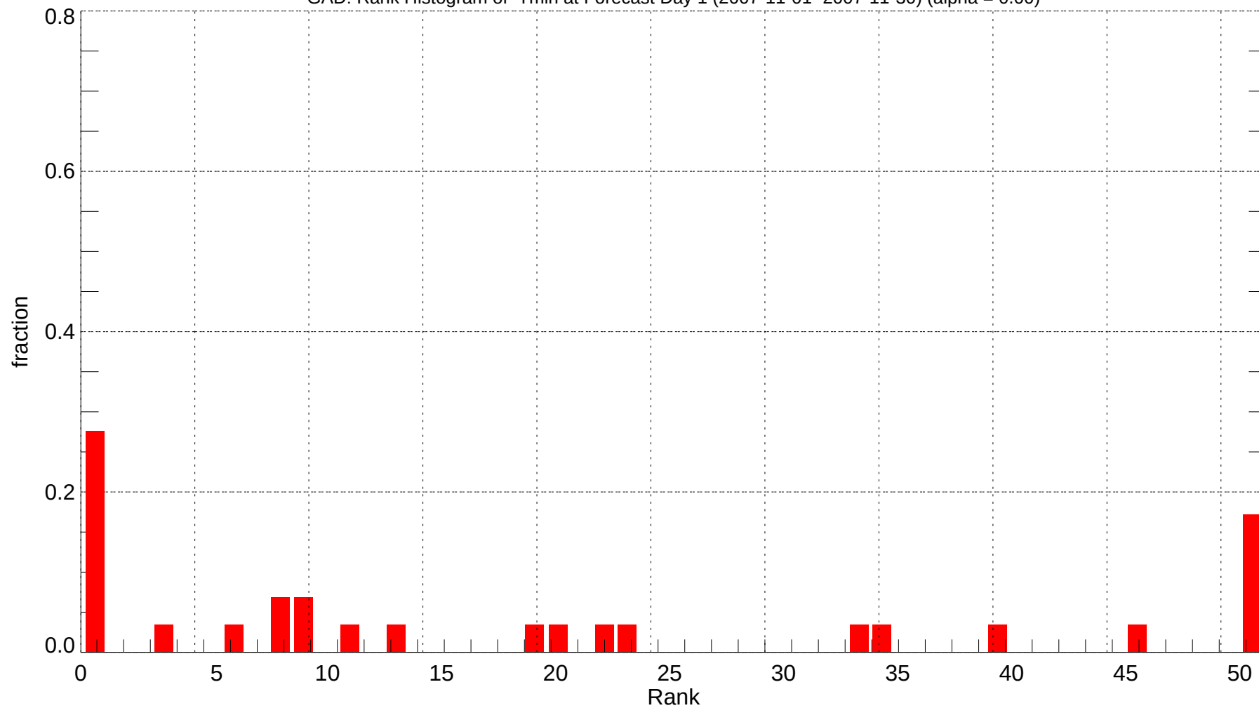
GAD: Rank Histogram of Tmin at Forecast Day 1 (2007-11-01~2007-11-30) (alpha = 0.00)
