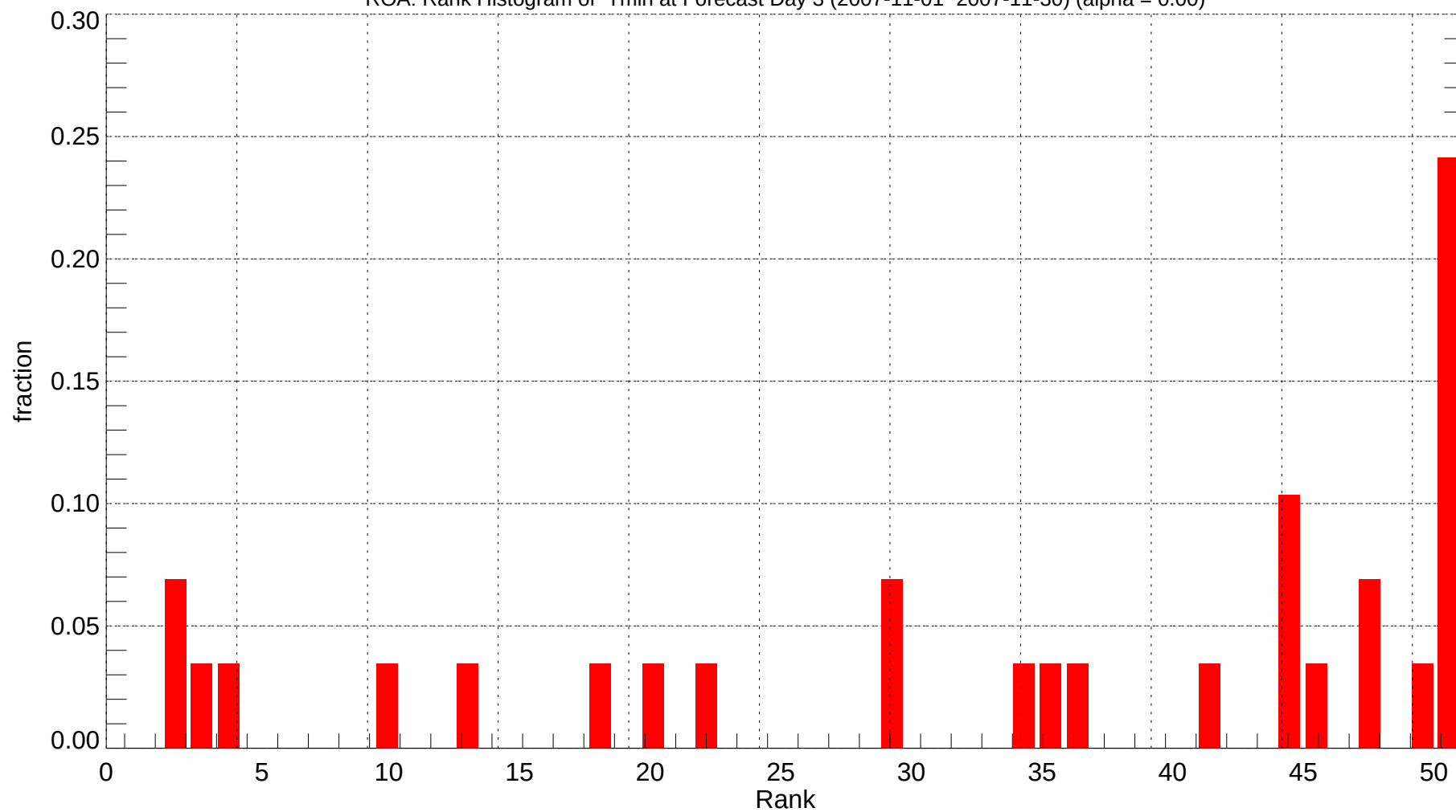
ROA: Rank Histogram of Tmin at Forecast Day 3 (2007-11-01~2007-11-30) (alpha = 0.00)
