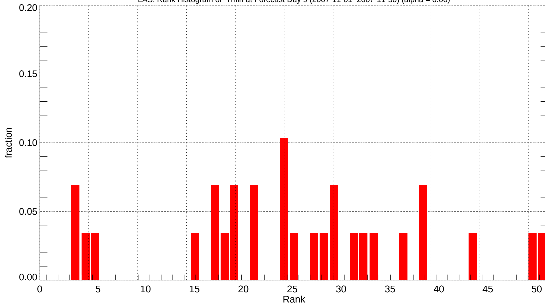
LAS: Rank Histogram of Tmin at Forecast Day 9 (2007-11-01~2007-11-30) (alpha = 0.00)
