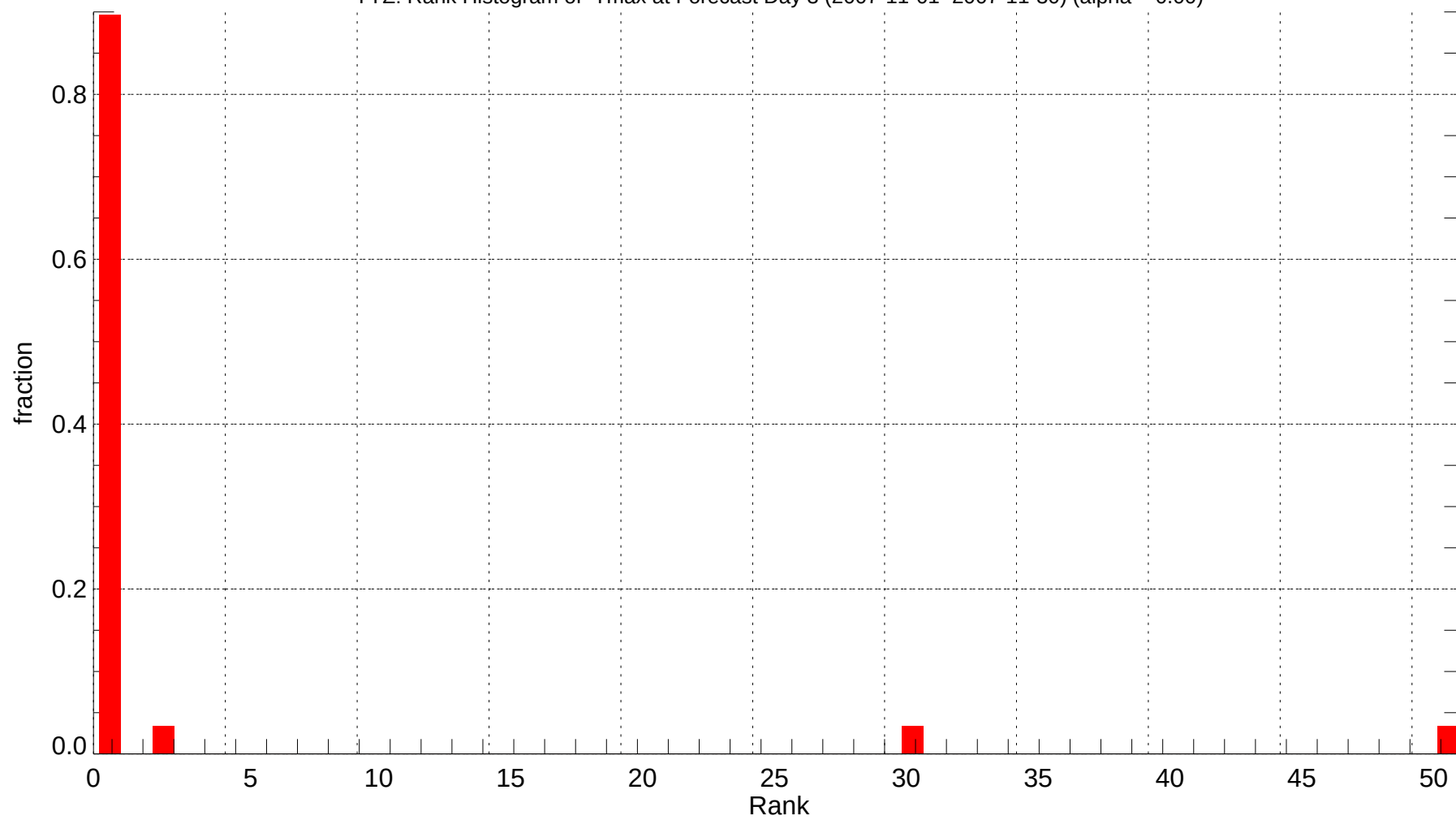
YYZ: Rank Histogram of Tmax at Forecast Day 3 (2007-11-01~2007-11-30) (alpha = 0.00)
