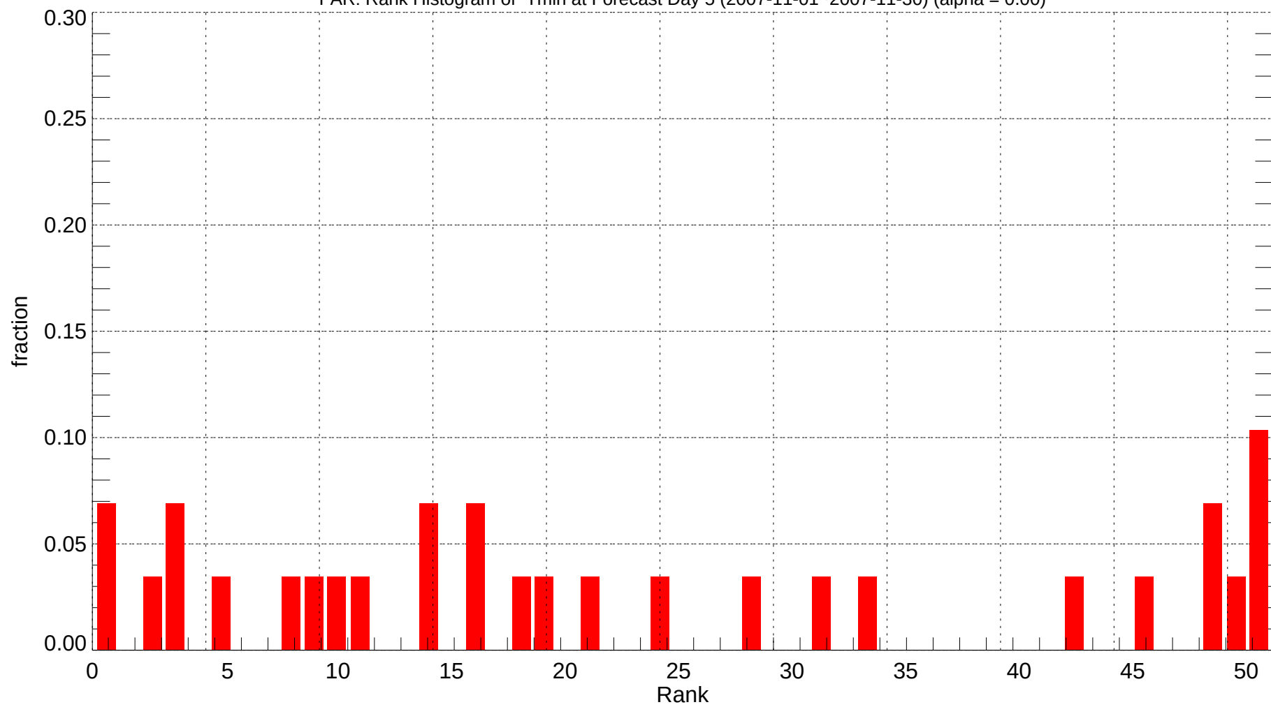
FAR: Rank Histogram of Tmin at Forecast Day 5 (2007-11-01~2007-11-30) (alpha = 0.00)
