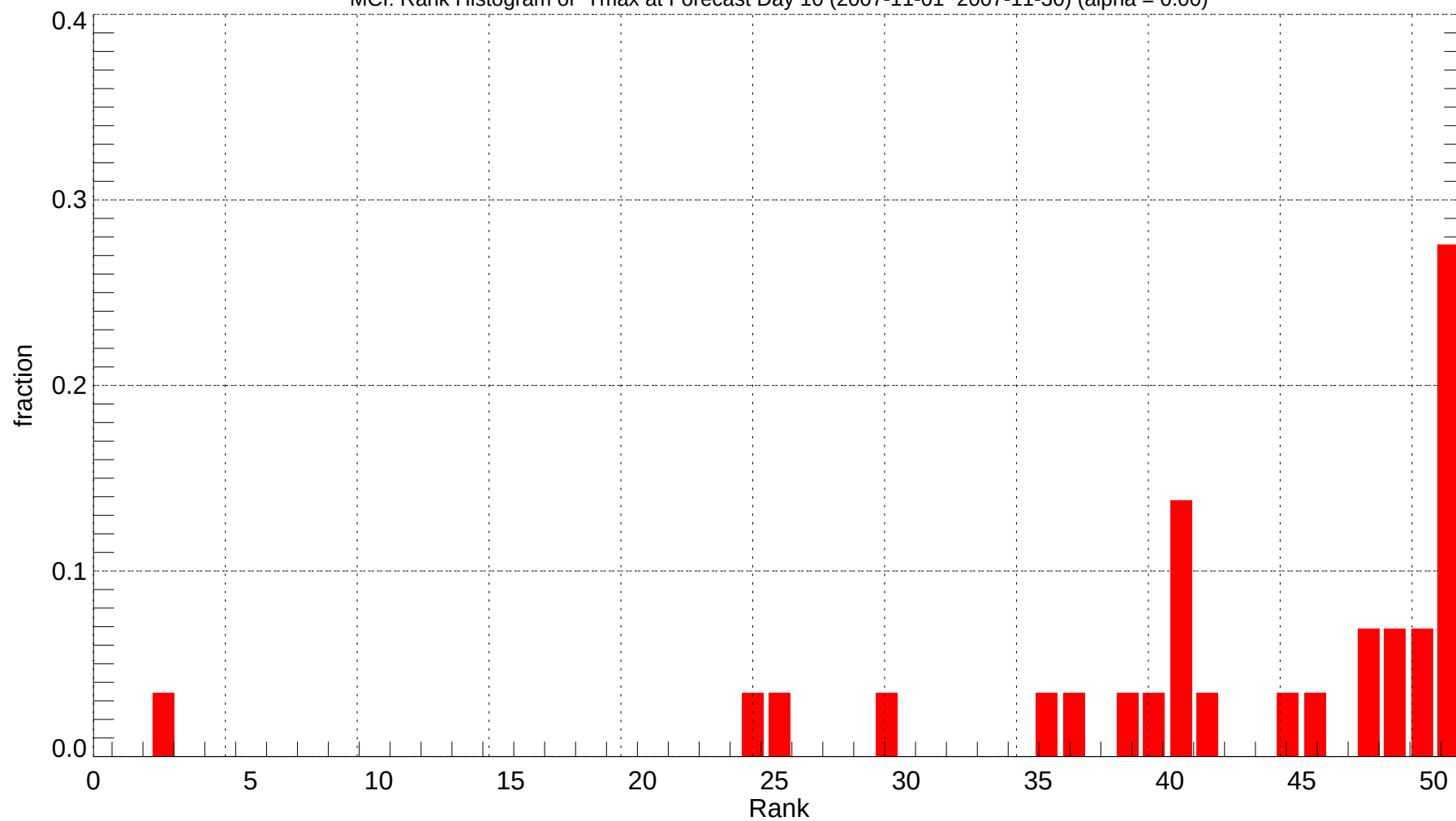
MCI: Rank Histogram of Tmax at Forecast Day 10 (2007-11-01~2007-11-30) (alpha = 0.00)
