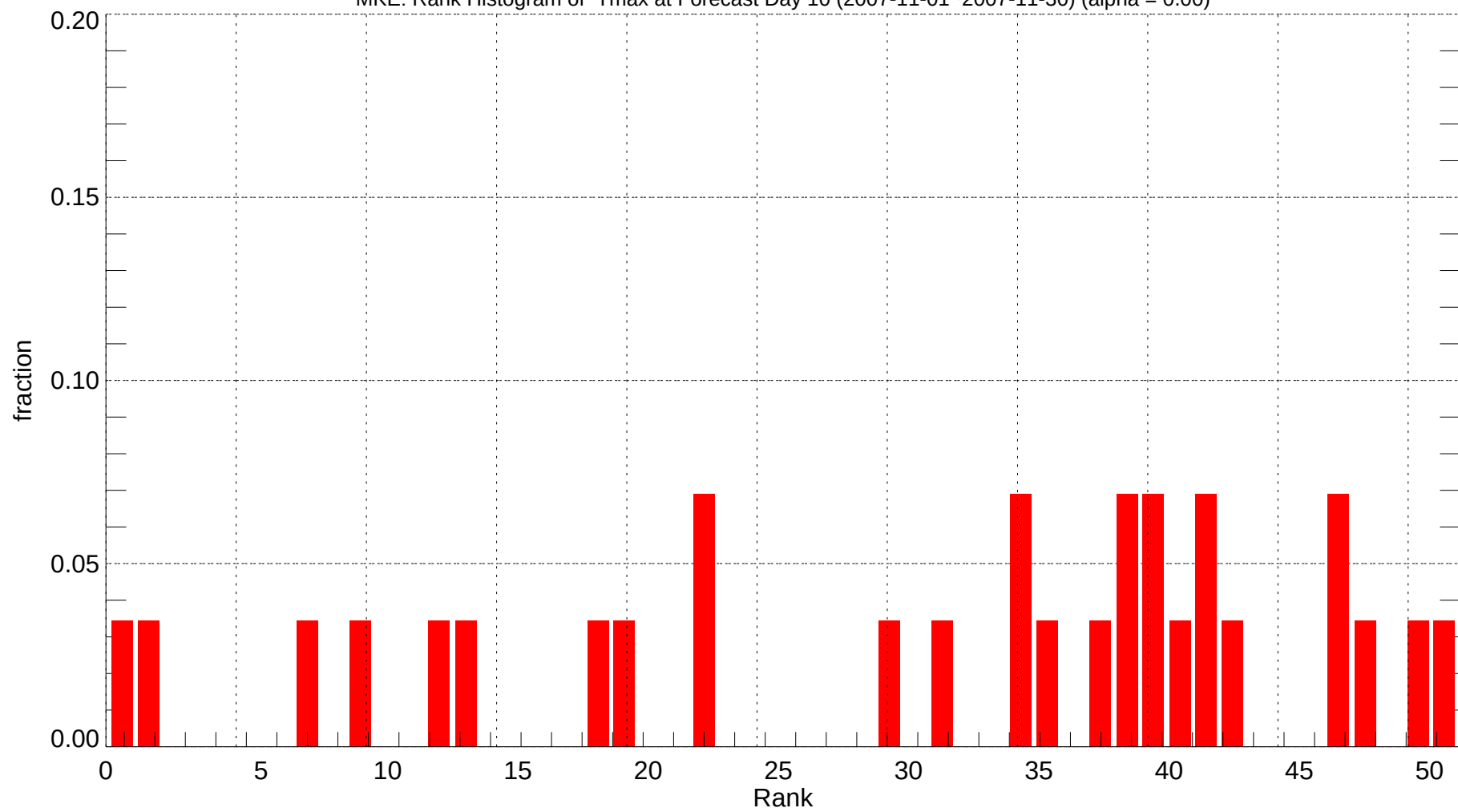
MKE: Rank Histogram of Tmax at Forecast Day 10 (2007-11-01~2007-11-30) (alpha = 0.00)
