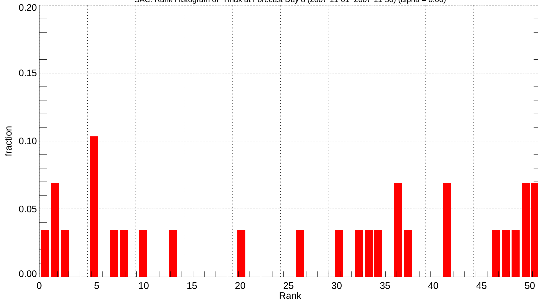
SAC: Rank Histogram of Tmax at Forecast Day 8 (2007-11-01~2007-11-30) (alpha = 0.00)
