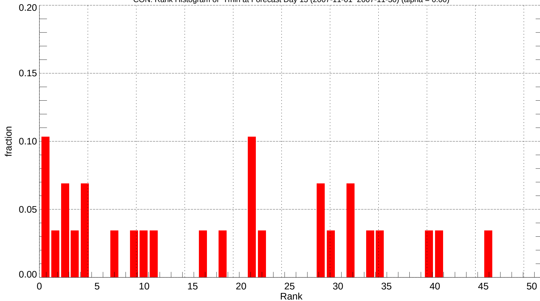
CON: Rank Histogram of Tmin at Forecast Day 13 (2007-11-01~2007-11-30) (alpha = 0.00)
