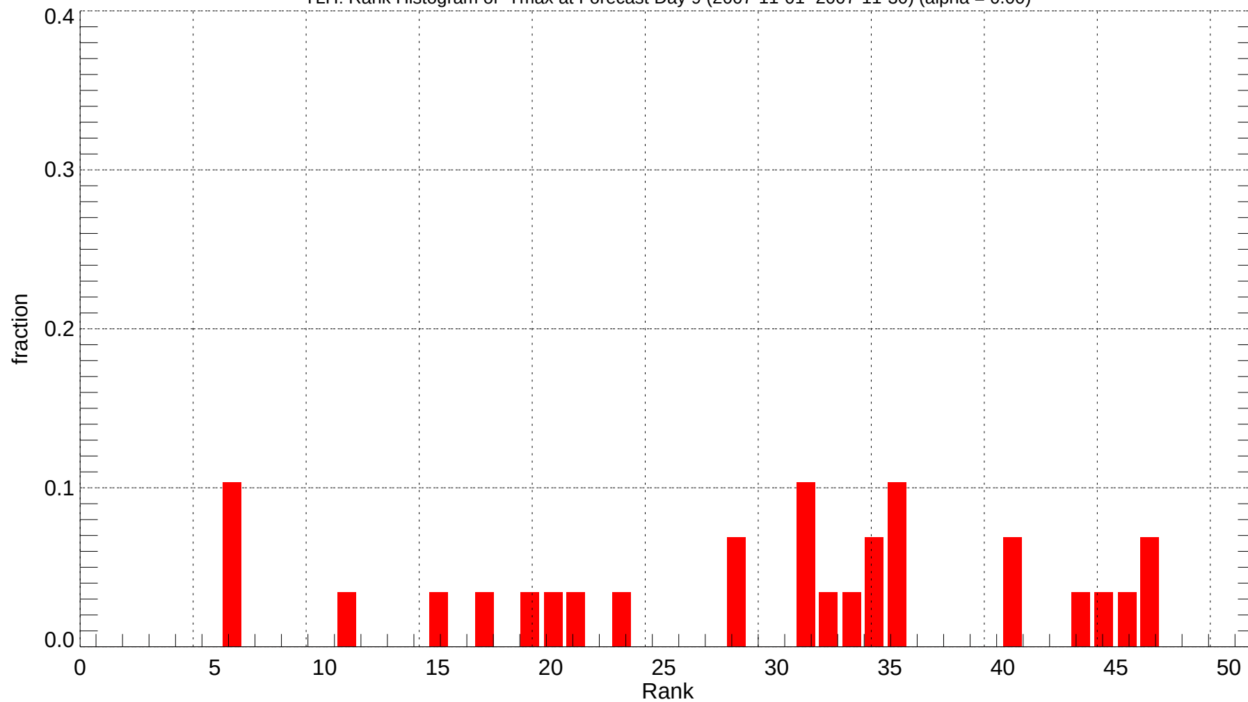
TLH: Rank Histogram of Tmax at Forecast Day 9 (2007-11-01~2007-11-30) (alpha = 0.00)
