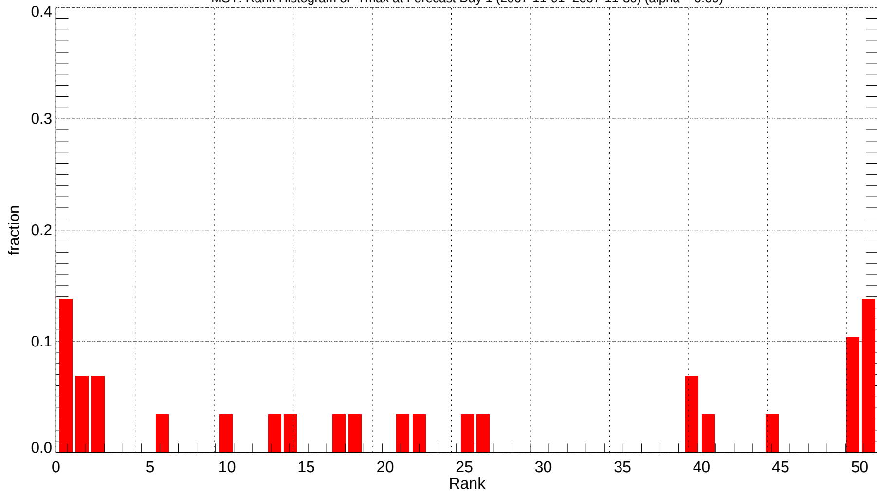
MSY: Rank Histogram of Tmax at Forecast Day 1 (2007-11-01~2007-11-30) (alpha = 0.00)
