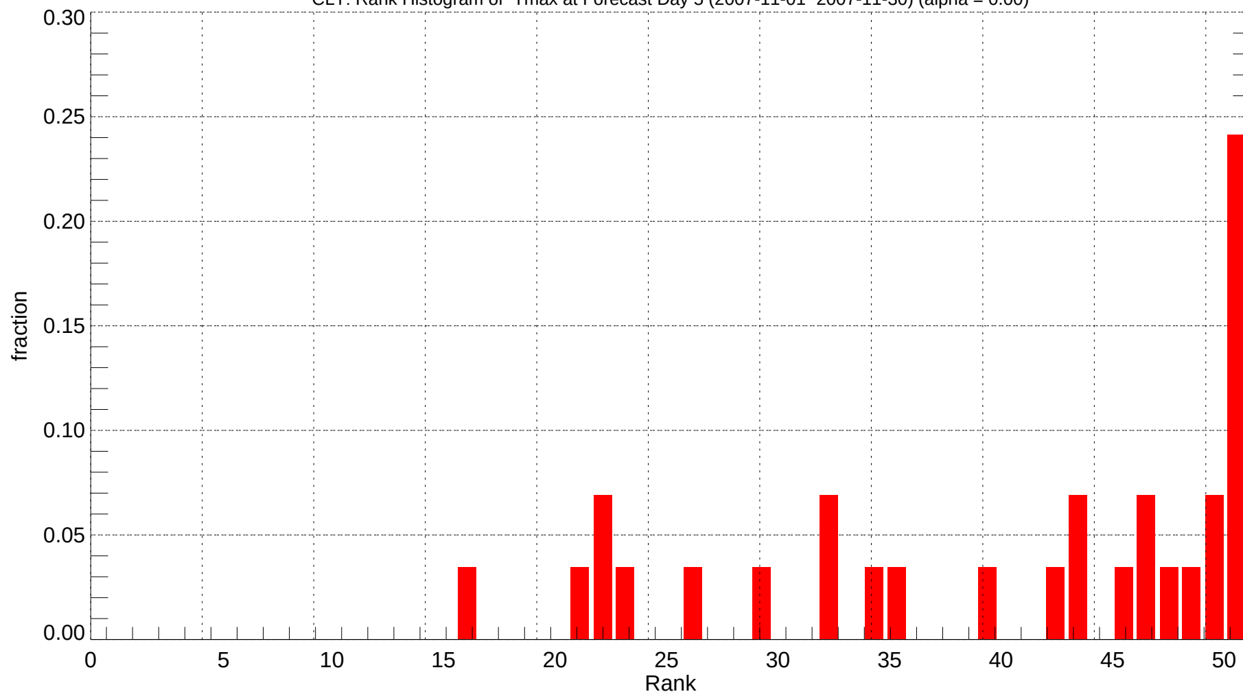
CLT: Rank Histogram of Tmax at Forecast Day 5 (2007-11-01~2007-11-30) (alpha = 0.00)
