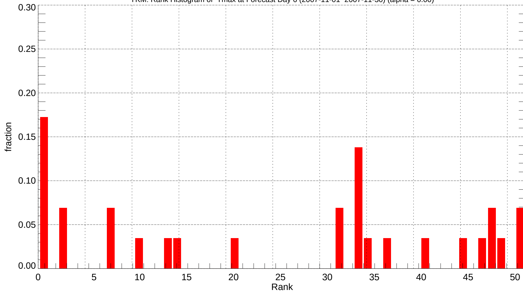
YKM: Rank Histogram of Tmax at Forecast Day 6 (2007-11-01~2007-11-30) (alpha = 0.00)
