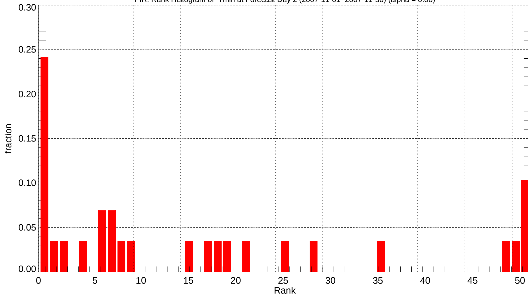
PIR: Rank Histogram of Tmin at Forecast Day 2 (2007-11-01~2007-11-30) (alpha = 0.00)
