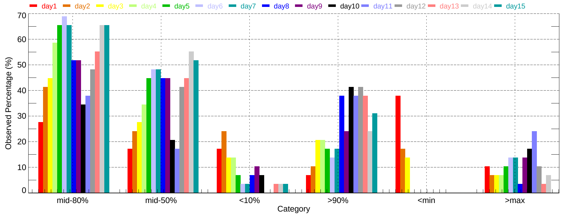
Observed Percentage of Ensembles - FSD: Min Temperature (2007-11-01~2007-11-30)
