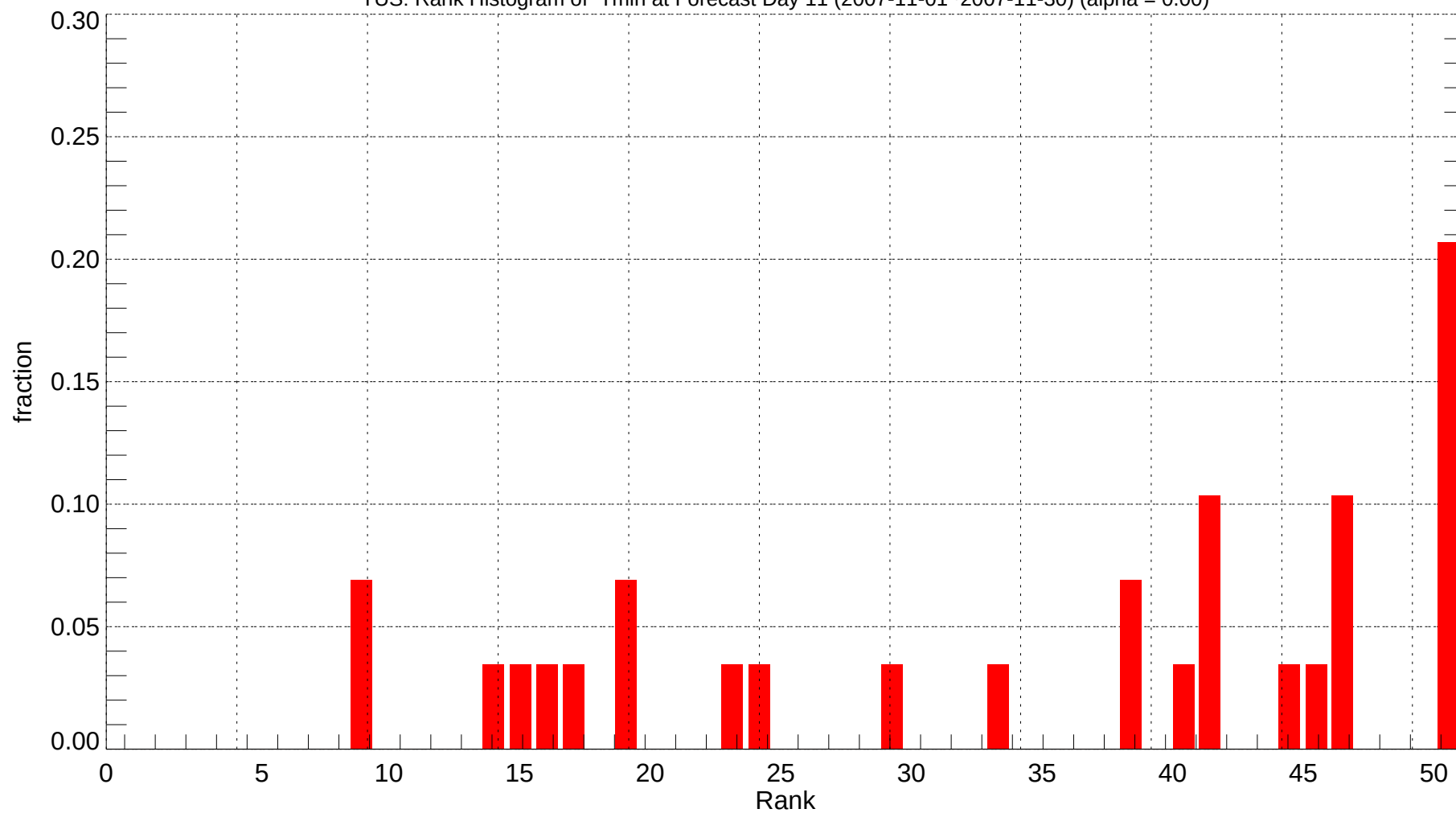
TUS: Rank Histogram of Tmin at Forecast Day 11 (2007-11-01~2007-11-30) (alpha = 0.00)
