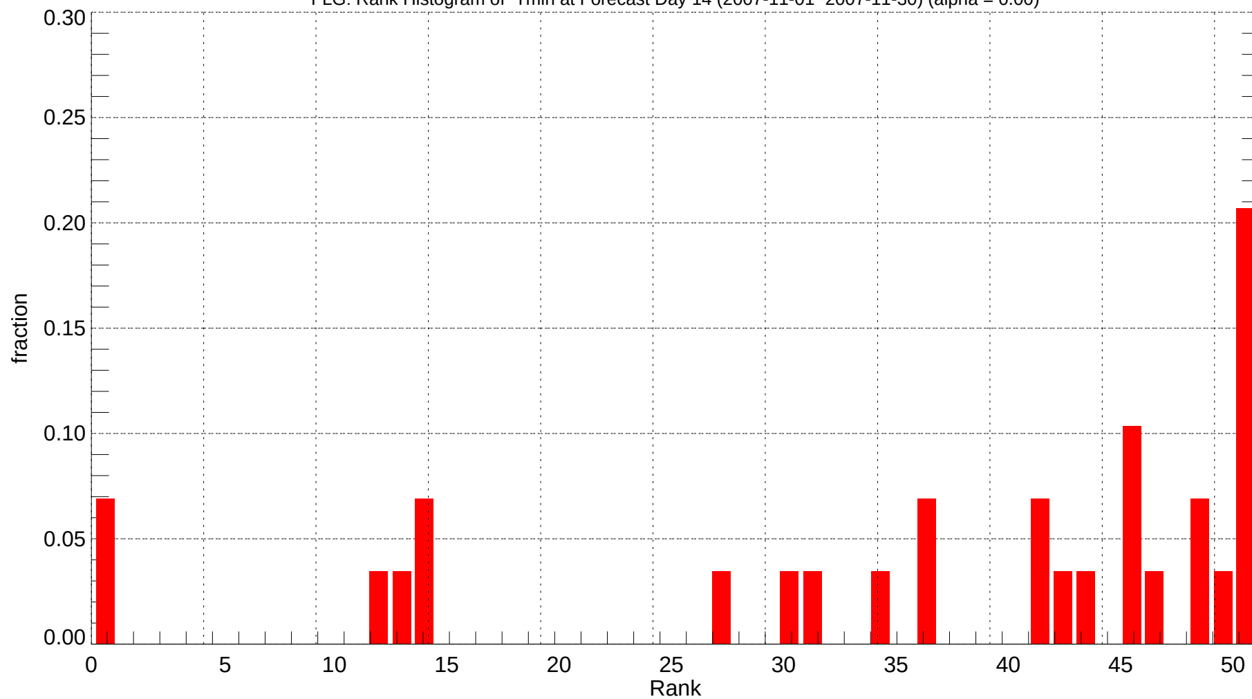
FLG: Rank Histogram of Tmin at Forecast Day 14 (2007-11-01~2007-11-30) (alpha = 0.00)
