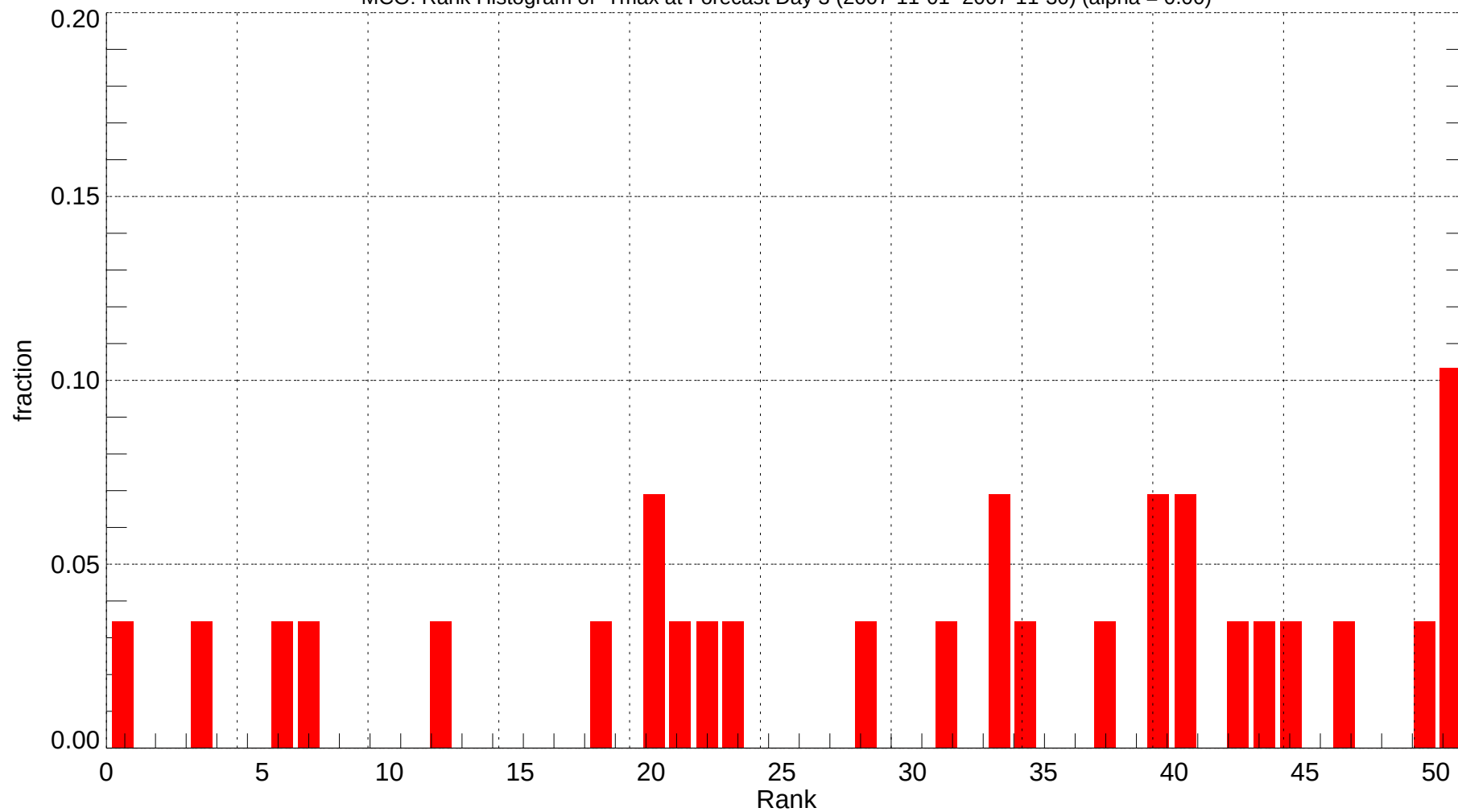
MCO: Rank Histogram of Tmax at Forecast Day 3 (2007-11-01~2007-11-30) (alpha = 0.00)
