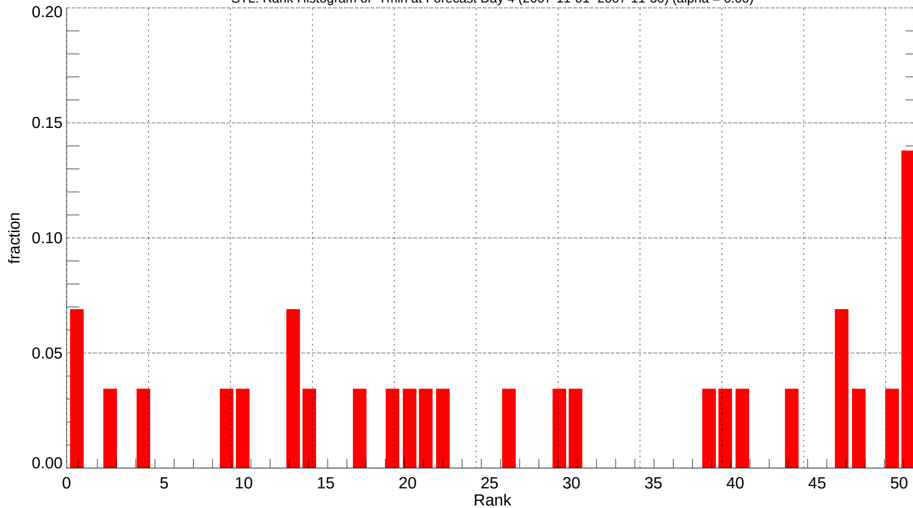
STL: Rank Histogram of Tmin at Forecast Day 4 (2007-11-01~2007-11-30) (alpha = 0.00)
