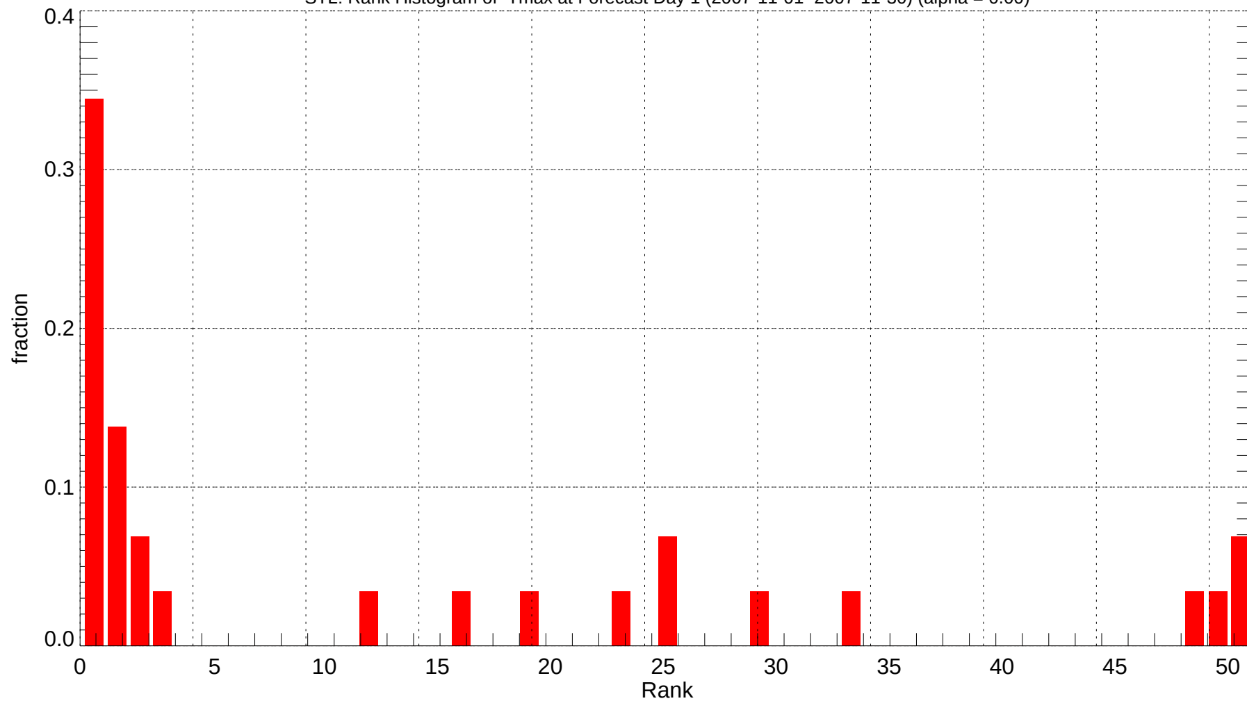
STL: Rank Histogram of Tmax at Forecast Day 1 (2007-11-01~2007-11-30) (alpha = 0.00)
