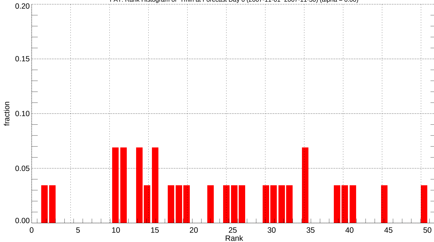
FAT: Rank Histogram of Tmin at Forecast Day 6 (2007-11-01~2007-11-30) (alpha = 0.00)
