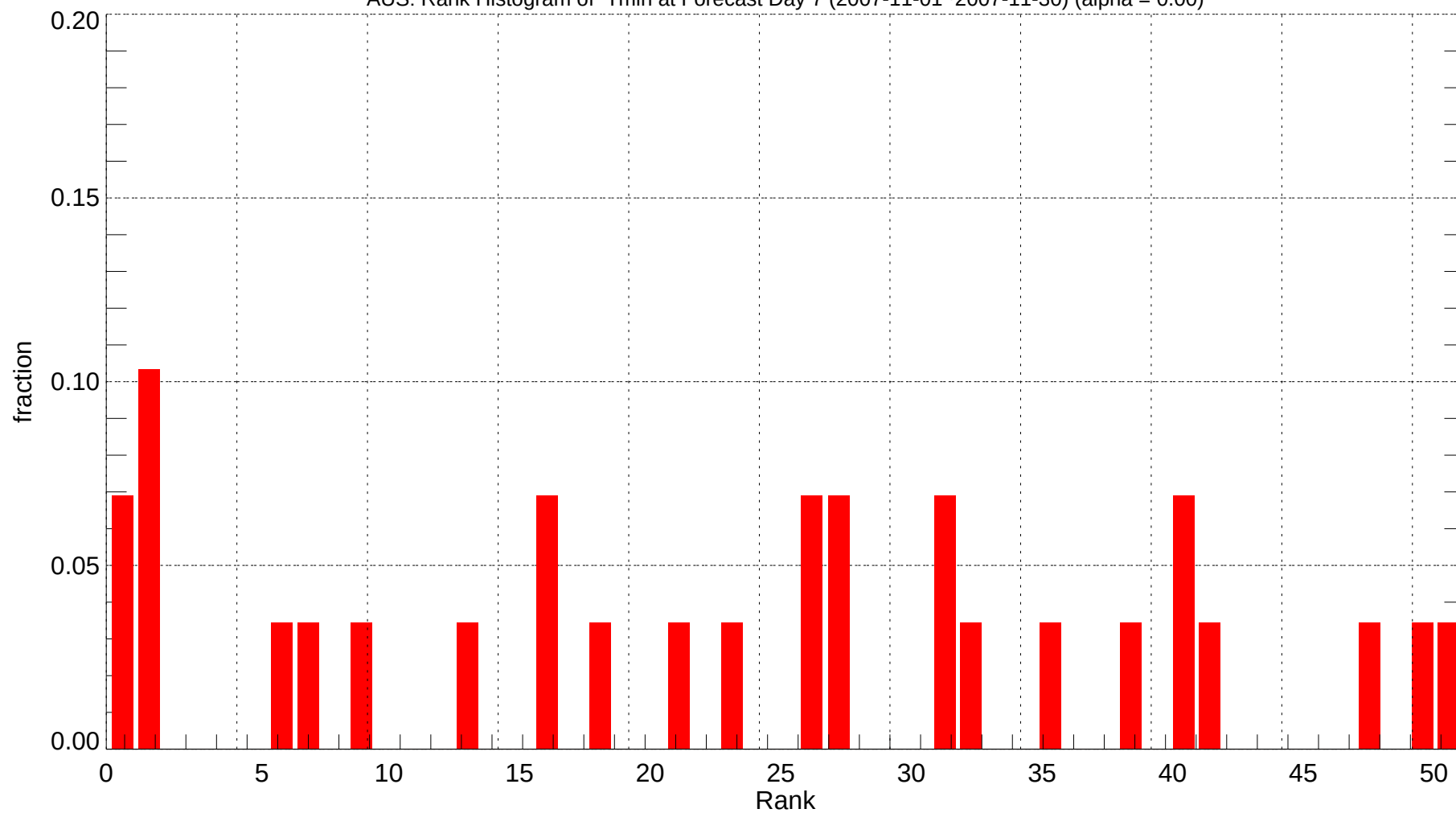
AUS: Rank Histogram of Tmin at Forecast Day 7 (2007-11-01~2007-11-30) (alpha = 0.00)
