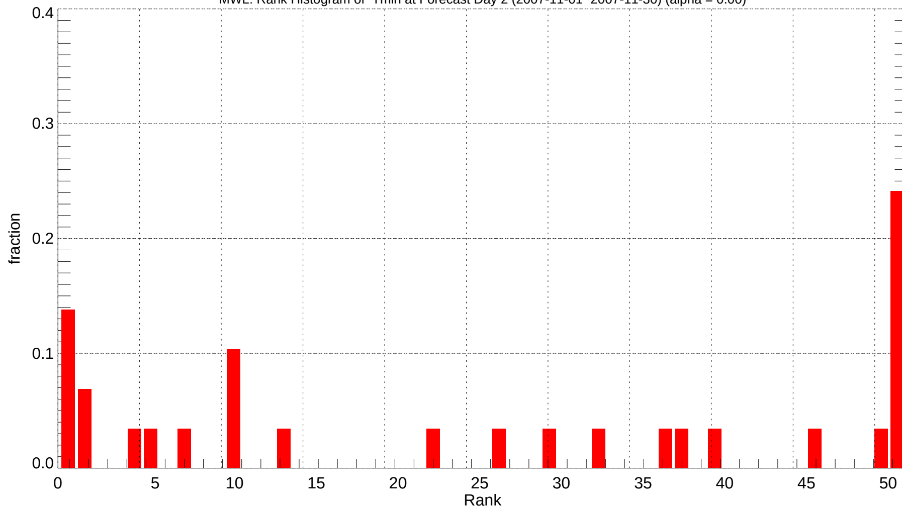
MWL: Rank Histogram of Tmin at Forecast Day 2 (2007-11-01~2007-11-30) (alpha = 0.00)
