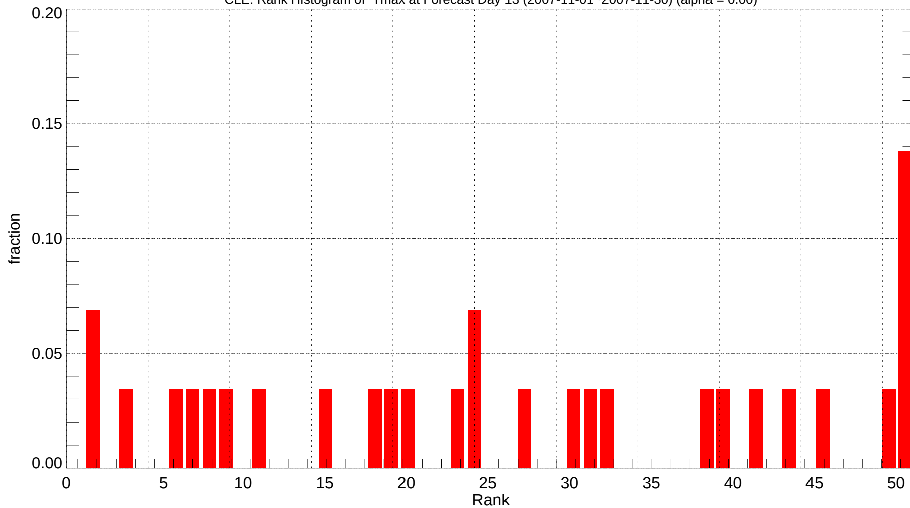
CLE: Rank Histogram of Tmax at Forecast Day 13 (2007-11-01~2007-11-30) (alpha = 0.00)
