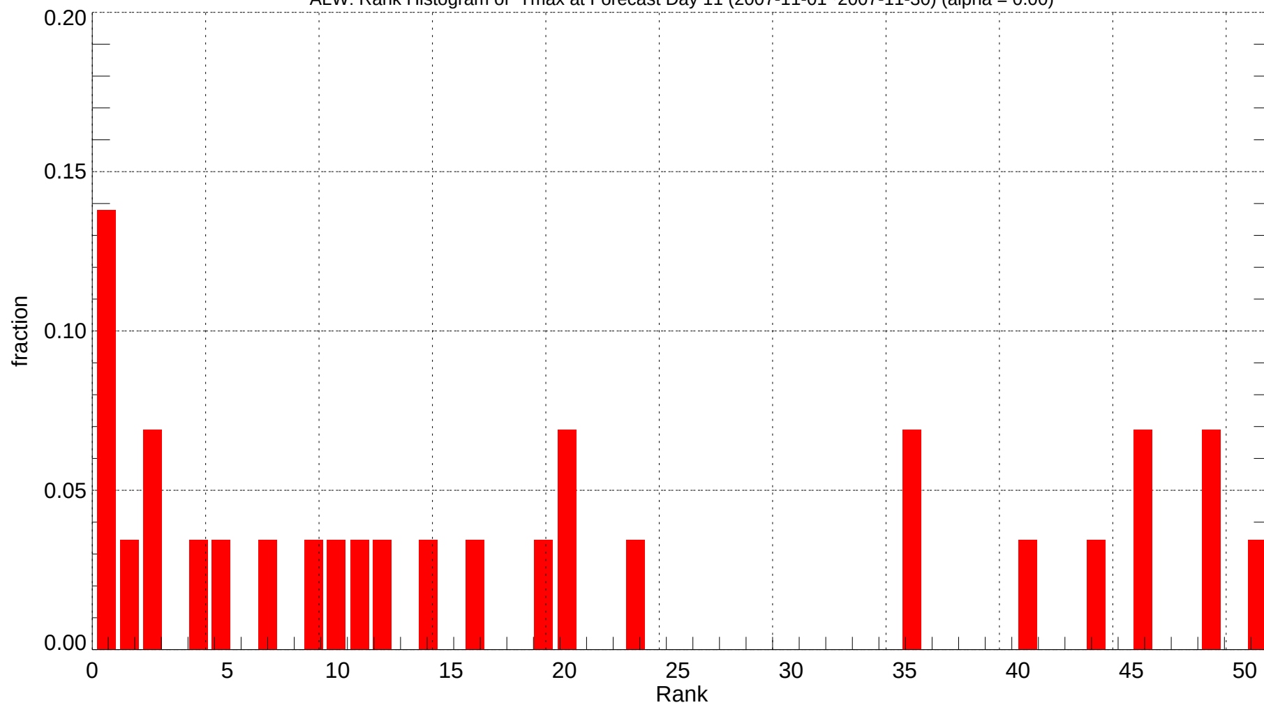
ALW: Rank Histogram of Tmax at Forecast Day 11 (2007-11-01~2007-11-30) (alpha = 0.00)
