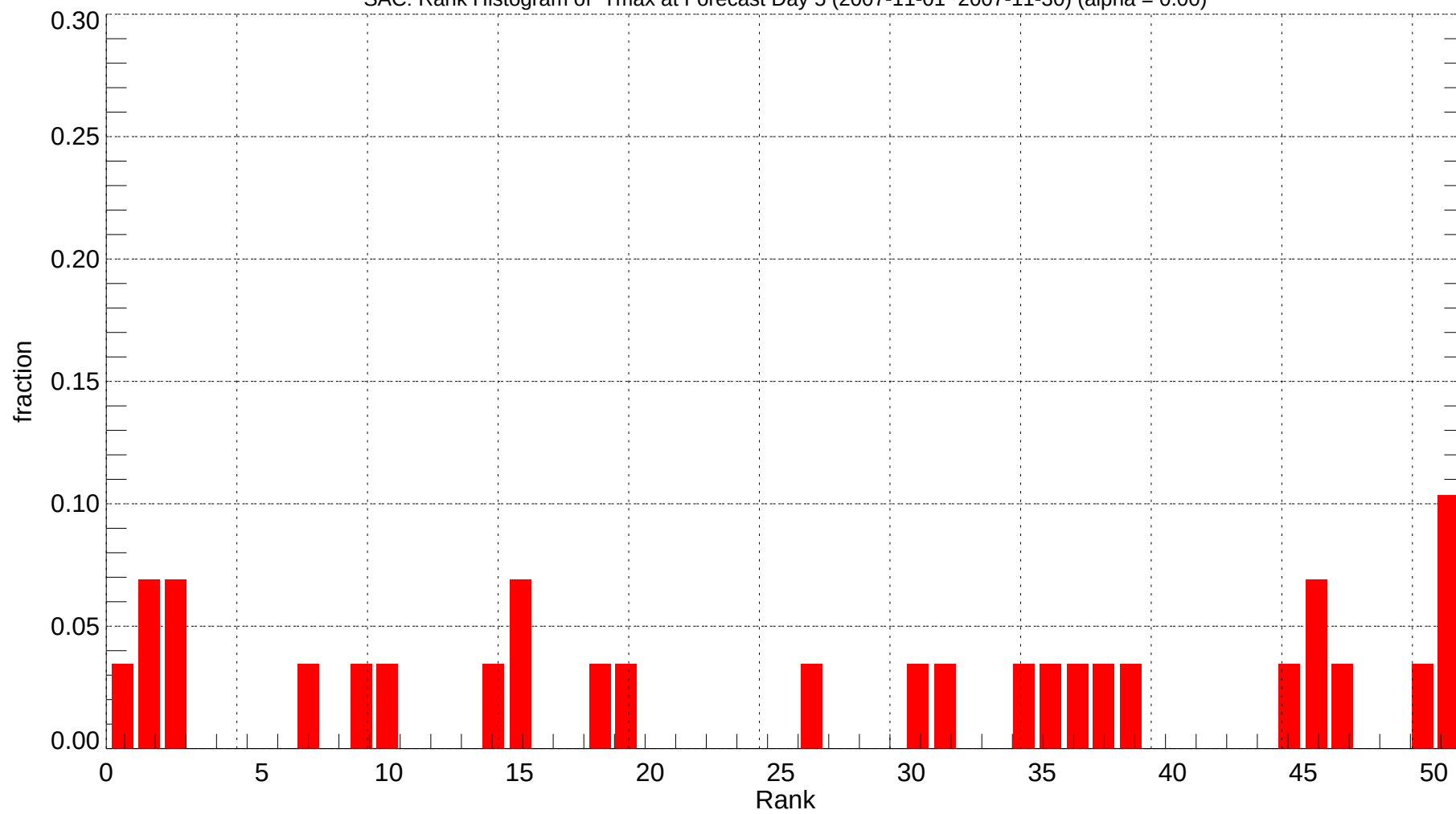
SAC: Rank Histogram of Tmax at Forecast Day 5 (2007-11-01~2007-11-30) (alpha = 0.00)
