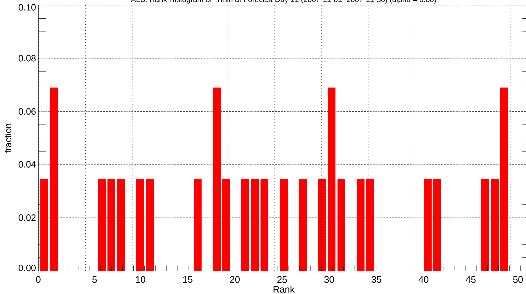
ALB: Rank Histogram of Tmin at Forecast Day 11 (2007-11-01~2007-11-30) (alpha = 0.00)
