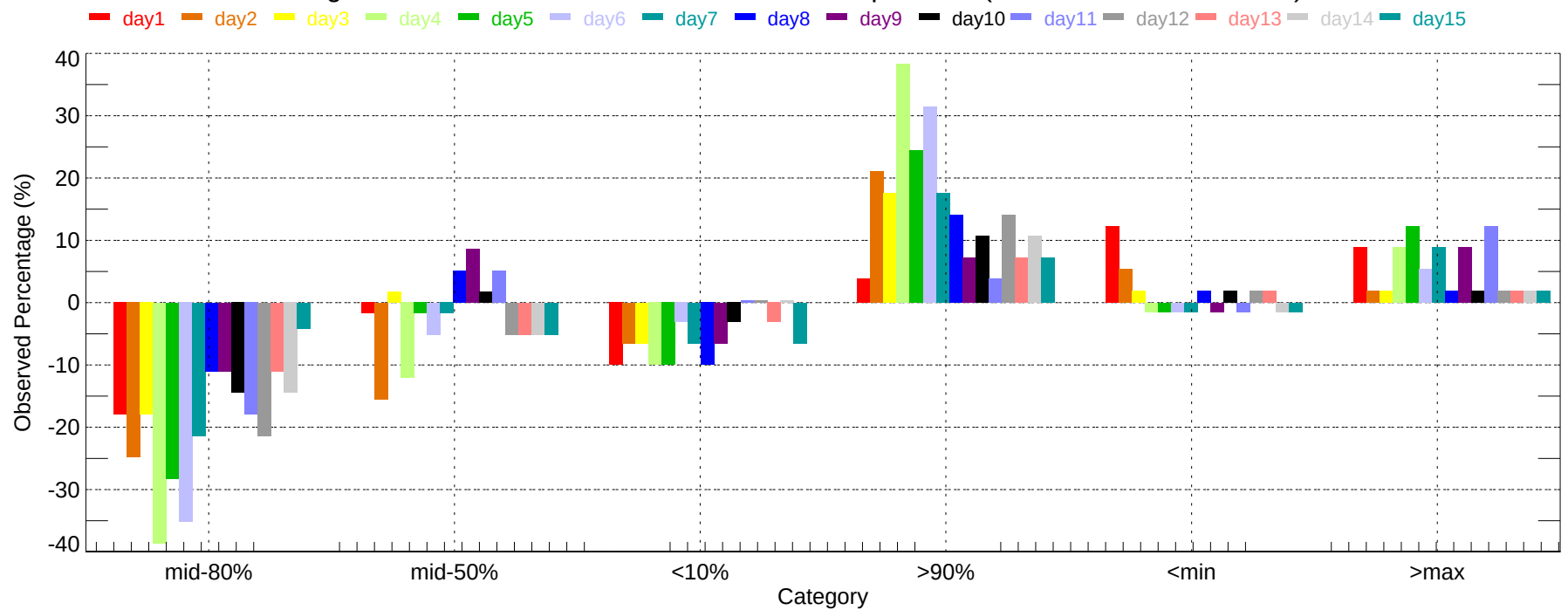
Observed Percentage Deviation of Ensembles - SAV: Max Temperature (2007-11-01~2007-11-30)
