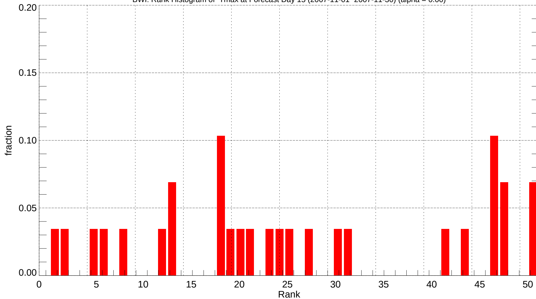
BWI: Rank Histogram of Tmax at Forecast Day 15 (2007-11-01~2007-11-30) (alpha = 0.00)
