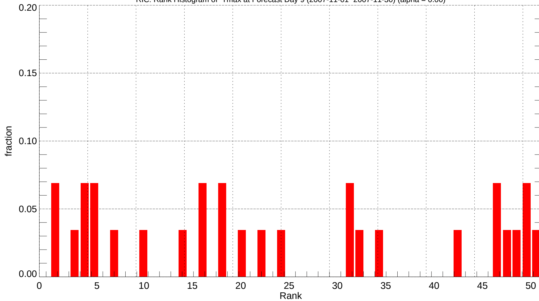
RIC: Rank Histogram of Tmax at Forecast Day 9 (2007-11-01~2007-11-30) (alpha = 0.00)
