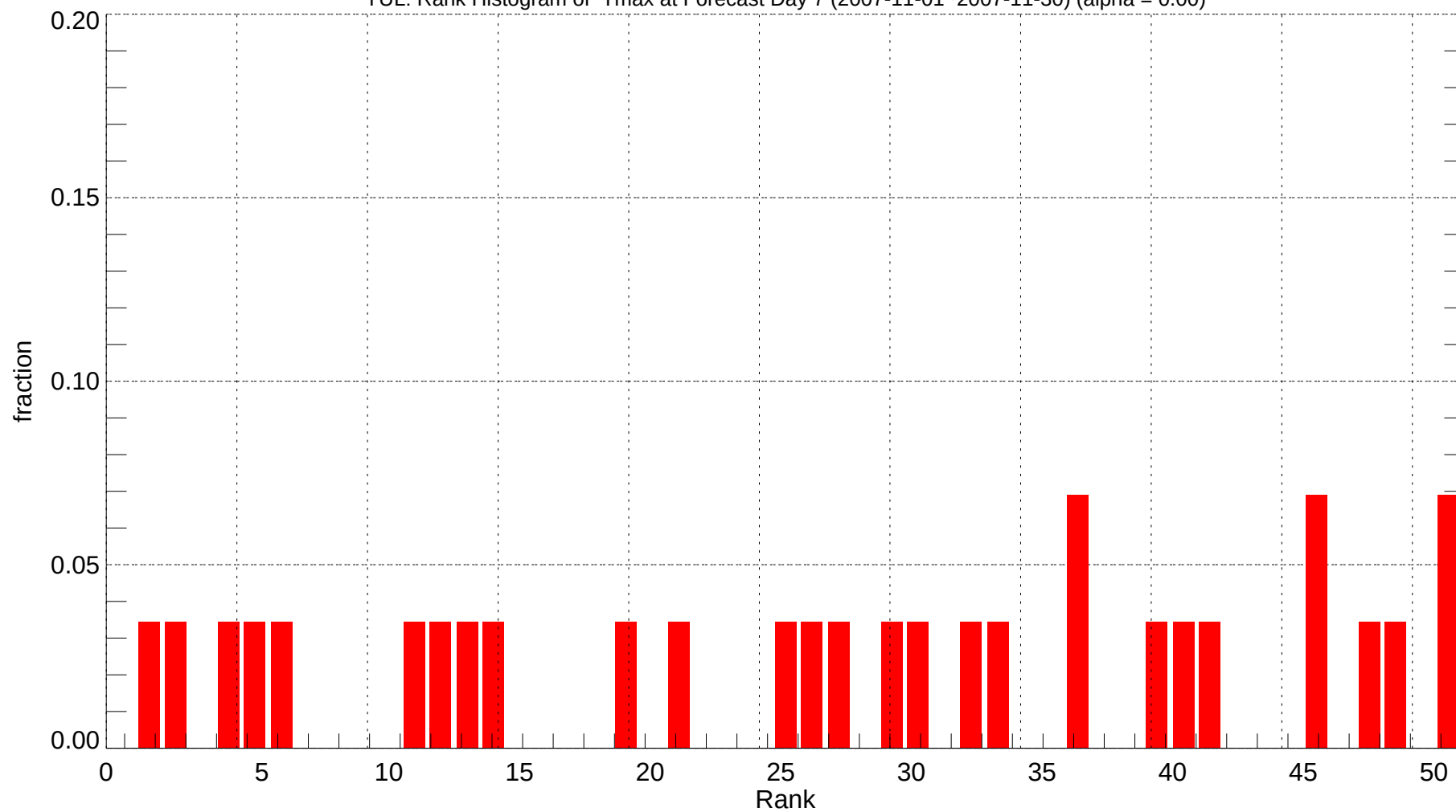
YUL: Rank Histogram of Tmax at Forecast Day 7 (2007-11-01~2007-11-30) (alpha = 0.00)
