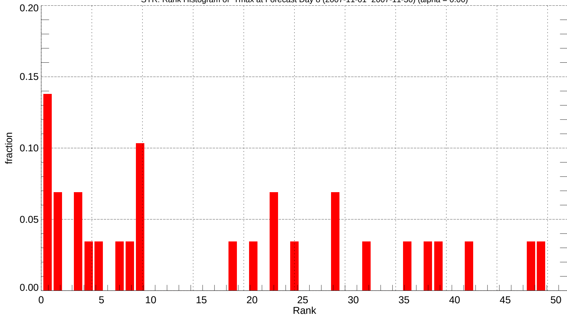
SYR: Rank Histogram of Tmax at Forecast Day 8 (2007-11-01~2007-11-30) (alpha = 0.00)
