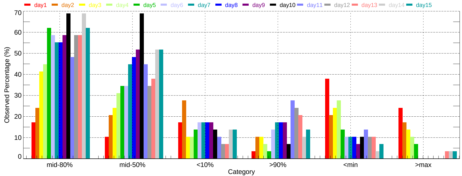
Observed Percentage of Ensembles - BUF: Max Temperature (2007-11-01~2007-11-30)
