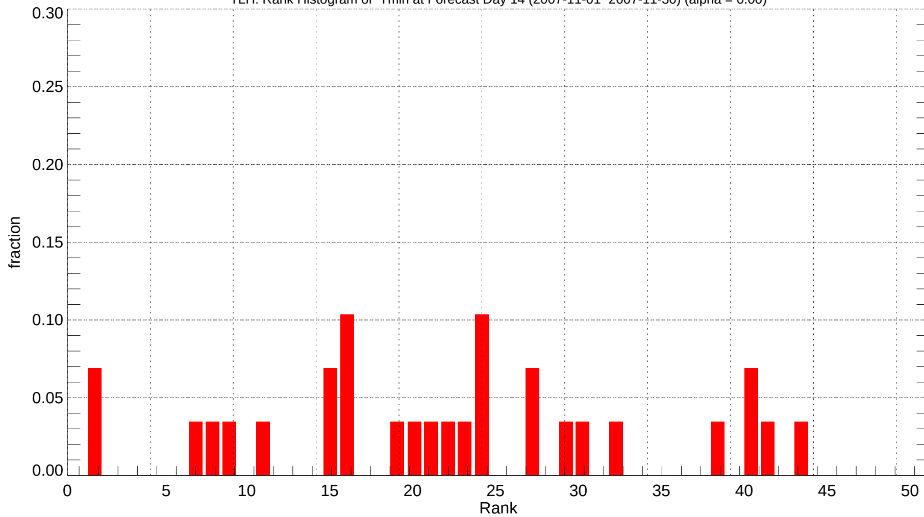
TLH: Rank Histogram of Tmin at Forecast Day 14 (2007-11-01~2007-11-30) (alpha = 0.00)
