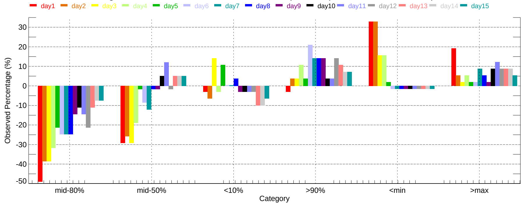
Observed Percentage Deviation of Ensembles - FWA: Min Temperature (2007-11-01~2007-11-30)
