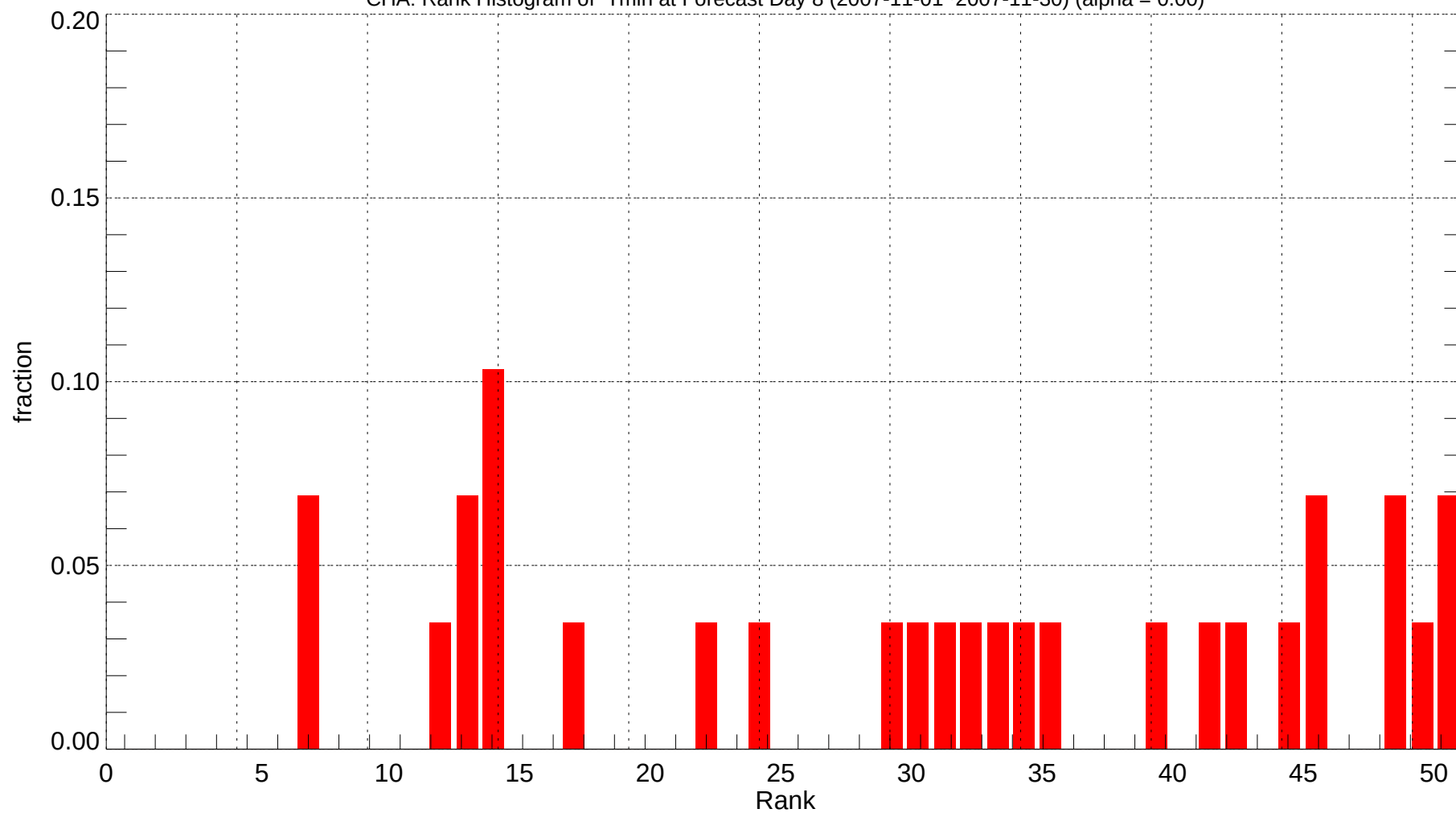
CHA: Rank Histogram of Tmin at Forecast Day 8 (2007-11-01~2007-11-30) (alpha = 0.00)
