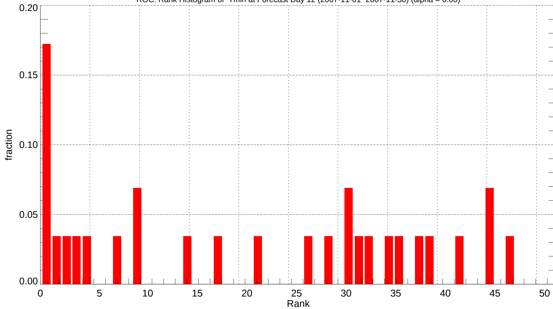
ROC: Rank Histogram of Tmin at Forecast Day 12 (2007-11-01~2007-11-30) (alpha = 0.00)
