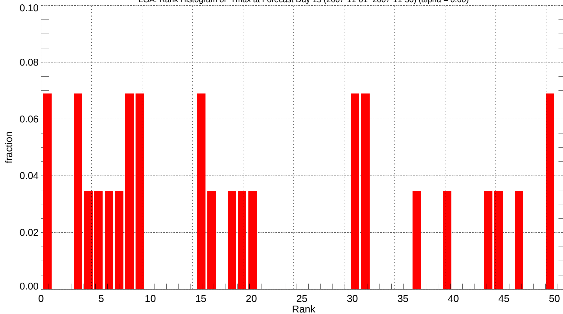
LGA: Rank Histogram of Tmax at Forecast Day 15 (2007-11-01~2007-11-30) (alpha = 0.00)
