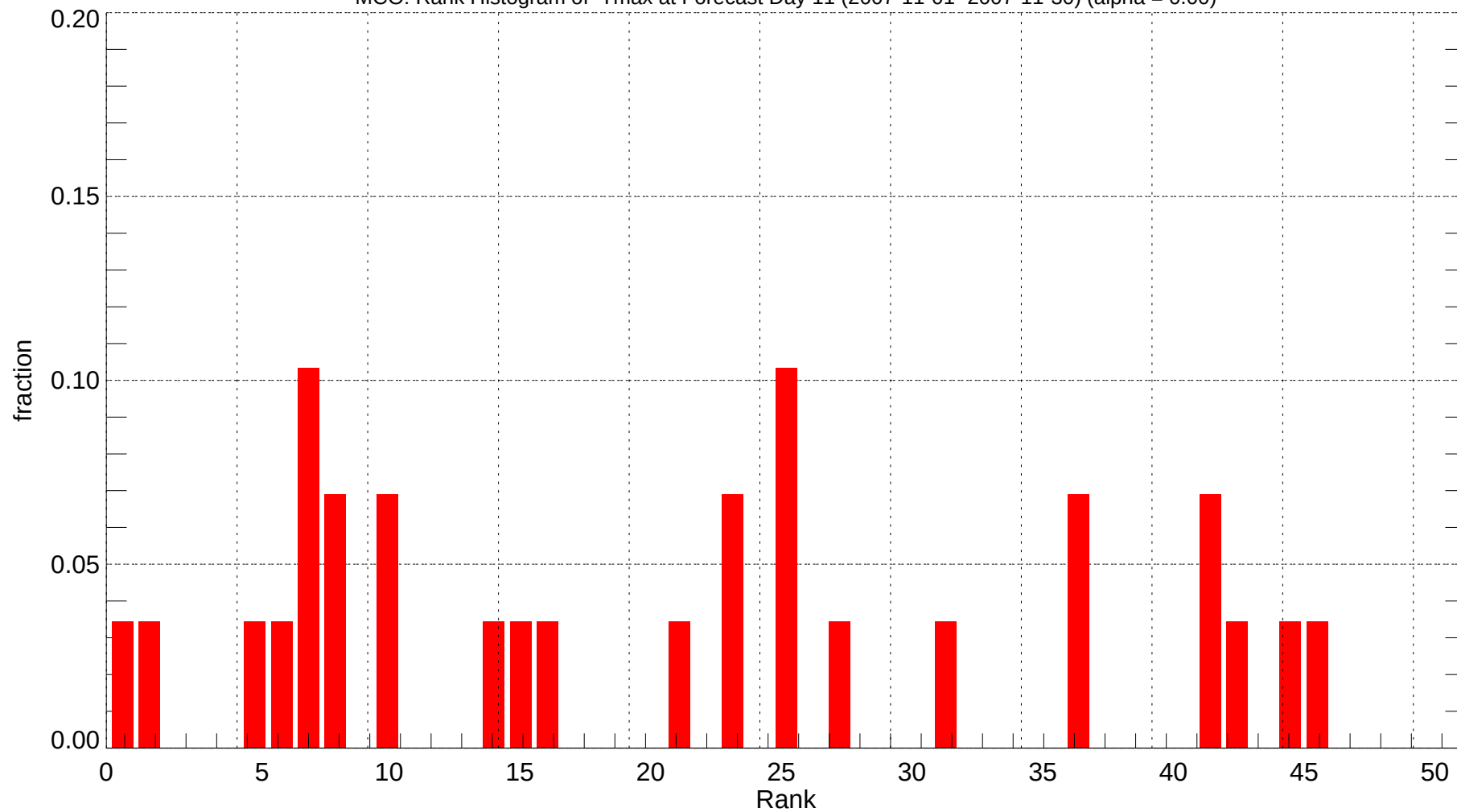
MCO: Rank Histogram of Tmax at Forecast Day 11 (2007-11-01~2007-11-30) (alpha = 0.00)
