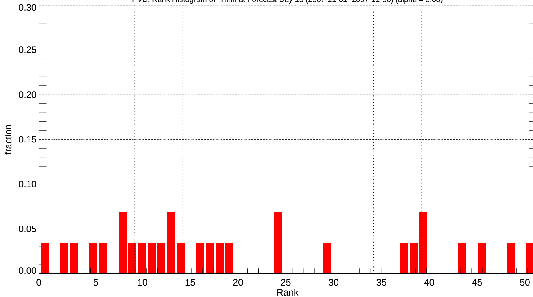
PVD: Rank Histogram of Tmin at Forecast Day 10 (2007-11-01~2007-11-30) (alpha = 0.00)
