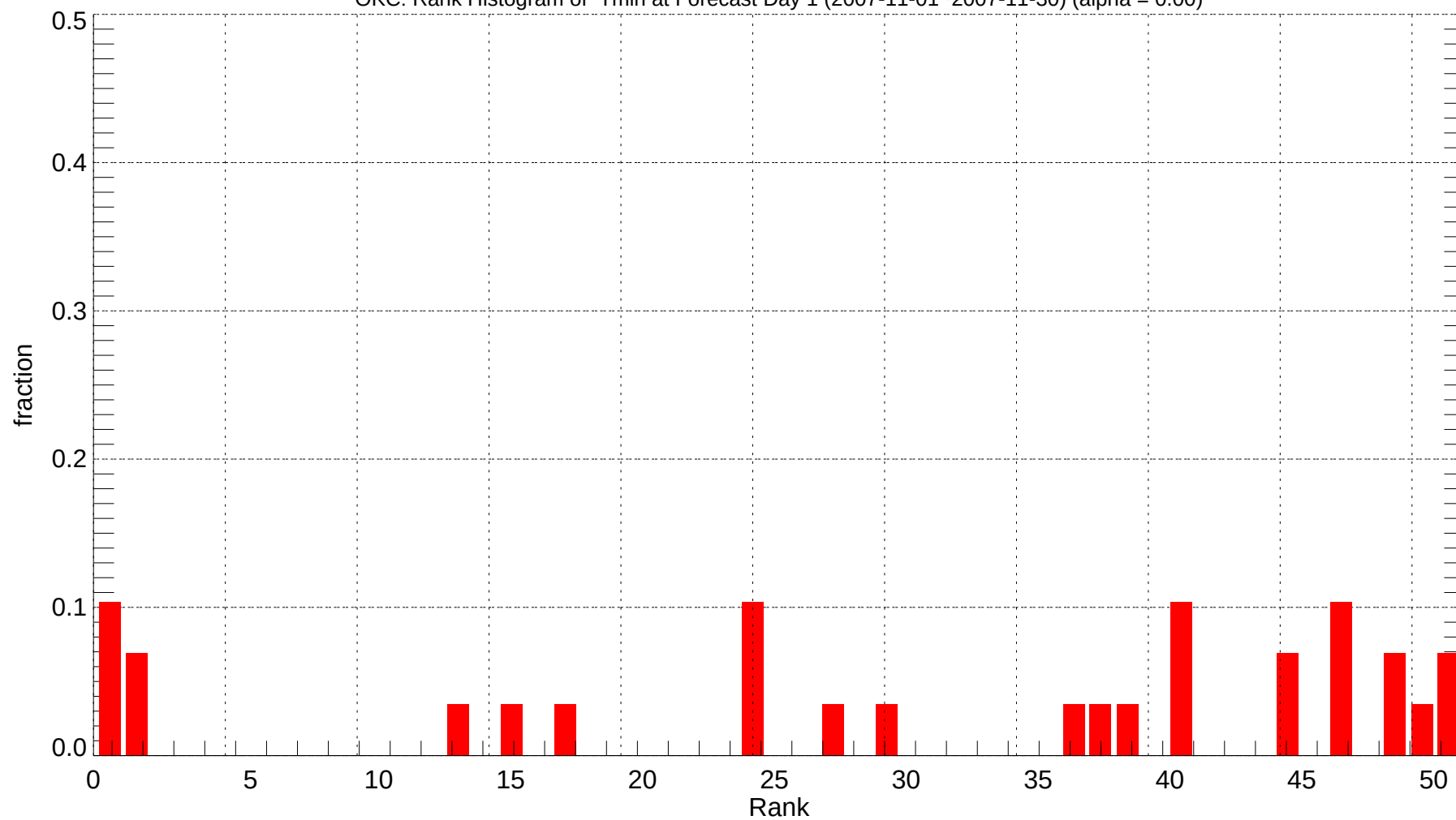
OKC: Rank Histogram of Tmin at Forecast Day 1 (2007-11-01~2007-11-30) (alpha = 0.00)
