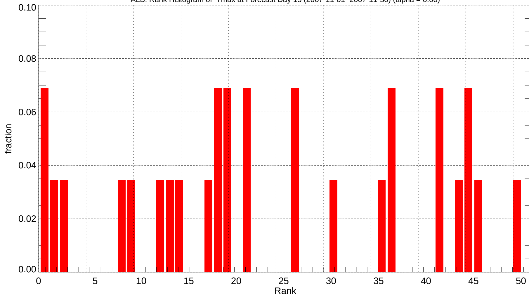
ALB: Rank Histogram of Tmax at Forecast Day 13 (2007-11-01~2007-11-30) (alpha = 0.00)
