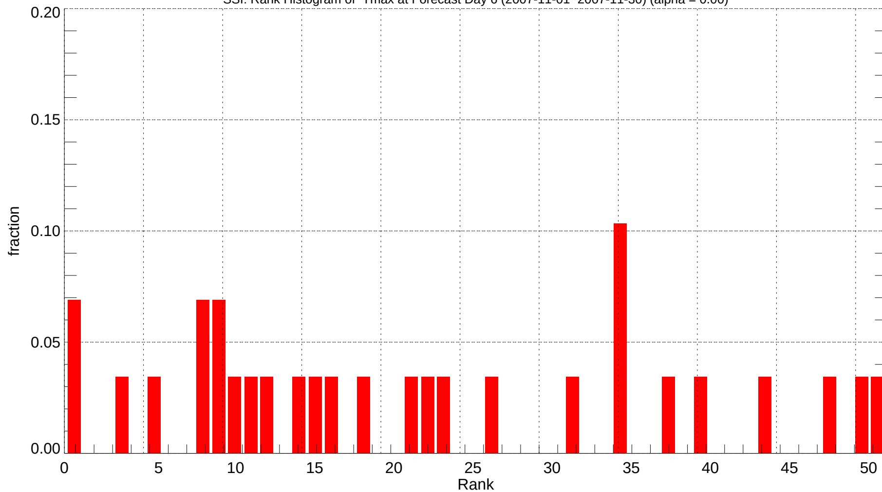
SSI: Rank Histogram of Tmax at Forecast Day 6 (2007-11-01~2007-11-30) (alpha = 0.00)
