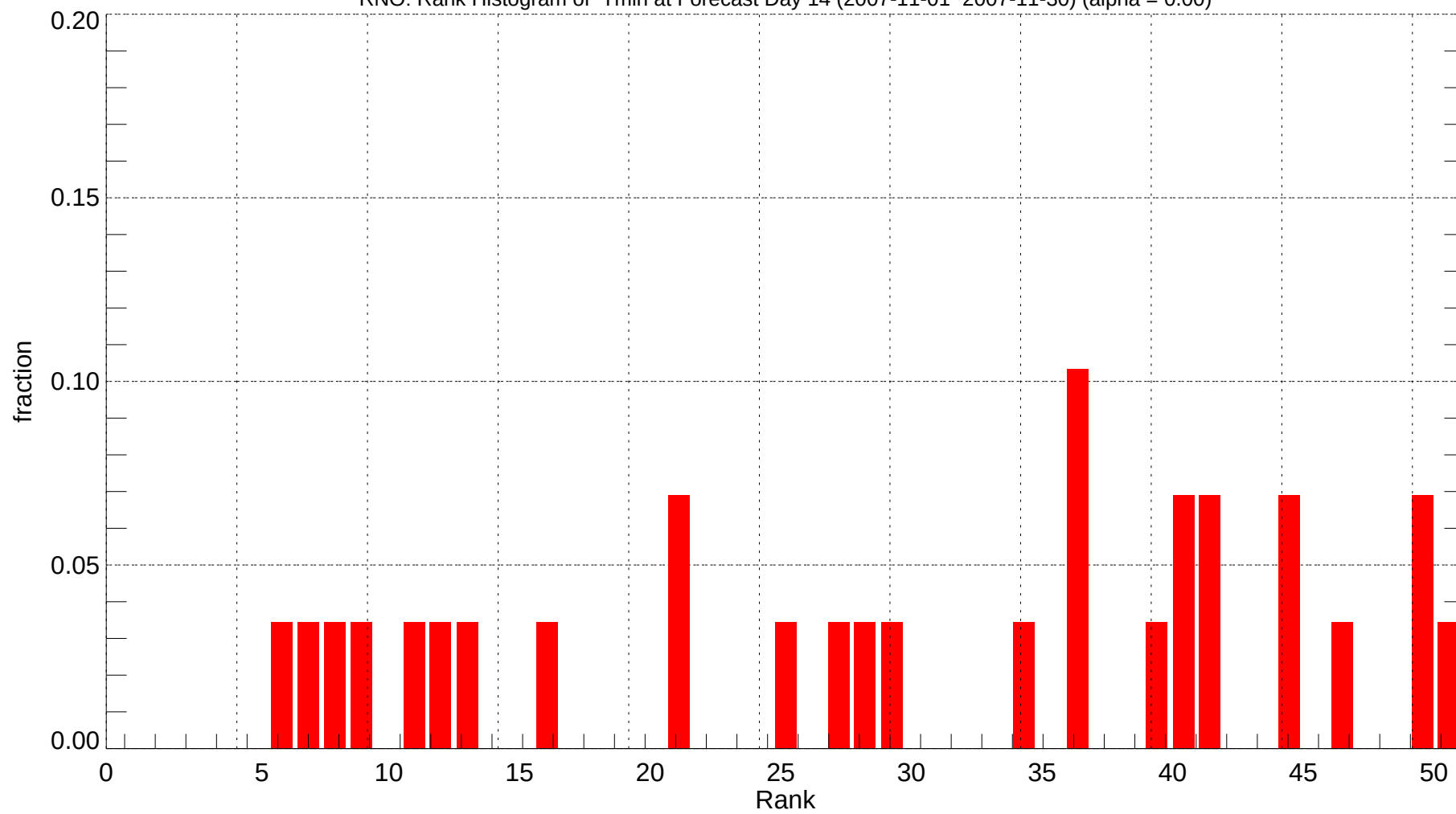
RNO: Rank Histogram of Tmin at Forecast Day 14 (2007-11-01~2007-11-30) (alpha = 0.00)
