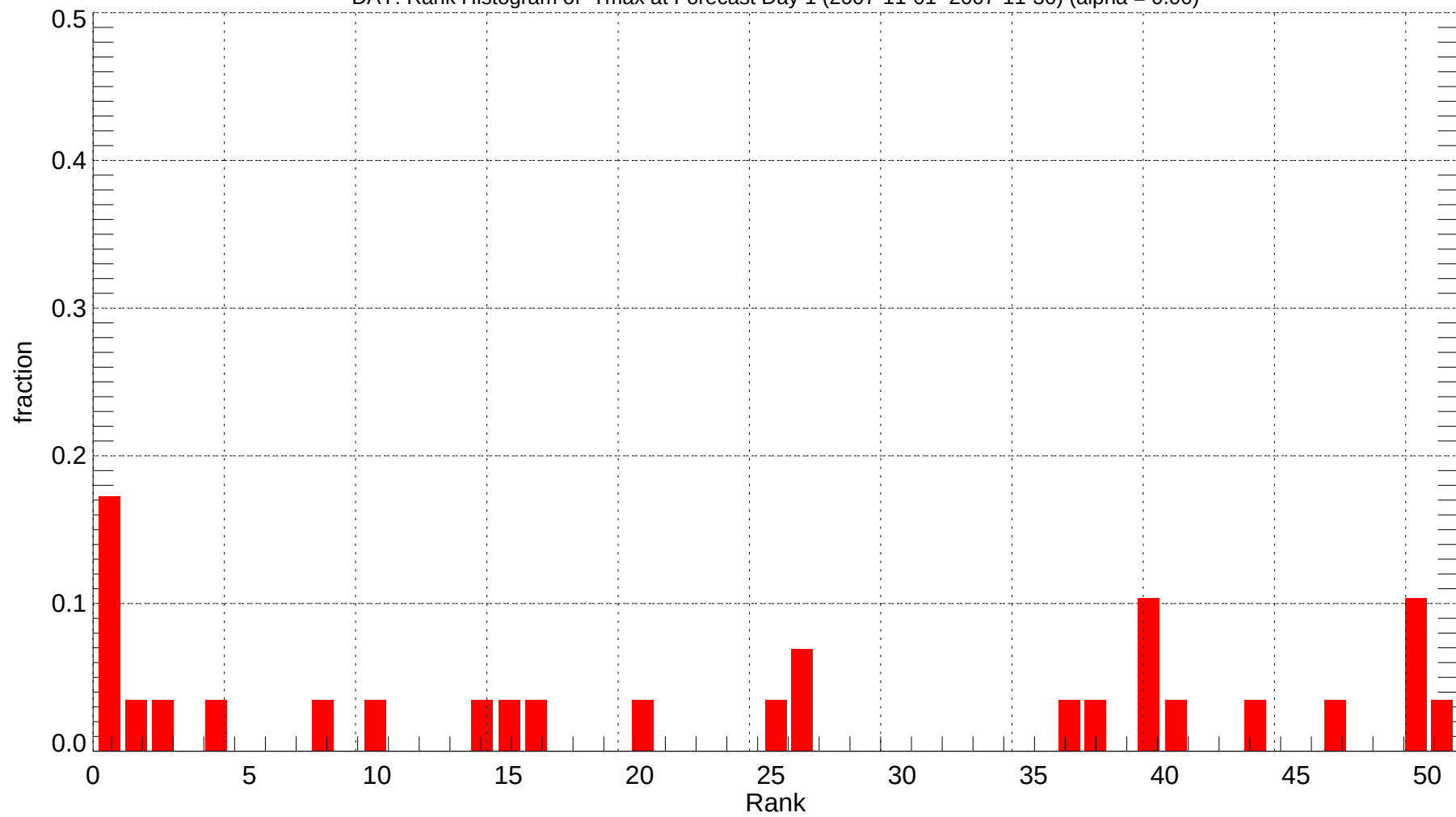
DAY: Rank Histogram of Tmax at Forecast Day 1 (2007-11-01~2007-11-30) (alpha = 0.00)
