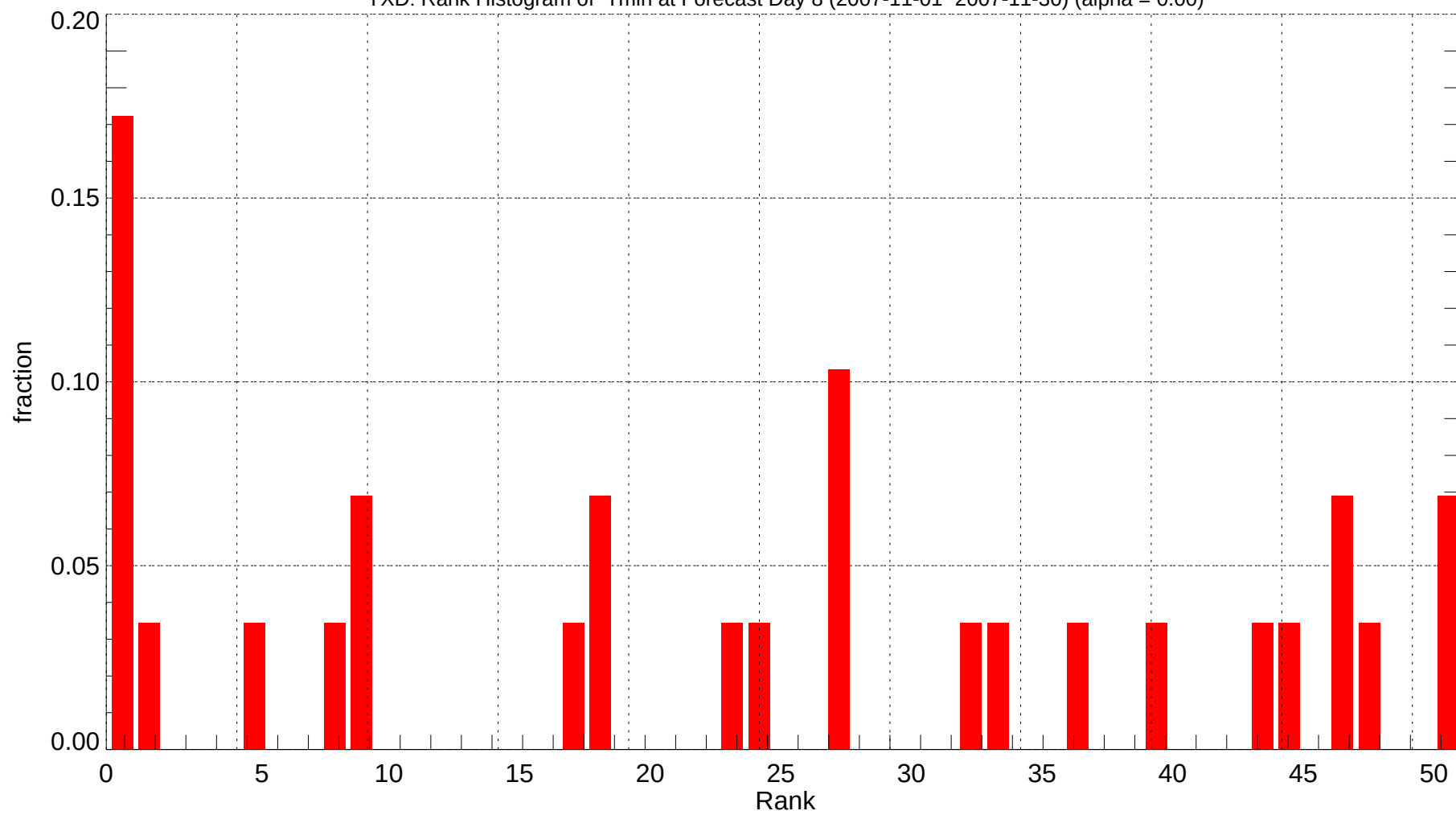
YXD: Rank Histogram of Tmin at Forecast Day 8 (2007-11-01~2007-11-30) (alpha = 0.00)
