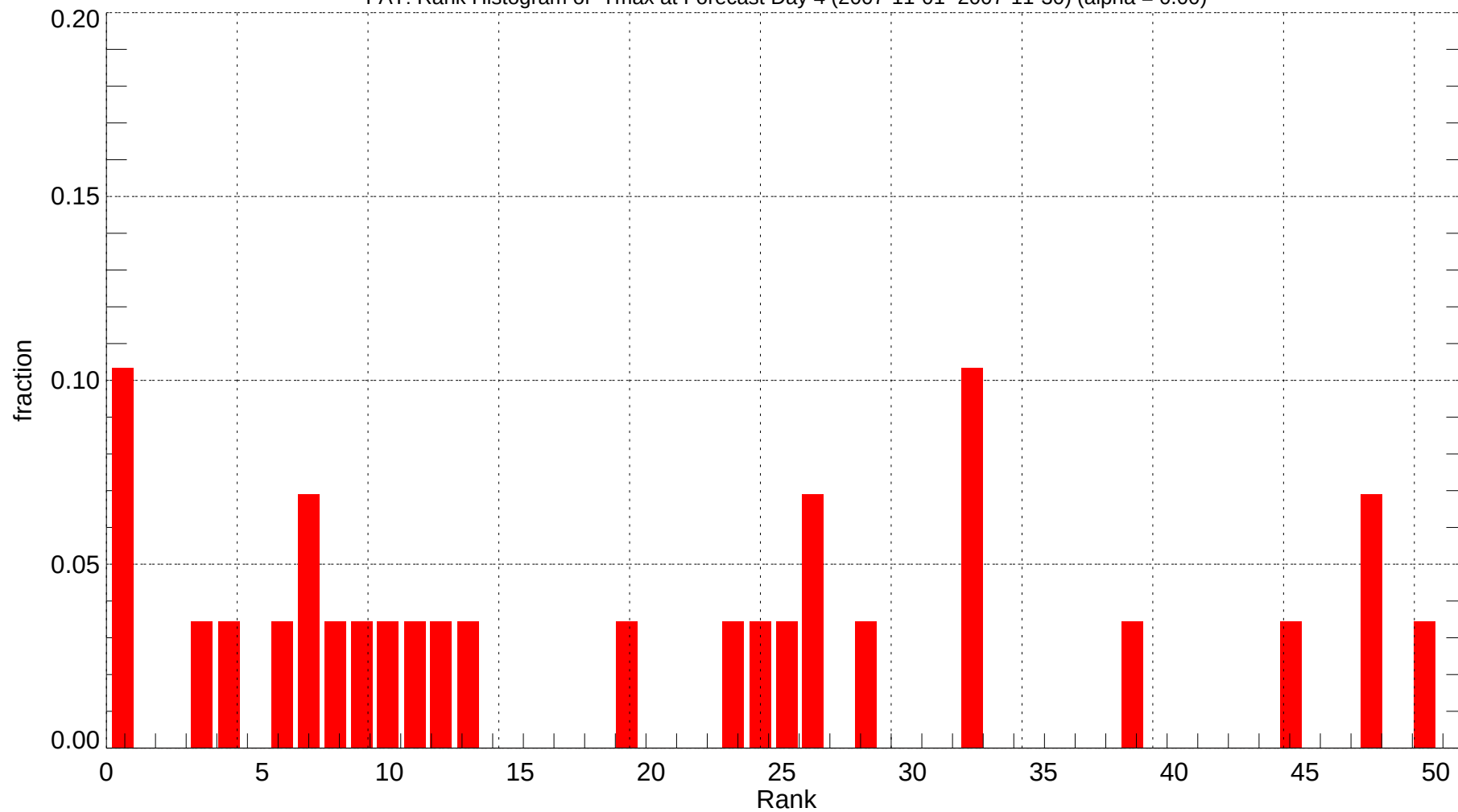
FAT: Rank Histogram of Tmax at Forecast Day 4 (2007-11-01~2007-11-30) (alpha = 0.00)
