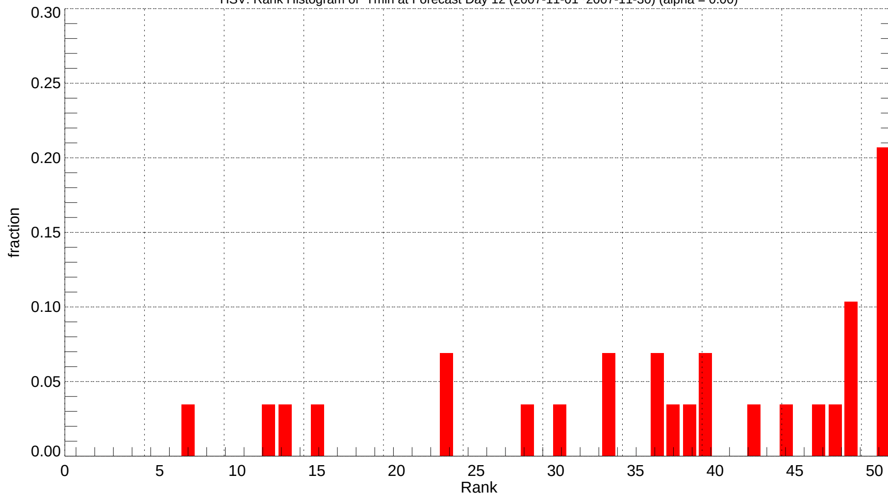
HSV: Rank Histogram of Tmin at Forecast Day 12 (2007-11-01~2007-11-30) (alpha = 0.00)
