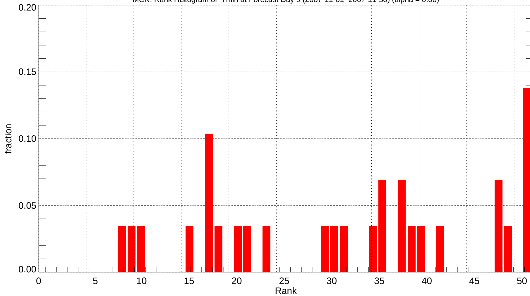
MCN: Rank Histogram of Tmin at Forecast Day 9 (2007-11-01~2007-11-30) (alpha = 0.00)
