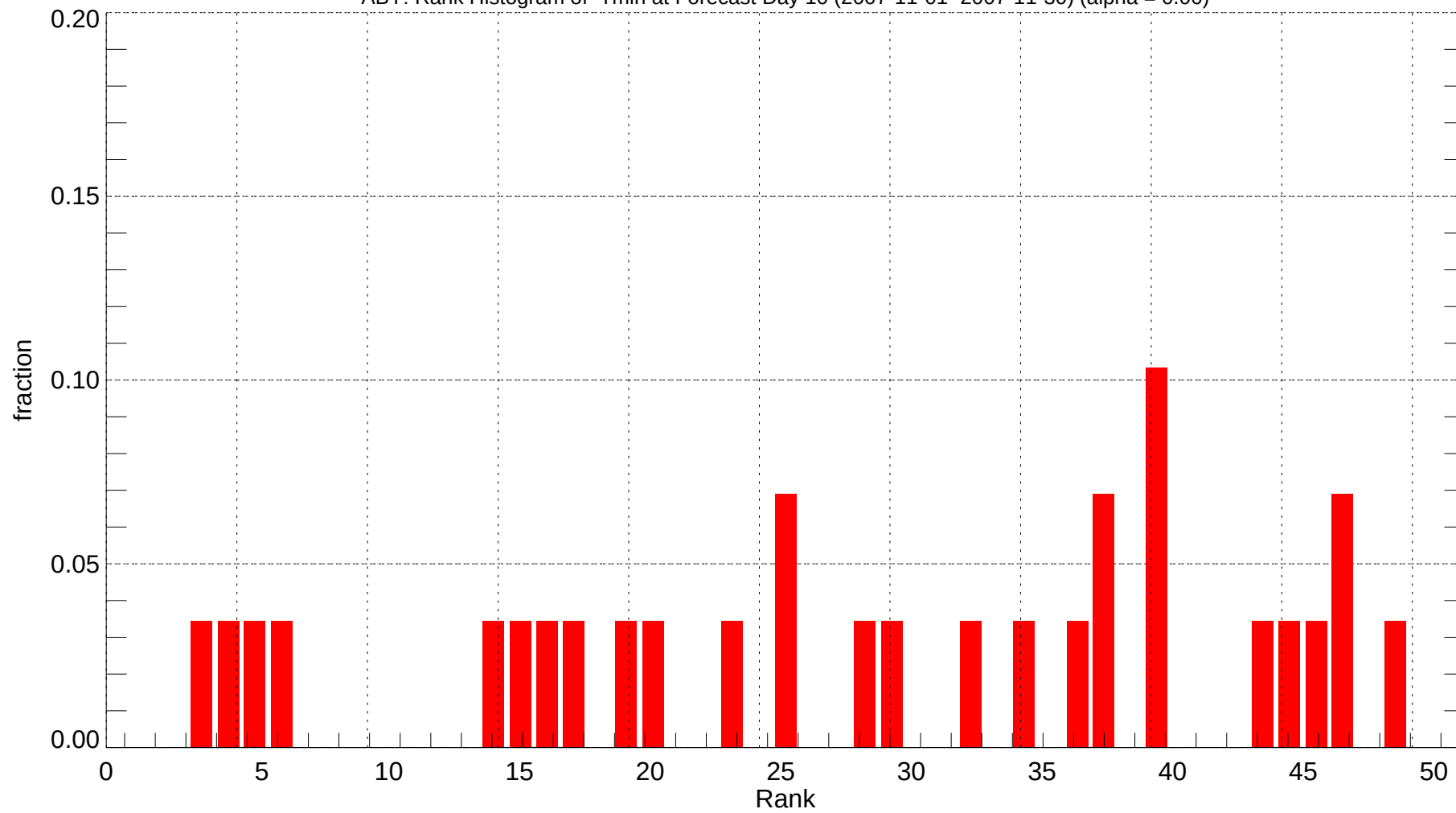
ABY: Rank Histogram of Tmin at Forecast Day 10 (2007-11-01~2007-11-30) (alpha = 0.00)
