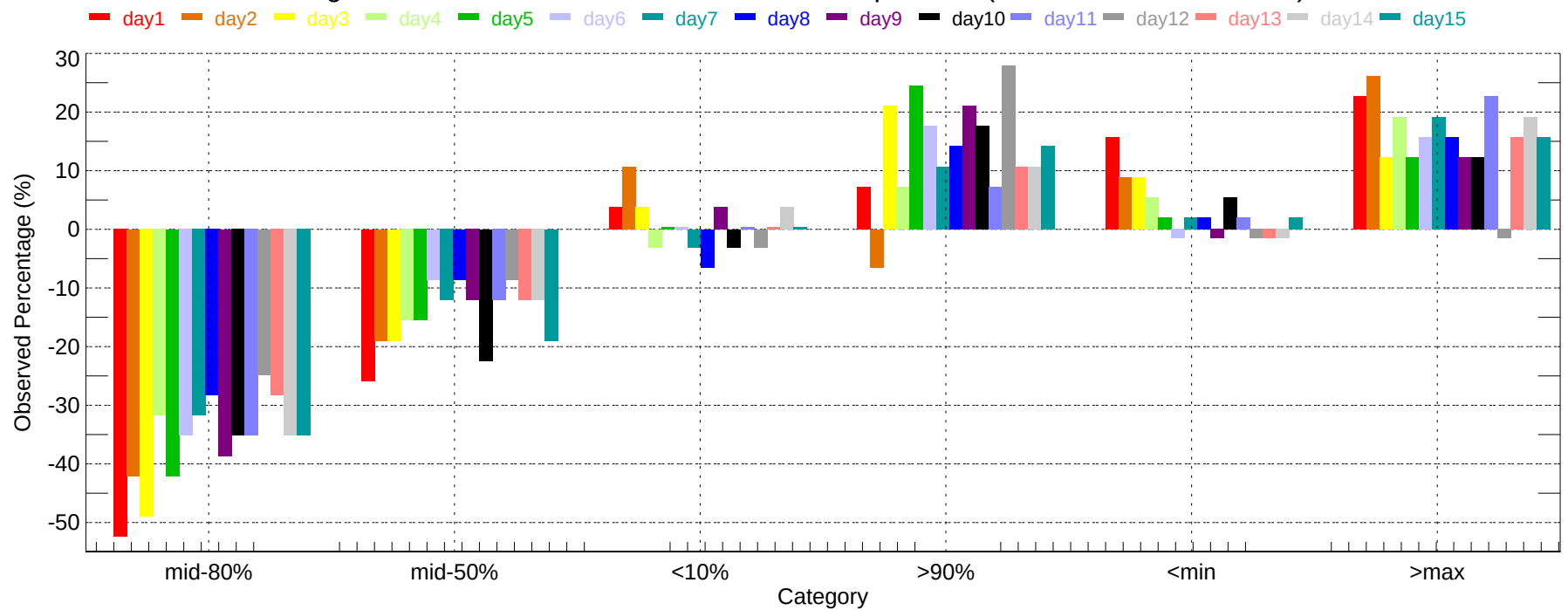
Observed Percentage Deviation of Ensembles - DEN: Max Temperature (2007-11-01~2007-11-30)
