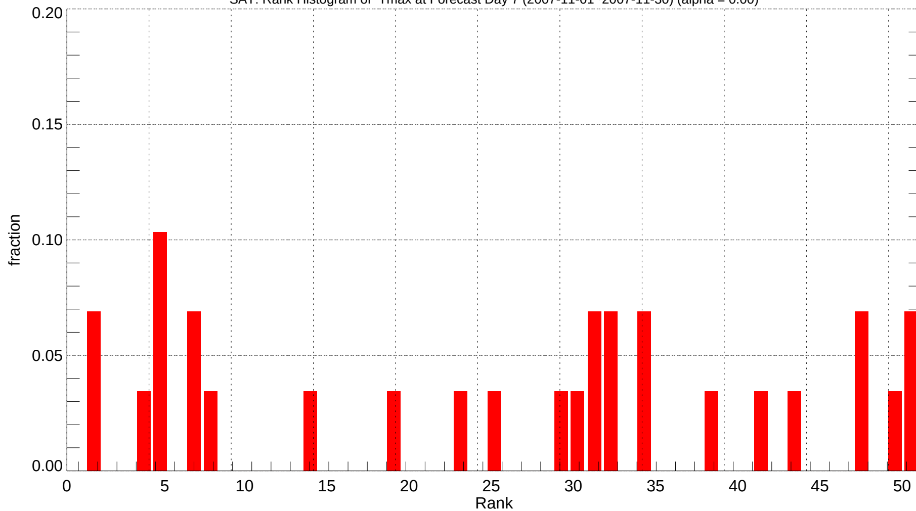
SAT: Rank Histogram of Tmax at Forecast Day 7 (2007-11-01~2007-11-30) (alpha = 0.00)
