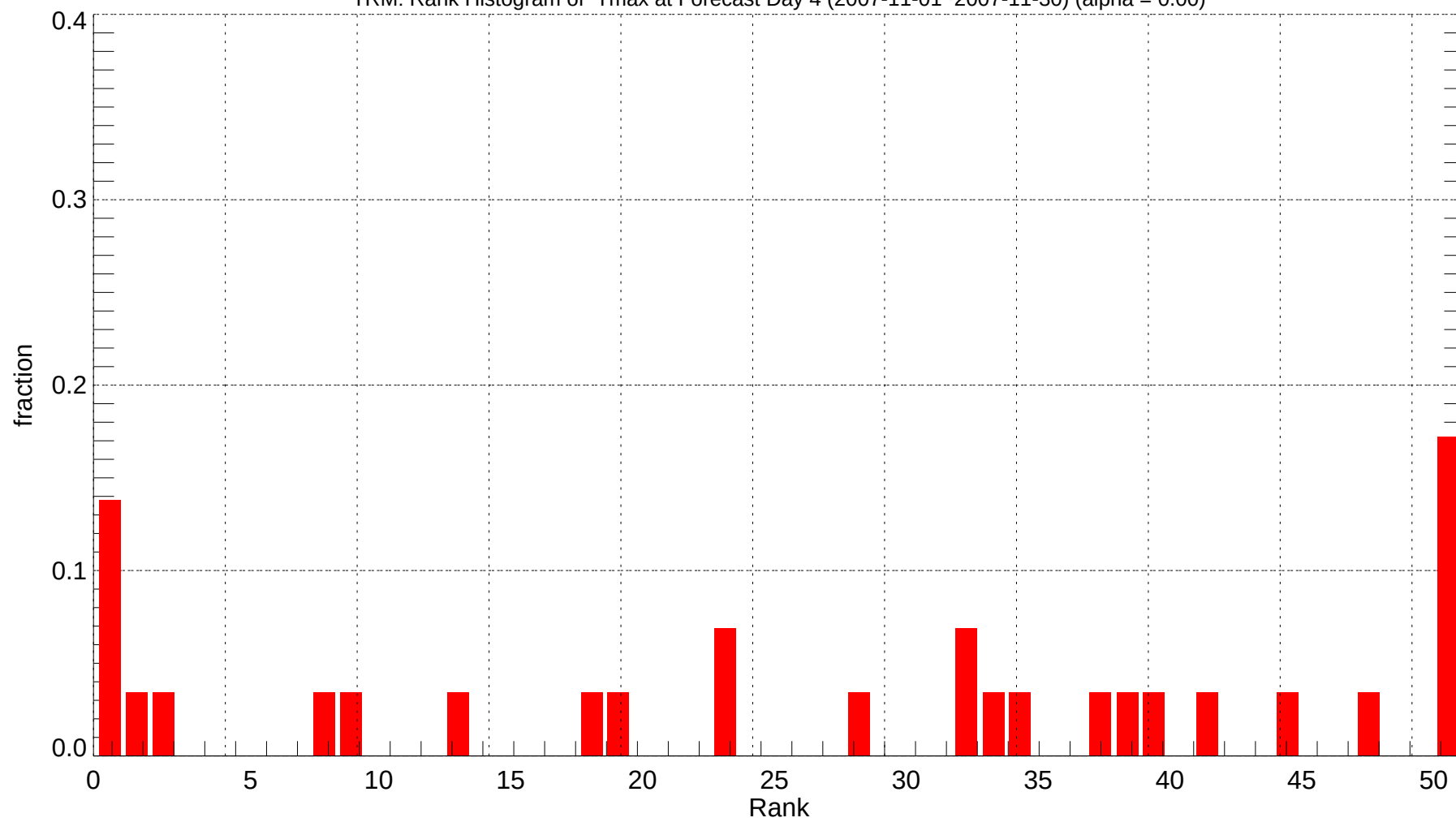
TRM: Rank Histogram of Tmax at Forecast Day 4 (2007-11-01~2007-11-30) (alpha = 0.00)
