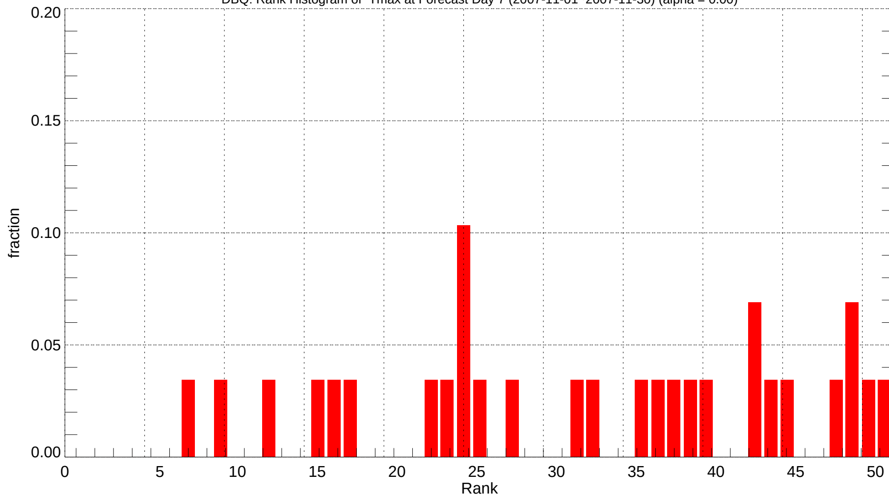
DBQ: Rank Histogram of Tmax at Forecast Day 7 (2007-11-01~2007-11-30) (alpha = 0.00)
