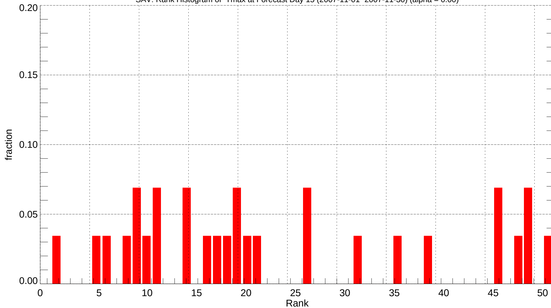
SAV: Rank Histogram of Tmax at Forecast Day 15 (2007-11-01~2007-11-30) (alpha = 0.00)
