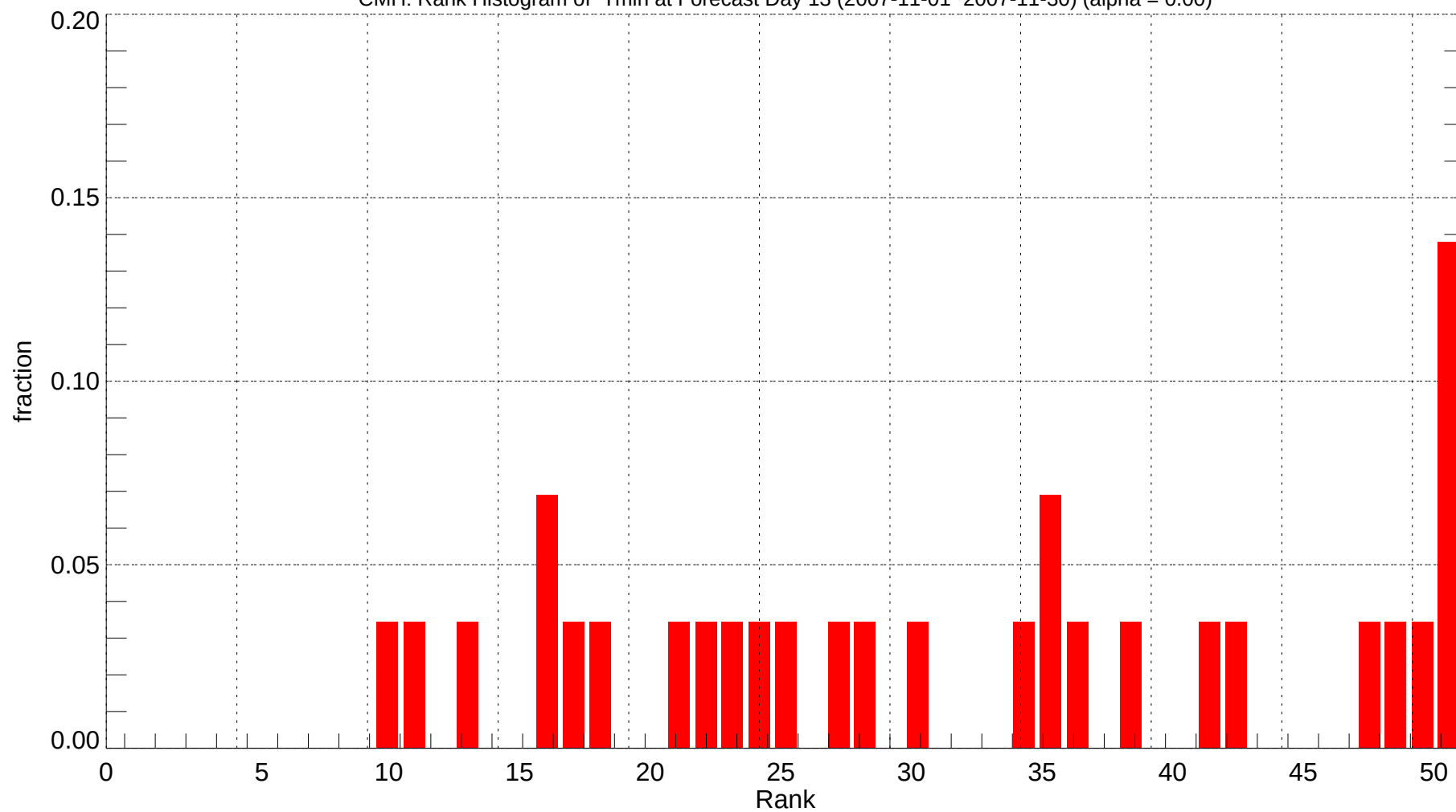
CMH: Rank Histogram of Tmin at Forecast Day 13 (2007-11-01~2007-11-30) (alpha = 0.00)
