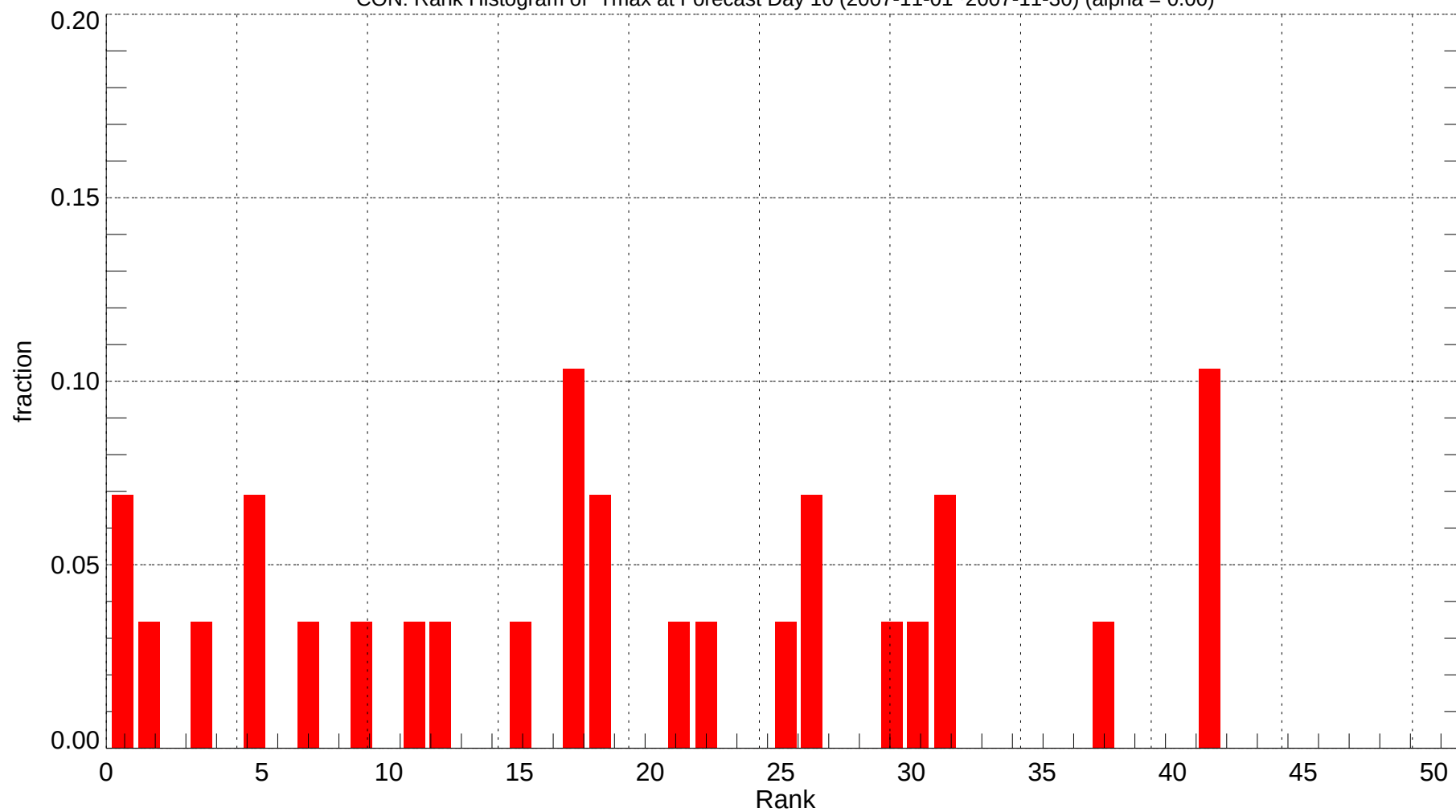
CON: Rank Histogram of Tmax at Forecast Day 10 (2007-11-01~2007-11-30) (alpha = 0.00)
