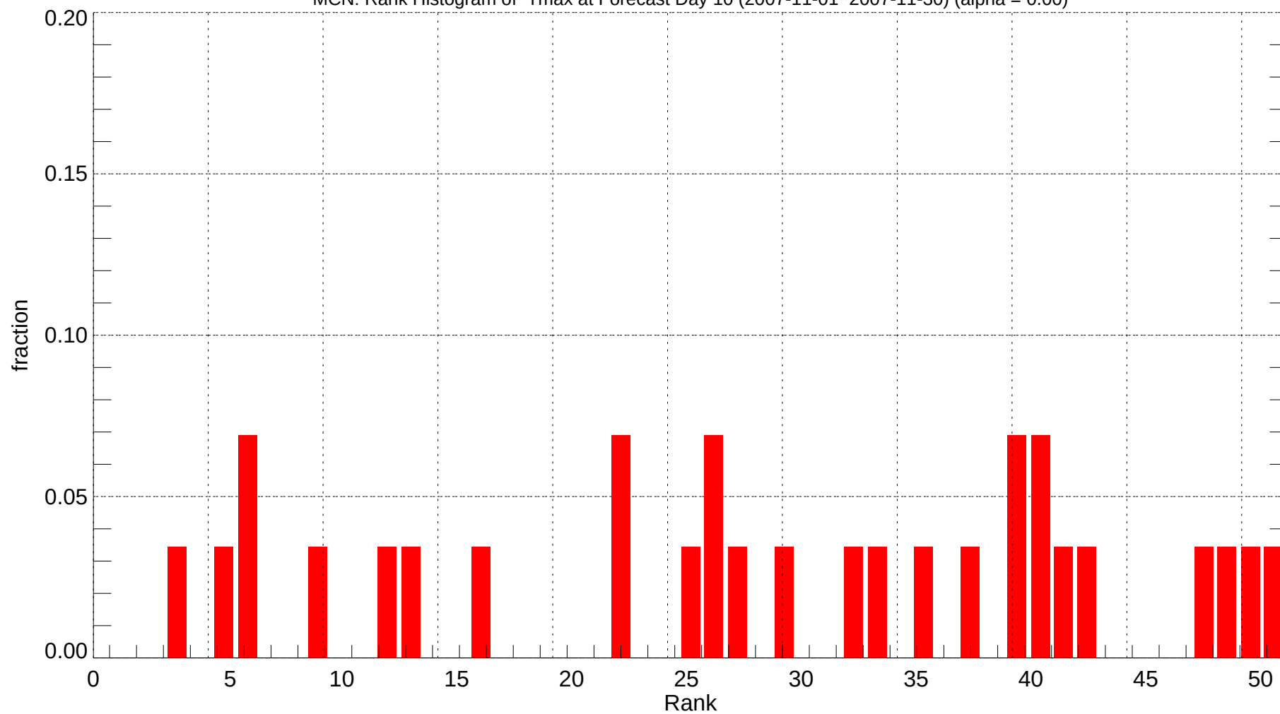
MCN: Rank Histogram of Tmax at Forecast Day 10 (2007-11-01~2007-11-30) (alpha = 0.00)
