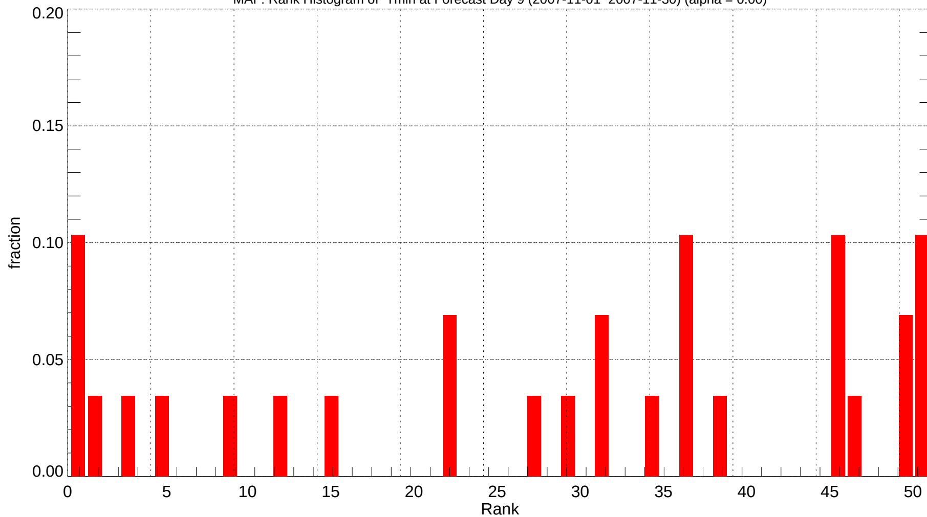
MAF: Rank Histogram of Tmin at Forecast Day 9 (2007-11-01~2007-11-30) (alpha = 0.00)
