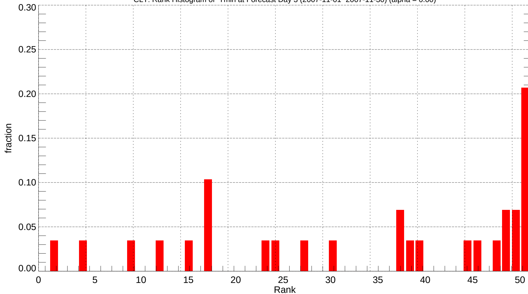
CLT: Rank Histogram of Tmin at Forecast Day 3 (2007-11-01~2007-11-30) (alpha = 0.00)
