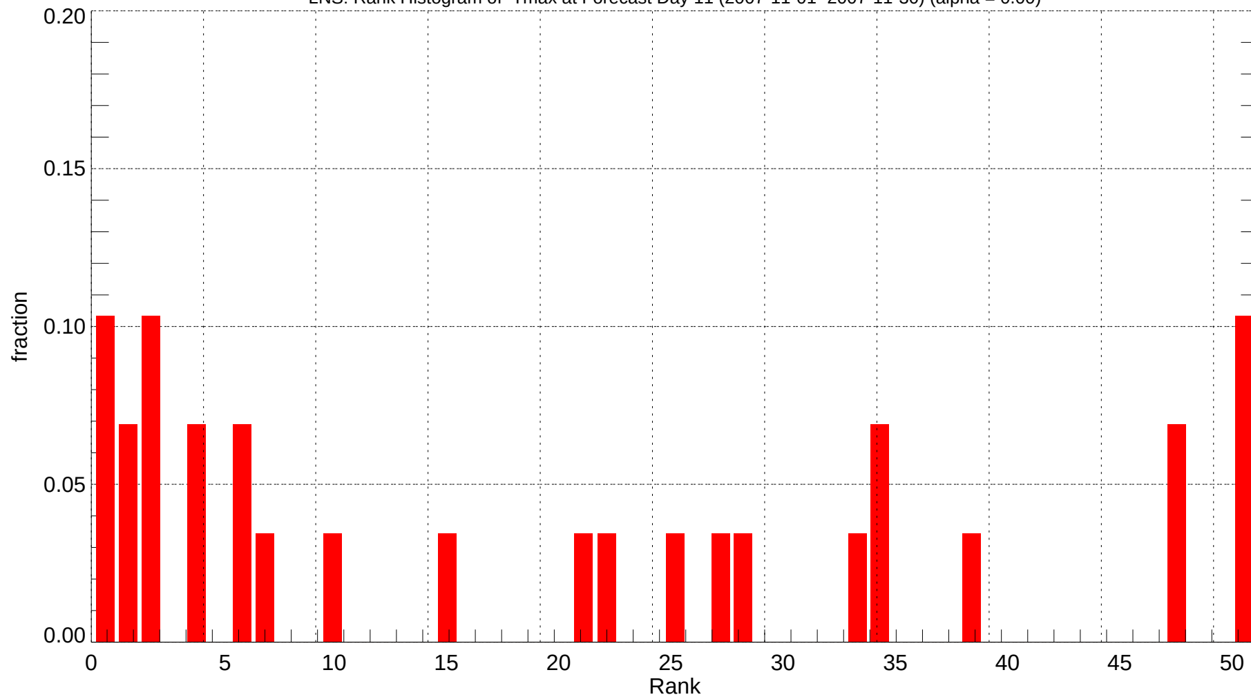
LNS: Rank Histogram of Tmax at Forecast Day 11 (2007-11-01~2007-11-30) (alpha = 0.00)
