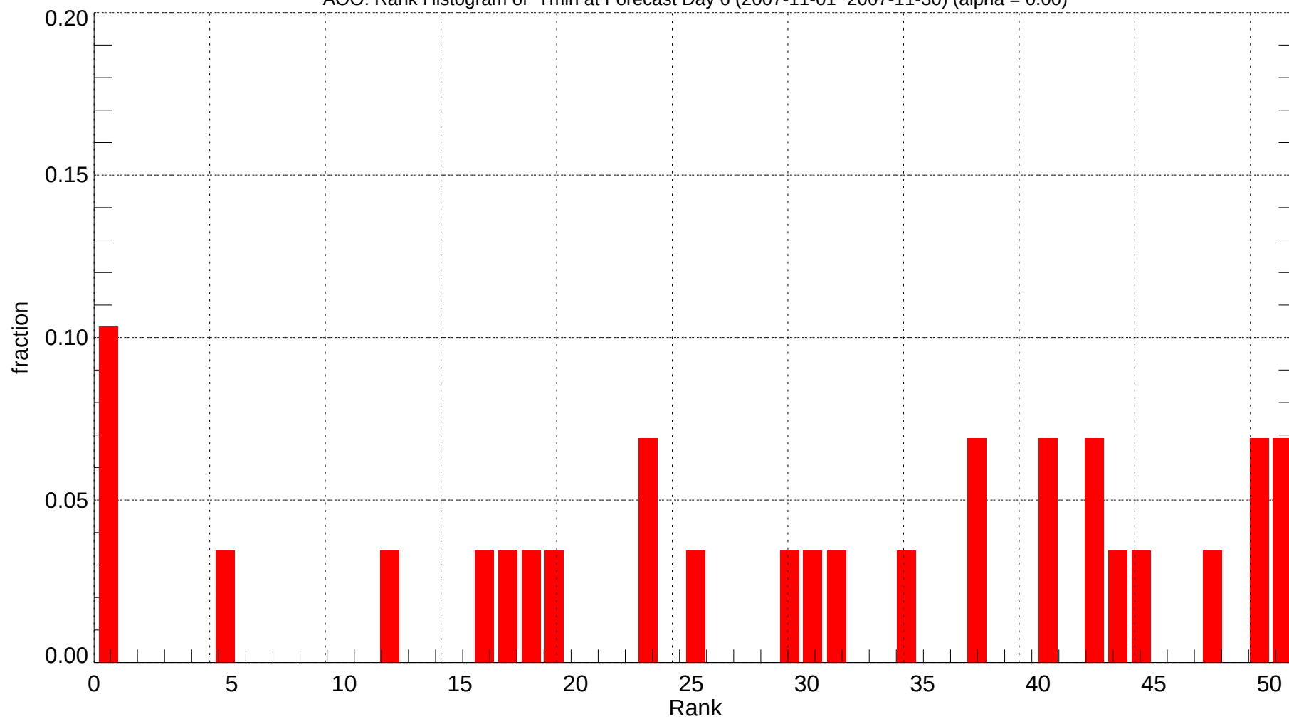
AOO: Rank Histogram of Tmin at Forecast Day 6 (2007-11-01~2007-11-30) (alpha = 0.00)
