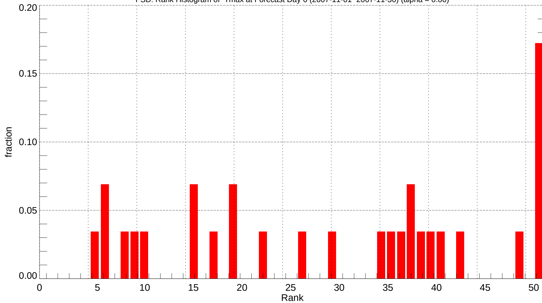
FSD: Rank Histogram of Tmax at Forecast Day 6 (2007-11-01~2007-11-30) (alpha = 0.00)
