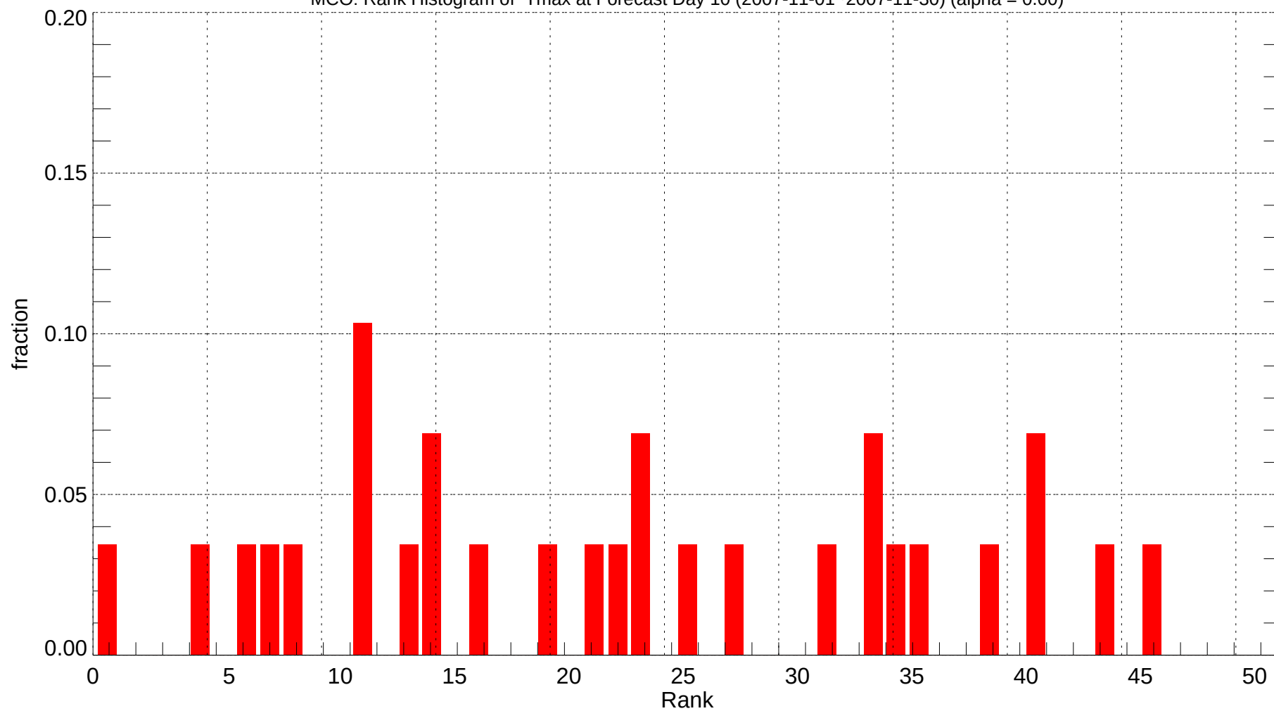
MCO: Rank Histogram of Tmax at Forecast Day 10 (2007-11-01~2007-11-30) (alpha = 0.00)
