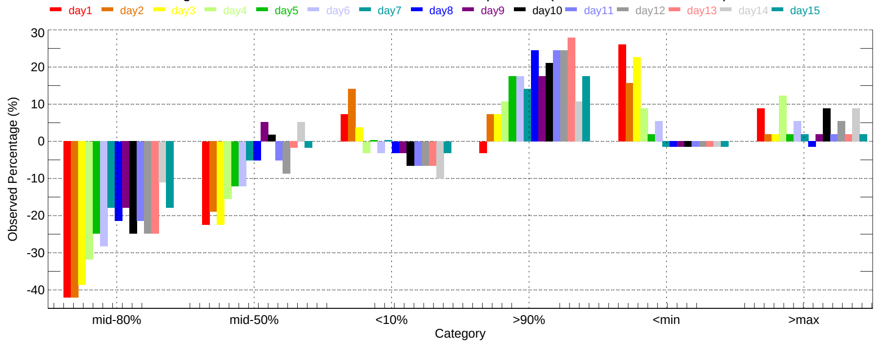
Observed Percentage Deviation of Ensembles - DSM: Min Temperature (2007-11-01~2007-11-30)
