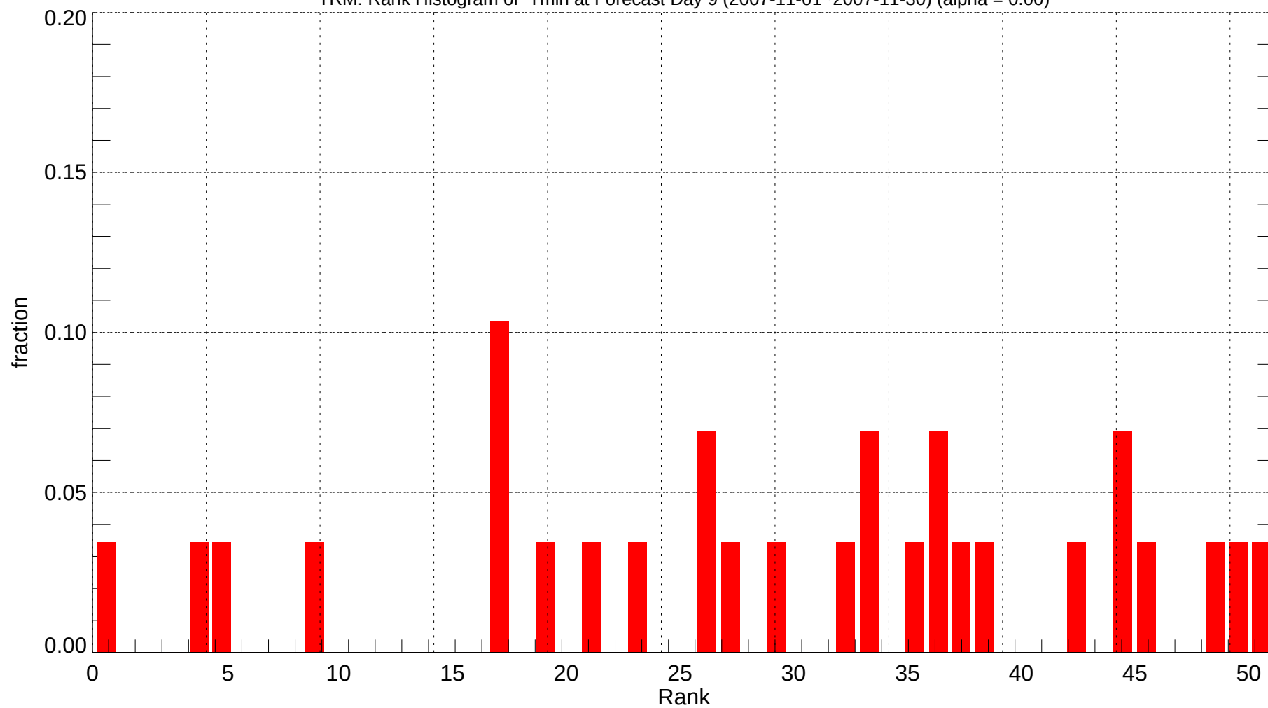
TRM: Rank Histogram of Tmin at Forecast Day 9 (2007-11-01~2007-11-30) (alpha = 0.00)
