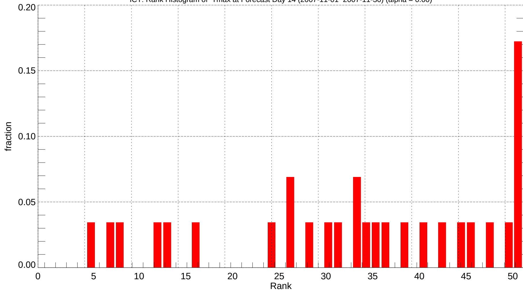
ICT: Rank Histogram of Tmax at Forecast Day 14 (2007-11-01~2007-11-30) (alpha = 0.00)
