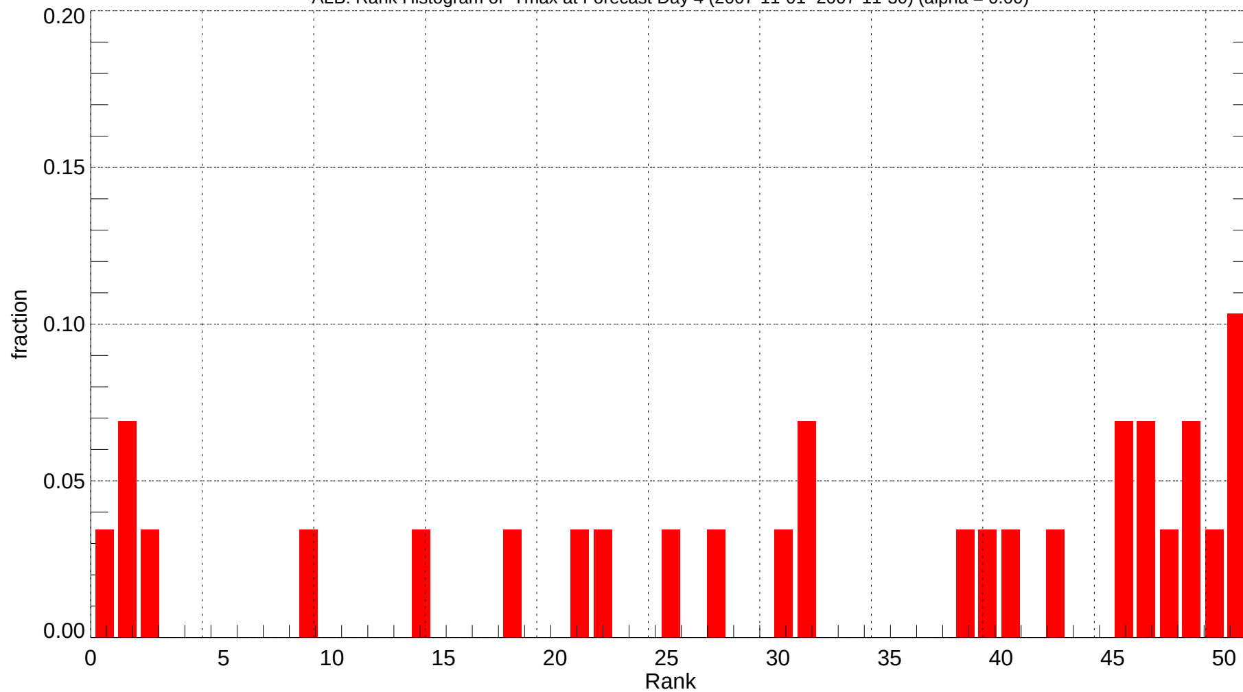
ALB: Rank Histogram of Tmax at Forecast Day 4 (2007-11-01~2007-11-30) (alpha = 0.00)
