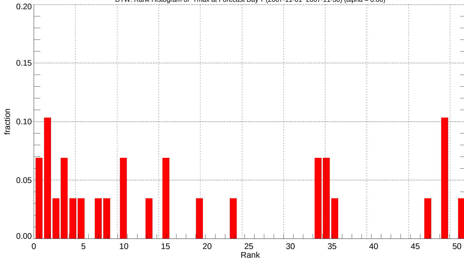
DTW: Rank Histogram of Tmax at Forecast Day 7 (2007-11-01~2007-11-30) (alpha = 0.00)
