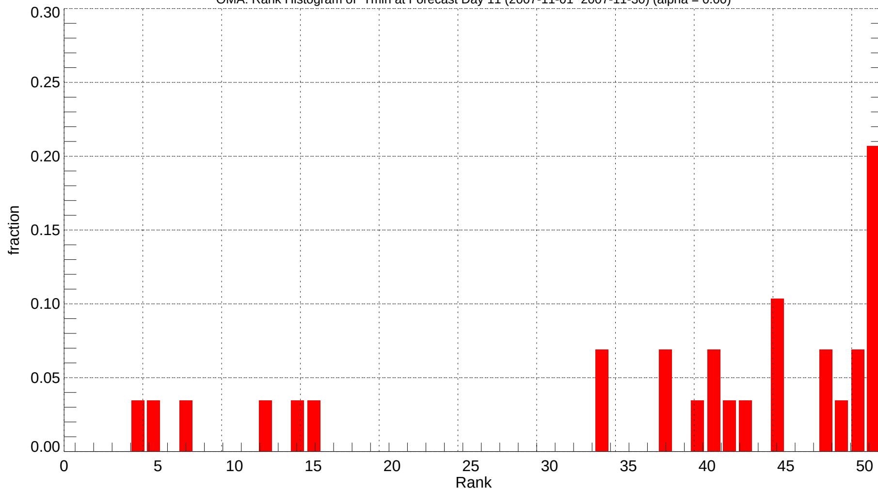
OMA: Rank Histogram of Tmin at Forecast Day 11 (2007-11-01~2007-11-30) (alpha = 0.00)
