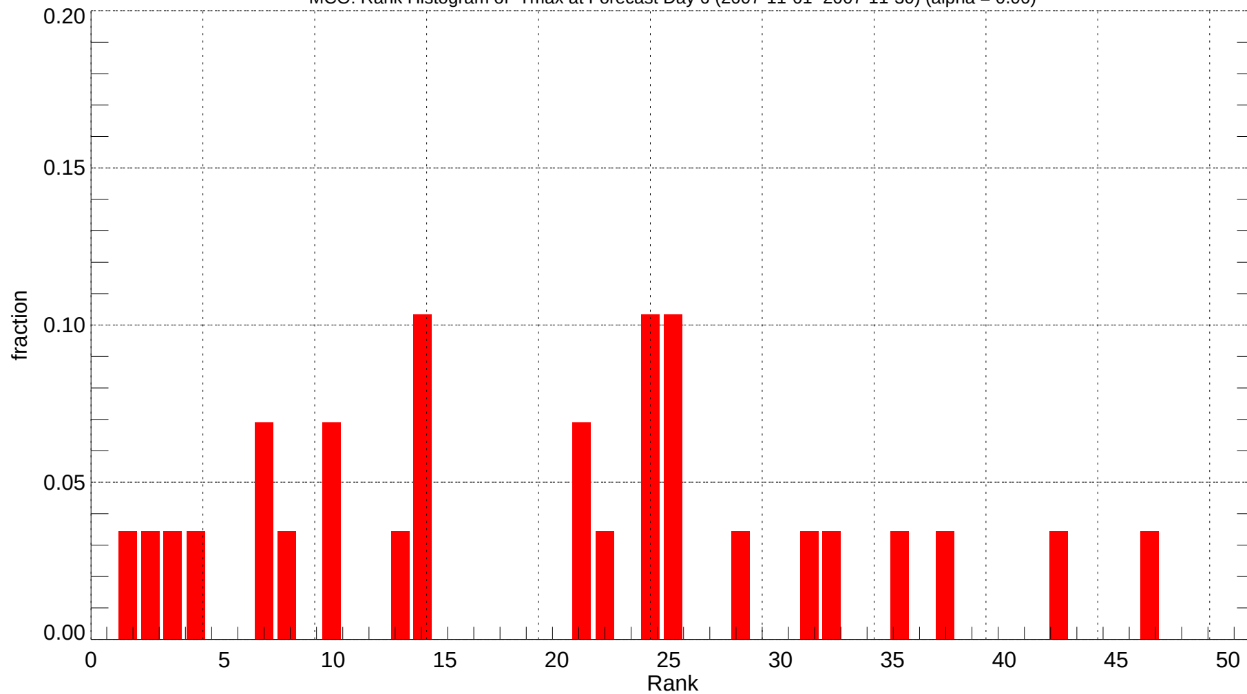
MCO: Rank Histogram of Tmax at Forecast Day 6 (2007-11-01~2007-11-30) (alpha = 0.00)
