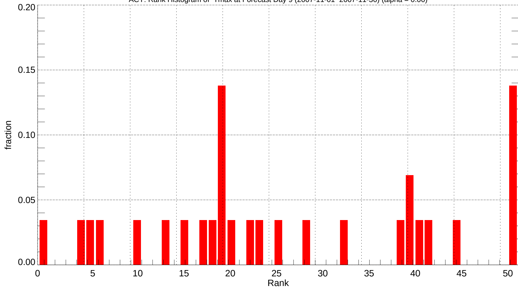
ACY: Rank Histogram of Tmax at Forecast Day 9 (2007-11-01~2007-11-30) (alpha = 0.00)
