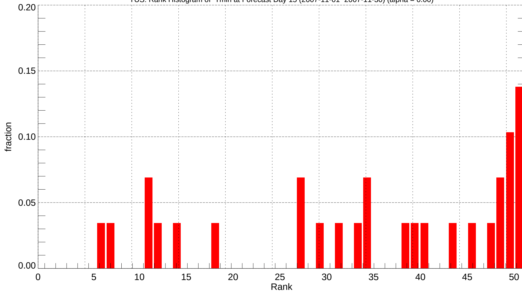
TUS: Rank Histogram of Tmin at Forecast Day 15 (2007-11-01~2007-11-30) (alpha = 0.00)
