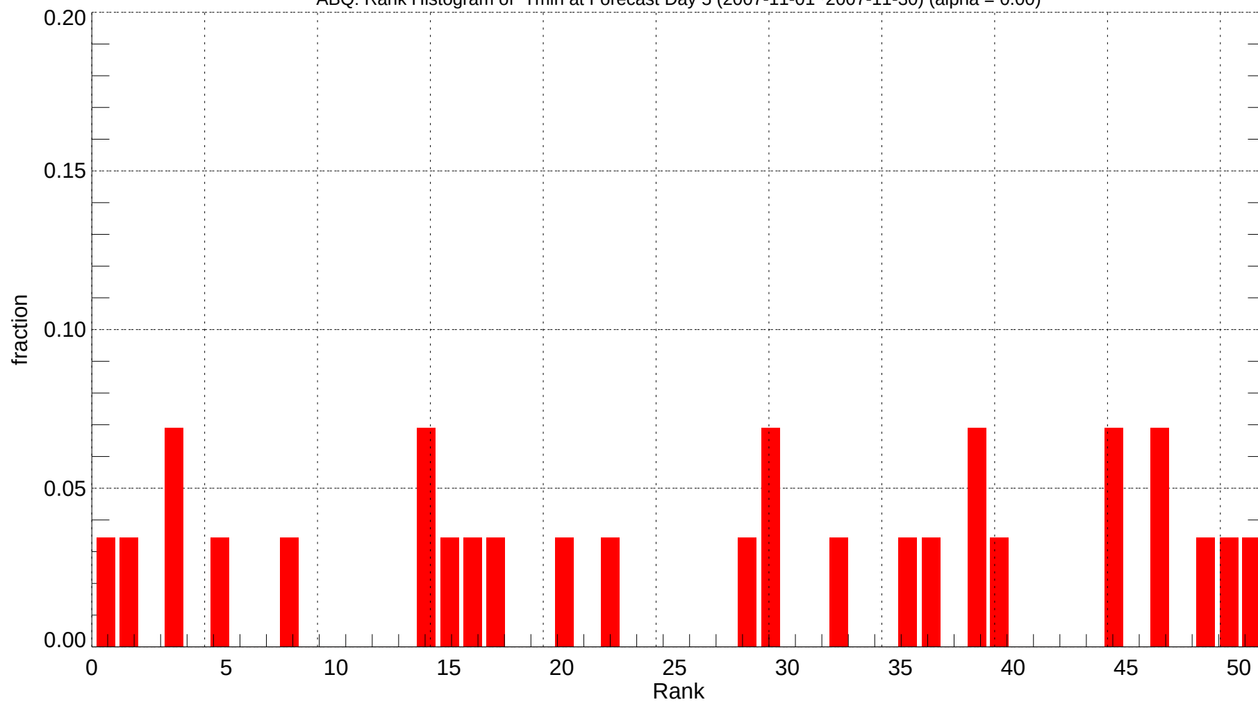
ABQ: Rank Histogram of Tmin at Forecast Day 5 (2007-11-01~2007-11-30) (alpha = 0.00)
