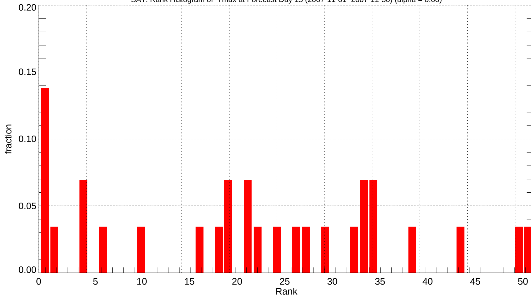
SAT: Rank Histogram of Tmax at Forecast Day 15 (2007-11-01~2007-11-30) (alpha = 0.00)
