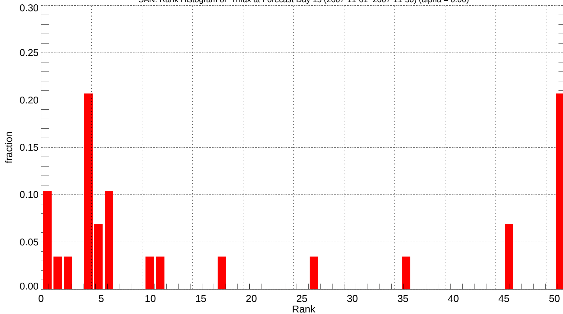
SAN: Rank Histogram of Tmax at Forecast Day 13 (2007-11-01~2007-11-30) (alpha = 0.00)
