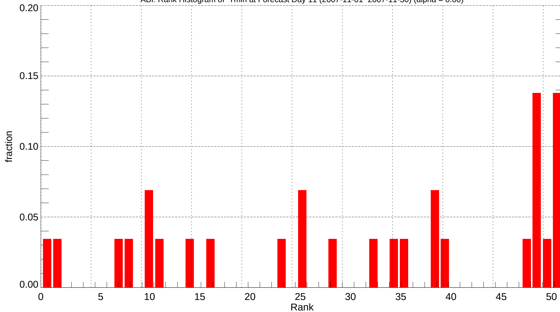
ABI: Rank Histogram of Tmin at Forecast Day 11 (2007-11-01~2007-11-30) (alpha = 0.00)
