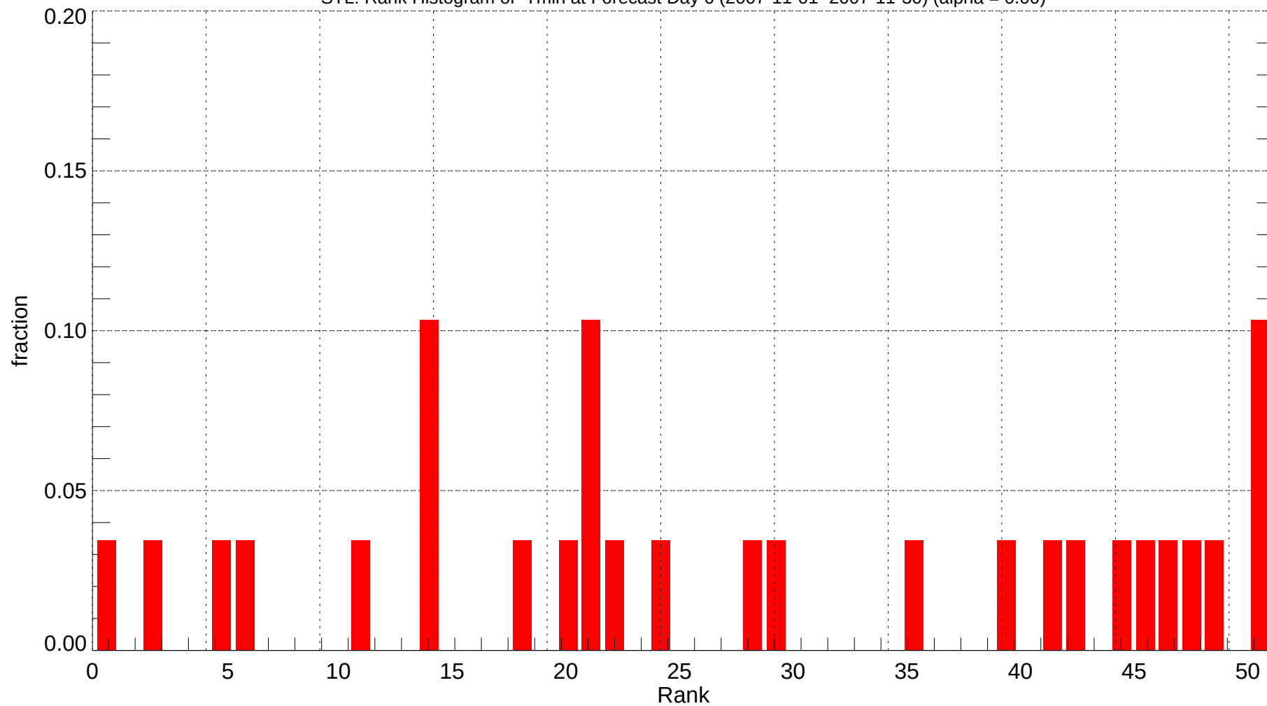
STL: Rank Histogram of Tmin at Forecast Day 6 (2007-11-01~2007-11-30) (alpha = 0.00)
