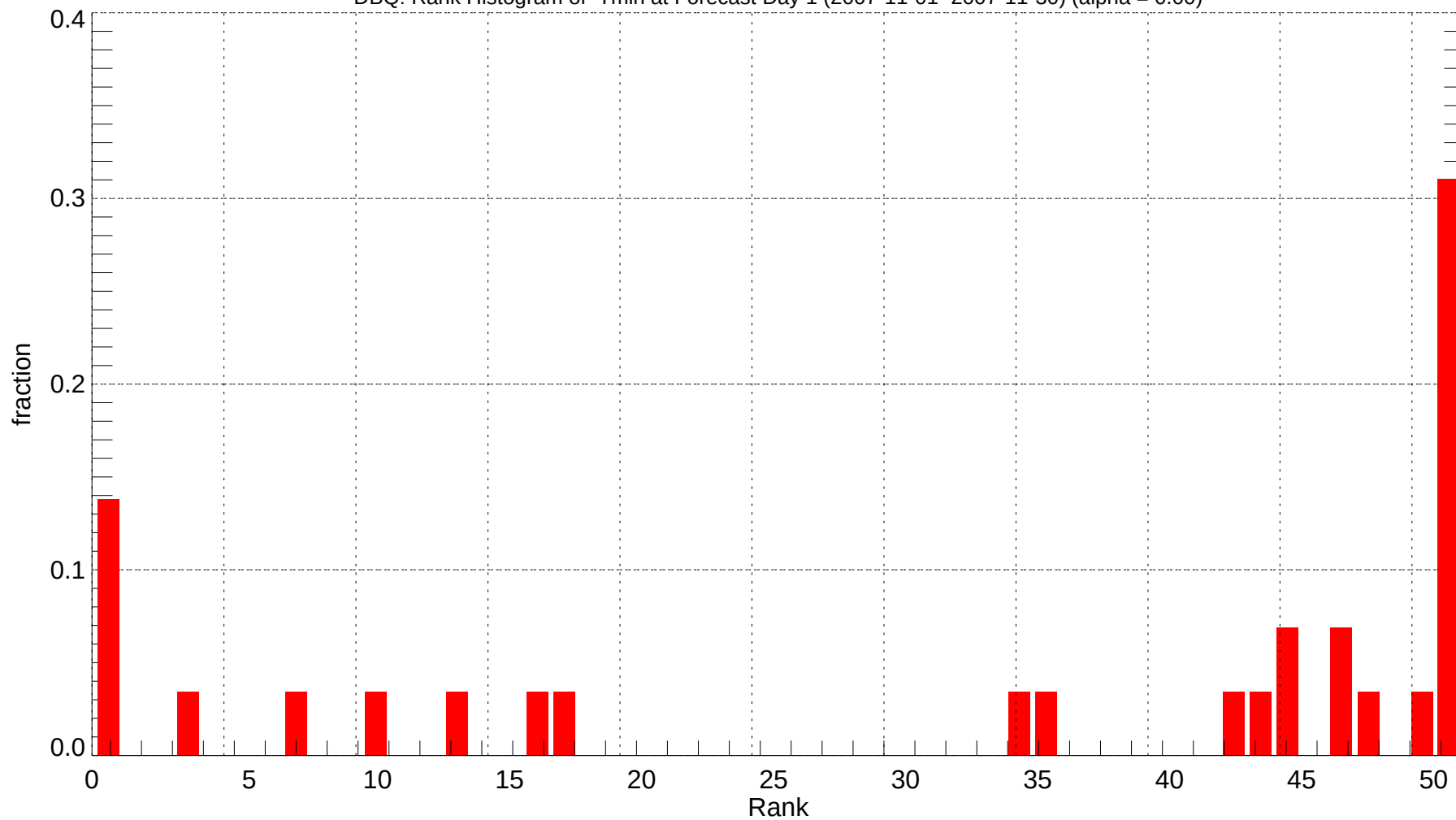
DBQ: Rank Histogram of Tmin at Forecast Day 1 (2007-11-01~2007-11-30) (alpha = 0.00)
