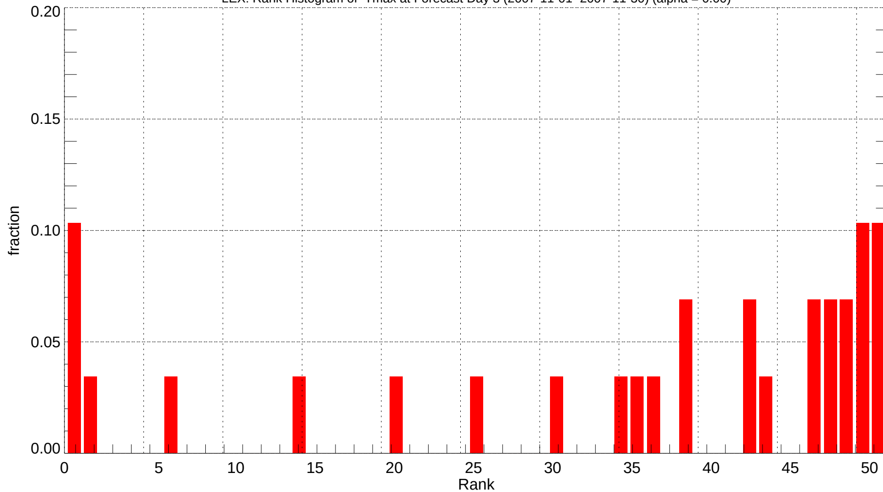
LEX: Rank Histogram of Tmax at Forecast Day 3 (2007-11-01~2007-11-30) (alpha = 0.00)
