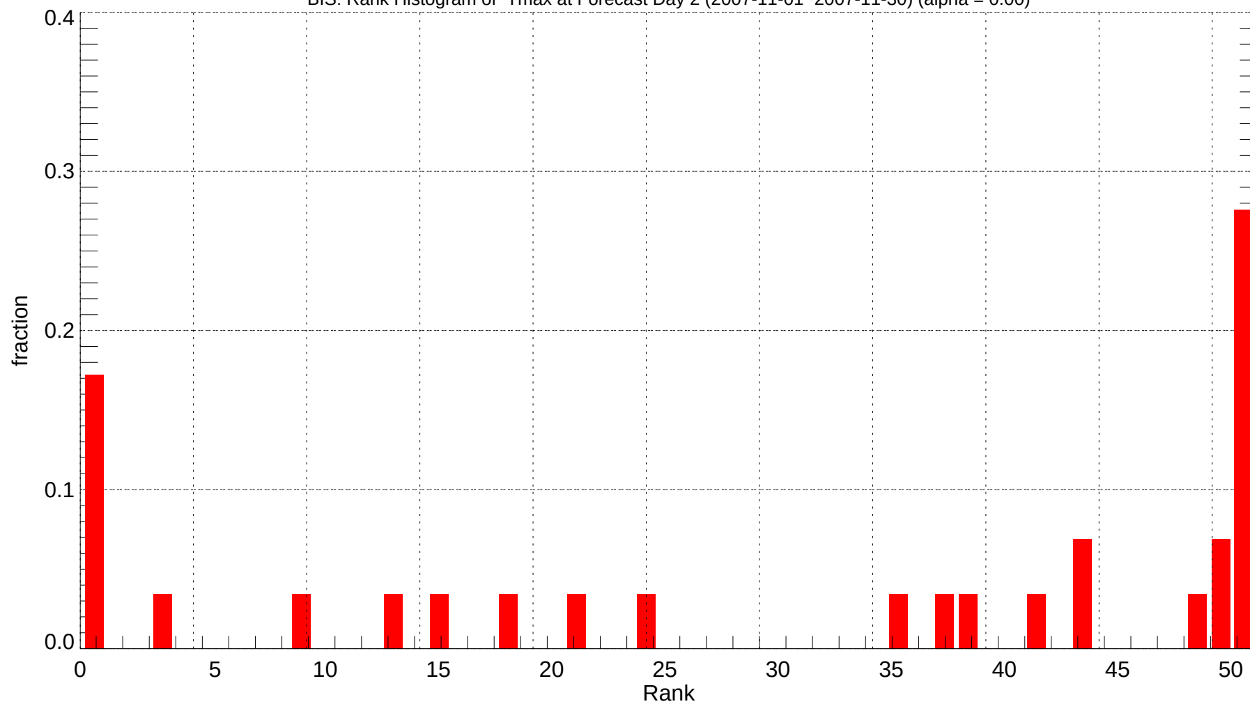
BIS: Rank Histogram of Tmax at Forecast Day 2 (2007-11-01~2007-11-30) (alpha = 0.00)
