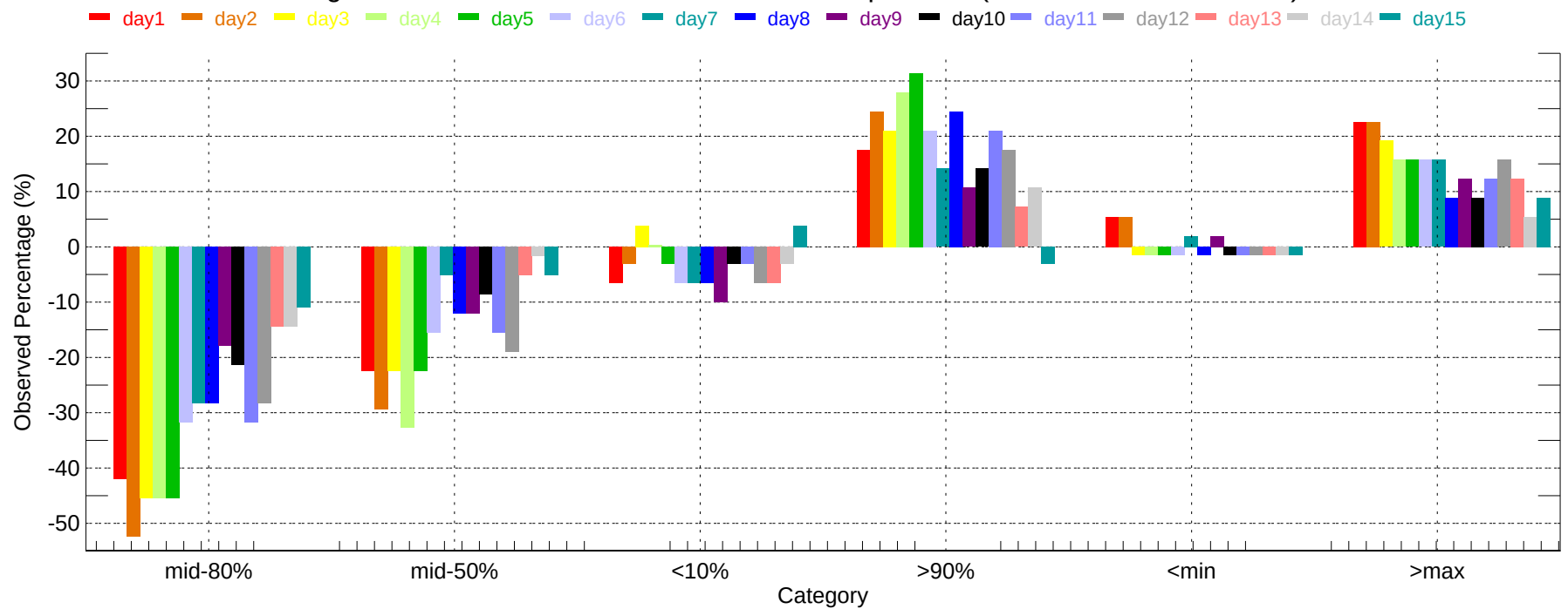
Observed Percentage Deviation of Ensembles - ROA: Min Temperature (2007-11-01~2007-11-30)
