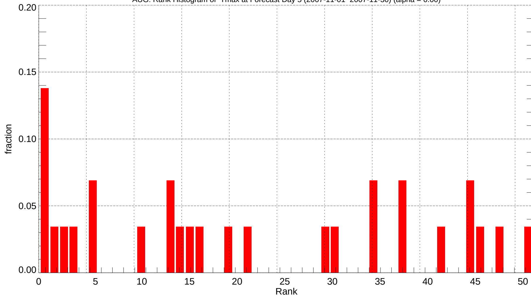
AUG: Rank Histogram of Tmax at Forecast Day 5 (2007-11-01~2007-11-30) (alpha = 0.00)
