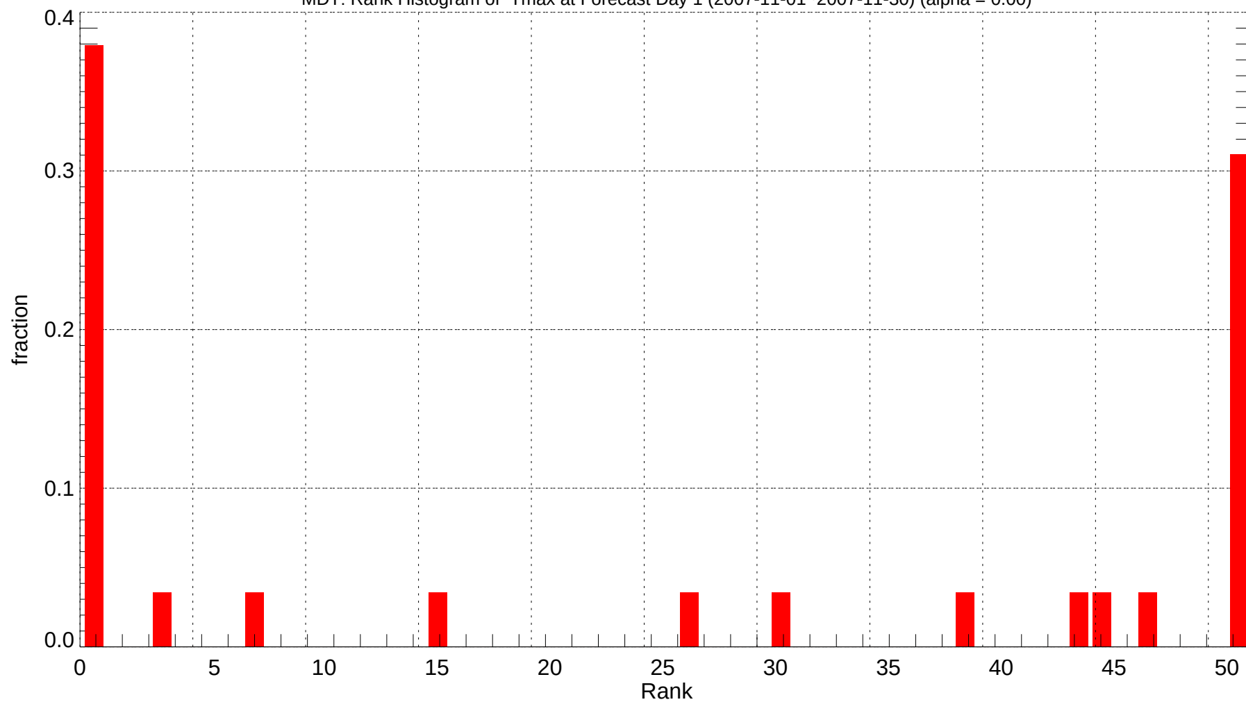
MDT: Rank Histogram of Tmax at Forecast Day 1 (2007-11-01~2007-11-30) (alpha = 0.00)
