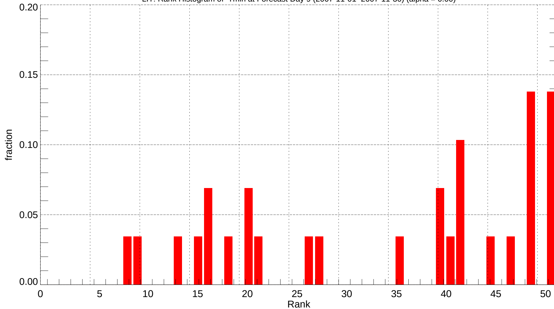
LIT: Rank Histogram of Tmin at Forecast Day 9 (2007-11-01~2007-11-30) (alpha = 0.00)
