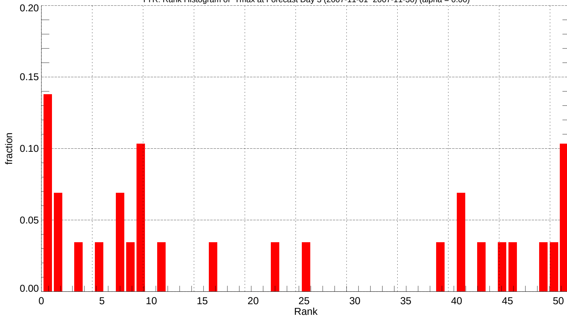
TYR: Rank Histogram of Tmax at Forecast Day 3 (2007-11-01~2007-11-30) (alpha = 0.00)
