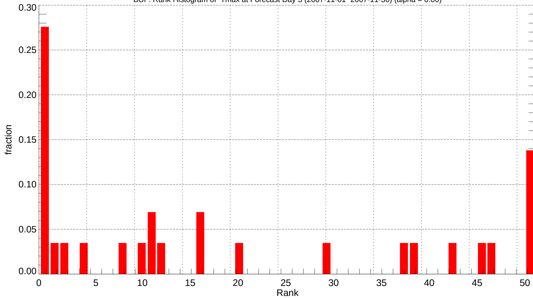
BUF: Rank Histogram of Tmax at Forecast Day 3 (2007-11-01~2007-11-30) (alpha = 0.00)
