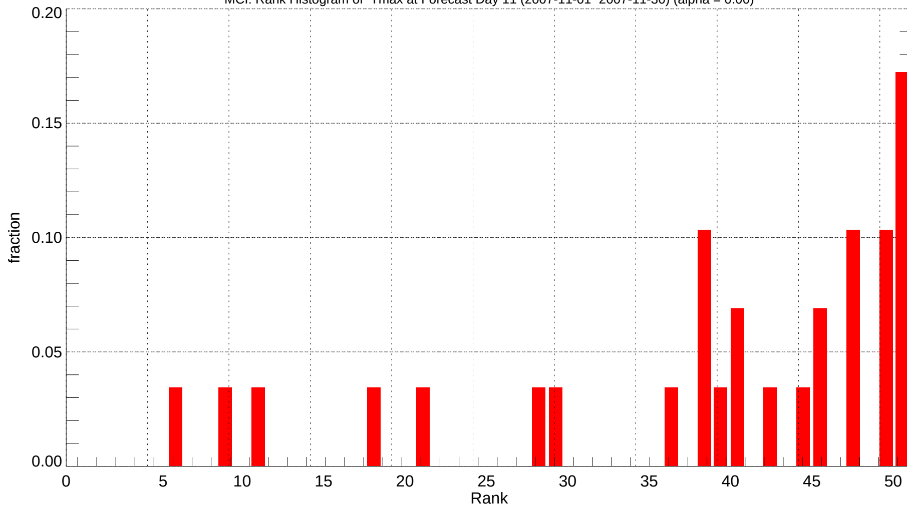
MCI: Rank Histogram of Tmax at Forecast Day 11 (2007-11-01~2007-11-30) (alpha = 0.00)
