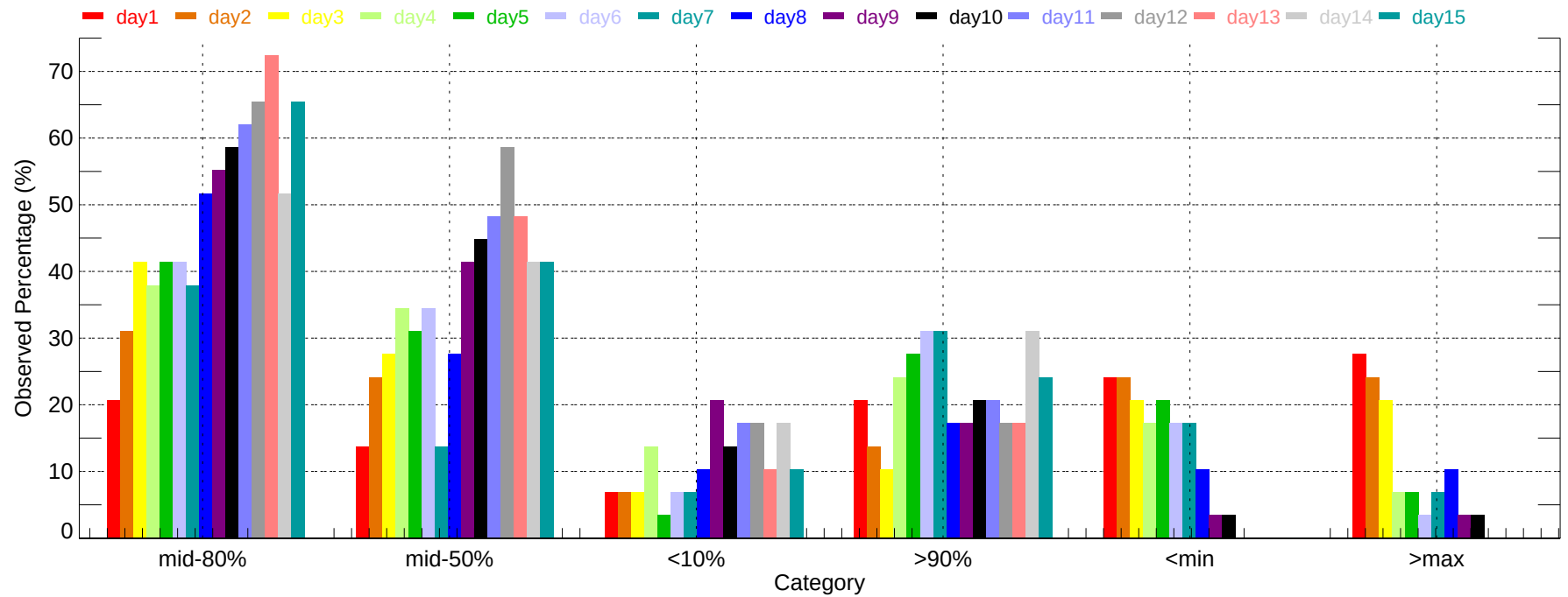
Observed Percentage of Ensembles - GTF: Max Temperature (2007-11-01~2007-11-30)
