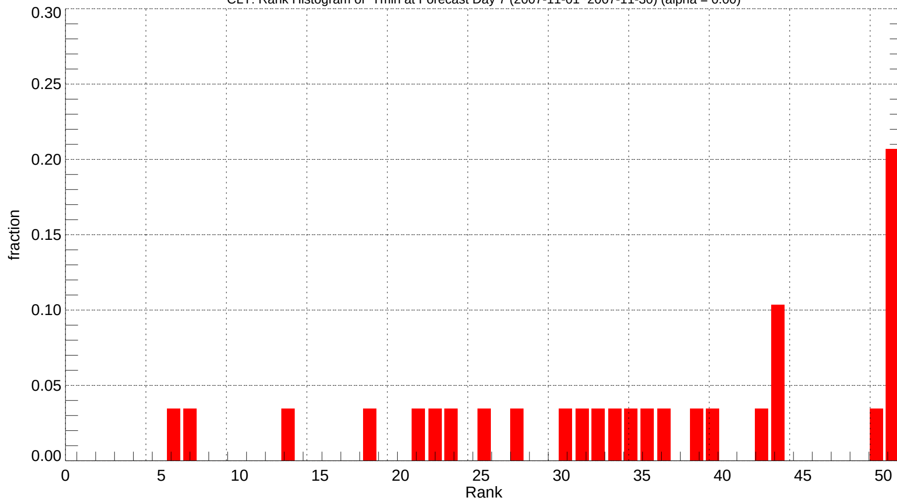
CLT: Rank Histogram of Tmin at Forecast Day 7 (2007-11-01~2007-11-30) (alpha = 0.00)
