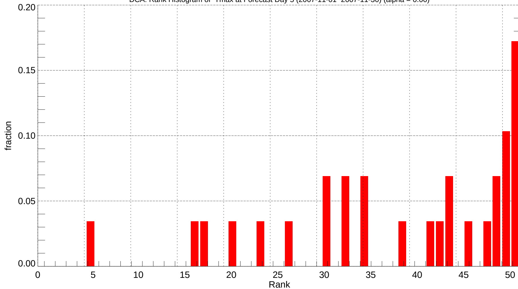
DCA: Rank Histogram of Tmax at Forecast Day 5 (2007-11-01~2007-11-30) (alpha = 0.00)
