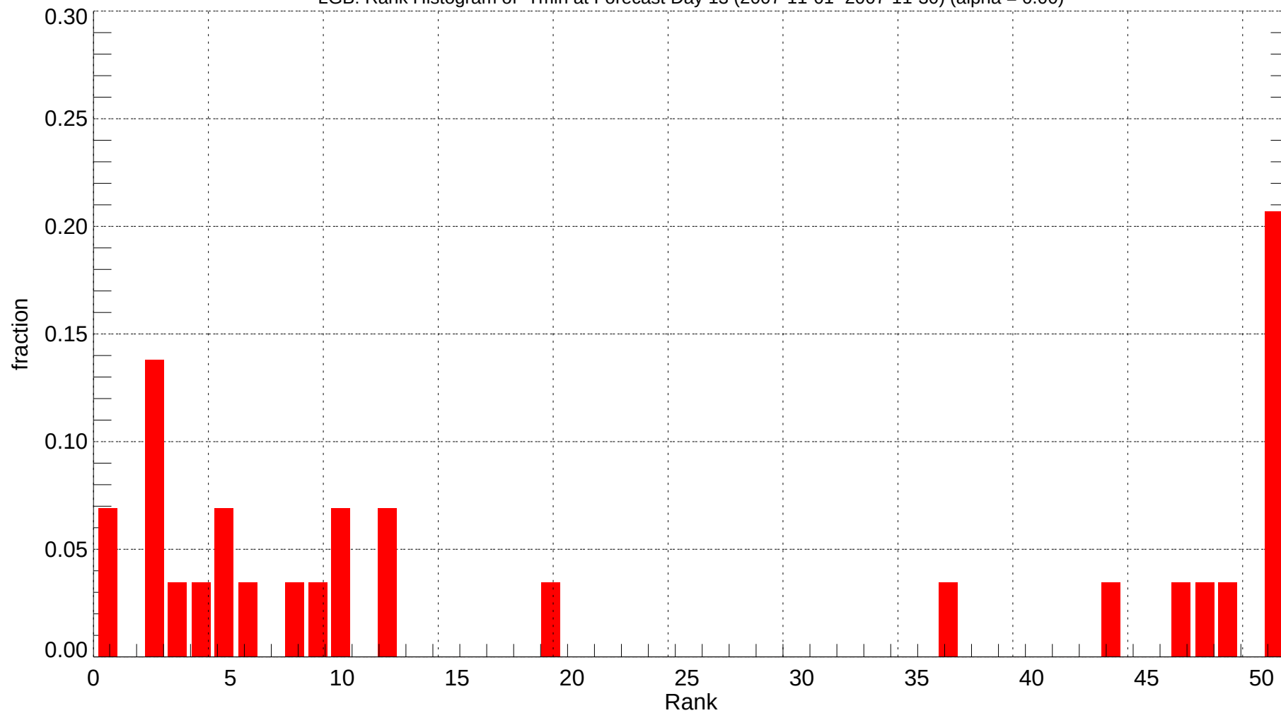
LGB: Rank Histogram of Tmin at Forecast Day 13 (2007-11-01~2007-11-30) (alpha = 0.00)
