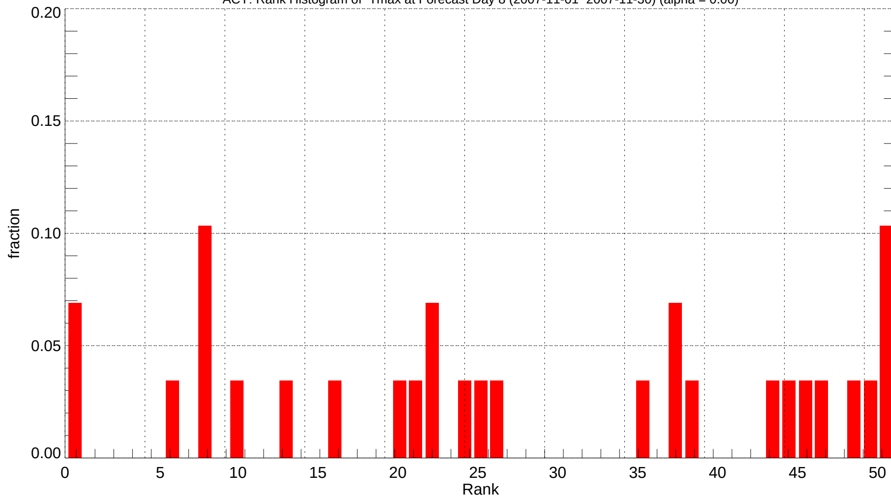
ACY: Rank Histogram of Tmax at Forecast Day 8 (2007-11-01~2007-11-30) (alpha = 0.00)
