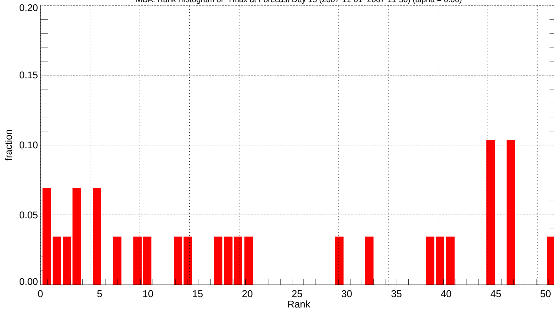
MBA: Rank Histogram of Tmax at Forecast Day 13 (2007-11-01~2007-11-30) (alpha = 0.00)
