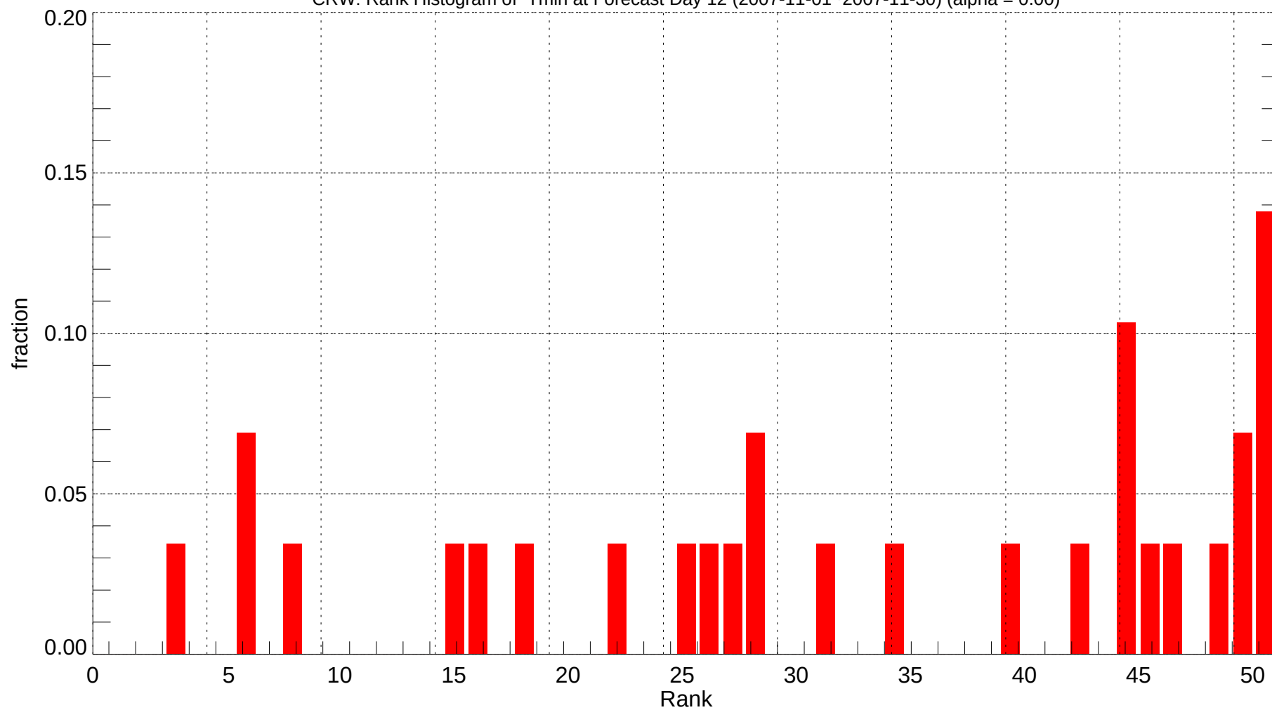
CRW: Rank Histogram of Tmin at Forecast Day 12 (2007-11-01~2007-11-30) (alpha = 0.00)
