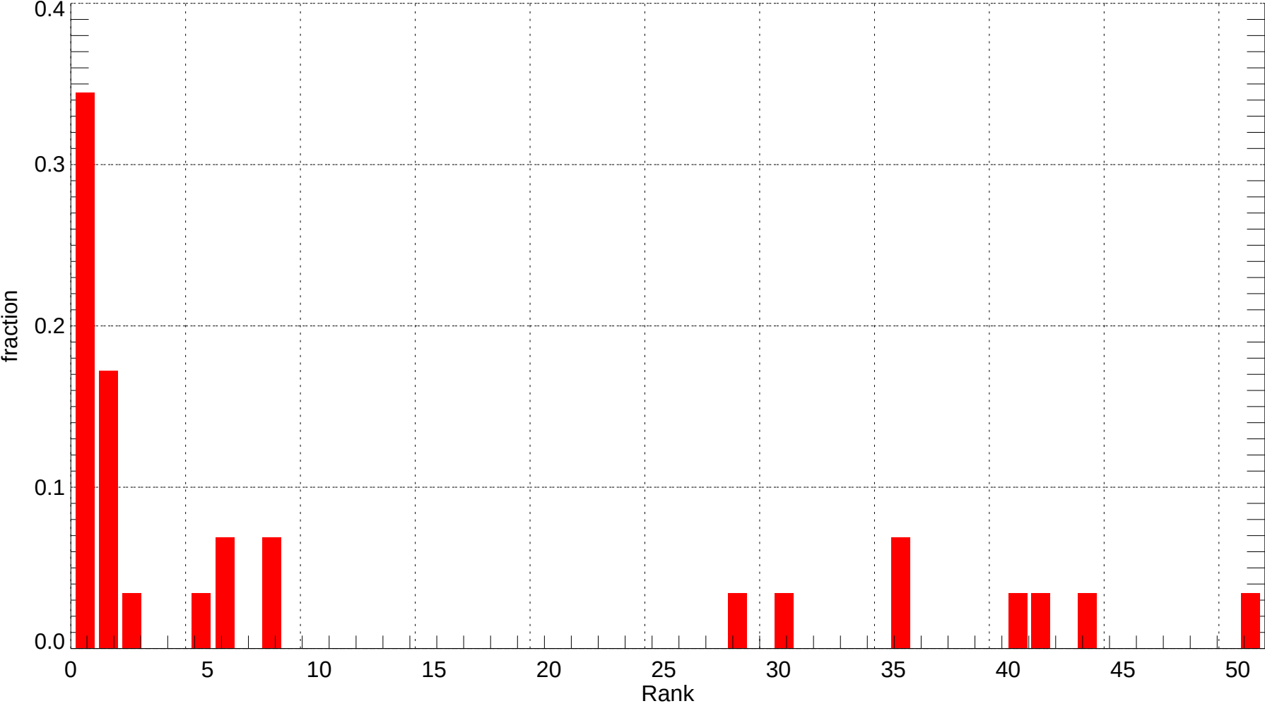
BFL: Rank Histogram of Tmin at Forecast Day 2 (2007-11-01~2007-11-30) (alpha = 0.00)
