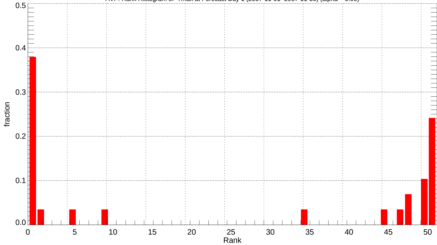
AVP: Rank Histogram of Tmax at Forecast Day 1 (2007-11-01~2007-11-30) (alpha = 0.00)
