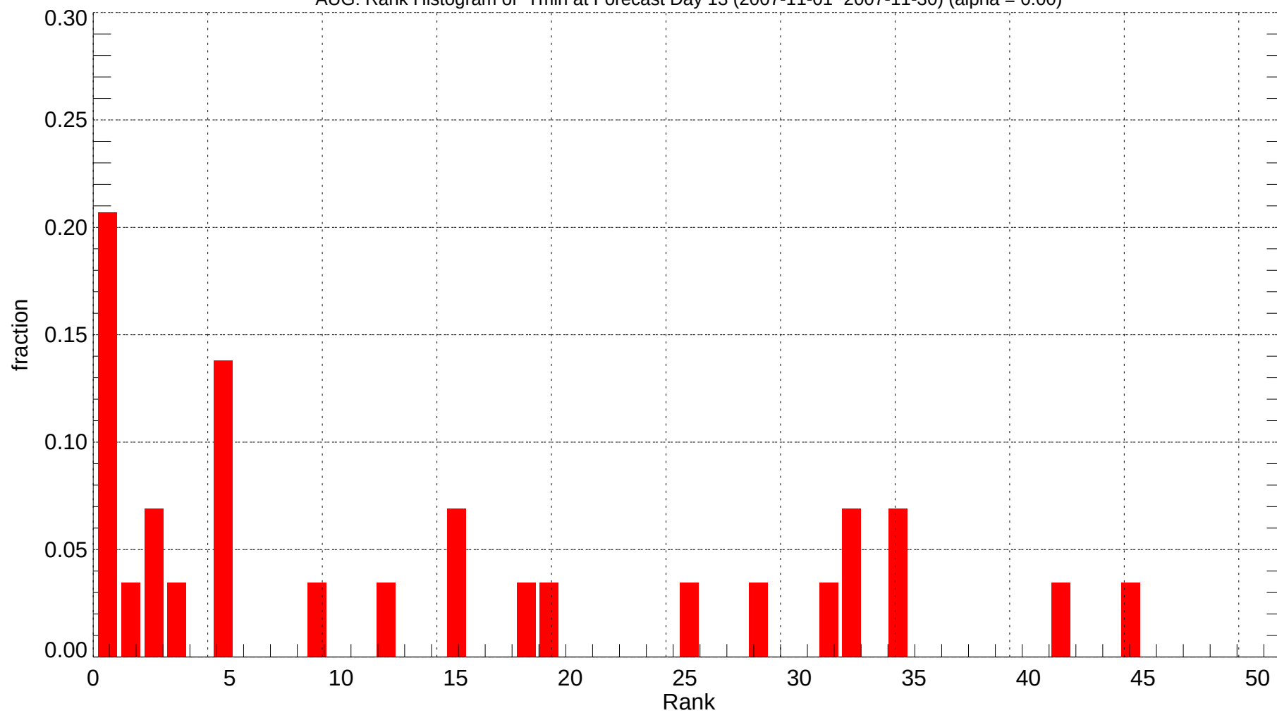
AUG: Rank Histogram of Tmin at Forecast Day 13 (2007-11-01~2007-11-30) (alpha = 0.00)
