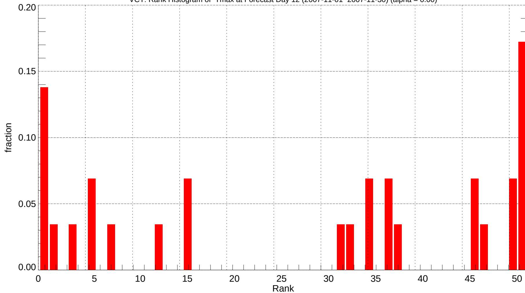
VCT: Rank Histogram of Tmax at Forecast Day 12 (2007-11-01~2007-11-30) (alpha = 0.00)
