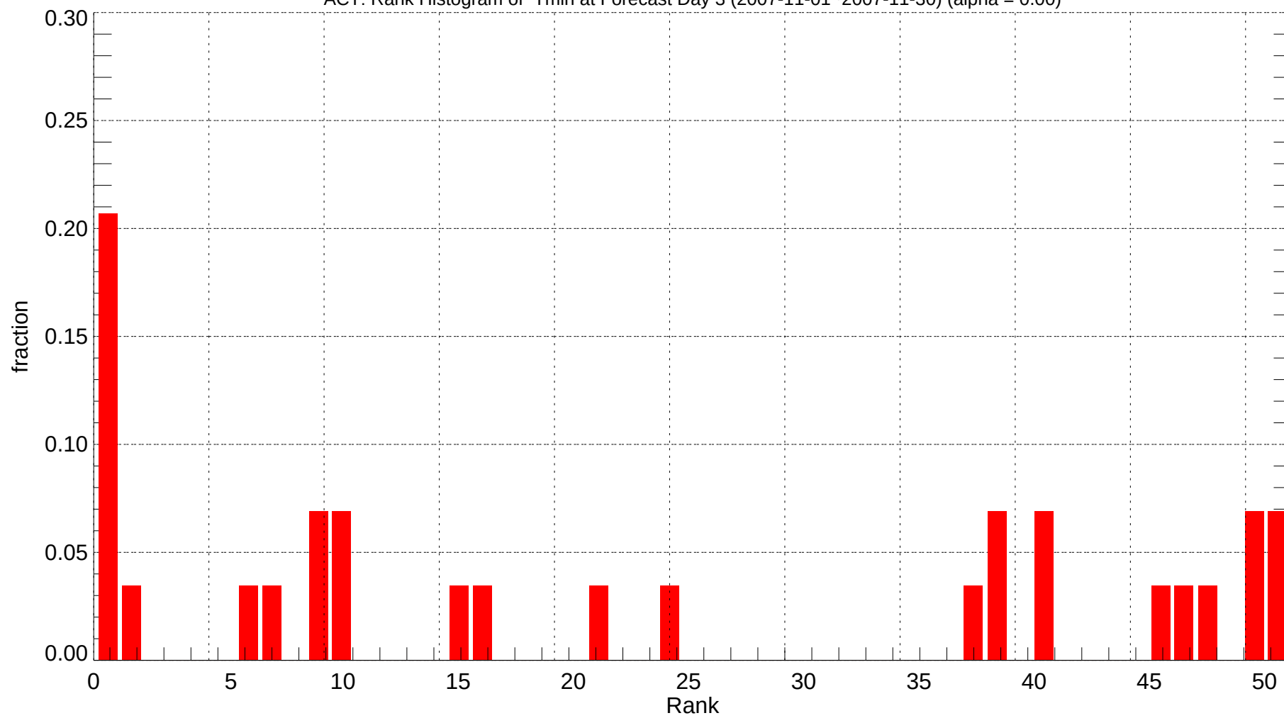
ACT: Rank Histogram of Tmin at Forecast Day 3 (2007-11-01~2007-11-30) (alpha = 0.00)
