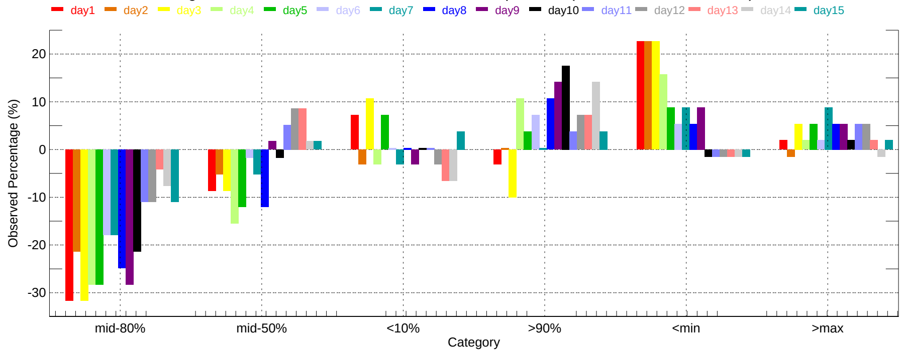
Observed Percentage Deviation of Ensembles - ORD: Max Temperature (2007-11-01~2007-11-30)
