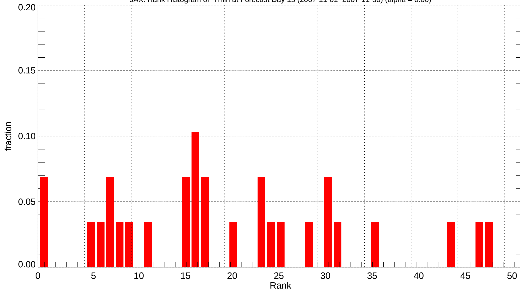
JAX: Rank Histogram of Tmin at Forecast Day 15 (2007-11-01~2007-11-30) (alpha = 0.00)
