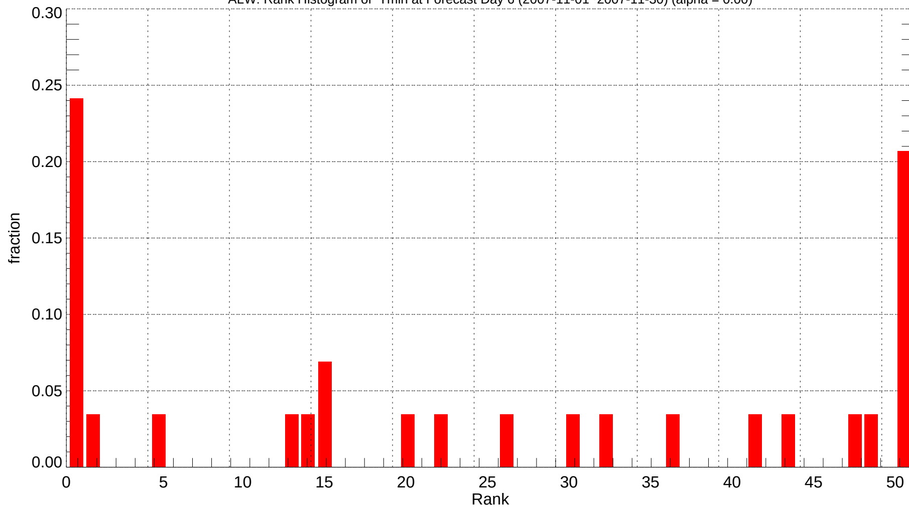
ALW: Rank Histogram of Tmin at Forecast Day 6 (2007-11-01~2007-11-30) (alpha = 0.00)
