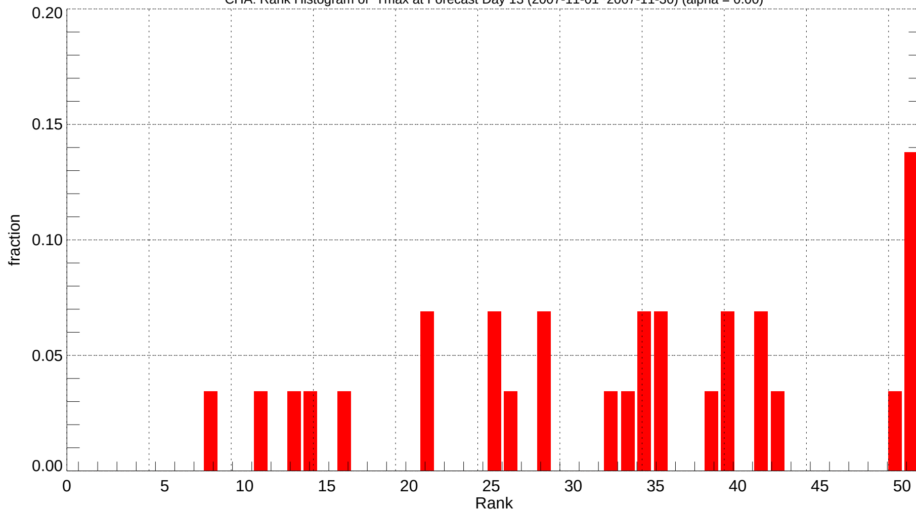
CHA: Rank Histogram of Tmax at Forecast Day 13 (2007-11-01~2007-11-30) (alpha = 0.00)
