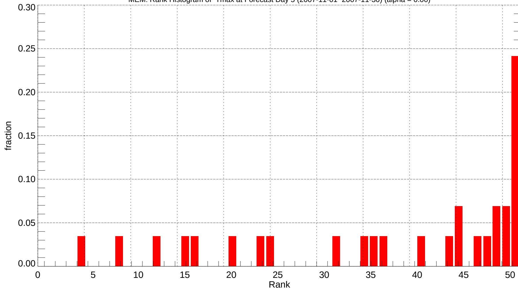
MEM: Rank Histogram of Tmax at Forecast Day 5 (2007-11-01~2007-11-30) (alpha = 0.00)
