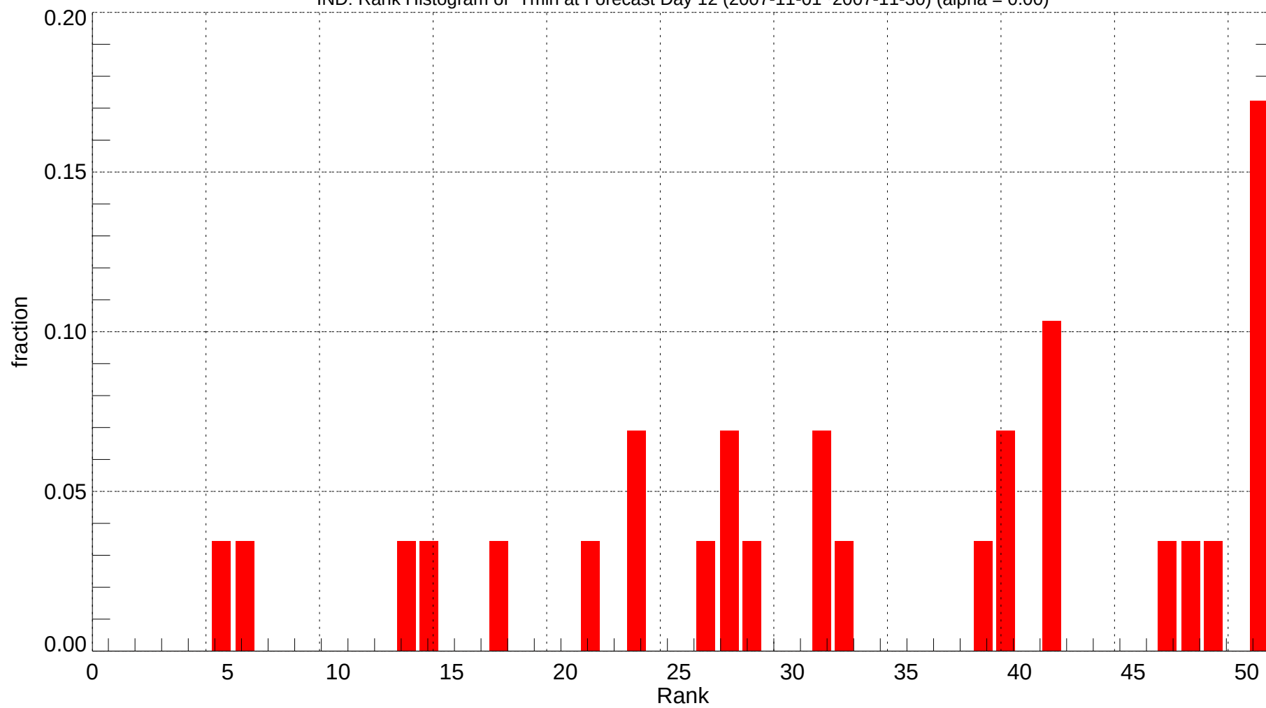
IND: Rank Histogram of Tmin at Forecast Day 12 (2007-11-01~2007-11-30) (alpha = 0.00)
