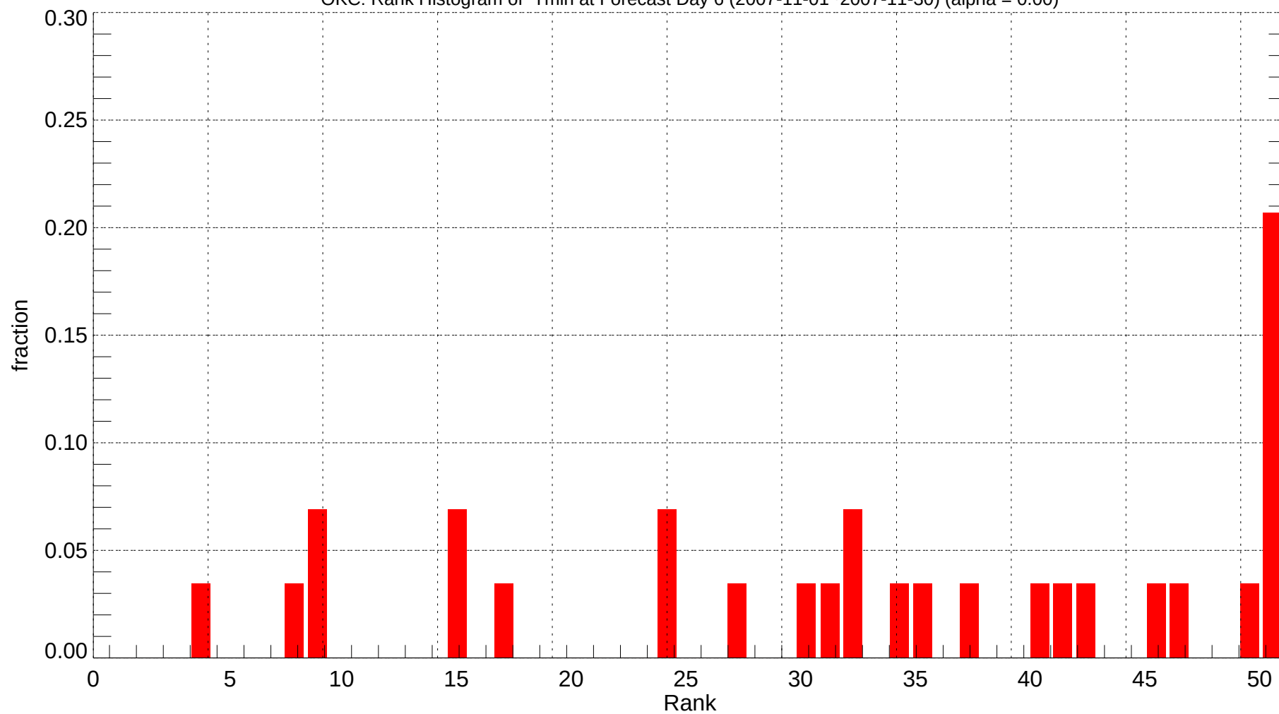
OKC: Rank Histogram of Tmin at Forecast Day 6 (2007-11-01~2007-11-30) (alpha = 0.00)
