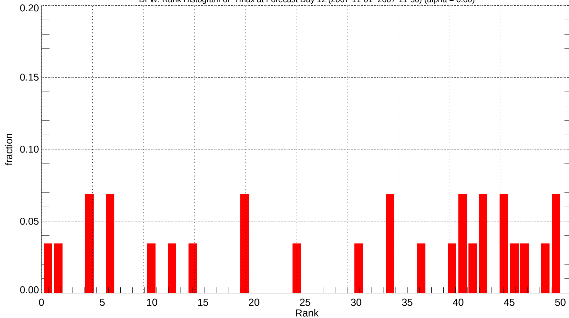
DFW: Rank Histogram of Tmax at Forecast Day 12 (2007-11-01~2007-11-30) (alpha = 0.00)
