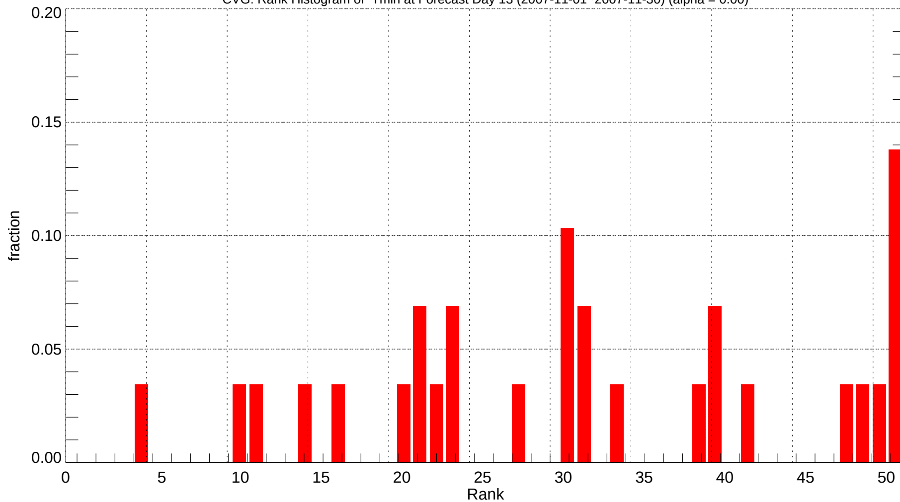
CVG: Rank Histogram of Tmin at Forecast Day 13 (2007-11-01~2007-11-30) (alpha = 0.00)
