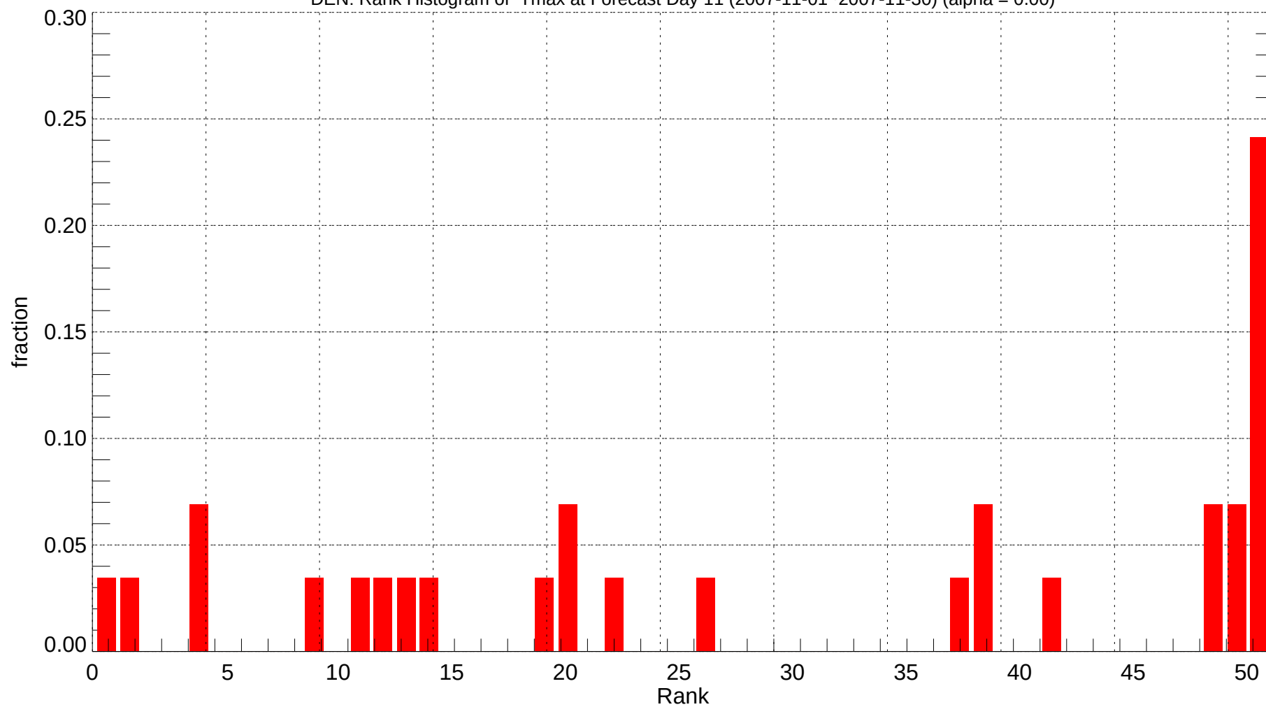
DEN: Rank Histogram of Tmax at Forecast Day 11 (2007-11-01~2007-11-30) (alpha = 0.00)
