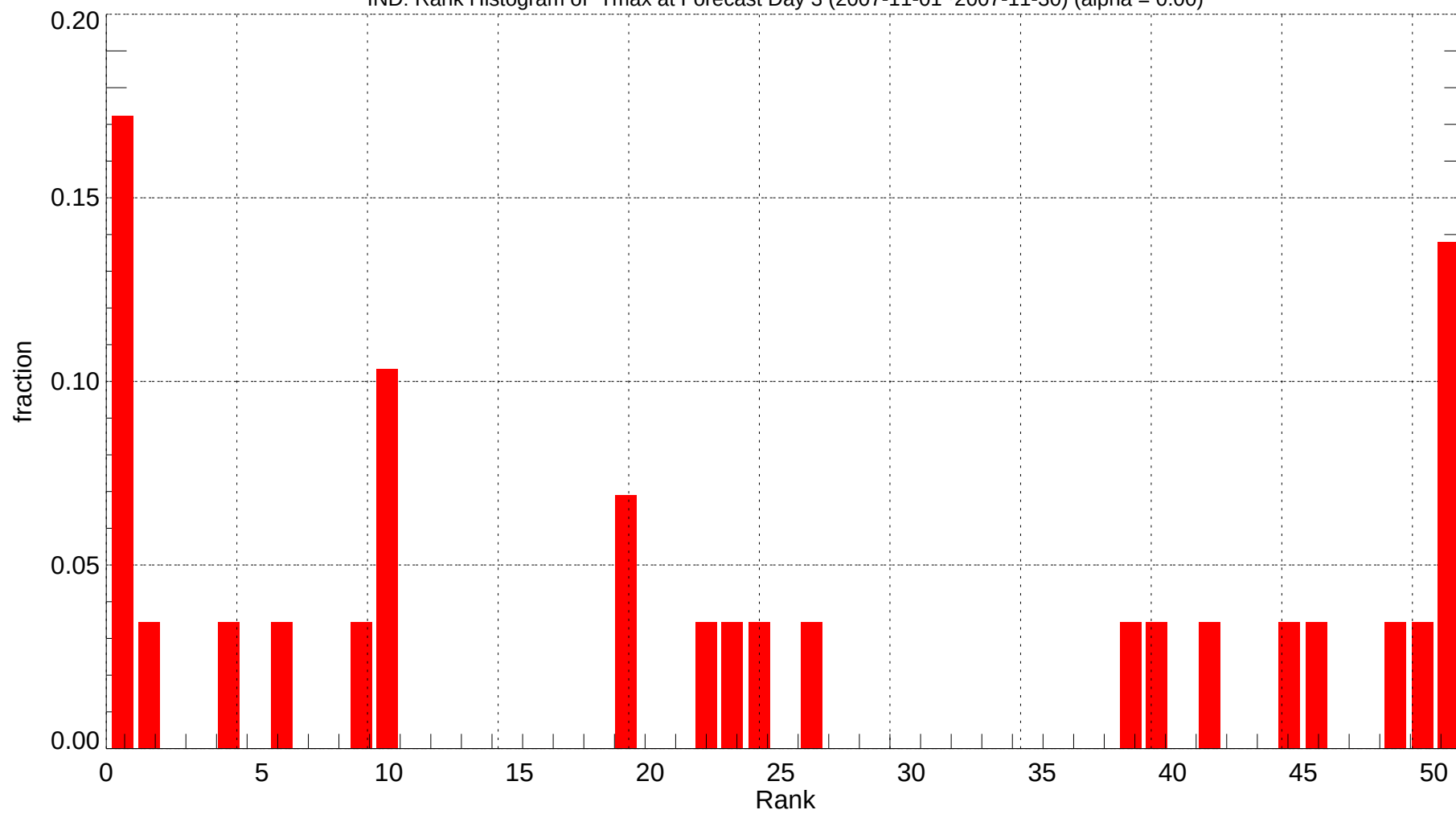
IND: Rank Histogram of Tmax at Forecast Day 3 (2007-11-01~2007-11-30) (alpha = 0.00)
