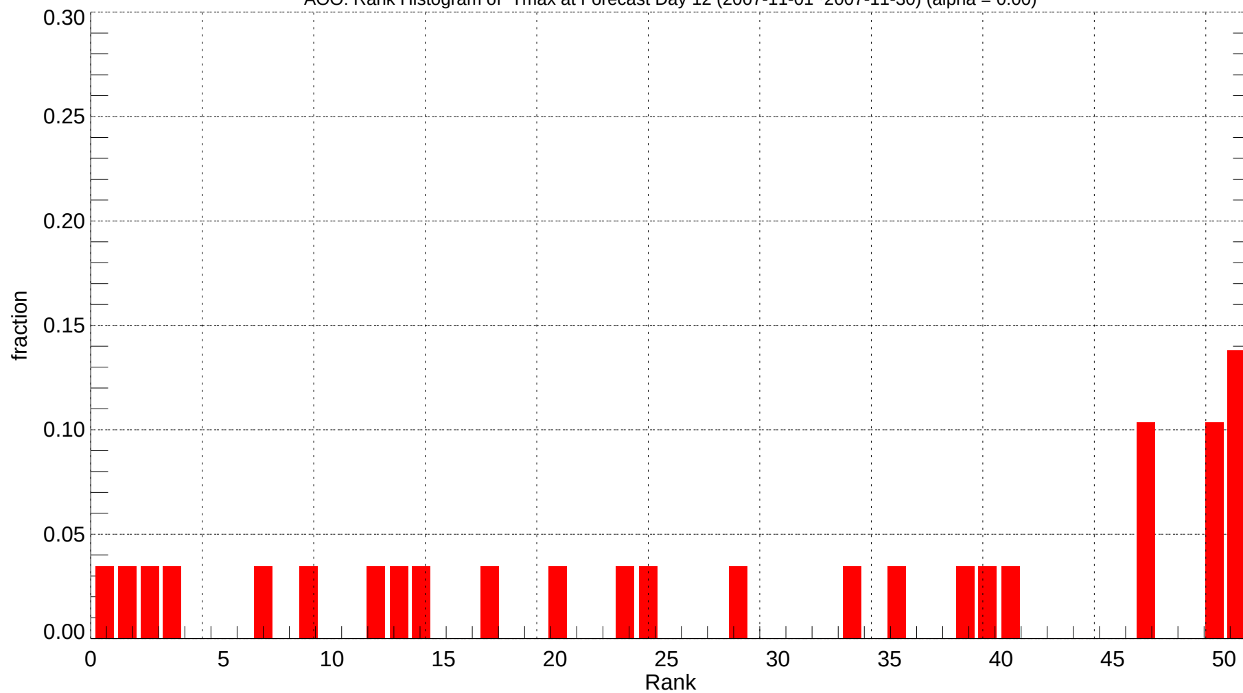
AOO: Rank Histogram of Tmax at Forecast Day 12 (2007-11-01~2007-11-30) (alpha = 0.00)
