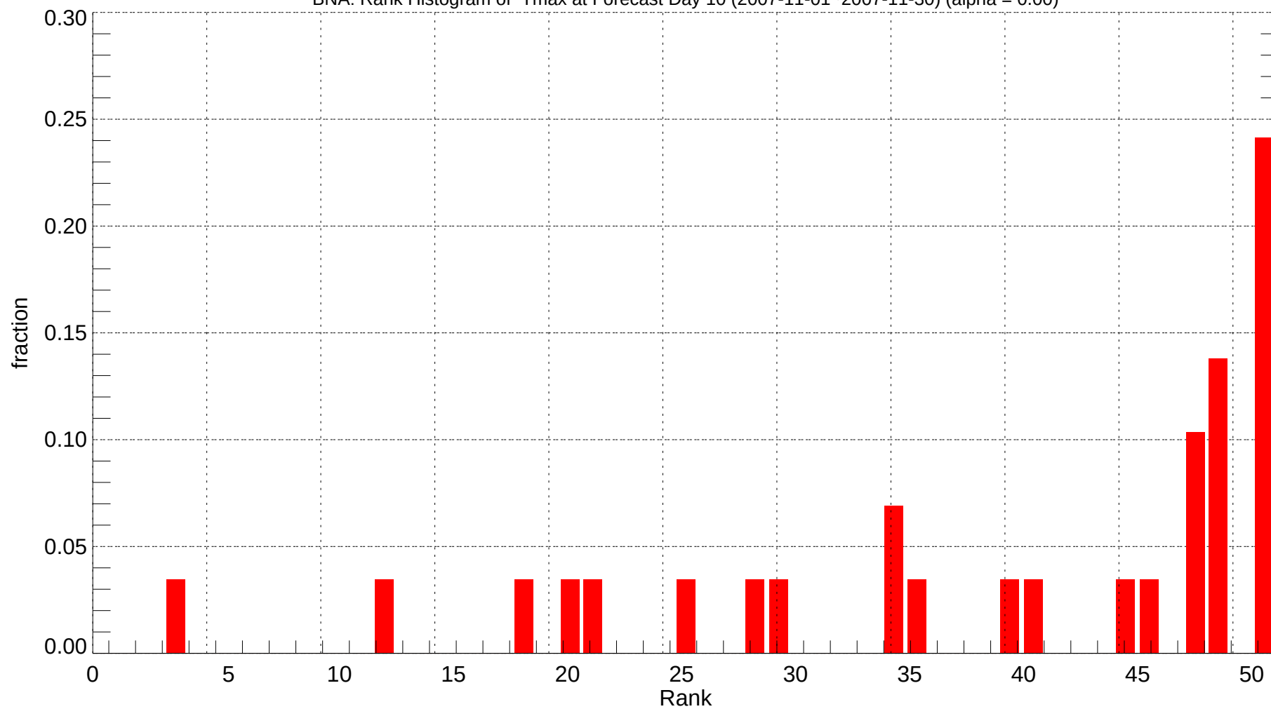
BNA: Rank Histogram of Tmax at Forecast Day 10 (2007-11-01~2007-11-30) (alpha = 0.00)
