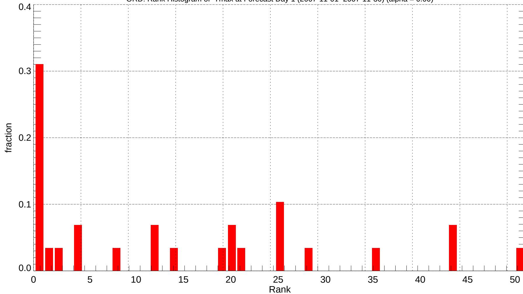
ORD: Rank Histogram of Tmax at Forecast Day 1 (2007-11-01~2007-11-30) (alpha = 0.00)
