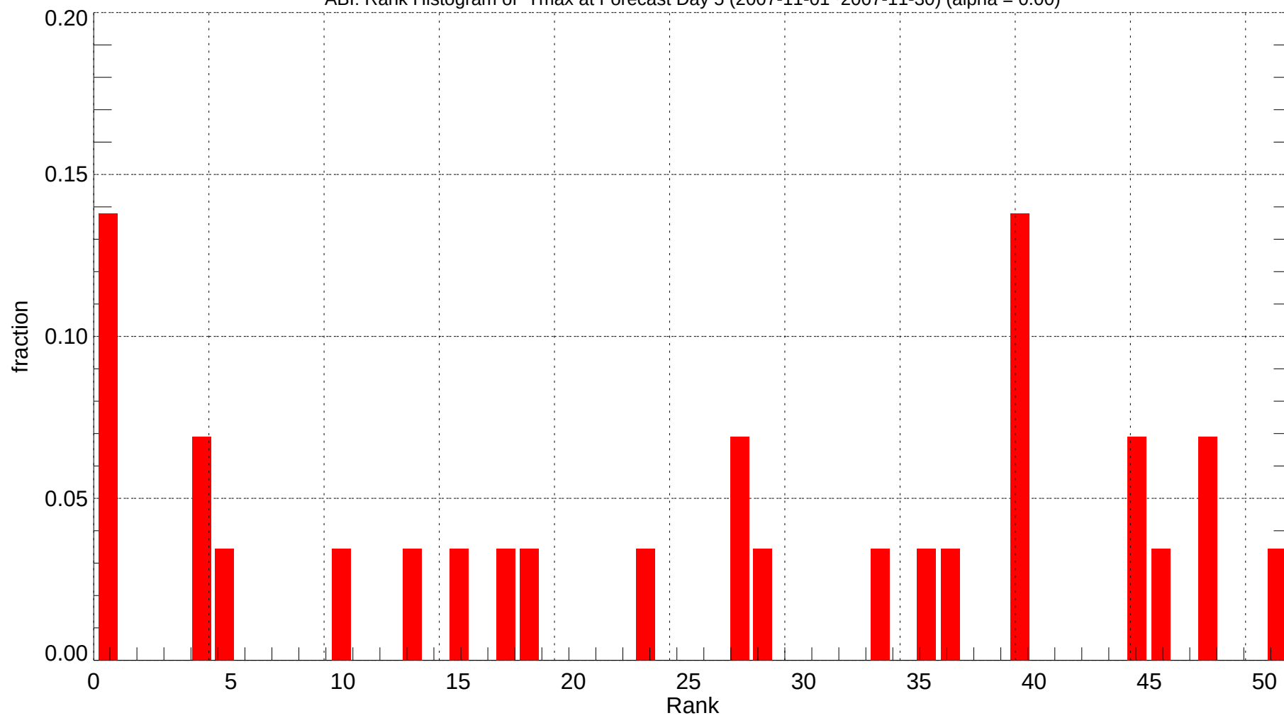
ABI: Rank Histogram of Tmax at Forecast Day 5 (2007-11-01~2007-11-30) (alpha = 0.00)
