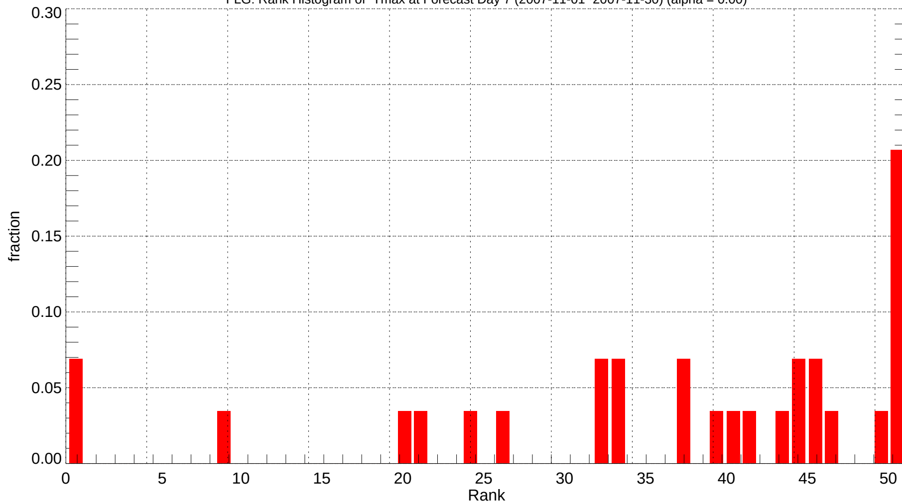
FLG: Rank Histogram of Tmax at Forecast Day 7 (2007-11-01~2007-11-30) (alpha = 0.00)
