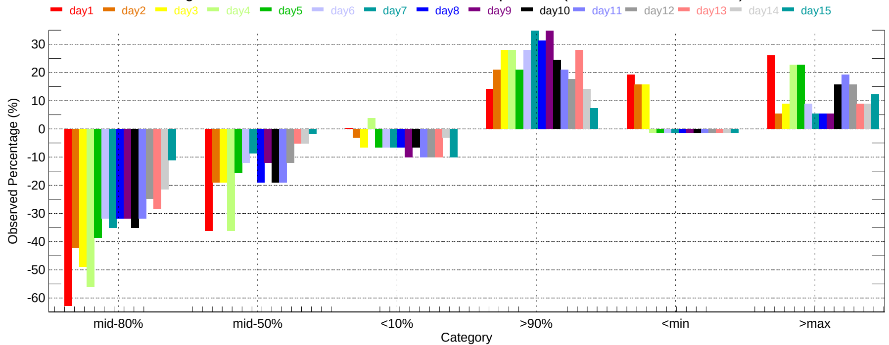
Observed Percentage Deviation of Ensembles - MEM: Max Temperature (2007-11-01~2007-11-30)
