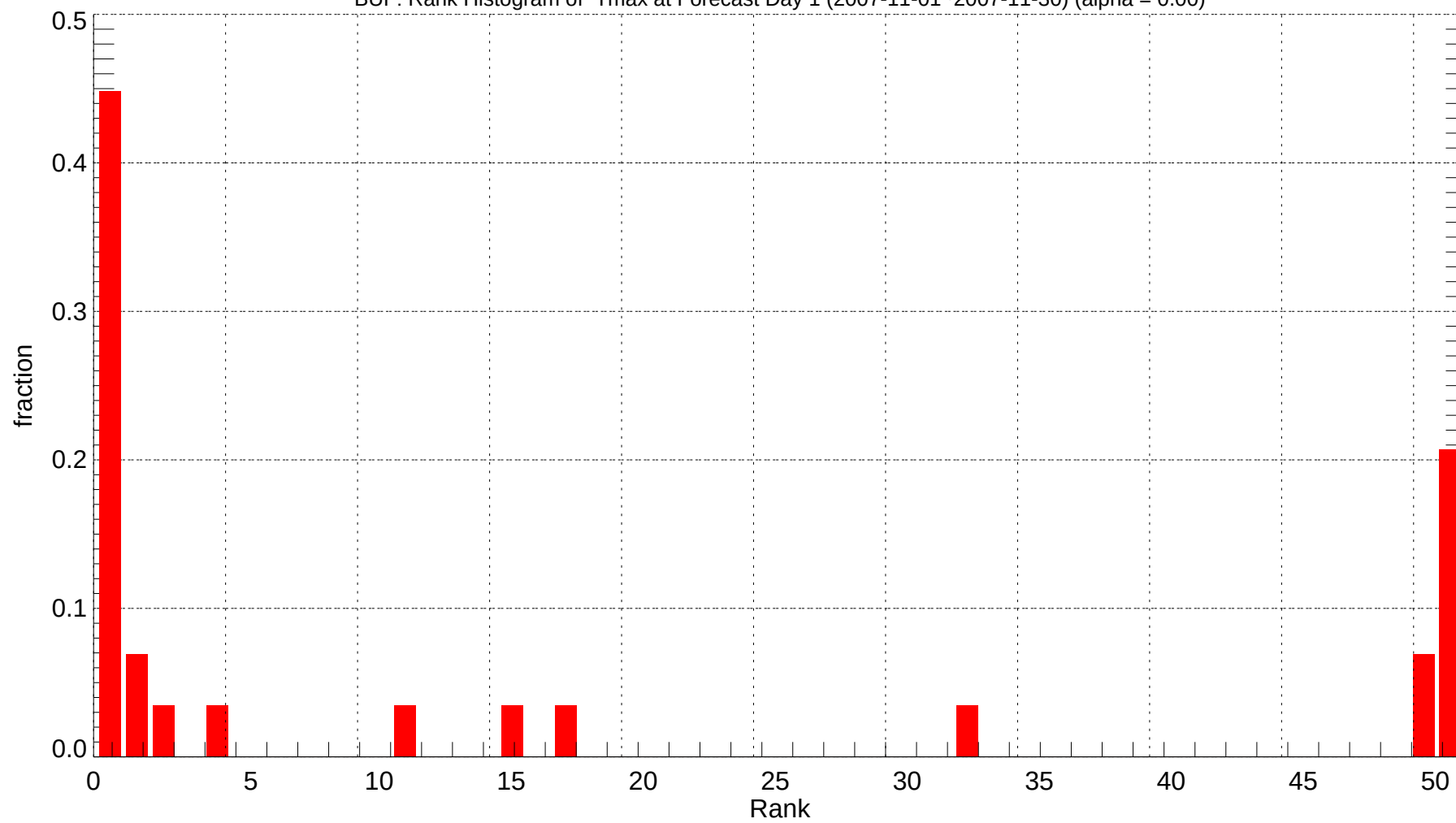
BUF: Rank Histogram of Tmax at Forecast Day 1 (2007-11-01~2007-11-30) (alpha = 0.00)
