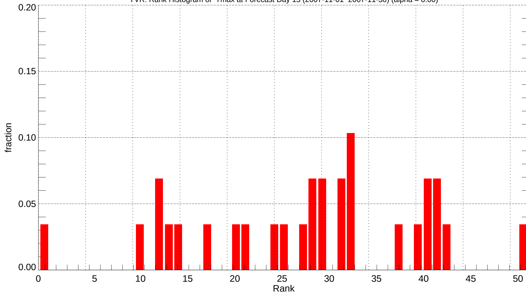
YVR: Rank Histogram of Tmax at Forecast Day 15 (2007-11-01~2007-11-30) (alpha = 0.00)
