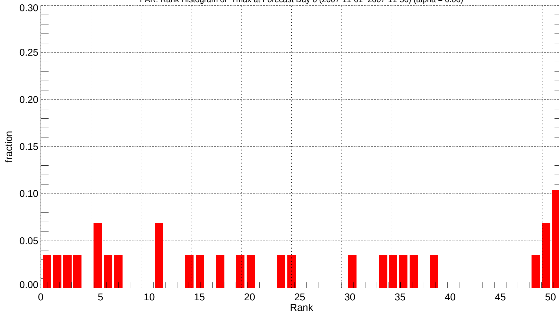
FAR: Rank Histogram of Tmax at Forecast Day 6 (2007-11-01~2007-11-30) (alpha = 0.00)
