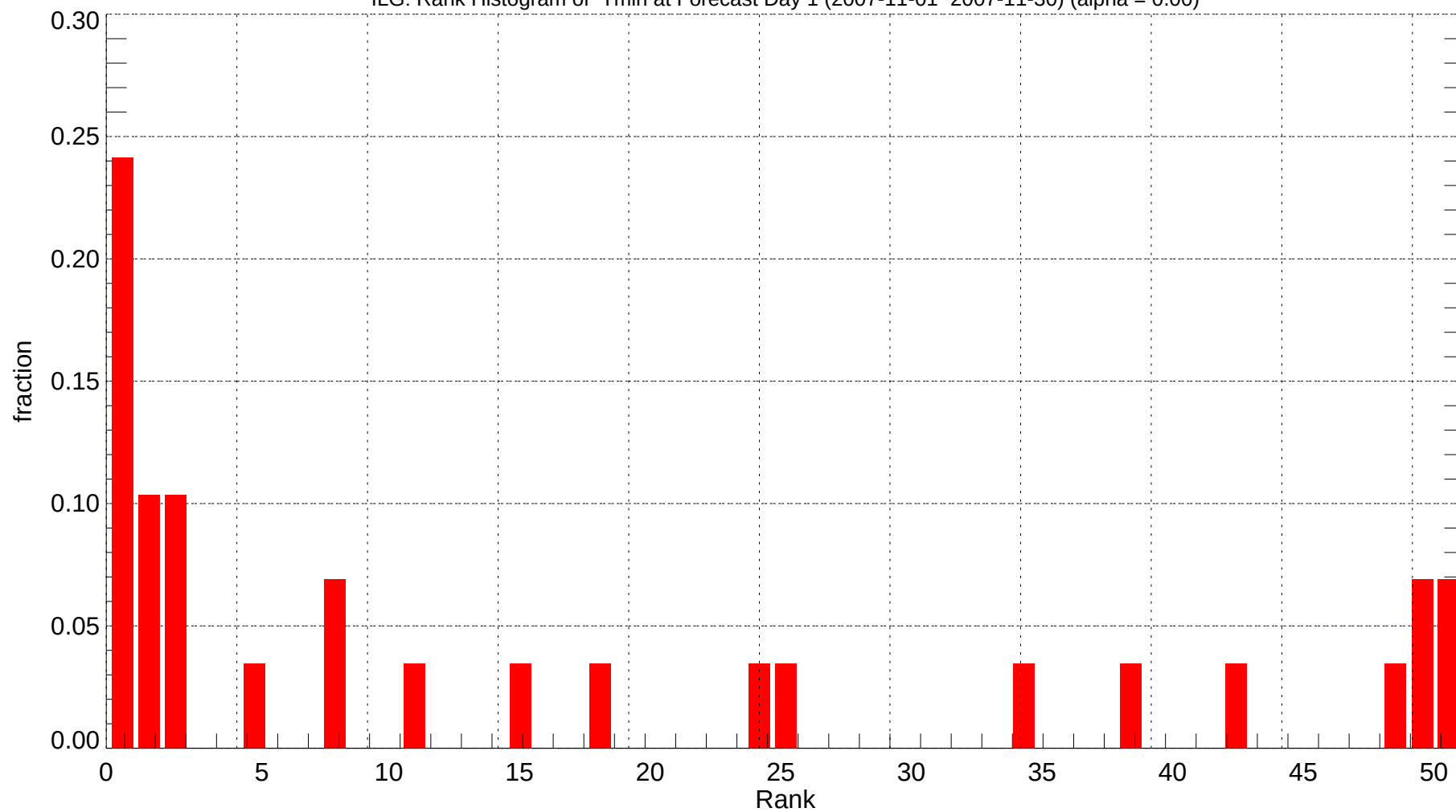
ILG: Rank Histogram of Tmin at Forecast Day 1 (2007-11-01~2007-11-30) (alpha = 0.00)
