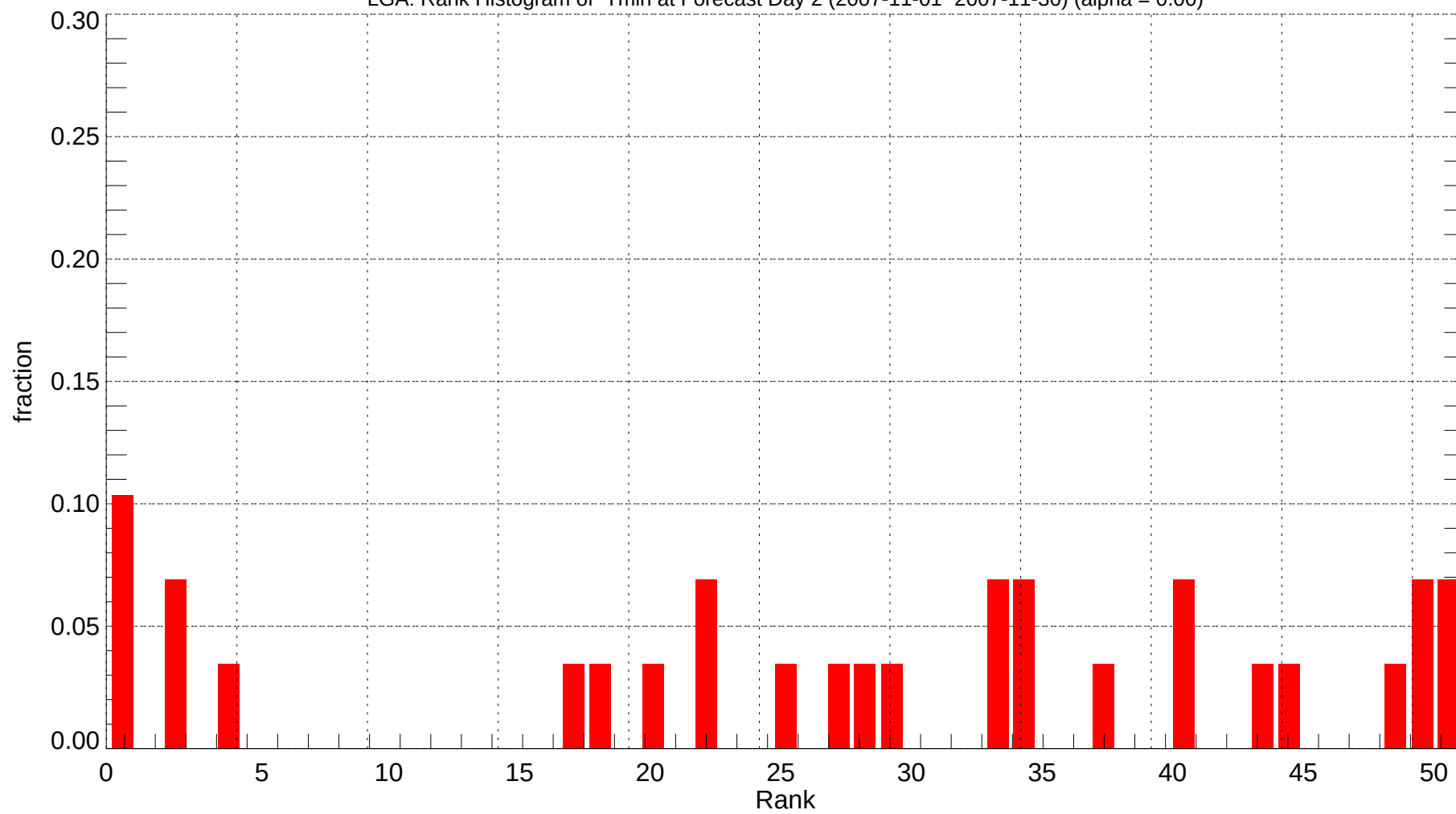
LGA: Rank Histogram of Tmin at Forecast Day 2 (2007-11-01~2007-11-30) (alpha = 0.00)
