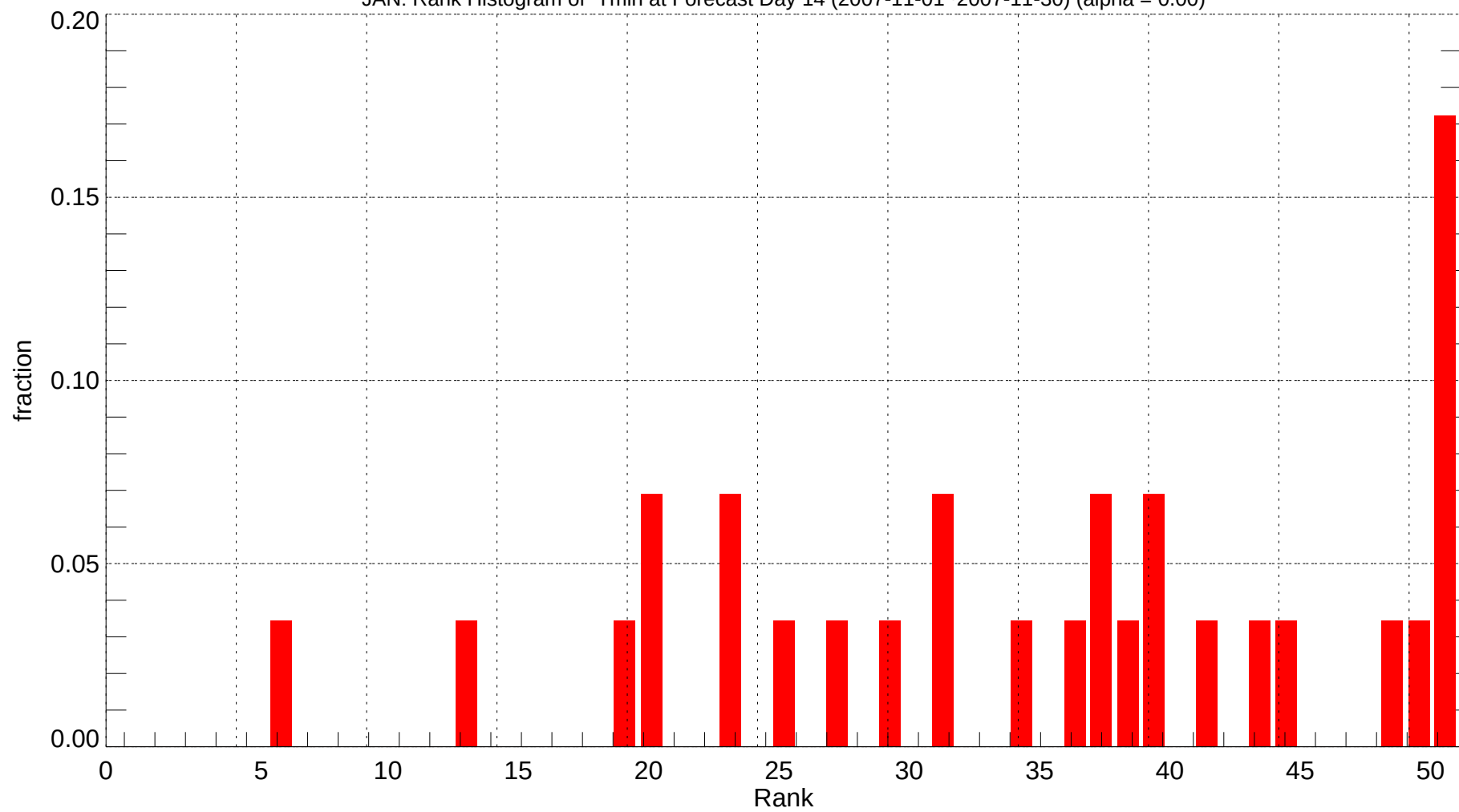
JAN: Rank Histogram of Tmin at Forecast Day 14 (2007-11-01~2007-11-30) (alpha = 0.00)
