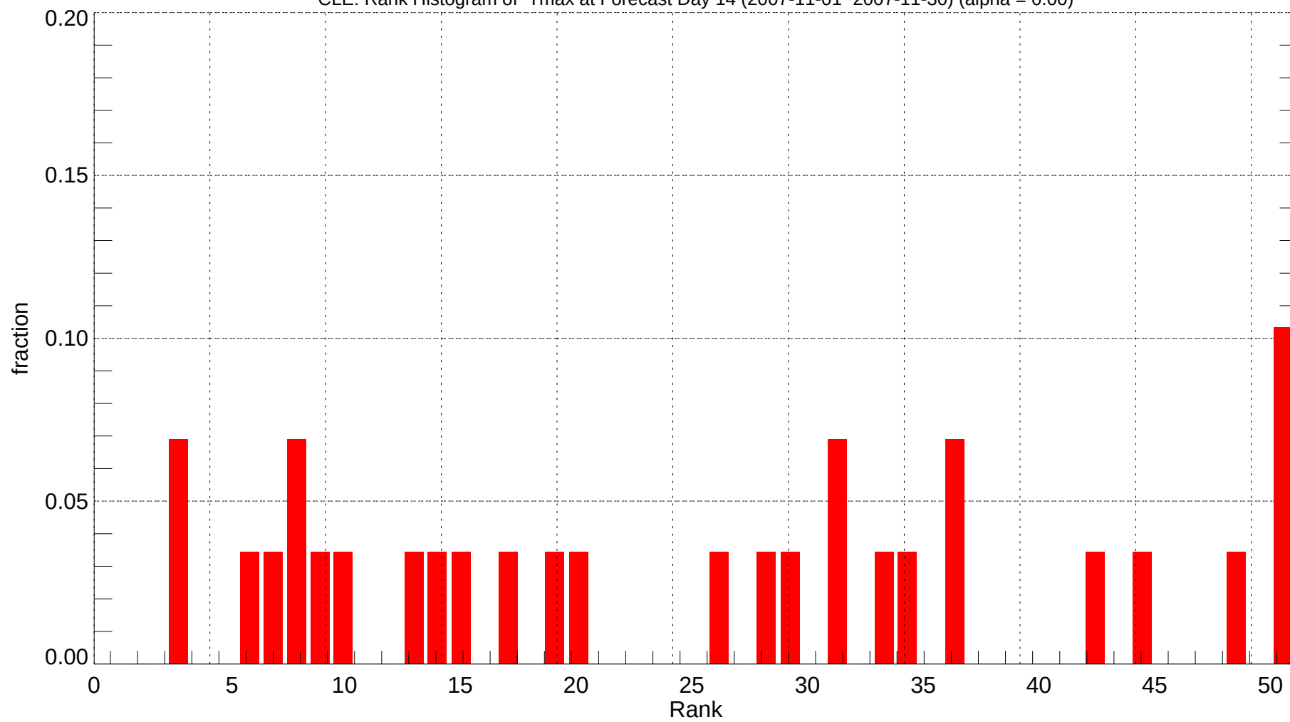
CLE: Rank Histogram of Tmax at Forecast Day 14 (2007-11-01~2007-11-30) (alpha = 0.00)
