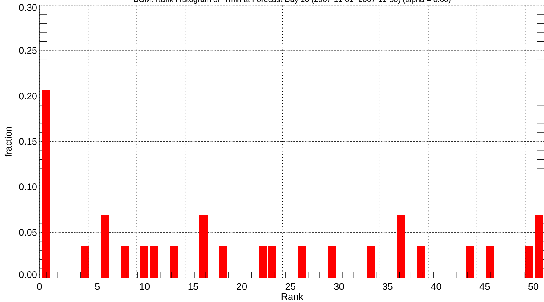
BGM: Rank Histogram of Tmin at Forecast Day 10 (2007-11-01~2007-11-30) (alpha = 0.00)
