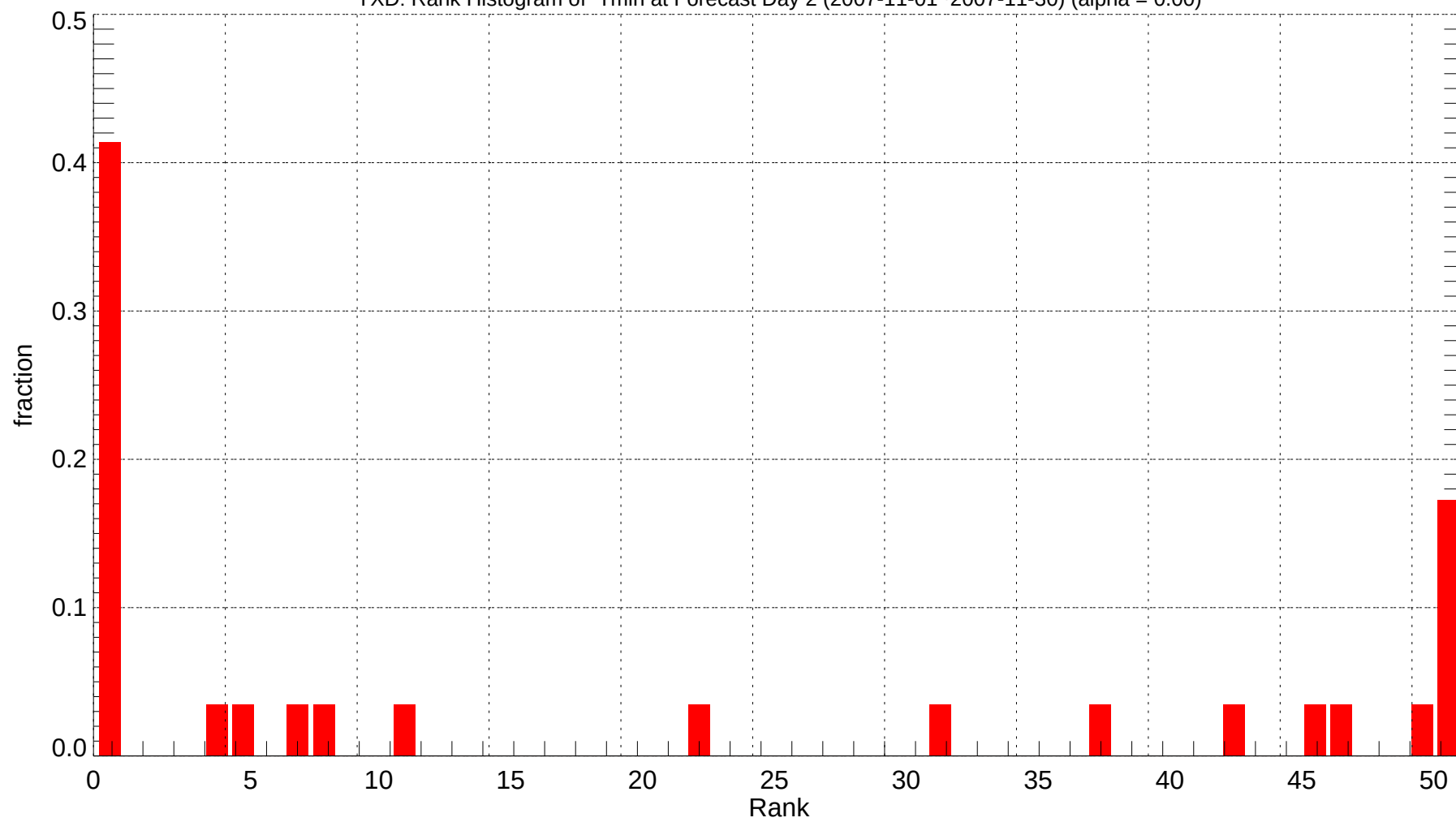
YXD: Rank Histogram of Tmin at Forecast Day 2 (2007-11-01~2007-11-30) (alpha = 0.00)
