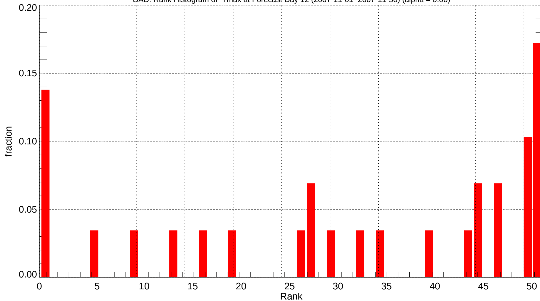
GAD: Rank Histogram of Tmax at Forecast Day 12 (2007-11-01~2007-11-30) (alpha = 0.00)
