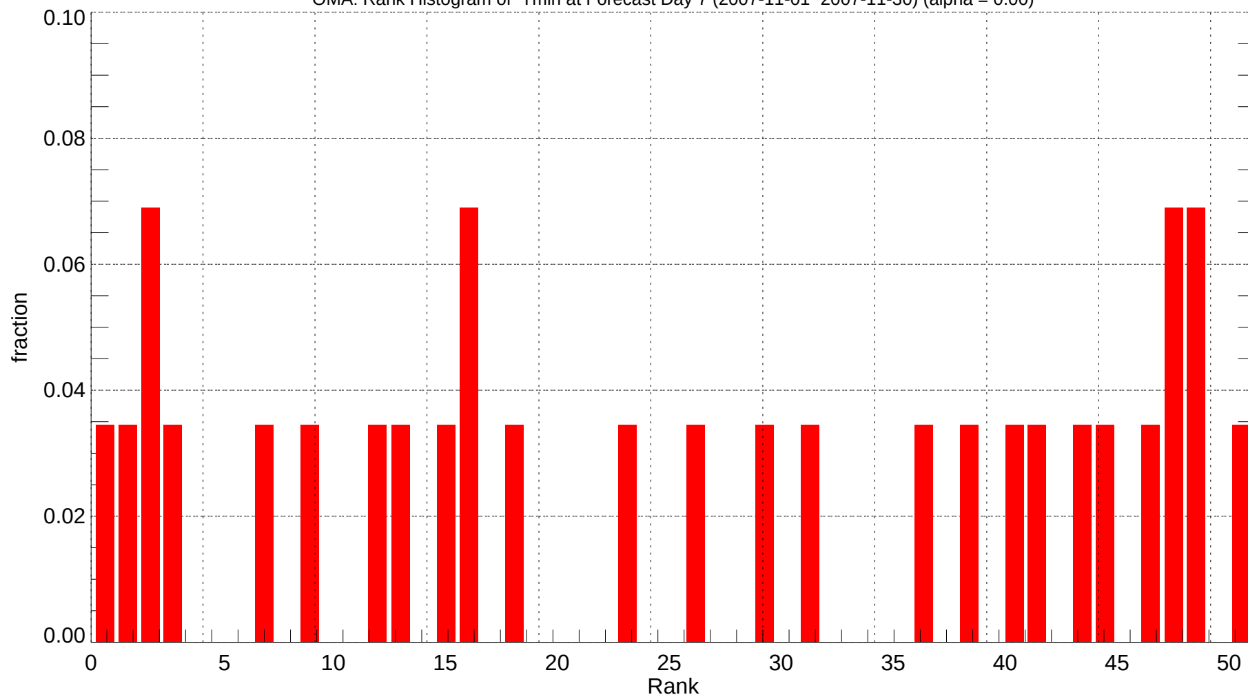
OMA: Rank Histogram of Tmin at Forecast Day 7 (2007-11-01~2007-11-30) (alpha = 0.00)
