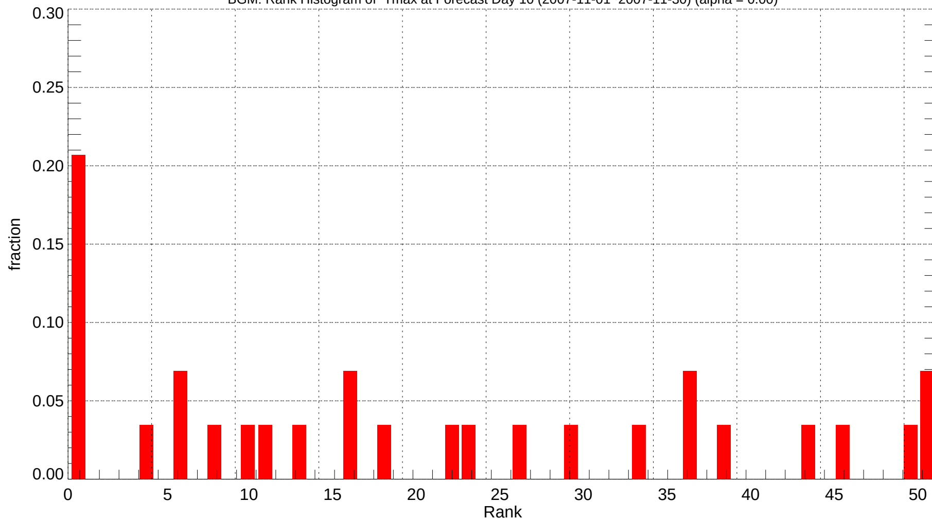
BGM: Rank Histogram of Tmax at Forecast Day 10 (2007-11-01~2007-11-30) (alpha = 0.00)
