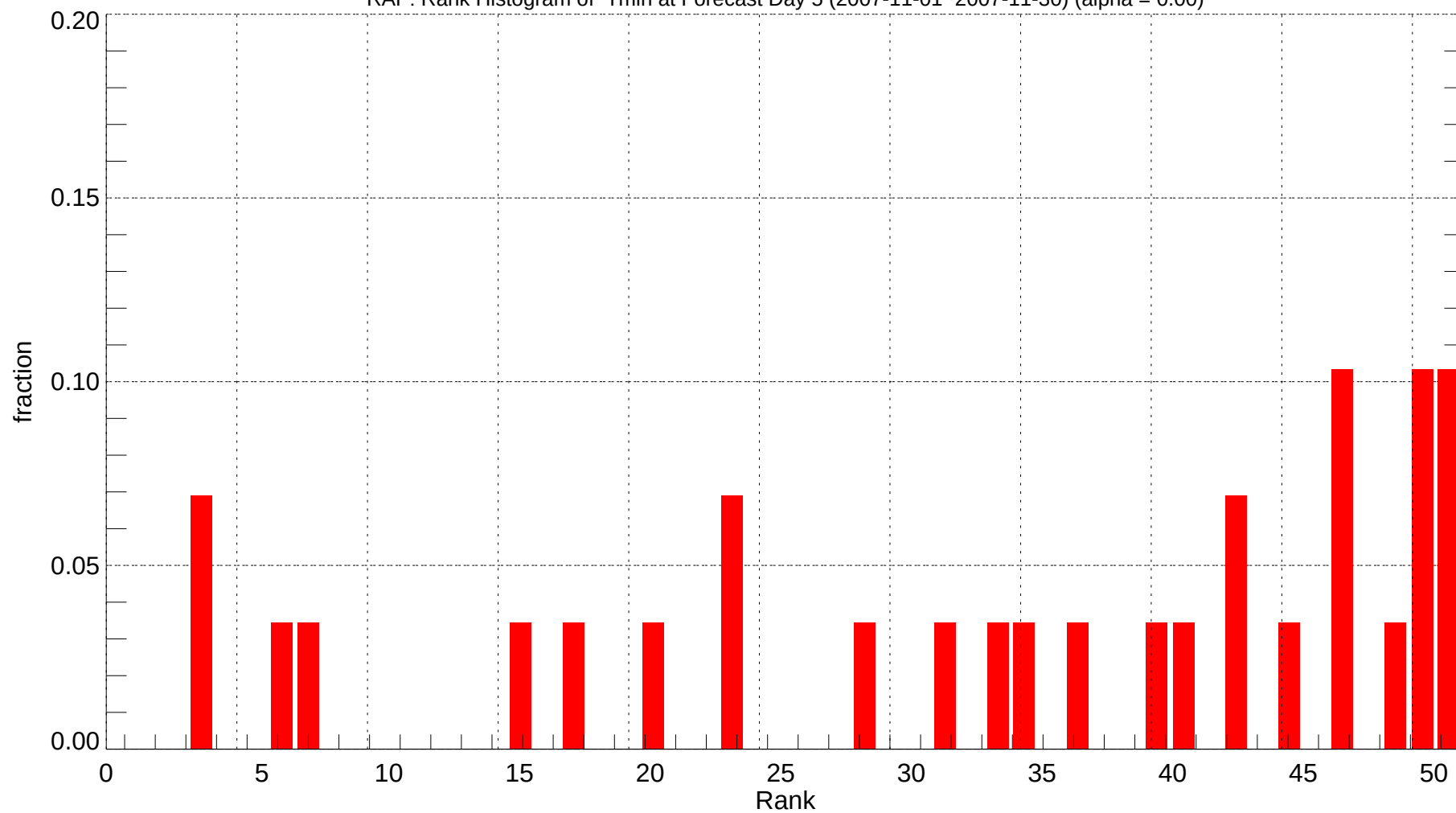
RAP: Rank Histogram of Tmin at Forecast Day 5 (2007-11-01~2007-11-30) (alpha = 0.00)
