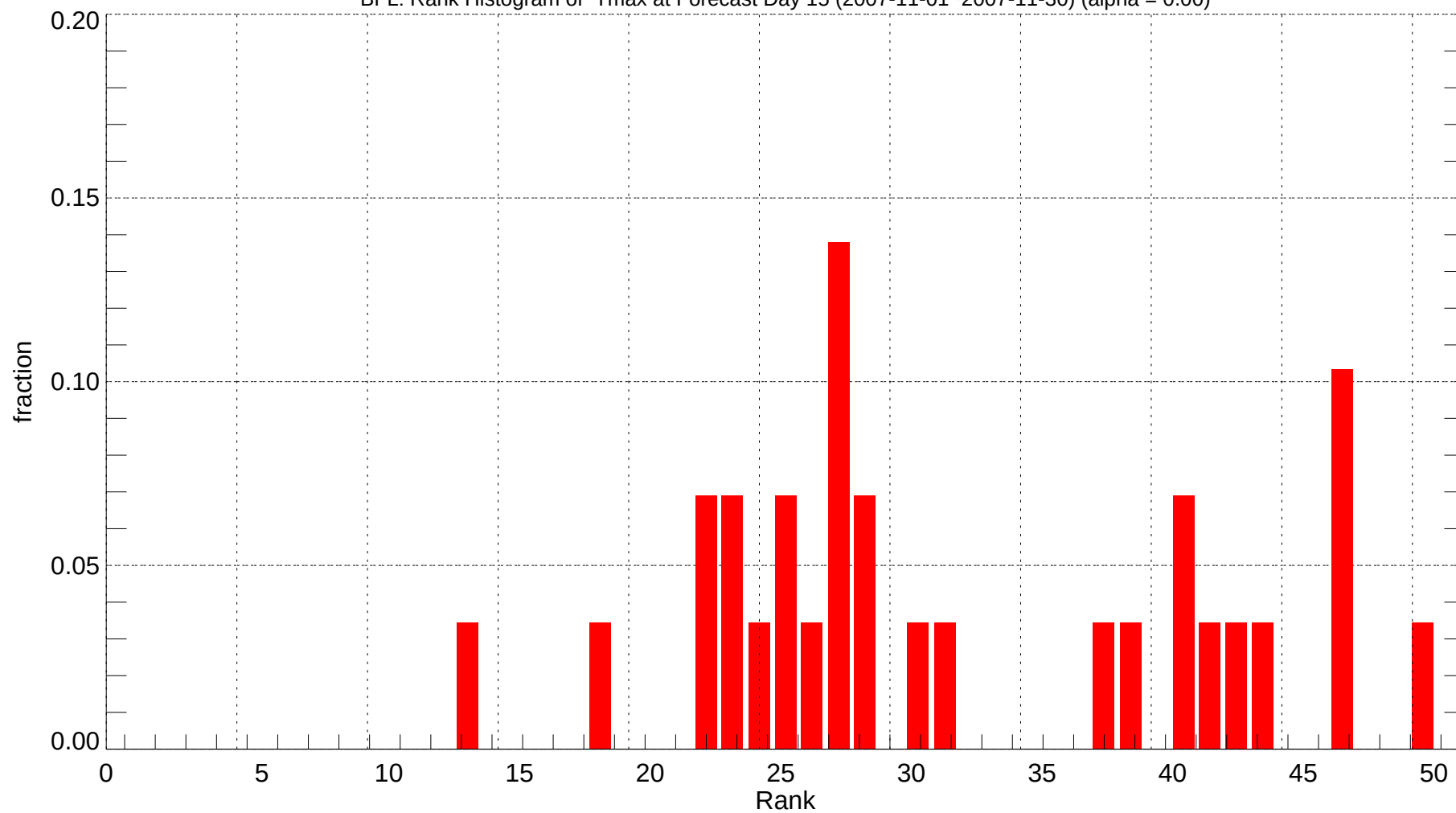
BFL: Rank Histogram of Tmax at Forecast Day 15 (2007-11-01~2007-11-30) (alpha = 0.00)
