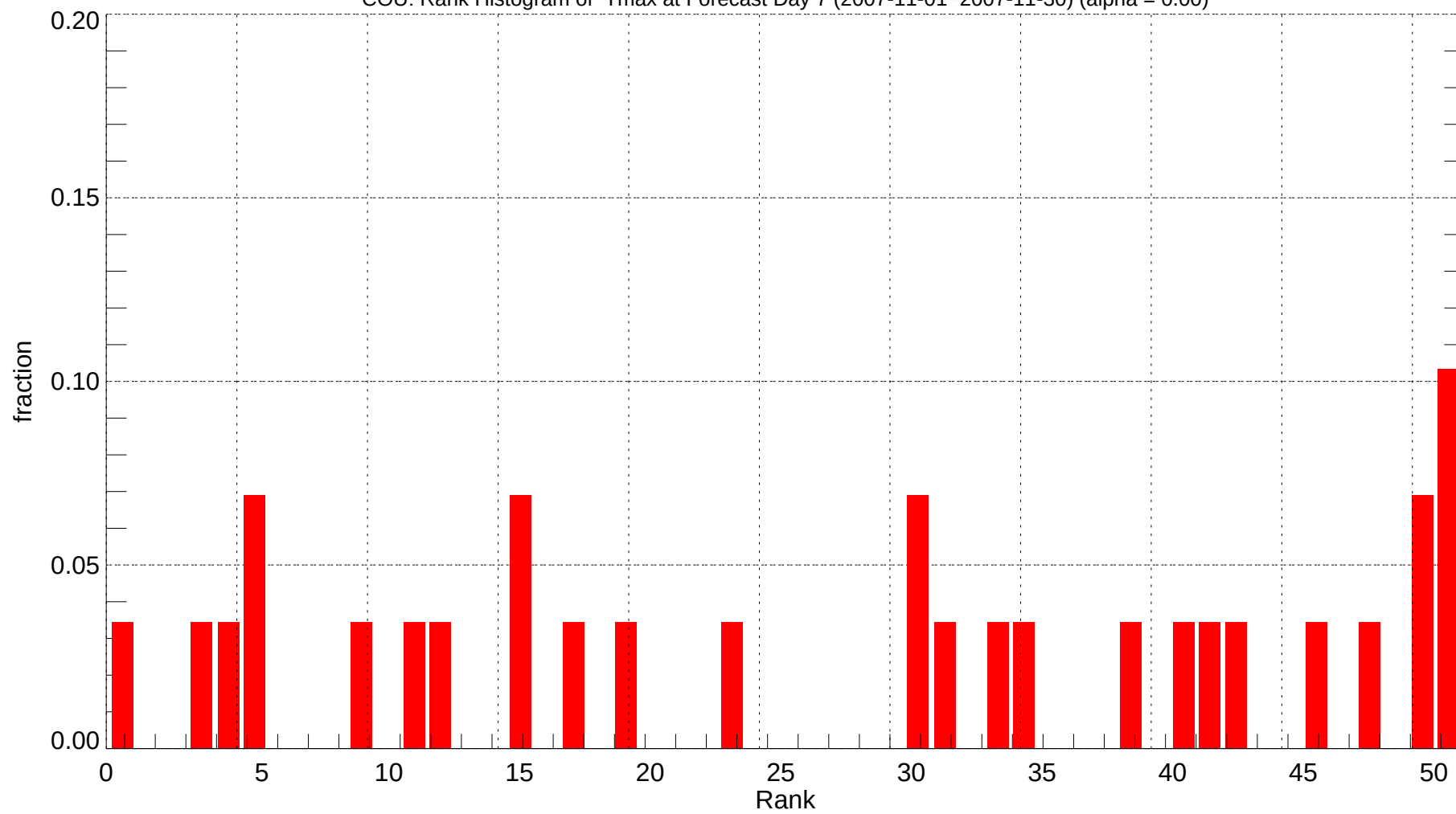
COU: Rank Histogram of Tmax at Forecast Day 7 (2007-11-01~2007-11-30) (alpha = 0.00)
