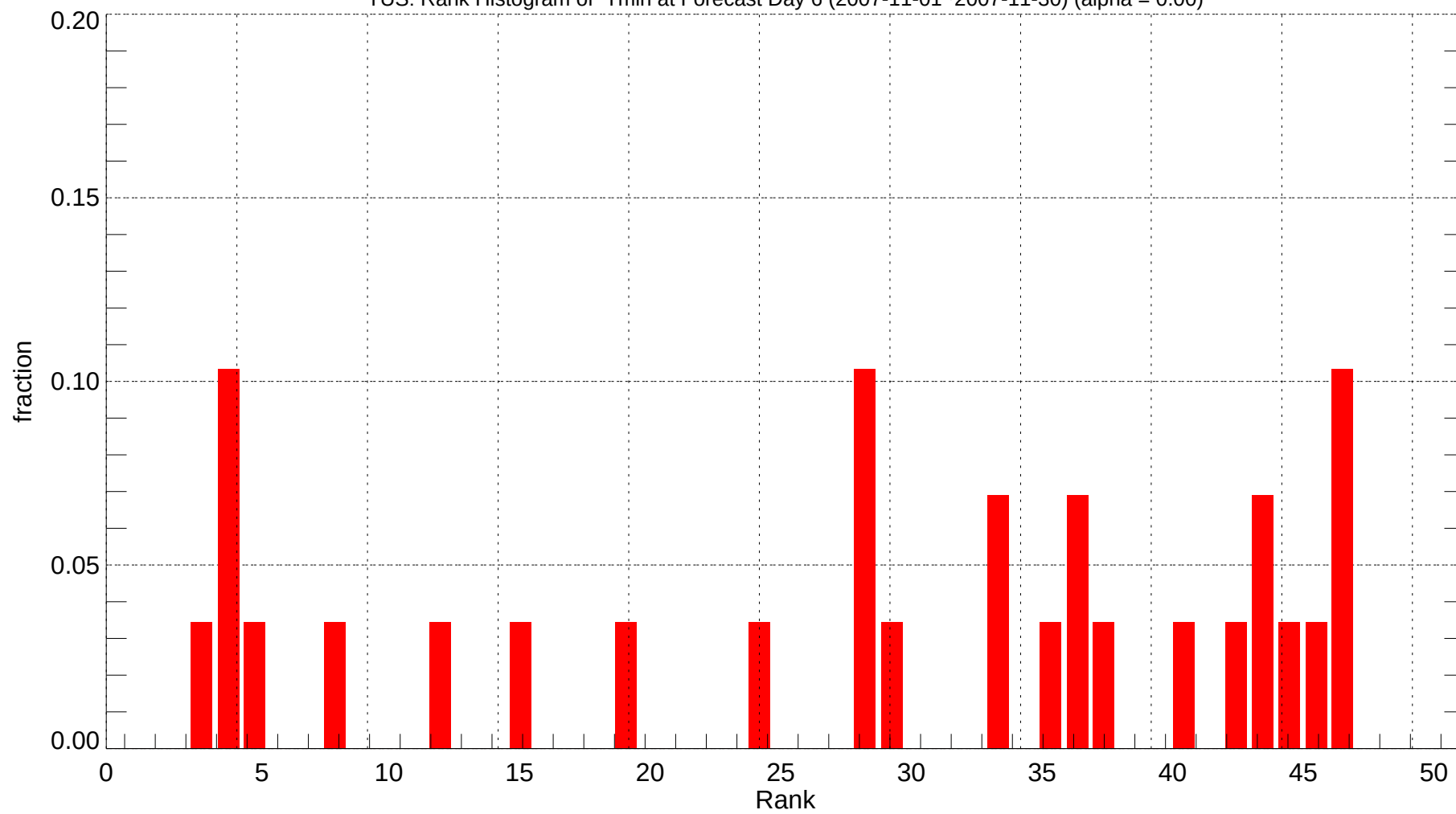
TUS: Rank Histogram of Tmin at Forecast Day 6 (2007-11-01~2007-11-30) (alpha = 0.00)
