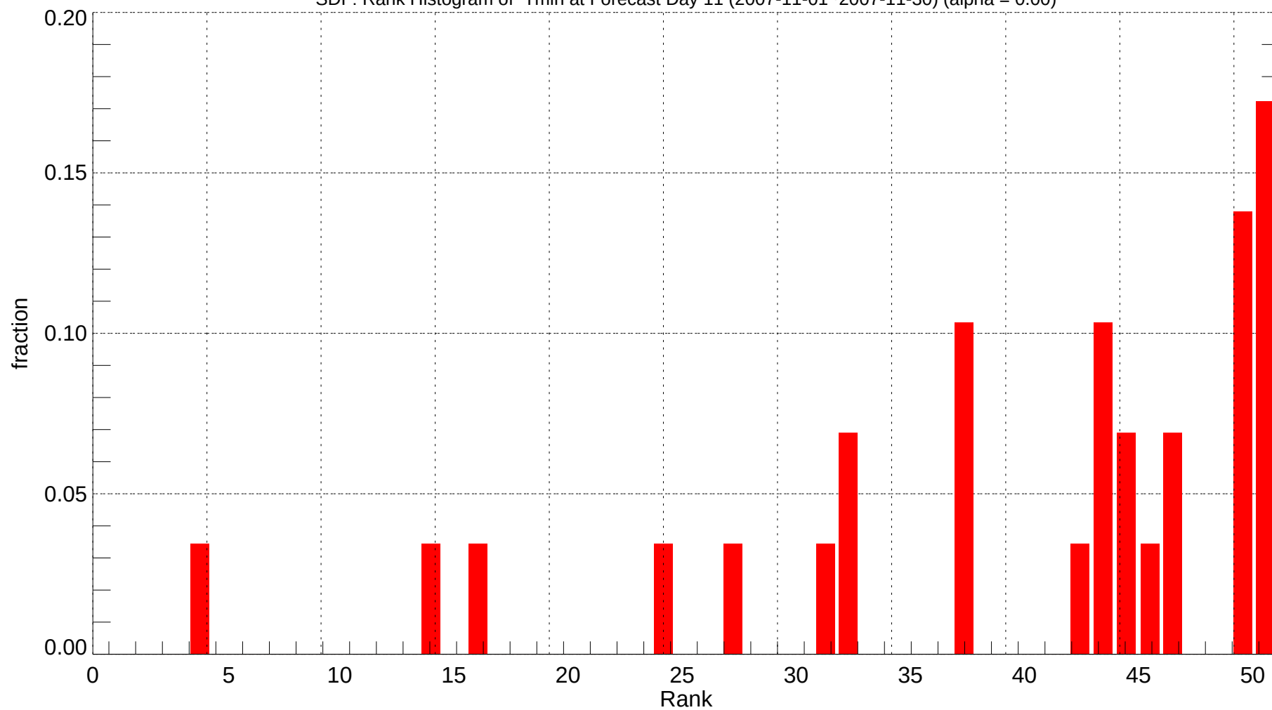
SDF: Rank Histogram of Tmin at Forecast Day 11 (2007-11-01~2007-11-30) (alpha = 0.00)
