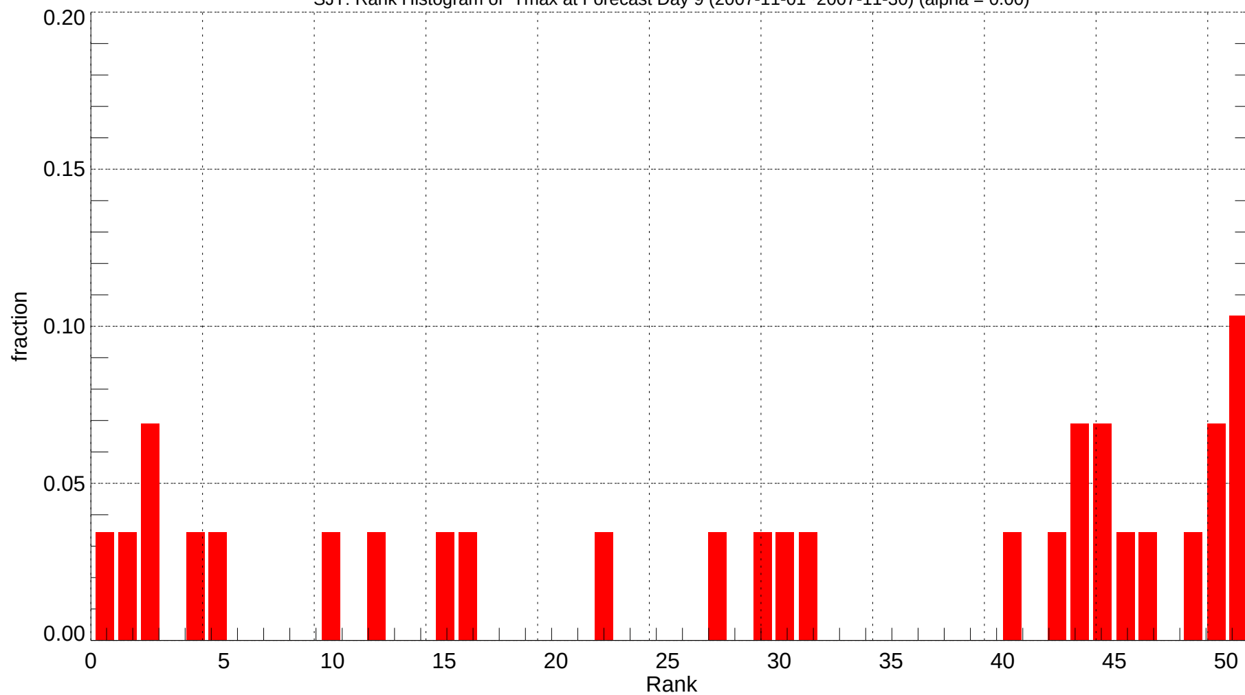
SJT: Rank Histogram of Tmax at Forecast Day 9 (2007-11-01~2007-11-30) (alpha = 0.00)
