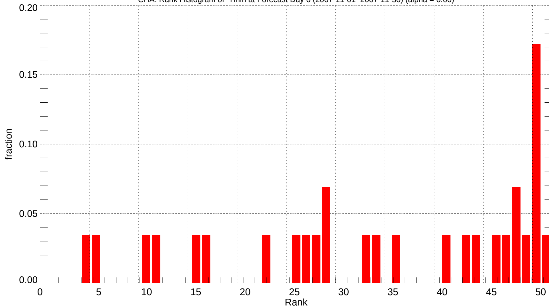
CHA: Rank Histogram of Tmin at Forecast Day 6 (2007-11-01~2007-11-30) (alpha = 0.00)
