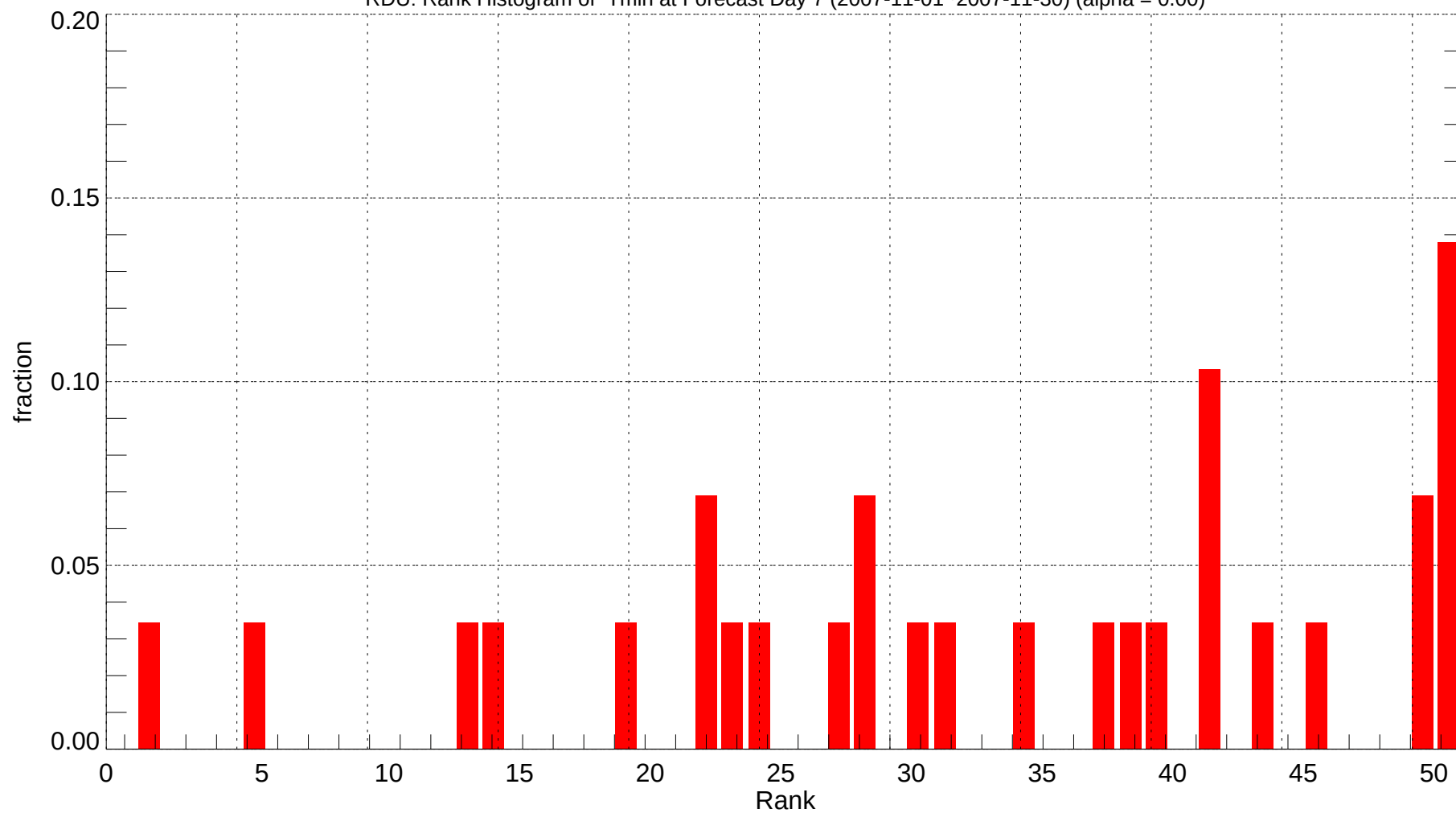
RDU: Rank Histogram of Tmin at Forecast Day 7 (2007-11-01~2007-11-30) (alpha = 0.00)
