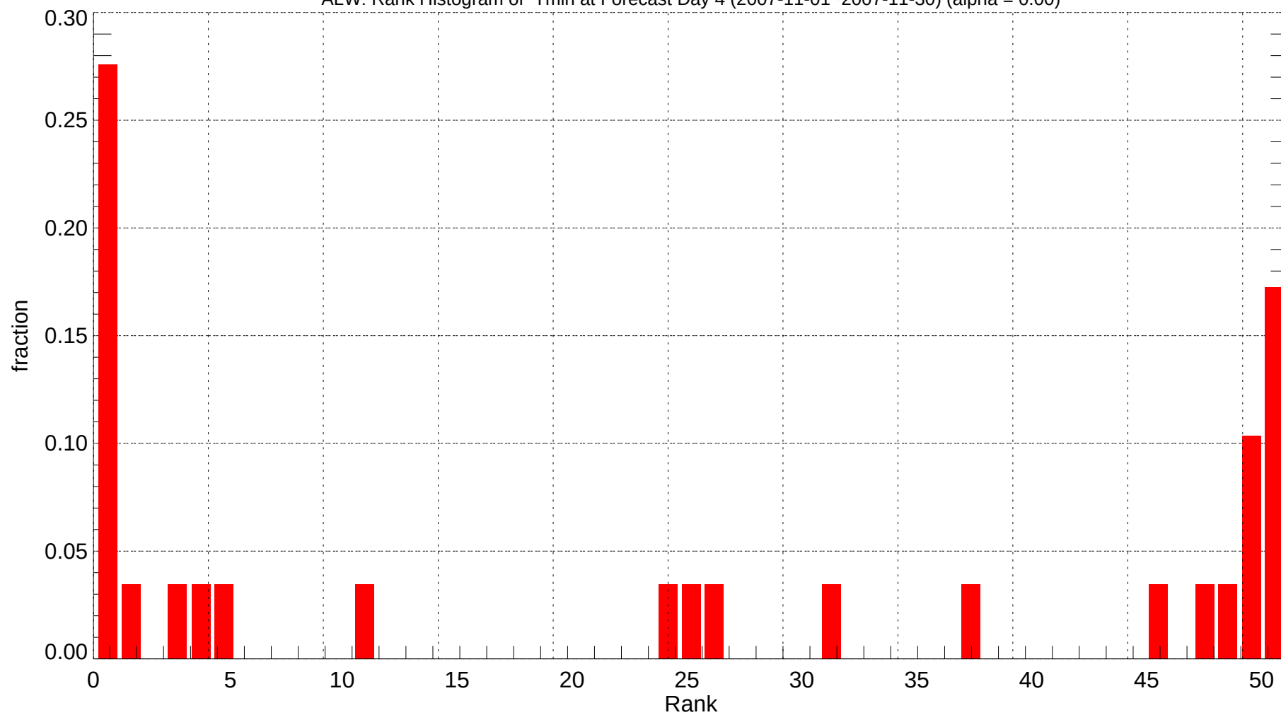
ALW: Rank Histogram of Tmin at Forecast Day 4 (2007-11-01~2007-11-30) (alpha = 0.00)
