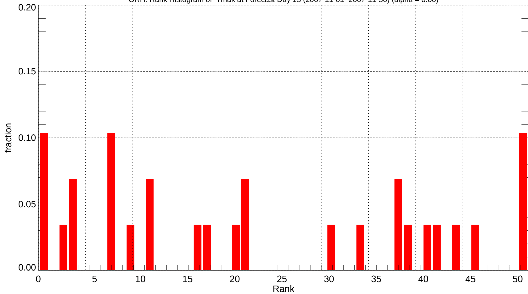
ORH: Rank Histogram of Tmax at Forecast Day 13 (2007-11-01~2007-11-30) (alpha = 0.00)
