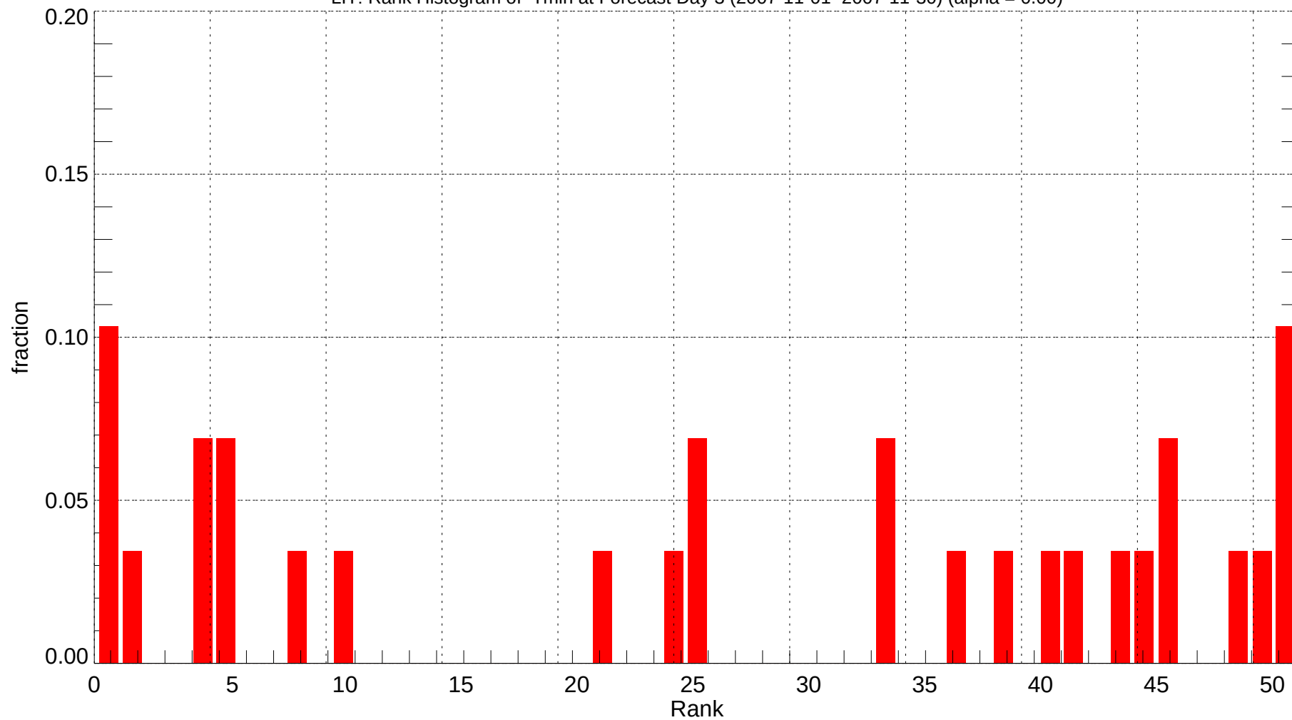
LIT: Rank Histogram of Tmin at Forecast Day 3 (2007-11-01~2007-11-30) (alpha = 0.00)
