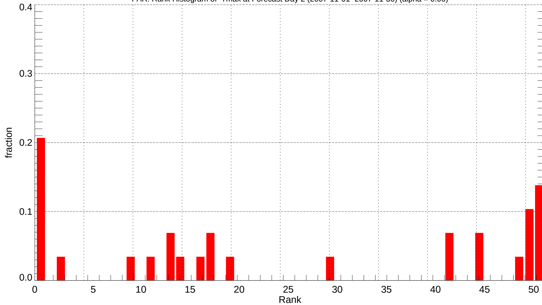
FAR: Rank Histogram of Tmax at Forecast Day 2 (2007-11-01~2007-11-30) (alpha = 0.00)
