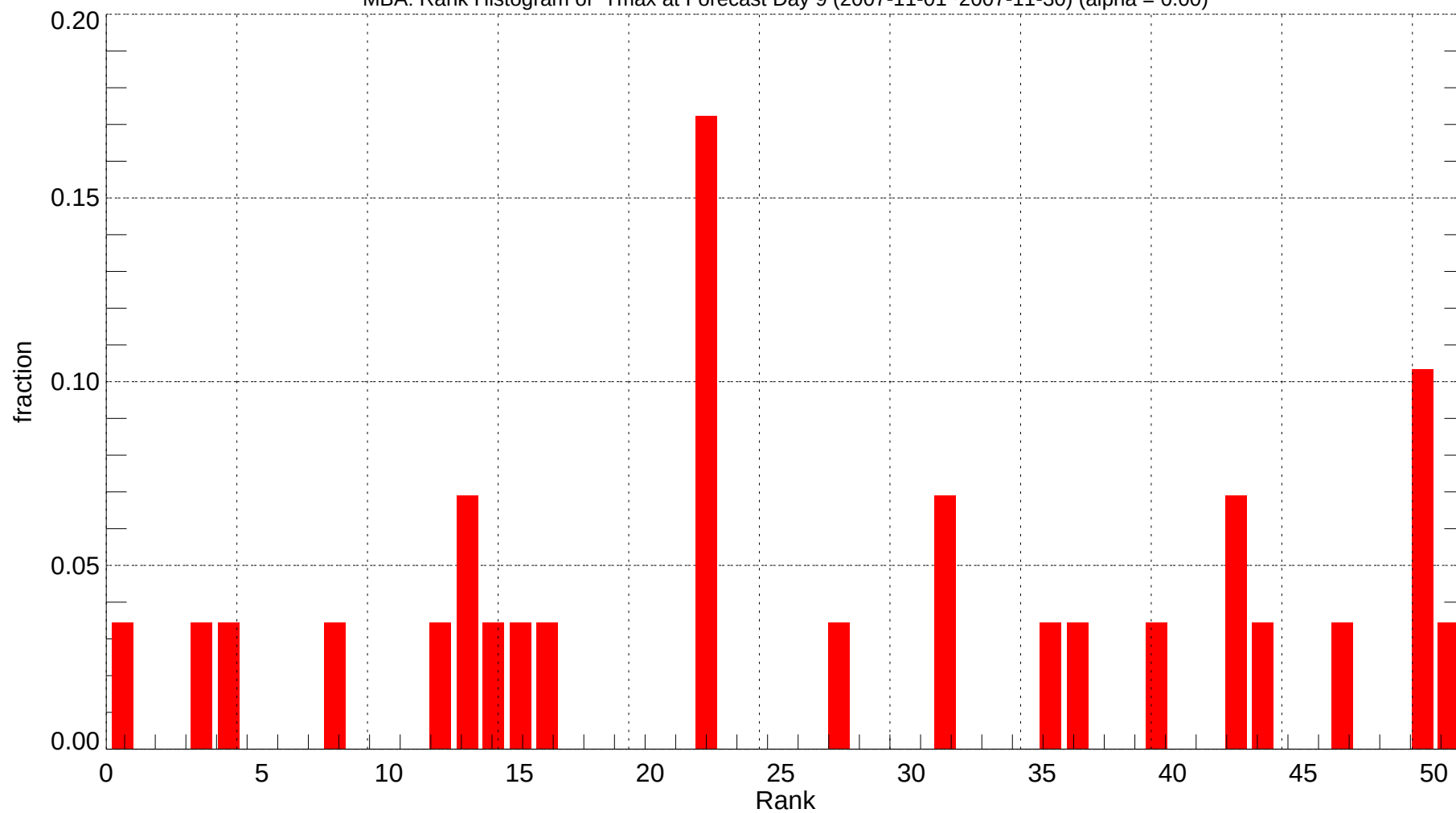
MBA: Rank Histogram of Tmax at Forecast Day 9 (2007-11-01~2007-11-30) (alpha = 0.00)
