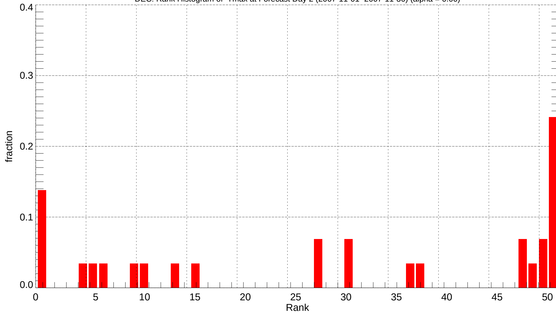
DEC: Rank Histogram of Tmax at Forecast Day 2 (2007-11-01~2007-11-30) (alpha = 0.00)
