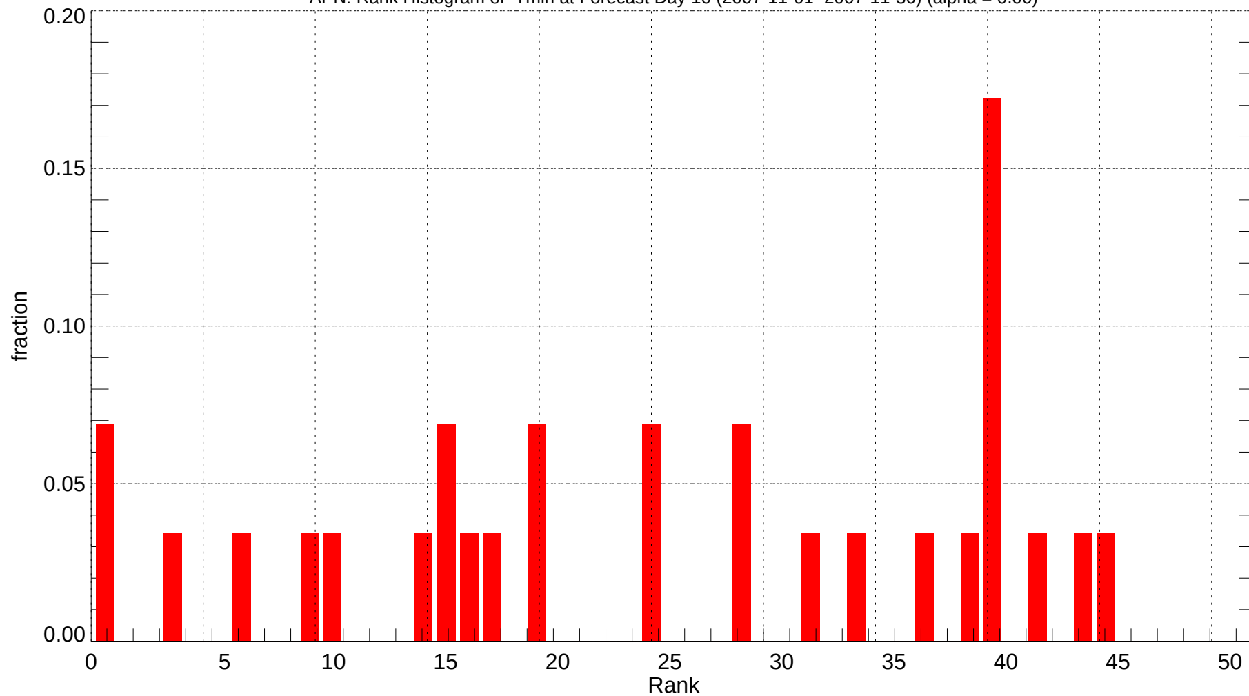
APN: Rank Histogram of Tmin at Forecast Day 10 (2007-11-01~2007-11-30) (alpha = 0.00)
