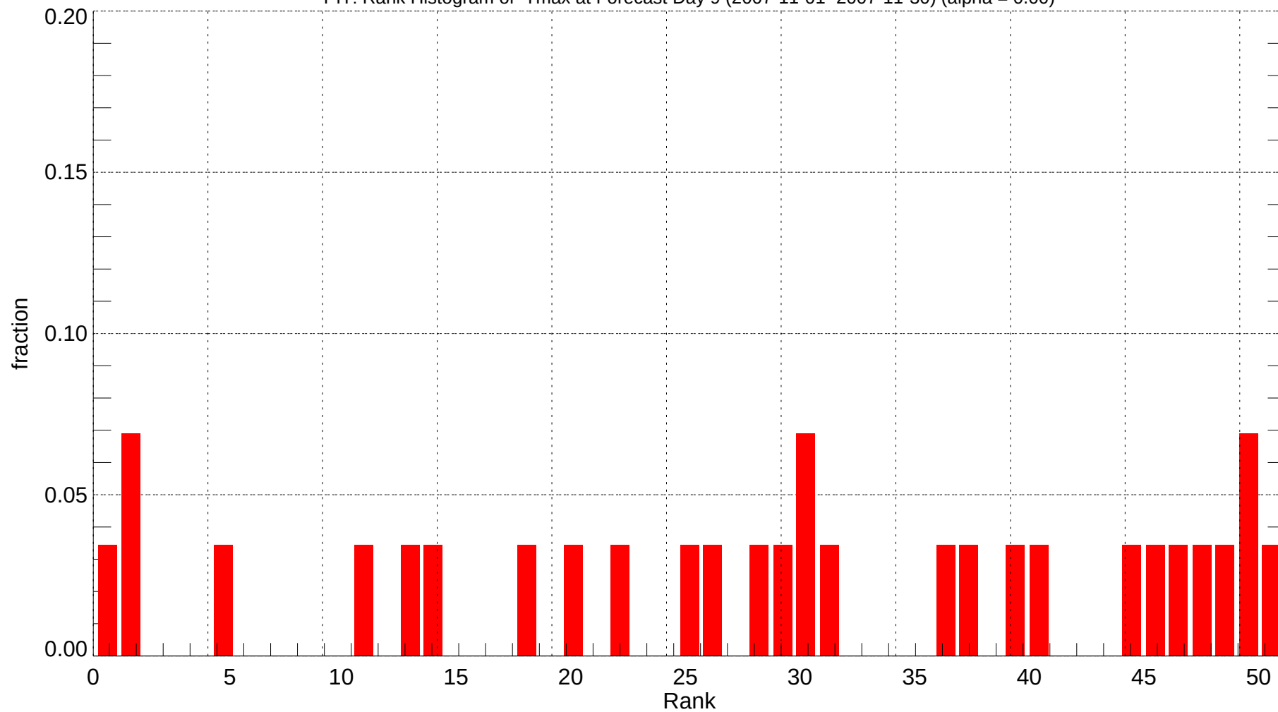
PIT: Rank Histogram of Tmax at Forecast Day 9 (2007-11-01~2007-11-30) (alpha = 0.00)
