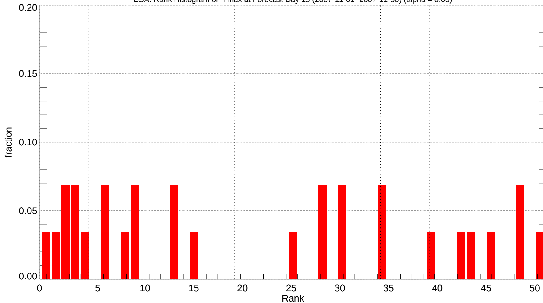
LGA: Rank Histogram of Tmax at Forecast Day 13 (2007-11-01~2007-11-30) (alpha = 0.00)
