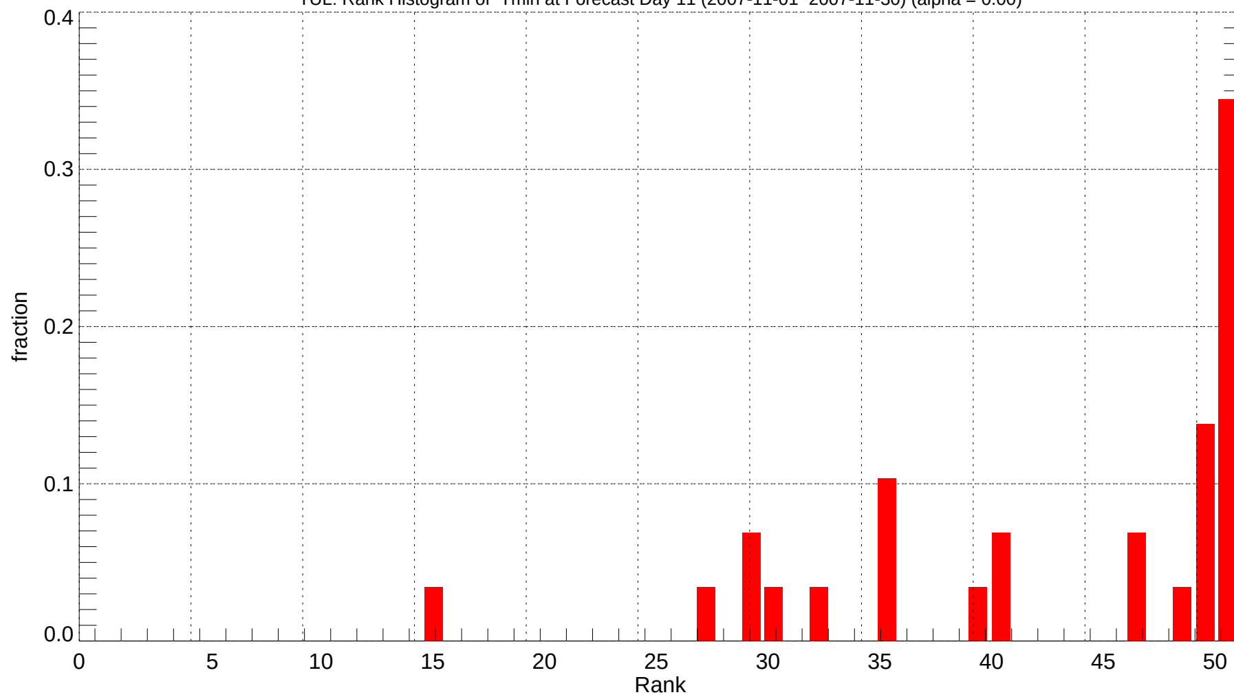
TUL: Rank Histogram of Tmin at Forecast Day 11 (2007-11-01~2007-11-30) (alpha = 0.00)
