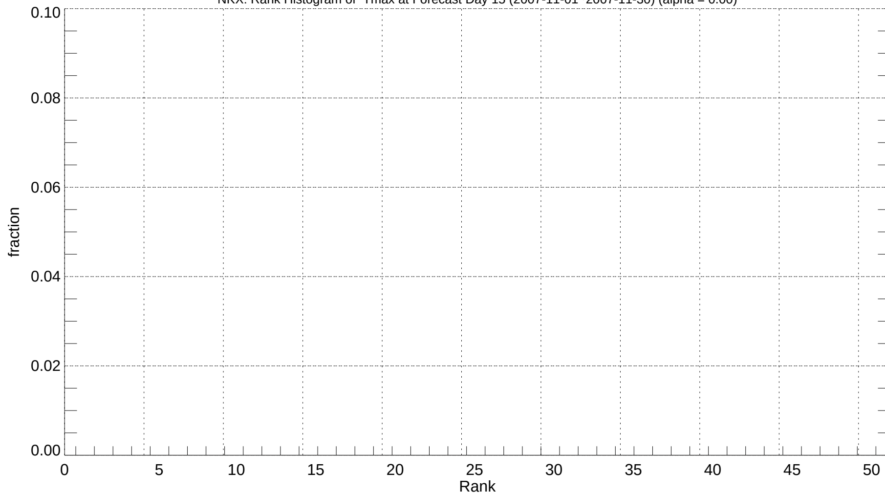
NKX: Rank Histogram of Tmax at Forecast Day 15 (2007-11-01~2007-11-30) (alpha = 0.00)
