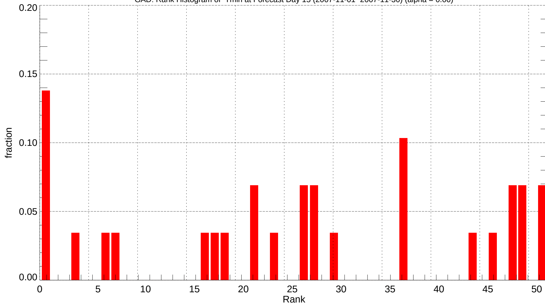
GAD: Rank Histogram of Tmin at Forecast Day 15 (2007-11-01~2007-11-30) (alpha = 0.00)
