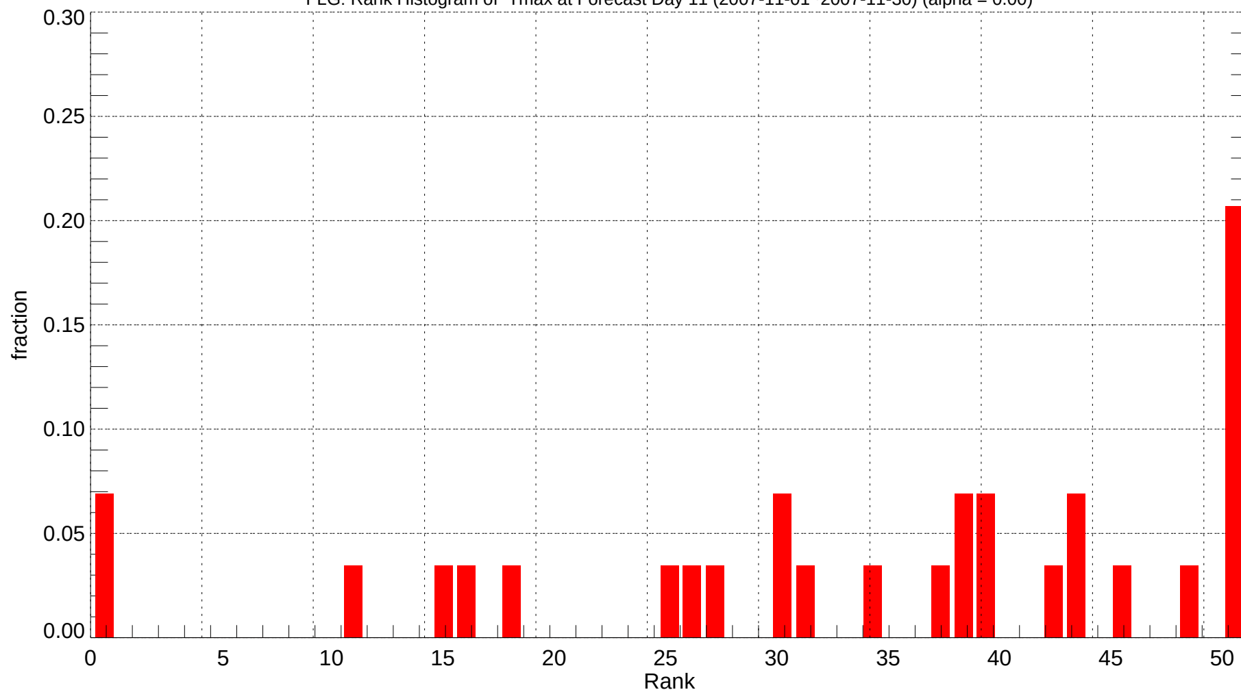
FLG: Rank Histogram of Tmax at Forecast Day 11 (2007-11-01~2007-11-30) (alpha = 0.00)
