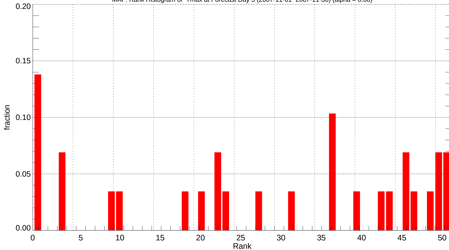
MAF: Rank Histogram of Tmax at Forecast Day 5 (2007-11-01~2007-11-30) (alpha = 0.00)
