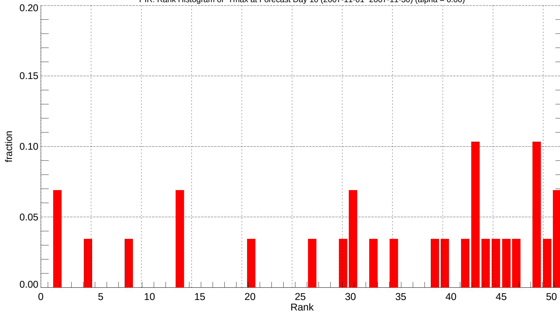
PIR: Rank Histogram of Tmax at Forecast Day 10 (2007-11-01~2007-11-30) (alpha = 0.00)
