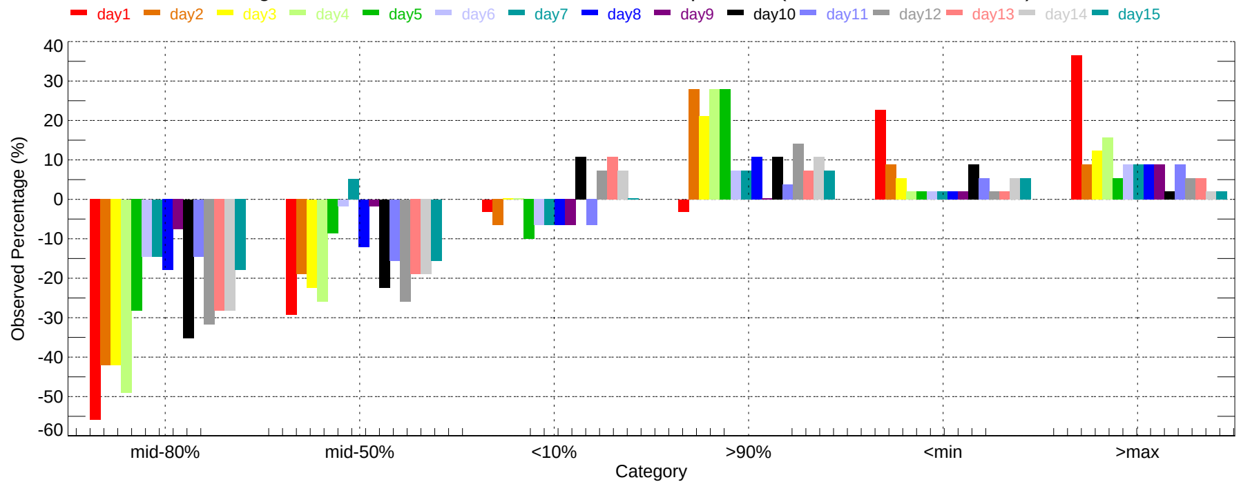
Observed Percentage Deviation of Ensembles - ACY: Max Temperature (2007-11-01~2007-11-30)
