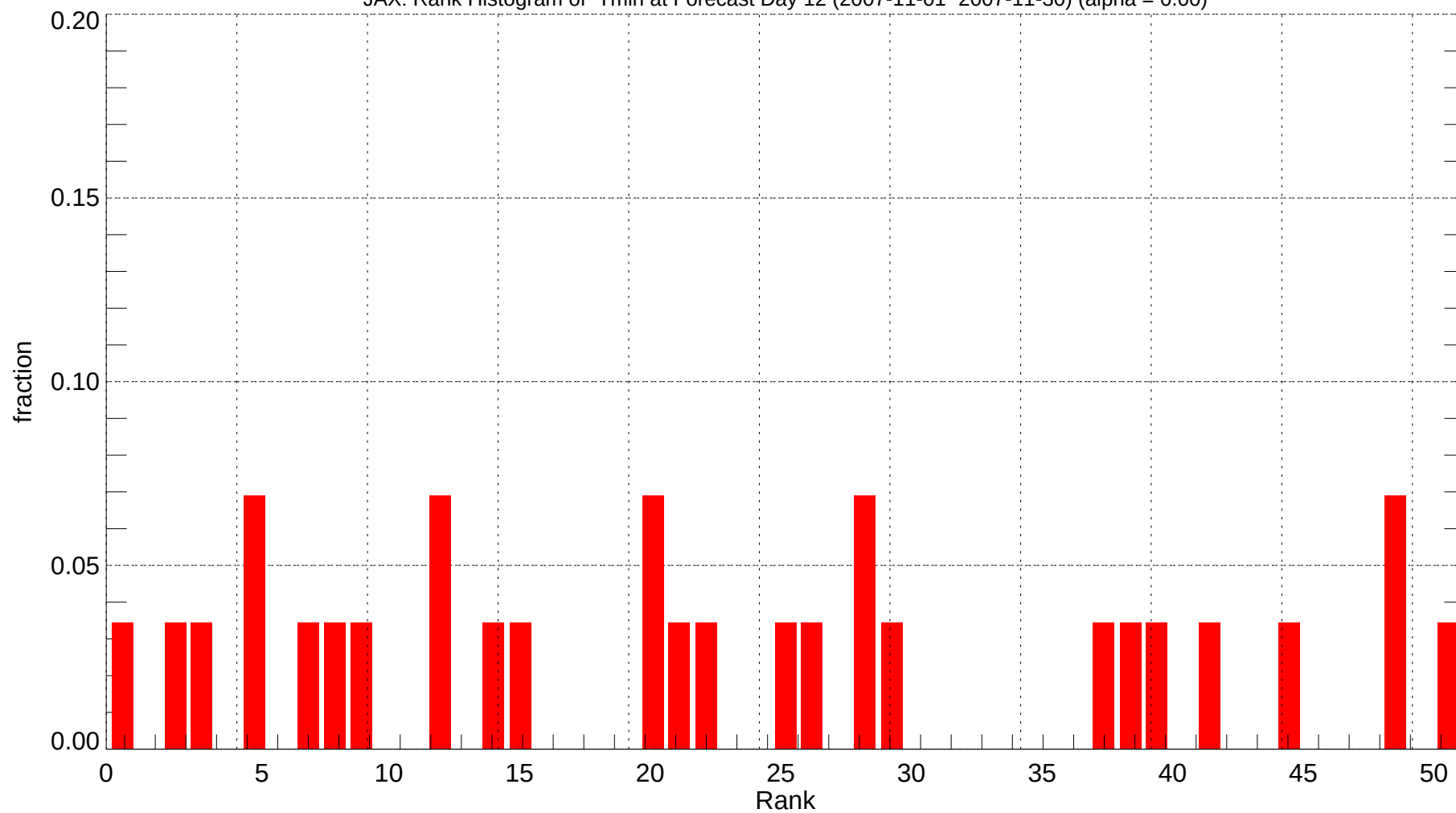
JAX: Rank Histogram of Tmin at Forecast Day 12 (2007-11-01~2007-11-30) (alpha = 0.00)
