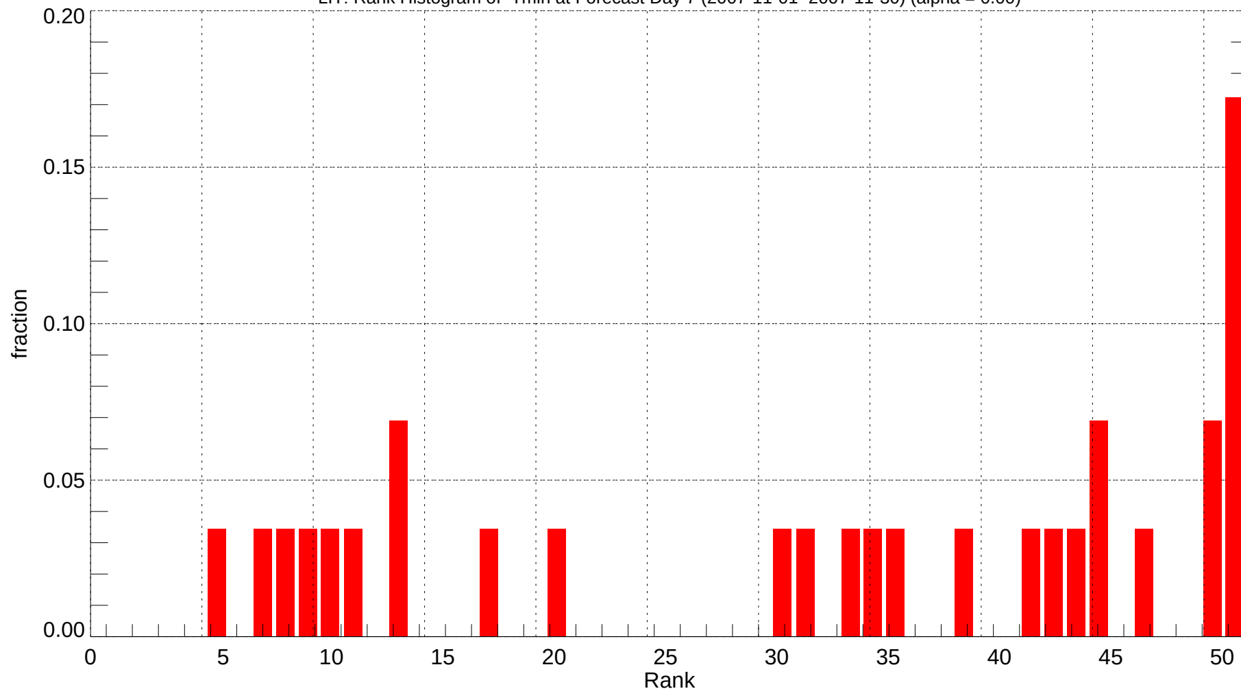
LIT: Rank Histogram of Tmin at Forecast Day 7 (2007-11-01~2007-11-30) (alpha = 0.00)
