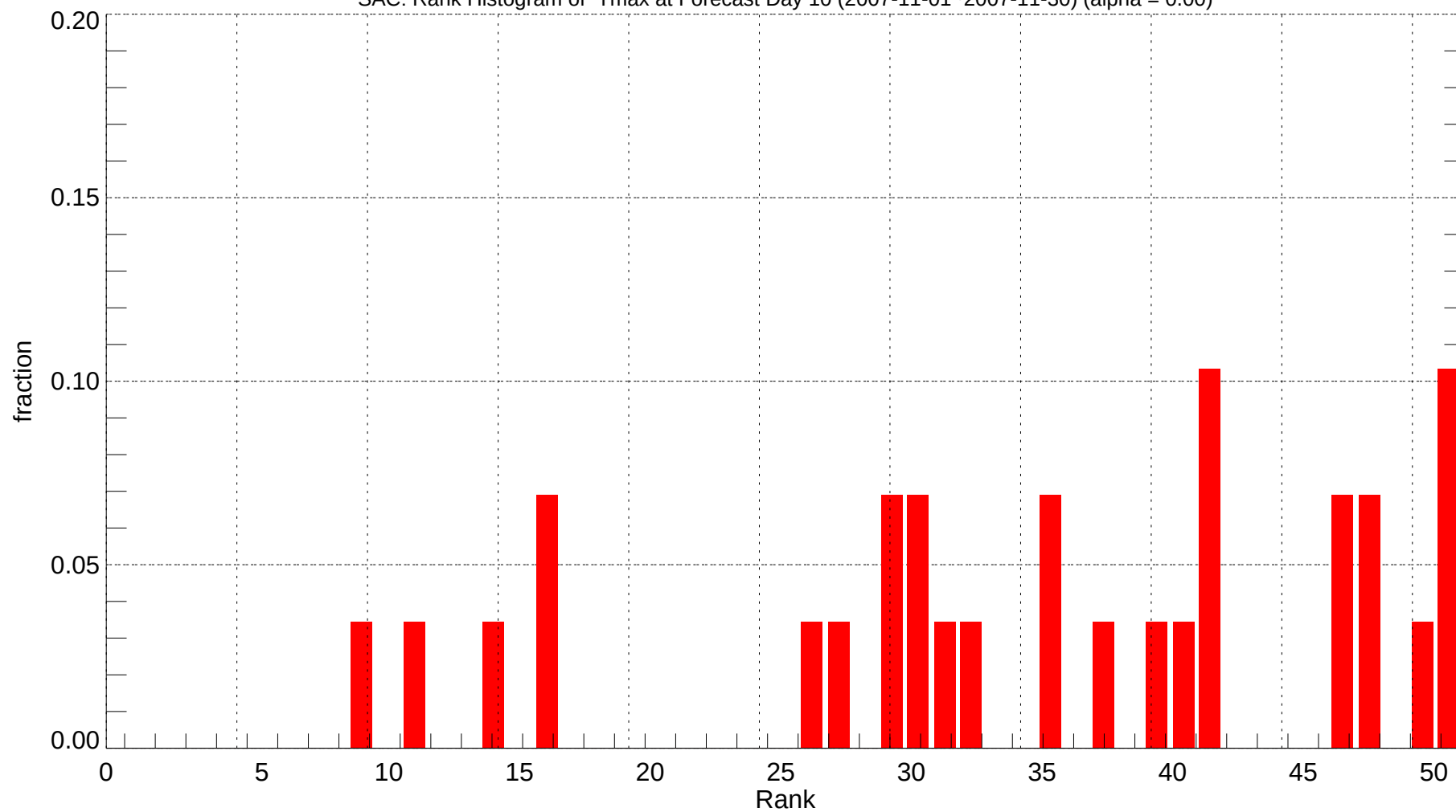
SAC: Rank Histogram of Tmax at Forecast Day 10 (2007-11-01~2007-11-30) (alpha = 0.00)
