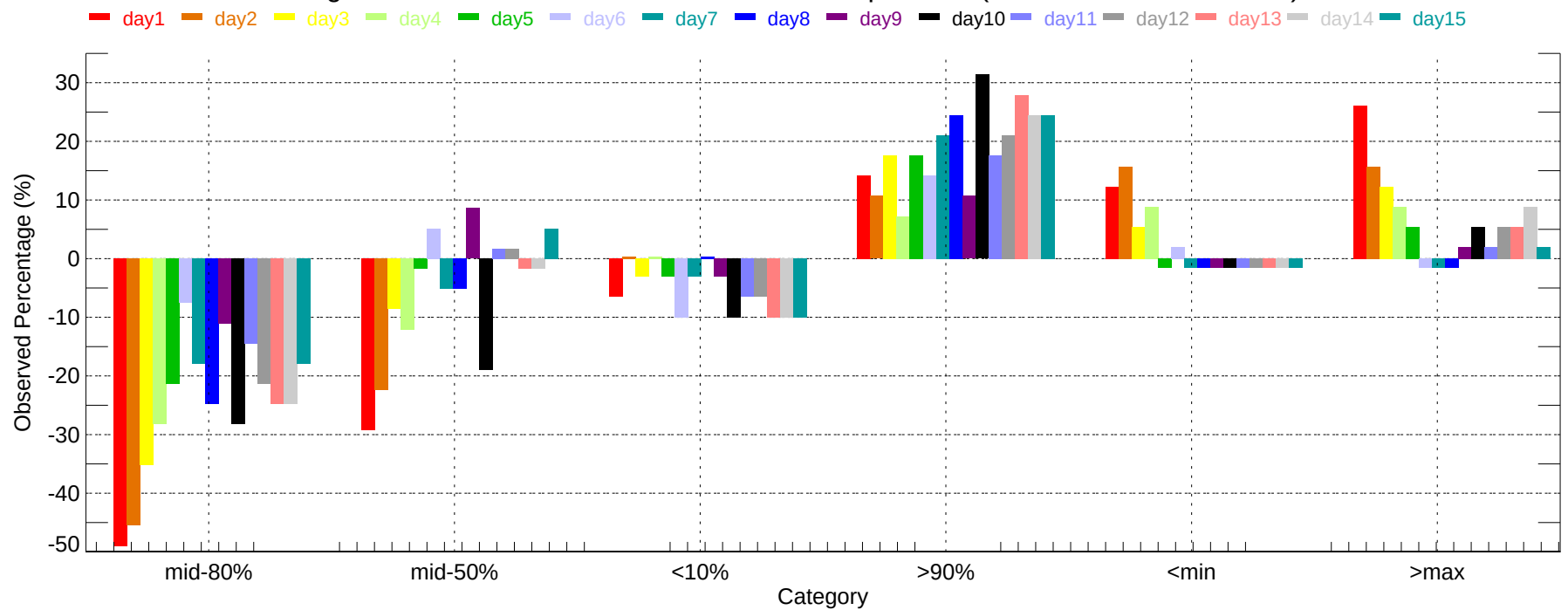
Observed Percentage Deviation of Ensembles - TRM: Min Temperature (2007-11-01~2007-11-30)
