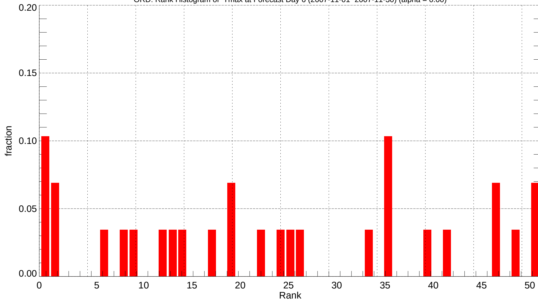
ORD: Rank Histogram of Tmax at Forecast Day 6 (2007-11-01~2007-11-30) (alpha = 0.00)
