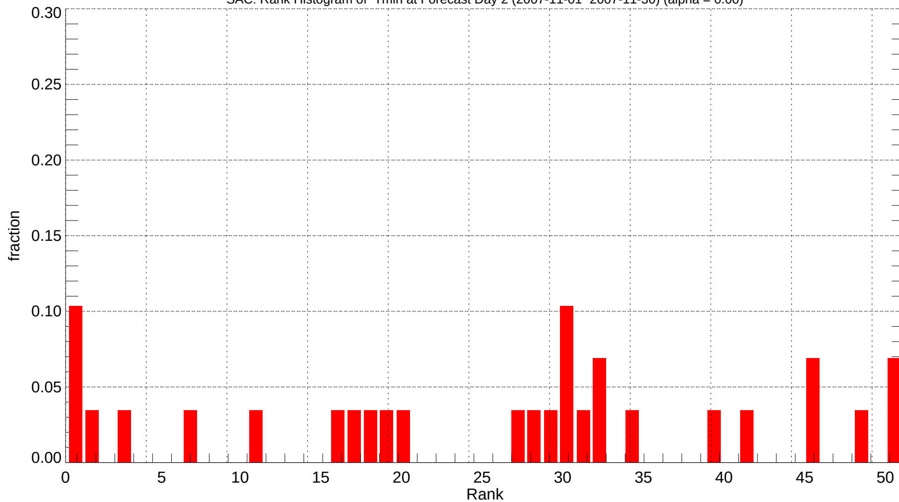
SAC: Rank Histogram of Tmin at Forecast Day 2 (2007-11-01~2007-11-30) (alpha = 0.00)
