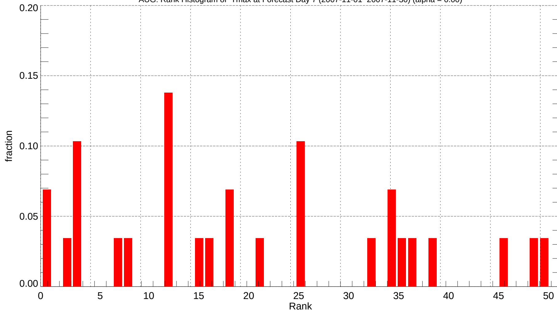
AUG: Rank Histogram of Tmax at Forecast Day 7 (2007-11-01~2007-11-30) (alpha = 0.00)
