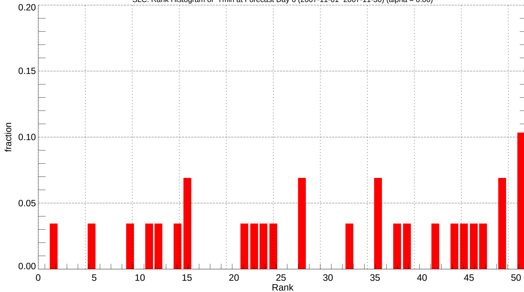
SLC: Rank Histogram of Tmin at Forecast Day 6 (2007-11-01~2007-11-30) (alpha = 0.00)
