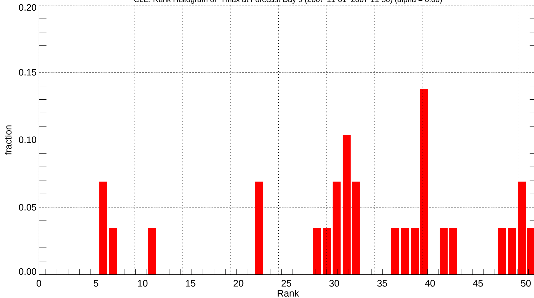
CLE: Rank Histogram of Tmax at Forecast Day 9 (2007-11-01~2007-11-30) (alpha = 0.00)
