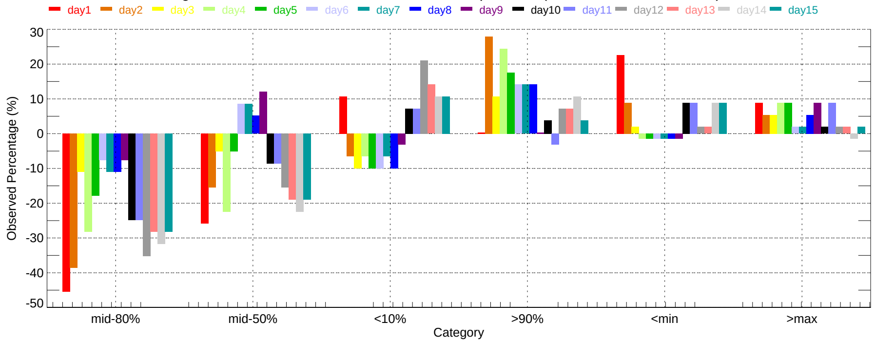
Observed Percentage Deviation of Ensembles - ILG: Max Temperature (2007-11-01~2007-11-30)
