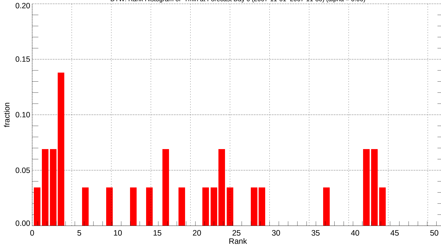
DTW: Rank Histogram of Tmin at Forecast Day 6 (2007-11-01~2007-11-30) (alpha = 0.00)
