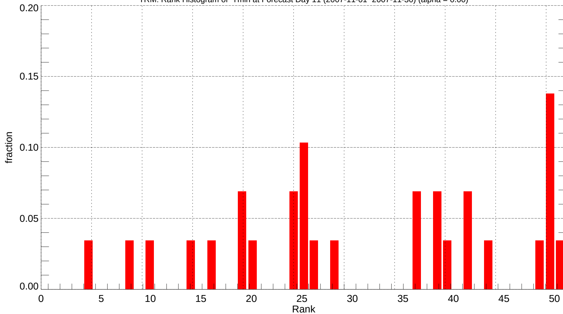
TRM: Rank Histogram of Tmin at Forecast Day 11 (2007-11-01~2007-11-30) (alpha = 0.00)
