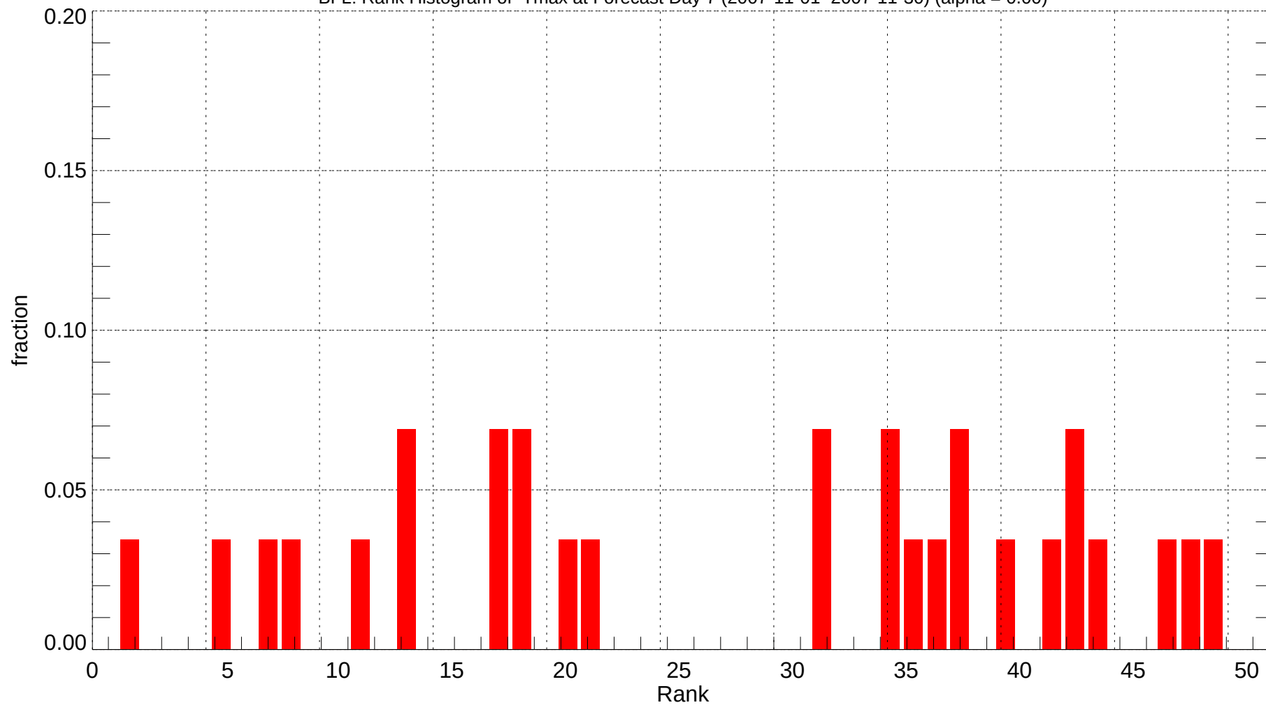
BFL: Rank Histogram of Tmax at Forecast Day 7 (2007-11-01~2007-11-30) (alpha = 0.00)
