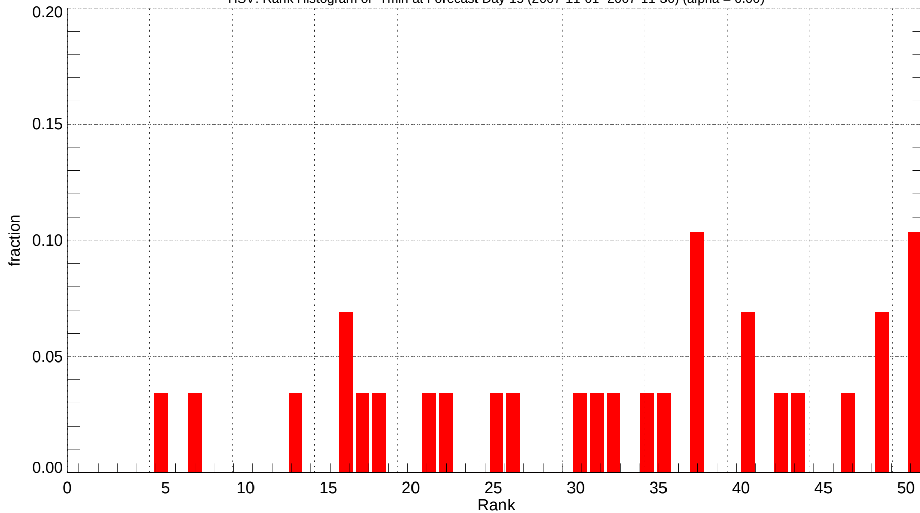
HSV: Rank Histogram of Tmin at Forecast Day 15 (2007-11-01~2007-11-30) (alpha = 0.00)
