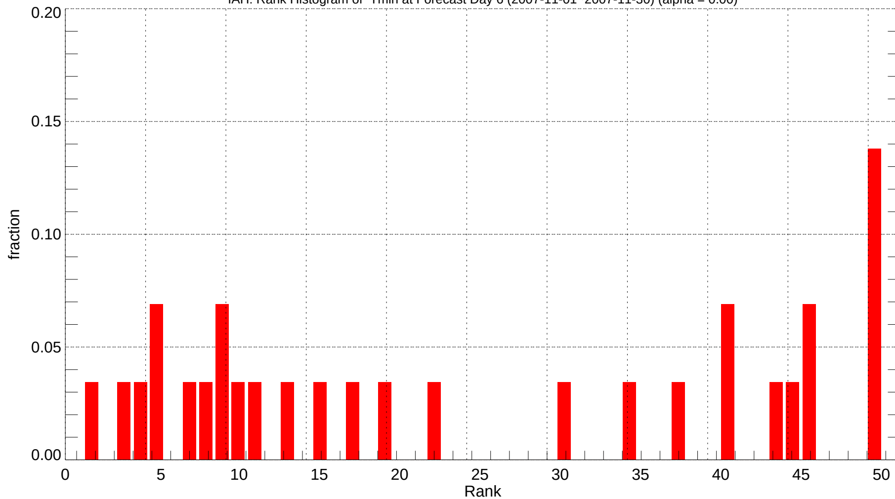
IAH: Rank Histogram of Tmin at Forecast Day 6 (2007-11-01~2007-11-30) (alpha = 0.00)
