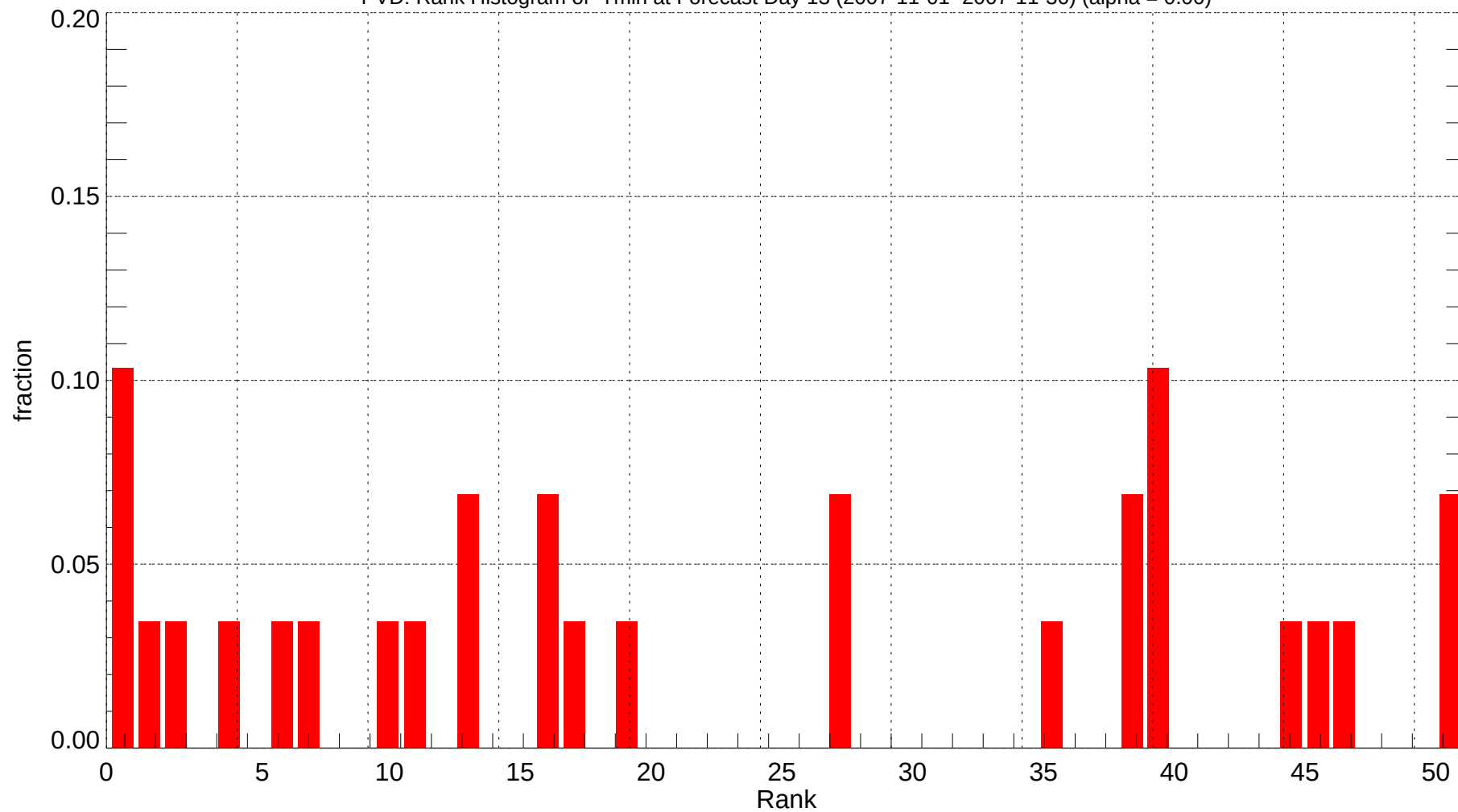
PVD: Rank Histogram of Tmin at Forecast Day 13 (2007-11-01~2007-11-30) (alpha = 0.00)
