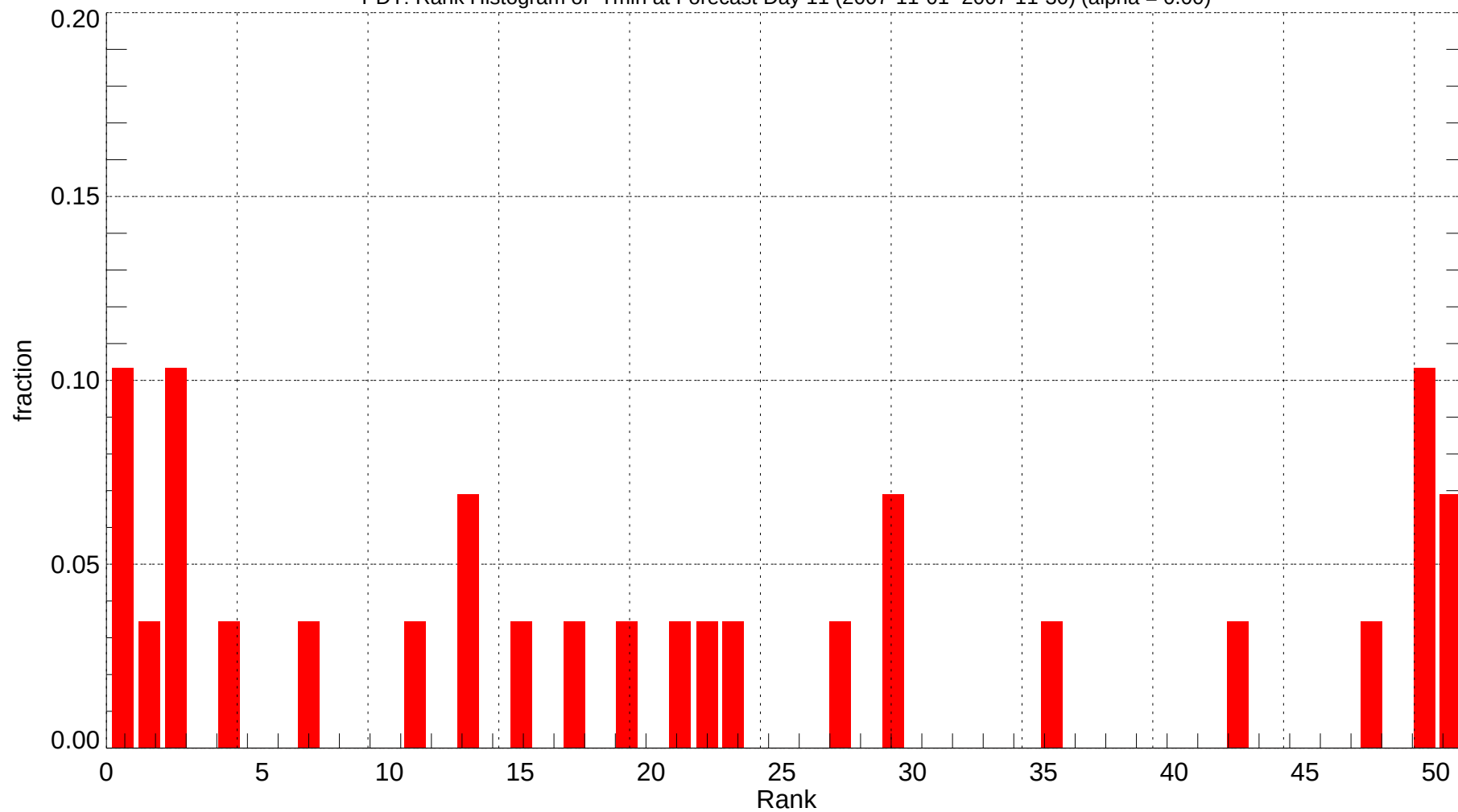
PDT: Rank Histogram of Tmin at Forecast Day 11 (2007-11-01~2007-11-30) (alpha = 0.00)
