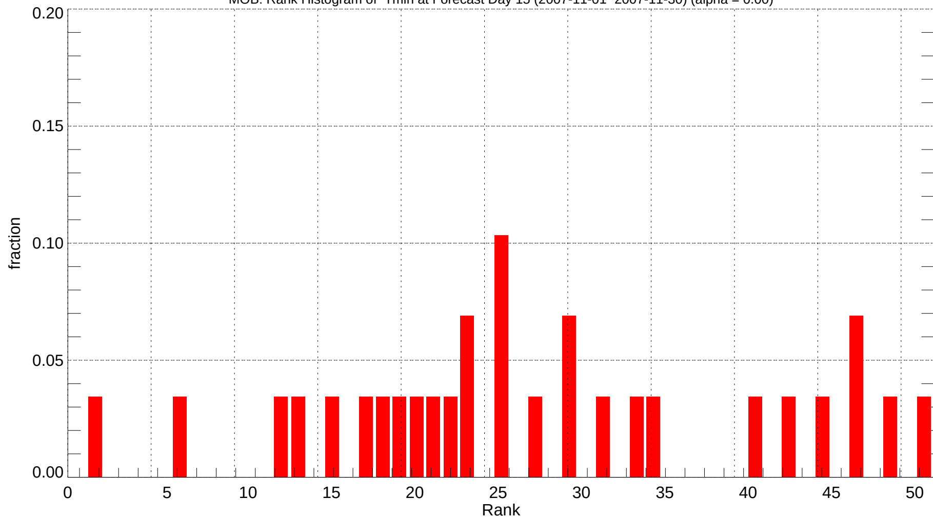
MOB: Rank Histogram of Tmin at Forecast Day 15 (2007-11-01~2007-11-30) (alpha = 0.00)
