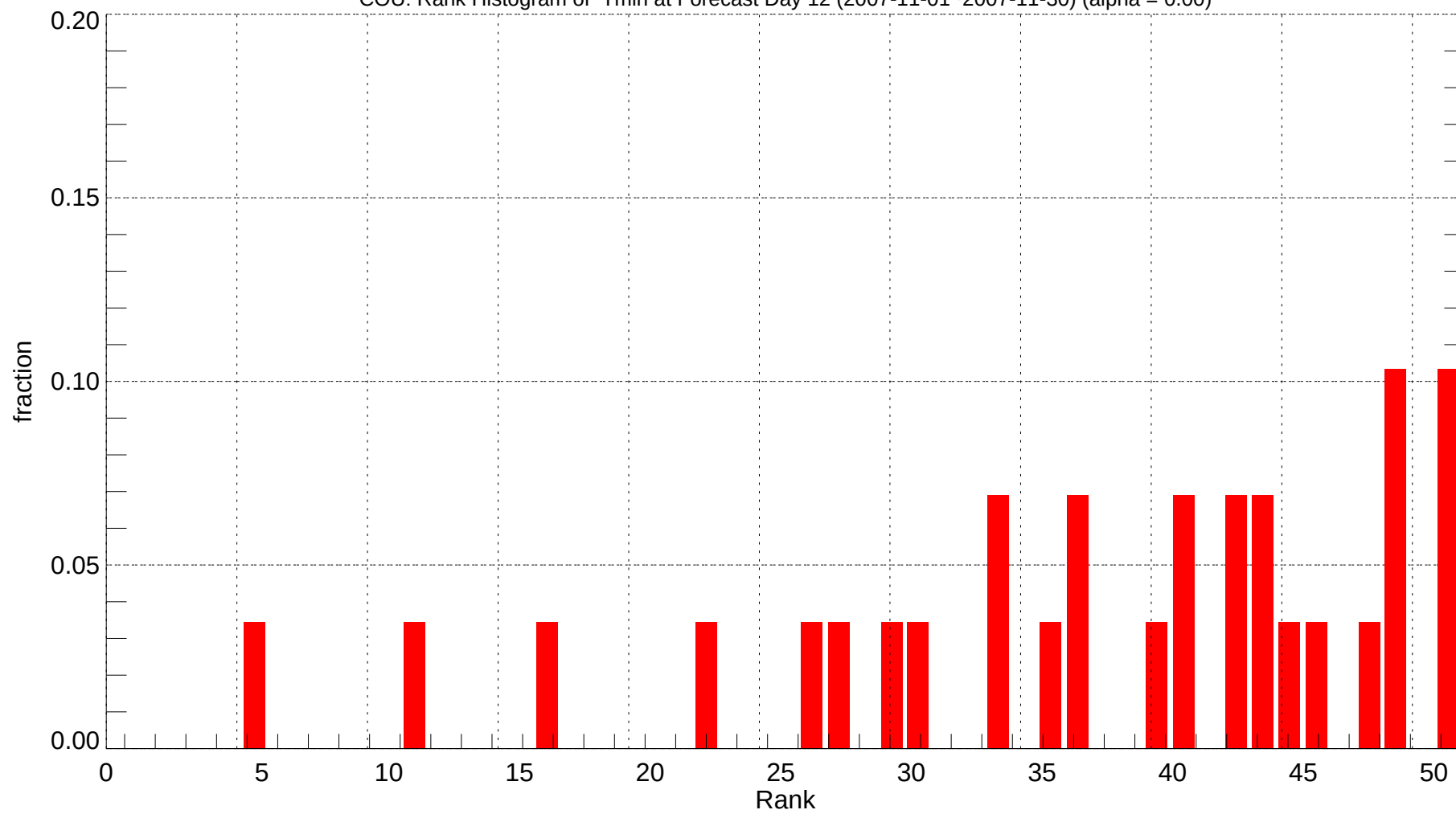
COU: Rank Histogram of Tmin at Forecast Day 12 (2007-11-01~2007-11-30) (alpha = 0.00)
