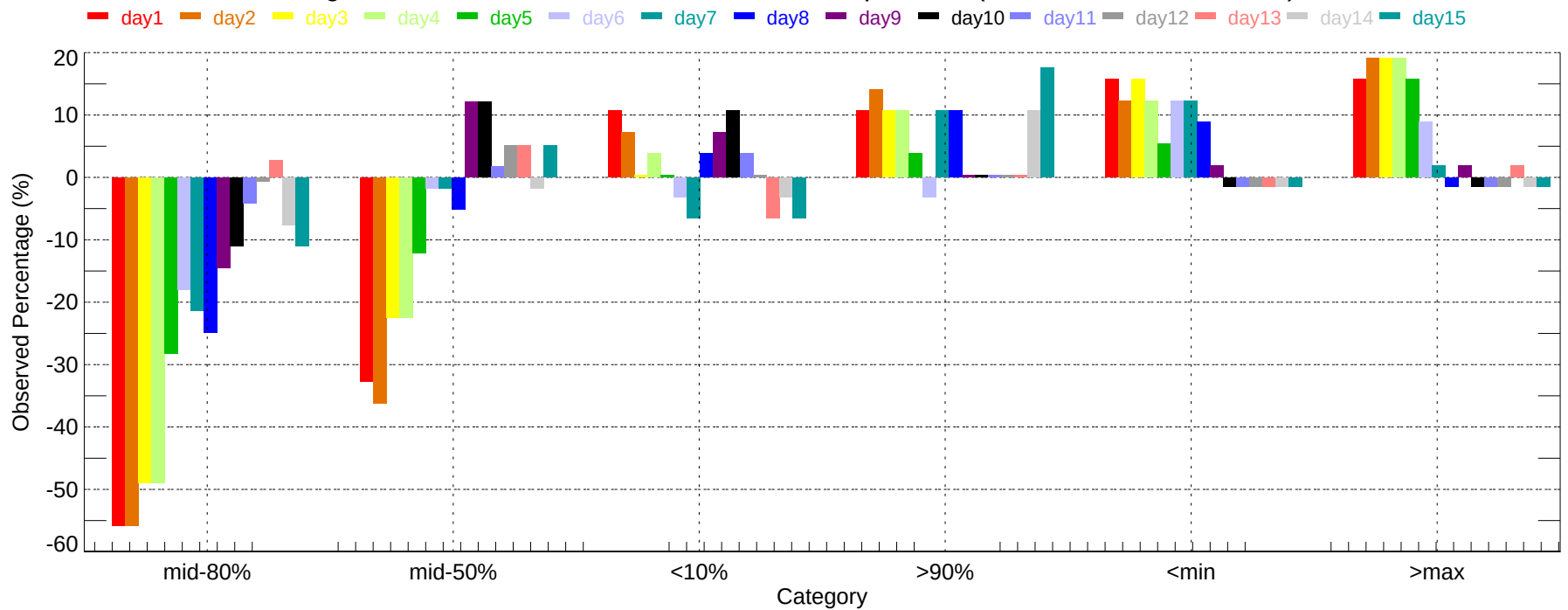
Observed Percentage Deviation of Ensembles - PDX: Min Temperature (2007-11-01~2007-11-30)
