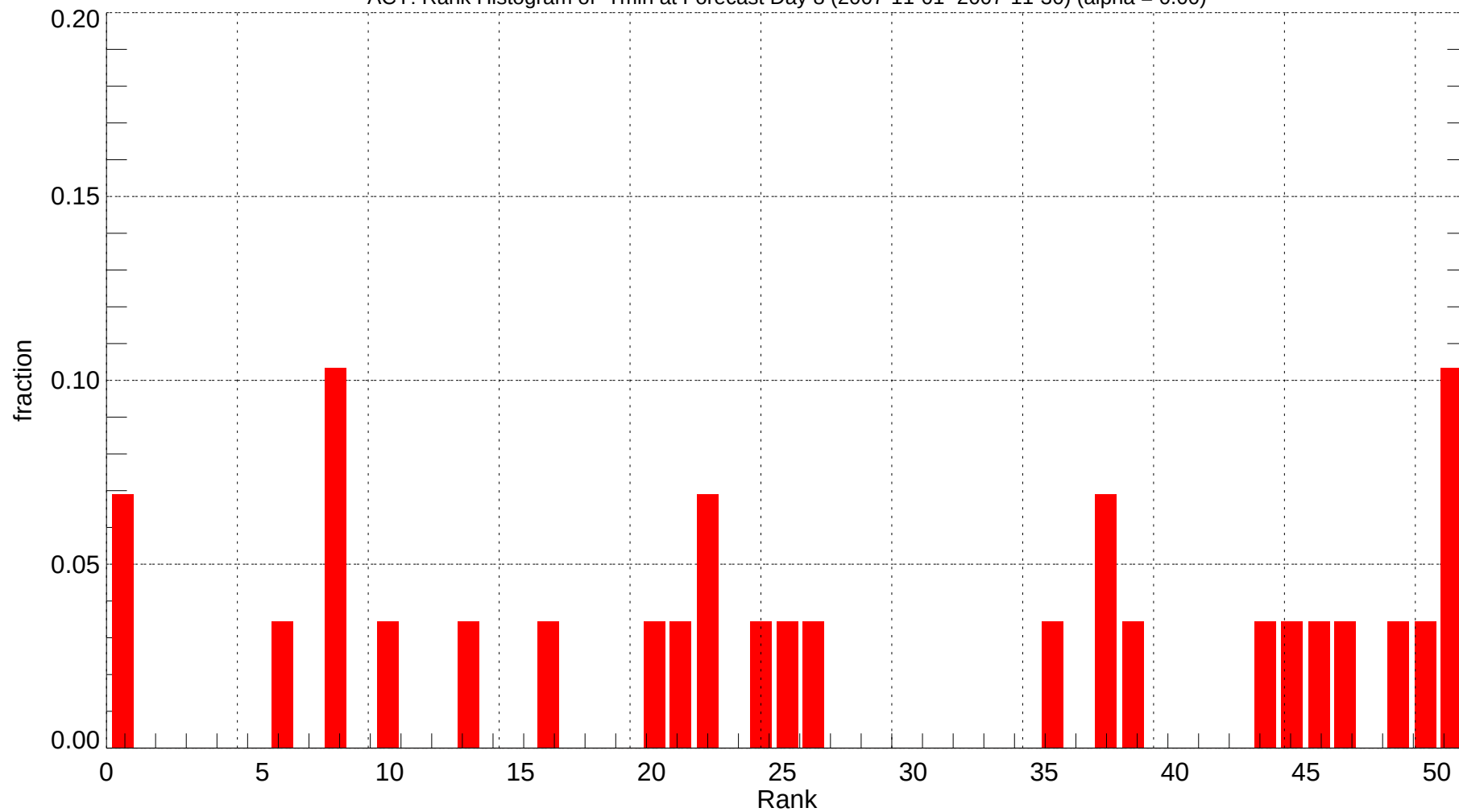
ACY: Rank Histogram of Tmin at Forecast Day 8 (2007-11-01~2007-11-30) (alpha = 0.00)
