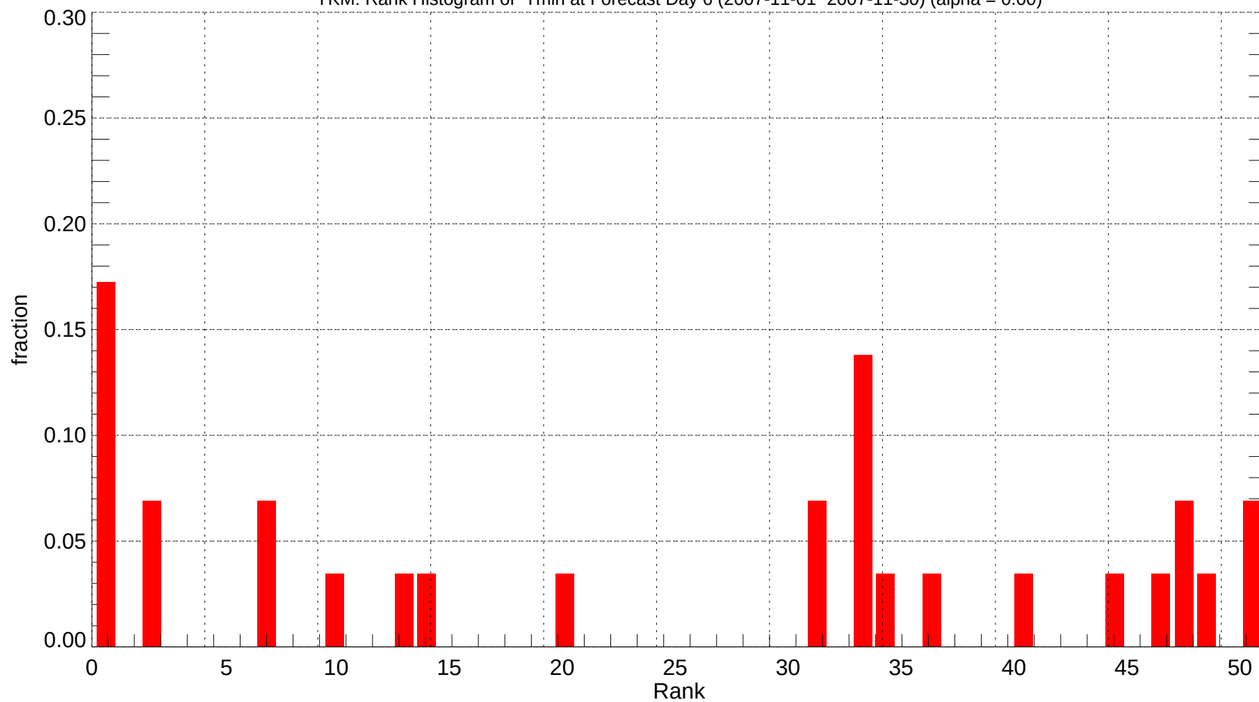
YKM: Rank Histogram of Tmin at Forecast Day 6 (2007-11-01~2007-11-30) (alpha = 0.00)
