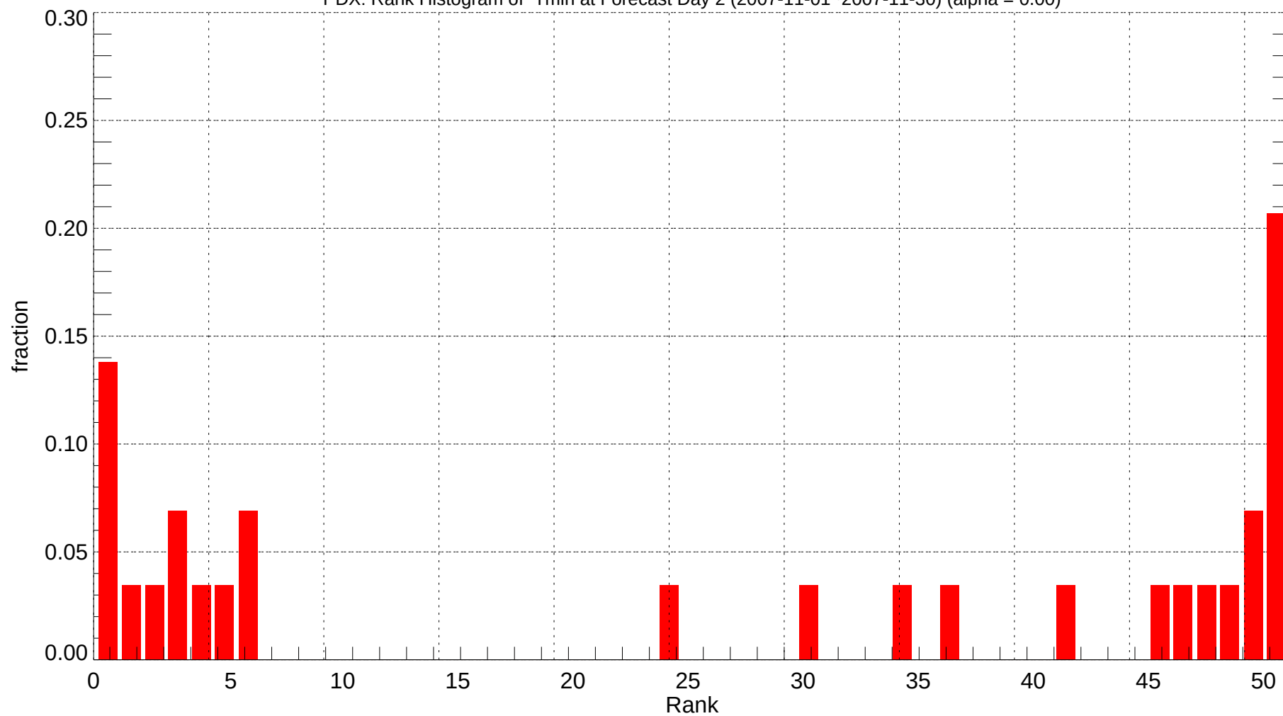
PDX: Rank Histogram of Tmin at Forecast Day 2 (2007-11-01~2007-11-30) (alpha = 0.00)
