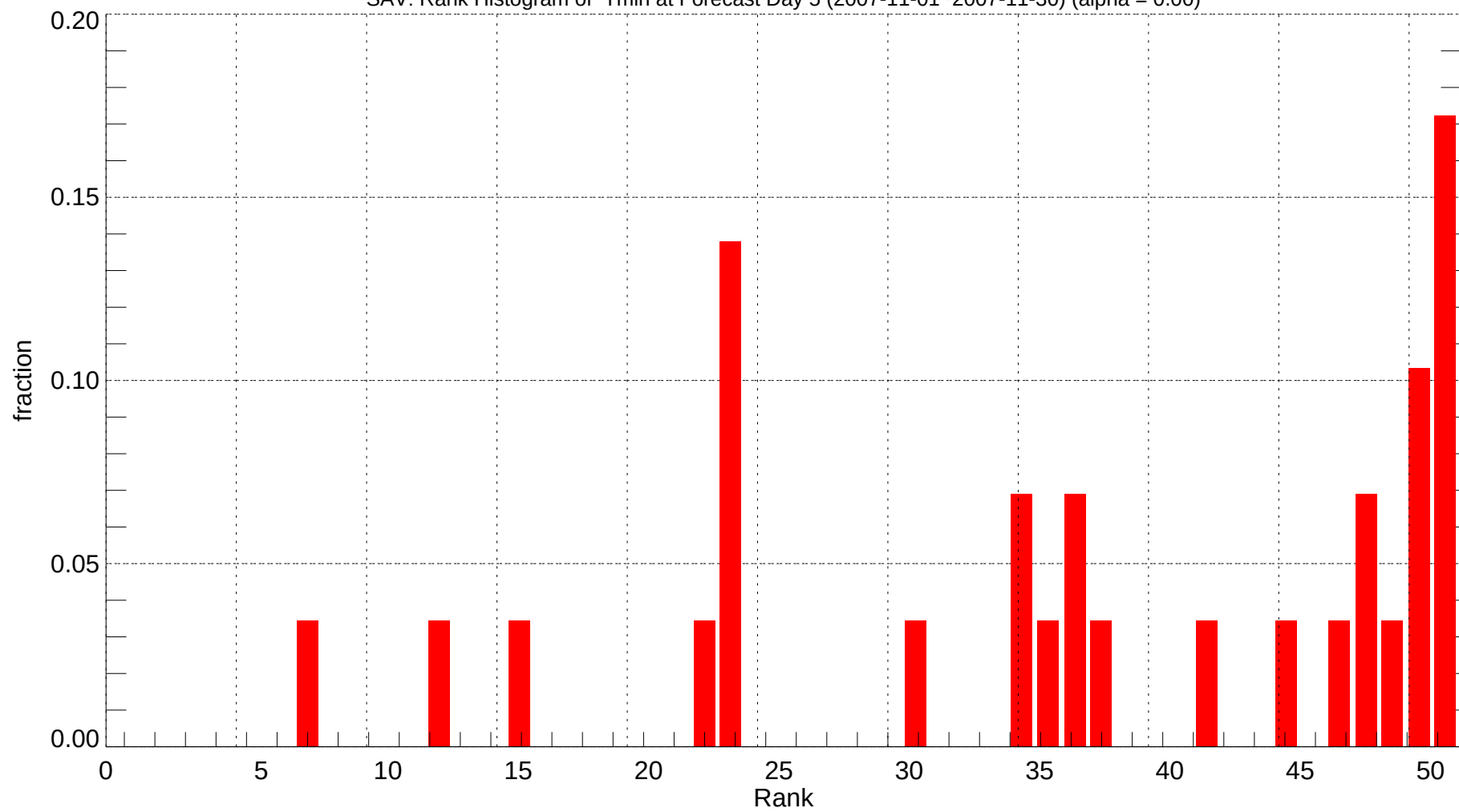
SAV: Rank Histogram of Tmin at Forecast Day 5 (2007-11-01~2007-11-30) (alpha = 0.00)
