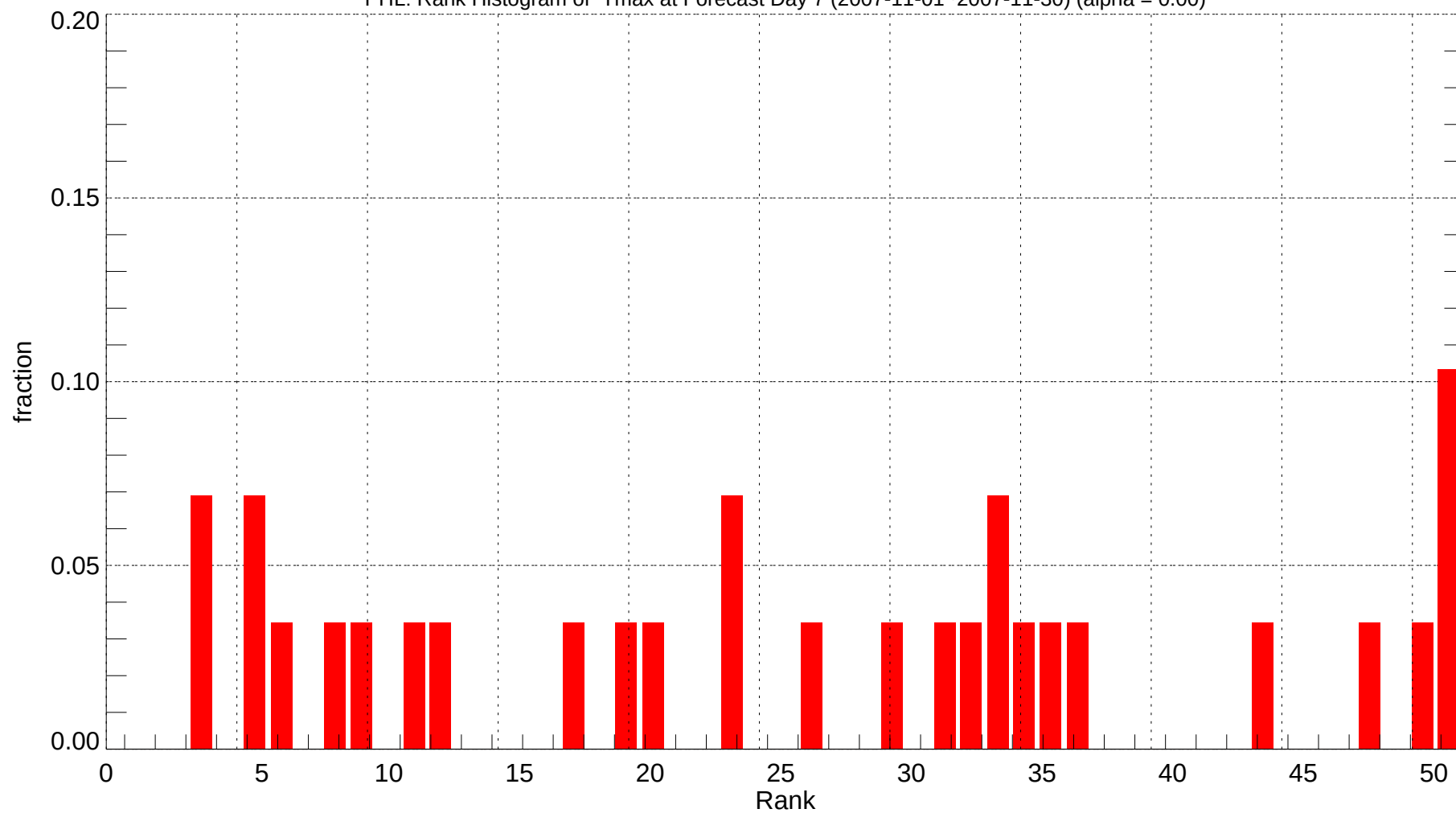
PHL: Rank Histogram of Tmax at Forecast Day 7 (2007-11-01~2007-11-30) (alpha = 0.00)
