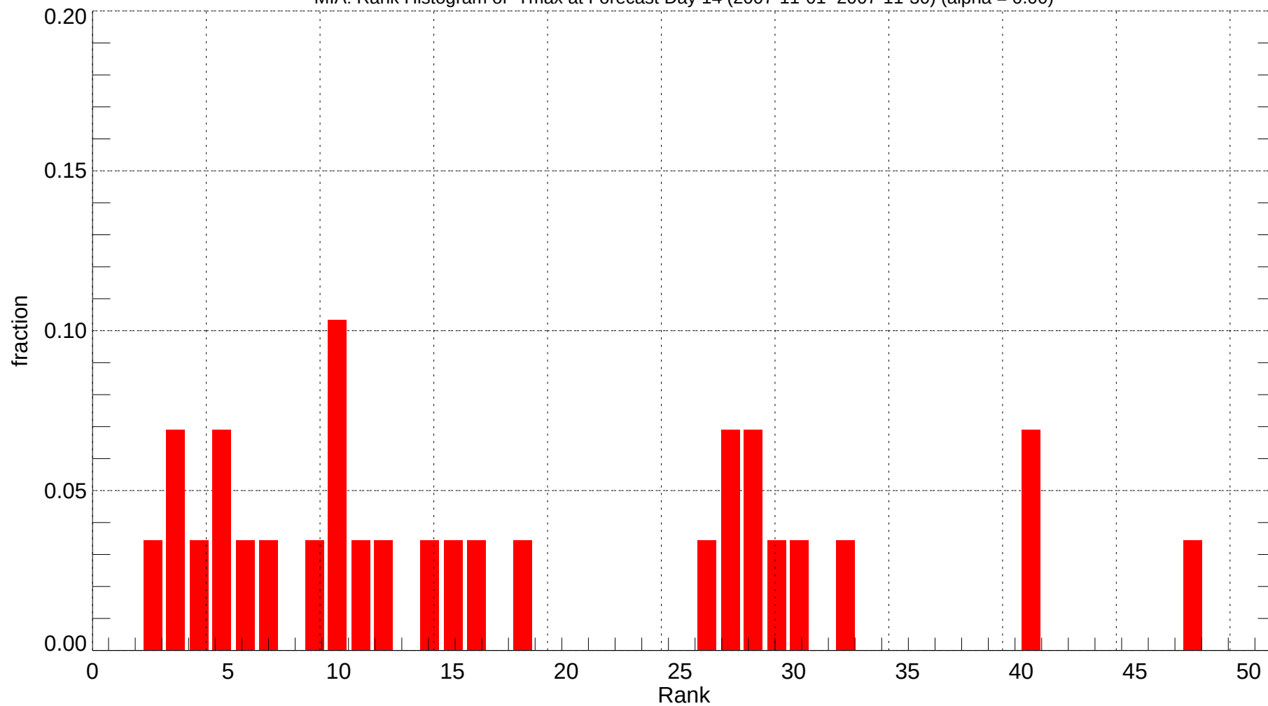
MIA: Rank Histogram of Tmax at Forecast Day 14 (2007-11-01~2007-11-30) (alpha = 0.00)
