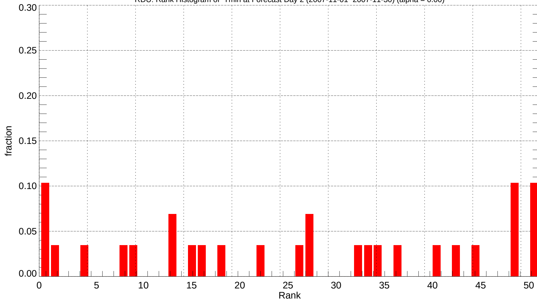
RDU: Rank Histogram of Tmin at Forecast Day 2 (2007-11-01~2007-11-30) (alpha = 0.00)
