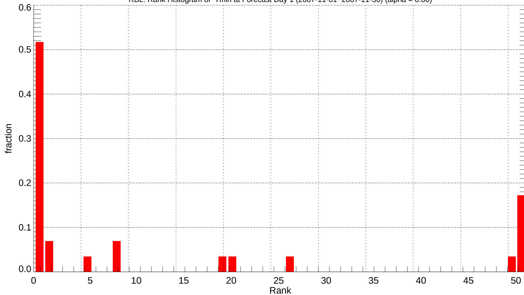
RBL: Rank Histogram of Tmin at Forecast Day 1 (2007-11-01~2007-11-30) (alpha = 0.00)
