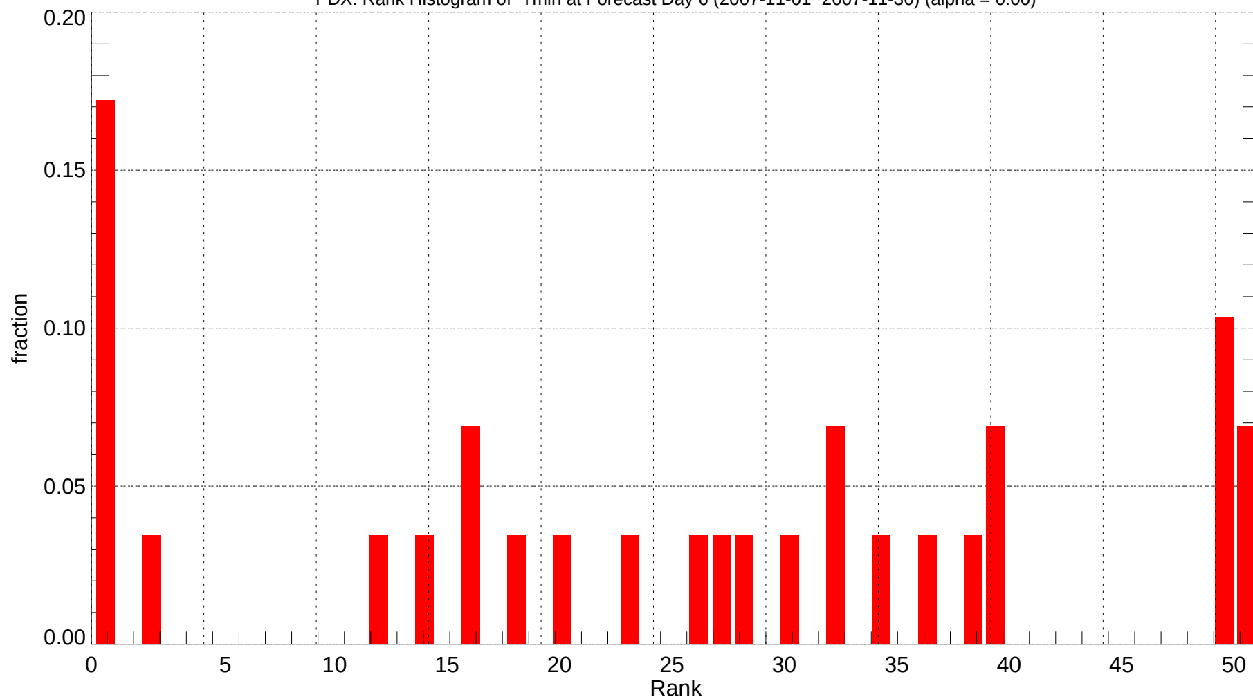
PDX: Rank Histogram of Tmin at Forecast Day 6 (2007-11-01~2007-11-30) (alpha = 0.00)
