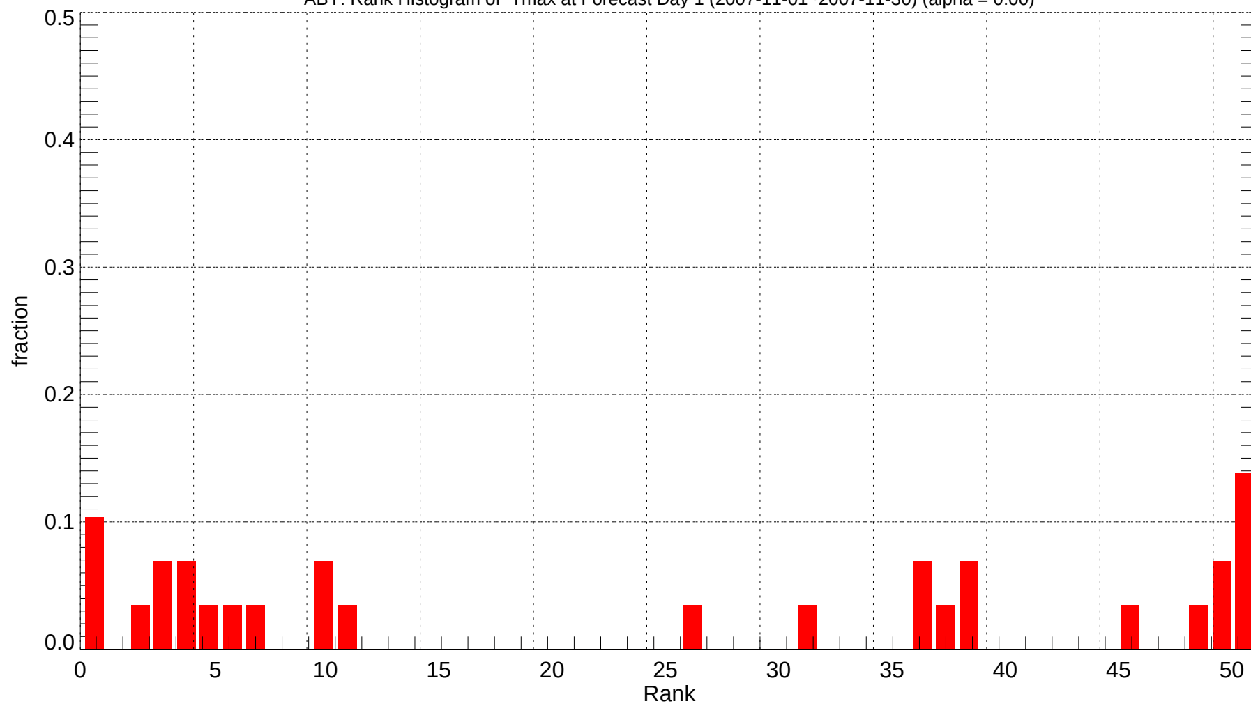
ABY: Rank Histogram of Tmax at Forecast Day 1 (2007-11-01~2007-11-30) (alpha = 0.00)
