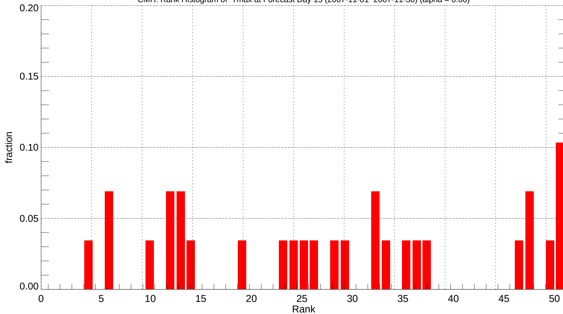
CMH: Rank Histogram of Tmax at Forecast Day 15 (2007-11-01~2007-11-30) (alpha = 0.00)
