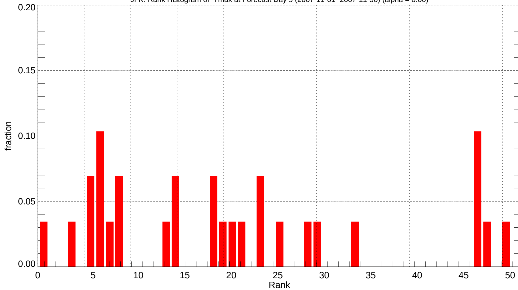
JFK: Rank Histogram of Tmax at Forecast Day 9 (2007-11-01~2007-11-30) (alpha = 0.00)
