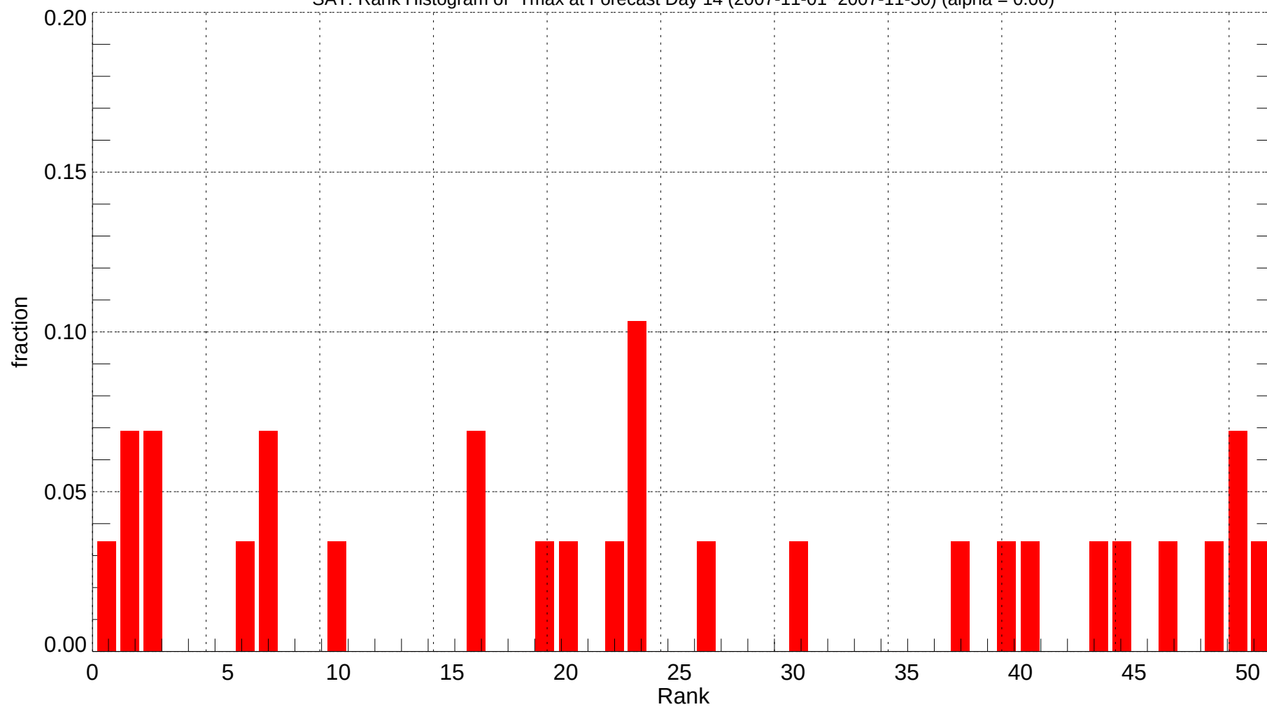
SAT: Rank Histogram of Tmax at Forecast Day 14 (2007-11-01~2007-11-30) (alpha = 0.00)
