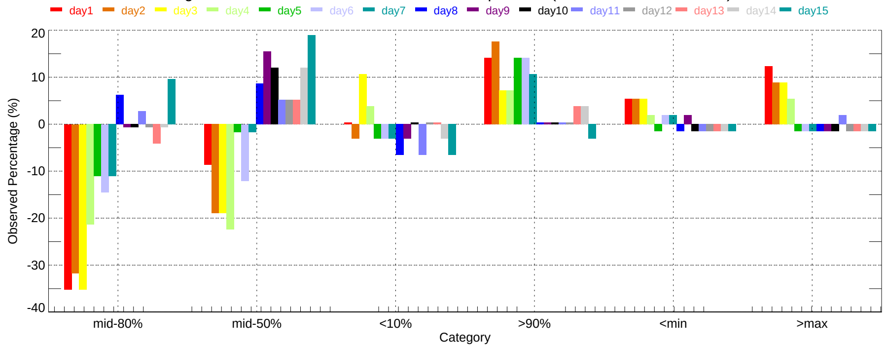
Observed Percentage Deviation of Ensembles - BOI: Max Temperature (2007-11-01~2007-11-30)
