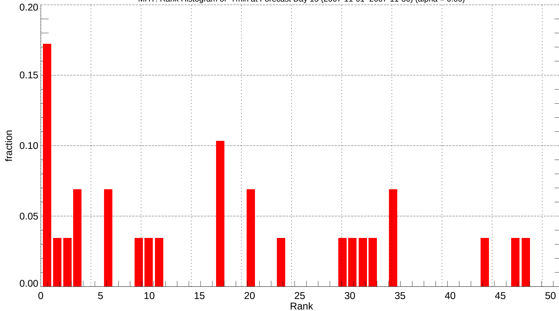
MHT: Rank Histogram of Tmin at Forecast Day 15 (2007-11-01~2007-11-30) (alpha = 0.00)
