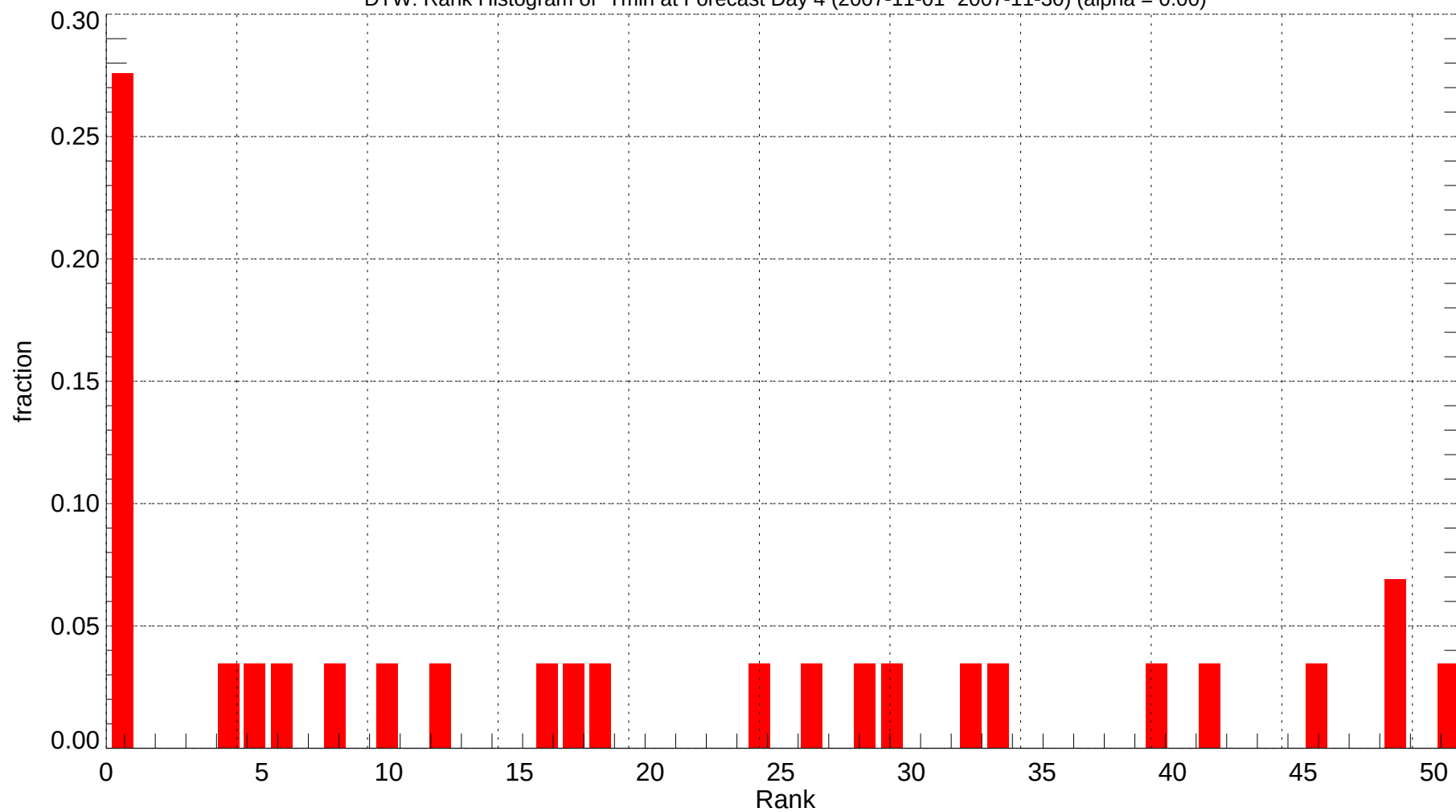
DTW: Rank Histogram of Tmin at Forecast Day 4 (2007-11-01~2007-11-30) (alpha = 0.00)
