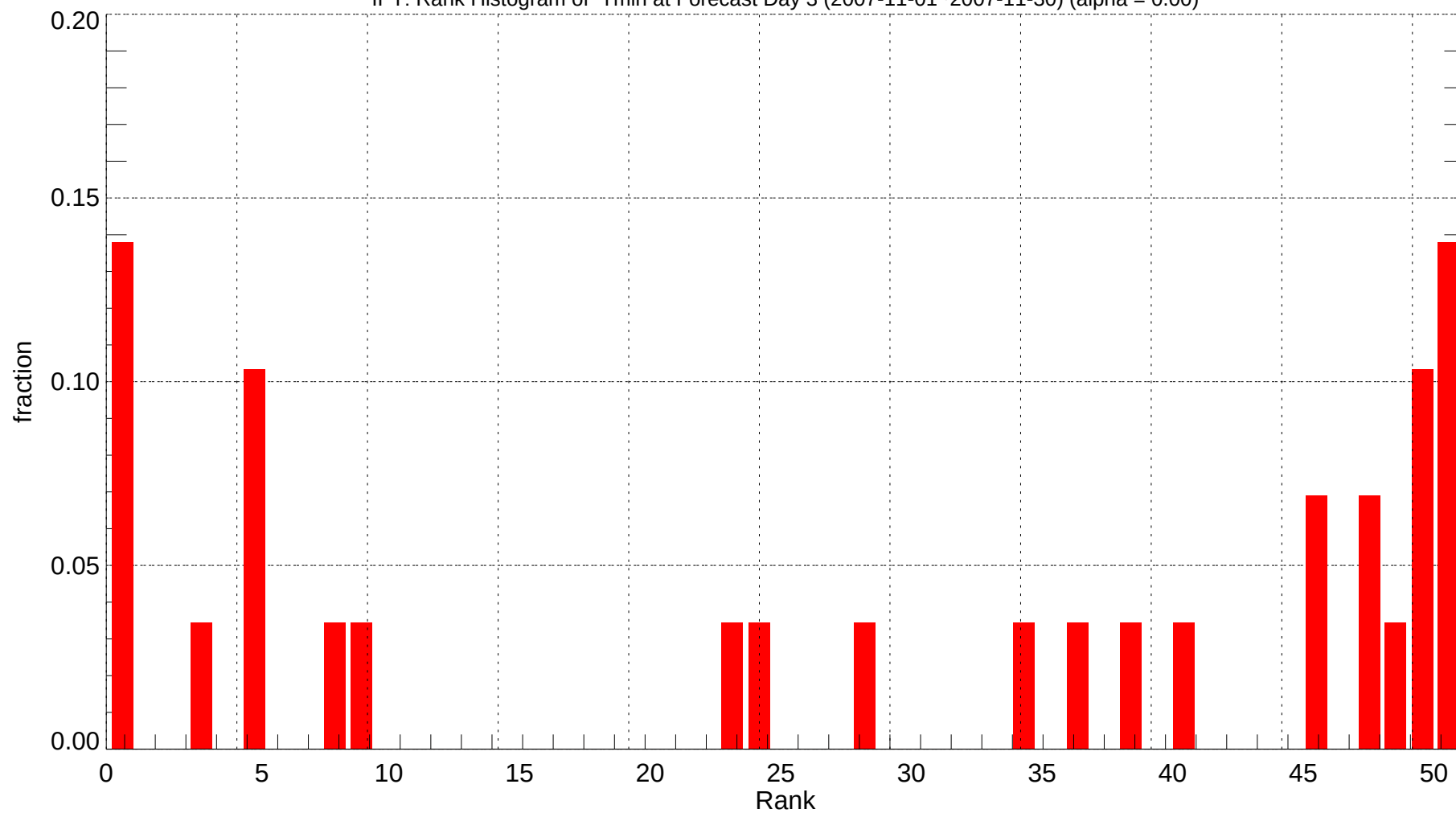
IPT: Rank Histogram of Tmin at Forecast Day 3 (2007-11-01~2007-11-30) (alpha = 0.00)
