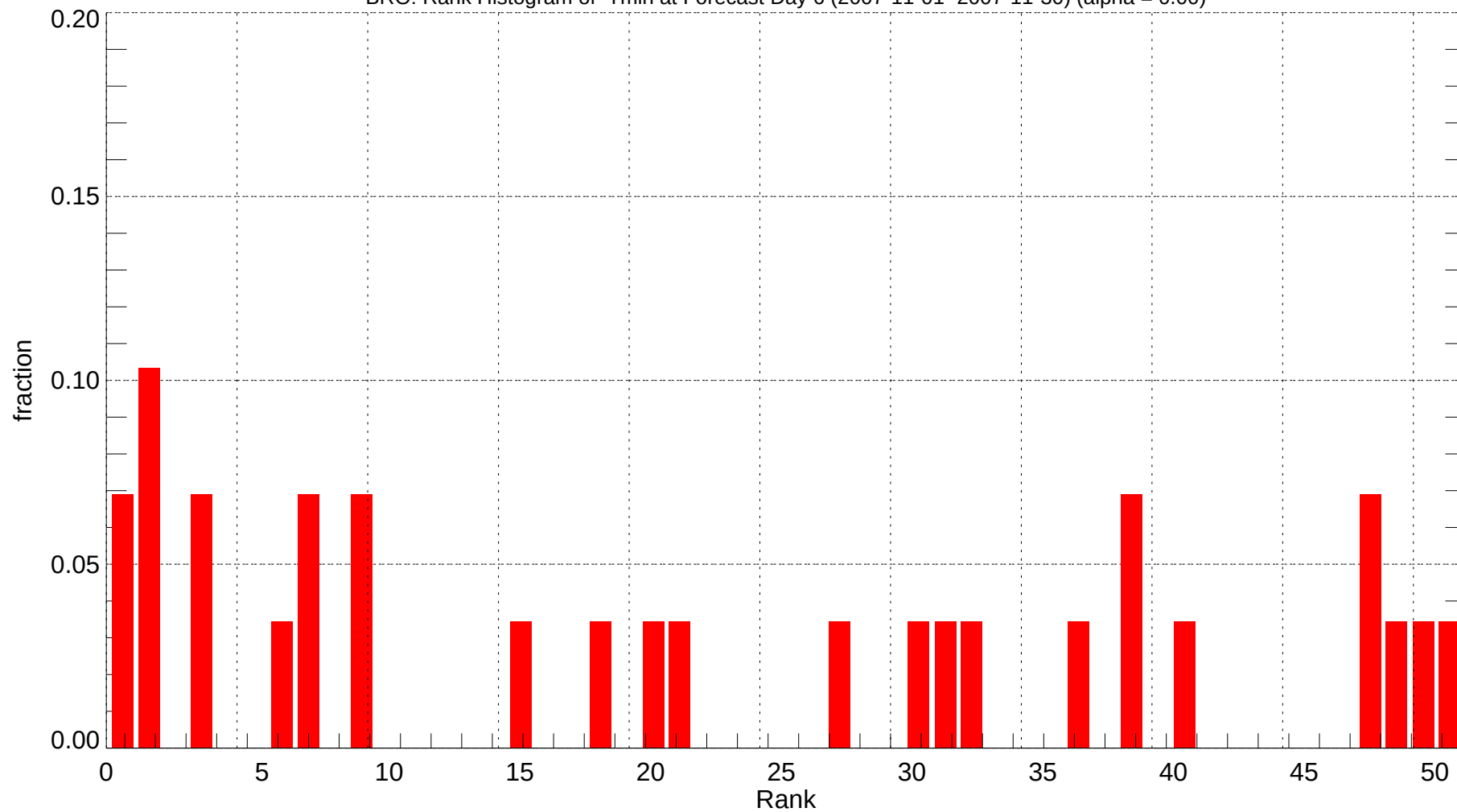
BRO: Rank Histogram of Tmin at Forecast Day 6 (2007-11-01~2007-11-30) (alpha = 0.00)
