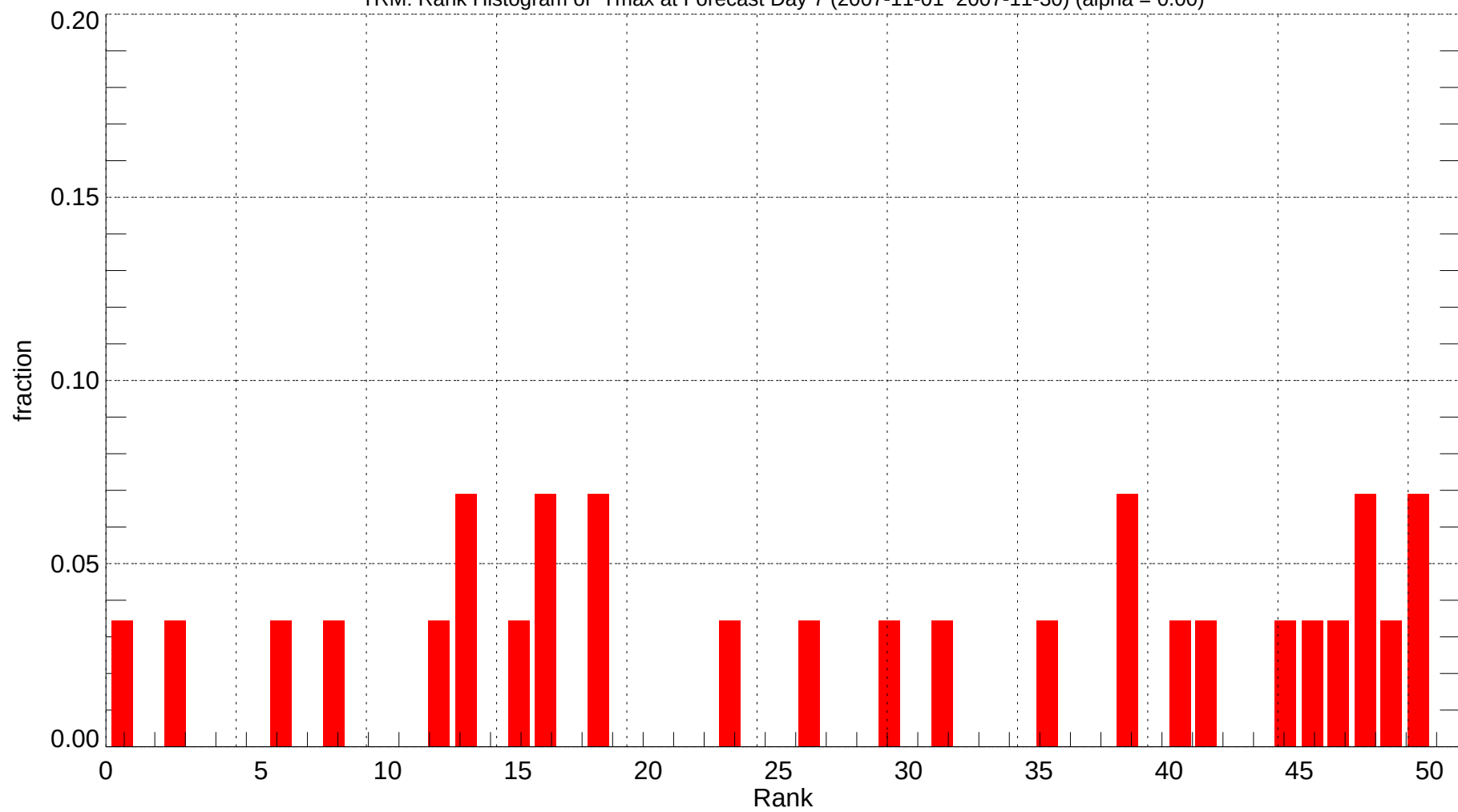
TRM: Rank Histogram of Tmax at Forecast Day 7 (2007-11-01~2007-11-30) (alpha = 0.00)
