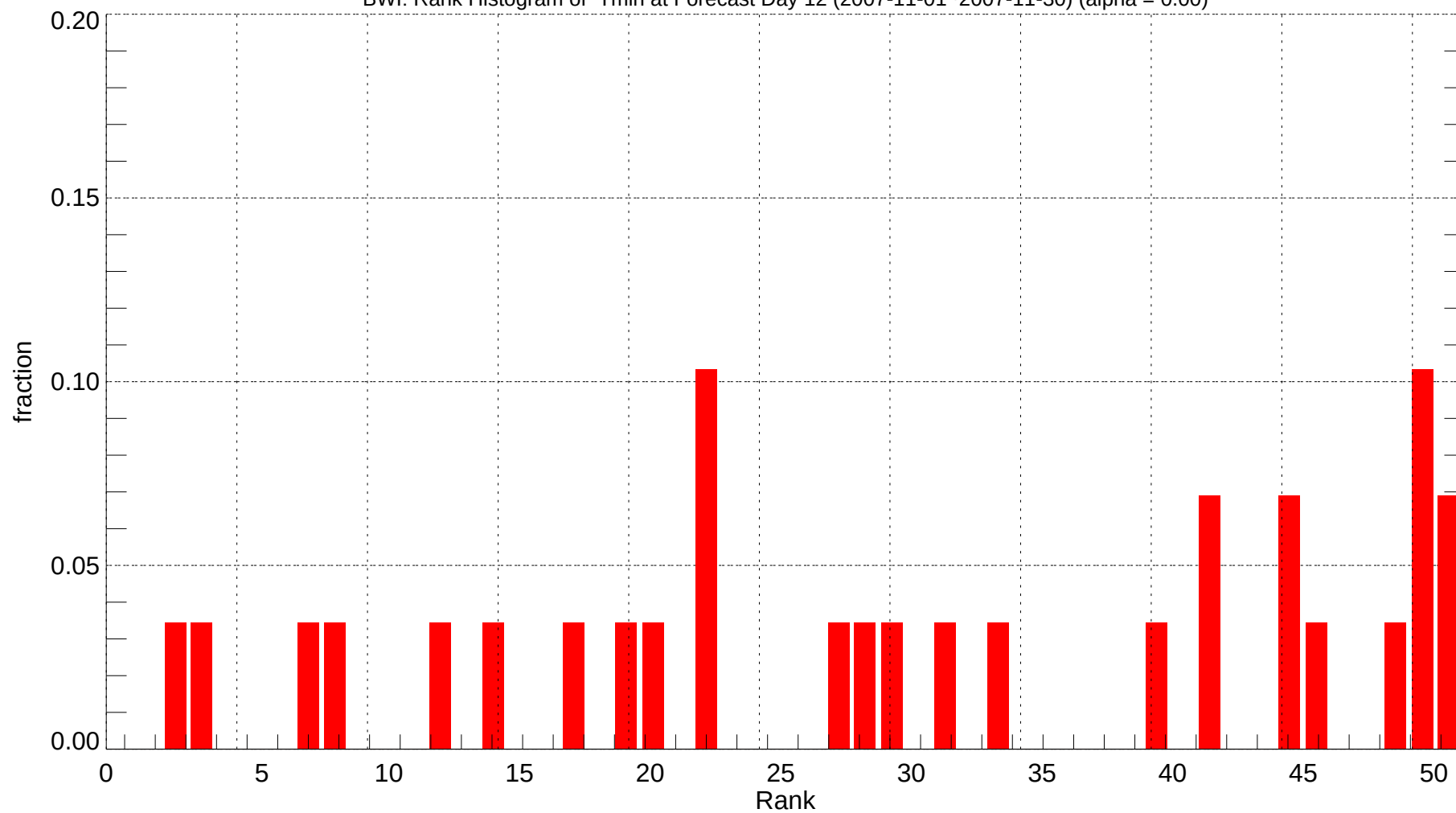
BWl: Rank Histogram of Tmin at Forecast Day 12 (2007-11-01~2007-11-30) (alpha = 0.00)
