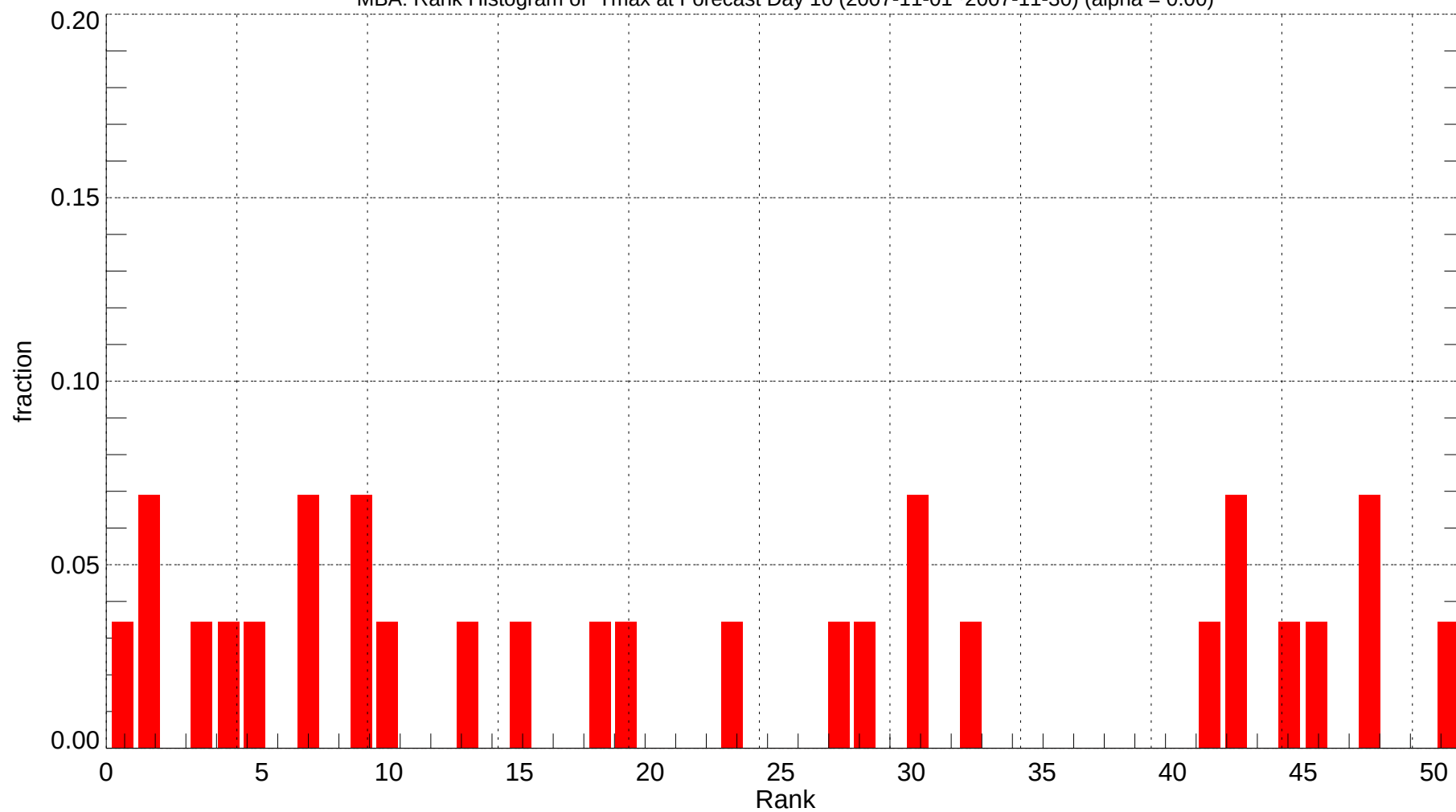
MBA: Rank Histogram of Tmax at Forecast Day 10 (2007-11-01~2007-11-30) (alpha = 0.00)
