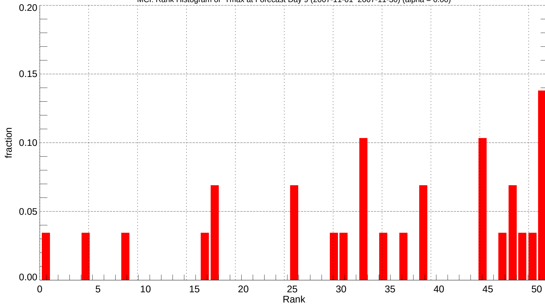
MCI: Rank Histogram of Tmax at Forecast Day 9 (2007-11-01~2007-11-30) (alpha = 0.00)
