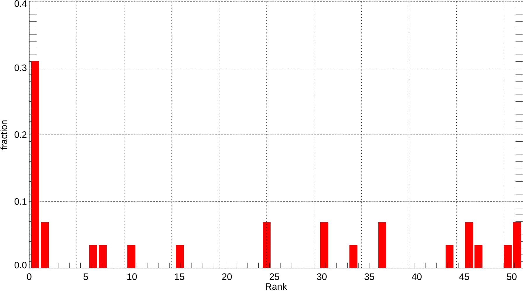
LFK: Rank Histogram of Tmin at Forecast Day 4 (2007-11-01~2007-11-30) (alpha = 0.00)
