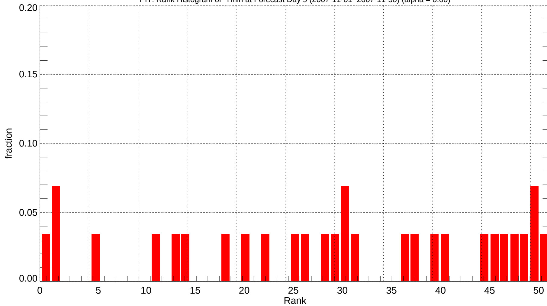
PIT: Rank Histogram of Tmin at Forecast Day 9 (2007-11-01~2007-11-30) (alpha = 0.00)
