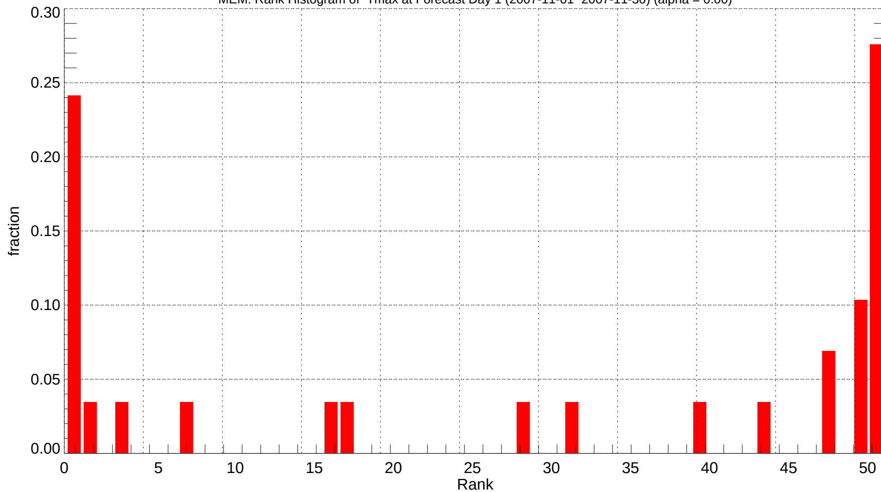
MEM: Rank Histogram of Tmax at Forecast Day 1 (2007-11-01~2007-11-30) (alpha = 0.00)
