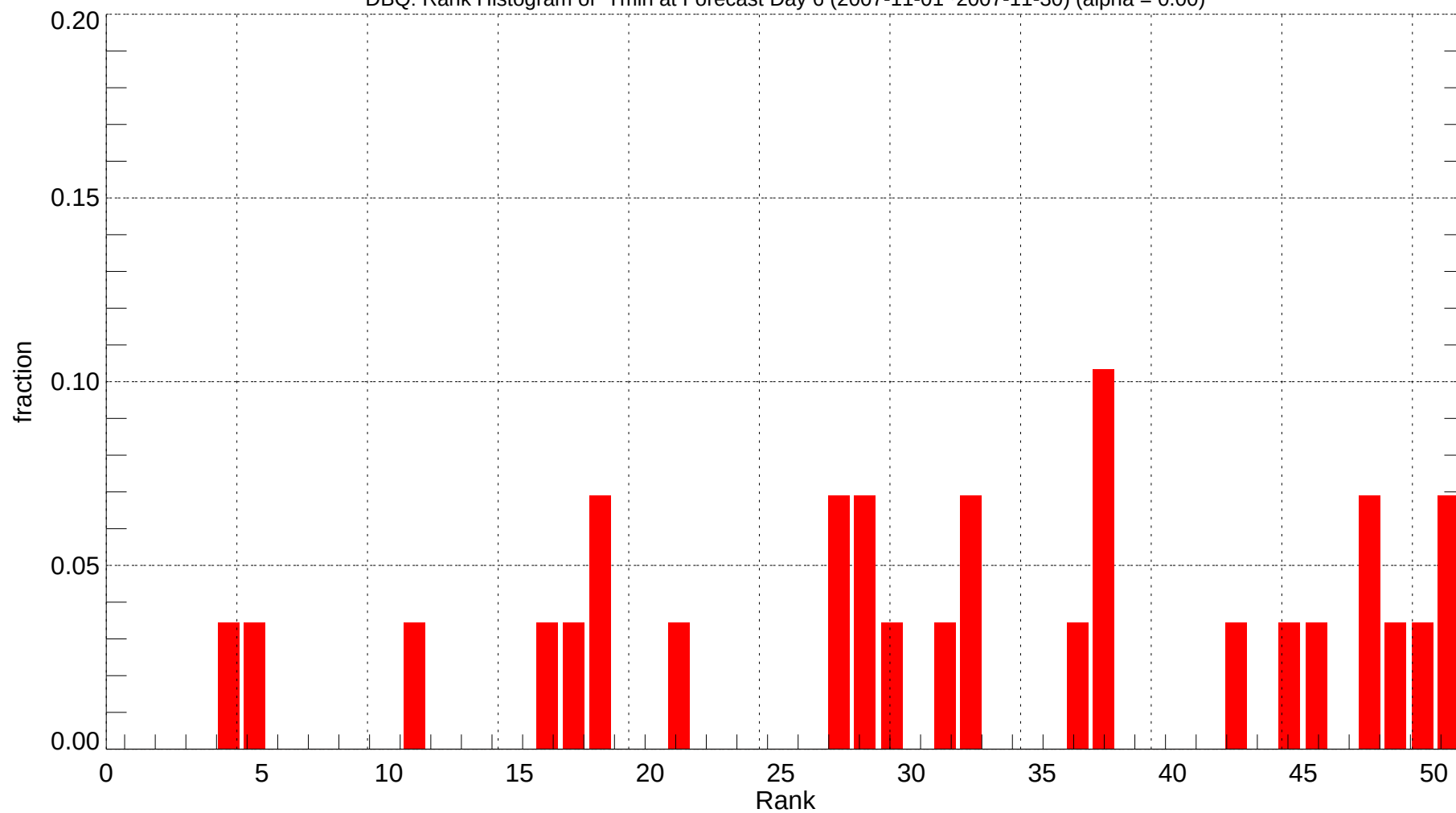
DBQ: Rank Histogram of Tmin at Forecast Day 6 (2007-11-01~2007-11-30) (alpha = 0.00)
