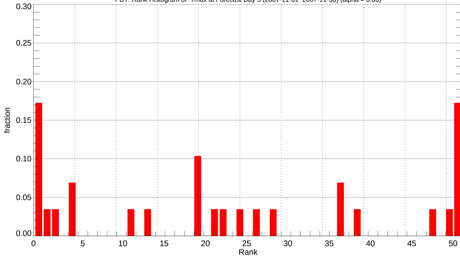
PDT: Rank Histogram of Tmax at Forecast Day 3 (2007-11-01~2007-11-30) (alpha = 0.00)
