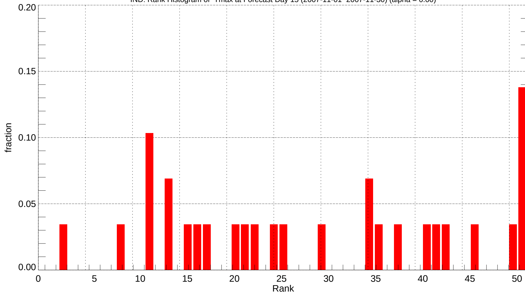
IND: Rank Histogram of Tmax at Forecast Day 15 (2007-11-01~2007-11-30) (alpha = 0.00)
