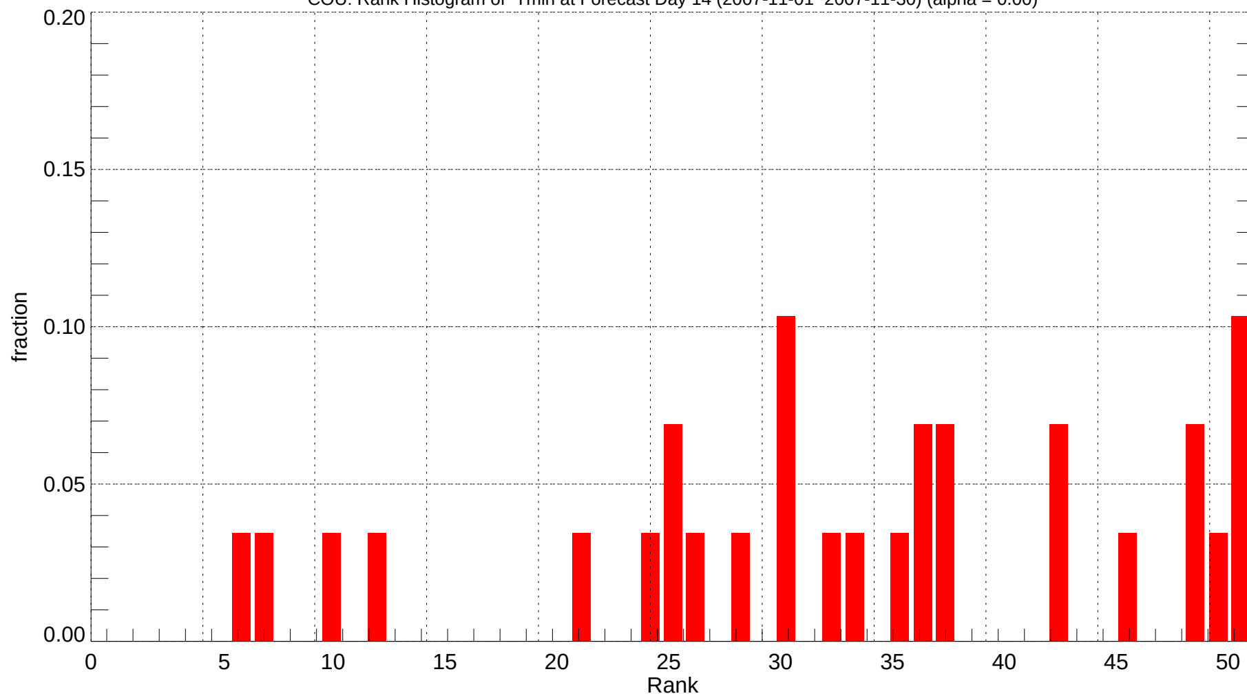
COU: Rank Histogram of Tmin at Forecast Day 14 (2007-11-01~2007-11-30) (alpha = 0.00)
