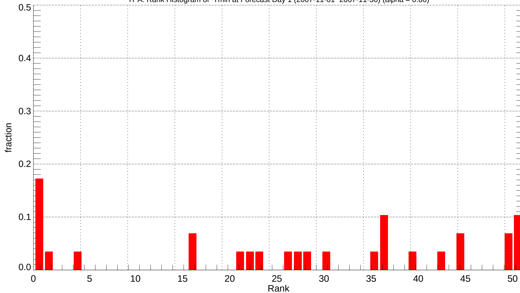
TPA: Rank Histogram of Tmin at Forecast Day 1 (2007-11-01~2007-11-30) (alpha = 0.00)
