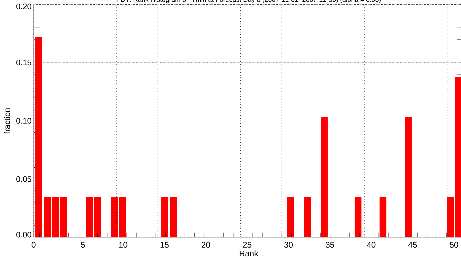
PDT: Rank Histogram of Tmin at Forecast Day 8 (2007-11-01~2007-11-30) (alpha = 0.00)
