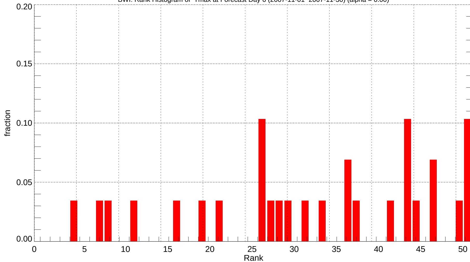
BWI: Rank Histogram of Tmax at Forecast Day 6 (2007-11-01~2007-11-30) (alpha = 0.00)
