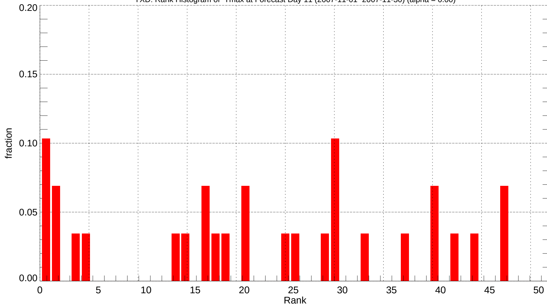
YXD: Rank Histogram of Tmax at Forecast Day 11 (2007-11-01~2007-11-30) (alpha = 0.00)
