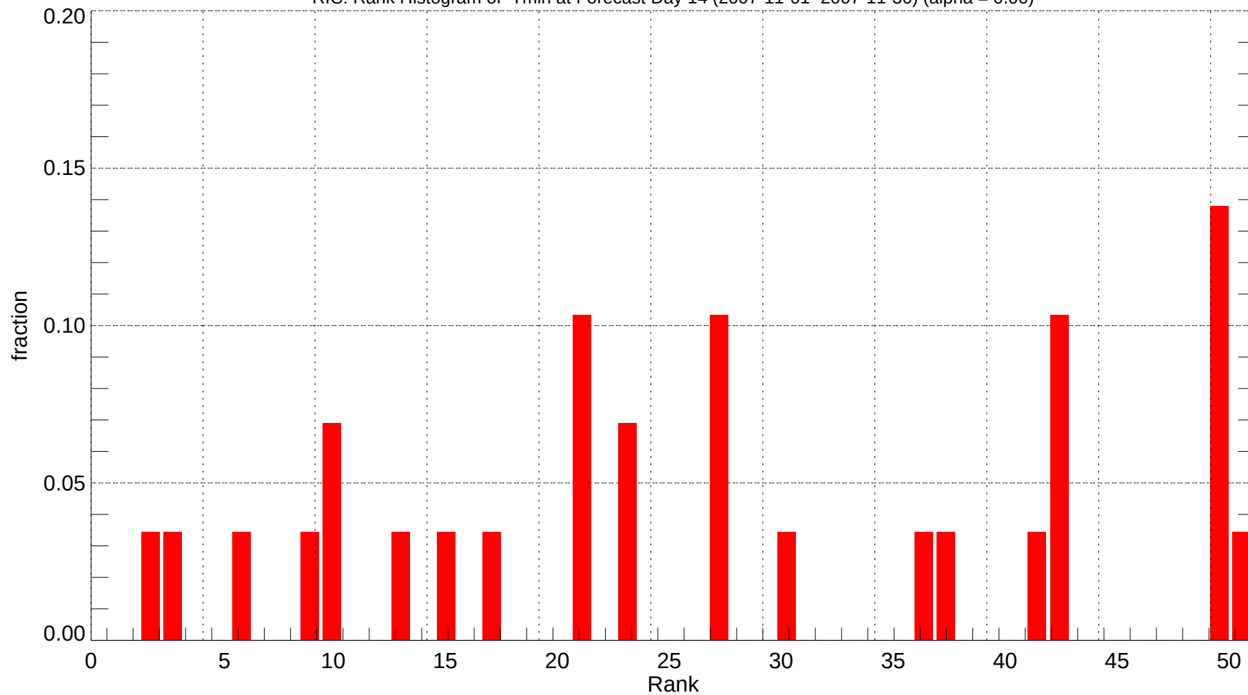
RIC: Rank Histogram of Tmin at Forecast Day 14 (2007-11-01~2007-11-30) (alpha = 0.00)
