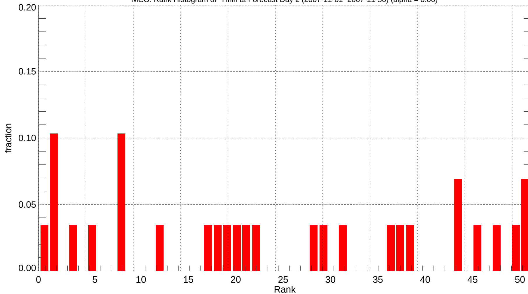
MCO: Rank Histogram of Tmin at Forecast Day 2 (2007-11-01~2007-11-30) (alpha = 0.00)
