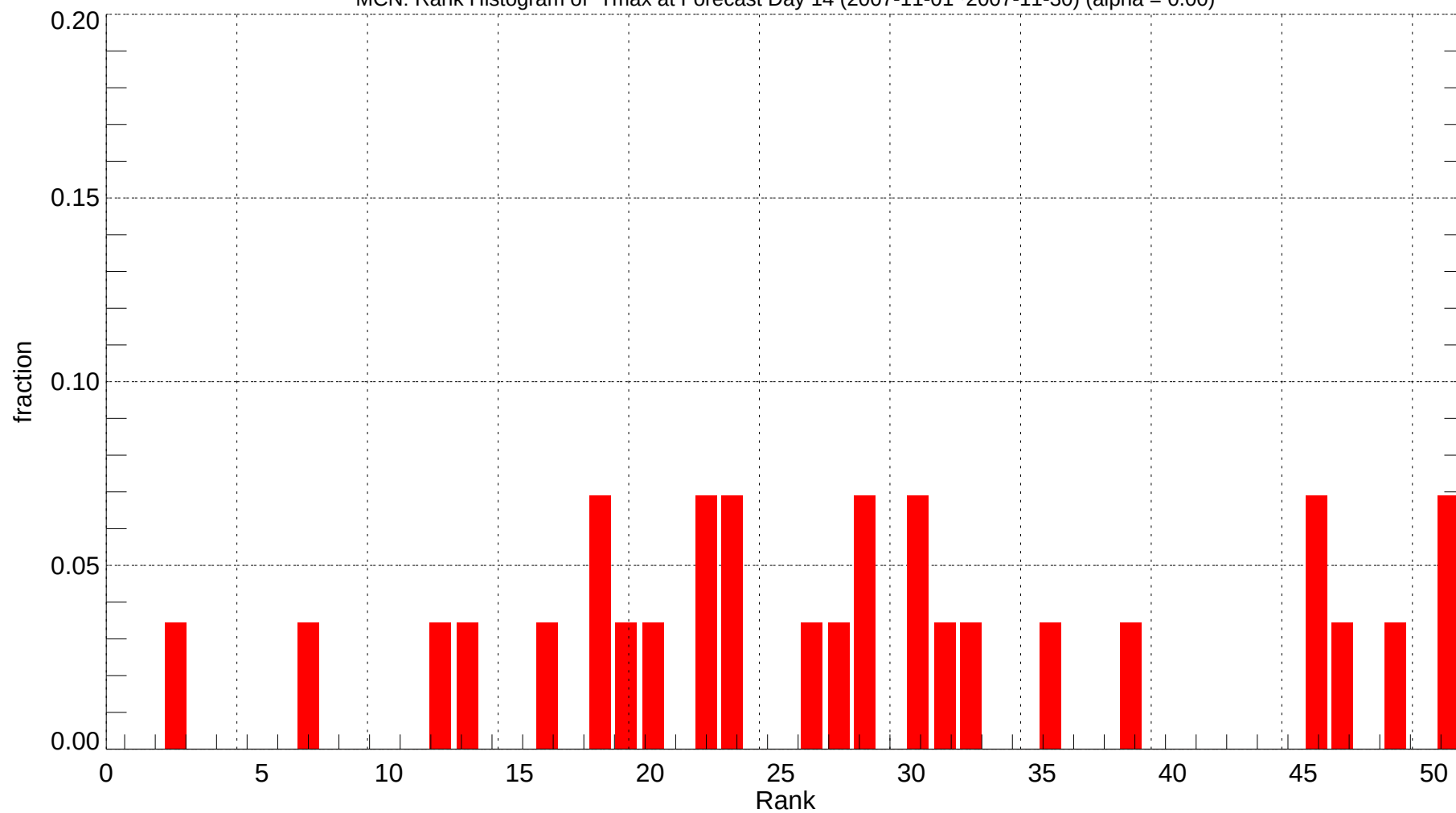
MCN: Rank Histogram of Tmax at Forecast Day 14 (2007-11-01~2007-11-30) (alpha = 0.00)
