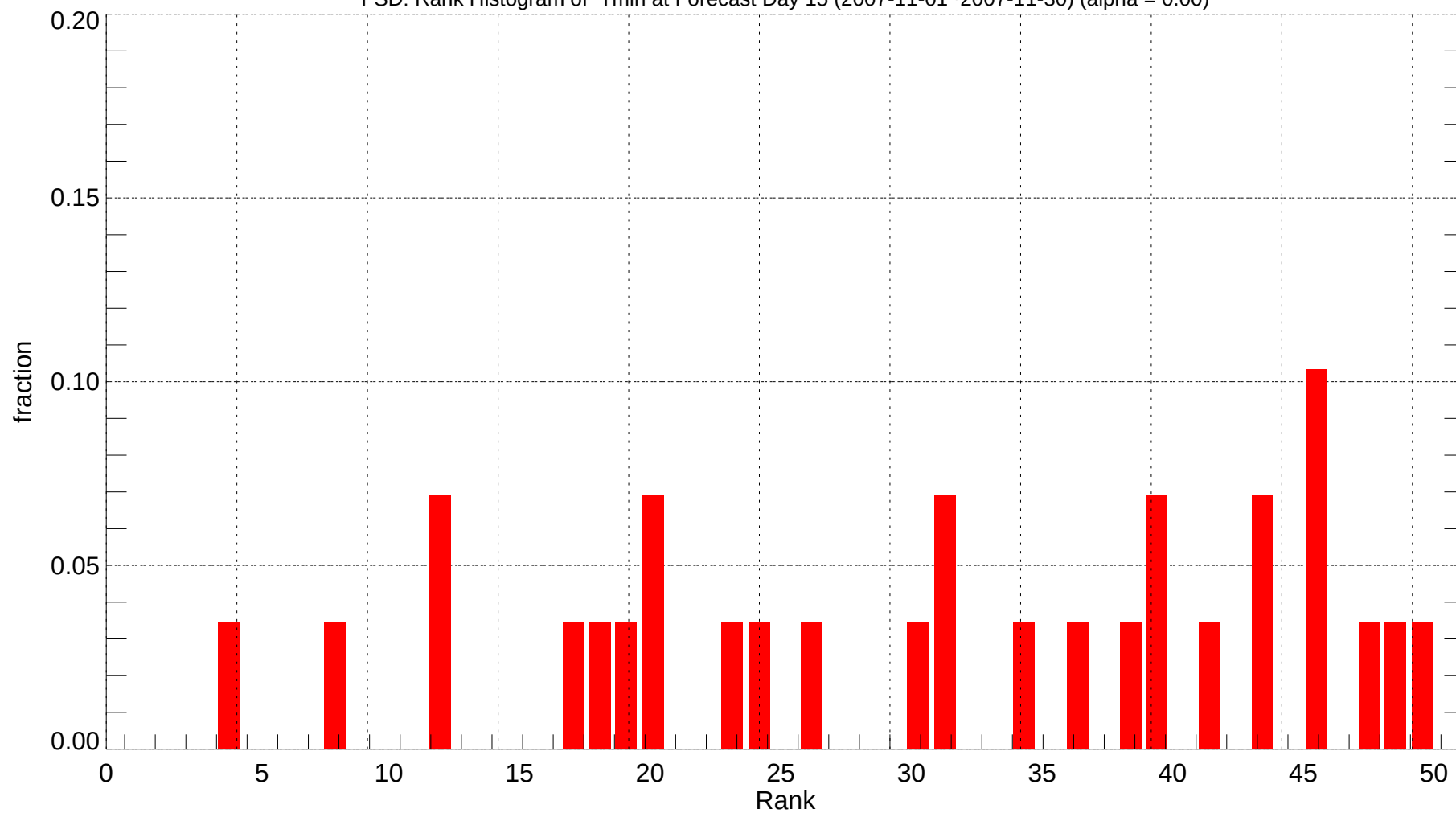
FSD: Rank Histogram of Tmin at Forecast Day 15 (2007-11-01~2007-11-30) (alpha = 0.00)
