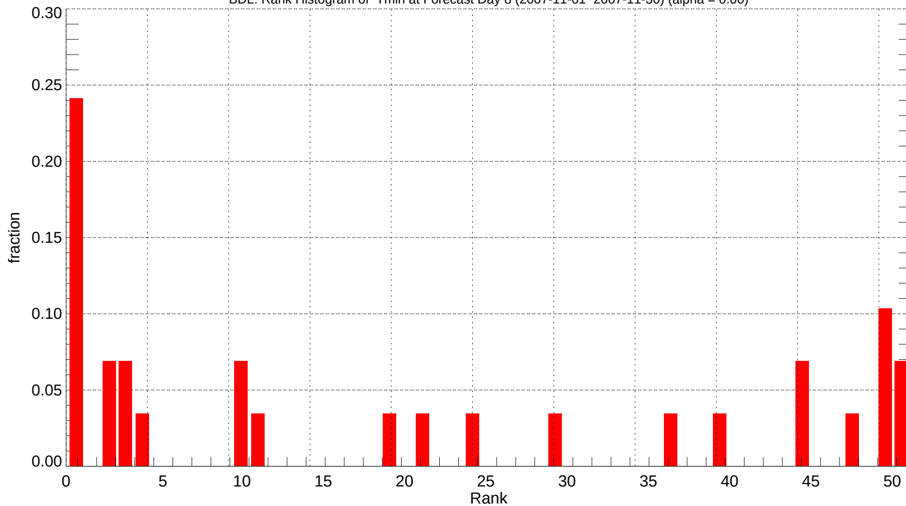
BDL: Rank Histogram of Tmin at Forecast Day 8 (2007-11-01~2007-11-30) (alpha = 0.00)
