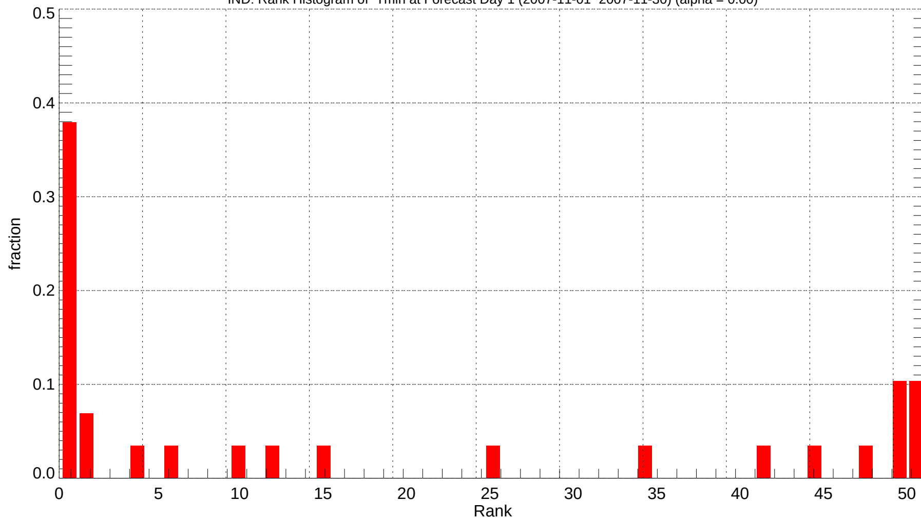
IND: Rank Histogram of Tmin at Forecast Day 1 (2007-11-01~2007-11-30) (alpha = 0.00)
