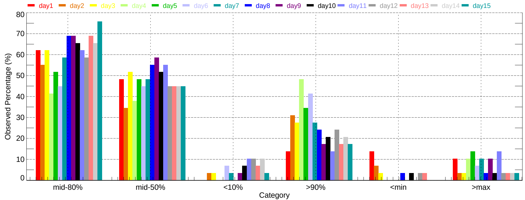
Observed Percentage of Ensembles - SAV: Max Temperature (2007-11-01~2007-11-30)
