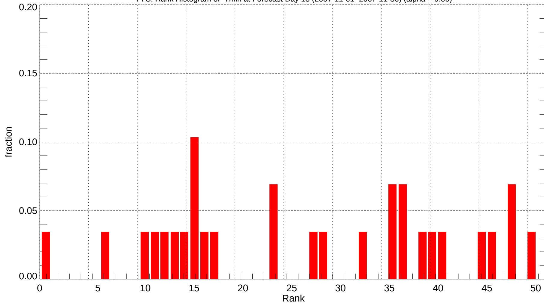
YYC: Rank Histogram of Tmin at Forecast Day 13 (2007-11-01~2007-11-30) (alpha = 0.00)
