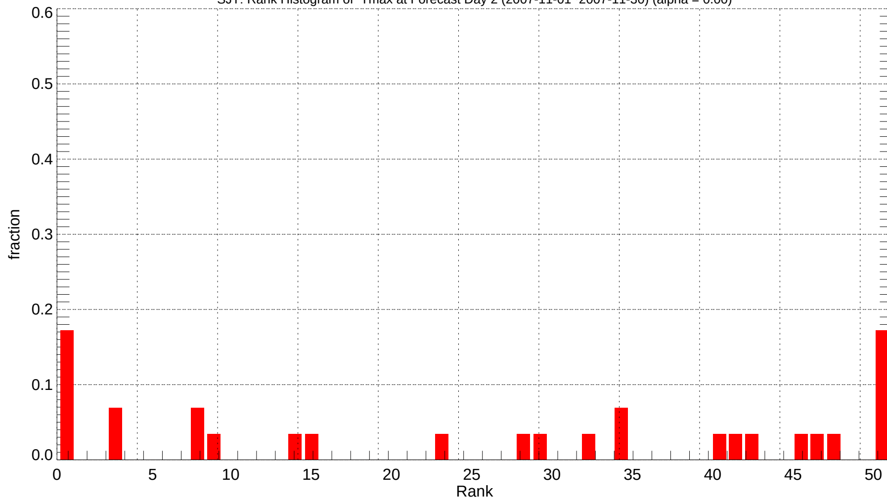
SJT: Rank Histogram of Tmax at Forecast Day 2 (2007-11-01~2007-11-30) (alpha = 0.00)
