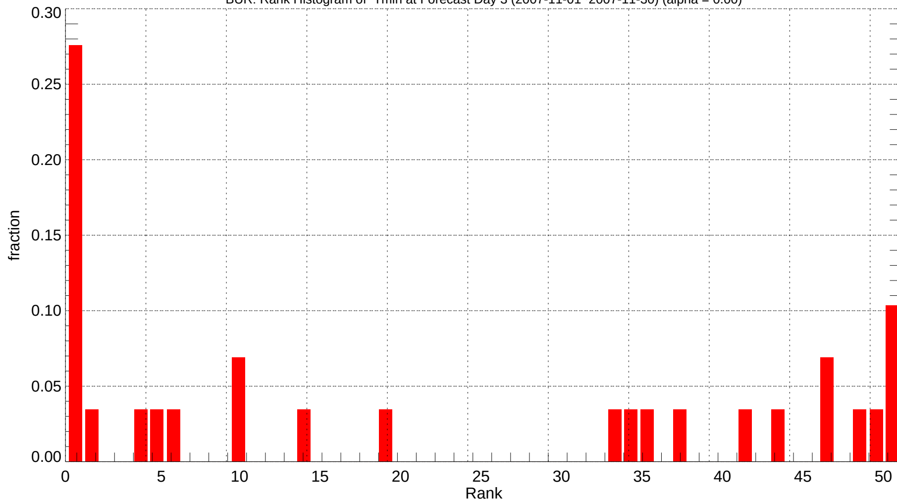
BUR: Rank Histogram of Tmin at Forecast Day 3 (2007-11-01~2007-11-30) (alpha = 0.00)
