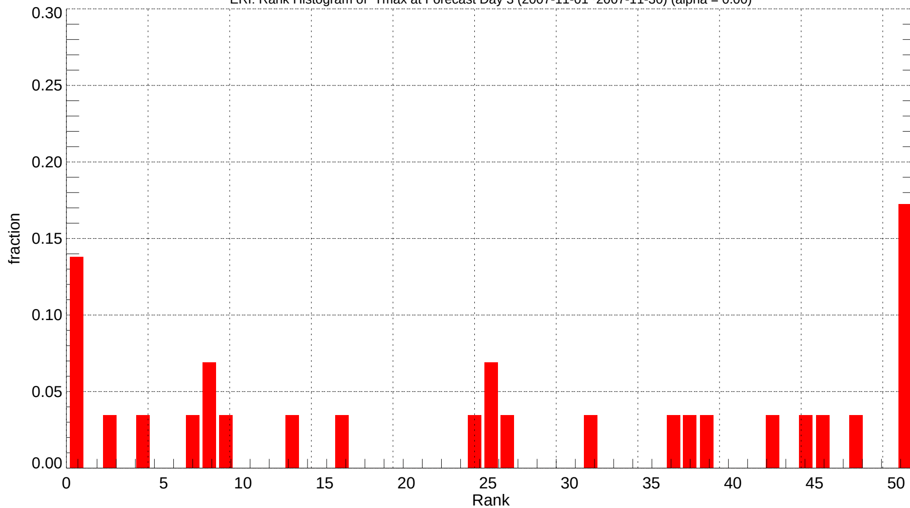
ERI: Rank Histogram of Tmax at Forecast Day 3 (2007-11-01~2007-11-30) (alpha = 0.00)
