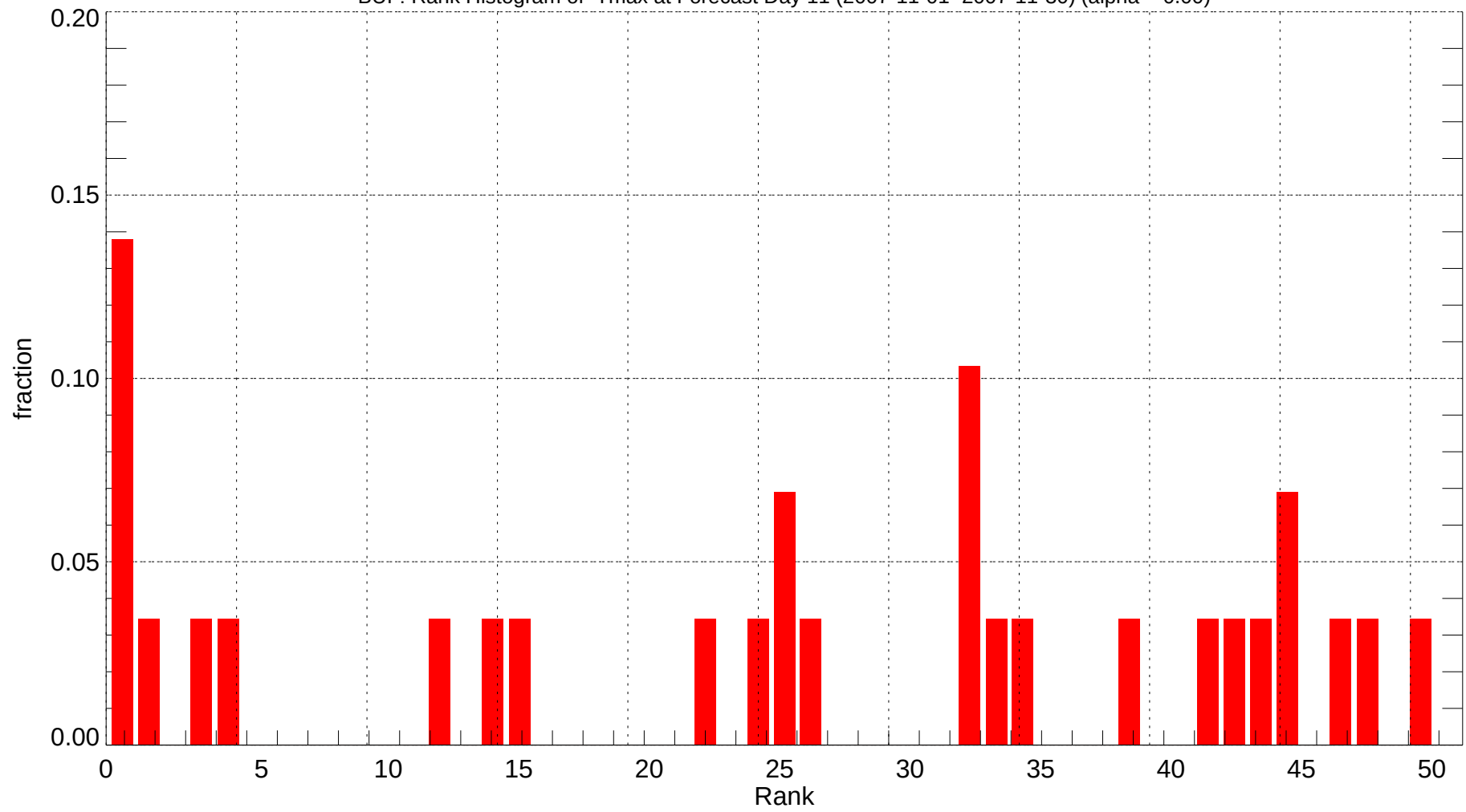
BUF: Rank Histogram of Tmax at Forecast Day 11 (2007-11-01~2007-11-30) (alpha = 0.00)
