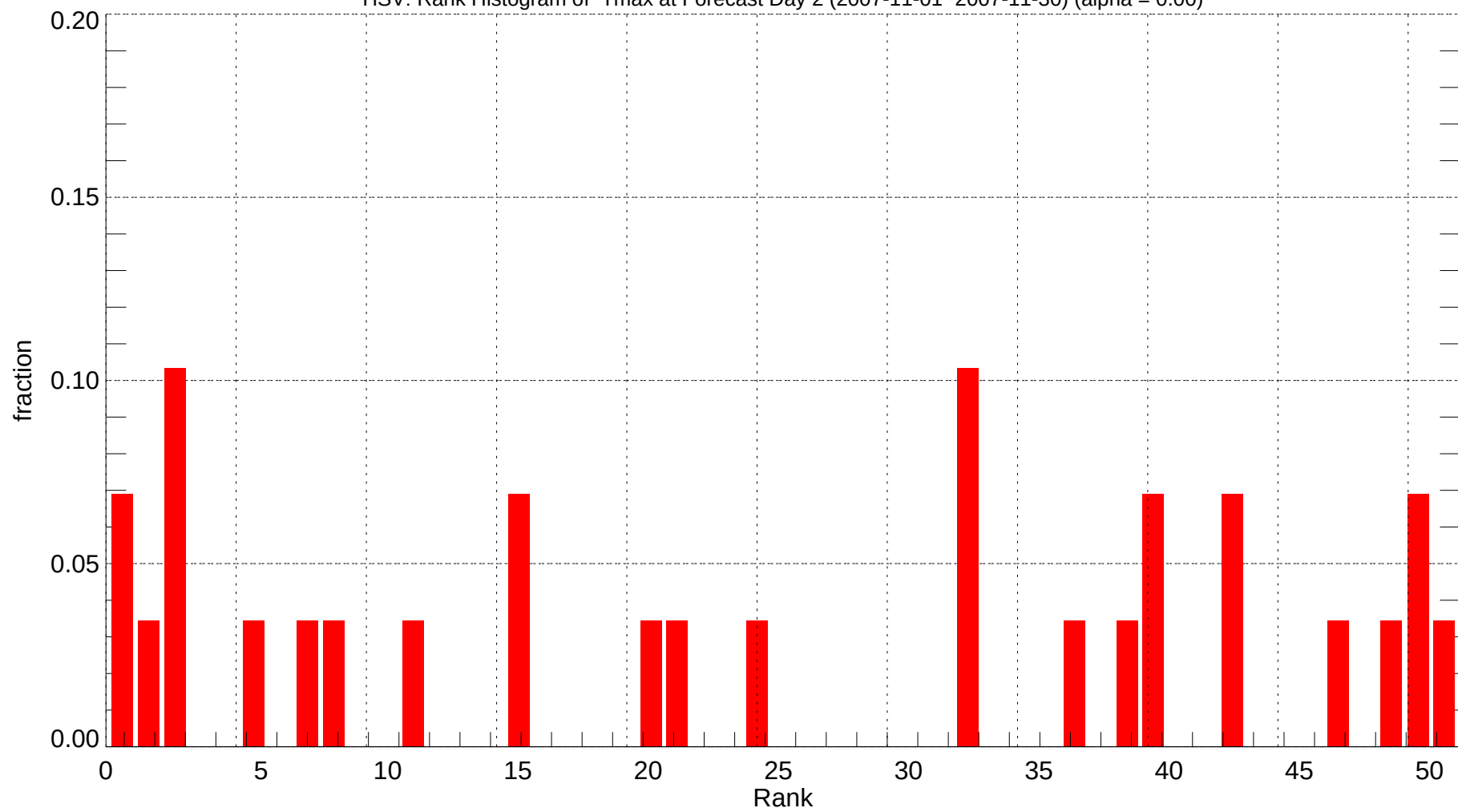
HSV: Rank Histogram of Tmax at Forecast Day 2 (2007-11-01~2007-11-30) (alpha = 0.00)
