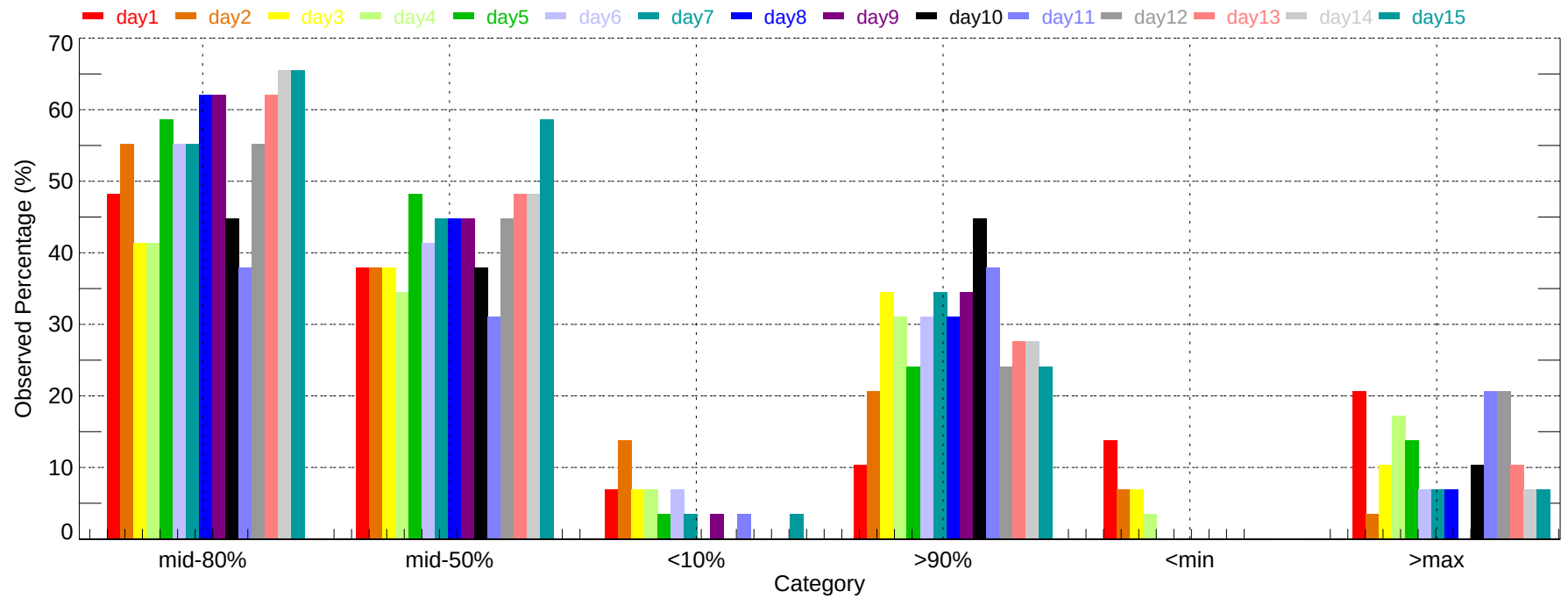
Observed Percentage of Ensembles - HSV: Min Temperature (2007-11-01~2007-11-30)
