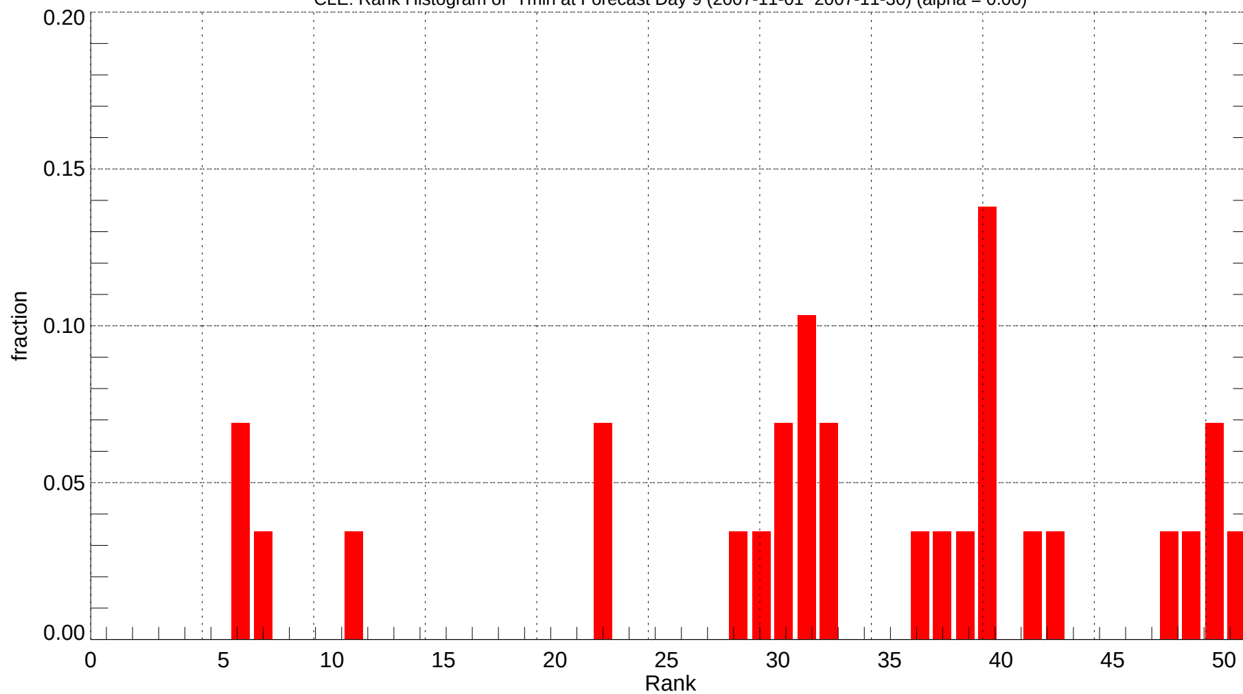
CLE: Rank Histogram of Tmin at Forecast Day 9 (2007-11-01~2007-11-30) (alpha = 0.00)
