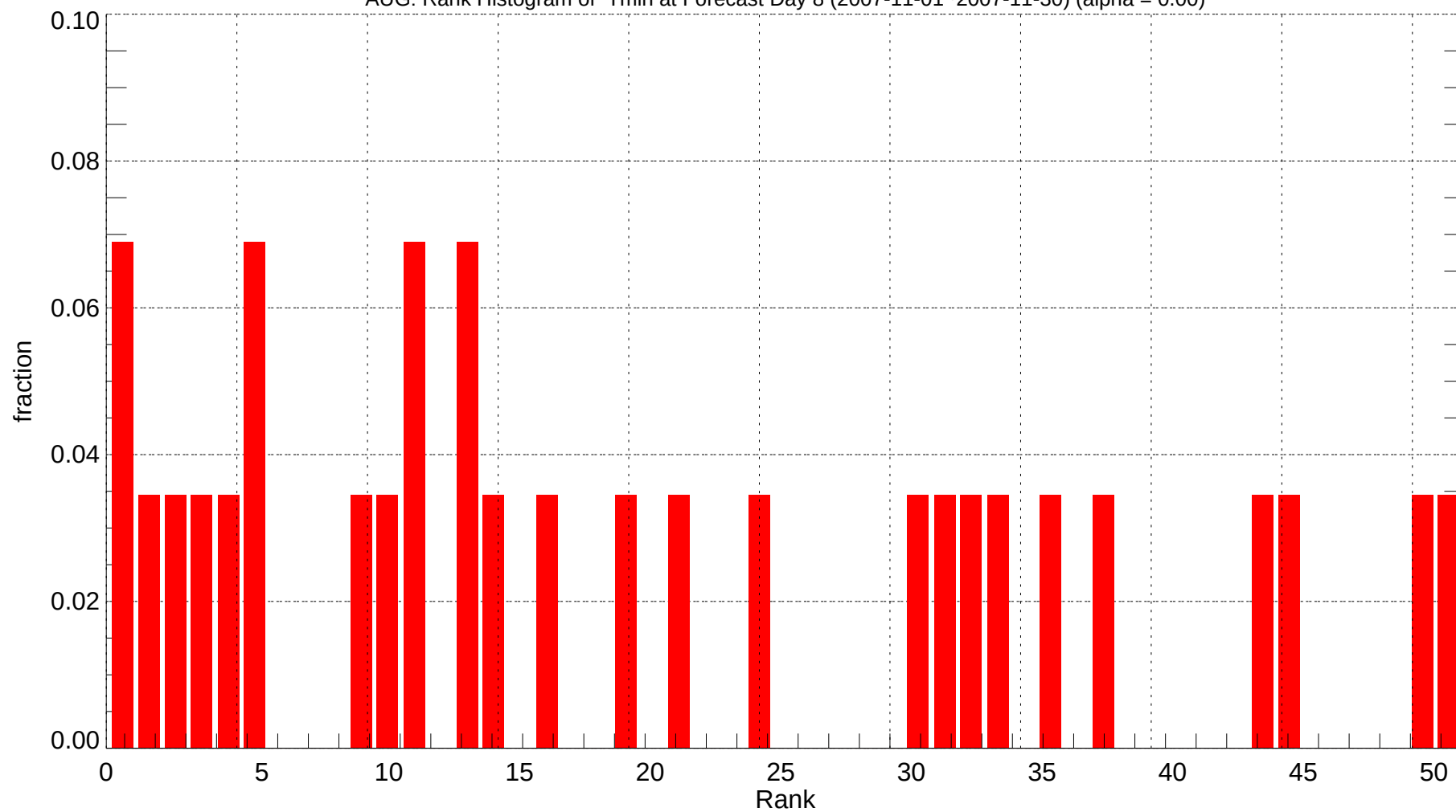
AUG: Rank Histogram of Tmin at Forecast Day 8 (2007-11-01~2007-11-30) (alpha = 0.00)
