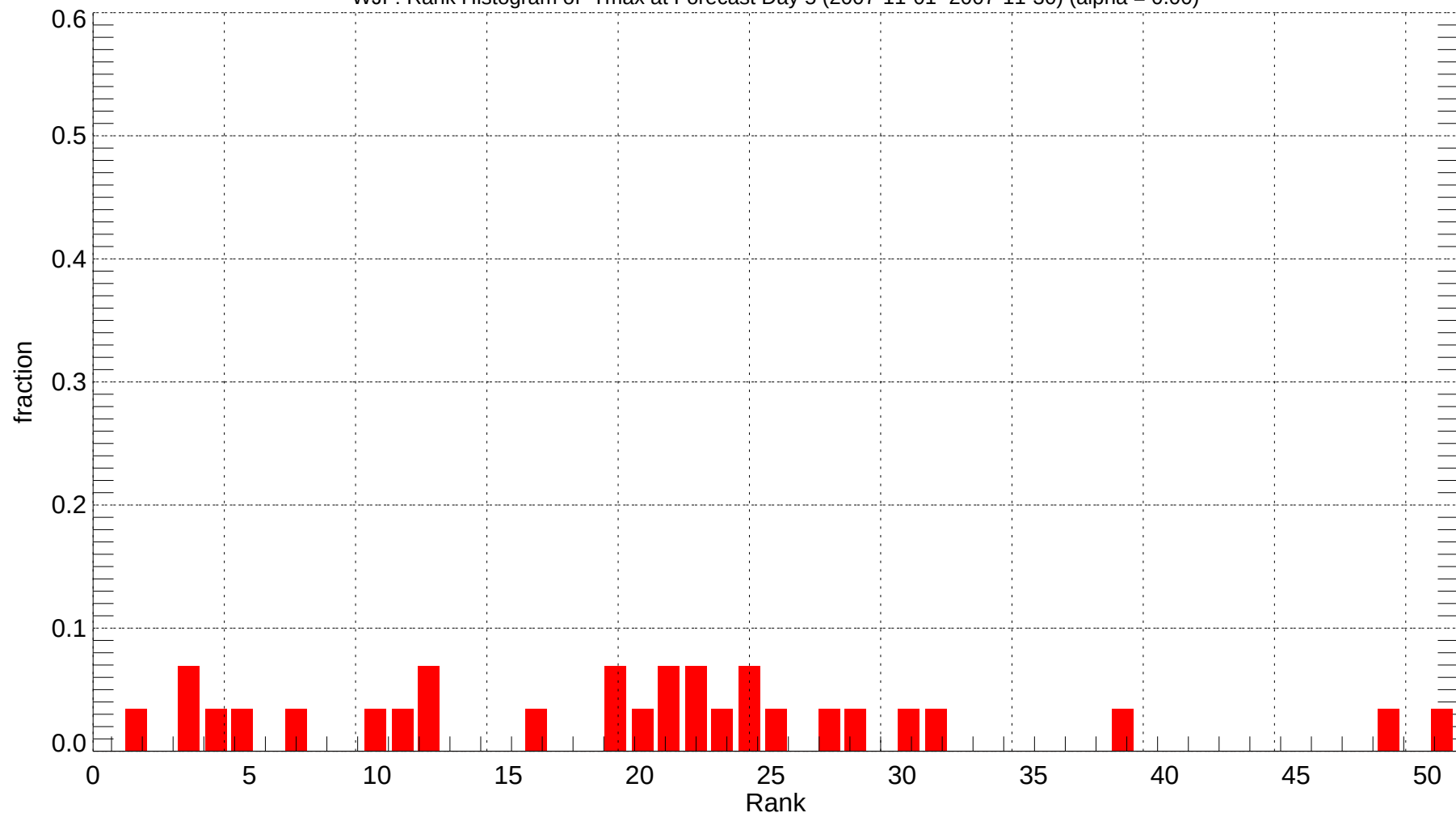
WJF: Rank Histogram of Tmax at Forecast Day 5 (2007-11-01~2007-11-30) (alpha = 0.00)
