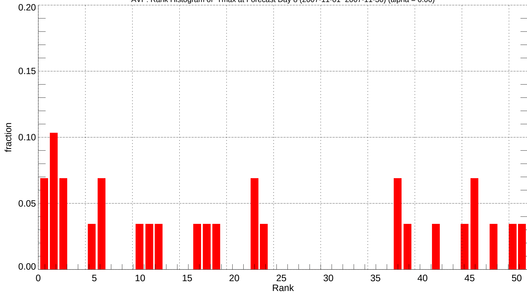
AVP: Rank Histogram of Tmax at Forecast Day 8 (2007-11-01~2007-11-30) (alpha = 0.00)
