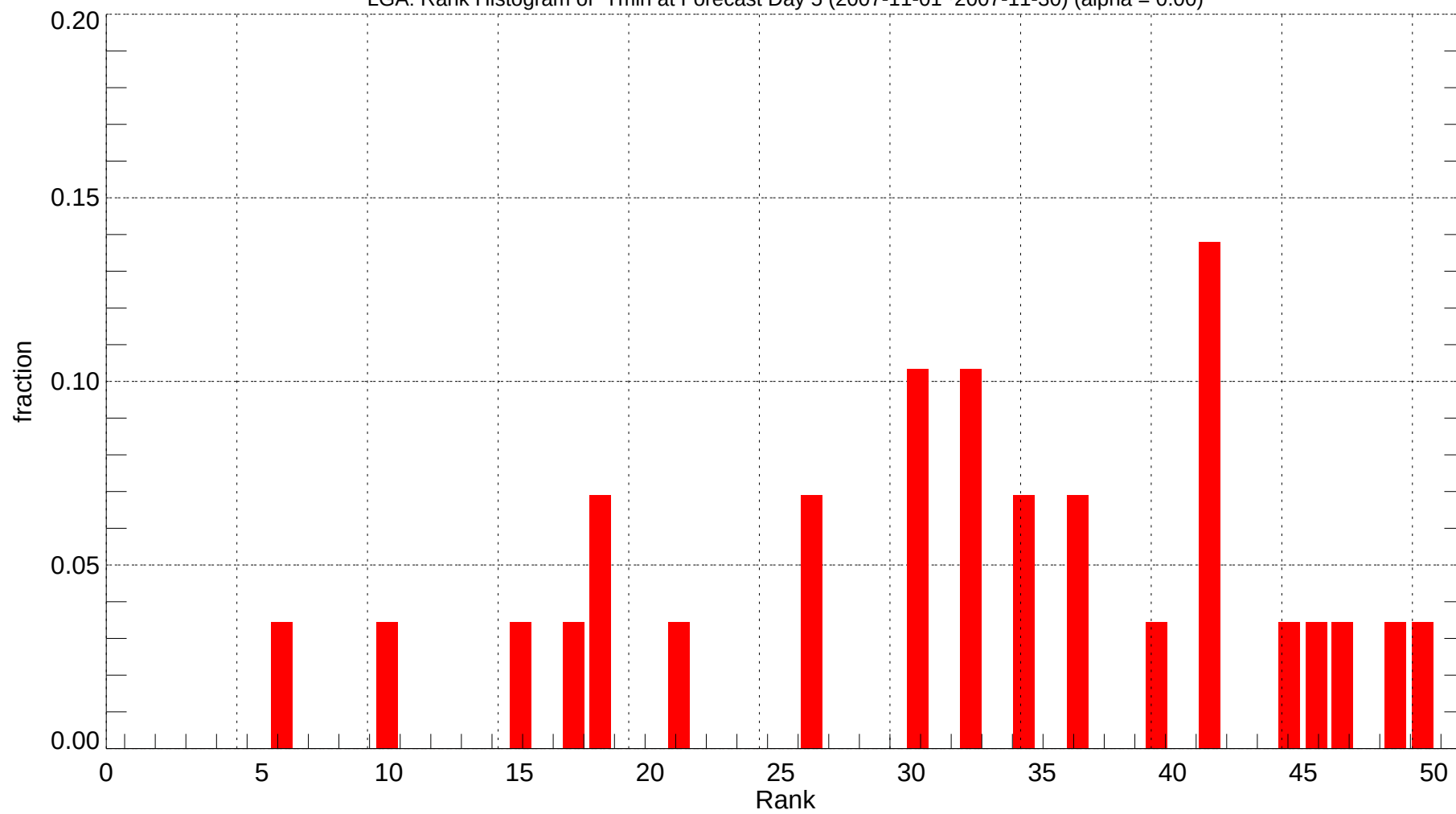
LGA: Rank Histogram of Tmin at Forecast Day 5 (2007-11-01~2007-11-30) (alpha = 0.00)
