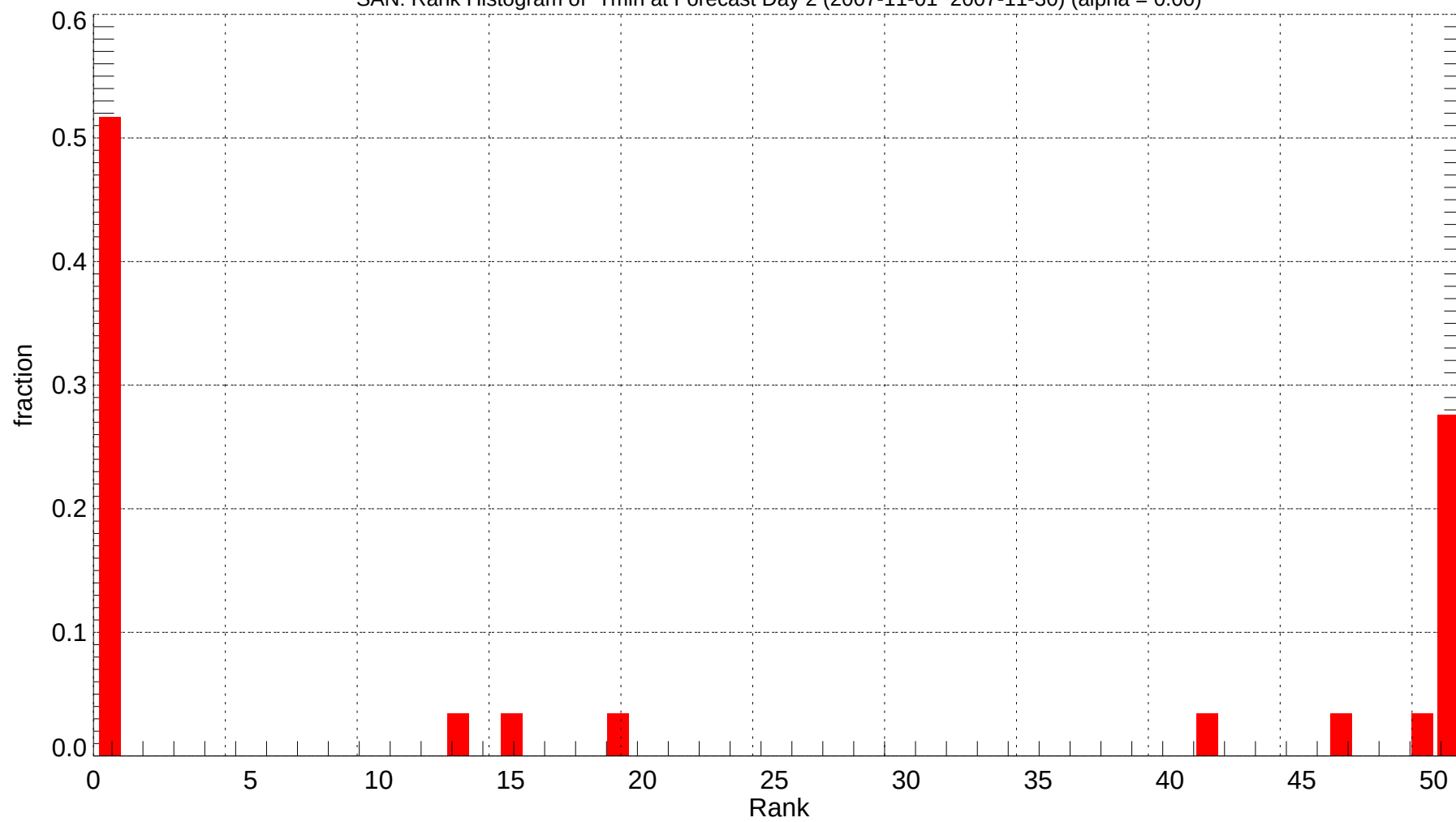
SAN: Rank Histogram of Tmin at Forecast Day 2 (2007-11-01~2007-11-30) (alpha = 0.00)
