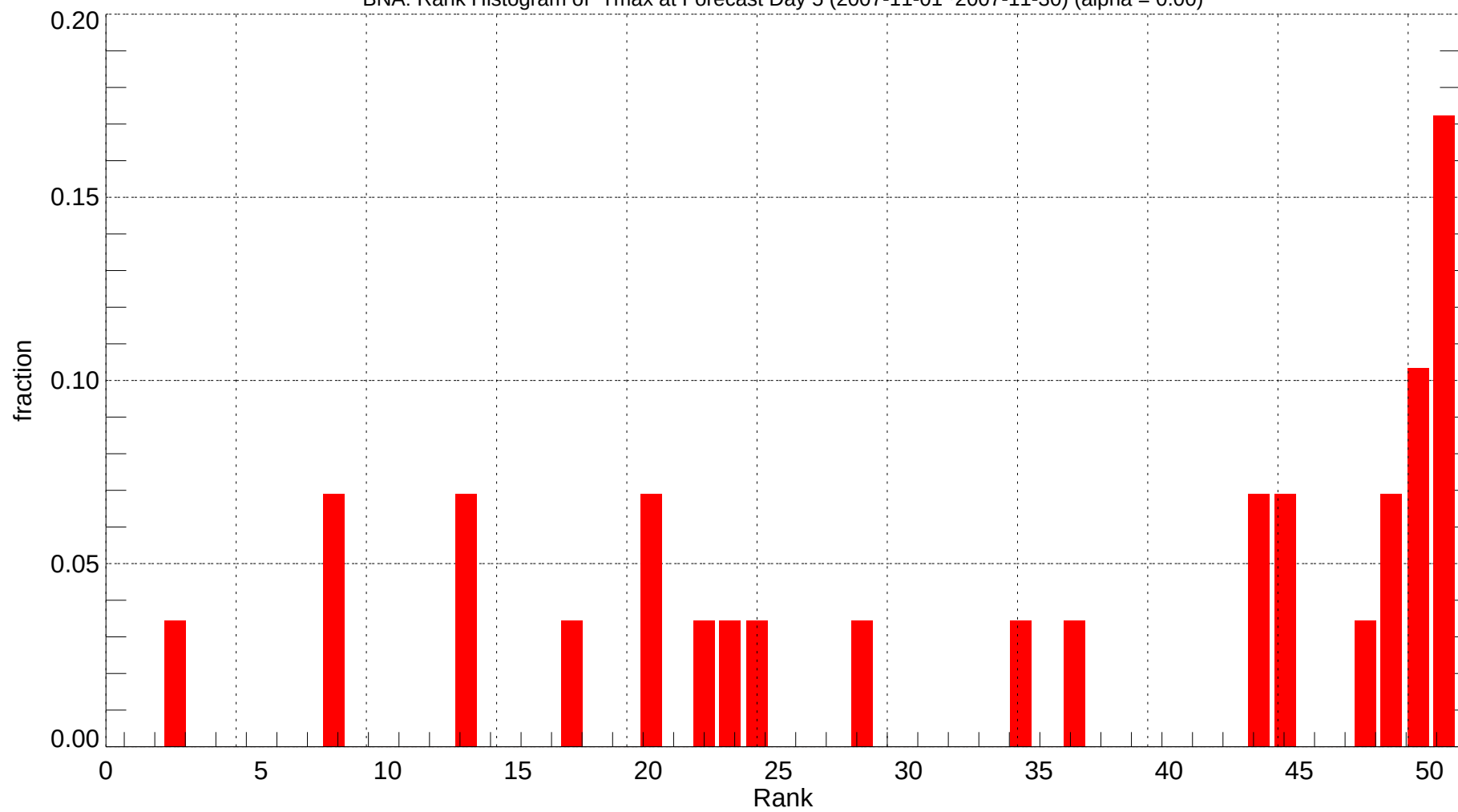
BNA: Rank Histogram of Tmax at Forecast Day 5 (2007-11-01~2007-11-30) (alpha = 0.00)
