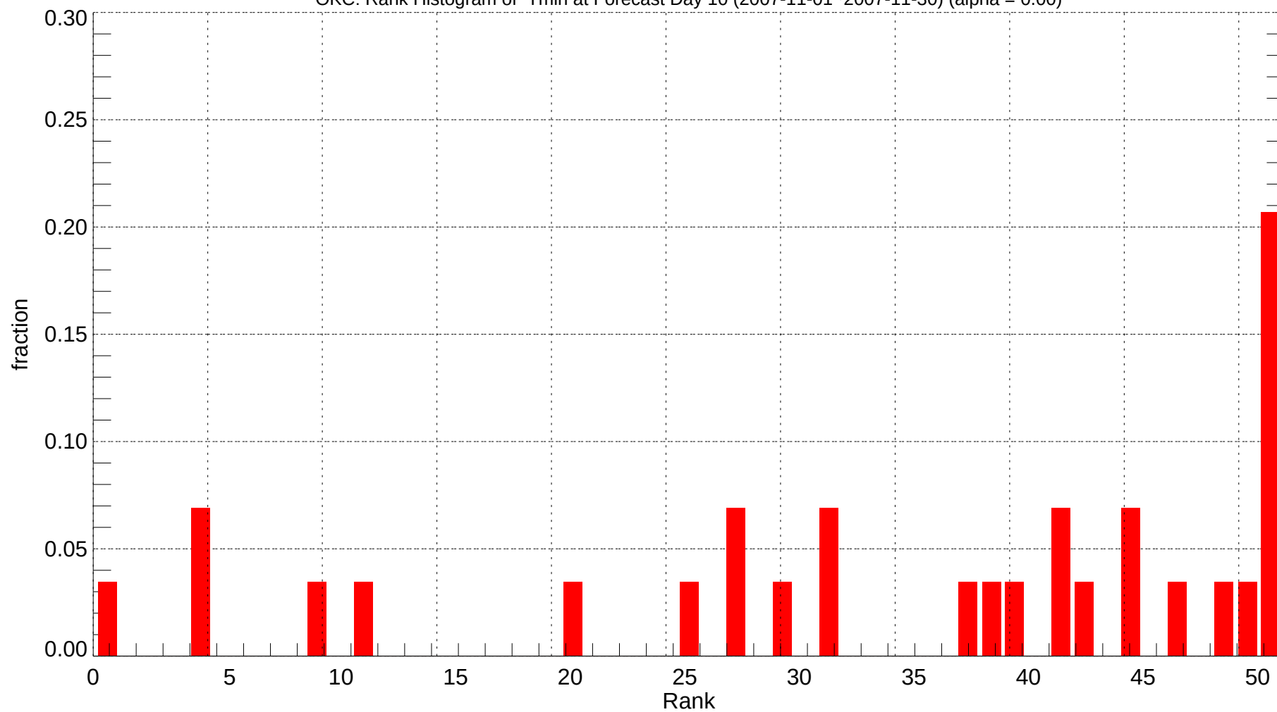
OKC: Rank Histogram of Tmin at Forecast Day 10 (2007-11-01~2007-11-30) (alpha = 0.00)
