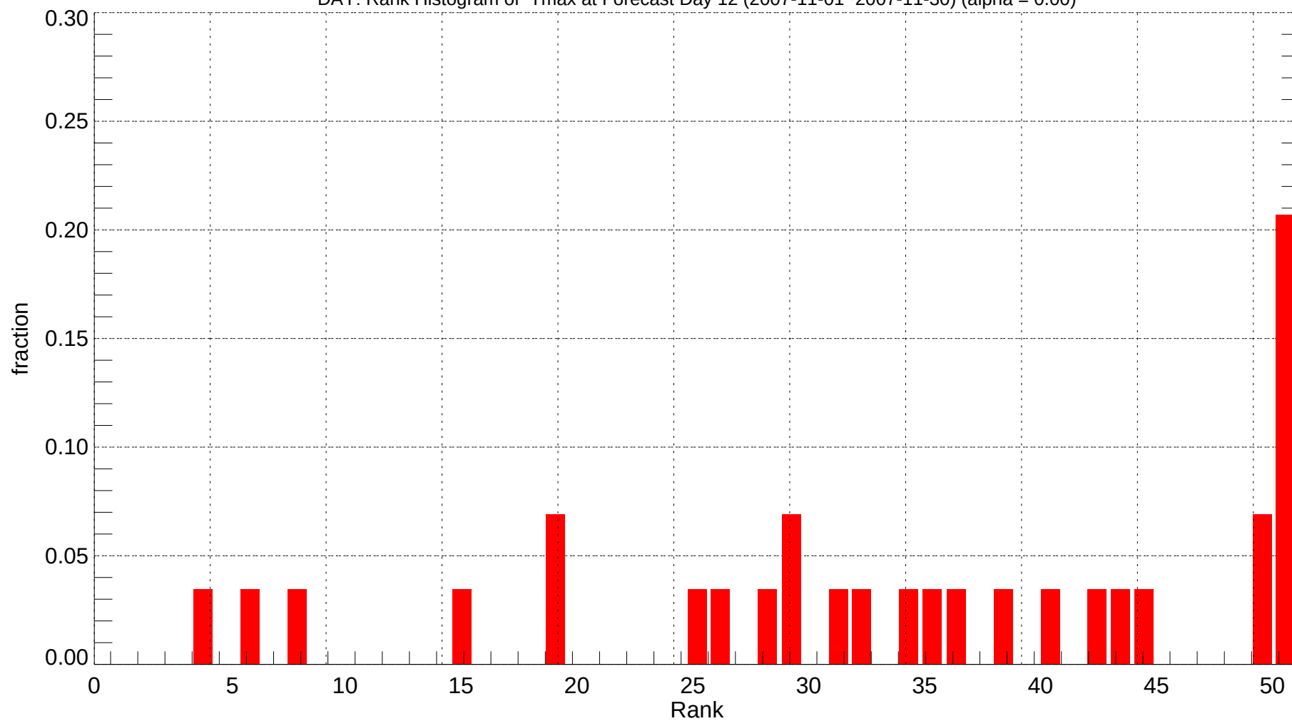
DAY: Rank Histogram of Tmax at Forecast Day 12 (2007-11-01~2007-11-30) (alpha = 0.00)
