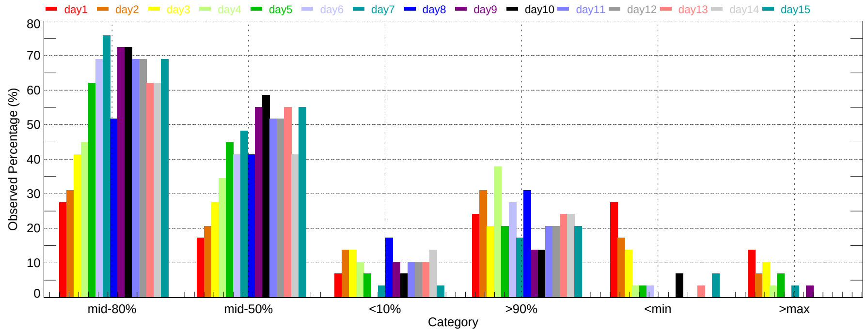
Observed Percentage of Ensembles - ALB: Max Temperature (2007-11-01~2007-11-30)
