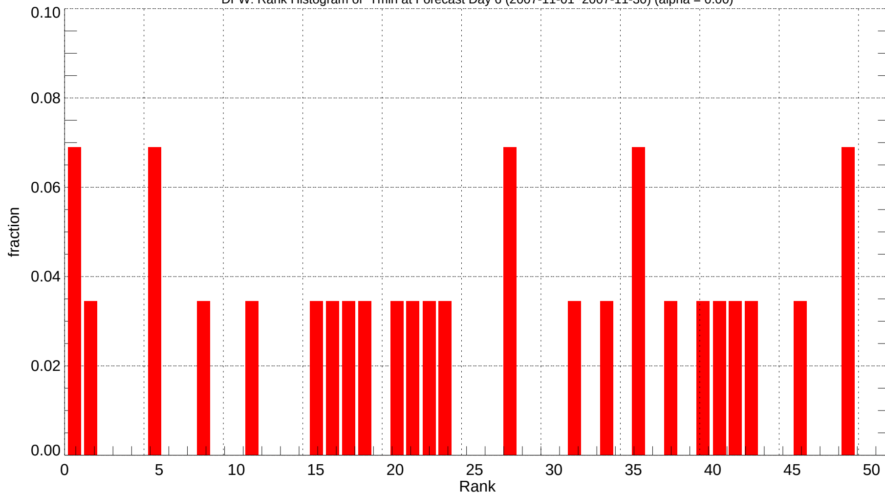
DFW: Rank Histogram of Tmin at Forecast Day 6 (2007-11-01~2007-11-30) (alpha = 0.00)
