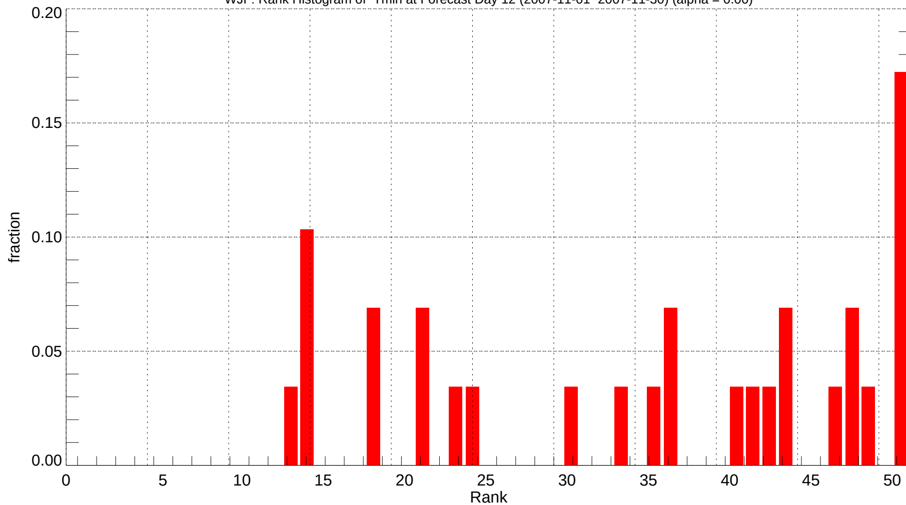
WJF: Rank Histogram of Tmin at Forecast Day 12 (2007-11-01~2007-11-30) (alpha = 0.00)
