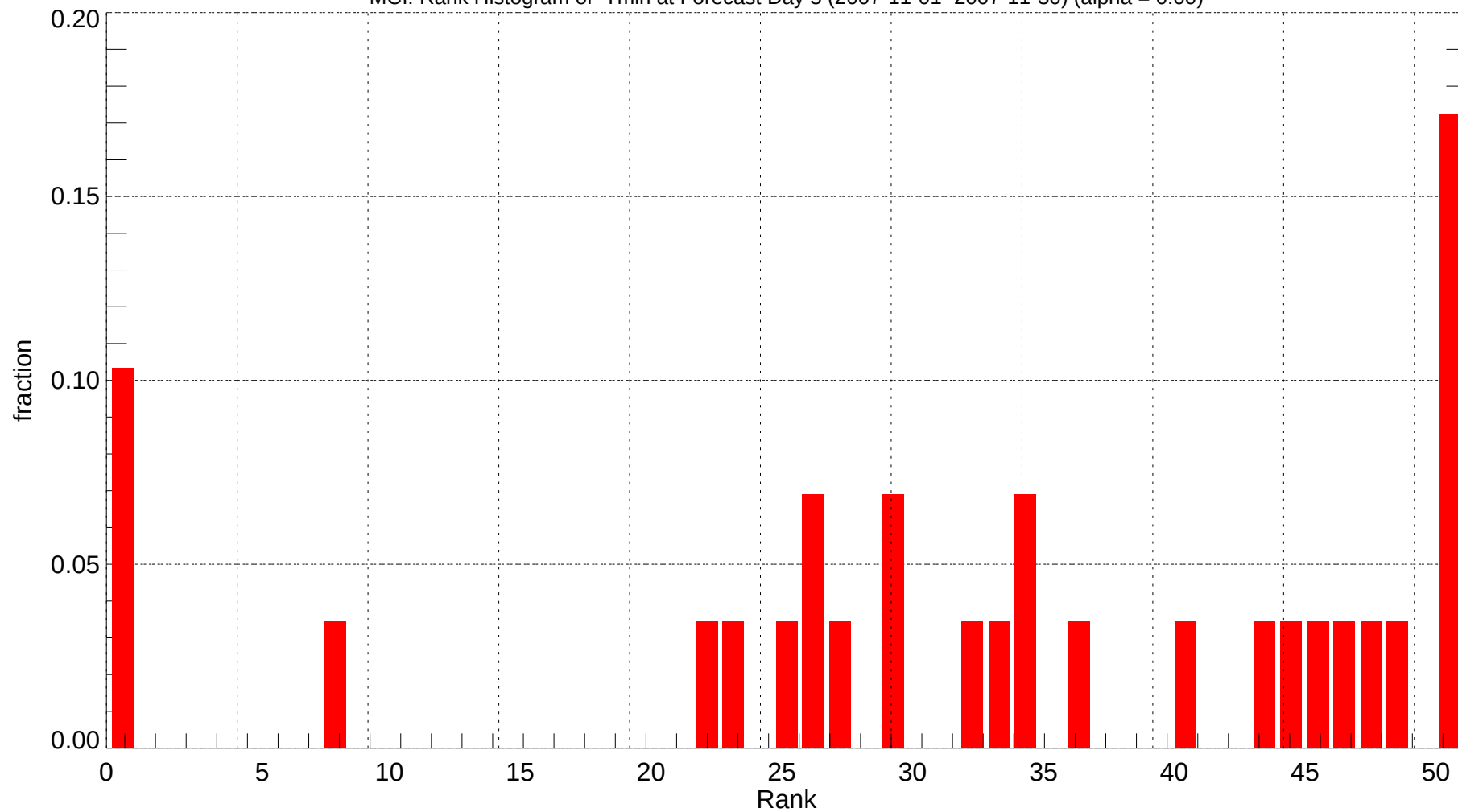
MCI: Rank Histogram of Tmin at Forecast Day 5 (2007-11-01~2007-11-30) (alpha = 0.00)
