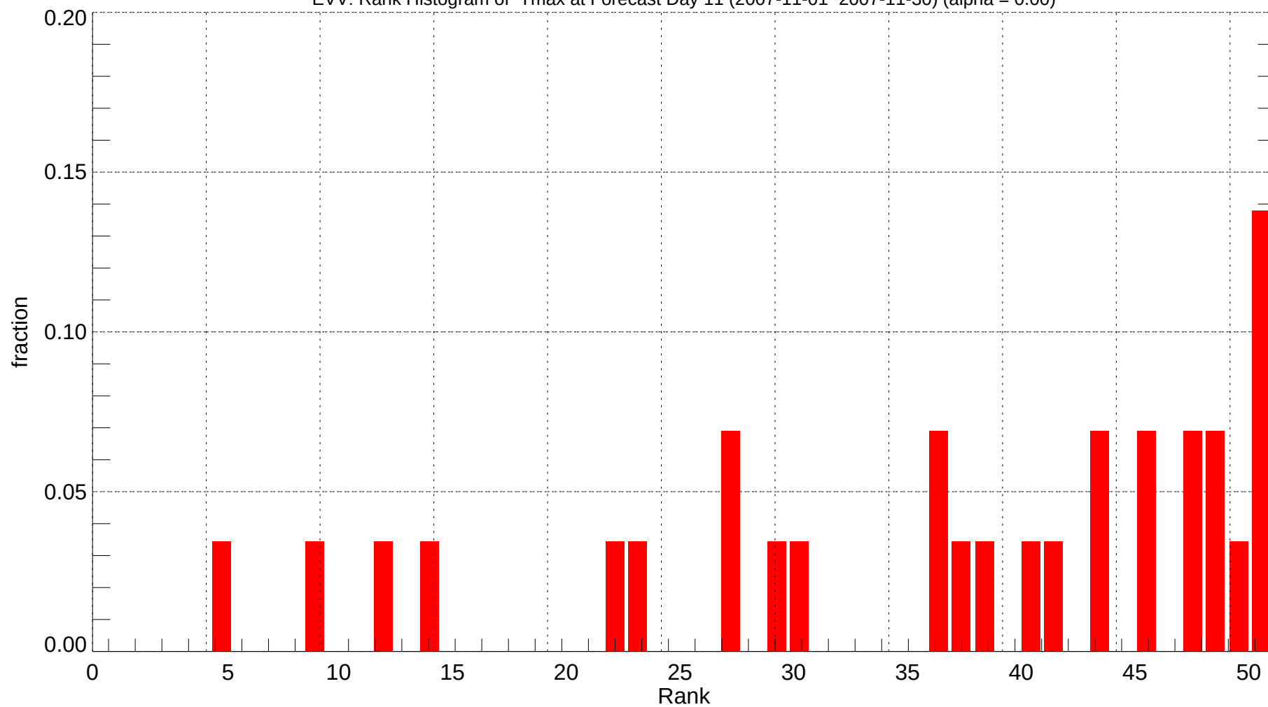
EVV: Rank Histogram of Tmax at Forecast Day 11 (2007-11-01~2007-11-30) (alpha = 0.00)
