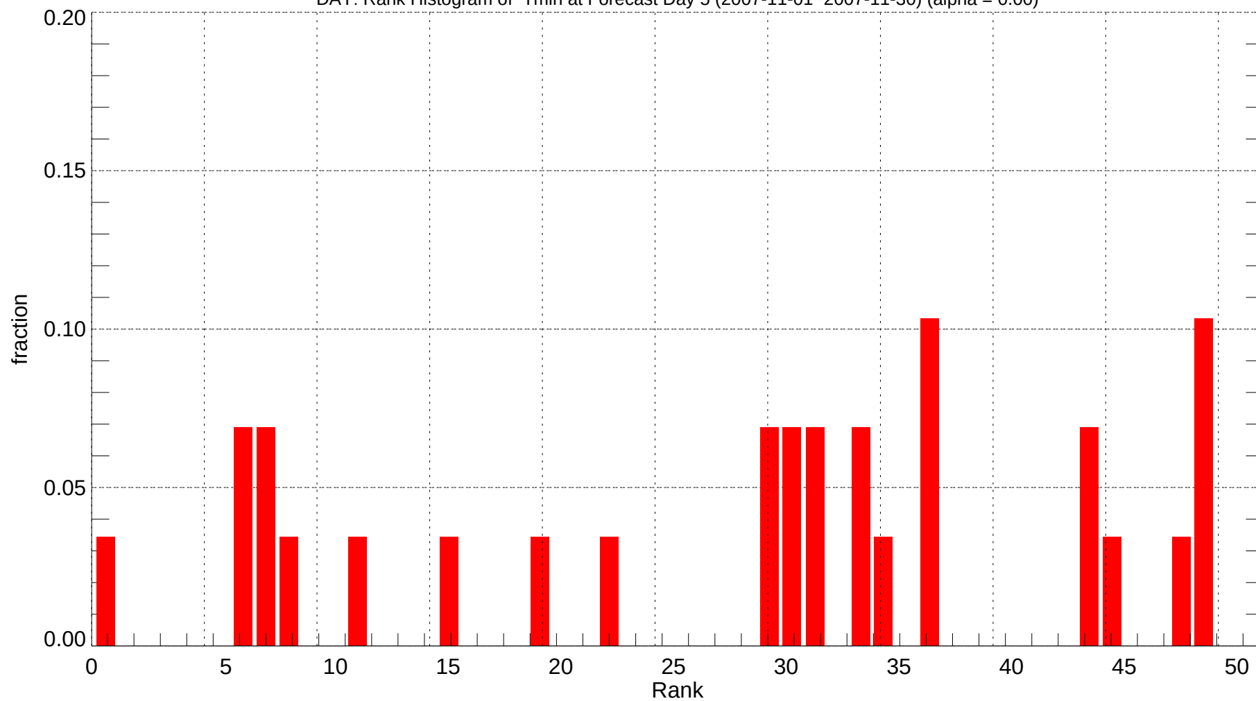
DAY: Rank Histogram of Tmin at Forecast Day 5 (2007-11-01~2007-11-30) (alpha = 0.00)
