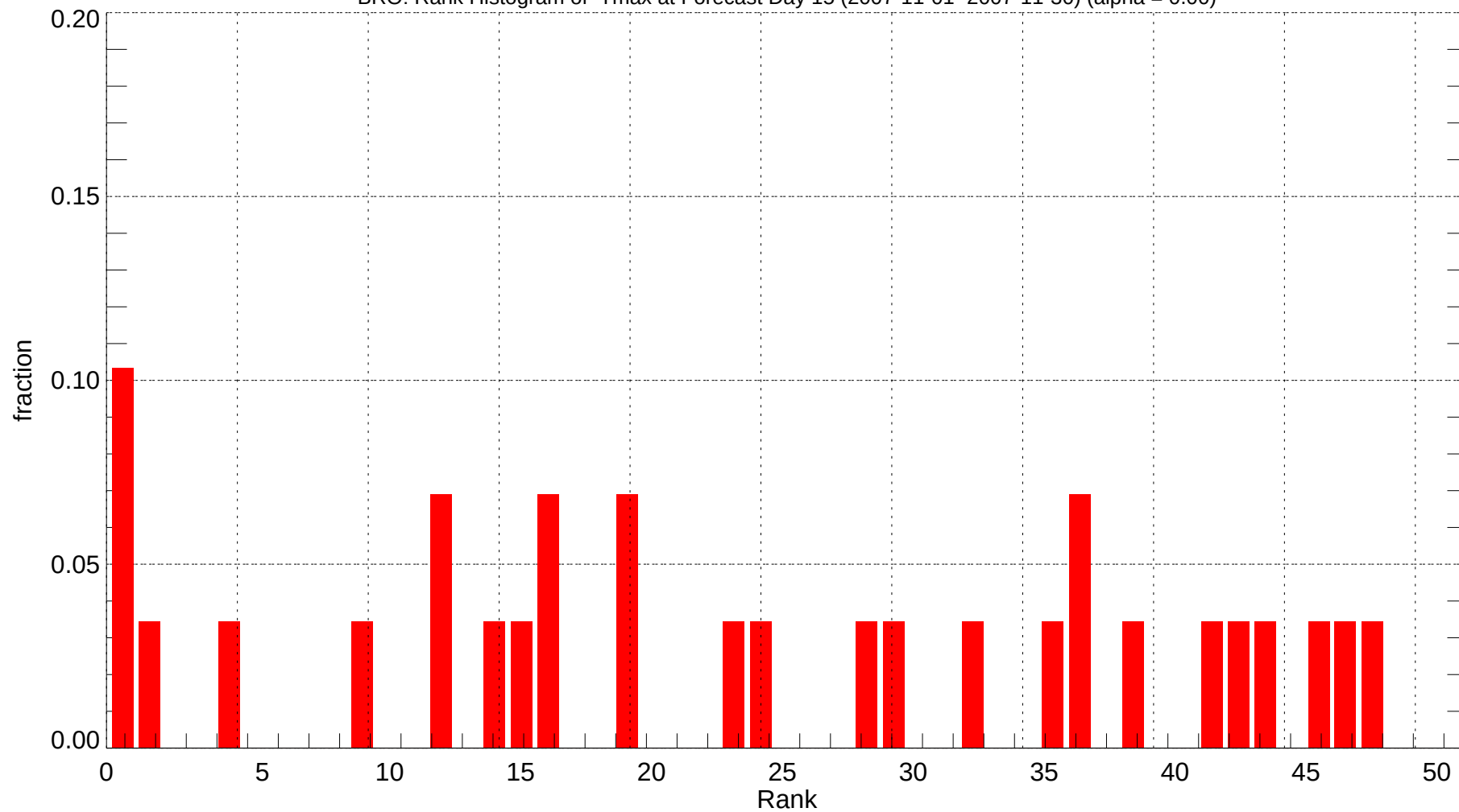
BRO: Rank Histogram of Tmax at Forecast Day 15 (2007-11-01~2007-11-30) (alpha = 0.00)
