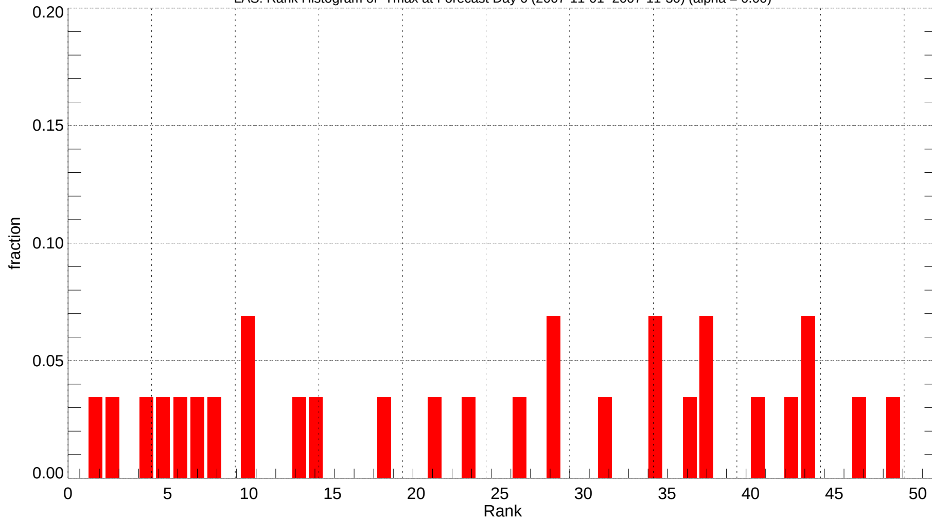
LAS: Rank Histogram of Tmax at Forecast Day 6 (2007-11-01~2007-11-30) (alpha = 0.00)
