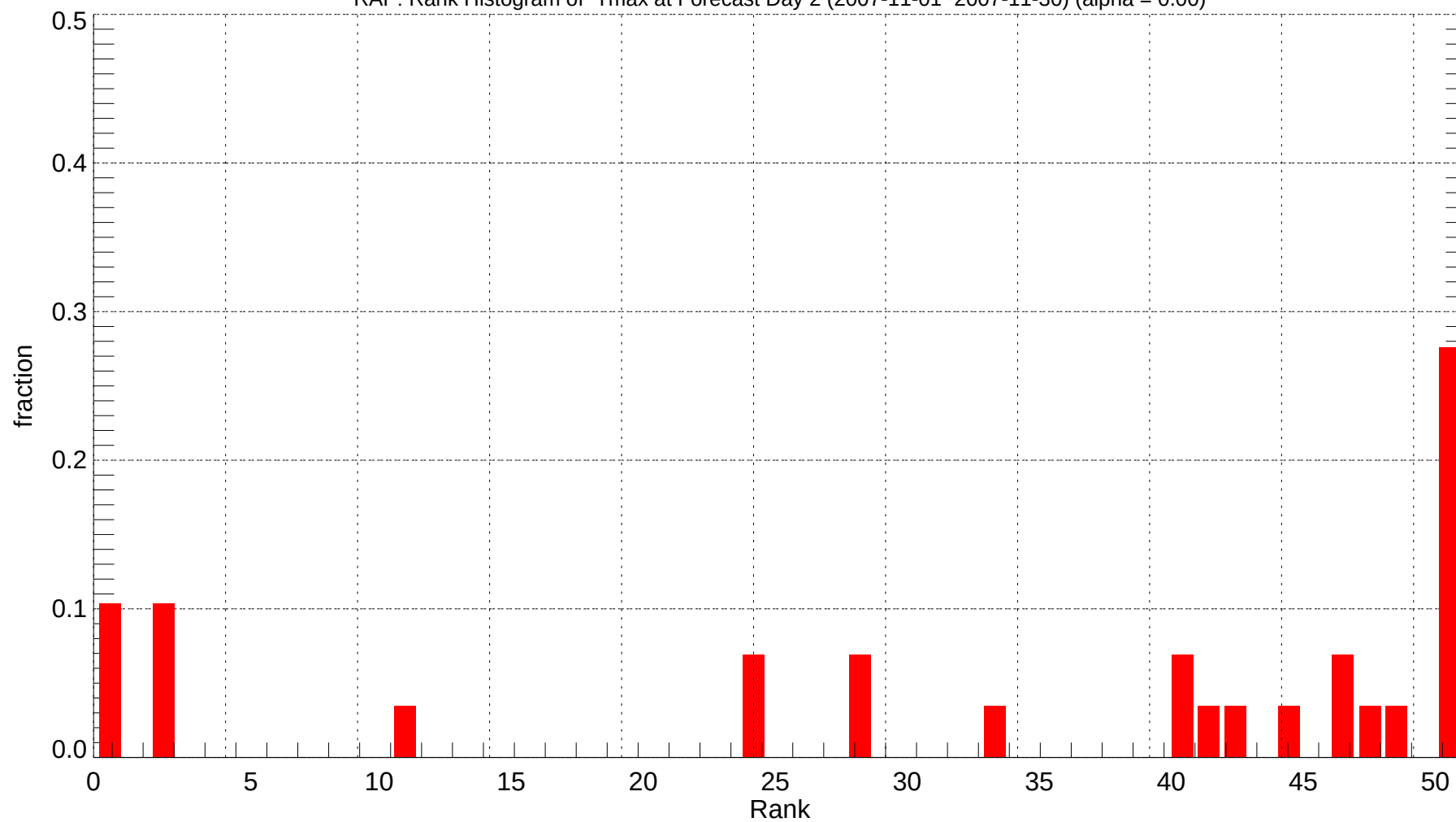
RAP: Rank Histogram of Tmax at Forecast Day 2 (2007-11-01~2007-11-30) (alpha = 0.00)
