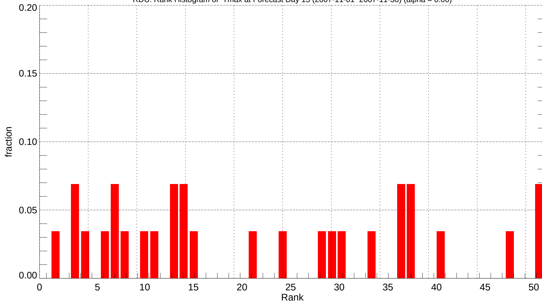
RDU: Rank Histogram of Tmax at Forecast Day 15 (2007-11-01~2007-11-30) (alpha = 0.00)
