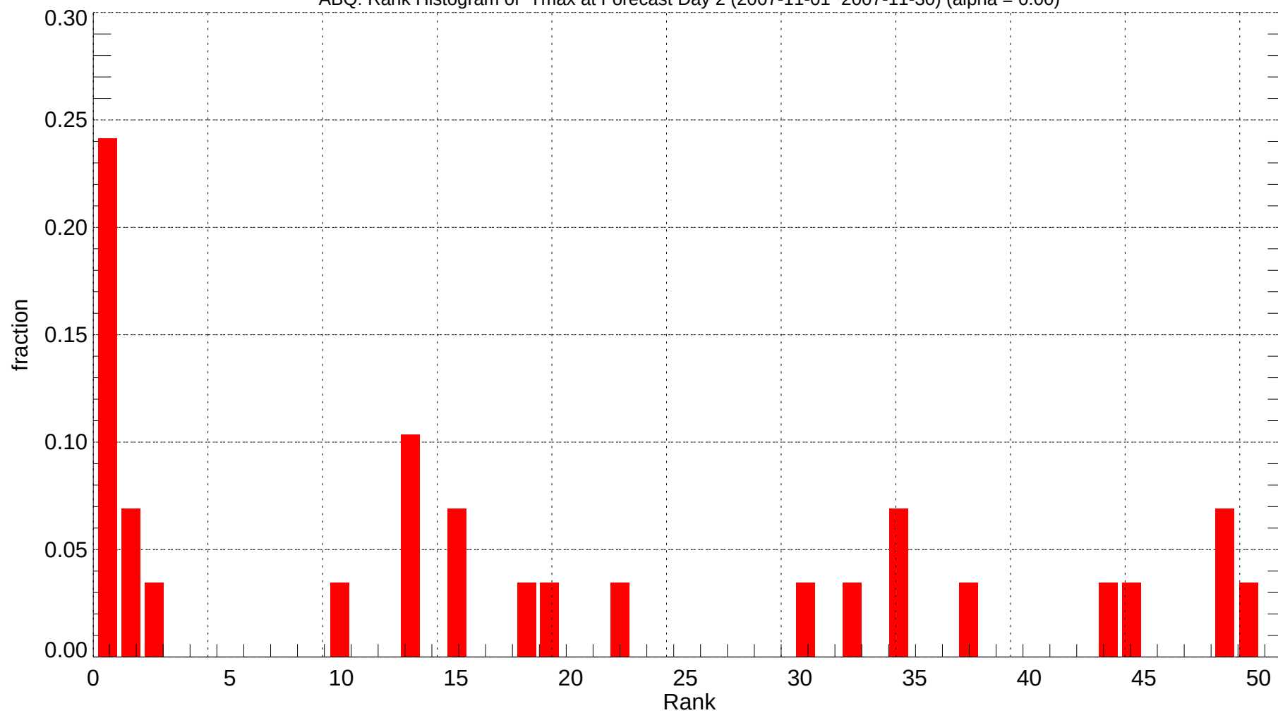
ABQ: Rank Histogram of Tmax at Forecast Day 2 (2007-11-01~2007-11-30) (alpha = 0.00)
