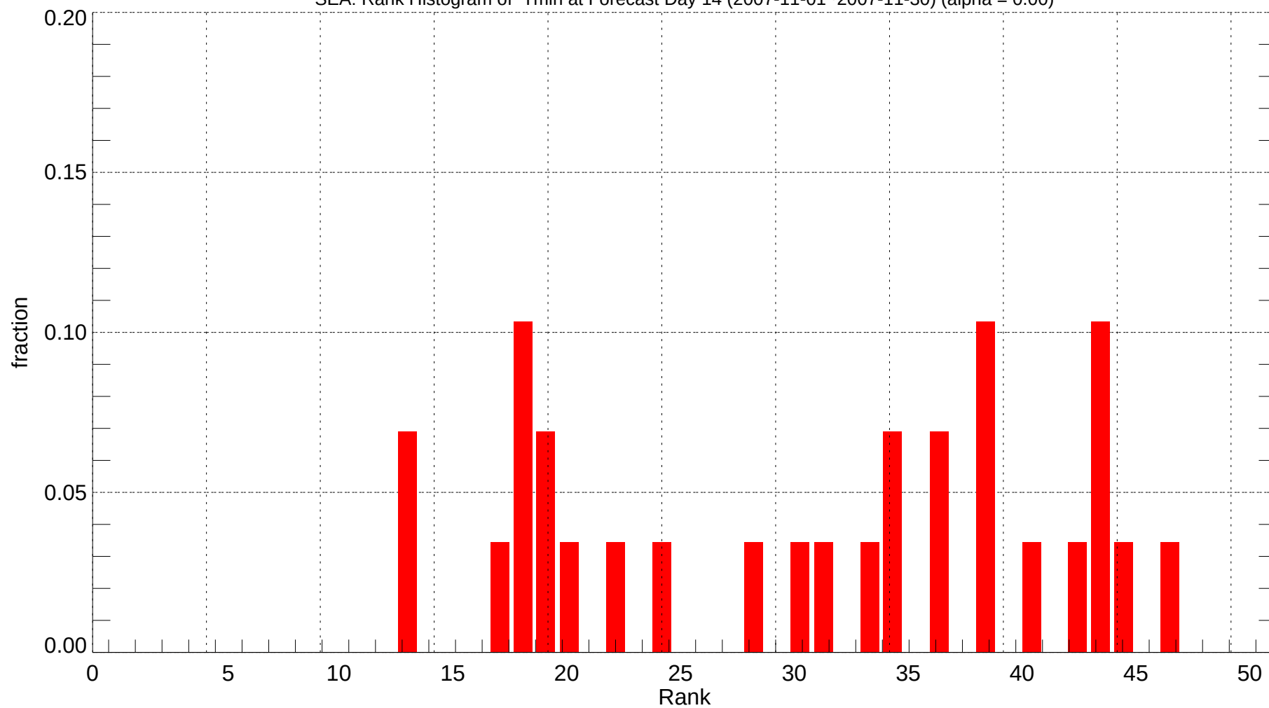
SEA: Rank Histogram of Tmin at Forecast Day 14 (2007-11-01~2007-11-30) (alpha = 0.00)
