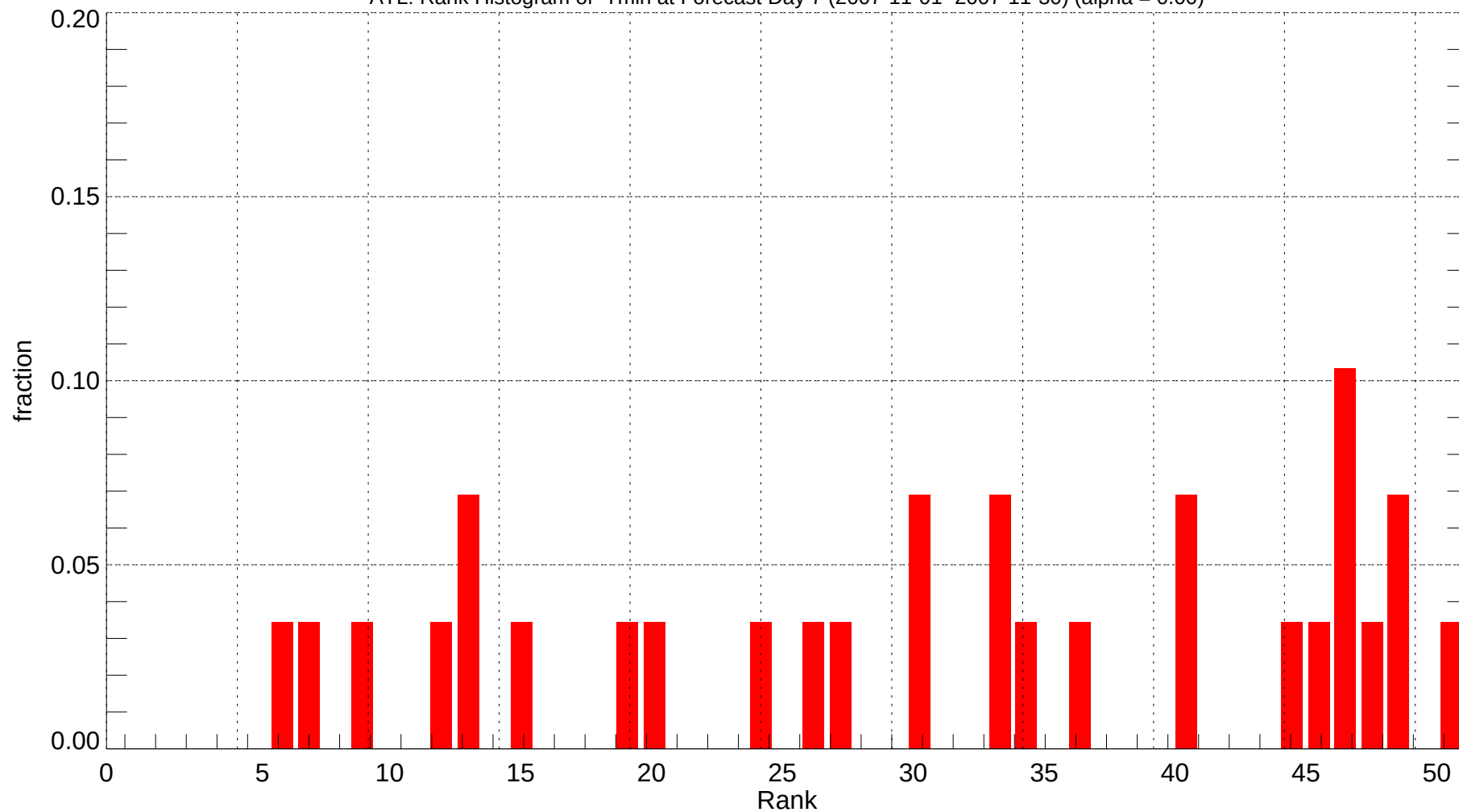
ATL: Rank Histogram of Tmin at Forecast Day 7 (2007-11-01~2007-11-30) (alpha = 0.00)
