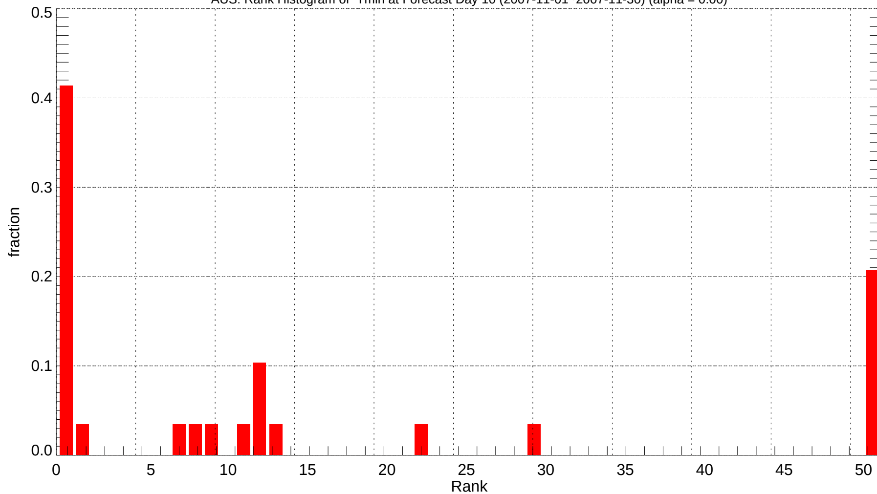
AUS: Rank Histogram of Tmin at Forecast Day 10 (2007-11-01~2007-11-30) (alpha = 0.00)
