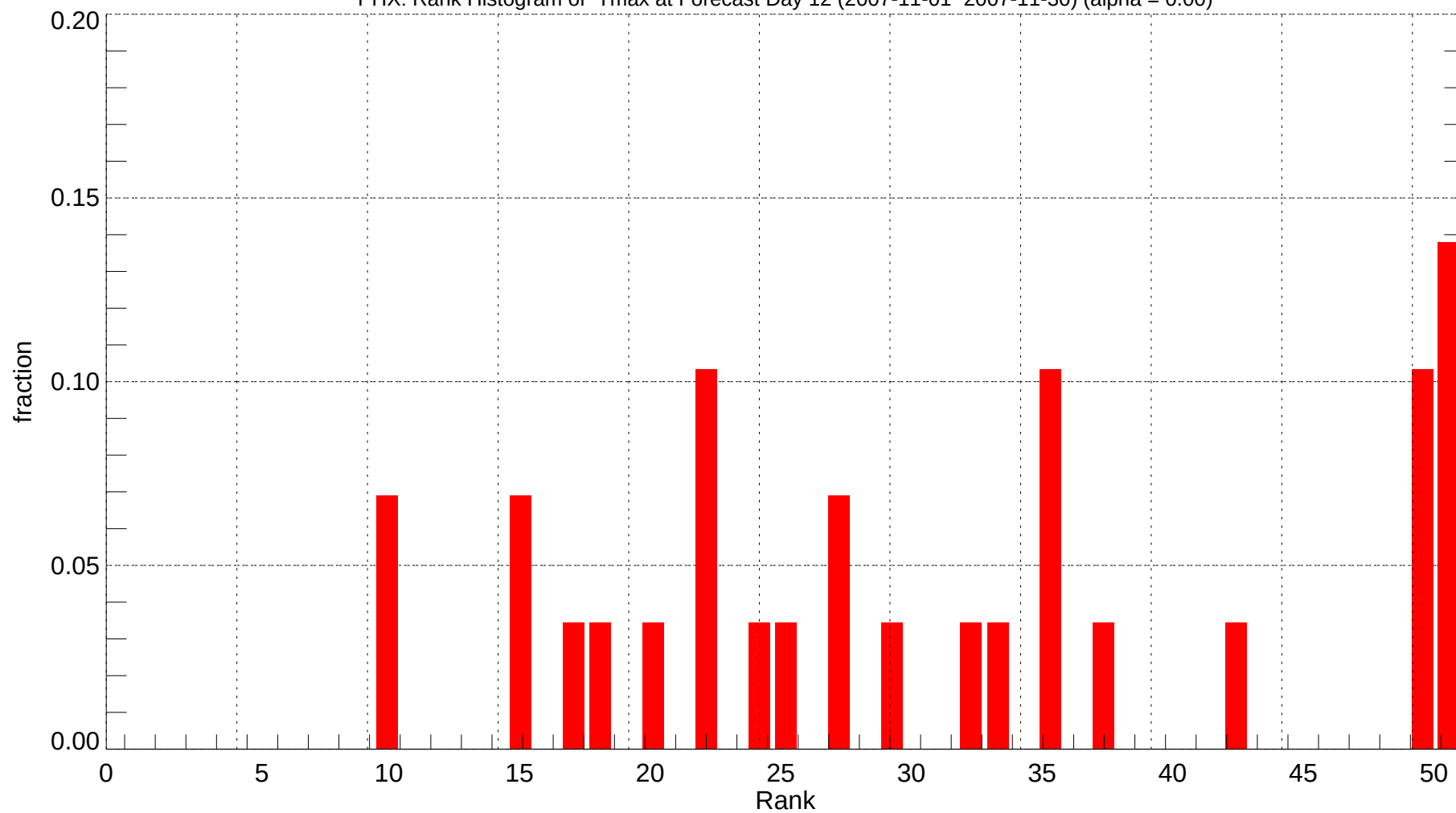
PHX: Rank Histogram of Tmax at Forecast Day 12 (2007-11-01~2007-11-30) (alpha = 0.00)
