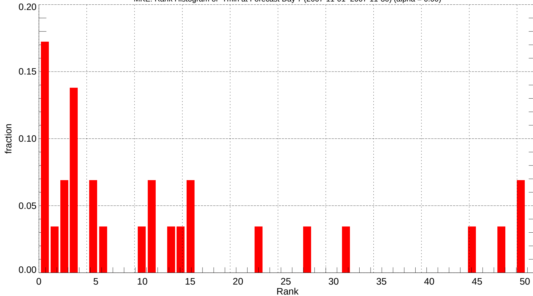
MKE: Rank Histogram of Tmin at Forecast Day 7 (2007-11-01~2007-11-30) (alpha = 0.00)
