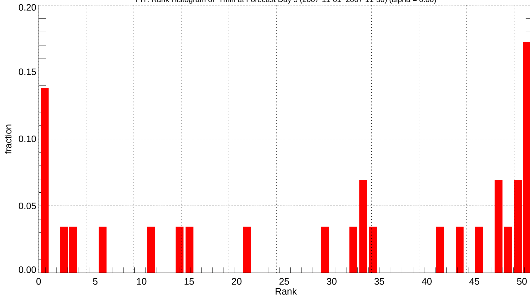
PIT: Rank Histogram of Tmin at Forecast Day 3 (2007-11-01~2007-11-30) (alpha = 0.00)
