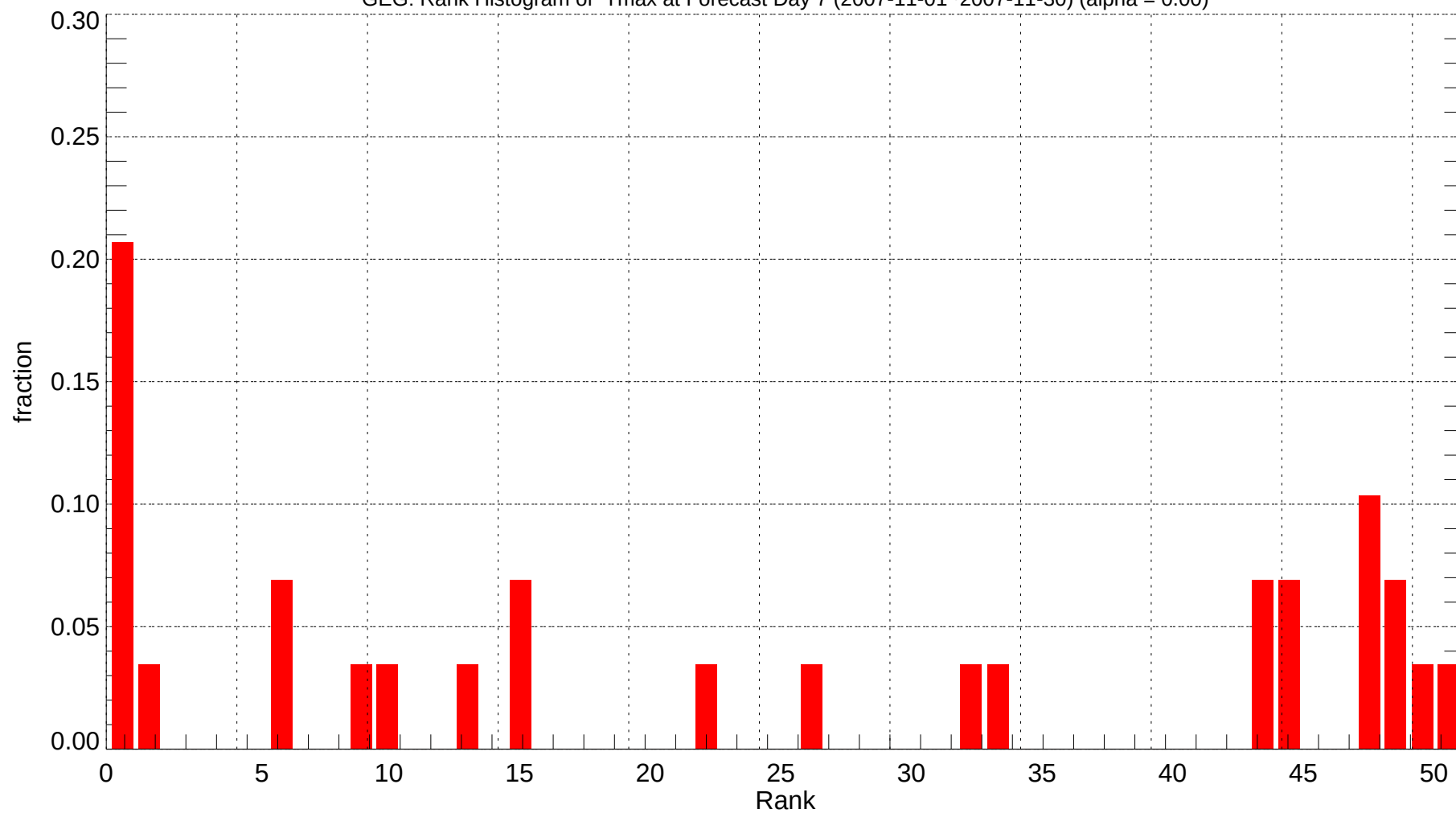
GEG: Rank Histogram of Tmax at Forecast Day 7 (2007-11-01~2007-11-30) (alpha = 0.00)
