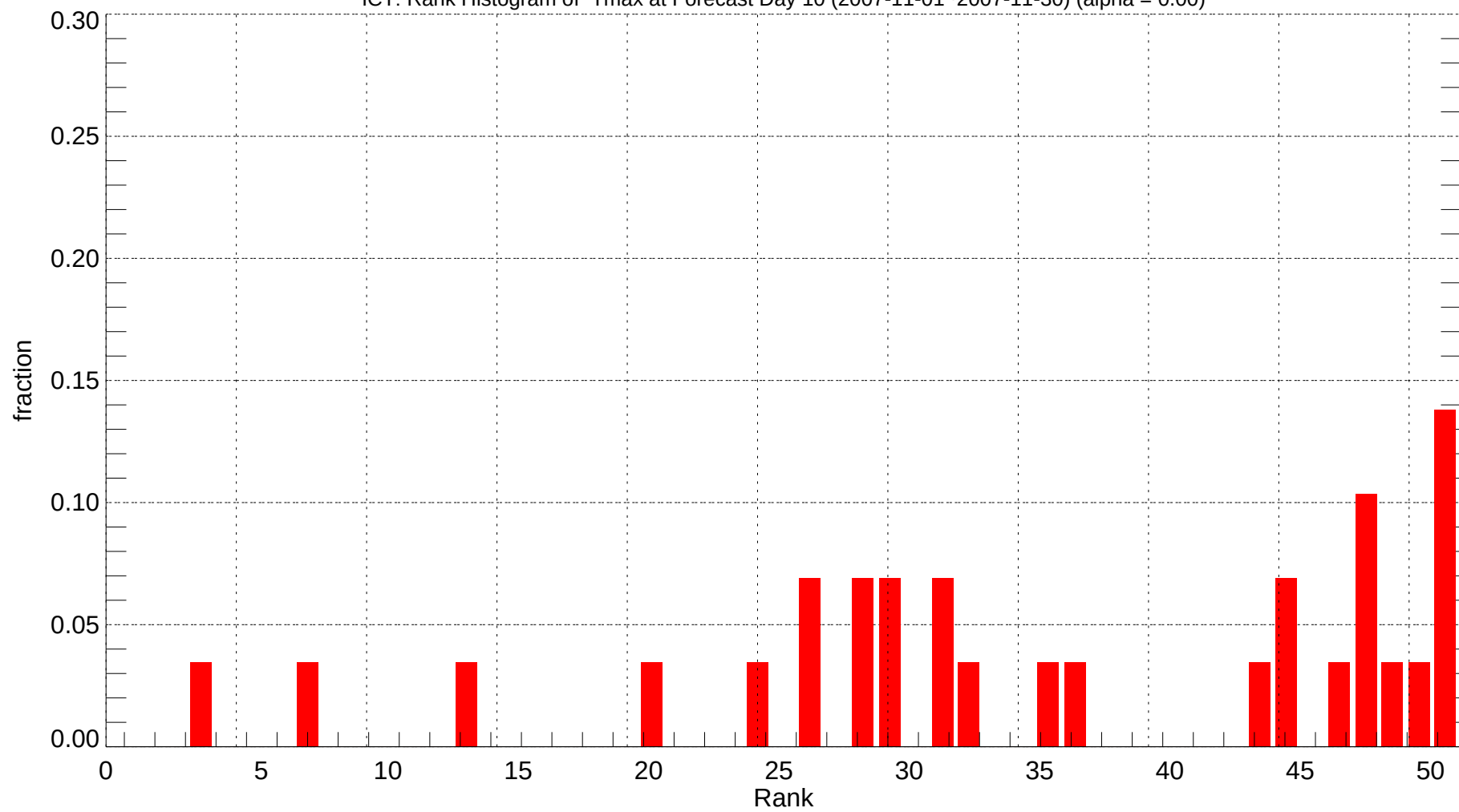
ICT: Rank Histogram of Tmax at Forecast Day 10 (2007-11-01~2007-11-30) (alpha = 0.00)
