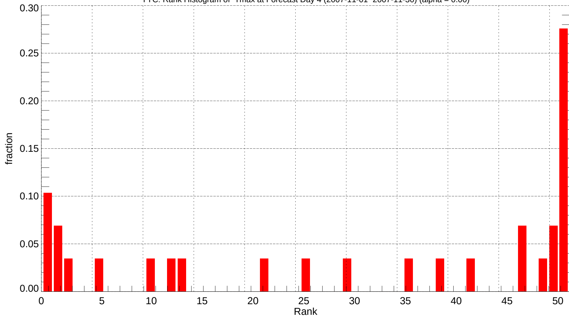
YYC: Rank Histogram of Tmax at Forecast Day 4 (2007-11-01~2007-11-30) (alpha = 0.00)
