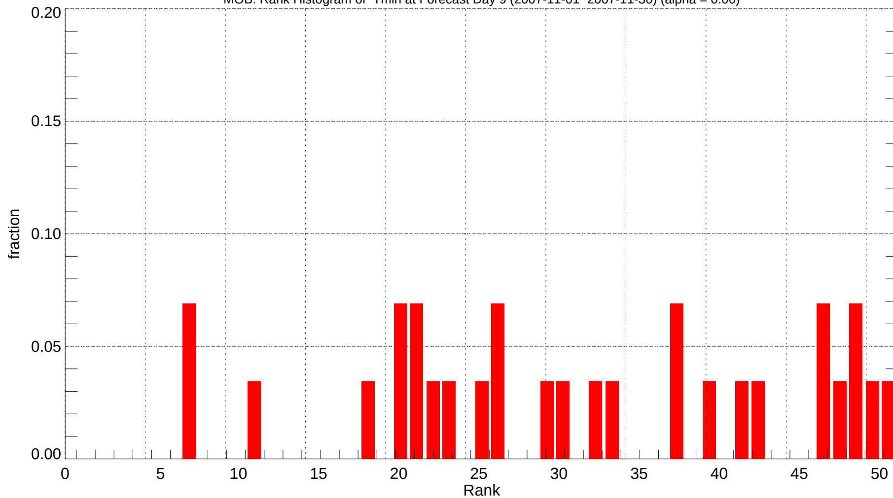
MOB: Rank Histogram of Tmin at Forecast Day 9 (2007-11-01~2007-11-30) (alpha = 0.00)
