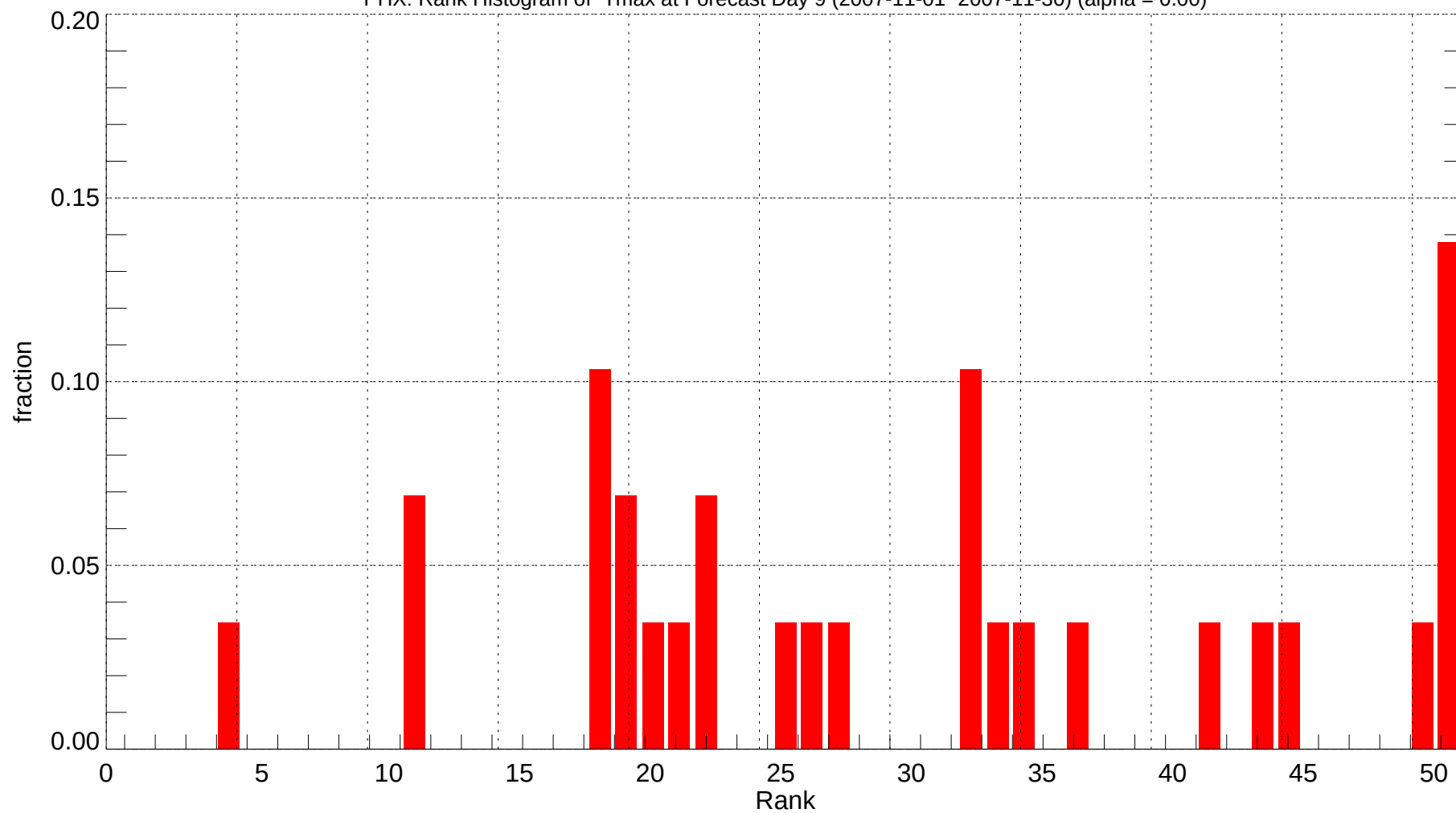
PHX: Rank Histogram of Tmax at Forecast Day 9 (2007-11-01~2007-11-30) (alpha = 0.00)
