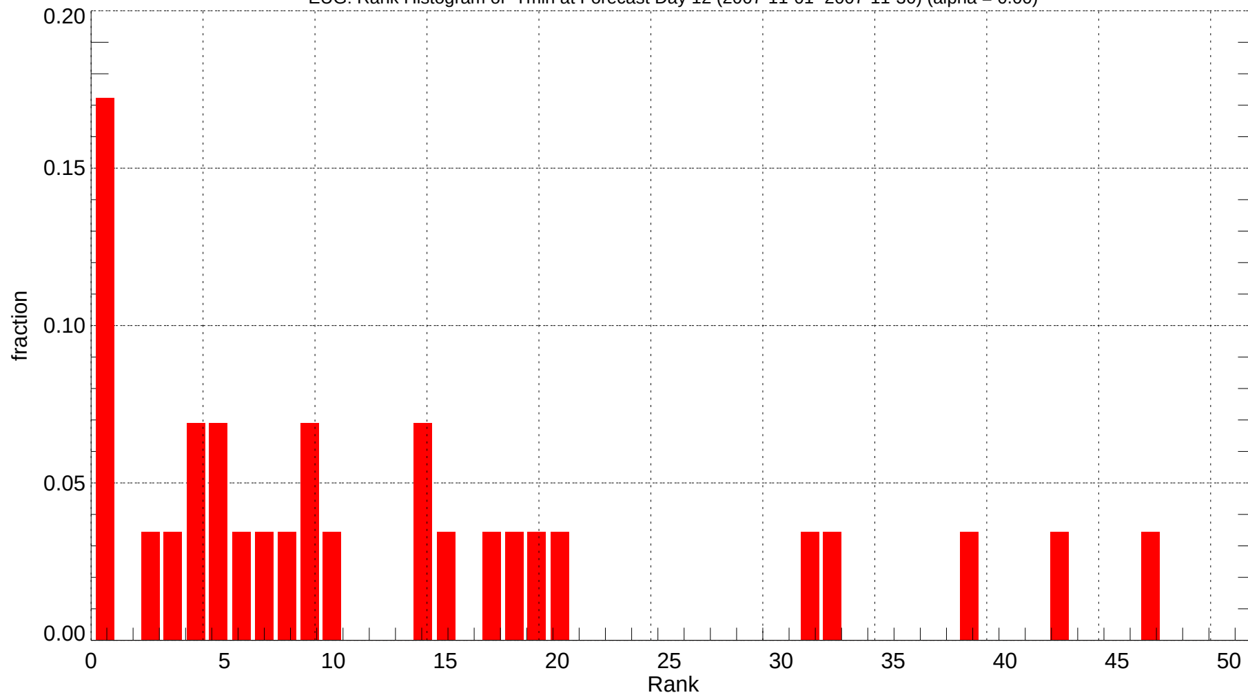
EUG: Rank Histogram of Tmin at Forecast Day 12 (2007-11-01~2007-11-30) (alpha = 0.00)
