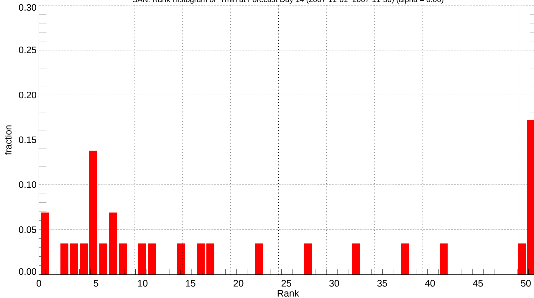
SAN: Rank Histogram of Tmin at Forecast Day 14 (2007-11-01~2007-11-30) (alpha = 0.00)
