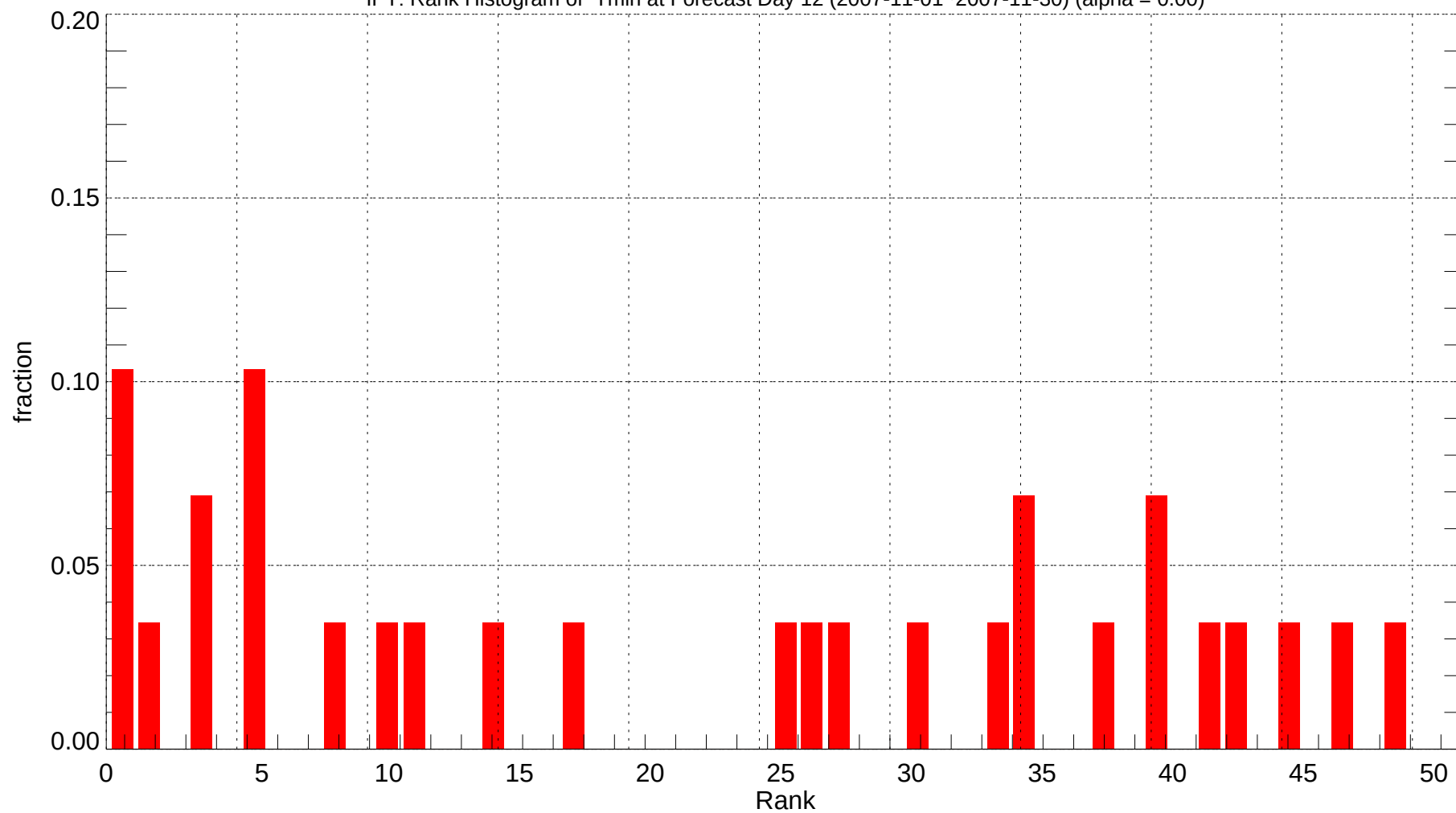
IPT: Rank Histogram of Tmin at Forecast Day 12 (2007-11-01~2007-11-30) (alpha = 0.00)
