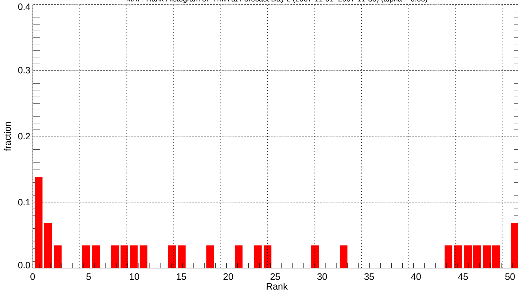
MAF: Rank Histogram of Tmin at Forecast Day 2 (2007-11-01~2007-11-30) (alpha = 0.00)
