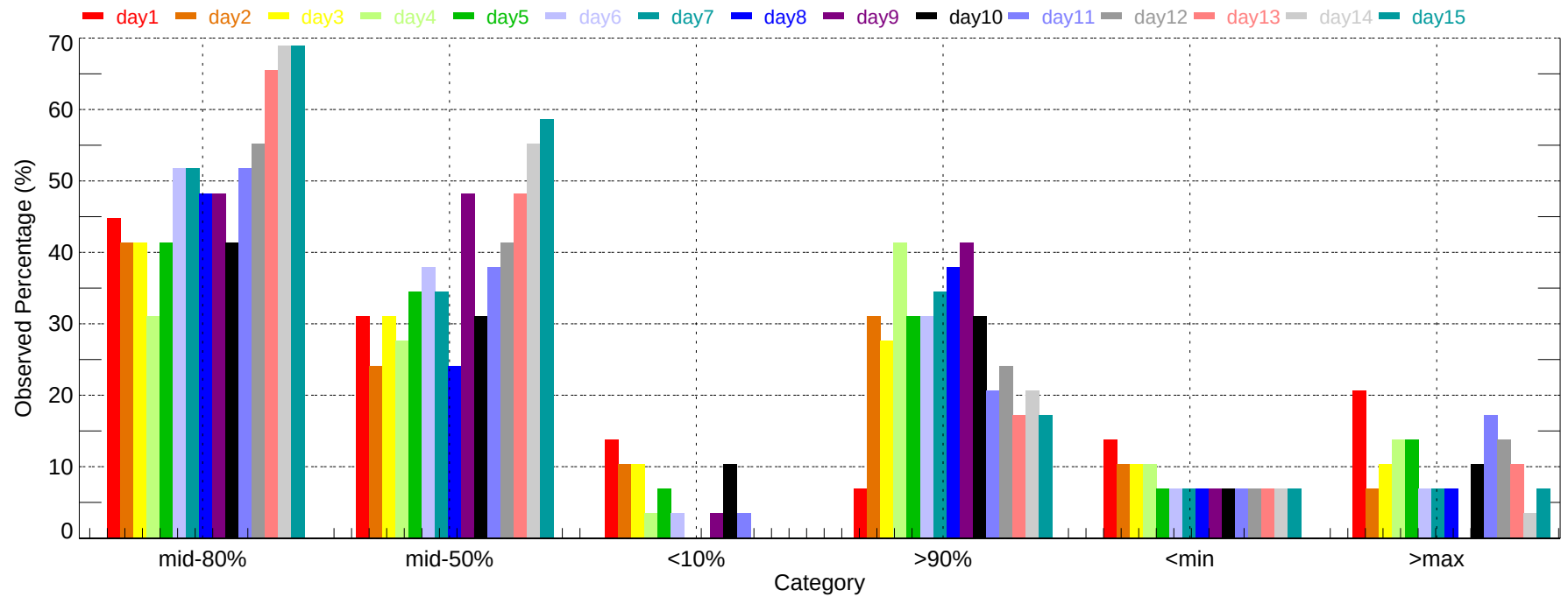
Observed Percentage of Ensembles - MSY: Max Temperature (2007-11-01~2007-11-30)
