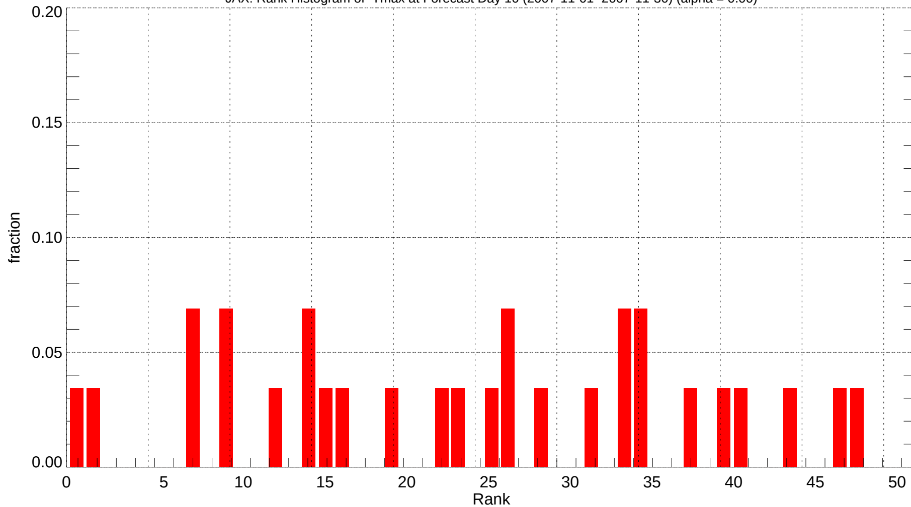
JAX: Rank Histogram of Tmax at Forecast Day 10 (2007-11-01~2007-11-30) (alpha = 0.00)
