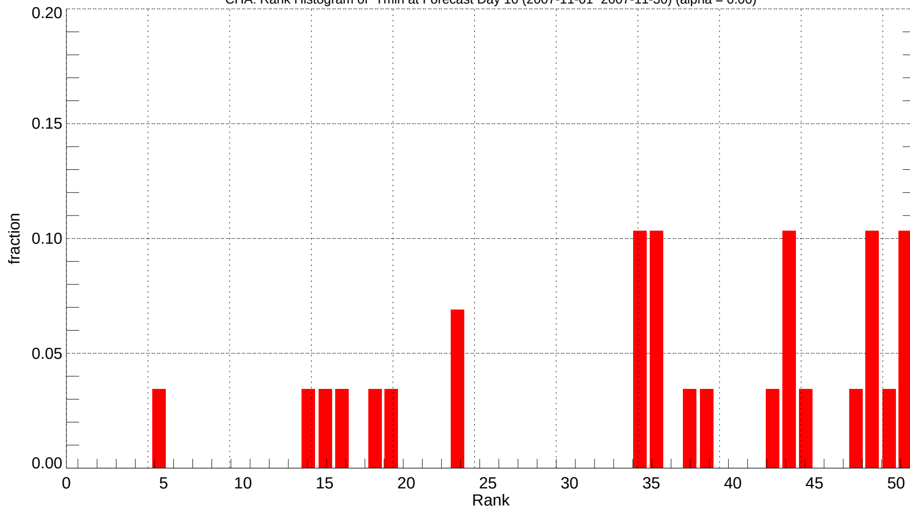
CHA: Rank Histogram of Tmin at Forecast Day 10 (2007-11-01~2007-11-30) (alpha = 0.00)
