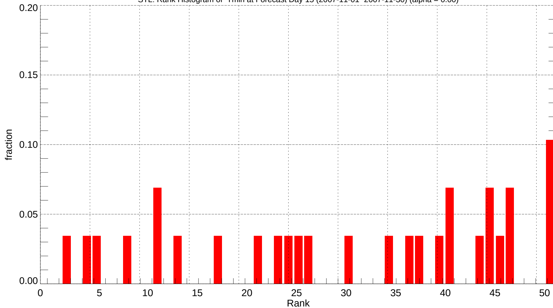
STL: Rank Histogram of Tmin at Forecast Day 15 (2007-11-01~2007-11-30) (alpha = 0.00)
