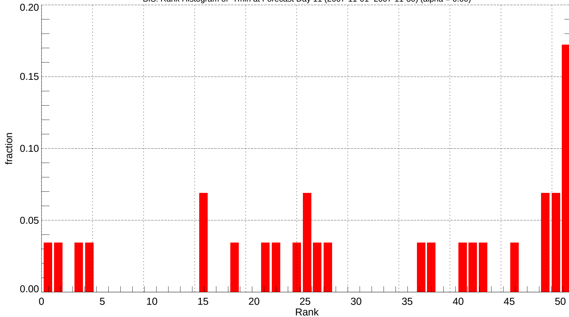
BIS: Rank Histogram of Tmin at Forecast Day 11 (2007-11-01~2007-11-30) (alpha = 0.00)
