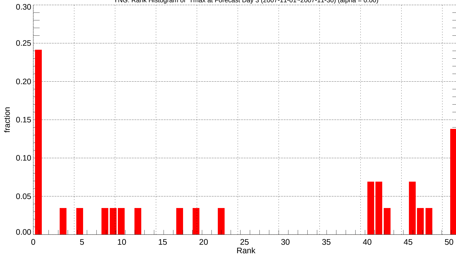
YNG: Rank Histogram of Tmax at Forecast Day 3 (2007-11-01~2007-11-30) (alpha = 0.00)
