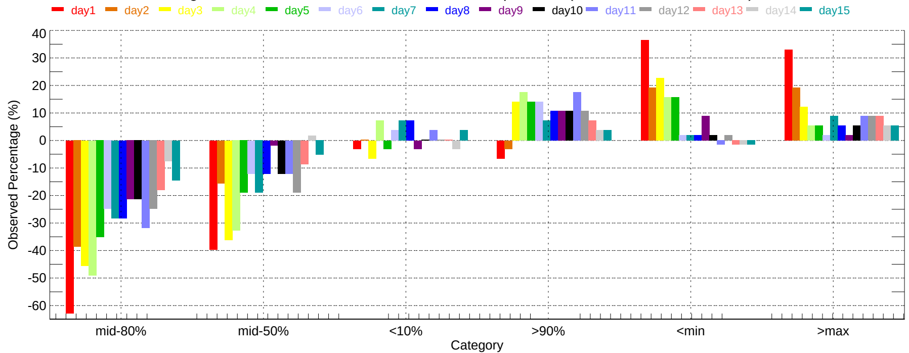
Observed Percentage Deviation of Ensembles - YNG: Min Temperature (2007-11-01~2007-11-30)
