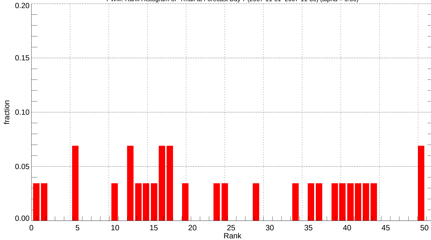
PWM: Rank Histogram of Tmax at Forecast Day 7 (2007-11-01~2007-11-30) (alpha = 0.00)
