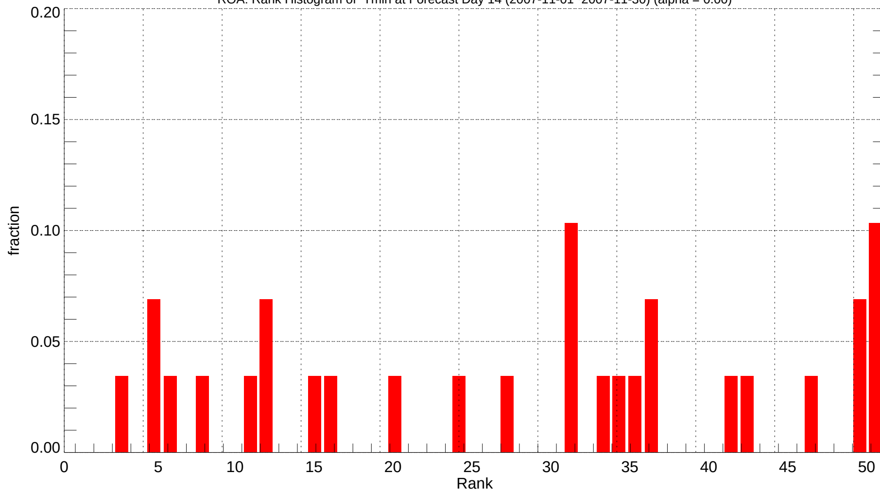
ROA: Rank Histogram of Tmin at Forecast Day 14 (2007-11-01~2007-11-30) (alpha = 0.00)
