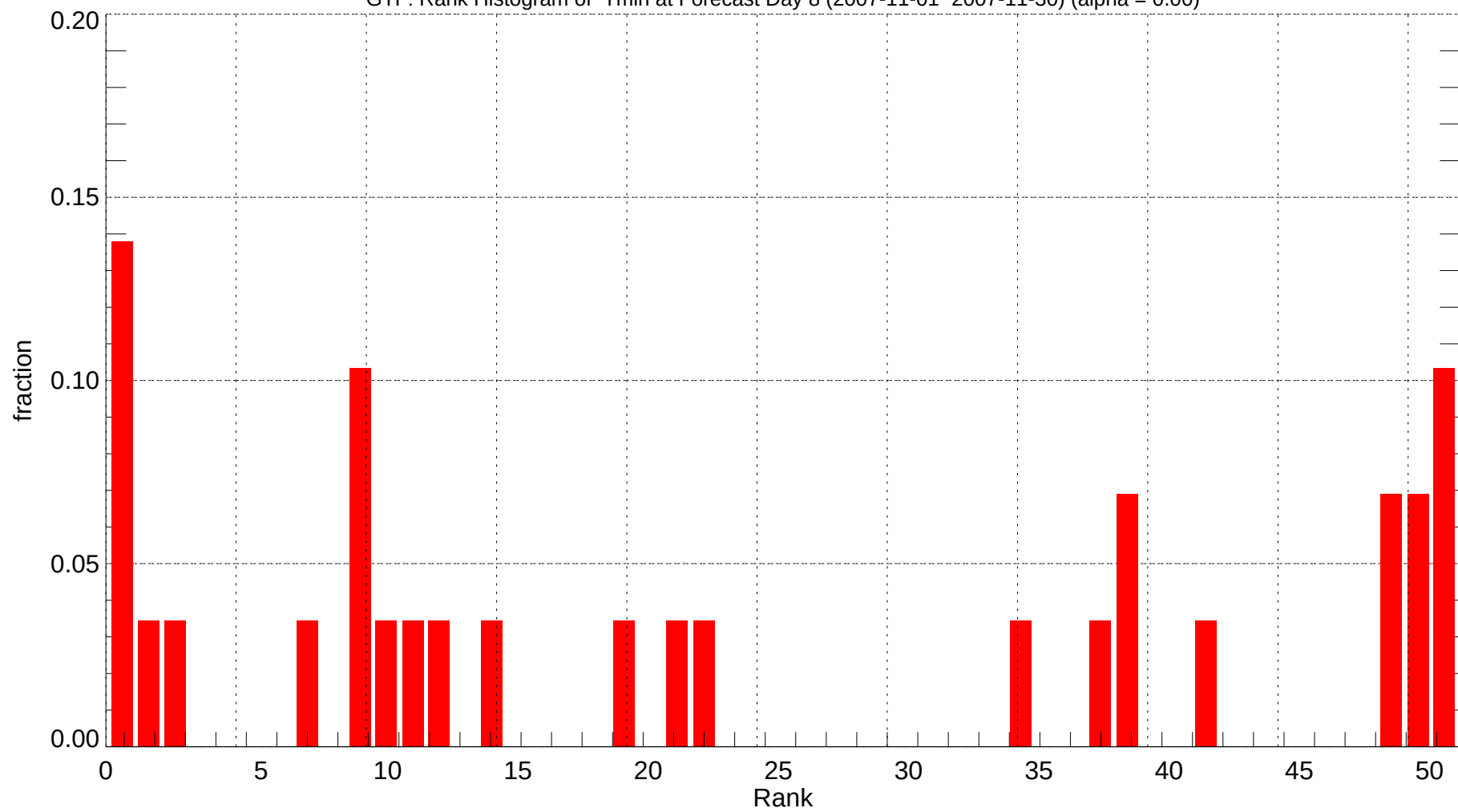
GTF: Rank Histogram of Tmin at Forecast Day 8 (2007-11-01~2007-11-30) (alpha = 0.00)
