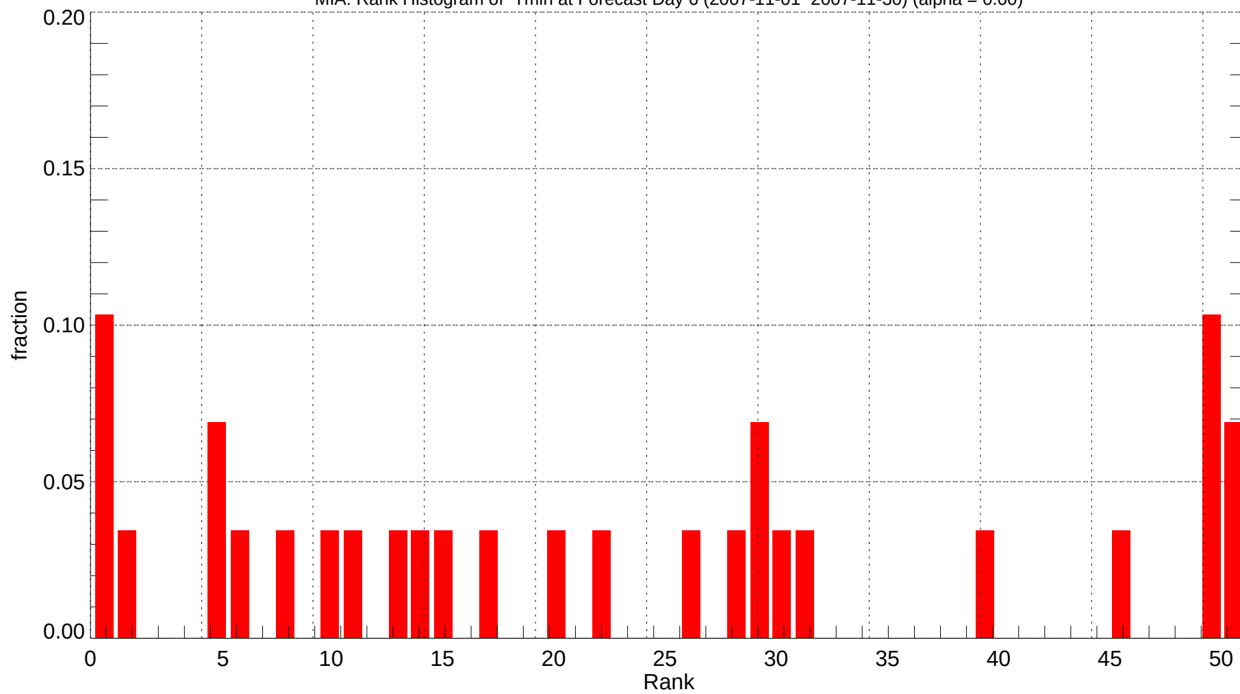
MIA: Rank Histogram of Tmin at Forecast Day 6 (2007-11-01~2007-11-30) (alpha = 0.00)
