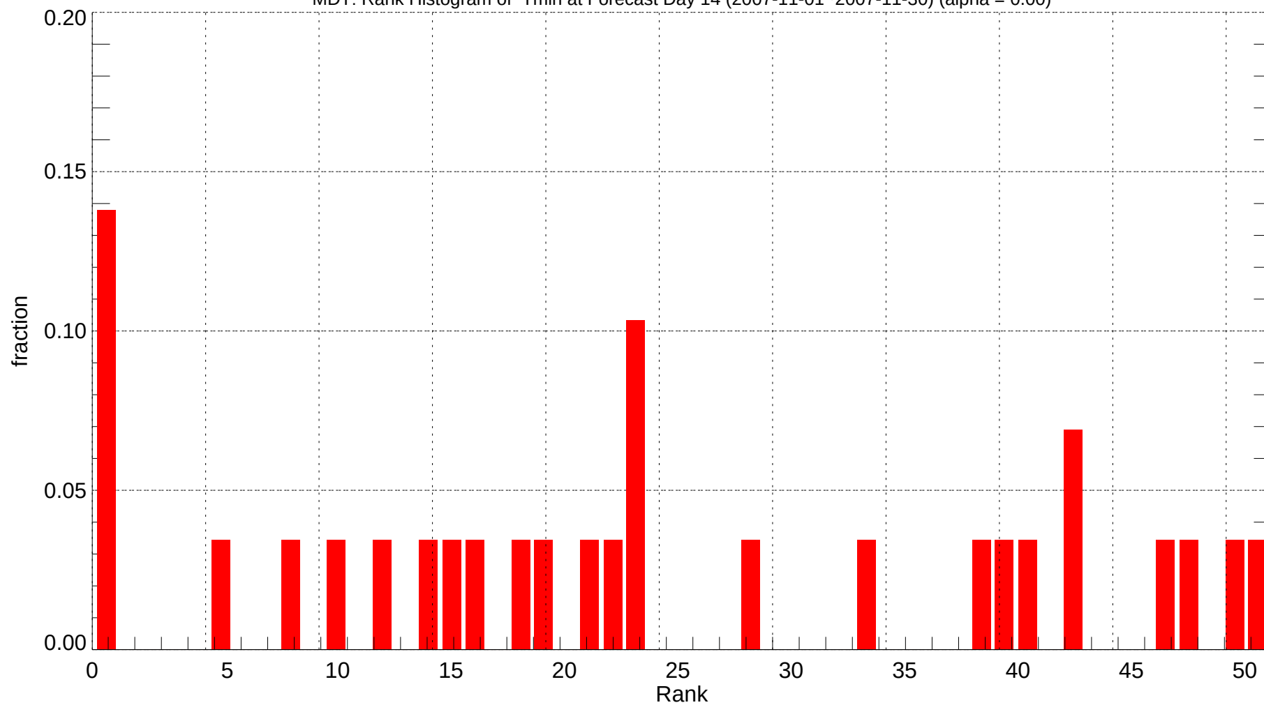
MDT: Rank Histogram of Tmin at Forecast Day 14 (2007-11-01~2007-11-30) (alpha = 0.00)
