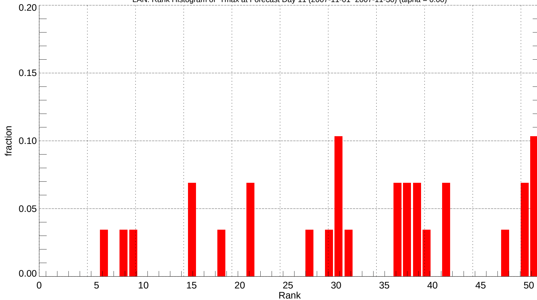
LAN: Rank Histogram of Tmax at Forecast Day 11 (2007-11-01~2007-11-30) (alpha = 0.00)
