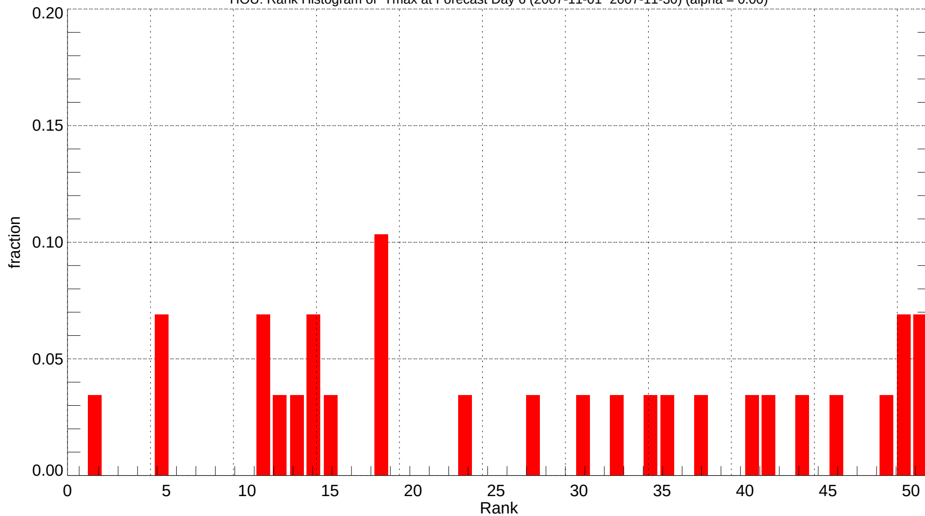
HOU: Rank Histogram of Tmax at Forecast Day 6 (2007-11-01~2007-11-30) (alpha = 0.00)
