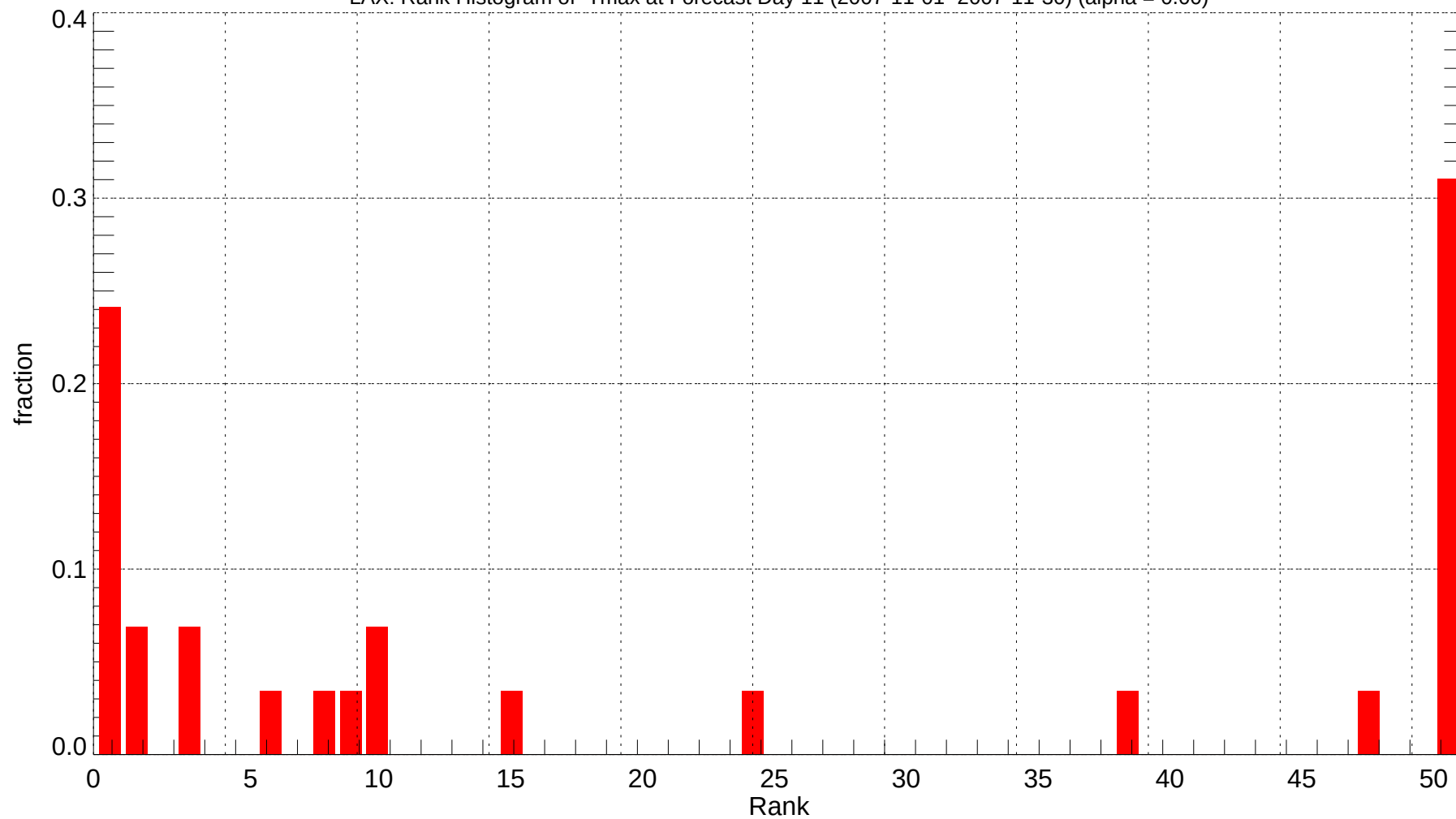
LAX: Rank Histogram of Tmax at Forecast Day 11 (2007-11-01~2007-11-30) (alpha = 0.00)
