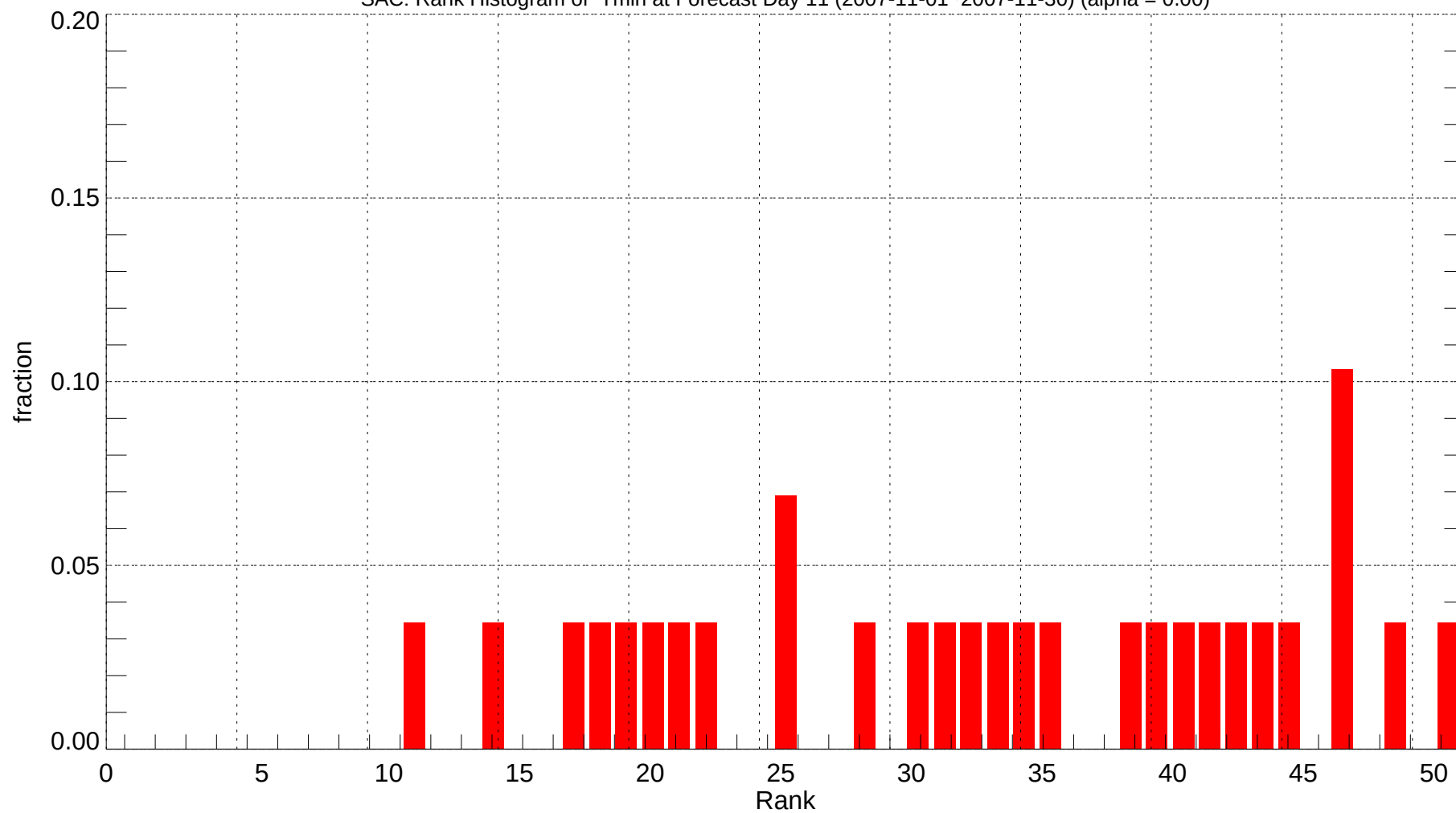
SAC: Rank Histogram of Tmin at Forecast Day 11 (2007-11-01~2007-11-30) (alpha = 0.00)
