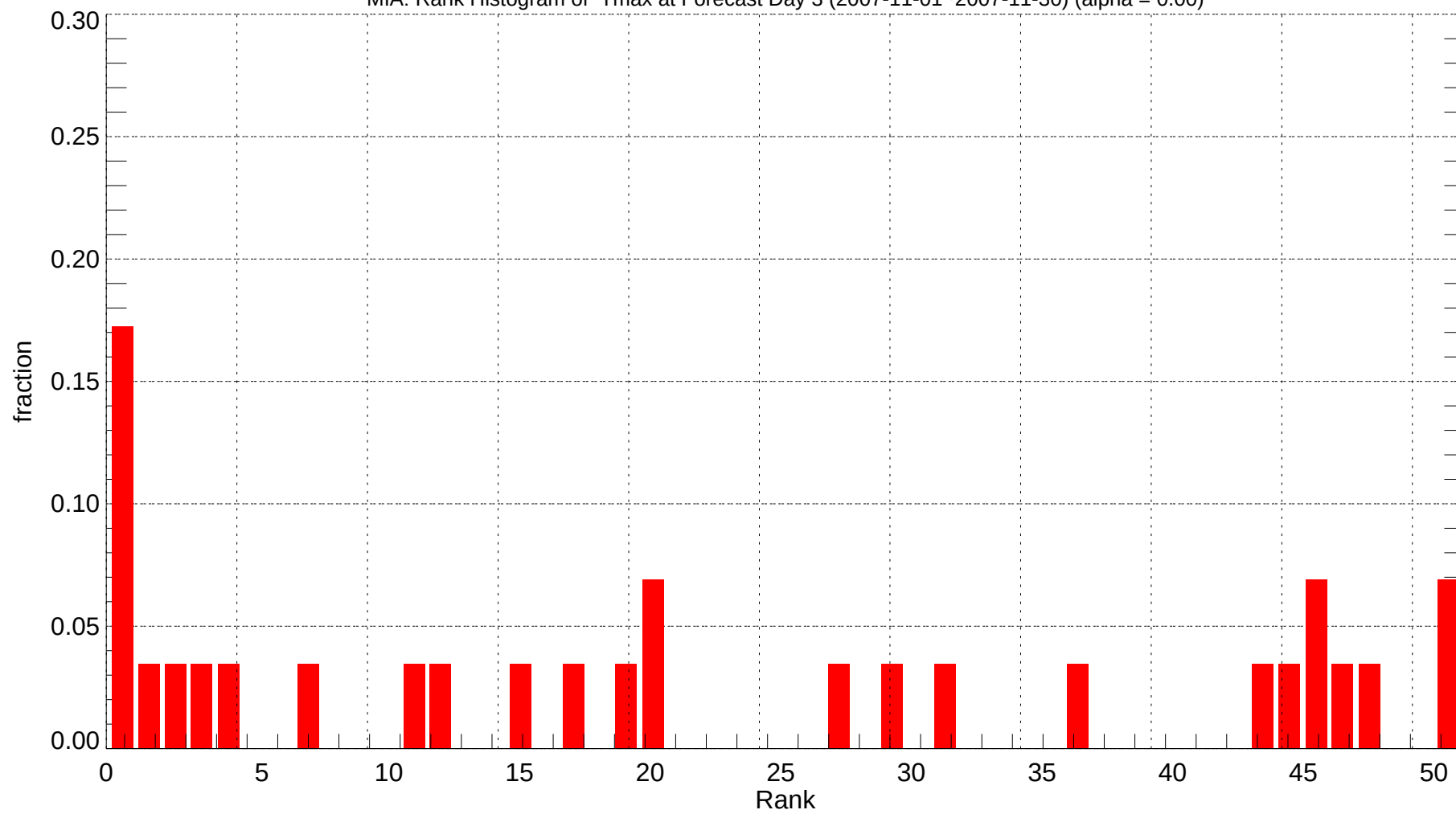
MIA: Rank Histogram of Tmax at Forecast Day 3 (2007-11-01~2007-11-30) (alpha = 0.00)
