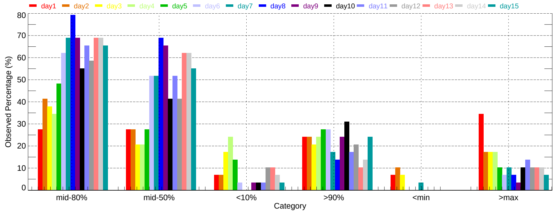
Observed Percentage of Ensembles - SLC: Max Temperature (2007-11-01~2007-11-30)
