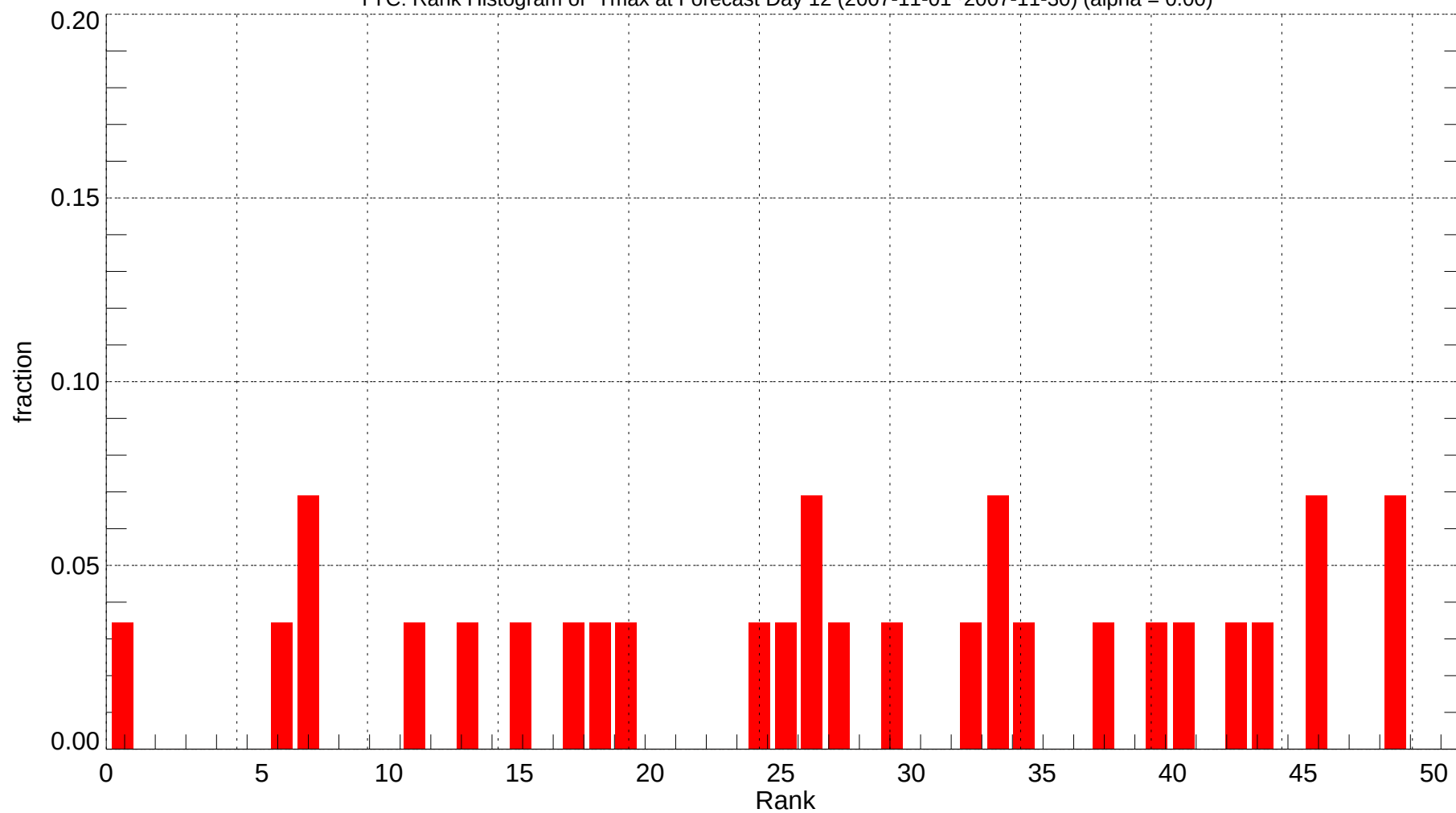
YYC: Rank Histogram of Tmax at Forecast Day 12 (2007-11-01~2007-11-30) (alpha = 0.00)
