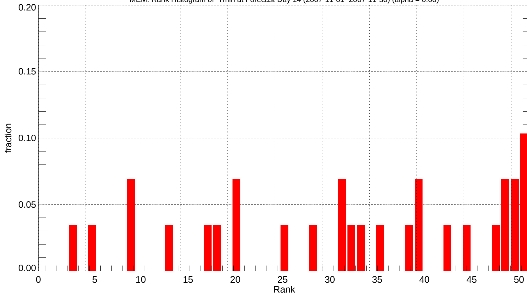
MEM: Rank Histogram of Tmin at Forecast Day 14 (2007-11-01~2007-11-30) (alpha = 0.00)
