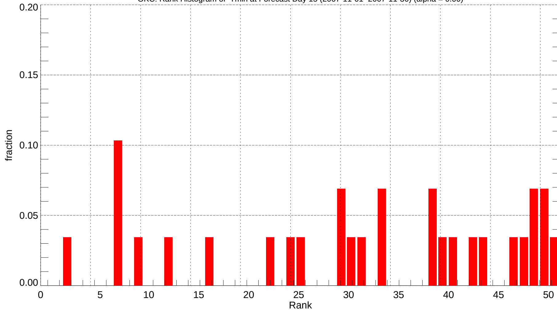
OKC: Rank Histogram of Tmin at Forecast Day 15 (2007-11-01~2007-11-30) (alpha = 0.00)
