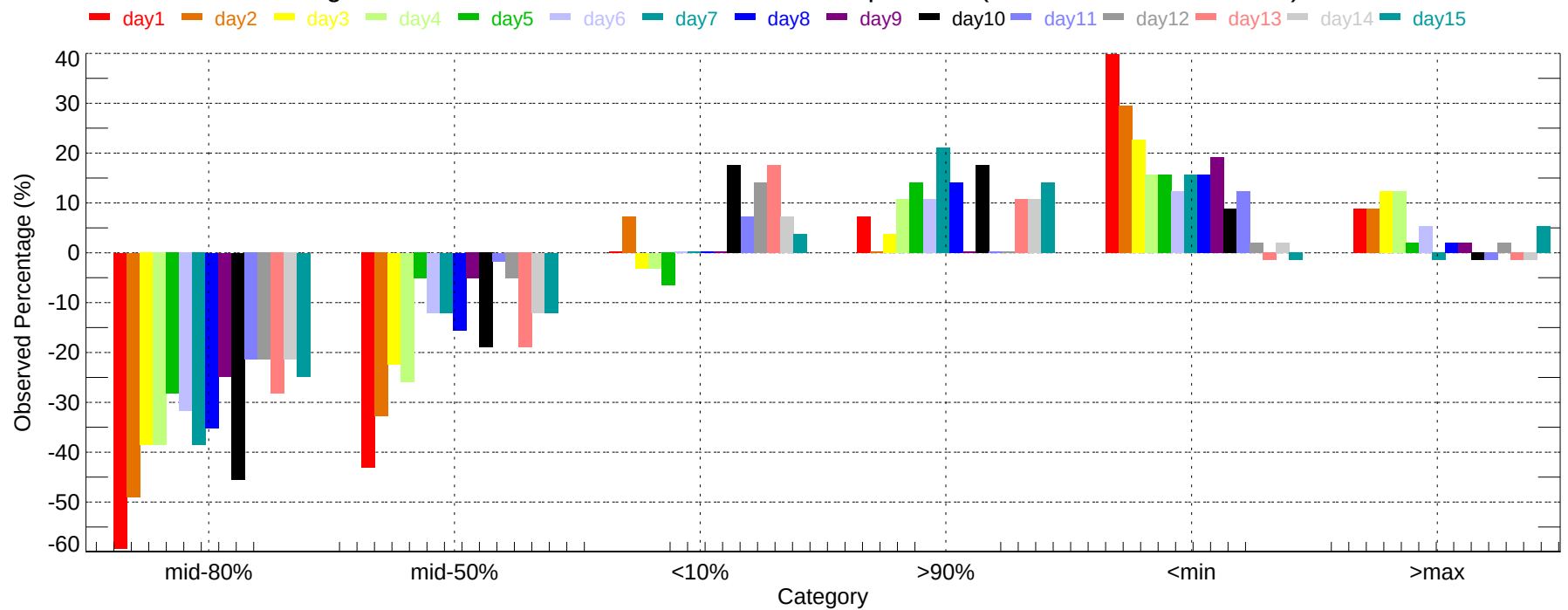
Observed Percentage Deviation of Ensembles - YKM: Min Temperature (2007-11-01~2007-11-30)
