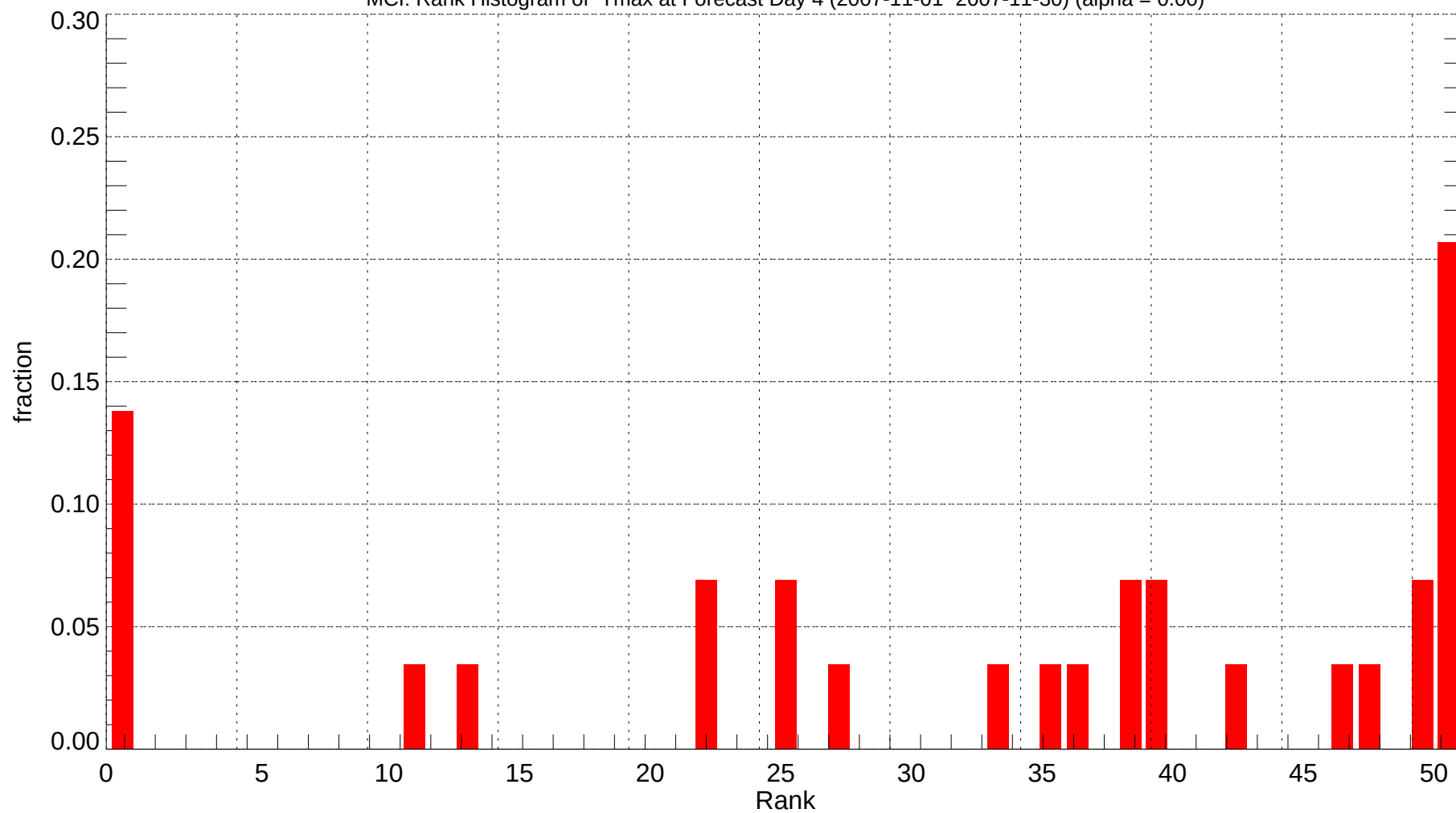
MCI: Rank Histogram of Tmax at Forecast Day 4 (2007-11-01~2007-11-30) (alpha = 0.00)
