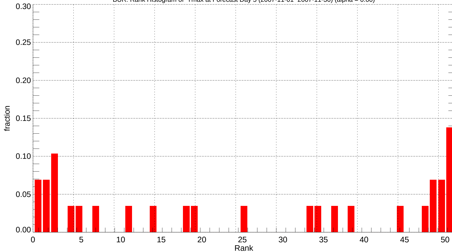
BUR: Rank Histogram of Tmax at Forecast Day 5 (2007-11-01~2007-11-30) (alpha = 0.00)
