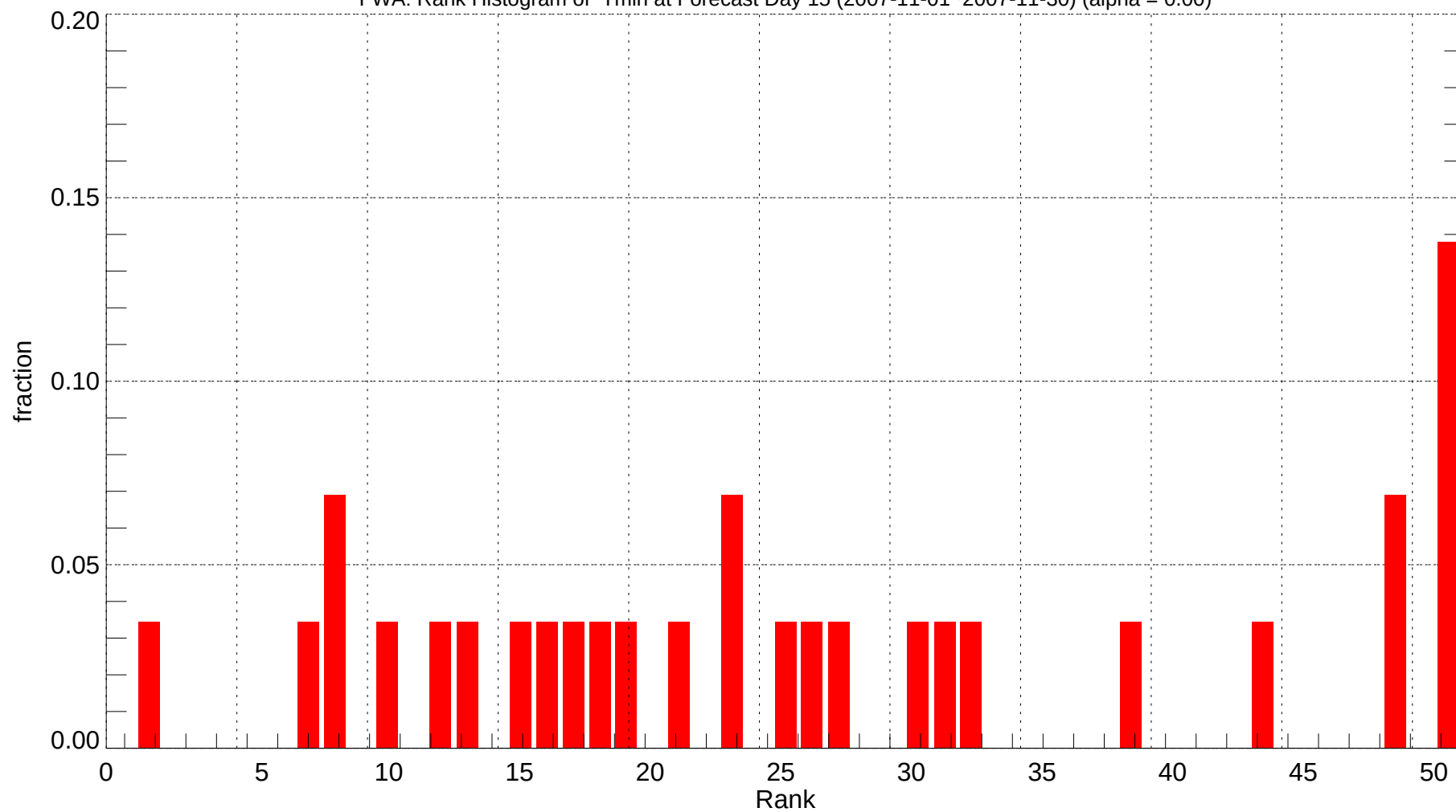
FWA: Rank Histogram of Tmin at Forecast Day 15 (2007-11-01~2007-11-30) (alpha = 0.00)
