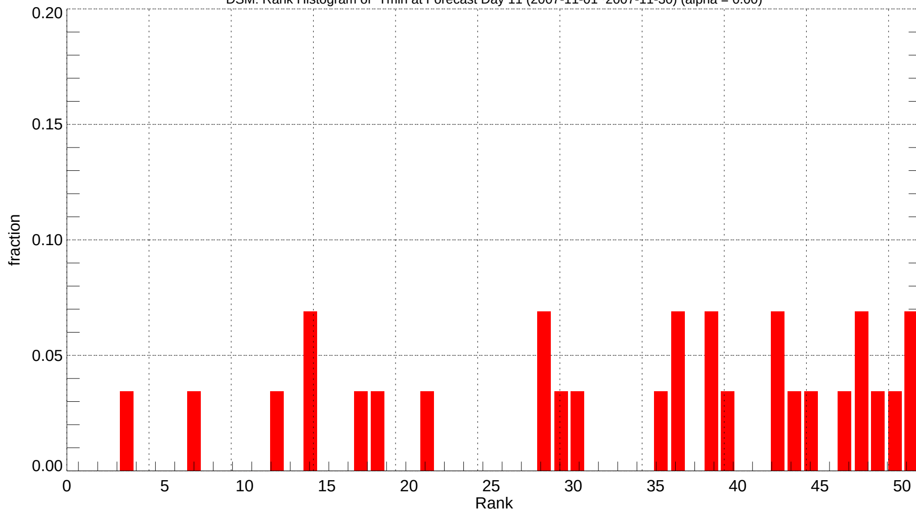
DSM: Rank Histogram of Tmin at Forecast Day 11 (2007-11-01~2007-11-30) (alpha = 0.00)
