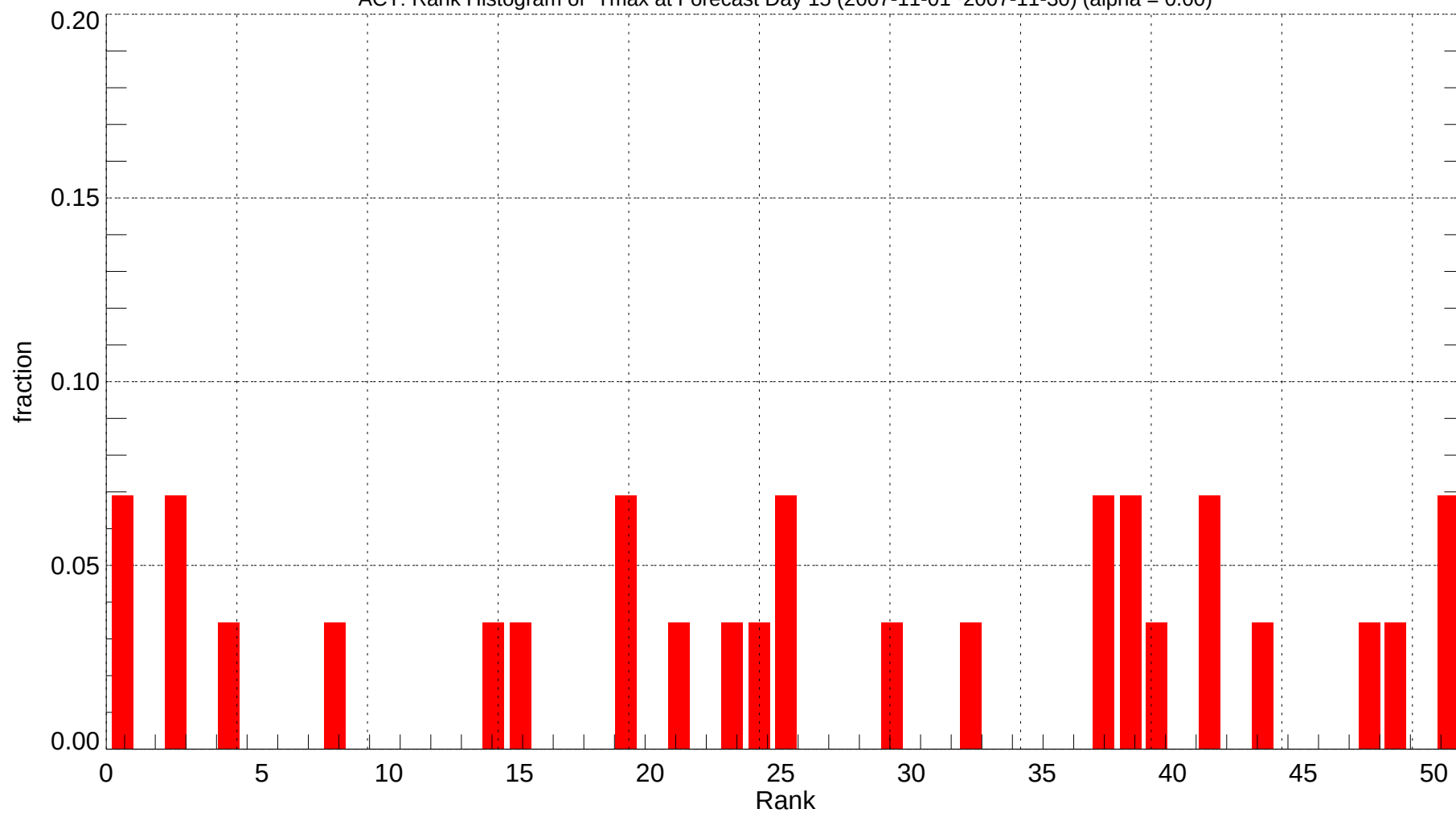
ACT: Rank Histogram of Tmax at Forecast Day 15 (2007-11-01~2007-11-30) (alpha = 0.00)
