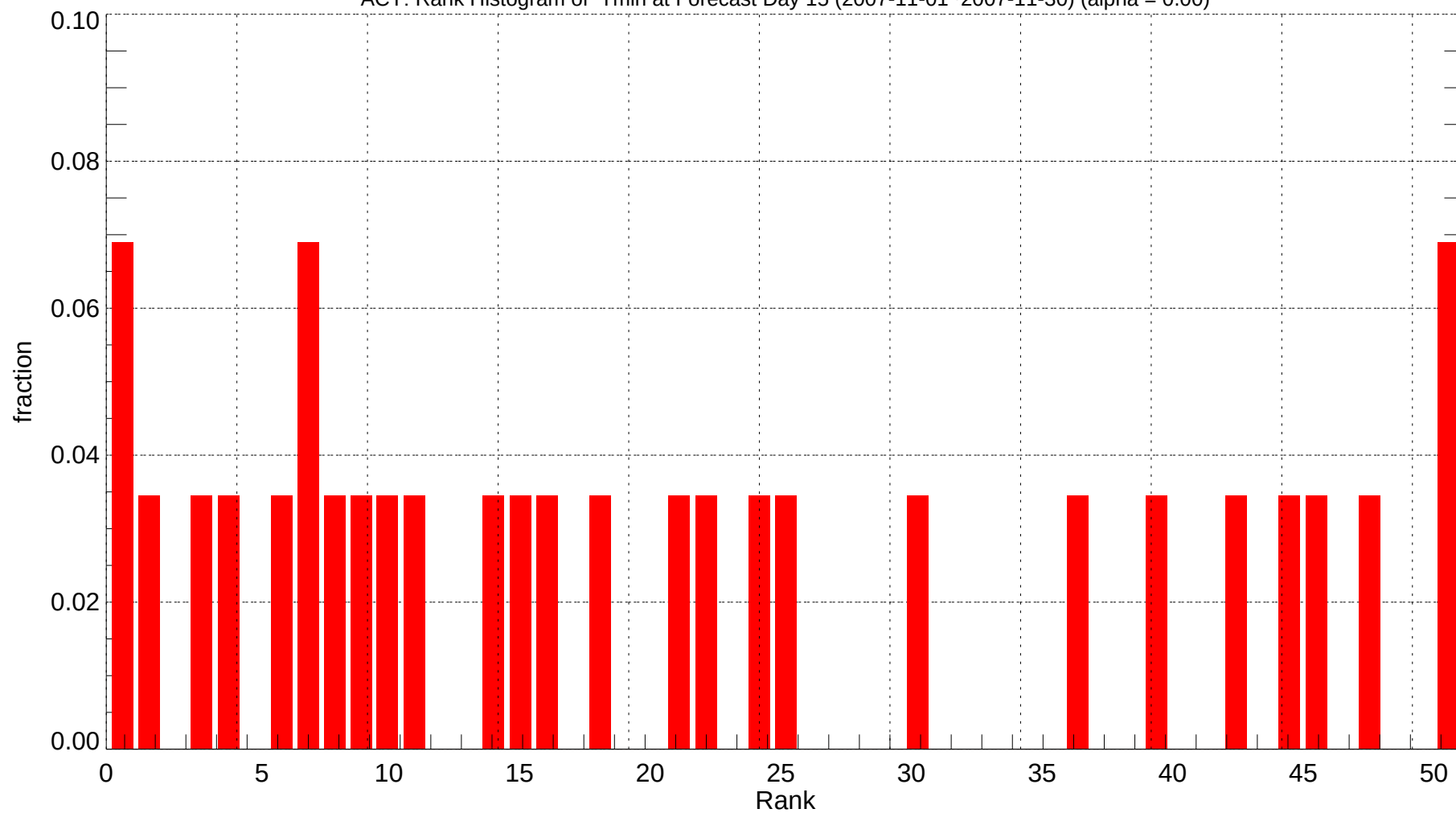
ACY: Rank Histogram of Tmin at Forecast Day 15 (2007-11-01~2007-11-30) (alpha = 0.00)
