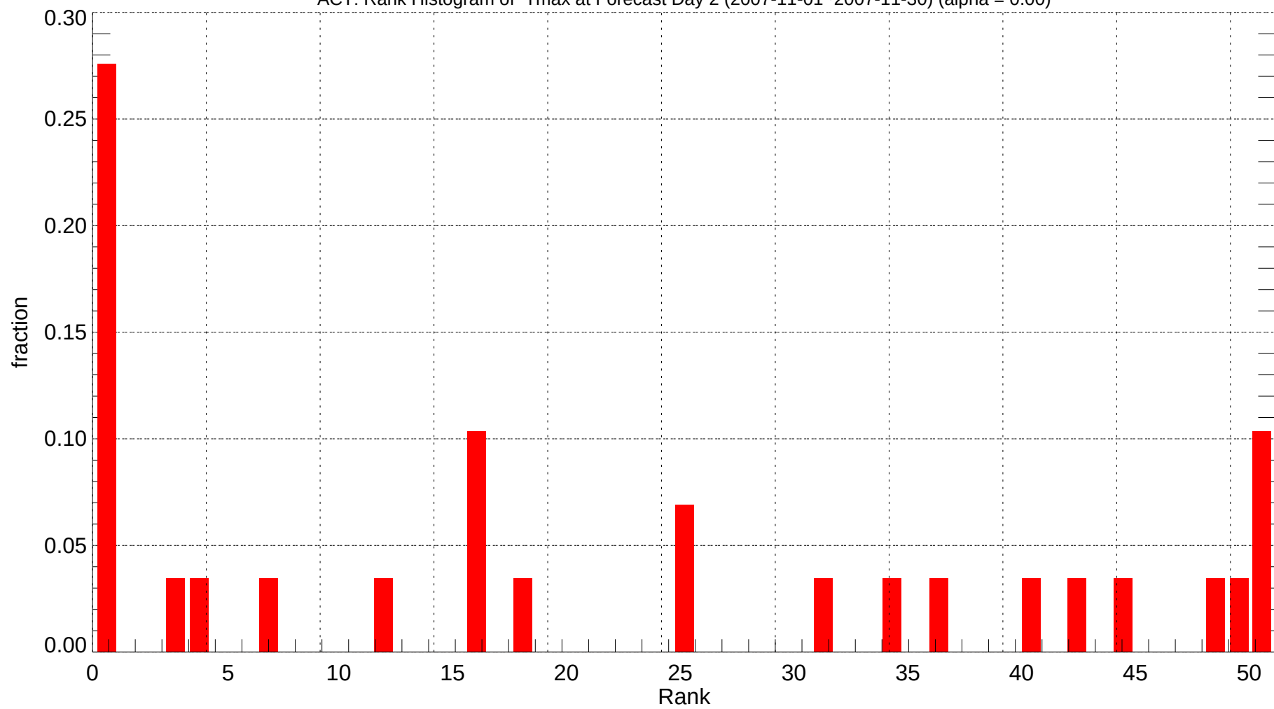
ACT: Rank Histogram of Tmax at Forecast Day 2 (2007-11-01~2007-11-30) (alpha = 0.00)
