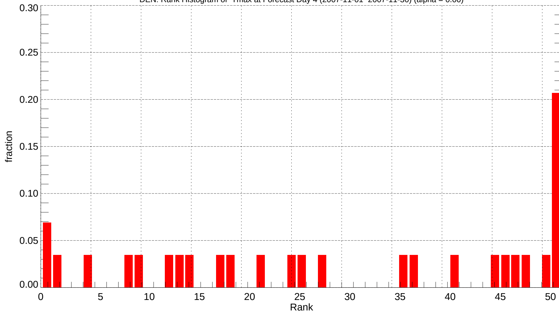
DEN: Rank Histogram of Tmax at Forecast Day 4 (2007-11-01~2007-11-30) (alpha = 0.00)
