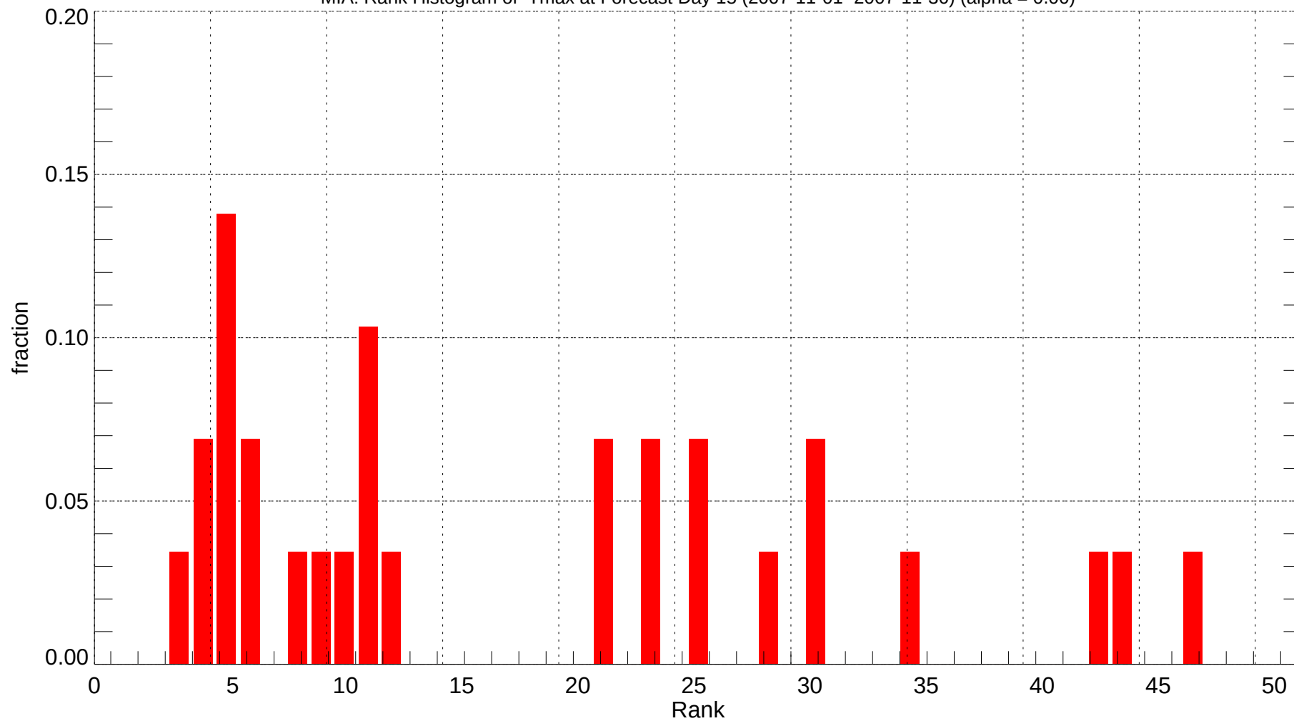
MIA: Rank Histogram of Tmax at Forecast Day 15 (2007-11-01~2007-11-30) (alpha = 0.00)
