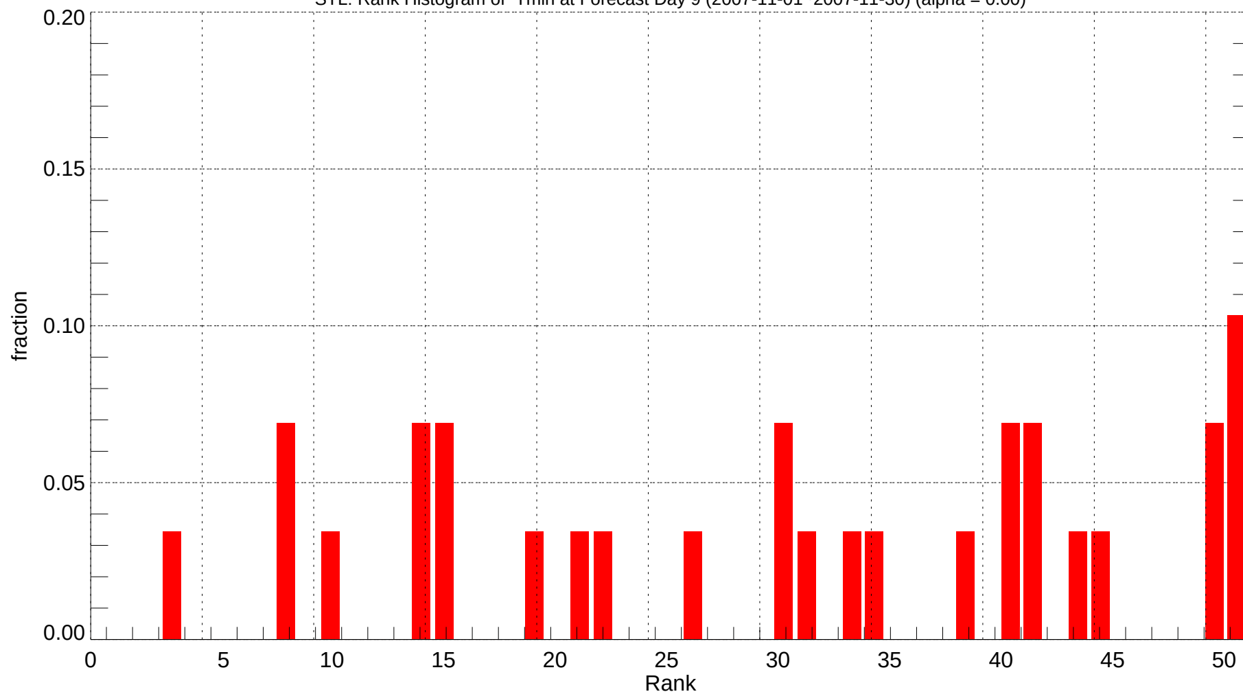
STL: Rank Histogram of Tmin at Forecast Day 9 (2007-11-01~2007-11-30) (alpha = 0.00)
