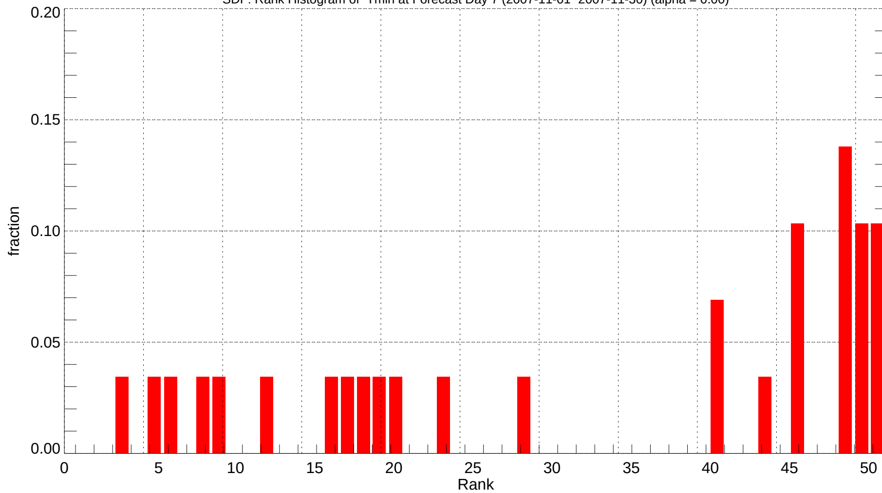
SDF: Rank Histogram of Tmin at Forecast Day 7 (2007-11-01~2007-11-30) (alpha = 0.00)
