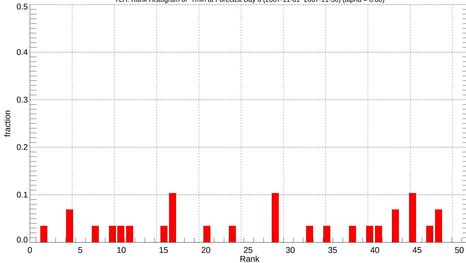
TLH: Rank Histogram of Tmin at Forecast Day 6 (2007-11-01~2007-11-30) (alpha = 0.00)
