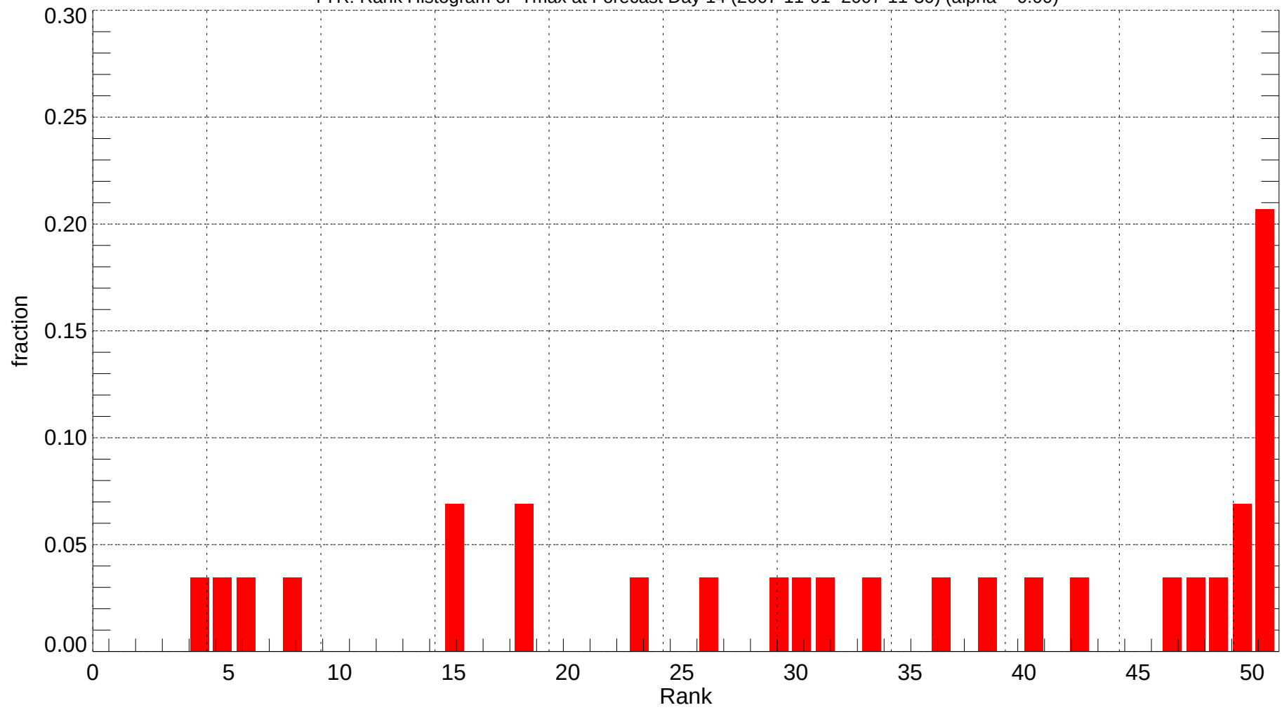
TYR: Rank Histogram of Tmax at Forecast Day 14 (2007-11-01~2007-11-30) (alpha = 0.00)
