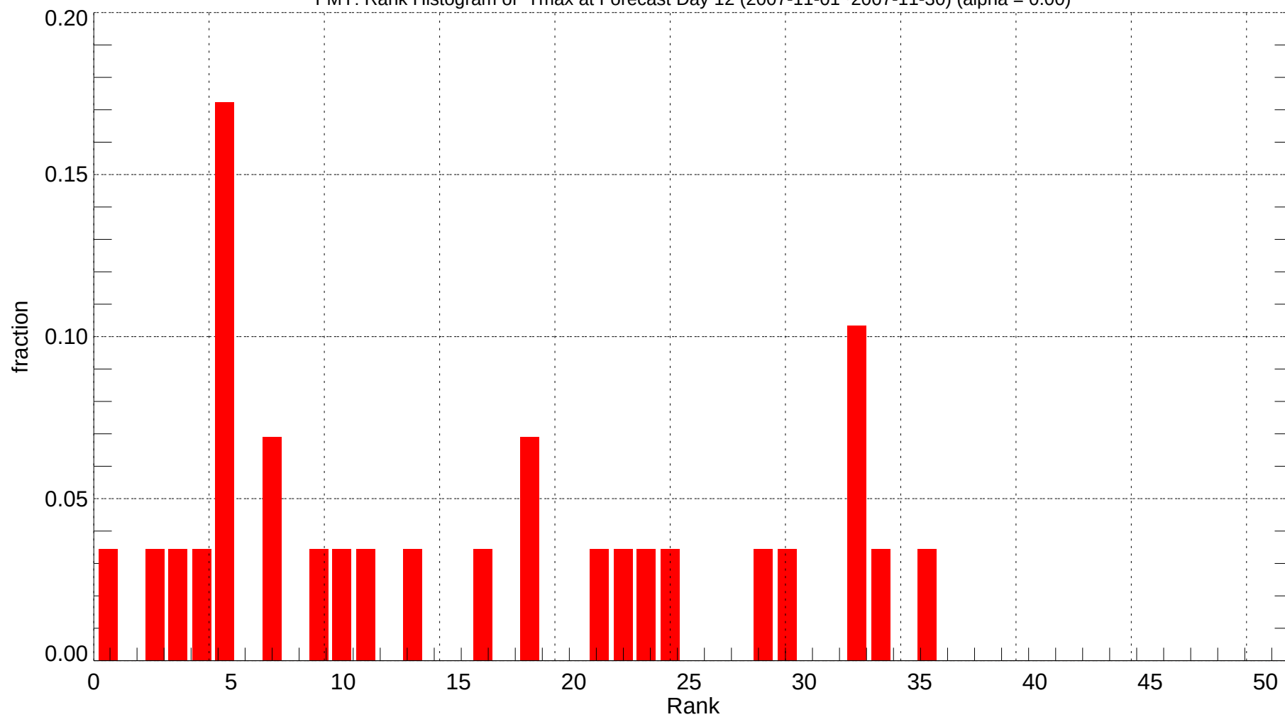
FMY: Rank Histogram of Tmax at Forecast Day 12 (2007-11-01~2007-11-30) (alpha = 0.00)
