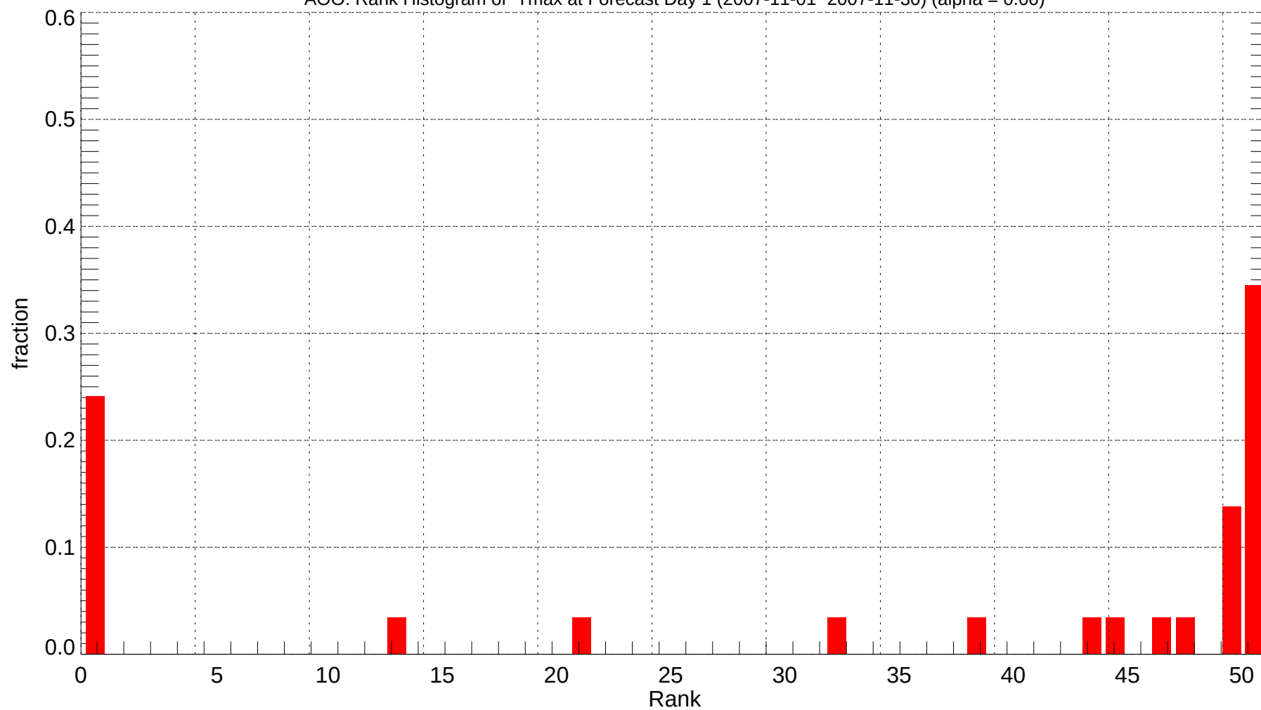
AOO: Rank Histogram of Tmax at Forecast Day 1 (2007-11-01~2007-11-30) (alpha = 0.00)
