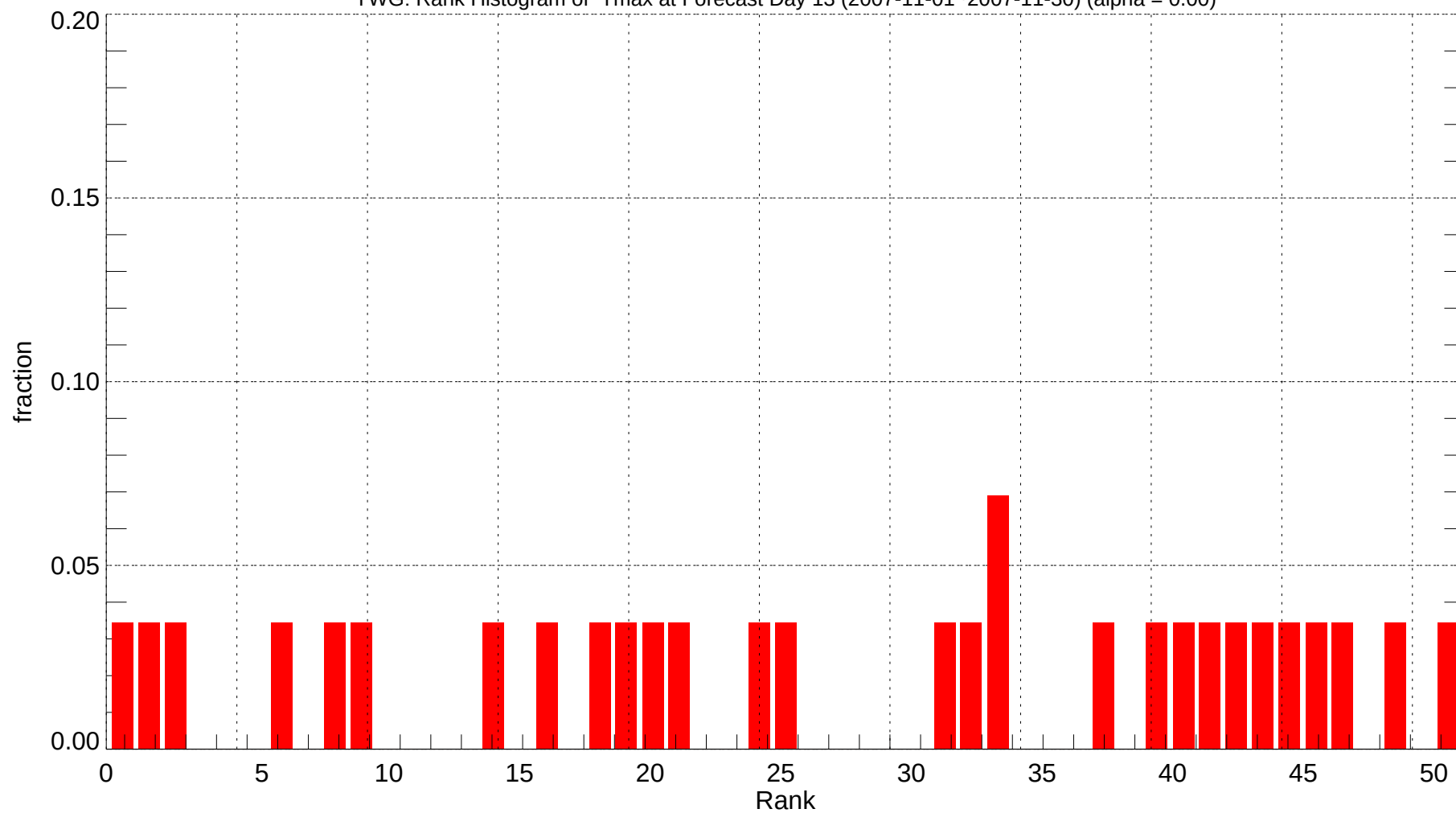
YWG: Rank Histogram of Tmax at Forecast Day 13 (2007-11-01~2007-11-30) (alpha = 0.00)
