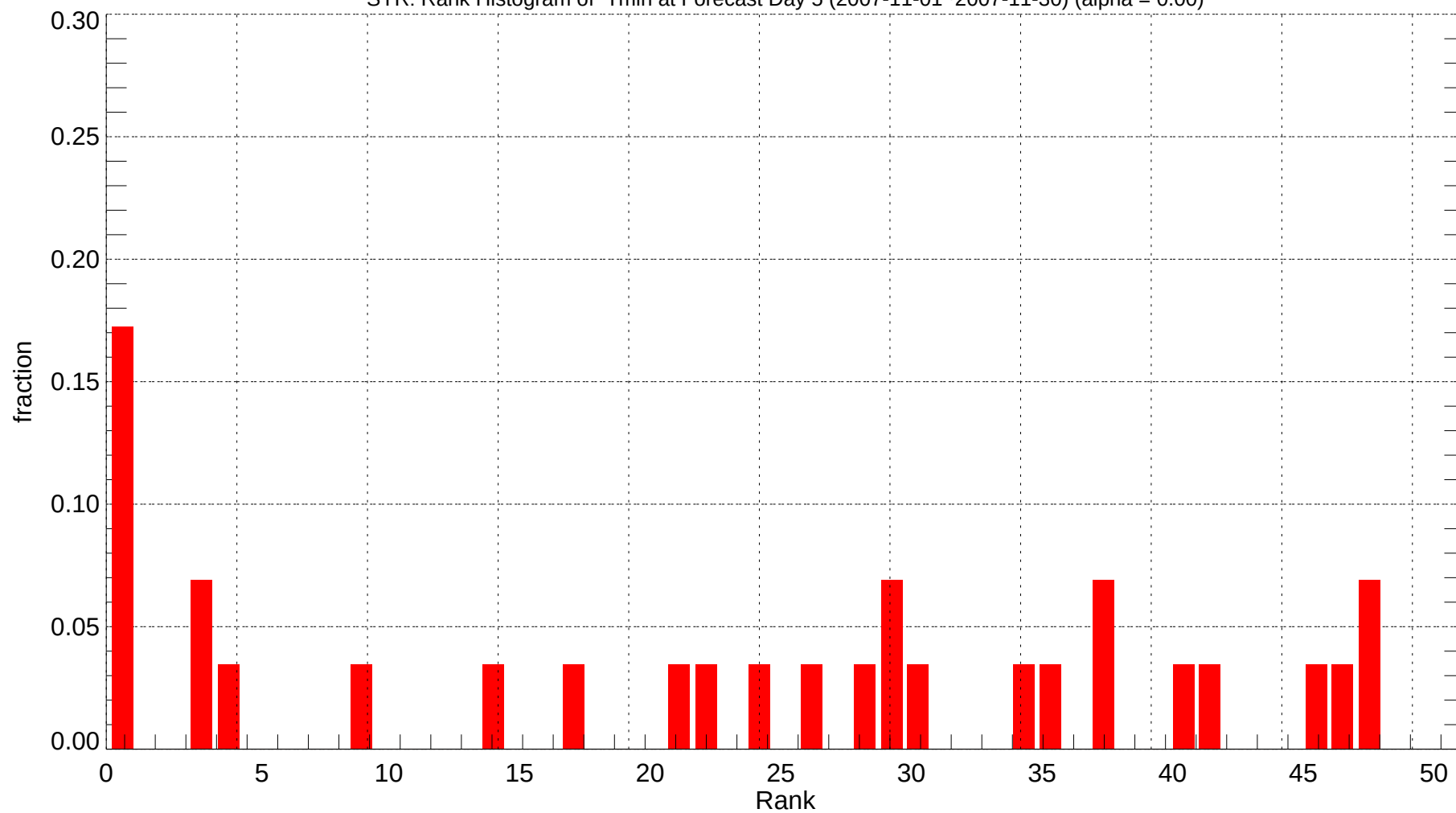
SYR: Rank Histogram of Tmin at Forecast Day 5 (2007-11-01~2007-11-30) (alpha = 0.00)
