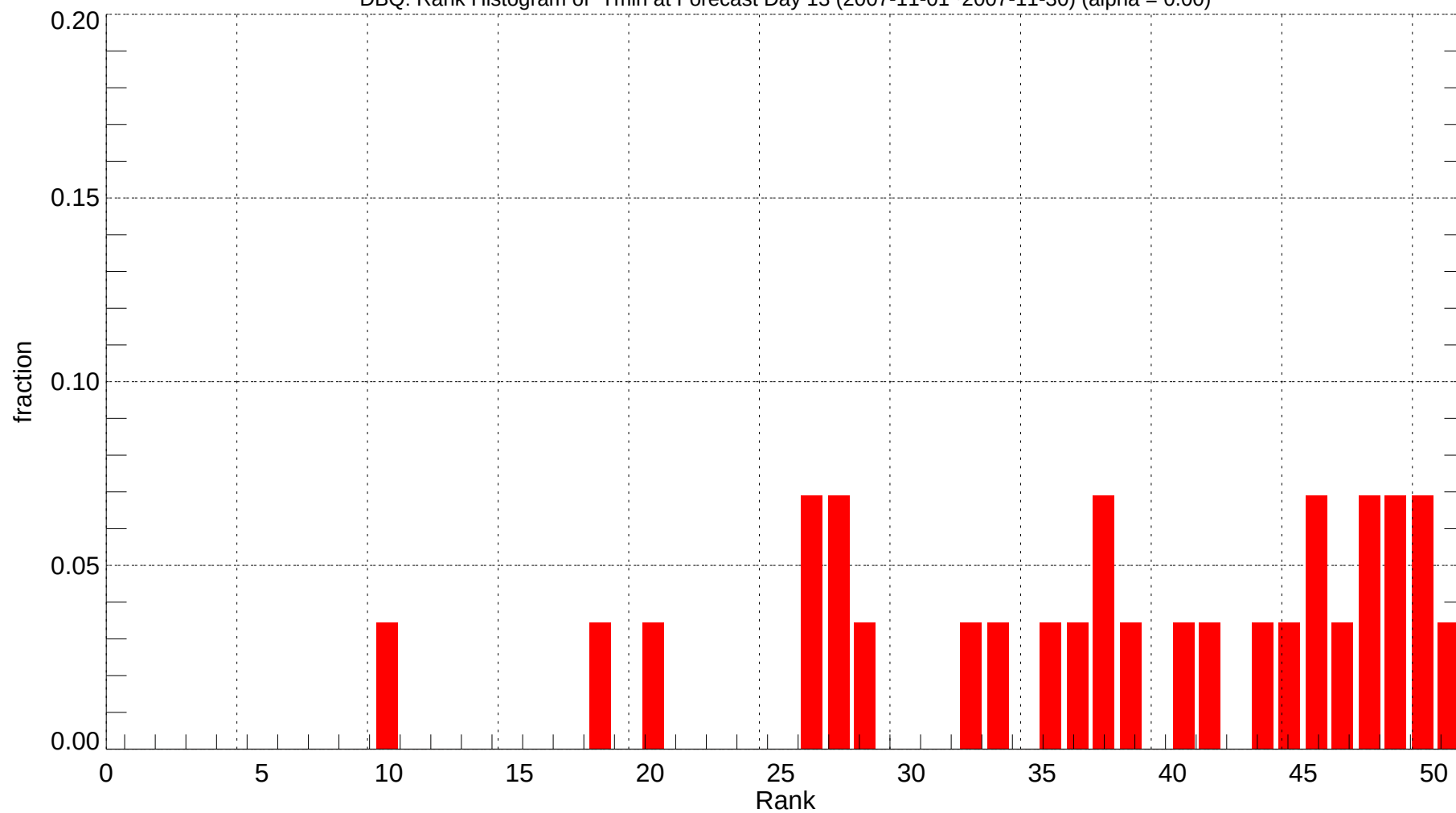
DBQ: Rank Histogram of Tmin at Forecast Day 13 (2007-11-01~2007-11-30) (alpha = 0.00)
