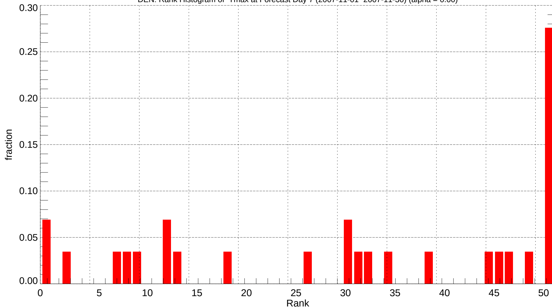
DEN: Rank Histogram of Tmax at Forecast Day 7 (2007-11-01~2007-11-30) (alpha = 0.00)
