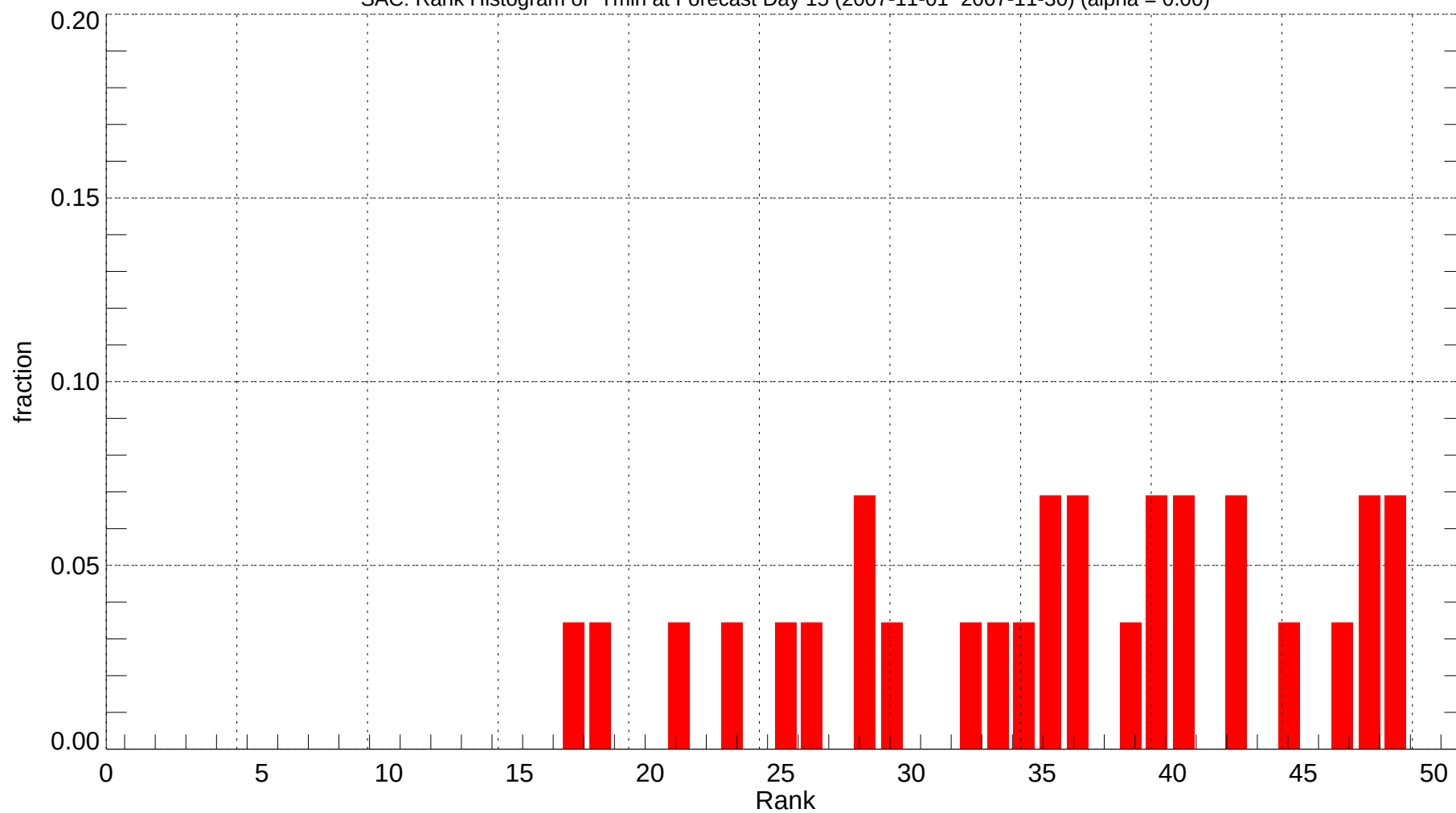
SAC: Rank Histogram of Tmin at Forecast Day 15 (2007-11-01~2007-11-30) (alpha = 0.00)
