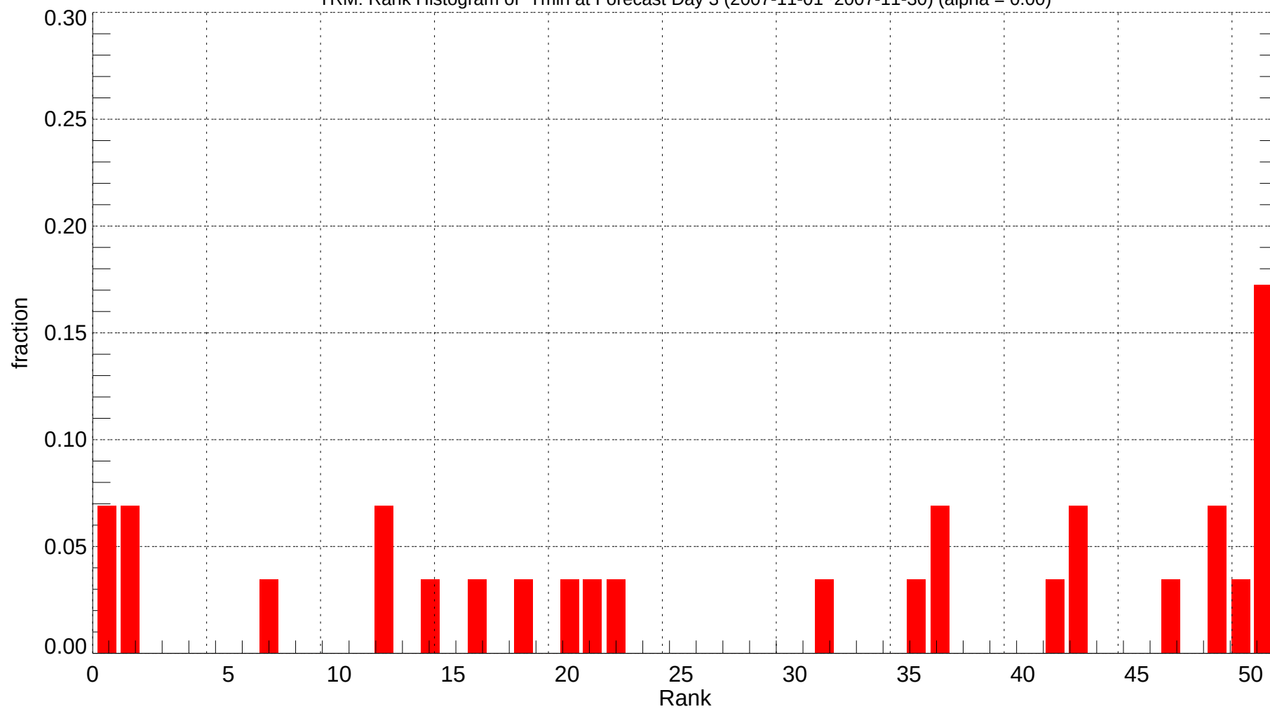
TRM: Rank Histogram of Tmin at Forecast Day 3 (2007-11-01~2007-11-30) (alpha = 0.00)
