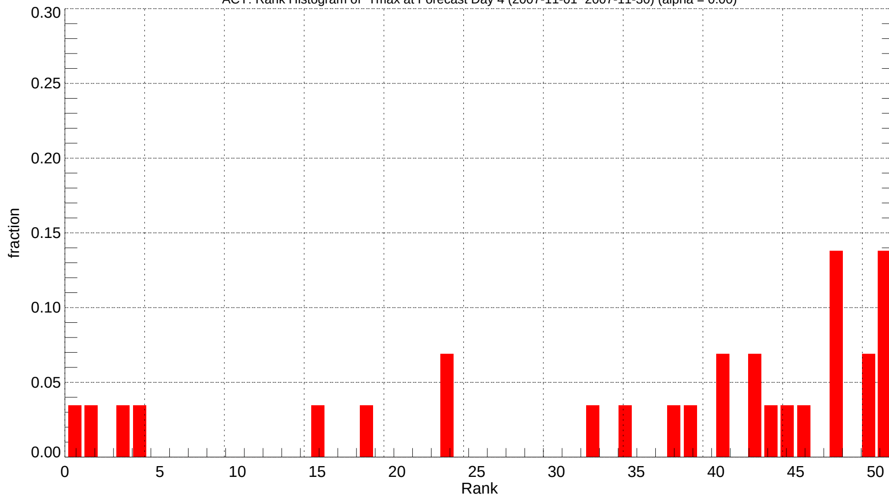
ACY: Rank Histogram of Tmax at Forecast Day 4 (2007-11-01~2007-11-30) (alpha = 0.00)
