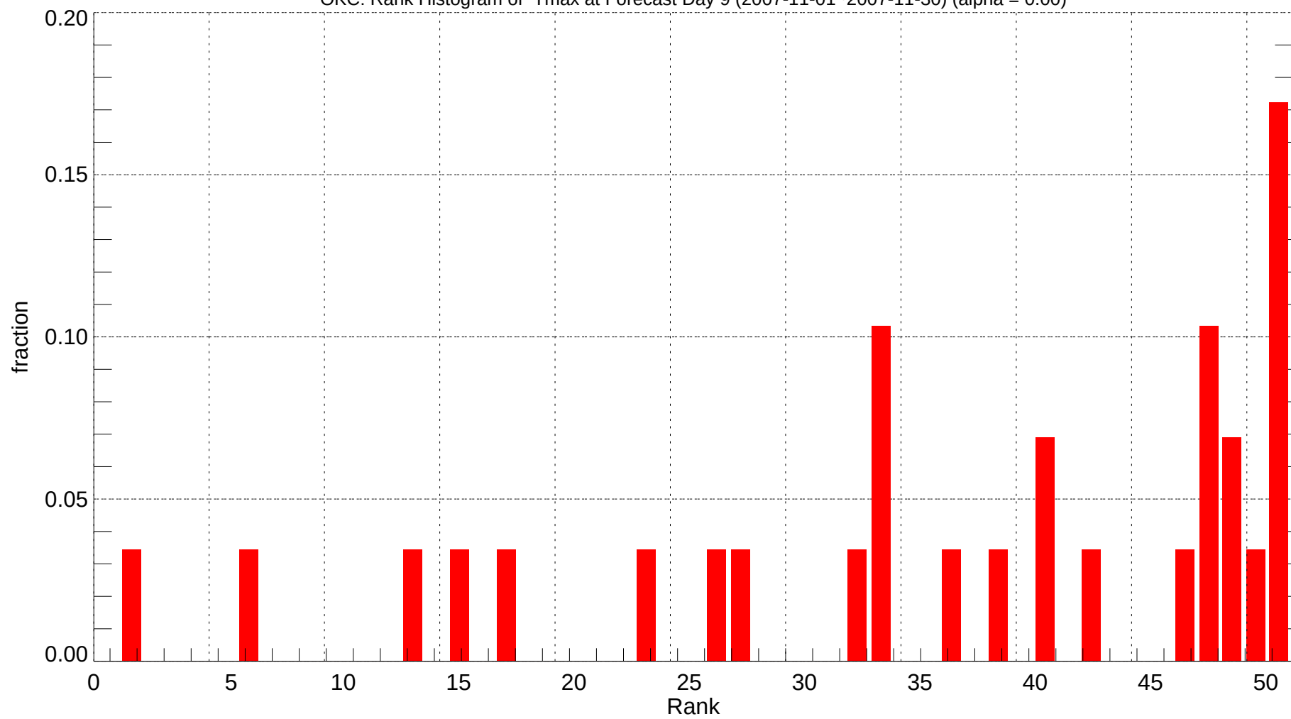
OKC: Rank Histogram of Tmax at Forecast Day 9 (2007-11-01~2007-11-30) (alpha = 0.00)
