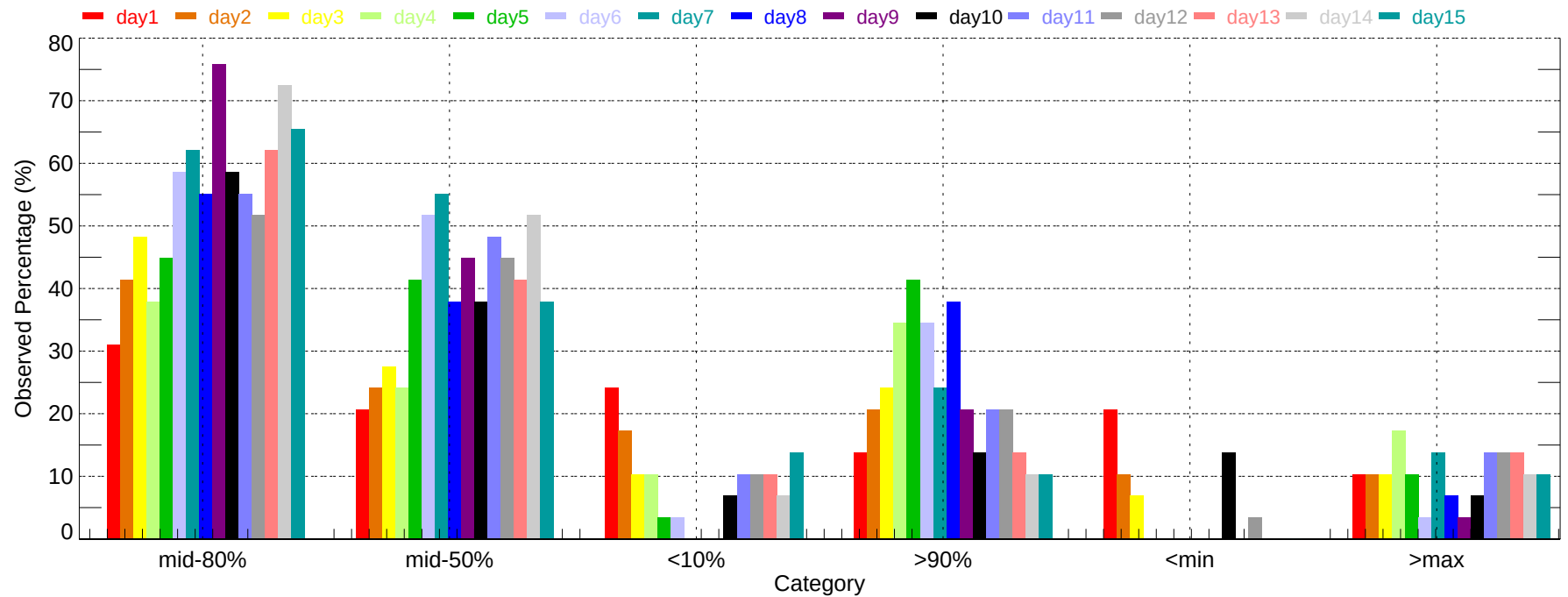
Observed Percentage of Ensembles - CLE: Max Temperature (2007-11-01~2007-11-30)
