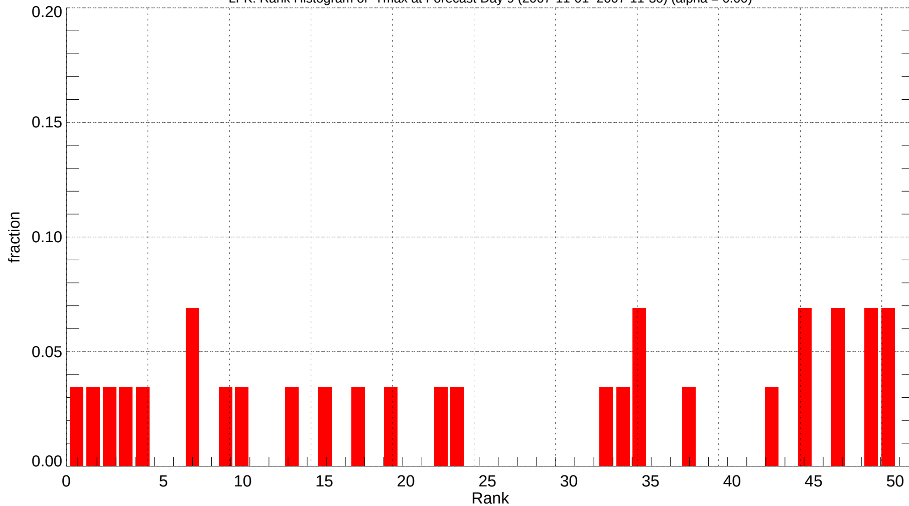
LFK: Rank Histogram of Tmax at Forecast Day 9 (2007-11-01~2007-11-30) (alpha = 0.00)
