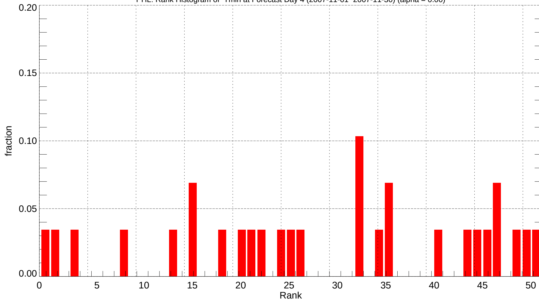
PHL: Rank Histogram of Tmin at Forecast Day 4 (2007-11-01~2007-11-30) (alpha = 0.00)
