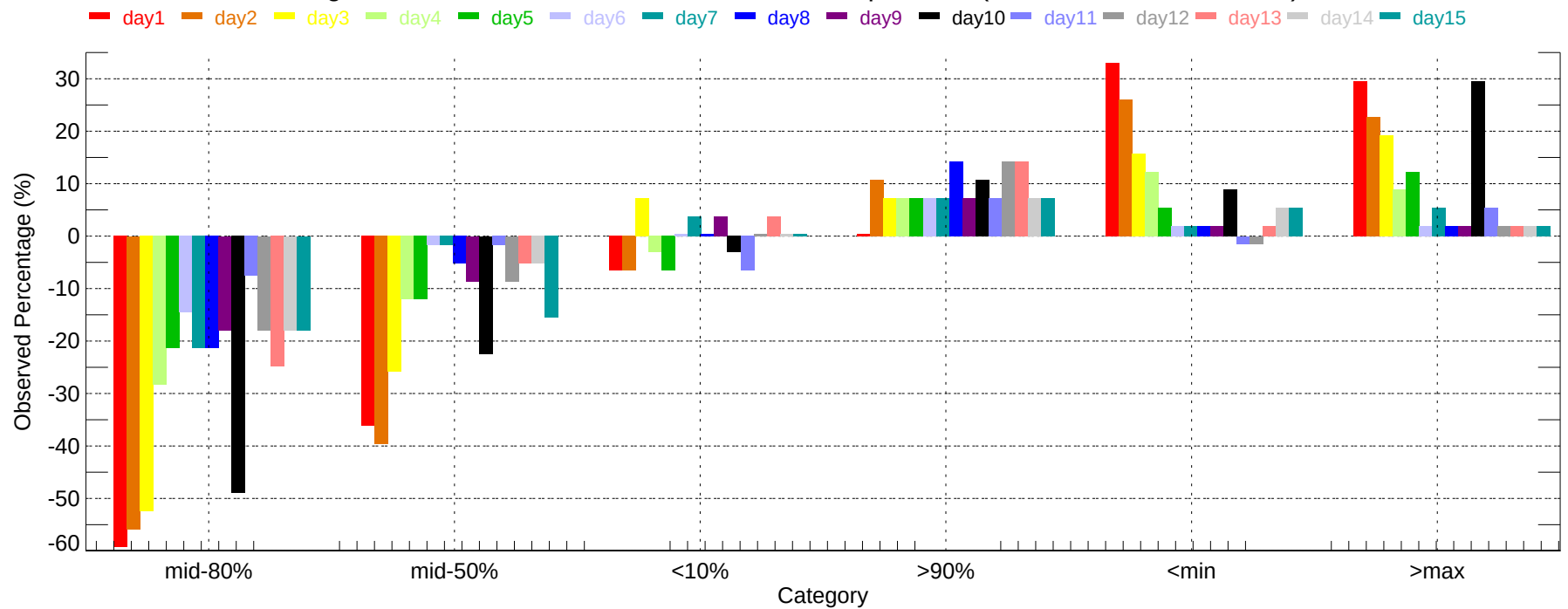
Observed Percentage Deviation of Ensembles - MDT: Min Temperature (2007-11-01~2007-11-30)
