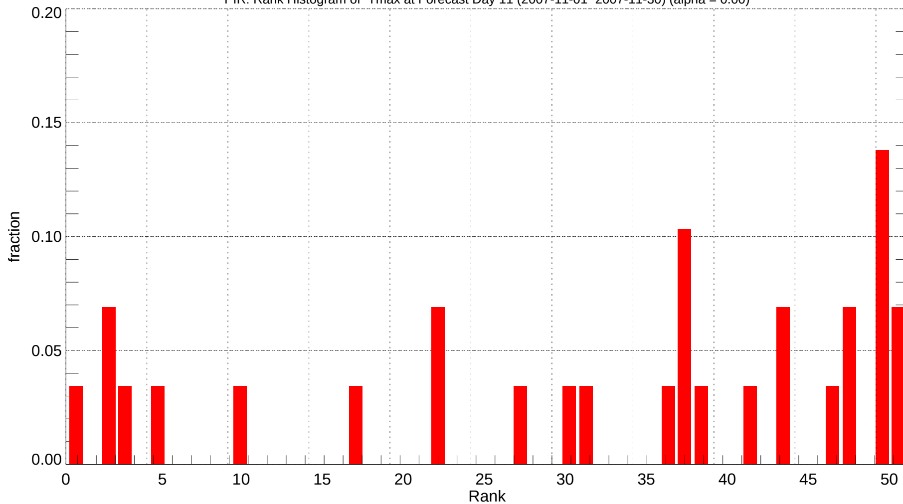
PIR: Rank Histogram of Tmax at Forecast Day 11 (2007-11-01~2007-11-30) (alpha = 0.00)
