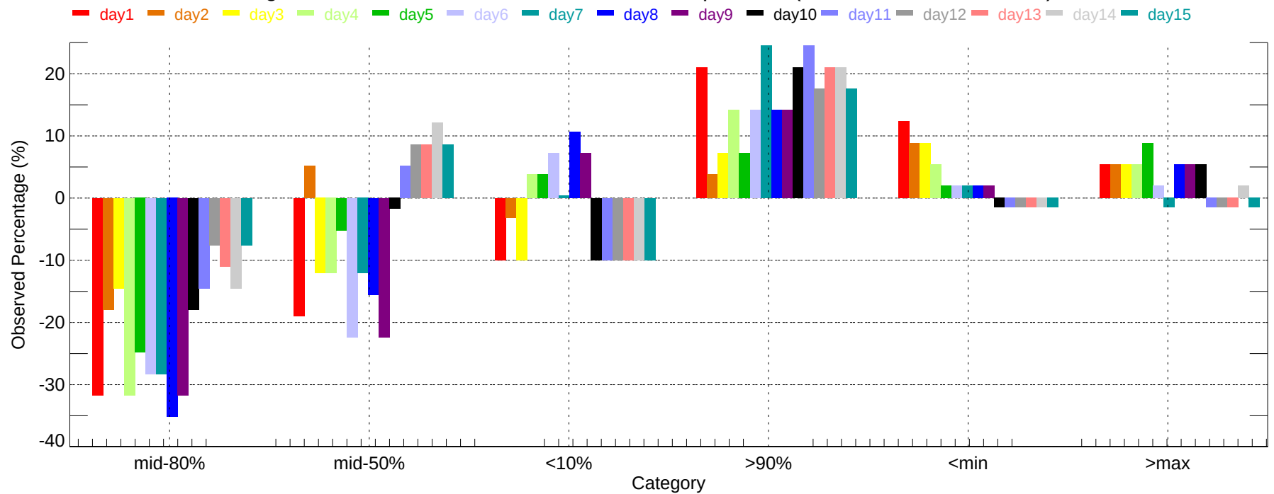
Observed Percentage Deviation of Ensembles - SAC: Min Temperature (2007-11-01~2007-11-30)
