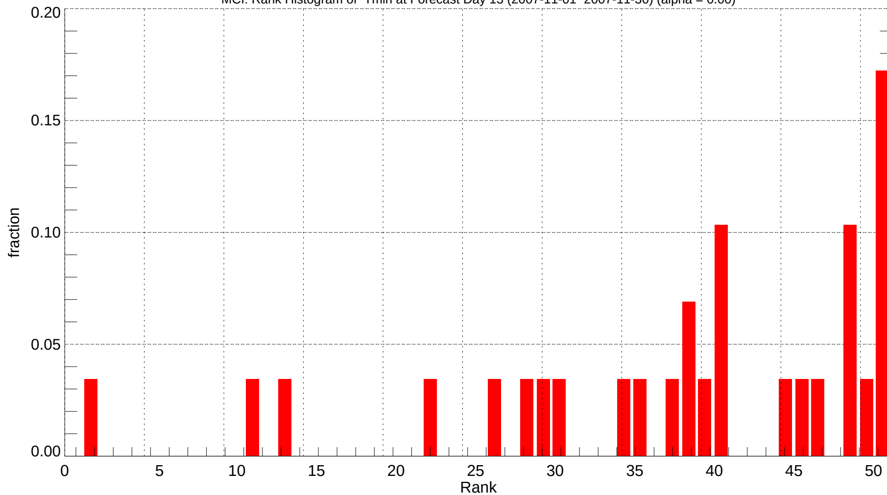
MCI: Rank Histogram of Tmin at Forecast Day 13 (2007-11-01~2007-11-30) (alpha = 0.00)
