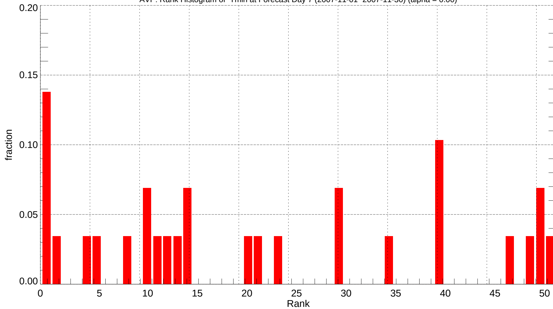
AVP: Rank Histogram of Tmin at Forecast Day 7 (2007-11-01~2007-11-30) (alpha = 0.00)
