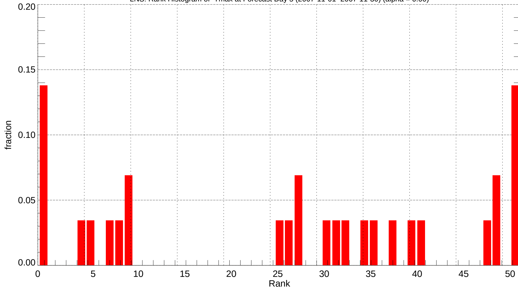
LNS: Rank Histogram of Tmax at Forecast Day 5 (2007-11-01~2007-11-30) (alpha = 0.00)
