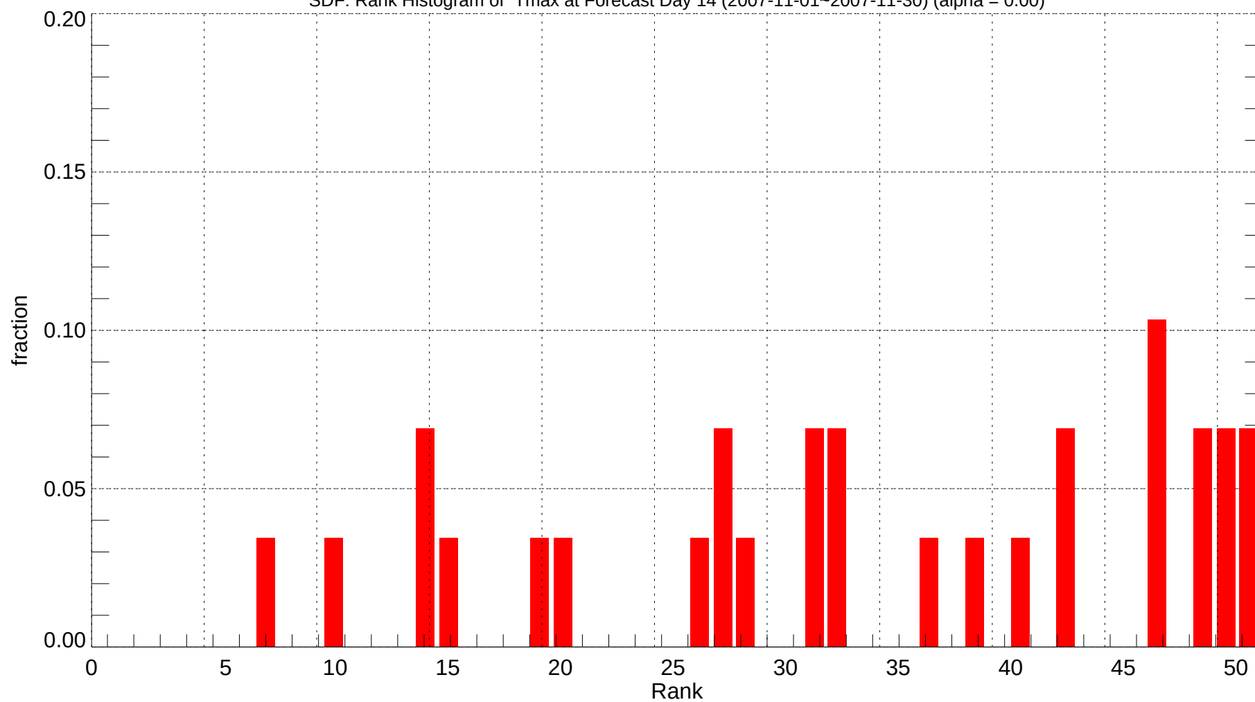
SDF: Rank Histogram of Tmax at Forecast Day 14 (2007-11-01~2007-11-30) (alpha = 0.00)
