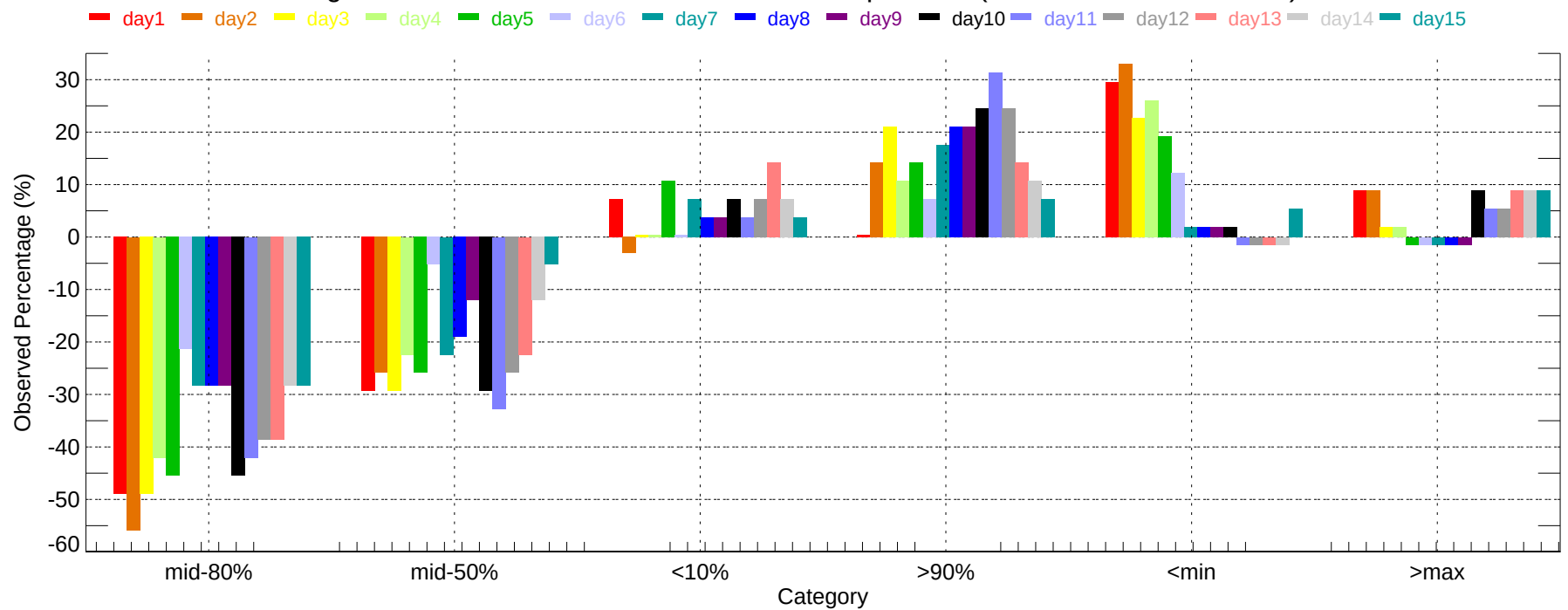
Observed Percentage Deviation of Ensembles - LFK: Max Temperature (2007-11-01~2007-11-30)
