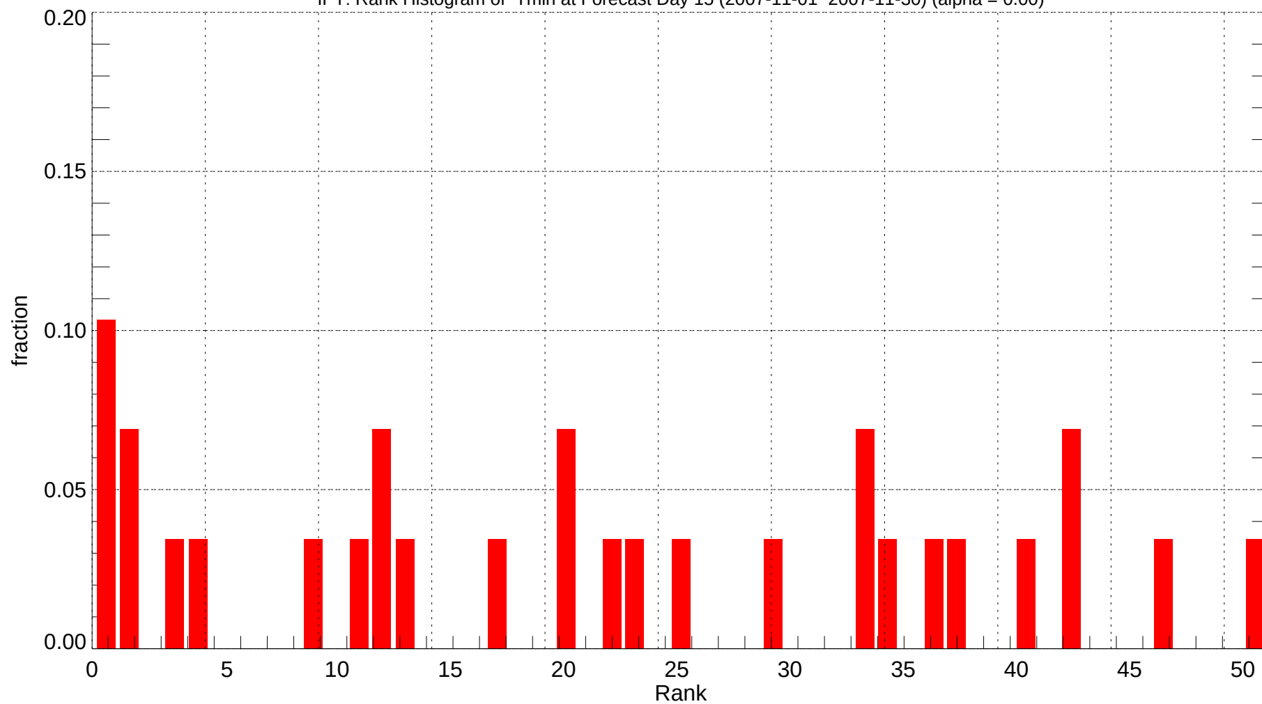
IPT: Rank Histogram of Tmin at Forecast Day 15 (2007-11-01~2007-11-30) (alpha = 0.00)
