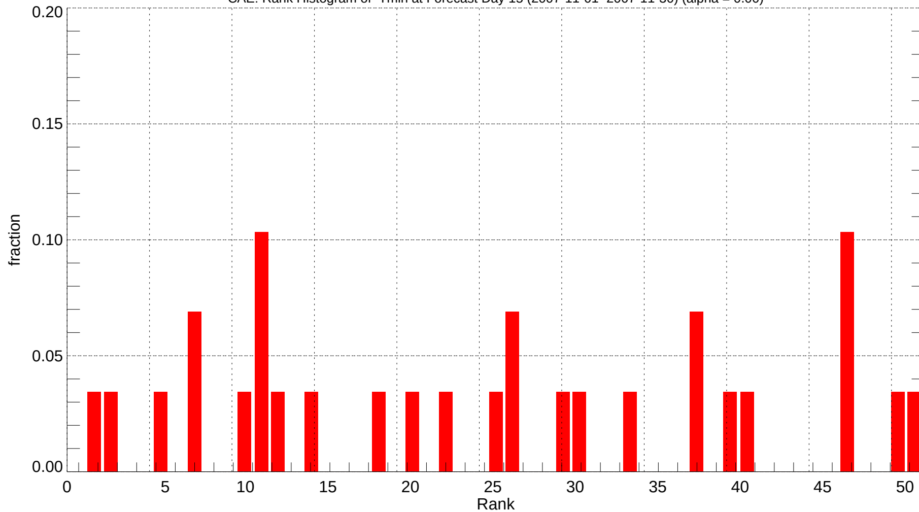
CAE: Rank Histogram of Tmin at Forecast Day 15 (2007-11-01~2007-11-30) (alpha = 0.00)
