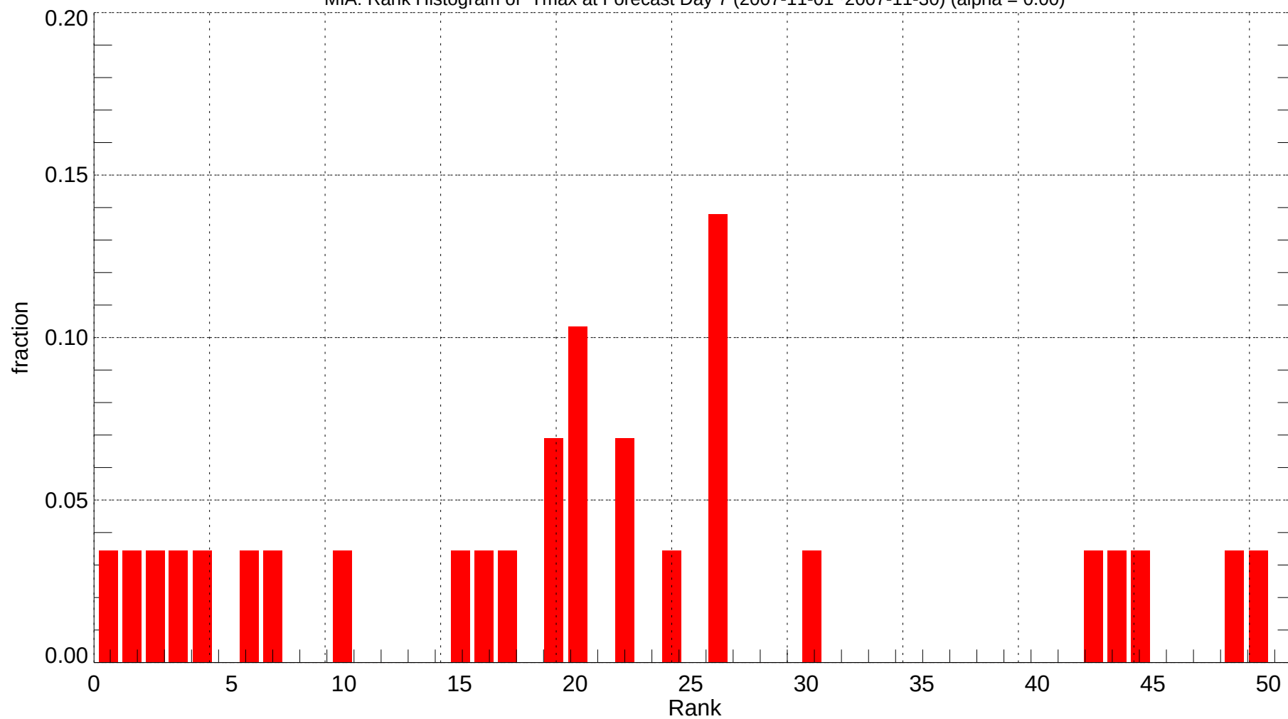
MIA: Rank Histogram of Tmax at Forecast Day 7 (2007-11-01~2007-11-30) (alpha = 0.00)
