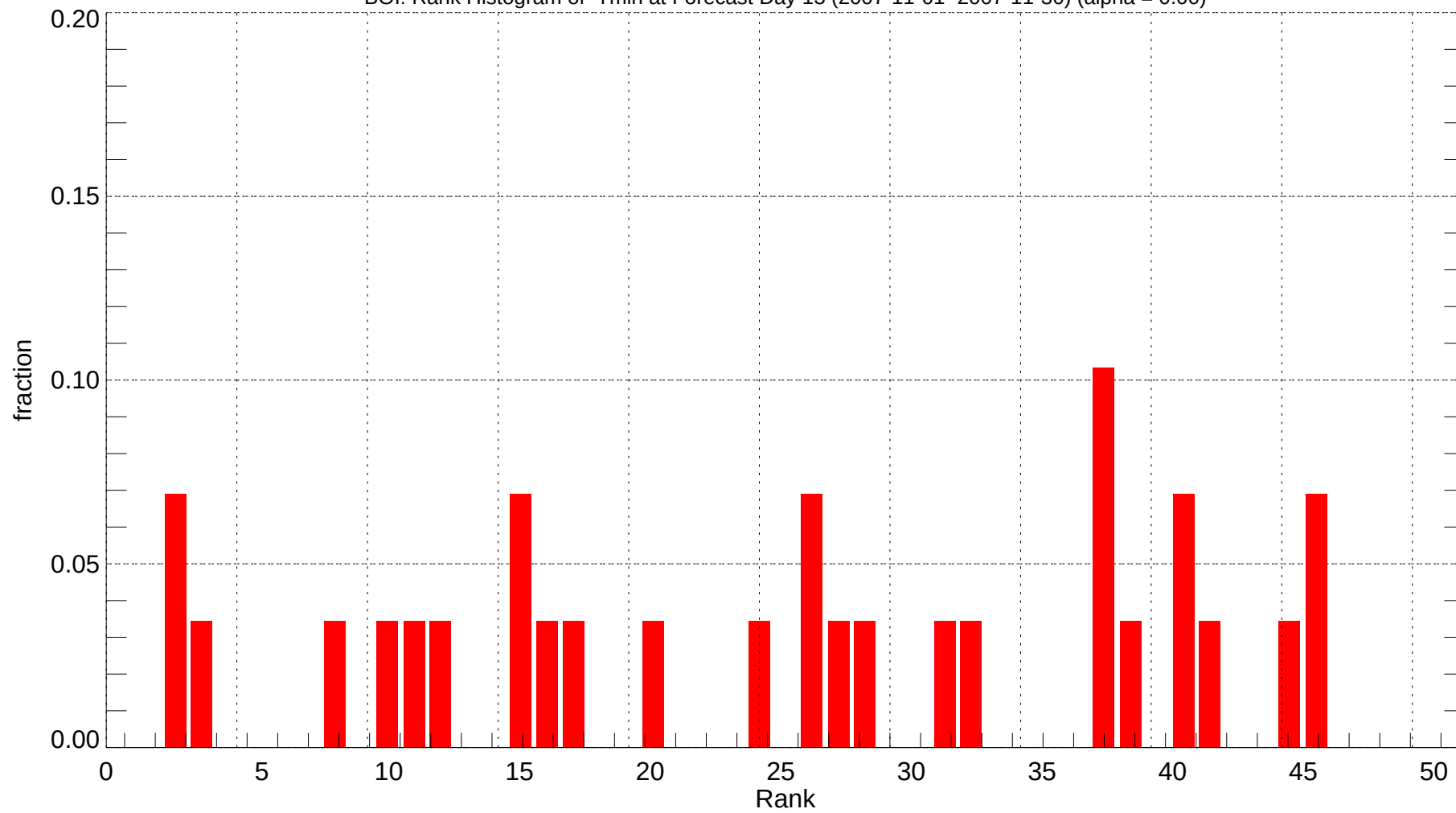
BOI: Rank Histogram of Tmin at Forecast Day 13 (2007-11-01~2007-11-30) (alpha = 0.00)
