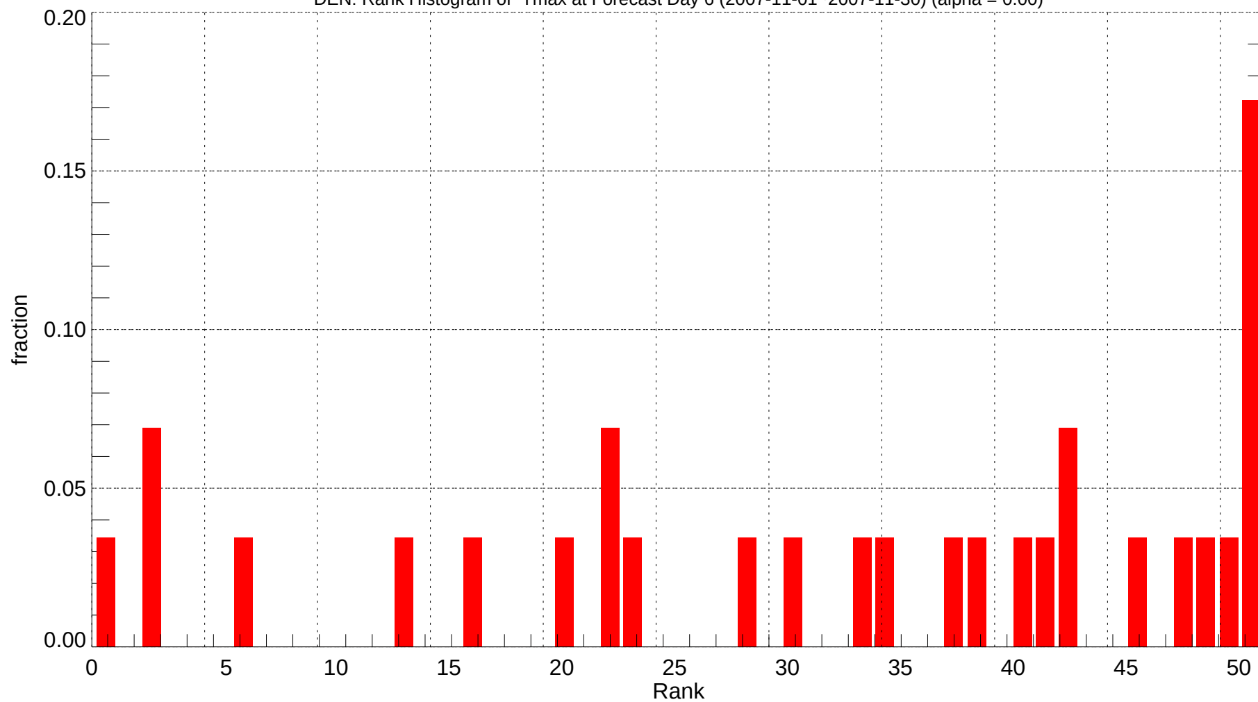
DEN: Rank Histogram of Tmax at Forecast Day 6 (2007-11-01~2007-11-30) (alpha = 0.00)
