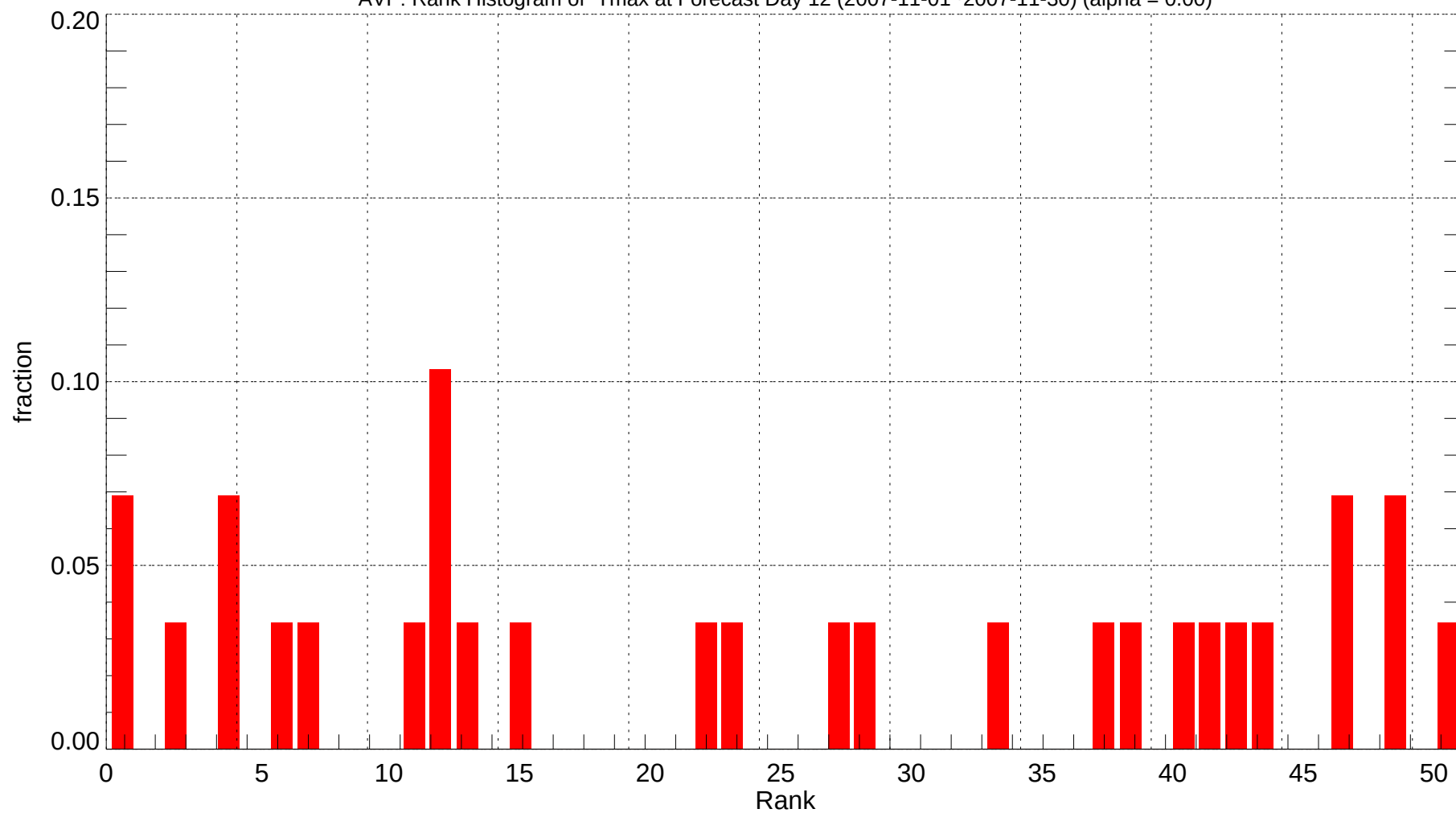
AVP: Rank Histogram of Tmax at Forecast Day 12 (2007-11-01~2007-11-30) (alpha = 0.00)
