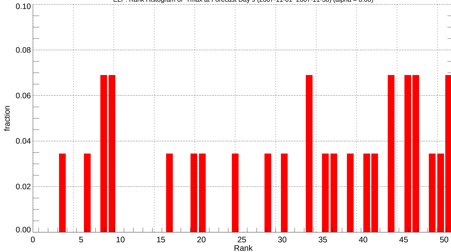
ELP: Rank Histogram of Tmax at Forecast Day 9 (2007-11-01~2007-11-30) (alpha = 0.00)
