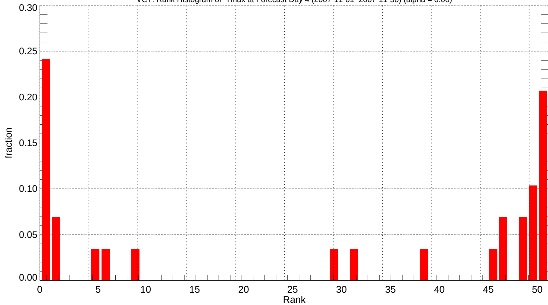
VCT: Rank Histogram of Tmax at Forecast Day 4 (2007-11-01~2007-11-30) (alpha = 0.00)
