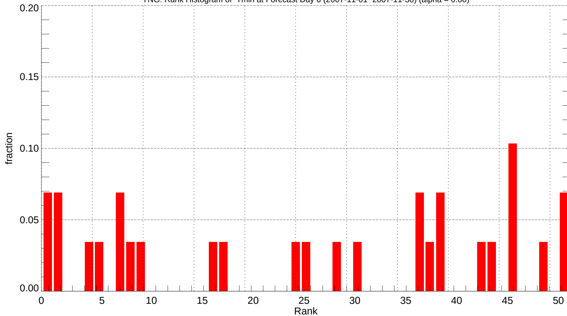
YNG: Rank Histogram of Tmin at Forecast Day 6 (2007-11-01~2007-11-30) (alpha = 0.00)
