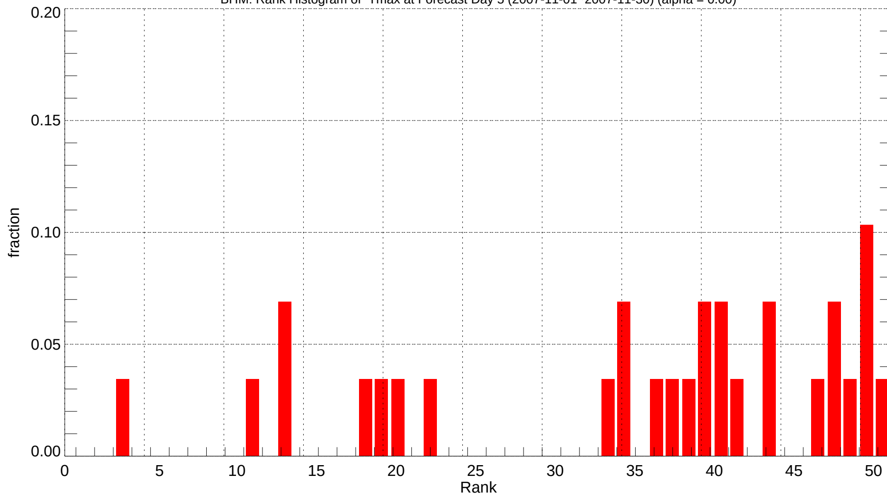
BHM: Rank Histogram of Tmax at Forecast Day 5 (2007-11-01~2007-11-30) (alpha = 0.00)
