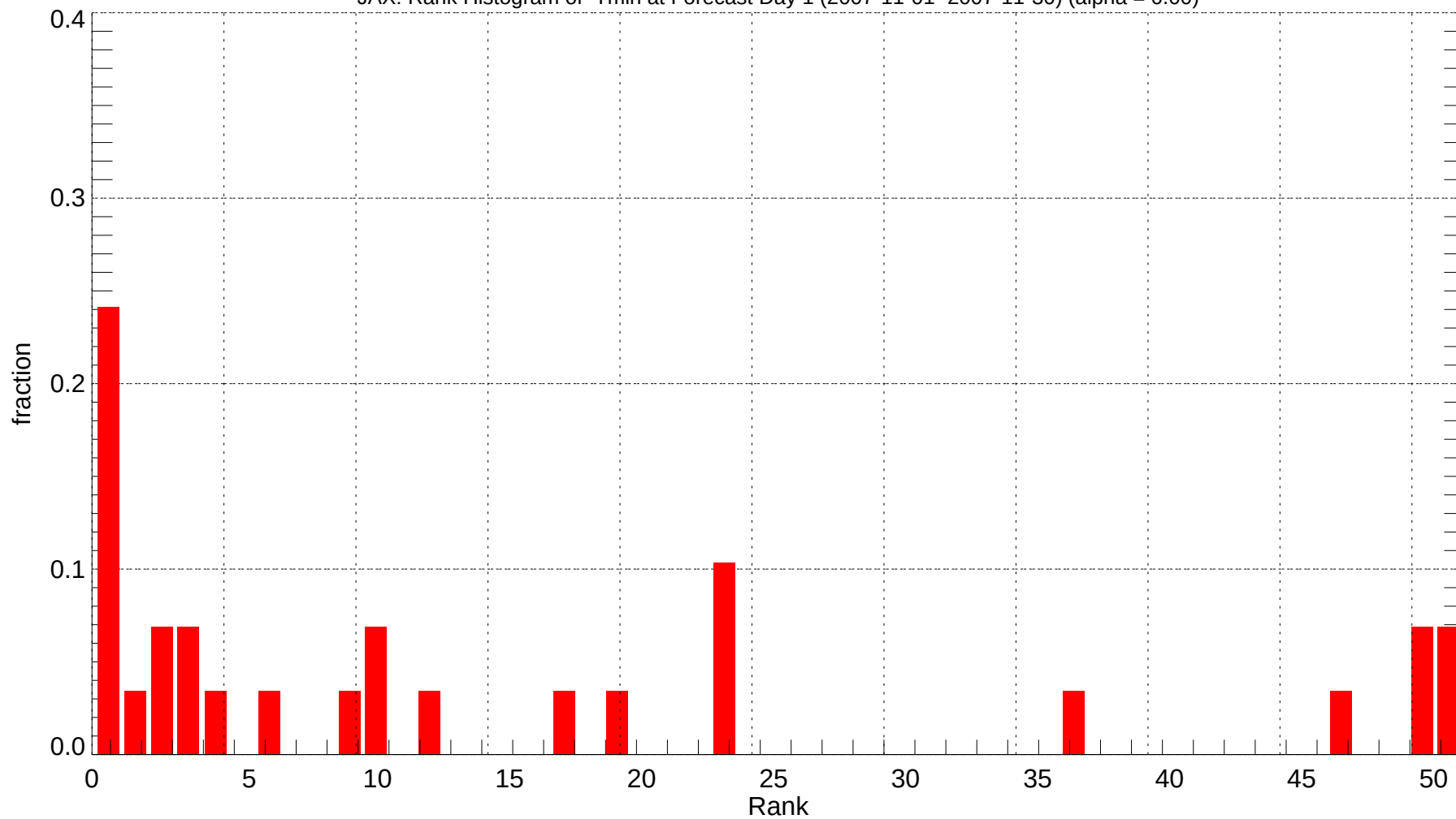
JAX: Rank Histogram of Tmin at Forecast Day 1 (2007-11-01~2007-11-30) (alpha = 0.00)
