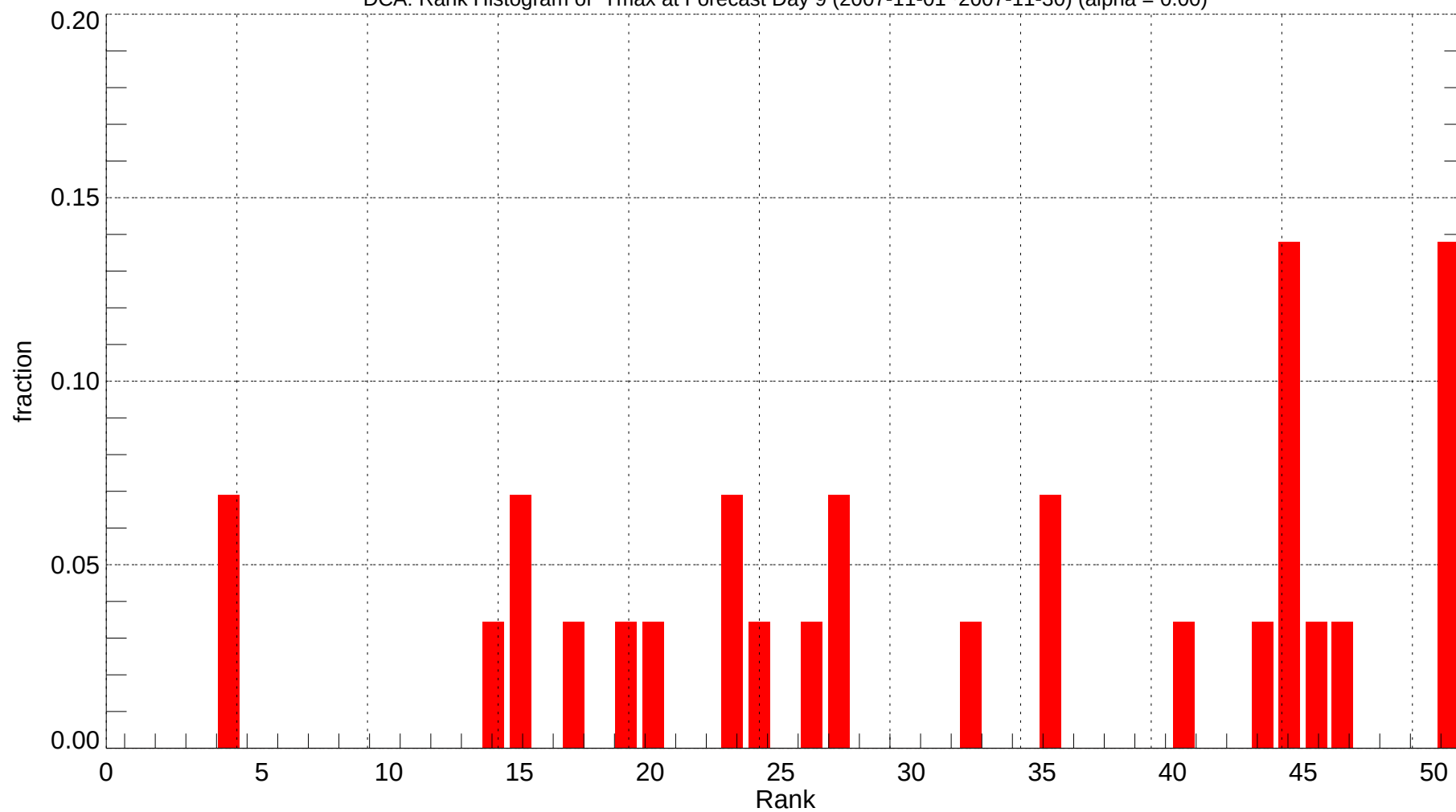
DCA: Rank Histogram of Tmax at Forecast Day 9 (2007-11-01~2007-11-30) (alpha = 0.00)
