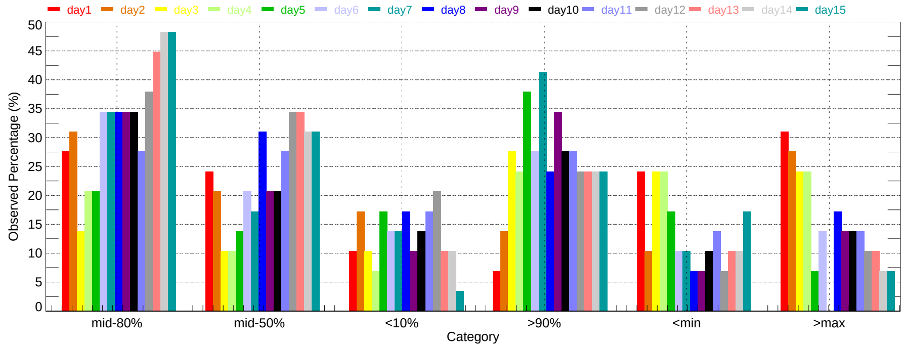
Observed Percentage of Ensembles - VCT: Min Temperature (2007-11-01~2007-11-30)
