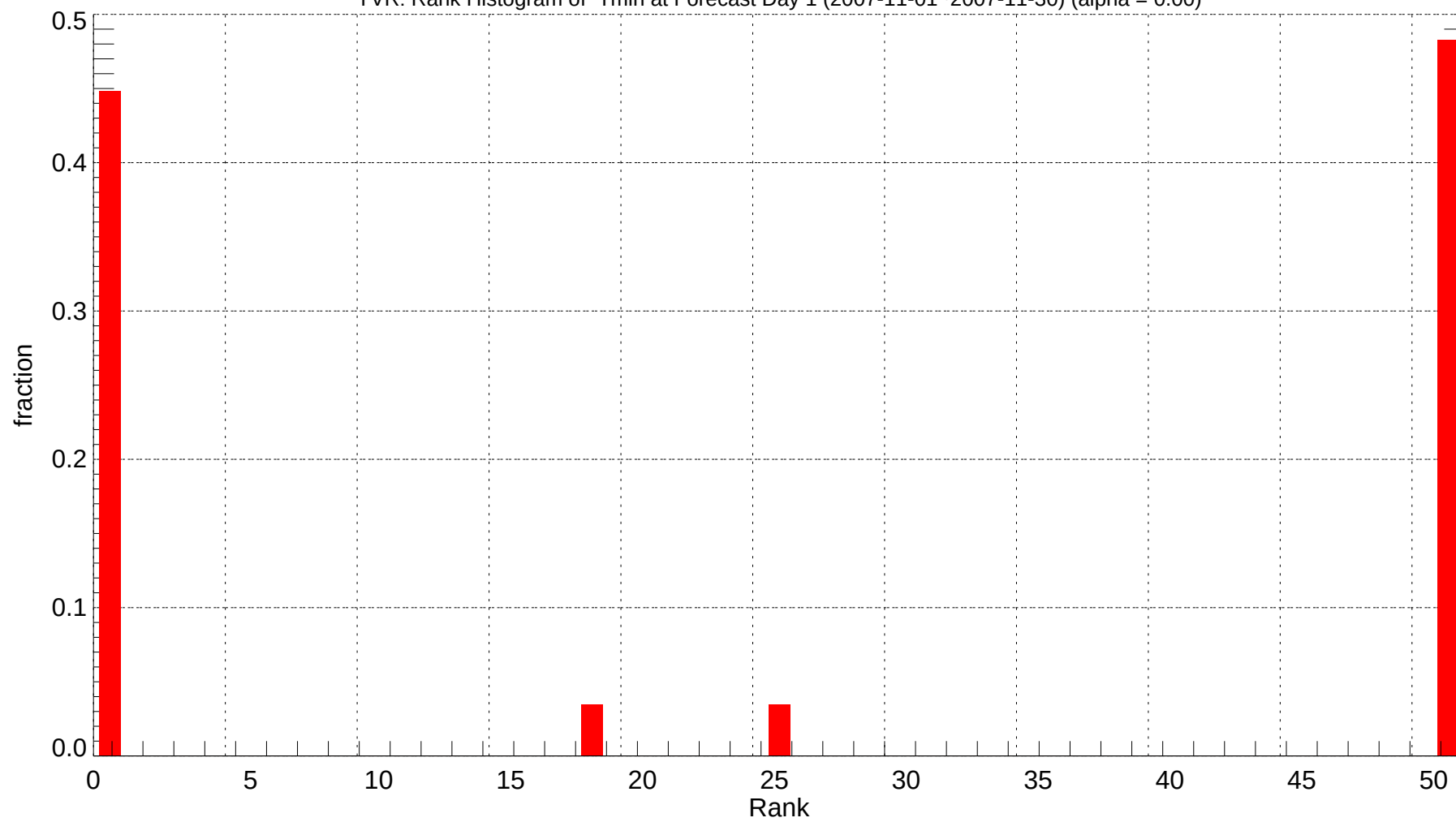
YVR: Rank Histogram of Tmin at Forecast Day 1 (2007-11-01~2007-11-30) (alpha = 0.00)
