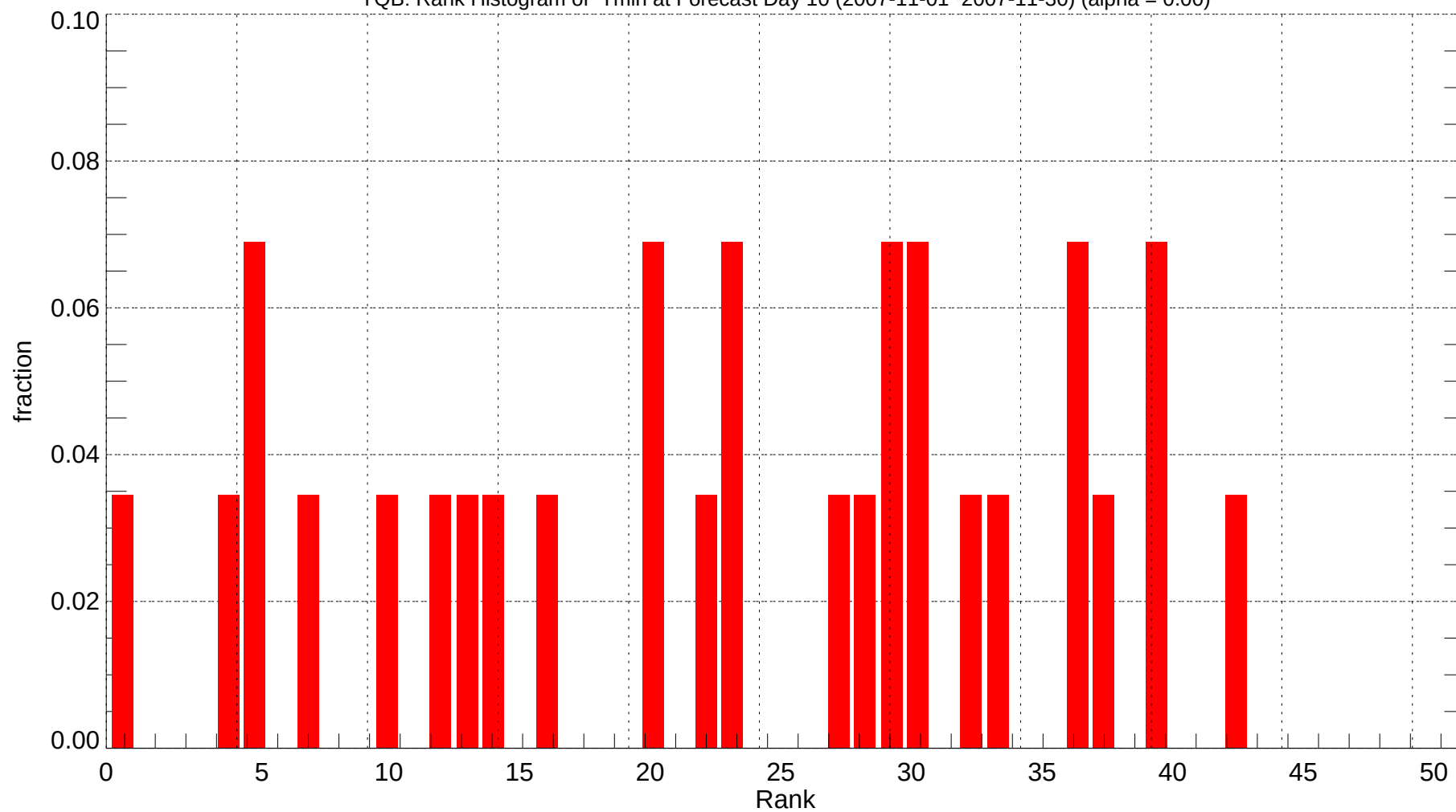
YQB: Rank Histogram of Tmin at Forecast Day 10 (2007-11-01~2007-11-30) (alpha = 0.00)
