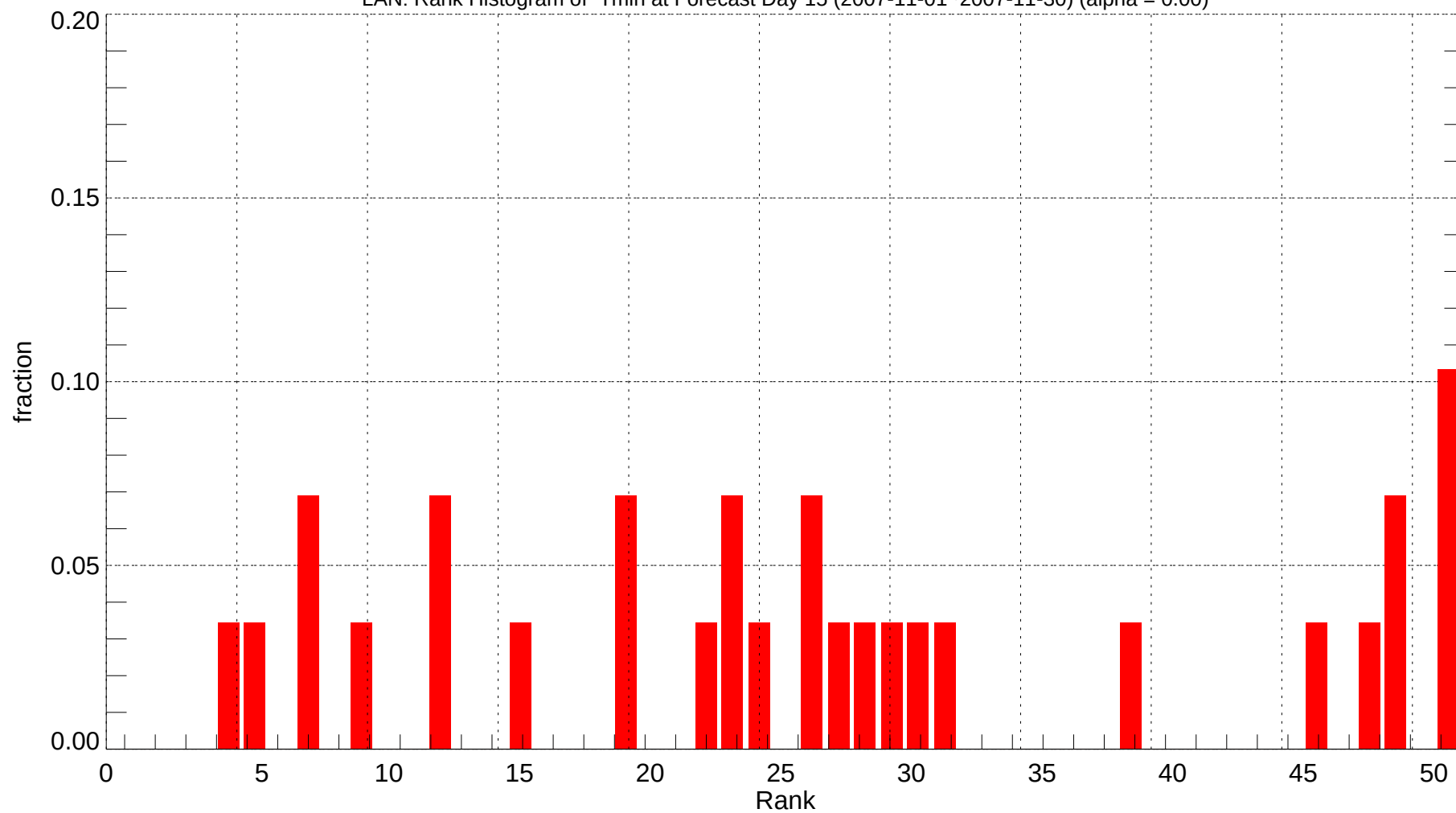
LAN: Rank Histogram of Tmin at Forecast Day 15 (2007-11-01~2007-11-30) (alpha = 0.00)
