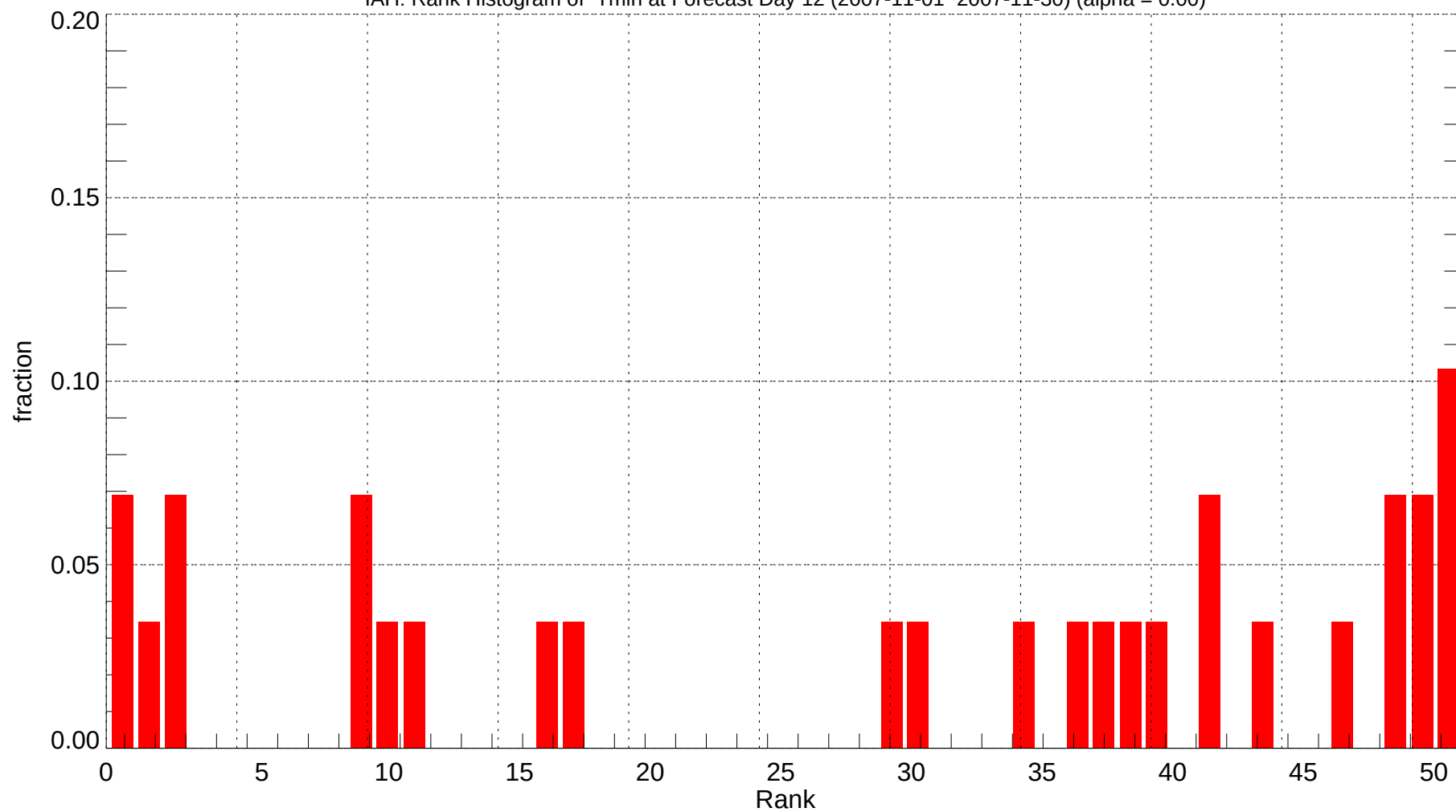
IAH: Rank Histogram of Tmin at Forecast Day 12 (2007-11-01~2007-11-30) (alpha = 0.00)
