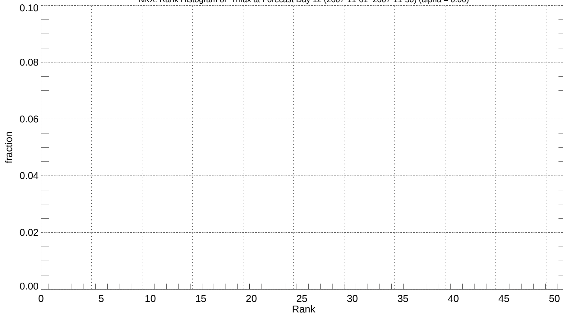
NKX: Rank Histogram of Tmax at Forecast Day 12 (2007-11-01~2007-11-30) (alpha = 0.00)
