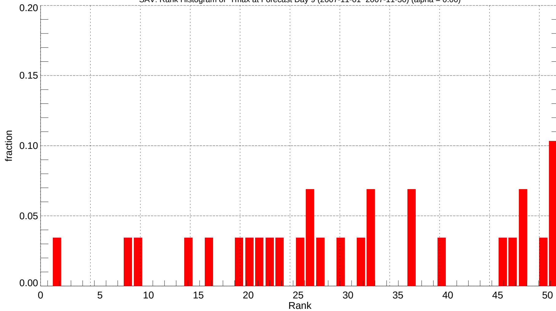
SAV: Rank Histogram of Tmax at Forecast Day 9 (2007-11-01~2007-11-30) (alpha = 0.00)
