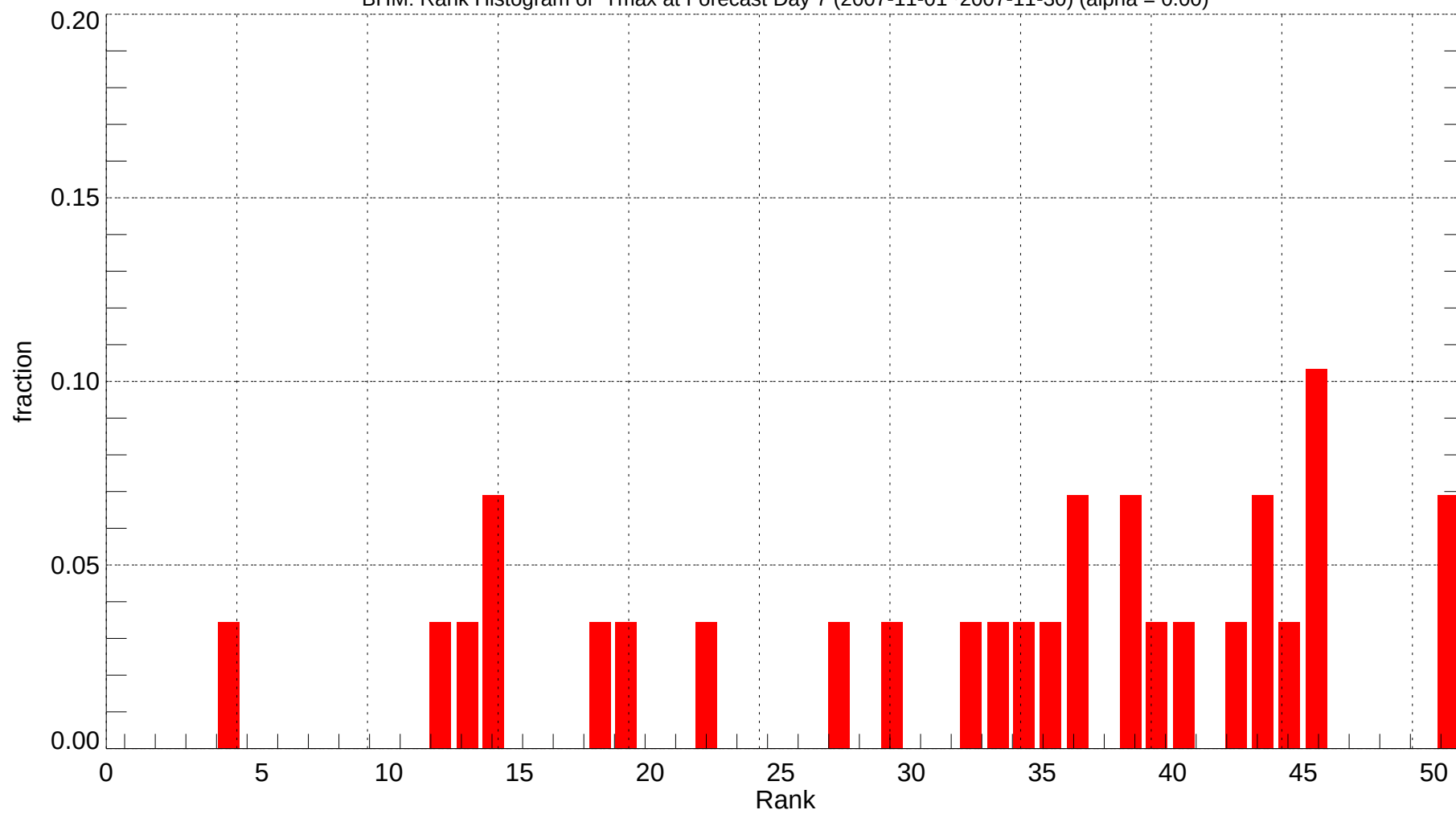
BHM: Rank Histogram of Tmax at Forecast Day 7 (2007-11-01~2007-11-30) (alpha = 0.00)
