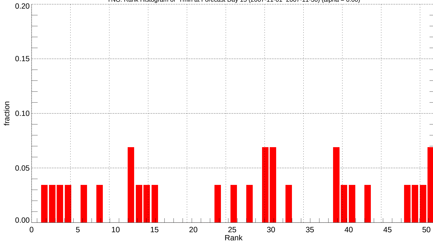
YNG: Rank Histogram of Tmin at Forecast Day 15 (2007-11-01~2007-11-30) (alpha = 0.00)
