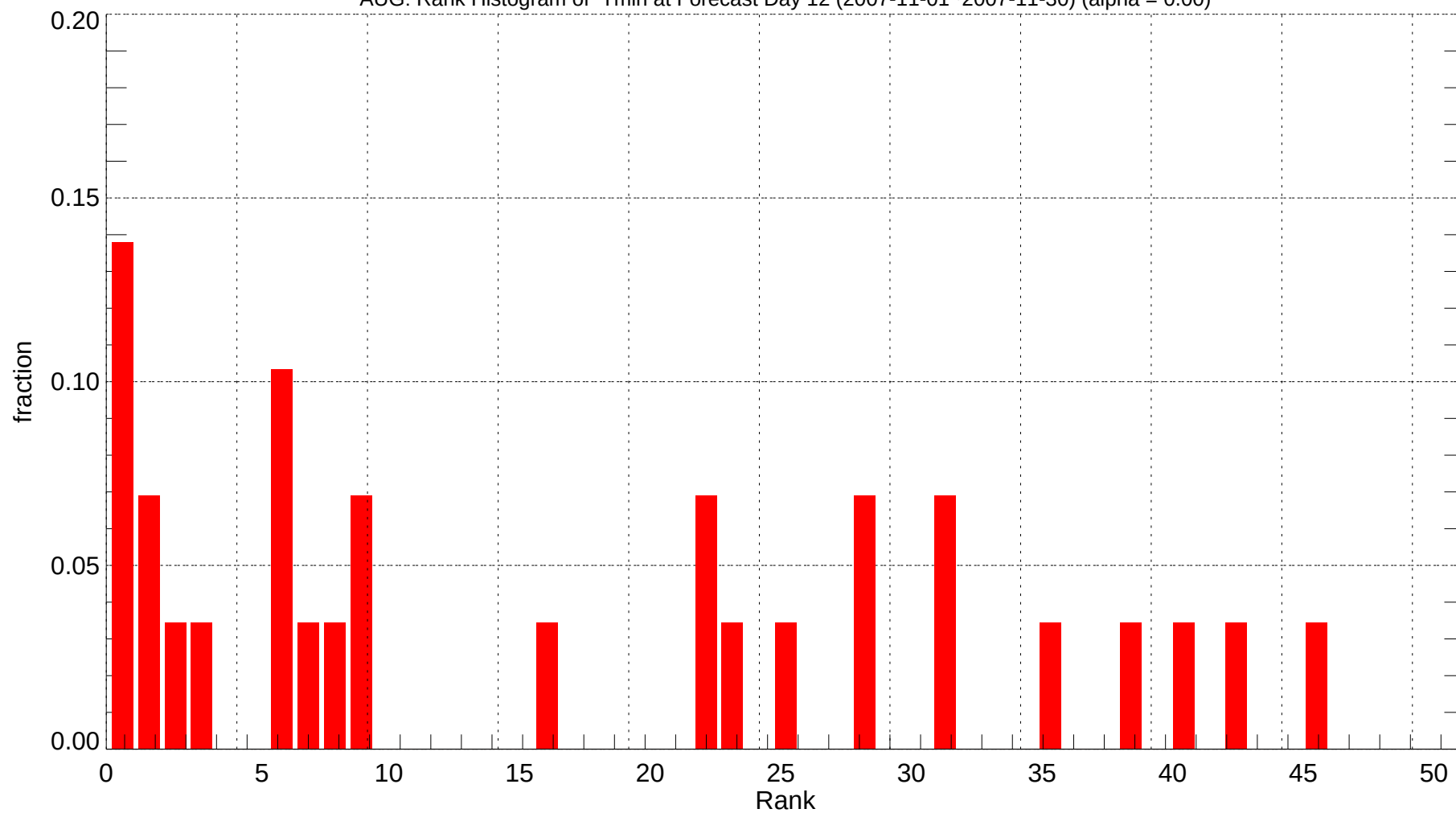
AUG: Rank Histogram of Tmin at Forecast Day 12 (2007-11-01~2007-11-30) (alpha = 0.00)
