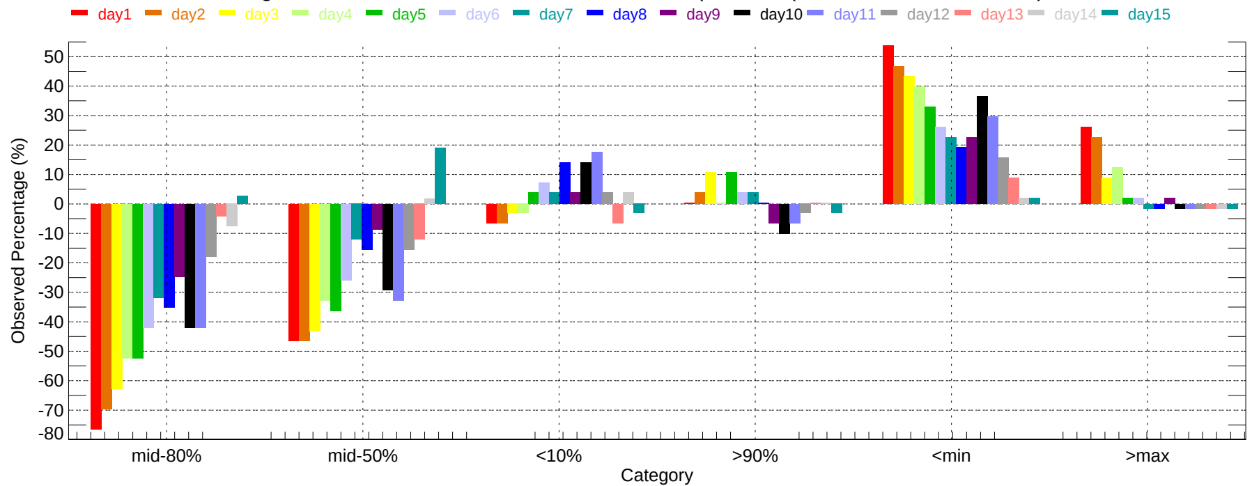
Observed Percentage Deviation of Ensembles - EUG: Max Temperature (2007-11-01~2007-11-30)
