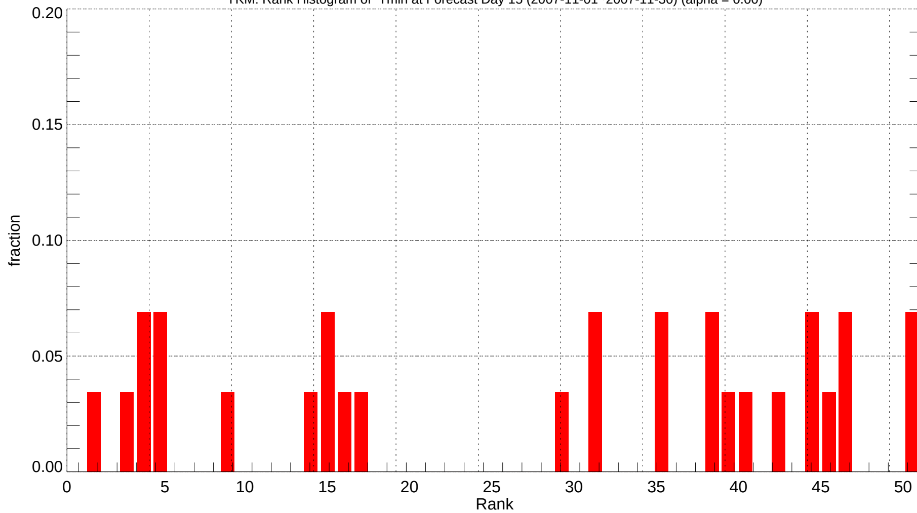
YKM: Rank Histogram of Tmin at Forecast Day 15 (2007-11-01~2007-11-30) (alpha = 0.00)
