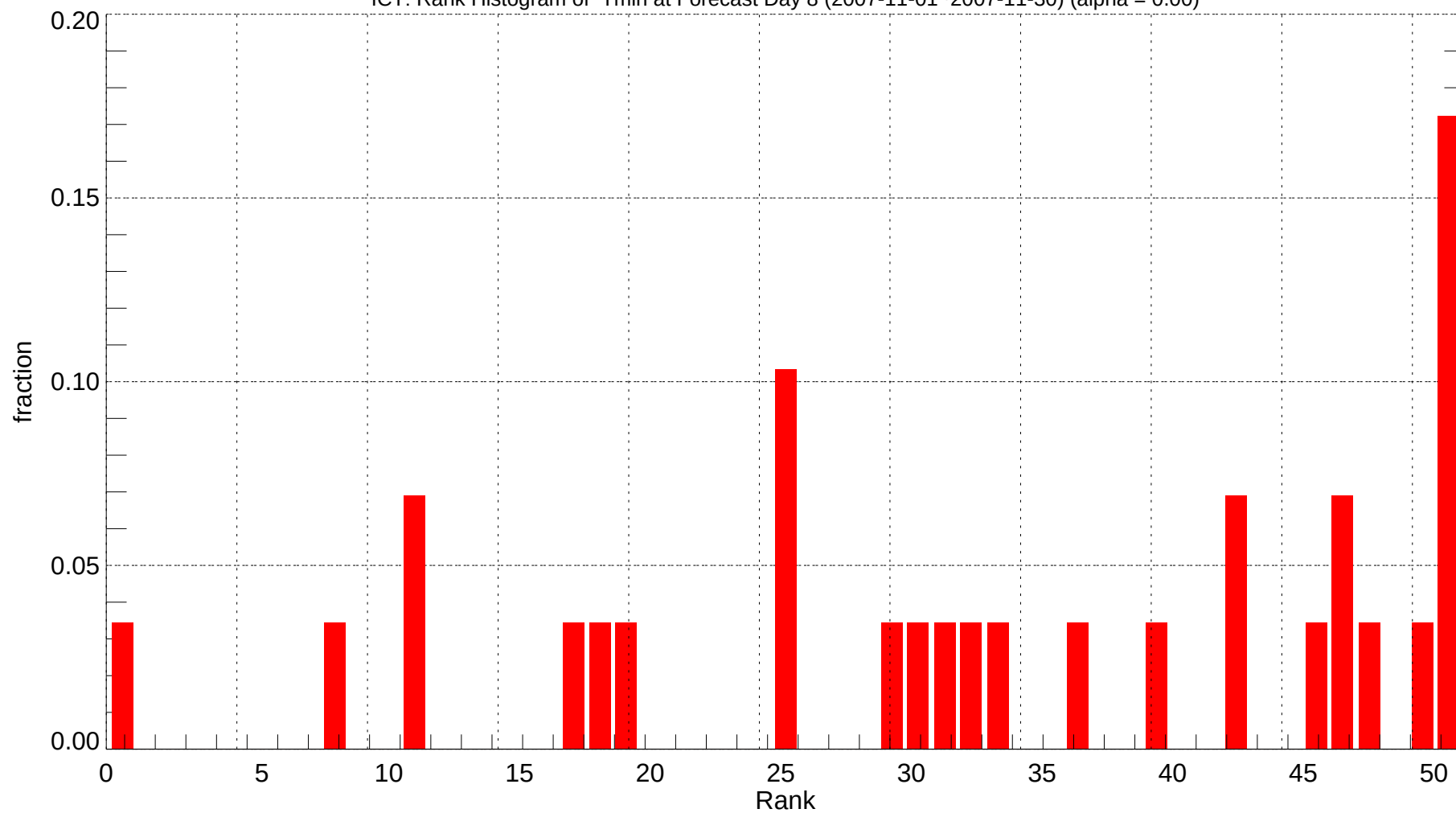
ICT: Rank Histogram of Tmin at Forecast Day 8 (2007-11-01~2007-11-30) (alpha = 0.00)
