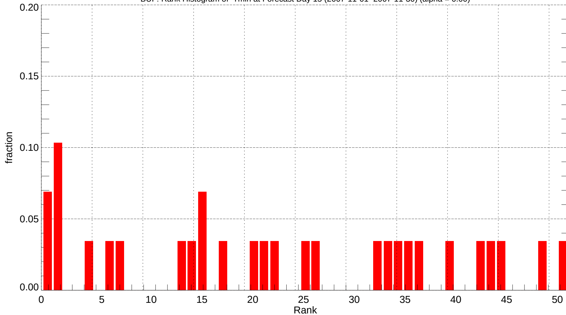
BUF: Rank Histogram of Tmin at Forecast Day 15 (2007-11-01~2007-11-30) (alpha = 0.00)
