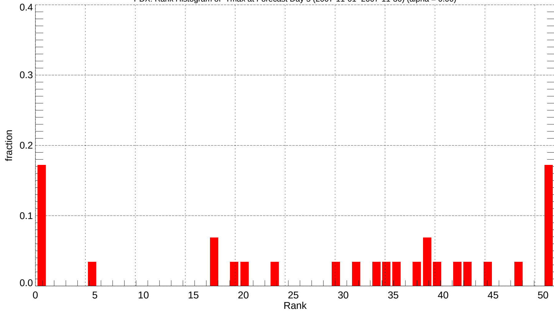
PDX: Rank Histogram of Tmax at Forecast Day 5 (2007-11-01~2007-11-30) (alpha = 0.00)
