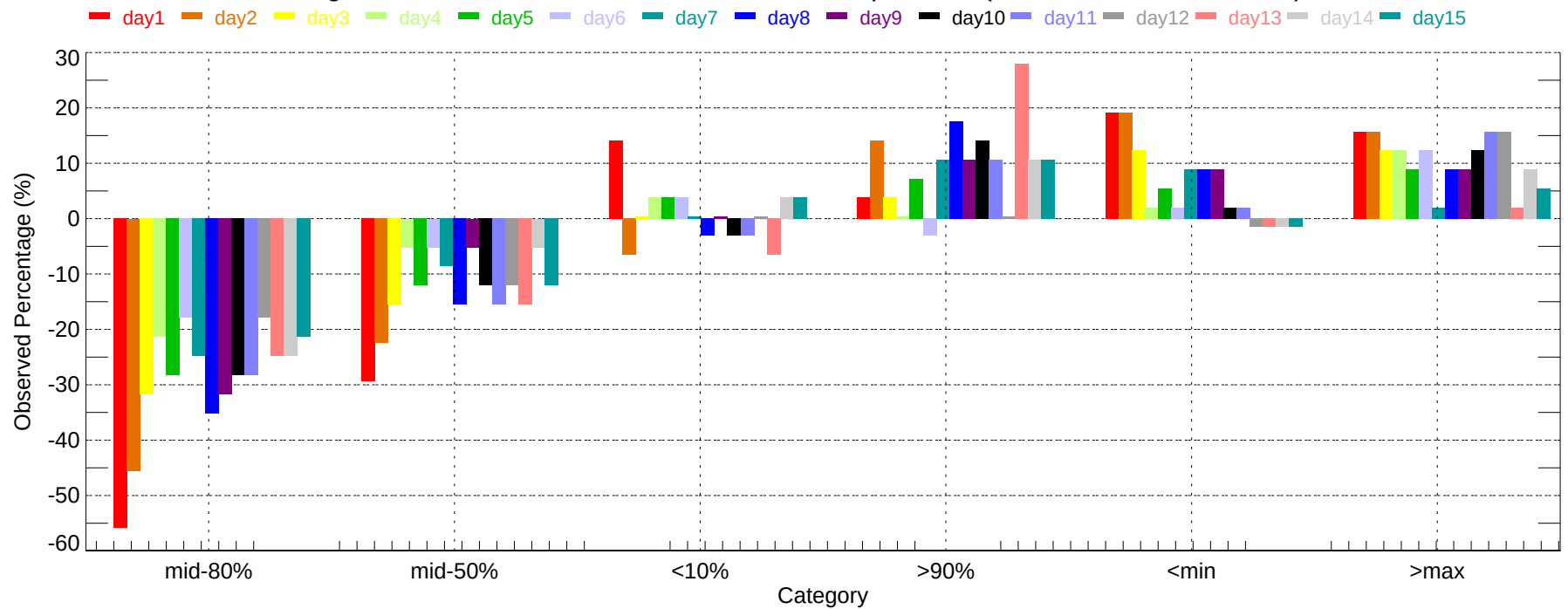
Observed Percentage Deviation of Ensembles - FAR: Max Temperature (2007-11-01~2007-11-30)
