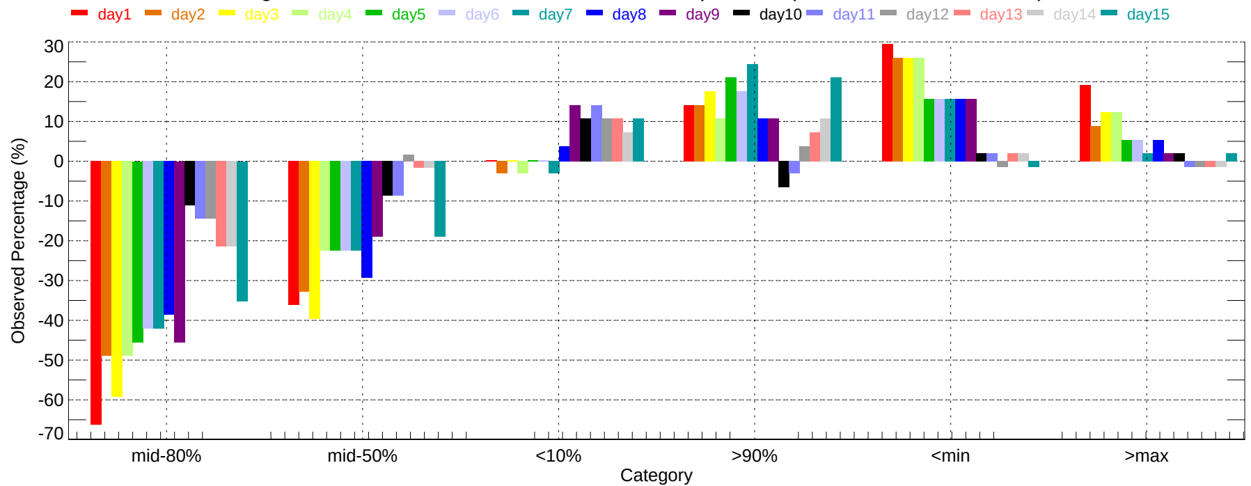
Observed Percentage Deviation of Ensembles - GEG: Max Temperature (2007-11-01~2007-11-30)
