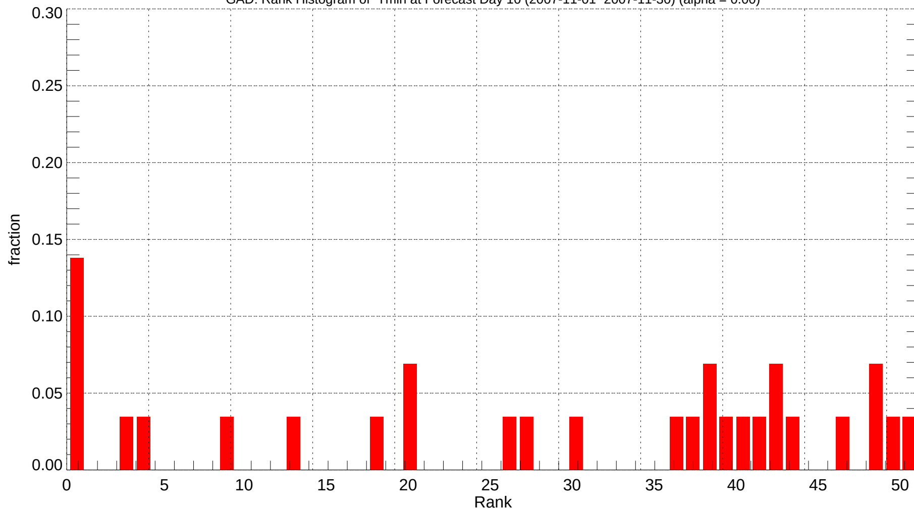
GAD: Rank Histogram of Tmin at Forecast Day 10 (2007-11-01~2007-11-30) (alpha = 0.00)
