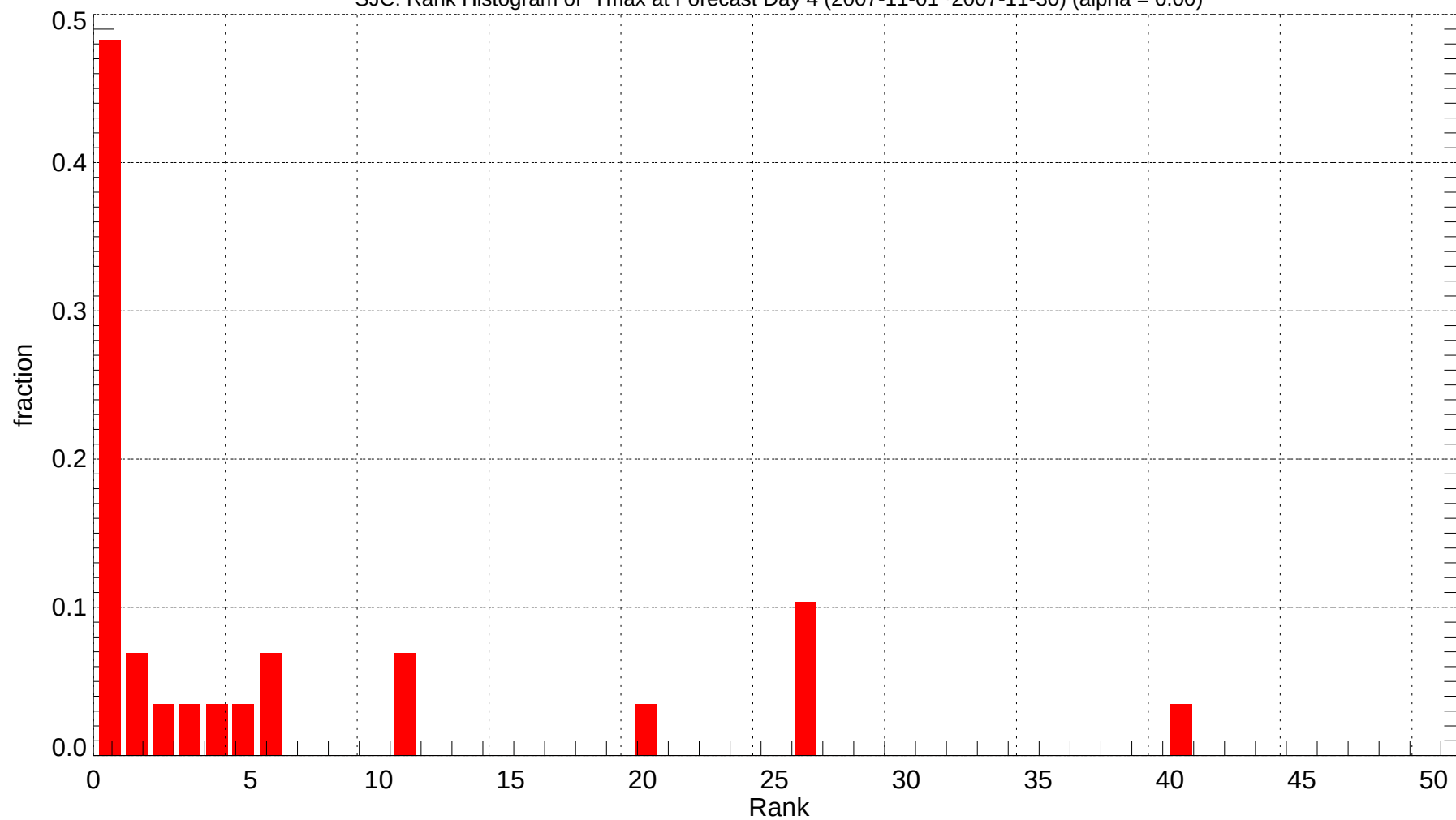
SJC: Rank Histogram of Tmax at Forecast Day 4 (2007-11-01~2007-11-30) (alpha = 0.00)
