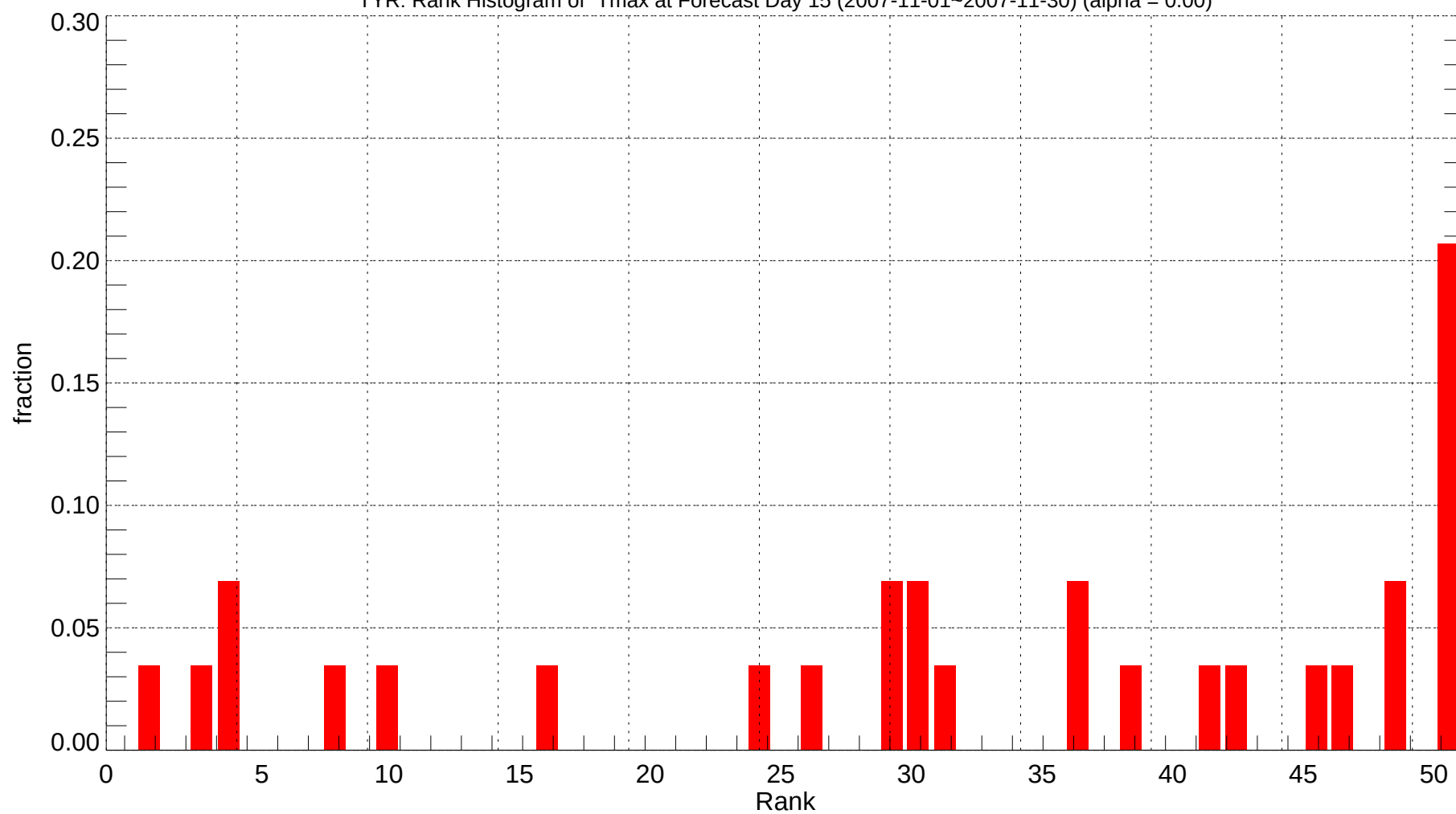
TYR: Rank Histogram of Tmax at Forecast Day 15 (2007-11-01~2007-11-30) (alpha = 0.00)
