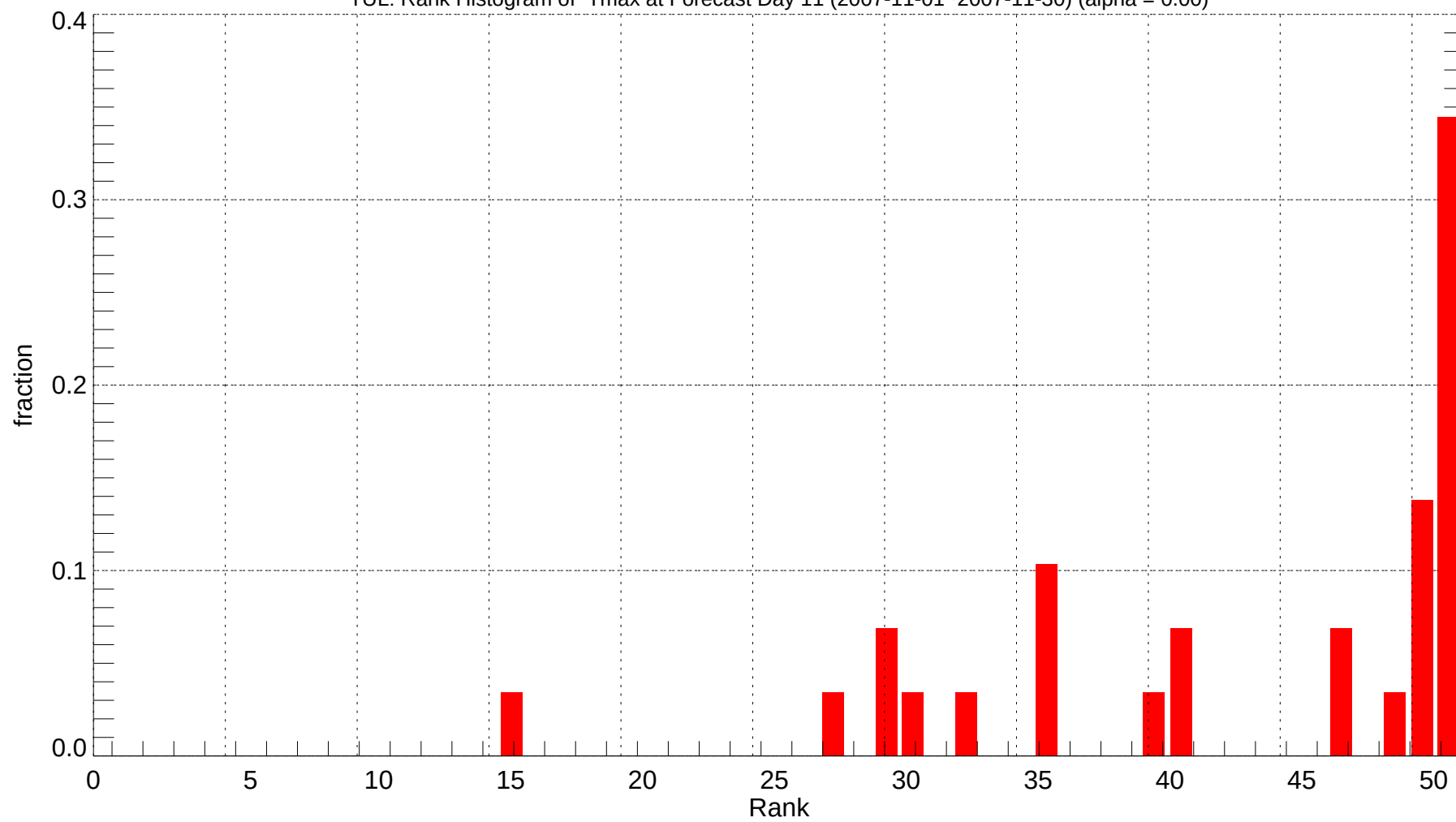
TUL: Rank Histogram of Tmax at Forecast Day 11 (2007-11-01~2007-11-30) (alpha = 0.00)
