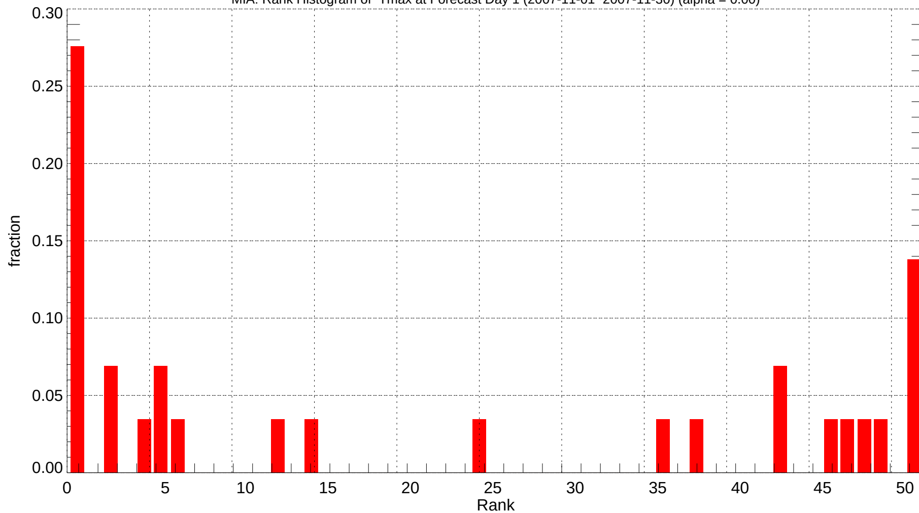
MIA: Rank Histogram of Tmax at Forecast Day 1 (2007-11-01~2007-11-30) (alpha = 0.00)
