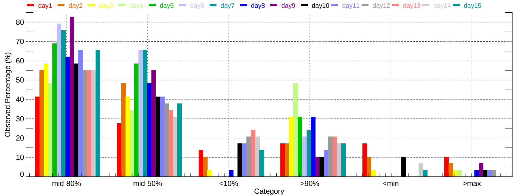
Observed Percentage of Ensembles - LGA: Max Temperature (2007-11-01~2007-11-30)
