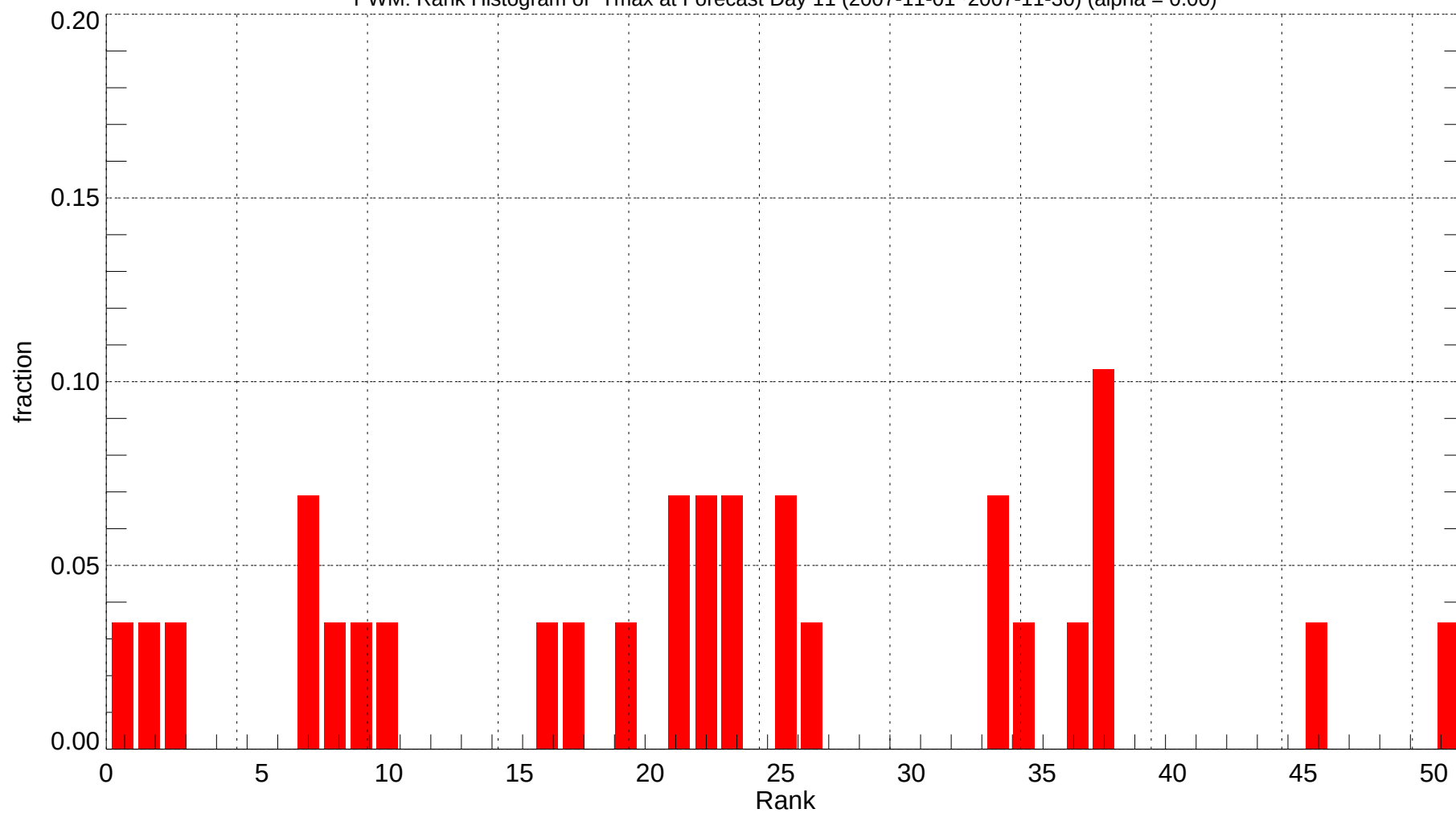
PWM: Rank Histogram of Tmax at Forecast Day 11 (2007-11-01~2007-11-30) (alpha = 0.00)
