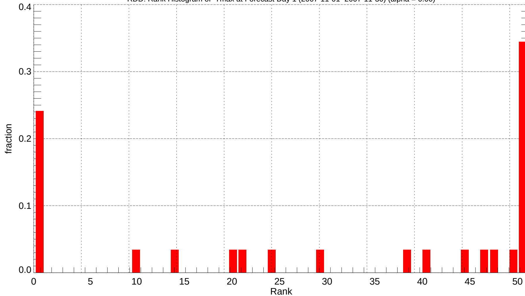
RDD: Rank Histogram of Tmax at Forecast Day 1 (2007-11-01~2007-11-30) (alpha = 0.00)
