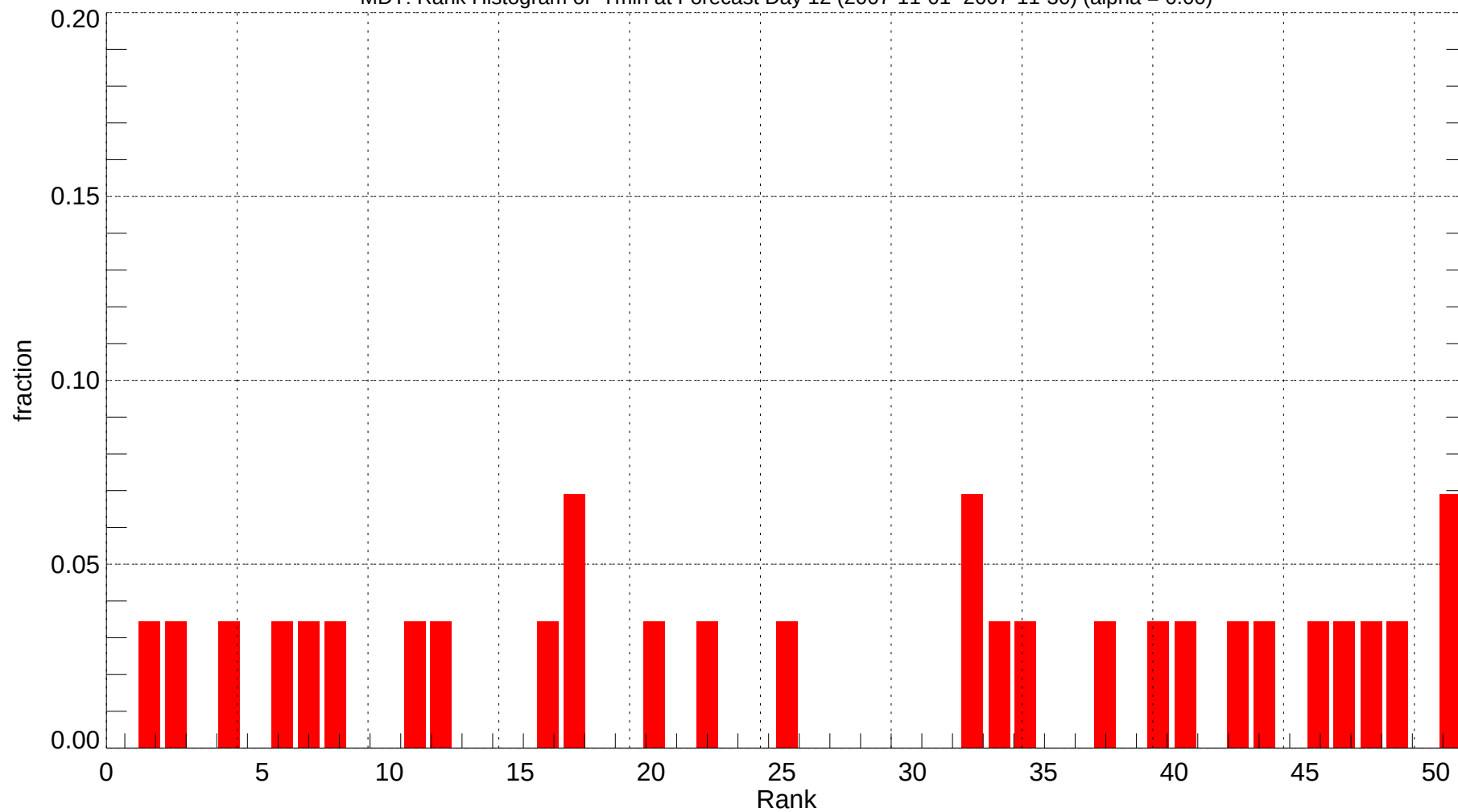
MDT: Rank Histogram of Tmin at Forecast Day 12 (2007-11-01~2007-11-30) (alpha = 0.00)
