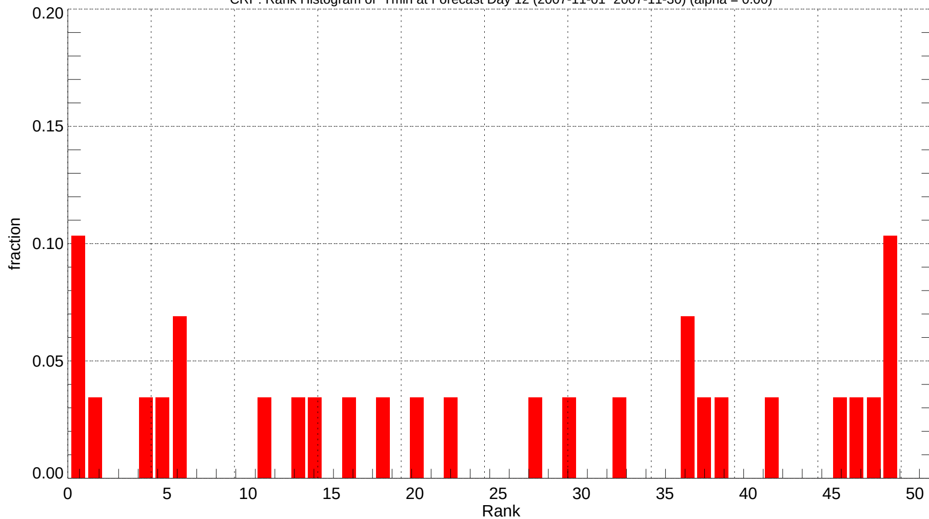
CRP: Rank Histogram of Tmin at Forecast Day 12 (2007-11-01~2007-11-30) (alpha = 0.00)
