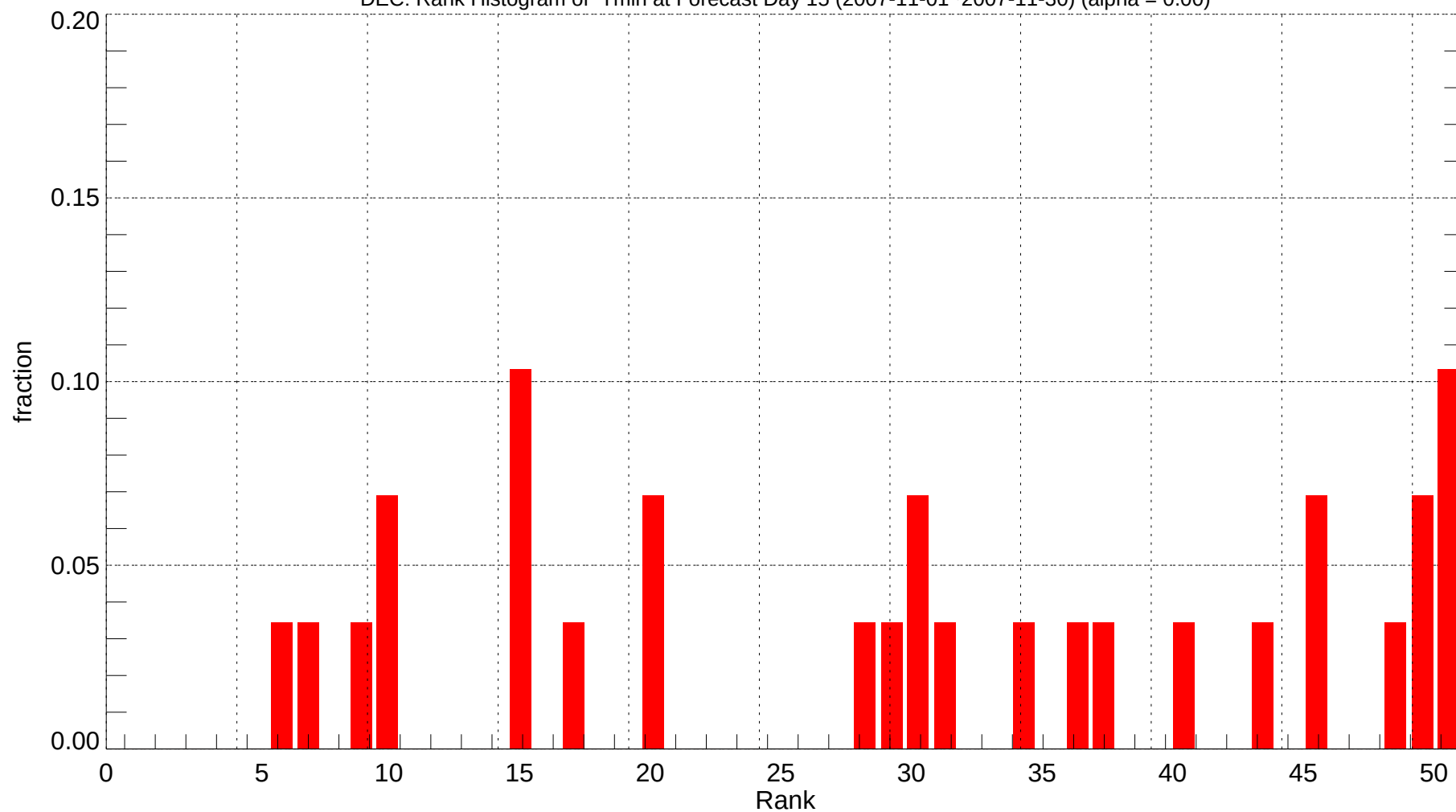
DEC: Rank Histogram of Tmin at Forecast Day 15 (2007-11-01~2007-11-30) (alpha = 0.00)
