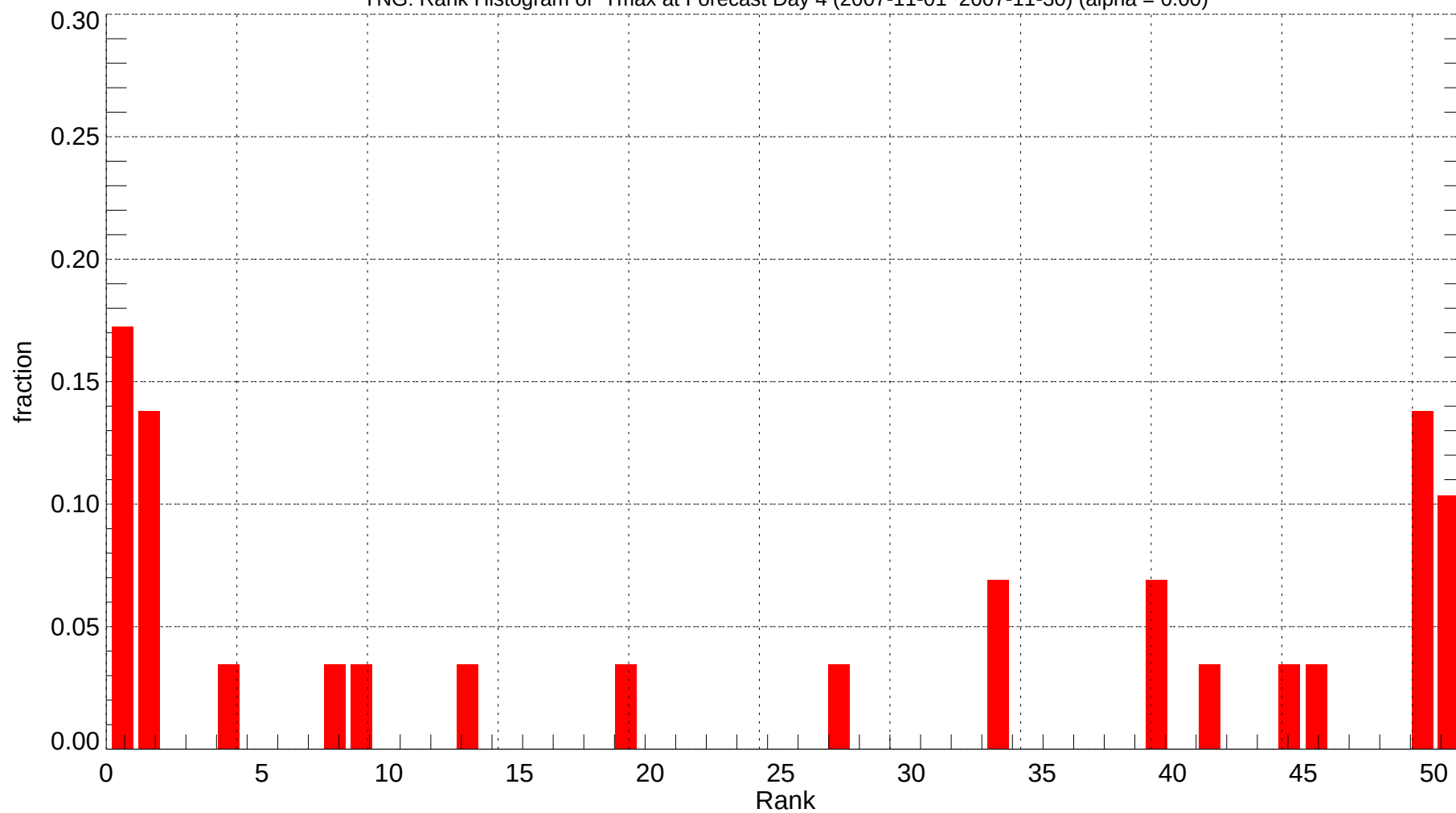
YNG: Rank Histogram of Tmax at Forecast Day 4 (2007-11-01~2007-11-30) (alpha = 0.00)
