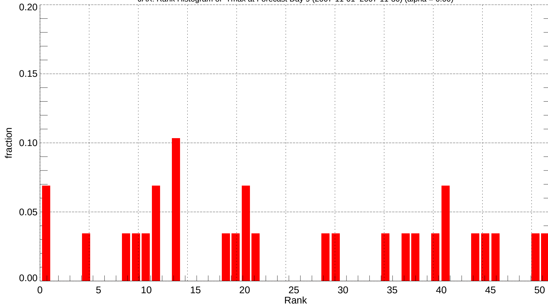
JAX: Rank Histogram of Tmax at Forecast Day 9 (2007-11-01~2007-11-30) (alpha = 0.00)
