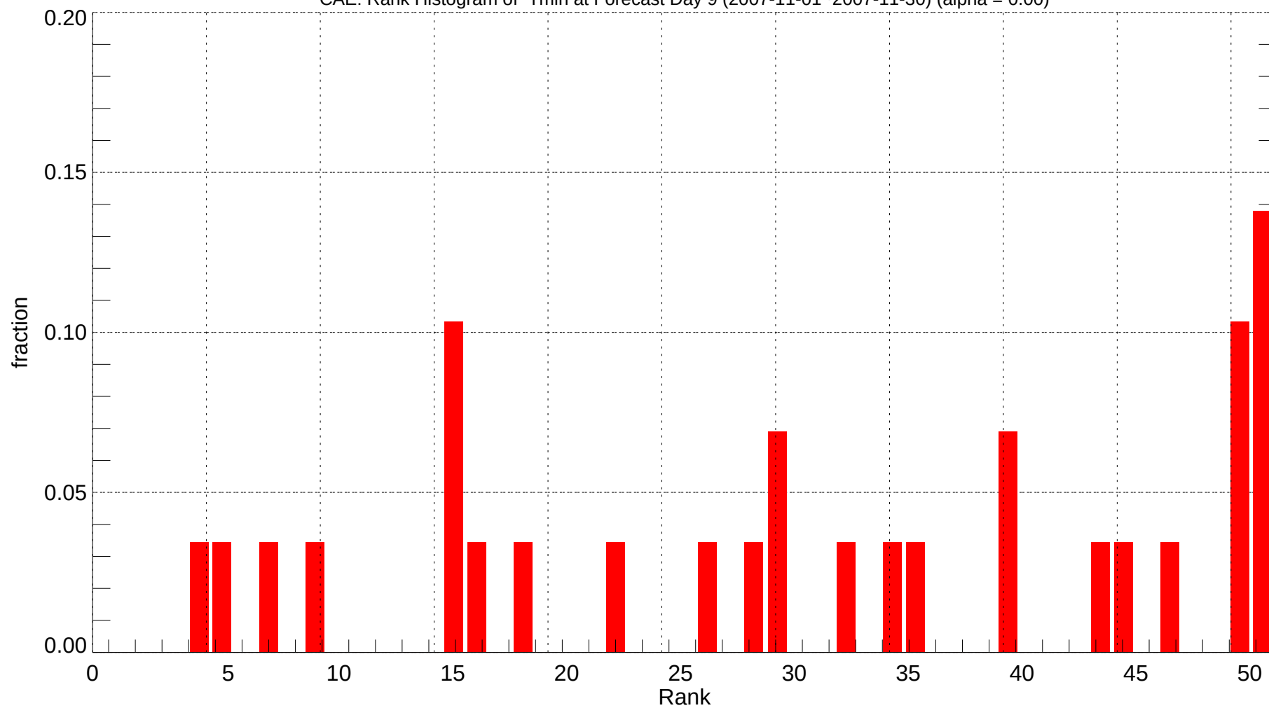
CAE: Rank Histogram of Tmin at Forecast Day 9 (2007-11-01~2007-11-30) (alpha = 0.00)
