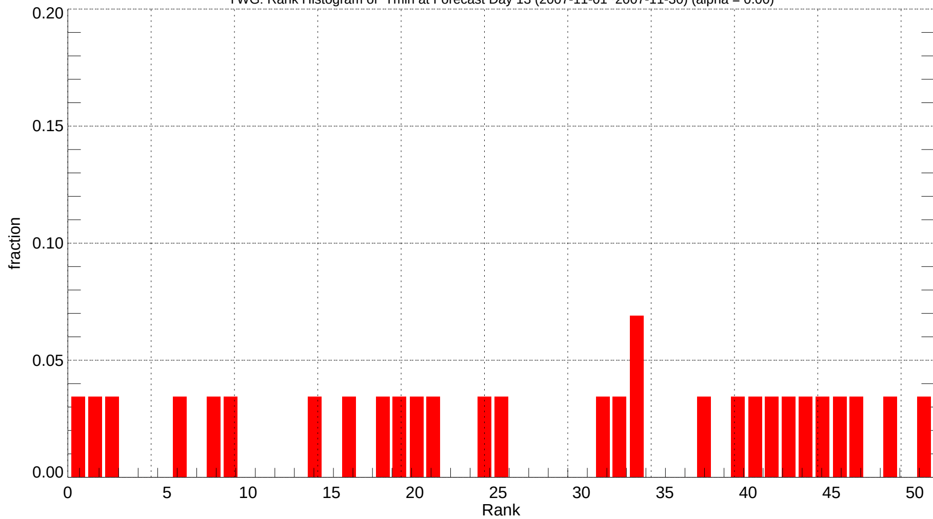
YWG: Rank Histogram of Tmin at Forecast Day 13 (2007-11-01~2007-11-30) (alpha = 0.00)
