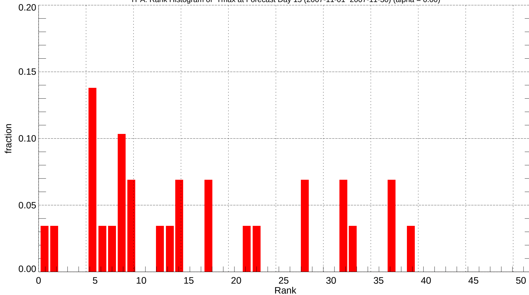
TPA: Rank Histogram of Tmax at Forecast Day 15 (2007-11-01~2007-11-30) (alpha = 0.00)
