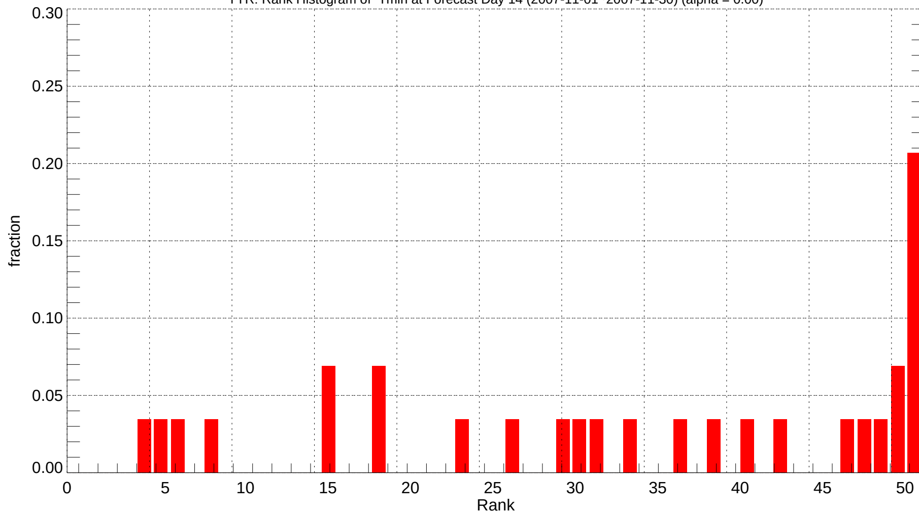
TYR: Rank Histogram of Tmin at Forecast Day 14 (2007-11-01~2007-11-30) (alpha = 0.00)
