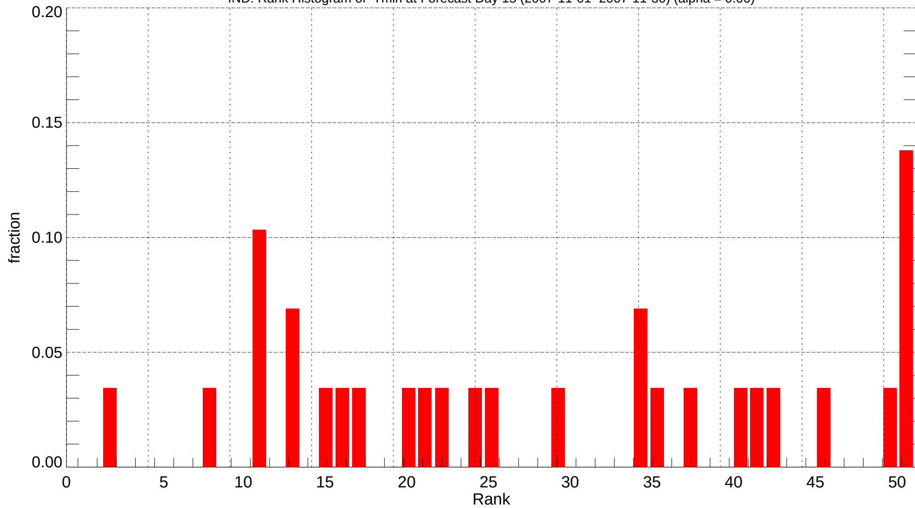
IND: Rank Histogram of Tmin at Forecast Day 15 (2007-11-01~2007-11-30) (alpha = 0.00)
