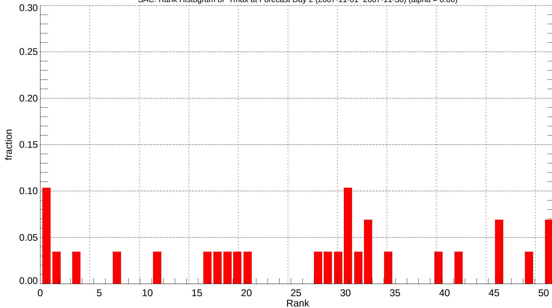
SAC: Rank Histogram of Tmax at Forecast Day 2 (2007-11-01~2007-11-30) (alpha = 0.00)
