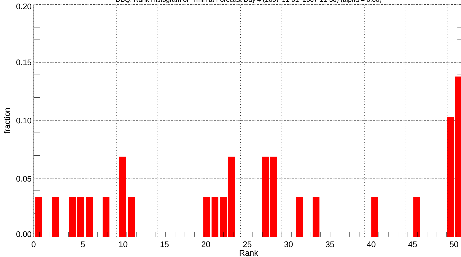
DBQ: Rank Histogram of Tmin at Forecast Day 4 (2007-11-01~2007-11-30) (alpha = 0.00)
