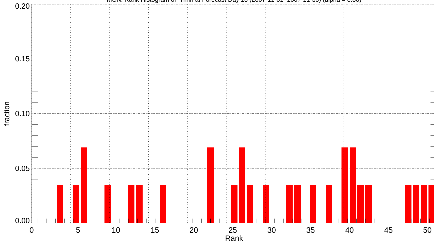
MCN: Rank Histogram of Tmin at Forecast Day 10 (2007-11-01~2007-11-30) (alpha = 0.00)
