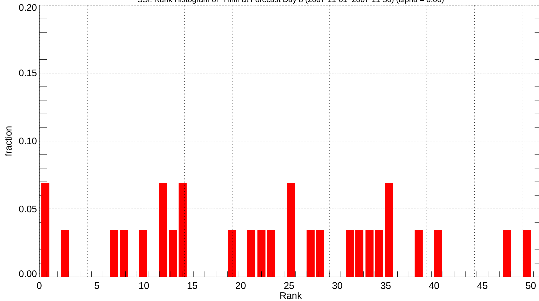
SSI: Rank Histogram of Tmin at Forecast Day 8 (2007-11-01~2007-11-30) (alpha = 0.00)
