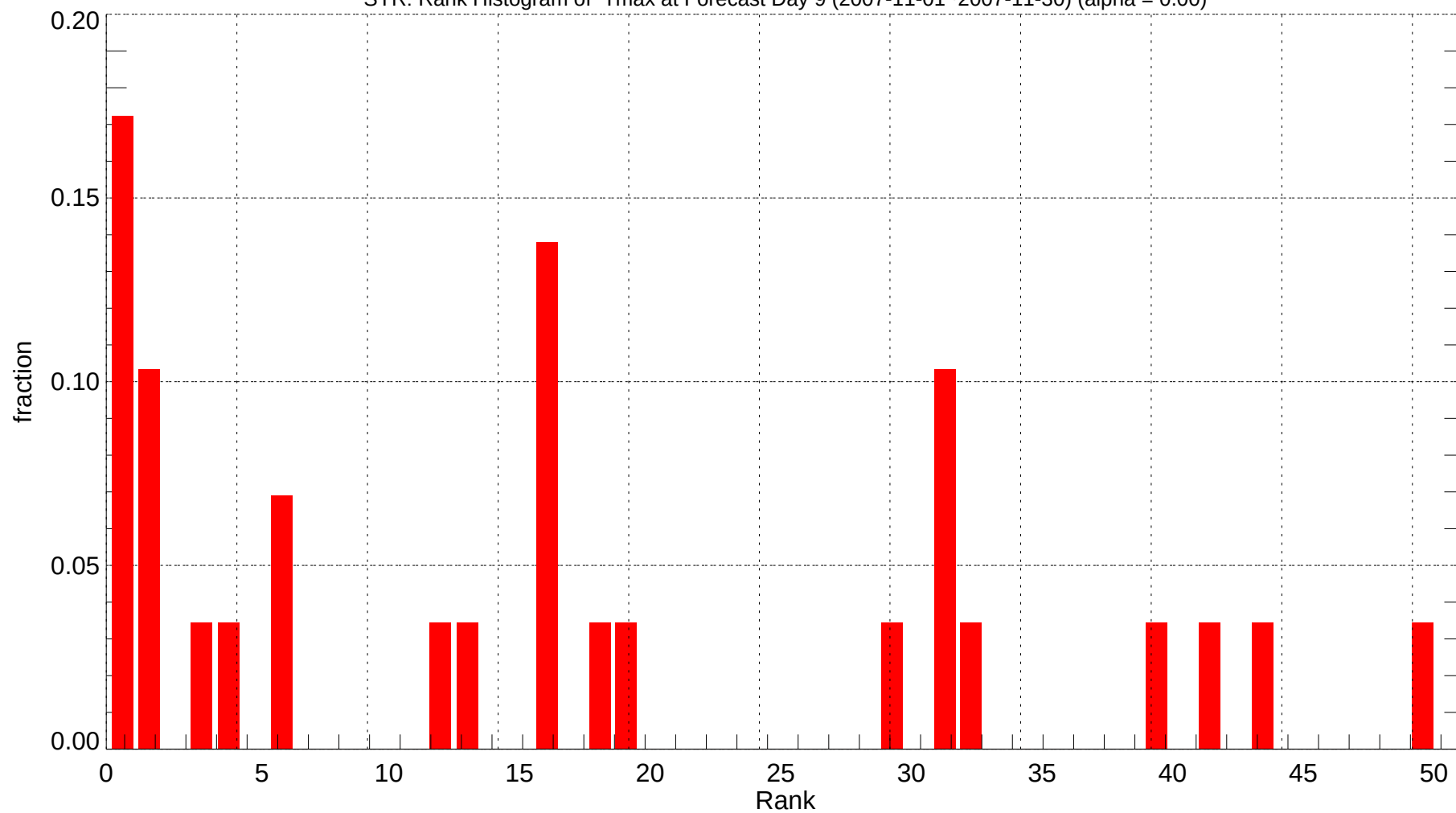
SYR: Rank Histogram of Tmax at Forecast Day 9 (2007-11-01~2007-11-30) (alpha = 0.00)
