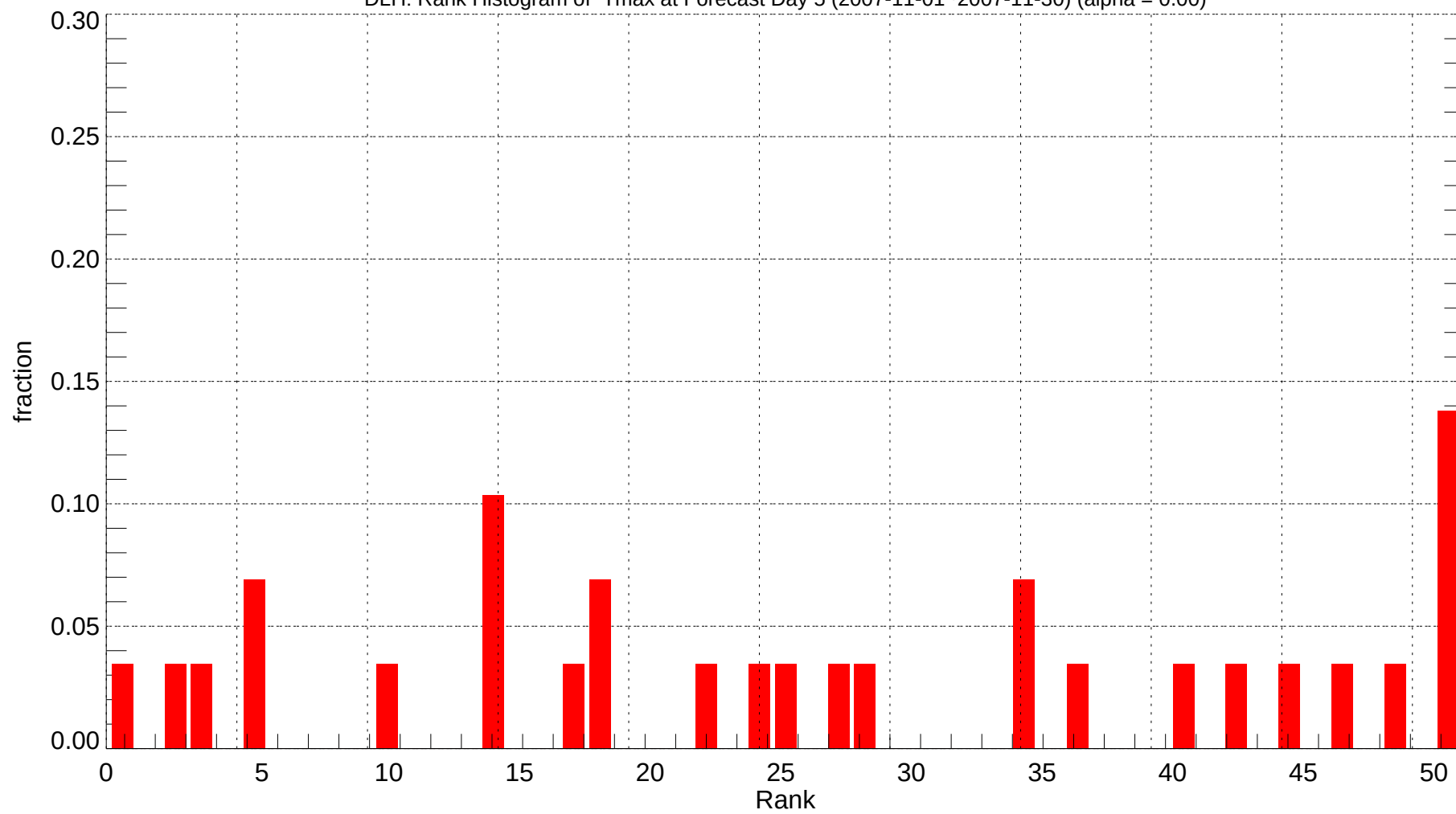
DLH: Rank Histogram of Tmax at Forecast Day 5 (2007-11-01~2007-11-30) (alpha = 0.00)
