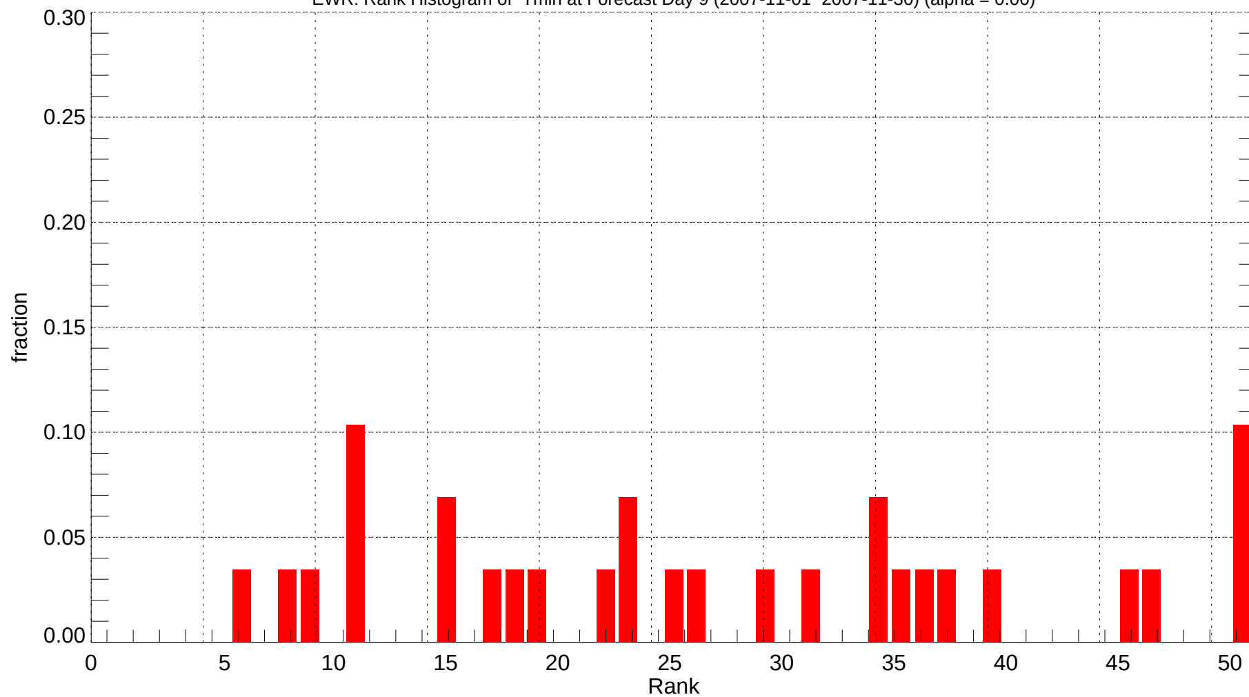
EWR: Rank Histogram of Tmin at Forecast Day 9 (2007-11-01~2007-11-30) (alpha = 0.00)
