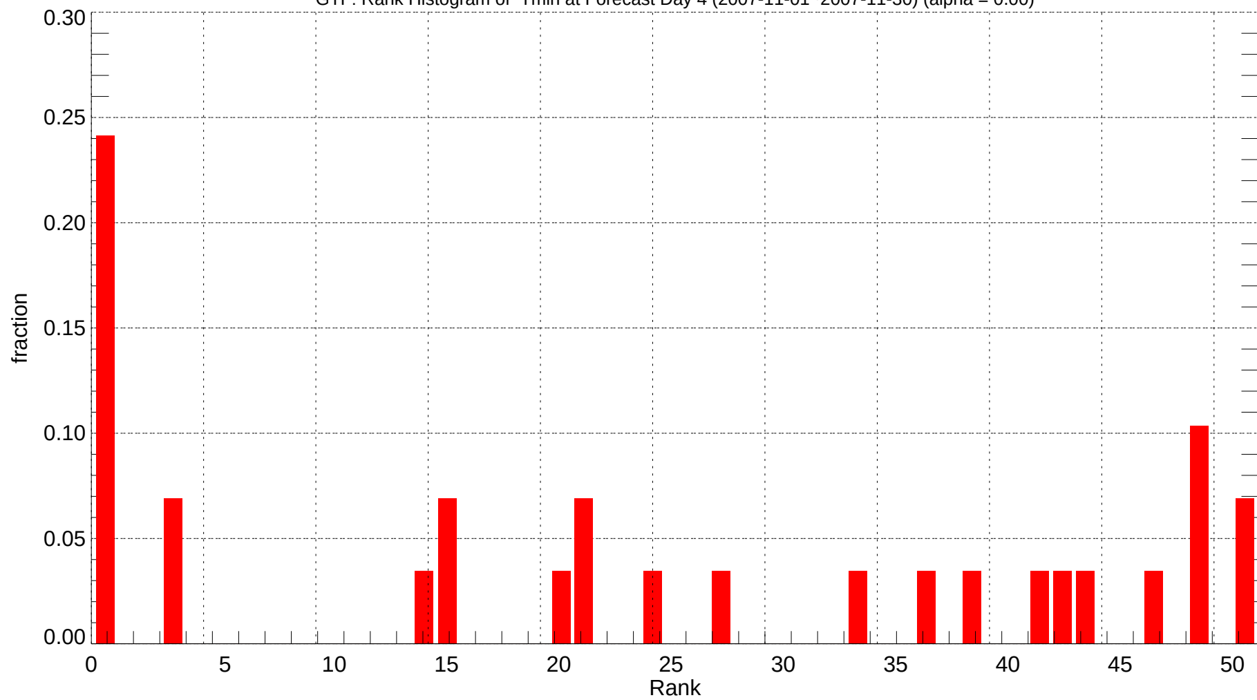
GTF: Rank Histogram of Tmin at Forecast Day 4 (2007-11-01~2007-11-30) (alpha = 0.00)
