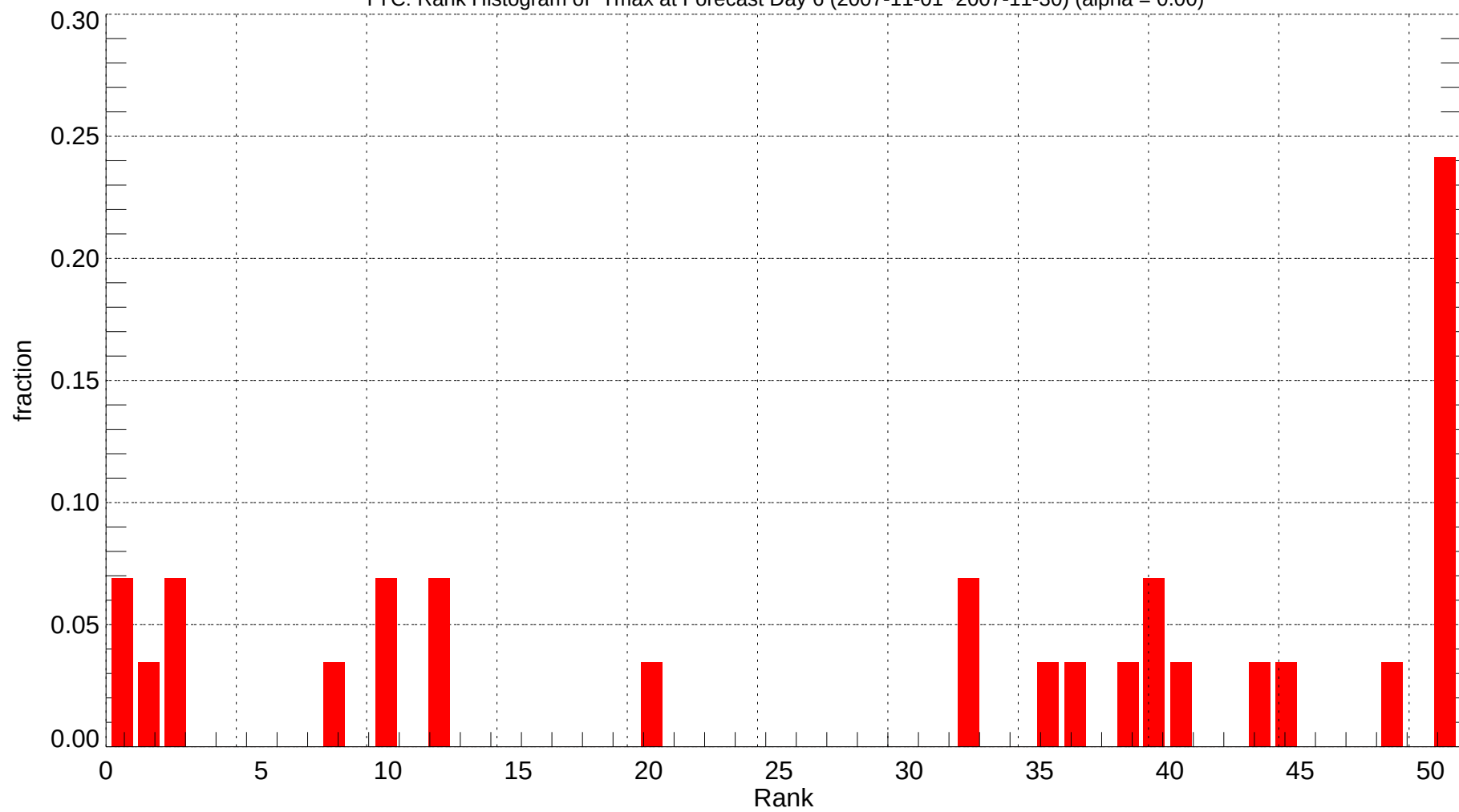
YYC: Rank Histogram of Tmax at Forecast Day 6 (2007-11-01~2007-11-30) (alpha = 0.00)
