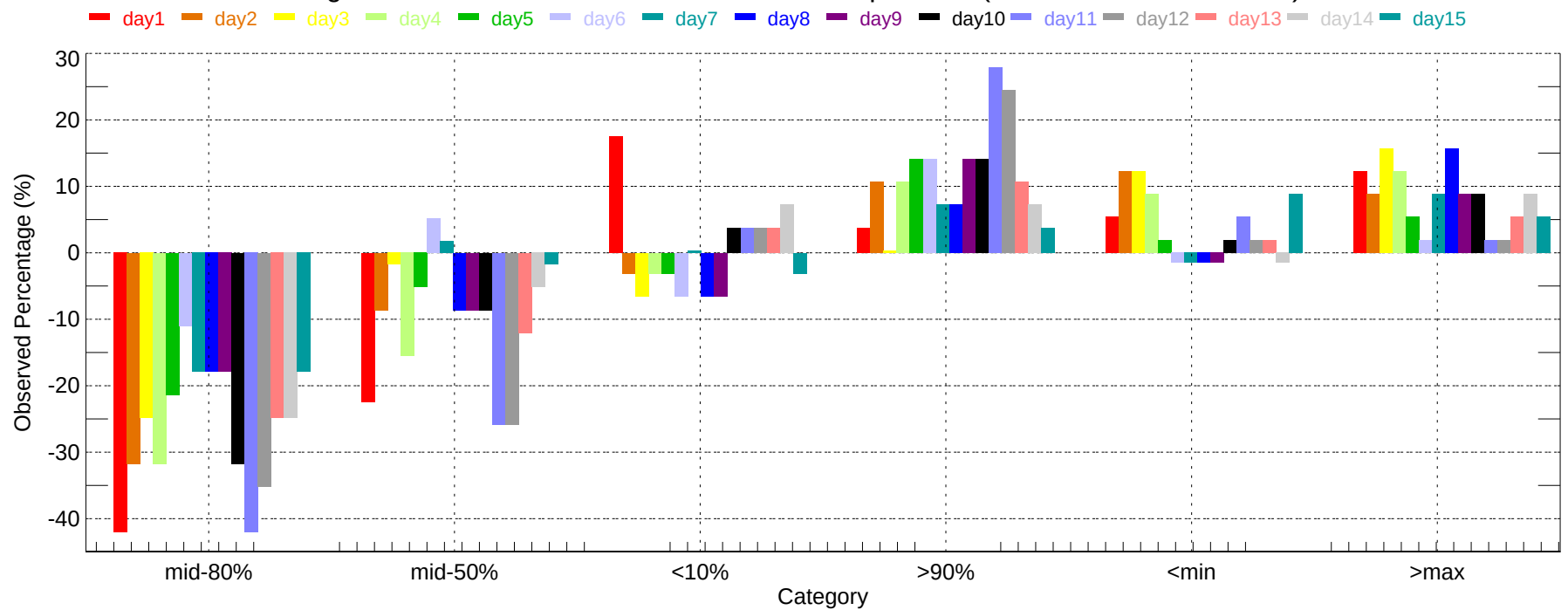
Observed Percentage Deviation of Ensembles - HOU: Min Temperature (2007-11-01~2007-11-30)
