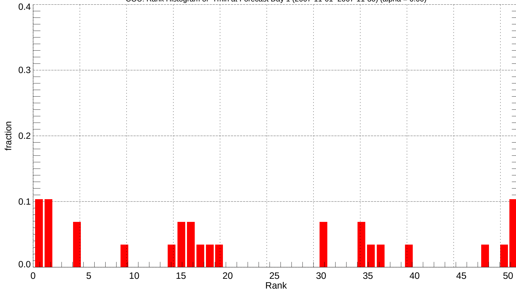
COU: Rank Histogram of Tmin at Forecast Day 1 (2007-11-01~2007-11-30) (alpha = 0.00)
