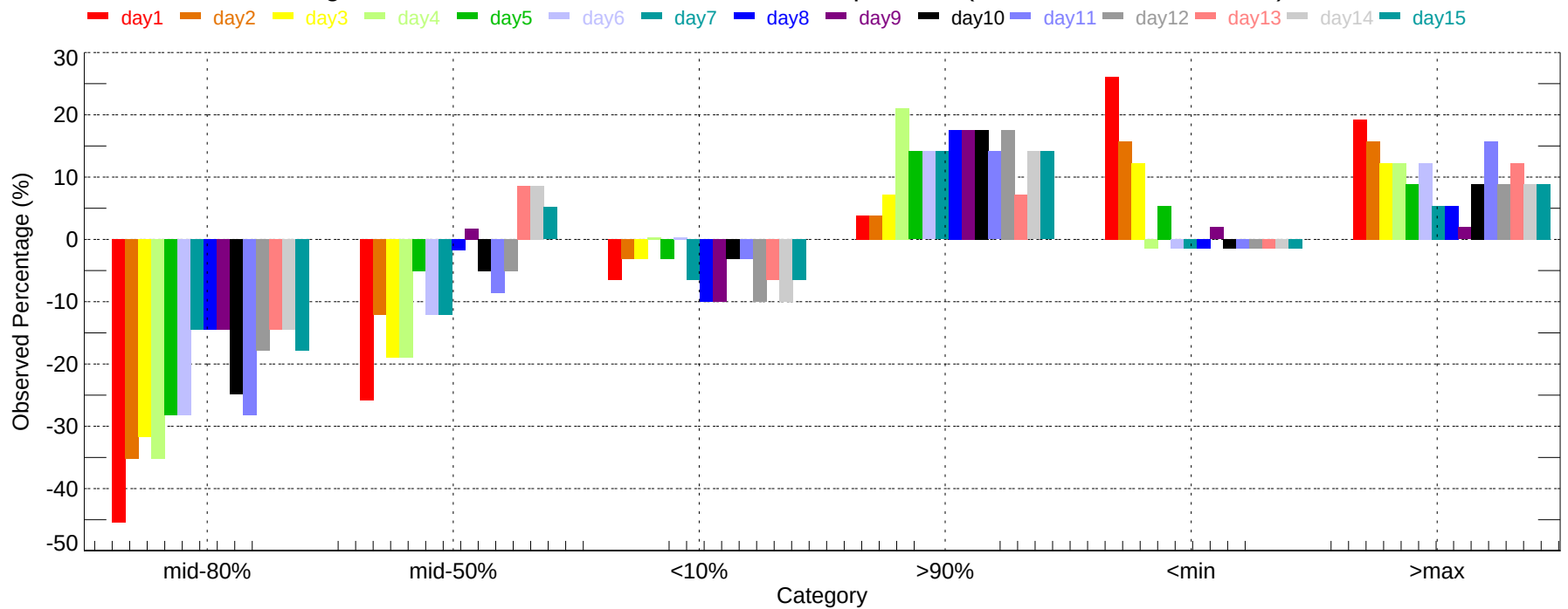
Observed Percentage Deviation of Ensembles - ERI: Min Temperature (2007-11-01~2007-11-30)
