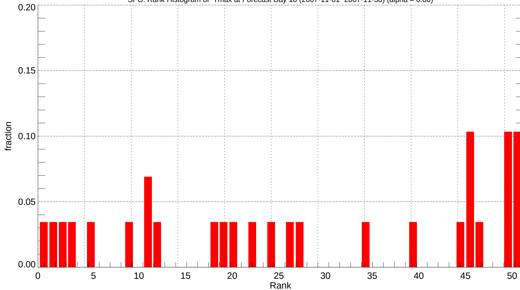
SFO: Rank Histogram of Tmax at Forecast Day 10 (2007-11-01~2007-11-30) (alpha = 0.00)
