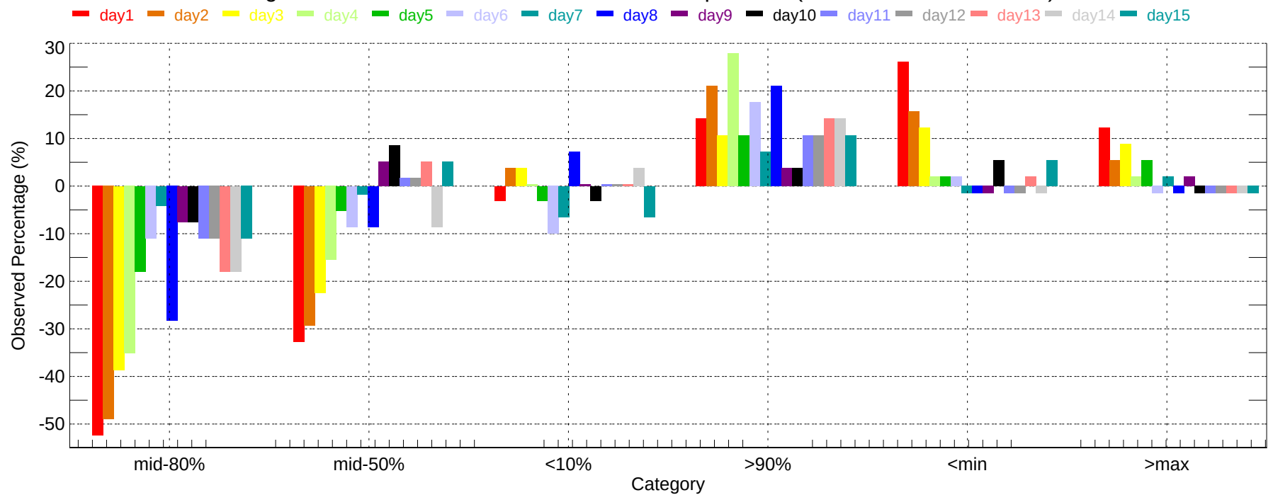
Observed Percentage Deviation of Ensembles - ALB: Max Temperature (2007-11-01~2007-11-30)
