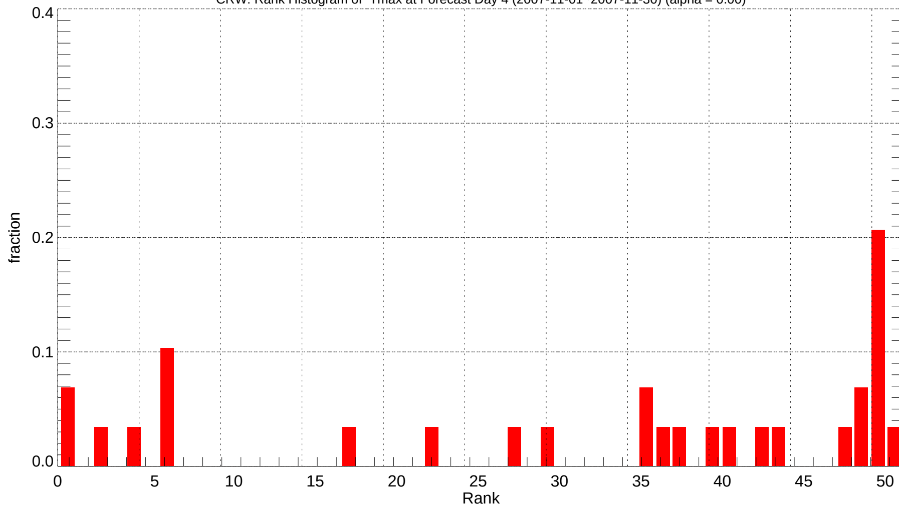
CRW: Rank Histogram of Tmax at Forecast Day 4 (2007-11-01~2007-11-30) (alpha = 0.00)
