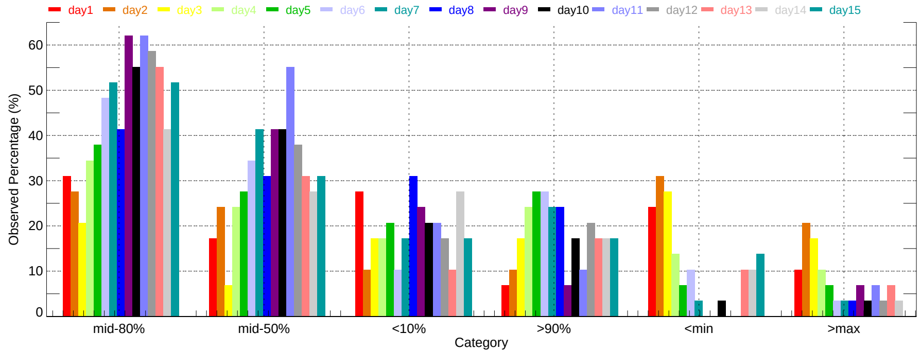
Observed Percentage of Ensembles - ORH: Max Temperature (2007-11-01~2007-11-30)
