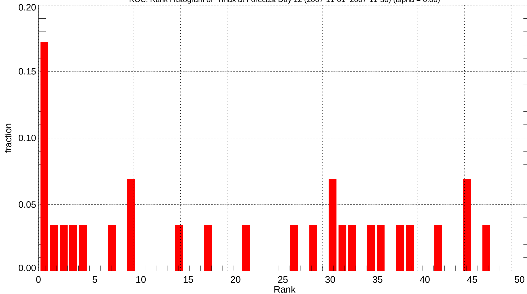
ROC: Rank Histogram of Tmax at Forecast Day 12 (2007-11-01~2007-11-30) (alpha = 0.00)
