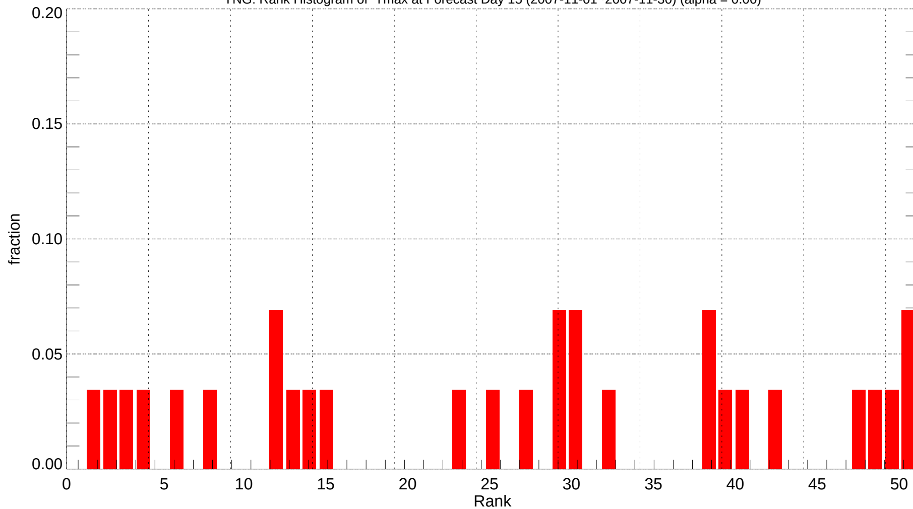
YNG: Rank Histogram of Tmax at Forecast Day 15 (2007-11-01~2007-11-30) (alpha = 0.00)
