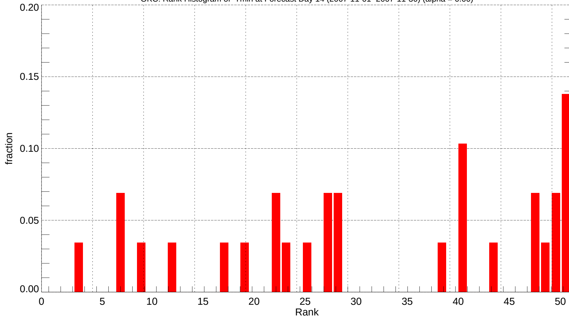
OKC: Rank Histogram of Tmin at Forecast Day 14 (2007-11-01~2007-11-30) (alpha = 0.00)
