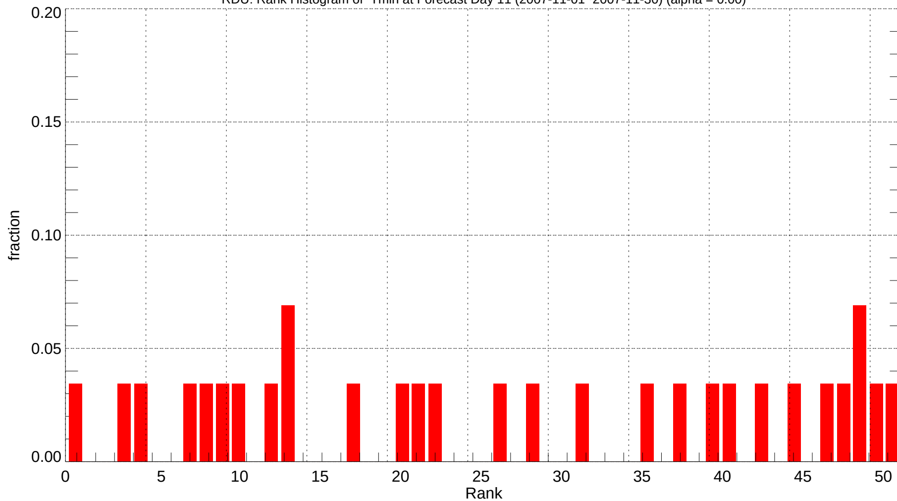
RDU: Rank Histogram of Tmin at Forecast Day 11 (2007-11-01~2007-11-30) (alpha = 0.00)
