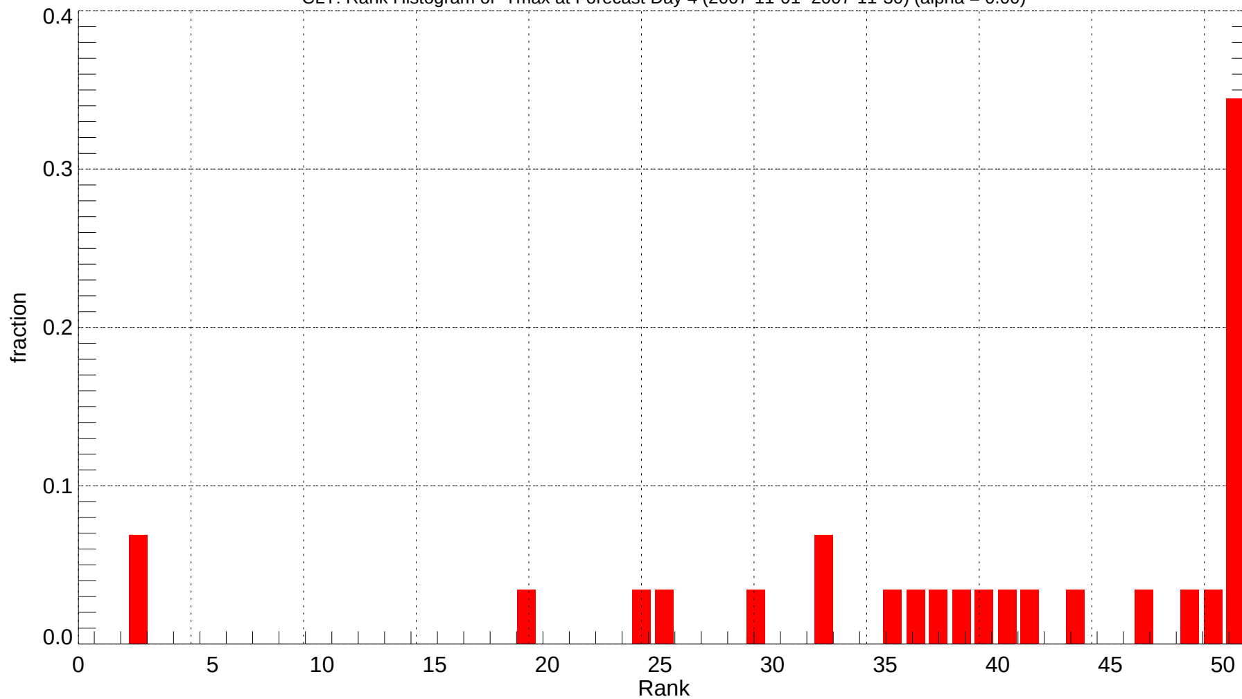
CLT: Rank Histogram of Tmax at Forecast Day 4 (2007-11-01~2007-11-30) (alpha = 0.00)
