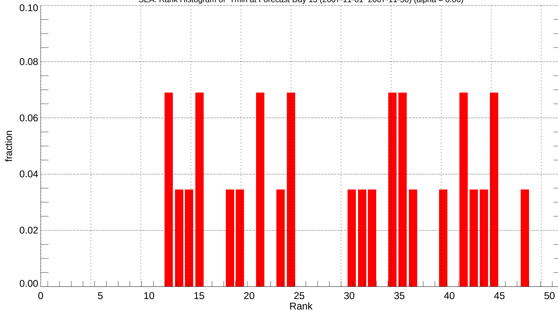
SEA: Rank Histogram of Tmin at Forecast Day 13 (2007-11-01~2007-11-30) (alpha = 0.00)
