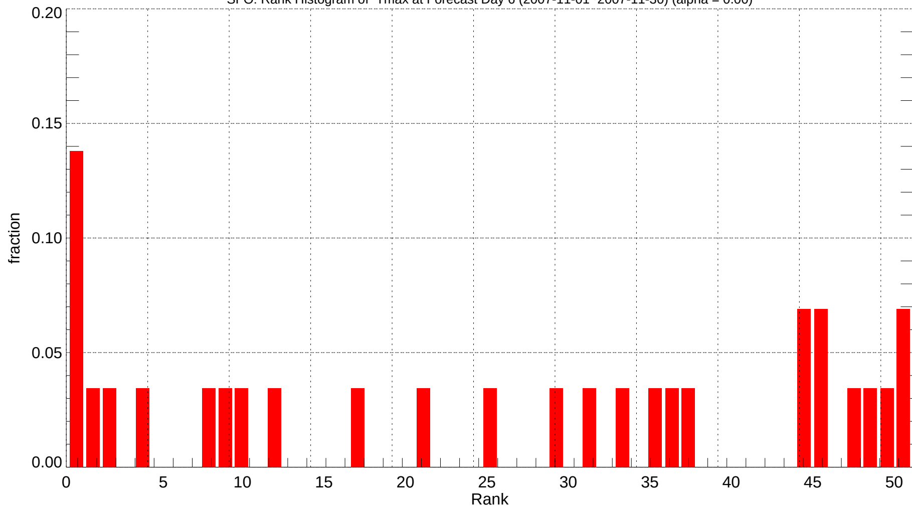
SFO: Rank Histogram of Tmax at Forecast Day 6 (2007-11-01~2007-11-30) (alpha = 0.00)
