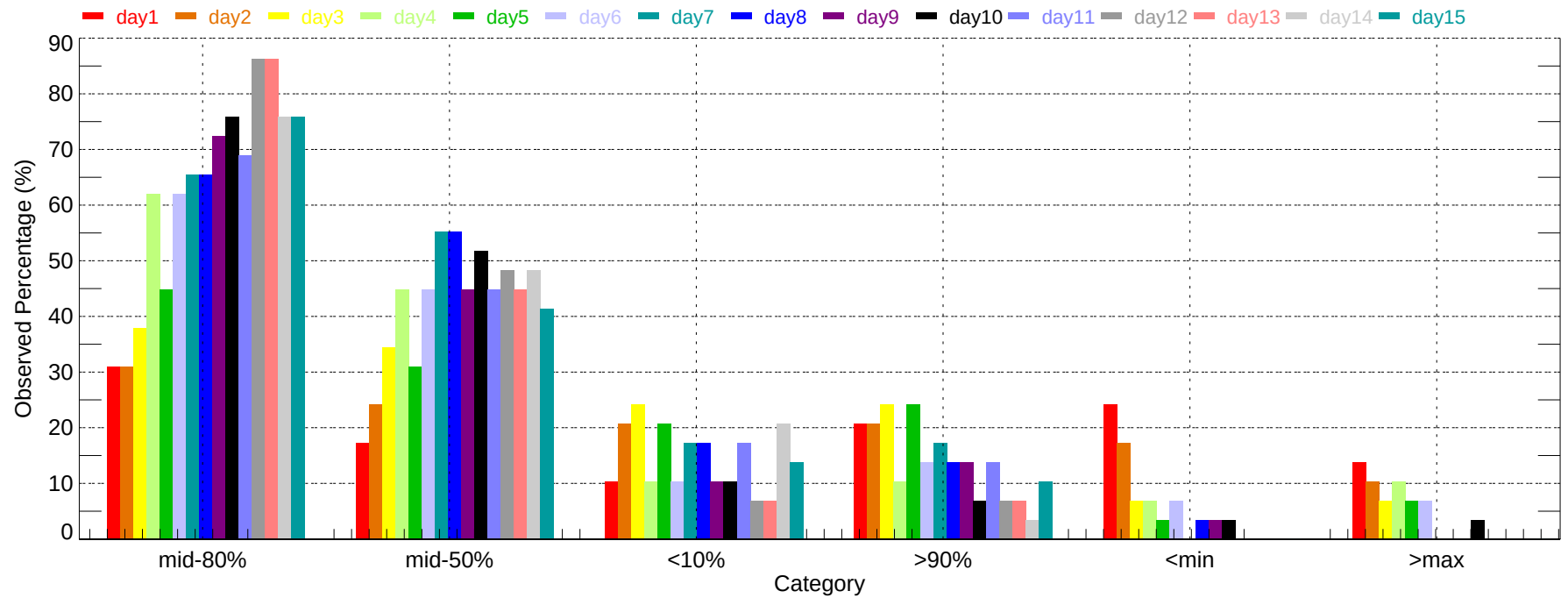
Observed Percentage of Ensembles - MIA: Min Temperature (2007-11-01~2007-11-30)
