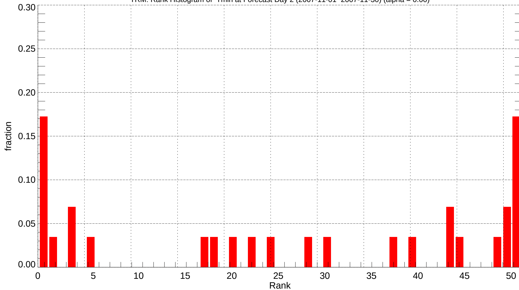
TRM: Rank Histogram of Tmin at Forecast Day 2 (2007-11-01~2007-11-30) (alpha = 0.00)
