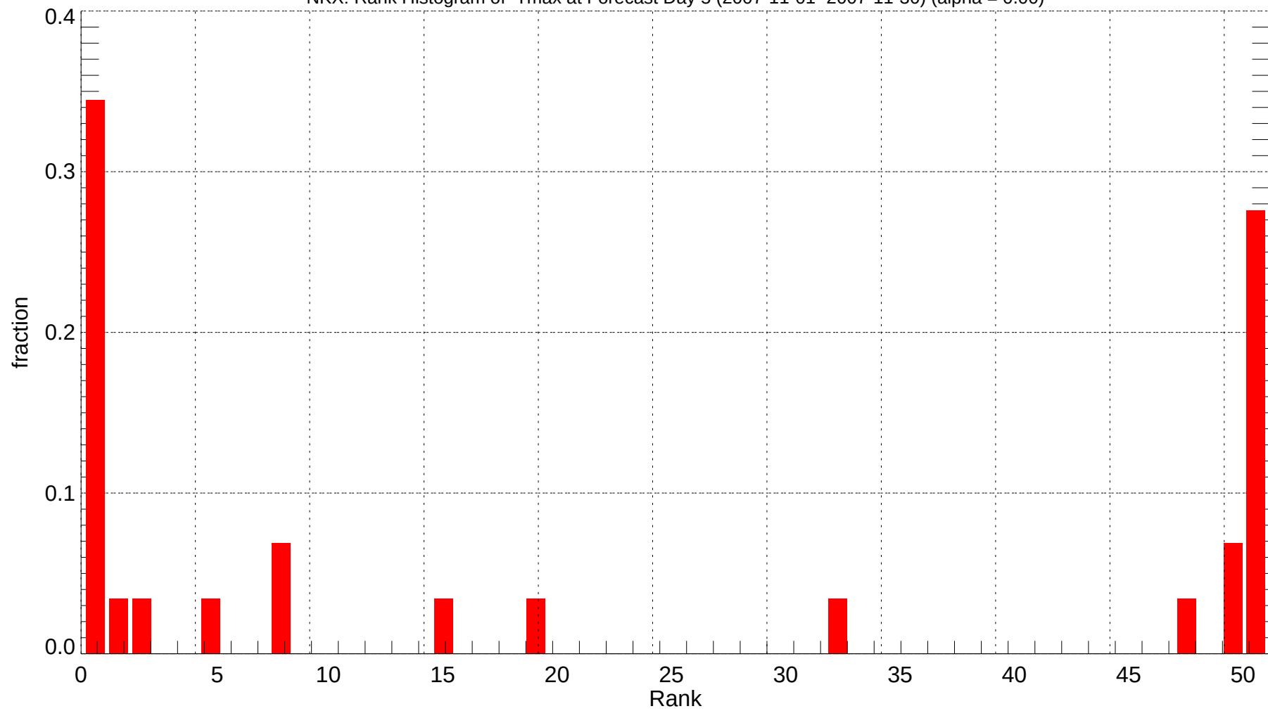
NKX: Rank Histogram of Tmax at Forecast Day 5 (2007-11-01~2007-11-30) (alpha = 0.00)
