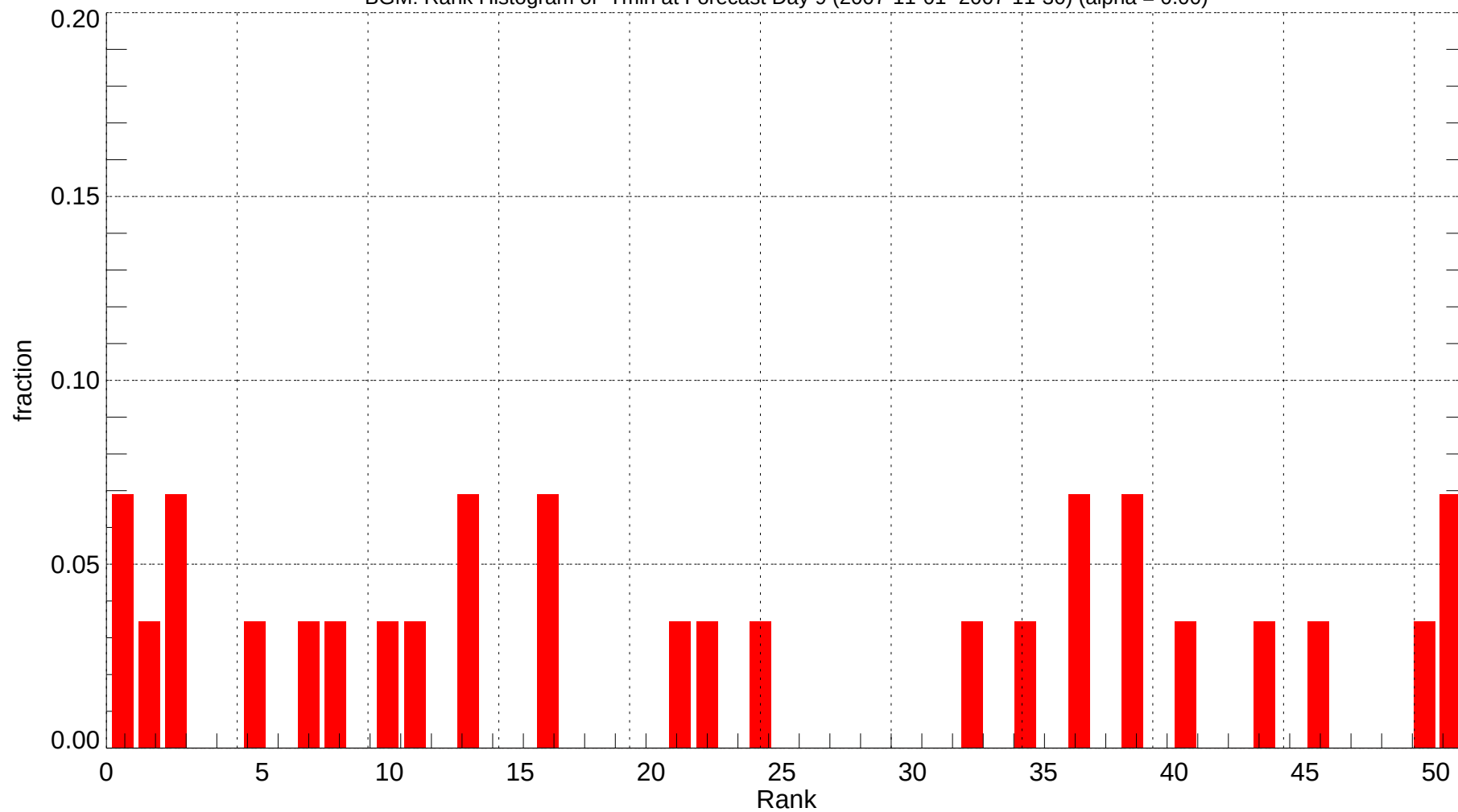
BGM: Rank Histogram of Tmin at Forecast Day 9 (2007-11-01~2007-11-30) (alpha = 0.00)
