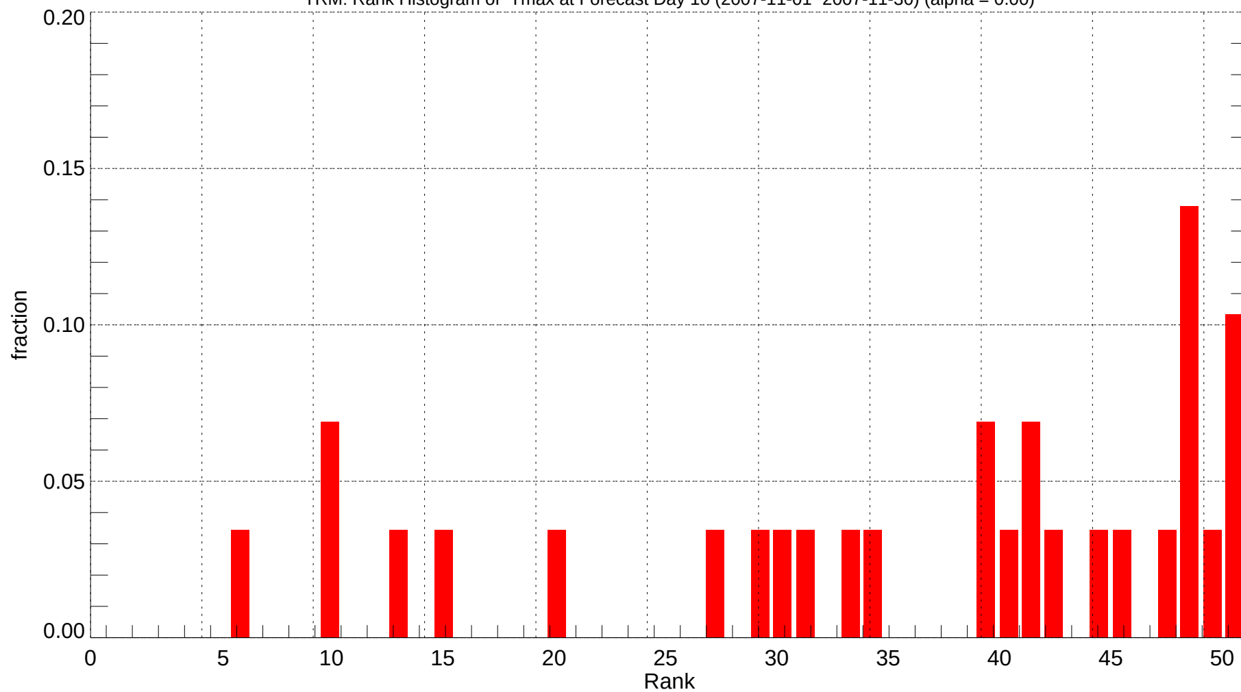
TRM: Rank Histogram of Tmax at Forecast Day 10 (2007-11-01~2007-11-30) (alpha = 0.00)
