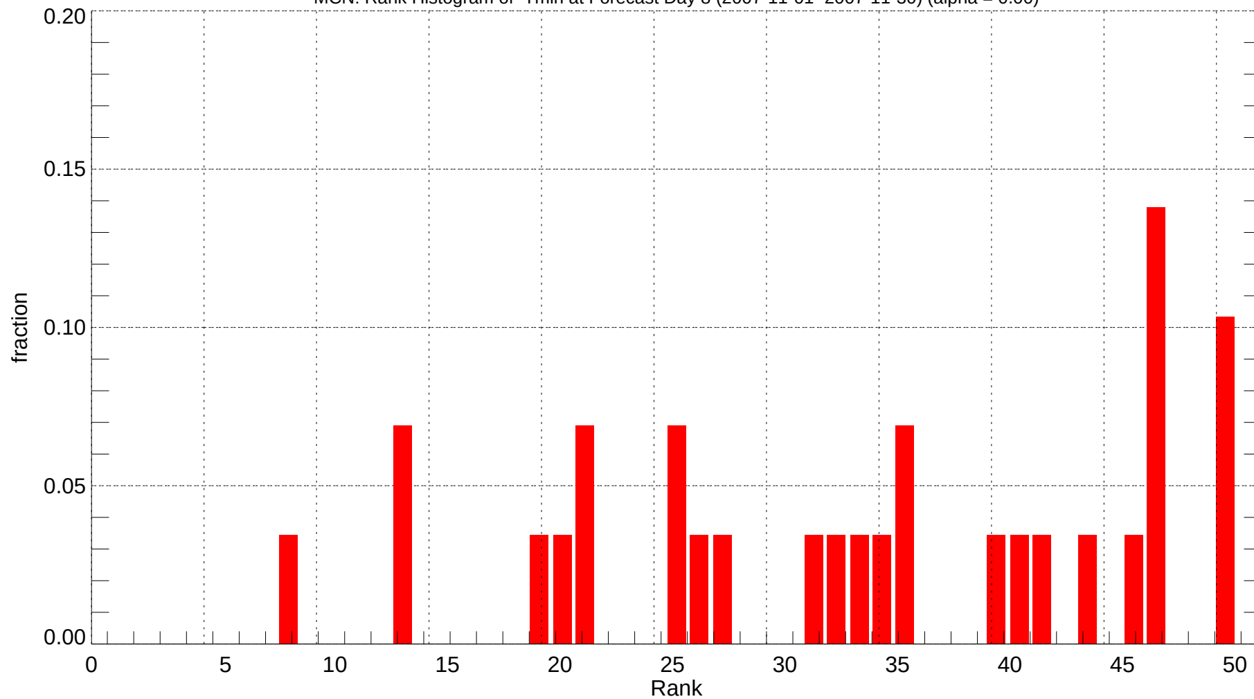
MCN: Rank Histogram of Tmin at Forecast Day 8 (2007-11-01~2007-11-30) (alpha = 0.00)
