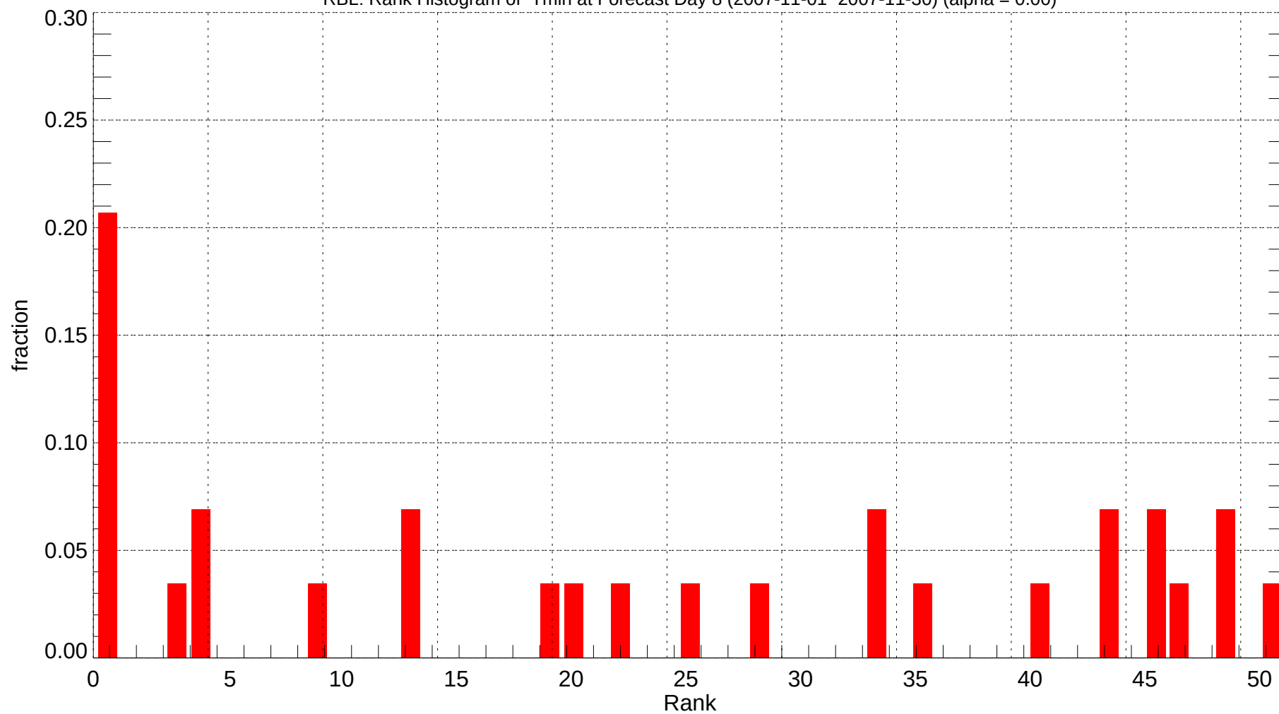
RBL: Rank Histogram of Tmin at Forecast Day 8 (2007-11-01~2007-11-30) (alpha = 0.00)
