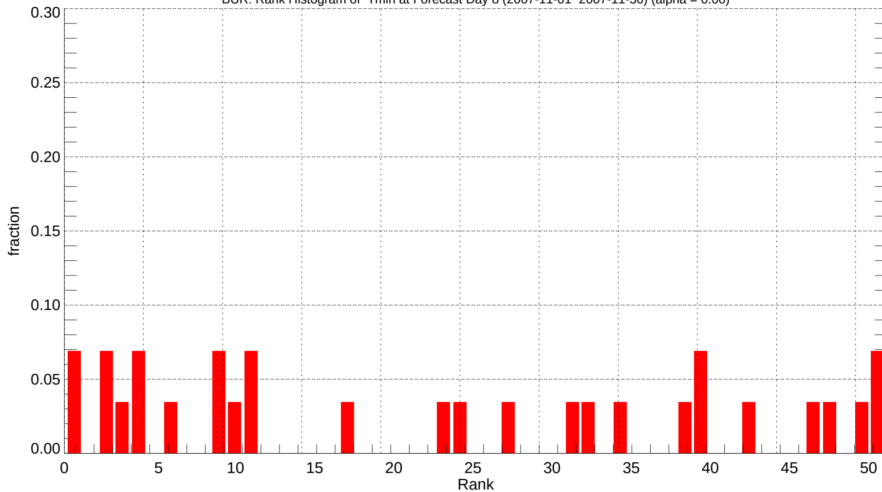
BUR: Rank Histogram of Tmin at Forecast Day 8 (2007-11-01~2007-11-30) (alpha = 0.00)
