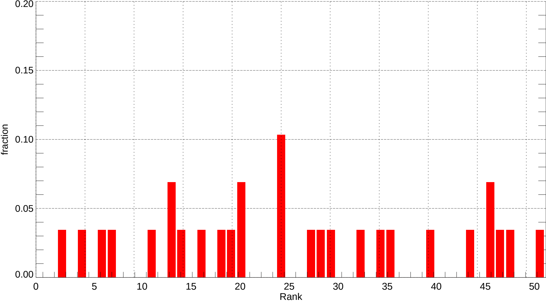
BFL: Rank Histogram of Tmin at Forecast Day 9 (2007-11-01~2007-11-30) (alpha = 0.00)
