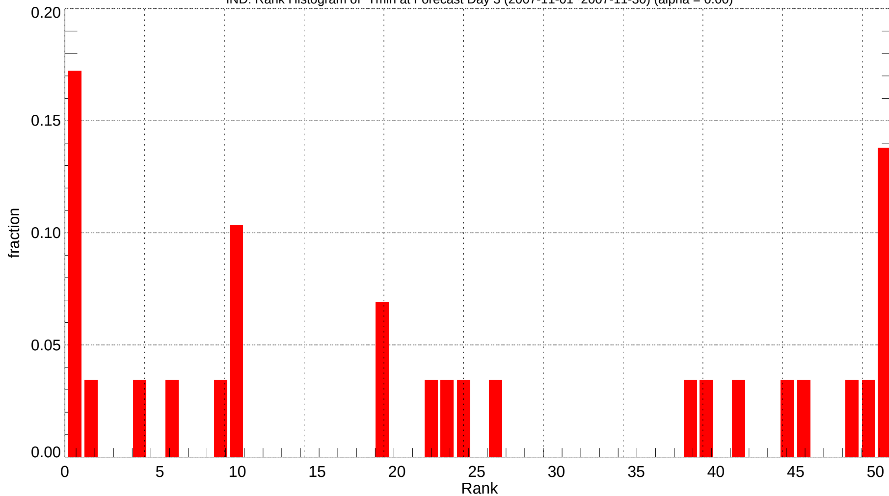
IND: Rank Histogram of Tmin at Forecast Day 3 (2007-11-01~2007-11-30) (alpha = 0.00)
