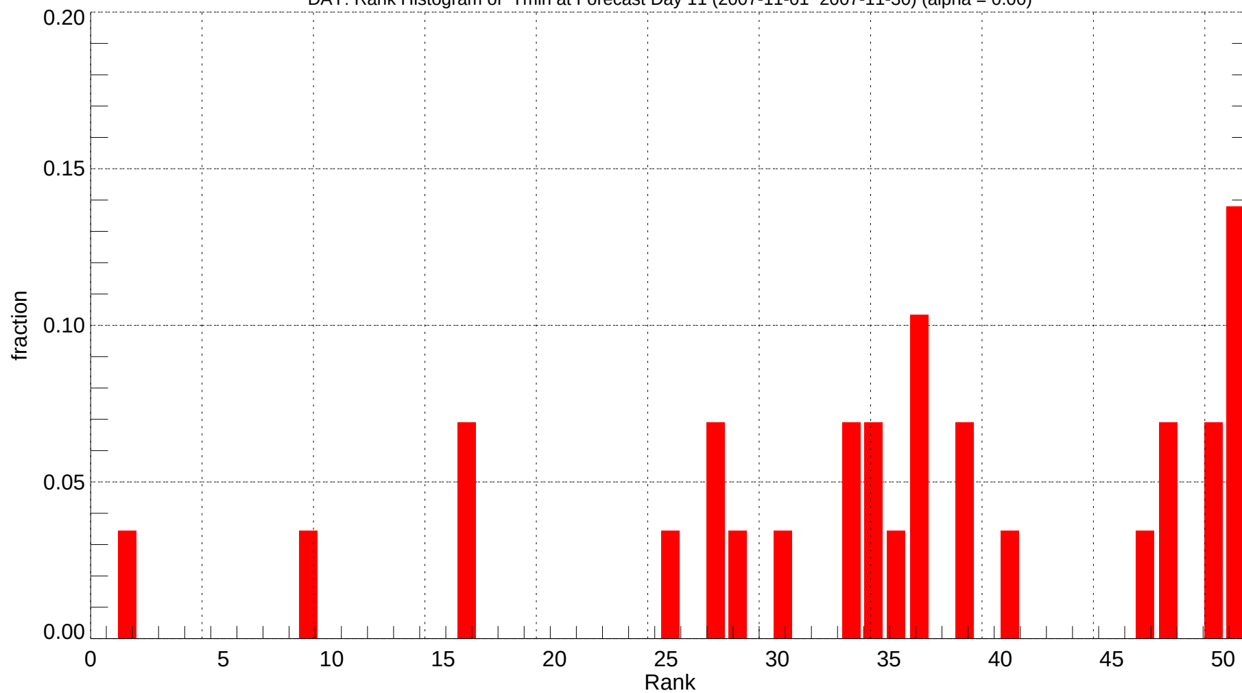
DAY: Rank Histogram of Tmin at Forecast Day 11 (2007-11-01~2007-11-30) (alpha = 0.00)
