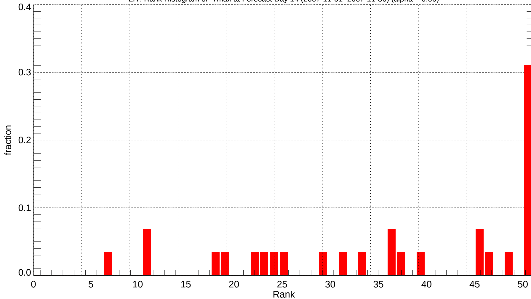
LIT: Rank Histogram of Tmax at Forecast Day 14 (2007-11-01~2007-11-30) (alpha = 0.00)
