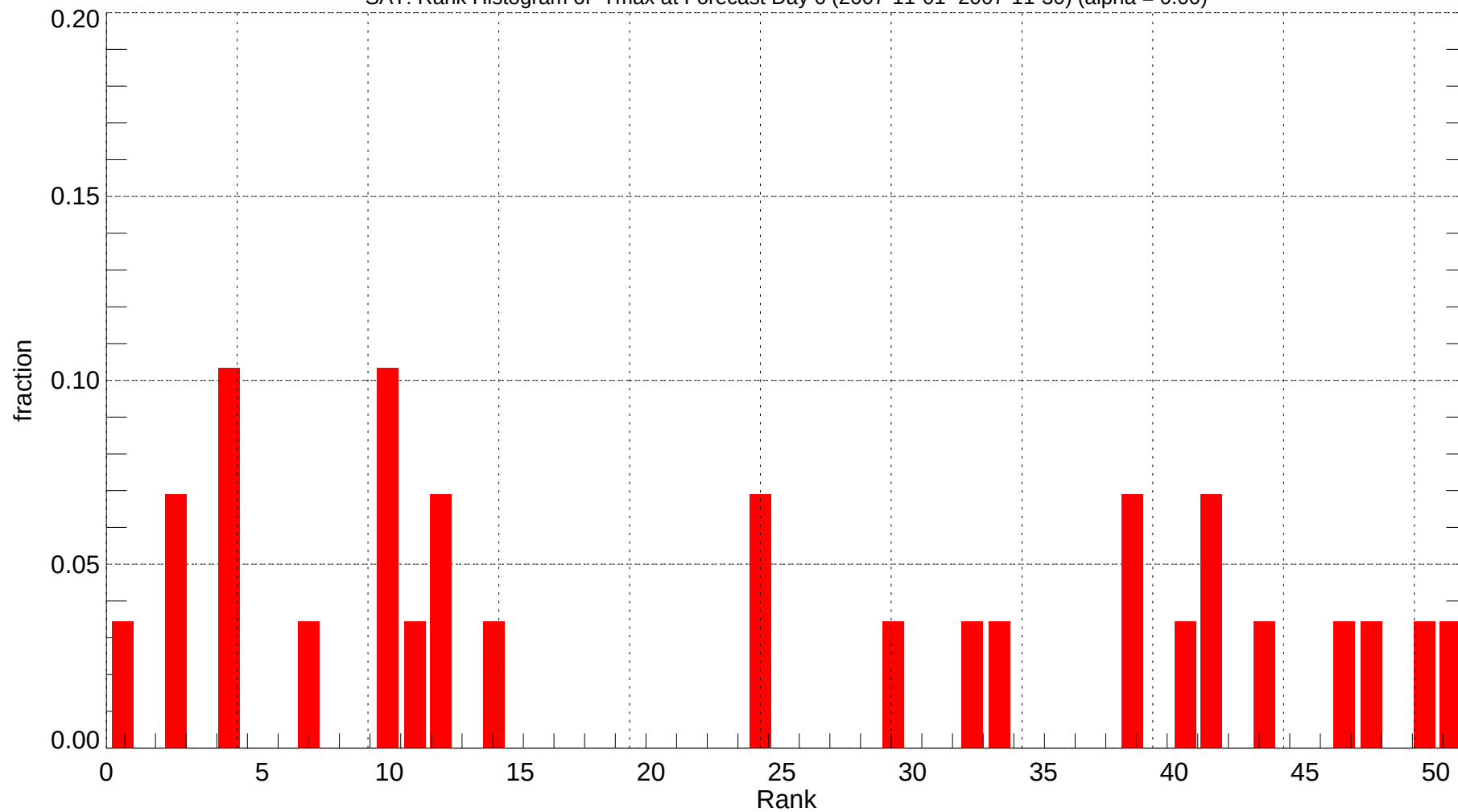
SAT: Rank Histogram of Tmax at Forecast Day 6 (2007-11-01~2007-11-30) (alpha = 0.00)
