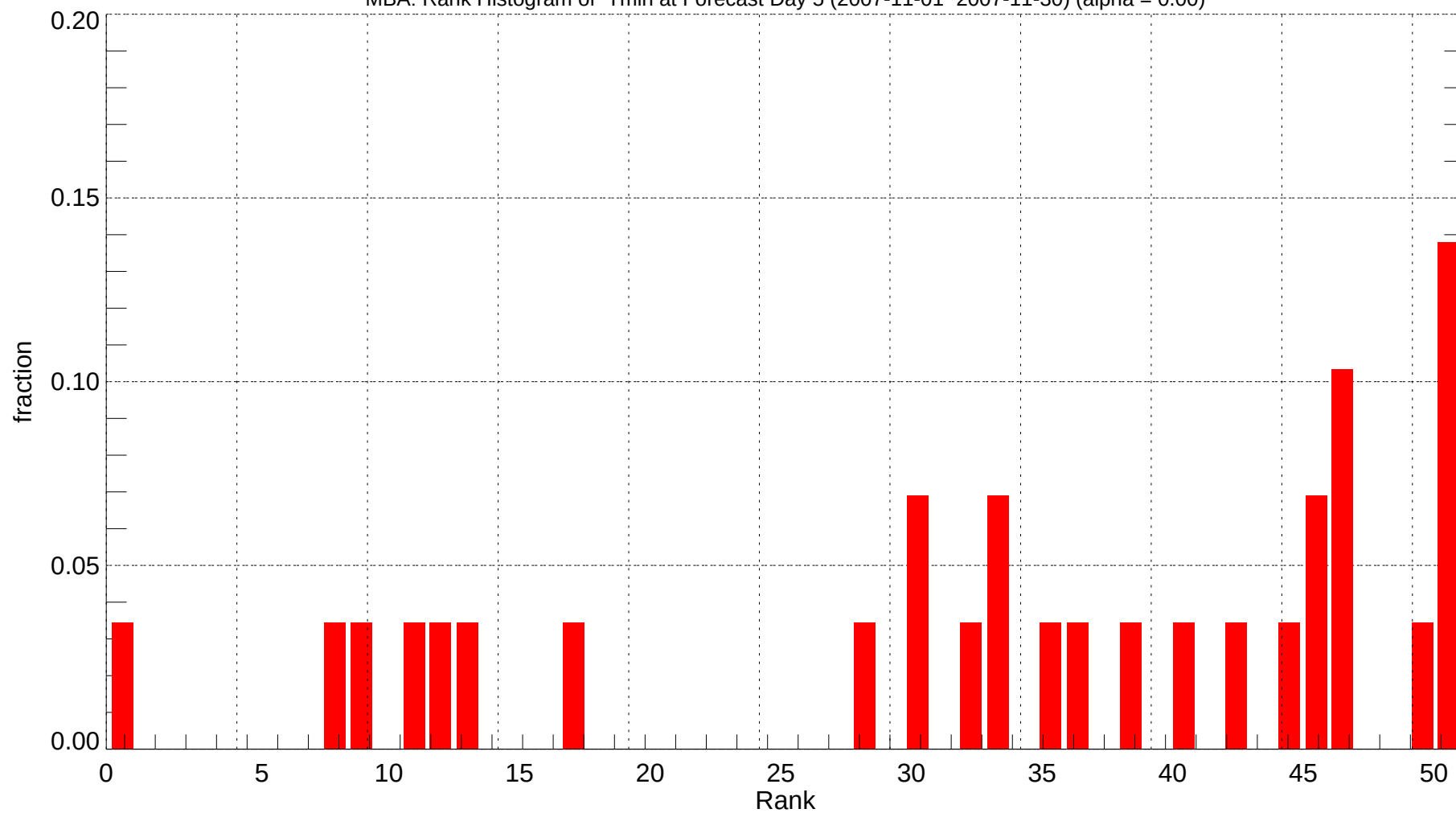
MBA: Rank Histogram of Tmin at Forecast Day 5 (2007-11-01~2007-11-30) (alpha = 0.00)
