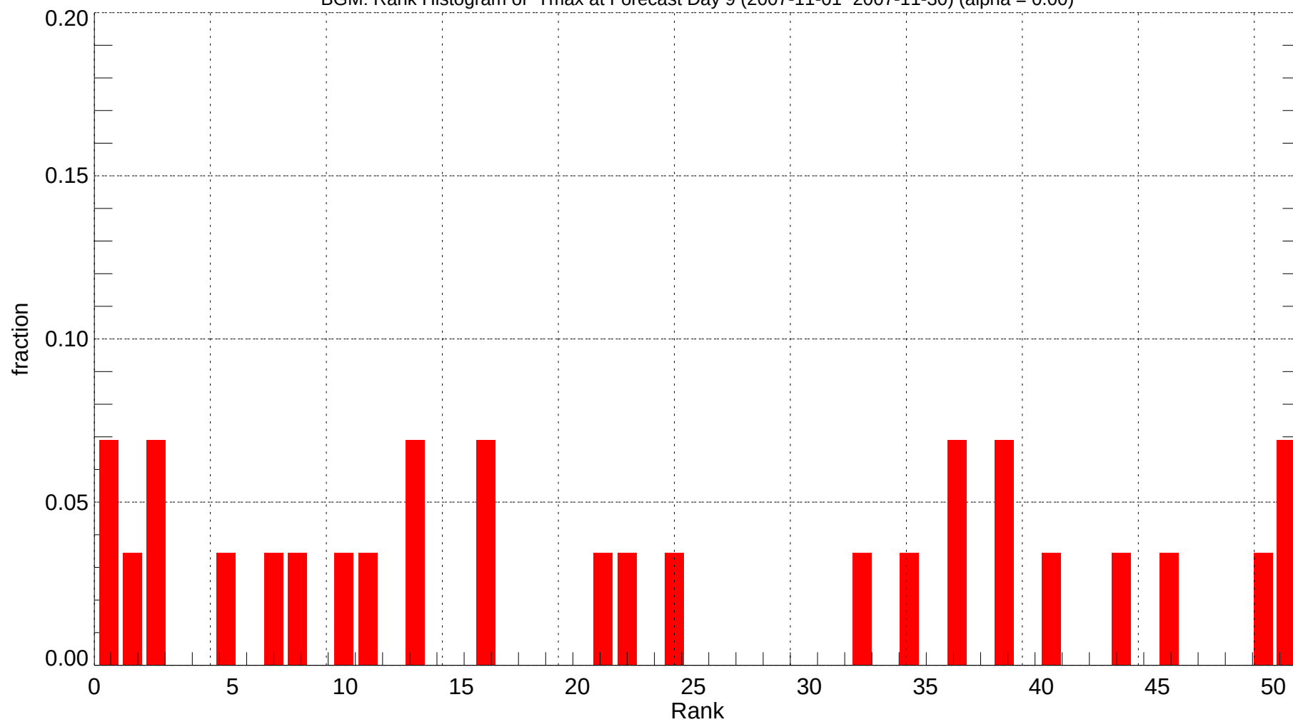
BGM: Rank Histogram of Tmax at Forecast Day 9 (2007-11-01~2007-11-30) (alpha = 0.00)
