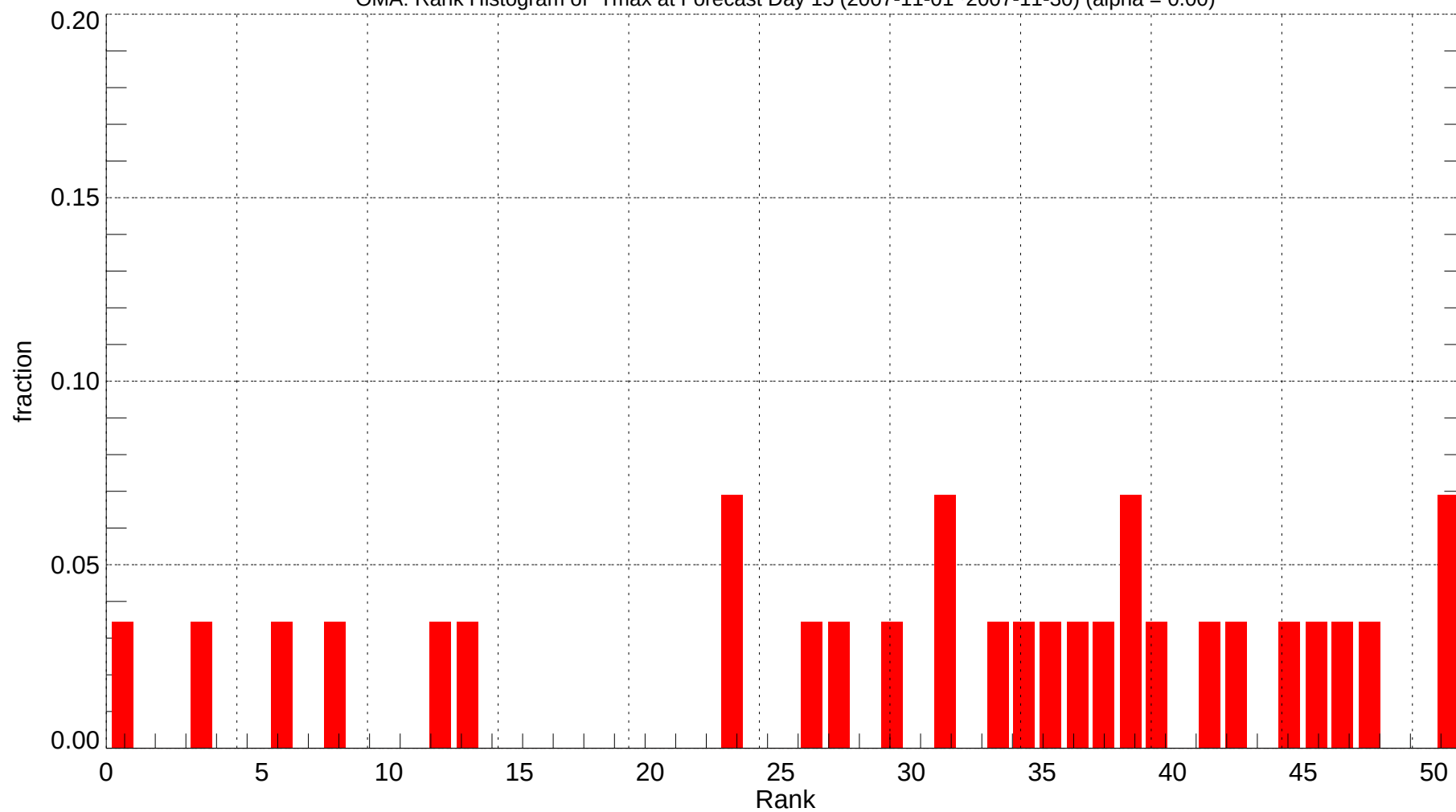
OMA: Rank Histogram of Tmax at Forecast Day 15 (2007-11-01~2007-11-30) (alpha = 0.00)
