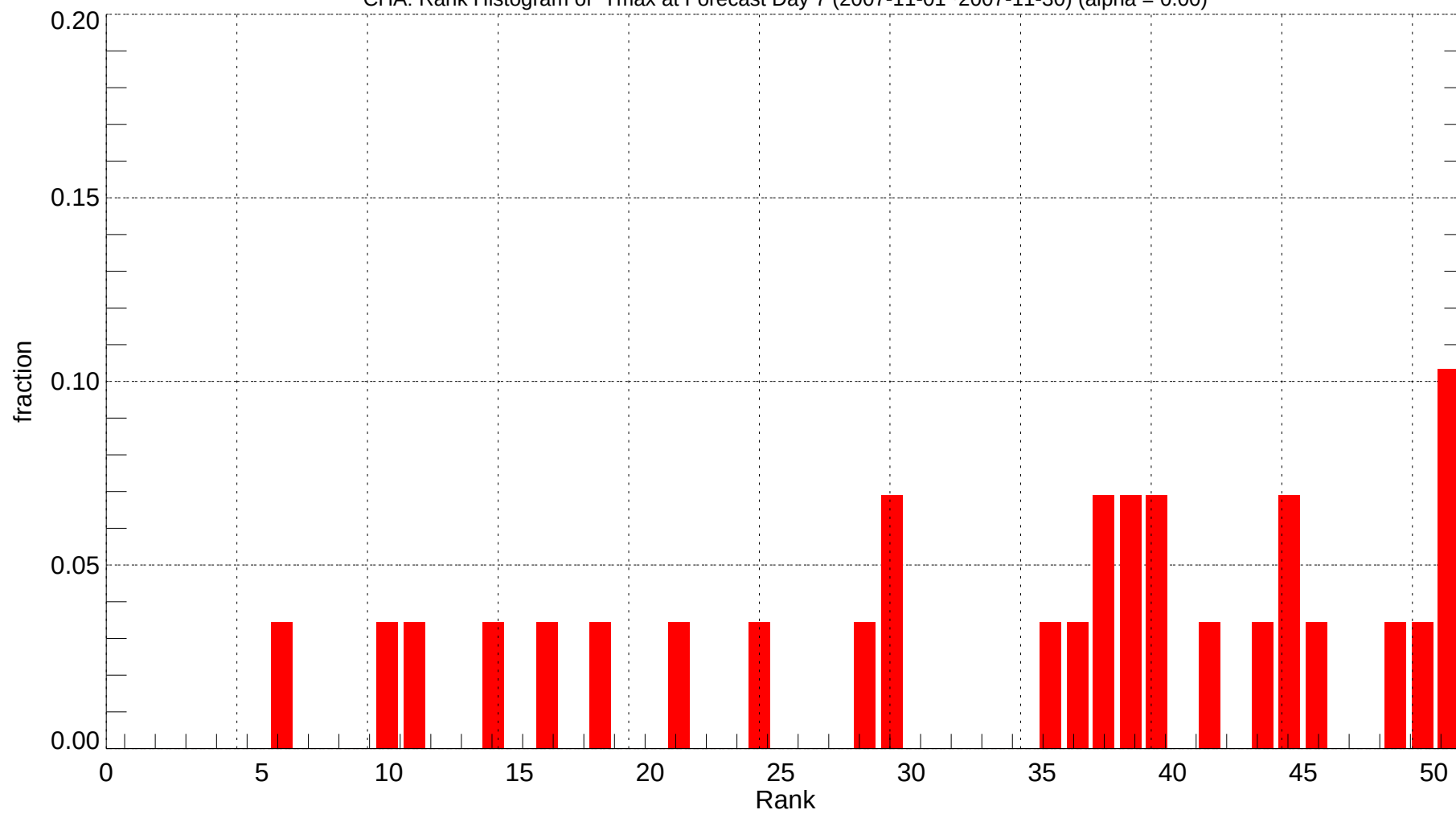
CHA: Rank Histogram of Tmax at Forecast Day 7 (2007-11-01~2007-11-30) (alpha = 0.00)
