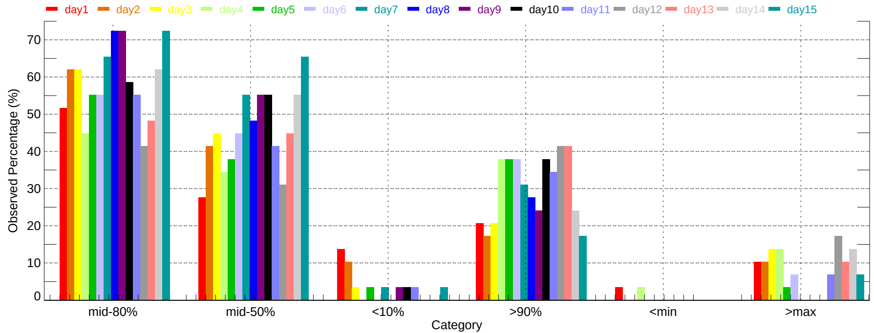
Observed Percentage of Ensembles - BHM: Max Temperature (2007-11-01~2007-11-30)
