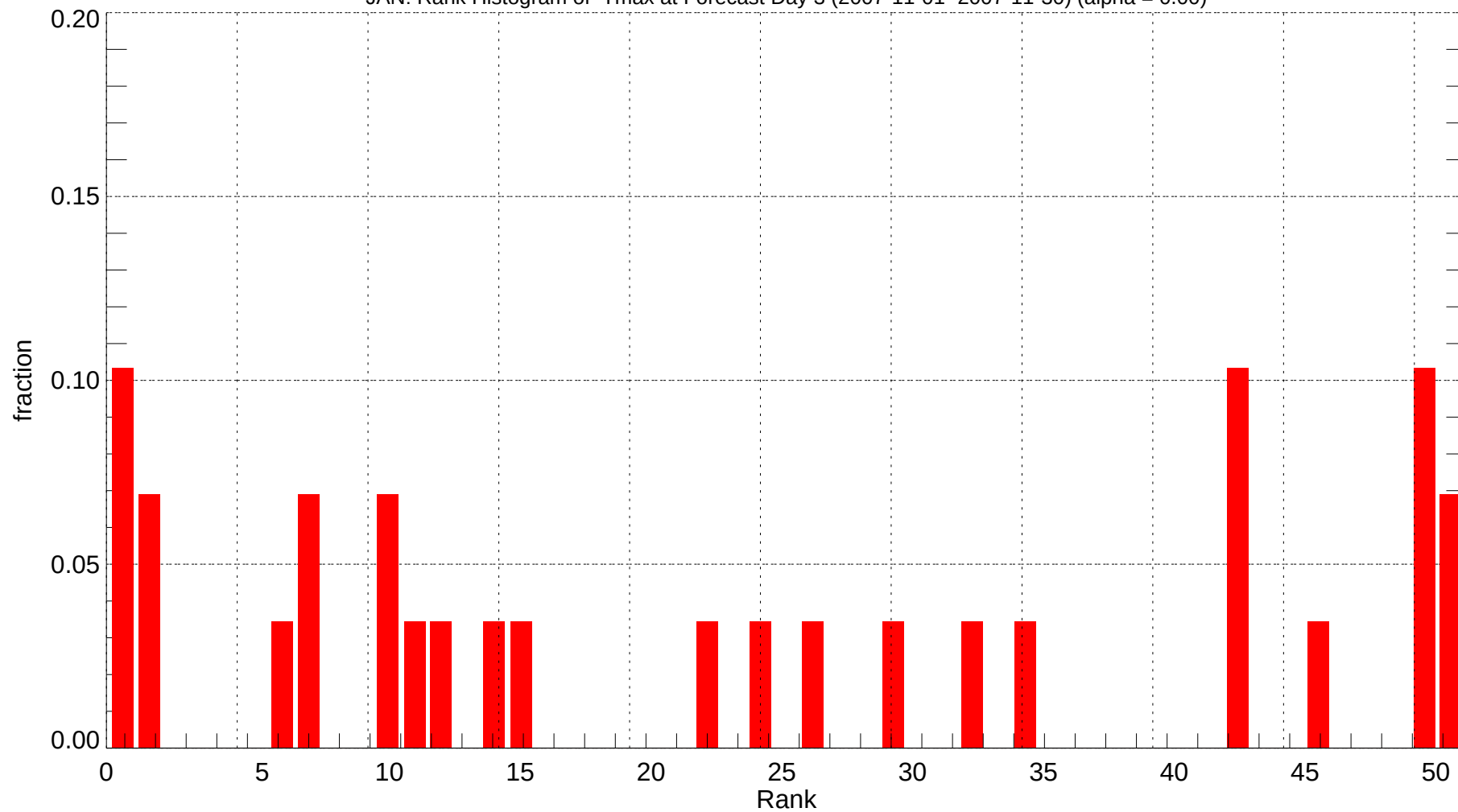
JAN: Rank Histogram of Tmax at Forecast Day 3 (2007-11-01~2007-11-30) (alpha = 0.00)
