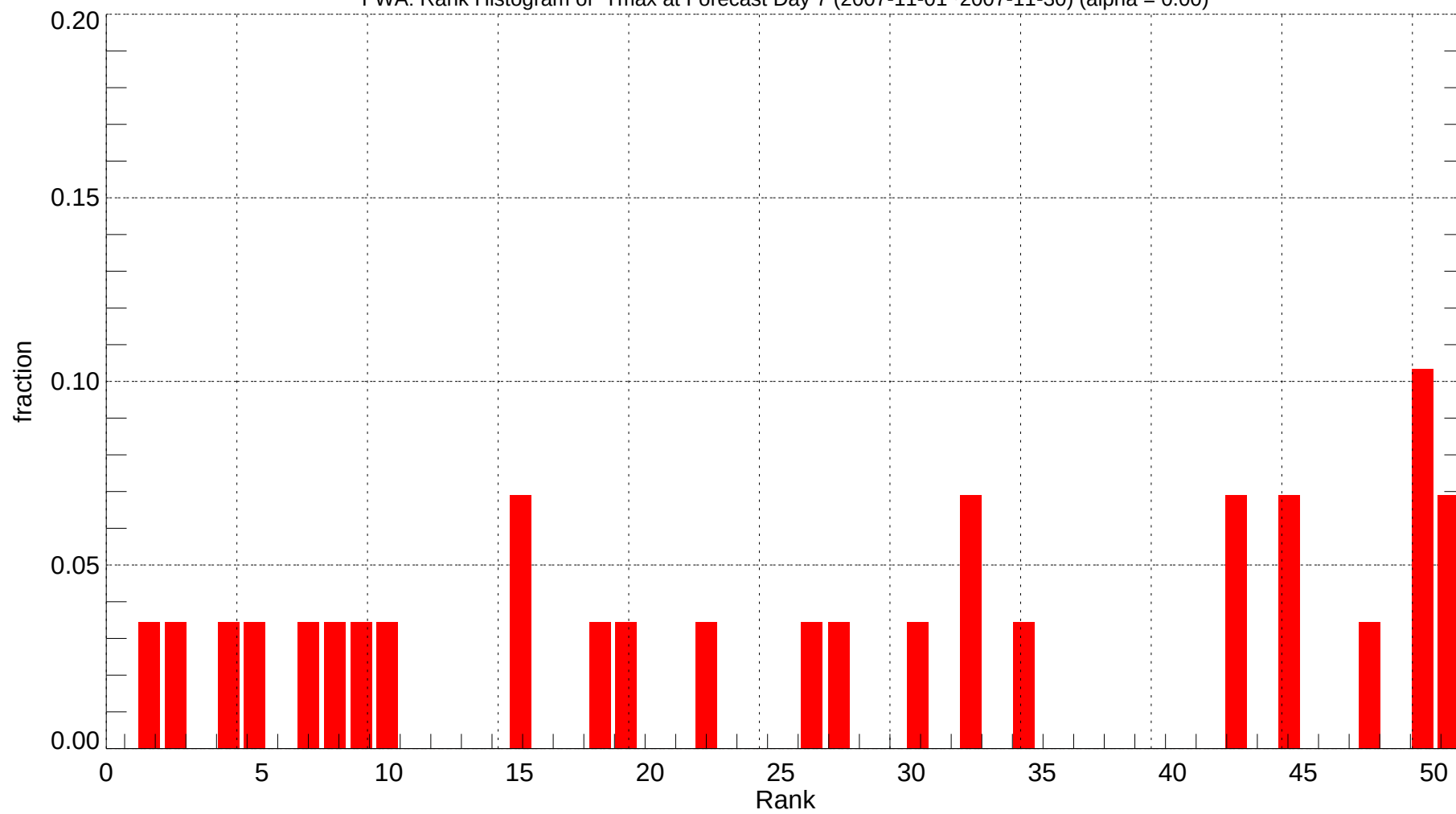
FWA: Rank Histogram of Tmax at Forecast Day 7 (2007-11-01~2007-11-30) (alpha = 0.00)
