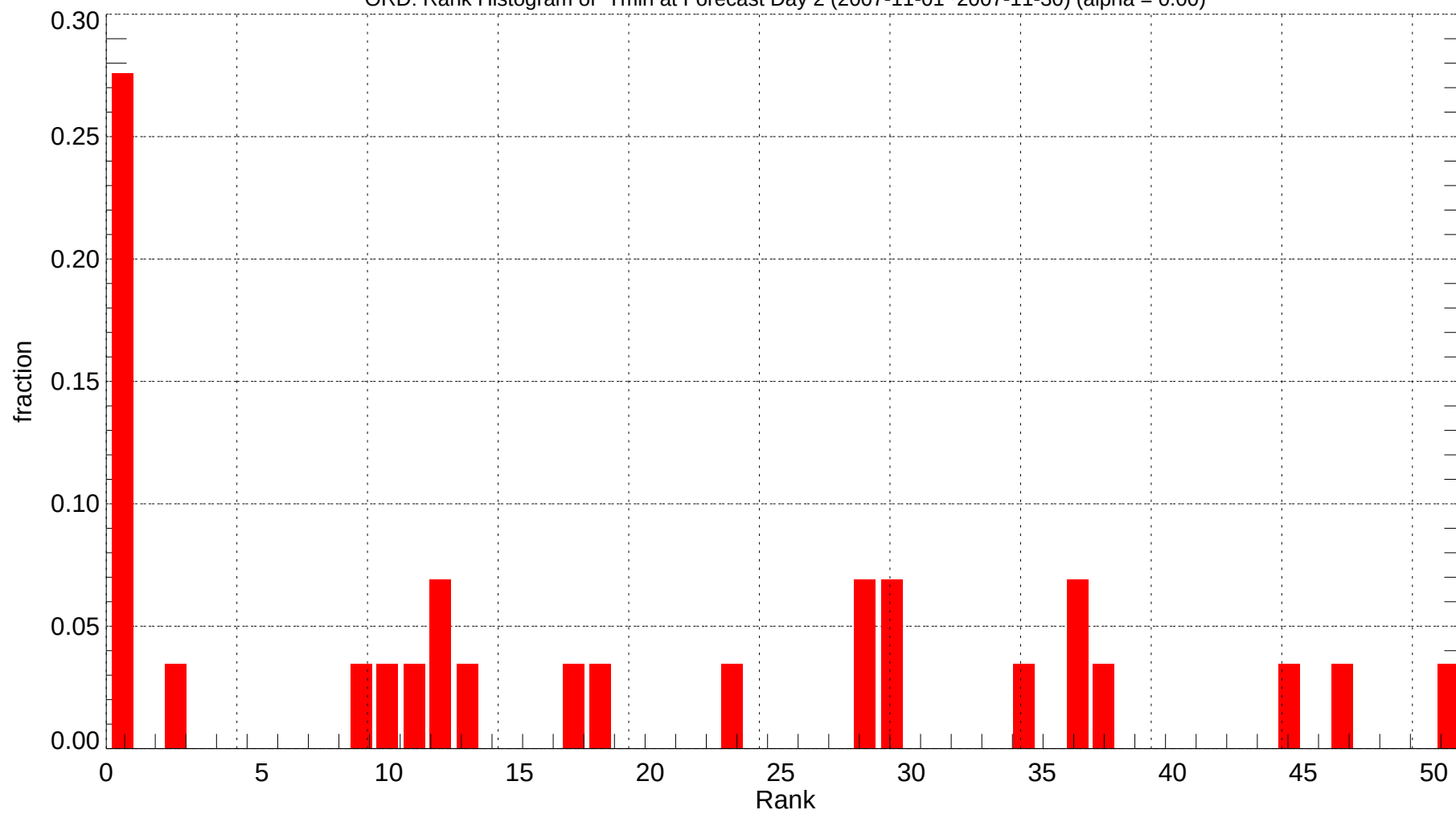
ORD: Rank Histogram of Tmin at Forecast Day 2 (2007-11-01~2007-11-30) (alpha = 0.00)
