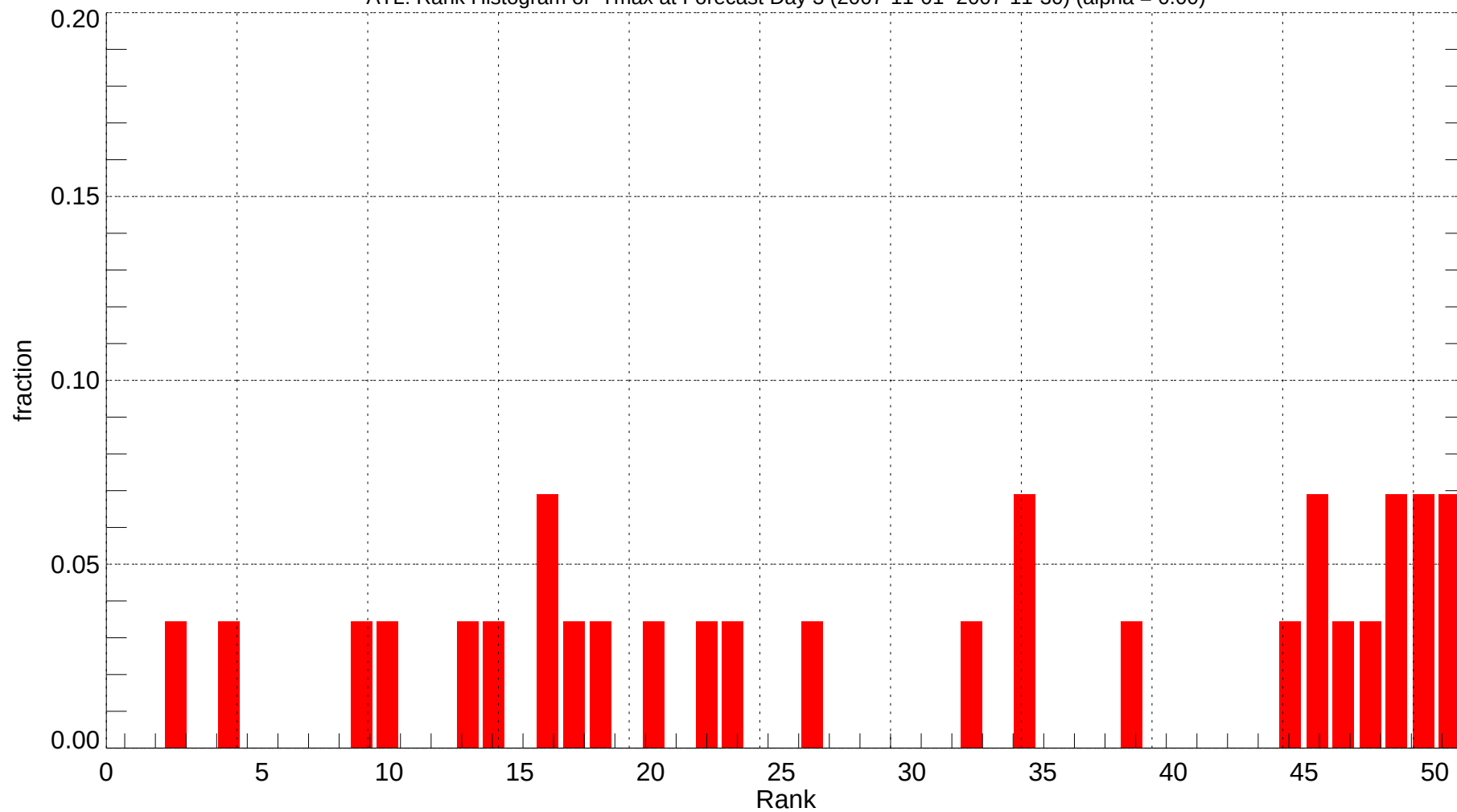
ATL: Rank Histogram of Tmax at Forecast Day 3 (2007-11-01~2007-11-30) (alpha = 0.00)
