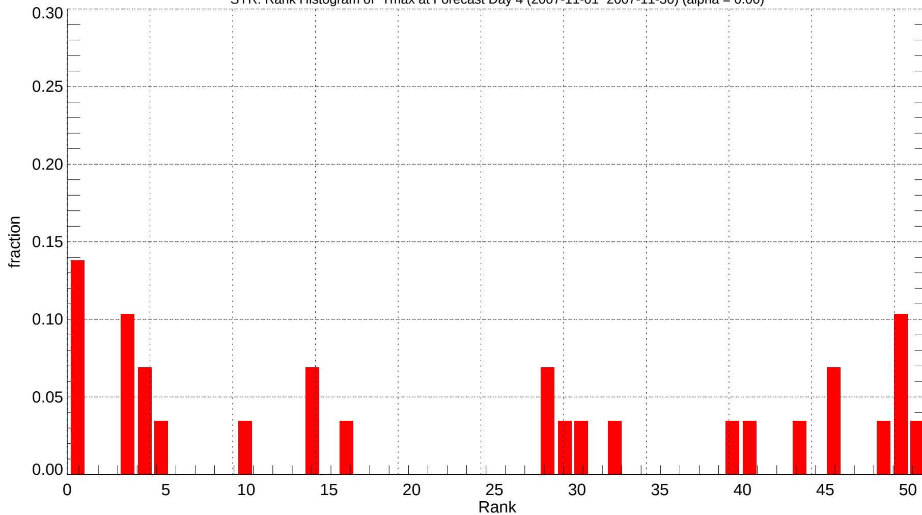
SYR: Rank Histogram of Tmax at Forecast Day 4 (2007-11-01~2007-11-30) (alpha = 0.00)
