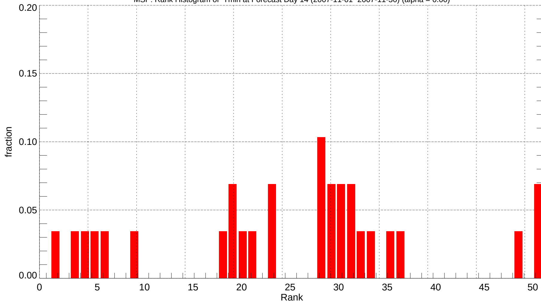
MSP: Rank Histogram of Tmin at Forecast Day 14 (2007-11-01~2007-11-30) (alpha = 0.00)
