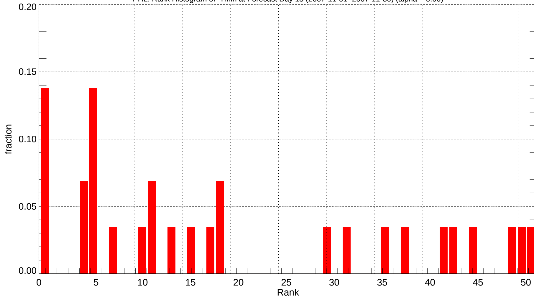
PHL: Rank Histogram of Tmin at Forecast Day 15 (2007-11-01~2007-11-30) (alpha = 0.00)
