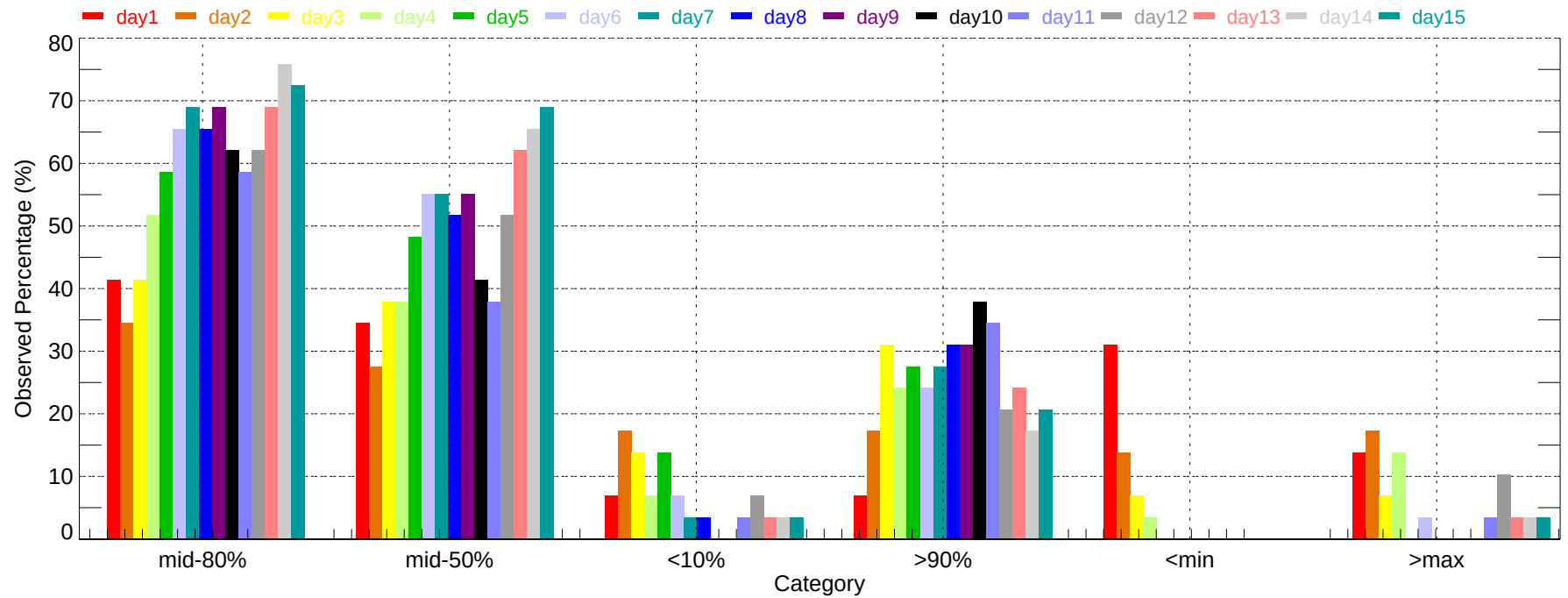
Observed Percentage of Ensembles - MOB: Max Temperature (2007-11-01~2007-11-30)
