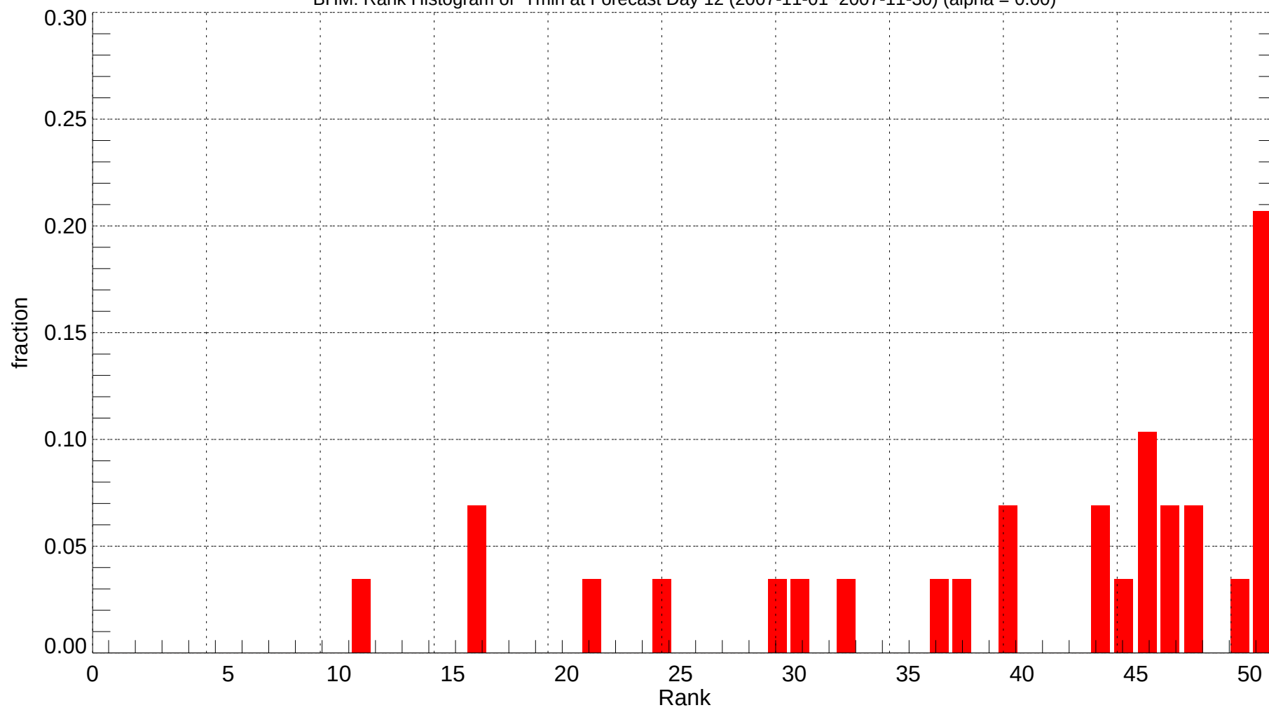
BHM: Rank Histogram of Tmin at Forecast Day 12 (2007-11-01~2007-11-30) (alpha = 0.00)
