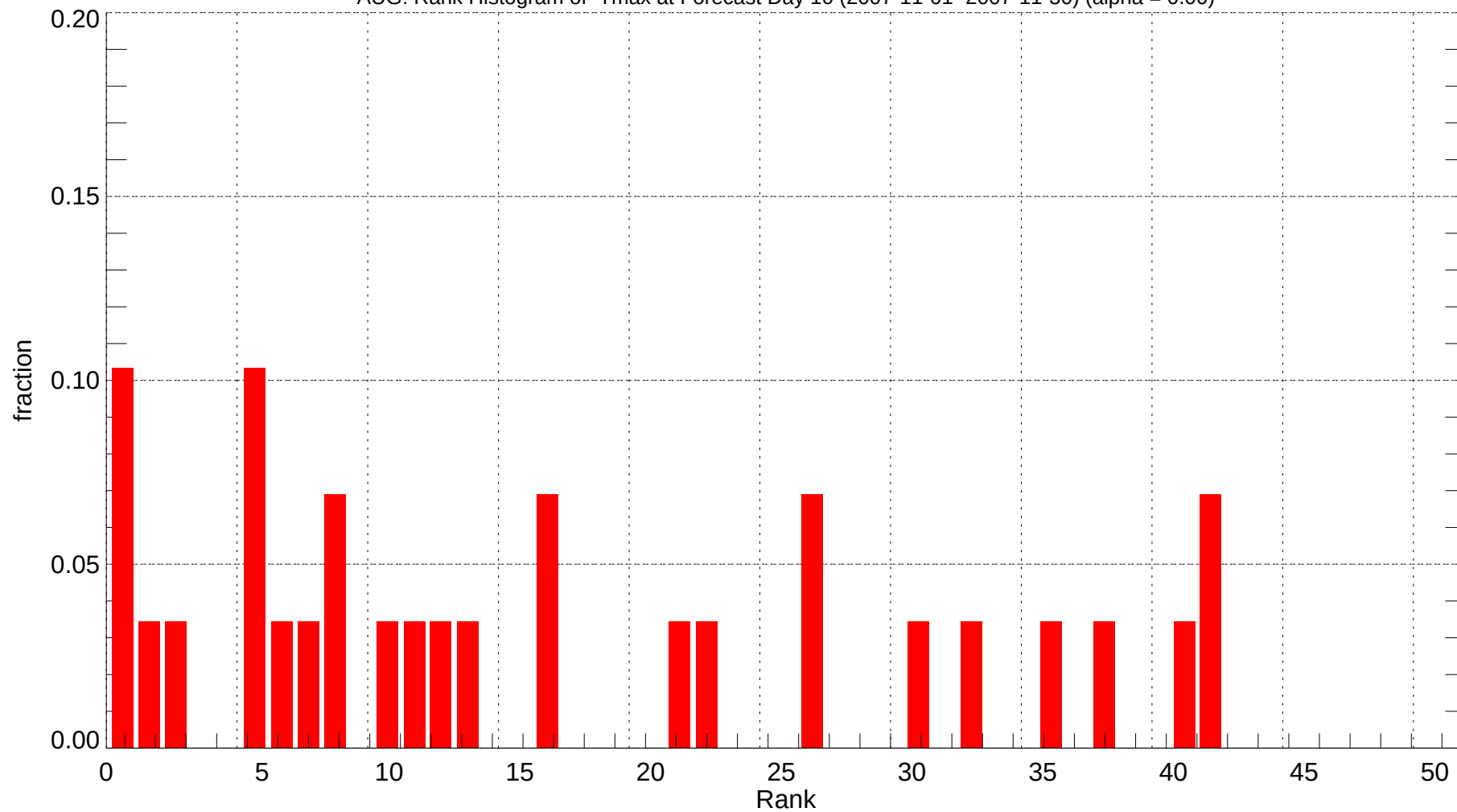
AUG: Rank Histogram of Tmax at Forecast Day 10 (2007-11-01~2007-11-30) (alpha = 0.00)
