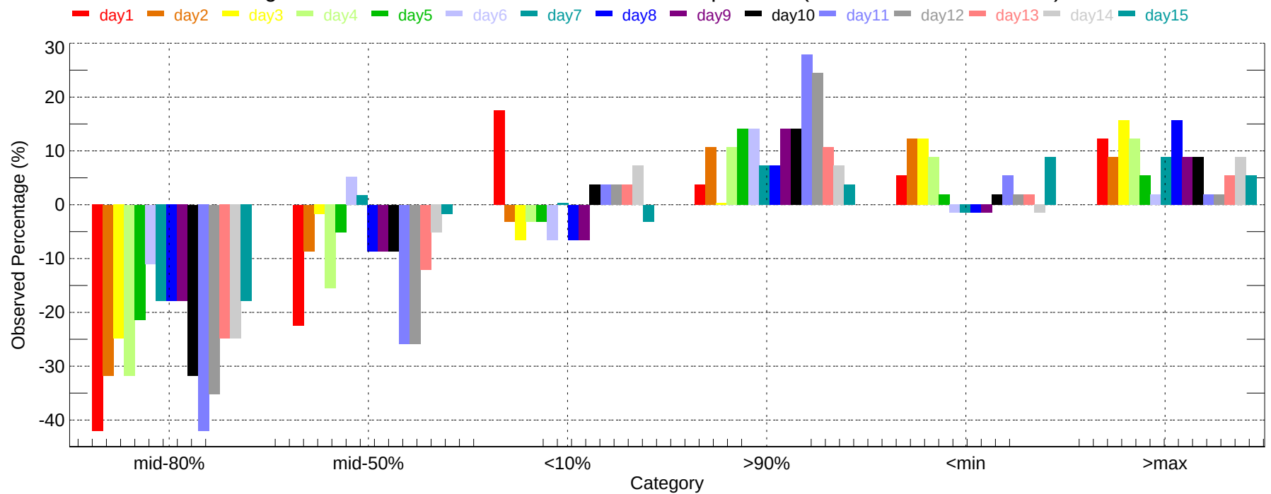
Observed Percentage Deviation of Ensembles - HOU: Max Temperature (2007-11-01~2007-11-30)
