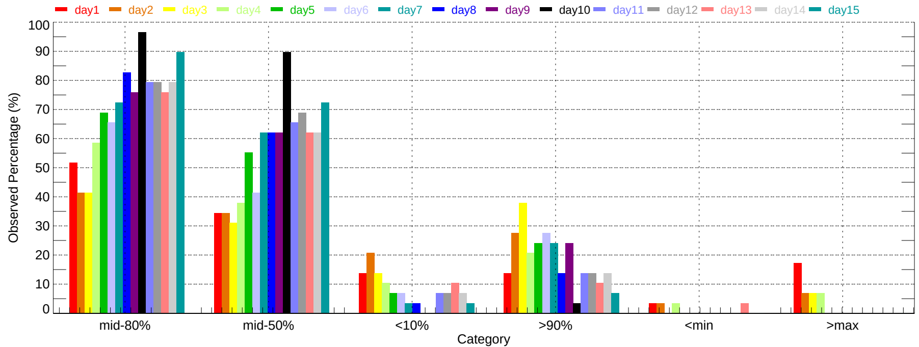
Observed Percentage of Ensembles - TLH: Min Temperature (2007-11-01~2007-11-30)
