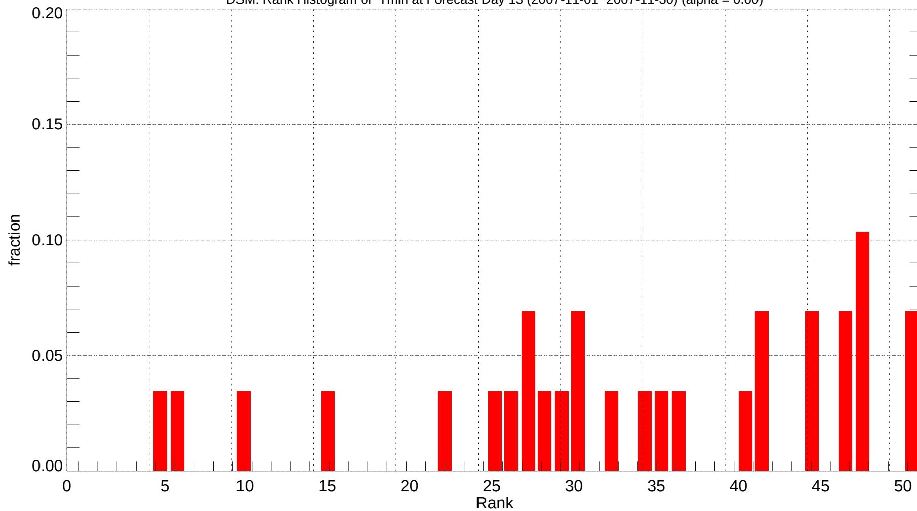
DSM: Rank Histogram of Tmin at Forecast Day 13 (2007-11-01~2007-11-30) (alpha = 0.00)
