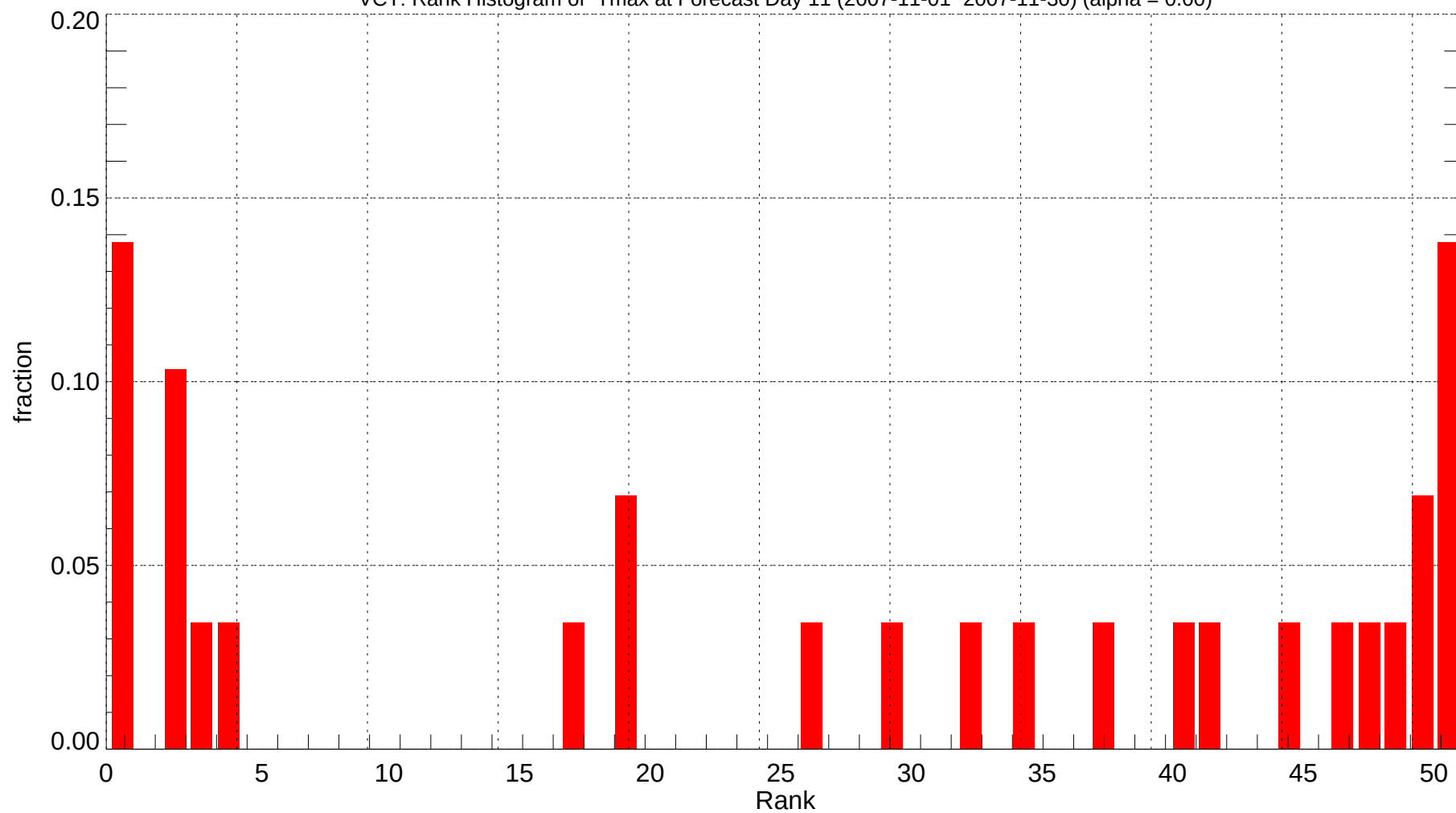
VCT: Rank Histogram of Tmax at Forecast Day 11 (2007-11-01~2007-11-30) (alpha = 0.00)
