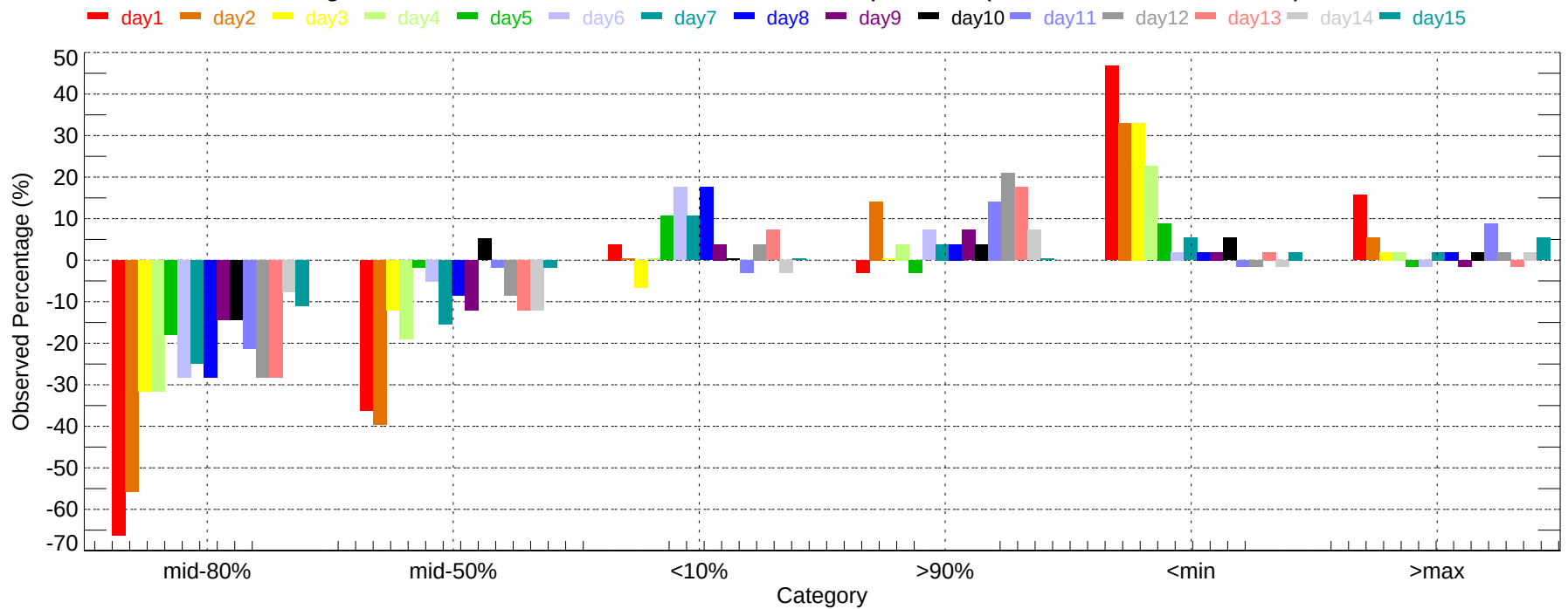
Observed Percentage Deviation of Ensembles - DTW: Min Temperature (2007-11-01~2007-11-30)
