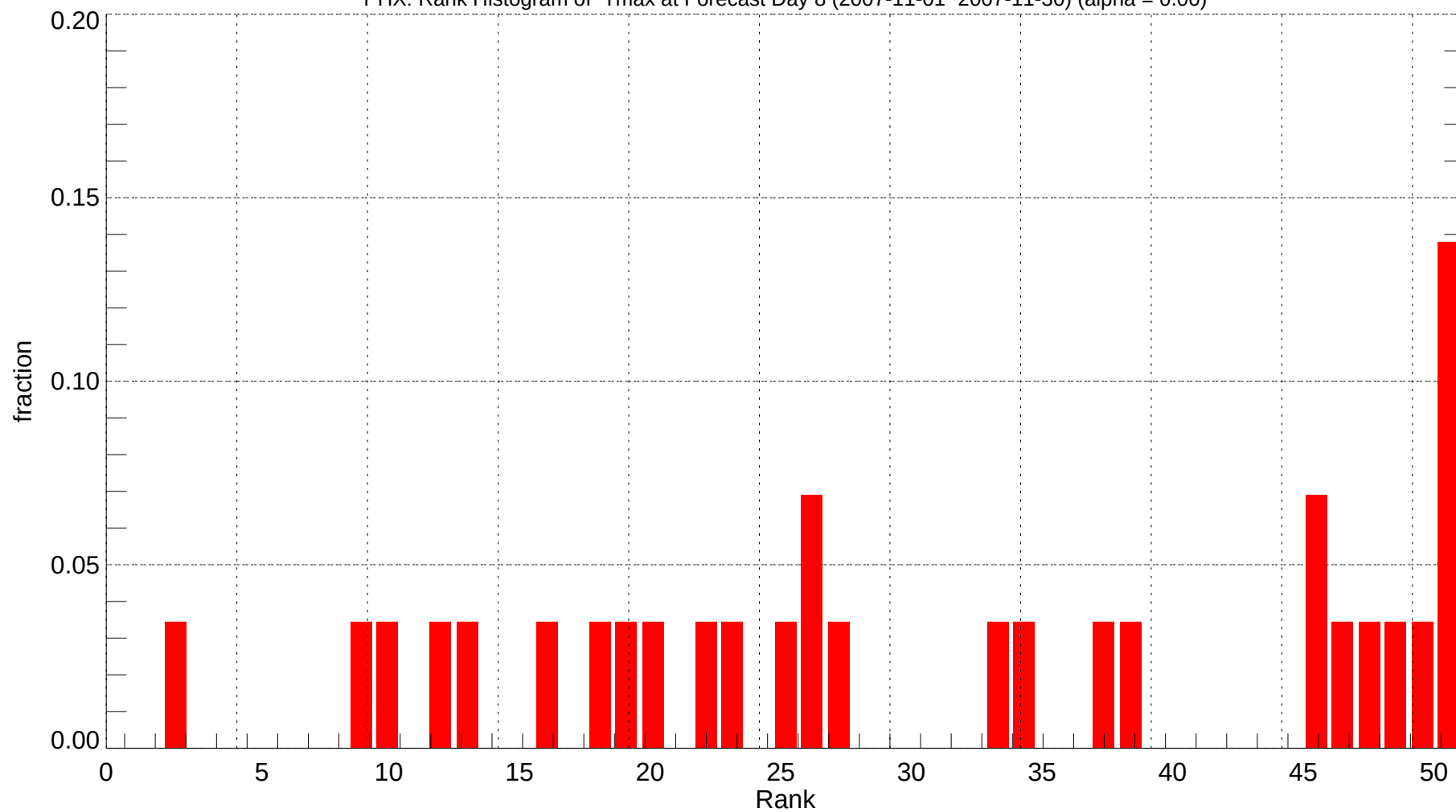
PHX: Rank Histogram of Tmax at Forecast Day 8 (2007-11-01~2007-11-30) (alpha = 0.00)
