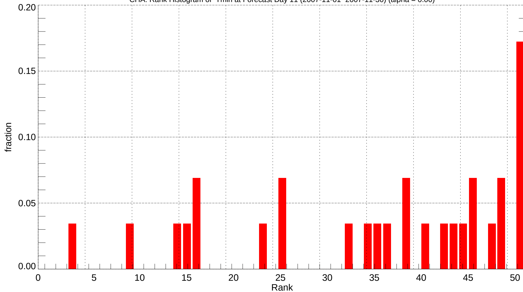
CHA: Rank Histogram of Tmin at Forecast Day 11 (2007-11-01~2007-11-30) (alpha = 0.00)
