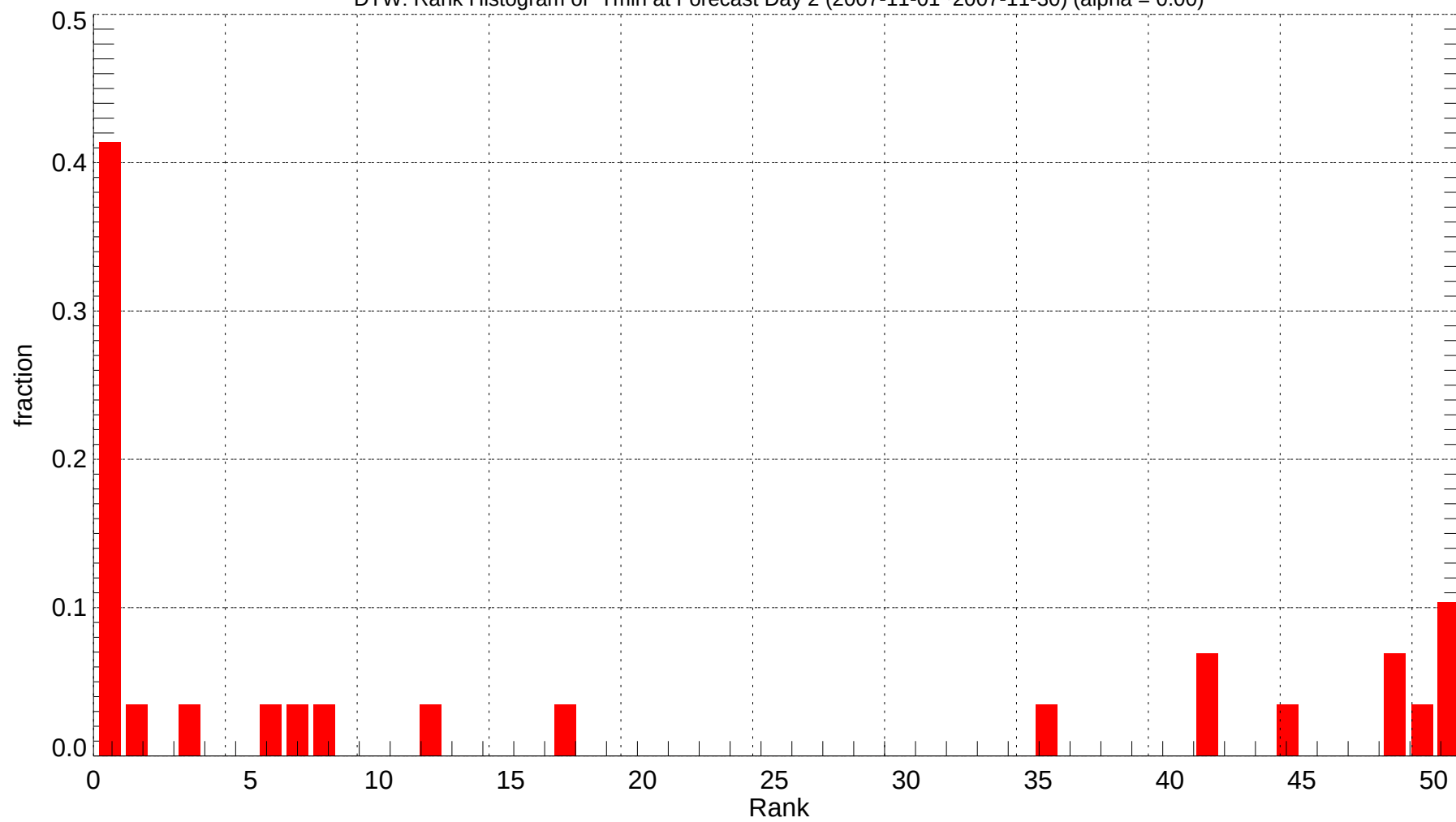
DTW: Rank Histogram of Tmin at Forecast Day 2 (2007-11-01~2007-11-30) (alpha = 0.00)
