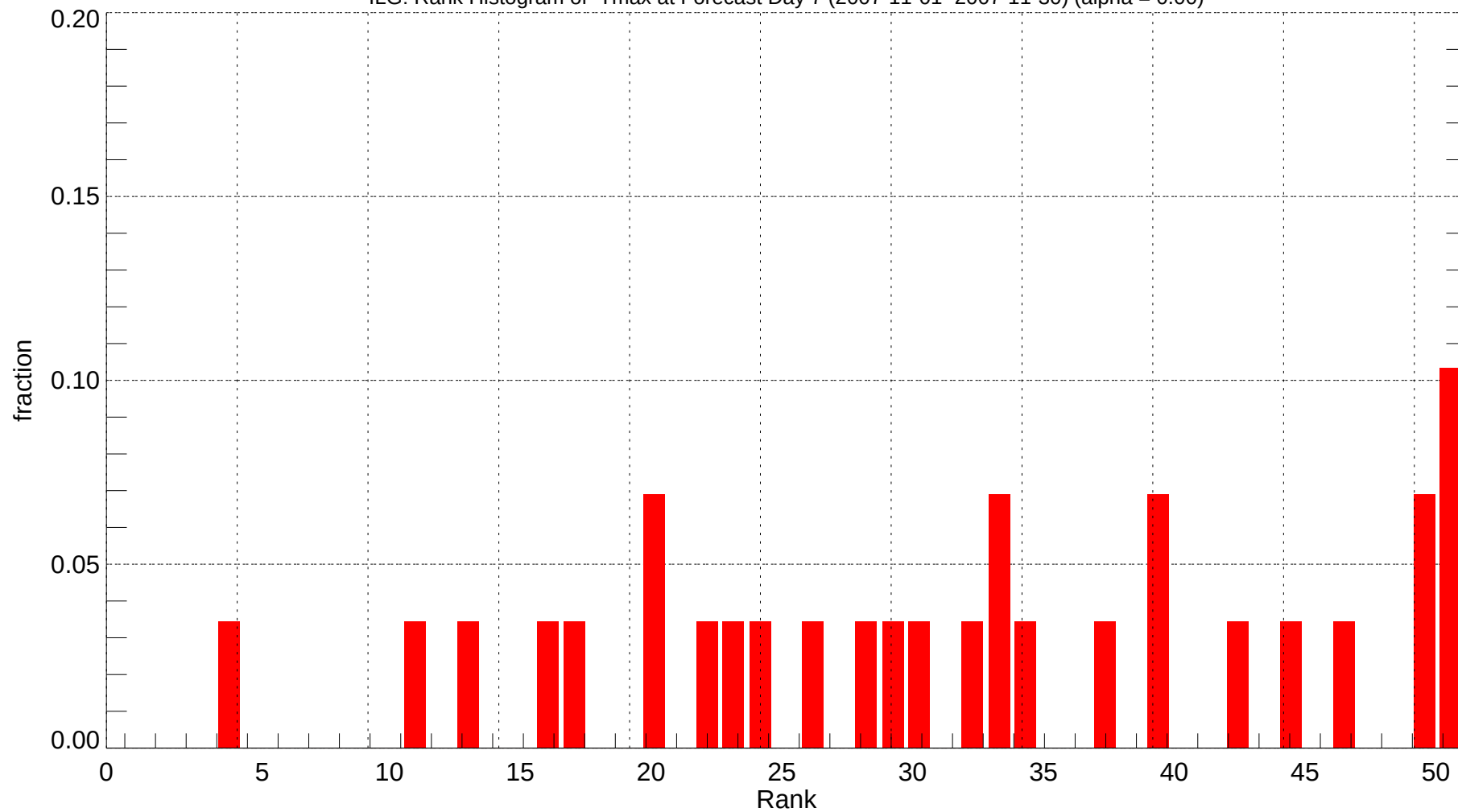
ILG: Rank Histogram of Tmax at Forecast Day 7 (2007-11-01~2007-11-30) (alpha = 0.00)
