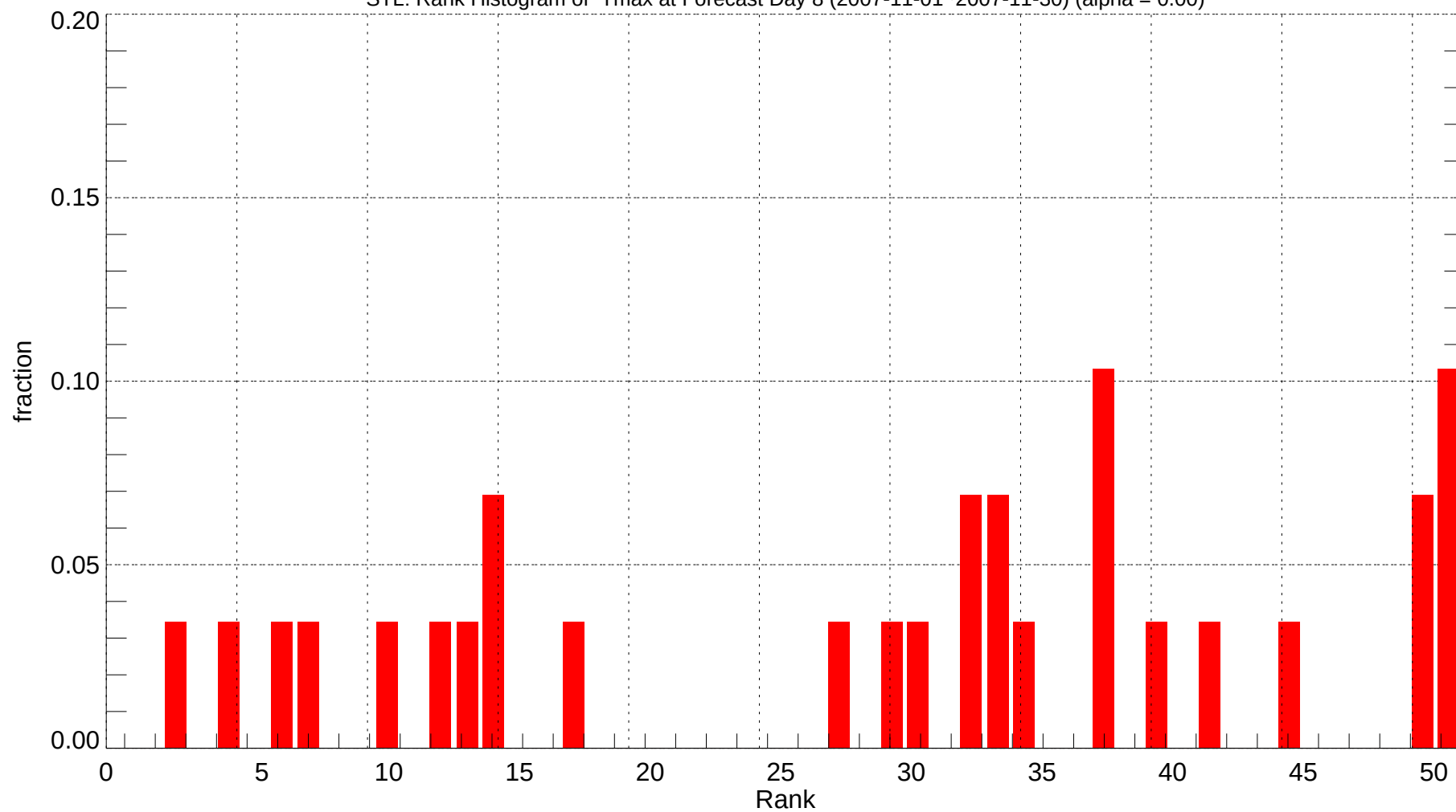
STL: Rank Histogram of Tmax at Forecast Day 8 (2007-11-01~2007-11-30) (alpha = 0.00)
