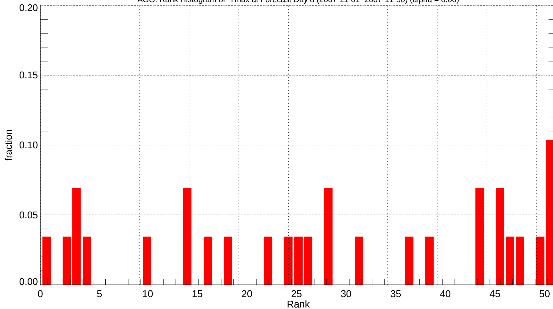
AOO: Rank Histogram of Tmax at Forecast Day 8 (2007-11-01~2007-11-30) (alpha = 0.00)
