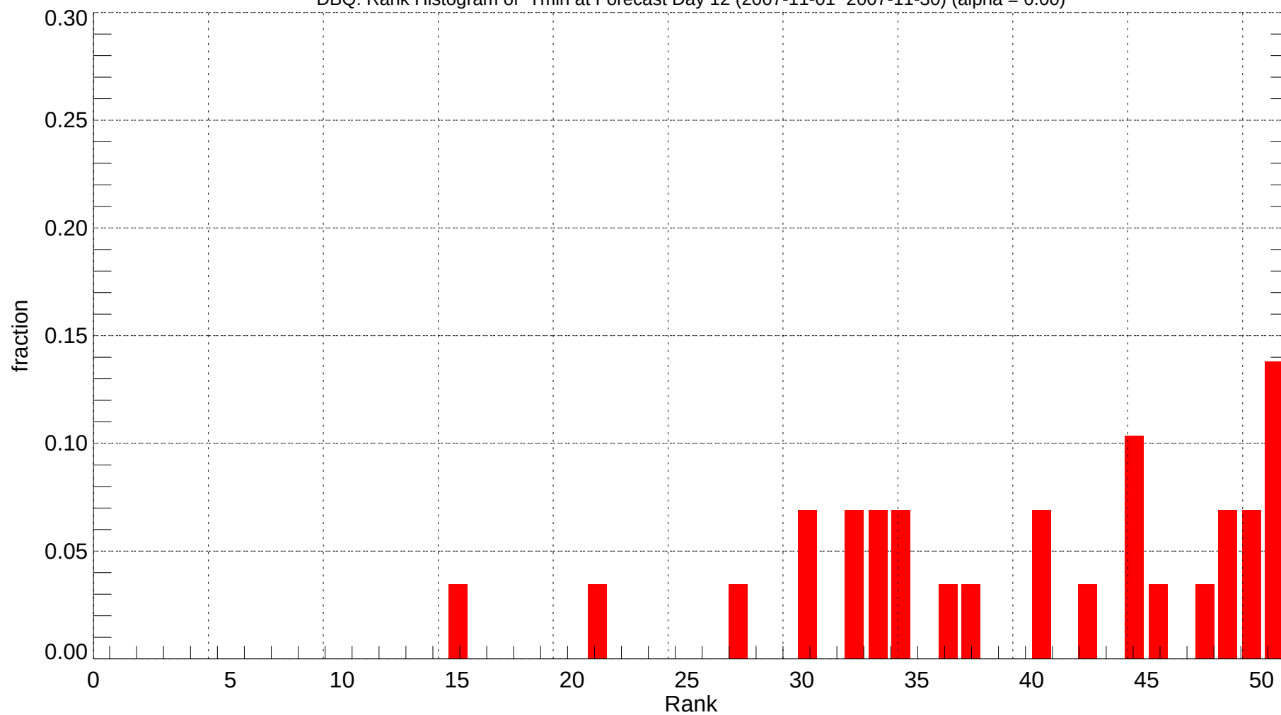
DBQ: Rank Histogram of Tmin at Forecast Day 12 (2007-11-01~2007-11-30) (alpha = 0.00)
