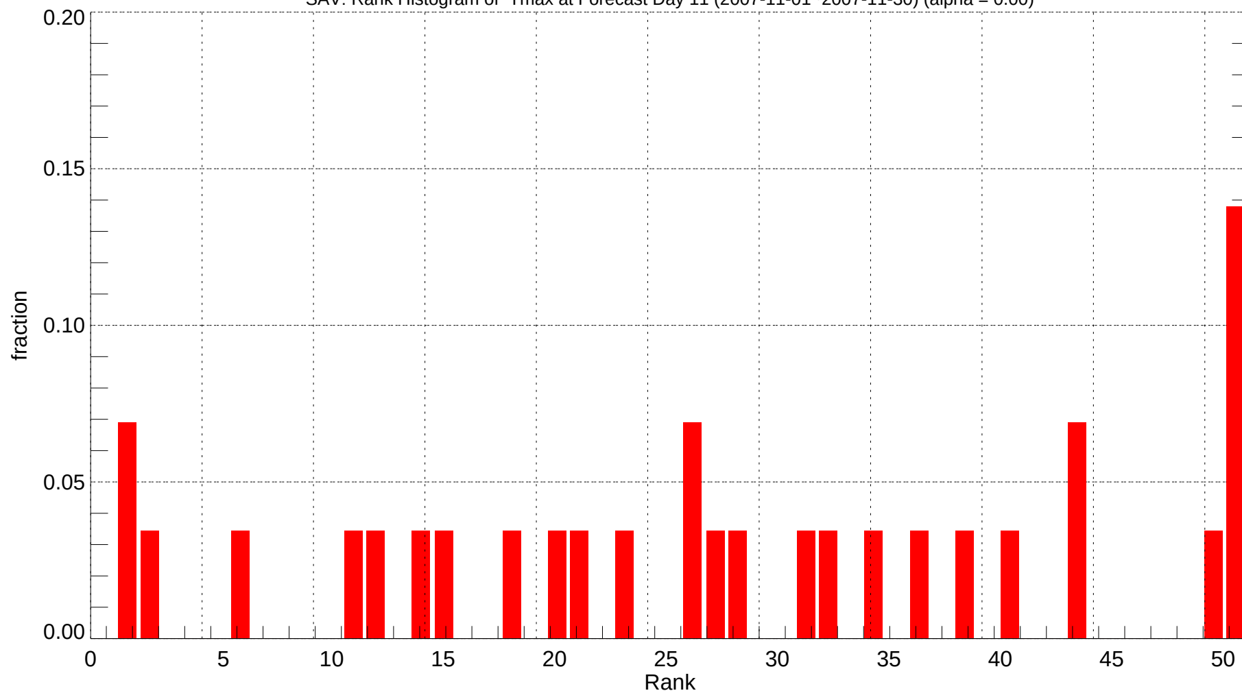
SAV: Rank Histogram of Tmax at Forecast Day 11 (2007-11-01~2007-11-30) (alpha = 0.00)
