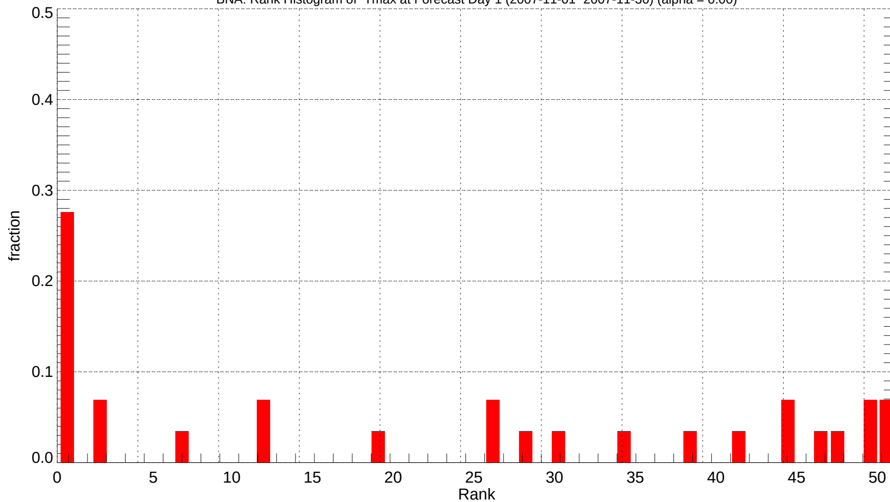
BNA: Rank Histogram of Tmax at Forecast Day 1 (2007-11-01~2007-11-30) (alpha = 0.00)
