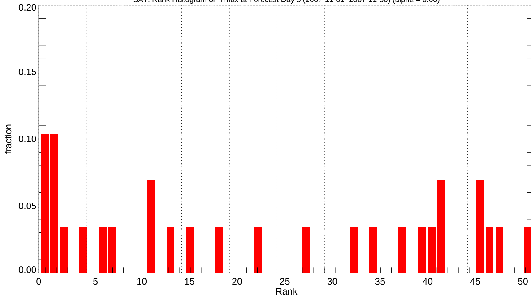
SAT: Rank Histogram of Tmax at Forecast Day 5 (2007-11-01~2007-11-30) (alpha = 0.00)
