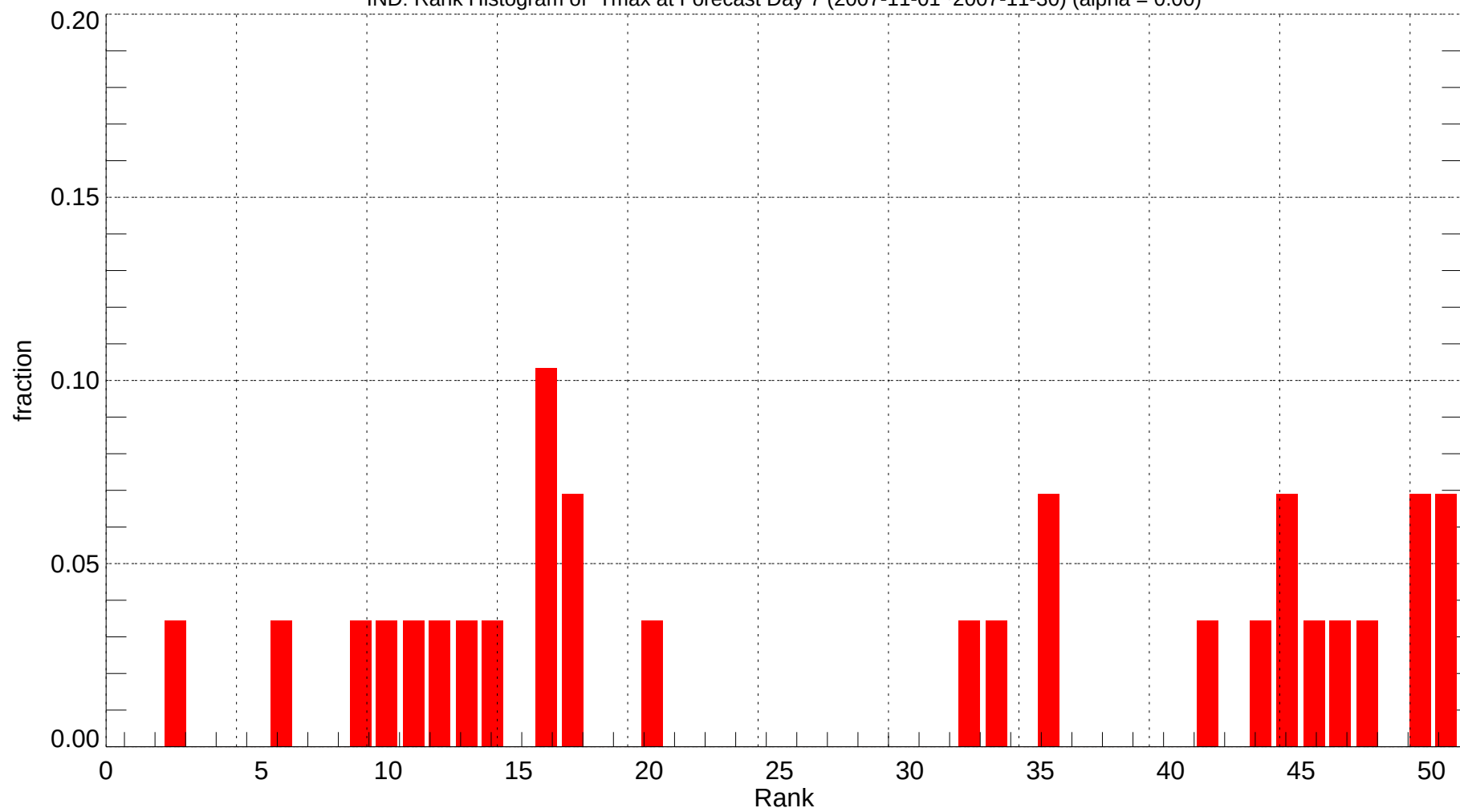
IND: Rank Histogram of Tmax at Forecast Day 7 (2007-11-01~2007-11-30) (alpha = 0.00)
