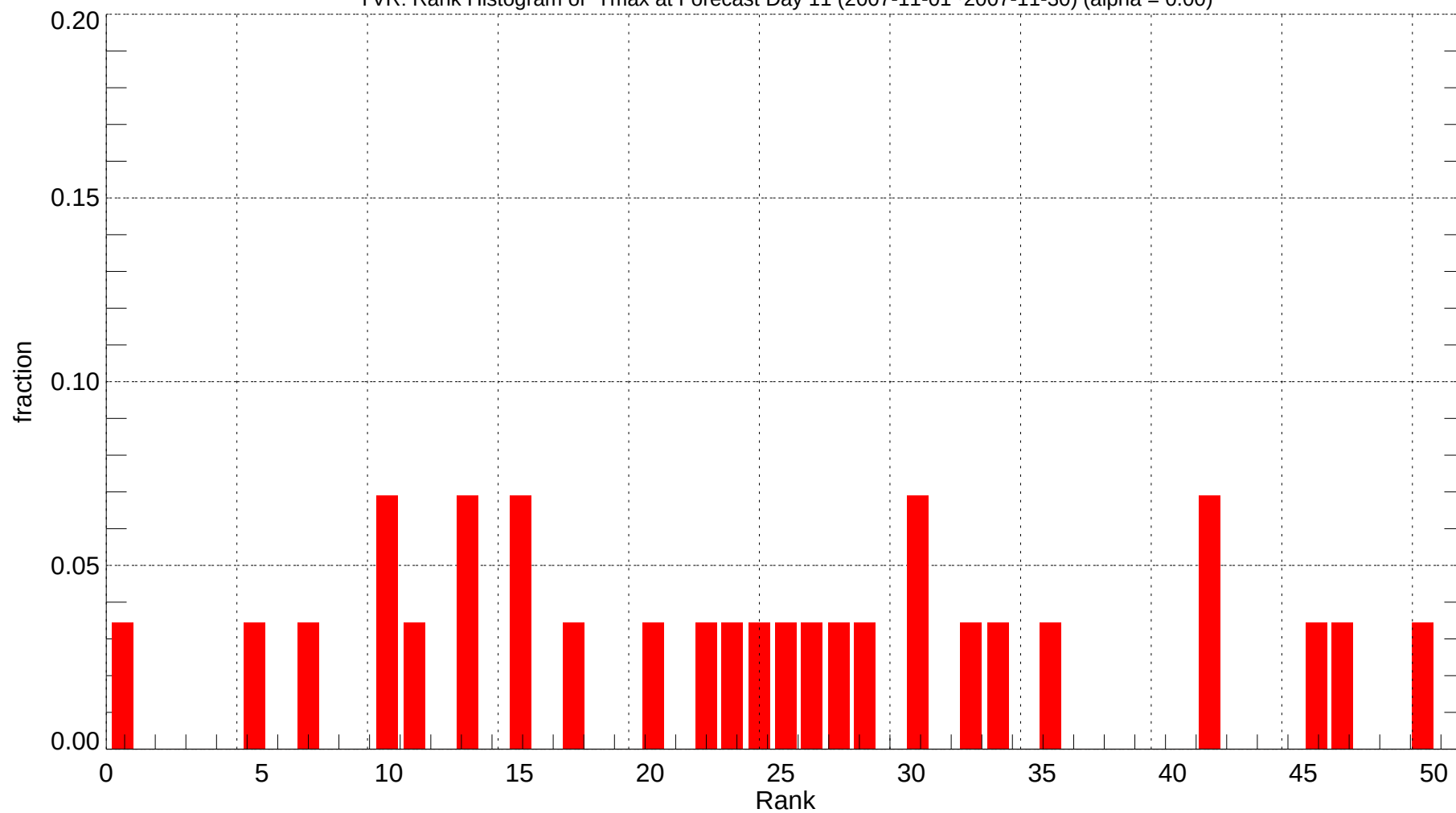
YVR: Rank Histogram of Tmax at Forecast Day 11 (2007-11-01~2007-11-30) (alpha = 0.00)
