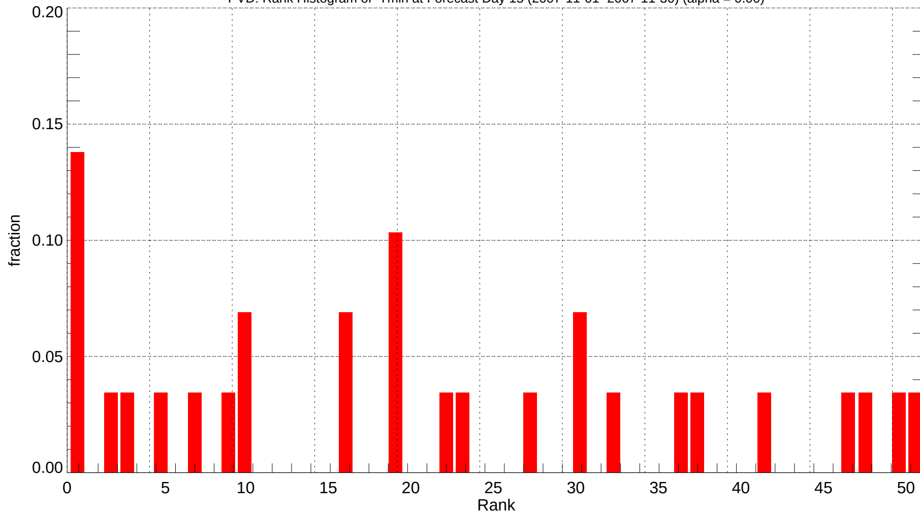
PVD: Rank Histogram of Tmin at Forecast Day 15 (2007-11-01~2007-11-30) (alpha = 0.00)
