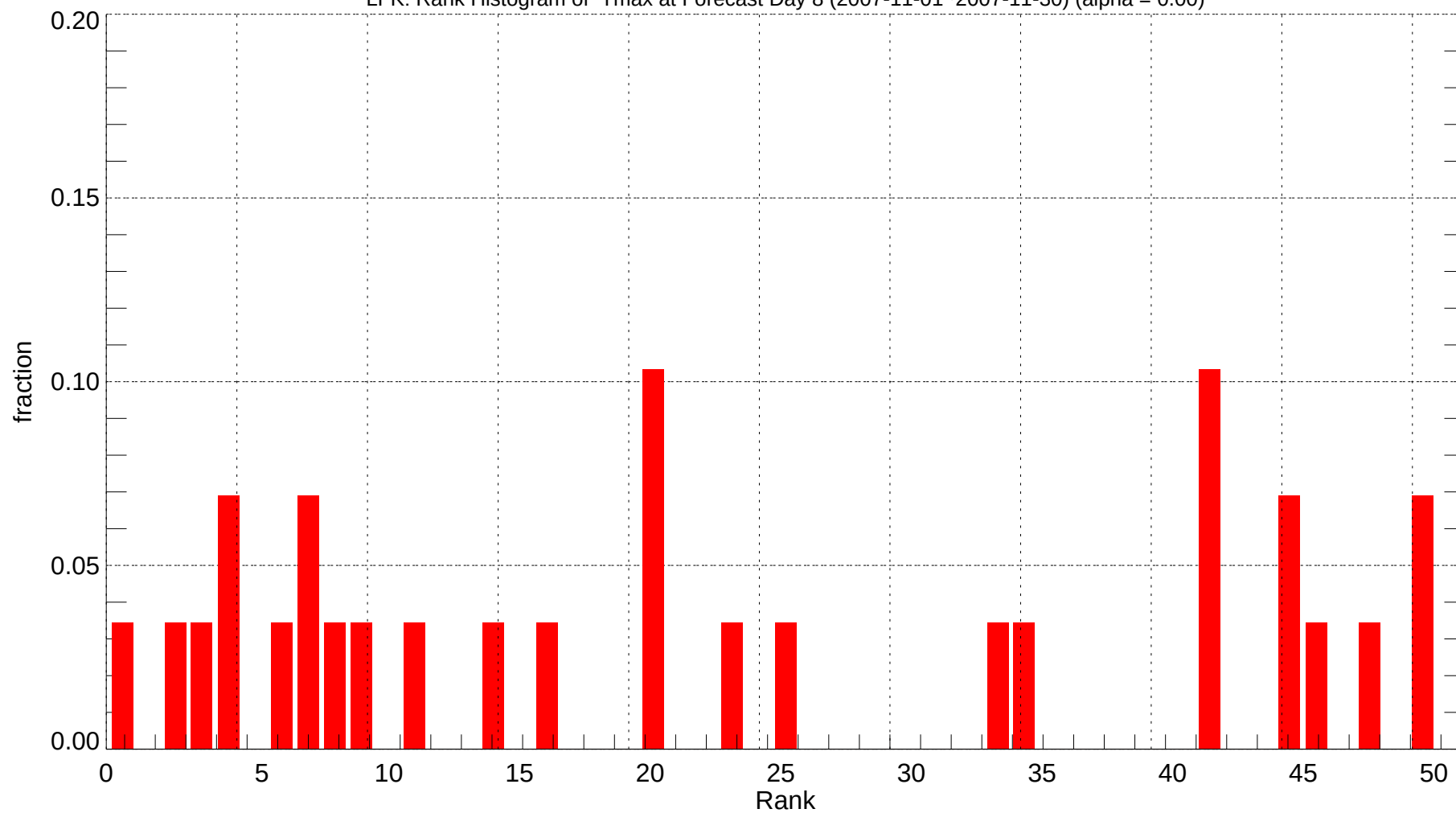
LFK: Rank Histogram of Tmax at Forecast Day 8 (2007-11-01~2007-11-30) (alpha = 0.00)
