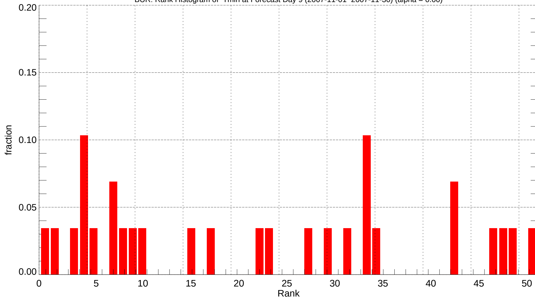
BUR: Rank Histogram of Tmin at Forecast Day 9 (2007-11-01~2007-11-30) (alpha = 0.00)
