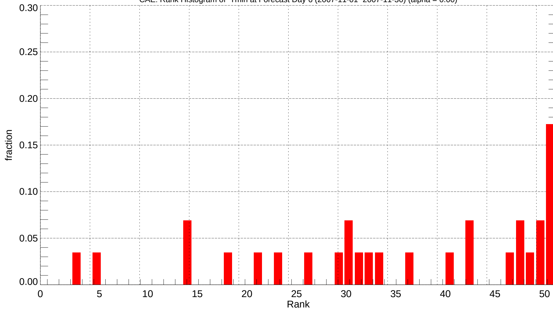
CAE: Rank Histogram of Tmin at Forecast Day 6 (2007-11-01~2007-11-30) (alpha = 0.00)
