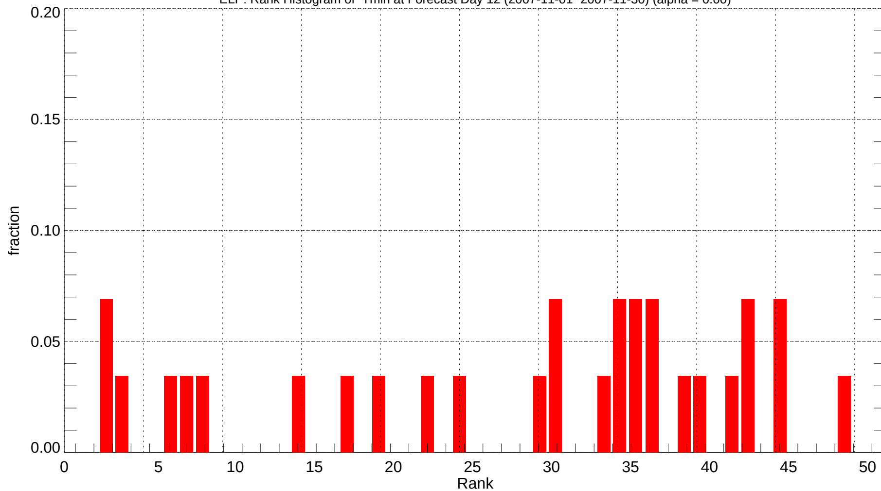
ELP: Rank Histogram of Tmin at Forecast Day 12 (2007-11-01~2007-11-30) (alpha = 0.00)
