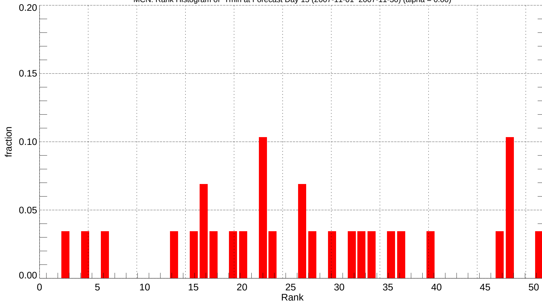
MCN: Rank Histogram of Tmin at Forecast Day 15 (2007-11-01~2007-11-30) (alpha = 0.00)
