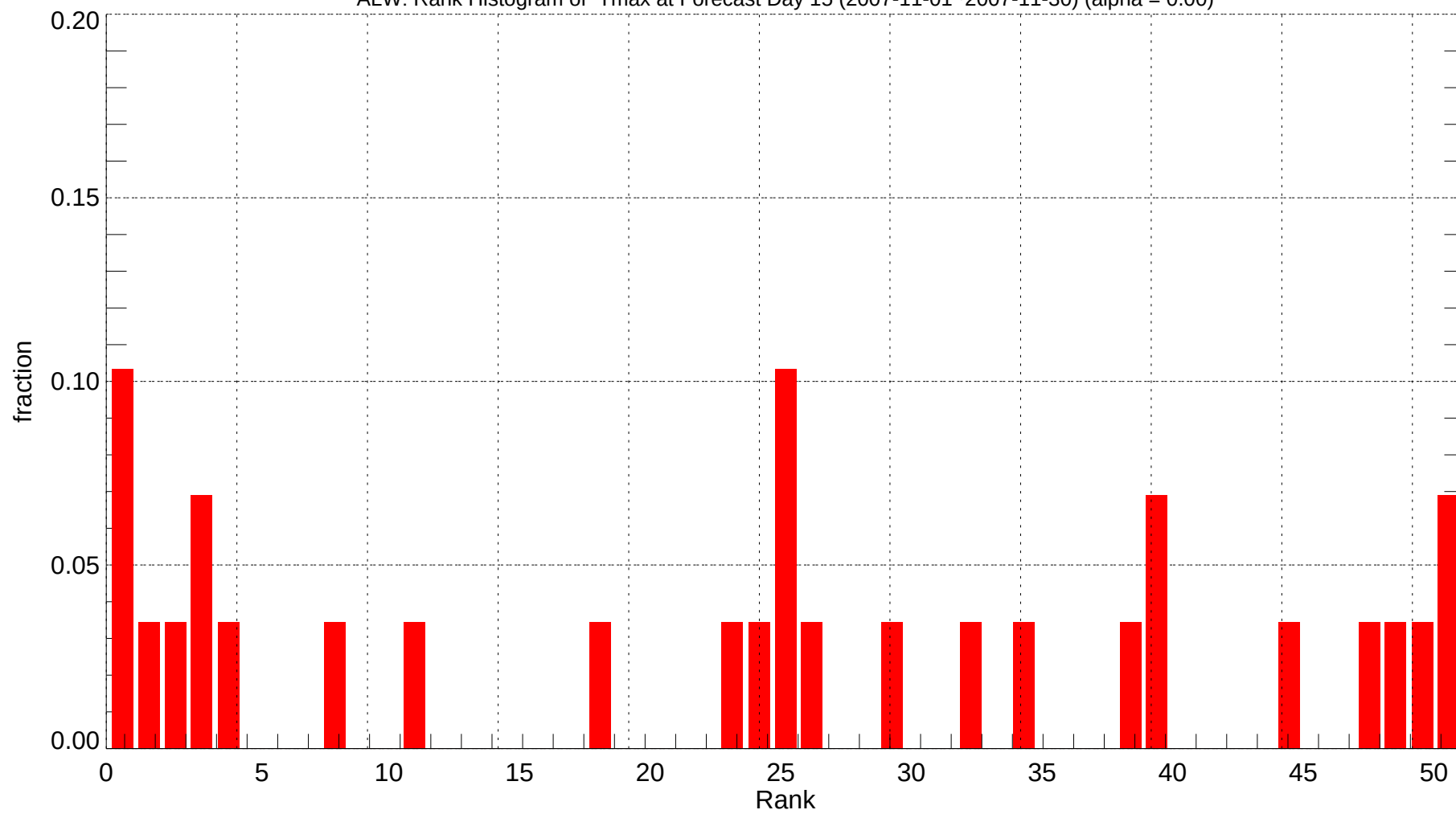
ALW: Rank Histogram of Tmax at Forecast Day 15 (2007-11-01~2007-11-30) (alpha = 0.00)
