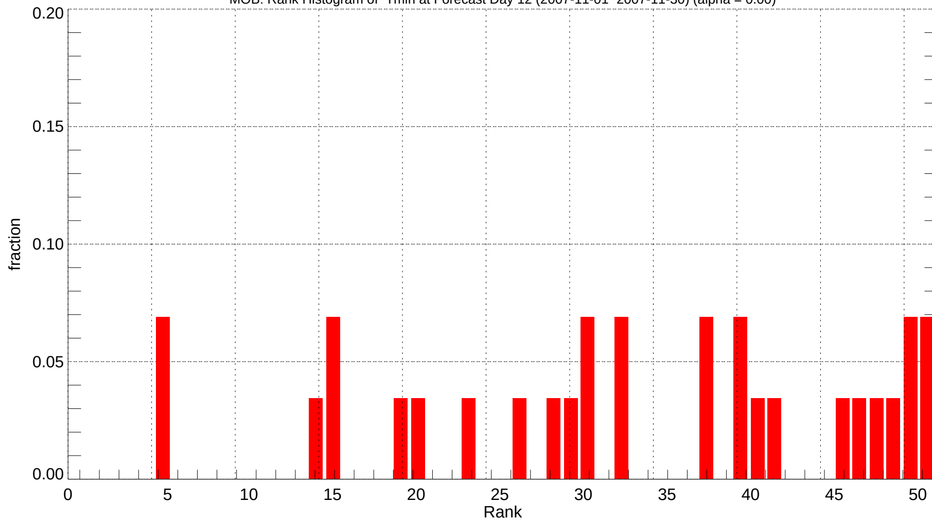
MOB: Rank Histogram of Tmin at Forecast Day 12 (2007-11-01~2007-11-30) (alpha = 0.00)
