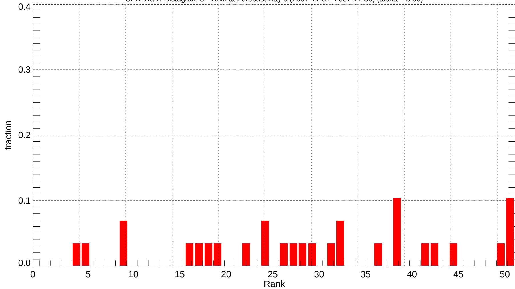
SEA: Rank Histogram of Tmin at Forecast Day 5 (2007-11-01~2007-11-30) (alpha = 0.00)
