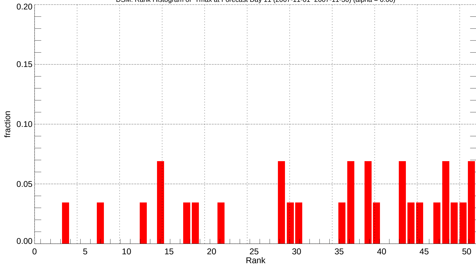
DSM: Rank Histogram of Tmax at Forecast Day 11 (2007-11-01~2007-11-30) (alpha = 0.00)
