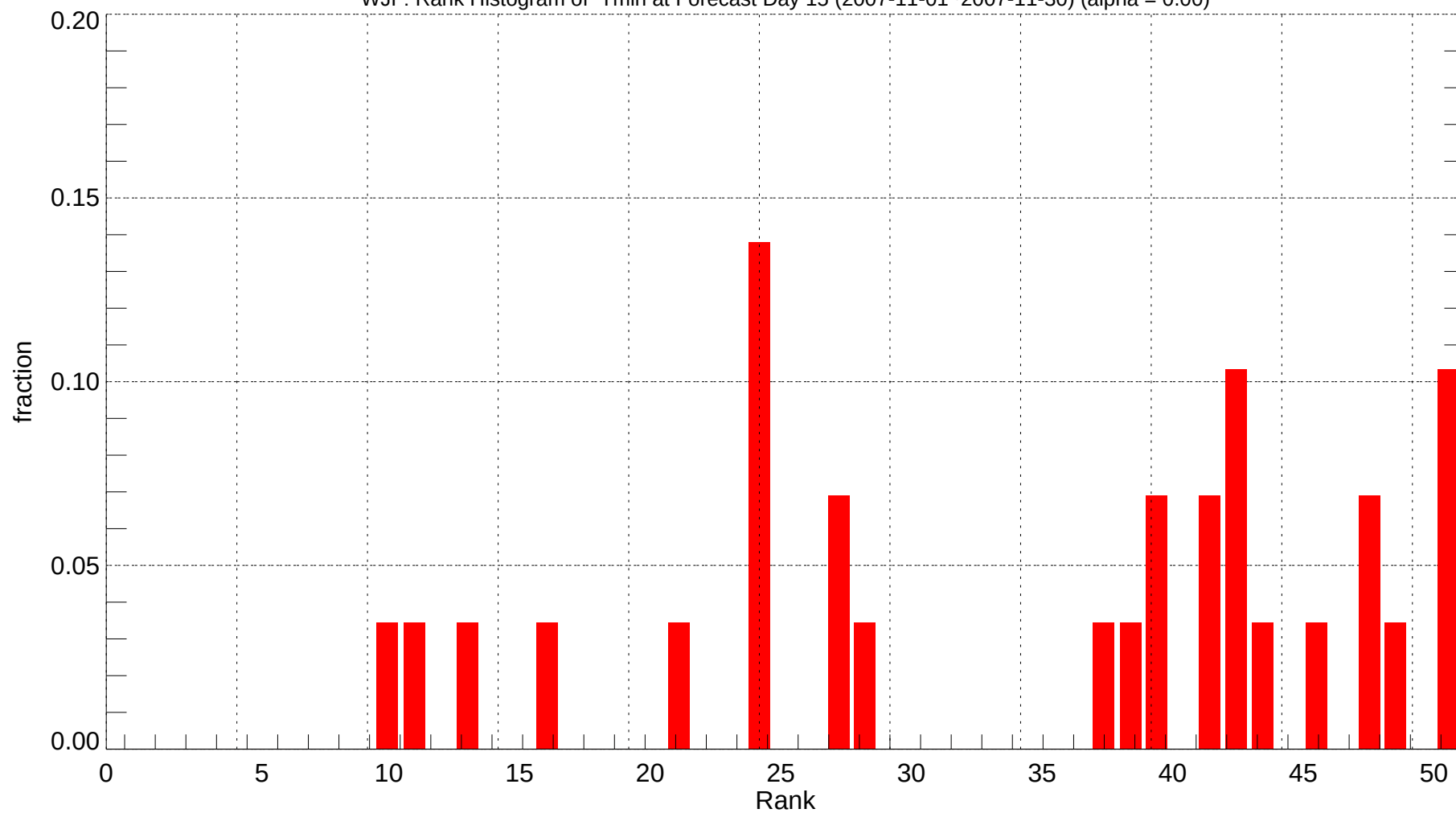
WJF: Rank Histogram of Tmin at Forecast Day 15 (2007-11-01~2007-11-30) (alpha = 0.00)
