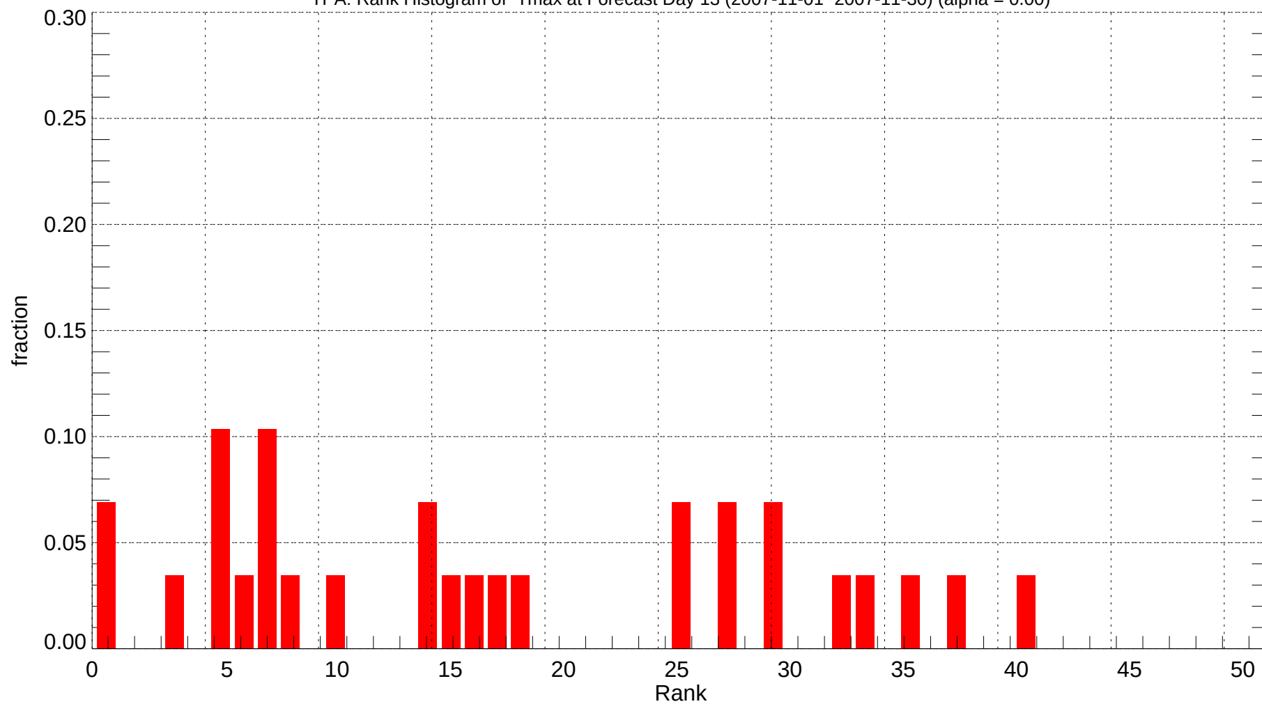
TPA: Rank Histogram of Tmax at Forecast Day 13 (2007-11-01~2007-11-30) (alpha = 0.00)
