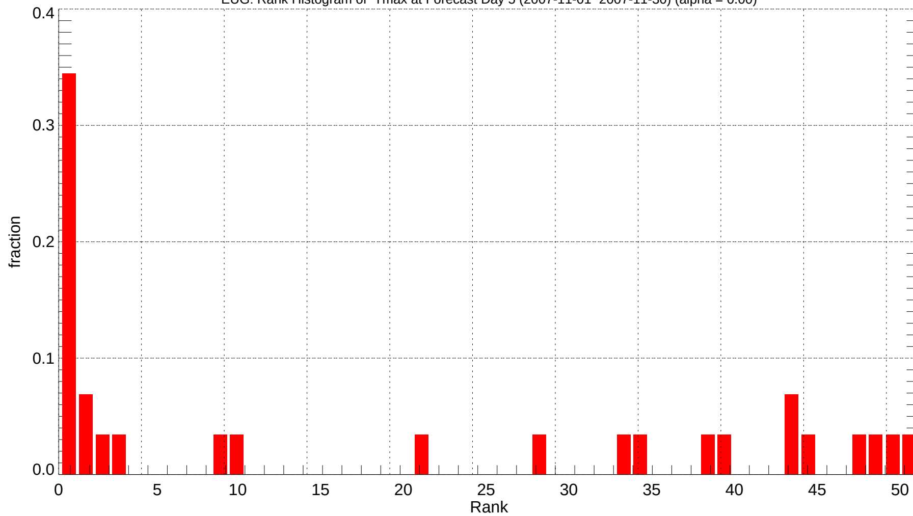
EUG: Rank Histogram of Tmax at Forecast Day 5 (2007-11-01~2007-11-30) (alpha = 0.00)
