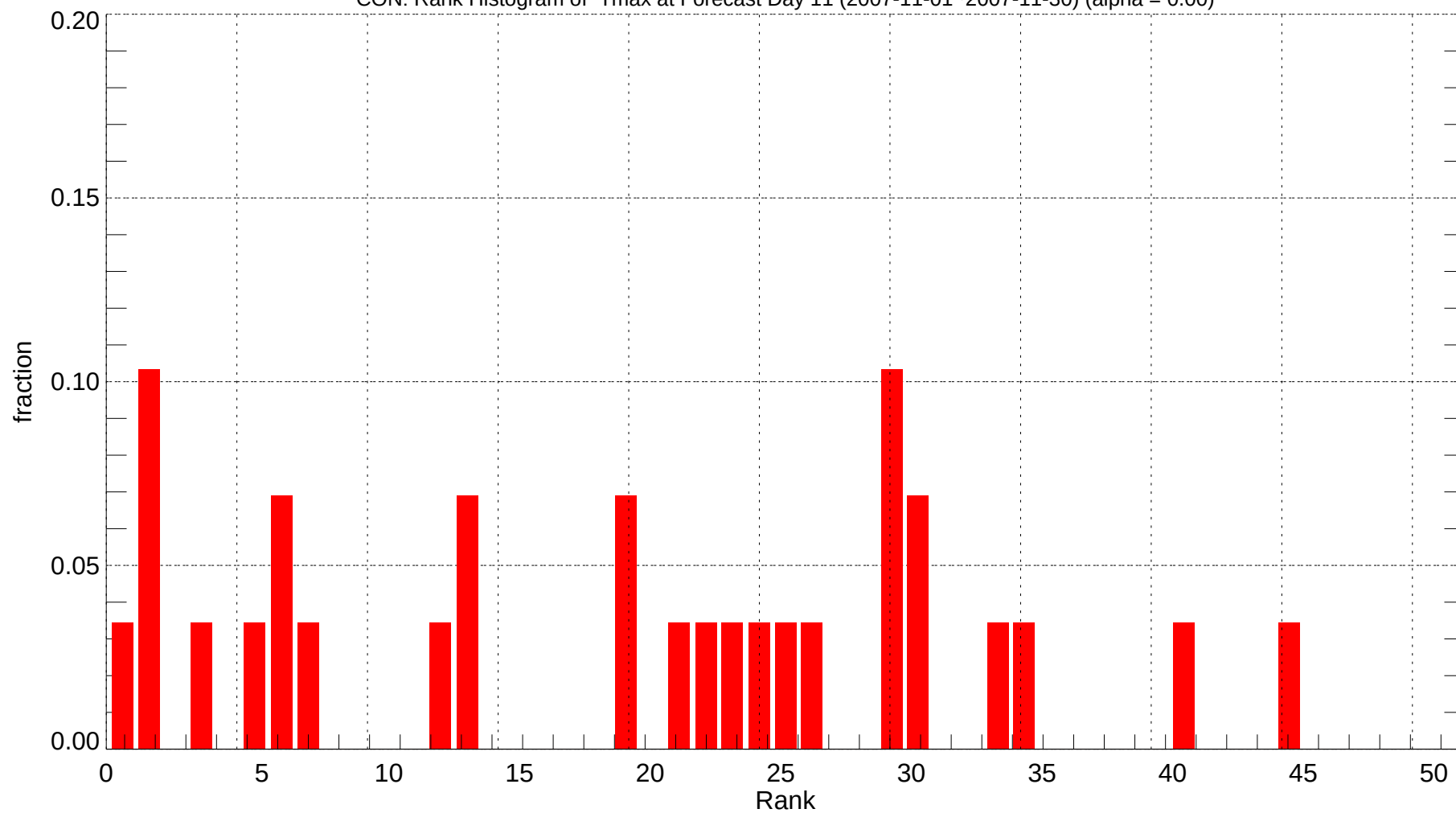
CON: Rank Histogram of Tmax at Forecast Day 11 (2007-11-01~2007-11-30) (alpha = 0.00)
