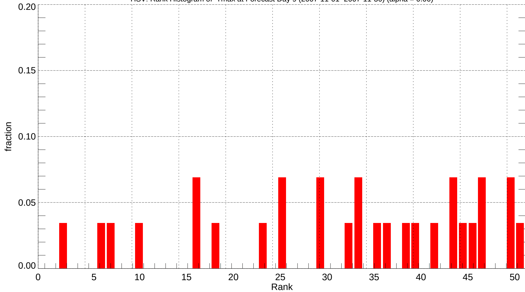
HSV: Rank Histogram of Tmax at Forecast Day 9 (2007-11-01~2007-11-30) (alpha = 0.00)
