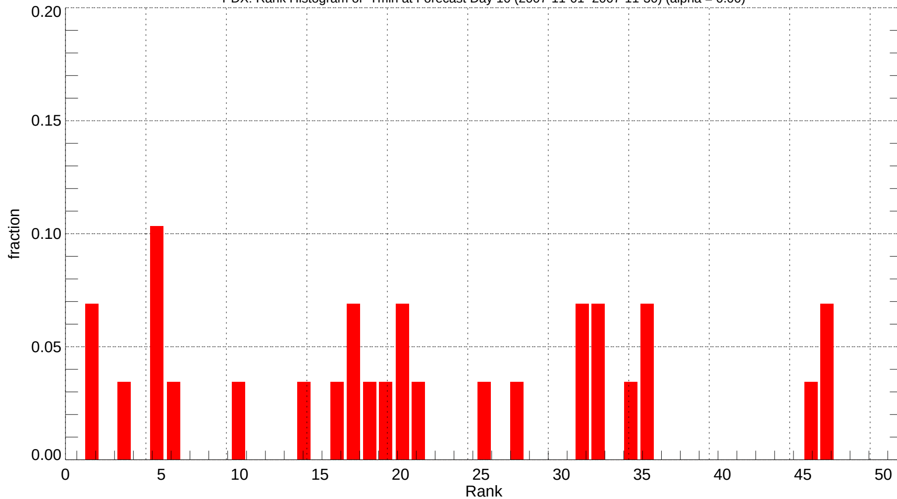
PDX: Rank Histogram of Tmin at Forecast Day 10 (2007-11-01~2007-11-30) (alpha = 0.00)
