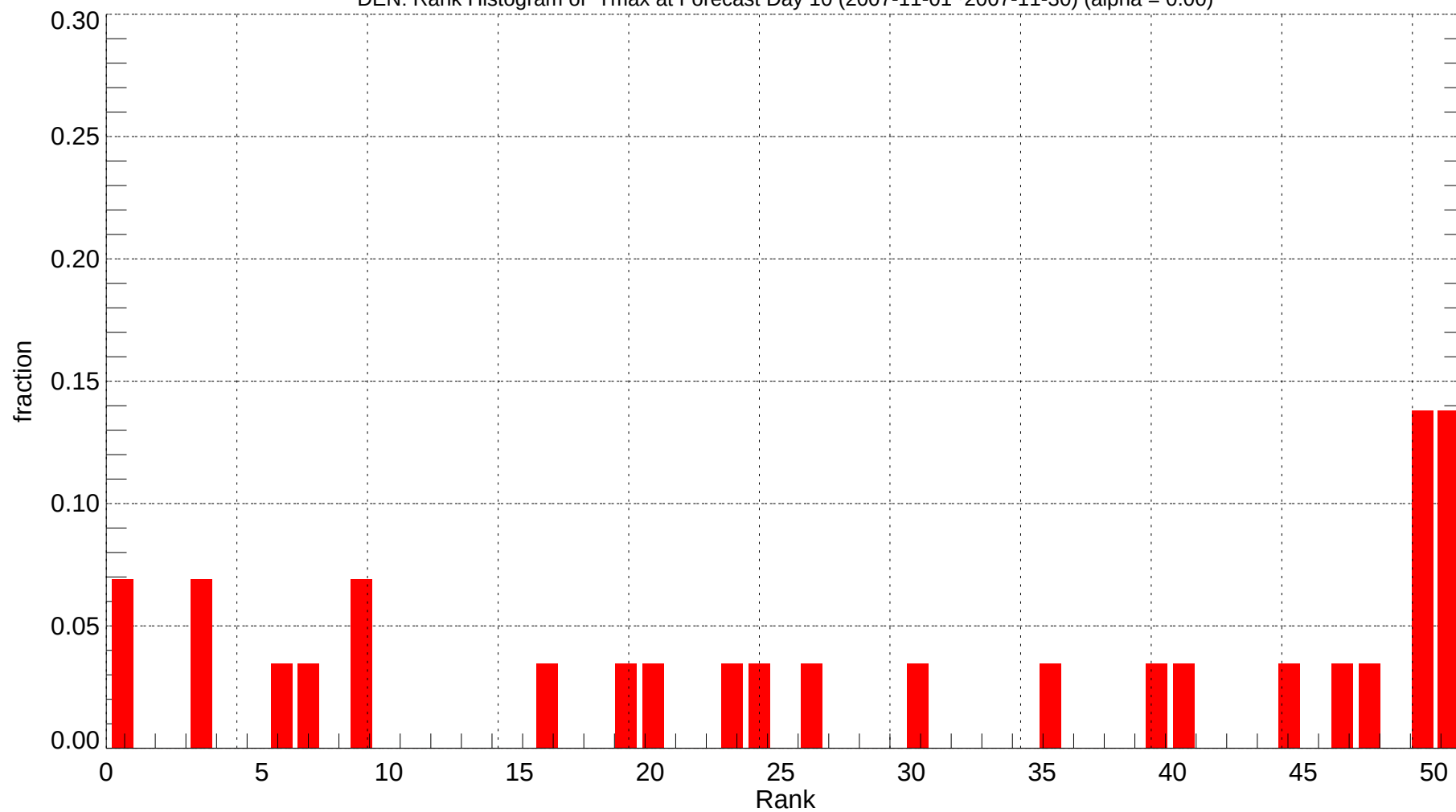
DEN: Rank Histogram of Tmax at Forecast Day 10 (2007-11-01~2007-11-30) (alpha = 0.00)
