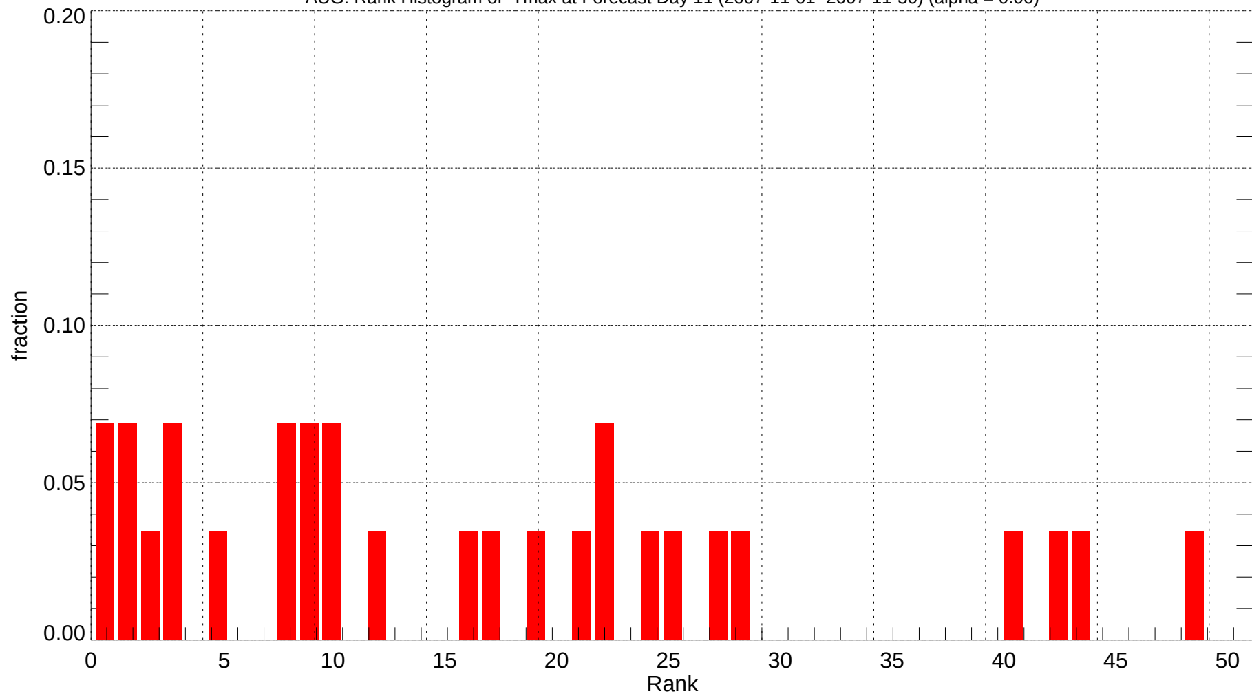
AUG: Rank Histogram of Tmax at Forecast Day 11 (2007-11-01~2007-11-30) (alpha = 0.00)
