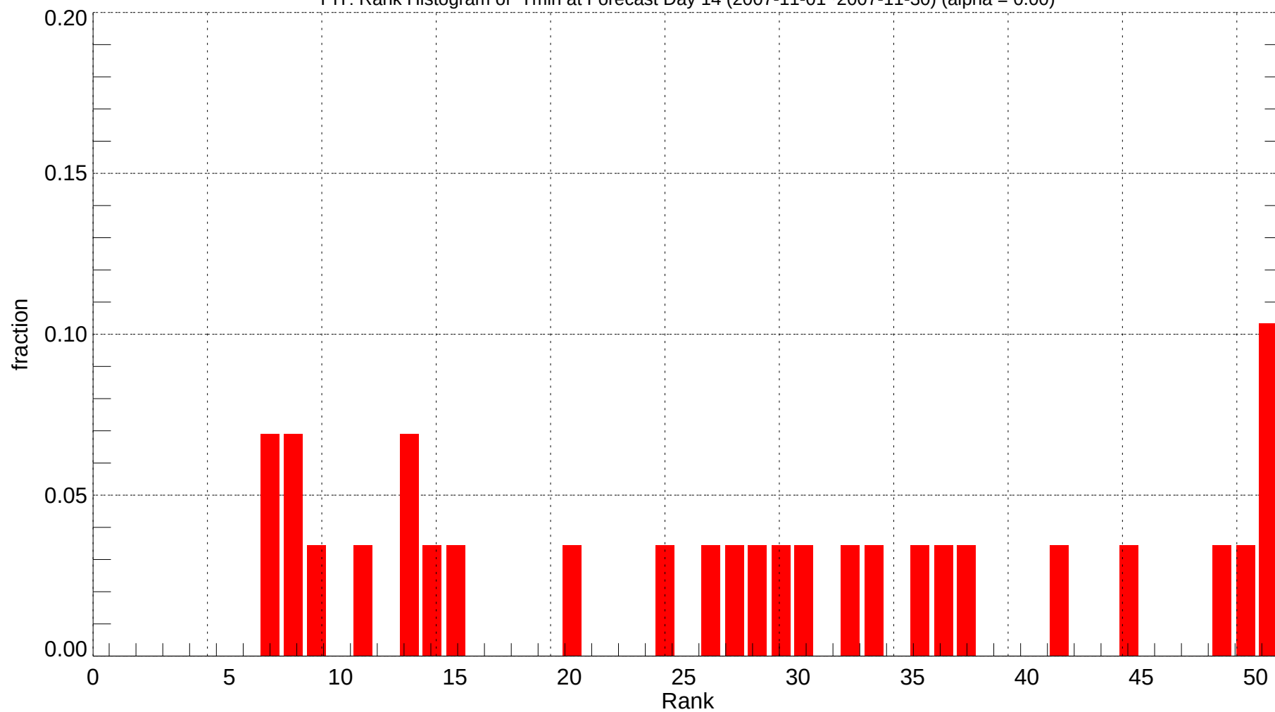
PIT: Rank Histogram of Tmin at Forecast Day 14 (2007-11-01~2007-11-30) (alpha = 0.00)
