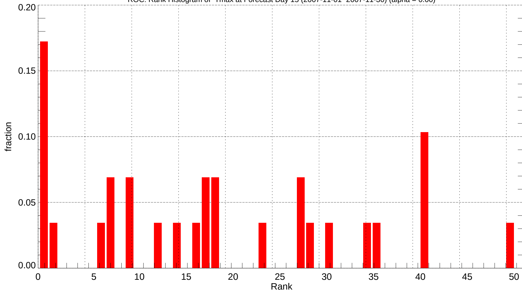
ROC: Rank Histogram of Tmax at Forecast Day 15 (2007-11-01~2007-11-30) (alpha = 0.00)
