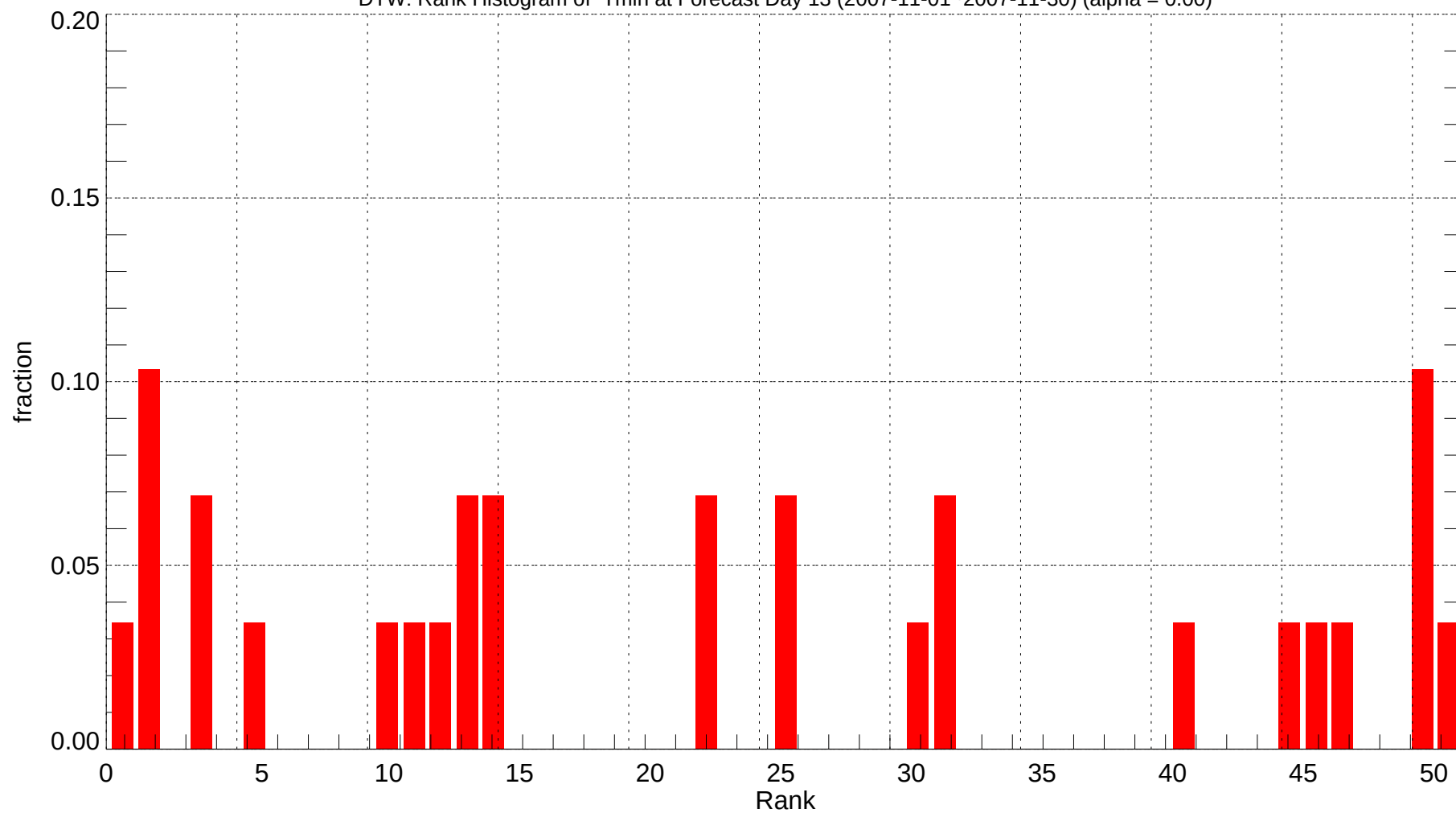
DTW: Rank Histogram of Tmin at Forecast Day 13 (2007-11-01~2007-11-30) (alpha = 0.00)
