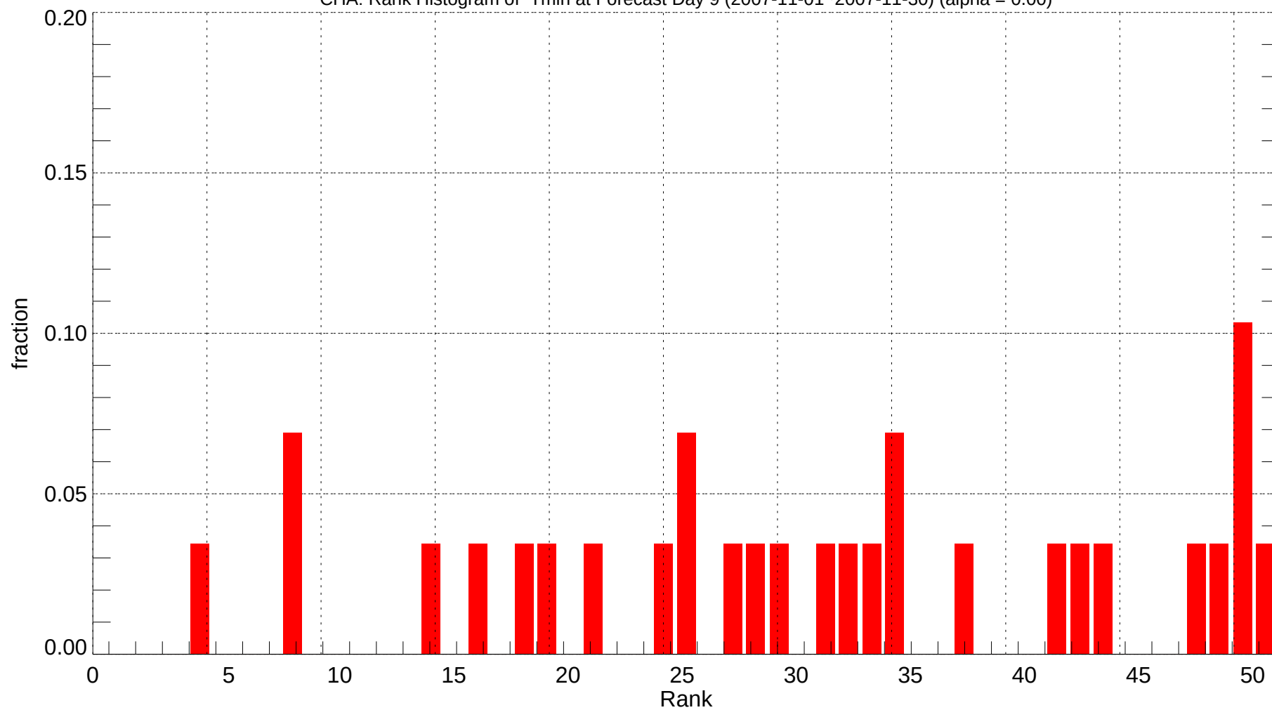
CHA: Rank Histogram of Tmin at Forecast Day 9 (2007-11-01~2007-11-30) (alpha = 0.00)
