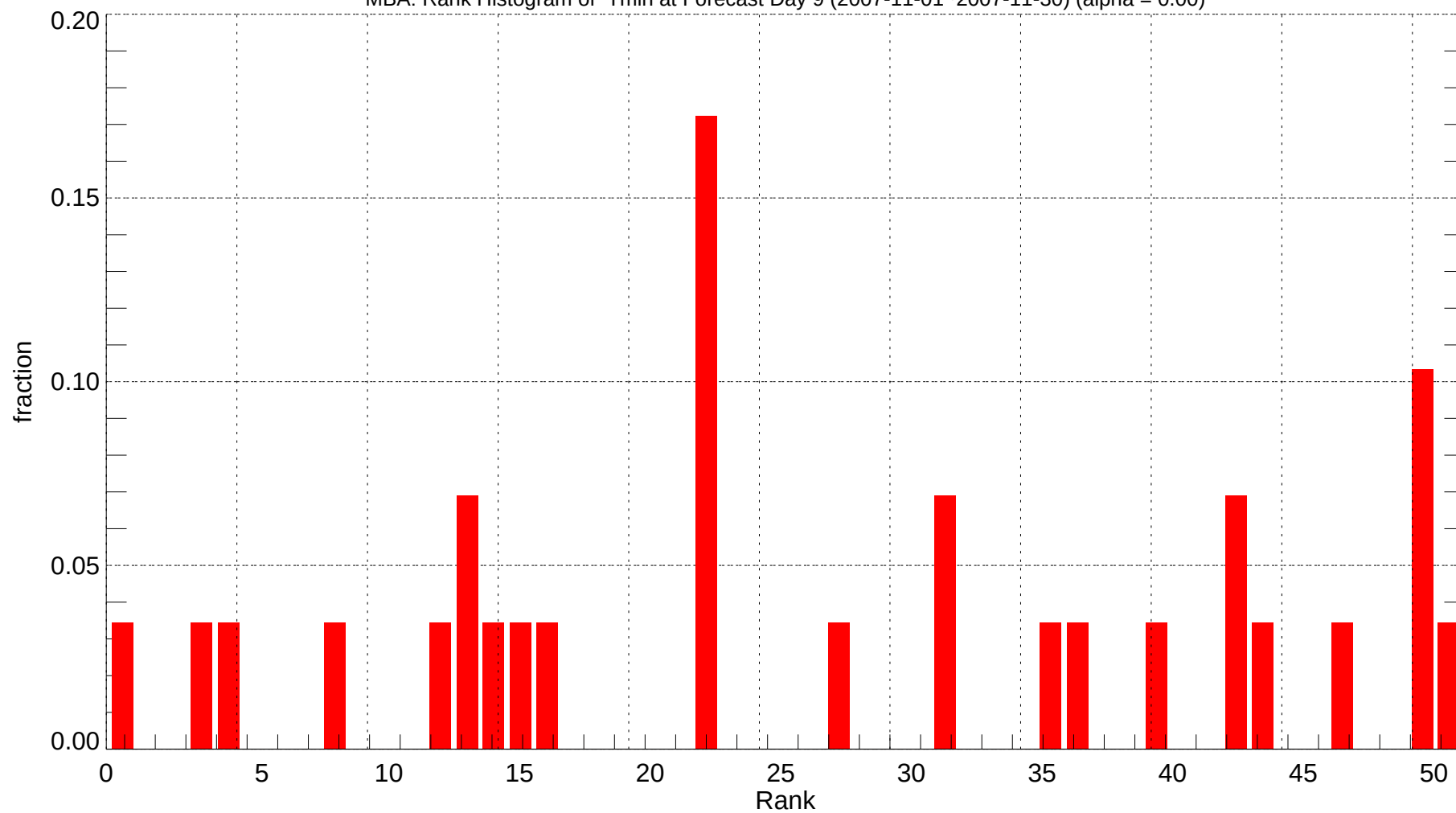
MBA: Rank Histogram of Tmin at Forecast Day 9 (2007-11-01~2007-11-30) (alpha = 0.00)
