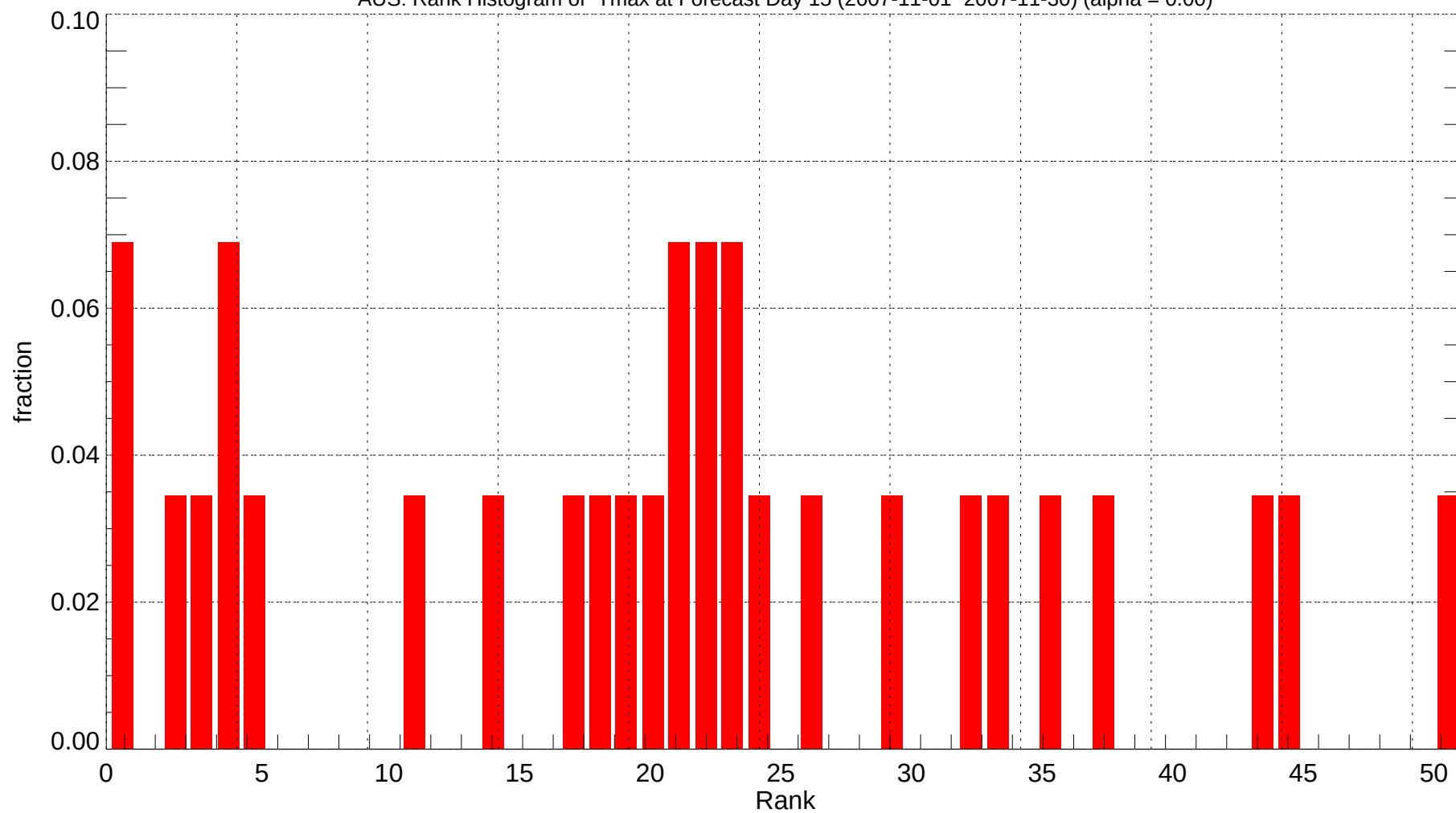
AUS: Rank Histogram of Tmax at Forecast Day 15 (2007-11-01~2007-11-30) (alpha = 0.00)
