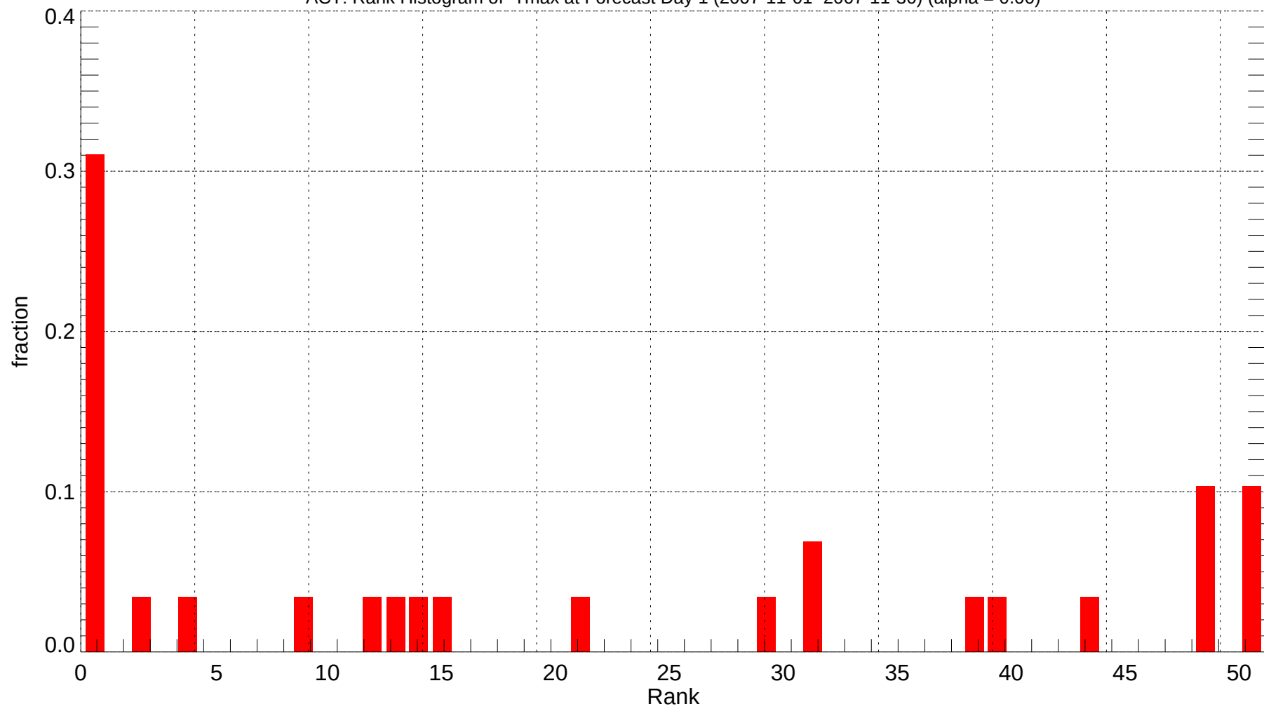
ACT: Rank Histogram of Tmax at Forecast Day 1 (2007-11-01~2007-11-30) (alpha = 0.00)
