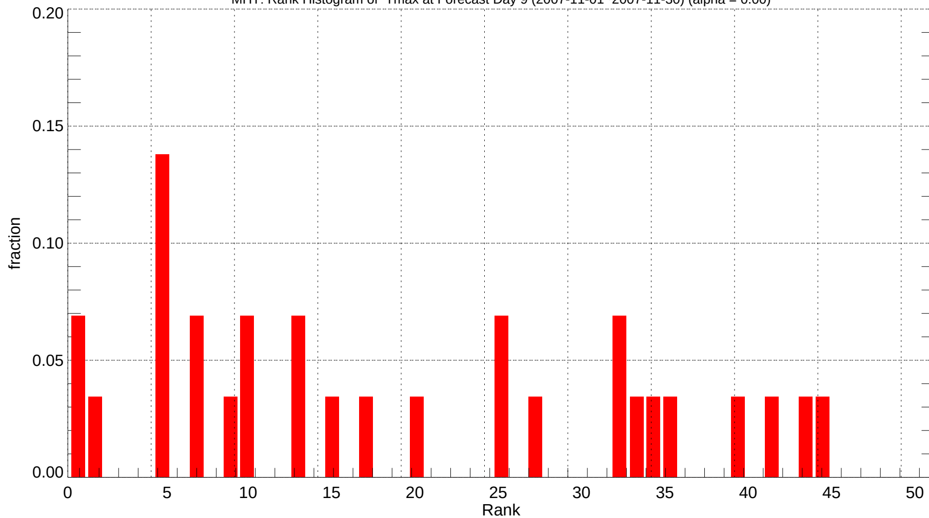
MHT: Rank Histogram of Tmax at Forecast Day 9 (2007-11-01~2007-11-30) (alpha = 0.00)
