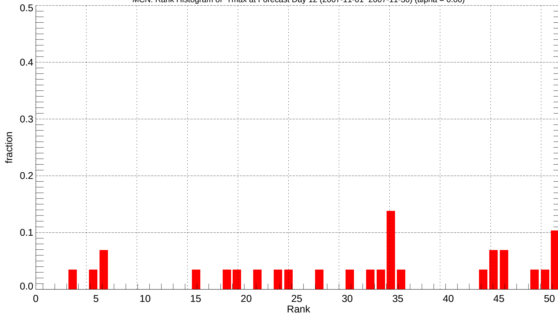
MCN: Rank Histogram of Tmax at Forecast Day 12 (2007-11-01~2007-11-30) (alpha = 0.00)
