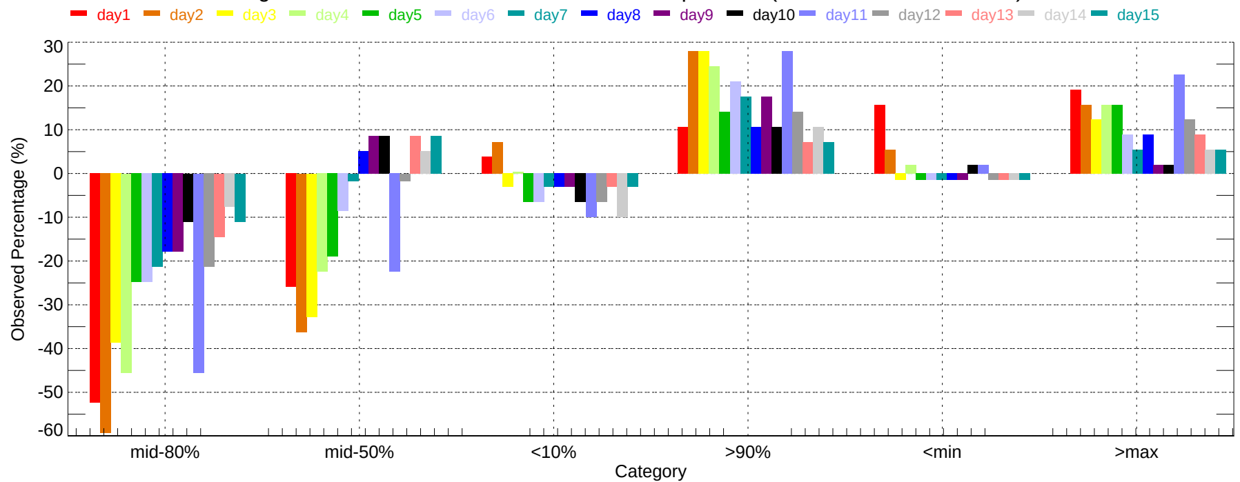
Observed Percentage Deviation of Ensembles - TYS: Min Temperature (2007-11-01~2007-11-30)
