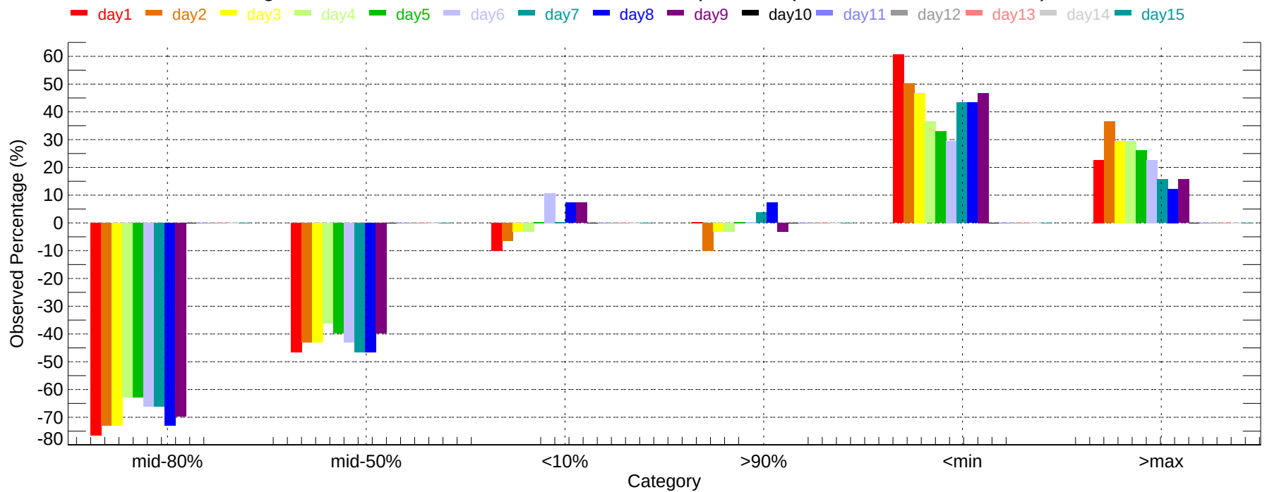
Observed Percentage Deviation of Ensembles - NKX: Min Temperature (2007-11-01~2007-11-30)
