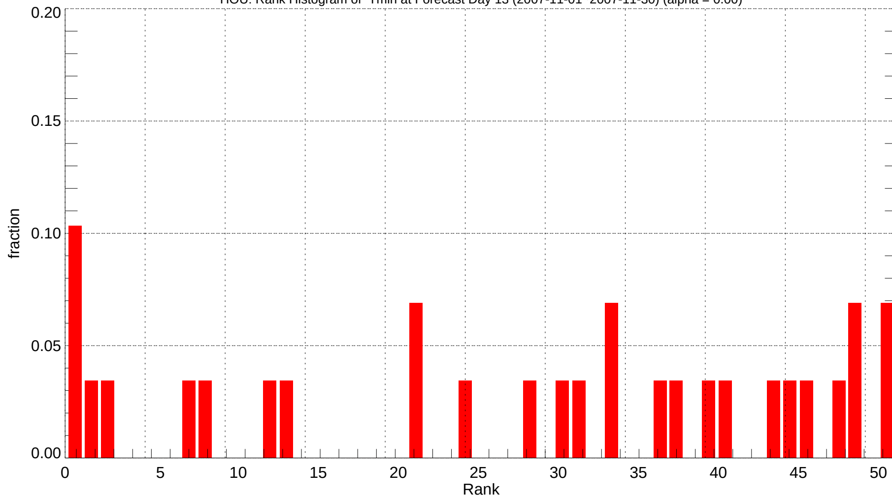
HOU: Rank Histogram of Tmin at Forecast Day 13 (2007-11-01~2007-11-30) (alpha = 0.00)
