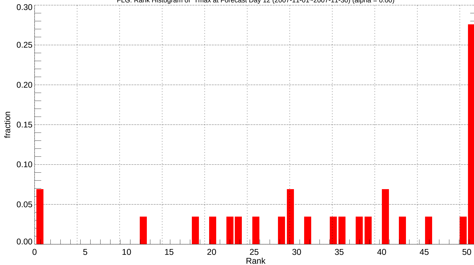
FLG: Rank Histogram of Tmax at Forecast Day 12 (2007-11-01~2007-11-30) (alpha = 0.00)
