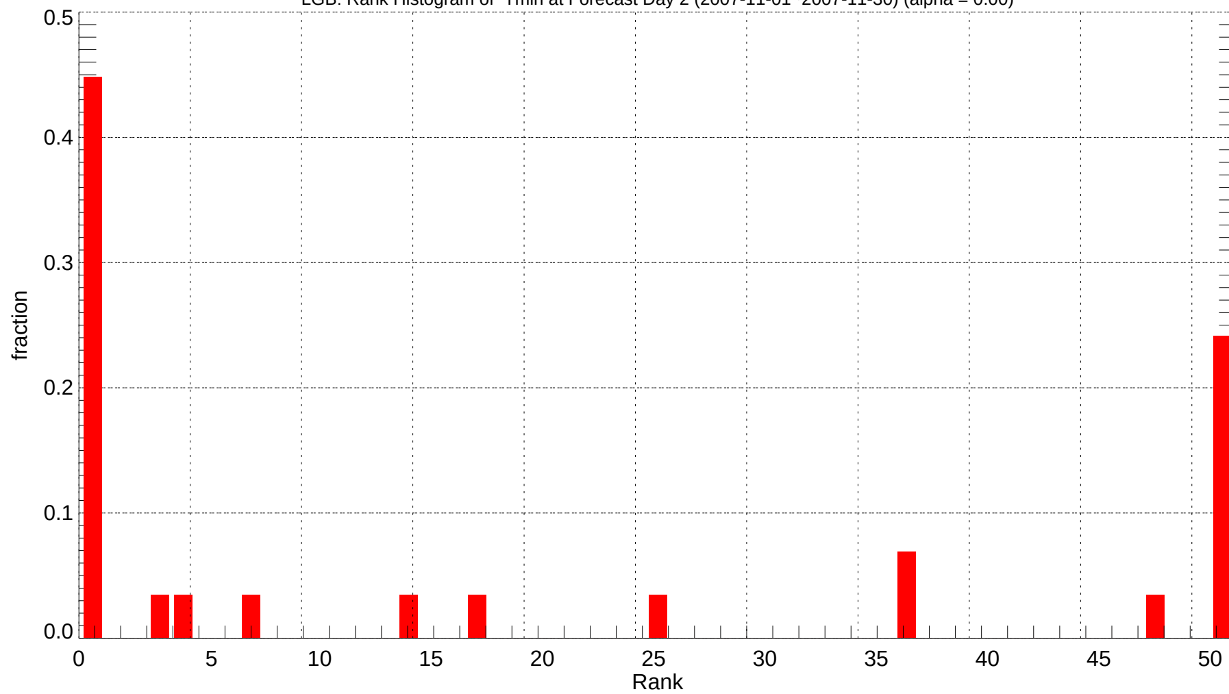
LGB: Rank Histogram of Tmin at Forecast Day 2 (2007-11-01~2007-11-30) (alpha = 0.00)
