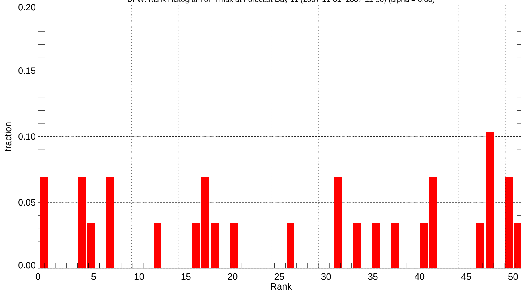
DFW: Rank Histogram of Tmax at Forecast Day 11 (2007-11-01~2007-11-30) (alpha = 0.00)
