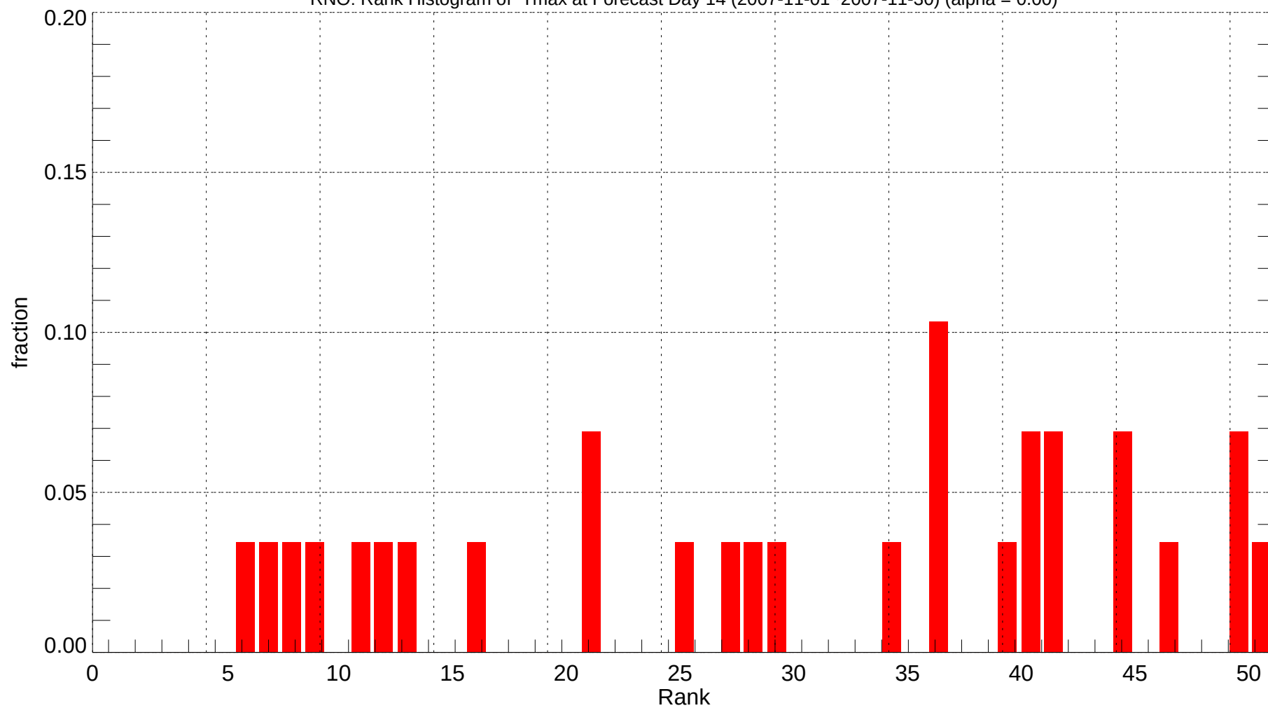
RNO: Rank Histogram of Tmax at Forecast Day 14 (2007-11-01~2007-11-30) (alpha = 0.00)
