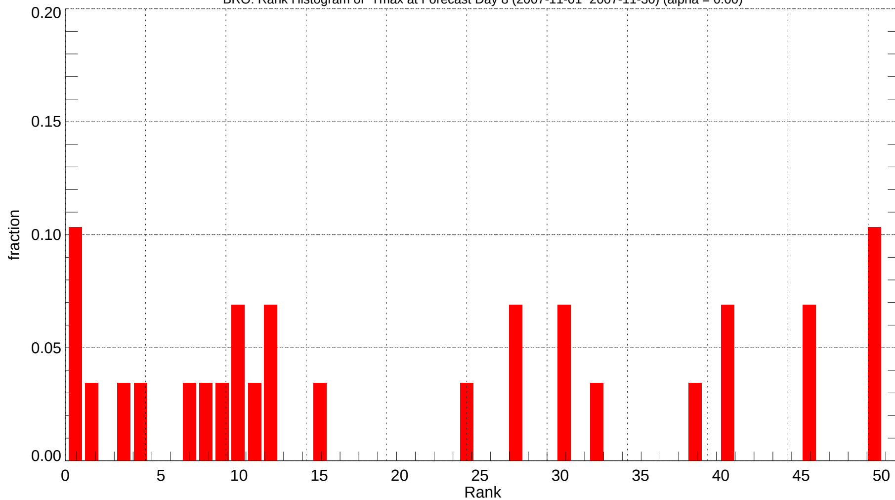
BRO: Rank Histogram of Tmax at Forecast Day 8 (2007-11-01~2007-11-30) (alpha = 0.00)
