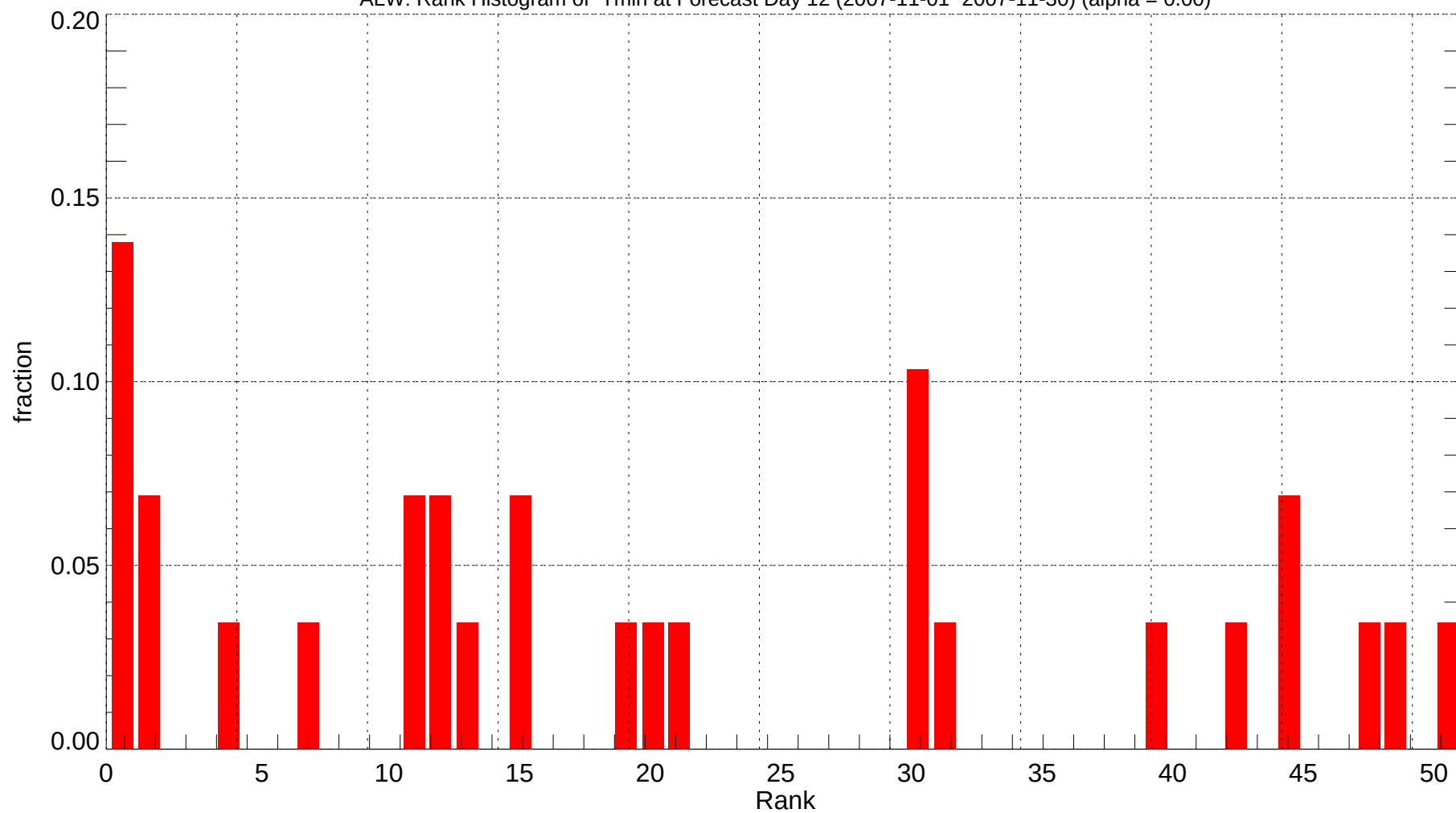
ALW: Rank Histogram of Tmin at Forecast Day 12 (2007-11-01~2007-11-30) (alpha = 0.00)
