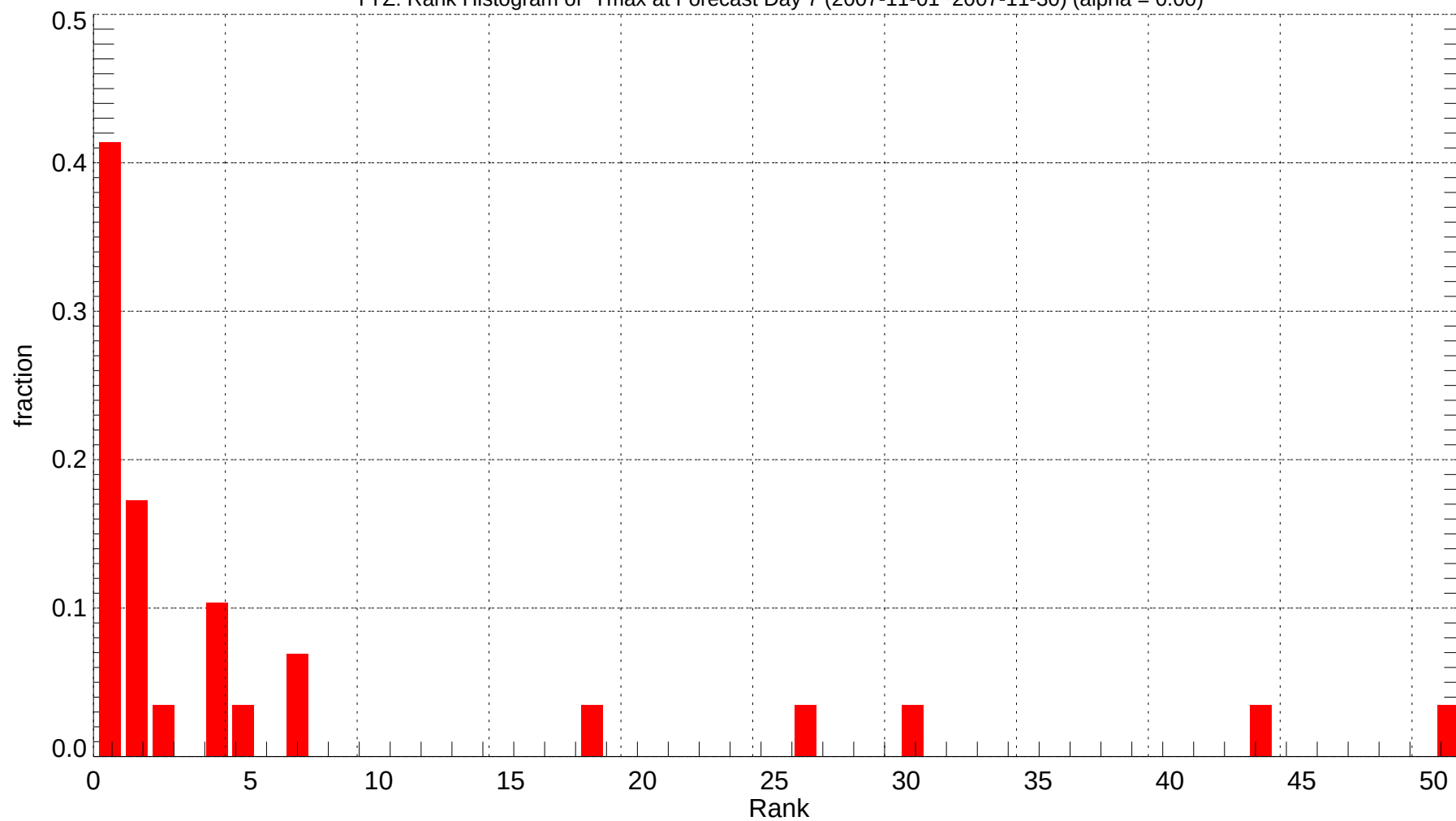
YYZ: Rank Histogram of Tmax at Forecast Day 7 (2007-11-01~2007-11-30) (alpha = 0.00)
