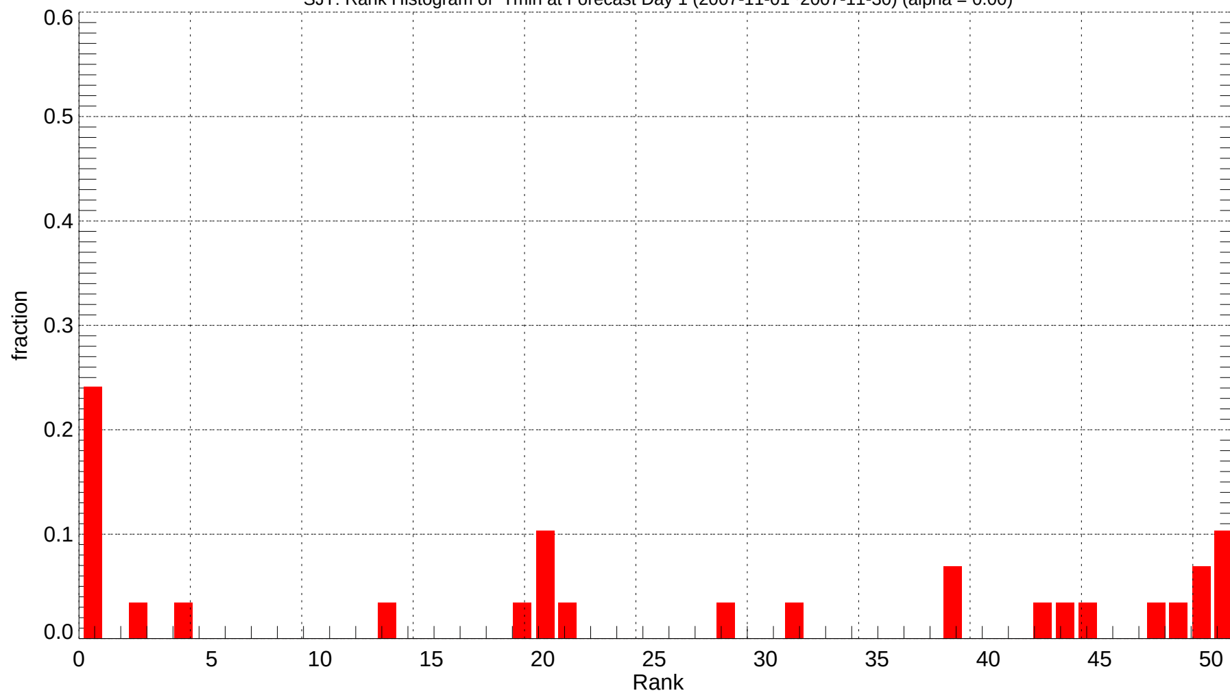
SJT: Rank Histogram of Tmin at Forecast Day 1 (2007-11-01~2007-11-30) (alpha = 0.00)
