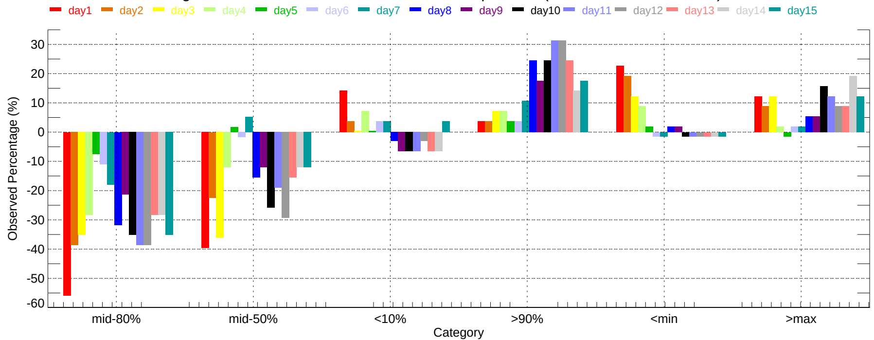
Observed Percentage Deviation of Ensembles - TYR: Min Temperature (2007-11-01~2007-11-30)
