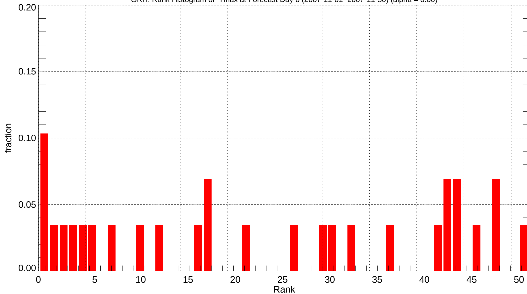
ORH: Rank Histogram of Tmax at Forecast Day 6 (2007-11-01~2007-11-30) (alpha = 0.00)
