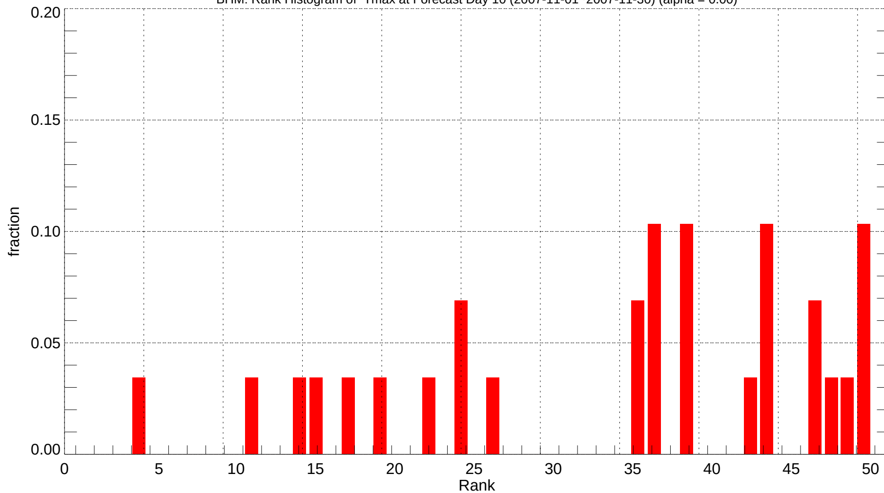
BHM: Rank Histogram of Tmax at Forecast Day 10 (2007-11-01~2007-11-30) (alpha = 0.00)
