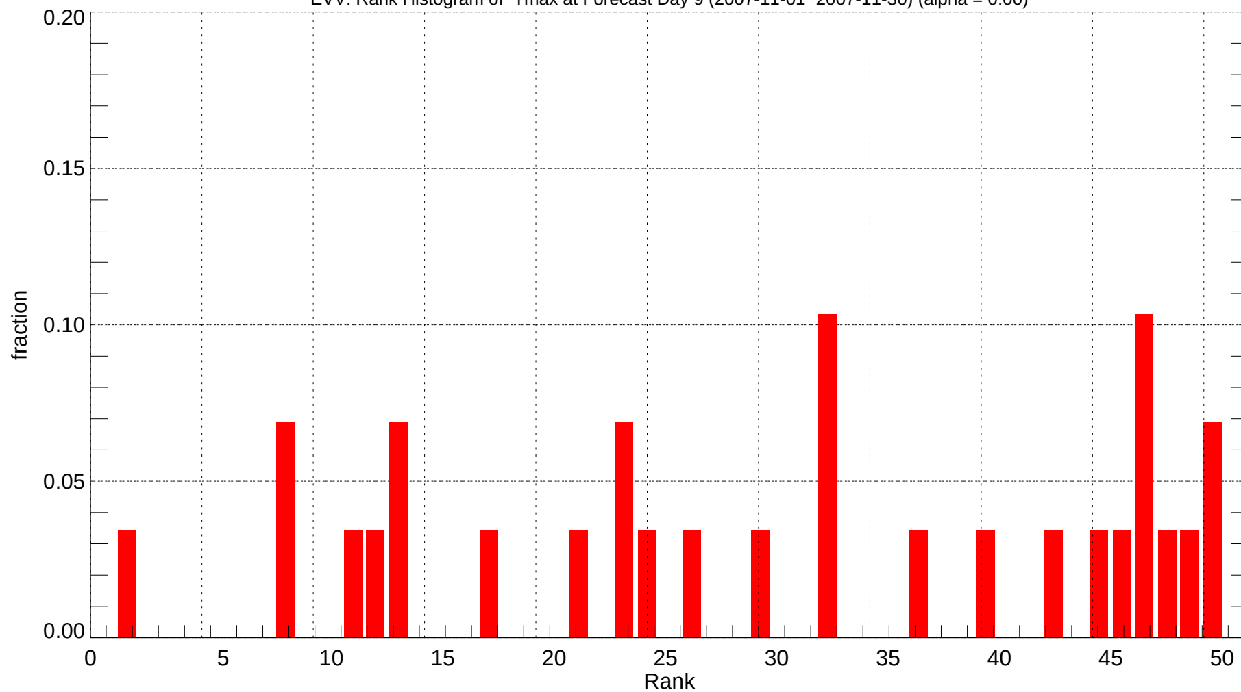
EVV: Rank Histogram of Tmax at Forecast Day 9 (2007-11-01~2007-11-30) (alpha = 0.00)
