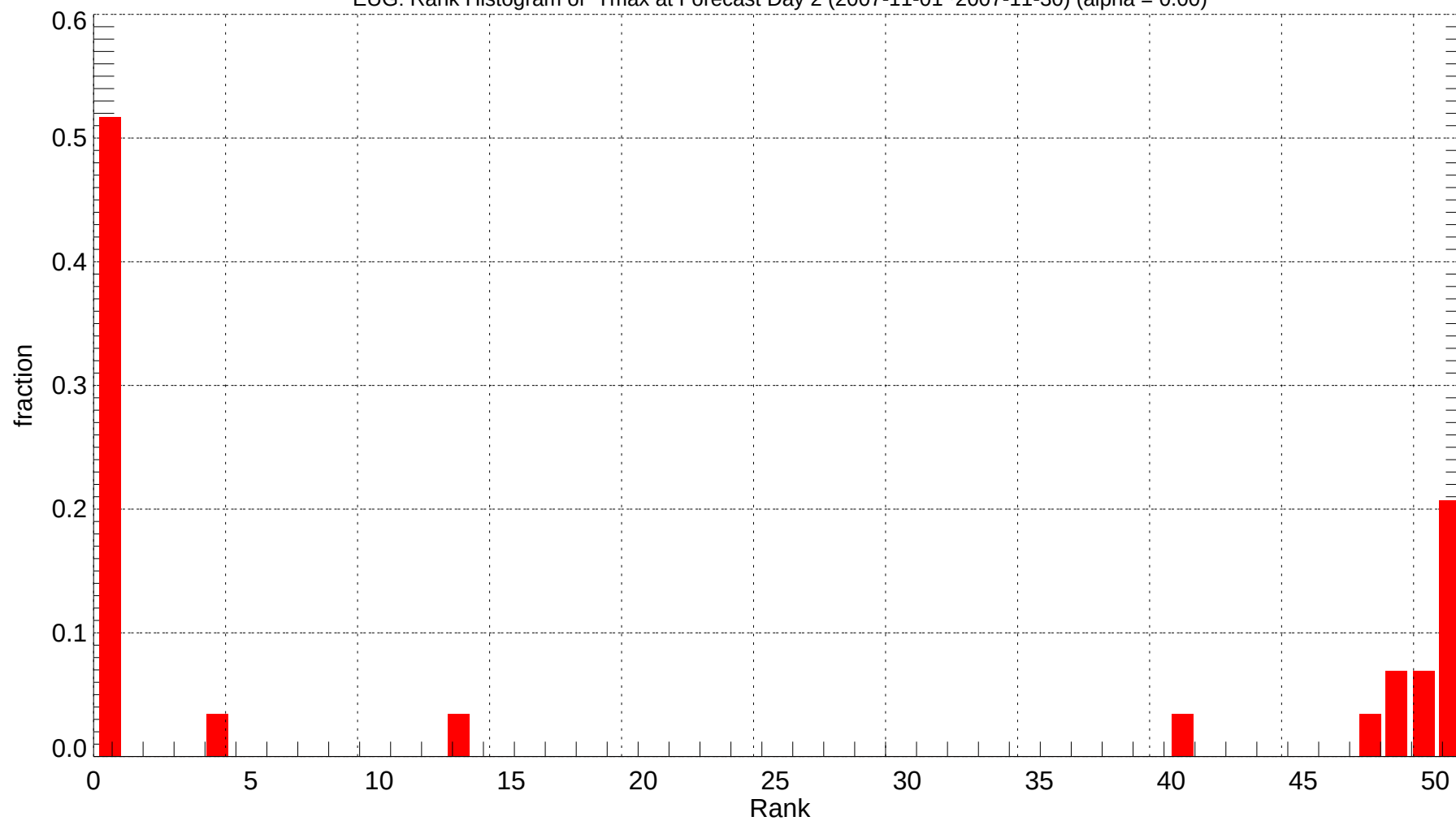
EUG: Rank Histogram of Tmax at Forecast Day 2 (2007-11-01~2007-11-30) (alpha = 0.00)
