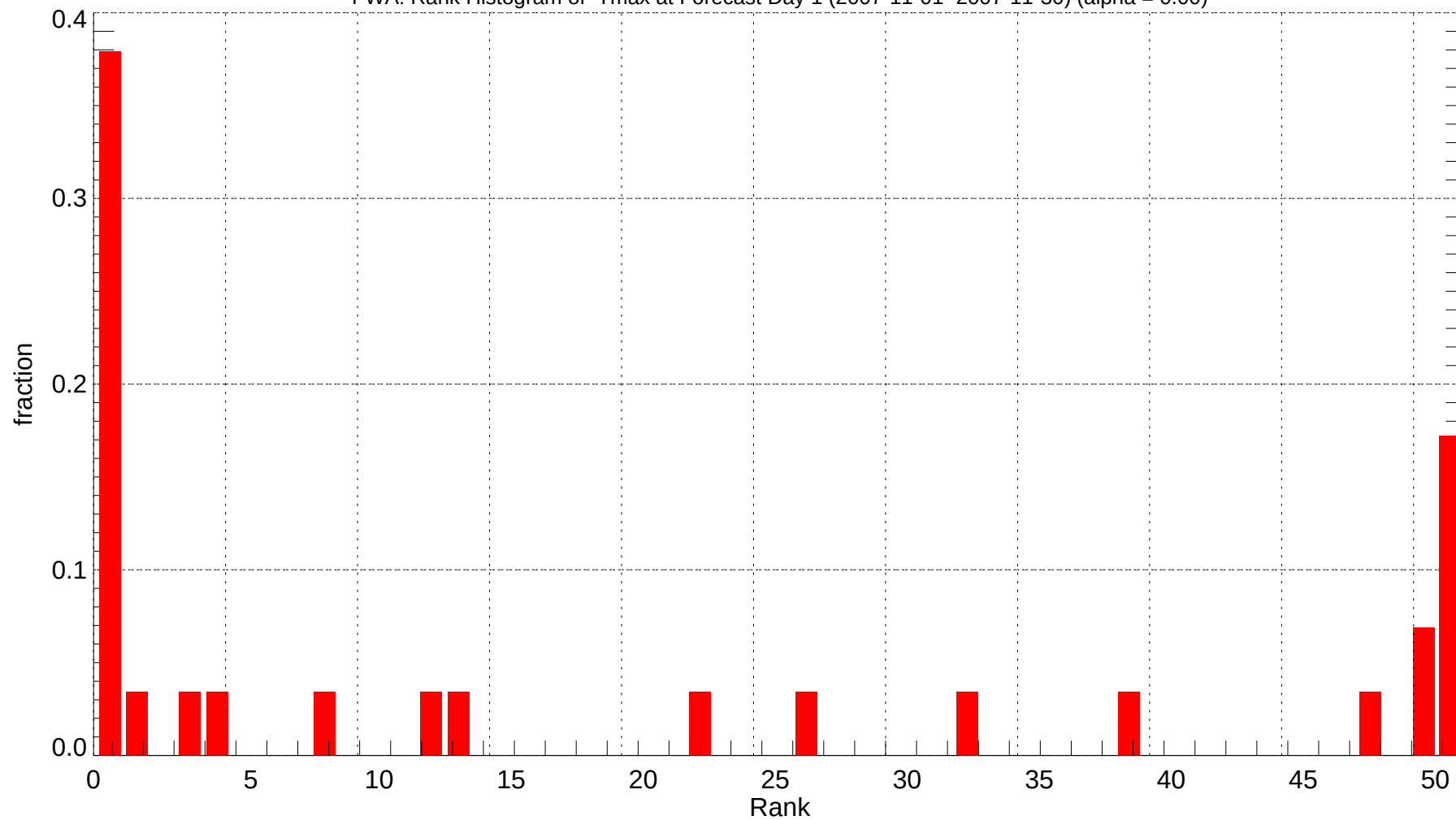
FWA: Rank Histogram of Tmax at Forecast Day 1 (2007-11-01~2007-11-30) (alpha = 0.00)
