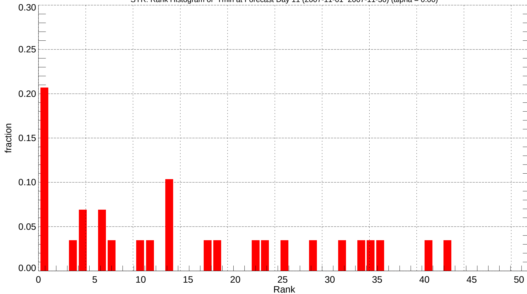
SYR: Rank Histogram of Tmin at Forecast Day 11 (2007-11-01~2007-11-30) (alpha = 0.00)
