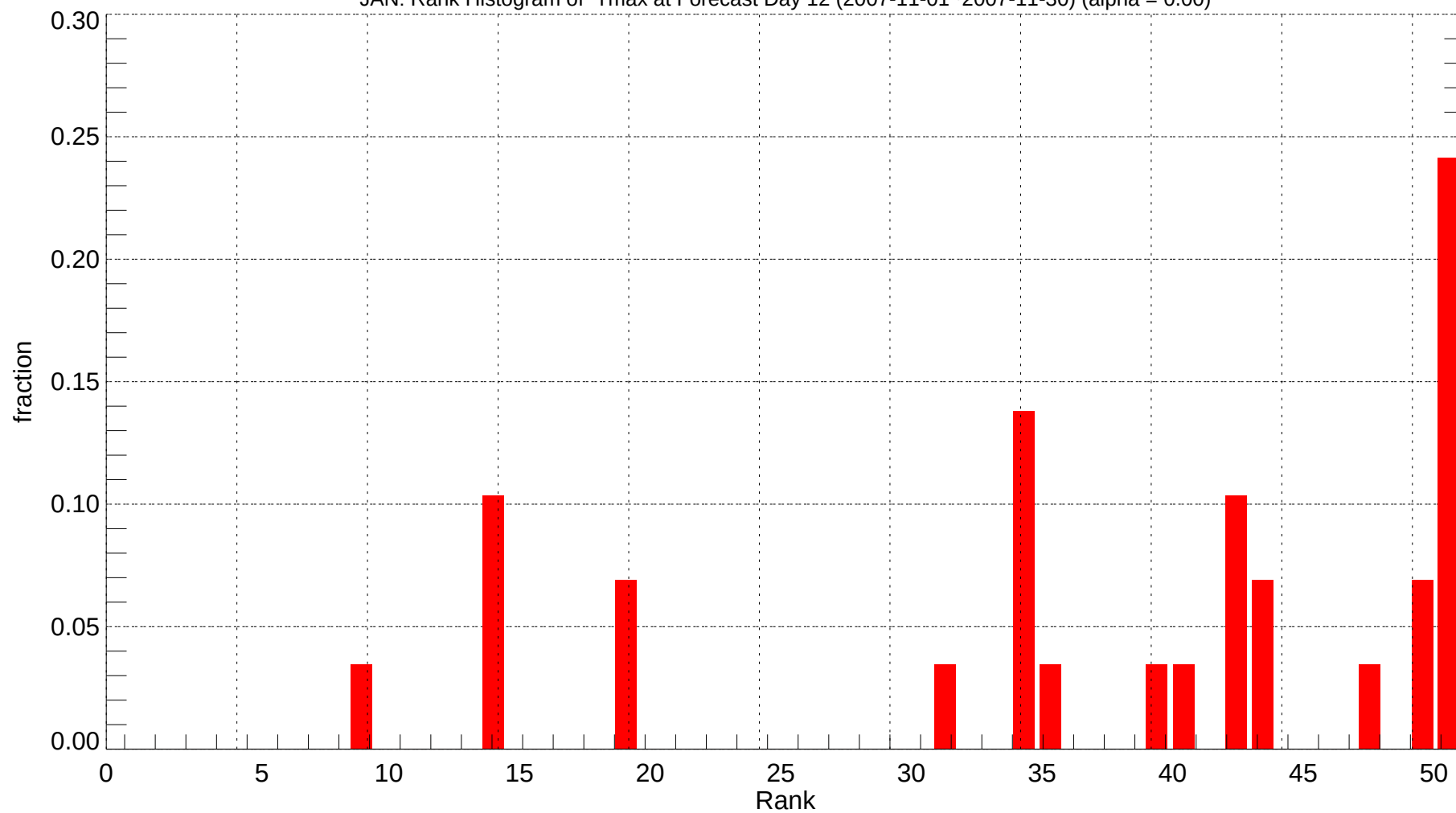
JAN: Rank Histogram of Tmax at Forecast Day 12 (2007-11-01~2007-11-30) (alpha = 0.00)
