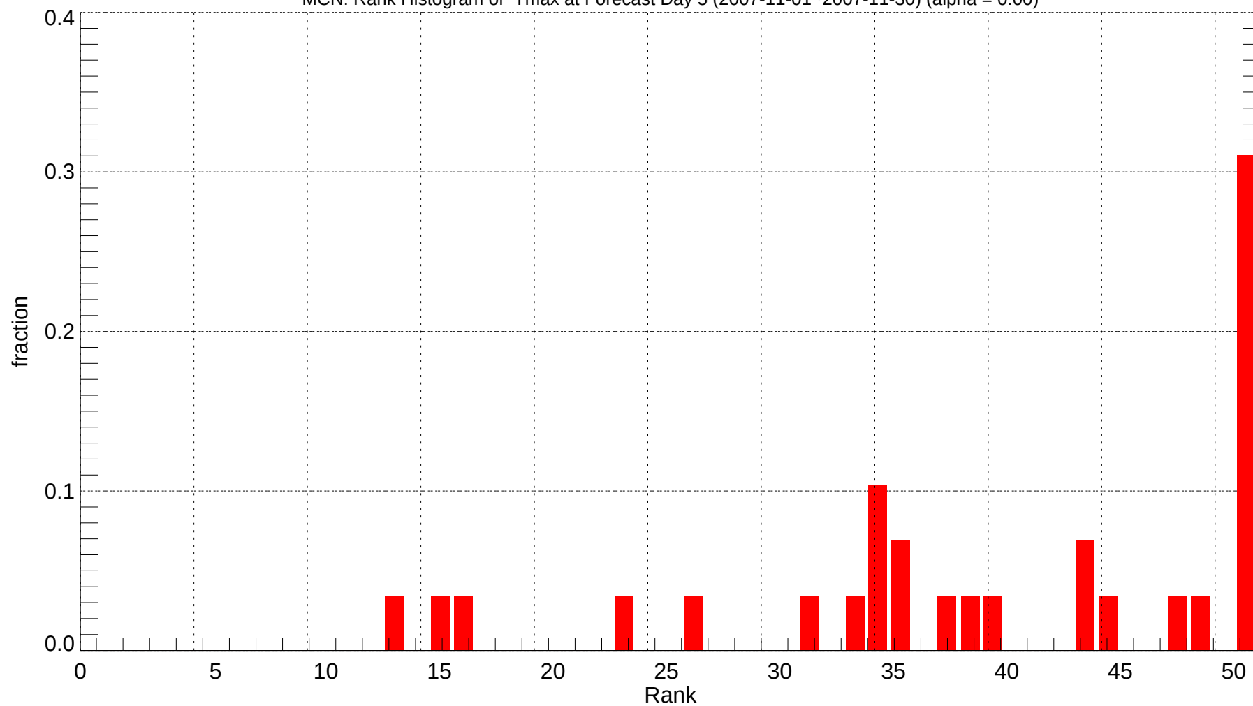
MCN: Rank Histogram of Tmax at Forecast Day 5 (2007-11-01~2007-11-30) (alpha = 0.00)
