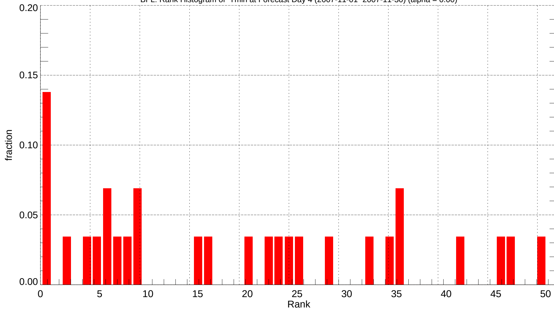
BFL: Rank Histogram of Tmin at Forecast Day 4 (2007-11-01~2007-11-30) (alpha = 0.00)
