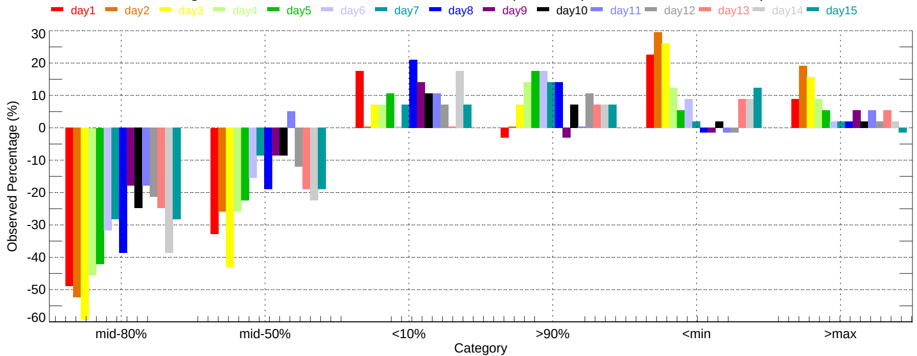
Observed Percentage Deviation of Ensembles - ORH: Max Temperature (2007-11-01~2007-11-30)
