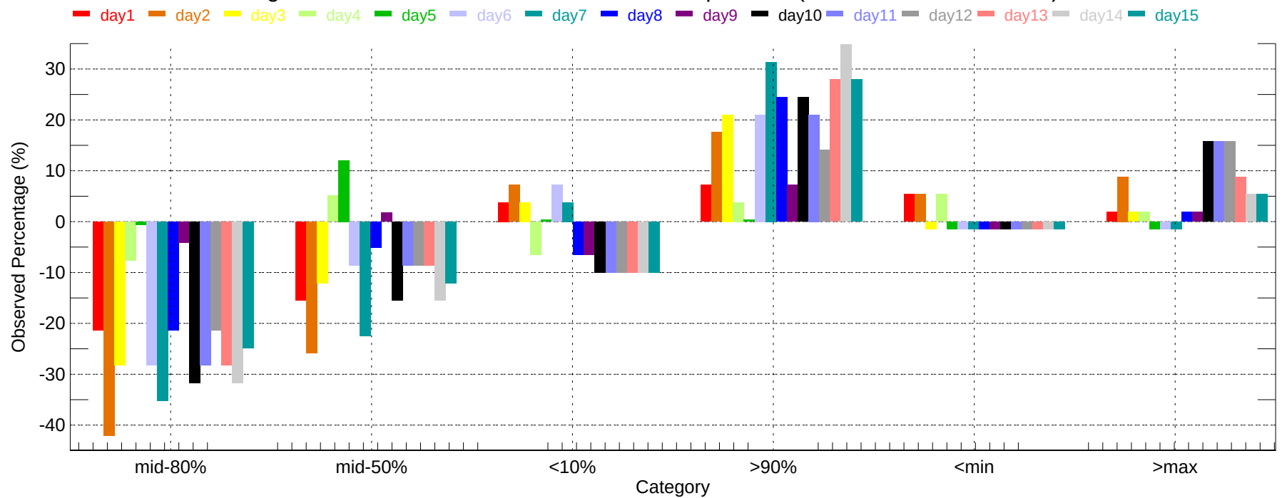
Observed Percentage Deviation of Ensembles - TUS: Min Temperature (2007-11-01~2007-11-30)
