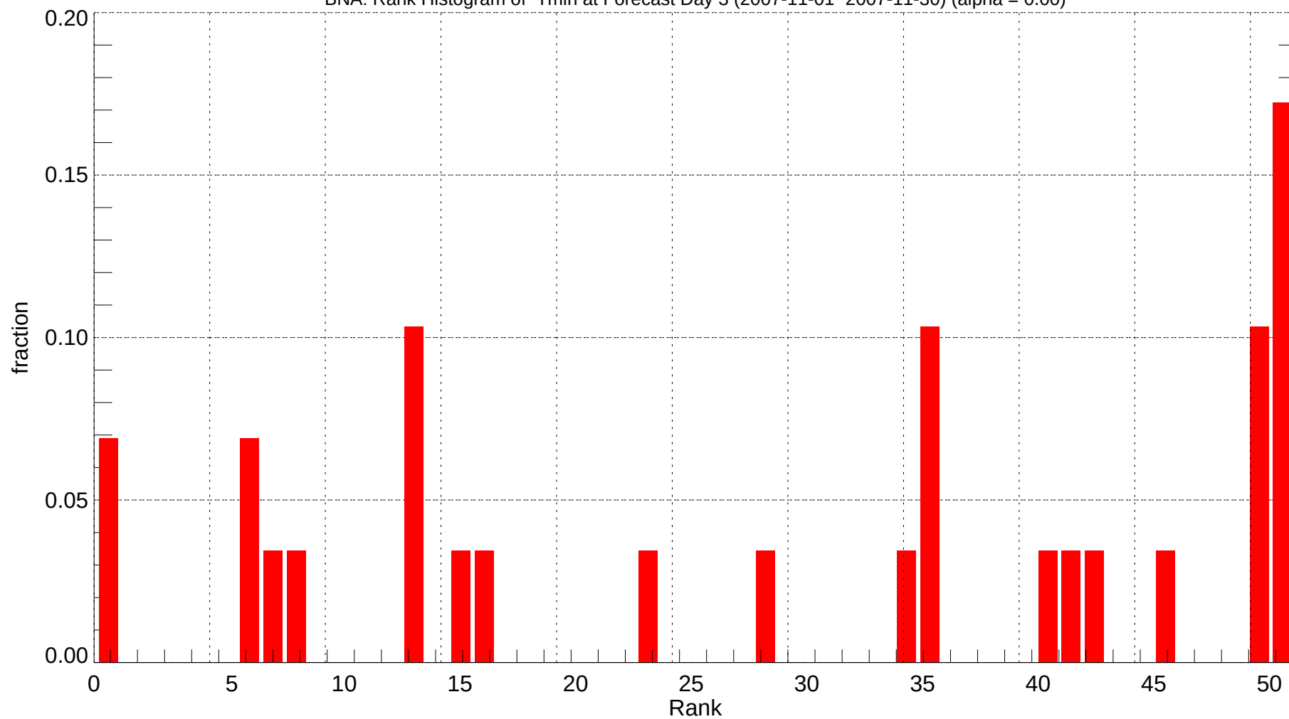
BNA: Rank Histogram of Tmin at Forecast Day 3 (2007-11-01~2007-11-30) (alpha = 0.00)
