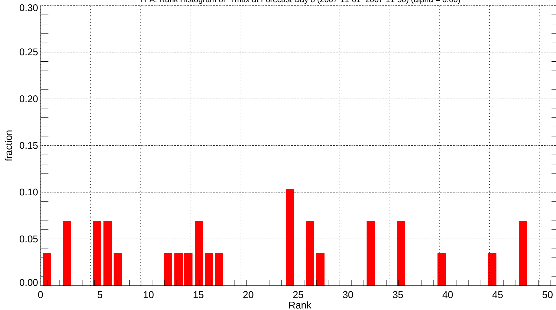
TPA: Rank Histogram of Tmax at Forecast Day 8 (2007-11-01~2007-11-30) (alpha = 0.00)
