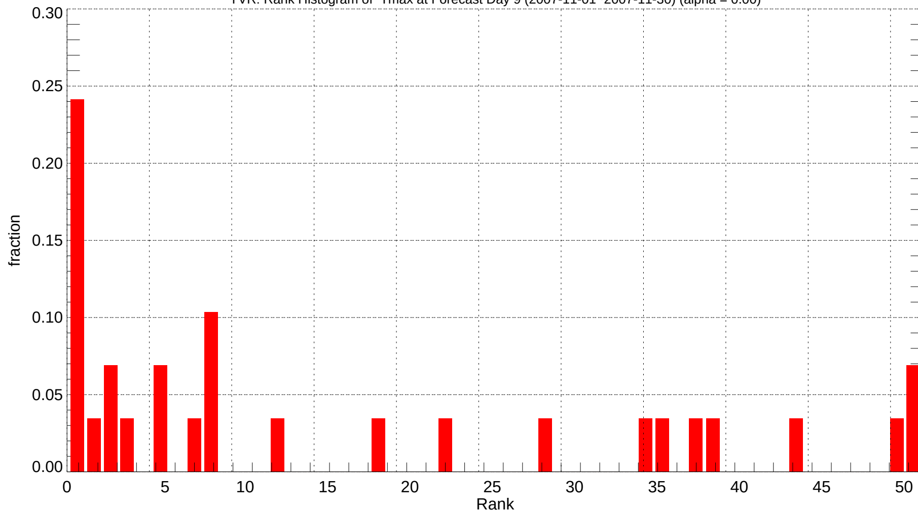
YVR: Rank Histogram of Tmax at Forecast Day 9 (2007-11-01~2007-11-30) (alpha = 0.00)
