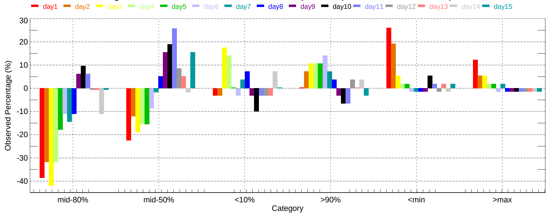
Observed Percentage Deviation of Ensembles - BTV: Min Temperature (2007-11-01~2007-11-30)
