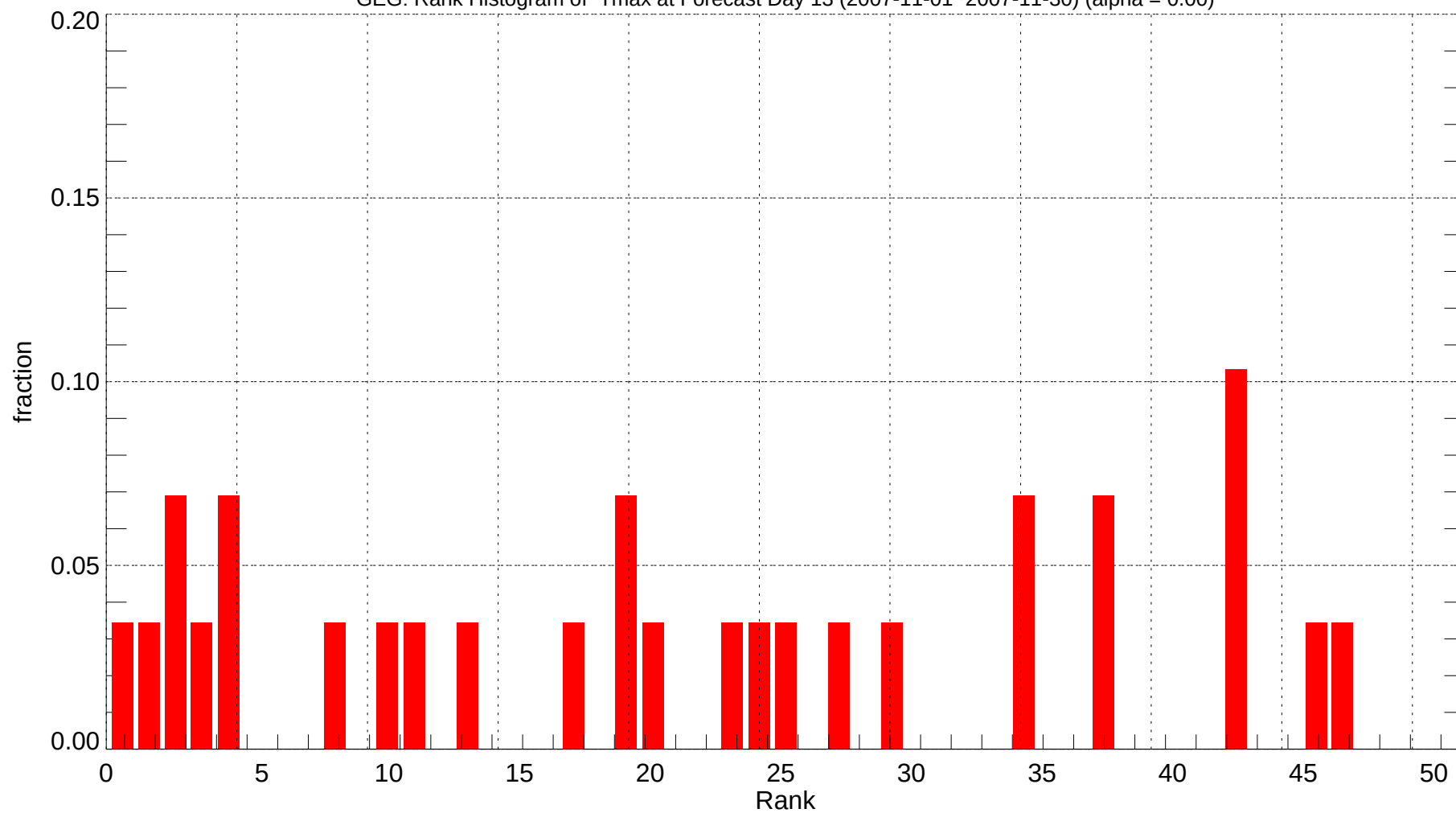
GEG: Rank Histogram of Tmax at Forecast Day 13 (2007-11-01~2007-11-30) (alpha = 0.00)
