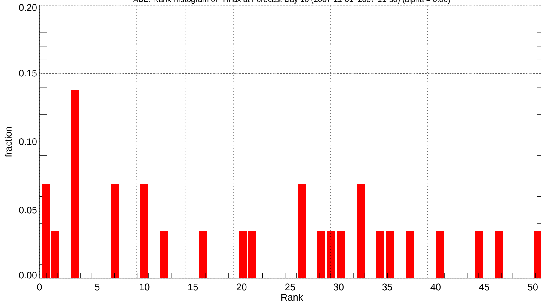
ABE: Rank Histogram of Tmax at Forecast Day 10 (2007-11-01~2007-11-30) (alpha = 0.00)
