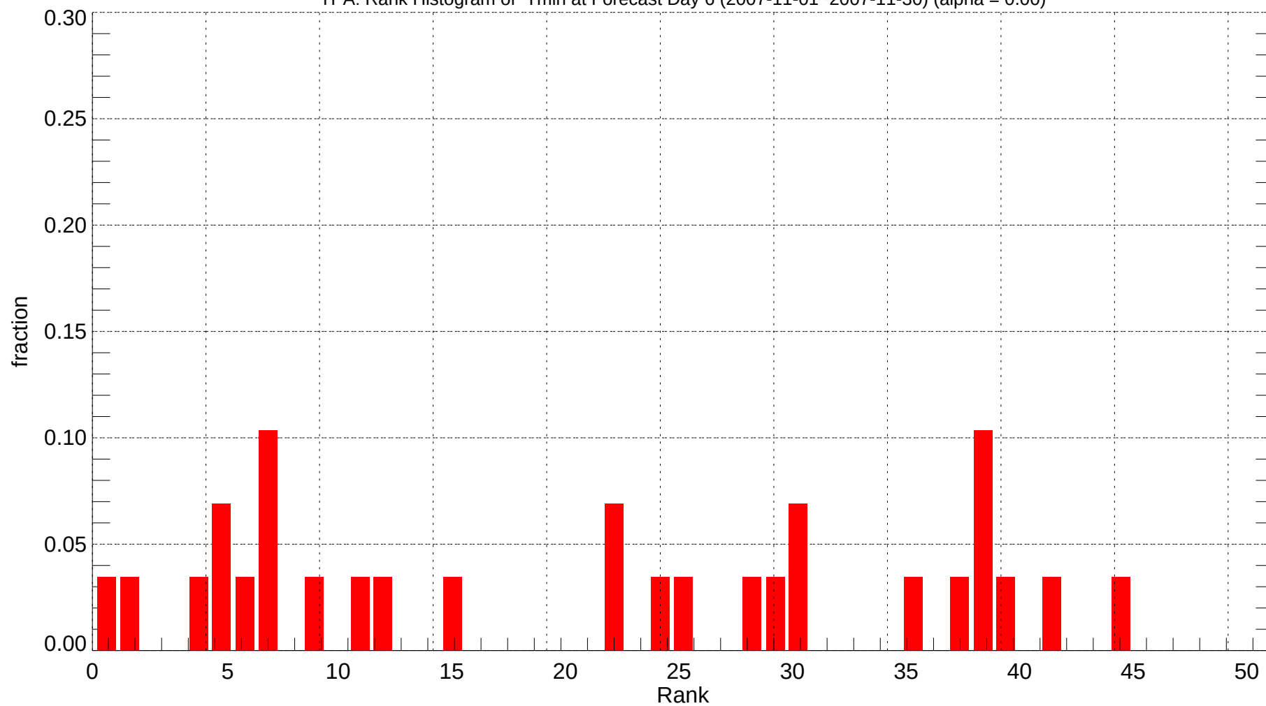
TPA: Rank Histogram of Tmin at Forecast Day 6 (2007-11-01~2007-11-30) (alpha = 0.00)
