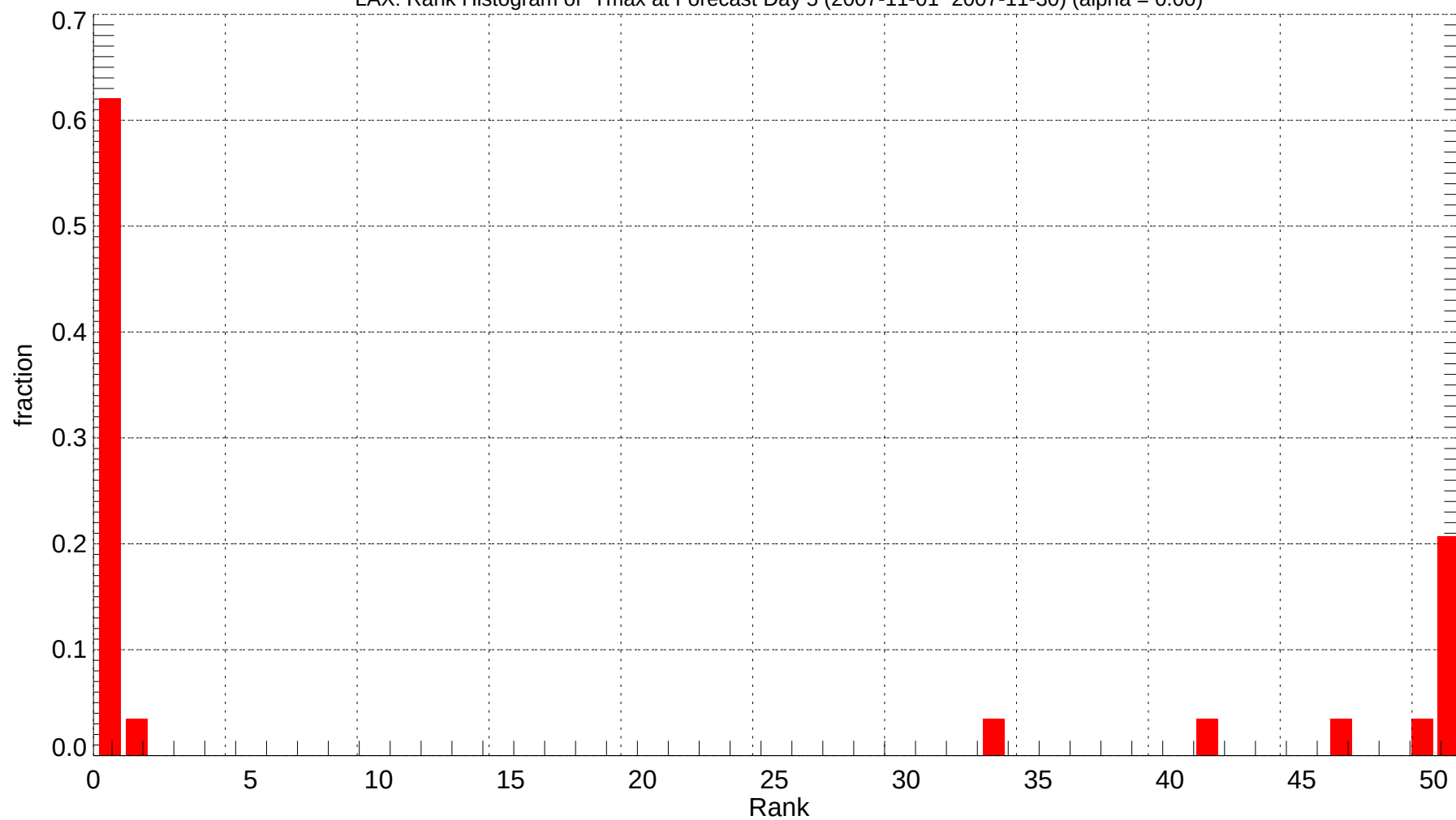
LAX: Rank Histogram of Tmax at Forecast Day 5 (2007-11-01~2007-11-30) (alpha = 0.00)
