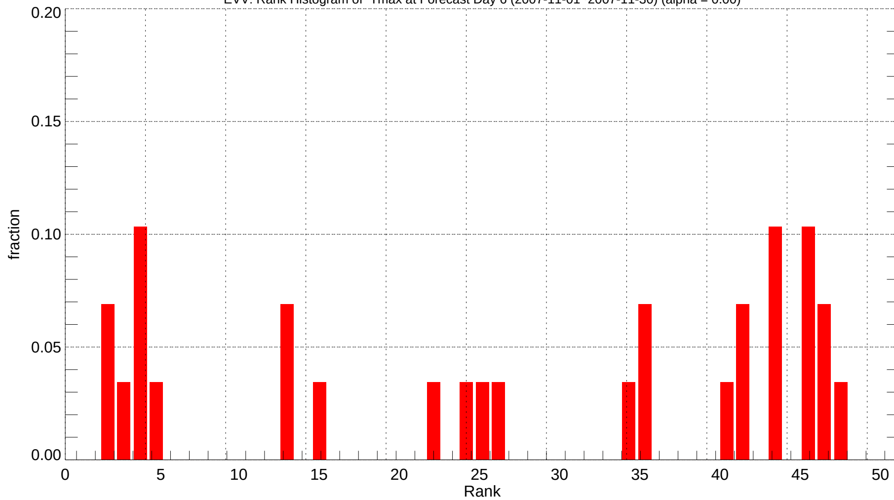
EVV: Rank Histogram of Tmax at Forecast Day 6 (2007-11-01~2007-11-30) (alpha = 0.00)
