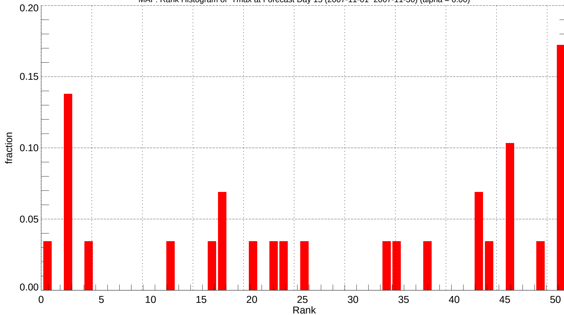
MAF: Rank Histogram of Tmax at Forecast Day 15 (2007-11-01~2007-11-30) (alpha = 0.00)
