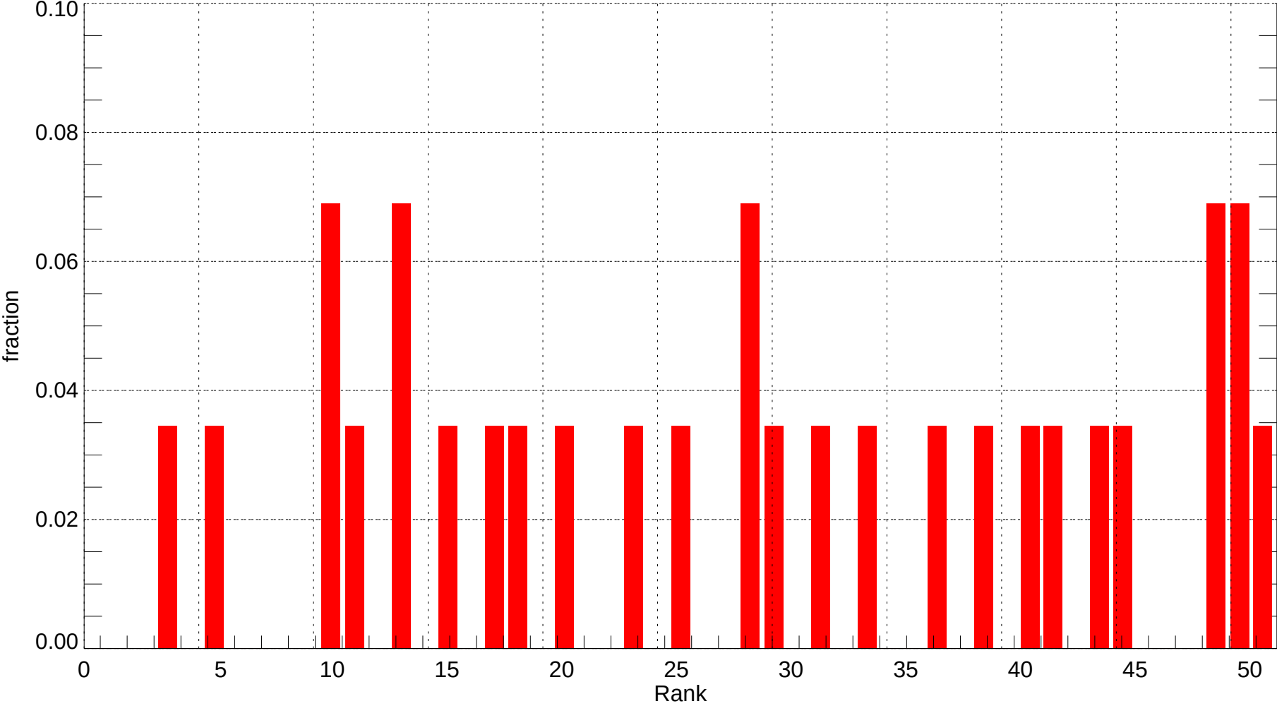
ATL: Rank Histogram of Tmin at Forecast Day 8 (2007-11-01~2007-11-30) (alpha = 0.00)
