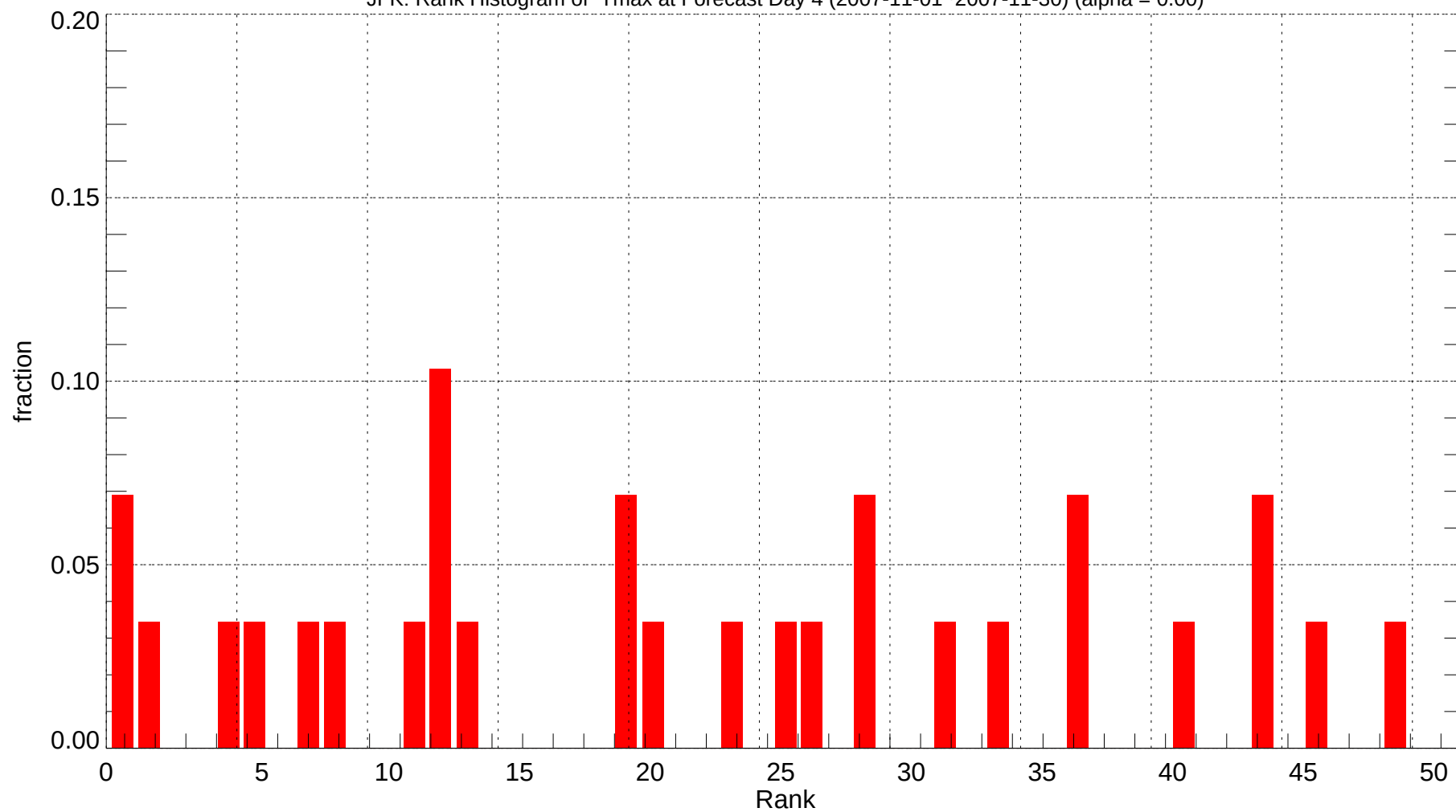
JFK: Rank Histogram of Tmax at Forecast Day 4 (2007-11-01~2007-11-30) (alpha = 0.00)
