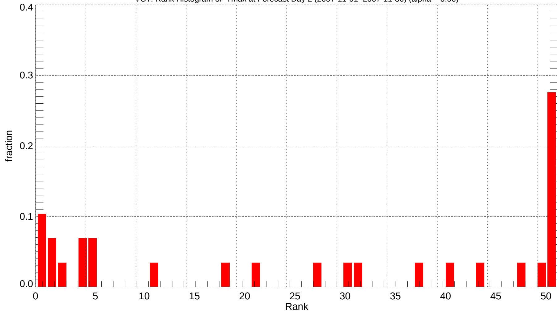
VCT: Rank Histogram of Tmax at Forecast Day 2 (2007-11-01~2007-11-30) (alpha = 0.00)
