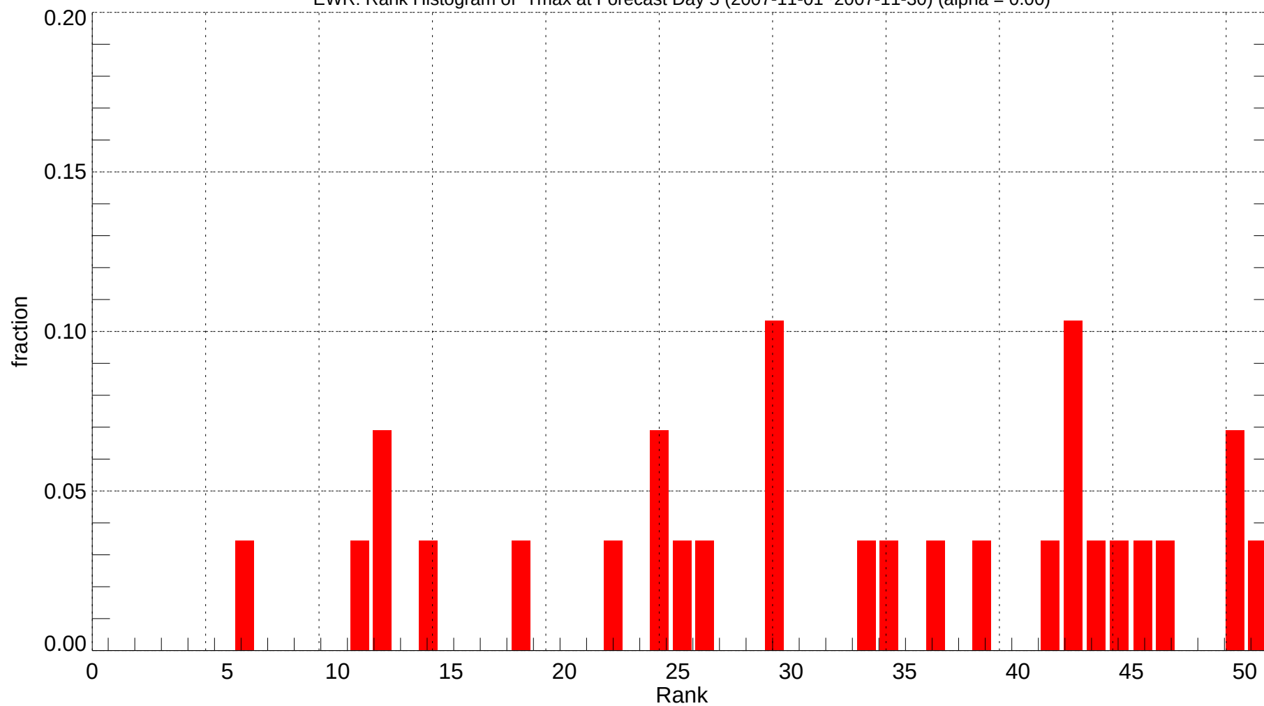
EWR: Rank Histogram of Tmax at Forecast Day 5 (2007-11-01~2007-11-30) (alpha = 0.00)
