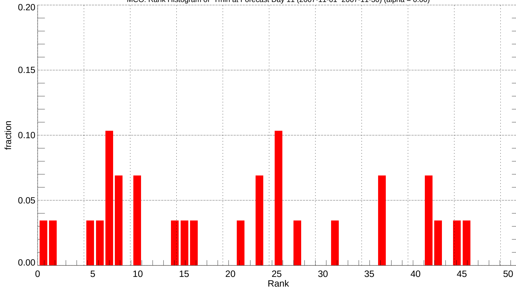
MCO: Rank Histogram of Tmin at Forecast Day 11 (2007-11-01~2007-11-30) (alpha = 0.00)
