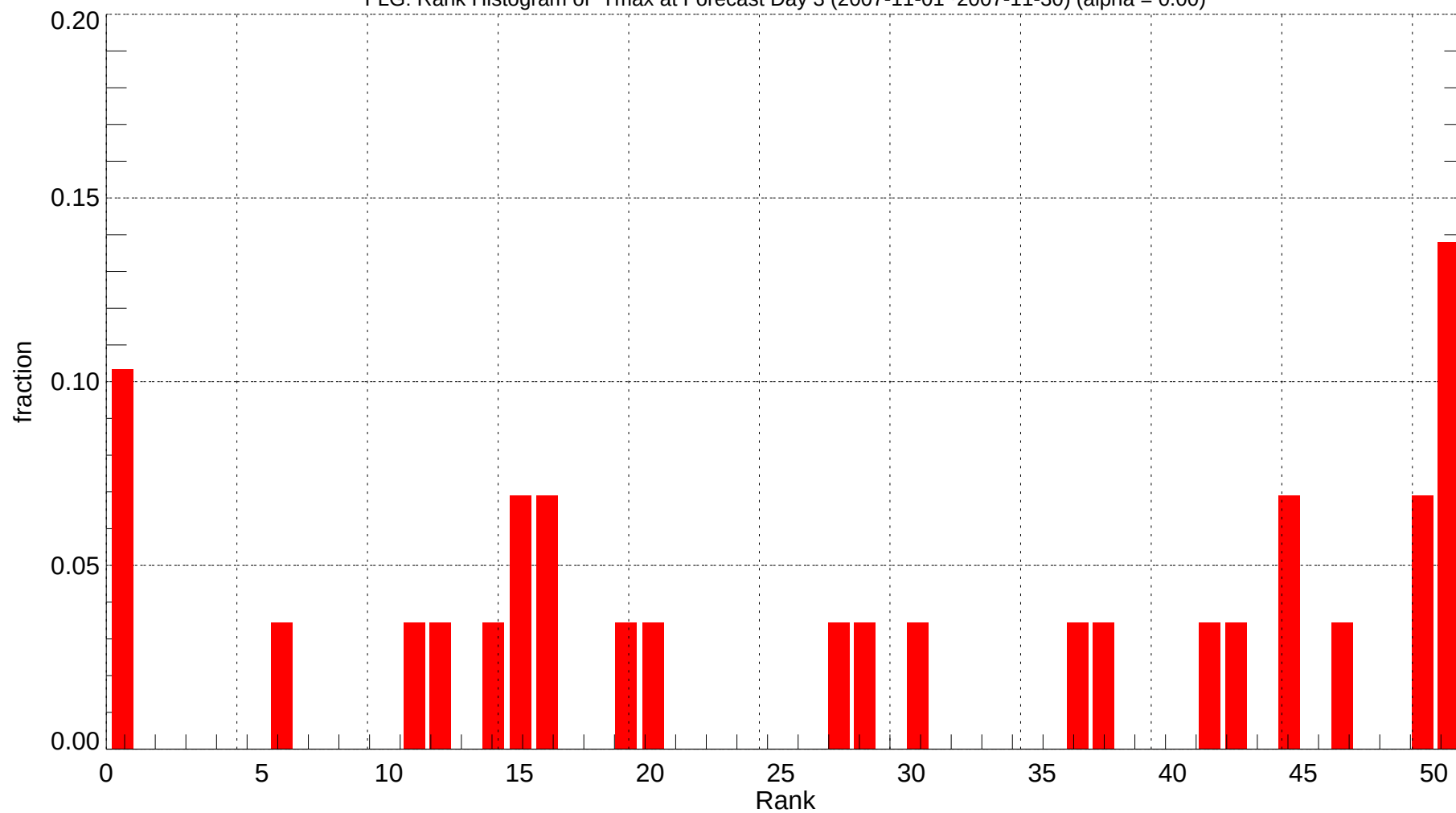
FLG: Rank Histogram of Tmax at Forecast Day 3 (2007-11-01~2007-11-30) (alpha = 0.00)
