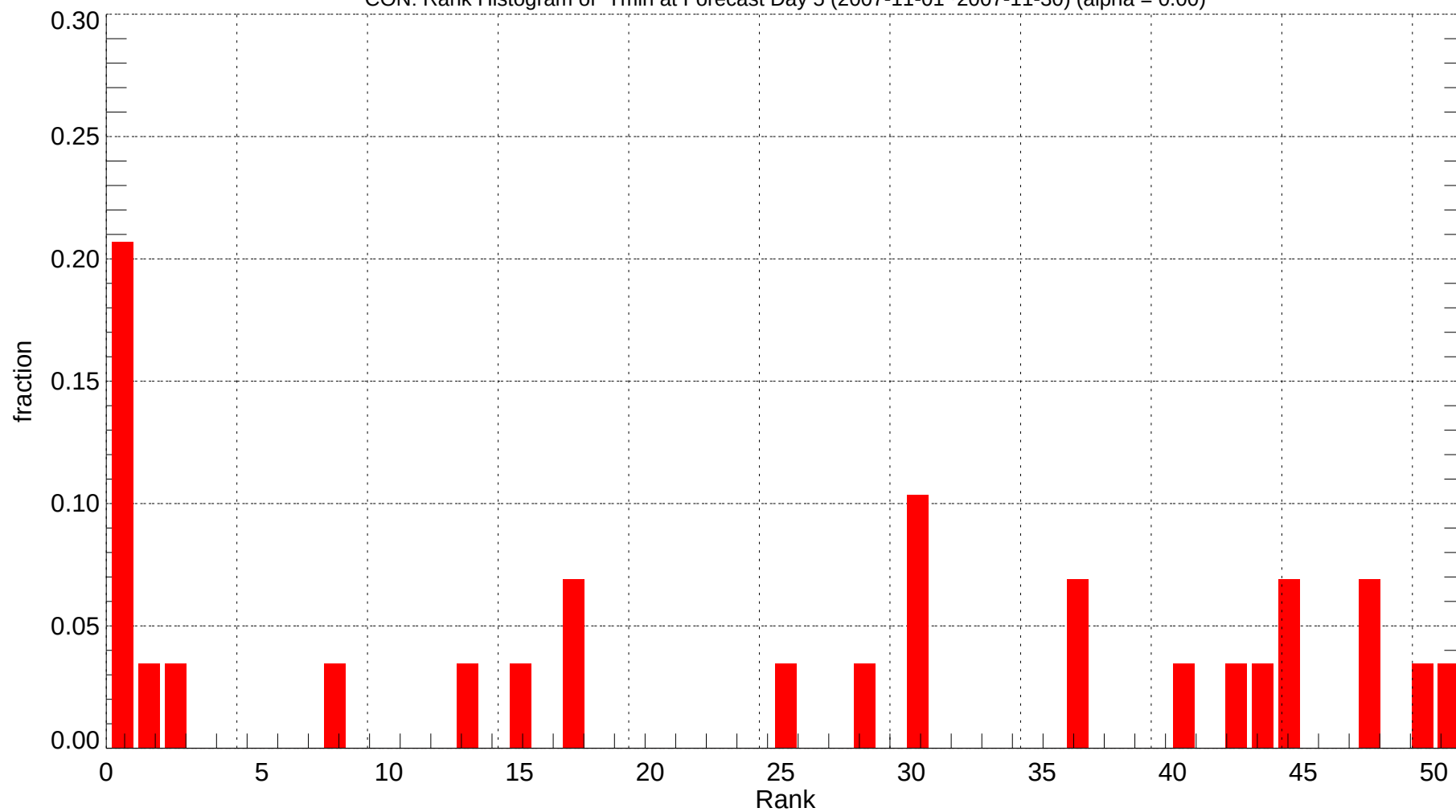
CON: Rank Histogram of Tmin at Forecast Day 5 (2007-11-01~2007-11-30) (alpha = 0.00)
