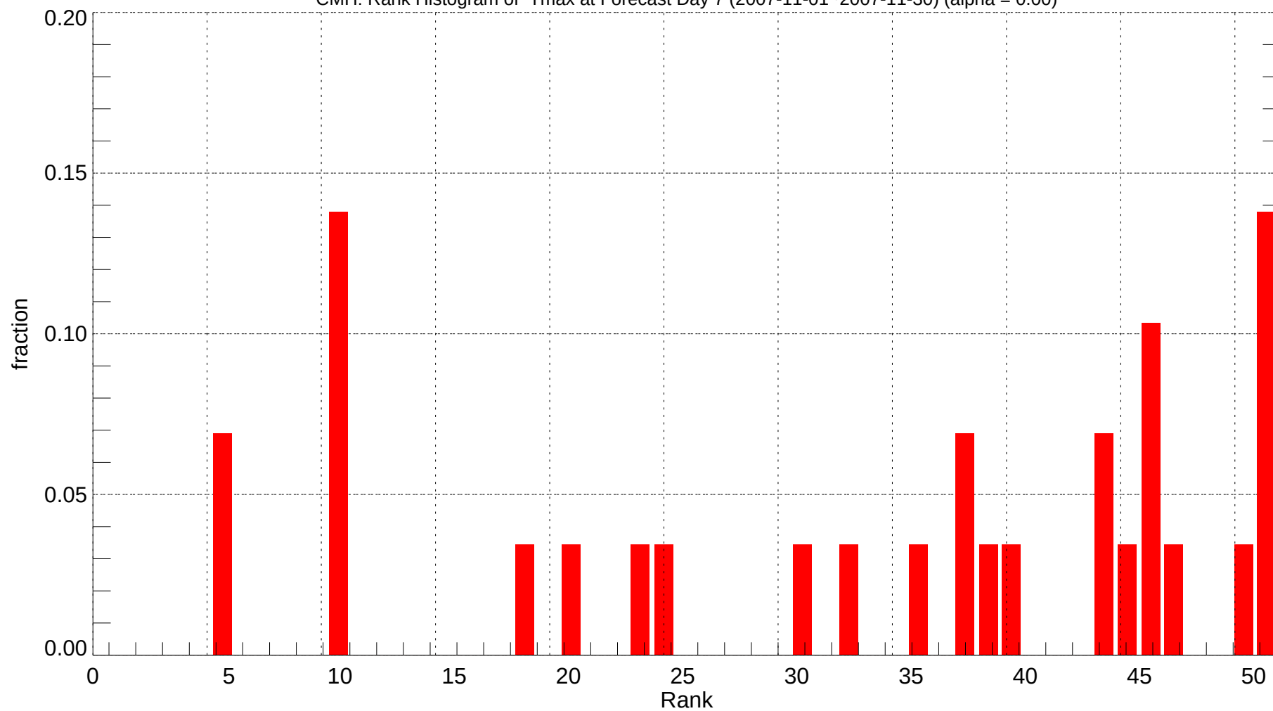
CMH: Rank Histogram of Tmax at Forecast Day 7 (2007-11-01~2007-11-30) (alpha = 0.00)
