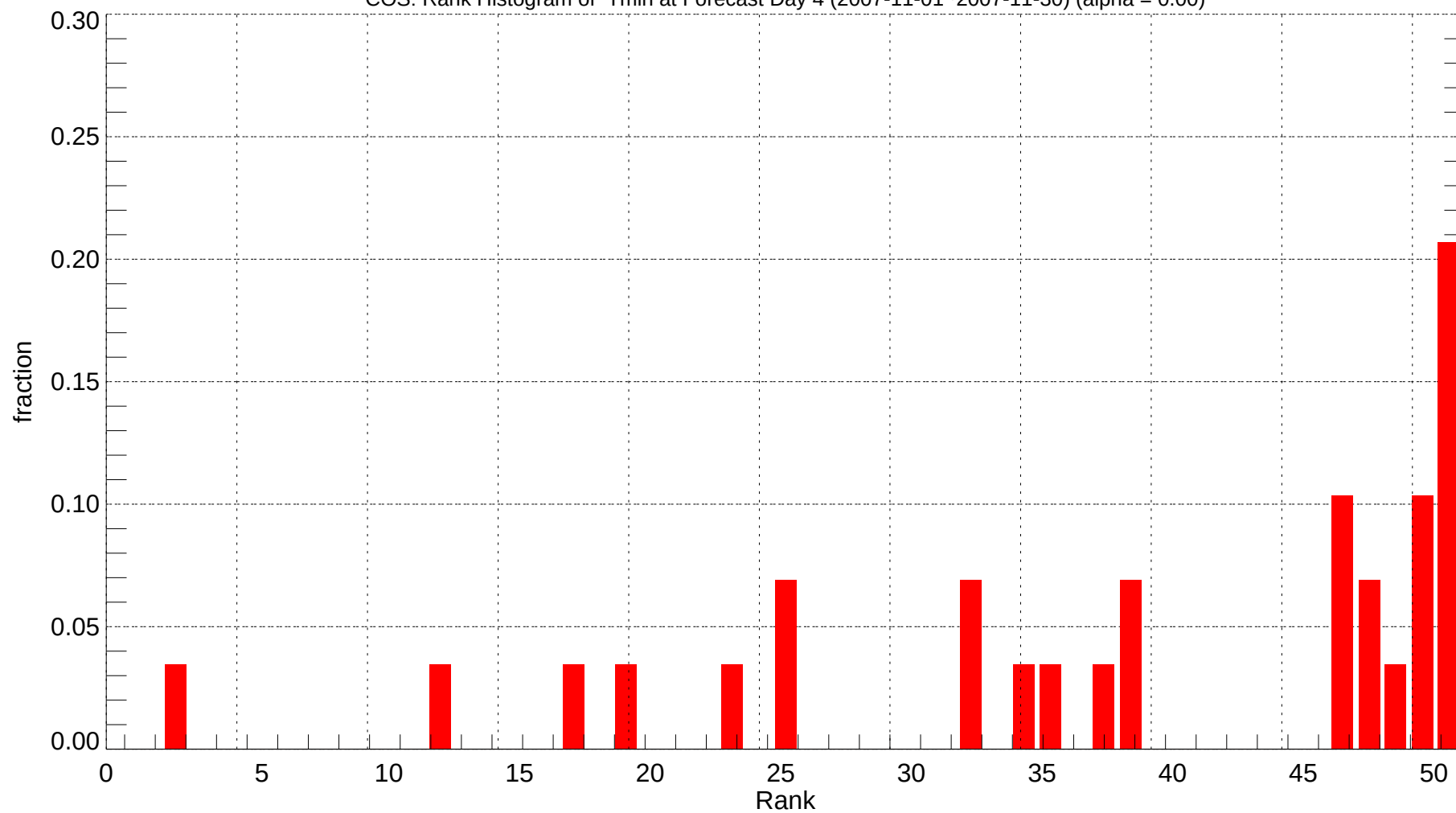
COS: Rank Histogram of Tmin at Forecast Day 4 (2007-11-01~2007-11-30) (alpha = 0.00)
