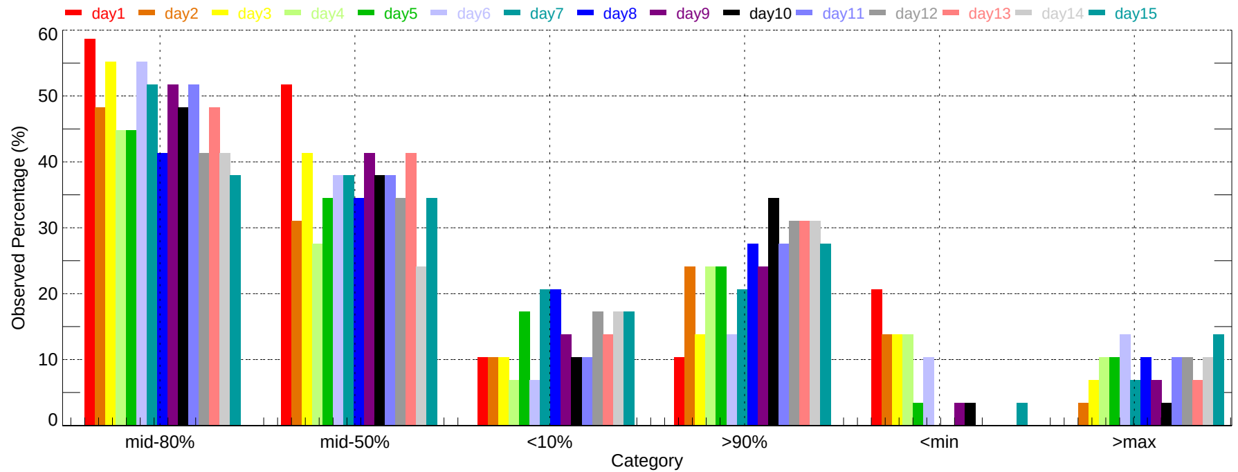
Observed Percentage of Ensembles - MAF: Max Temperature (2007-11-01~2007-11-30)
