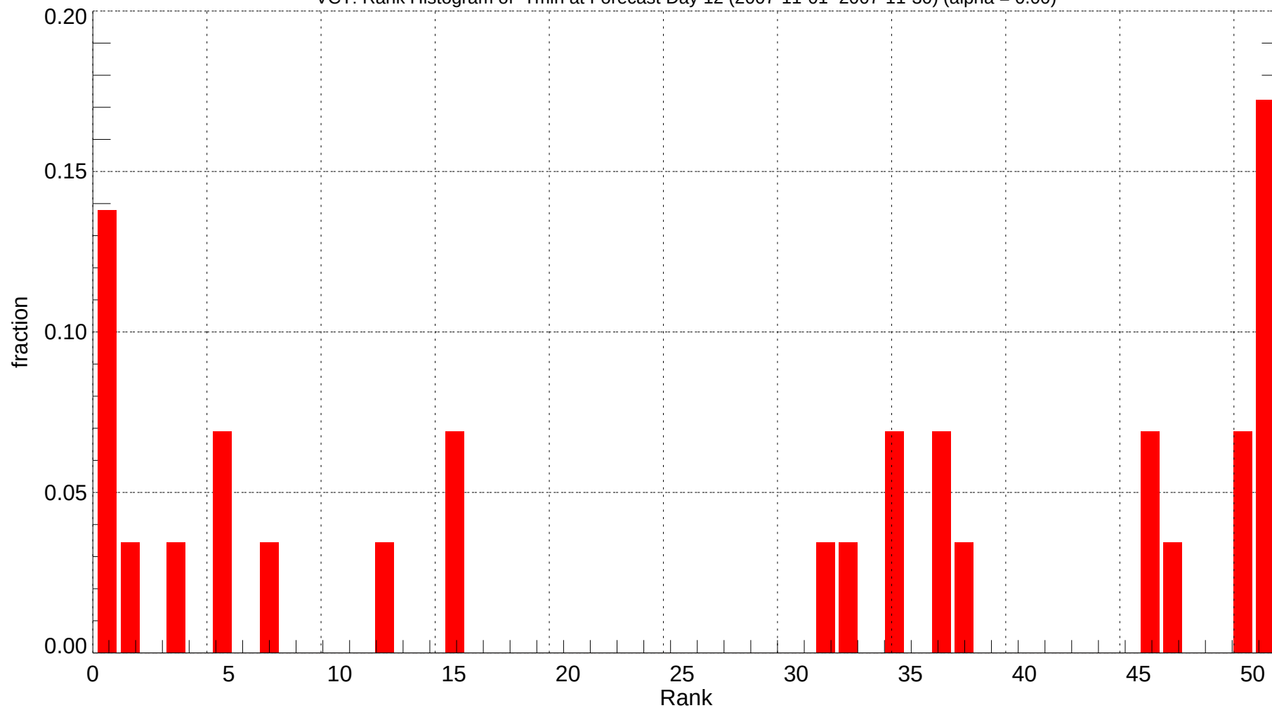
VCT: Rank Histogram of Tmin at Forecast Day 12 (2007-11-01~2007-11-30) (alpha = 0.00)
