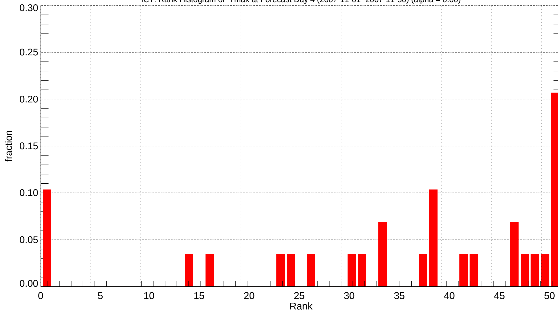
ICT: Rank Histogram of Tmax at Forecast Day 4 (2007-11-01~2007-11-30) (alpha = 0.00)
