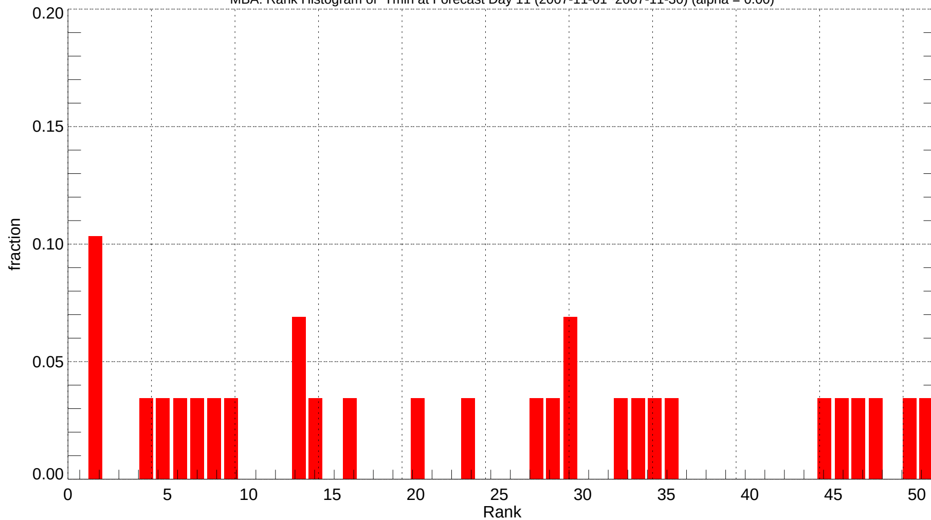
MBA: Rank Histogram of Tmin at Forecast Day 11 (2007-11-01~2007-11-30) (alpha = 0.00)
