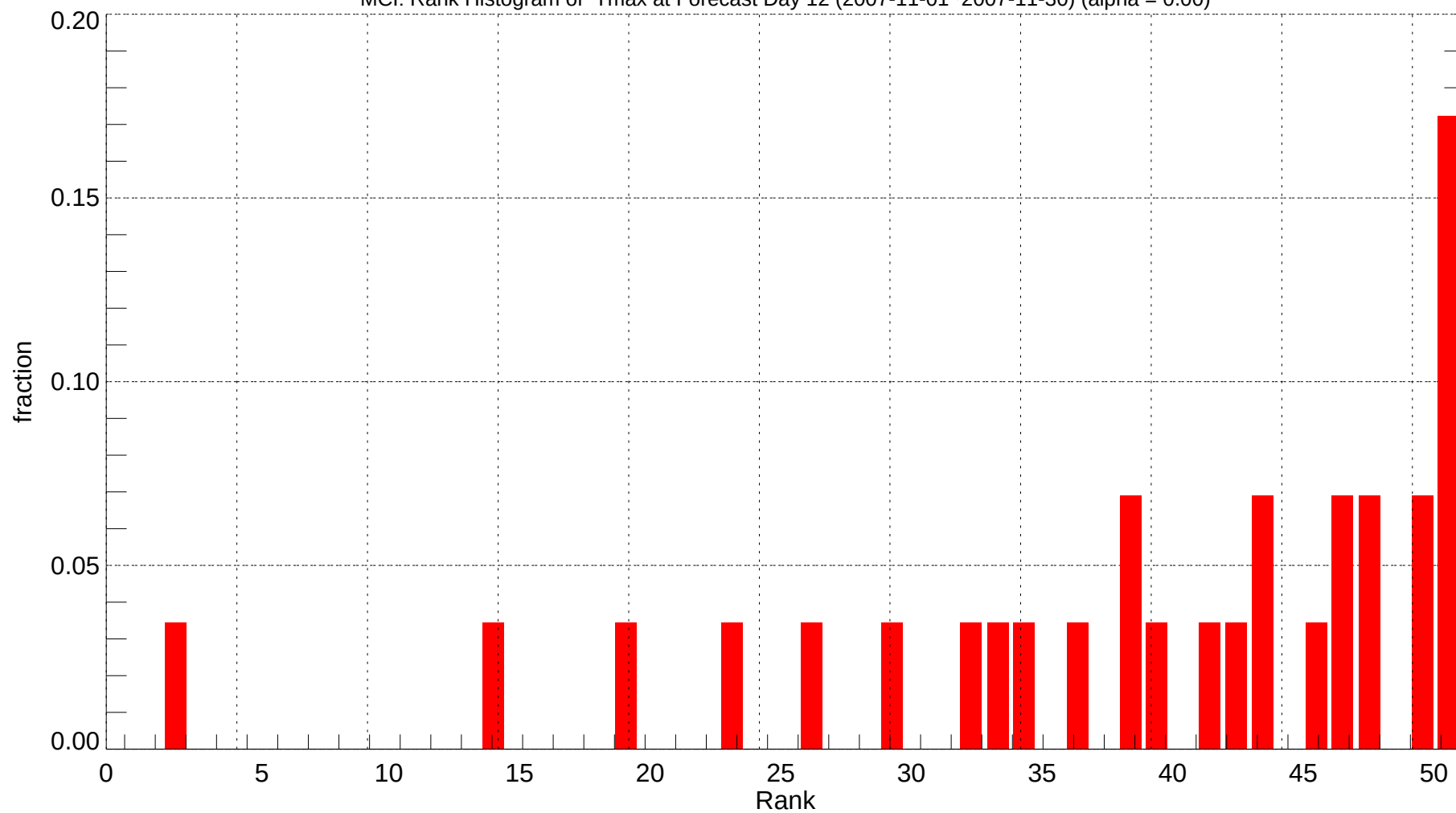
MCI: Rank Histogram of Tmax at Forecast Day 12 (2007-11-01~2007-11-30) (alpha = 0.00)
