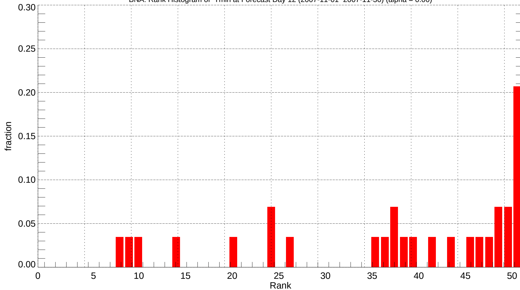
BNA: Rank Histogram of Tmin at Forecast Day 12 (2007-11-01~2007-11-30) (alpha = 0.00)
