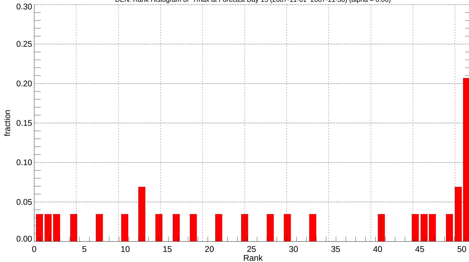
DEN: Rank Histogram of Tmax at Forecast Day 15 (2007-11-01~2007-11-30) (alpha = 0.00)
