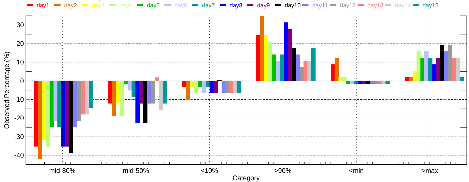
Observed Percentage Deviation of Ensembles - OKC: Max Temperature (2007-11-01~2007-11-30)
