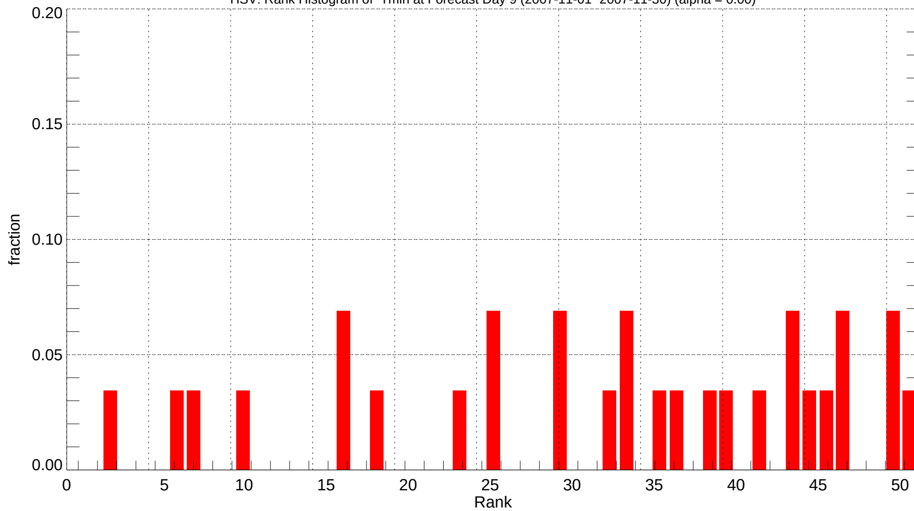
HSV: Rank Histogram of Tmin at Forecast Day 9 (2007-11-01~2007-11-30) (alpha = 0.00)
