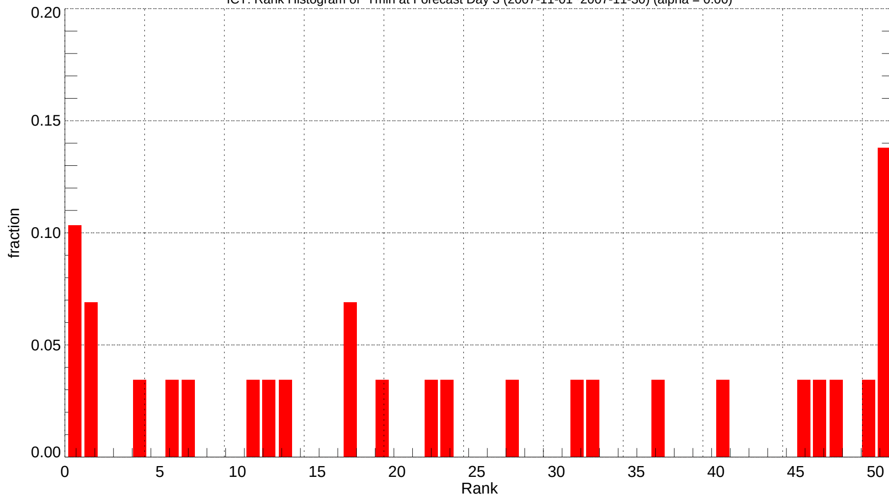
ICT: Rank Histogram of Tmin at Forecast Day 3 (2007-11-01~2007-11-30) (alpha = 0.00)
