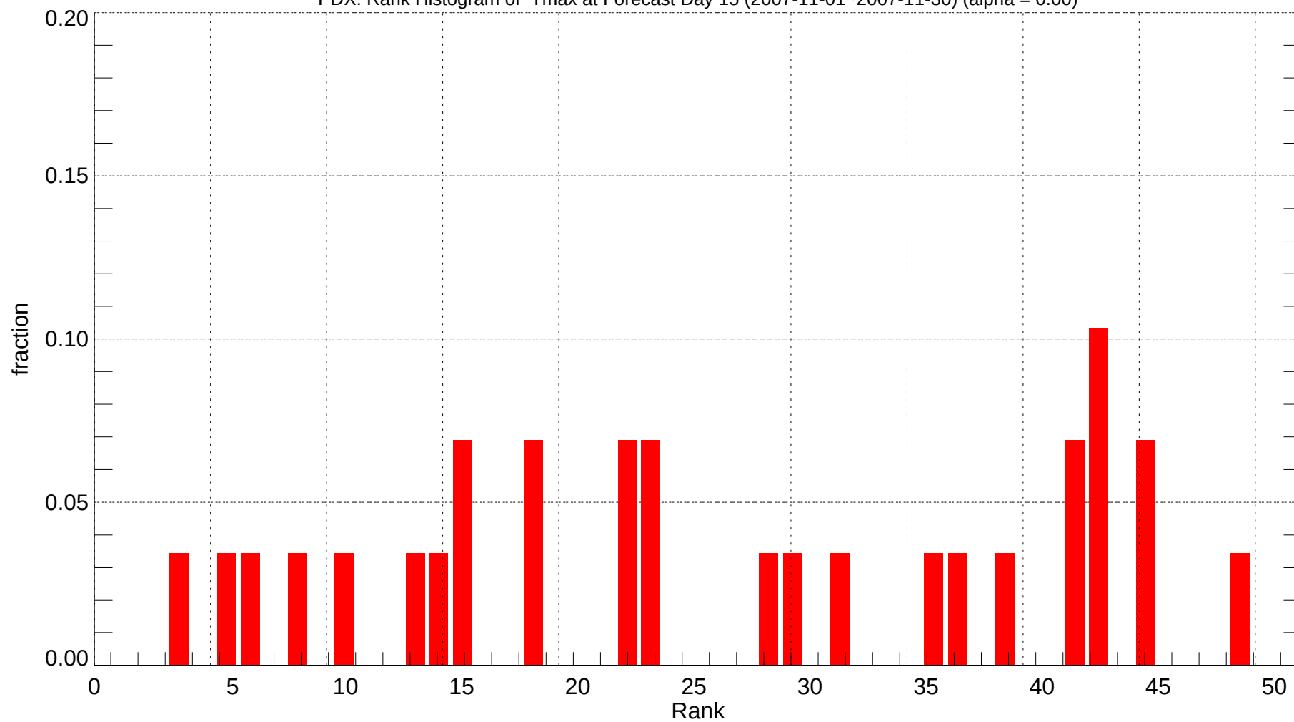
PDX: Rank Histogram of Tmax at Forecast Day 15 (2007-11-01~2007-11-30) (alpha = 0.00)
