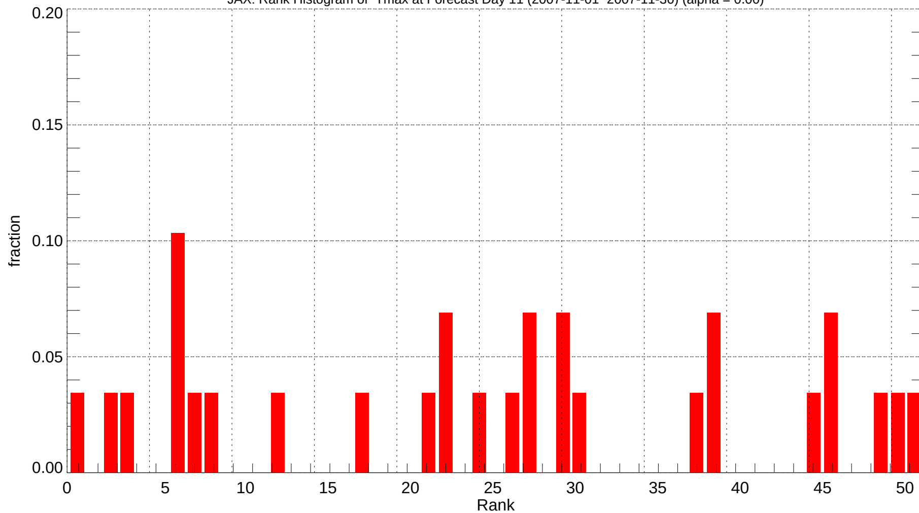
JAX: Rank Histogram of Tmax at Forecast Day 11 (2007-11-01~2007-11-30) (alpha = 0.00)
