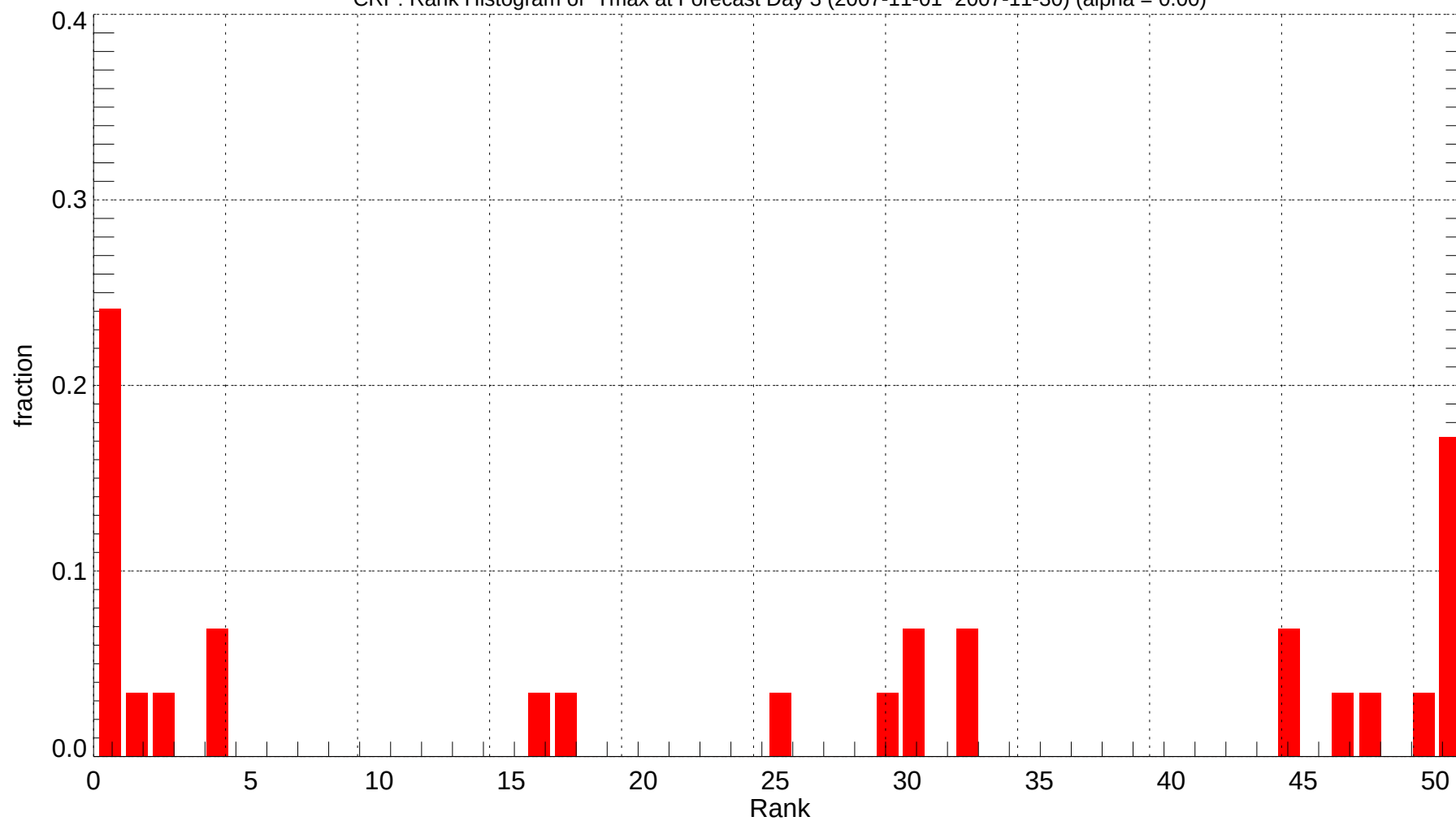
CRP: Rank Histogram of Tmax at Forecast Day 3 (2007-11-01~2007-11-30) (alpha = 0.00)
