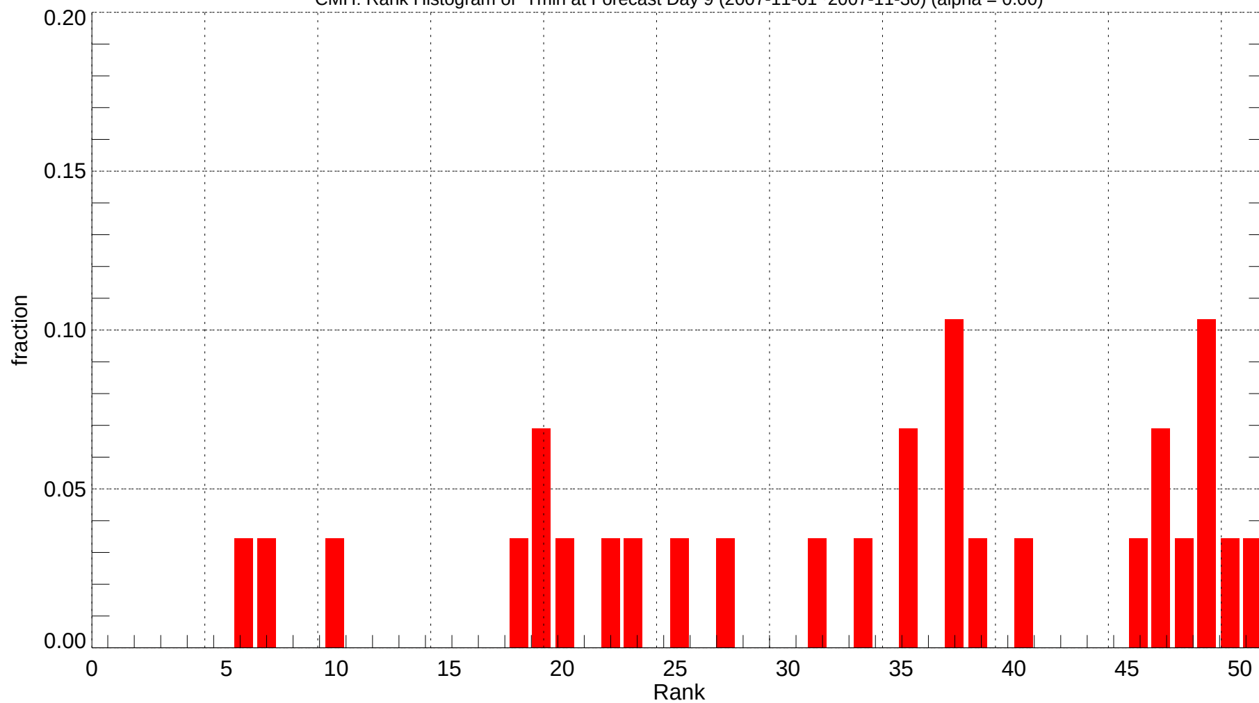
CMH: Rank Histogram of Tmin at Forecast Day 9 (2007-11-01~2007-11-30) (alpha = 0.00)
