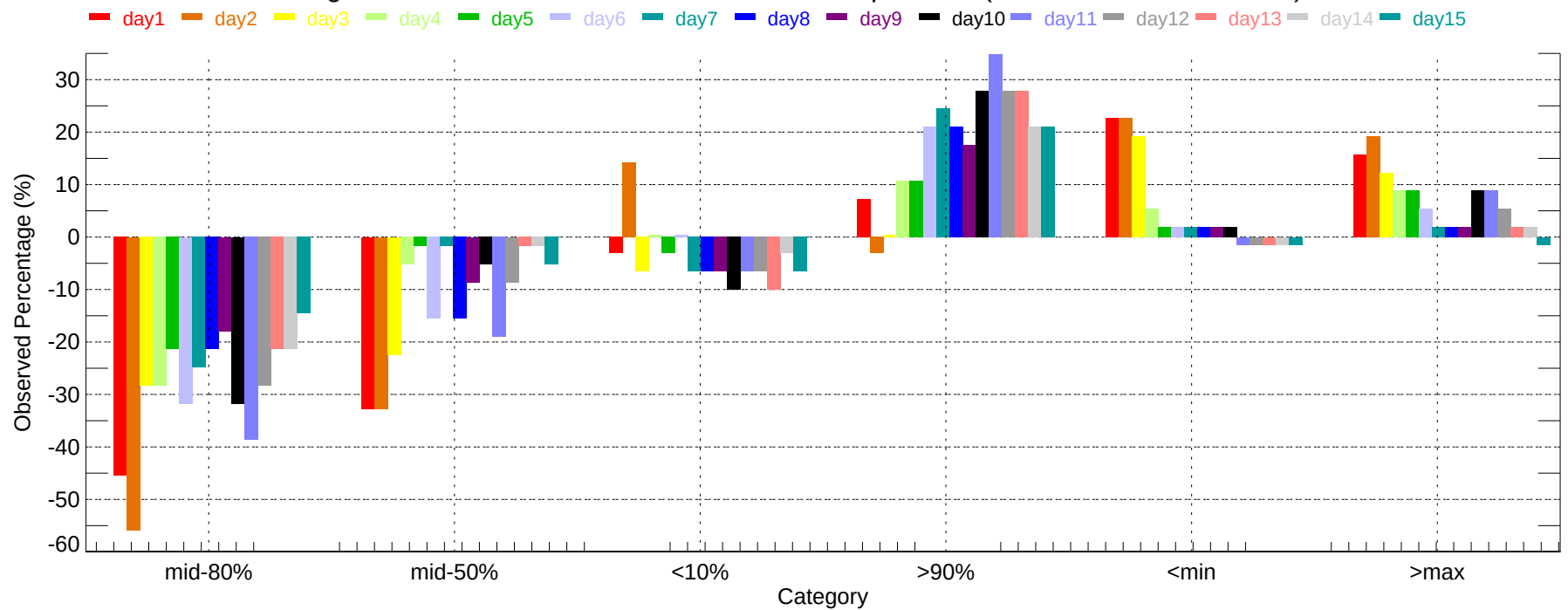
Observed Percentage Deviation of Ensembles - DLH: Max Temperature (2007-11-01~2007-11-30)
