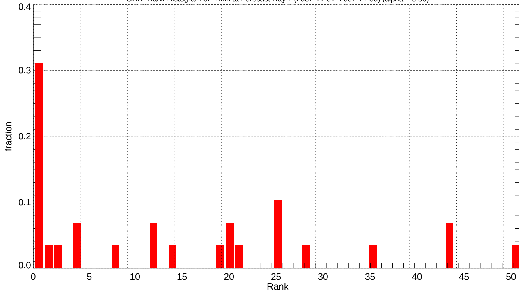
ORD: Rank Histogram of Tmin at Forecast Day 1 (2007-11-01~2007-11-30) (alpha = 0.00)
