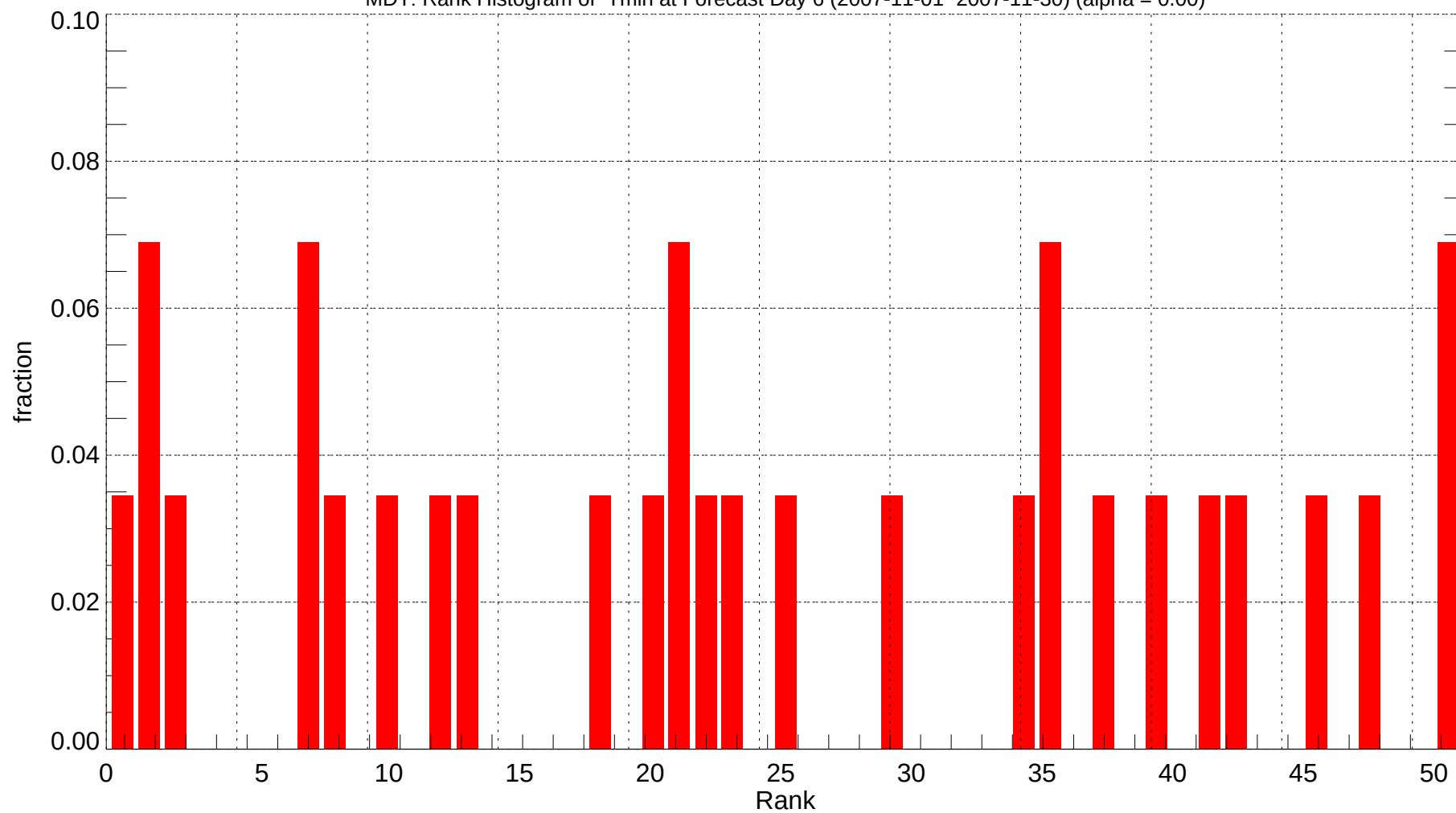
MDT: Rank Histogram of Tmin at Forecast Day 6 (2007-11-01~2007-11-30) (alpha = 0.00)
