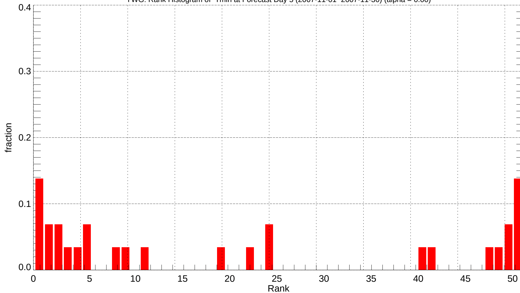
YWG: Rank Histogram of Tmin at Forecast Day 5 (2007-11-01~2007-11-30) (alpha = 0.00)
