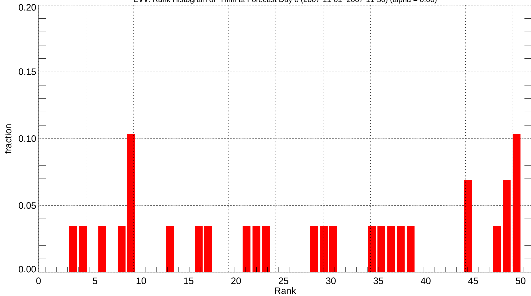
EVV: Rank Histogram of Tmin at Forecast Day 8 (2007-11-01~2007-11-30) (alpha = 0.00)
