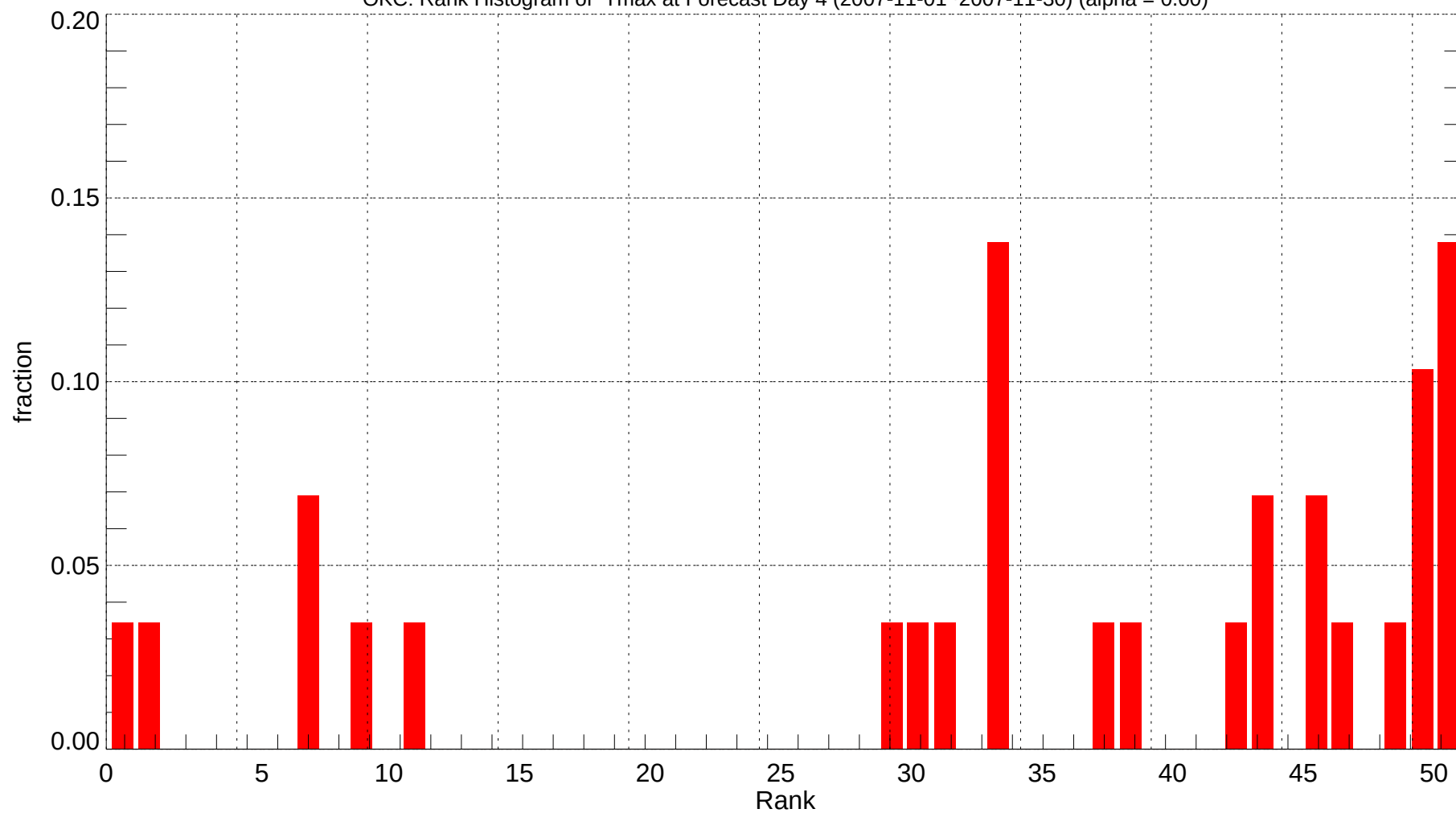
OKC: Rank Histogram of Tmax at Forecast Day 4 (2007-11-01~2007-11-30) (alpha = 0.00)
