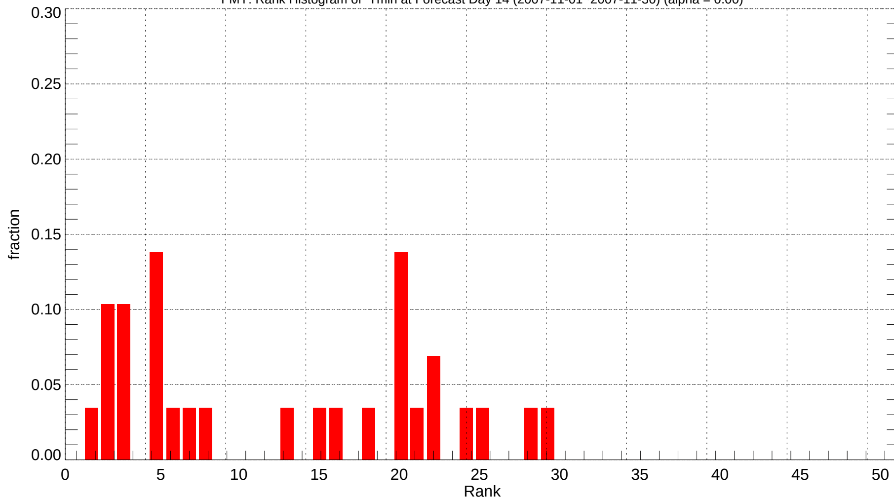
FMY: Rank Histogram of Tmin at Forecast Day 14 (2007-11-01~2007-11-30) (alpha = 0.00)
