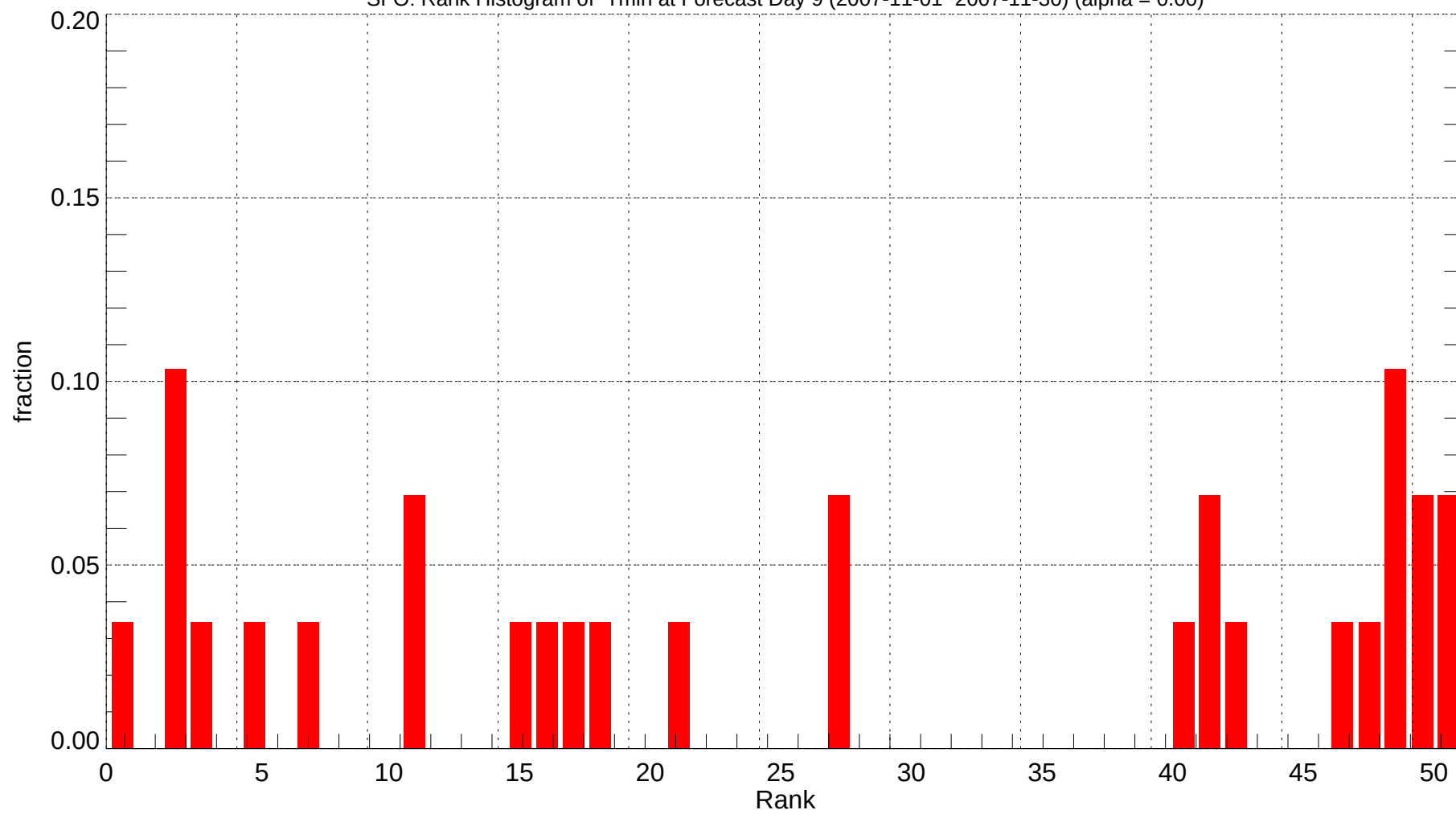
SFO: Rank Histogram of Tmin at Forecast Day 9 (2007-11-01~2007-11-30) (alpha = 0.00)
