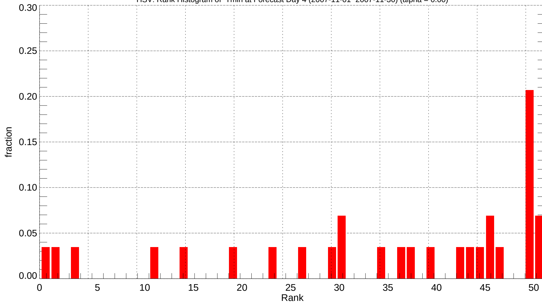
HSV: Rank Histogram of Tmin at Forecast Day 4 (2007-11-01~2007-11-30) (alpha = 0.00)
