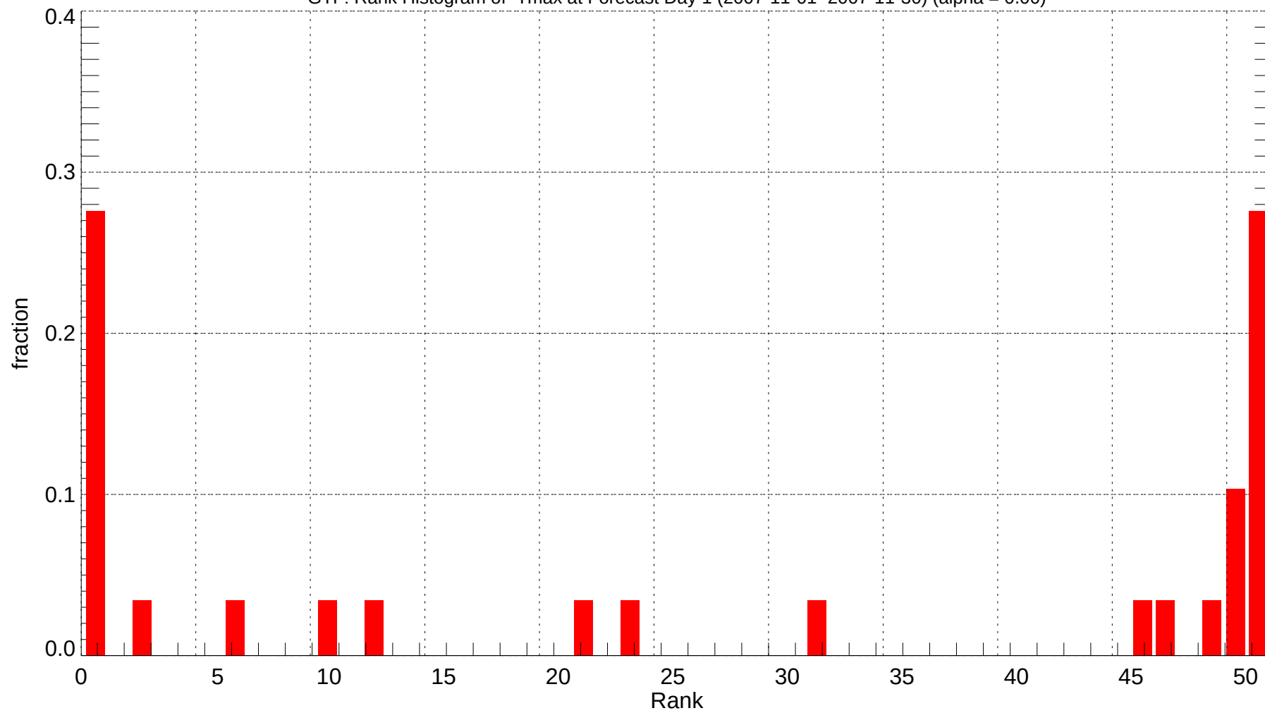
GTF: Rank Histogram of Tmax at Forecast Day 1 (2007-11-01~2007-11-30) (alpha = 0.00)
