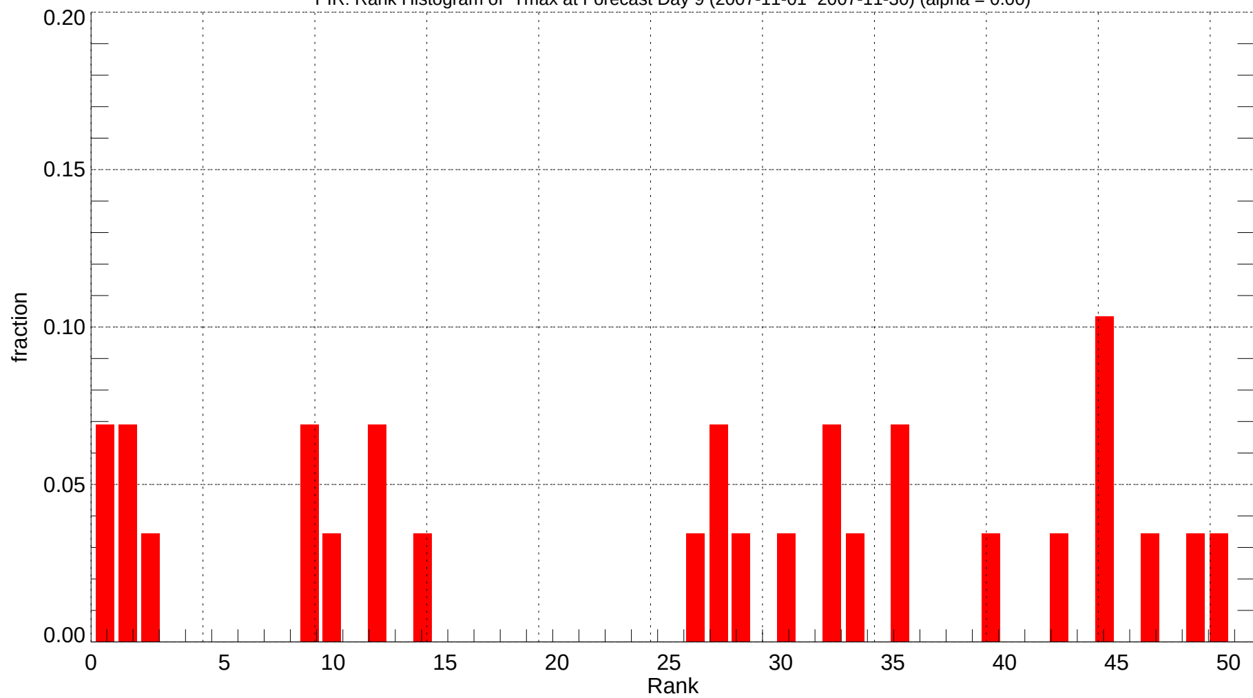
PIR: Rank Histogram of Tmax at Forecast Day 9 (2007-11-01~2007-11-30) (alpha = 0.00)
