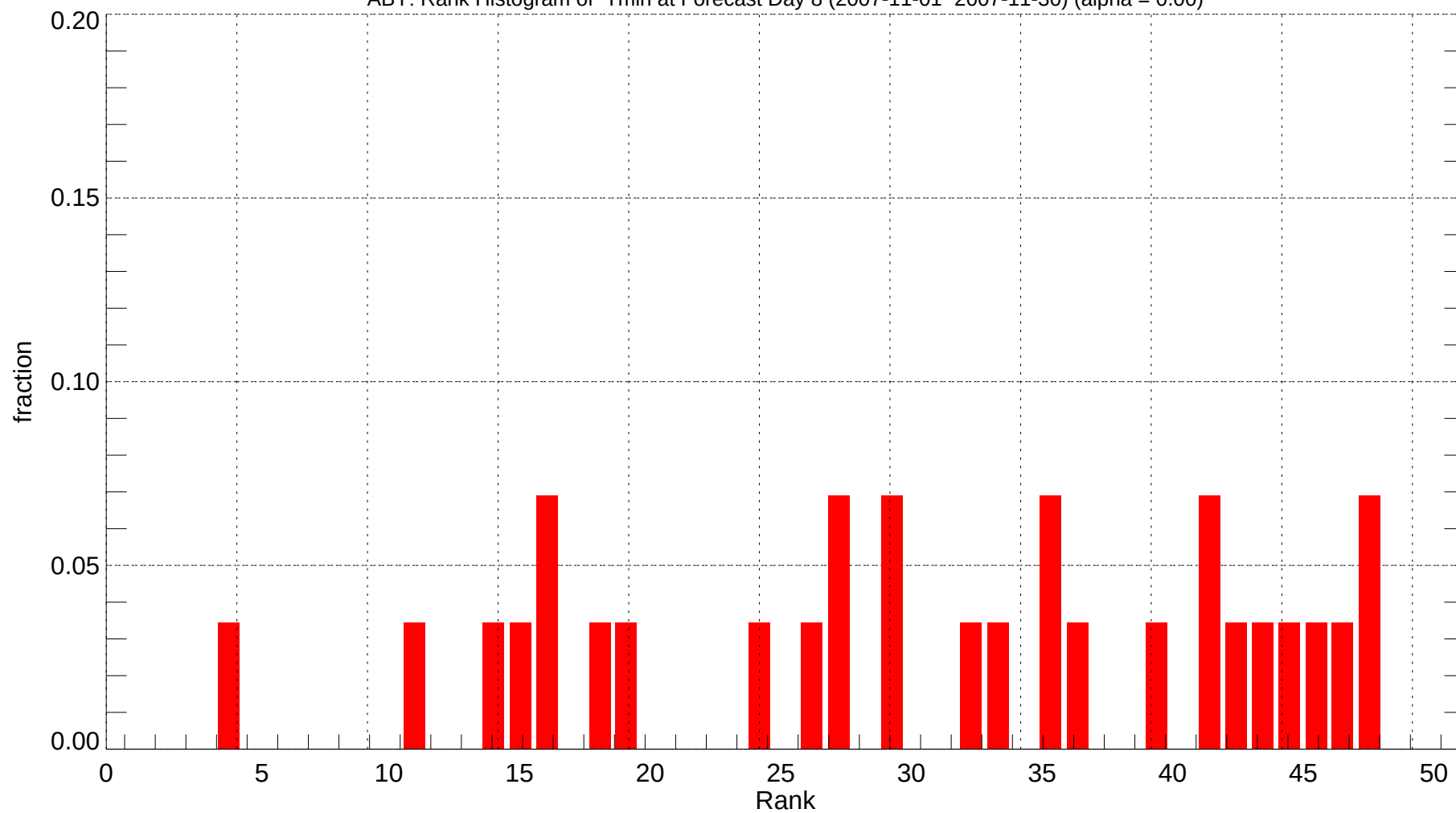
ABY: Rank Histogram of Tmin at Forecast Day 8 (2007-11-01~2007-11-30) (alpha = 0.00)
