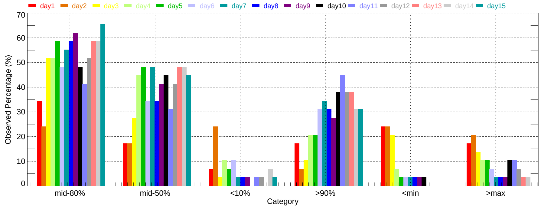
Observed Percentage of Ensembles - DLH: Max Temperature (2007-11-01~2007-11-30)
