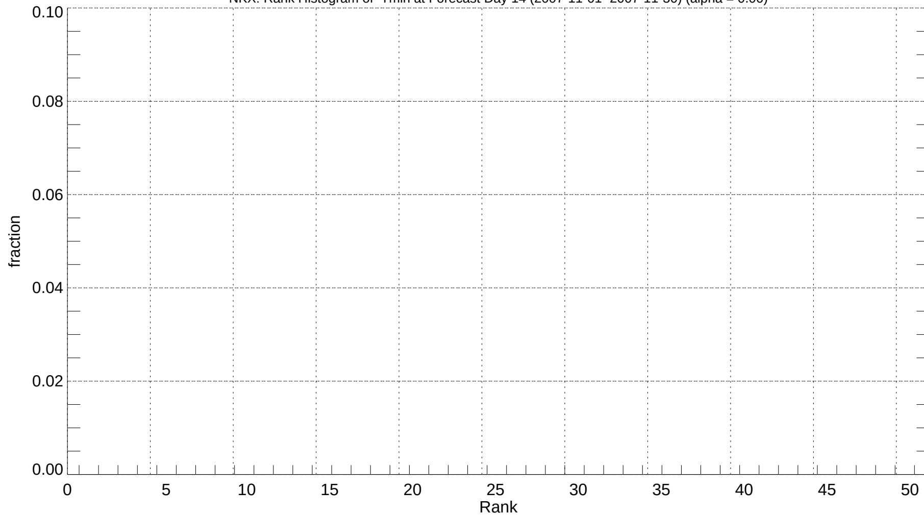
NKX: Rank Histogram of Tmin at Forecast Day 14 (2007-11-01~2007-11-30) (alpha = 0.00)
