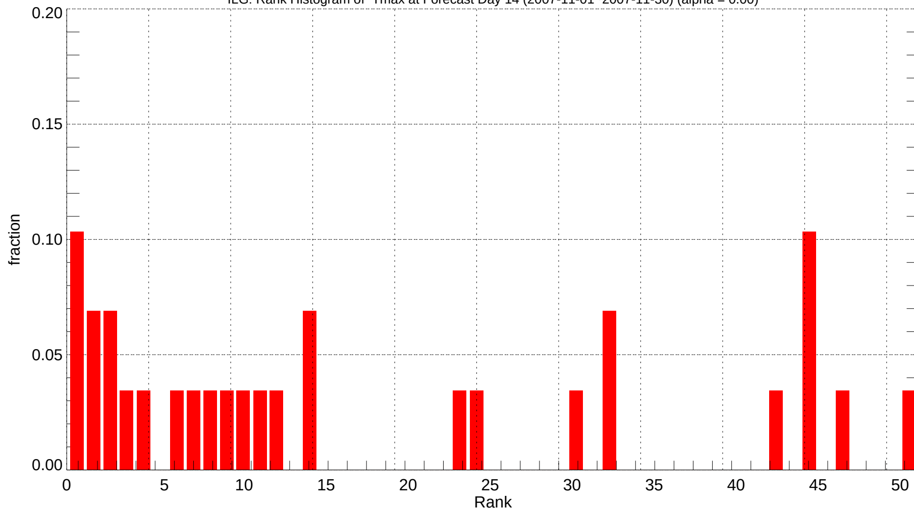
ILG: Rank Histogram of Tmax at Forecast Day 14 (2007-11-01~2007-11-30) (alpha = 0.00)
