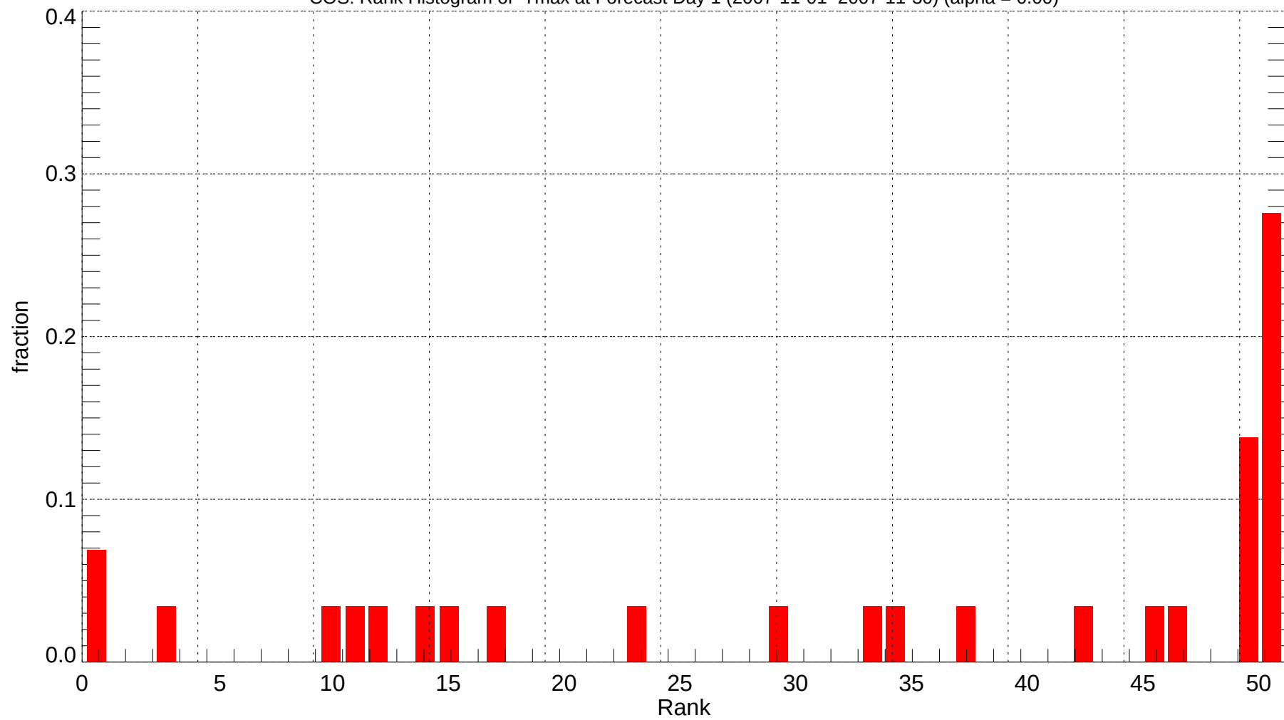
COS: Rank Histogram of Tmax at Forecast Day 1 (2007-11-01~2007-11-30) (alpha = 0.00)
