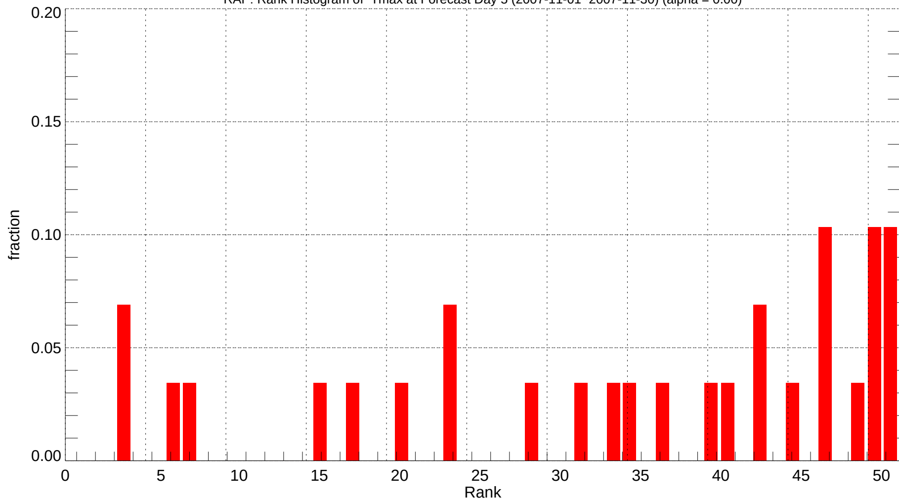
RAP: Rank Histogram of Tmax at Forecast Day 5 (2007-11-01~2007-11-30) (alpha = 0.00)
