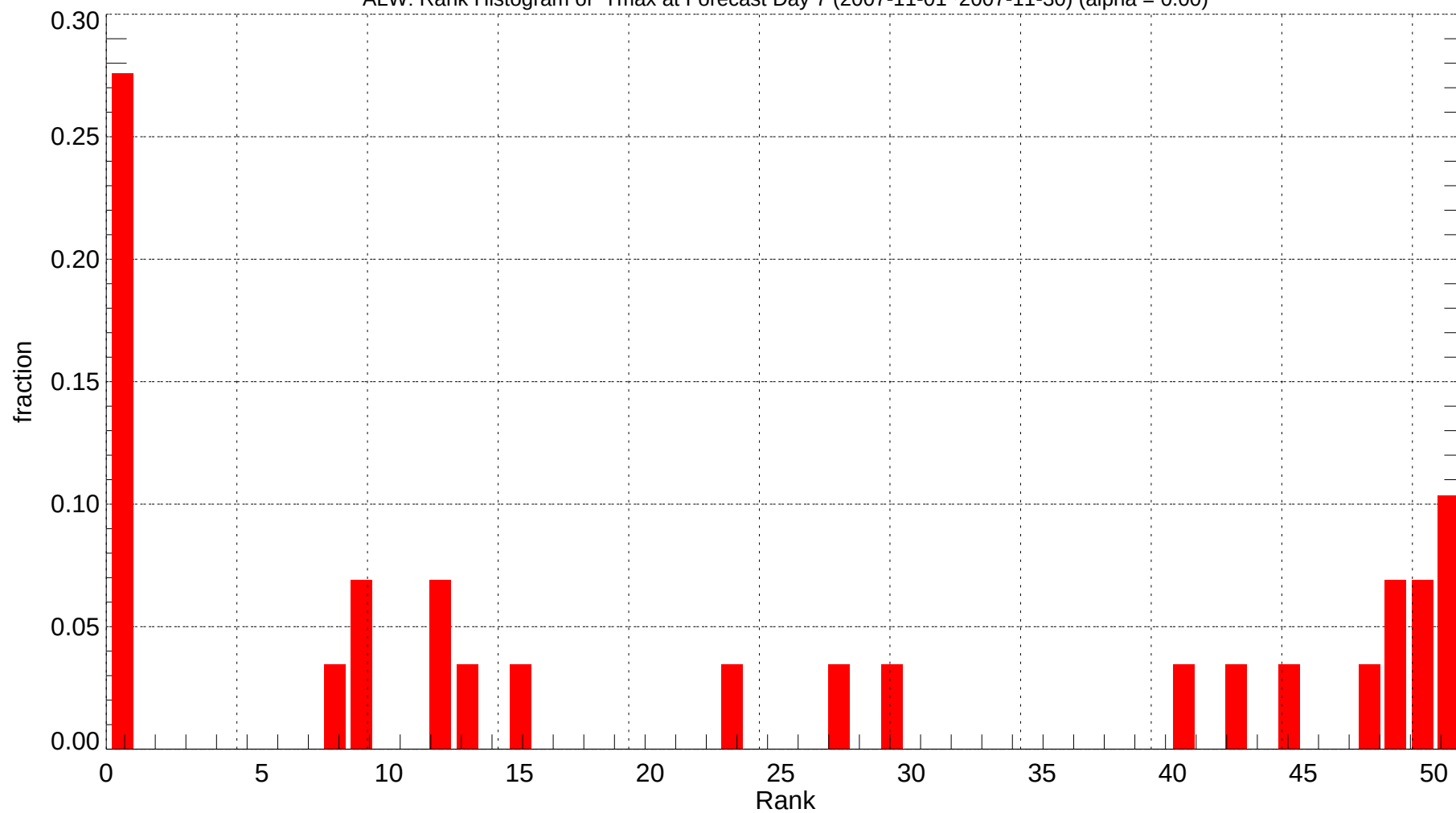
ALW: Rank Histogram of Tmax at Forecast Day 7 (2007-11-01~2007-11-30) (alpha = 0.00)
