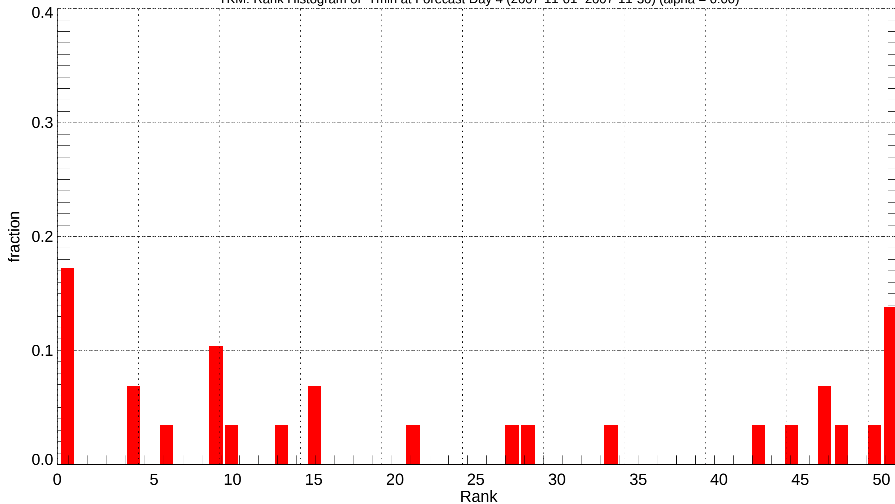
YKM: Rank Histogram of Tmin at Forecast Day 4 (2007-11-01~2007-11-30) (alpha = 0.00)
