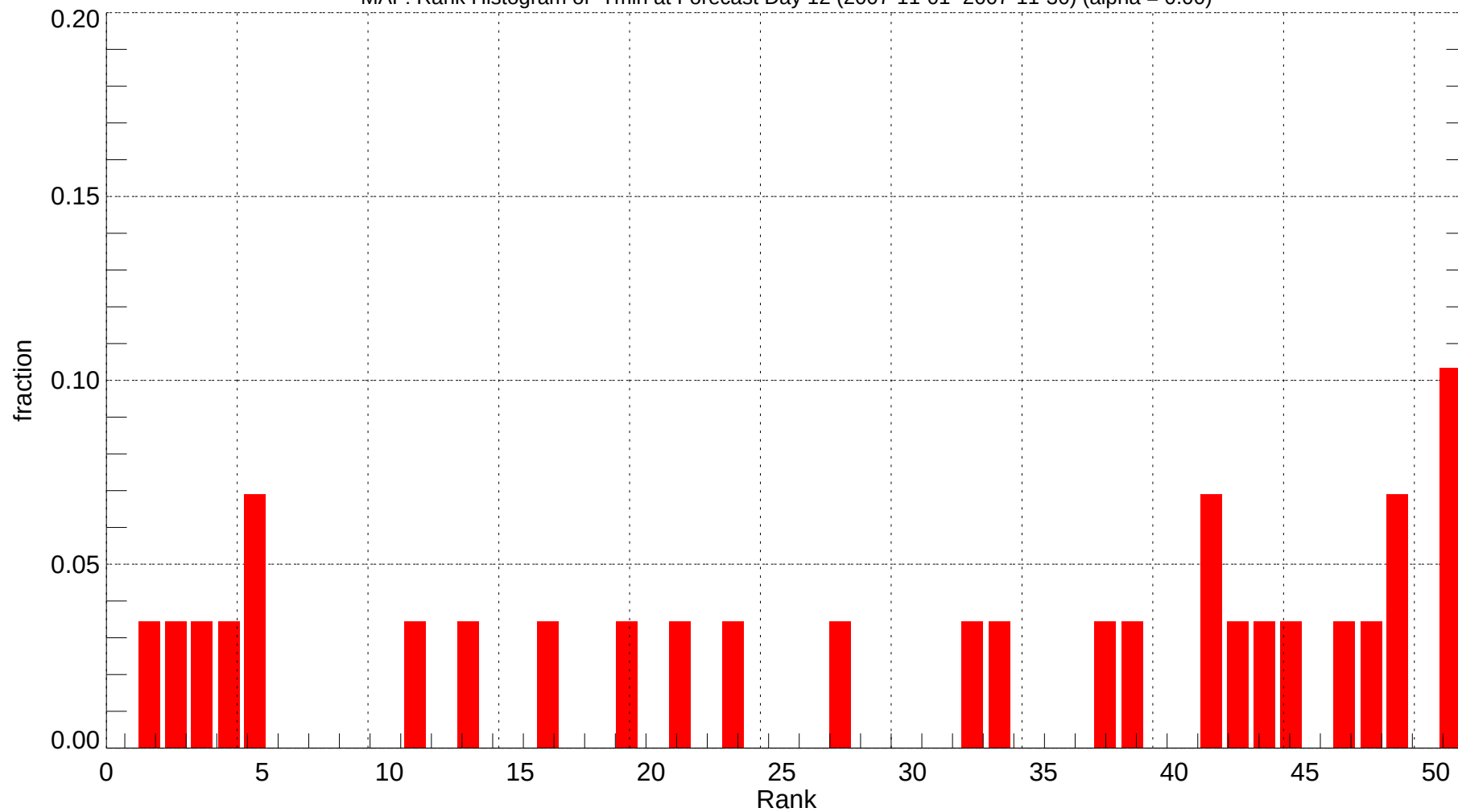
MAF: Rank Histogram of Tmin at Forecast Day 12 (2007-11-01~2007-11-30) (alpha = 0.00)
