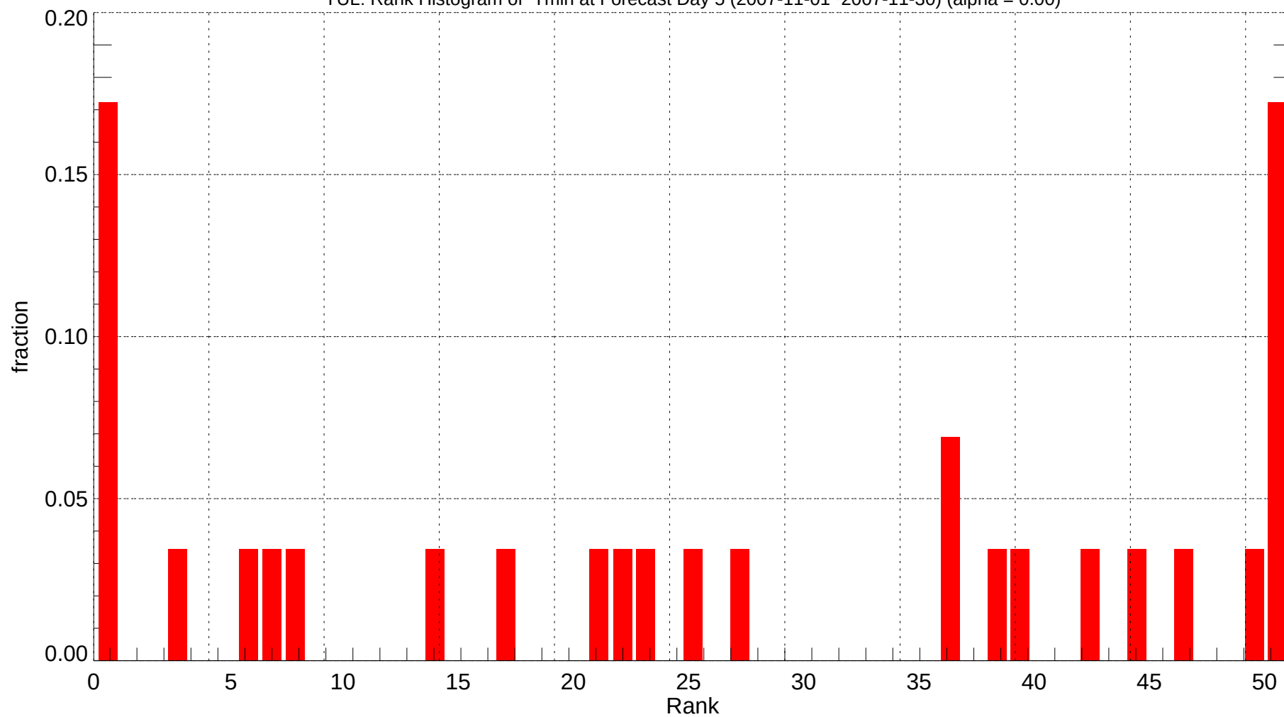
YUL: Rank Histogram of Tmin at Forecast Day 5 (2007-11-01~2007-11-30) (alpha = 0.00)
