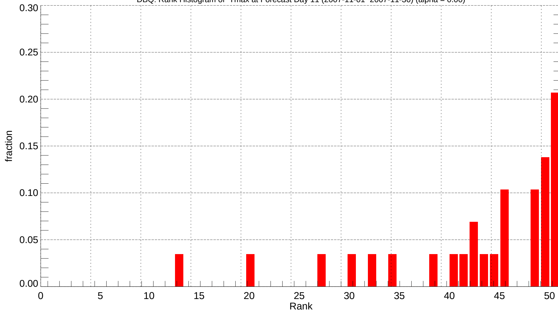
DBQ: Rank Histogram of Tmax at Forecast Day 11 (2007-11-01~2007-11-30) (alpha = 0.00)
