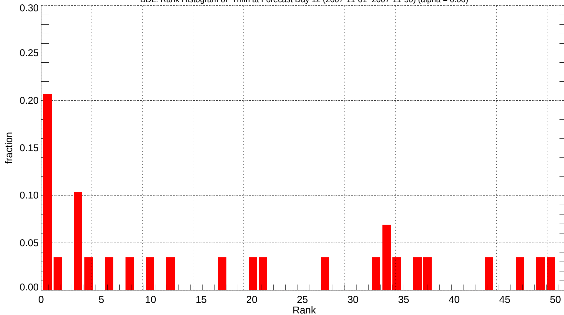
BDL: Rank Histogram of Tmin at Forecast Day 12 (2007-11-01~2007-11-30) (alpha = 0.00)
