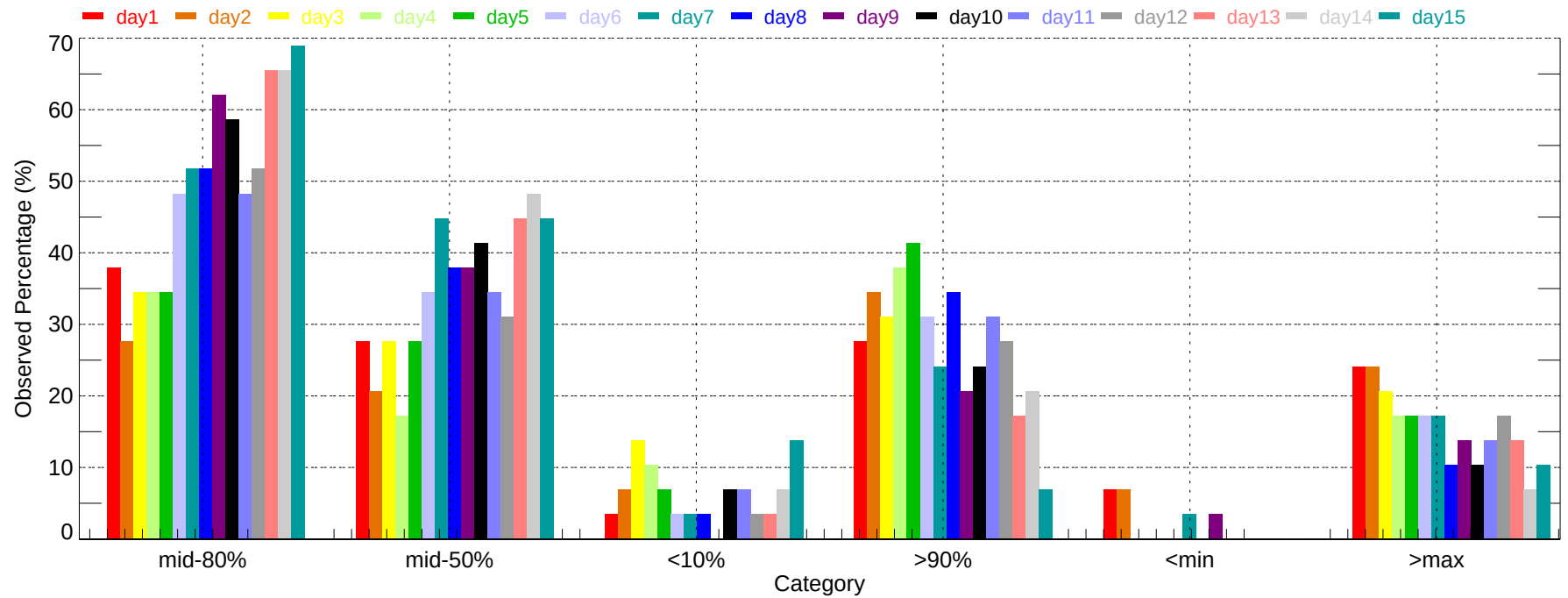
Observed Percentage of Ensembles - ROA: Max Temperature (2007-11-01~2007-11-30)
