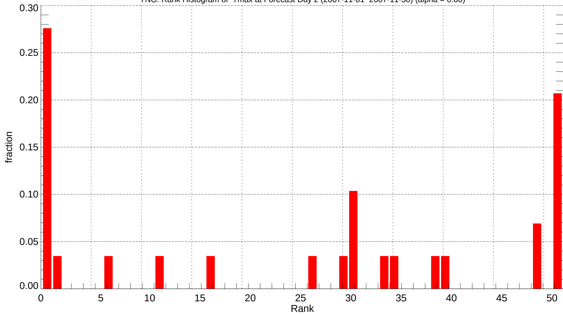
YNG: Rank Histogram of Tmax at Forecast Day 2 (2007-11-01~2007-11-30) (alpha = 0.00)
