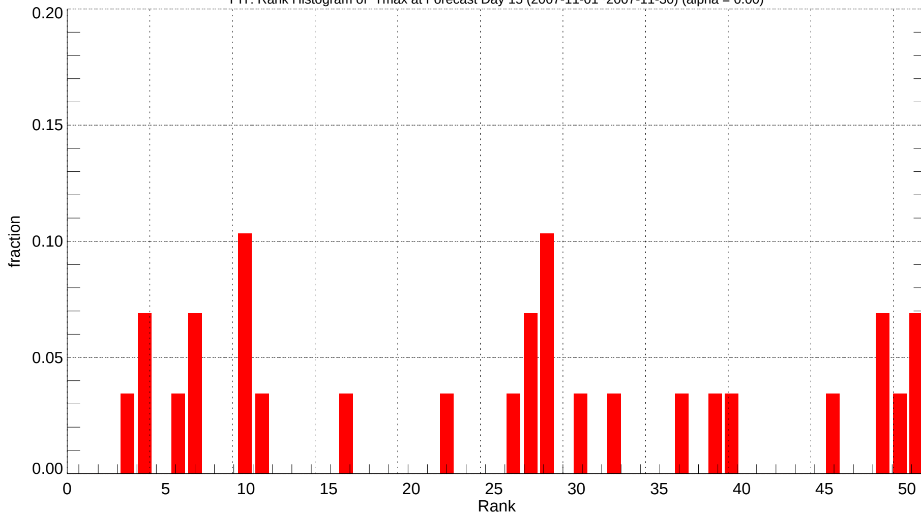
PIT: Rank Histogram of Tmax at Forecast Day 15 (2007-11-01~2007-11-30) (alpha = 0.00)
