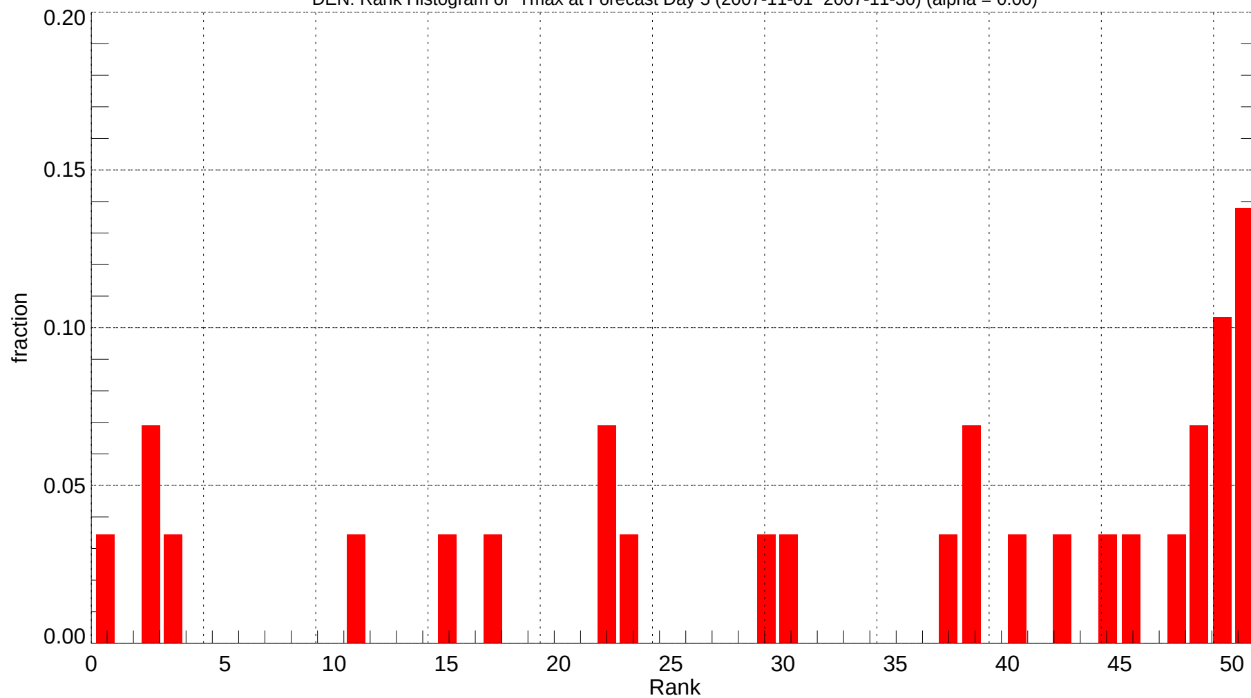
DEN: Rank Histogram of Tmax at Forecast Day 5 (2007-11-01~2007-11-30) (alpha = 0.00)
