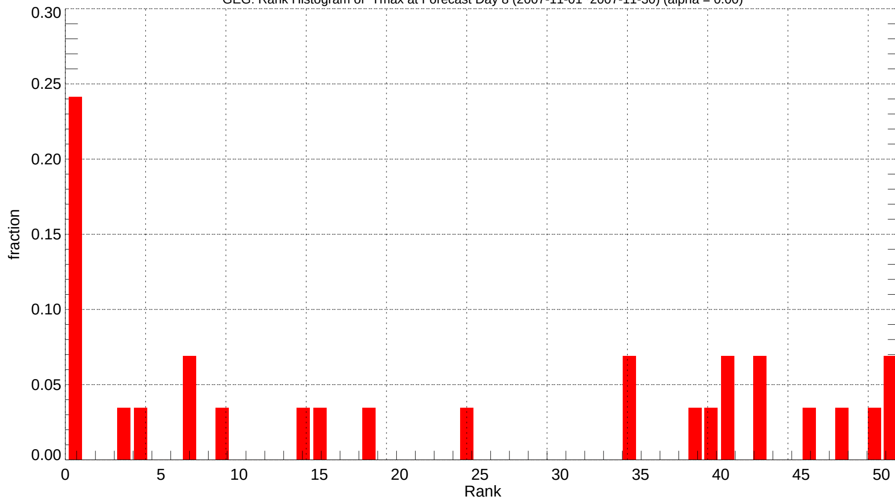
GEG: Rank Histogram of Tmax at Forecast Day 8 (2007-11-01~2007-11-30) (alpha = 0.00)
