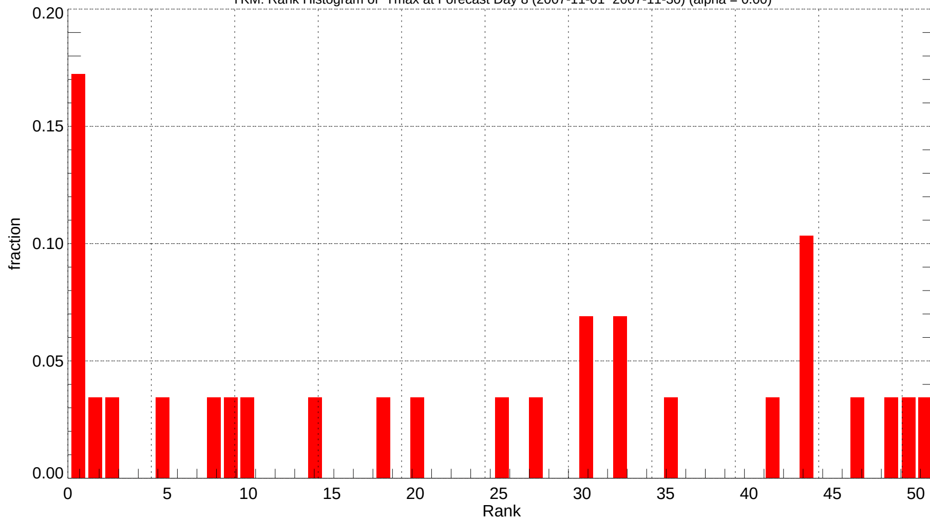
YKM: Rank Histogram of Tmax at Forecast Day 8 (2007-11-01~2007-11-30) (alpha = 0.00)
