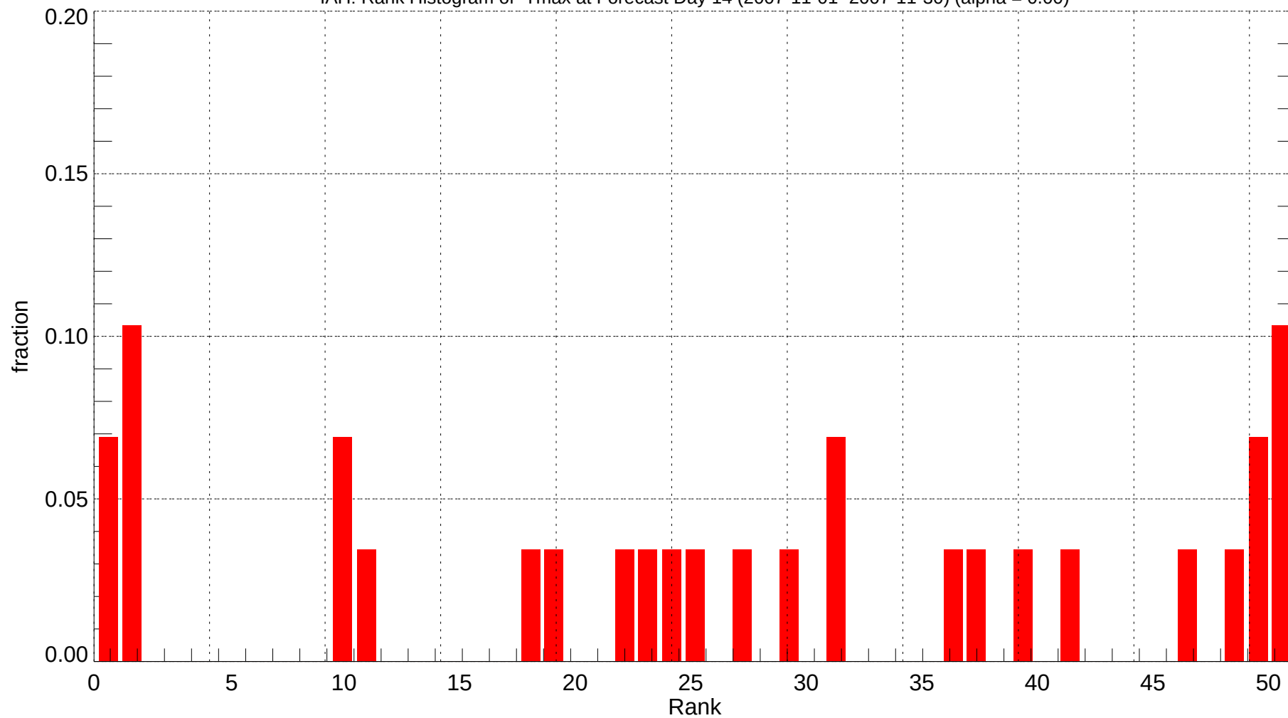
IAH: Rank Histogram of Tmax at Forecast Day 14 (2007-11-01~2007-11-30) (alpha = 0.00)
