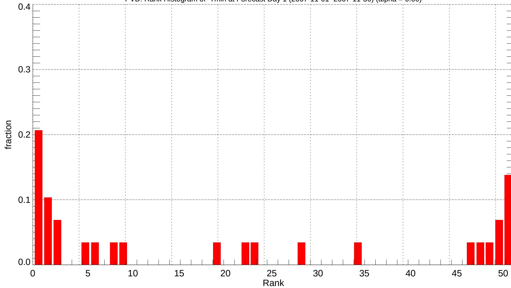
PVD: Rank Histogram of Tmin at Forecast Day 1 (2007-11-01~2007-11-30) (alpha = 0.00)
