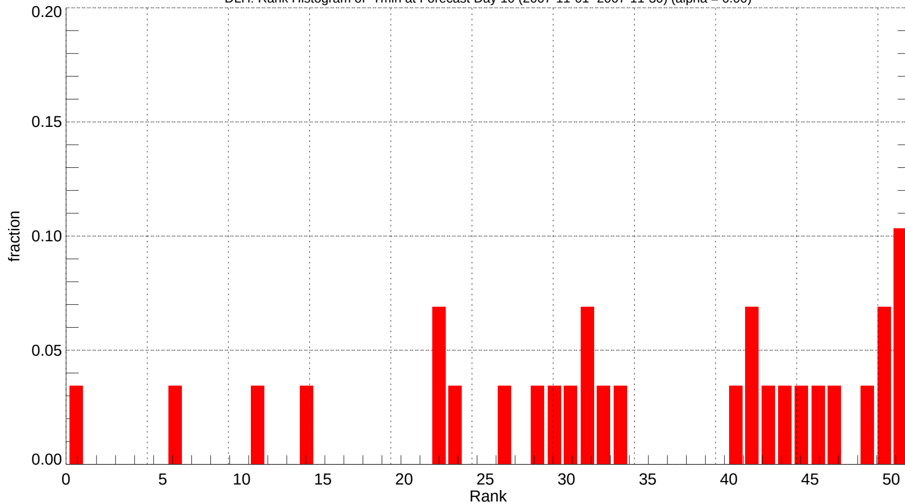
DLH: Rank Histogram of Tmin at Forecast Day 10 (2007-11-01~2007-11-30) (alpha = 0.00)
