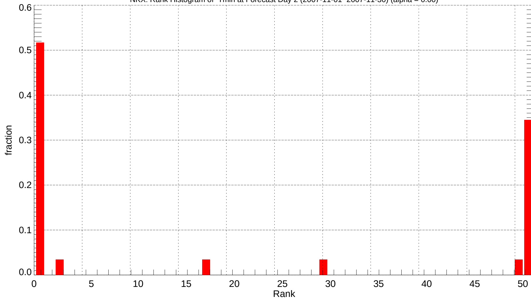
NKX: Rank Histogram of Tmin at Forecast Day 2 (2007-11-01~2007-11-30) (alpha = 0.00)
