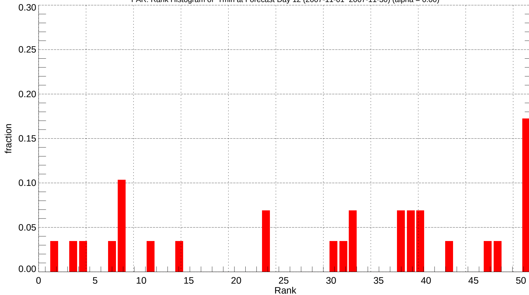
FAR: Rank Histogram of Tmin at Forecast Day 12 (2007-11-01~2007-11-30) (alpha = 0.00)
