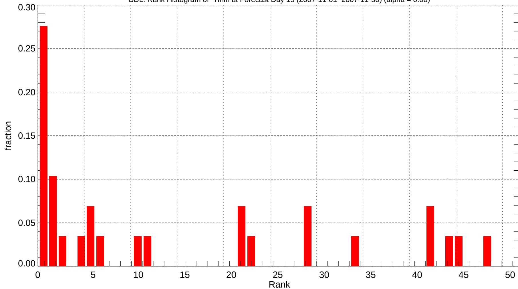
BDL: Rank Histogram of Tmin at Forecast Day 15 (2007-11-01~2007-11-30) (alpha = 0.00)
