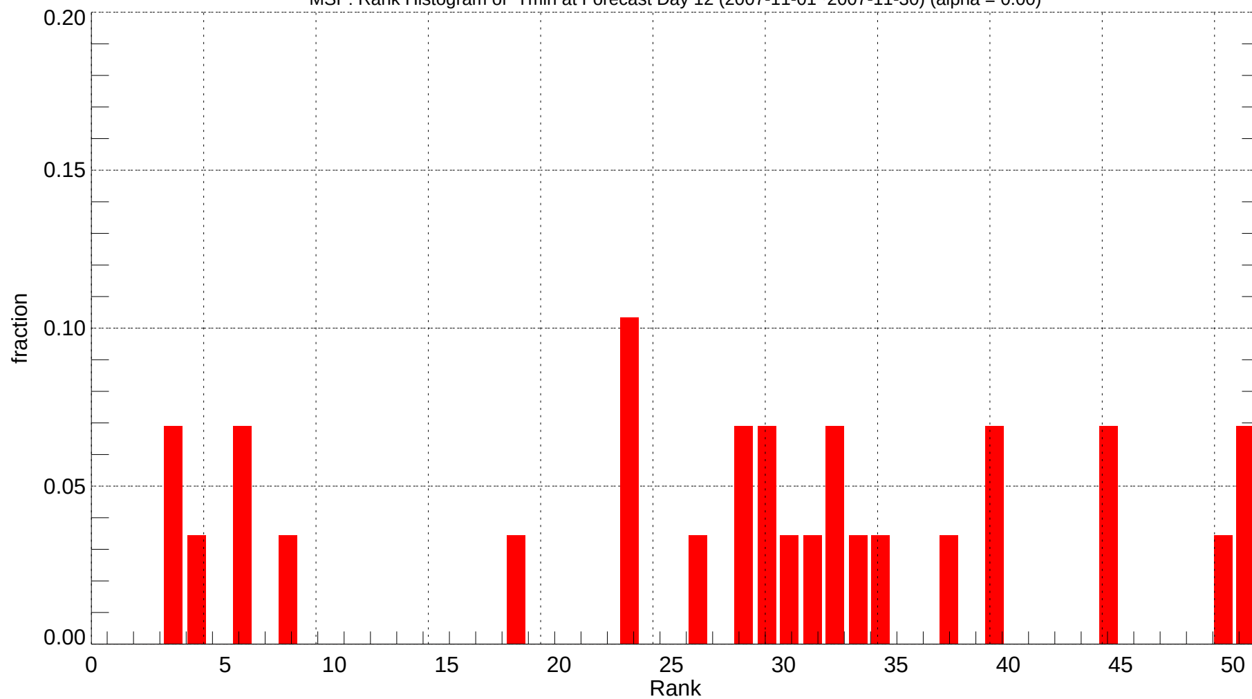
MSP: Rank Histogram of Tmin at Forecast Day 12 (2007-11-01~2007-11-30) (alpha = 0.00)
