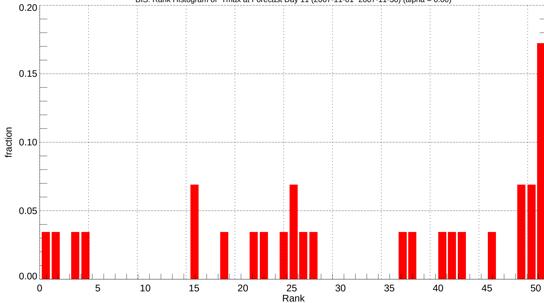
BIS: Rank Histogram of Tmax at Forecast Day 11 (2007-11-01~2007-11-30) (alpha = 0.00)
