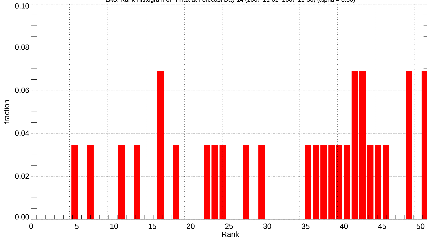
LAS: Rank Histogram of Tmax at Forecast Day 14 (2007-11-01~2007-11-30) (alpha = 0.00)
