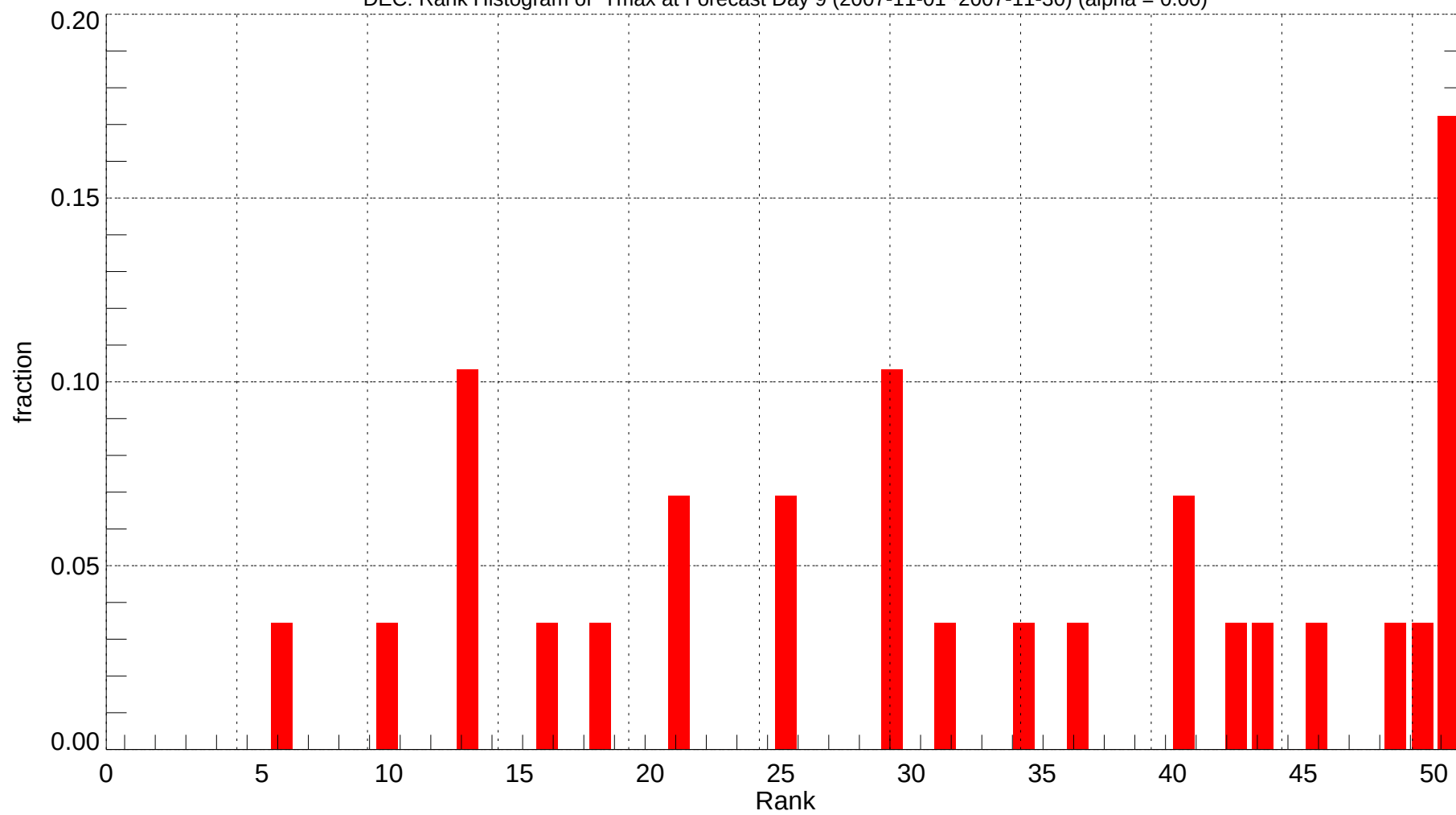
DEC: Rank Histogram of Tmax at Forecast Day 9 (2007-11-01~2007-11-30) (alpha = 0.00)
