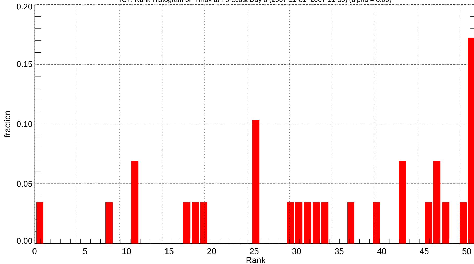
ICT: Rank Histogram of Tmax at Forecast Day 8 (2007-11-01~2007-11-30) (alpha = 0.00)
