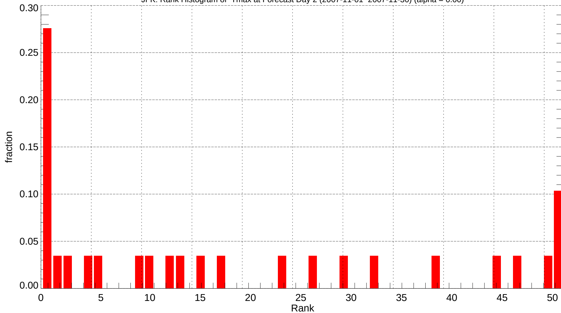
JFK: Rank Histogram of Tmax at Forecast Day 2 (2007-11-01~2007-11-30) (alpha = 0.00)
