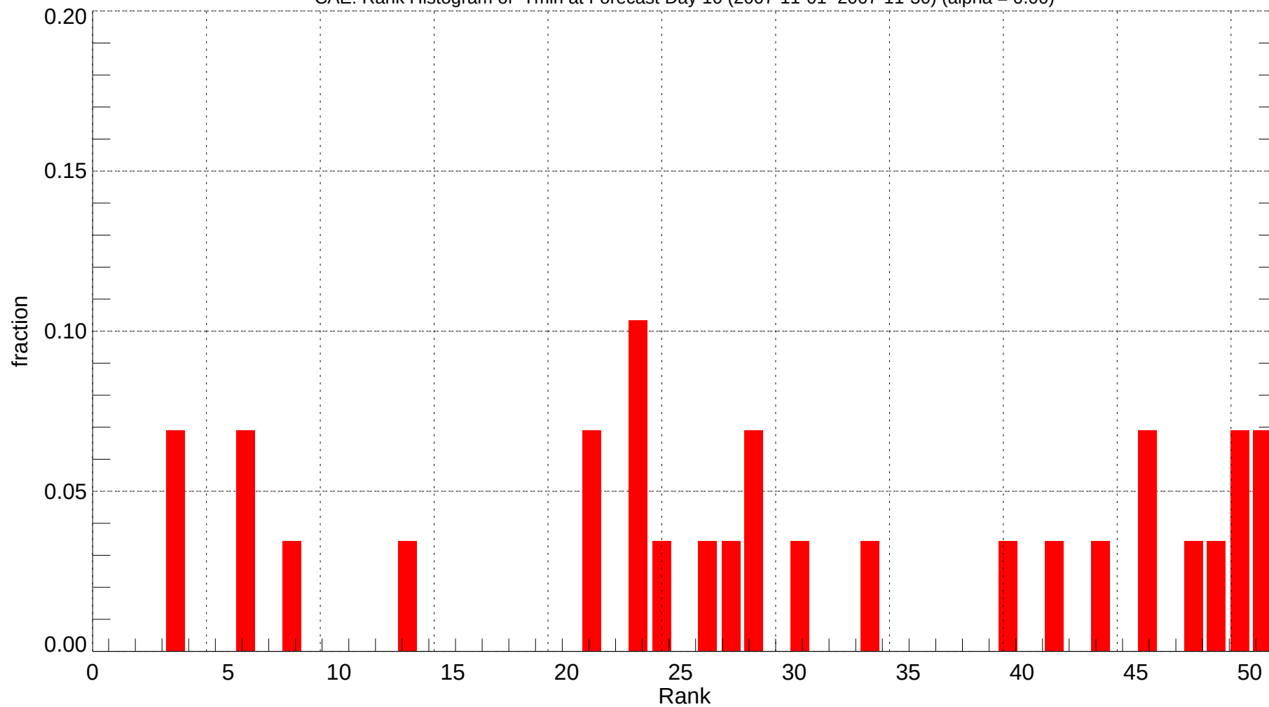
CAE: Rank Histogram of Tmin at Forecast Day 10 (2007-11-01~2007-11-30) (alpha = 0.00)
