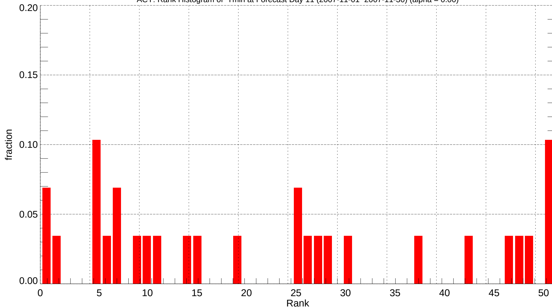
ACY: Rank Histogram of Tmin at Forecast Day 11 (2007-11-01~2007-11-30) (alpha = 0.00)
