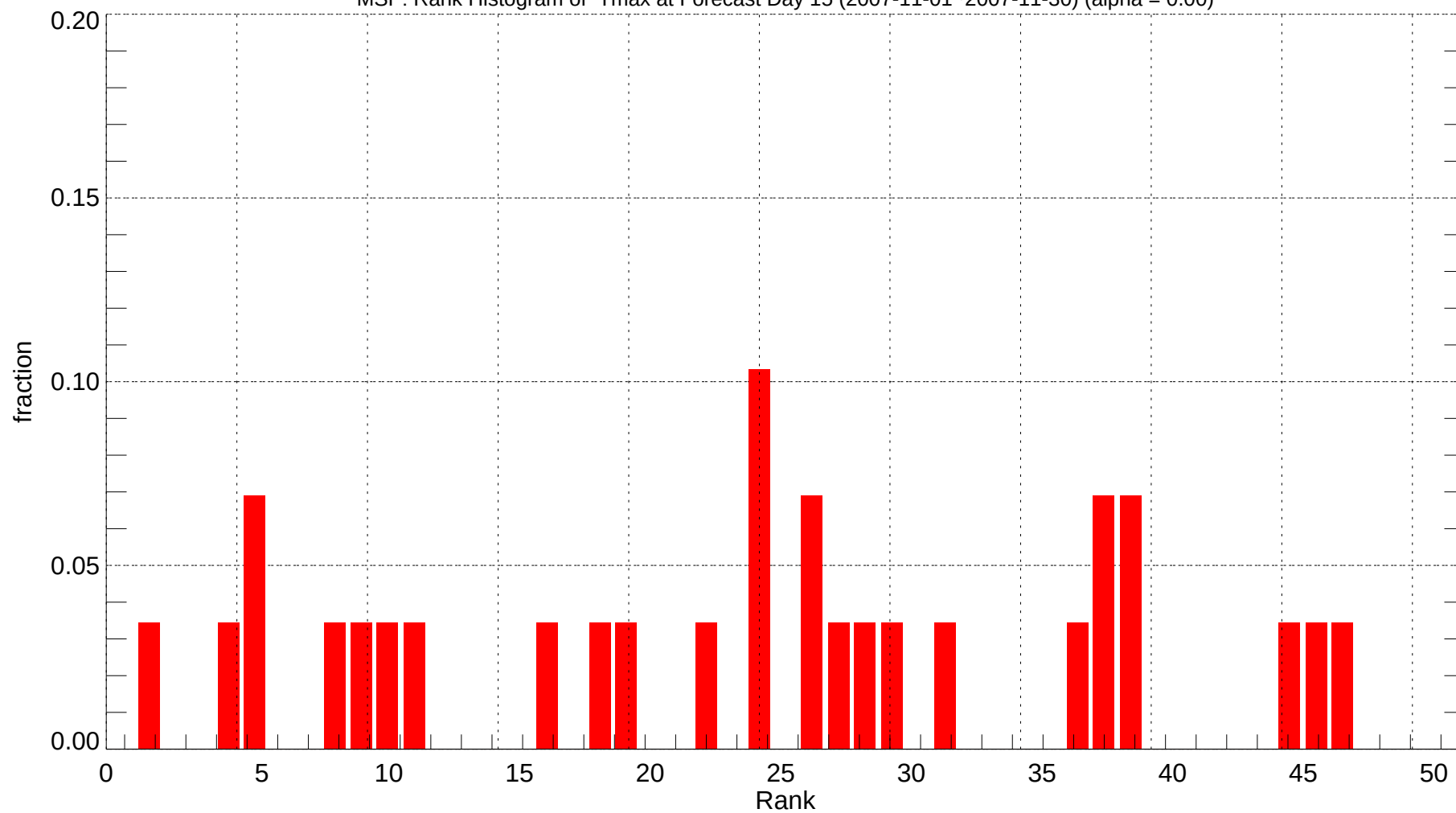
MSP: Rank Histogram of Tmax at Forecast Day 15 (2007-11-01~2007-11-30) (alpha = 0.00)
