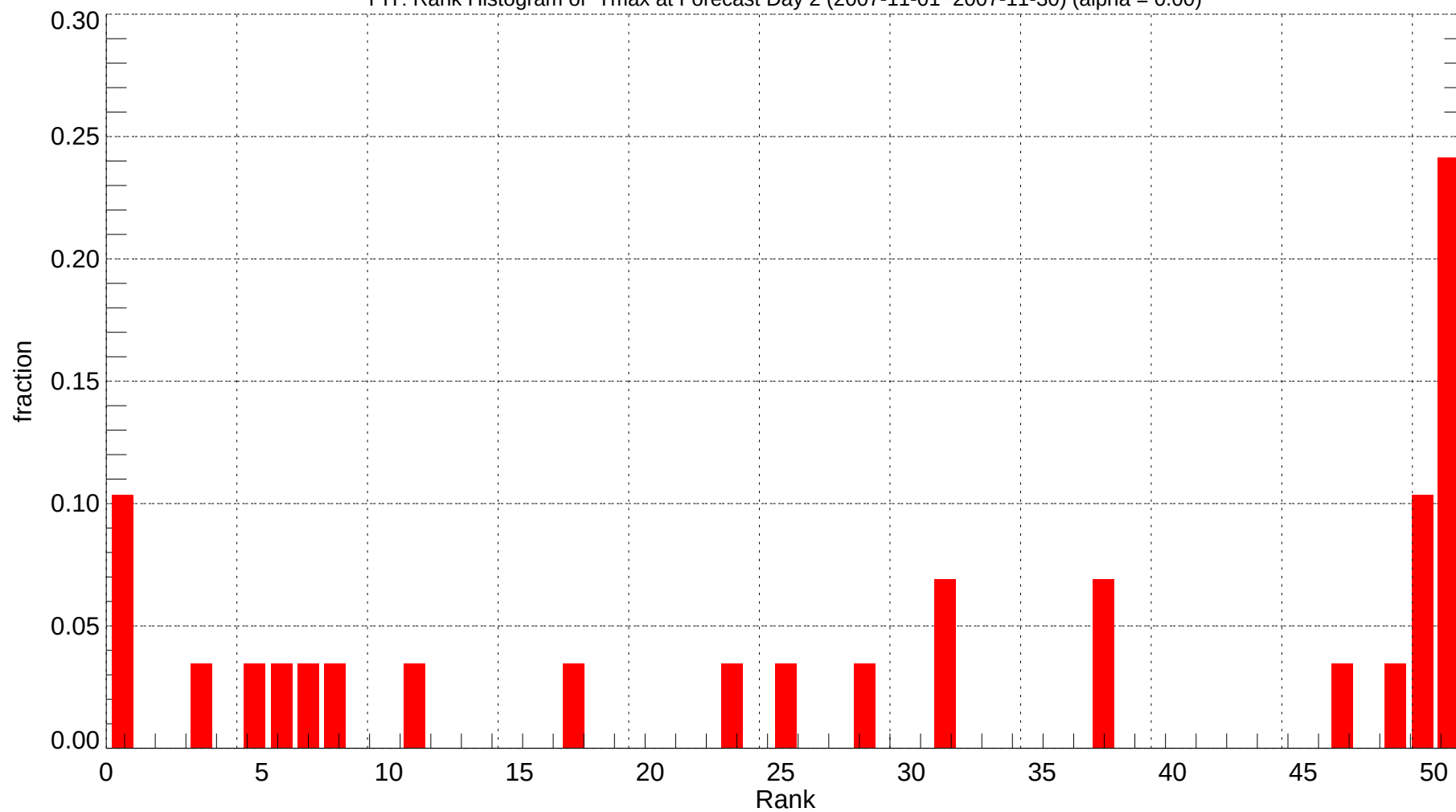
PIT: Rank Histogram of Tmax at Forecast Day 2 (2007-11-01~2007-11-30) (alpha = 0.00)
