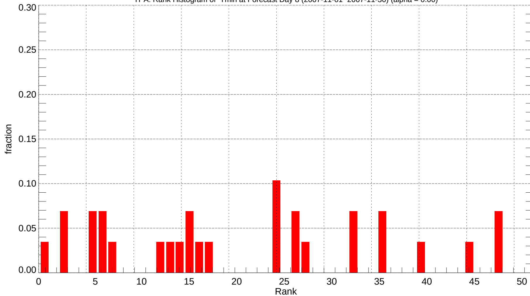
TPA: Rank Histogram of Tmin at Forecast Day 8 (2007-11-01~2007-11-30) (alpha = 0.00)
