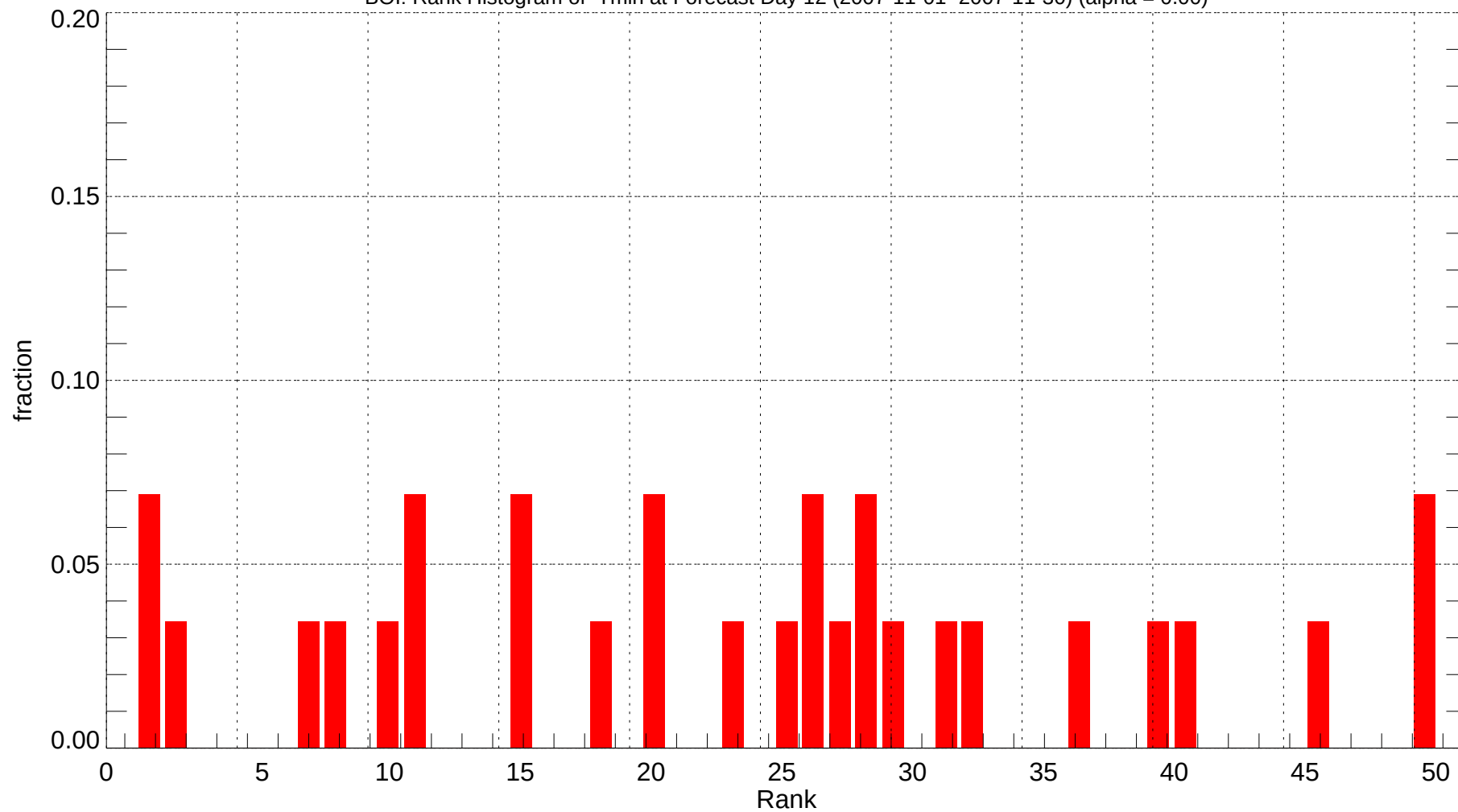
BOI: Rank Histogram of Tmin at Forecast Day 12 (2007-11-01~2007-11-30) (alpha = 0.00)
