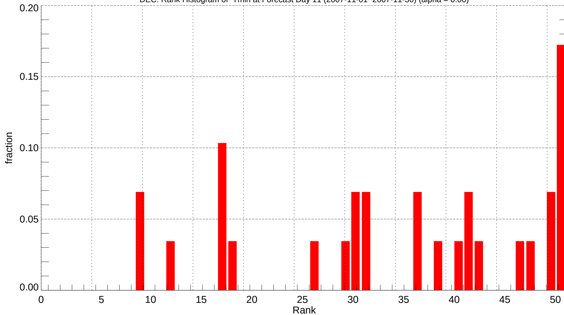
DEC: Rank Histogram of Tmin at Forecast Day 11 (2007-11-01~2007-11-30) (alpha = 0.00)
