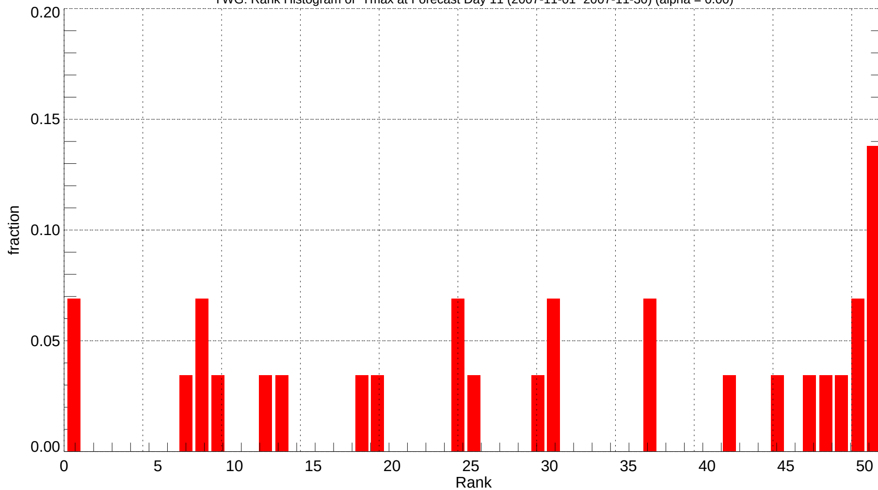
YWG: Rank Histogram of Tmax at Forecast Day 11 (2007-11-01~2007-11-30) (alpha = 0.00)
