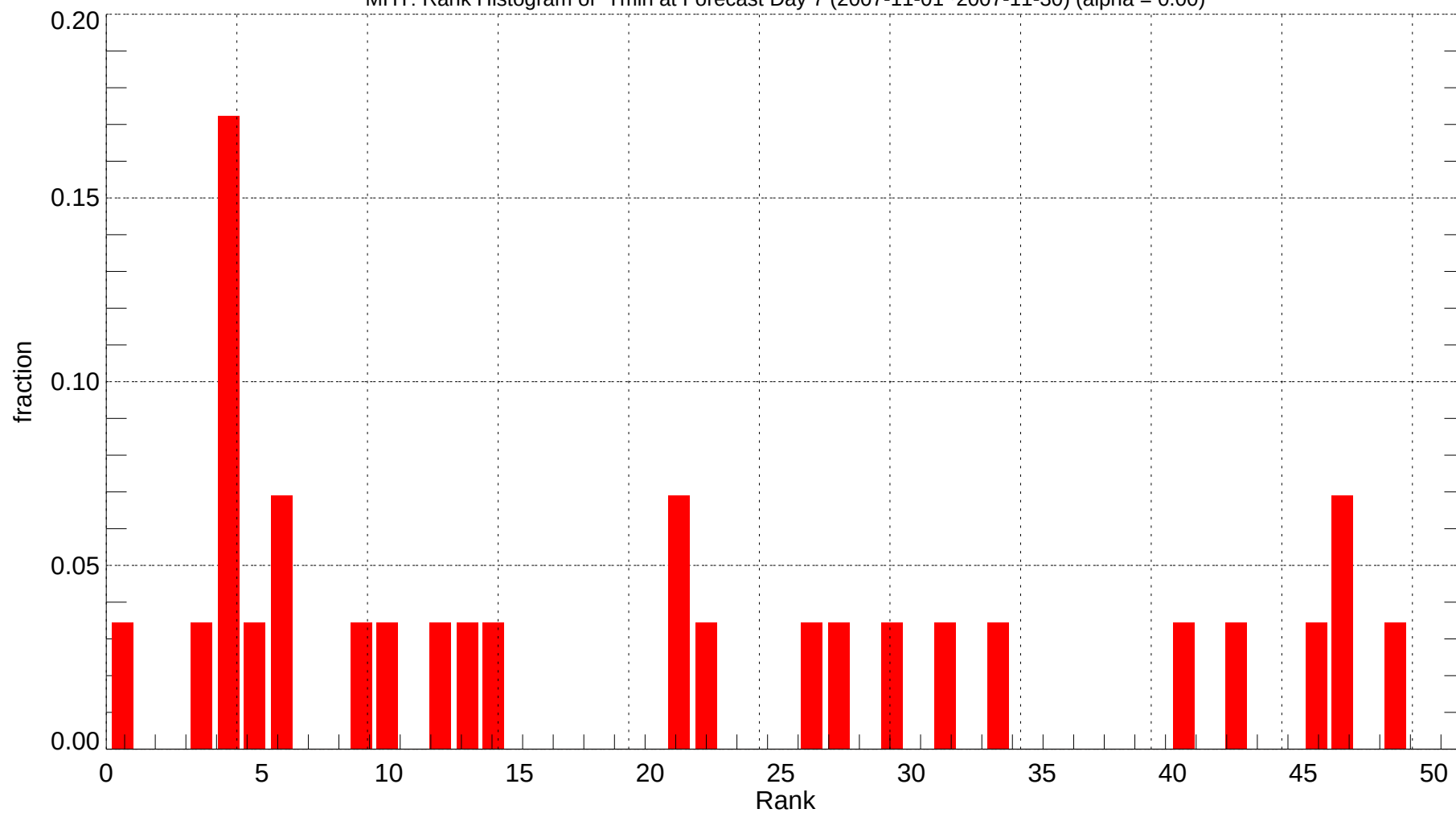
MHT: Rank Histogram of Tmin at Forecast Day 7 (2007-11-01~2007-11-30) (alpha = 0.00)
