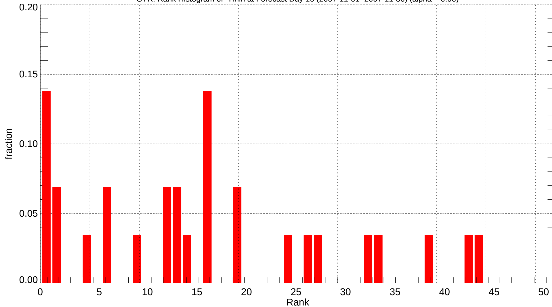
SYR: Rank Histogram of Tmin at Forecast Day 10 (2007-11-01~2007-11-30) (alpha = 0.00)
