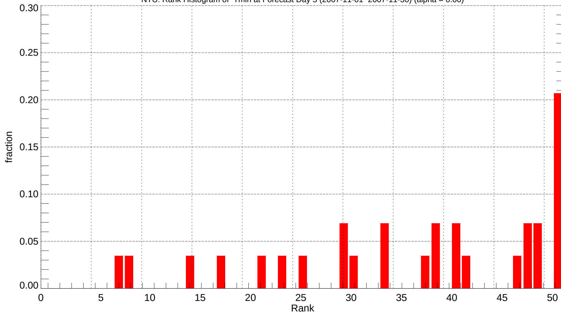
NTU: Rank Histogram of Tmin at Forecast Day 5 (2007-11-01~2007-11-30) (alpha = 0.00)
