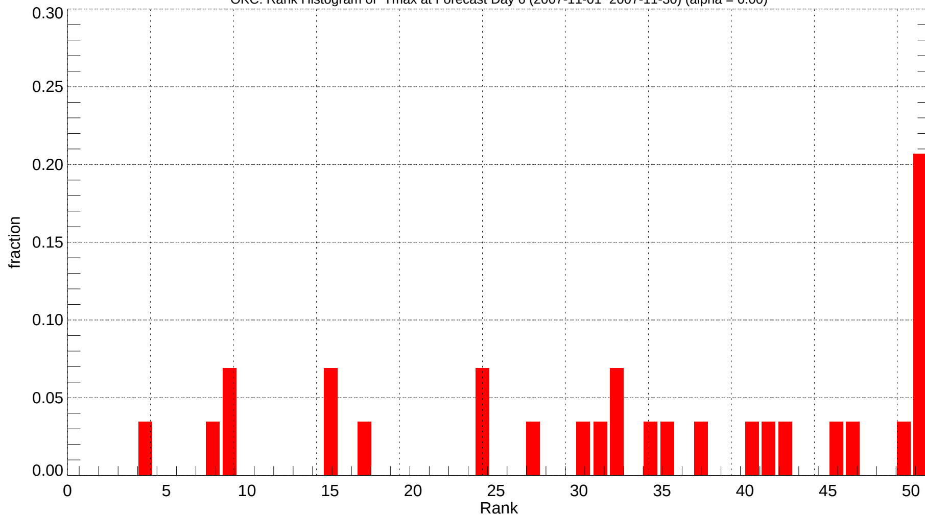
OKC: Rank Histogram of Tmax at Forecast Day 6 (2007-11-01~2007-11-30) (alpha = 0.00)
