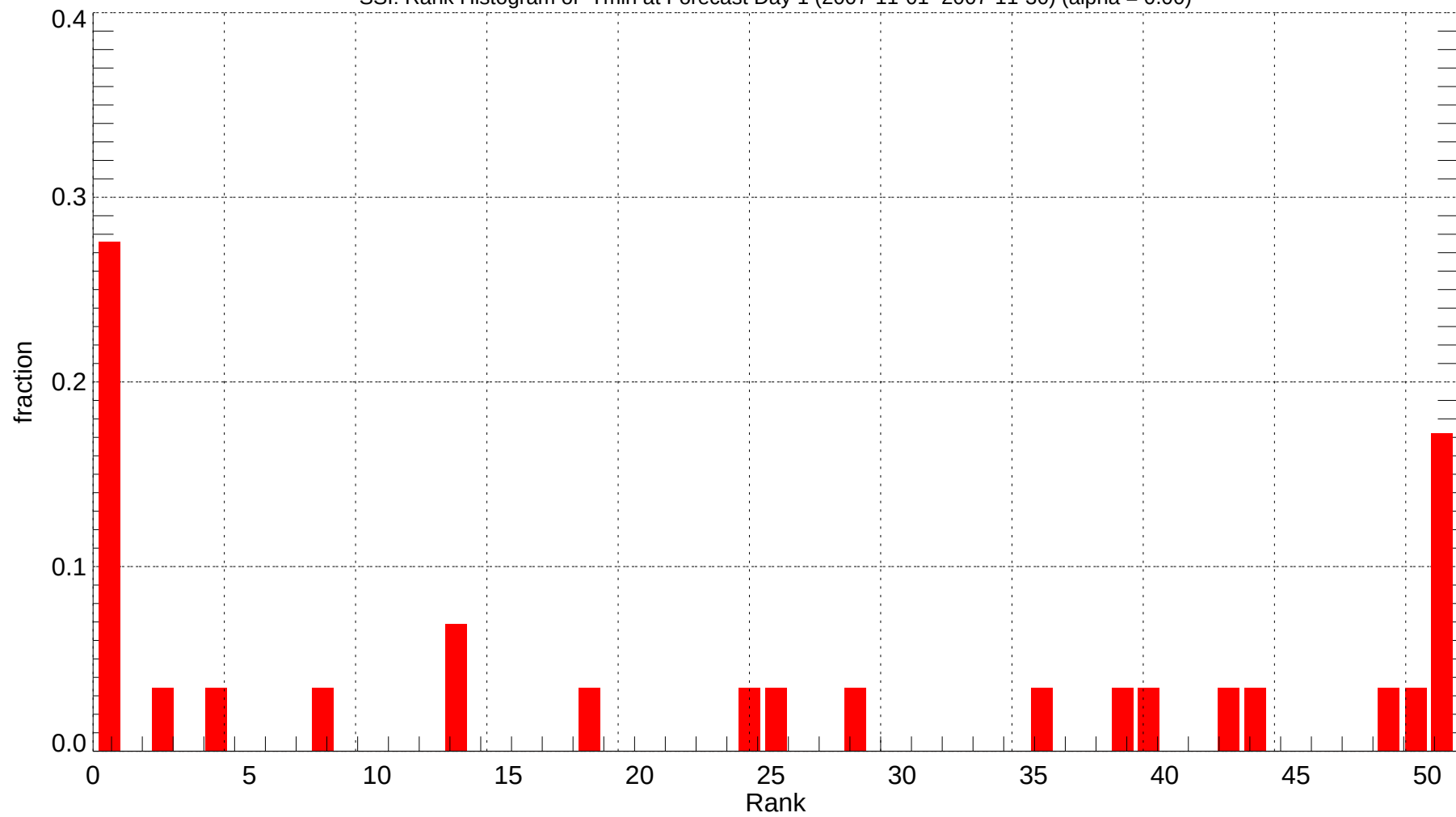
SSI: Rank Histogram of Tmin at Forecast Day 1 (2007-11-01~2007-11-30) (alpha = 0.00)
