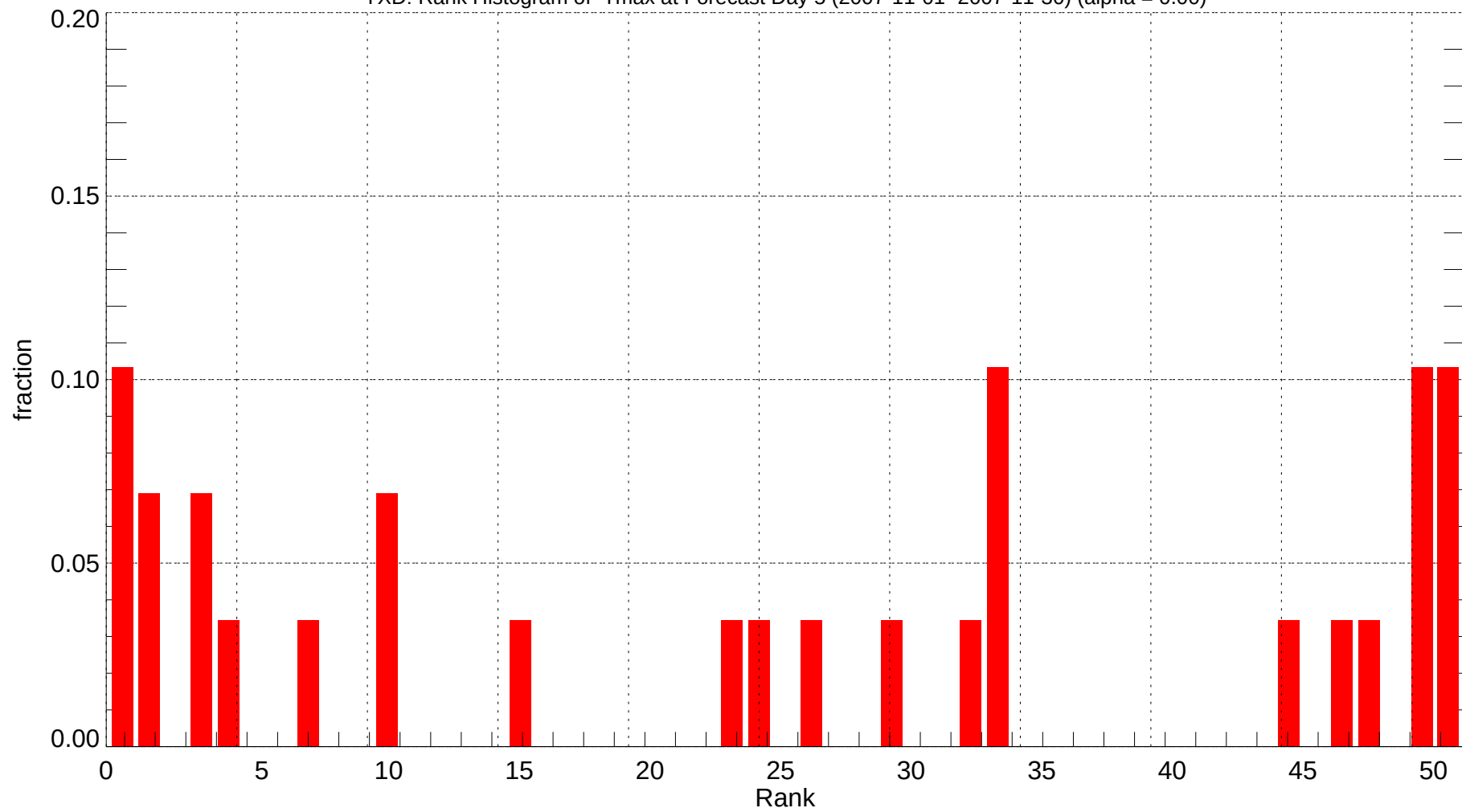
YXD: Rank Histogram of Tmax at Forecast Day 5 (2007-11-01~2007-11-30) (alpha = 0.00)
