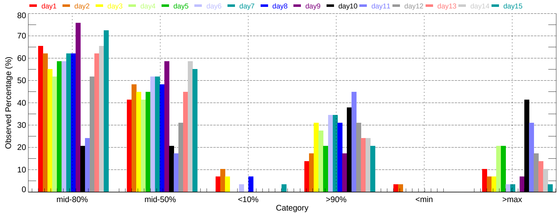
Observed Percentage of Ensembles - ATL: Max Temperature (2007-11-01~2007-11-30)
