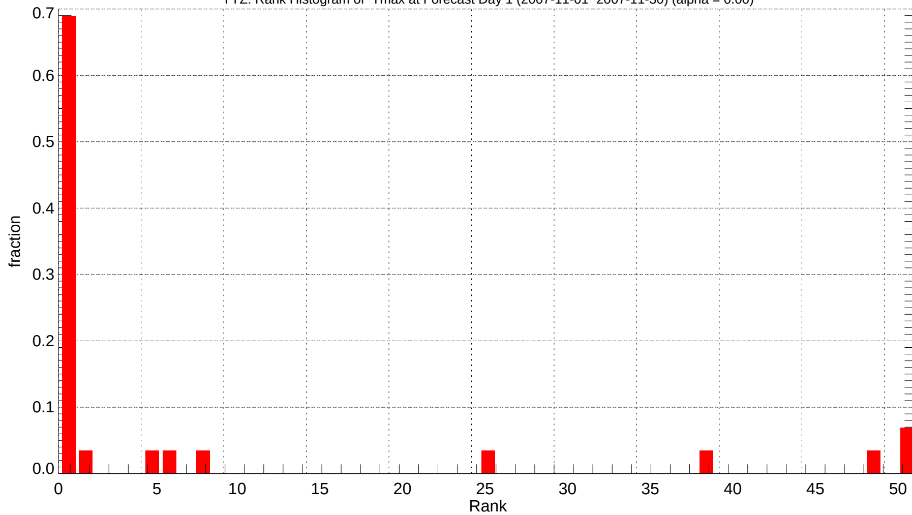
YYZ: Rank Histogram of Tmax at Forecast Day 1 (2007-11-01~2007-11-30) (alpha = 0.00)
