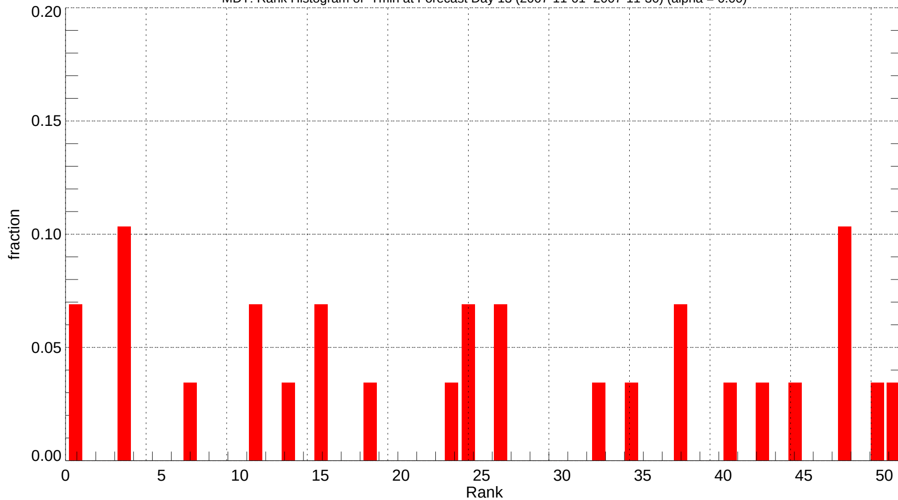
MDT: Rank Histogram of Tmin at Forecast Day 13 (2007-11-01~2007-11-30) (alpha = 0.00)
