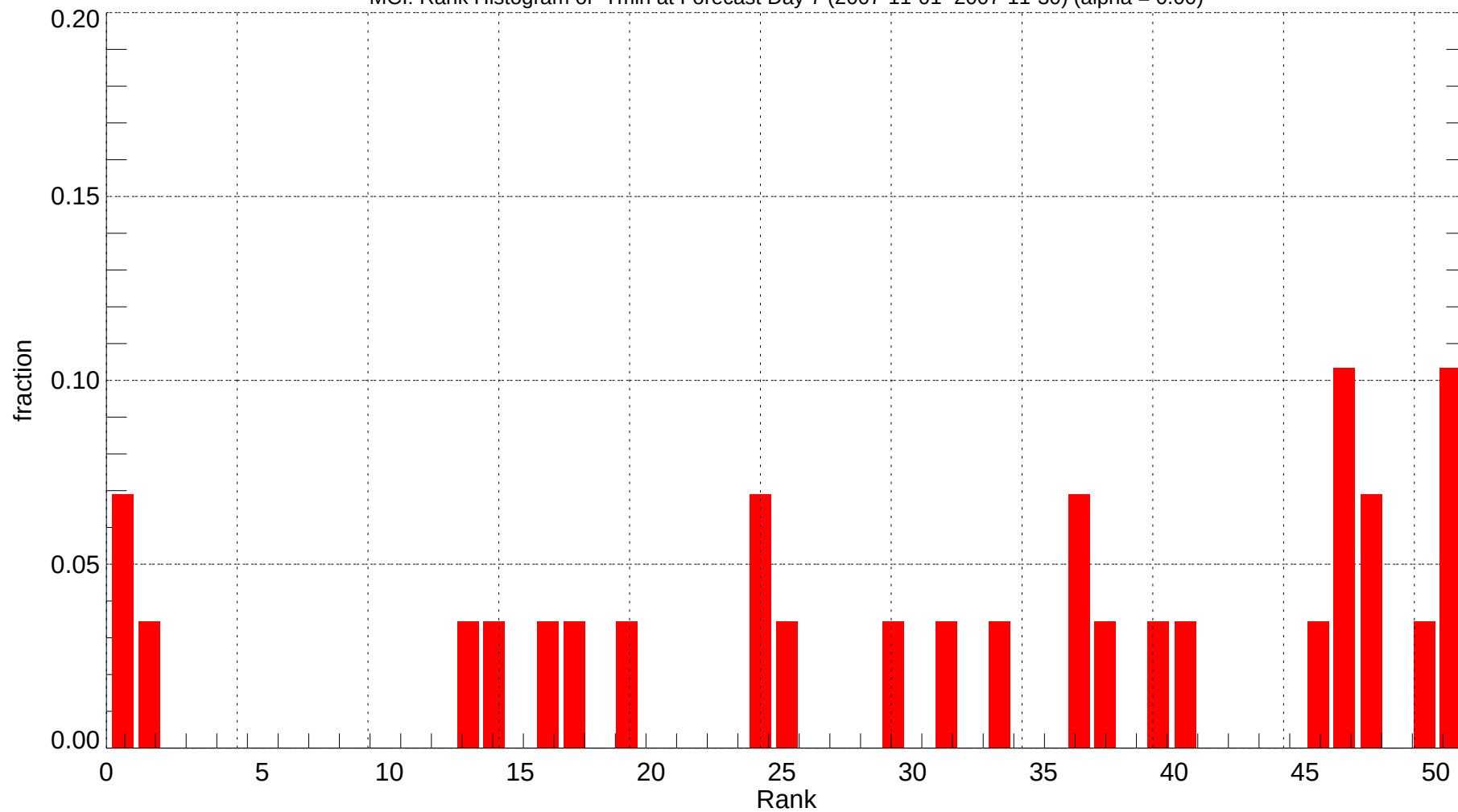
MCI: Rank Histogram of Tmin at Forecast Day 7 (2007-11-01~2007-11-30) (alpha = 0.00)
