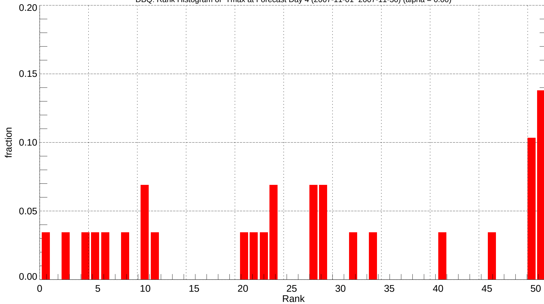
DBQ: Rank Histogram of Tmax at Forecast Day 4 (2007-11-01~2007-11-30) (alpha = 0.00)
