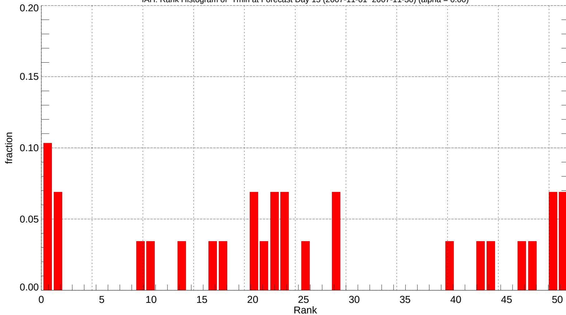
IAH: Rank Histogram of Tmin at Forecast Day 15 (2007-11-01~2007-11-30) (alpha = 0.00)
