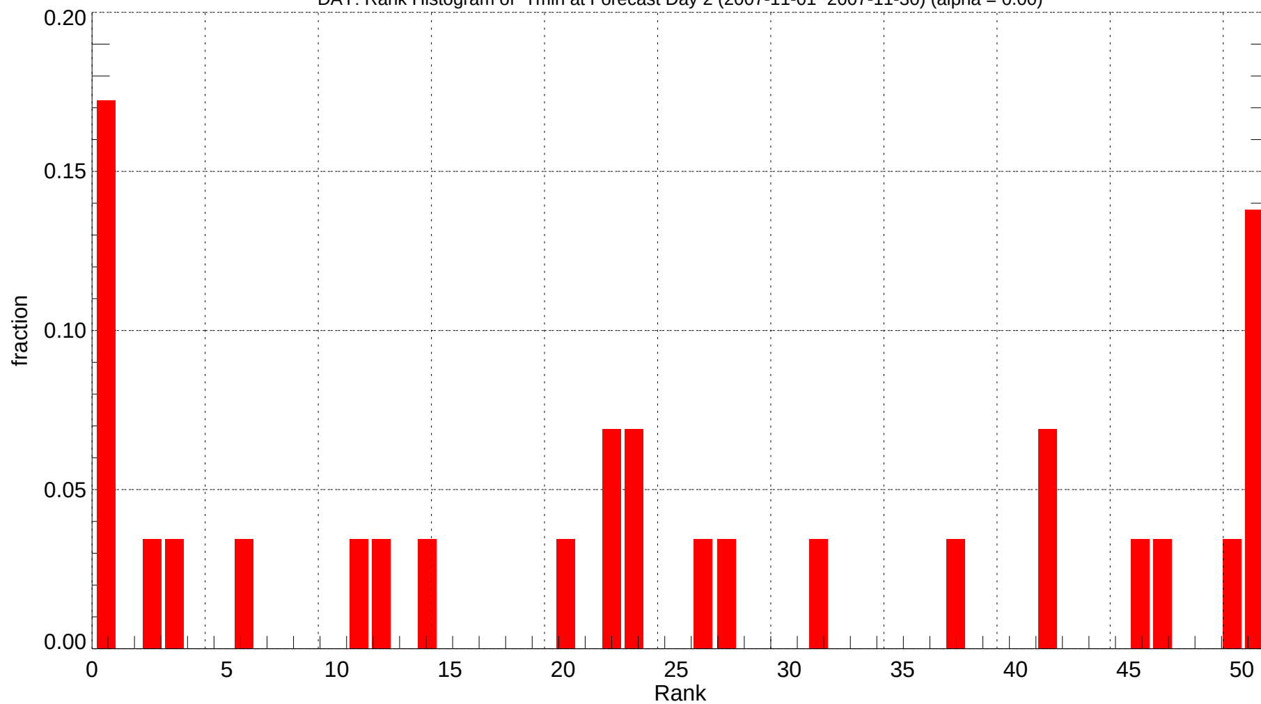
DAY: Rank Histogram of Tmin at Forecast Day 2 (2007-11-01~2007-11-30) (alpha = 0.00)
