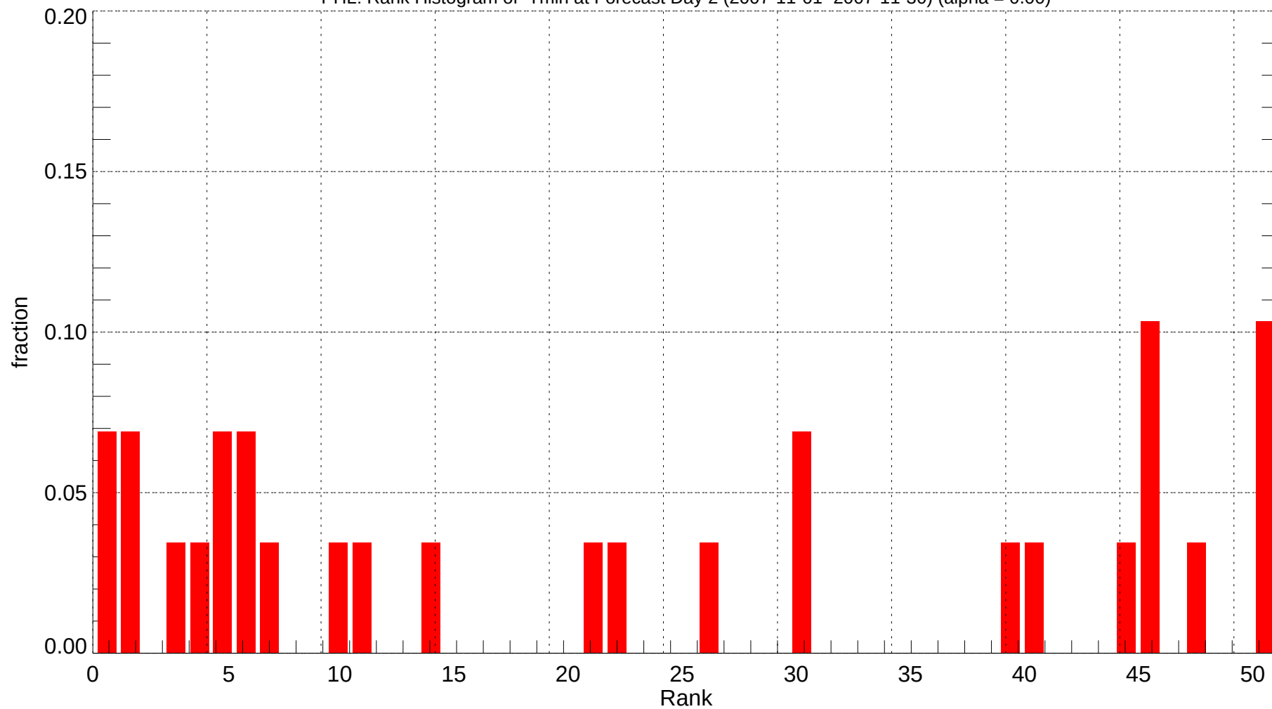
PHL: Rank Histogram of Tmin at Forecast Day 2 (2007-11-01~2007-11-30) (alpha = 0.00)
