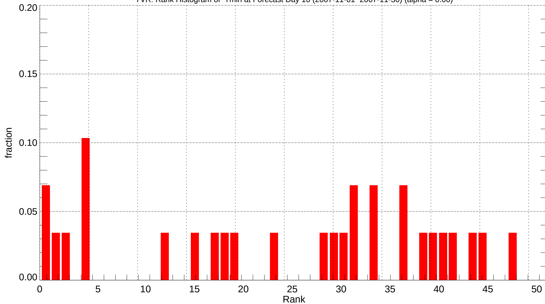
YVR: Rank Histogram of Tmin at Forecast Day 10 (2007-11-01~2007-11-30) (alpha = 0.00)
