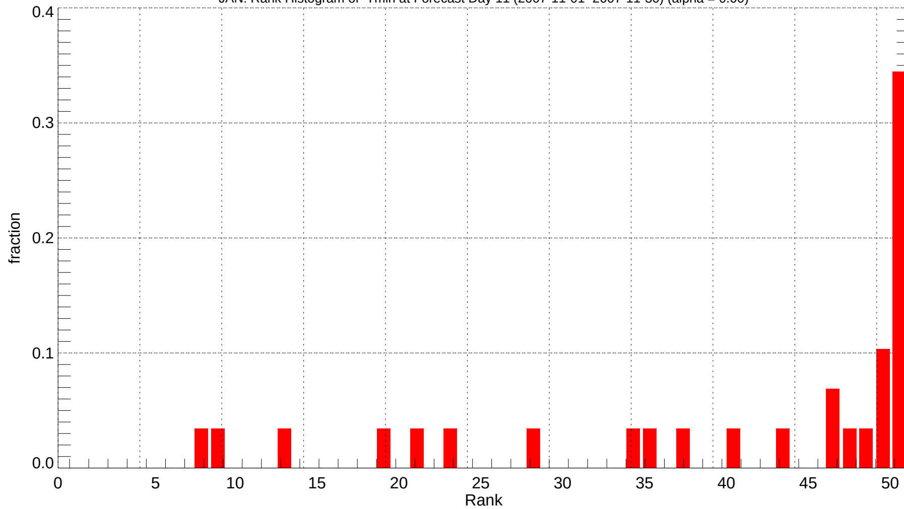
JAN: Rank Histogram of Tmin at Forecast Day 11 (2007-11-01~2007-11-30) (alpha = 0.00)
