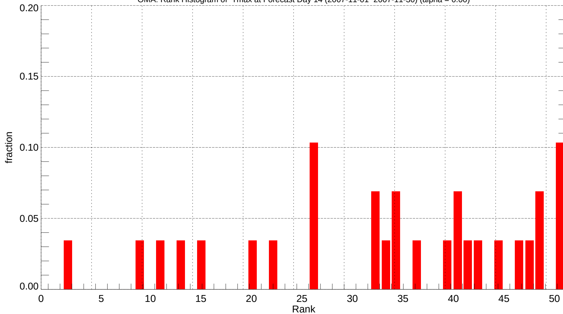
OMA: Rank Histogram of Tmax at Forecast Day 14 (2007-11-01~2007-11-30) (alpha = 0.00)
