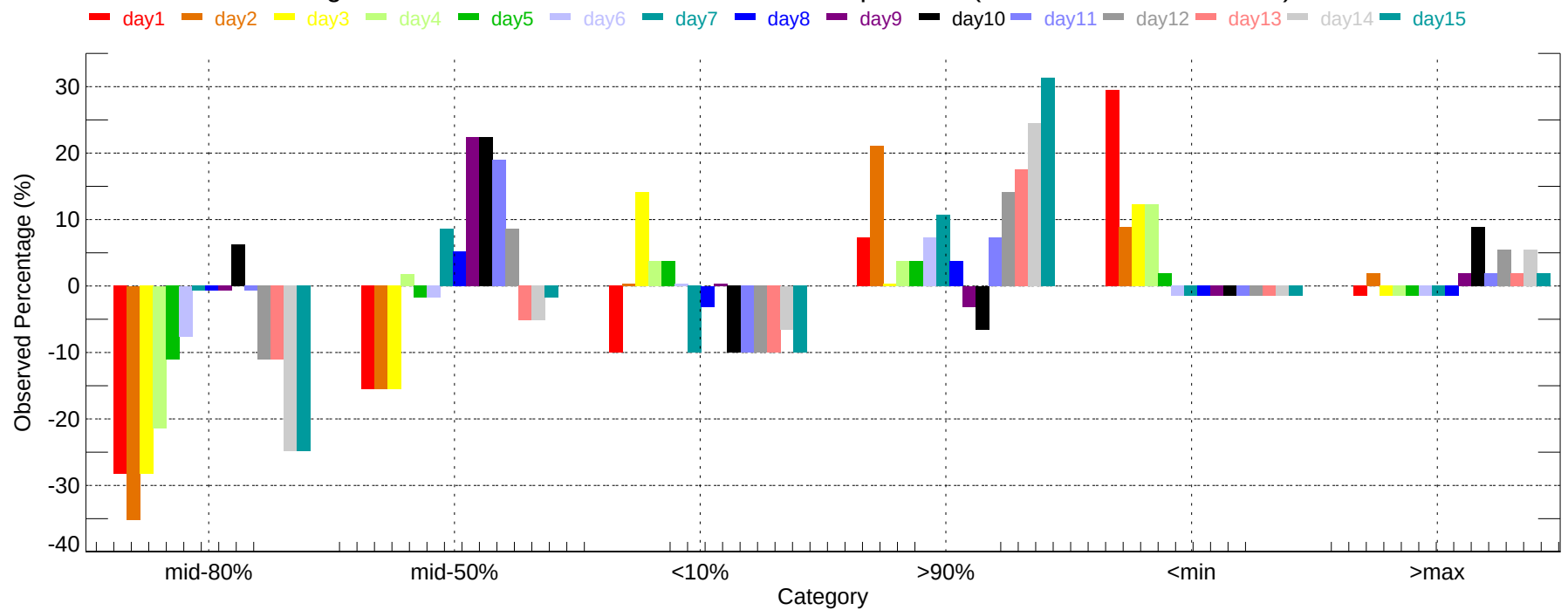
Observed Percentage Deviation of Ensembles - LAS: Min Temperature (2007-11-01~2007-11-30)
