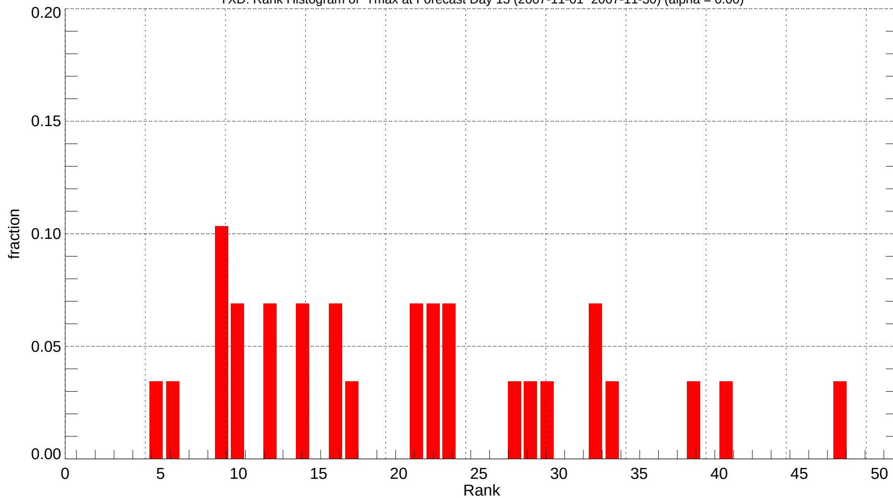
YXD: Rank Histogram of Tmax at Forecast Day 13 (2007-11-01~2007-11-30) (alpha = 0.00)
