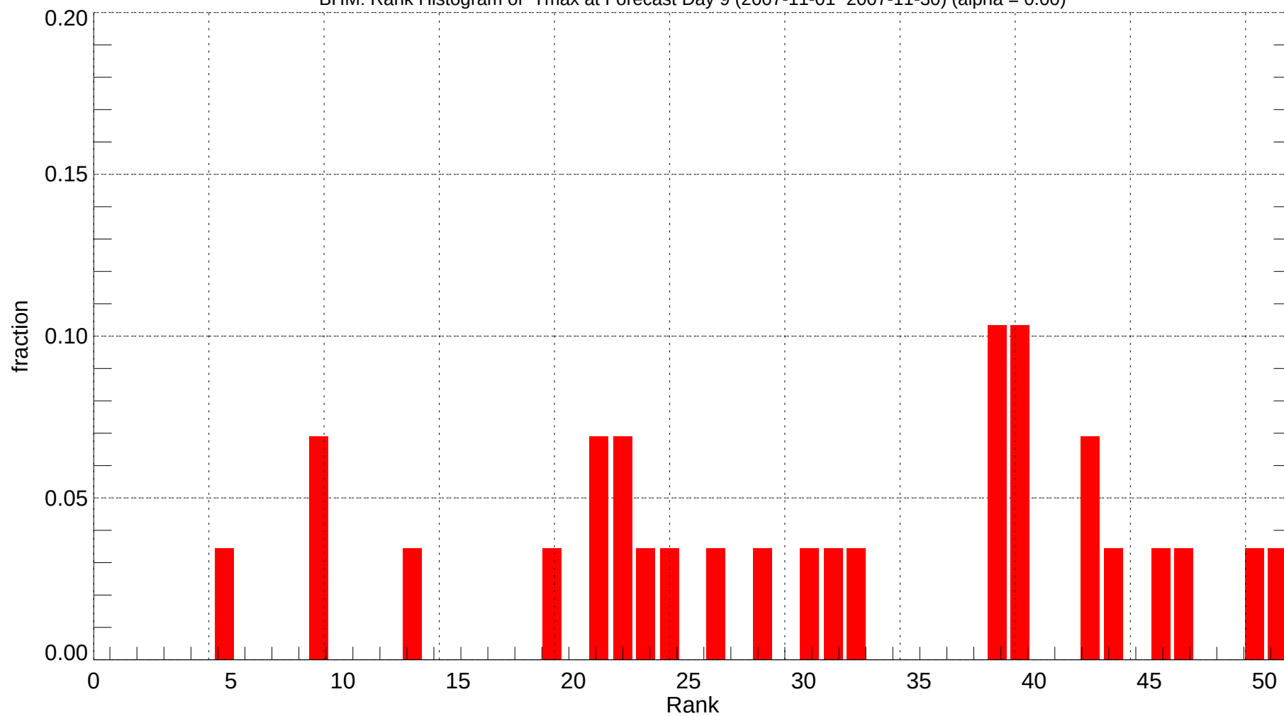
BHM: Rank Histogram of Tmax at Forecast Day 9 (2007-11-01~2007-11-30) (alpha = 0.00)
