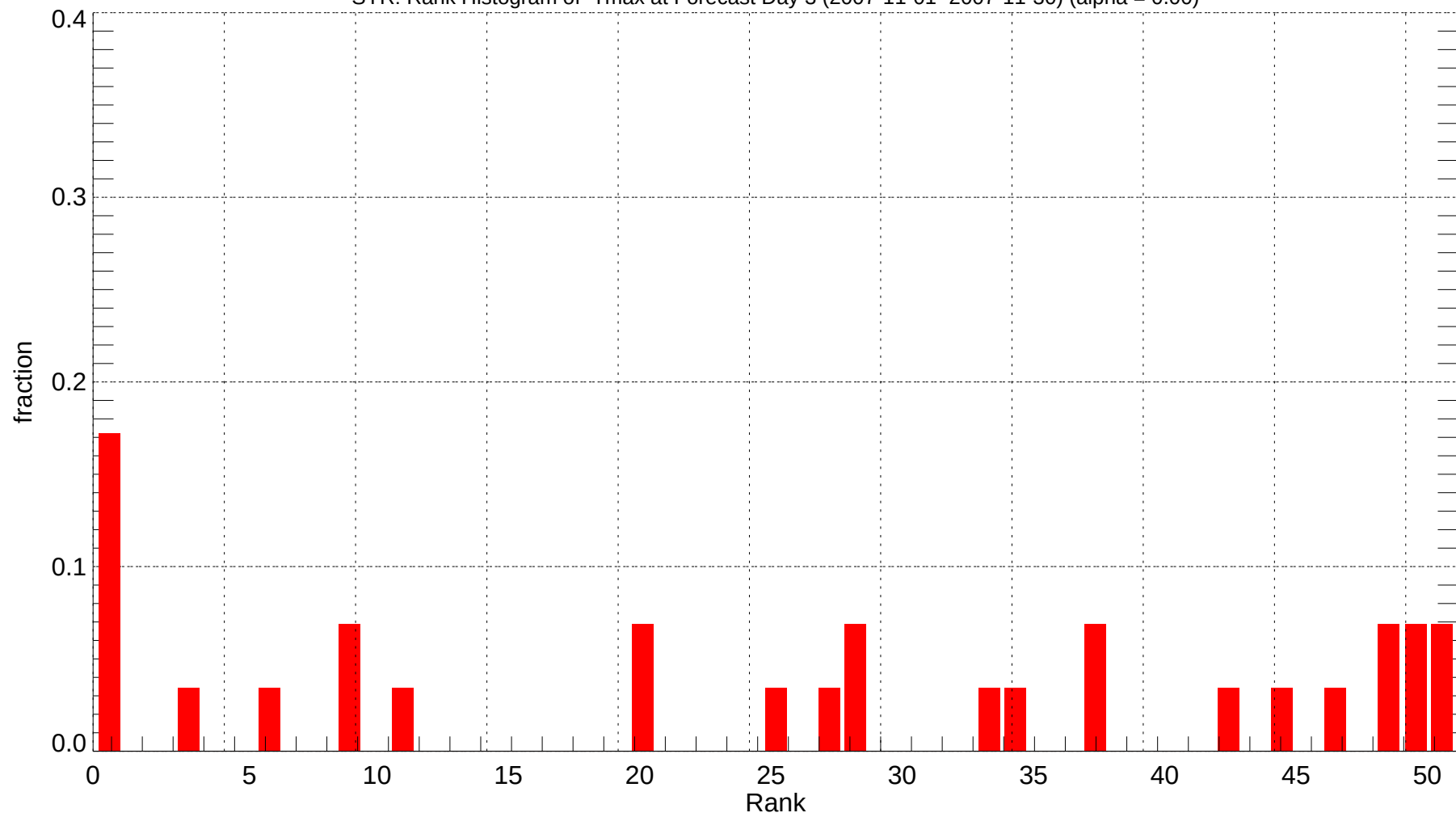
SYR: Rank Histogram of Tmax at Forecast Day 3 (2007-11-01~2007-11-30) (alpha = 0.00)
