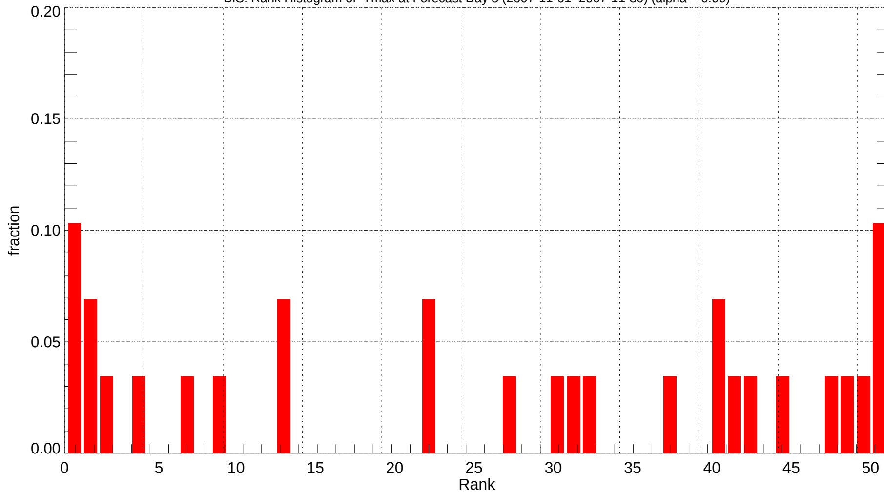
BIS: Rank Histogram of Tmax at Forecast Day 5 (2007-11-01~2007-11-30) (alpha = 0.00)
