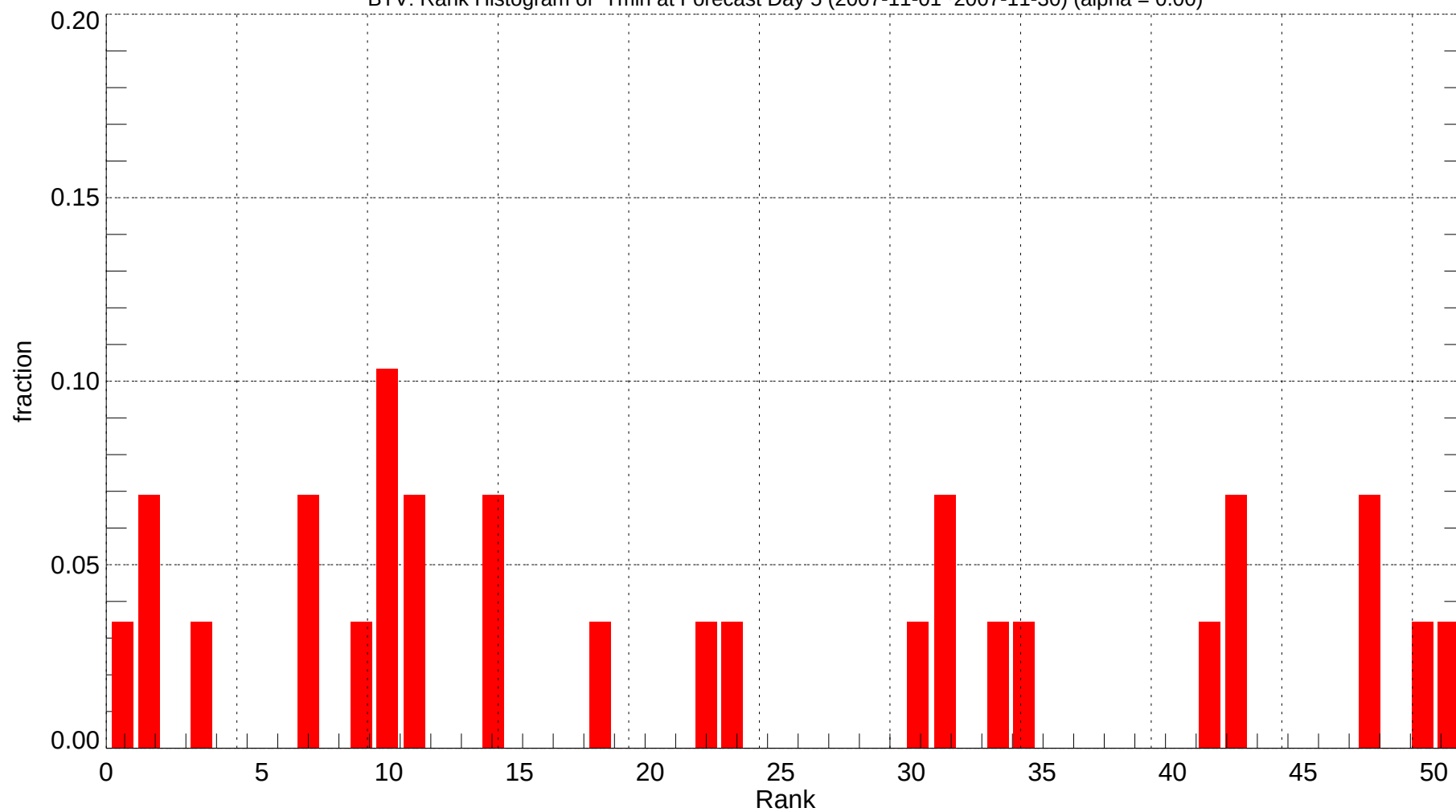
BTV: Rank Histogram of Tmin at Forecast Day 5 (2007-11-01~2007-11-30) (alpha = 0.00)
