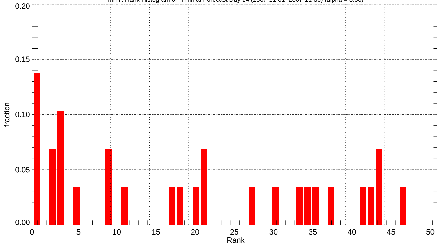
MHT: Rank Histogram of Tmin at Forecast Day 14 (2007-11-01~2007-11-30) (alpha = 0.00)
