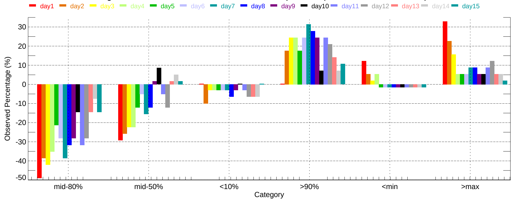
Observed Percentage Deviation of Ensembles - CRW: Min Temperature (2007-11-01~2007-11-30)
