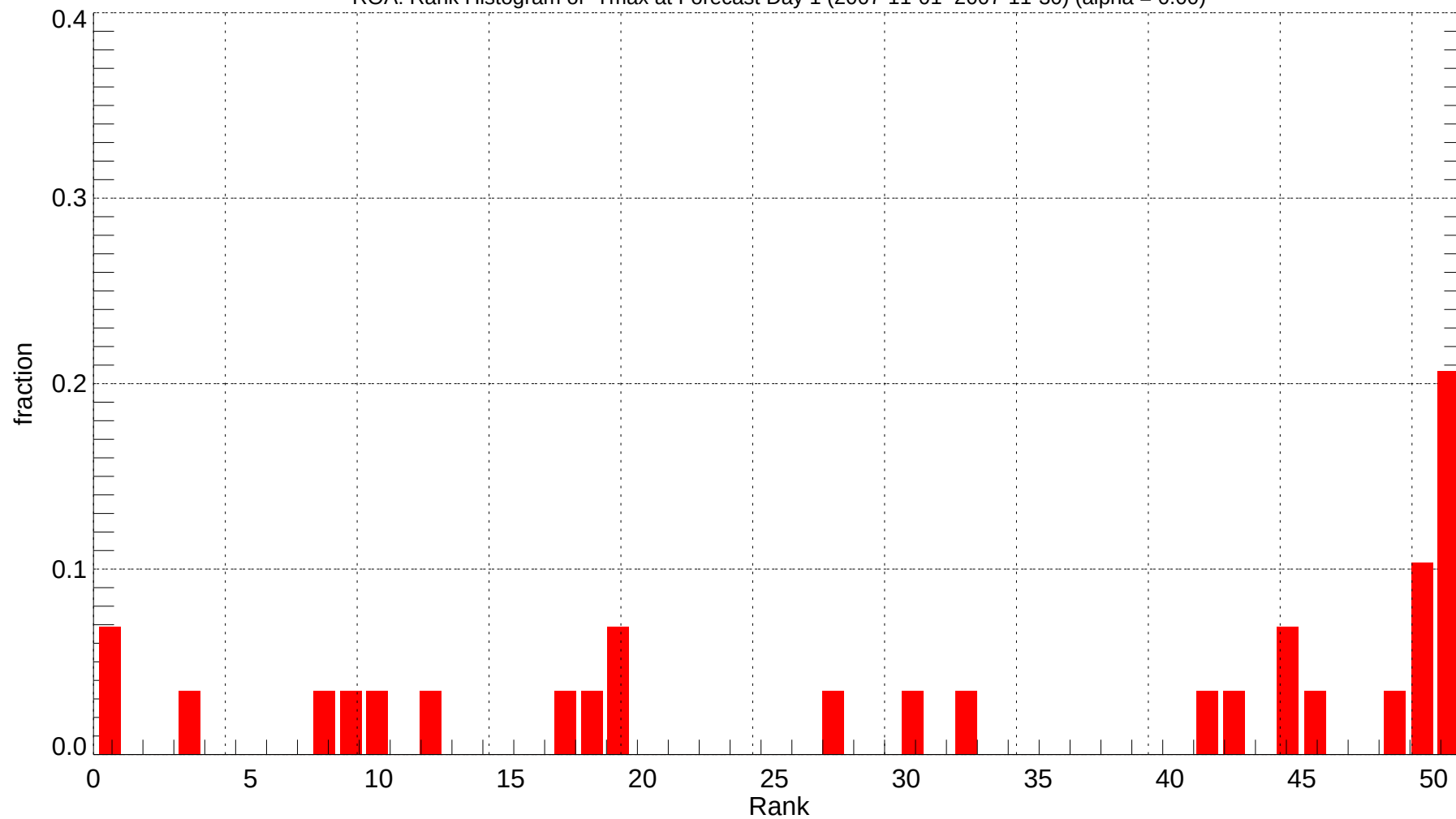
ROA: Rank Histogram of Tmax at Forecast Day 1 (2007-11-01~2007-11-30) (alpha = 0.00)
