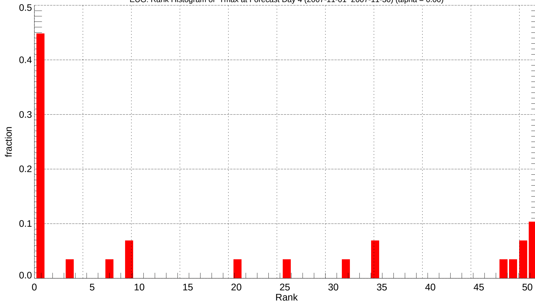
EUG: Rank Histogram of Tmax at Forecast Day 4 (2007-11-01~2007-11-30) (alpha = 0.00)
