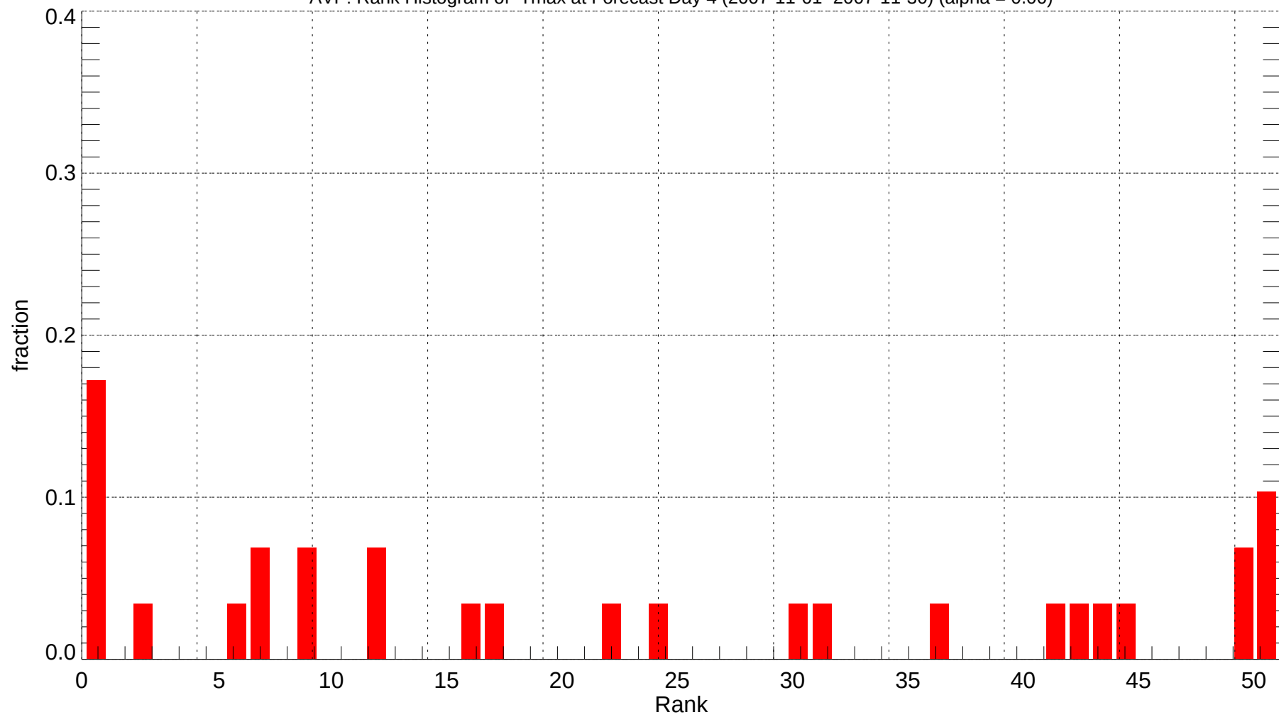
AVP: Rank Histogram of Tmax at Forecast Day 4 (2007-11-01~2007-11-30) (alpha = 0.00)
