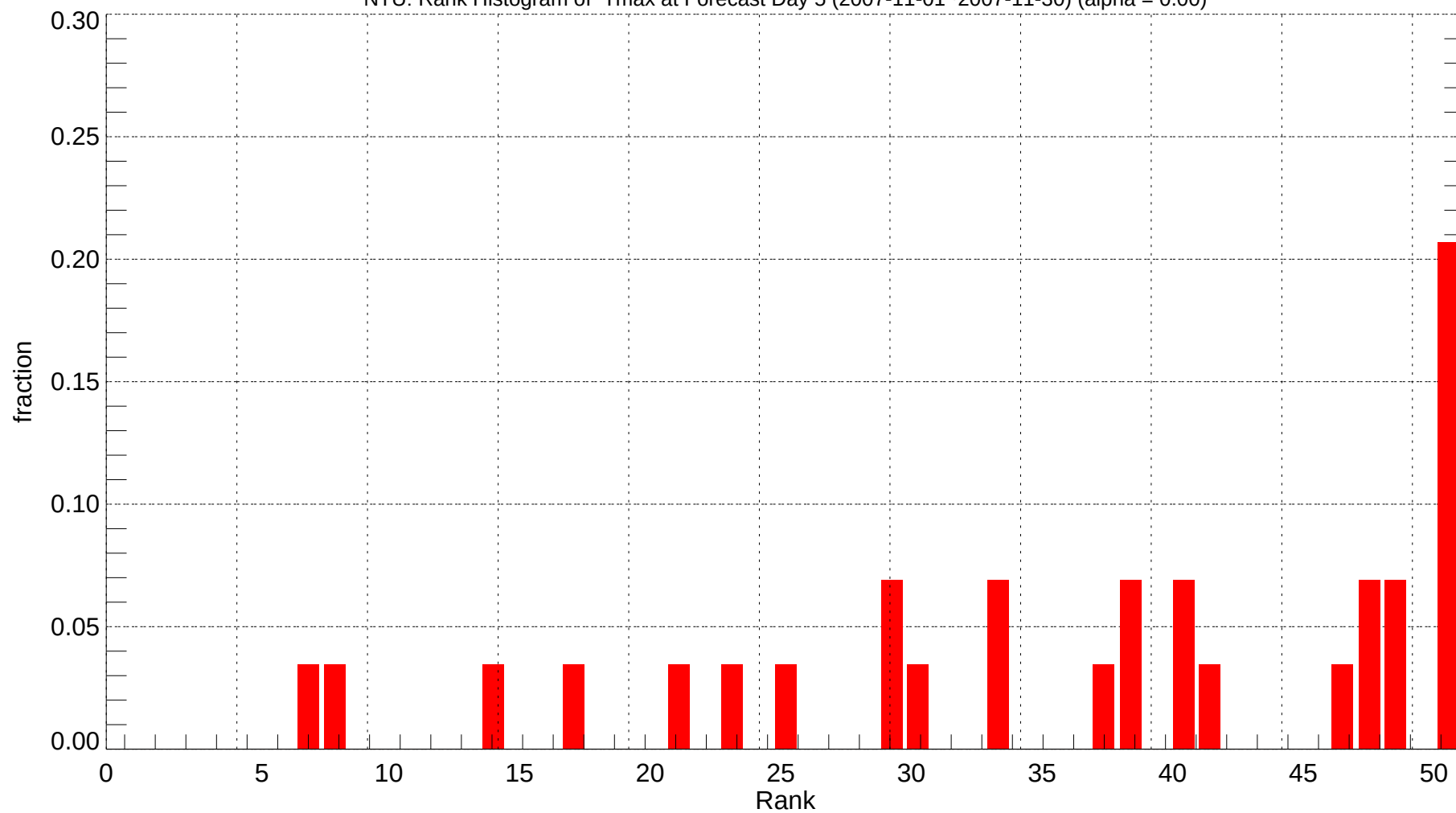
NTU: Rank Histogram of Tmax at Forecast Day 5 (2007-11-01~2007-11-30) (alpha = 0.00)
