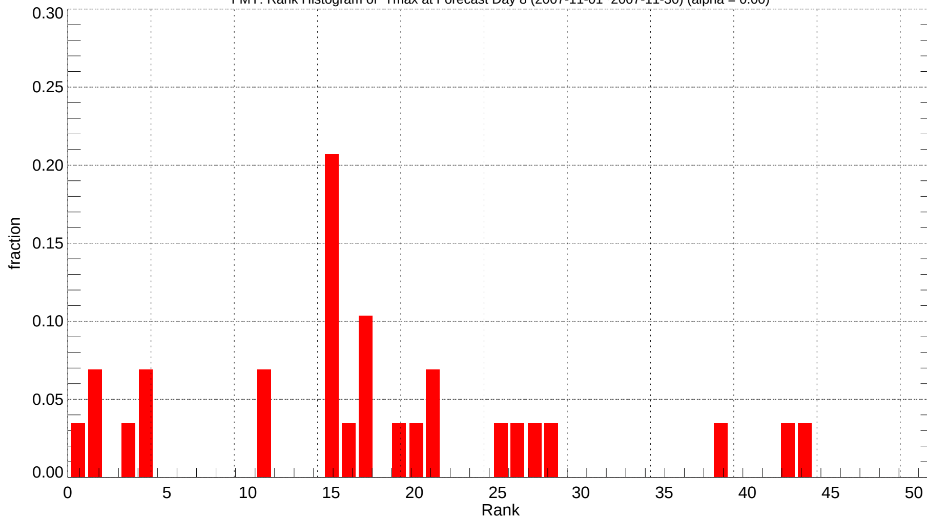
FMY: Rank Histogram of Tmax at Forecast Day 8 (2007-11-01~2007-11-30) (alpha = 0.00)
