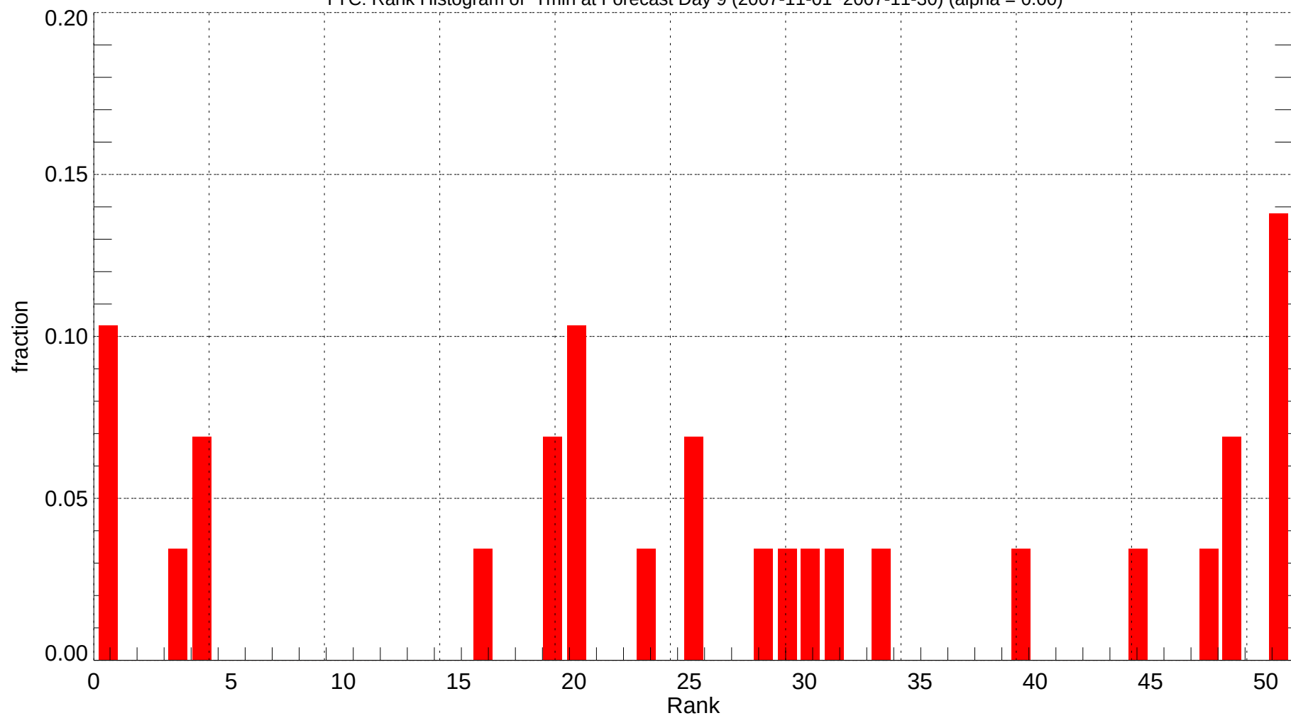
YYC: Rank Histogram of Tmin at Forecast Day 9 (2007-11-01~2007-11-30) (alpha = 0.00)
