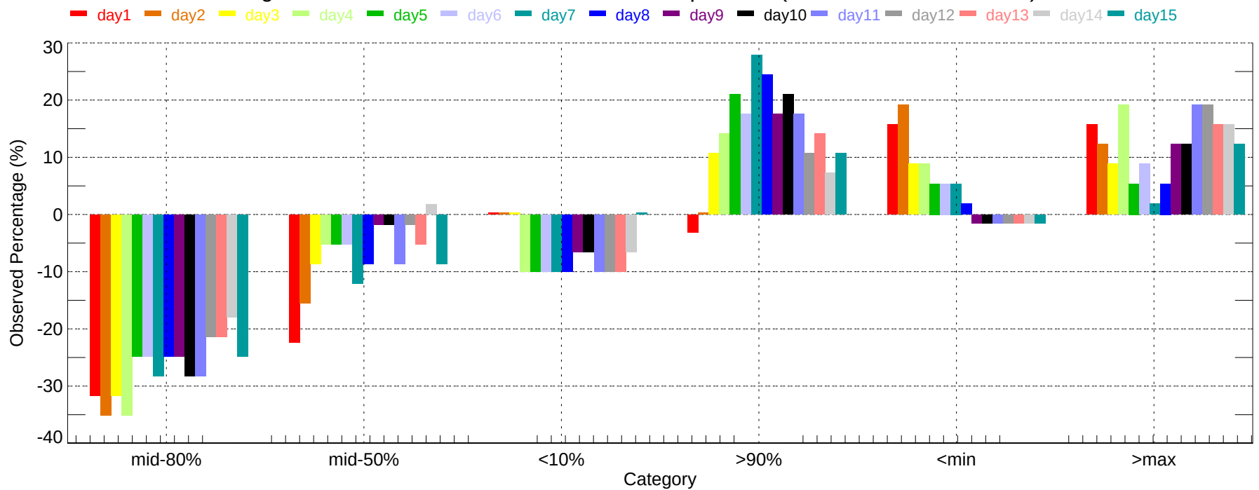
Observed Percentage Deviation of Ensembles - ICT: Max Temperature (2007-11-01~2007-11-30)
