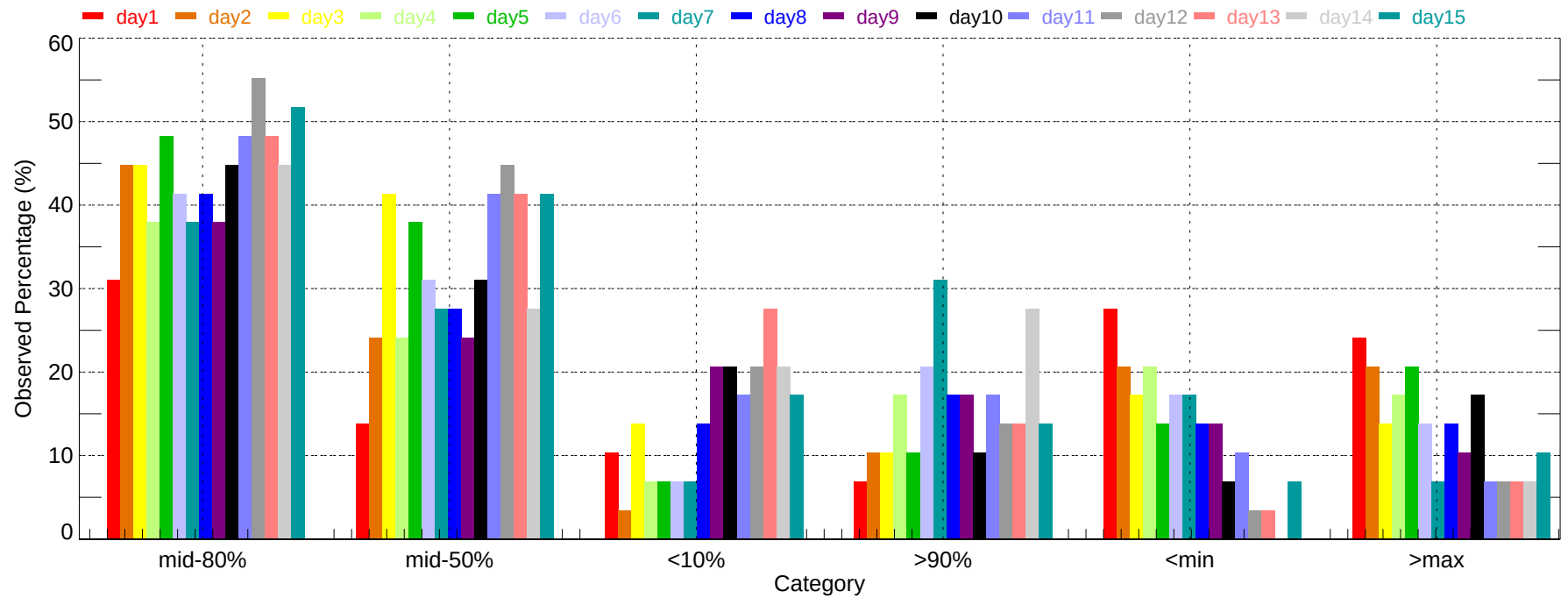
Observed Percentage of Ensembles - PDT: Min Temperature (2007-11-01~2007-11-30)
