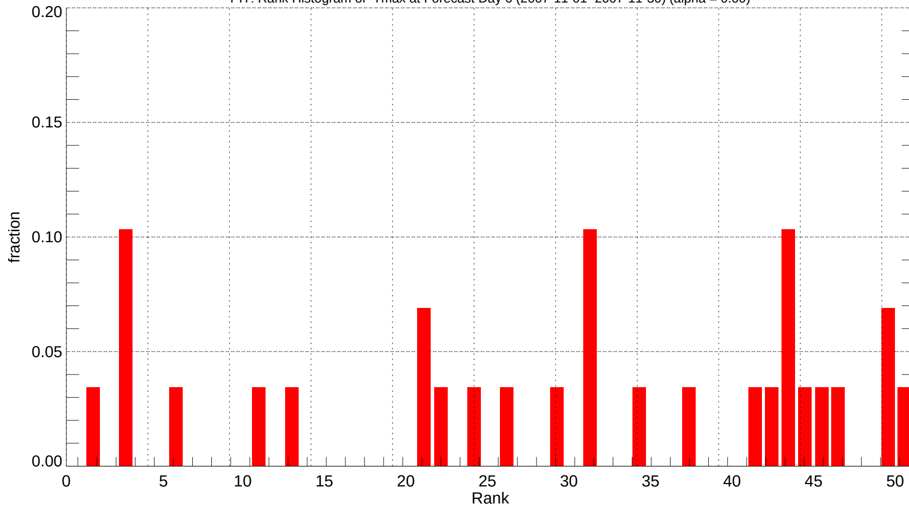
PIT: Rank Histogram of Tmax at Forecast Day 6 (2007-11-01~2007-11-30) (alpha = 0.00)
