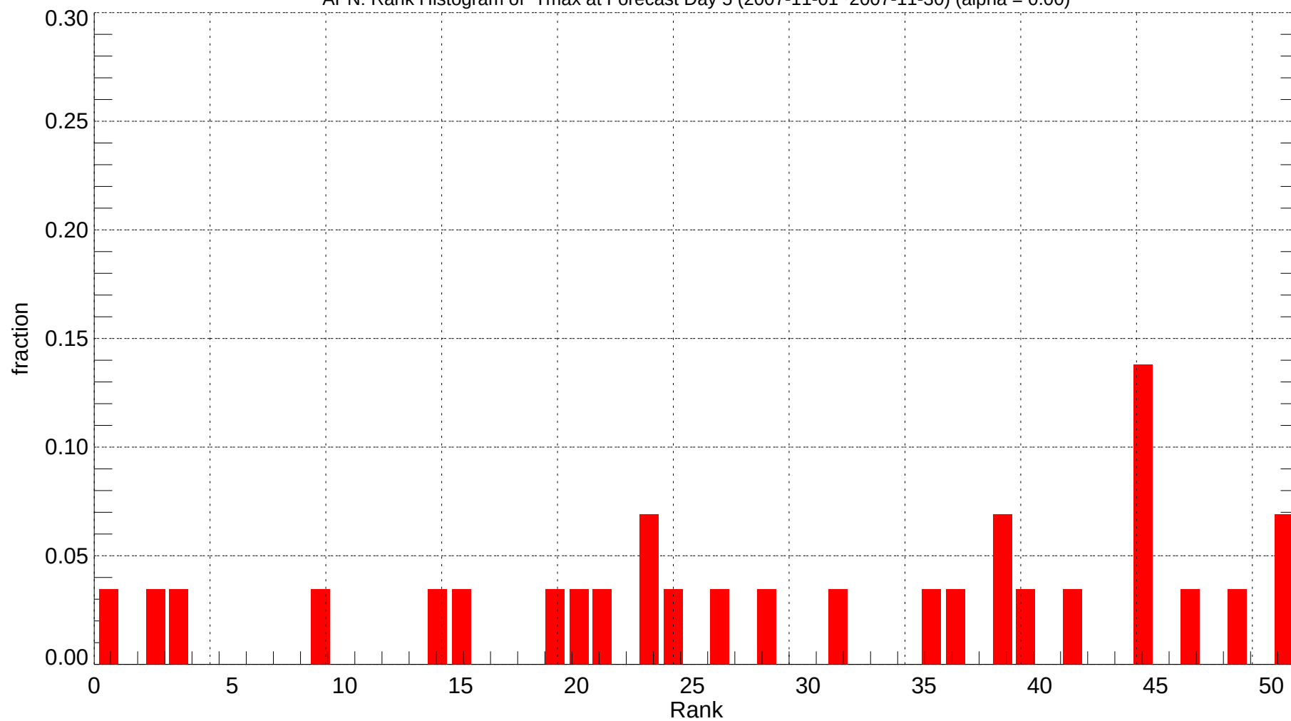
APN: Rank Histogram of Tmax at Forecast Day 5 (2007-11-01~2007-11-30) (alpha = 0.00)
