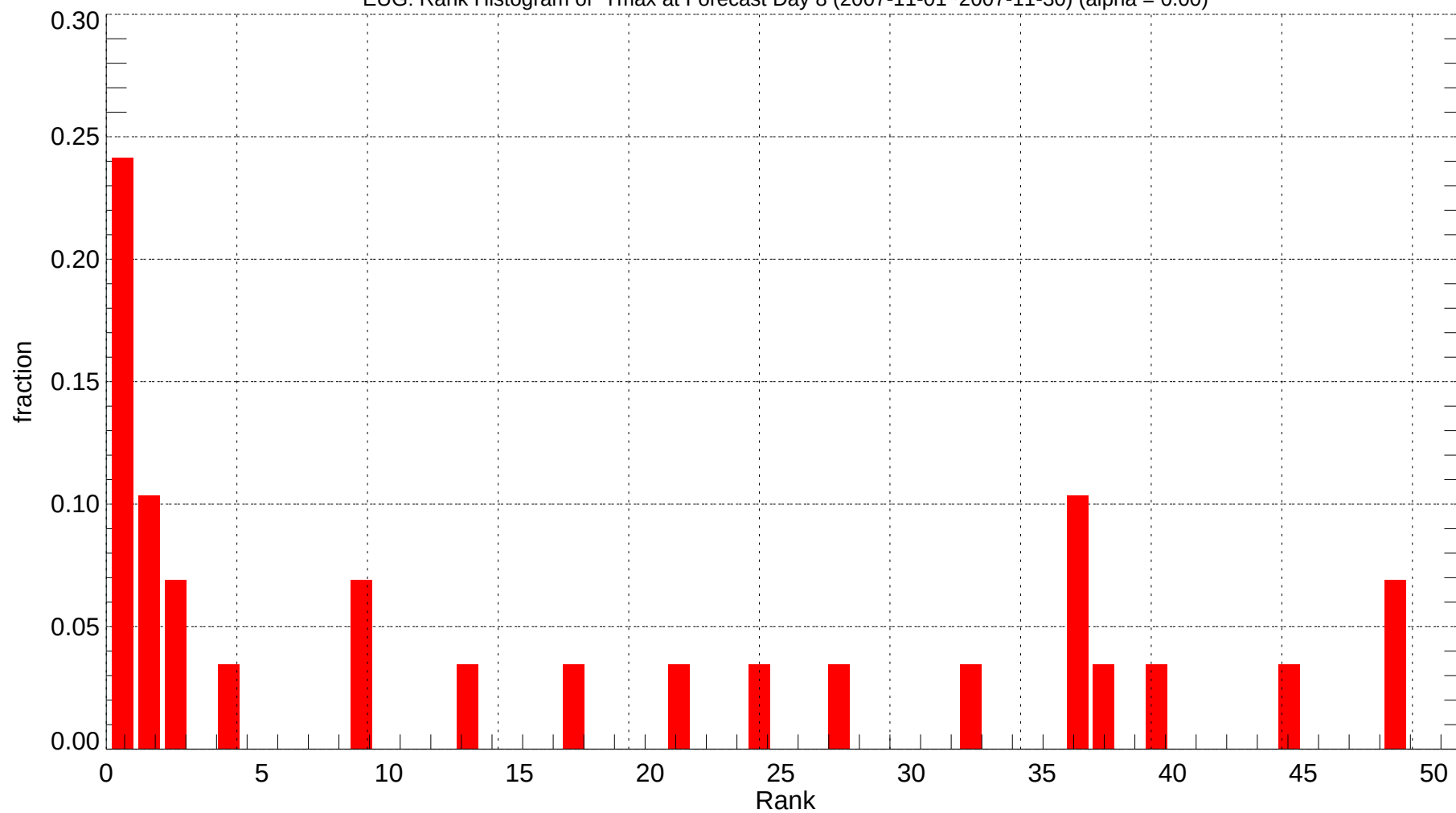
EUG: Rank Histogram of Tmax at Forecast Day 8 (2007-11-01~2007-11-30) (alpha = 0.00)
