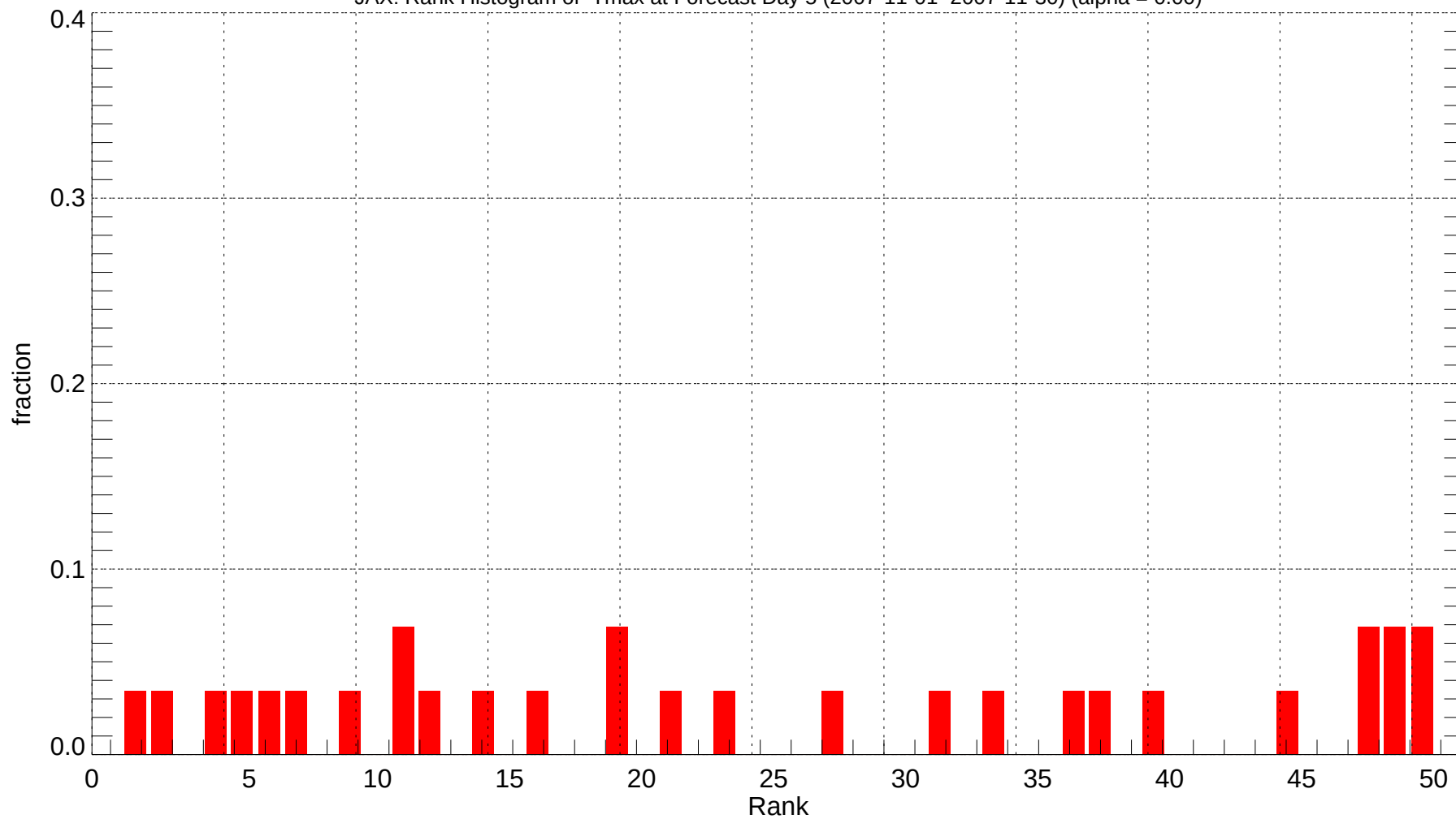
JAX: Rank Histogram of Tmax at Forecast Day 5 (2007-11-01~2007-11-30) (alpha = 0.00)
