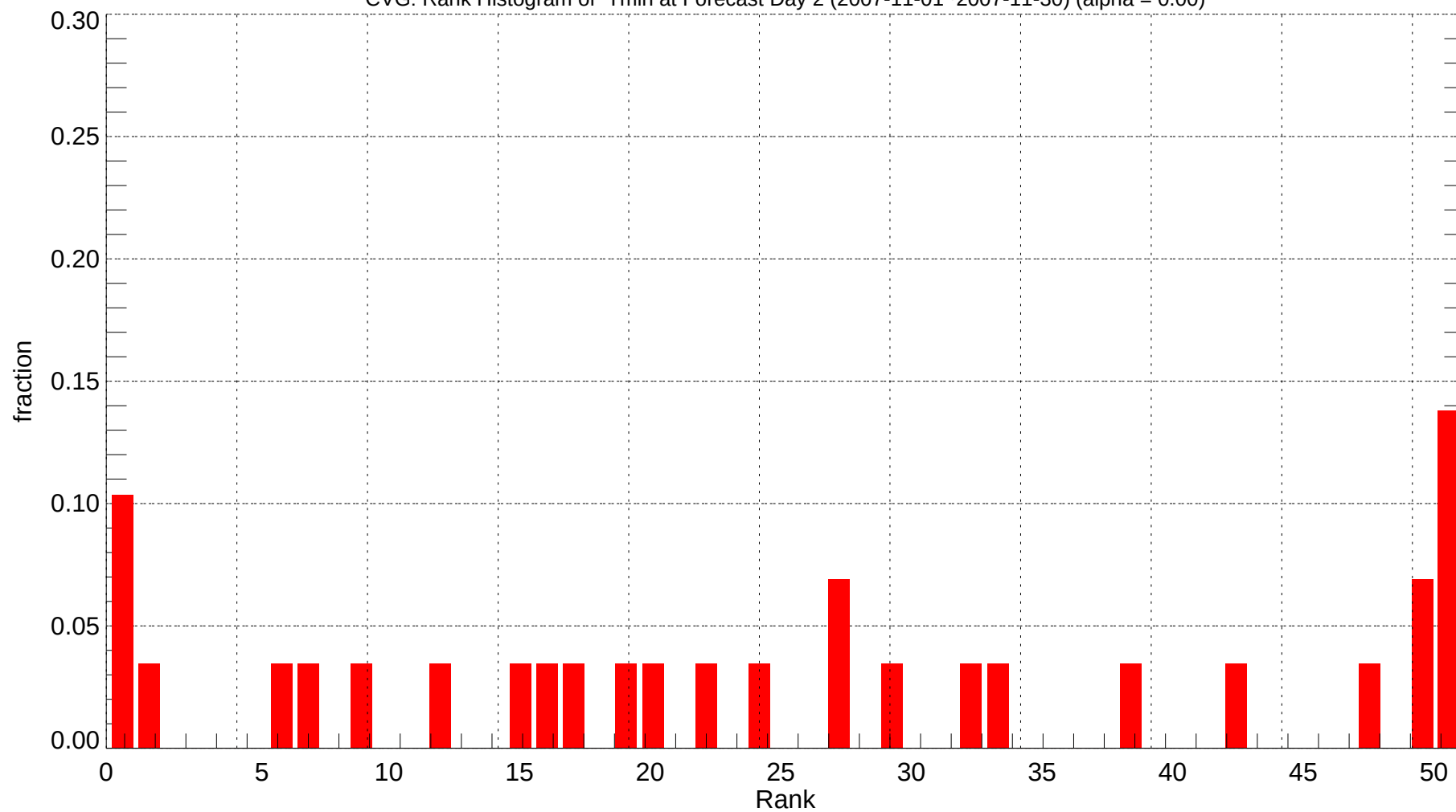
CVG: Rank Histogram of Tmin at Forecast Day 2 (2007-11-01~2007-11-30) (alpha = 0.00)
