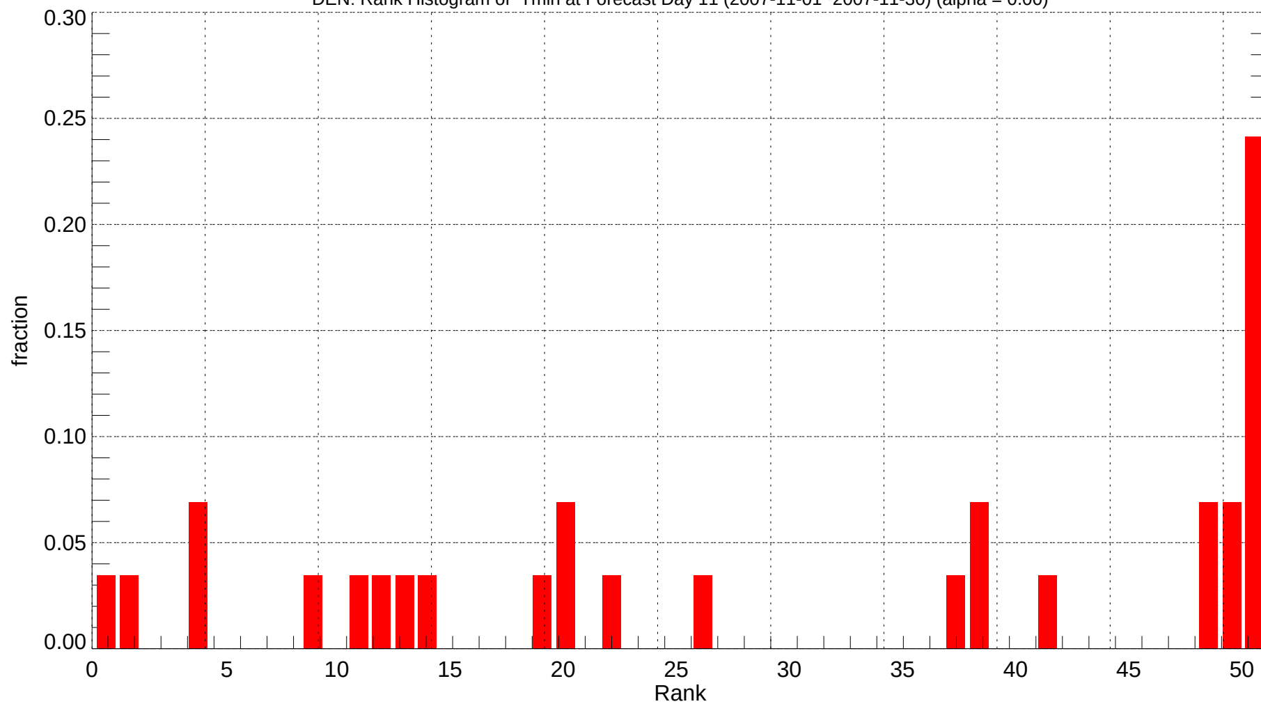
DEN: Rank Histogram of Tmin at Forecast Day 11 (2007-11-01~2007-11-30) (alpha = 0.00)
