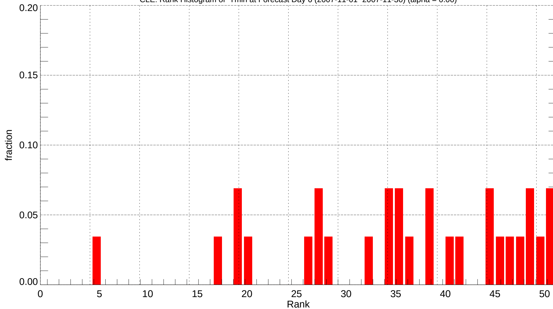
CLE: Rank Histogram of Tmin at Forecast Day 6 (2007-11-01~2007-11-30) (alpha = 0.00)
