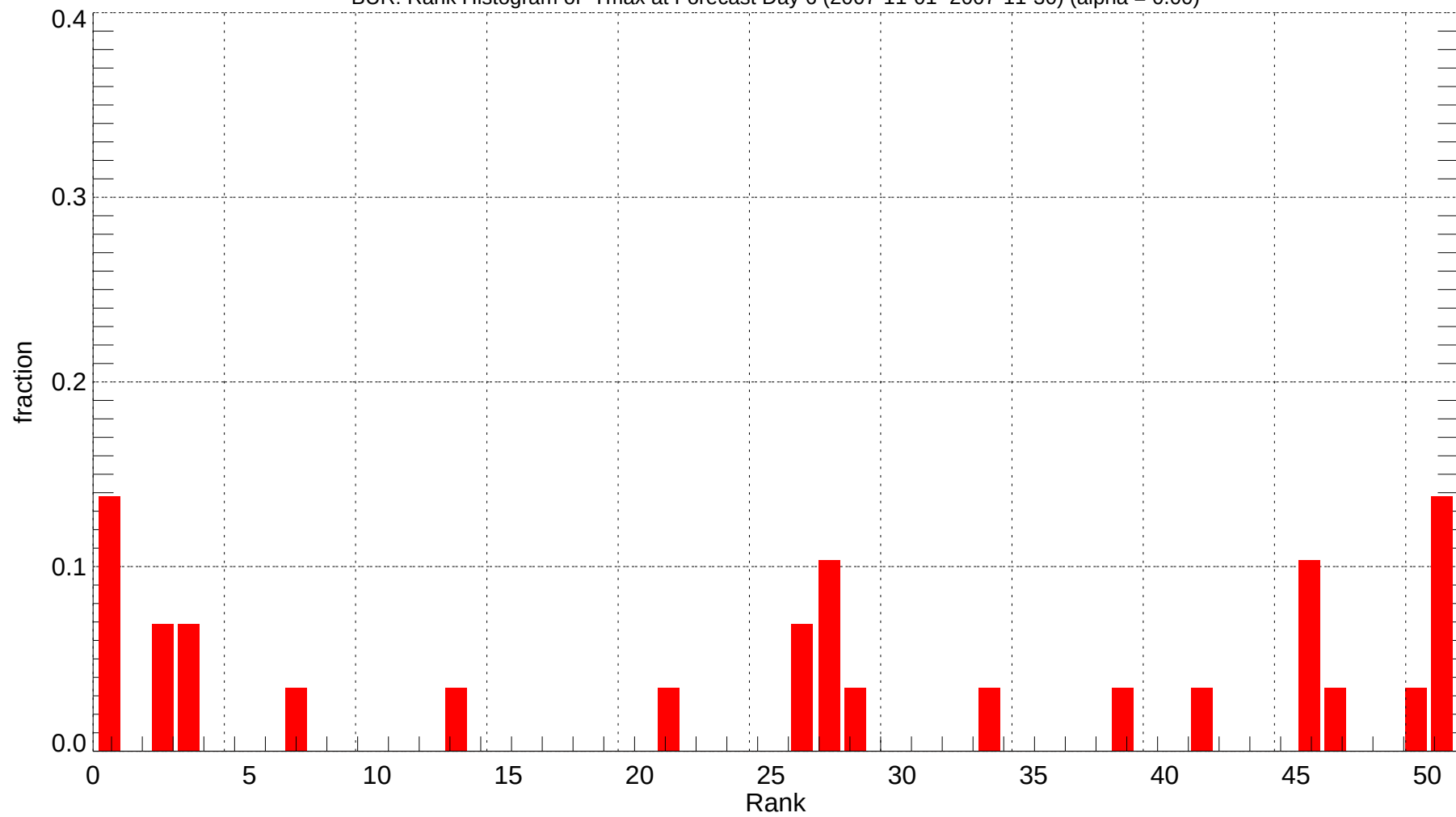
BUR: Rank Histogram of Tmax at Forecast Day 6 (2007-11-01~2007-11-30) (alpha = 0.00)
