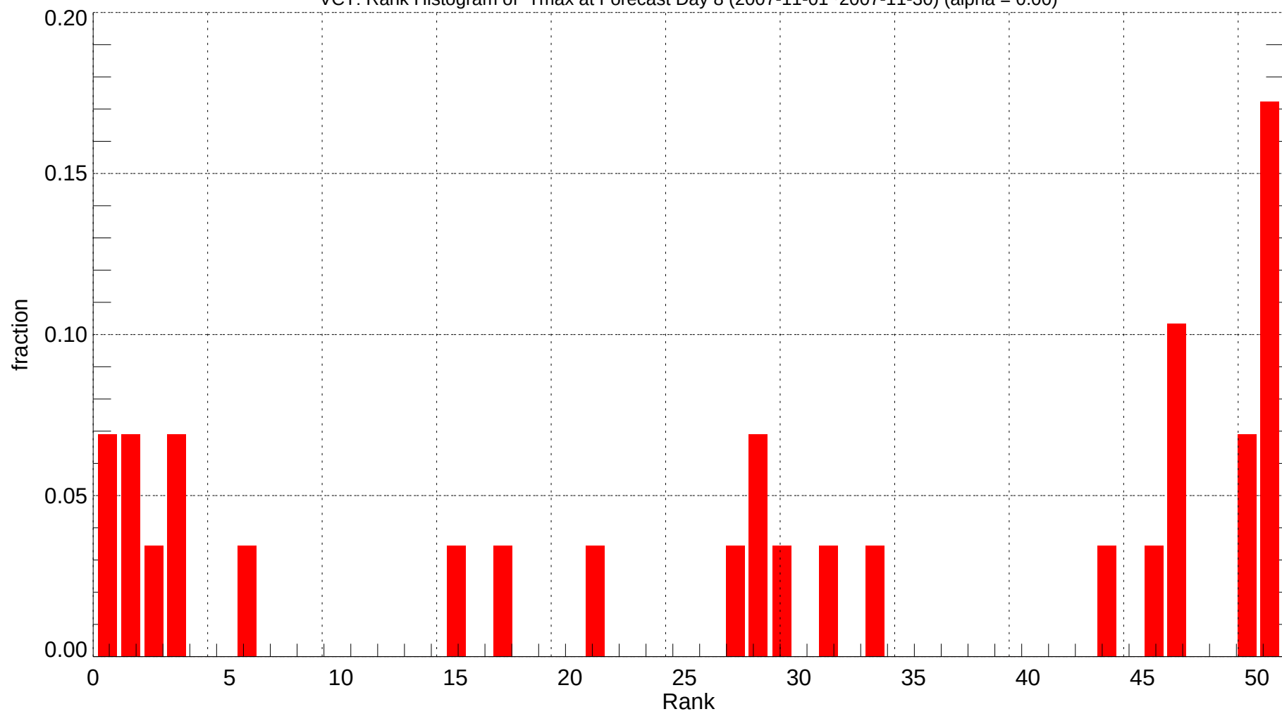
VCT: Rank Histogram of Tmax at Forecast Day 8 (2007-11-01~2007-11-30) (alpha = 0.00)
