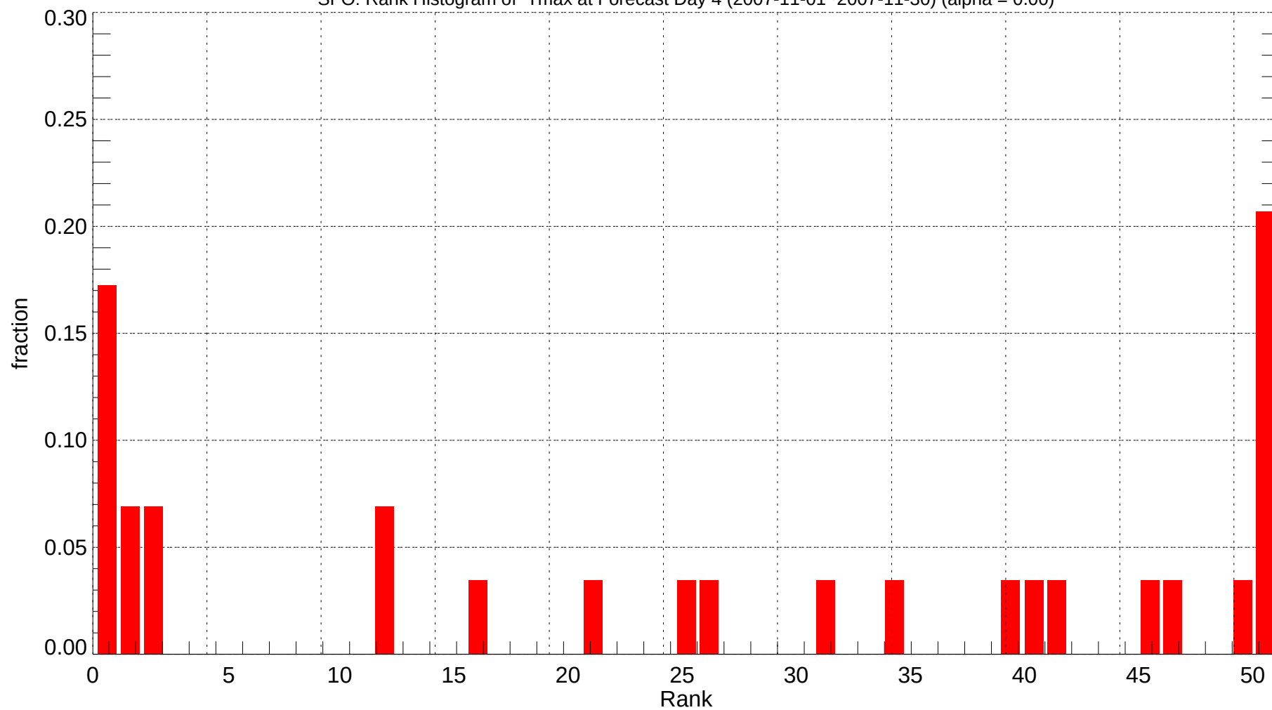
SFO: Rank Histogram of Tmax at Forecast Day 4 (2007-11-01~2007-11-30) (alpha = 0.00)
