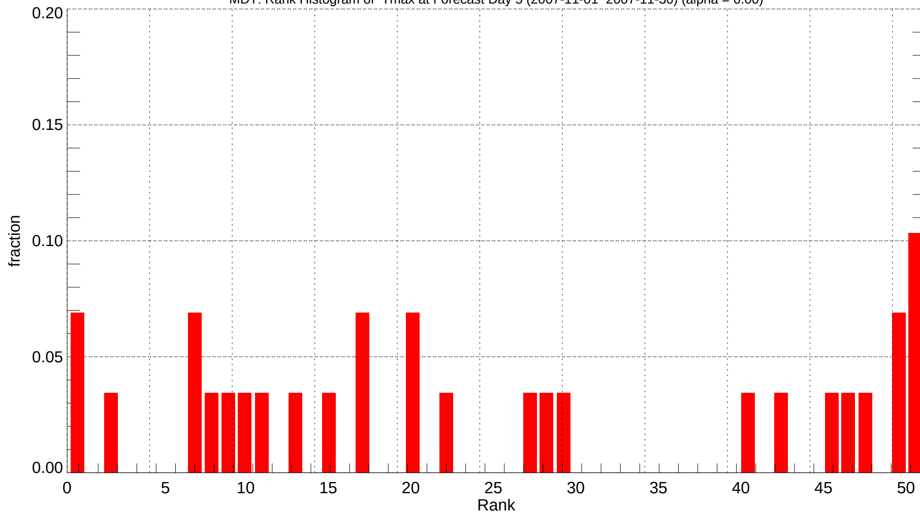
MDT: Rank Histogram of Tmax at Forecast Day 5 (2007-11-01~2007-11-30) (alpha = 0.00)
