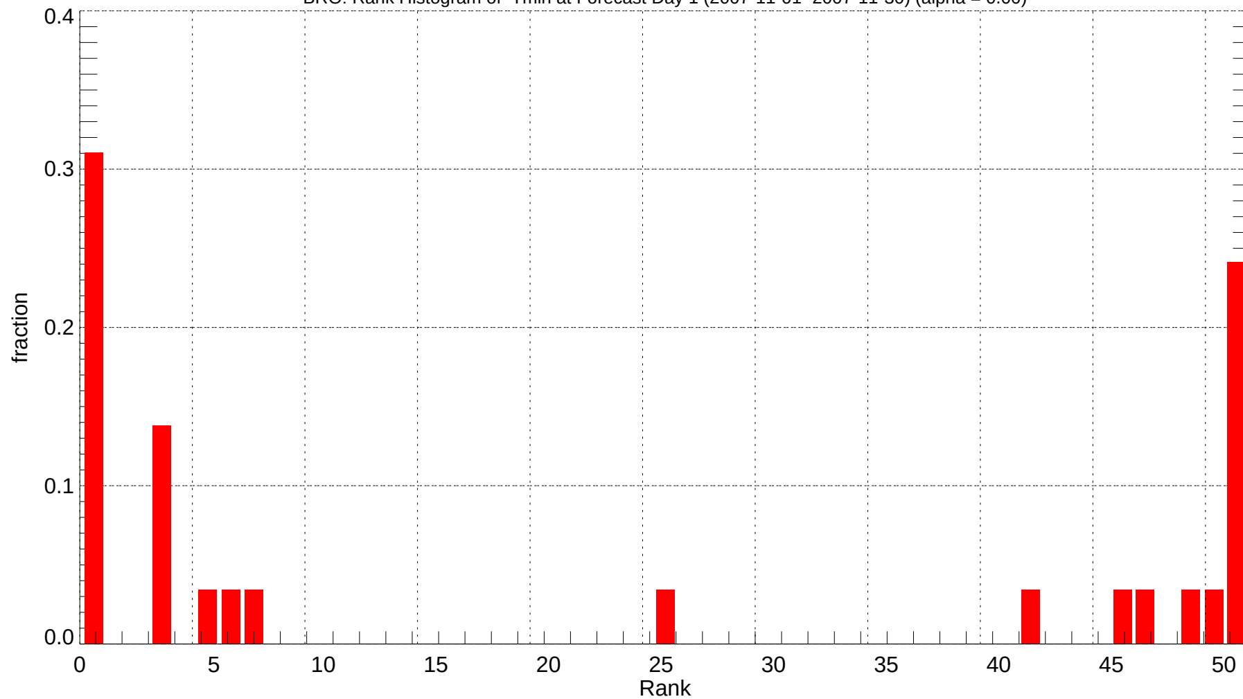
BRO: Rank Histogram of Tmin at Forecast Day 1 (2007-11-01~2007-11-30) (alpha = 0.00)
