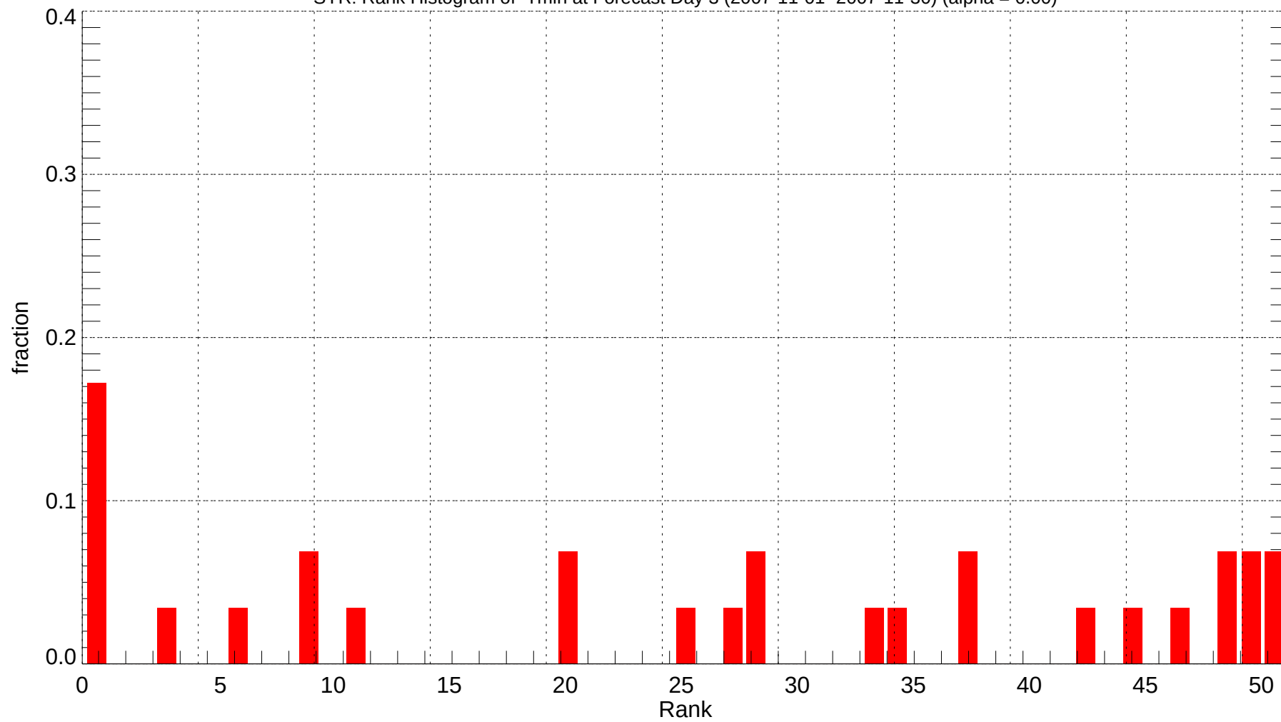
SYR: Rank Histogram of Tmin at Forecast Day 3 (2007-11-01~2007-11-30) (alpha = 0.00)
