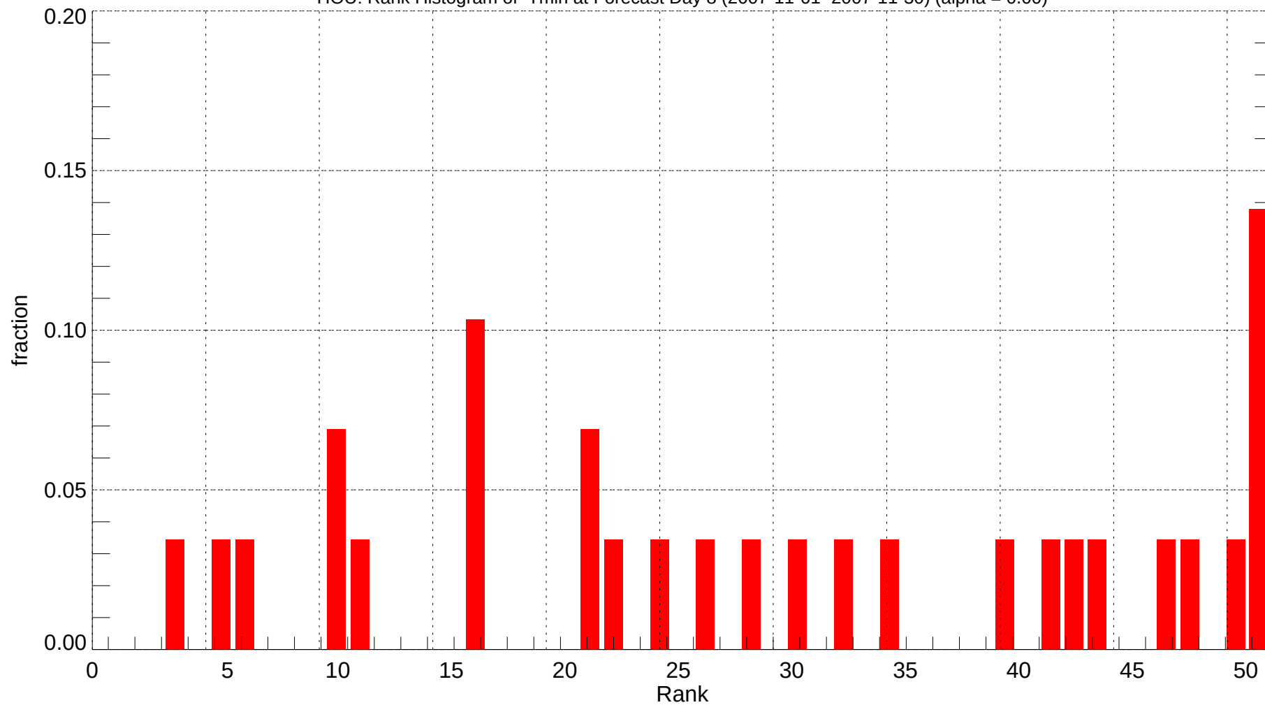
HOU: Rank Histogram of Tmin at Forecast Day 8 (2007-11-01~2007-11-30) (alpha = 0.00)
