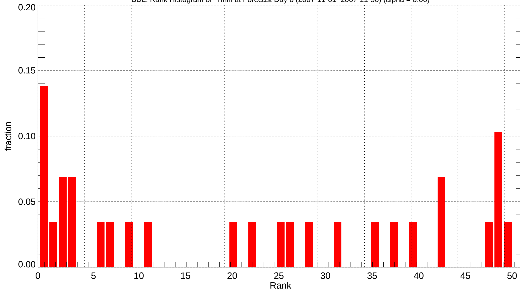
BDL: Rank Histogram of Tmin at Forecast Day 6 (2007-11-01~2007-11-30) (alpha = 0.00)
