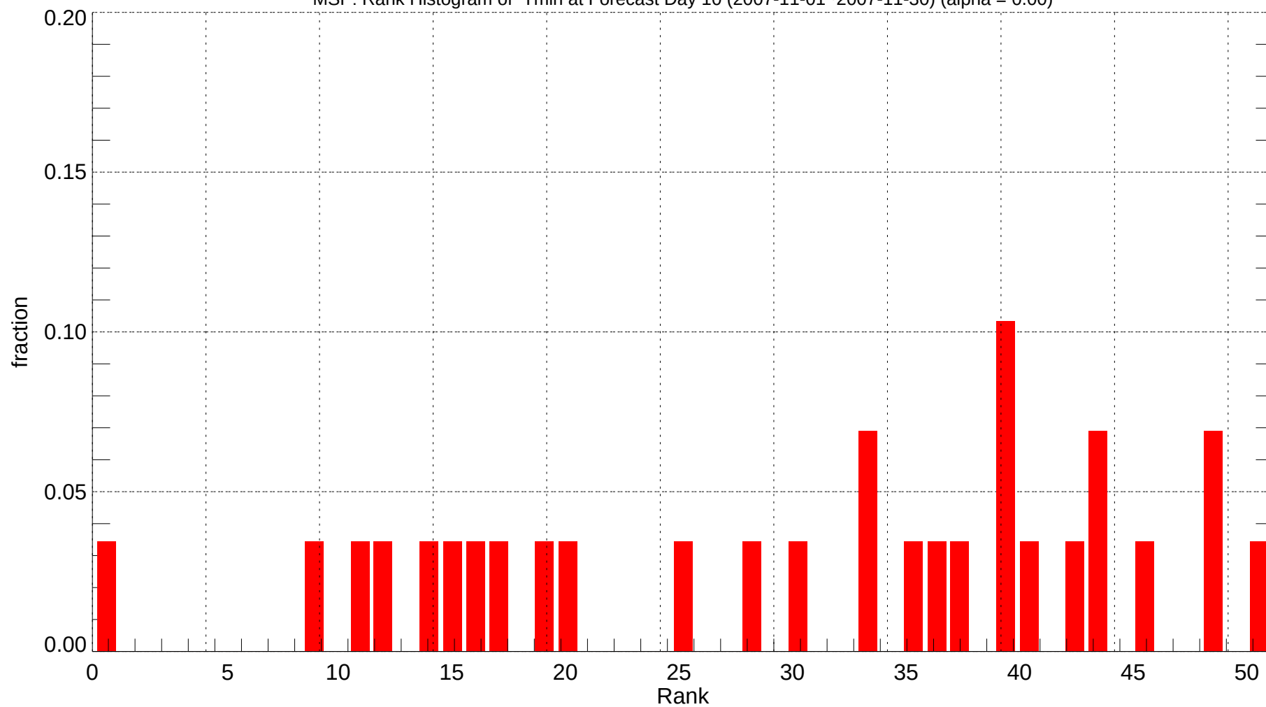
MSP: Rank Histogram of Tmin at Forecast Day 10 (2007-11-01~2007-11-30) (alpha = 0.00)
