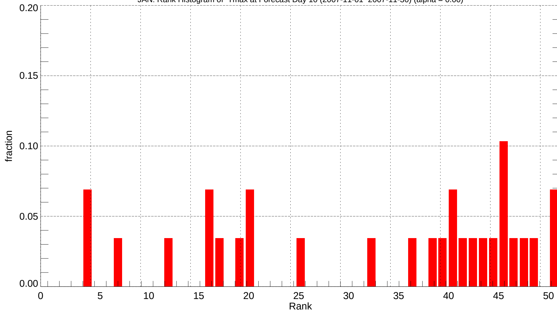
JAN: Rank Histogram of Tmax at Forecast Day 10 (2007-11-01~2007-11-30) (alpha = 0.00)
