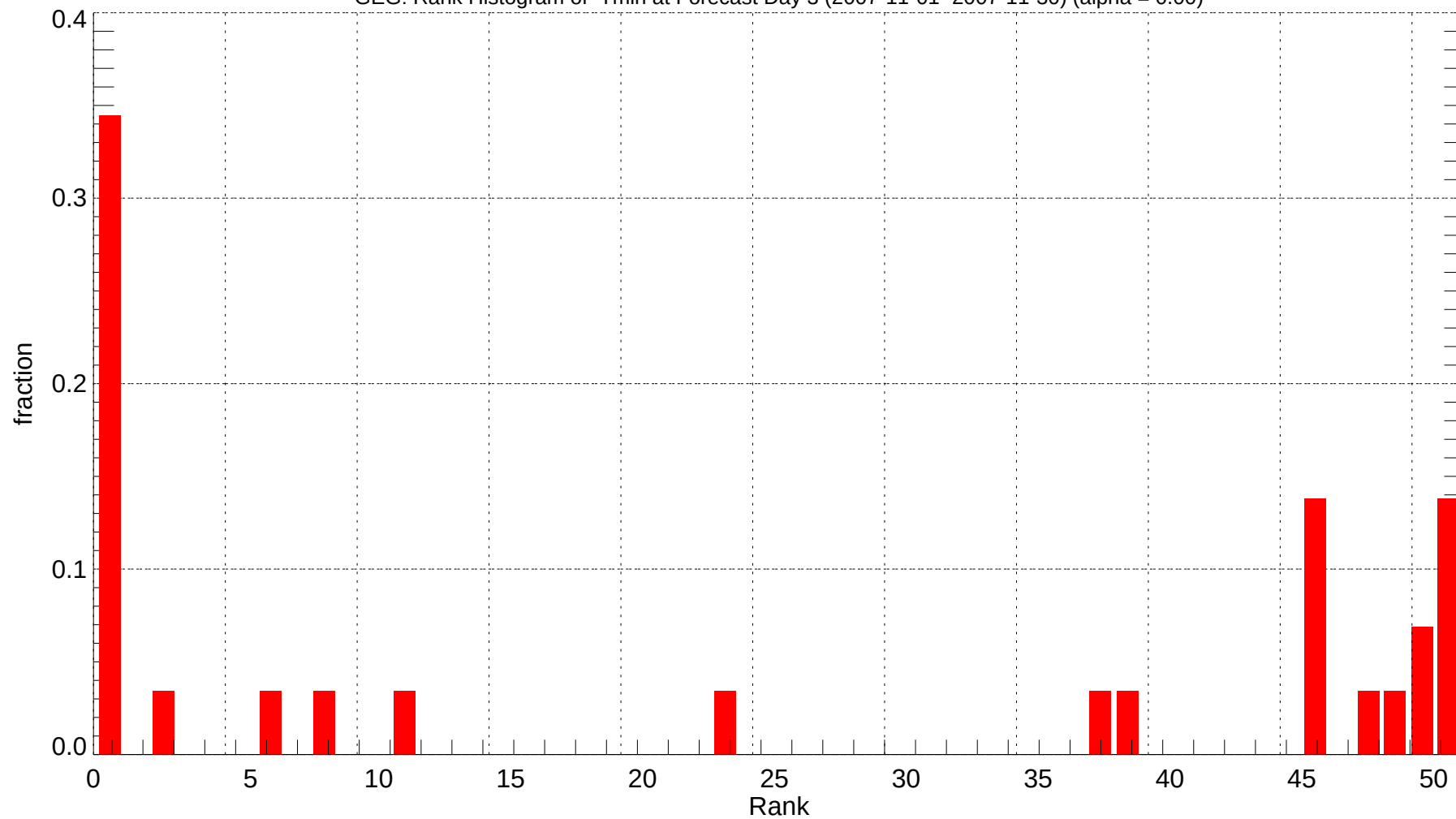
GEG: Rank Histogram of Tmin at Forecast Day 3 (2007-11-01~2007-11-30) (alpha = 0.00)
