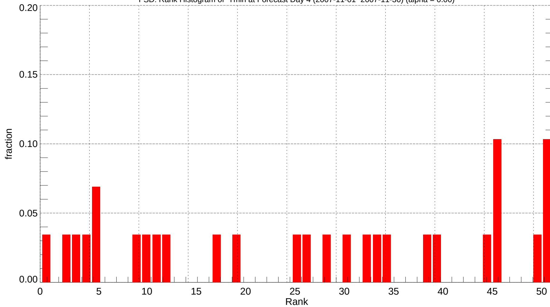
FSD: Rank Histogram of Tmin at Forecast Day 4 (2007-11-01~2007-11-30) (alpha = 0.00)
