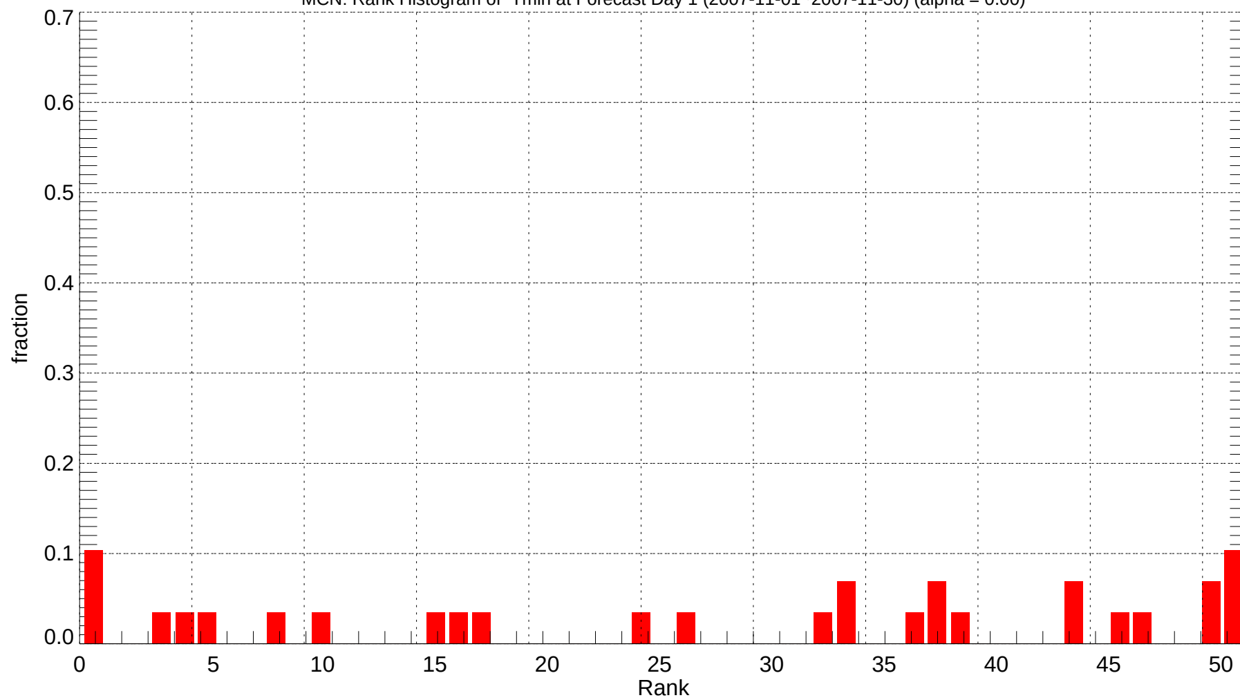
MCN: Rank Histogram of Tmin at Forecast Day 1 (2007-11-01~2007-11-30) (alpha = 0.00)
