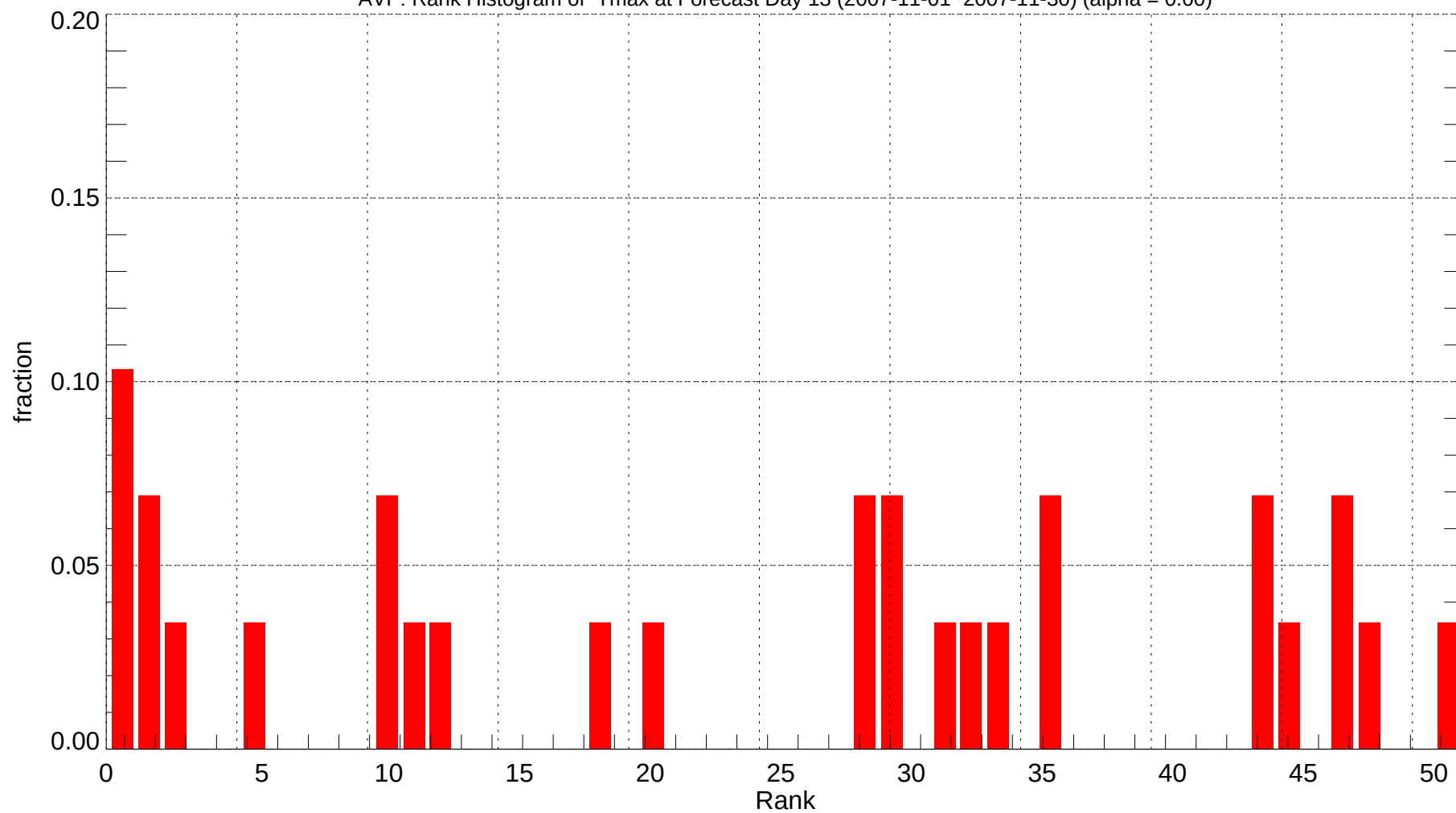
AVP: Rank Histogram of Tmax at Forecast Day 13 (2007-11-01~2007-11-30) (alpha = 0.00)
