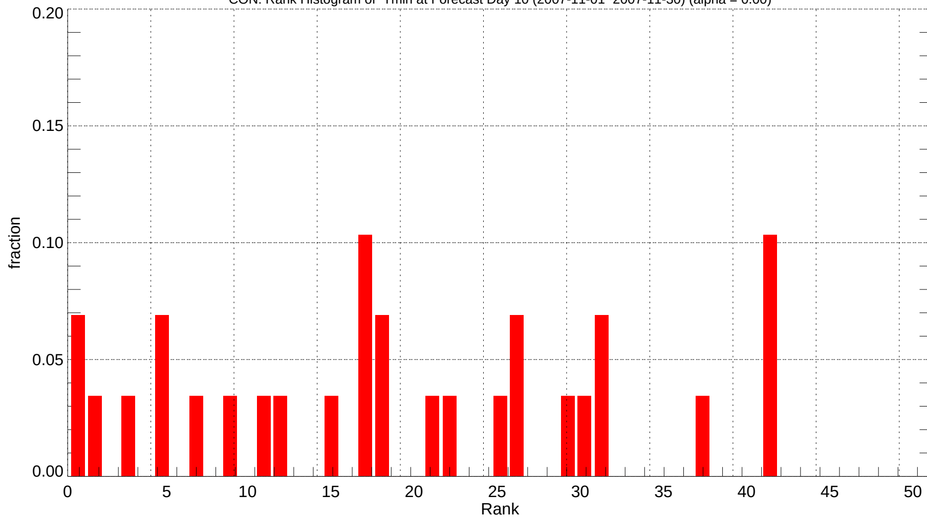
CON: Rank Histogram of Tmin at Forecast Day 10 (2007-11-01~2007-11-30) (alpha = 0.00)
