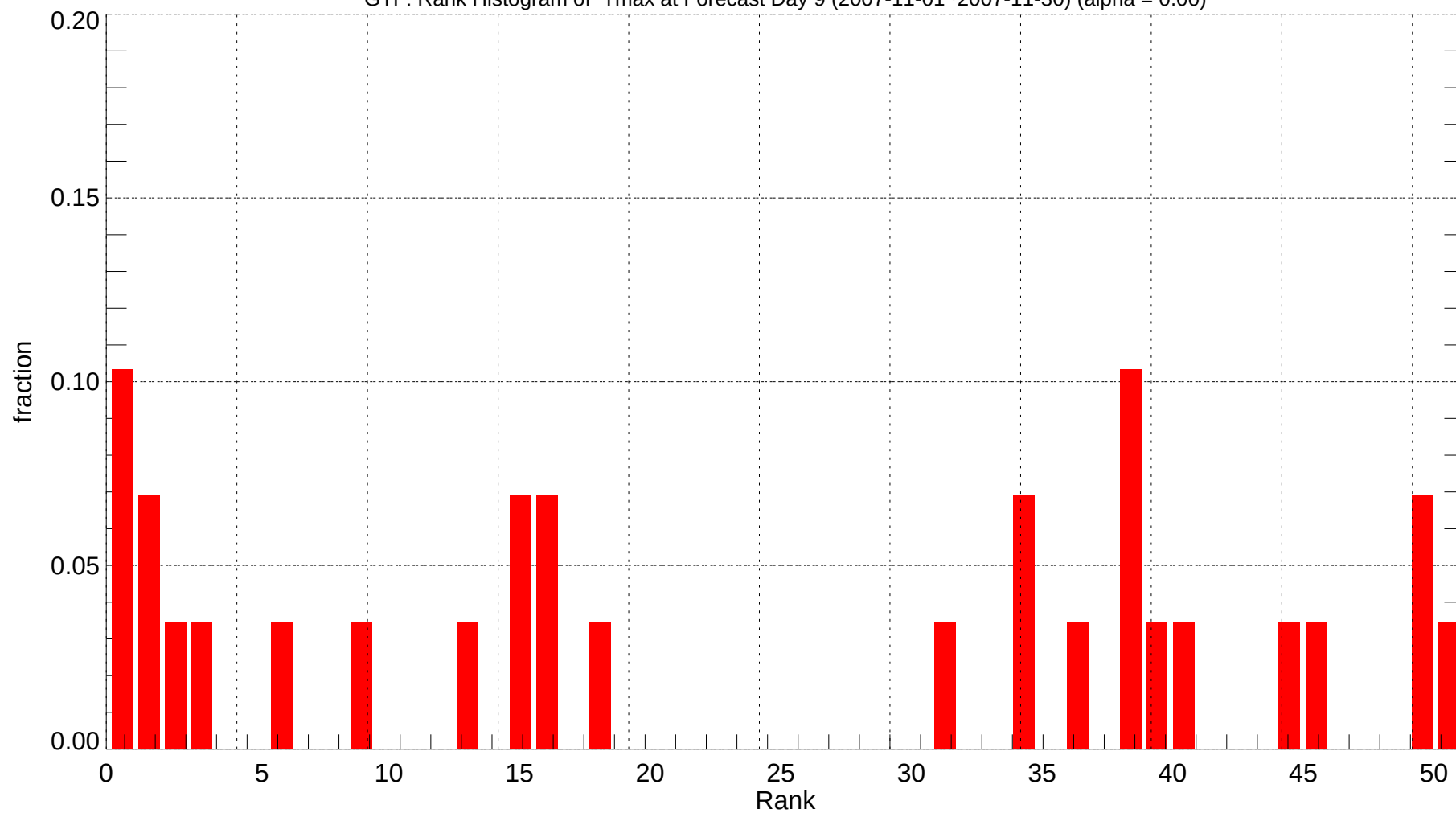
GTF: Rank Histogram of Tmax at Forecast Day 9 (2007-11-01~2007-11-30) (alpha = 0.00)
