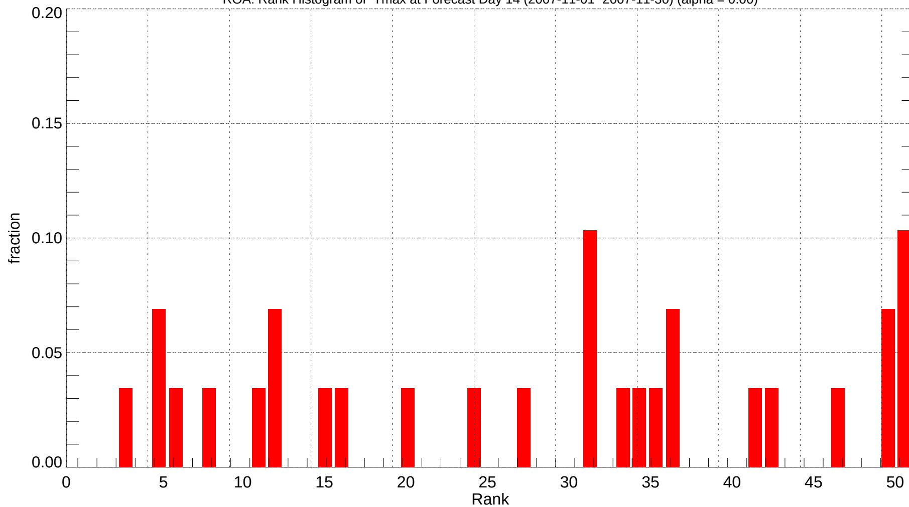
ROA: Rank Histogram of Tmax at Forecast Day 14 (2007-11-01~2007-11-30) (alpha = 0.00)
