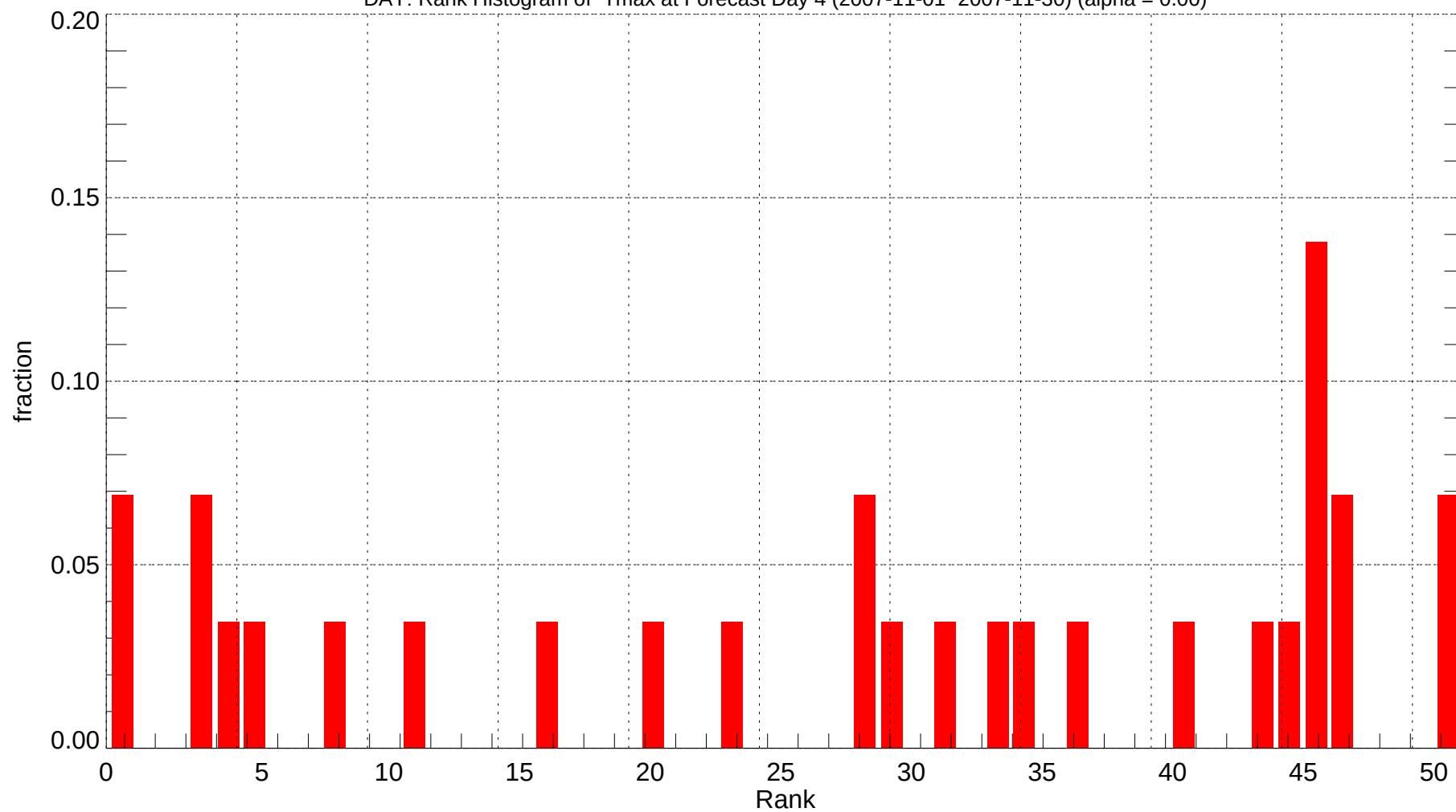
DAY: Rank Histogram of Tmax at Forecast Day 4 (2007-11-01~2007-11-30) (alpha = 0.00)
