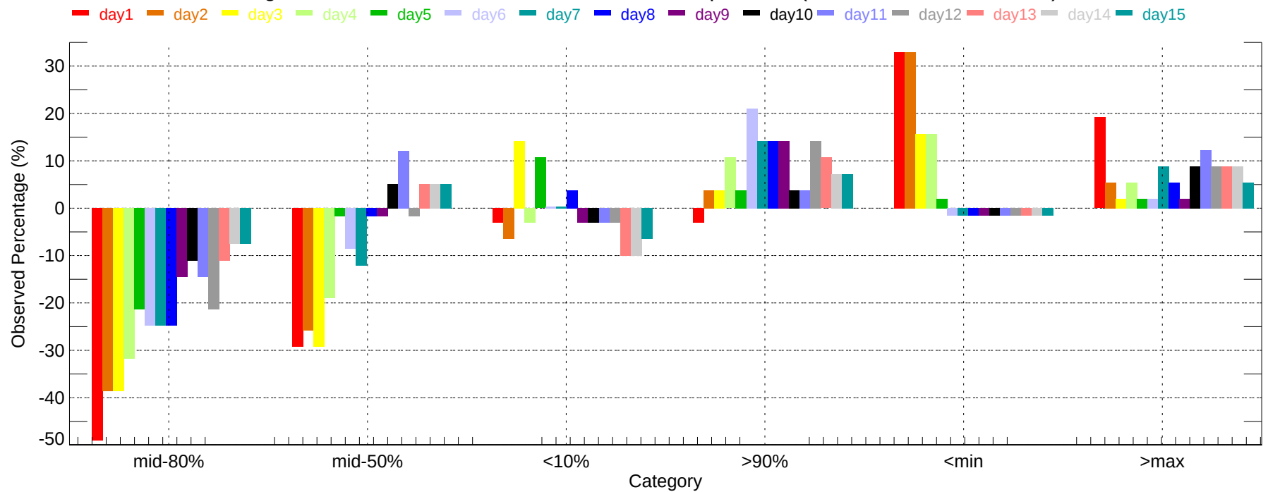
Observed Percentage Deviation of Ensembles - FWA: Max Temperature (2007-11-01~2007-11-30)
