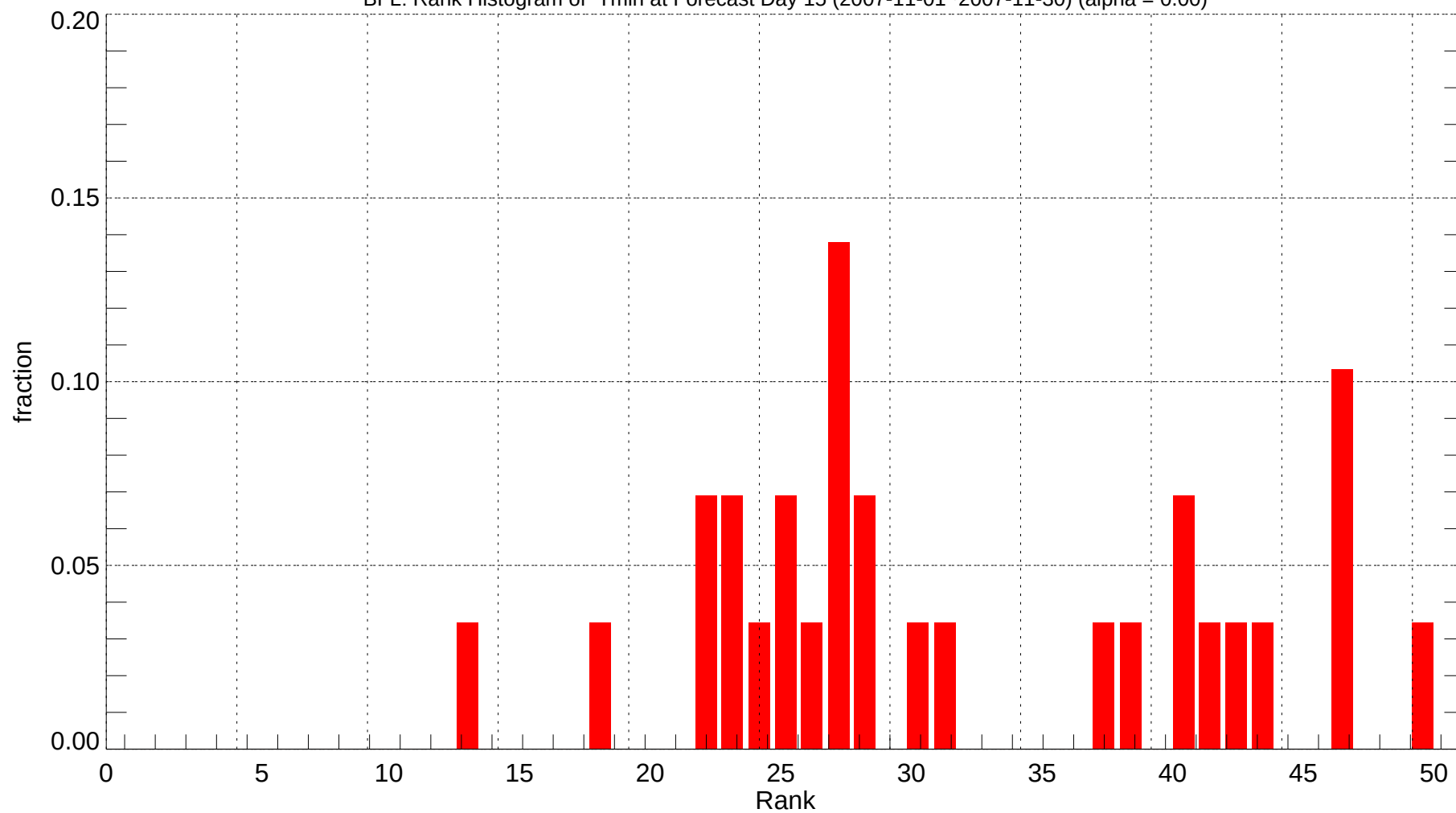
BFL: Rank Histogram of Tmin at Forecast Day 15 (2007-11-01~2007-11-30) (alpha = 0.00)
