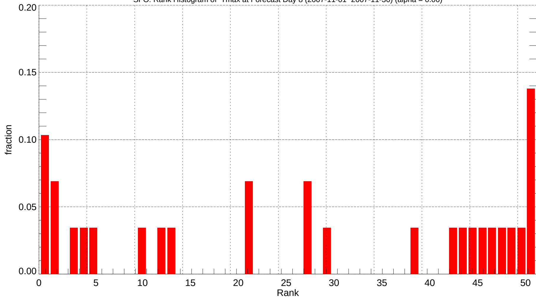
SFO: Rank Histogram of Tmax at Forecast Day 8 (2007-11-01~2007-11-30) (alpha = 0.00)
