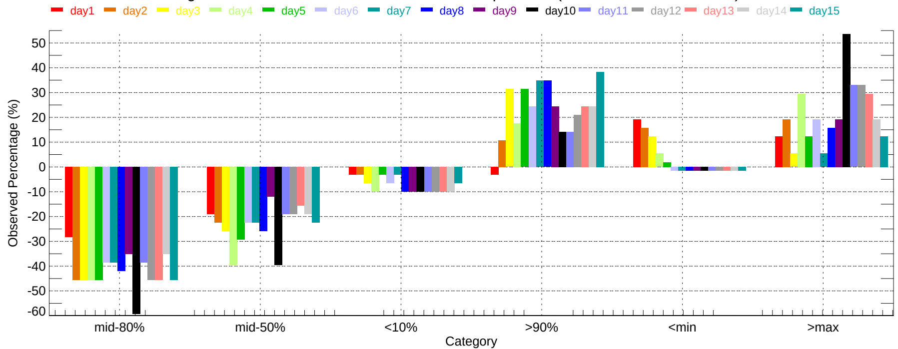
Observed Percentage Deviation of Ensembles - TUL: Min Temperature (2007-11-01~2007-11-30)
