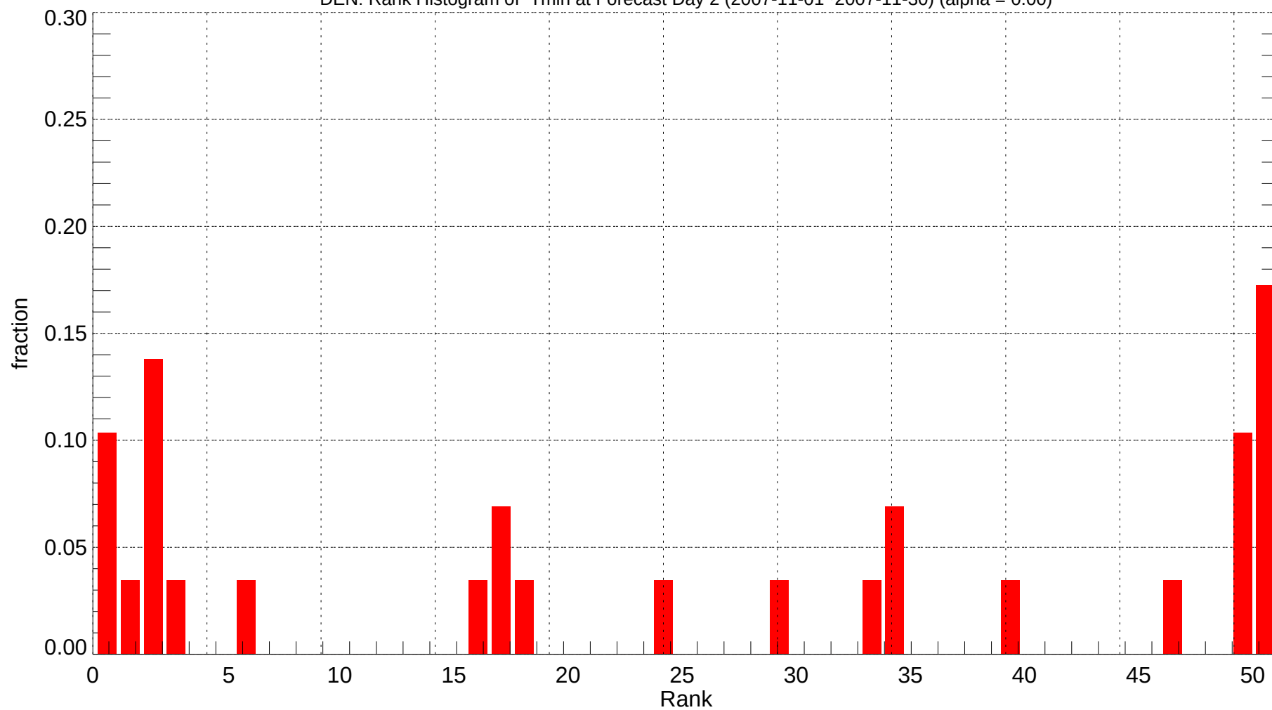
DEN: Rank Histogram of Tmin at Forecast Day 2 (2007-11-01~2007-11-30) (alpha = 0.00)
