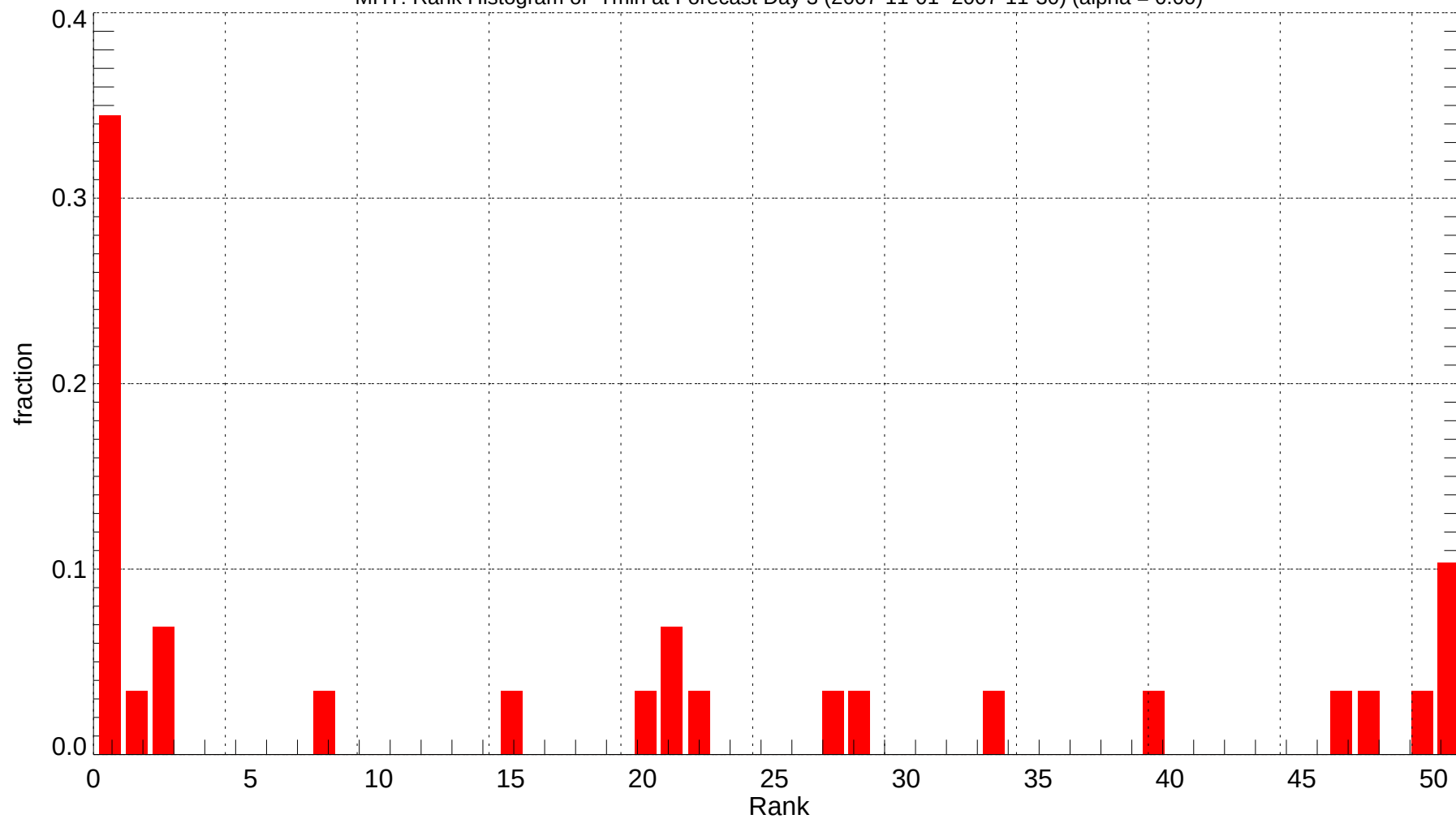
MHT: Rank Histogram of Tmin at Forecast Day 3 (2007-11-01~2007-11-30) (alpha = 0.00)
