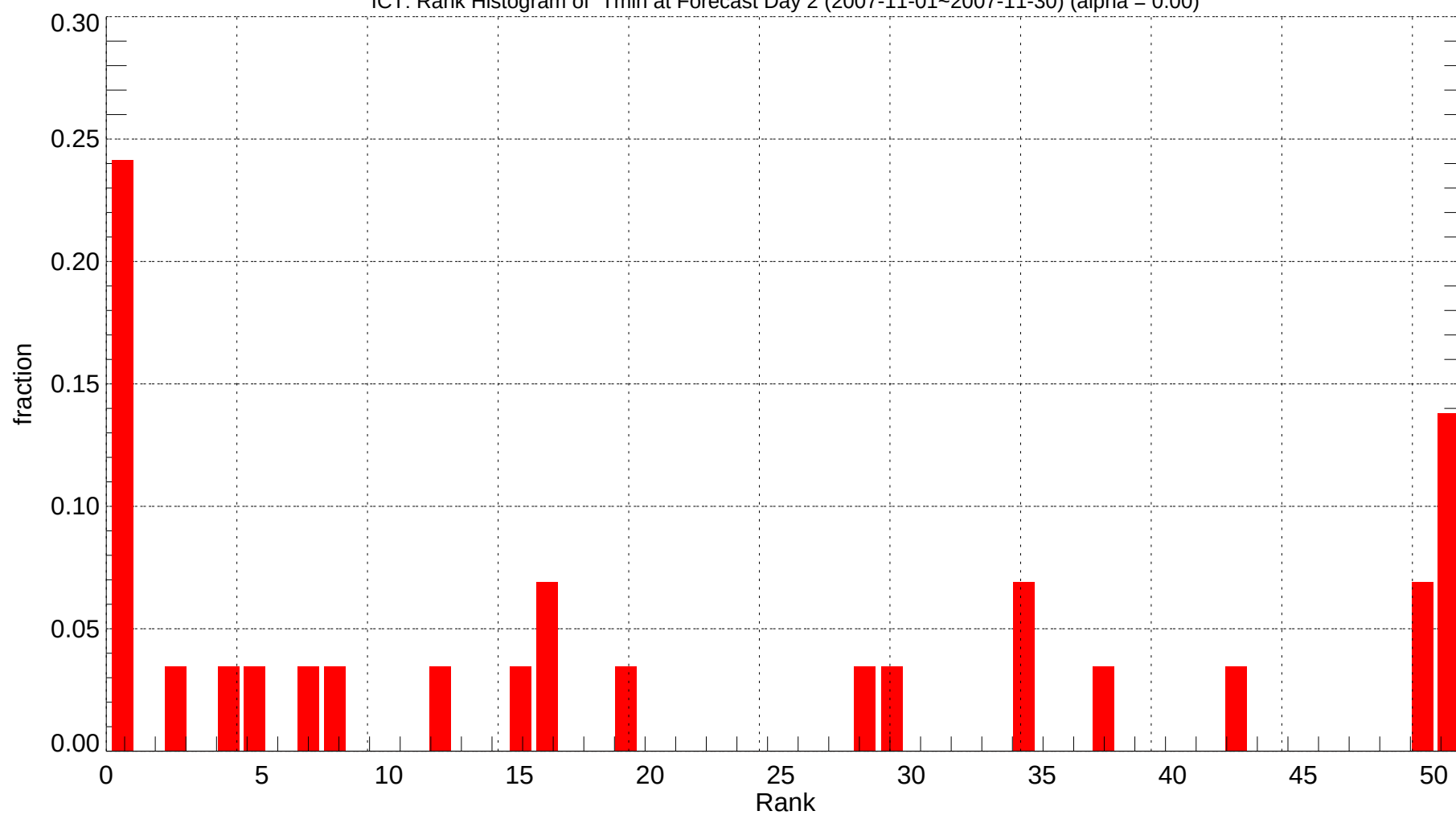
ICT: Rank Histogram of Tmin at Forecast Day 2 (2007-11-01~2007-11-30) (alpha = 0.00)
