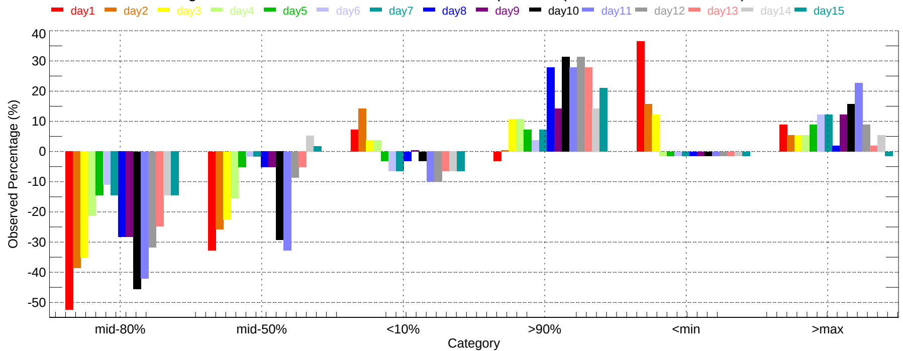
Observed Percentage Deviation of Ensembles - FSD: Min Temperature (2007-11-01~2007-11-30)
