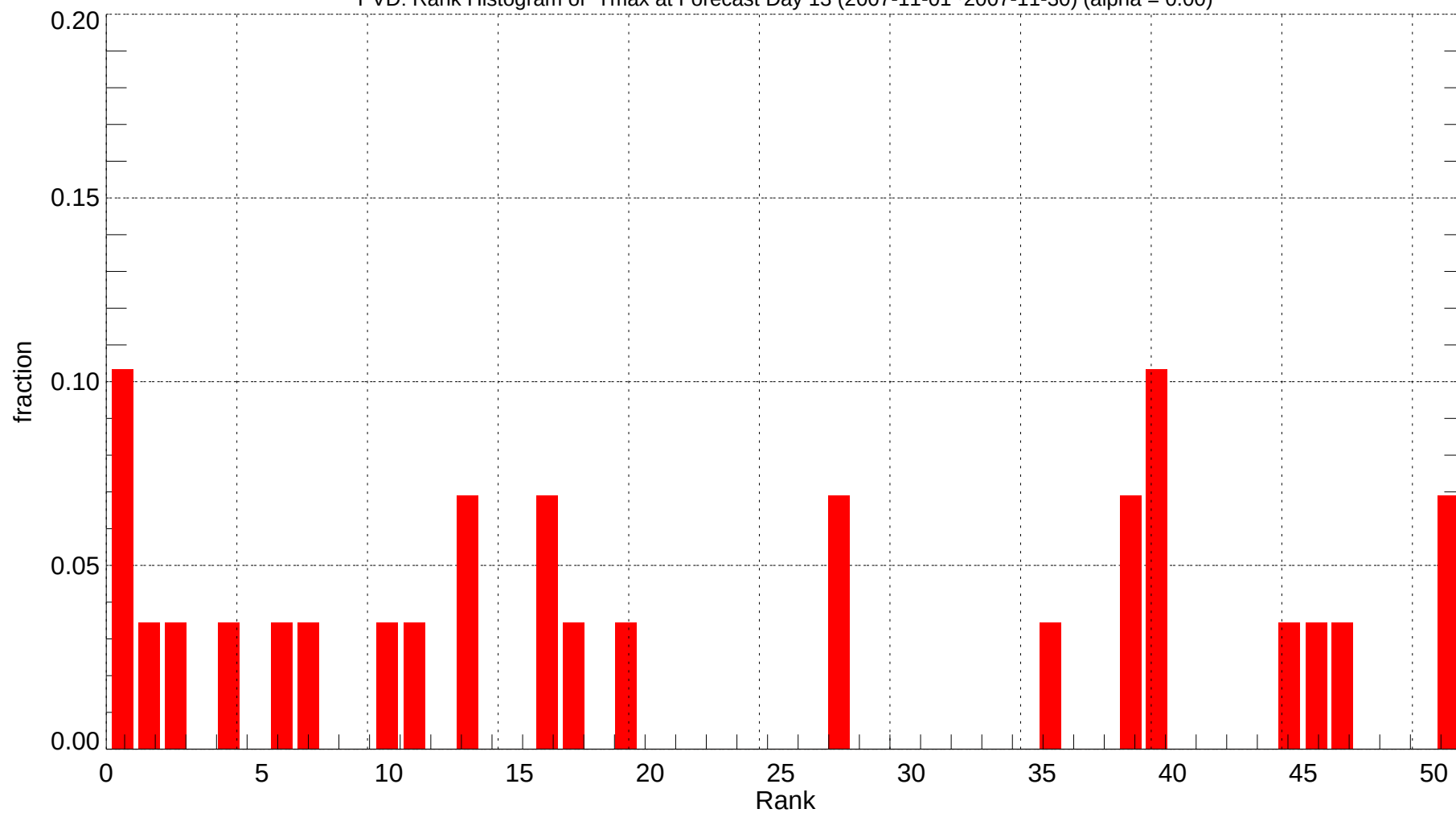
PVD: Rank Histogram of Tmax at Forecast Day 13 (2007-11-01~2007-11-30) (alpha = 0.00)
