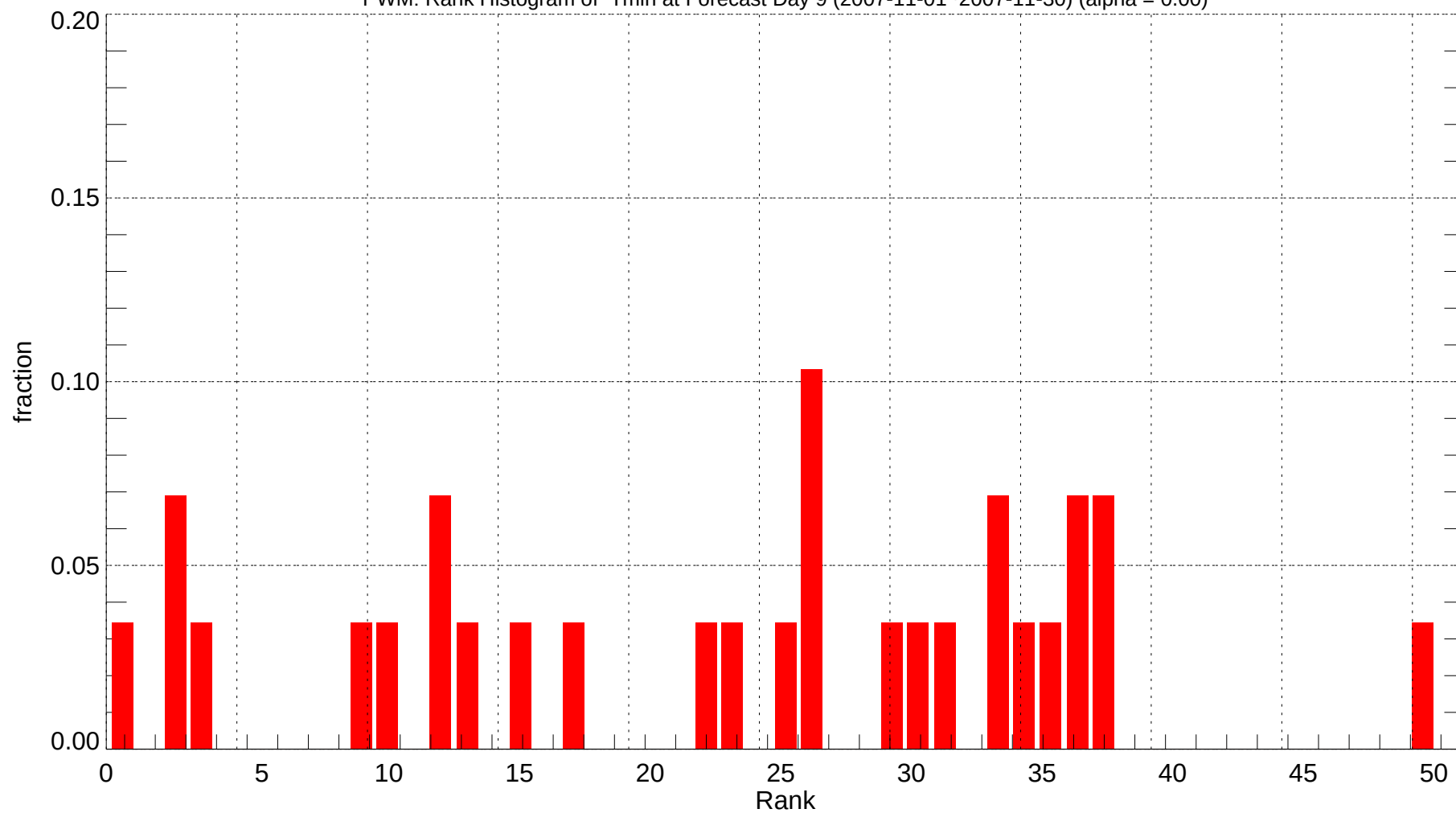
PWM: Rank Histogram of Tmin at Forecast Day 9 (2007-11-01~2007-11-30) (alpha = 0.00)
