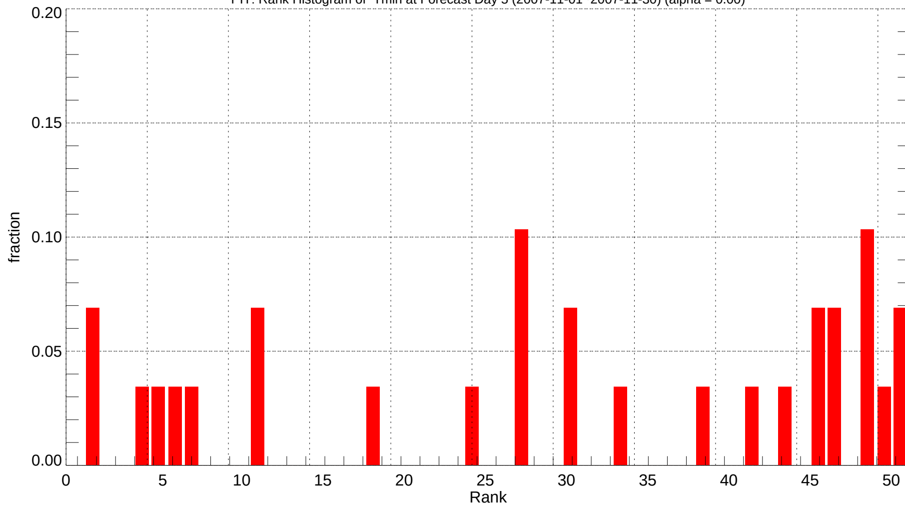
PIT: Rank Histogram of Tmin at Forecast Day 5 (2007-11-01~2007-11-30) (alpha = 0.00)
