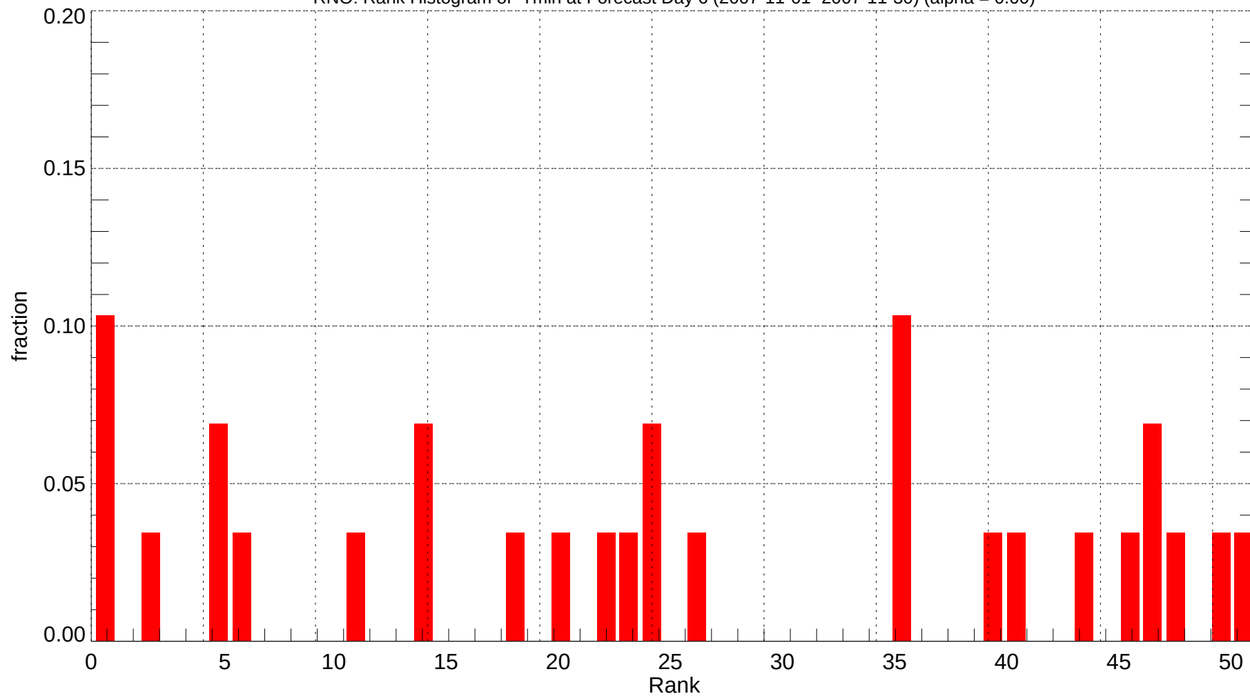
RNO: Rank Histogram of Tmin at Forecast Day 6 (2007-11-01~2007-11-30) (alpha = 0.00)
