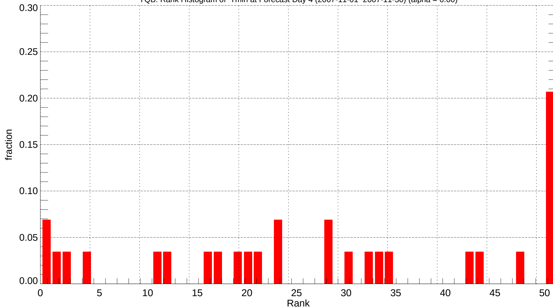
YQB: Rank Histogram of Tmin at Forecast Day 4 (2007-11-01~2007-11-30) (alpha = 0.00)
