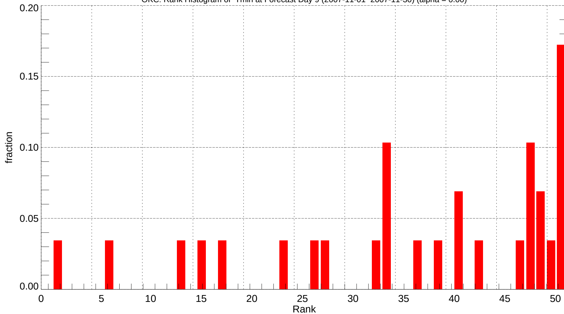
OKC: Rank Histogram of Tmin at Forecast Day 9 (2007-11-01~2007-11-30) (alpha = 0.00)
