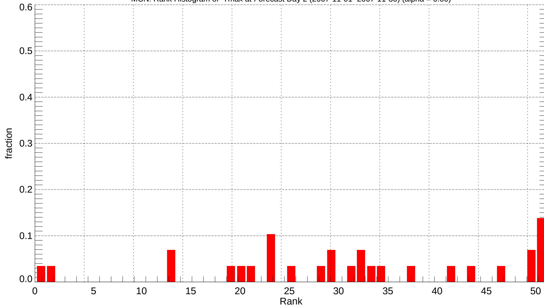
MCN: Rank Histogram of Tmax at Forecast Day 2 (2007-11-01~2007-11-30) (alpha = 0.00)
