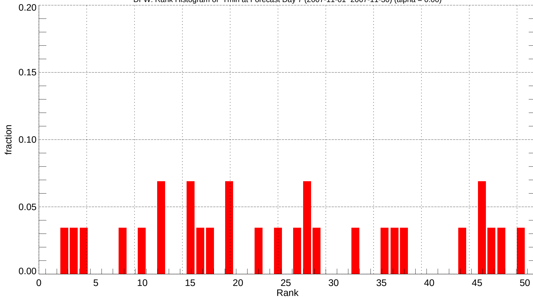
DFW: Rank Histogram of Tmin at Forecast Day 7 (2007-11-01~2007-11-30) (alpha = 0.00)
