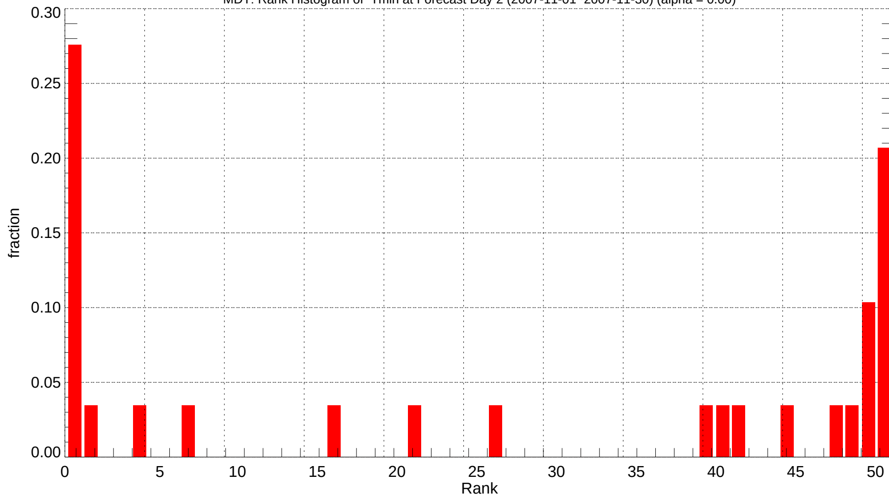
MDT: Rank Histogram of Tmin at Forecast Day 2 (2007-11-01~2007-11-30) (alpha = 0.00)
