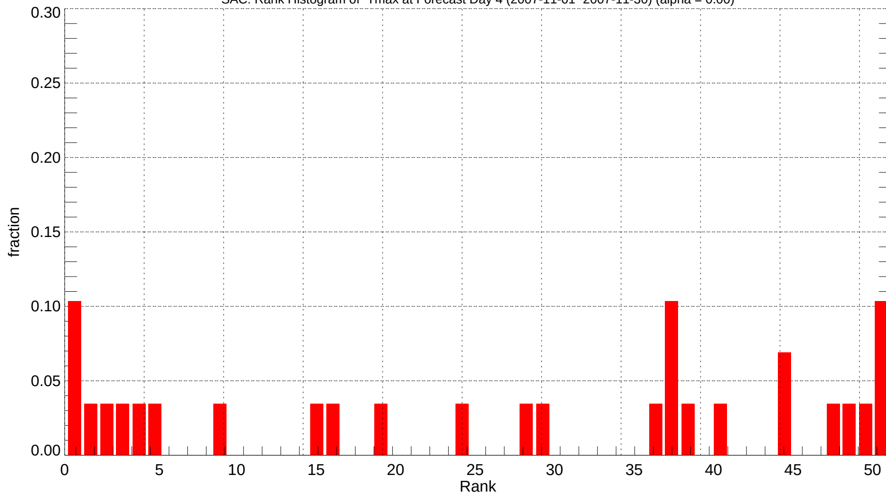
SAC: Rank Histogram of Tmax at Forecast Day 4 (2007-11-01~2007-11-30) (alpha = 0.00)
