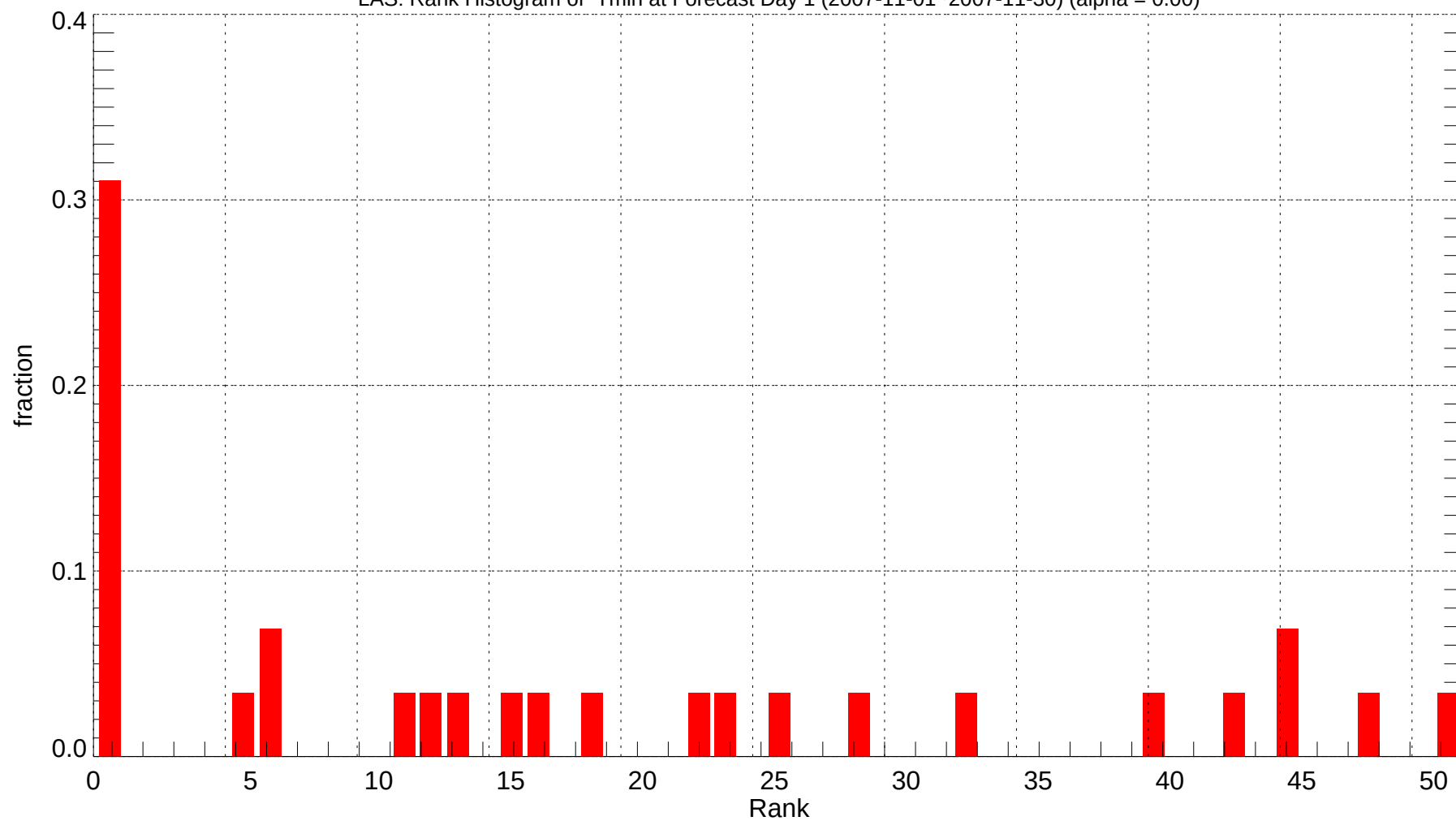
LAS: Rank Histogram of Tmin at Forecast Day 1 (2007-11-01~2007-11-30) (alpha = 0.00)
