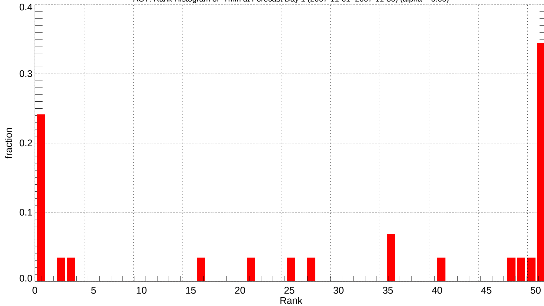
ACY: Rank Histogram of Tmin at Forecast Day 1 (2007-11-01~2007-11-30) (alpha = 0.00)
