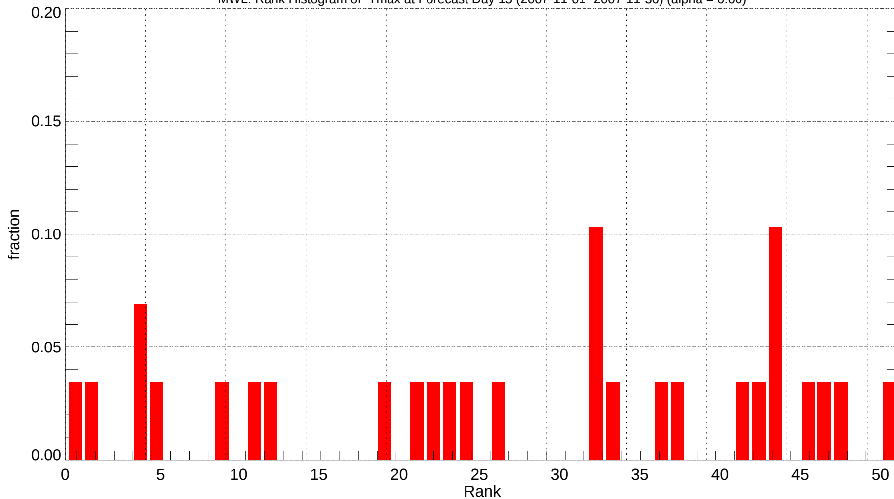
MWL: Rank Histogram of Tmax at Forecast Day 15 (2007-11-01~2007-11-30) (alpha = 0.00)
