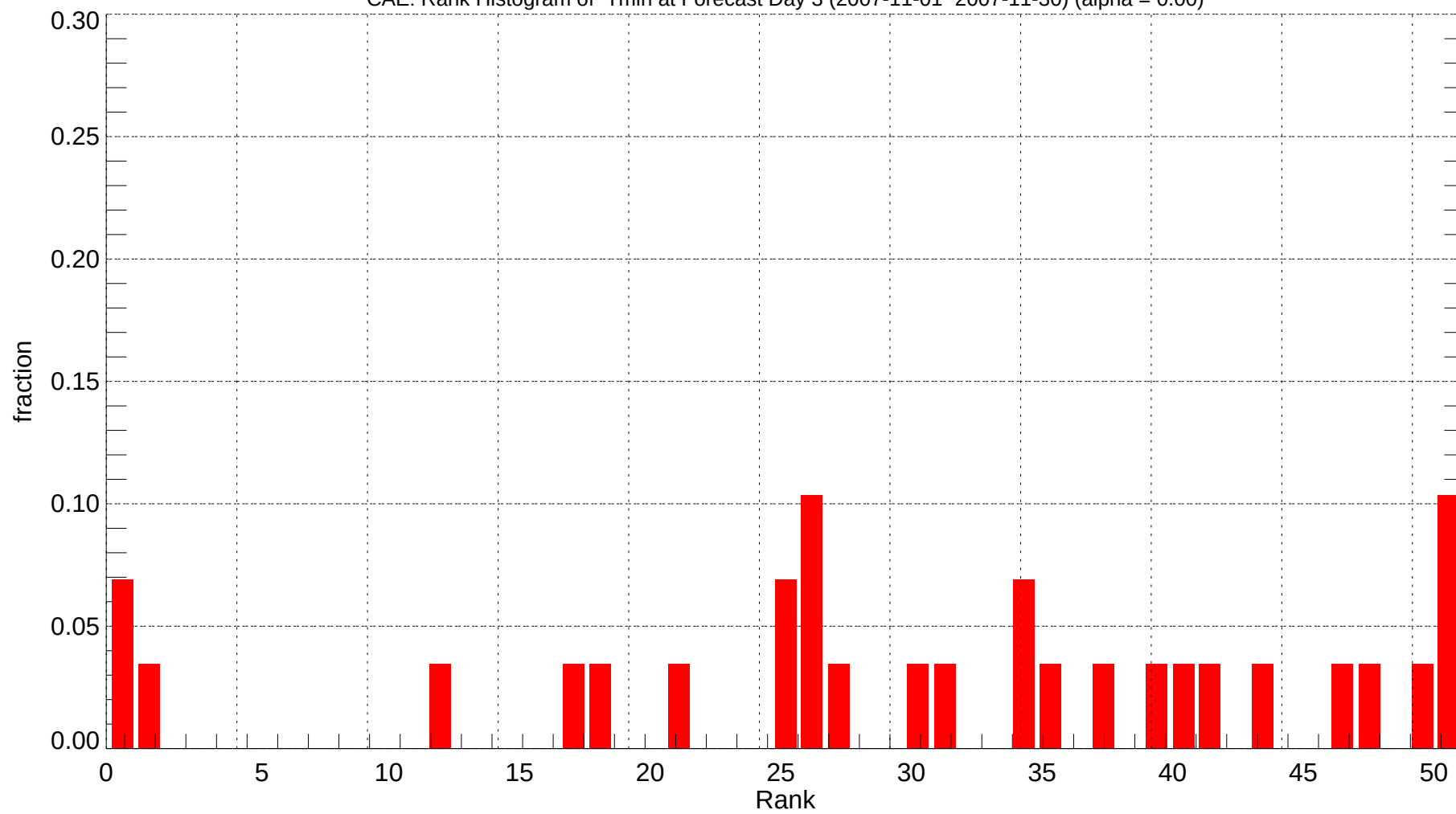
CAE: Rank Histogram of Tmin at Forecast Day 3 (2007-11-01~2007-11-30) (alpha = 0.00)
