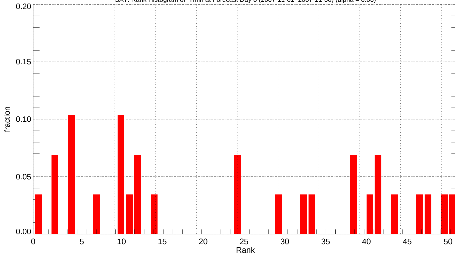
SAT: Rank Histogram of Tmin at Forecast Day 6 (2007-11-01~2007-11-30) (alpha = 0.00)
