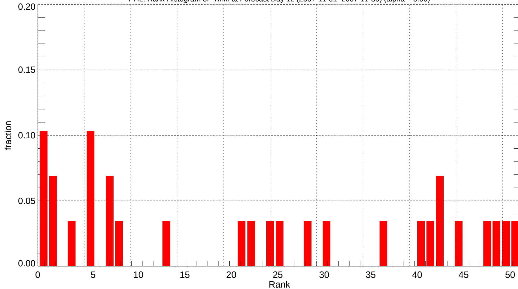
PHL: Rank Histogram of Tmin at Forecast Day 12 (2007-11-01~2007-11-30) (alpha = 0.00)
