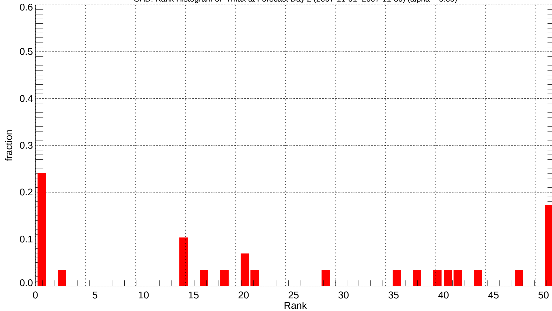
GAD: Rank Histogram of Tmax at Forecast Day 2 (2007-11-01~2007-11-30) (alpha = 0.00)
