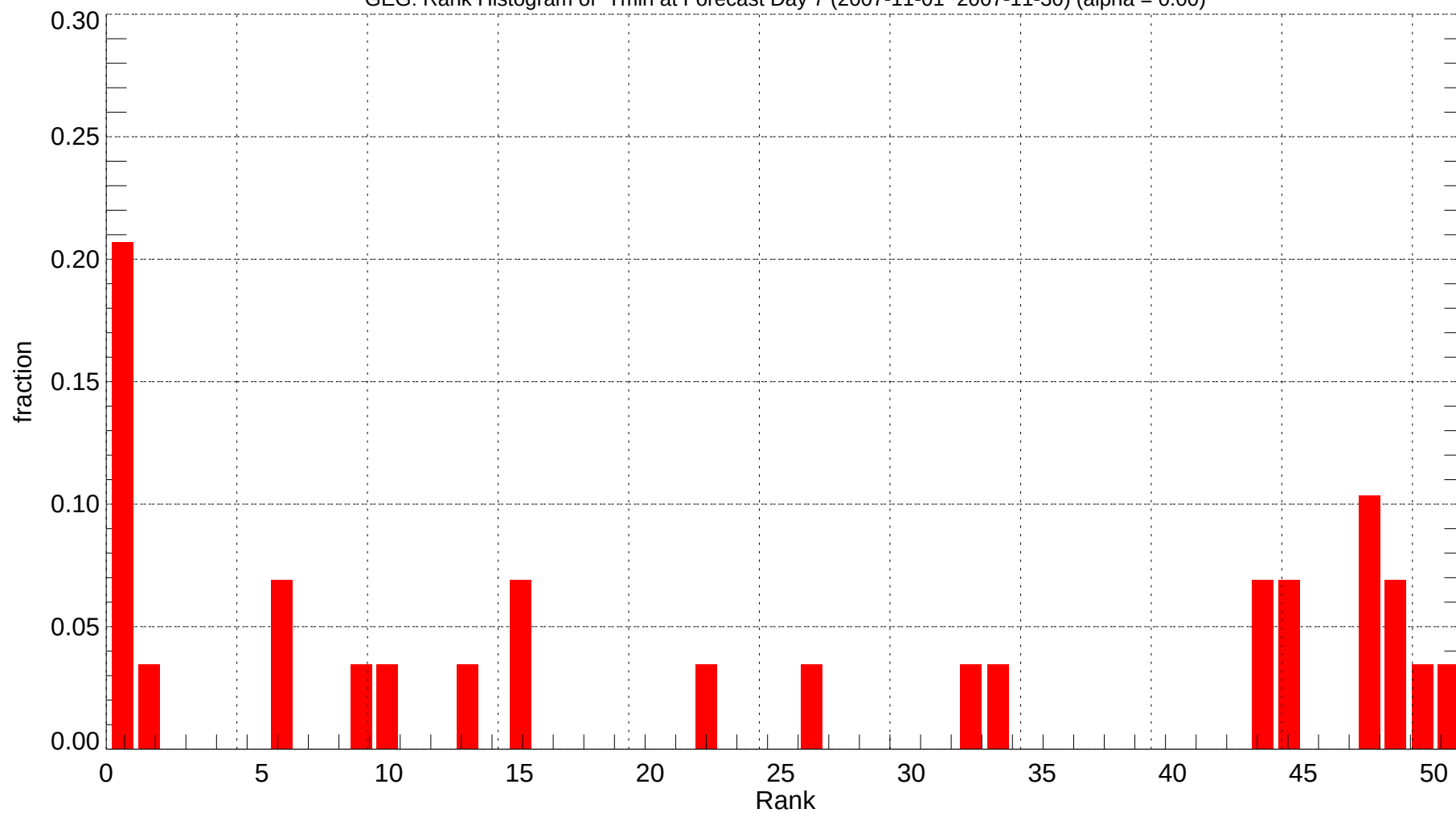
GEG: Rank Histogram of Tmin at Forecast Day 7 (2007-11-01~2007-11-30) (alpha = 0.00)
