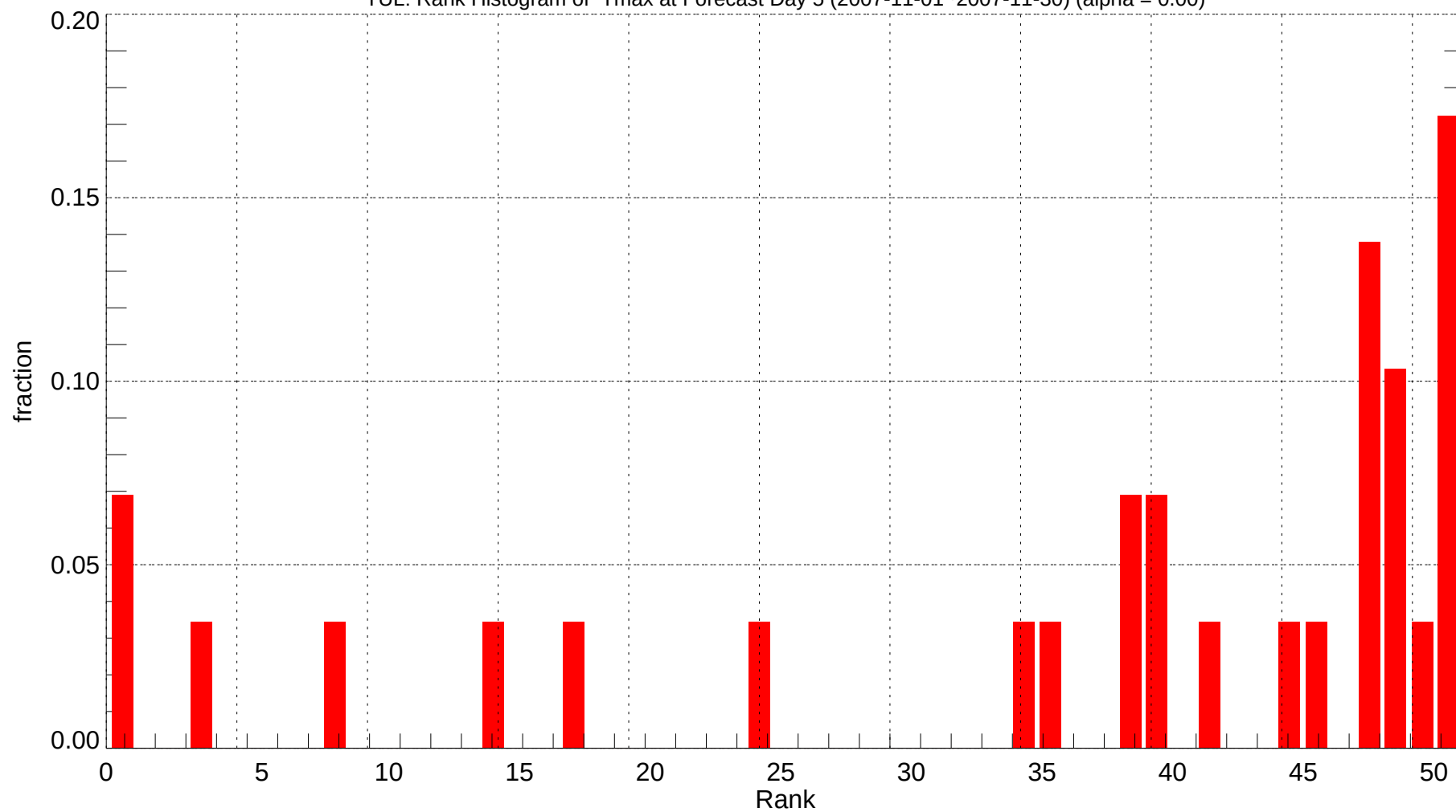
TUL: Rank Histogram of Tmax at Forecast Day 5 (2007-11-01~2007-11-30) (alpha = 0.00)
