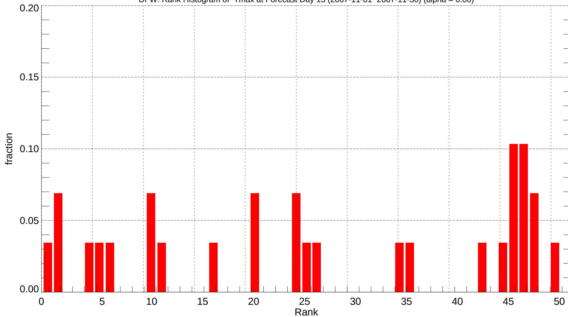
DFW: Rank Histogram of Tmax at Forecast Day 13 (2007-11-01~2007-11-30) (alpha = 0.00)
