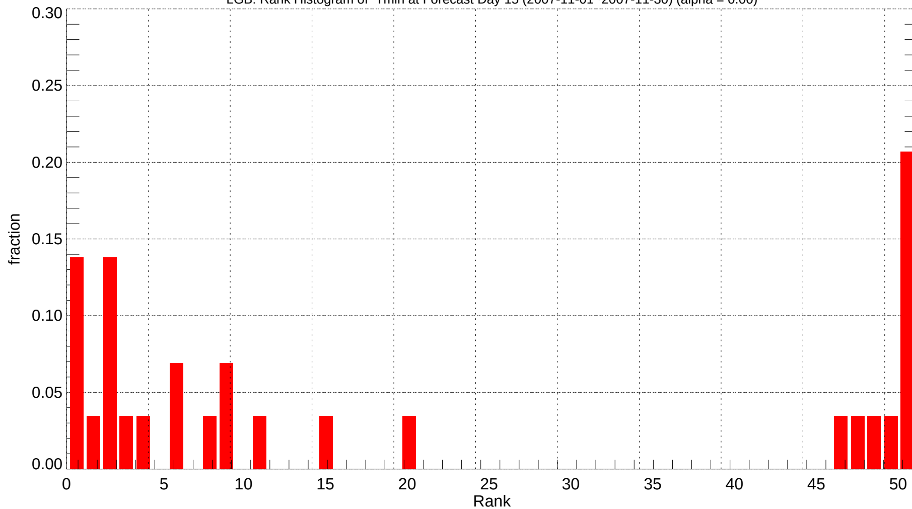
LGB: Rank Histogram of Tmin at Forecast Day 15 (2007-11-01~2007-11-30) (alpha = 0.00)
