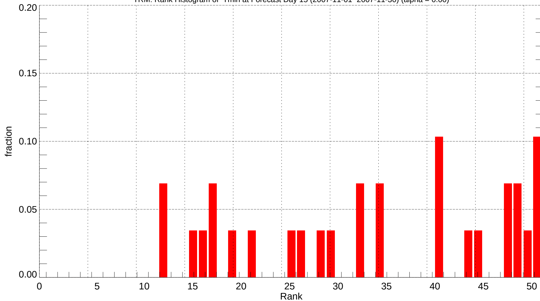
TRM: Rank Histogram of Tmin at Forecast Day 15 (2007-11-01~2007-11-30) (alpha = 0.00)
