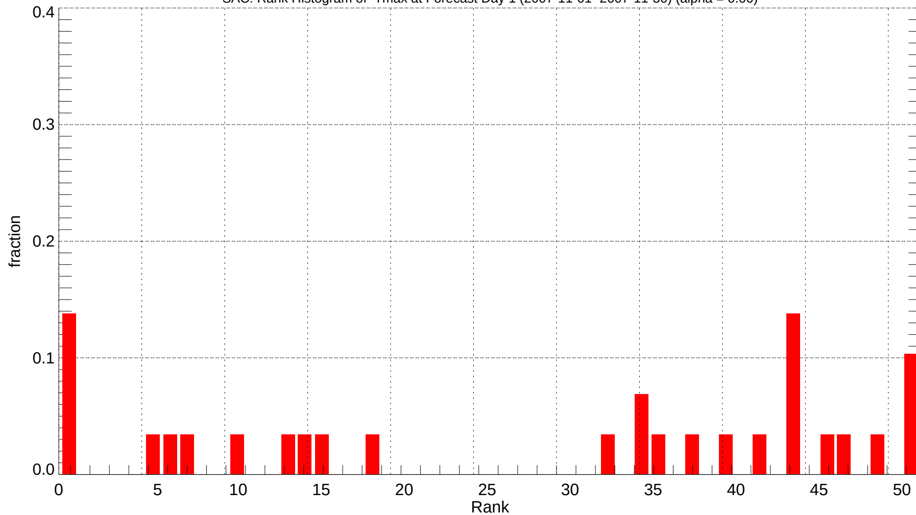
SAC: Rank Histogram of Tmax at Forecast Day 1 (2007-11-01~2007-11-30) (alpha = 0.00)
