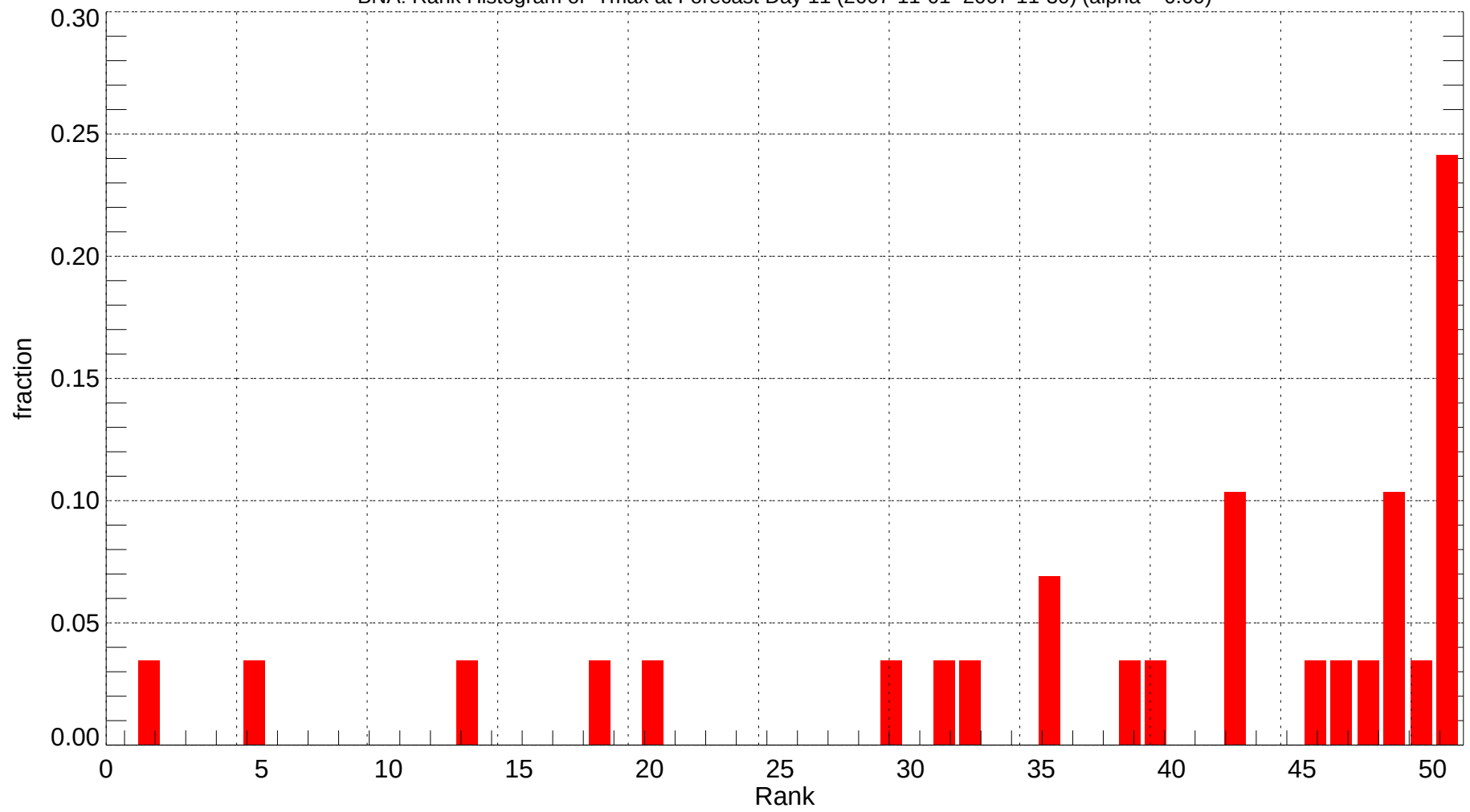
BNA: Rank Histogram of Tmax at Forecast Day 11 (2007-11-01~2007-11-30) (alpha = 0.00)
