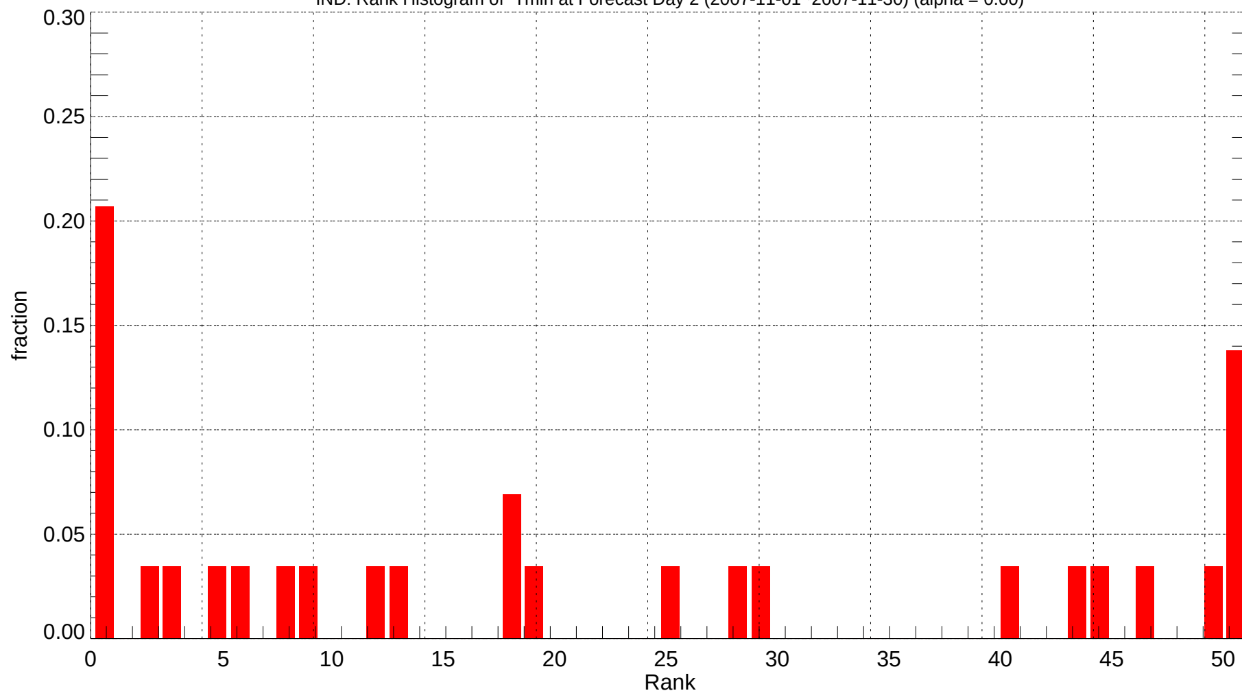
IND: Rank Histogram of Tmin at Forecast Day 2 (2007-11-01~2007-11-30) (alpha = 0.00)
