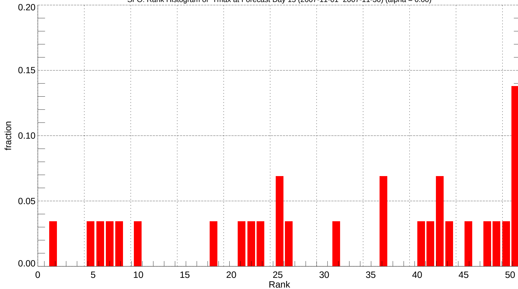
SFO: Rank Histogram of Tmax at Forecast Day 15 (2007-11-01~2007-11-30) (alpha = 0.00)
