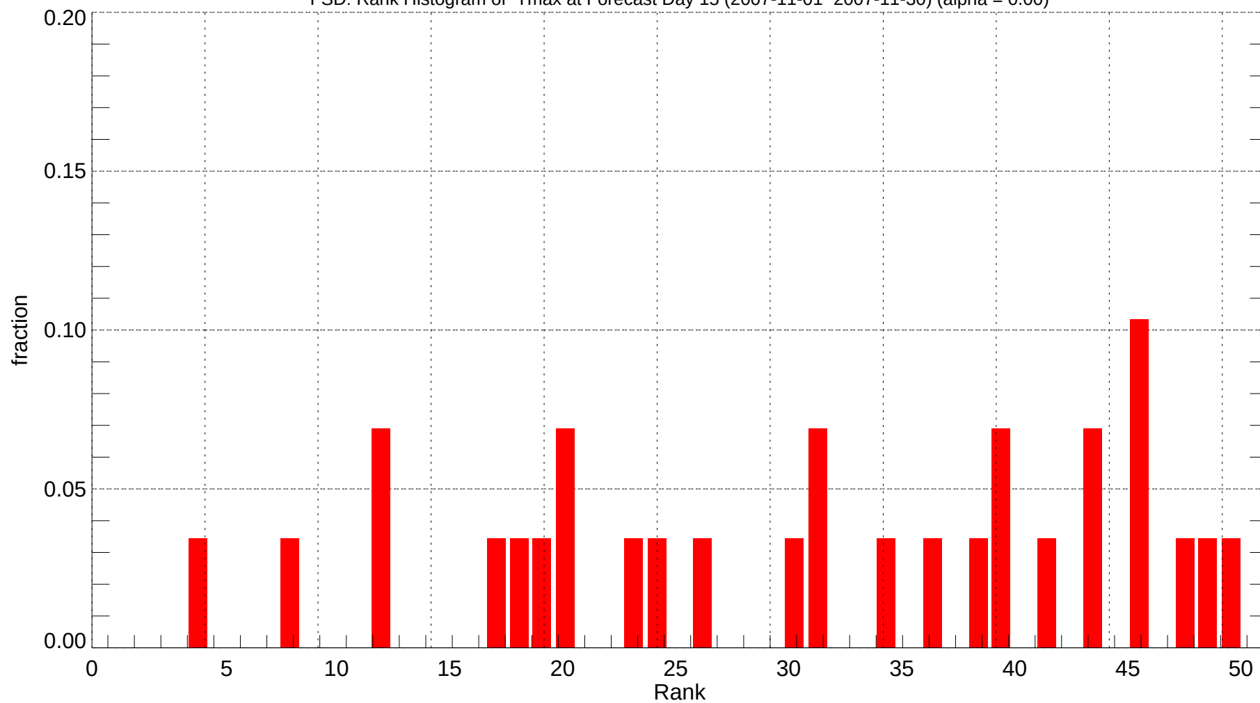
FSD: Rank Histogram of Tmax at Forecast Day 15 (2007-11-01~2007-11-30) (alpha = 0.00)
