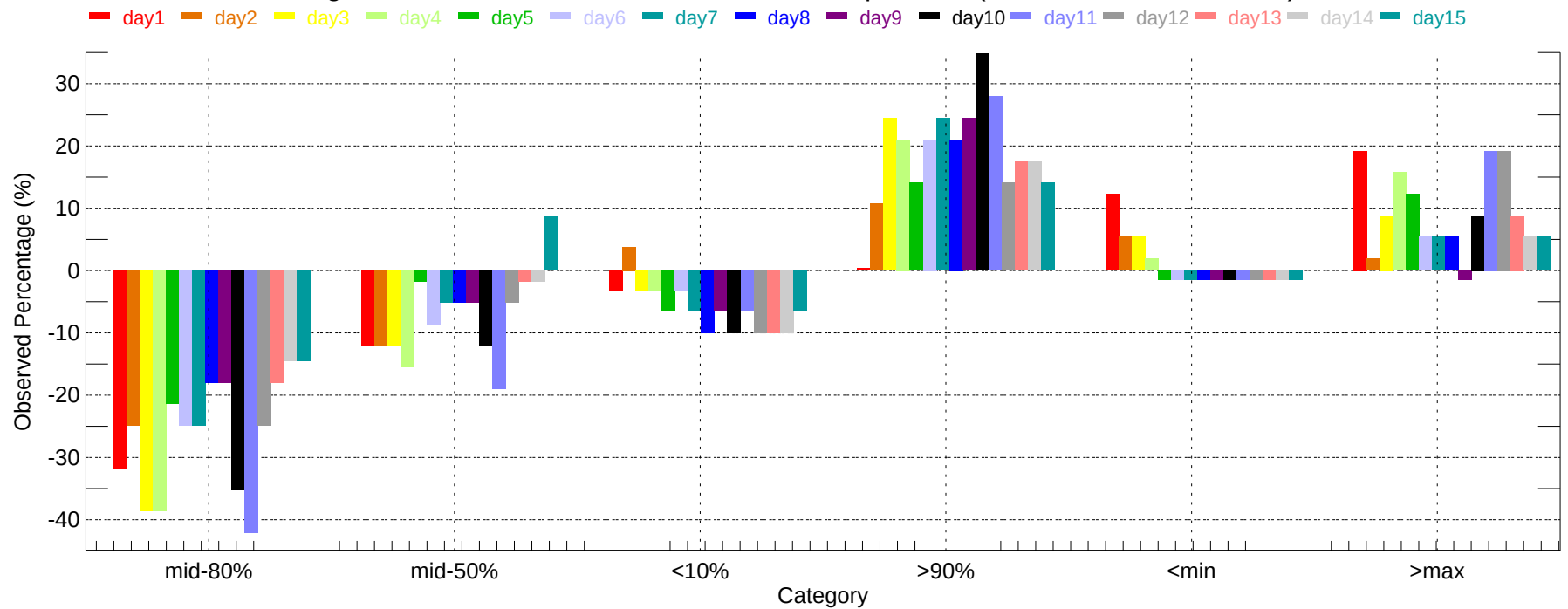
Observed Percentage Deviation of Ensembles - HSV: Min Temperature (2007-11-01~2007-11-30)
