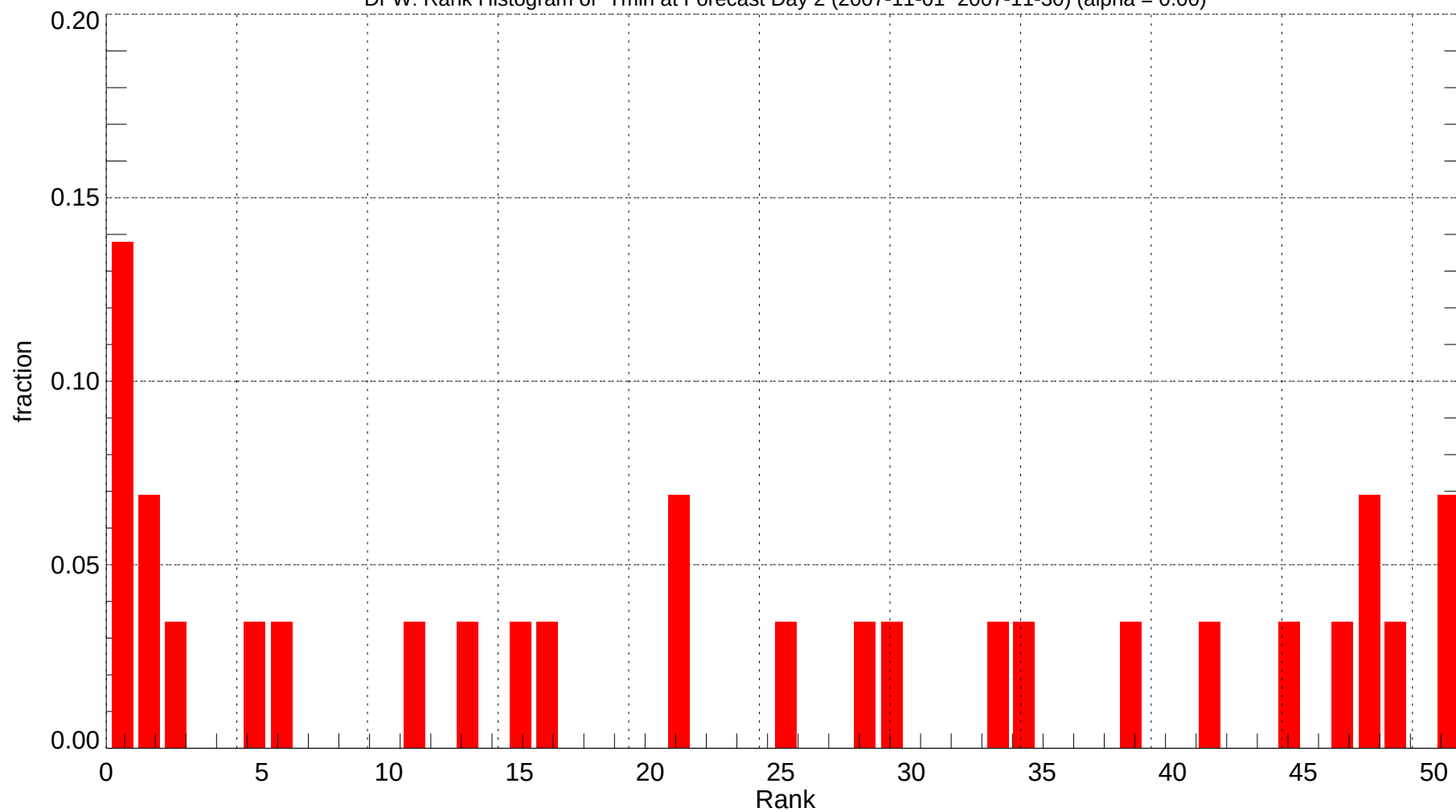
DFW: Rank Histogram of Tmin at Forecast Day 2 (2007-11-01~2007-11-30) (alpha = 0.00)
