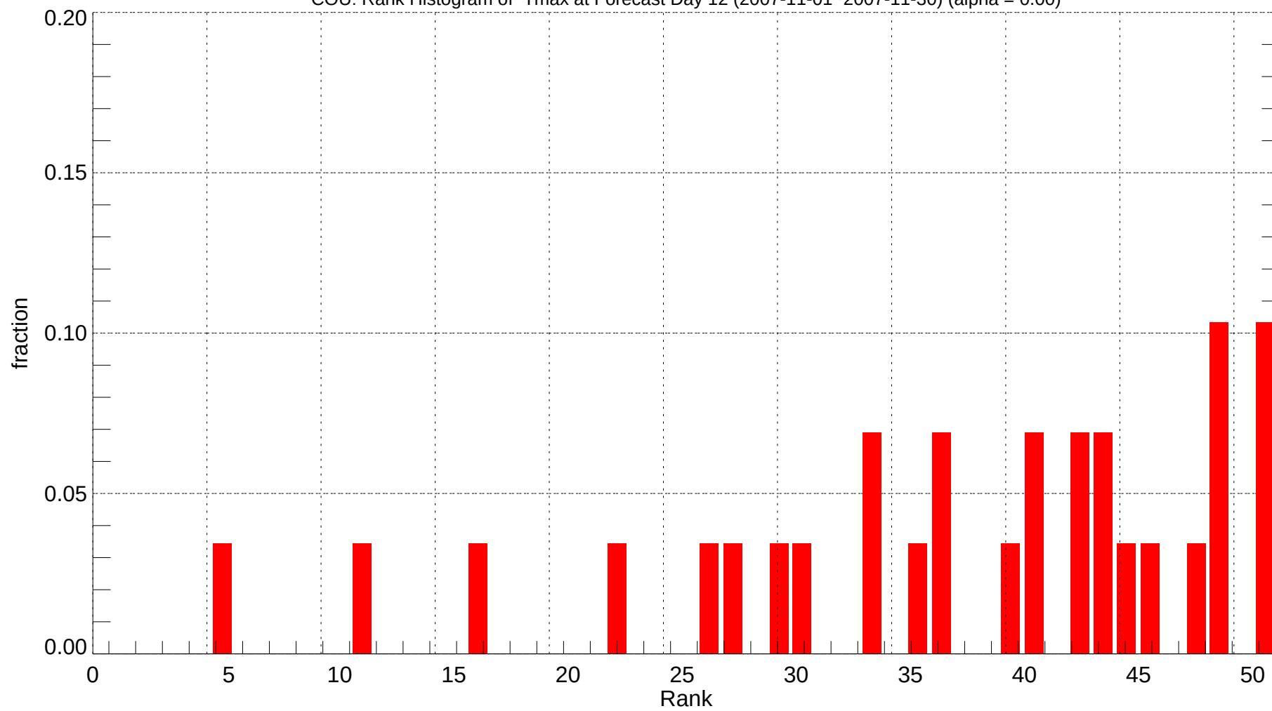
COU: Rank Histogram of Tmax at Forecast Day 12 (2007-11-01~2007-11-30) (alpha = 0.00)
