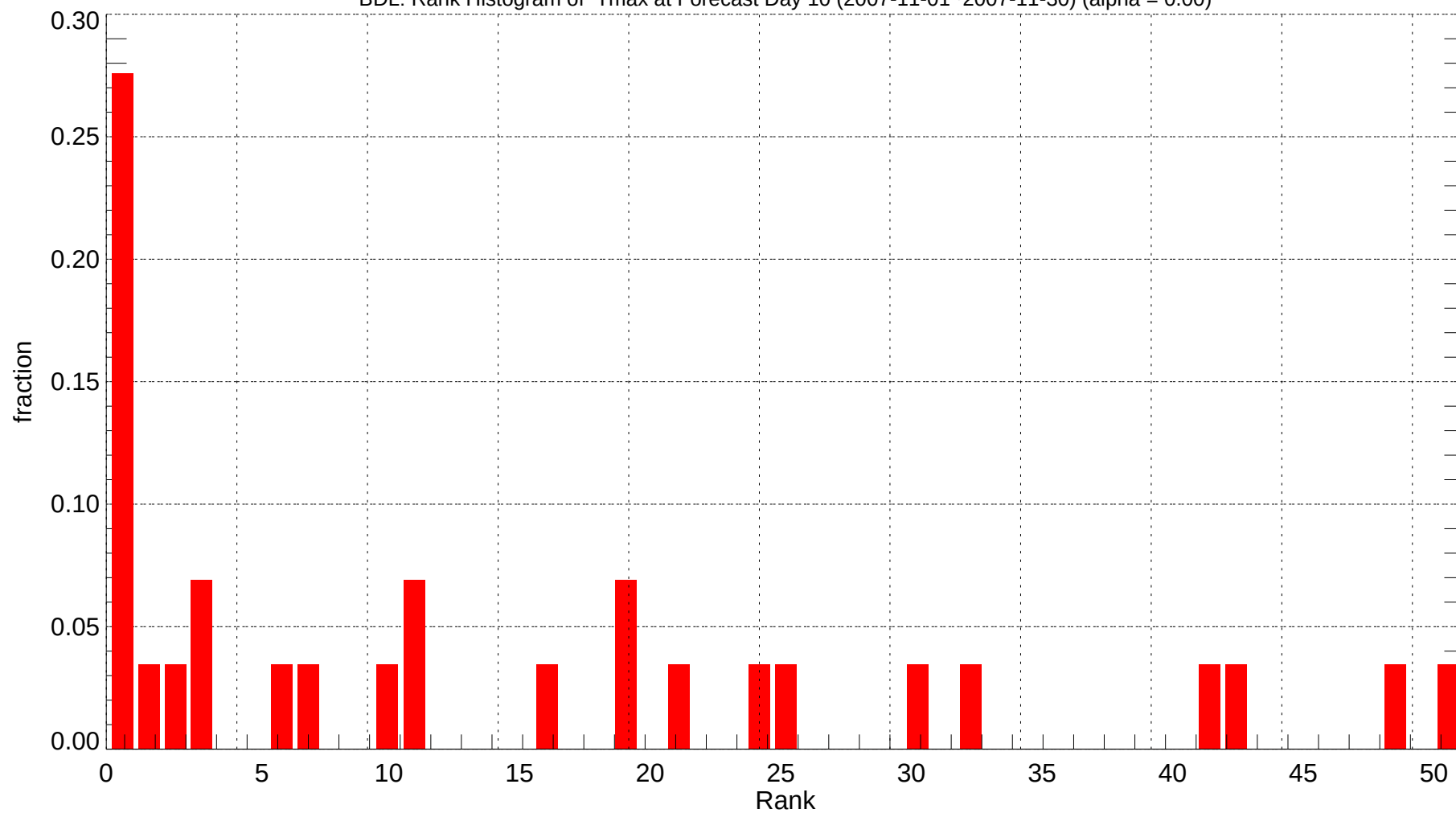
BDL: Rank Histogram of Tmax at Forecast Day 10 (2007-11-01~2007-11-30) (alpha = 0.00)
