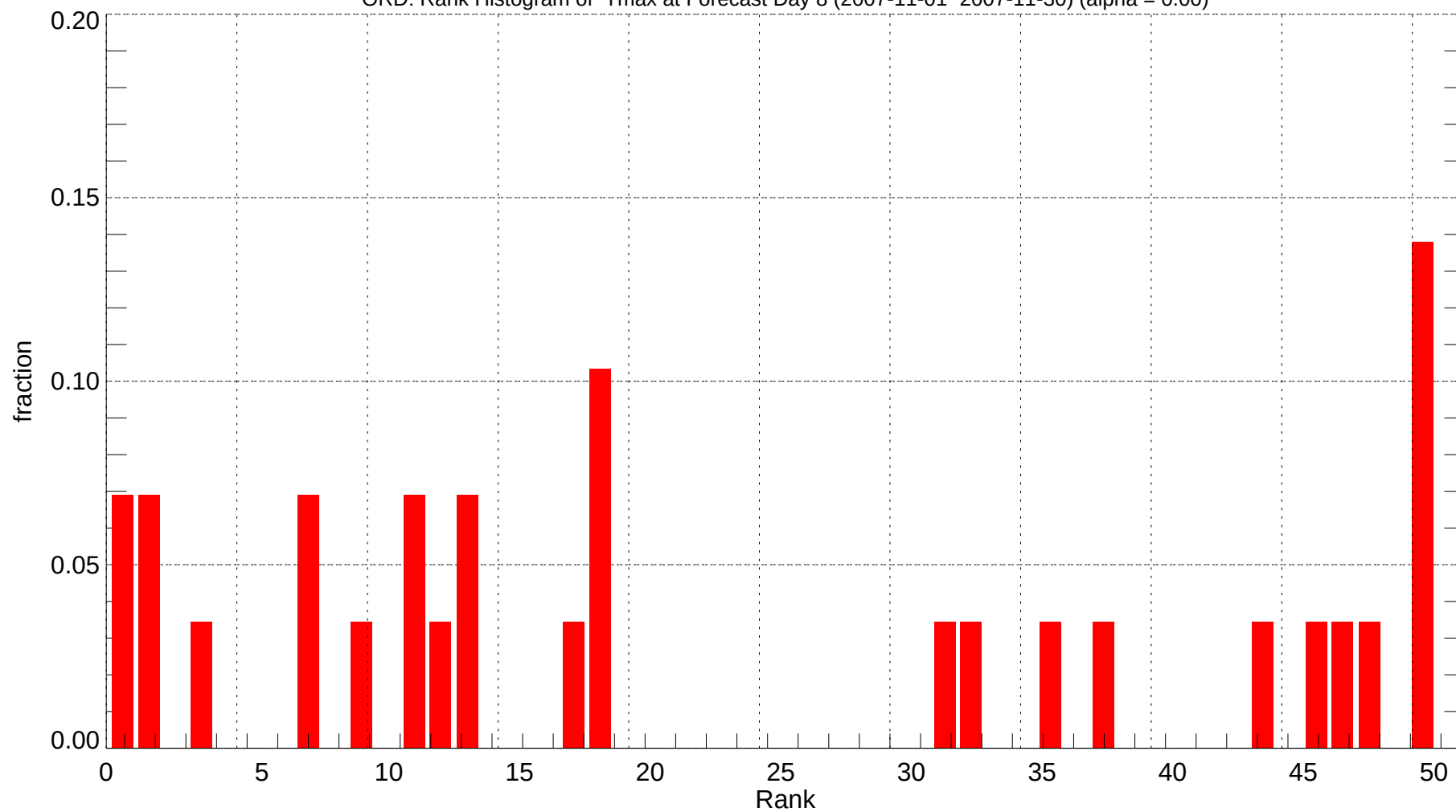
ORD: Rank Histogram of Tmax at Forecast Day 8 (2007-11-01~2007-11-30) (alpha = 0.00)
