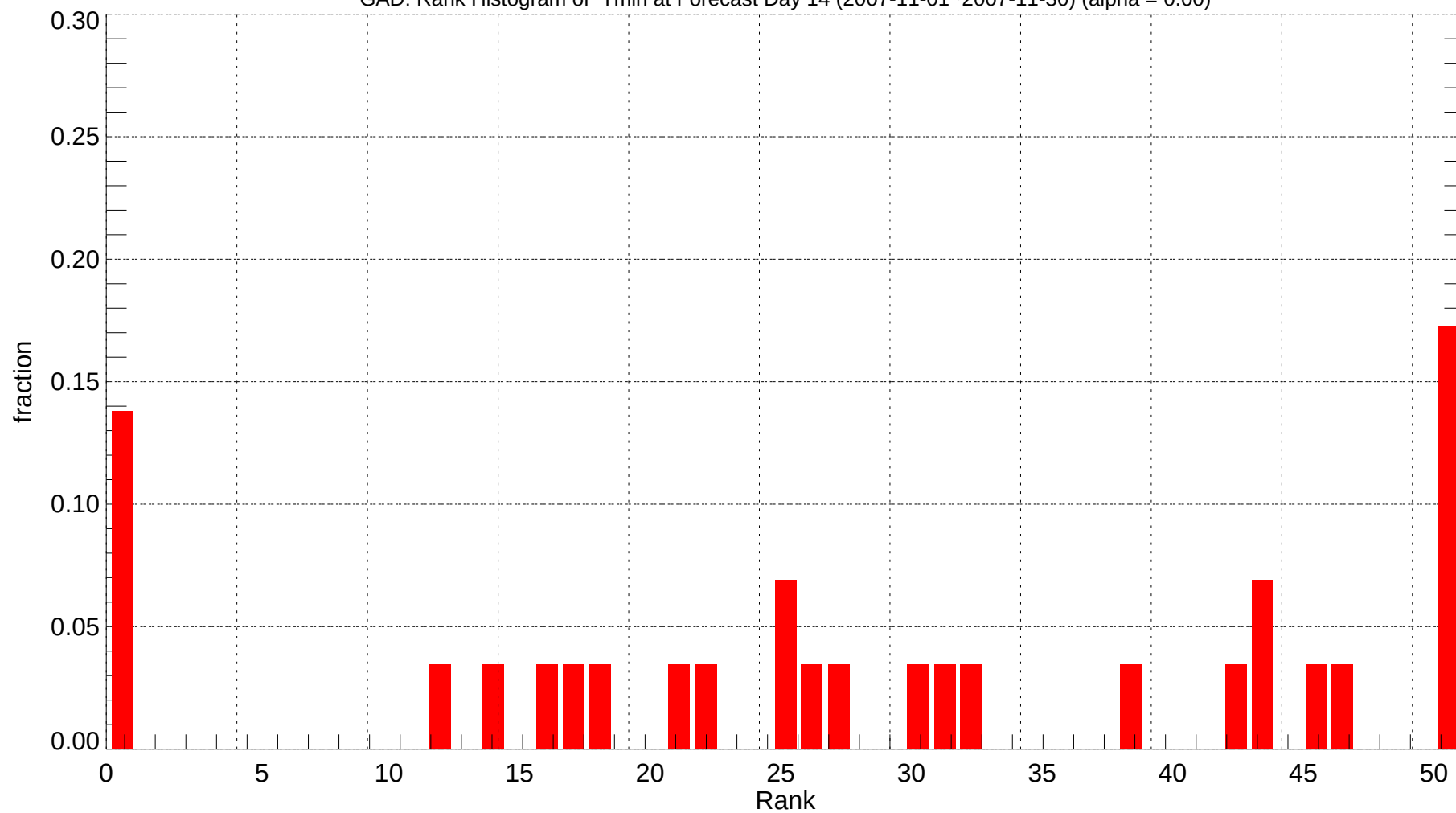
GAD: Rank Histogram of Tmin at Forecast Day 14 (2007-11-01~2007-11-30) (alpha = 0.00)
