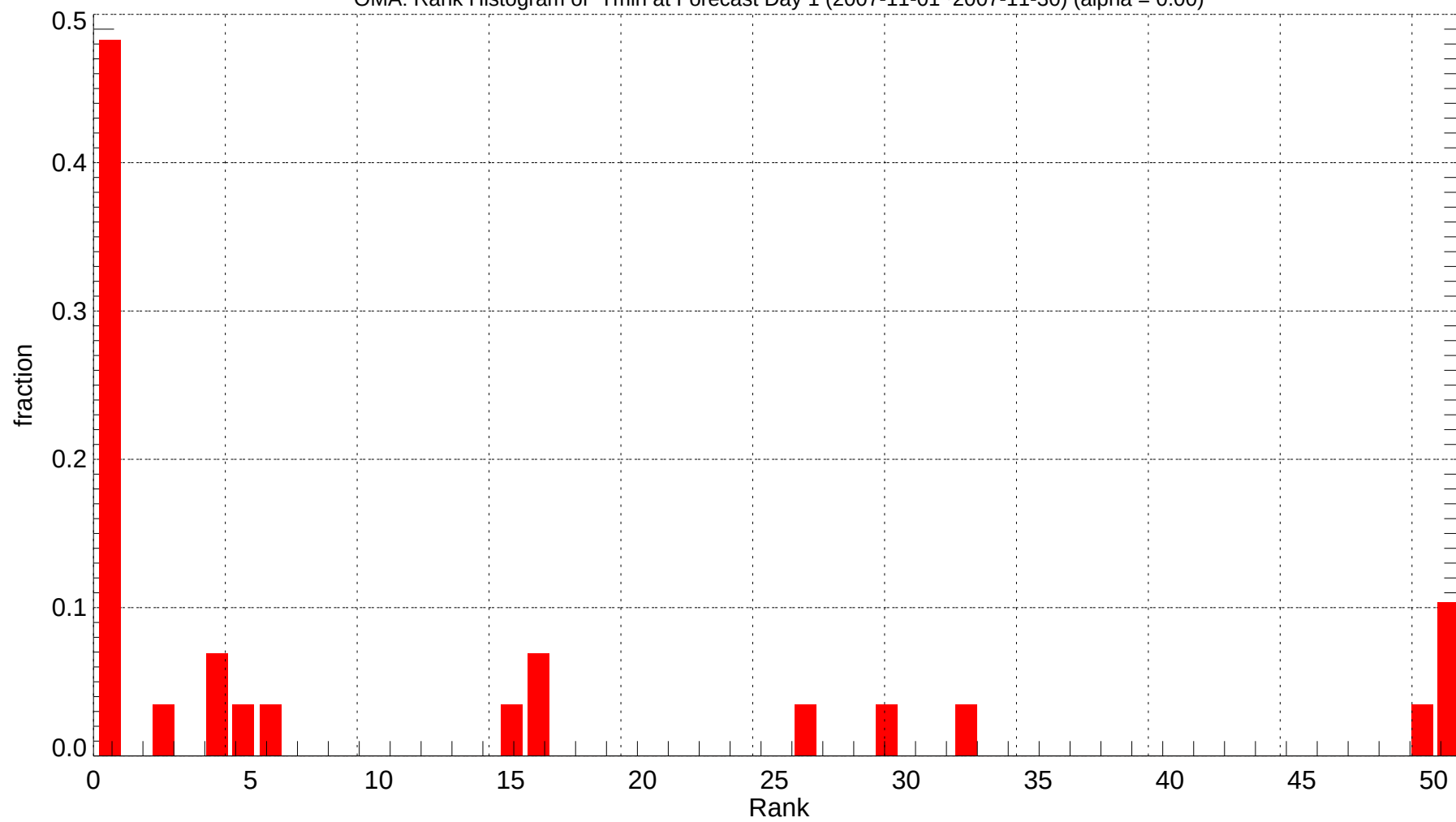
OMA: Rank Histogram of Tmin at Forecast Day 1 (2007-11-01~2007-11-30) (alpha = 0.00)
