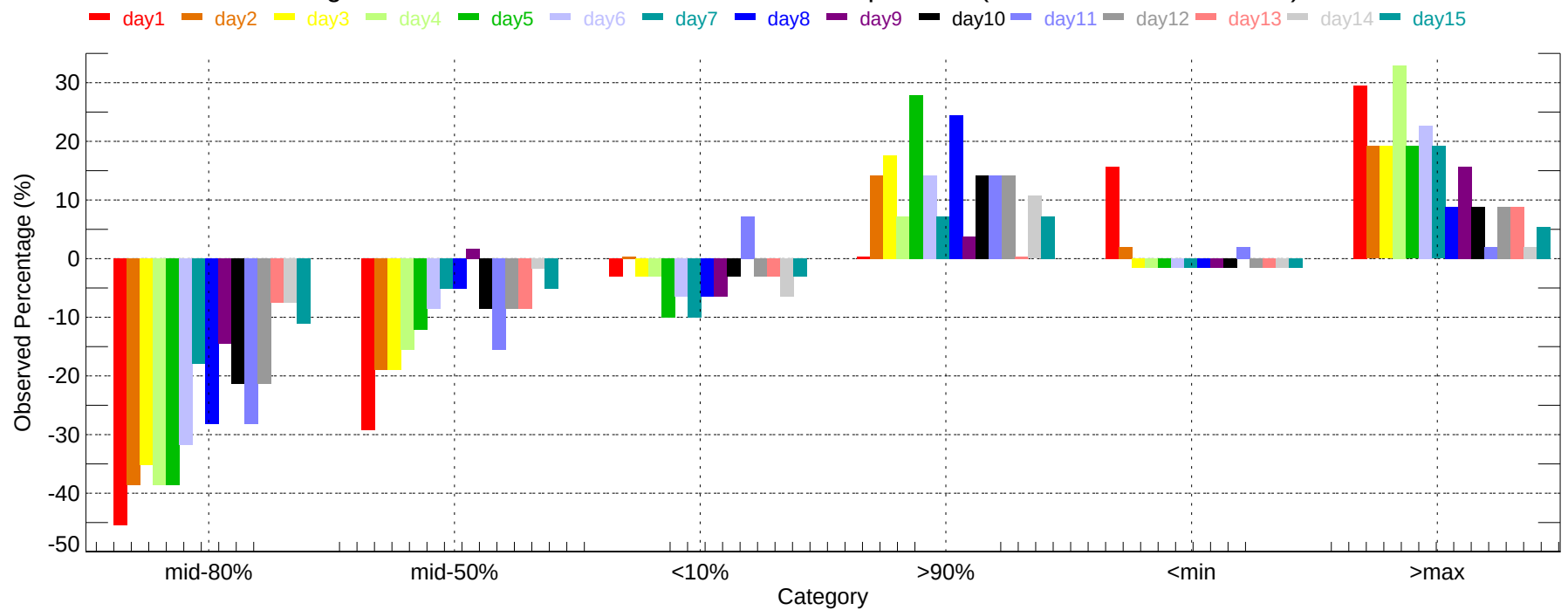
Observed Percentage Deviation of Ensembles - CLT: Max Temperature (2007-11-01~2007-11-30)
