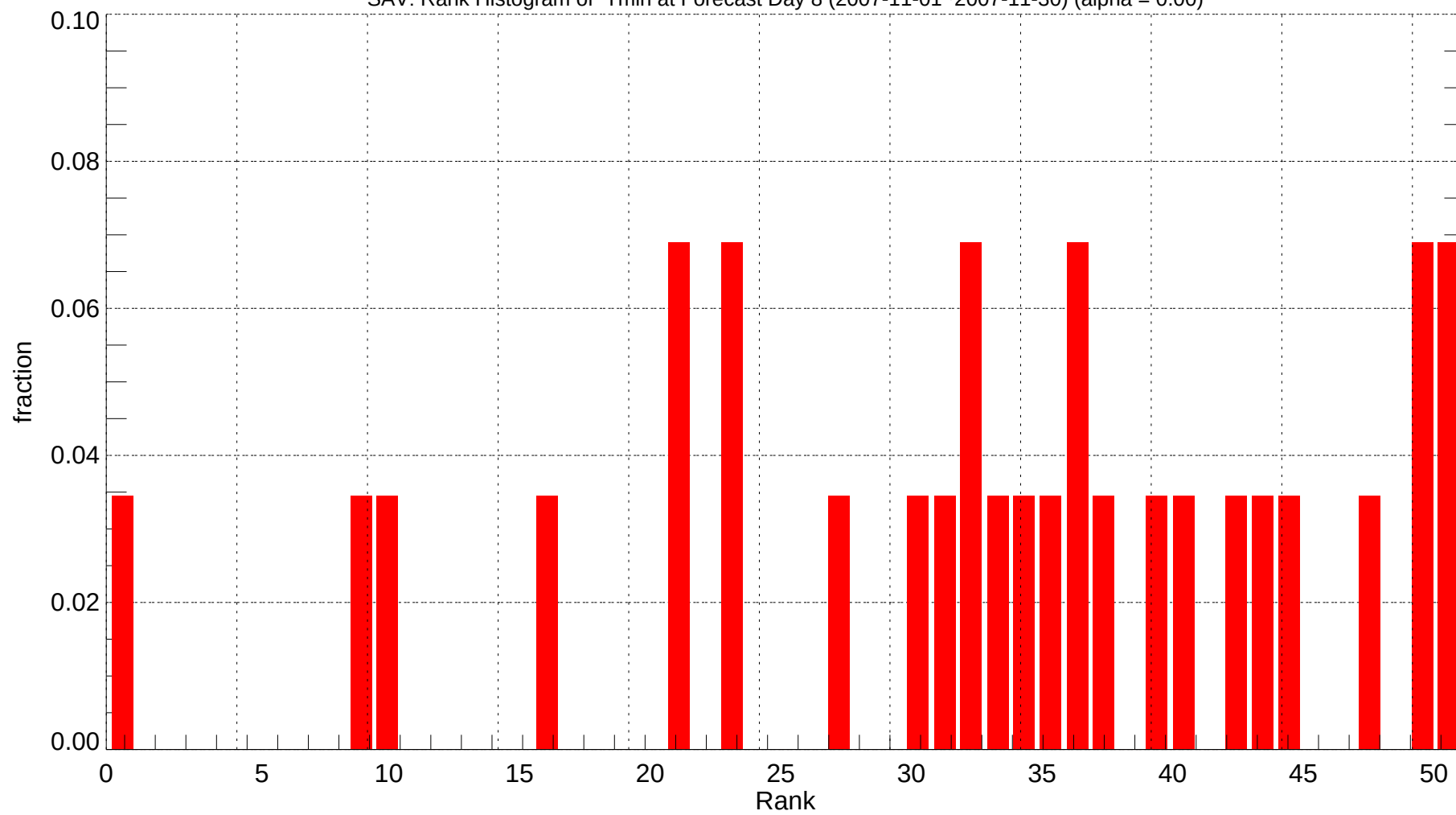
SAV: Rank Histogram of Tmin at Forecast Day 8 (2007-11-01~2007-11-30) (alpha = 0.00)
