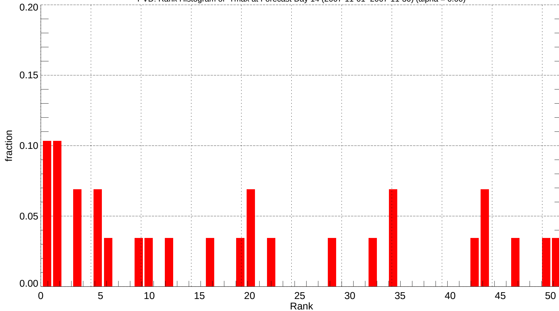
PVD: Rank Histogram of Tmax at Forecast Day 14 (2007-11-01~2007-11-30) (alpha = 0.00)
