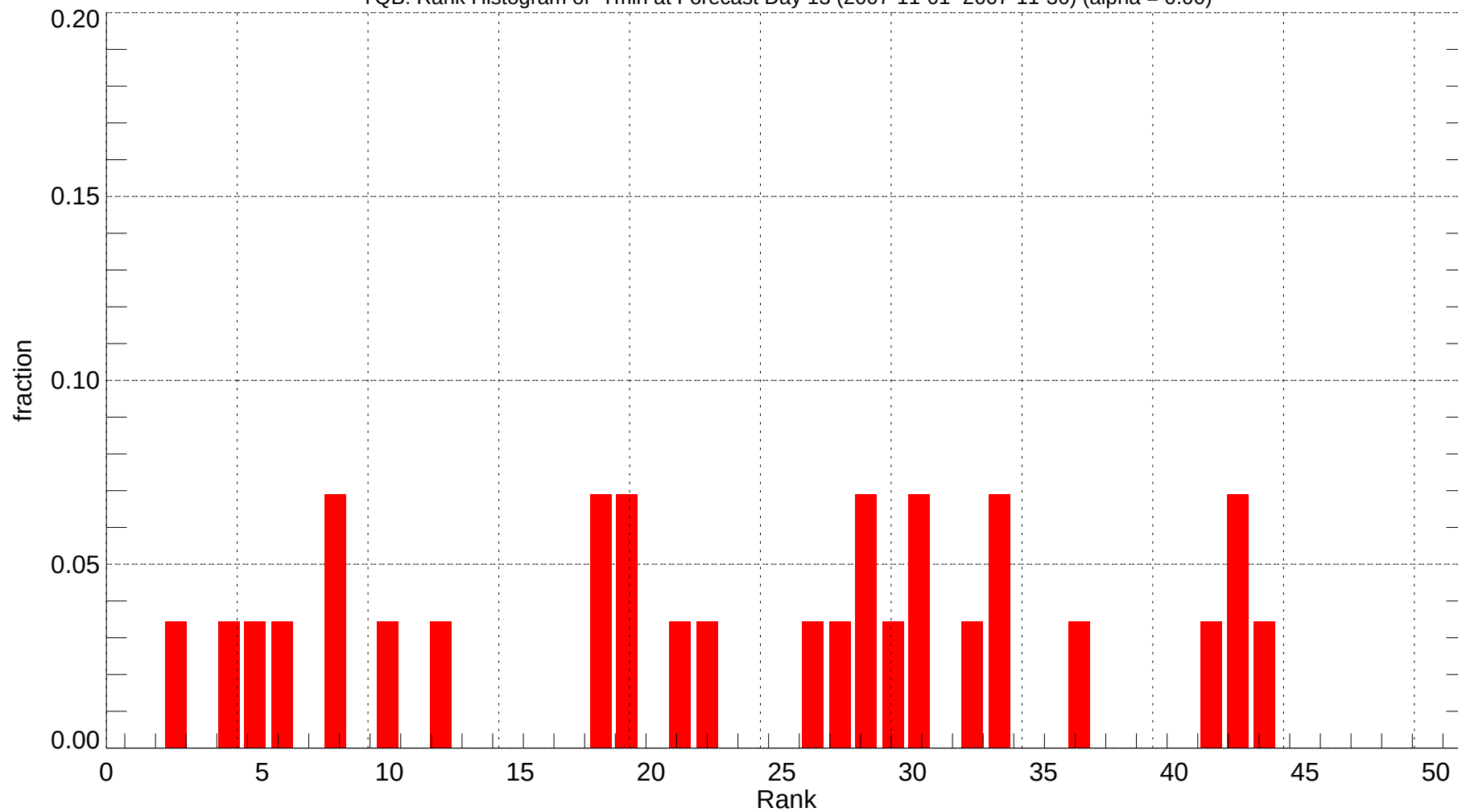
YQB: Rank Histogram of Tmin at Forecast Day 13 (2007-11-01~2007-11-30) (alpha = 0.00)
