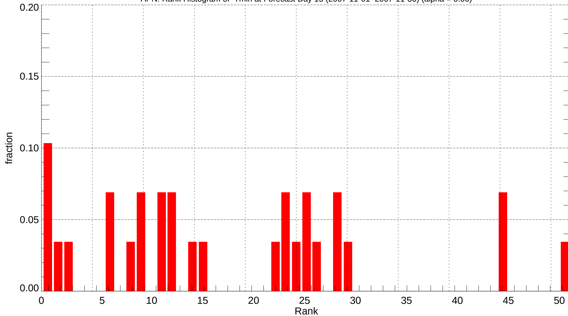
APN: Rank Histogram of Tmin at Forecast Day 15 (2007-11-01~2007-11-30) (alpha = 0.00)
