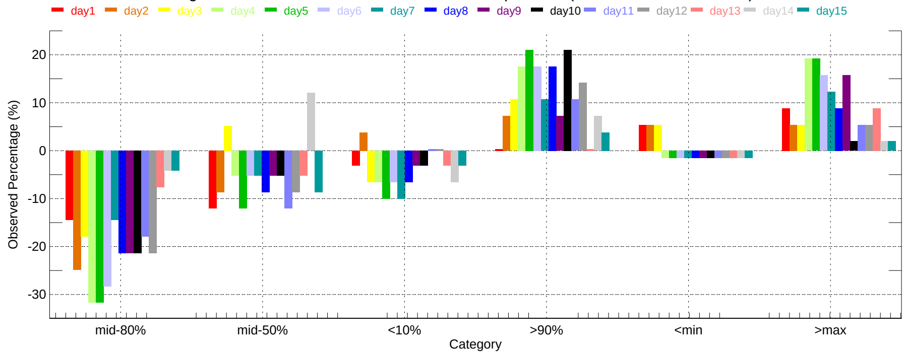
Observed Percentage Deviation of Ensembles - CAE: Max Temperature (2007-11-01~2007-11-30)
