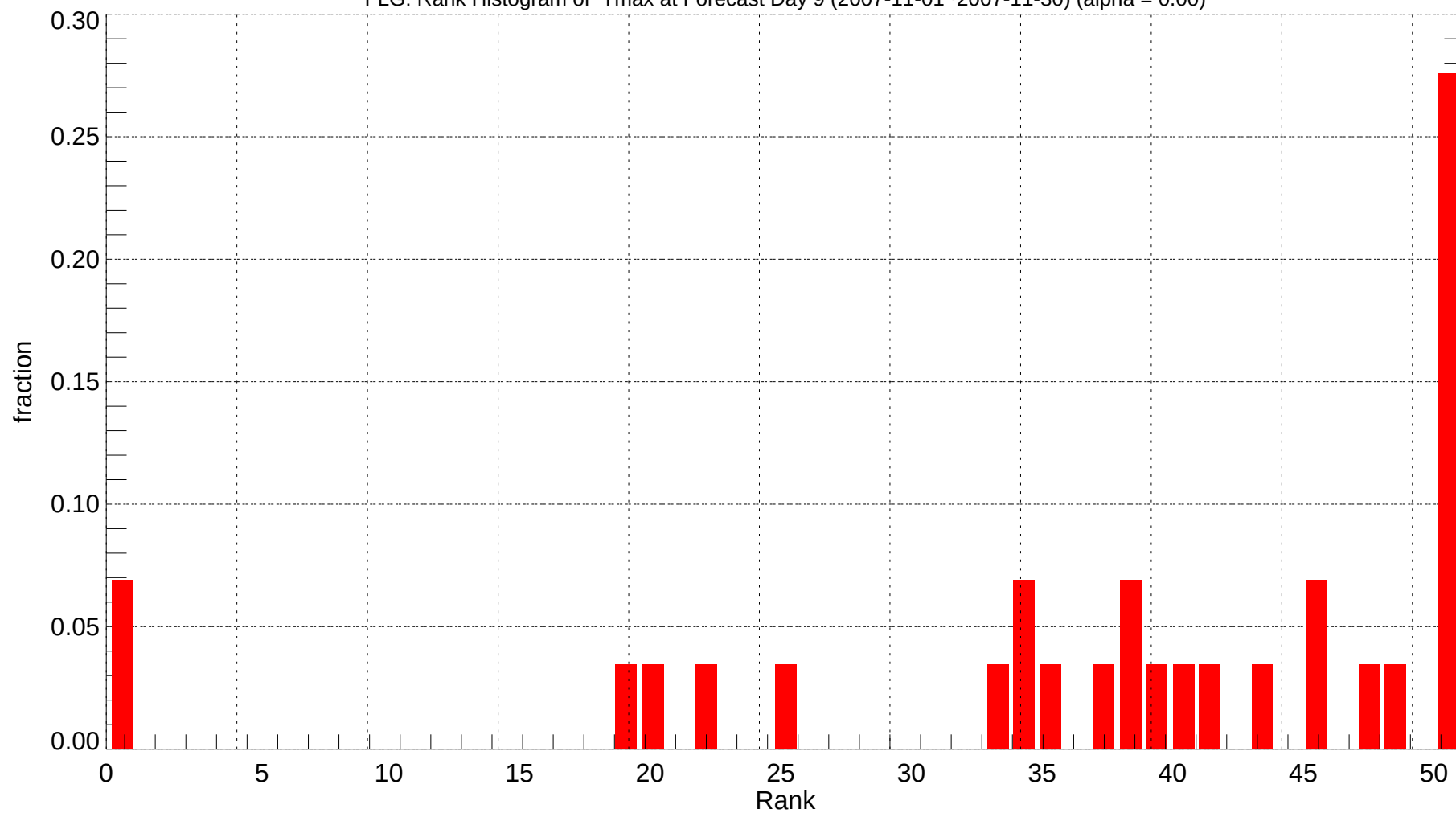
FLG: Rank Histogram of Tmax at Forecast Day 9 (2007-11-01~2007-11-30) (alpha = 0.00)
