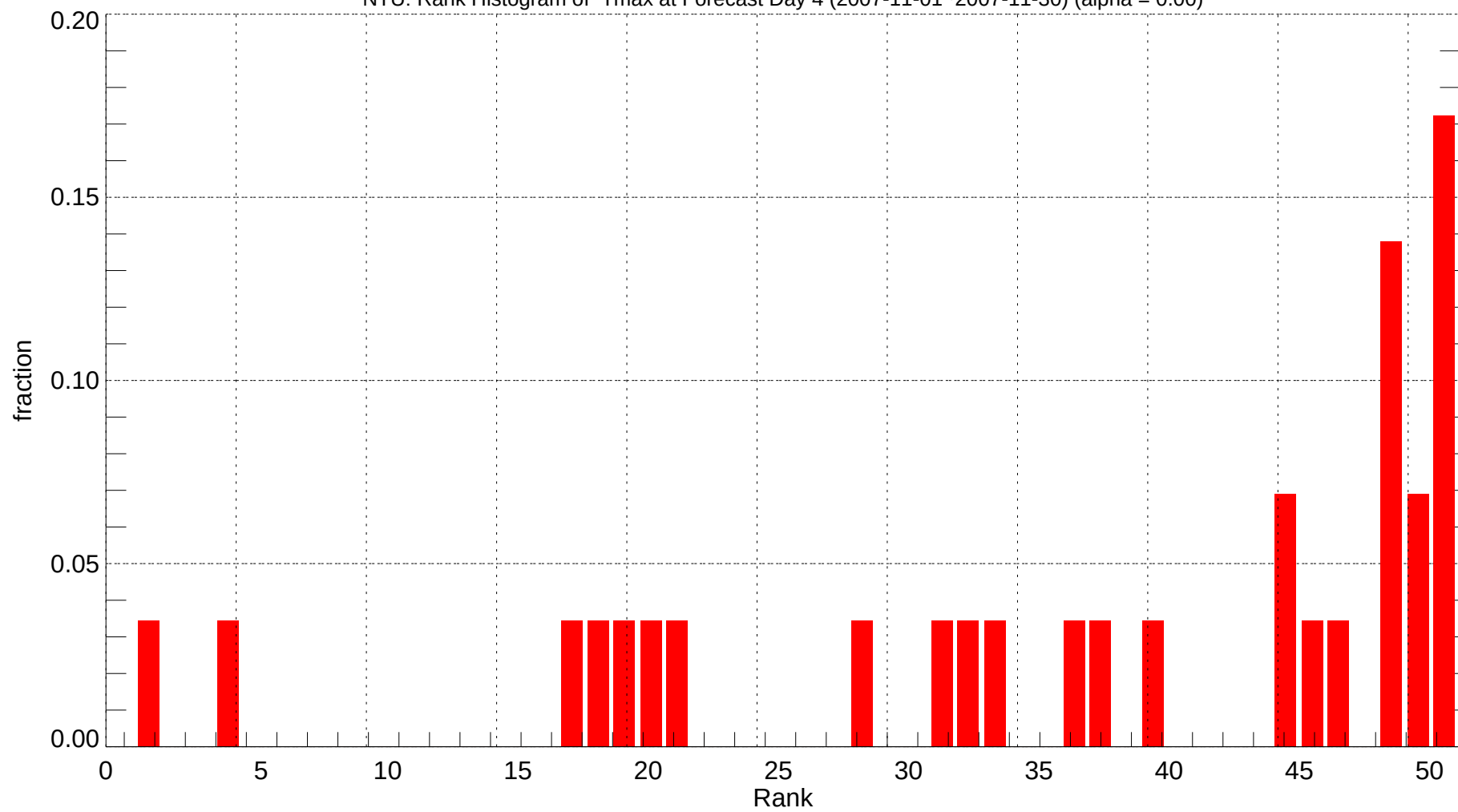
NTU: Rank Histogram of Tmax at Forecast Day 4 (2007-11-01~2007-11-30) (alpha = 0.00)
