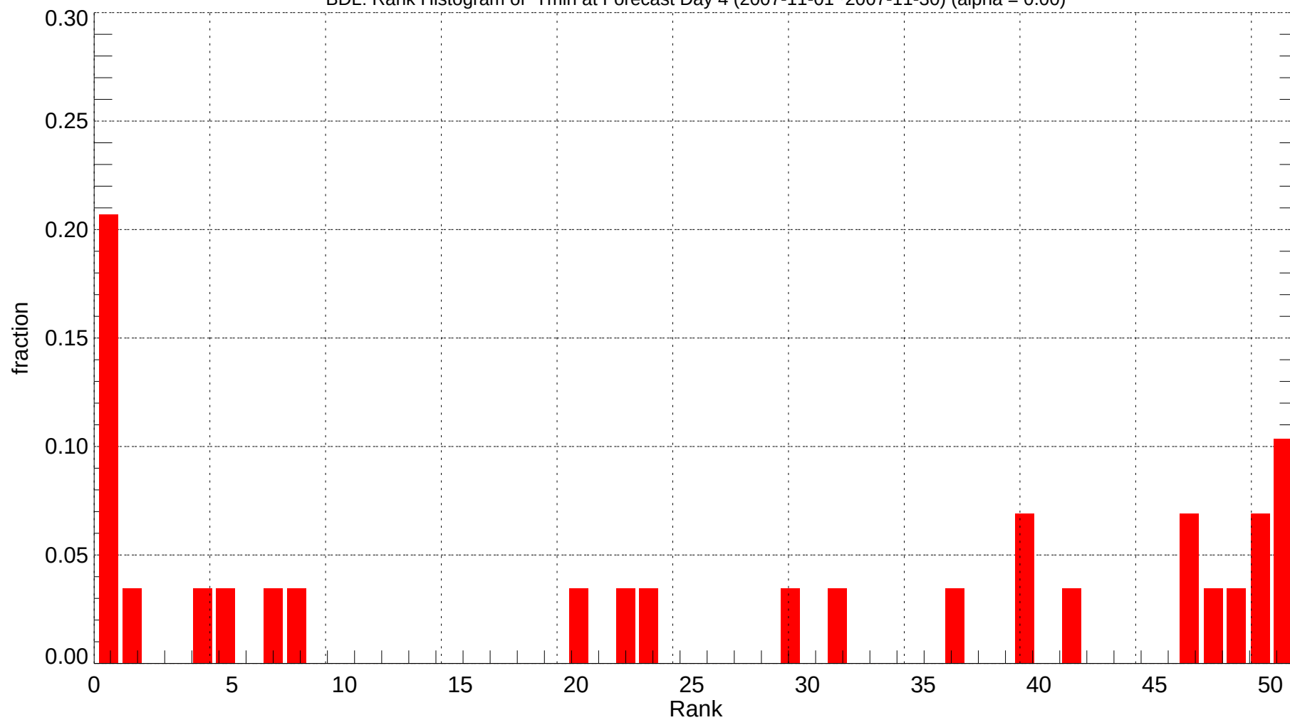
BDL: Rank Histogram of Tmin at Forecast Day 4 (2007-11-01~2007-11-30) (alpha = 0.00)
