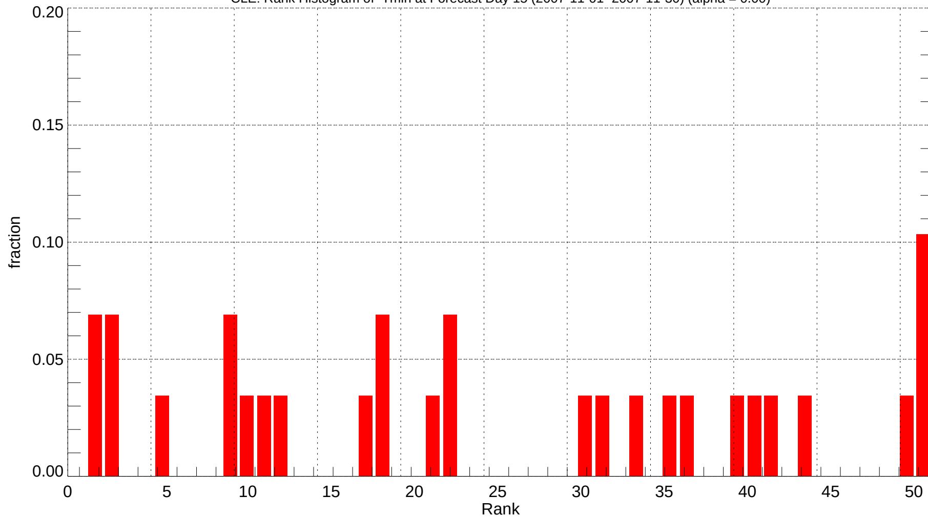
CLE: Rank Histogram of Tmin at Forecast Day 15 (2007-11-01~2007-11-30) (alpha = 0.00)
