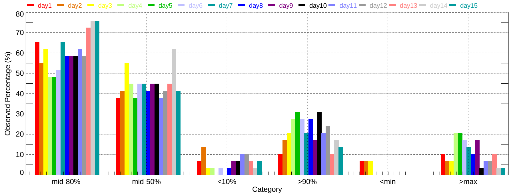
Observed Percentage of Ensembles - CAE: Max Temperature (2007-11-01~2007-11-30)
