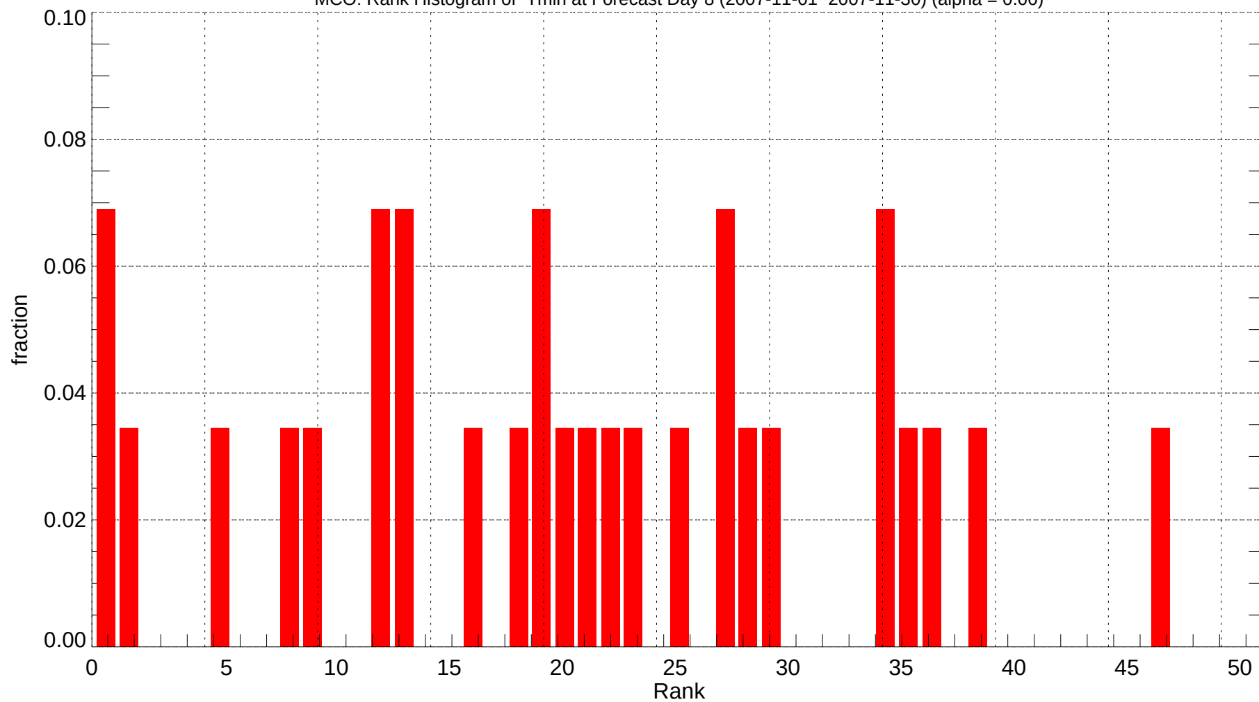
MCO: Rank Histogram of Tmin at Forecast Day 8 (2007-11-01~2007-11-30) (alpha = 0.00)
