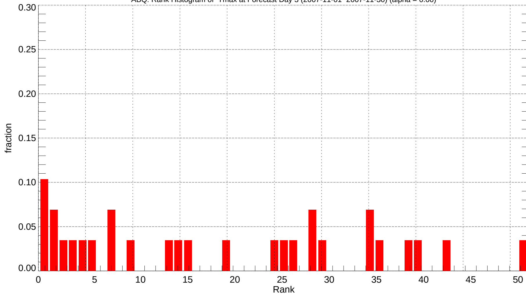
ABQ: Rank Histogram of Tmax at Forecast Day 3 (2007-11-01~2007-11-30) (alpha = 0.00)
