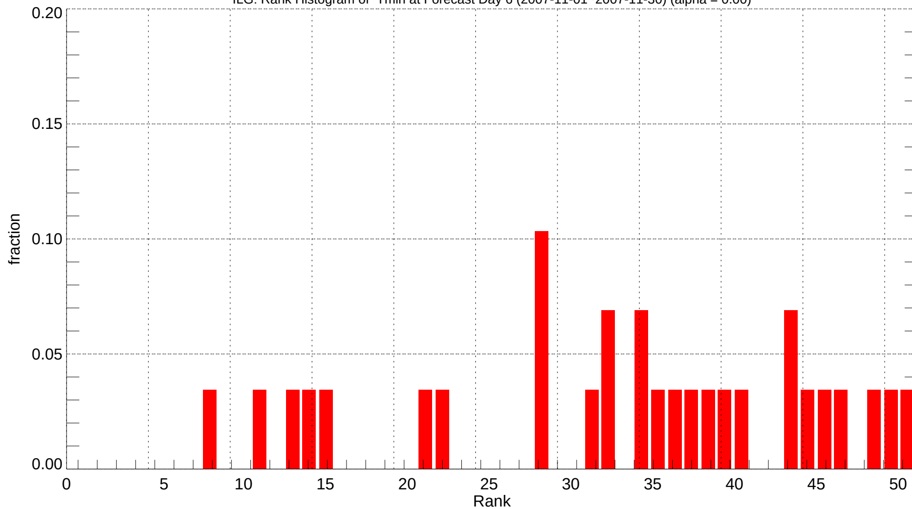
ILG: Rank Histogram of Tmin at Forecast Day 6 (2007-11-01~2007-11-30) (alpha = 0.00)
