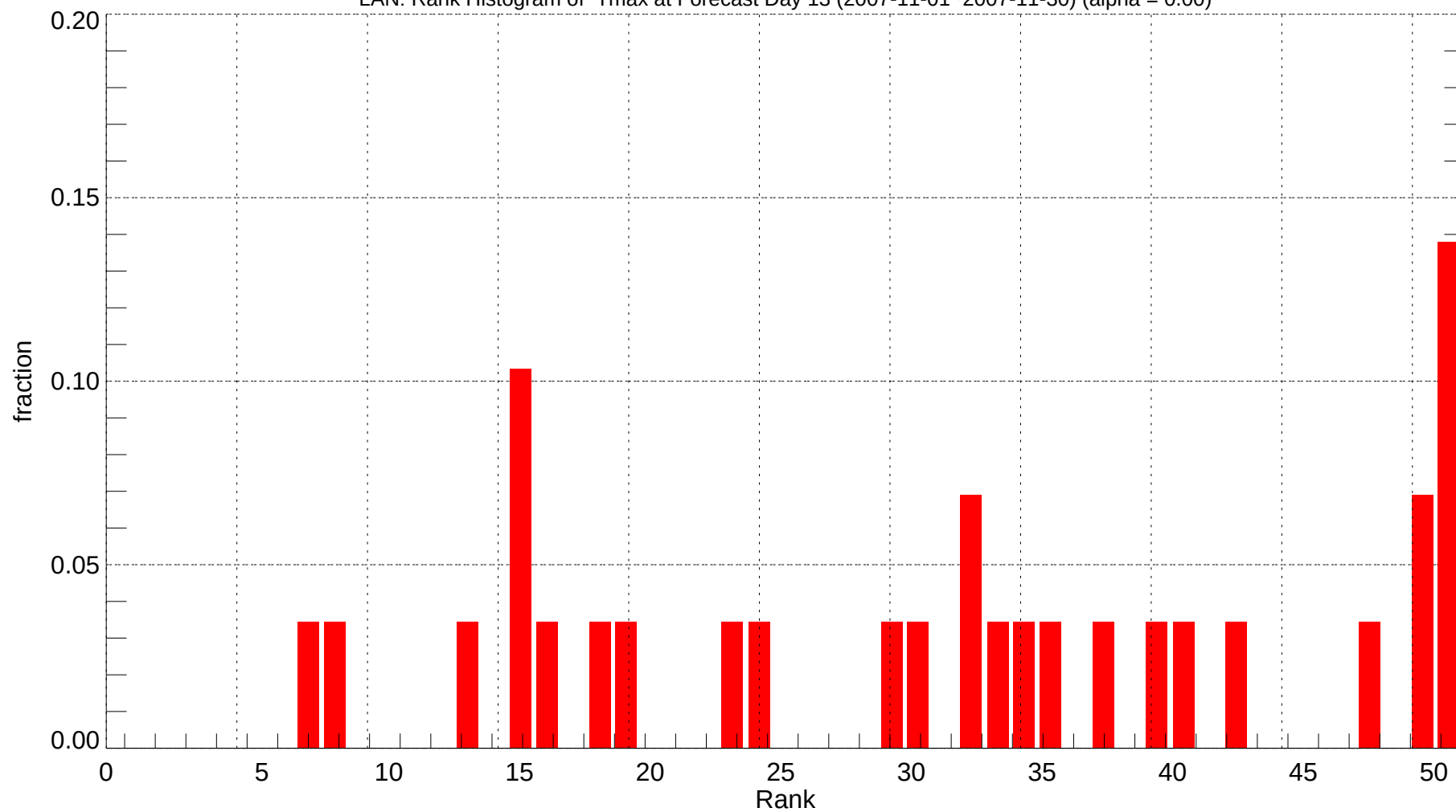
LAN: Rank Histogram of Tmax at Forecast Day 13 (2007-11-01~2007-11-30) (alpha = 0.00)
