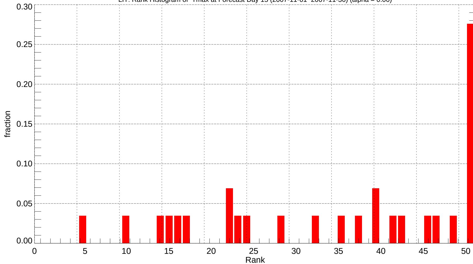
LIT: Rank Histogram of Tmax at Forecast Day 15 (2007-11-01~2007-11-30) (alpha = 0.00)
