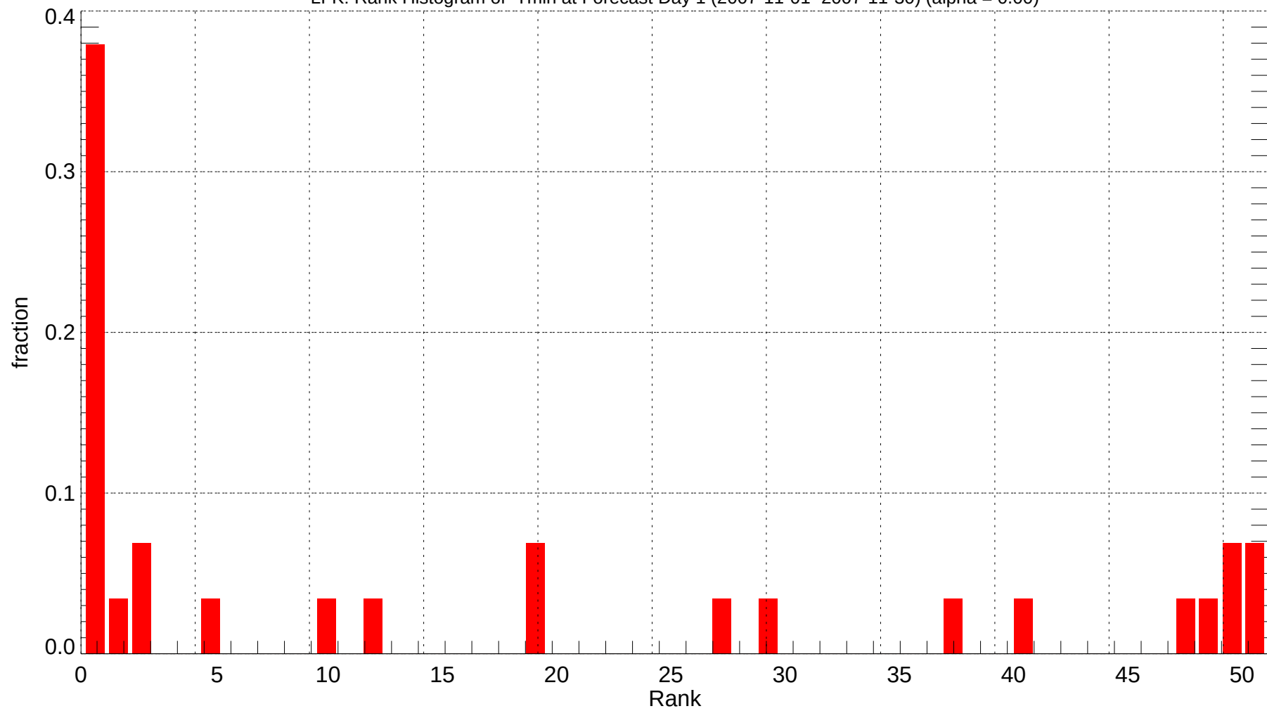
LFK: Rank Histogram of Tmin at Forecast Day 1 (2007-11-01~2007-11-30) (alpha = 0.00)
