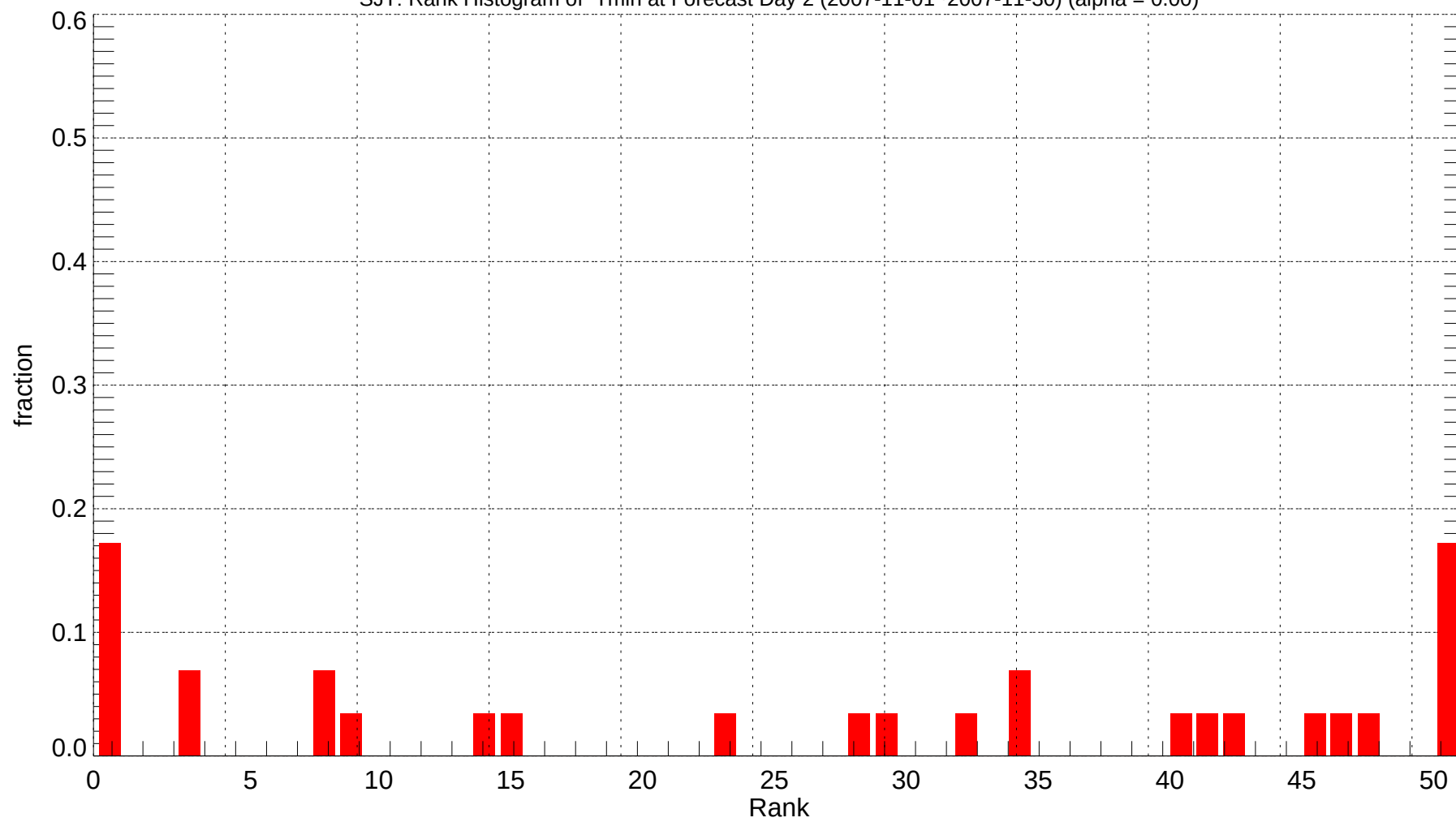
SJT: Rank Histogram of Tmin at Forecast Day 2 (2007-11-01~2007-11-30) (alpha = 0.00)
