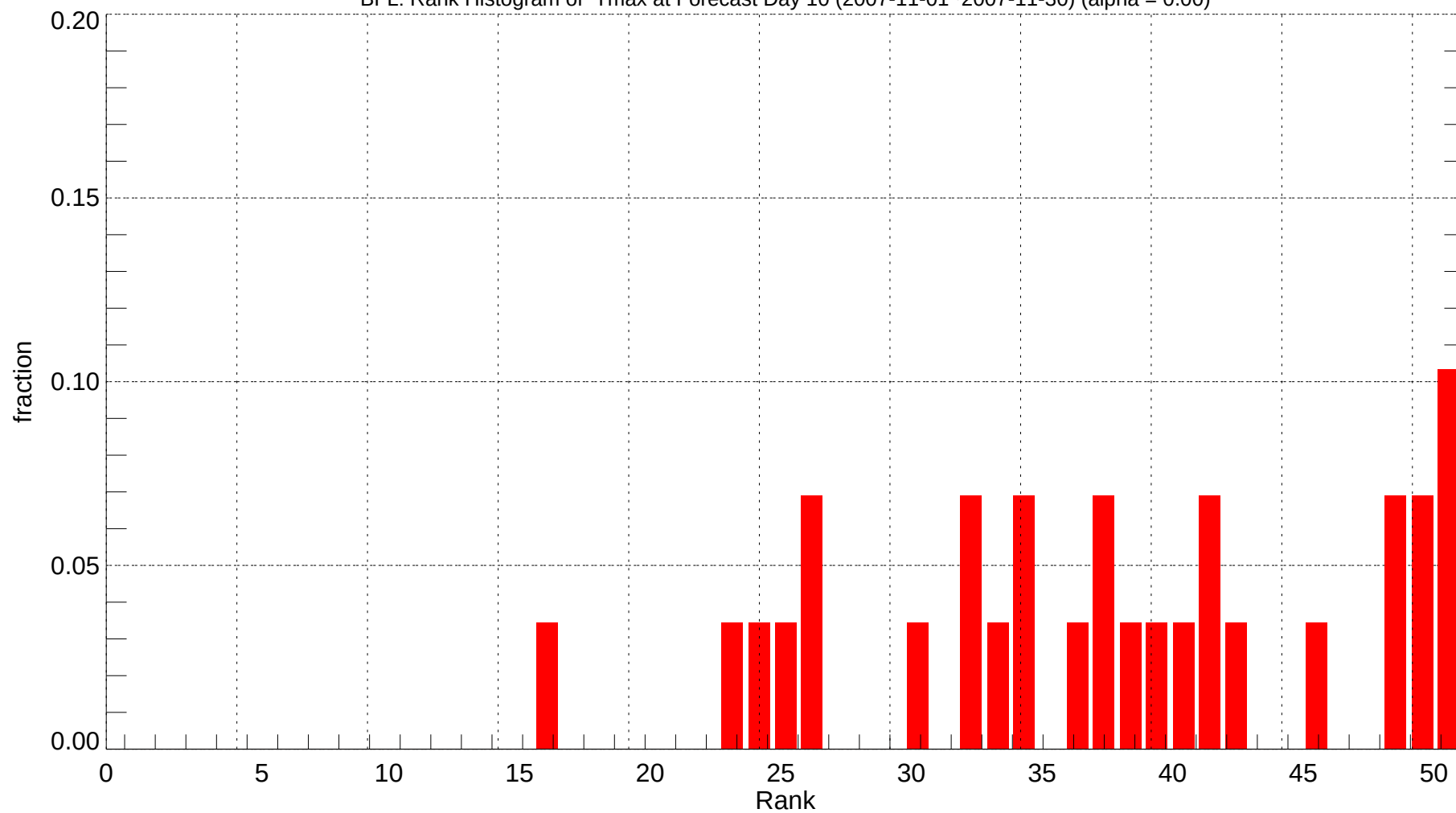
BFL: Rank Histogram of Tmax at Forecast Day 10 (2007-11-01~2007-11-30) (alpha = 0.00)
