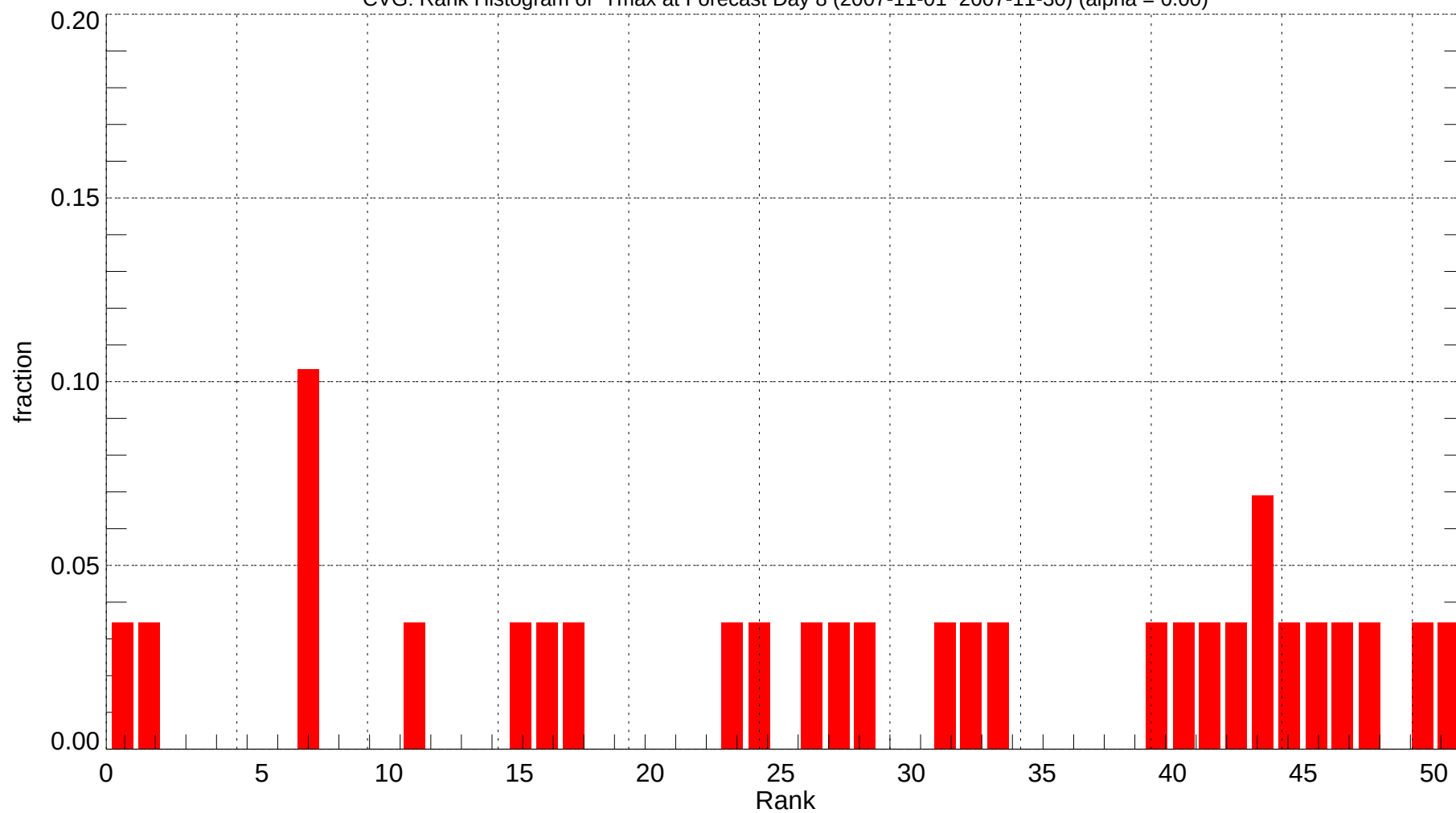
CVG: Rank Histogram of Tmax at Forecast Day 8 (2007-11-01~2007-11-30) (alpha = 0.00)
