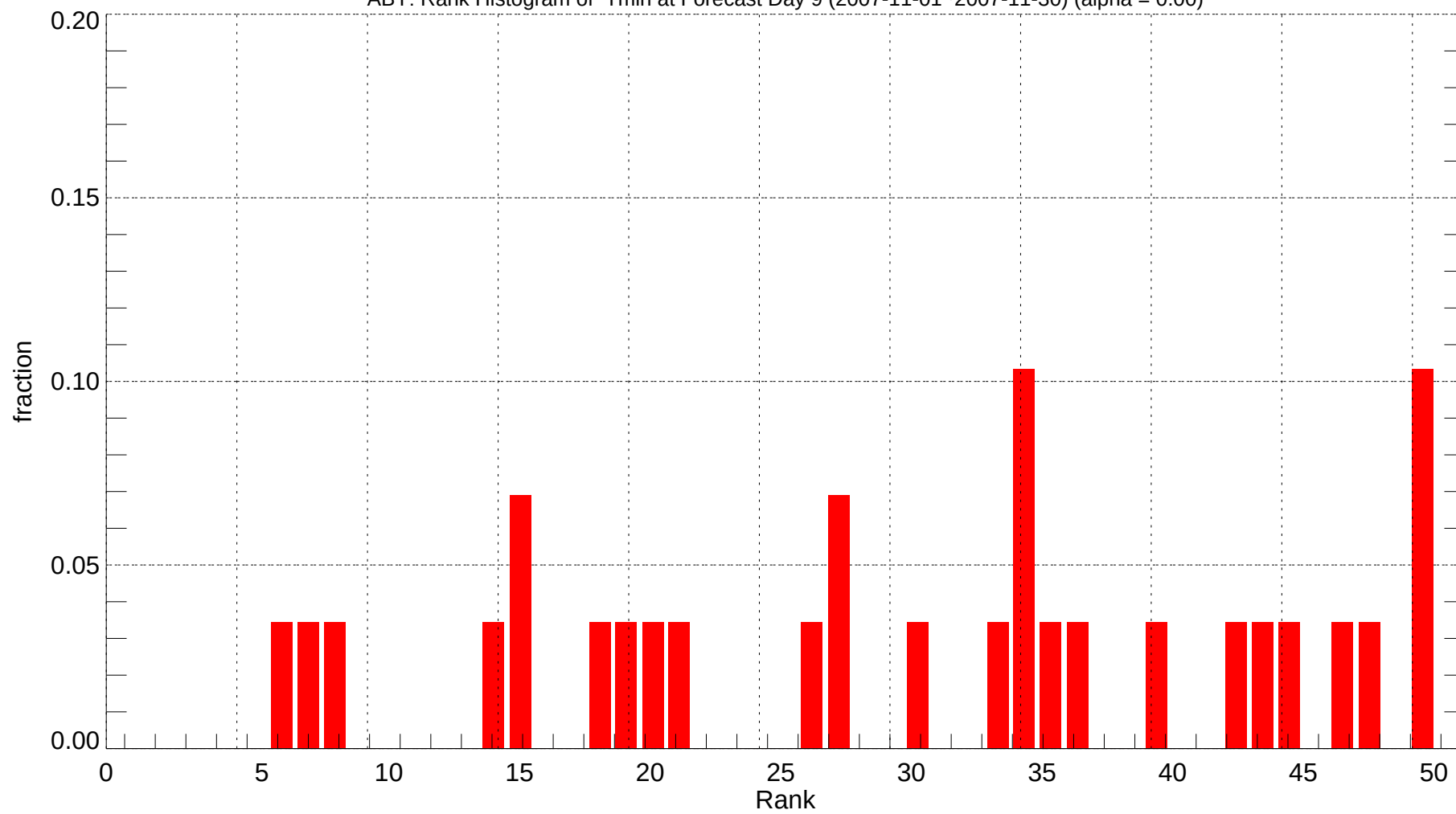
ABY: Rank Histogram of Tmin at Forecast Day 9 (2007-11-01~2007-11-30) (alpha = 0.00)
