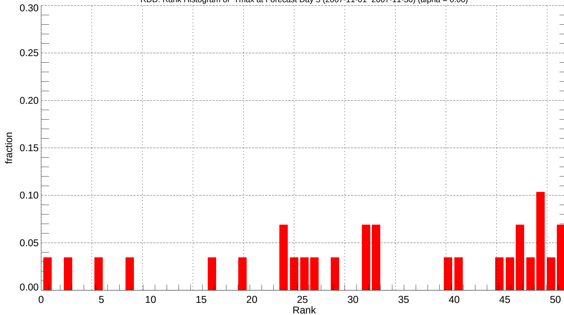
RDD: Rank Histogram of Tmax at Forecast Day 5 (2007-11-01~2007-11-30) (alpha = 0.00)
