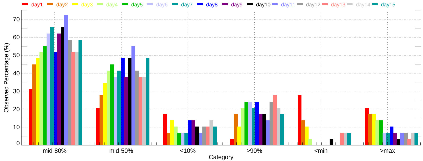
Observed Percentage of Ensembles - BOS: Min Temperature (2007-11-01~2007-11-30)
