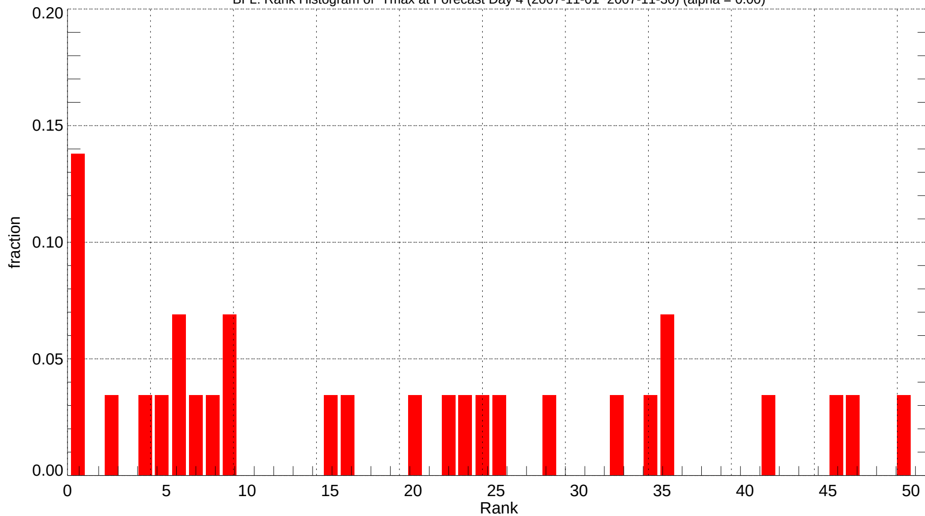
BFL: Rank Histogram of Tmax at Forecast Day 4 (2007-11-01~2007-11-30) (alpha = 0.00)
