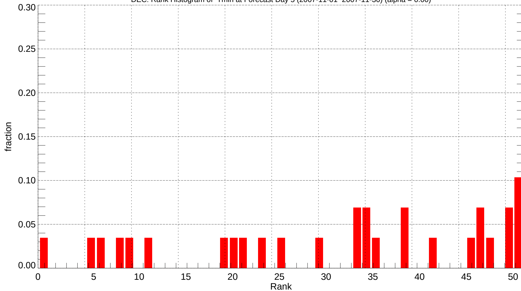
DEC: Rank Histogram of Tmin at Forecast Day 5 (2007-11-01~2007-11-30) (alpha = 0.00)
