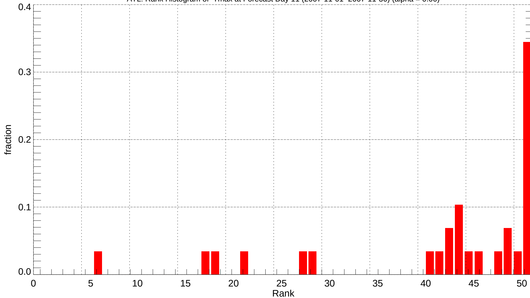
ATL: Rank Histogram of Tmax at Forecast Day 11 (2007-11-01~2007-11-30) (alpha = 0.00)
