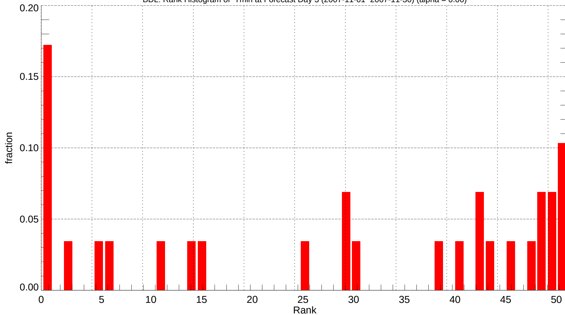
BDL: Rank Histogram of Tmin at Forecast Day 3 (2007-11-01~2007-11-30) (alpha = 0.00)
