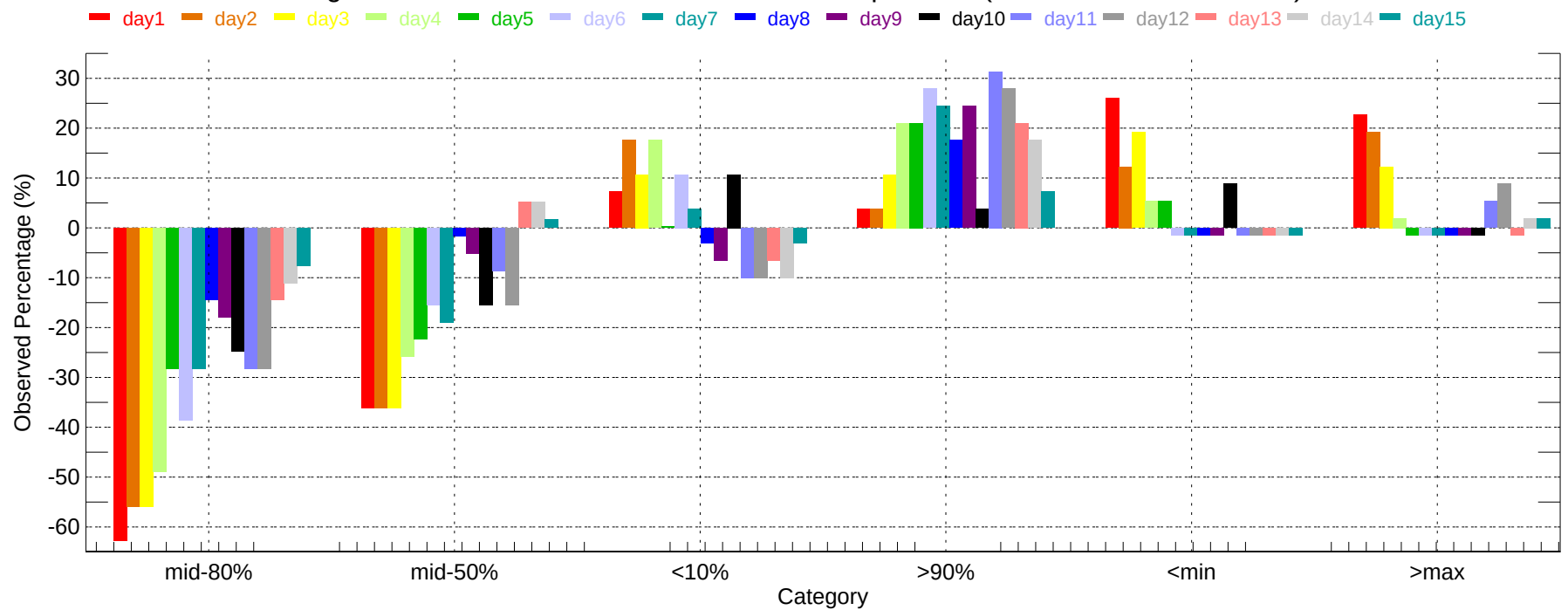
Observed Percentage Deviation of Ensembles - EVV: Max Temperature (2007-11-01~2007-11-30)
