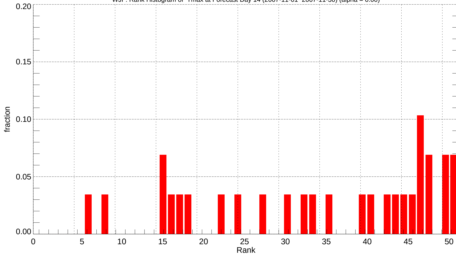
WJF: Rank Histogram of Tmax at Forecast Day 14 (2007-11-01~2007-11-30) (alpha = 0.00)
