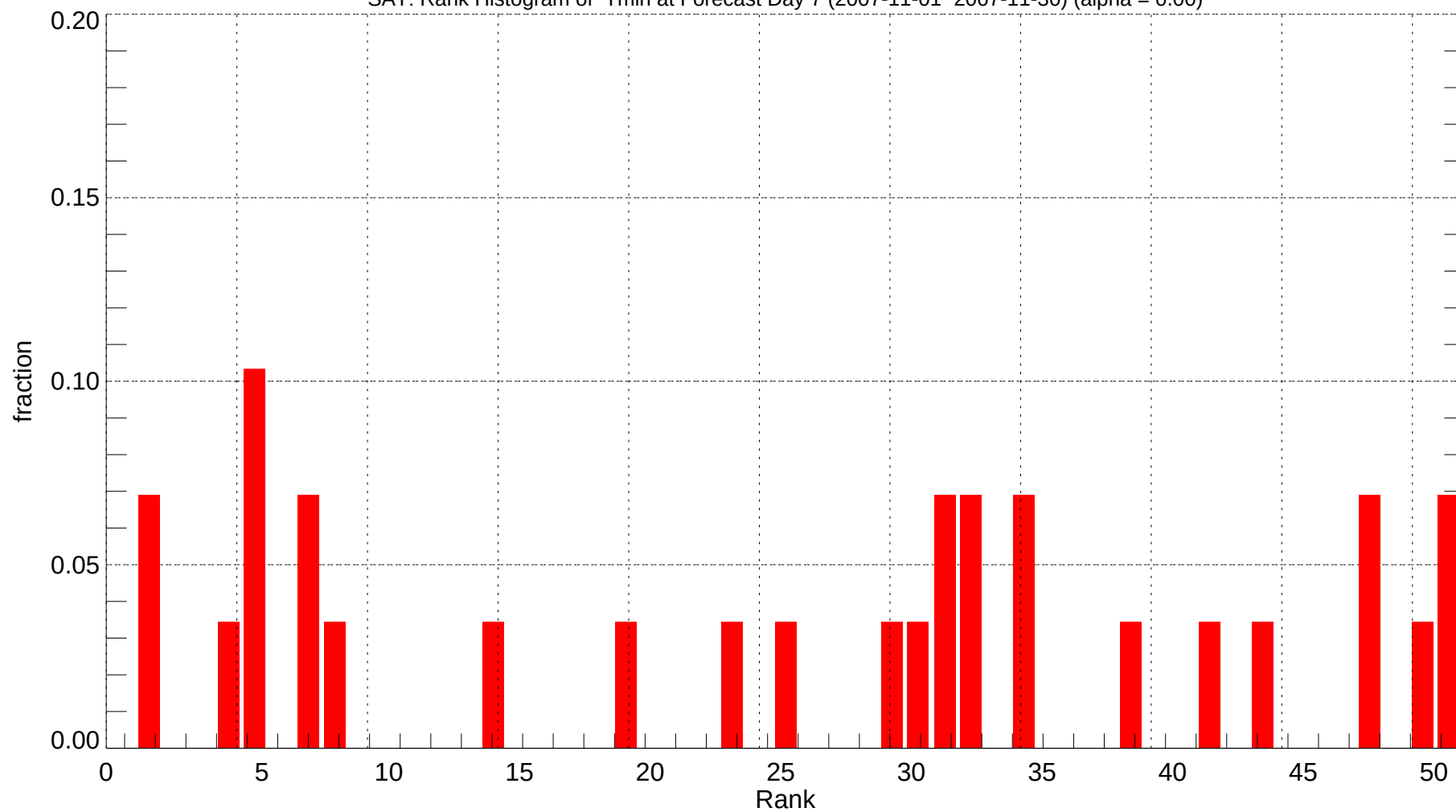
SAT: Rank Histogram of Tmin at Forecast Day 7 (2007-11-01~2007-11-30) (alpha = 0.00)
