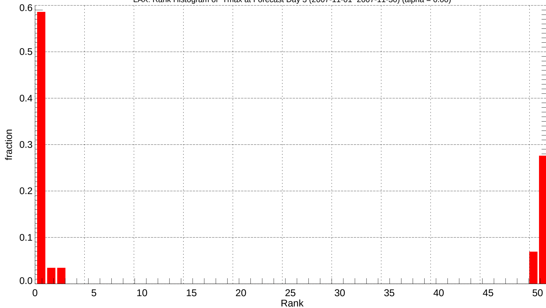
LAX: Rank Histogram of Tmax at Forecast Day 3 (2007-11-01~2007-11-30) (alpha = 0.00)
