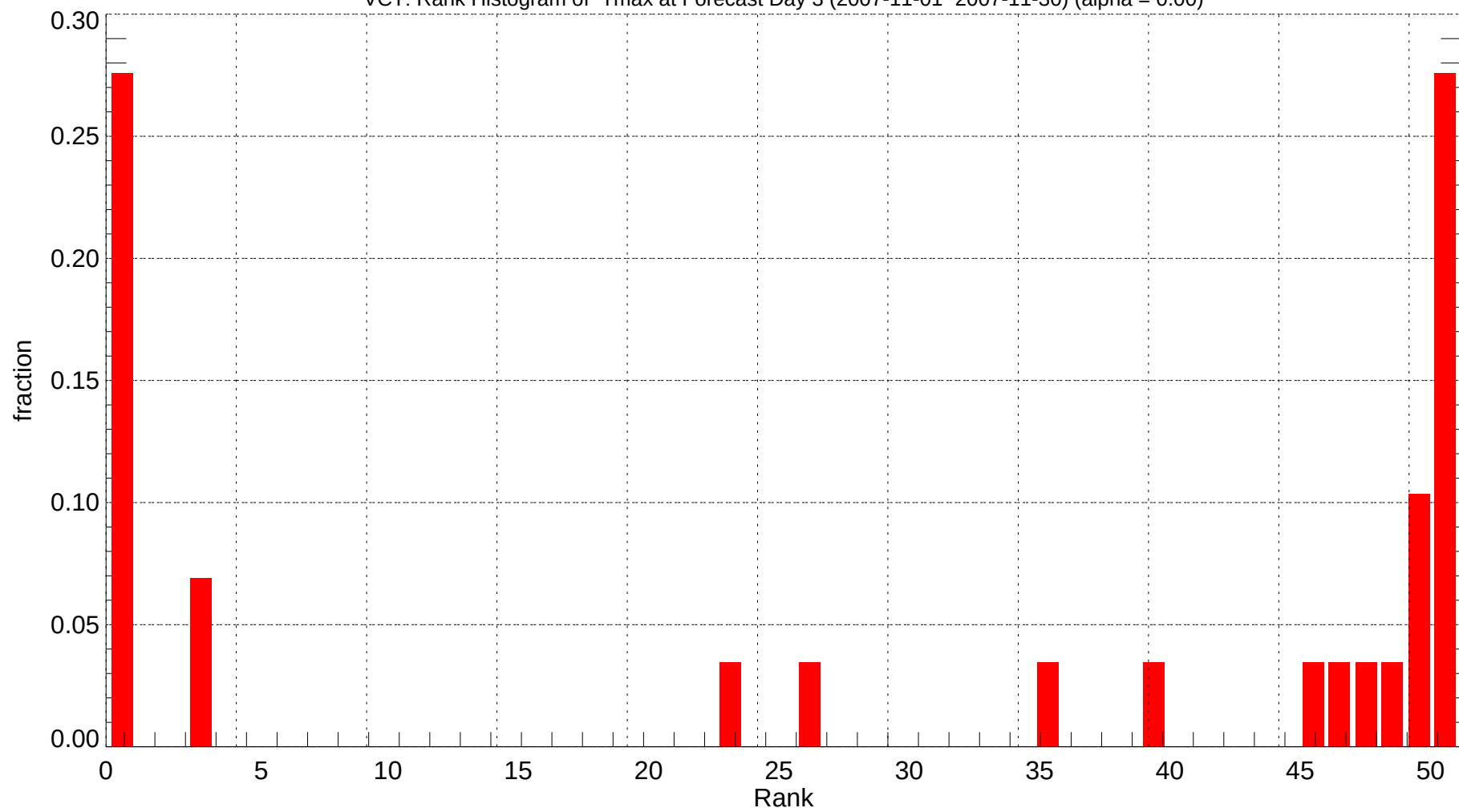
VCT: Rank Histogram of Tmax at Forecast Day 3 (2007-11-01~2007-11-30) (alpha = 0.00)
