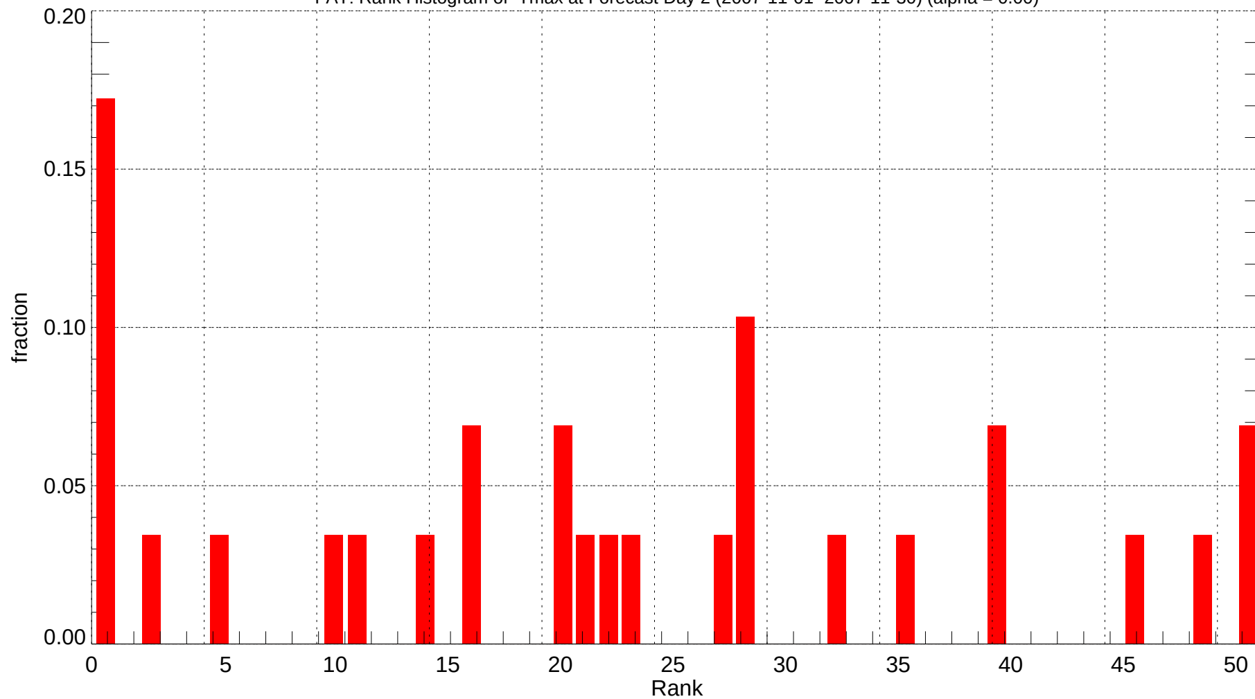
FAT: Rank Histogram of Tmax at Forecast Day 2 (2007-11-01~2007-11-30) (alpha = 0.00)
