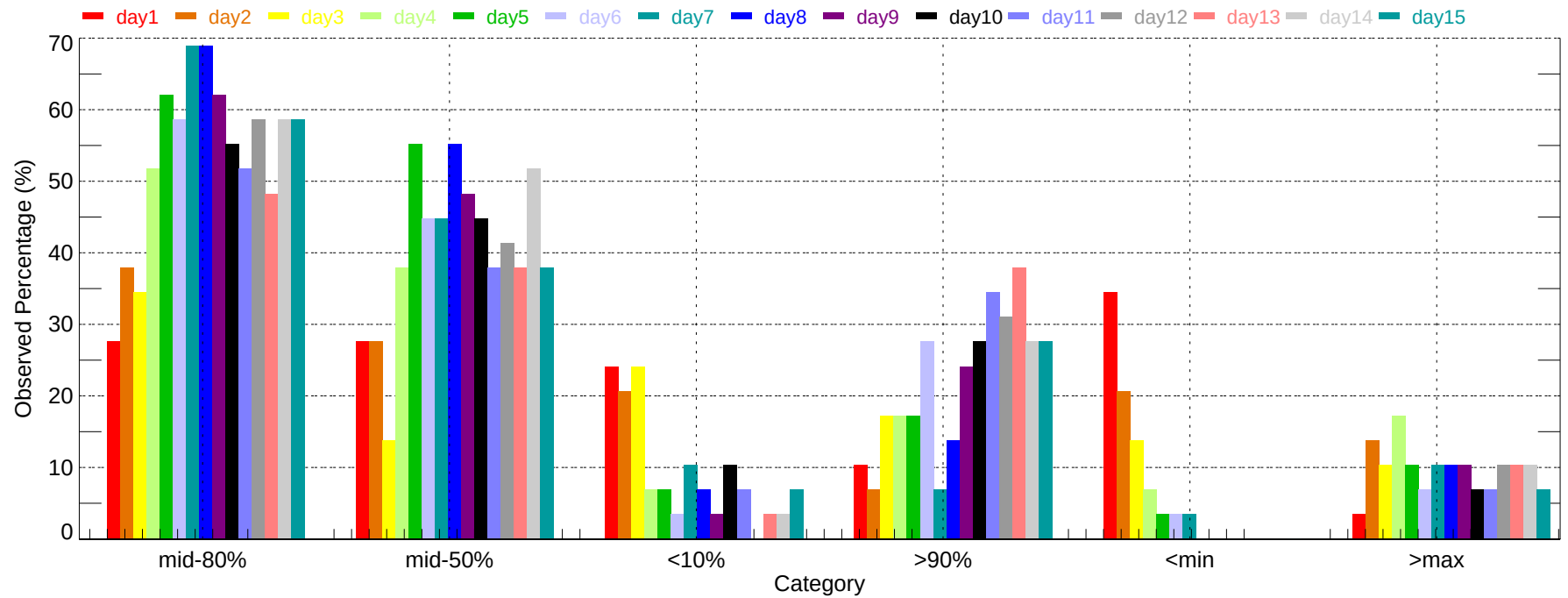
Observed Percentage of Ensembles - STL: Max Temperature (2007-11-01~2007-11-30)
