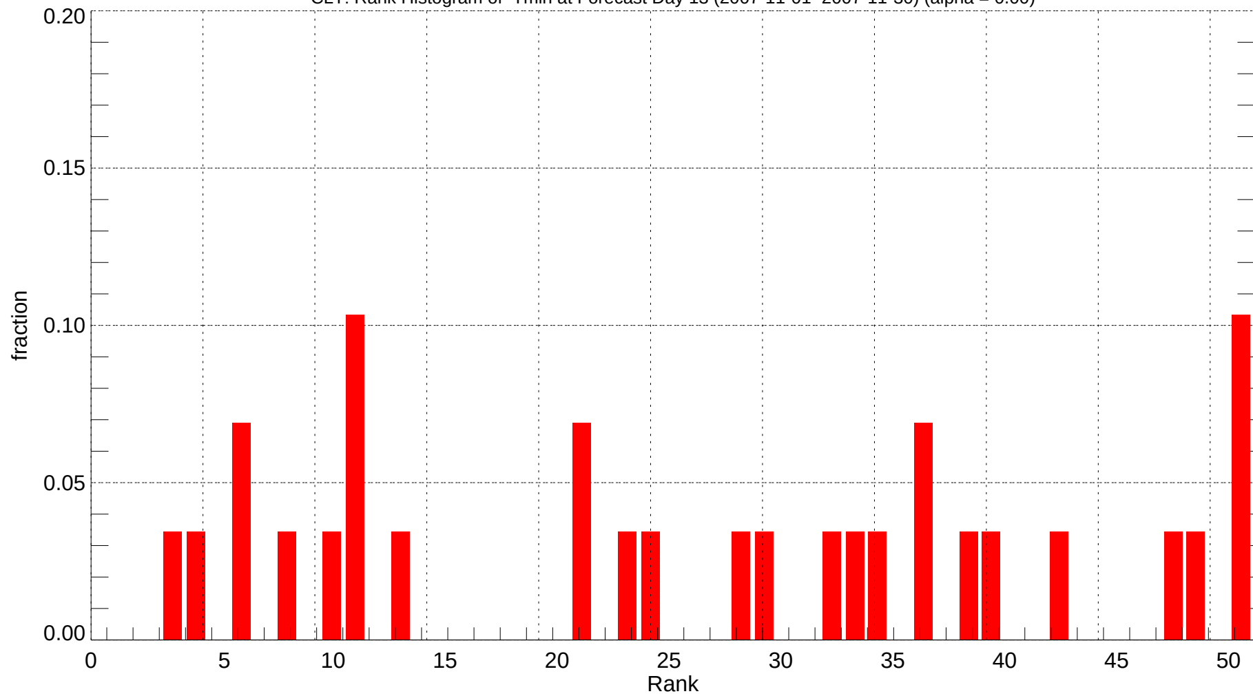
CLT: Rank Histogram of Tmin at Forecast Day 13 (2007-11-01~2007-11-30) (alpha = 0.00)
