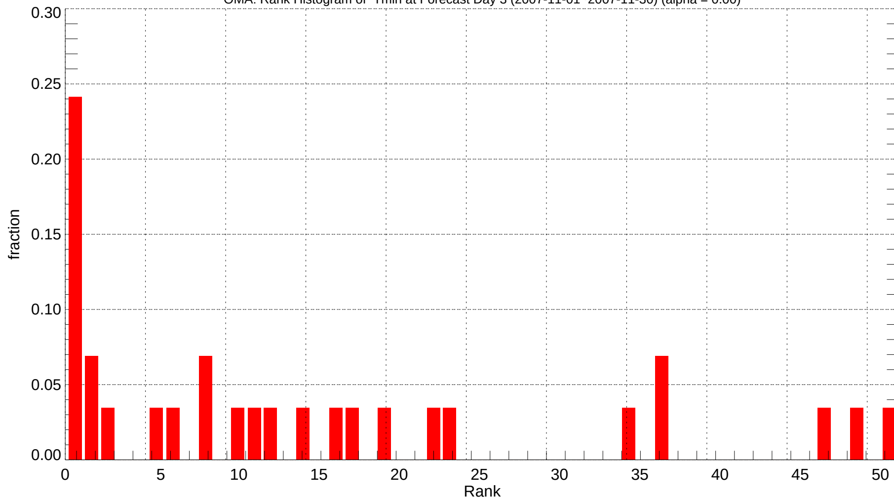
OMA: Rank Histogram of Tmin at Forecast Day 3 (2007-11-01~2007-11-30) (alpha = 0.00)
