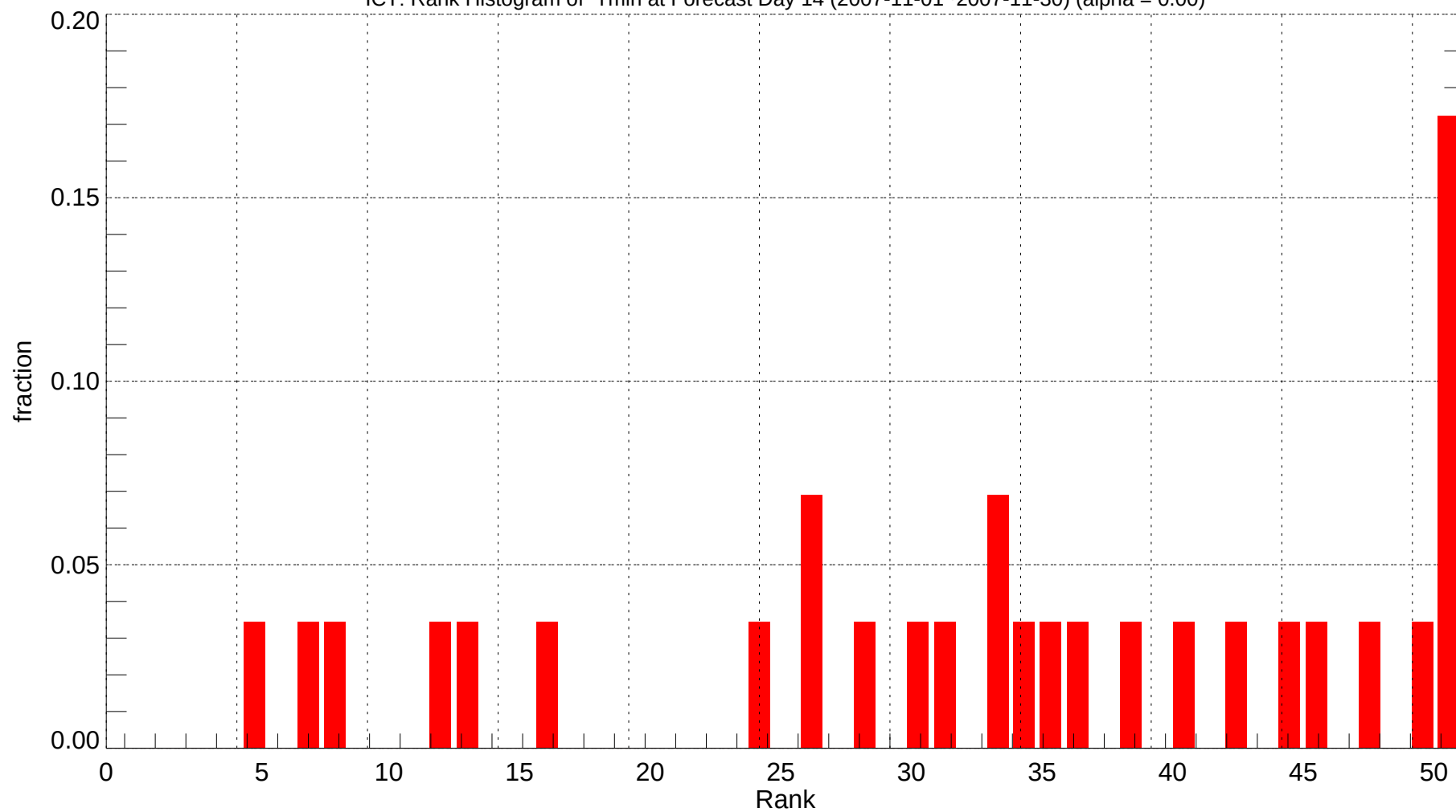
ICT: Rank Histogram of Tmin at Forecast Day 14 (2007-11-01~2007-11-30) (alpha = 0.00)
