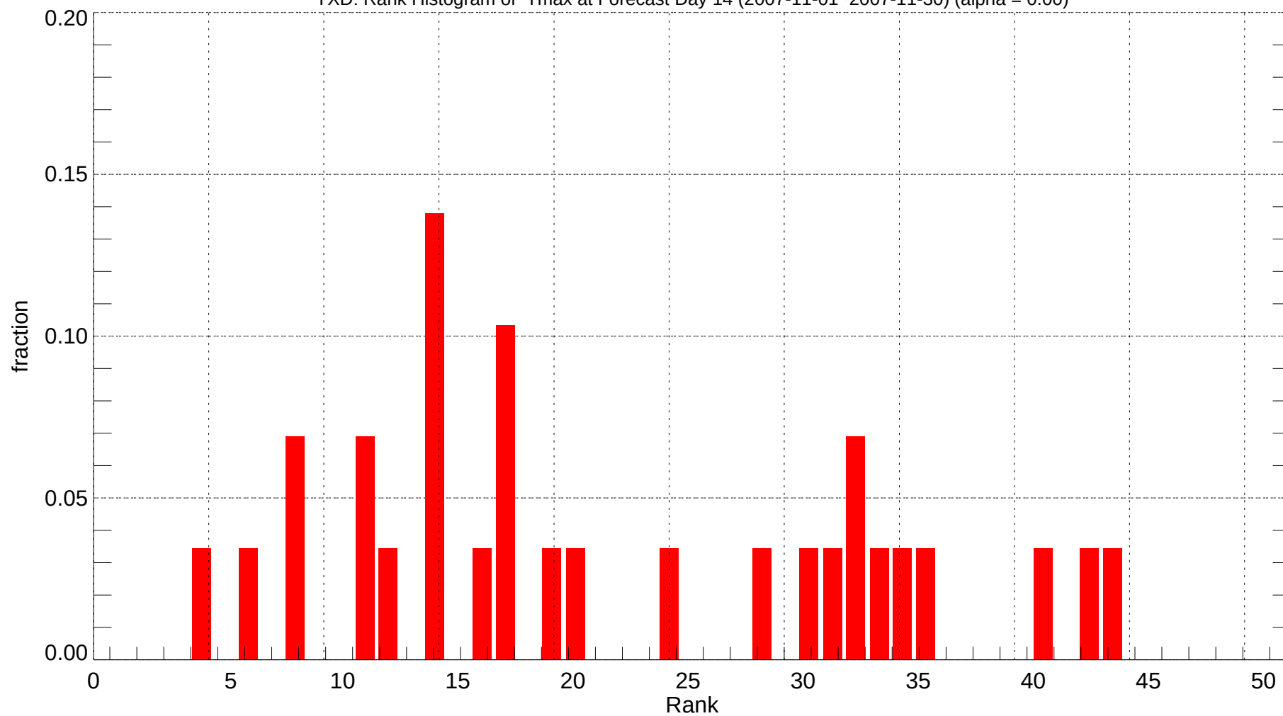
YXD: Rank Histogram of Tmax at Forecast Day 14 (2007-11-01~2007-11-30) (alpha = 0.00)
