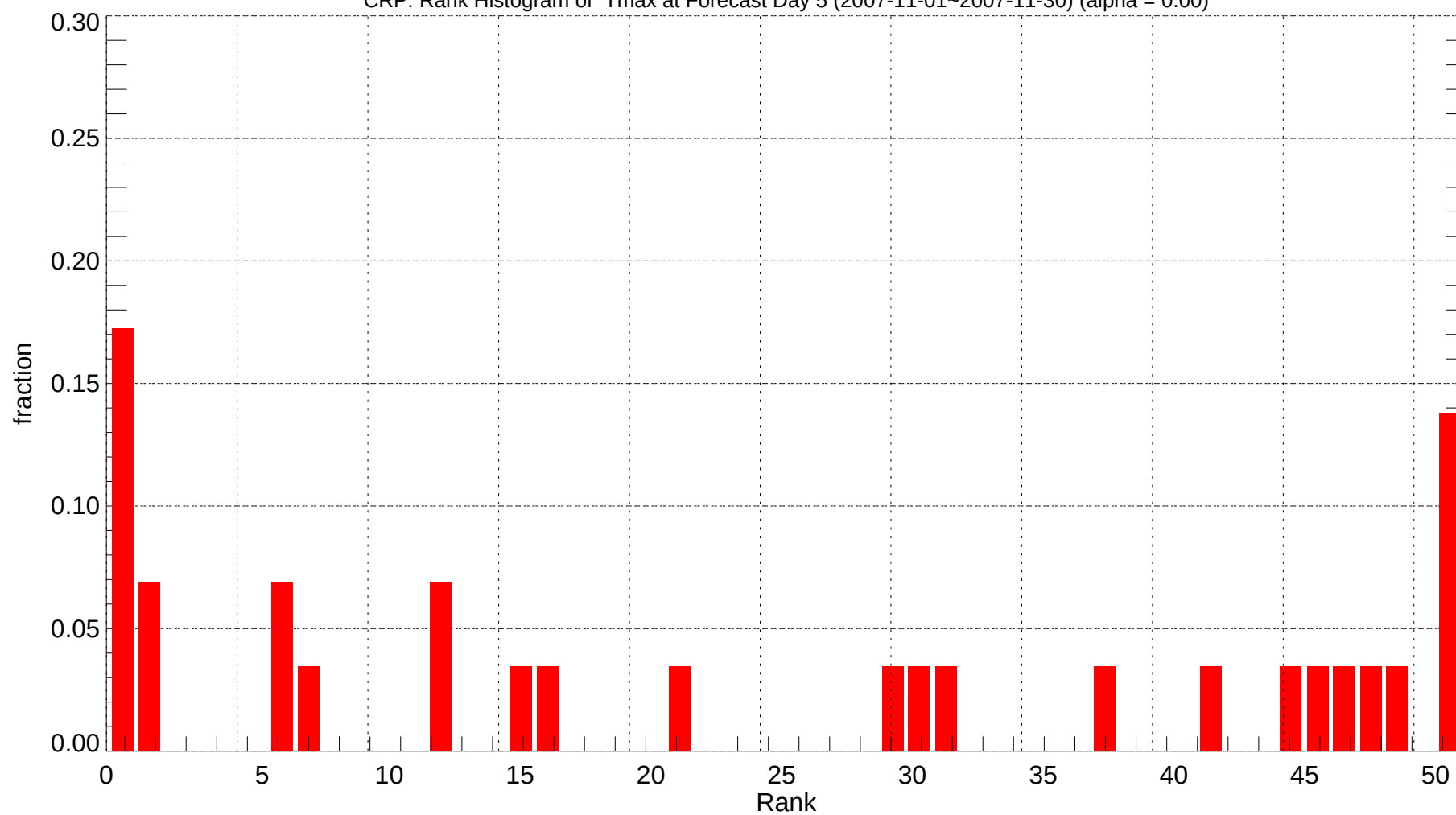
CRP: Rank Histogram of Tmax at Forecast Day 5 (2007-11-01~2007-11-30) (alpha = 0.00)
