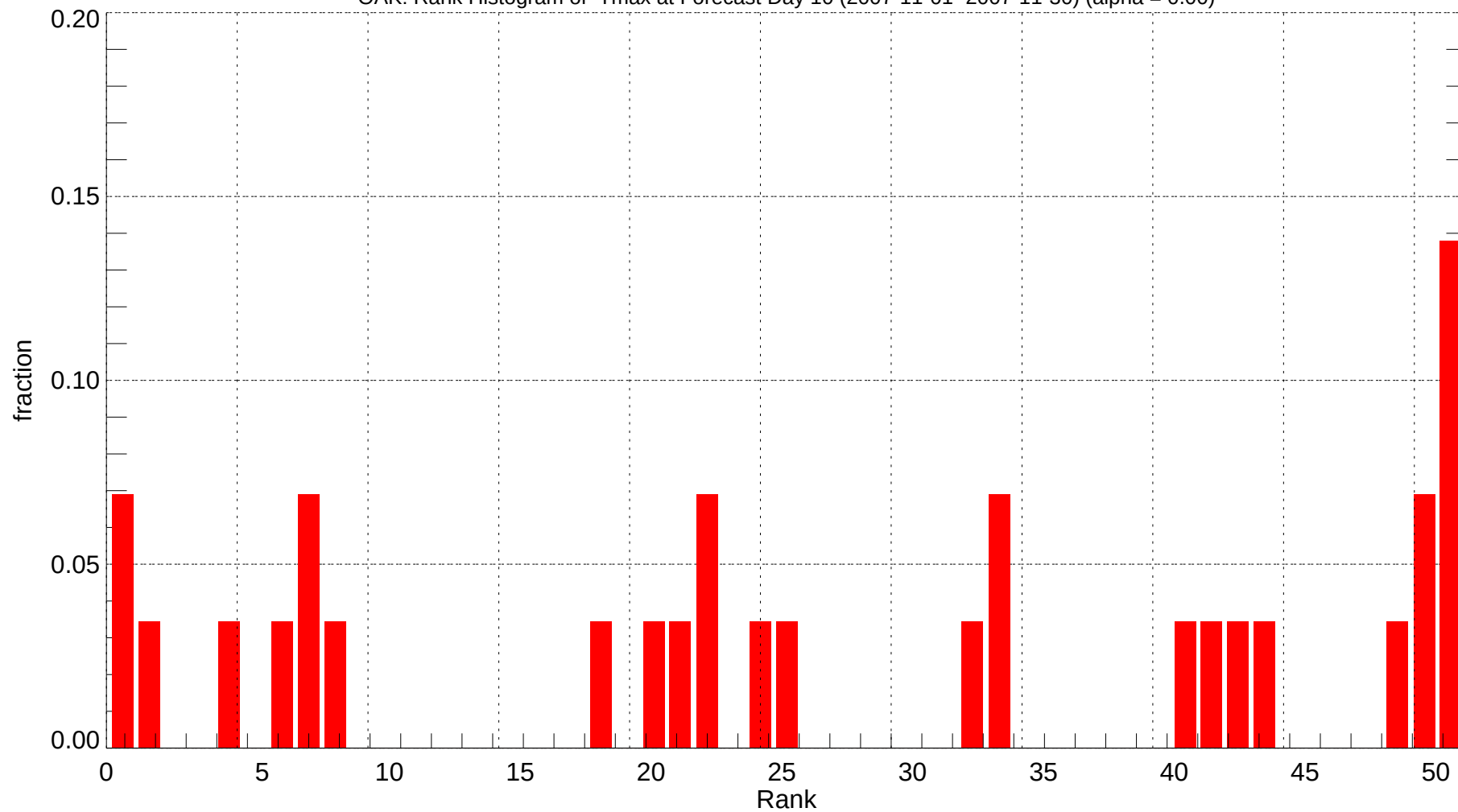
OAK: Rank Histogram of Tmax at Forecast Day 10 (2007-11-01~2007-11-30) (alpha = 0.00)
