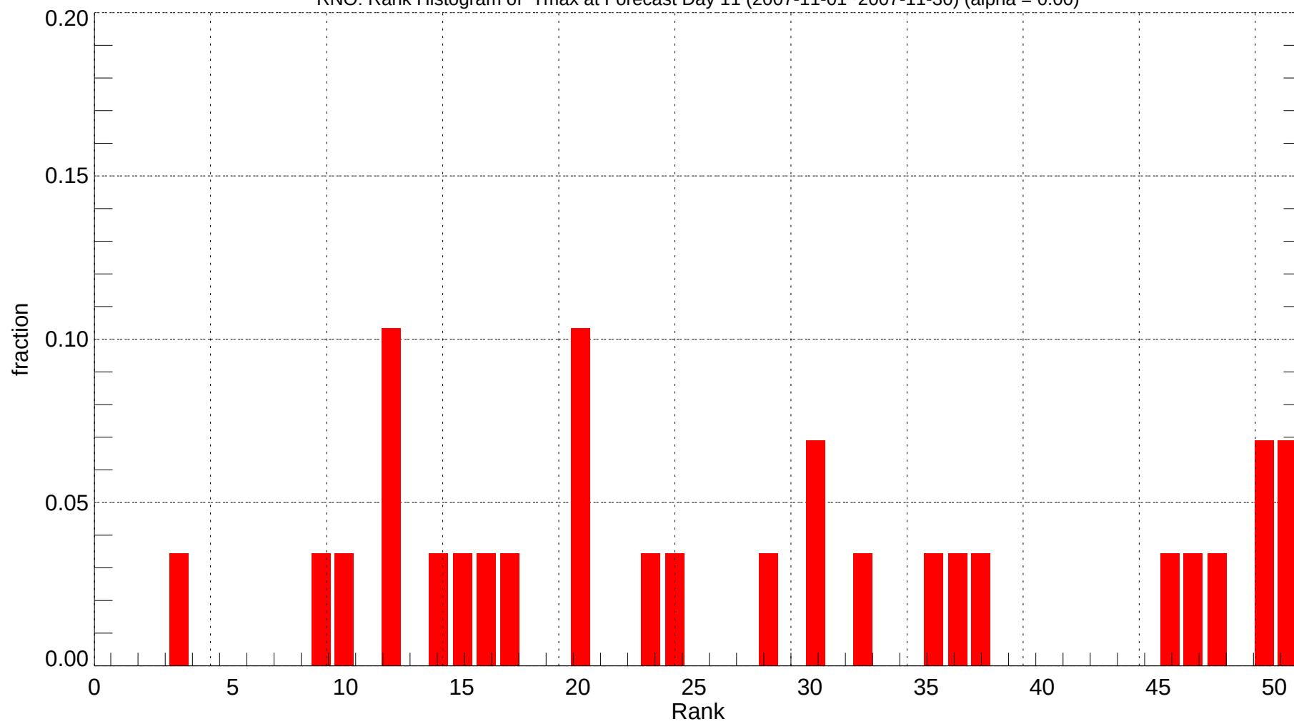
RNO: Rank Histogram of Tmax at Forecast Day 11 (2007-11-01~2007-11-30) (alpha = 0.00)
