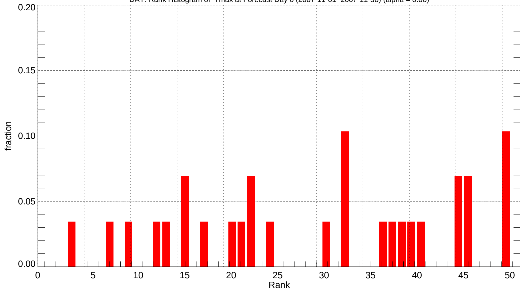
DAY: Rank Histogram of Tmax at Forecast Day 6 (2007-11-01~2007-11-30) (alpha = 0.00)
