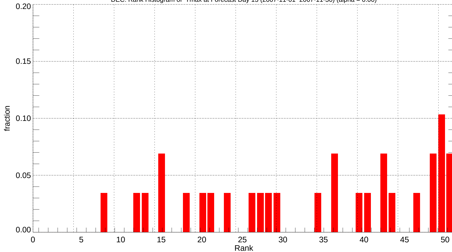
DEC: Rank Histogram of Tmax at Forecast Day 13 (2007-11-01~2007-11-30) (alpha = 0.00)
