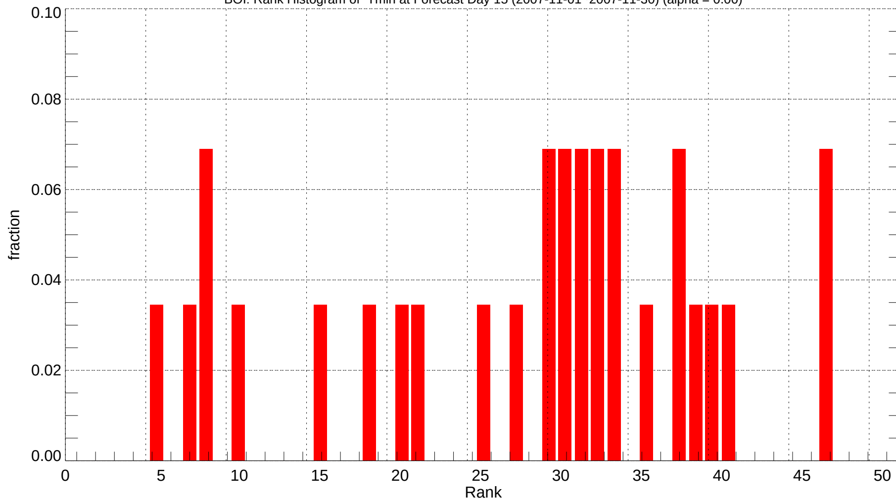
BOI: Rank Histogram of Tmin at Forecast Day 15 (2007-11-01~2007-11-30) (alpha = 0.00)
