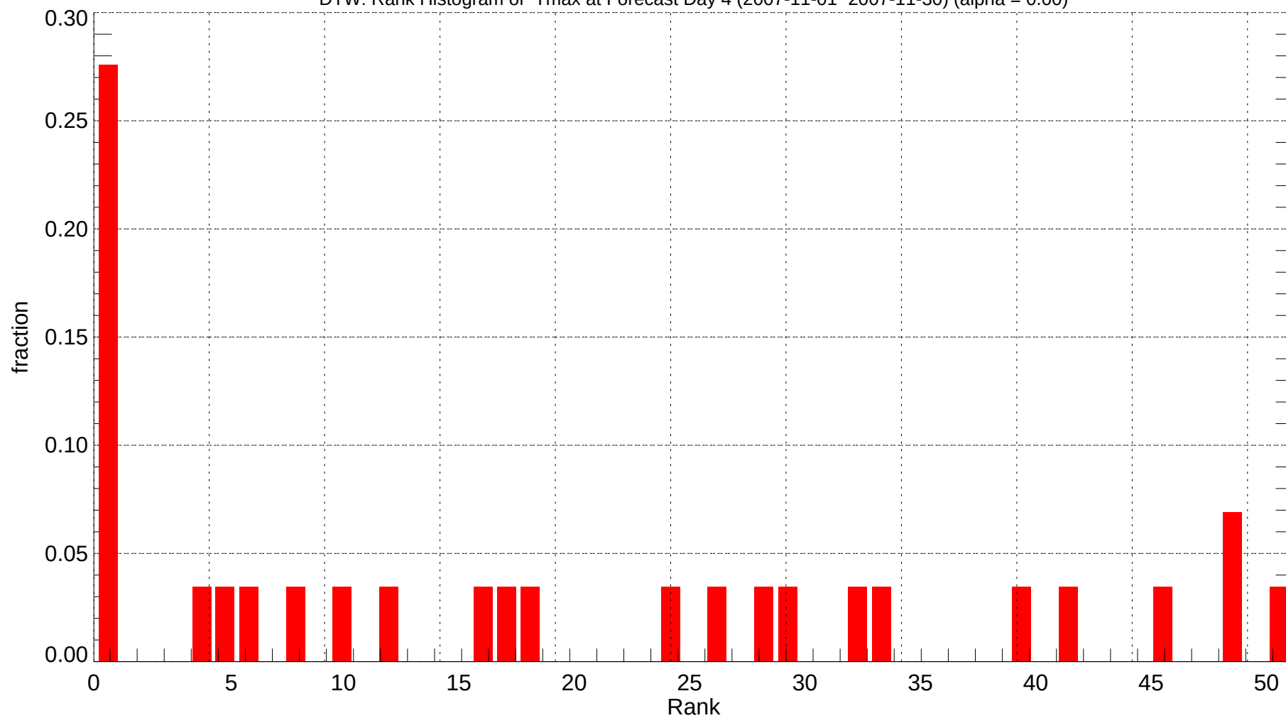
DTW: Rank Histogram of Tmax at Forecast Day 4 (2007-11-01~2007-11-30) (alpha = 0.00)
