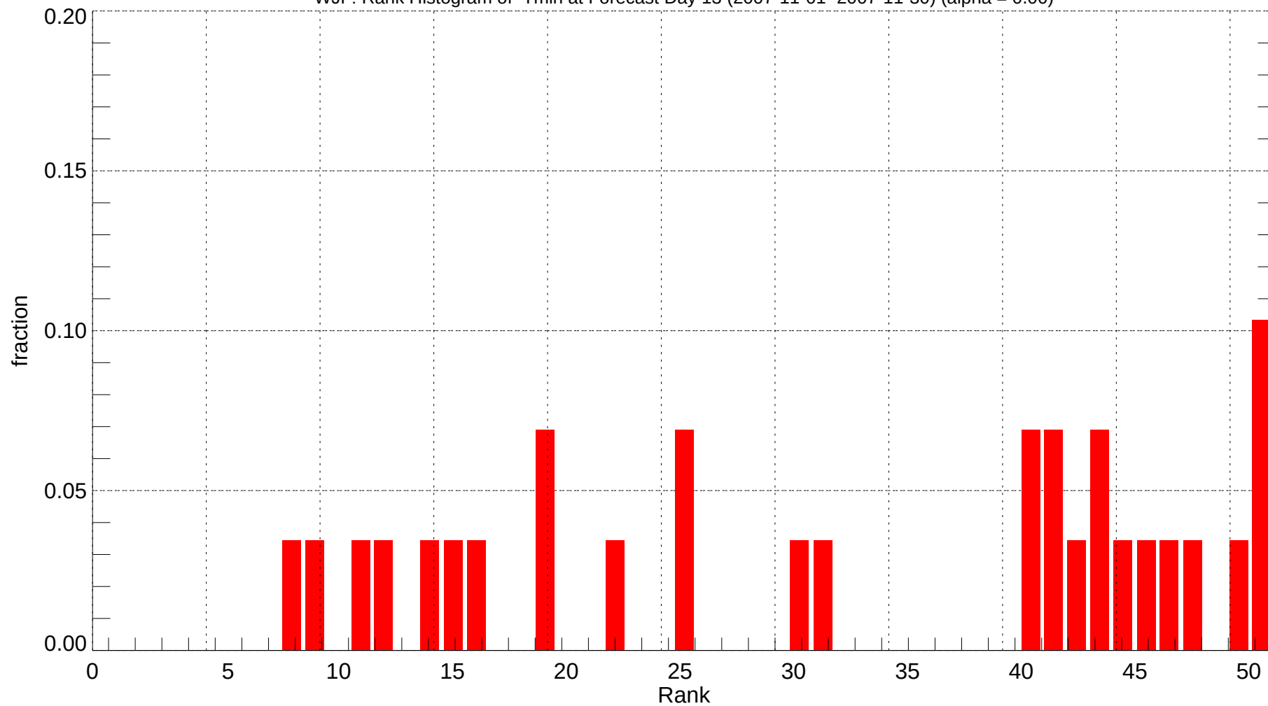
WJF: Rank Histogram of Tmin at Forecast Day 13 (2007-11-01~2007-11-30) (alpha = 0.00)
