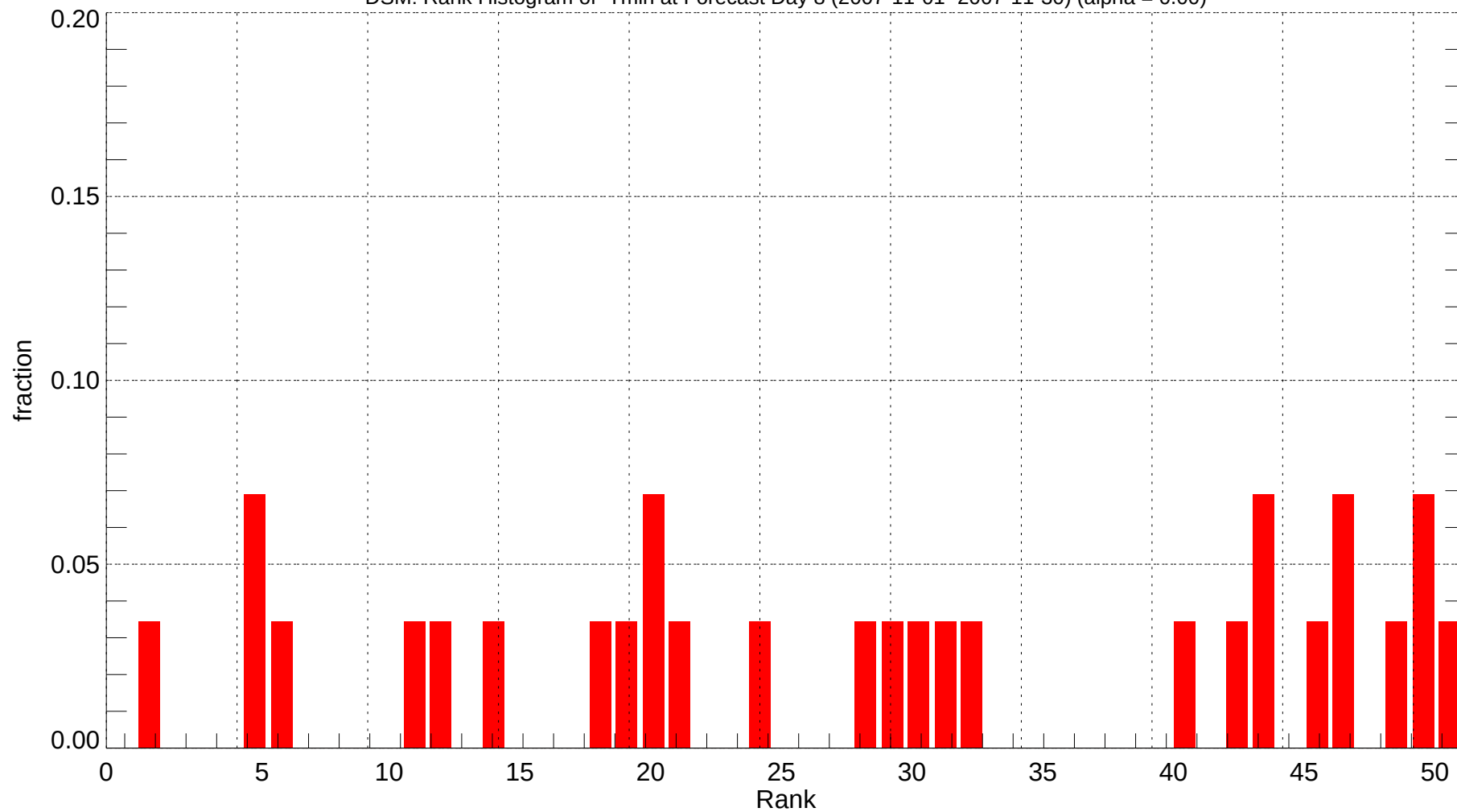
DSM: Rank Histogram of Tmin at Forecast Day 8 (2007-11-01~2007-11-30) (alpha = 0.00)
