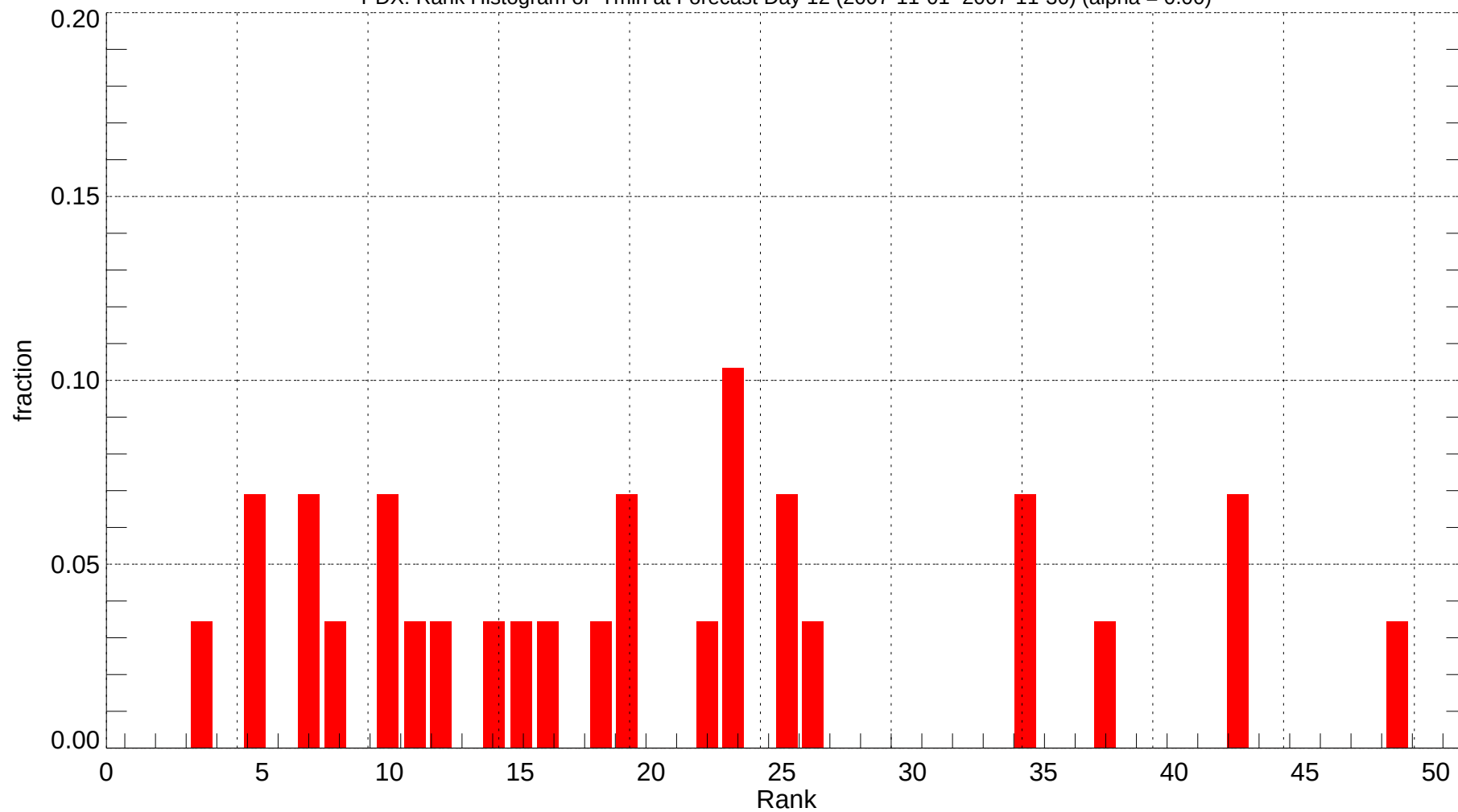
PDX: Rank Histogram of Tmin at Forecast Day 12 (2007-11-01~2007-11-30) (alpha = 0.00)
