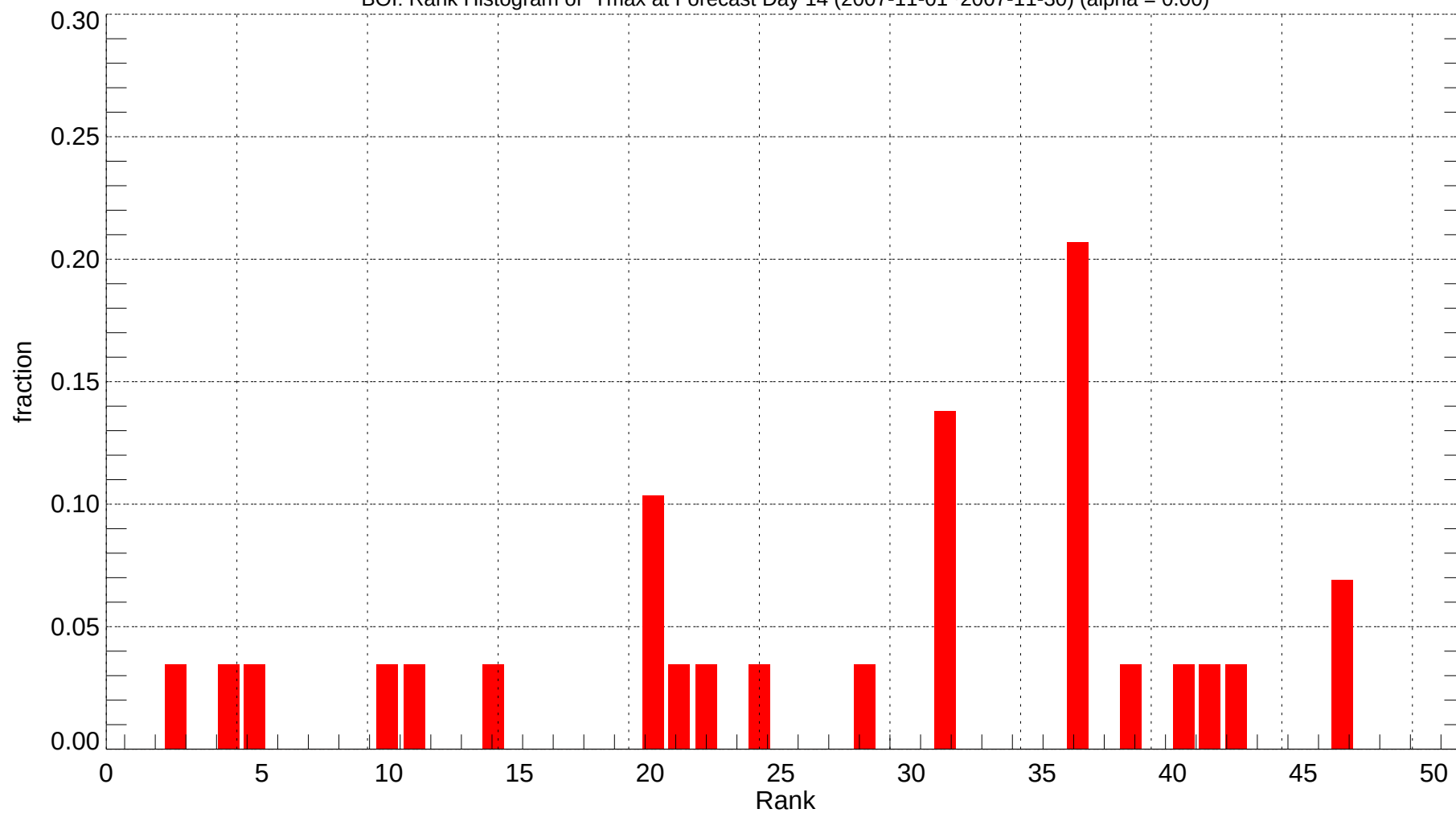
BOI: Rank Histogram of Tmax at Forecast Day 14 (2007-11-01~2007-11-30) (alpha = 0.00)
