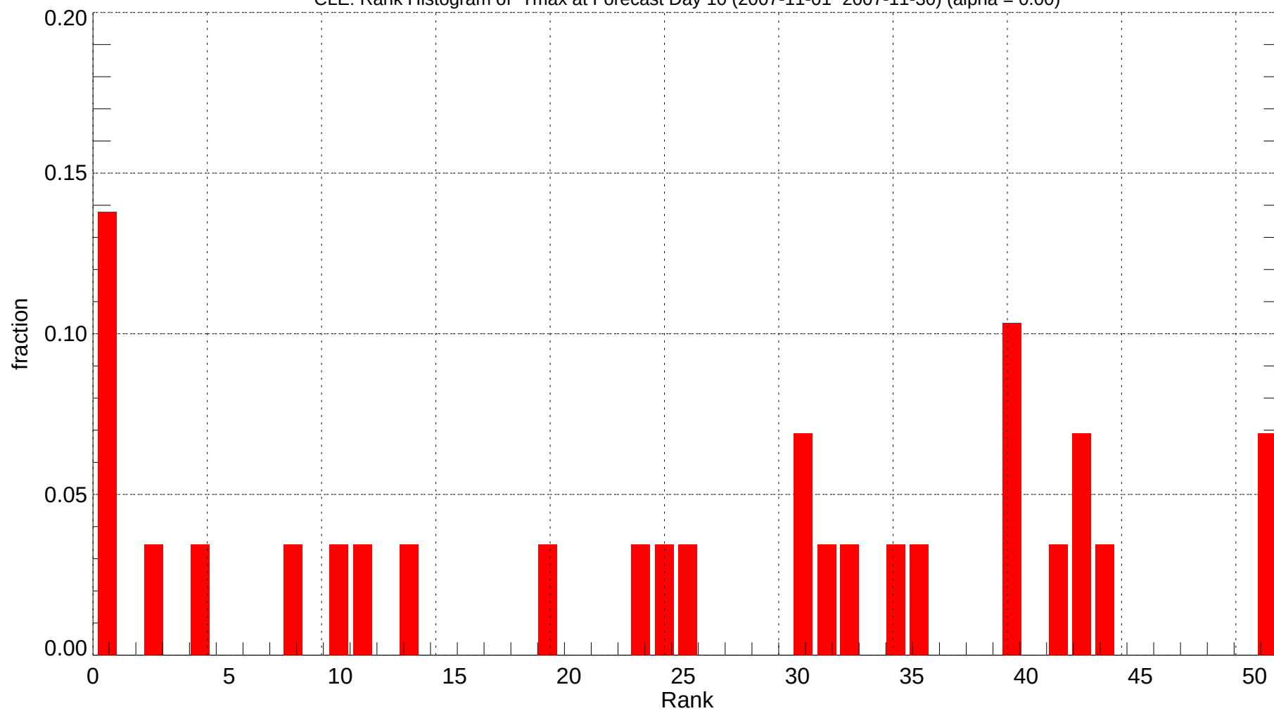
CLE: Rank Histogram of Tmax at Forecast Day 10 (2007-11-01~2007-11-30) (alpha = 0.00)
