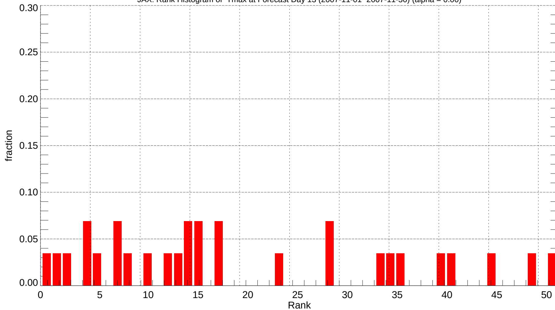
JAX: Rank Histogram of Tmax at Forecast Day 13 (2007-11-01~2007-11-30) (alpha = 0.00)
