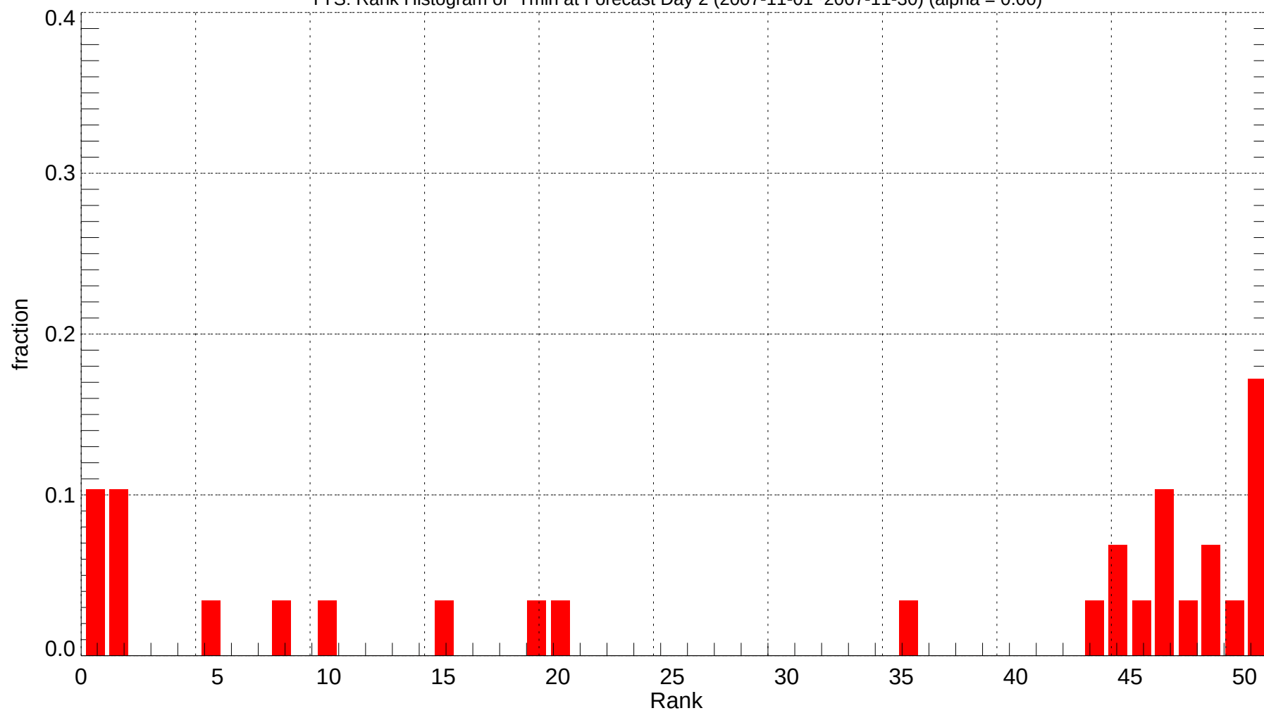
TYS: Rank Histogram of Tmin at Forecast Day 2 (2007-11-01~2007-11-30) (alpha = 0.00)
