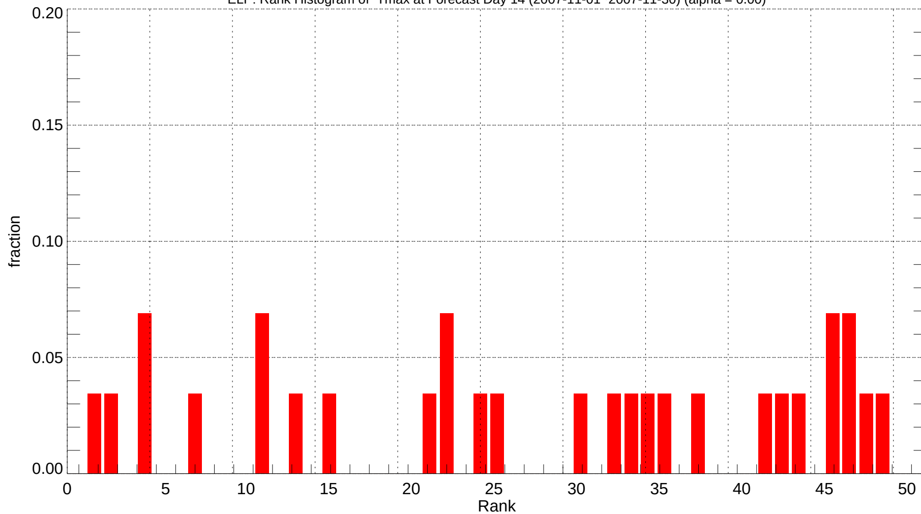
ELP: Rank Histogram of Tmax at Forecast Day 14 (2007-11-01~2007-11-30) (alpha = 0.00)
