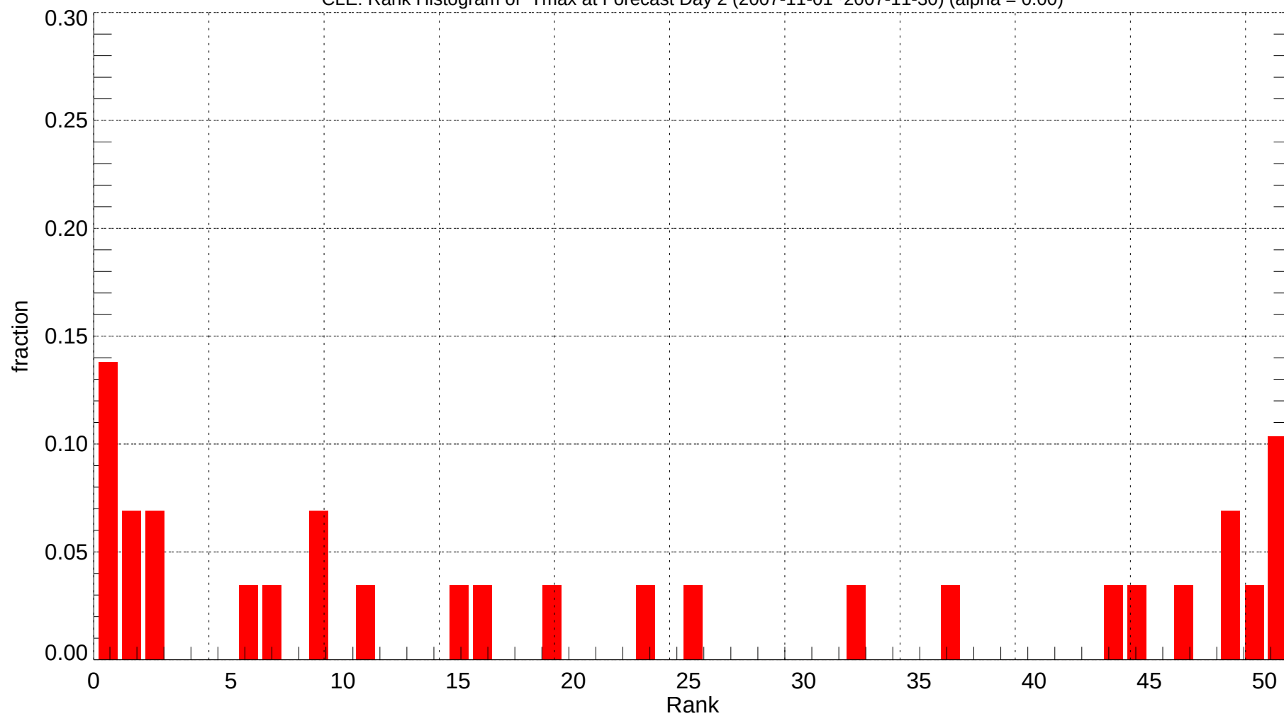
CLE: Rank Histogram of Tmax at Forecast Day 2 (2007-11-01~2007-11-30) (alpha = 0.00)
