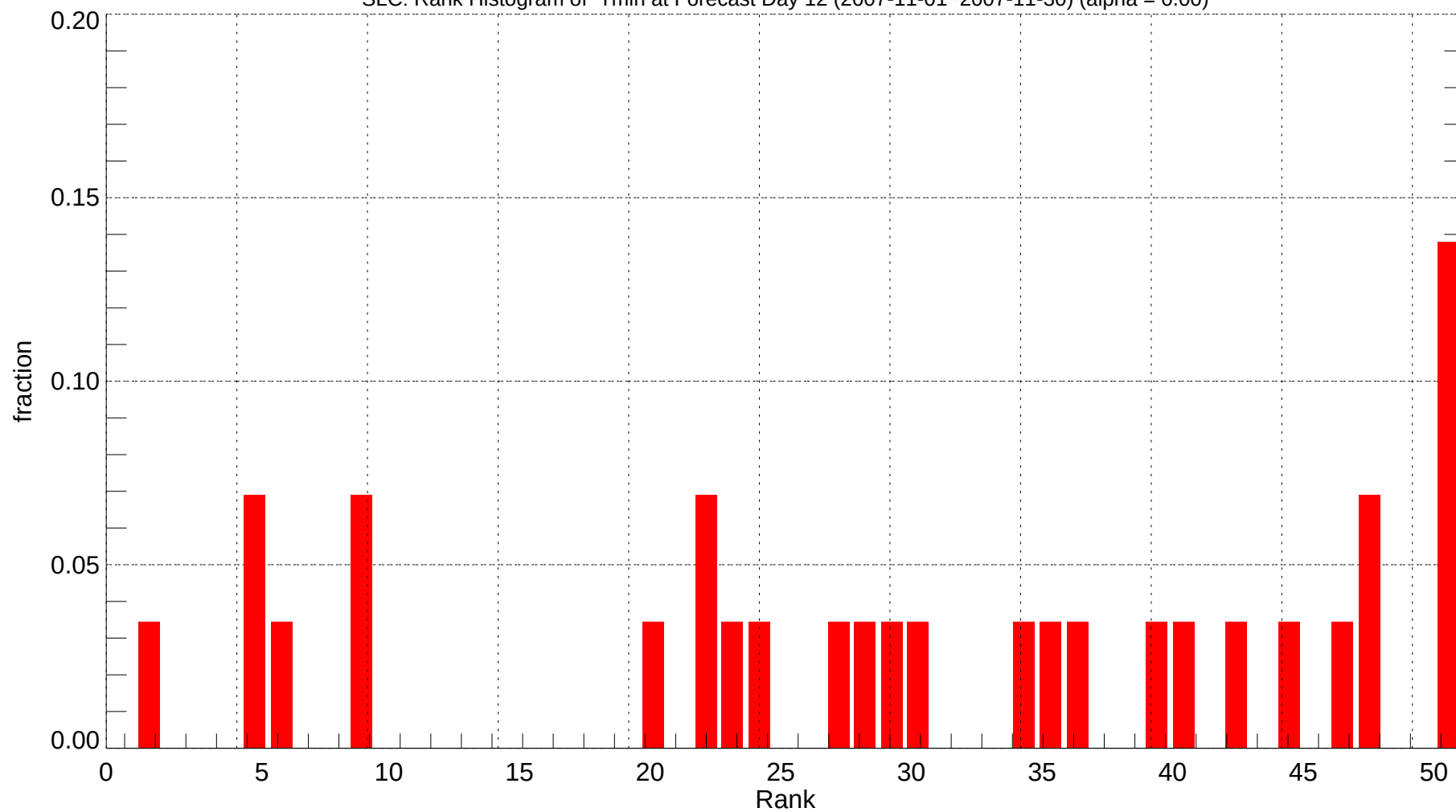
SLC: Rank Histogram of Tmin at Forecast Day 12 (2007-11-01~2007-11-30) (alpha = 0.00)
