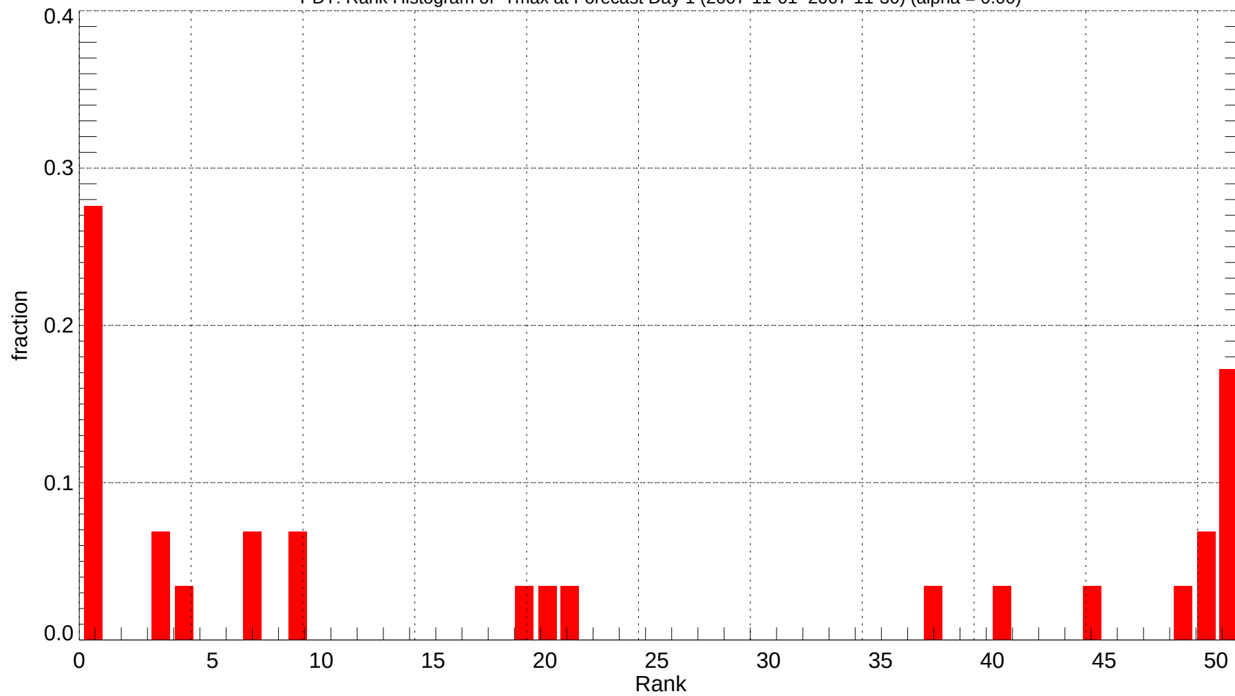
PDT: Rank Histogram of Tmax at Forecast Day 1 (2007-11-01~2007-11-30) (alpha = 0.00)
