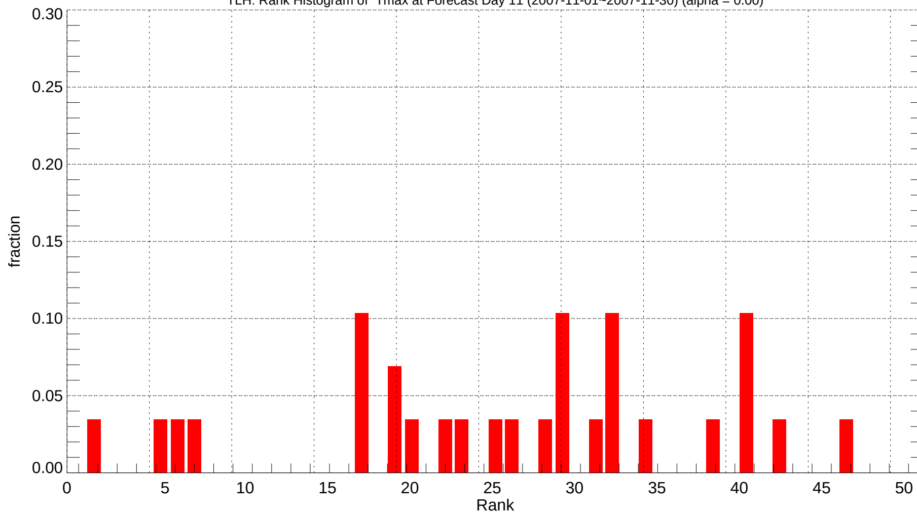
TLH: Rank Histogram of Tmax at Forecast Day 11 (2007-11-01~2007-11-30) (alpha = 0.00)
