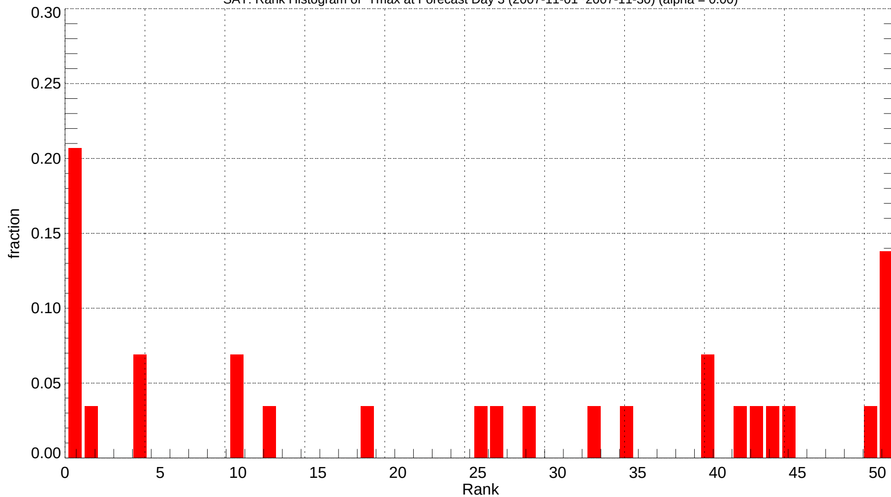
SAT: Rank Histogram of Tmax at Forecast Day 3 (2007-11-01~2007-11-30) (alpha = 0.00)
