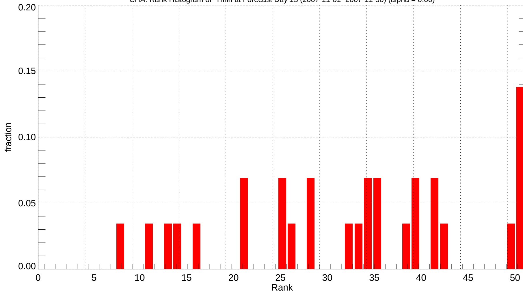
CHA: Rank Histogram of Tmin at Forecast Day 13 (2007-11-01~2007-11-30) (alpha = 0.00)
