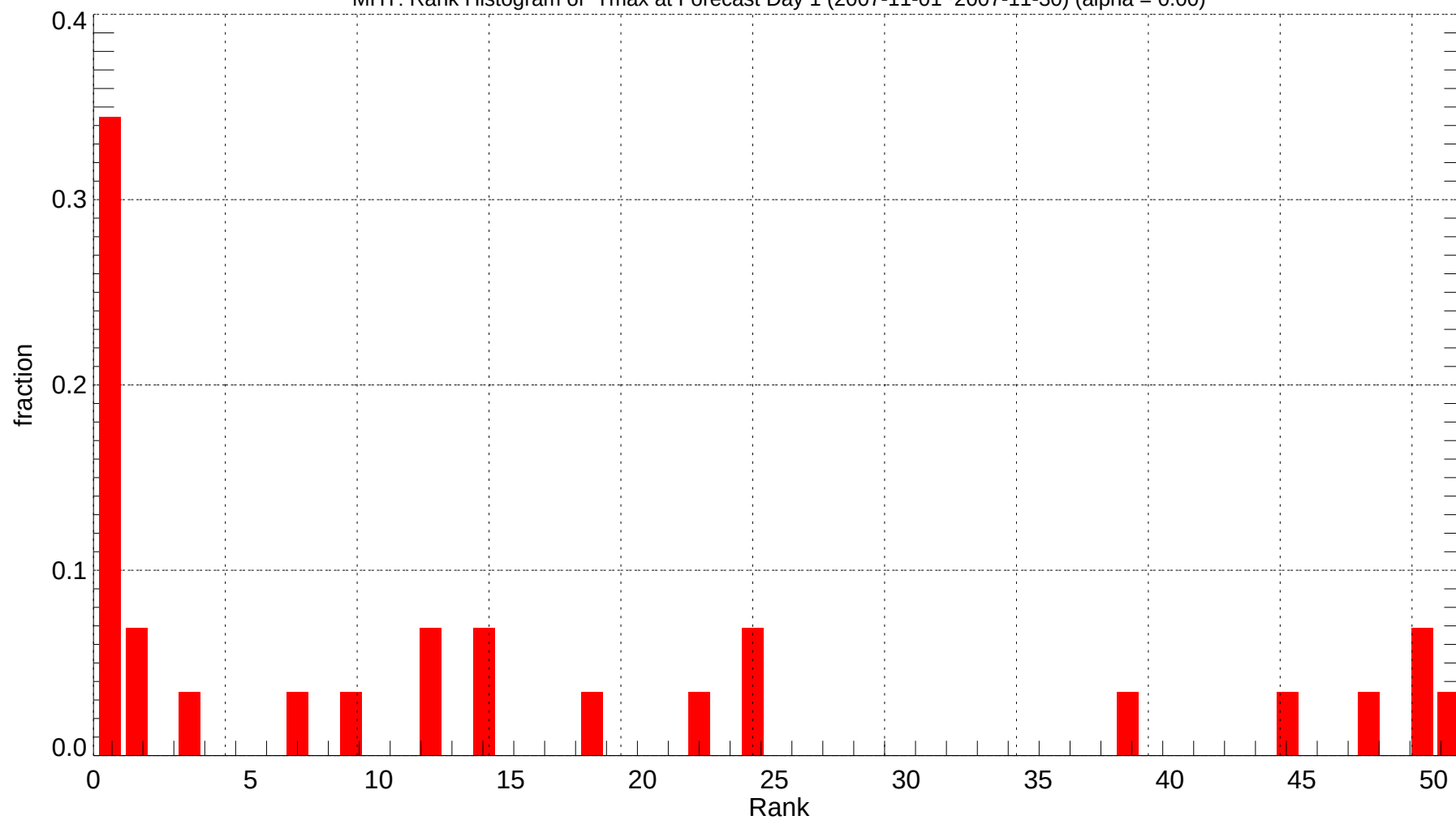
MHT: Rank Histogram of Tmax at Forecast Day 1 (2007-11-01~2007-11-30) (alpha = 0.00)
