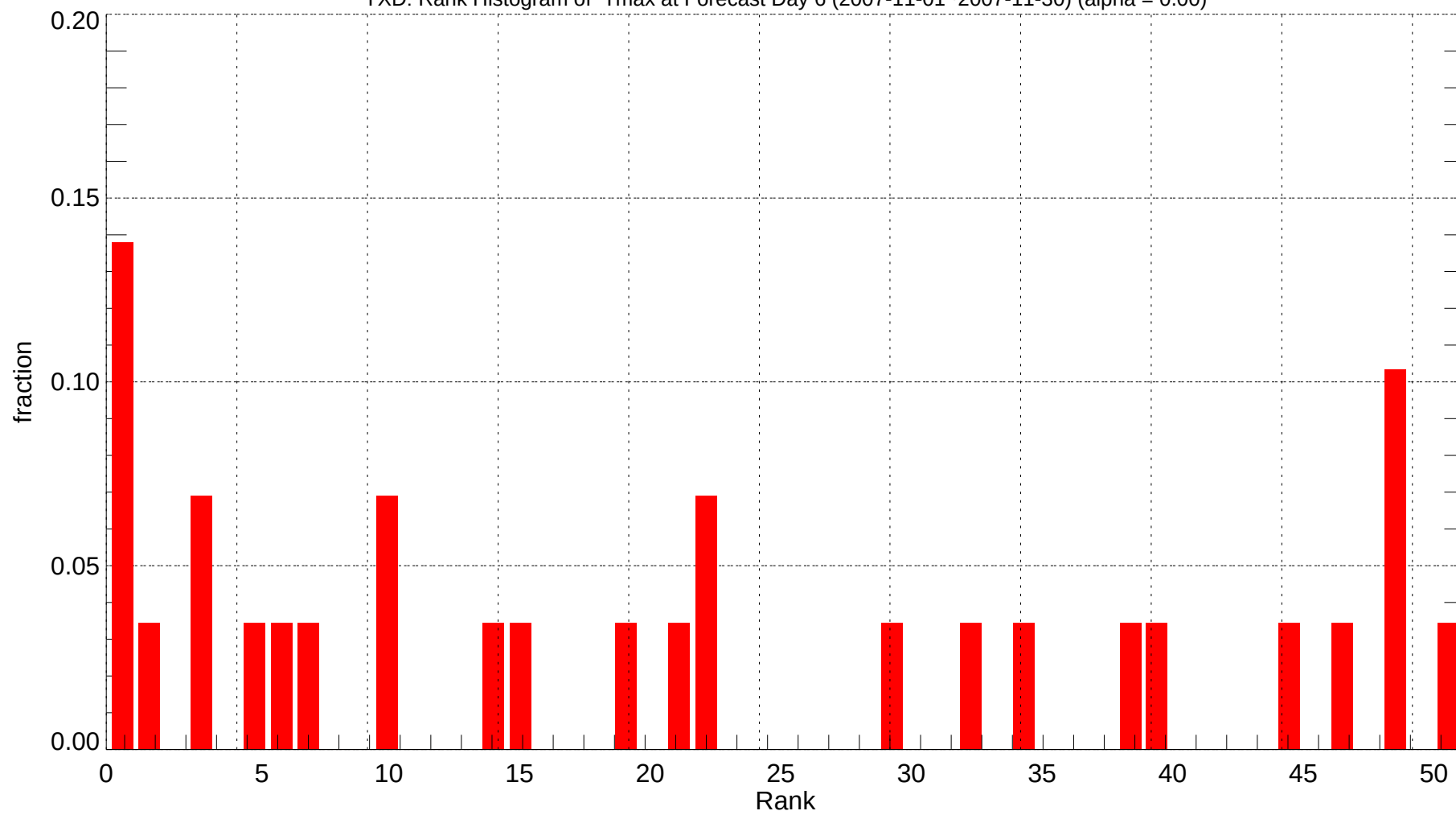
YXD: Rank Histogram of Tmax at Forecast Day 6 (2007-11-01~2007-11-30) (alpha = 0.00)
