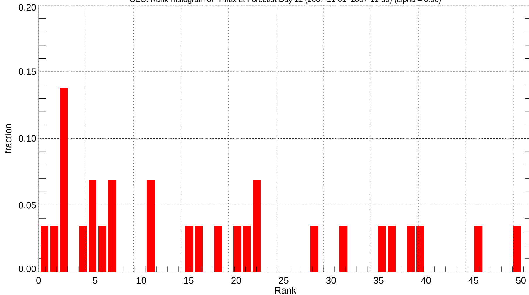
GEG: Rank Histogram of Tmax at Forecast Day 11 (2007-11-01~2007-11-30) (alpha = 0.00)
