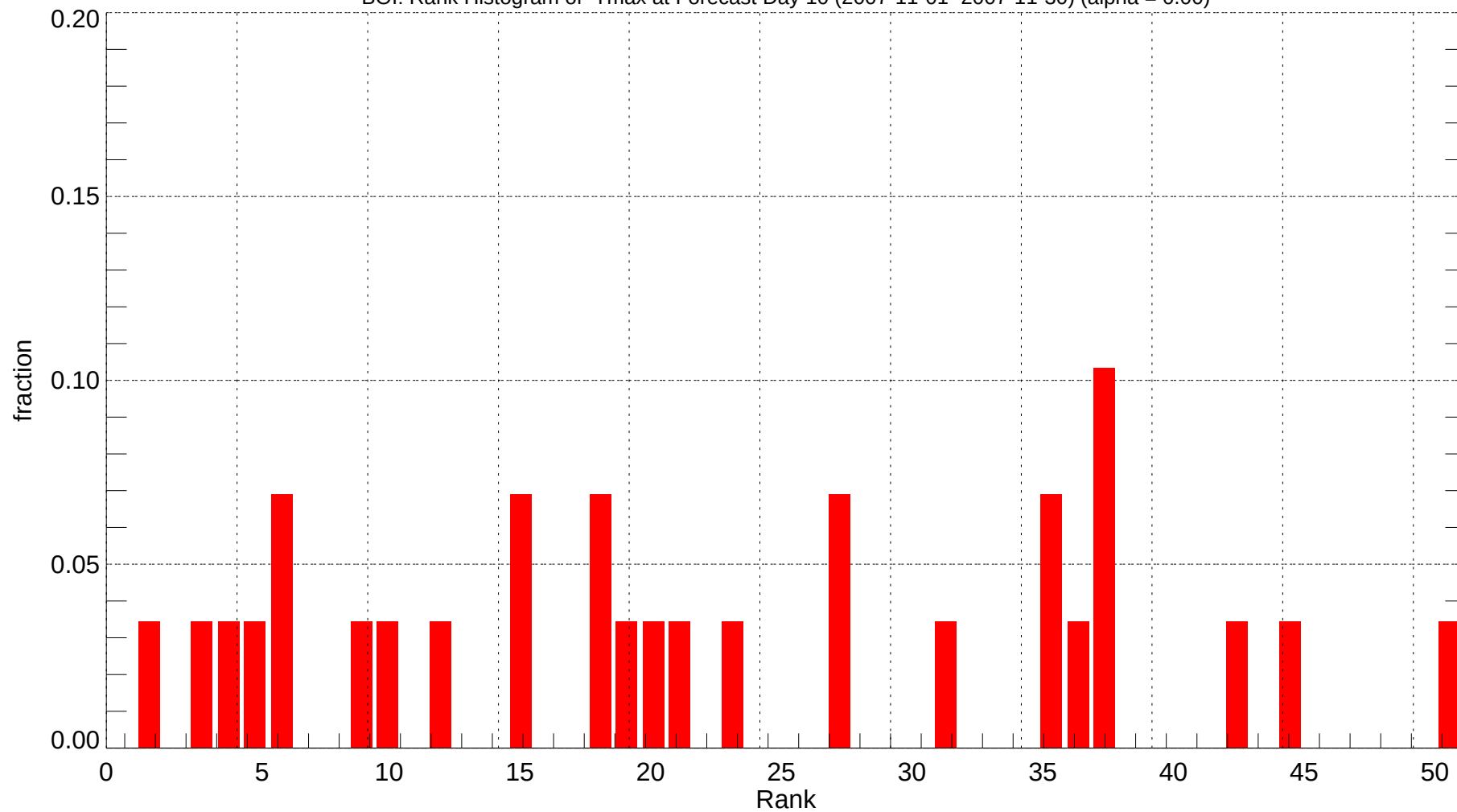
BOI: Rank Histogram of Tmax at Forecast Day 10 (2007-11-01~2007-11-30) (alpha = 0.00)
