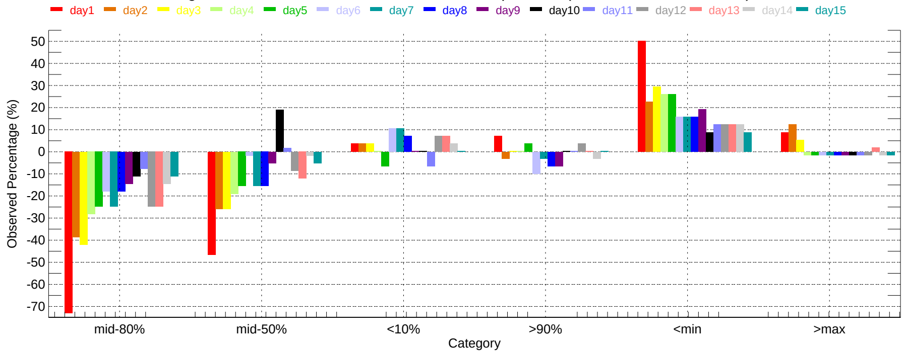
Observed Percentage Deviation of Ensembles - ROC: Min Temperature (2007-11-01~2007-11-30)
