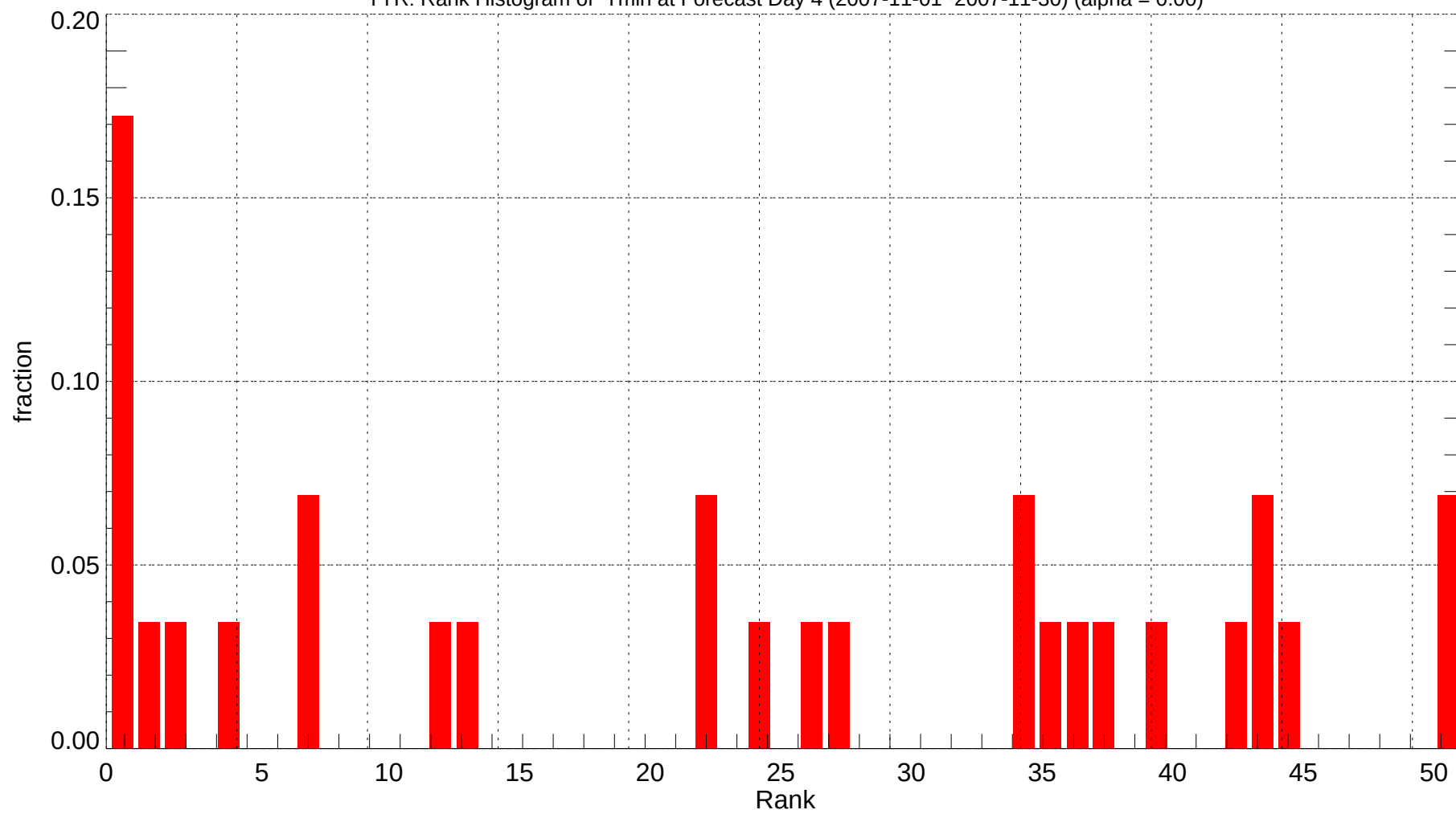
TYR: Rank Histogram of Tmin at Forecast Day 4 (2007-11-01~2007-11-30) (alpha = 0.00)
