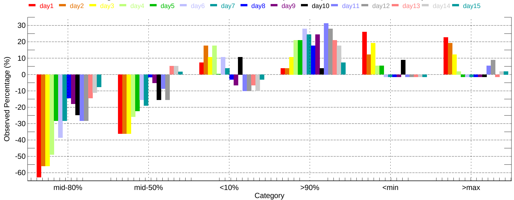
Observed Percentage Deviation of Ensembles - EVV: Min Temperature (2007-11-01~2007-11-30)
