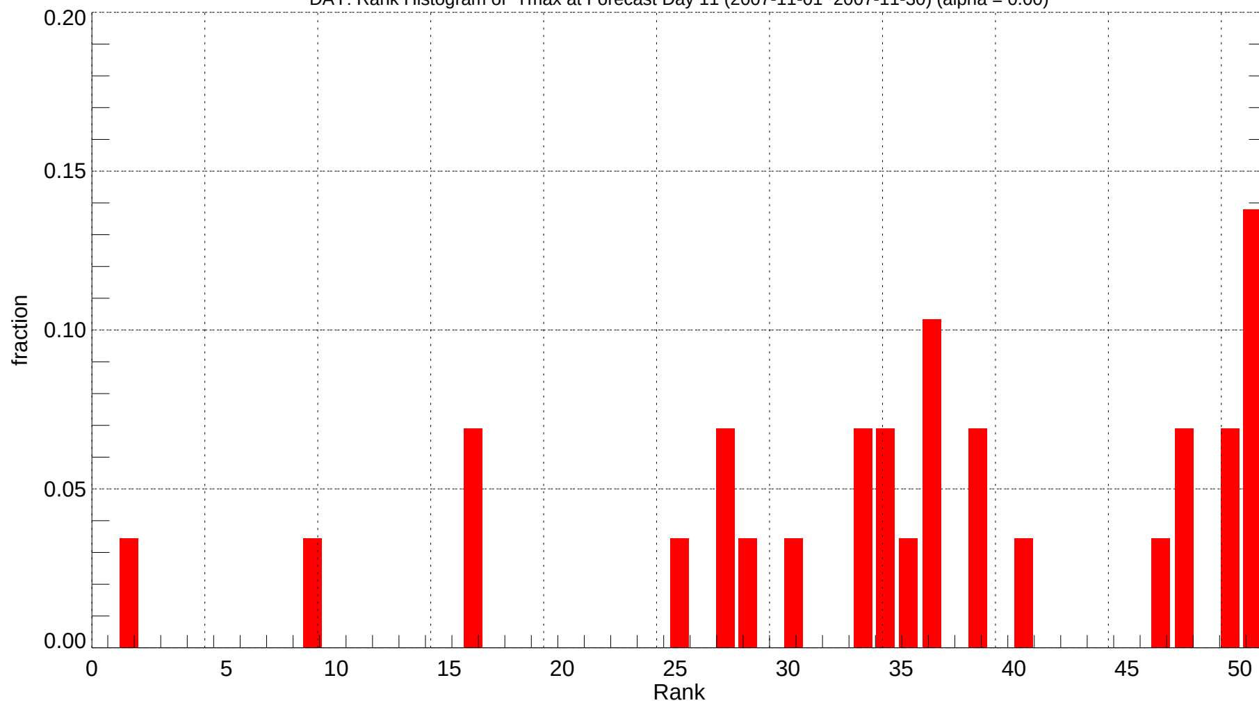
DAY: Rank Histogram of Tmax at Forecast Day 11 (2007-11-01~2007-11-30) (alpha = 0.00)
