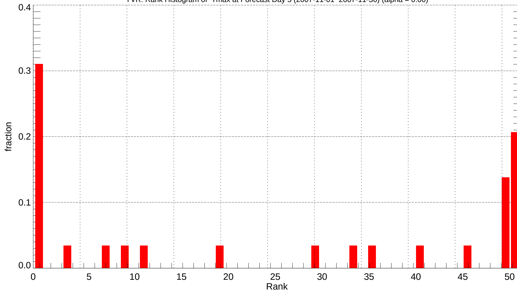
YVR: Rank Histogram of Tmax at Forecast Day 5 (2007-11-01~2007-11-30) (alpha = 0.00)
