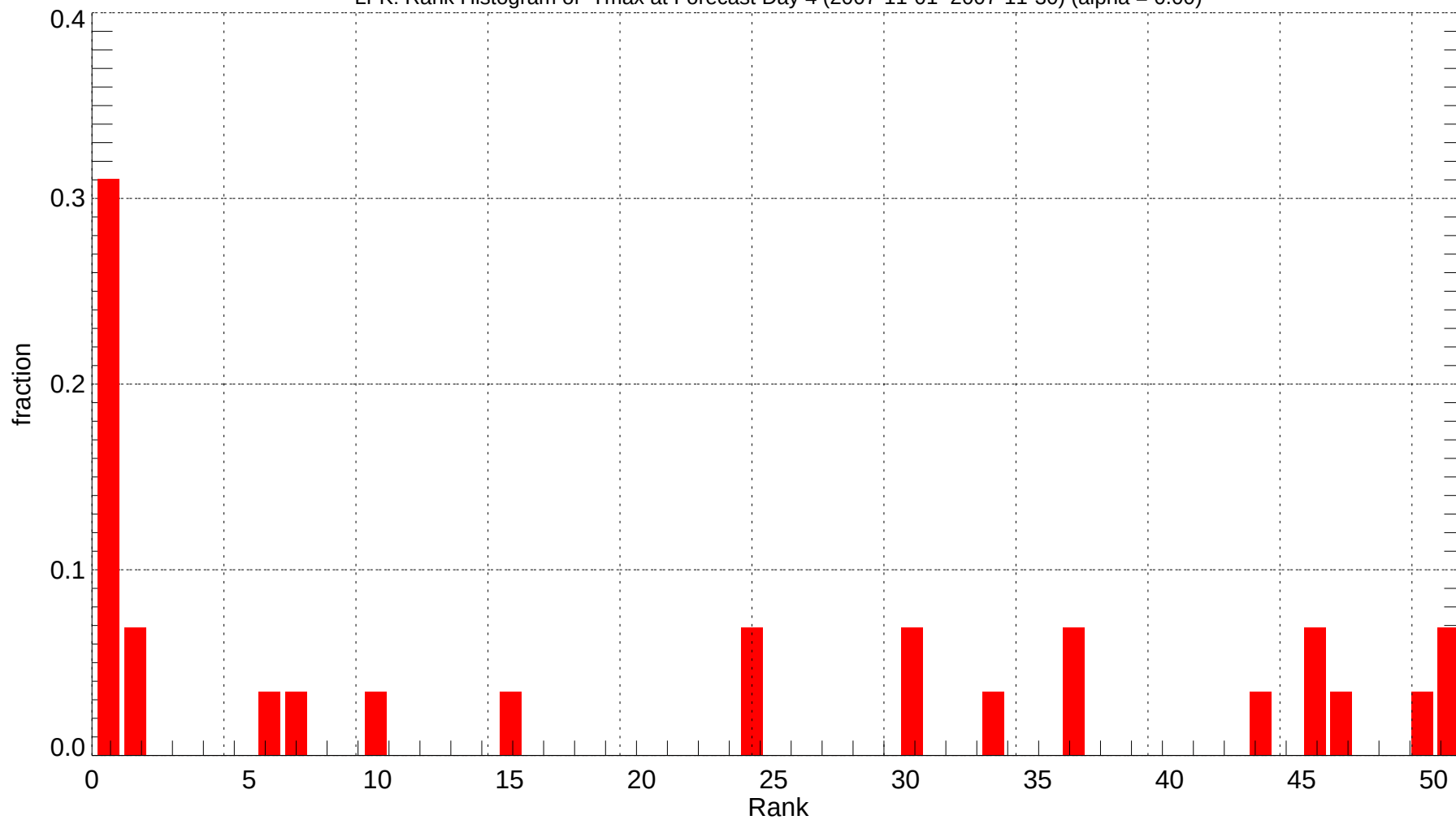
LFK: Rank Histogram of Tmax at Forecast Day 4 (2007-11-01~2007-11-30) (alpha = 0.00)
