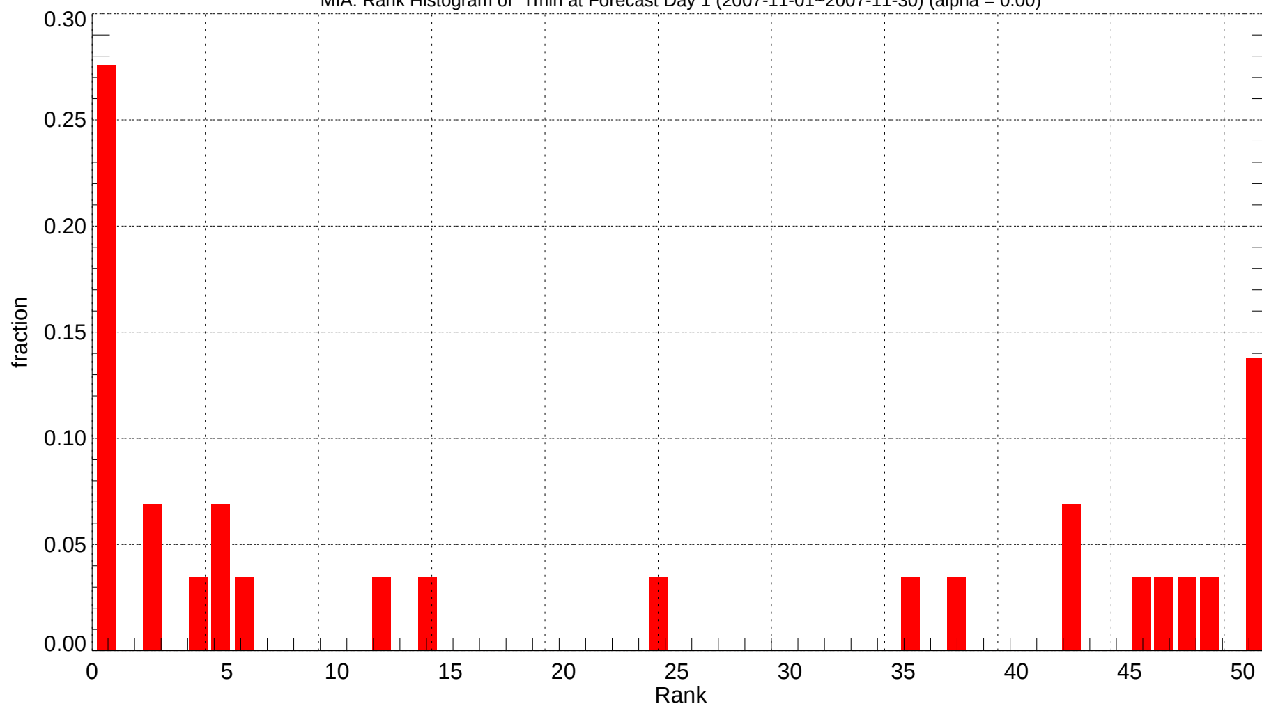
MIA: Rank Histogram of Tmin at Forecast Day 1 (2007-11-01~2007-11-30) (alpha = 0.00)
