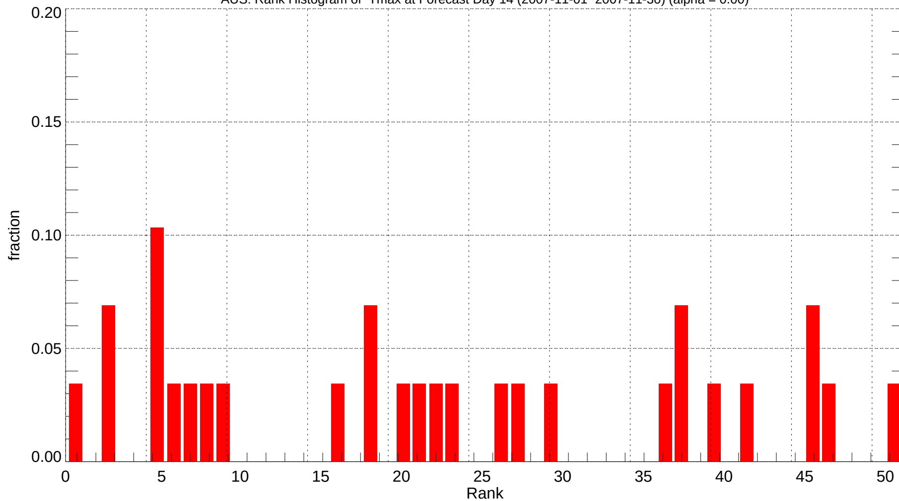
AUS: Rank Histogram of Tmax at Forecast Day 14 (2007-11-01~2007-11-30) (alpha = 0.00)
