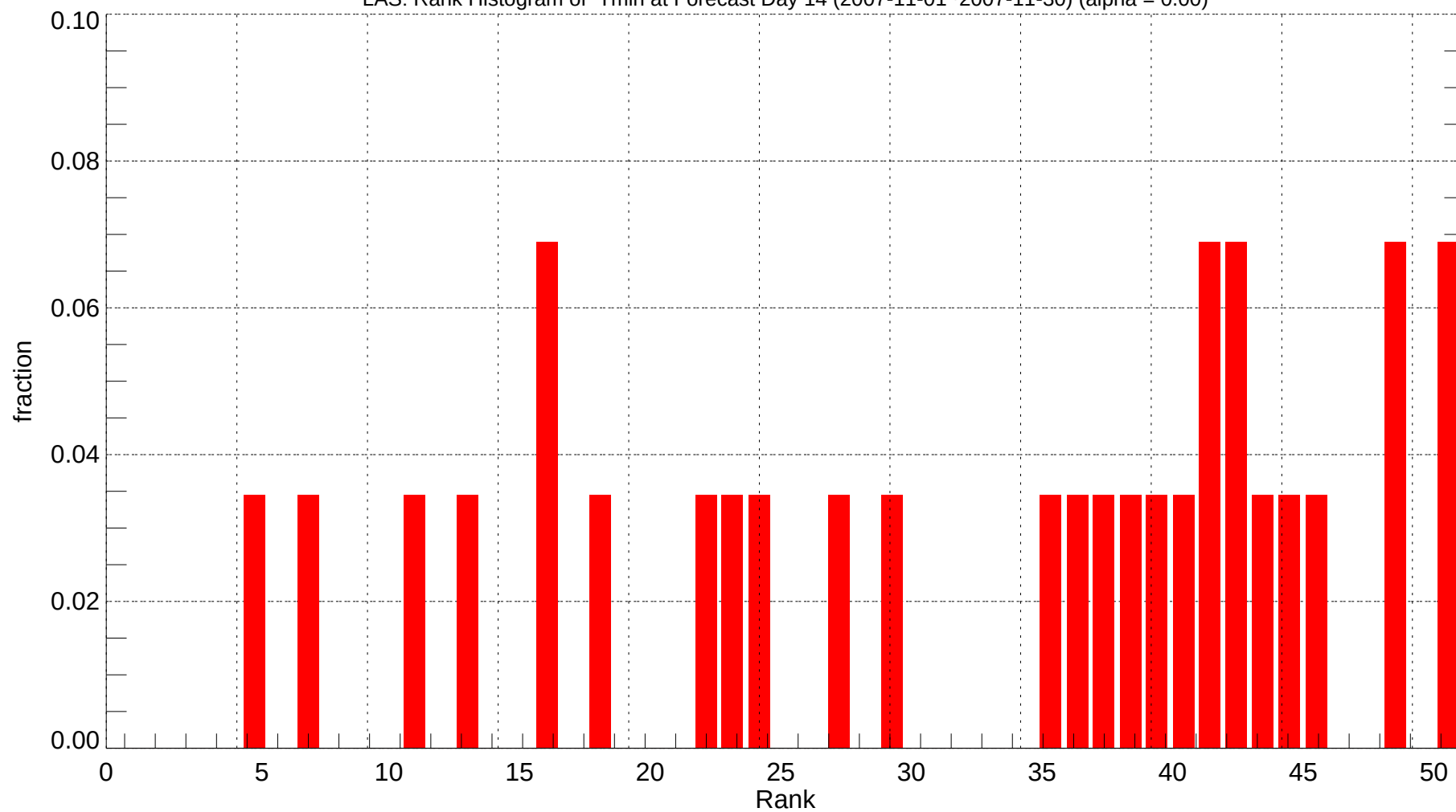
LAS: Rank Histogram of Tmin at Forecast Day 14 (2007-11-01~2007-11-30) (alpha = 0.00)
