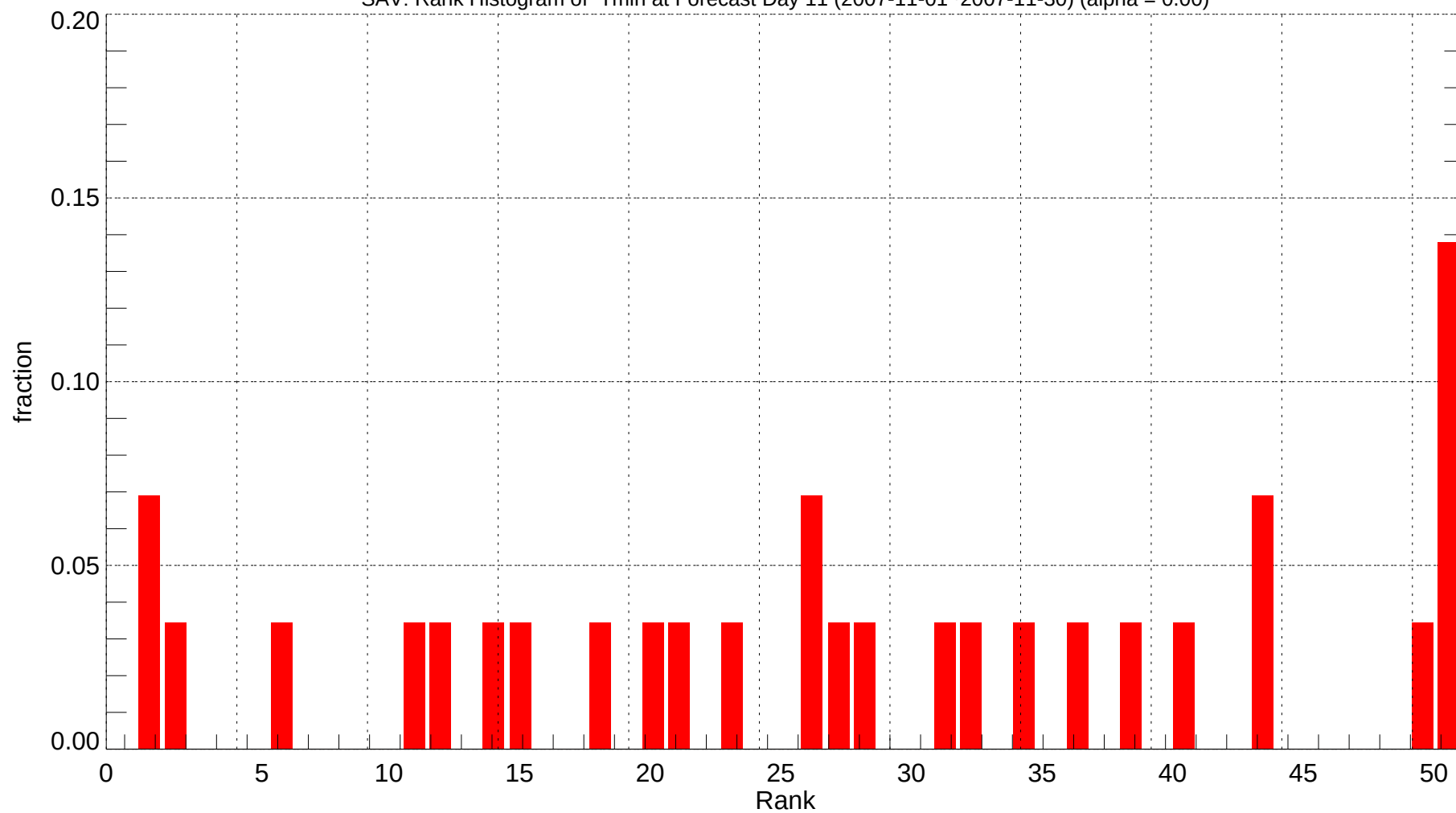
SAV: Rank Histogram of Tmin at Forecast Day 11 (2007-11-01~2007-11-30) (alpha = 0.00)
