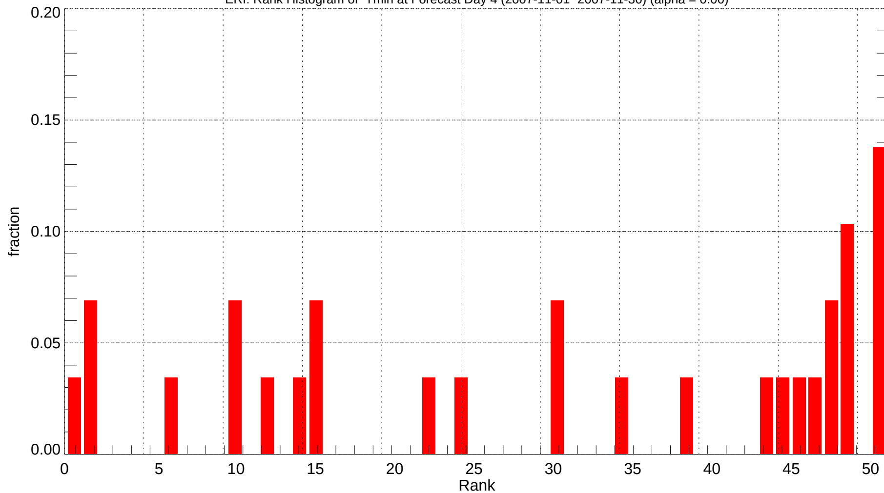
ERI: Rank Histogram of Tmin at Forecast Day 4 (2007-11-01~2007-11-30) (alpha = 0.00)
