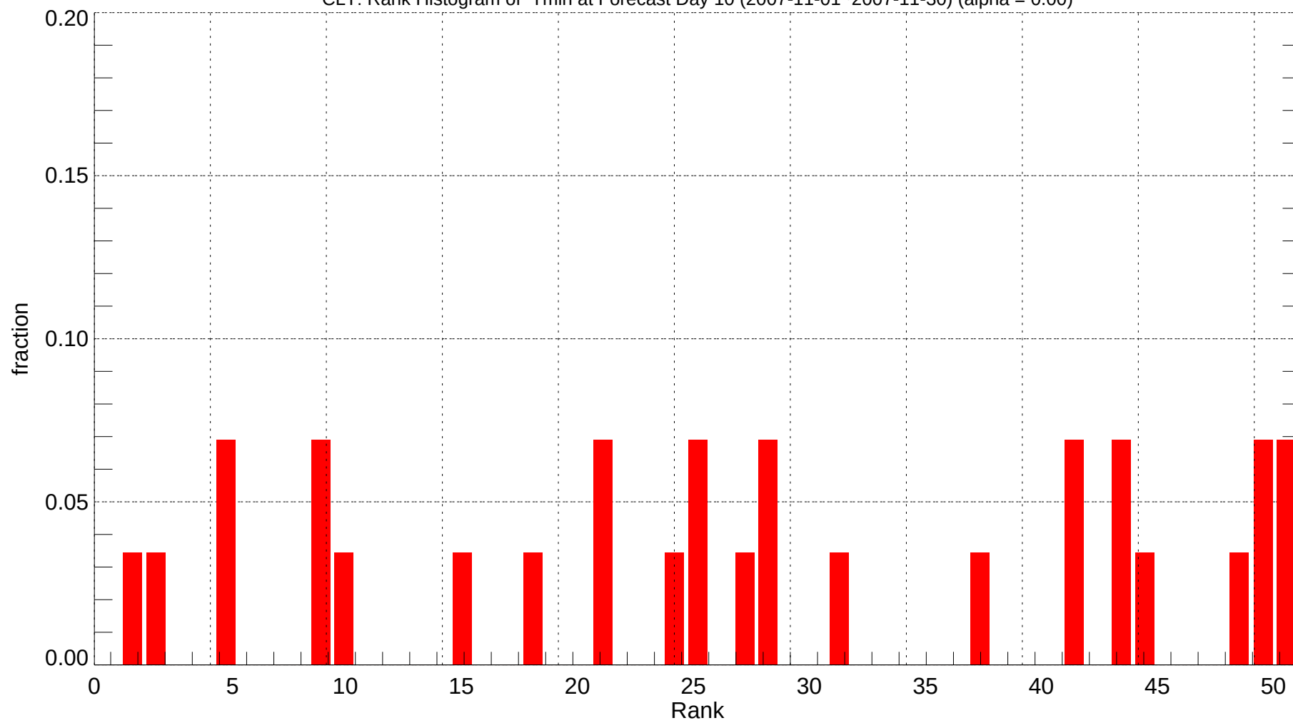
CLT: Rank Histogram of Tmin at Forecast Day 10 (2007-11-01~2007-11-30) (alpha = 0.00)
