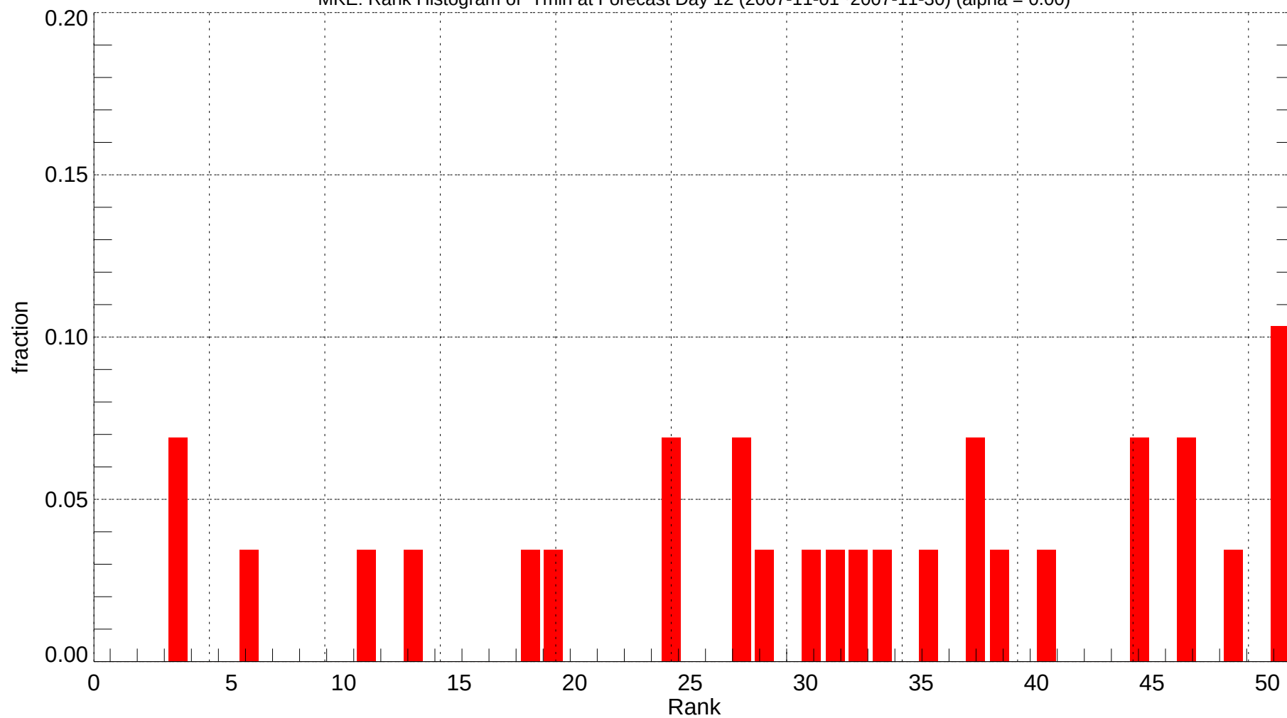
MKE: Rank Histogram of Tmin at Forecast Day 12 (2007-11-01~2007-11-30) (alpha = 0.00)
