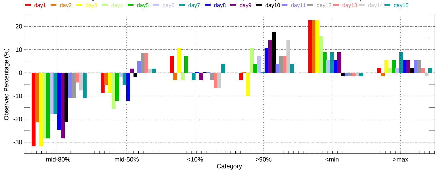
Observed Percentage Deviation of Ensembles - ORD: Min Temperature (2007-11-01~2007-11-30)
