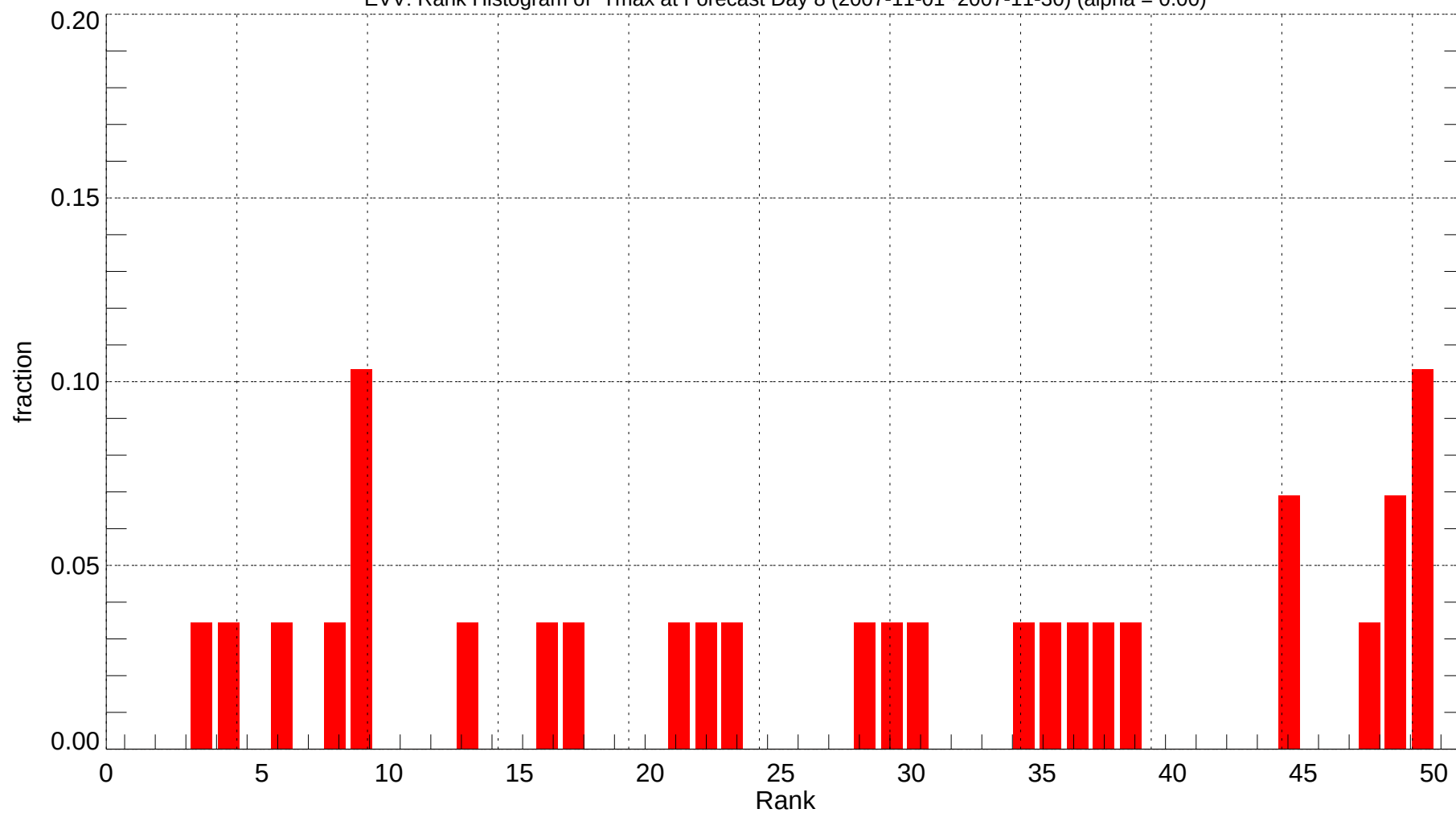
EVV: Rank Histogram of Tmax at Forecast Day 8 (2007-11-01~2007-11-30) (alpha = 0.00)
