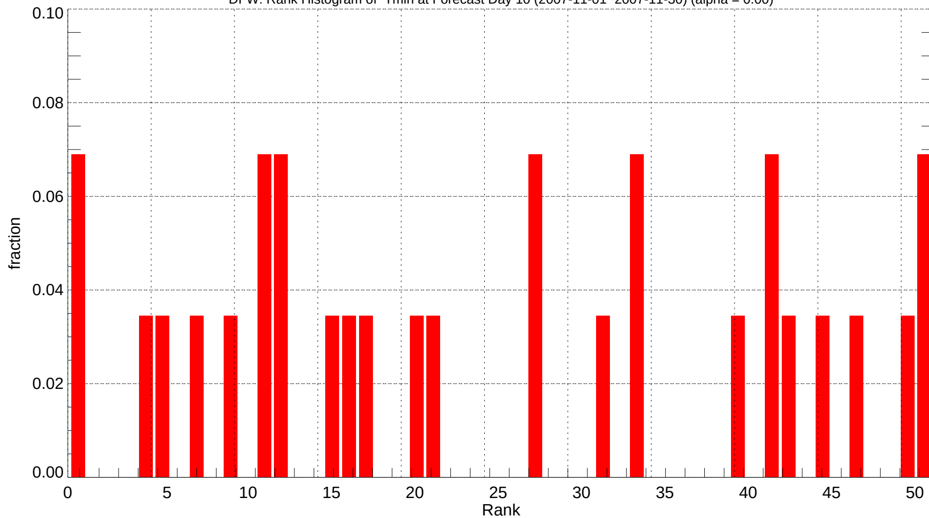
DFW: Rank Histogram of Tmin at Forecast Day 10 (2007-11-01~2007-11-30) (alpha = 0.00)
