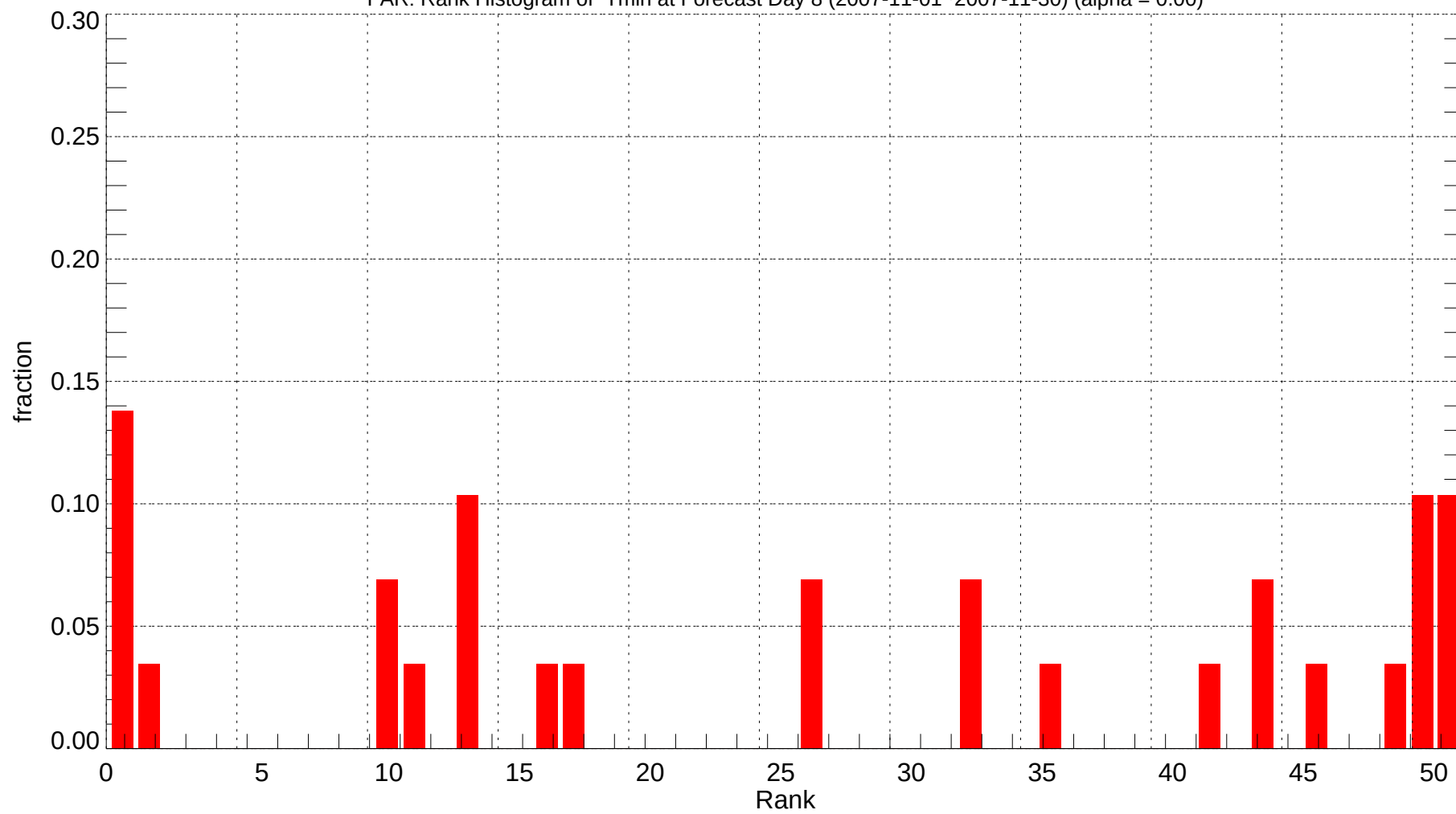
FAR: Rank Histogram of Tmin at Forecast Day 8 (2007-11-01~2007-11-30) (alpha = 0.00)
