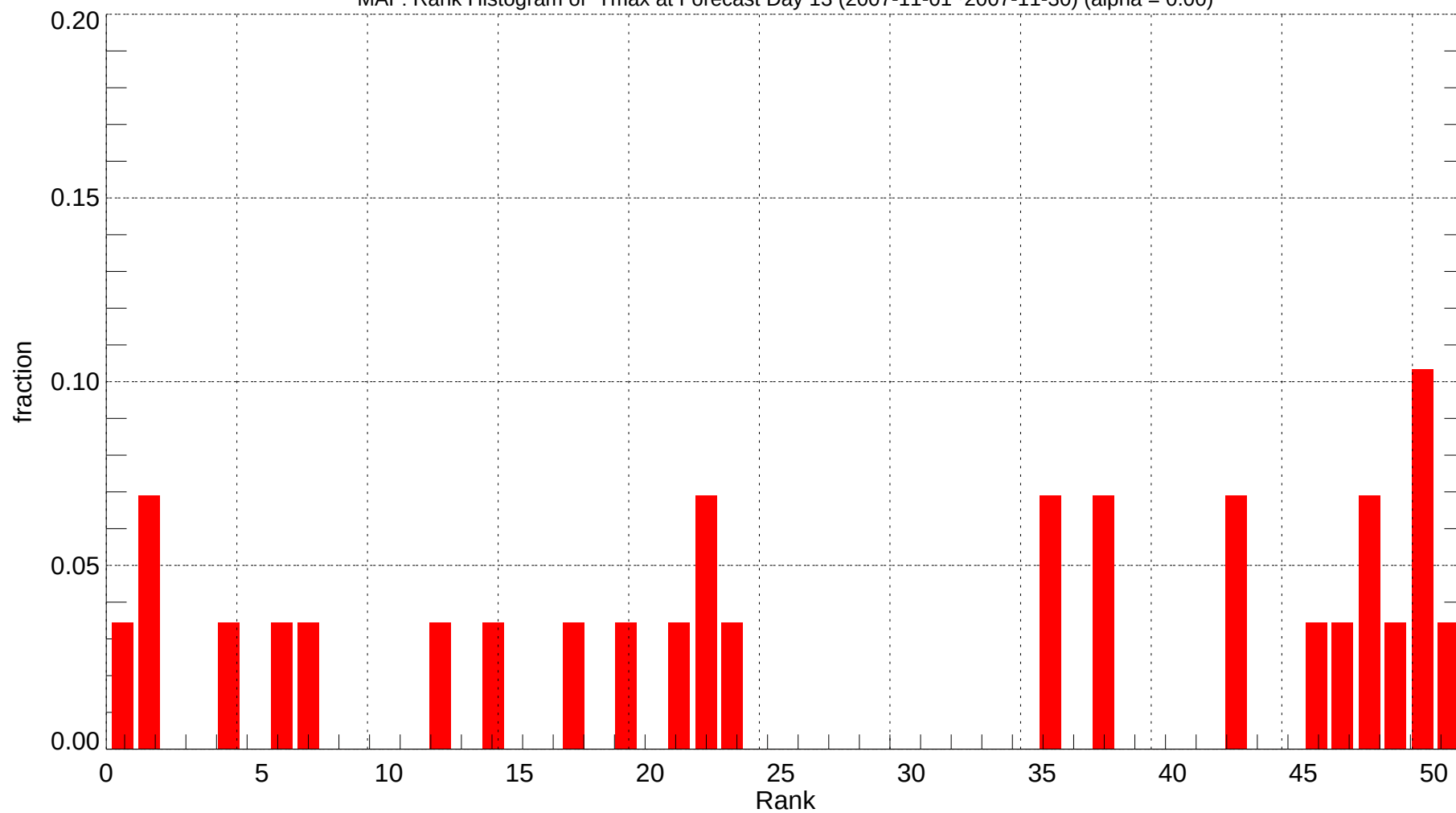
MAF: Rank Histogram of Tmax at Forecast Day 13 (2007-11-01~2007-11-30) (alpha = 0.00)
