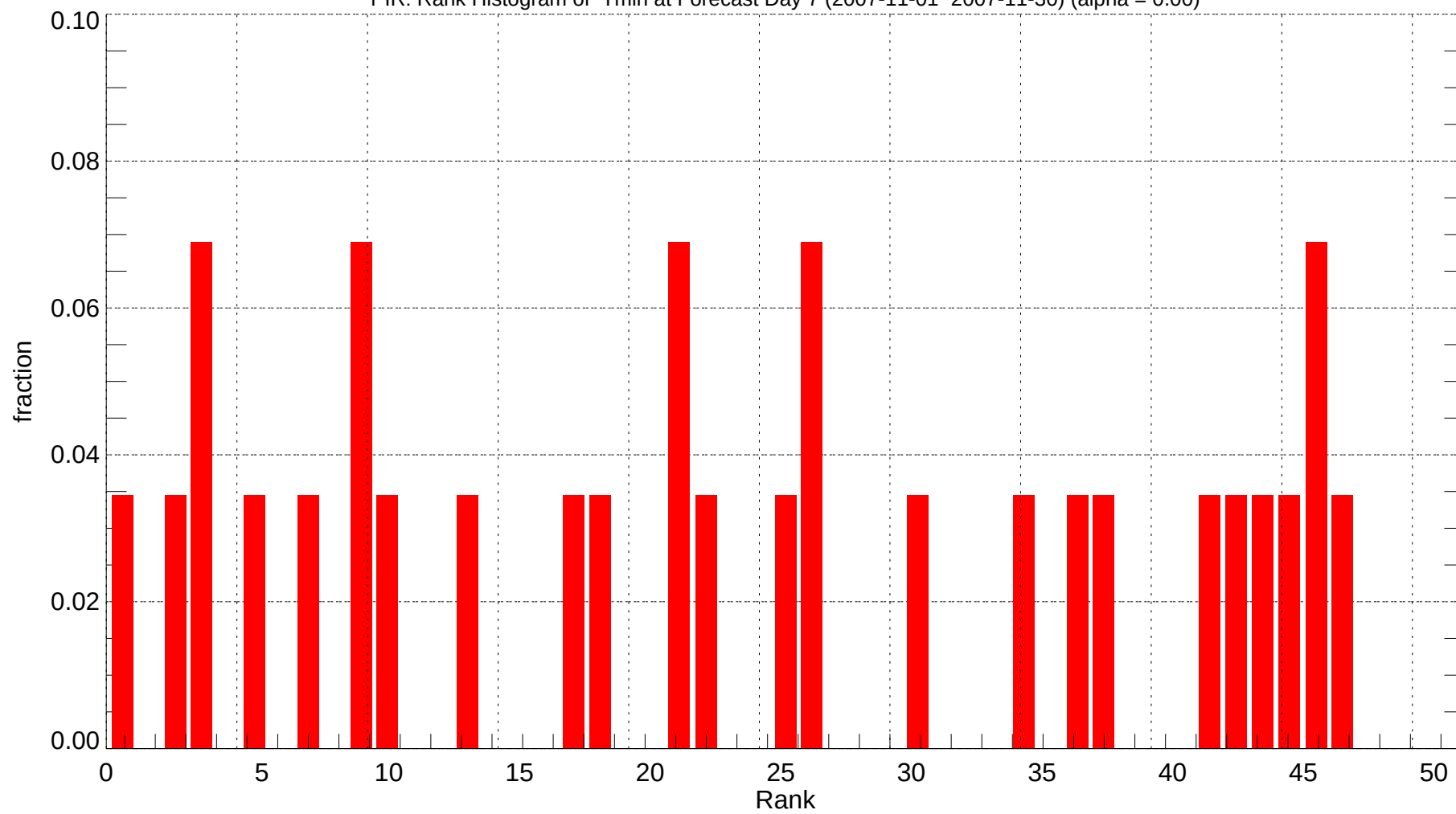
PIR: Rank Histogram of Tmin at Forecast Day 7 (2007-11-01~2007-11-30) (alpha = 0.00)
