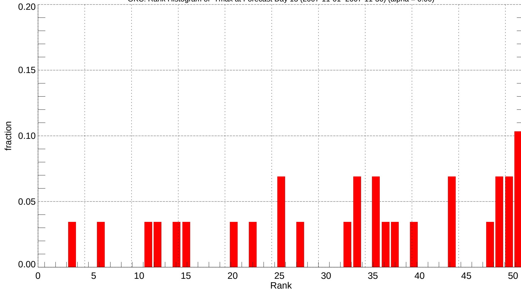
OKC: Rank Histogram of Tmax at Forecast Day 13 (2007-11-01~2007-11-30) (alpha = 0.00)
