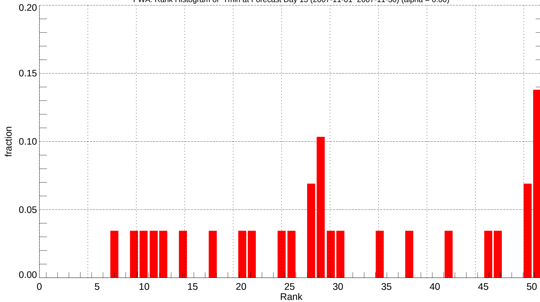
FWA: Rank Histogram of Tmin at Forecast Day 13 (2007-11-01~2007-11-30) (alpha = 0.00)
