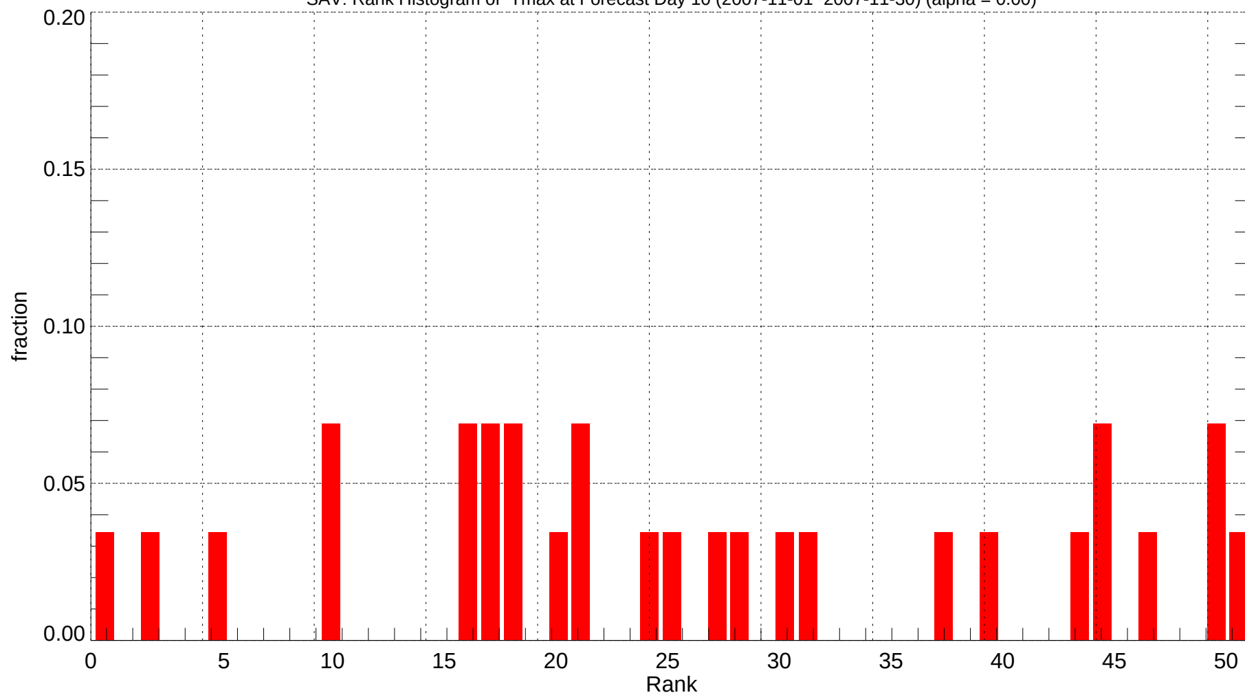
SAV: Rank Histogram of Tmax at Forecast Day 10 (2007-11-01~2007-11-30) (alpha = 0.00)
