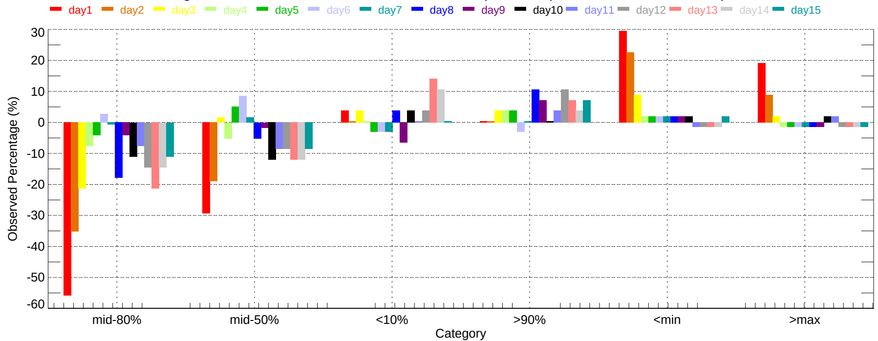
Observed Percentage Deviation of Ensembles - JFK: Max Temperature (2007-11-01~2007-11-30)
