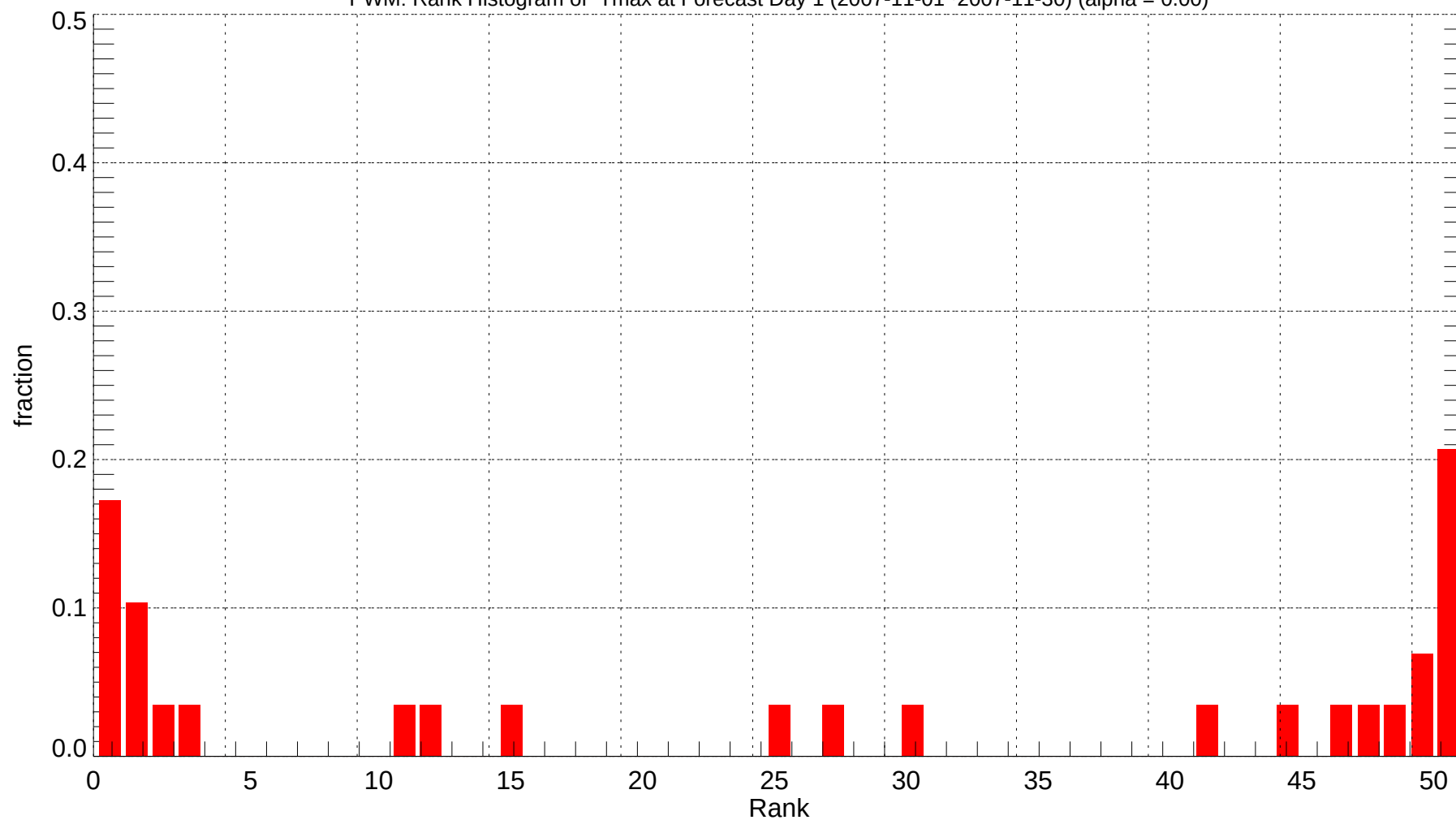
PWM: Rank Histogram of Tmax at Forecast Day 1 (2007-11-01~2007-11-30) (alpha = 0.00)
