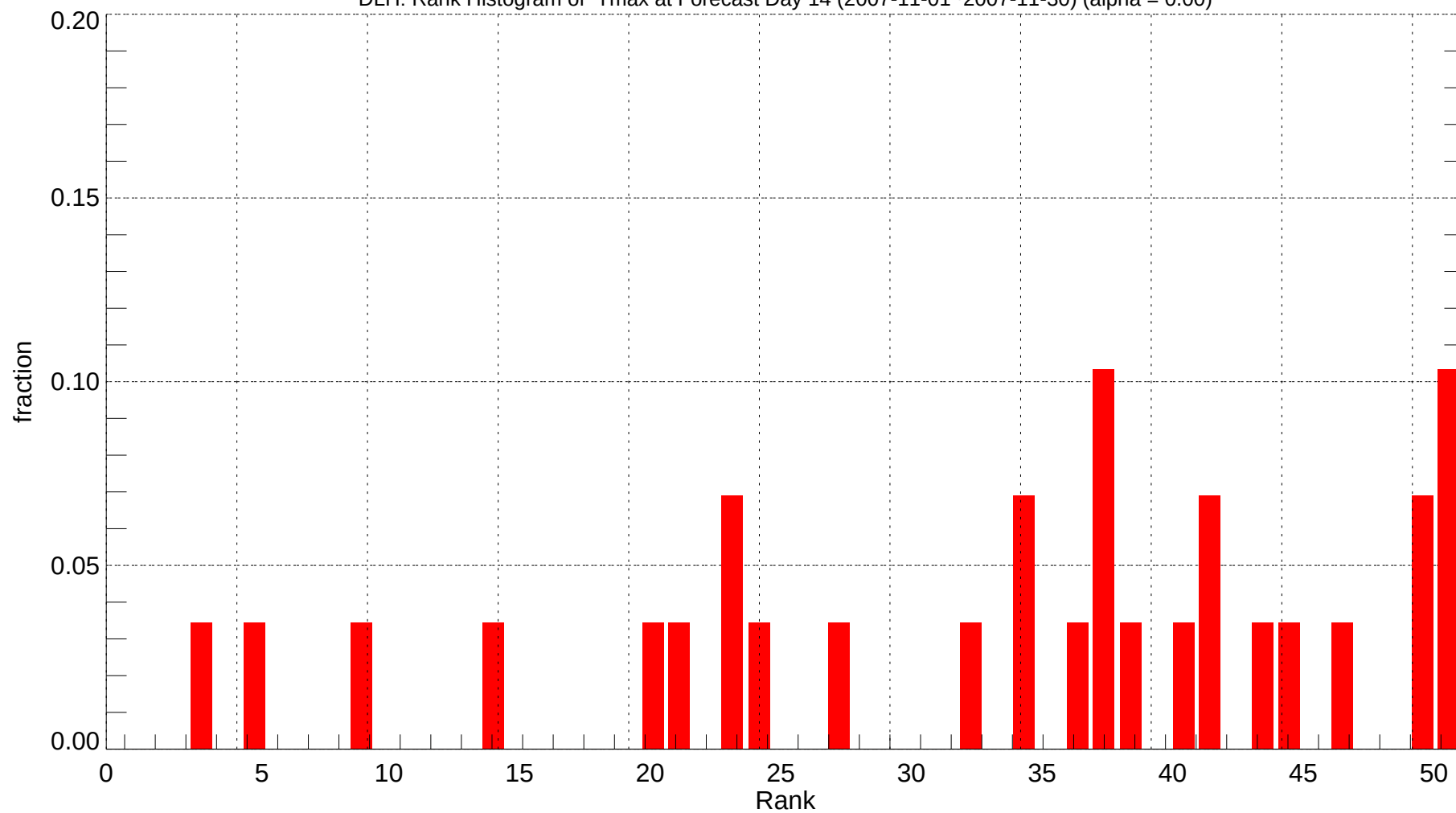
DLH: Rank Histogram of Tmax at Forecast Day 14 (2007-11-01~2007-11-30) (alpha = 0.00)
