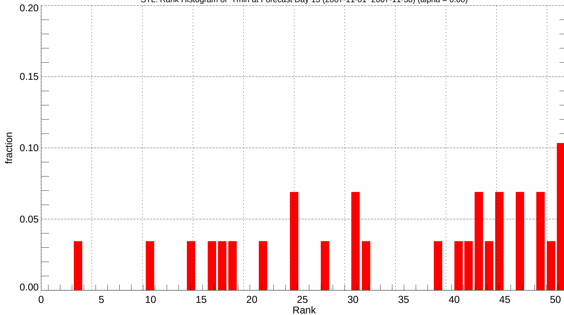
STL: Rank Histogram of Tmin at Forecast Day 13 (2007-11-01~2007-11-30) (alpha = 0.00)
