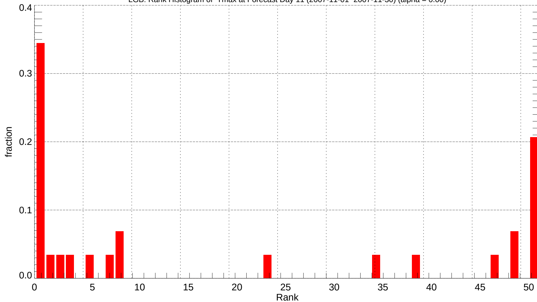
LGB: Rank Histogram of Tmax at Forecast Day 11 (2007-11-01~2007-11-30) (alpha = 0.00)
