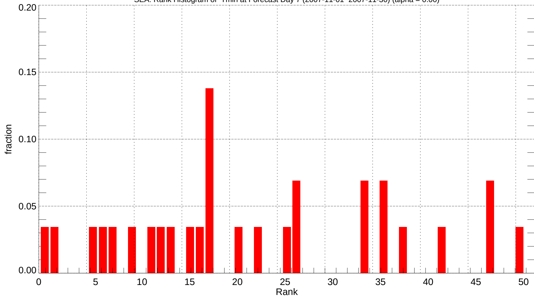
SEA: Rank Histogram of Tmin at Forecast Day 7 (2007-11-01~2007-11-30) (alpha = 0.00)
