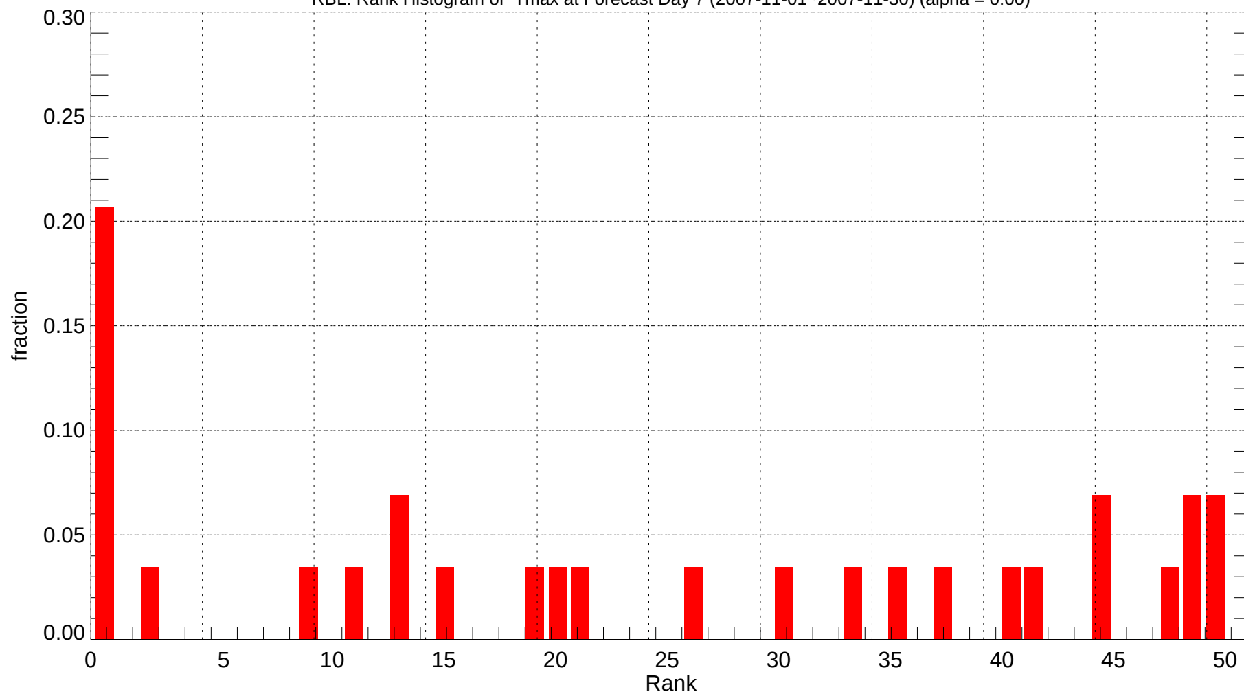
RBL: Rank Histogram of Tmax at Forecast Day 7 (2007-11-01~2007-11-30) (alpha = 0.00)
