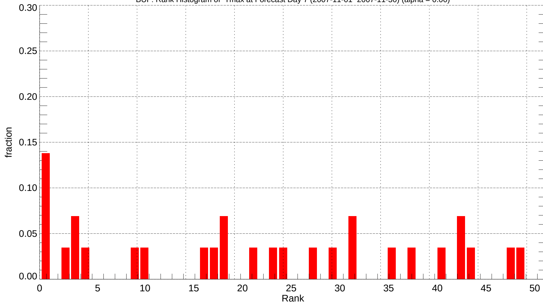
BUF: Rank Histogram of Tmax at Forecast Day 7 (2007-11-01~2007-11-30) (alpha = 0.00)
