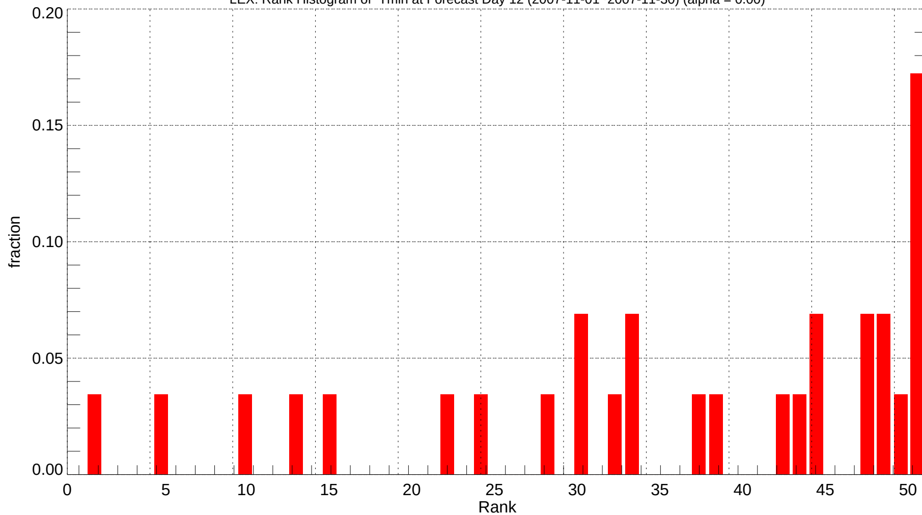
LEX: Rank Histogram of Tmin at Forecast Day 12 (2007-11-01~2007-11-30) (alpha = 0.00)
