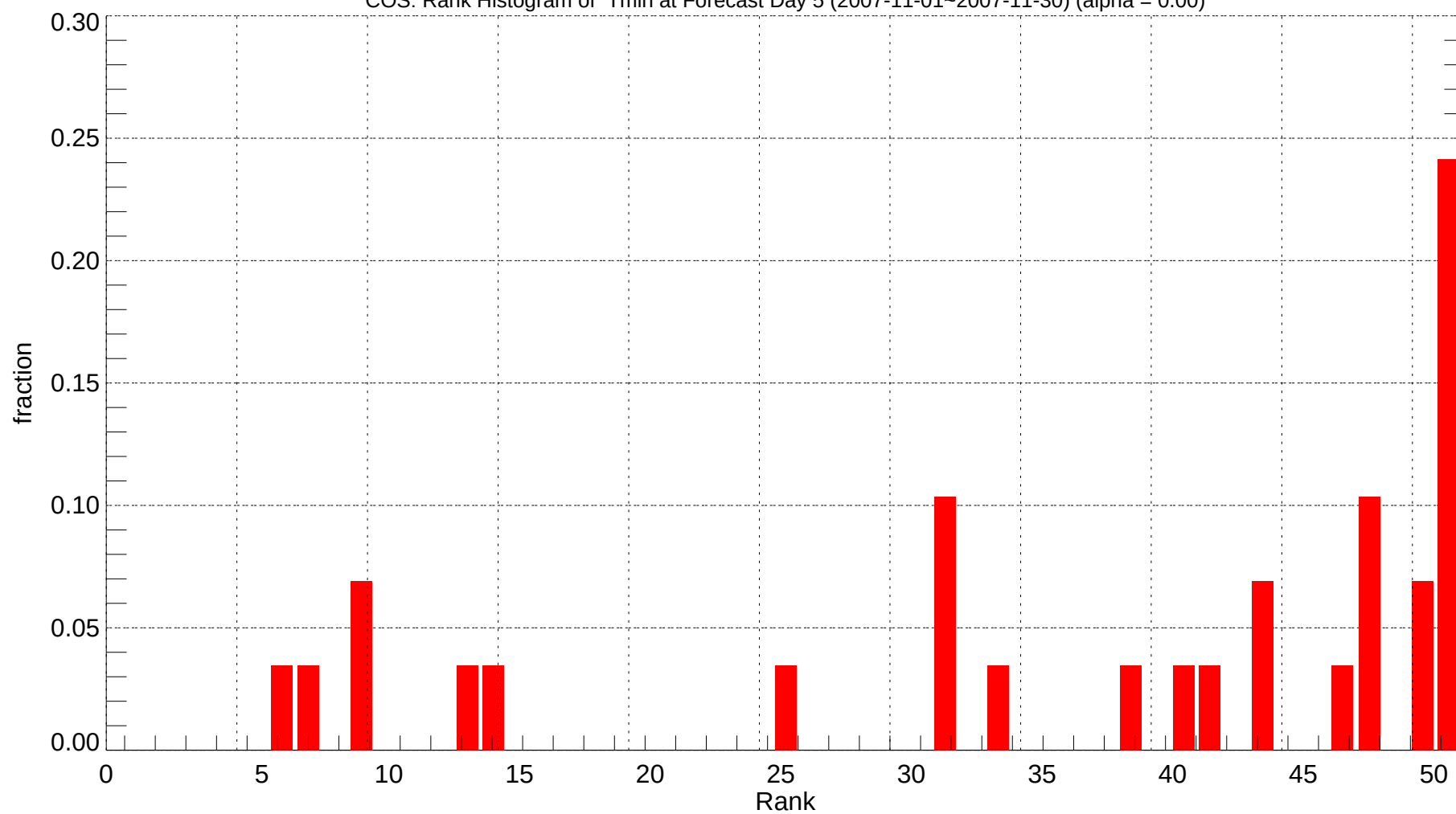
COS: Rank Histogram of Tmin at Forecast Day 5 (2007-11-01~2007-11-30) (alpha = 0.00)
