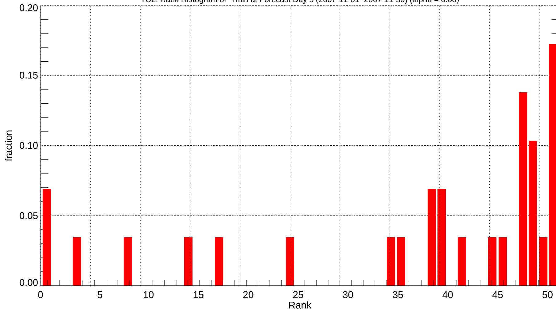
TUL: Rank Histogram of Tmin at Forecast Day 5 (2007-11-01~2007-11-30) (alpha = 0.00)
