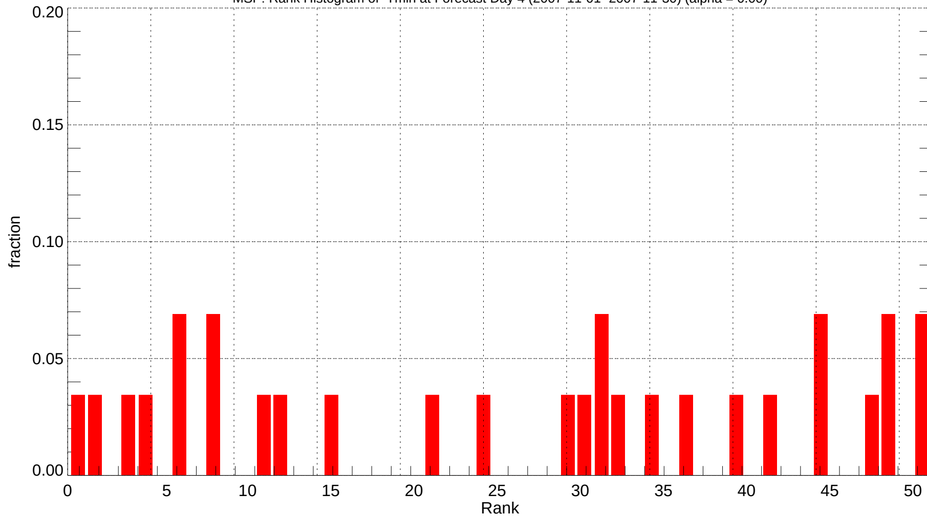
MSP: Rank Histogram of Tmin at Forecast Day 4 (2007-11-01~2007-11-30) (alpha = 0.00)
