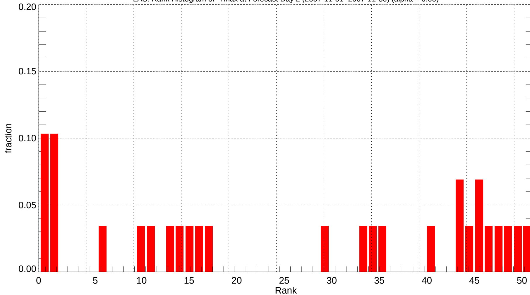
LAS: Rank Histogram of Tmax at Forecast Day 2 (2007-11-01~2007-11-30) (alpha = 0.00)
