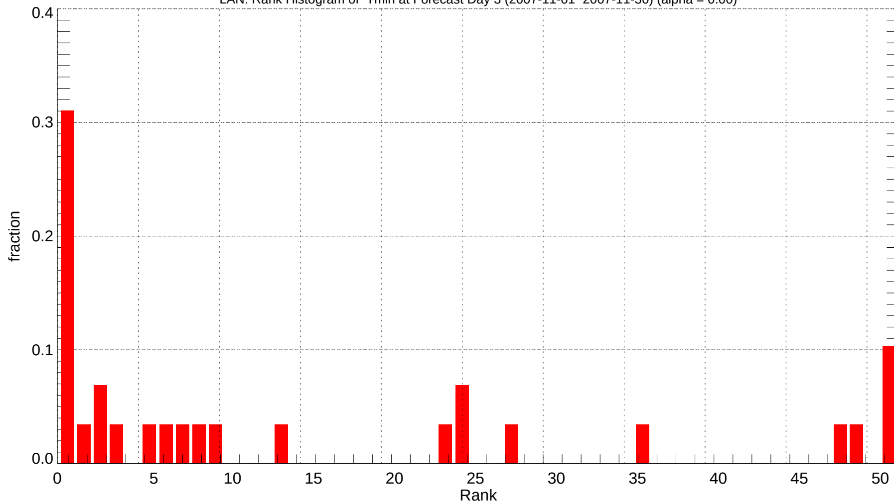
LAN: Rank Histogram of Tmin at Forecast Day 3 (2007-11-01~2007-11-30) (alpha = 0.00)
