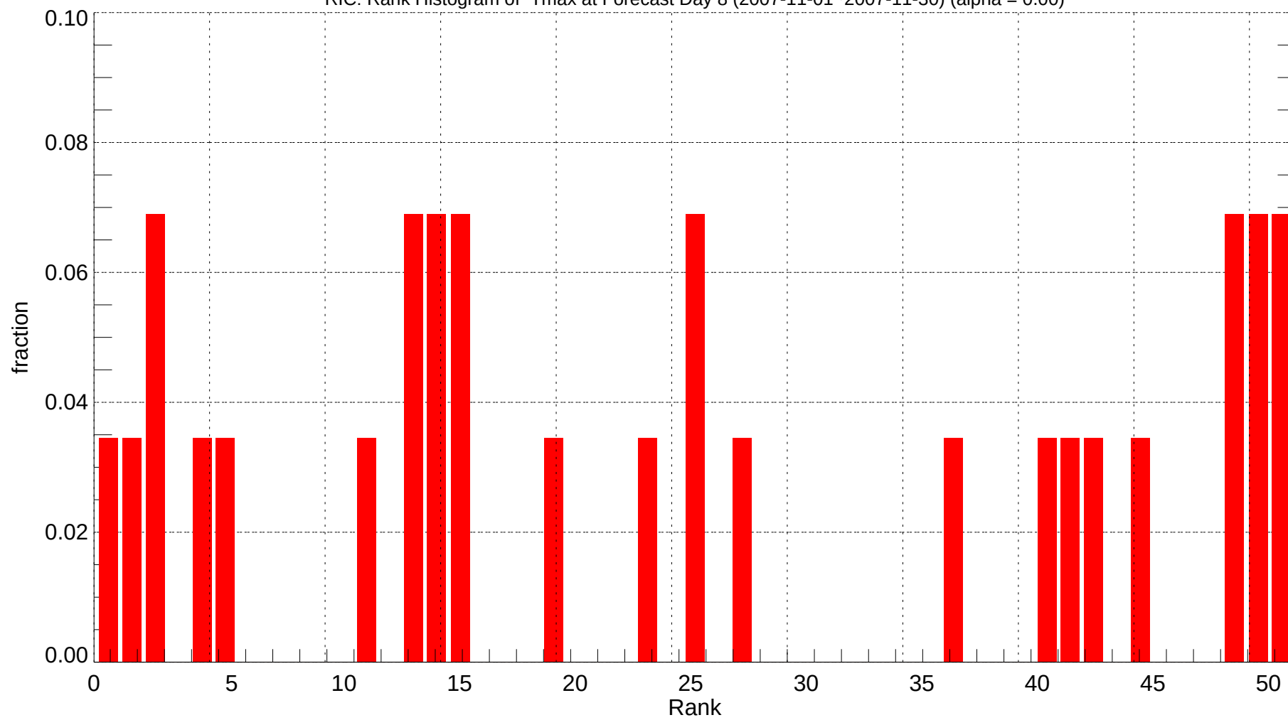
RIC: Rank Histogram of Tmax at Forecast Day 8 (2007-11-01~2007-11-30) (alpha = 0.00)
