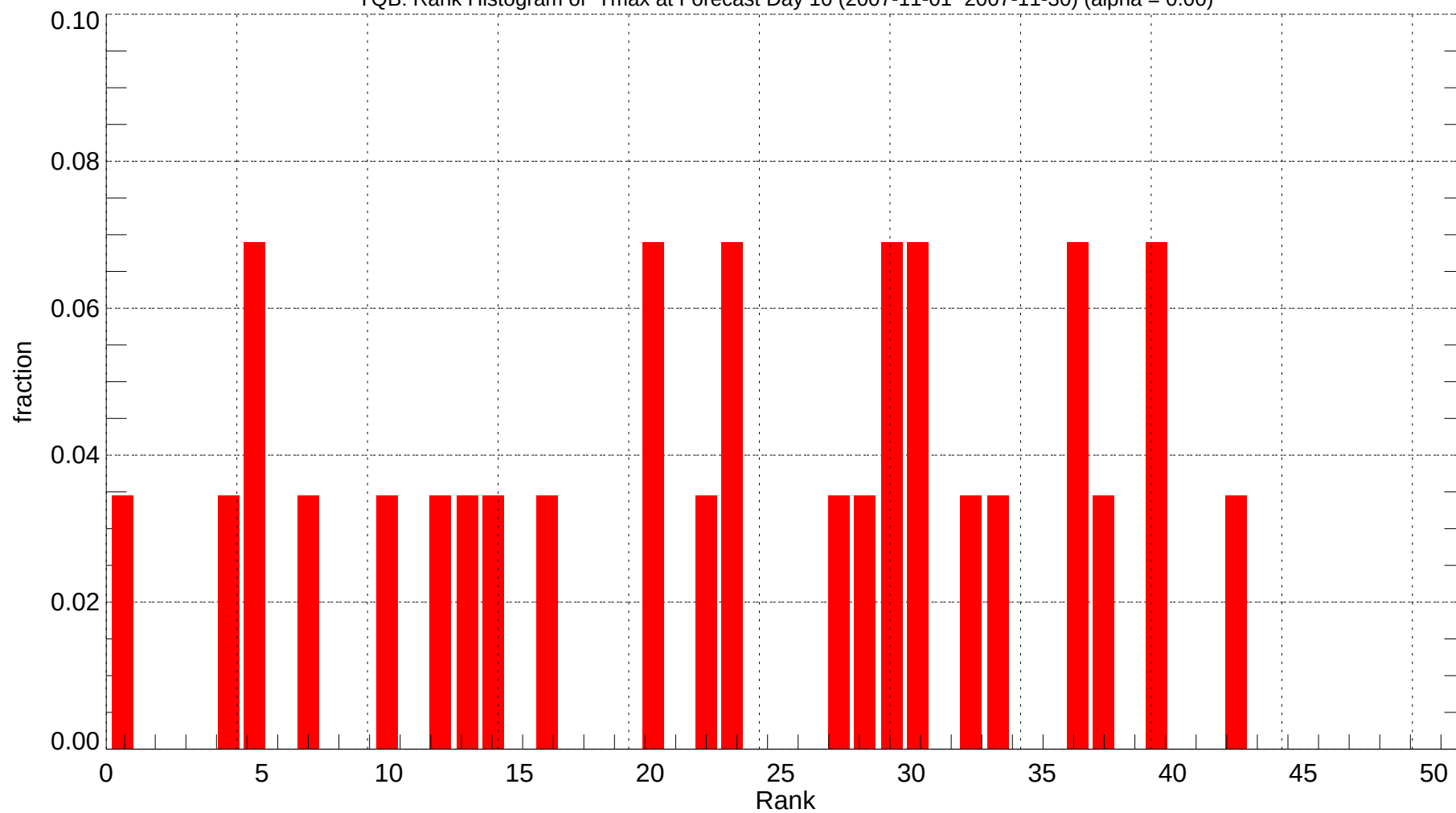
YQB: Rank Histogram of Tmax at Forecast Day 10 (2007-11-01~2007-11-30) (alpha = 0.00)
