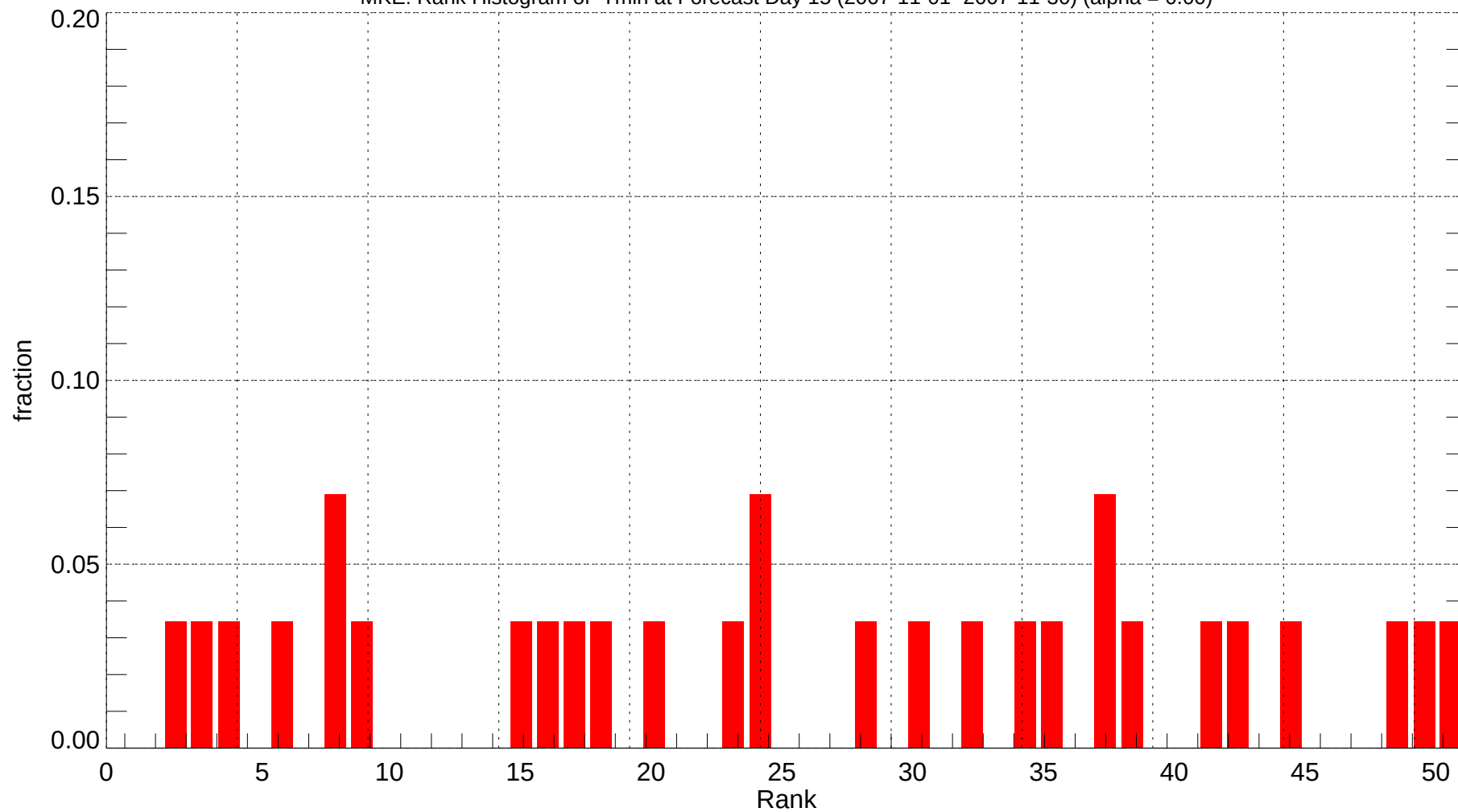
MKE: Rank Histogram of Tmin at Forecast Day 15 (2007-11-01~2007-11-30) (alpha = 0.00)
