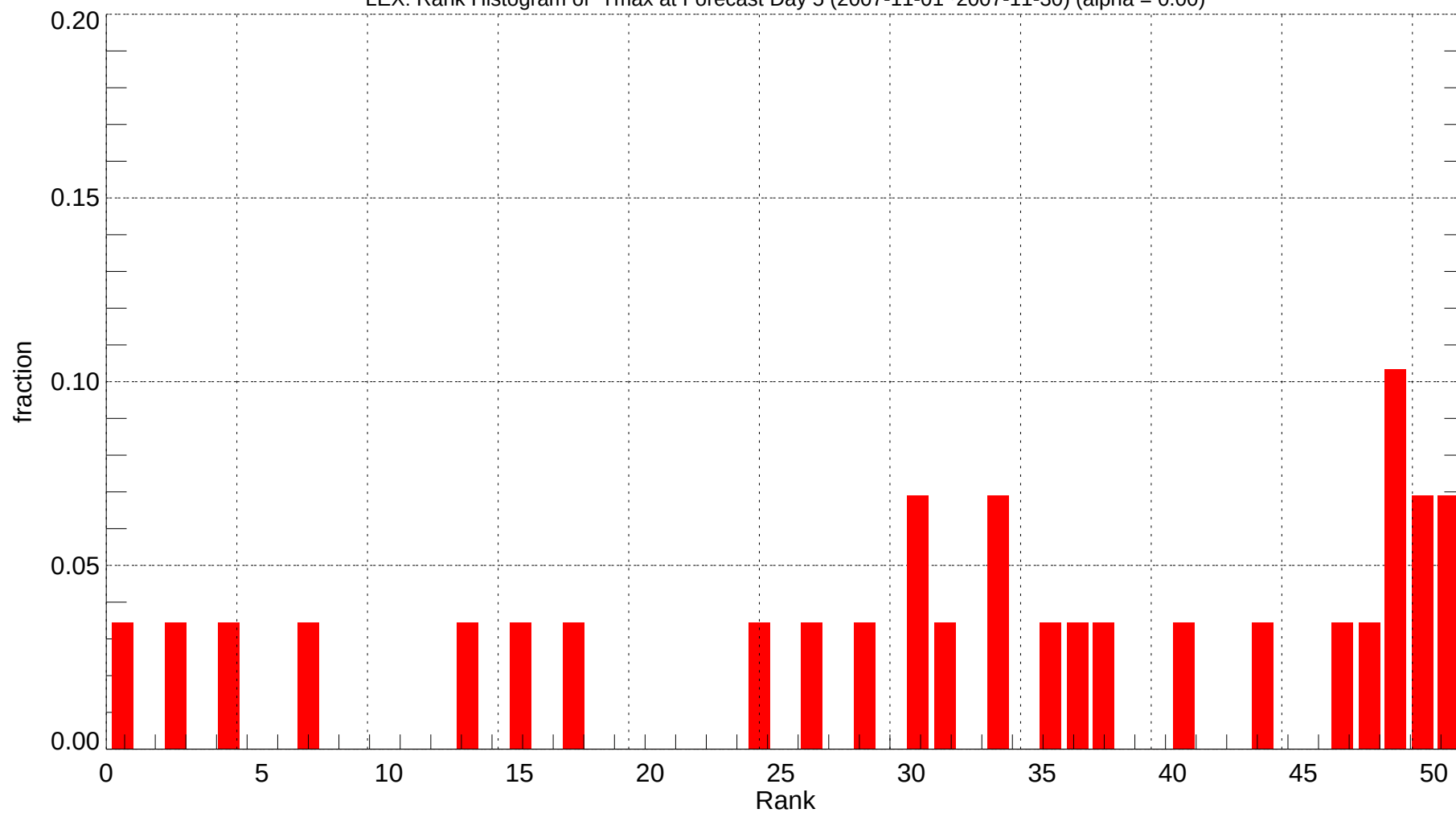
LEX: Rank Histogram of Tmax at Forecast Day 5 (2007-11-01~2007-11-30) (alpha = 0.00)
