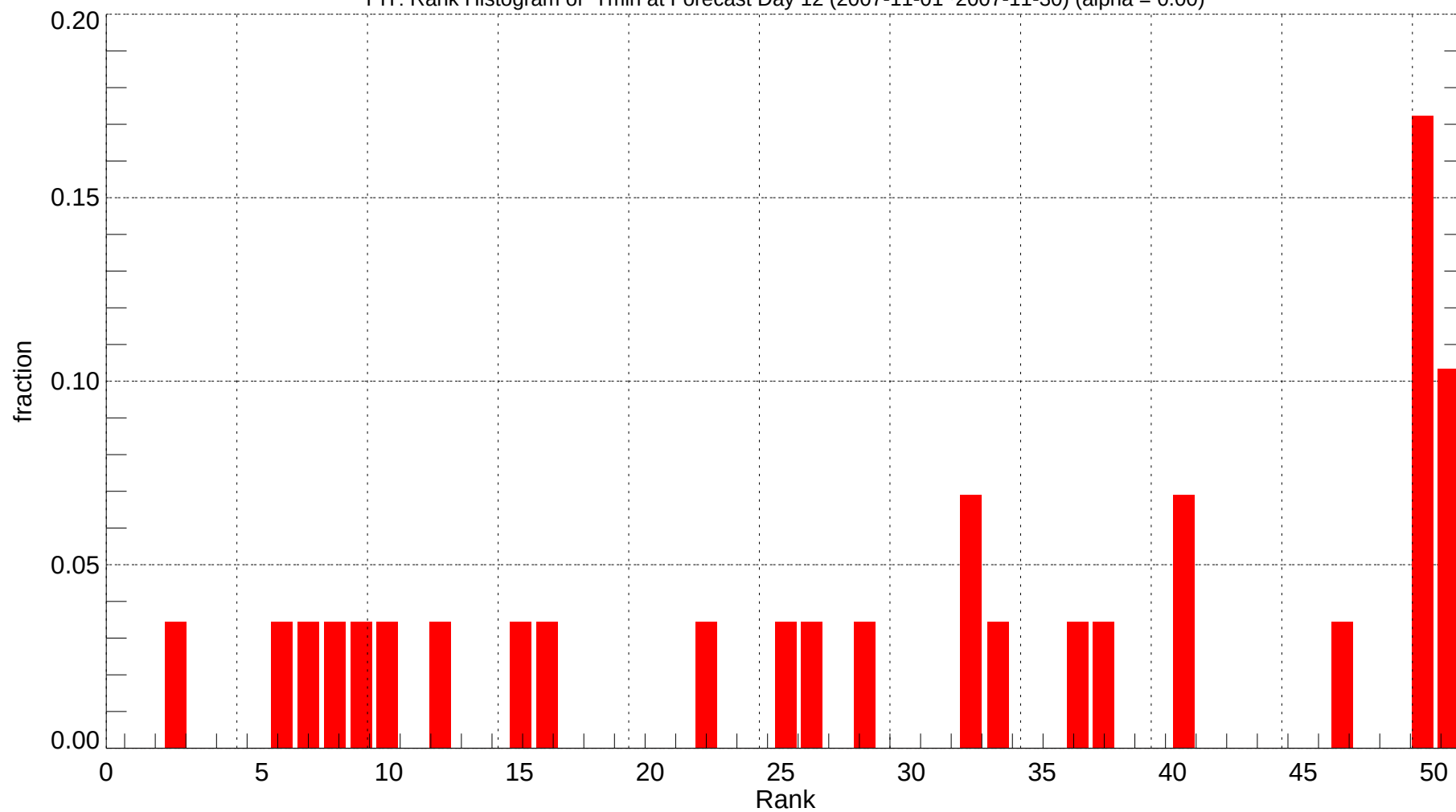
PIT: Rank Histogram of Tmin at Forecast Day 12 (2007-11-01~2007-11-30) (alpha = 0.00)
