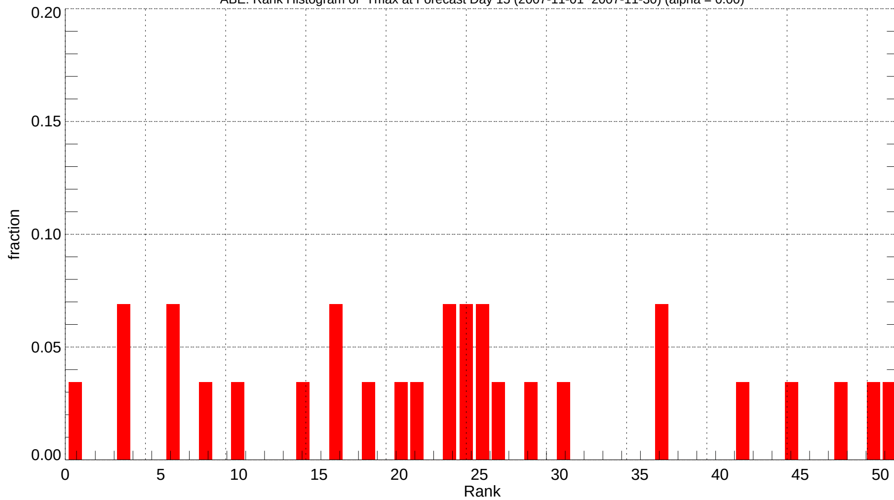
ABE: Rank Histogram of Tmax at Forecast Day 15 (2007-11-01~2007-11-30) (alpha = 0.00)
