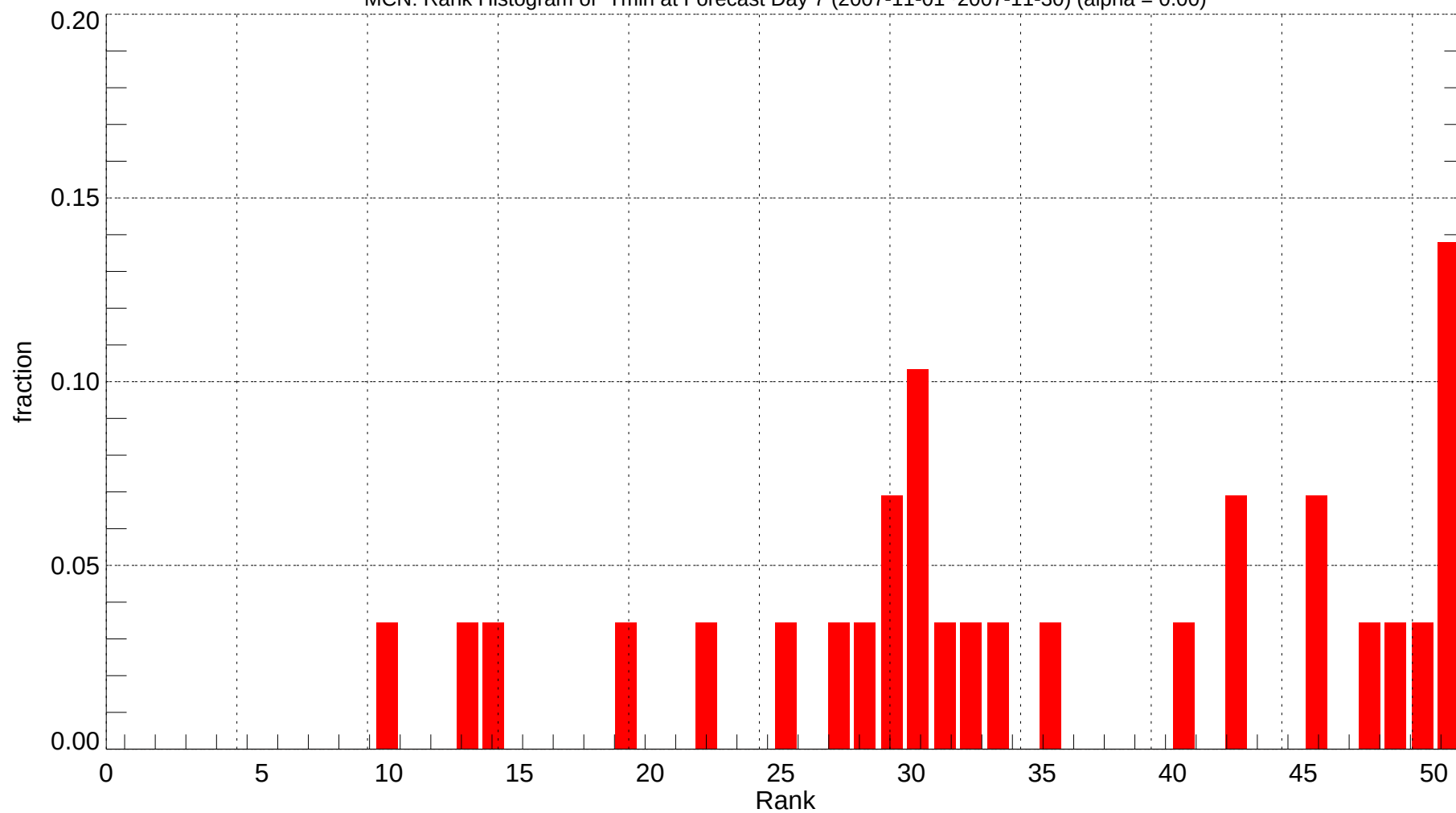
MCN: Rank Histogram of Tmin at Forecast Day 7 (2007-11-01~2007-11-30) (alpha = 0.00)
