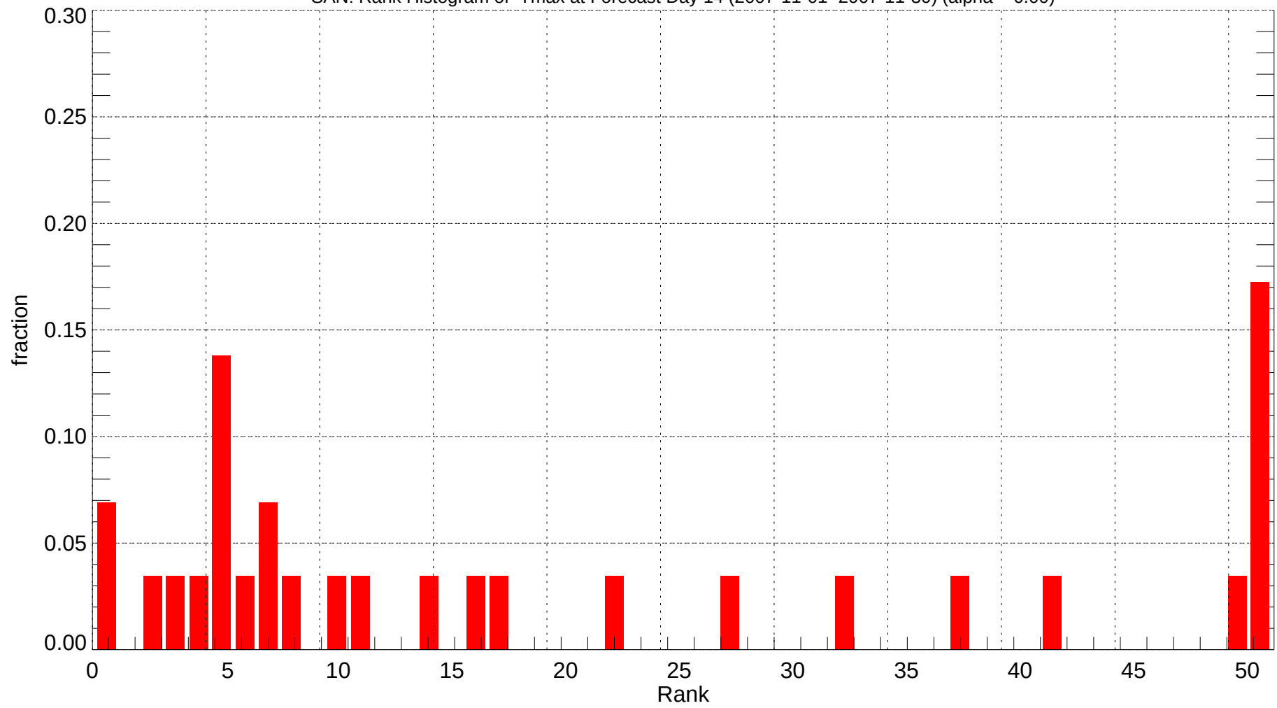
SAN: Rank Histogram of Tmax at Forecast Day 14 (2007-11-01~2007-11-30) (alpha = 0.00)
