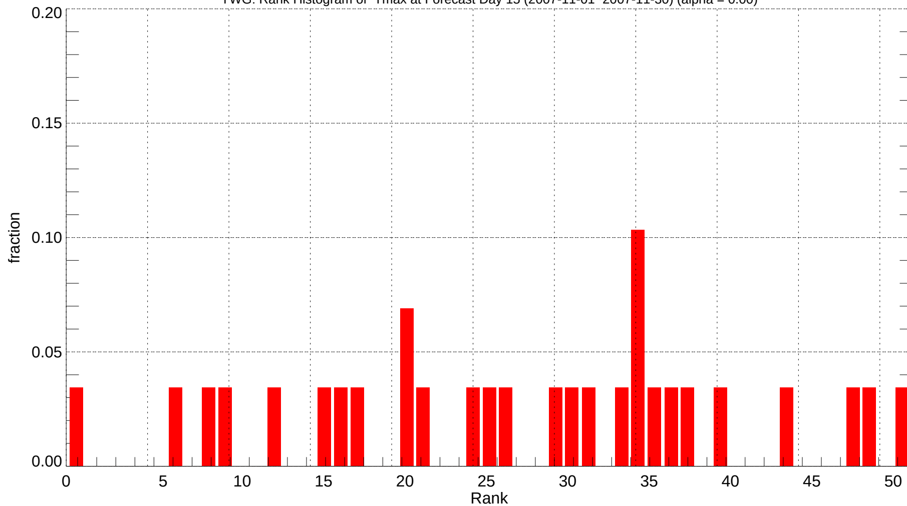
YWG: Rank Histogram of Tmax at Forecast Day 15 (2007-11-01~2007-11-30) (alpha = 0.00)
