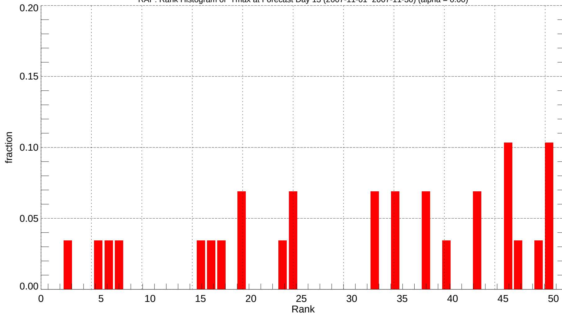
RAP: Rank Histogram of Tmax at Forecast Day 13 (2007-11-01~2007-11-30) (alpha = 0.00)
