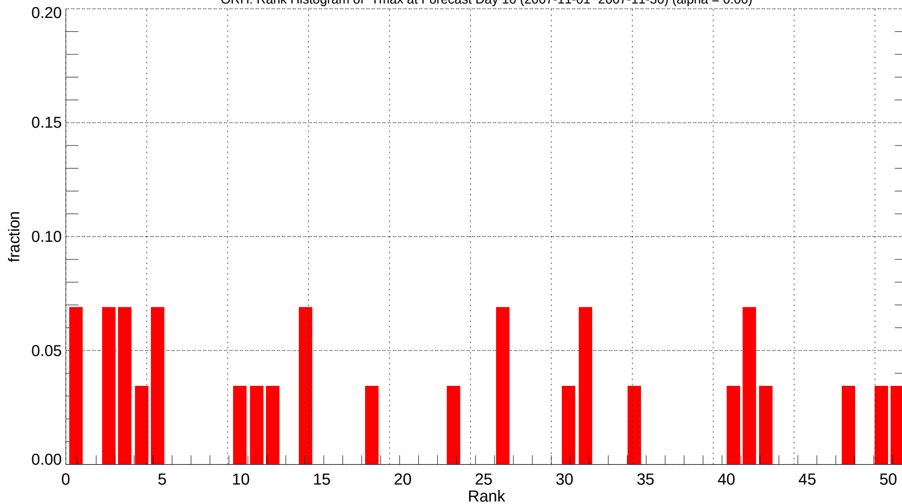
ORH: Rank Histogram of Tmax at Forecast Day 10 (2007-11-01~2007-11-30) (alpha = 0.00)
