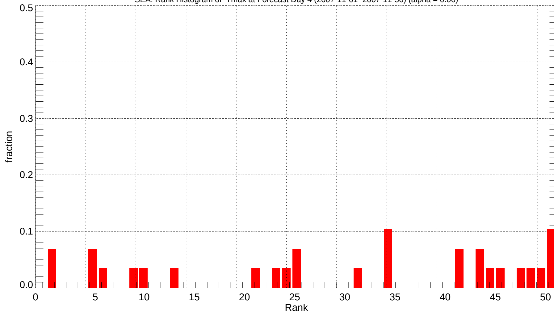
SEA: Rank Histogram of Tmax at Forecast Day 4 (2007-11-01~2007-11-30) (alpha = 0.00)
