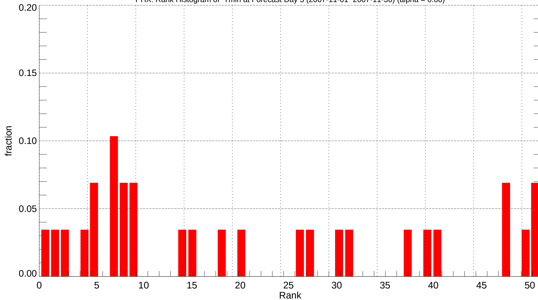
PHX: Rank Histogram of Tmin at Forecast Day 3 (2007-11-01~2007-11-30) (alpha = 0.00)
