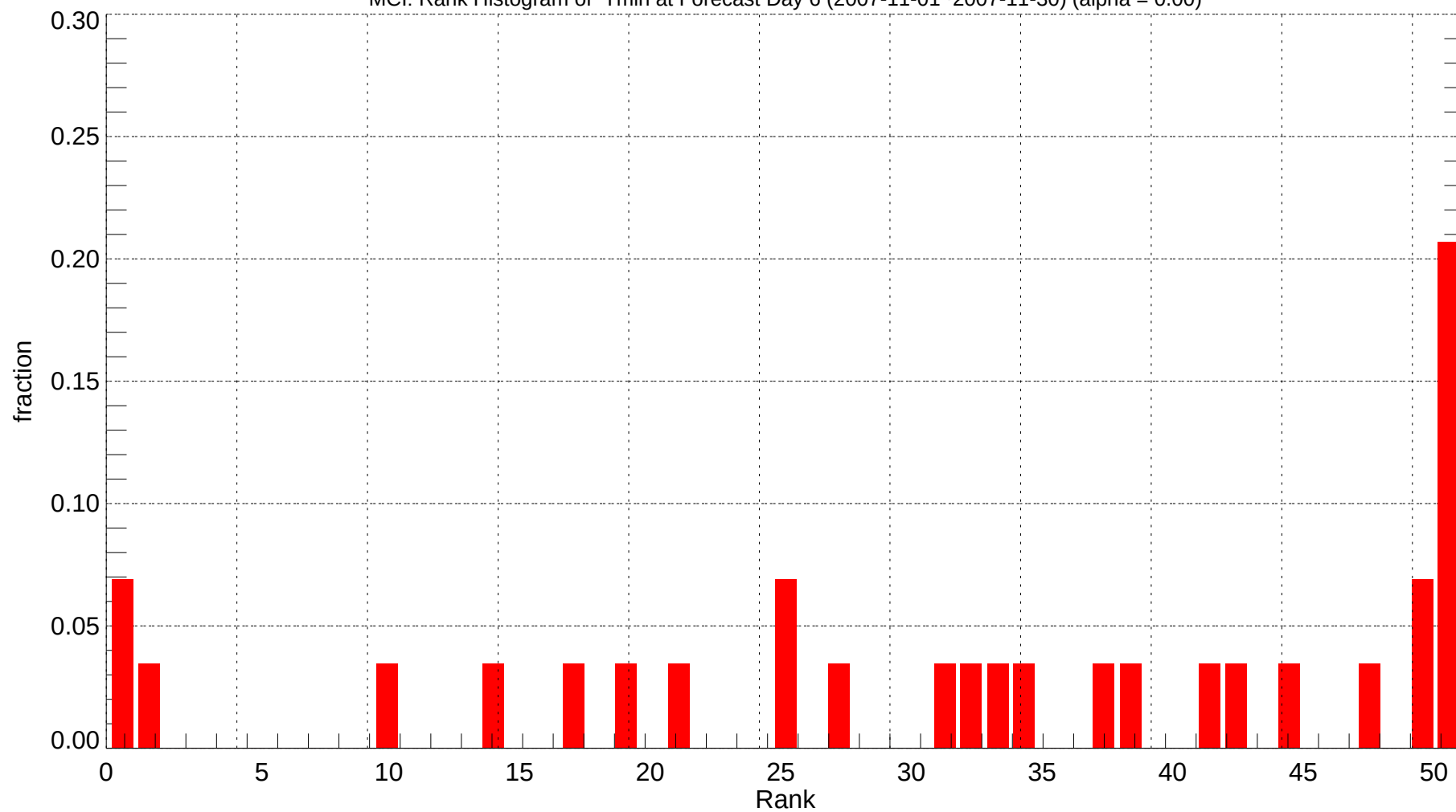
MCI: Rank Histogram of Tmin at Forecast Day 6 (2007-11-01~2007-11-30) (alpha = 0.00)
