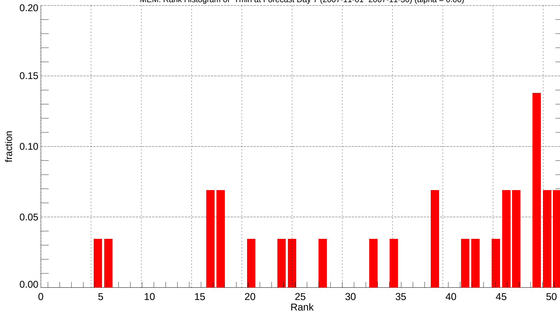
MEM: Rank Histogram of Tmin at Forecast Day 7 (2007-11-01~2007-11-30) (alpha = 0.00)
