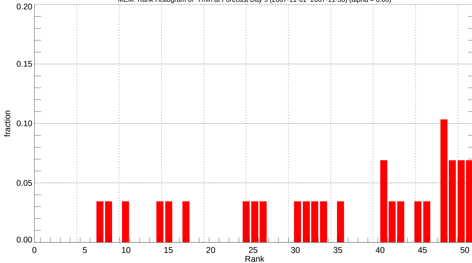
MEM: Rank Histogram of Tmin at Forecast Day 9 (2007-11-01~2007-11-30) (alpha = 0.00)
