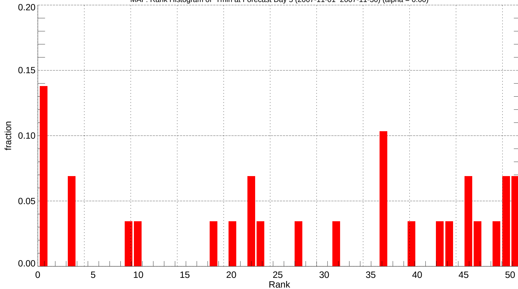
MAF: Rank Histogram of Tmin at Forecast Day 5 (2007-11-01~2007-11-30) (alpha = 0.00)
