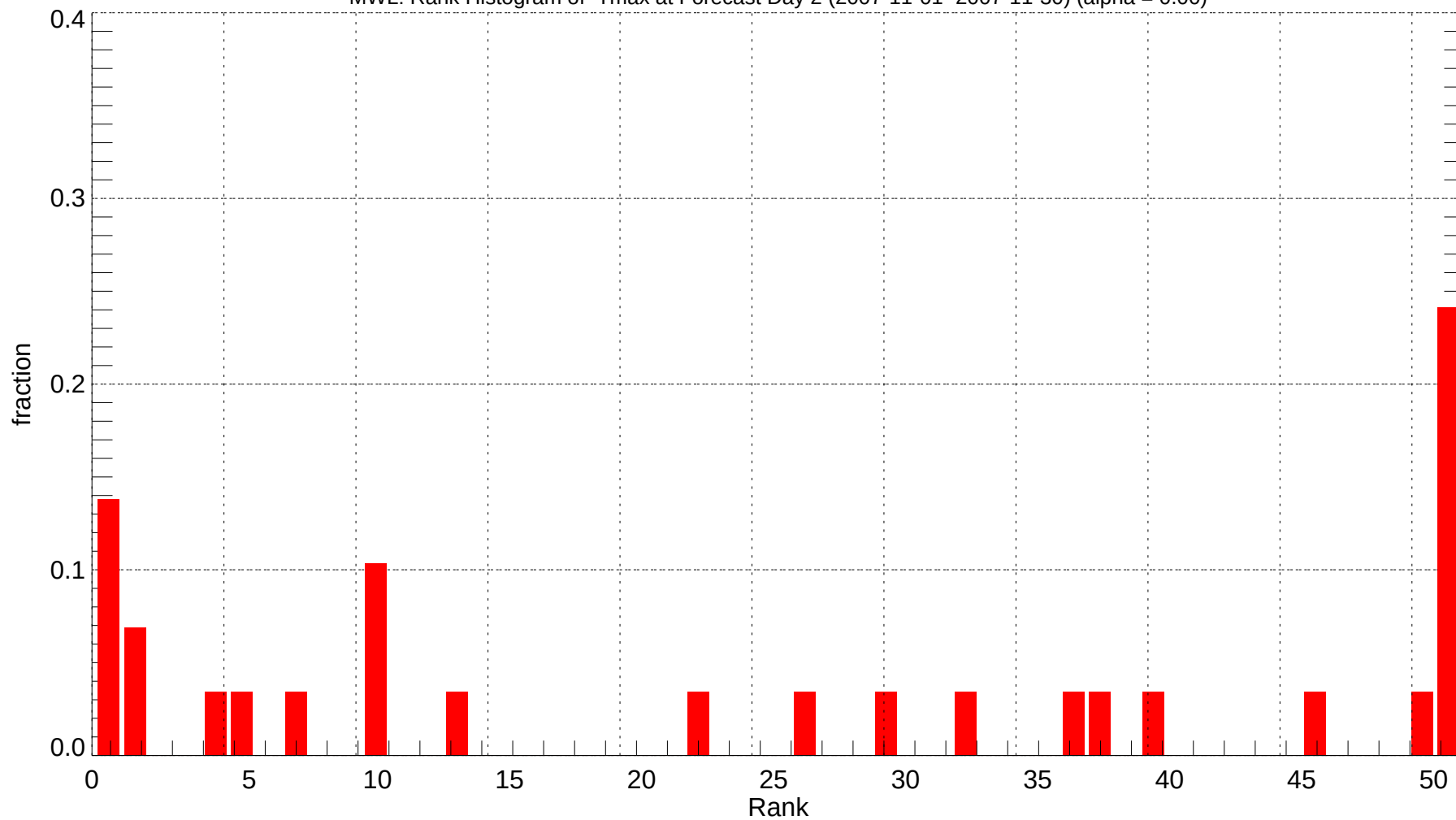
MWL: Rank Histogram of Tmax at Forecast Day 2 (2007-11-01~2007-11-30) (alpha = 0.00)
