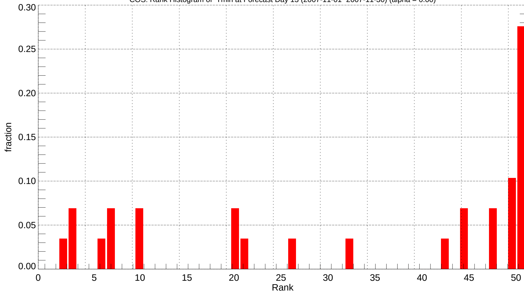
COS: Rank Histogram of Tmin at Forecast Day 13 (2007-11-01~2007-11-30) (alpha = 0.00)
