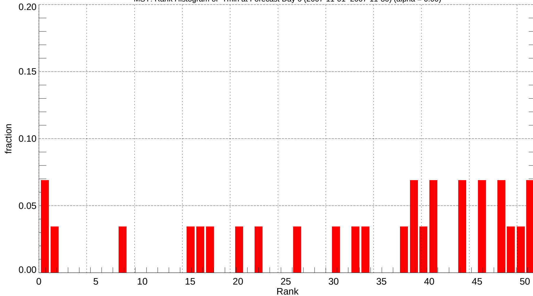
MSY: Rank Histogram of Tmin at Forecast Day 6 (2007-11-01~2007-11-30) (alpha = 0.00)
