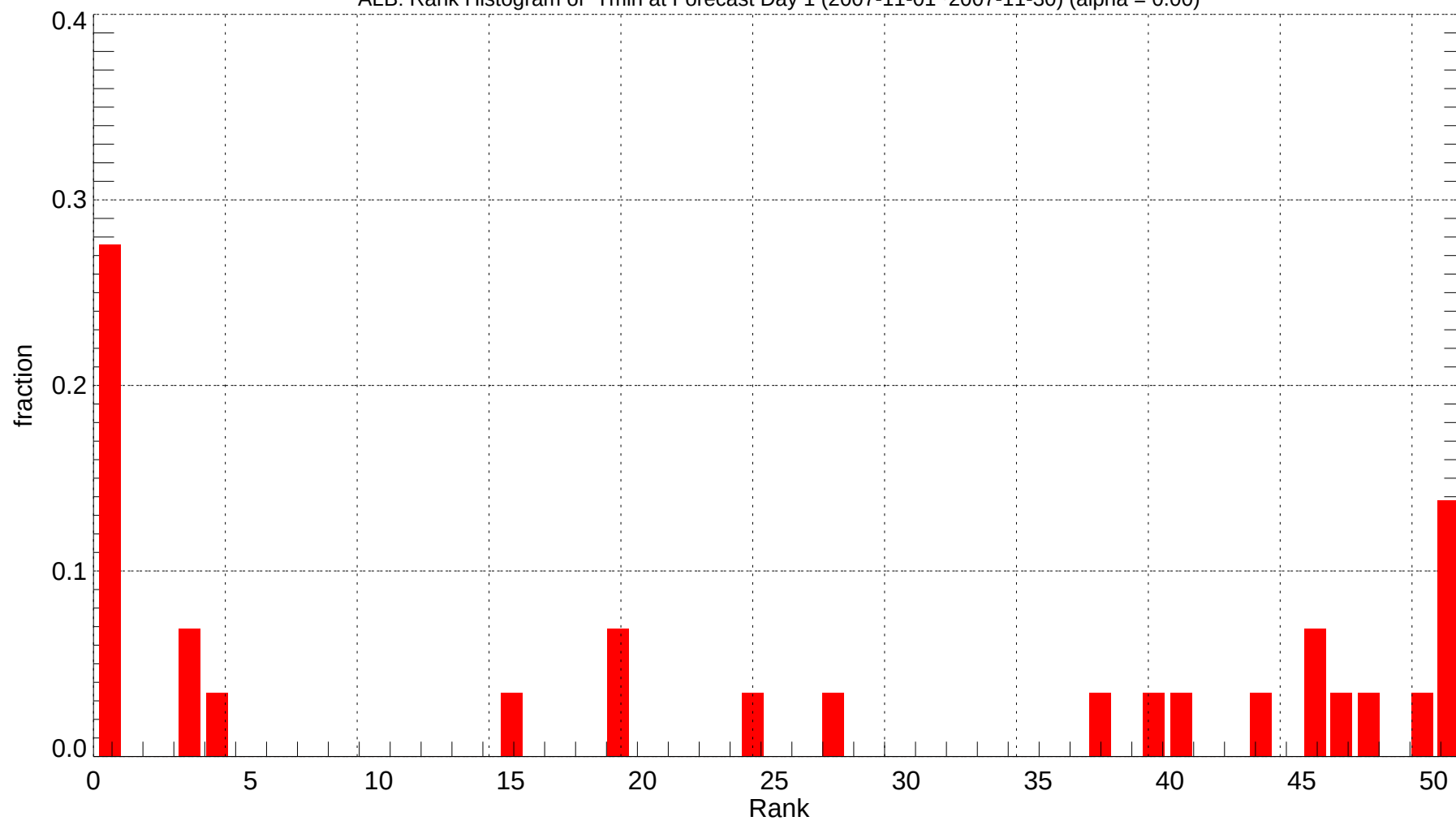
ALB: Rank Histogram of Tmin at Forecast Day 1 (2007-11-01~2007-11-30) (alpha = 0.00)
