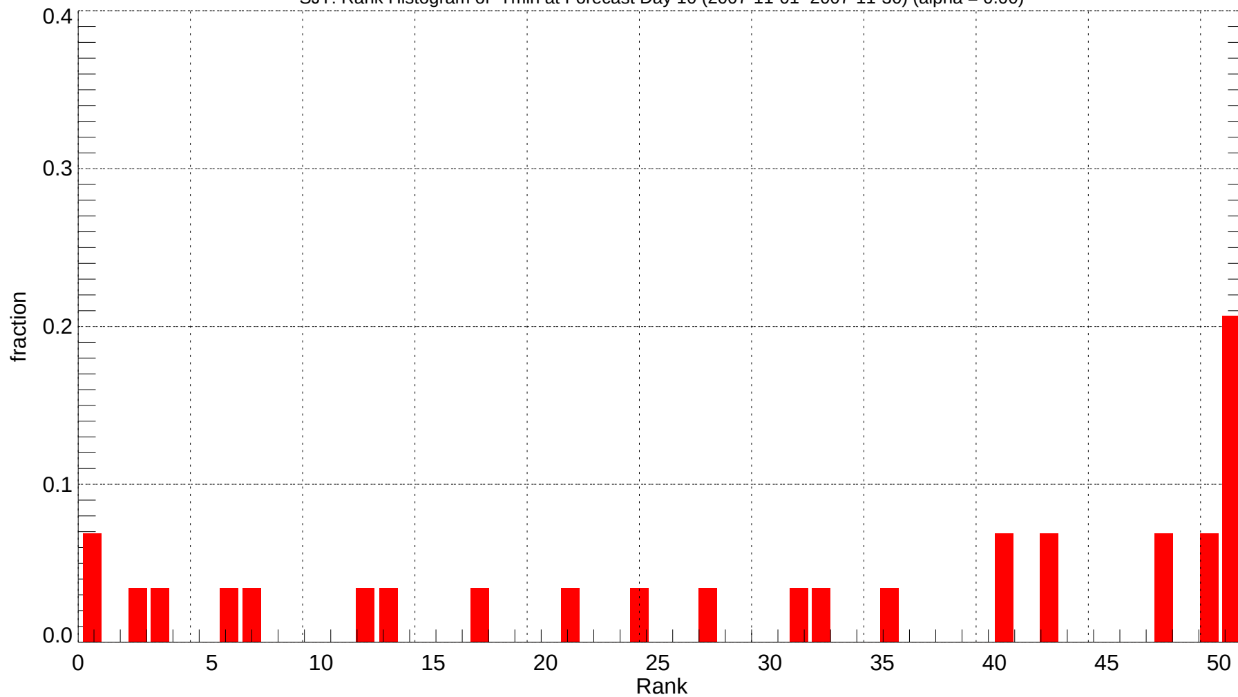
SJT: Rank Histogram of Tmin at Forecast Day 10 (2007-11-01~2007-11-30) (alpha = 0.00)
