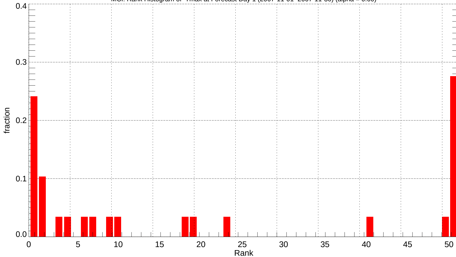
MCI: Rank Histogram of Tmax at Forecast Day 1 (2007-11-01~2007-11-30) (alpha = 0.00)
