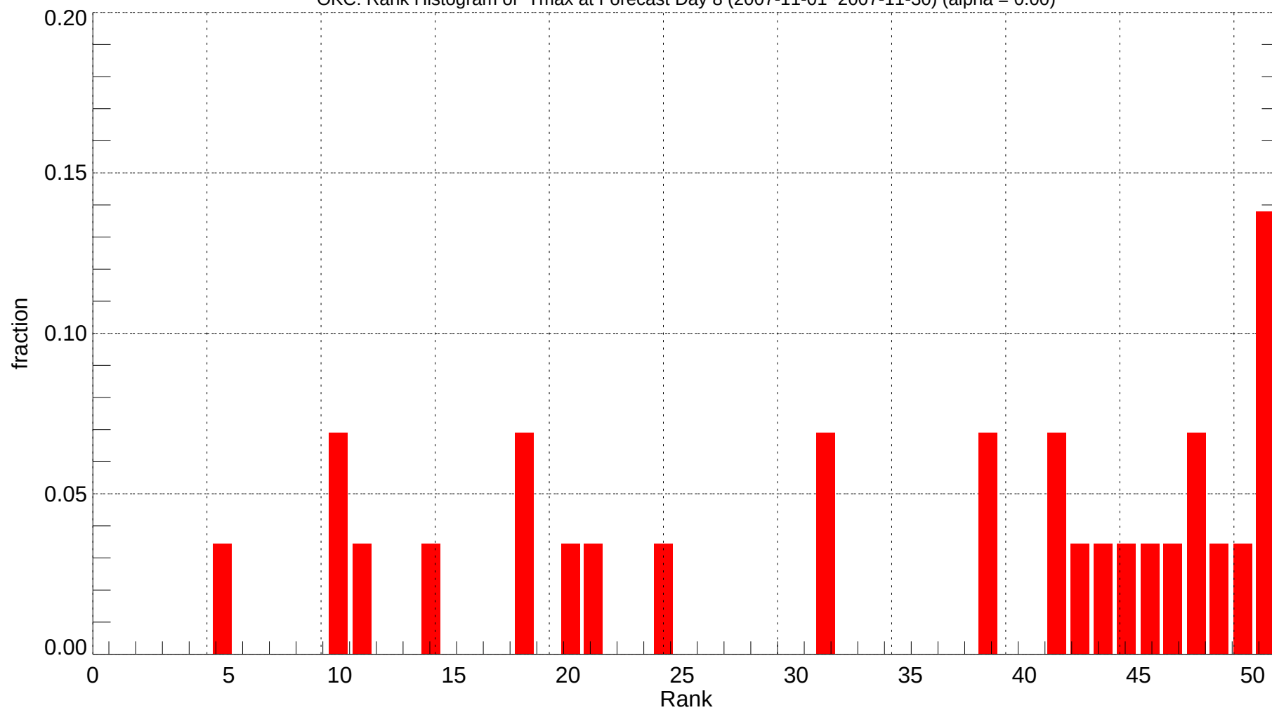
OKC: Rank Histogram of Tmax at Forecast Day 8 (2007-11-01~2007-11-30) (alpha = 0.00)
