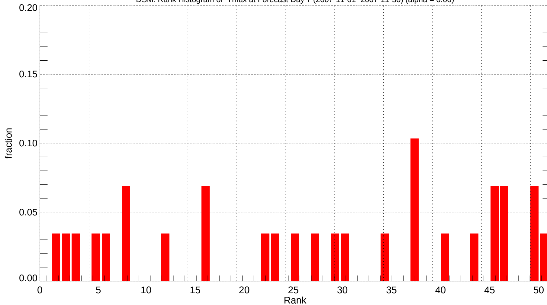
DSM: Rank Histogram of Tmax at Forecast Day 7 (2007-11-01~2007-11-30) (alpha = 0.00)
