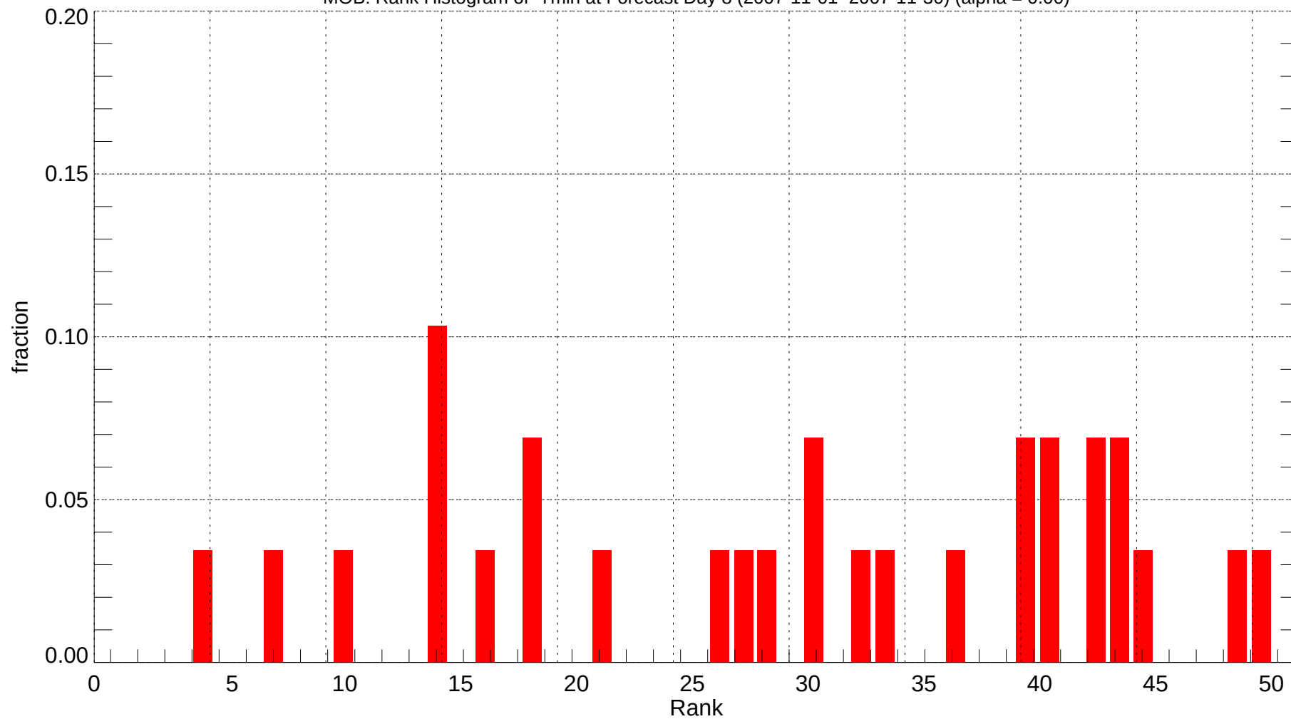
MOB: Rank Histogram of Tmin at Forecast Day 8 (2007-11-01~2007-11-30) (alpha = 0.00)
