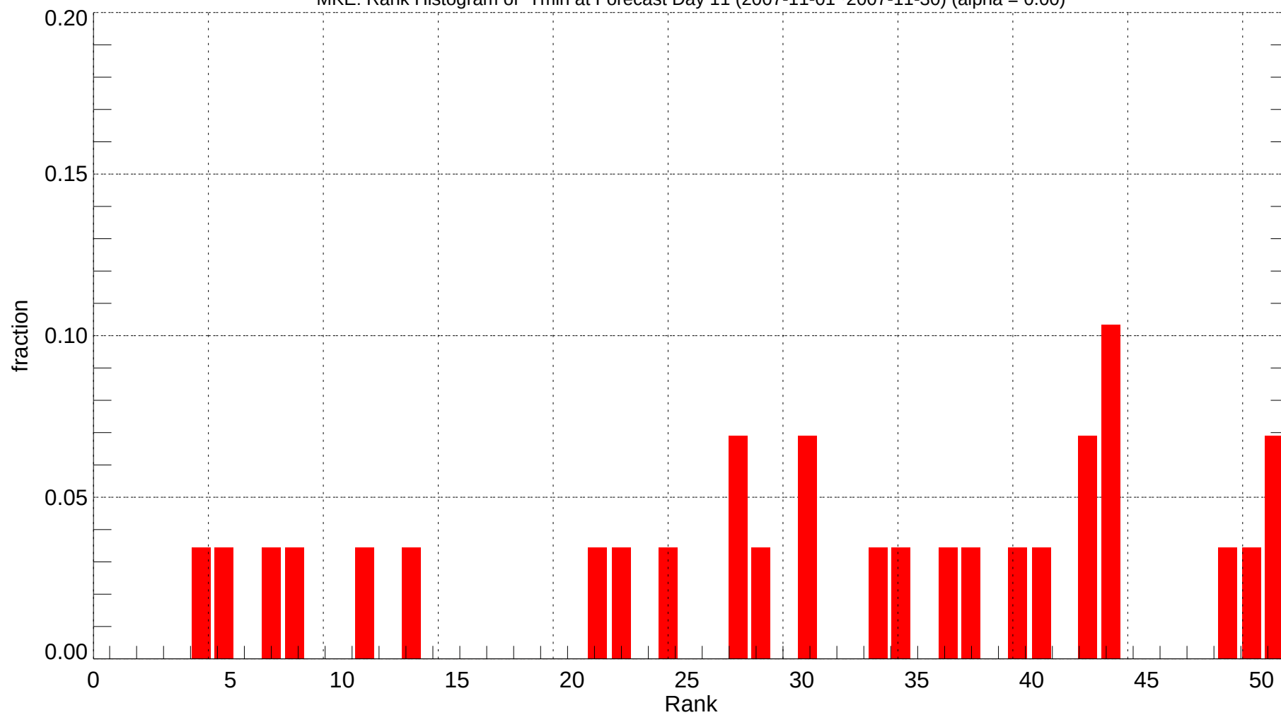
MKE: Rank Histogram of Tmin at Forecast Day 11 (2007-11-01~2007-11-30) (alpha = 0.00)
