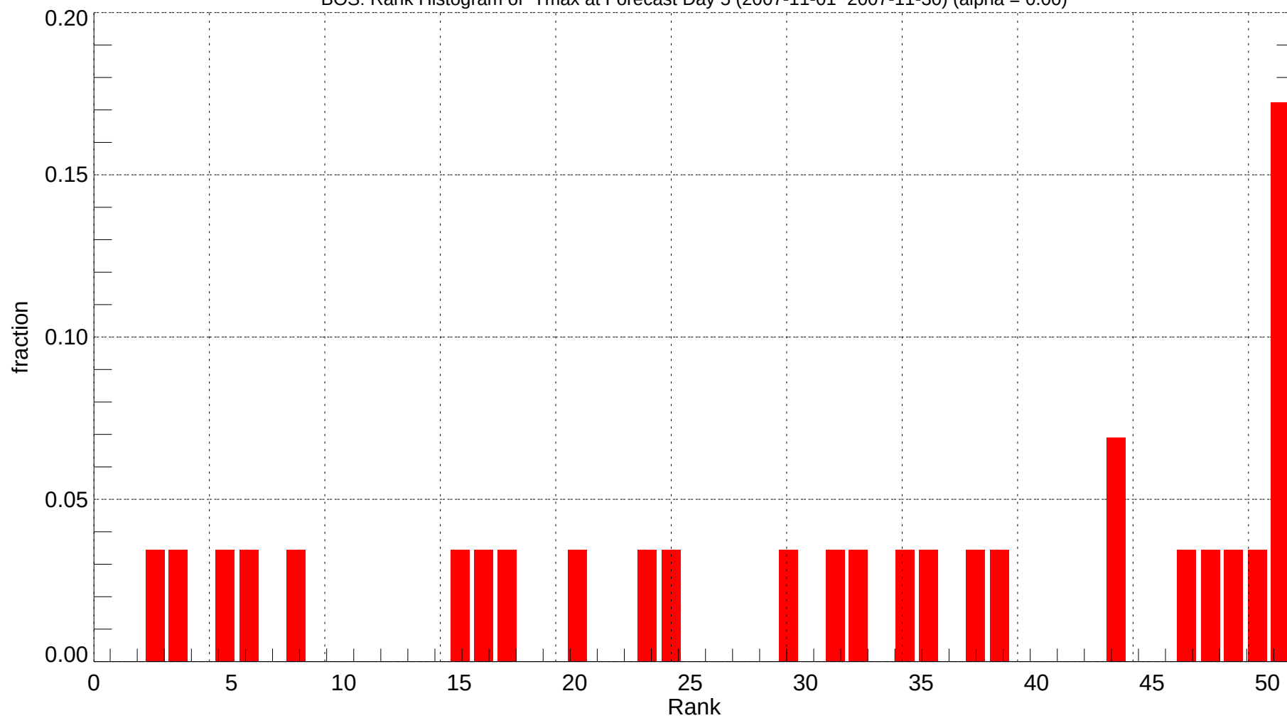
BOS: Rank Histogram of Tmax at Forecast Day 5 (2007-11-01~2007-11-30) (alpha = 0.00)
