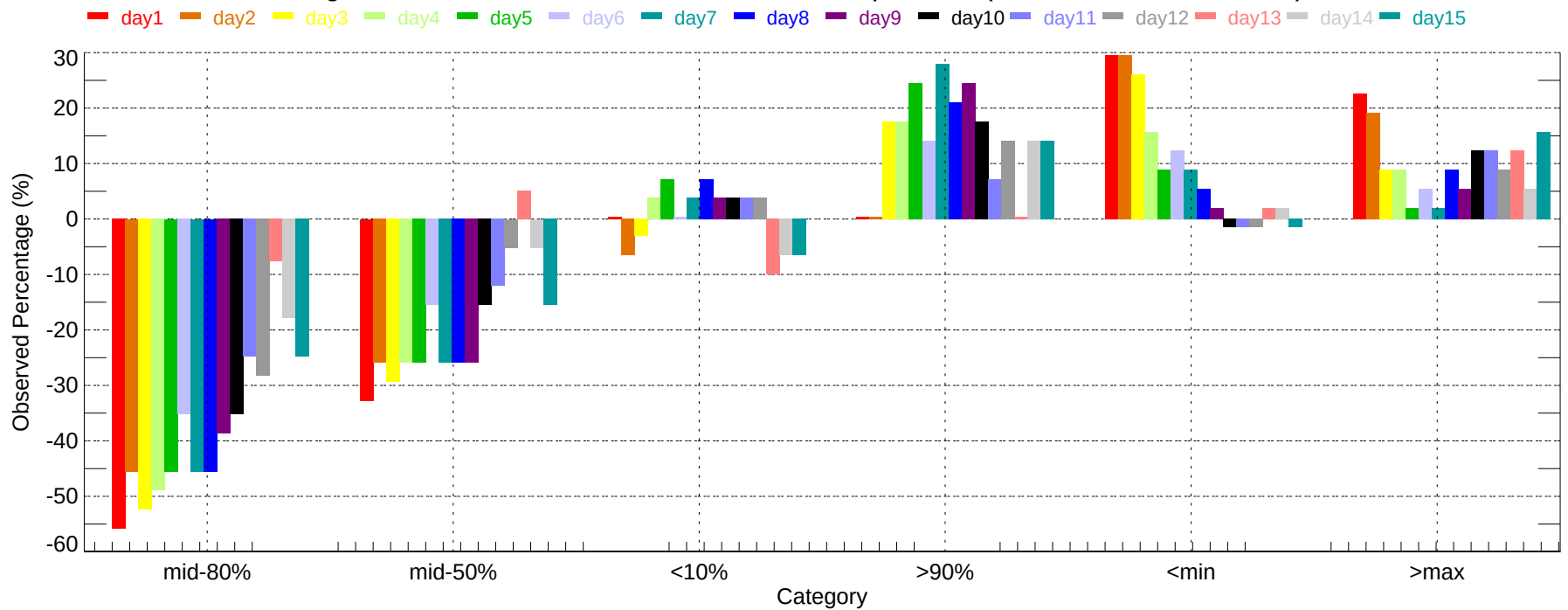
Observed Percentage Deviation of Ensembles - SFO: Max Temperature (2007-11-01~2007-11-30)
