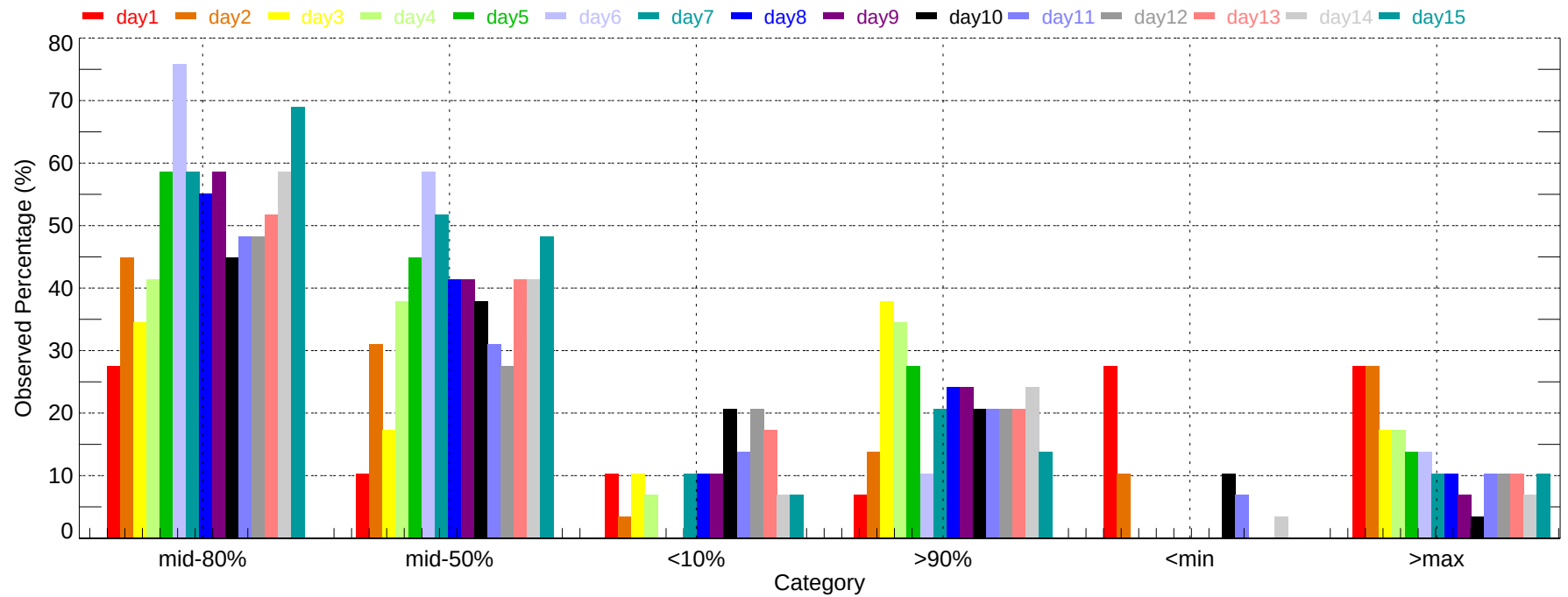
Observed Percentage of Ensembles - NTU: Min Temperature (2007-11-01~2007-11-30)
