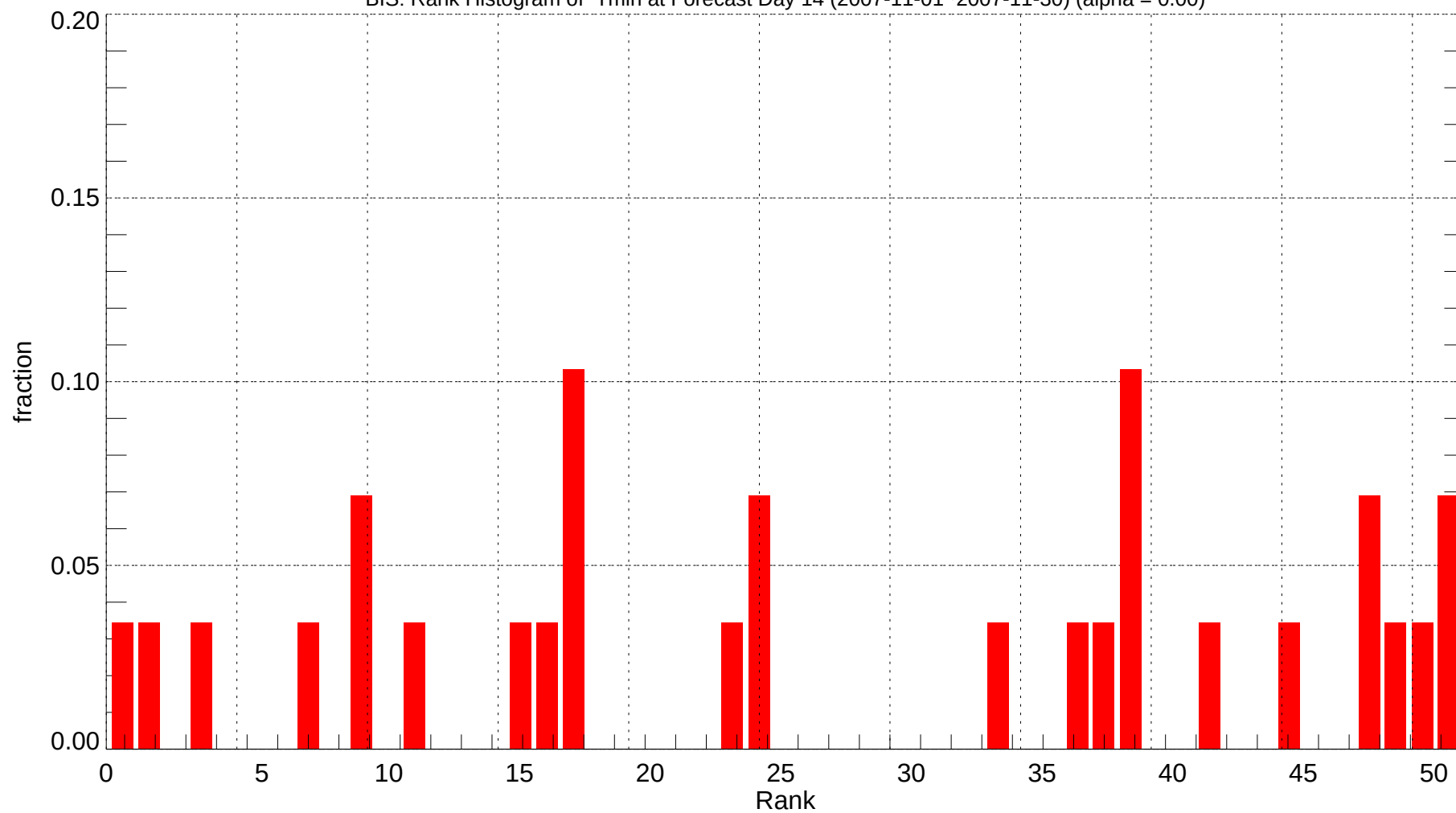
BIS: Rank Histogram of Tmin at Forecast Day 14 (2007-11-01~2007-11-30) (alpha = 0.00)
