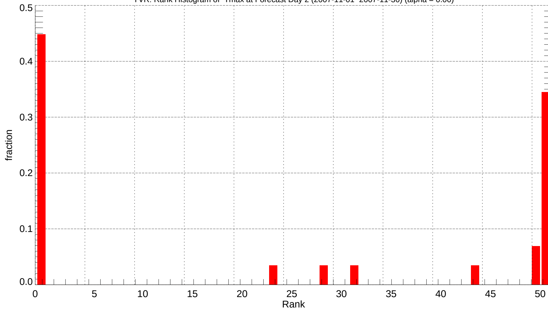
YVR: Rank Histogram of Tmax at Forecast Day 2 (2007-11-01~2007-11-30) (alpha = 0.00)
