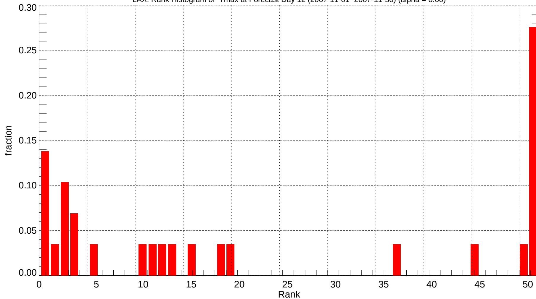
LAX: Rank Histogram of Tmax at Forecast Day 12 (2007-11-01~2007-11-30) (alpha = 0.00)
