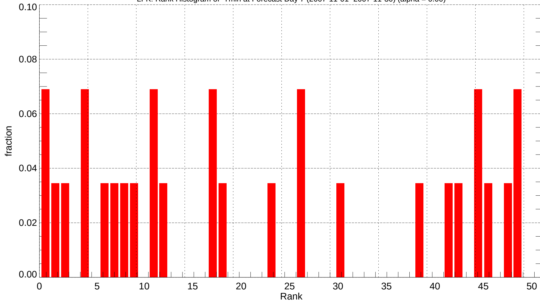
LFK: Rank Histogram of Tmin at Forecast Day 7 (2007-11-01~2007-11-30) (alpha = 0.00)
