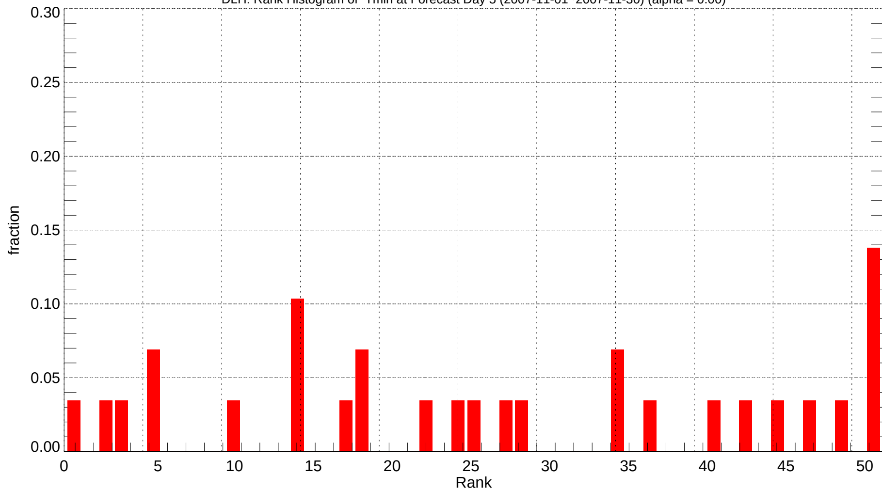
DLH: Rank Histogram of Tmin at Forecast Day 5 (2007-11-01~2007-11-30) (alpha = 0.00)
