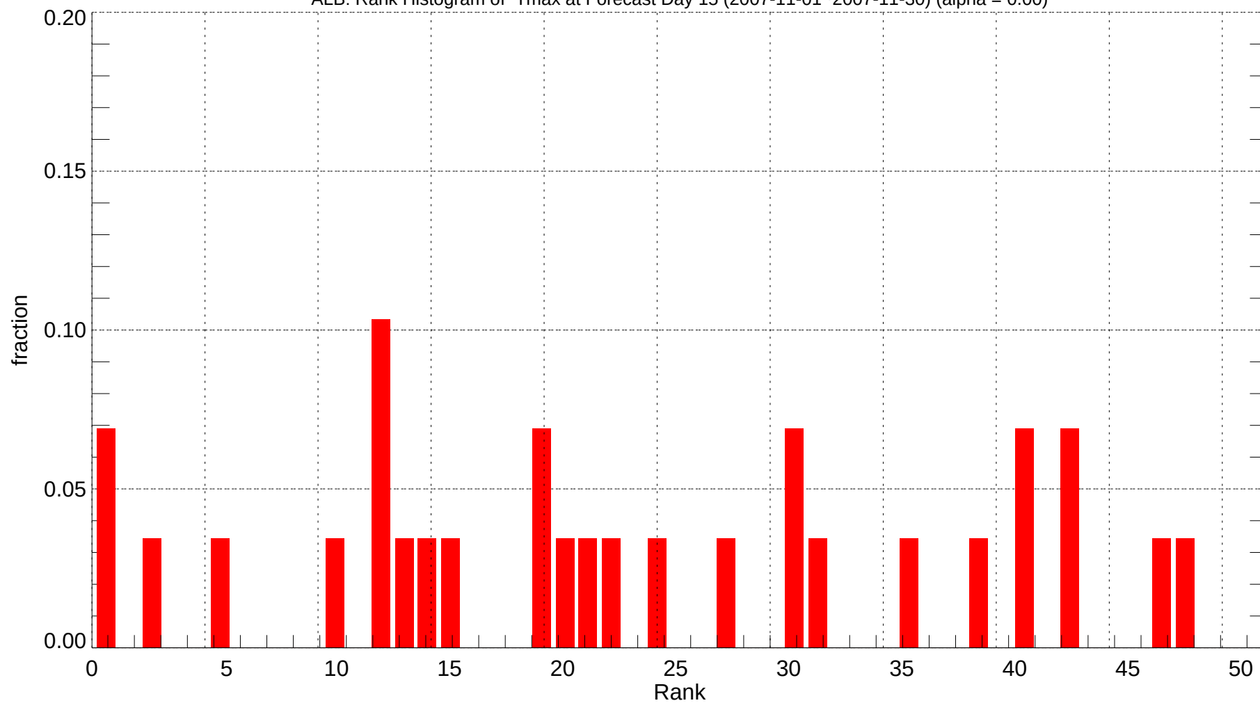
ALB: Rank Histogram of Tmax at Forecast Day 15 (2007-11-01~2007-11-30) (alpha = 0.00)
