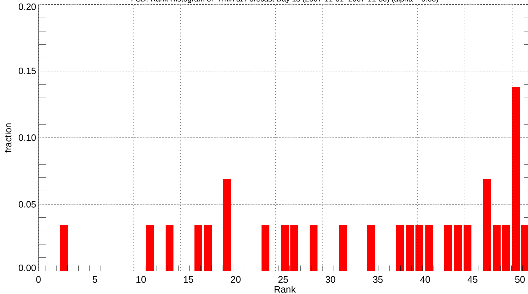
FSD: Rank Histogram of Tmin at Forecast Day 13 (2007-11-01~2007-11-30) (alpha = 0.00)
