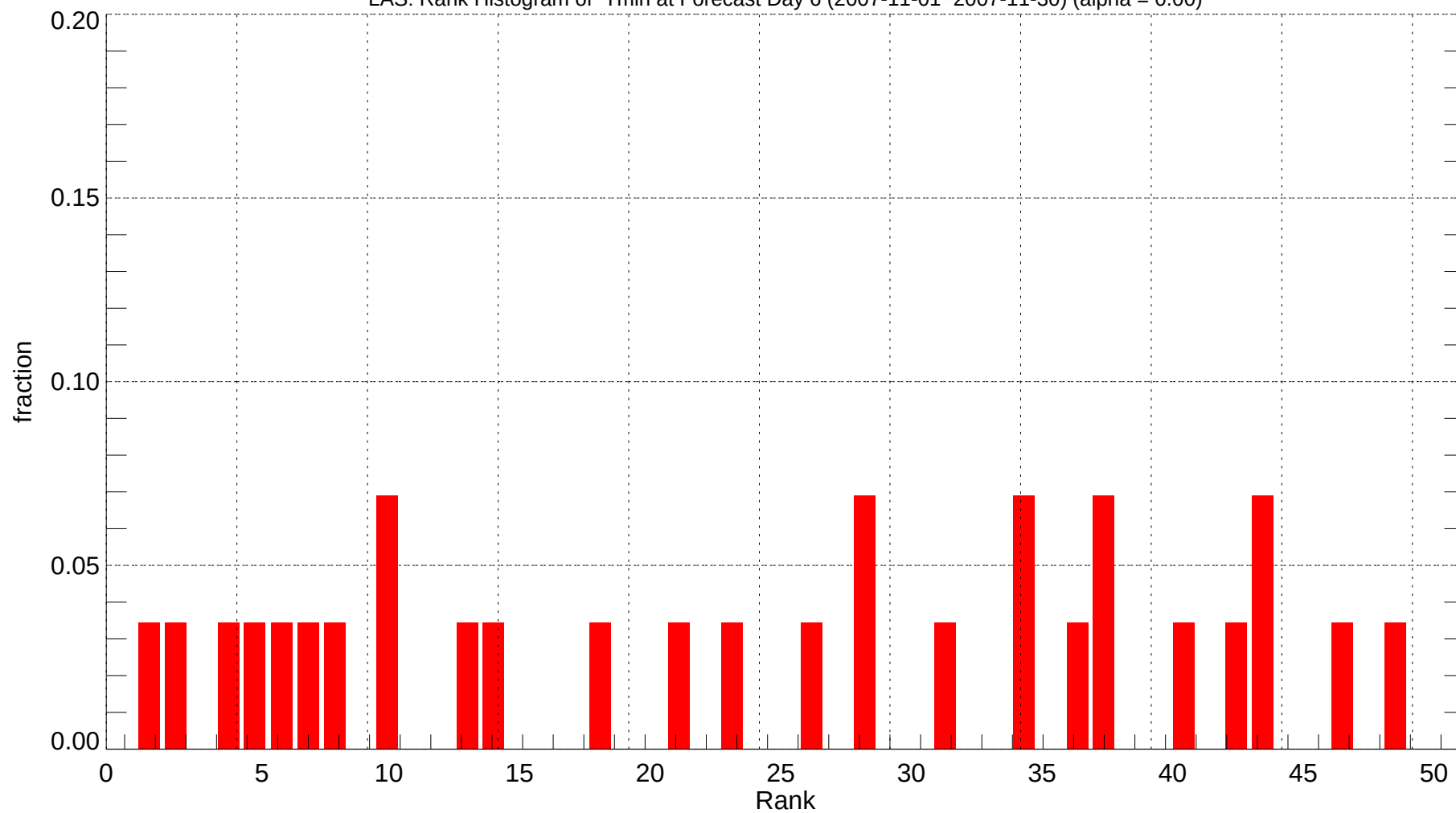
LAS: Rank Histogram of Tmin at Forecast Day 6 (2007-11-01~2007-11-30) (alpha = 0.00)
