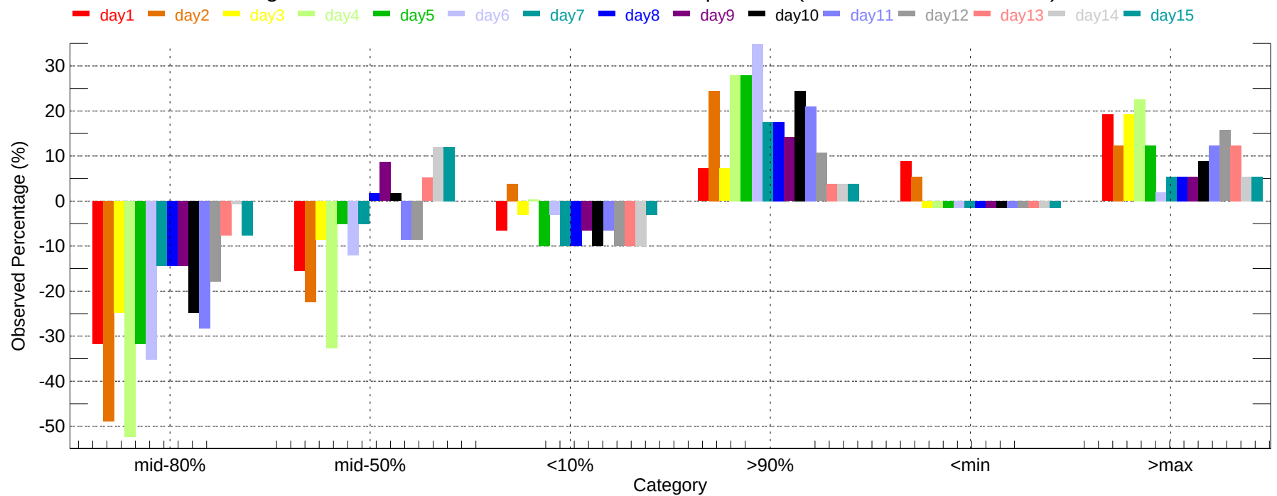
Observed Percentage Deviation of Ensembles - CHA: Min Temperature (2007-11-01~2007-11-30)
