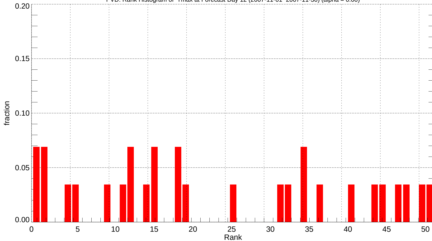
PVD: Rank Histogram of Tmax at Forecast Day 12 (2007-11-01~2007-11-30) (alpha = 0.00)
