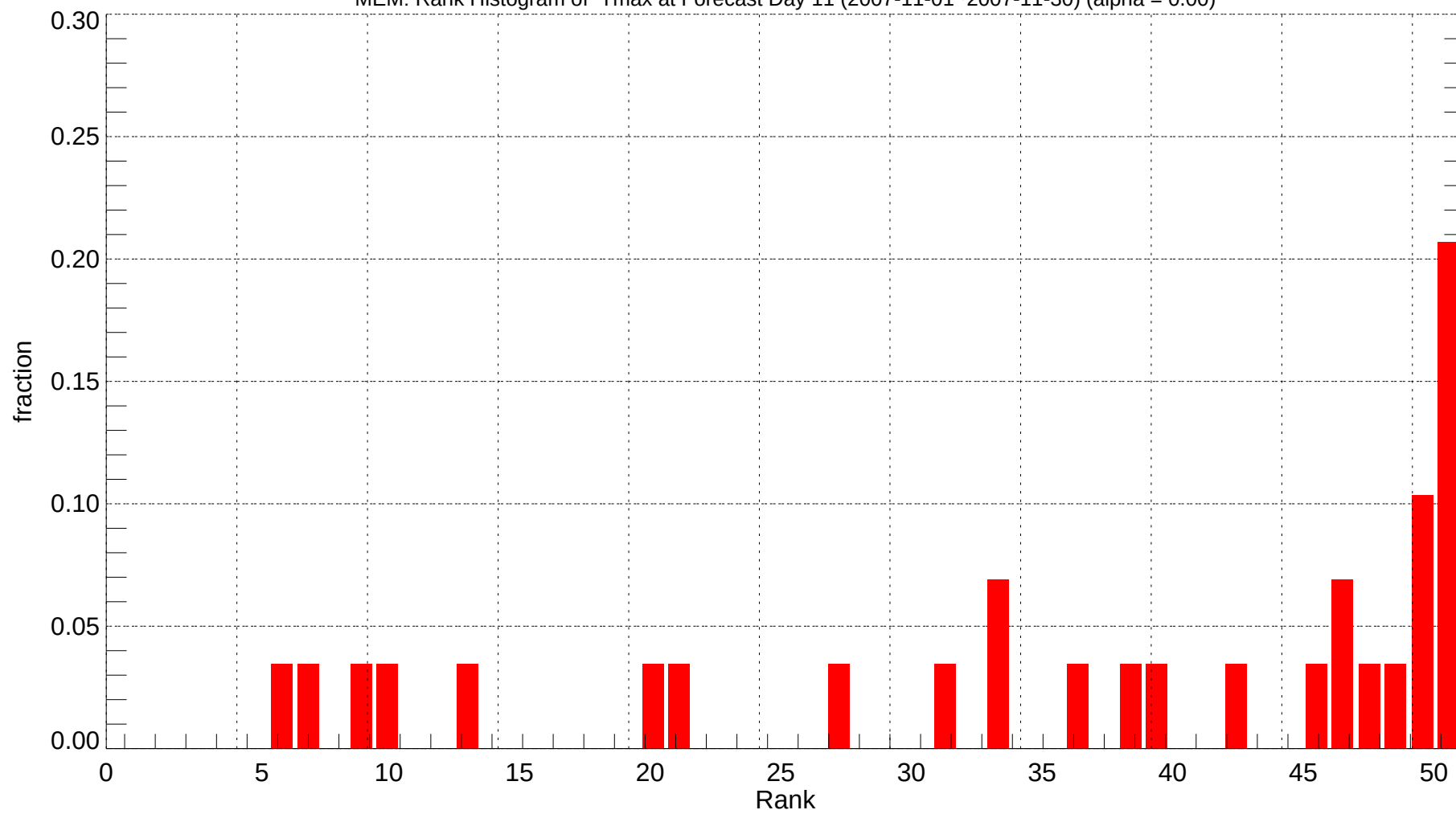
MEM: Rank Histogram of Tmax at Forecast Day 11 (2007-11-01~2007-11-30) (alpha = 0.00)
