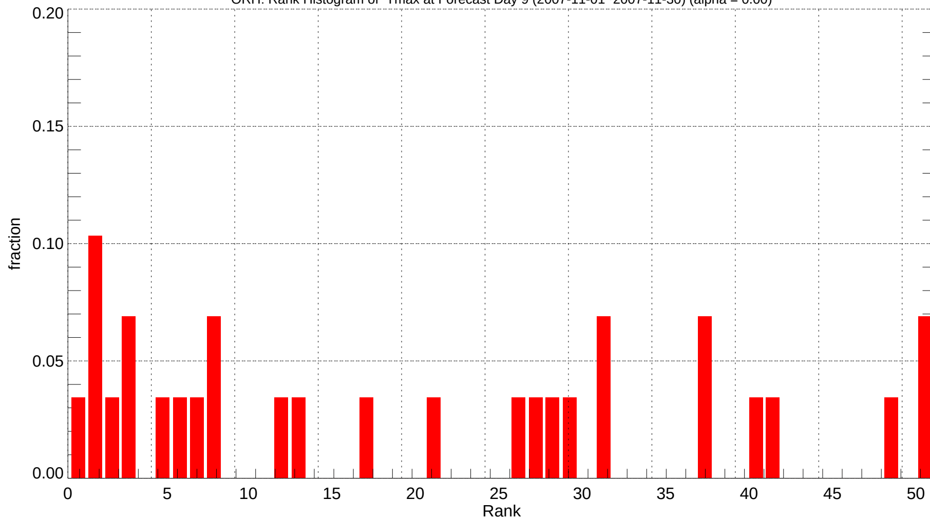
ORH: Rank Histogram of Tmax at Forecast Day 9 (2007-11-01~2007-11-30) (alpha = 0.00)
