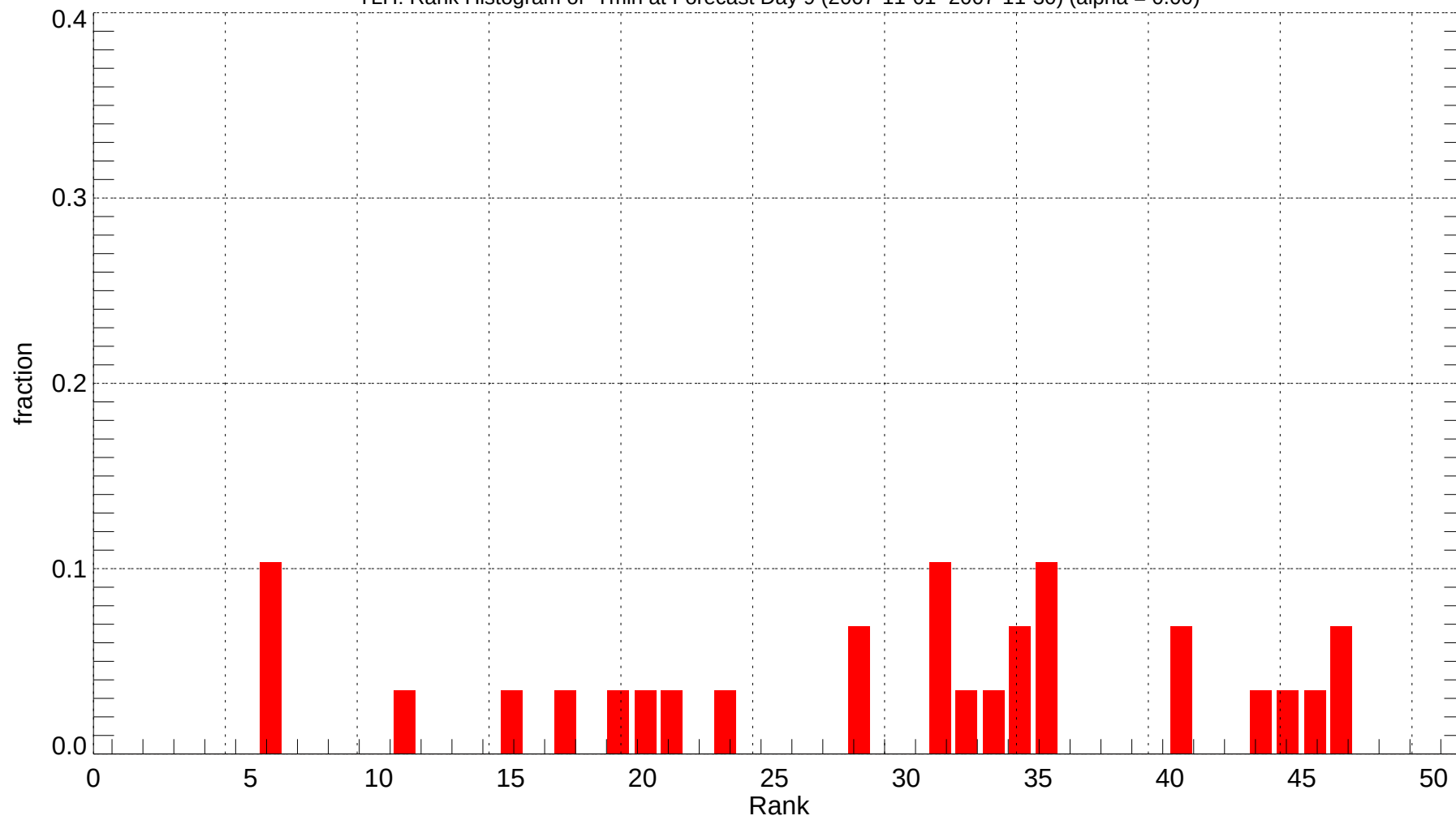
TLH: Rank Histogram of Tmin at Forecast Day 9 (2007-11-01~2007-11-30) (alpha = 0.00)
