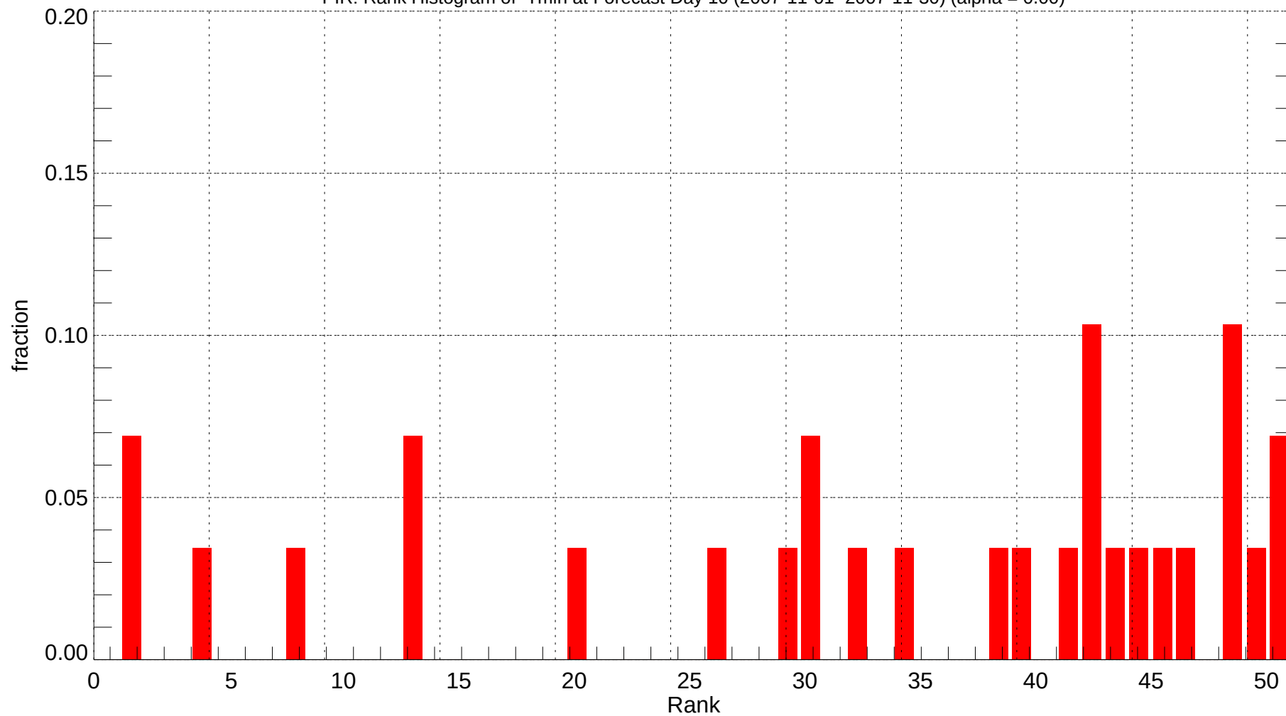
PIR: Rank Histogram of Tmin at Forecast Day 10 (2007-11-01~2007-11-30) (alpha = 0.00)
