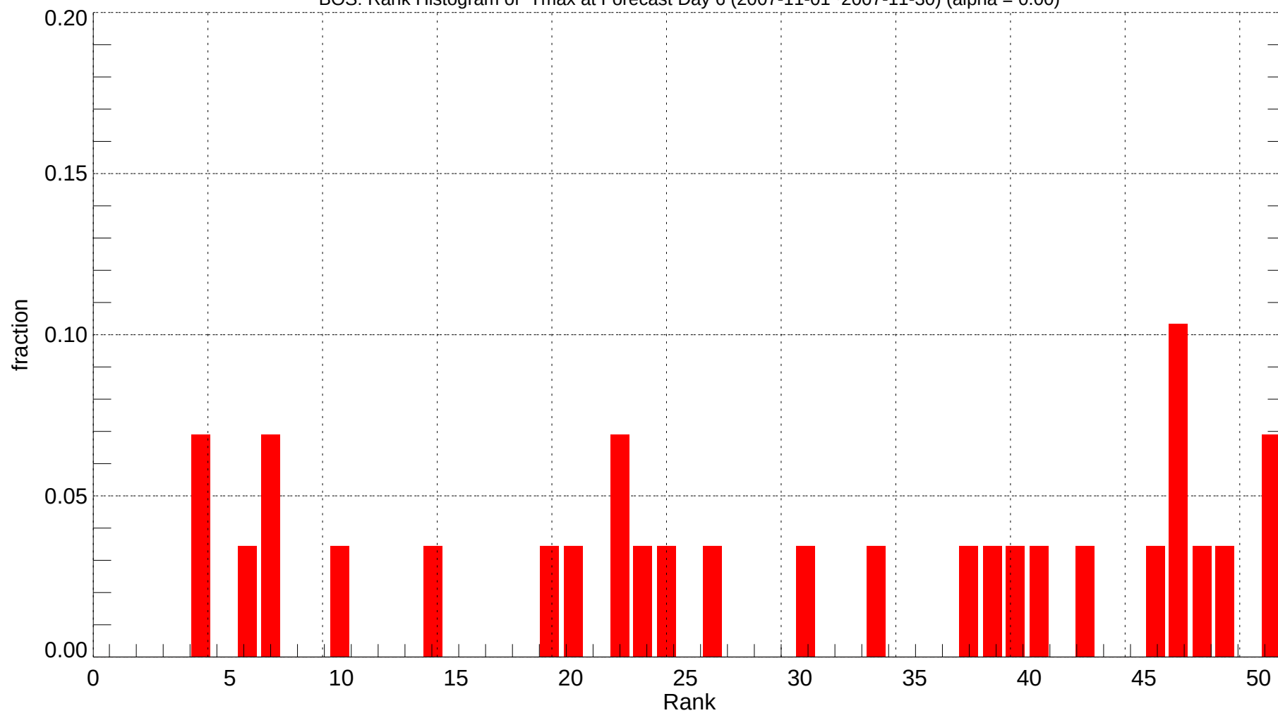
BOS: Rank Histogram of Tmax at Forecast Day 6 (2007-11-01~2007-11-30) (alpha = 0.00)
