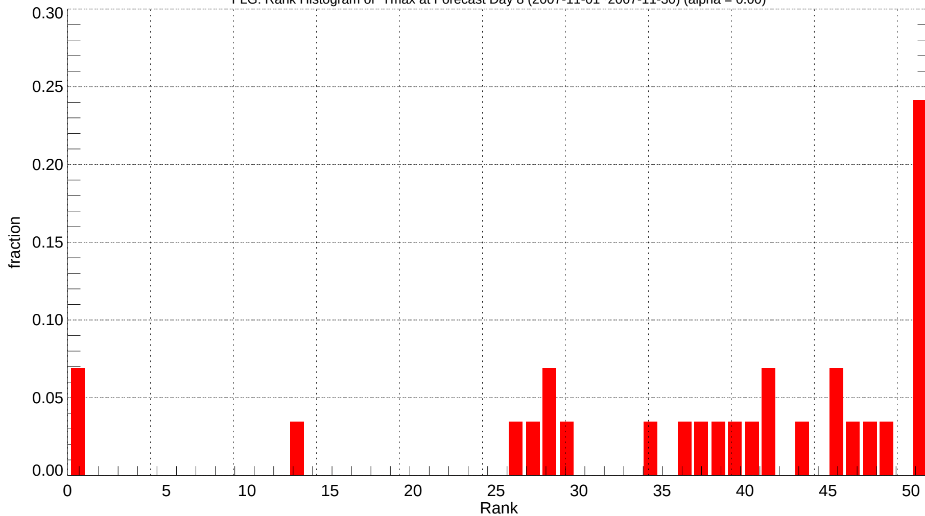
FLG: Rank Histogram of Tmax at Forecast Day 8 (2007-11-01~2007-11-30) (alpha = 0.00)
