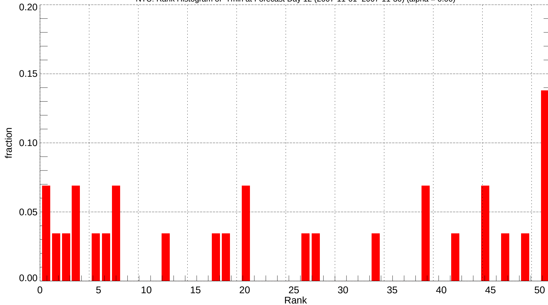
NTU: Rank Histogram of Tmin at Forecast Day 12 (2007-11-01~2007-11-30) (alpha = 0.00)
