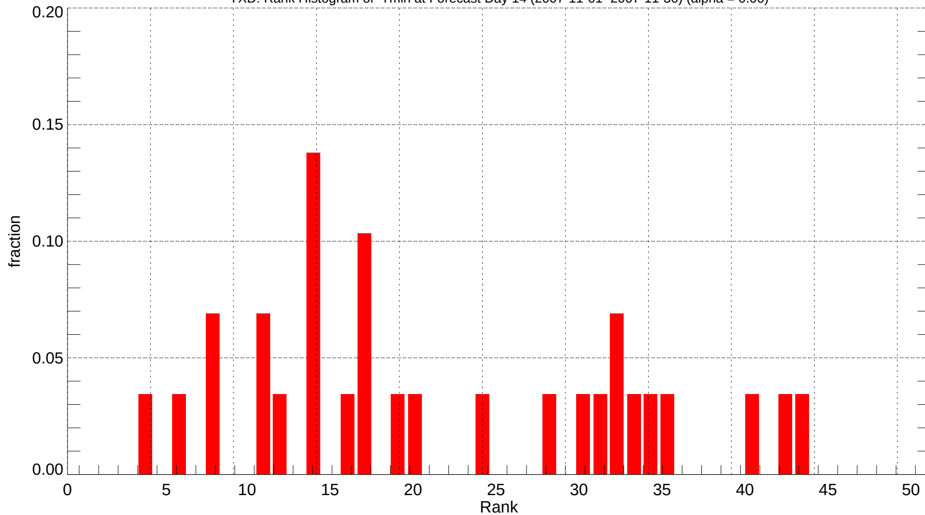
YXD: Rank Histogram of Tmin at Forecast Day 14 (2007-11-01~2007-11-30) (alpha = 0.00)
