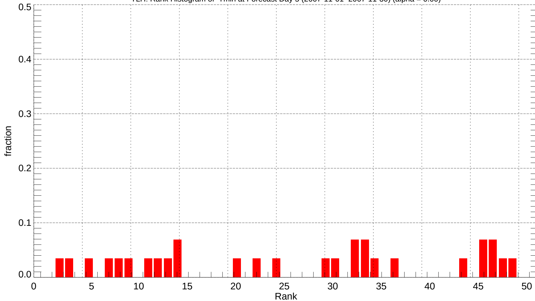
TLH: Rank Histogram of Tmin at Forecast Day 5 (2007-11-01~2007-11-30) (alpha = 0.00)
