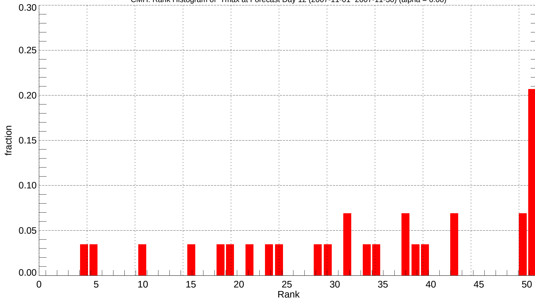
CMH: Rank Histogram of Tmax at Forecast Day 12 (2007-11-01~2007-11-30) (alpha = 0.00)
