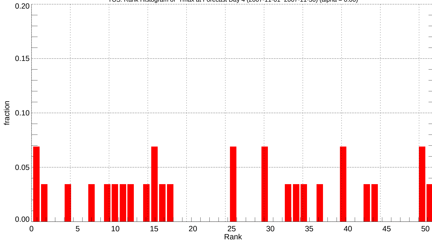
TUS: Rank Histogram of Tmax at Forecast Day 4 (2007-11-01~2007-11-30) (alpha = 0.00)
