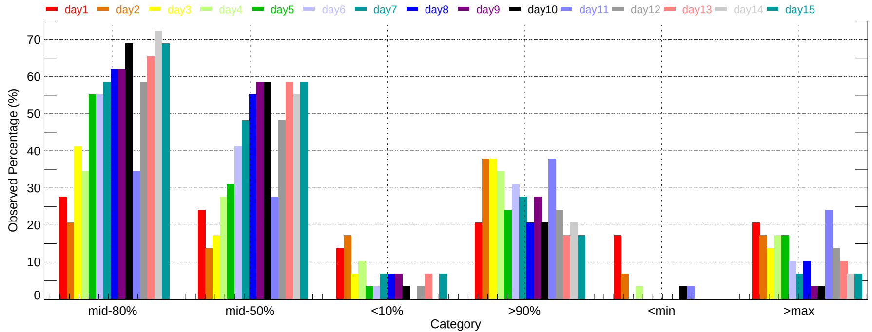
Observed Percentage of Ensembles - TYS: Max Temperature (2007-11-01~2007-11-30)
