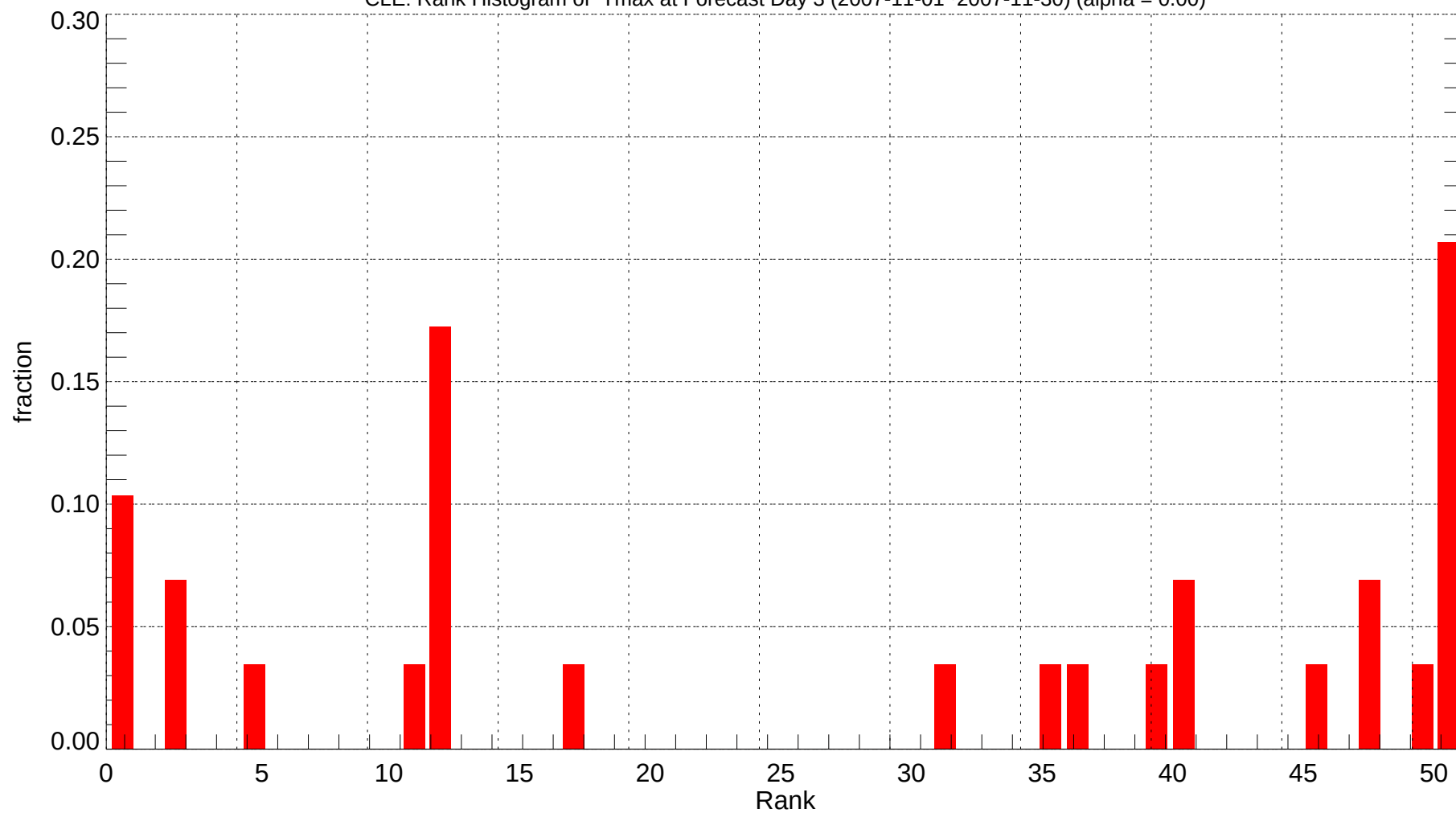
CLE: Rank Histogram of Tmax at Forecast Day 3 (2007-11-01~2007-11-30) (alpha = 0.00)
