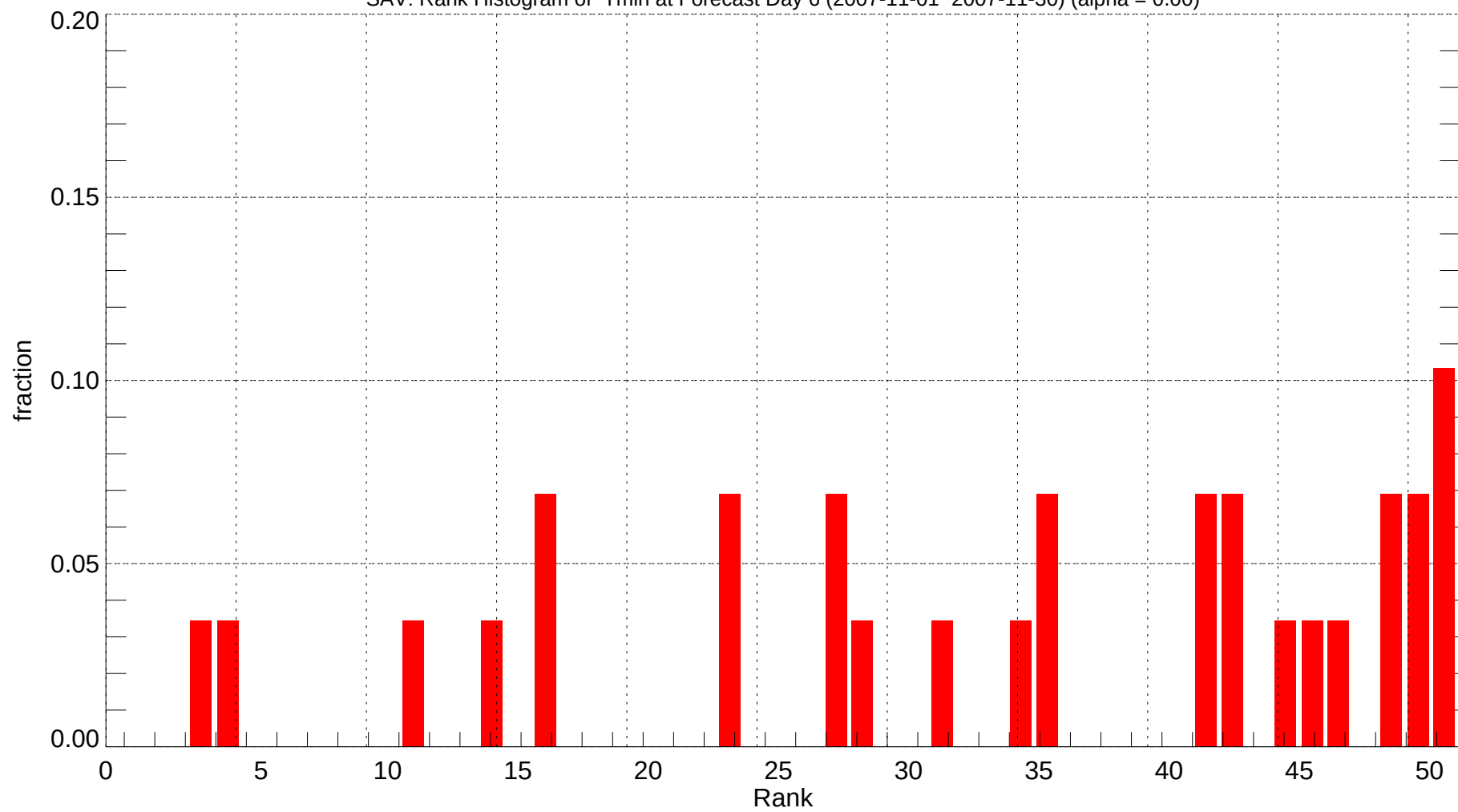
SAV: Rank Histogram of Tmin at Forecast Day 6 (2007-11-01~2007-11-30) (alpha = 0.00)
