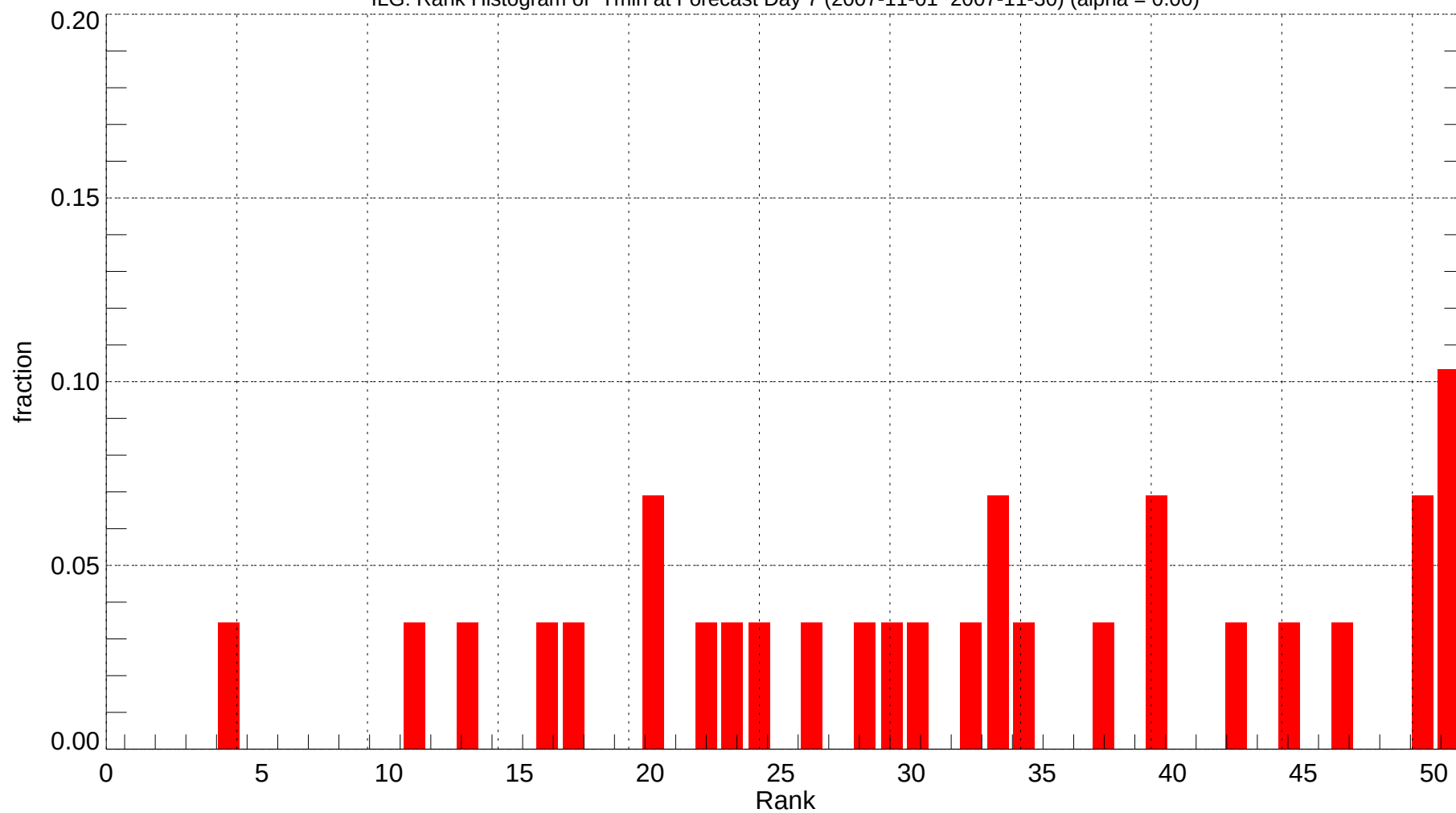
ILG: Rank Histogram of Tmin at Forecast Day 7 (2007-11-01~2007-11-30) (alpha = 0.00)
