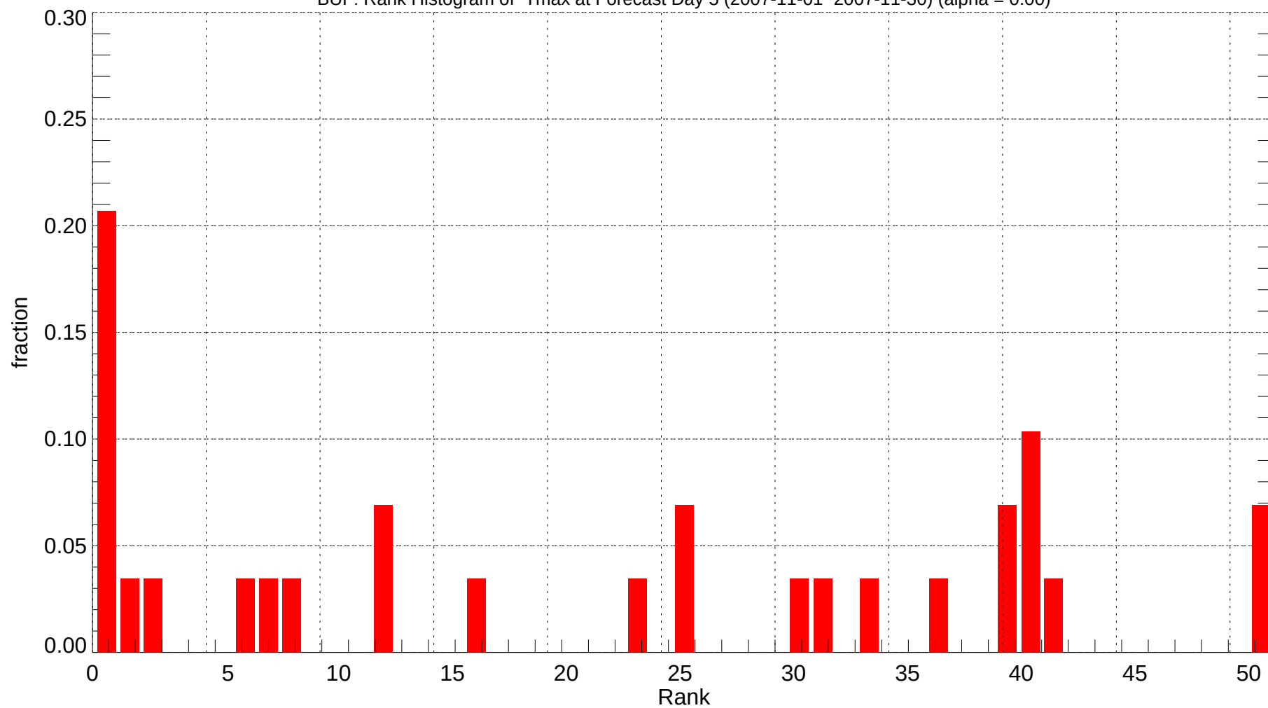
BUF: Rank Histogram of Tmax at Forecast Day 5 (2007-11-01~2007-11-30) (alpha = 0.00)
