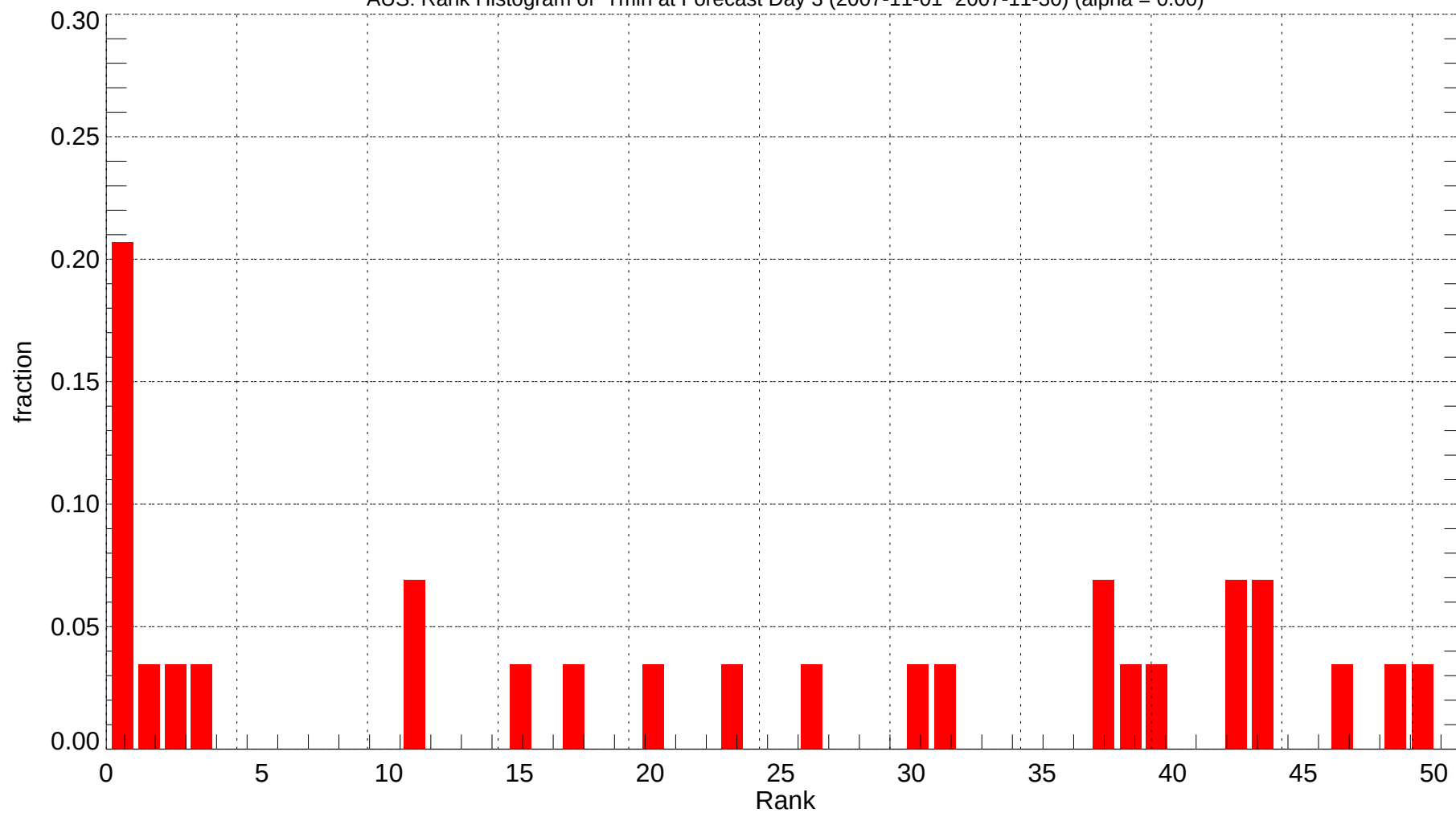
AUS: Rank Histogram of Tmin at Forecast Day 3 (2007-11-01~2007-11-30) (alpha = 0.00)
