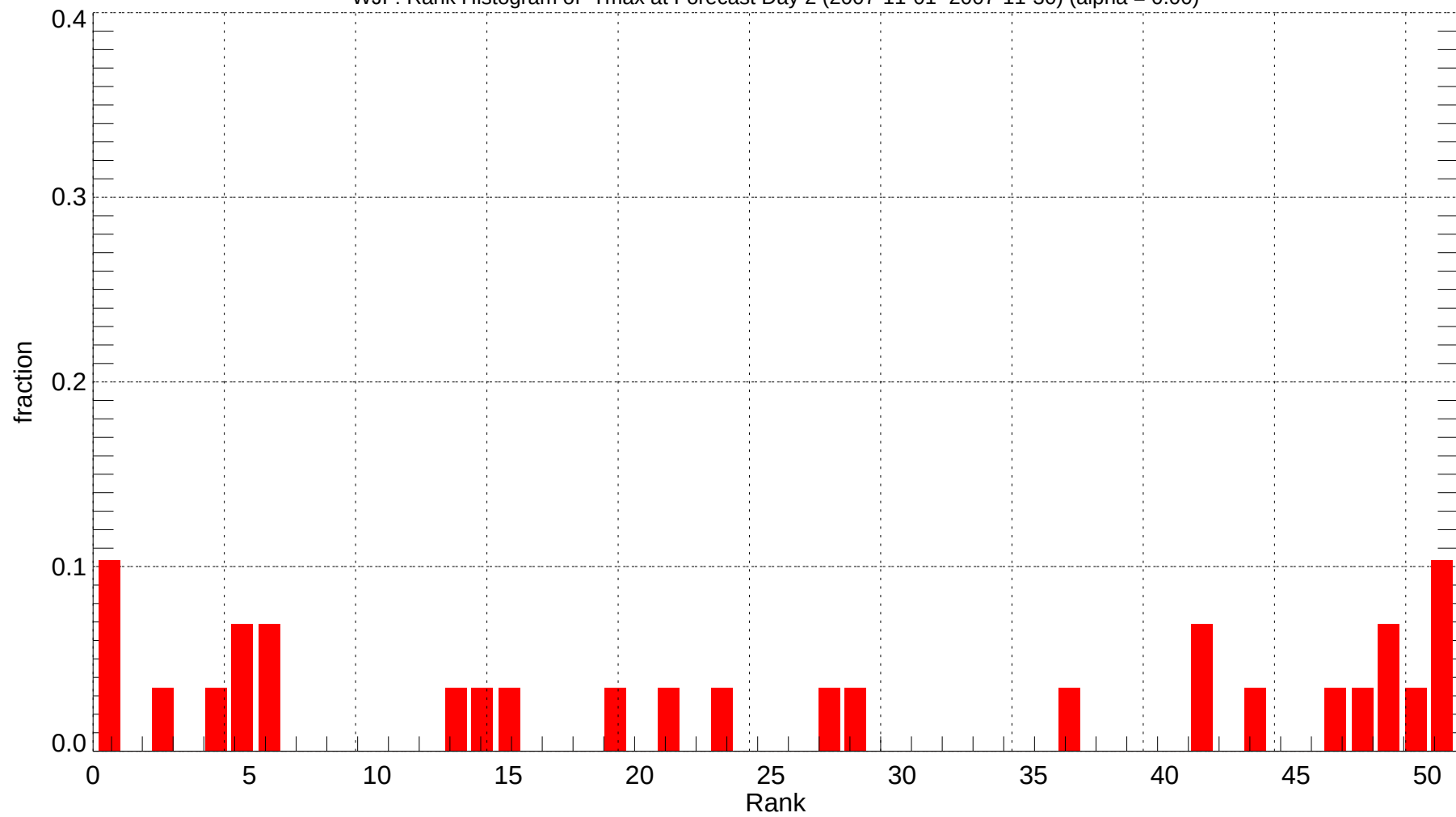
WJF: Rank Histogram of Tmax at Forecast Day 2 (2007-11-01~2007-11-30) (alpha = 0.00)
