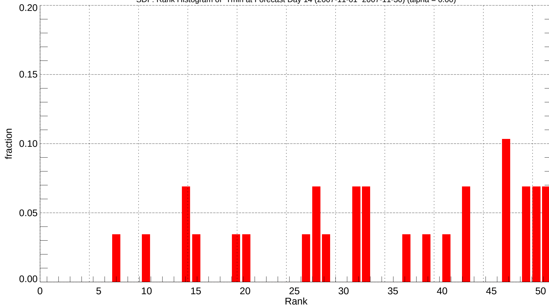
SDF: Rank Histogram of Tmin at Forecast Day 14 (2007-11-01~2007-11-30) (alpha = 0.00)
