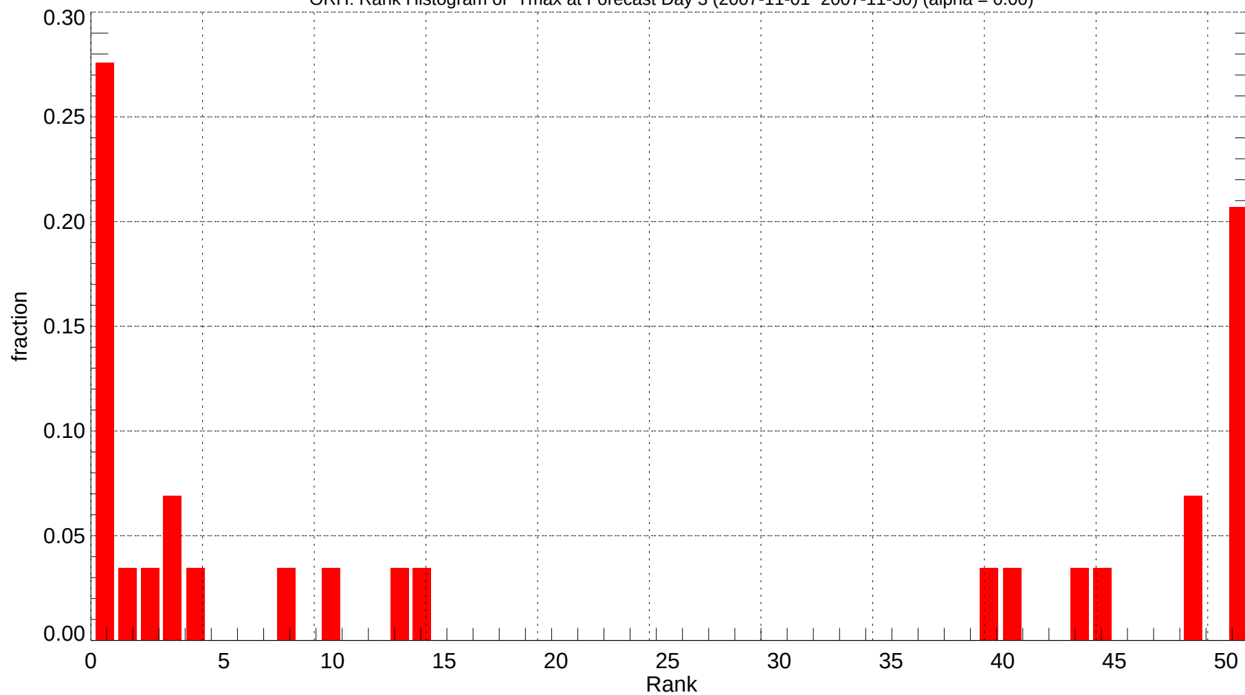
ORH: Rank Histogram of Tmax at Forecast Day 3 (2007-11-01~2007-11-30) (alpha = 0.00)
