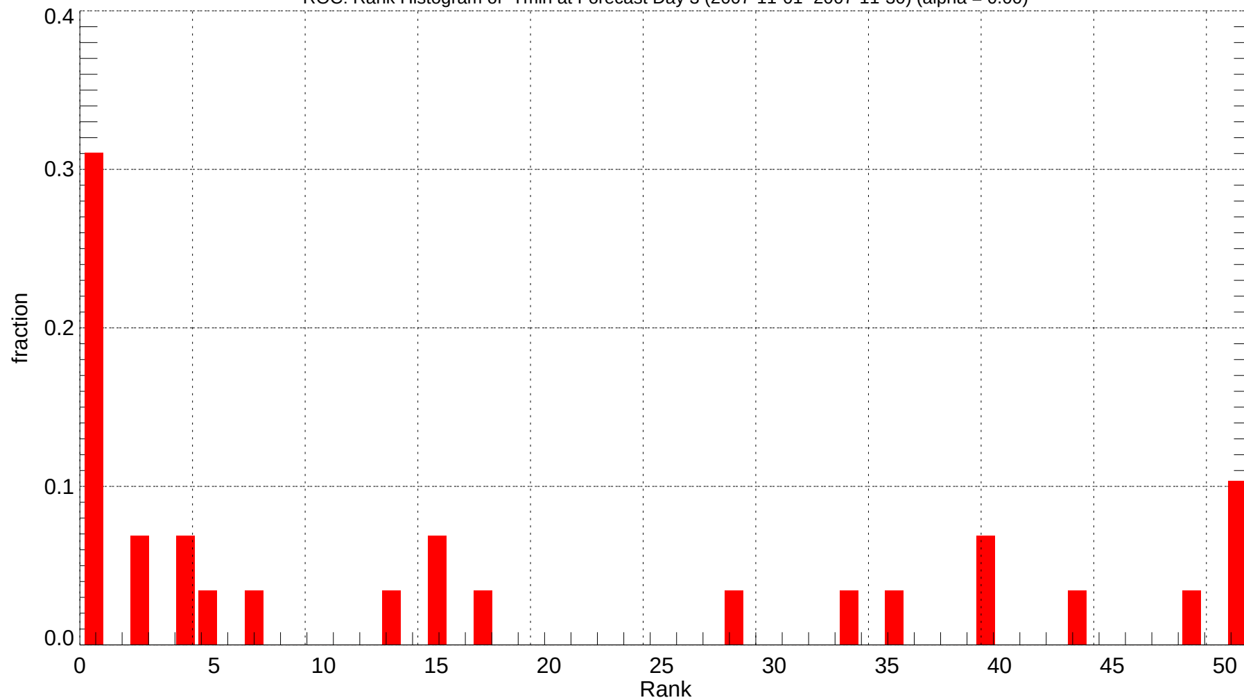
ROC: Rank Histogram of Tmin at Forecast Day 3 (2007-11-01~2007-11-30) (alpha = 0.00)
