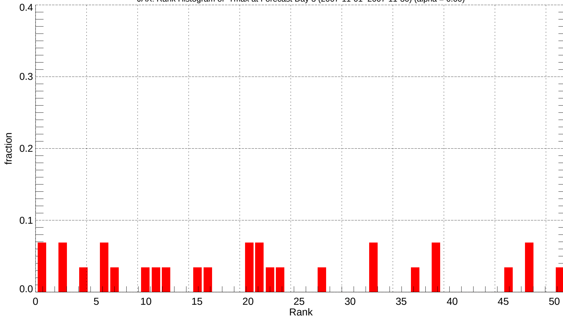
JAX: Rank Histogram of Tmax at Forecast Day 3 (2007-11-01~2007-11-30) (alpha = 0.00)
