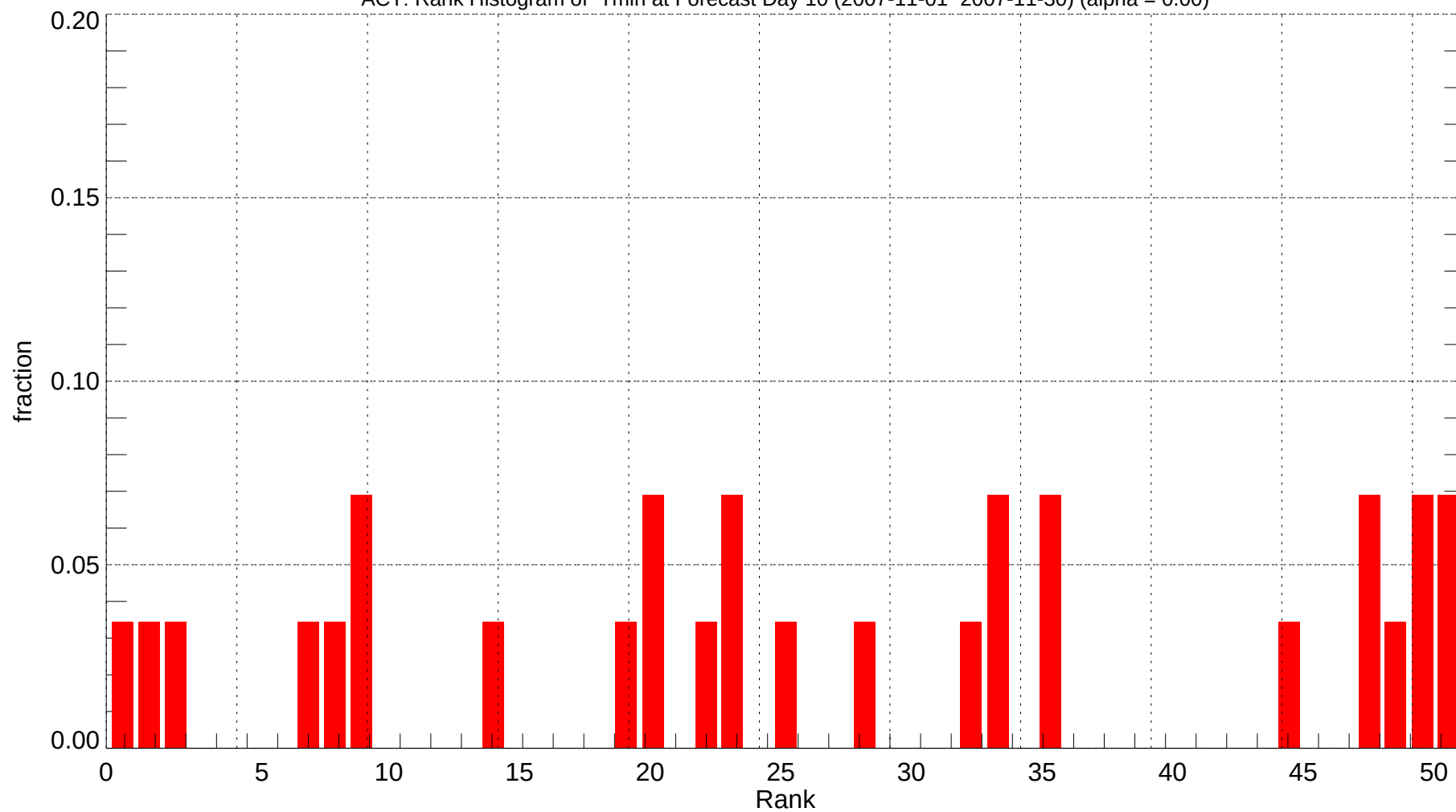
ACT: Rank Histogram of Tmin at Forecast Day 10 (2007-11-01~2007-11-30) (alpha = 0.00)
