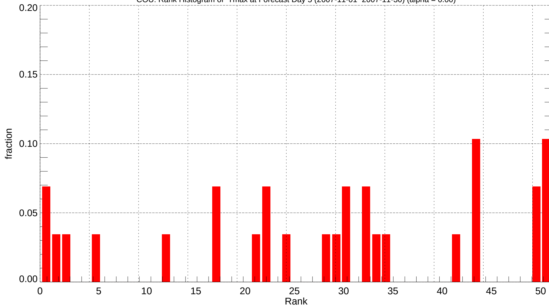
COU: Rank Histogram of Tmax at Forecast Day 5 (2007-11-01~2007-11-30) (alpha = 0.00)
