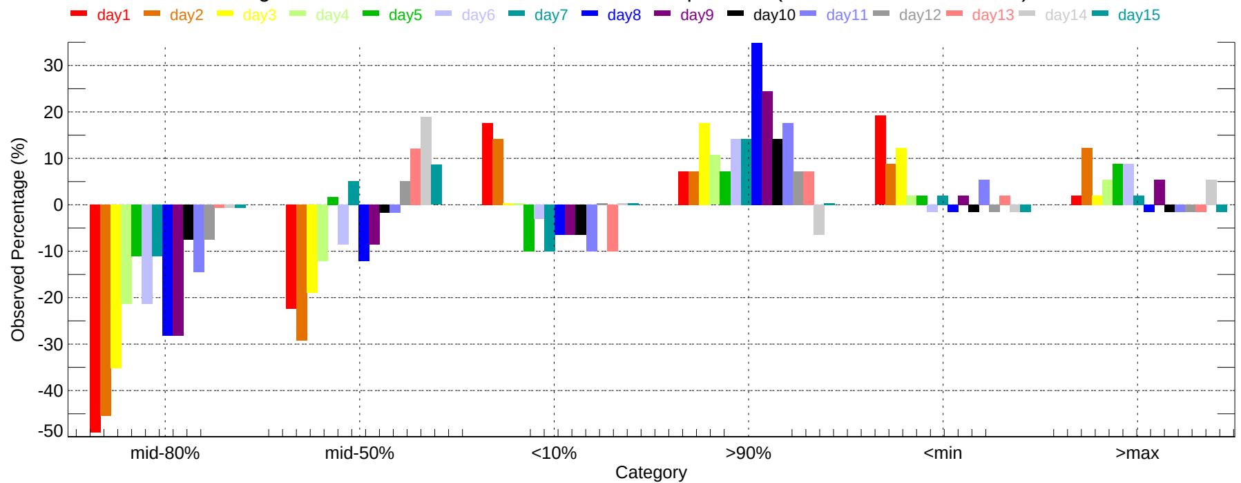
Observed Percentage Deviation of Ensembles - MSP: Min Temperature (2007-11-01~2007-11-30)
