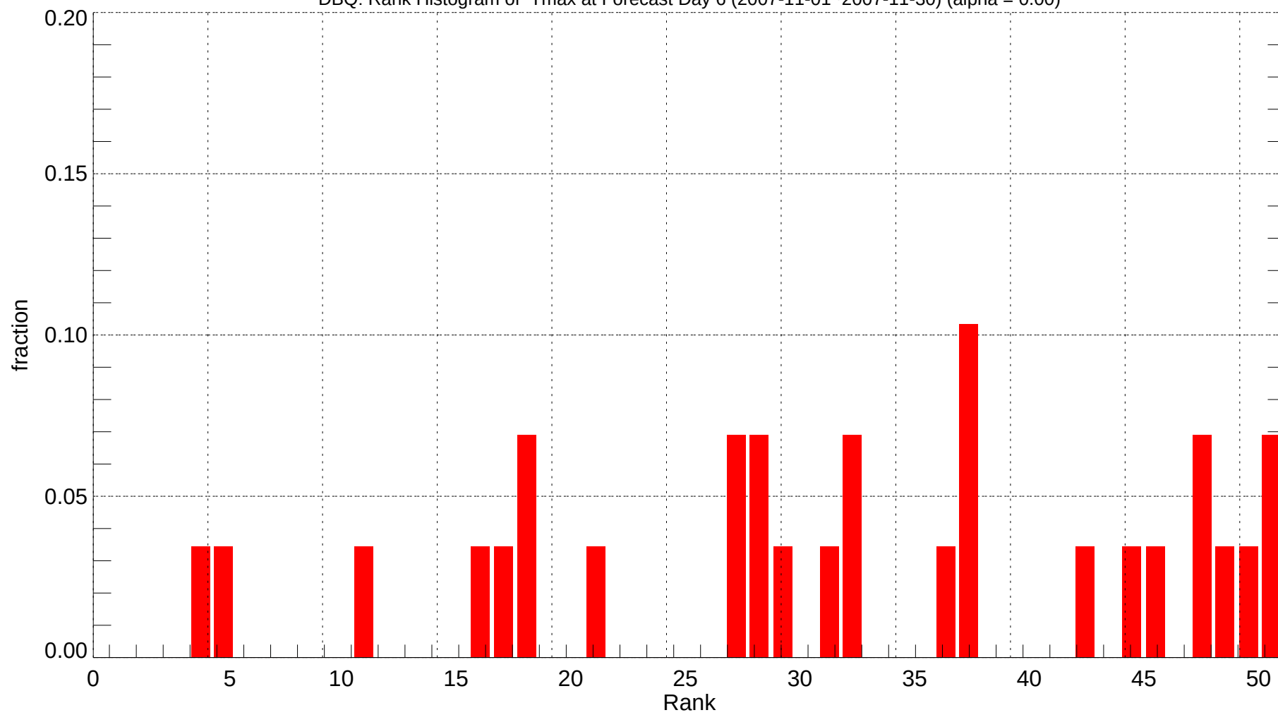
DBQ: Rank Histogram of Tmax at Forecast Day 6 (2007-11-01~2007-11-30) (alpha = 0.00)
