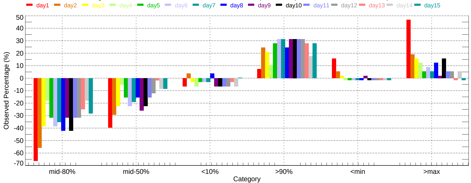
Observed Percentage Deviation of Ensembles - RAP: Min Temperature (2007-11-01~2007-11-30)
