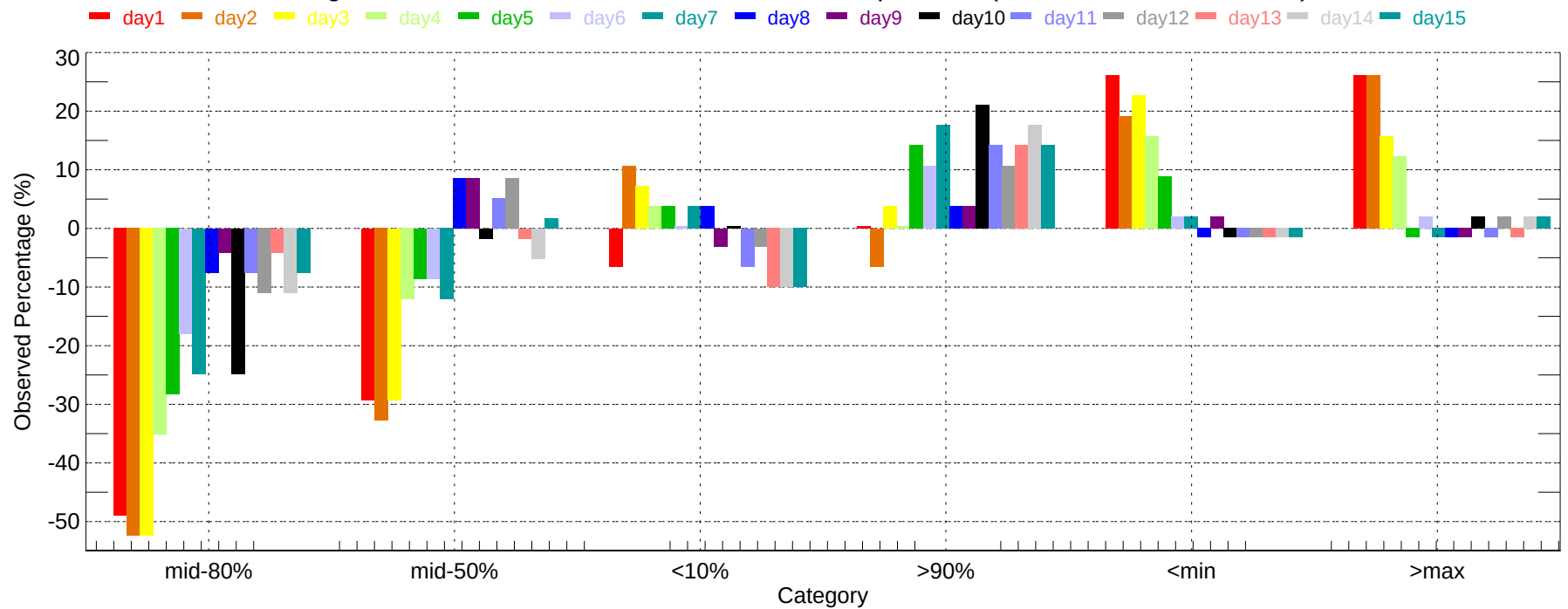
Observed Percentage Deviation of Ensembles - RNO: Max Temperature (2007-11-01~2007-11-30)
