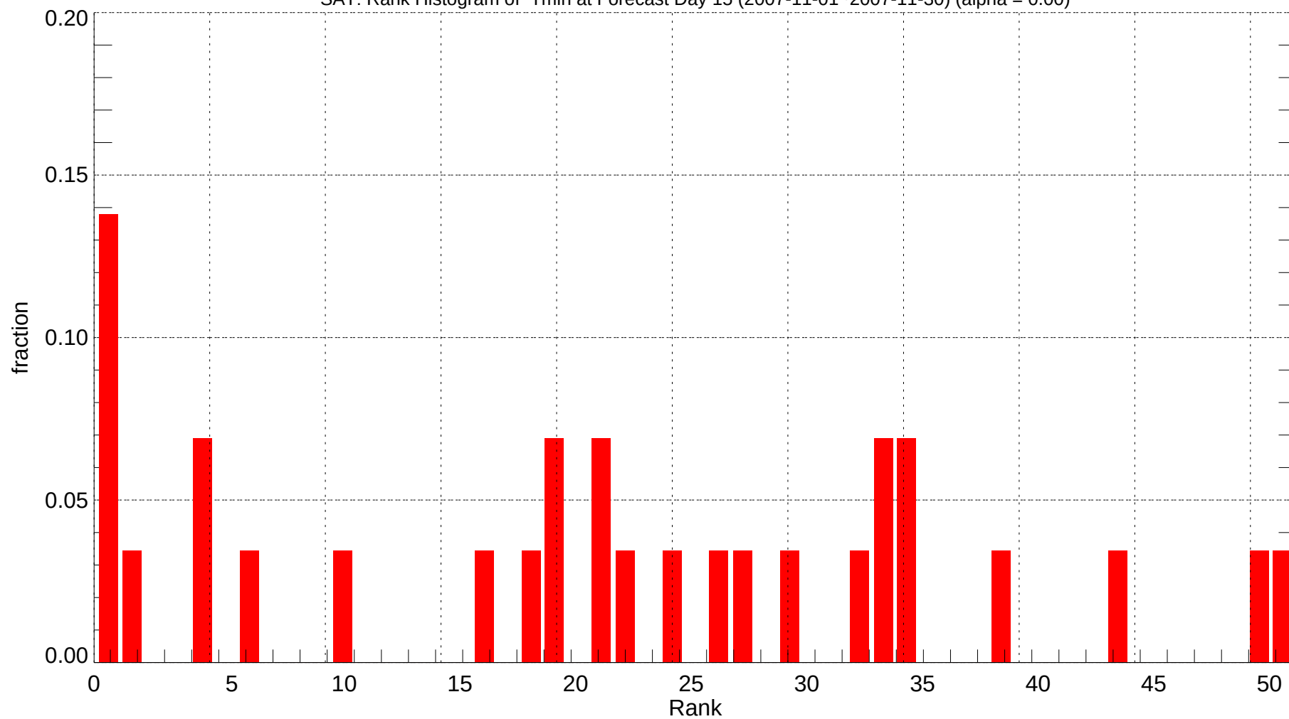
SAT: Rank Histogram of Tmin at Forecast Day 15 (2007-11-01~2007-11-30) (alpha = 0.00)
