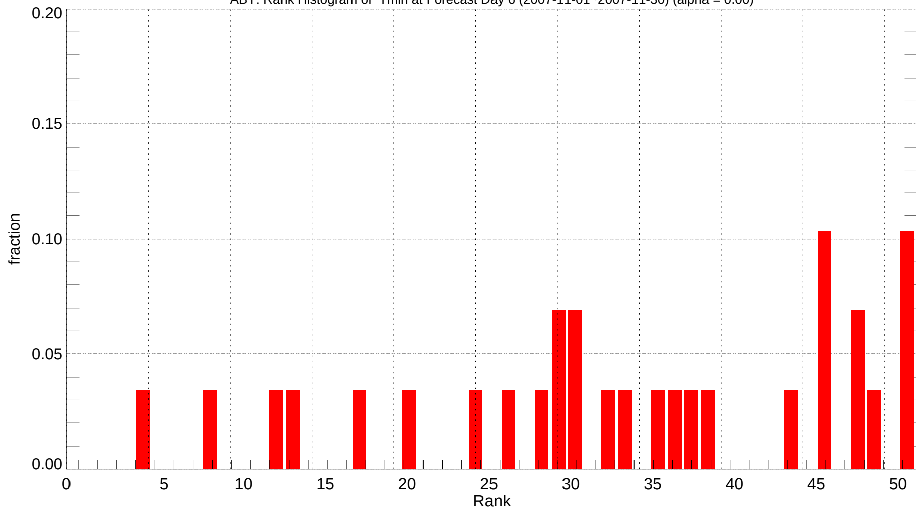
ABY: Rank Histogram of Tmin at Forecast Day 6 (2007-11-01~2007-11-30) (alpha = 0.00)
