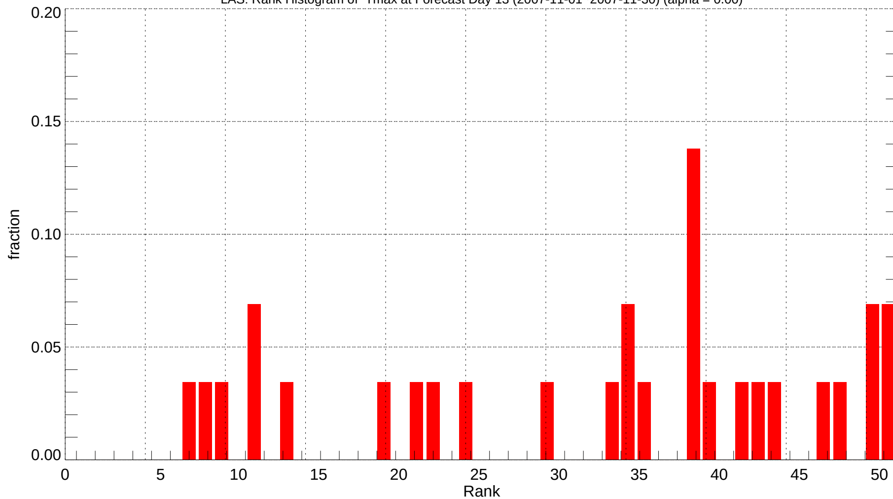
LAS: Rank Histogram of Tmax at Forecast Day 13 (2007-11-01~2007-11-30) (alpha = 0.00)
