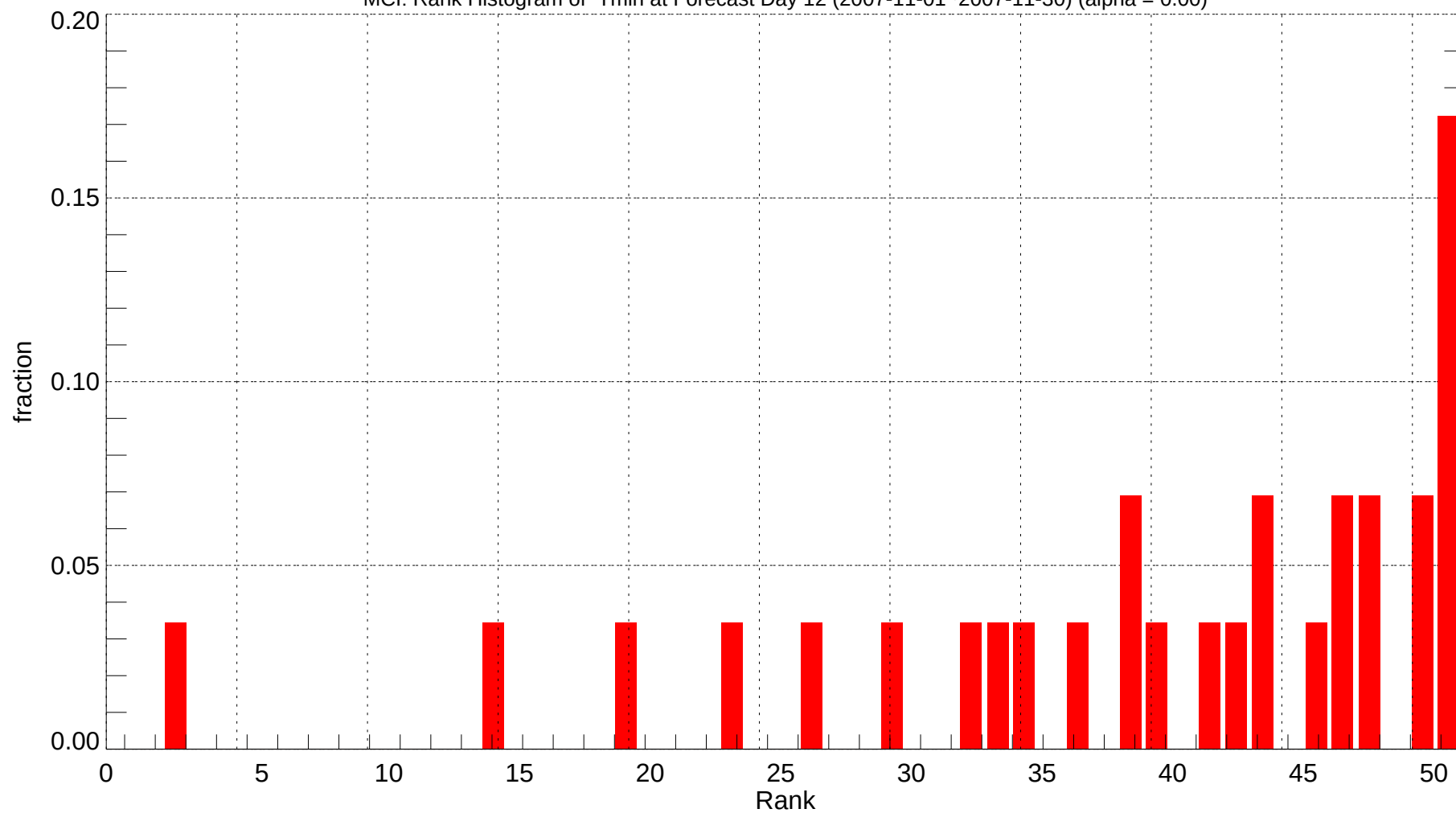
MCI: Rank Histogram of Tmin at Forecast Day 12 (2007-11-01~2007-11-30) (alpha = 0.00)
