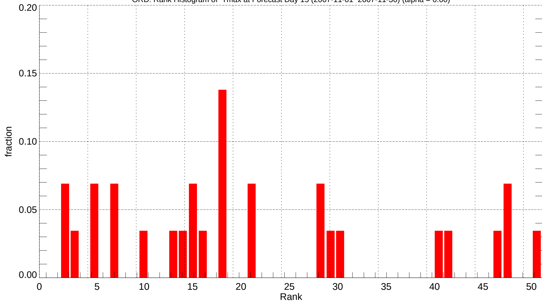
ORD: Rank Histogram of Tmax at Forecast Day 15 (2007-11-01~2007-11-30) (alpha = 0.00)
