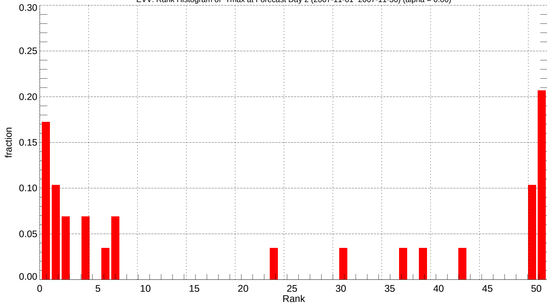
EVV: Rank Histogram of Tmax at Forecast Day 2 (2007-11-01~2007-11-30) (alpha = 0.00)
