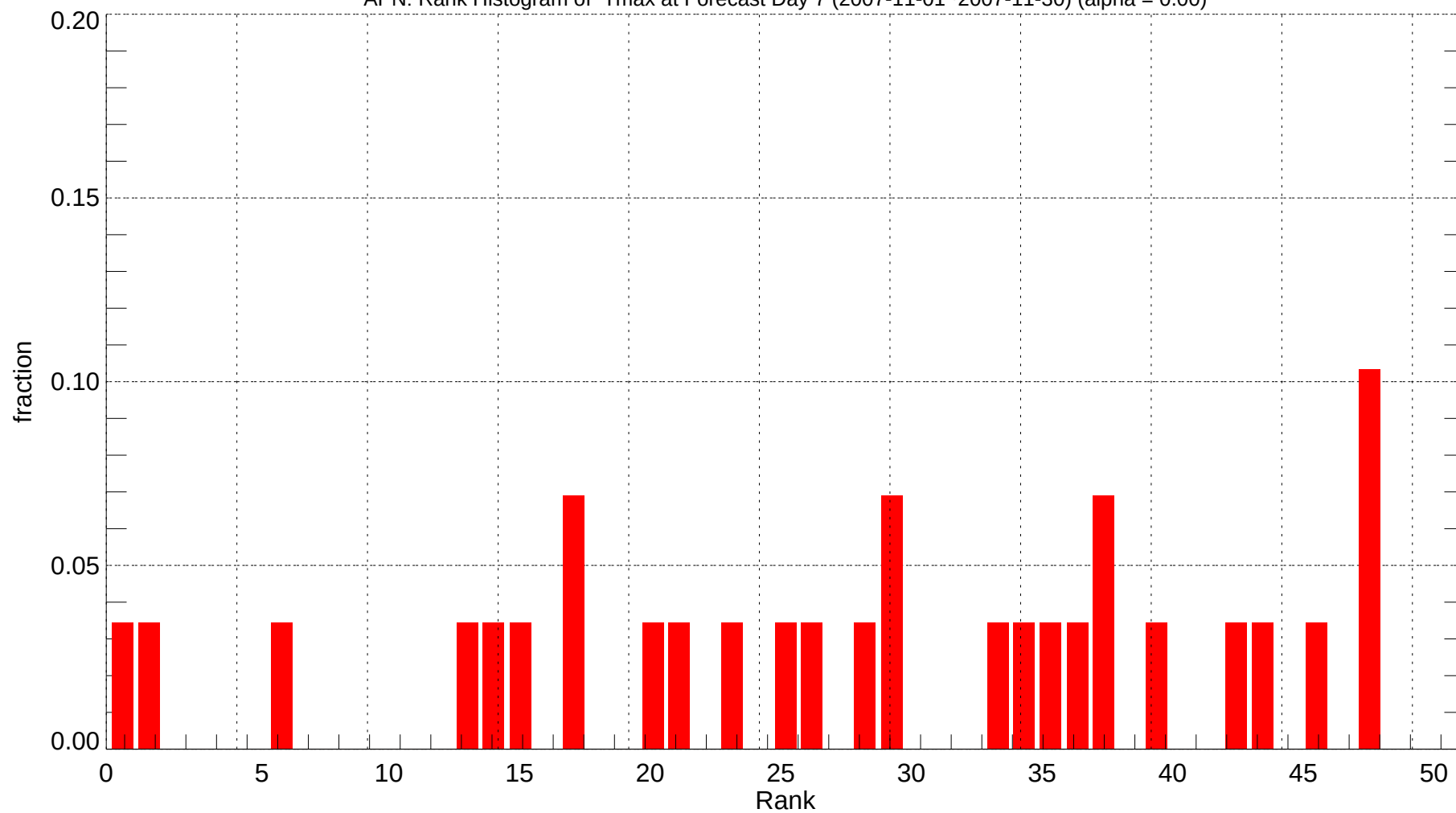
APN: Rank Histogram of Tmax at Forecast Day 7 (2007-11-01~2007-11-30) (alpha = 0.00)
