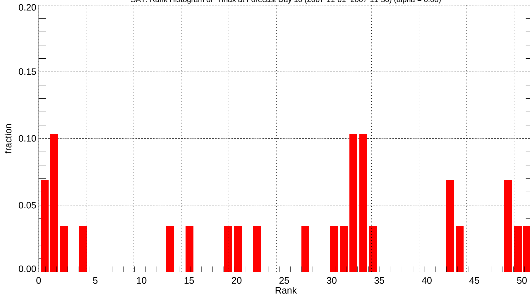
SAT: Rank Histogram of Tmax at Forecast Day 10 (2007-11-01~2007-11-30) (alpha = 0.00)
