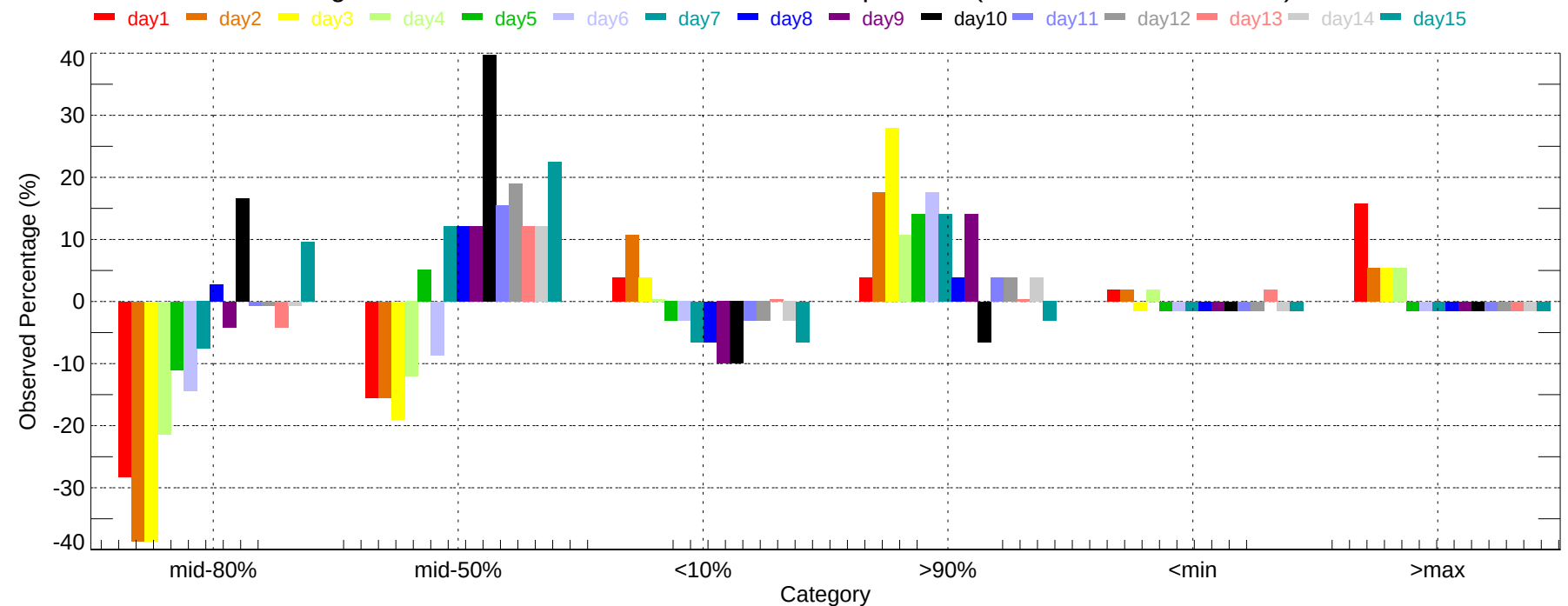
Observed Percentage Deviation of Ensembles - TLH: Min Temperature (2007-11-01~2007-11-30)
