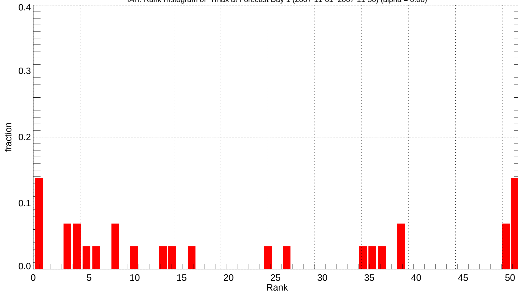
IAH: Rank Histogram of Tmax at Forecast Day 1 (2007-11-01~2007-11-30) (alpha = 0.00)
