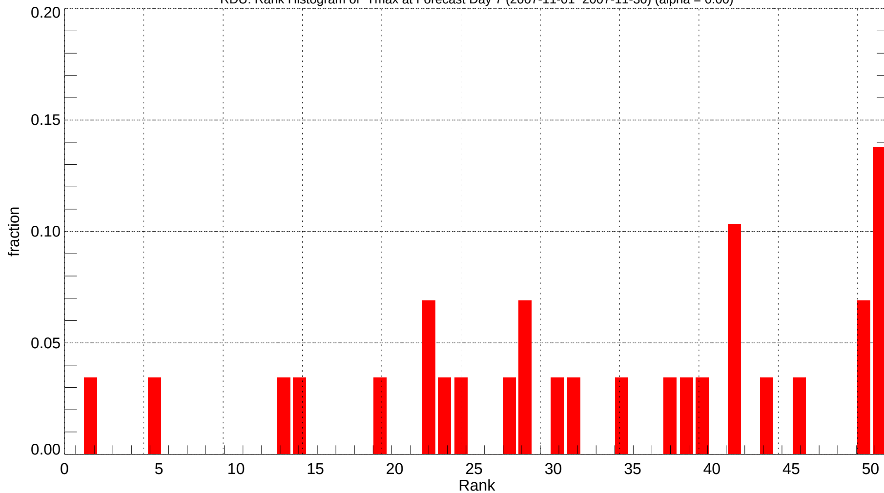
RDU: Rank Histogram of Tmax at Forecast Day 7 (2007-11-01~2007-11-30) (alpha = 0.00)
