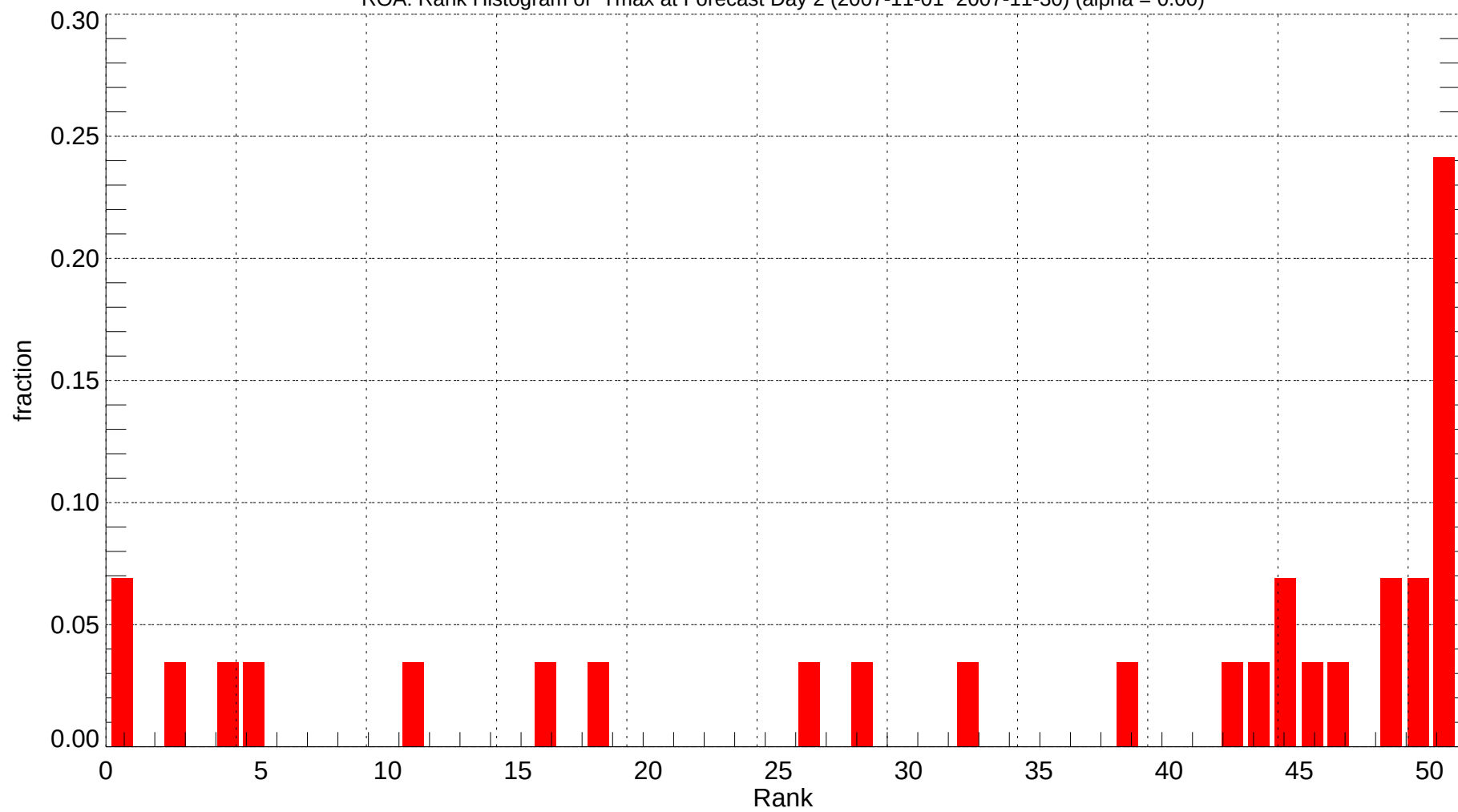
ROA: Rank Histogram of Tmax at Forecast Day 2 (2007-11-01~2007-11-30) (alpha = 0.00)
