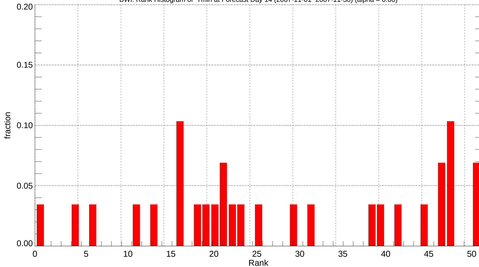
BWl: Rank Histogram of Tmin at Forecast Day 14 (2007-11-01~2007-11-30) (alpha = 0.00)
