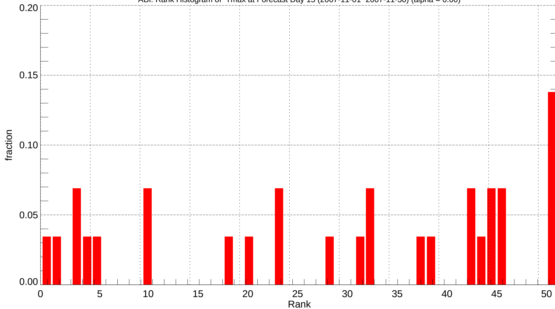
ABI: Rank Histogram of Tmax at Forecast Day 15 (2007-11-01~2007-11-30) (alpha = 0.00)
