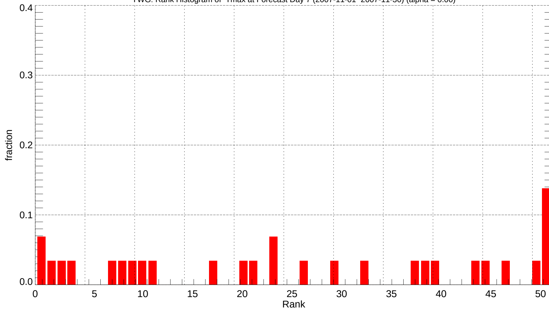
YWG: Rank Histogram of Tmax at Forecast Day 7 (2007-11-01~2007-11-30) (alpha = 0.00)
