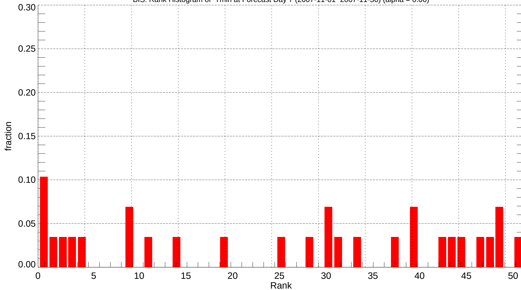
BIS: Rank Histogram of Tmin at Forecast Day 7 (2007-11-01~2007-11-30) (alpha = 0.00)
