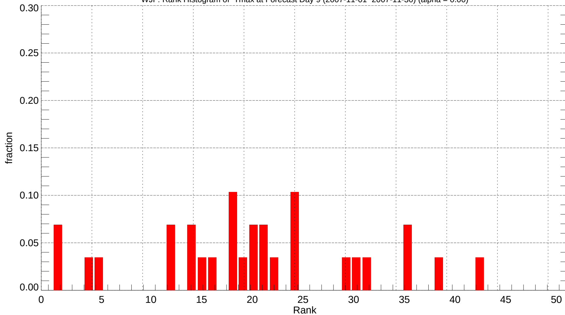
WJF: Rank Histogram of Tmax at Forecast Day 9 (2007-11-01~2007-11-30) (alpha = 0.00)
