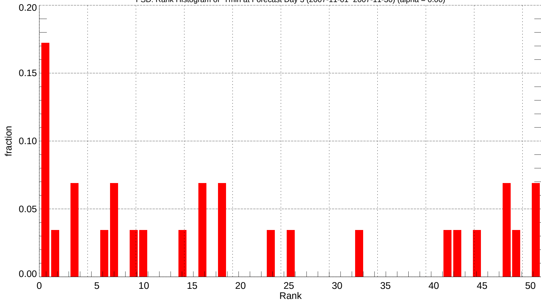
FSD: Rank Histogram of Tmin at Forecast Day 3 (2007-11-01~2007-11-30) (alpha = 0.00)
