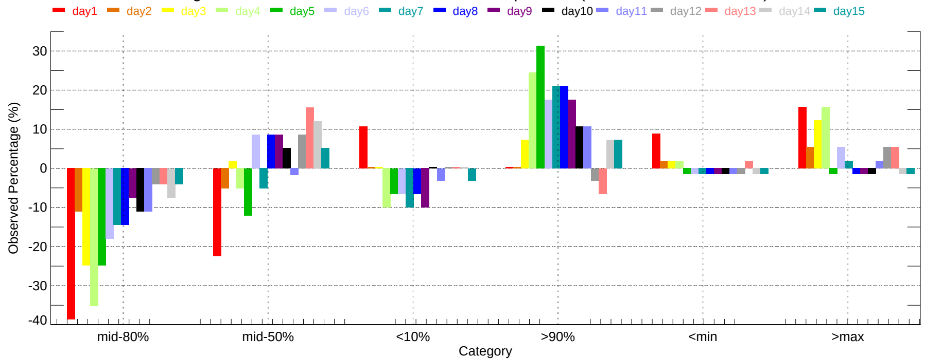
Observed Percentage Deviation of Ensembles - ABY: Max Temperature (2007-11-01~2007-11-30)
