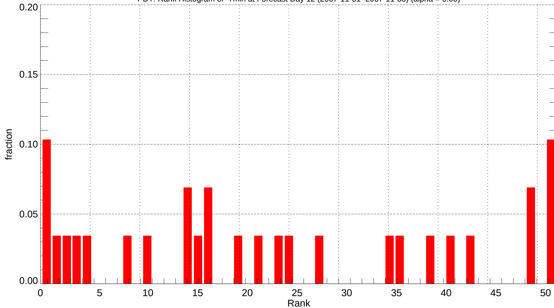
PDT: Rank Histogram of Tmin at Forecast Day 12 (2007-11-01~2007-11-30) (alpha = 0.00)
