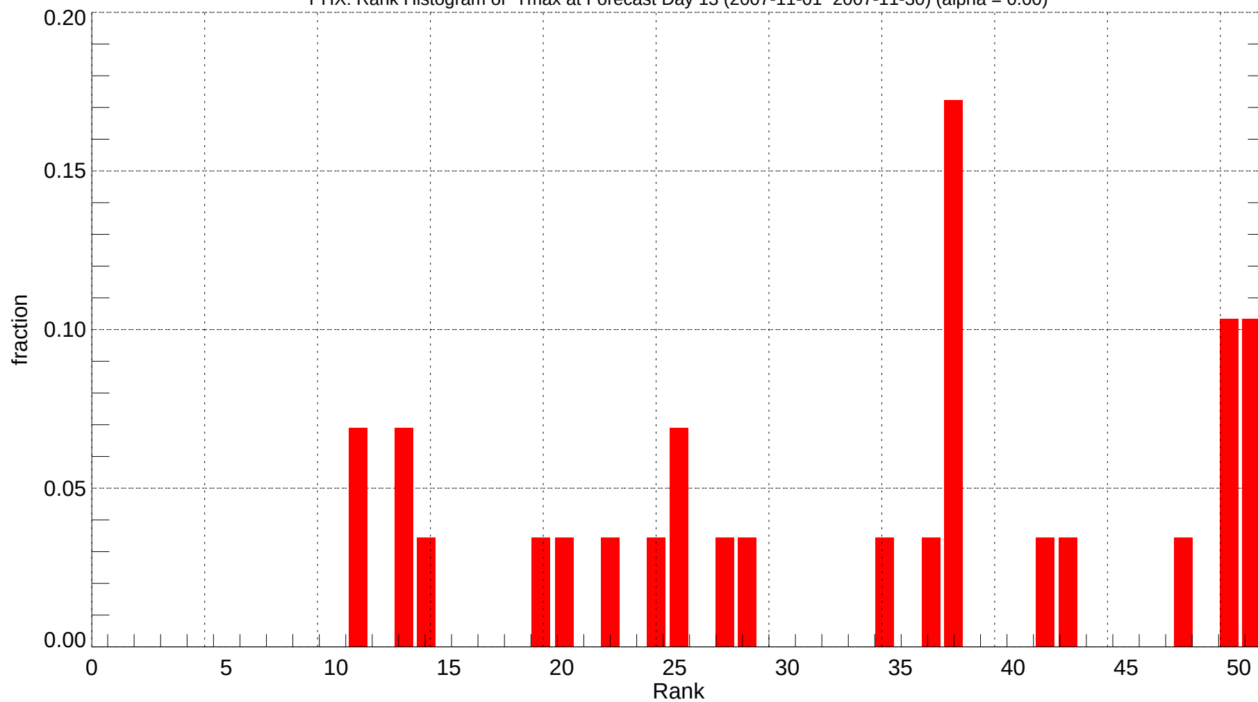
PHX: Rank Histogram of Tmax at Forecast Day 13 (2007-11-01~2007-11-30) (alpha = 0.00)
