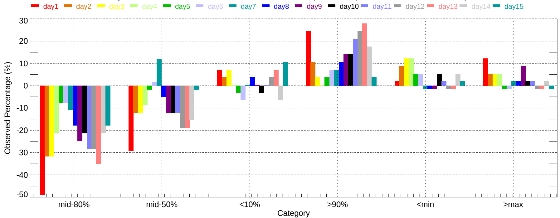
Observed Percentage Deviation of Ensembles - DFW: Max Temperature (2007-11-01~2007-11-30)
