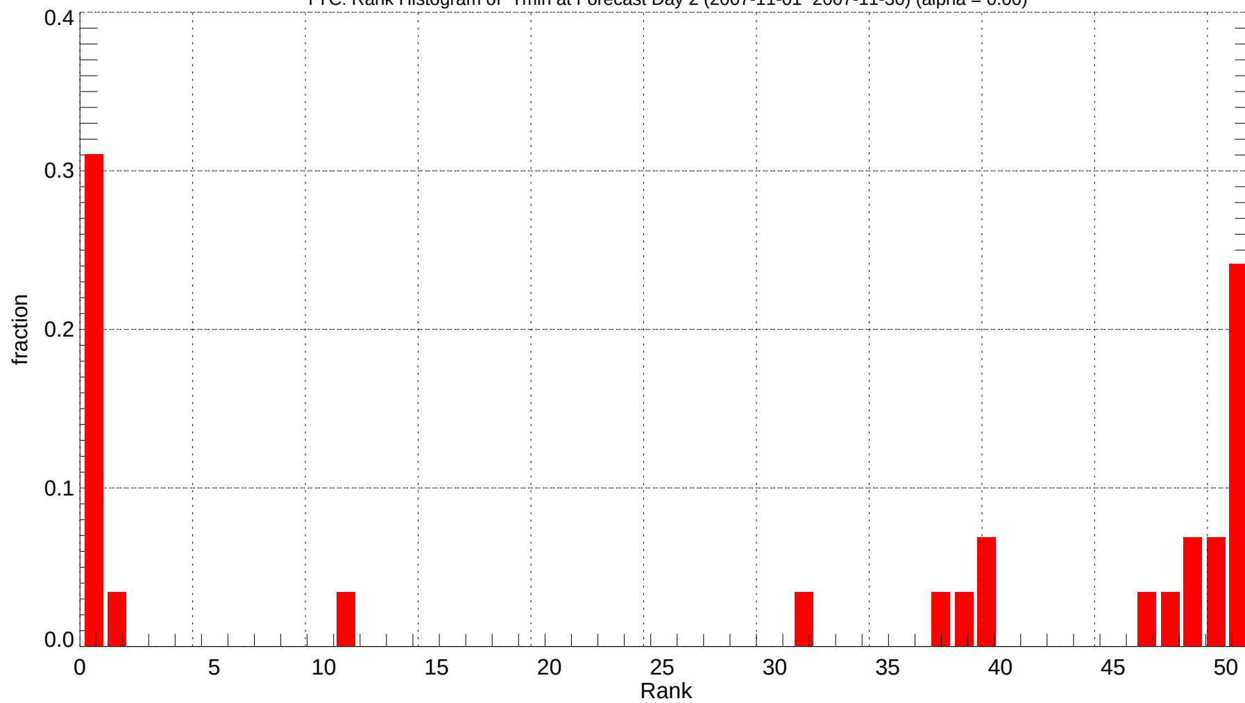
YYC: Rank Histogram of Tmin at Forecast Day 2 (2007-11-01~2007-11-30) (alpha = 0.00)
