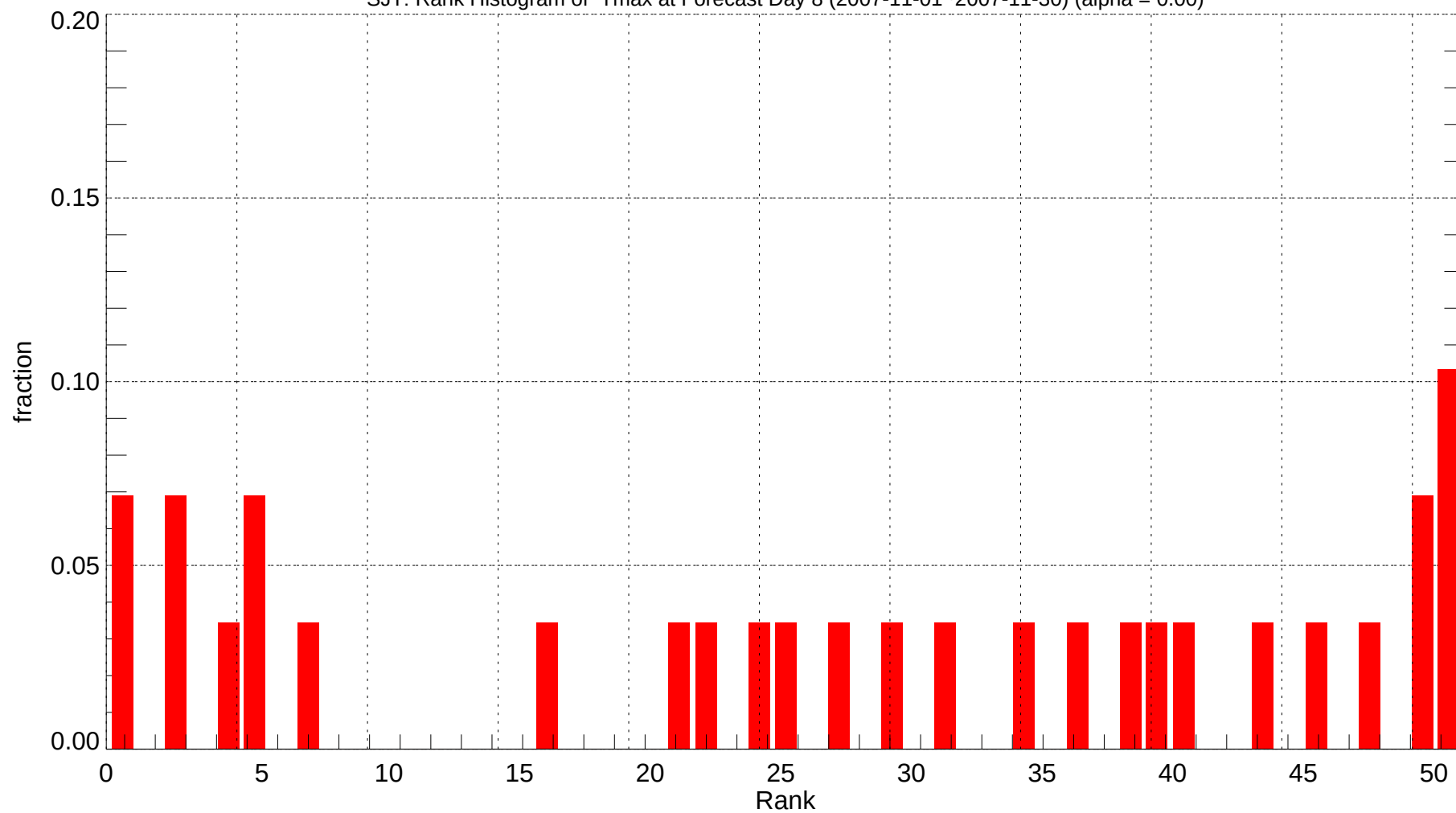
SJT: Rank Histogram of Tmax at Forecast Day 8 (2007-11-01~2007-11-30) (alpha = 0.00)
