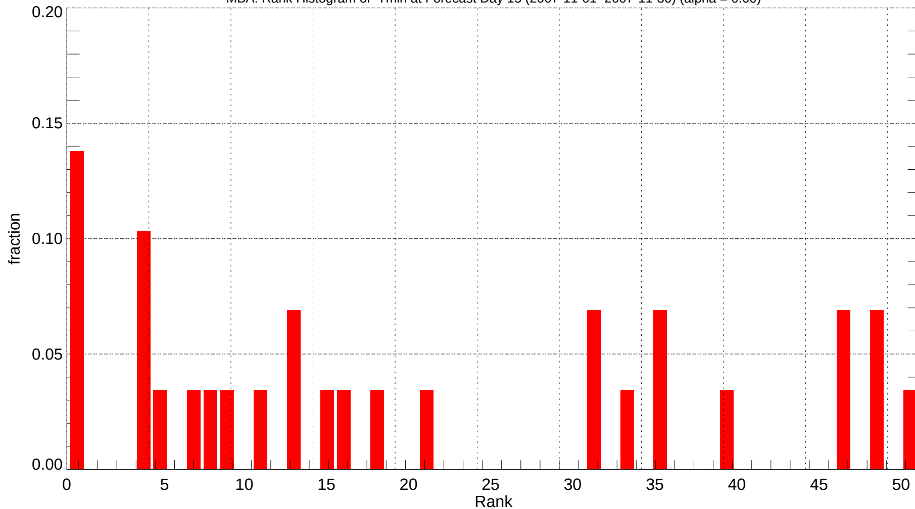
MBA: Rank Histogram of Tmin at Forecast Day 15 (2007-11-01~2007-11-30) (alpha = 0.00)
