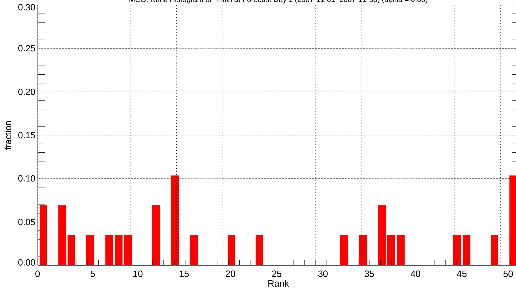
MCO: Rank Histogram of Tmin at Forecast Day 1 (2007-11-01~2007-11-30) (alpha = 0.00)
