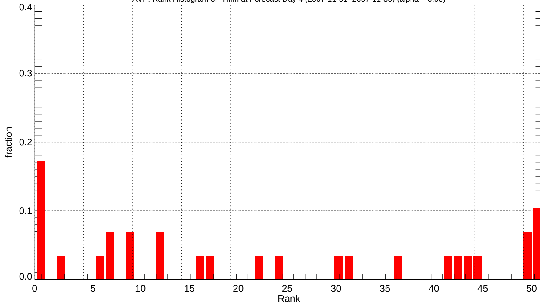
AVP: Rank Histogram of Tmin at Forecast Day 4 (2007-11-01~2007-11-30) (alpha = 0.00)
