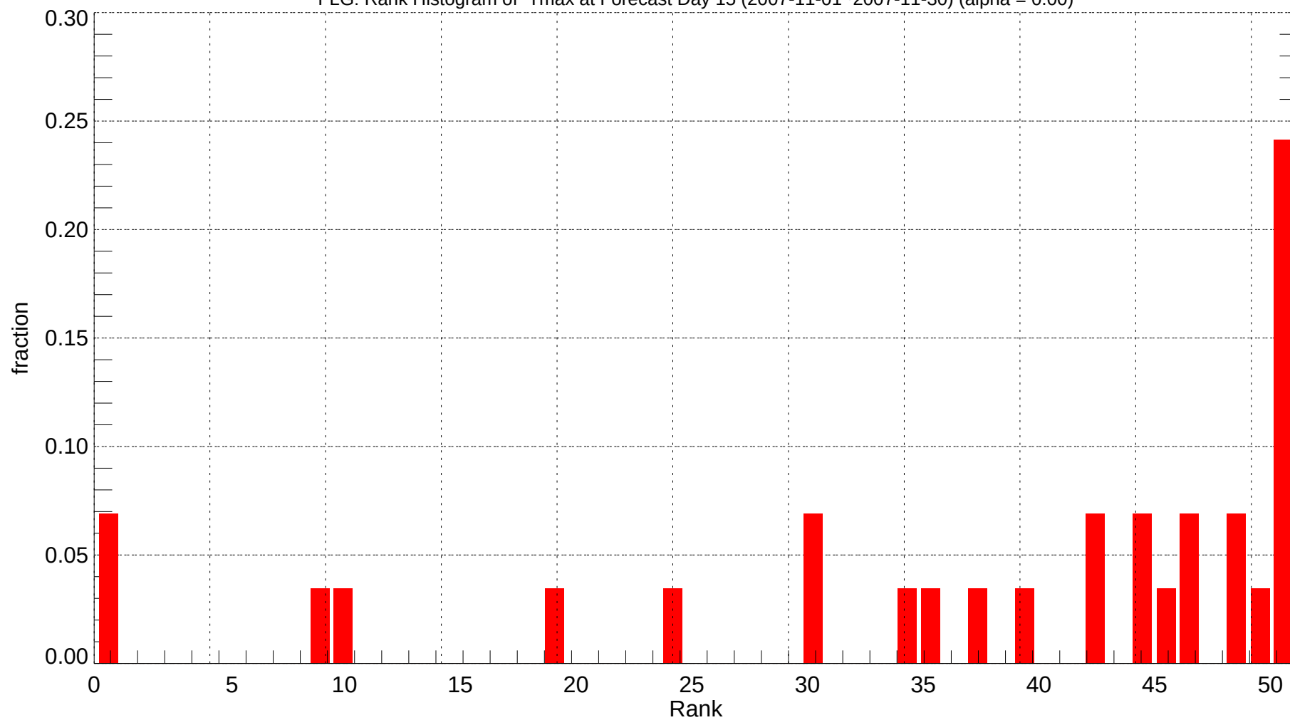
FLG: Rank Histogram of Tmax at Forecast Day 15 (2007-11-01~2007-11-30) (alpha = 0.00)
