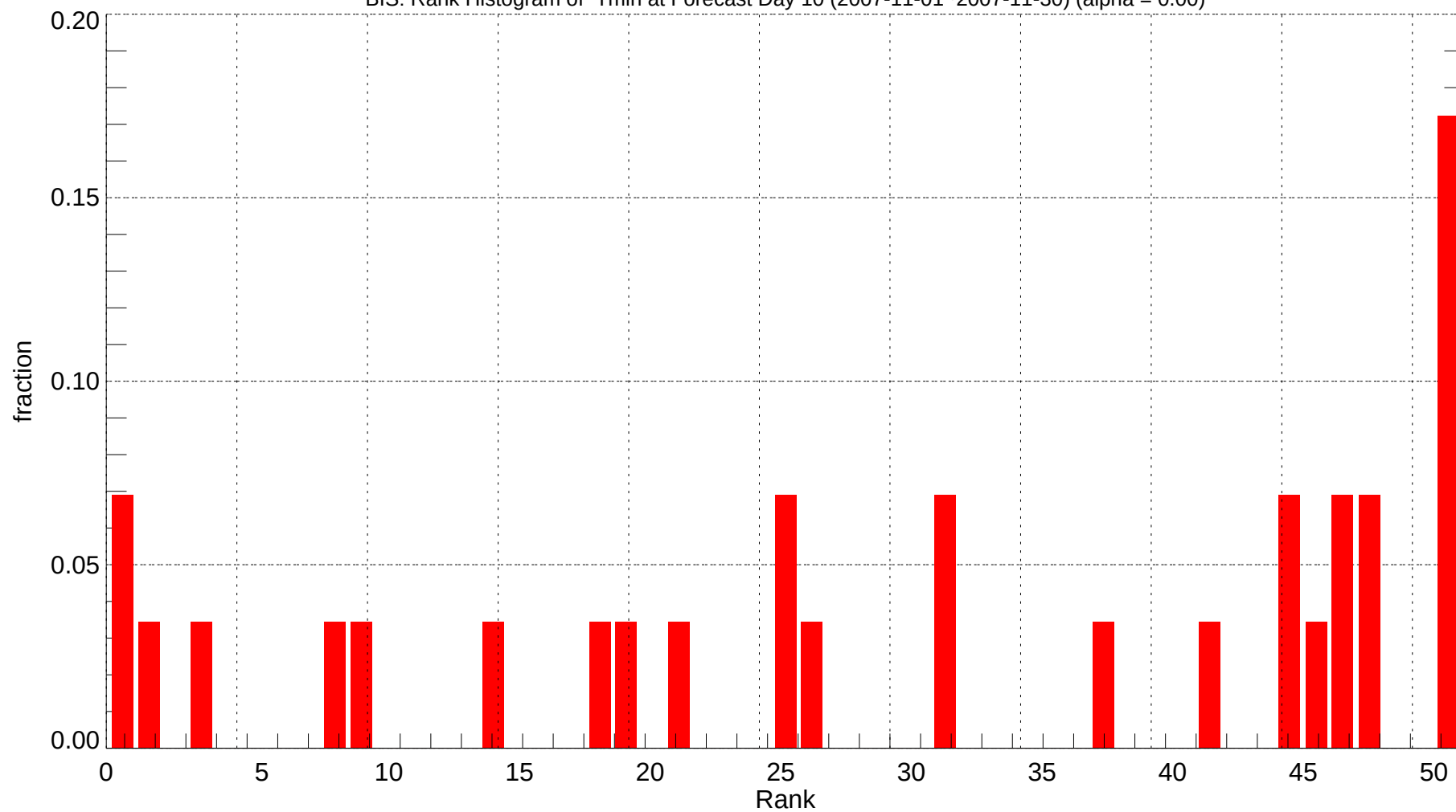
BIS: Rank Histogram of Tmin at Forecast Day 10 (2007-11-01~2007-11-30) (alpha = 0.00)
