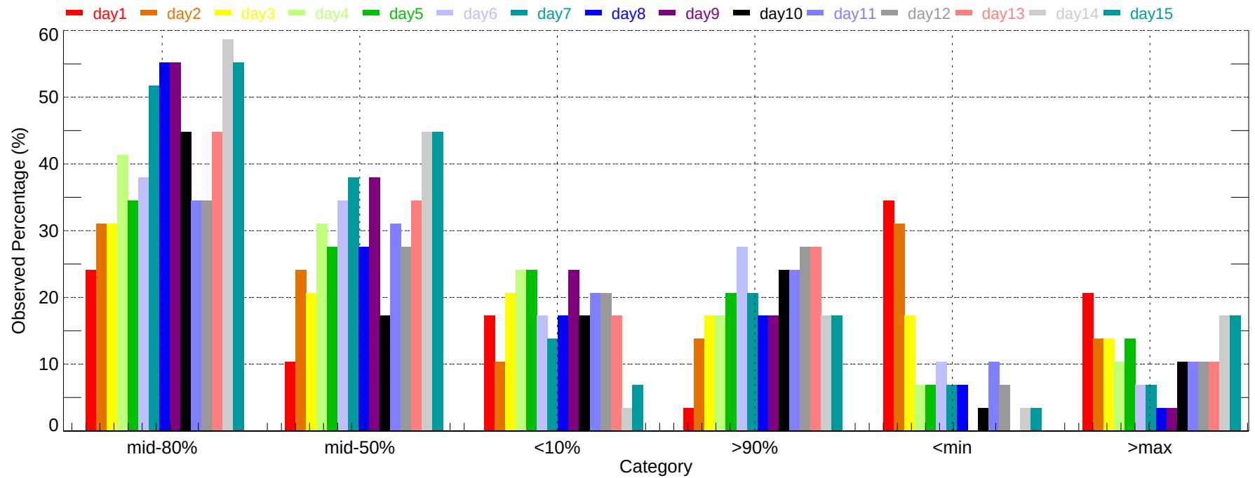
Observed Percentage of Ensembles - BUR: Min Temperature (2007-11-01~2007-11-30)
