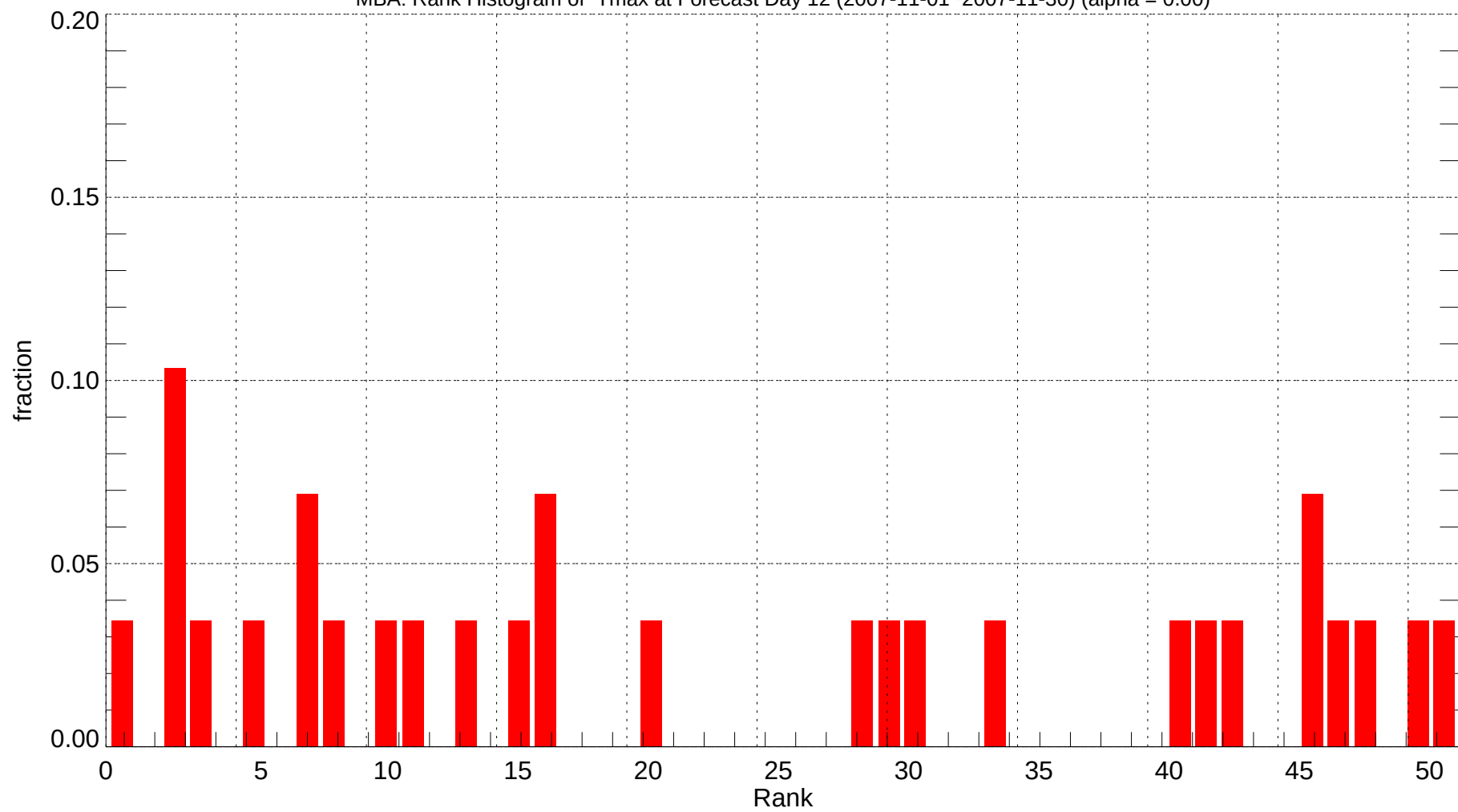
MBA: Rank Histogram of Tmax at Forecast Day 12 (2007-11-01~2007-11-30) (alpha = 0.00)
