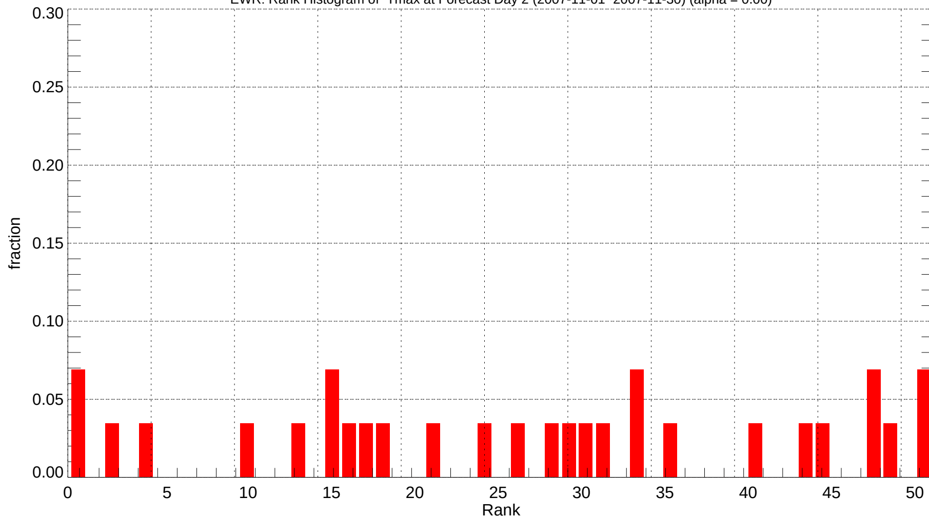
EWR: Rank Histogram of Tmax at Forecast Day 2 (2007-11-01~2007-11-30) (alpha = 0.00)
