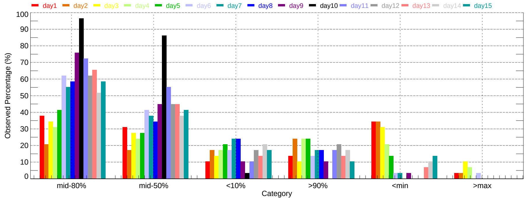
Observed Percentage of Ensembles - MHT: Min Temperature (2007-11-01~2007-11-30)
