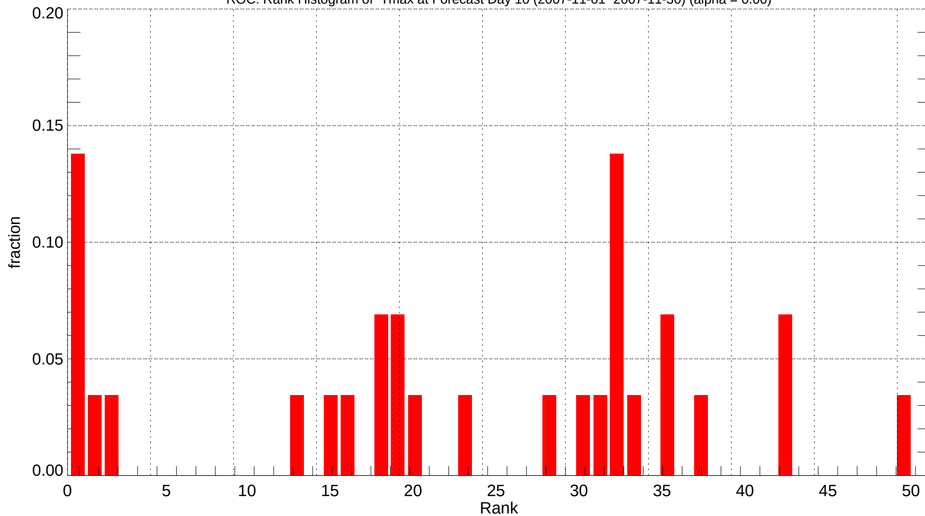
ROC: Rank Histogram of Tmax at Forecast Day 10 (2007-11-01~2007-11-30) (alpha = 0.00)
