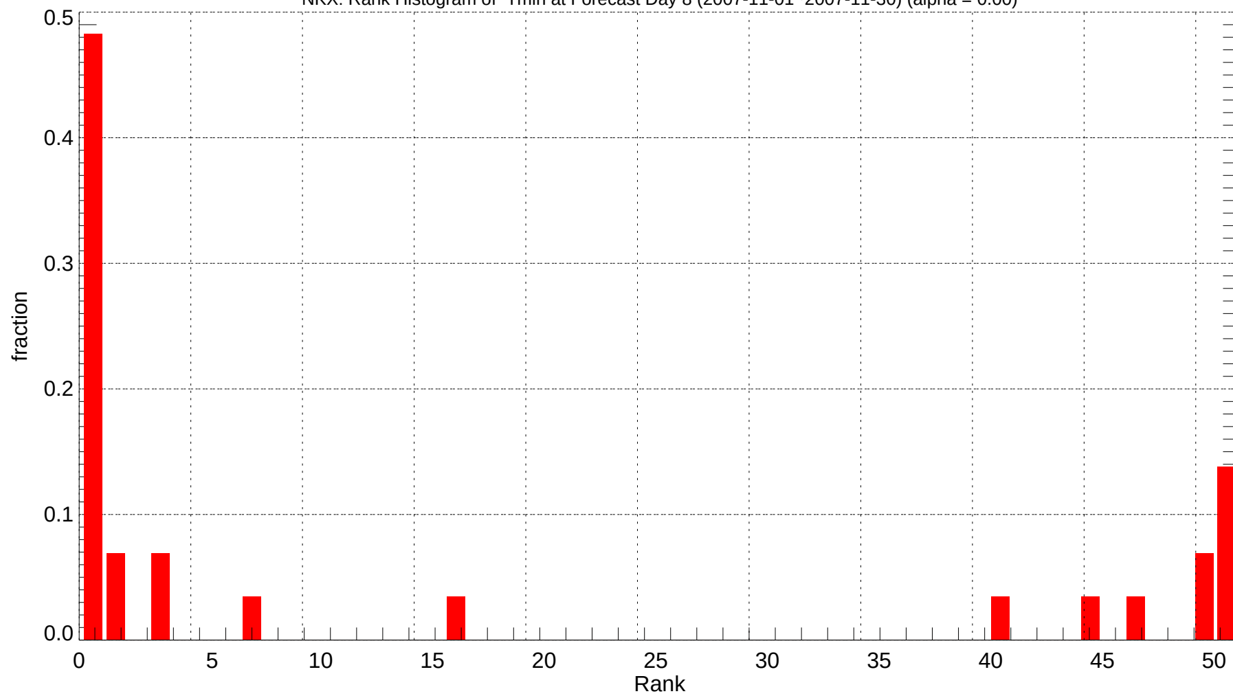
NKX: Rank Histogram of Tmin at Forecast Day 8 (2007-11-01~2007-11-30) (alpha = 0.00)
