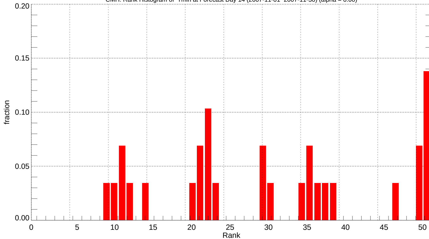
CMH: Rank Histogram of Tmin at Forecast Day 14 (2007-11-01~2007-11-30) (alpha = 0.00)
