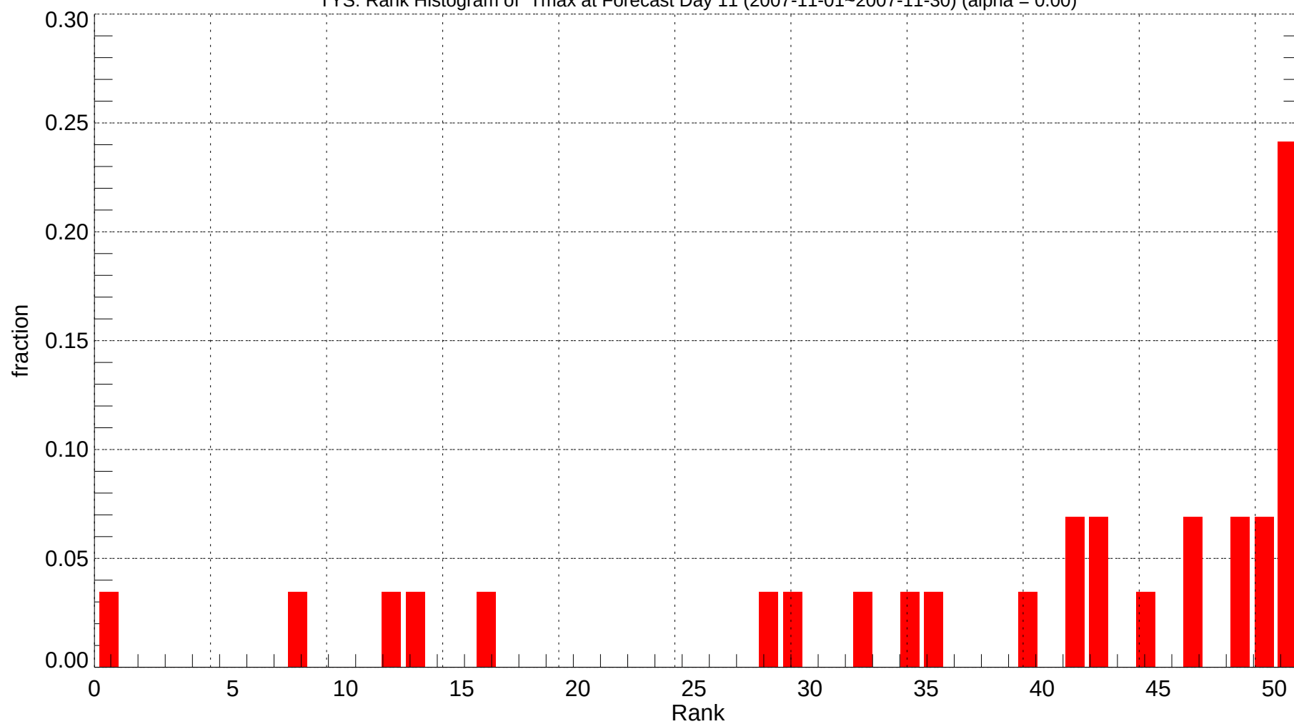
TYS: Rank Histogram of Tmax at Forecast Day 11 (2007-11-01~2007-11-30) (alpha = 0.00)
