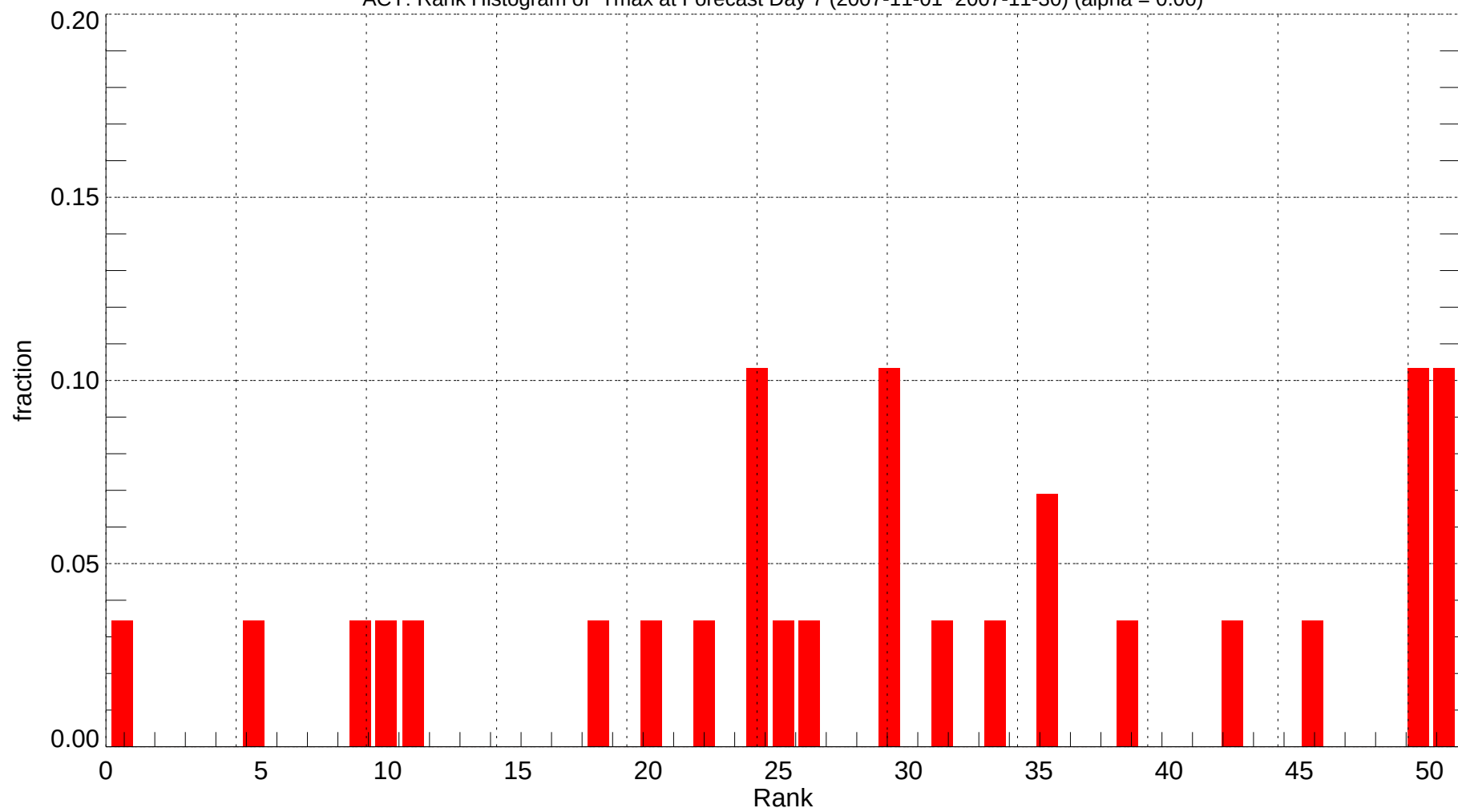
ACY: Rank Histogram of Tmax at Forecast Day 7 (2007-11-01~2007-11-30) (alpha = 0.00)
