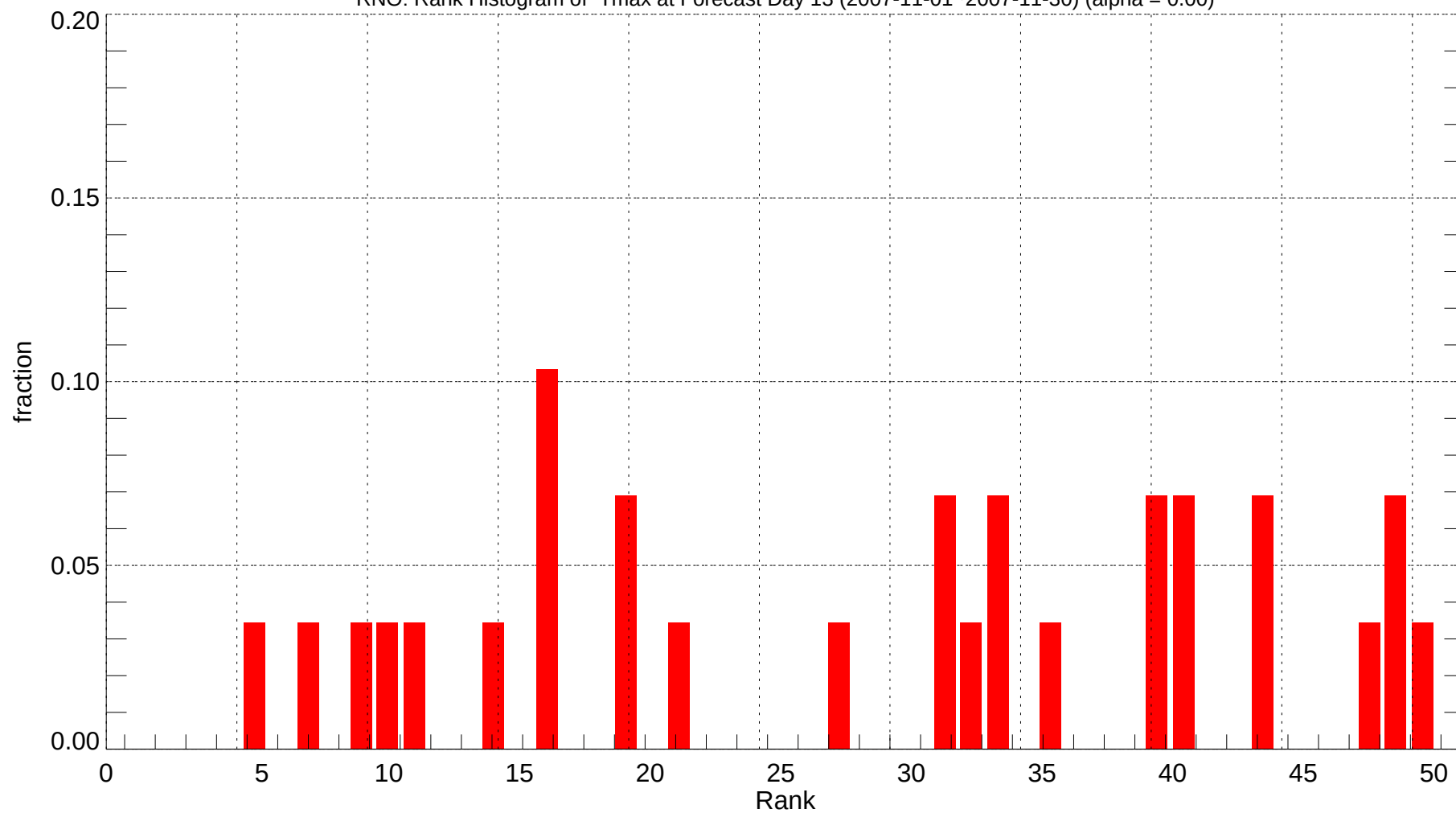
RNO: Rank Histogram of Tmax at Forecast Day 13 (2007-11-01~2007-11-30) (alpha = 0.00)
