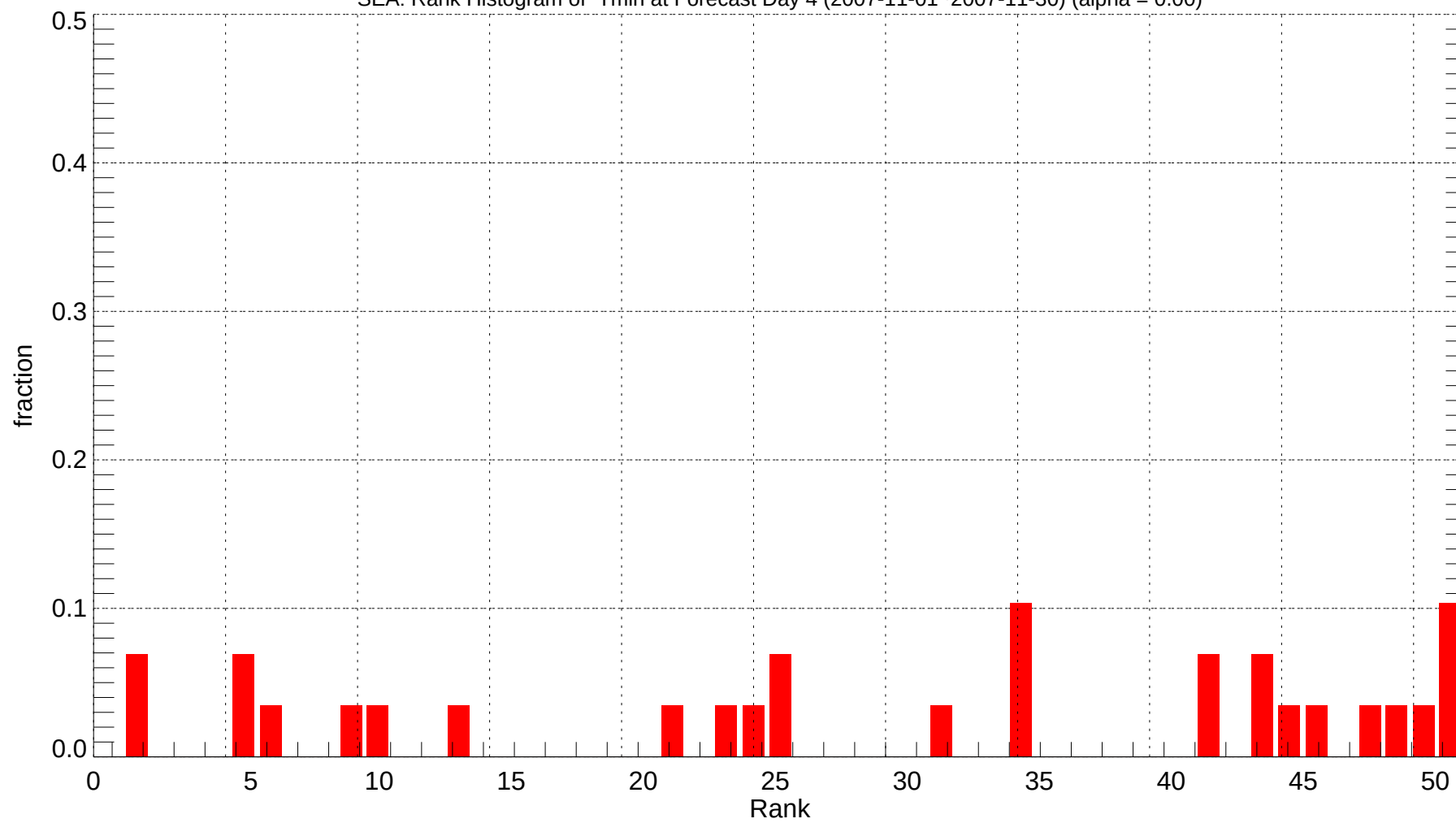
SEA: Rank Histogram of Tmin at Forecast Day 4 (2007-11-01~2007-11-30) (alpha = 0.00)
