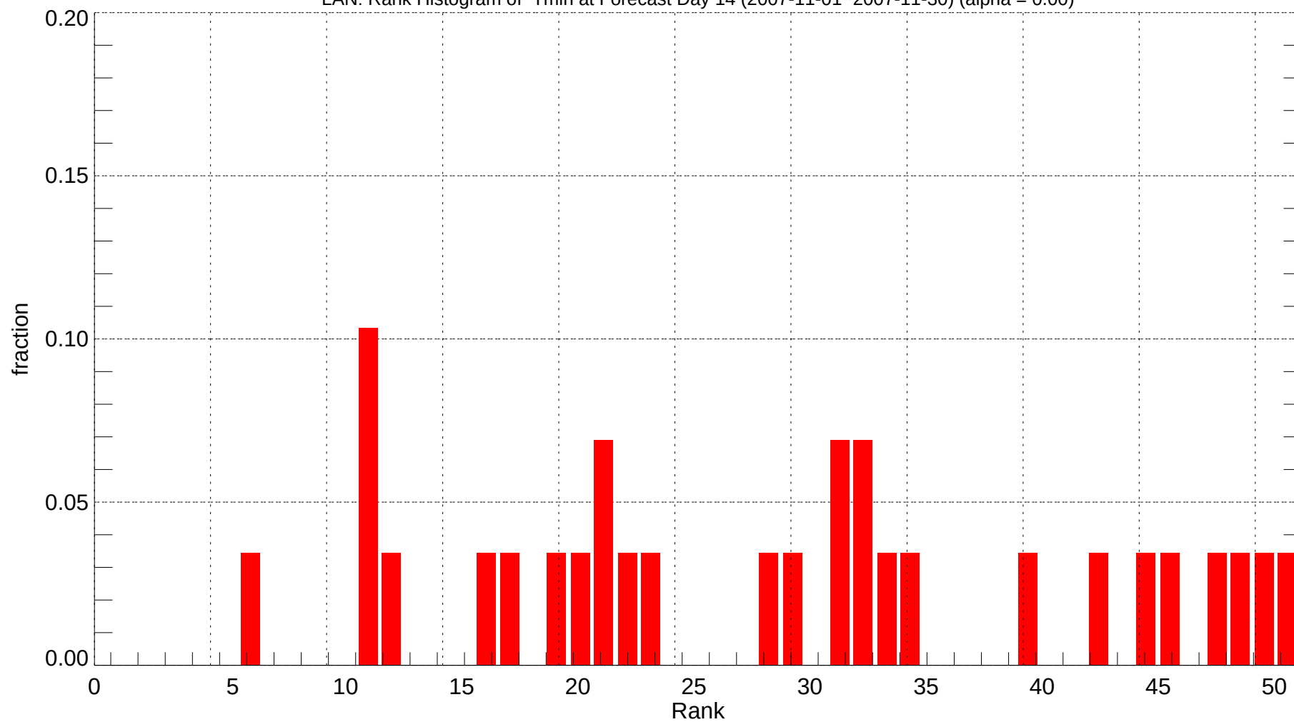
LAN: Rank Histogram of Tmin at Forecast Day 14 (2007-11-01~2007-11-30) (alpha = 0.00)
