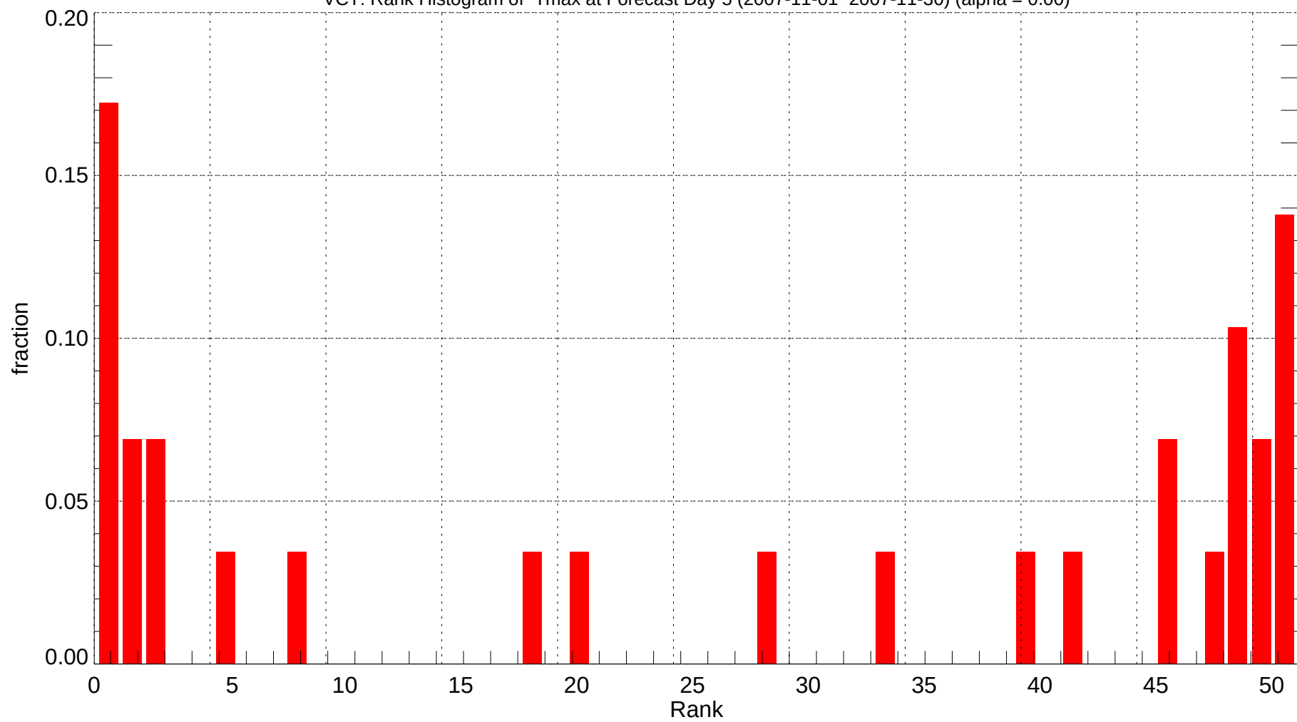
VCT: Rank Histogram of Tmax at Forecast Day 5 (2007-11-01~2007-11-30) (alpha = 0.00)
