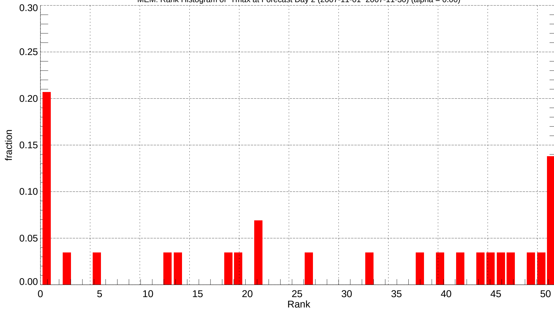
MEM: Rank Histogram of Tmax at Forecast Day 2 (2007-11-01~2007-11-30) (alpha = 0.00)
