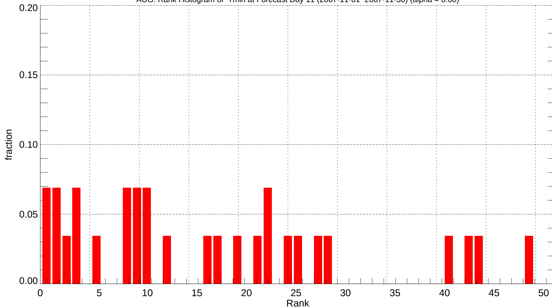
AUG: Rank Histogram of Tmin at Forecast Day 11 (2007-11-01~2007-11-30) (alpha = 0.00)
