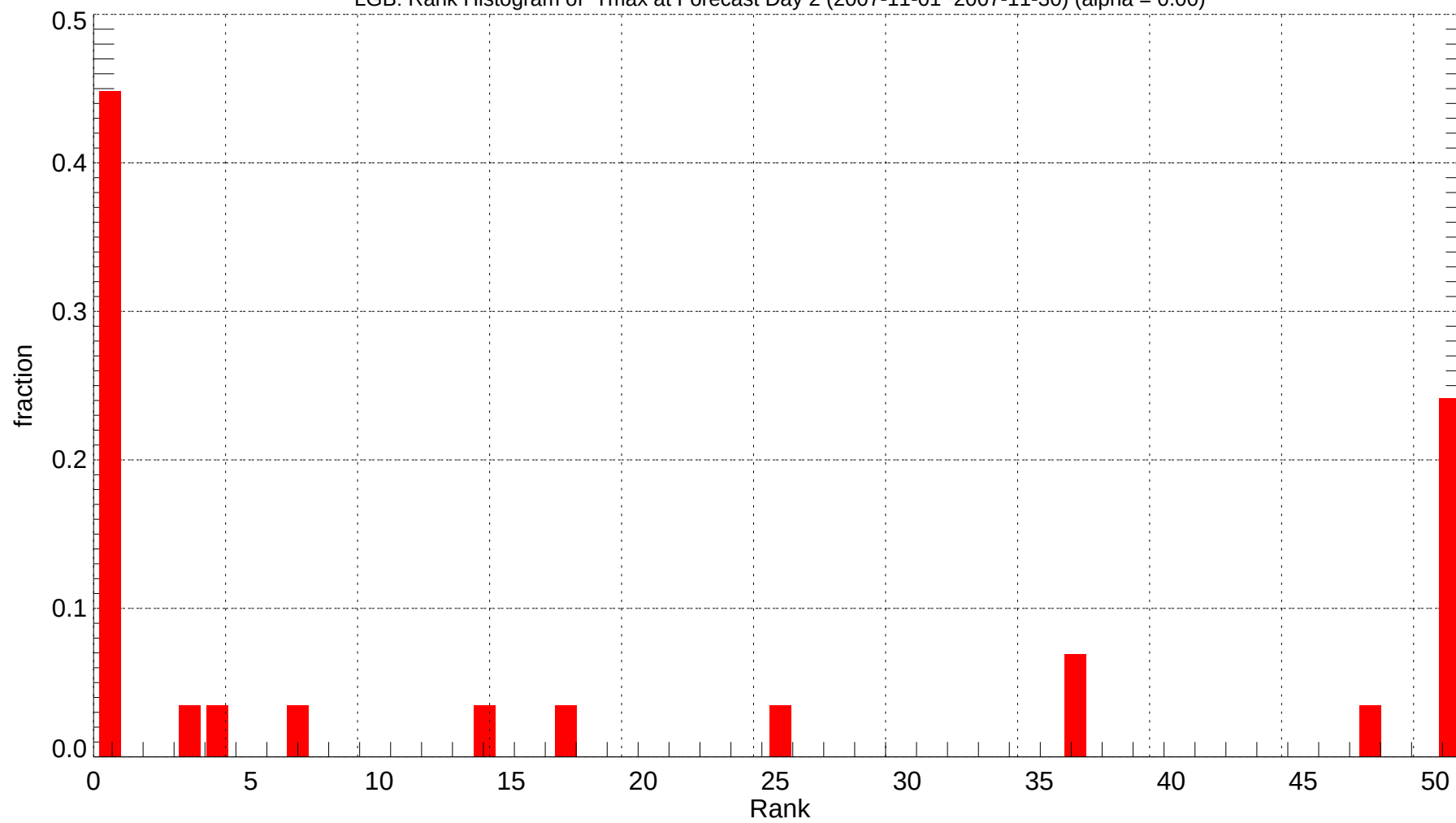
LGB: Rank Histogram of Tmax at Forecast Day 2 (2007-11-01~2007-11-30) (alpha = 0.00)
