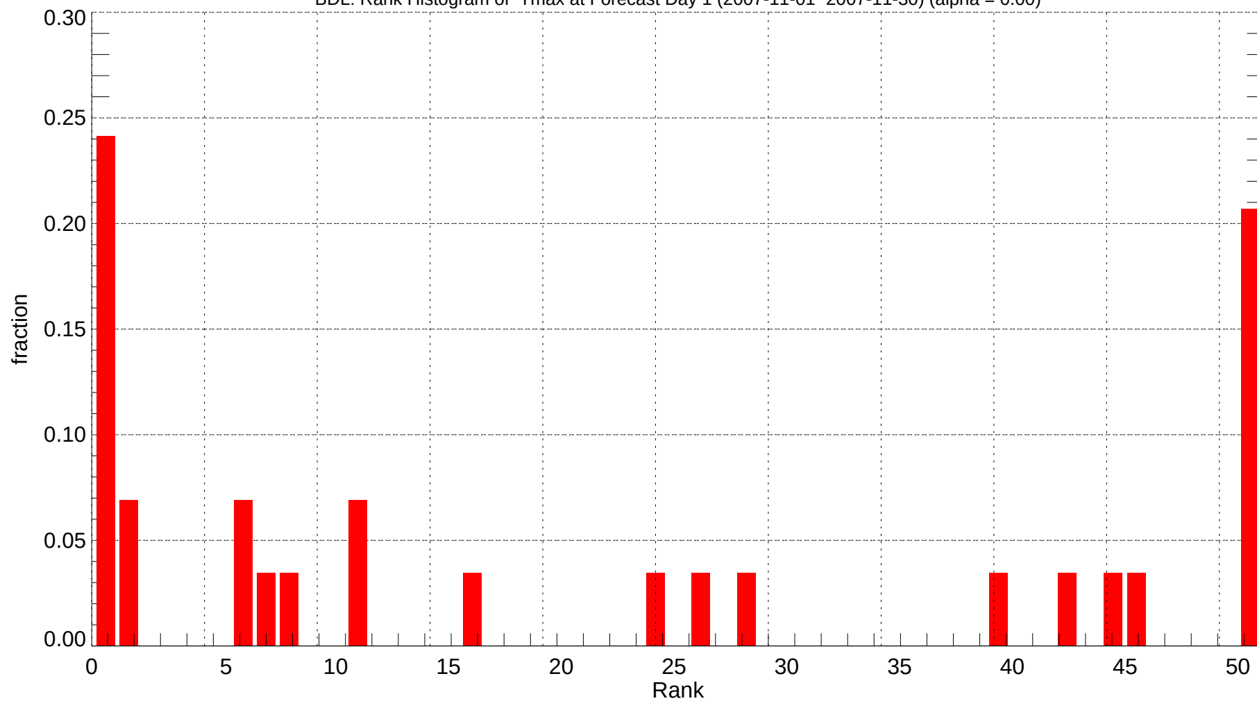
BDL: Rank Histogram of Tmax at Forecast Day 1 (2007-11-01~2007-11-30) (alpha = 0.00)
