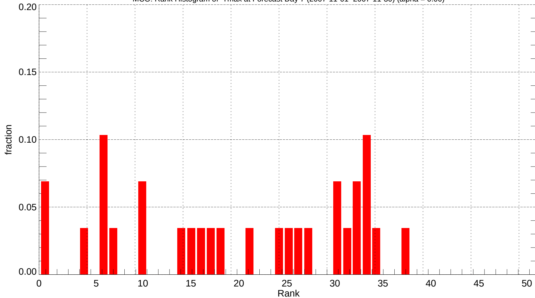
MCO: Rank Histogram of Tmax at Forecast Day 7 (2007-11-01~2007-11-30) (alpha = 0.00)
