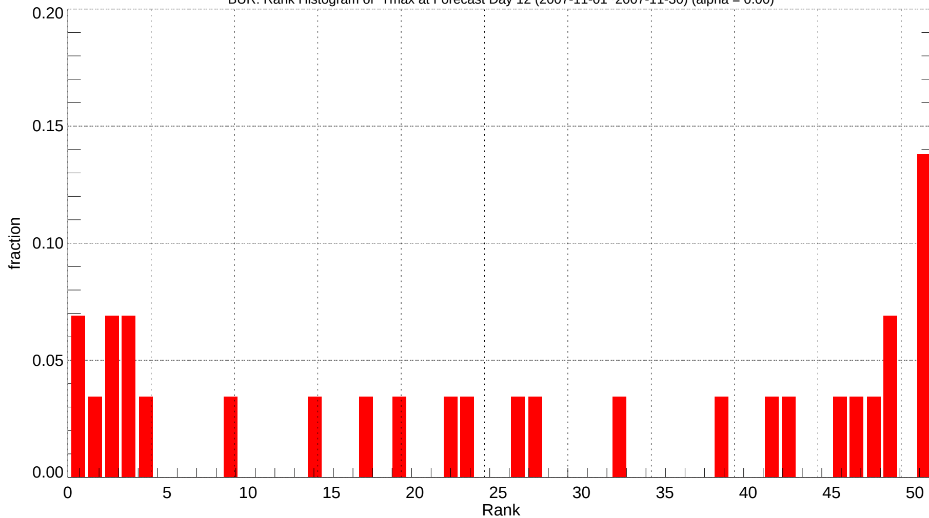
BUR: Rank Histogram of Tmax at Forecast Day 12 (2007-11-01~2007-11-30) (alpha = 0.00)
