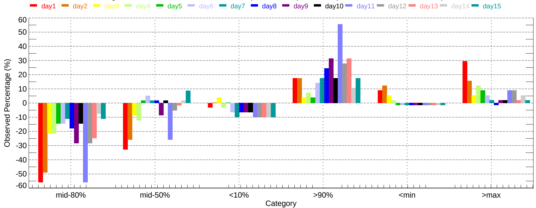
Observed Percentage Deviation of Ensembles - DBQ: Min Temperature (2007-11-01~2007-11-30)
