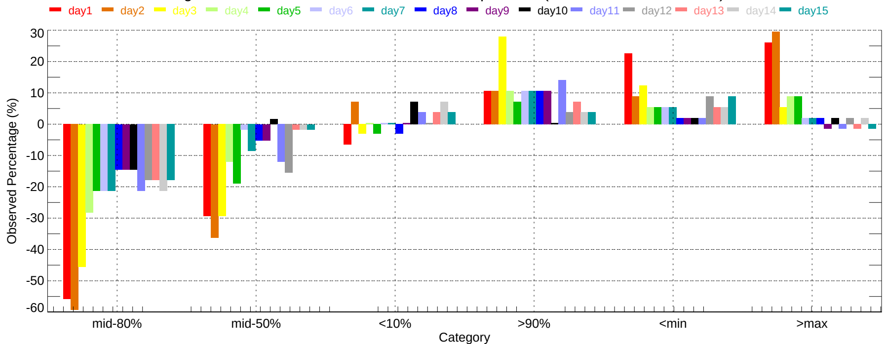
Observed Percentage Deviation of Ensembles - IPT: Min Temperature (2007-11-01~2007-11-30)
