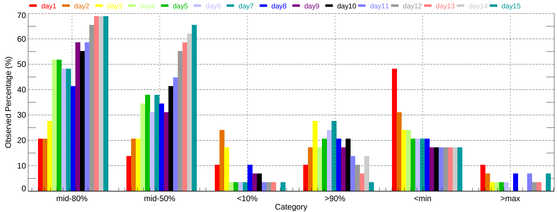
Observed Percentage of Ensembles - RBL: Min Temperature (2007-11-01~2007-11-30)
