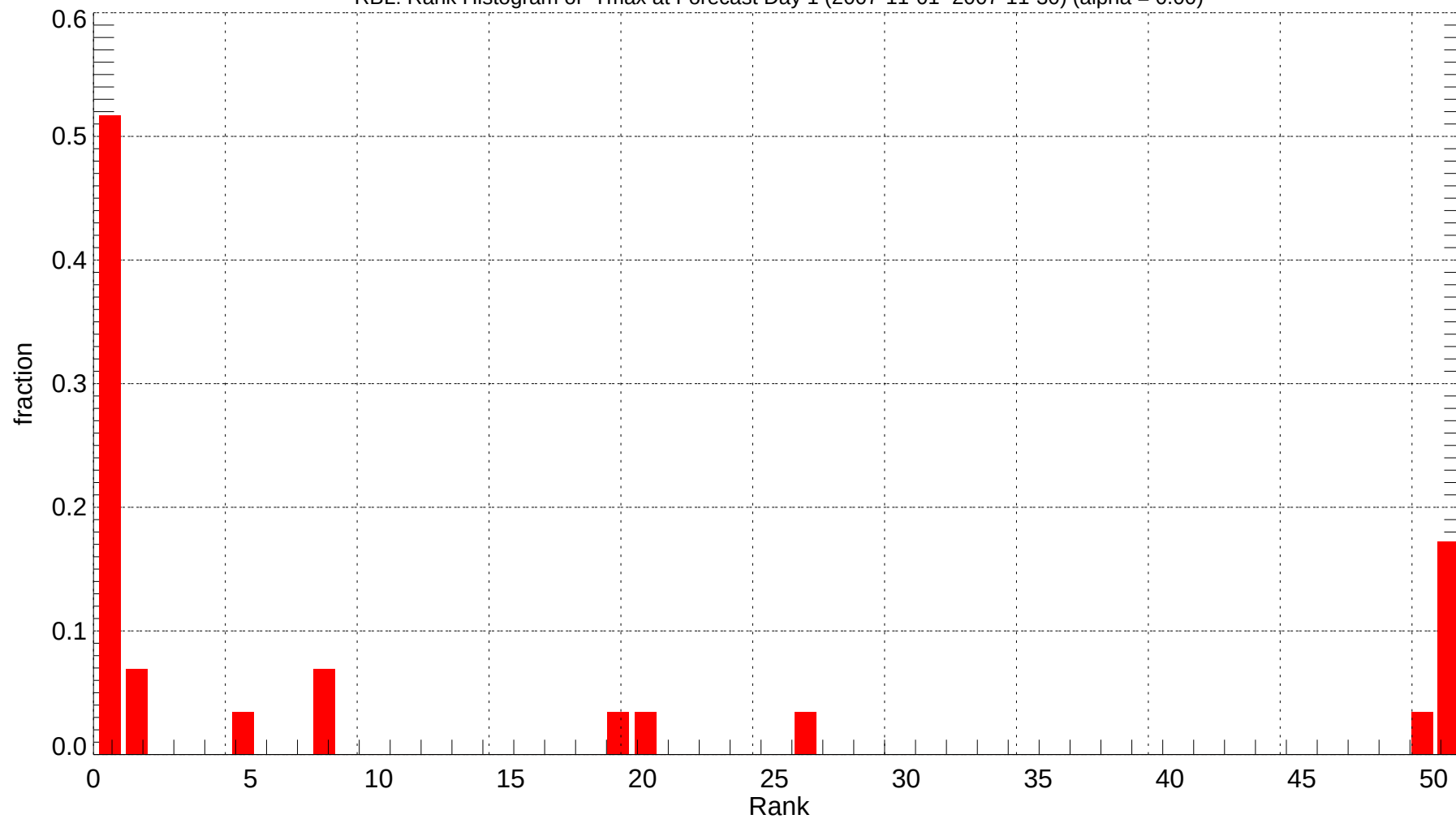
RBL: Rank Histogram of Tmax at Forecast Day 1 (2007-11-01~2007-11-30) (alpha = 0.00)
