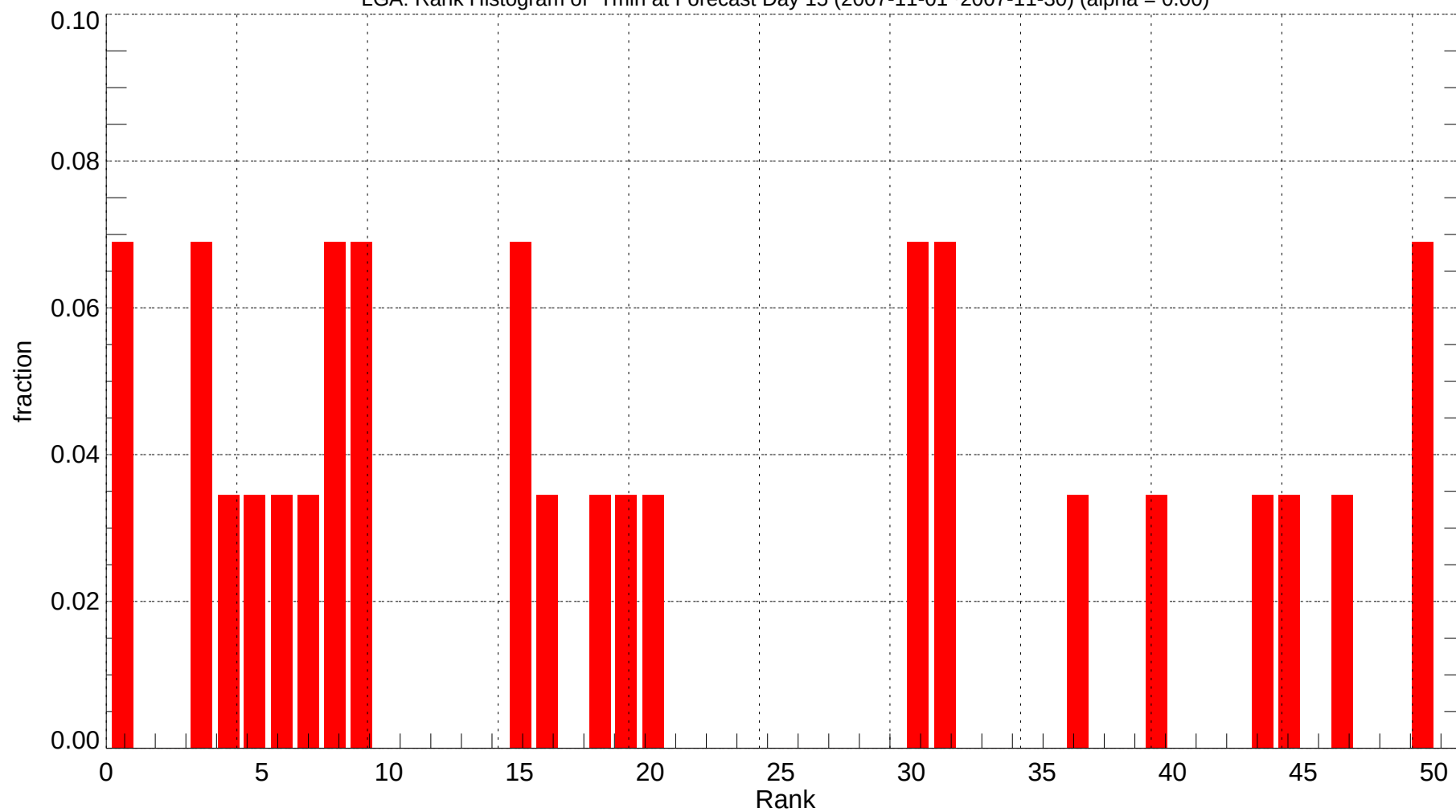
LGA: Rank Histogram of Tmin at Forecast Day 15 (2007-11-01~2007-11-30) (alpha = 0.00)
