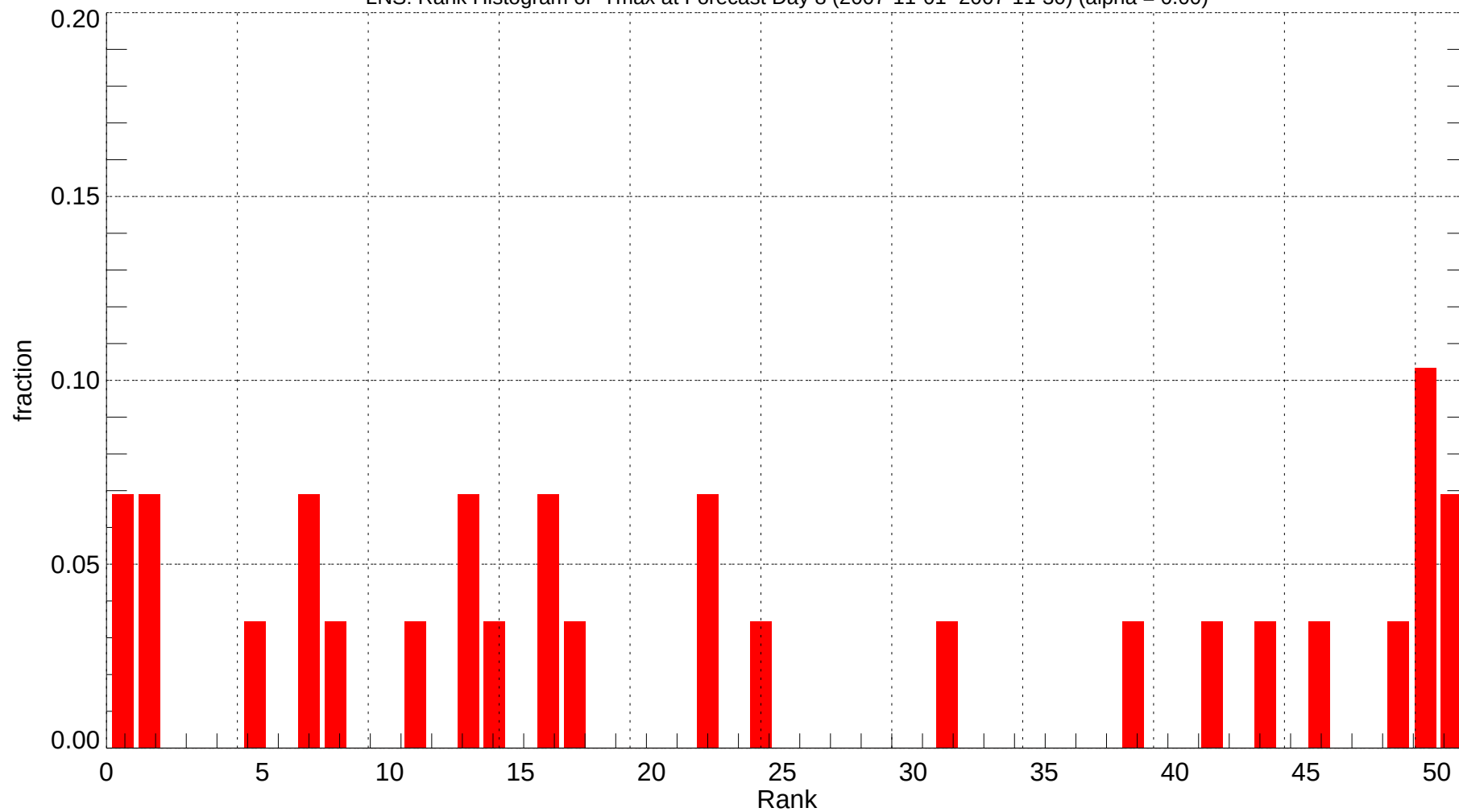
LNS: Rank Histogram of Tmax at Forecast Day 8 (2007-11-01~2007-11-30) (alpha = 0.00)
