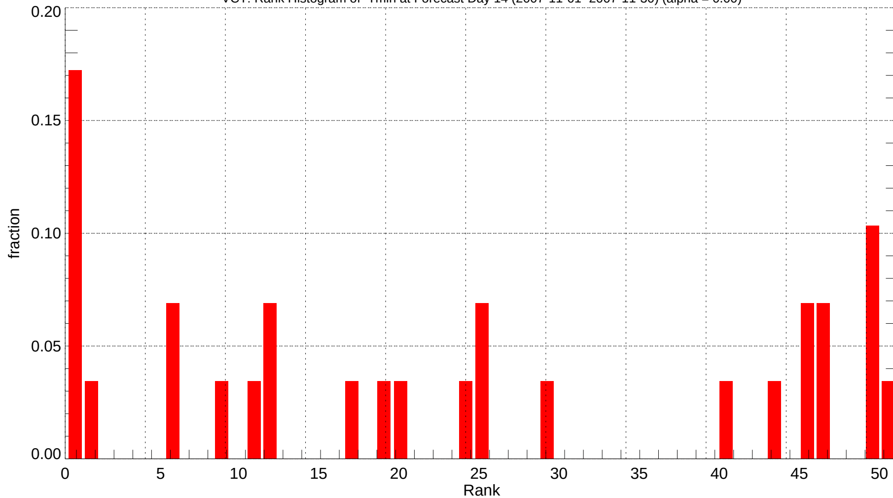
VCT: Rank Histogram of Tmin at Forecast Day 14 (2007-11-01~2007-11-30) (alpha = 0.00)
