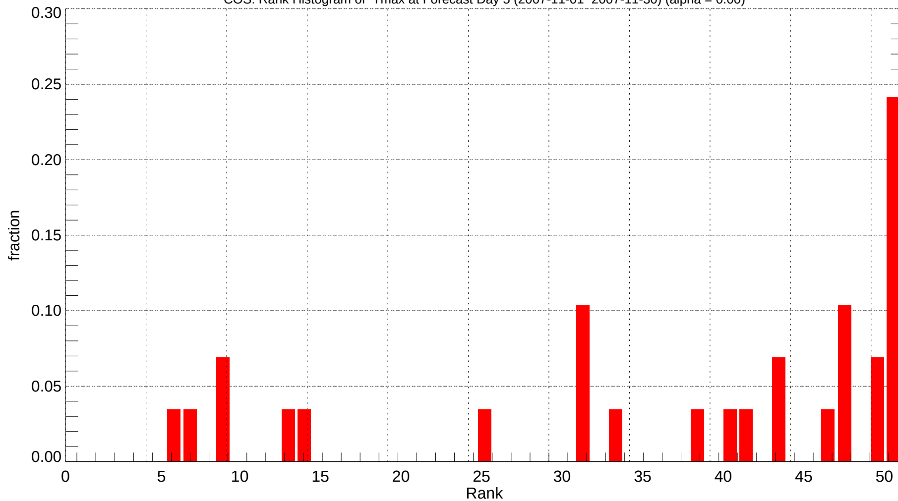
COS: Rank Histogram of Tmax at Forecast Day 5 (2007-11-01~2007-11-30) (alpha = 0.00)
