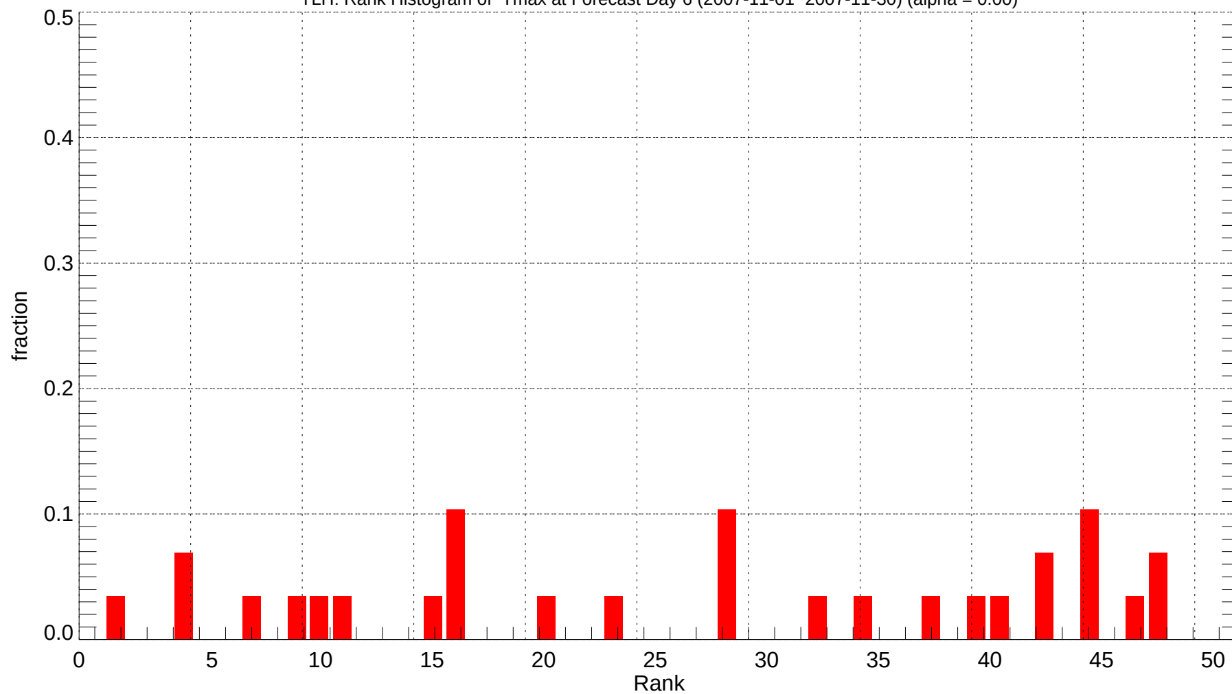
TLH: Rank Histogram of Tmax at Forecast Day 6 (2007-11-01~2007-11-30) (alpha = 0.00)
