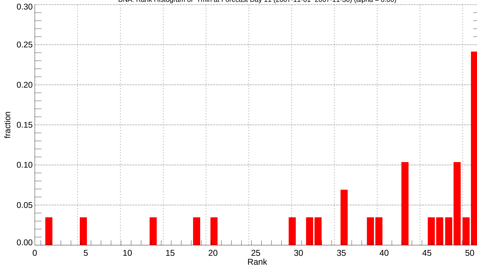
BNA: Rank Histogram of Tmin at Forecast Day 11 (2007-11-01~2007-11-30) (alpha = 0.00)
