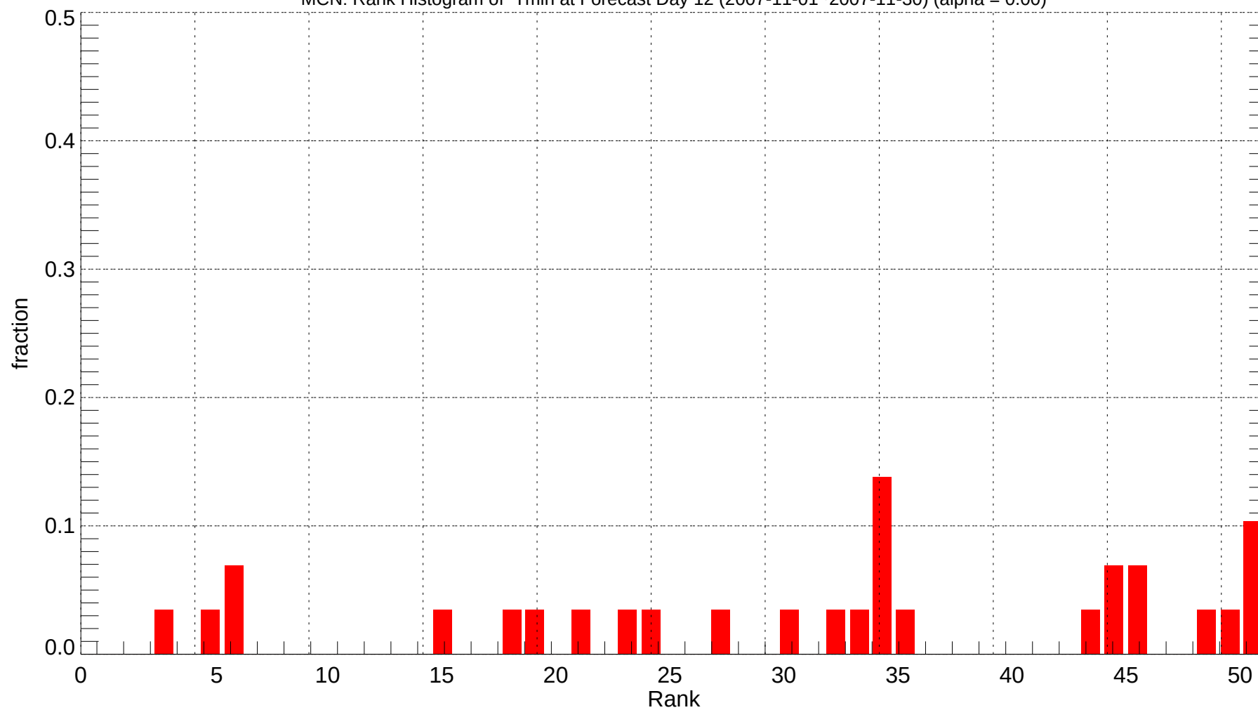
MCN: Rank Histogram of Tmin at Forecast Day 12 (2007-11-01~2007-11-30) (alpha = 0.00)
