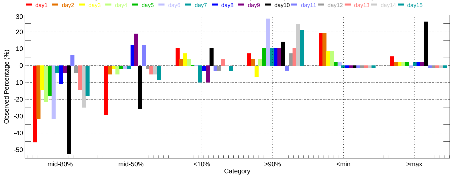
Observed Percentage Deviation of Ensembles - ABQ: Min Temperature (2007-11-01~2007-11-30)
