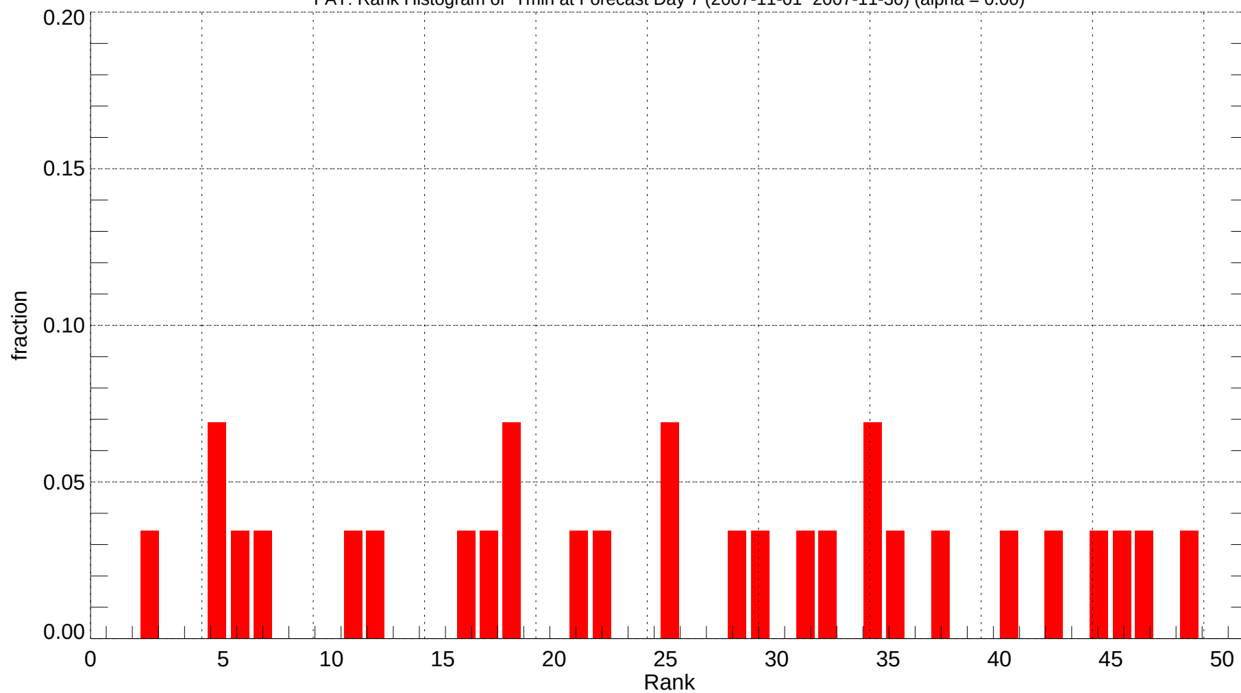
FAT: Rank Histogram of Tmin at Forecast Day 7 (2007-11-01~2007-11-30) (alpha = 0.00)
