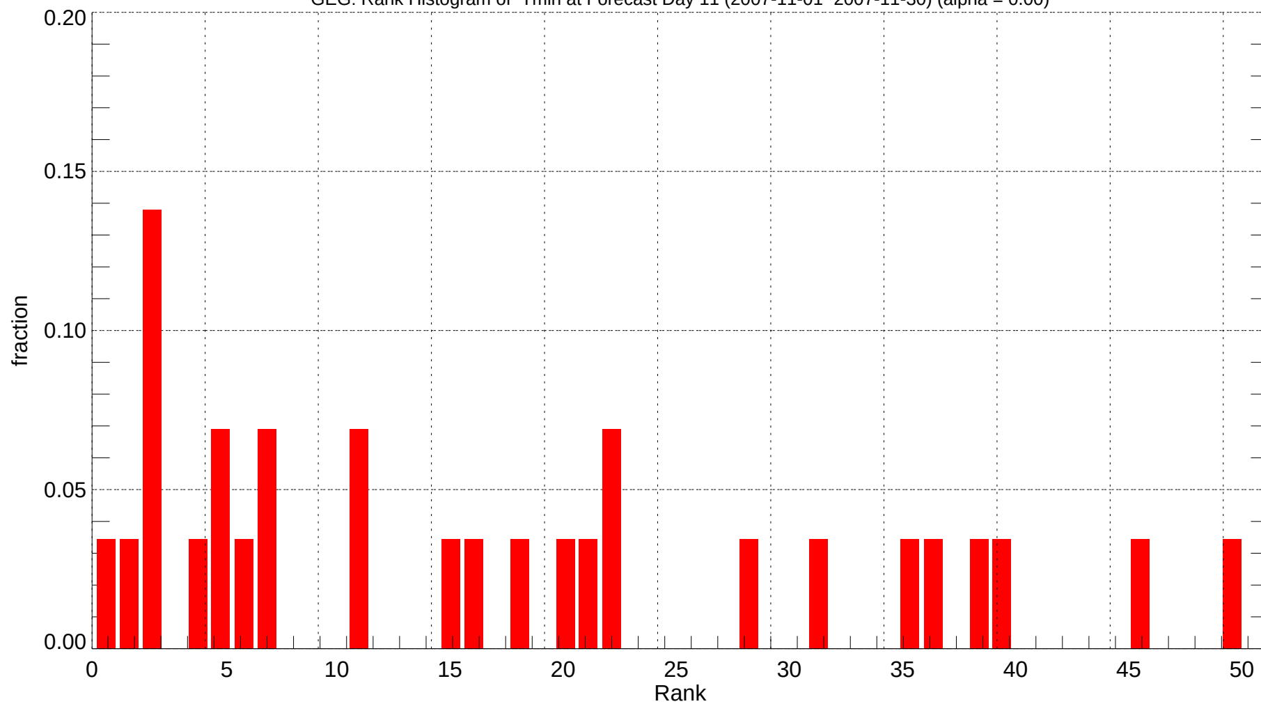
GEG: Rank Histogram of Tmin at Forecast Day 11 (2007-11-01~2007-11-30) (alpha = 0.00)
