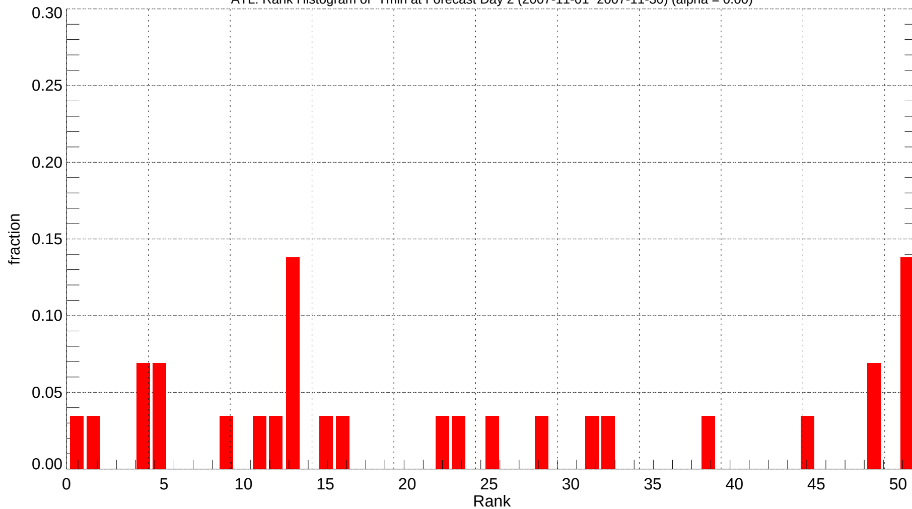
ATL: Rank Histogram of Tmin at Forecast Day 2 (2007-11-01~2007-11-30) (alpha = 0.00)
