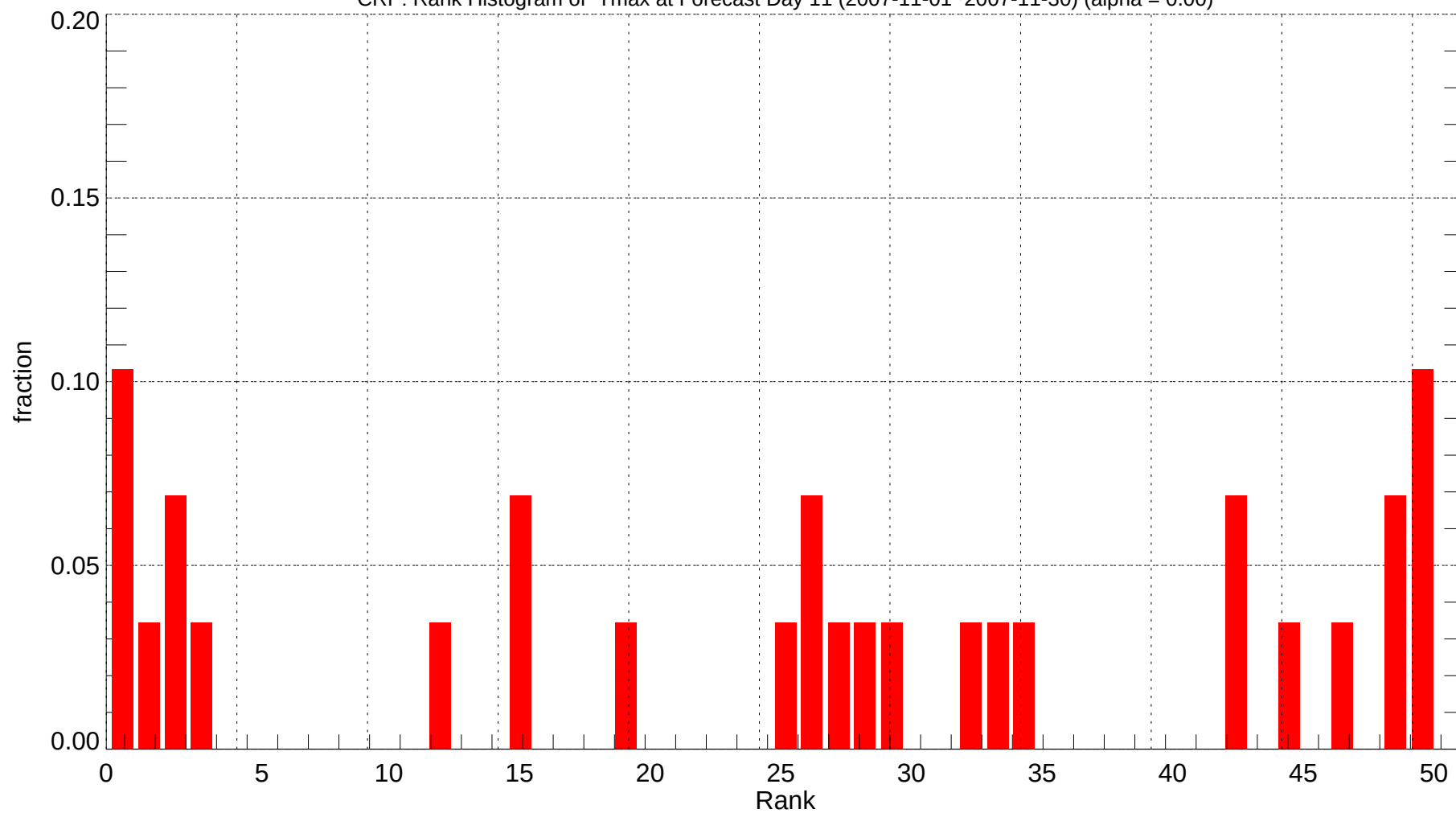
CRP: Rank Histogram of Tmax at Forecast Day 11 (2007-11-01~2007-11-30) (alpha = 0.00)
