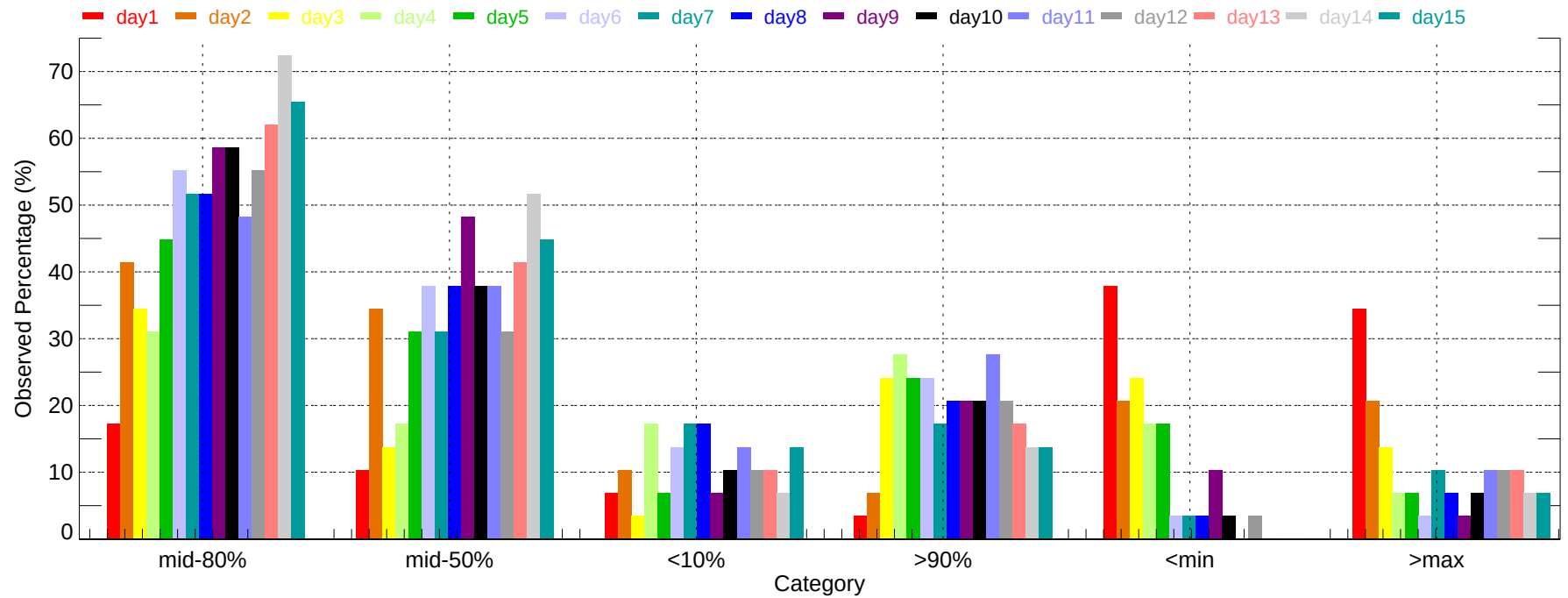
Observed Percentage of Ensembles - YNG: Min Temperature (2007-11-01~2007-11-30)
