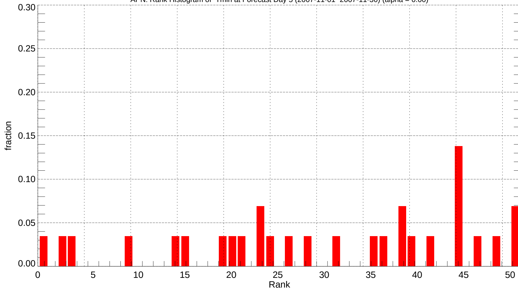
APN: Rank Histogram of Tmin at Forecast Day 5 (2007-11-01~2007-11-30) (alpha = 0.00)
