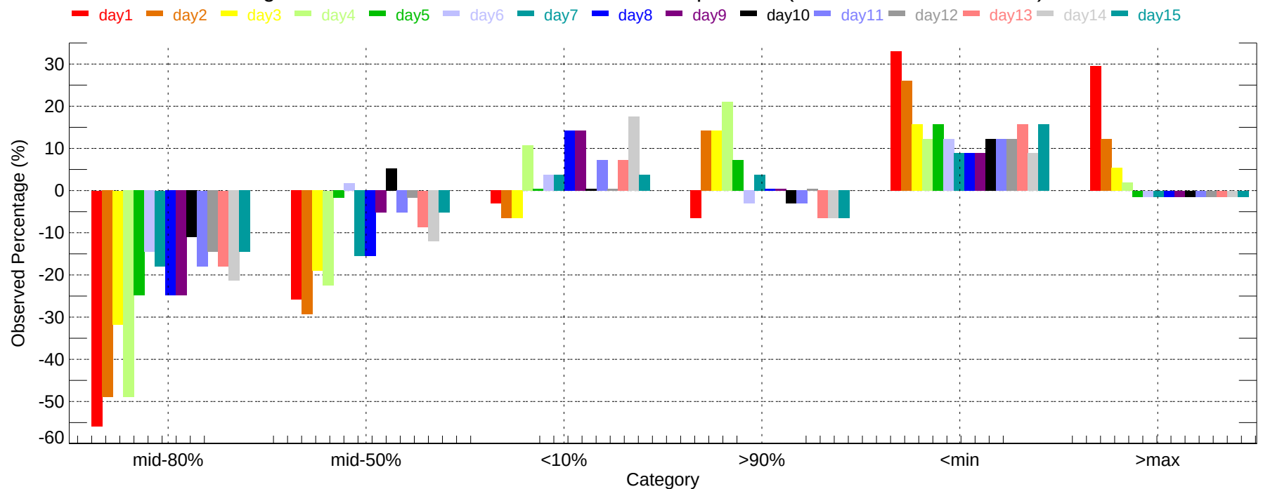
Observed Percentage Deviation of Ensembles - SYR: Min Temperature (2007-11-01~2007-11-30)
