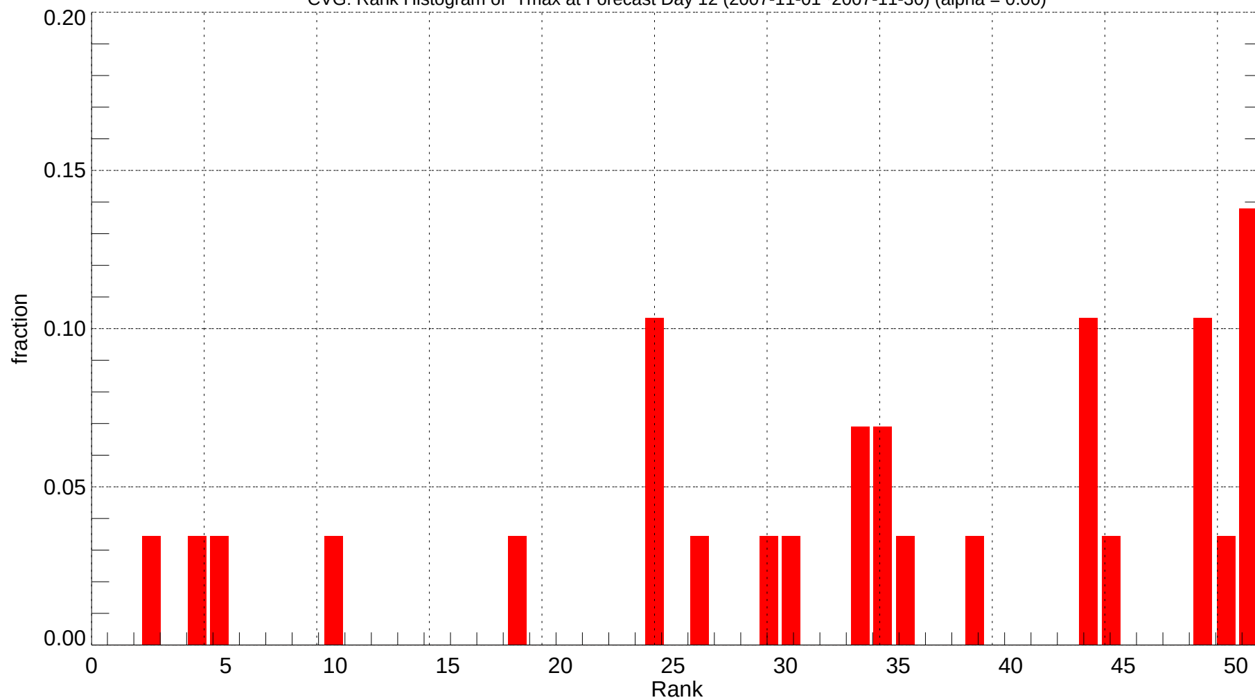
CVG: Rank Histogram of Tmax at Forecast Day 12 (2007-11-01~2007-11-30) (alpha = 0.00)
