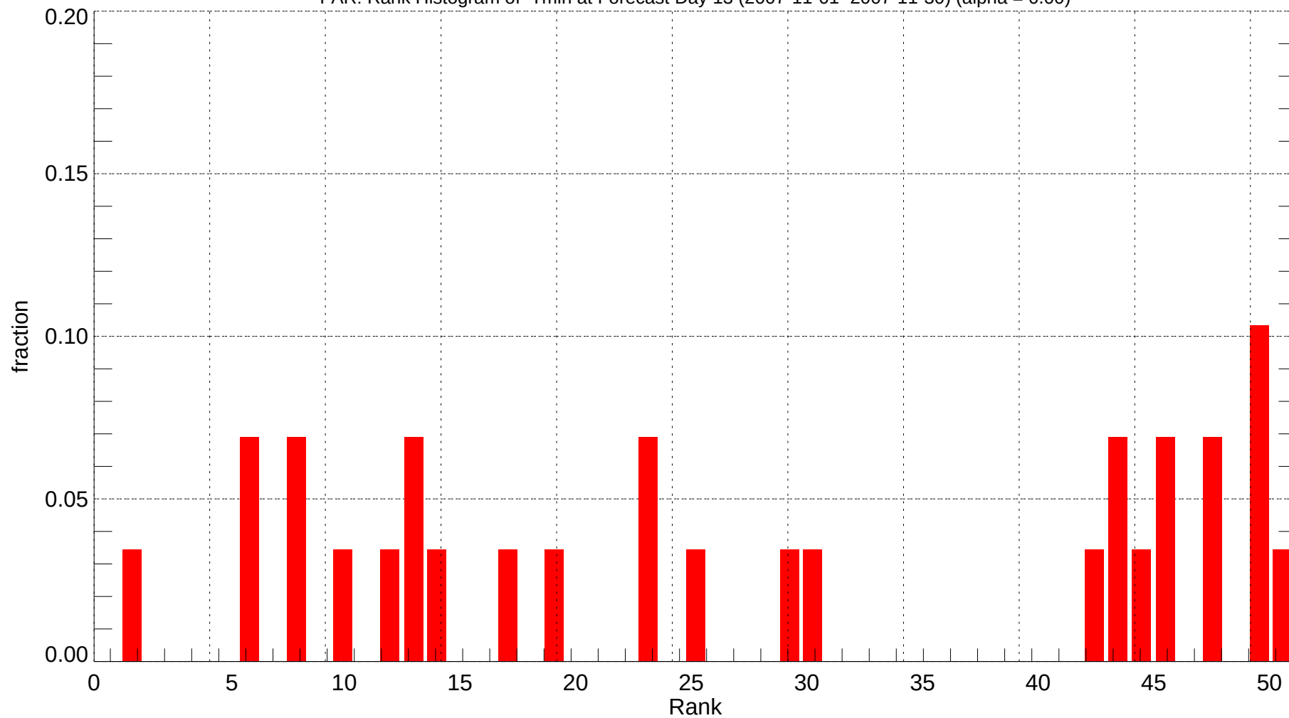
FAR: Rank Histogram of Tmin at Forecast Day 13 (2007-11-01~2007-11-30) (alpha = 0.00)
