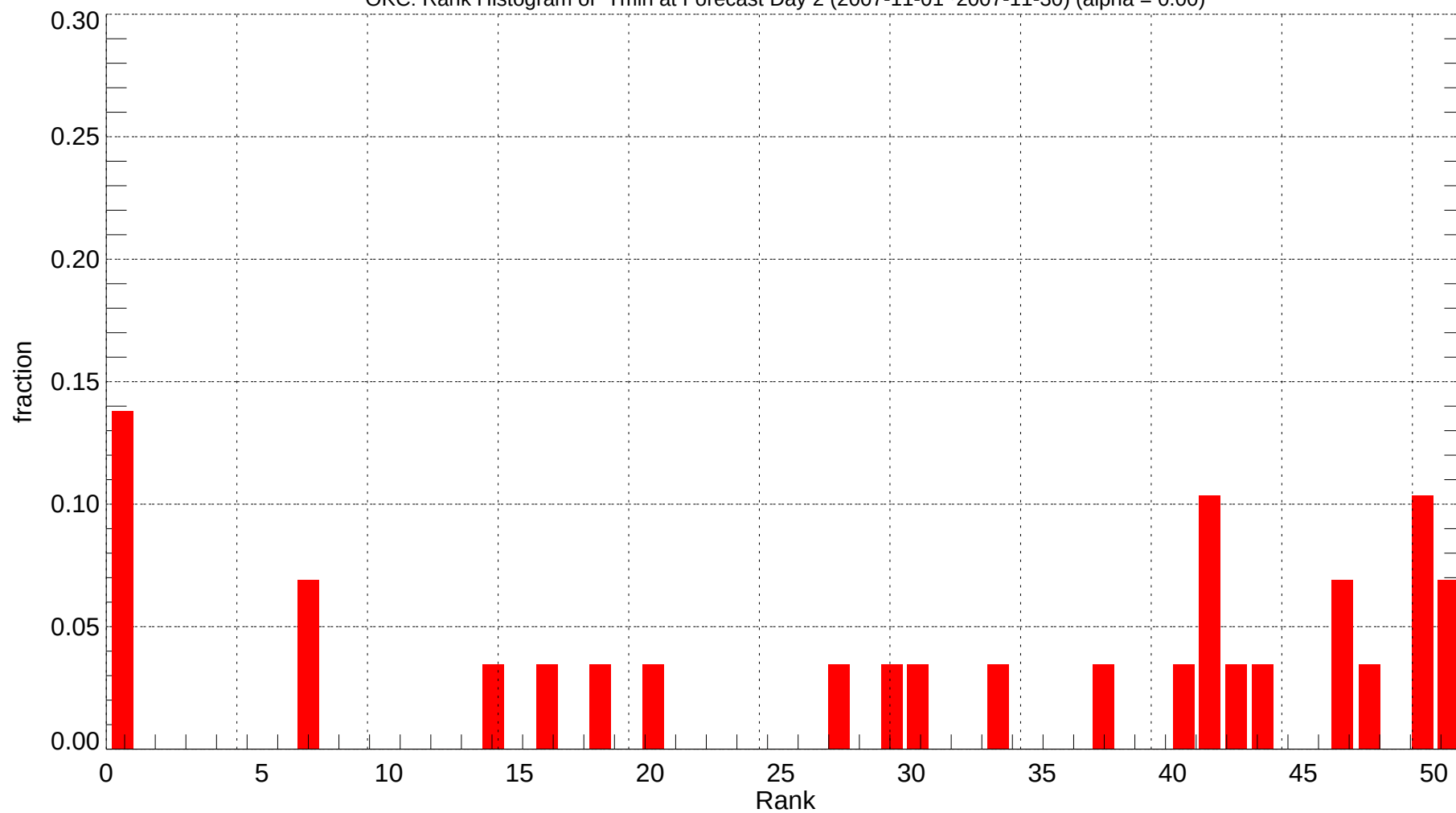
OKC: Rank Histogram of Tmin at Forecast Day 2 (2007-11-01~2007-11-30) (alpha = 0.00)
