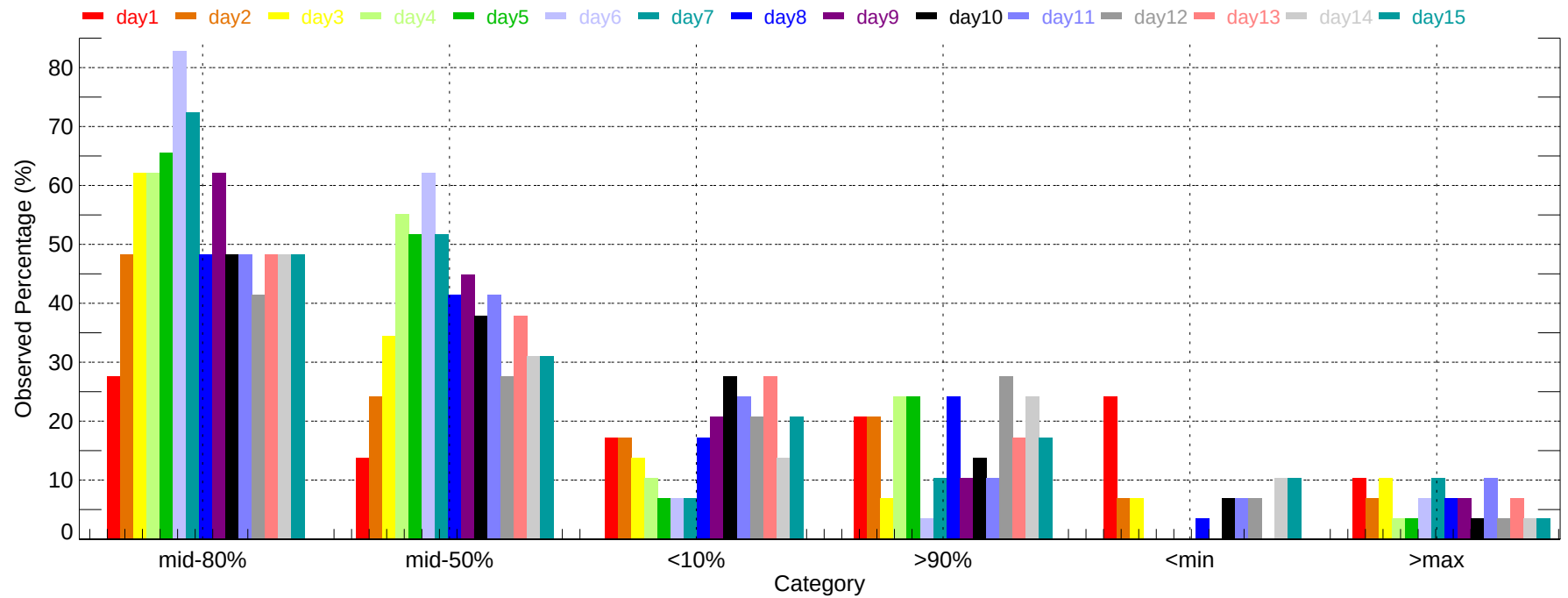
Observed Percentage of Ensembles - PHL: Max Temperature (2007-11-01~2007-11-30)
