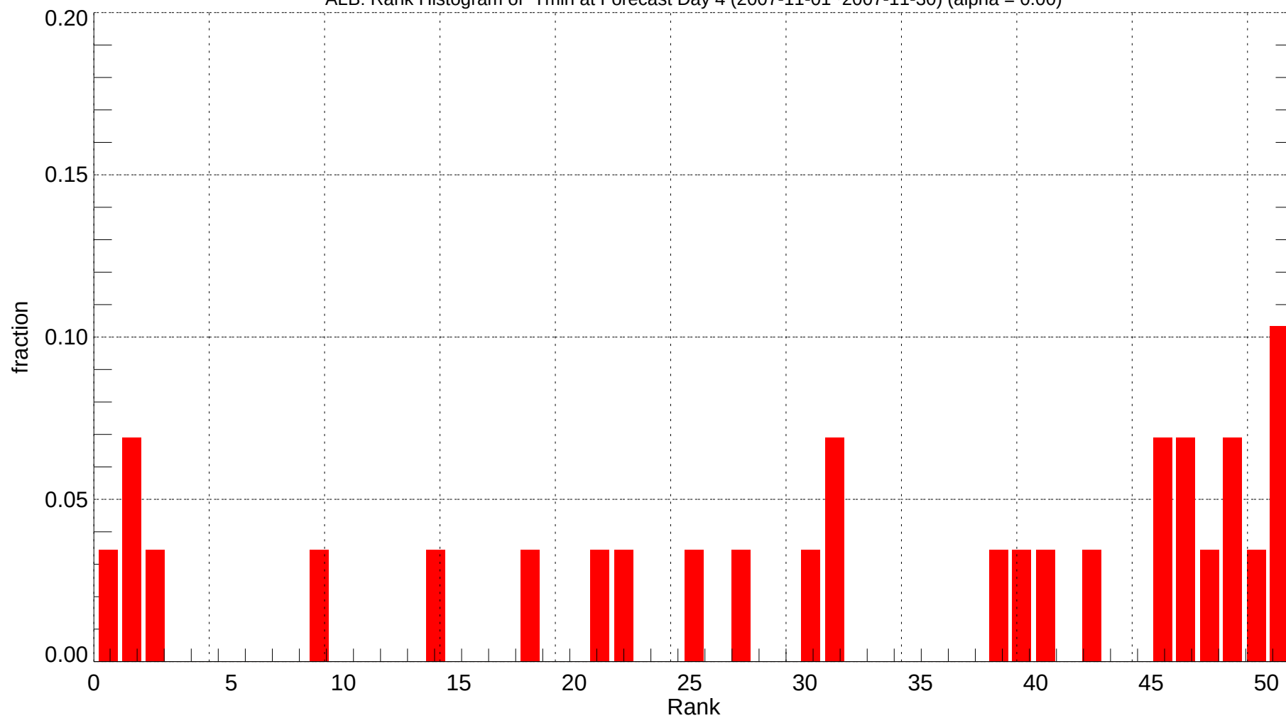
ALB: Rank Histogram of Tmin at Forecast Day 4 (2007-11-01~2007-11-30) (alpha = 0.00)
