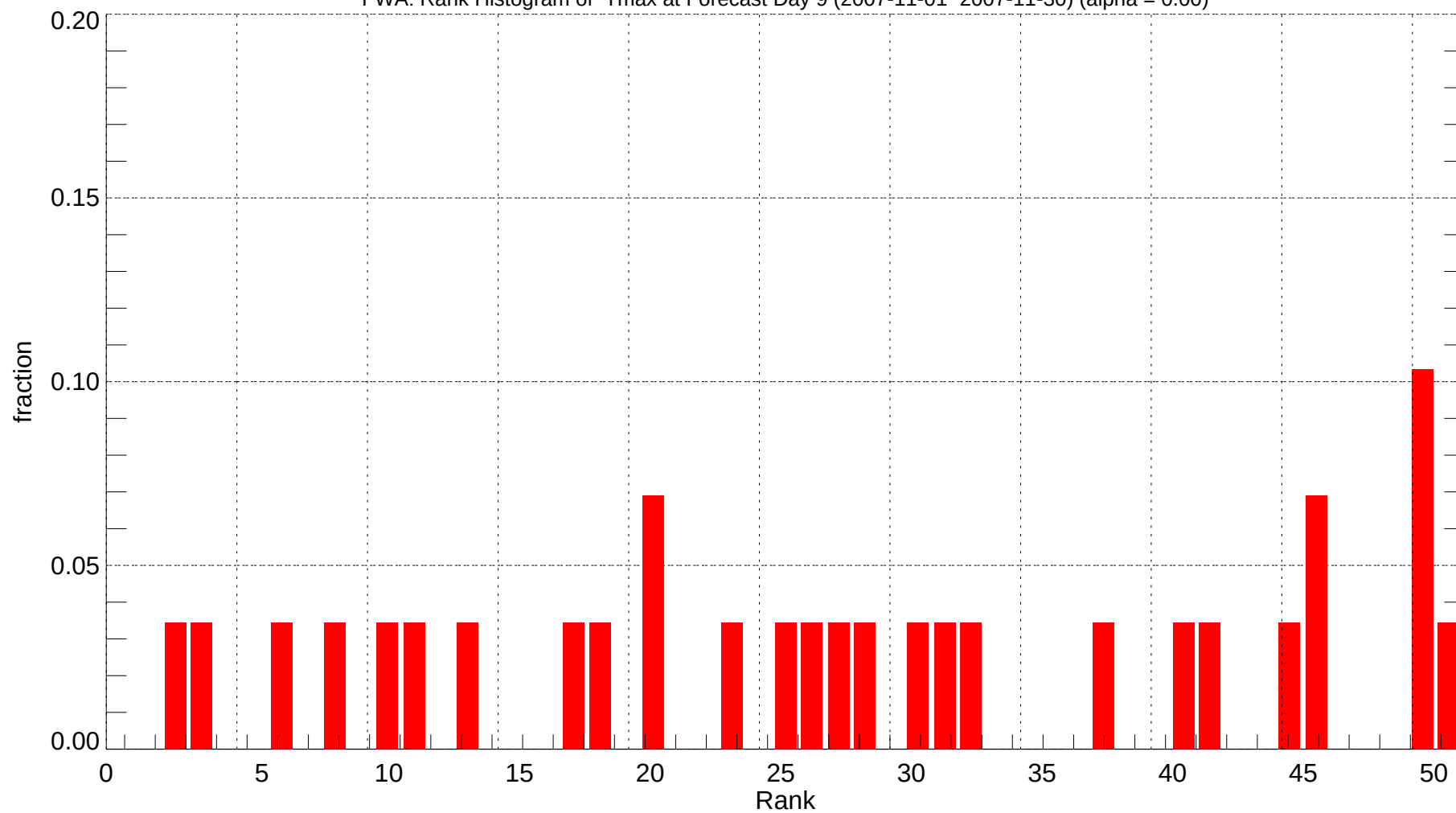
FWA: Rank Histogram of Tmax at Forecast Day 9 (2007-11-01~2007-11-30) (alpha = 0.00)
