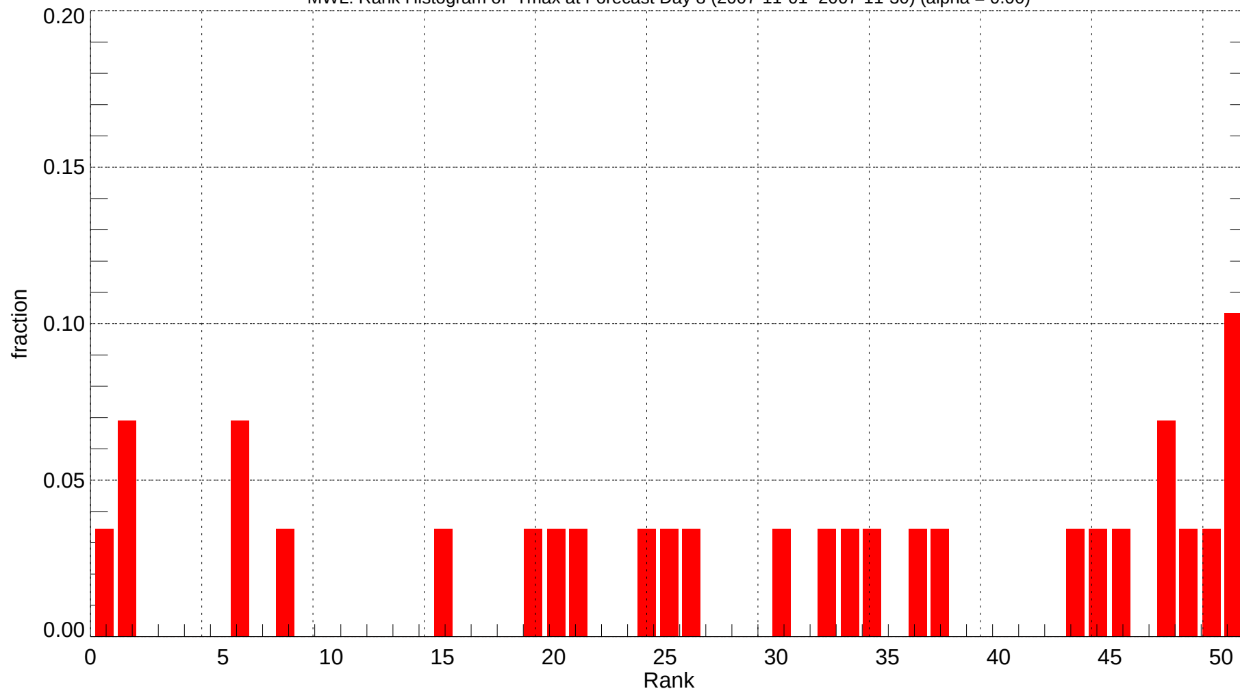
MWL: Rank Histogram of Tmax at Forecast Day 8 (2007-11-01~2007-11-30) (alpha = 0.00)
