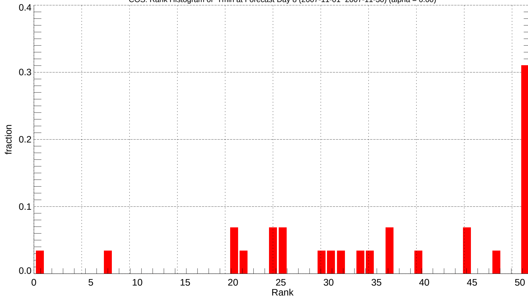
COS: Rank Histogram of Tmin at Forecast Day 8 (2007-11-01~2007-11-30) (alpha = 0.00)
