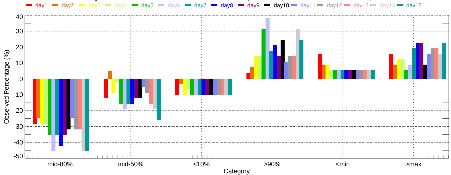
Observed Percentage Deviation of Ensembles - FLG: Min Temperature (2007-11-01~2007-11-30)
