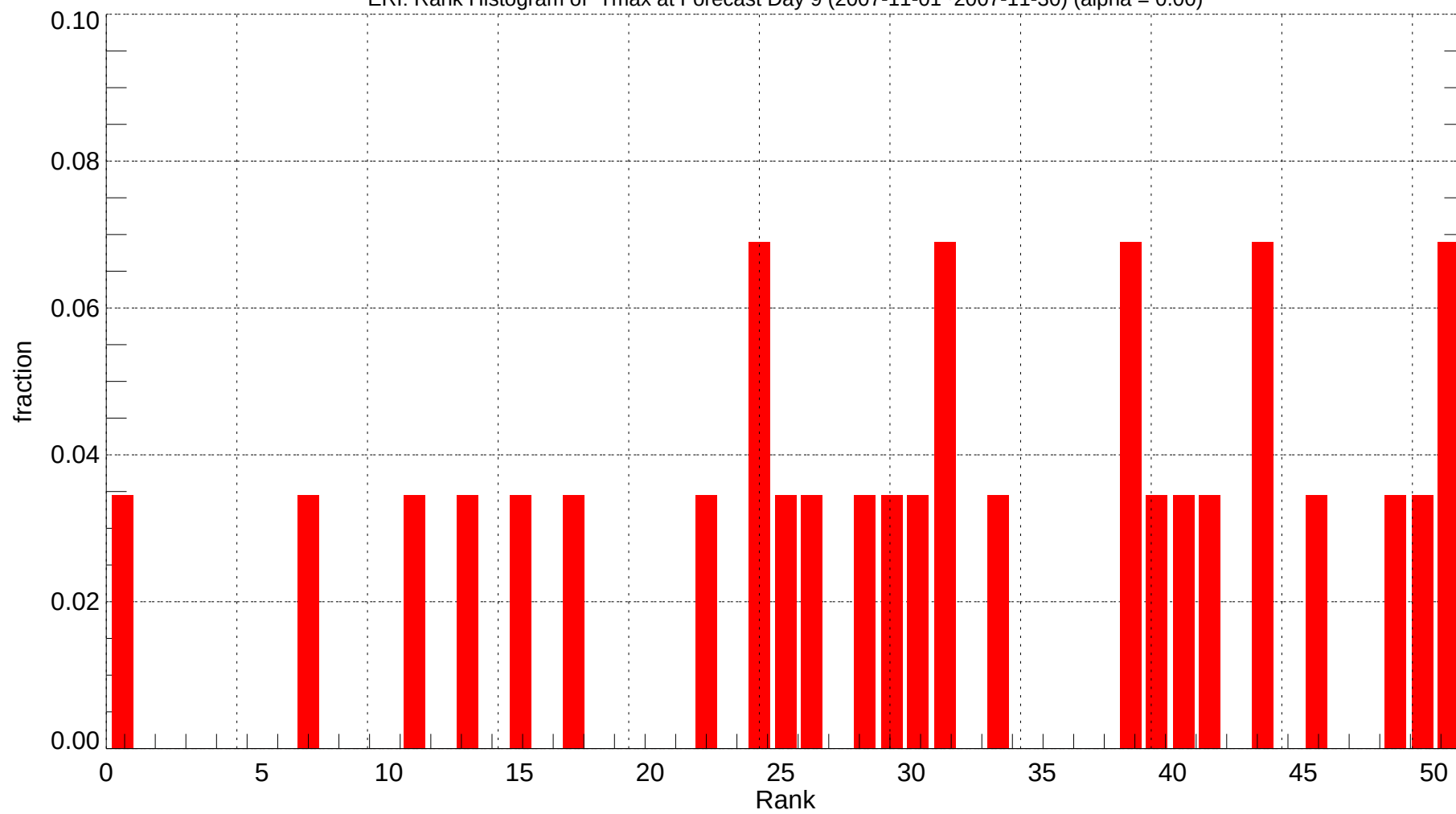
ERI: Rank Histogram of Tmax at Forecast Day 9 (2007-11-01~2007-11-30) (alpha = 0.00)
