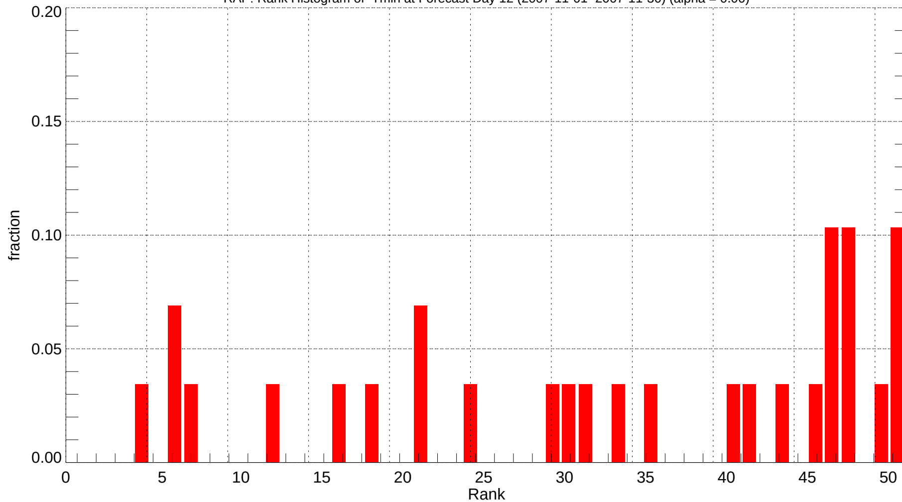
RAP: Rank Histogram of Tmin at Forecast Day 12 (2007-11-01~2007-11-30) (alpha = 0.00)
