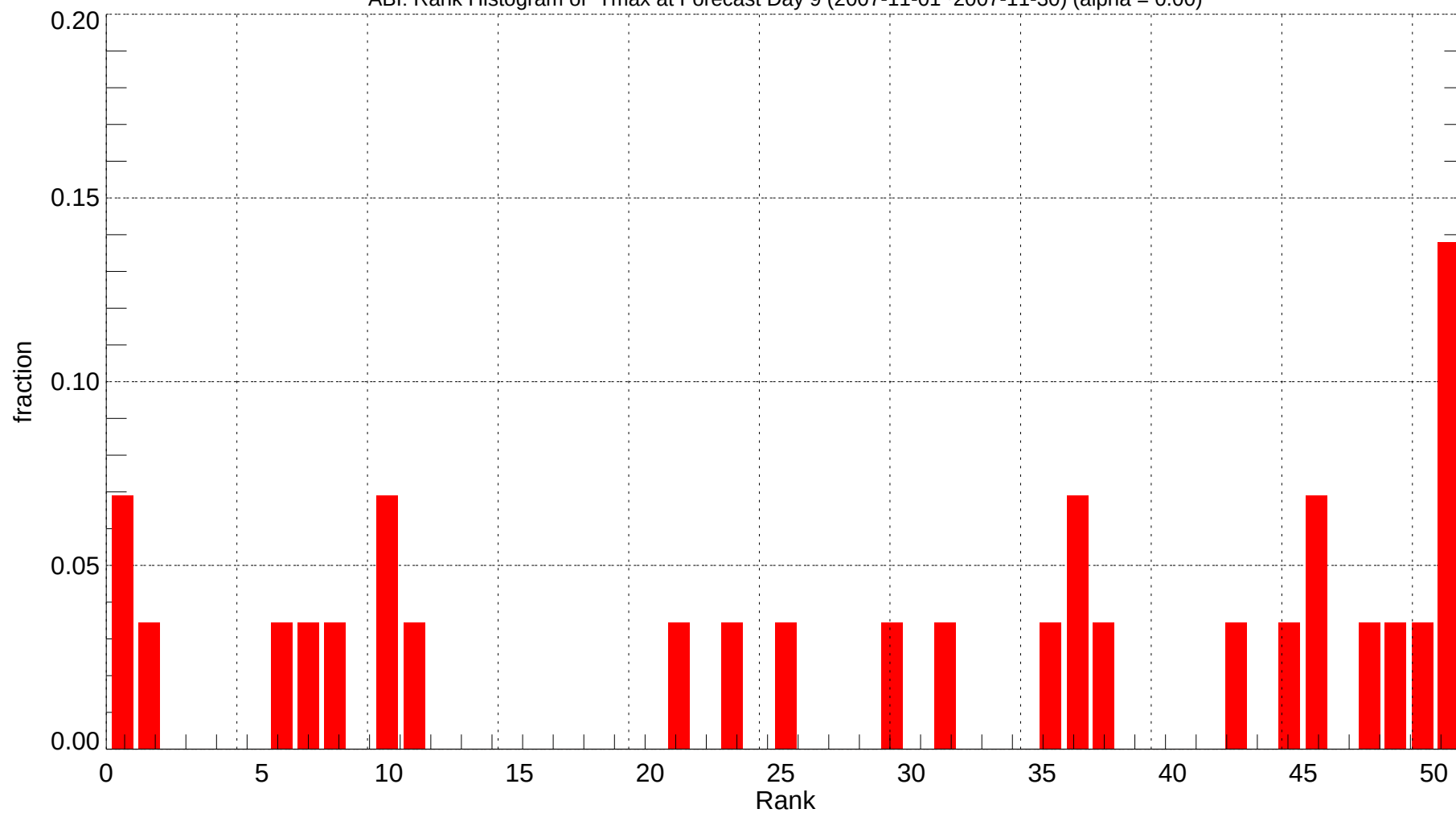
ABI: Rank Histogram of Tmax at Forecast Day 9 (2007-11-01~2007-11-30) (alpha = 0.00)
