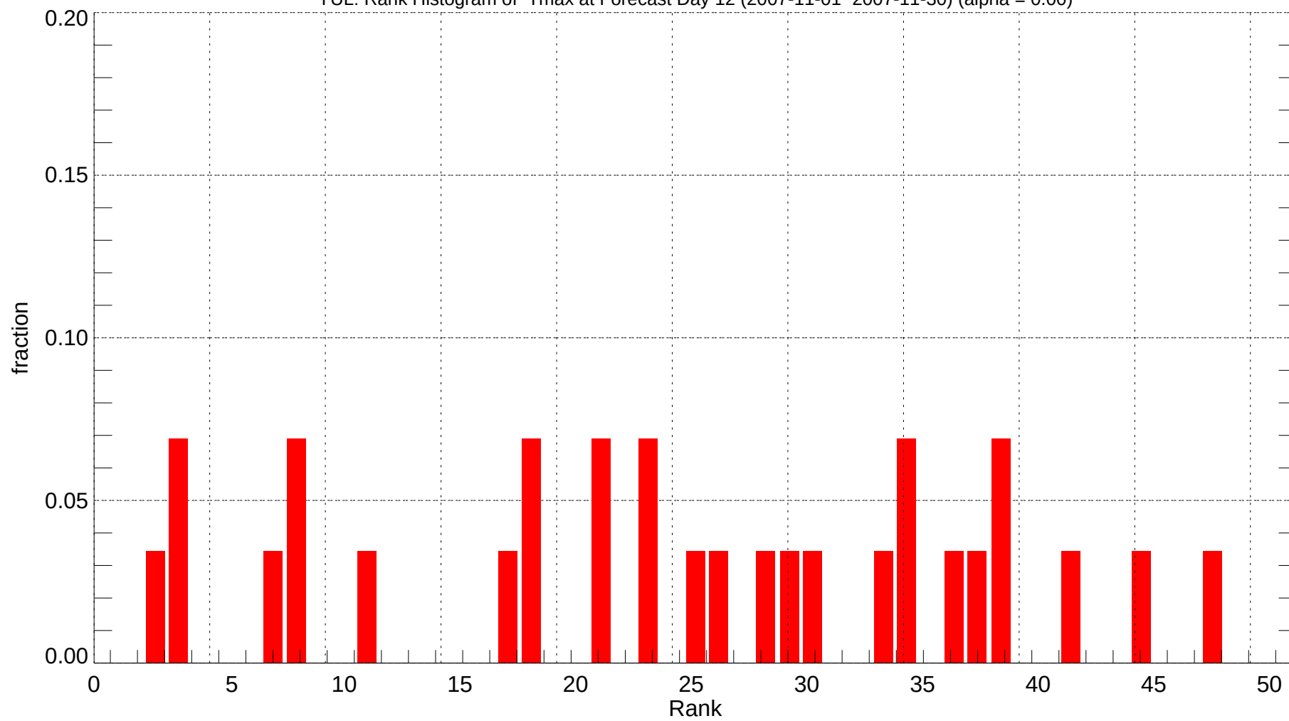
YUL: Rank Histogram of Tmax at Forecast Day 12 (2007-11-01~2007-11-30) (alpha = 0.00)
