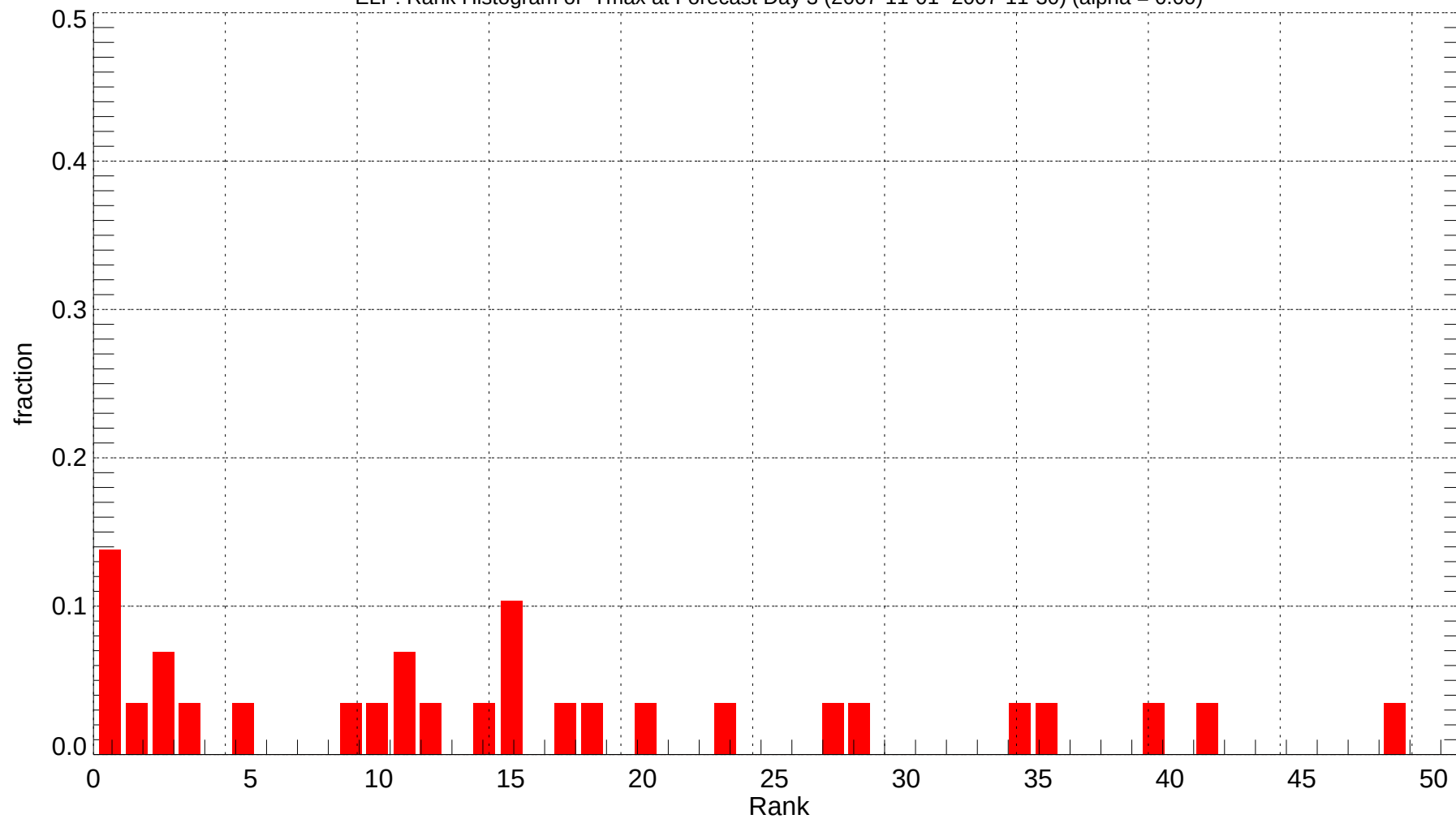
ELP: Rank Histogram of Tmax at Forecast Day 3 (2007-11-01~2007-11-30) (alpha = 0.00)
