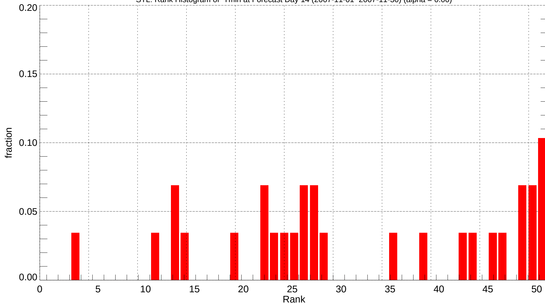
STL: Rank Histogram of Tmin at Forecast Day 14 (2007-11-01~2007-11-30) (alpha = 0.00)
