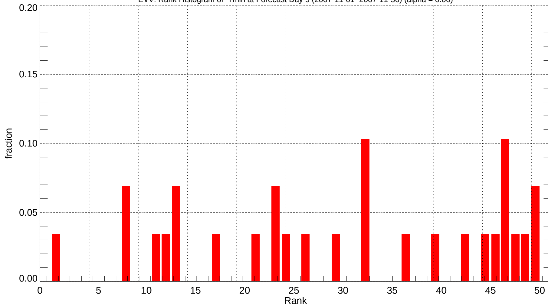
EVV: Rank Histogram of Tmin at Forecast Day 9 (2007-11-01~2007-11-30) (alpha = 0.00)
