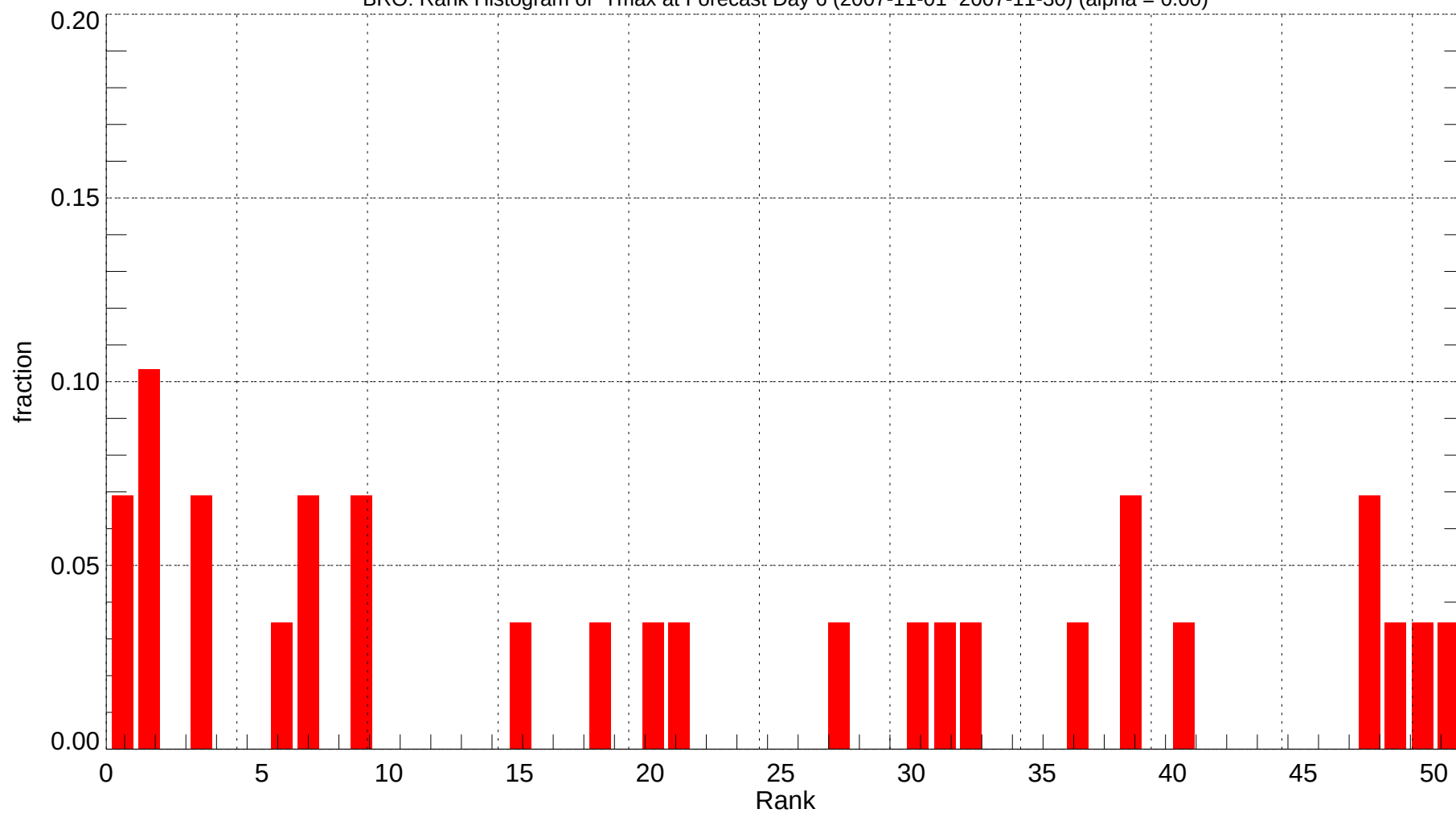
BRO: Rank Histogram of Tmax at Forecast Day 6 (2007-11-01~2007-11-30) (alpha = 0.00)
