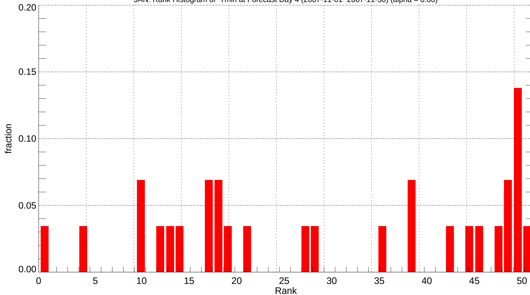
JAN: Rank Histogram of Tmin at Forecast Day 4 (2007-11-01~2007-11-30) (alpha = 0.00)
