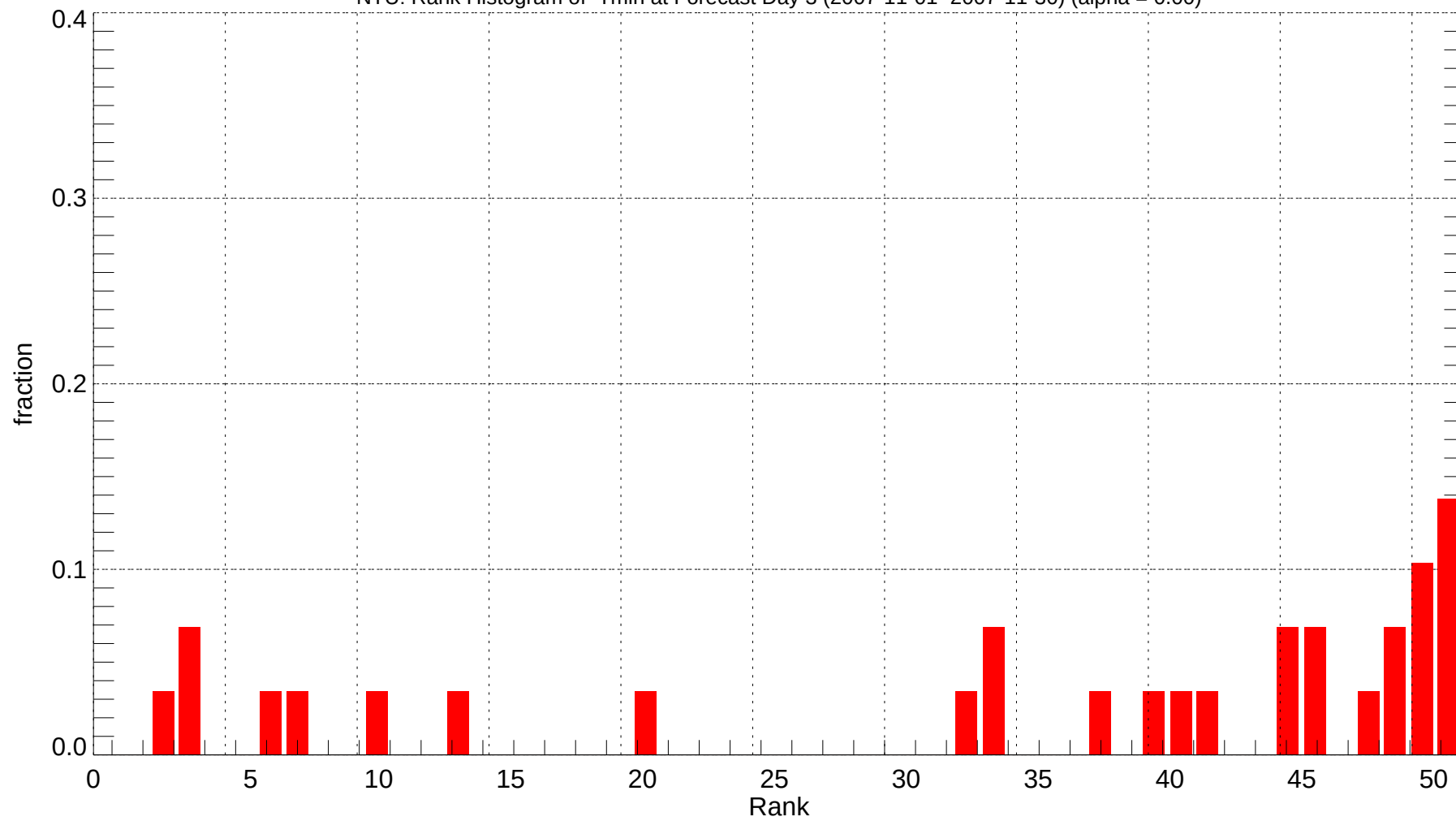
NTU: Rank Histogram of Tmin at Forecast Day 3 (2007-11-01~2007-11-30) (alpha = 0.00)
