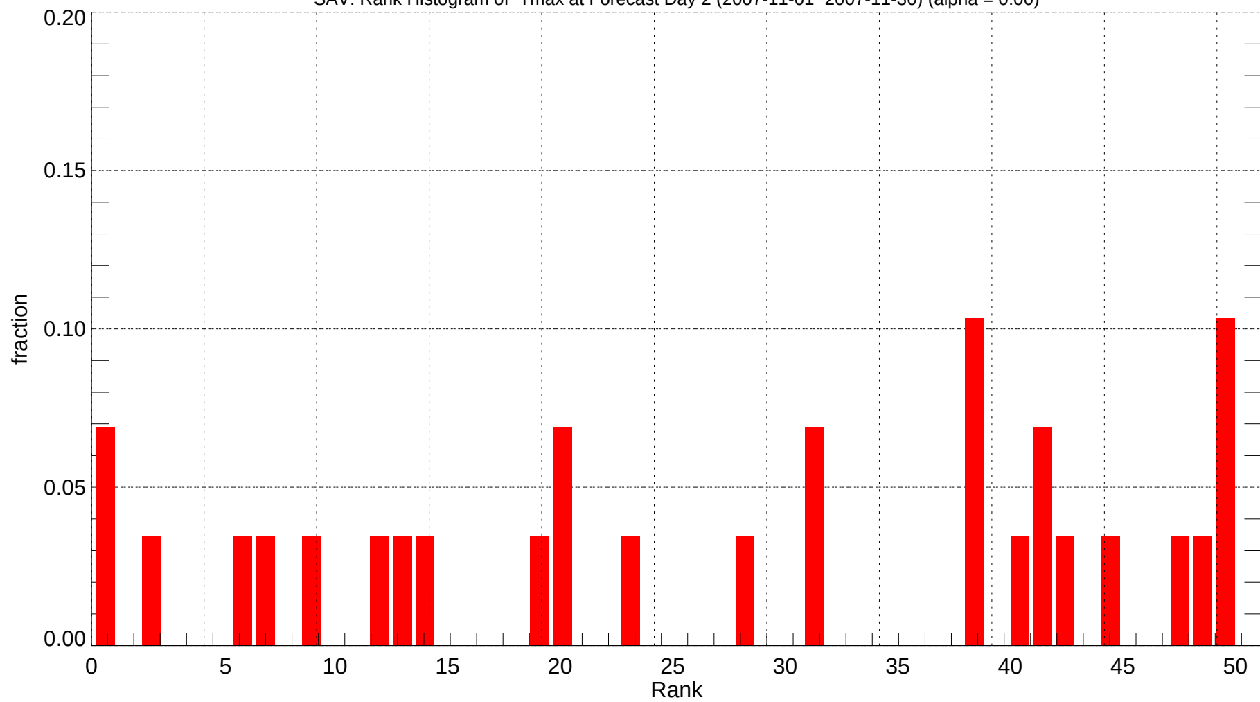
SAV: Rank Histogram of Tmax at Forecast Day 2 (2007-11-01~2007-11-30) (alpha = 0.00)
