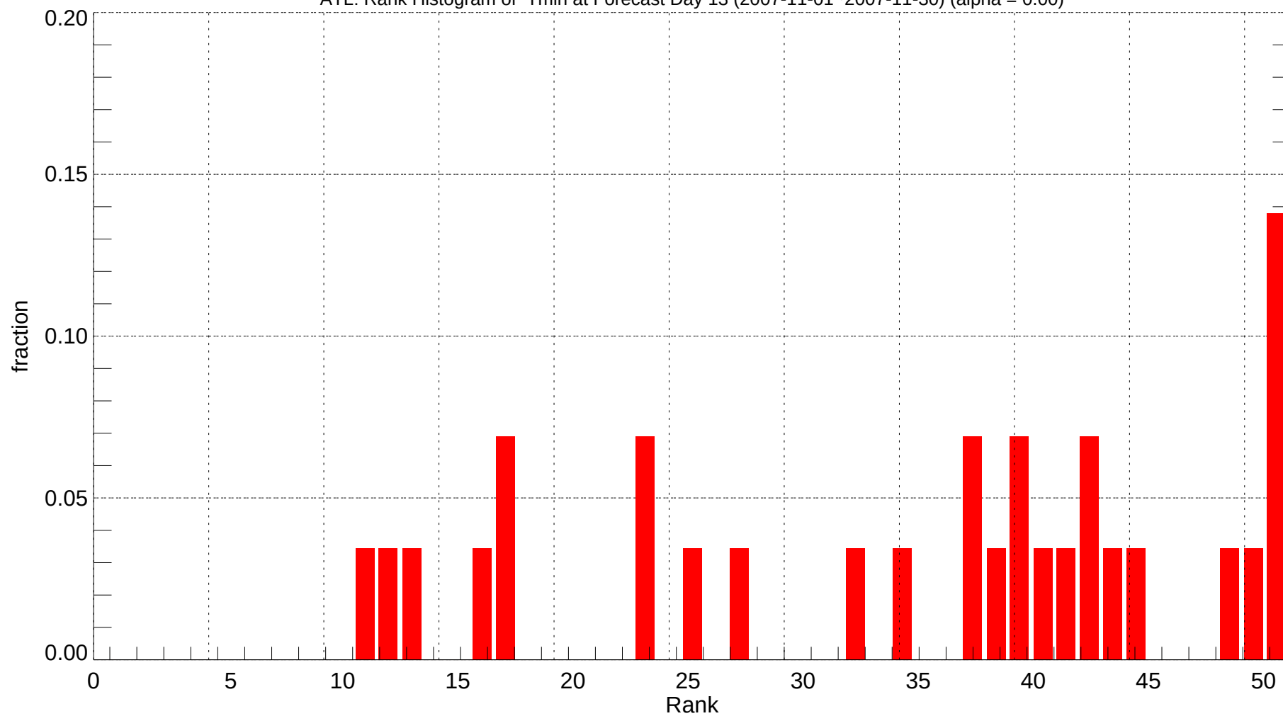
ATL: Rank Histogram of Tmin at Forecast Day 13 (2007-11-01~2007-11-30) (alpha = 0.00)
