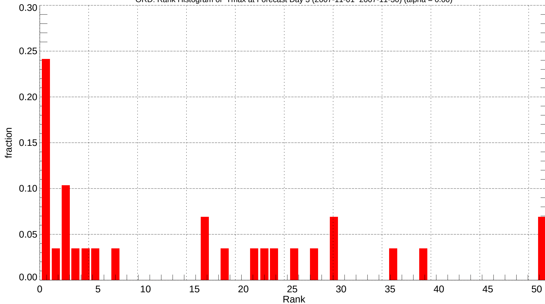
ORD: Rank Histogram of Tmax at Forecast Day 3 (2007-11-01~2007-11-30) (alpha = 0.00)
