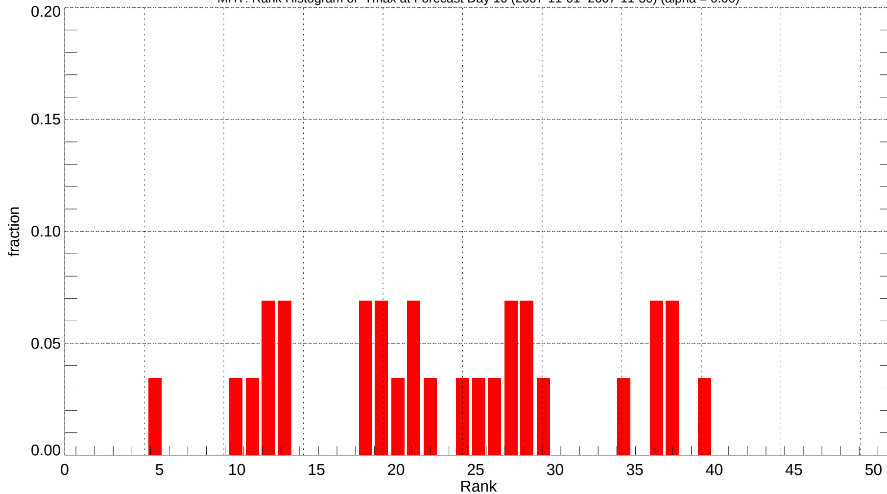
MHT: Rank Histogram of Tmax at Forecast Day 10 (2007-11-01~2007-11-30) (alpha = 0.00)
