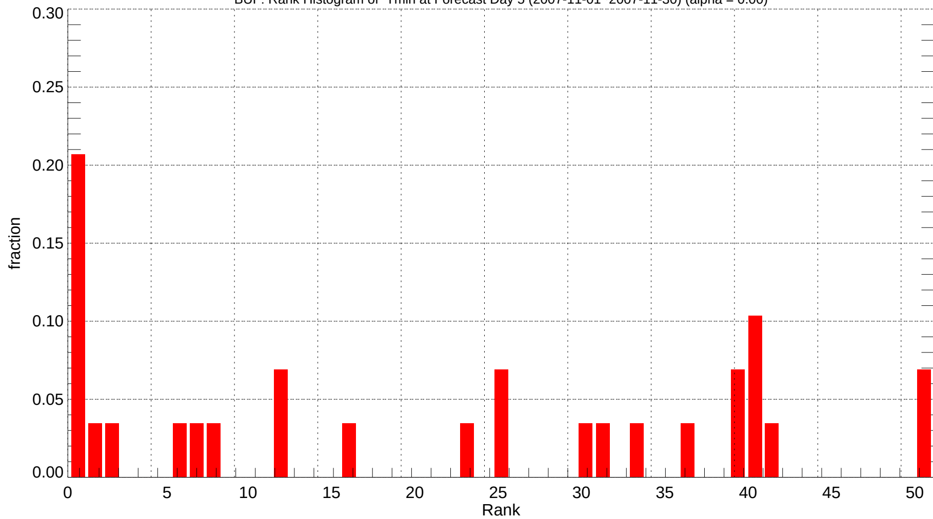
BUF: Rank Histogram of Tmin at Forecast Day 5 (2007-11-01~2007-11-30) (alpha = 0.00)
