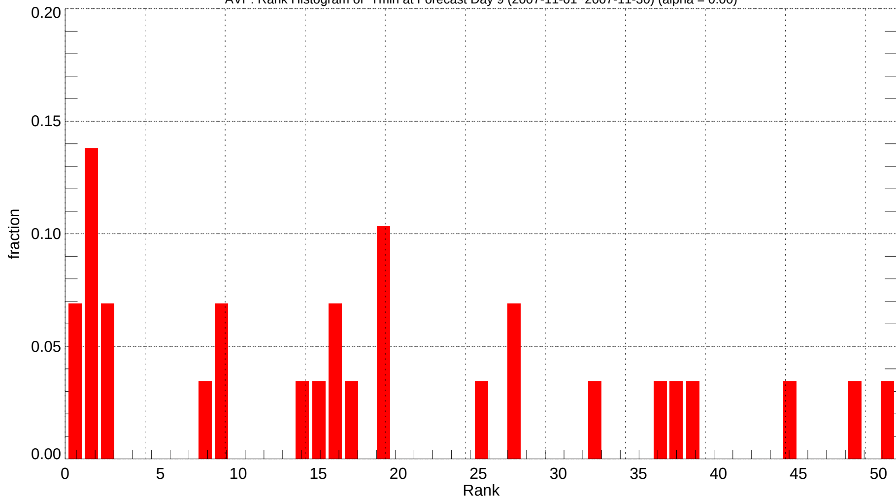
AVP: Rank Histogram of Tmin at Forecast Day 9 (2007-11-01~2007-11-30) (alpha = 0.00)
