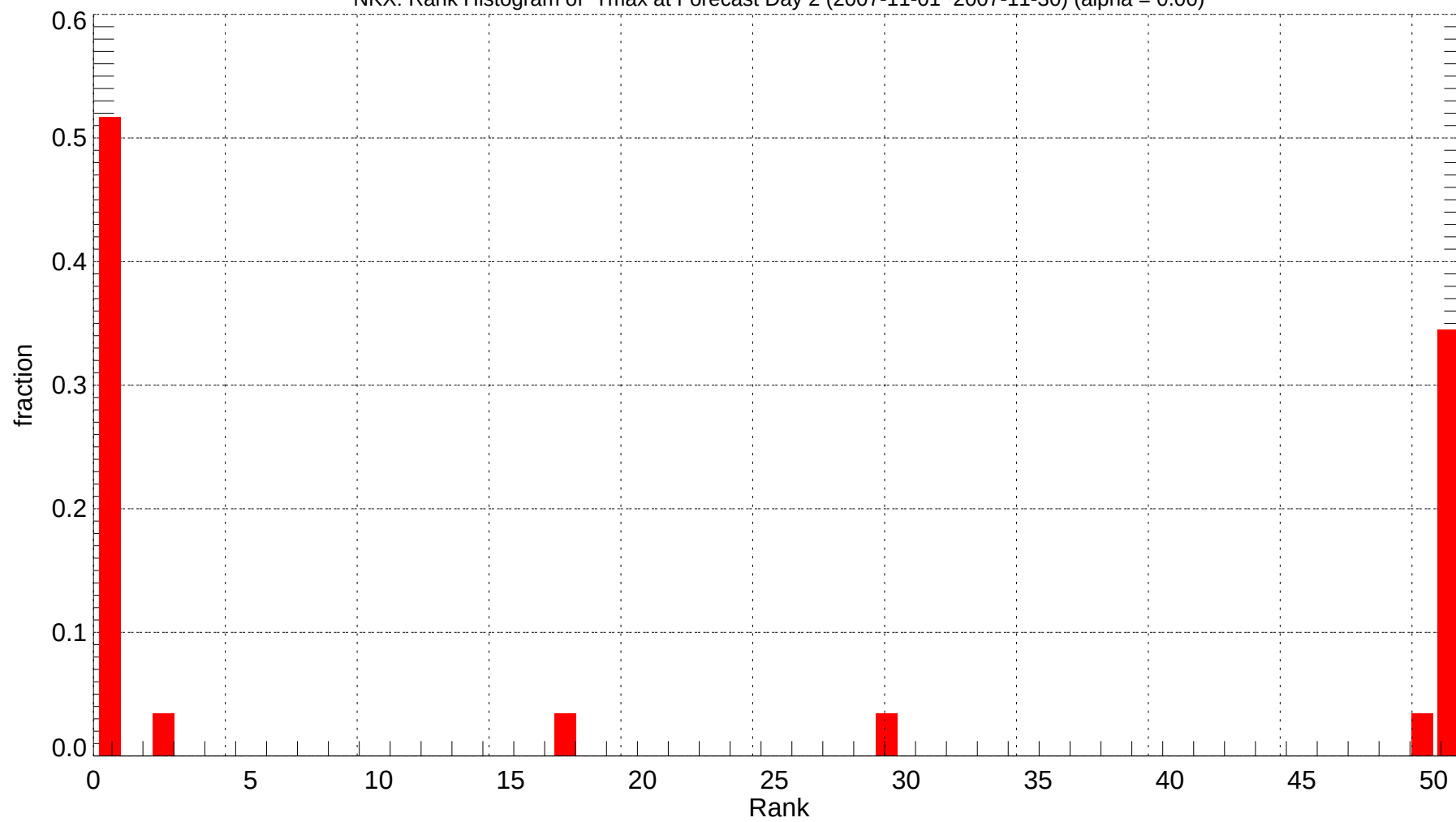
NKX: Rank Histogram of Tmax at Forecast Day 2 (2007-11-01~2007-11-30) (alpha = 0.00)
