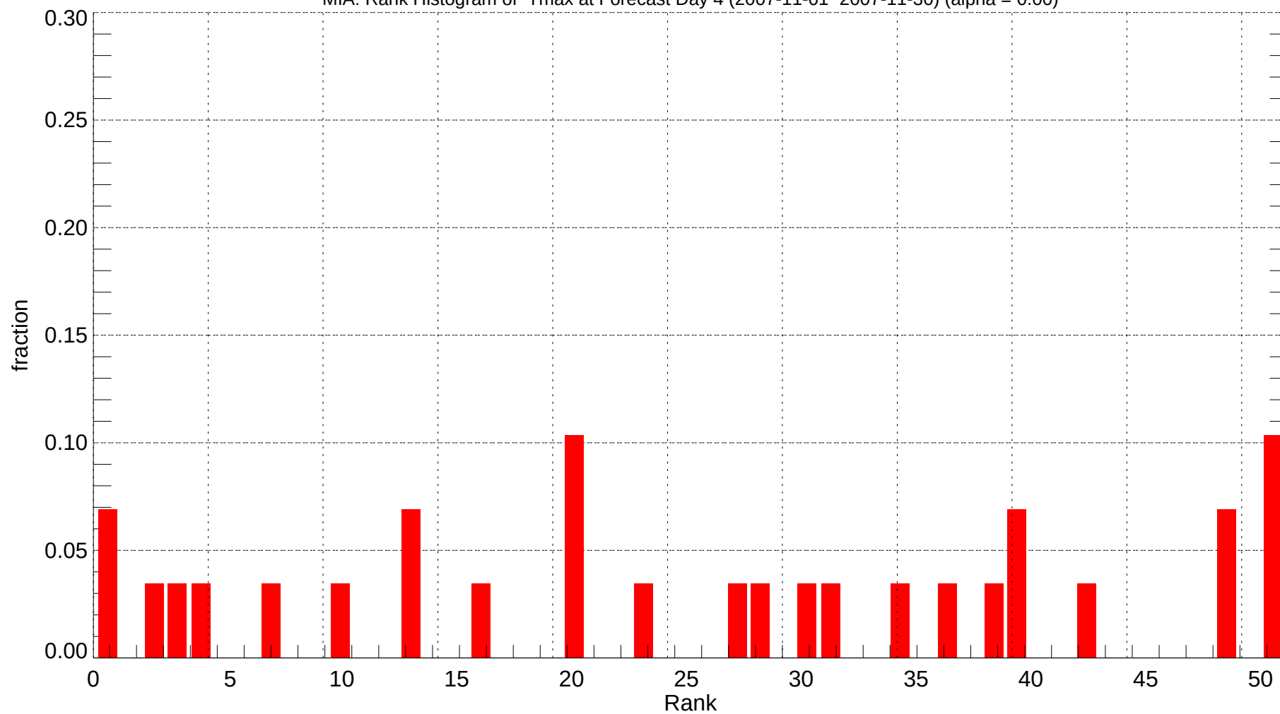
MIA: Rank Histogram of Tmax at Forecast Day 4 (2007-11-01~2007-11-30) (alpha = 0.00)
