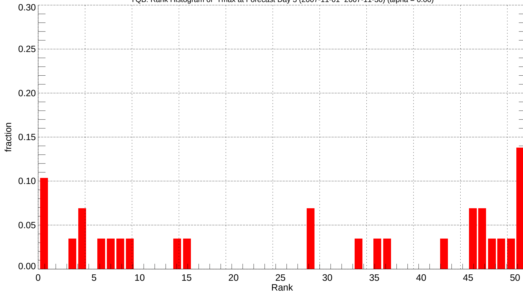
YQB: Rank Histogram of Tmax at Forecast Day 3 (2007-11-01~2007-11-30) (alpha = 0.00)
