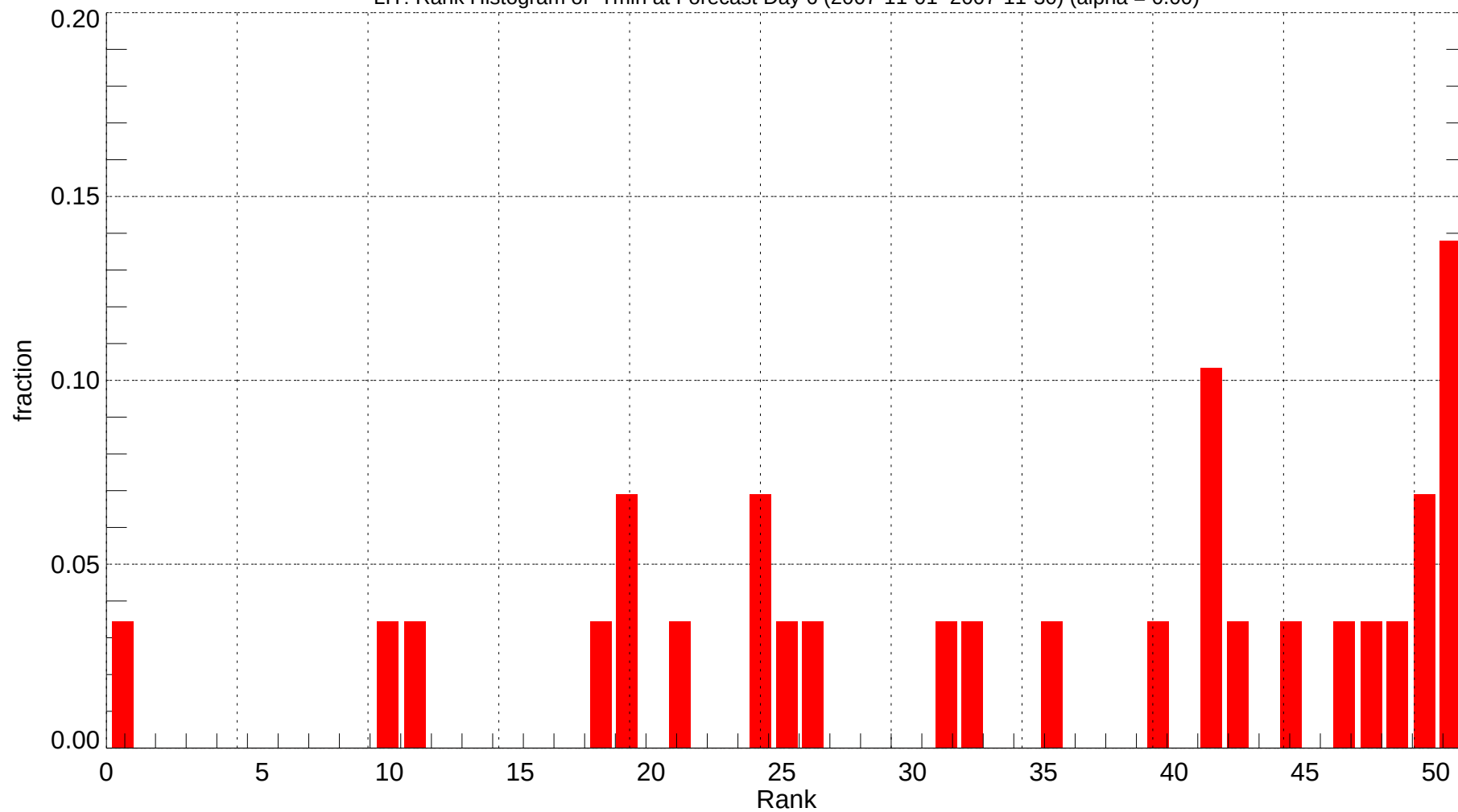
LIT: Rank Histogram of Tmin at Forecast Day 6 (2007-11-01~2007-11-30) (alpha = 0.00)
