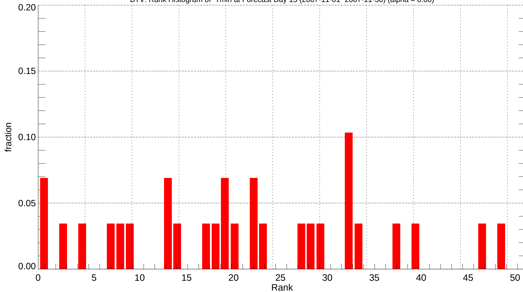
BTV: Rank Histogram of Tmin at Forecast Day 15 (2007-11-01~2007-11-30) (alpha = 0.00)
