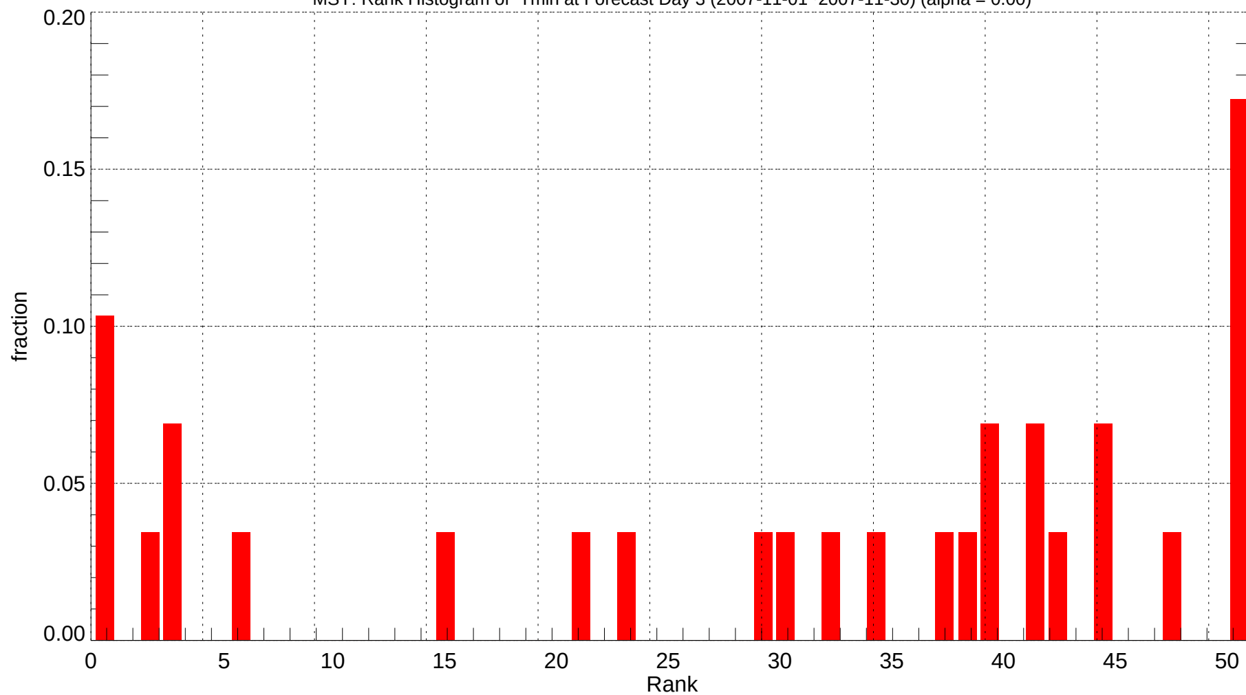
MSY: Rank Histogram of Tmin at Forecast Day 3 (2007-11-01~2007-11-30) (alpha = 0.00)
