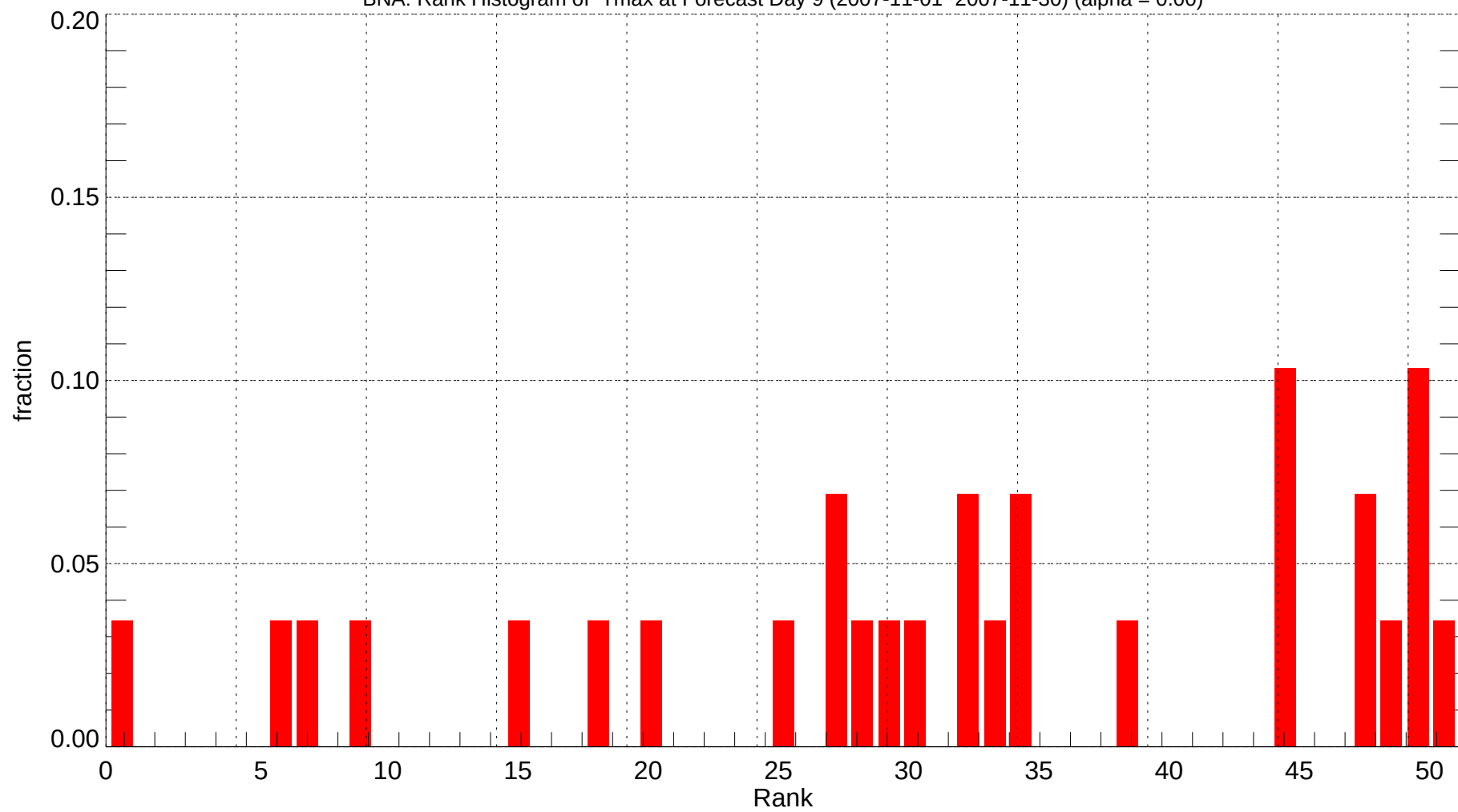
BNA: Rank Histogram of Tmax at Forecast Day 9 (2007-11-01~2007-11-30) (alpha = 0.00)
