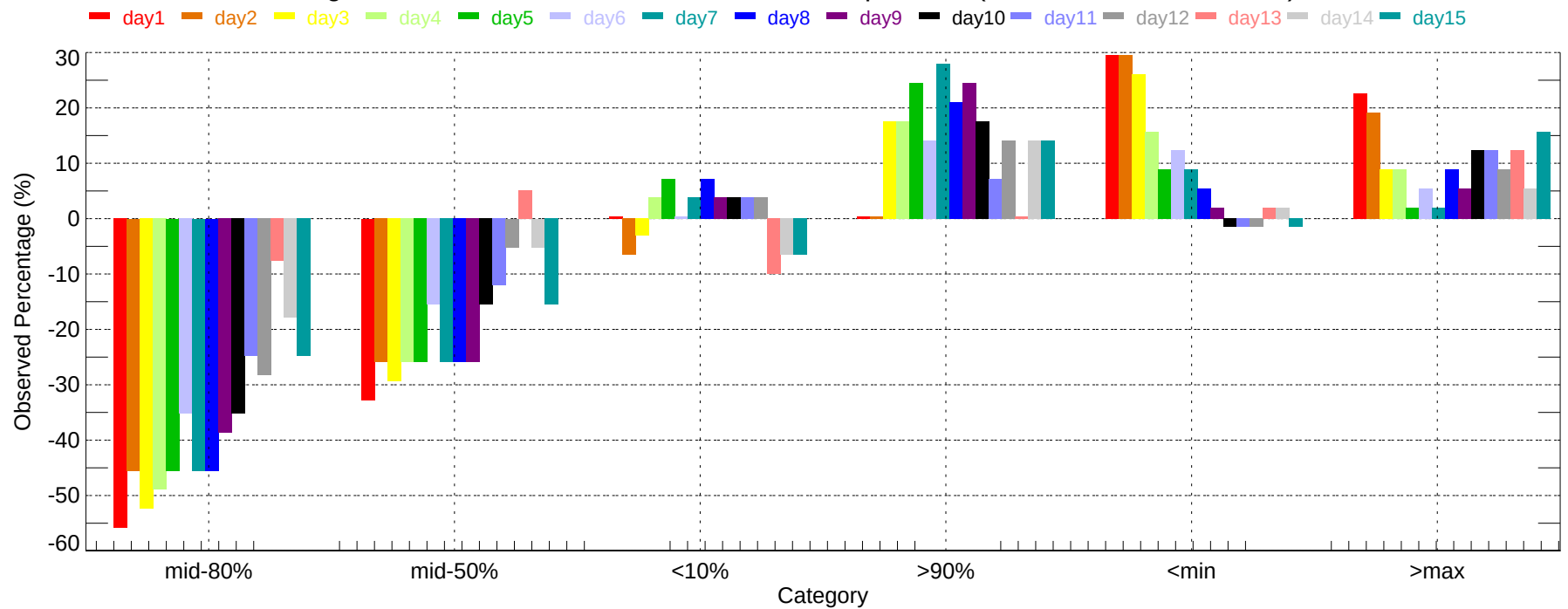
Observed Percentage Deviation of Ensembles - SFO: Min Temperature (2007-11-01~2007-11-30)
