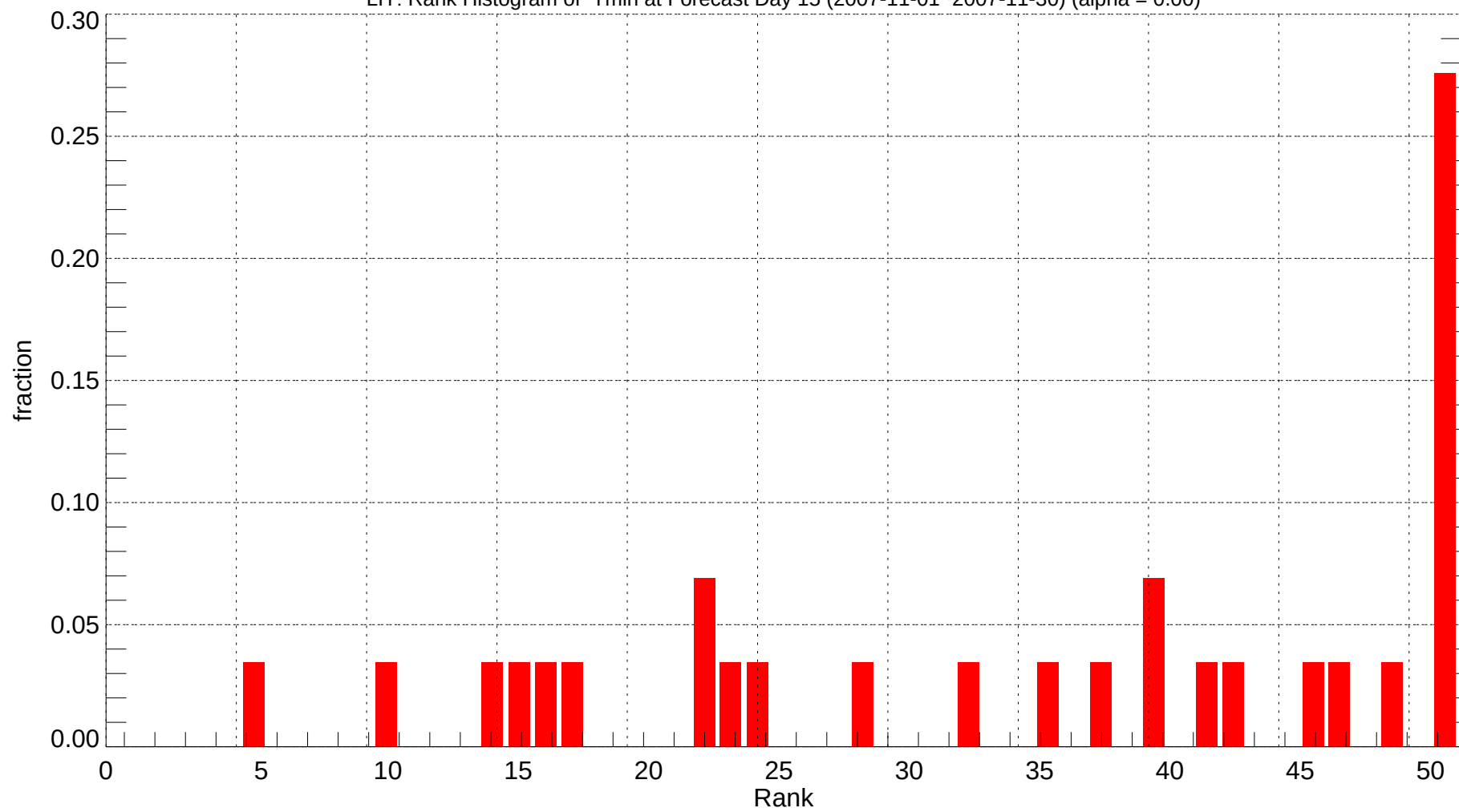
LIT: Rank Histogram of Tmin at Forecast Day 15 (2007-11-01~2007-11-30) (alpha = 0.00)
