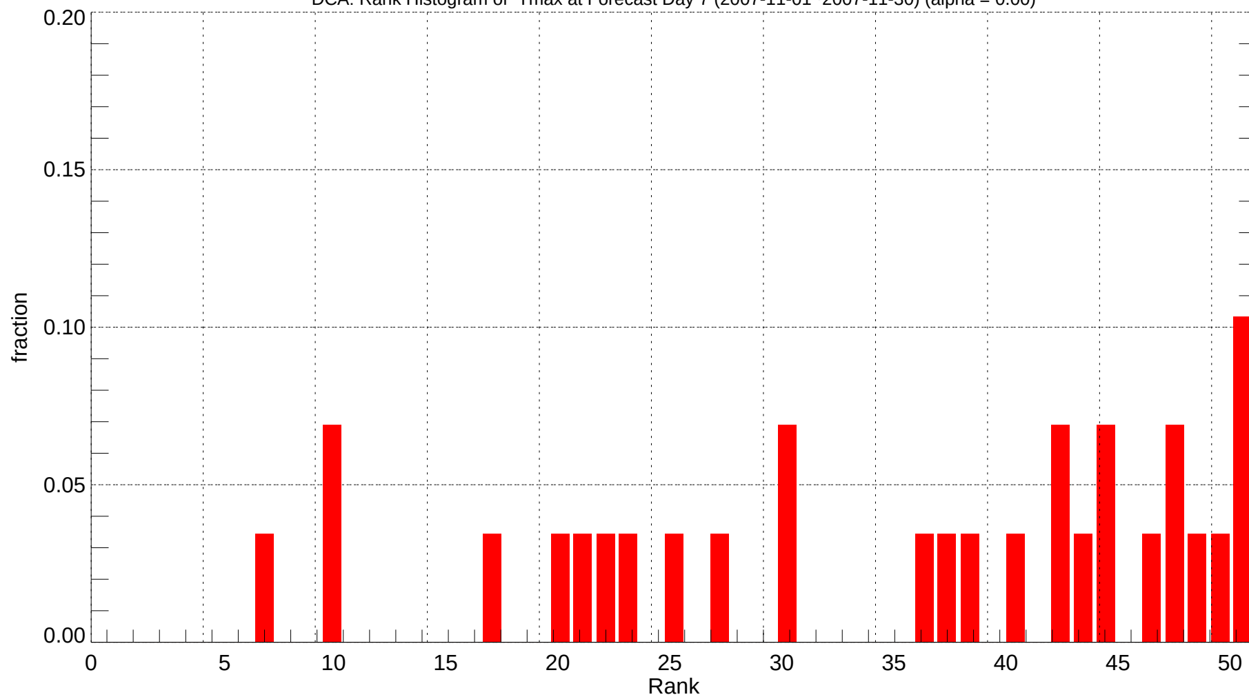
DCA: Rank Histogram of Tmax at Forecast Day 7 (2007-11-01~2007-11-30) (alpha = 0.00)
