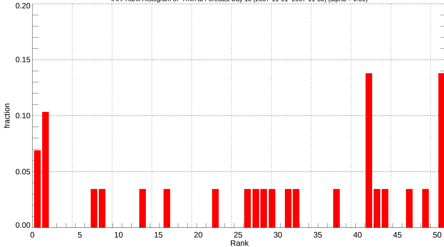
IAH: Rank Histogram of Tmin at Forecast Day 10 (2007-11-01~2007-11-30) (alpha = 0.00)
