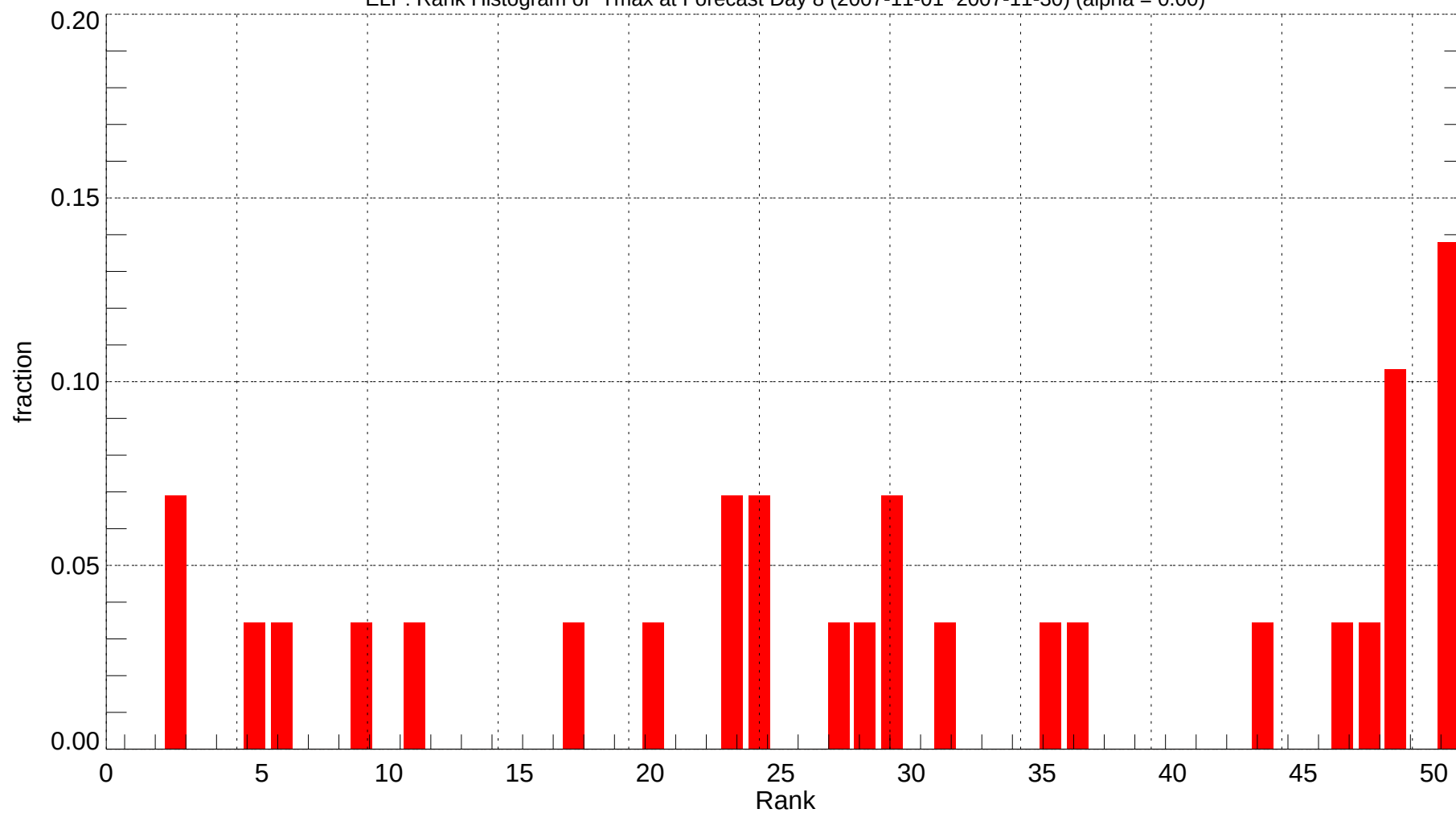
ELP: Rank Histogram of Tmax at Forecast Day 8 (2007-11-01~2007-11-30) (alpha = 0.00)
