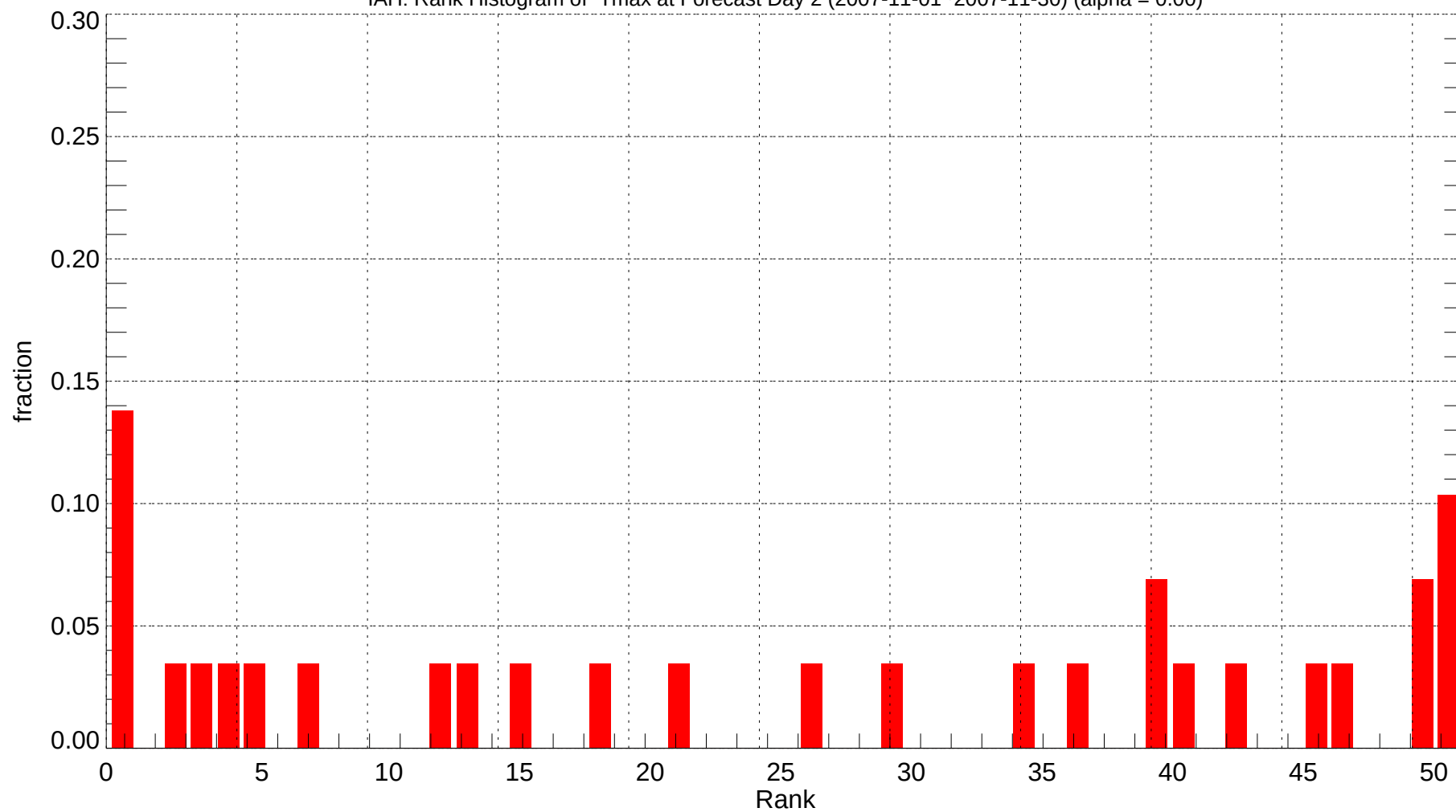
IAH: Rank Histogram of Tmax at Forecast Day 2 (2007-11-01~2007-11-30) (alpha = 0.00)
