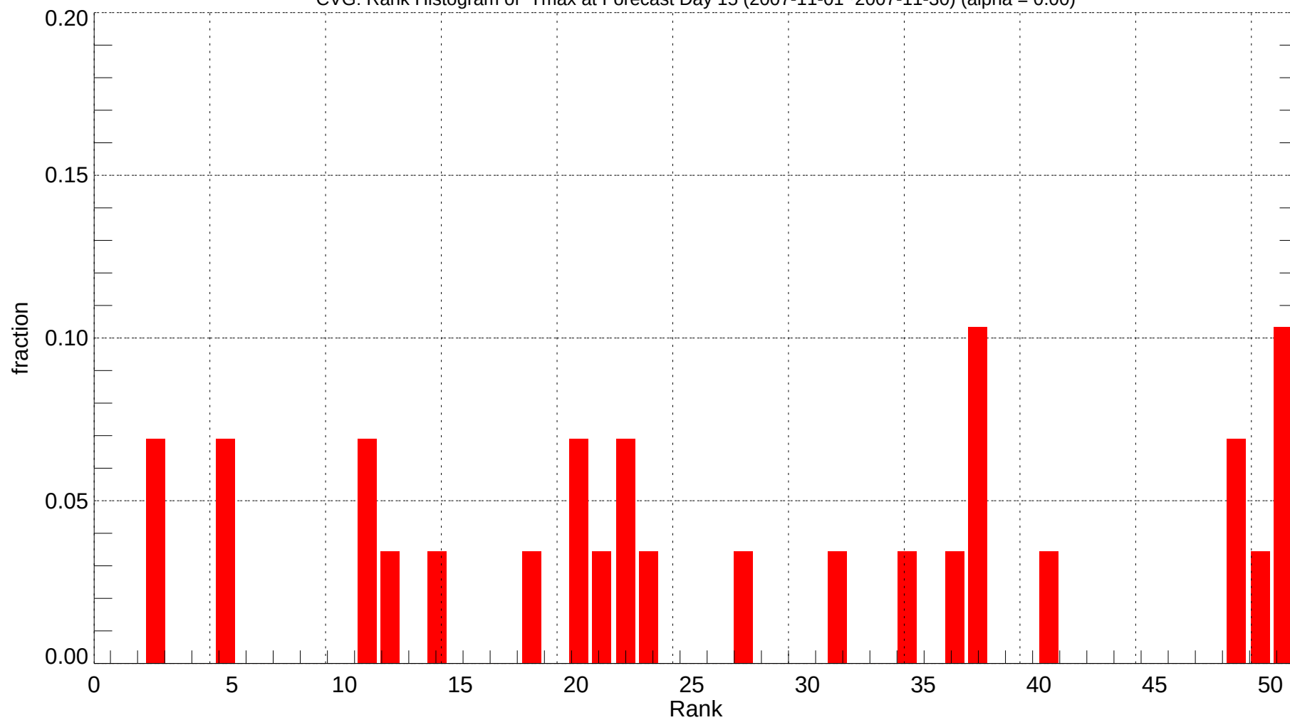
CVG: Rank Histogram of Tmax at Forecast Day 15 (2007-11-01~2007-11-30) (alpha = 0.00)
