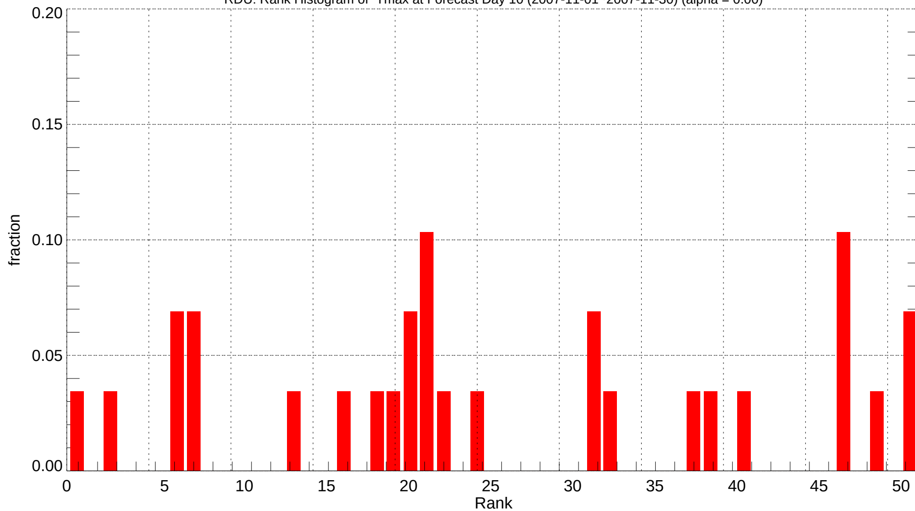
RDU: Rank Histogram of Tmax at Forecast Day 10 (2007-11-01~2007-11-30) (alpha = 0.00)
