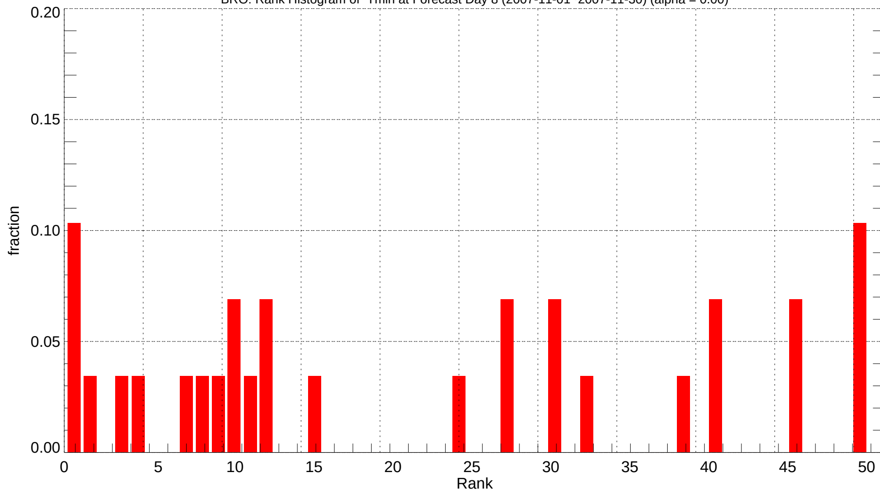
BRO: Rank Histogram of Tmin at Forecast Day 8 (2007-11-01~2007-11-30) (alpha = 0.00)
