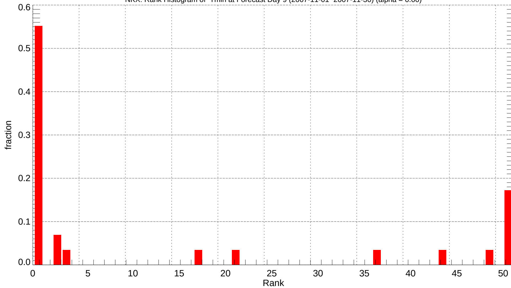
NKX: Rank Histogram of Tmin at Forecast Day 9 (2007-11-01~2007-11-30) (alpha = 0.00)
