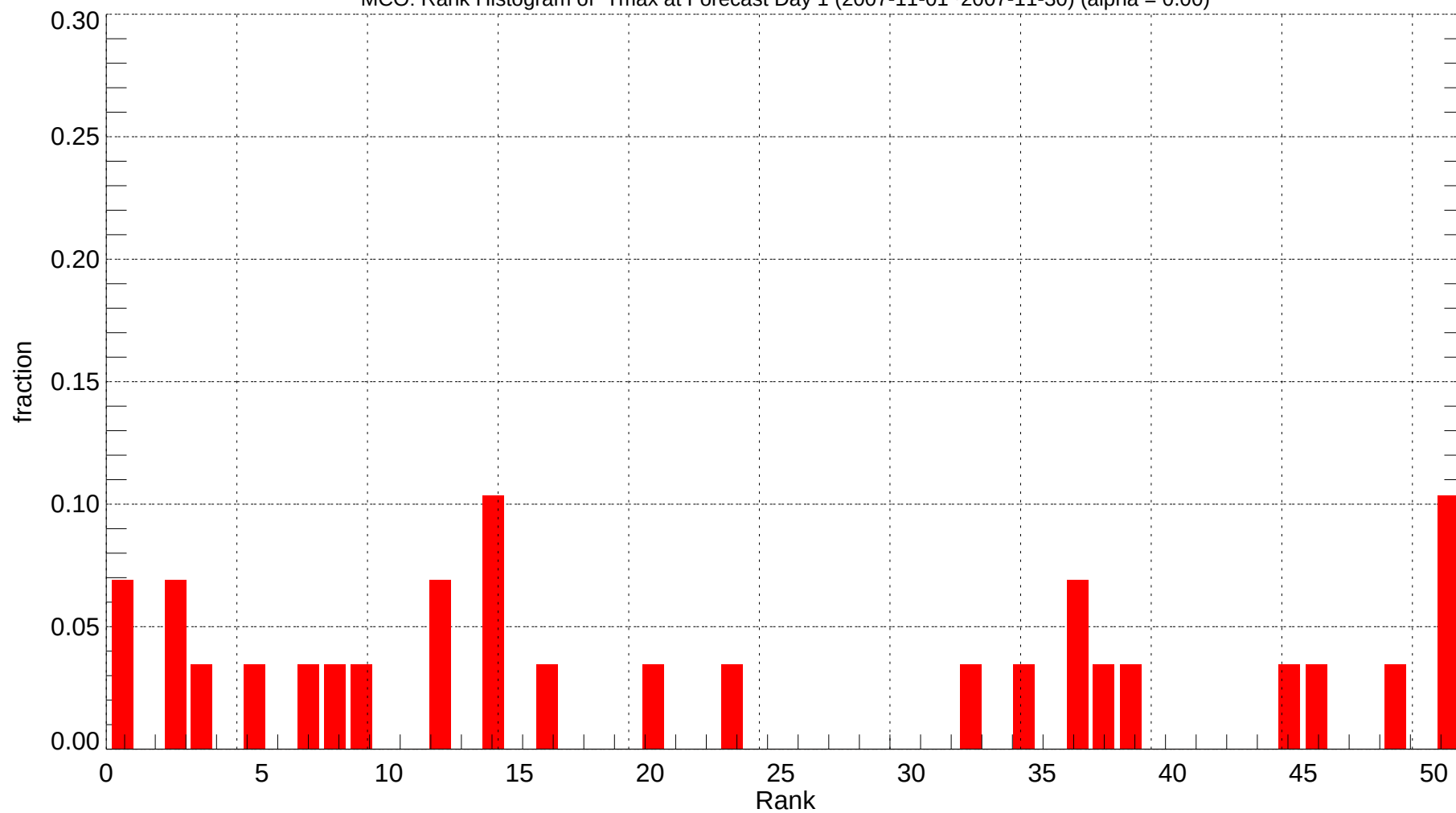
MCO: Rank Histogram of Tmax at Forecast Day 1 (2007-11-01~2007-11-30) (alpha = 0.00)
