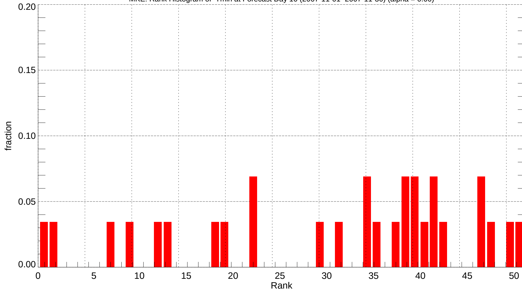
MKE: Rank Histogram of Tmin at Forecast Day 10 (2007-11-01~2007-11-30) (alpha = 0.00)
