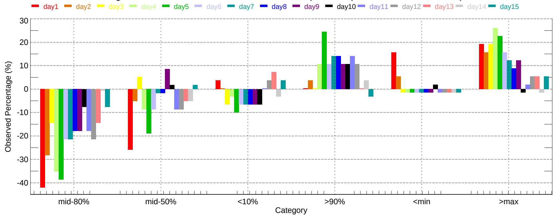
Observed Percentage Deviation of Ensembles - RDU: Max Temperature (2007-11-01~2007-11-30)
