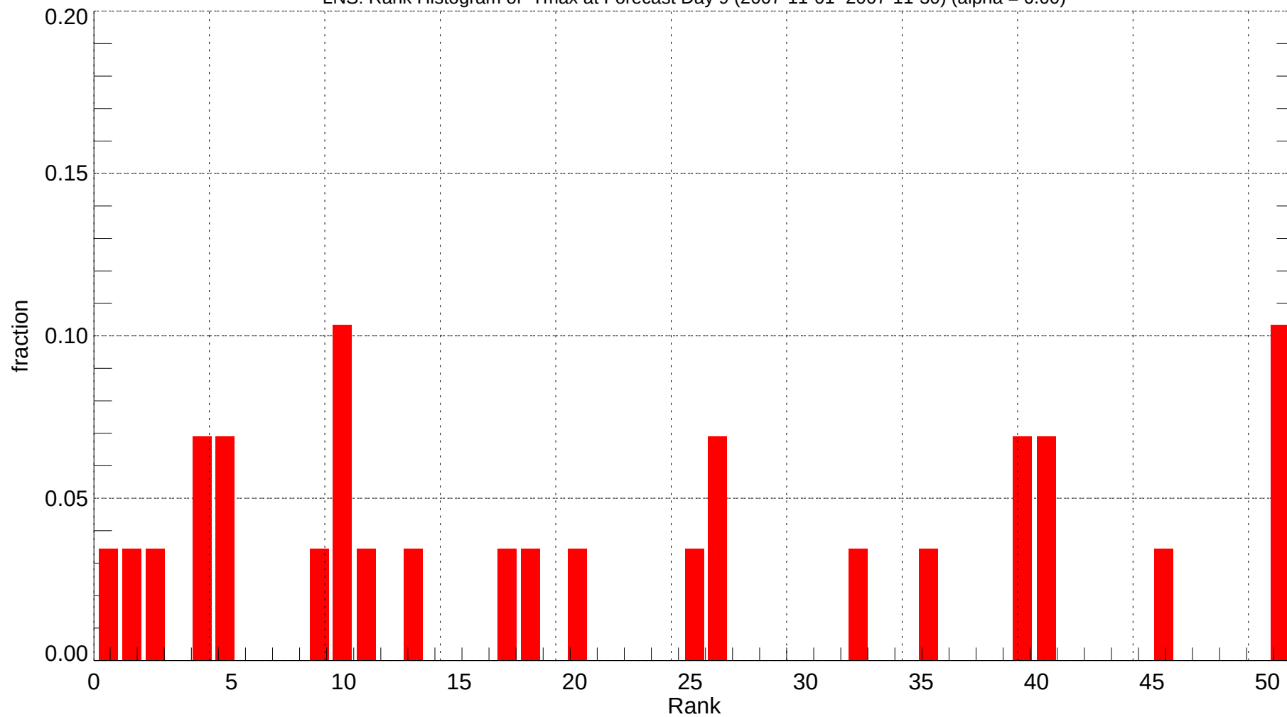
LNS: Rank Histogram of Tmax at Forecast Day 9 (2007-11-01~2007-11-30) (alpha = 0.00)
