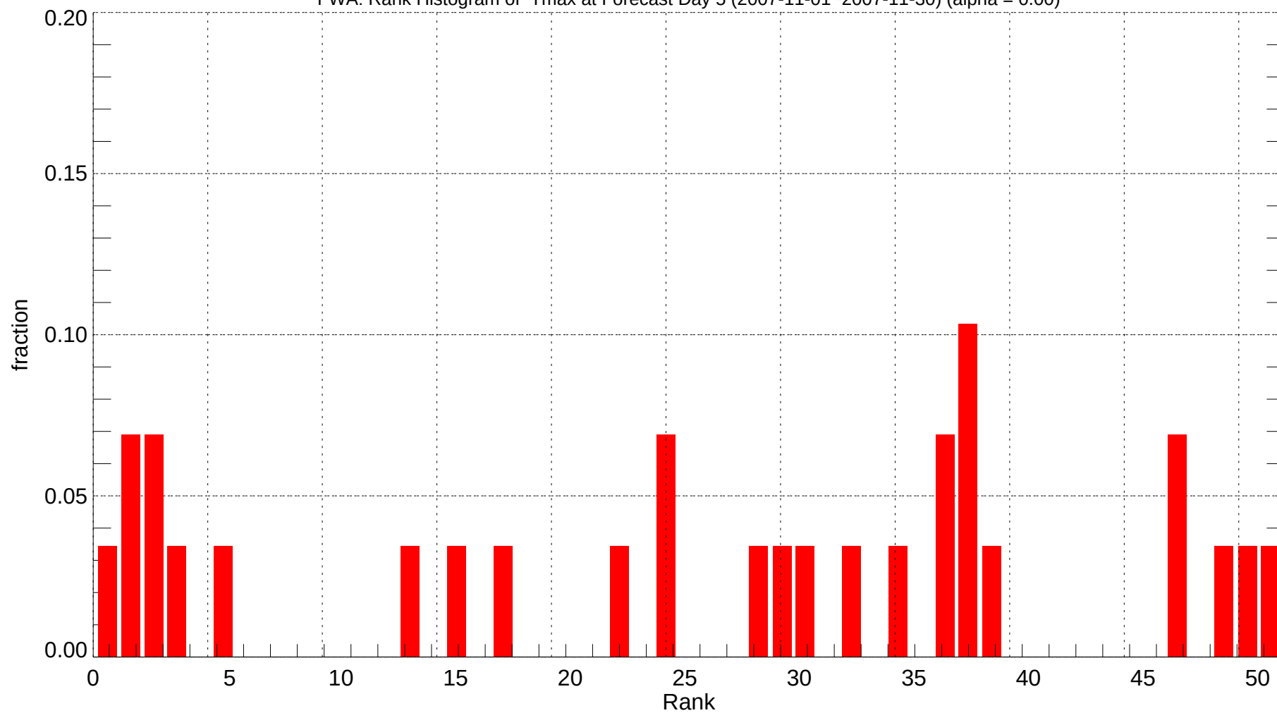
FWA: Rank Histogram of Tmax at Forecast Day 5 (2007-11-01~2007-11-30) (alpha = 0.00)
