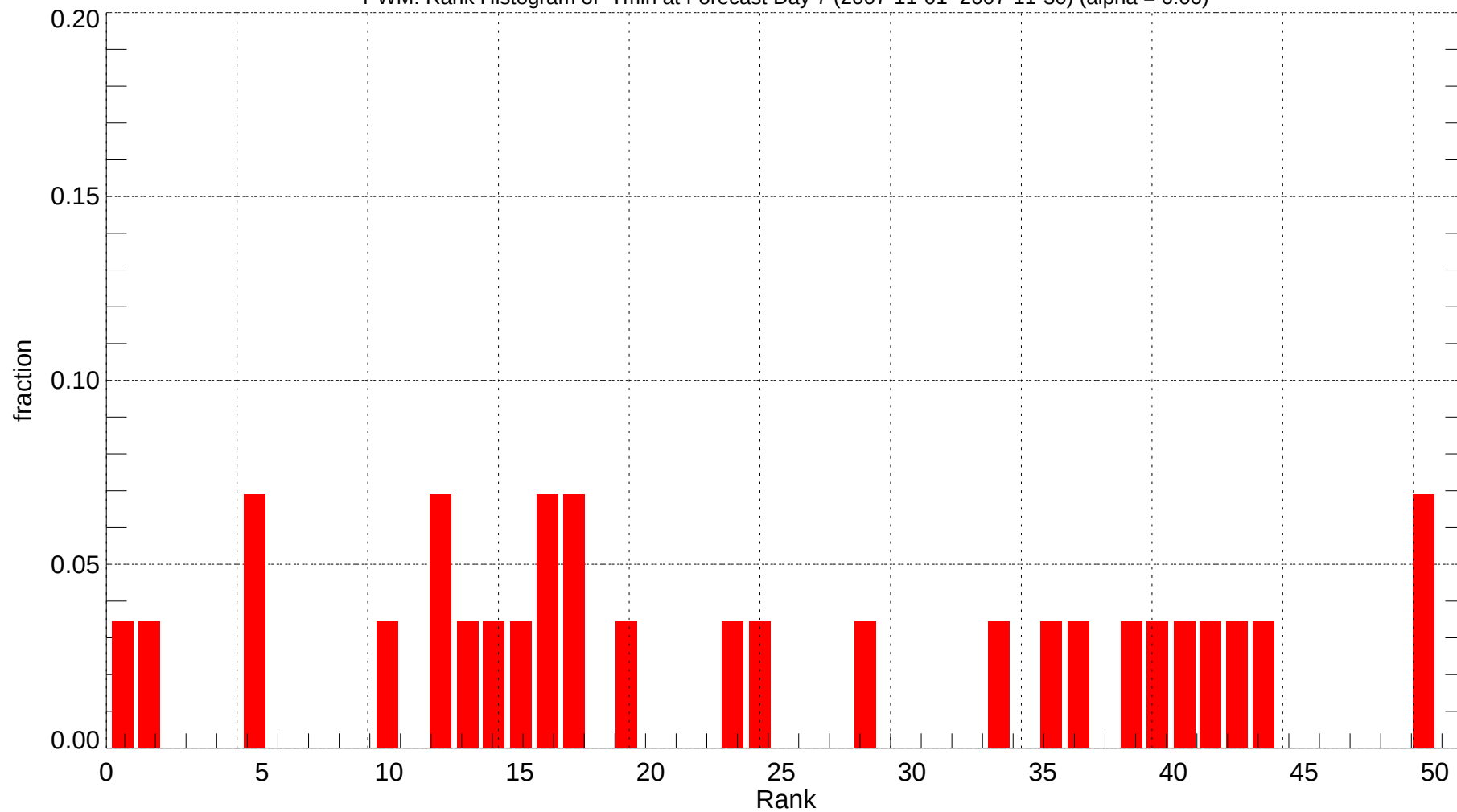
PWM: Rank Histogram of Tmin at Forecast Day 7 (2007-11-01~2007-11-30) (alpha = 0.00)
