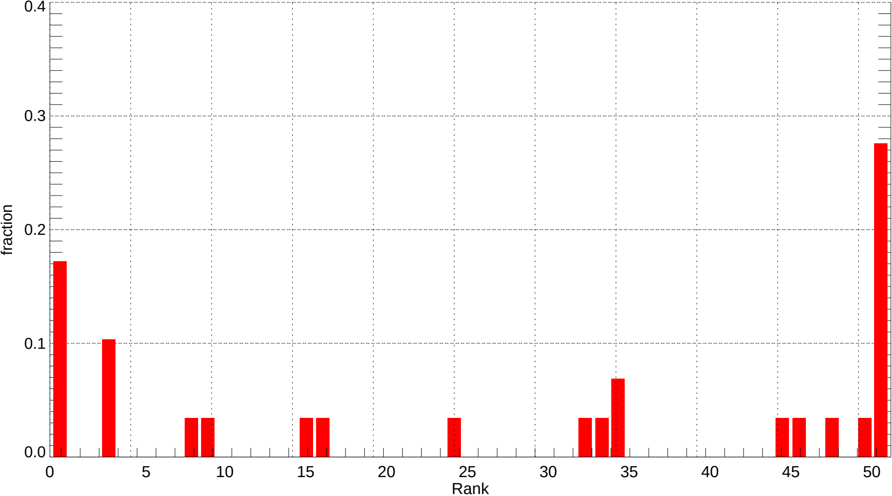
SDF: Rank Histogram of Tmin at Forecast Day 1 (2007-11-01~2007-11-30) (alpha = 0.00)
