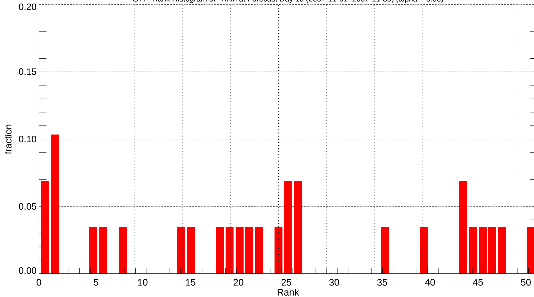
GTF: Rank Histogram of Tmin at Forecast Day 10 (2007-11-01~2007-11-30) (alpha = 0.00)
