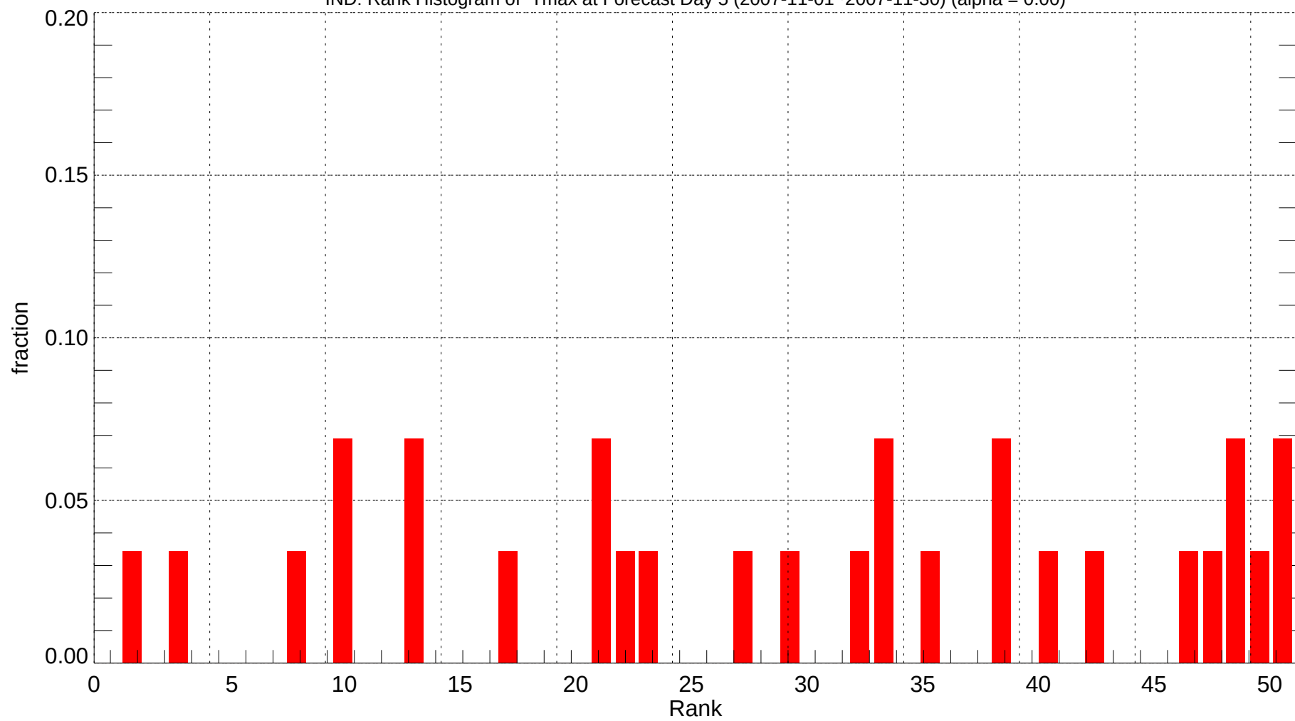
IND: Rank Histogram of Tmax at Forecast Day 5 (2007-11-01~2007-11-30) (alpha = 0.00)
