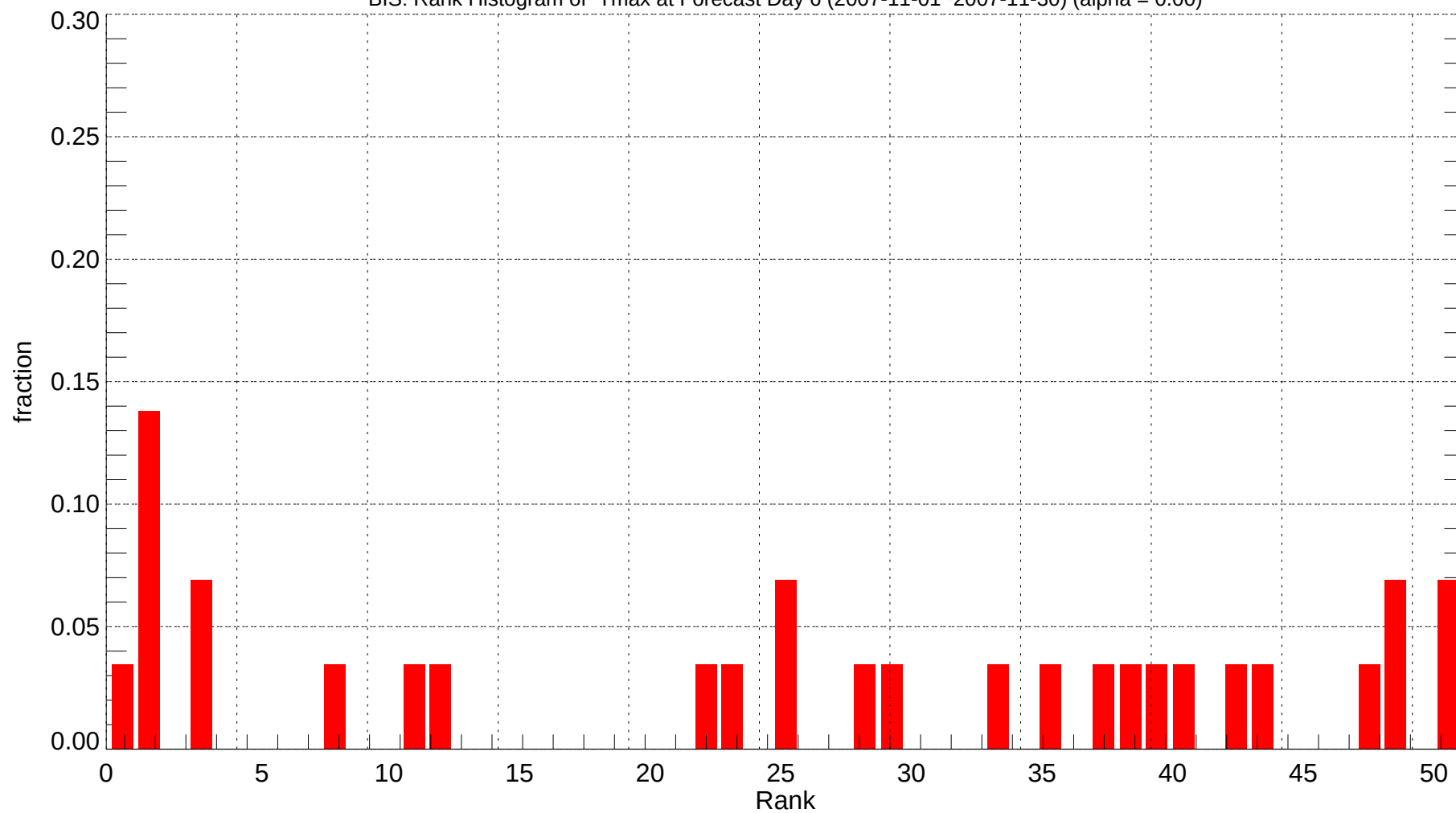
BIS: Rank Histogram of Tmax at Forecast Day 6 (2007-11-01~2007-11-30) (alpha = 0.00)
