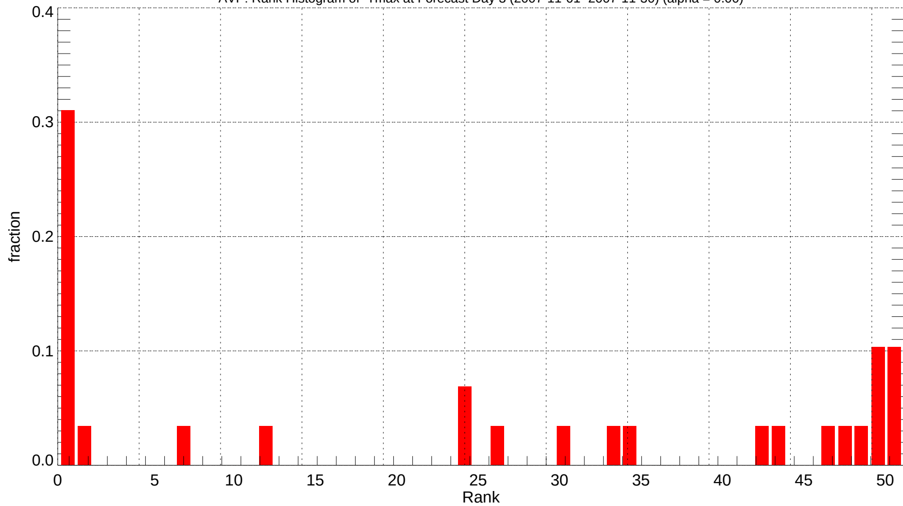
AVP: Rank Histogram of Tmax at Forecast Day 3 (2007-11-01~2007-11-30) (alpha = 0.00)
