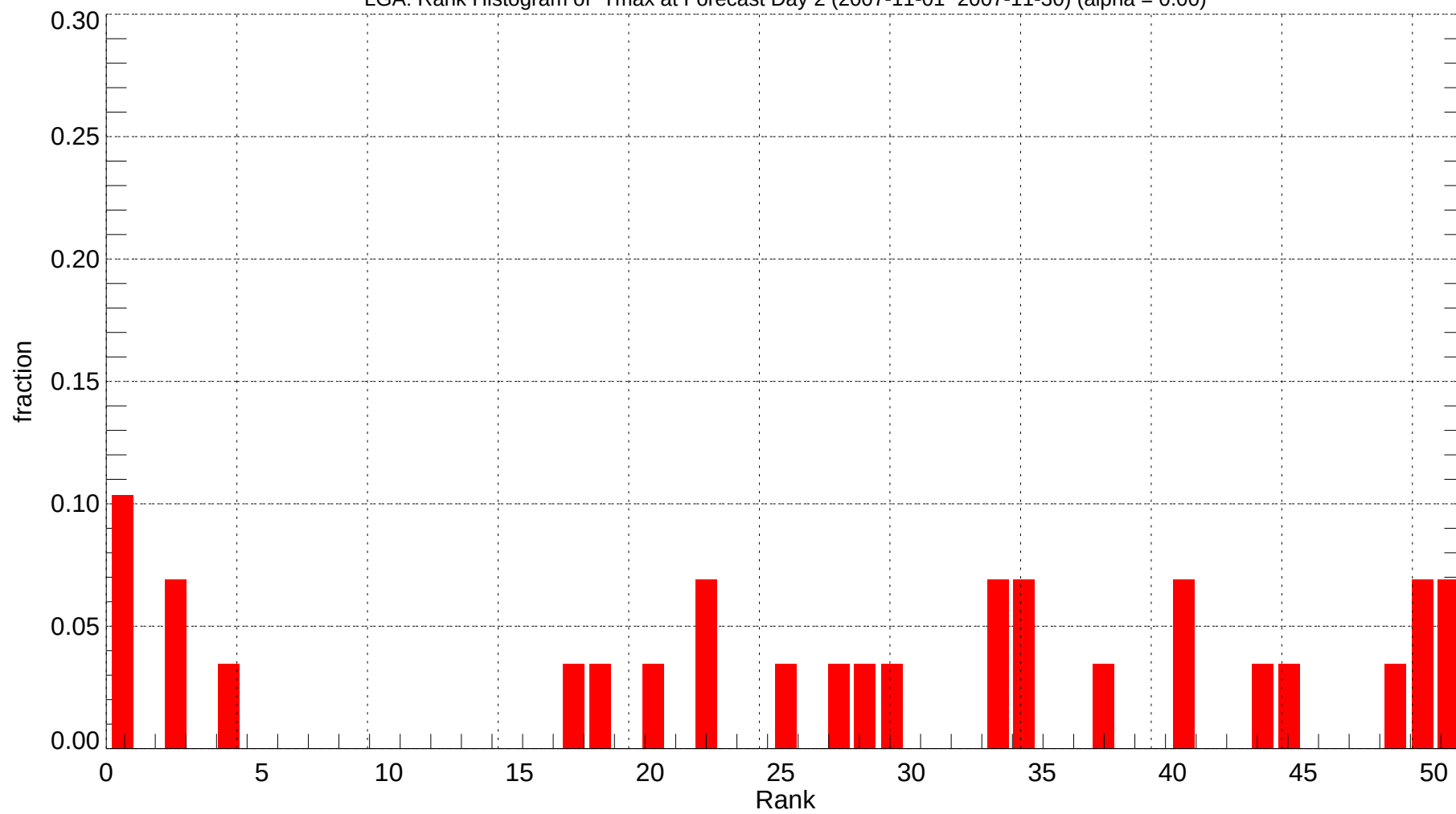
LGA: Rank Histogram of Tmax at Forecast Day 2 (2007-11-01~2007-11-30) (alpha = 0.00)
