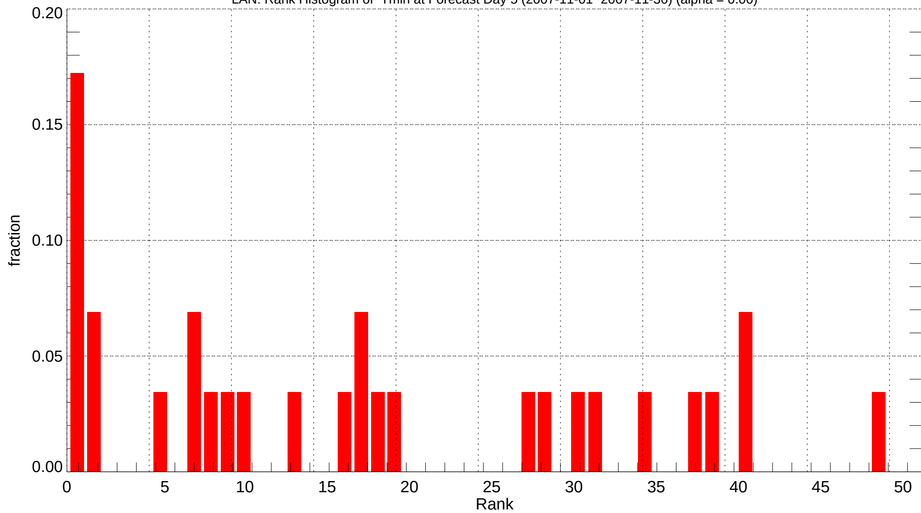
LAN: Rank Histogram of Tmin at Forecast Day 5 (2007-11-01~2007-11-30) (alpha = 0.00)
