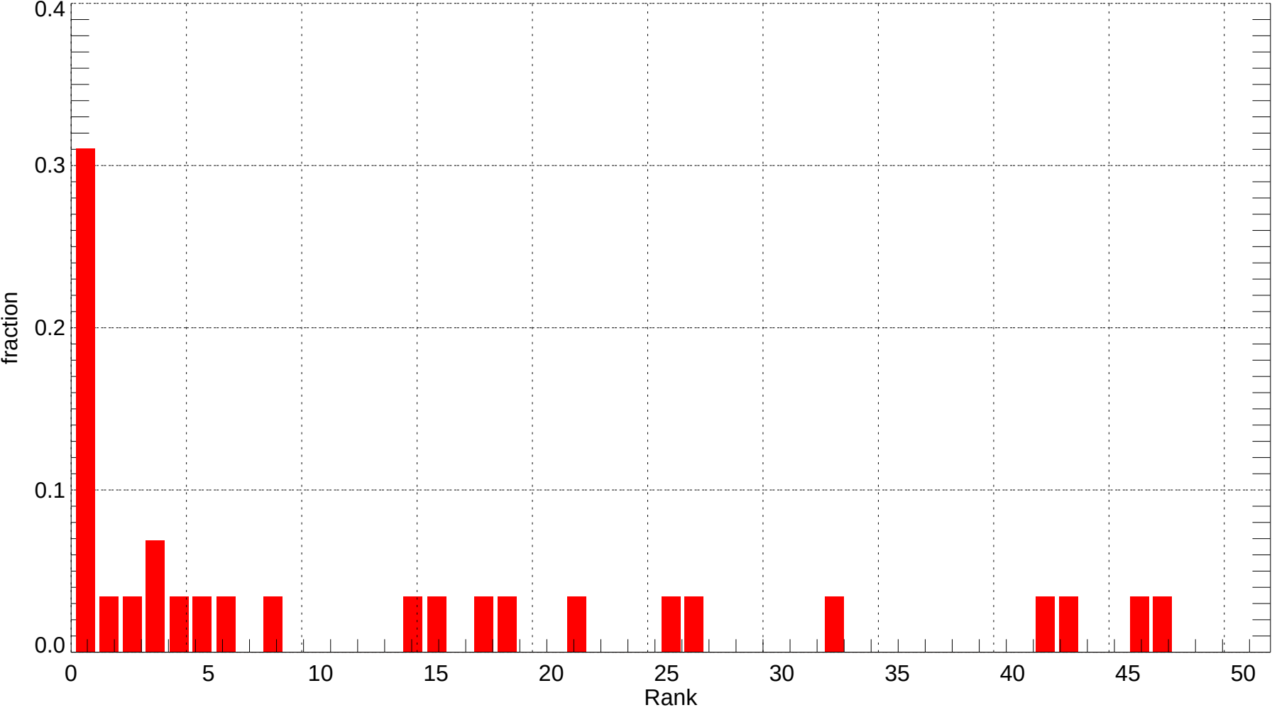
BFL: Rank Histogram of Tmin at Forecast Day 3 (2007-11-01~2007-11-30) (alpha = 0.00)
