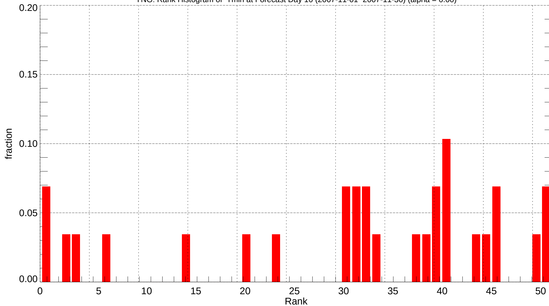
YNG: Rank Histogram of Tmin at Forecast Day 10 (2007-11-01~2007-11-30) (alpha = 0.00)
