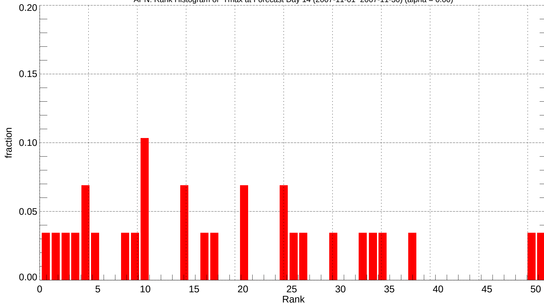
APN: Rank Histogram of Tmax at Forecast Day 14 (2007-11-01~2007-11-30) (alpha = 0.00)
