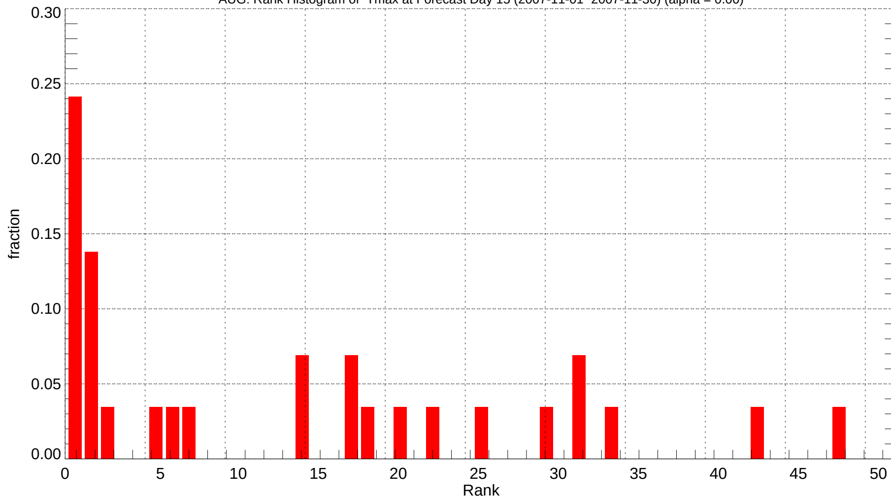
AUG: Rank Histogram of Tmax at Forecast Day 15 (2007-11-01~2007-11-30) (alpha = 0.00)
