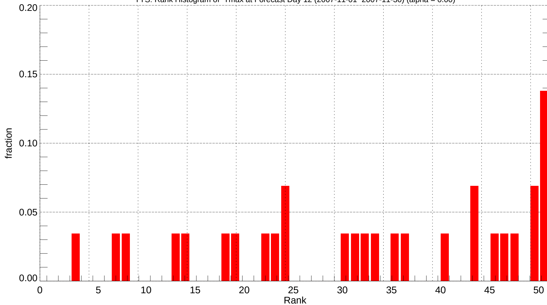
TYS: Rank Histogram of Tmax at Forecast Day 12 (2007-11-01~2007-11-30) (alpha = 0.00)
