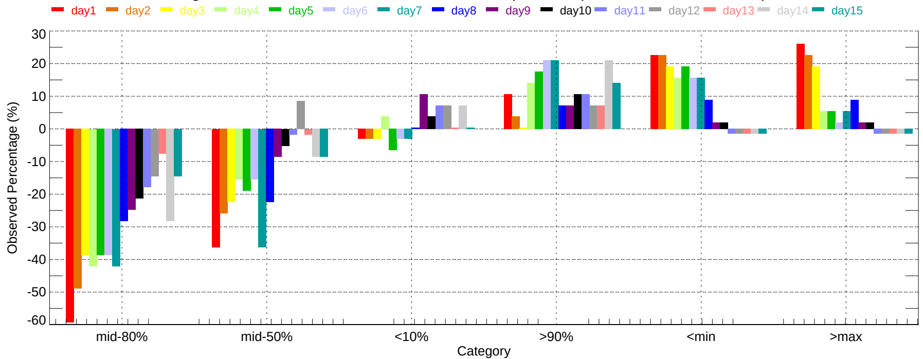
Observed Percentage Deviation of Ensembles - GTF: Max Temperature (2007-11-01~2007-11-30)
