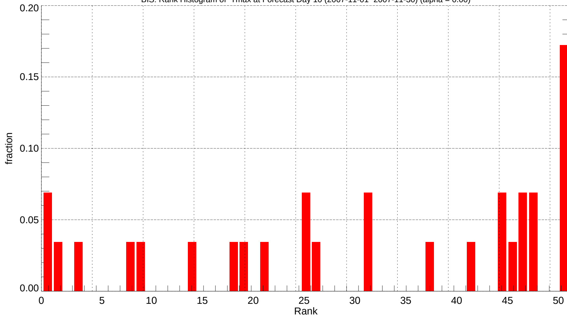
BIS: Rank Histogram of Tmax at Forecast Day 10 (2007-11-01~2007-11-30) (alpha = 0.00)
