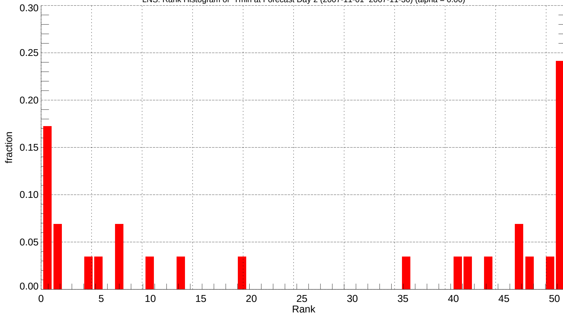
LNS: Rank Histogram of Tmin at Forecast Day 2 (2007-11-01~2007-11-30) (alpha = 0.00)
