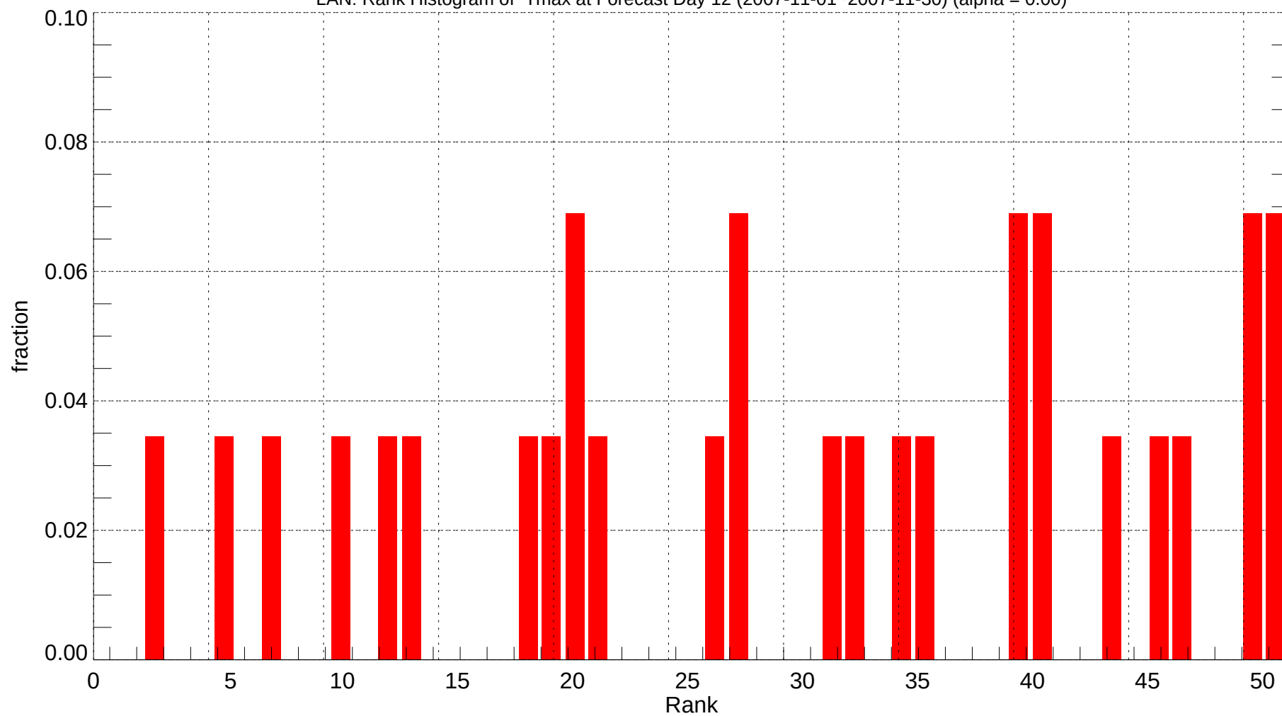
LAN: Rank Histogram of Tmax at Forecast Day 12 (2007-11-01~2007-11-30) (alpha = 0.00)
