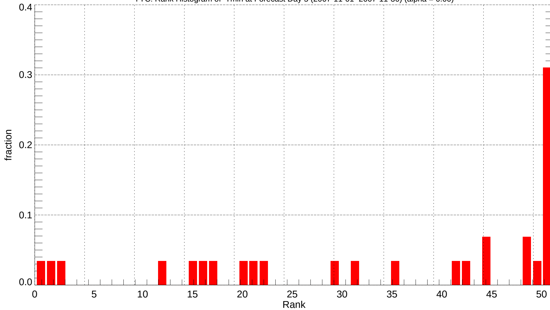
YYC: Rank Histogram of Tmin at Forecast Day 5 (2007-11-01~2007-11-30) (alpha = 0.00)
