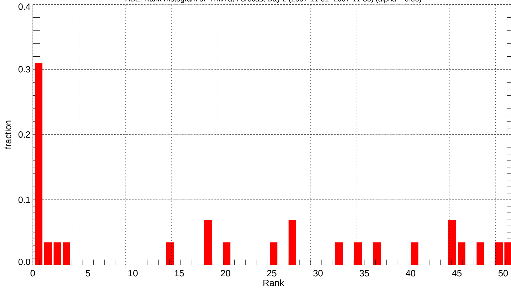
ABE: Rank Histogram of Tmin at Forecast Day 2 (2007-11-01~2007-11-30) (alpha = 0.00)
