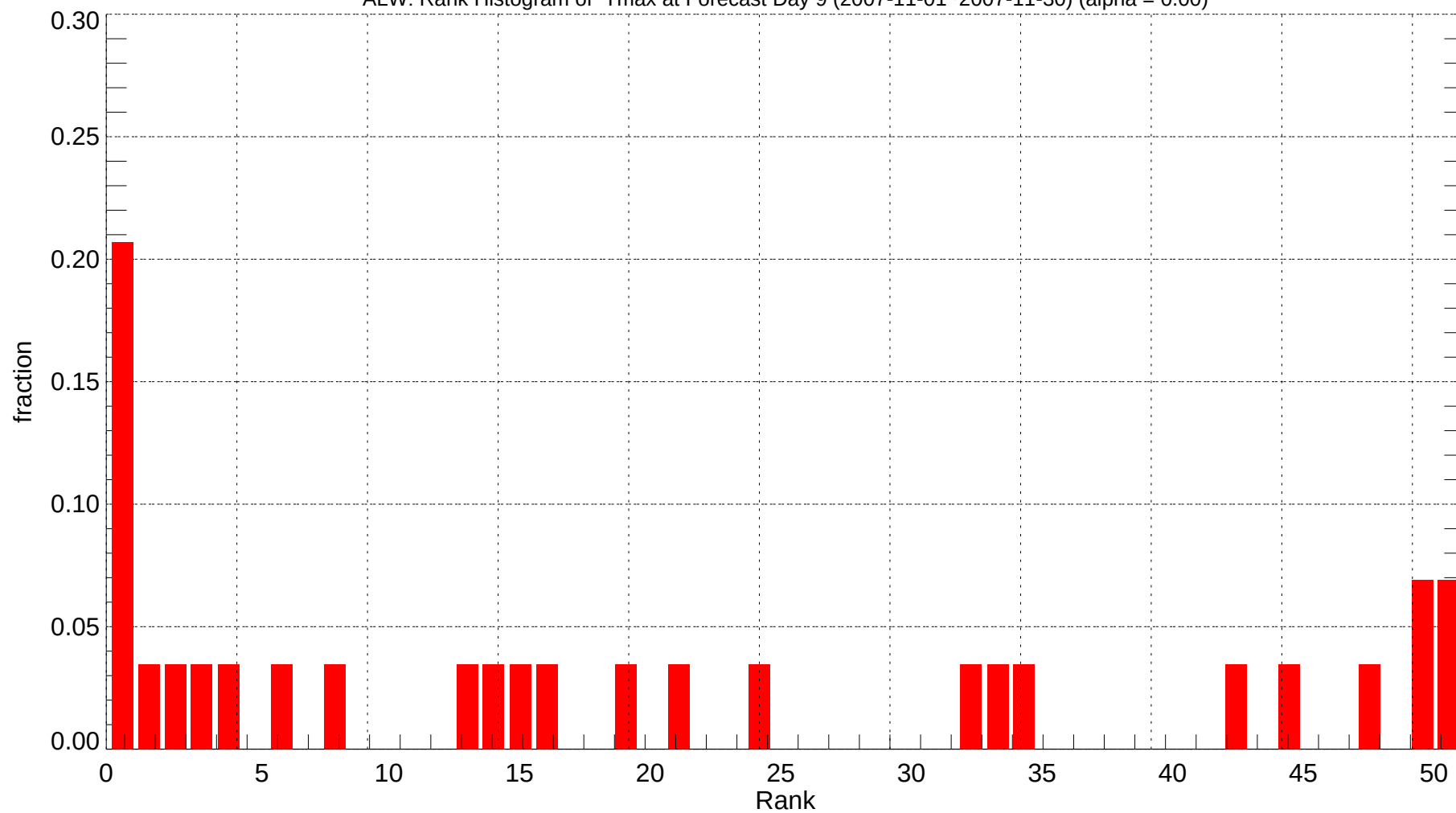
ALW: Rank Histogram of Tmax at Forecast Day 9 (2007-11-01~2007-11-30) (alpha = 0.00)
