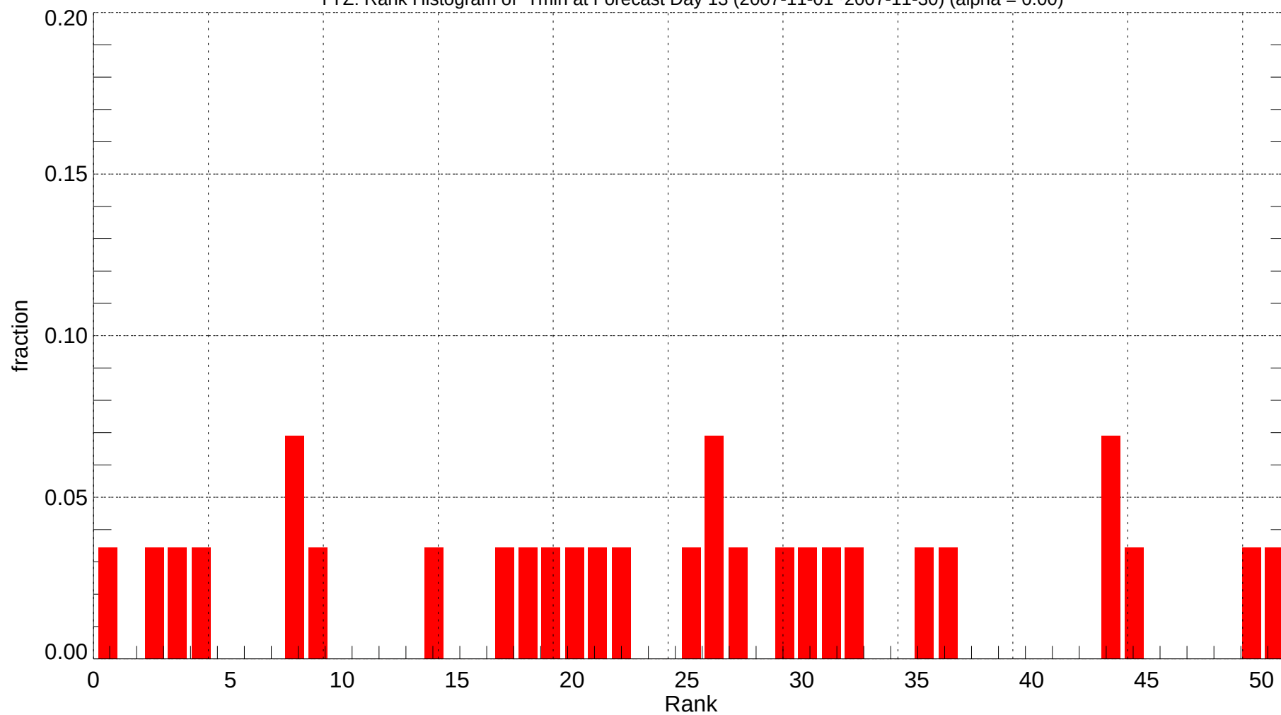
YYZ: Rank Histogram of Tmin at Forecast Day 13 (2007-11-01~2007-11-30) (alpha = 0.00)
