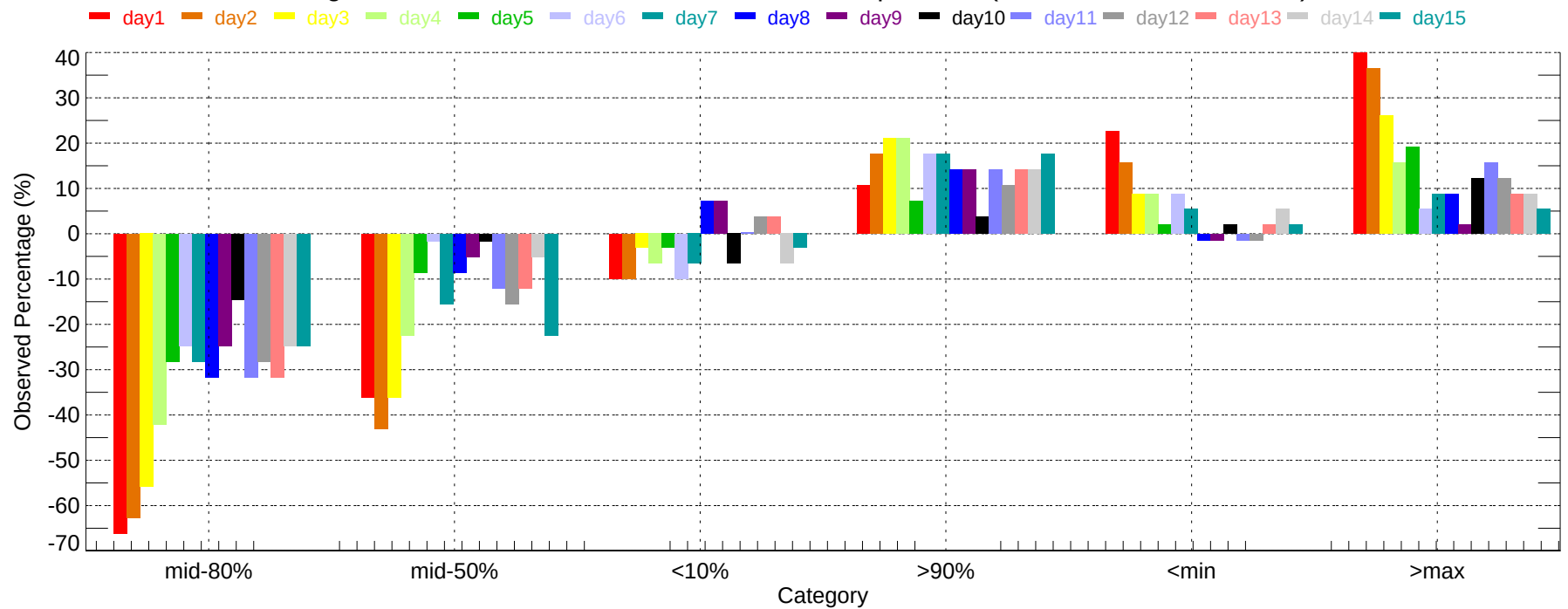
Observed Percentage Deviation of Ensembles - AOO: Max Temperature (2007-11-01~2007-11-30)
