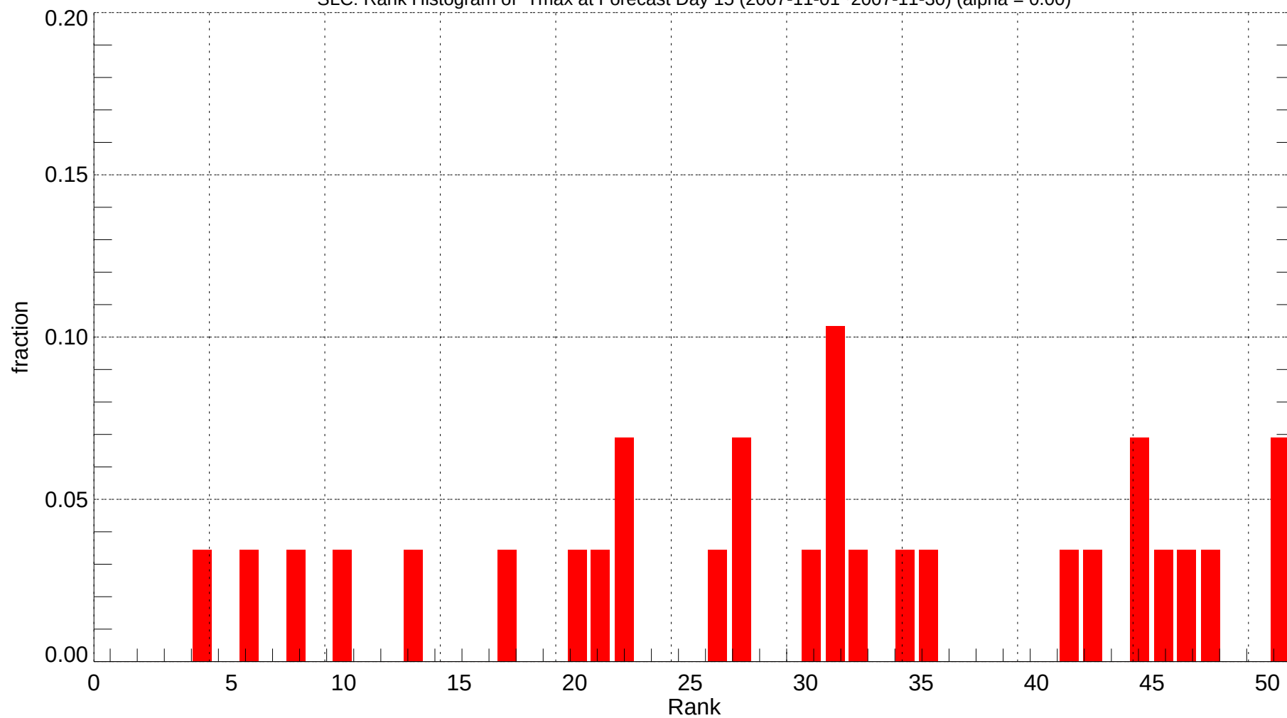
SLC: Rank Histogram of Tmax at Forecast Day 15 (2007-11-01~2007-11-30) (alpha = 0.00)
