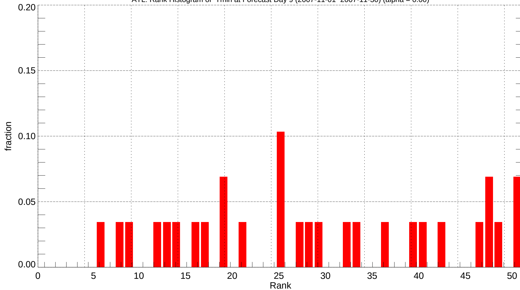
ATL: Rank Histogram of Tmin at Forecast Day 9 (2007-11-01~2007-11-30) (alpha = 0.00)
