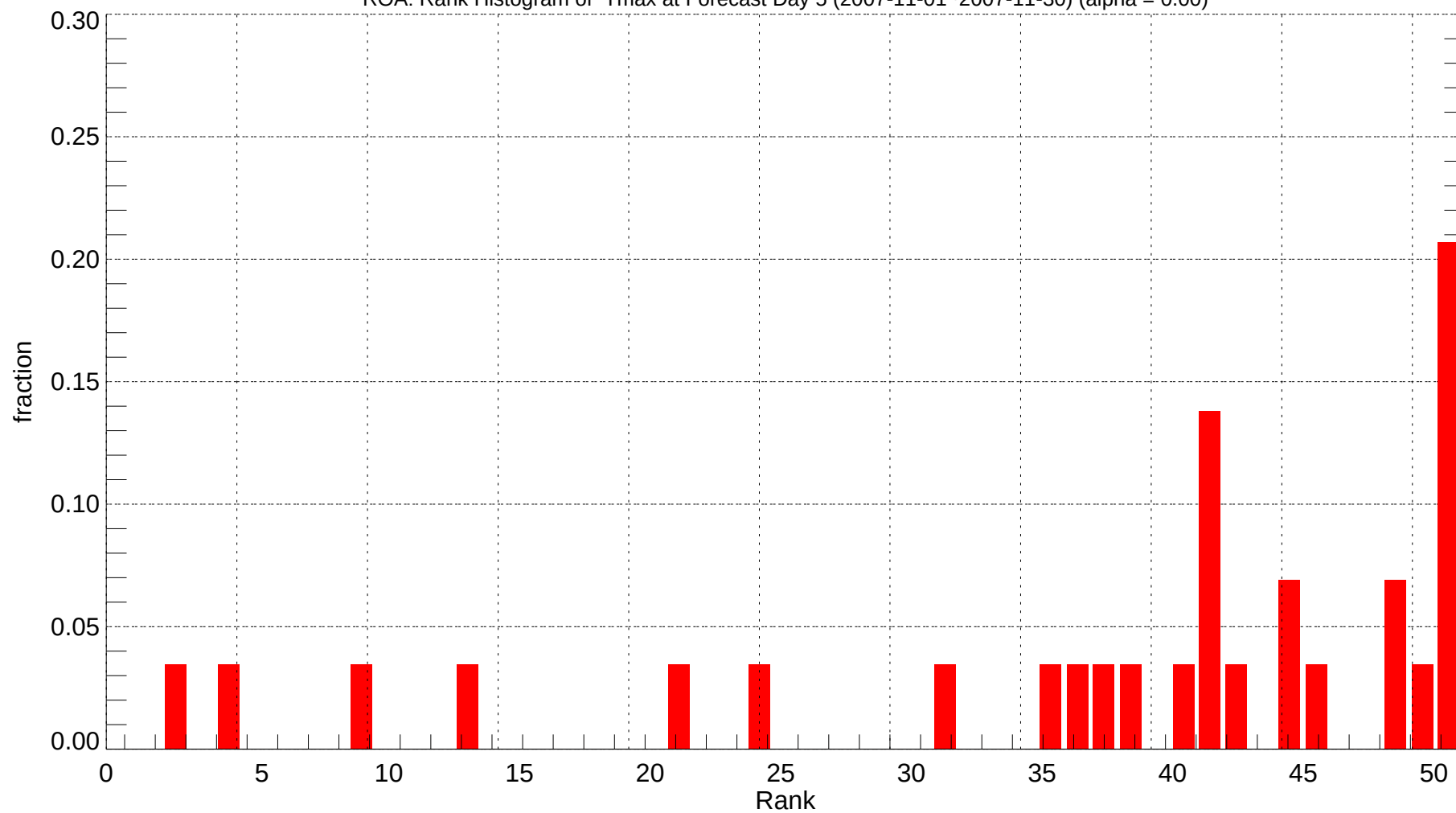
ROA: Rank Histogram of Tmax at Forecast Day 5 (2007-11-01~2007-11-30) (alpha = 0.00)
