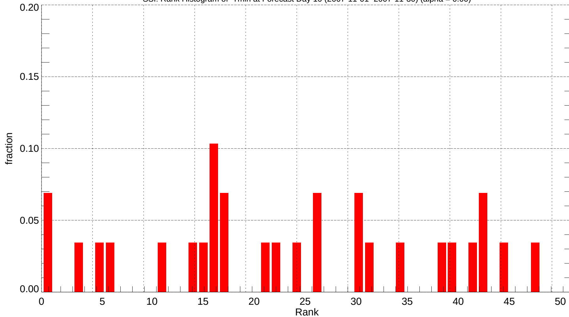
SSI: Rank Histogram of Tmin at Forecast Day 10 (2007-11-01~2007-11-30) (alpha = 0.00)
