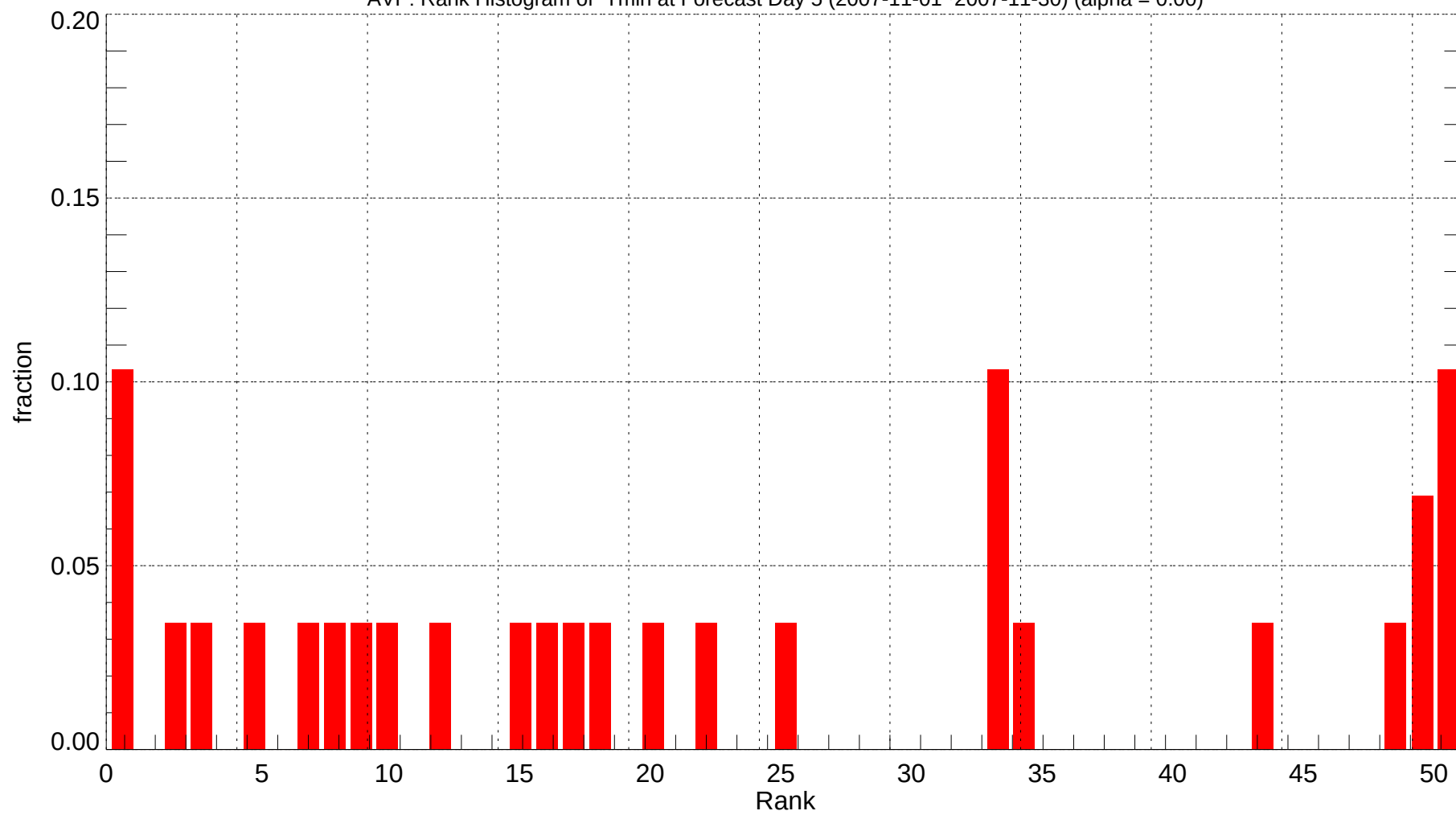
AVP: Rank Histogram of Tmin at Forecast Day 5 (2007-11-01~2007-11-30) (alpha = 0.00)
