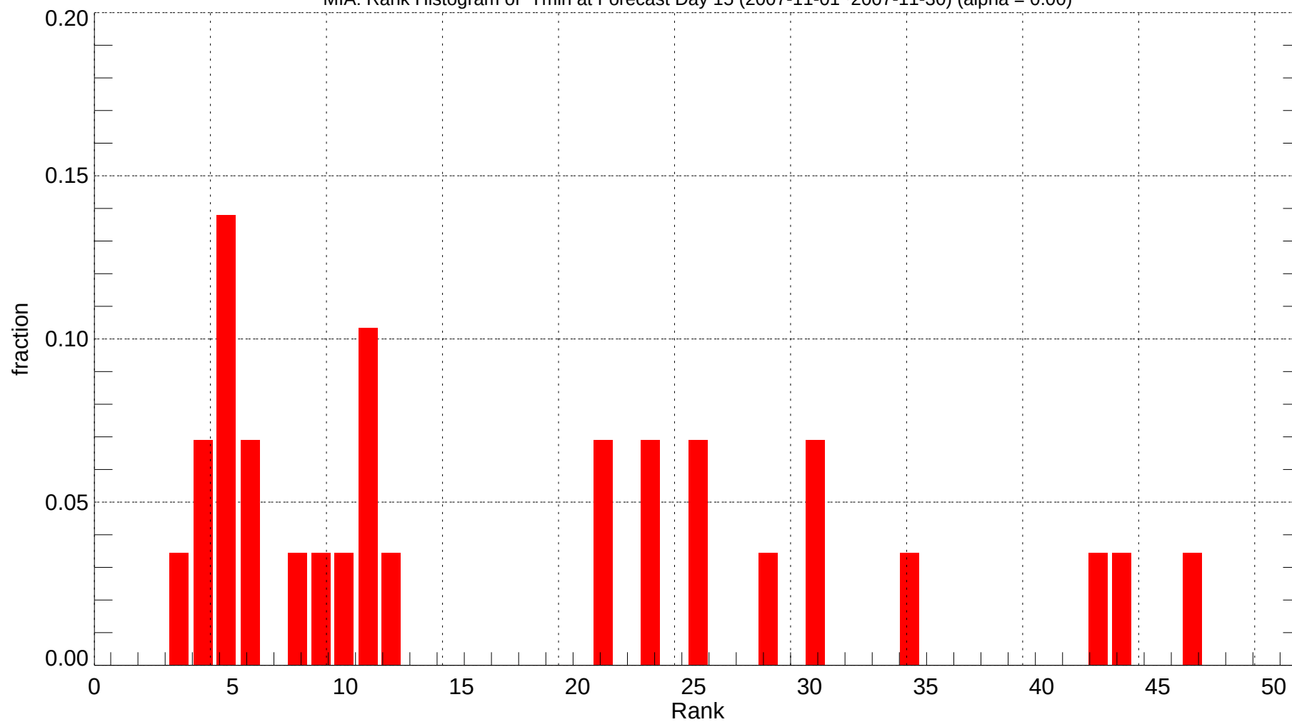
MIA: Rank Histogram of Tmin at Forecast Day 15 (2007-11-01~2007-11-30) (alpha = 0.00)
