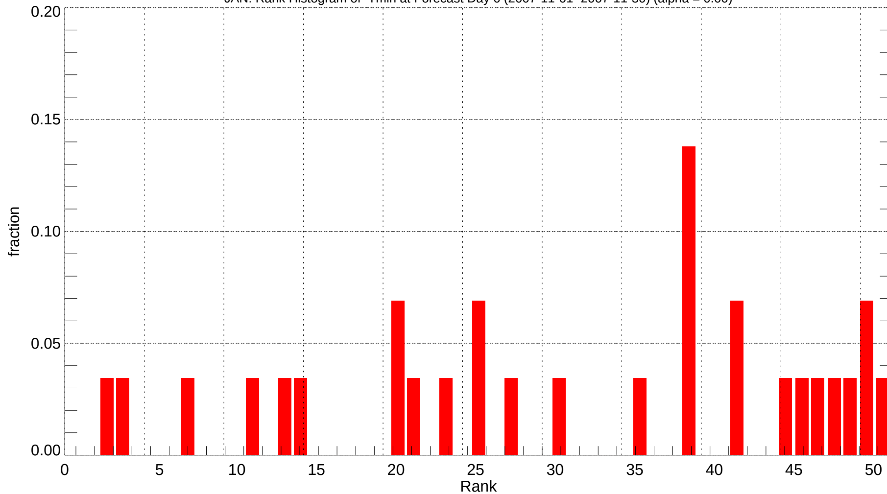
JAN: Rank Histogram of Tmin at Forecast Day 6 (2007-11-01~2007-11-30) (alpha = 0.00)
