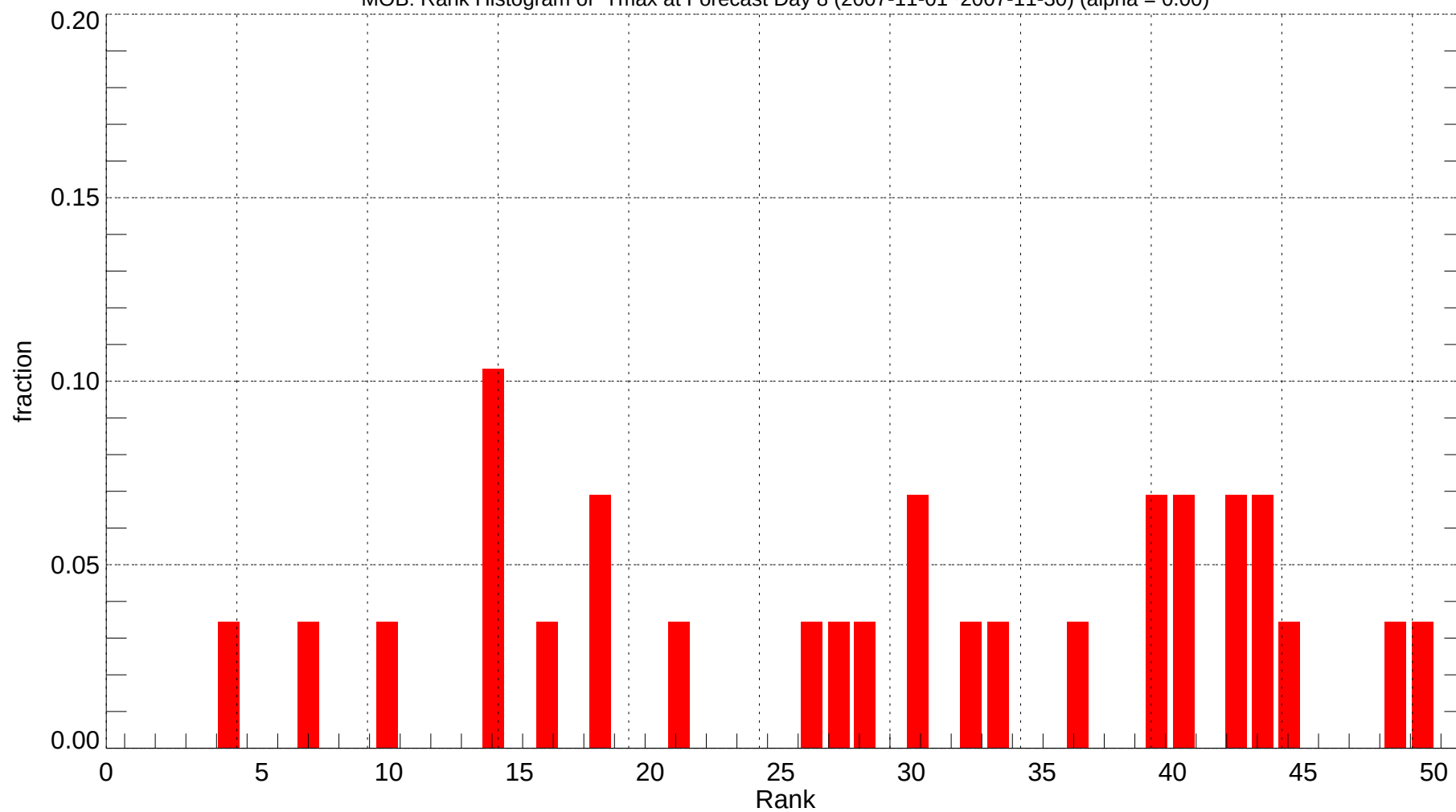
MOB: Rank Histogram of Tmax at Forecast Day 8 (2007-11-01~2007-11-30) (alpha = 0.00)
