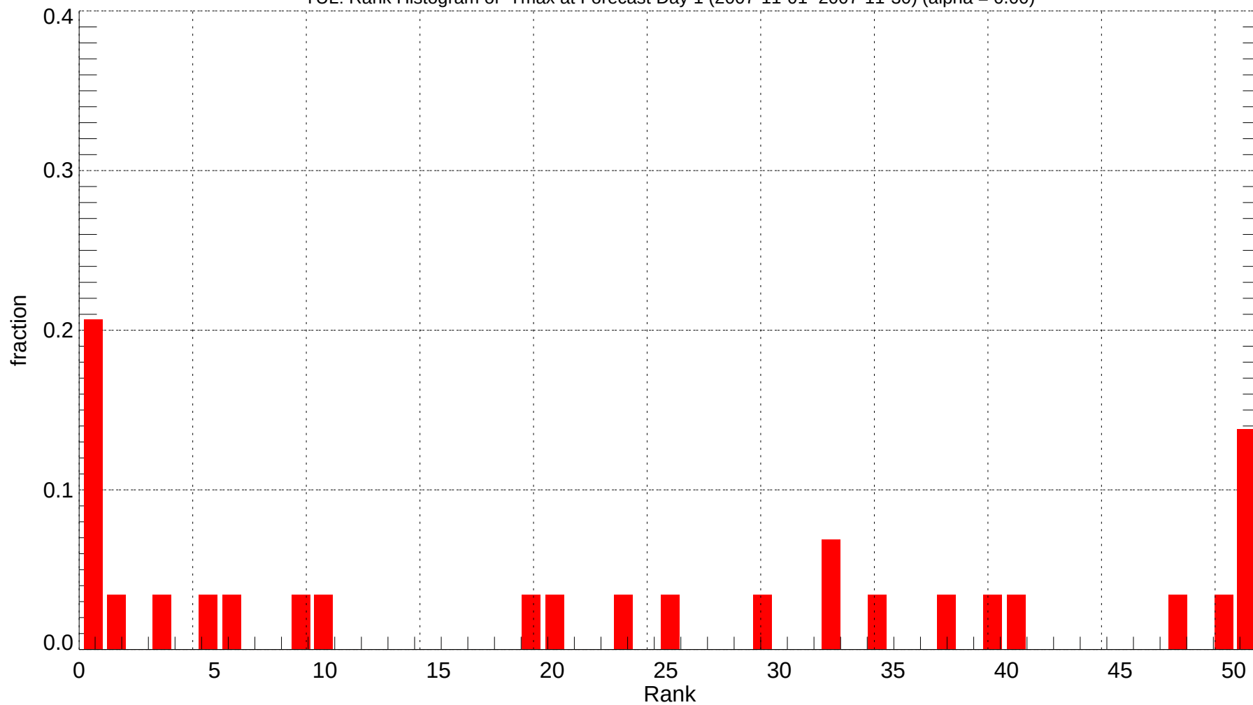
TUL: Rank Histogram of Tmax at Forecast Day 1 (2007-11-01~2007-11-30) (alpha = 0.00)
