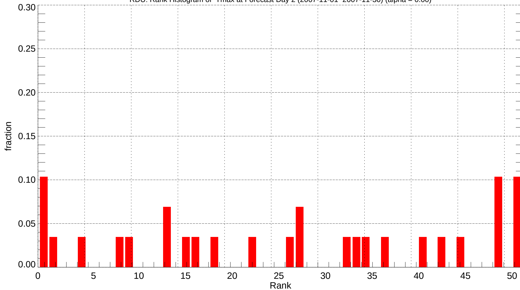
RDU: Rank Histogram of Tmax at Forecast Day 2 (2007-11-01~2007-11-30) (alpha = 0.00)
