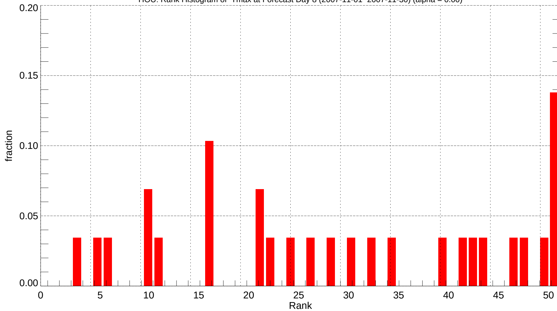
HOU: Rank Histogram of Tmax at Forecast Day 8 (2007-11-01~2007-11-30) (alpha = 0.00)
