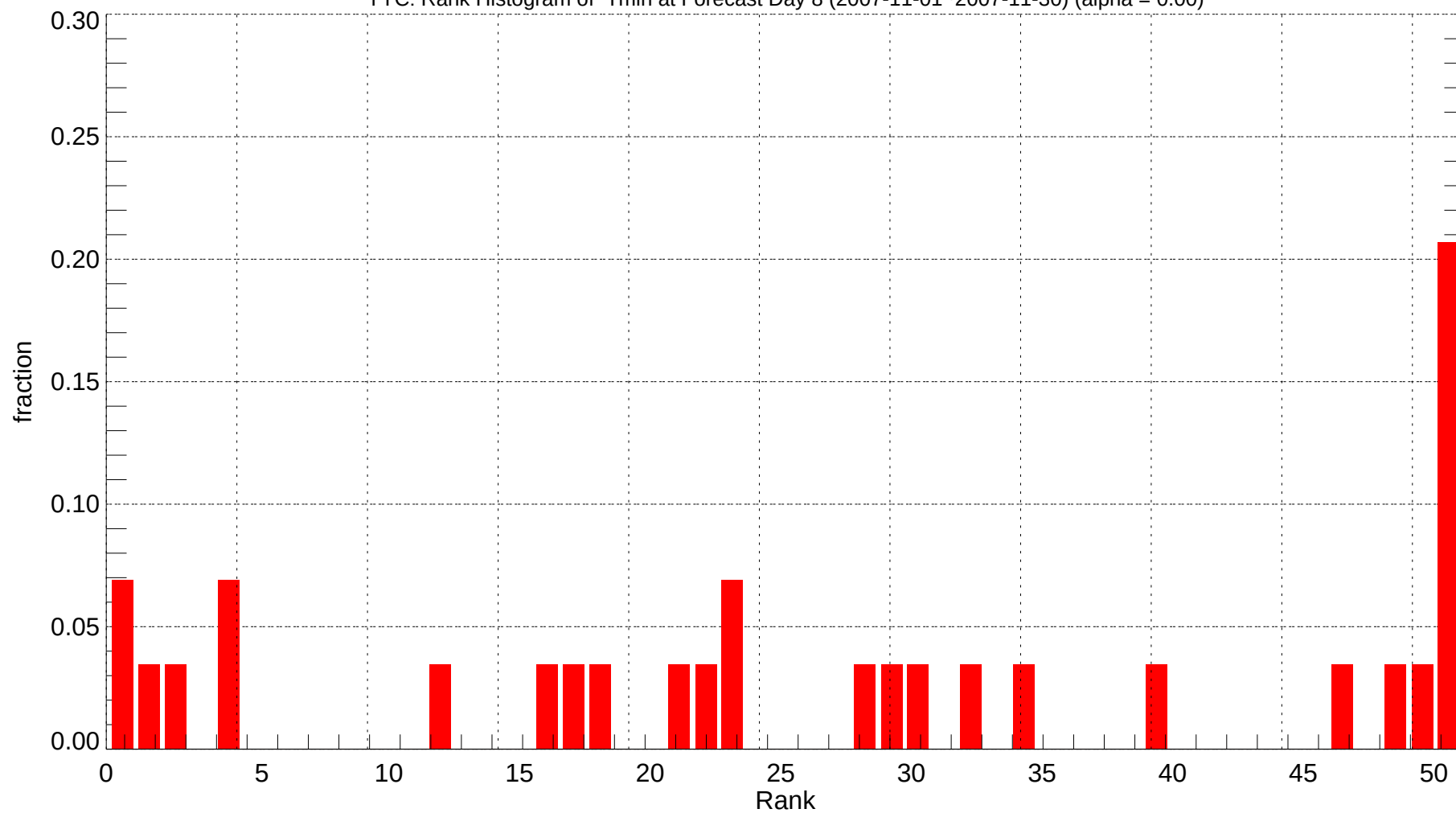
YYC: Rank Histogram of Tmin at Forecast Day 8 (2007-11-01~2007-11-30) (alpha = 0.00)
