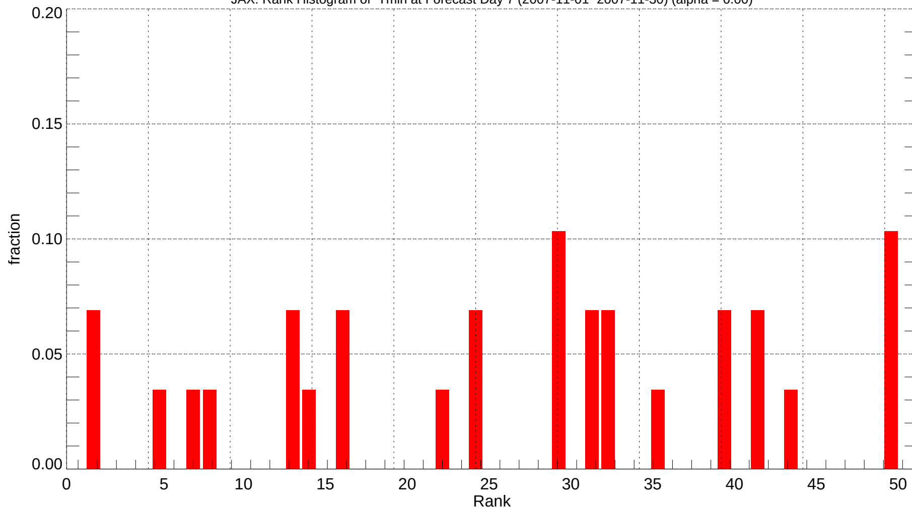
JAX: Rank Histogram of Tmin at Forecast Day 7 (2007-11-01~2007-11-30) (alpha = 0.00)
