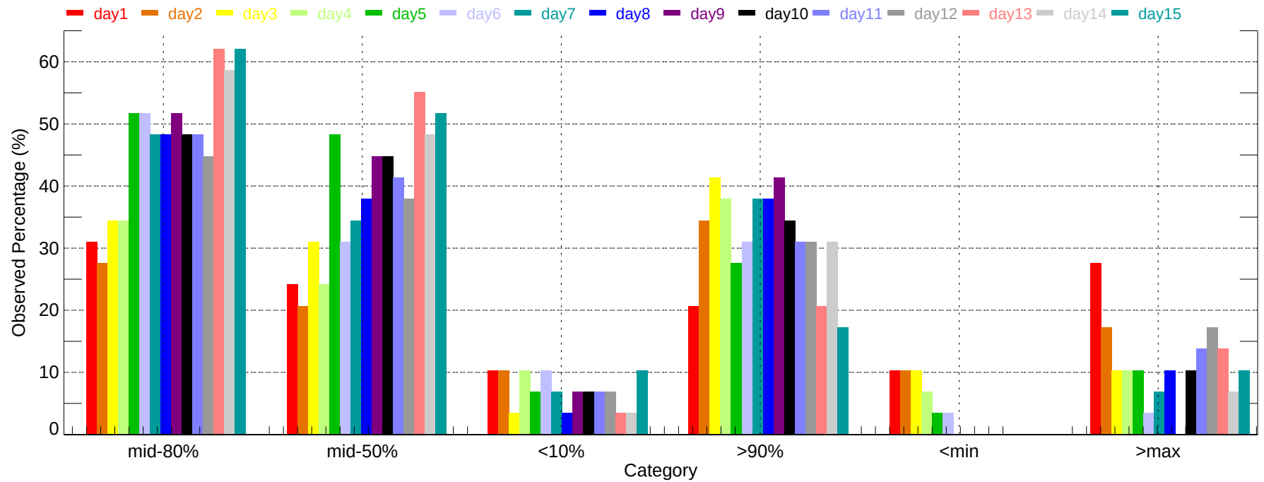
Observed Percentage of Ensembles - LEX: Max Temperature (2007-11-01~2007-11-30)
