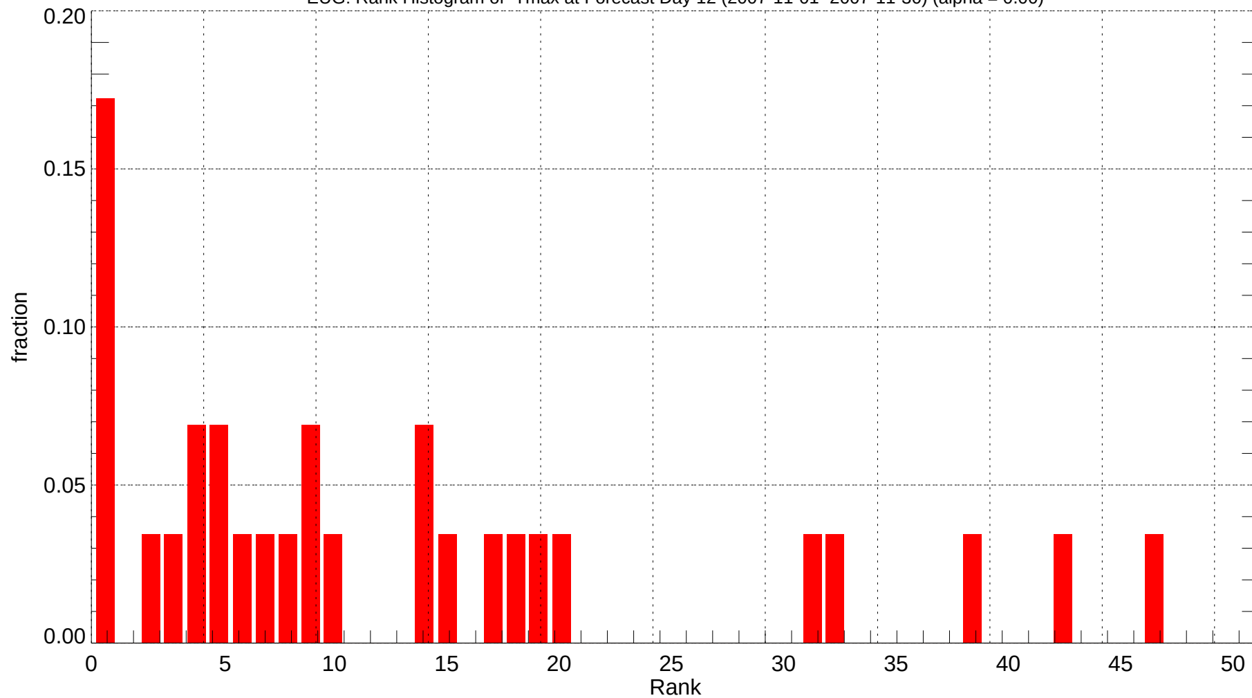
EUG: Rank Histogram of Tmax at Forecast Day 12 (2007-11-01~2007-11-30) (alpha = 0.00)
