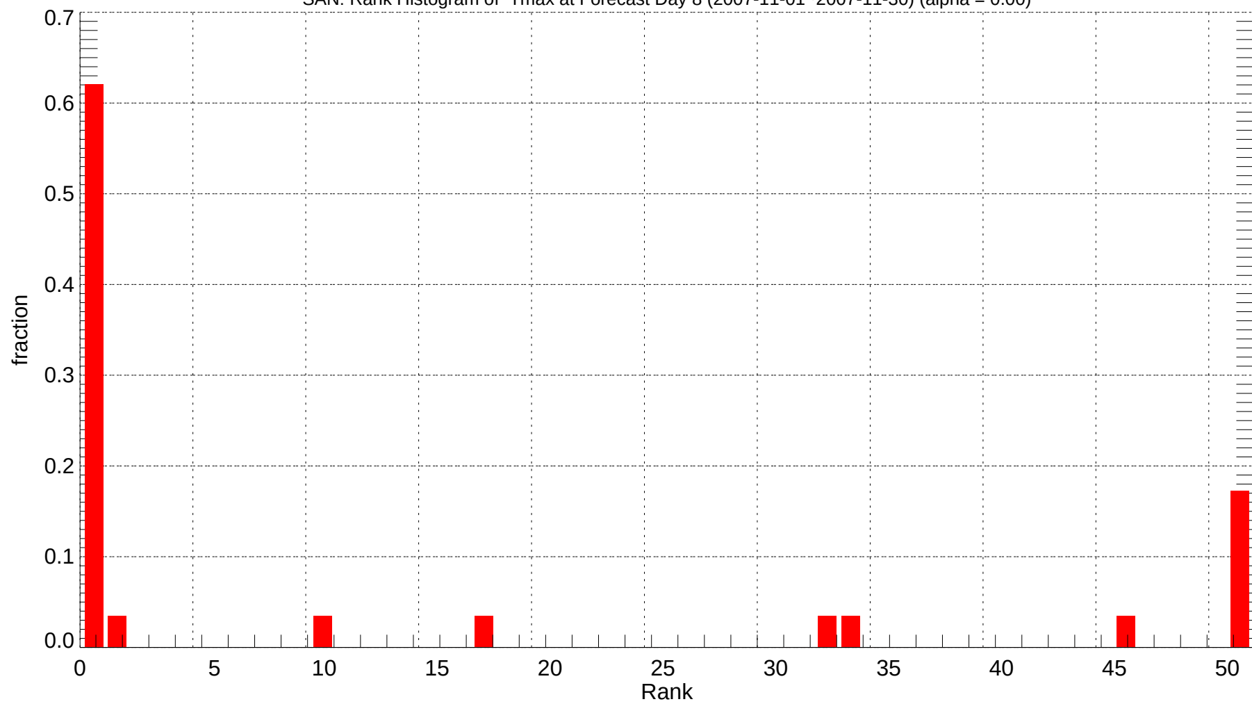
SAN: Rank Histogram of Tmax at Forecast Day 8 (2007-11-01~2007-11-30) (alpha = 0.00)
