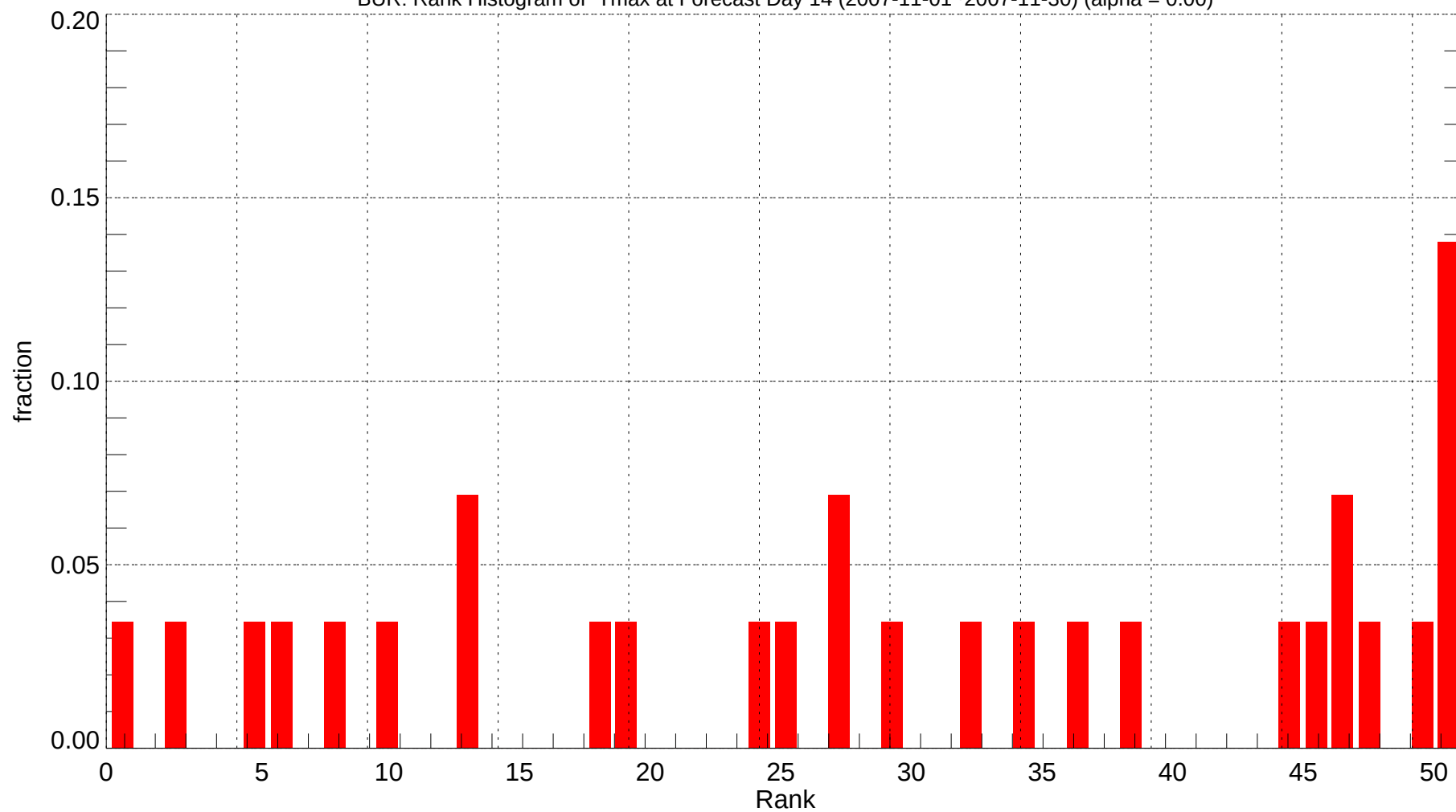
BUR: Rank Histogram of Tmax at Forecast Day 14 (2007-11-01~2007-11-30) (alpha = 0.00)
