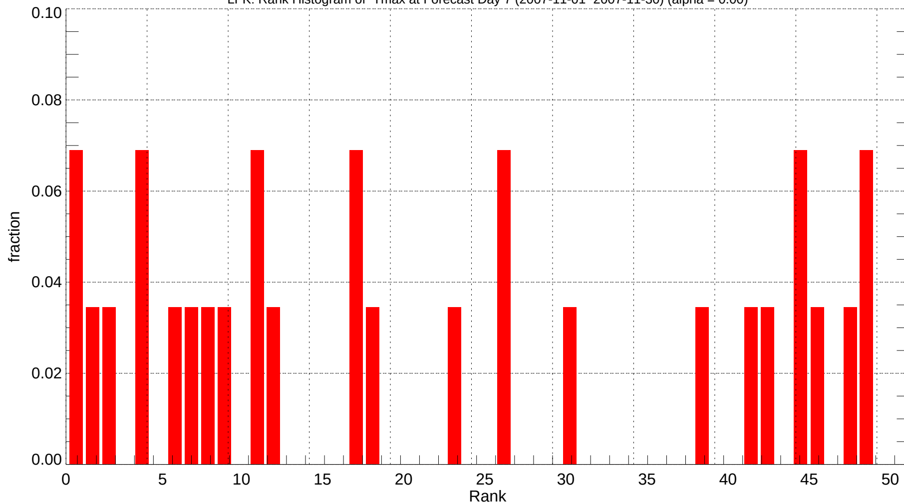
LFK: Rank Histogram of Tmax at Forecast Day 7 (2007-11-01~2007-11-30) (alpha = 0.00)
