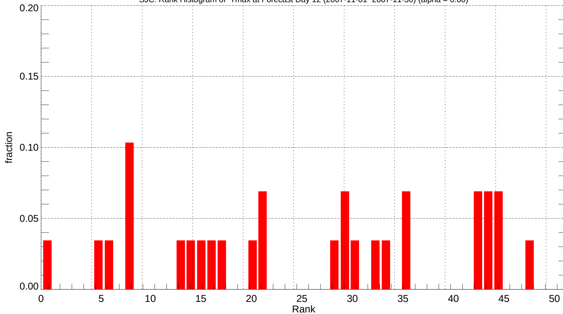
SJC: Rank Histogram of Tmax at Forecast Day 12 (2007-11-01~2007-11-30) (alpha = 0.00)
