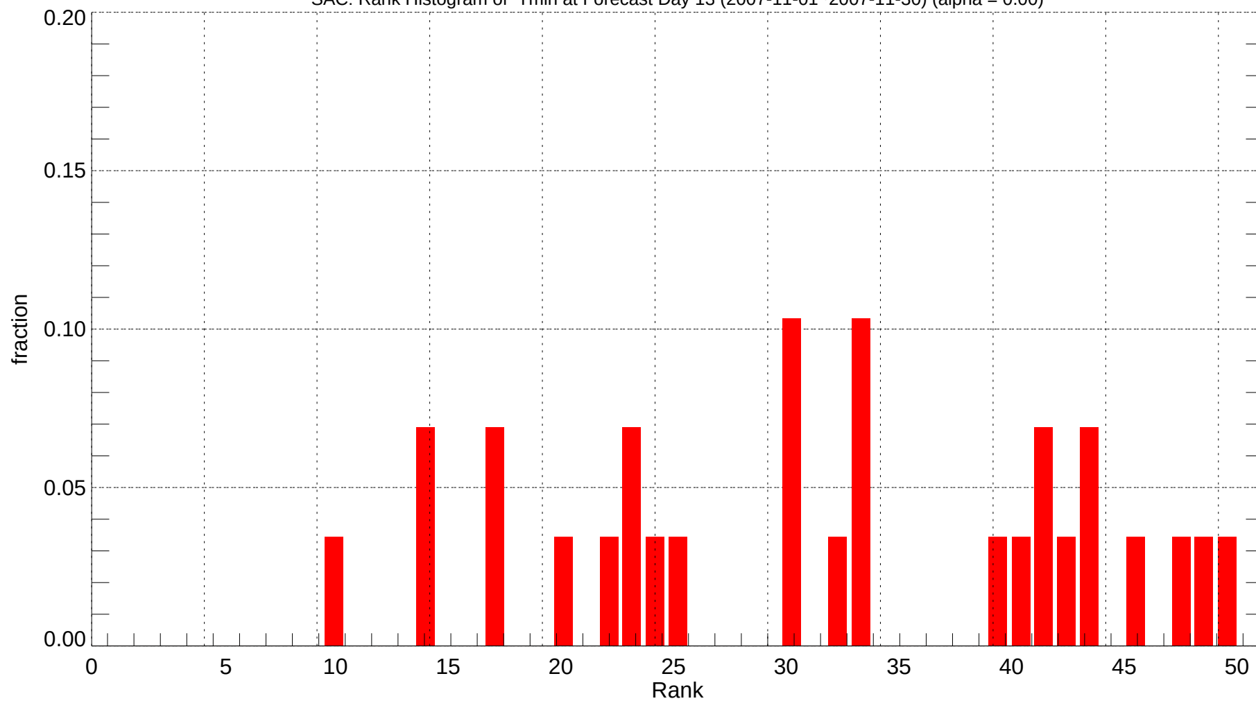
SAC: Rank Histogram of Tmin at Forecast Day 13 (2007-11-01~2007-11-30) (alpha = 0.00)
