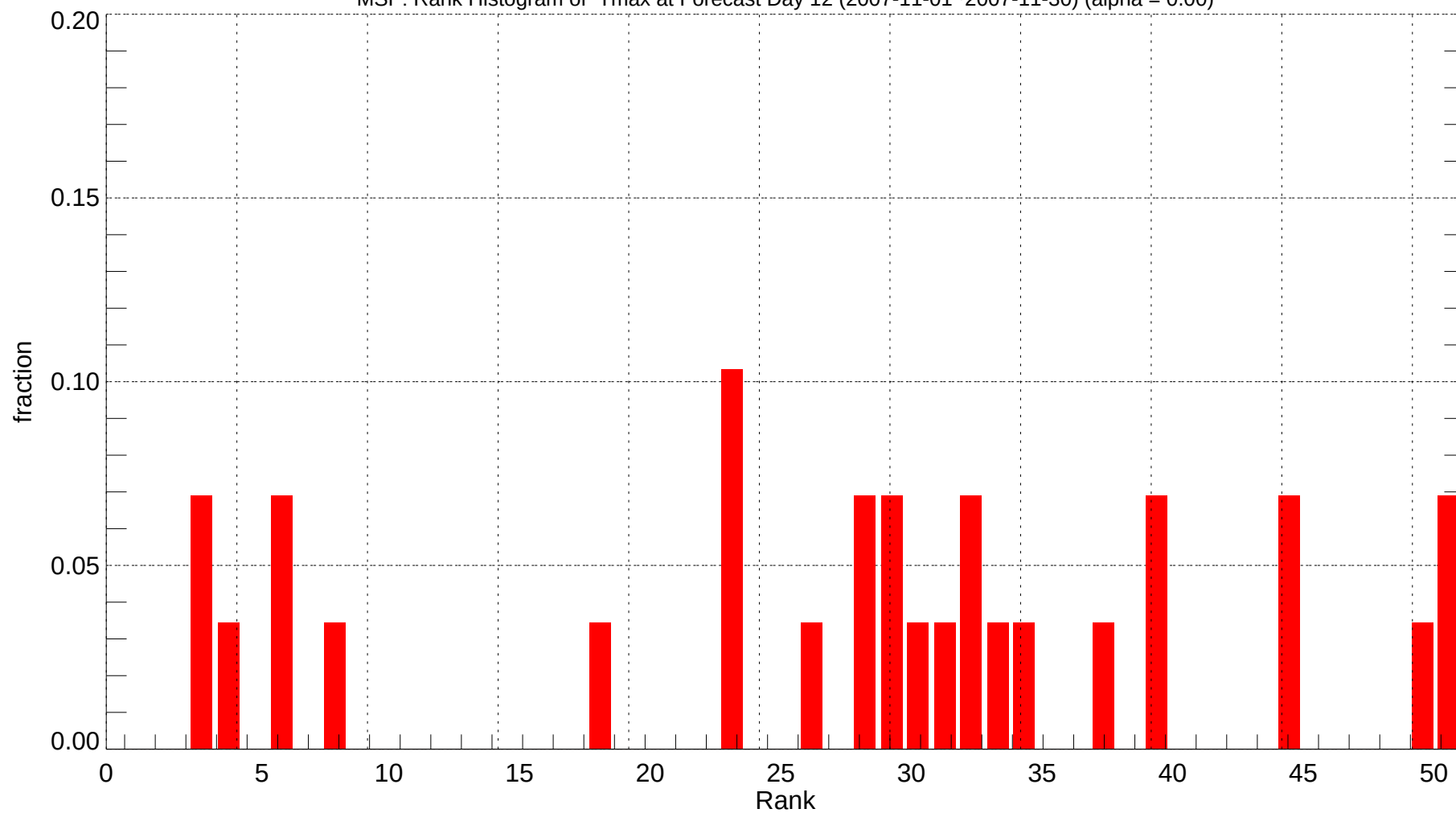
MSP: Rank Histogram of Tmax at Forecast Day 12 (2007-11-01~2007-11-30) (alpha = 0.00)
