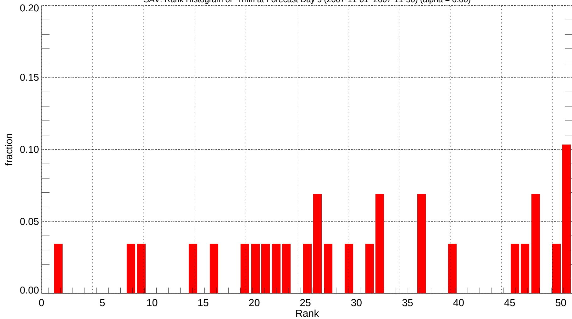
SAV: Rank Histogram of Tmin at Forecast Day 9 (2007-11-01~2007-11-30) (alpha = 0.00)
