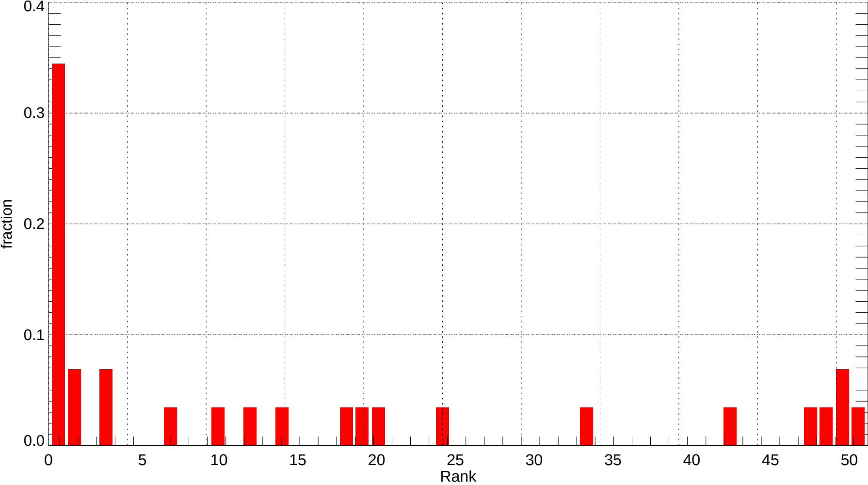
SJC: Rank Histogram of Tmin at Forecast Day 2 (2007-11-01~2007-11-30) (alpha = 0.00)
