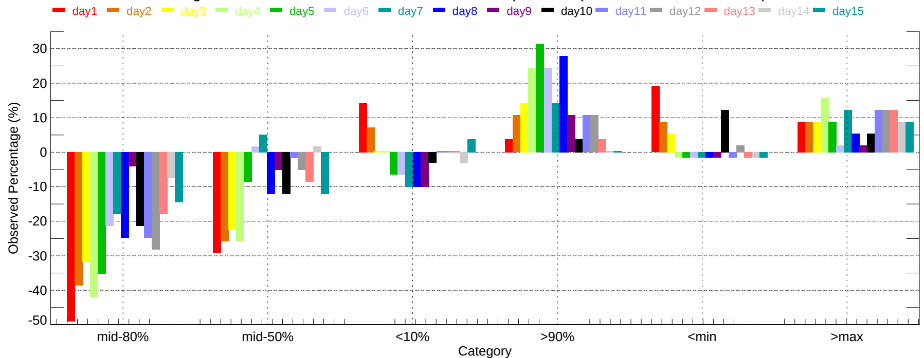
Observed Percentage Deviation of Ensembles - CLE: Max Temperature (2007-11-01~2007-11-30)
