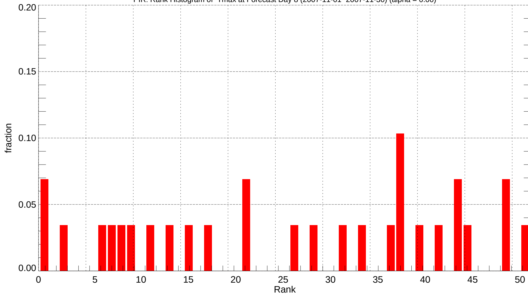
PIR: Rank Histogram of Tmax at Forecast Day 8 (2007-11-01~2007-11-30) (alpha = 0.00)
