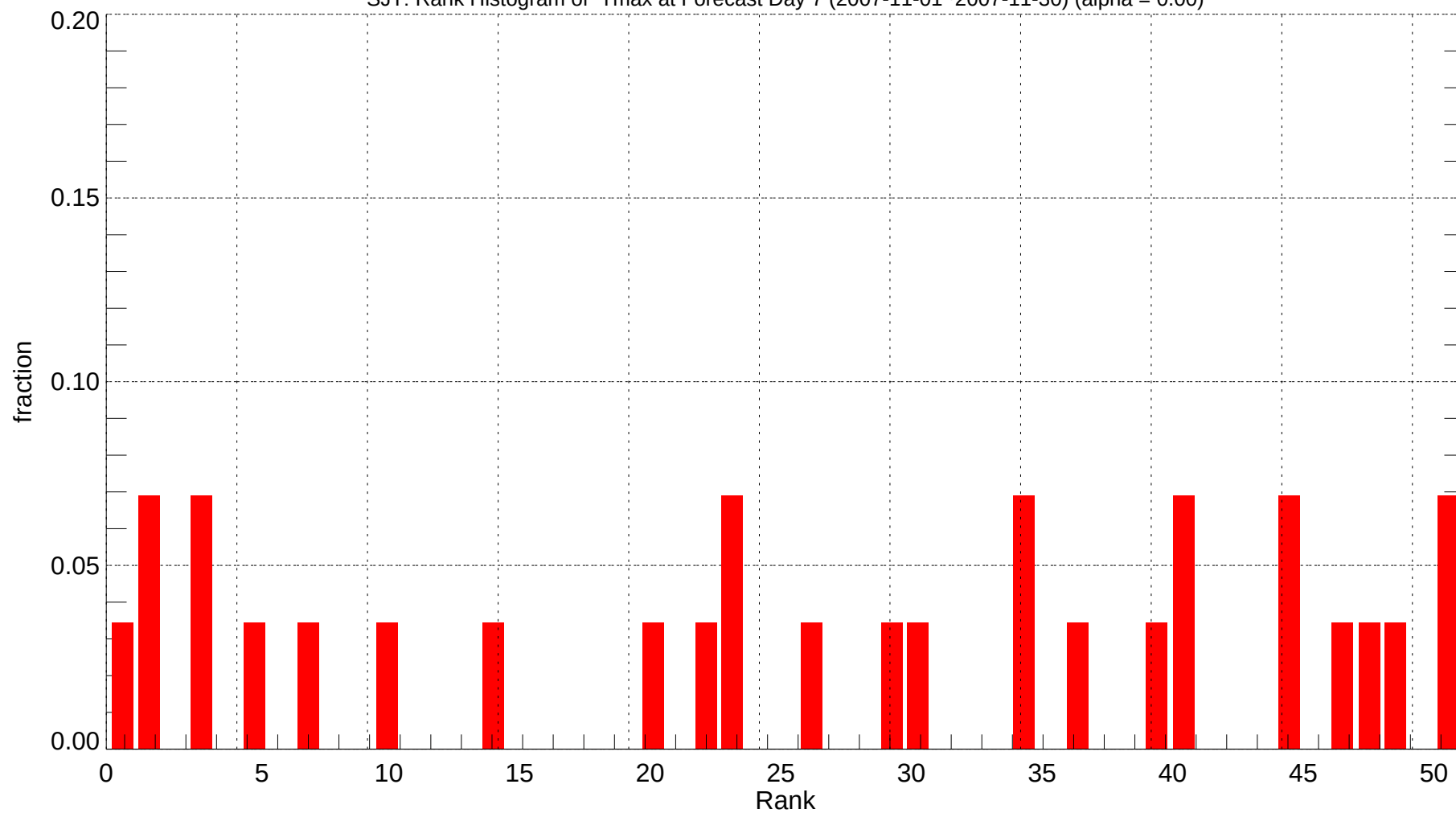
SJT: Rank Histogram of Tmax at Forecast Day 7 (2007-11-01~2007-11-30) (alpha = 0.00)
