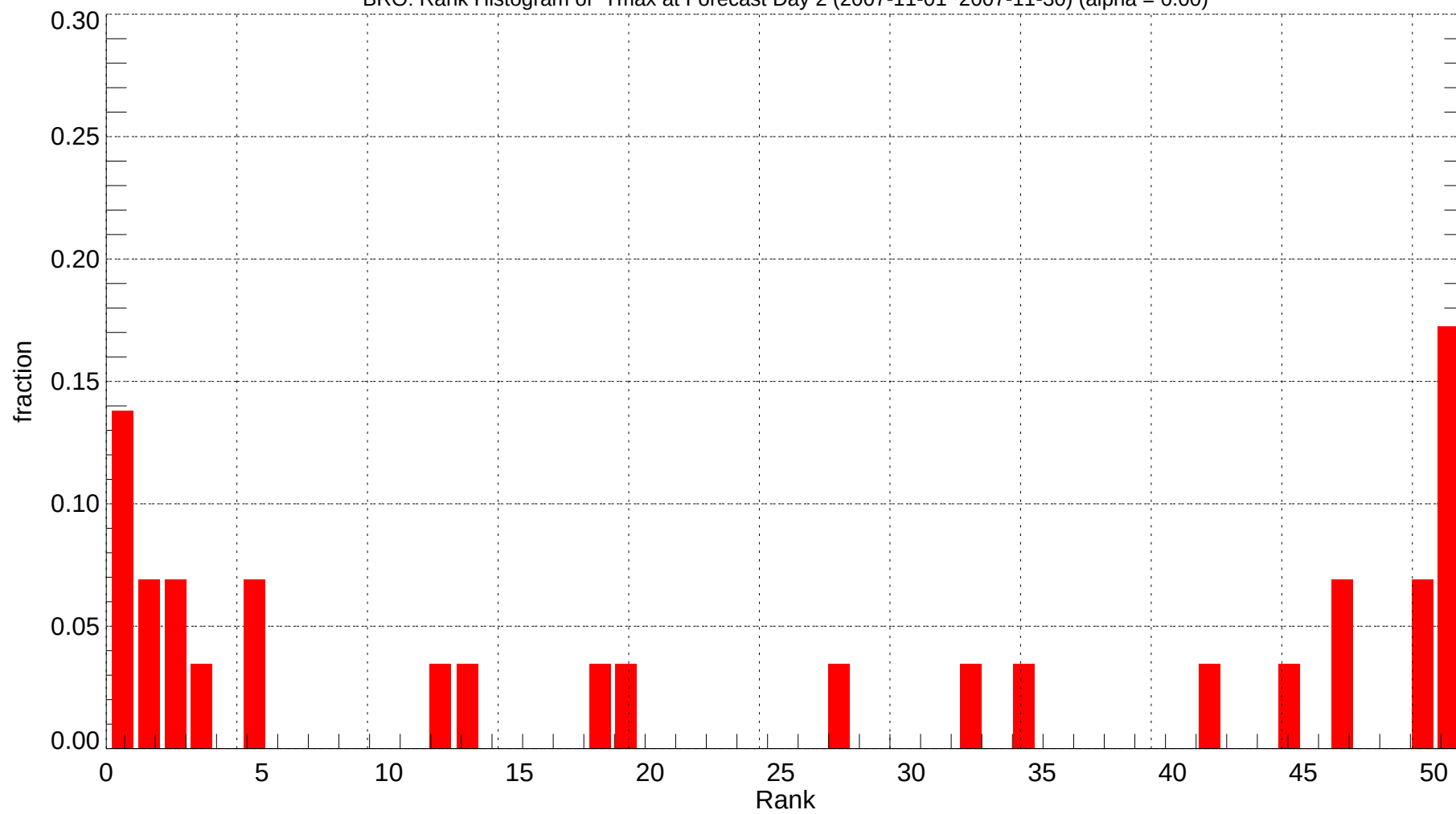
BRO: Rank Histogram of Tmax at Forecast Day 2 (2007-11-01~2007-11-30) (alpha = 0.00)
