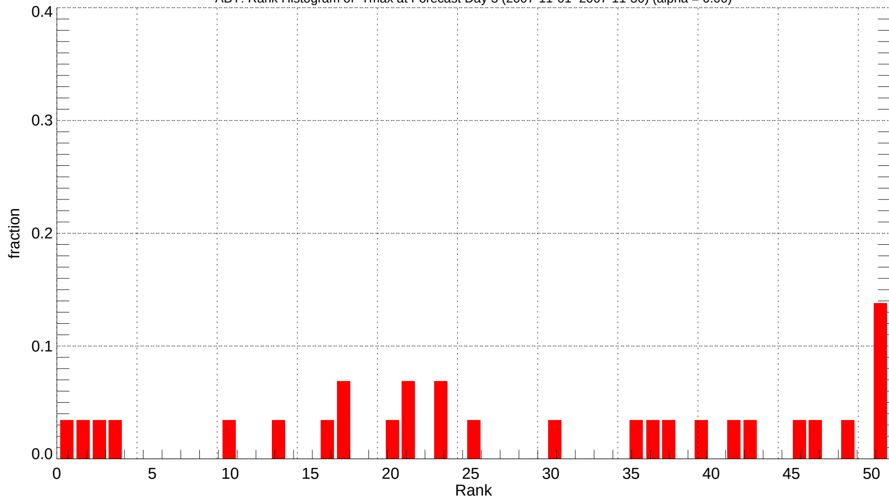
ABY: Rank Histogram of Tmax at Forecast Day 3 (2007-11-01~2007-11-30) (alpha = 0.00)
