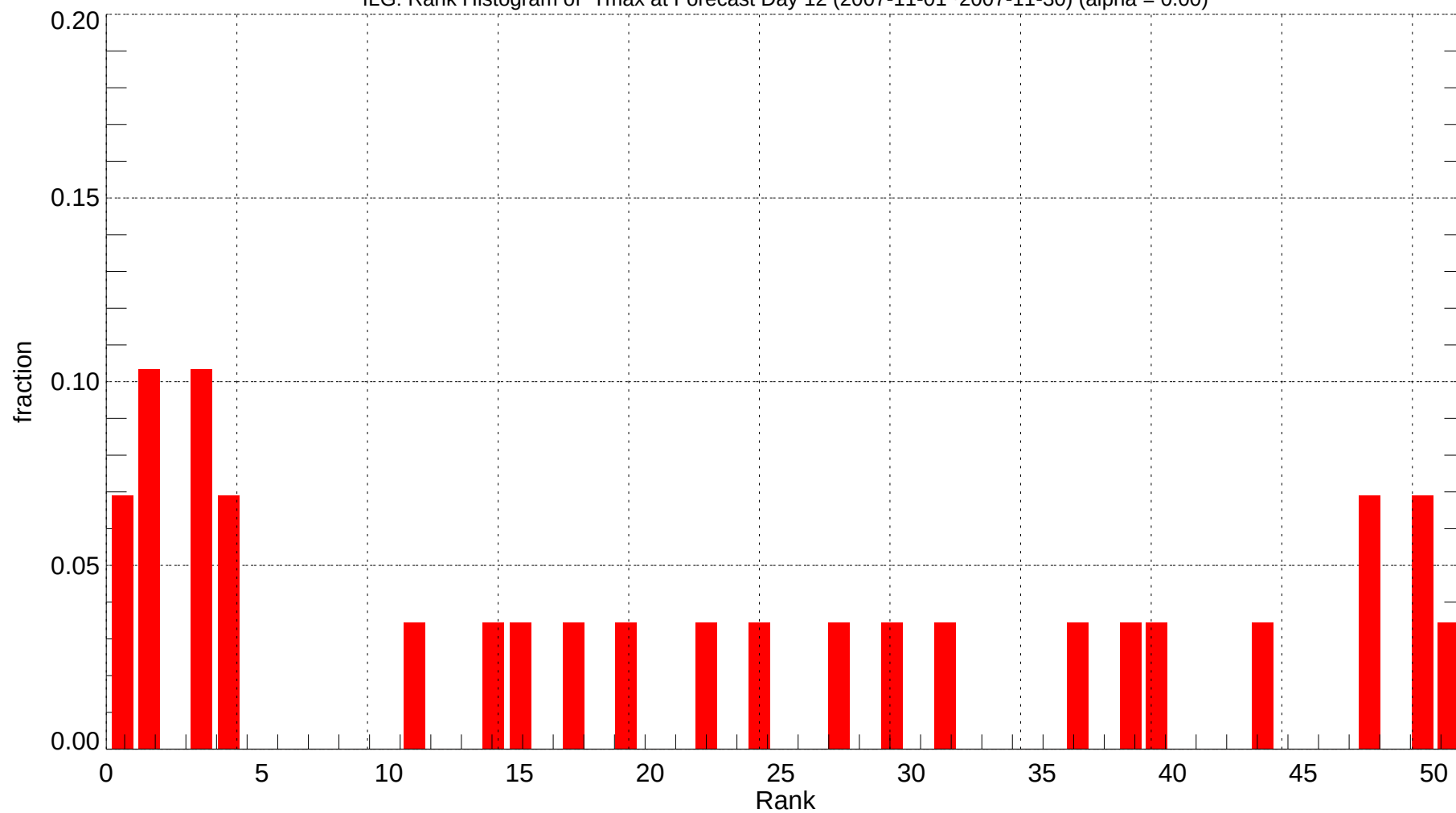
ILG: Rank Histogram of Tmax at Forecast Day 12 (2007-11-01~2007-11-30) (alpha = 0.00)
