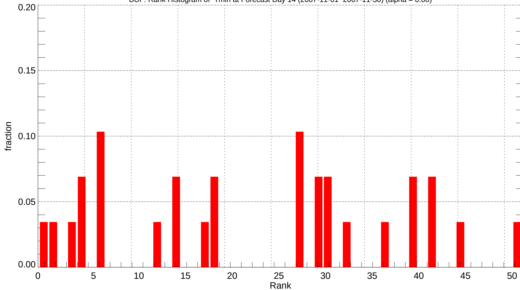
BUF: Rank Histogram of Tmin at Forecast Day 14 (2007-11-01~2007-11-30) (alpha = 0.00)
