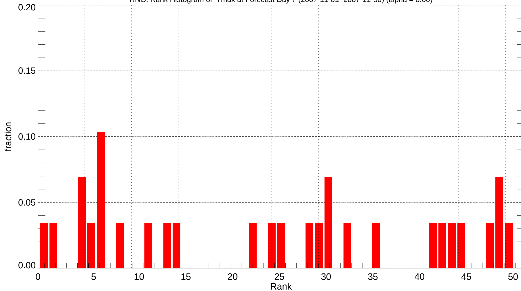
RNO: Rank Histogram of Tmax at Forecast Day 7 (2007-11-01~2007-11-30) (alpha = 0.00)
