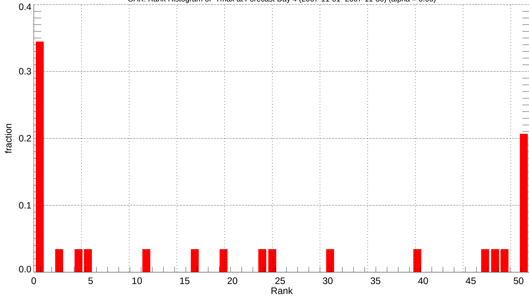
OAK: Rank Histogram of Tmax at Forecast Day 4 (2007-11-01~2007-11-30) (alpha = 0.00)
