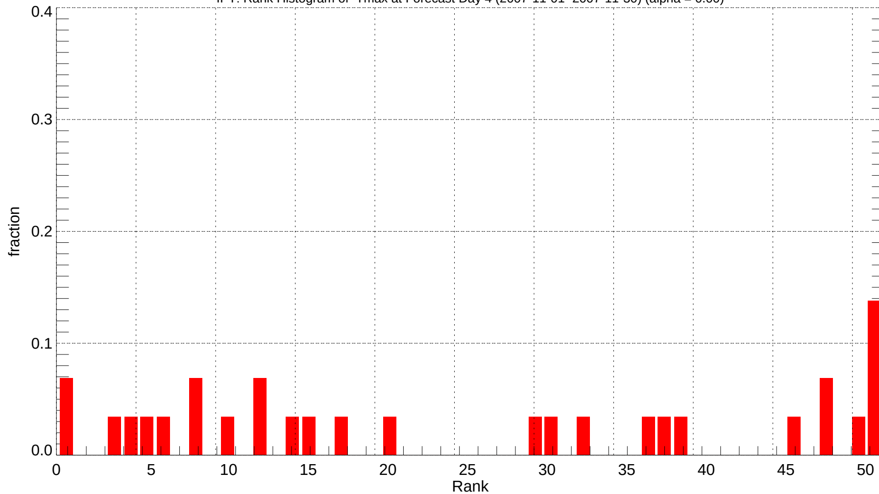
IPT: Rank Histogram of Tmax at Forecast Day 4 (2007-11-01~2007-11-30) (alpha = 0.00)
