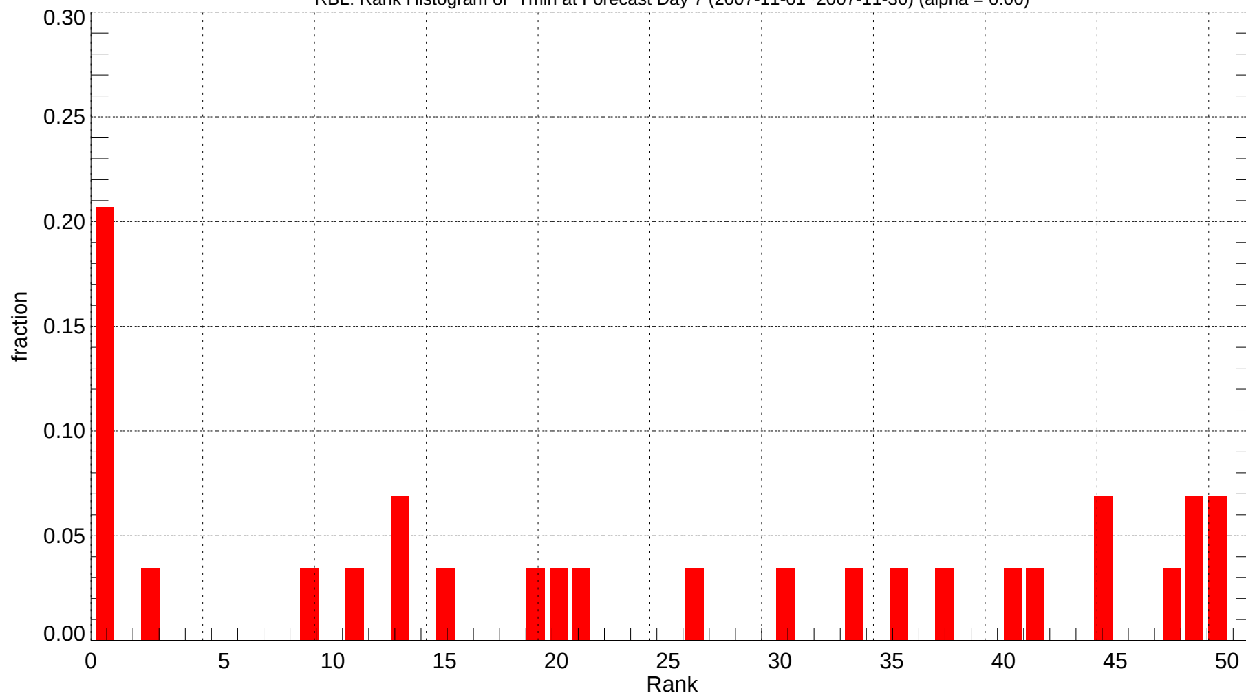
RBL: Rank Histogram of Tmin at Forecast Day 7 (2007-11-01~2007-11-30) (alpha = 0.00)
