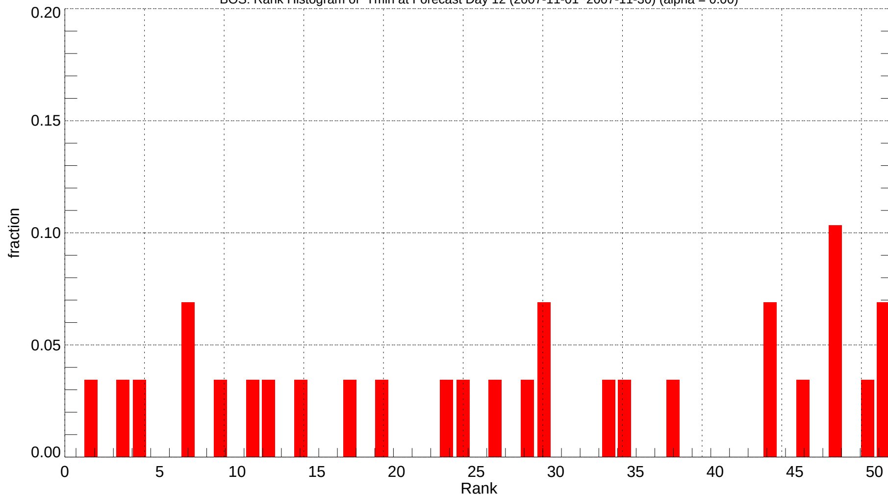
BOS: Rank Histogram of Tmin at Forecast Day 12 (2007-11-01~2007-11-30) (alpha = 0.00)
