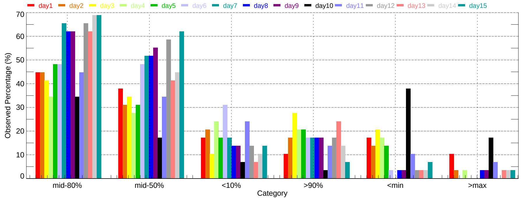
Observed Percentage of Ensembles - AUS: Max Temperature (2007-11-01~2007-11-30)
