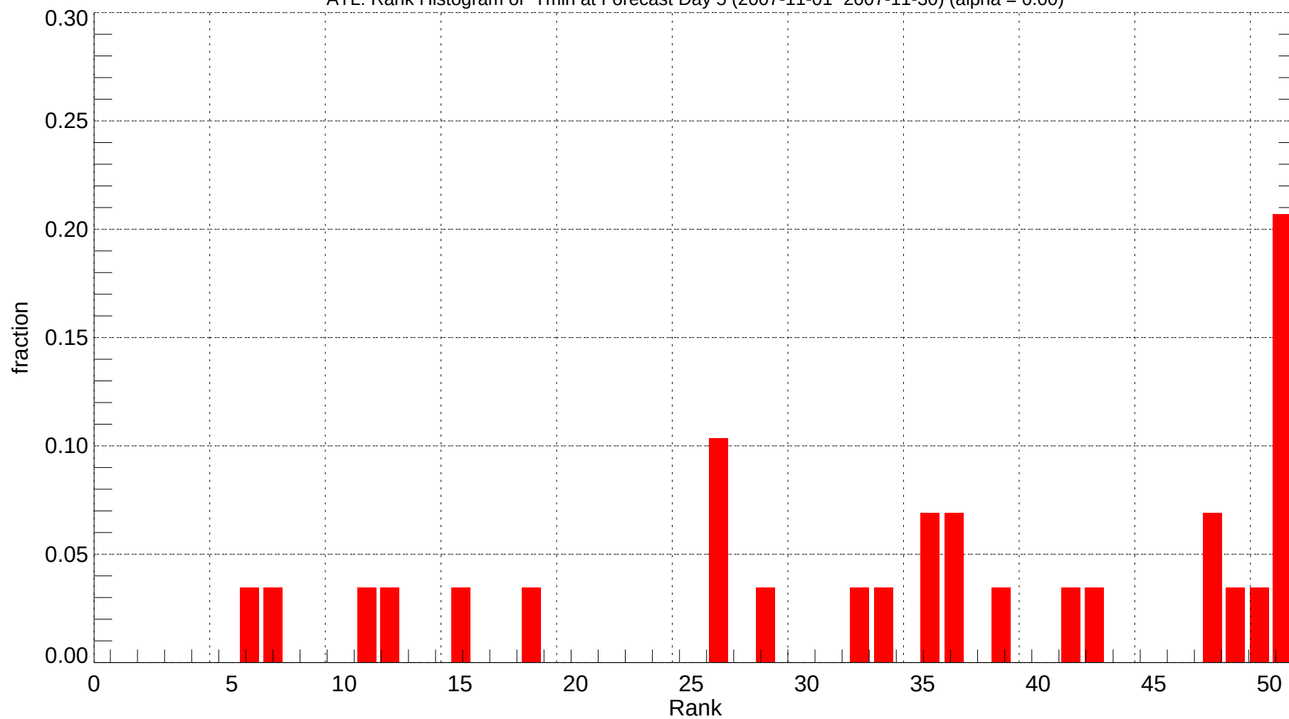
ATL: Rank Histogram of Tmin at Forecast Day 5 (2007-11-01~2007-11-30) (alpha = 0.00)
