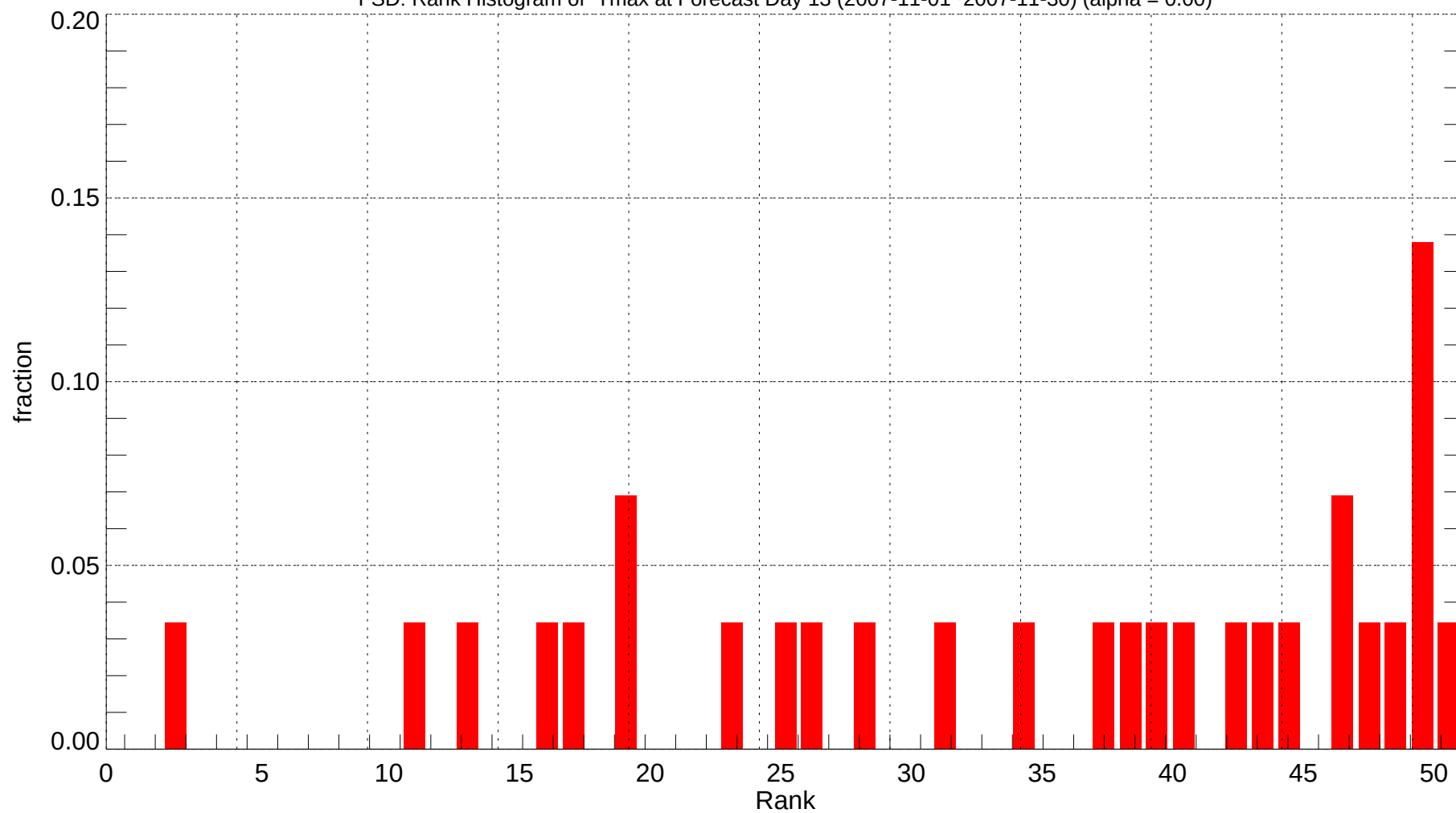
FSD: Rank Histogram of Tmax at Forecast Day 13 (2007-11-01~2007-11-30) (alpha = 0.00)
