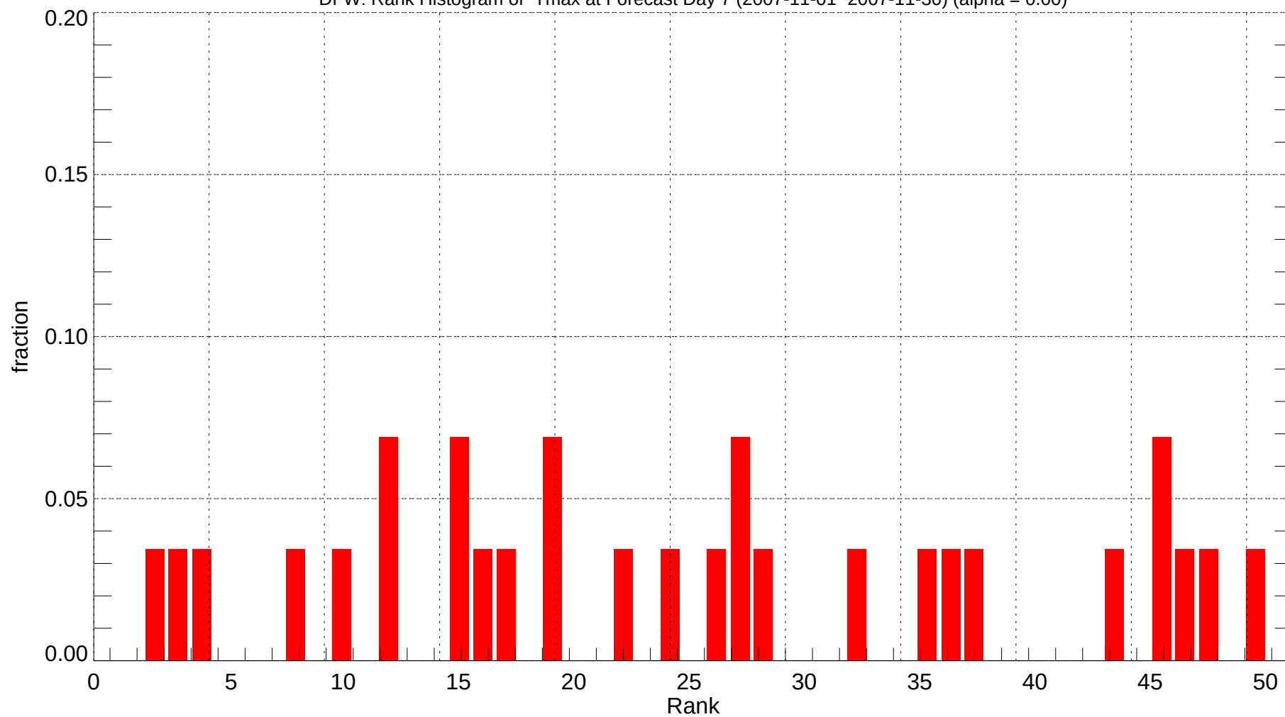
DFW: Rank Histogram of Tmax at Forecast Day 7 (2007-11-01~2007-11-30) (alpha = 0.00)
