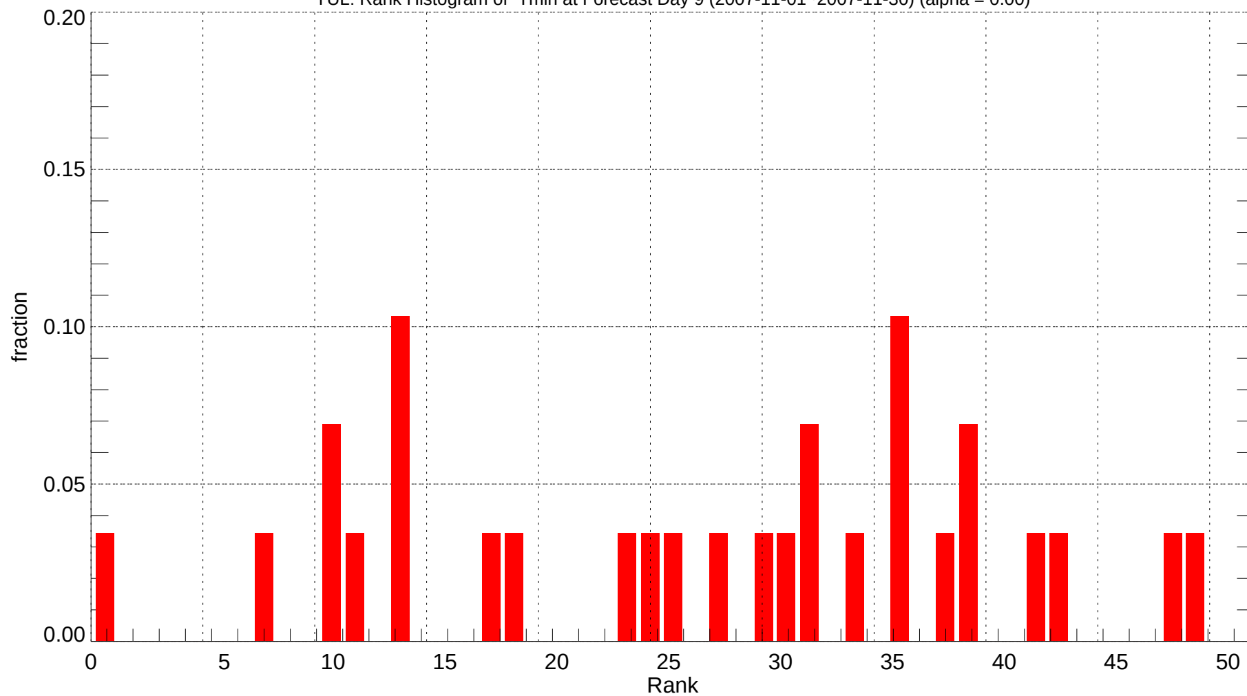
YUL: Rank Histogram of Tmin at Forecast Day 9 (2007-11-01~2007-11-30) (alpha = 0.00)
