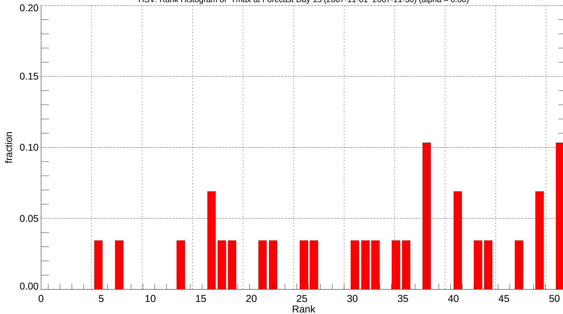
HSV: Rank Histogram of Tmax at Forecast Day 15 (2007-11-01~2007-11-30) (alpha = 0.00)
