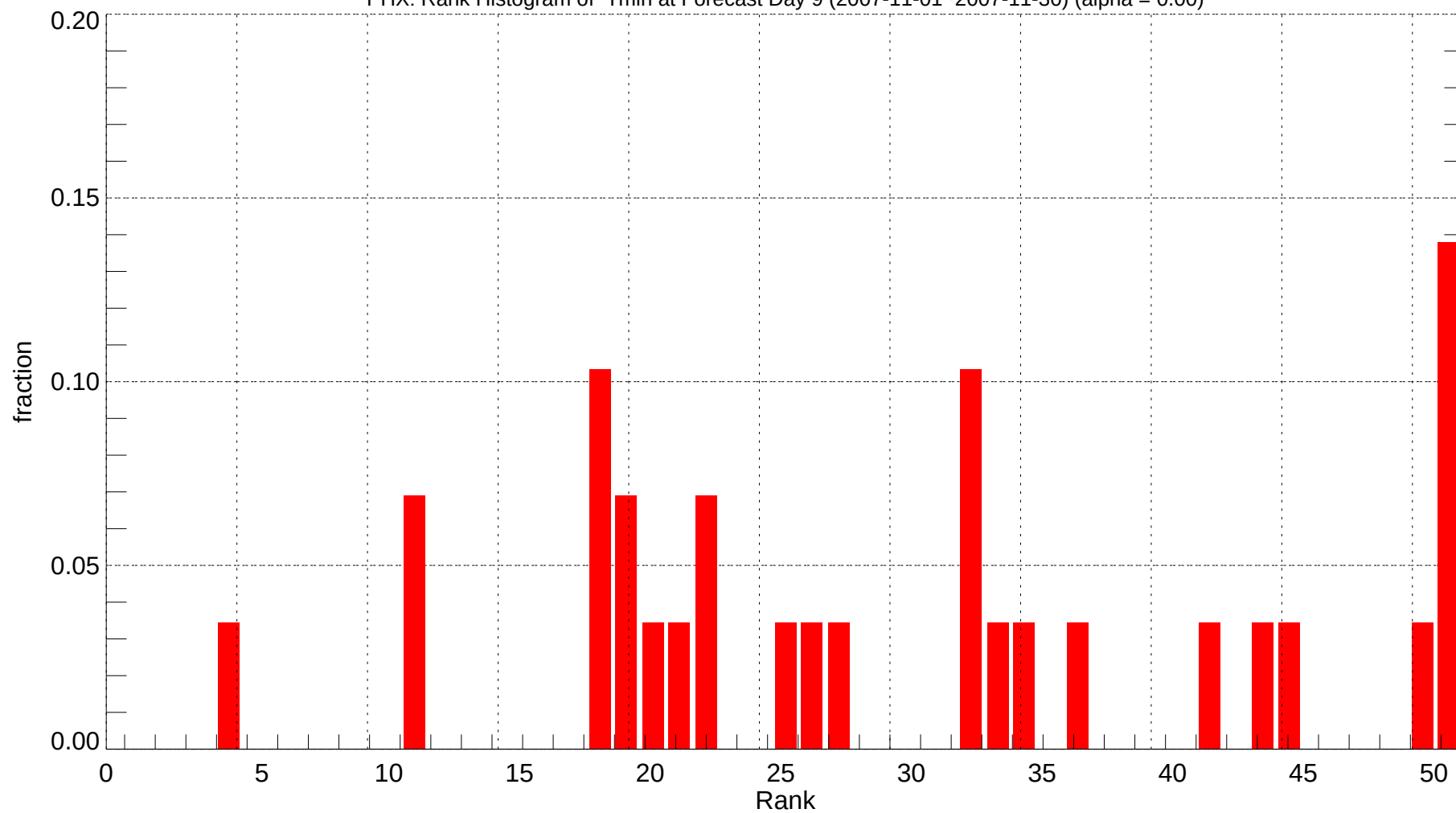
PHX: Rank Histogram of Tmin at Forecast Day 9 (2007-11-01~2007-11-30) (alpha = 0.00)
