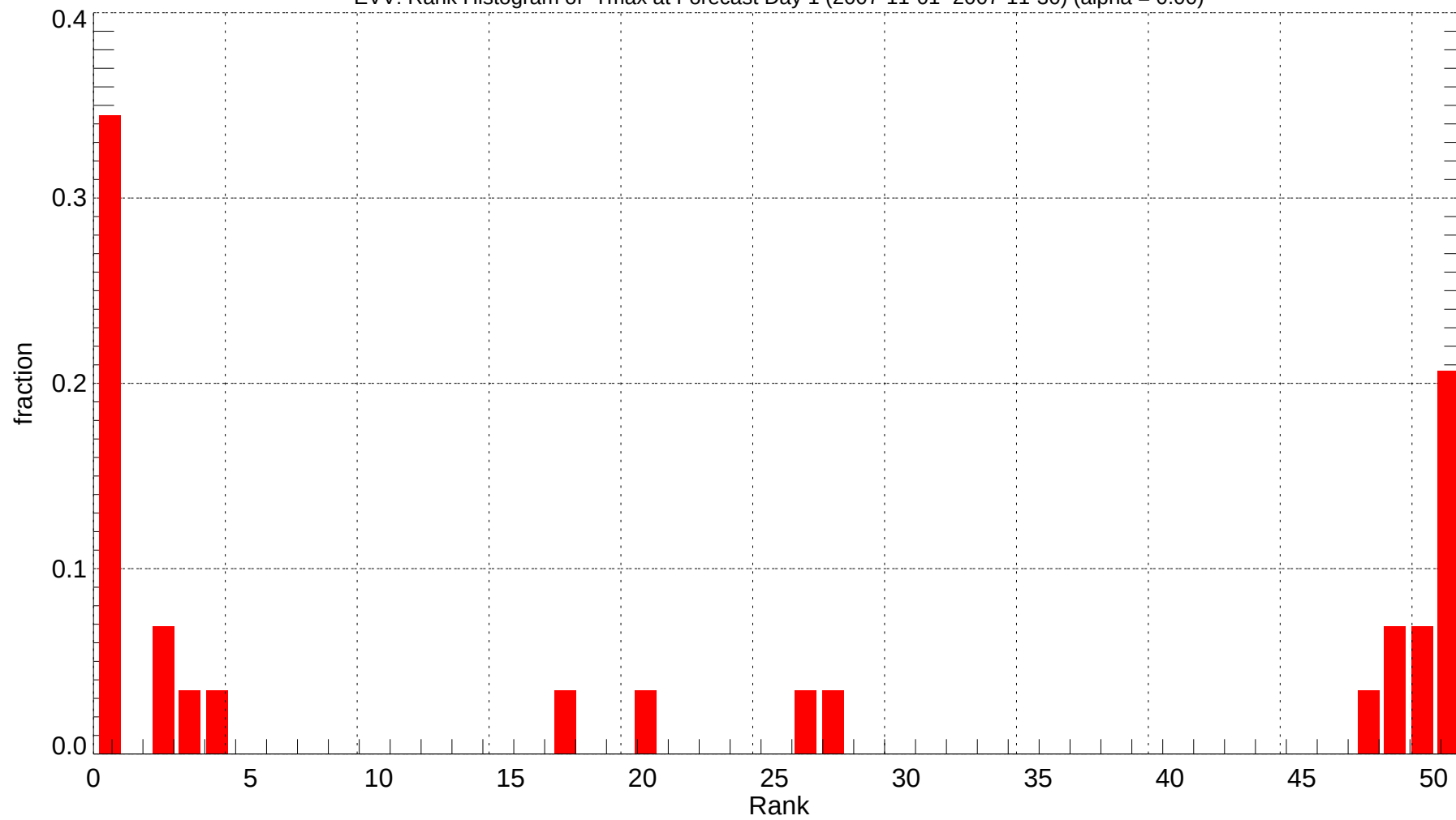
EVV: Rank Histogram of Tmax at Forecast Day 1 (2007-11-01~2007-11-30) (alpha = 0.00)
