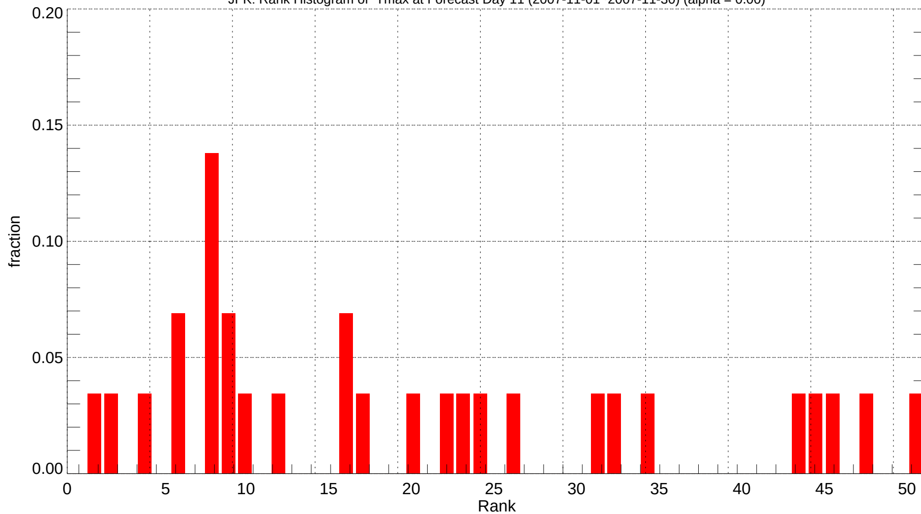
JFK: Rank Histogram of Tmax at Forecast Day 11 (2007-11-01~2007-11-30) (alpha = 0.00)
