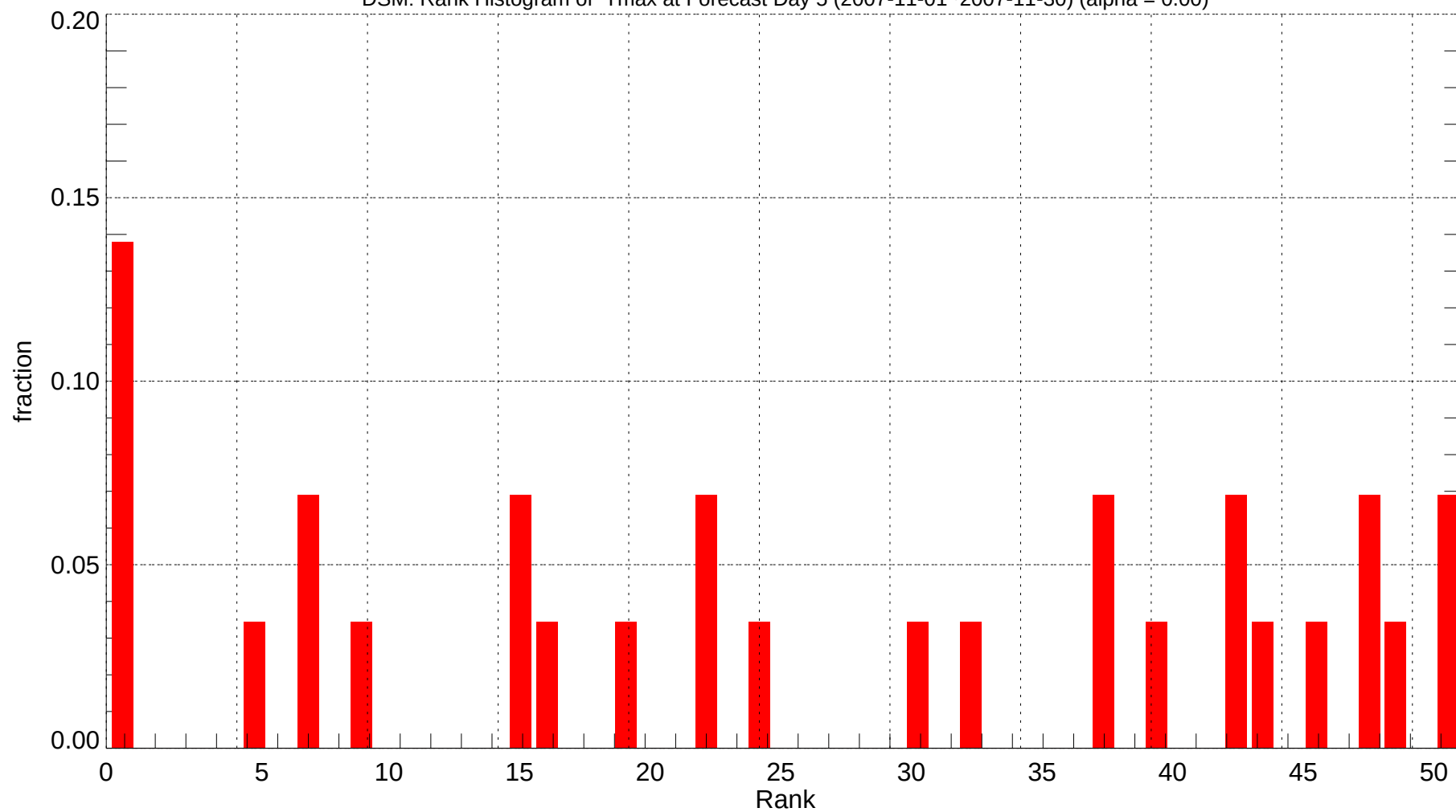
DSM: Rank Histogram of Tmax at Forecast Day 5 (2007-11-01~2007-11-30) (alpha = 0.00)
