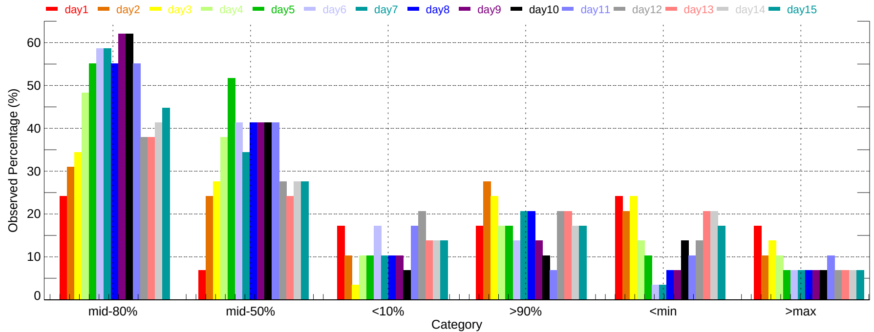
Observed Percentage of Ensembles - BGM: Min Temperature (2007-11-01~2007-11-30)
