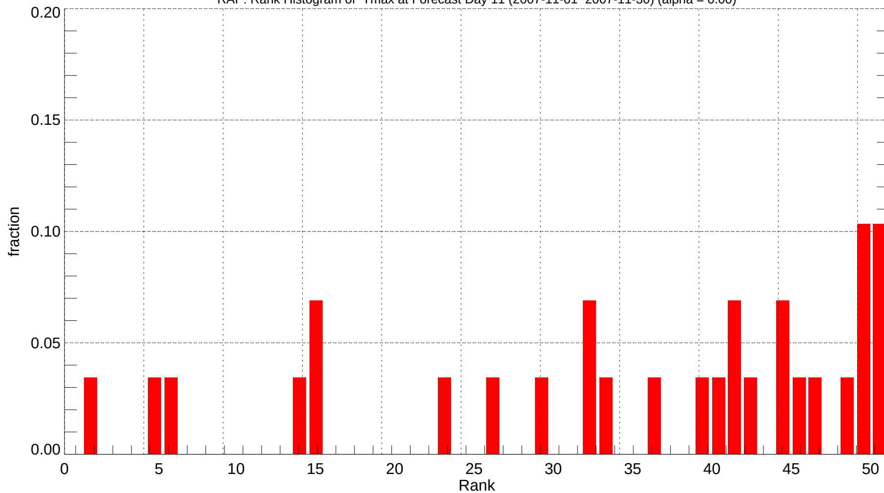
RAP: Rank Histogram of Tmax at Forecast Day 11 (2007-11-01~2007-11-30) (alpha = 0.00)
