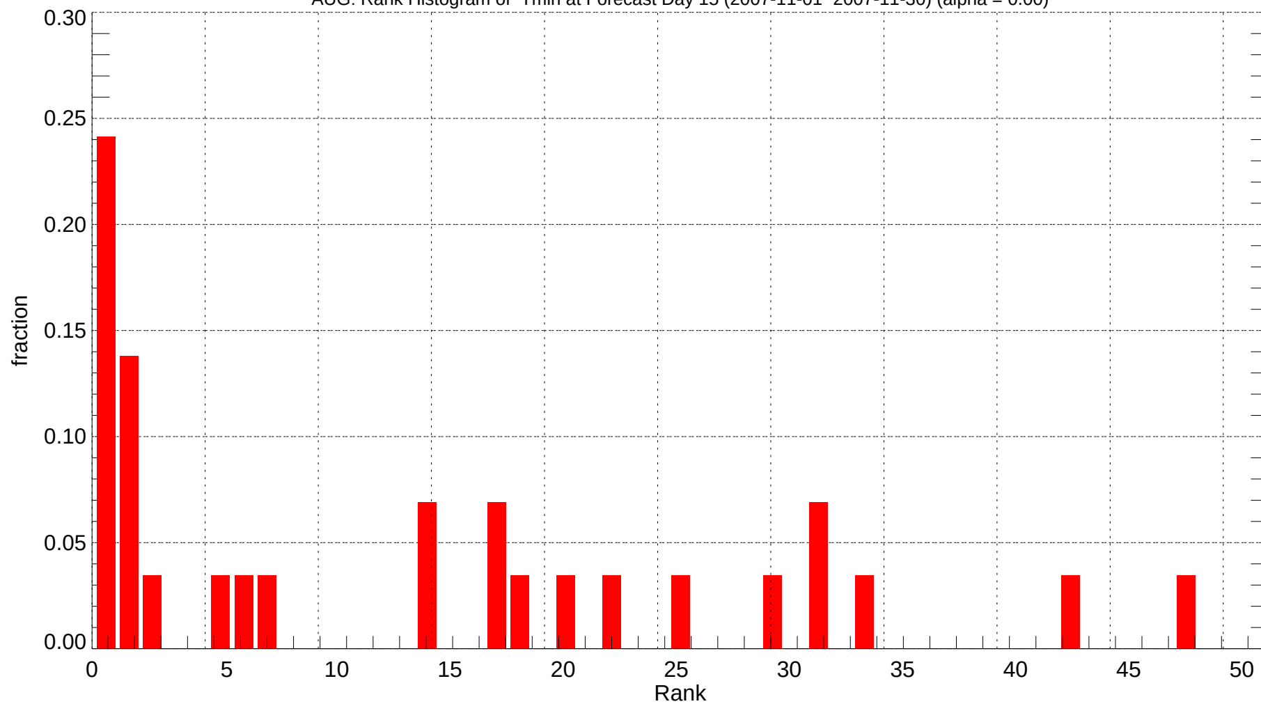
AUG: Rank Histogram of Tmin at Forecast Day 15 (2007-11-01~2007-11-30) (alpha = 0.00)
