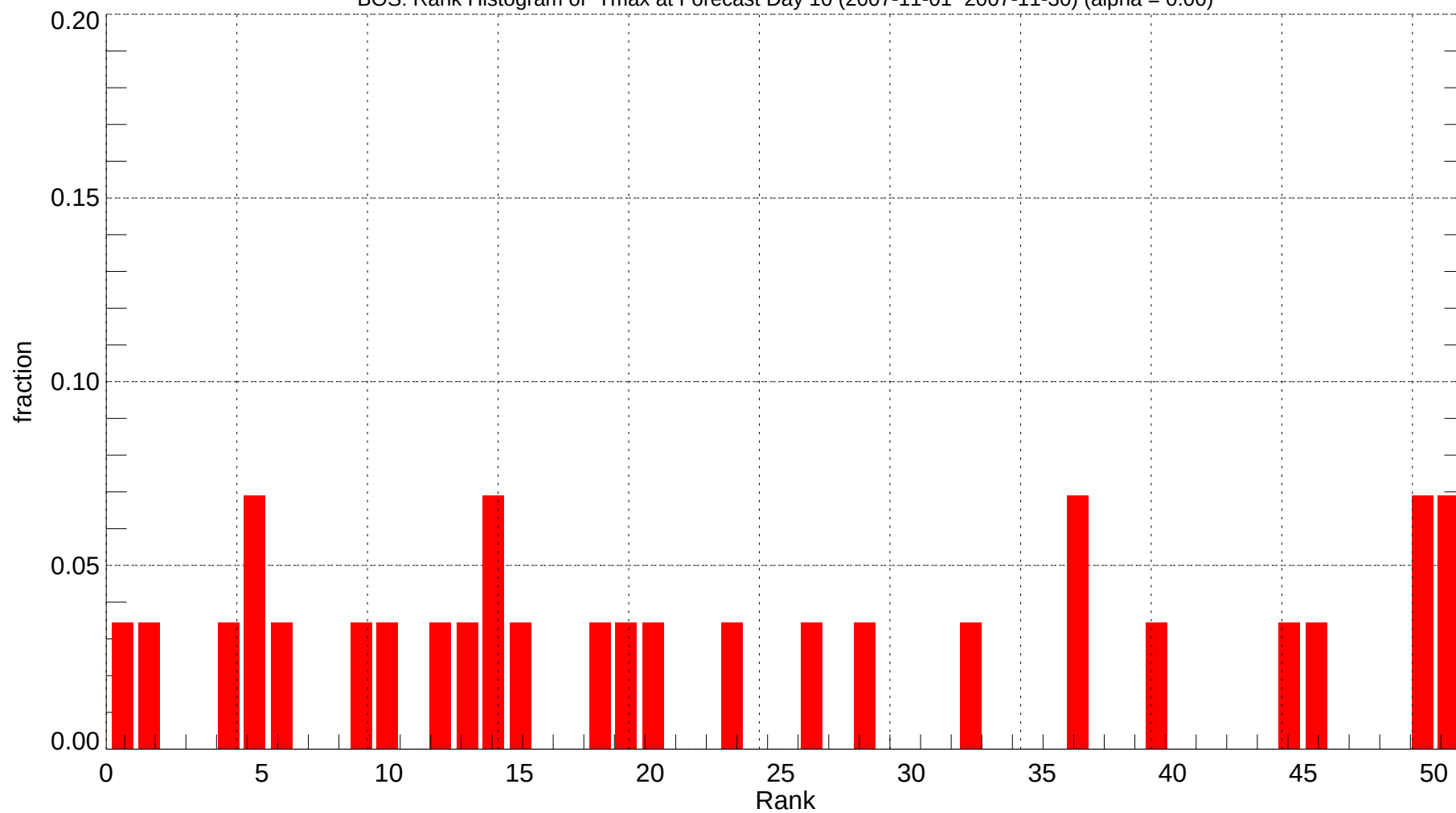
BOS: Rank Histogram of Tmax at Forecast Day 10 (2007-11-01~2007-11-30) (alpha = 0.00)
