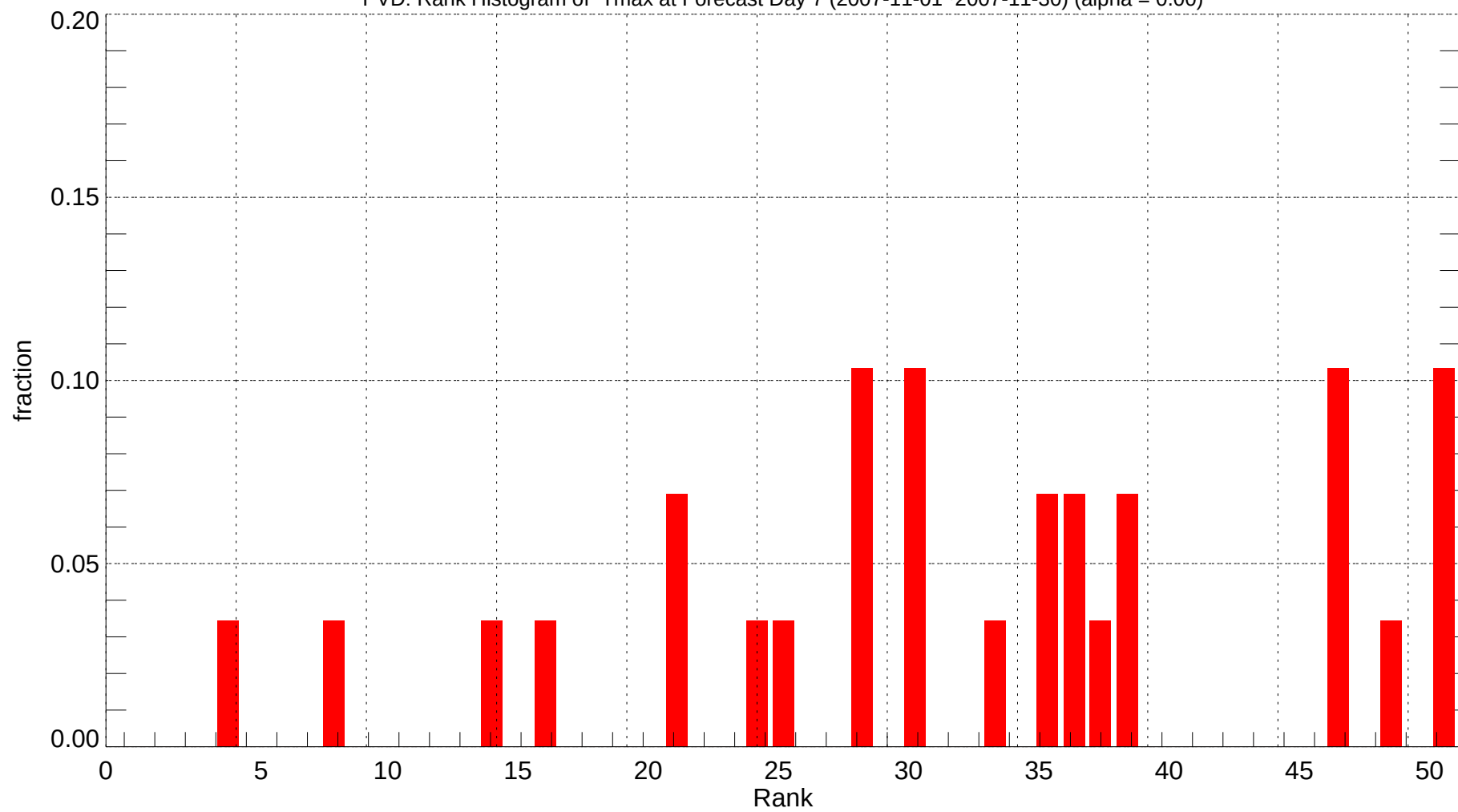
PVD: Rank Histogram of Tmax at Forecast Day 7 (2007-11-01~2007-11-30) (alpha = 0.00)
