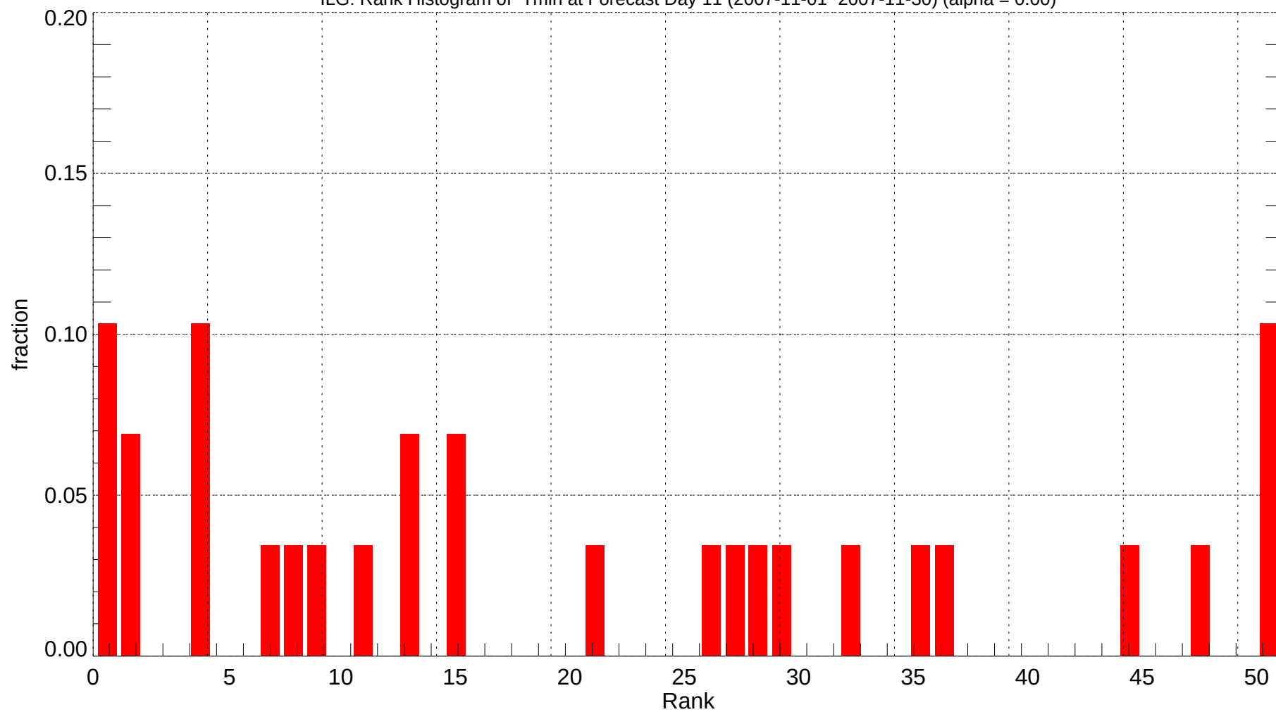
ILG: Rank Histogram of Tmin at Forecast Day 11 (2007-11-01~2007-11-30) (alpha = 0.00)
