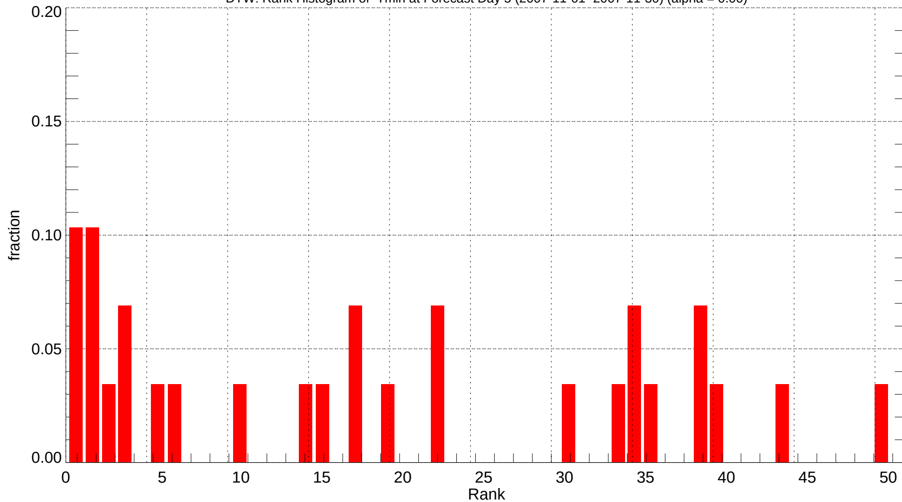
DTW: Rank Histogram of Tmin at Forecast Day 5 (2007-11-01~2007-11-30) (alpha = 0.00)
