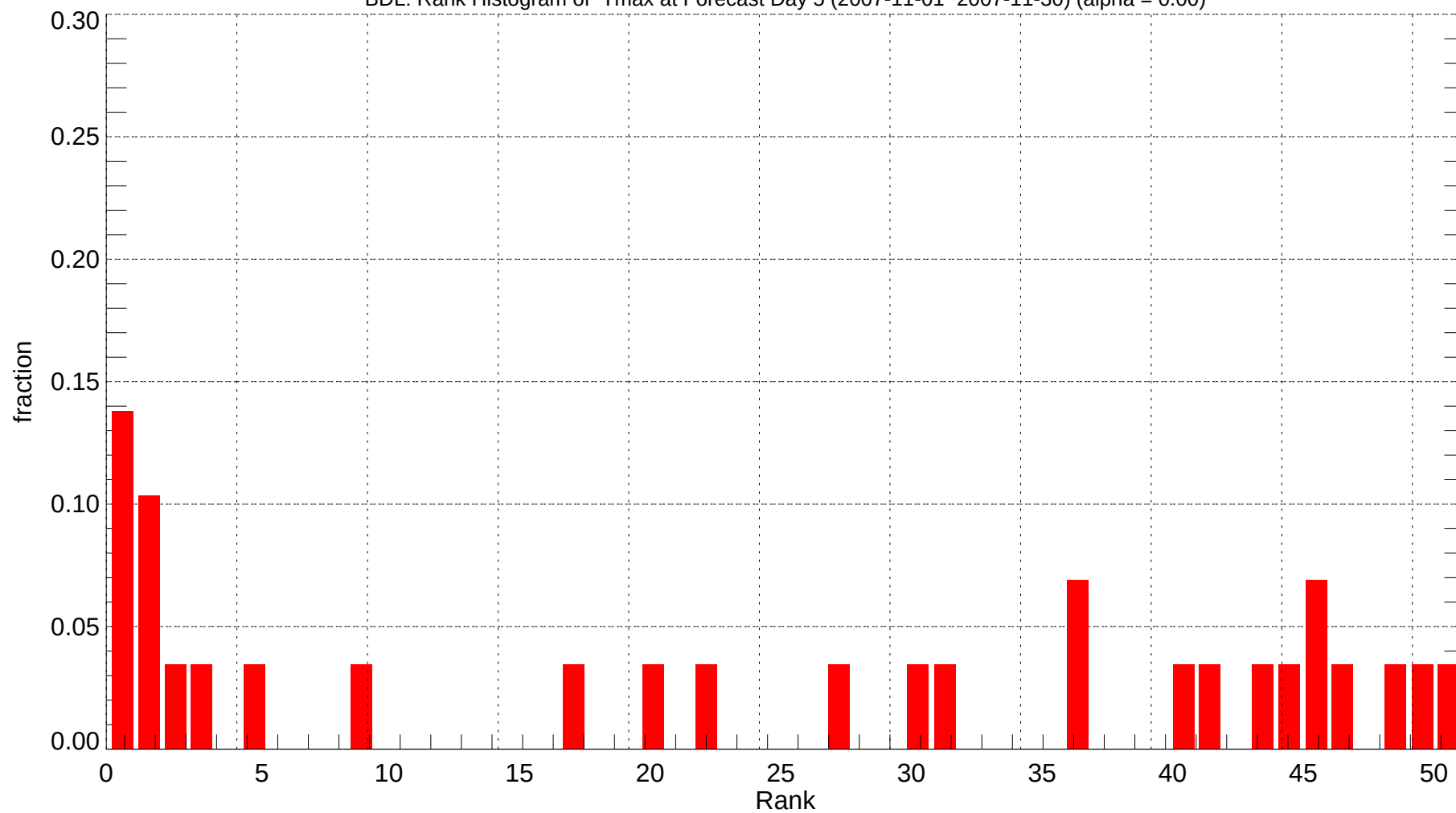
BDL: Rank Histogram of Tmax at Forecast Day 5 (2007-11-01~2007-11-30) (alpha = 0.00)
