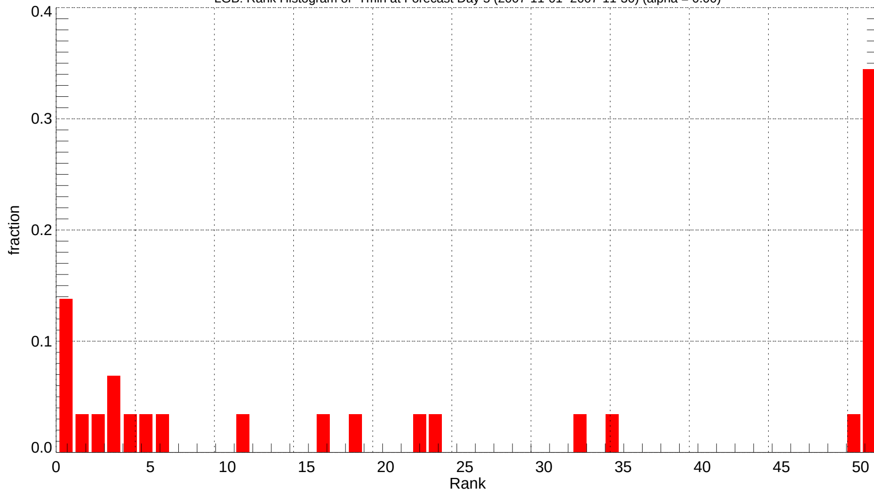
LGB: Rank Histogram of Tmin at Forecast Day 5 (2007-11-01~2007-11-30) (alpha = 0.00)
