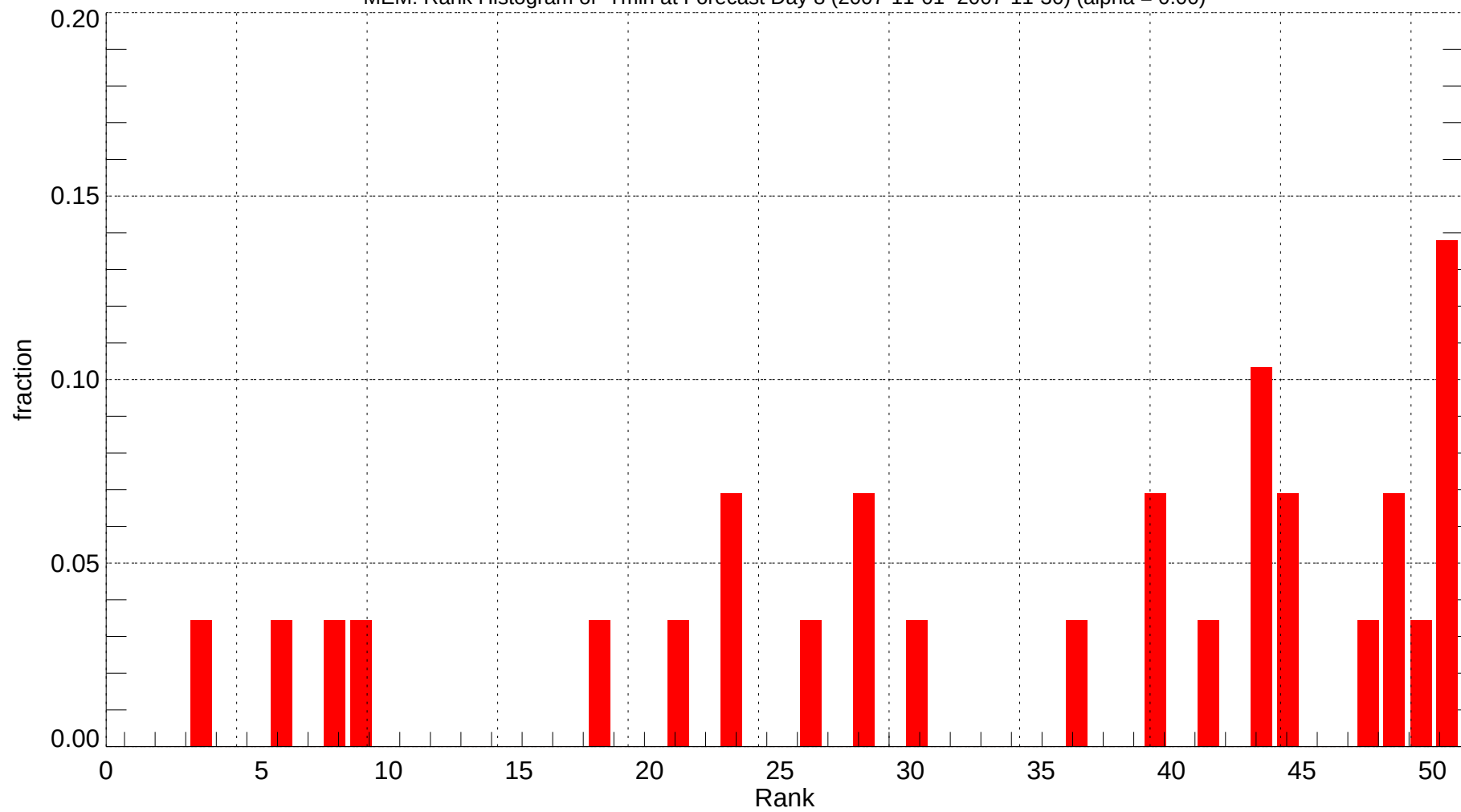
MEM: Rank Histogram of Tmin at Forecast Day 8 (2007-11-01~2007-11-30) (alpha = 0.00)
