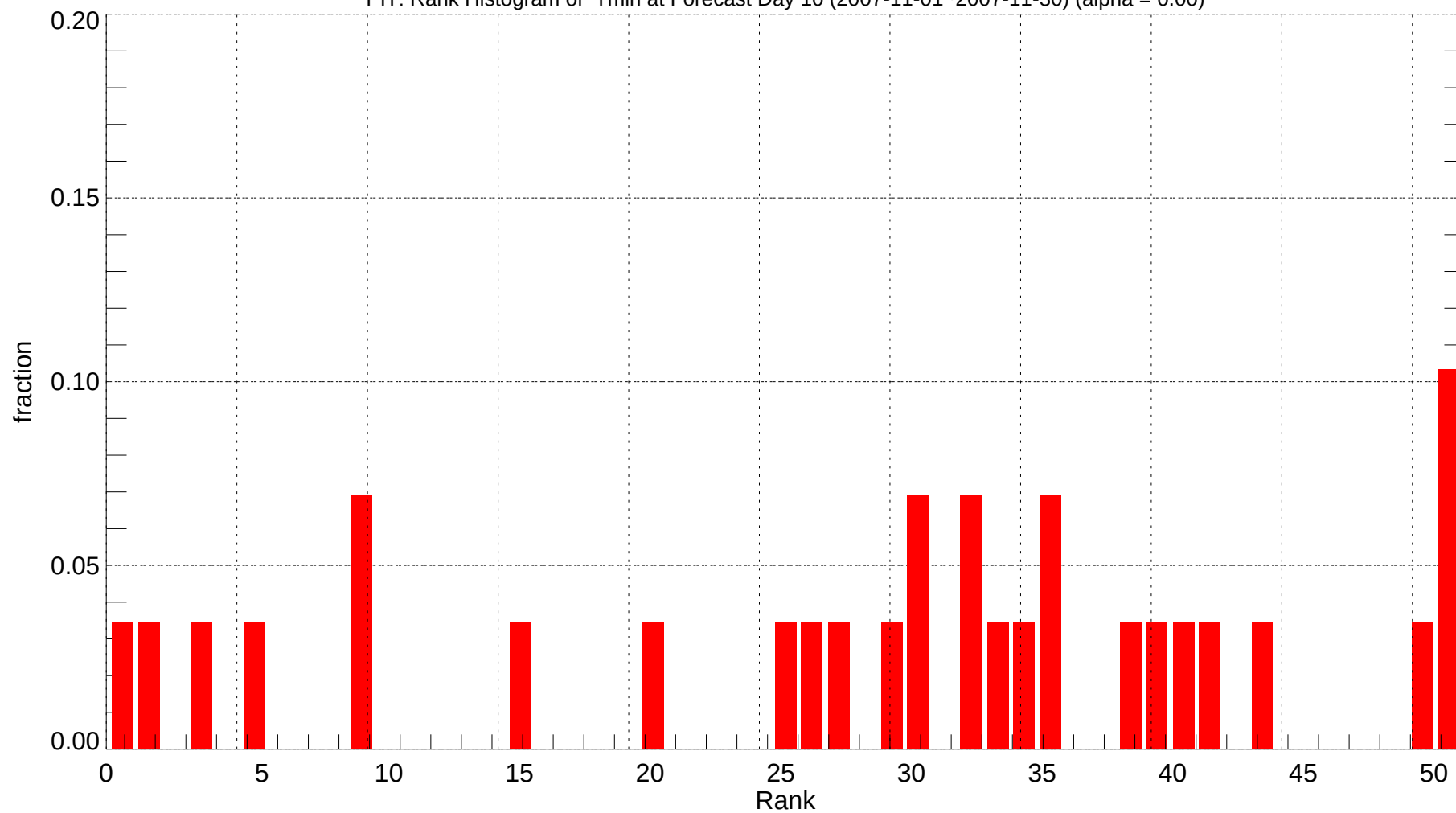
PIT: Rank Histogram of Tmin at Forecast Day 10 (2007-11-01~2007-11-30) (alpha = 0.00)
