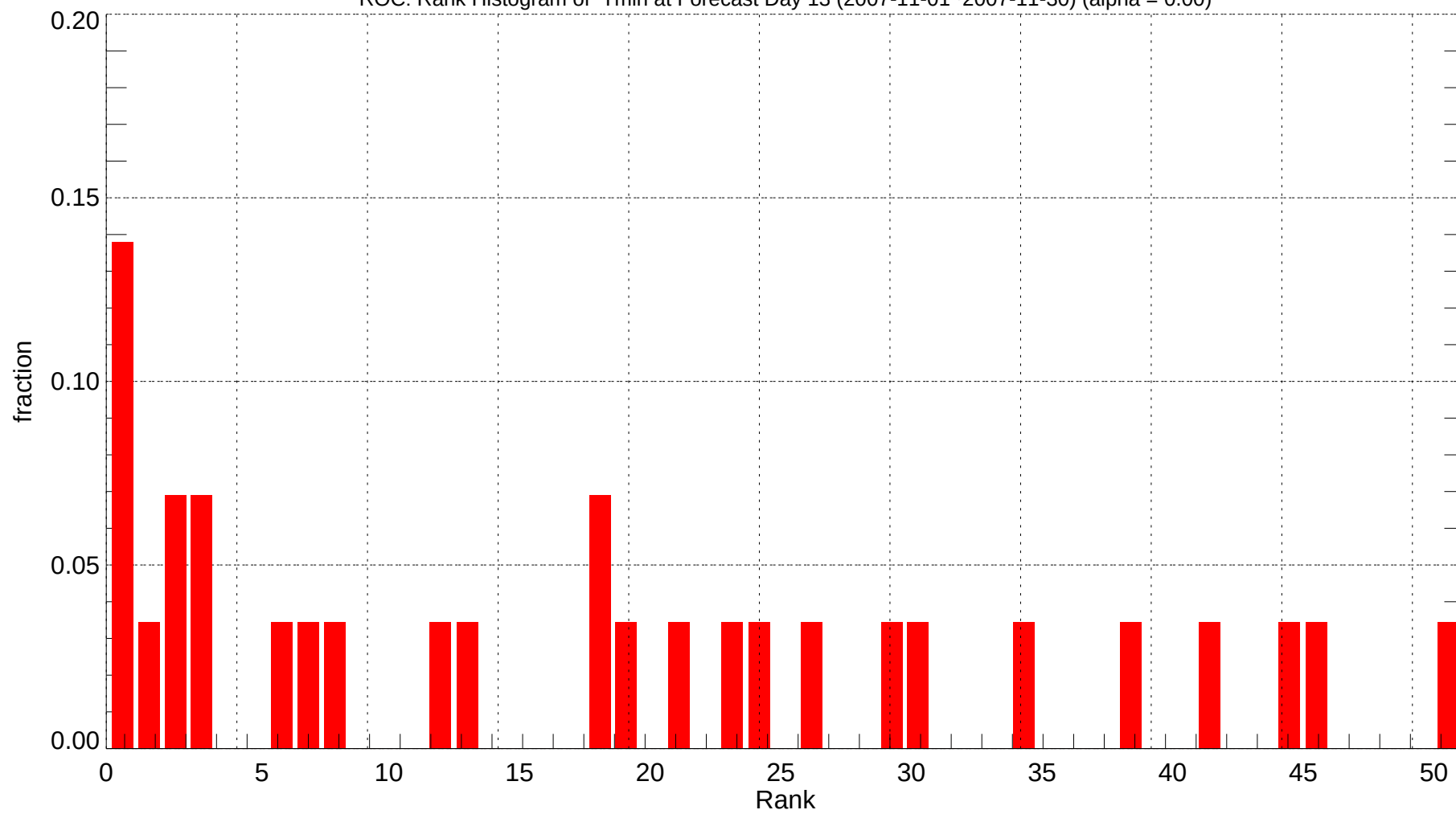
ROC: Rank Histogram of Tmin at Forecast Day 13 (2007-11-01~2007-11-30) (alpha = 0.00)
