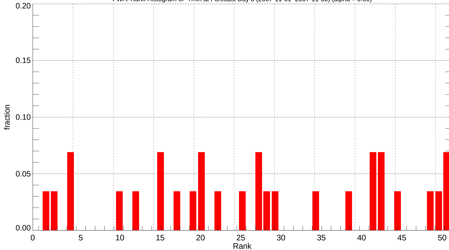
FWA: Rank Histogram of Tmin at Forecast Day 8 (2007-11-01~2007-11-30) (alpha = 0.00)
