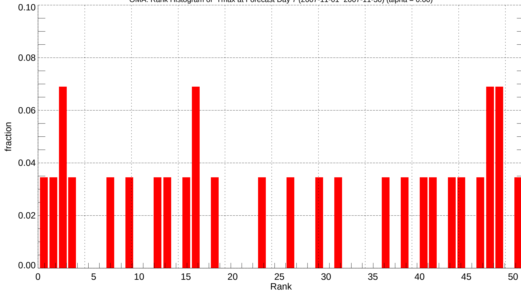
OMA: Rank Histogram of Tmax at Forecast Day 7 (2007-11-01~2007-11-30) (alpha = 0.00)
