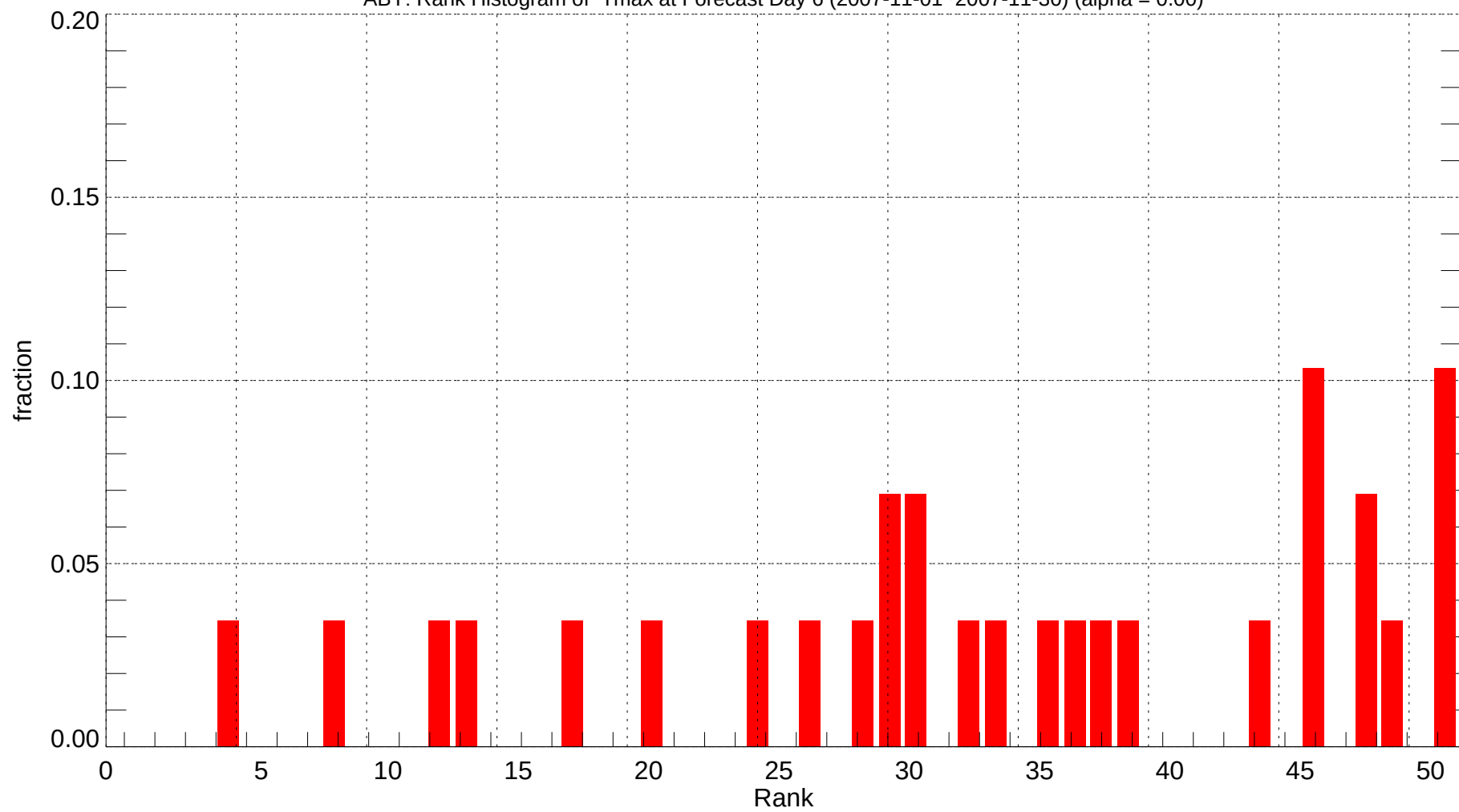
ABY: Rank Histogram of Tmax at Forecast Day 6 (2007-11-01~2007-11-30) (alpha = 0.00)
