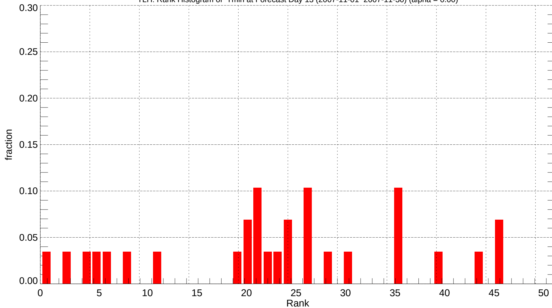
TLH: Rank Histogram of Tmin at Forecast Day 13 (2007-11-01~2007-11-30) (alpha = 0.00)
