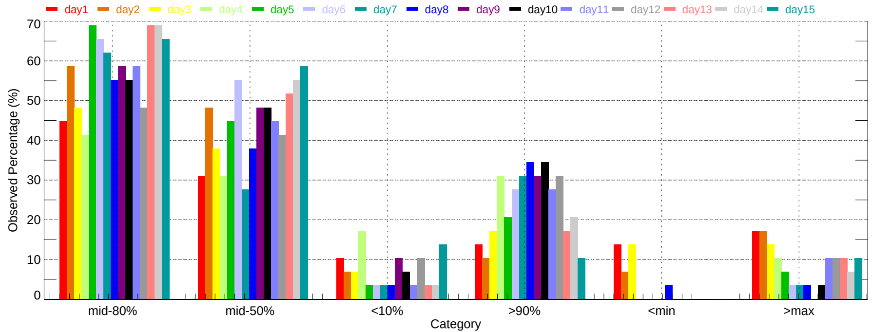
Observed Percentage of Ensembles - CVG: Min Temperature (2007-11-01~2007-11-30)
