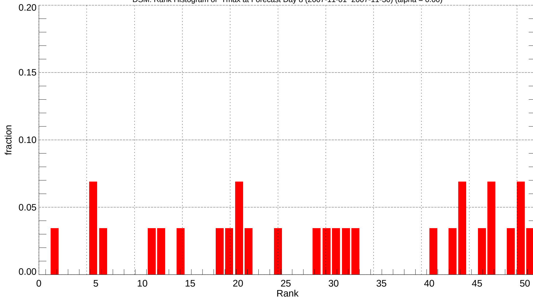
DSM: Rank Histogram of Tmax at Forecast Day 8 (2007-11-01~2007-11-30) (alpha = 0.00)
