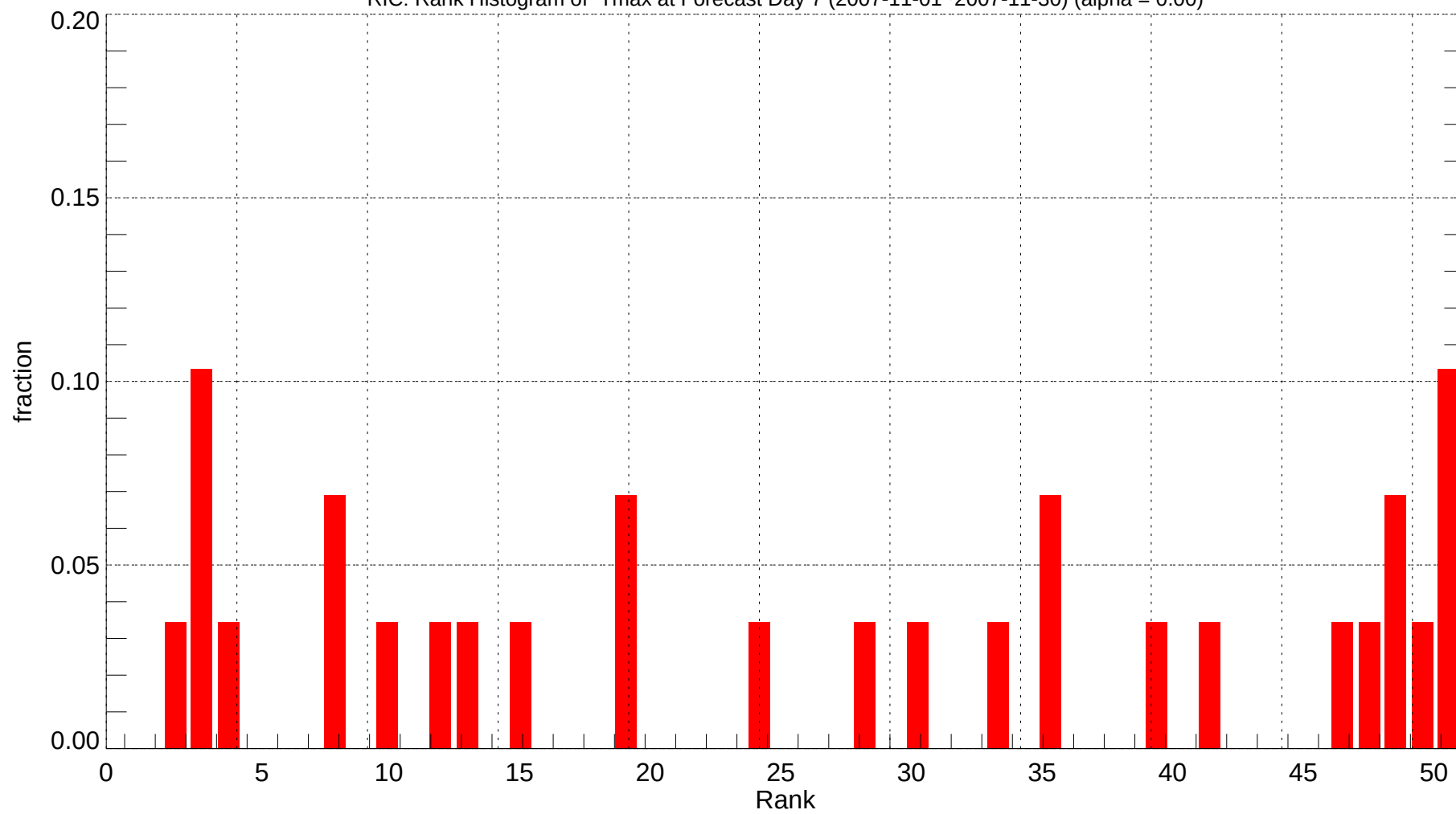
RIC: Rank Histogram of Tmax at Forecast Day 7 (2007-11-01~2007-11-30) (alpha = 0.00)
