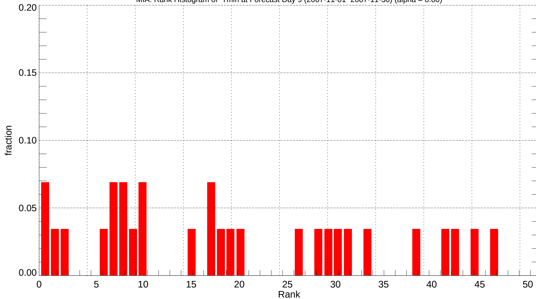
MIA: Rank Histogram of Tmin at Forecast Day 9 (2007-11-01~2007-11-30) (alpha = 0.00)
