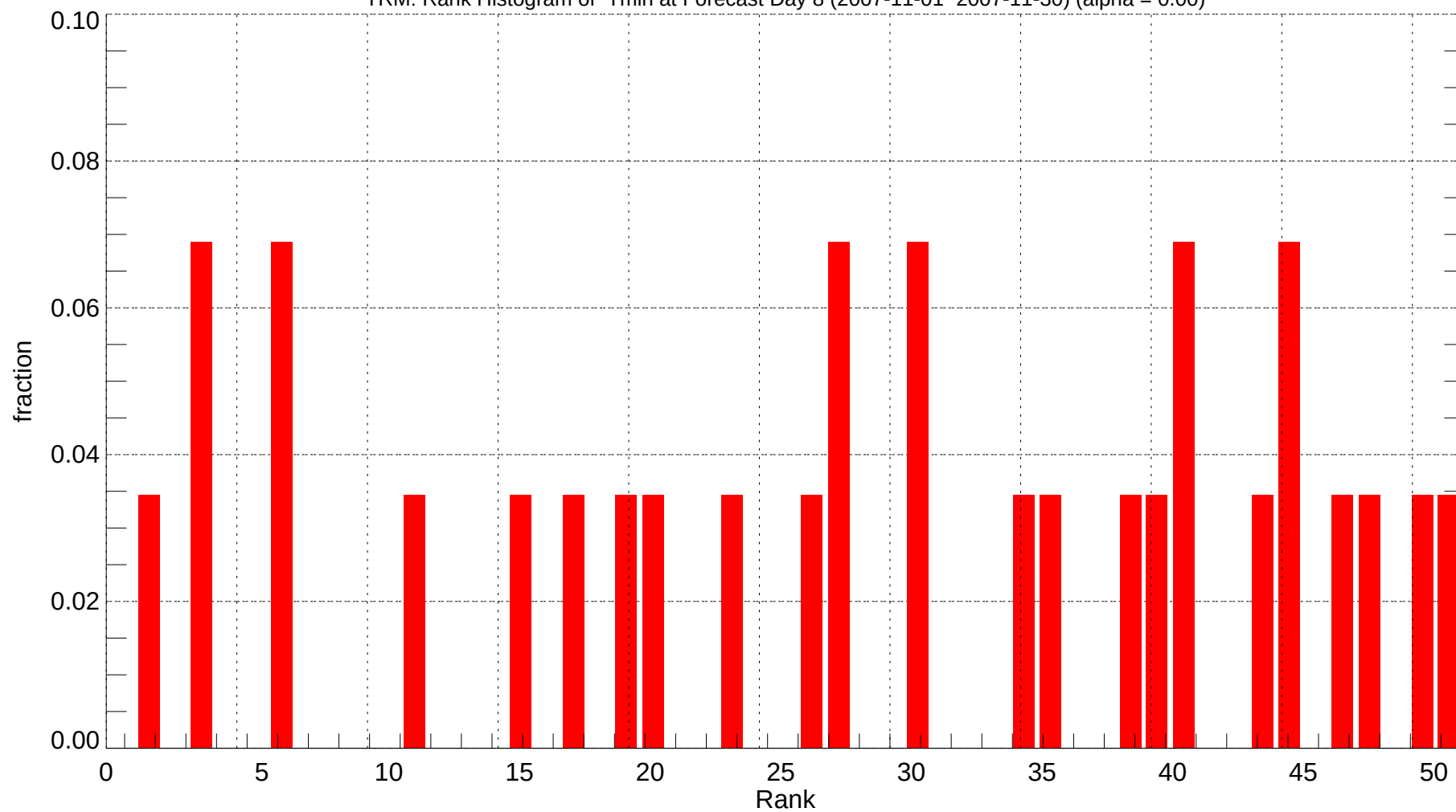
TRM: Rank Histogram of Tmin at Forecast Day 8 (2007-11-01~2007-11-30) (alpha = 0.00)
