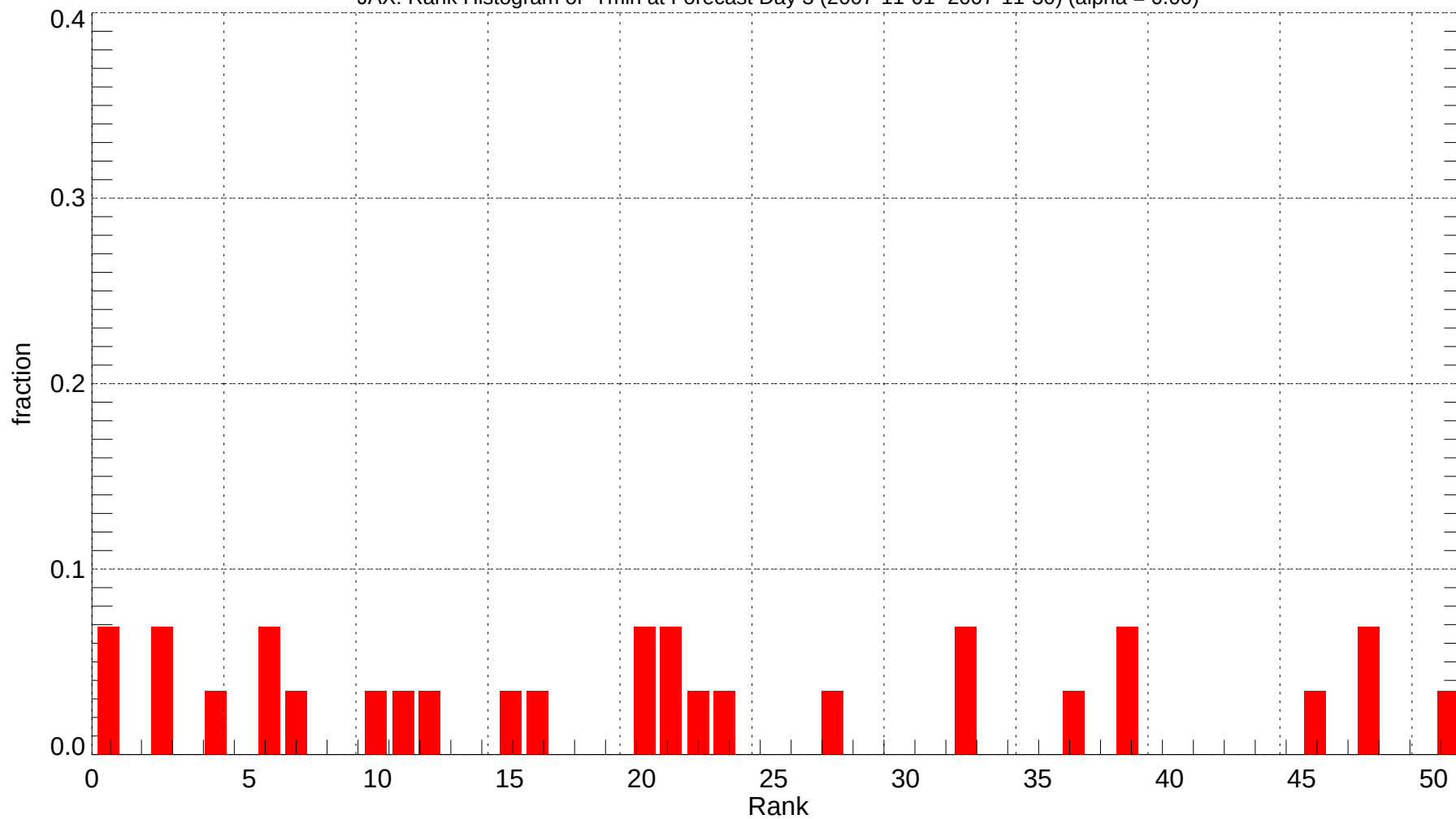
JAX: Rank Histogram of Tmin at Forecast Day 3 (2007-11-01~2007-11-30) (alpha = 0.00)
