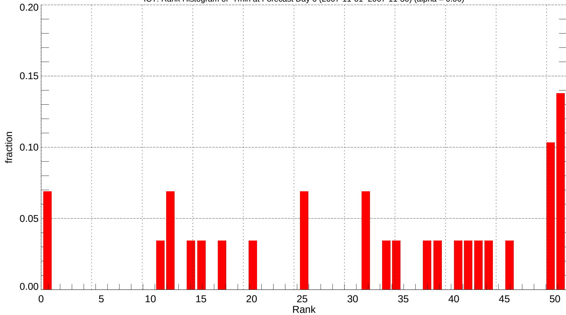
ICT: Rank Histogram of Tmin at Forecast Day 6 (2007-11-01~2007-11-30) (alpha = 0.00)
