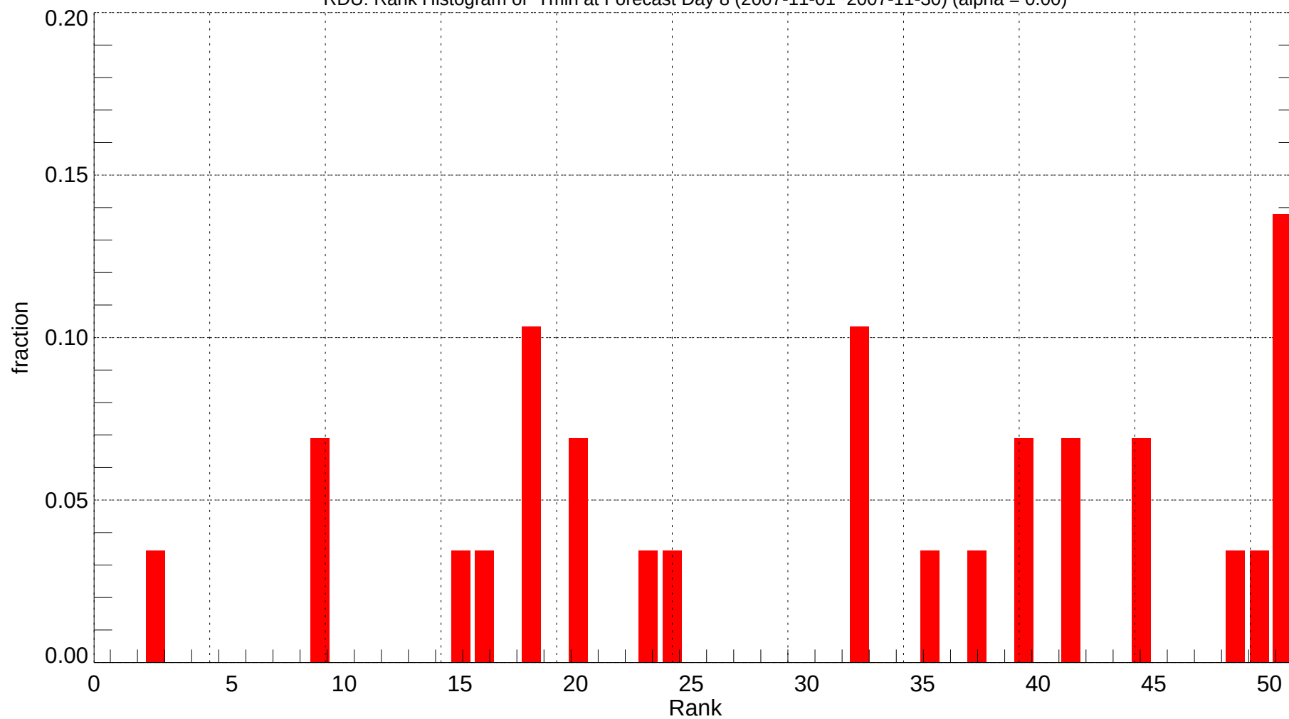
RDU: Rank Histogram of Tmin at Forecast Day 8 (2007-11-01~2007-11-30) (alpha = 0.00)
