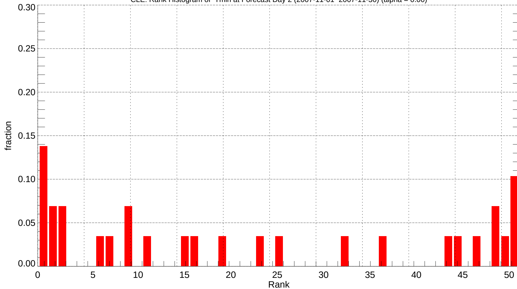
CLE: Rank Histogram of Tmin at Forecast Day 2 (2007-11-01~2007-11-30) (alpha = 0.00)
