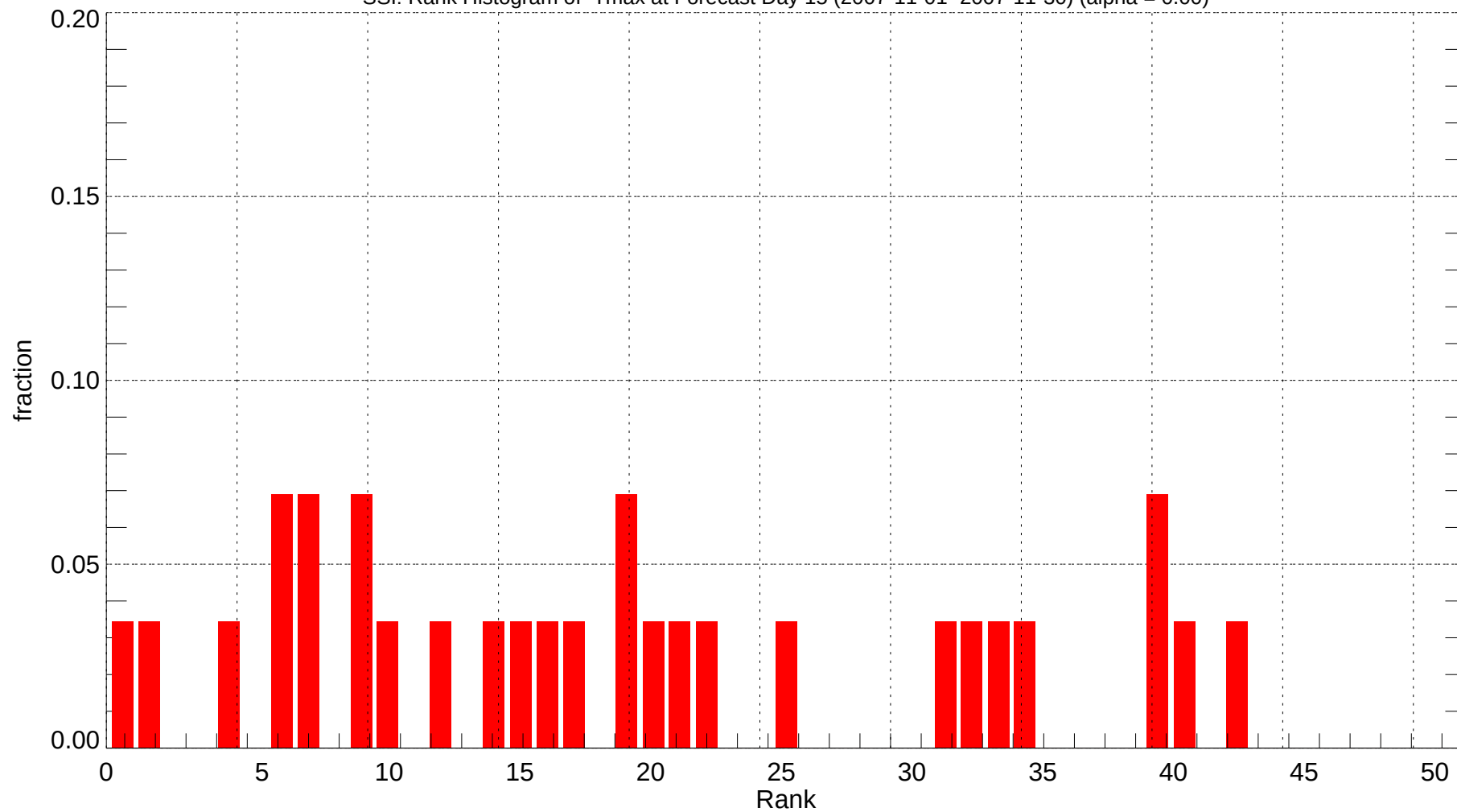
SSI: Rank Histogram of Tmax at Forecast Day 15 (2007-11-01~2007-11-30) (alpha = 0.00)
