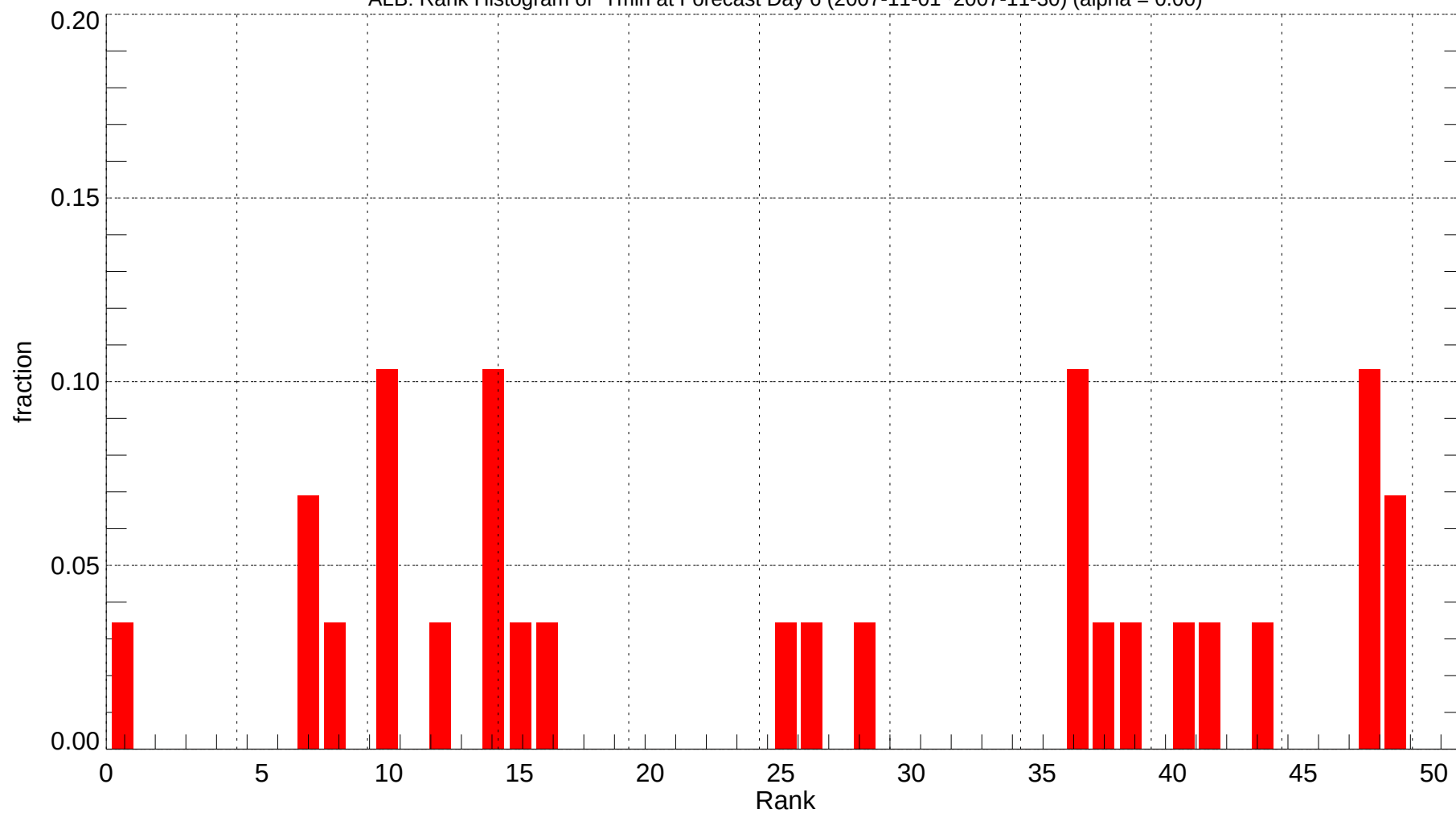
ALB: Rank Histogram of Tmin at Forecast Day 6 (2007-11-01~2007-11-30) (alpha = 0.00)
