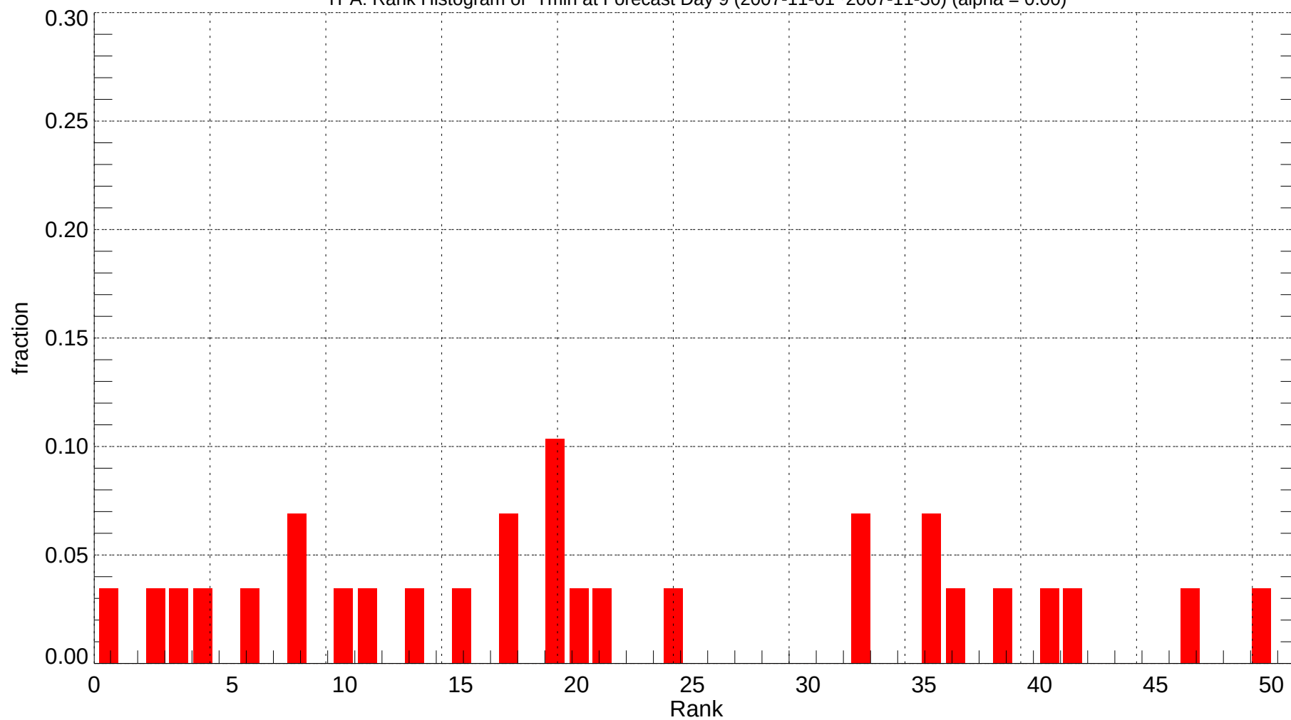
TPA: Rank Histogram of Tmin at Forecast Day 9 (2007-11-01~2007-11-30) (alpha = 0.00)
