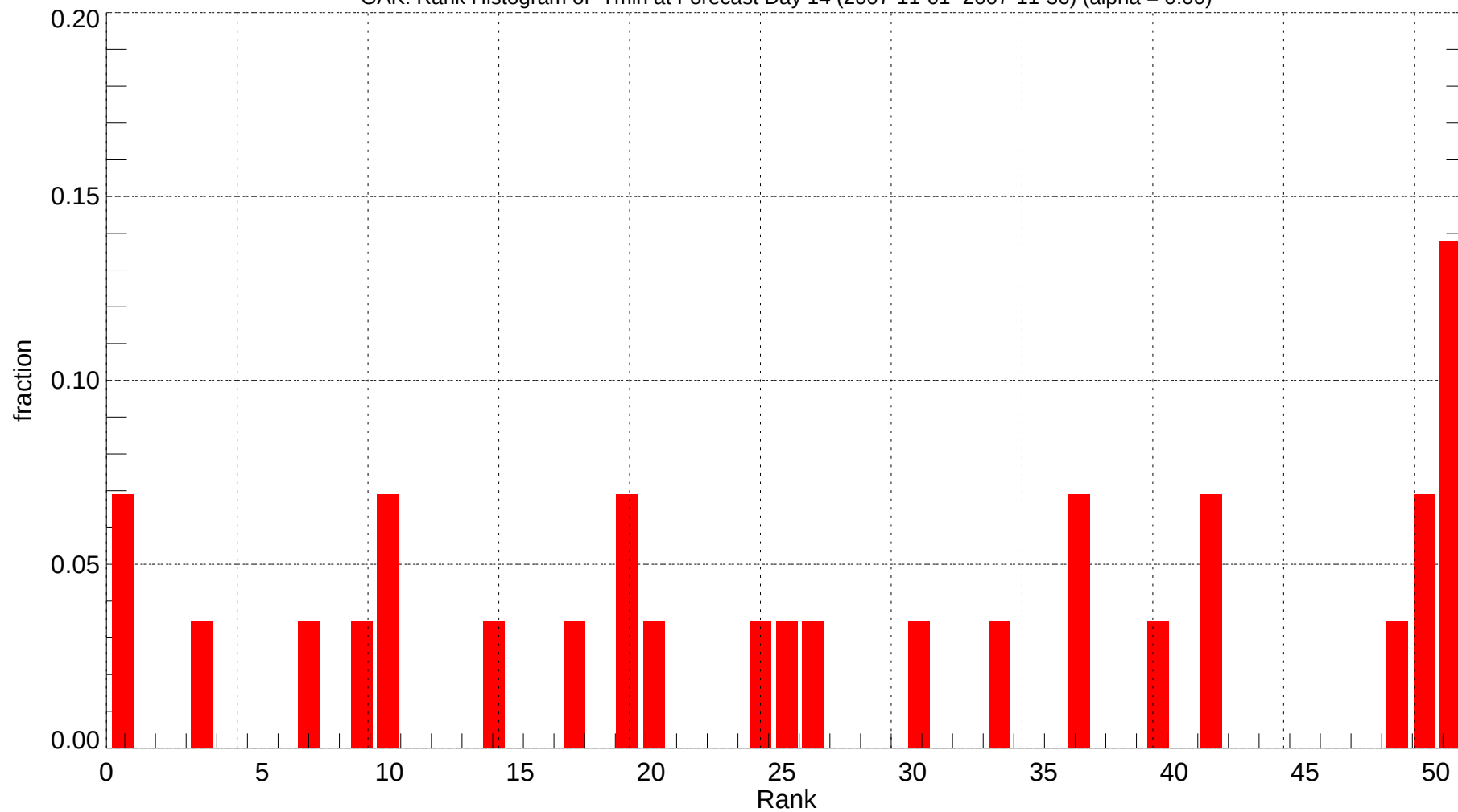
OAK: Rank Histogram of Tmin at Forecast Day 14 (2007-11-01~2007-11-30) (alpha = 0.00)
