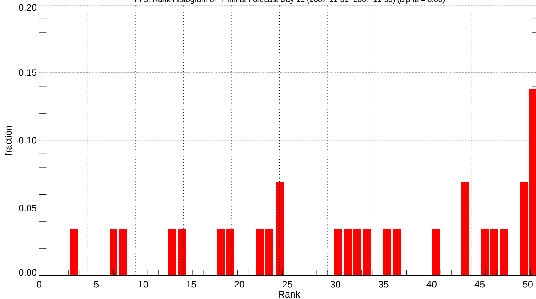
TYS: Rank Histogram of Tmin at Forecast Day 12 (2007-11-01~2007-11-30) (alpha = 0.00)
