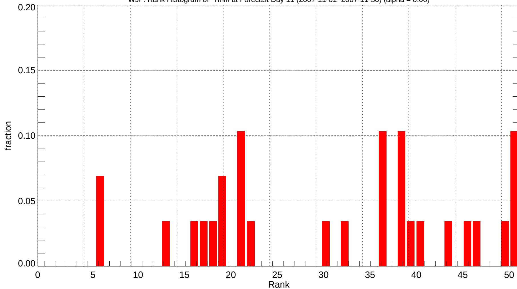
WJF: Rank Histogram of Tmin at Forecast Day 11 (2007-11-01~2007-11-30) (alpha = 0.00)
