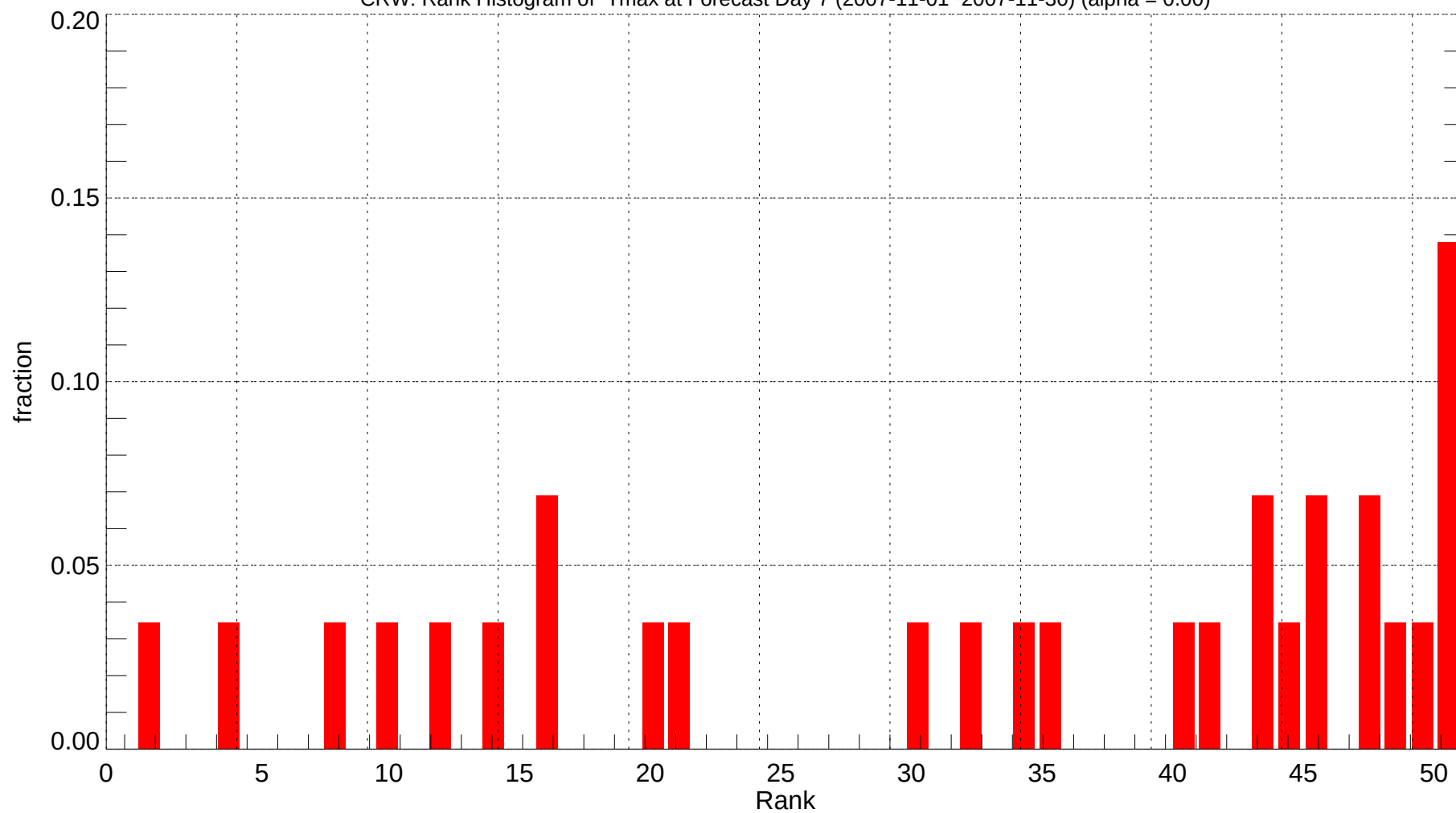
CRW: Rank Histogram of Tmax at Forecast Day 7 (2007-11-01~2007-11-30) (alpha = 0.00)
