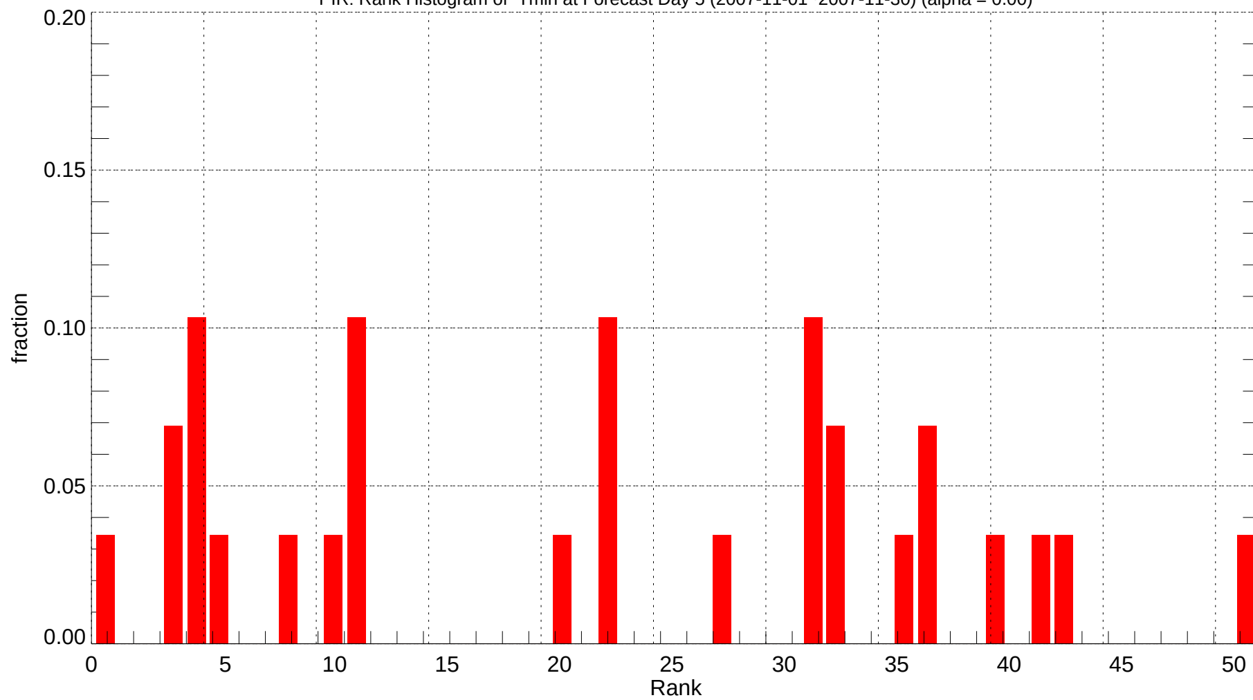
PIR: Rank Histogram of Tmin at Forecast Day 5 (2007-11-01~2007-11-30) (alpha = 0.00)
