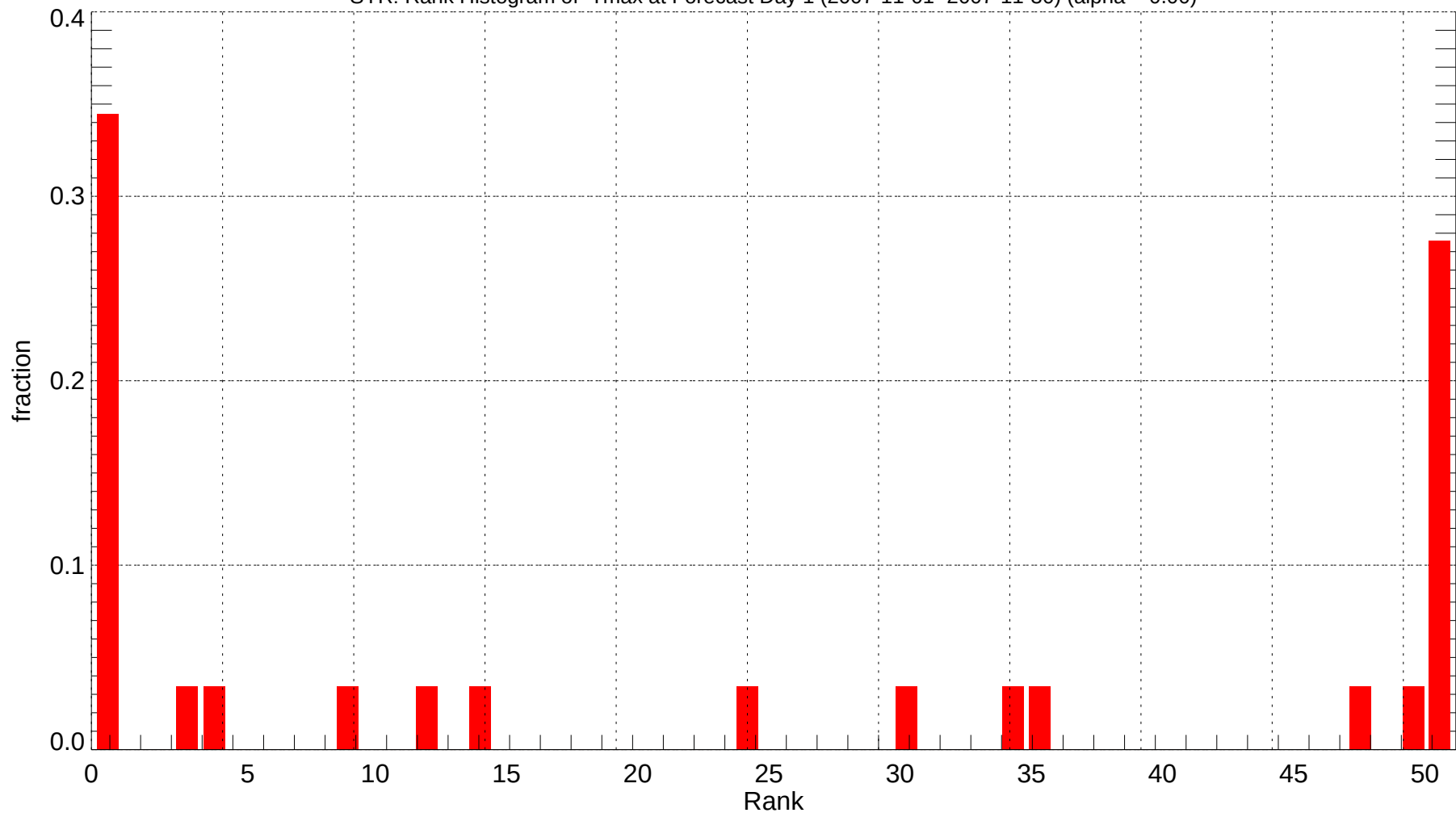
SYR: Rank Histogram of Tmax at Forecast Day 1 (2007-11-01~2007-11-30) (alpha = 0.00)
