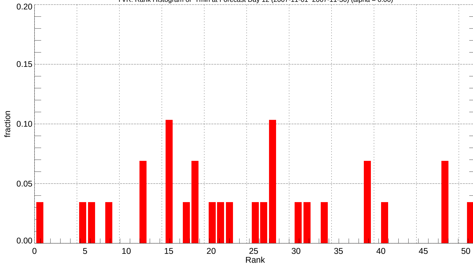
YVR: Rank Histogram of Tmin at Forecast Day 12 (2007-11-01~2007-11-30) (alpha = 0.00)
