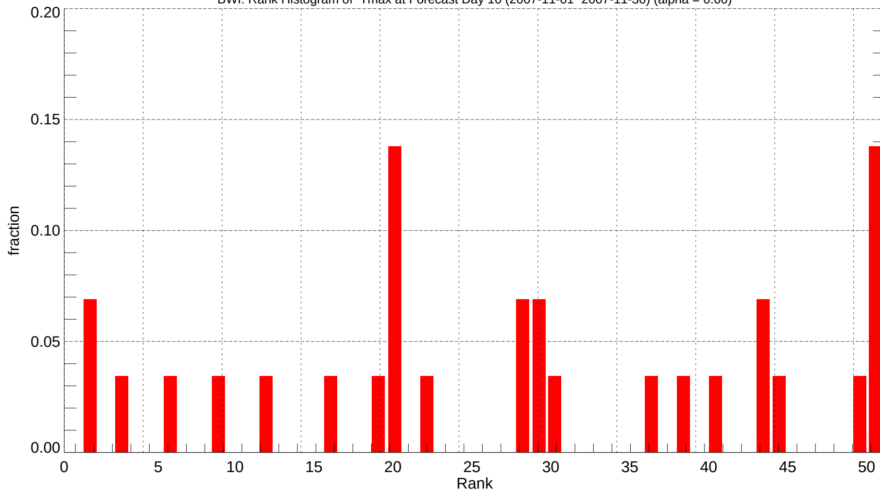
BWI: Rank Histogram of Tmax at Forecast Day 10 (2007-11-01~2007-11-30) (alpha = 0.00)
