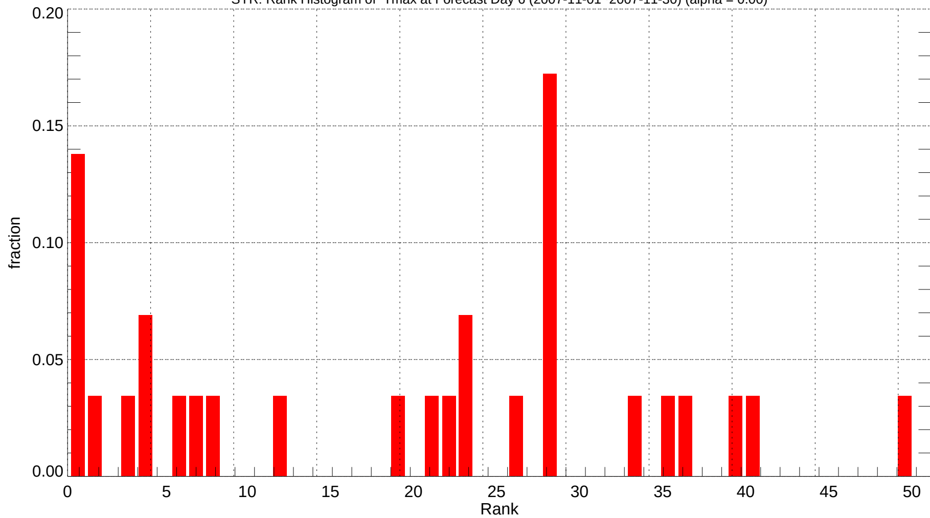
SYR: Rank Histogram of Tmax at Forecast Day 6 (2007-11-01~2007-11-30) (alpha = 0.00)
