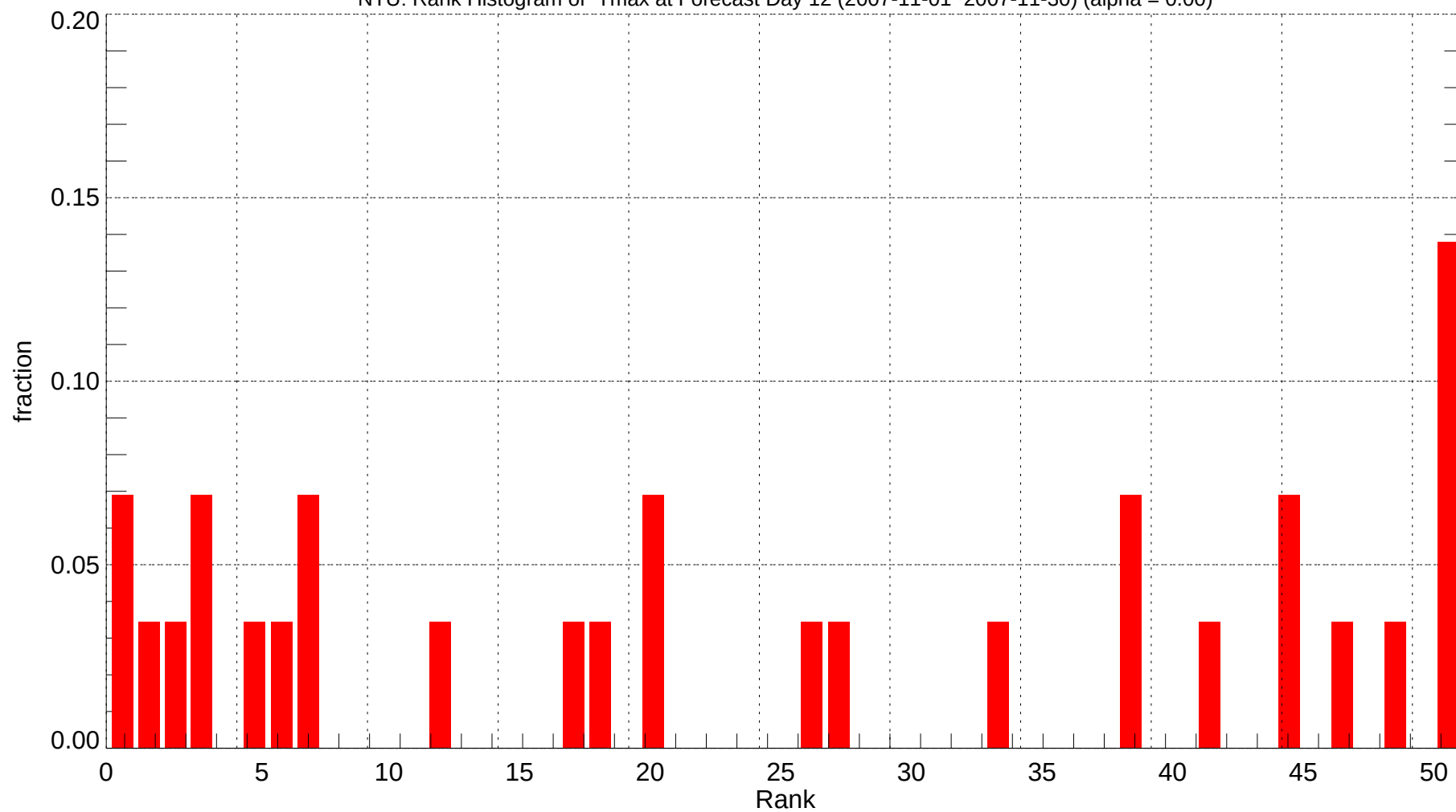
NTU: Rank Histogram of Tmax at Forecast Day 12 (2007-11-01~2007-11-30) (alpha = 0.00)
