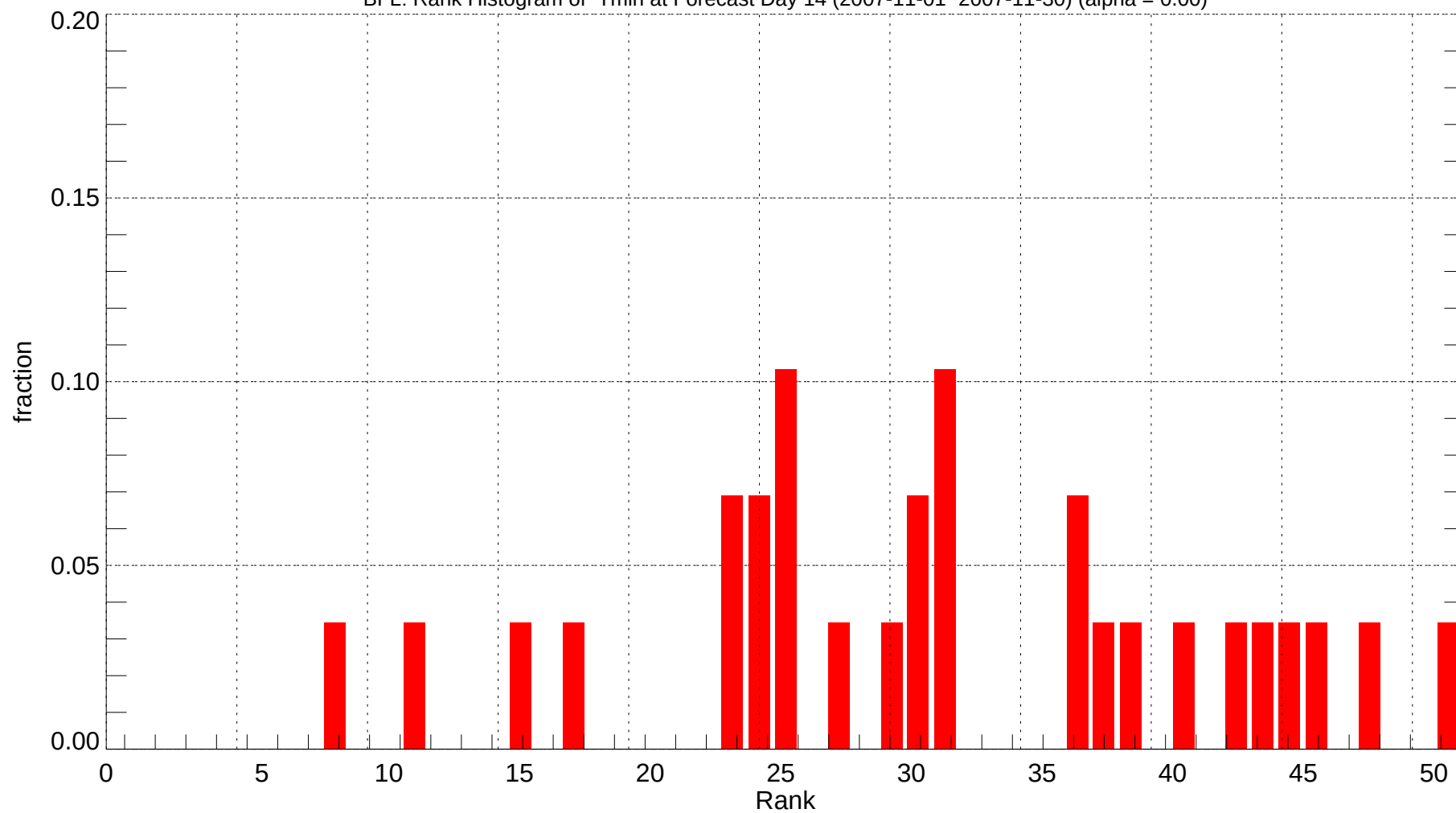
BFL: Rank Histogram of Tmin at Forecast Day 14 (2007-11-01~2007-11-30) (alpha = 0.00)
