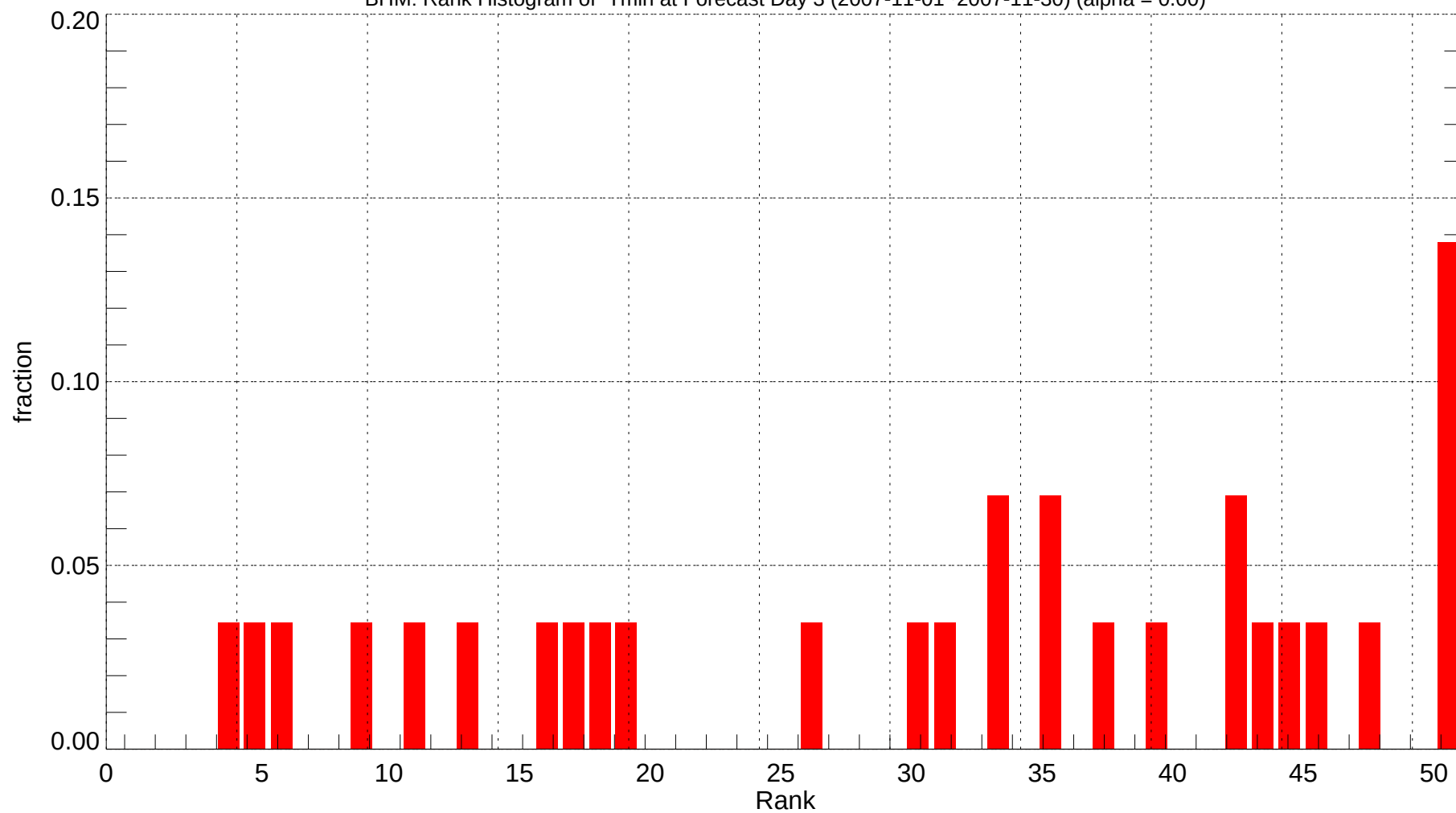
BHM: Rank Histogram of Tmin at Forecast Day 3 (2007-11-01~2007-11-30) (alpha = 0.00)
