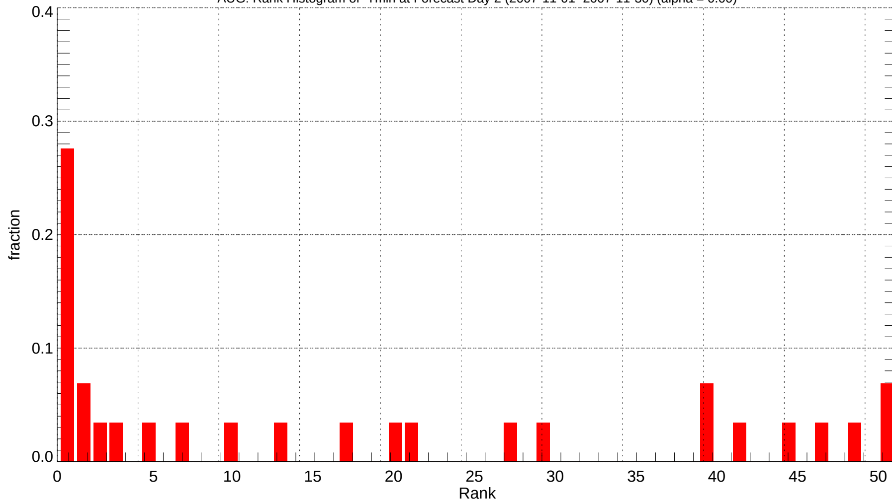
AUG: Rank Histogram of Tmin at Forecast Day 2 (2007-11-01~2007-11-30) (alpha = 0.00)
