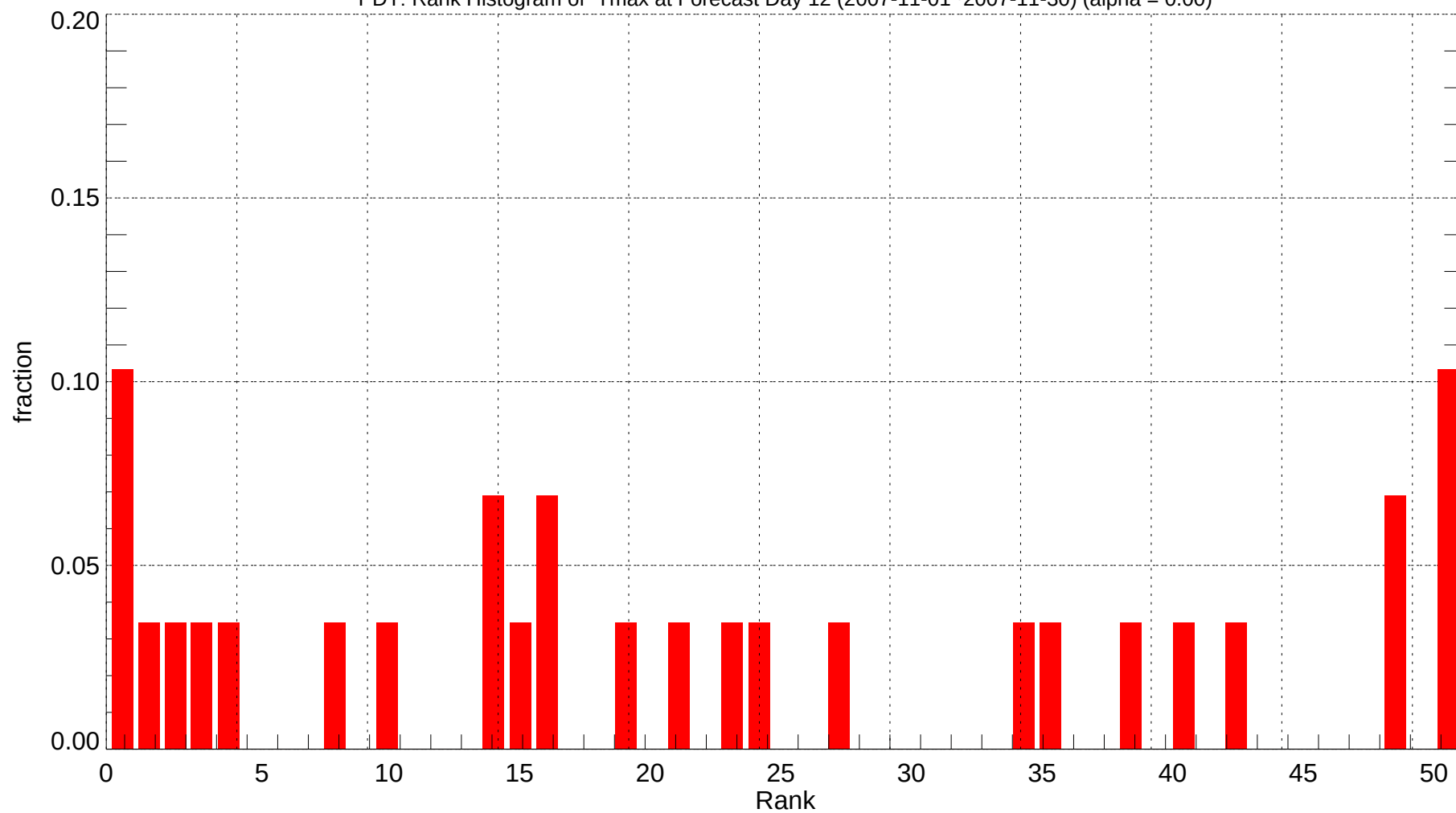
PDT: Rank Histogram of Tmax at Forecast Day 12 (2007-11-01~2007-11-30) (alpha = 0.00)
