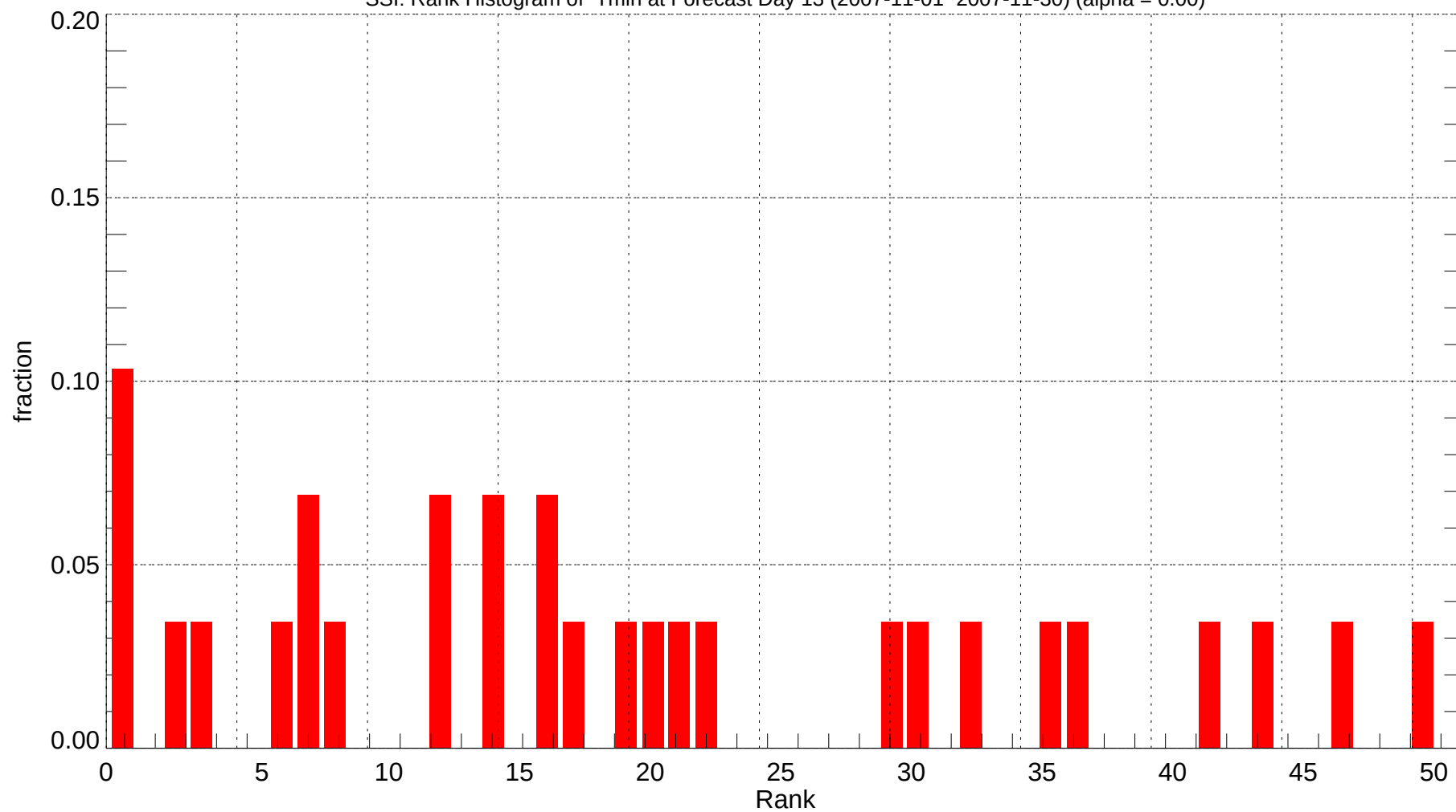
SSI: Rank Histogram of Tmin at Forecast Day 13 (2007-11-01~2007-11-30) (alpha = 0.00)
