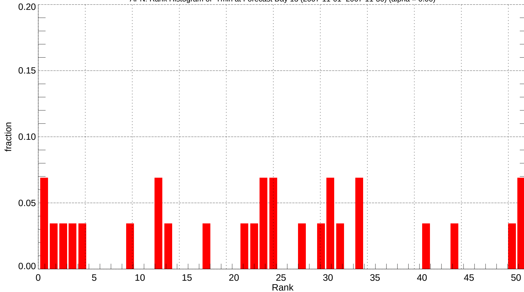
APN: Rank Histogram of Tmin at Forecast Day 13 (2007-11-01~2007-11-30) (alpha = 0.00)
