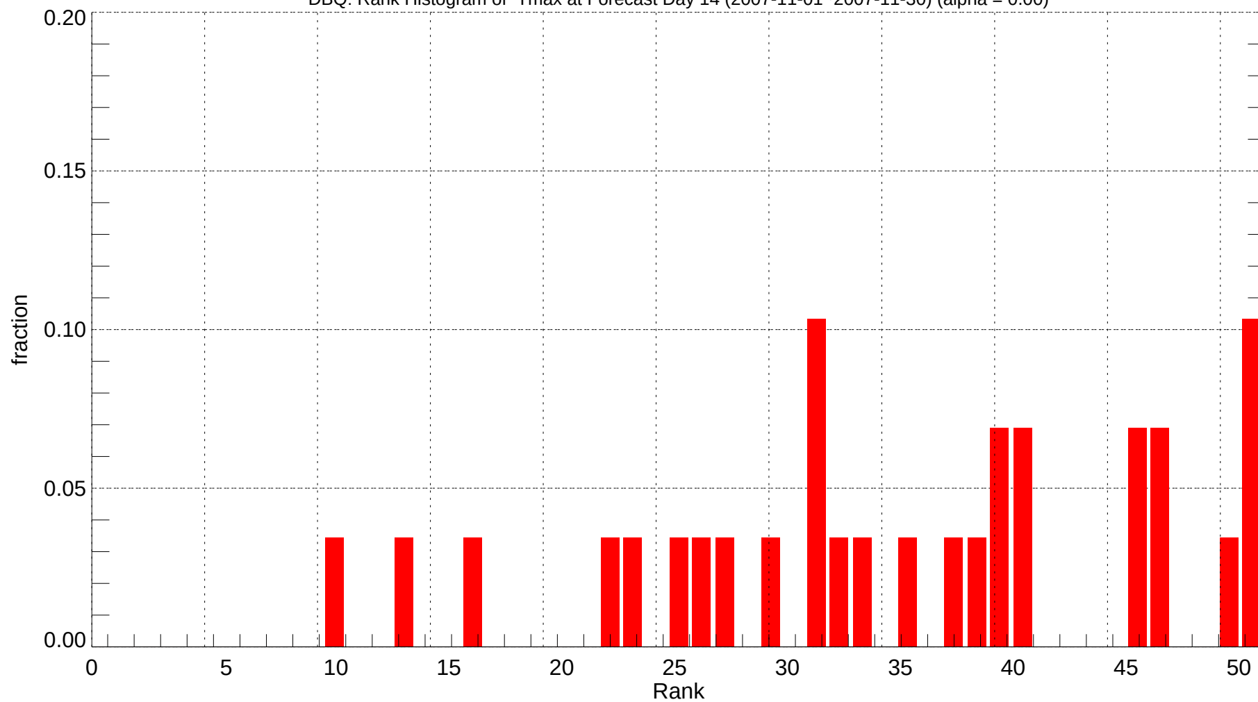
DBQ: Rank Histogram of Tmax at Forecast Day 14 (2007-11-01~2007-11-30) (alpha = 0.00)
