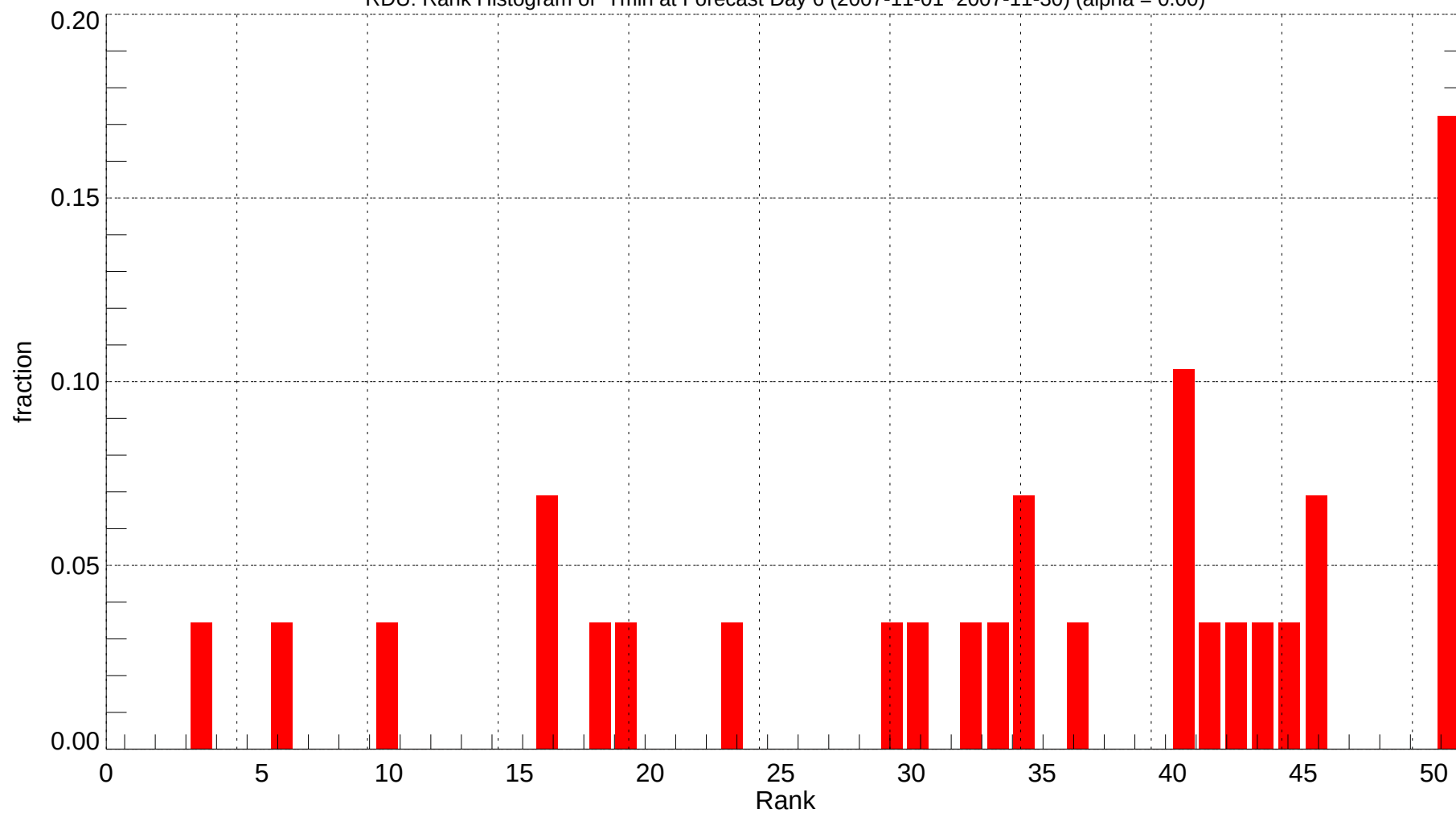
RDU: Rank Histogram of Tmin at Forecast Day 6 (2007-11-01~2007-11-30) (alpha = 0.00)
