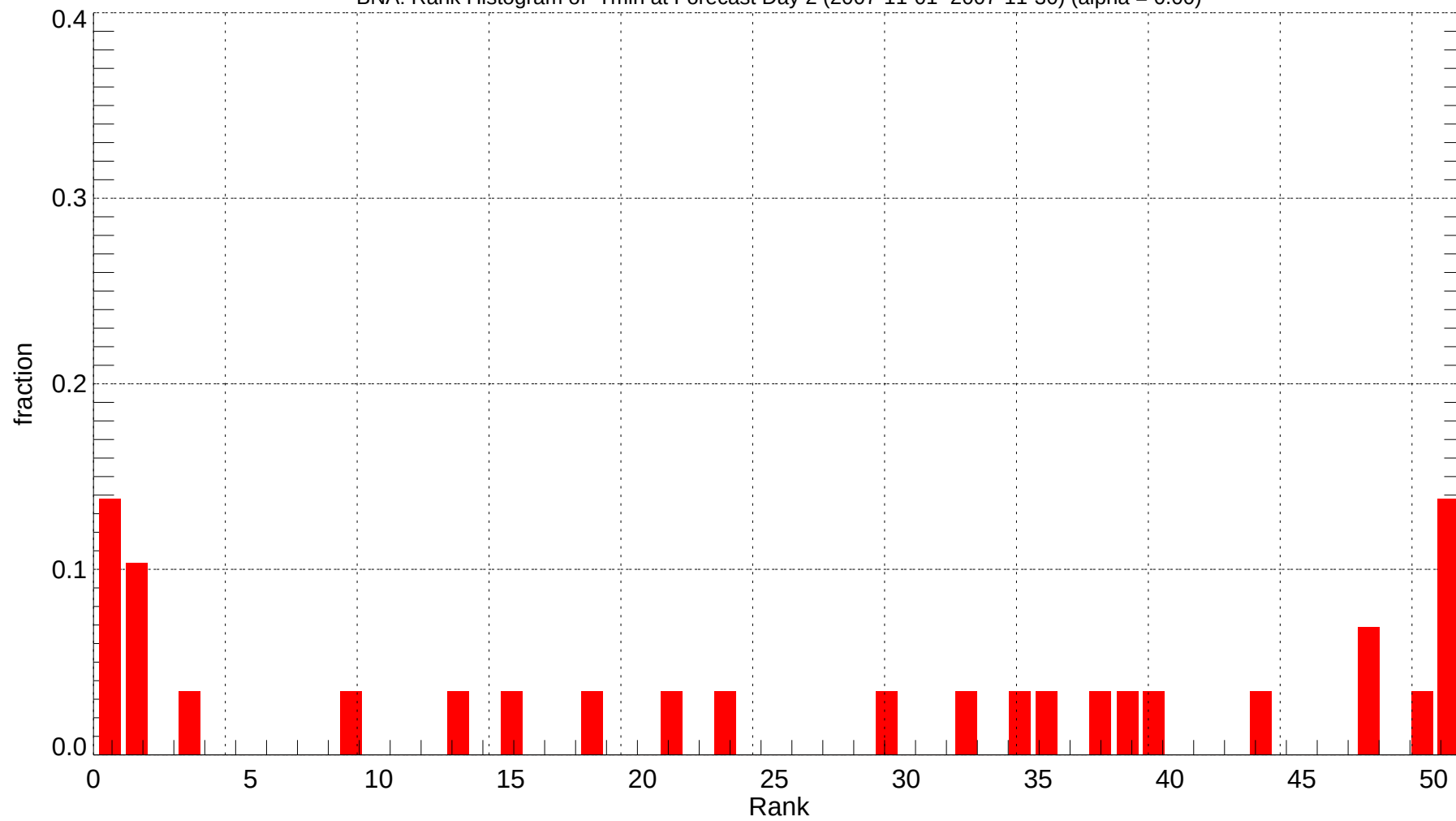
BNA: Rank Histogram of Tmin at Forecast Day 2 (2007-11-01~2007-11-30) (alpha = 0.00)
