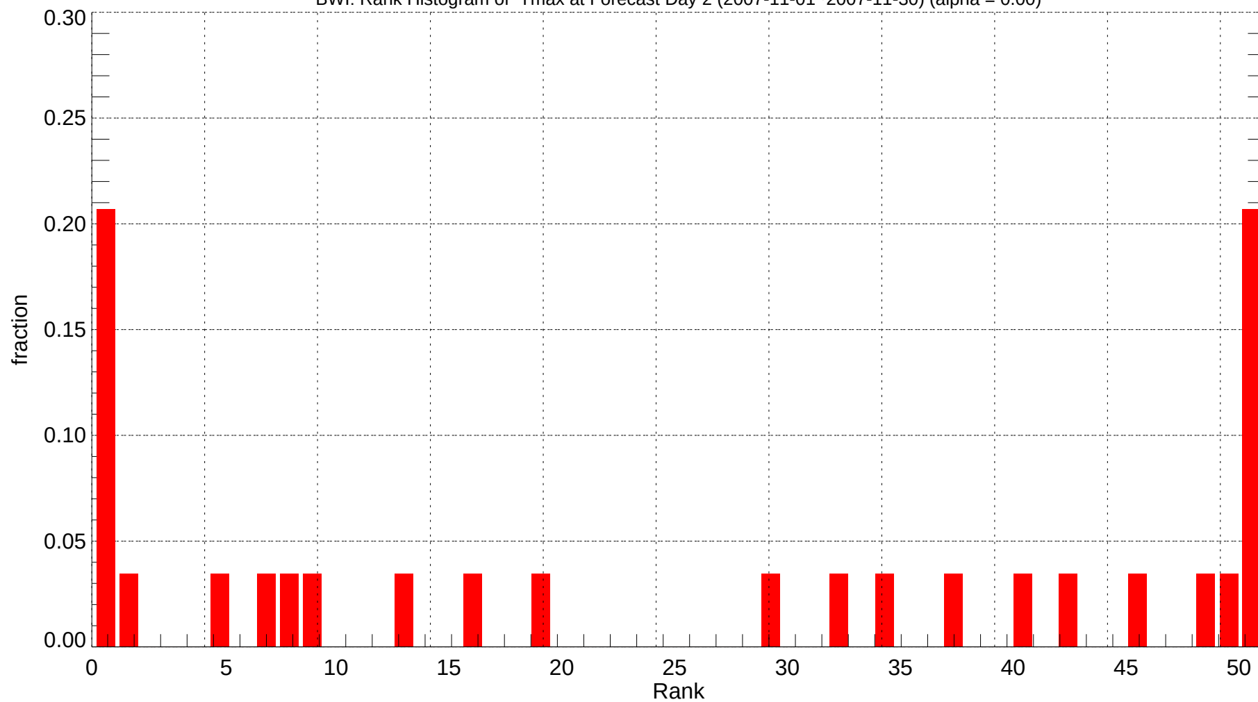
BWI: Rank Histogram of Tmax at Forecast Day 2 (2007-11-01~2007-11-30) (alpha = 0.00)
