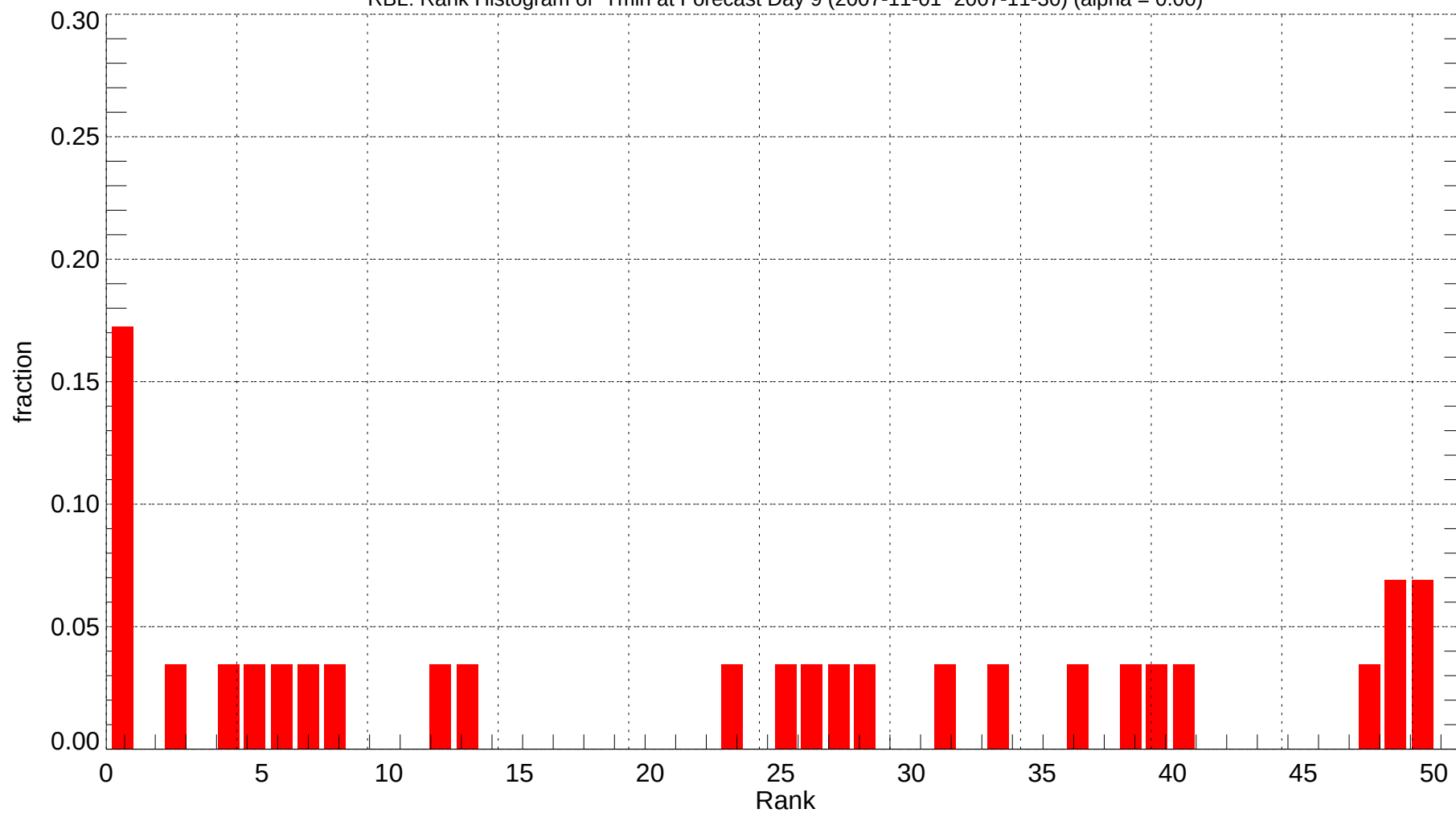
RBL: Rank Histogram of Tmin at Forecast Day 9 (2007-11-01~2007-11-30) (alpha = 0.00)
