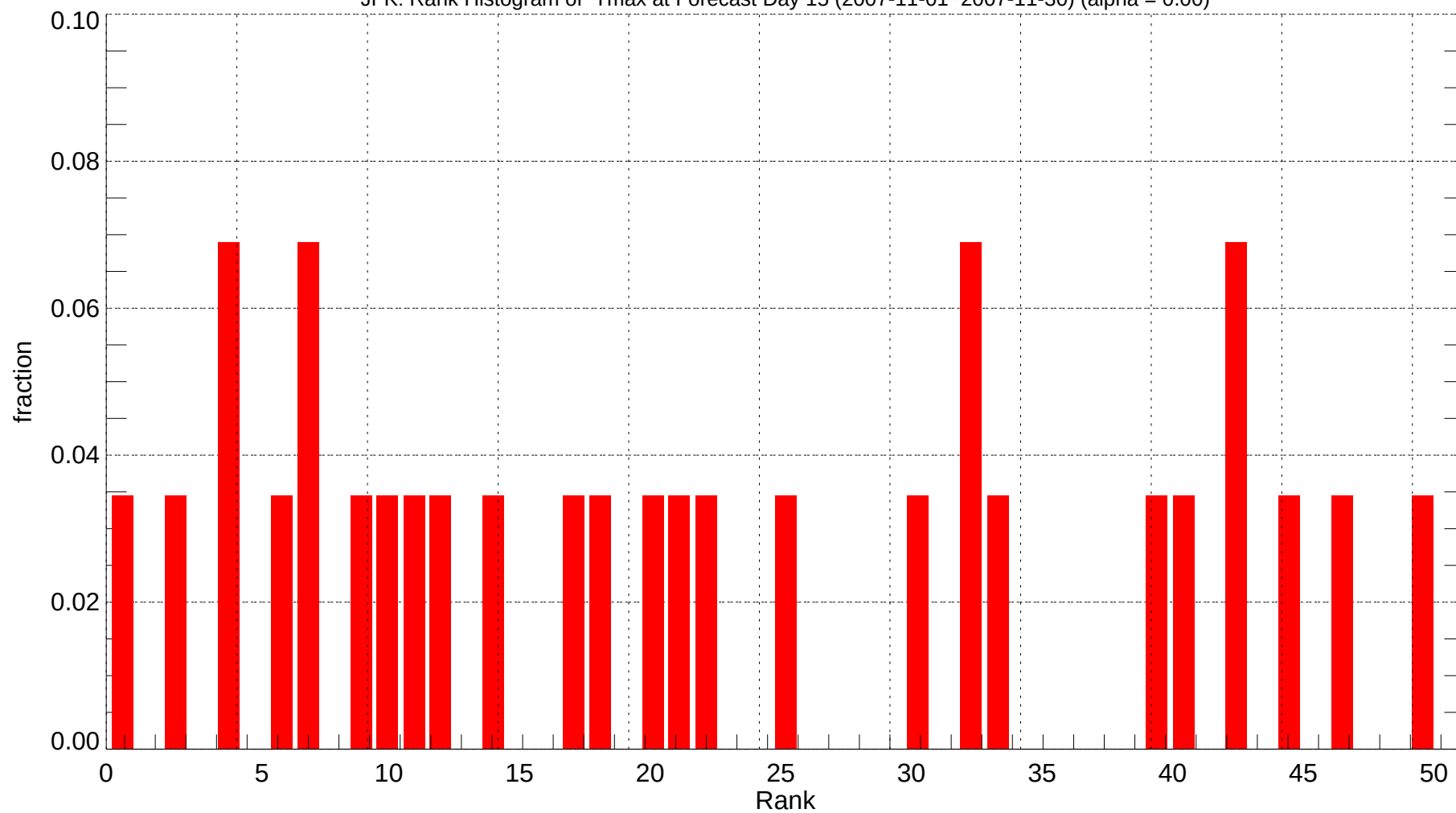
JFK: Rank Histogram of Tmax at Forecast Day 15 (2007-11-01~2007-11-30) (alpha = 0.00)
