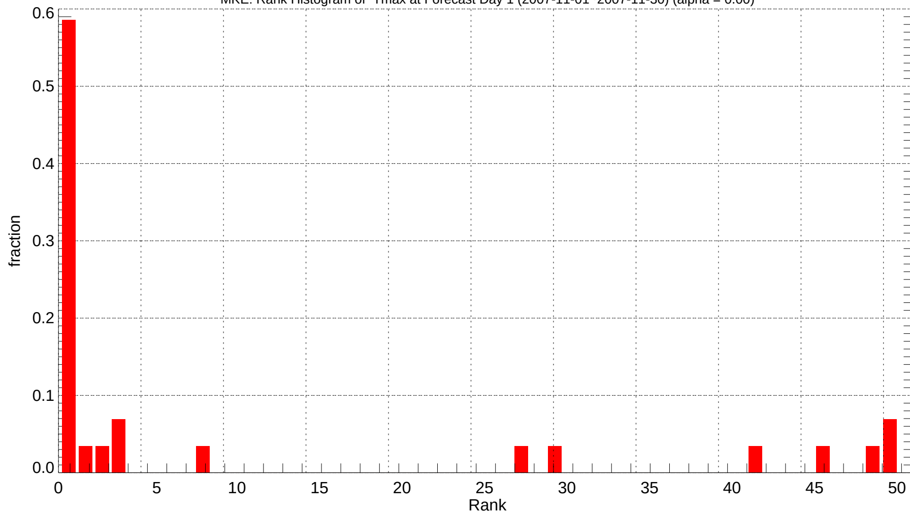
MKE: Rank Histogram of Tmax at Forecast Day 1 (2007-11-01~2007-11-30) (alpha = 0.00)
