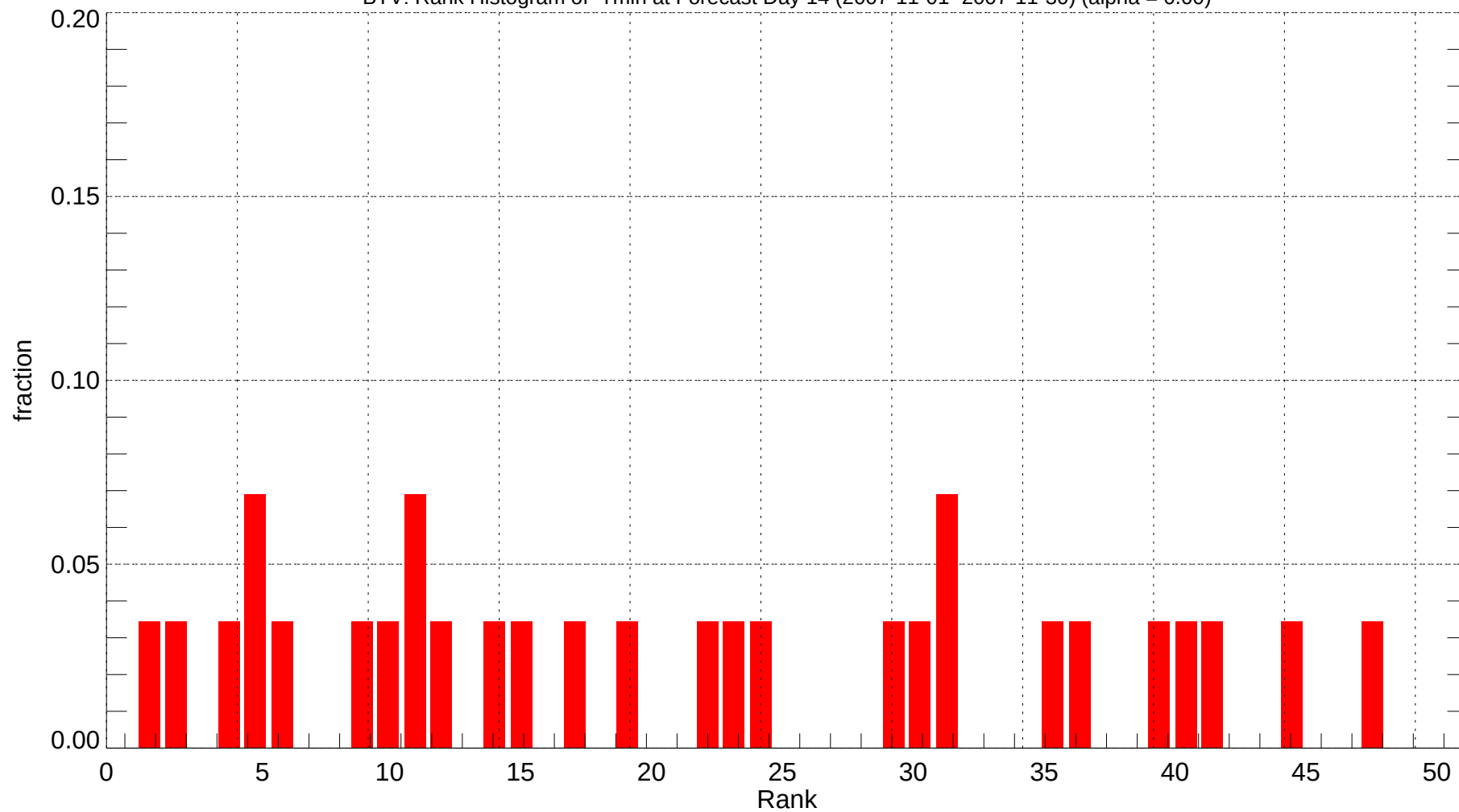
BTV: Rank Histogram of Tmin at Forecast Day 14 (2007-11-01~2007-11-30) (alpha = 0.00)
