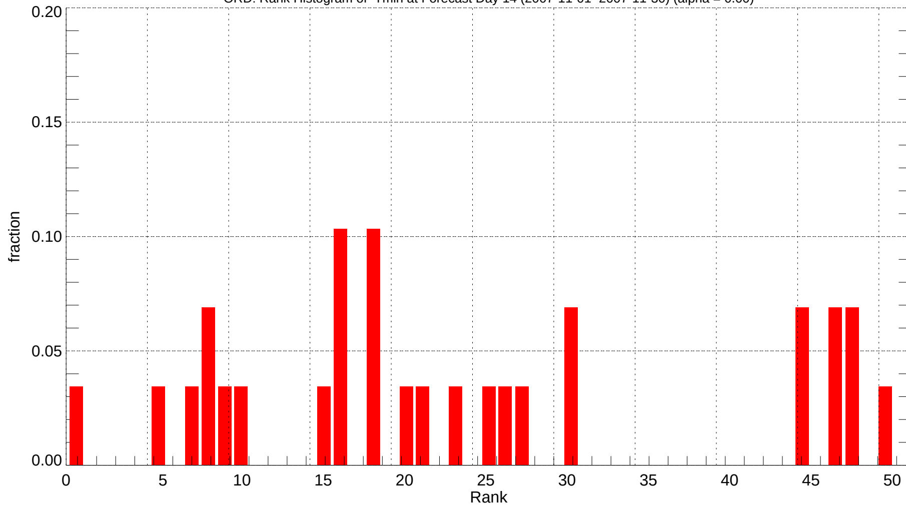
ORD: Rank Histogram of Tmin at Forecast Day 14 (2007-11-01~2007-11-30) (alpha = 0.00)
