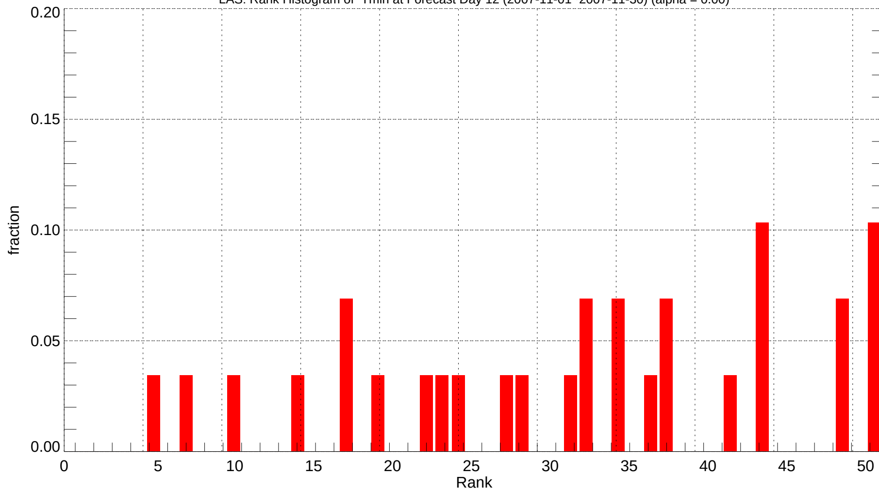
LAS: Rank Histogram of Tmin at Forecast Day 12 (2007-11-01~2007-11-30) (alpha = 0.00)
