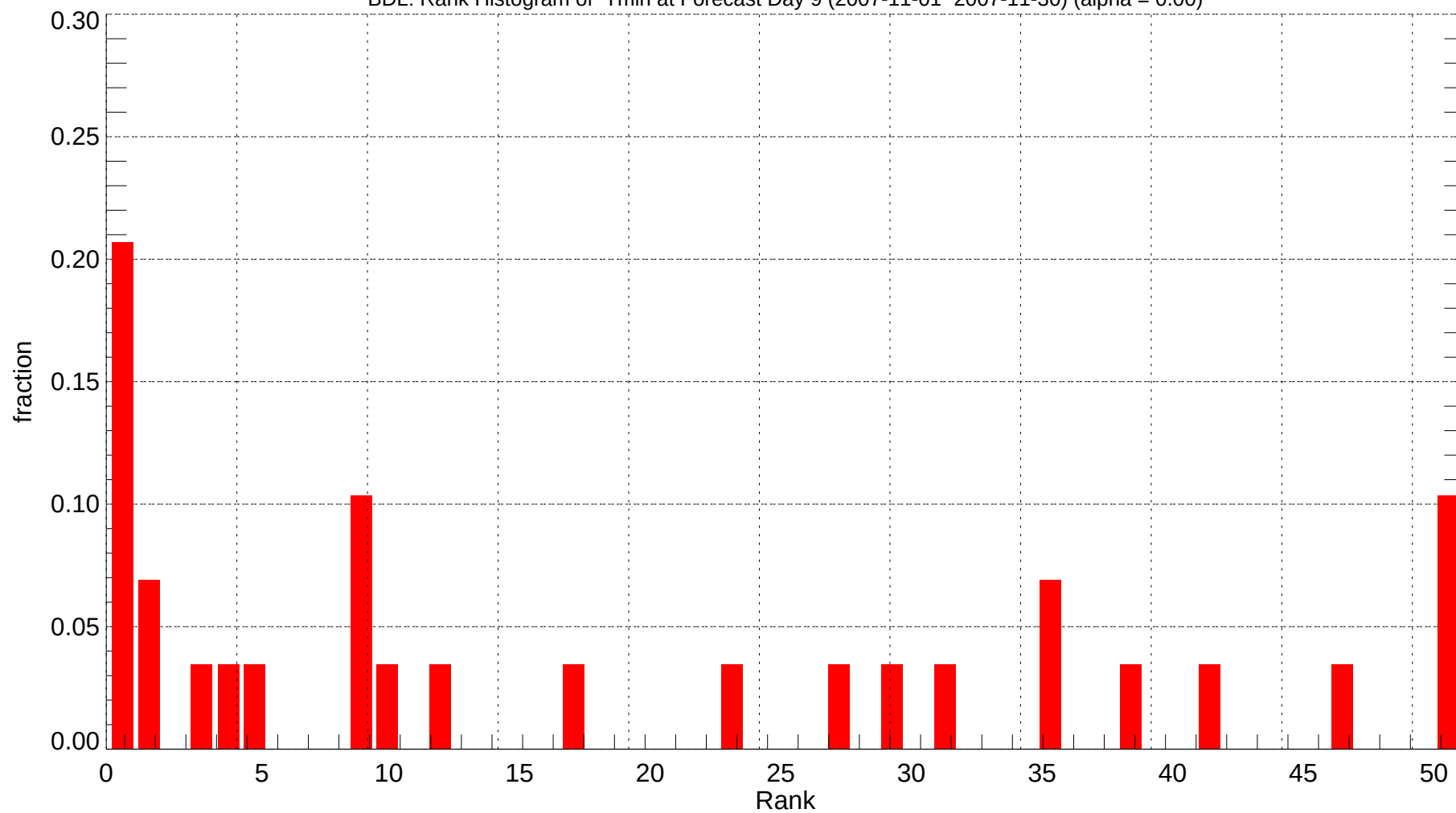
BDL: Rank Histogram of Tmin at Forecast Day 9 (2007-11-01~2007-11-30) (alpha = 0.00)
