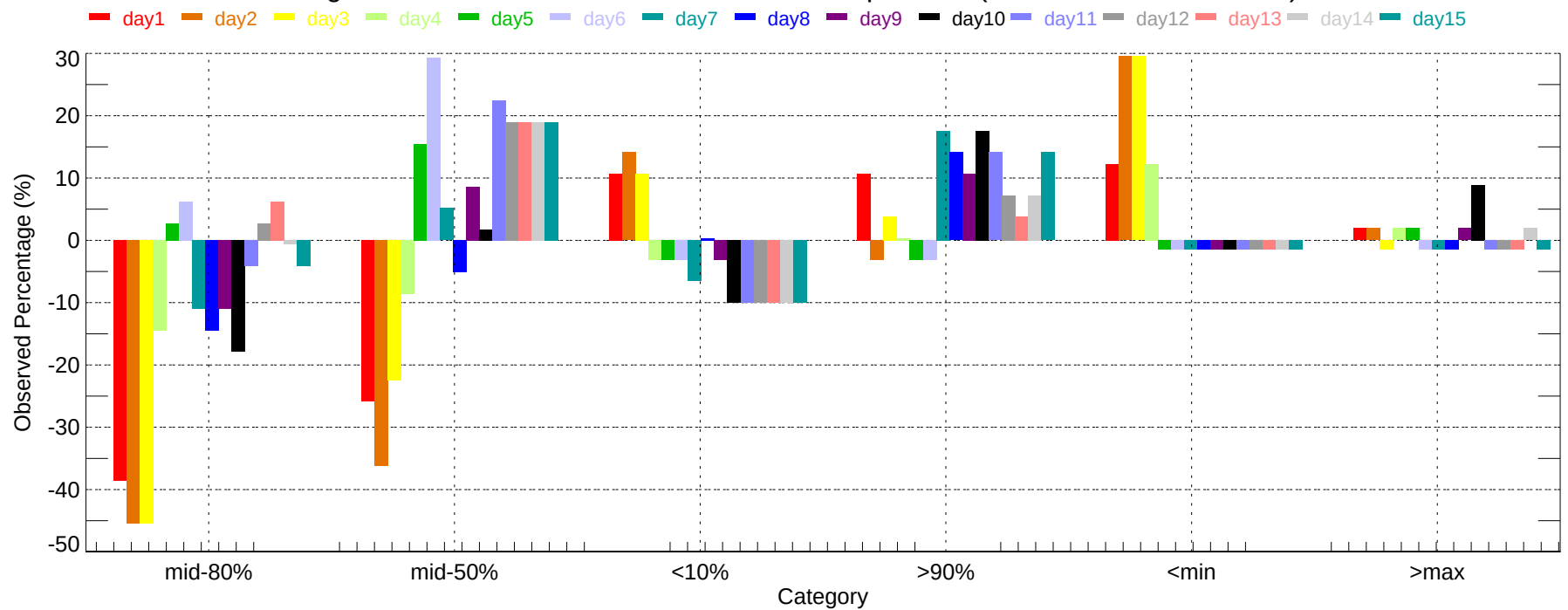
Observed Percentage Deviation of Ensembles - BFL: Max Temperature (2007-11-01~2007-11-30)
