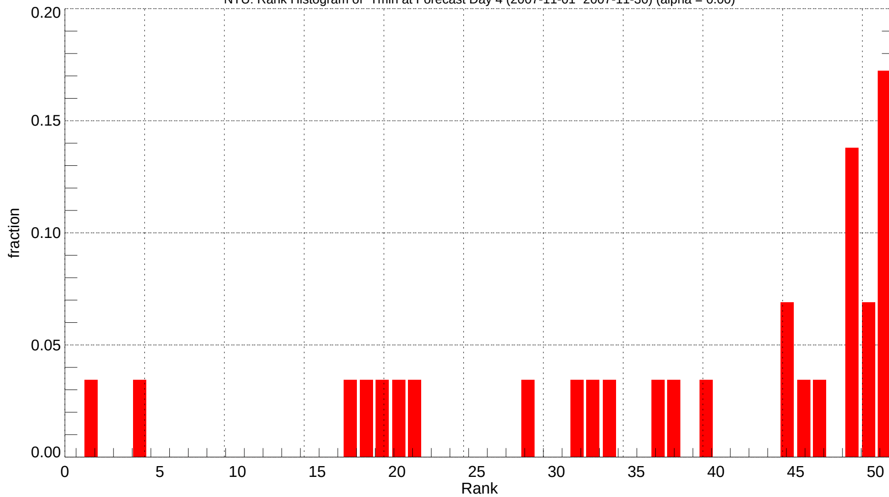
NTU: Rank Histogram of Tmin at Forecast Day 4 (2007-11-01~2007-11-30) (alpha = 0.00)
