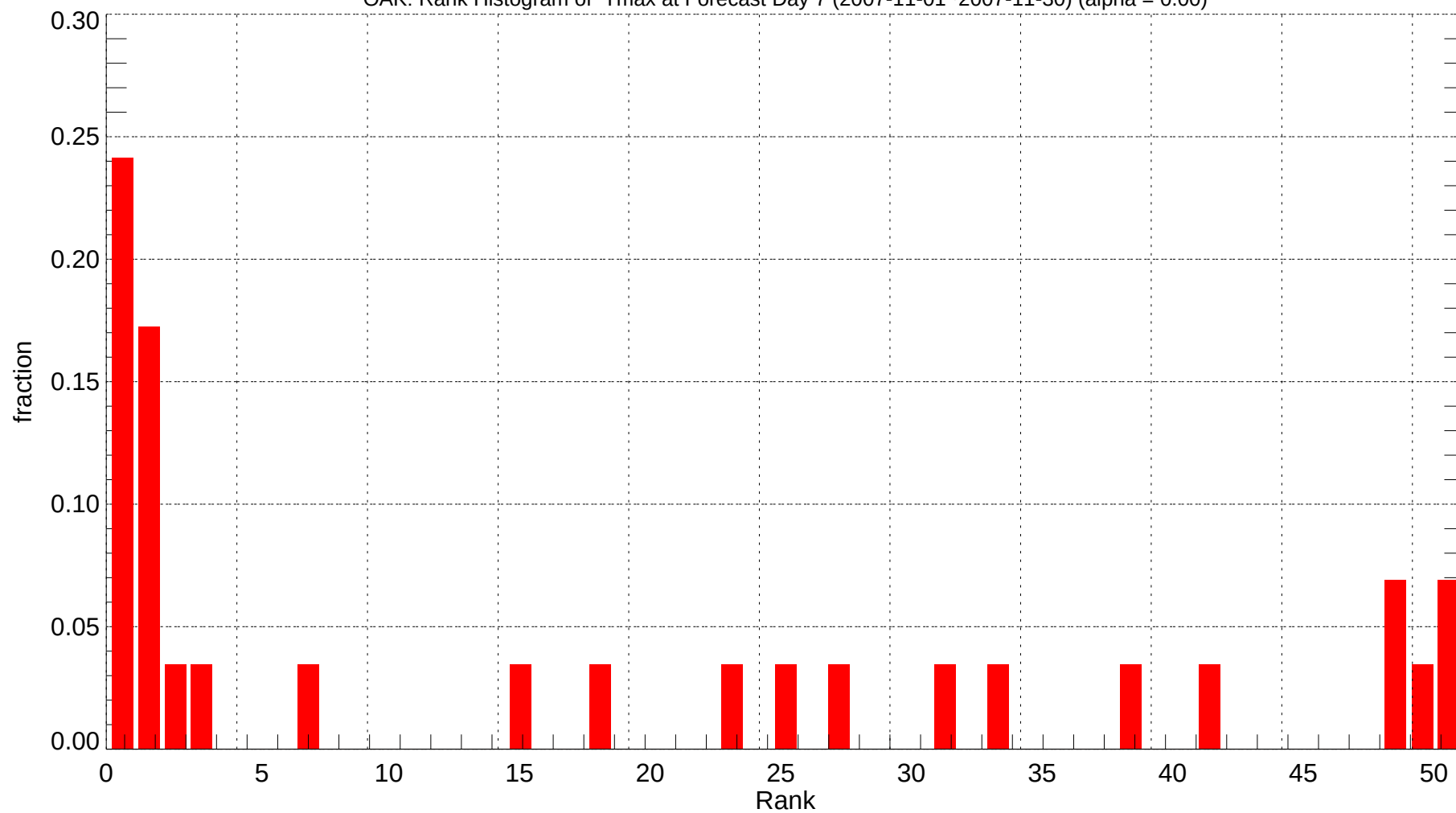
OAK: Rank Histogram of Tmax at Forecast Day 7 (2007-11-01~2007-11-30) (alpha = 0.00)
