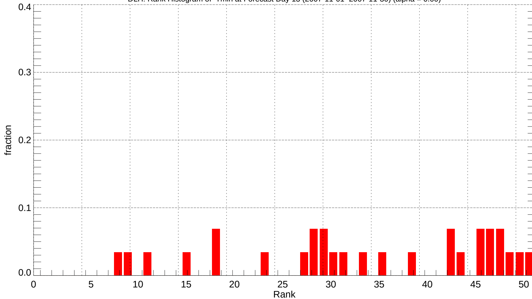
DLH: Rank Histogram of Tmin at Forecast Day 13 (2007-11-01~2007-11-30) (alpha = 0.00)
