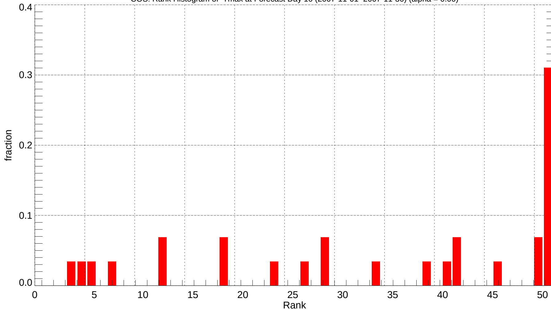
COS: Rank Histogram of Tmax at Forecast Day 10 (2007-11-01~2007-11-30) (alpha = 0.00)
