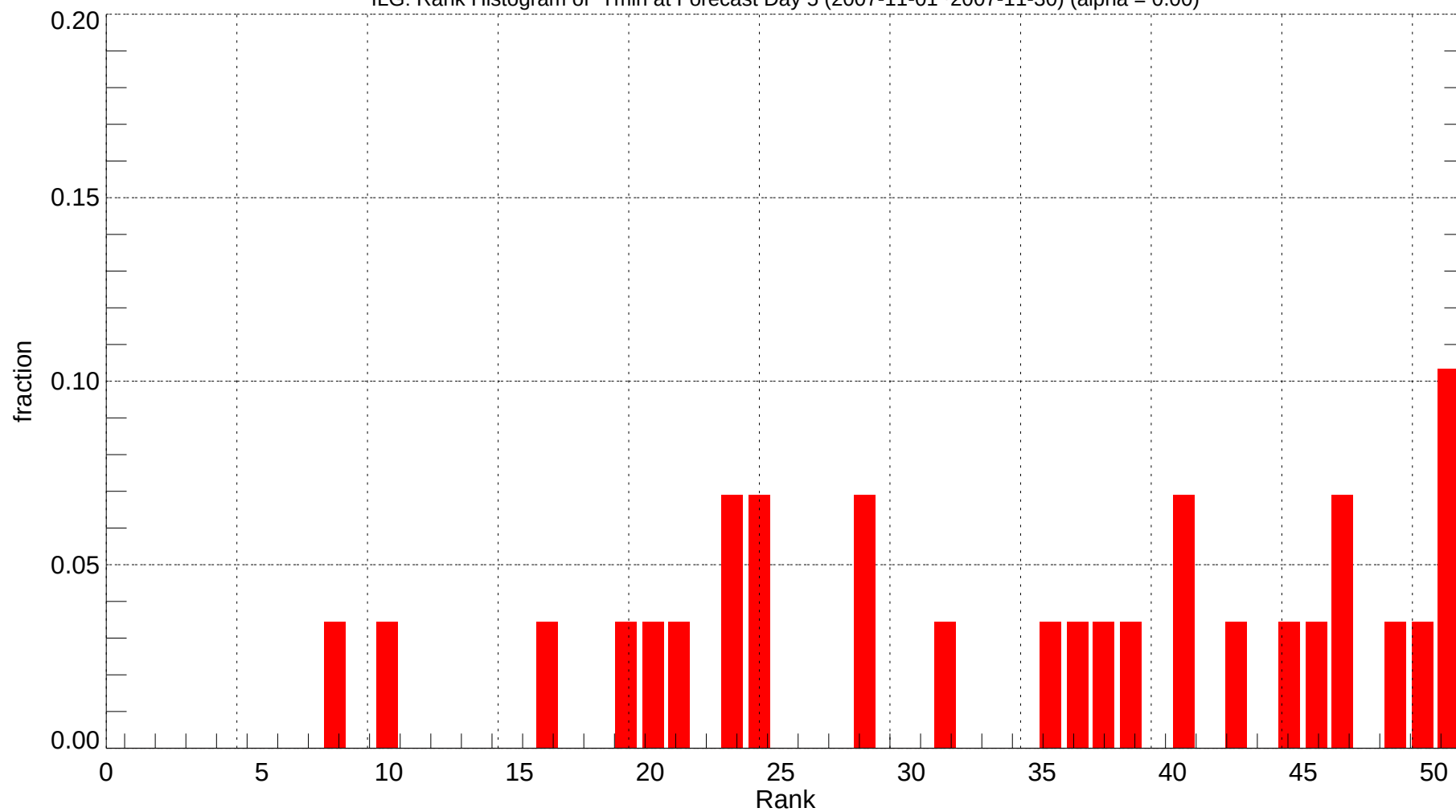
ILG: Rank Histogram of Tmin at Forecast Day 5 (2007-11-01~2007-11-30) (alpha = 0.00)
