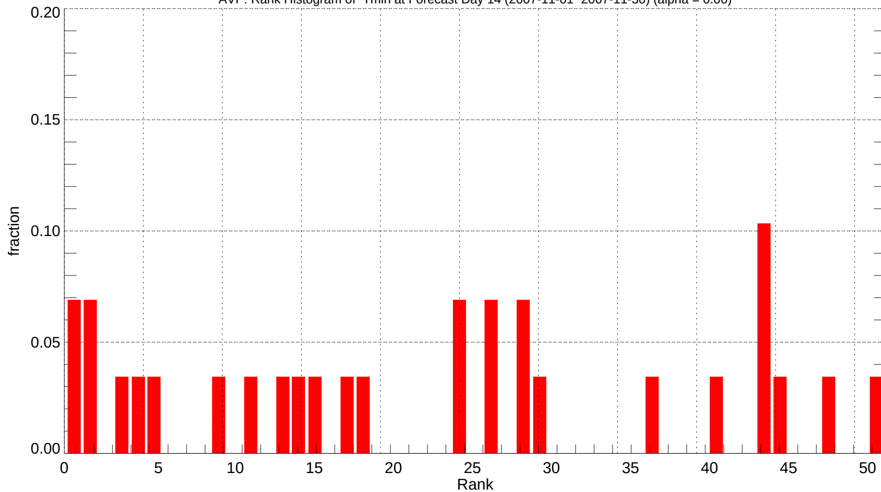
AVP: Rank Histogram of Tmin at Forecast Day 14 (2007-11-01~2007-11-30) (alpha = 0.00)
