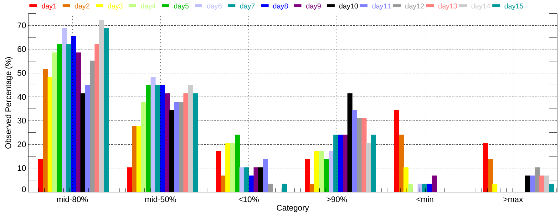
Observed Percentage of Ensembles - PIR: Min Temperature (2007-11-01~2007-11-30)
