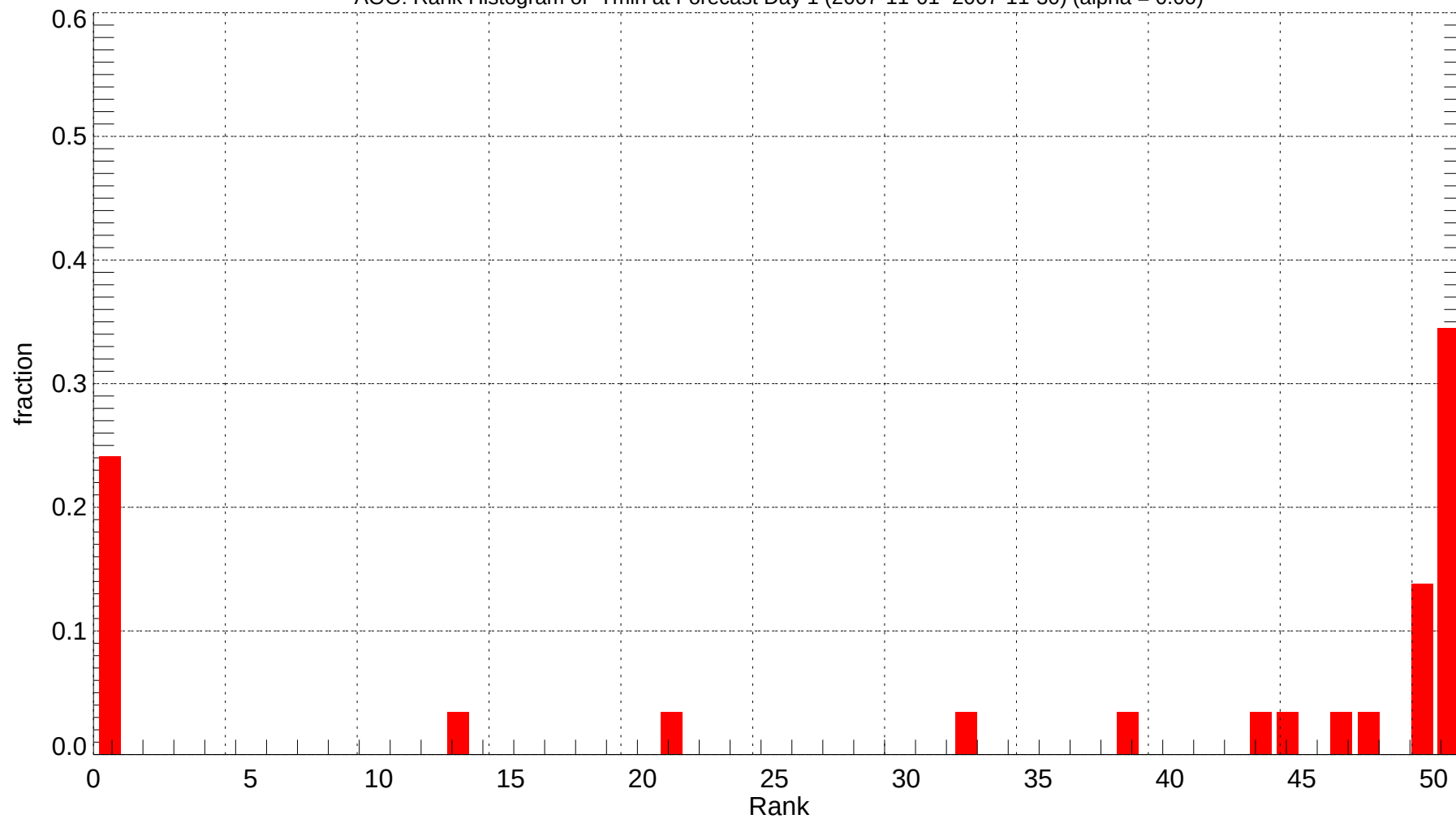
AOO: Rank Histogram of Tmin at Forecast Day 1 (2007-11-01~2007-11-30) (alpha = 0.00)
