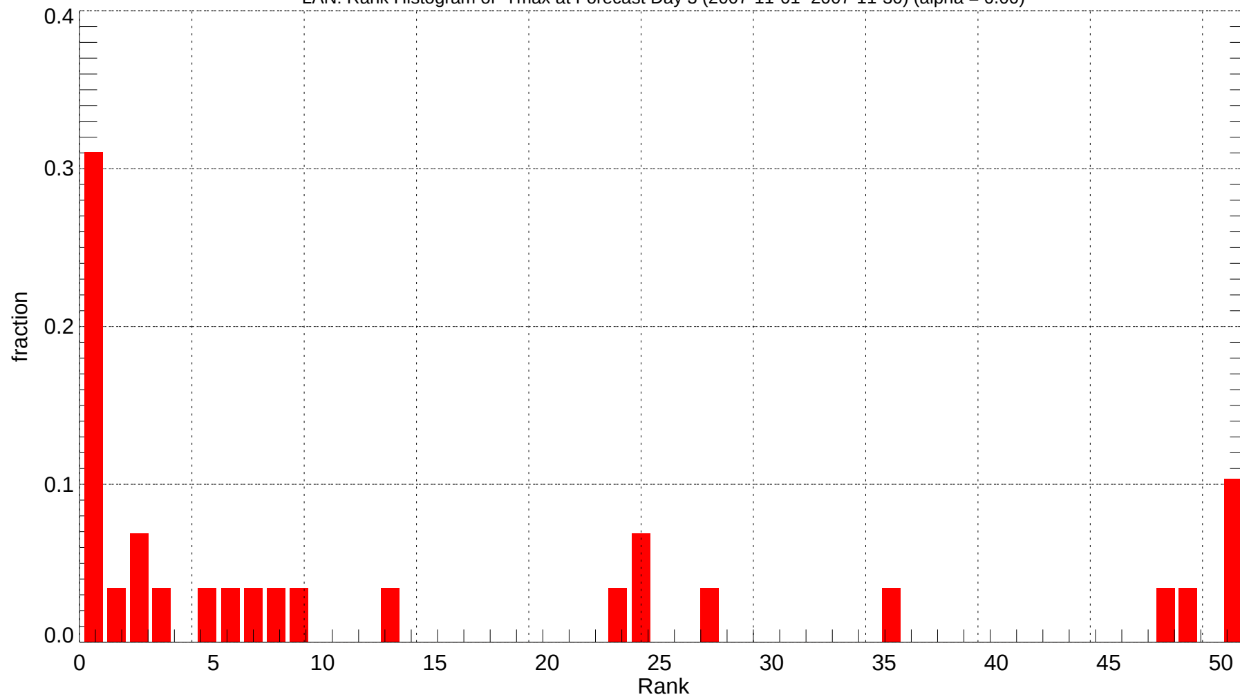
LAN: Rank Histogram of Tmax at Forecast Day 3 (2007-11-01~2007-11-30) (alpha = 0.00)
