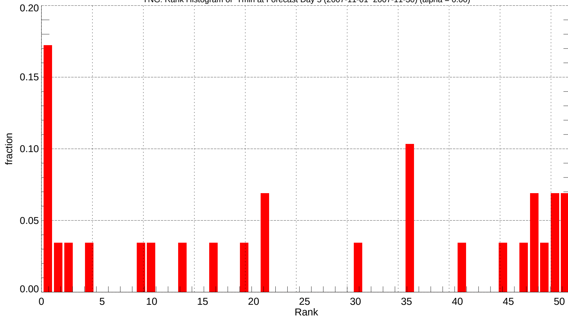
YNG: Rank Histogram of Tmin at Forecast Day 5 (2007-11-01~2007-11-30) (alpha = 0.00)
