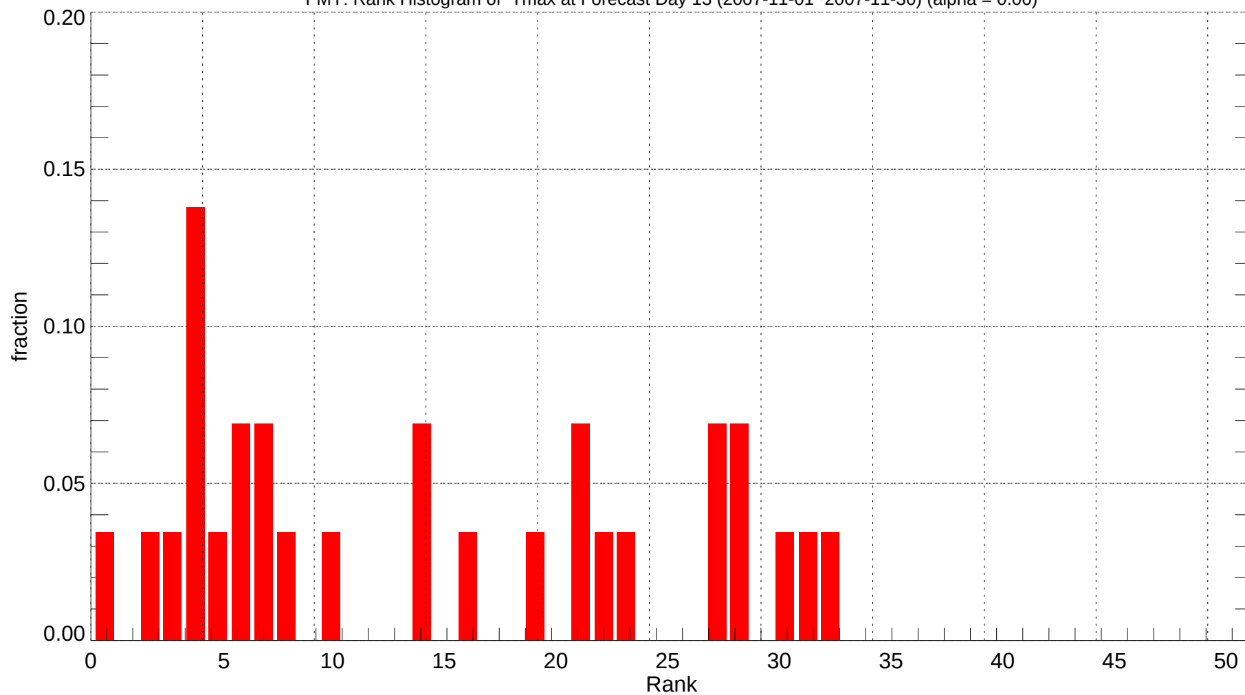
FMY: Rank Histogram of Tmax at Forecast Day 13 (2007-11-01~2007-11-30) (alpha = 0.00)
