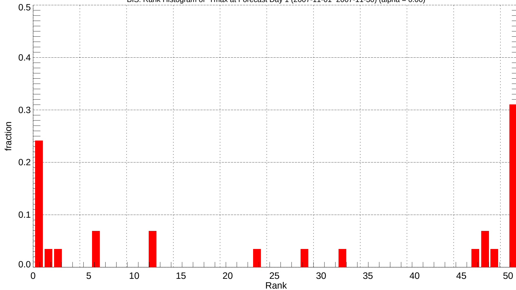
BIS: Rank Histogram of Tmax at Forecast Day 1 (2007-11-01~2007-11-30) (alpha = 0.00)
