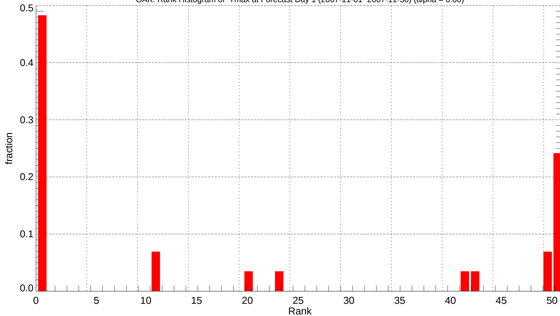
OAK: Rank Histogram of Tmax at Forecast Day 1 (2007-11-01~2007-11-30) (alpha = 0.00)
