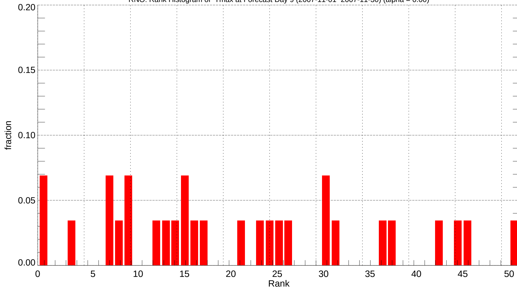
RNO: Rank Histogram of Tmax at Forecast Day 9 (2007-11-01~2007-11-30) (alpha = 0.00)
