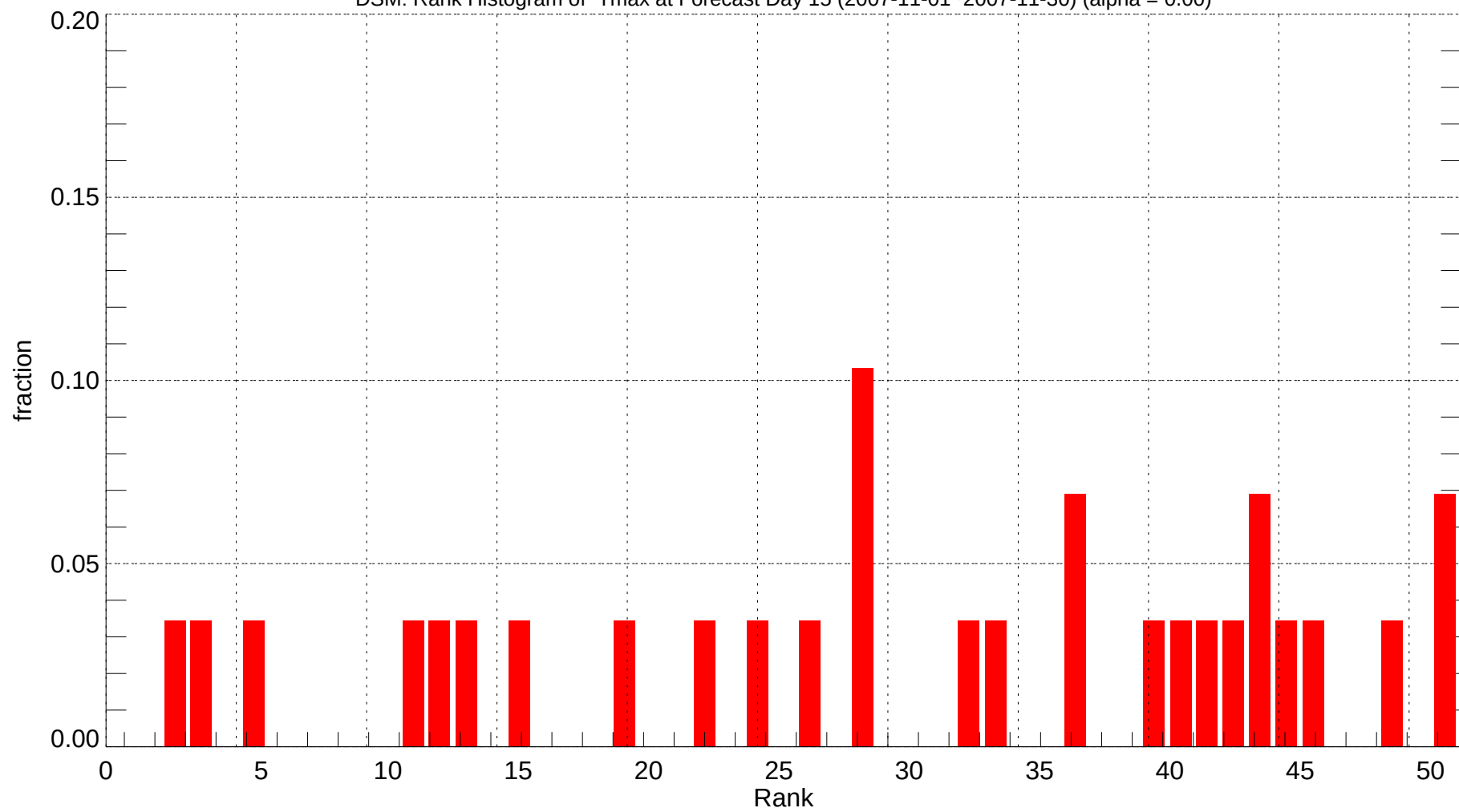
DSM: Rank Histogram of Tmax at Forecast Day 15 (2007-11-01~2007-11-30) (alpha = 0.00)
