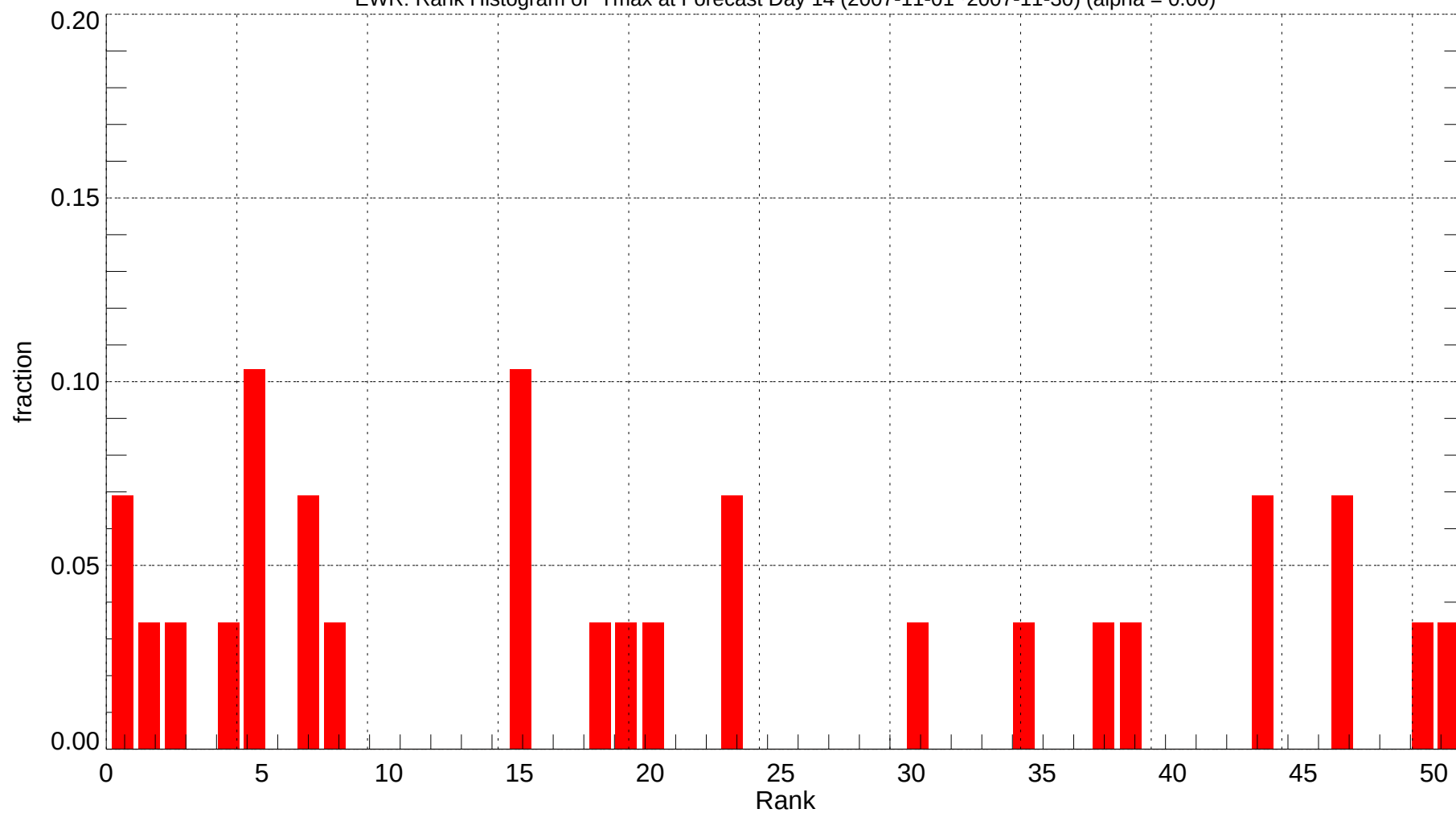
EWR: Rank Histogram of Tmax at Forecast Day 14 (2007-11-01~2007-11-30) (alpha = 0.00)
