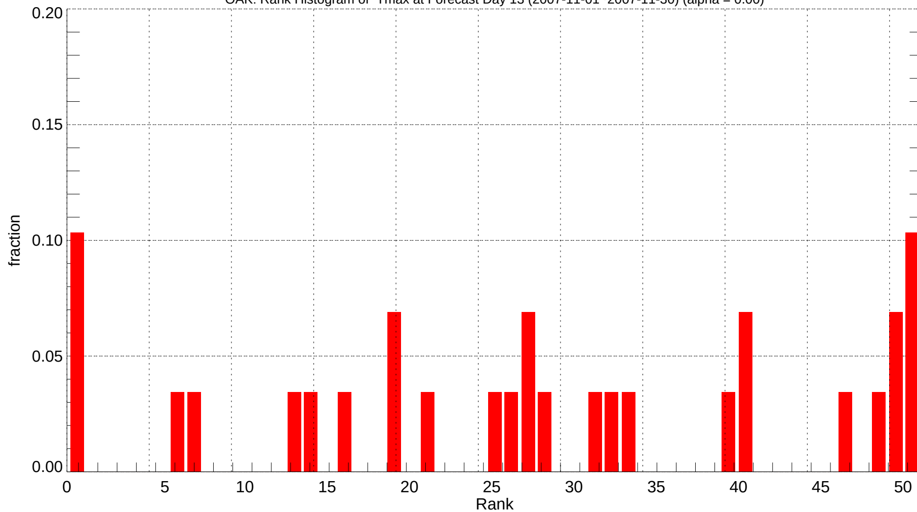
OAK: Rank Histogram of Tmax at Forecast Day 13 (2007-11-01~2007-11-30) (alpha = 0.00)
