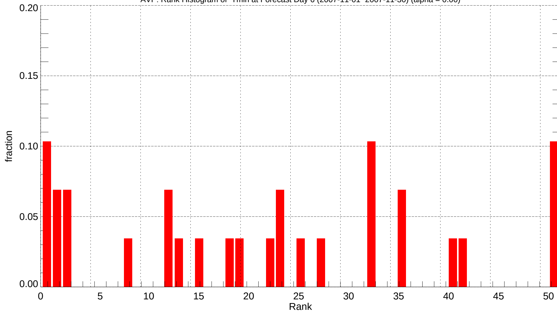
AVP: Rank Histogram of Tmin at Forecast Day 6 (2007-11-01~2007-11-30) (alpha = 0.00)
