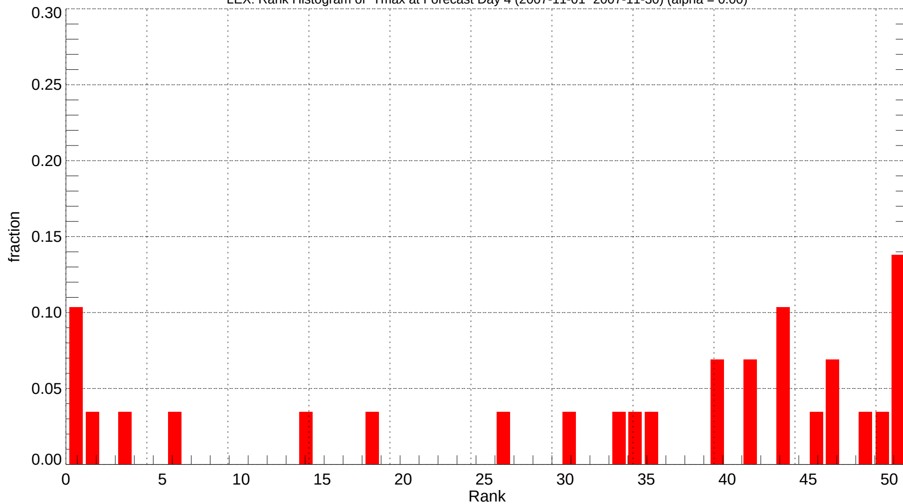
LEX: Rank Histogram of Tmax at Forecast Day 4 (2007-11-01~2007-11-30) (alpha = 0.00)
