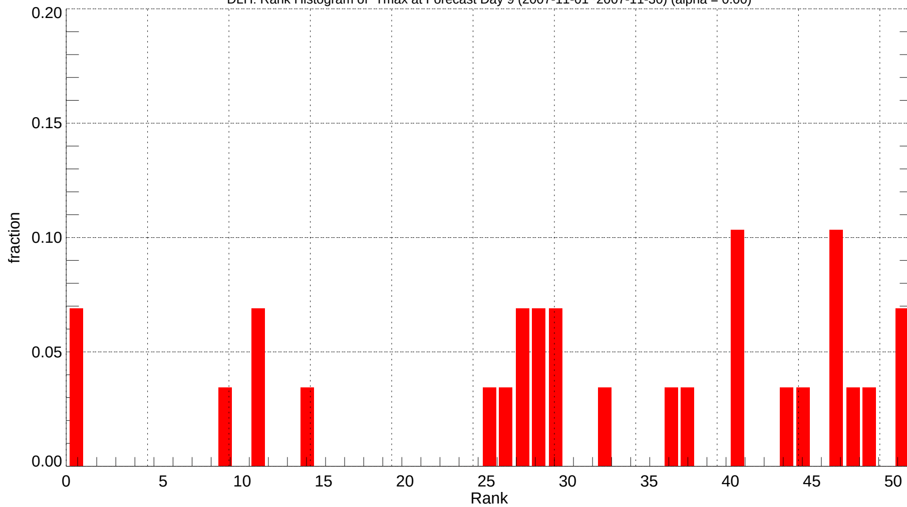
DLH: Rank Histogram of Tmax at Forecast Day 9 (2007-11-01~2007-11-30) (alpha = 0.00)
