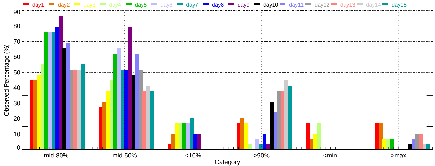
Observed Percentage of Ensembles - WJF: Min Temperature (2007-11-01~2007-11-30)
