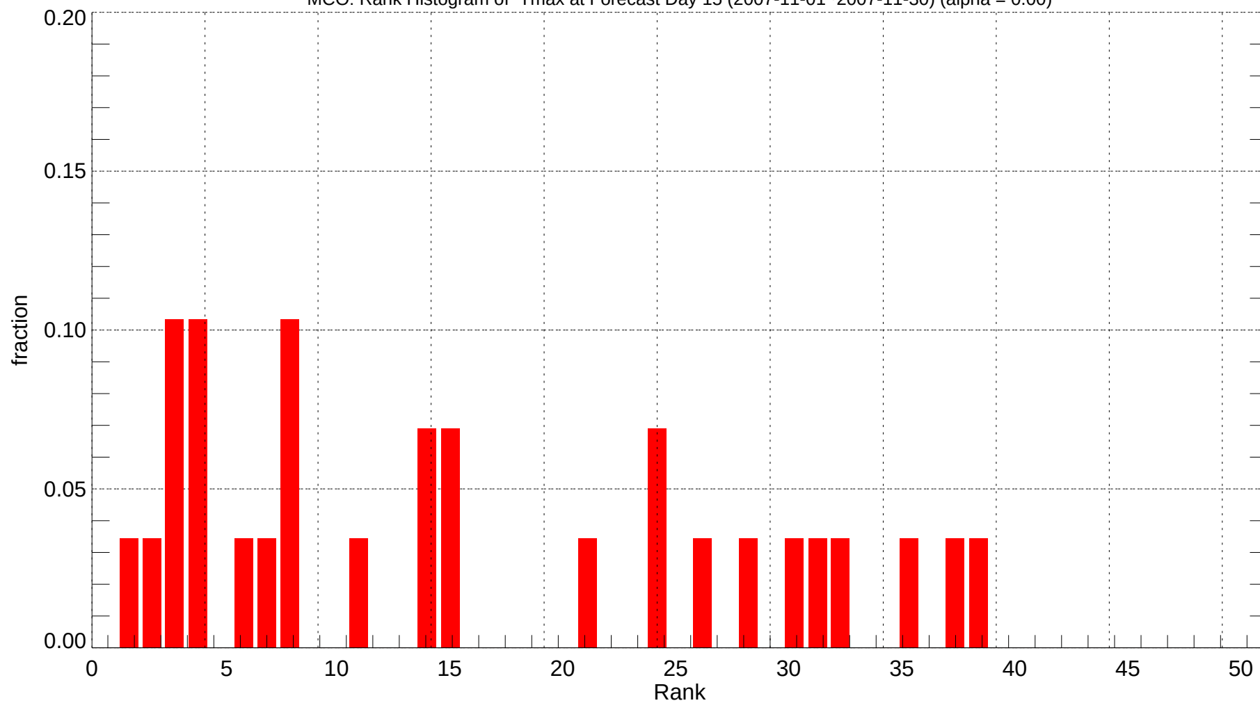
MCO: Rank Histogram of Tmax at Forecast Day 15 (2007-11-01~2007-11-30) (alpha = 0.00)
