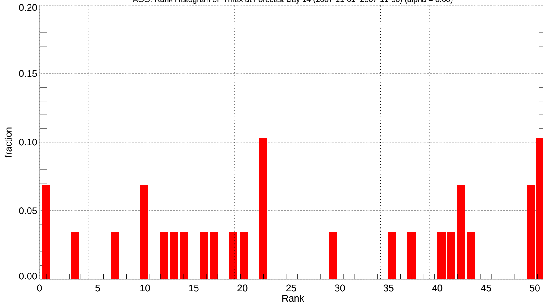
AOO: Rank Histogram of Tmax at Forecast Day 14 (2007-11-01~2007-11-30) (alpha = 0.00)
