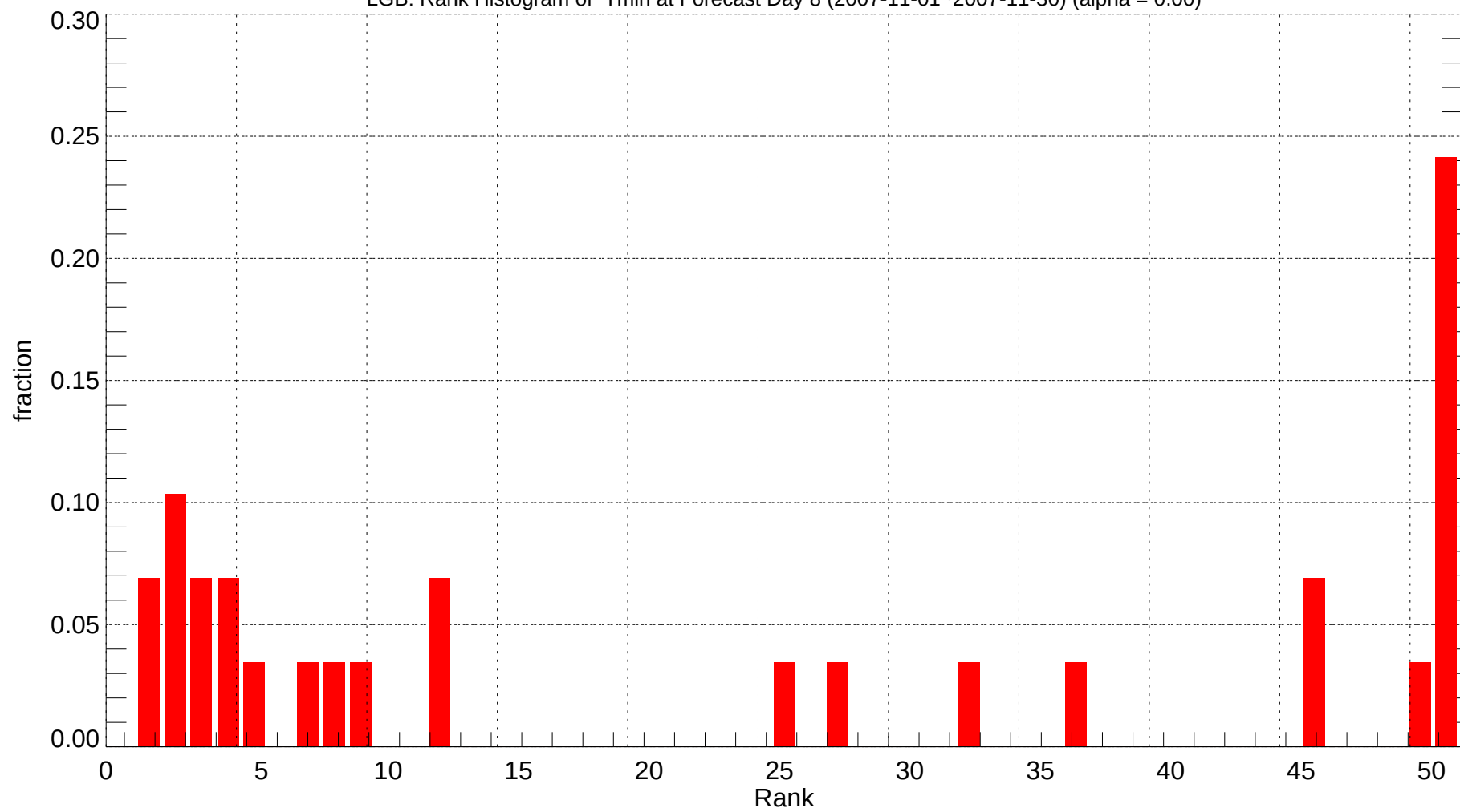
LGB: Rank Histogram of Tmin at Forecast Day 8 (2007-11-01~2007-11-30) (alpha = 0.00)
