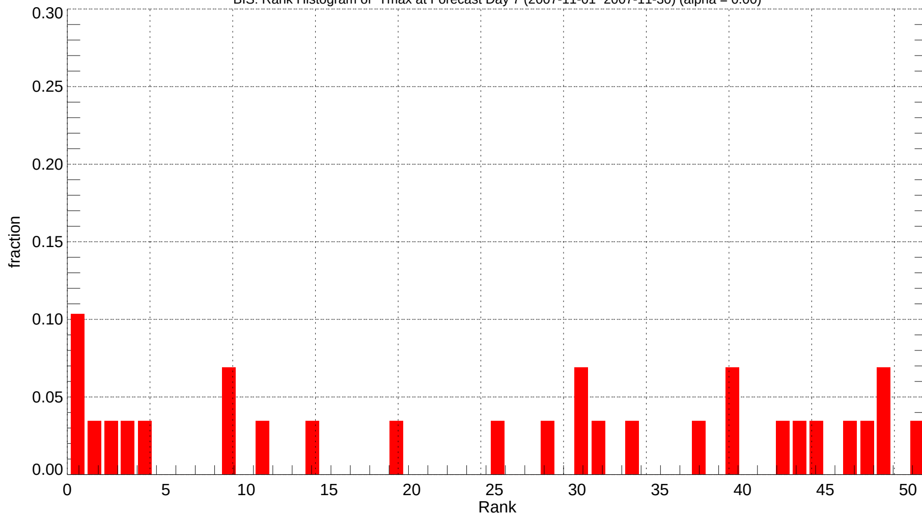
BIS: Rank Histogram of Tmax at Forecast Day 7 (2007-11-01~2007-11-30) (alpha = 0.00)
