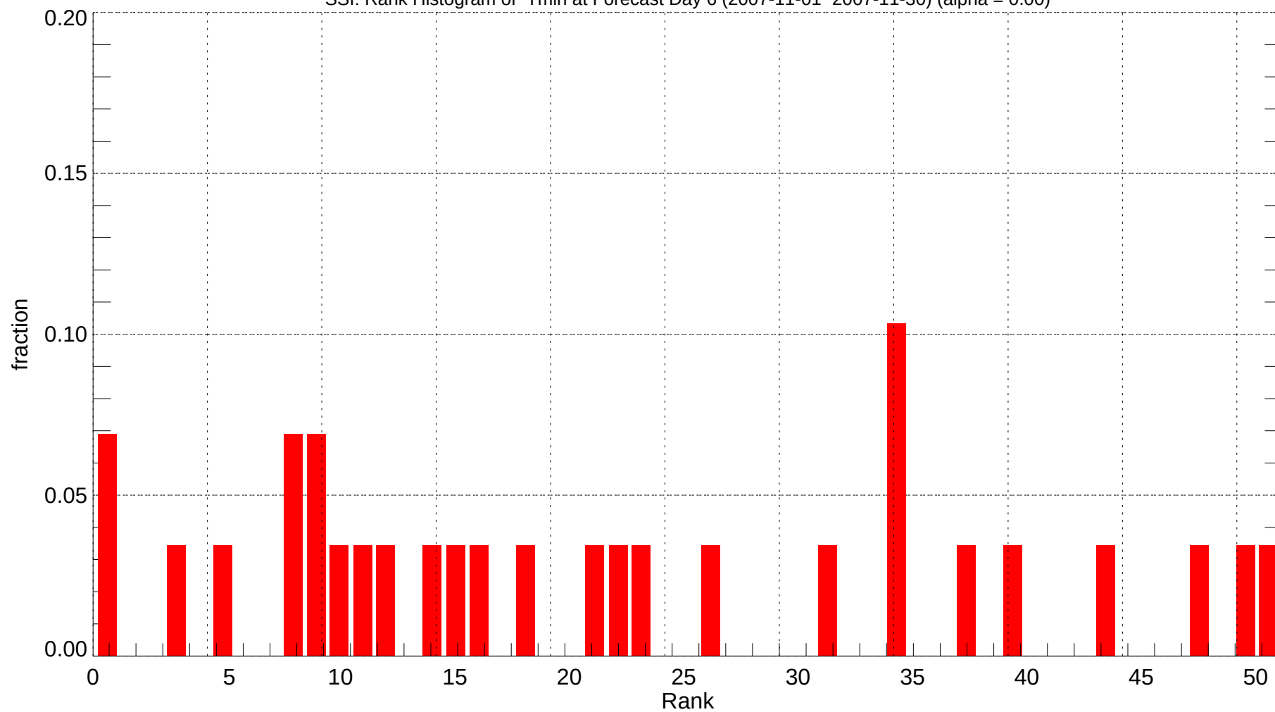
SSI: Rank Histogram of Tmin at Forecast Day 6 (2007-11-01~2007-11-30) (alpha = 0.00)
