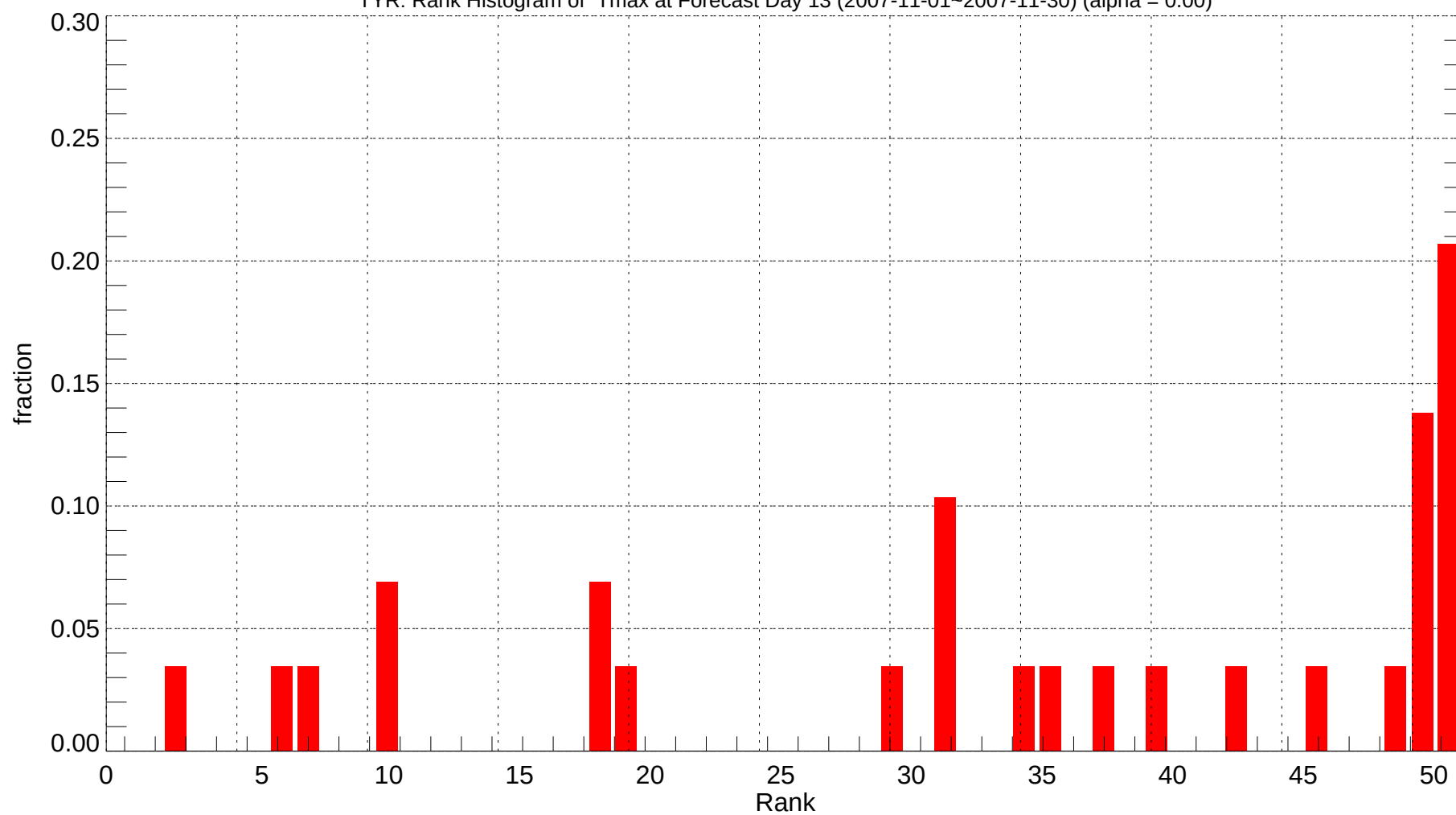
TYR: Rank Histogram of Tmax at Forecast Day 13 (2007-11-01~2007-11-30) (alpha = 0.00)
