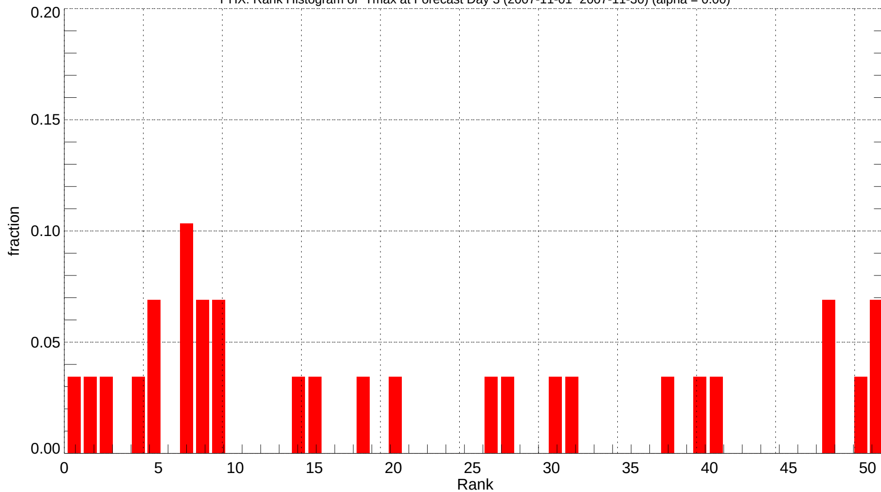
PHX: Rank Histogram of Tmax at Forecast Day 3 (2007-11-01~2007-11-30) (alpha = 0.00)
