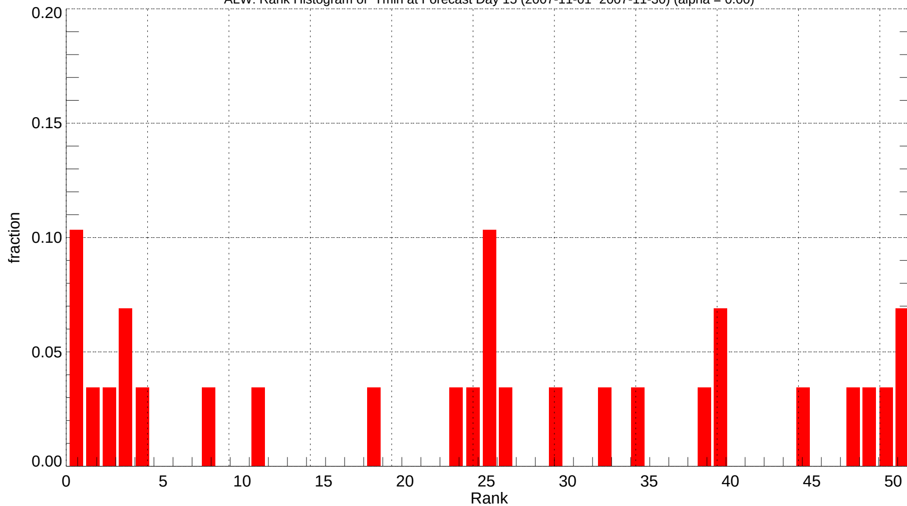
ALW: Rank Histogram of Tmin at Forecast Day 15 (2007-11-01~2007-11-30) (alpha = 0.00)
