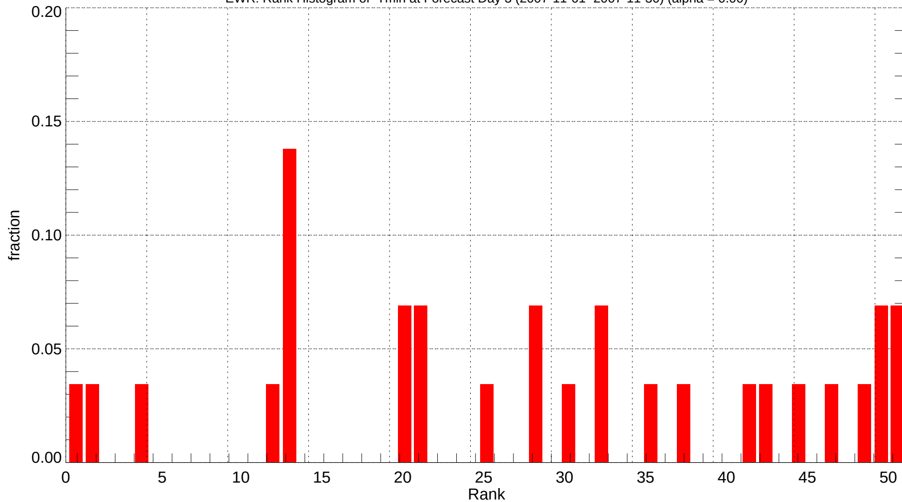
EWR: Rank Histogram of Tmin at Forecast Day 3 (2007-11-01~2007-11-30) (alpha = 0.00)
