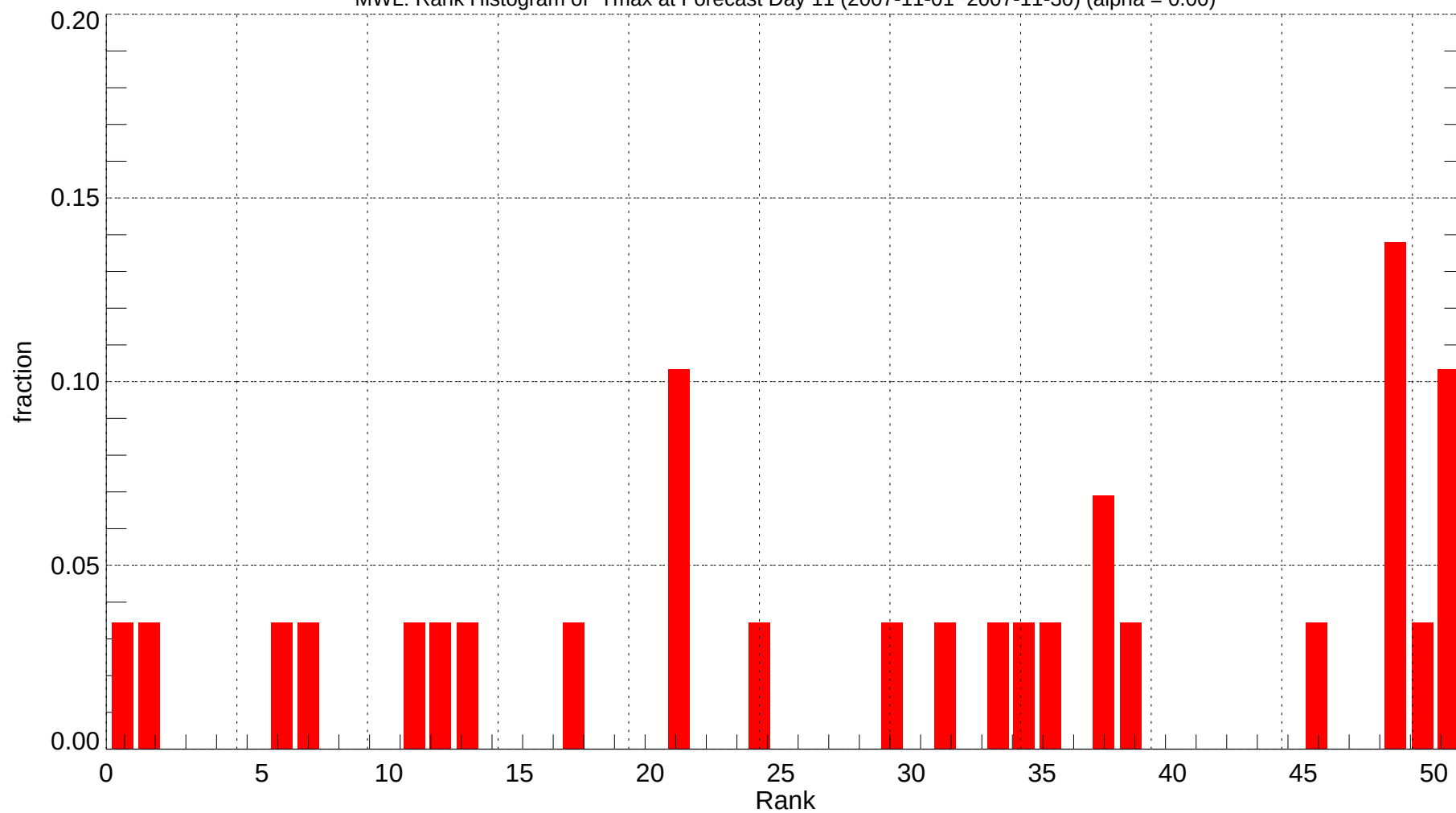
MWL: Rank Histogram of Tmax at Forecast Day 11 (2007-11-01~2007-11-30) (alpha = 0.00)
