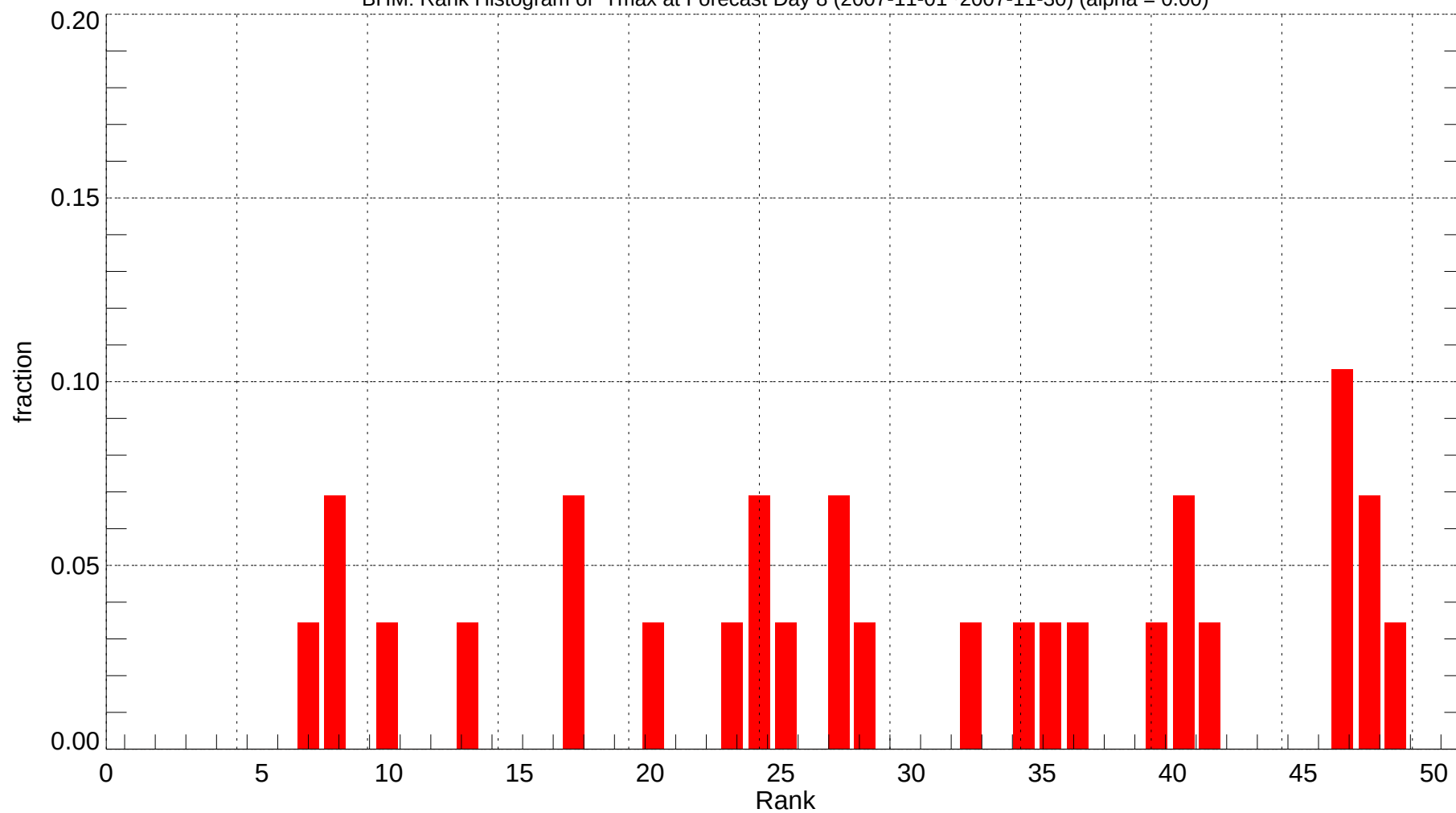
BHM: Rank Histogram of Tmax at Forecast Day 8 (2007-11-01~2007-11-30) (alpha = 0.00)
