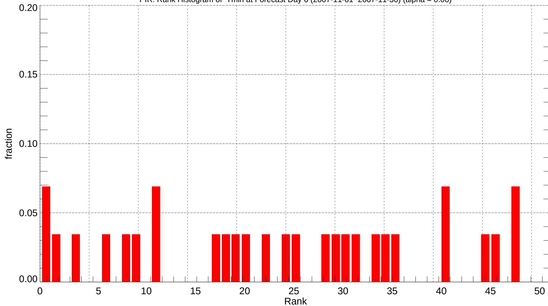
PIR: Rank Histogram of Tmin at Forecast Day 6 (2007-11-01~2007-11-30) (alpha = 0.00)
