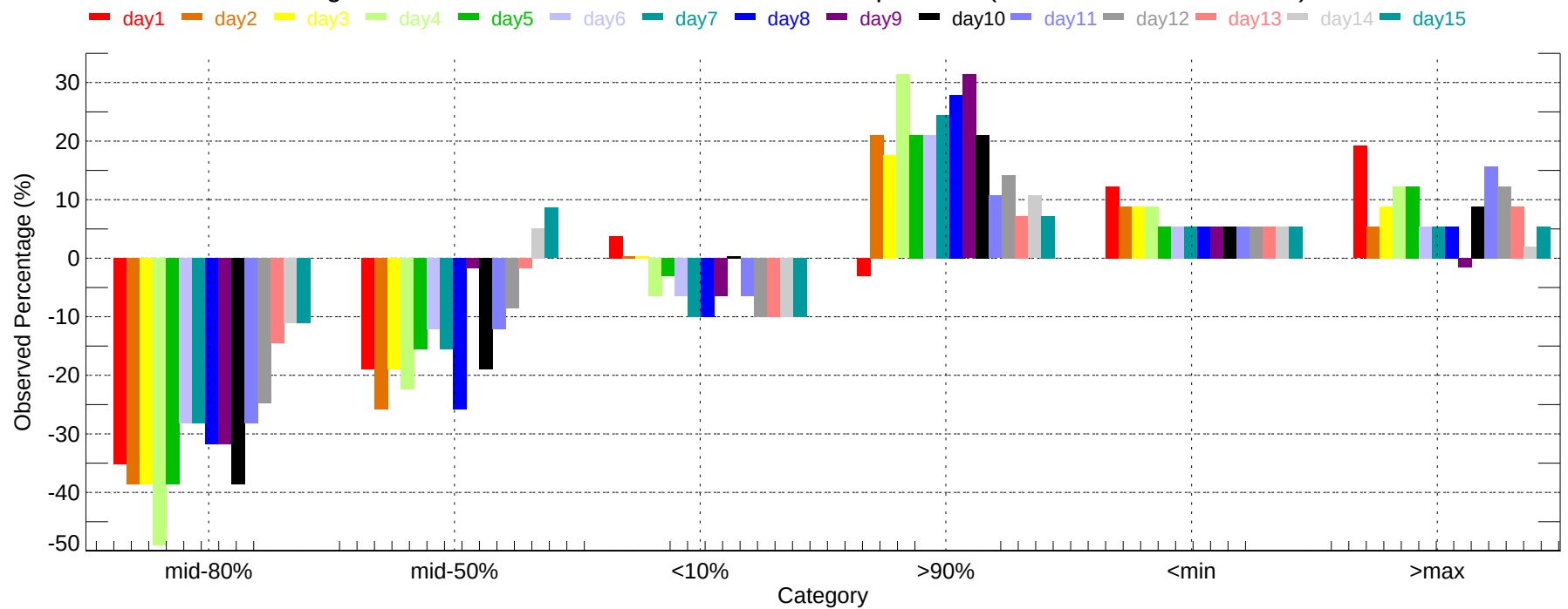
Observed Percentage Deviation of Ensembles - MSY: Max Temperature (2007-11-01~2007-11-30)
