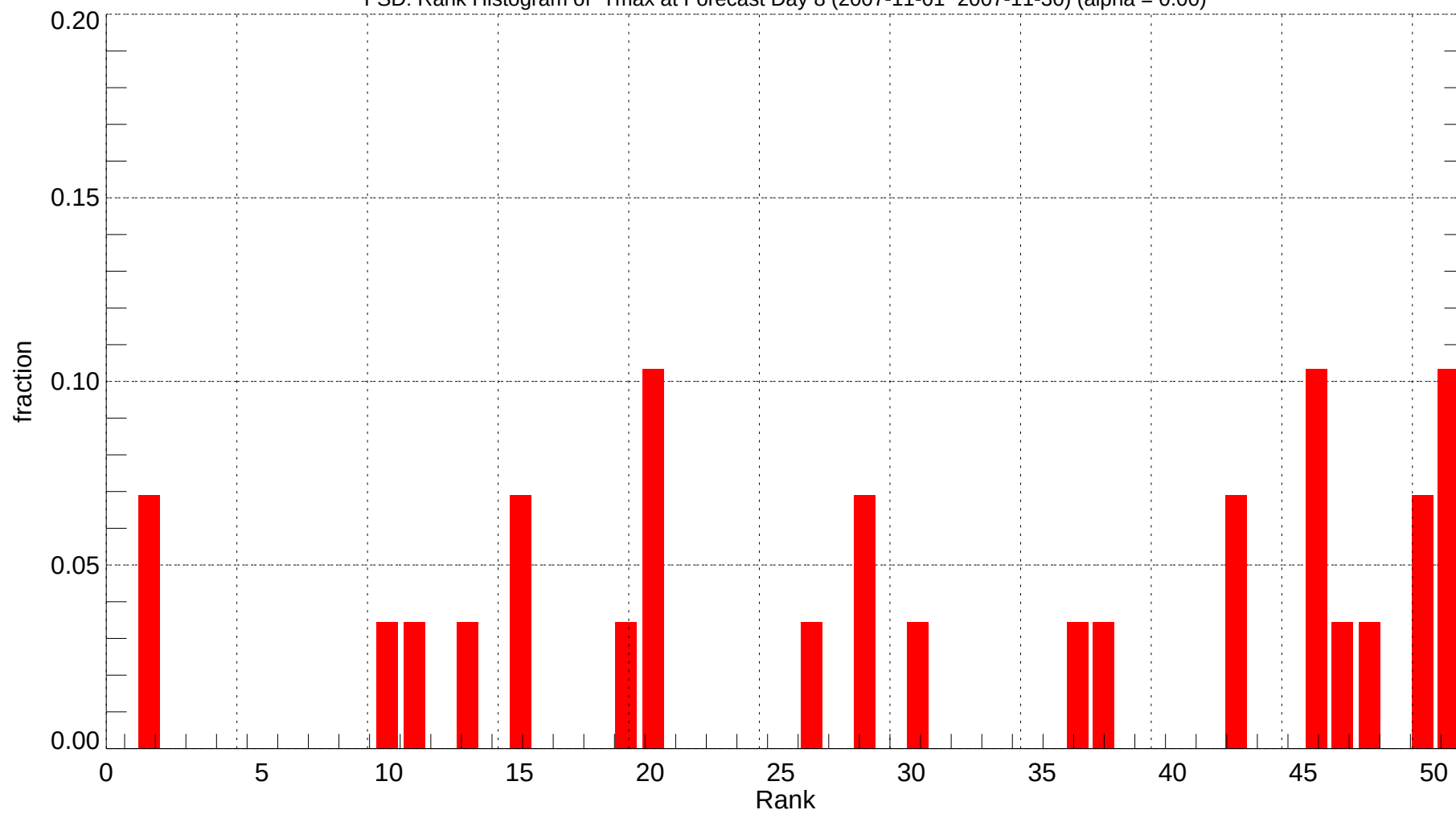
FSD: Rank Histogram of Tmax at Forecast Day 8 (2007-11-01~2007-11-30) (alpha = 0.00)
