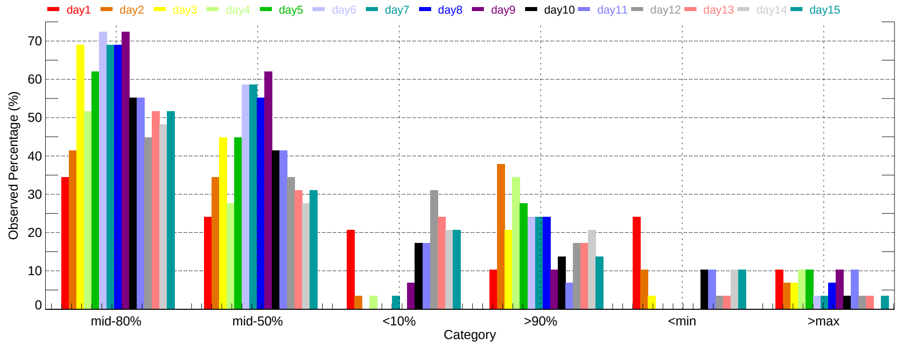
Observed Percentage of Ensembles - ILG: Min Temperature (2007-11-01~2007-11-30)
