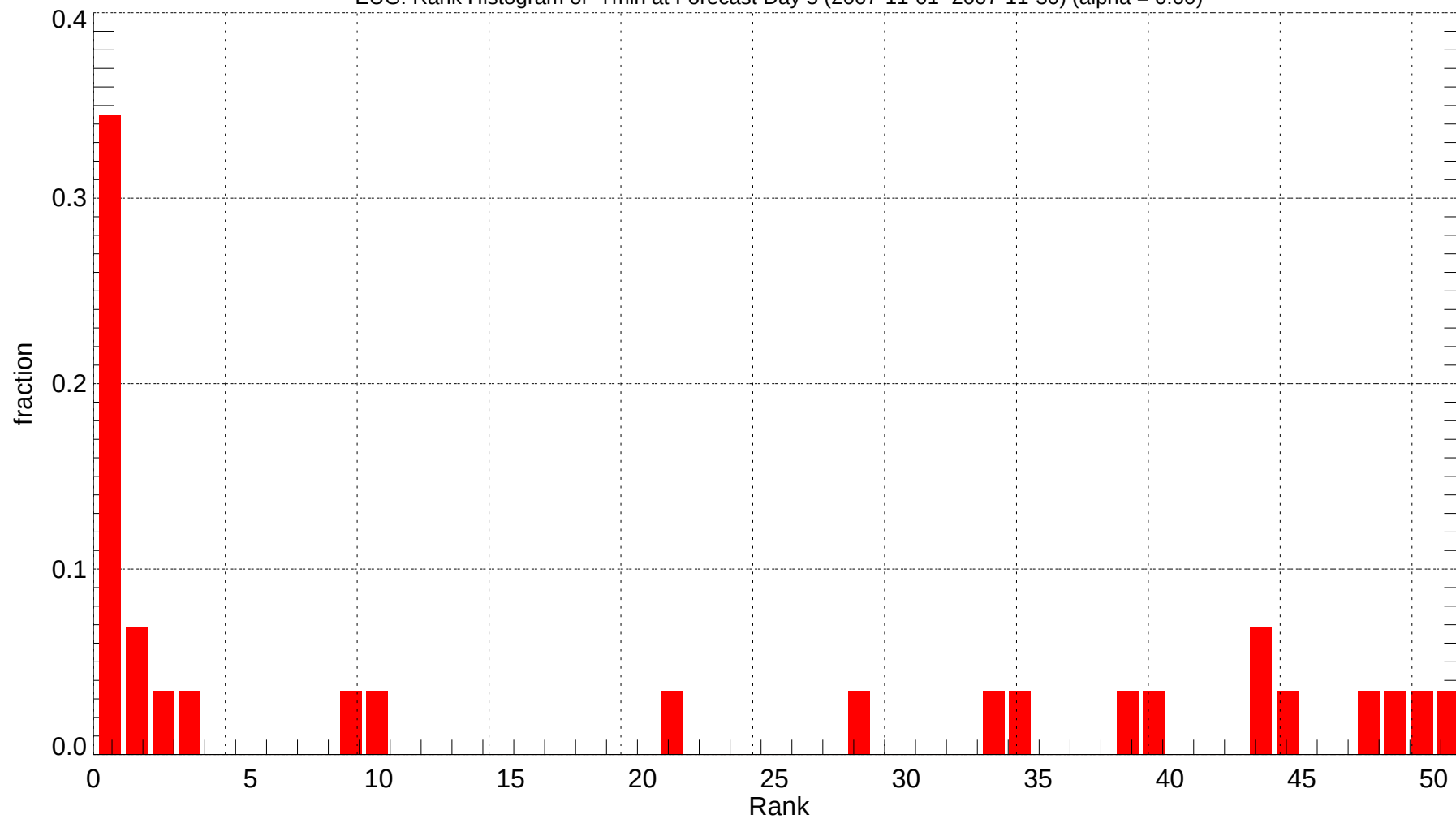
EUG: Rank Histogram of Tmin at Forecast Day 5 (2007-11-01~2007-11-30) (alpha = 0.00)
