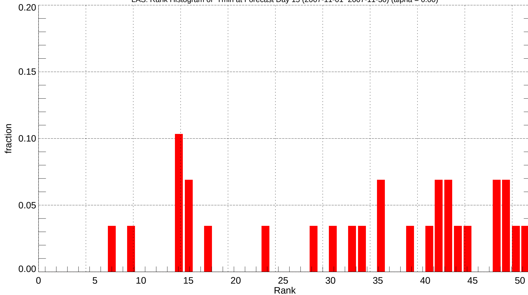
LAS: Rank Histogram of Tmin at Forecast Day 15 (2007-11-01~2007-11-30) (alpha = 0.00)
