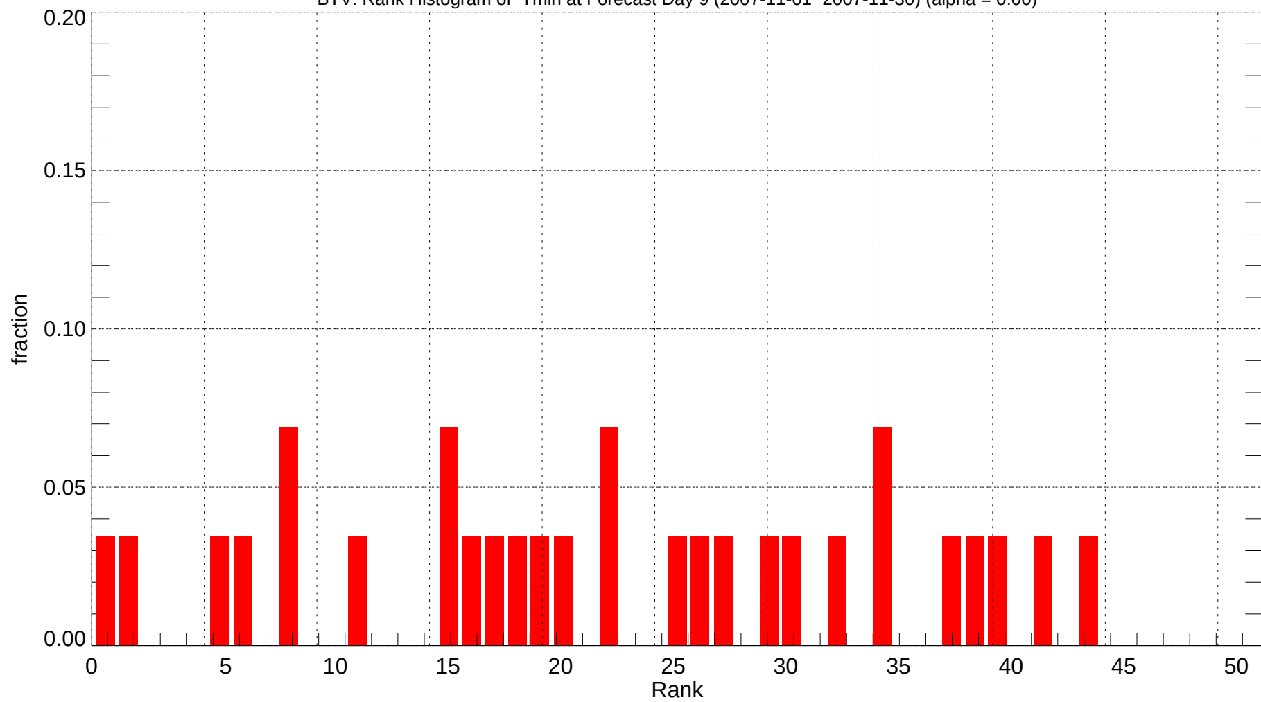
BTV: Rank Histogram of Tmin at Forecast Day 9 (2007-11-01~2007-11-30) (alpha = 0.00)
