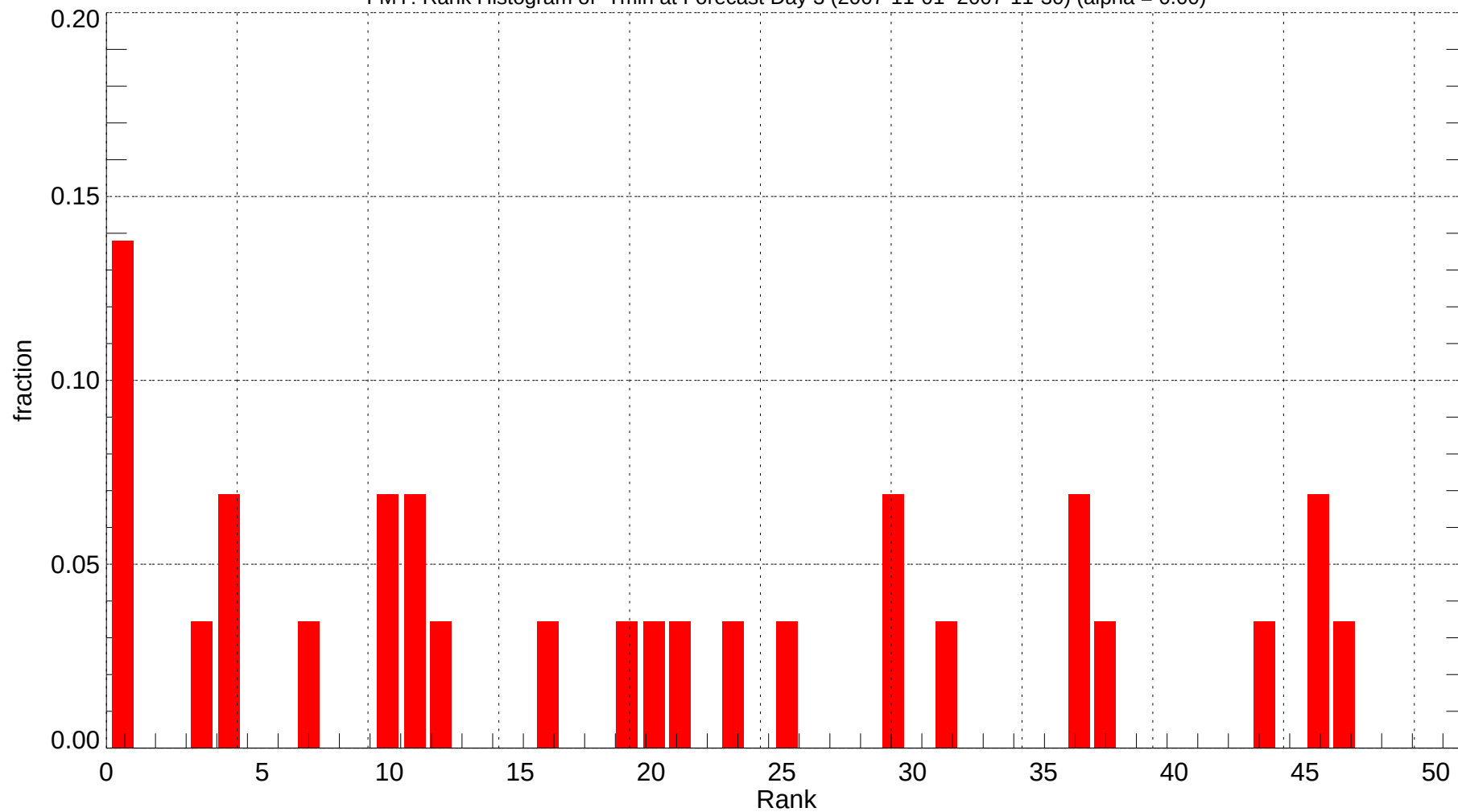
FMY: Rank Histogram of Tmin at Forecast Day 3 (2007-11-01~2007-11-30) (alpha = 0.00)
