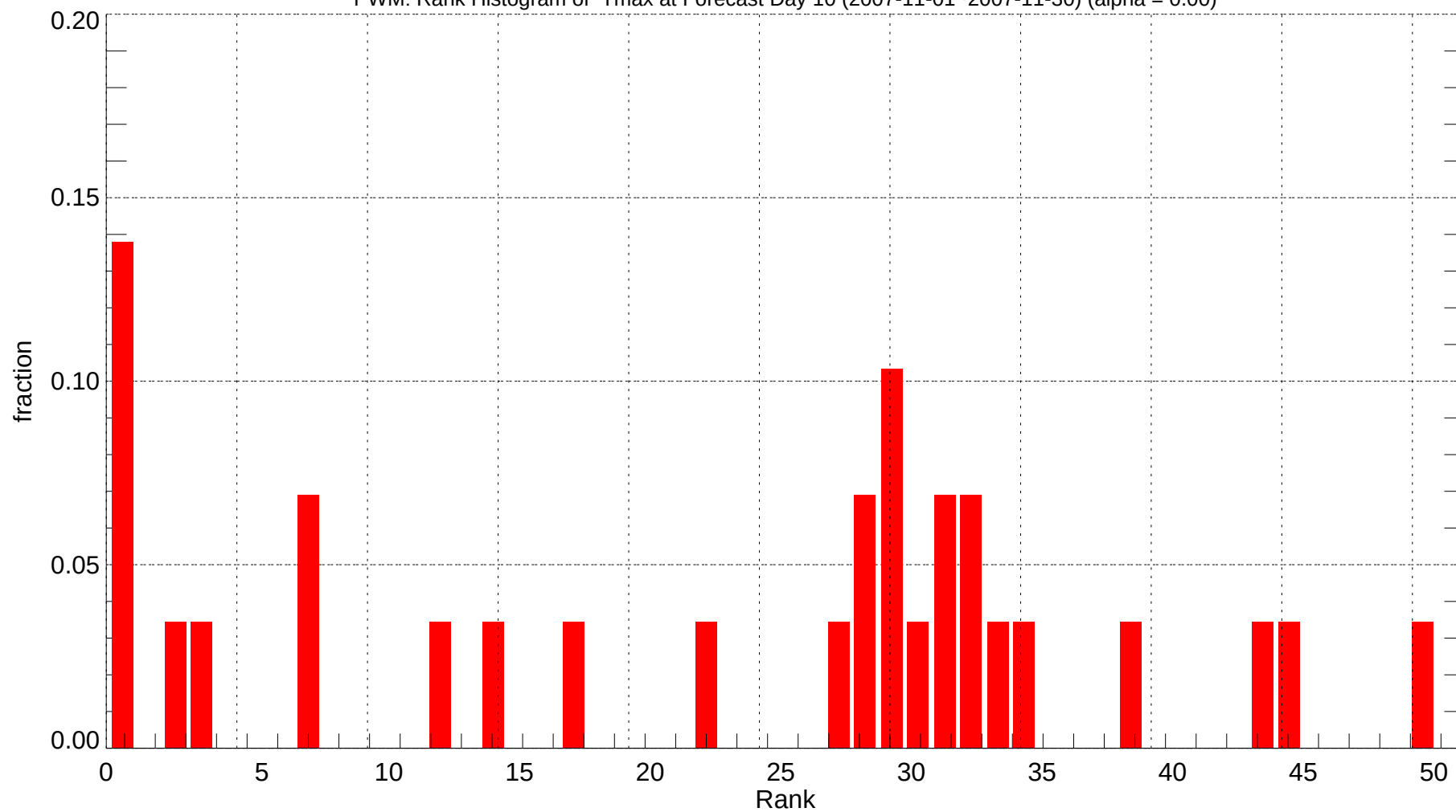
PWM: Rank Histogram of Tmax at Forecast Day 10 (2007-11-01~2007-11-30) (alpha = 0.00)
