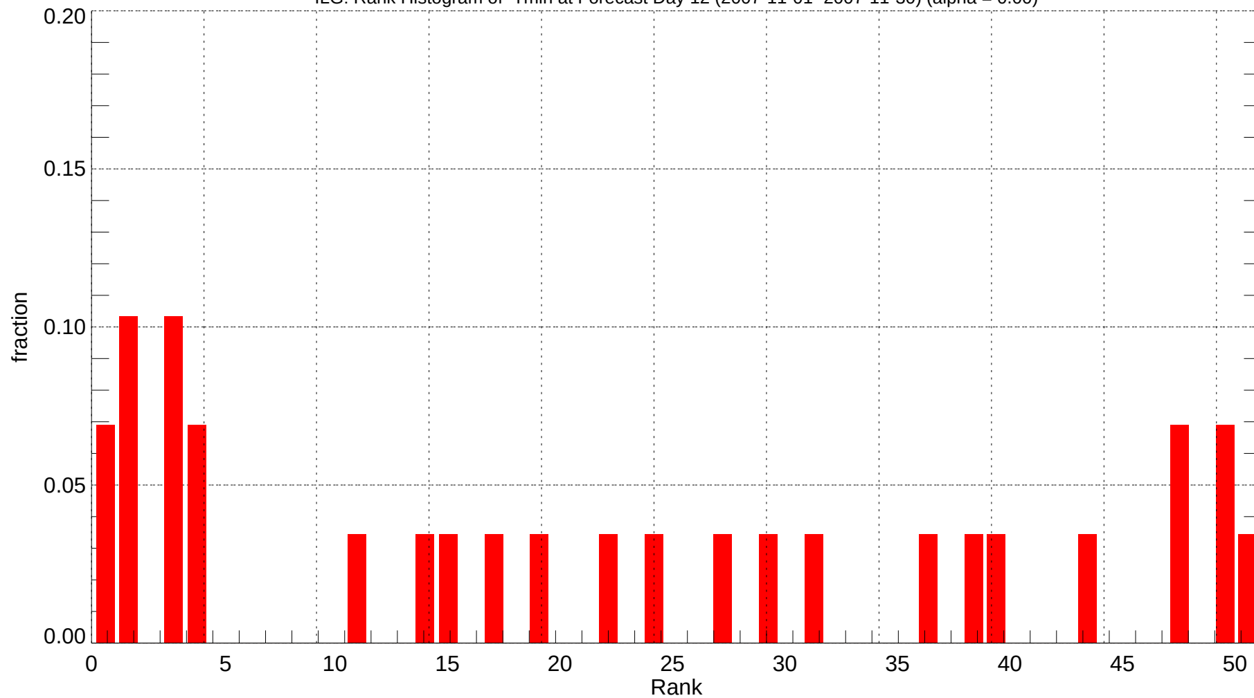
ILG: Rank Histogram of Tmin at Forecast Day 12 (2007-11-01~2007-11-30) (alpha = 0.00)
