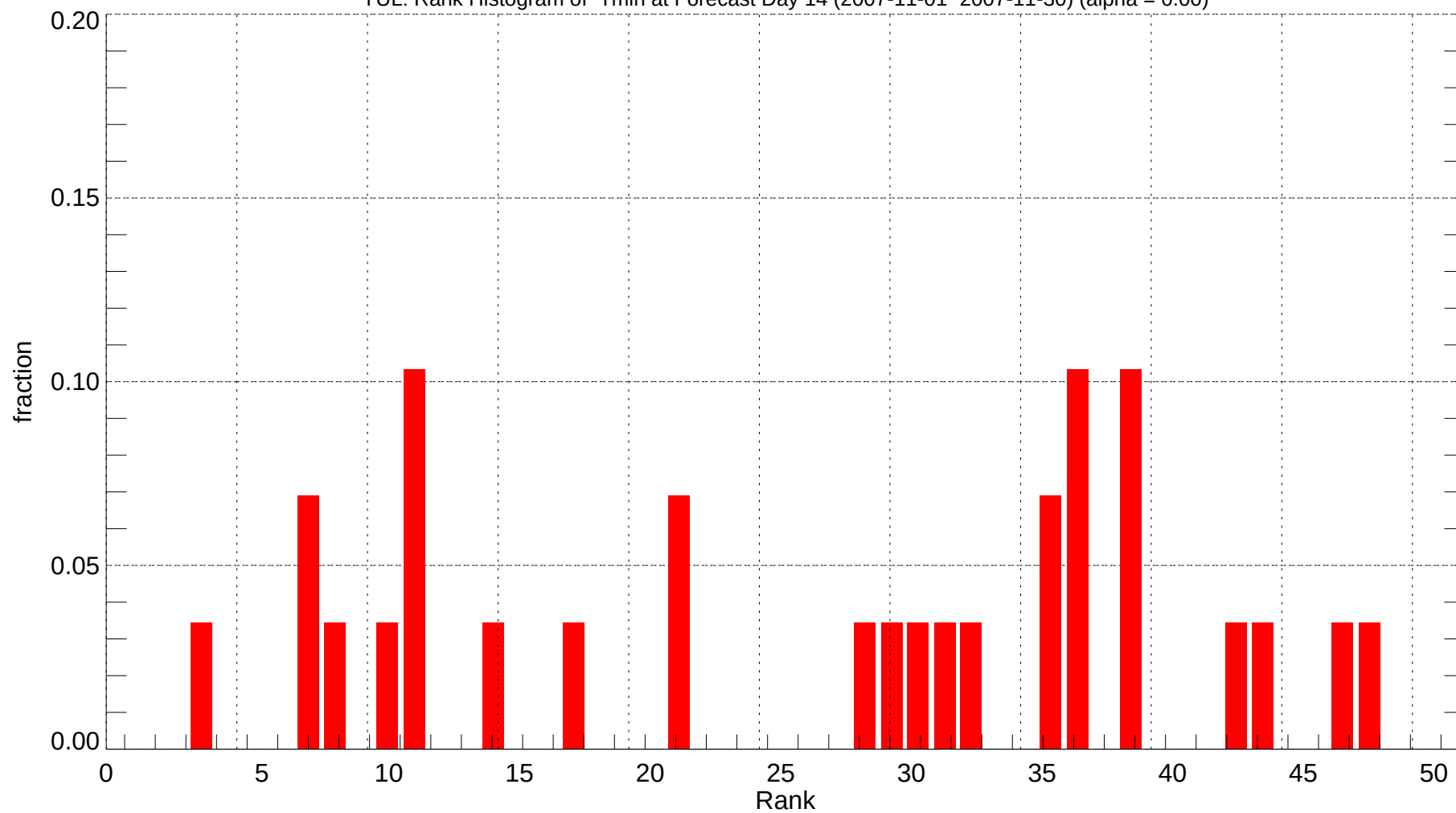
YUL: Rank Histogram of Tmin at Forecast Day 14 (2007-11-01~2007-11-30) (alpha = 0.00)
