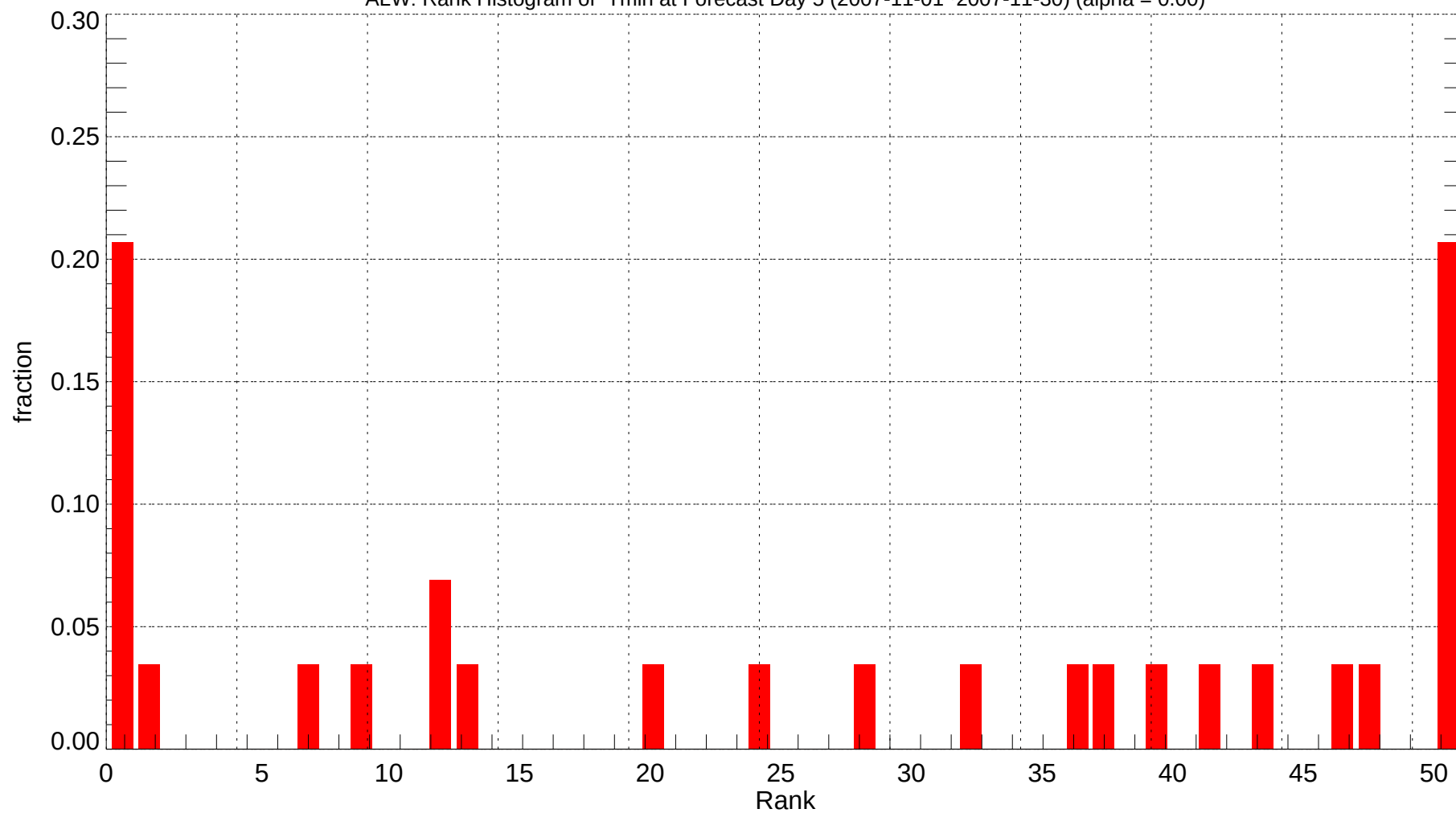
ALW: Rank Histogram of Tmin at Forecast Day 5 (2007-11-01~2007-11-30) (alpha = 0.00)
