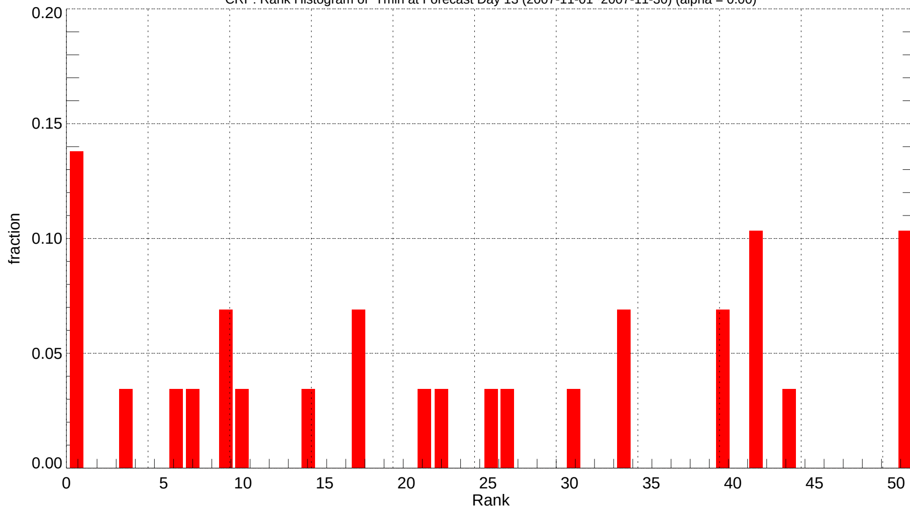
CRP: Rank Histogram of Tmin at Forecast Day 13 (2007-11-01~2007-11-30) (alpha = 0.00)
