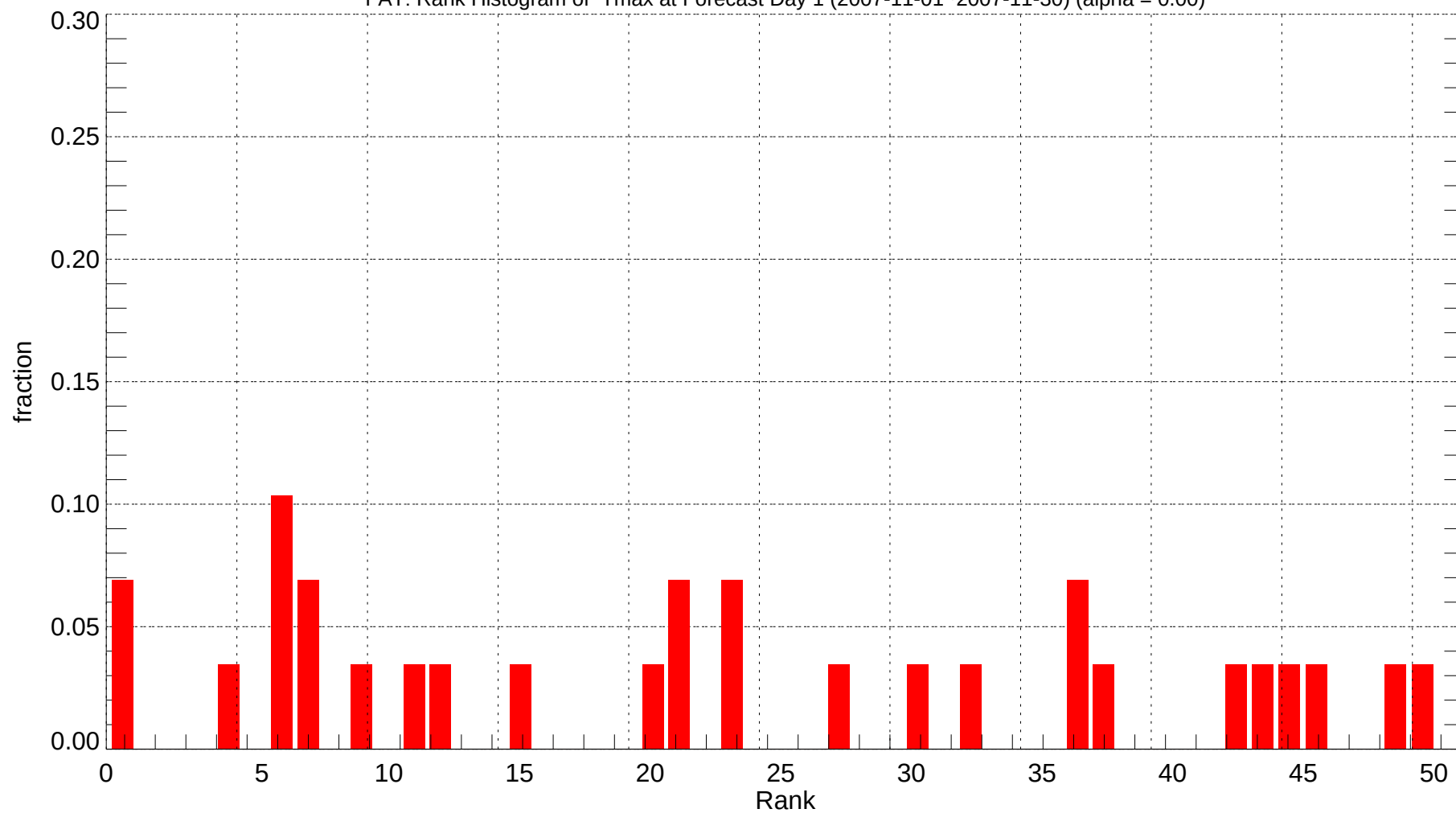
FAT: Rank Histogram of Tmax at Forecast Day 1 (2007-11-01~2007-11-30) (alpha = 0.00)
