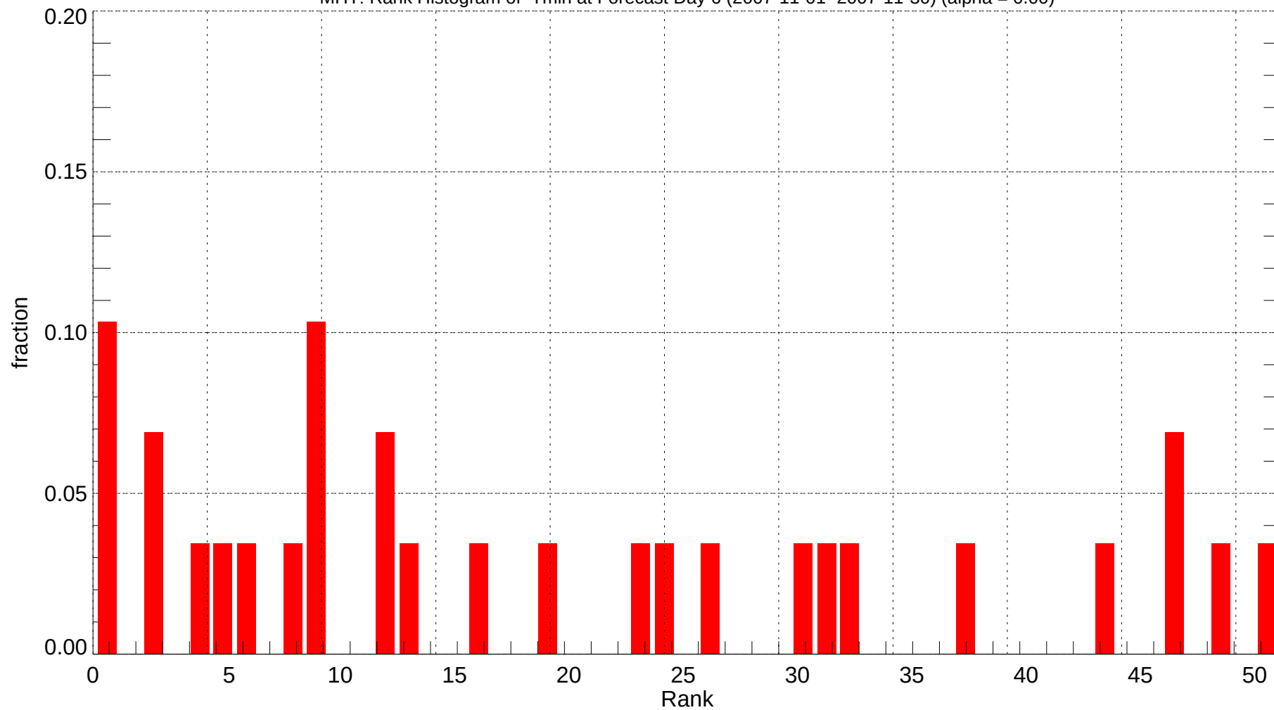
MHT: Rank Histogram of Tmin at Forecast Day 6 (2007-11-01~2007-11-30) (alpha = 0.00)
