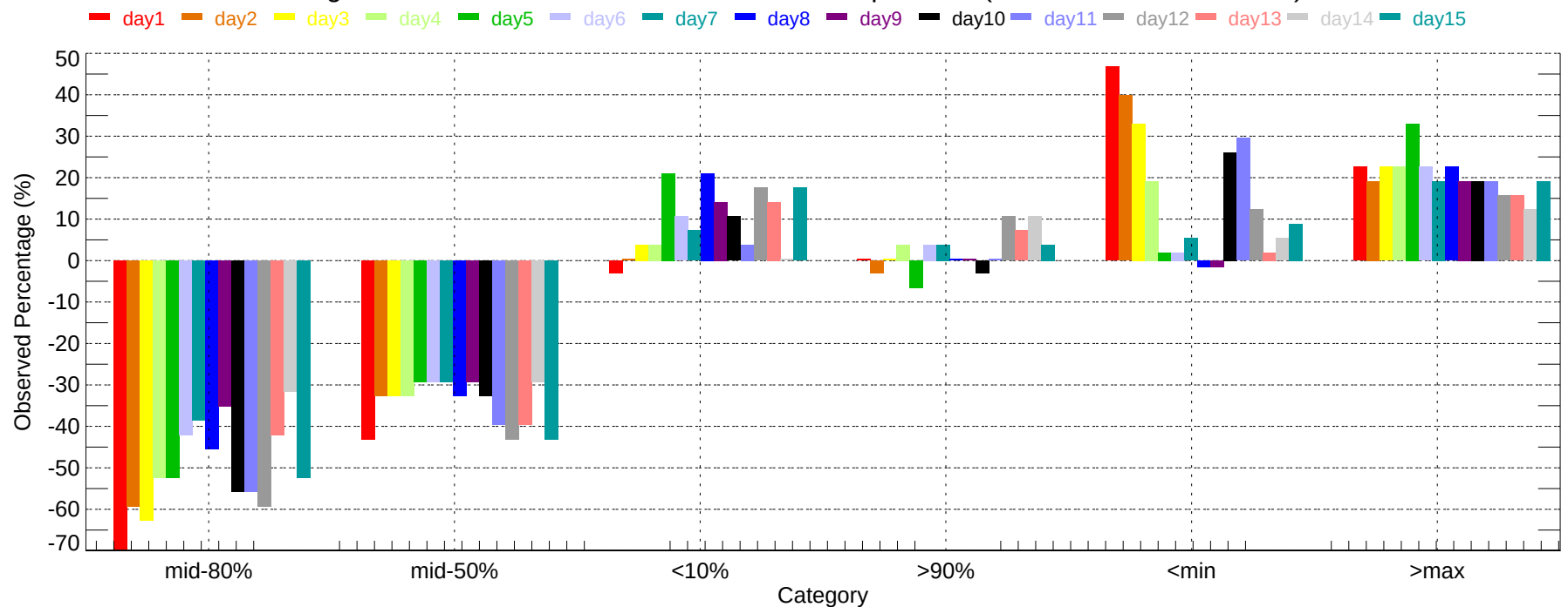
Observed Percentage Deviation of Ensembles - LGB: Max Temperature (2007-11-01~2007-11-30)
