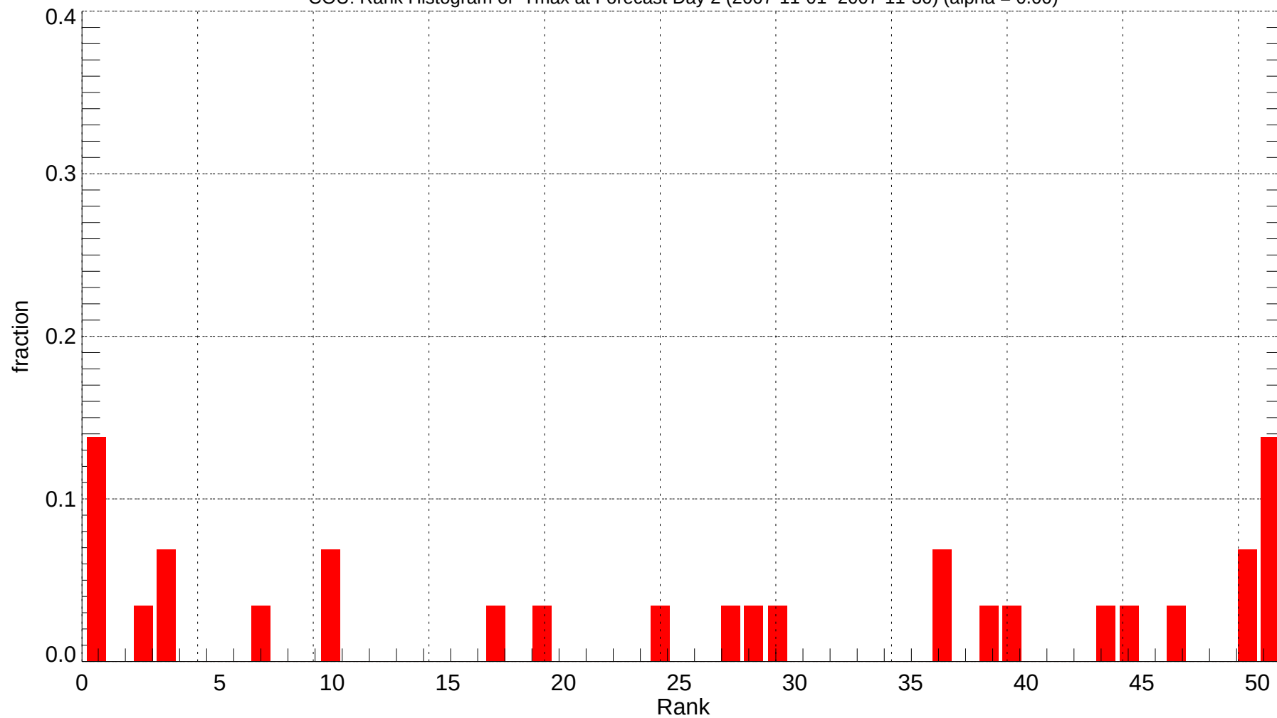
COU: Rank Histogram of Tmax at Forecast Day 2 (2007-11-01~2007-11-30) (alpha = 0.00)
