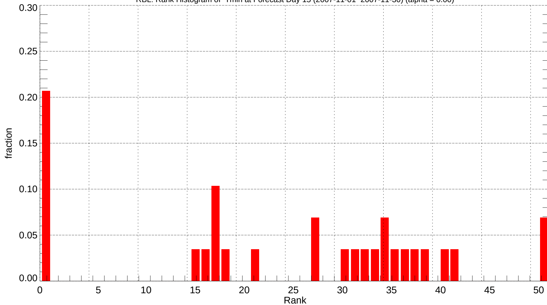
RBL: Rank Histogram of Tmin at Forecast Day 15 (2007-11-01~2007-11-30) (alpha = 0.00)
