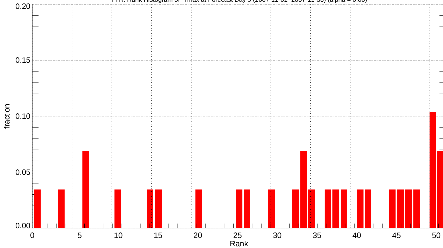
TYR: Rank Histogram of Tmax at Forecast Day 9 (2007-11-01~2007-11-30) (alpha = 0.00)
