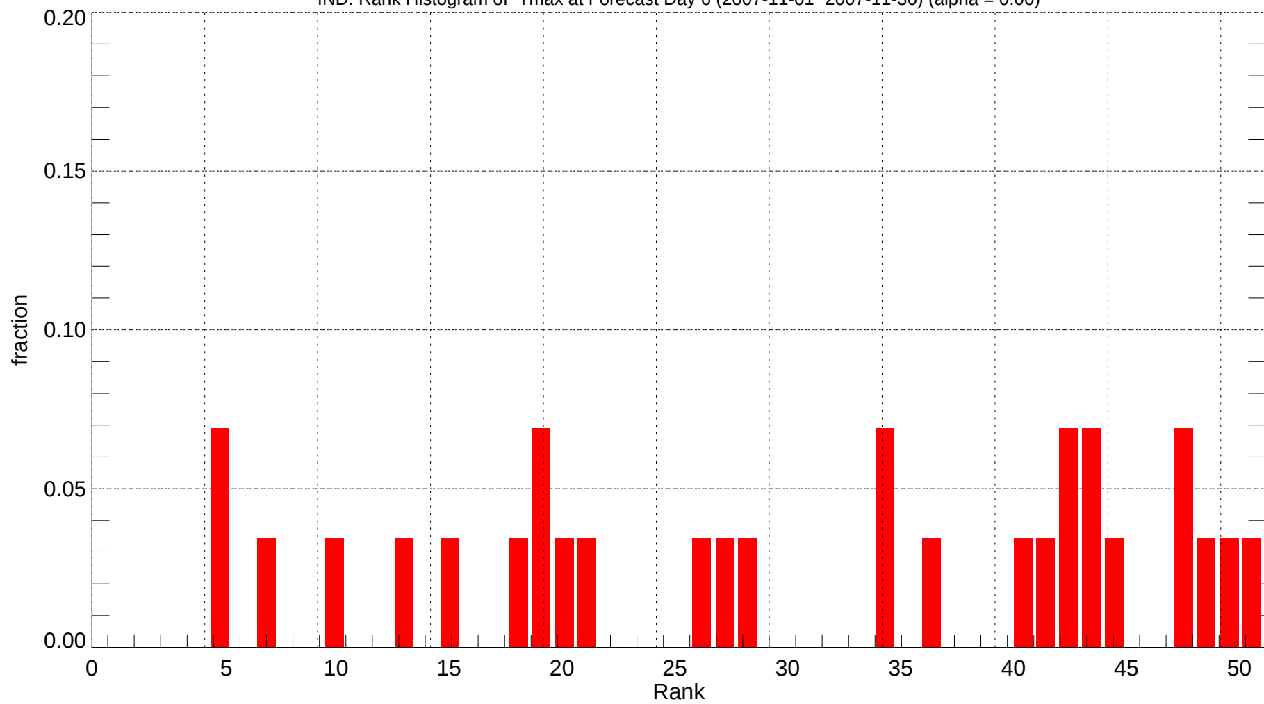
IND: Rank Histogram of Tmax at Forecast Day 6 (2007-11-01~2007-11-30) (alpha = 0.00)
