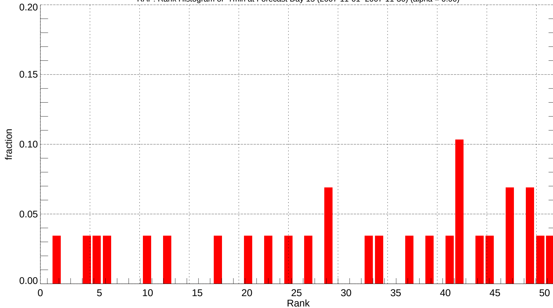
RAP: Rank Histogram of Tmin at Forecast Day 15 (2007-11-01~2007-11-30) (alpha = 0.00)
