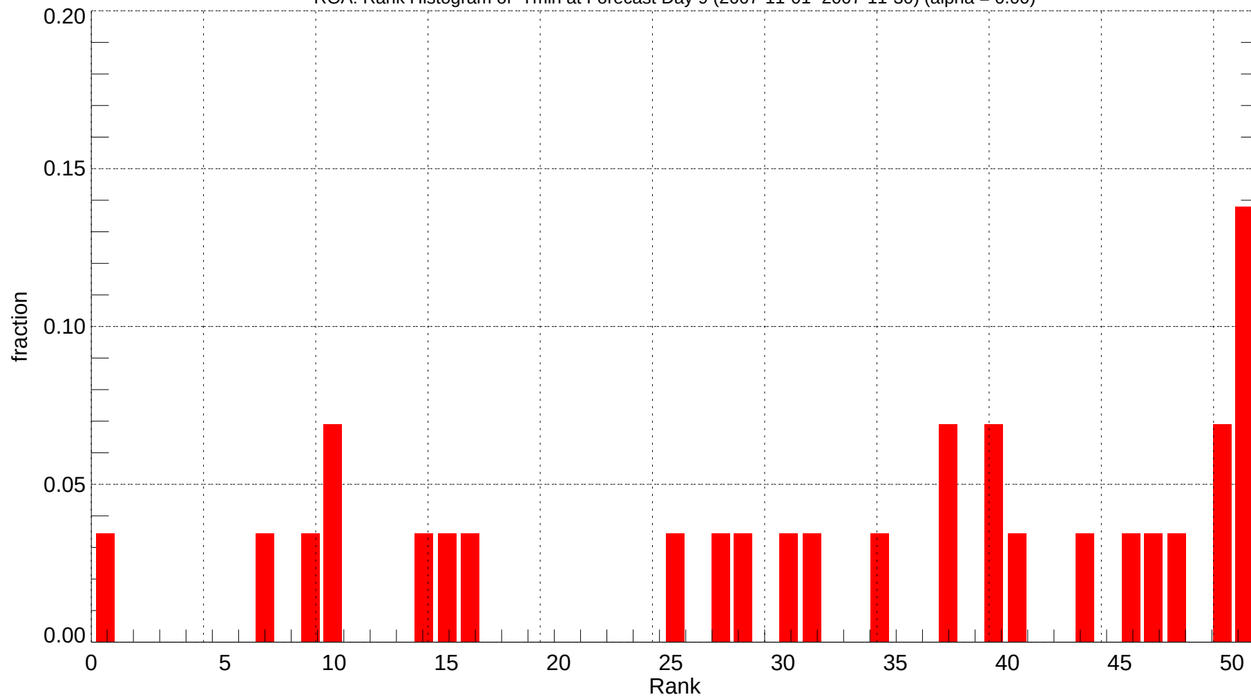
ROA: Rank Histogram of Tmin at Forecast Day 9 (2007-11-01~2007-11-30) (alpha = 0.00)
