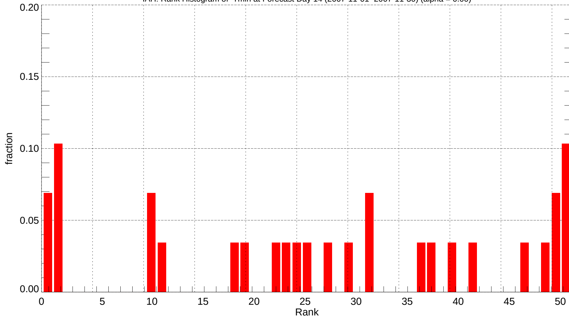
IAH: Rank Histogram of Tmin at Forecast Day 14 (2007-11-01~2007-11-30) (alpha = 0.00)
