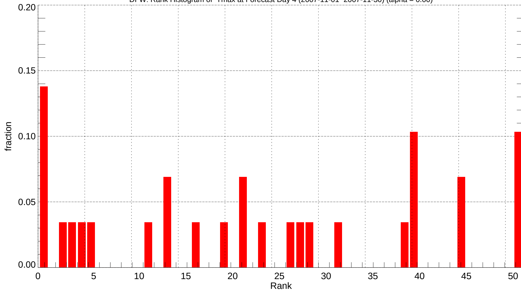
DFW: Rank Histogram of Tmax at Forecast Day 4 (2007-11-01~2007-11-30) (alpha = 0.00)
