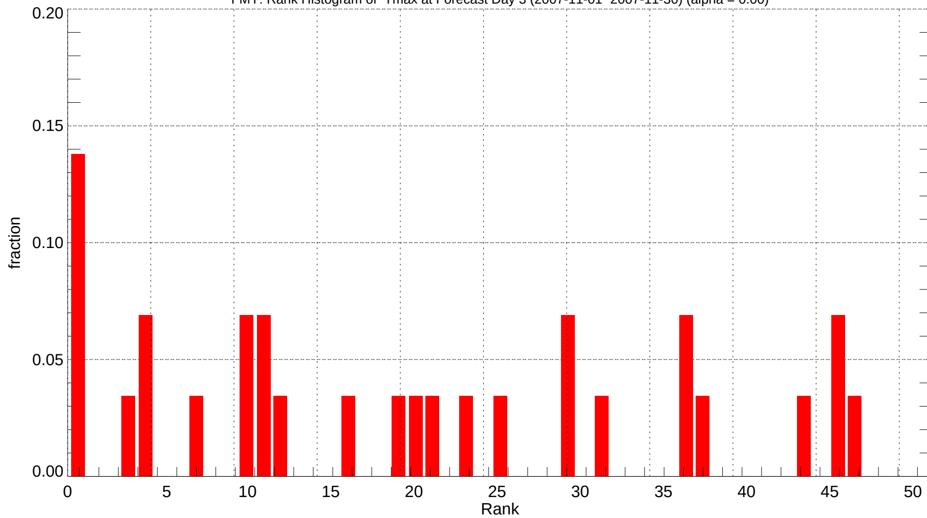
FMY: Rank Histogram of Tmax at Forecast Day 3 (2007-11-01~2007-11-30) (alpha = 0.00)
