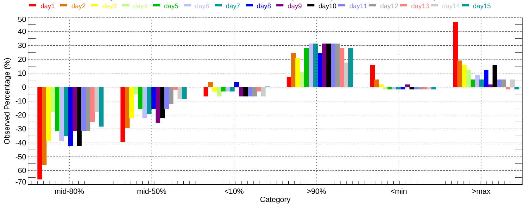
Observed Percentage Deviation of Ensembles - RAP: Max Temperature (2007-11-01~2007-11-30)
