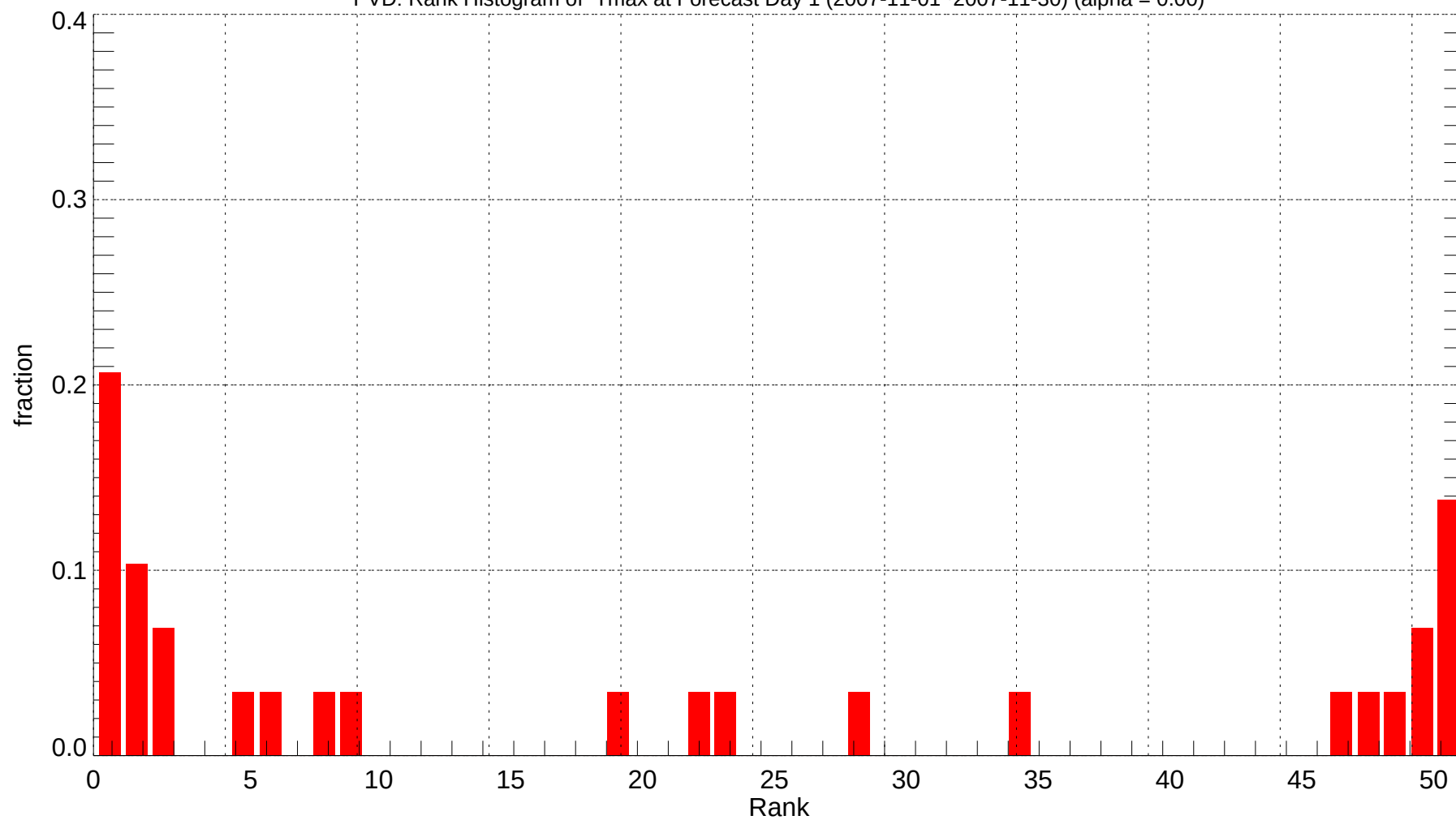
PVD: Rank Histogram of Tmax at Forecast Day 1 (2007-11-01~2007-11-30) (alpha = 0.00)
