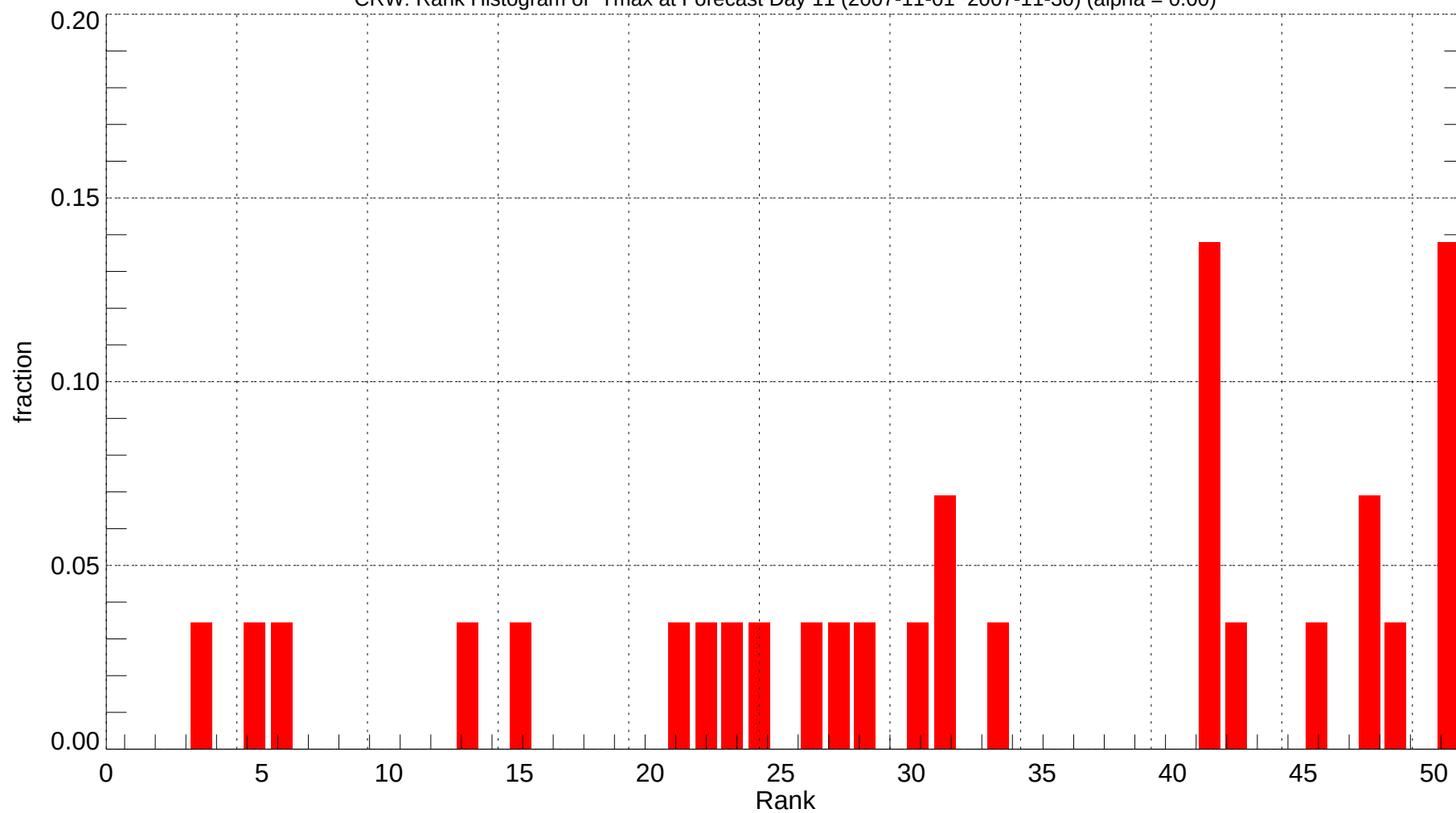
CRW: Rank Histogram of Tmax at Forecast Day 11 (2007-11-01~2007-11-30) (alpha = 0.00)
