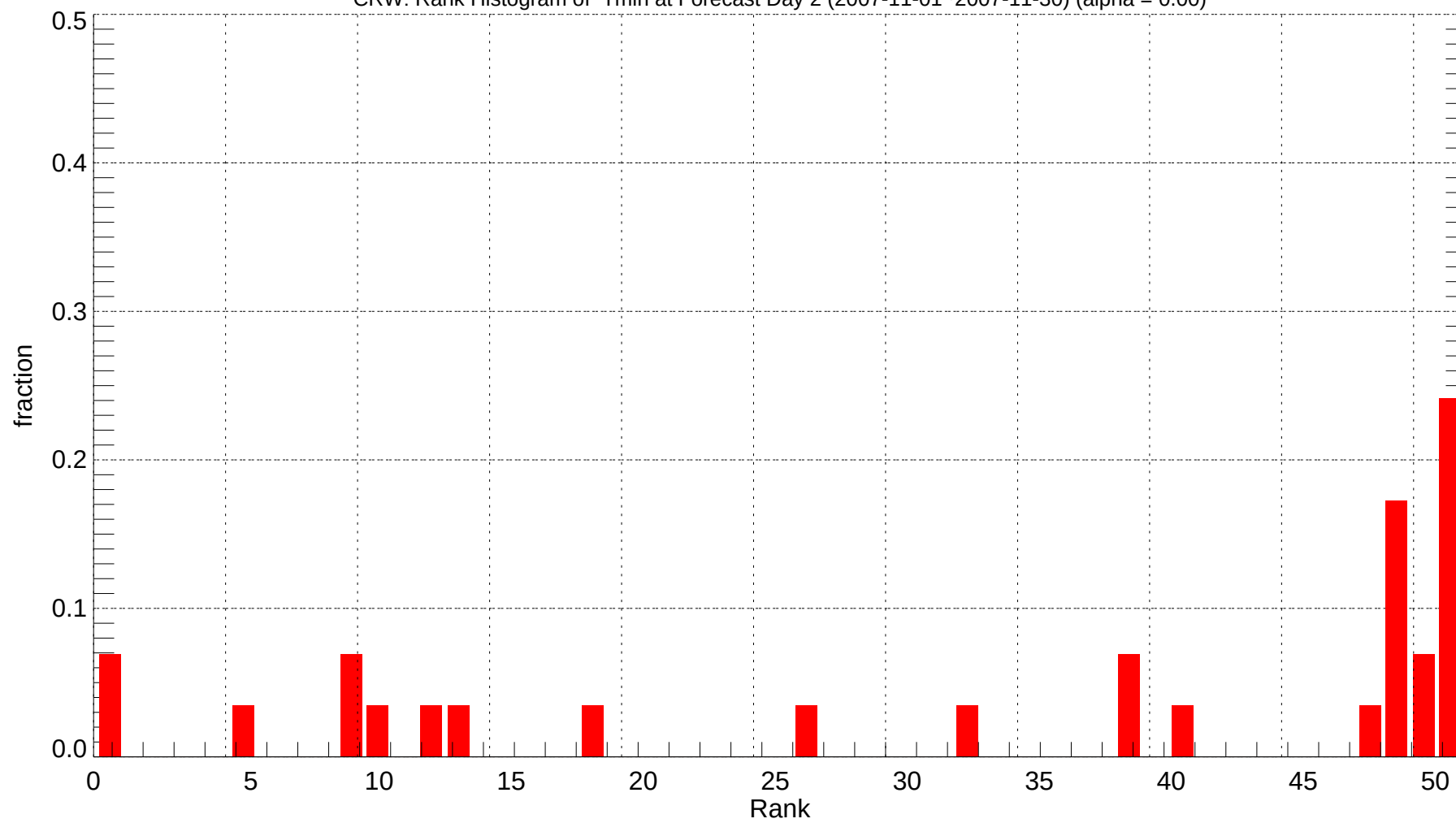
CRW: Rank Histogram of Tmin at Forecast Day 2 (2007-11-01~2007-11-30) (alpha = 0.00)
