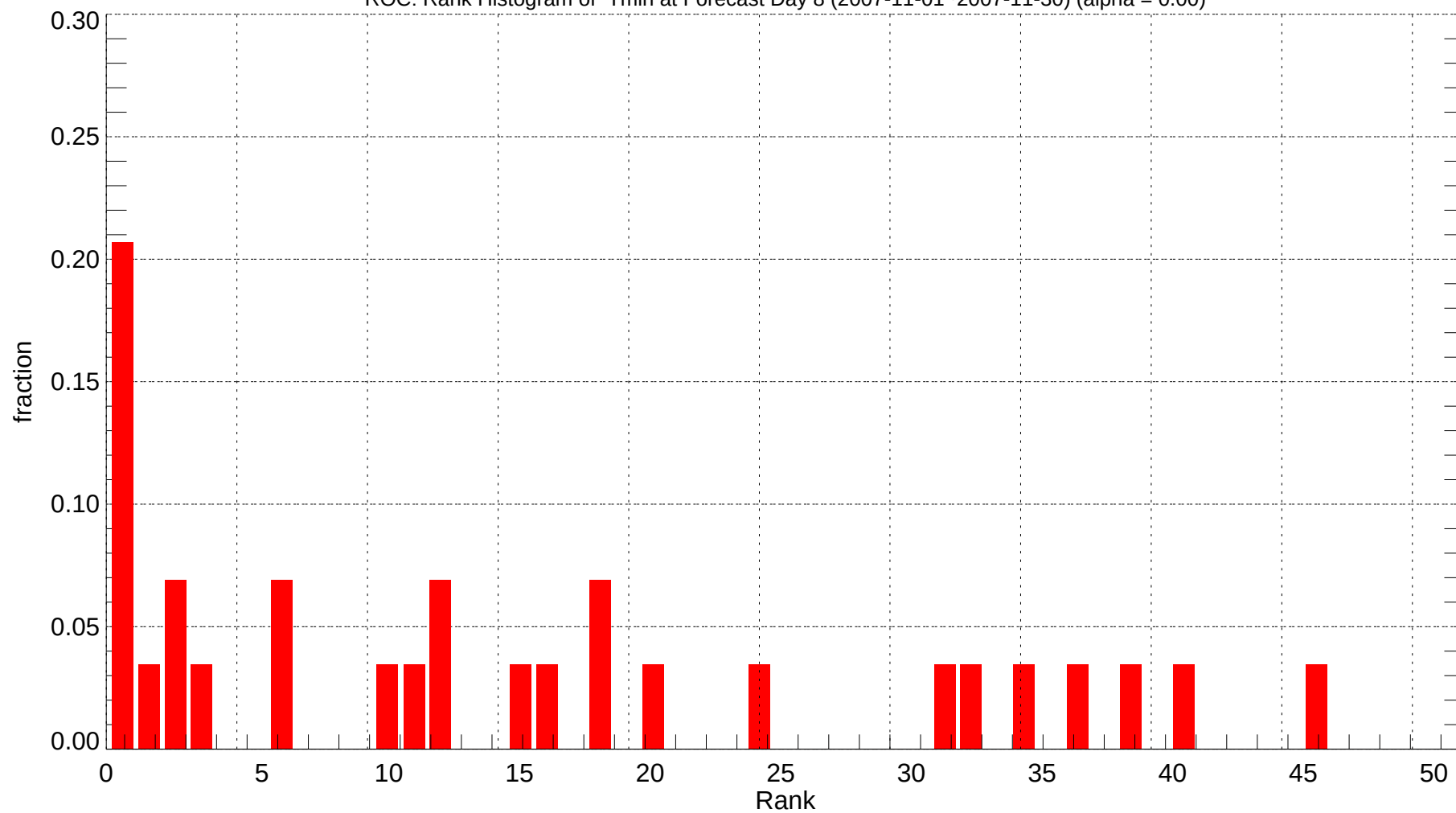
ROC: Rank Histogram of Tmin at Forecast Day 8 (2007-11-01~2007-11-30) (alpha = 0.00)
