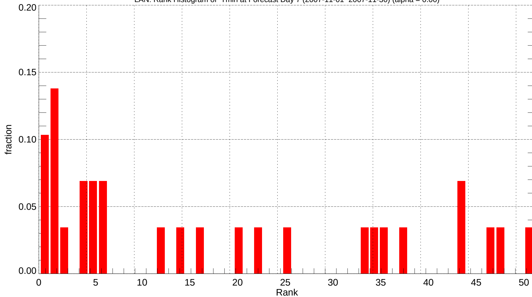
LAN: Rank Histogram of Tmin at Forecast Day 7 (2007-11-01~2007-11-30) (alpha = 0.00)
