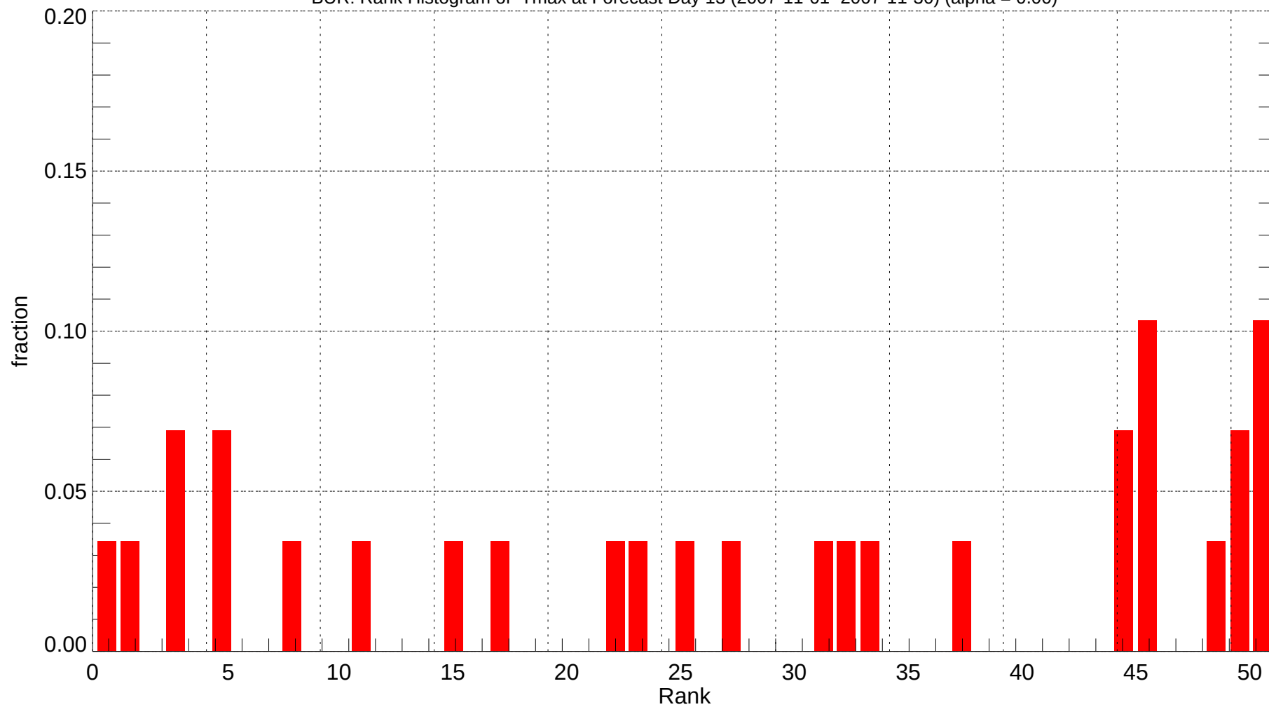
BUR: Rank Histogram of Tmax at Forecast Day 13 (2007-11-01~2007-11-30) (alpha = 0.00)
