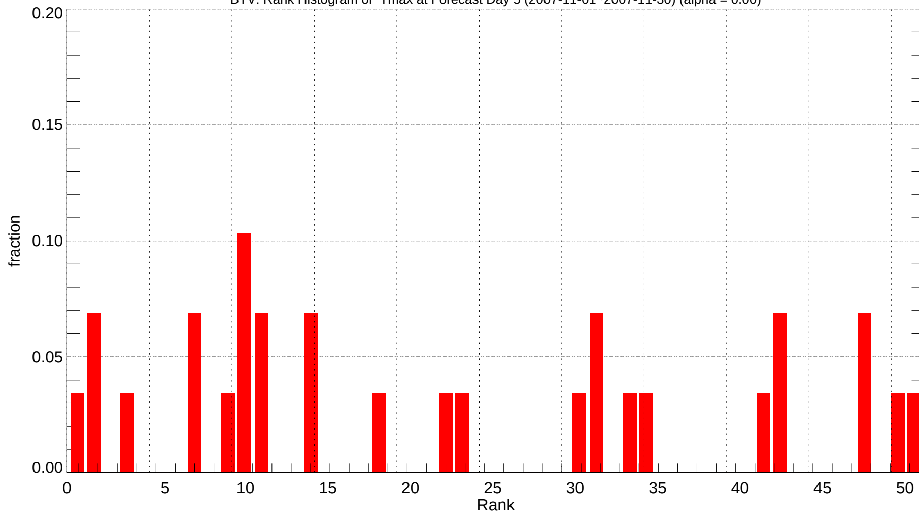
BTV: Rank Histogram of Tmax at Forecast Day 5 (2007-11-01~2007-11-30) (alpha = 0.00)
