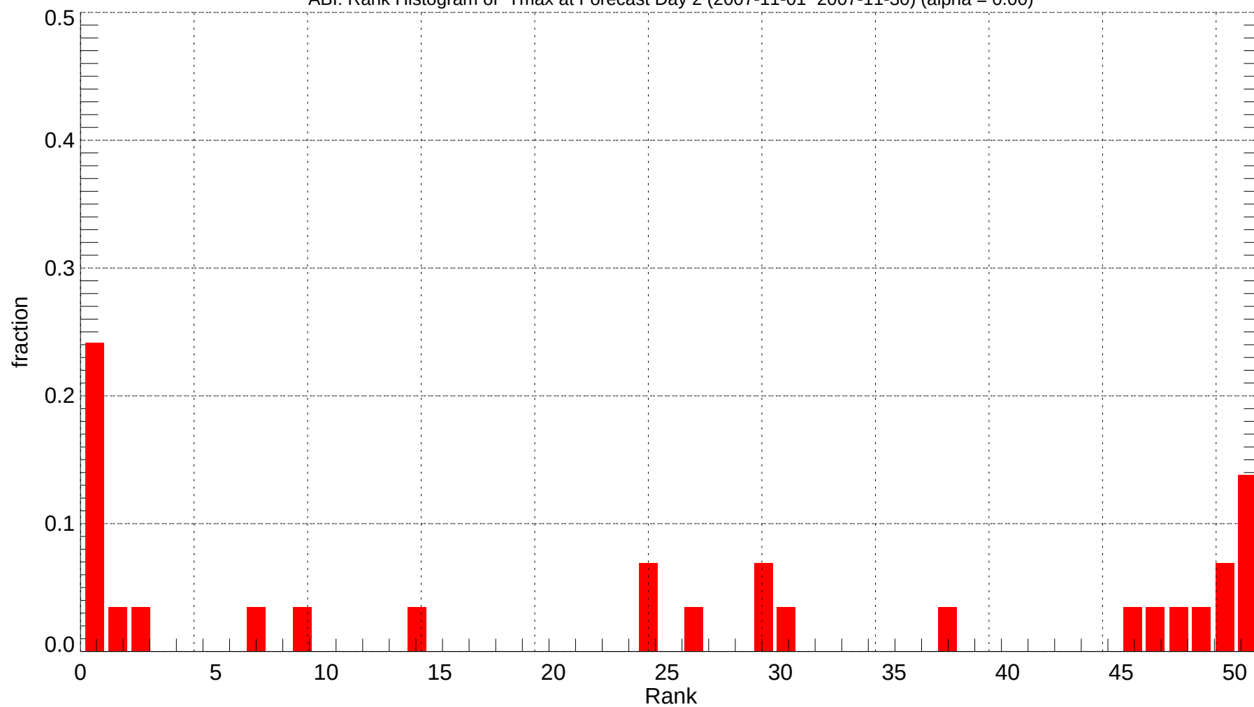
ABI: Rank Histogram of Tmax at Forecast Day 2 (2007-11-01~2007-11-30) (alpha = 0.00)
