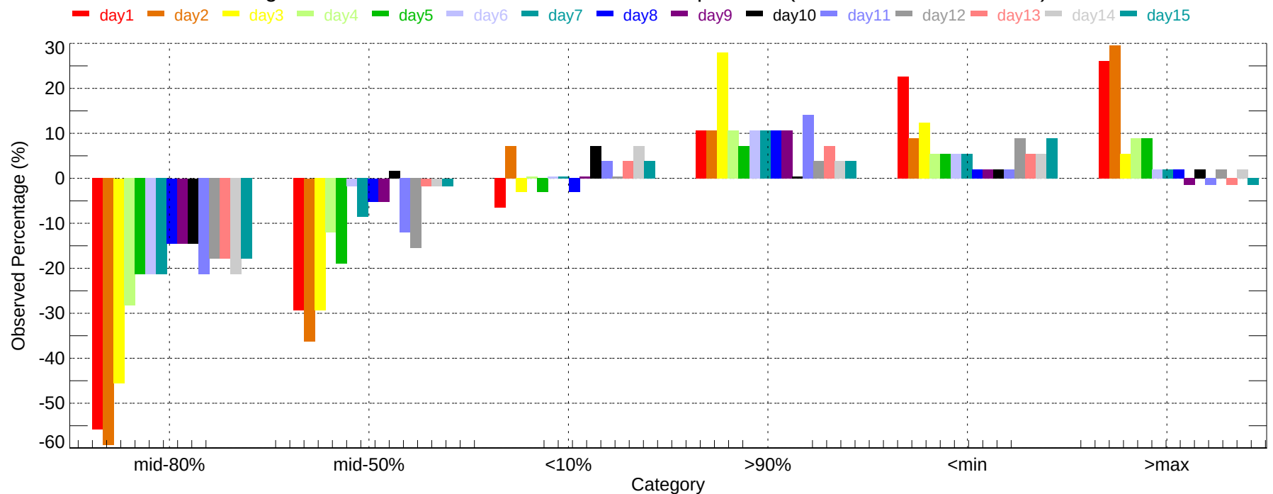
Observed Percentage Deviation of Ensembles - IPT: Max Temperature (2007-11-01~2007-11-30)
