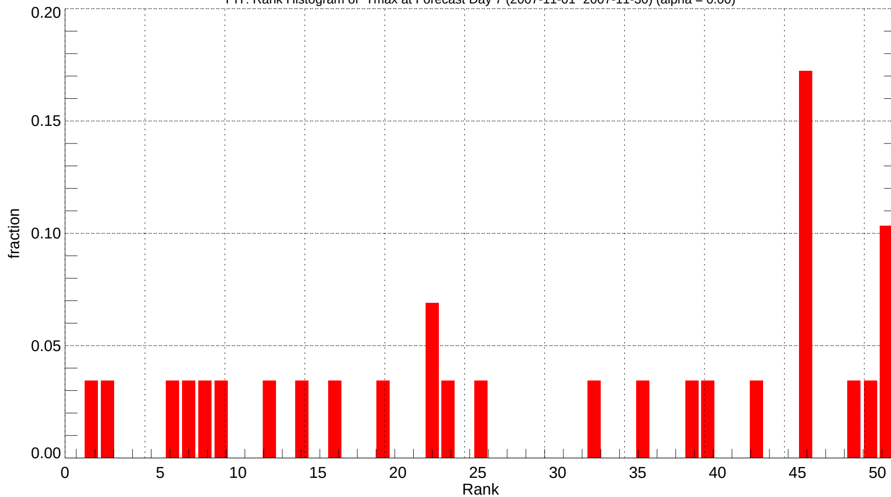
PIT: Rank Histogram of Tmax at Forecast Day 7 (2007-11-01~2007-11-30) (alpha = 0.00)
