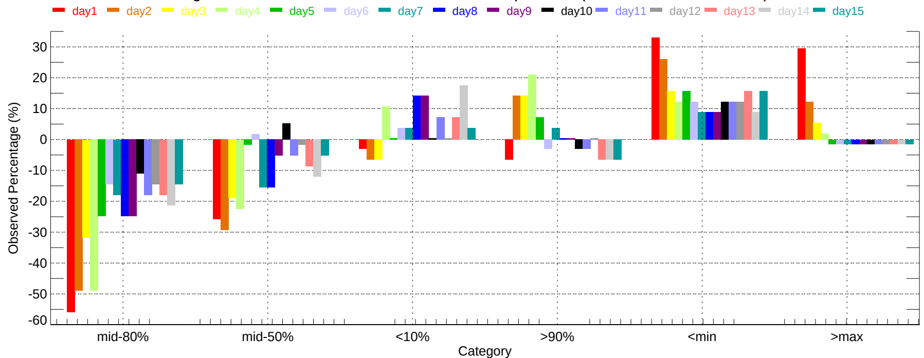
Observed Percentage Deviation of Ensembles - SYR: Max Temperature (2007-11-01~2007-11-30)
