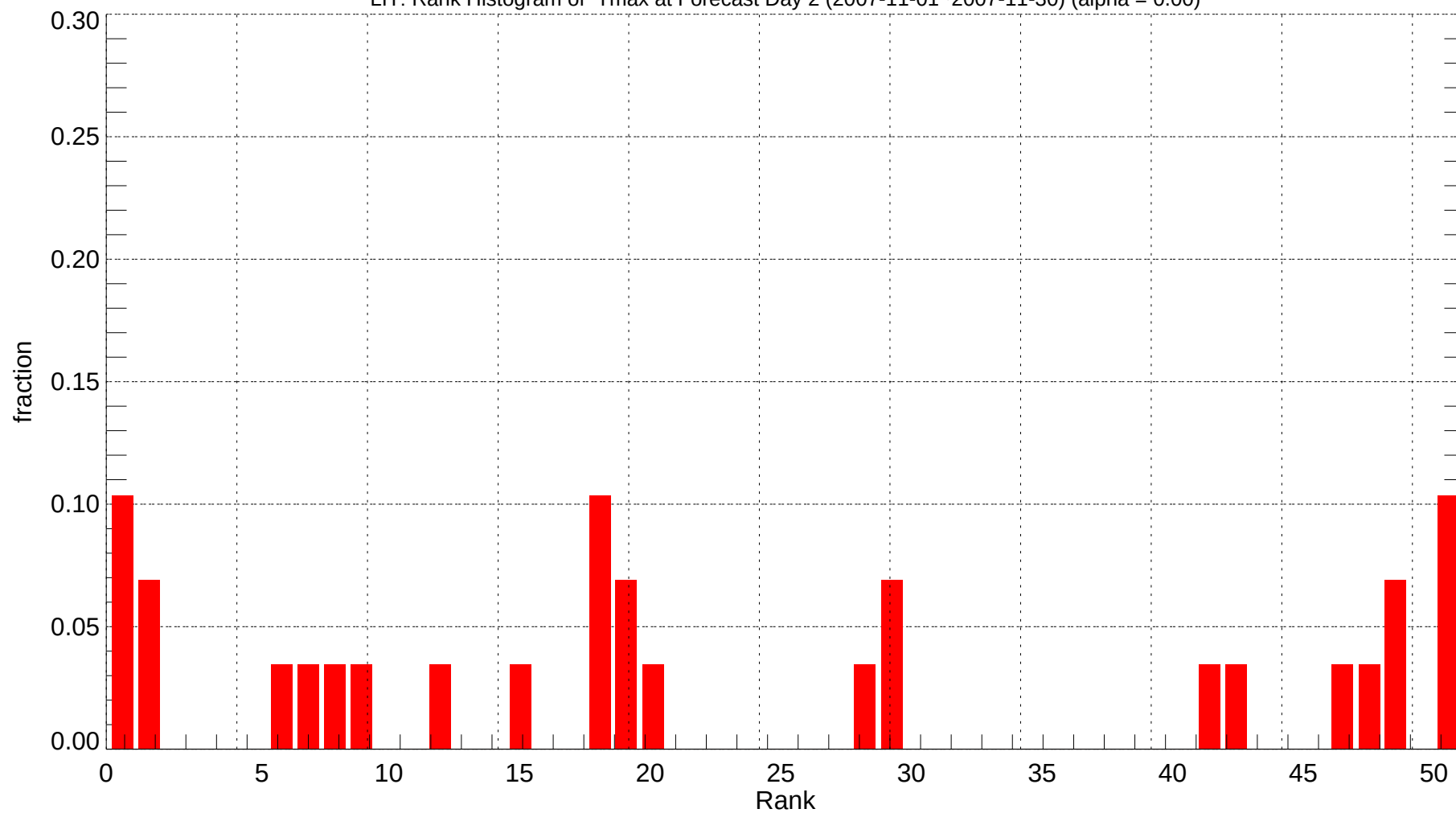
LIT: Rank Histogram of Tmax at Forecast Day 2 (2007-11-01~2007-11-30) (alpha = 0.00)
