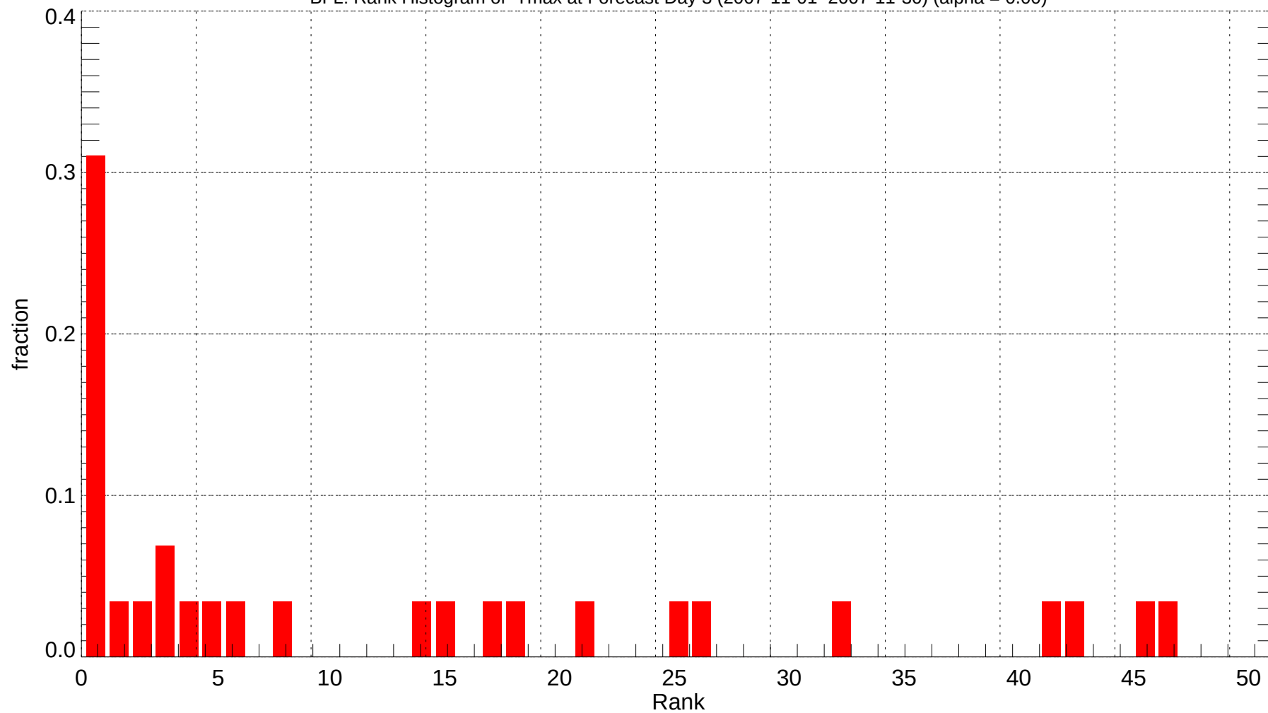
BFL: Rank Histogram of Tmax at Forecast Day 3 (2007-11-01~2007-11-30) (alpha = 0.00)
