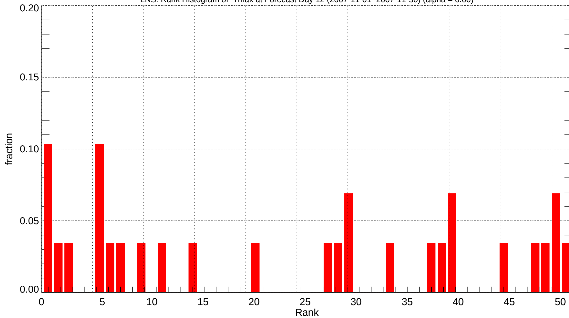
LNS: Rank Histogram of Tmax at Forecast Day 12 (2007-11-01~2007-11-30) (alpha = 0.00)
