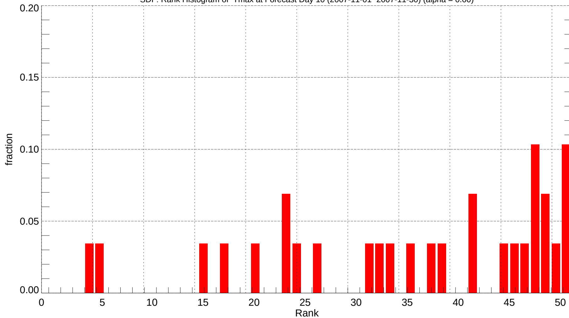
SDF: Rank Histogram of Tmax at Forecast Day 10 (2007-11-01~2007-11-30) (alpha = 0.00)
