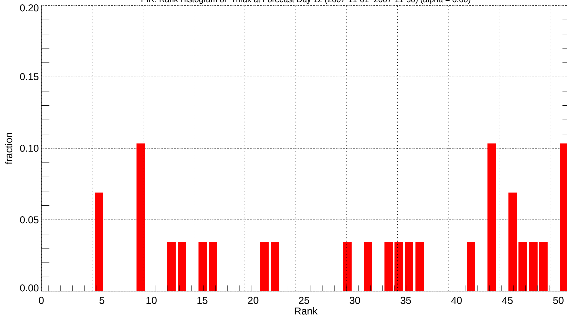
PIR: Rank Histogram of Tmax at Forecast Day 12 (2007-11-01~2007-11-30) (alpha = 0.00)
