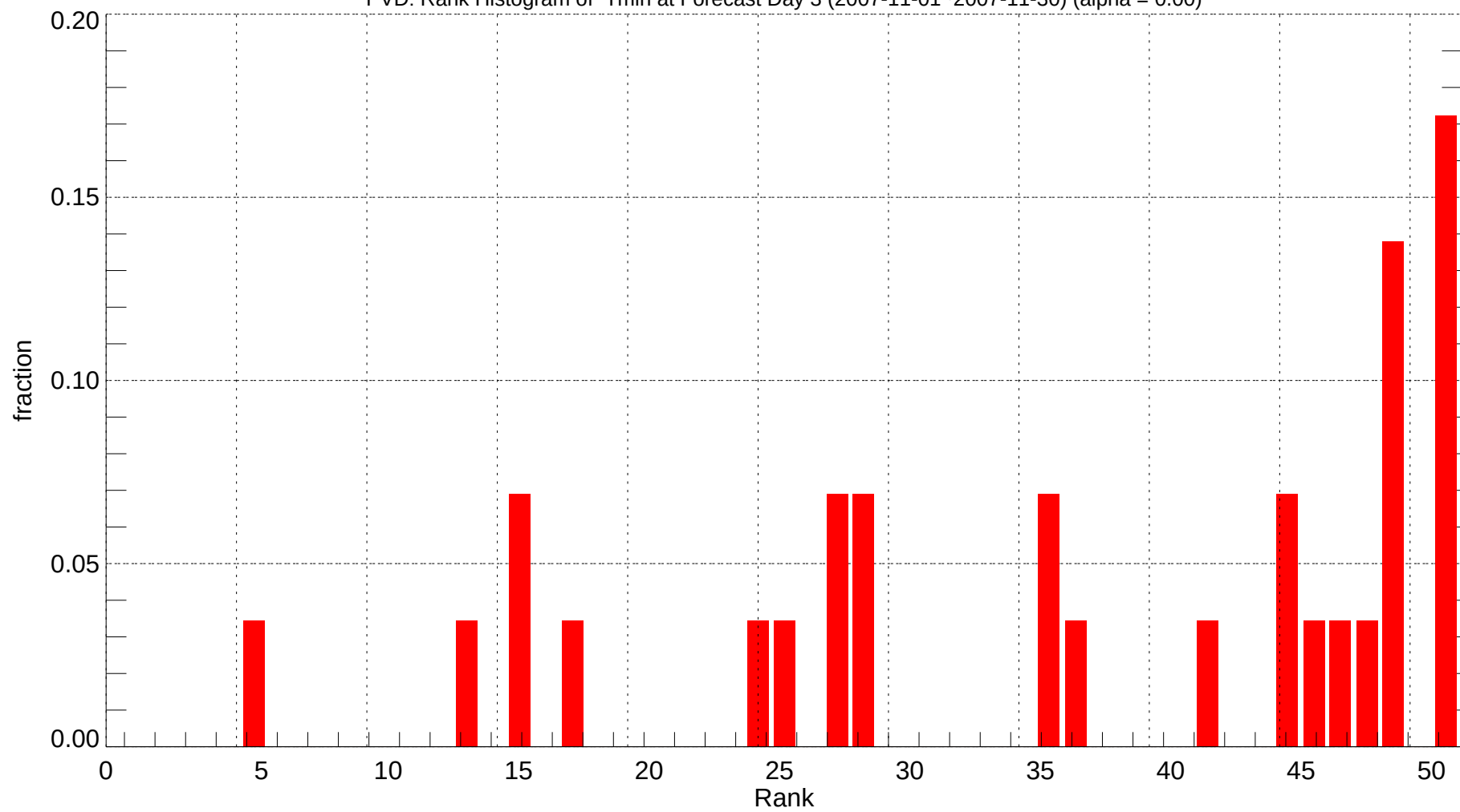
PVD: Rank Histogram of Tmin at Forecast Day 3 (2007-11-01~2007-11-30) (alpha = 0.00)
