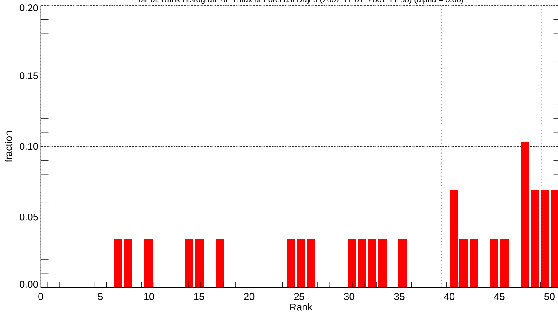
MEM: Rank Histogram of Tmax at Forecast Day 9 (2007-11-01~2007-11-30) (alpha = 0.00)
