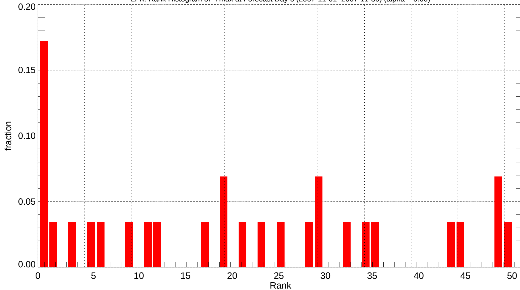
LFK: Rank Histogram of Tmax at Forecast Day 6 (2007-11-01~2007-11-30) (alpha = 0.00)
