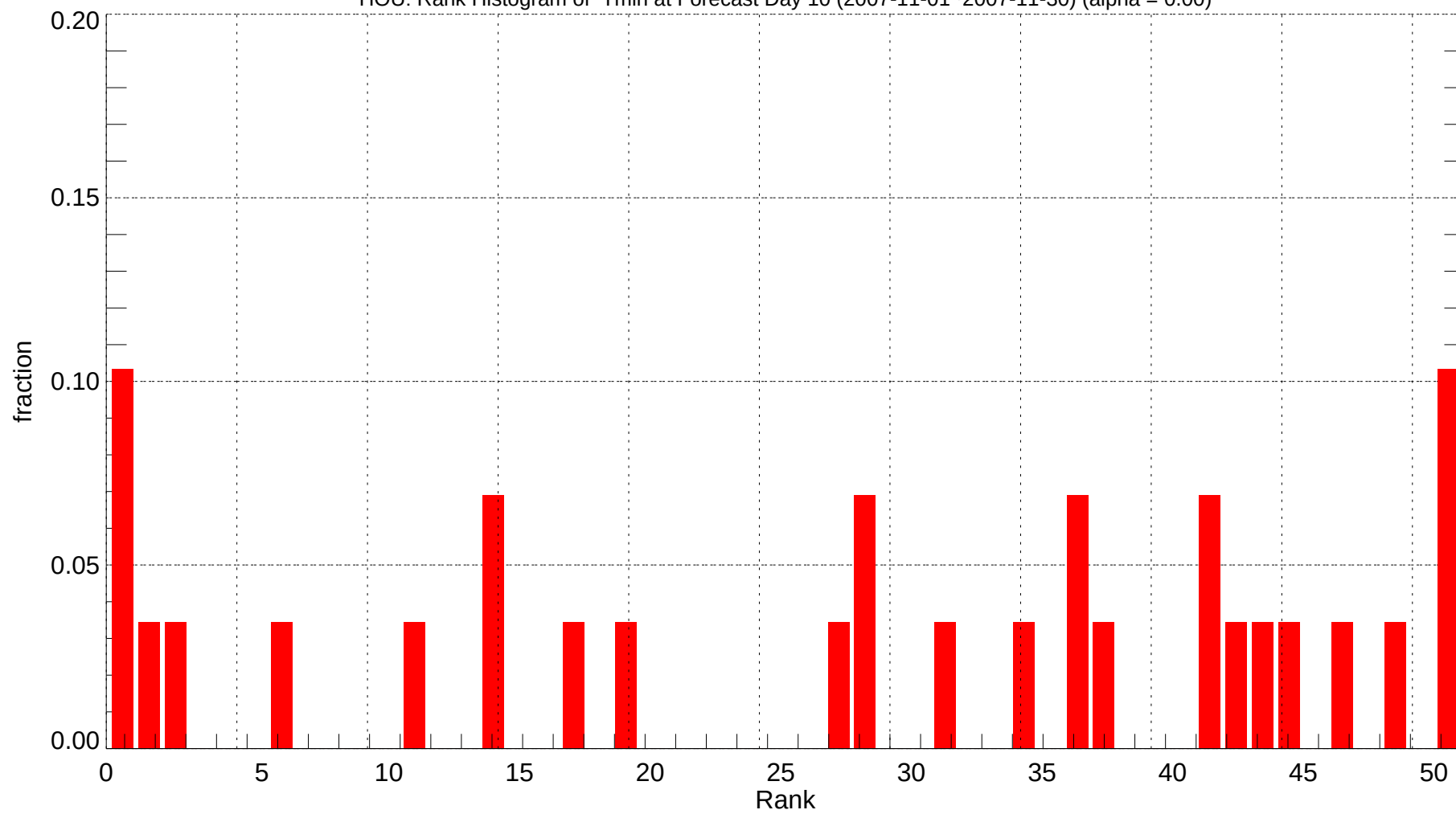
HOU: Rank Histogram of Tmin at Forecast Day 10 (2007-11-01~2007-11-30) (alpha = 0.00)
