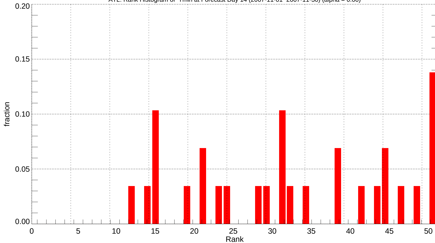
ATL: Rank Histogram of Tmin at Forecast Day 14 (2007-11-01~2007-11-30) (alpha = 0.00)
