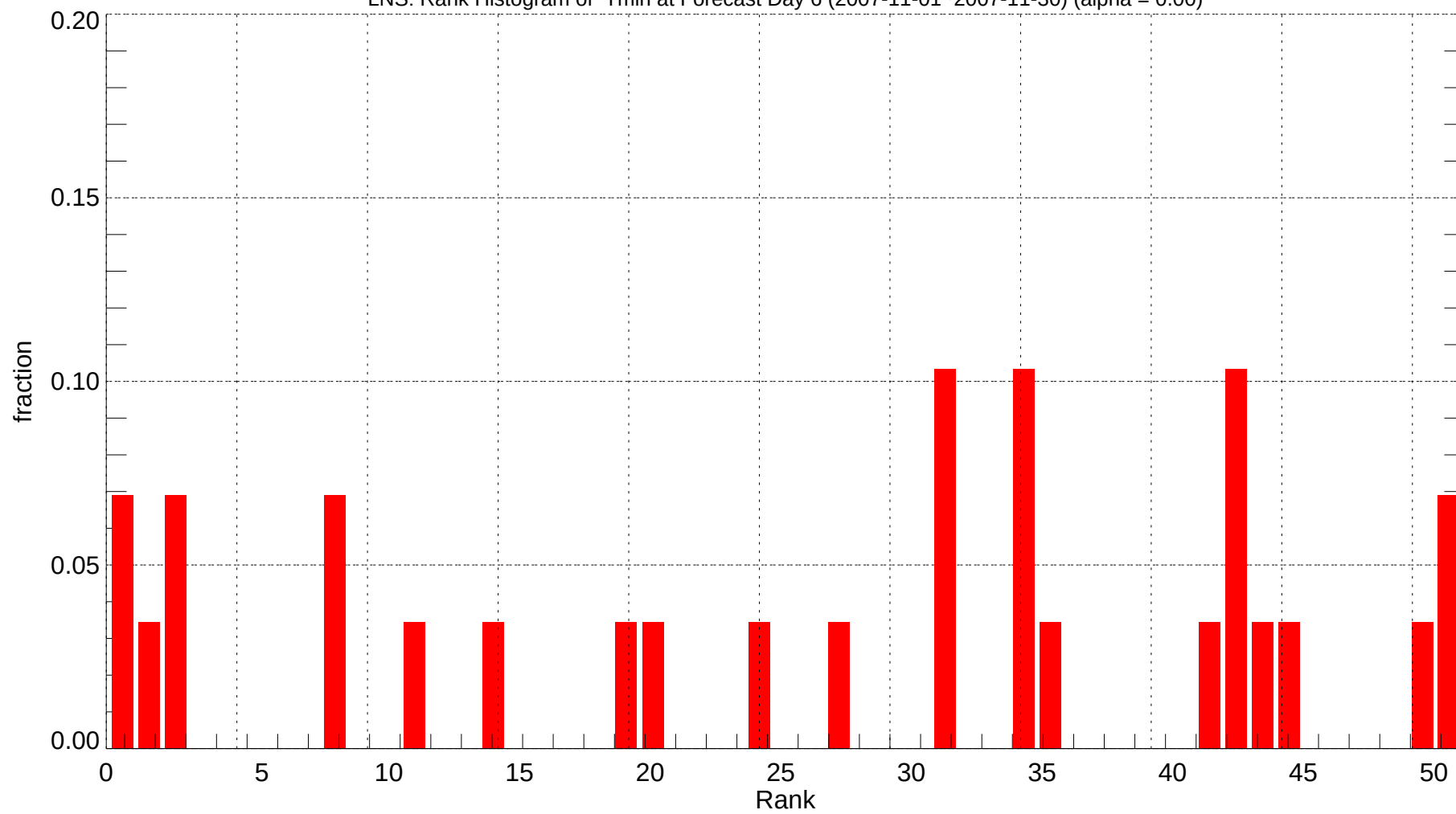
LNS: Rank Histogram of Tmin at Forecast Day 6 (2007-11-01~2007-11-30) (alpha = 0.00)
