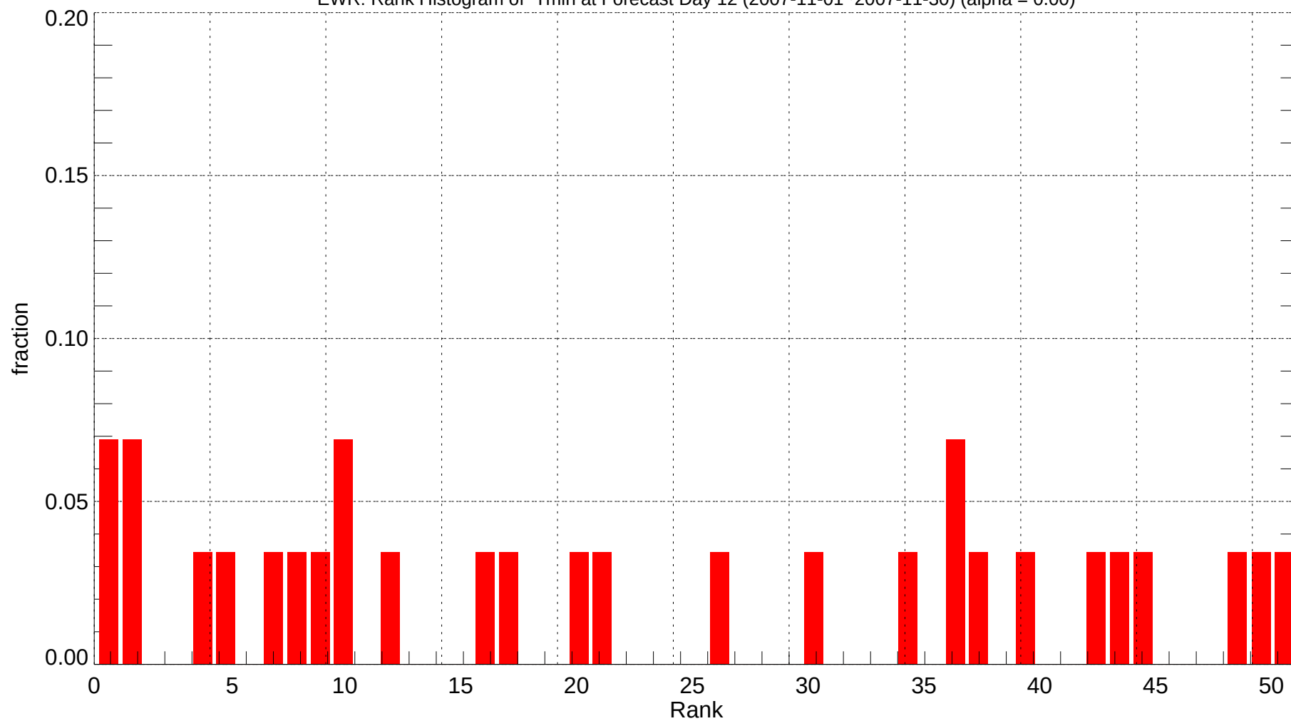
EWR: Rank Histogram of Tmin at Forecast Day 12 (2007-11-01~2007-11-30) (alpha = 0.00)
