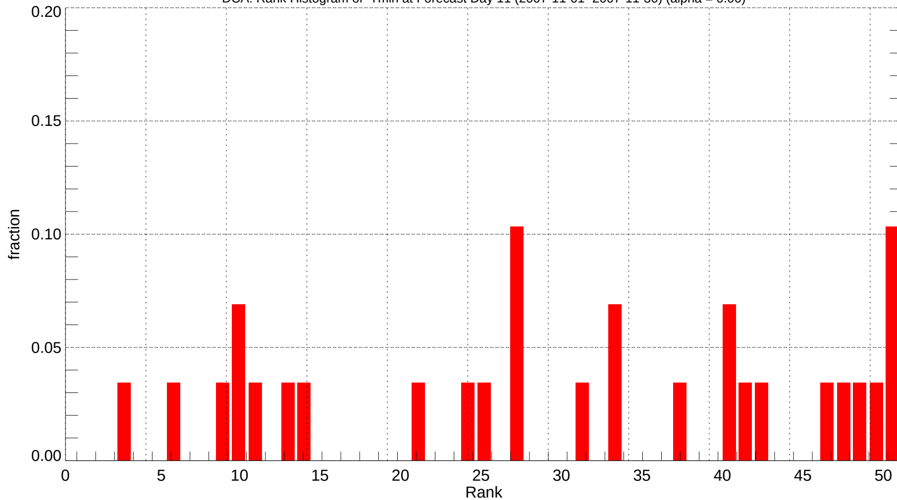
DCA: Rank Histogram of Tmin at Forecast Day 11 (2007-11-01~2007-11-30) (alpha = 0.00)
