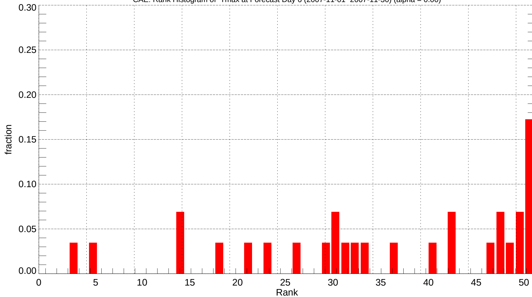
CAE: Rank Histogram of Tmax at Forecast Day 6 (2007-11-01~2007-11-30) (alpha = 0.00)
