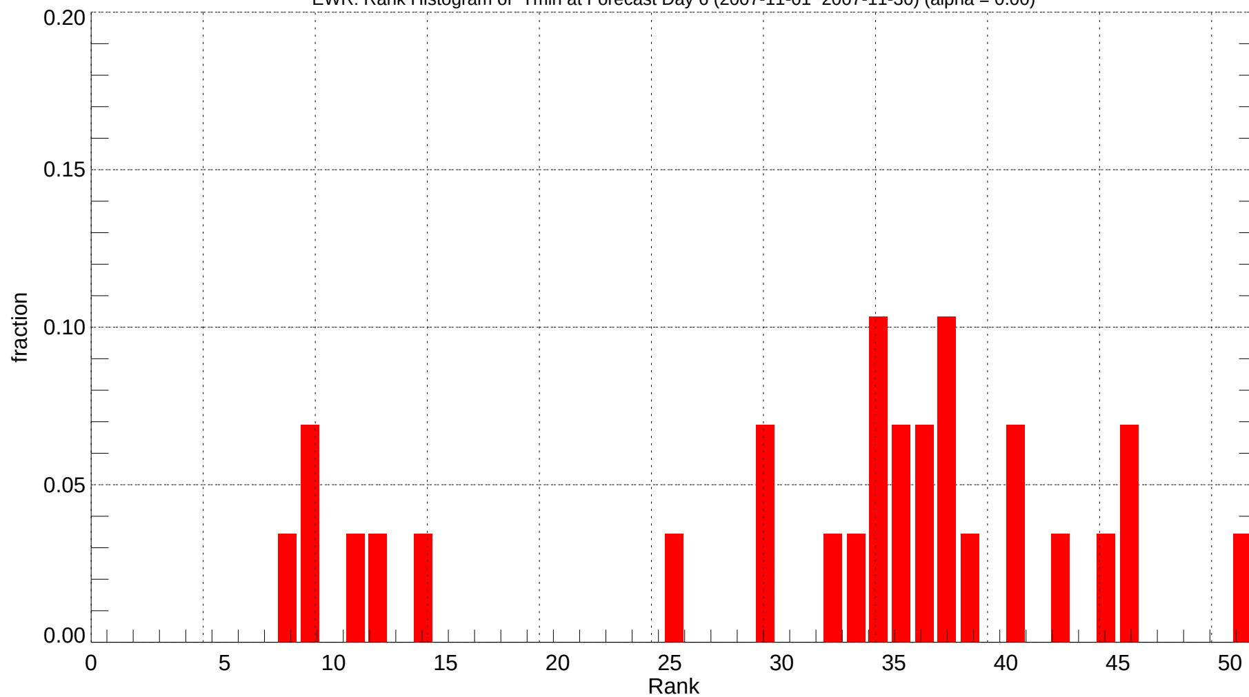
EWR: Rank Histogram of Tmin at Forecast Day 6 (2007-11-01~2007-11-30) (alpha = 0.00)
