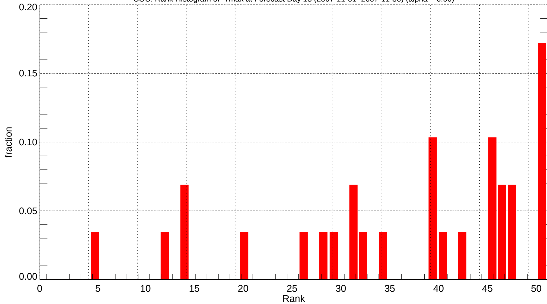
COU: Rank Histogram of Tmax at Forecast Day 13 (2007-11-01~2007-11-30) (alpha = 0.00)
