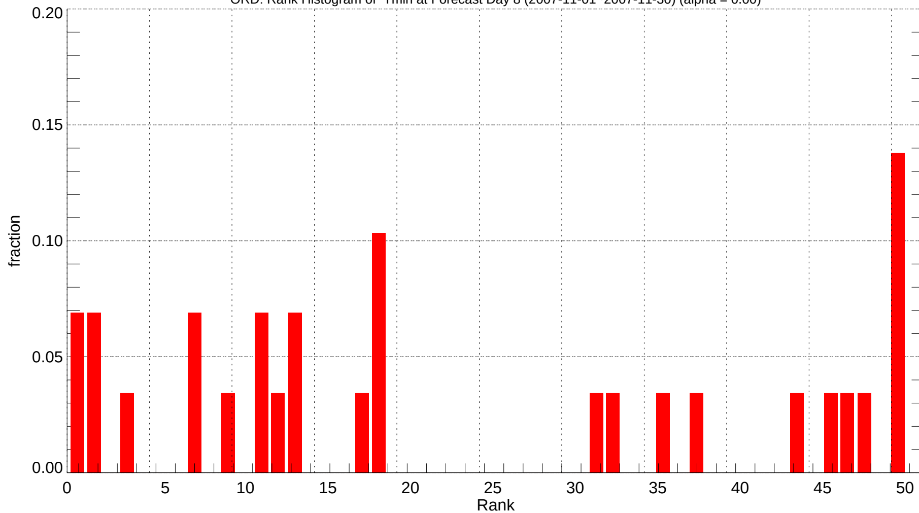
ORD: Rank Histogram of Tmin at Forecast Day 8 (2007-11-01~2007-11-30) (alpha = 0.00)
