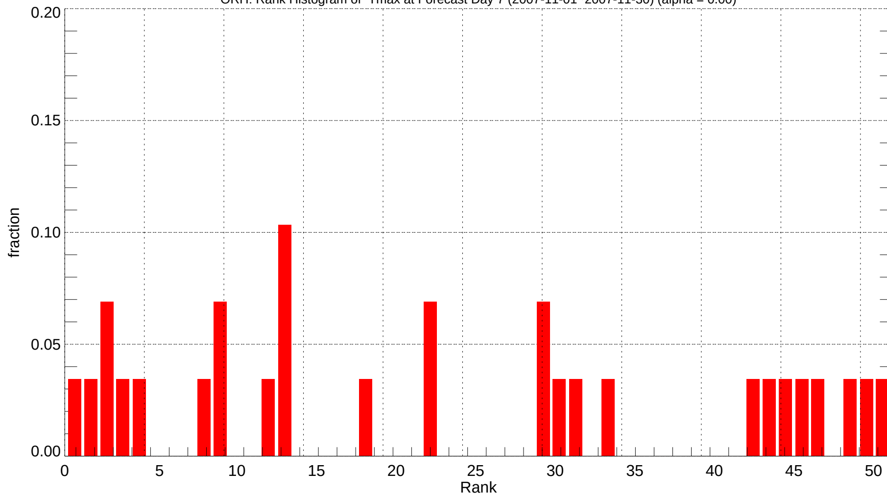
ORH: Rank Histogram of Tmax at Forecast Day 7 (2007-11-01~2007-11-30) (alpha = 0.00)
