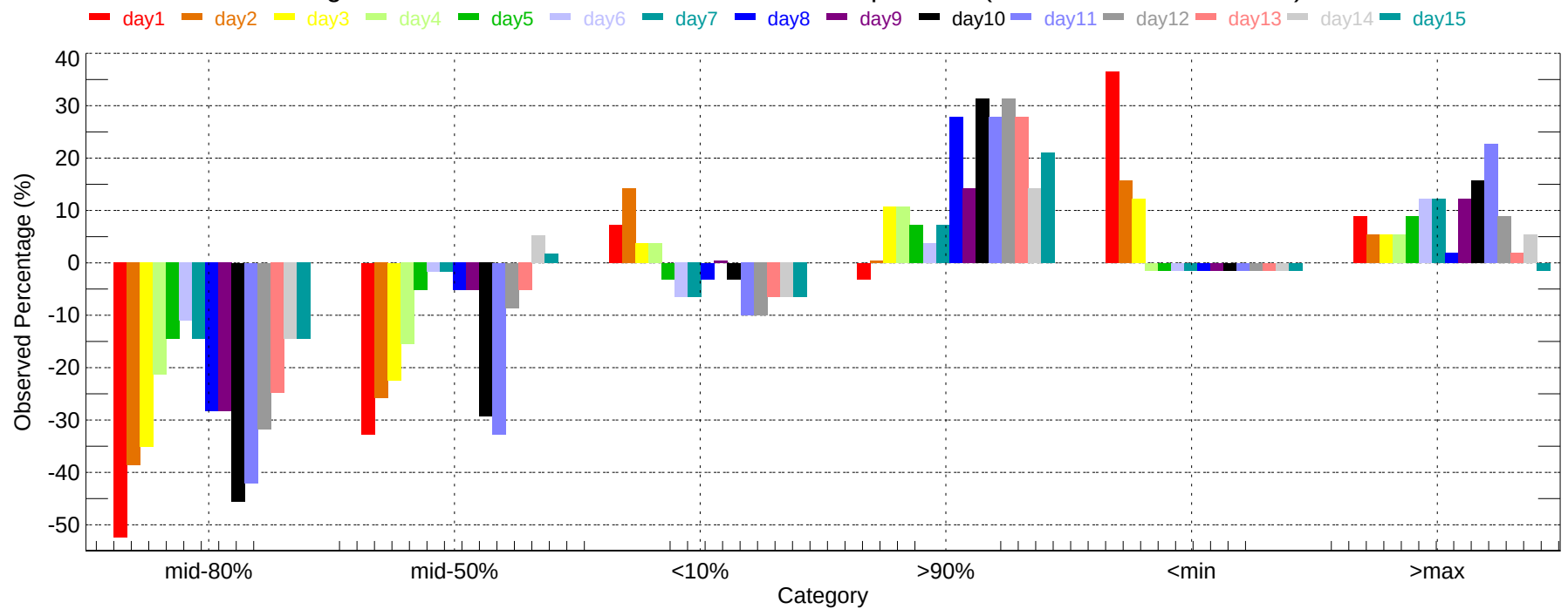
Observed Percentage Deviation of Ensembles - FSD: Max Temperature (2007-11-01~2007-11-30)
