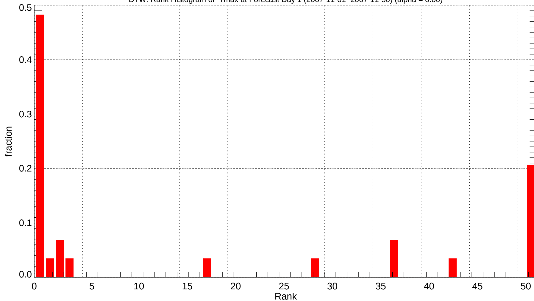
DTW: Rank Histogram of Tmax at Forecast Day 1 (2007-11-01~2007-11-30) (alpha = 0.00)
