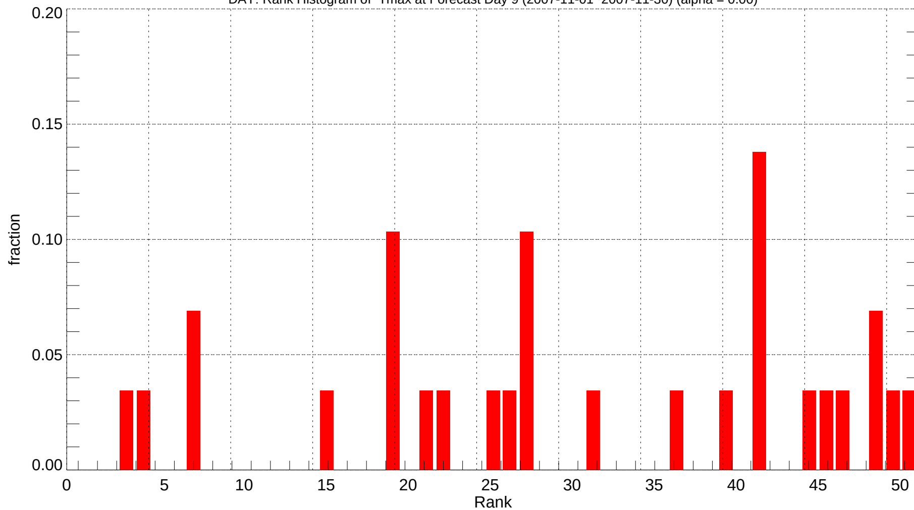
DAY: Rank Histogram of Tmax at Forecast Day 9 (2007-11-01~2007-11-30) (alpha = 0.00)
