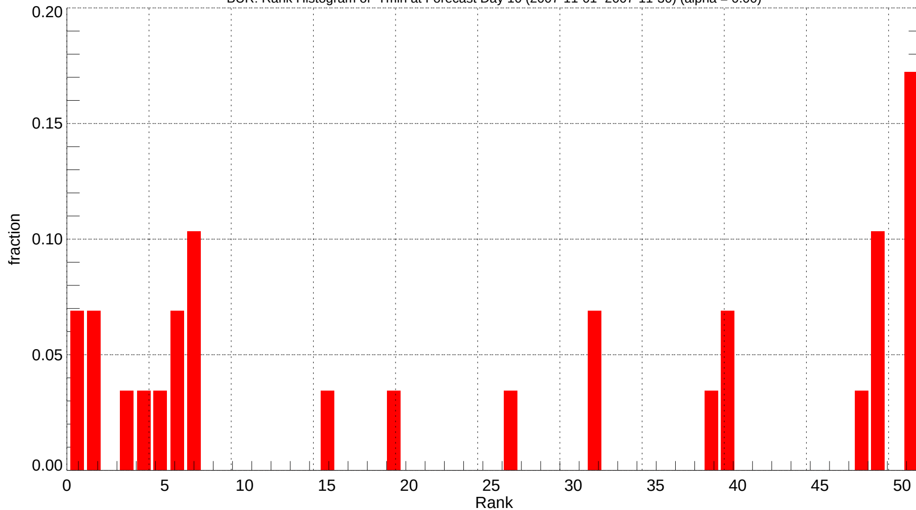
BUR: Rank Histogram of Tmin at Forecast Day 10 (2007-11-01~2007-11-30) (alpha = 0.00)
