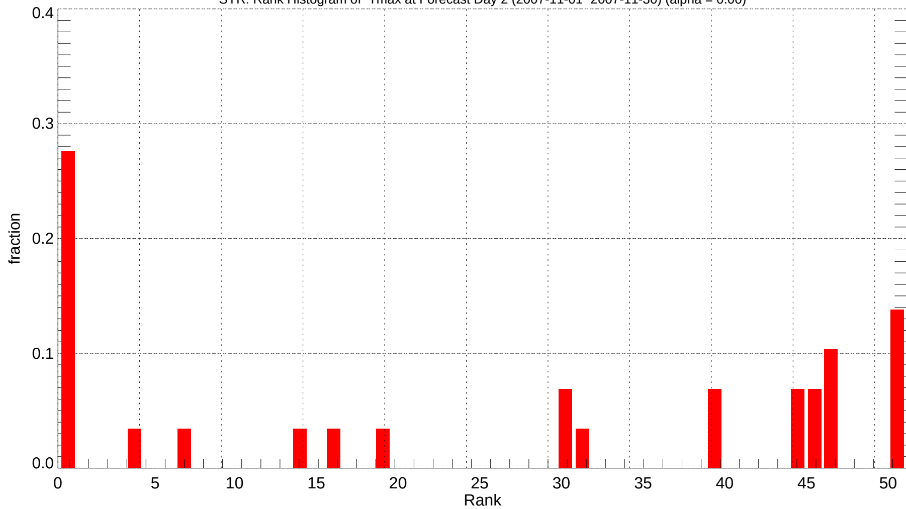
SYR: Rank Histogram of Tmax at Forecast Day 2 (2007-11-01~2007-11-30) (alpha = 0.00)
