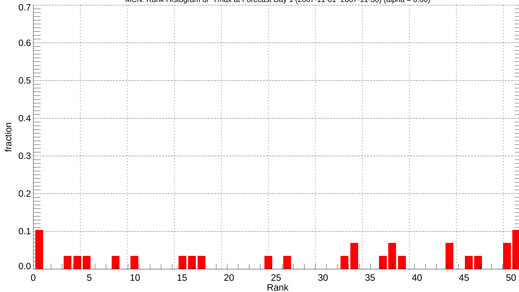
MCN: Rank Histogram of Tmax at Forecast Day 1 (2007-11-01~2007-11-30) (alpha = 0.00)
