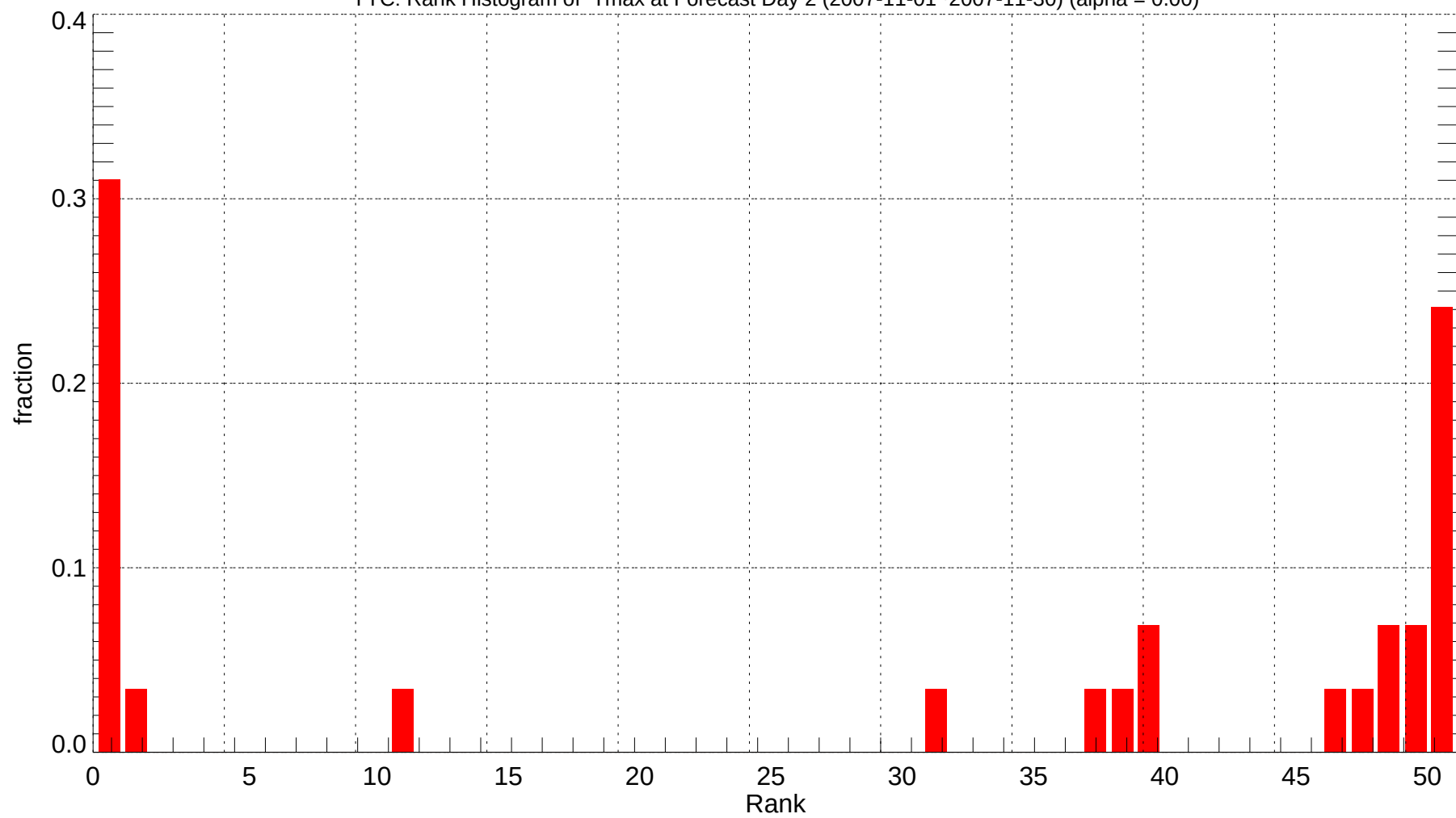
YYC: Rank Histogram of Tmax at Forecast Day 2 (2007-11-01~2007-11-30) (alpha = 0.00)
