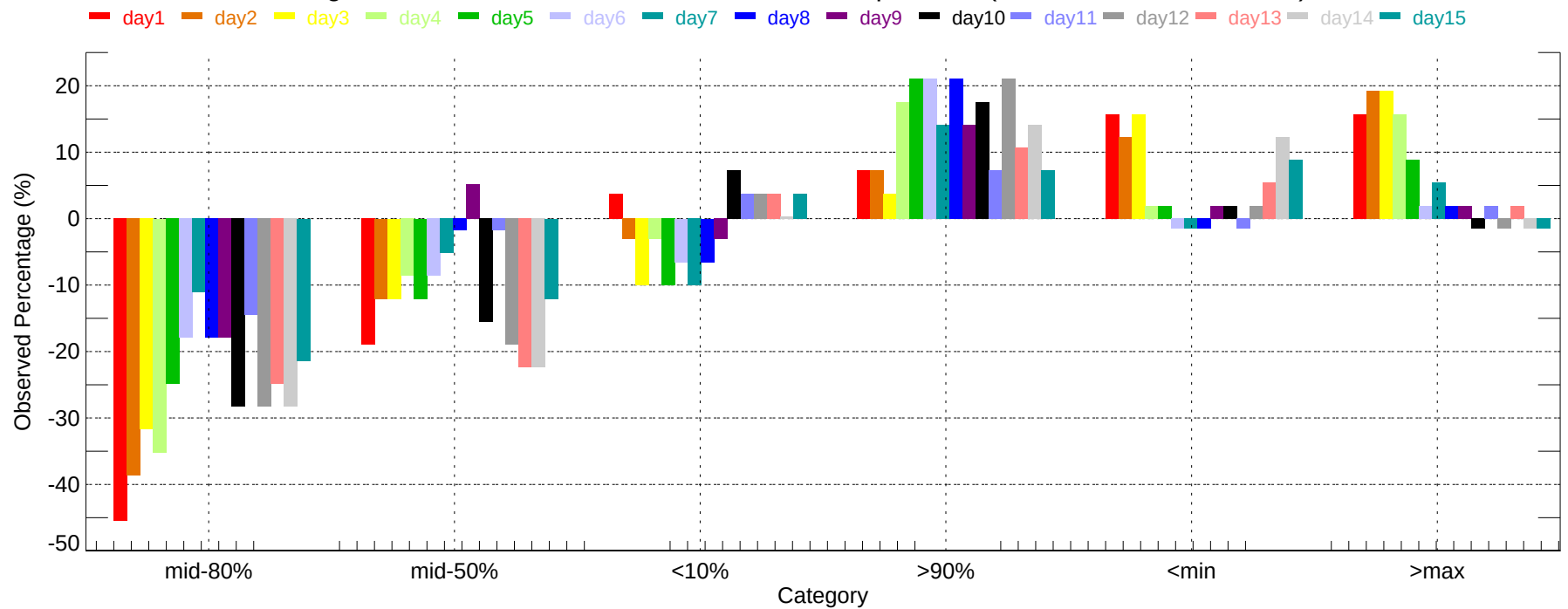
Observed Percentage Deviation of Ensembles - MBA: Max Temperature (2007-11-01~2007-11-30)
