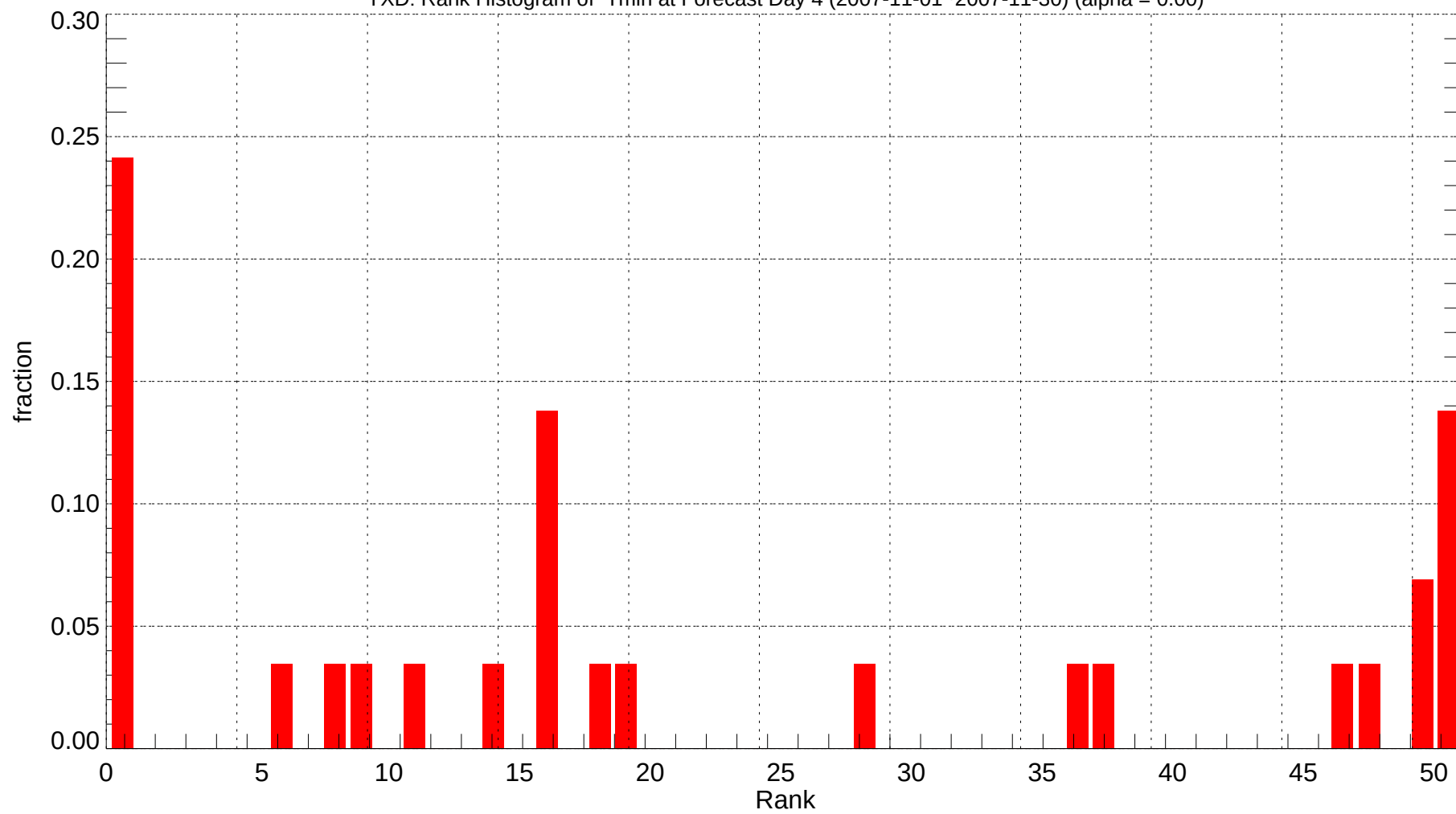
YXD: Rank Histogram of Tmin at Forecast Day 4 (2007-11-01~2007-11-30) (alpha = 0.00)
