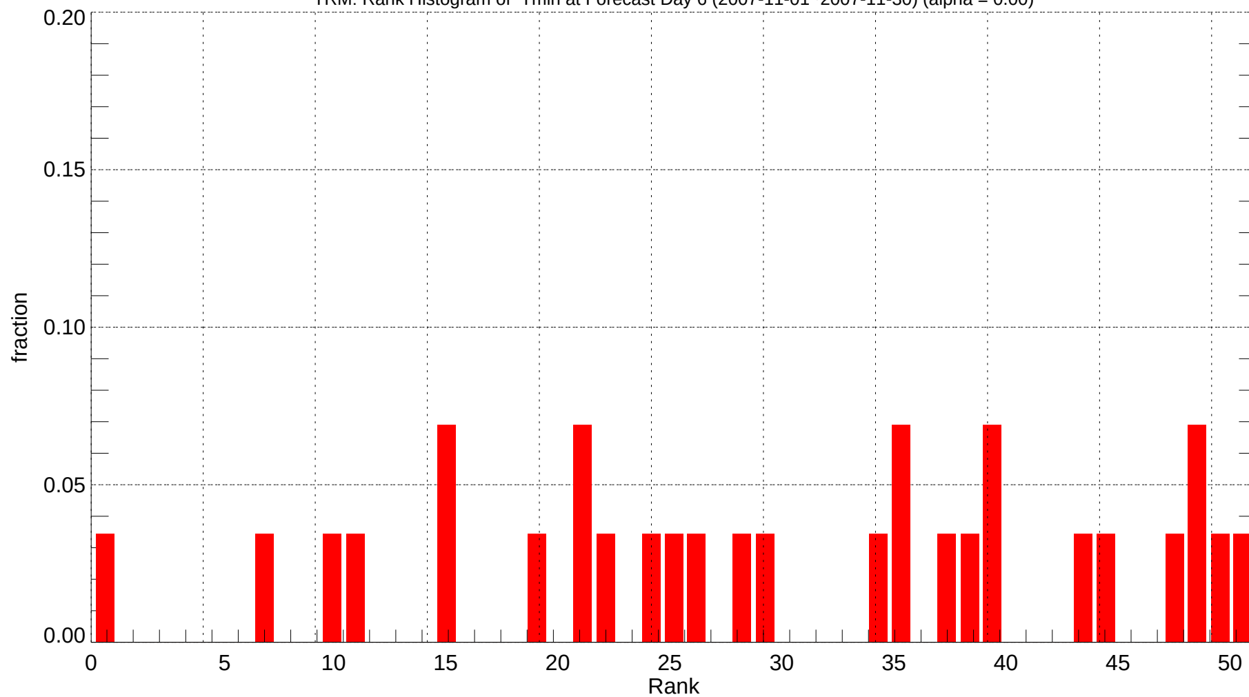
TRM: Rank Histogram of Tmin at Forecast Day 6 (2007-11-01~2007-11-30) (alpha = 0.00)
