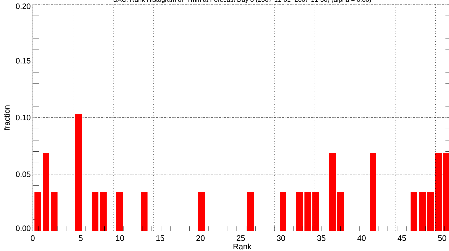
SAC: Rank Histogram of Tmin at Forecast Day 8 (2007-11-01~2007-11-30) (alpha = 0.00)
