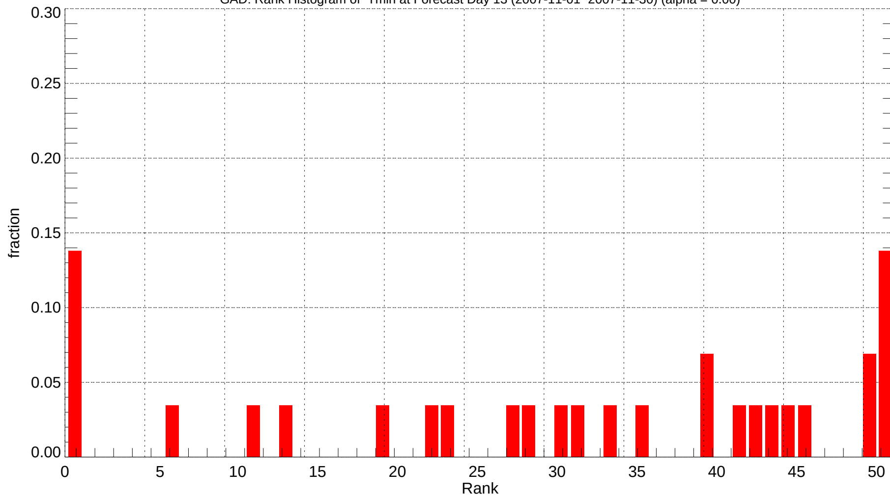
GAD: Rank Histogram of Tmin at Forecast Day 13 (2007-11-01~2007-11-30) (alpha = 0.00)
