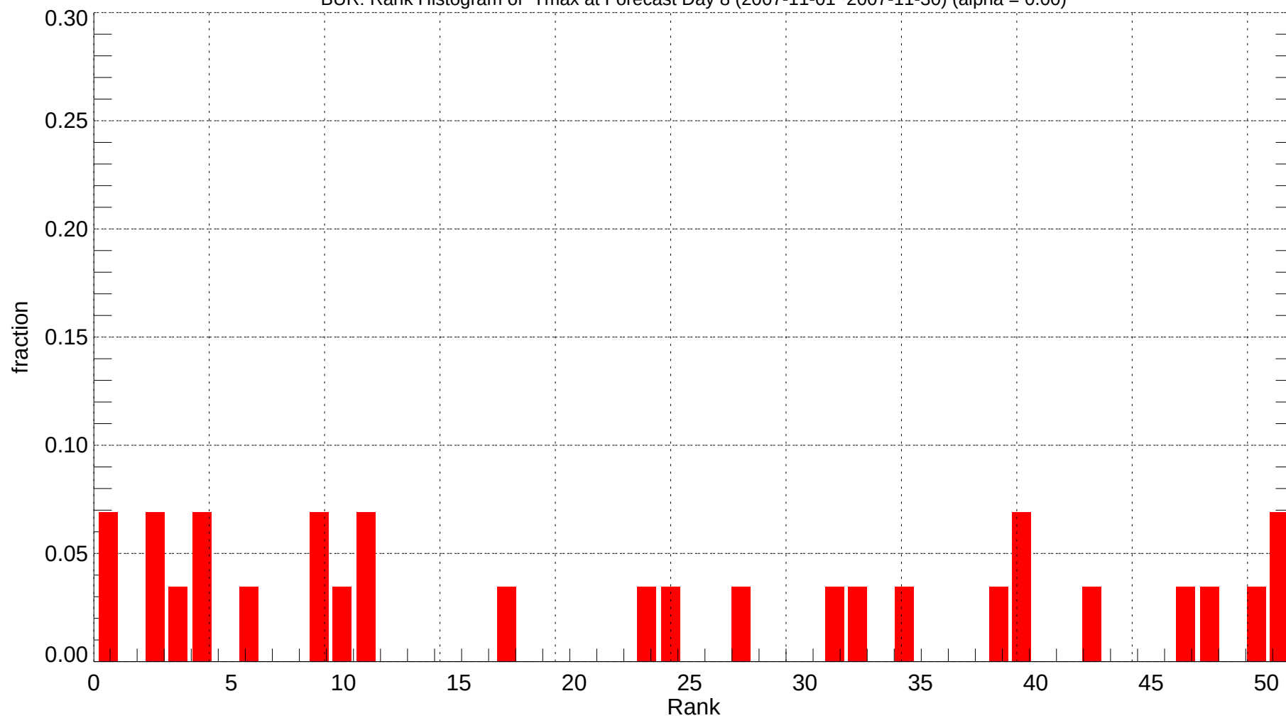
BUR: Rank Histogram of Tmax at Forecast Day 8 (2007-11-01~2007-11-30) (alpha = 0.00)
