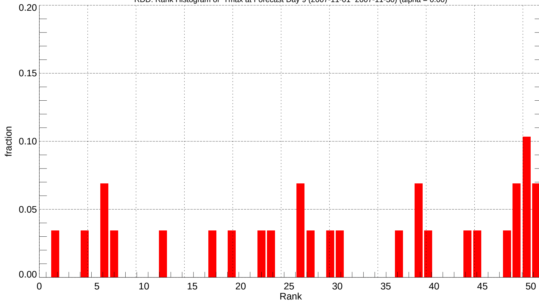
RDD: Rank Histogram of Tmax at Forecast Day 9 (2007-11-01~2007-11-30) (alpha = 0.00)
