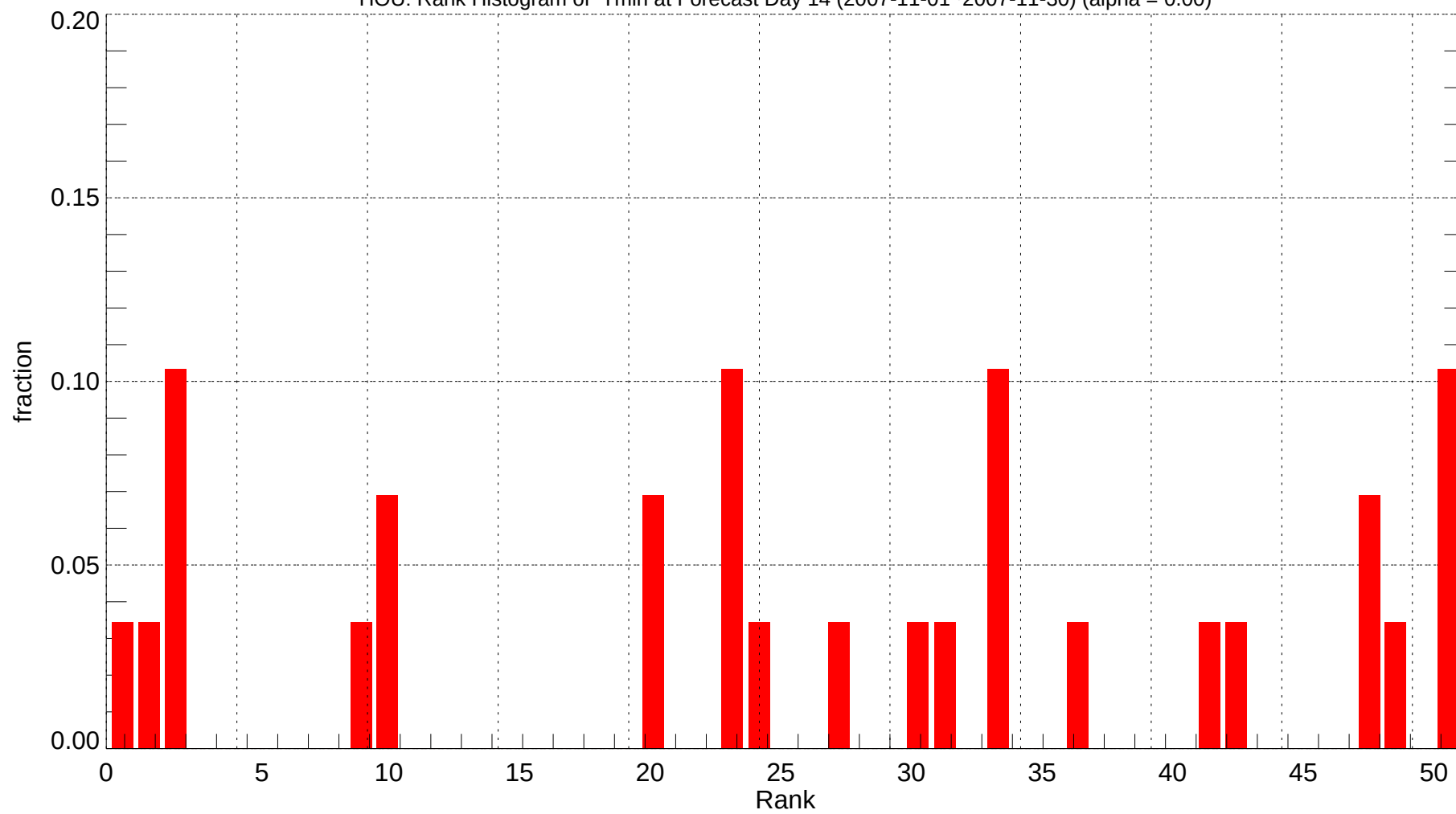
HOU: Rank Histogram of Tmin at Forecast Day 14 (2007-11-01~2007-11-30) (alpha = 0.00)
