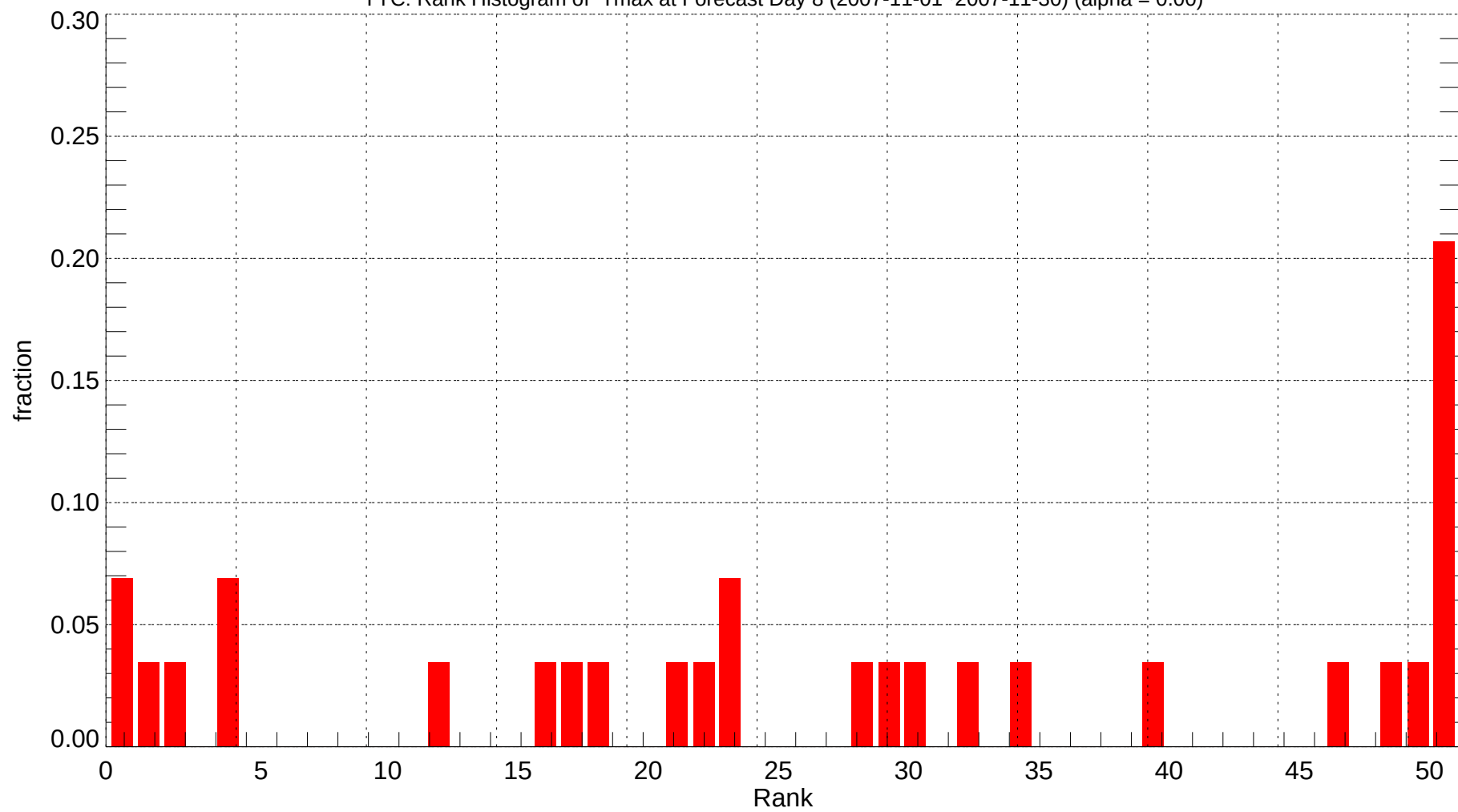
YYC: Rank Histogram of Tmax at Forecast Day 8 (2007-11-01~2007-11-30) (alpha = 0.00)
