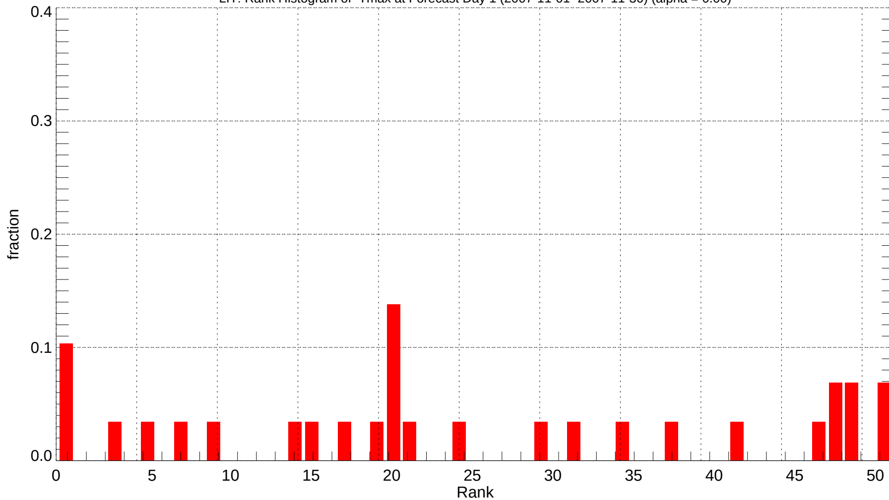
LIT: Rank Histogram of Tmax at Forecast Day 1 (2007-11-01~2007-11-30) (alpha = 0.00)
