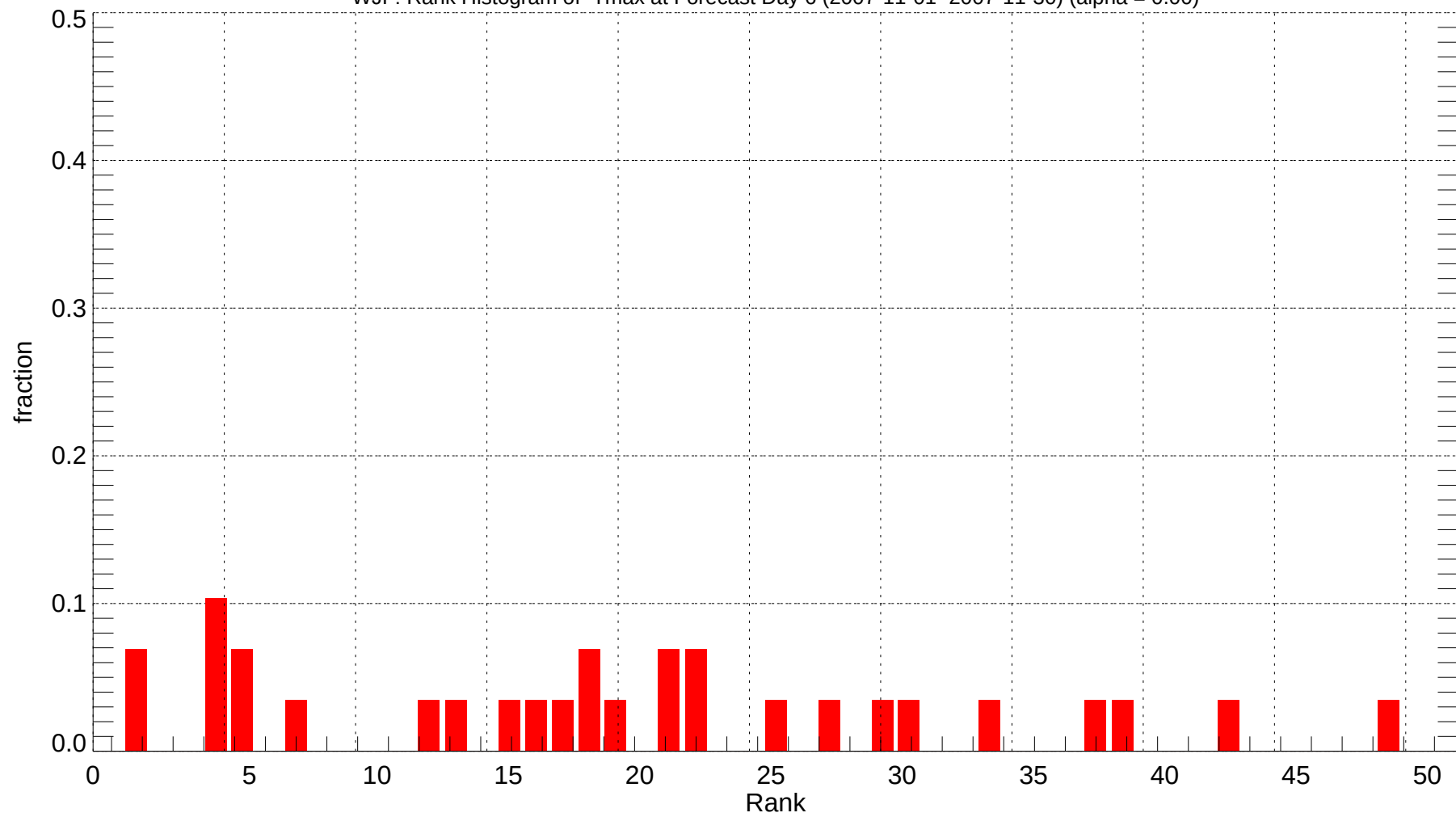
WJF: Rank Histogram of Tmax at Forecast Day 6 (2007-11-01~2007-11-30) (alpha = 0.00)
