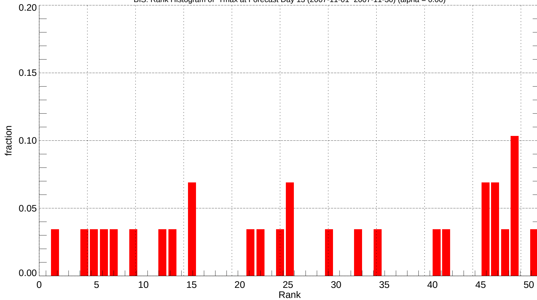
BIS: Rank Histogram of Tmax at Forecast Day 13 (2007-11-01~2007-11-30) (alpha = 0.00)
