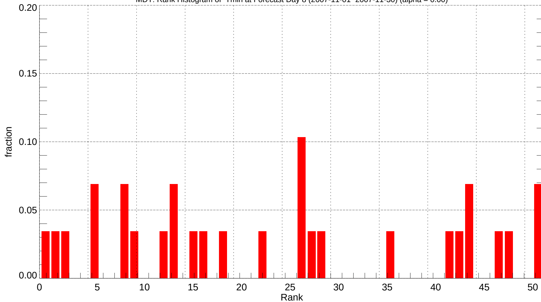
MDT: Rank Histogram of Tmin at Forecast Day 8 (2007-11-01~2007-11-30) (alpha = 0.00)
