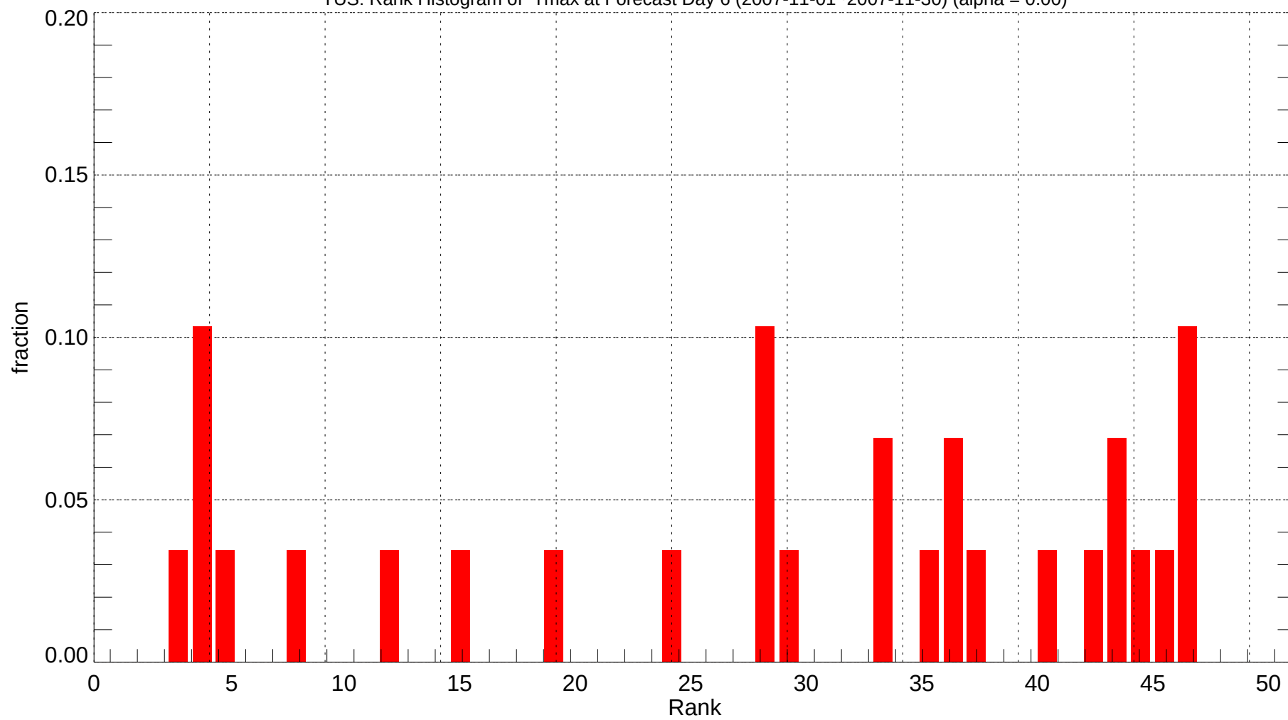
TUS: Rank Histogram of Tmax at Forecast Day 6 (2007-11-01~2007-11-30) (alpha = 0.00)
