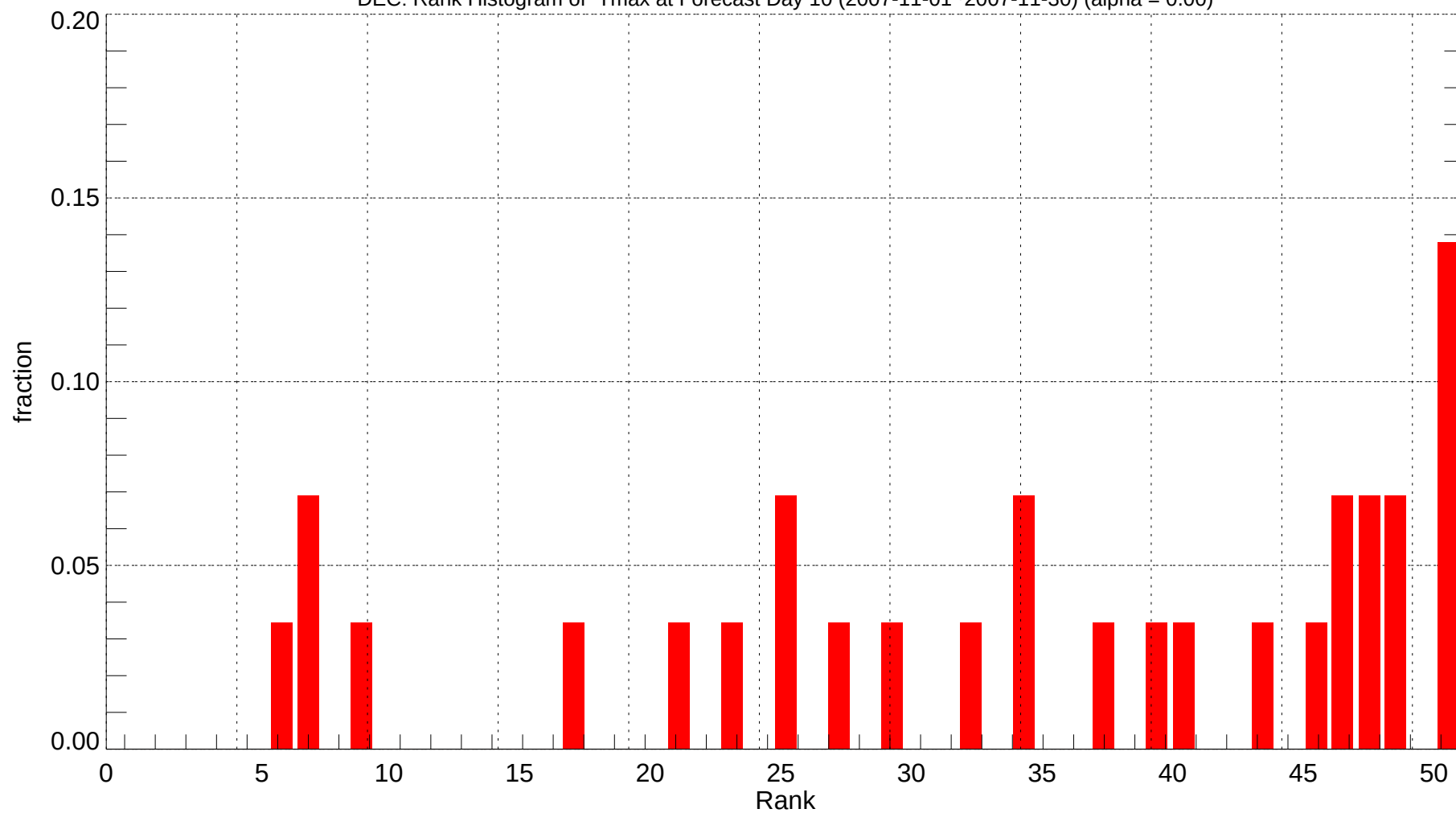
DEC: Rank Histogram of Tmax at Forecast Day 10 (2007-11-01~2007-11-30) (alpha = 0.00)
