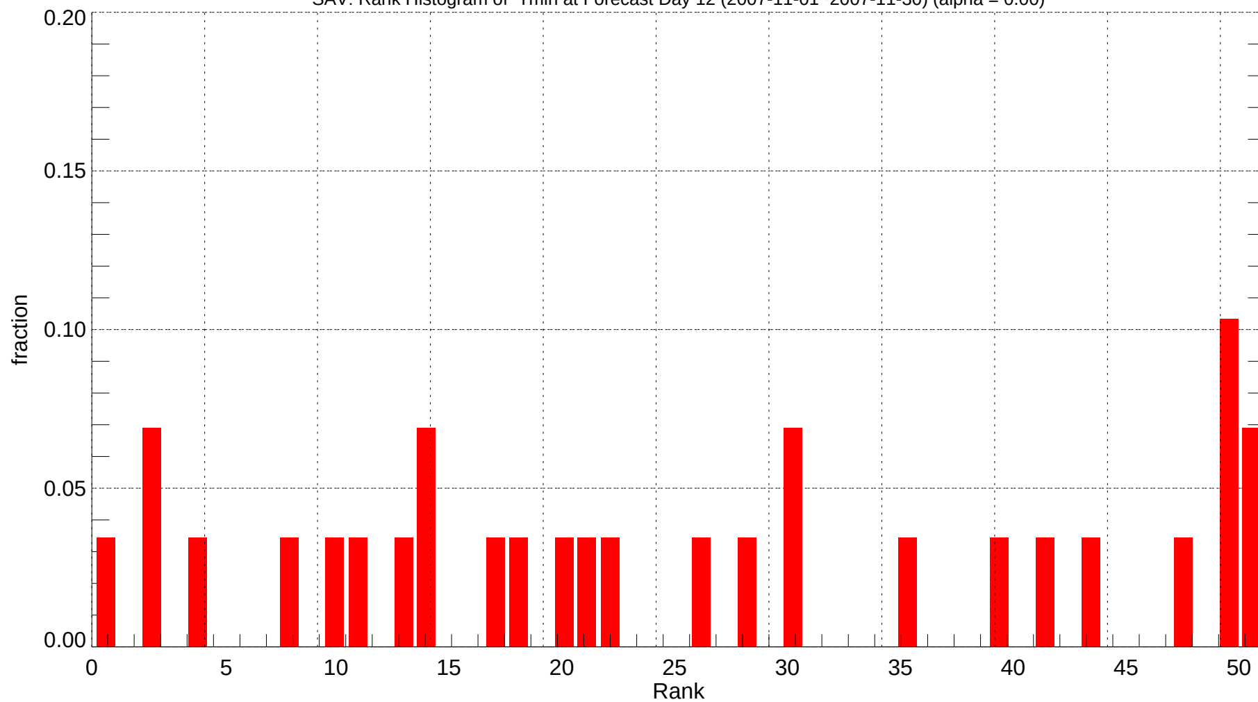
SAV: Rank Histogram of Tmin at Forecast Day 12 (2007-11-01~2007-11-30) (alpha = 0.00)
