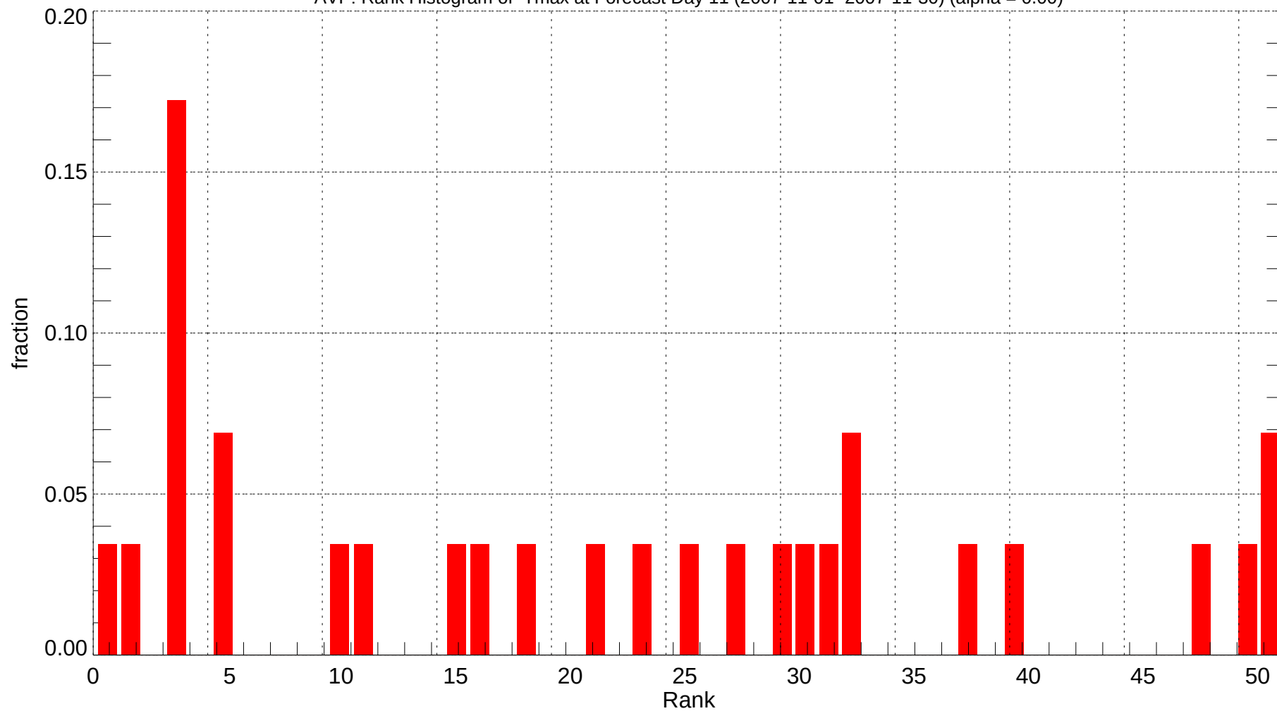
AVP: Rank Histogram of Tmax at Forecast Day 11 (2007-11-01~2007-11-30) (alpha = 0.00)
