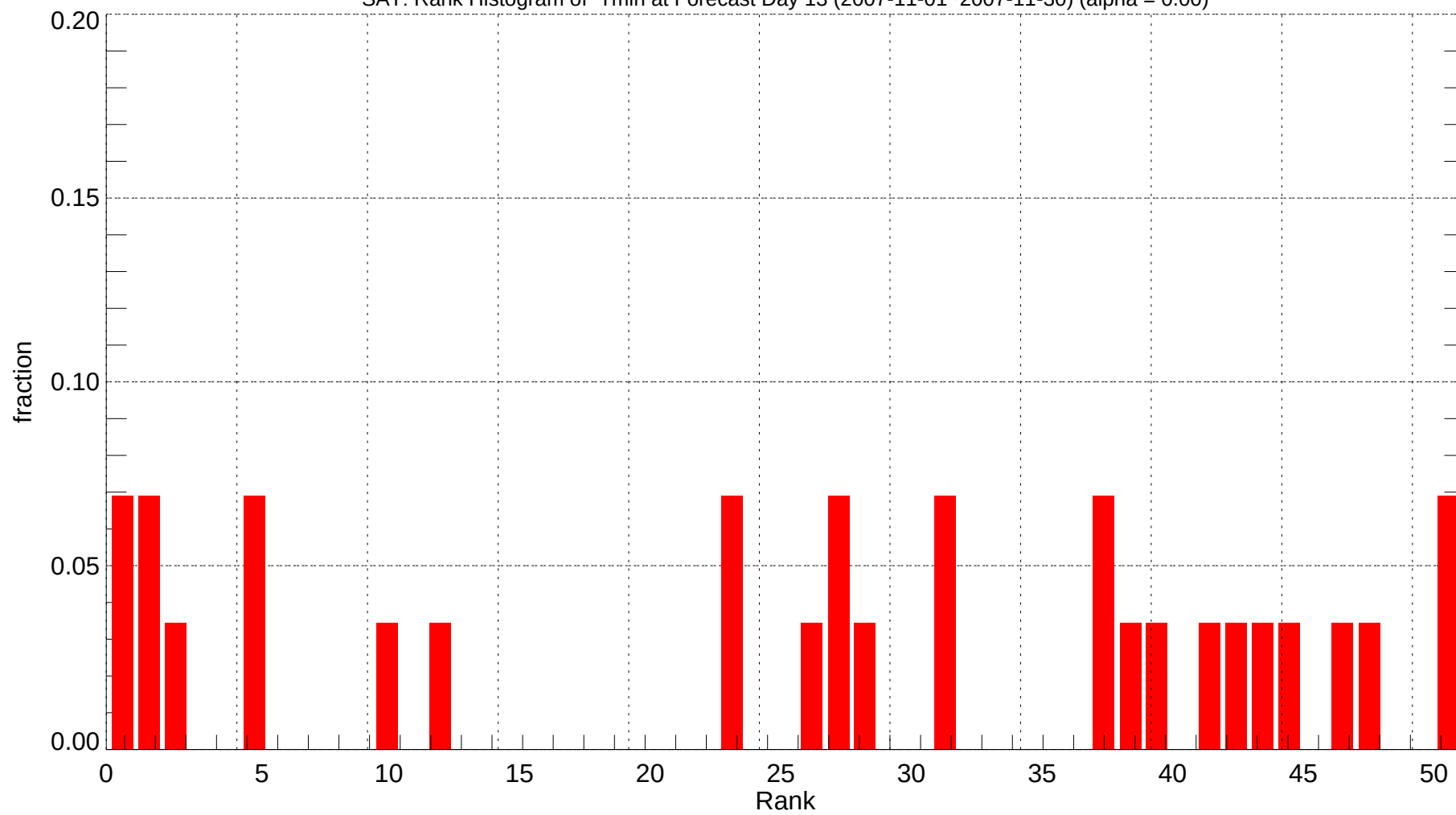
SAT: Rank Histogram of Tmin at Forecast Day 13 (2007-11-01~2007-11-30) (alpha = 0.00)
