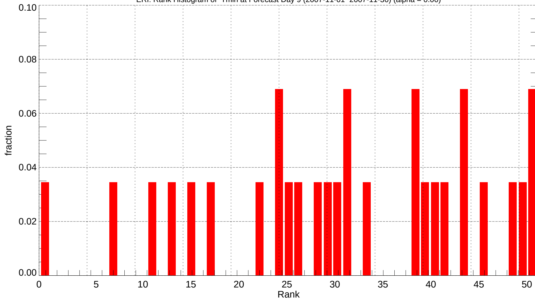
ERI: Rank Histogram of Tmin at Forecast Day 9 (2007-11-01~2007-11-30) (alpha = 0.00)
