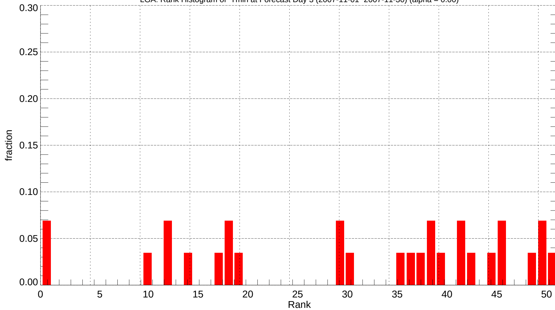
LGA: Rank Histogram of Tmin at Forecast Day 3 (2007-11-01~2007-11-30) (alpha = 0.00)
