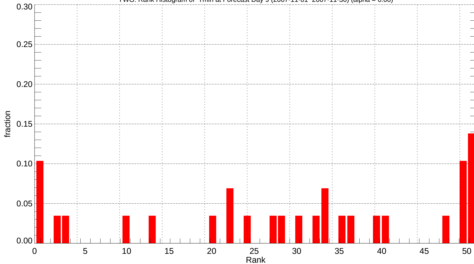
YWG: Rank Histogram of Tmin at Forecast Day 9 (2007-11-01~2007-11-30) (alpha = 0.00)
