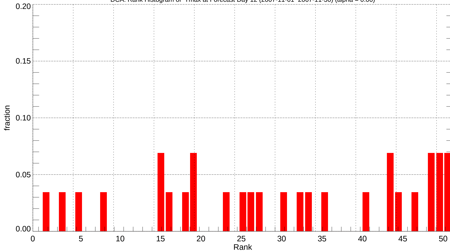
DCA: Rank Histogram of Tmax at Forecast Day 12 (2007-11-01~2007-11-30) (alpha = 0.00)
