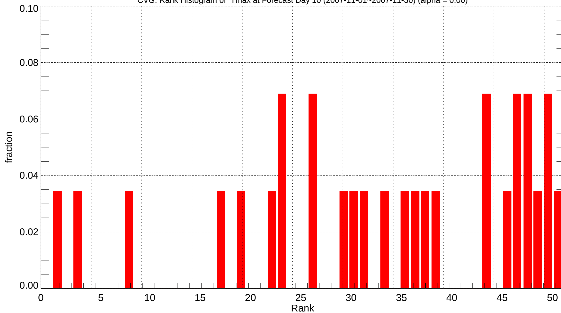
CVG: Rank Histogram of Tmax at Forecast Day 10 (2007-11-01~2007-11-30) (alpha = 0.00)
