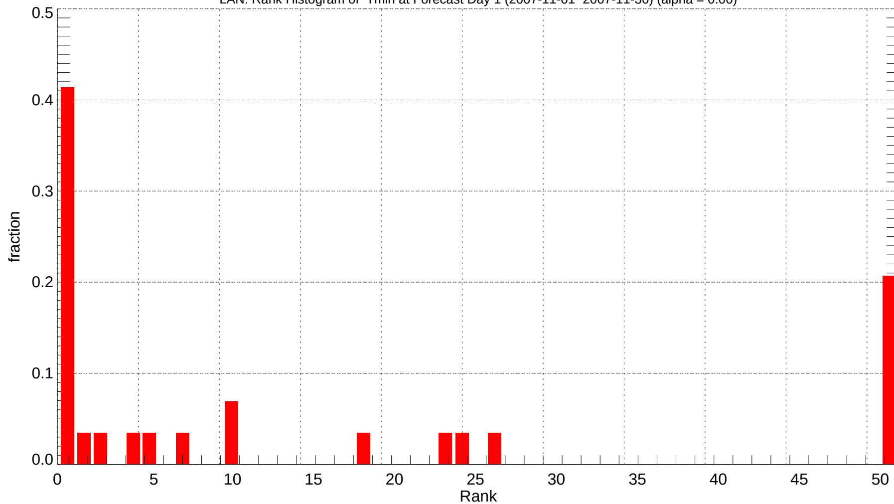
LAN: Rank Histogram of Tmin at Forecast Day 1 (2007-11-01~2007-11-30) (alpha = 0.00)
