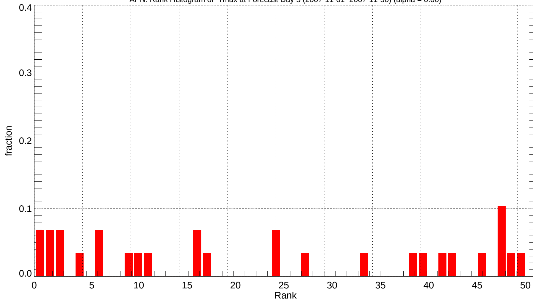
APN: Rank Histogram of Tmax at Forecast Day 3 (2007-11-01~2007-11-30) (alpha = 0.00)
