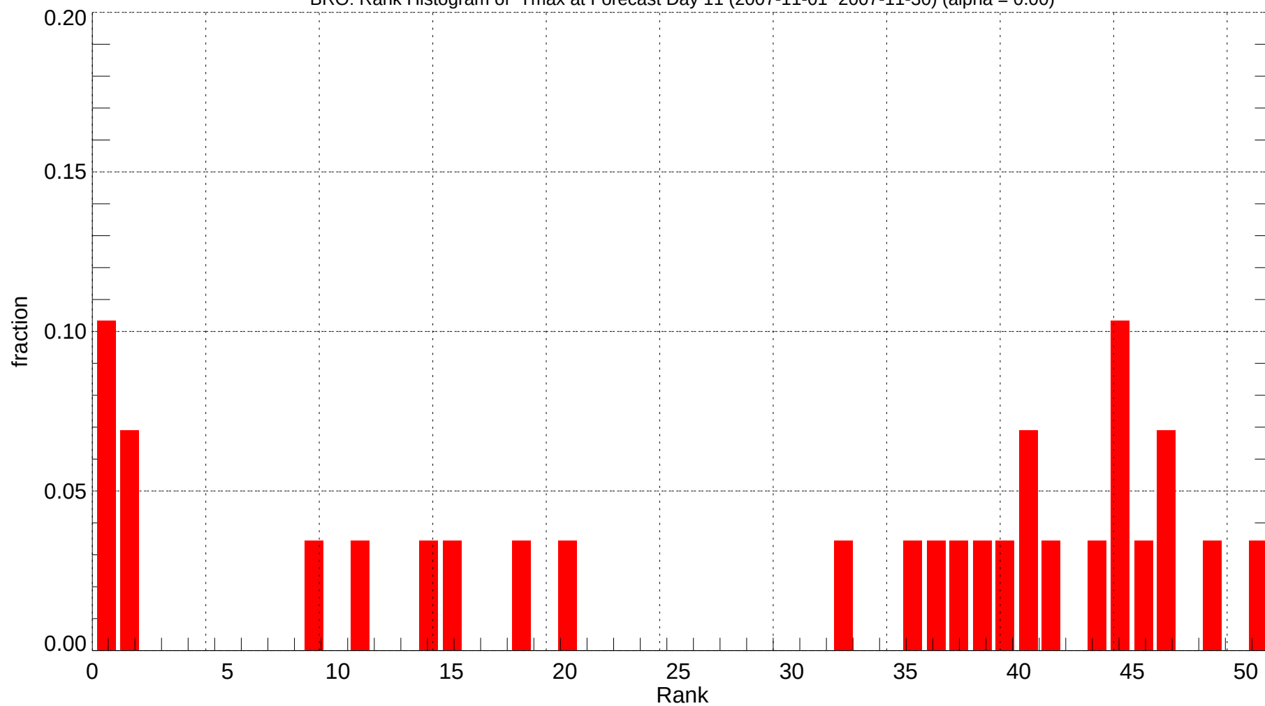
BRO: Rank Histogram of Tmax at Forecast Day 11 (2007-11-01~2007-11-30) (alpha = 0.00)
