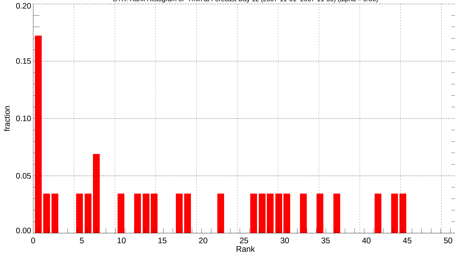
SYR: Rank Histogram of Tmin at Forecast Day 12 (2007-11-01~2007-11-30) (alpha = 0.00)
