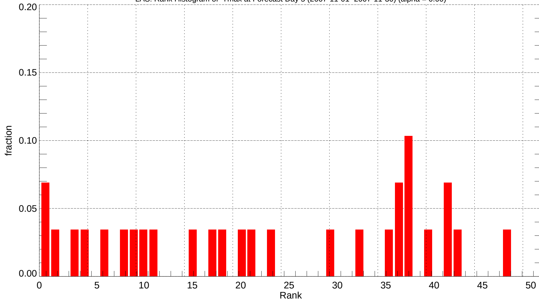
LAS: Rank Histogram of Tmax at Forecast Day 5 (2007-11-01~2007-11-30) (alpha = 0.00)
