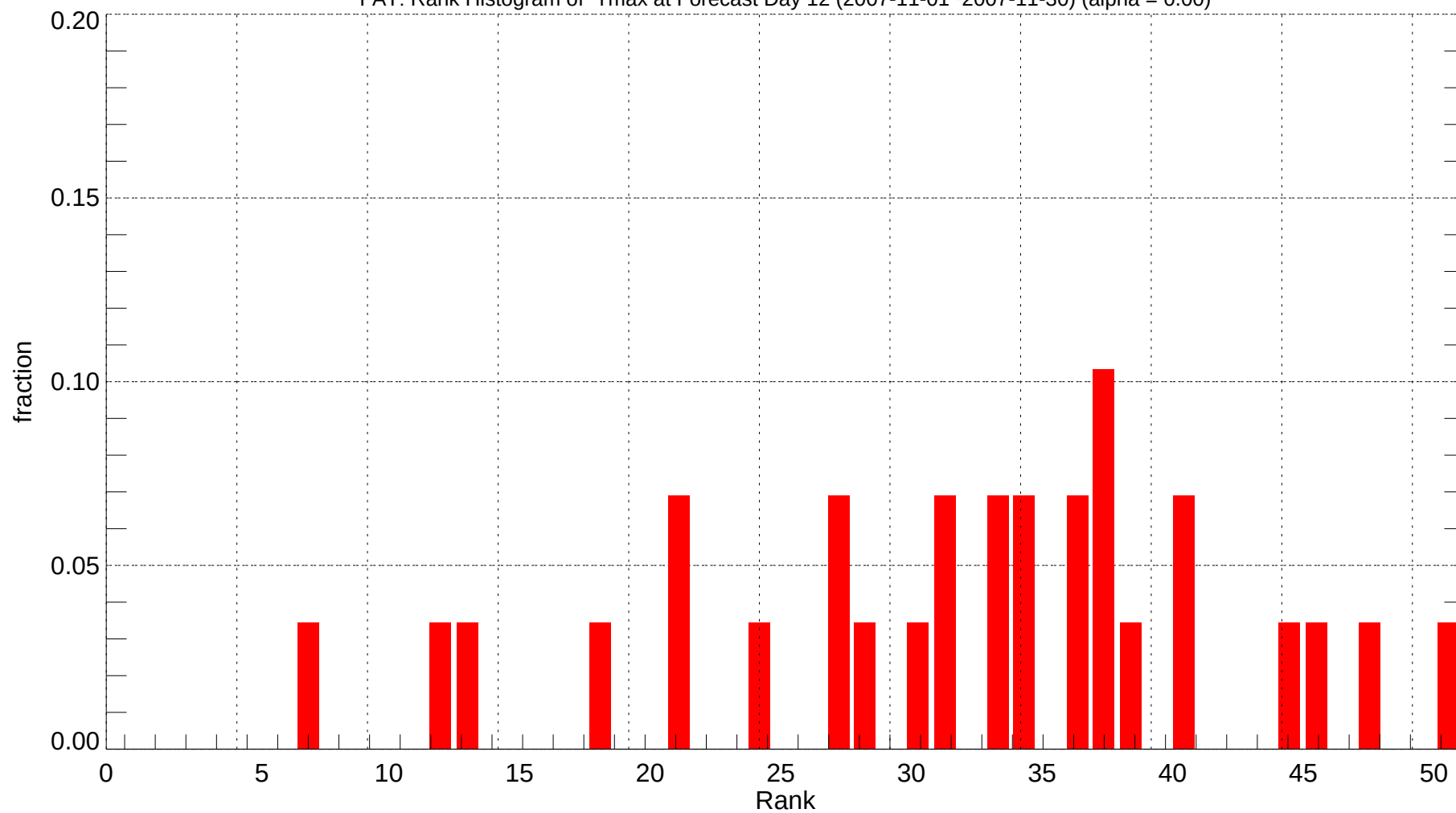
FAT: Rank Histogram of Tmax at Forecast Day 12 (2007-11-01~2007-11-30) (alpha = 0.00)
