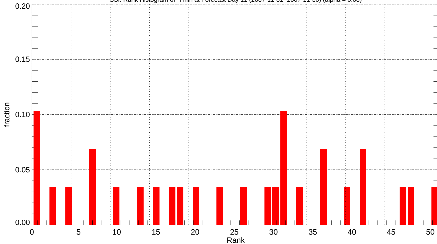
SSI: Rank Histogram of Tmin at Forecast Day 11 (2007-11-01~2007-11-30) (alpha = 0.00)
