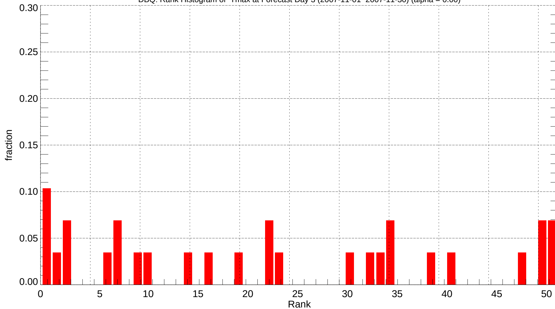
DBQ: Rank Histogram of Tmax at Forecast Day 3 (2007-11-01~2007-11-30) (alpha = 0.00)
