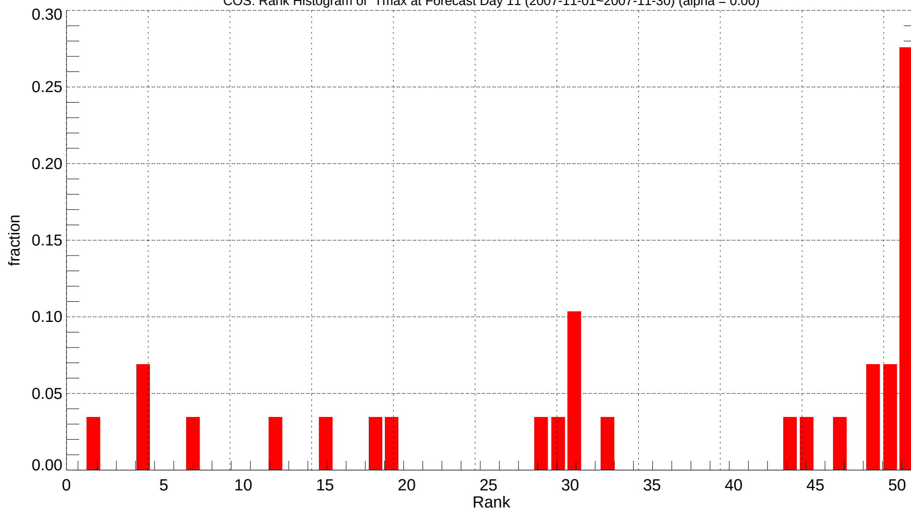
COS: Rank Histogram of Tmax at Forecast Day 11 (2007-11-01~2007-11-30) (alpha = 0.00)
