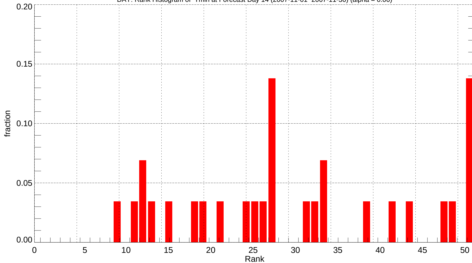
DAY: Rank Histogram of Tmin at Forecast Day 14 (2007-11-01~2007-11-30) (alpha = 0.00)
