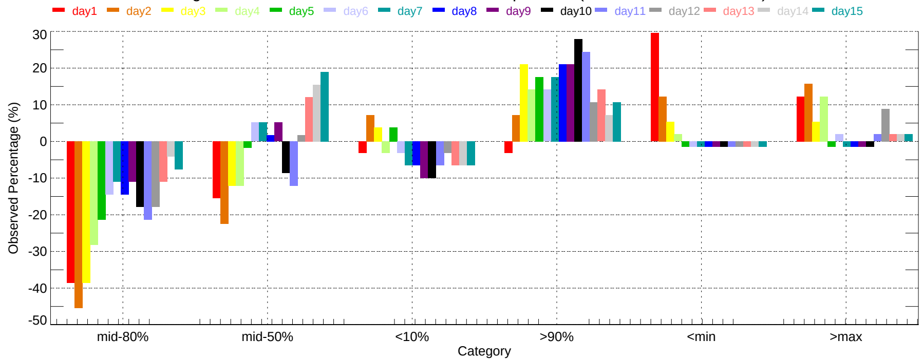
Observed Percentage Deviation of Ensembles - MOB: Min Temperature (2007-11-01~2007-11-30)
