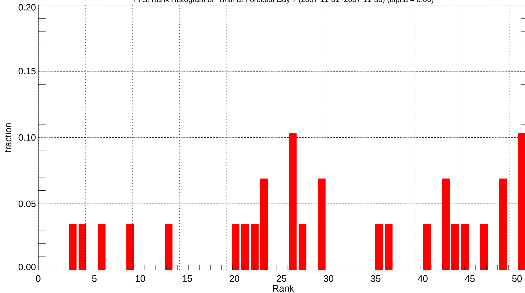
TYS: Rank Histogram of Tmin at Forecast Day 7 (2007-11-01~2007-11-30) (alpha = 0.00)
