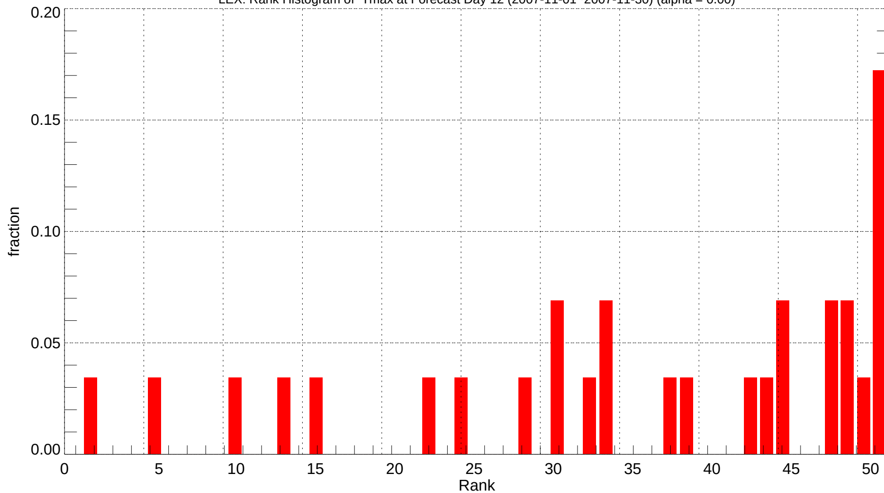
LEX: Rank Histogram of Tmax at Forecast Day 12 (2007-11-01~2007-11-30) (alpha = 0.00)
