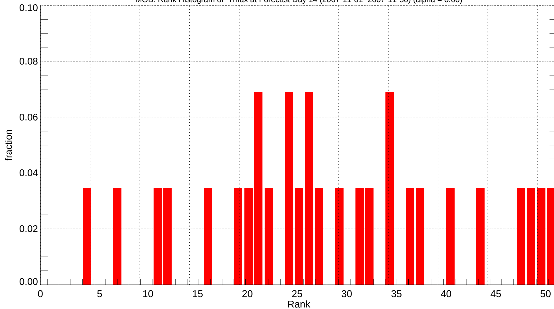
MOB: Rank Histogram of Tmax at Forecast Day 14 (2007-11-01~2007-11-30) (alpha = 0.00)
