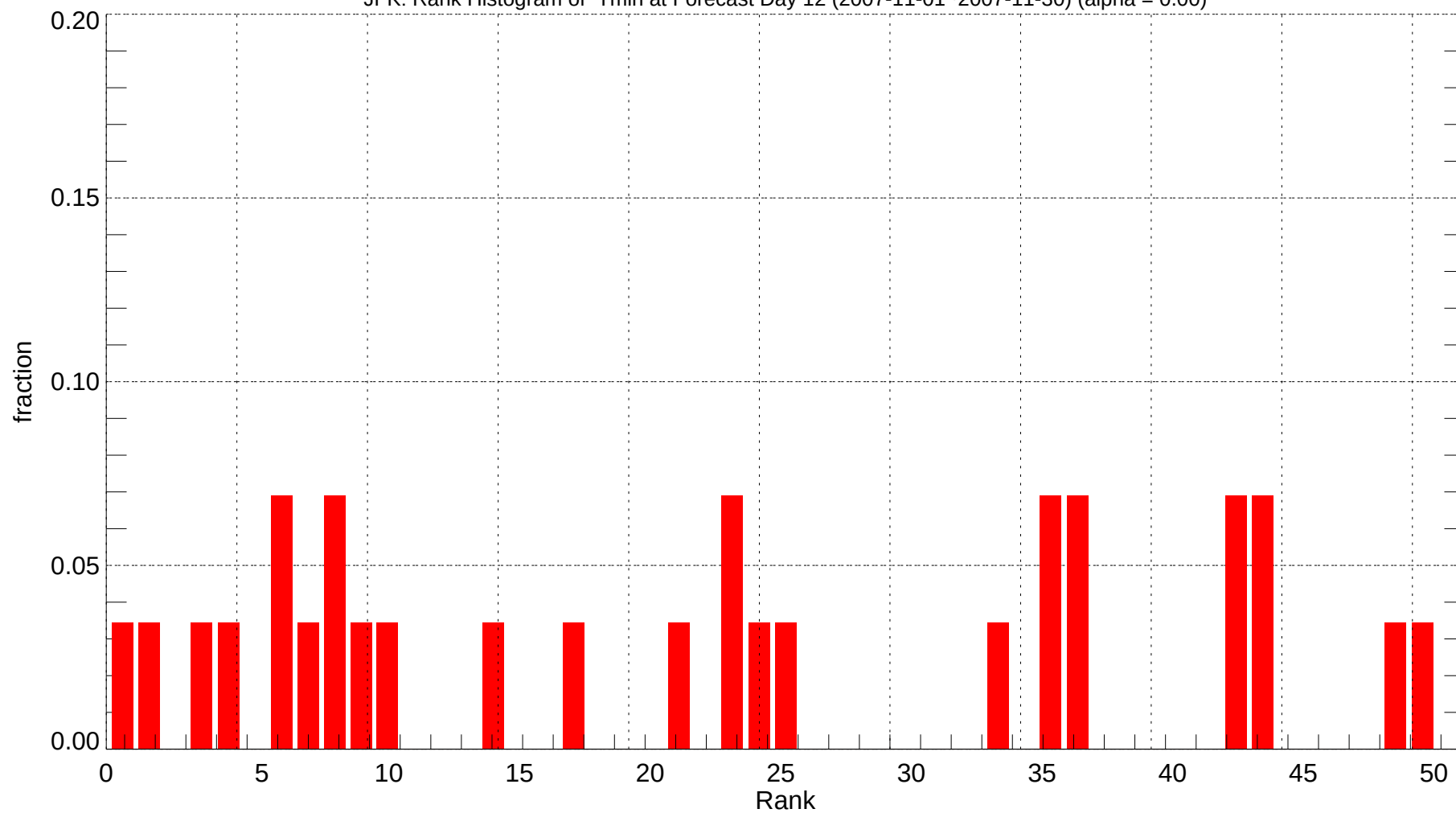
JFK: Rank Histogram of Tmin at Forecast Day 12 (2007-11-01~2007-11-30) (alpha = 0.00)
