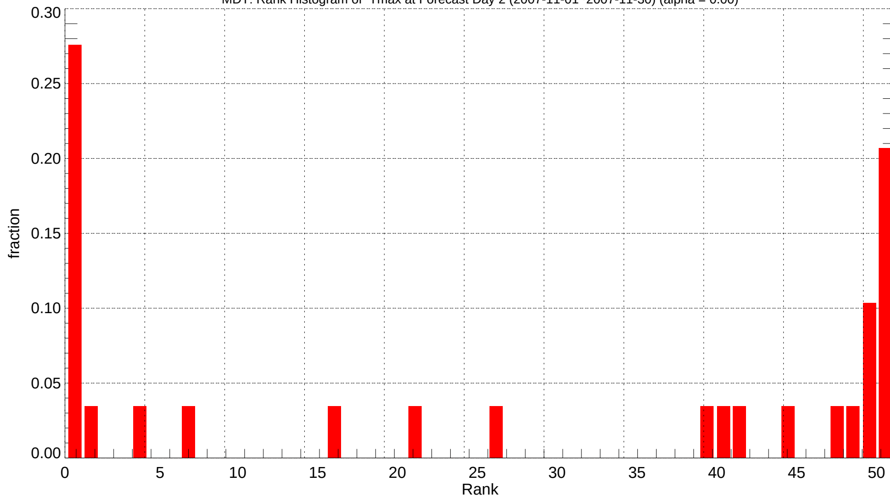
MDT: Rank Histogram of Tmax at Forecast Day 2 (2007-11-01~2007-11-30) (alpha = 0.00)
