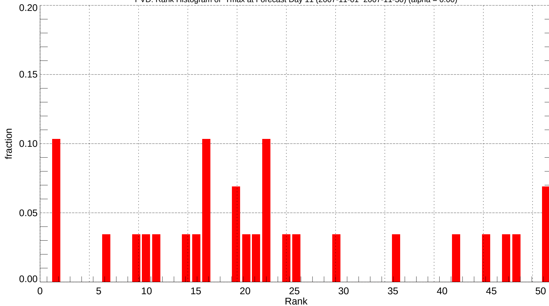
PVD: Rank Histogram of Tmax at Forecast Day 11 (2007-11-01~2007-11-30) (alpha = 0.00)
