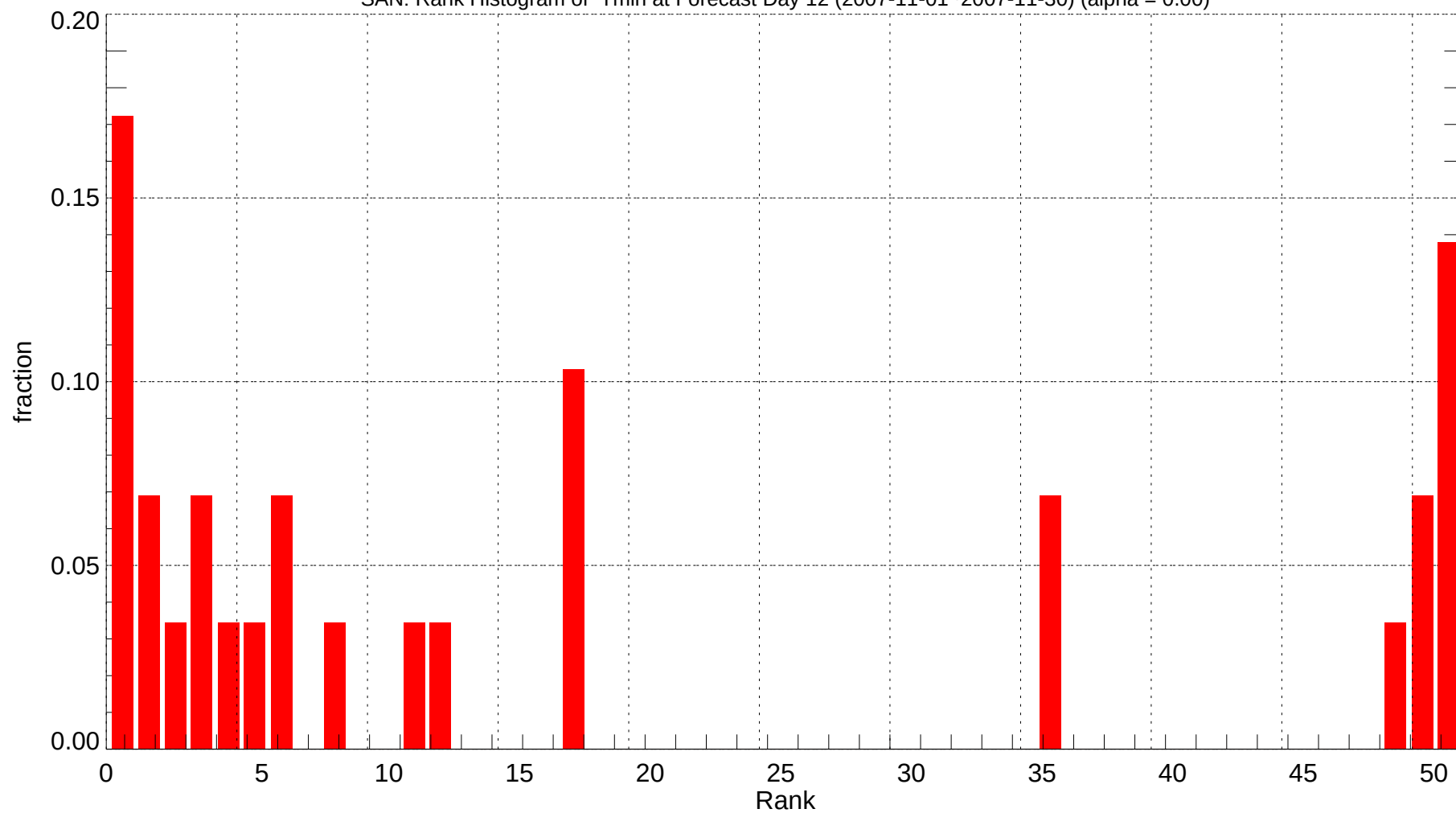
SAN: Rank Histogram of Tmin at Forecast Day 12 (2007-11-01~2007-11-30) (alpha = 0.00)
