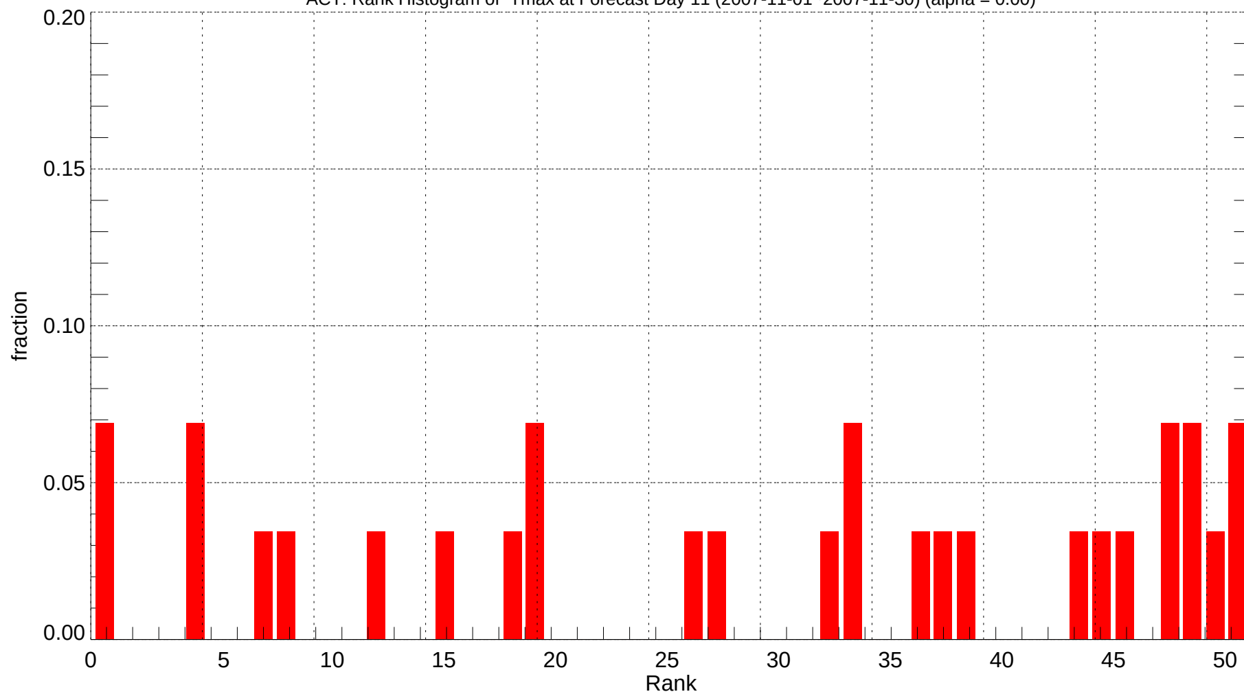
ACT: Rank Histogram of Tmax at Forecast Day 11 (2007-11-01~2007-11-30) (alpha = 0.00)
