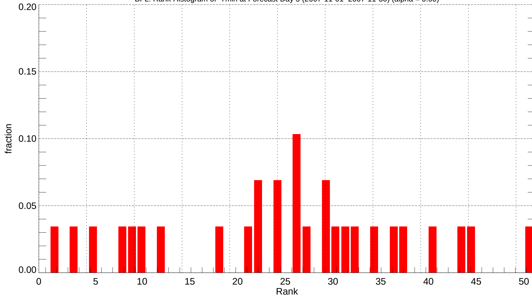
BFL: Rank Histogram of Tmin at Forecast Day 5 (2007-11-01~2007-11-30) (alpha = 0.00)
