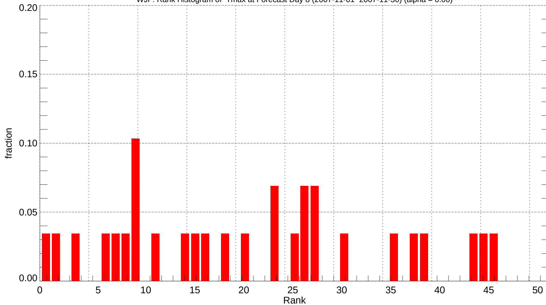
WJF: Rank Histogram of Tmax at Forecast Day 8 (2007-11-01~2007-11-30) (alpha = 0.00)
