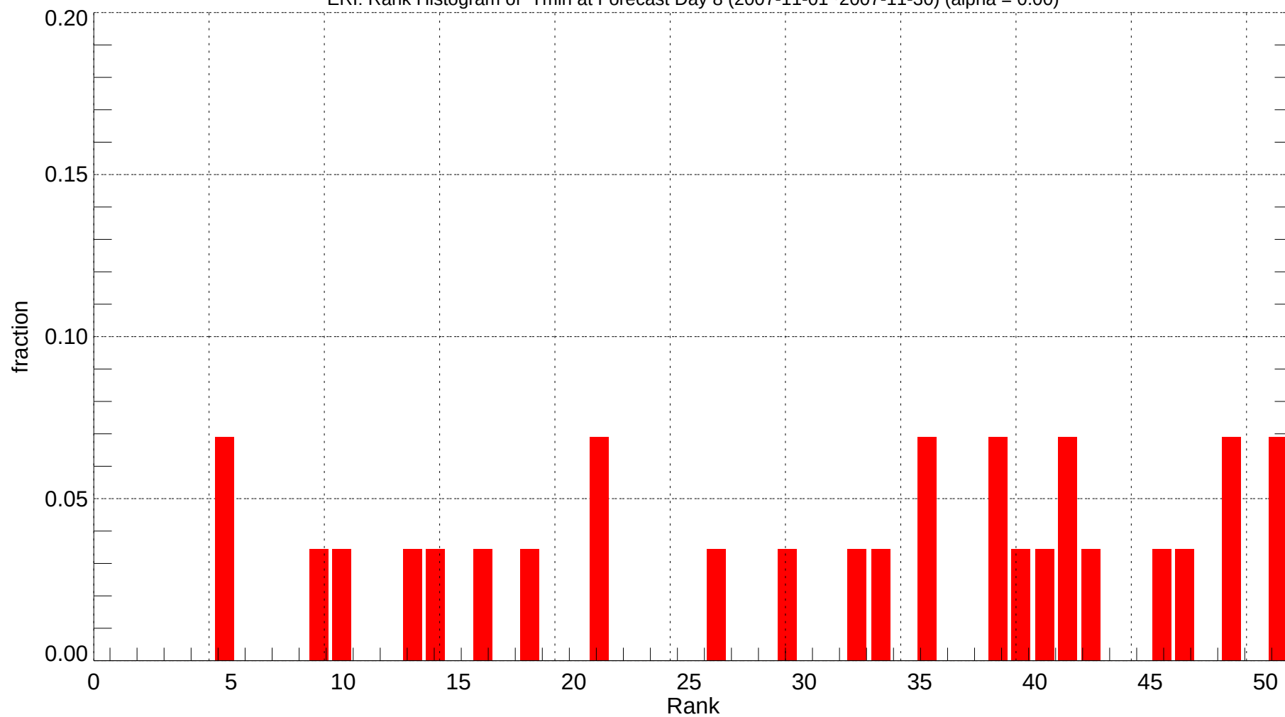
ERI: Rank Histogram of Tmin at Forecast Day 8 (2007-11-01~2007-11-30) (alpha = 0.00)
