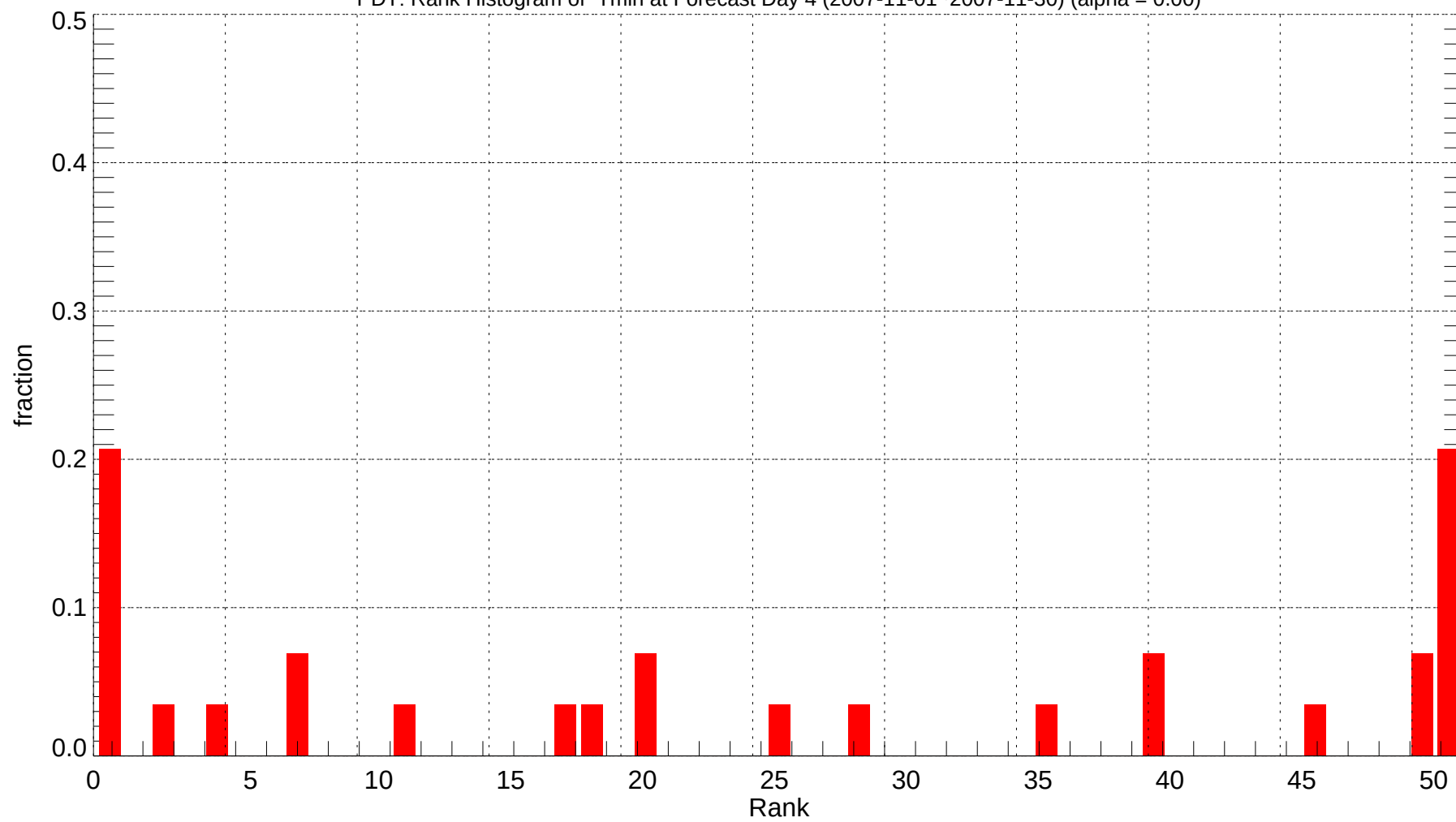
PDT: Rank Histogram of Tmin at Forecast Day 4 (2007-11-01~2007-11-30) (alpha = 0.00)
