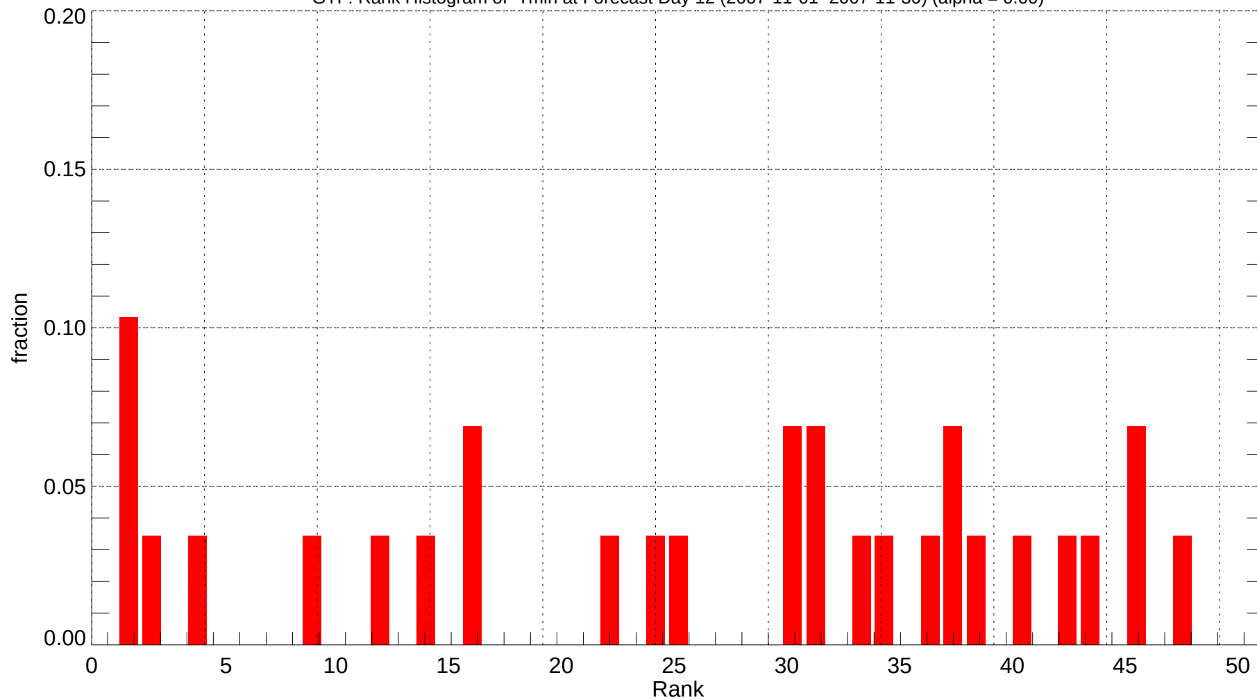
GTF: Rank Histogram of Tmin at Forecast Day 12 (2007-11-01~2007-11-30) (alpha = 0.00)
