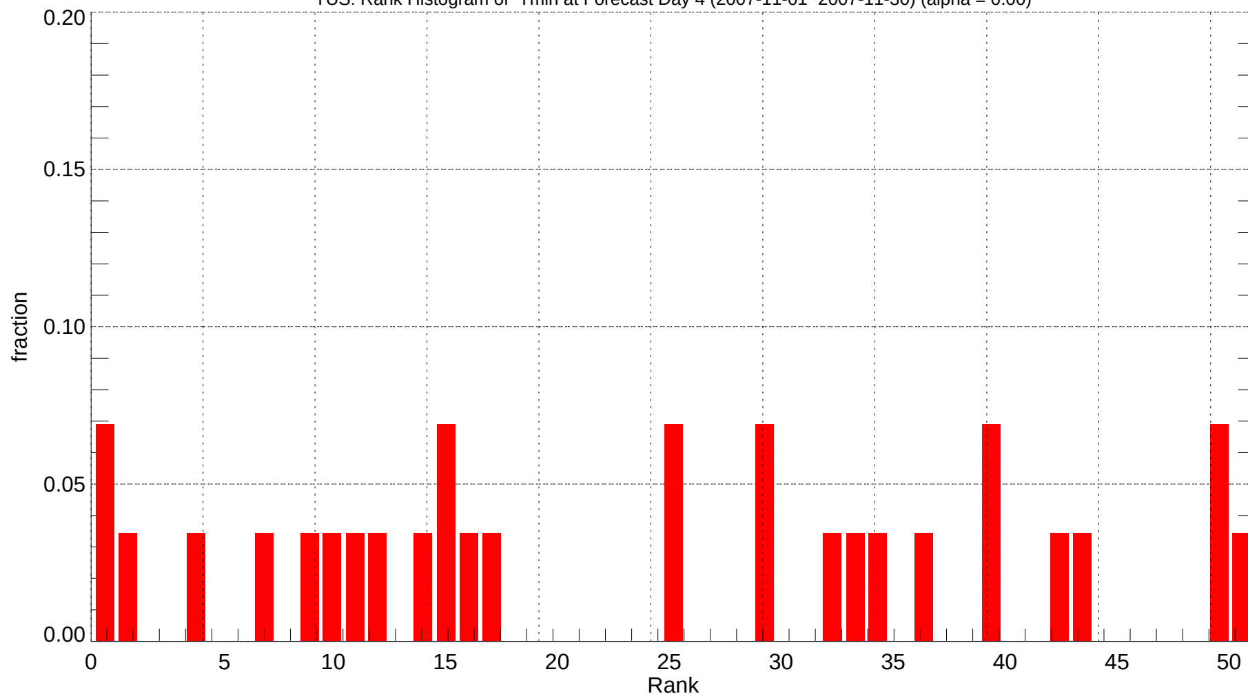
TUS: Rank Histogram of Tmin at Forecast Day 4 (2007-11-01~2007-11-30) (alpha = 0.00)
