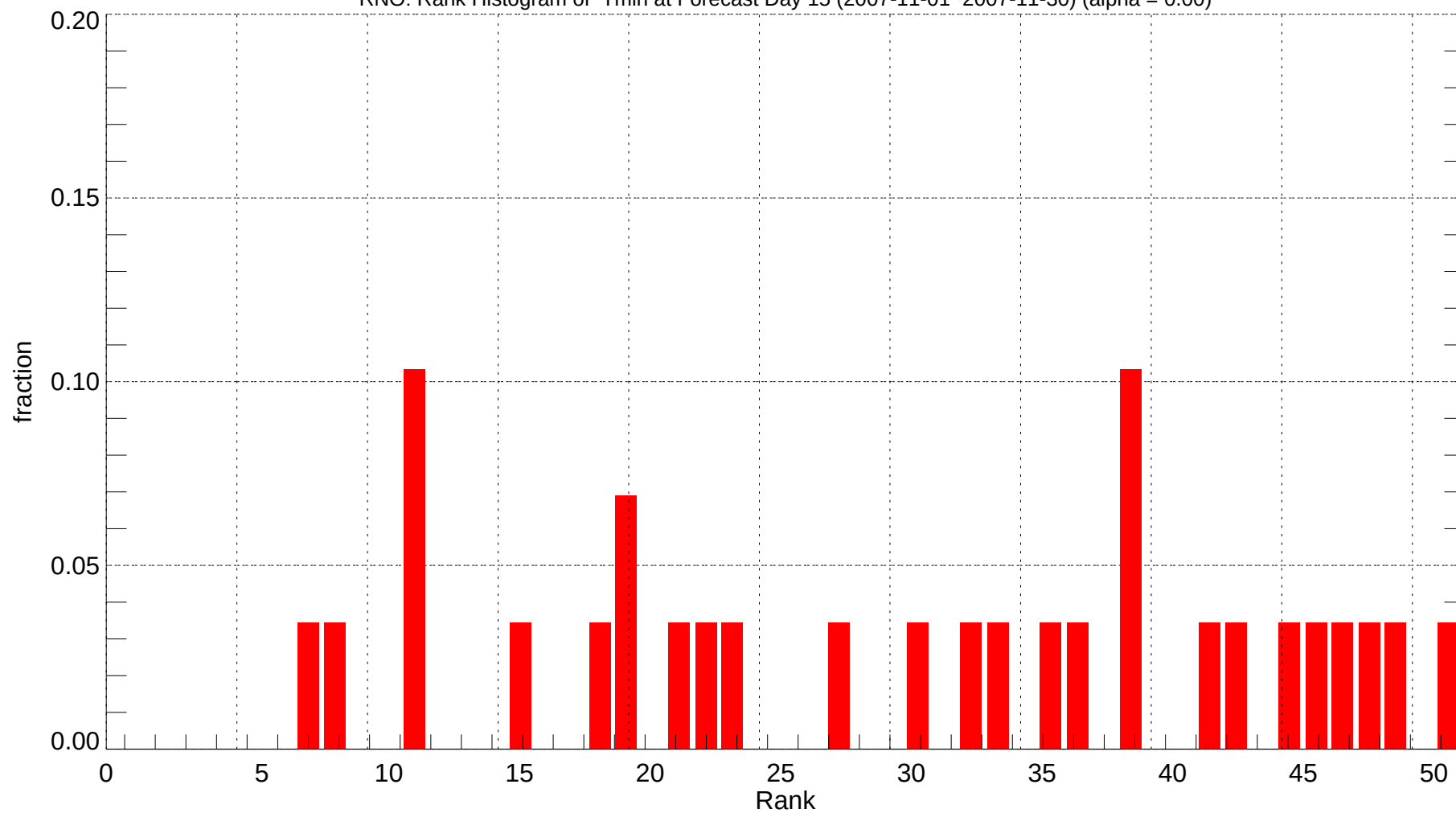
RNO: Rank Histogram of Tmin at Forecast Day 15 (2007-11-01~2007-11-30) (alpha = 0.00)
