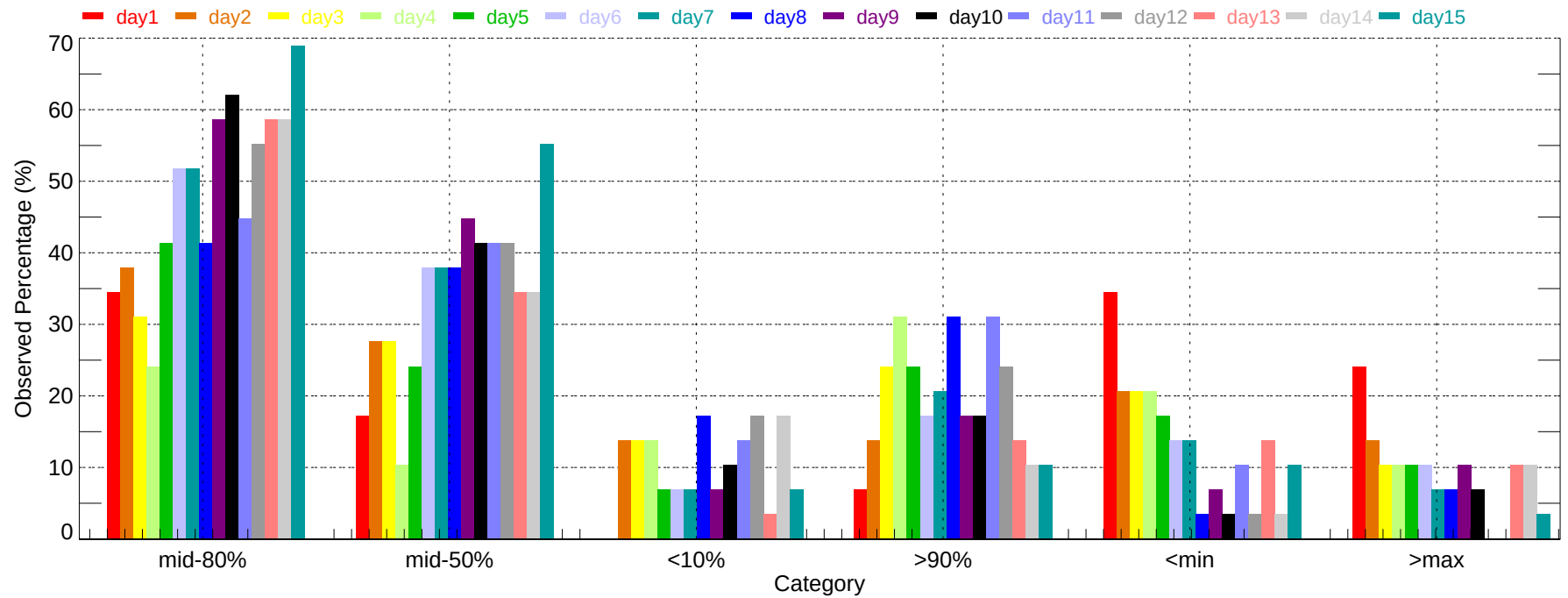
Observed Percentage of Ensembles - CRP: Max Temperature (2007-11-01~2007-11-30)
