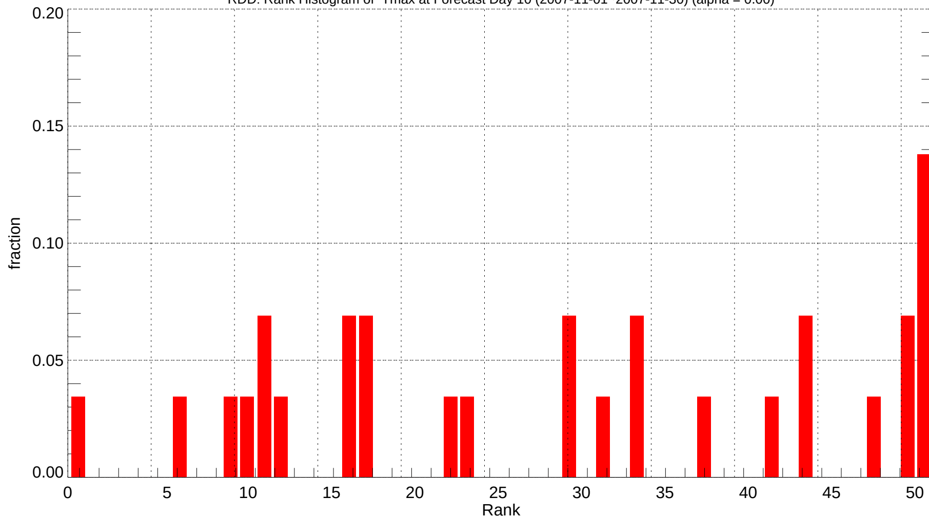
RDD: Rank Histogram of Tmax at Forecast Day 10 (2007-11-01~2007-11-30) (alpha = 0.00)
