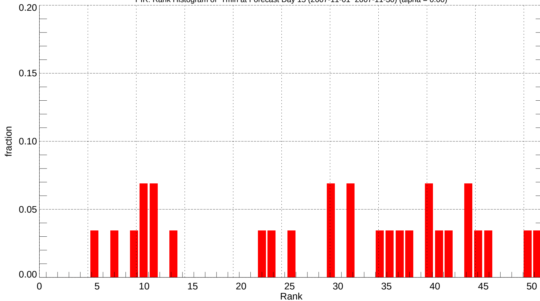
PIR: Rank Histogram of Tmin at Forecast Day 15 (2007-11-01~2007-11-30) (alpha = 0.00)
