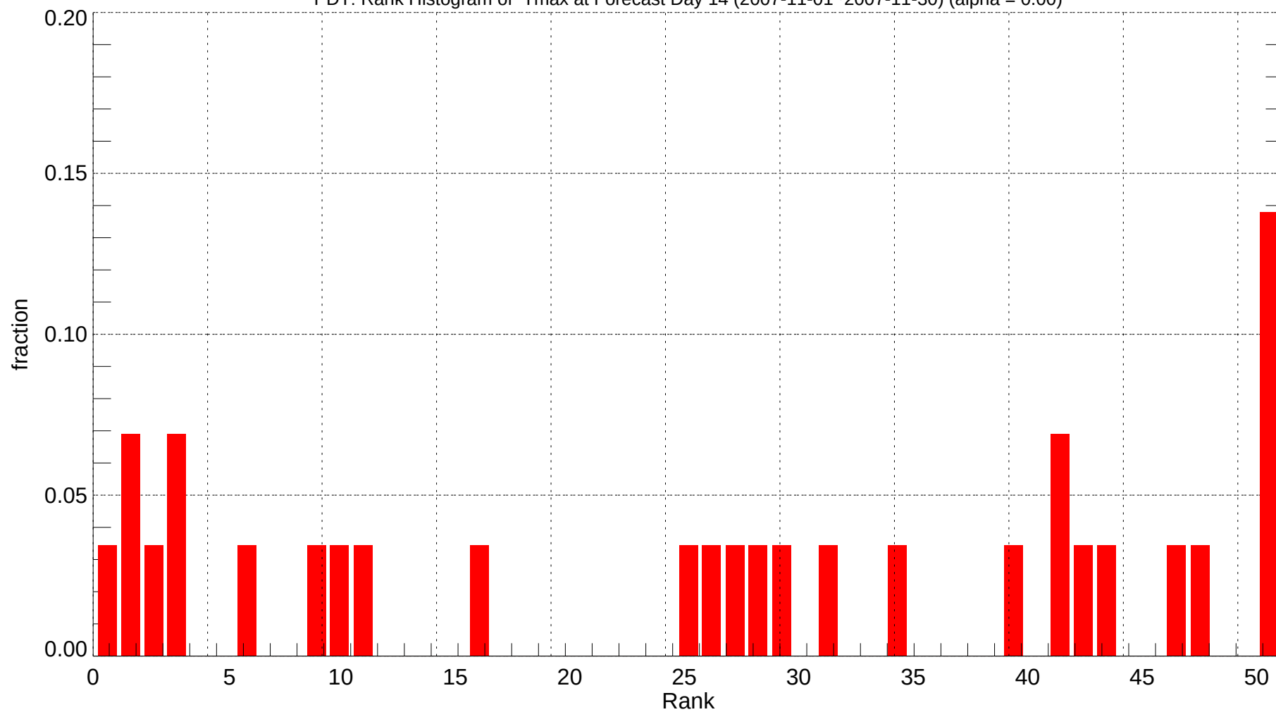
PDT: Rank Histogram of Tmax at Forecast Day 14 (2007-11-01~2007-11-30) (alpha = 0.00)
