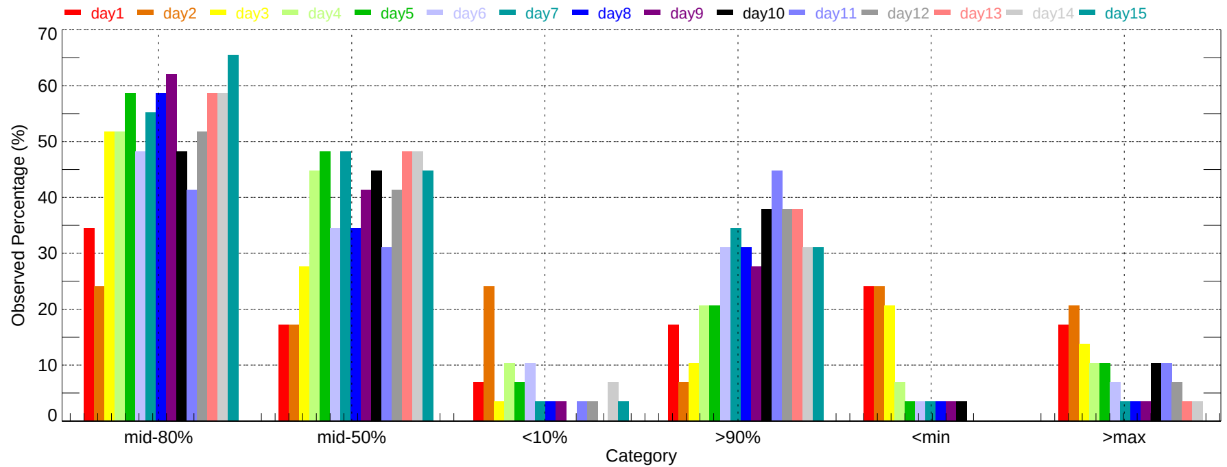
Observed Percentage of Ensembles - DLH: Min Temperature (2007-11-01~2007-11-30)
