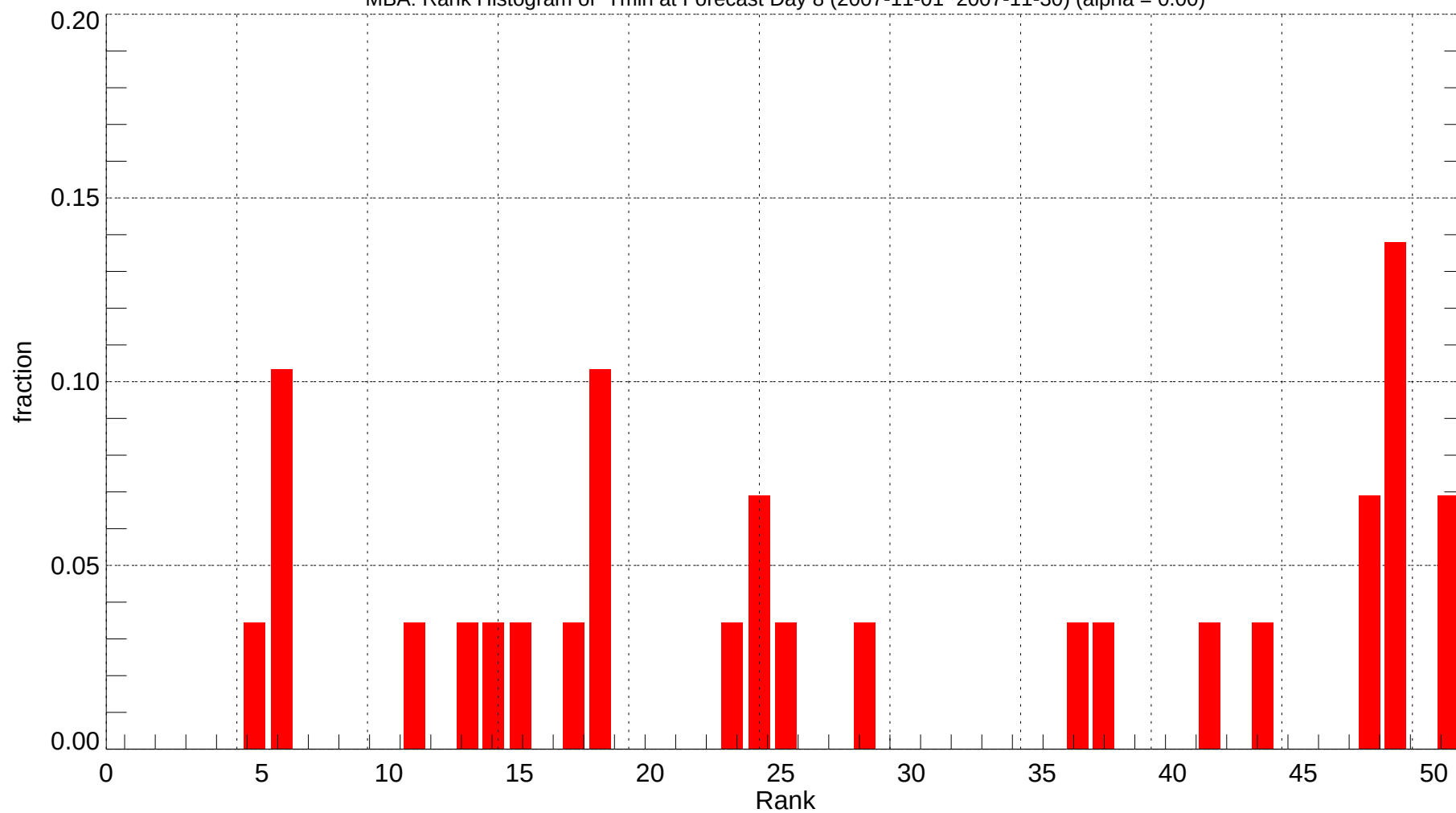
MBA: Rank Histogram of Tmin at Forecast Day 8 (2007-11-01~2007-11-30) (alpha = 0.00)
