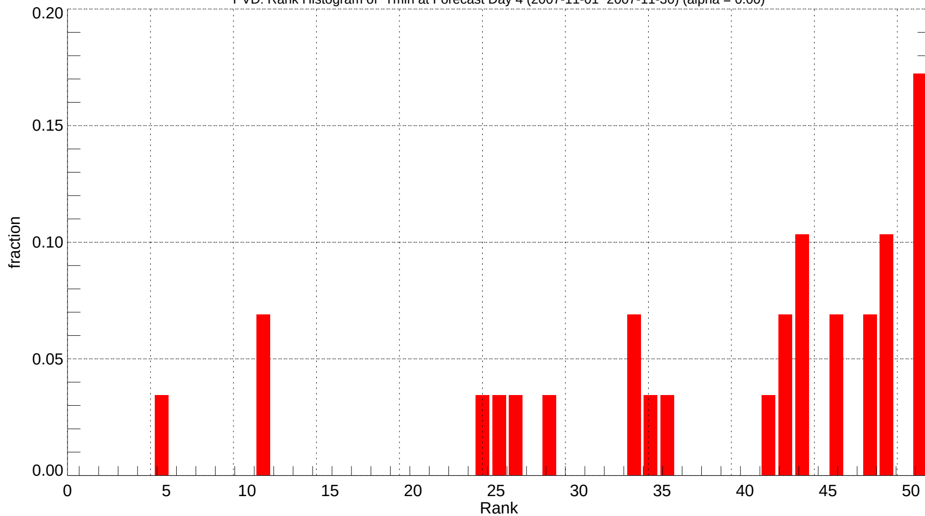
PVD: Rank Histogram of Tmin at Forecast Day 4 (2007-11-01~2007-11-30) (alpha = 0.00)
