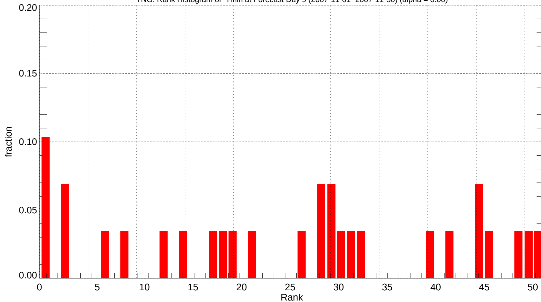
YNG: Rank Histogram of Tmin at Forecast Day 9 (2007-11-01~2007-11-30) (alpha = 0.00)
