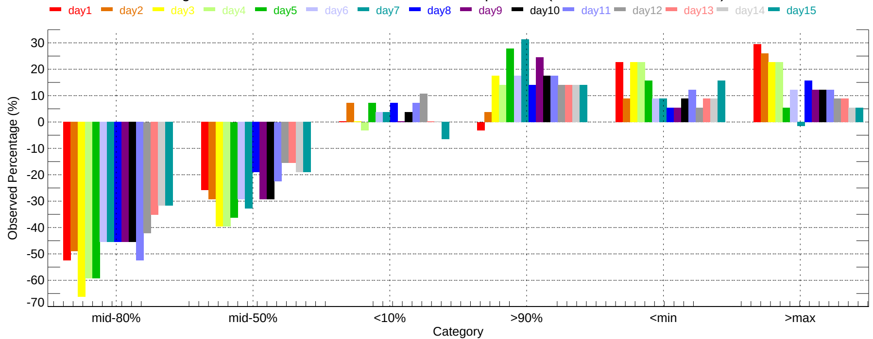
Observed Percentage Deviation of Ensembles - VCT: Max Temperature (2007-11-01~2007-11-30)
