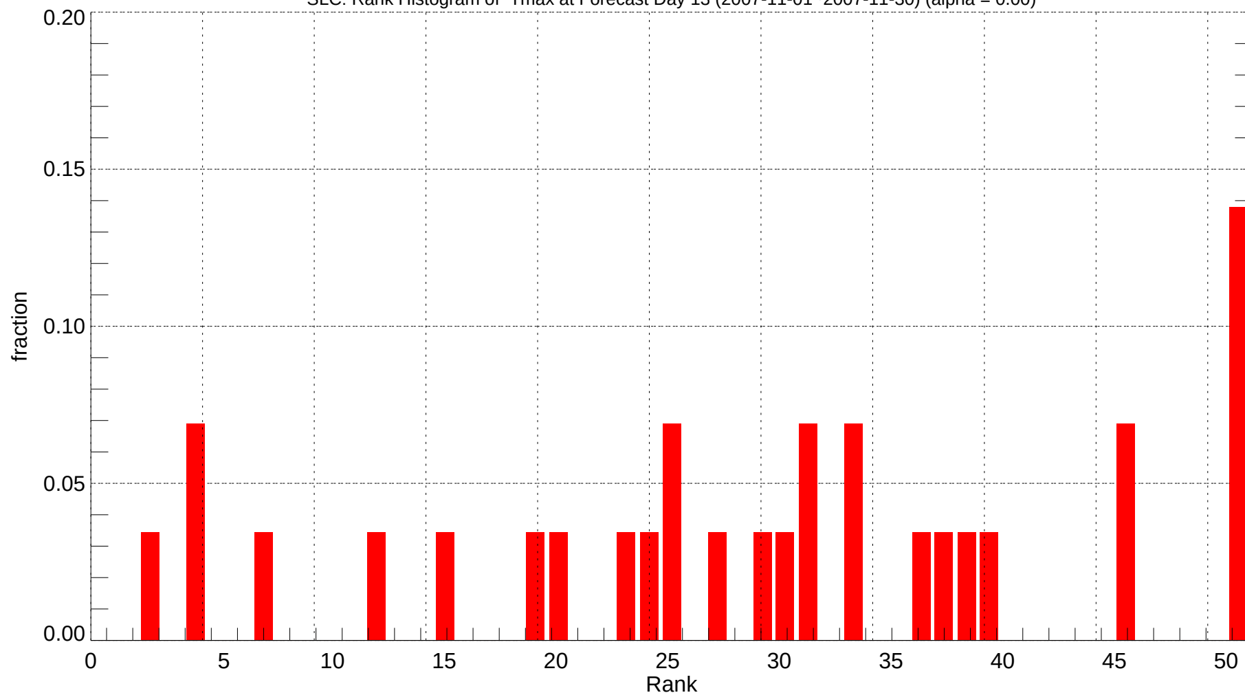
SLC: Rank Histogram of Tmax at Forecast Day 13 (2007-11-01~2007-11-30) (alpha = 0.00)
