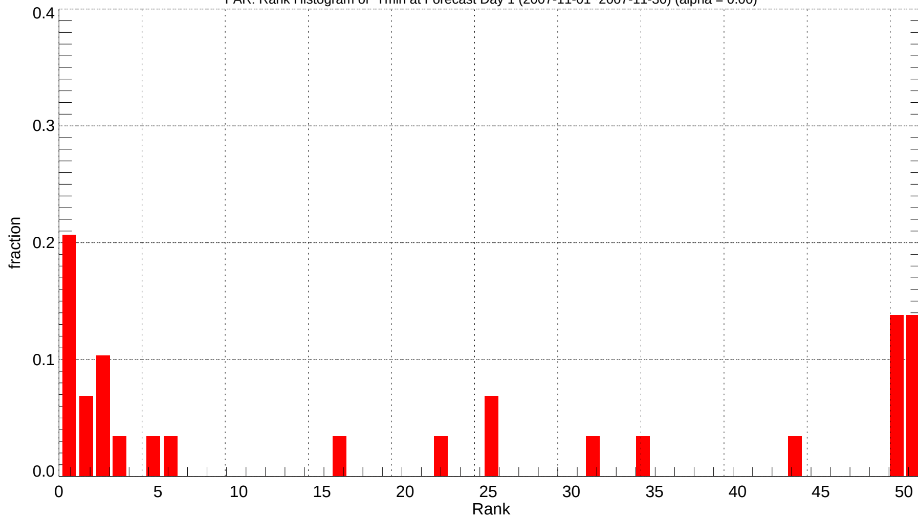
FAR: Rank Histogram of Tmin at Forecast Day 1 (2007-11-01~2007-11-30) (alpha = 0.00)
