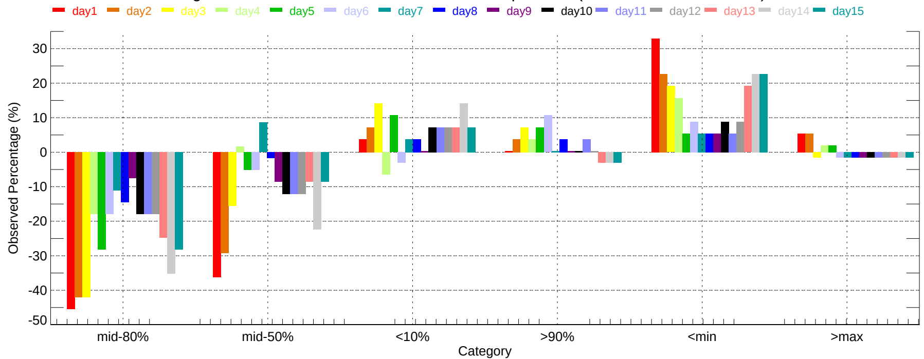
Observed Percentage Deviation of Ensembles - AUG: Min Temperature (2007-11-01~2007-11-30)
