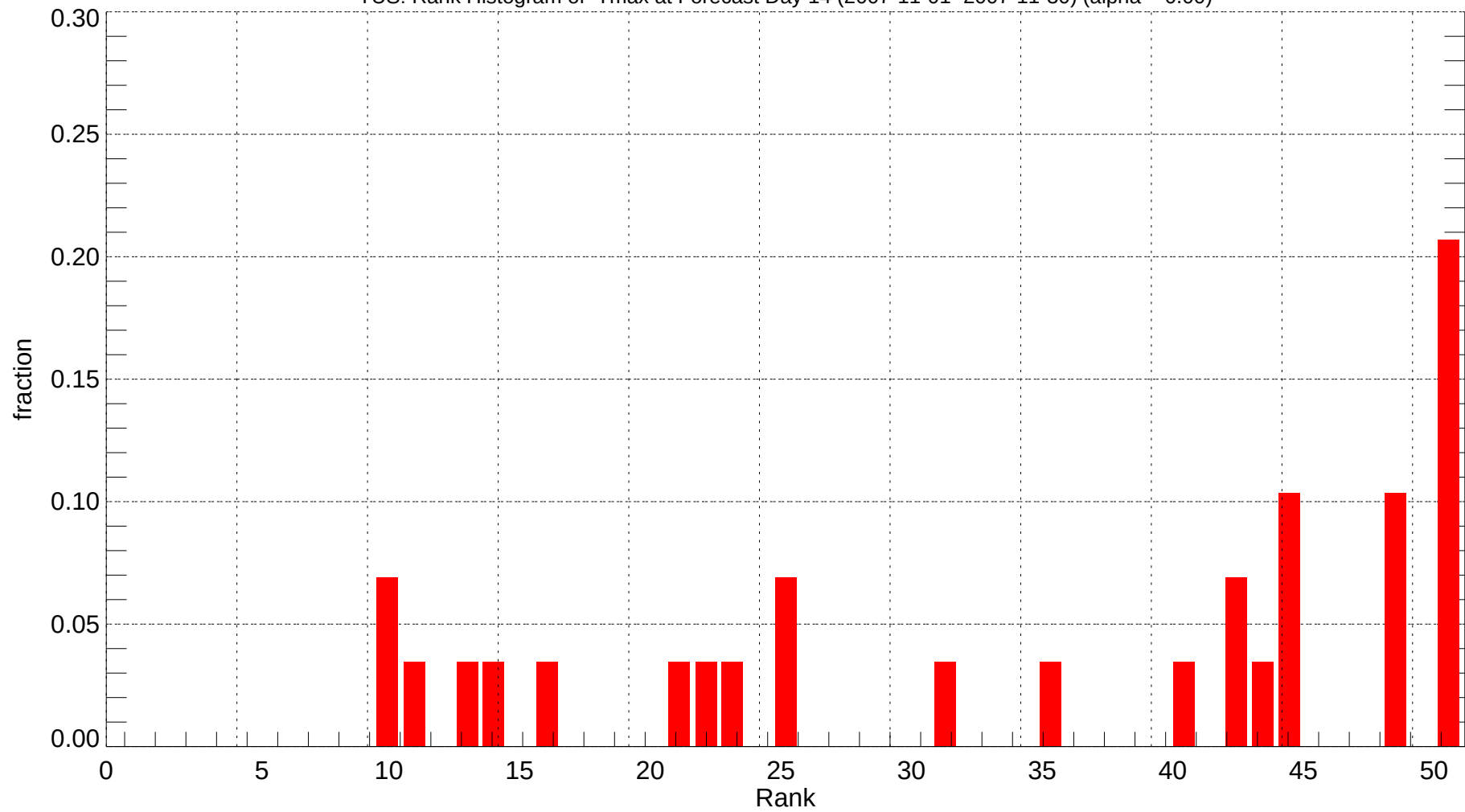
TUS: Rank Histogram of Tmax at Forecast Day 14 (2007-11-01~2007-11-30) (alpha = 0.00)
