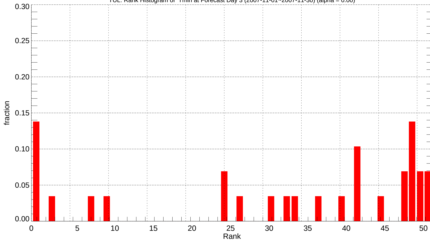
TUL: Rank Histogram of Tmin at Forecast Day 3 (2007-11-01~2007-11-30) (alpha = 0.00)
