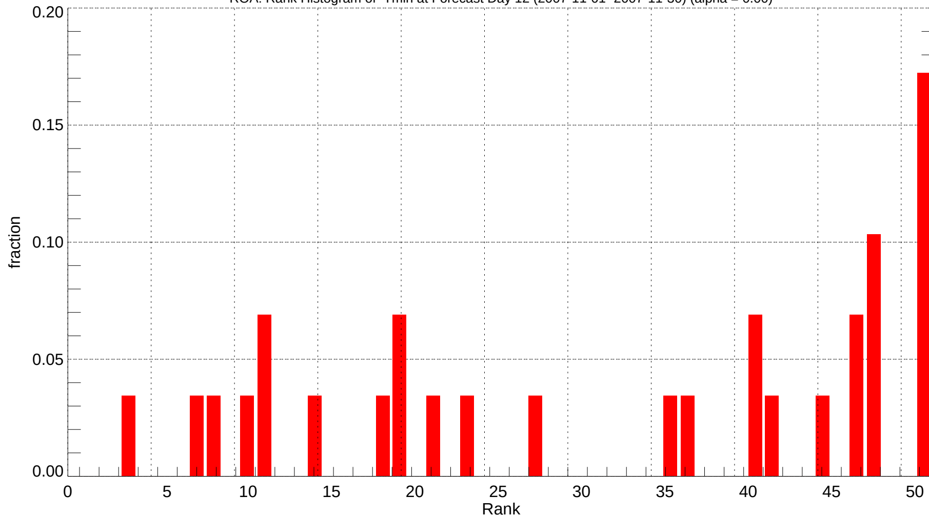
ROA: Rank Histogram of Tmin at Forecast Day 12 (2007-11-01~2007-11-30) (alpha = 0.00)
