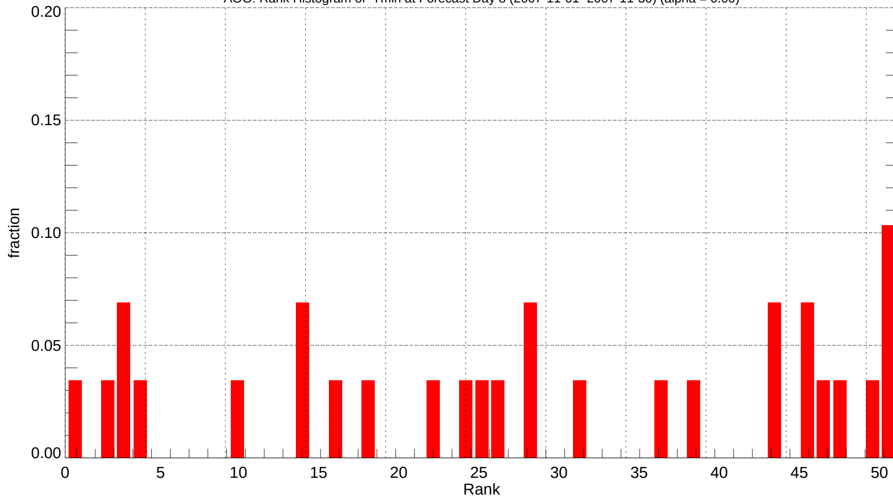
AOO: Rank Histogram of Tmin at Forecast Day 8 (2007-11-01~2007-11-30) (alpha = 0.00)
