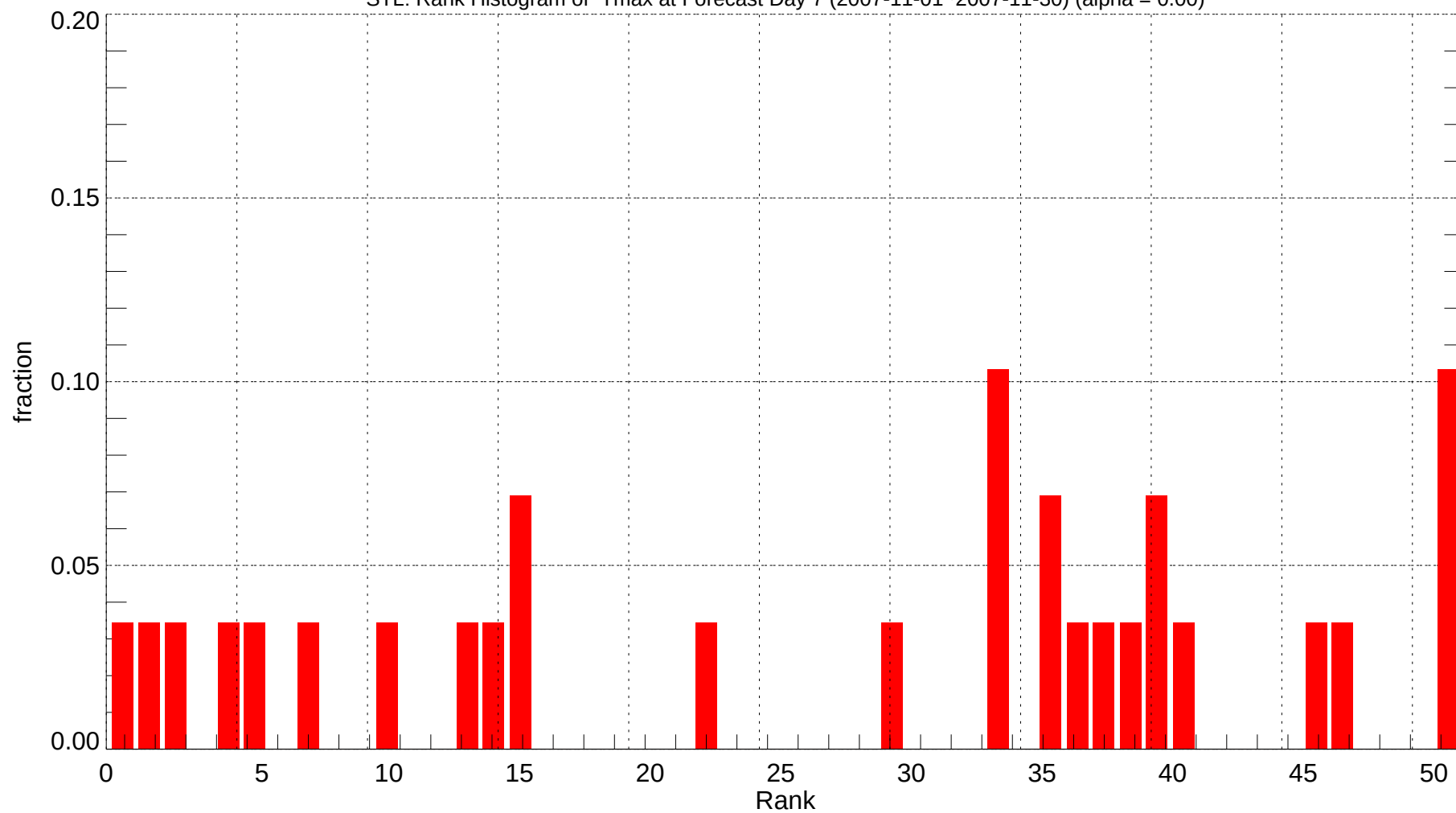
STL: Rank Histogram of Tmax at Forecast Day 7 (2007-11-01~2007-11-30) (alpha = 0.00)
