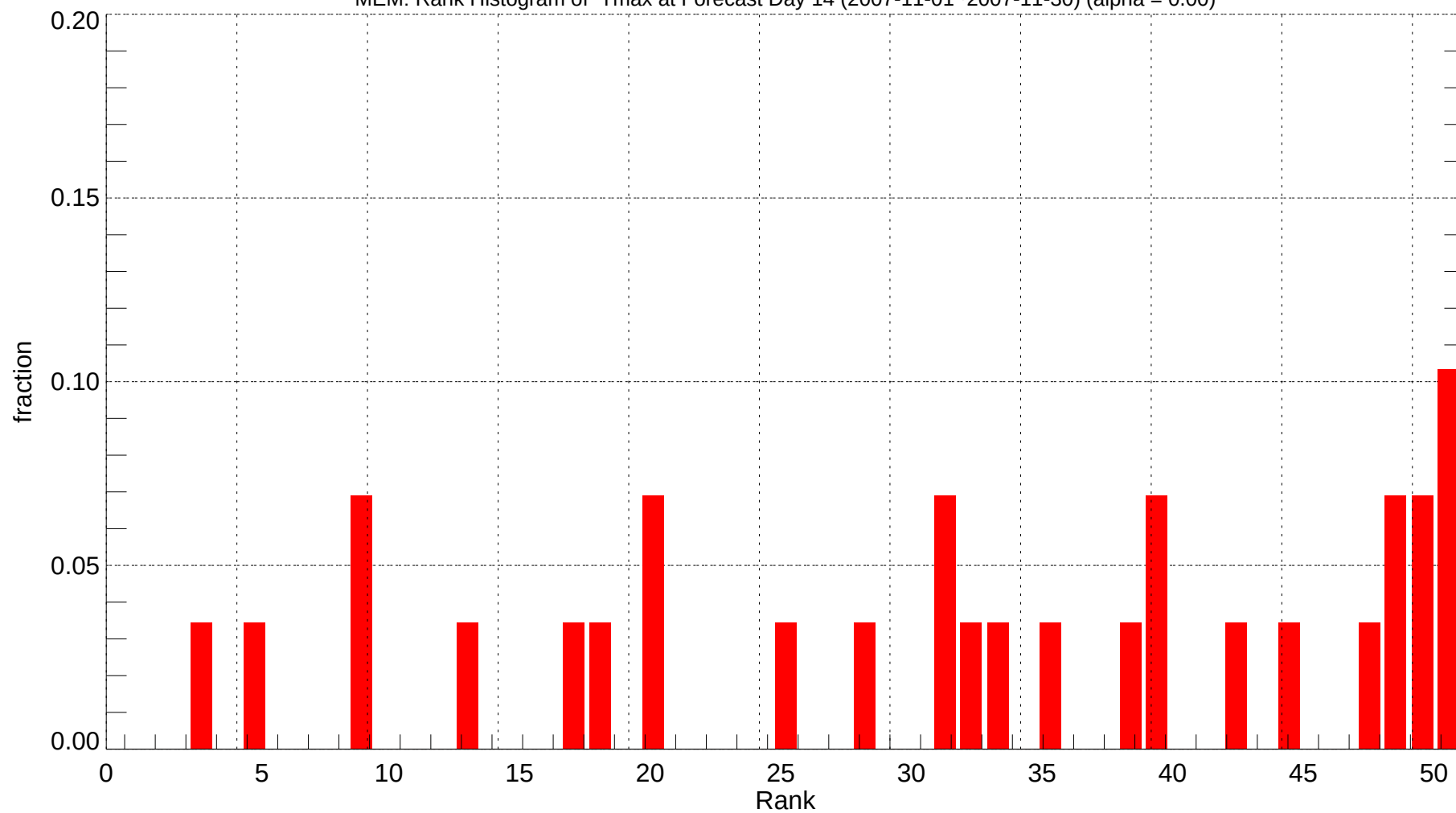
MEM: Rank Histogram of Tmax at Forecast Day 14 (2007-11-01~2007-11-30) (alpha = 0.00)
