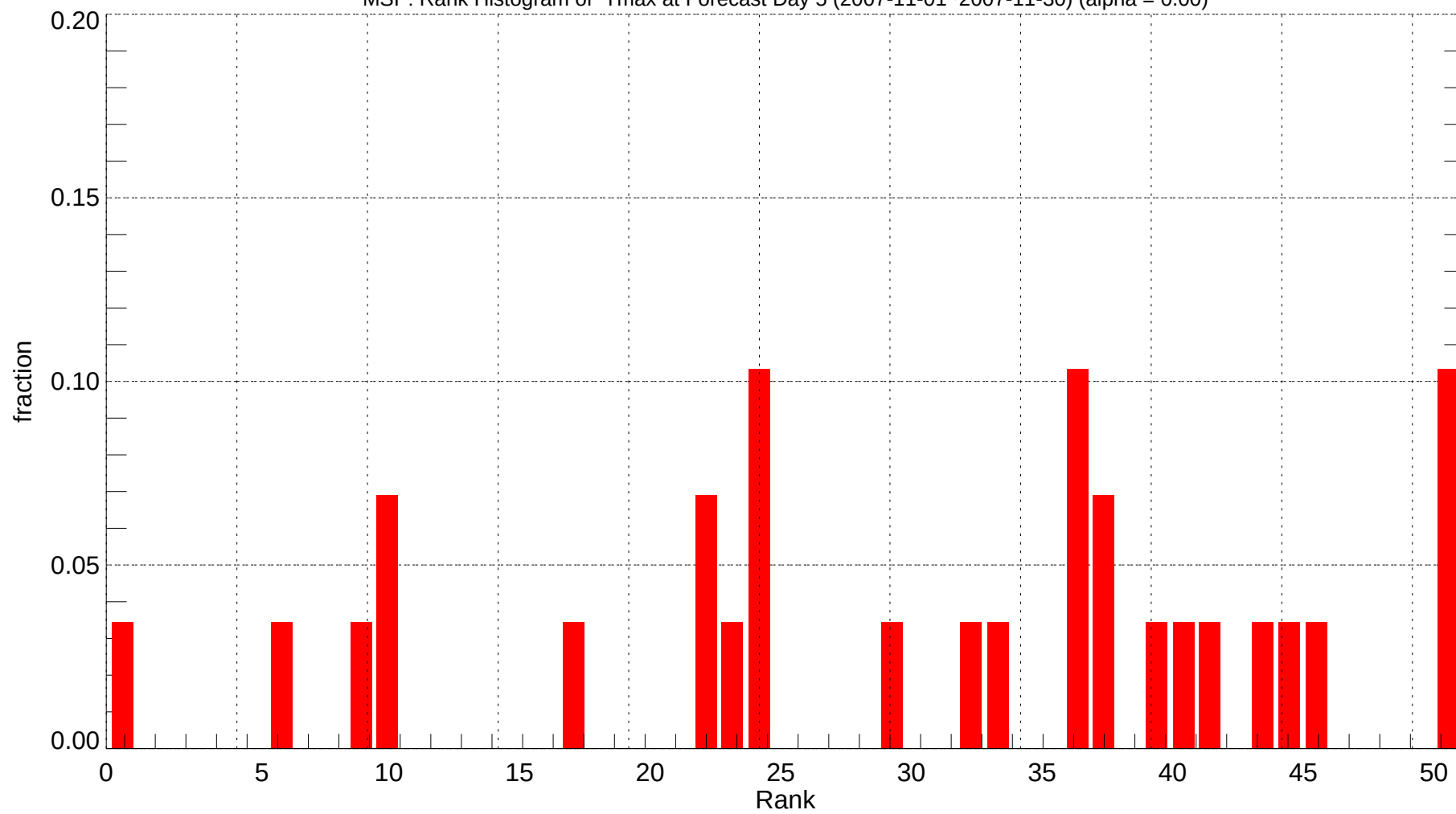
MSP: Rank Histogram of Tmax at Forecast Day 5 (2007-11-01~2007-11-30) (alpha = 0.00)
