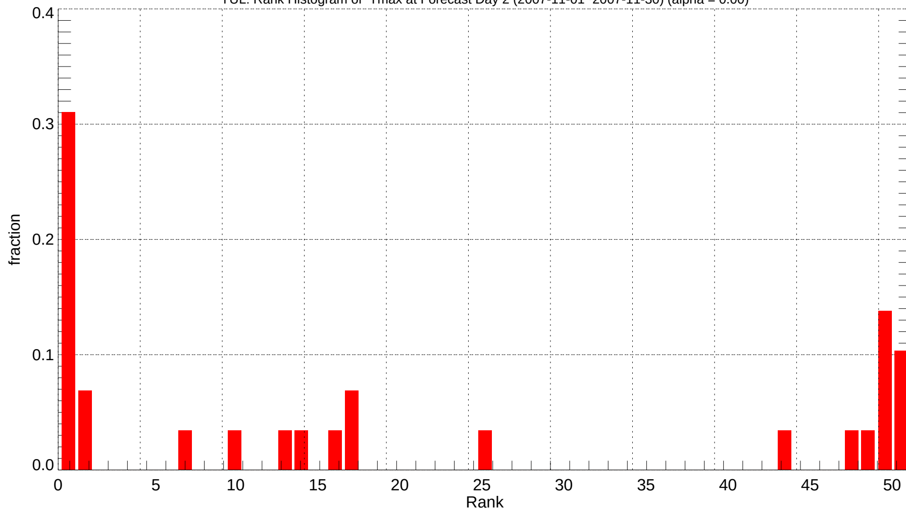
YUL: Rank Histogram of Tmax at Forecast Day 2 (2007-11-01~2007-11-30) (alpha = 0.00)
