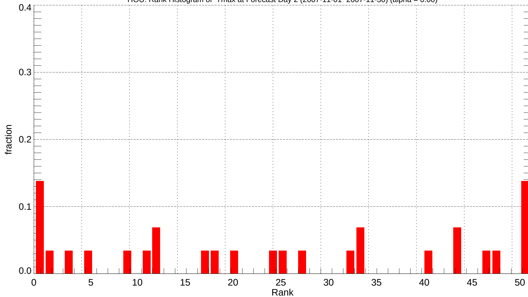
HOU: Rank Histogram of Tmax at Forecast Day 2 (2007-11-01~2007-11-30) (alpha = 0.00)
