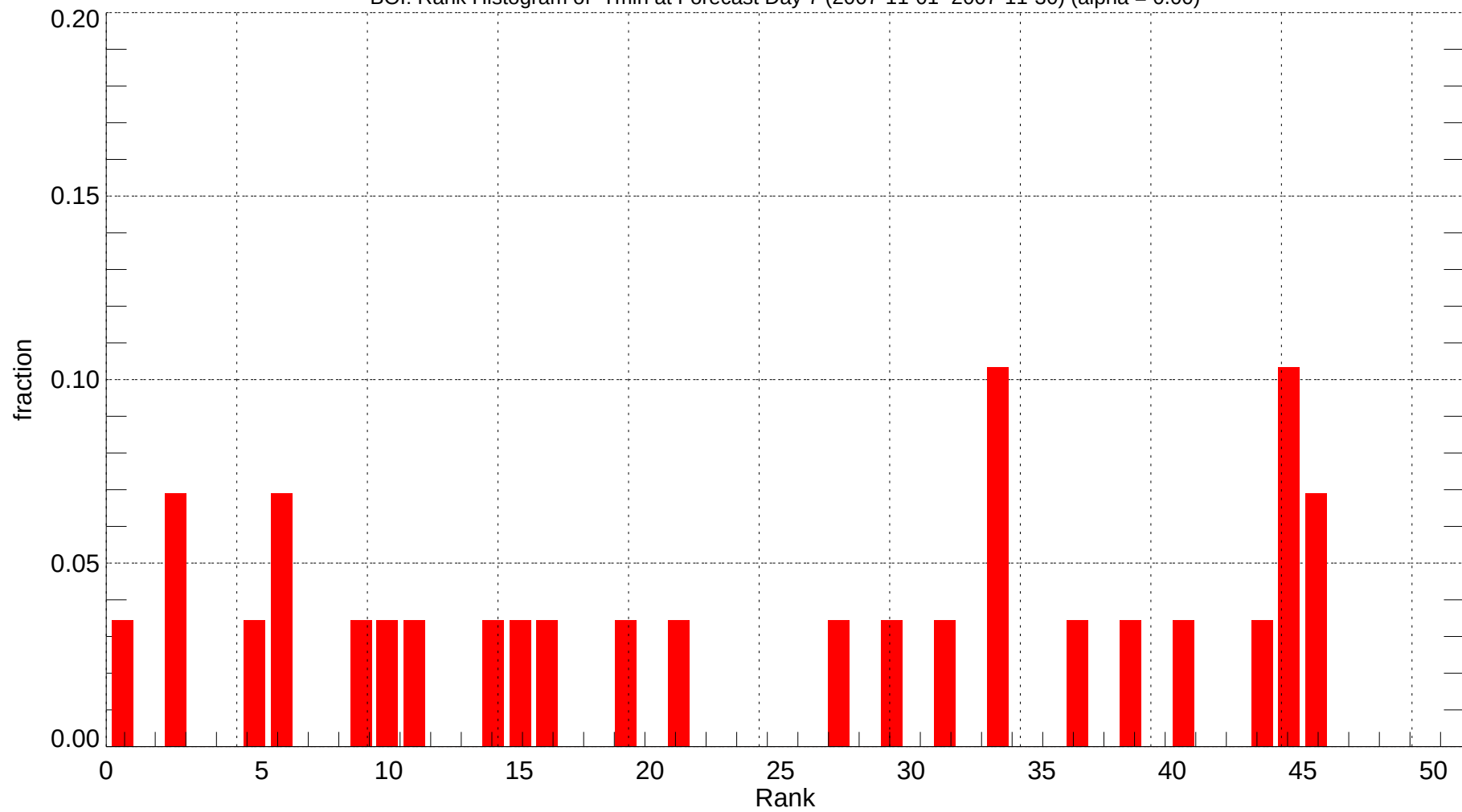
BOI: Rank Histogram of Tmin at Forecast Day 7 (2007-11-01~2007-11-30) (alpha = 0.00)
