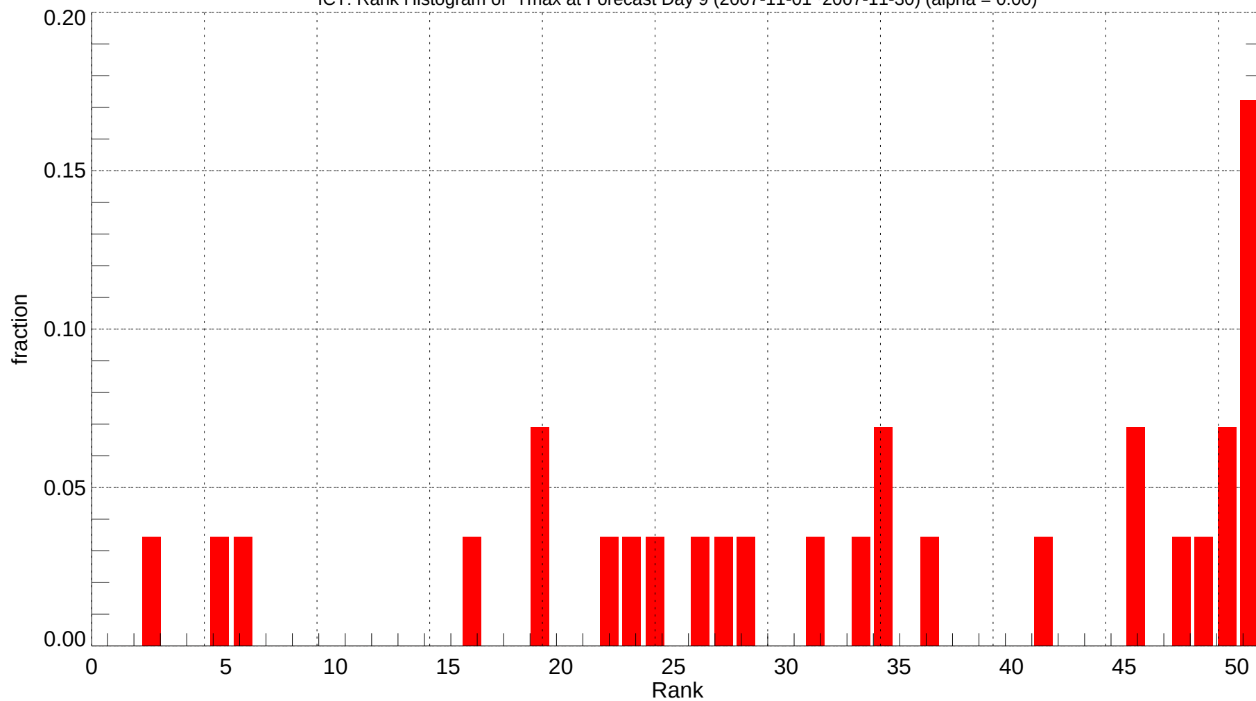
ICT: Rank Histogram of Tmax at Forecast Day 9 (2007-11-01~2007-11-30) (alpha = 0.00)
