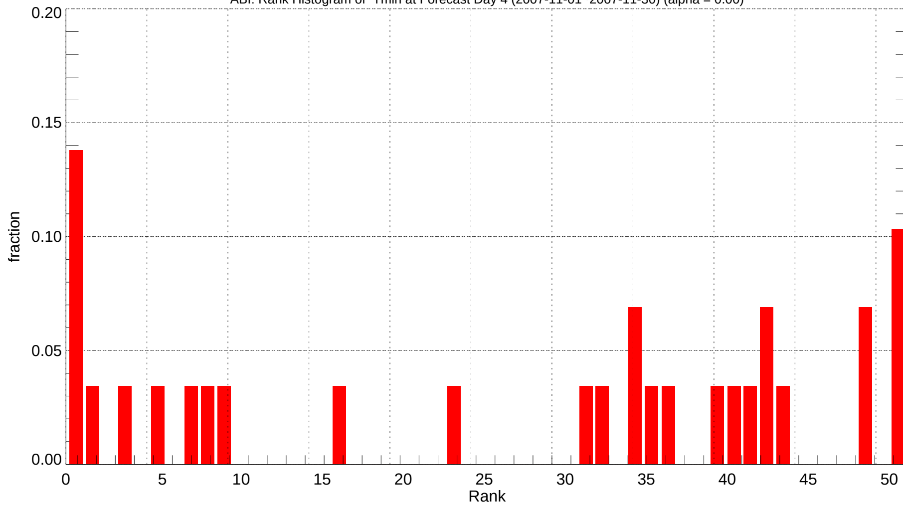
ABI: Rank Histogram of Tmin at Forecast Day 4 (2007-11-01~2007-11-30) (alpha = 0.00)
