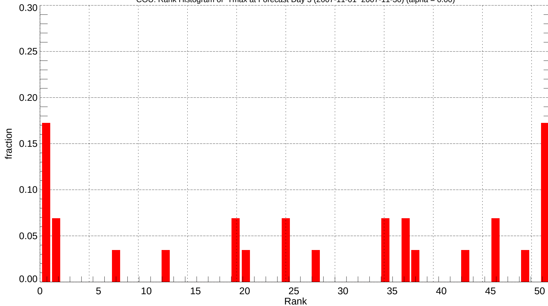
COU: Rank Histogram of Tmax at Forecast Day 3 (2007-11-01~2007-11-30) (alpha = 0.00)
