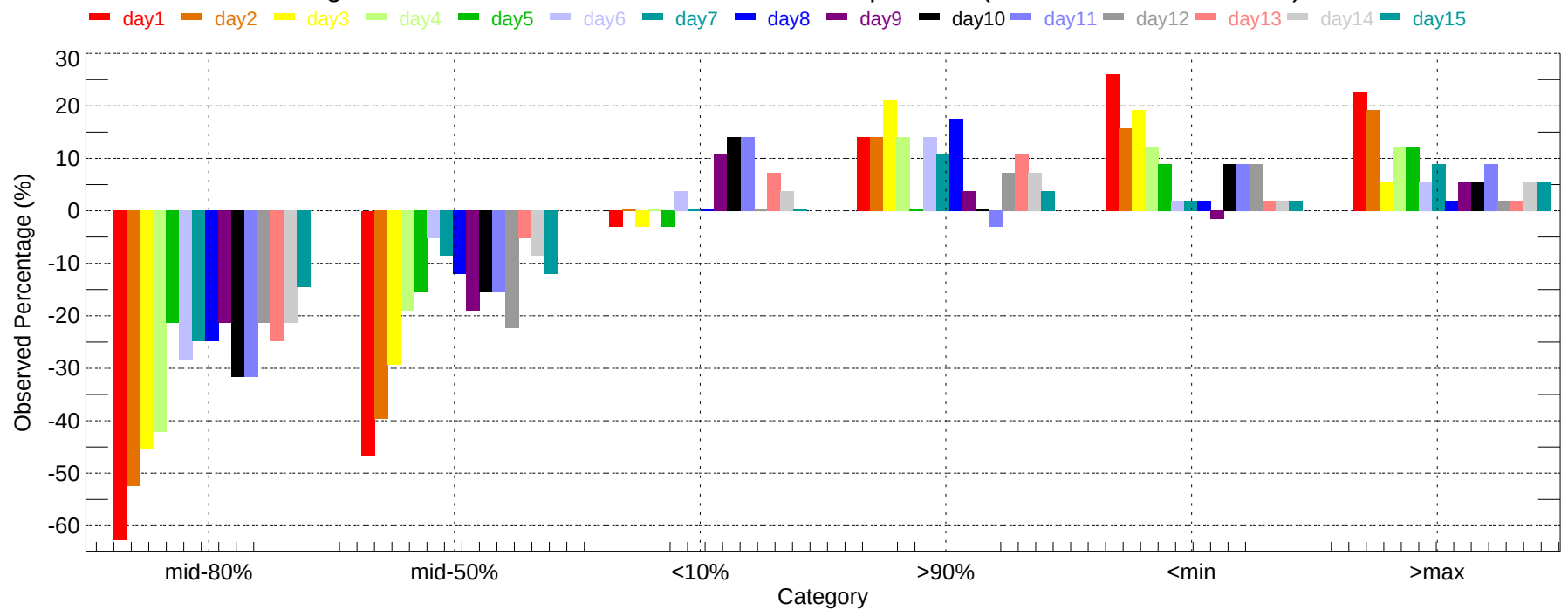
Observed Percentage Deviation of Ensembles - LNS: Max Temperature (2007-11-01~2007-11-30)
