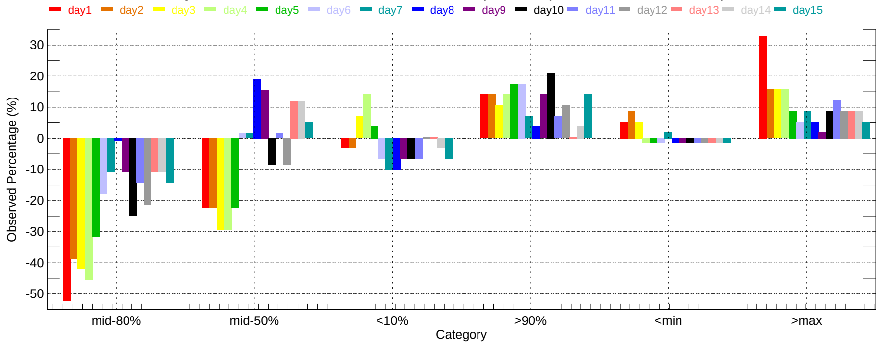
Observed Percentage Deviation of Ensembles - SLC: Min Temperature (2007-11-01~2007-11-30)
