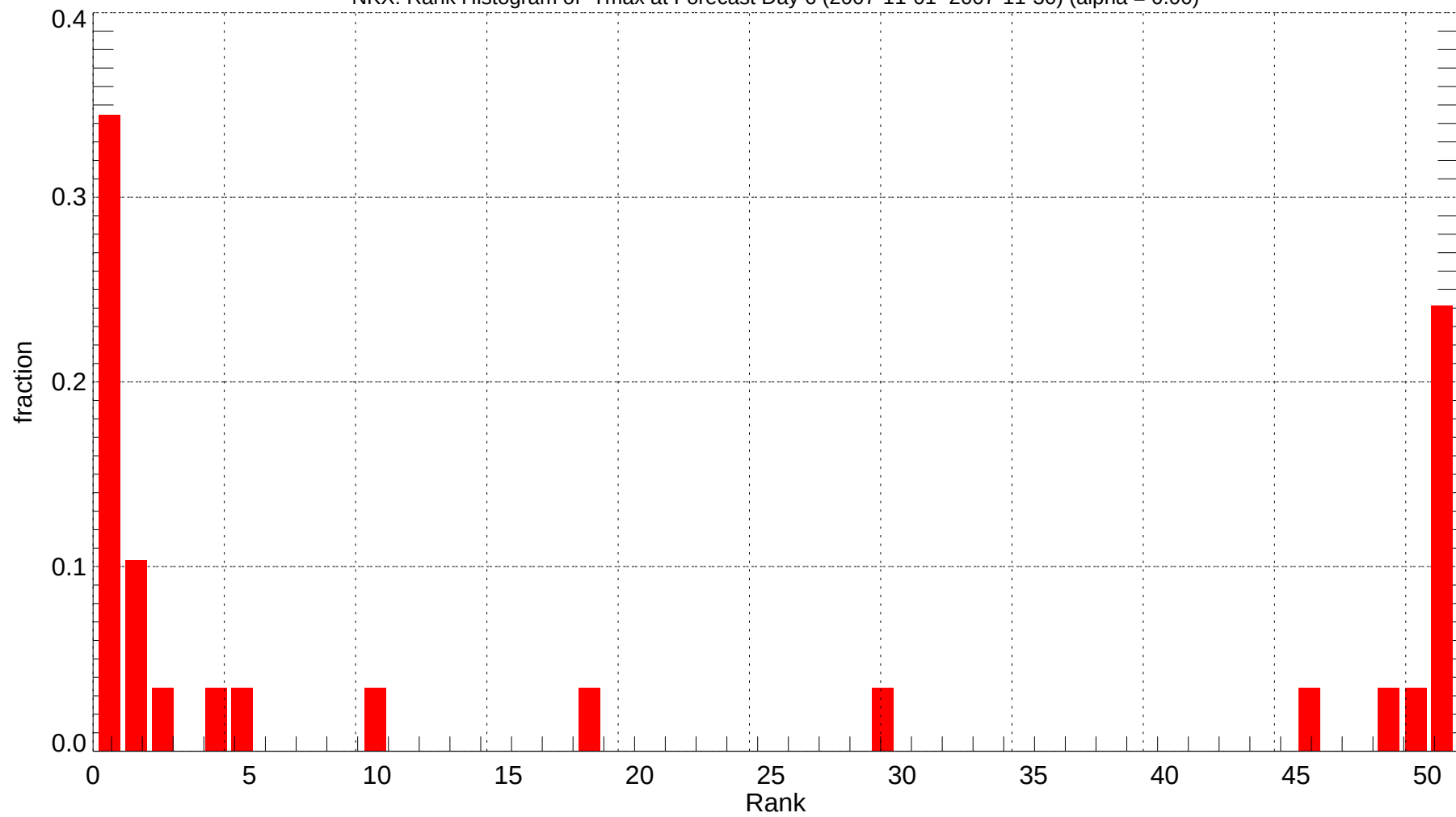
NKX: Rank Histogram of Tmax at Forecast Day 6 (2007-11-01~2007-11-30) (alpha = 0.00)
