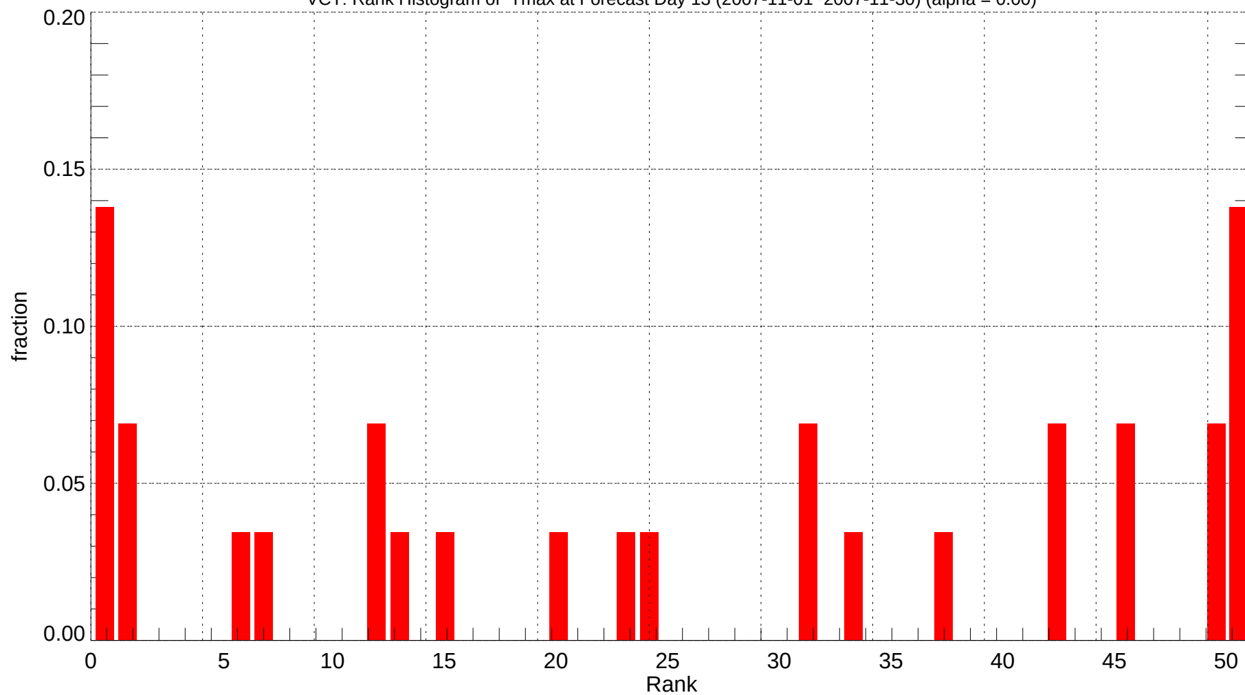
VCT: Rank Histogram of Tmax at Forecast Day 13 (2007-11-01~2007-11-30) (alpha = 0.00)
