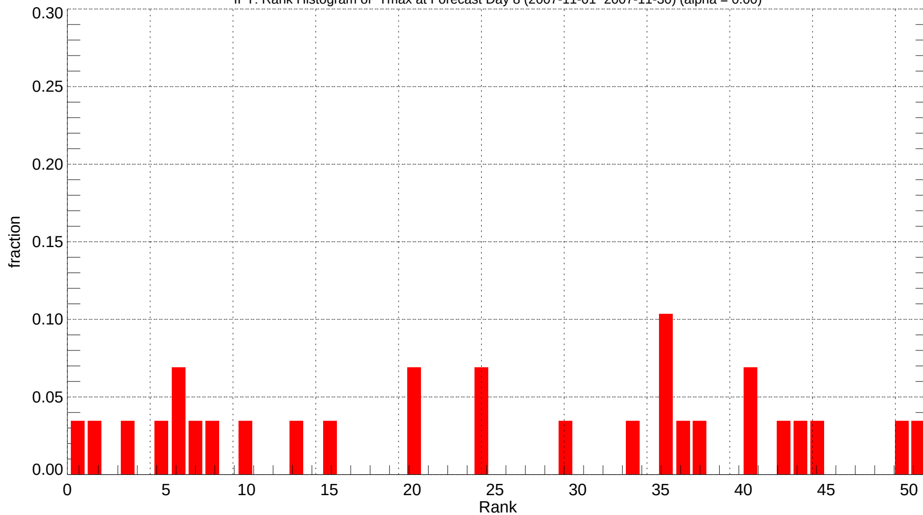
IPT: Rank Histogram of Tmax at Forecast Day 8 (2007-11-01~2007-11-30) (alpha = 0.00)
