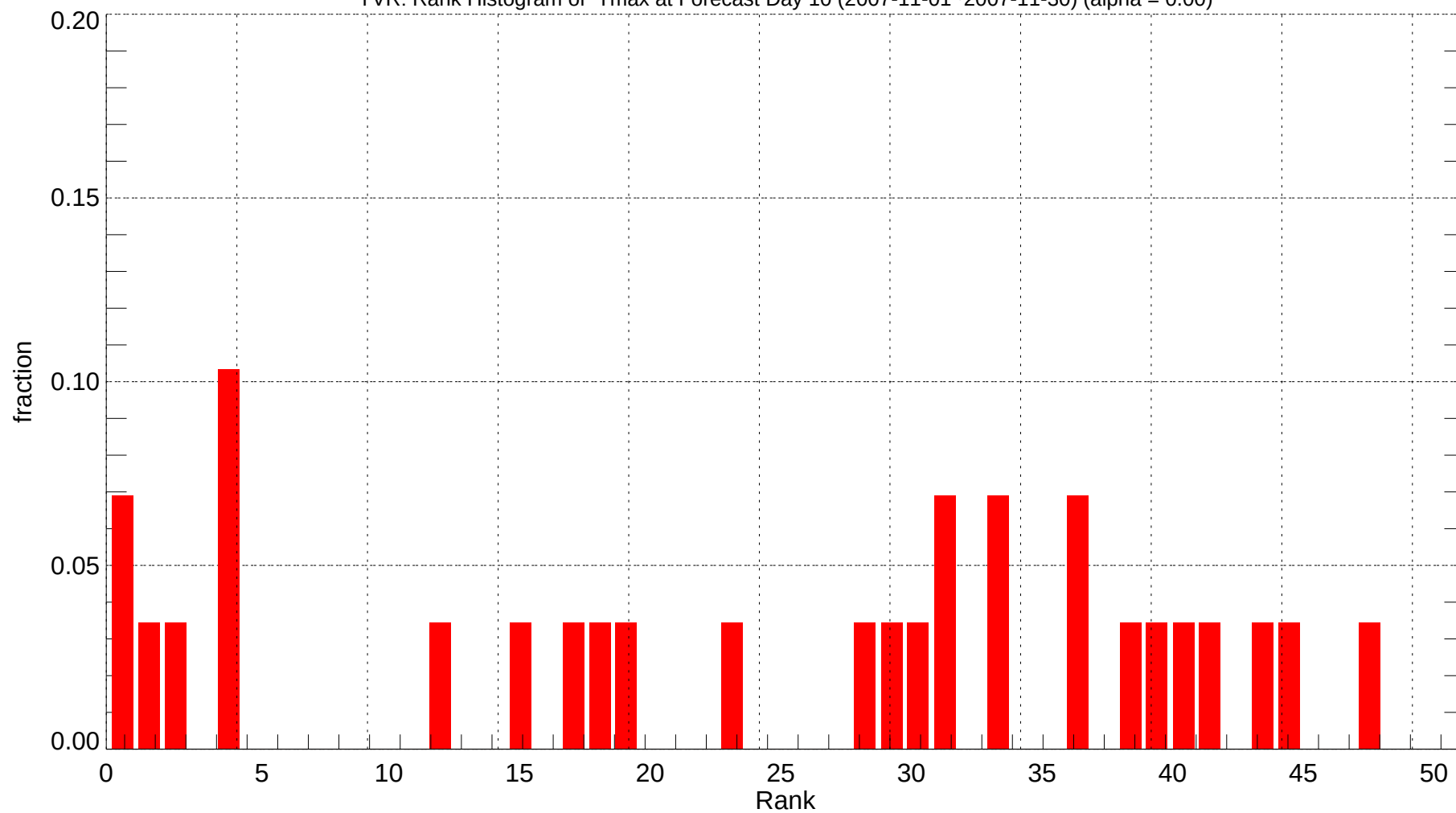
YVR: Rank Histogram of Tmax at Forecast Day 10 (2007-11-01~2007-11-30) (alpha = 0.00)
