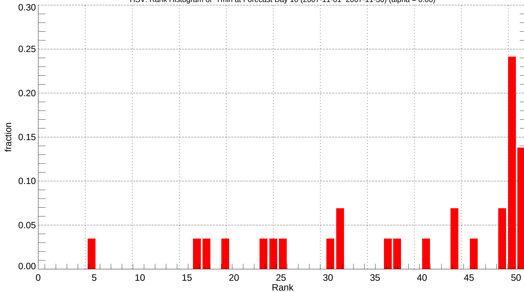
HSV: Rank Histogram of Tmin at Forecast Day 10 (2007-11-01~2007-11-30) (alpha = 0.00)
