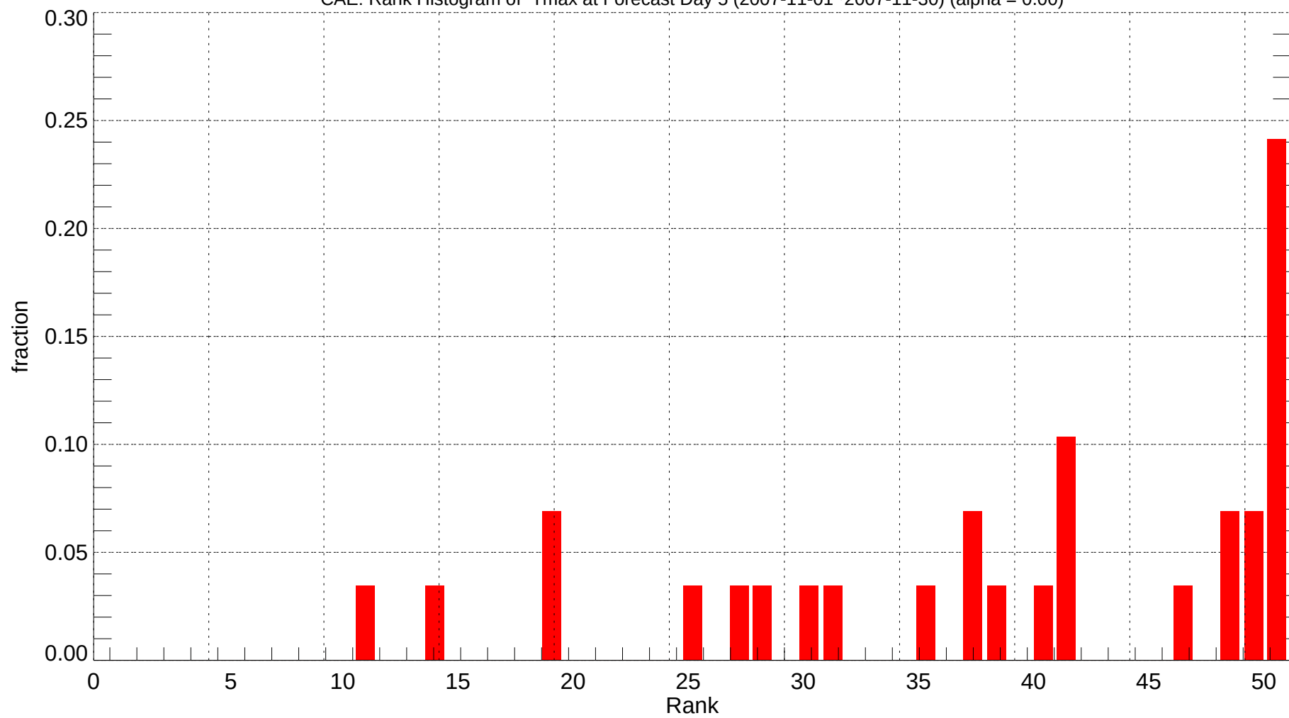
CAE: Rank Histogram of Tmax at Forecast Day 5 (2007-11-01~2007-11-30) (alpha = 0.00)
