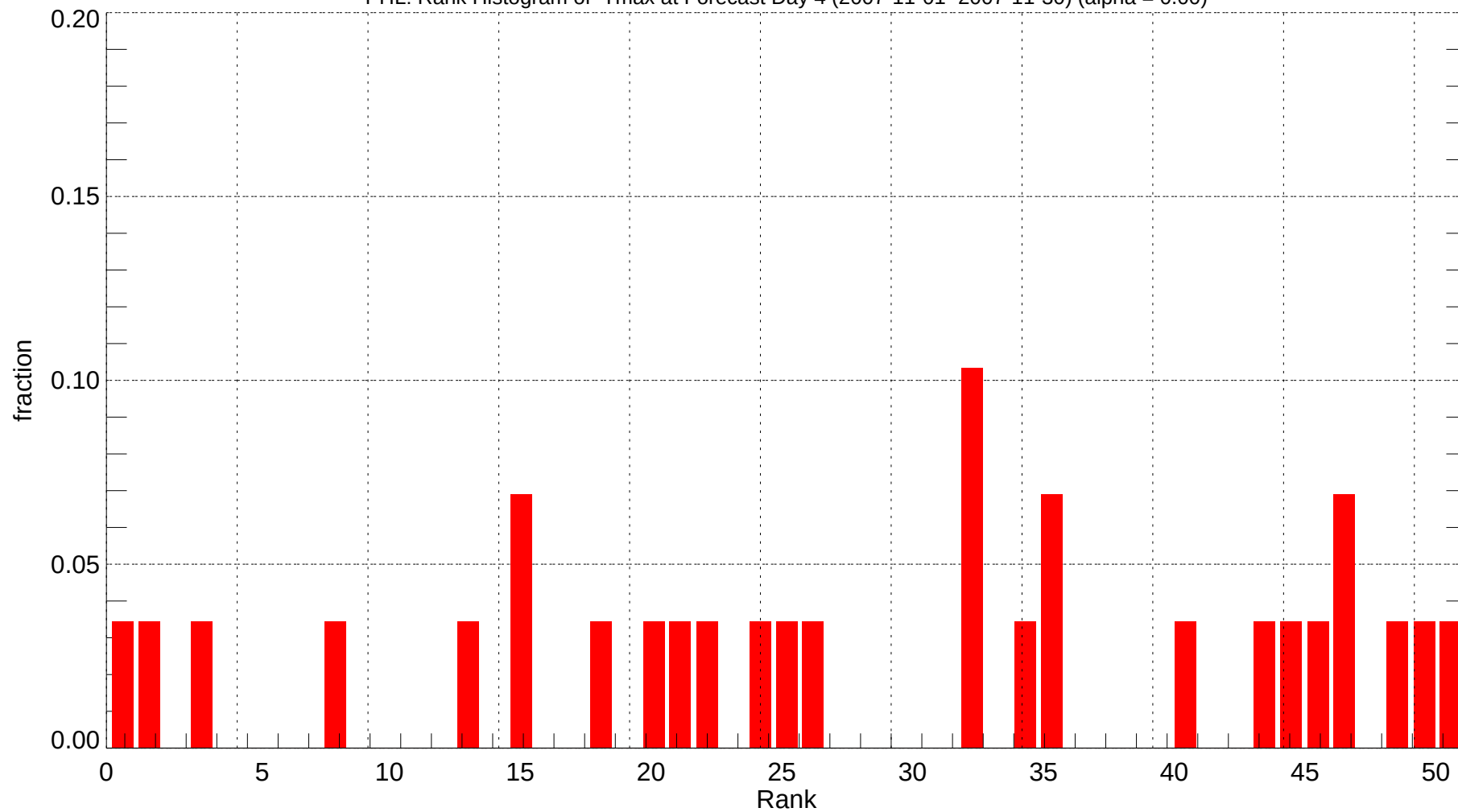
PHL: Rank Histogram of Tmax at Forecast Day 4 (2007-11-01~2007-11-30) (alpha = 0.00)
