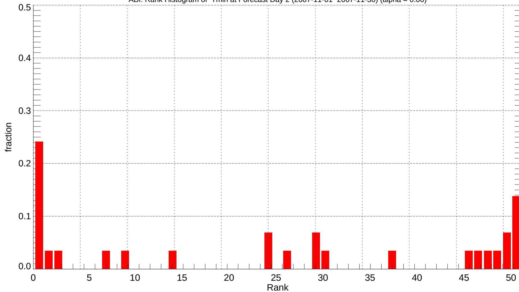
ABI: Rank Histogram of Tmin at Forecast Day 2 (2007-11-01~2007-11-30) (alpha = 0.00)
