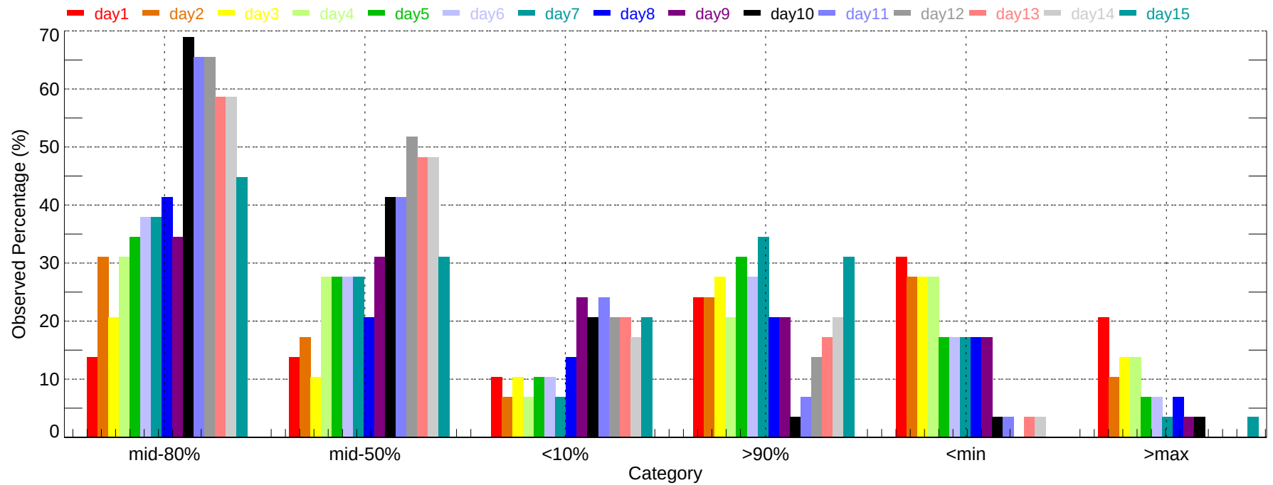
Observed Percentage of Ensembles - GEG: Max Temperature (2007-11-01~2007-11-30)
