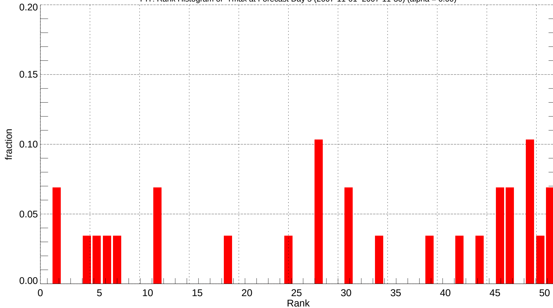
PIT: Rank Histogram of Tmax at Forecast Day 5 (2007-11-01~2007-11-30) (alpha = 0.00)
