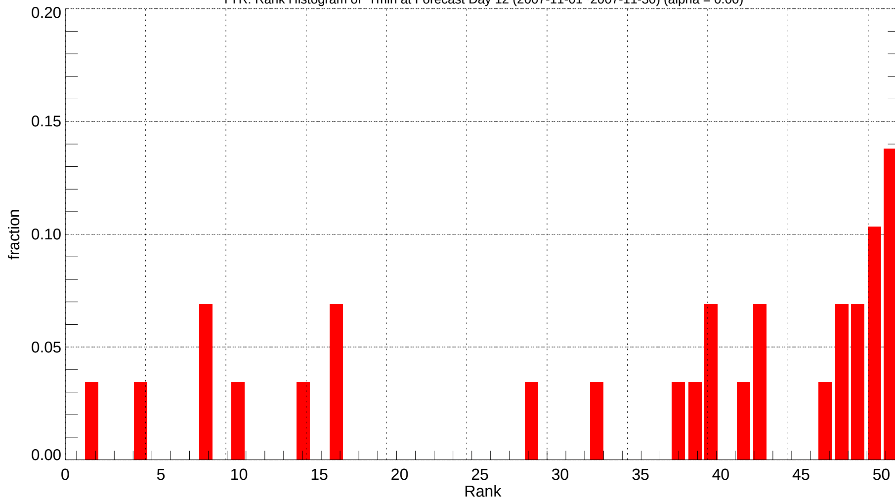
TYR: Rank Histogram of Tmin at Forecast Day 12 (2007-11-01~2007-11-30) (alpha = 0.00)
