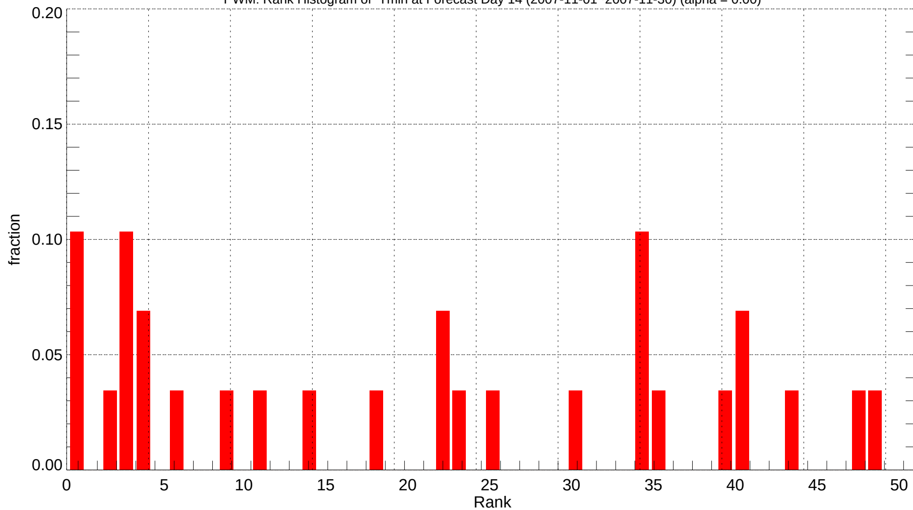
PWM: Rank Histogram of Tmin at Forecast Day 14 (2007-11-01~2007-11-30) (alpha = 0.00)
