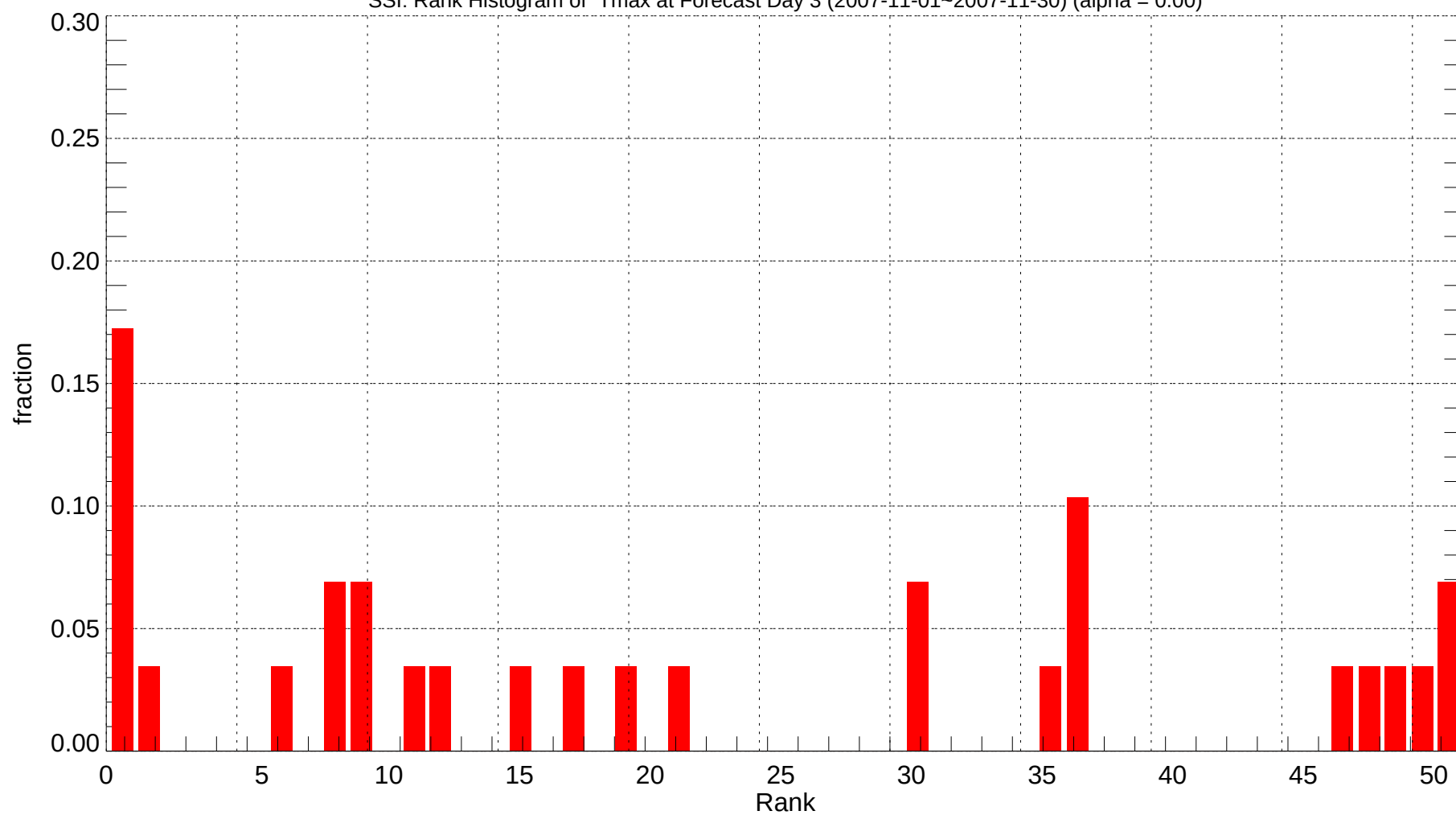
SSI: Rank Histogram of Tmax at Forecast Day 3 (2007-11-01~2007-11-30) (alpha = 0.00)
