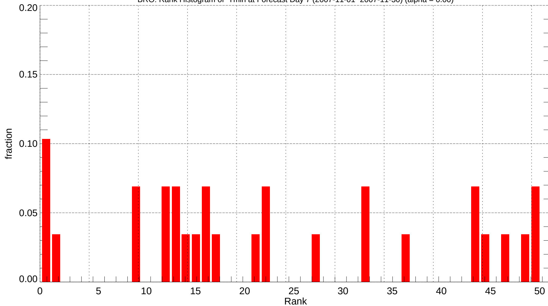
BRO: Rank Histogram of Tmin at Forecast Day 7 (2007-11-01~2007-11-30) (alpha = 0.00)
