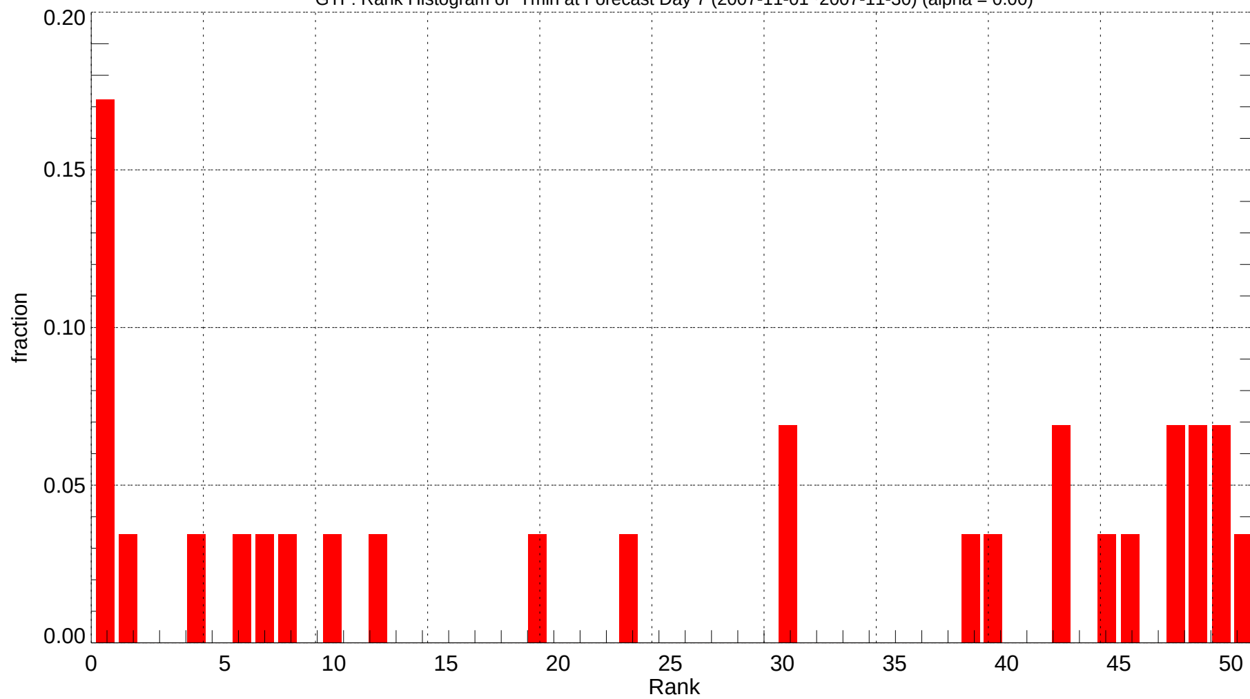
GTF: Rank Histogram of Tmin at Forecast Day 7 (2007-11-01~2007-11-30) (alpha = 0.00)
