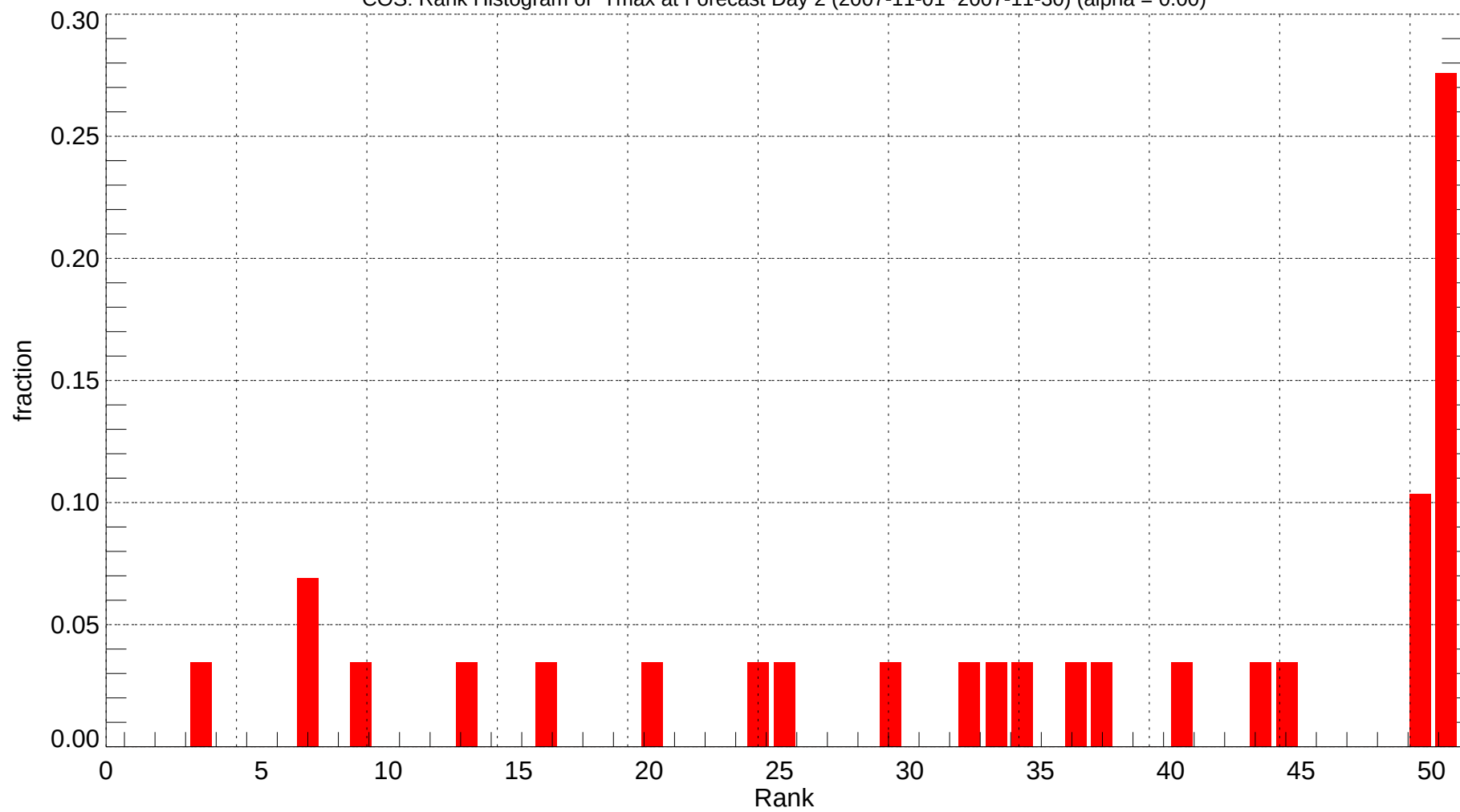
COS: Rank Histogram of Tmax at Forecast Day 2 (2007-11-01~2007-11-30) (alpha = 0.00)
