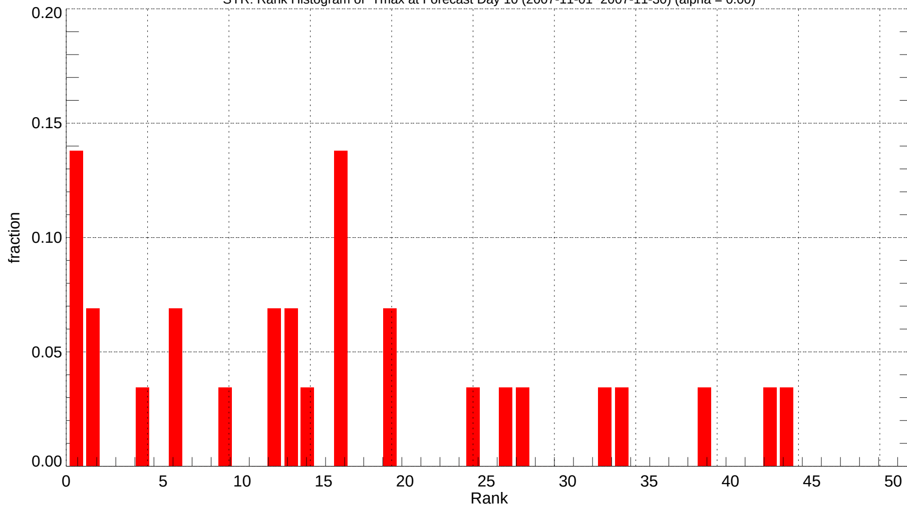
SYR: Rank Histogram of Tmax at Forecast Day 10 (2007-11-01~2007-11-30) (alpha = 0.00)
