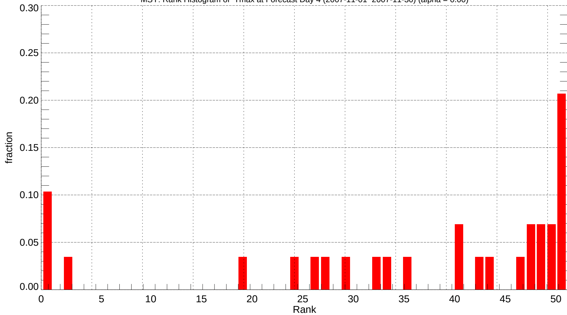
MSY: Rank Histogram of Tmax at Forecast Day 4 (2007-11-01~2007-11-30) (alpha = 0.00)
