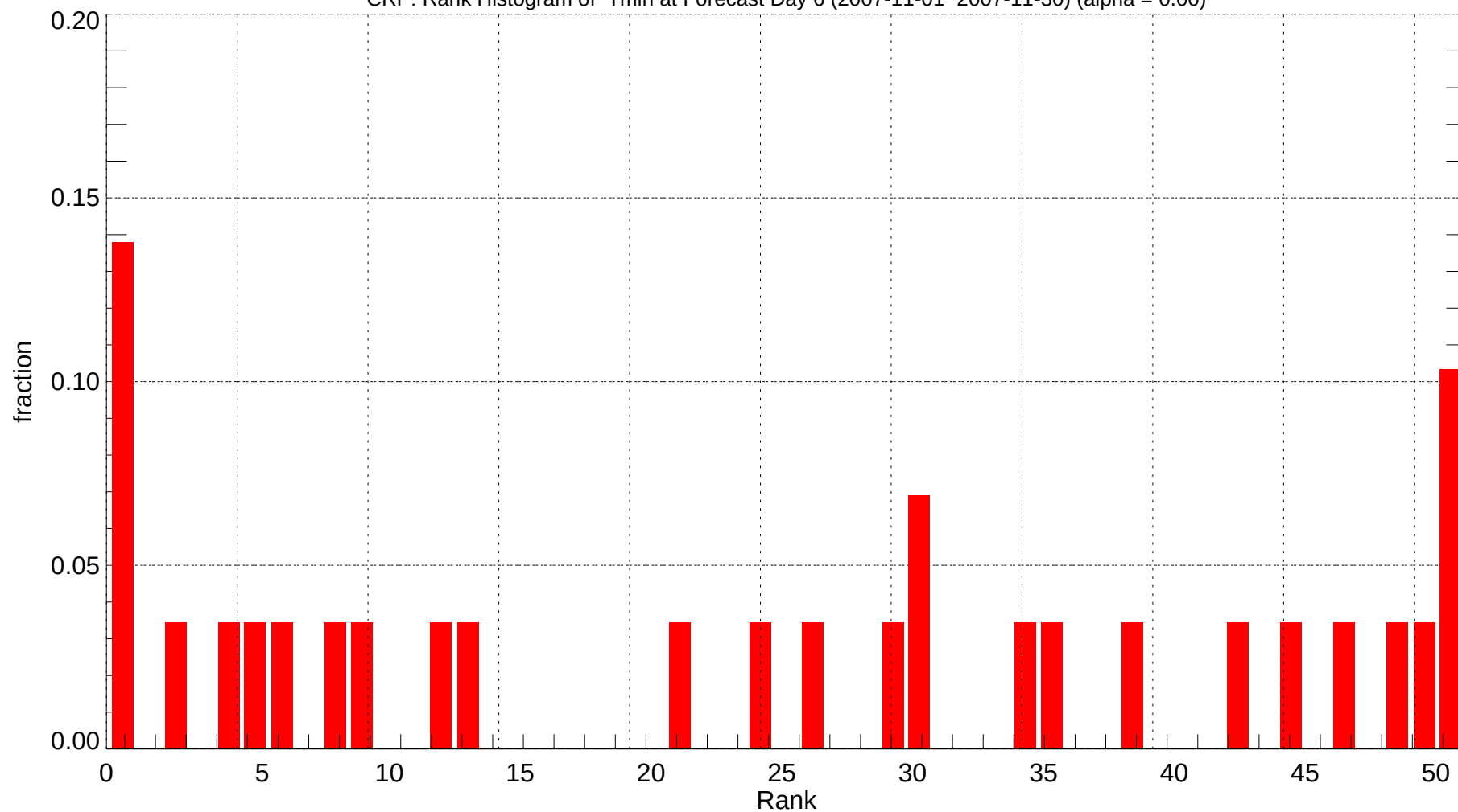
CRP: Rank Histogram of Tmin at Forecast Day 6 (2007-11-01~2007-11-30) (alpha = 0.00)
