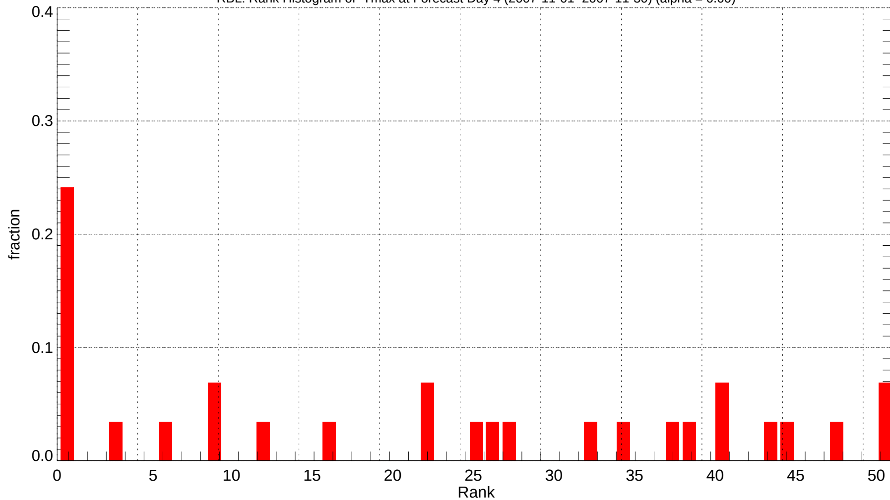
RBL: Rank Histogram of Tmax at Forecast Day 4 (2007-11-01~2007-11-30) (alpha = 0.00)
