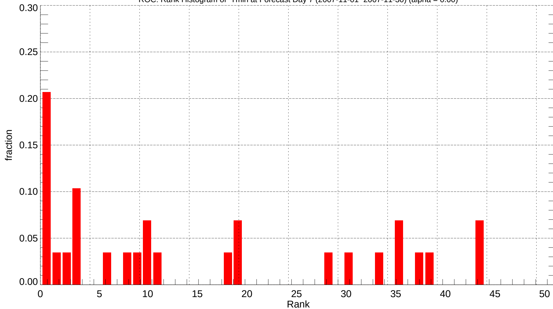
ROC: Rank Histogram of Tmin at Forecast Day 7 (2007-11-01~2007-11-30) (alpha = 0.00)
