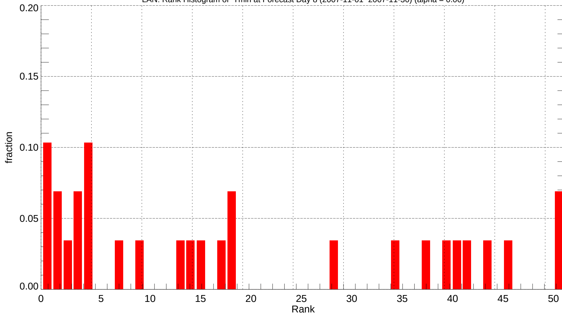
LAN: Rank Histogram of Tmin at Forecast Day 8 (2007-11-01~2007-11-30) (alpha = 0.00)
