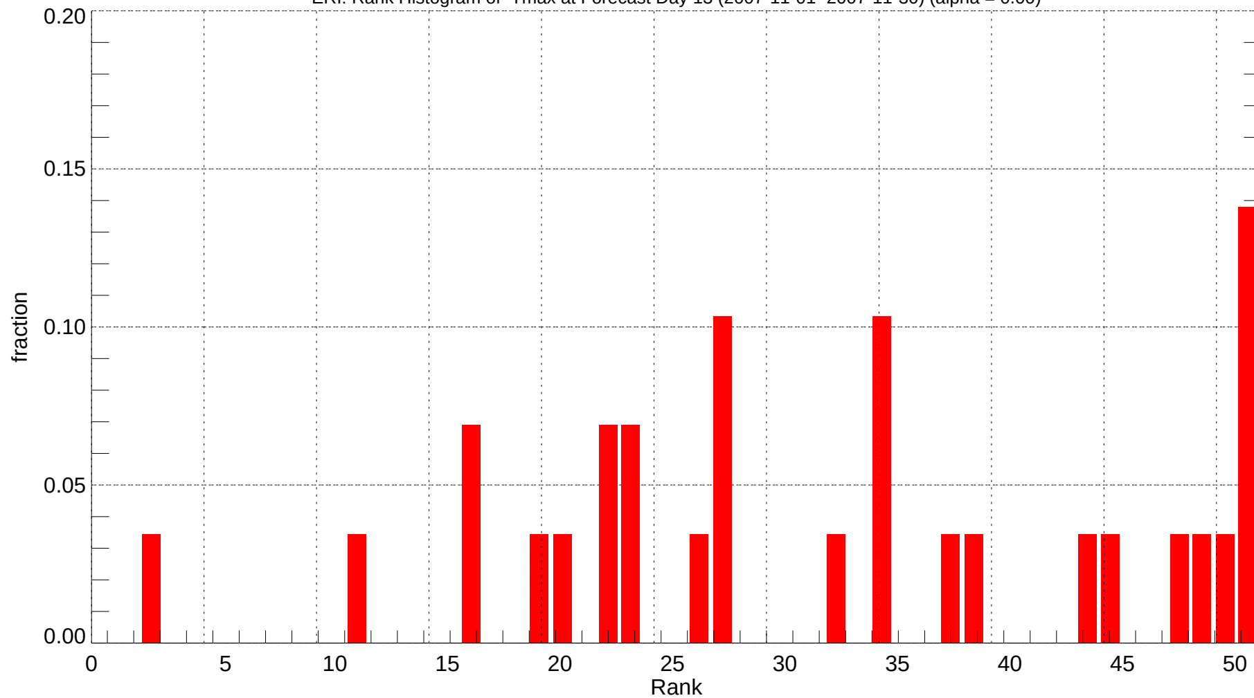
ERI: Rank Histogram of Tmax at Forecast Day 13 (2007-11-01~2007-11-30) (alpha = 0.00)
