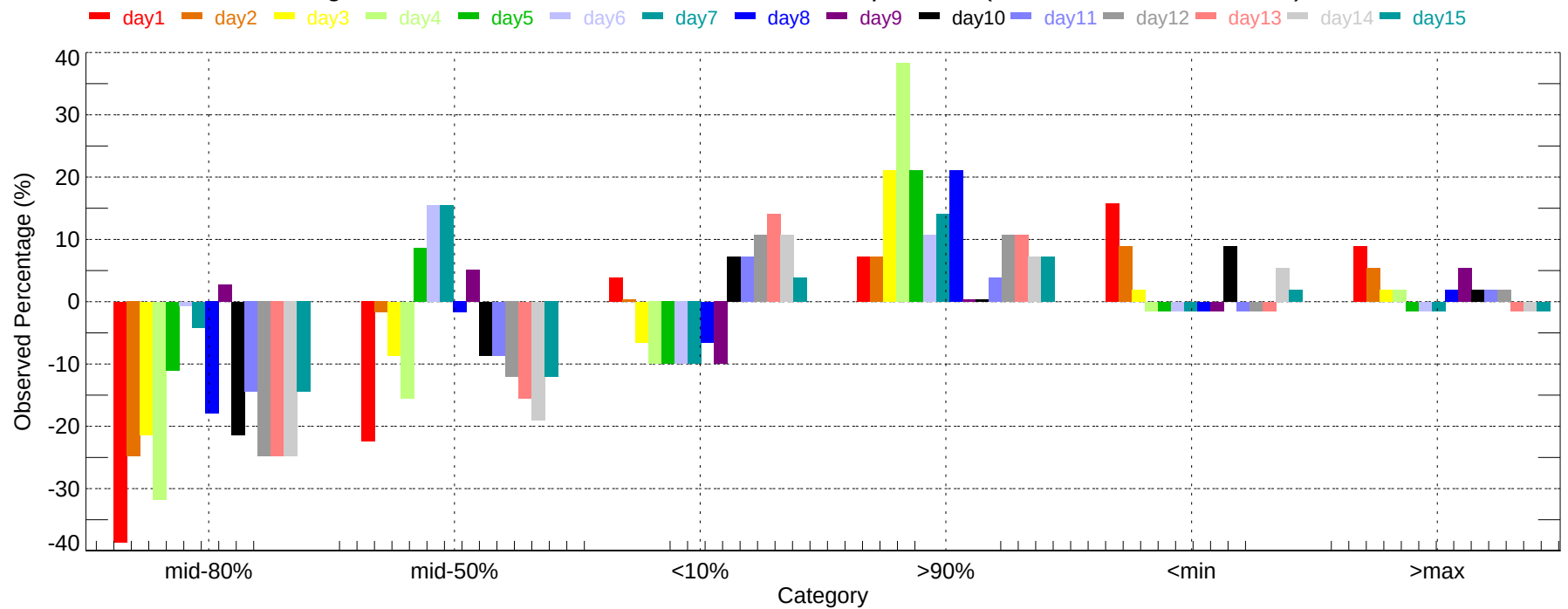
Observed Percentage Deviation of Ensembles - LGA: Max Temperature (2007-11-01~2007-11-30)
