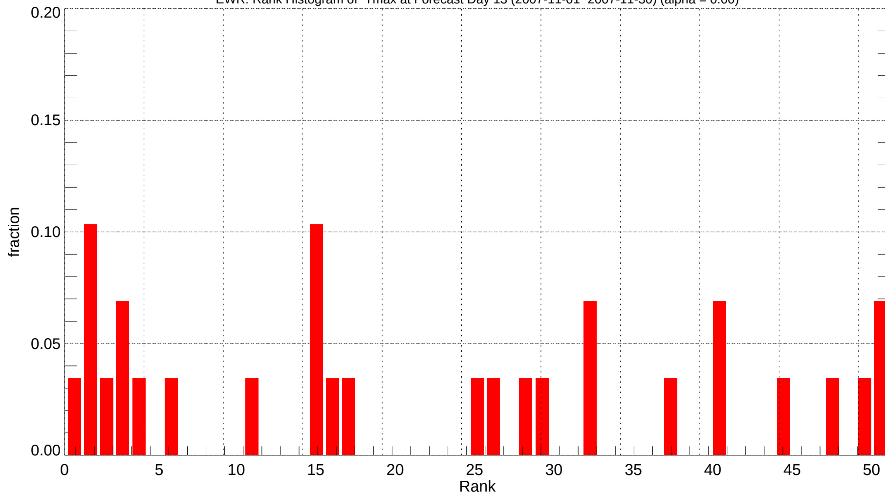
EWR: Rank Histogram of Tmax at Forecast Day 13 (2007-11-01~2007-11-30) (alpha = 0.00)
