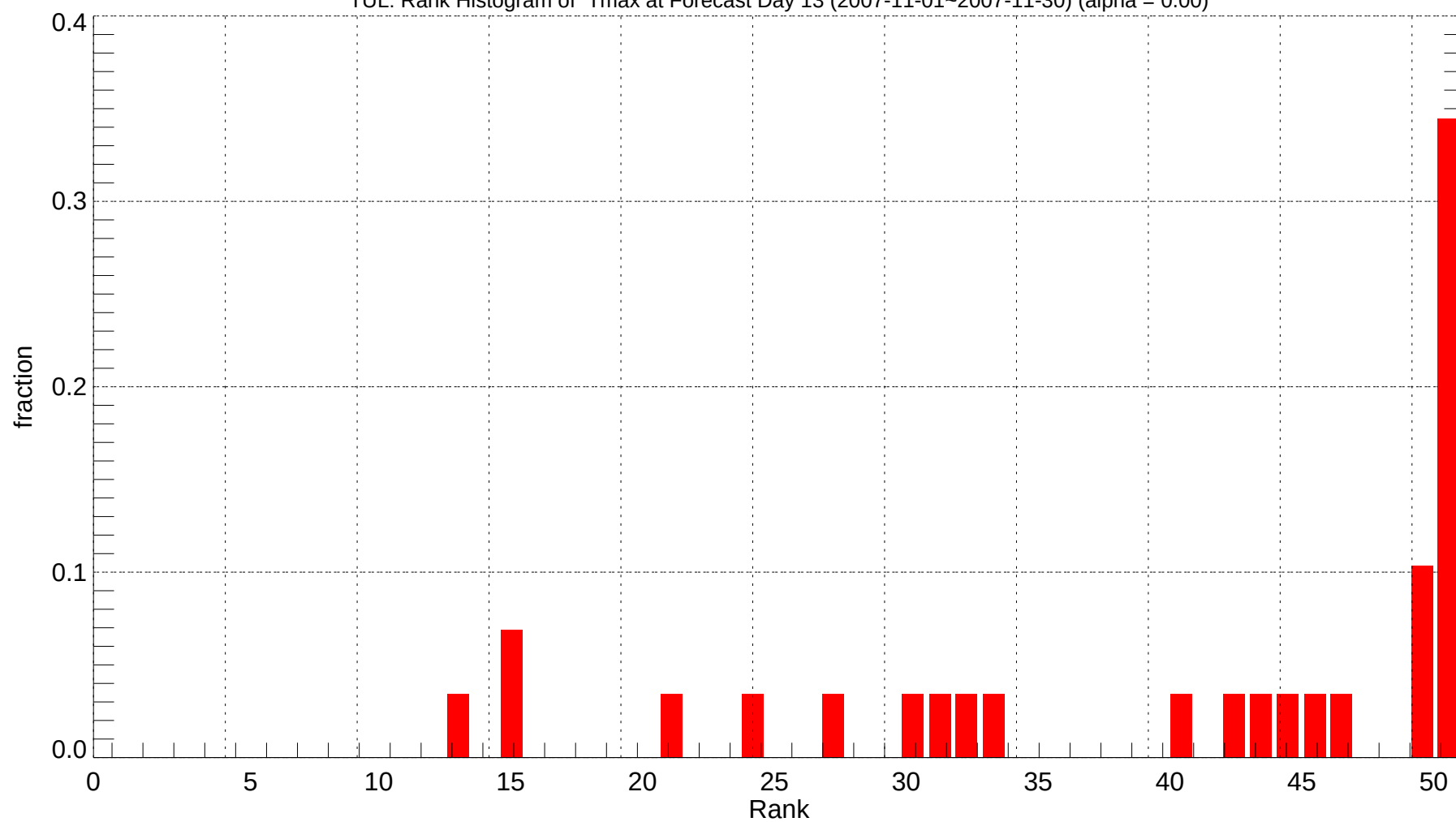
TUL: Rank Histogram of Tmax at Forecast Day 13 (2007-11-01~2007-11-30) (alpha = 0.00)
