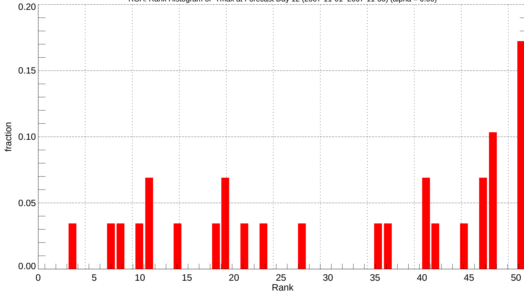
ROA: Rank Histogram of Tmax at Forecast Day 12 (2007-11-01~2007-11-30) (alpha = 0.00)
