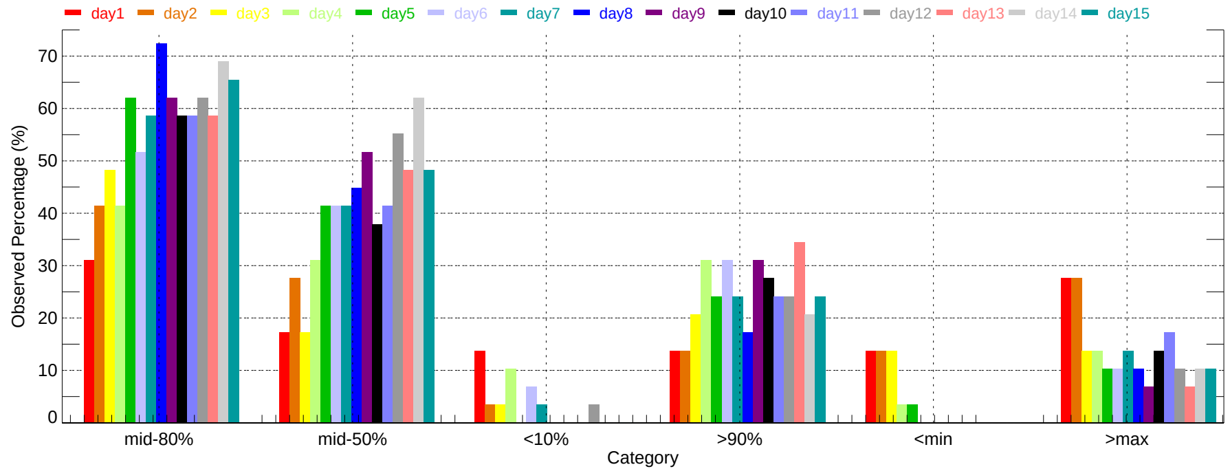
Observed Percentage of Ensembles - DEC: Min Temperature (2007-11-01~2007-11-30)
