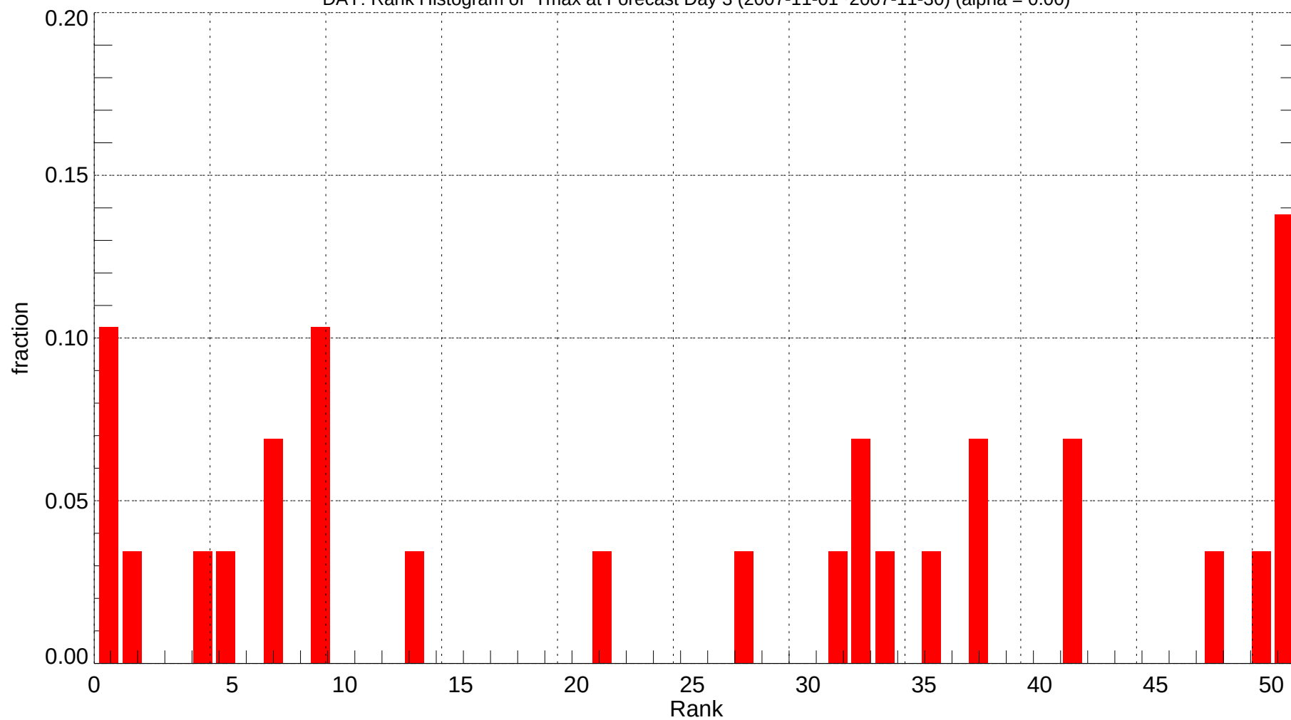
DAY: Rank Histogram of Tmax at Forecast Day 3 (2007-11-01~2007-11-30) (alpha = 0.00)
