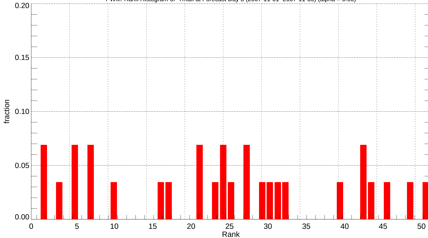
PWM: Rank Histogram of Tmax at Forecast Day 8 (2007-11-01~2007-11-30) (alpha = 0.00)
