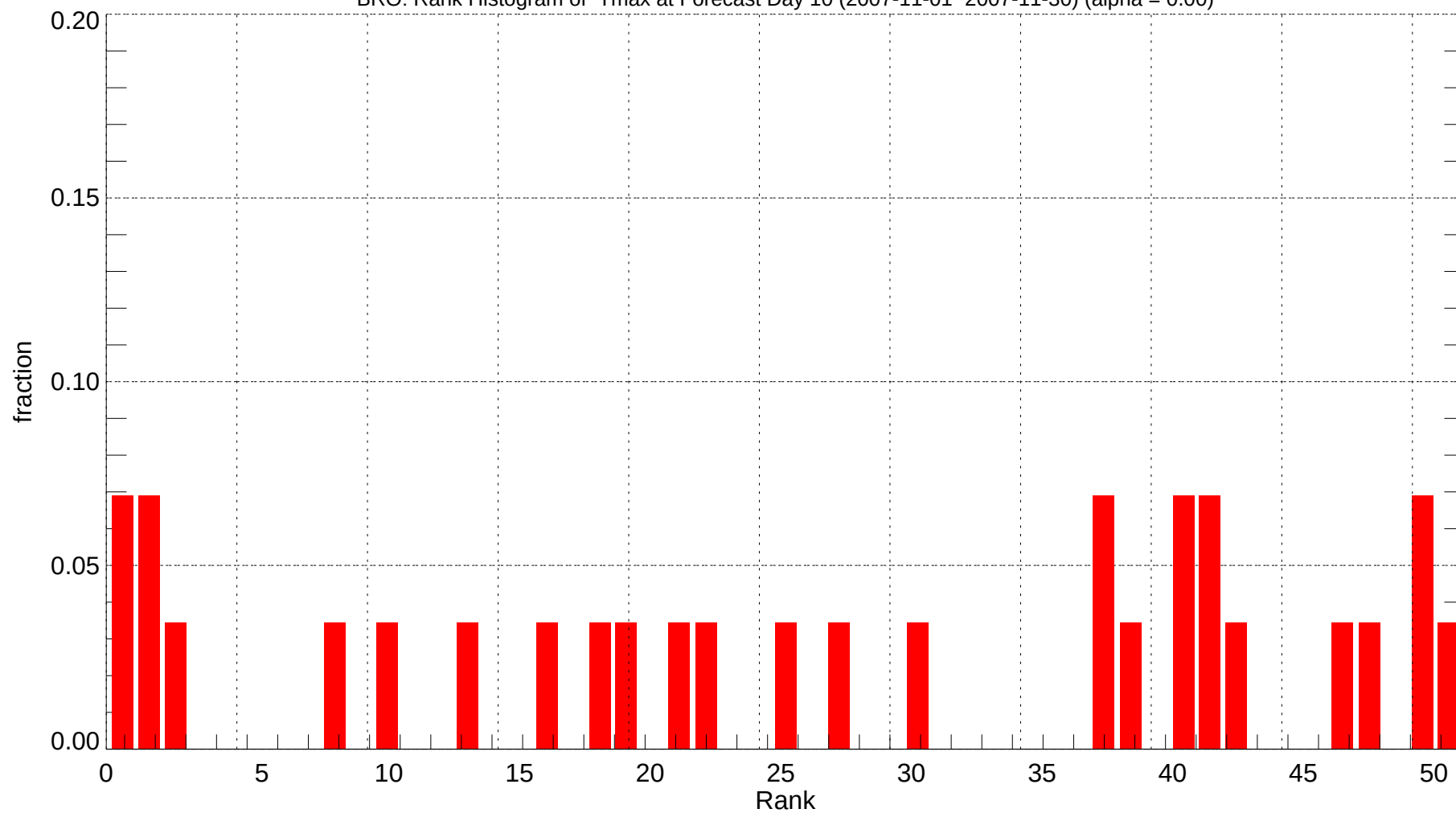
BRO: Rank Histogram of Tmax at Forecast Day 10 (2007-11-01~2007-11-30) (alpha = 0.00)
