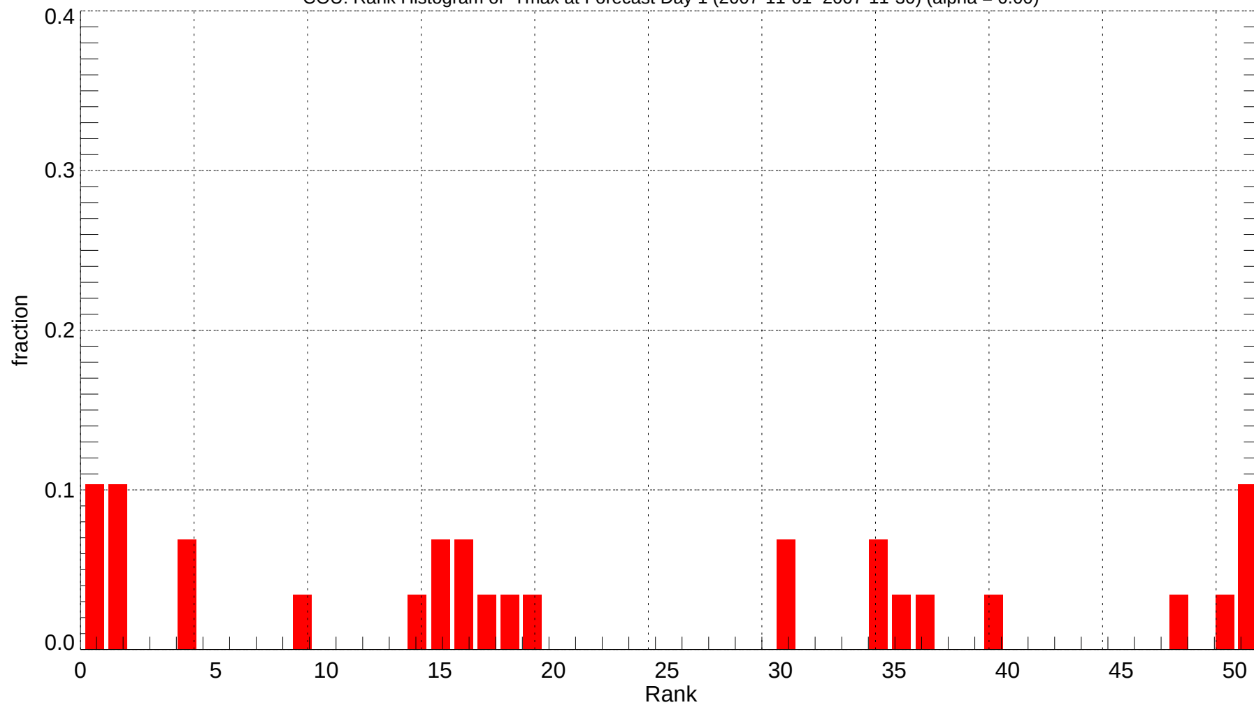
COU: Rank Histogram of Tmax at Forecast Day 1 (2007-11-01~2007-11-30) (alpha = 0.00)
