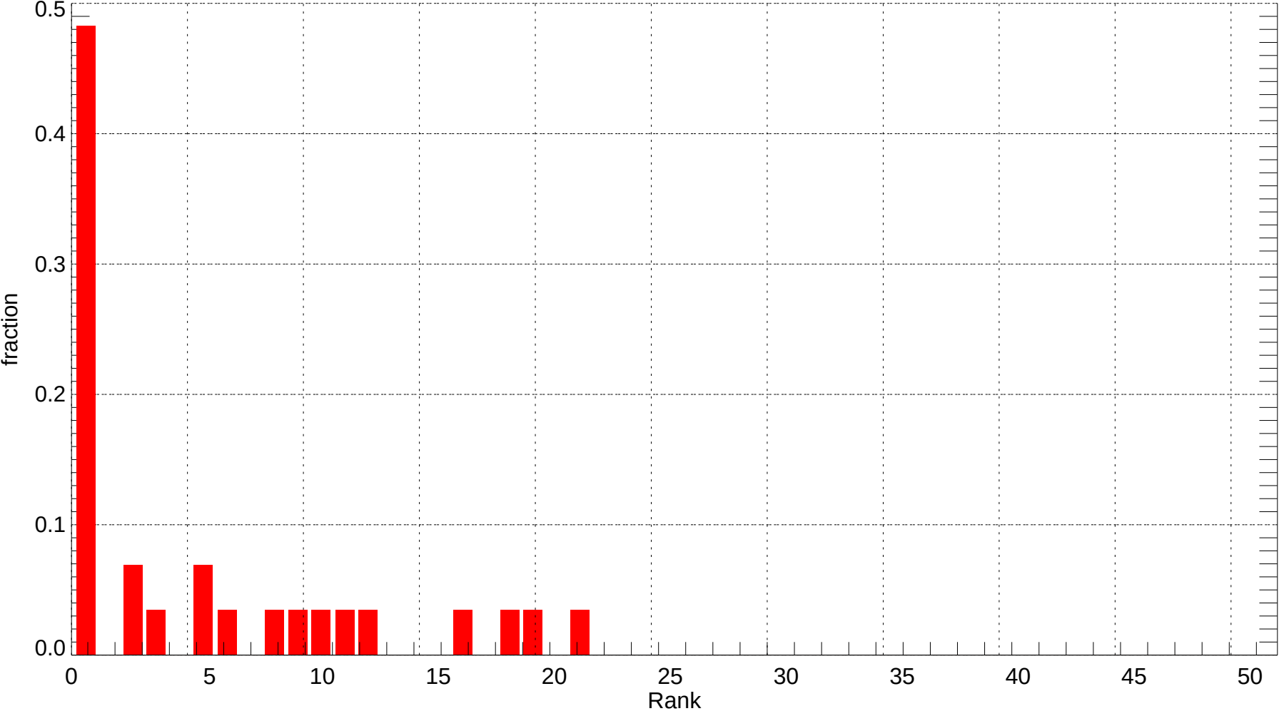
SJC: Rank Histogram of Tmin at Forecast Day 8 (2007-11-01~2007-11-30) (alpha = 0.00)
