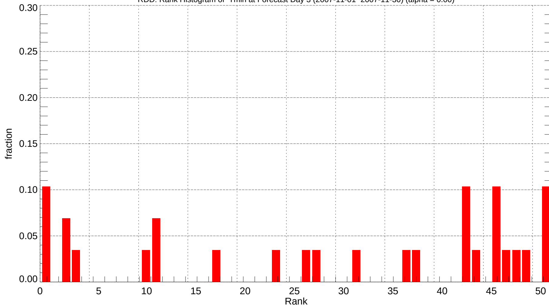
RDD: Rank Histogram of Tmin at Forecast Day 3 (2007-11-01~2007-11-30) (alpha = 0.00)
