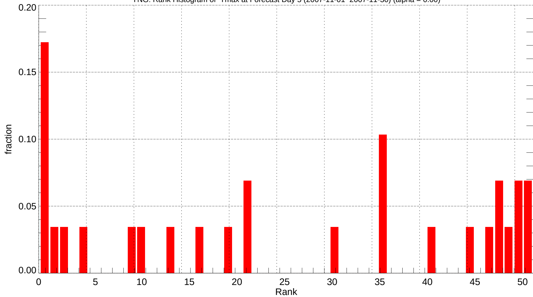
YNG: Rank Histogram of Tmax at Forecast Day 5 (2007-11-01~2007-11-30) (alpha = 0.00)
