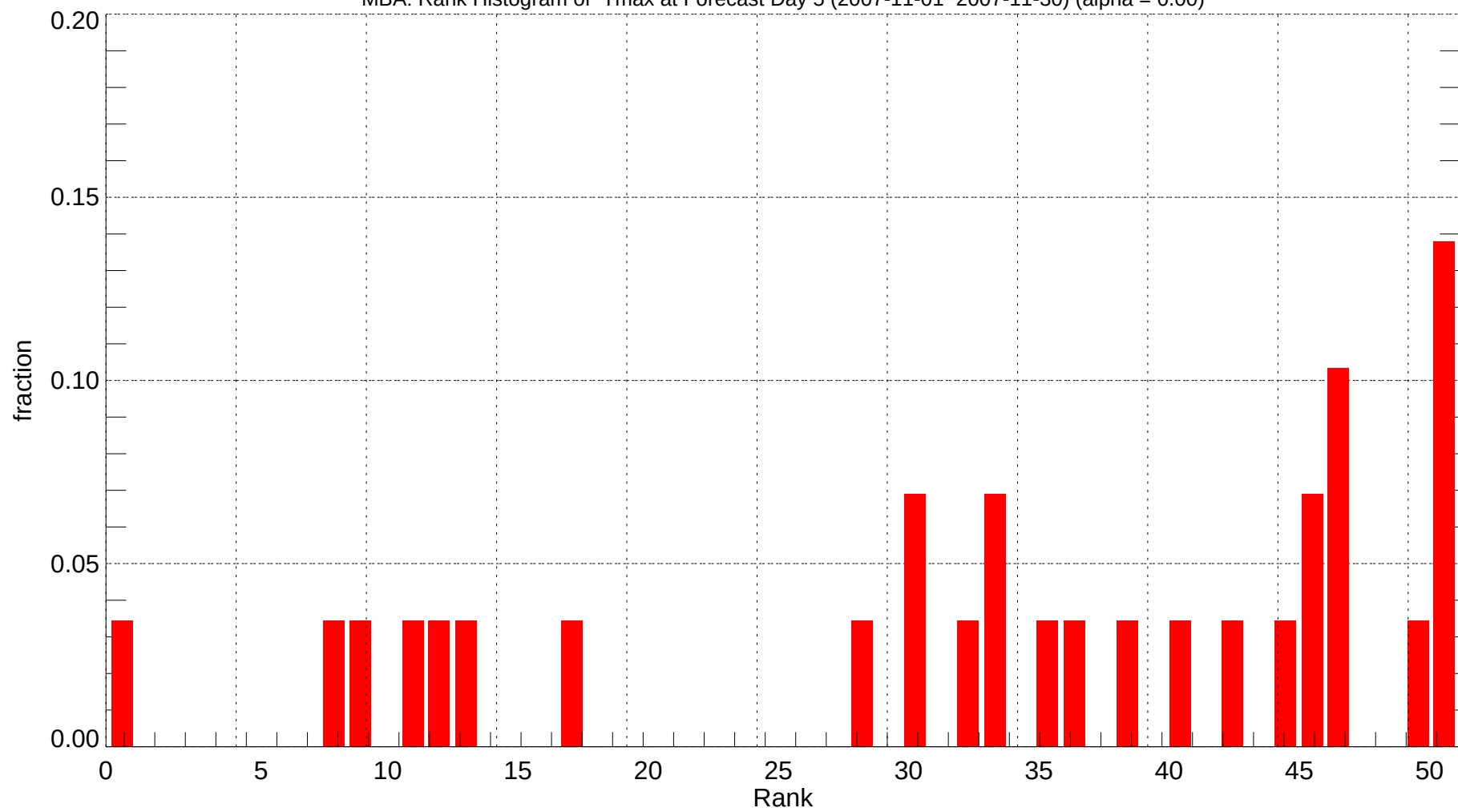
MBA: Rank Histogram of Tmax at Forecast Day 5 (2007-11-01~2007-11-30) (alpha = 0.00)
