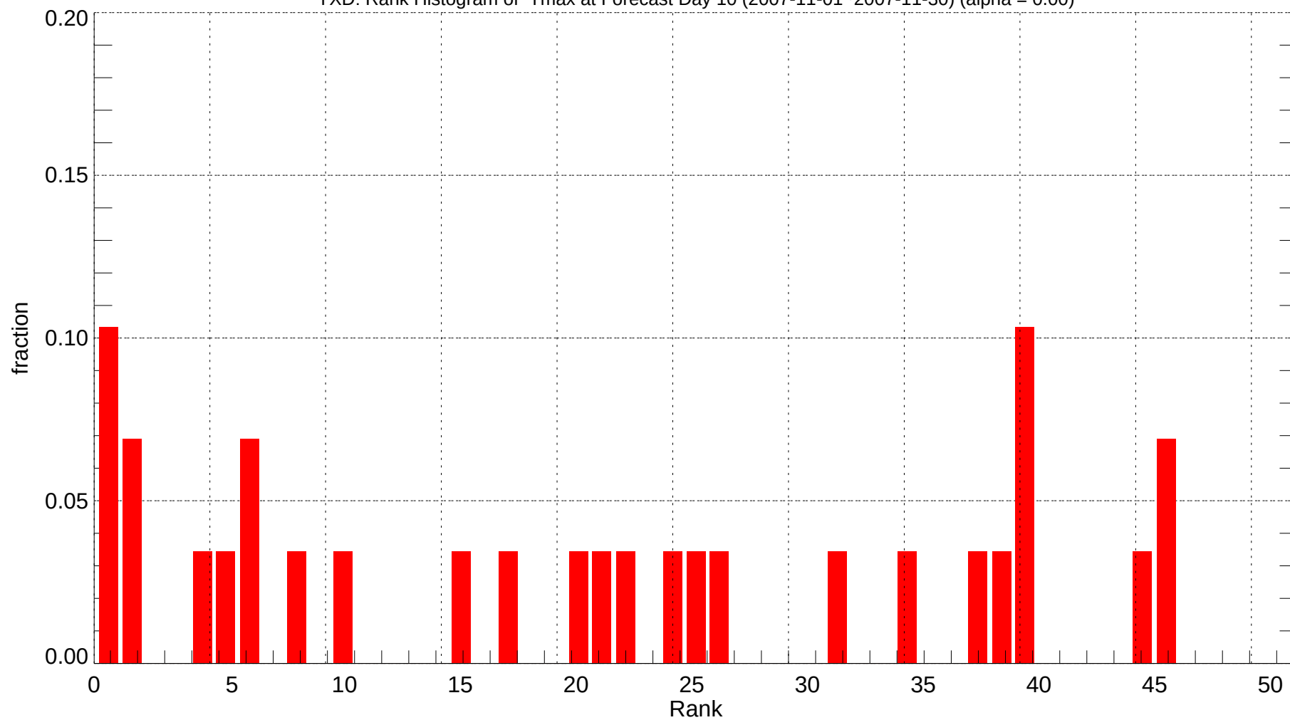
YXD: Rank Histogram of Tmax at Forecast Day 10 (2007-11-01~2007-11-30) (alpha = 0.00)
