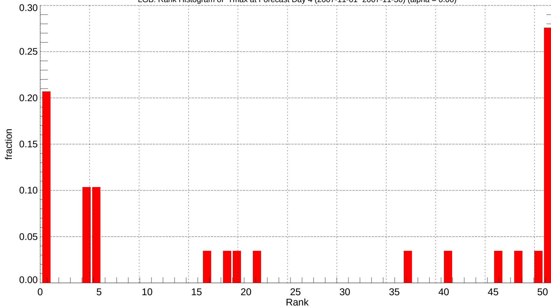
LGB: Rank Histogram of Tmax at Forecast Day 4 (2007-11-01~2007-11-30) (alpha = 0.00)
