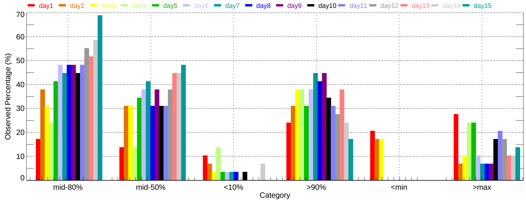
Observed Percentage of Ensembles - MEM: Min Temperature (2007-11-01~2007-11-30)
