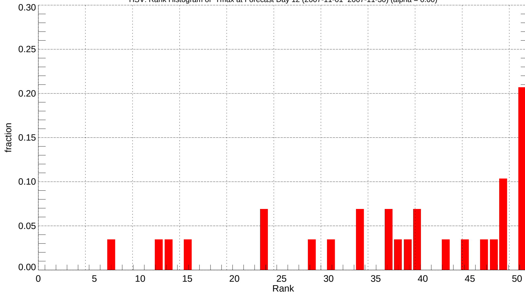
HSV: Rank Histogram of Tmax at Forecast Day 12 (2007-11-01~2007-11-30) (alpha = 0.00)
