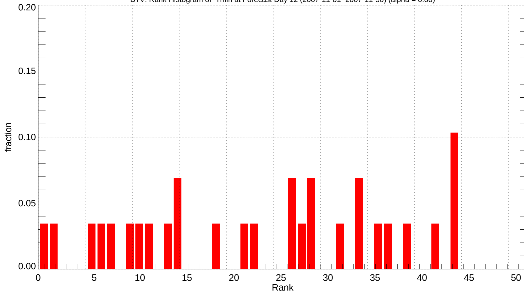
BTV: Rank Histogram of Tmin at Forecast Day 12 (2007-11-01~2007-11-30) (alpha = 0.00)
