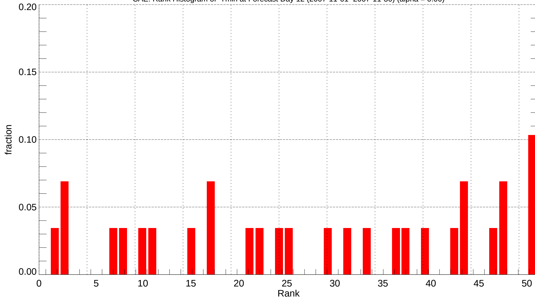
CAE: Rank Histogram of Tmin at Forecast Day 12 (2007-11-01~2007-11-30) (alpha = 0.00)
