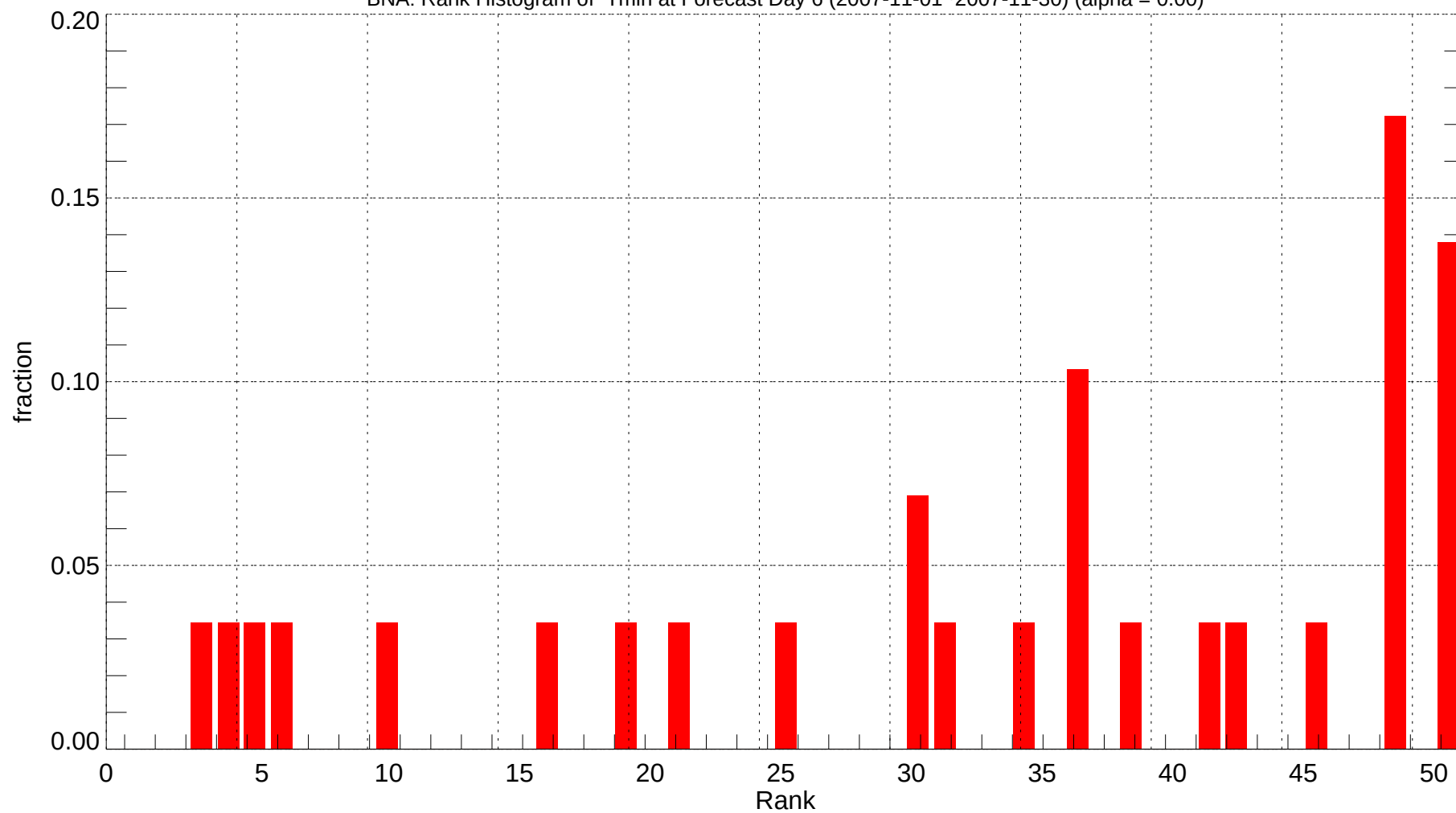
BNA: Rank Histogram of Tmin at Forecast Day 6 (2007-11-01~2007-11-30) (alpha = 0.00)
