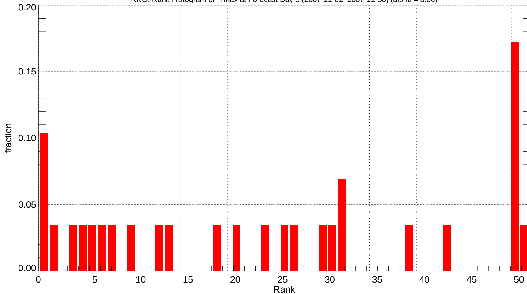
RNO: Rank Histogram of Tmax at Forecast Day 5 (2007-11-01~2007-11-30) (alpha = 0.00)
