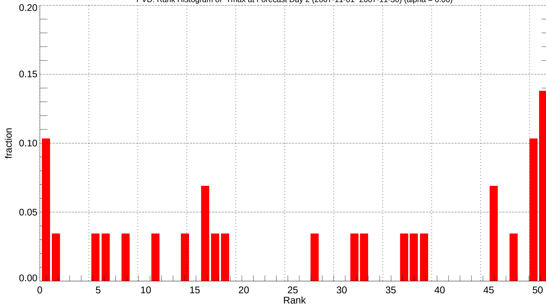
PVD: Rank Histogram of Tmax at Forecast Day 2 (2007-11-01~2007-11-30) (alpha = 0.00)
