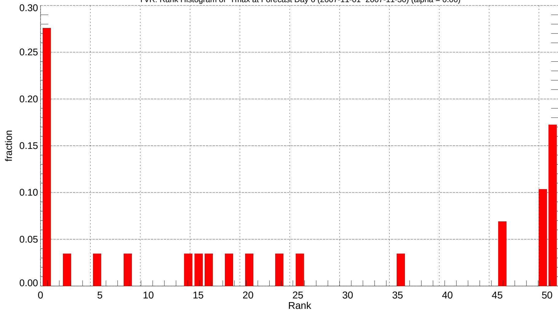
YVR: Rank Histogram of Tmax at Forecast Day 6 (2007-11-01~2007-11-30) (alpha = 0.00)
