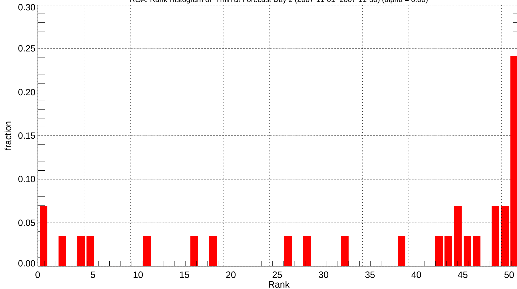
ROA: Rank Histogram of Tmin at Forecast Day 2 (2007-11-01~2007-11-30) (alpha = 0.00)
