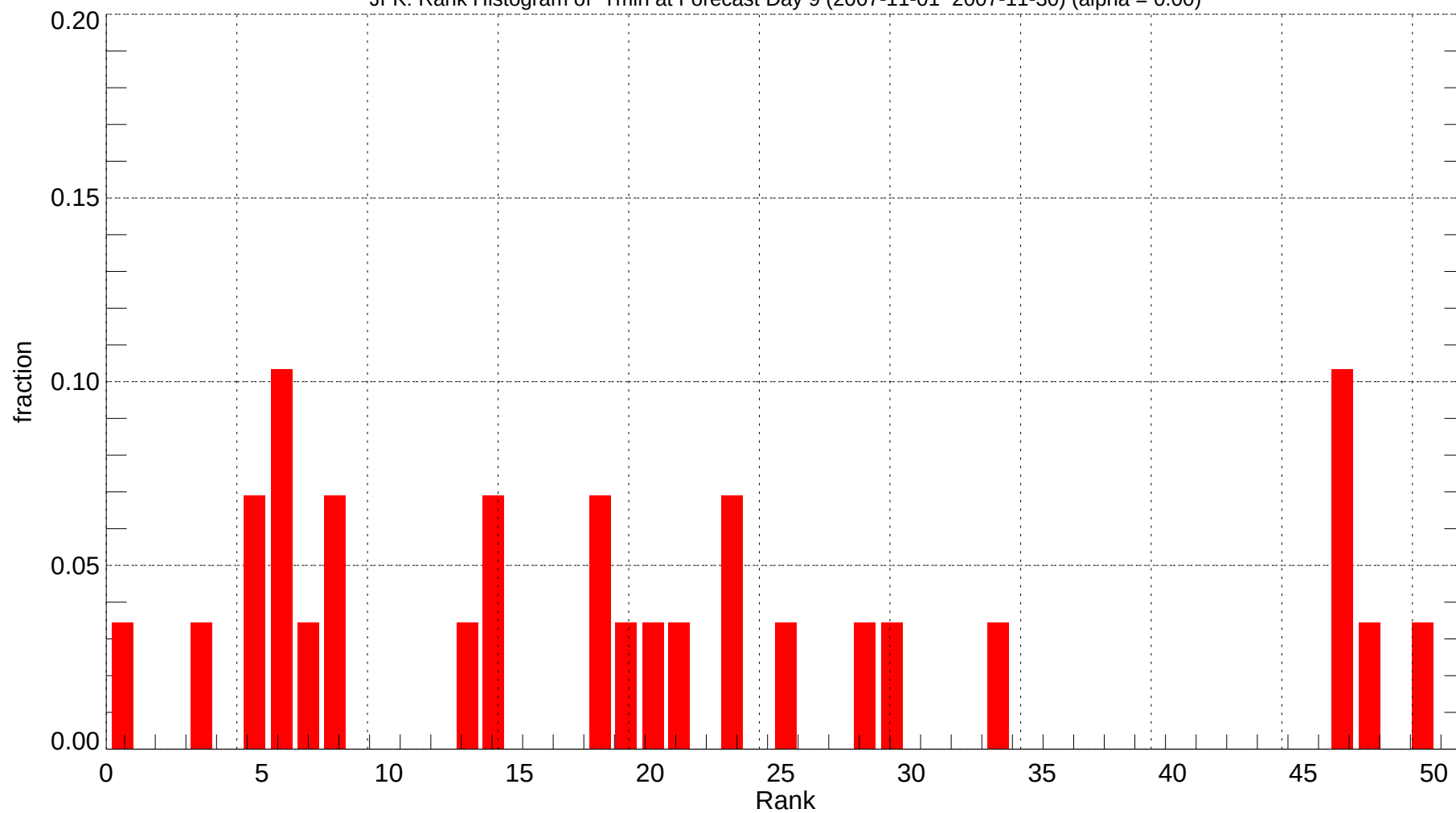
JFK: Rank Histogram of Tmin at Forecast Day 9 (2007-11-01~2007-11-30) (alpha = 0.00)
