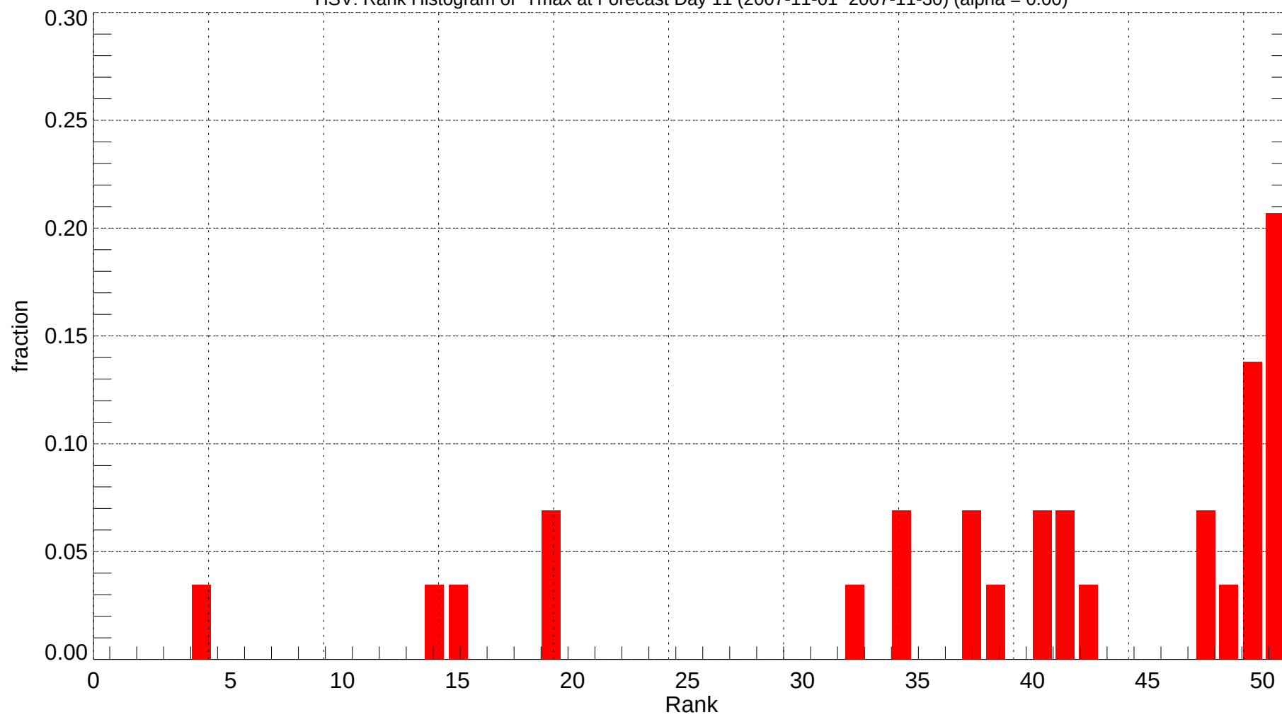
HSV: Rank Histogram of Tmax at Forecast Day 11 (2007-11-01~2007-11-30) (alpha = 0.00)
