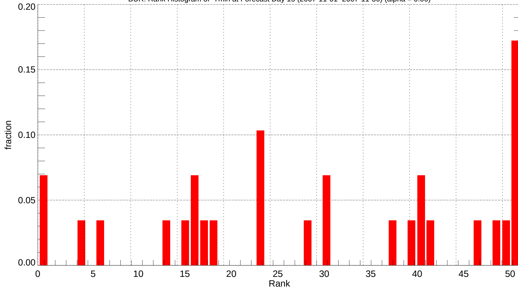
BUR: Rank Histogram of Tmin at Forecast Day 15 (2007-11-01~2007-11-30) (alpha = 0.00)
