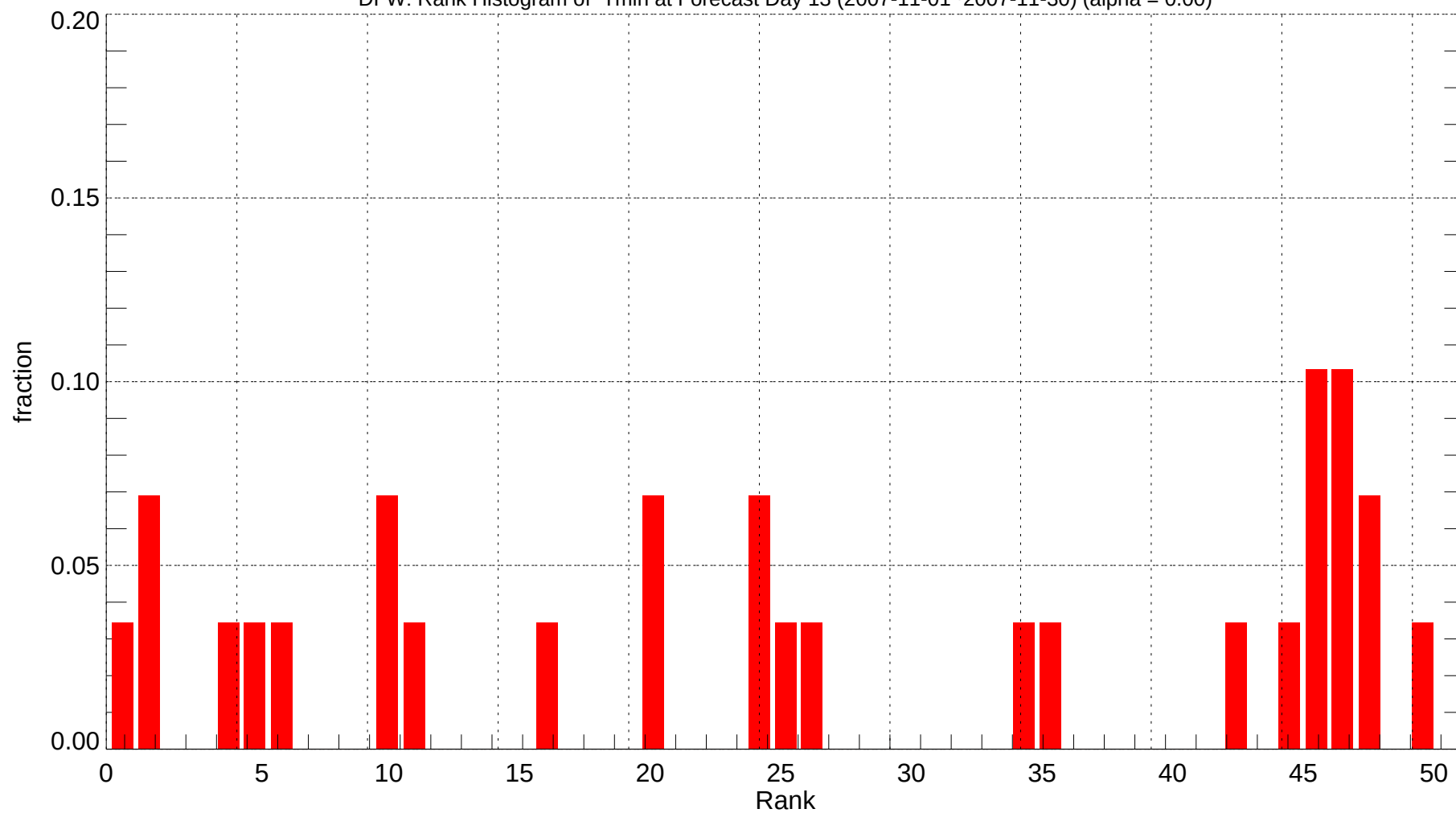
DFW: Rank Histogram of Tmin at Forecast Day 13 (2007-11-01~2007-11-30) (alpha = 0.00)
