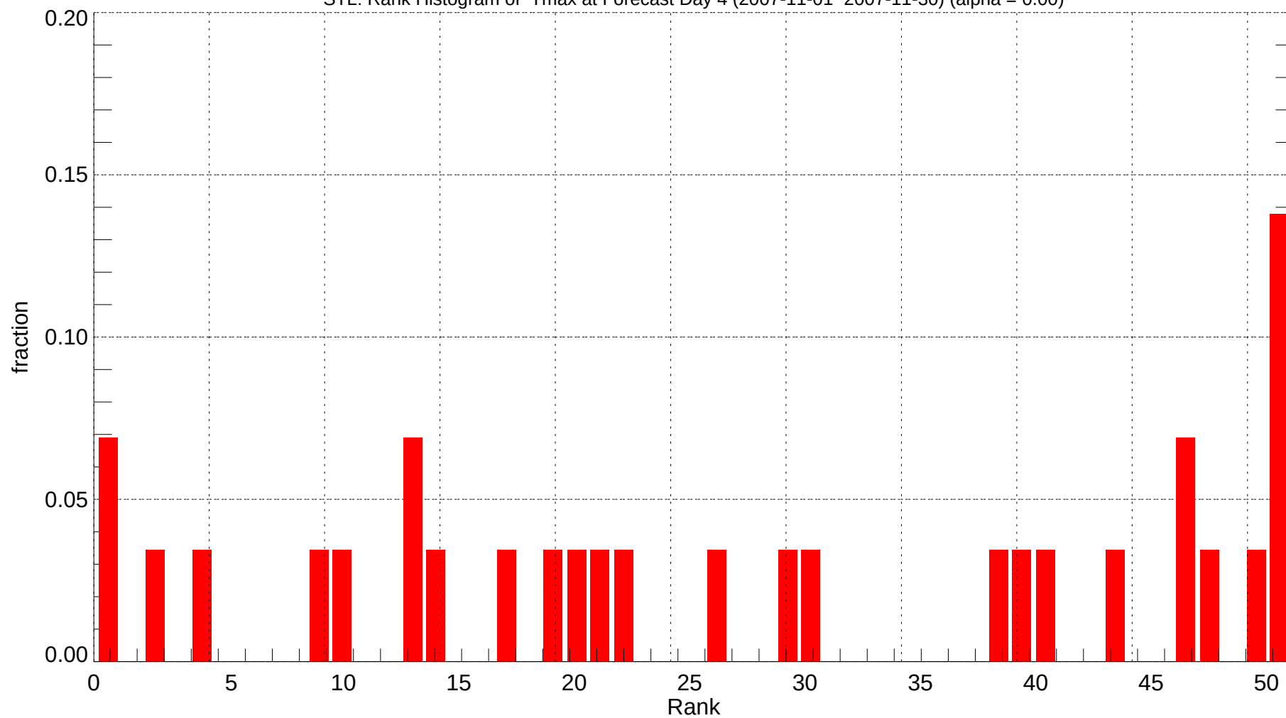
STL: Rank Histogram of Tmax at Forecast Day 4 (2007-11-01~2007-11-30) (alpha = 0.00)
