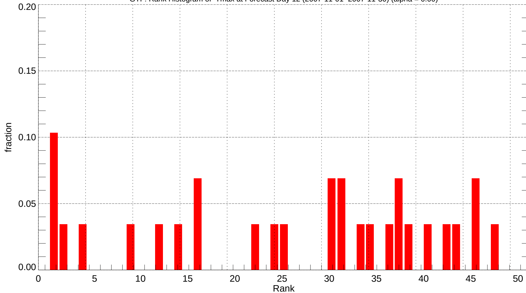
GTF: Rank Histogram of Tmax at Forecast Day 12 (2007-11-01~2007-11-30) (alpha = 0.00)
