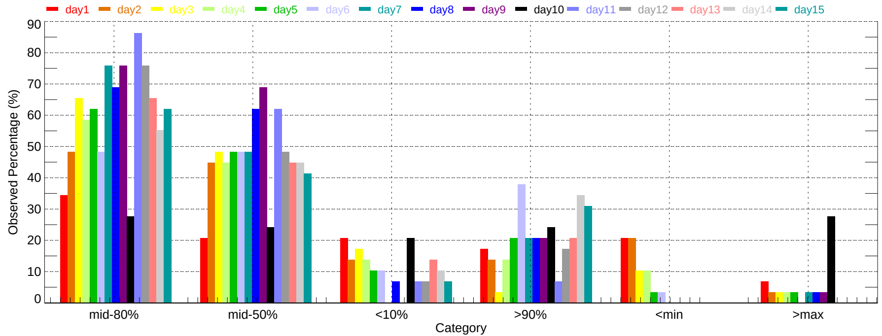
Observed Percentage of Ensembles - ABQ: Max Temperature (2007-11-01~2007-11-30)
