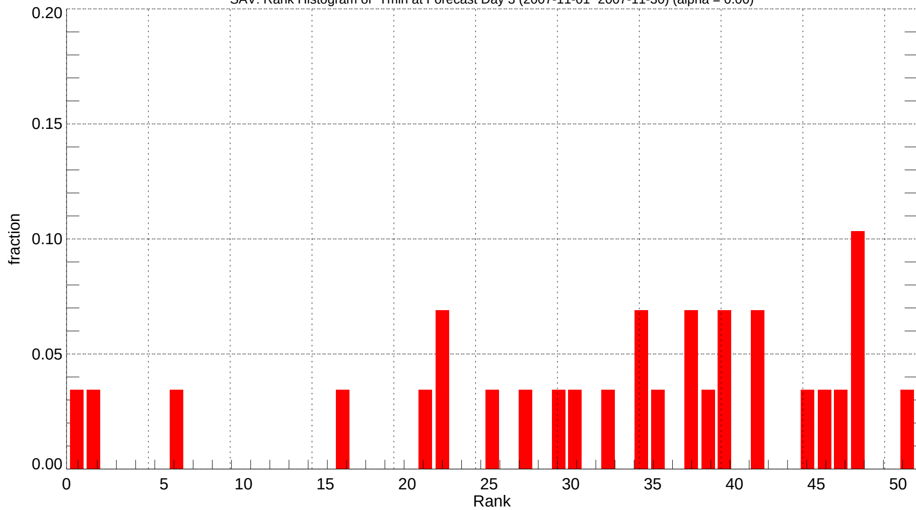
SAV: Rank Histogram of Tmin at Forecast Day 3 (2007-11-01~2007-11-30) (alpha = 0.00)
