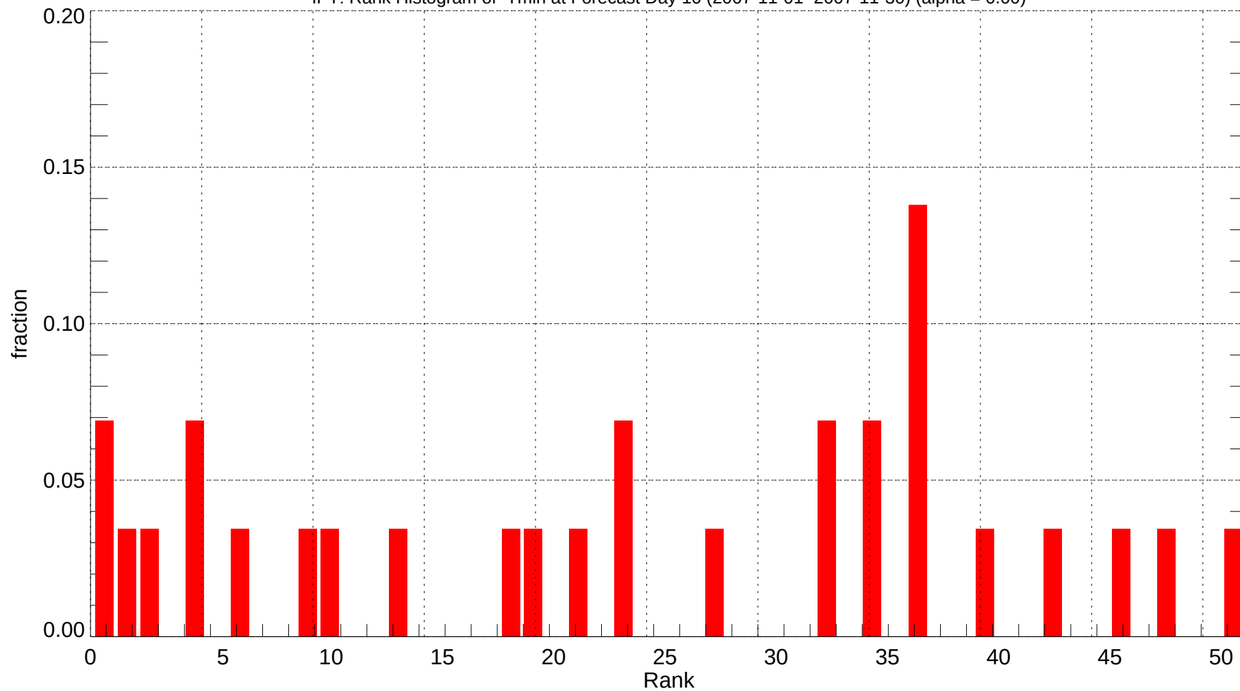
IPT: Rank Histogram of Tmin at Forecast Day 10 (2007-11-01~2007-11-30) (alpha = 0.00)
