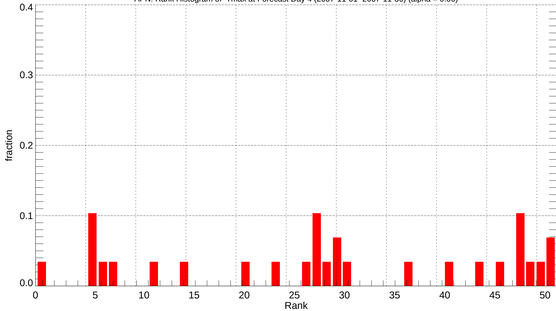
APN: Rank Histogram of Tmax at Forecast Day 4 (2007-11-01~2007-11-30) (alpha = 0.00)
