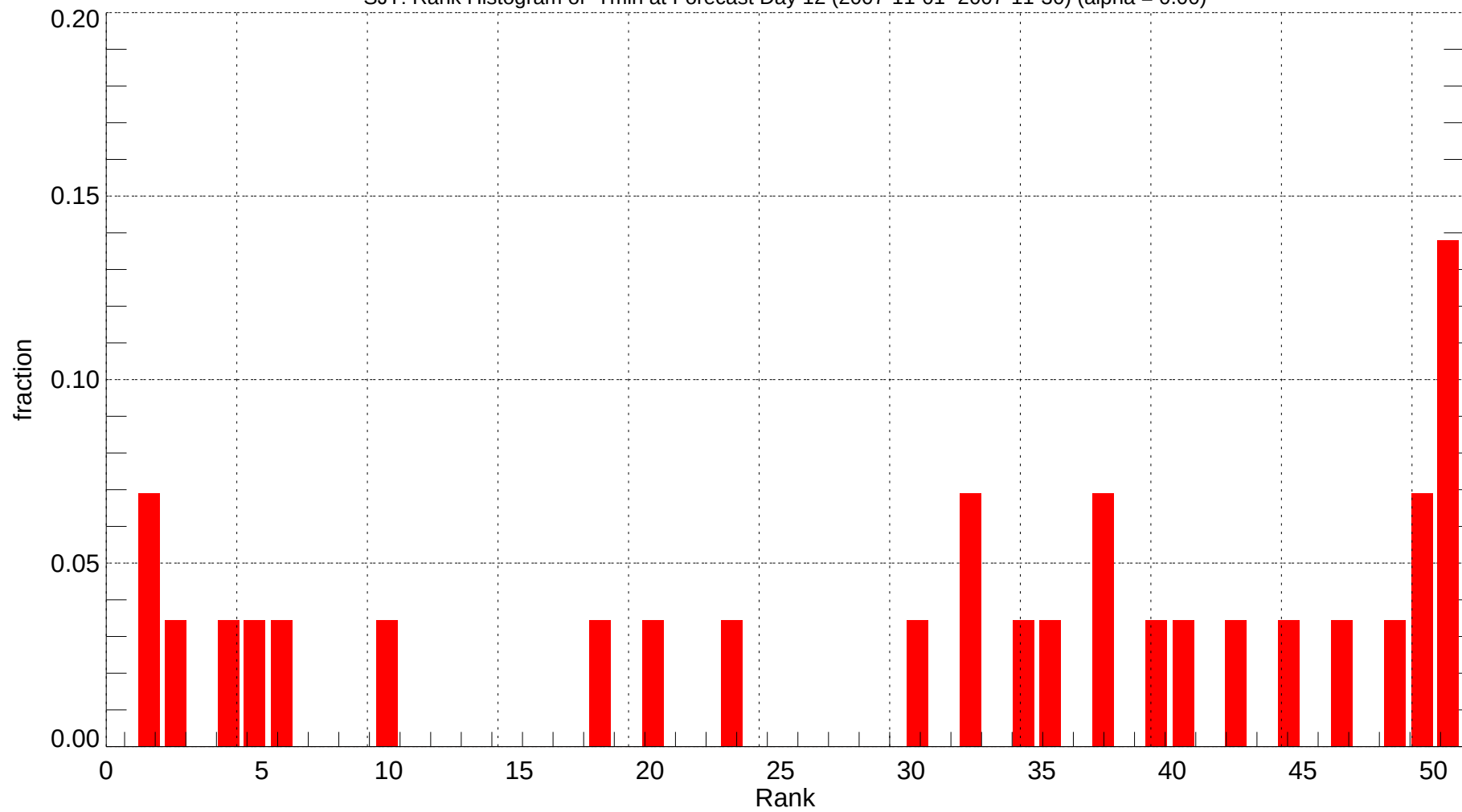
SJT: Rank Histogram of Tmin at Forecast Day 12 (2007-11-01~2007-11-30) (alpha = 0.00)
