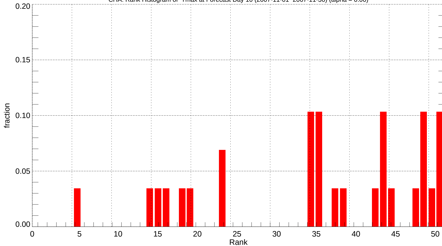
CHA: Rank Histogram of Tmax at Forecast Day 10 (2007-11-01~2007-11-30) (alpha = 0.00)
