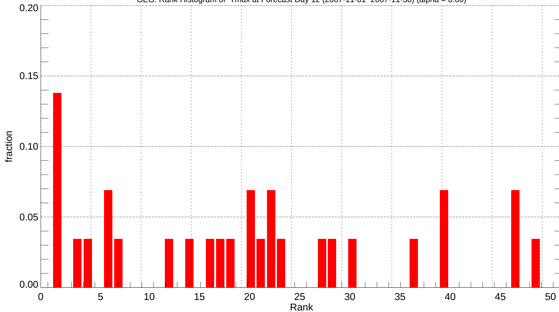
GEG: Rank Histogram of Tmax at Forecast Day 12 (2007-11-01~2007-11-30) (alpha = 0.00)
