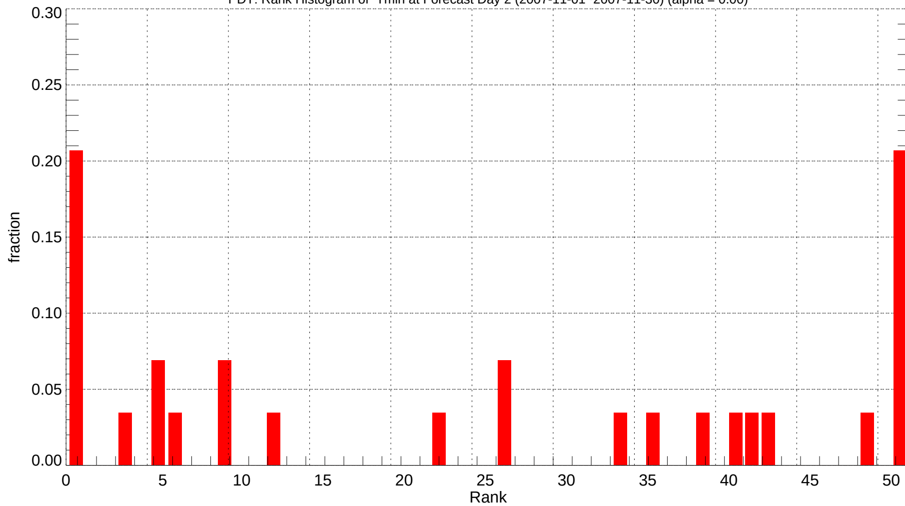
PDT: Rank Histogram of Tmin at Forecast Day 2 (2007-11-01~2007-11-30) (alpha = 0.00)
