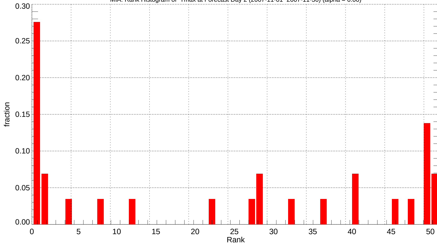
MIA: Rank Histogram of Tmax at Forecast Day 2 (2007-11-01~2007-11-30) (alpha = 0.00)
