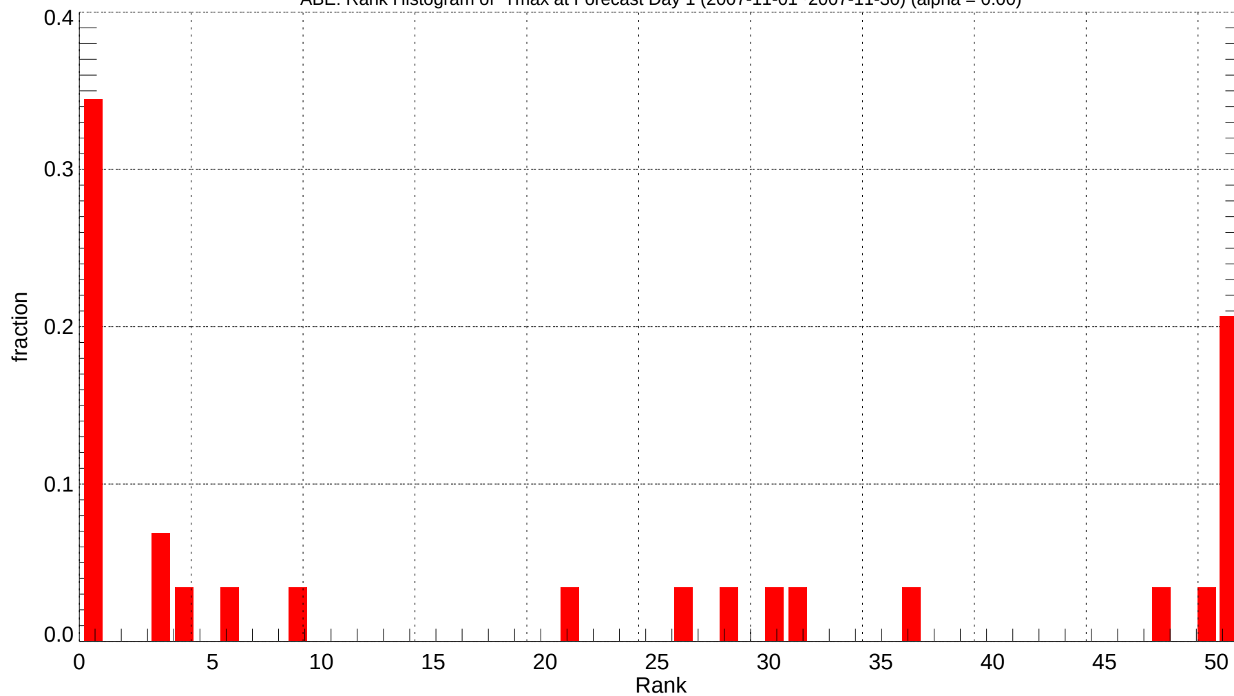
ABE: Rank Histogram of Tmax at Forecast Day 1 (2007-11-01~2007-11-30) (alpha = 0.00)
