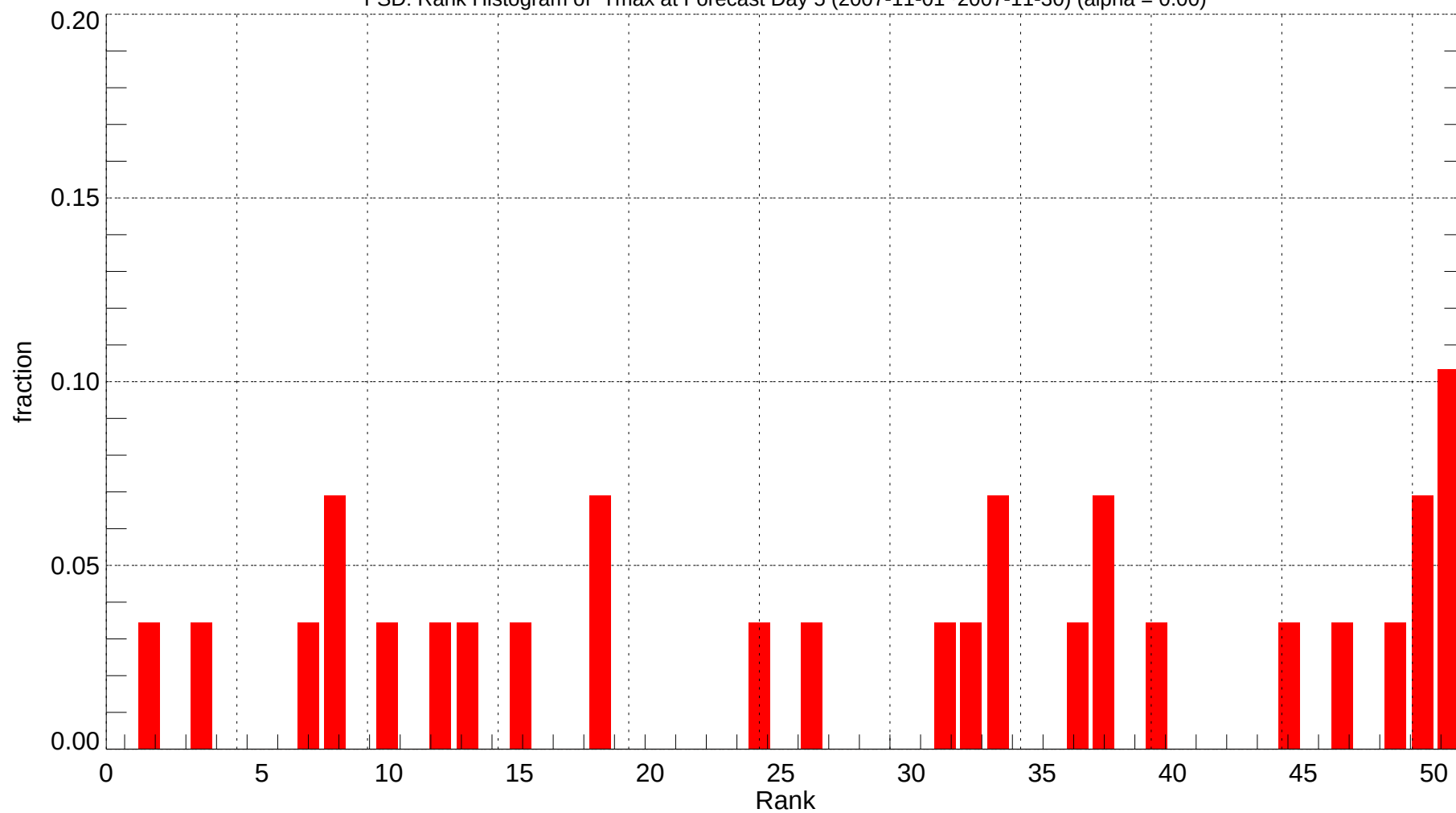
FSD: Rank Histogram of Tmax at Forecast Day 5 (2007-11-01~2007-11-30) (alpha = 0.00)
