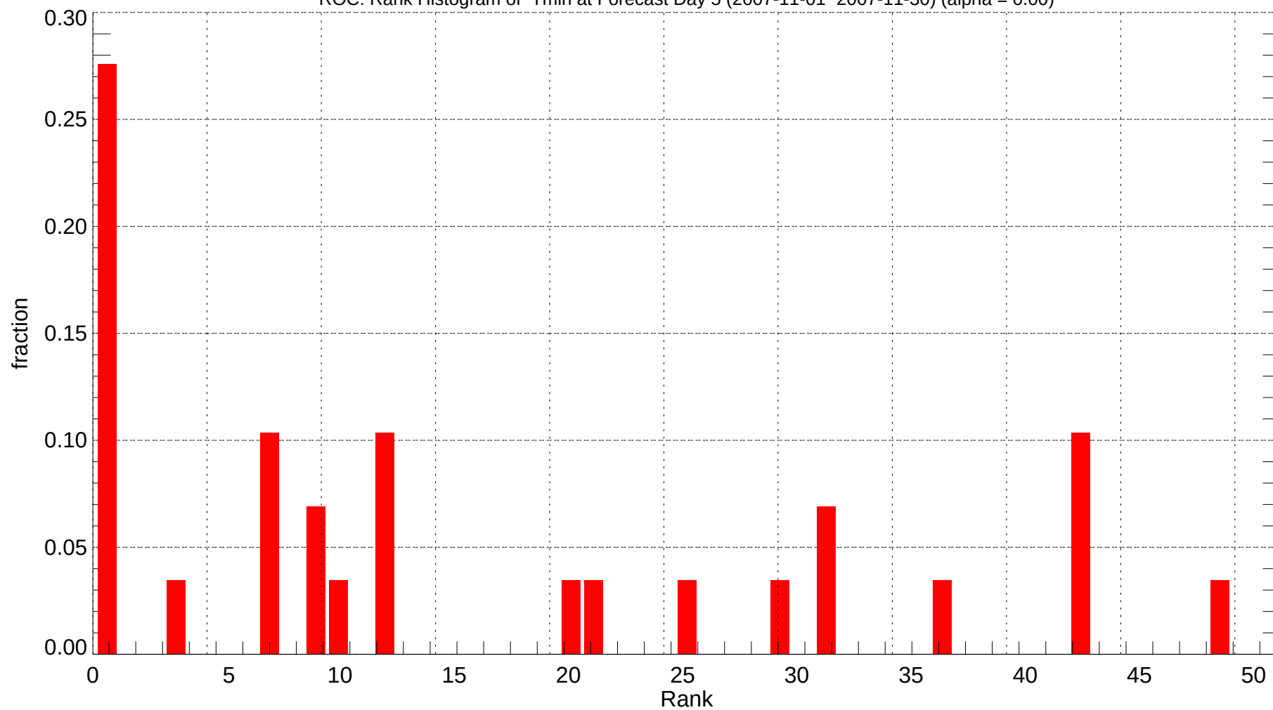
ROC: Rank Histogram of Tmin at Forecast Day 5 (2007-11-01~2007-11-30) (alpha = 0.00)
