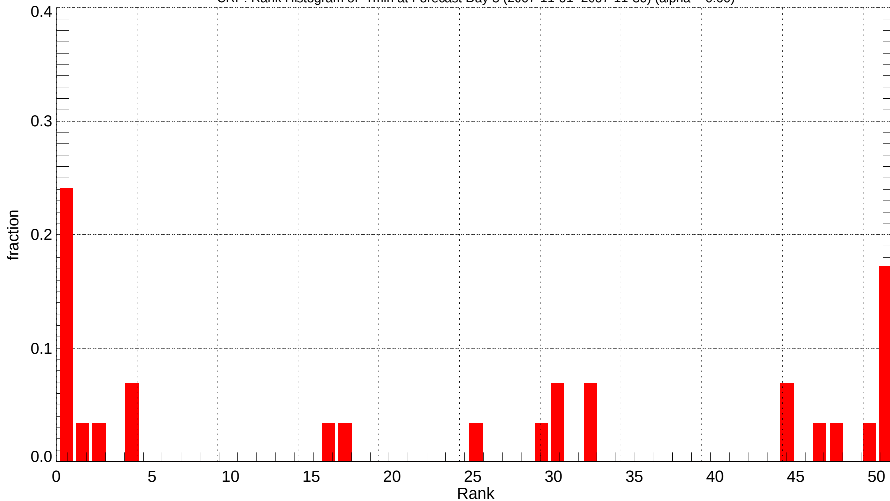
CRP: Rank Histogram of Tmin at Forecast Day 3 (2007-11-01~2007-11-30) (alpha = 0.00)
