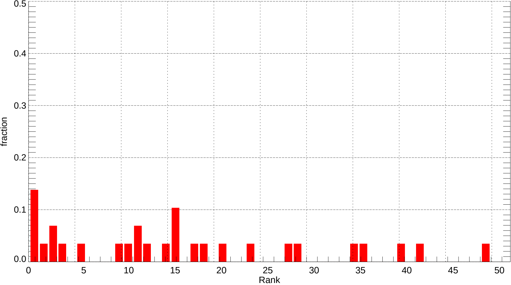
ELP: Rank Histogram of Tmin at Forecast Day 3 (2007-11-01~2007-11-30) (alpha = 0.00)
