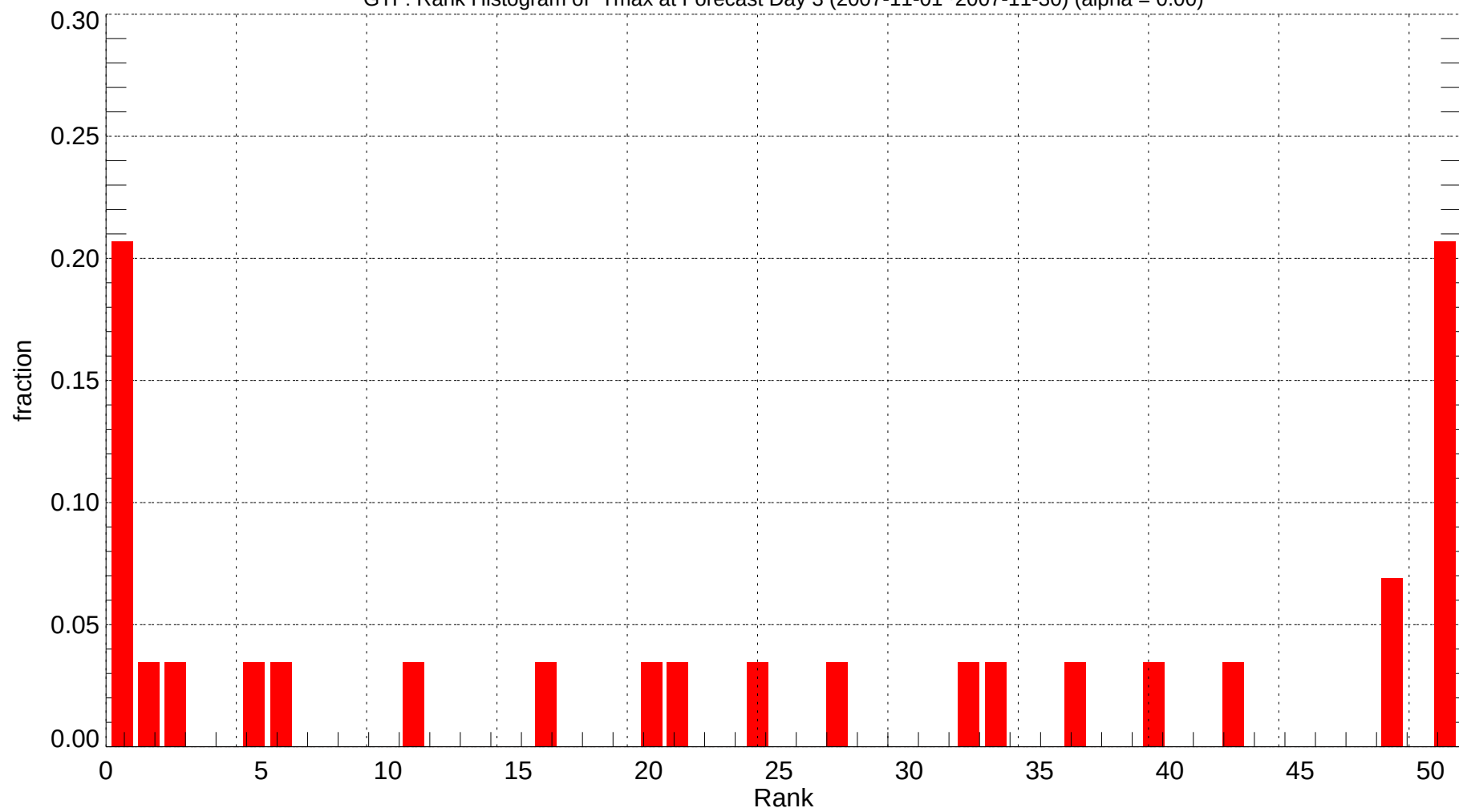
GTF: Rank Histogram of Tmax at Forecast Day 3 (2007-11-01~2007-11-30) (alpha = 0.00)
