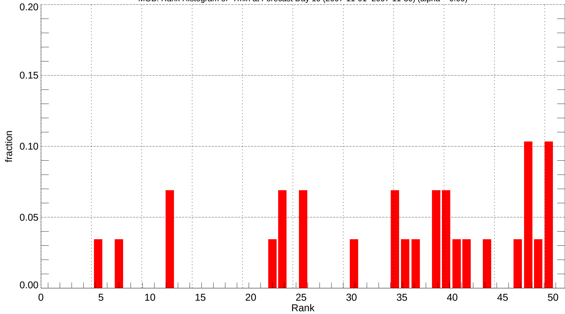
MOB: Rank Histogram of Tmin at Forecast Day 10 (2007-11-01~2007-11-30) (alpha = 0.00)
