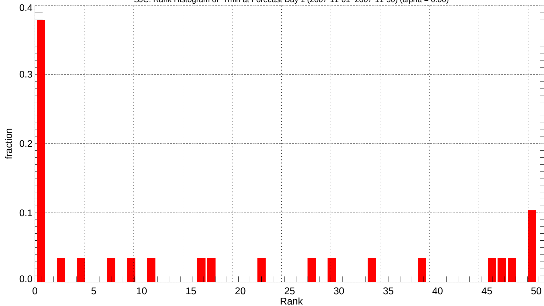
SJC: Rank Histogram of Tmin at Forecast Day 1 (2007-11-01~2007-11-30) (alpha = 0.00)
