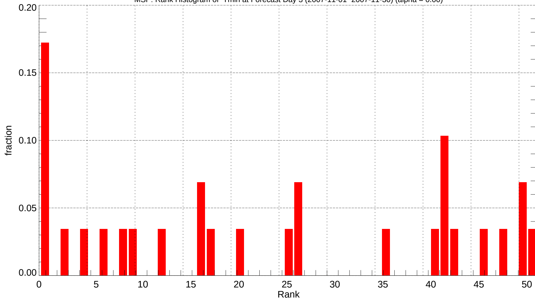
MSP: Rank Histogram of Tmin at Forecast Day 3 (2007-11-01~2007-11-30) (alpha = 0.00)
