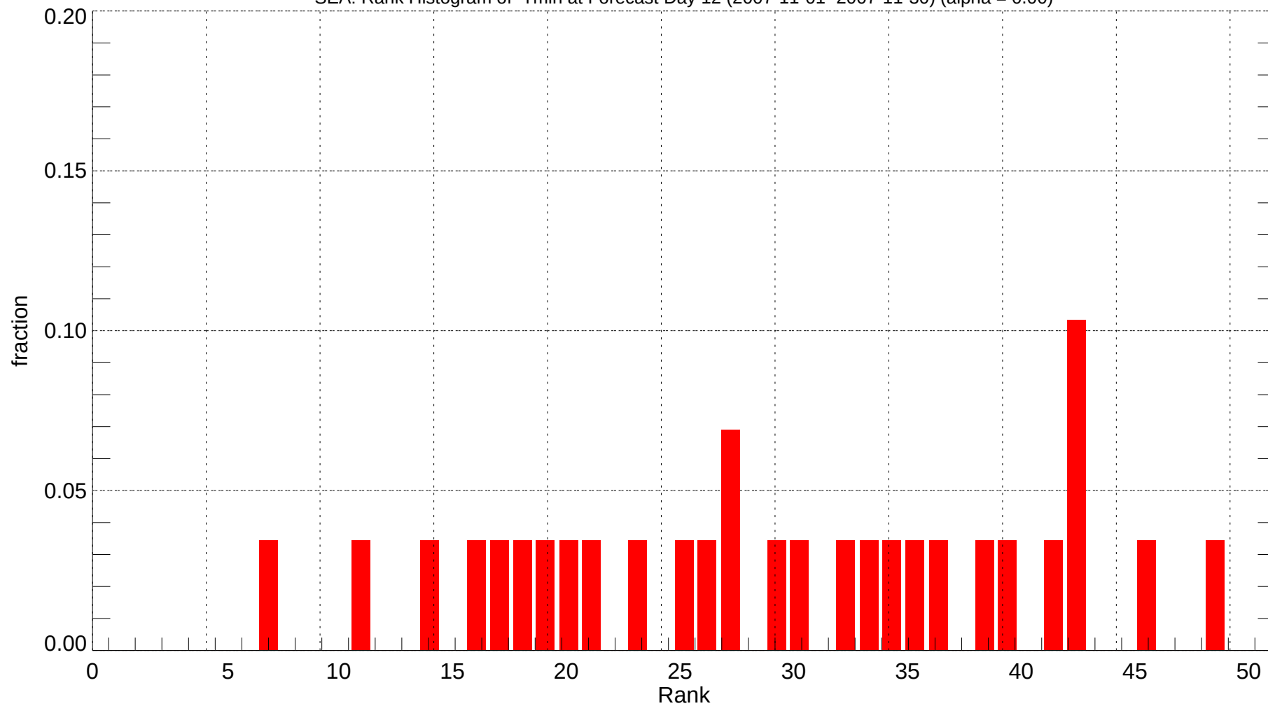
SEA: Rank Histogram of Tmin at Forecast Day 12 (2007-11-01~2007-11-30) (alpha = 0.00)
