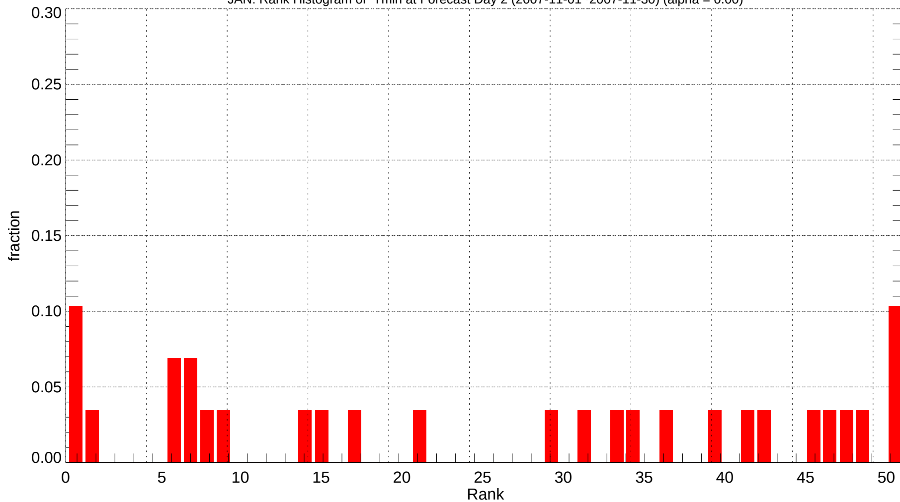
JAN: Rank Histogram of Tmin at Forecast Day 2 (2007-11-01~2007-11-30) (alpha = 0.00)
