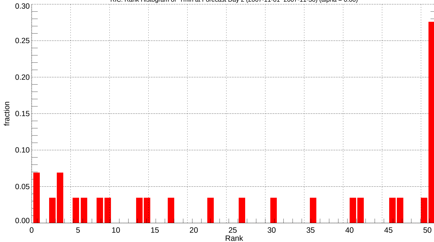
RIC: Rank Histogram of Tmin at Forecast Day 2 (2007-11-01~2007-11-30) (alpha = 0.00)
