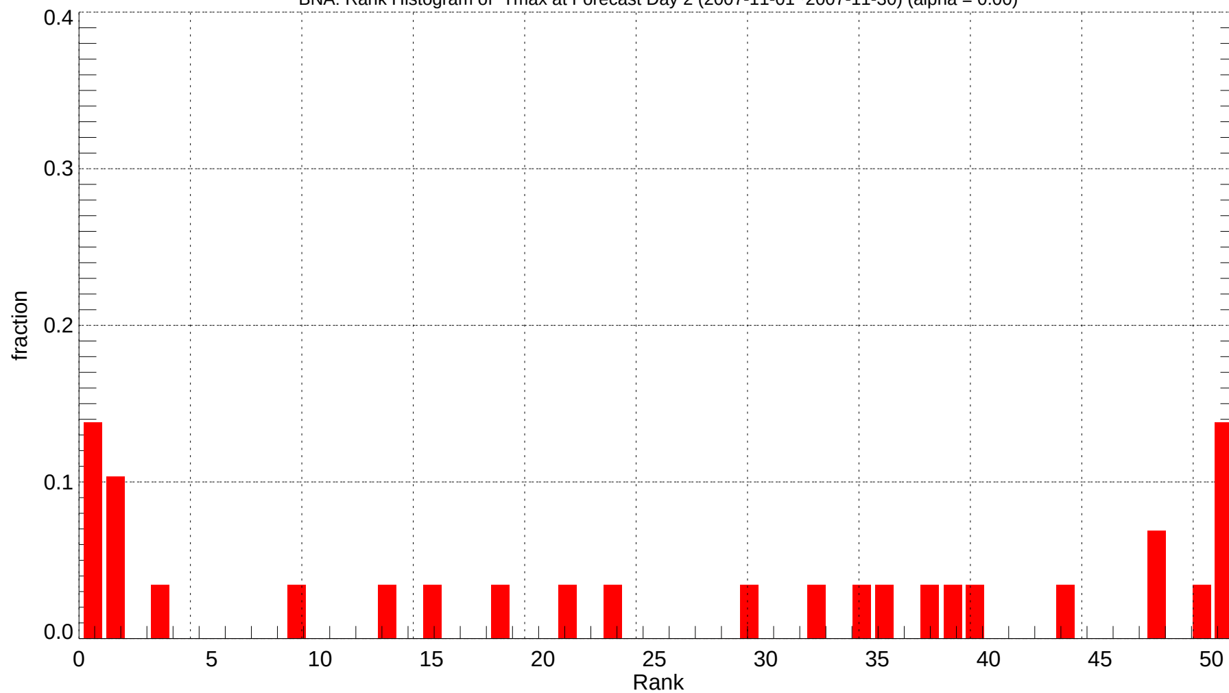
BNA: Rank Histogram of Tmax at Forecast Day 2 (2007-11-01~2007-11-30) (alpha = 0.00)
