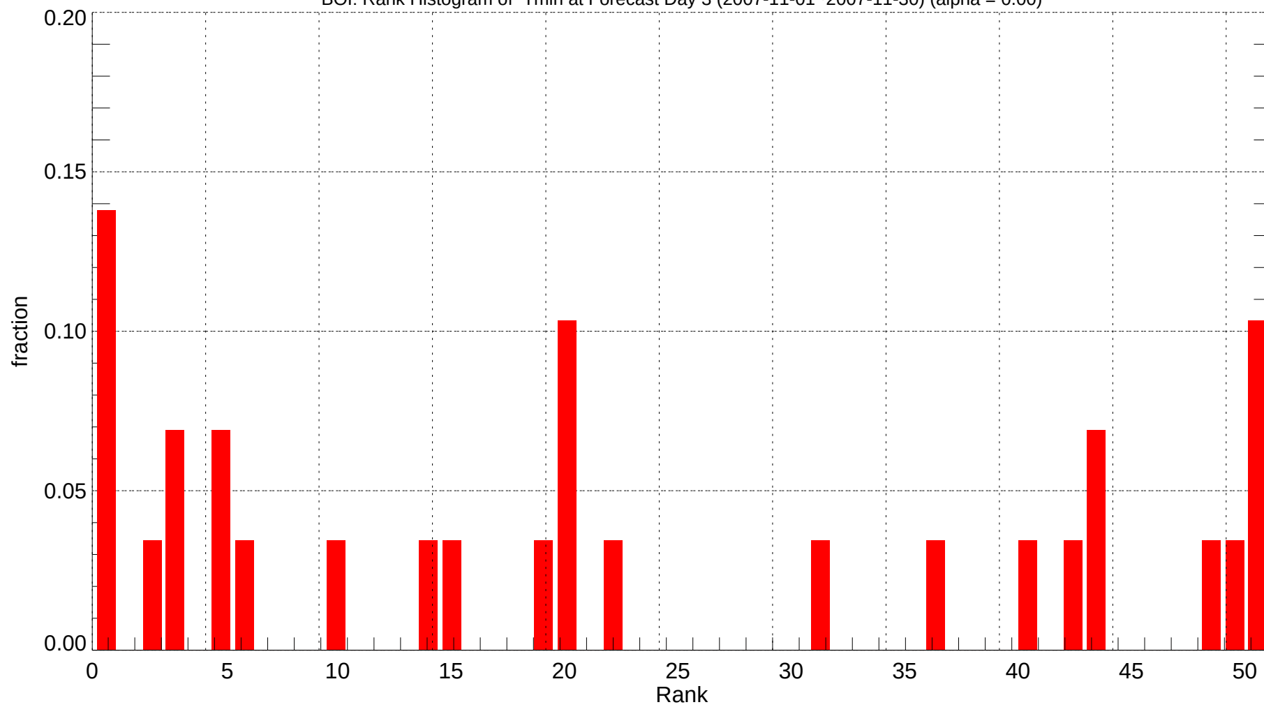
BOI: Rank Histogram of Tmin at Forecast Day 3 (2007-11-01~2007-11-30) (alpha = 0.00)
