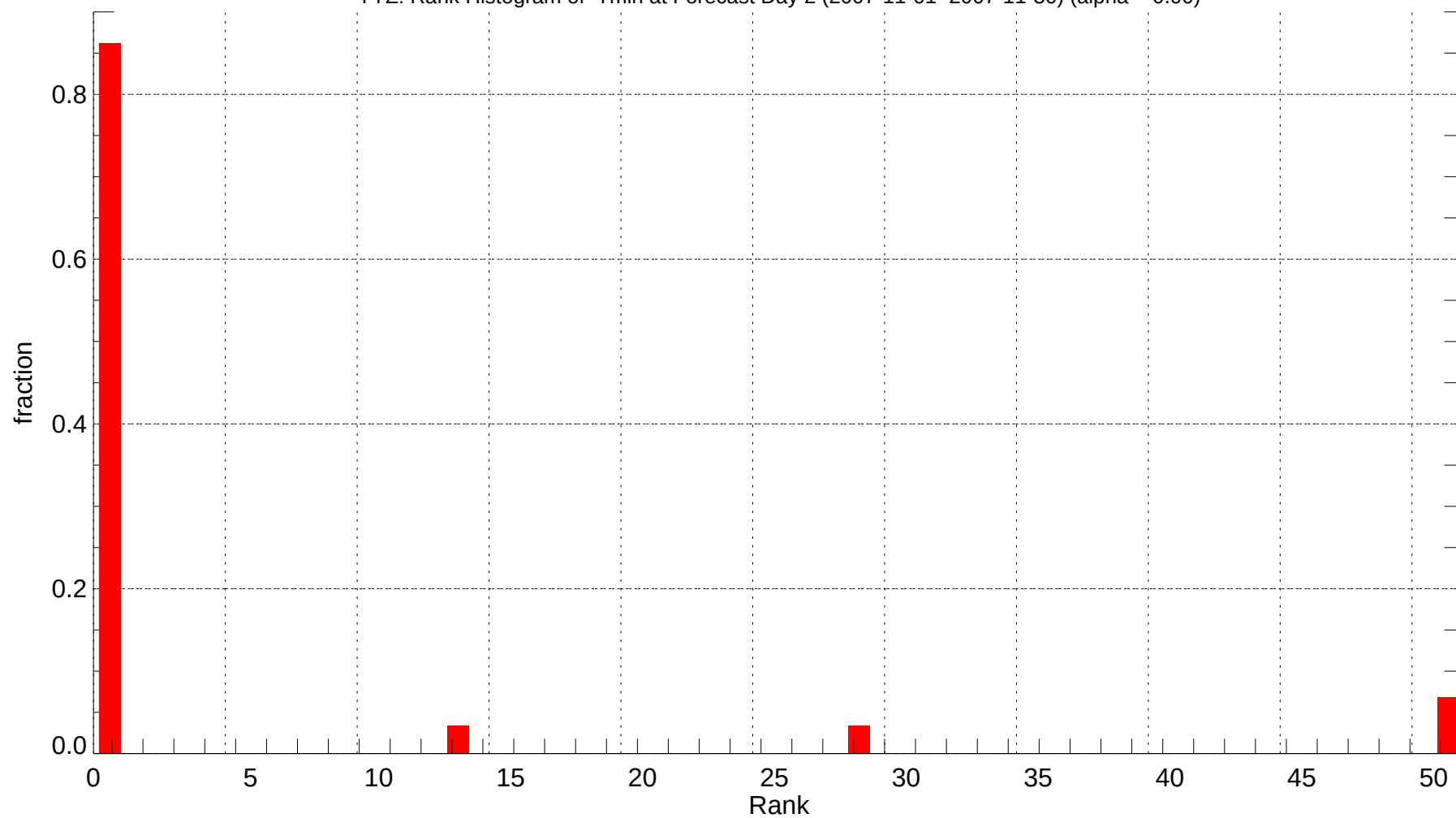
YYZ: Rank Histogram of Tmin at Forecast Day 2 (2007-11-01~2007-11-30) (alpha = 0.00)
