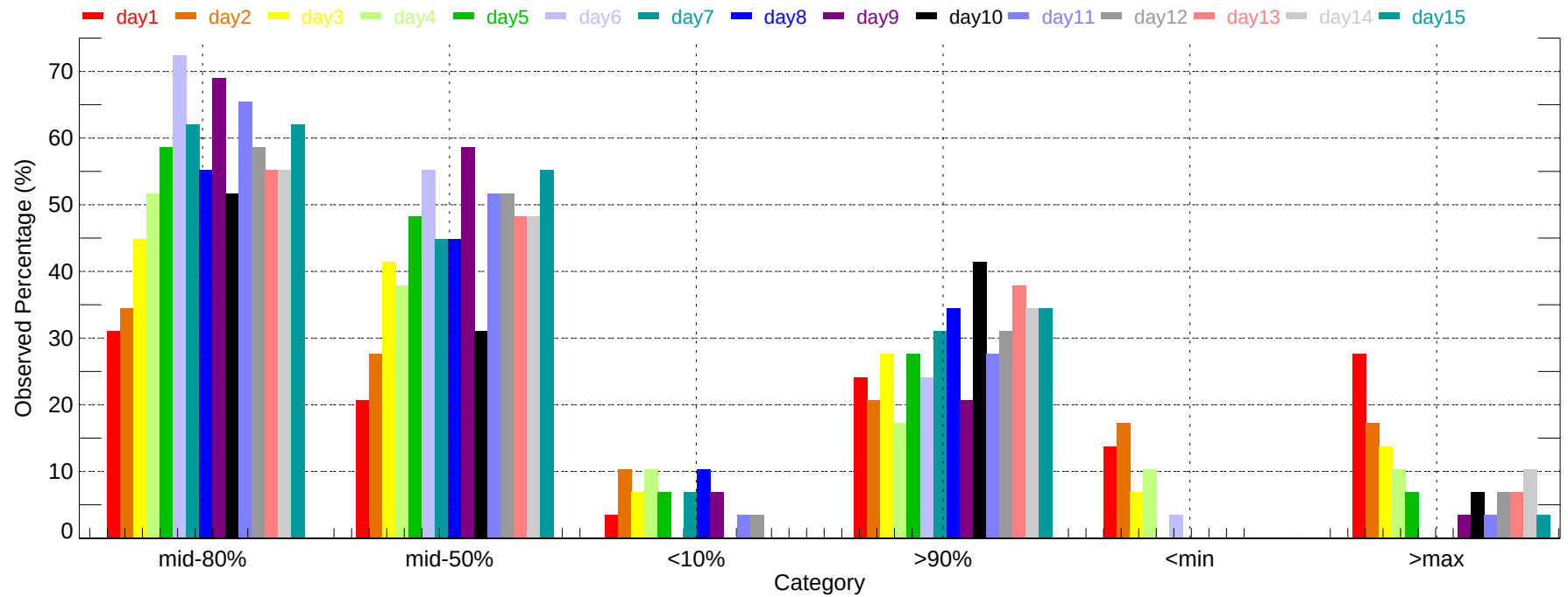
Observed Percentage of Ensembles - TRM: Min Temperature (2007-11-01~2007-11-30)
