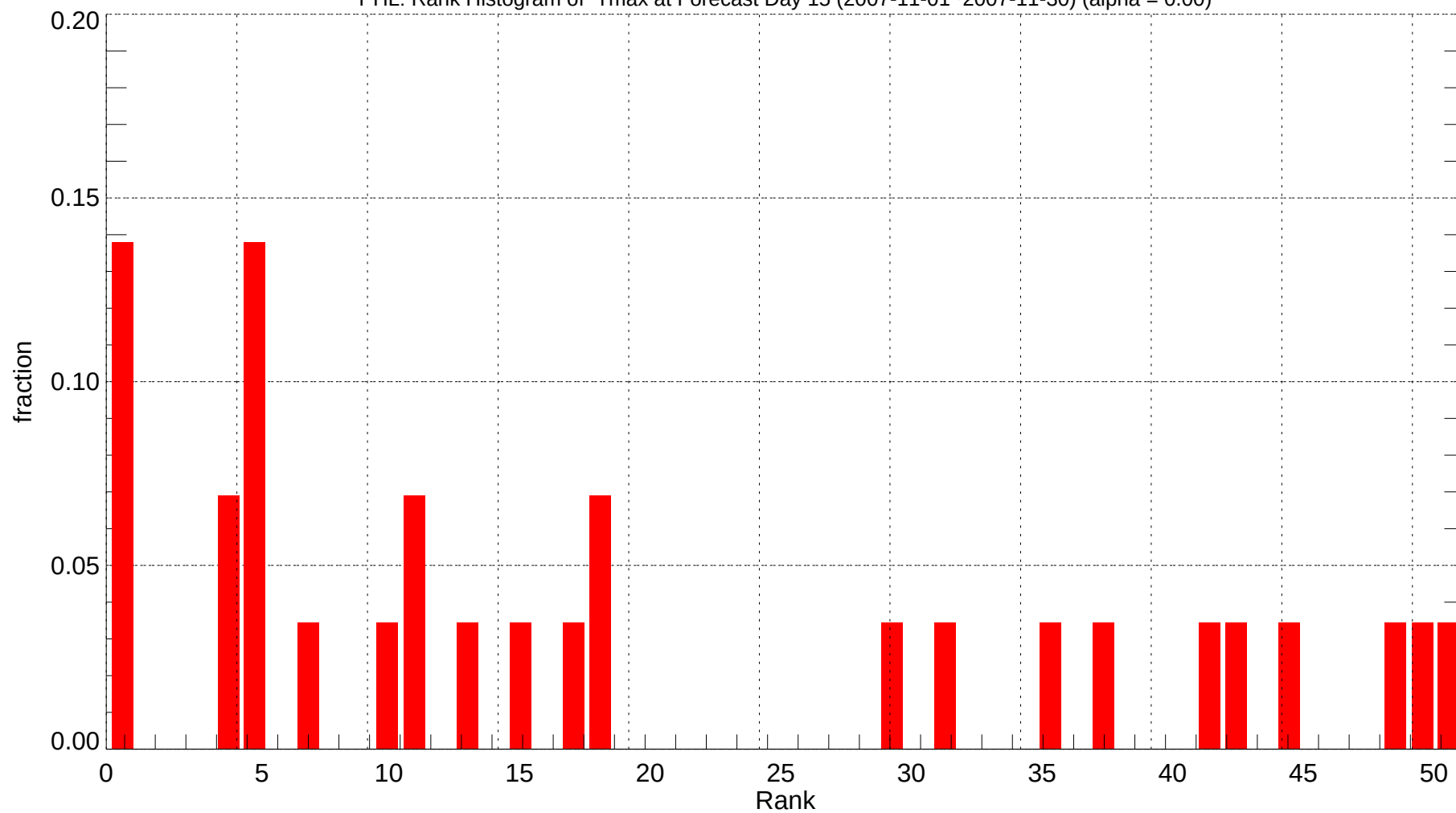
PHL: Rank Histogram of Tmax at Forecast Day 15 (2007-11-01~2007-11-30) (alpha = 0.00)
