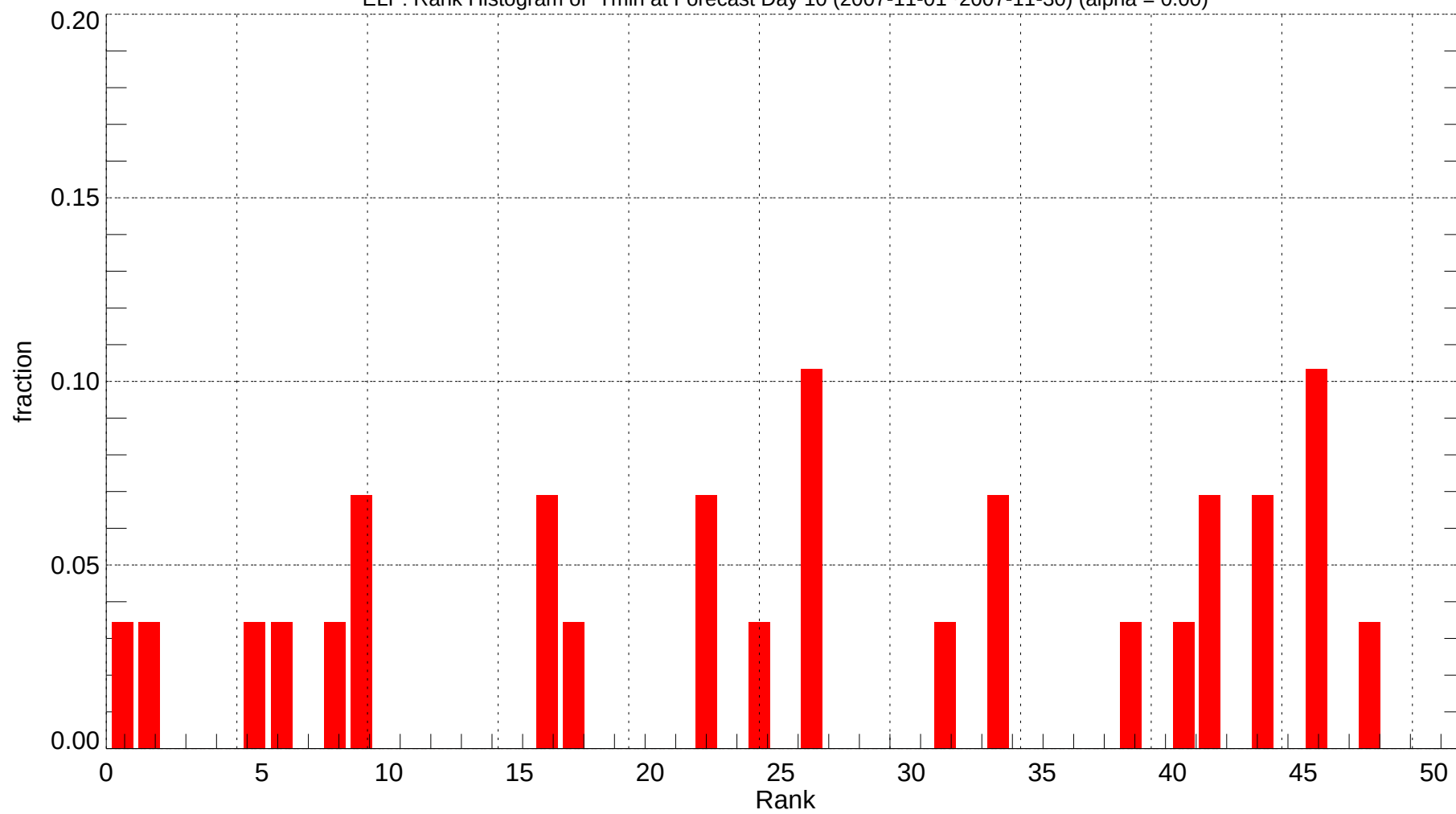
ELP: Rank Histogram of Tmin at Forecast Day 10 (2007-11-01~2007-11-30) (alpha = 0.00)
