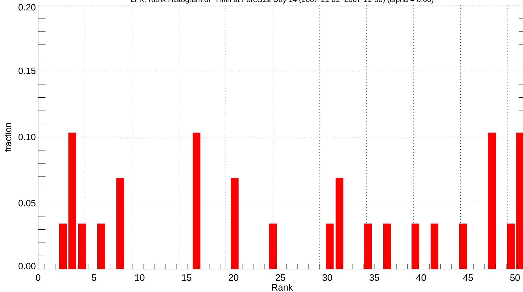
LFK: Rank Histogram of Tmin at Forecast Day 14 (2007-11-01~2007-11-30) (alpha = 0.00)
