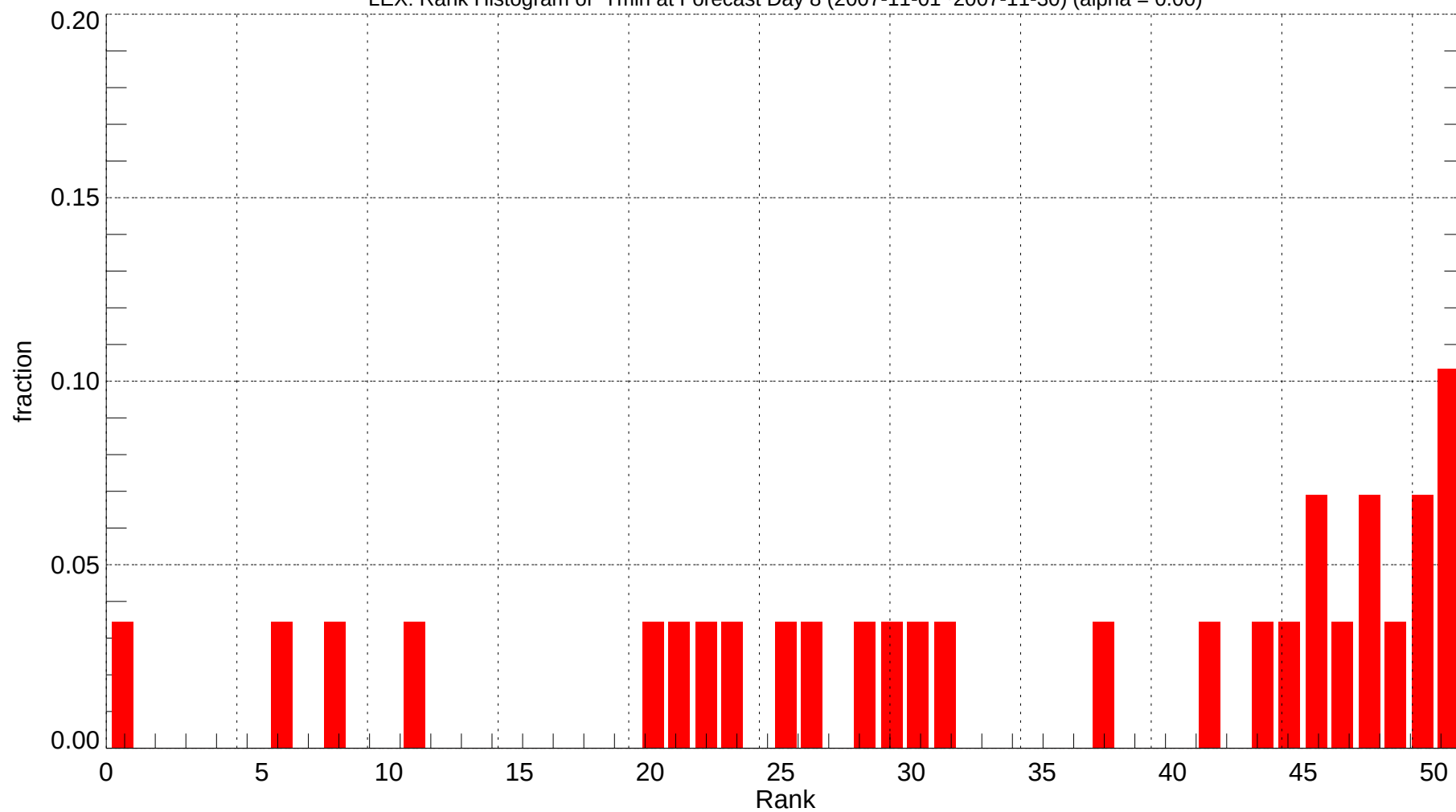
LEX: Rank Histogram of Tmin at Forecast Day 8 (2007-11-01~2007-11-30) (alpha = 0.00)
