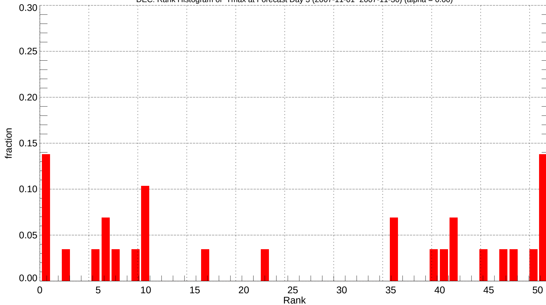
DEC: Rank Histogram of Tmax at Forecast Day 3 (2007-11-01~2007-11-30) (alpha = 0.00)
