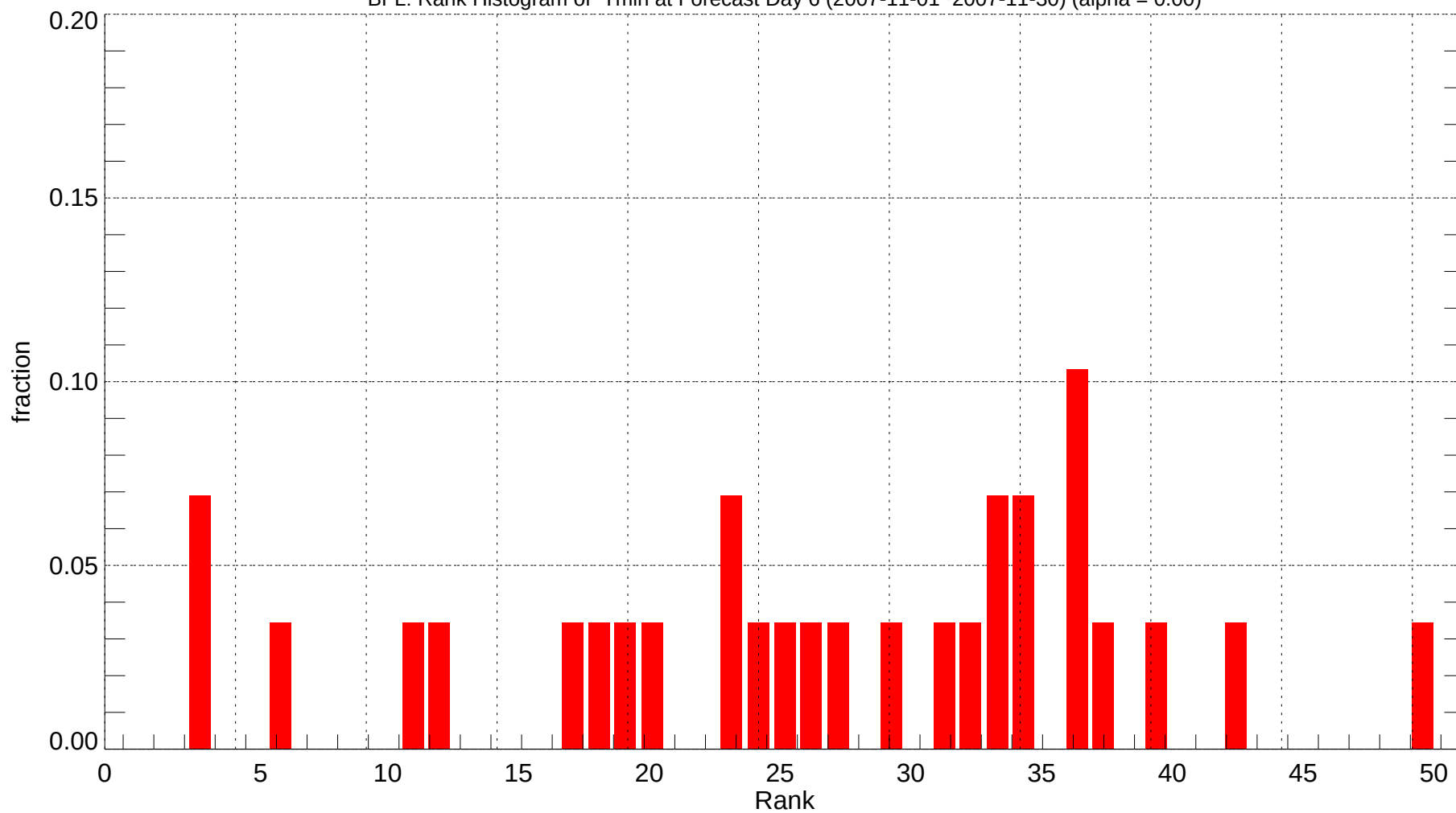
BFL: Rank Histogram of Tmin at Forecast Day 6 (2007-11-01~2007-11-30) (alpha = 0.00)
