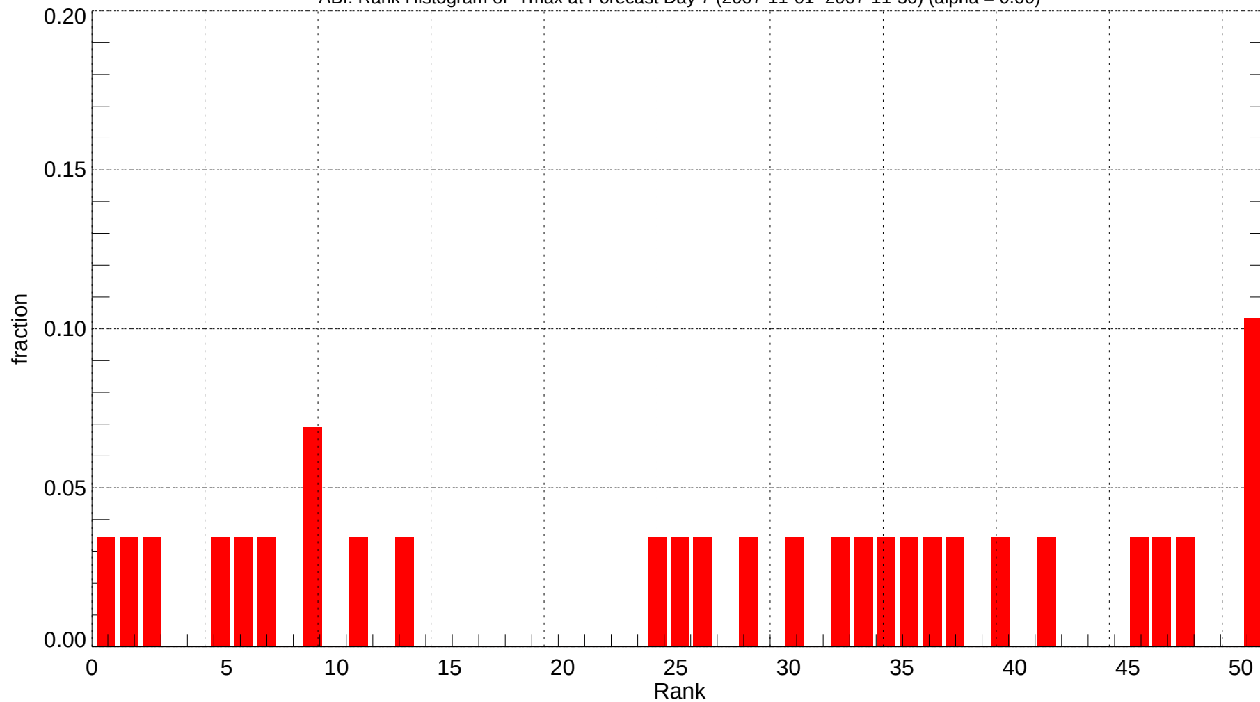
ABI: Rank Histogram of Tmax at Forecast Day 7 (2007-11-01~2007-11-30) (alpha = 0.00)
