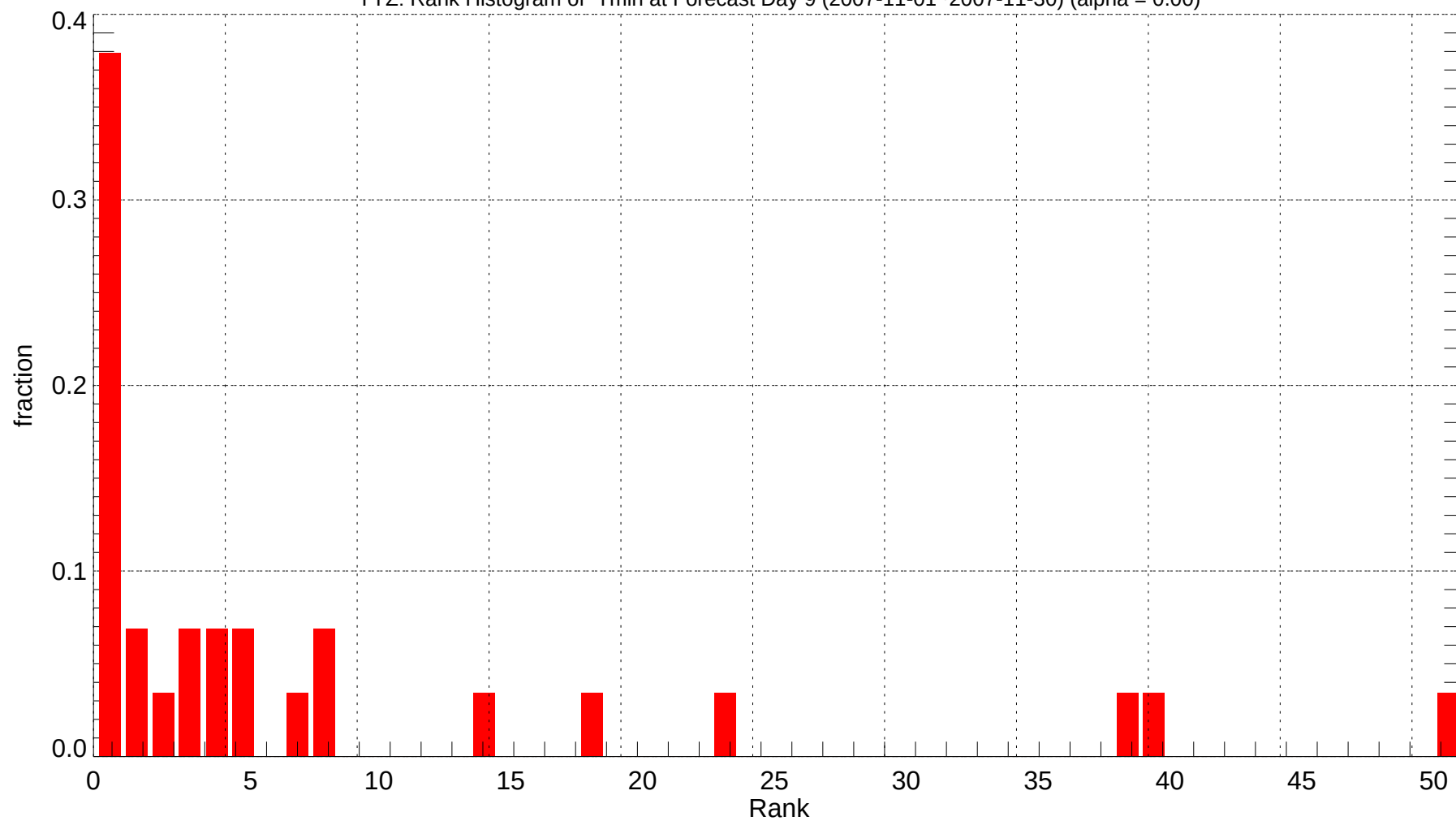
YYZ: Rank Histogram of Tmin at Forecast Day 9 (2007-11-01~2007-11-30) (alpha = 0.00)
