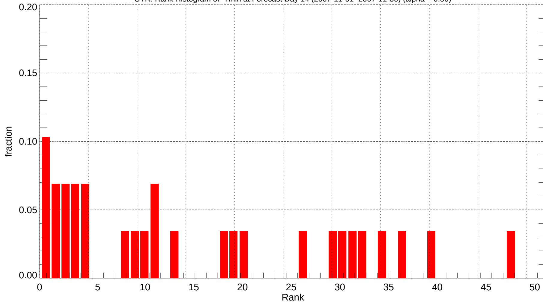
SYR: Rank Histogram of Tmin at Forecast Day 14 (2007-11-01~2007-11-30) (alpha = 0.00)
