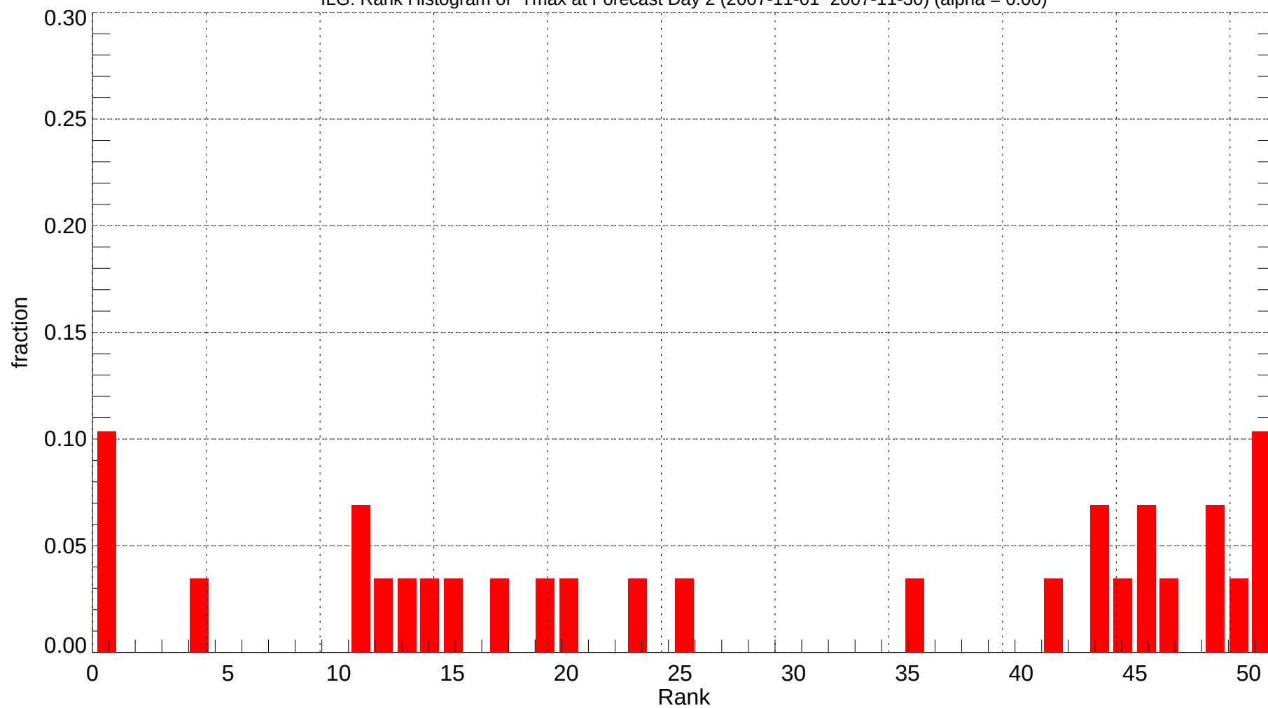
ILG: Rank Histogram of Tmax at Forecast Day 2 (2007-11-01~2007-11-30) (alpha = 0.00)
