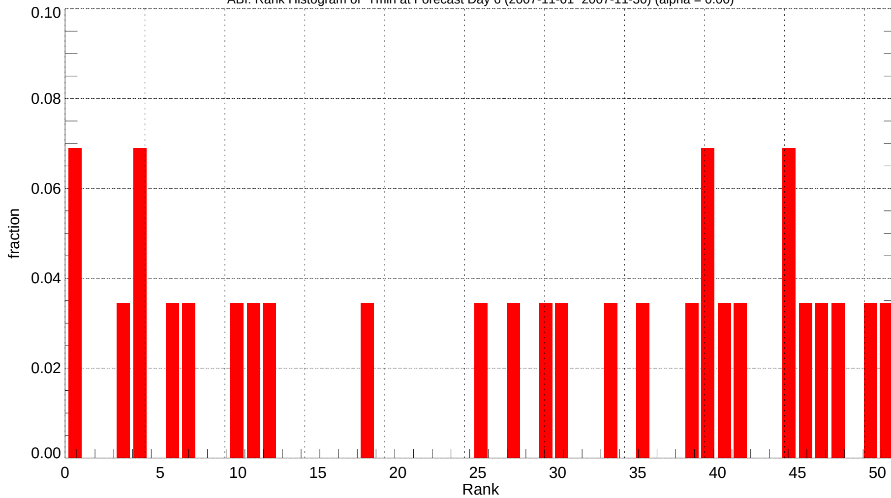
ABI: Rank Histogram of Tmin at Forecast Day 6 (2007-11-01~2007-11-30) (alpha = 0.00)
