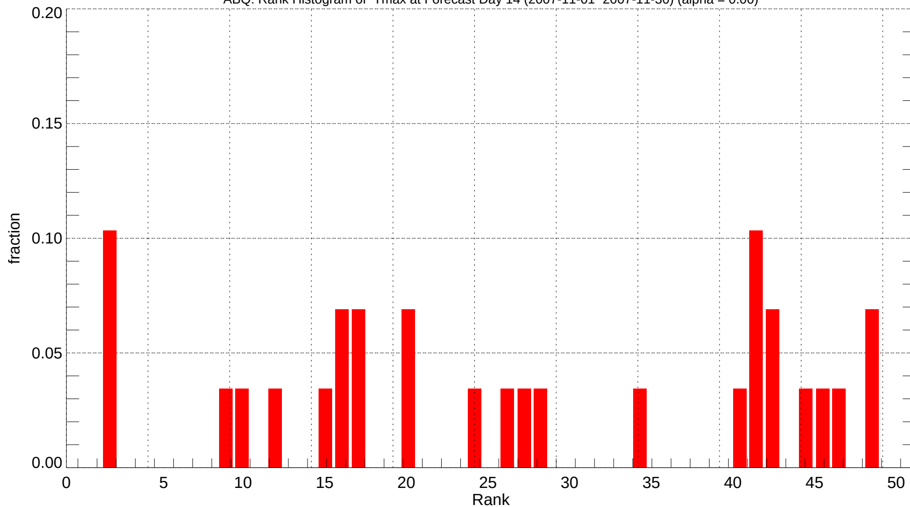
ABQ: Rank Histogram of Tmax at Forecast Day 14 (2007-11-01~2007-11-30) (alpha = 0.00)
