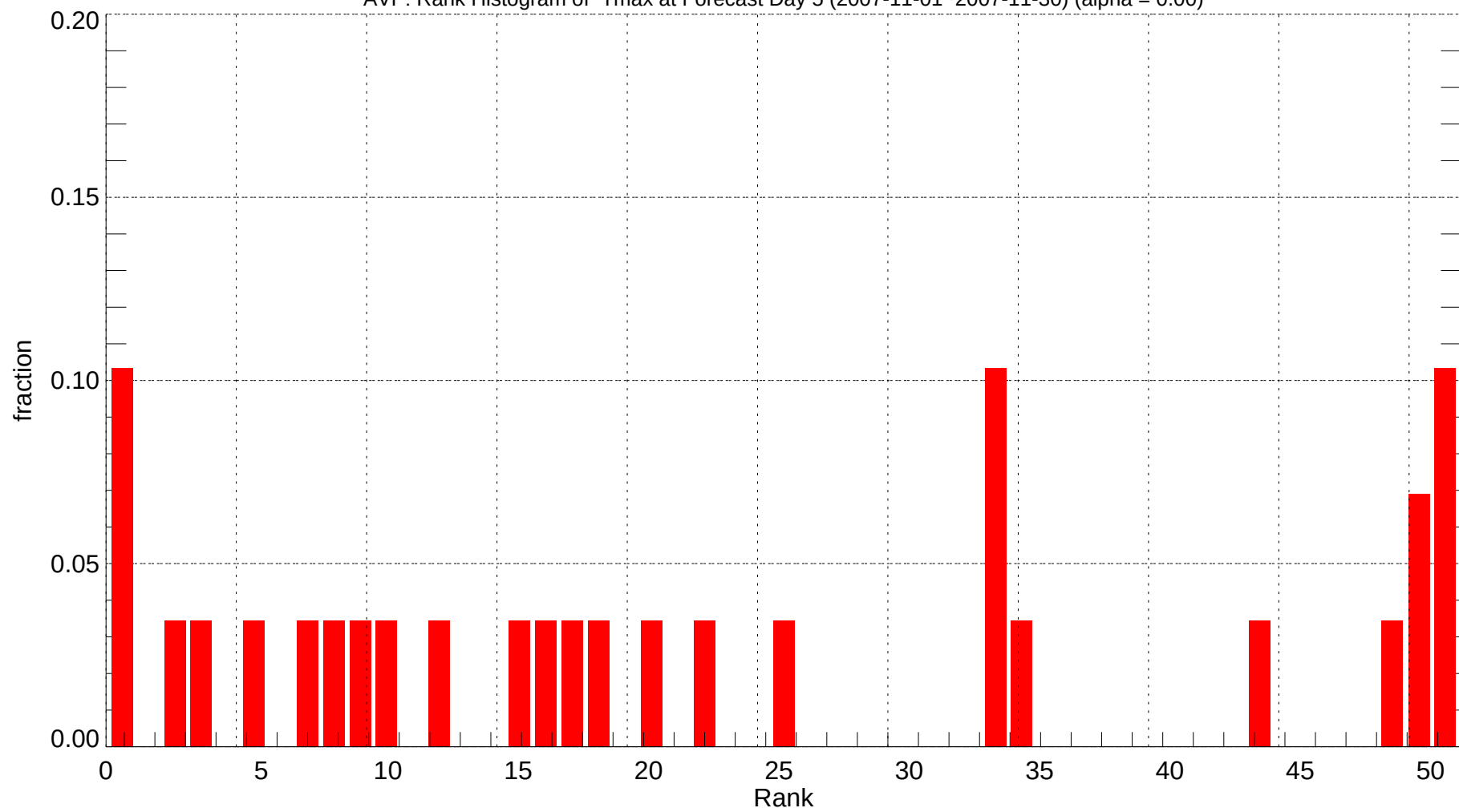
AVP: Rank Histogram of Tmax at Forecast Day 5 (2007-11-01~2007-11-30) (alpha = 0.00)
