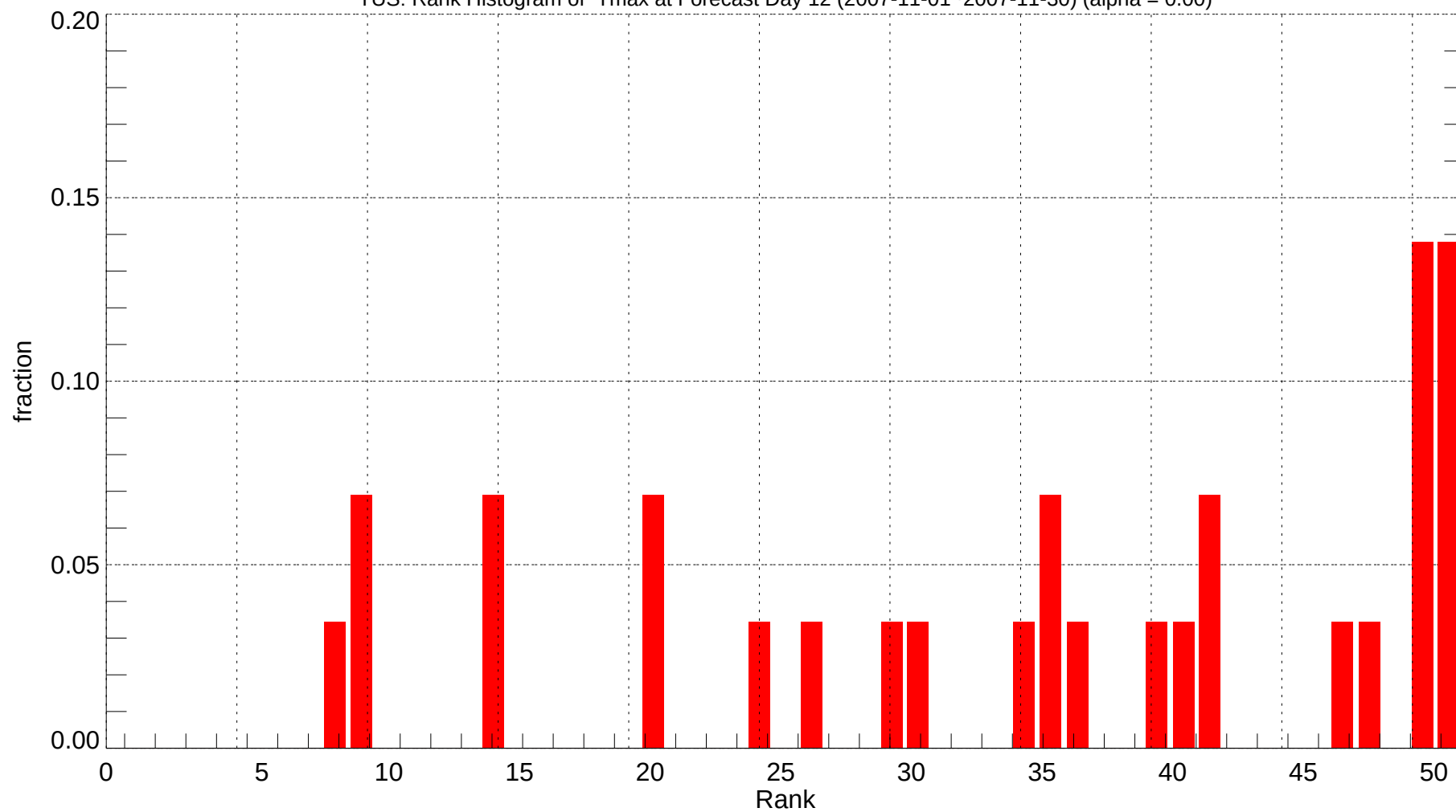
TUS: Rank Histogram of Tmax at Forecast Day 12 (2007-11-01~2007-11-30) (alpha = 0.00)
