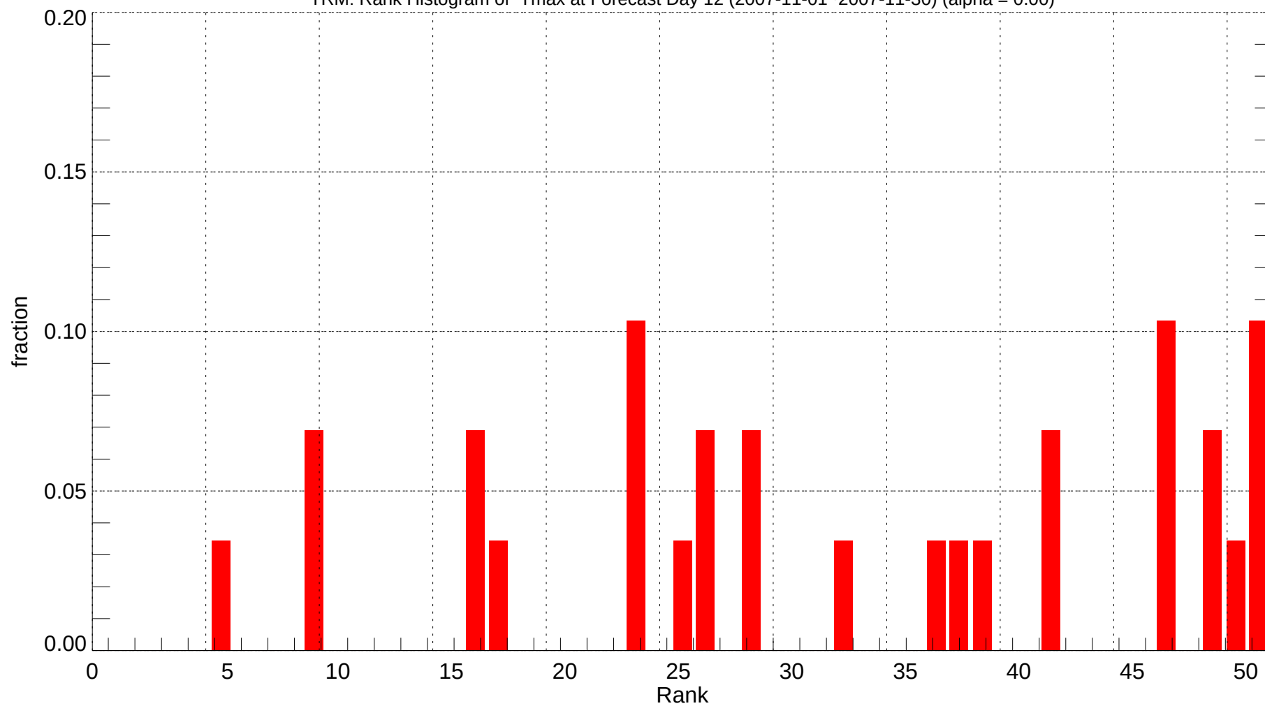
TRM: Rank Histogram of Tmax at Forecast Day 12 (2007-11-01~2007-11-30) (alpha = 0.00)
