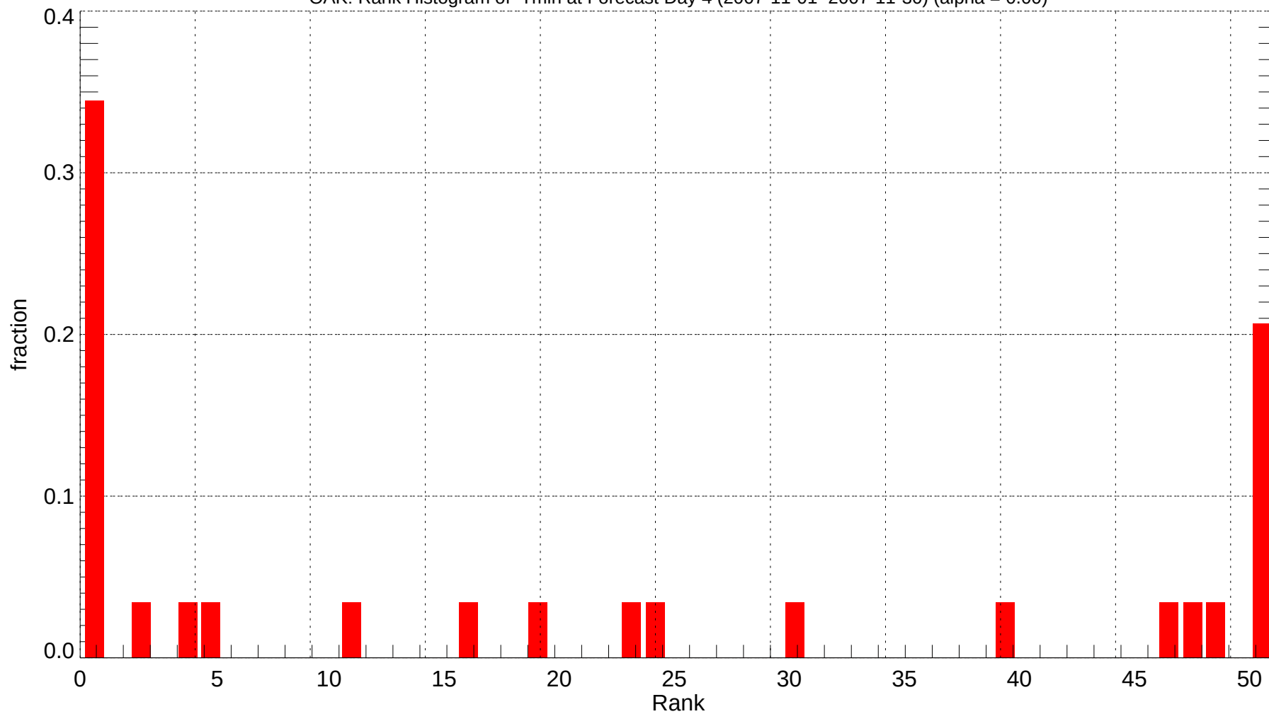
OAK: Rank Histogram of Tmin at Forecast Day 4 (2007-11-01~2007-11-30) (alpha = 0.00)
