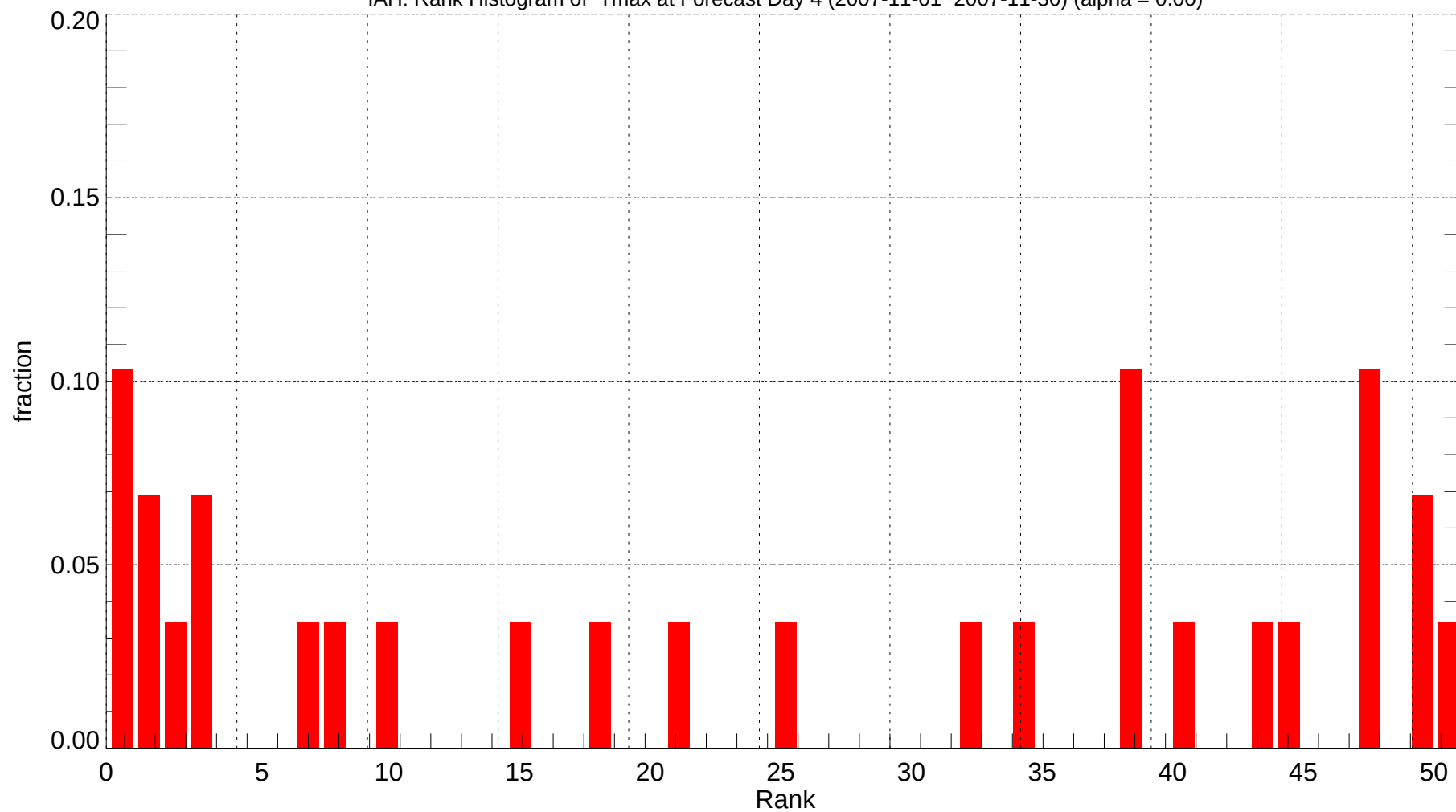
IAH: Rank Histogram of Tmax at Forecast Day 4 (2007-11-01~2007-11-30) (alpha = 0.00)
