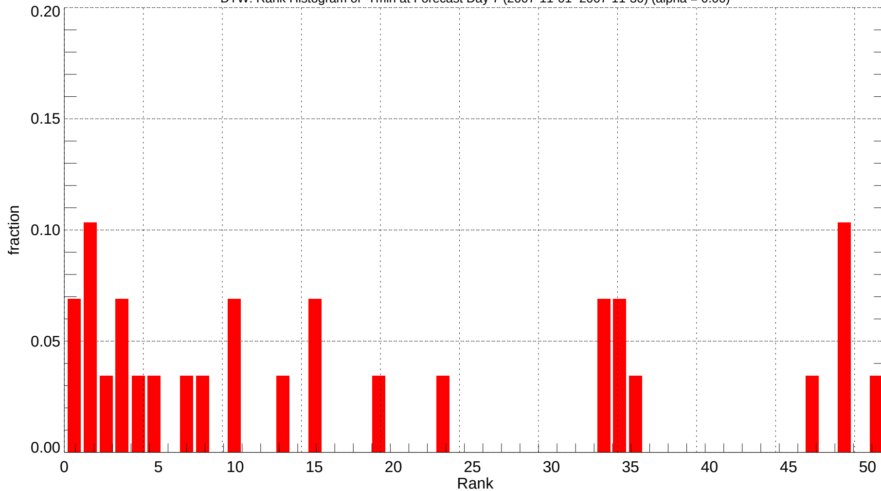
DTW: Rank Histogram of Tmin at Forecast Day 7 (2007-11-01~2007-11-30) (alpha = 0.00)
