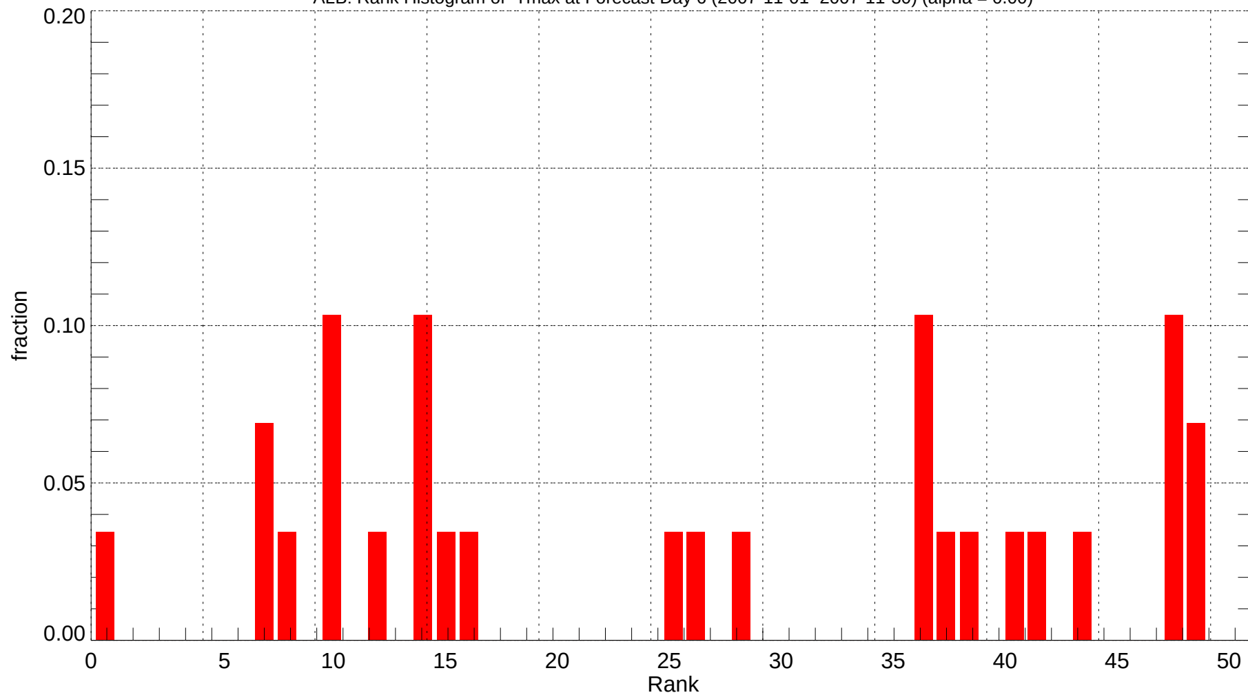
ALB: Rank Histogram of Tmax at Forecast Day 6 (2007-11-01~2007-11-30) (alpha = 0.00)
