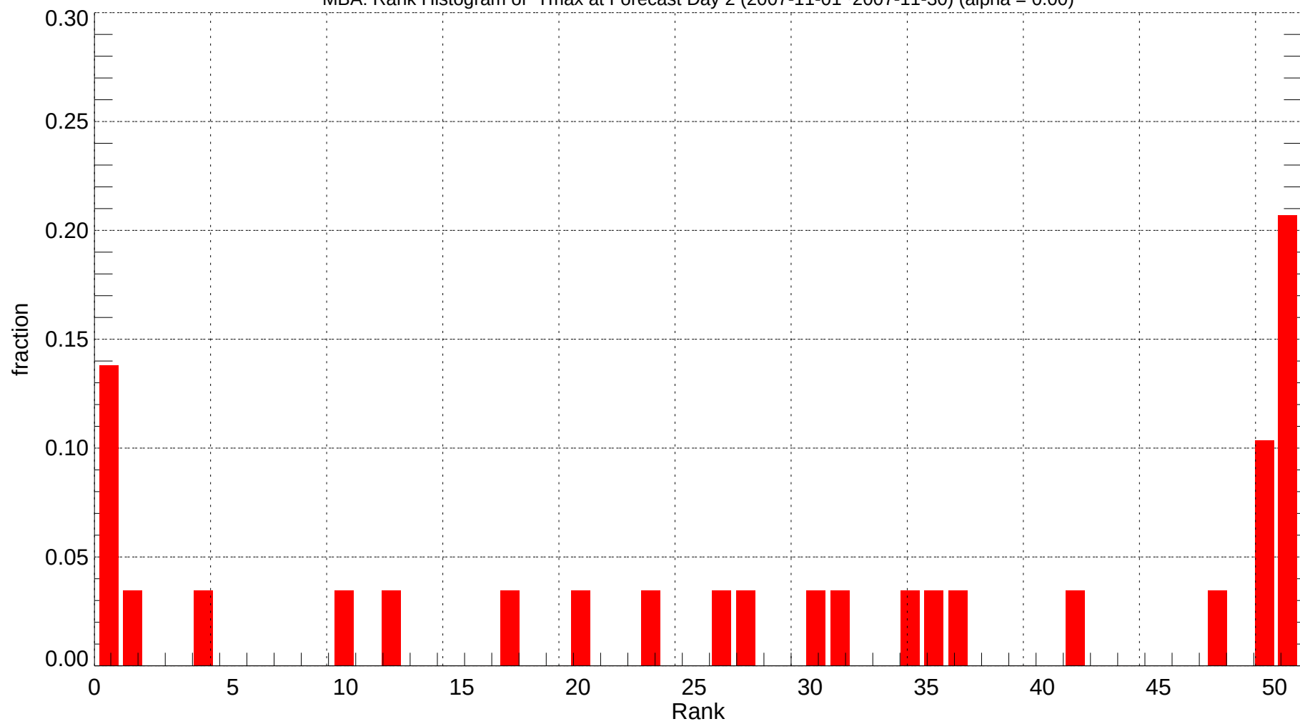
MBA: Rank Histogram of Tmax at Forecast Day 2 (2007-11-01~2007-11-30) (alpha = 0.00)
