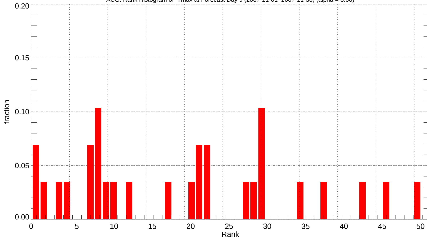
AUG: Rank Histogram of Tmax at Forecast Day 9 (2007-11-01~2007-11-30) (alpha = 0.00)
