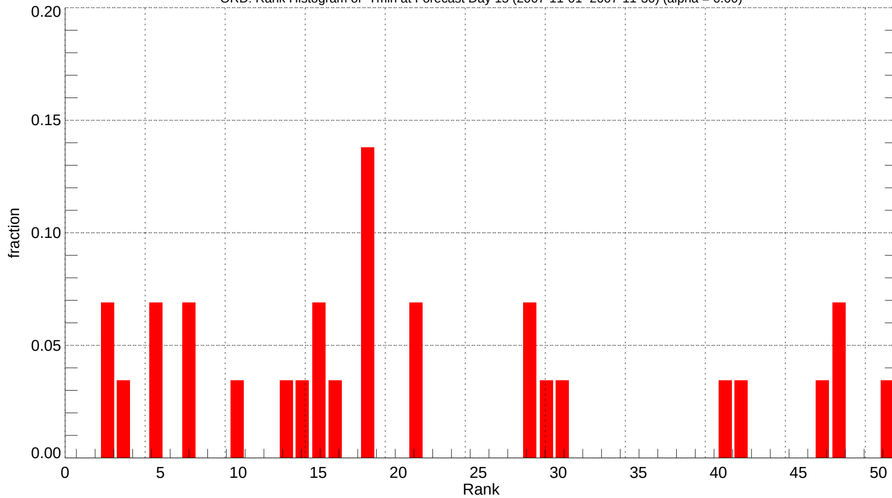
ORD: Rank Histogram of Tmin at Forecast Day 15 (2007-11-01~2007-11-30) (alpha = 0.00)
