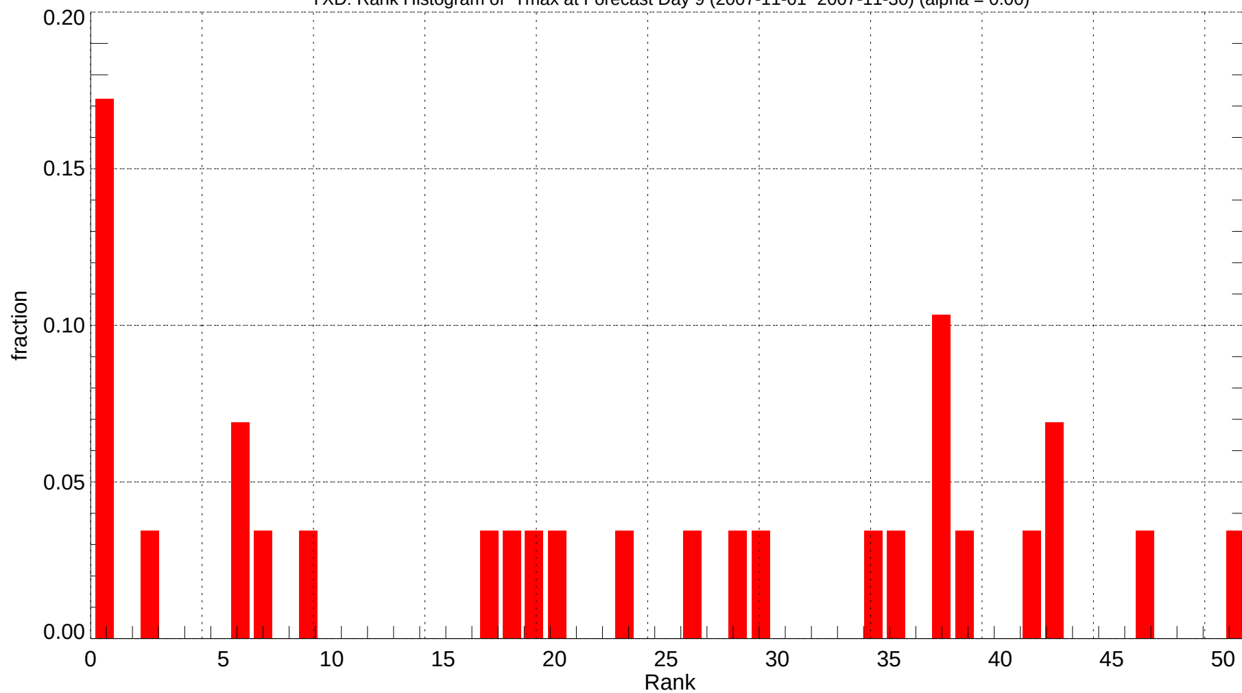
YXD: Rank Histogram of Tmax at Forecast Day 9 (2007-11-01~2007-11-30) (alpha = 0.00)
