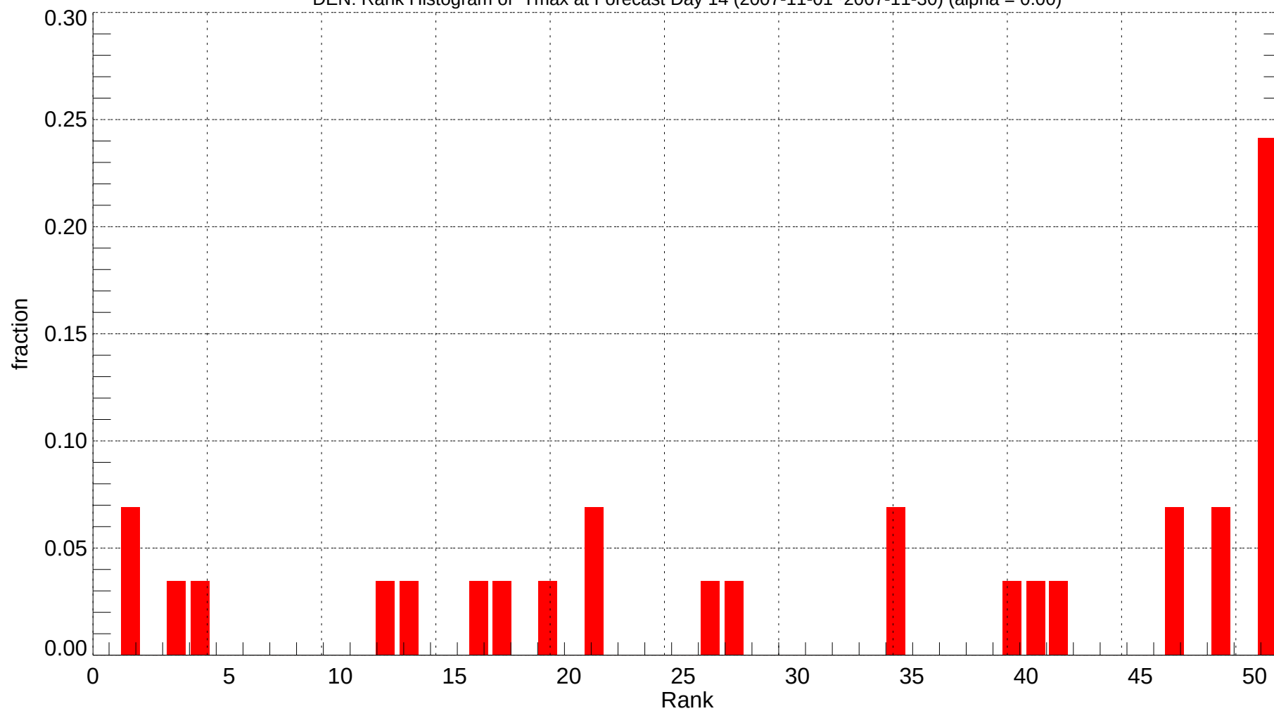
DEN: Rank Histogram of Tmax at Forecast Day 14 (2007-11-01~2007-11-30) (alpha = 0.00)
