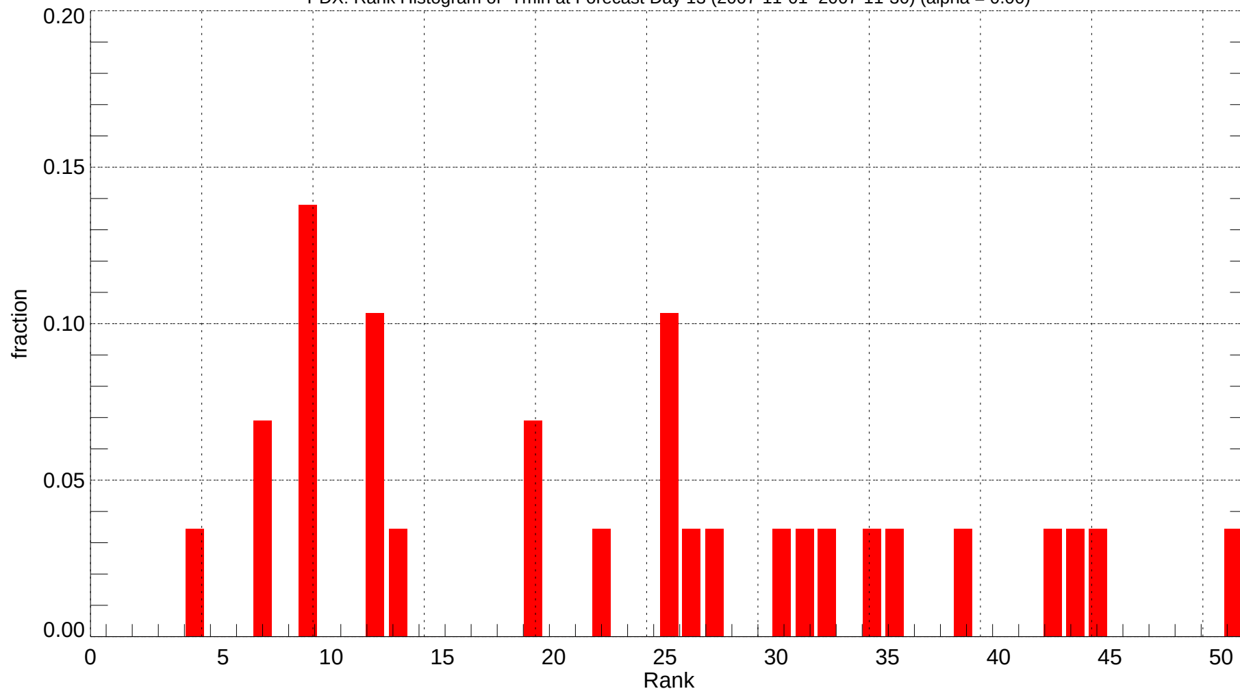
PDX: Rank Histogram of Tmin at Forecast Day 13 (2007-11-01~2007-11-30) (alpha = 0.00)
