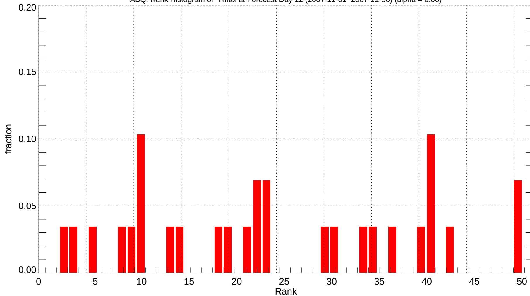
ABQ: Rank Histogram of Tmax at Forecast Day 12 (2007-11-01~2007-11-30) (alpha = 0.00)
