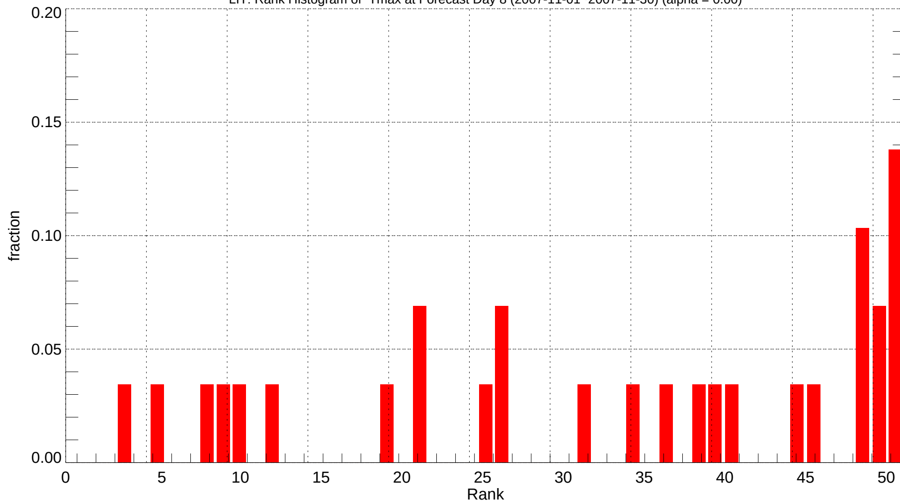
LIT: Rank Histogram of Tmax at Forecast Day 8 (2007-11-01~2007-11-30) (alpha = 0.00)
