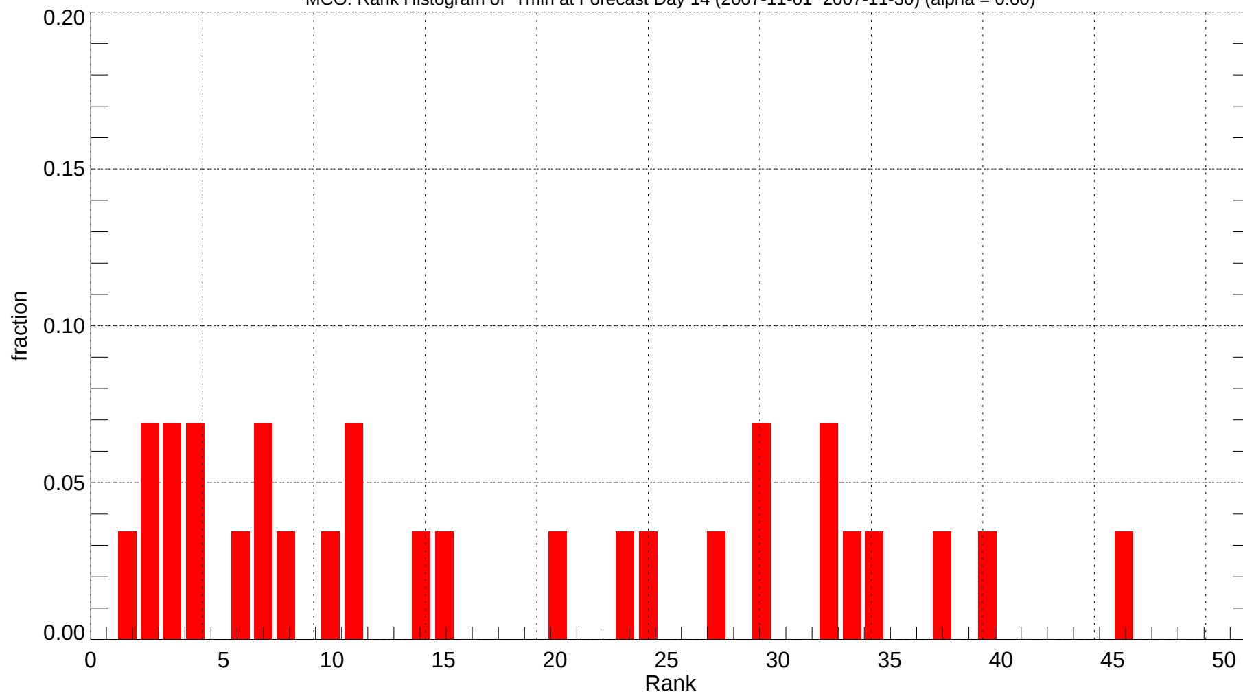
MCO: Rank Histogram of Tmin at Forecast Day 14 (2007-11-01~2007-11-30) (alpha = 0.00)
