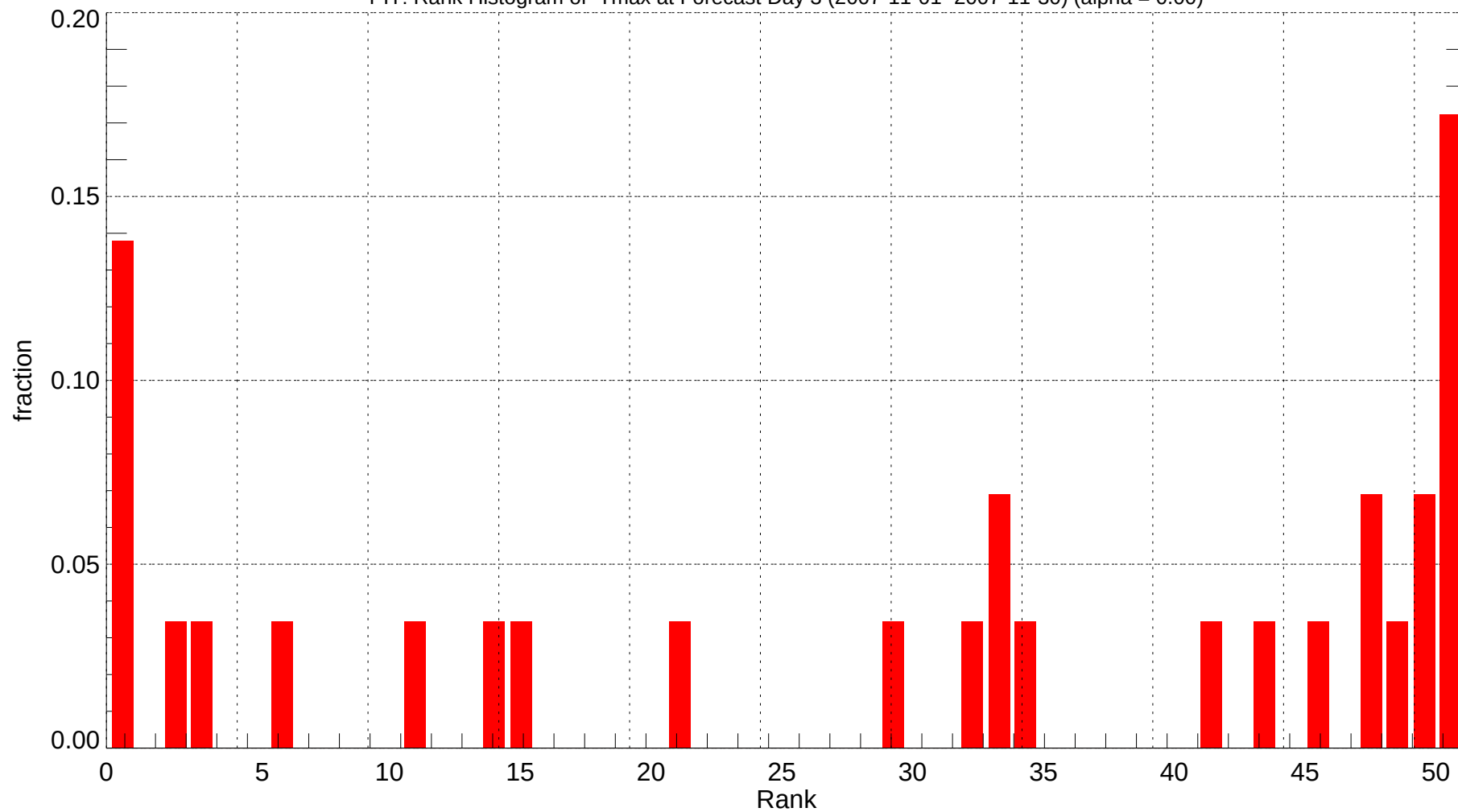
PIT: Rank Histogram of Tmax at Forecast Day 3 (2007-11-01~2007-11-30) (alpha = 0.00)
