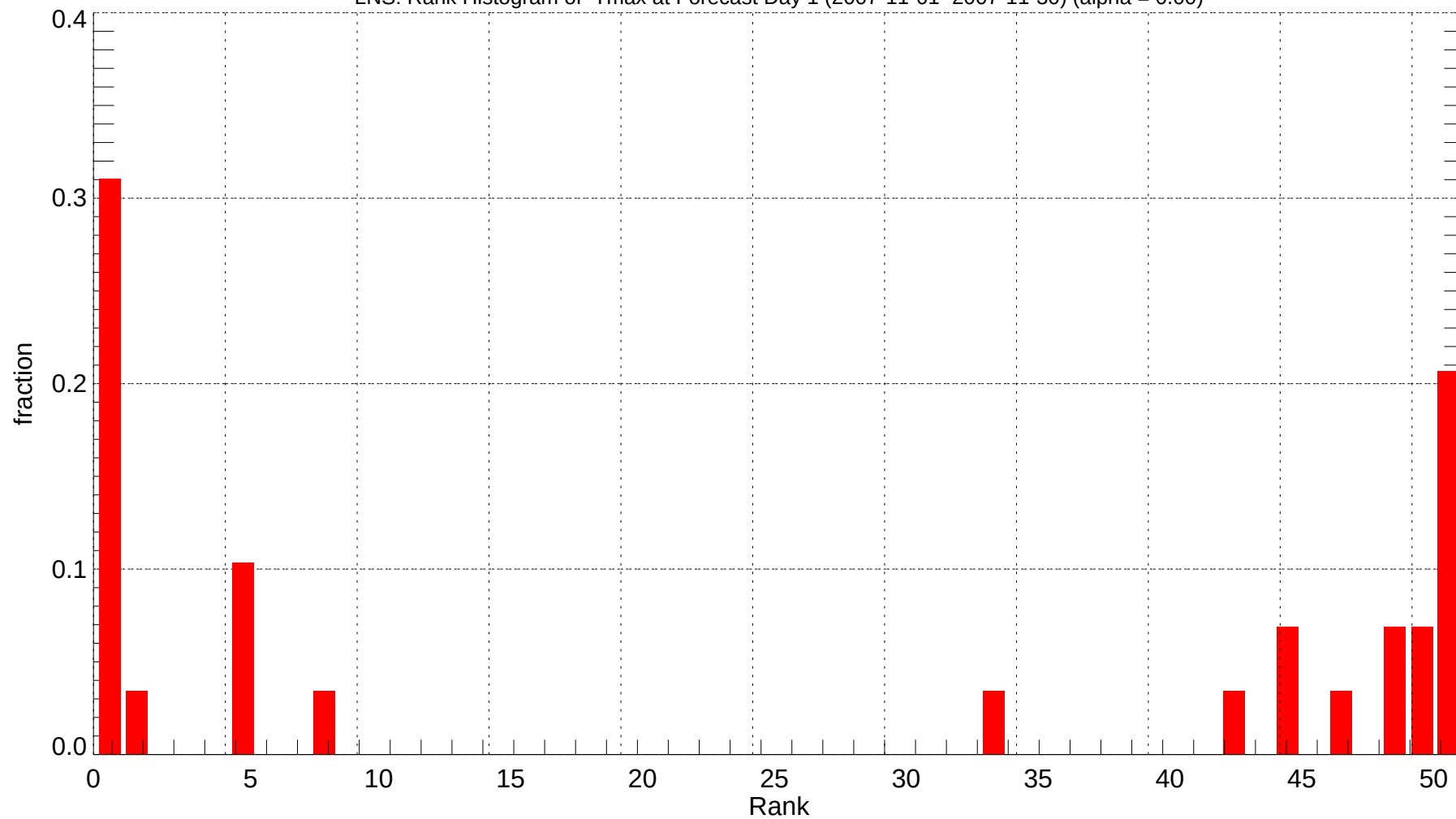
LNS: Rank Histogram of Tmax at Forecast Day 1 (2007-11-01~2007-11-30) (alpha = 0.00)
