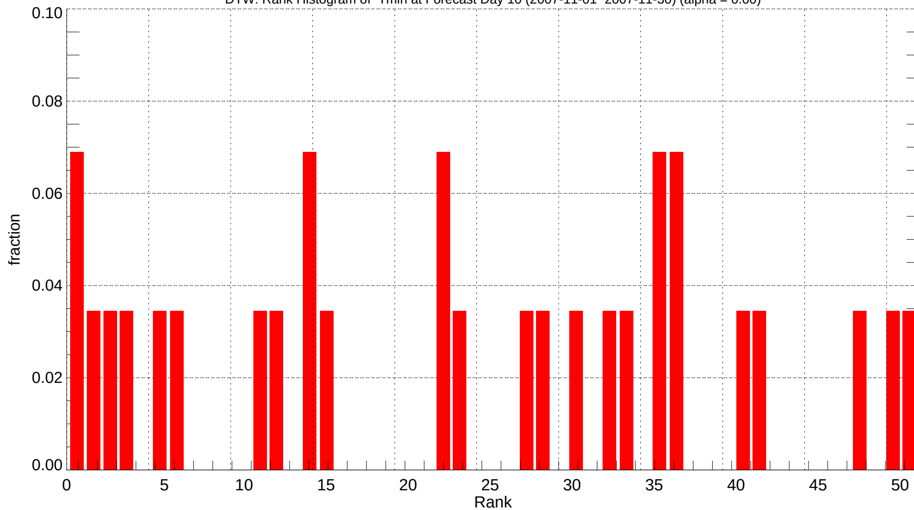
DTW: Rank Histogram of Tmin at Forecast Day 10 (2007-11-01~2007-11-30) (alpha = 0.00)
