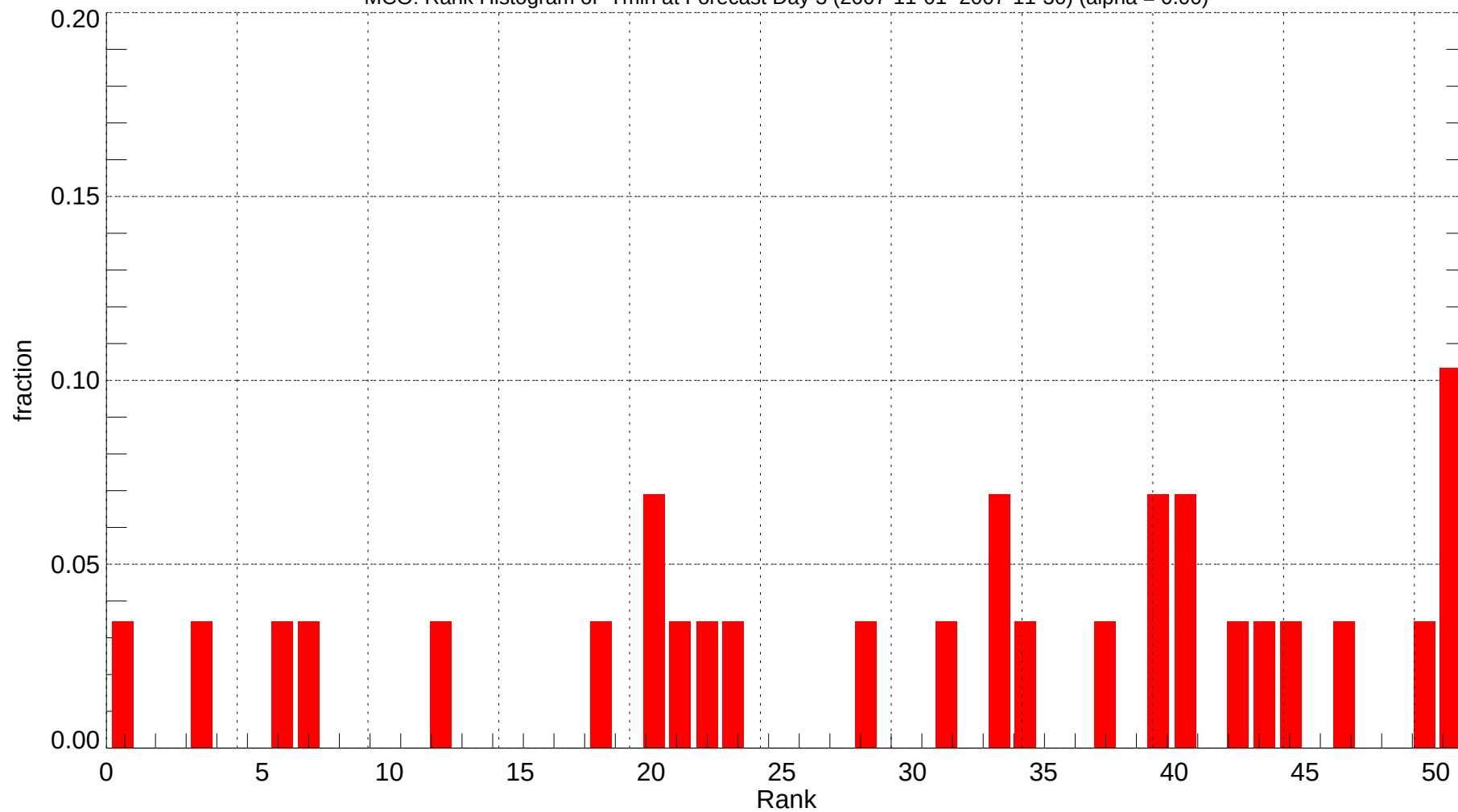
MCO: Rank Histogram of Tmin at Forecast Day 3 (2007-11-01~2007-11-30) (alpha = 0.00)
