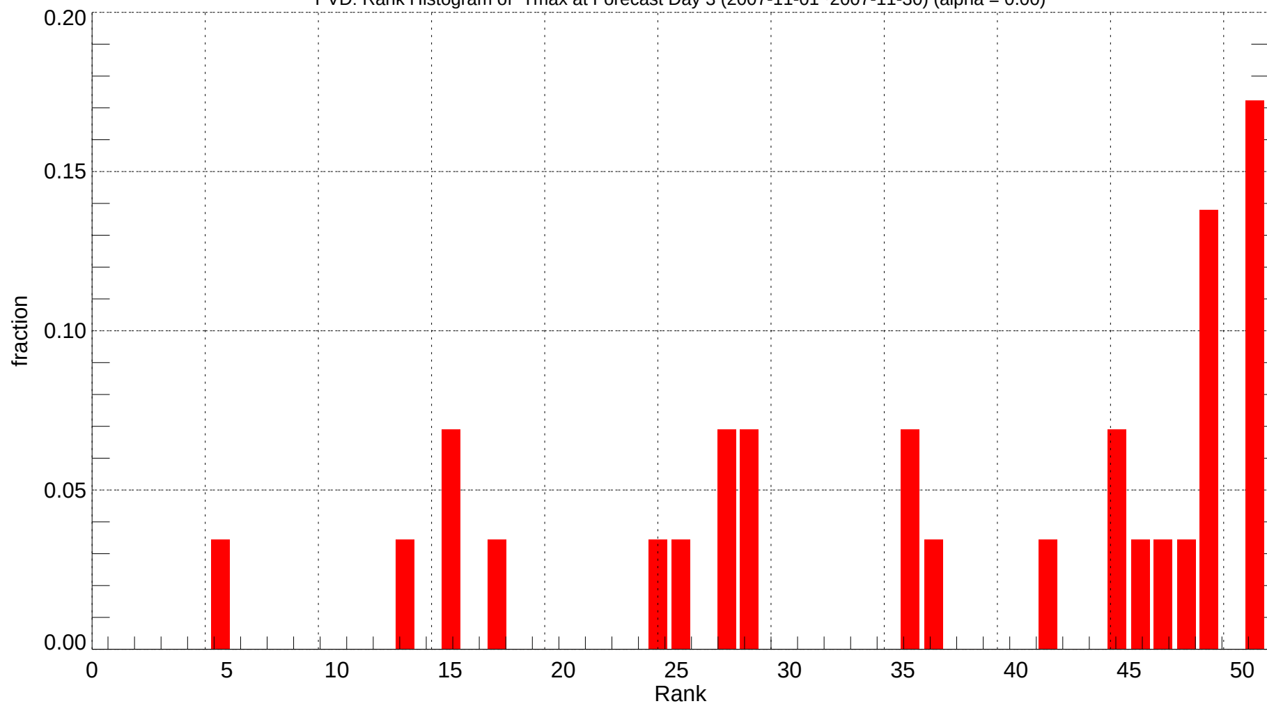
PVD: Rank Histogram of Tmax at Forecast Day 3 (2007-11-01~2007-11-30) (alpha = 0.00)
