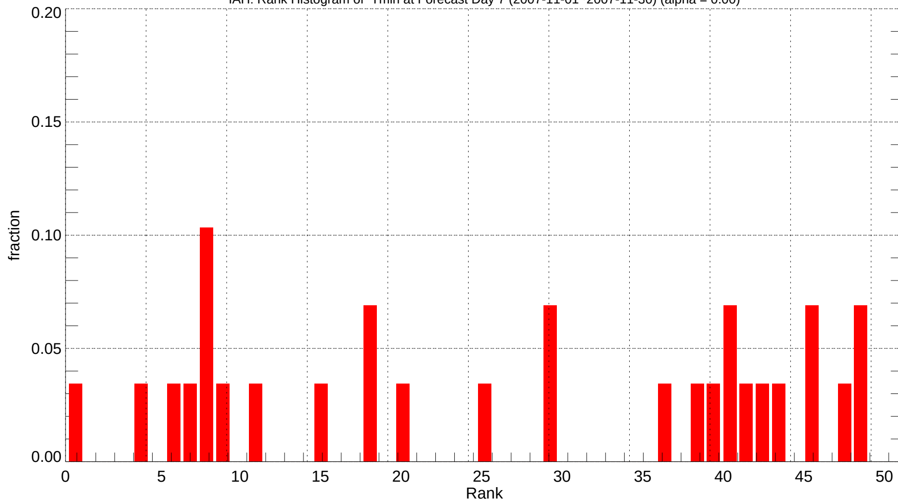
IAH: Rank Histogram of Tmin at Forecast Day 7 (2007-11-01~2007-11-30) (alpha = 0.00)
