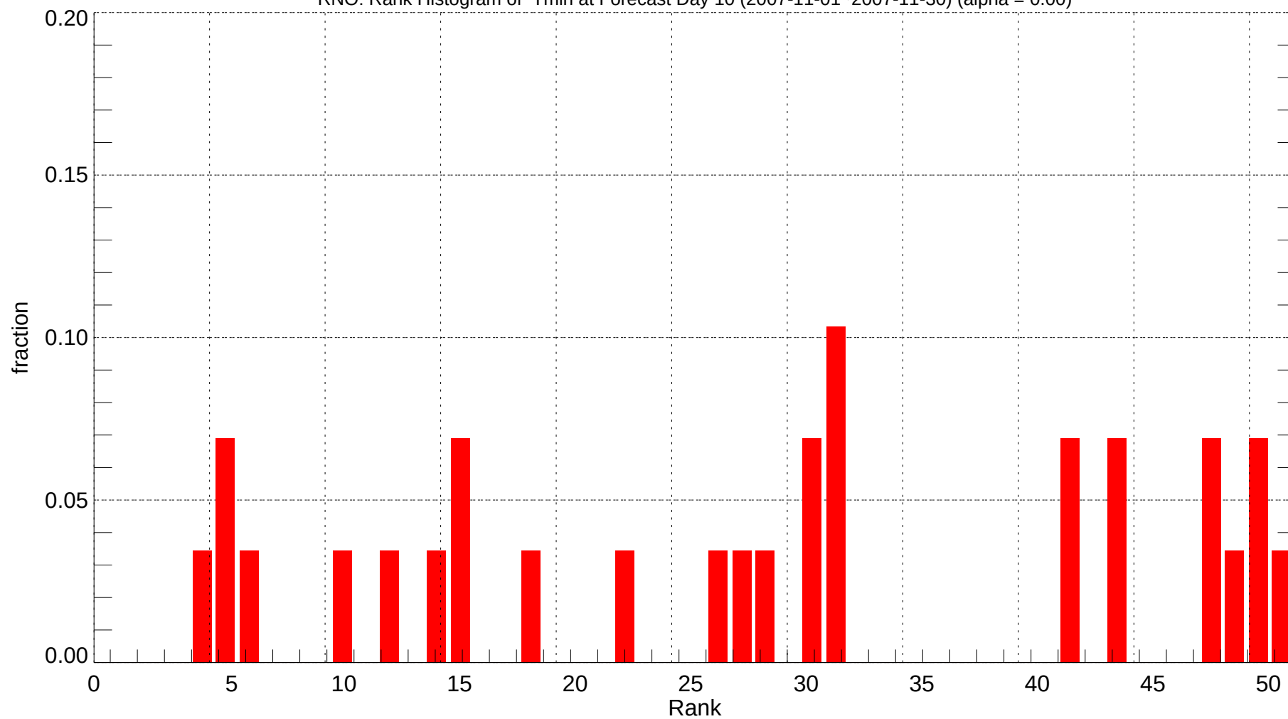
RNO: Rank Histogram of Tmin at Forecast Day 10 (2007-11-01~2007-11-30) (alpha = 0.00)
