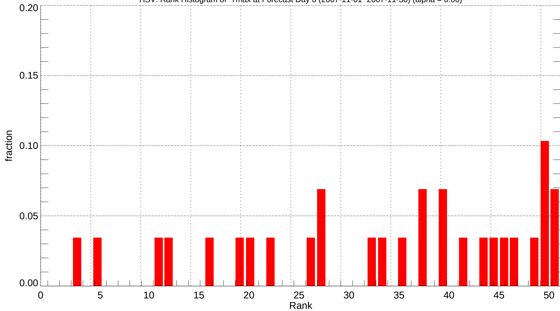
HSV: Rank Histogram of Tmax at Forecast Day 6 (2007-11-01~2007-11-30) (alpha = 0.00)
