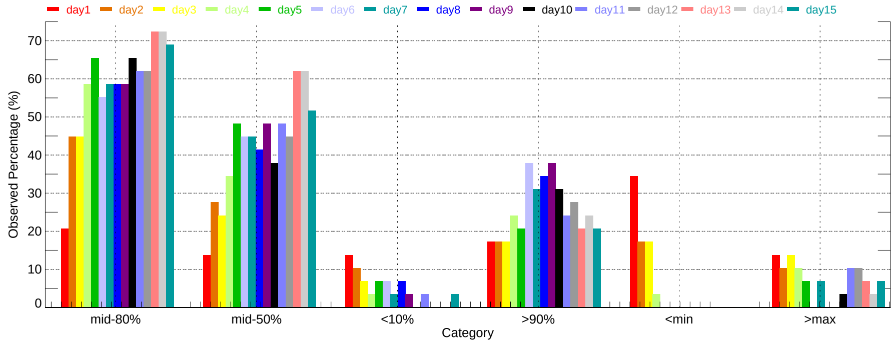
Observed Percentage of Ensembles - IND: Min Temperature (2007-11-01~2007-11-30)
