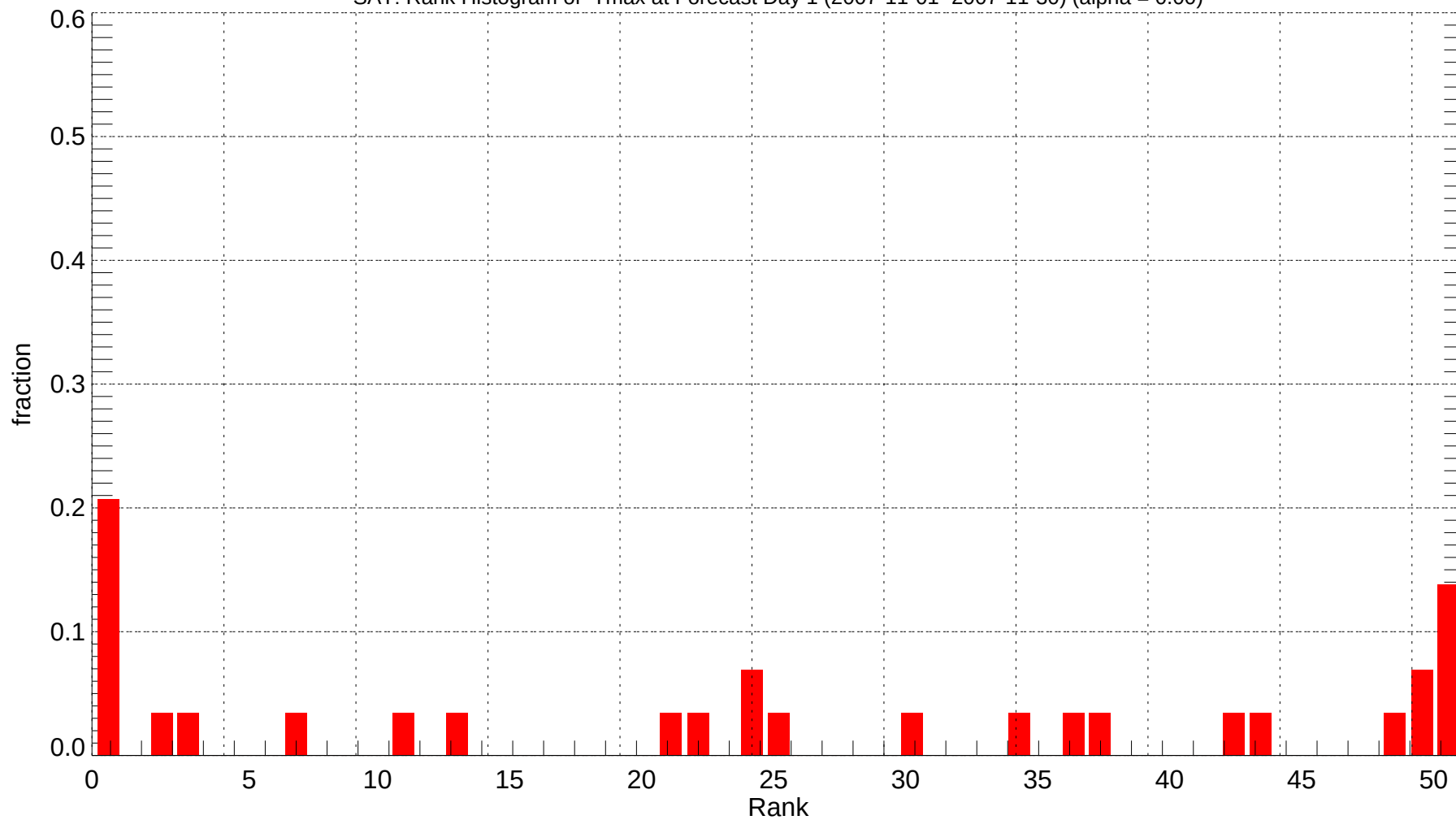
SAT: Rank Histogram of Tmax at Forecast Day 1 (2007-11-01~2007-11-30) (alpha = 0.00)
