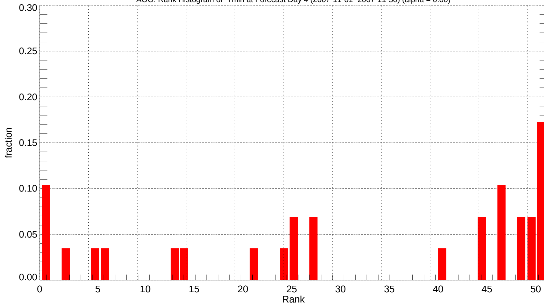
AOO: Rank Histogram of Tmin at Forecast Day 4 (2007-11-01~2007-11-30) (alpha = 0.00)
