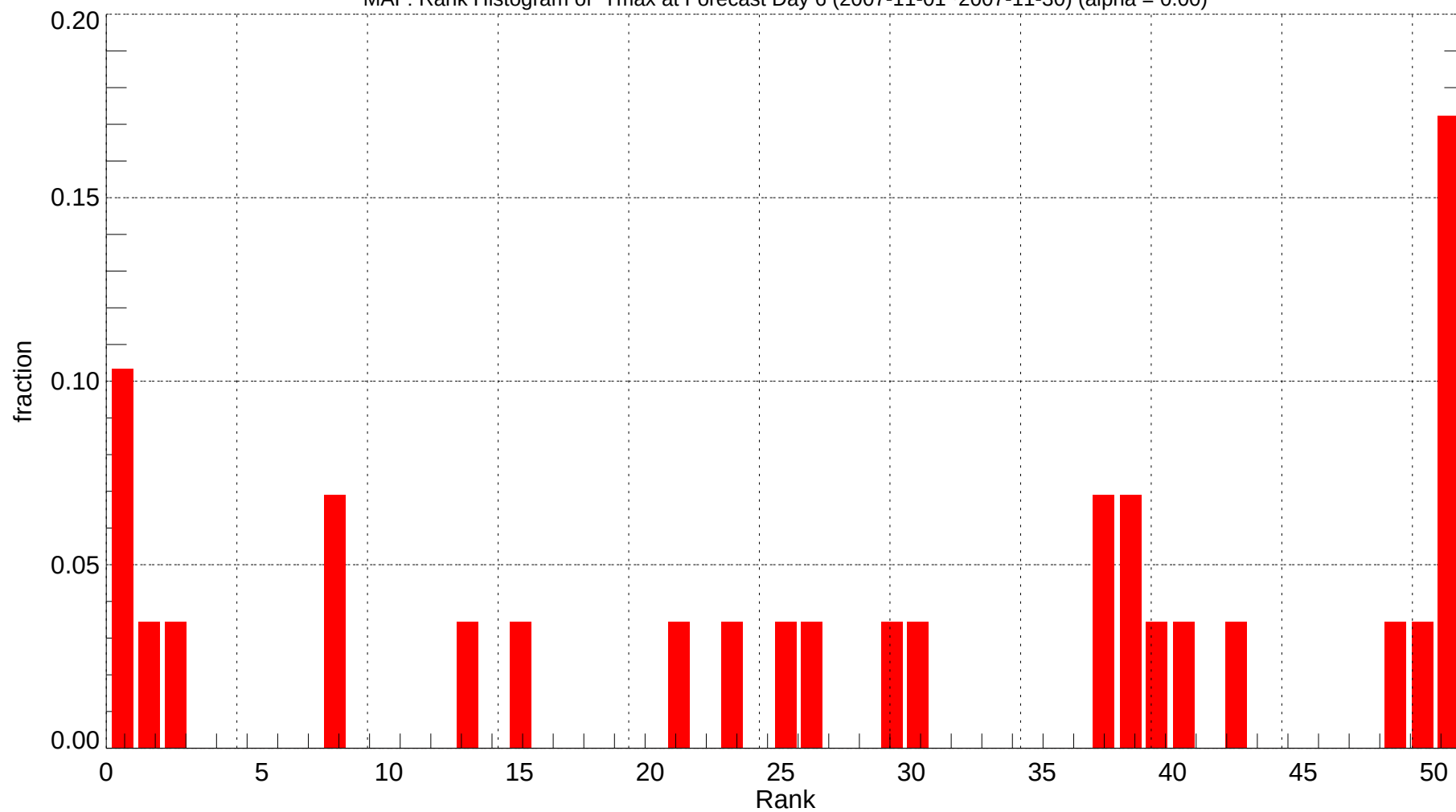
MAF: Rank Histogram of Tmax at Forecast Day 6 (2007-11-01~2007-11-30) (alpha = 0.00)
