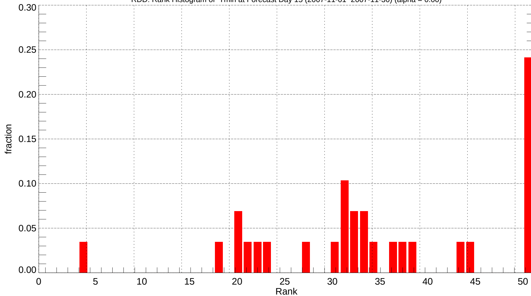
RDD: Rank Histogram of Tmin at Forecast Day 15 (2007-11-01~2007-11-30) (alpha = 0.00)
