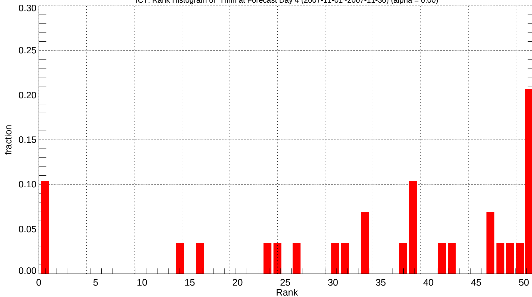
ICT: Rank Histogram of Tmin at Forecast Day 4 (2007-11-01~2007-11-30) (alpha = 0.00)
