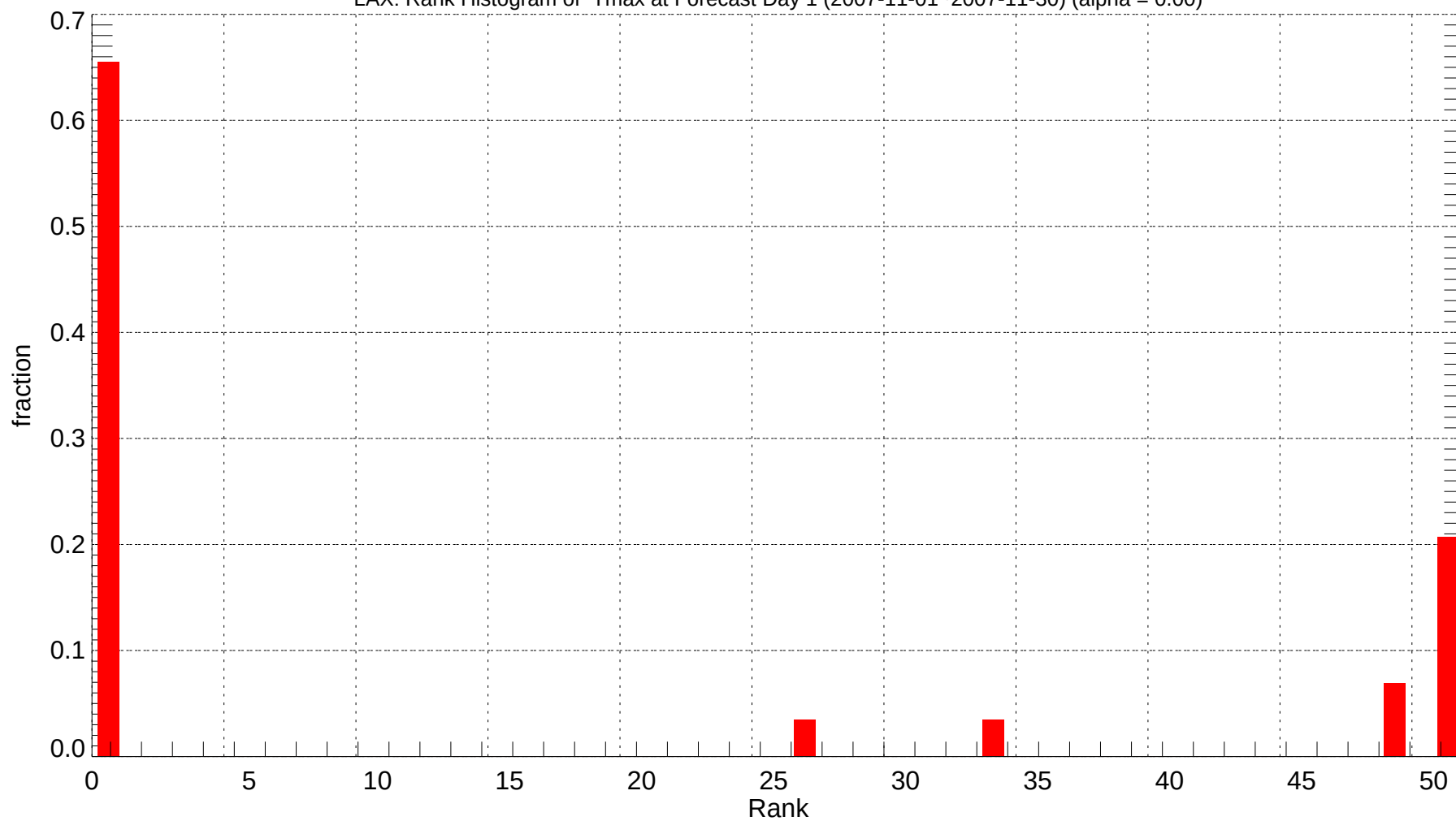
LAX: Rank Histogram of Tmax at Forecast Day 1 (2007-11-01~2007-11-30) (alpha = 0.00)
