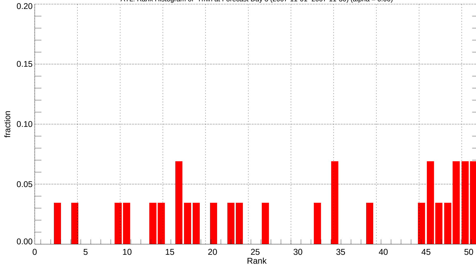
ATL: Rank Histogram of Tmin at Forecast Day 3 (2007-11-01~2007-11-30) (alpha = 0.00)
