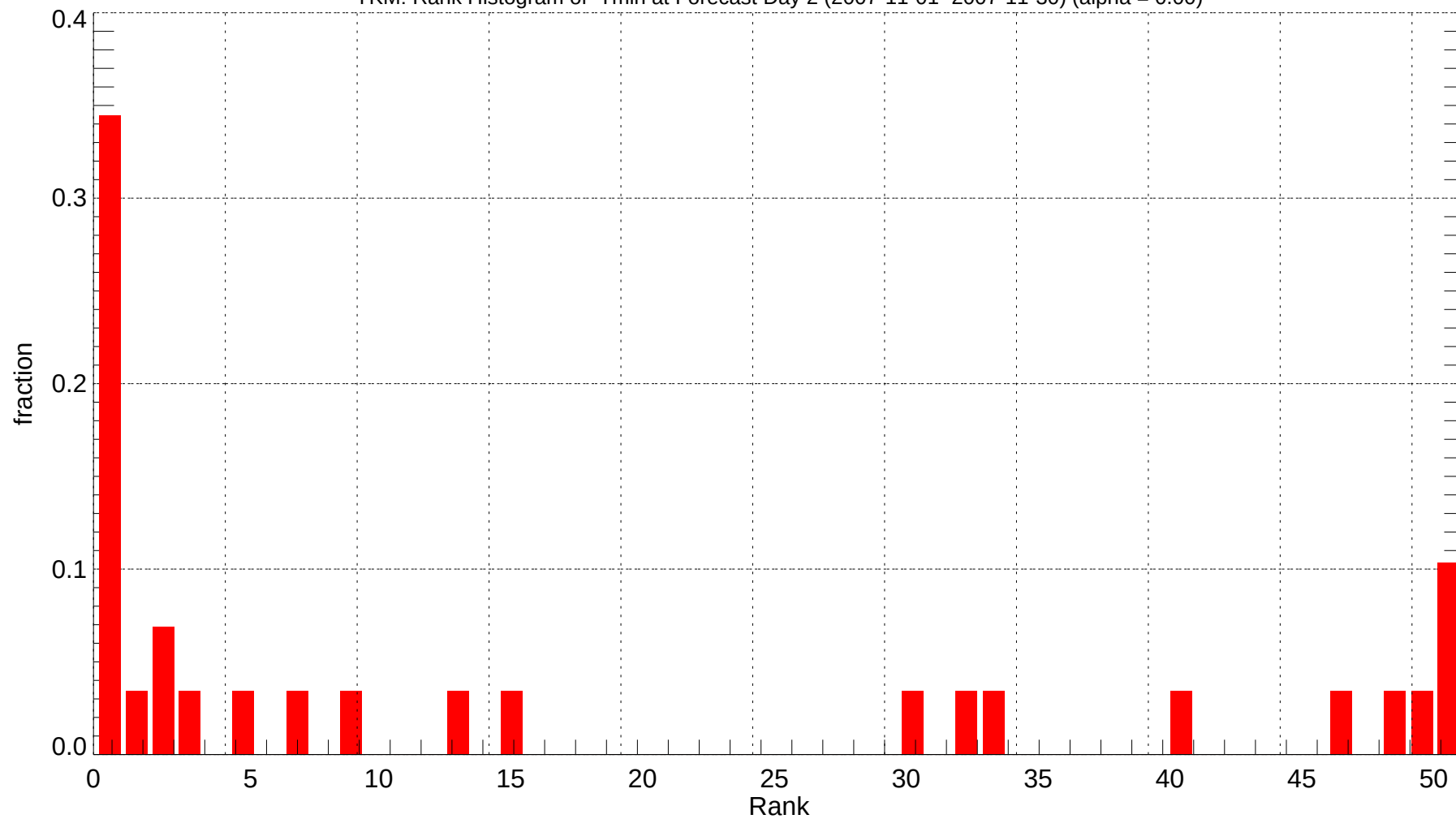
YKM: Rank Histogram of Tmin at Forecast Day 2 (2007-11-01~2007-11-30) (alpha = 0.00)
