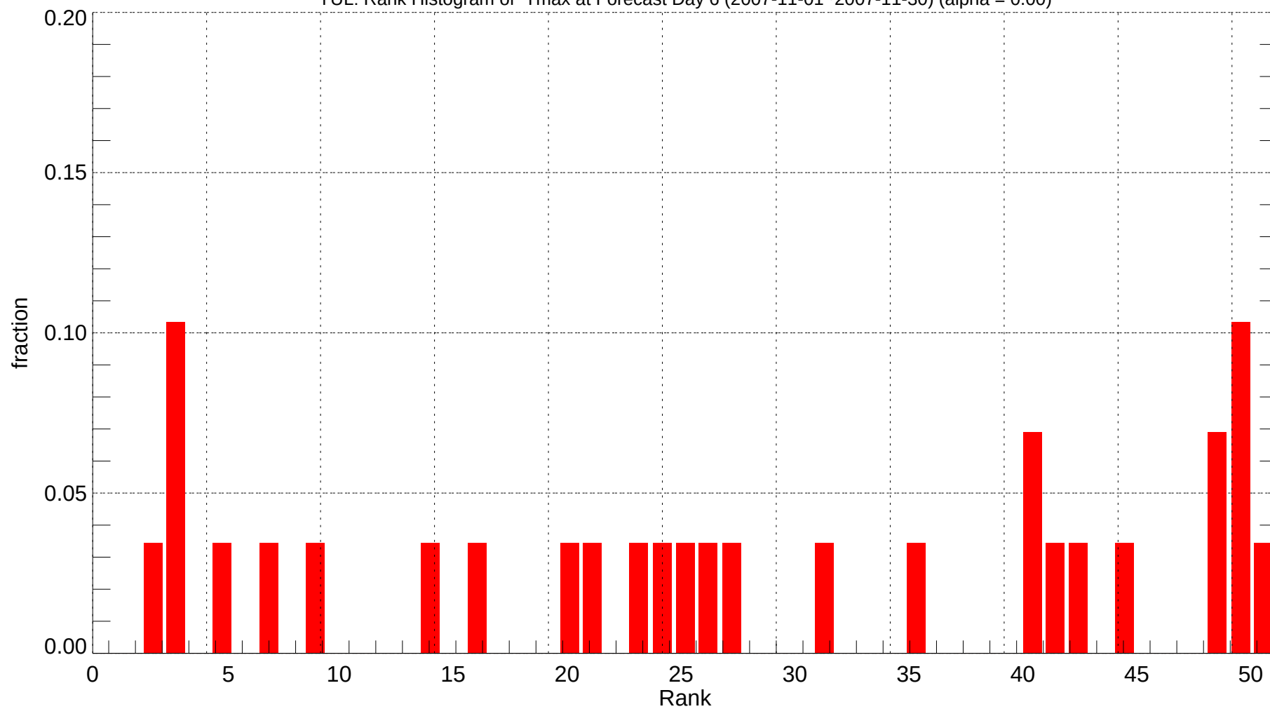
YUL: Rank Histogram of Tmax at Forecast Day 6 (2007-11-01~2007-11-30) (alpha = 0.00)
