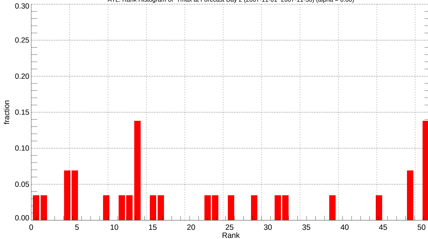
ATL: Rank Histogram of Tmax at Forecast Day 2 (2007-11-01~2007-11-30) (alpha = 0.00)
