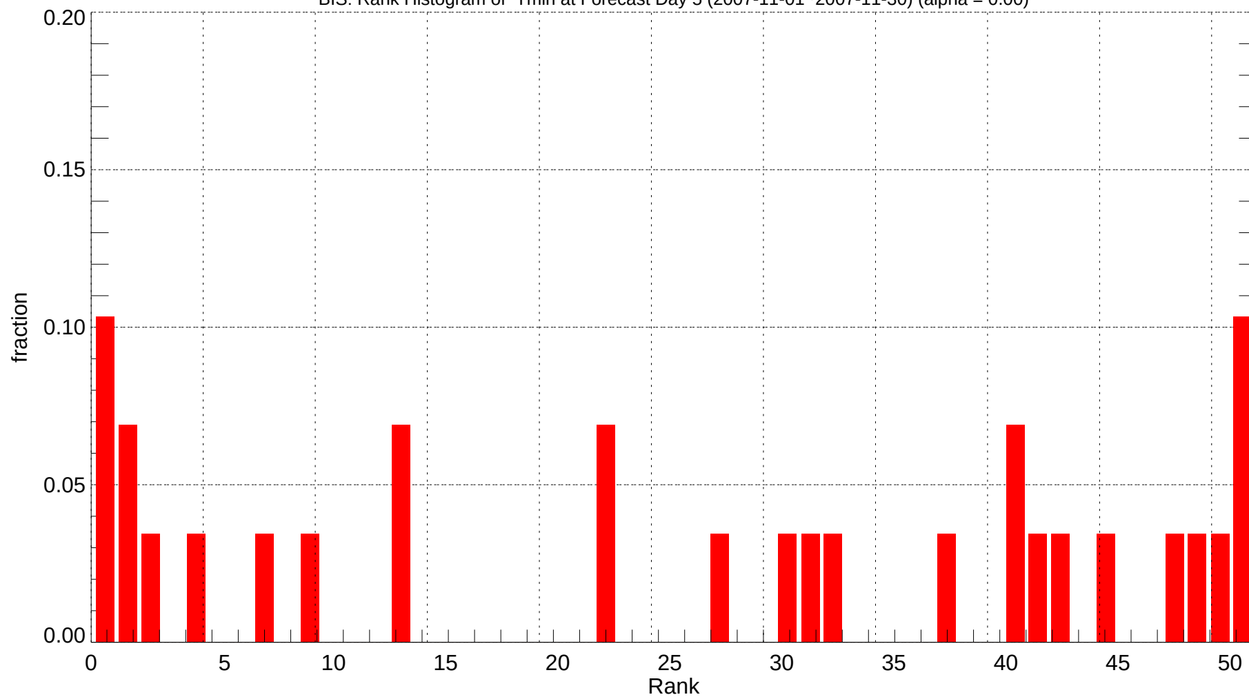
BIS: Rank Histogram of Tmin at Forecast Day 5 (2007-11-01~2007-11-30) (alpha = 0.00)
