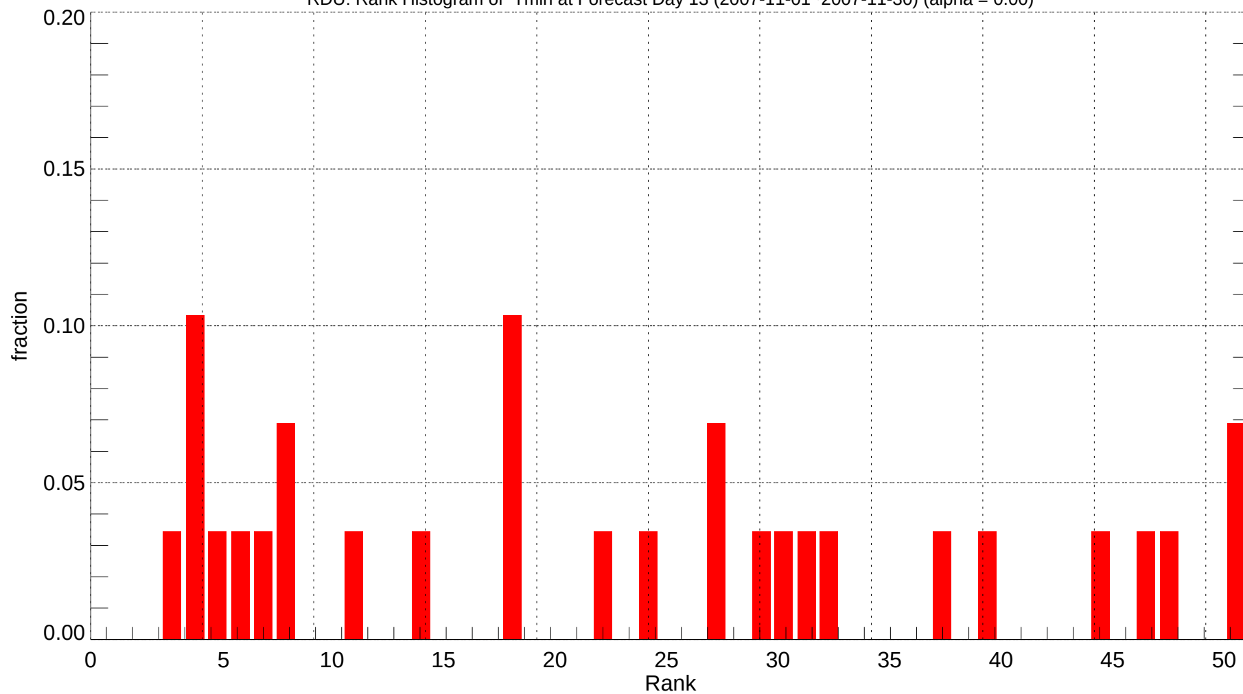
RDU: Rank Histogram of Tmin at Forecast Day 13 (2007-11-01~2007-11-30) (alpha = 0.00)
