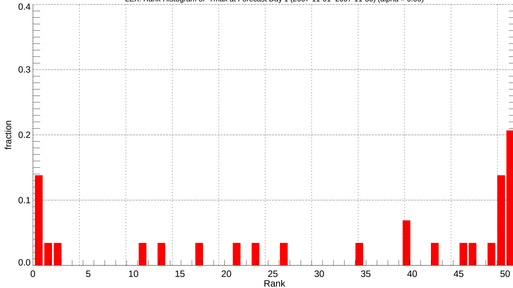
LEX: Rank Histogram of Tmax at Forecast Day 1 (2007-11-01~2007-11-30) (alpha = 0.00)
