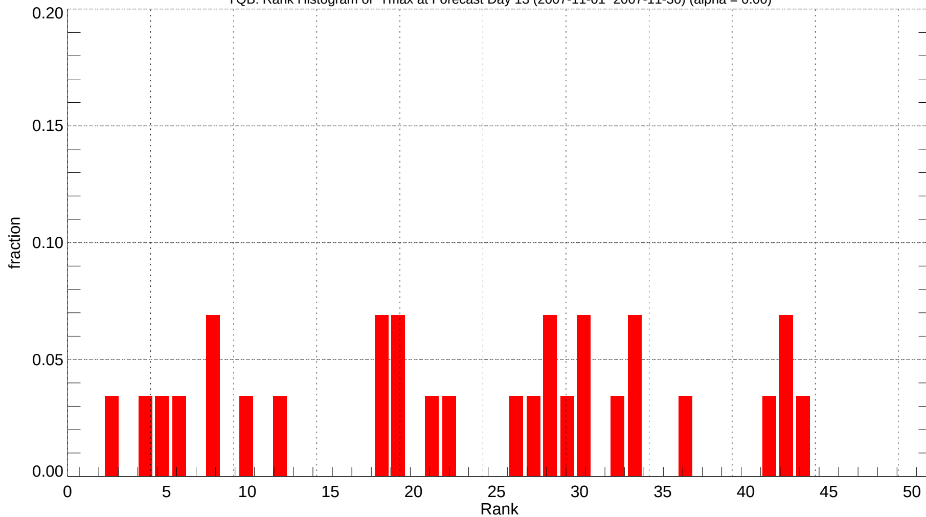
YQB: Rank Histogram of Tmax at Forecast Day 13 (2007-11-01~2007-11-30) (alpha = 0.00)
