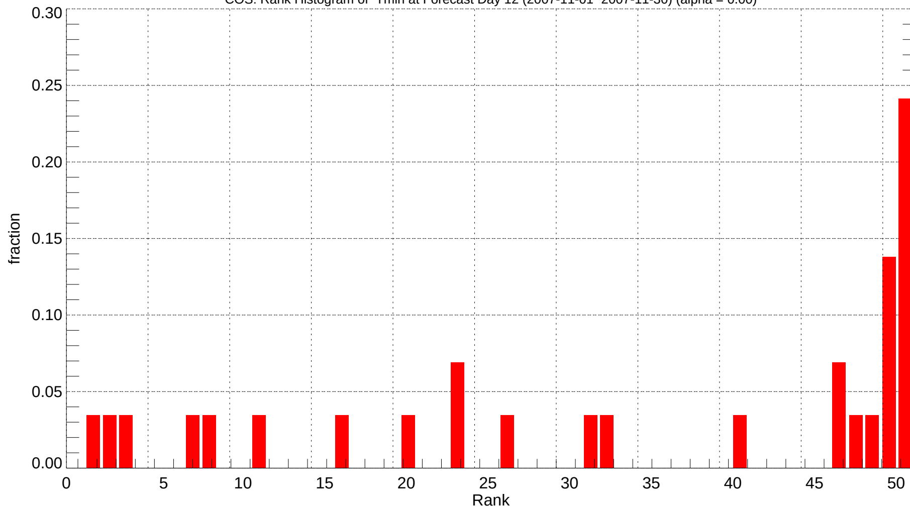
COS: Rank Histogram of Tmin at Forecast Day 12 (2007-11-01~2007-11-30) (alpha = 0.00)
