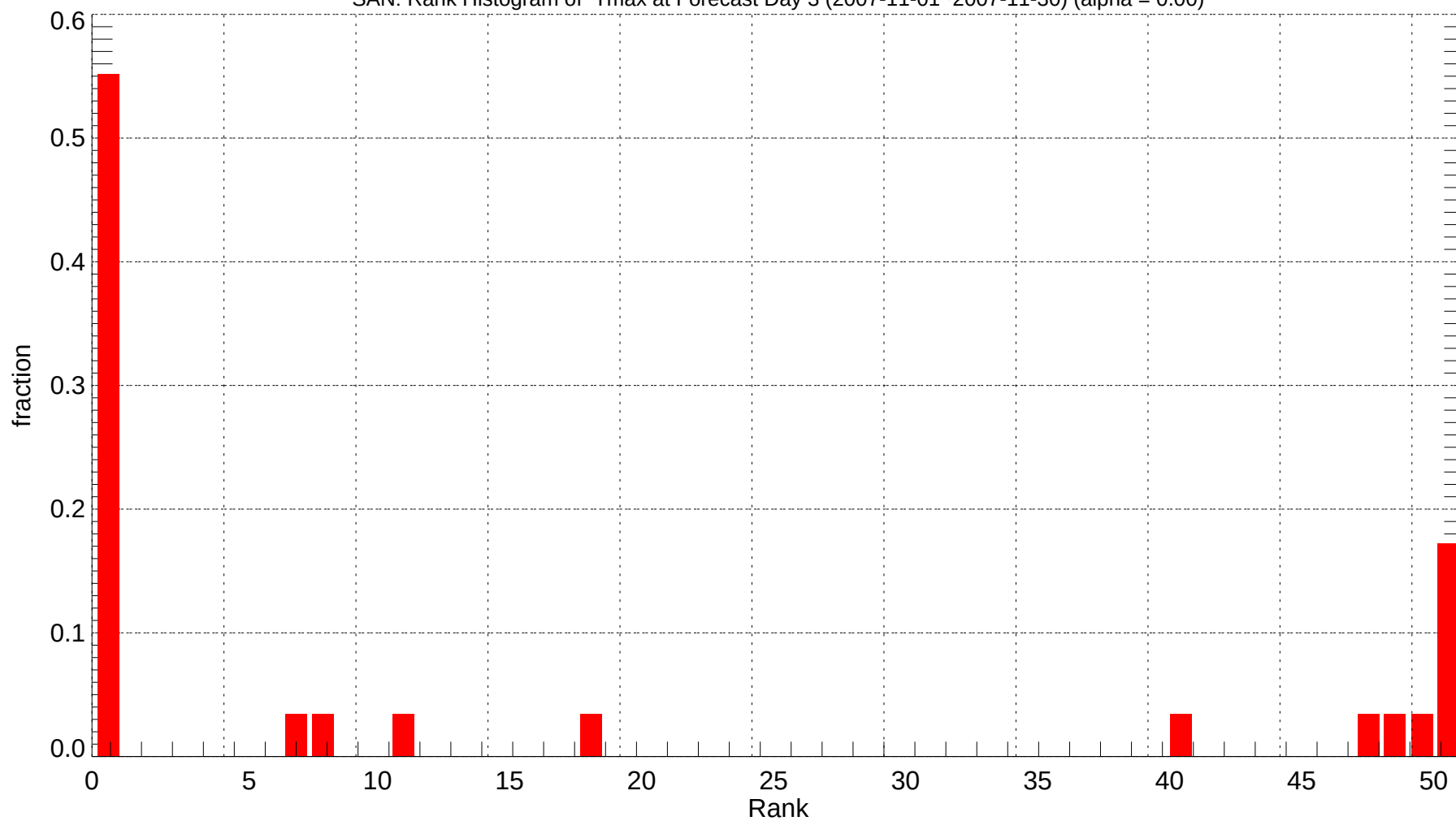
SAN: Rank Histogram of Tmax at Forecast Day 3 (2007-11-01~2007-11-30) (alpha = 0.00)
