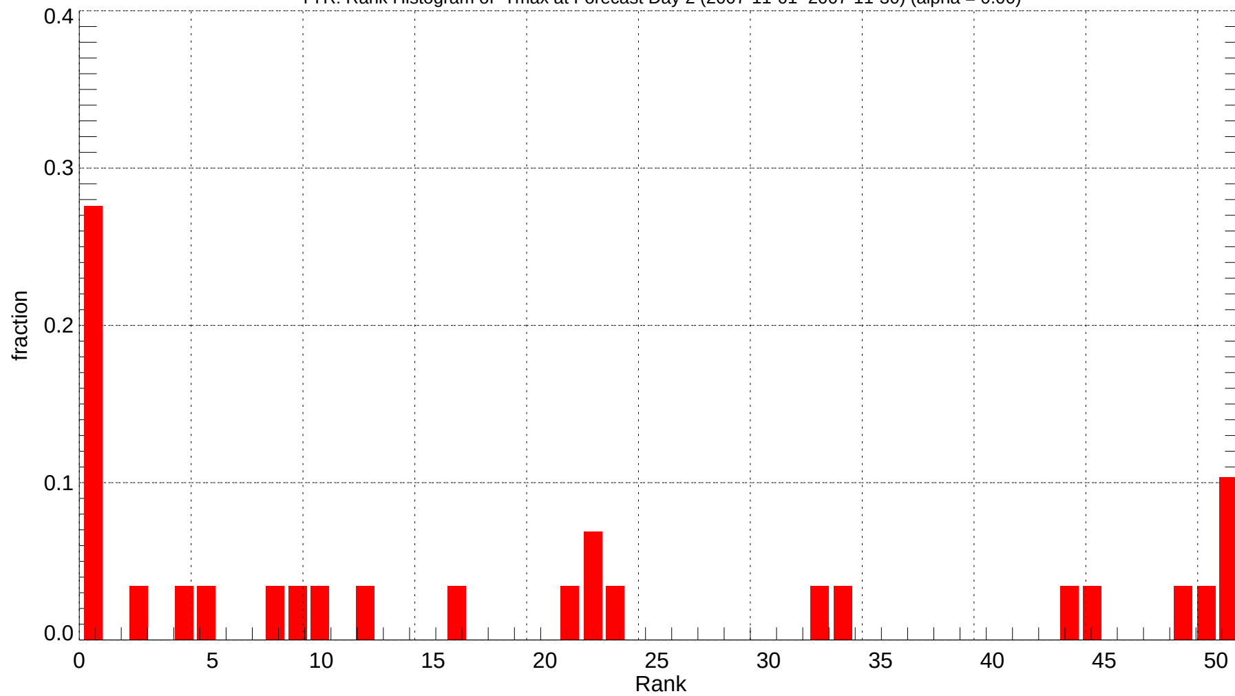
TYR: Rank Histogram of Tmax at Forecast Day 2 (2007-11-01~2007-11-30) (alpha = 0.00)
