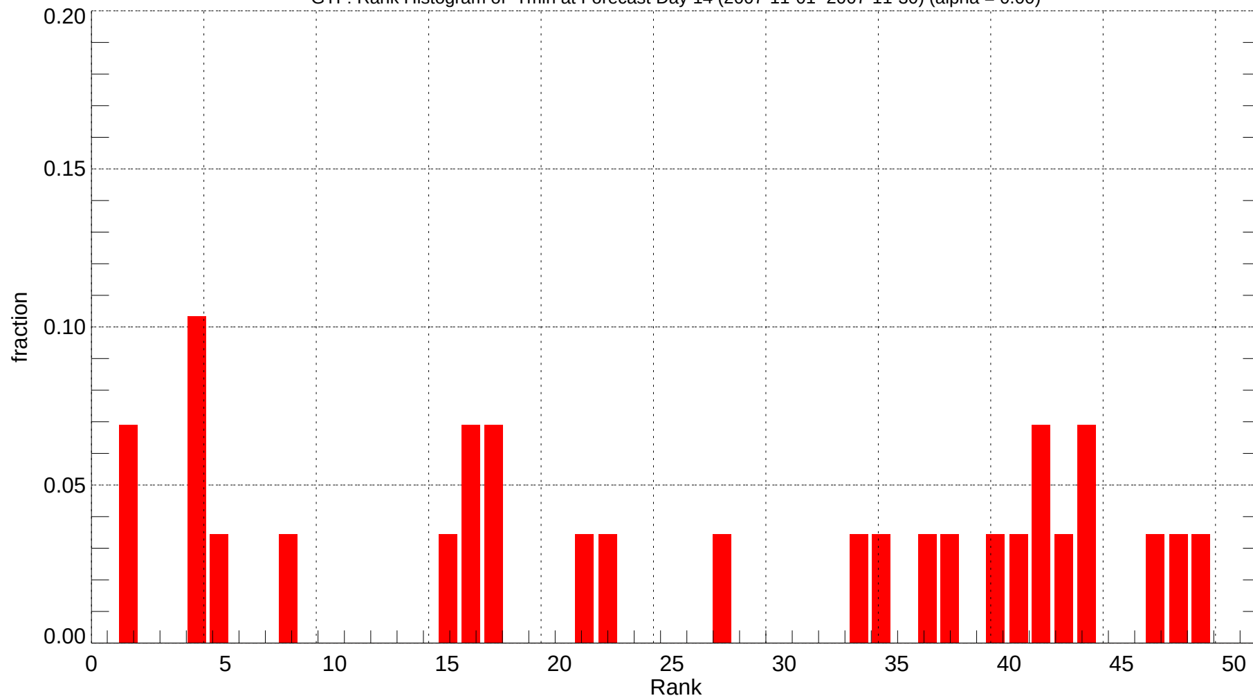
GTF: Rank Histogram of Tmin at Forecast Day 14 (2007-11-01~2007-11-30) (alpha = 0.00)
