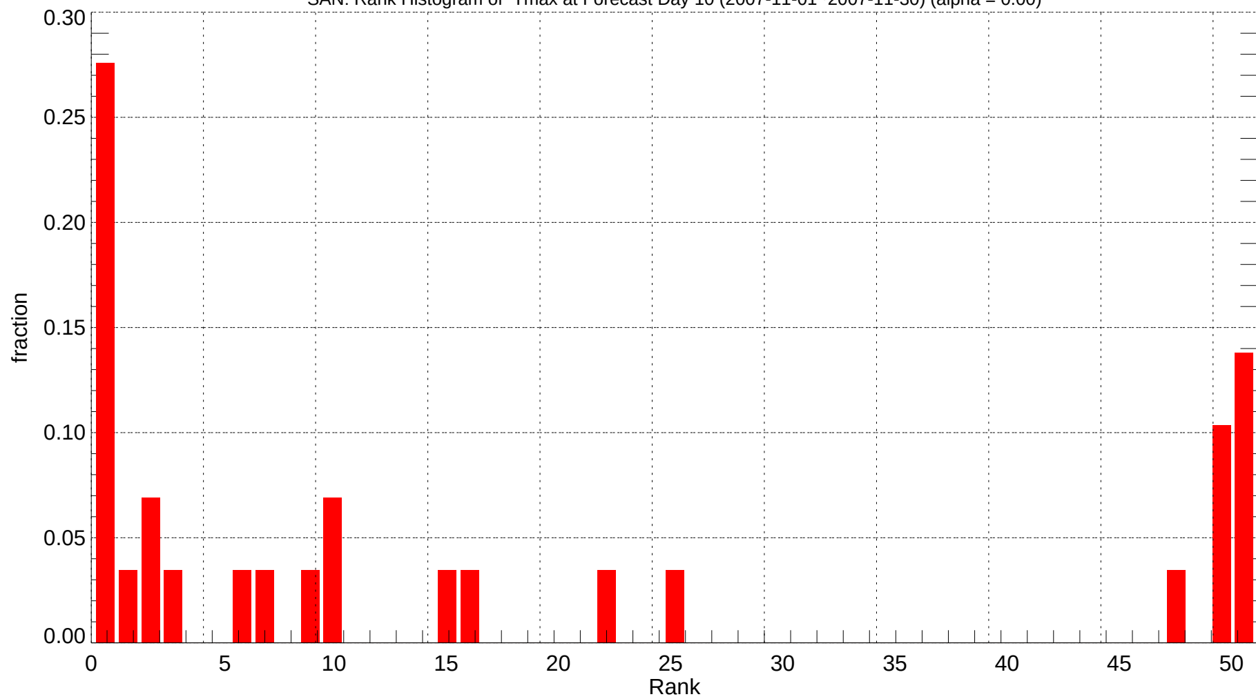
SAN: Rank Histogram of Tmax at Forecast Day 10 (2007-11-01~2007-11-30) (alpha = 0.00)
