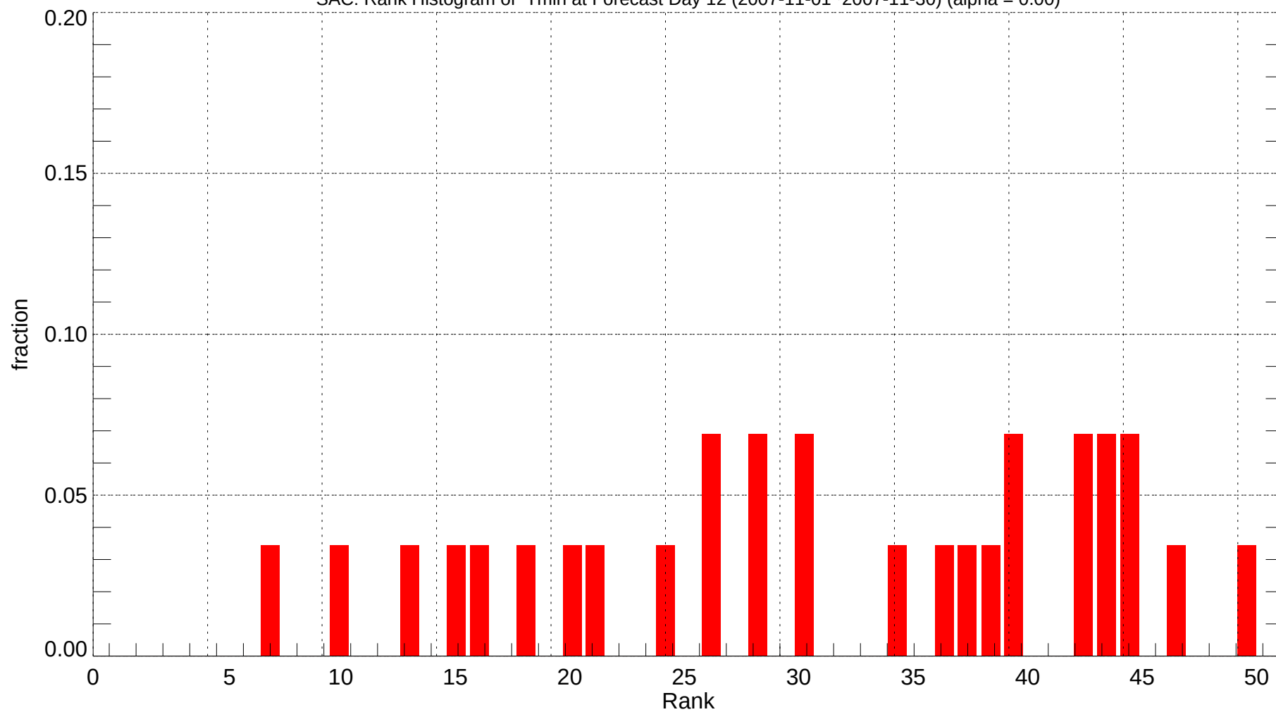
SAC: Rank Histogram of Tmin at Forecast Day 12 (2007-11-01~2007-11-30) (alpha = 0.00)
