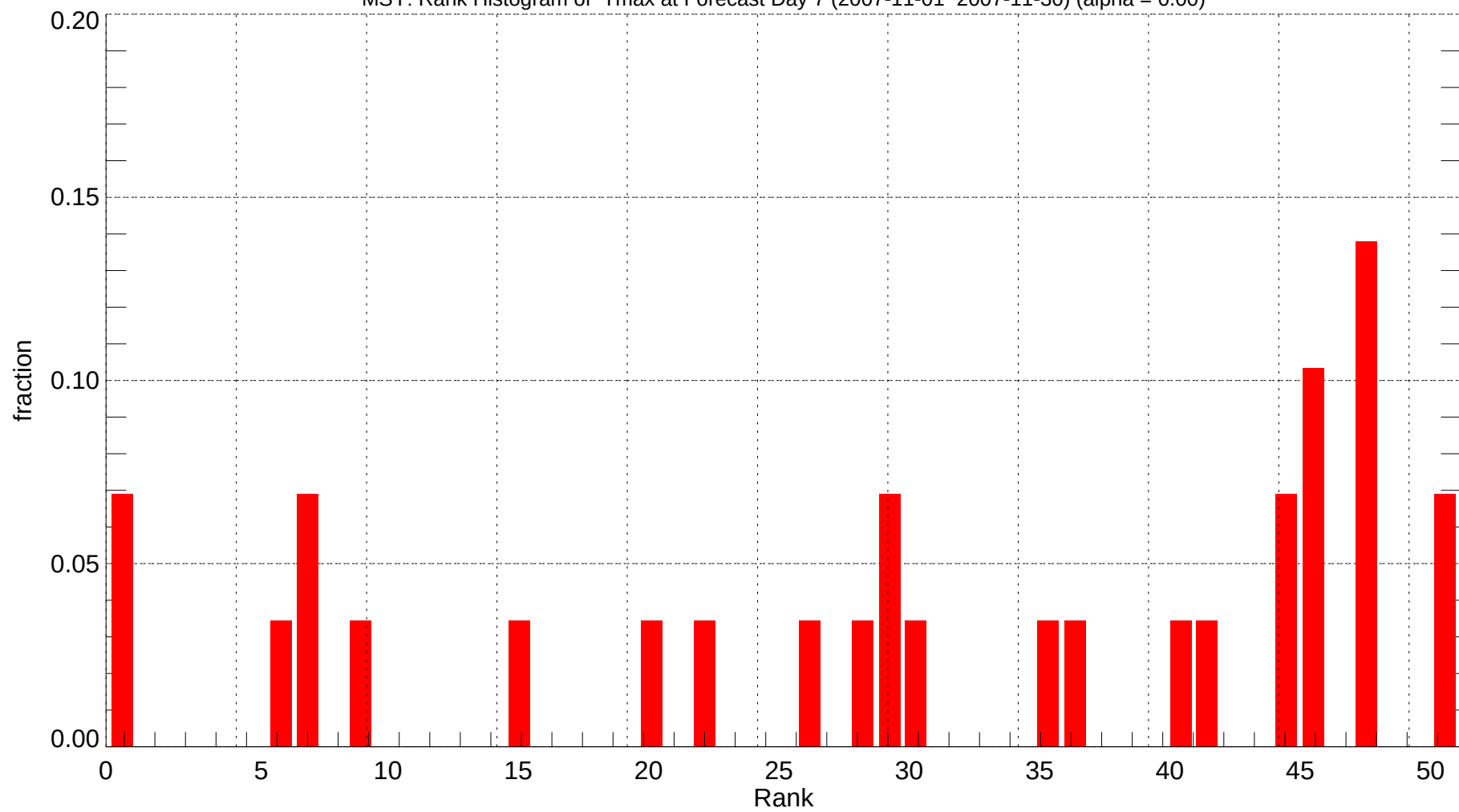
MSY: Rank Histogram of Tmax at Forecast Day 7 (2007-11-01~2007-11-30) (alpha = 0.00)
