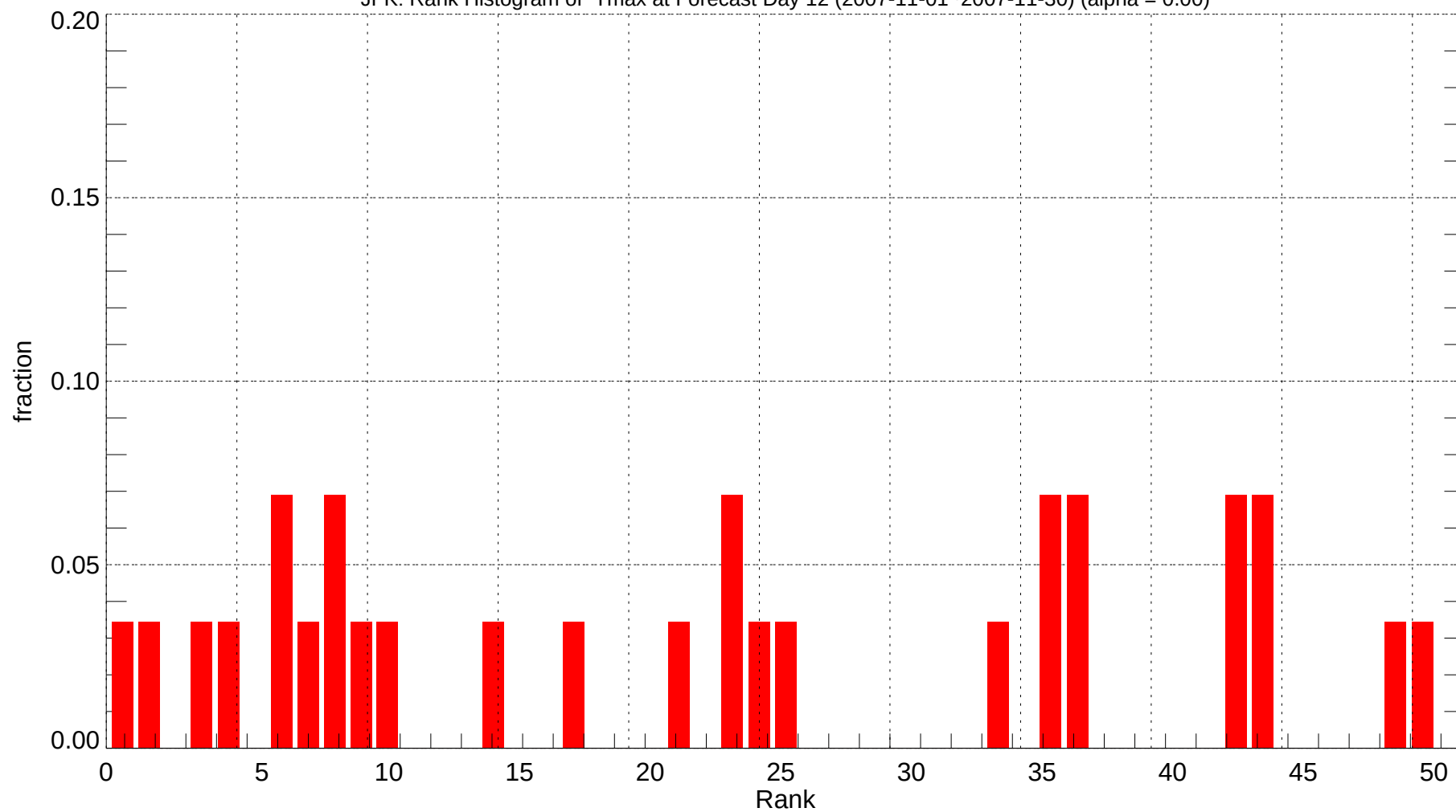
JFK: Rank Histogram of Tmax at Forecast Day 12 (2007-11-01~2007-11-30) (alpha = 0.00)
