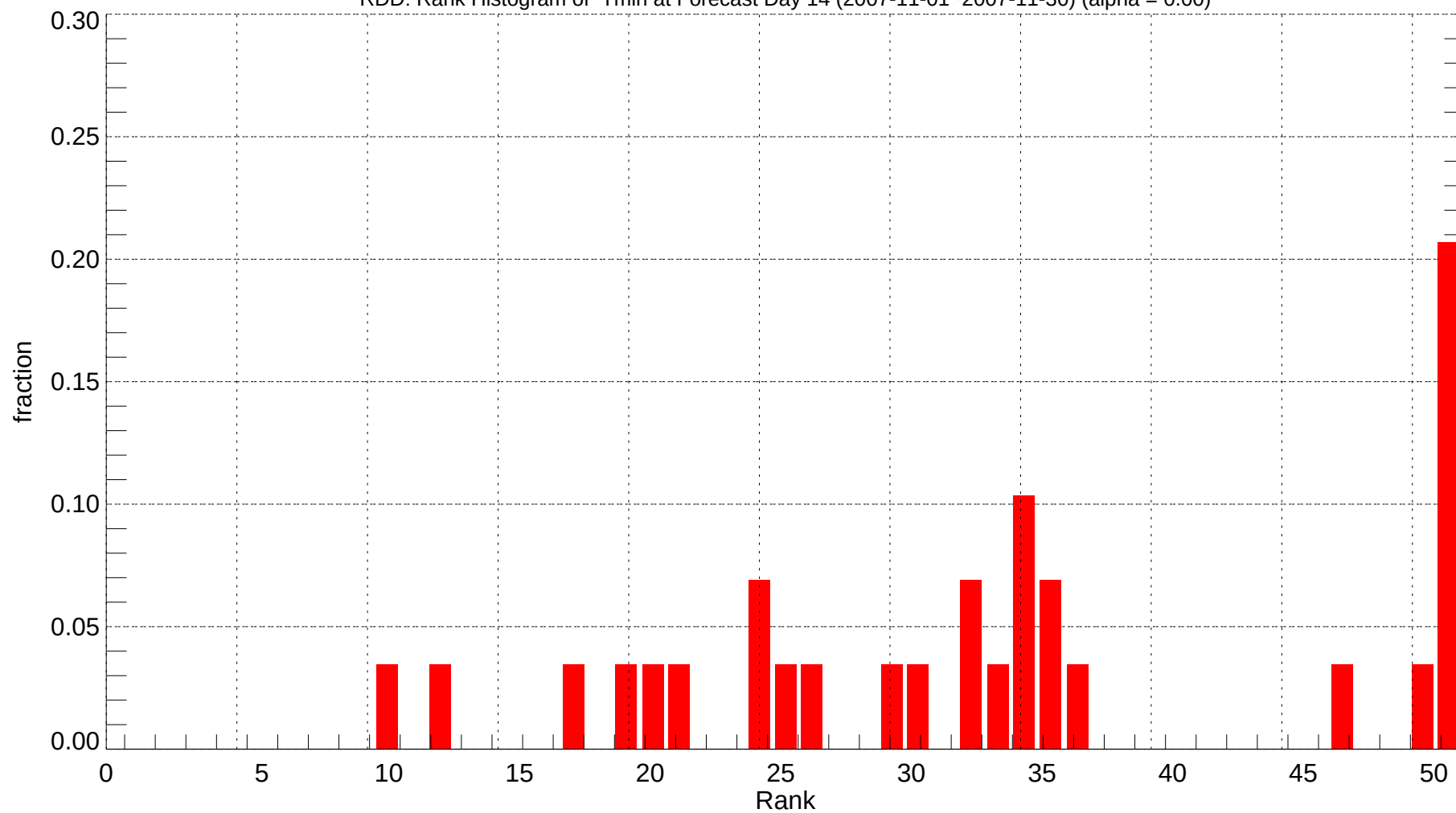
RDD: Rank Histogram of Tmin at Forecast Day 14 (2007-11-01~2007-11-30) (alpha = 0.00)
