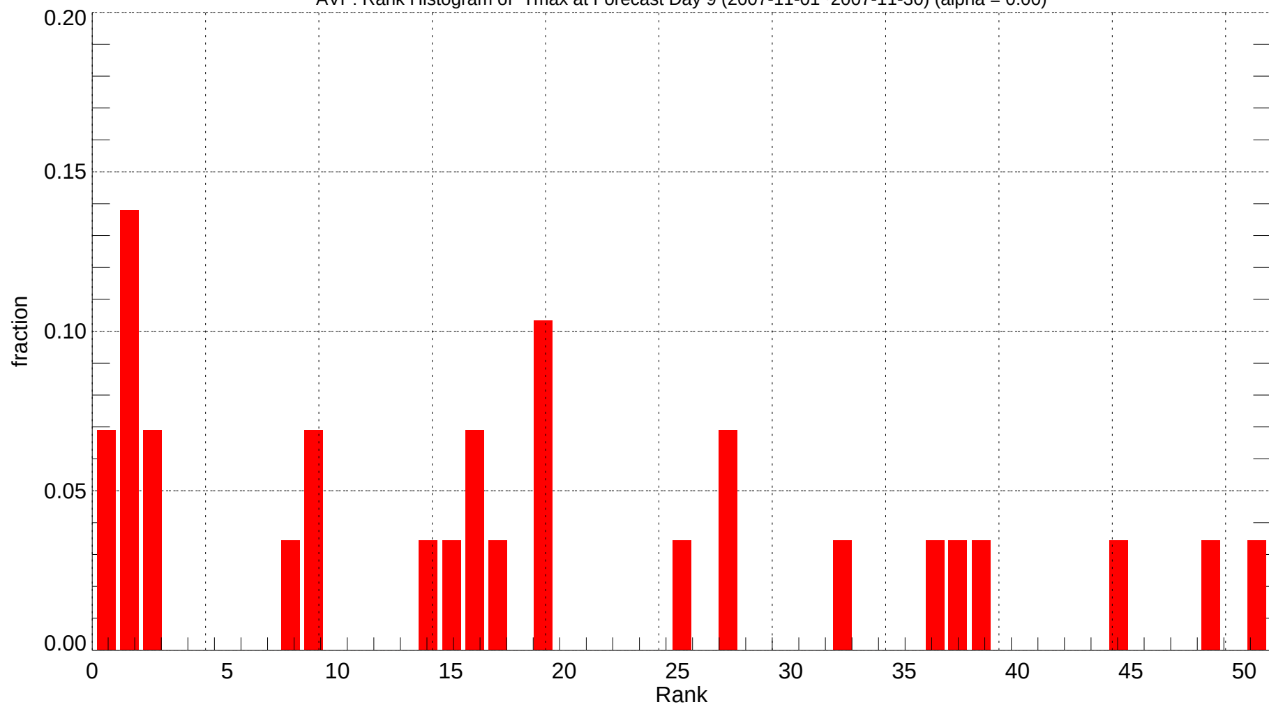
AVP: Rank Histogram of Tmax at Forecast Day 9 (2007-11-01~2007-11-30) (alpha = 0.00)
