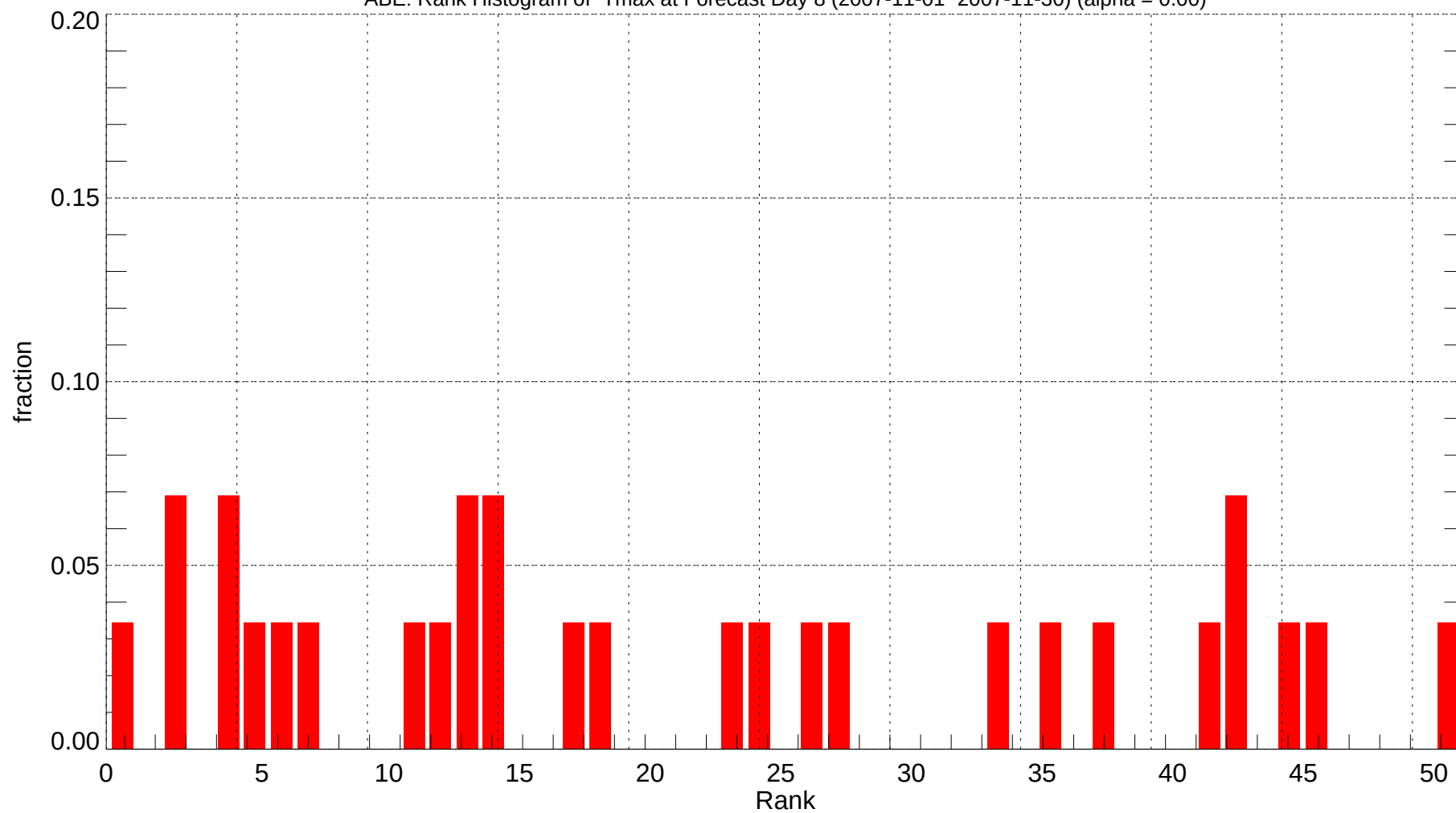
ABE: Rank Histogram of Tmax at Forecast Day 8 (2007-11-01~2007-11-30) (alpha = 0.00)
