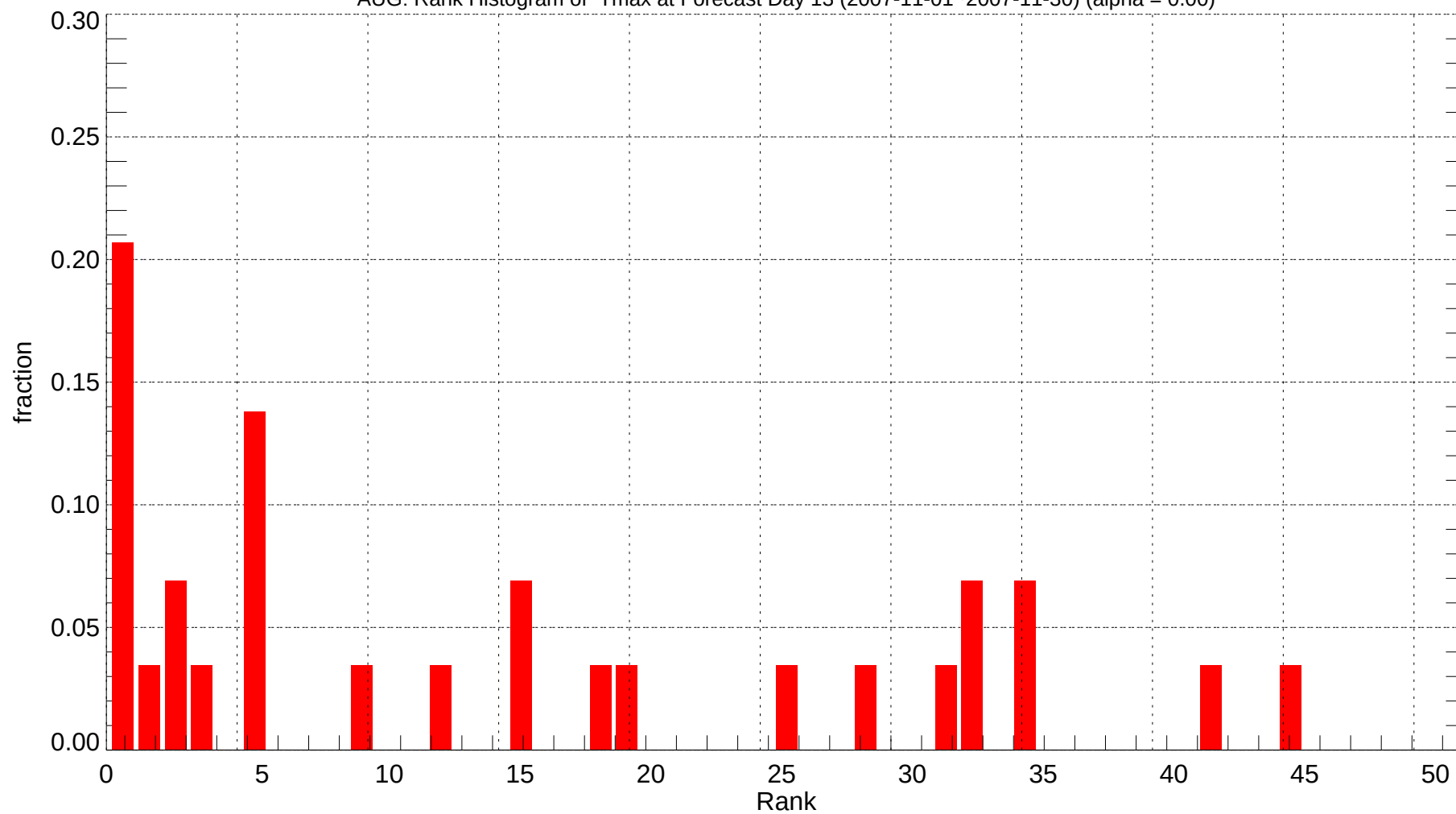
AUG: Rank Histogram of Tmax at Forecast Day 13 (2007-11-01~2007-11-30) (alpha = 0.00)
