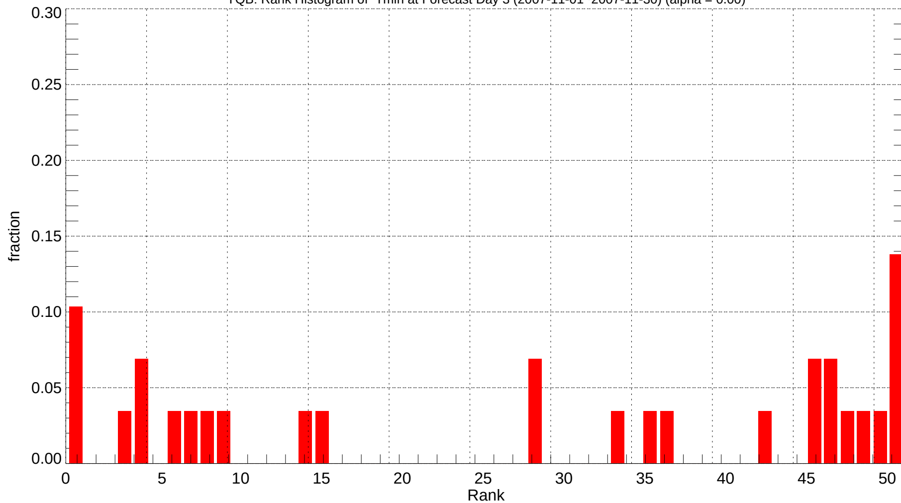
YQB: Rank Histogram of Tmin at Forecast Day 3 (2007-11-01~2007-11-30) (alpha = 0.00)
