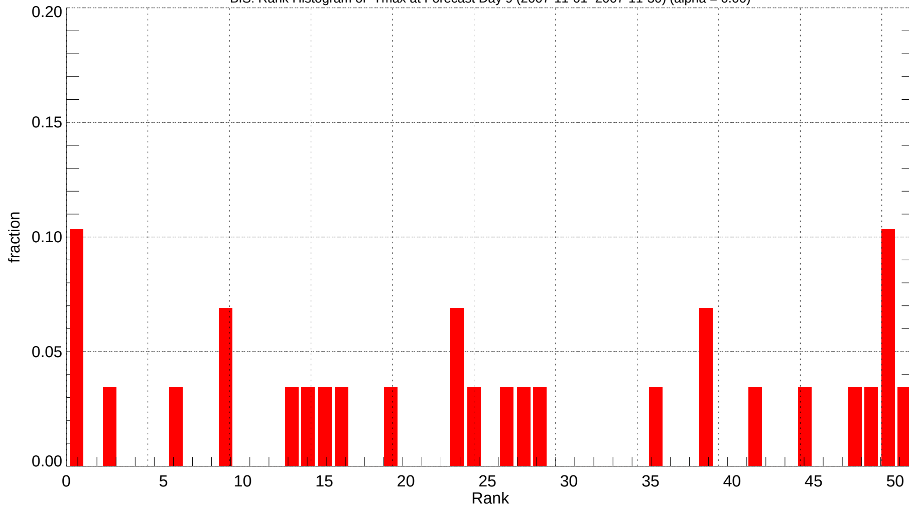
BIS: Rank Histogram of Tmax at Forecast Day 9 (2007-11-01~2007-11-30) (alpha = 0.00)
