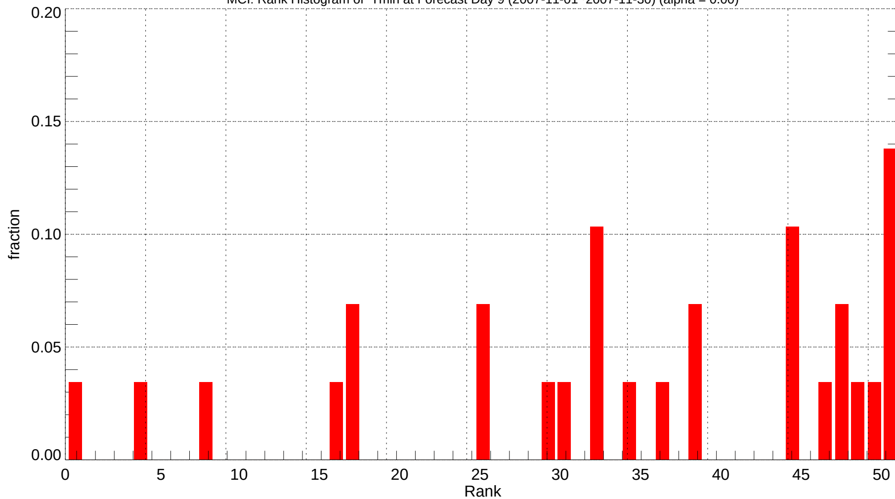
MCI: Rank Histogram of Tmin at Forecast Day 9 (2007-11-01~2007-11-30) (alpha = 0.00)
