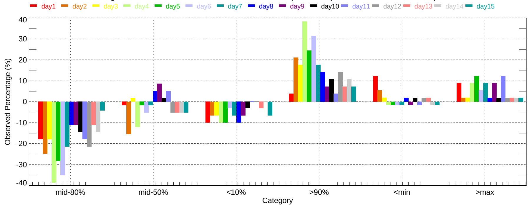
Observed Percentage Deviation of Ensembles - SAV: Min Temperature (2007-11-01~2007-11-30)
