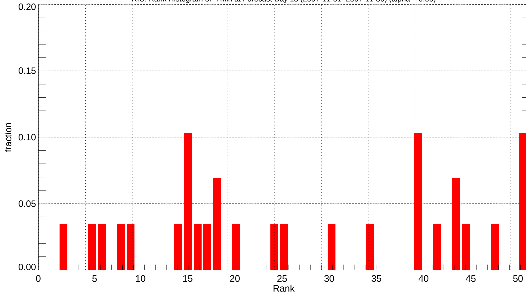
RIC: Rank Histogram of Tmin at Forecast Day 15 (2007-11-01~2007-11-30) (alpha = 0.00)
