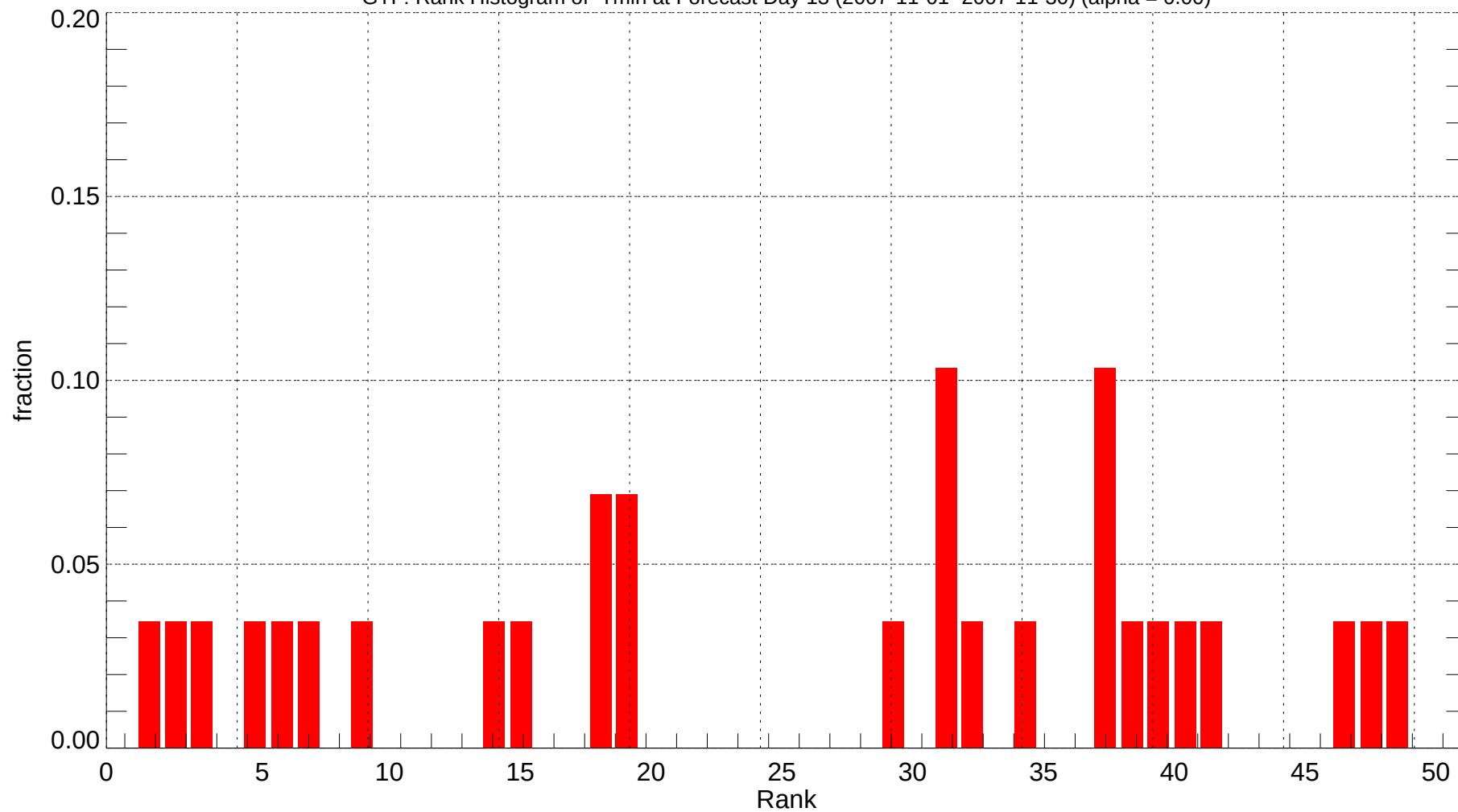
GTF: Rank Histogram of Tmin at Forecast Day 13 (2007-11-01~2007-11-30) (alpha = 0.00)
