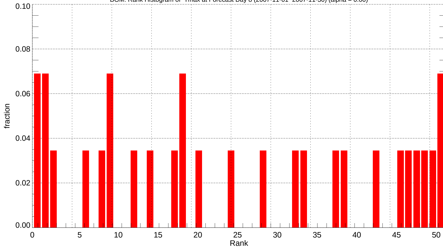
BGM: Rank Histogram of Tmax at Forecast Day 8 (2007-11-01~2007-11-30) (alpha = 0.00)
