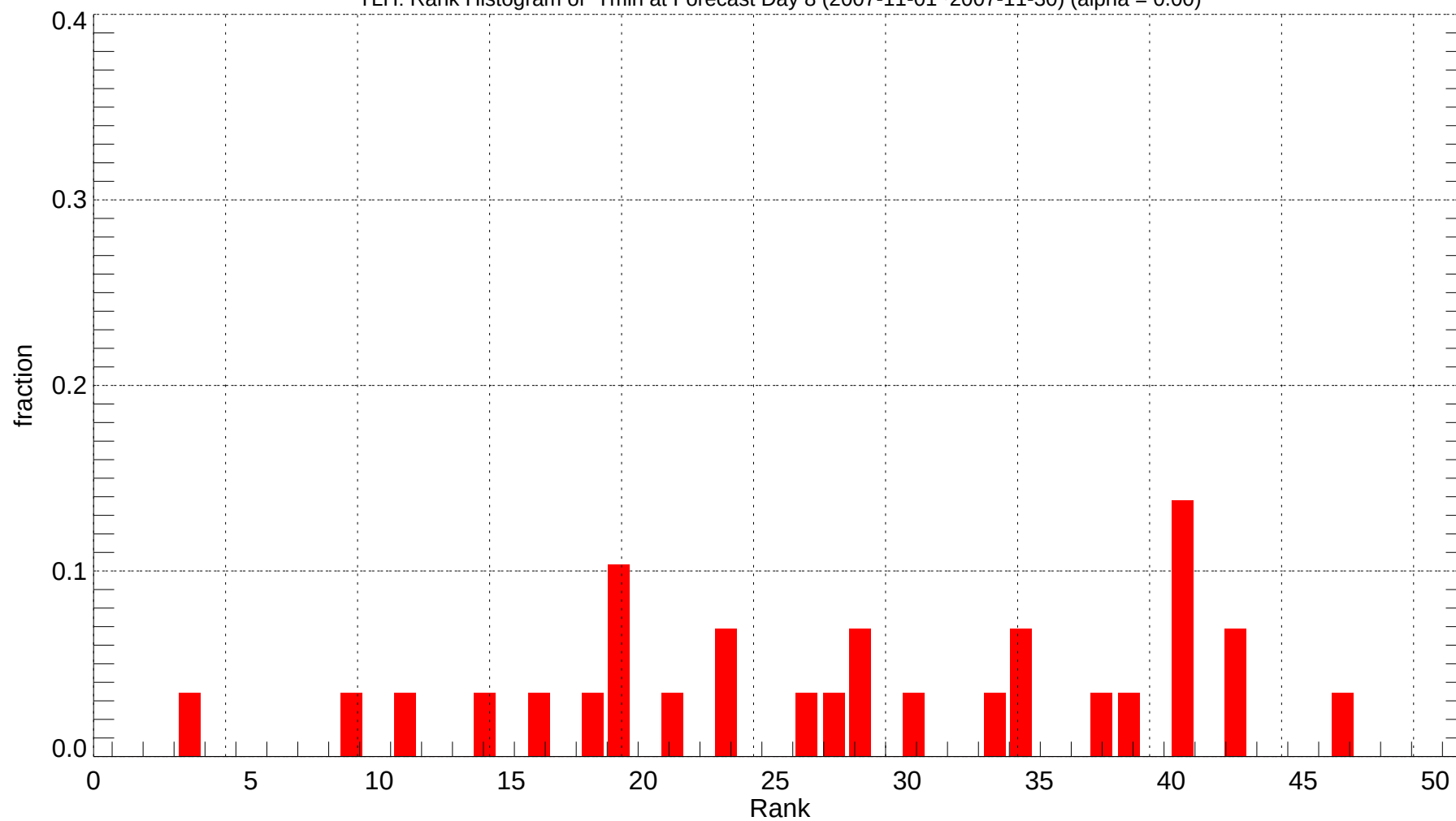
TLH: Rank Histogram of Tmin at Forecast Day 8 (2007-11-01~2007-11-30) (alpha = 0.00)
