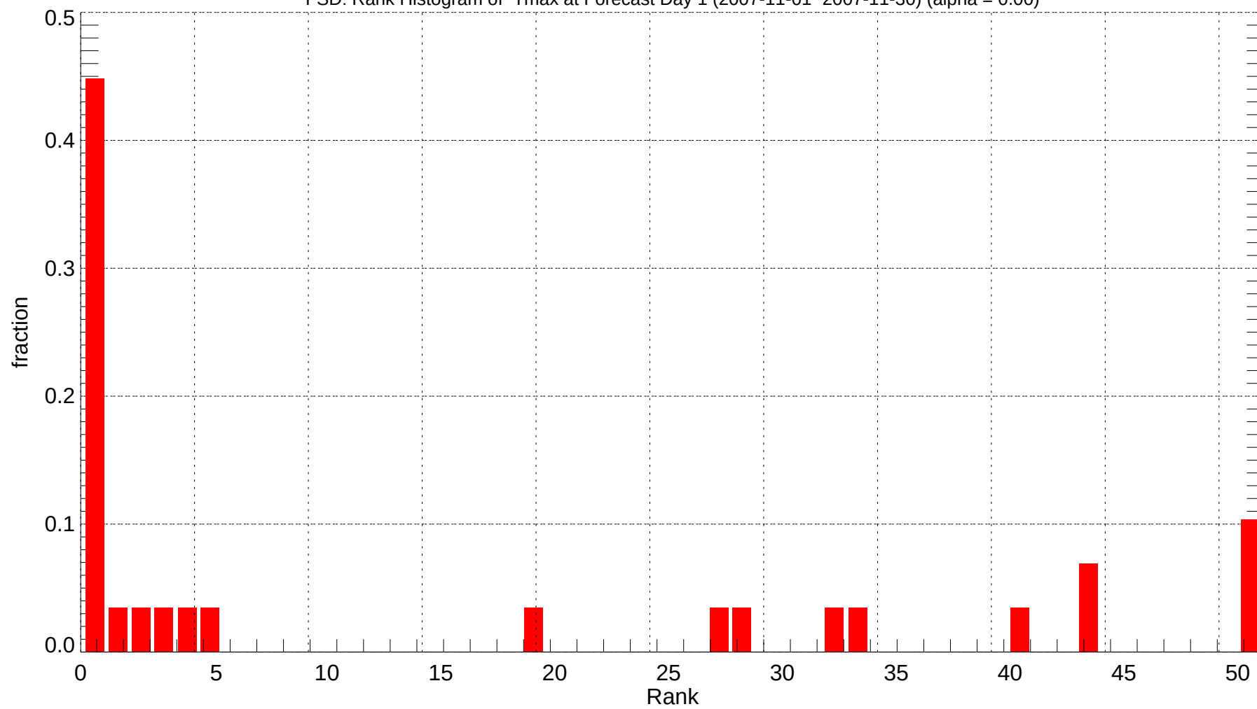
FSD: Rank Histogram of Tmax at Forecast Day 1 (2007-11-01~2007-11-30) (alpha = 0.00)
