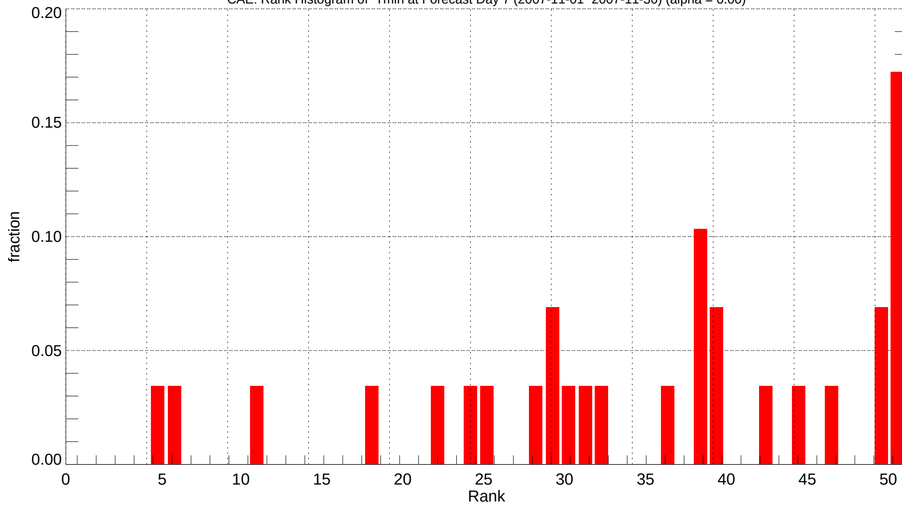
CAE: Rank Histogram of Tmin at Forecast Day 7 (2007-11-01~2007-11-30) (alpha = 0.00)
