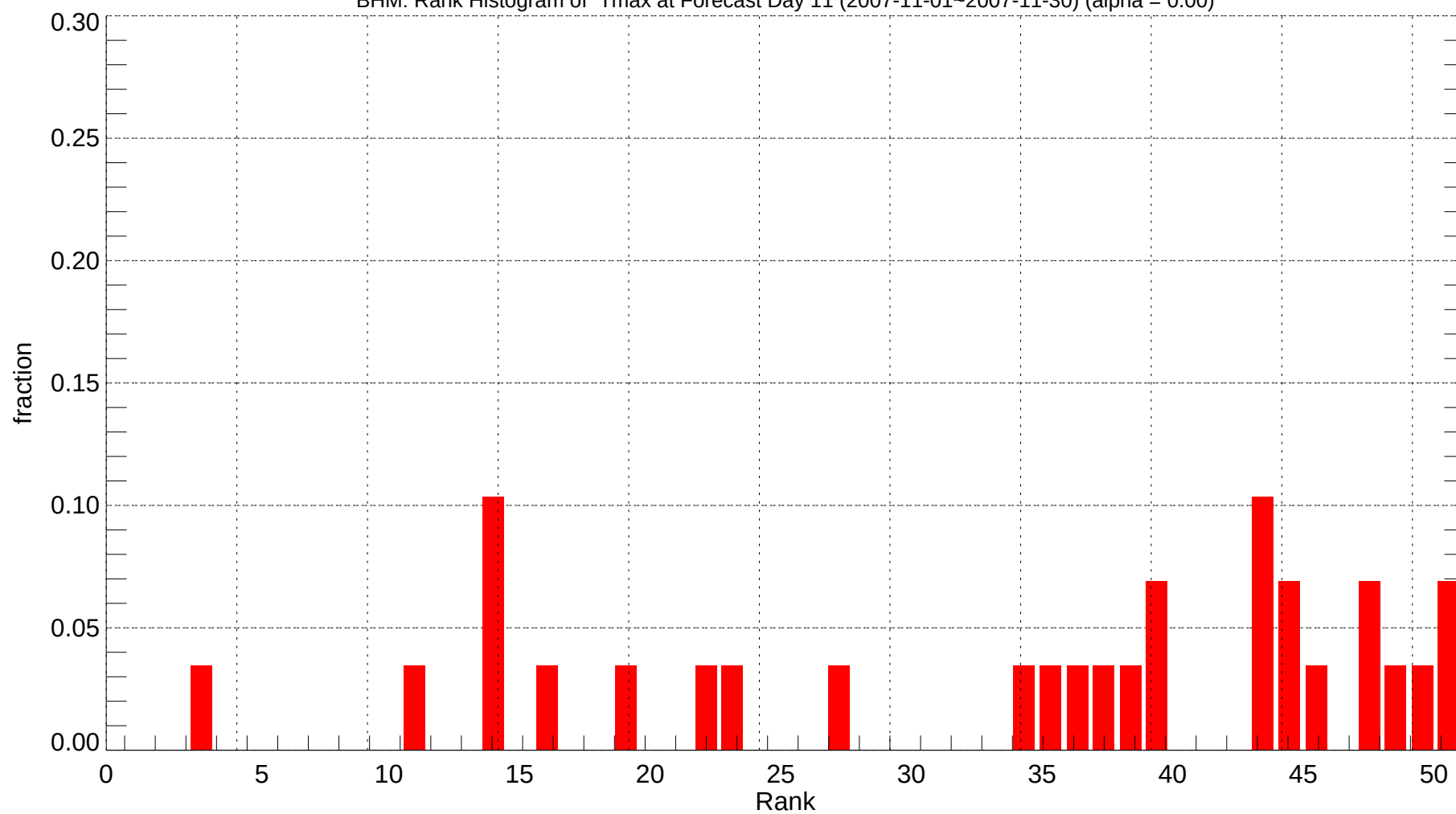
BHM: Rank Histogram of Tmax at Forecast Day 11 (2007-11-01~2007-11-30) (alpha = 0.00)
