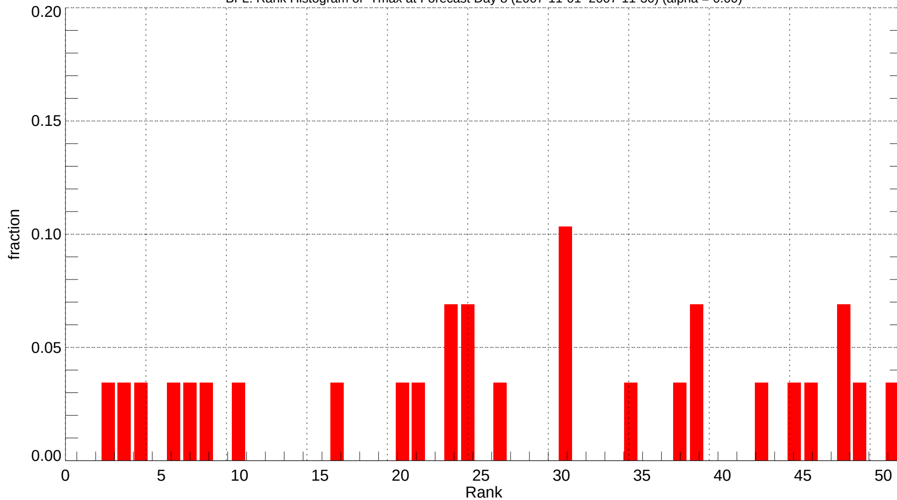
BFL: Rank Histogram of Tmax at Forecast Day 8 (2007-11-01~2007-11-30) (alpha = 0.00)
