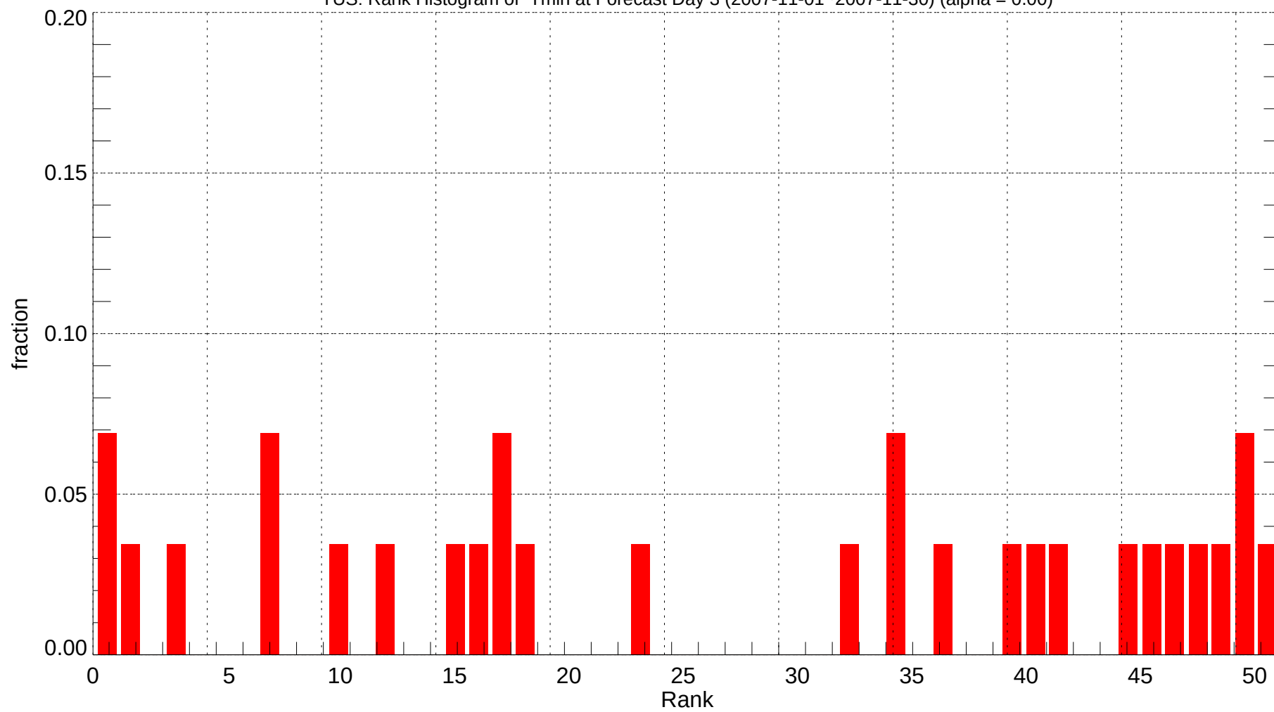
TUS: Rank Histogram of Tmin at Forecast Day 3 (2007-11-01~2007-11-30) (alpha = 0.00)
