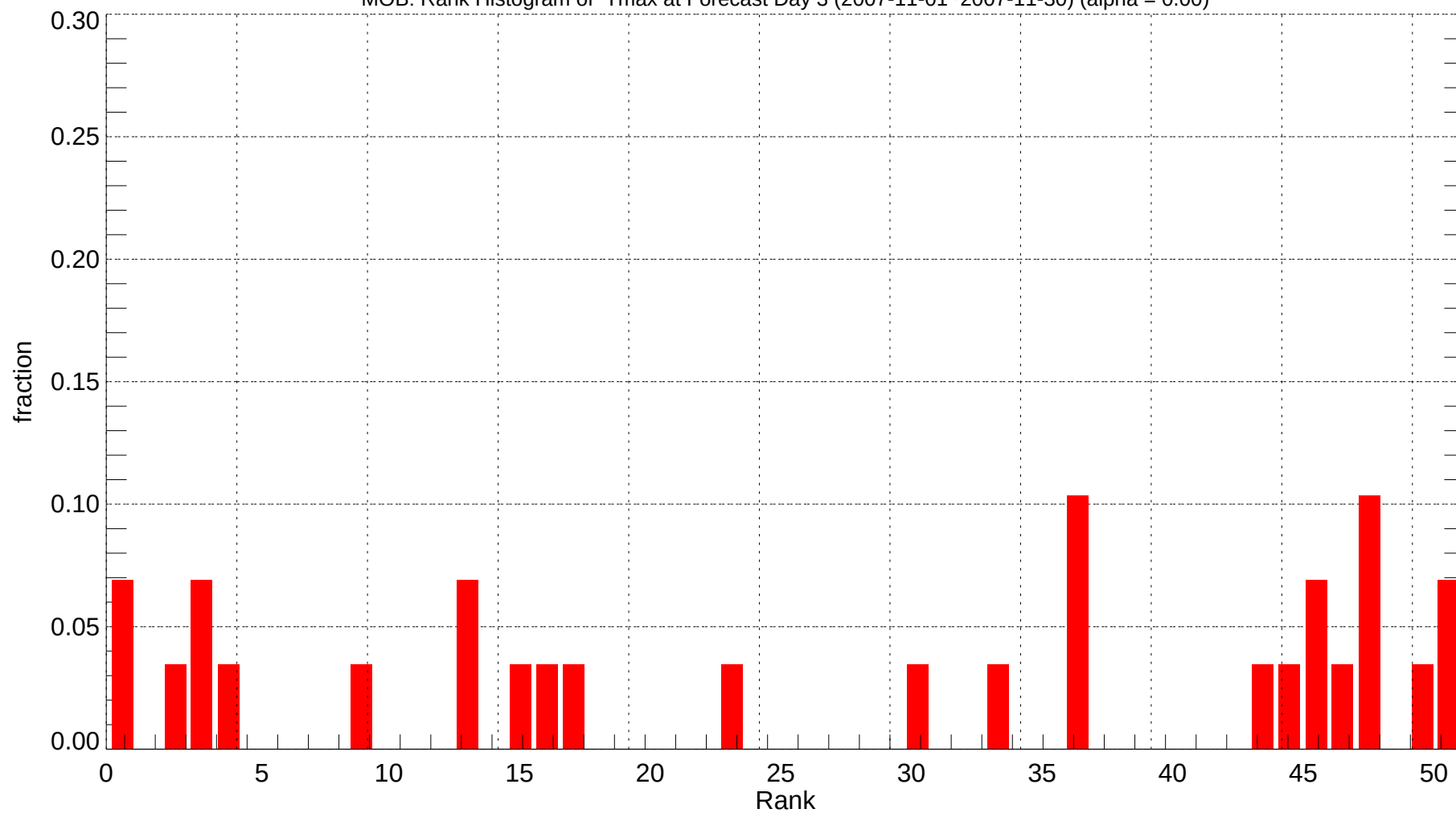
MOB: Rank Histogram of Tmax at Forecast Day 3 (2007-11-01~2007-11-30) (alpha = 0.00)
