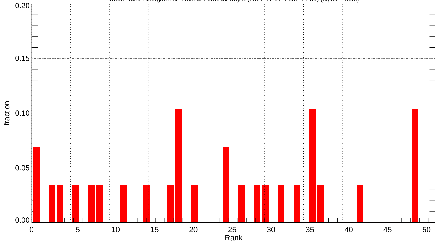
MCO: Rank Histogram of Tmin at Forecast Day 5 (2007-11-01~2007-11-30) (alpha = 0.00)
