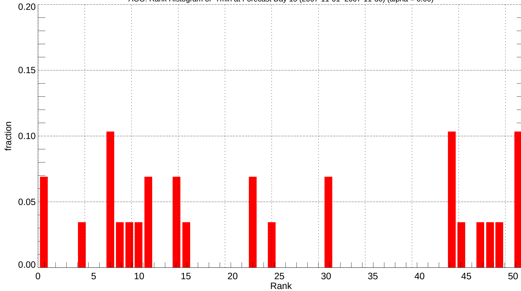
AOO: Rank Histogram of Tmin at Forecast Day 15 (2007-11-01~2007-11-30) (alpha = 0.00)
