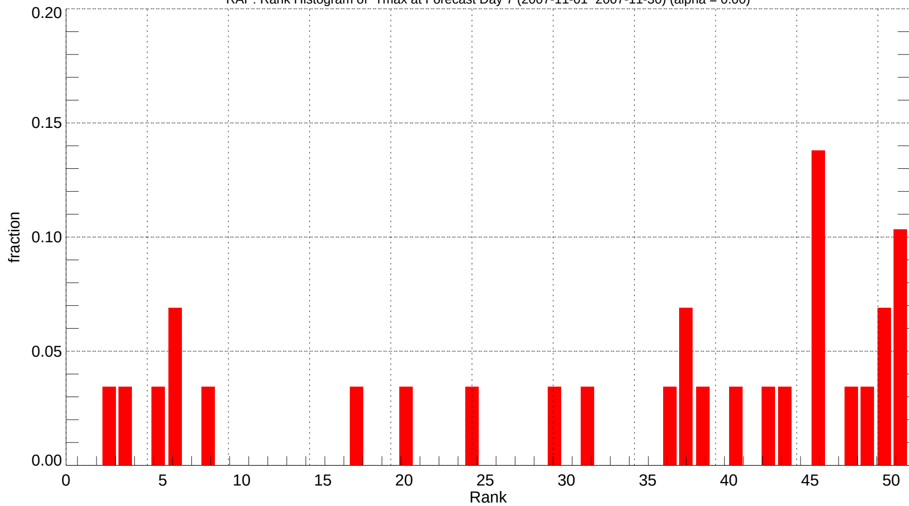
RAP: Rank Histogram of Tmax at Forecast Day 7 (2007-11-01~2007-11-30) (alpha = 0.00)
