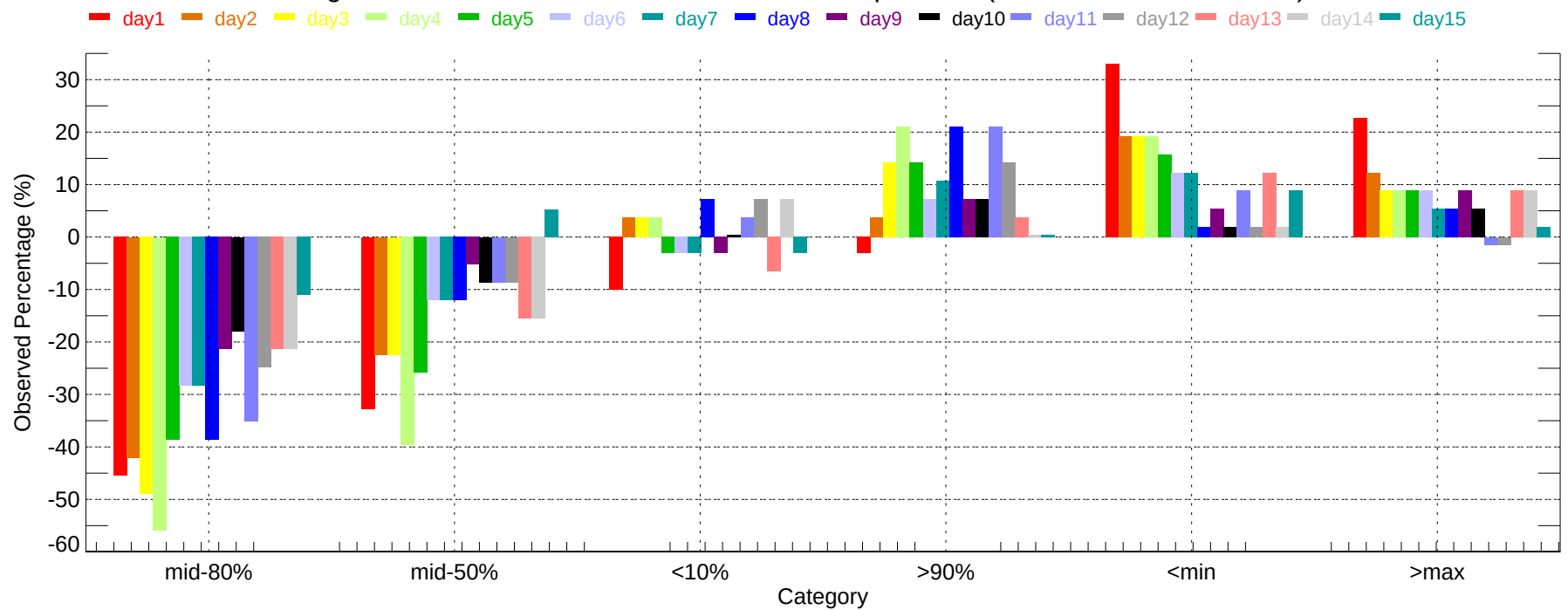
Observed Percentage Deviation of Ensembles - CRP: Max Temperature (2007-11-01~2007-11-30)
