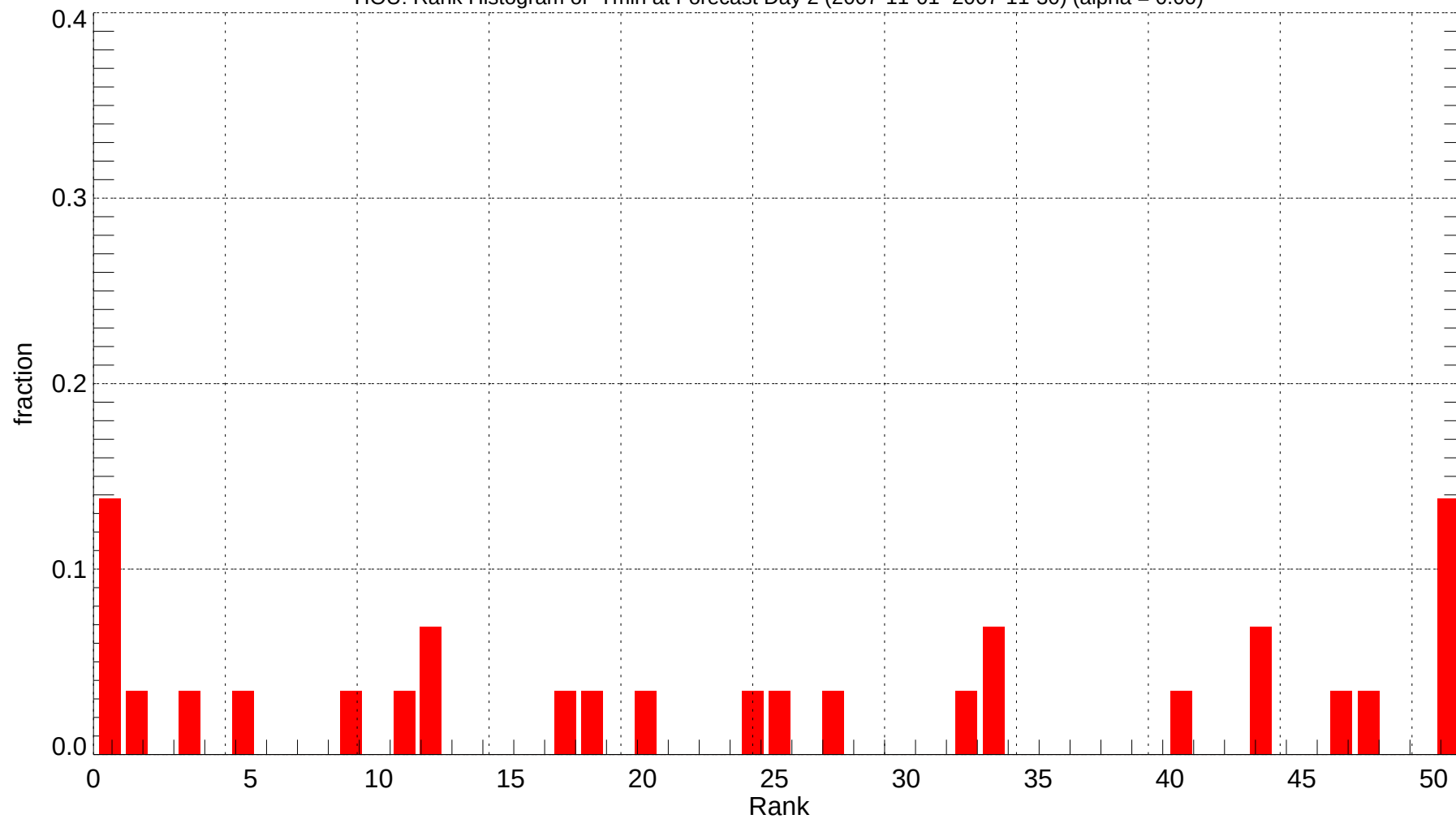
HOU: Rank Histogram of Tmin at Forecast Day 2 (2007-11-01~2007-11-30) (alpha = 0.00)
