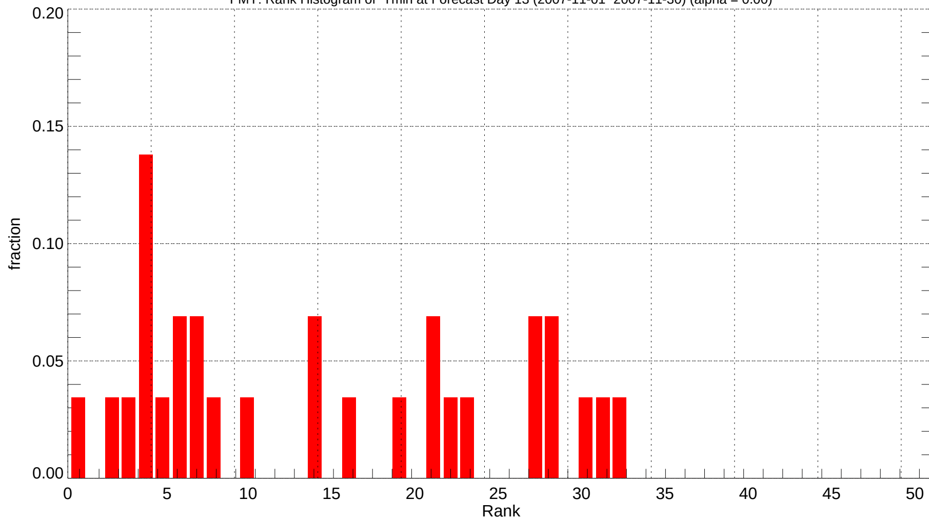
FMY: Rank Histogram of Tmin at Forecast Day 13 (2007-11-01~2007-11-30) (alpha = 0.00)
