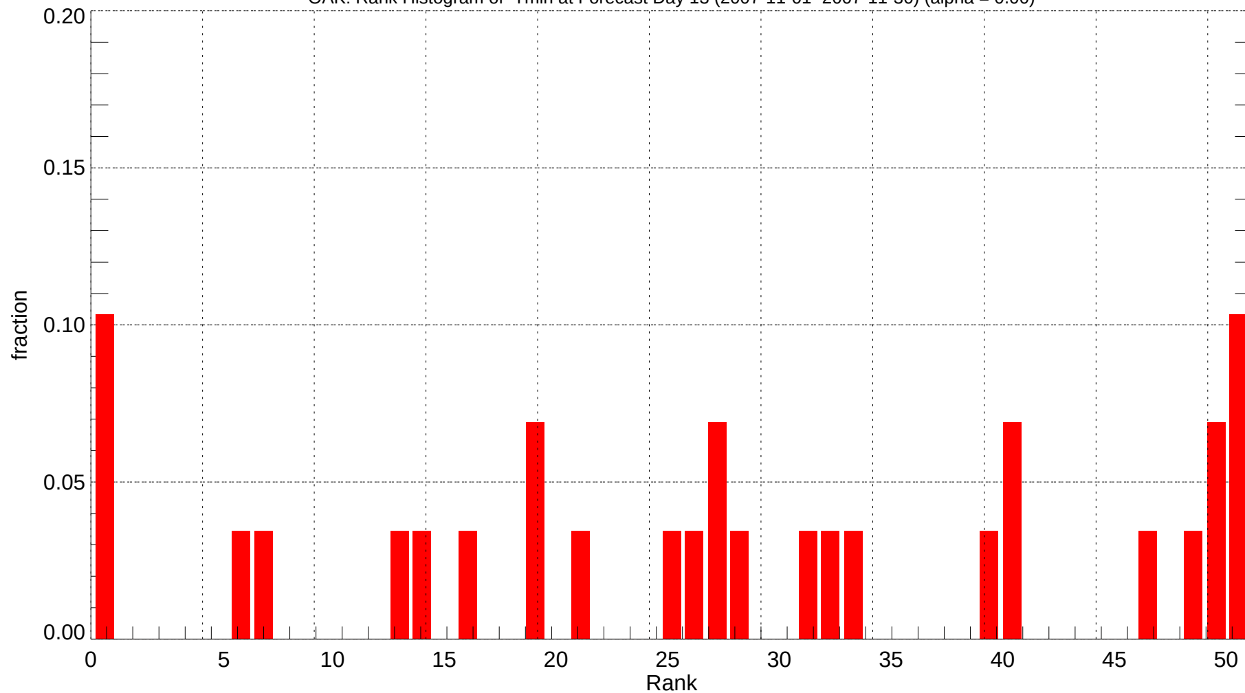
OAK: Rank Histogram of Tmin at Forecast Day 13 (2007-11-01~2007-11-30) (alpha = 0.00)
