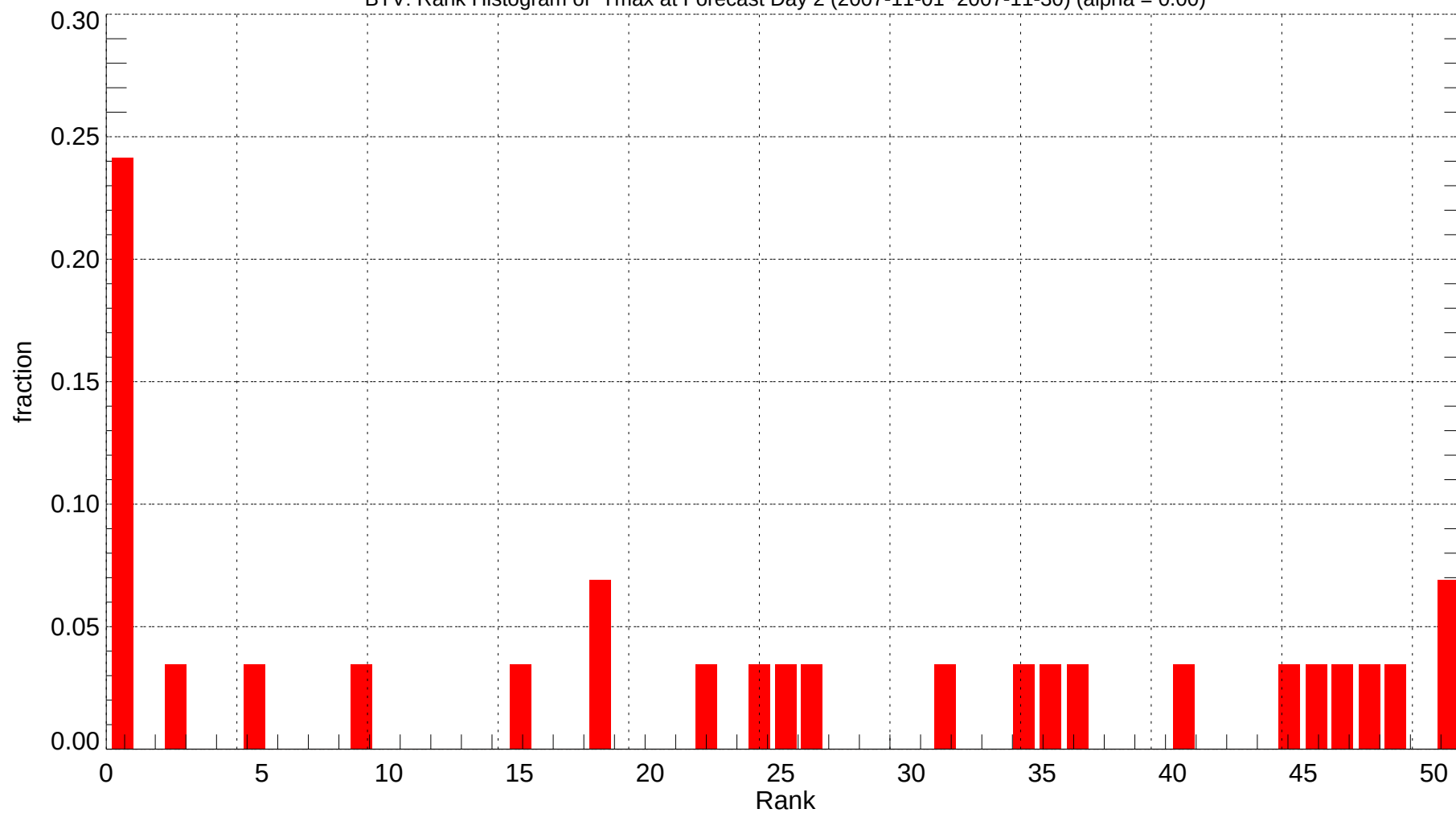
BTV: Rank Histogram of Tmax at Forecast Day 2 (2007-11-01~2007-11-30) (alpha = 0.00)
