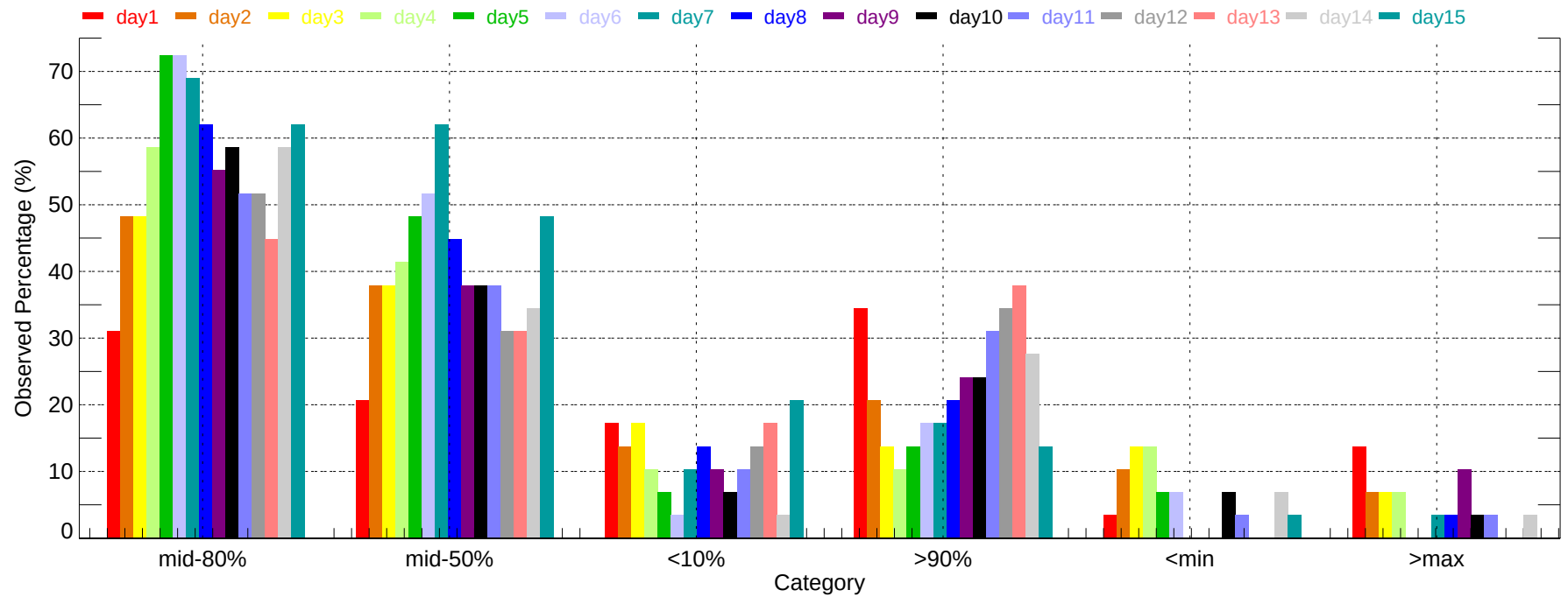
Observed Percentage of Ensembles - DFW: Min Temperature (2007-11-01~2007-11-30)
