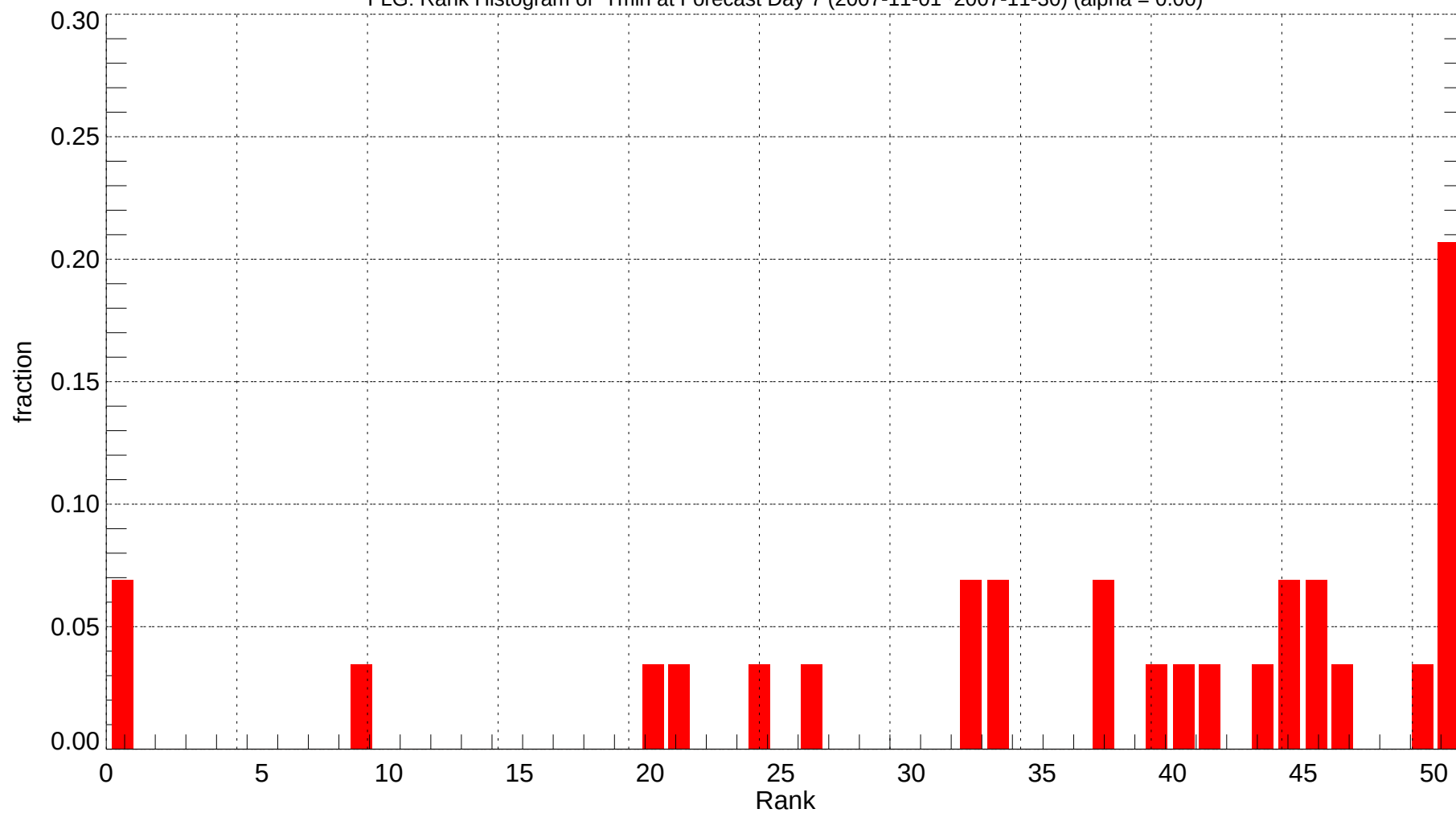
FLG: Rank Histogram of Tmin at Forecast Day 7 (2007-11-01~2007-11-30) (alpha = 0.00)
