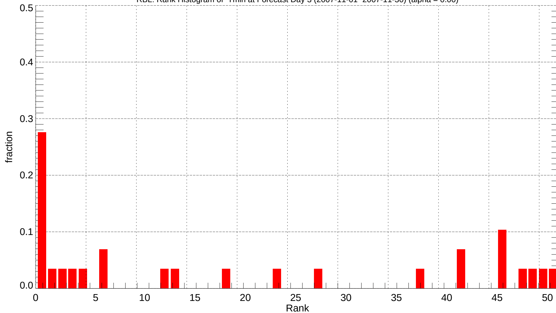
RBL: Rank Histogram of Tmin at Forecast Day 3 (2007-11-01~2007-11-30) (alpha = 0.00)
