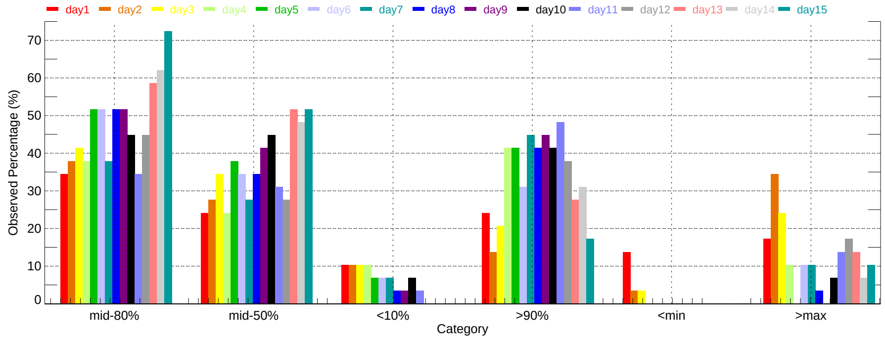
Observed Percentage of Ensembles - SDF: Max Temperature (2007-11-01~2007-11-30)
