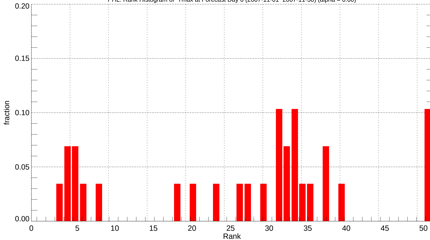
PHL: Rank Histogram of Tmax at Forecast Day 6 (2007-11-01~2007-11-30) (alpha = 0.00)
