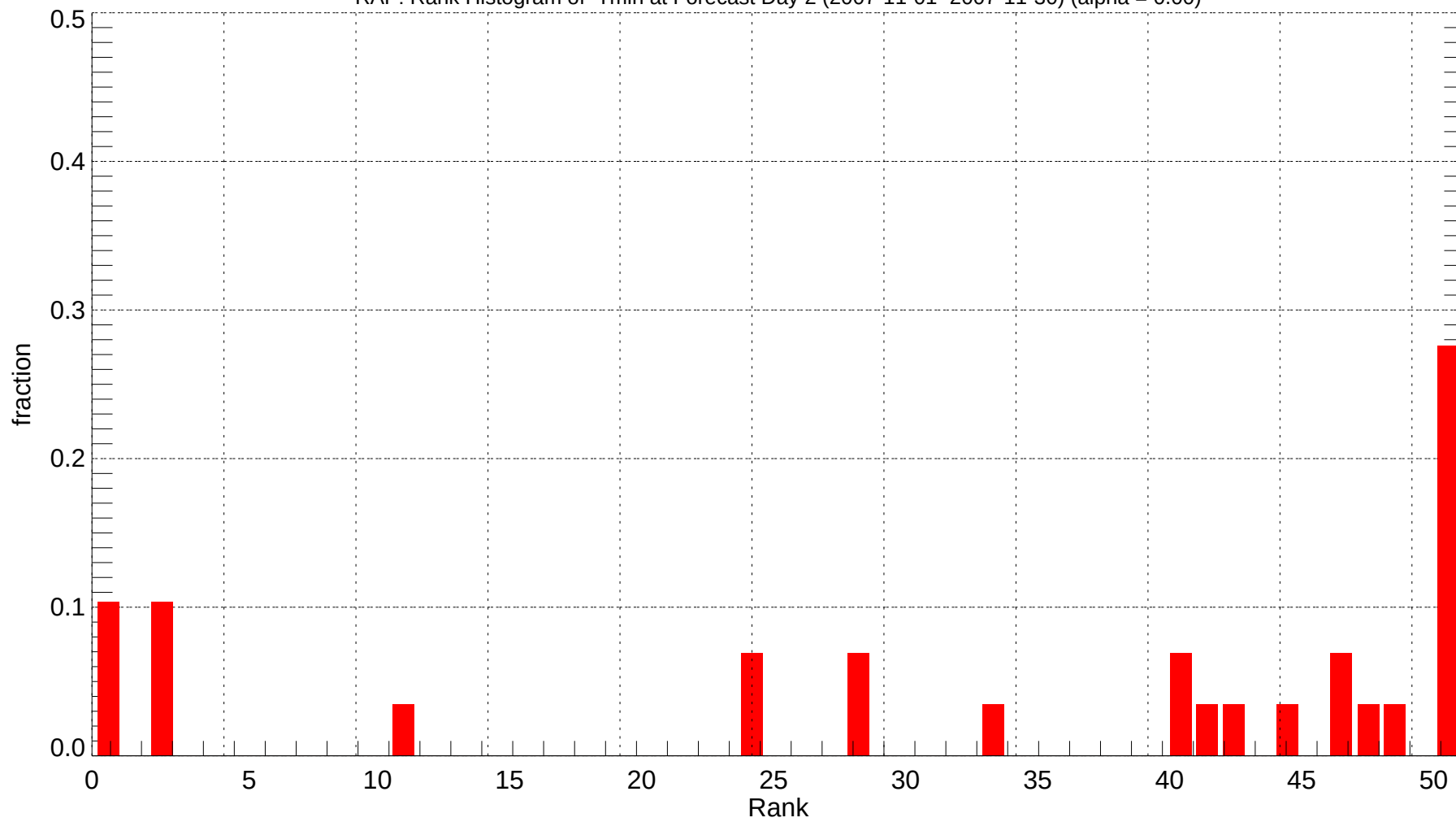
RAP: Rank Histogram of Tmin at Forecast Day 2 (2007-11-01~2007-11-30) (alpha = 0.00)
