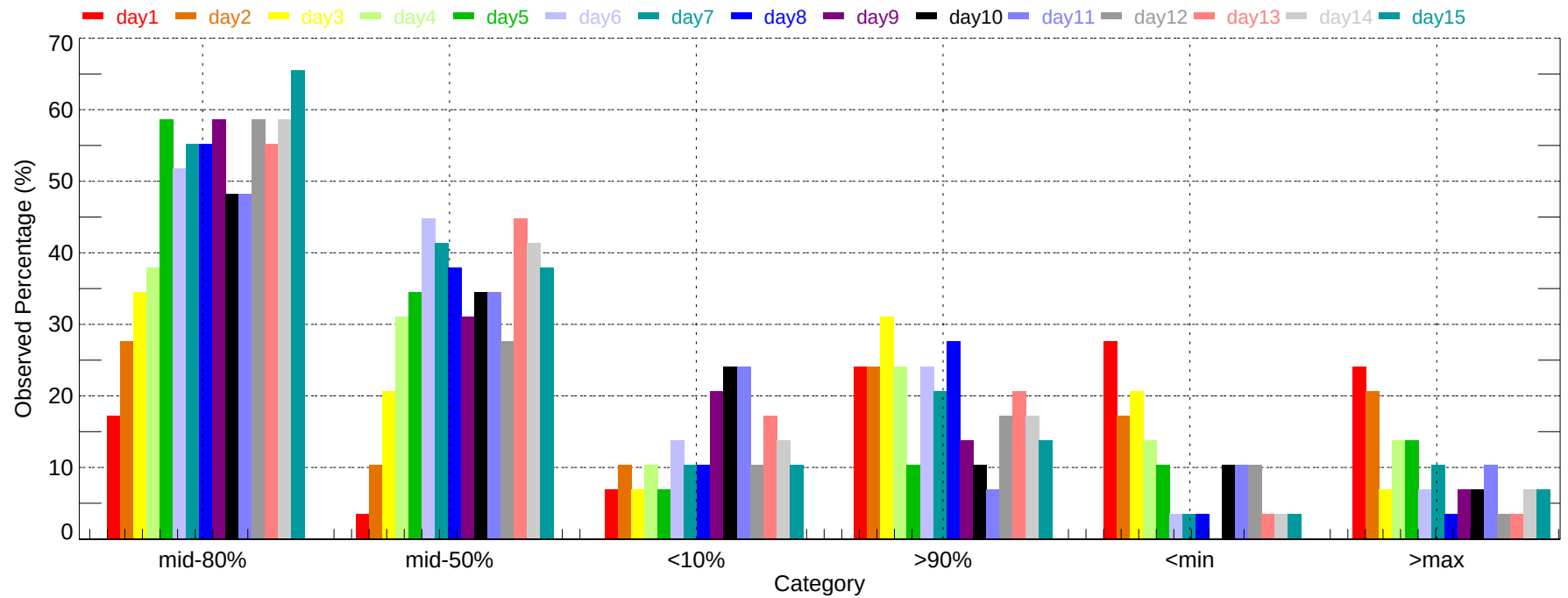
Observed Percentage of Ensembles - LNS: Max Temperature (2007-11-01~2007-11-30)
