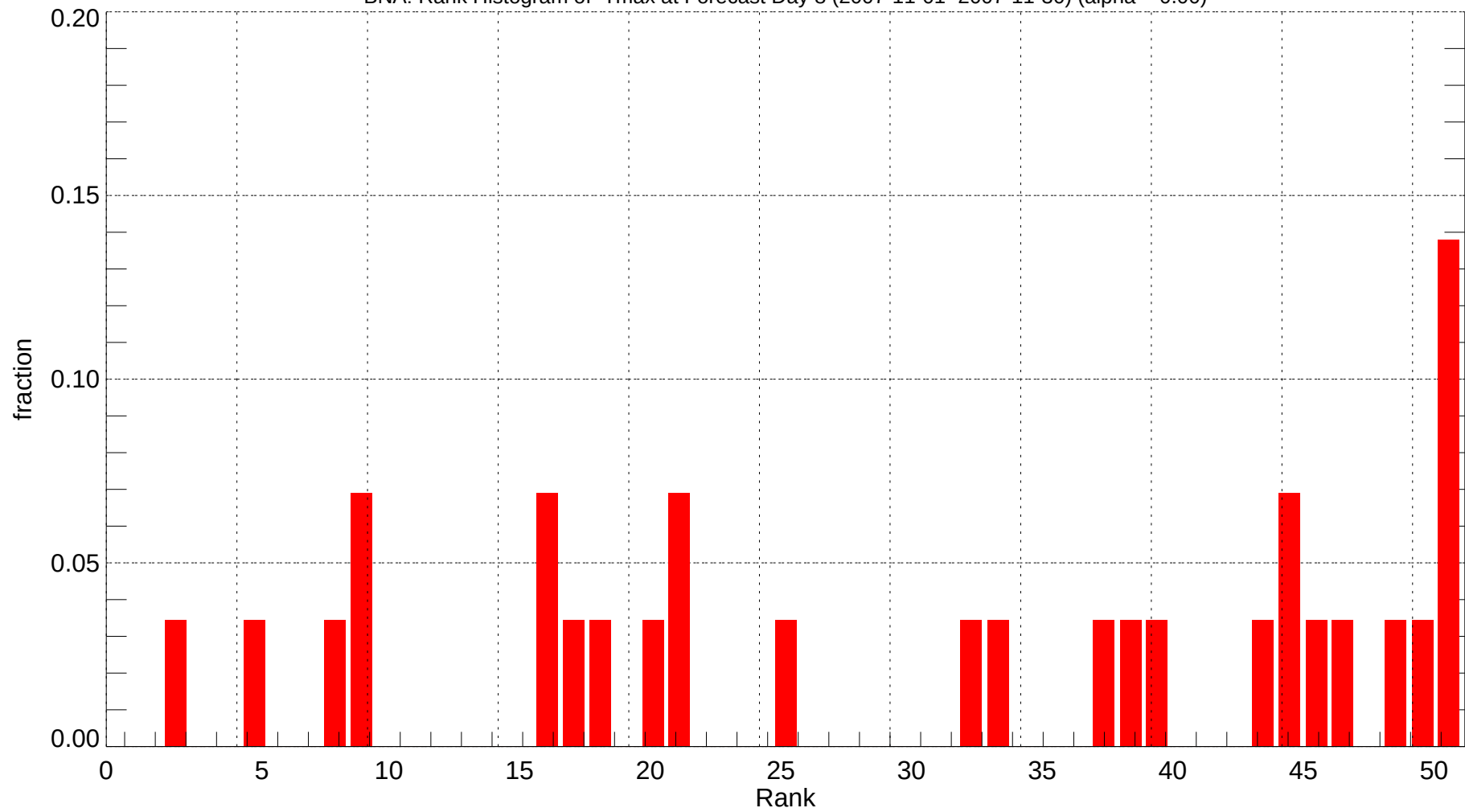
BNA: Rank Histogram of Tmax at Forecast Day 8 (2007-11-01~2007-11-30) (alpha = 0.00)
