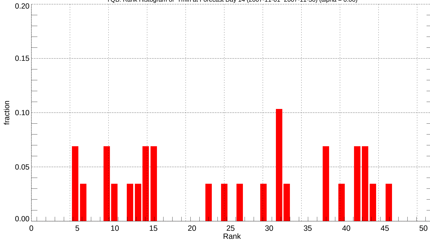
YQB: Rank Histogram of Tmin at Forecast Day 14 (2007-11-01~2007-11-30) (alpha = 0.00)
