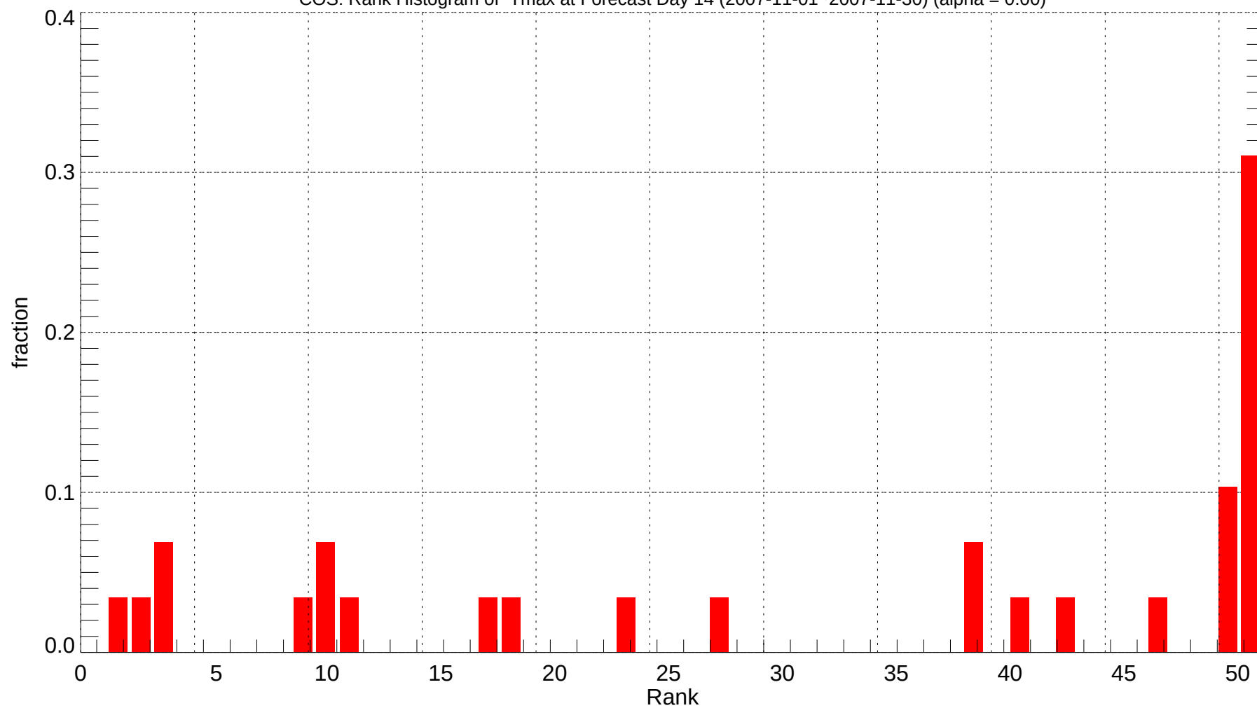
COS: Rank Histogram of Tmax at Forecast Day 14 (2007-11-01~2007-11-30) (alpha = 0.00)
