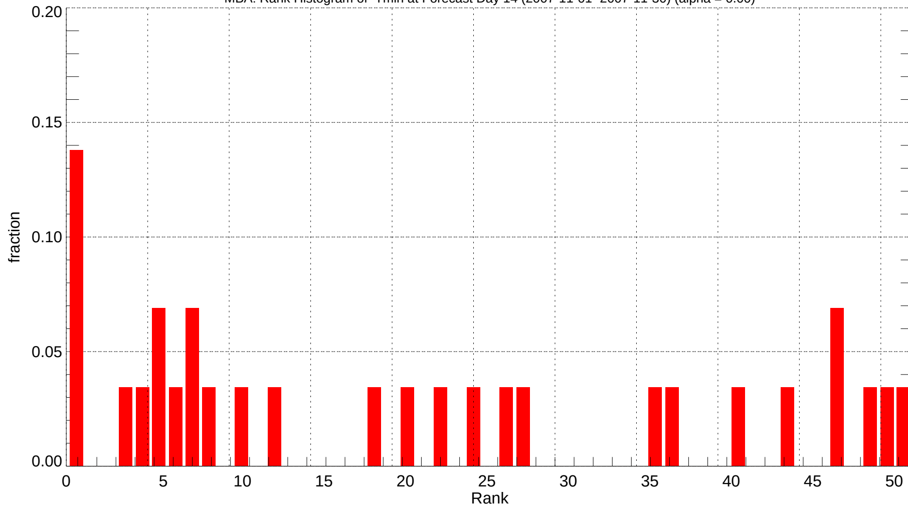
MBA: Rank Histogram of Tmin at Forecast Day 14 (2007-11-01~2007-11-30) (alpha = 0.00)
