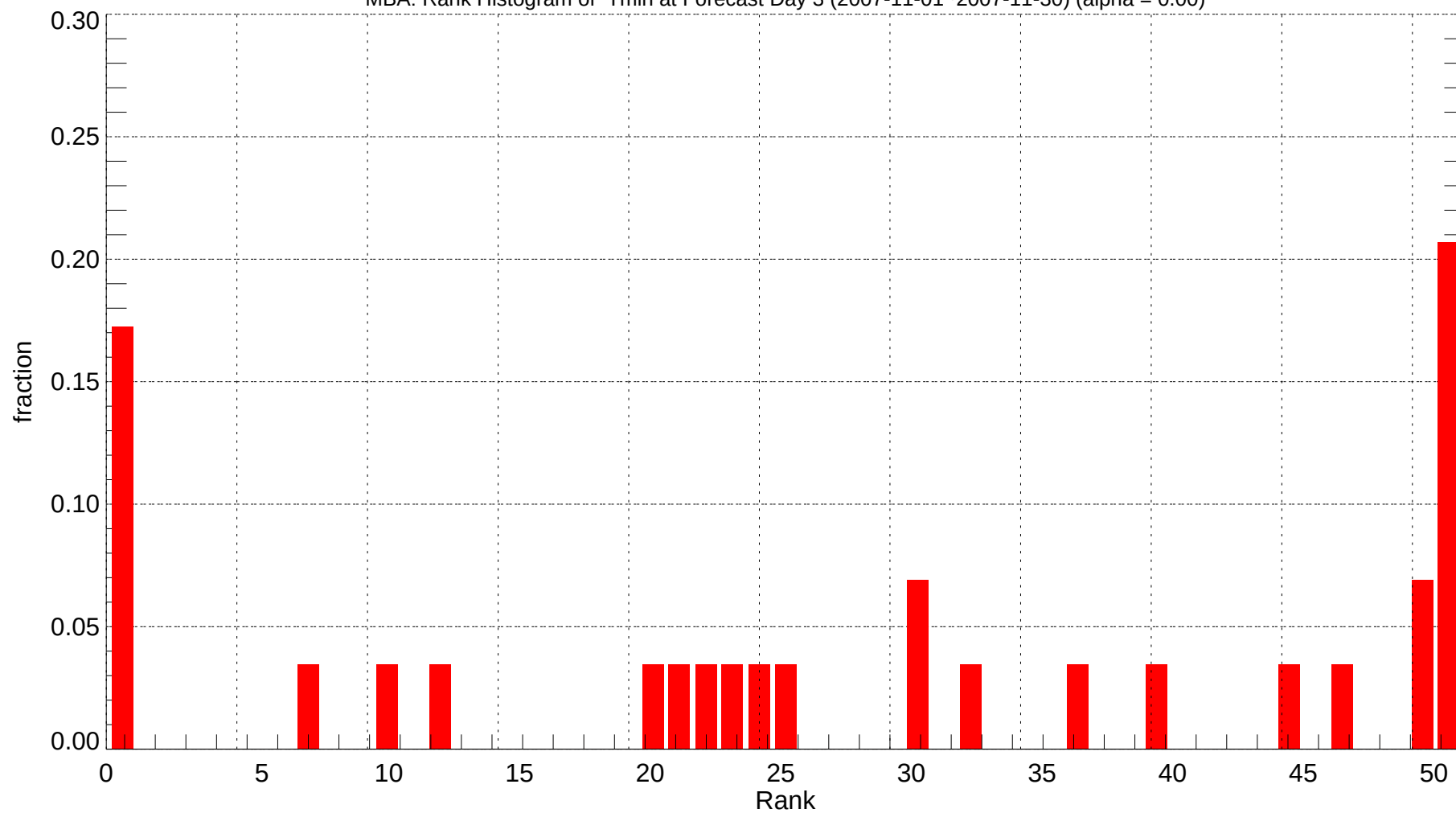
MBA: Rank Histogram of Tmin at Forecast Day 3 (2007-11-01~2007-11-30) (alpha = 0.00)
