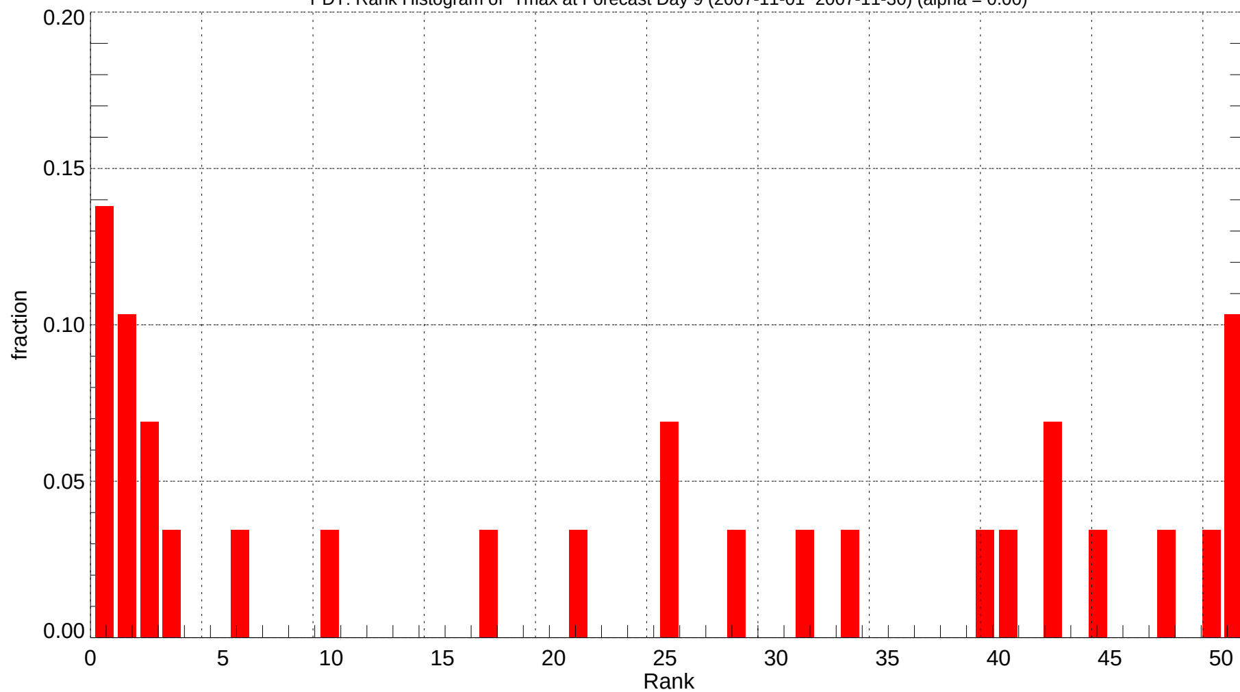
PDT: Rank Histogram of Tmax at Forecast Day 9 (2007-11-01~2007-11-30) (alpha = 0.00)
