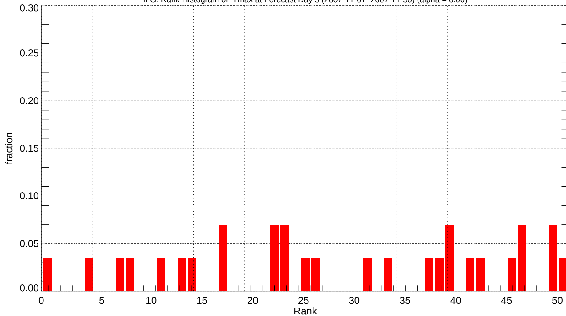
ILG: Rank Histogram of Tmax at Forecast Day 3 (2007-11-01~2007-11-30) (alpha = 0.00)
