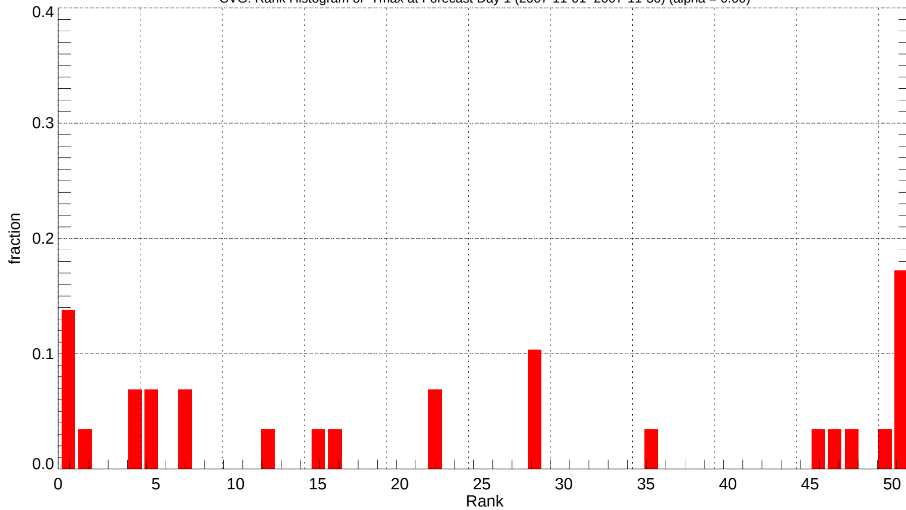
CVG: Rank Histogram of Tmax at Forecast Day 1 (2007-11-01~2007-11-30) (alpha = 0.00)
