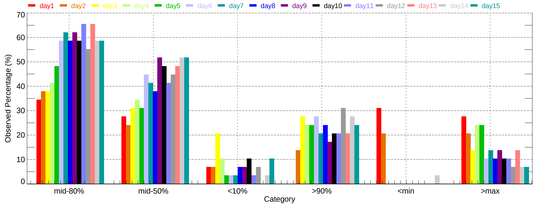
Observed Percentage of Ensembles - BWI: Min Temperature (2007-11-01~2007-11-30)
