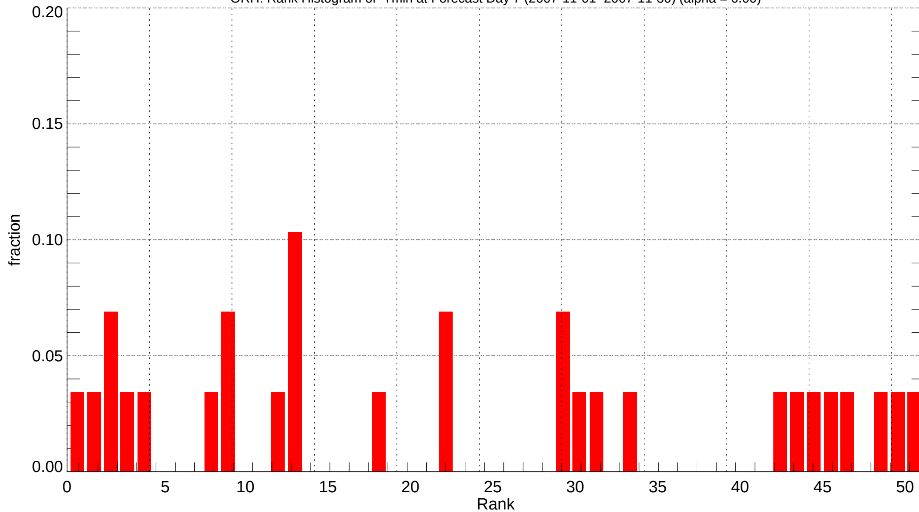
ORH: Rank Histogram of Tmin at Forecast Day 7 (2007-11-01~2007-11-30) (alpha = 0.00)
