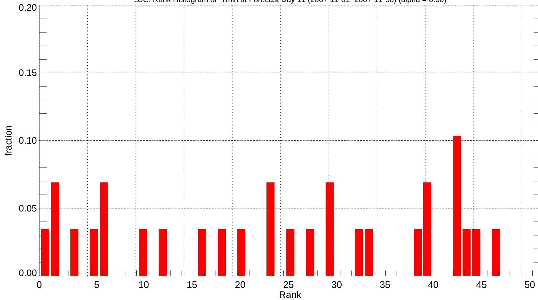
SJC: Rank Histogram of Tmin at Forecast Day 11 (2007-11-01~2007-11-30) (alpha = 0.00)
