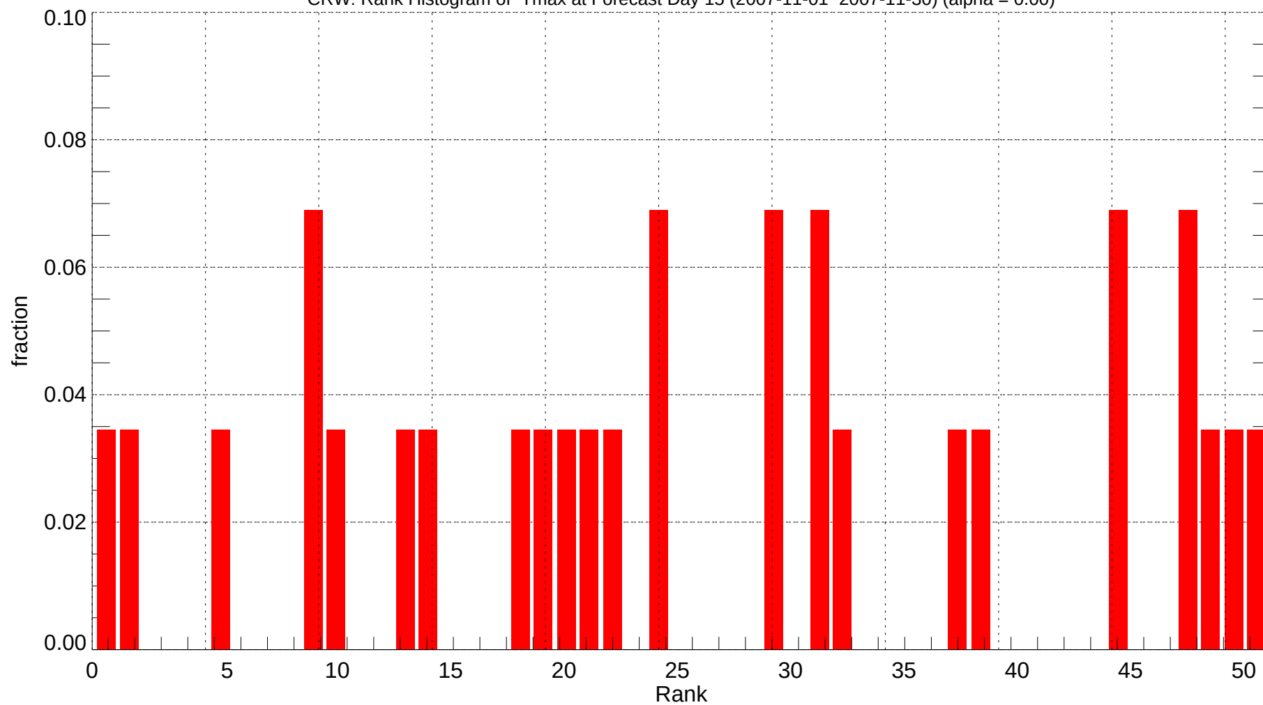
CRW: Rank Histogram of Tmax at Forecast Day 15 (2007-11-01~2007-11-30) (alpha = 0.00)
