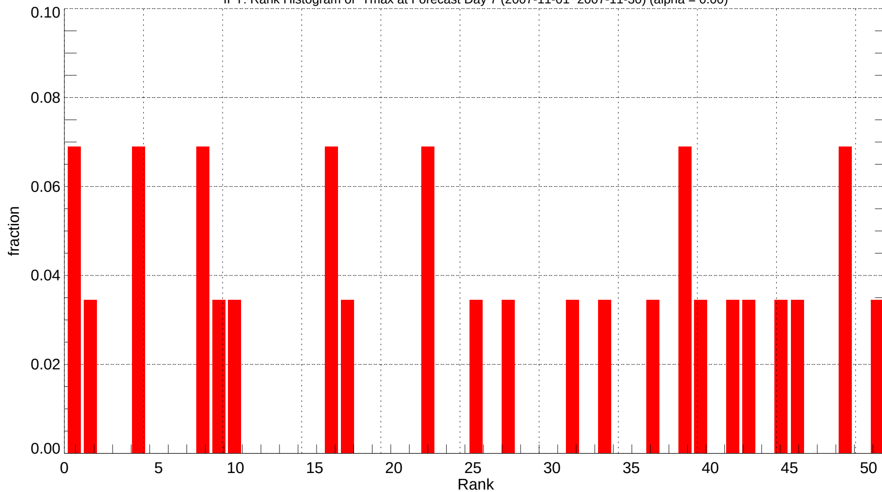
IPT: Rank Histogram of Tmax at Forecast Day 7 (2007-11-01~2007-11-30) (alpha = 0.00)
