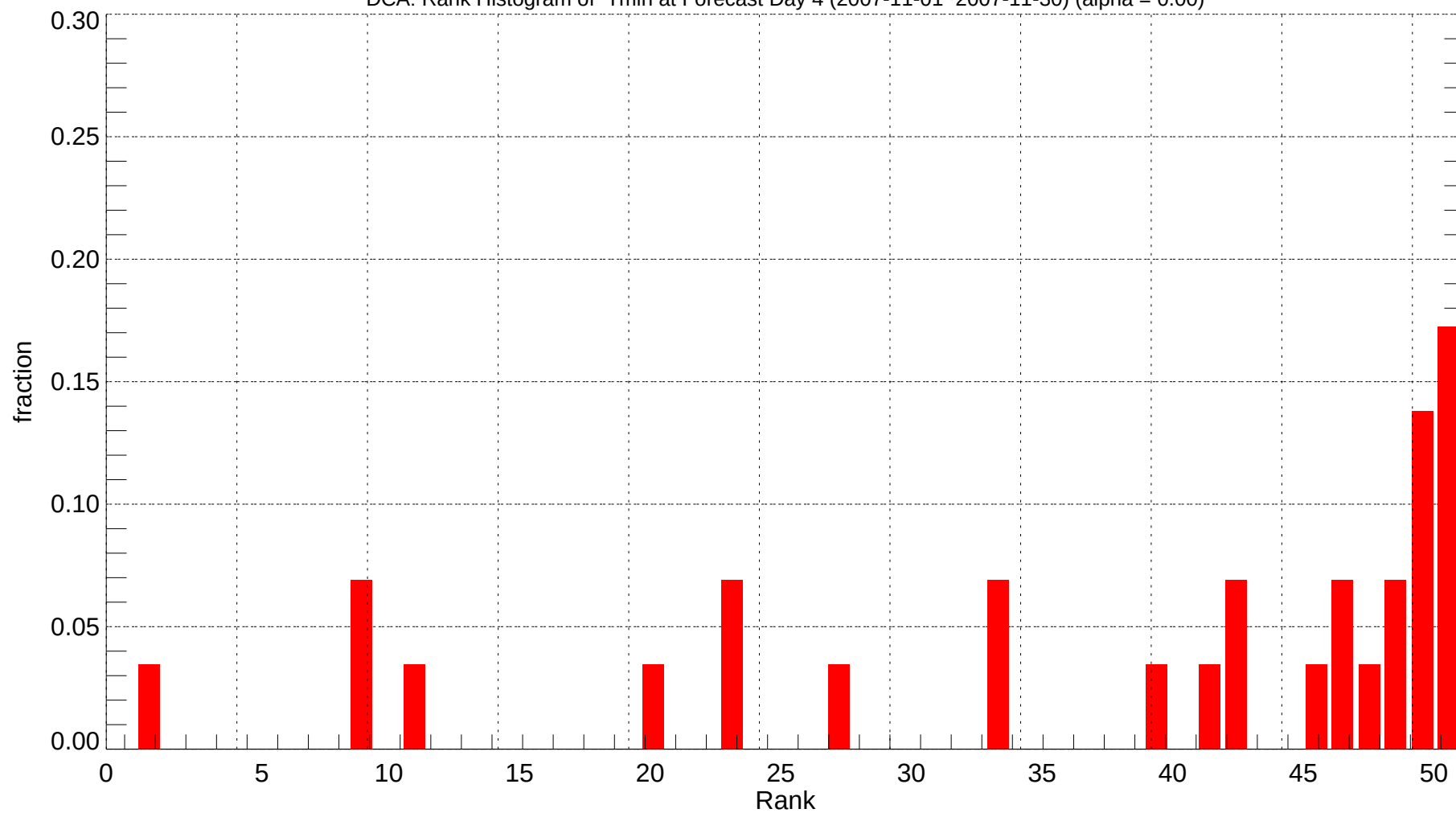
DCA: Rank Histogram of Tmin at Forecast Day 4 (2007-11-01~2007-11-30) (alpha = 0.00)
