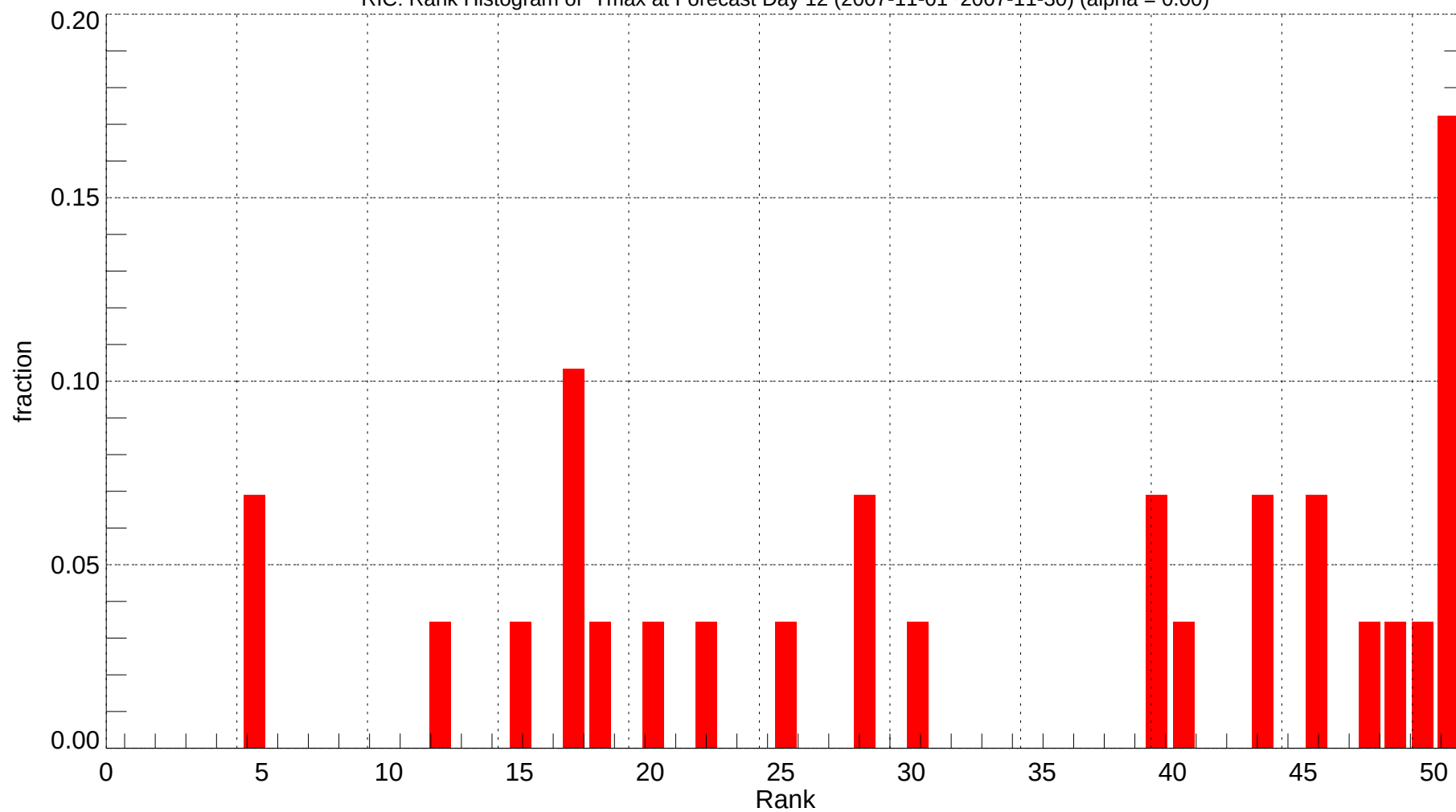
RIC: Rank Histogram of Tmax at Forecast Day 12 (2007-11-01~2007-11-30) (alpha = 0.00)
