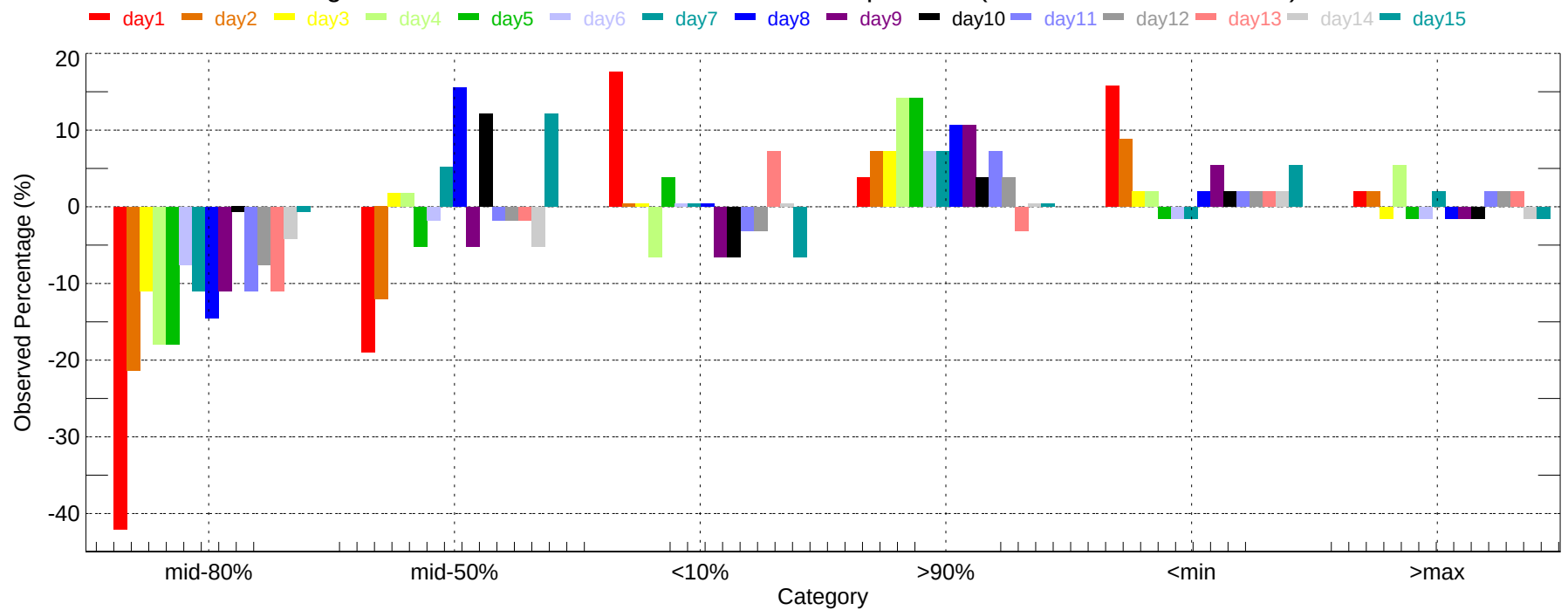
Observed Percentage Deviation of Ensembles - JAX: Max Temperature (2007-11-01~2007-11-30)
