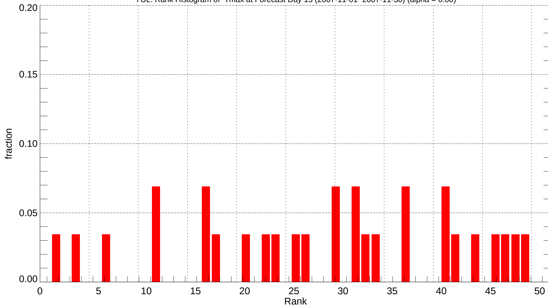
YUL: Rank Histogram of Tmax at Forecast Day 15 (2007-11-01~2007-11-30) (alpha = 0.00)
