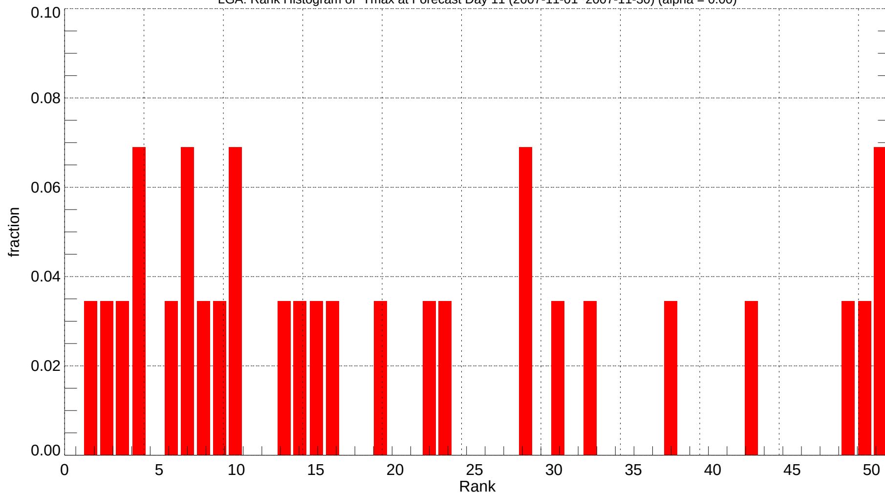
LGA: Rank Histogram of Tmax at Forecast Day 11 (2007-11-01~2007-11-30) (alpha = 0.00)
