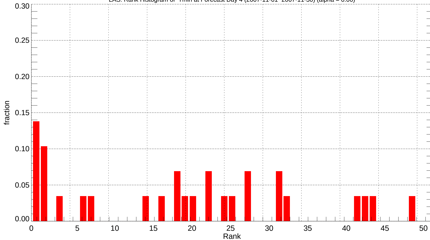
LAS: Rank Histogram of Tmin at Forecast Day 4 (2007-11-01~2007-11-30) (alpha = 0.00)
