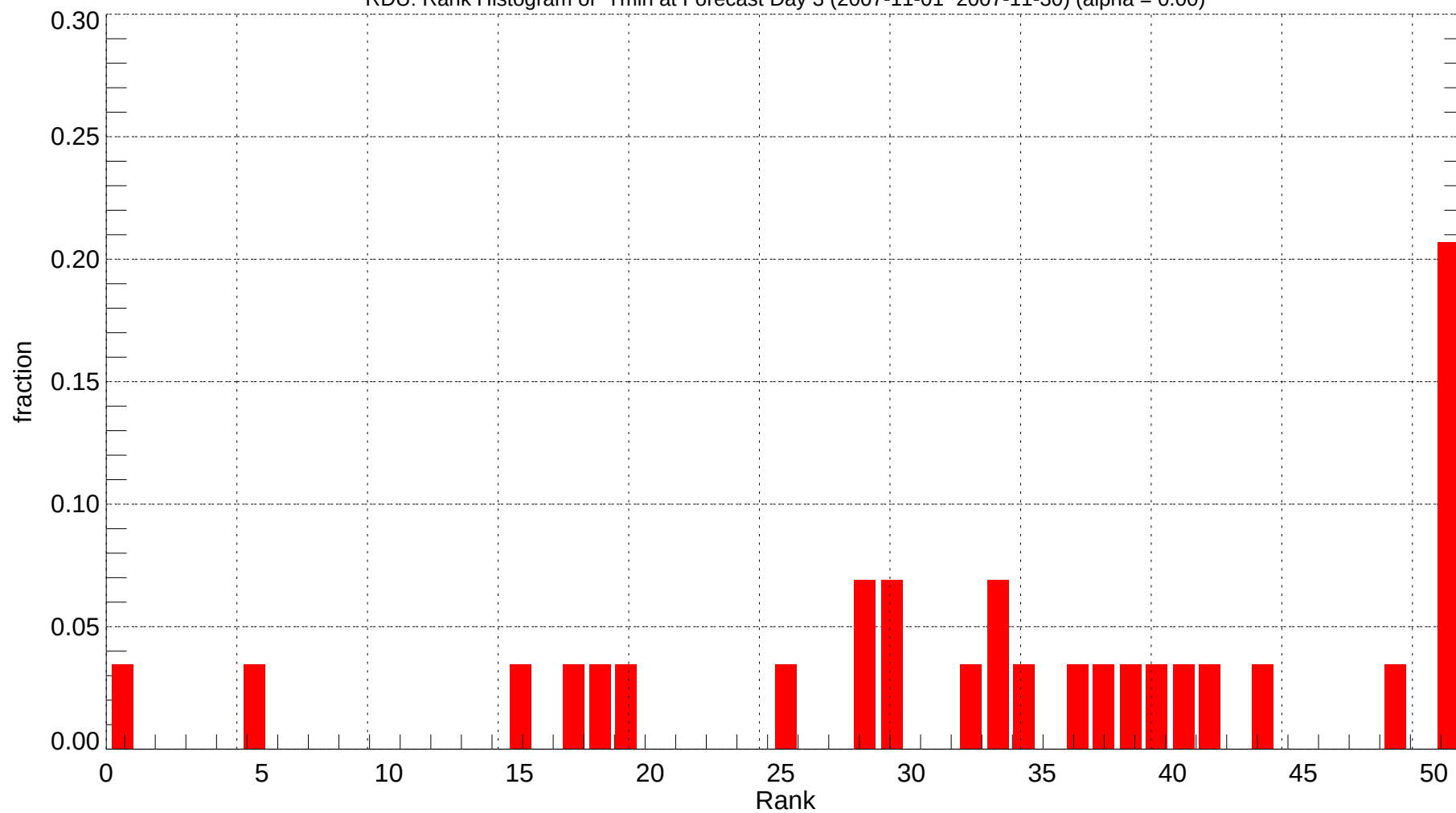
RDU: Rank Histogram of Tmin at Forecast Day 3 (2007-11-01~2007-11-30) (alpha = 0.00)
