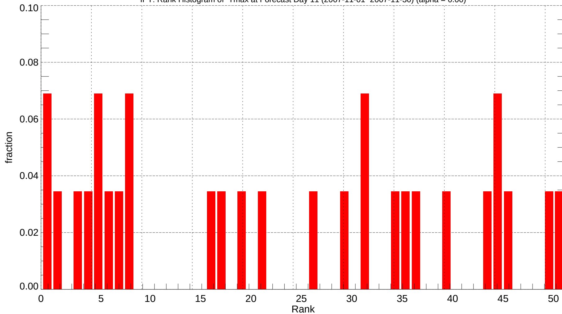
IPT: Rank Histogram of Tmax at Forecast Day 11 (2007-11-01~2007-11-30) (alpha = 0.00)
