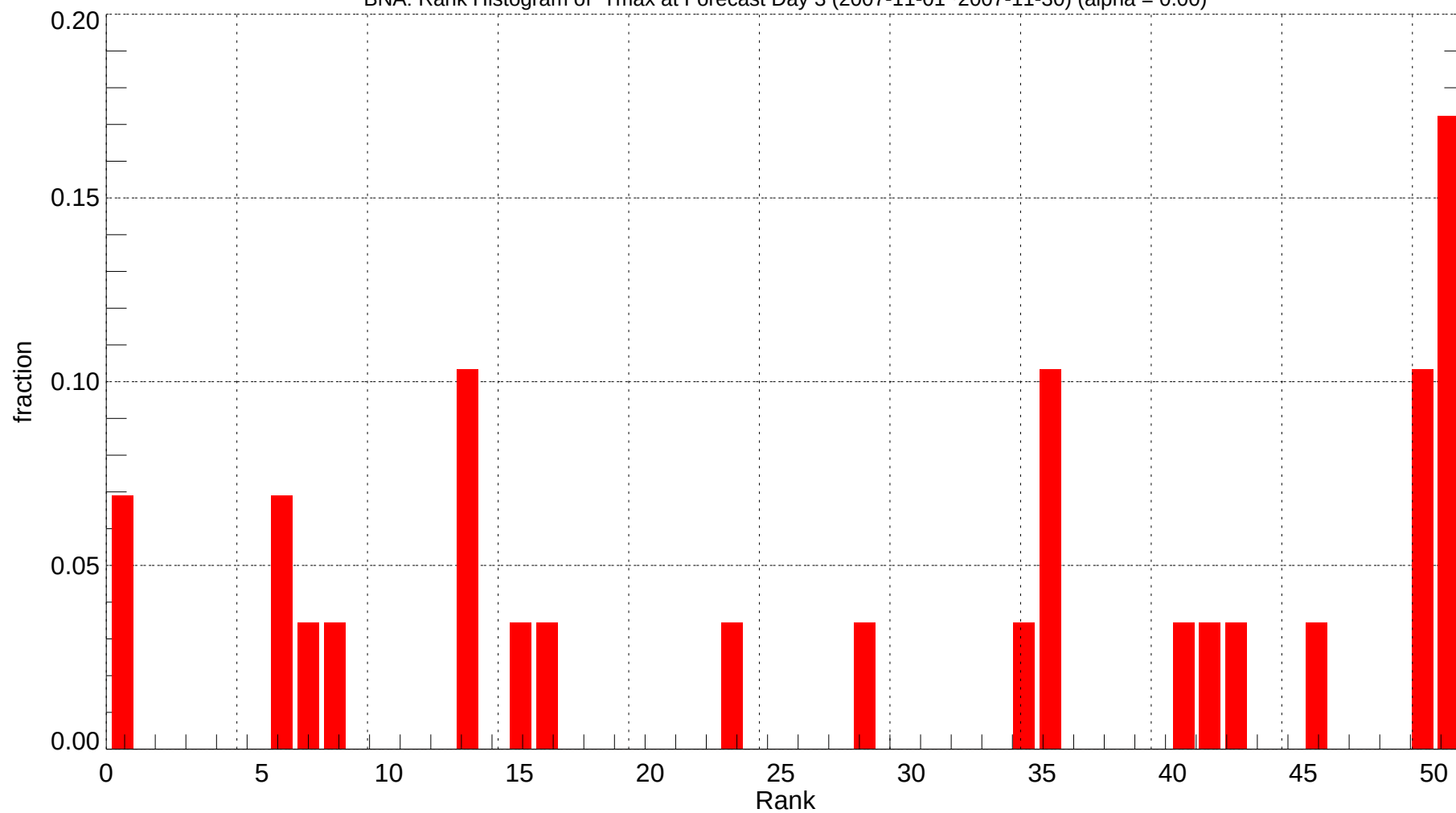
BNA: Rank Histogram of Tmax at Forecast Day 3 (2007-11-01~2007-11-30) (alpha = 0.00)
