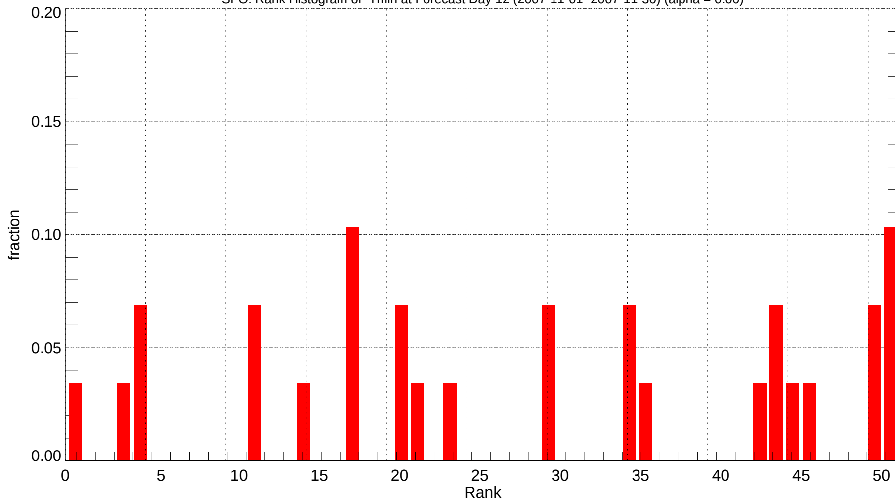
SFO: Rank Histogram of Tmin at Forecast Day 12 (2007-11-01~2007-11-30) (alpha = 0.00)
