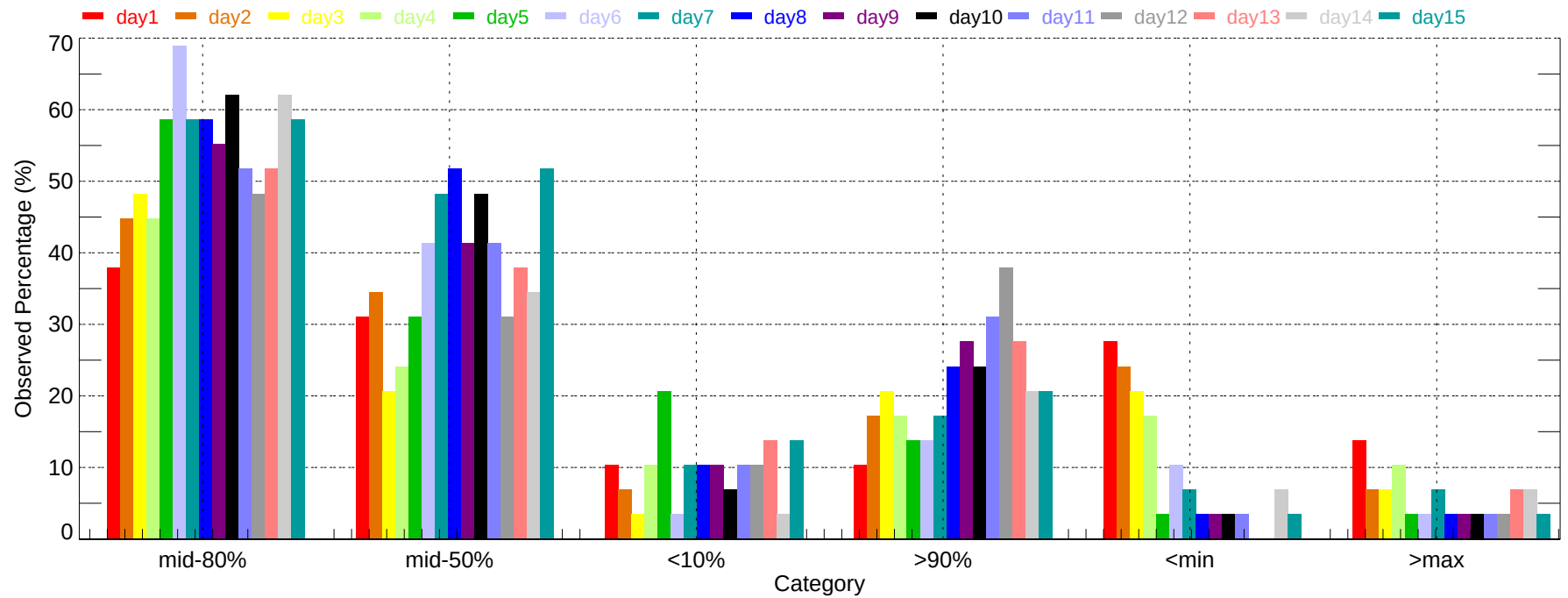
Observed Percentage of Ensembles - ACT: Min Temperature (2007-11-01~2007-11-30)
