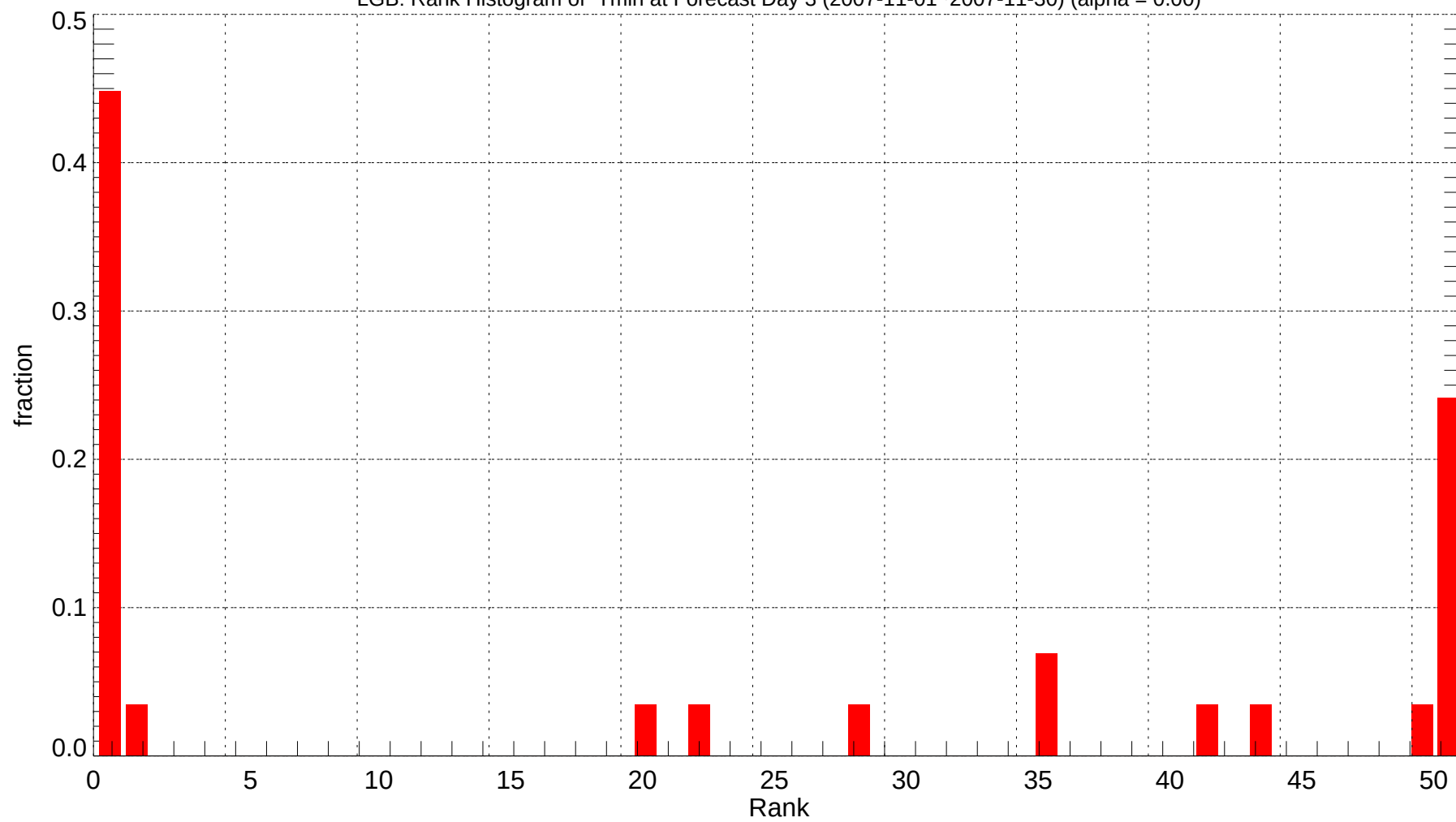
LGB: Rank Histogram of Tmin at Forecast Day 3 (2007-11-01~2007-11-30) (alpha = 0.00)
