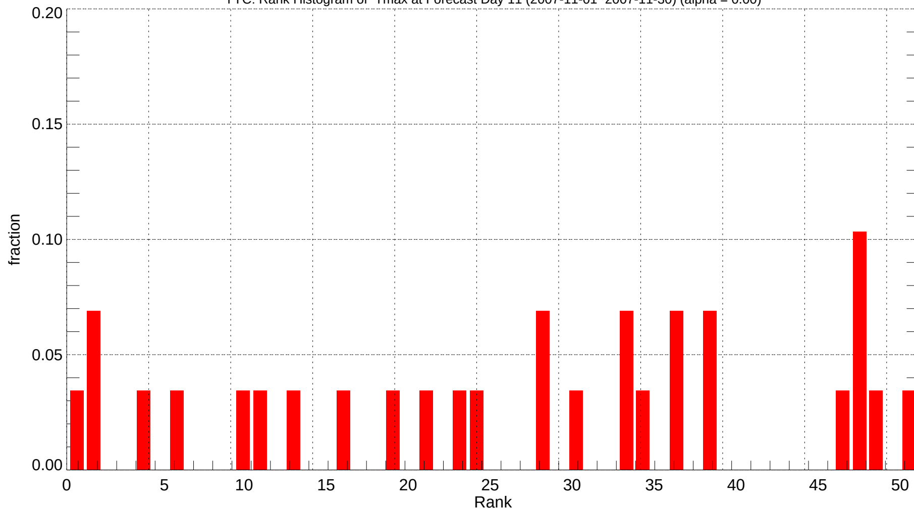
YYC: Rank Histogram of Tmax at Forecast Day 11 (2007-11-01~2007-11-30) (alpha = 0.00)
