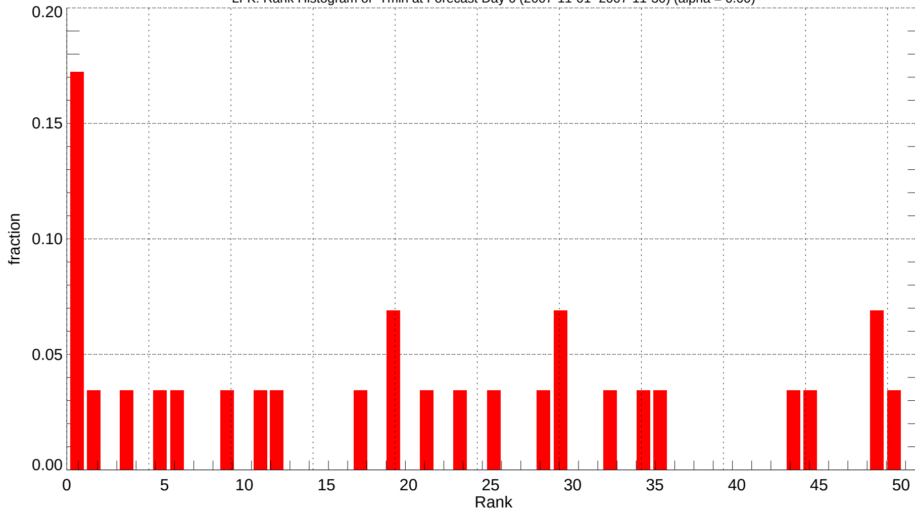
LFK: Rank Histogram of Tmin at Forecast Day 6 (2007-11-01~2007-11-30) (alpha = 0.00)
