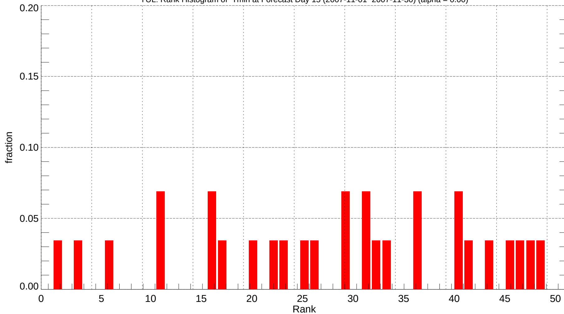
YUL: Rank Histogram of Tmin at Forecast Day 15 (2007-11-01~2007-11-30) (alpha = 0.00)
