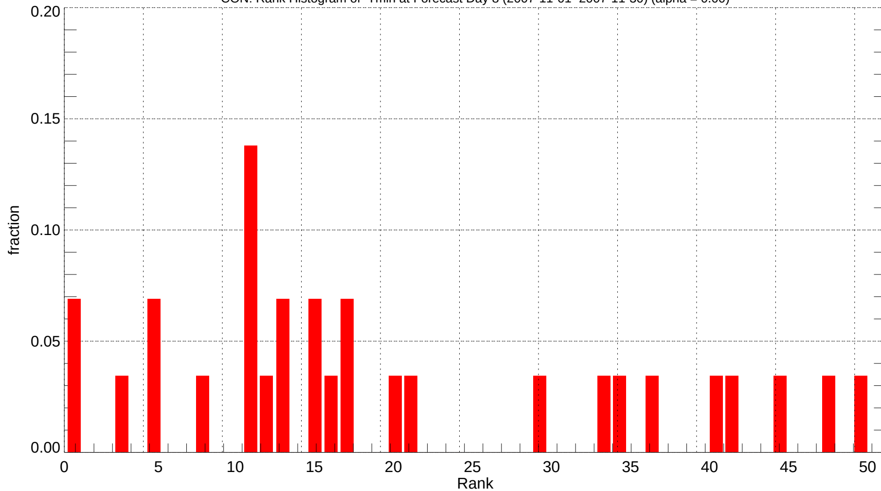
CON: Rank Histogram of Tmin at Forecast Day 8 (2007-11-01~2007-11-30) (alpha = 0.00)
