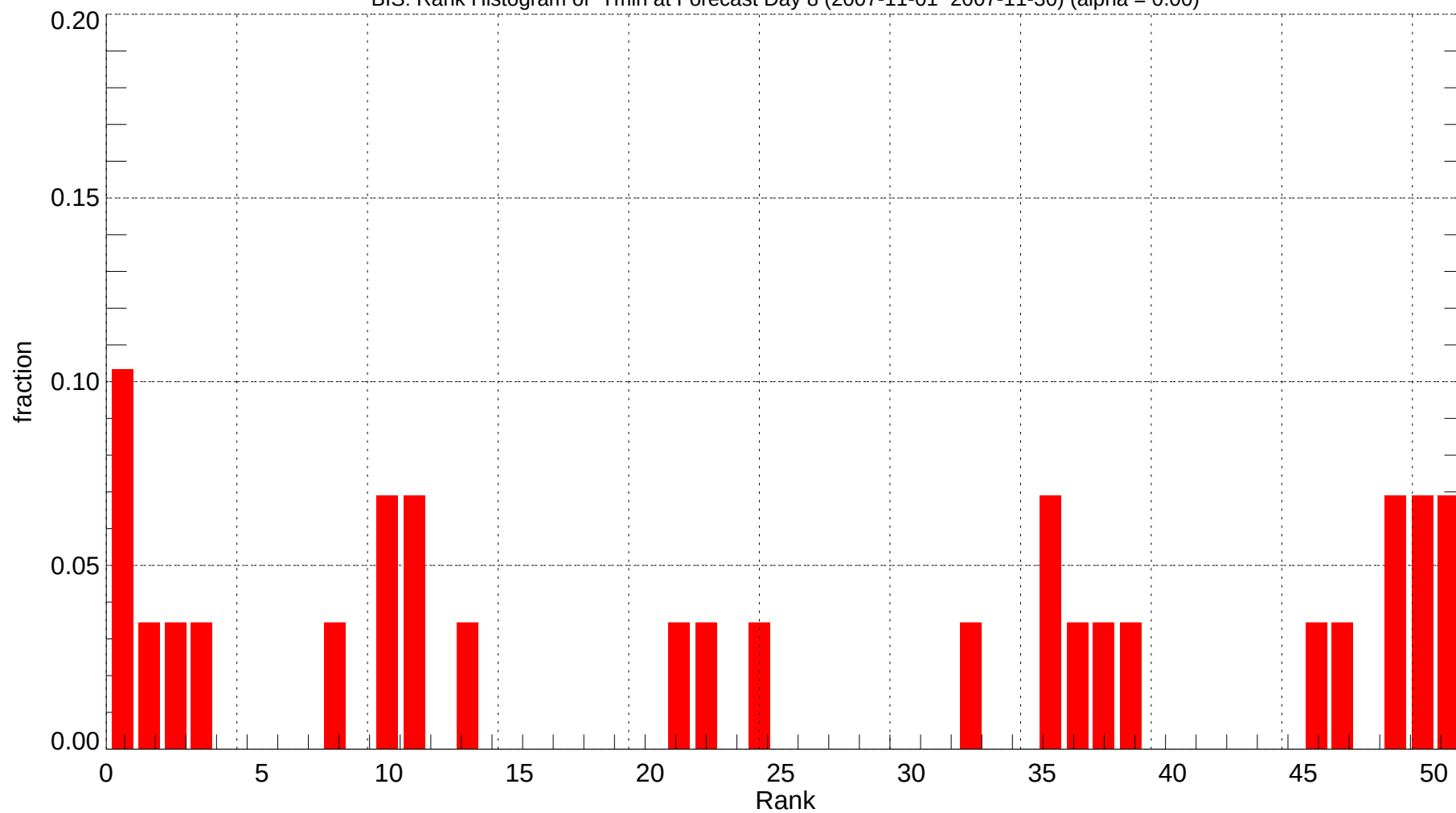
BIS: Rank Histogram of Tmin at Forecast Day 8 (2007-11-01~2007-11-30) (alpha = 0.00)
