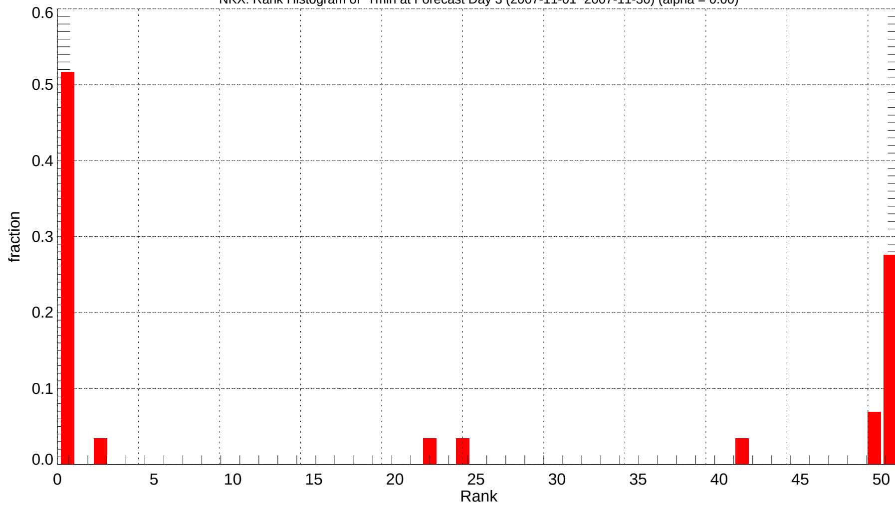
NKX: Rank Histogram of Tmin at Forecast Day 3 (2007-11-01~2007-11-30) (alpha = 0.00)
