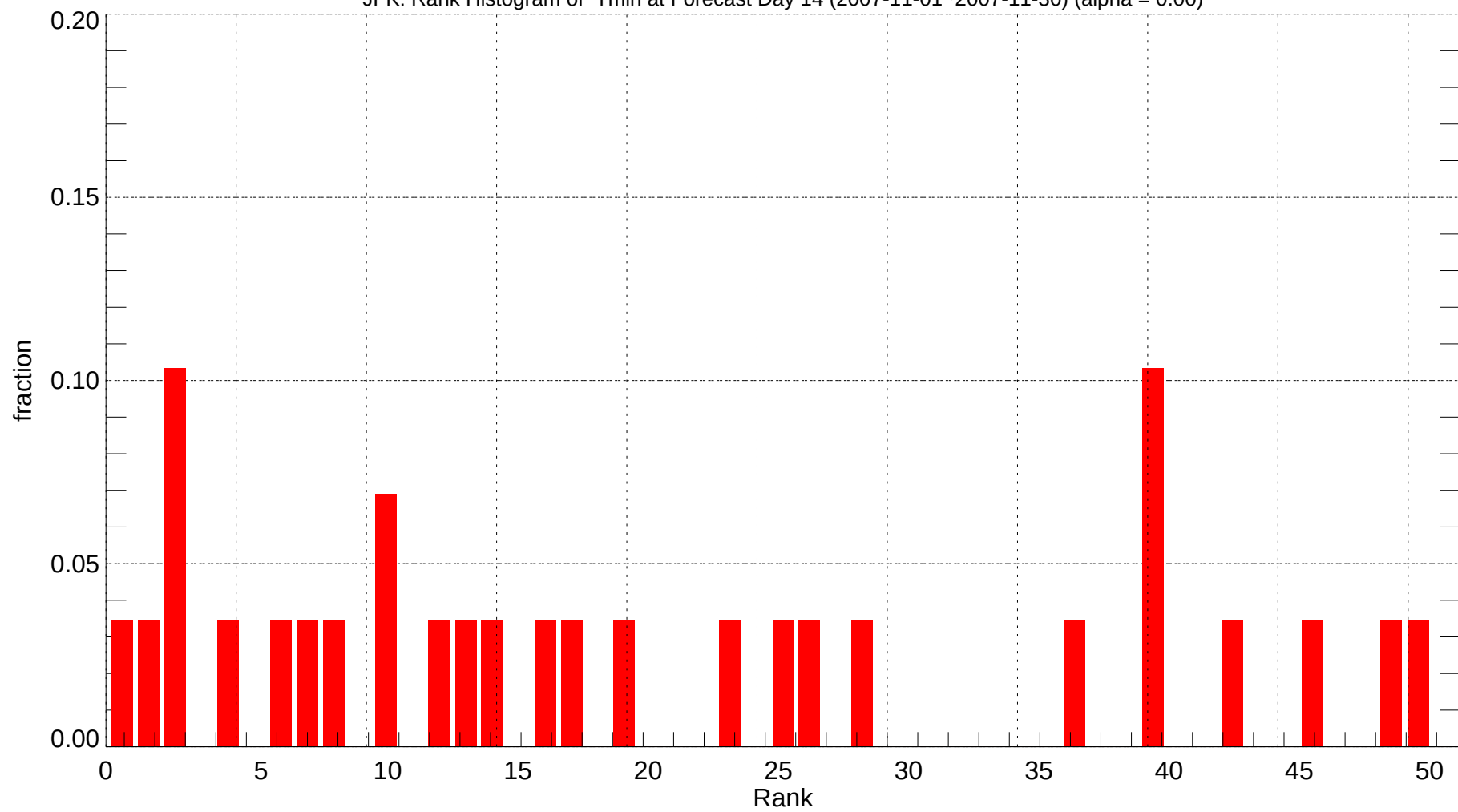
JFK: Rank Histogram of Tmin at Forecast Day 14 (2007-11-01~2007-11-30) (alpha = 0.00)
