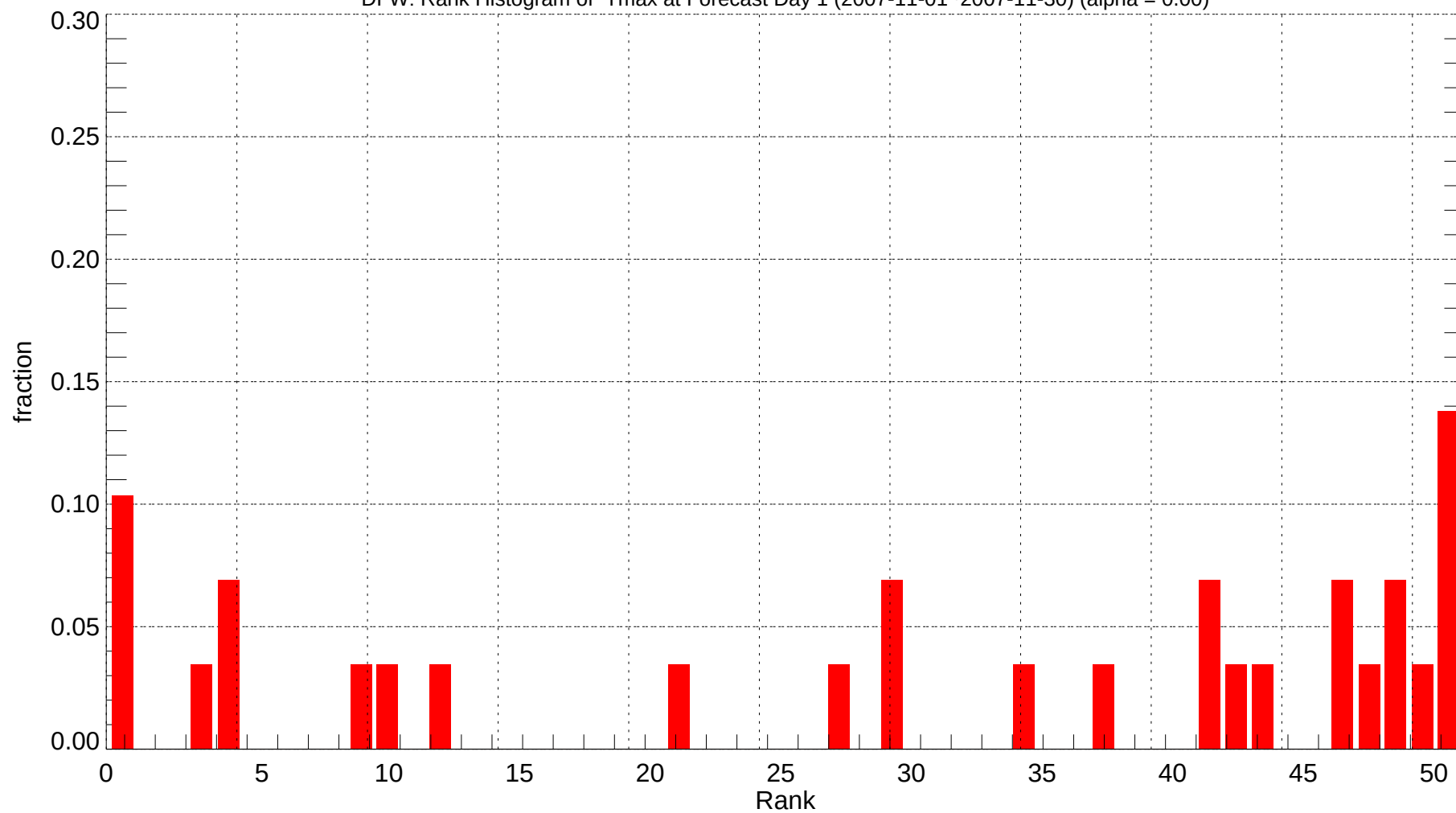
DFW: Rank Histogram of Tmax at Forecast Day 1 (2007-11-01~2007-11-30) (alpha = 0.00)
