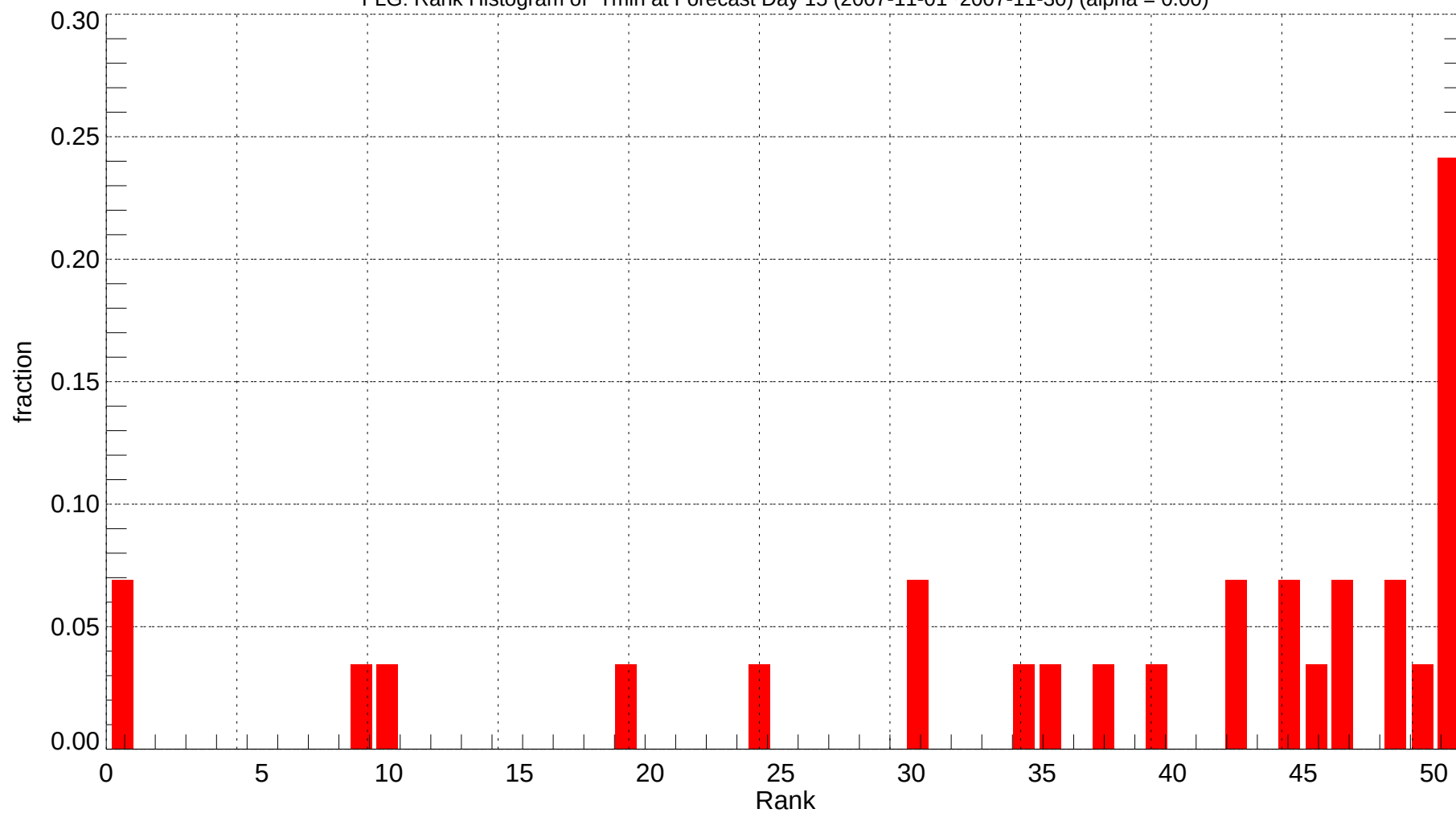
FLG: Rank Histogram of Tmin at Forecast Day 15 (2007-11-01~2007-11-30) (alpha = 0.00)
