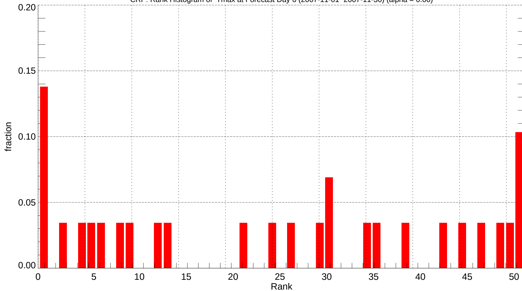
CRP: Rank Histogram of Tmax at Forecast Day 6 (2007-11-01~2007-11-30) (alpha = 0.00)
