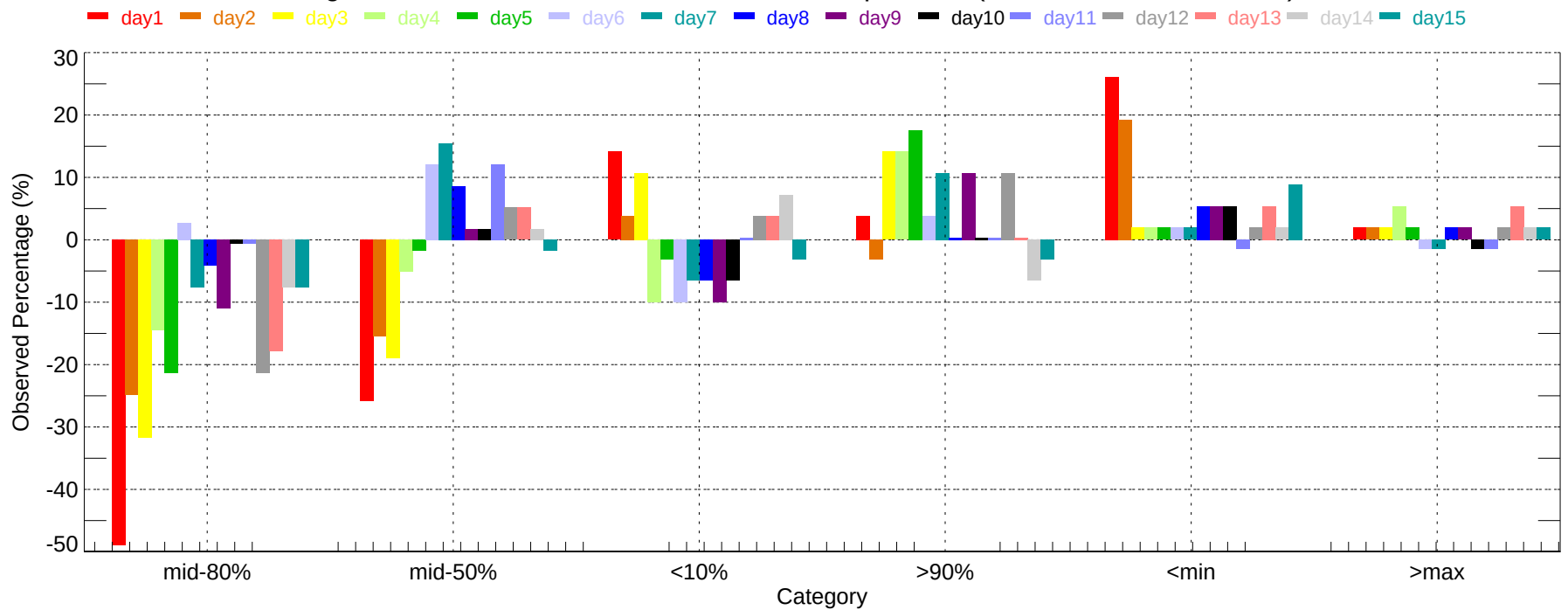
Observed Percentage Deviation of Ensembles - APN: Min Temperature (2007-11-01~2007-11-30)
