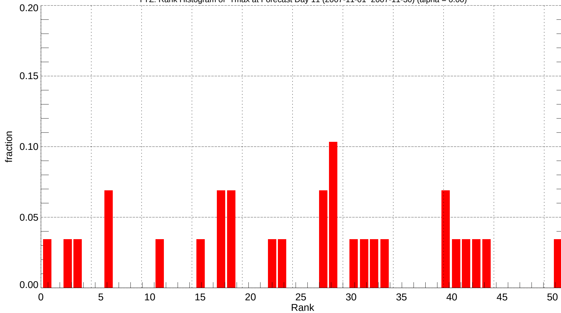
YYZ: Rank Histogram of Tmax at Forecast Day 11 (2007-11-01~2007-11-30) (alpha = 0.00)
