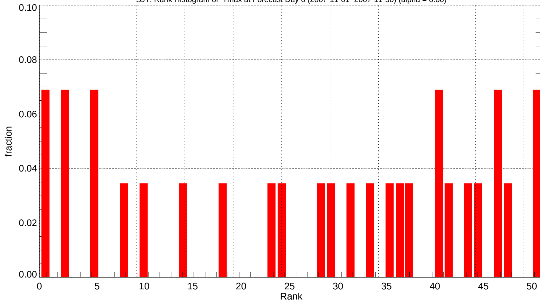
SJT: Rank Histogram of Tmax at Forecast Day 6 (2007-11-01~2007-11-30) (alpha = 0.00)
