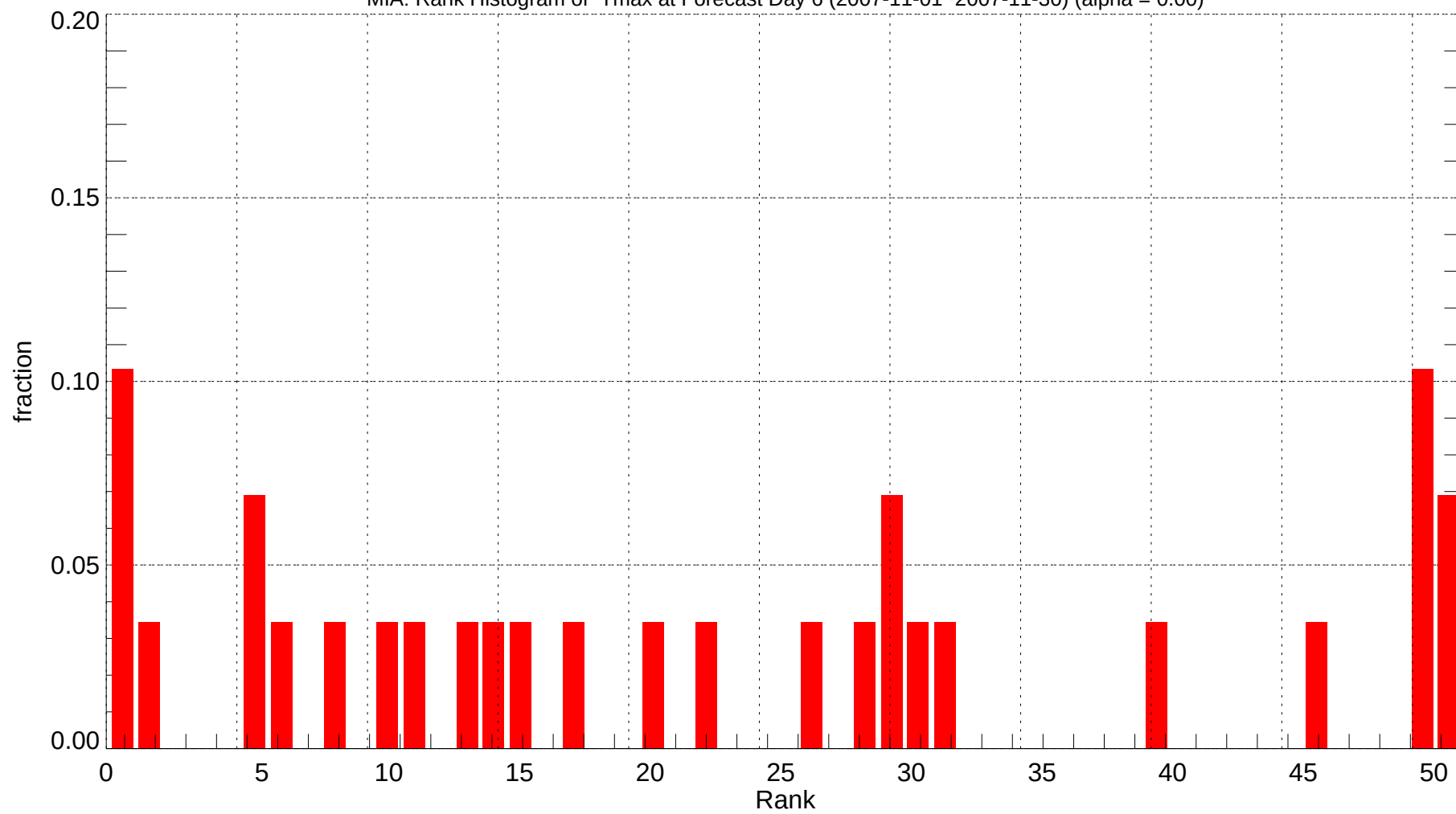
MIA: Rank Histogram of Tmax at Forecast Day 6 (2007-11-01~2007-11-30) (alpha = 0.00)
