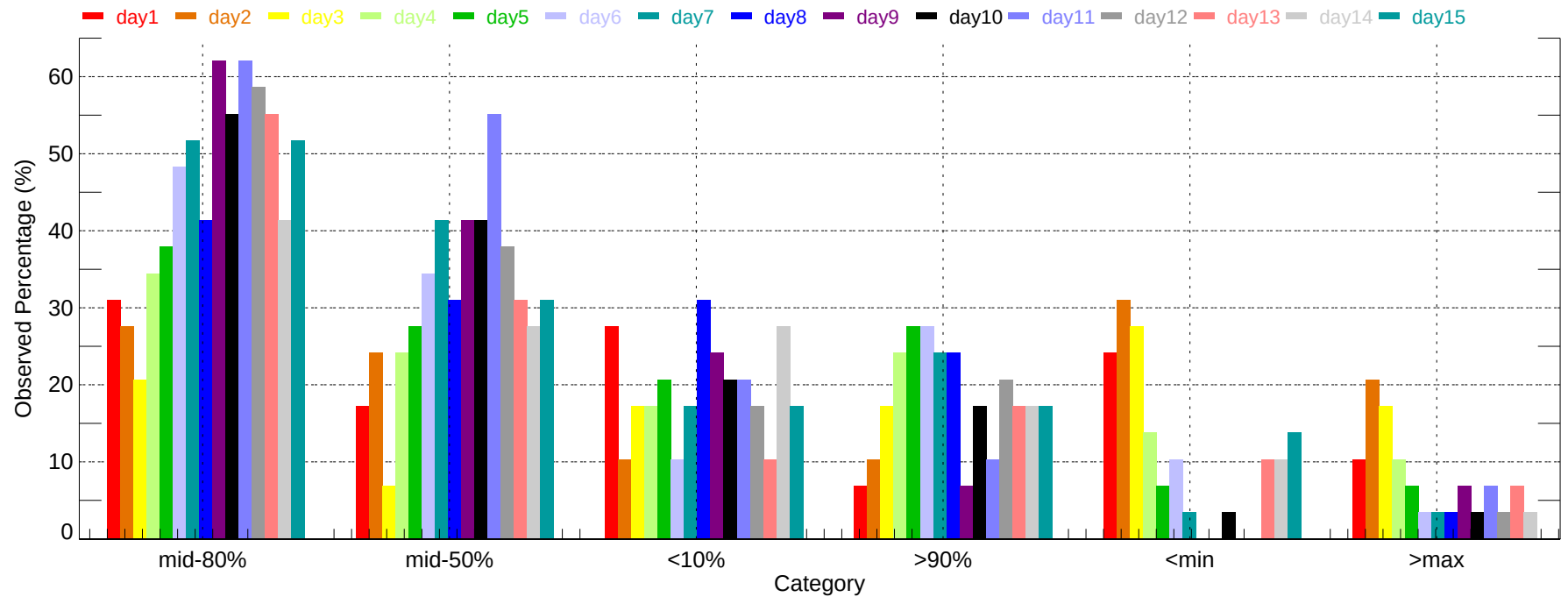
Observed Percentage of Ensembles - ORH: Min Temperature (2007-11-01~2007-11-30)
