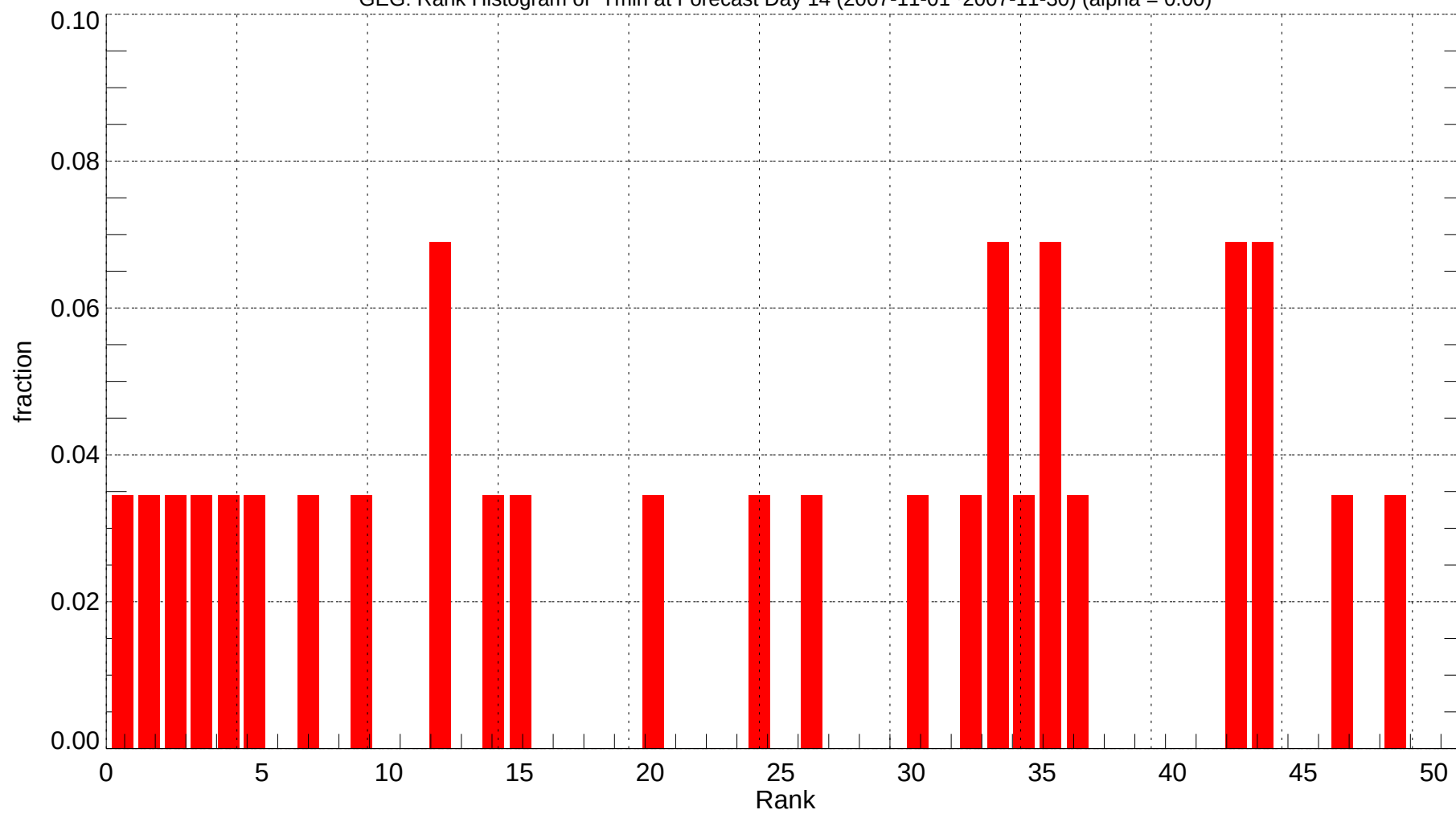
GEG: Rank Histogram of Tmin at Forecast Day 14 (2007-11-01~2007-11-30) (alpha = 0.00)
