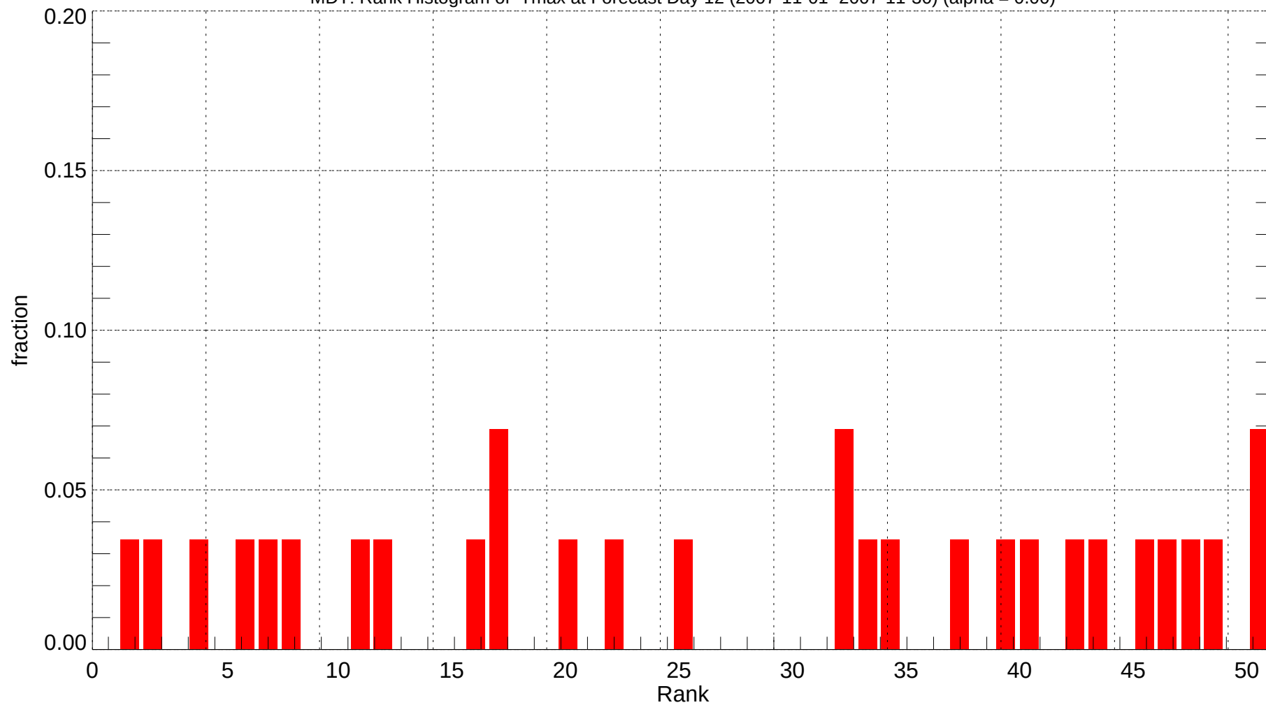
MDT: Rank Histogram of Tmax at Forecast Day 12 (2007-11-01~2007-11-30) (alpha = 0.00)
