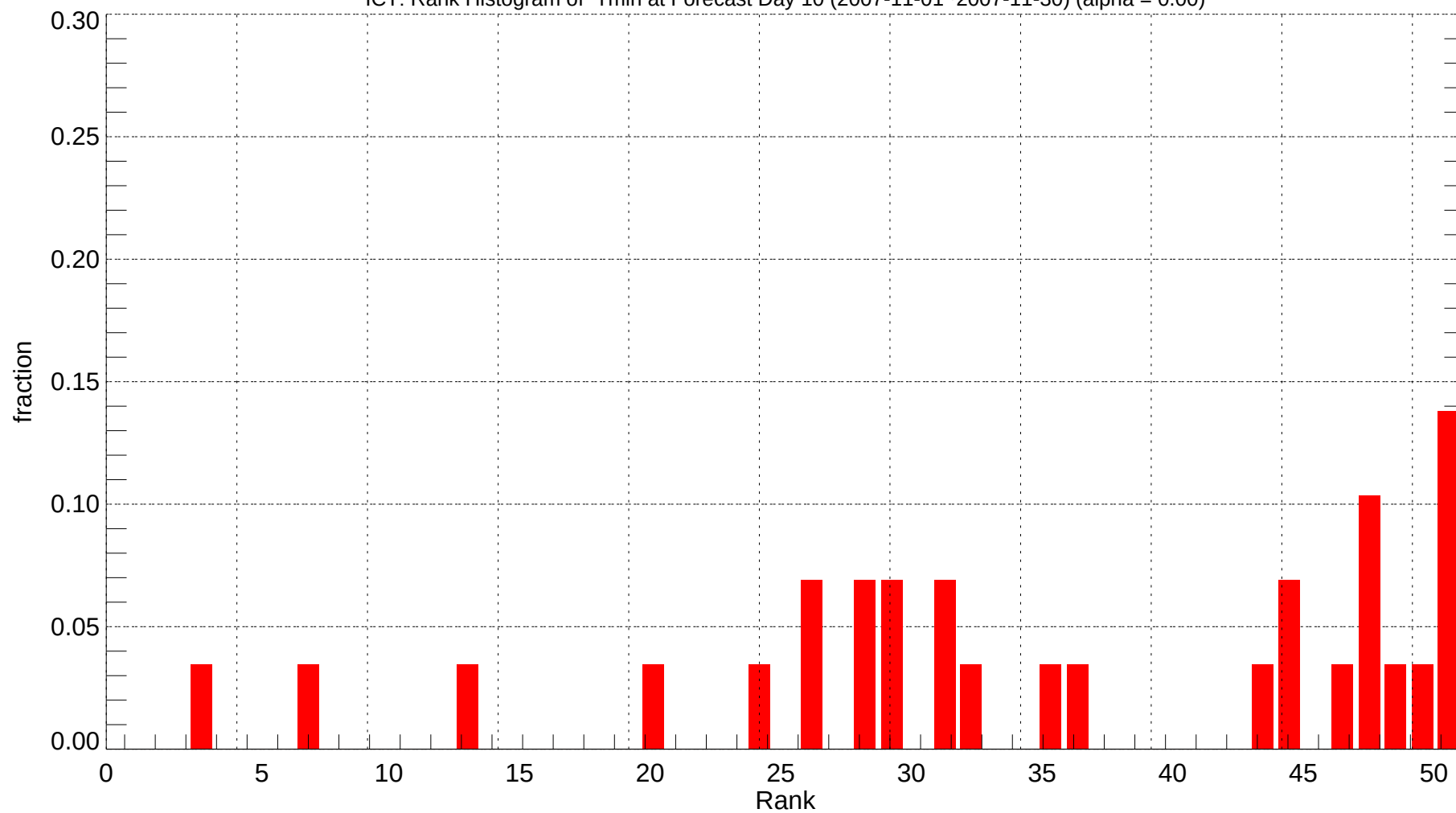
ICT: Rank Histogram of Tmin at Forecast Day 10 (2007-11-01~2007-11-30) (alpha = 0.00)
