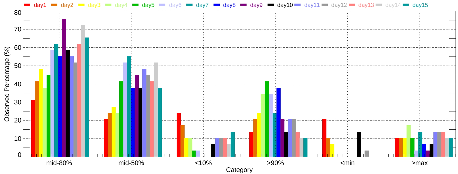
Observed Percentage of Ensembles - CLE: Min Temperature (2007-11-01~2007-11-30)
