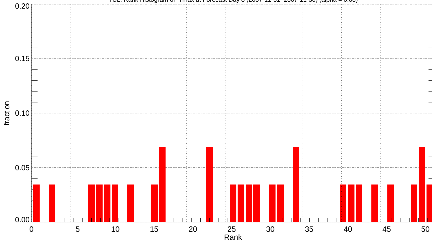
YUL: Rank Histogram of Tmax at Forecast Day 8 (2007-11-01~2007-11-30) (alpha = 0.00)
