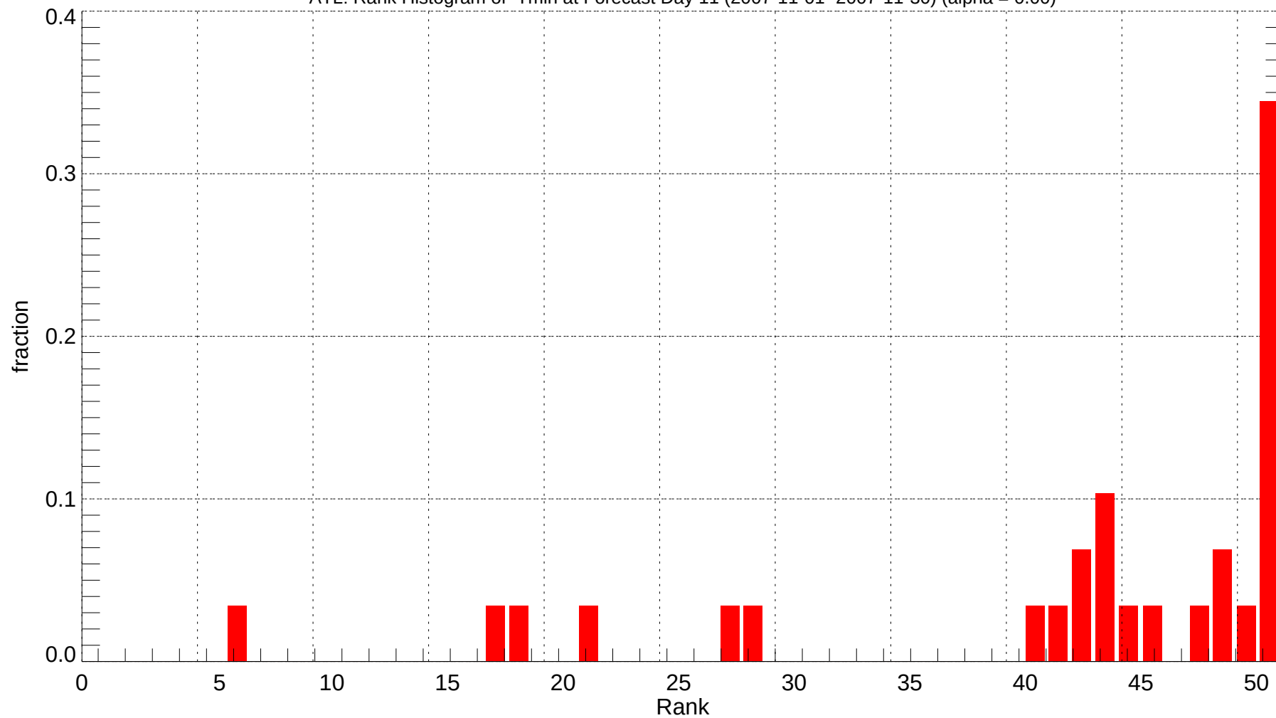
ATL: Rank Histogram of Tmin at Forecast Day 11 (2007-11-01~2007-11-30) (alpha = 0.00)
