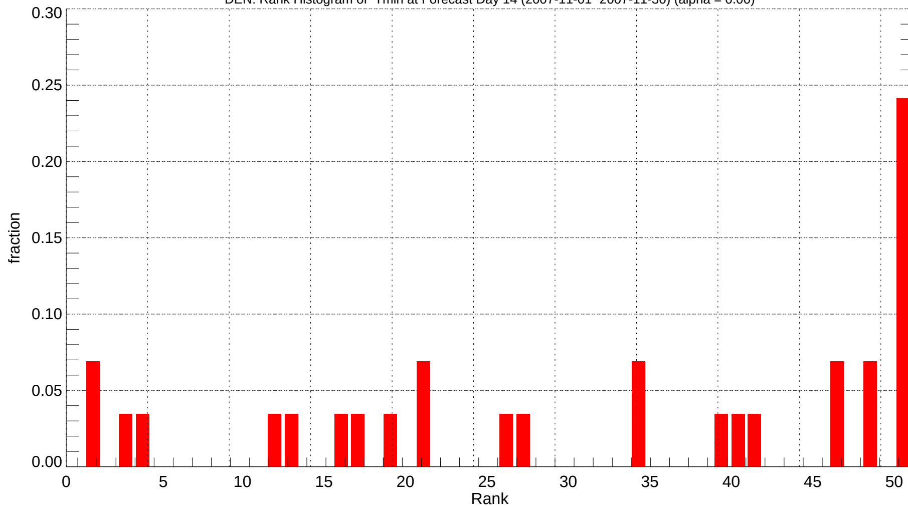
DEN: Rank Histogram of Tmin at Forecast Day 14 (2007-11-01~2007-11-30) (alpha = 0.00)
