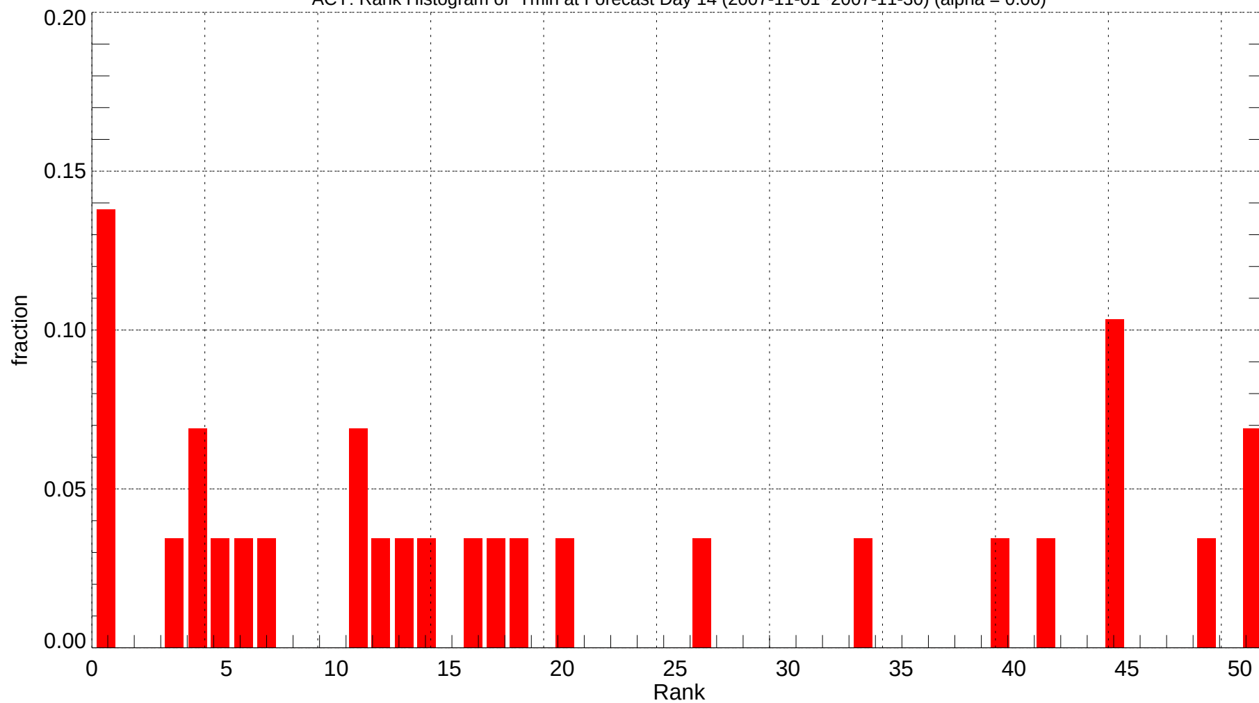
ACY: Rank Histogram of Tmin at Forecast Day 14 (2007-11-01~2007-11-30) (alpha = 0.00)
