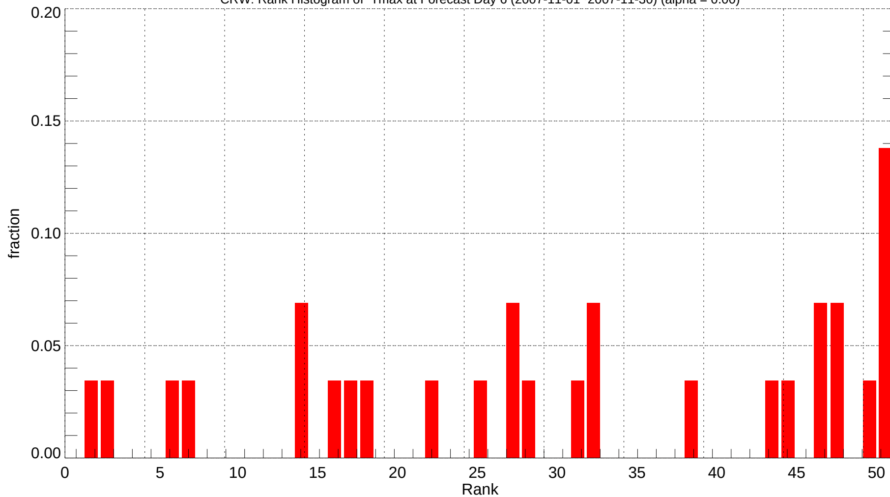
CRW: Rank Histogram of Tmax at Forecast Day 6 (2007-11-01~2007-11-30) (alpha = 0.00)
