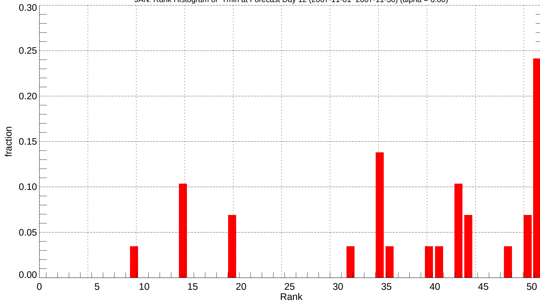
JAN: Rank Histogram of Tmin at Forecast Day 12 (2007-11-01~2007-11-30) (alpha = 0.00)
