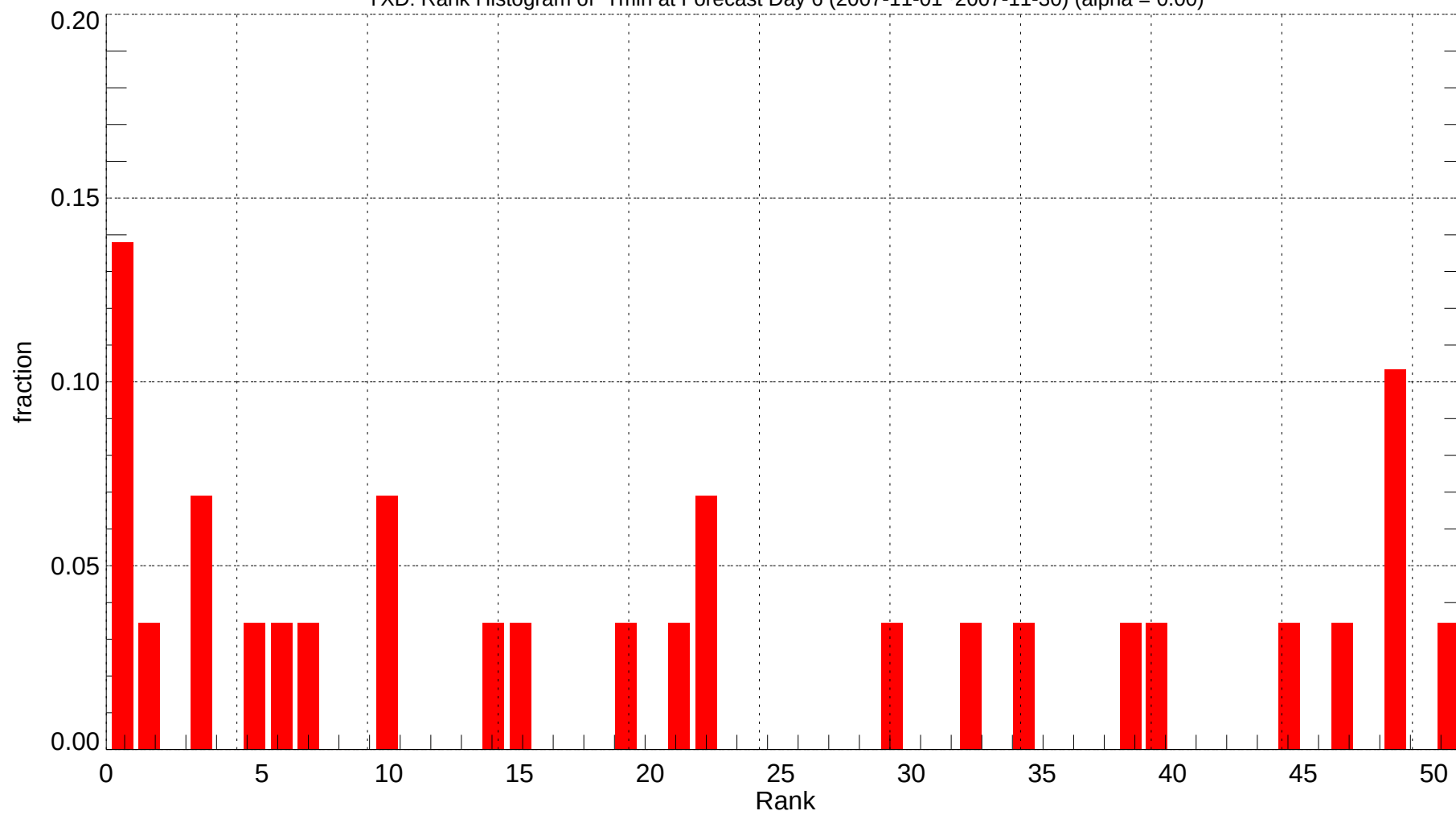
YXD: Rank Histogram of Tmin at Forecast Day 6 (2007-11-01~2007-11-30) (alpha = 0.00)
