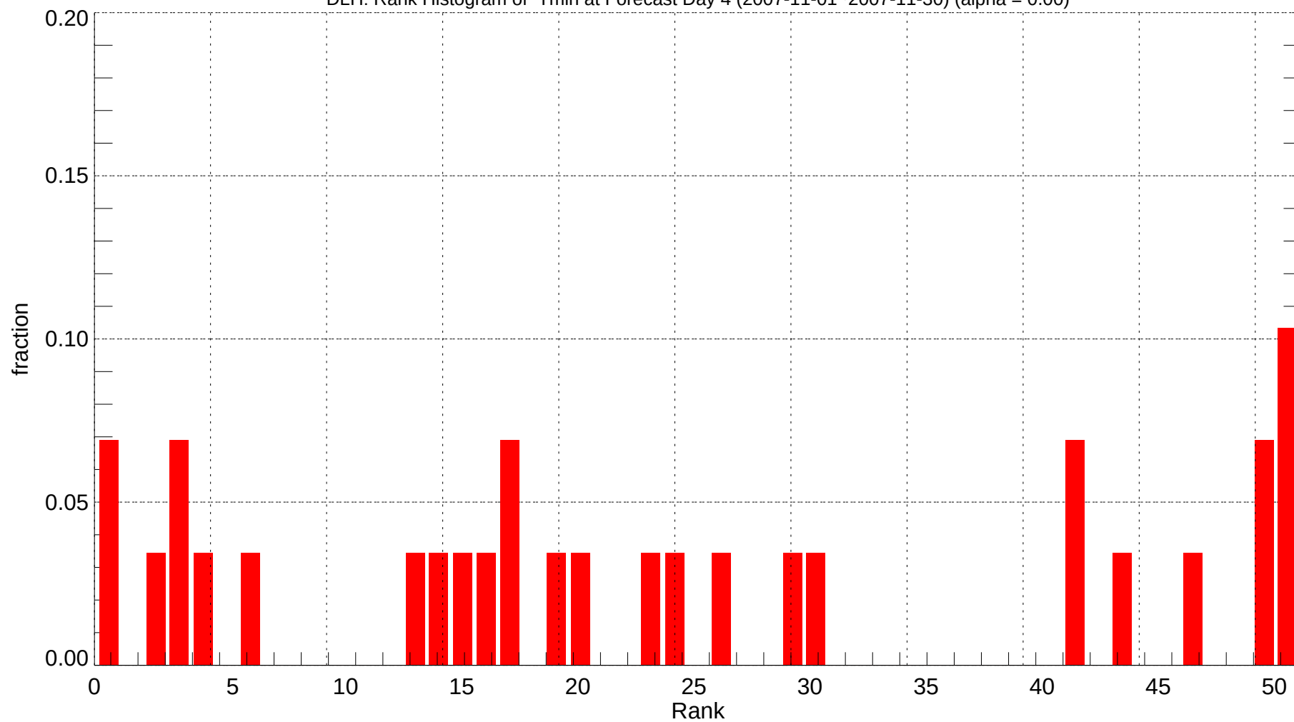
DLH: Rank Histogram of Tmin at Forecast Day 4 (2007-11-01~2007-11-30) (alpha = 0.00)
