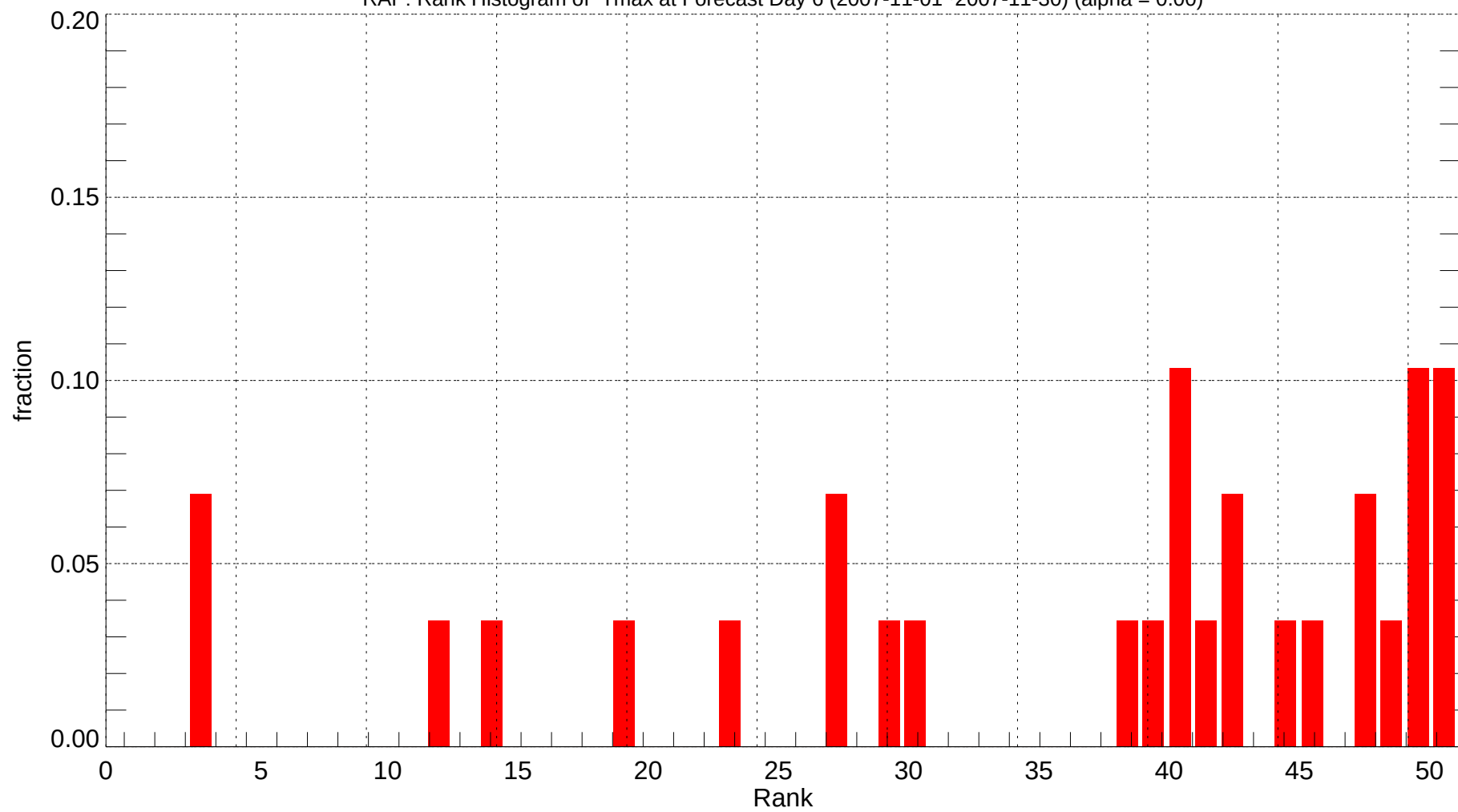
RAP: Rank Histogram of Tmax at Forecast Day 6 (2007-11-01~2007-11-30) (alpha = 0.00)
