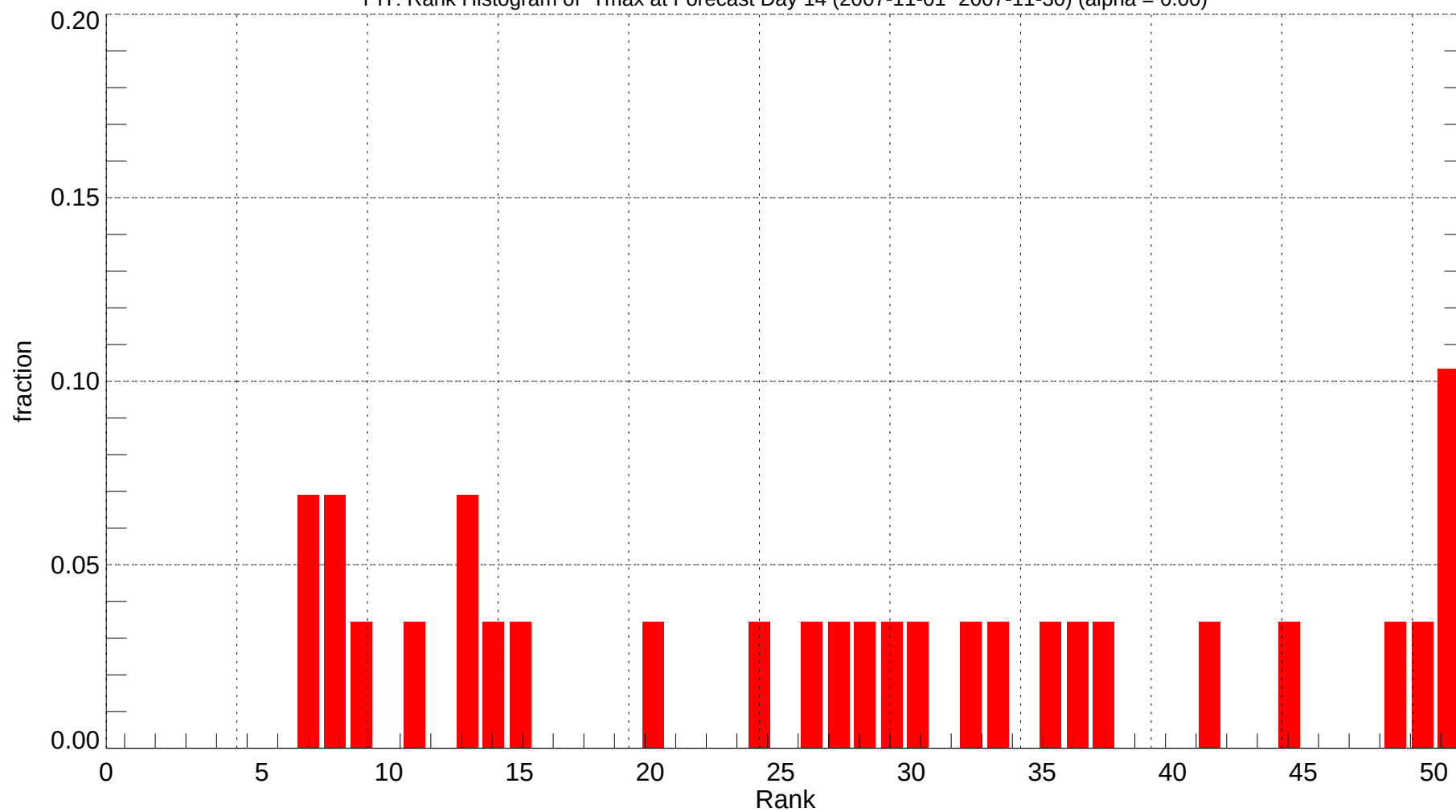
PIT: Rank Histogram of Tmax at Forecast Day 14 (2007-11-01~2007-11-30) (alpha = 0.00)
