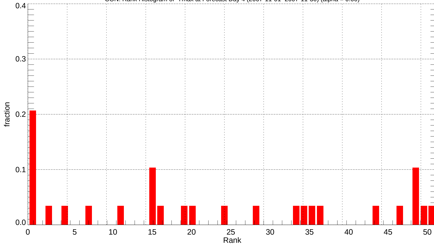
CON: Rank Histogram of Tmax at Forecast Day 4 (2007-11-01~2007-11-30) (alpha = 0.00)
