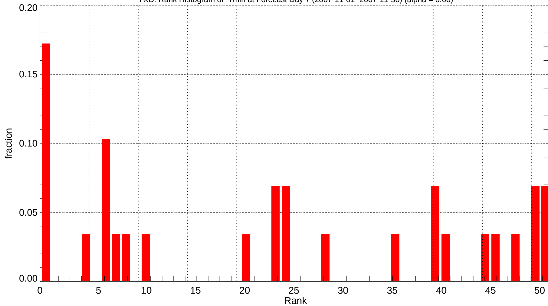
YXD: Rank Histogram of Tmin at Forecast Day 7 (2007-11-01~2007-11-30) (alpha = 0.00)
