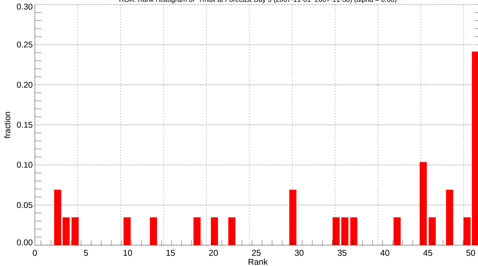
ROA: Rank Histogram of Tmax at Forecast Day 3 (2007-11-01~2007-11-30) (alpha = 0.00)
