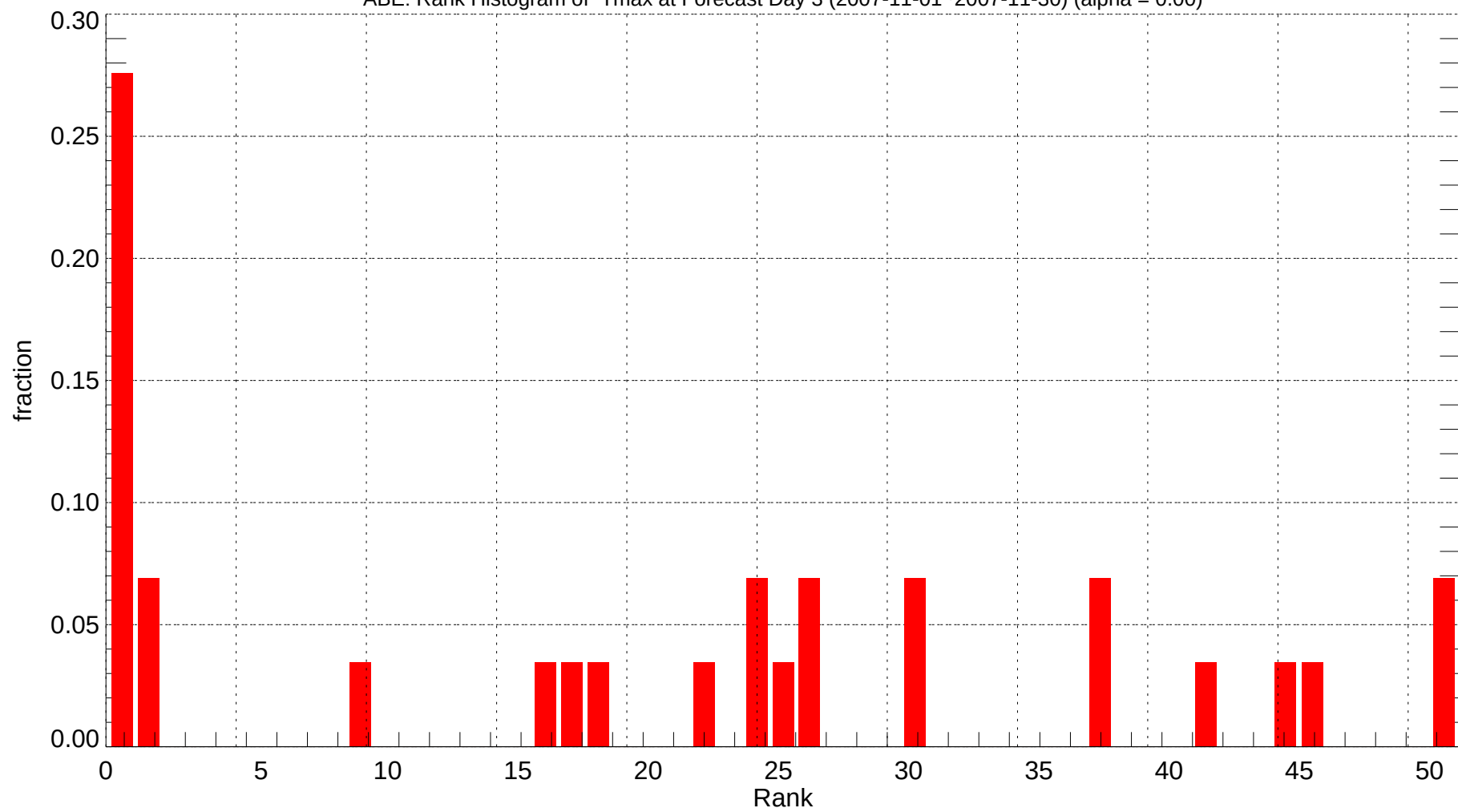
ABE: Rank Histogram of Tmax at Forecast Day 3 (2007-11-01~2007-11-30) (alpha = 0.00)
