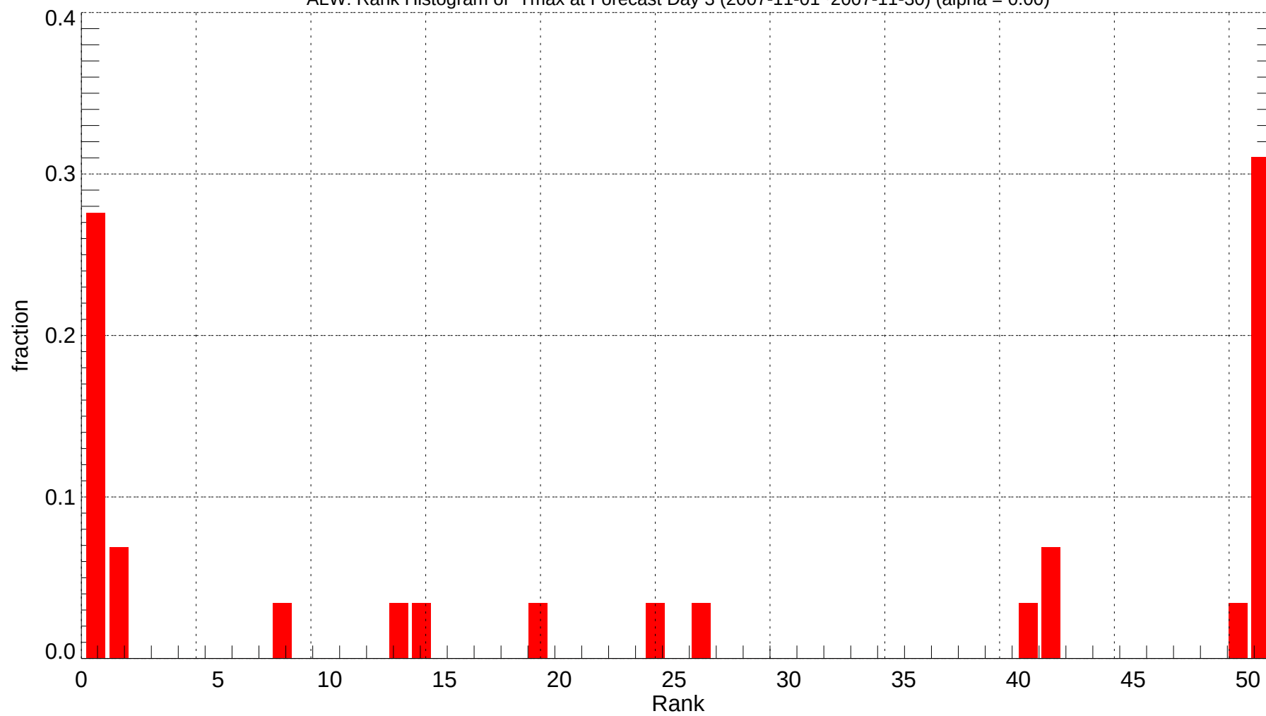
ALW: Rank Histogram of Tmax at Forecast Day 3 (2007-11-01~2007-11-30) (alpha = 0.00)
