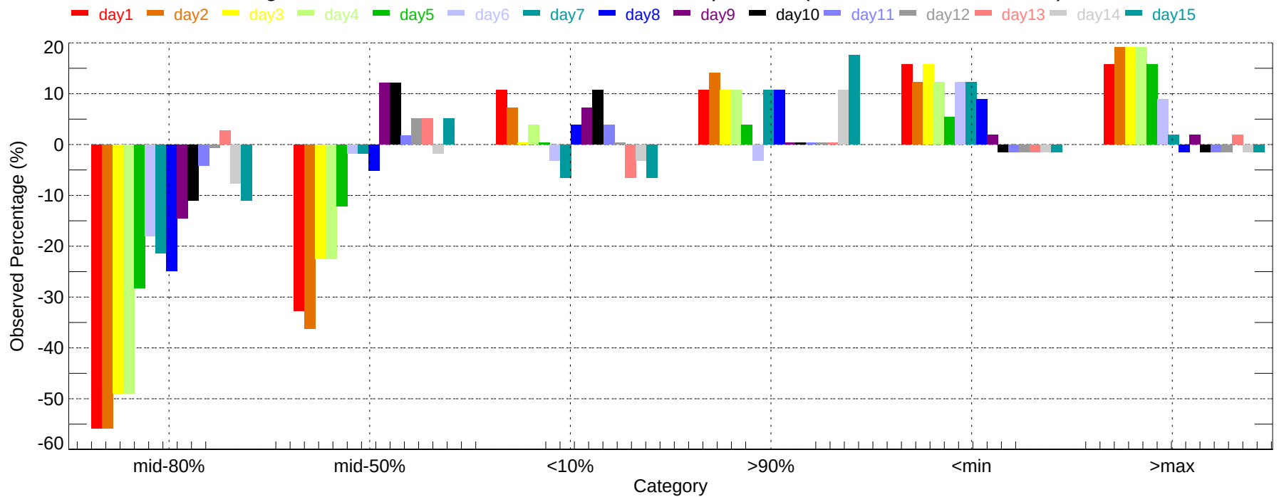
Observed Percentage Deviation of Ensembles - PDX: Max Temperature (2007-11-01~2007-11-30)
