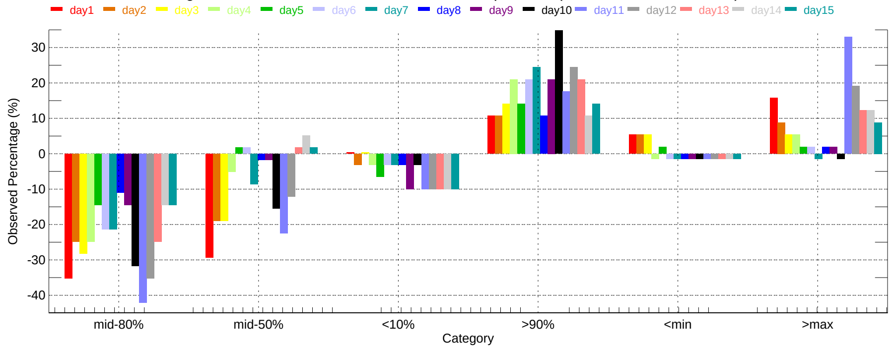
Observed Percentage Deviation of Ensembles - JAN: Max Temperature (2007-11-01~2007-11-30)
