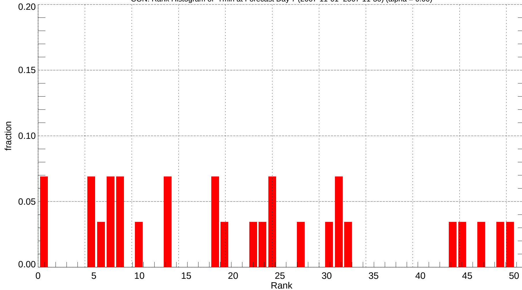
CON: Rank Histogram of Tmin at Forecast Day 7 (2007-11-01~2007-11-30) (alpha = 0.00)
