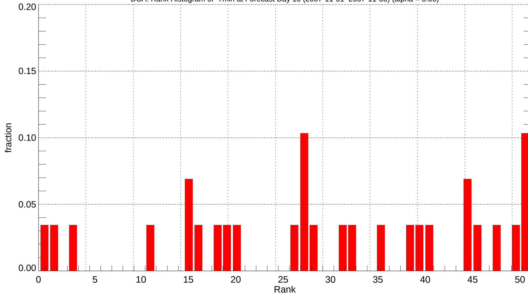
DCA: Rank Histogram of Tmin at Forecast Day 10 (2007-11-01~2007-11-30) (alpha = 0.00)
