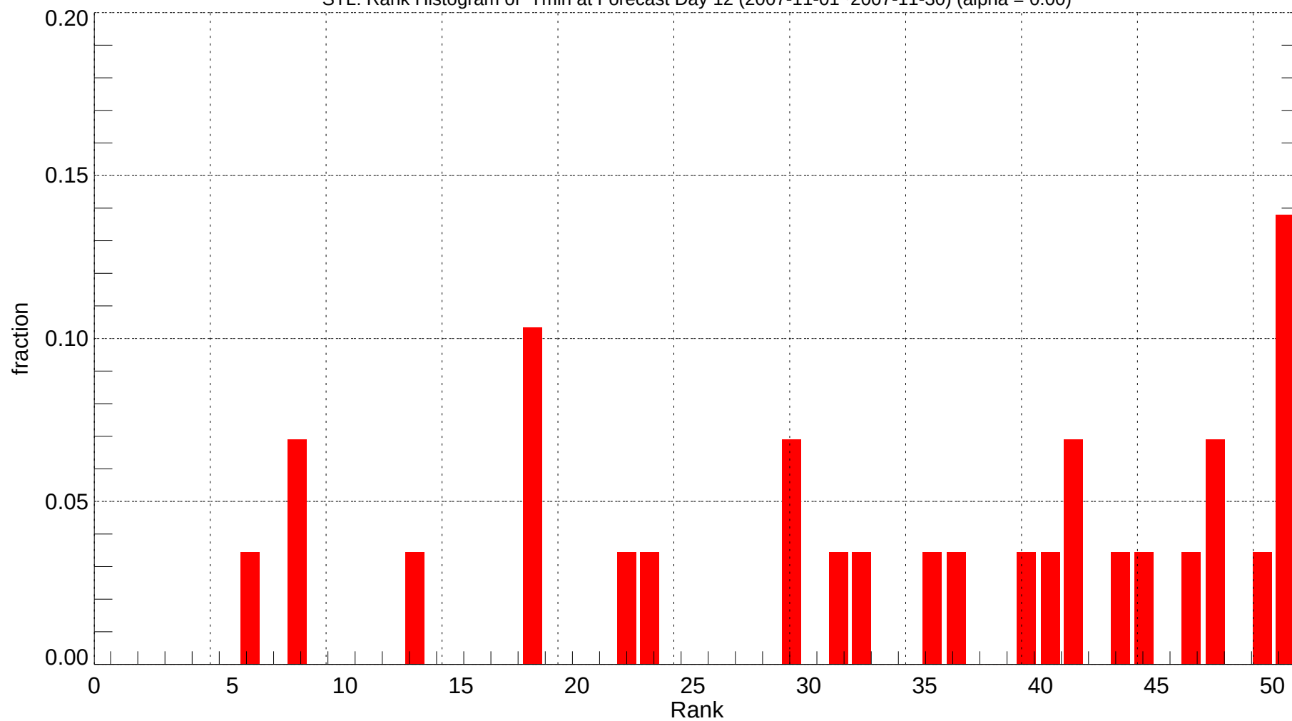
STL: Rank Histogram of Tmin at Forecast Day 12 (2007-11-01~2007-11-30) (alpha = 0.00)
