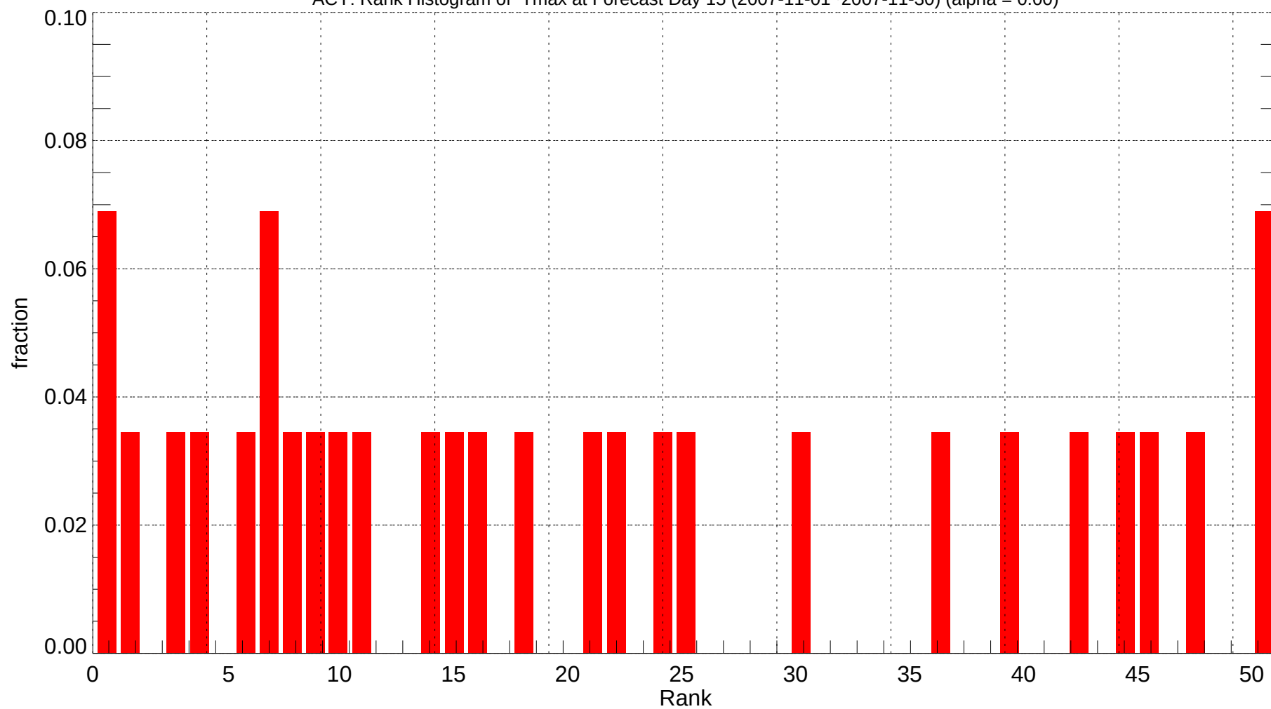
ACY: Rank Histogram of Tmax at Forecast Day 15 (2007-11-01~2007-11-30) (alpha = 0.00)
