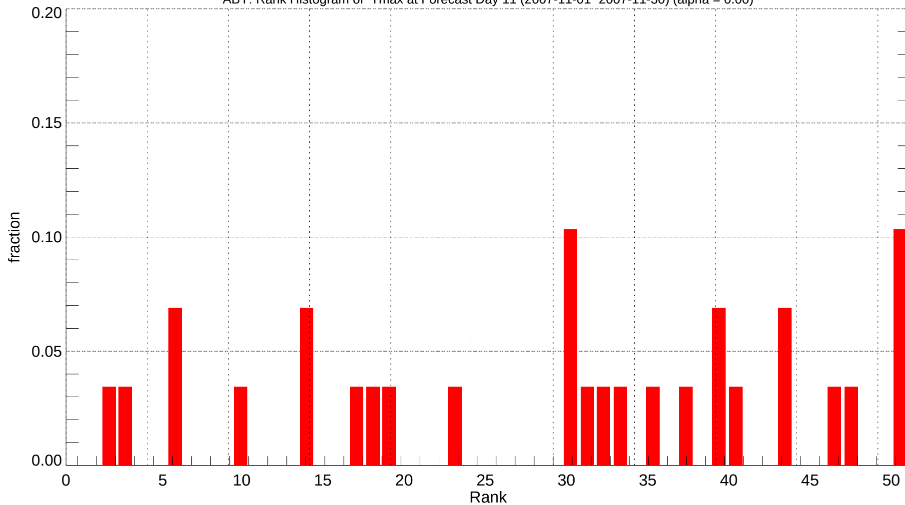
ABY: Rank Histogram of Tmax at Forecast Day 11 (2007-11-01~2007-11-30) (alpha = 0.00)
