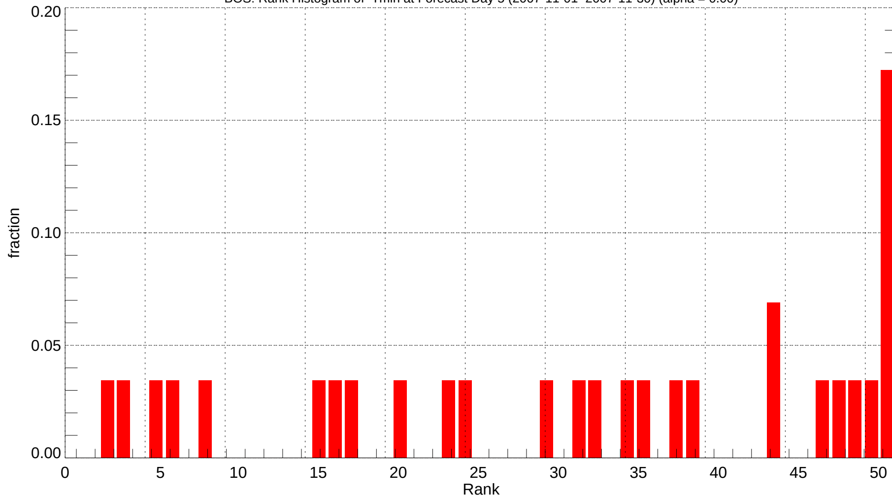
BOS: Rank Histogram of Tmin at Forecast Day 5 (2007-11-01~2007-11-30) (alpha = 0.00)
