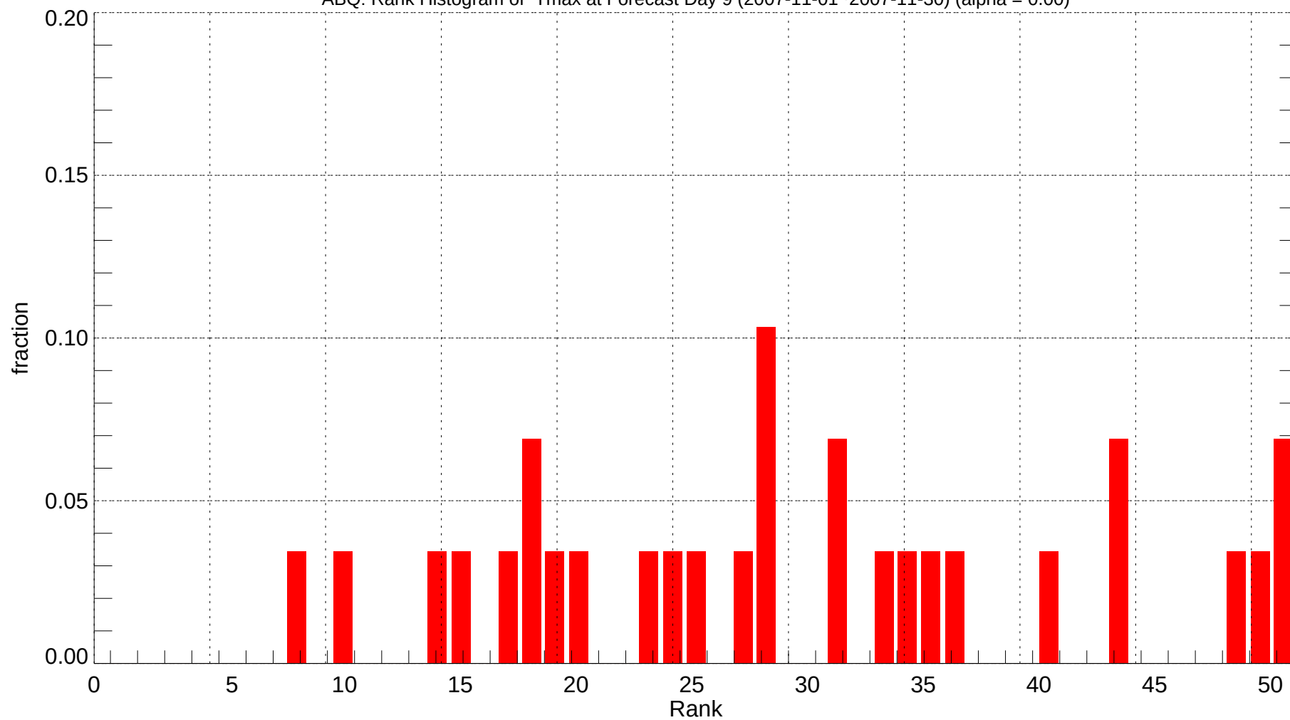
ABQ: Rank Histogram of Tmax at Forecast Day 9 (2007-11-01~2007-11-30) (alpha = 0.00)
