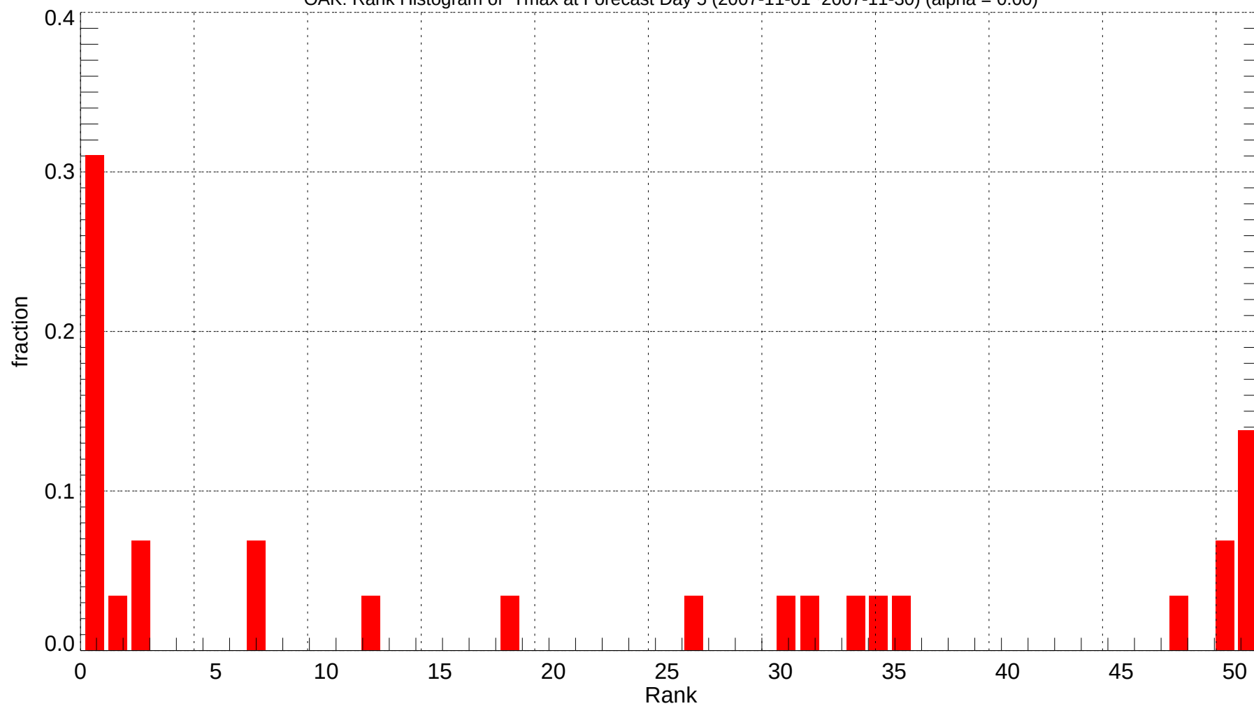
OAK: Rank Histogram of Tmax at Forecast Day 5 (2007-11-01~2007-11-30) (alpha = 0.00)
