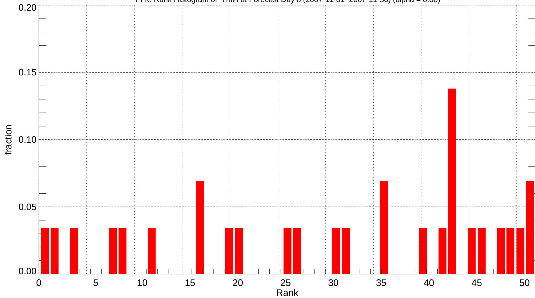
TYR: Rank Histogram of Tmin at Forecast Day 8 (2007-11-01~2007-11-30) (alpha = 0.00)
