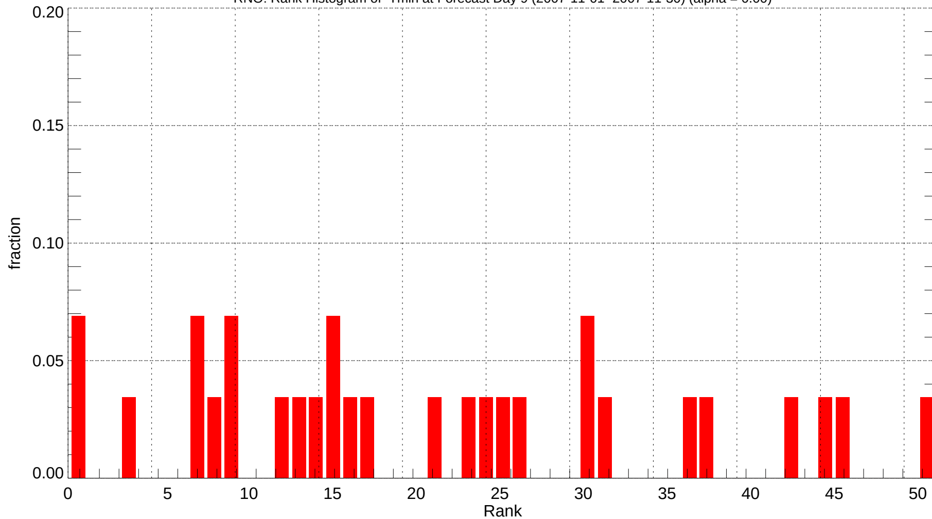
RNO: Rank Histogram of Tmin at Forecast Day 9 (2007-11-01~2007-11-30) (alpha = 0.00)
