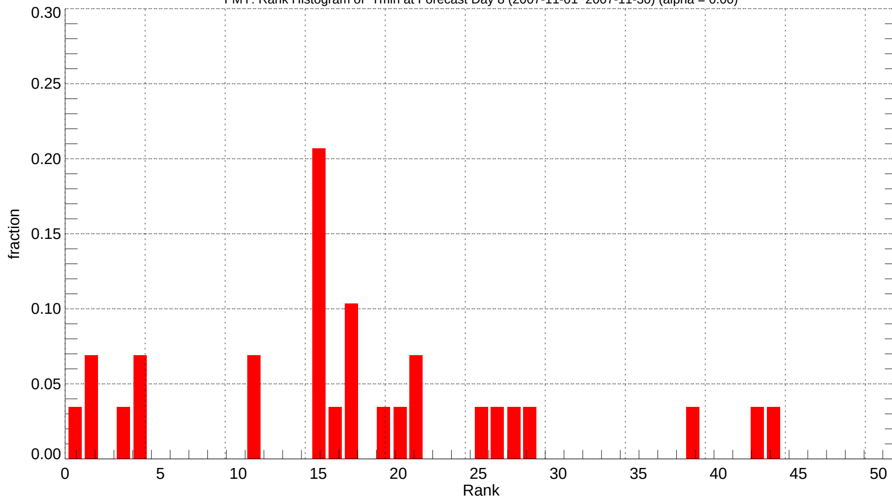
FMY: Rank Histogram of Tmin at Forecast Day 8 (2007-11-01~2007-11-30) (alpha = 0.00)
