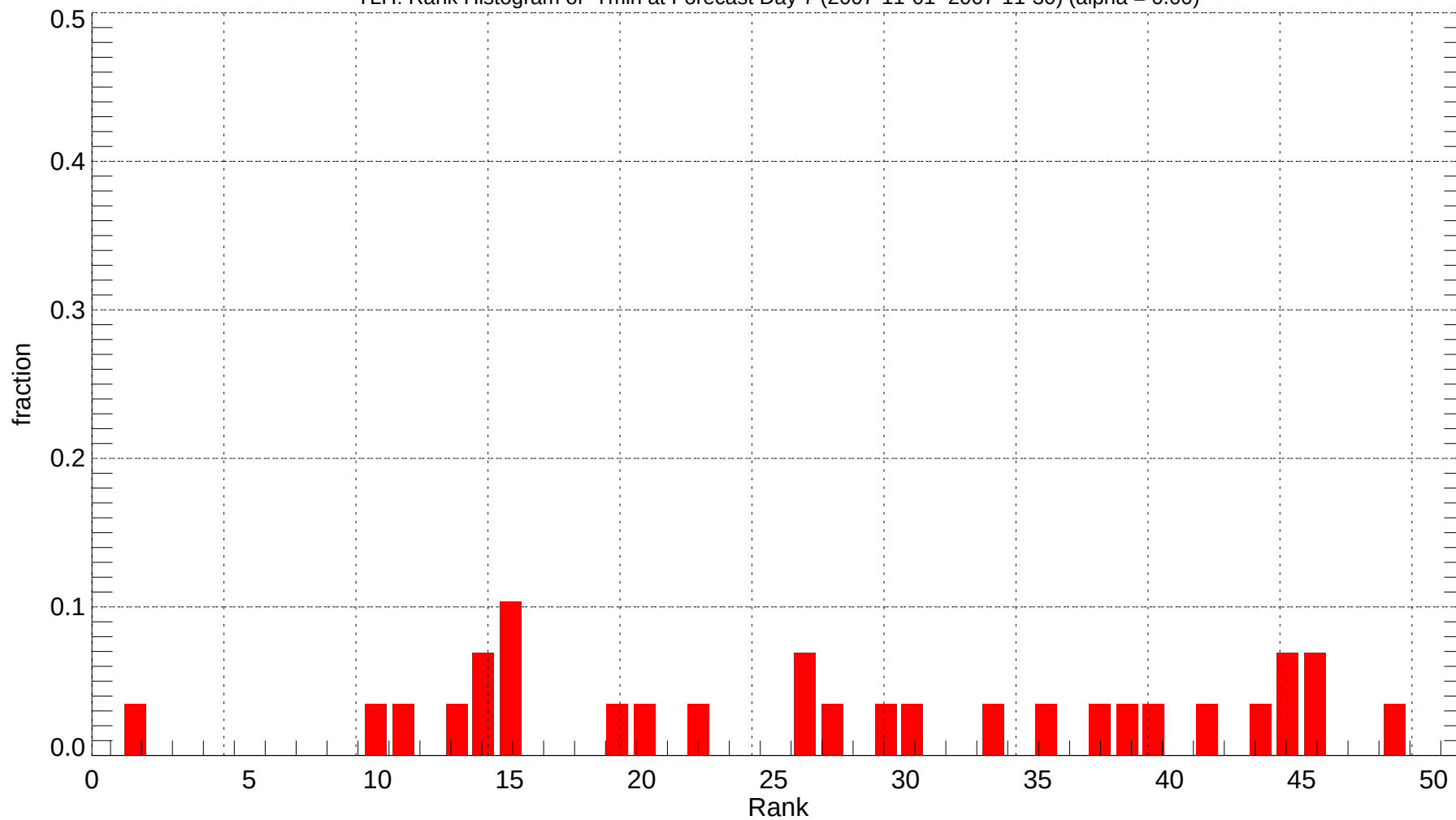
TLH: Rank Histogram of Tmin at Forecast Day 7 (2007-11-01~2007-11-30) (alpha = 0.00)
