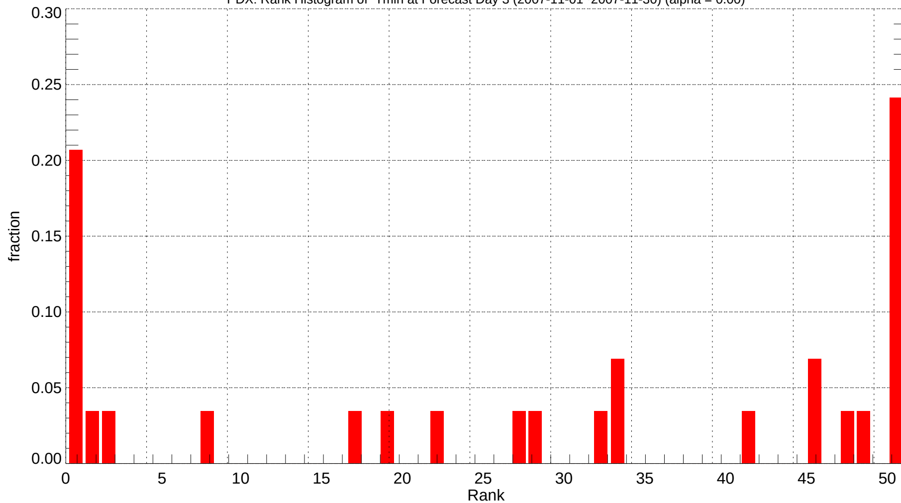
PDX: Rank Histogram of Tmin at Forecast Day 3 (2007-11-01~2007-11-30) (alpha = 0.00)
