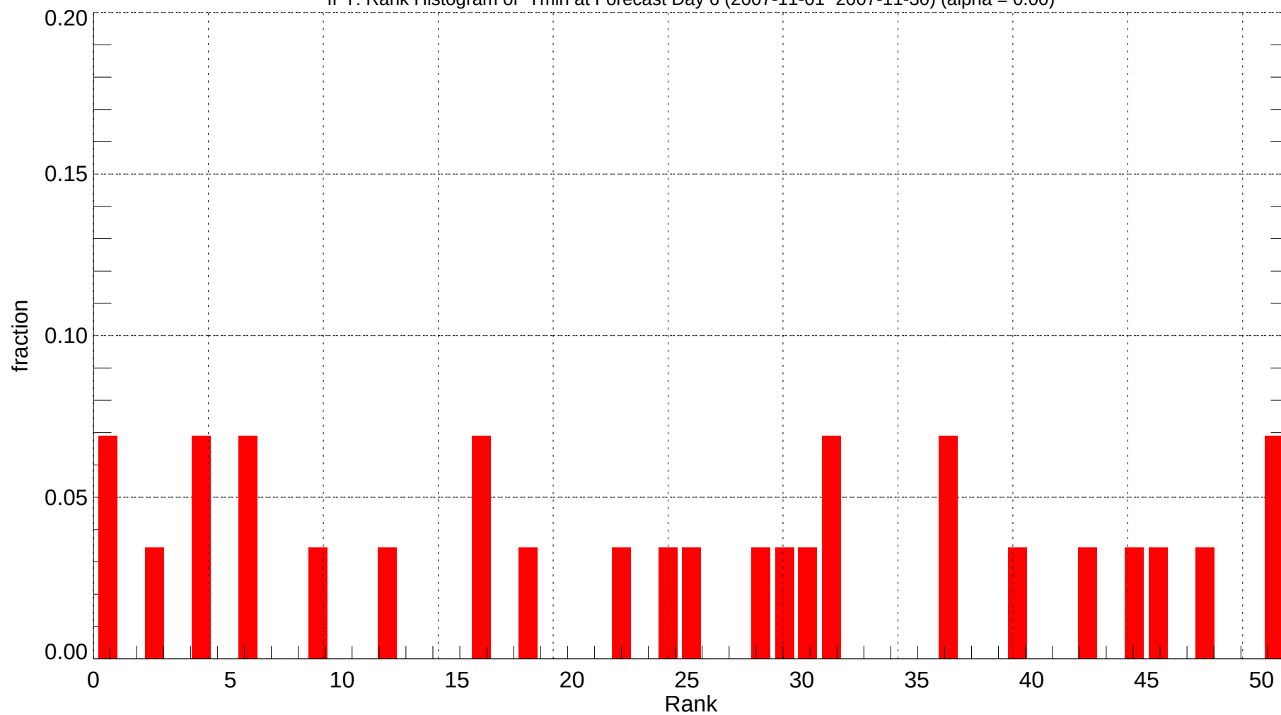
IPT: Rank Histogram of Tmin at Forecast Day 6 (2007-11-01~2007-11-30) (alpha = 0.00)
