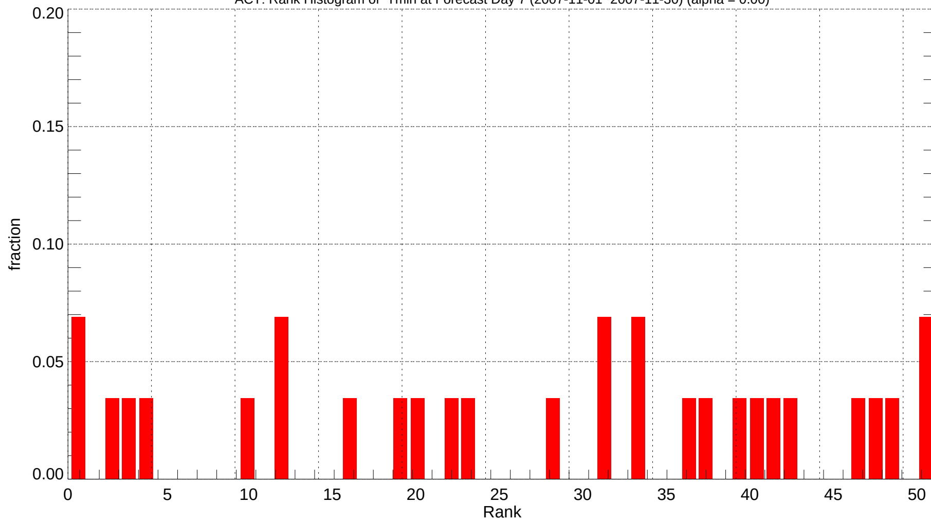
ACT: Rank Histogram of Tmin at Forecast Day 7 (2007-11-01~2007-11-30) (alpha = 0.00)
