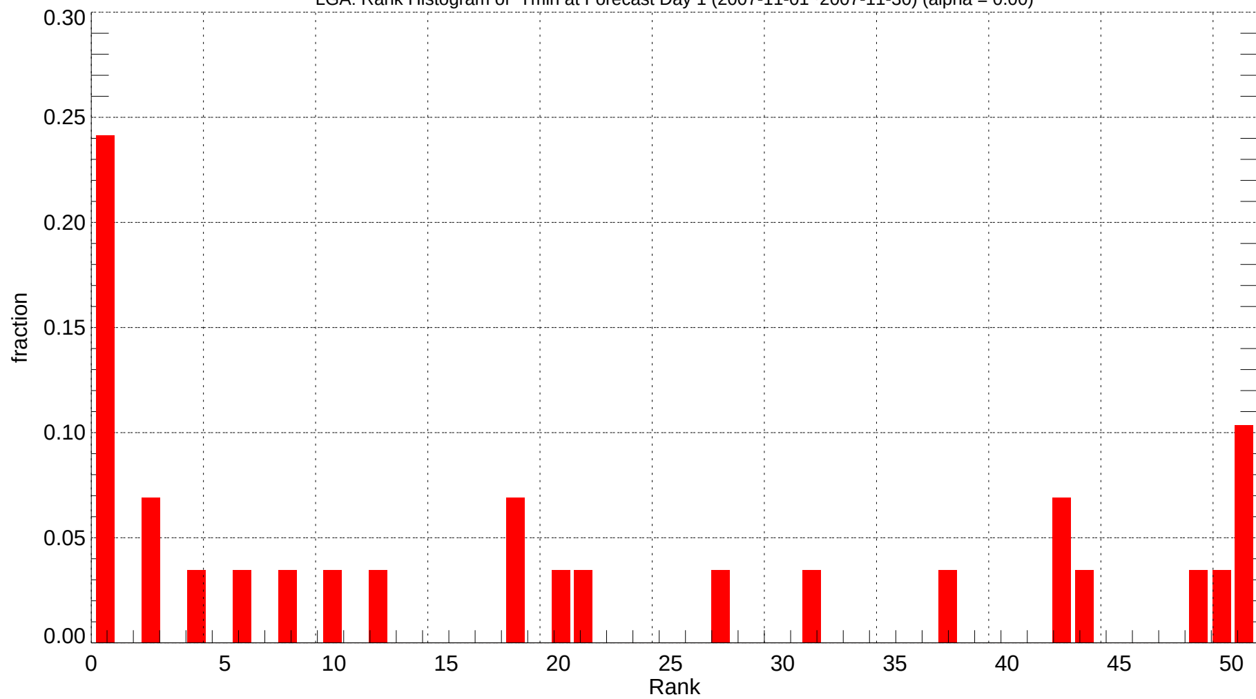
LGA: Rank Histogram of Tmin at Forecast Day 1 (2007-11-01~2007-11-30) (alpha = 0.00)
