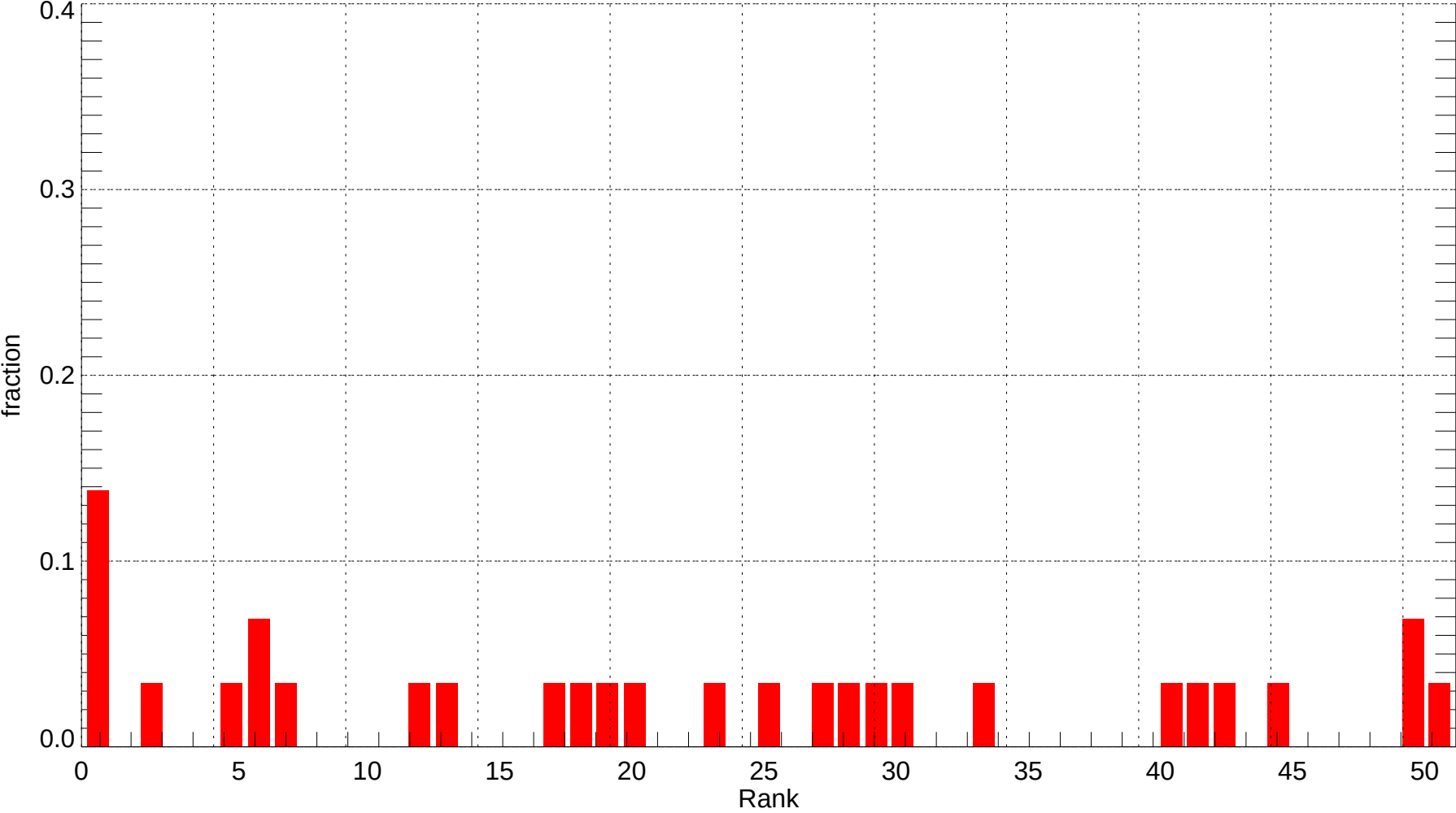
SSI: Rank Histogram of Tmax at Forecast Day 4 (2007-11-01~2007-11-30) (alpha = 0.00)
