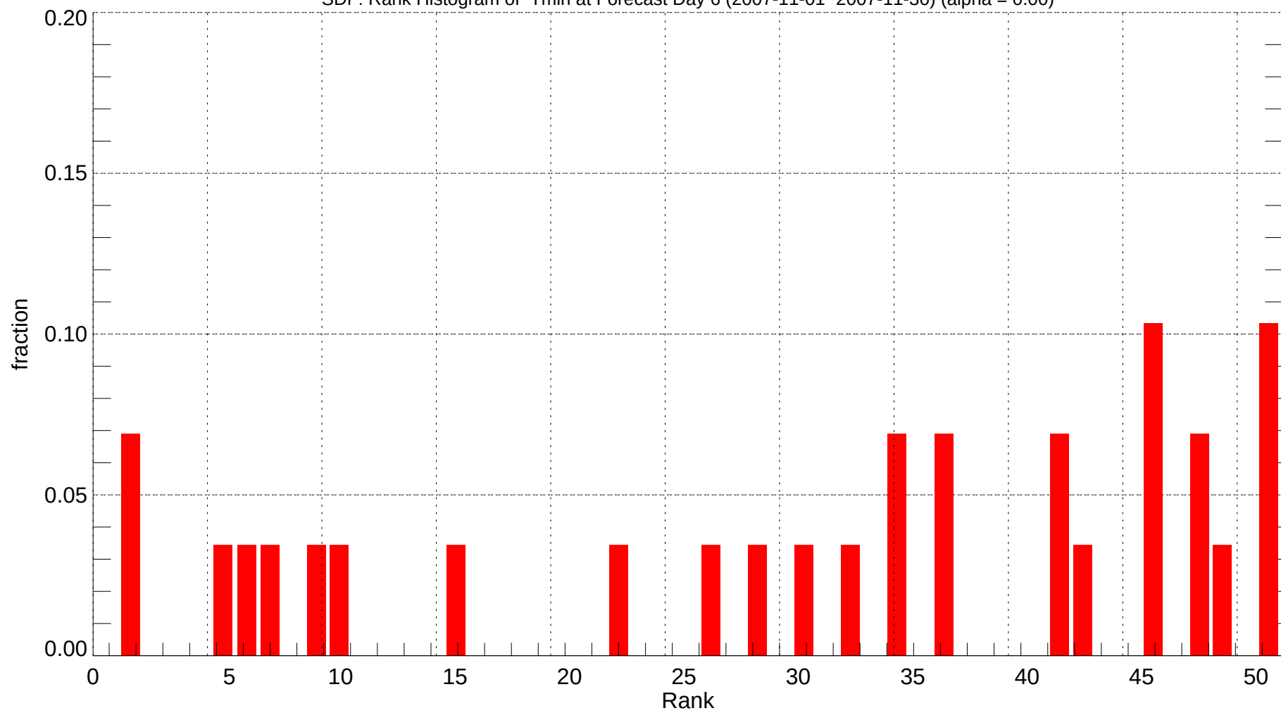
SDF: Rank Histogram of Tmin at Forecast Day 6 (2007-11-01~2007-11-30) (alpha = 0.00)
