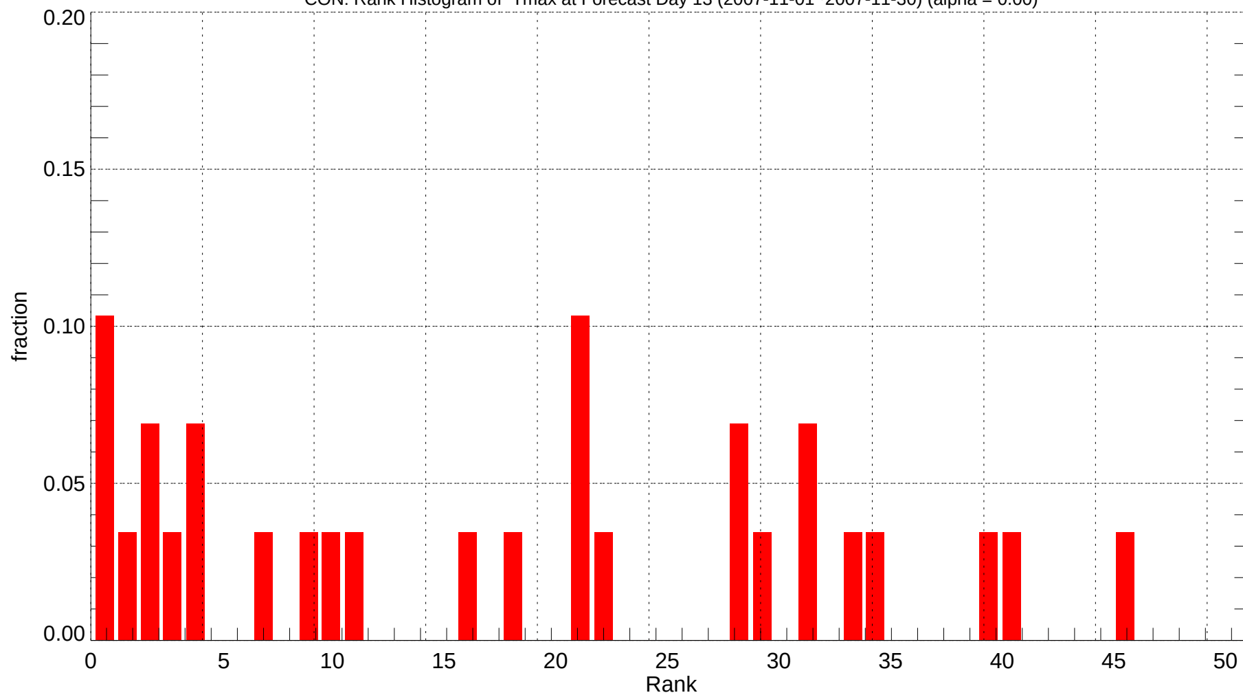
CON: Rank Histogram of Tmax at Forecast Day 13 (2007-11-01~2007-11-30) (alpha = 0.00)
