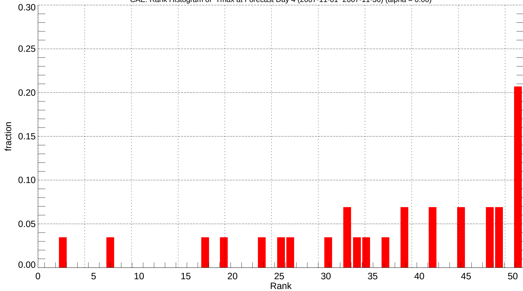
CAE: Rank Histogram of Tmax at Forecast Day 4 (2007-11-01~2007-11-30) (alpha = 0.00)
