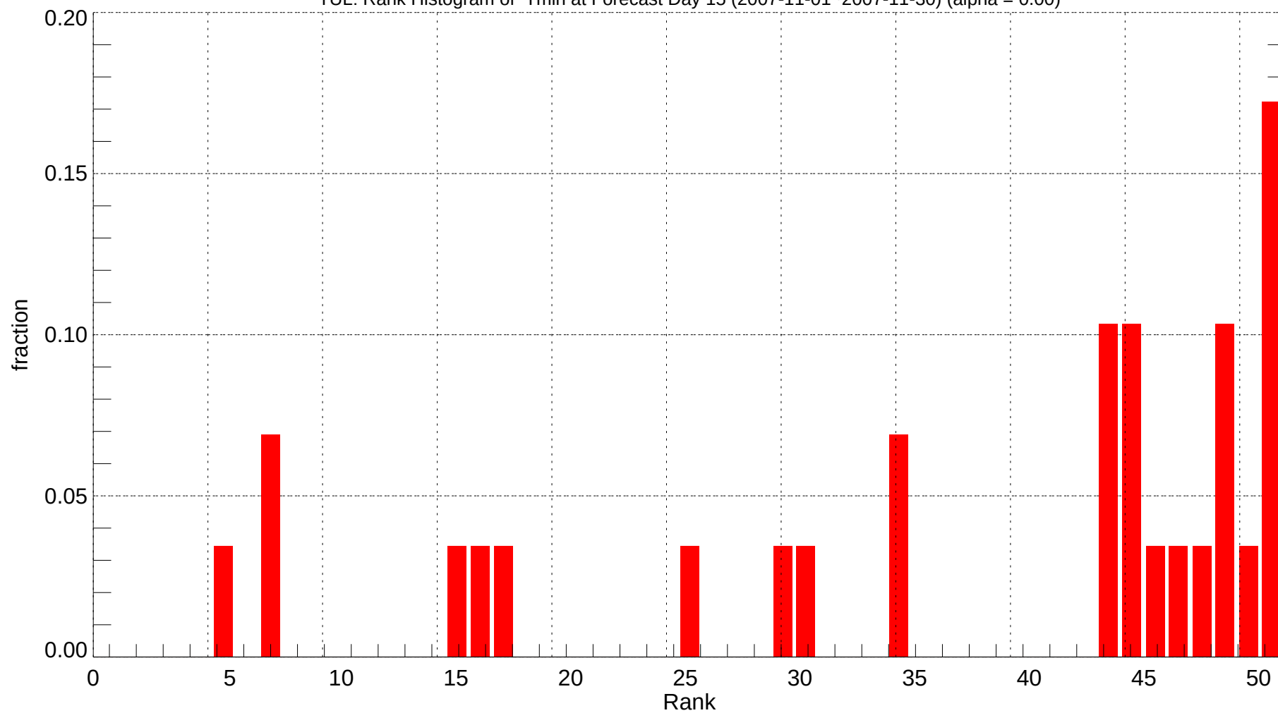
TUL: Rank Histogram of Tmin at Forecast Day 15 (2007-11-01~2007-11-30) (alpha = 0.00)
