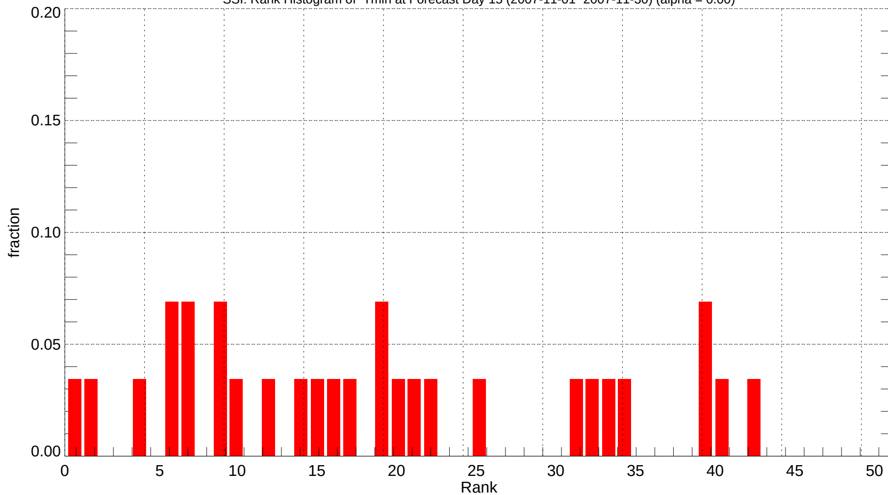
SSI: Rank Histogram of Tmin at Forecast Day 15 (2007-11-01~2007-11-30) (alpha = 0.00)
