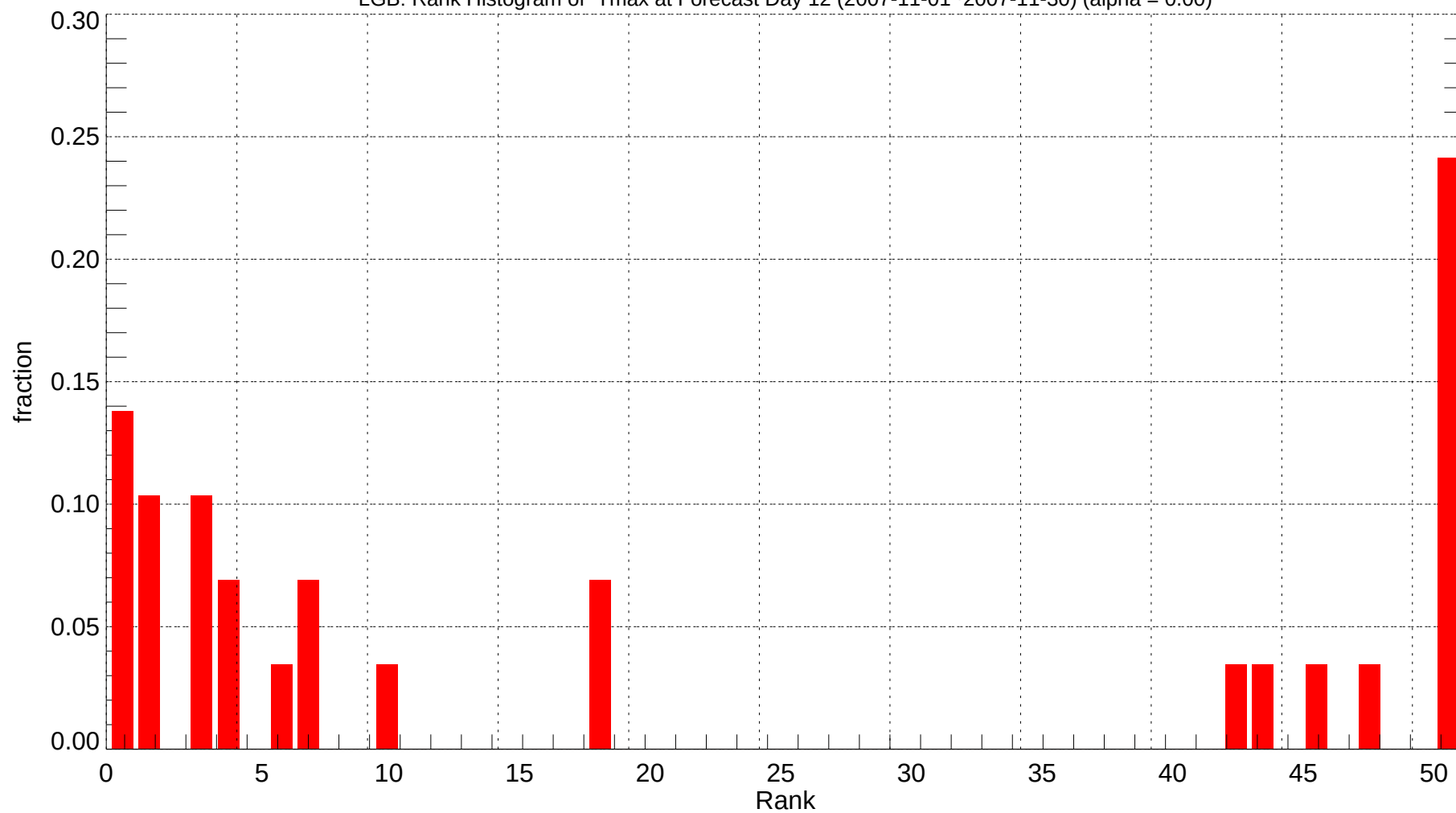
LGB: Rank Histogram of Tmax at Forecast Day 12 (2007-11-01~2007-11-30) (alpha = 0.00)
