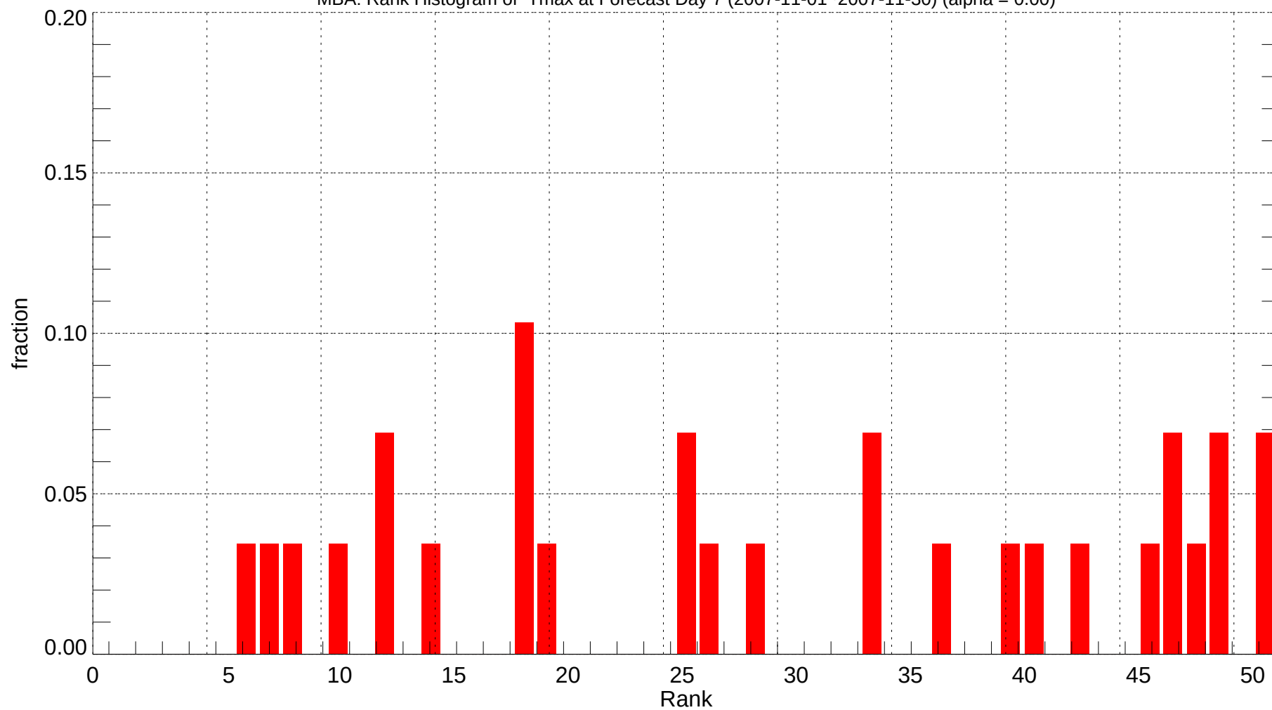
MBA: Rank Histogram of Tmax at Forecast Day 7 (2007-11-01~2007-11-30) (alpha = 0.00)
