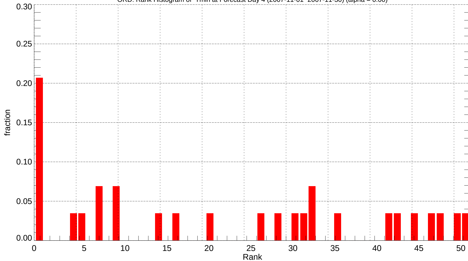
ORD: Rank Histogram of Tmin at Forecast Day 4 (2007-11-01~2007-11-30) (alpha = 0.00)
