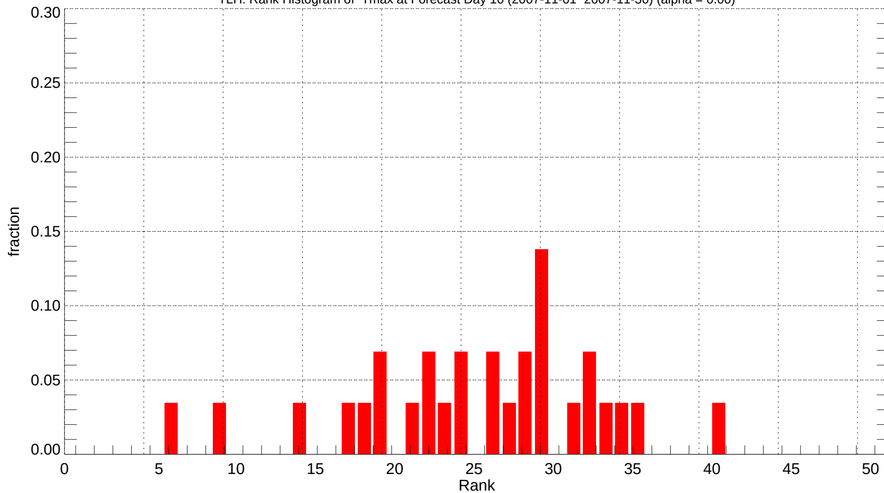
TLH: Rank Histogram of Tmax at Forecast Day 10 (2007-11-01~2007-11-30) (alpha = 0.00)
