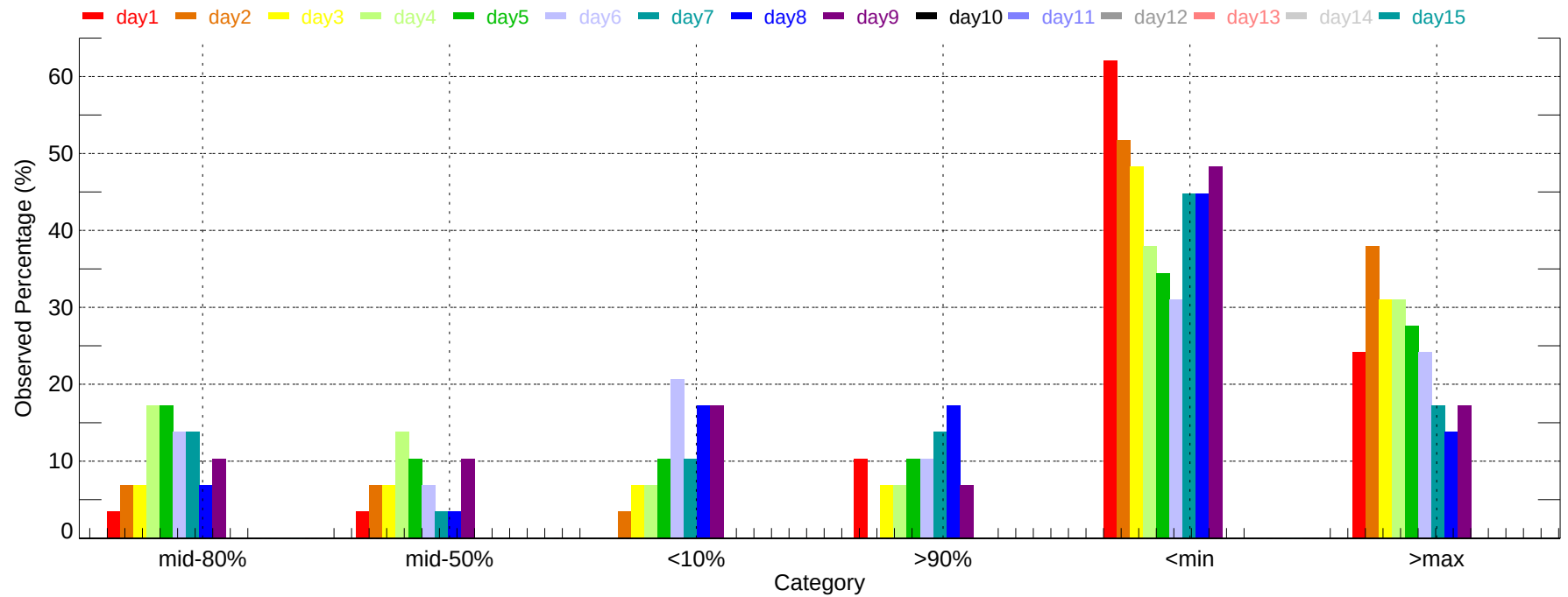
Observed Percentage of Ensembles - NKX: Min Temperature (2007-11-01~2007-11-30)
