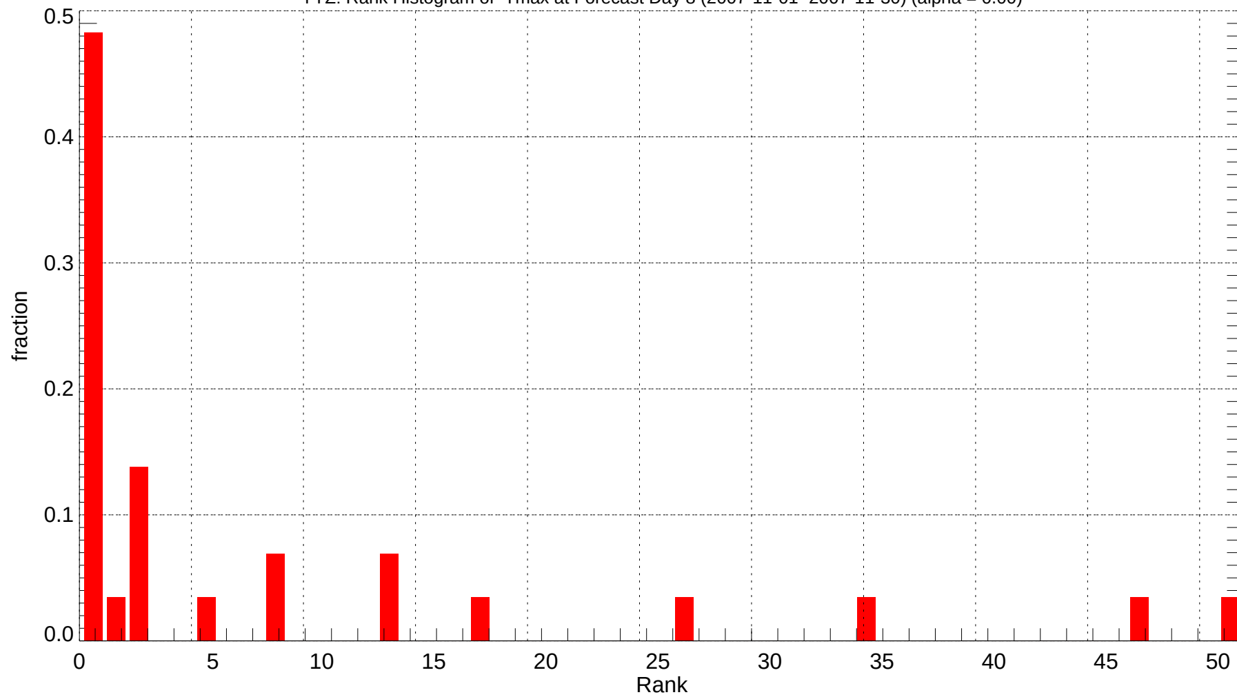
YYZ: Rank Histogram of Tmax at Forecast Day 8 (2007-11-01~2007-11-30) (alpha = 0.00)
