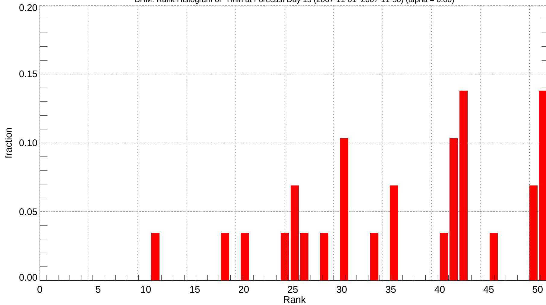
BHM: Rank Histogram of Tmin at Forecast Day 13 (2007-11-01~2007-11-30) (alpha = 0.00)
