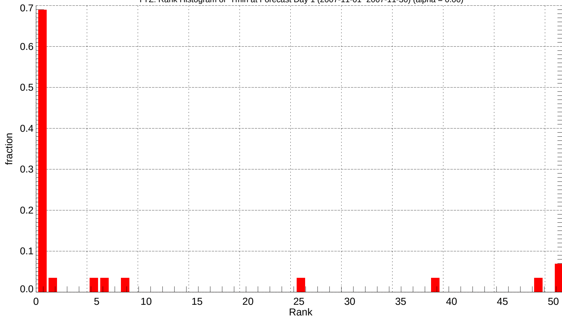
YYZ: Rank Histogram of Tmin at Forecast Day 1 (2007-11-01~2007-11-30) (alpha = 0.00)
