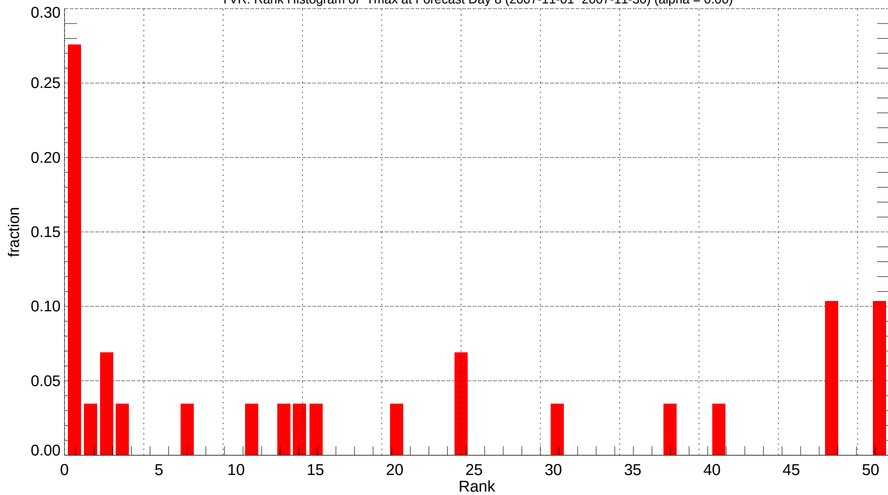
YVR: Rank Histogram of Tmax at Forecast Day 8 (2007-11-01~2007-11-30) (alpha = 0.00)
