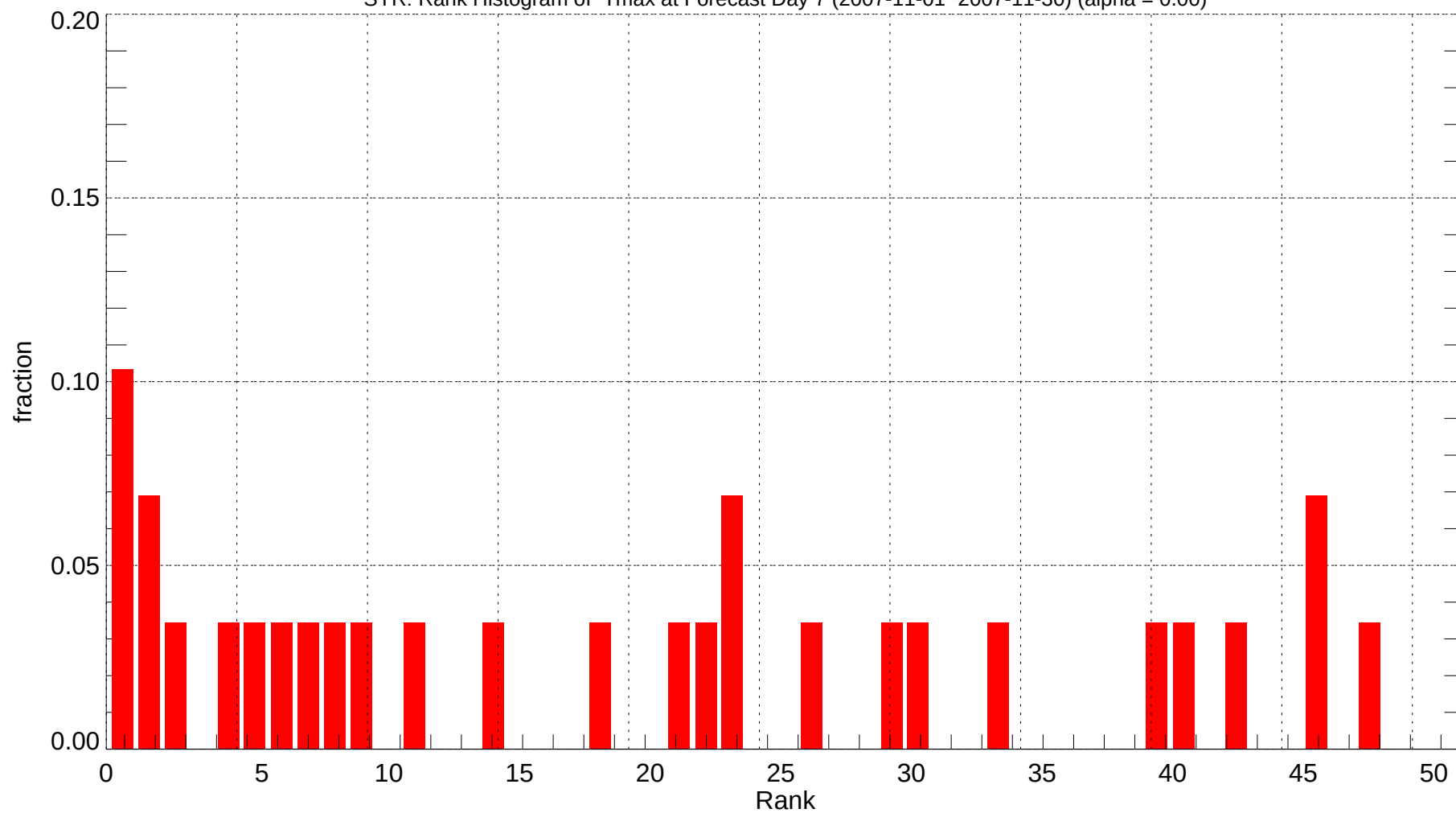
SYR: Rank Histogram of Tmax at Forecast Day 7 (2007-11-01~2007-11-30) (alpha = 0.00)
