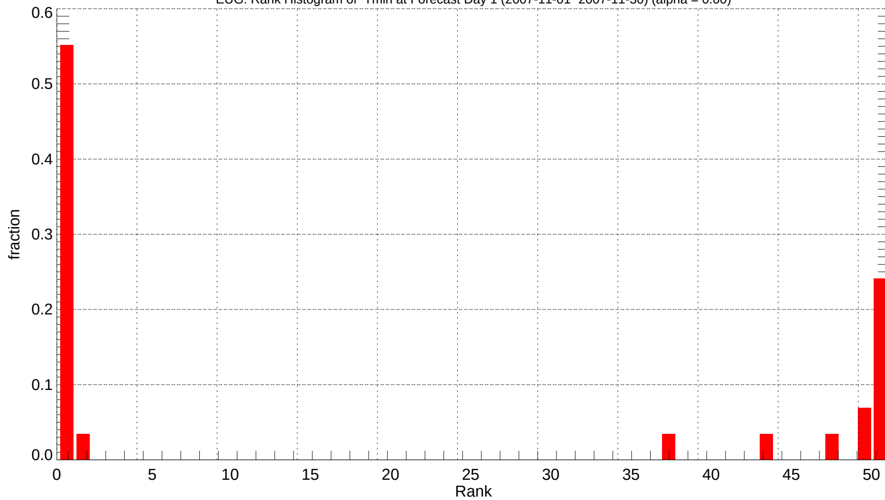
EUG: Rank Histogram of Tmin at Forecast Day 1 (2007-11-01~2007-11-30) (alpha = 0.00)
