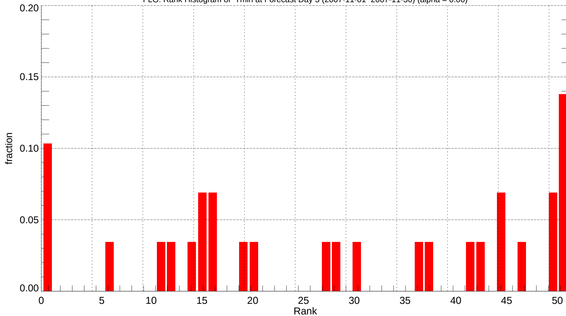
FLG: Rank Histogram of Tmin at Forecast Day 3 (2007-11-01~2007-11-30) (alpha = 0.00)
