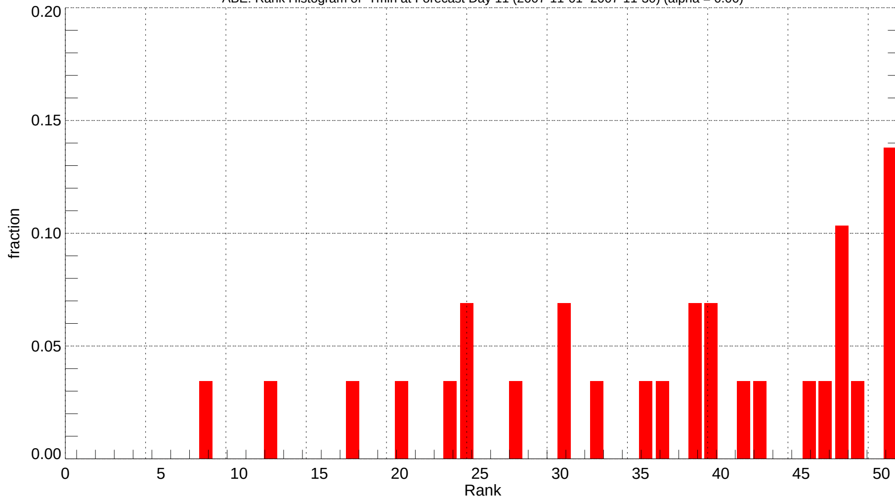
ABE: Rank Histogram of Tmin at Forecast Day 11 (2007-11-01~2007-11-30) (alpha = 0.00)
