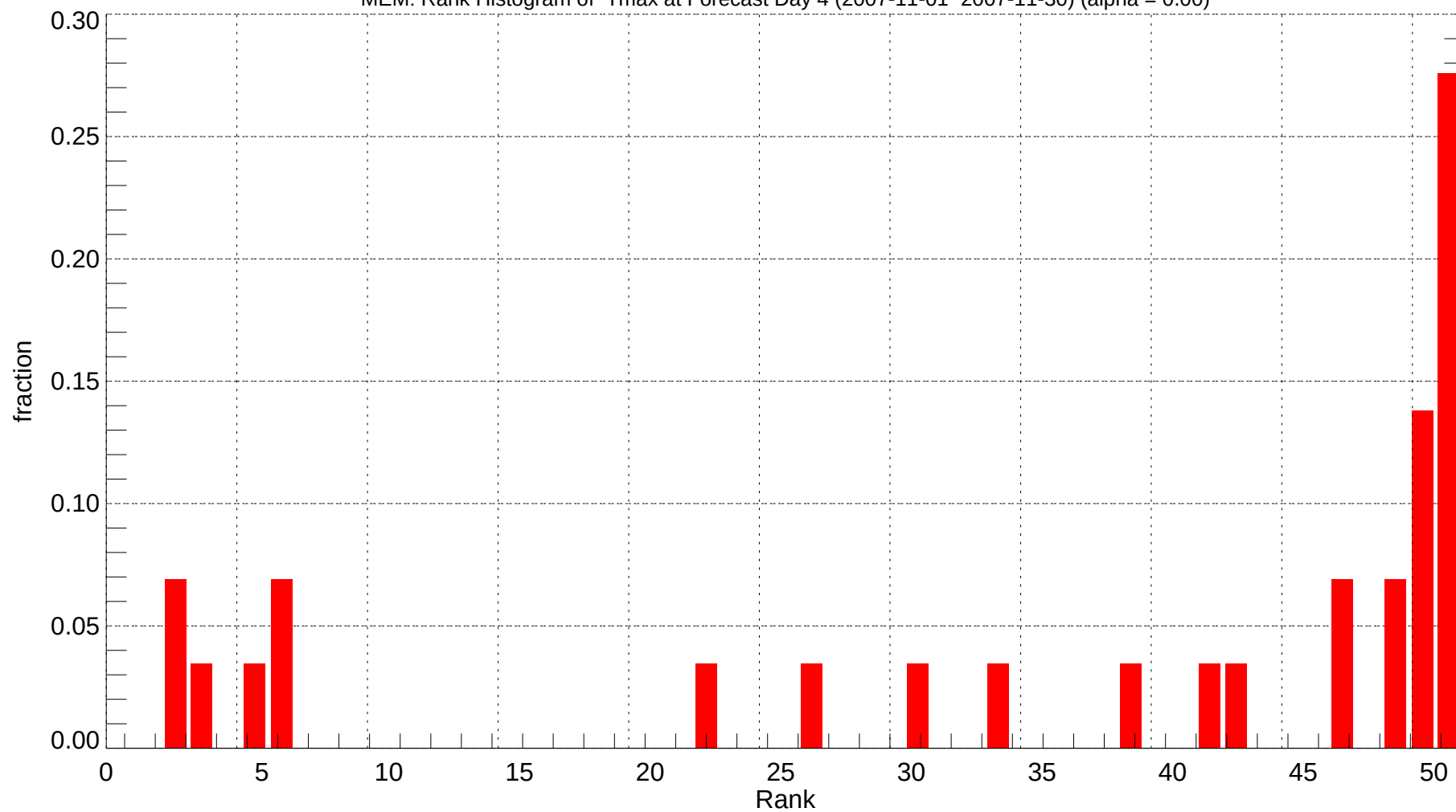
MEM: Rank Histogram of Tmax at Forecast Day 4 (2007-11-01~2007-11-30) (alpha = 0.00)
