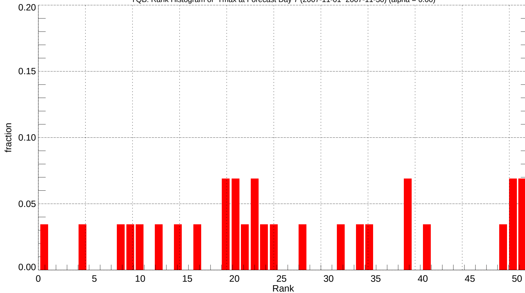
YQB: Rank Histogram of Tmax at Forecast Day 7 (2007-11-01~2007-11-30) (alpha = 0.00)
