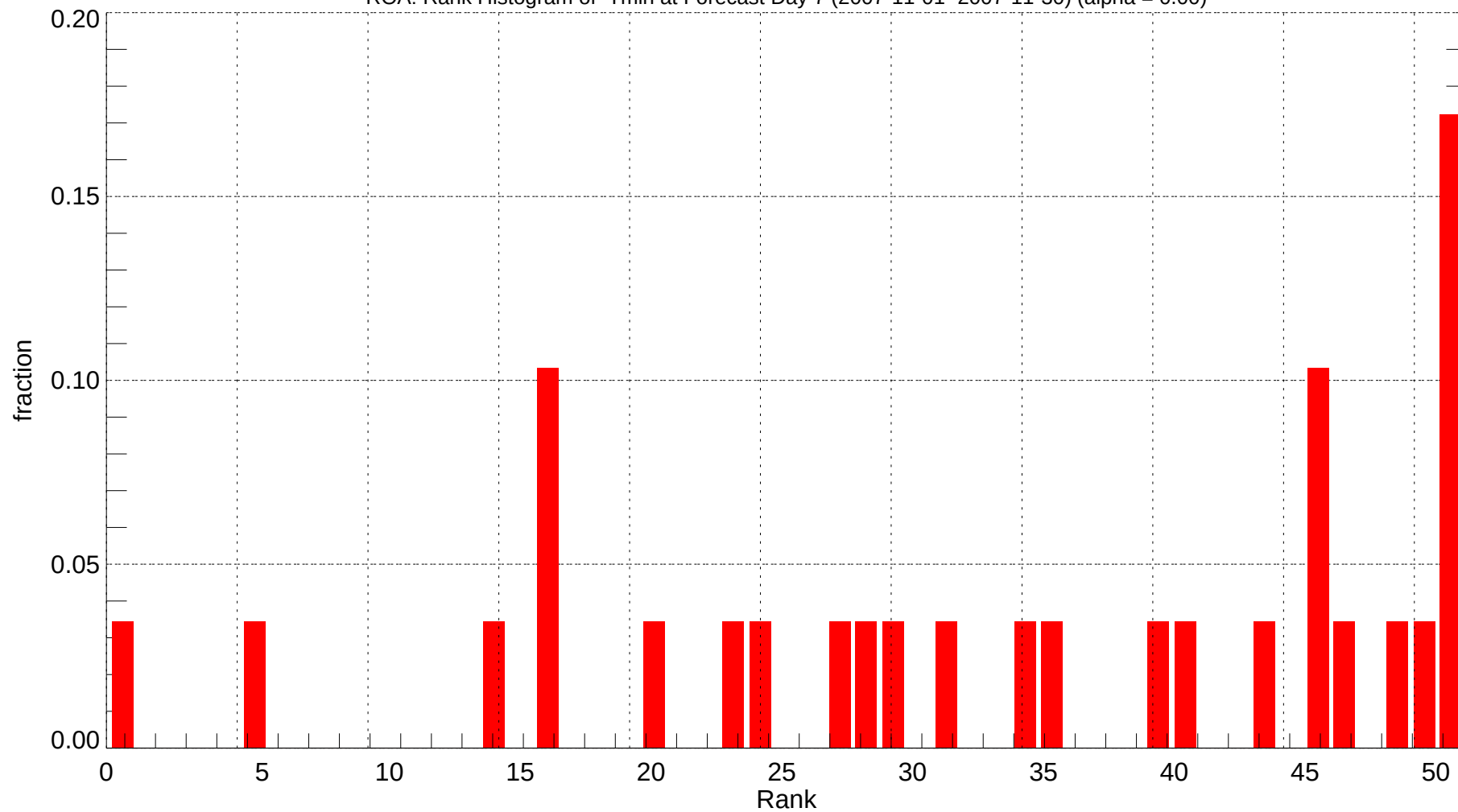
ROA: Rank Histogram of Tmin at Forecast Day 7 (2007-11-01~2007-11-30) (alpha = 0.00)
