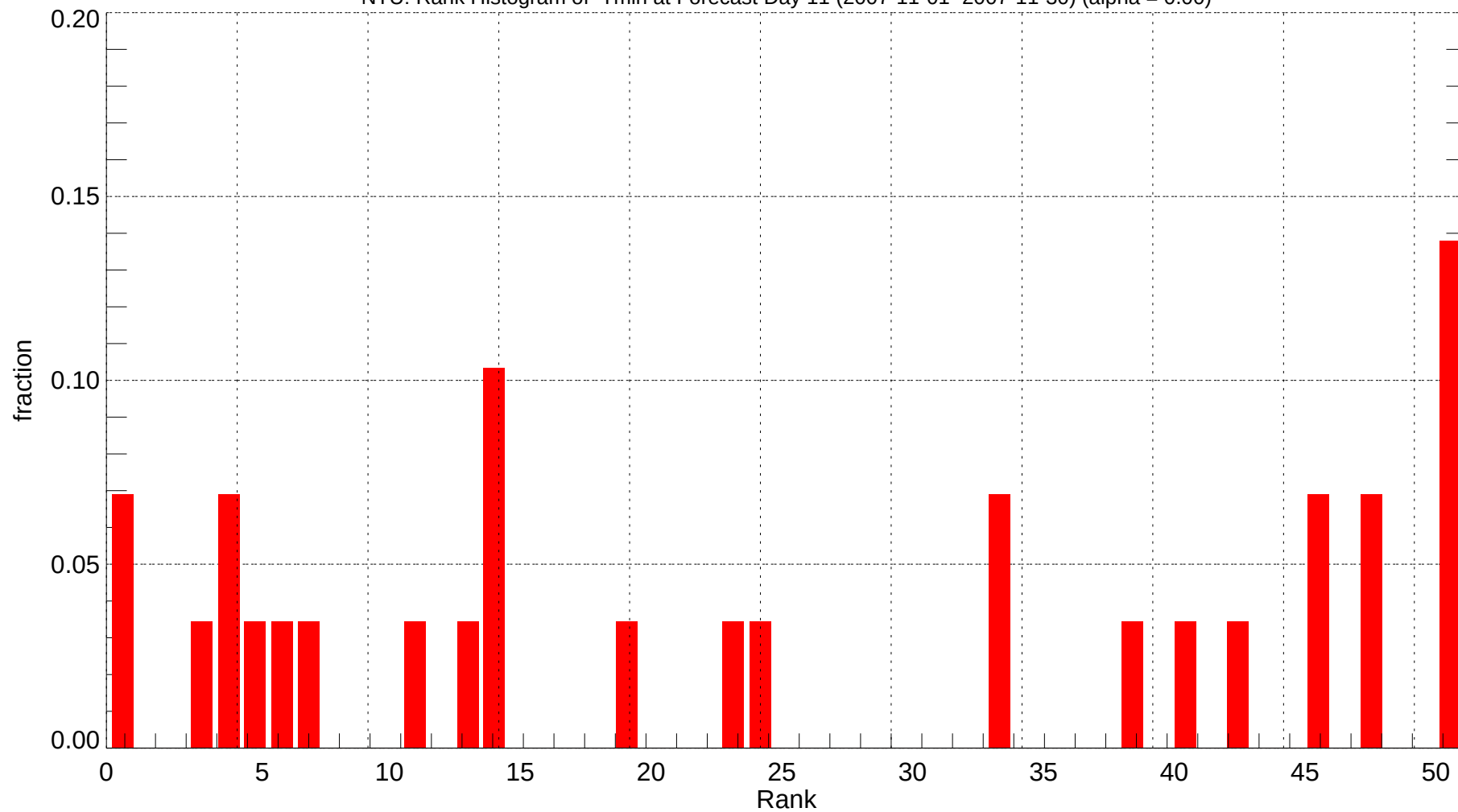
NTU: Rank Histogram of Tmin at Forecast Day 11 (2007-11-01~2007-11-30) (alpha = 0.00)
