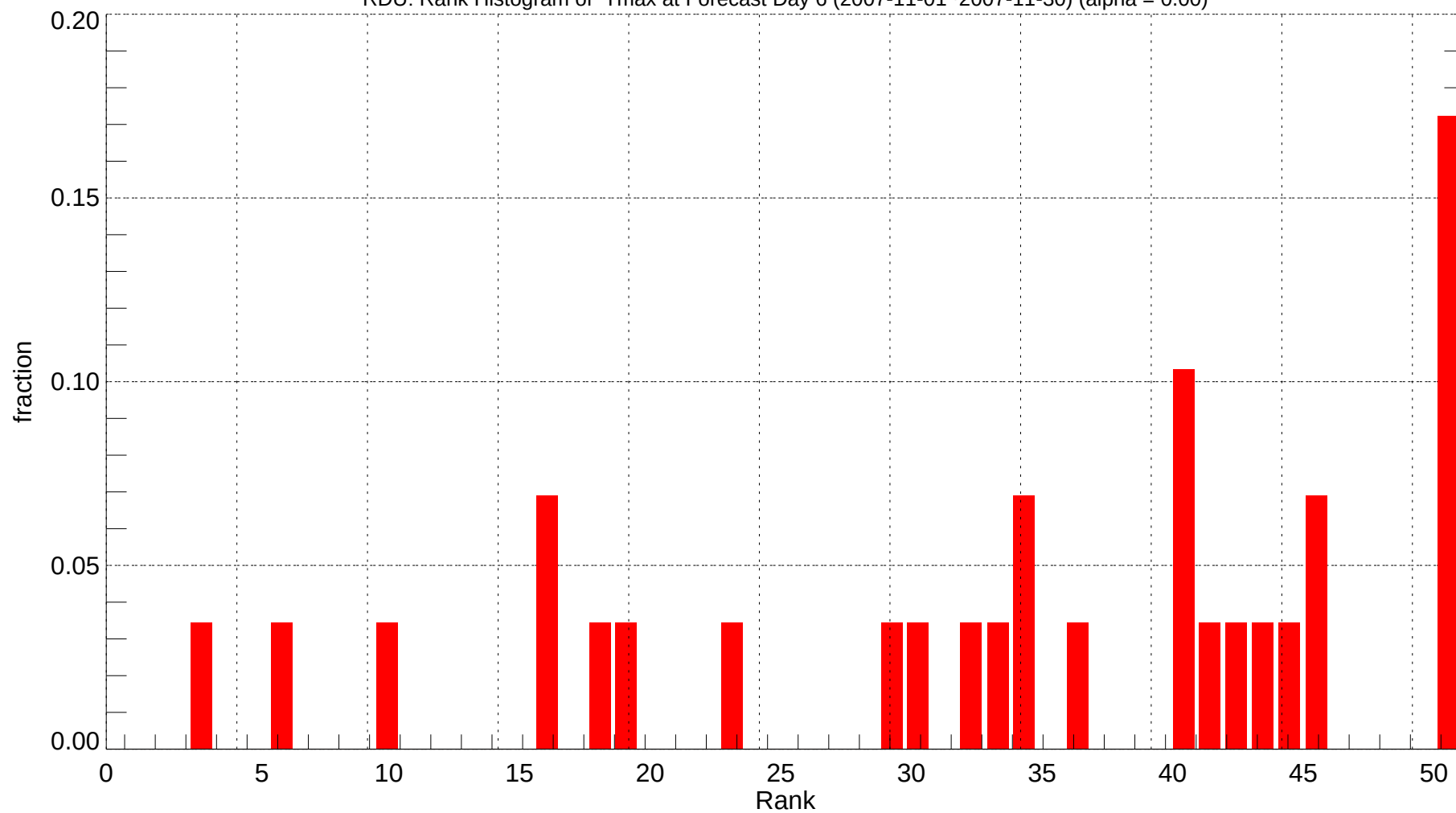
RDU: Rank Histogram of Tmax at Forecast Day 6 (2007-11-01~2007-11-30) (alpha = 0.00)
