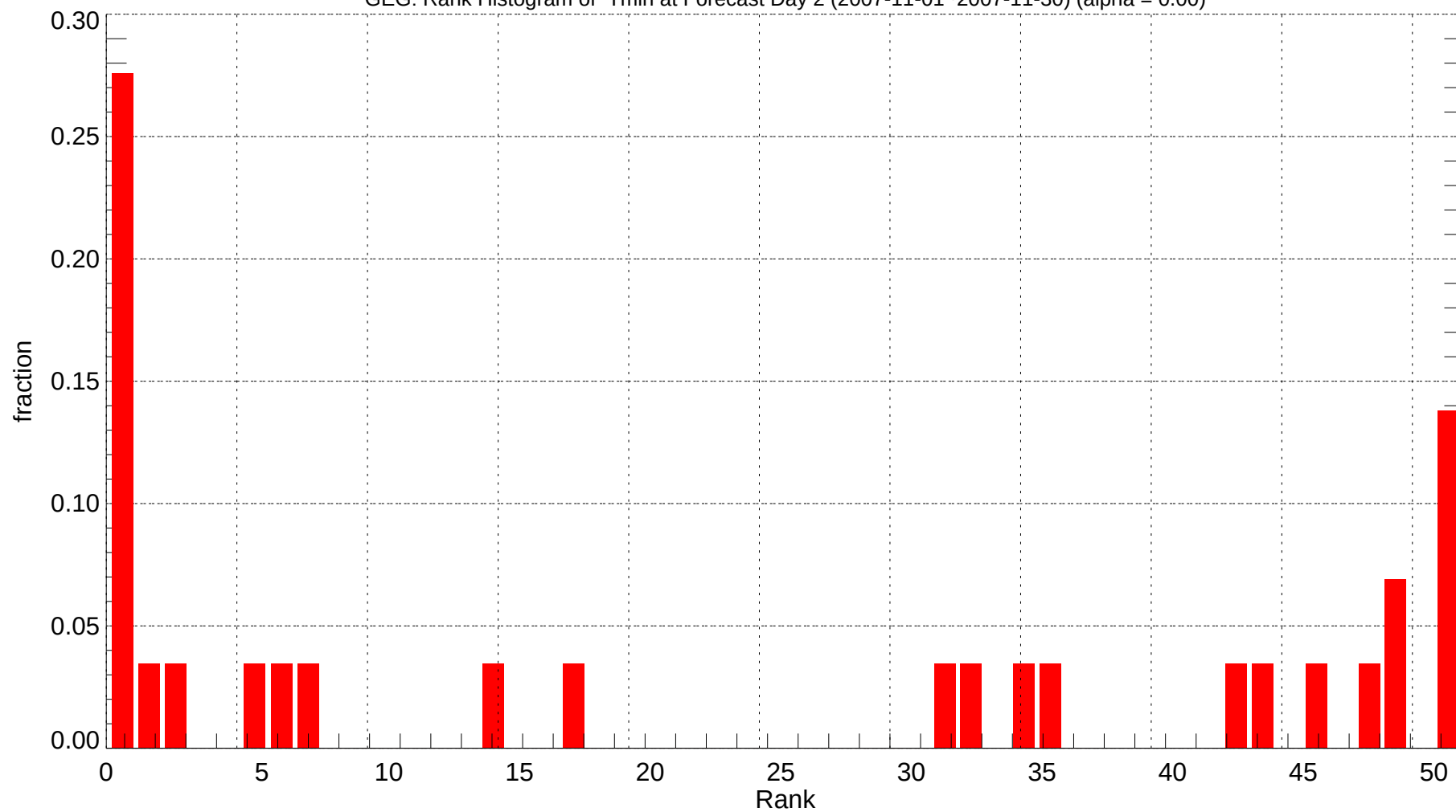
GEG: Rank Histogram of Tmin at Forecast Day 2 (2007-11-01~2007-11-30) (alpha = 0.00)
