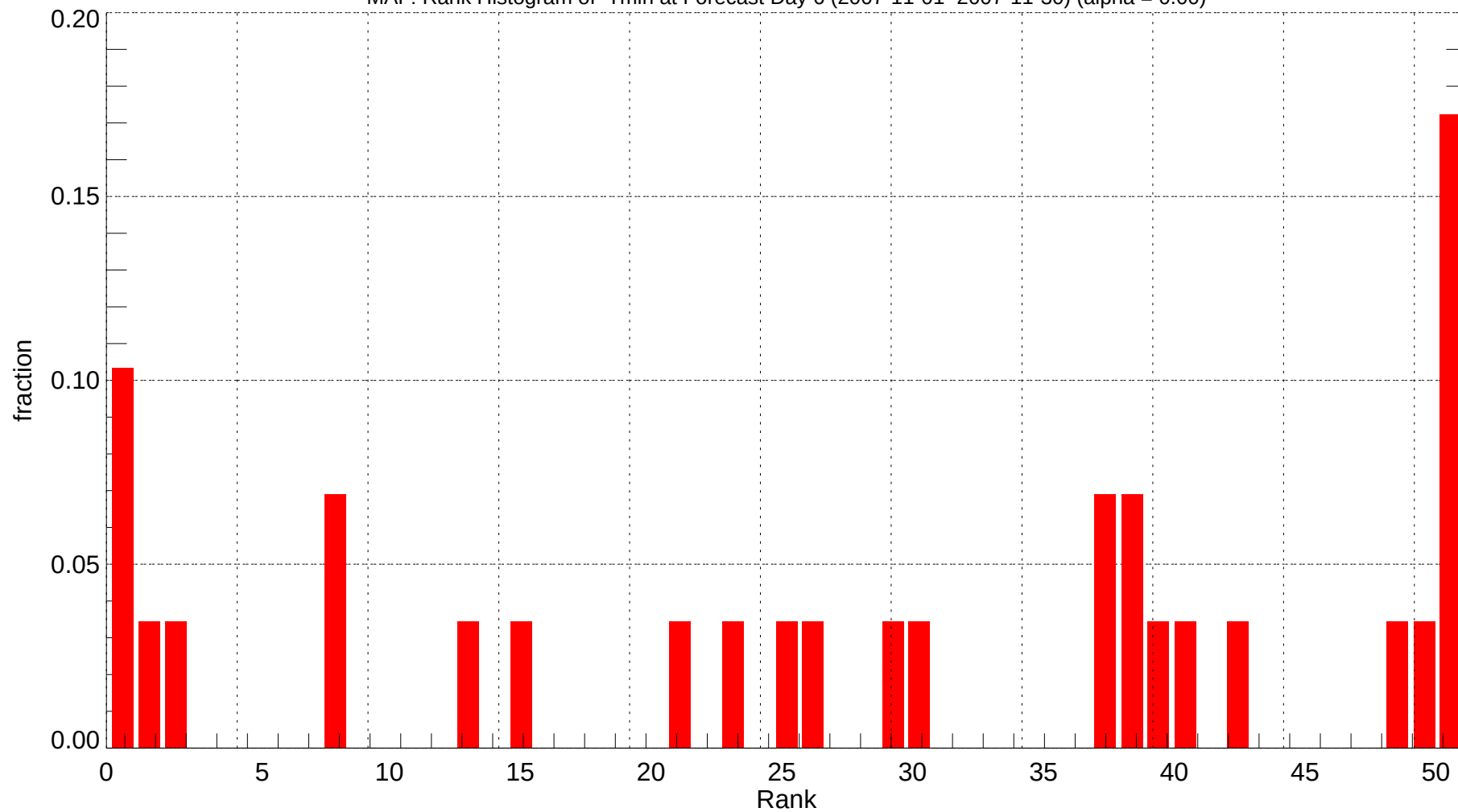
MAF: Rank Histogram of Tmin at Forecast Day 6 (2007-11-01~2007-11-30) (alpha = 0.00)
