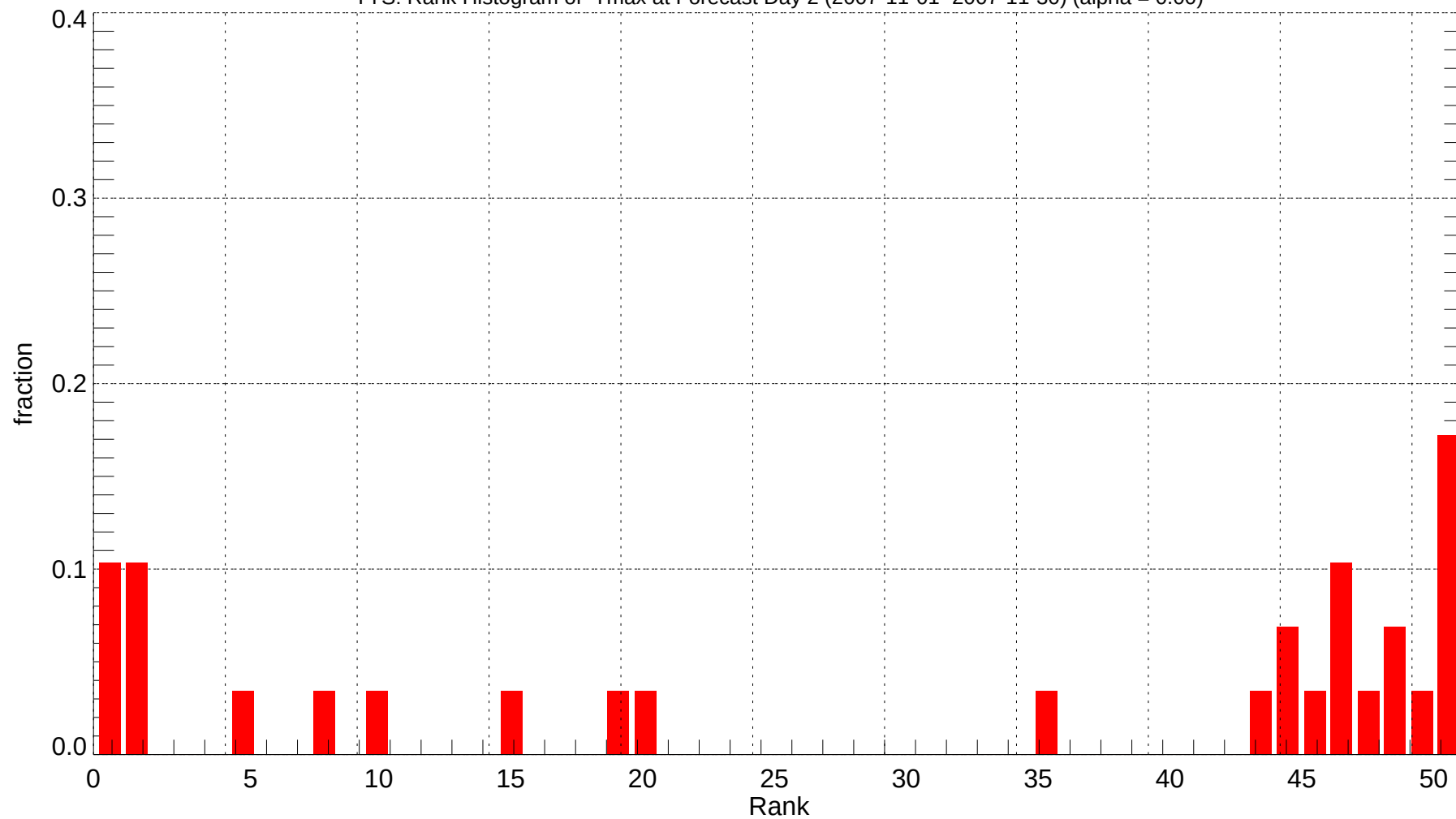
TYS: Rank Histogram of Tmax at Forecast Day 2 (2007-11-01~2007-11-30) (alpha = 0.00)
