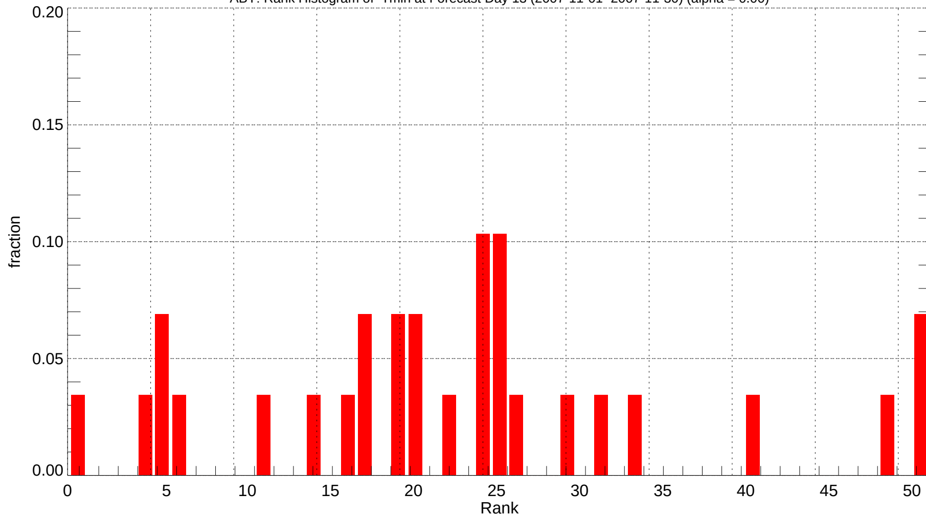
ABY: Rank Histogram of Tmin at Forecast Day 13 (2007-11-01~2007-11-30) (alpha = 0.00)
