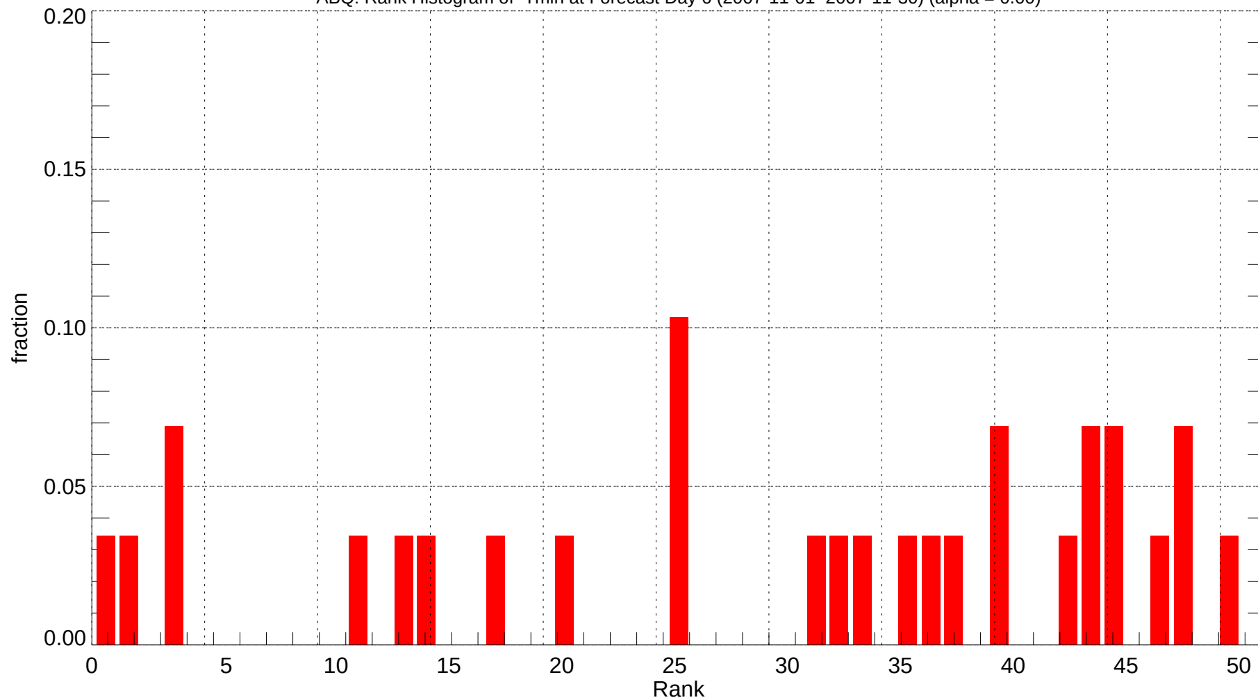
ABQ: Rank Histogram of Tmin at Forecast Day 6 (2007-11-01~2007-11-30) (alpha = 0.00)
