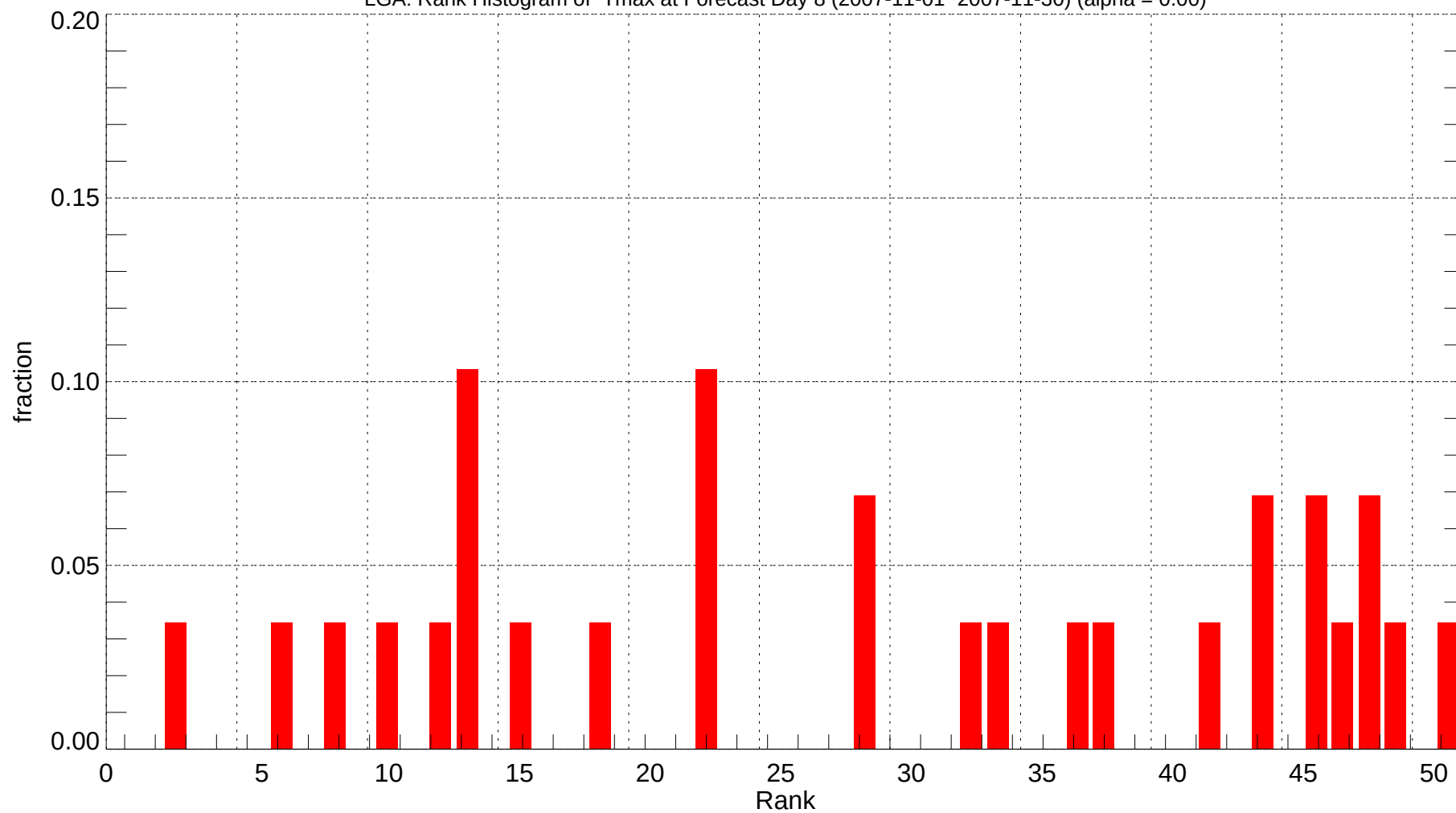
LGA: Rank Histogram of Tmax at Forecast Day 8 (2007-11-01~2007-11-30) (alpha = 0.00)
