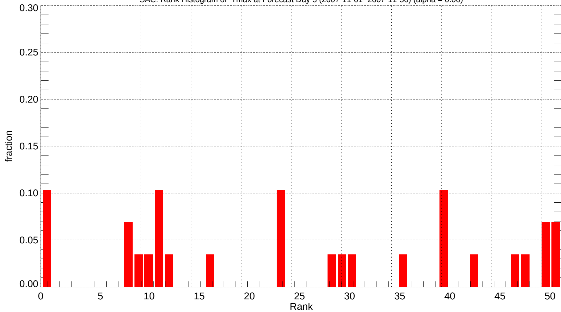
SAC: Rank Histogram of Tmax at Forecast Day 3 (2007-11-01~2007-11-30) (alpha = 0.00)
