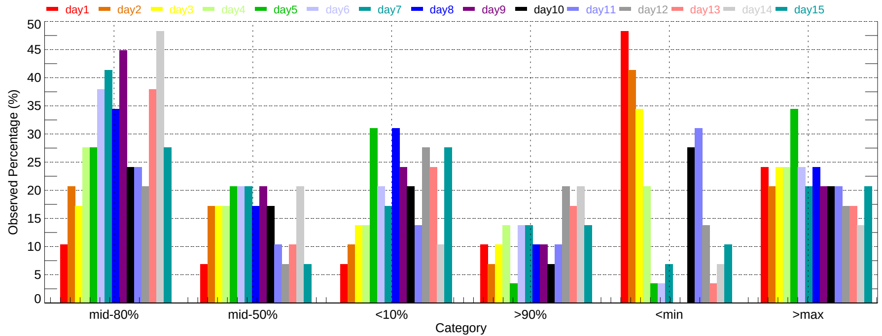
Observed Percentage of Ensembles - LGB: Min Temperature (2007-11-01~2007-11-30)
