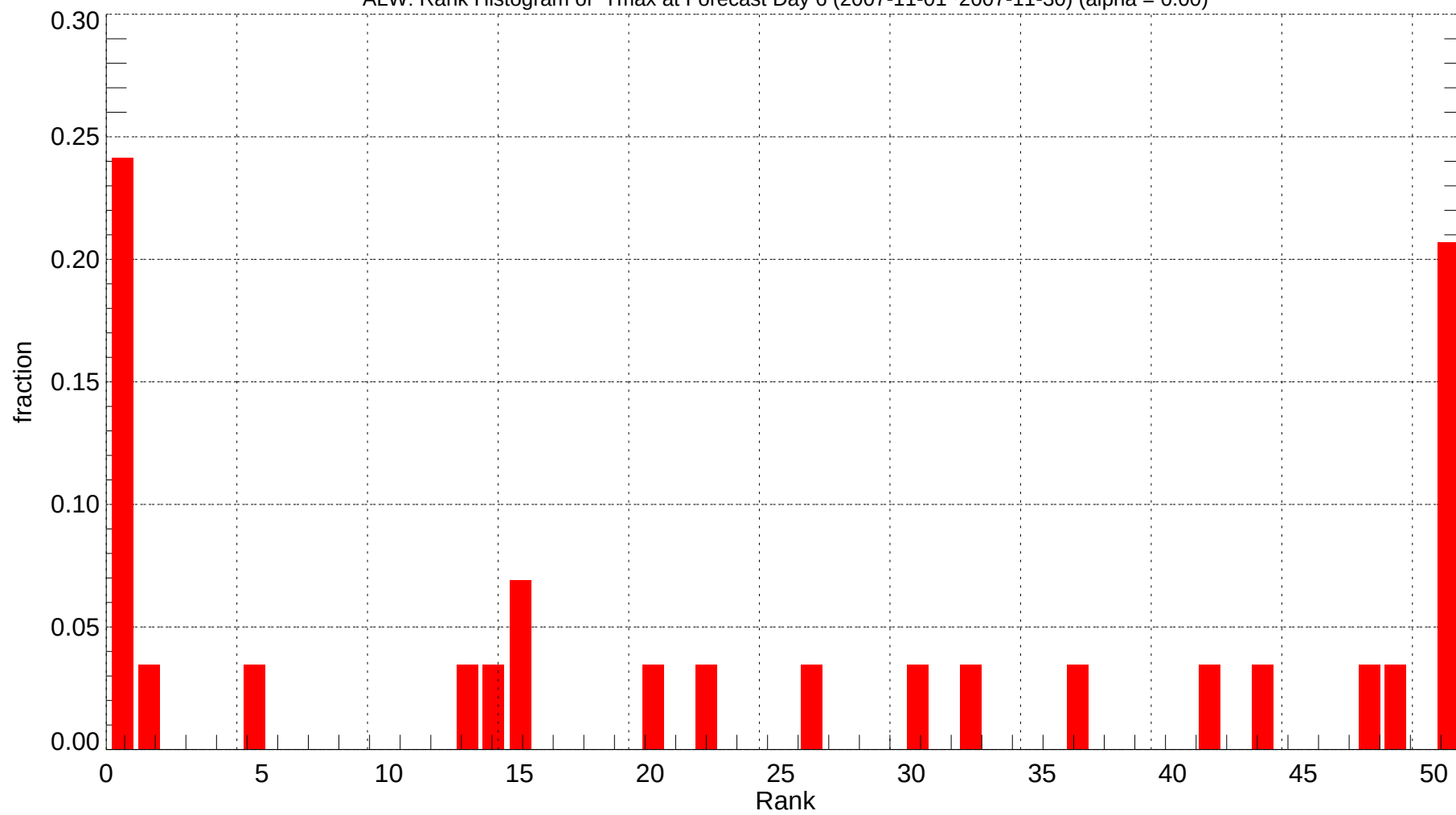
ALW: Rank Histogram of Tmax at Forecast Day 6 (2007-11-01~2007-11-30) (alpha = 0.00)
