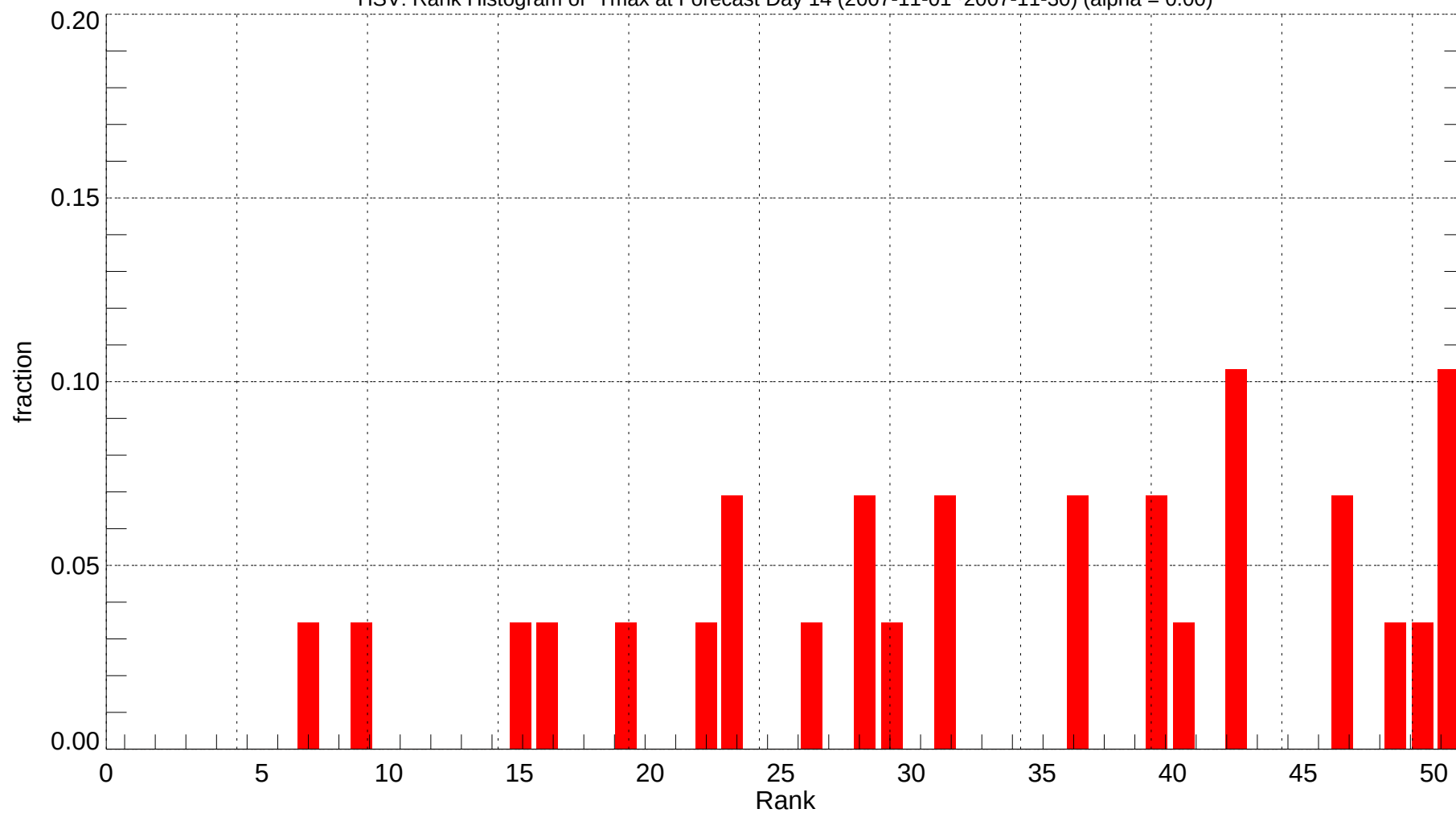
HSV: Rank Histogram of Tmax at Forecast Day 14 (2007-11-01~2007-11-30) (alpha = 0.00)
