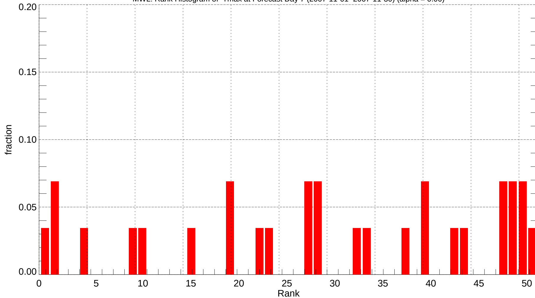
MWL: Rank Histogram of Tmax at Forecast Day 7 (2007-11-01~2007-11-30) (alpha = 0.00)
