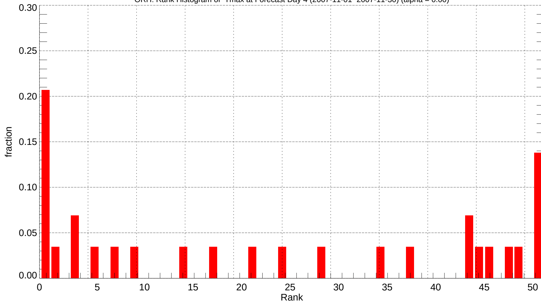
ORH: Rank Histogram of Tmax at Forecast Day 4 (2007-11-01~2007-11-30) (alpha = 0.00)
