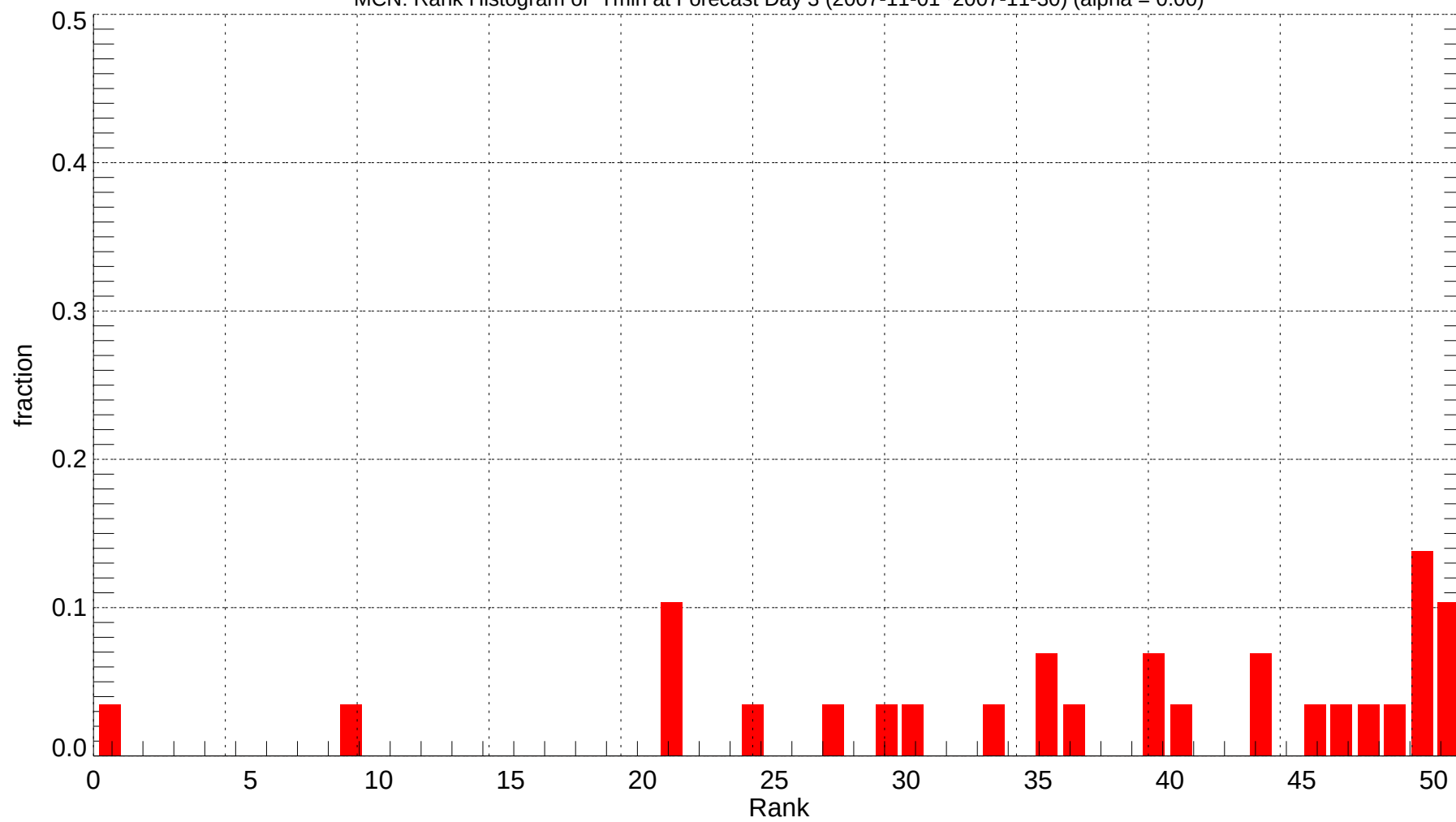
MCN: Rank Histogram of Tmin at Forecast Day 3 (2007-11-01~2007-11-30) (alpha = 0.00)
