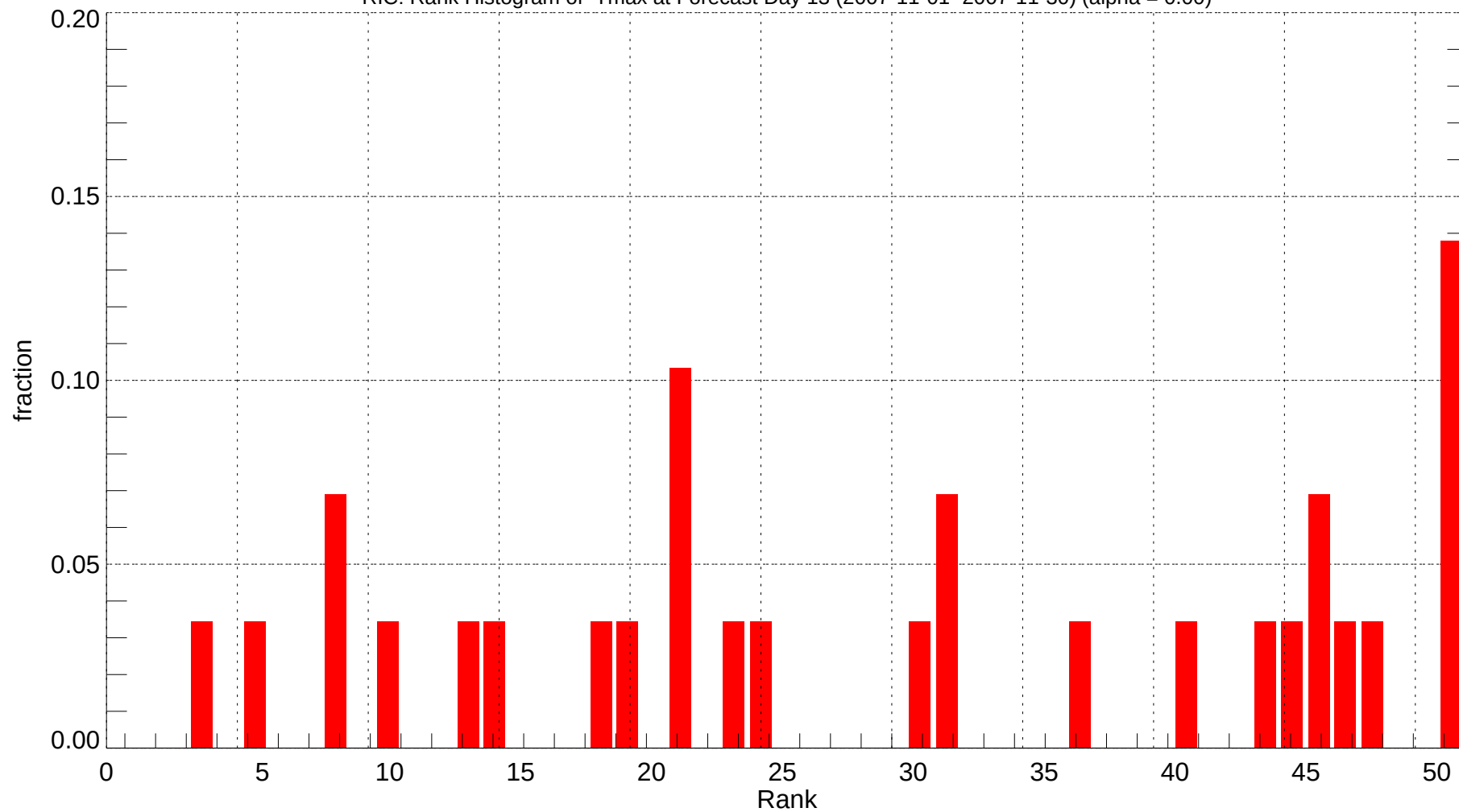
RIC: Rank Histogram of Tmax at Forecast Day 13 (2007-11-01~2007-11-30) (alpha = 0.00)
