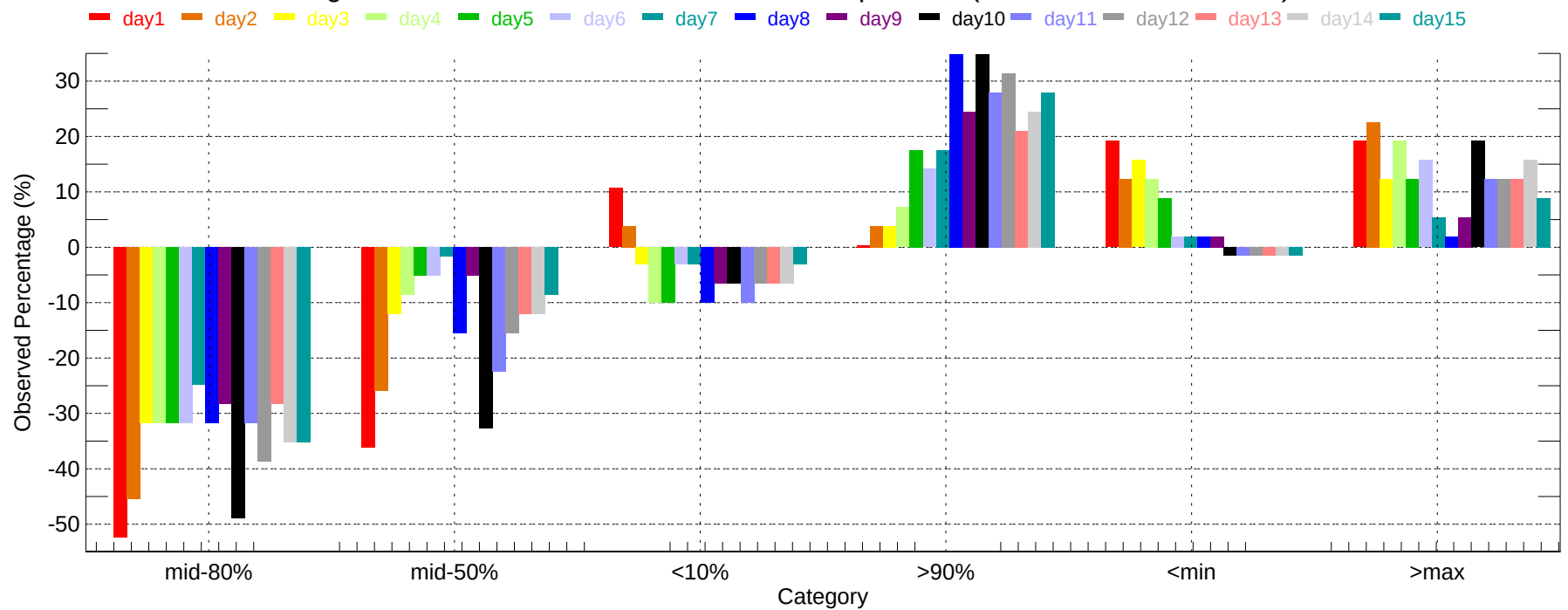
Observed Percentage Deviation of Ensembles - MCI: Min Temperature (2007-11-01~2007-11-30)
