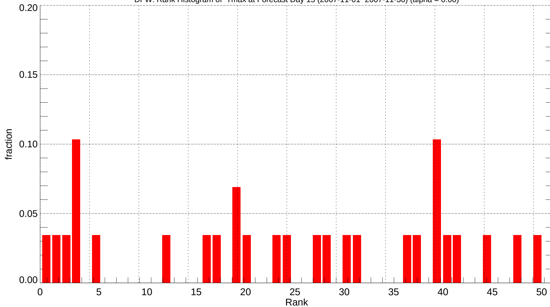
DFW: Rank Histogram of Tmax at Forecast Day 15 (2007-11-01~2007-11-30) (alpha = 0.00)
