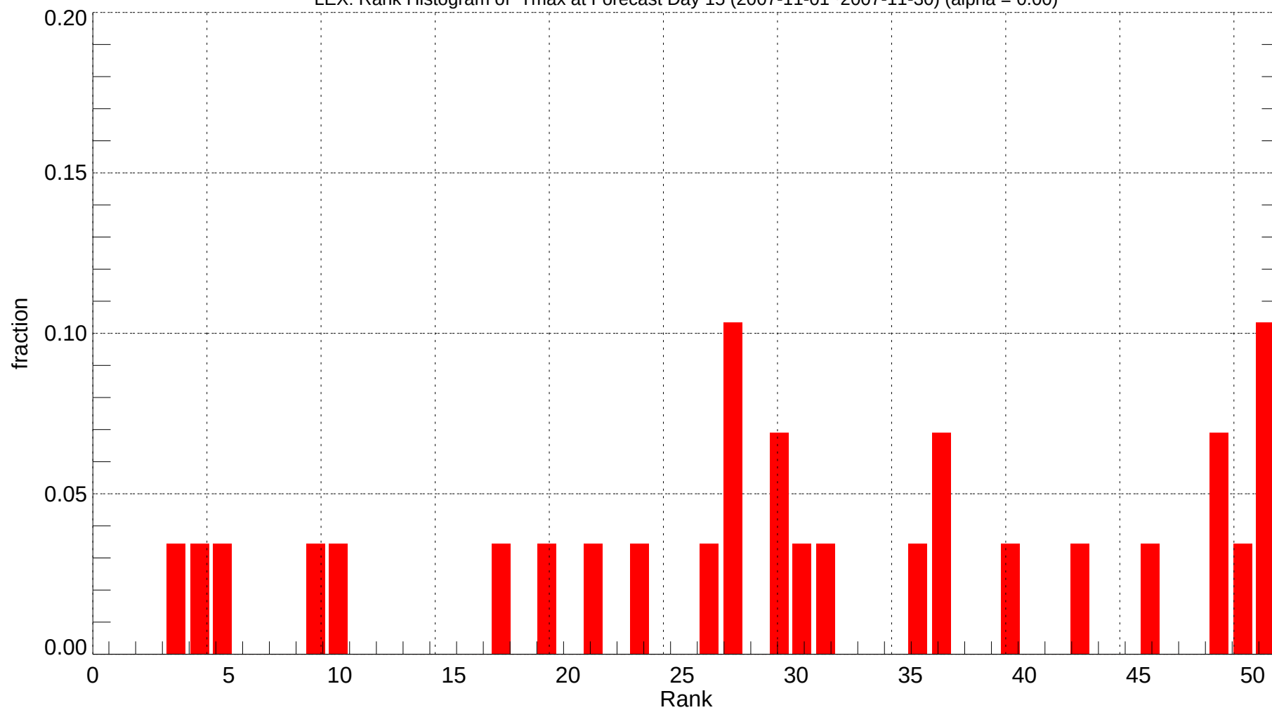
LEX: Rank Histogram of Tmax at Forecast Day 15 (2007-11-01~2007-11-30) (alpha = 0.00)
