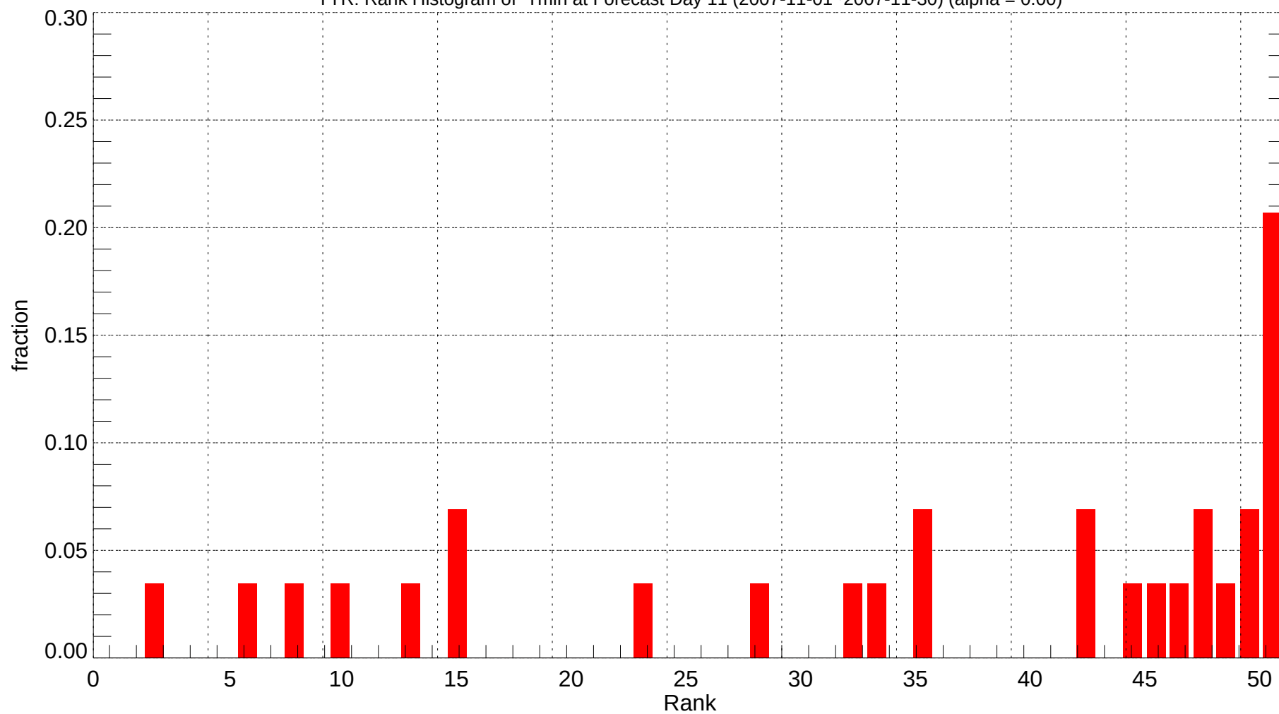
TYR: Rank Histogram of Tmin at Forecast Day 11 (2007-11-01~2007-11-30) (alpha = 0.00)
