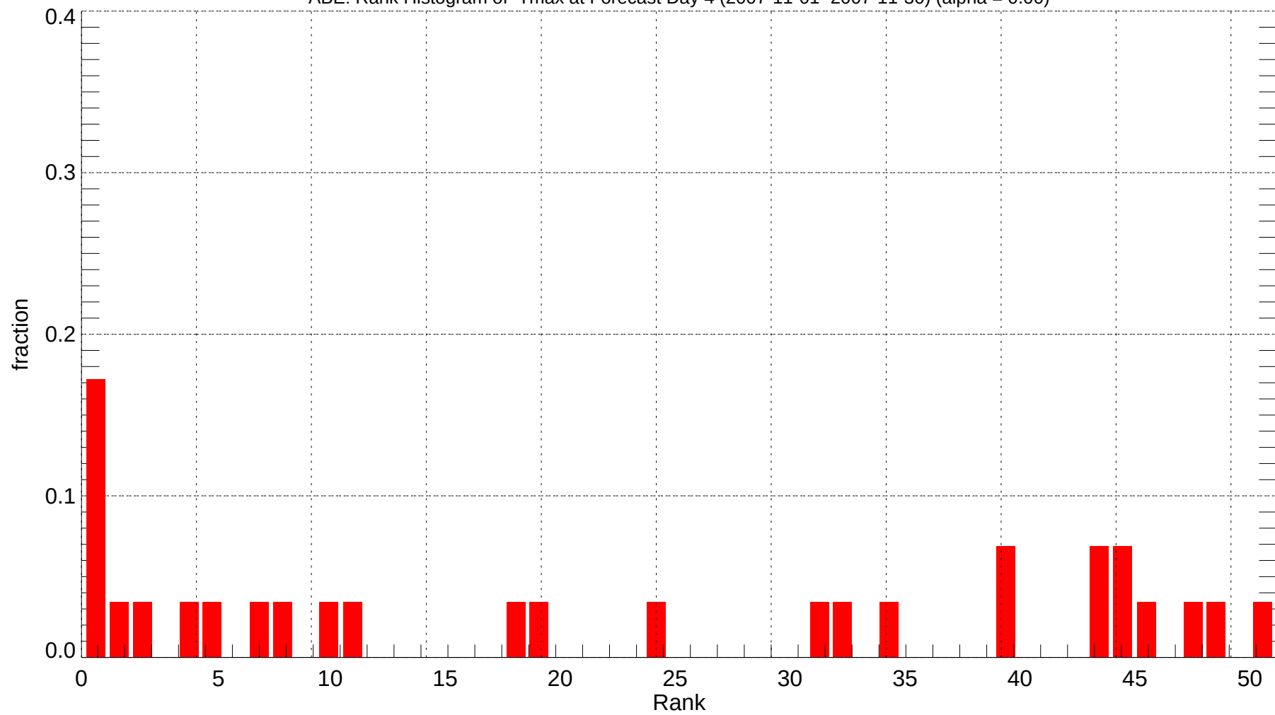
ABE: Rank Histogram of Tmax at Forecast Day 4 (2007-11-01~2007-11-30) (alpha = 0.00)
