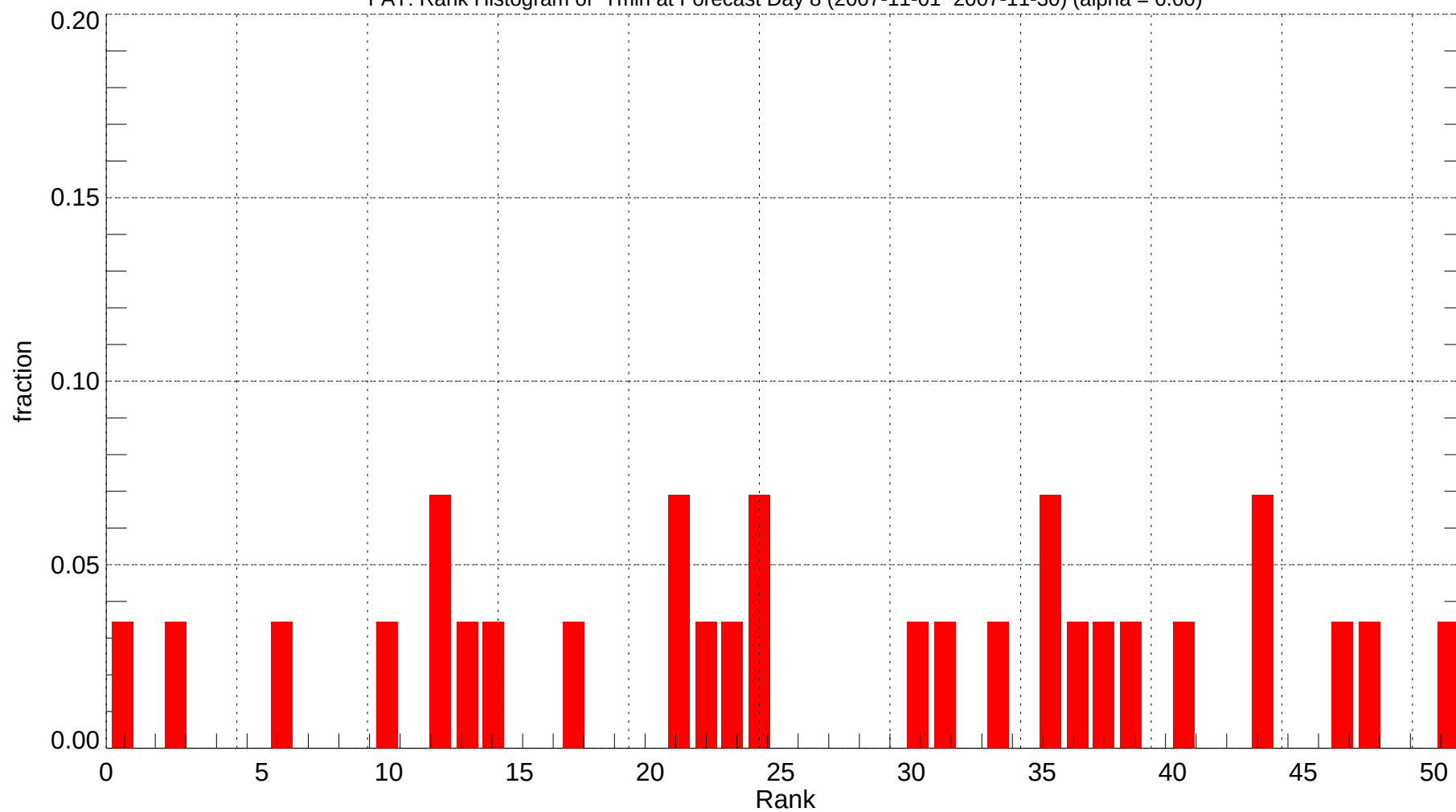
FAT: Rank Histogram of Tmin at Forecast Day 8 (2007-11-01~2007-11-30) (alpha = 0.00)
