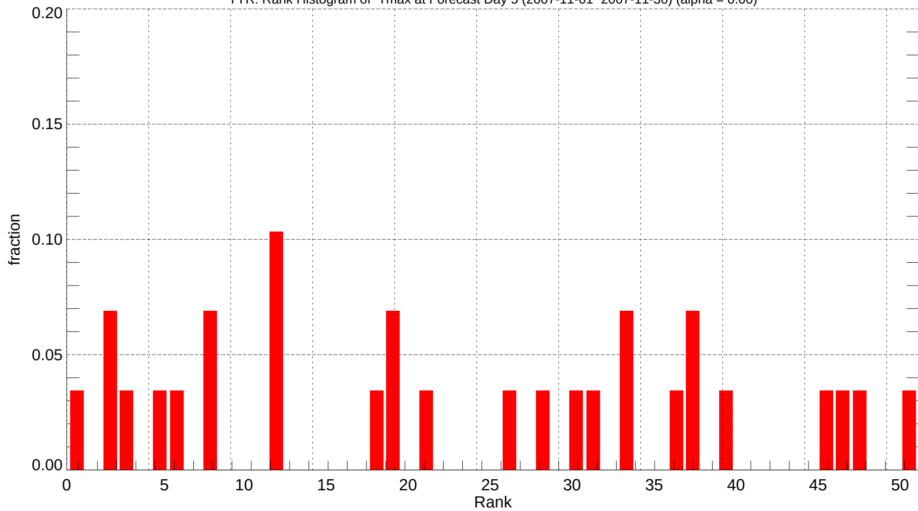
TYR: Rank Histogram of Tmax at Forecast Day 5 (2007-11-01~2007-11-30) (alpha = 0.00)
