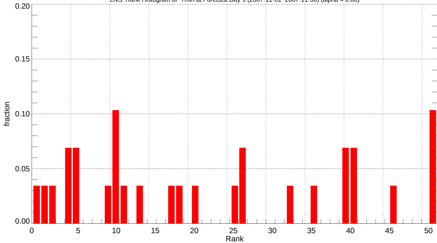
LNS: Rank Histogram of Tmin at Forecast Day 9 (2007-11-01~2007-11-30) (alpha = 0.00)
