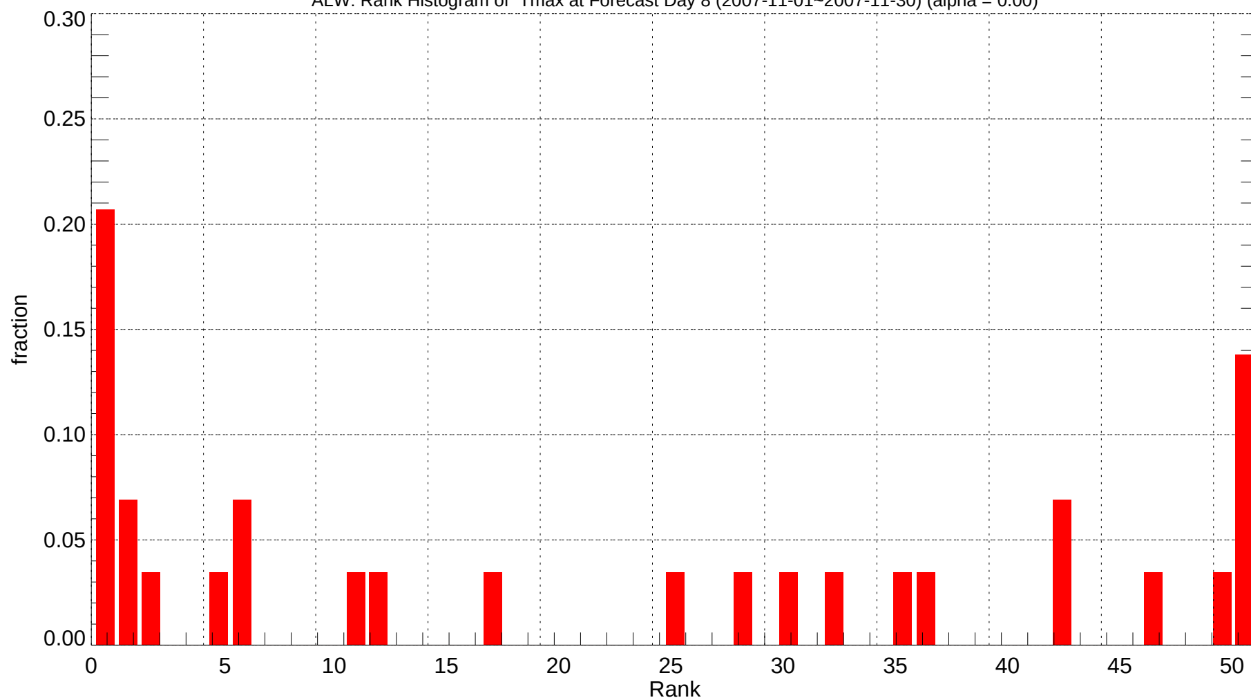
ALW: Rank Histogram of Tmax at Forecast Day 8 (2007-11-01~2007-11-30) (alpha = 0.00)
