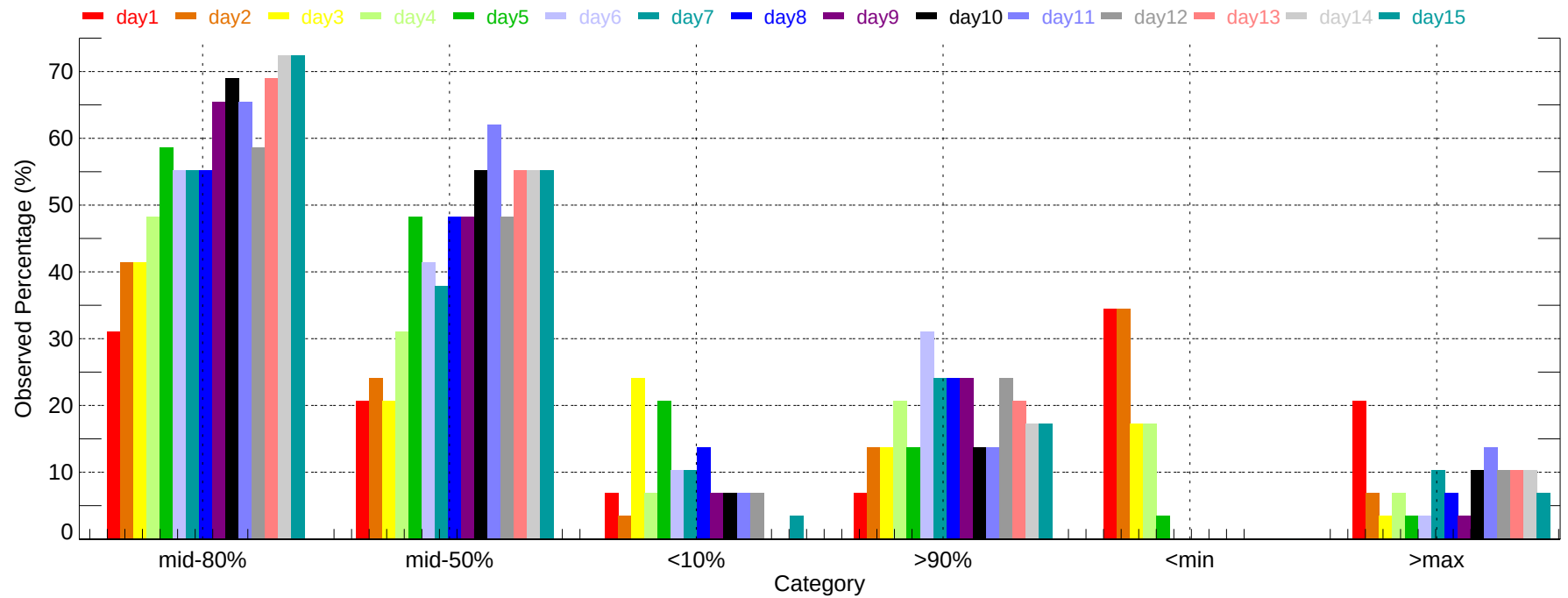
Observed Percentage of Ensembles - FWA: Min Temperature (2007-11-01~2007-11-30)
