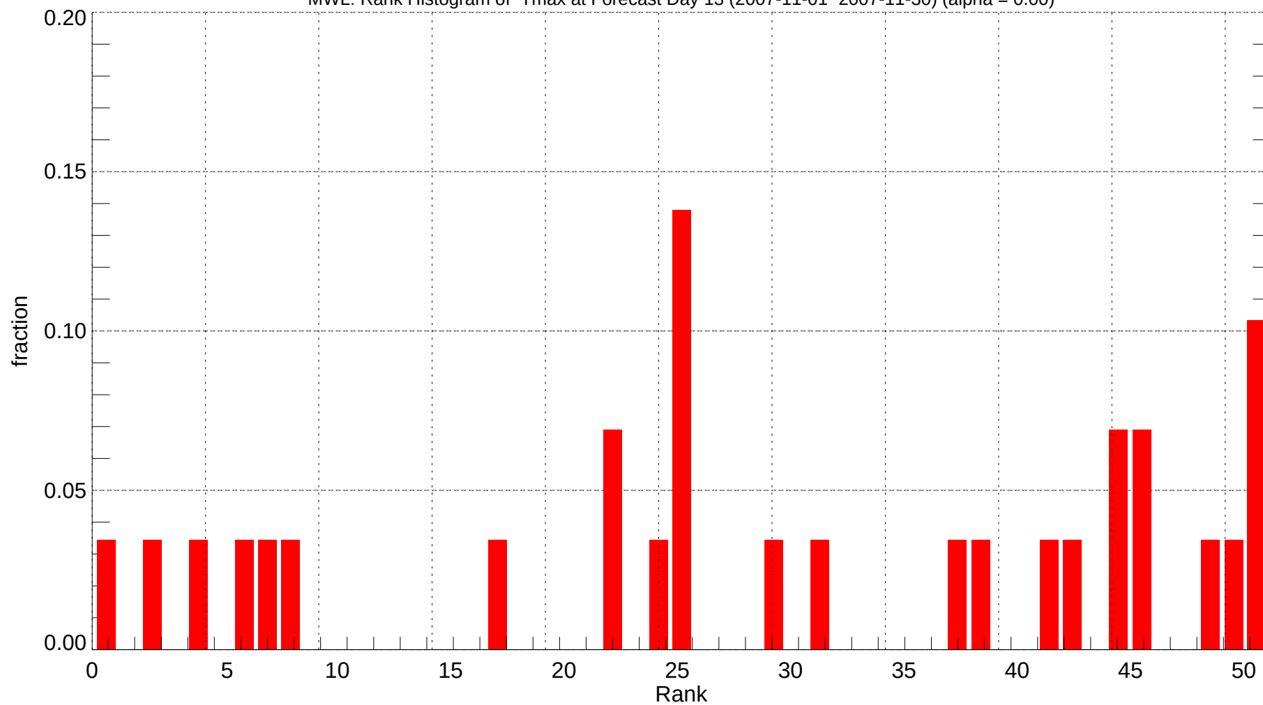
MWL: Rank Histogram of Tmax at Forecast Day 13 (2007-11-01~2007-11-30) (alpha = 0.00)
