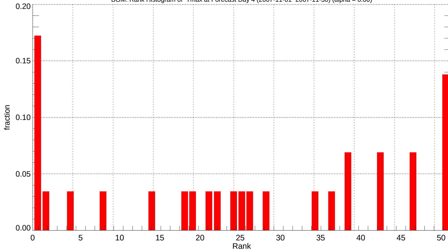
BGM: Rank Histogram of Tmax at Forecast Day 4 (2007-11-01~2007-11-30) (alpha = 0.00)
