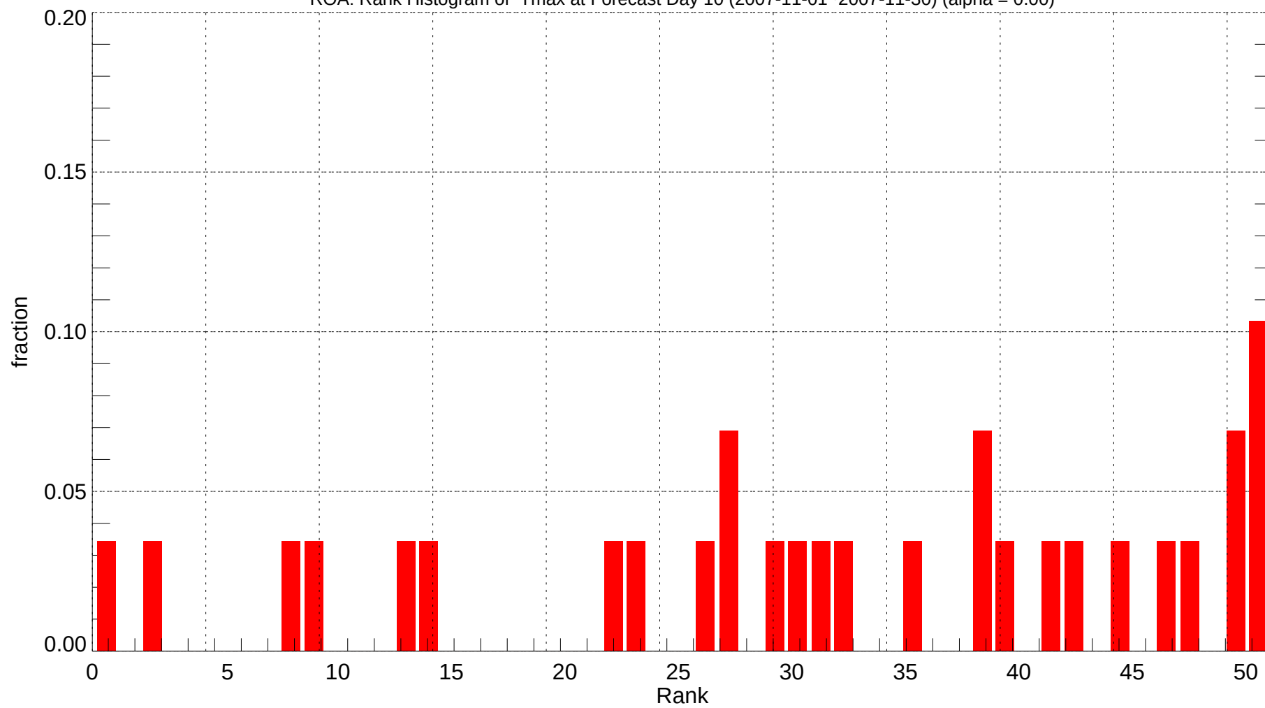
ROA: Rank Histogram of Tmax at Forecast Day 10 (2007-11-01~2007-11-30) (alpha = 0.00)
