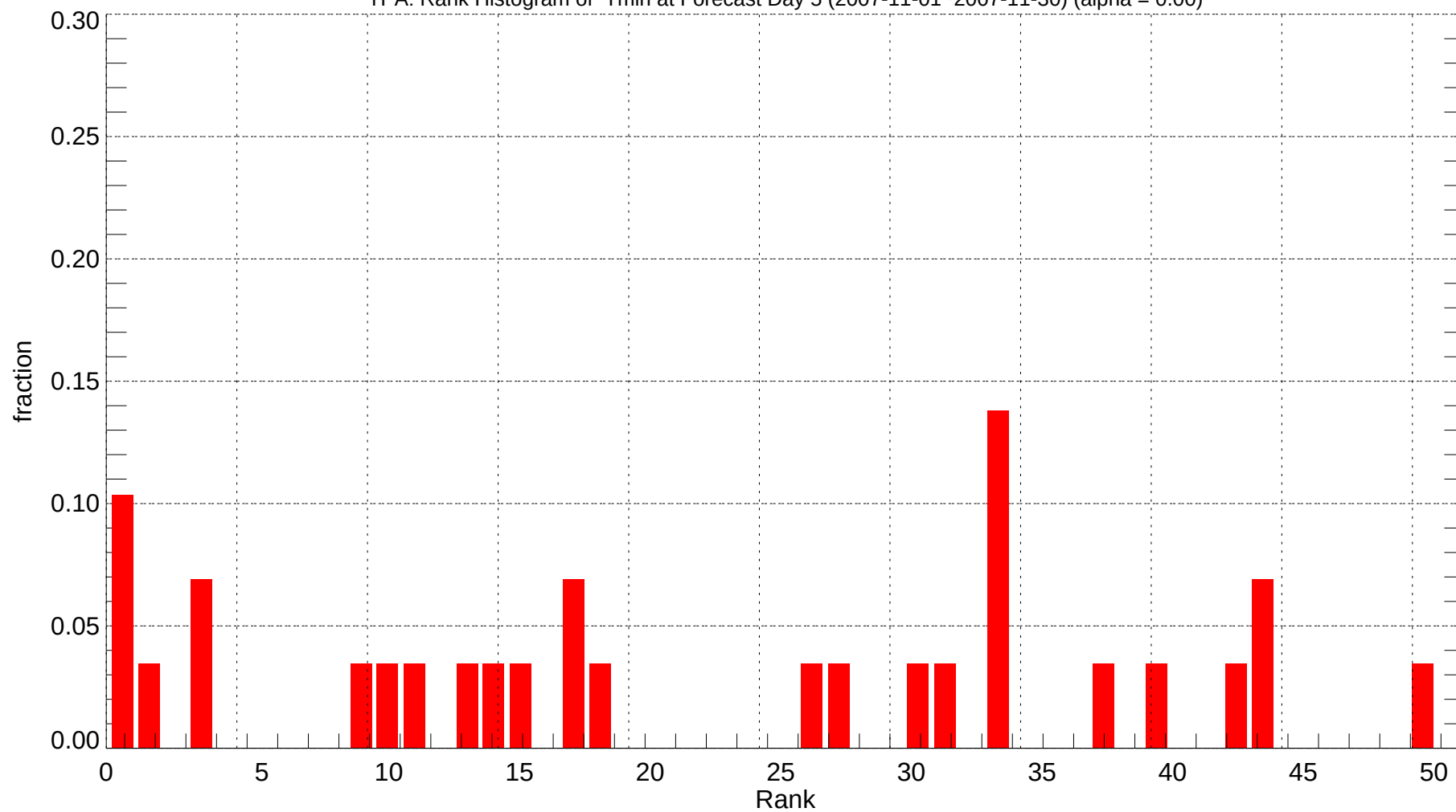
TPA: Rank Histogram of Tmin at Forecast Day 5 (2007-11-01~2007-11-30) (alpha = 0.00)
