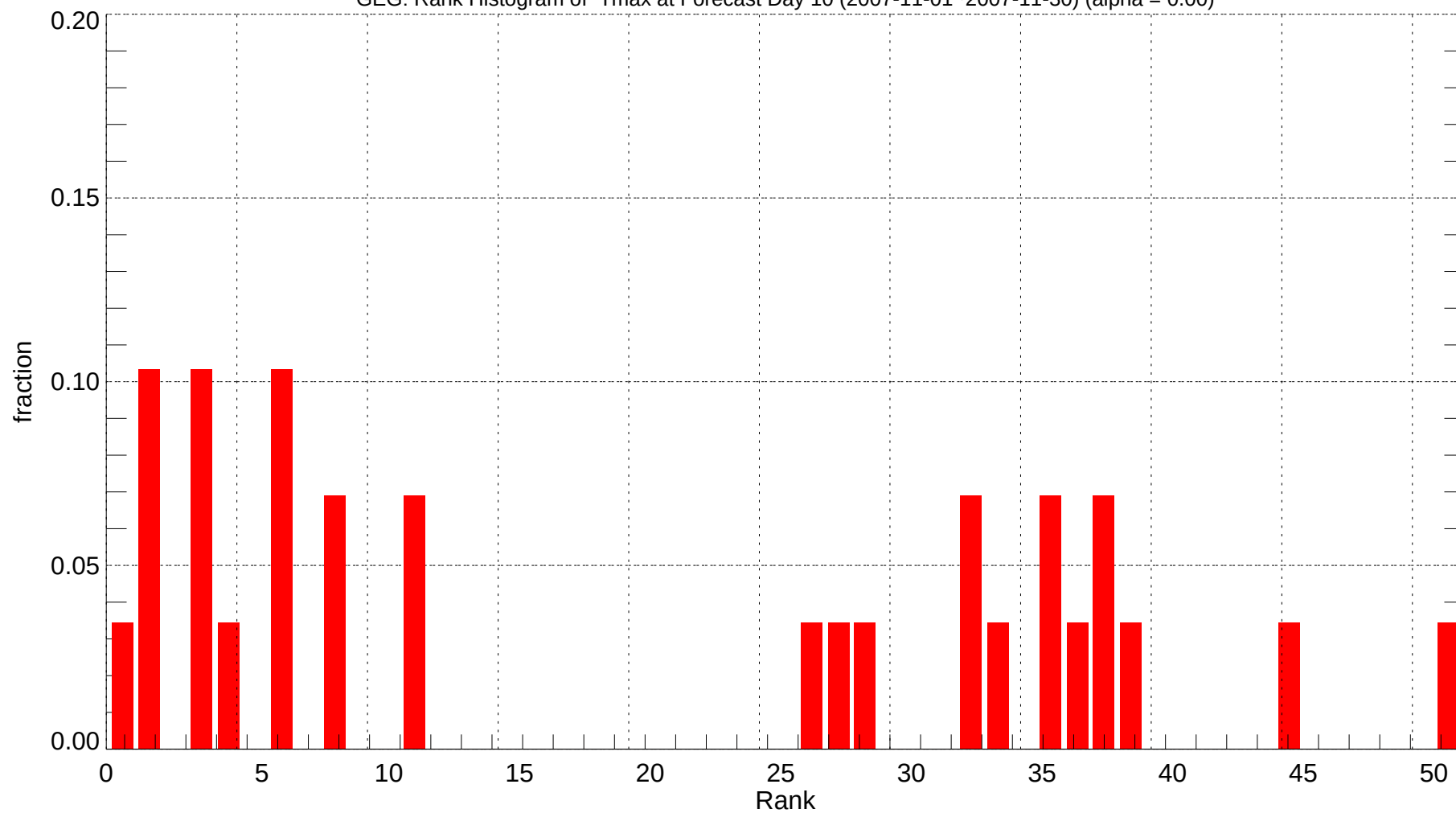
GEG: Rank Histogram of Tmax at Forecast Day 10 (2007-11-01~2007-11-30) (alpha = 0.00)
