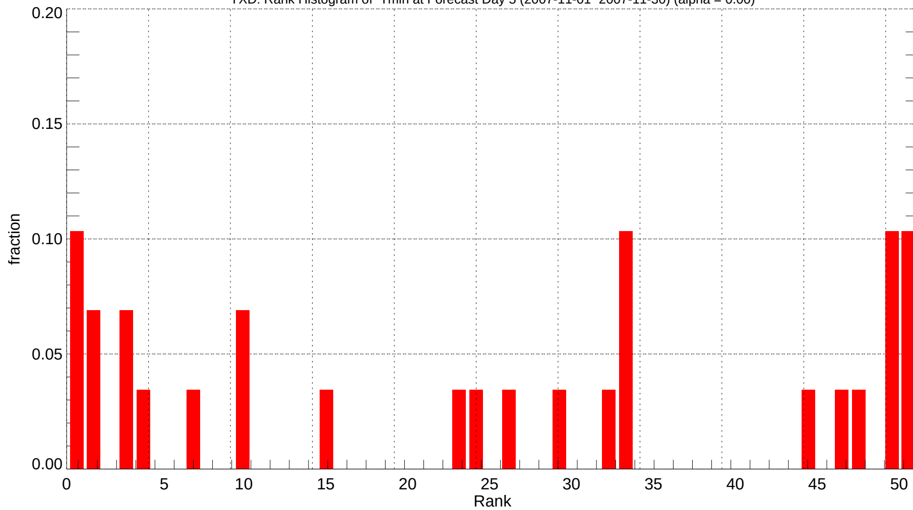
YXD: Rank Histogram of Tmin at Forecast Day 5 (2007-11-01~2007-11-30) (alpha = 0.00)
