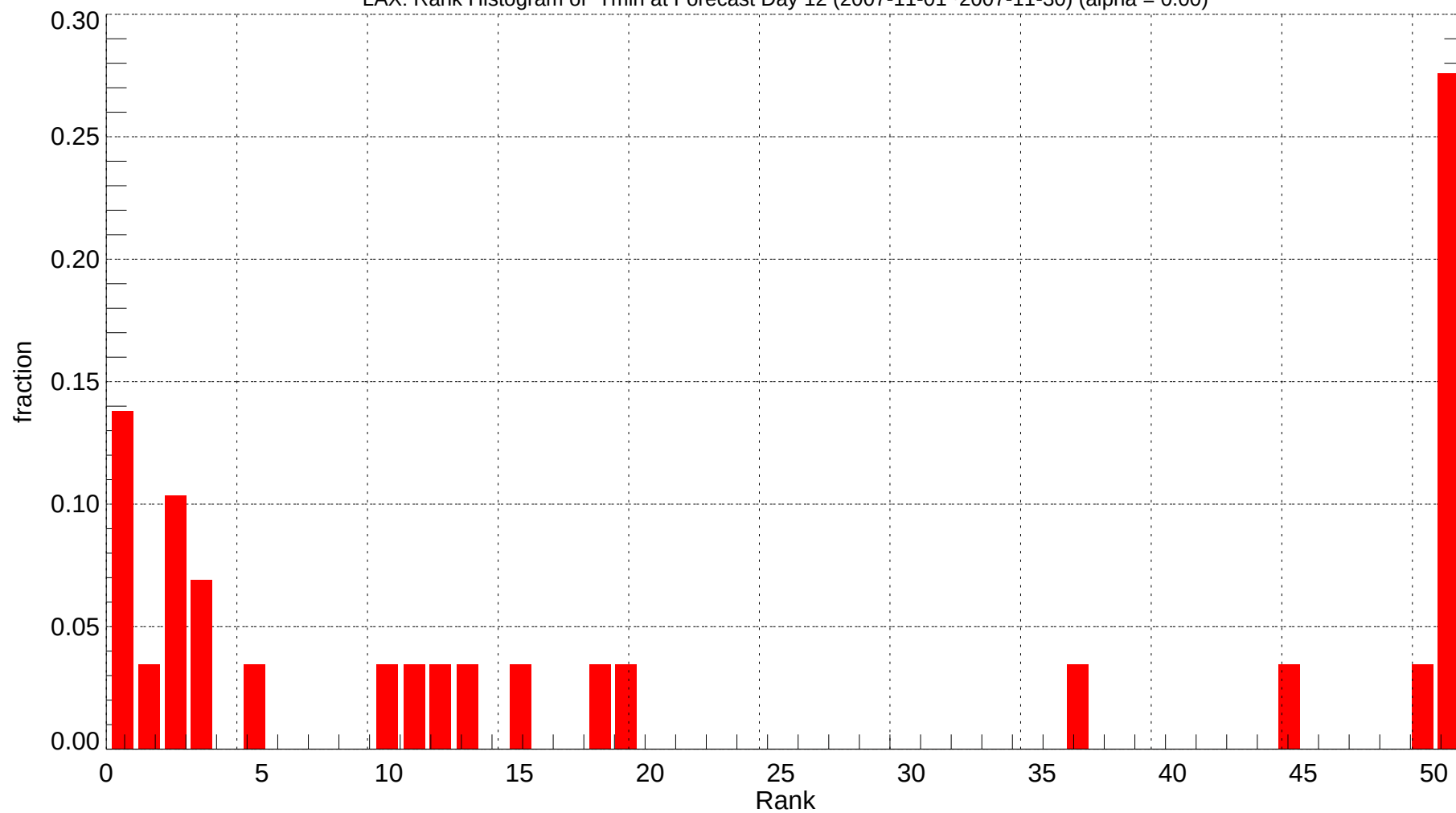
LAX: Rank Histogram of Tmin at Forecast Day 12 (2007-11-01~2007-11-30) (alpha = 0.00)
