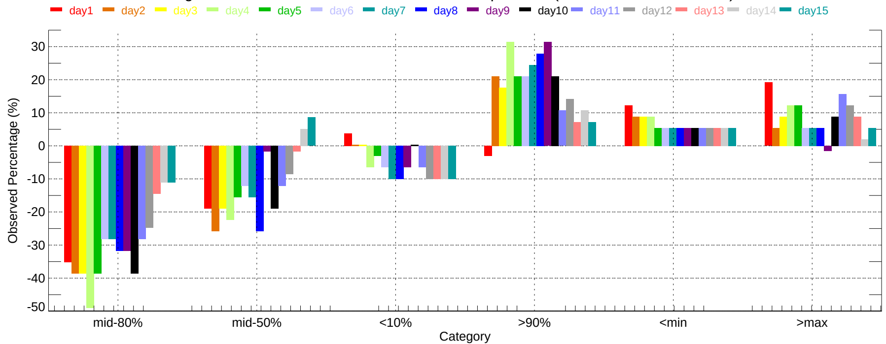
Observed Percentage Deviation of Ensembles - MSY: Min Temperature (2007-11-01~2007-11-30)
