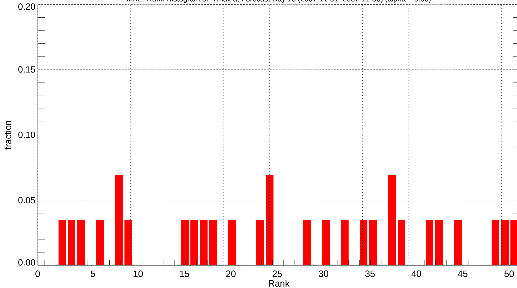
MKE: Rank Histogram of Tmax at Forecast Day 15 (2007-11-01~2007-11-30) (alpha = 0.00)
