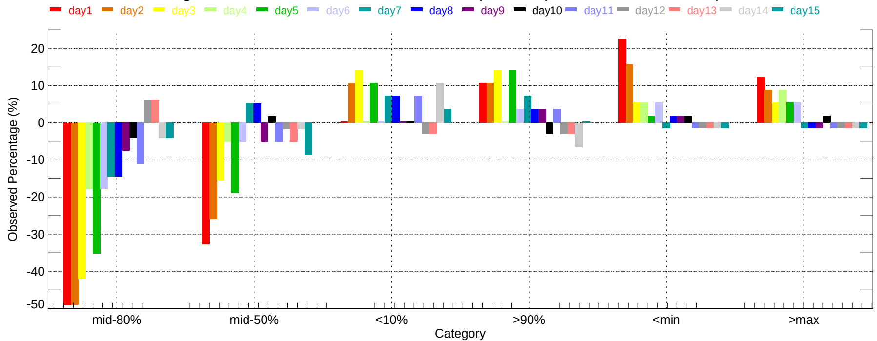
Observed Percentage Deviation of Ensembles - MIA: Min Temperature (2007-11-01~2007-11-30)
