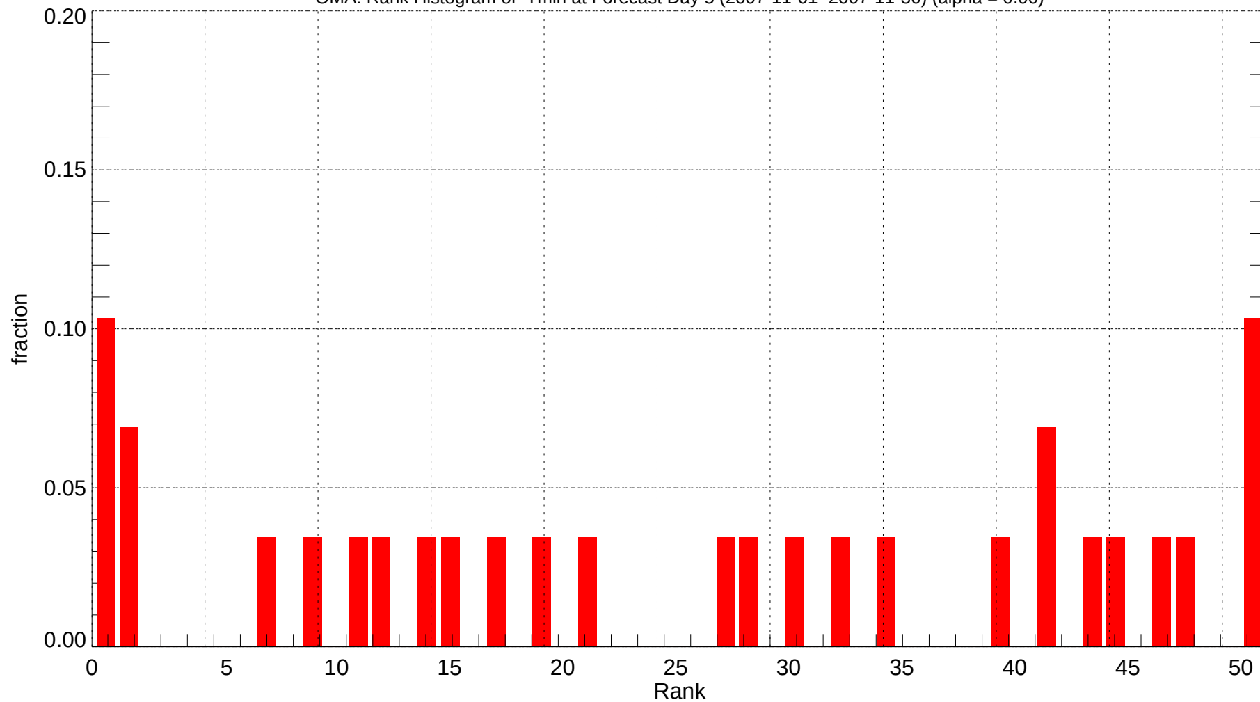
OMA: Rank Histogram of Tmin at Forecast Day 5 (2007-11-01~2007-11-30) (alpha = 0.00)
