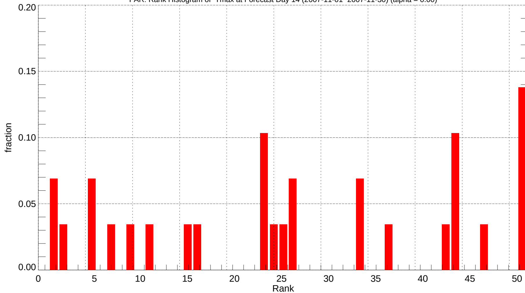
FAR: Rank Histogram of Tmax at Forecast Day 14 (2007-11-01~2007-11-30) (alpha = 0.00)
