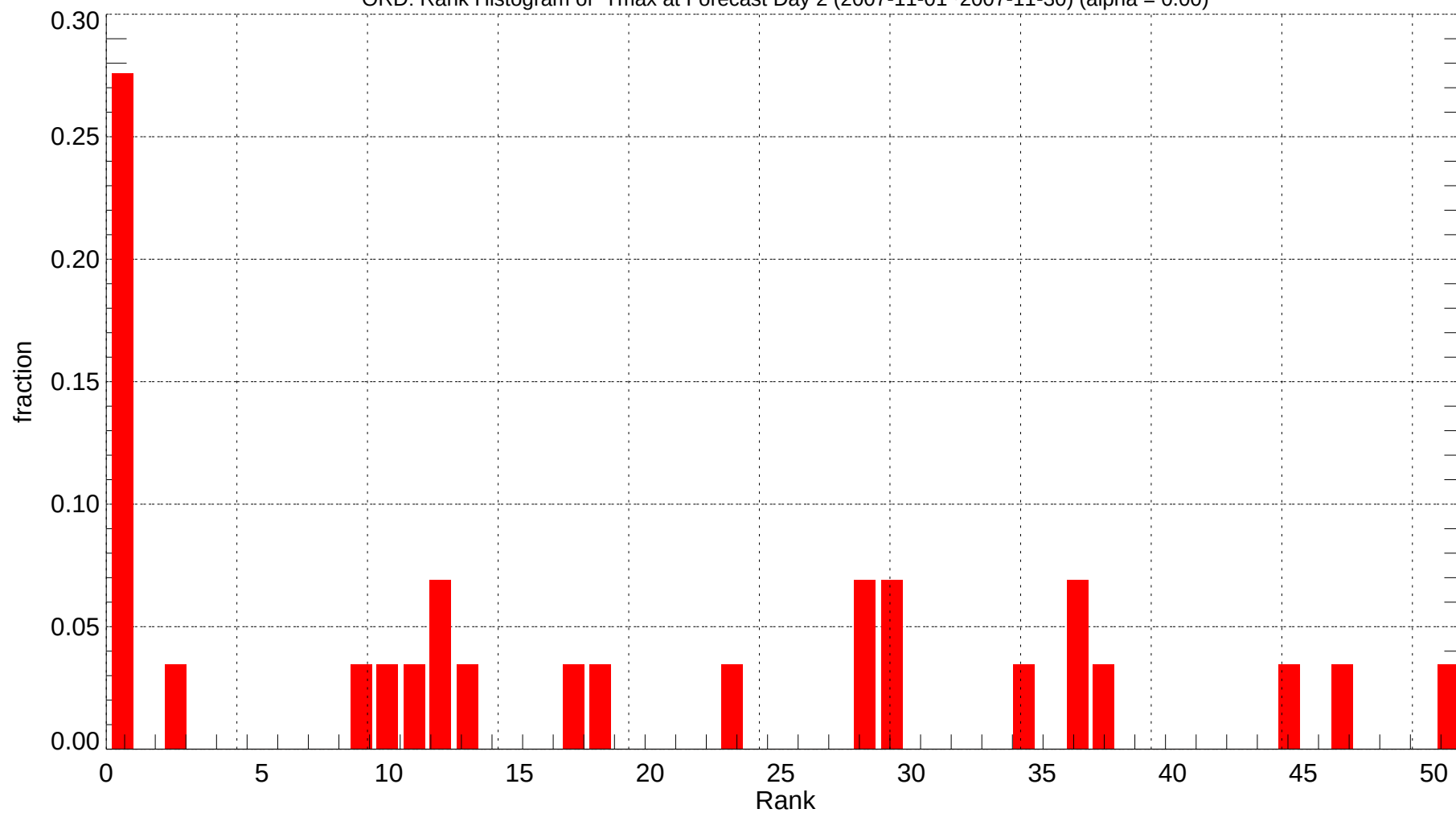
ORD: Rank Histogram of Tmax at Forecast Day 2 (2007-11-01~2007-11-30) (alpha = 0.00)
