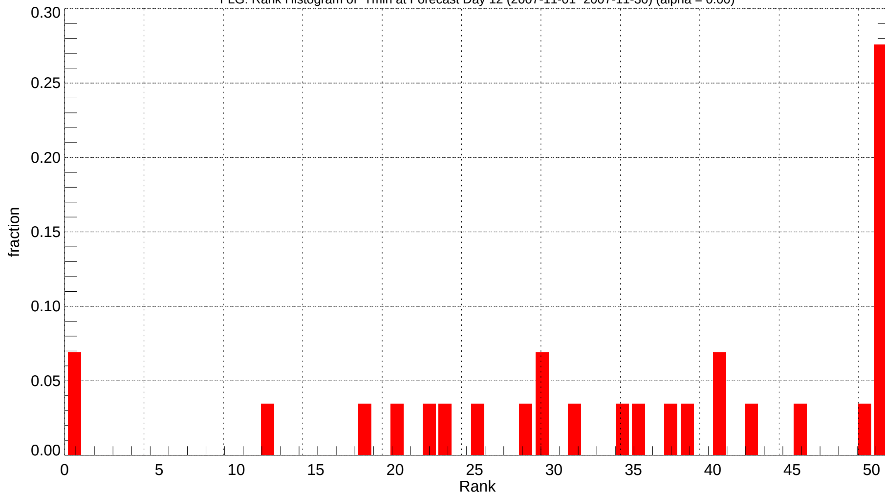
FLG: Rank Histogram of Tmin at Forecast Day 12 (2007-11-01~2007-11-30) (alpha = 0.00)
