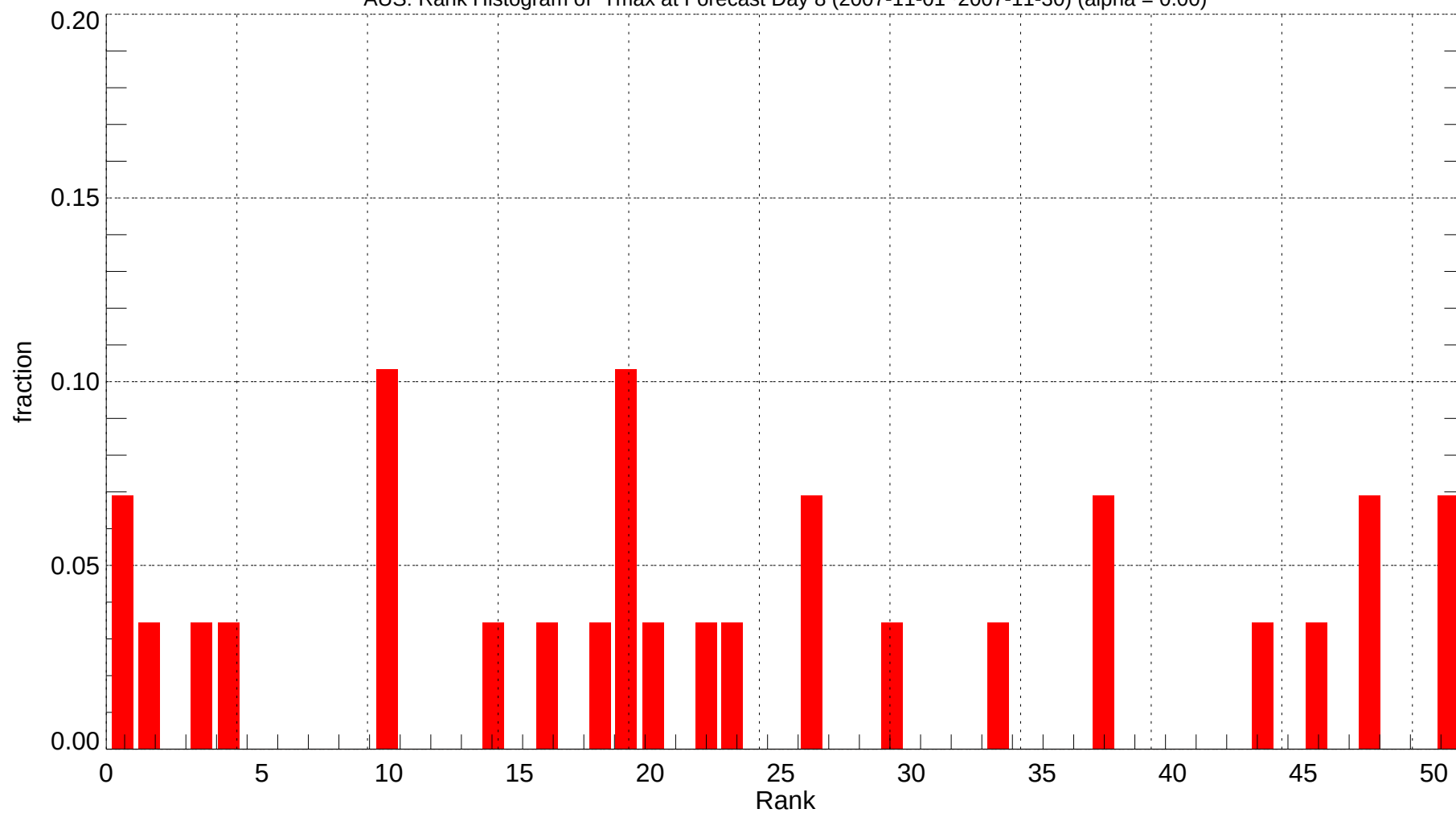
AUS: Rank Histogram of Tmax at Forecast Day 8 (2007-11-01~2007-11-30) (alpha = 0.00)
