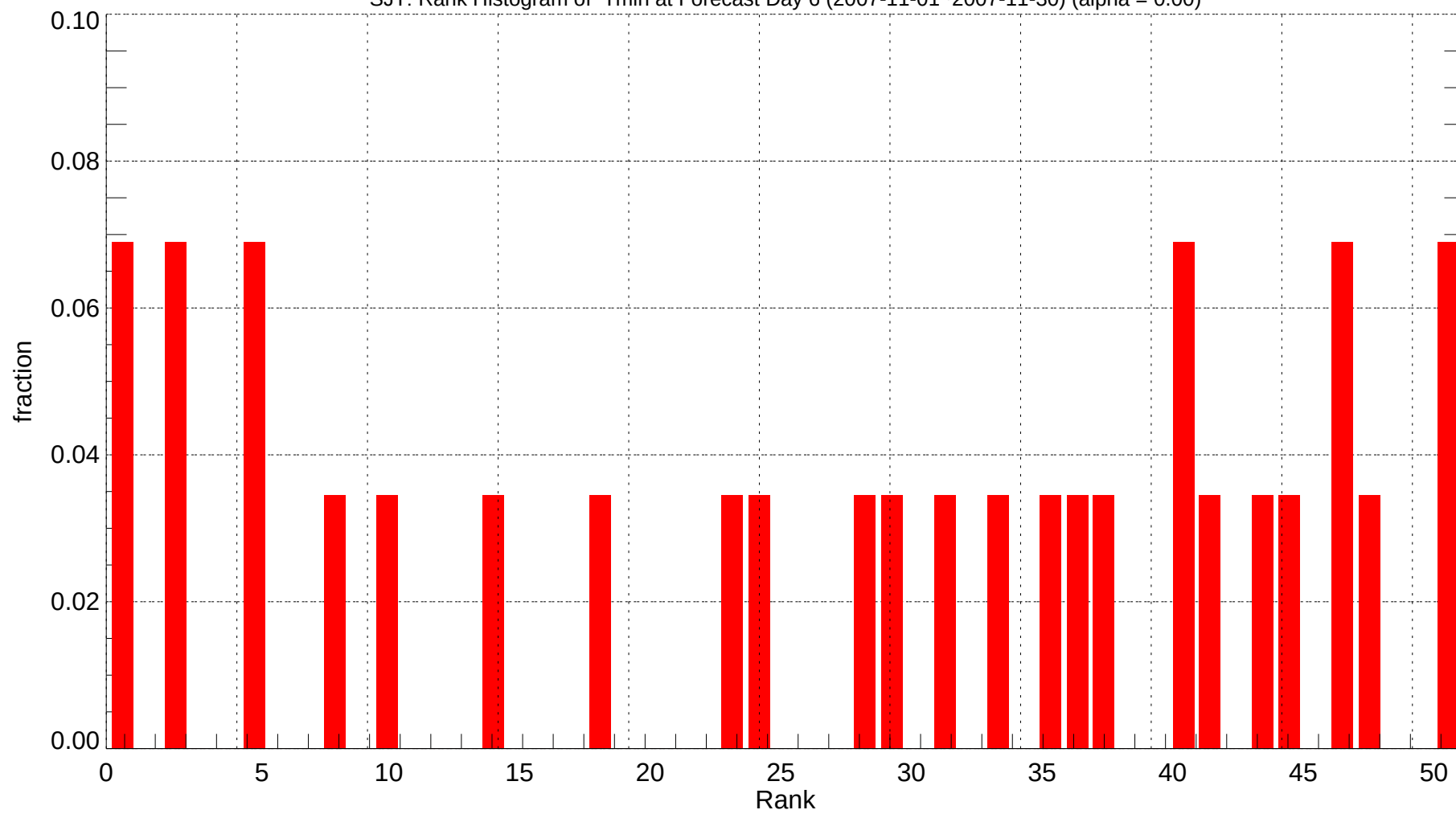
SJT: Rank Histogram of Tmin at Forecast Day 6 (2007-11-01~2007-11-30) (alpha = 0.00)
