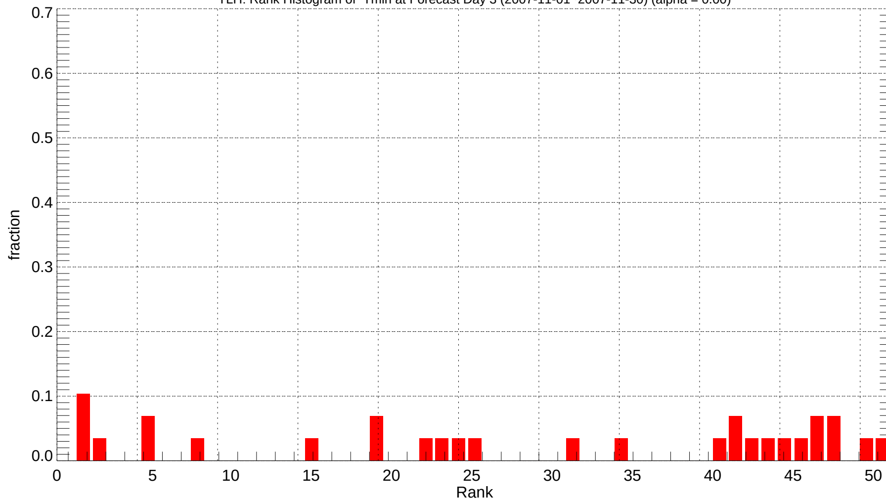
TLH: Rank Histogram of Tmin at Forecast Day 3 (2007-11-01~2007-11-30) (alpha = 0.00)
