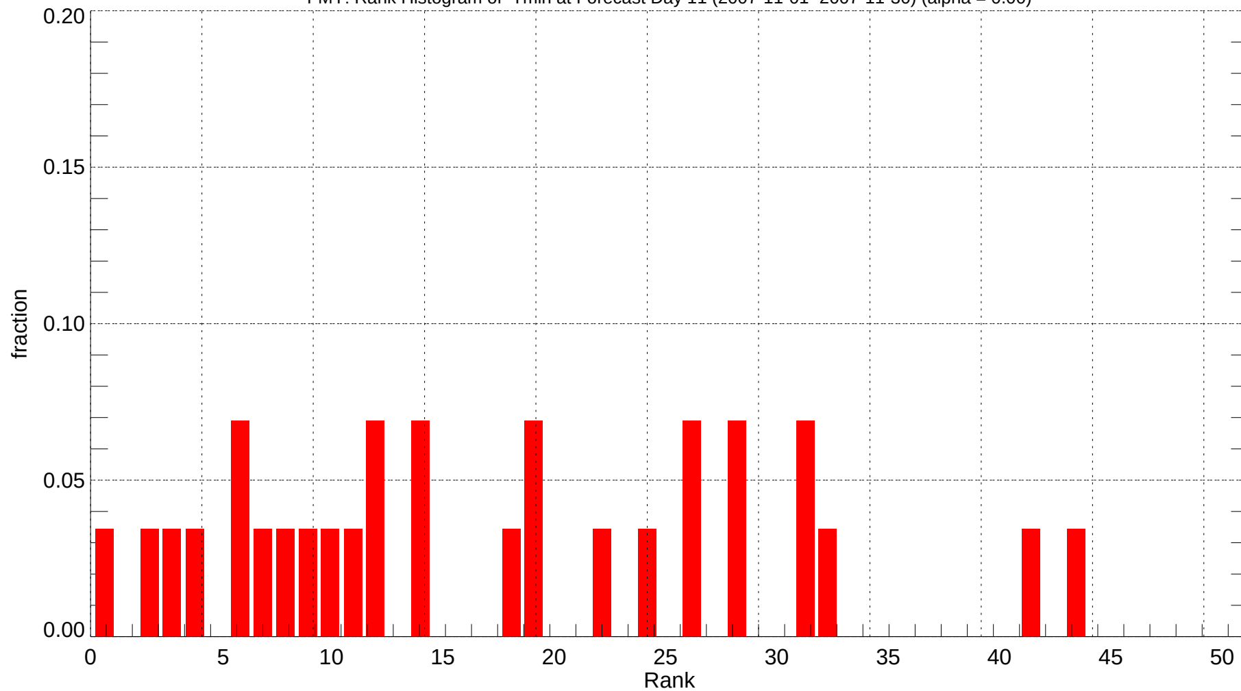
FMY: Rank Histogram of Tmin at Forecast Day 11 (2007-11-01~2007-11-30) (alpha = 0.00)
