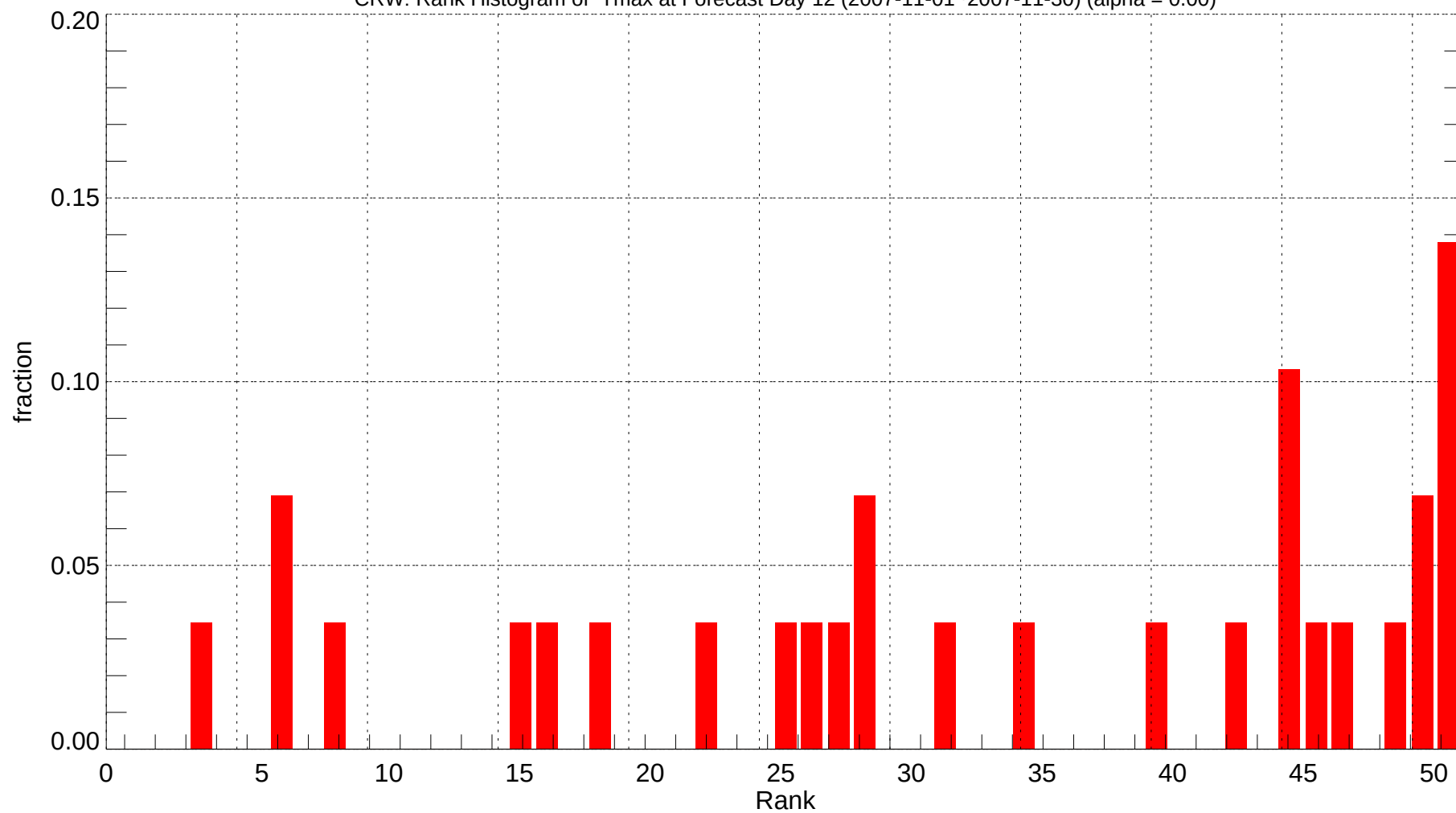
CRW: Rank Histogram of Tmax at Forecast Day 12 (2007-11-01~2007-11-30) (alpha = 0.00)
