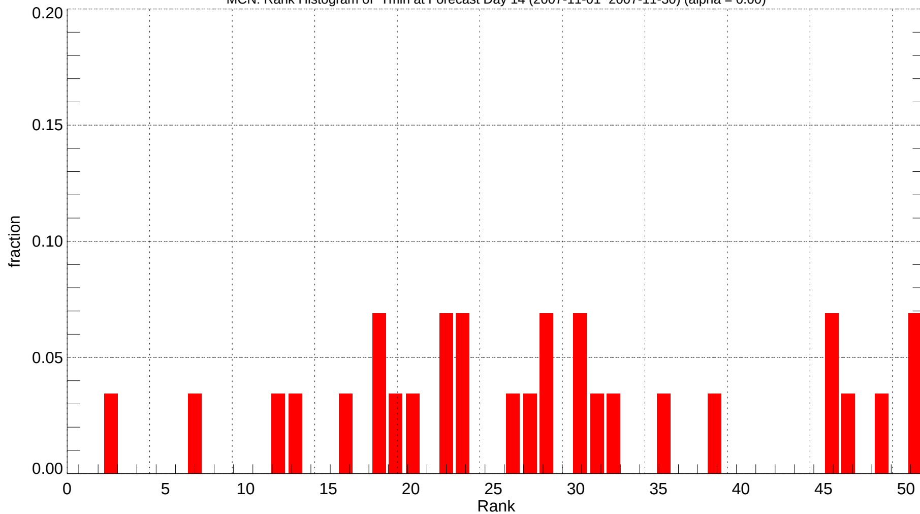
MCN: Rank Histogram of Tmin at Forecast Day 14 (2007-11-01~2007-11-30) (alpha = 0.00)
