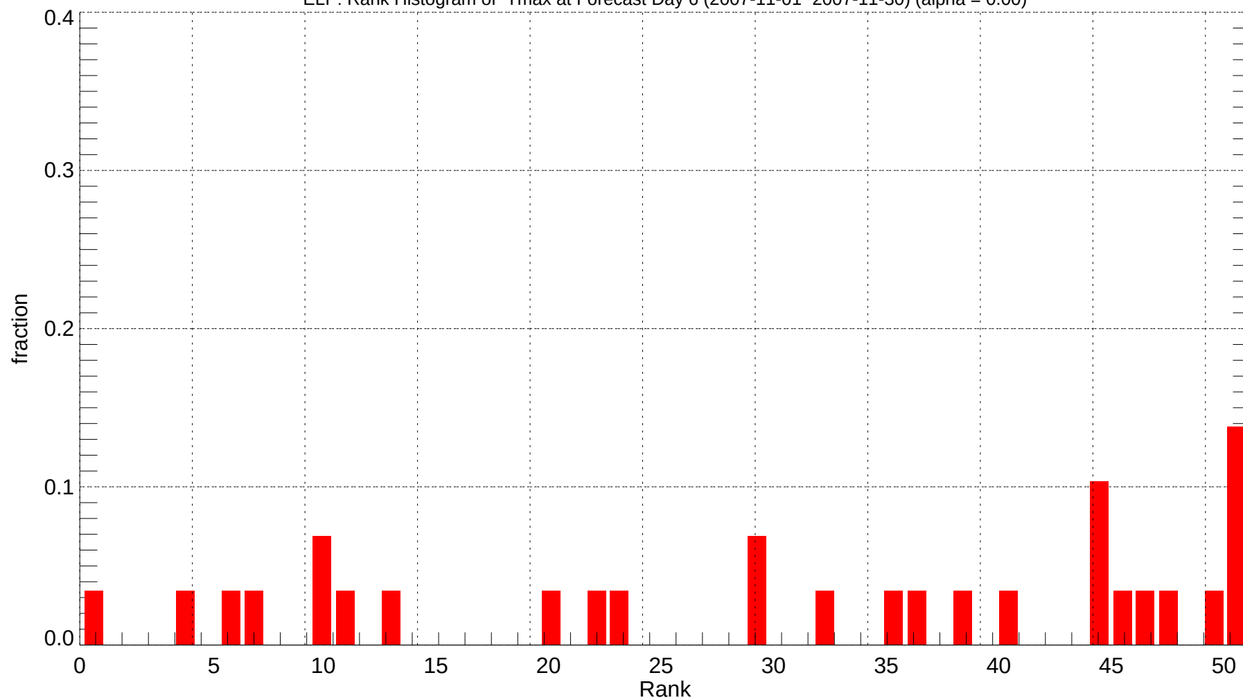
ELP: Rank Histogram of Tmax at Forecast Day 6 (2007-11-01~2007-11-30) (alpha = 0.00)
