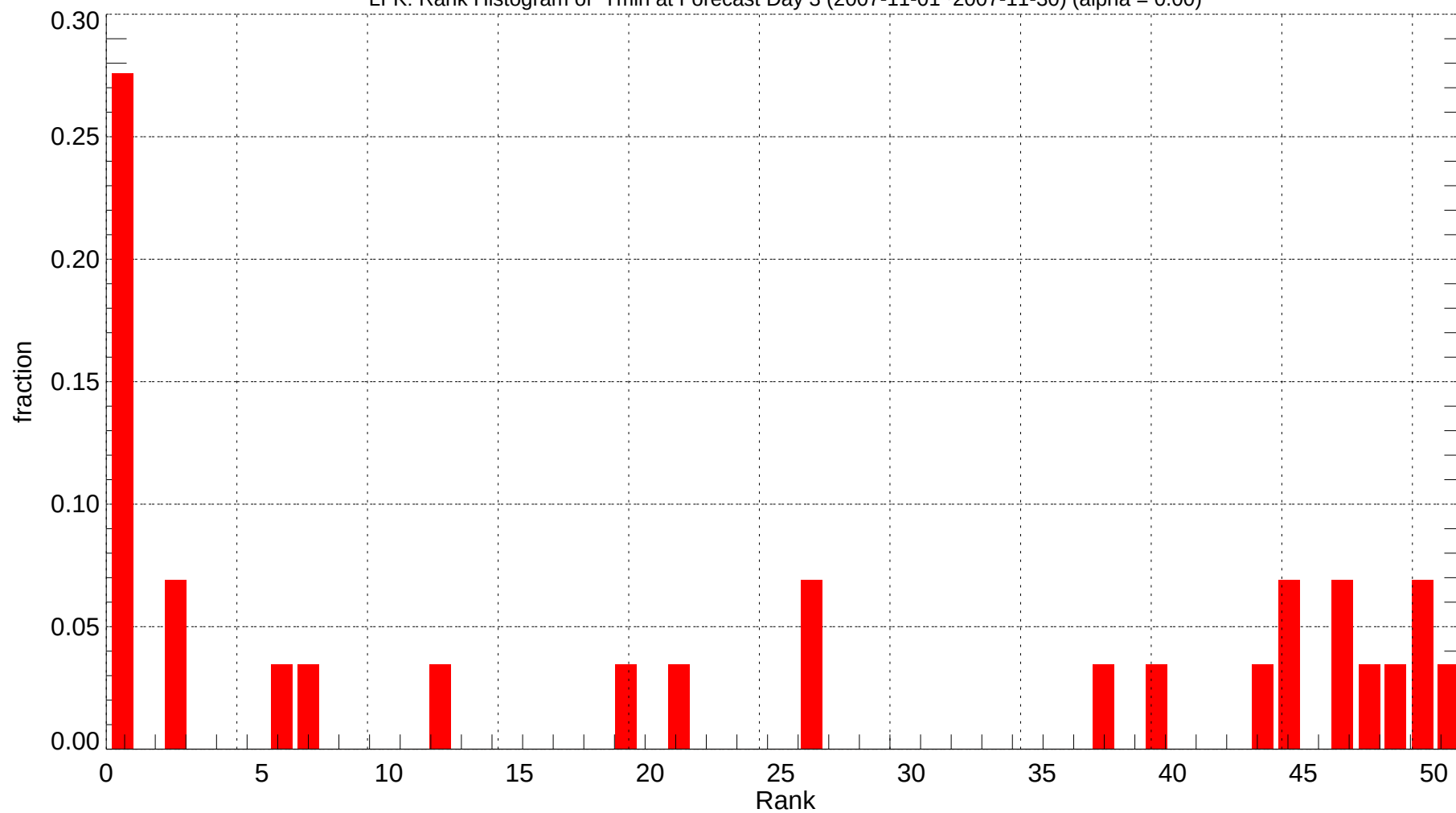
LFK: Rank Histogram of Tmin at Forecast Day 3 (2007-11-01~2007-11-30) (alpha = 0.00)
