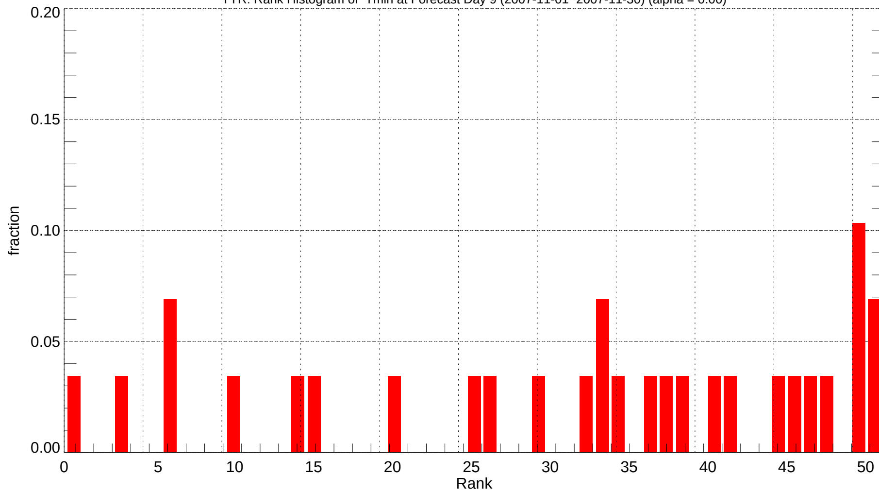
TYR: Rank Histogram of Tmin at Forecast Day 9 (2007-11-01~2007-11-30) (alpha = 0.00)
