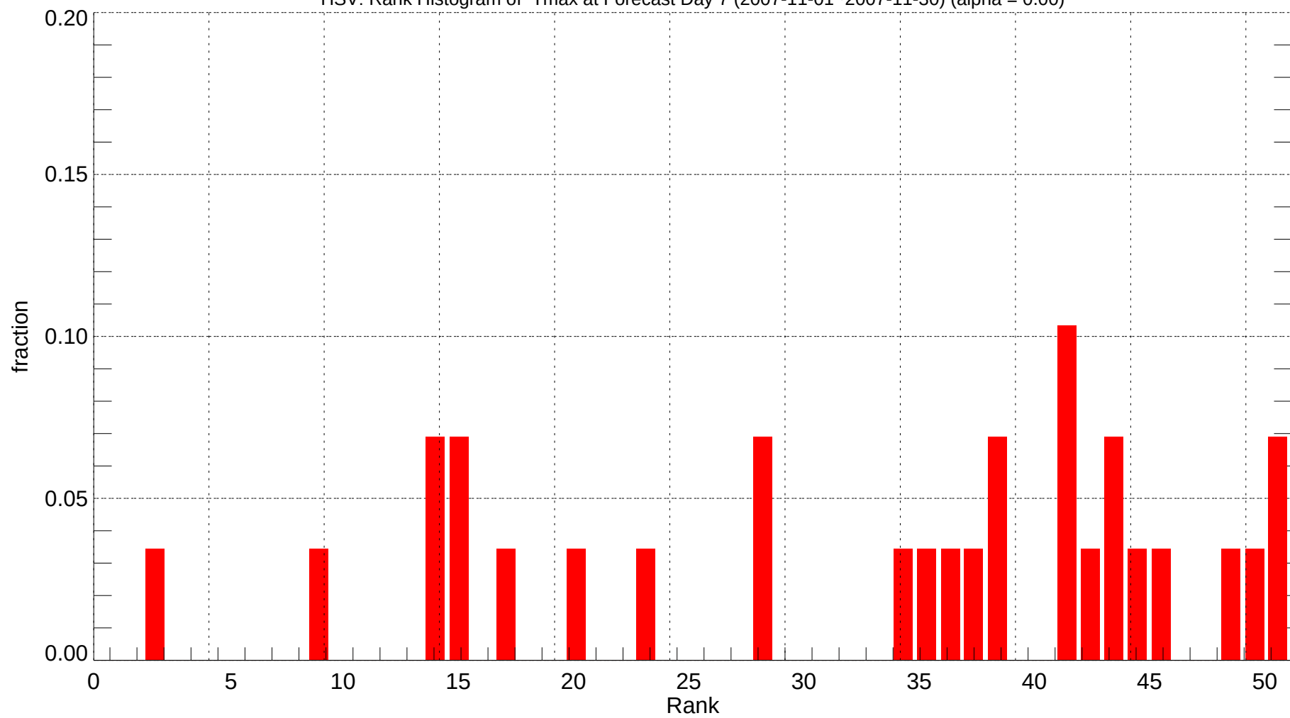
HSV: Rank Histogram of Tmax at Forecast Day 7 (2007-11-01~2007-11-30) (alpha = 0.00)
