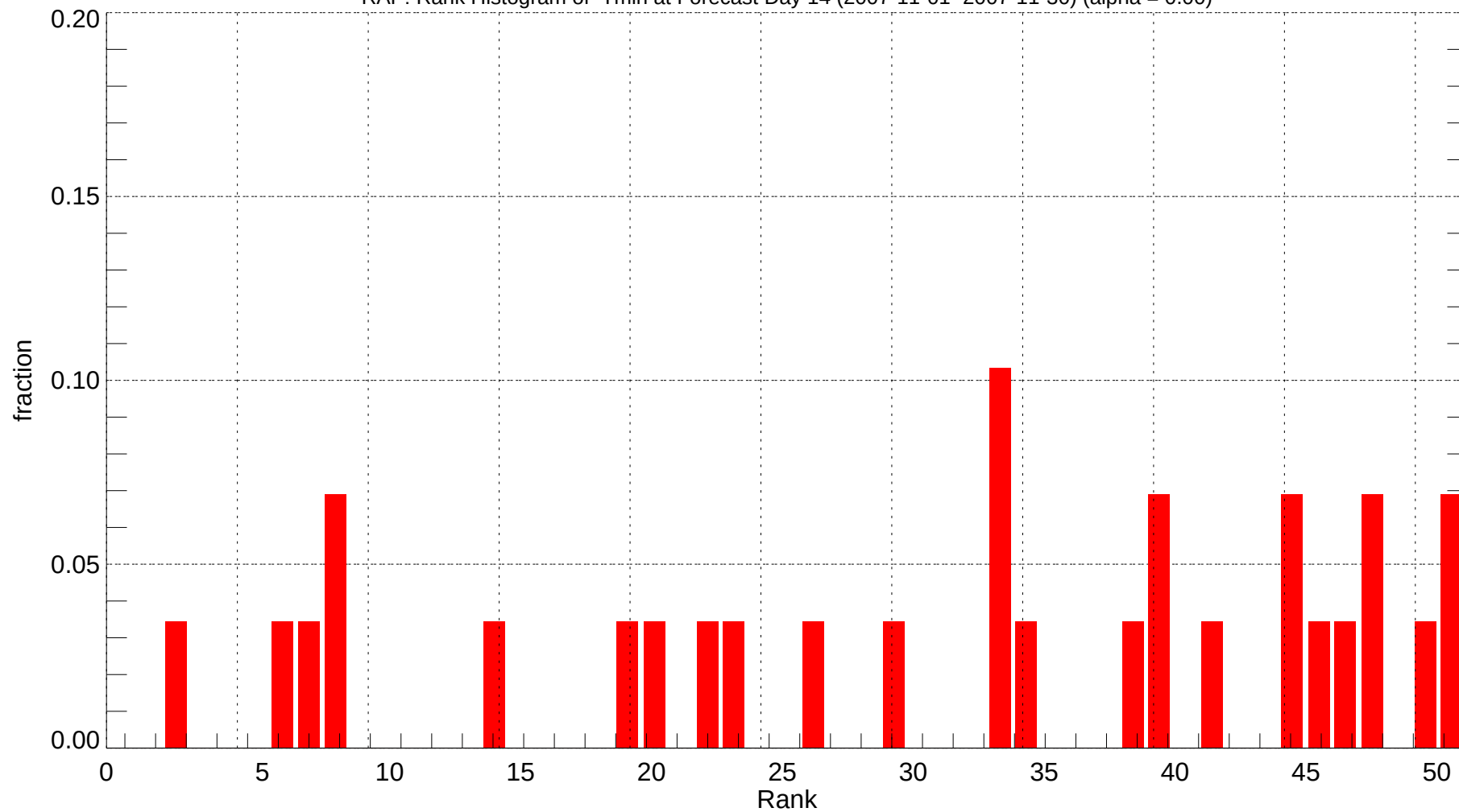
RAP: Rank Histogram of Tmin at Forecast Day 14 (2007-11-01~2007-11-30) (alpha = 0.00)
