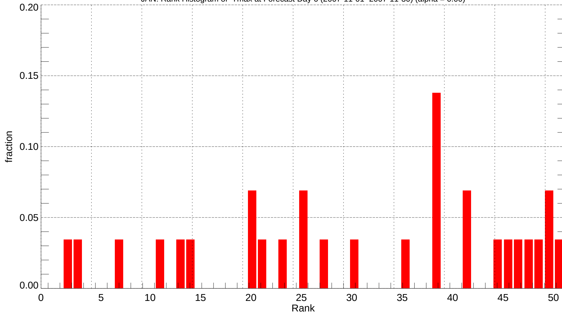
JAN: Rank Histogram of Tmax at Forecast Day 6 (2007-11-01~2007-11-30) (alpha = 0.00)
