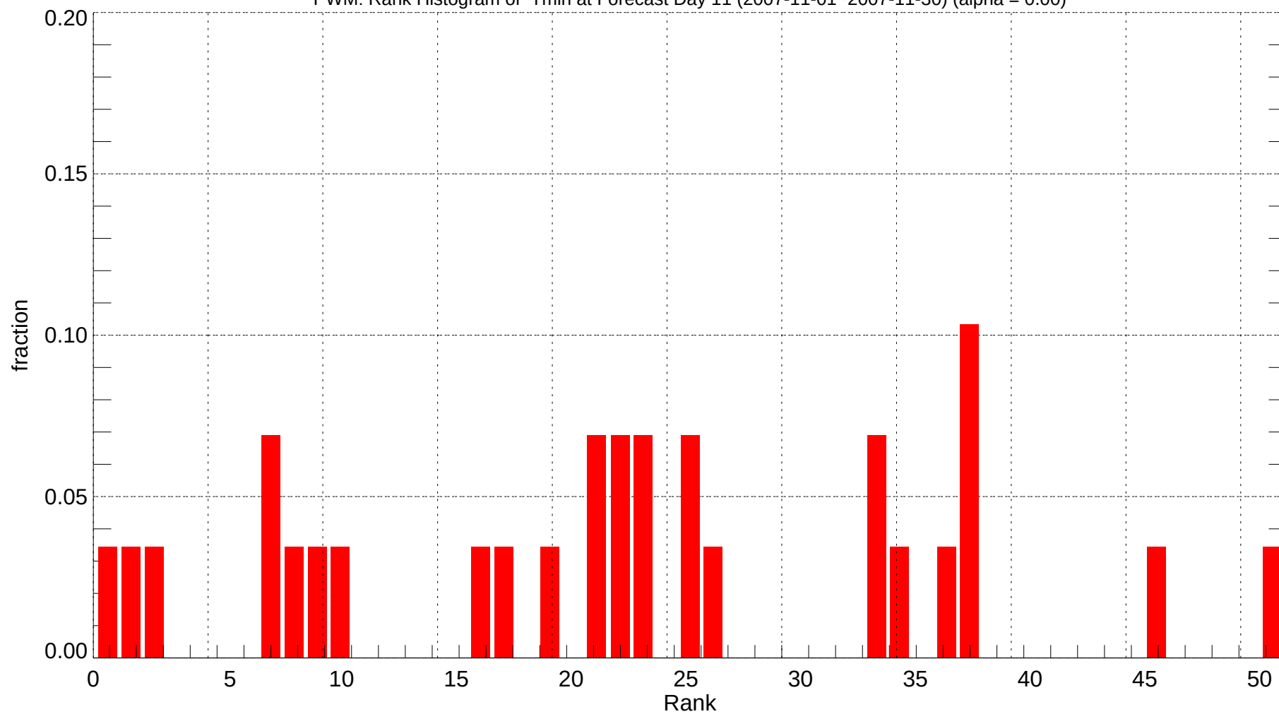
PWM: Rank Histogram of Tmin at Forecast Day 11 (2007-11-01~2007-11-30) (alpha = 0.00)
