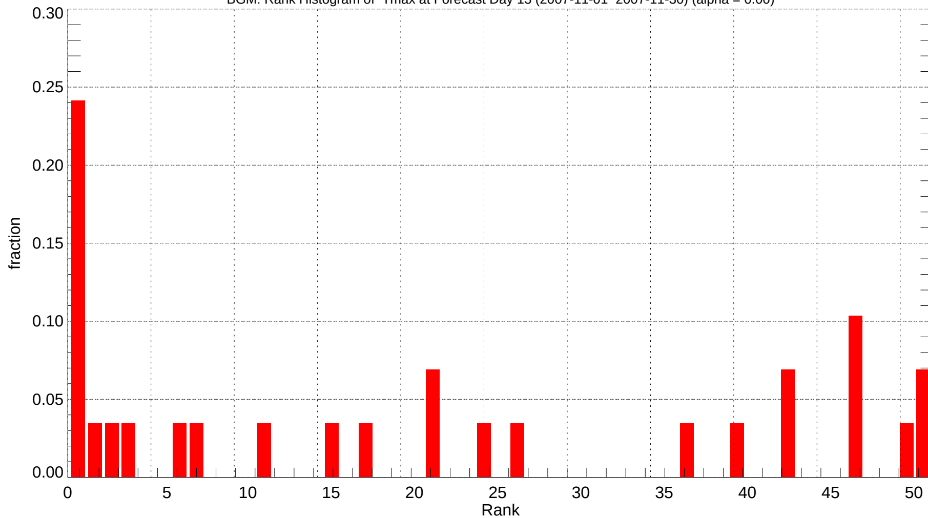
BGM: Rank Histogram of Tmax at Forecast Day 13 (2007-11-01~2007-11-30) (alpha = 0.00)
