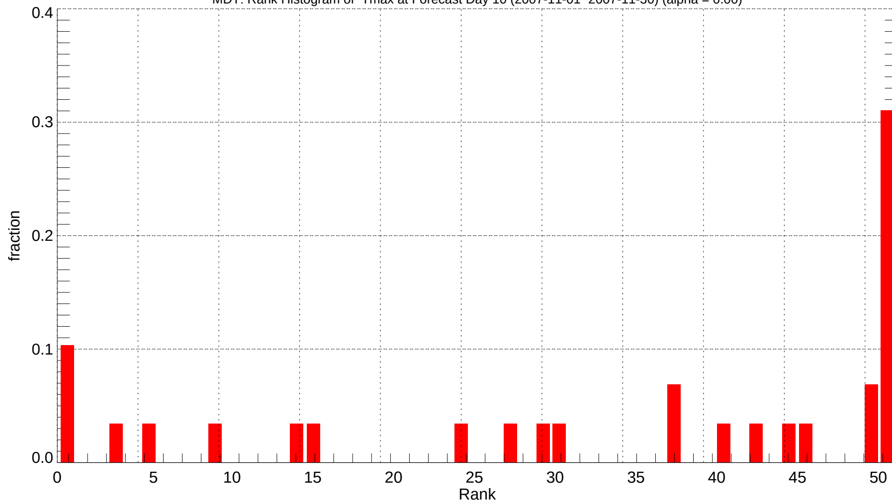
MDT: Rank Histogram of Tmax at Forecast Day 10 (2007-11-01~2007-11-30) (alpha = 0.00)
