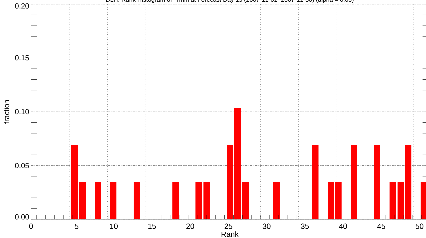
DLH: Rank Histogram of Tmin at Forecast Day 15 (2007-11-01~2007-11-30) (alpha = 0.00)
