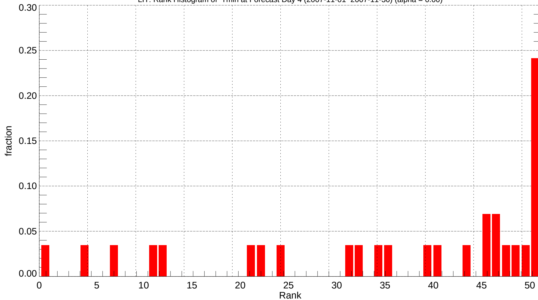
LIT: Rank Histogram of Tmin at Forecast Day 4 (2007-11-01~2007-11-30) (alpha = 0.00)
