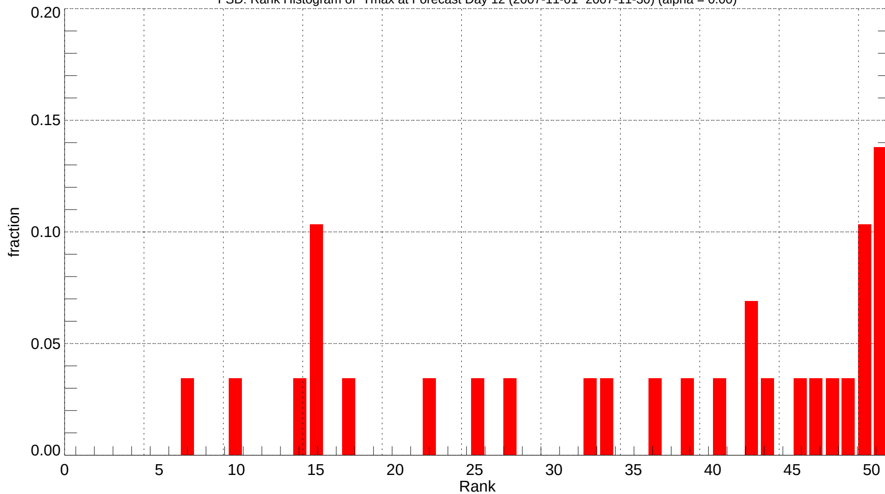
FSD: Rank Histogram of Tmax at Forecast Day 12 (2007-11-01~2007-11-30) (alpha = 0.00)
