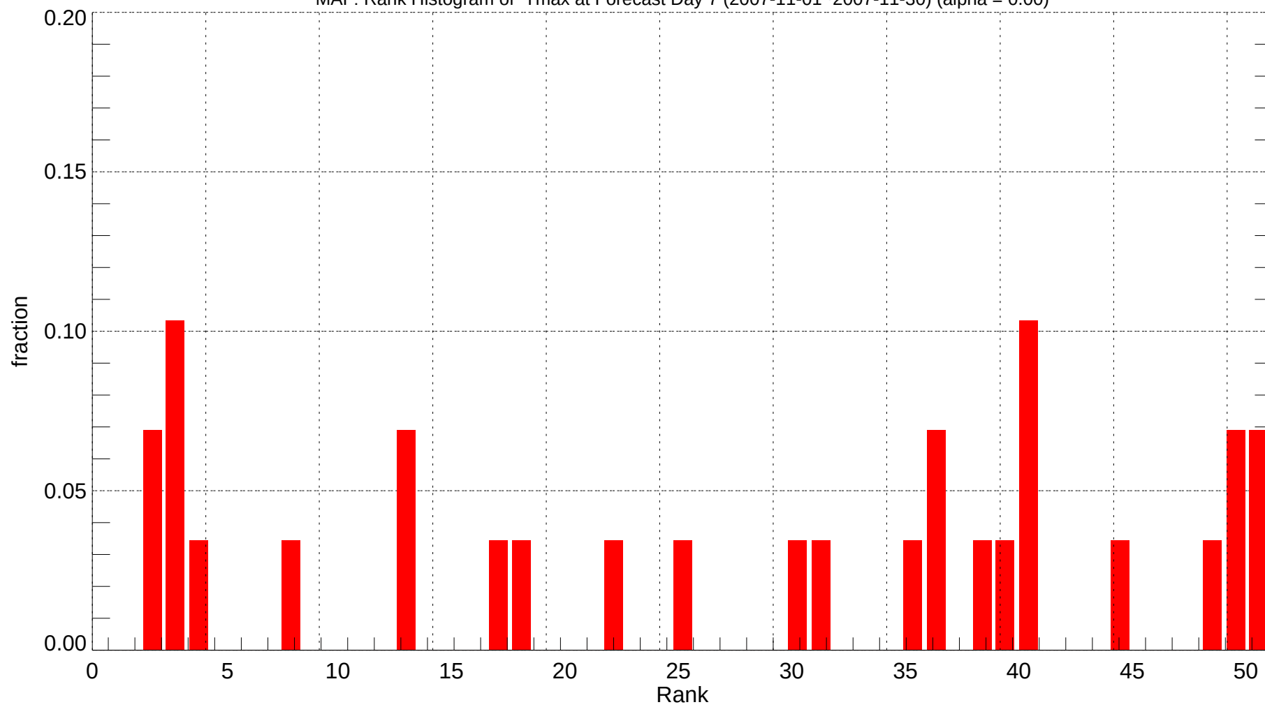
MAF: Rank Histogram of Tmax at Forecast Day 7 (2007-11-01~2007-11-30) (alpha = 0.00)
