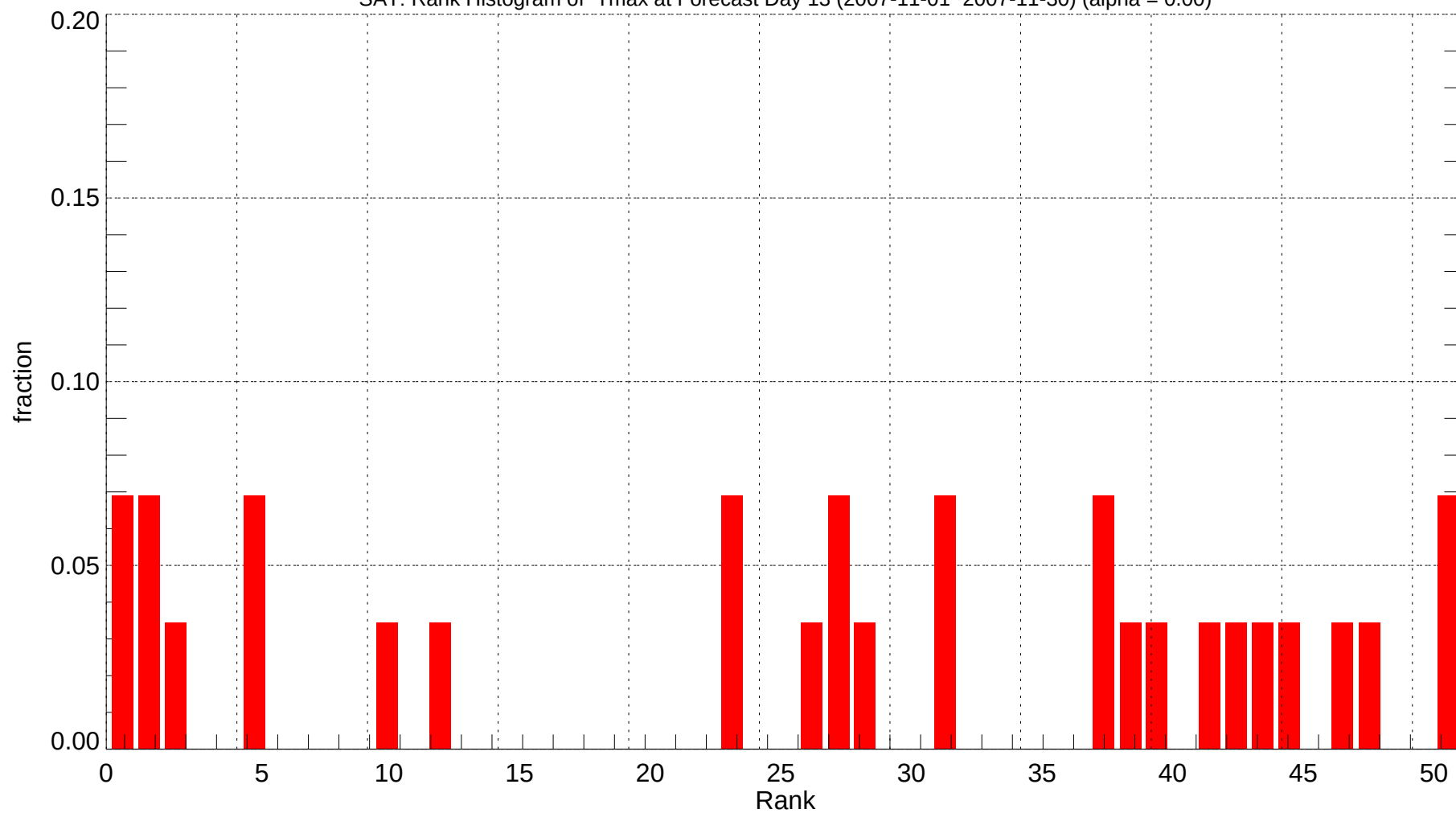
SAT: Rank Histogram of Tmax at Forecast Day 13 (2007-11-01~2007-11-30) (alpha = 0.00)
