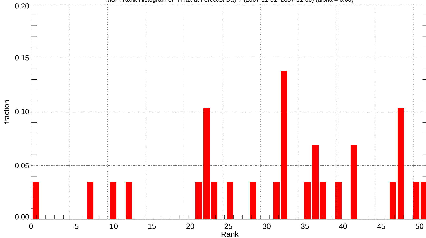
MSP: Rank Histogram of Tmax at Forecast Day 7 (2007-11-01~2007-11-30) (alpha = 0.00)
