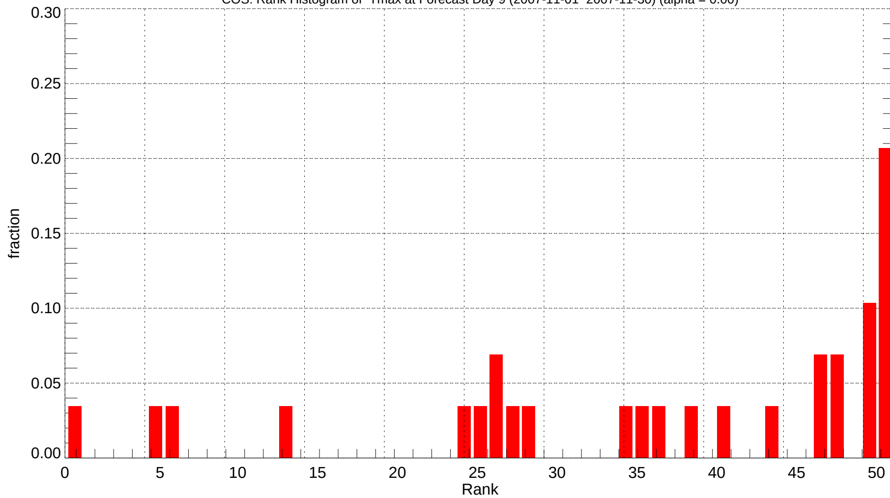
COS: Rank Histogram of Tmax at Forecast Day 9 (2007-11-01~2007-11-30) (alpha = 0.00)
