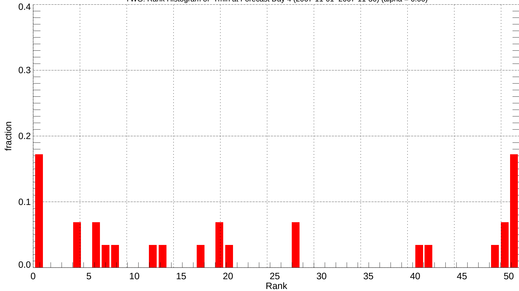
YWG: Rank Histogram of Tmin at Forecast Day 4 (2007-11-01~2007-11-30) (alpha = 0.00)
