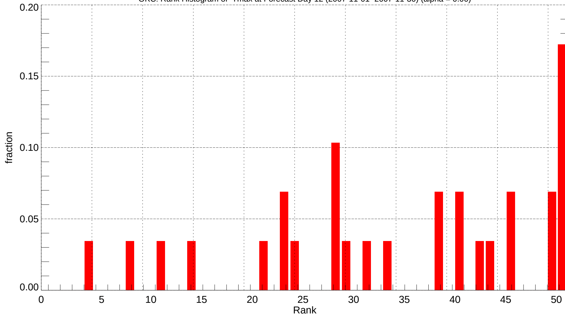
OKC: Rank Histogram of Tmax at Forecast Day 12 (2007-11-01~2007-11-30) (alpha = 0.00)
