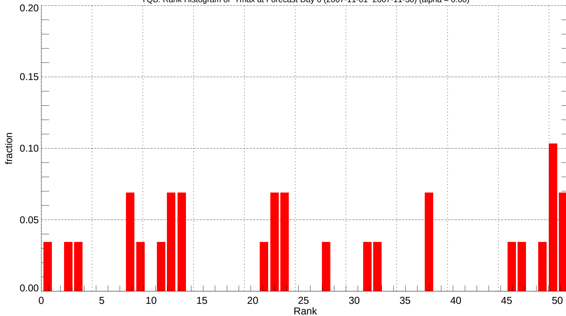
YQB: Rank Histogram of Tmax at Forecast Day 6 (2007-11-01~2007-11-30) (alpha = 0.00)
