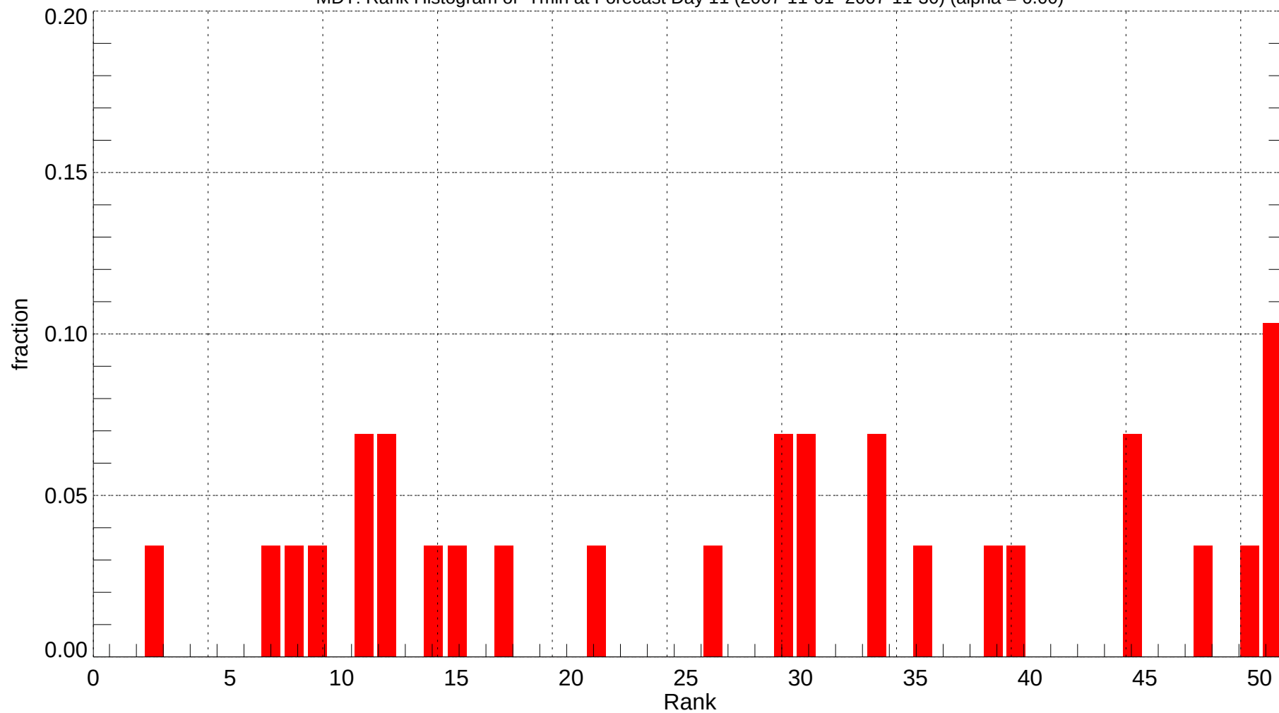
MDT: Rank Histogram of Tmin at Forecast Day 11 (2007-11-01~2007-11-30) (alpha = 0.00)
