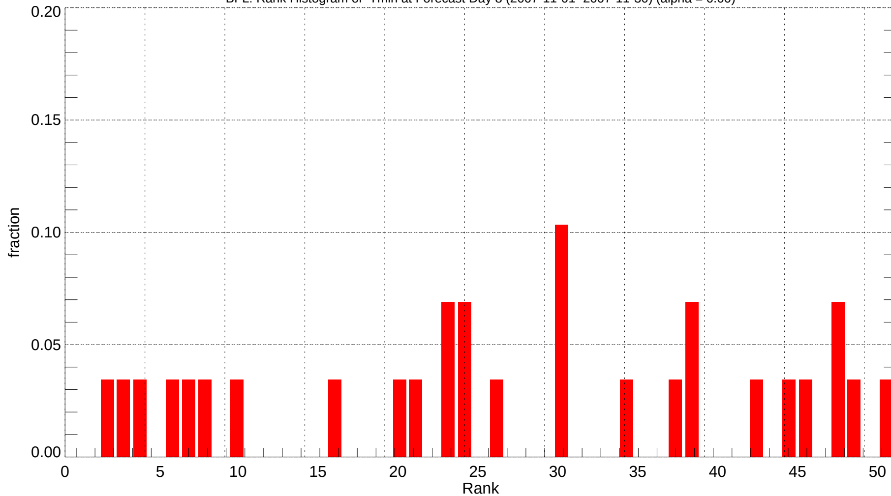
BFL: Rank Histogram of Tmin at Forecast Day 8 (2007-11-01~2007-11-30) (alpha = 0.00)
