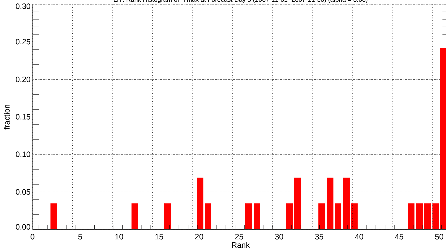
LIT: Rank Histogram of Tmax at Forecast Day 5 (2007-11-01~2007-11-30) (alpha = 0.00)
