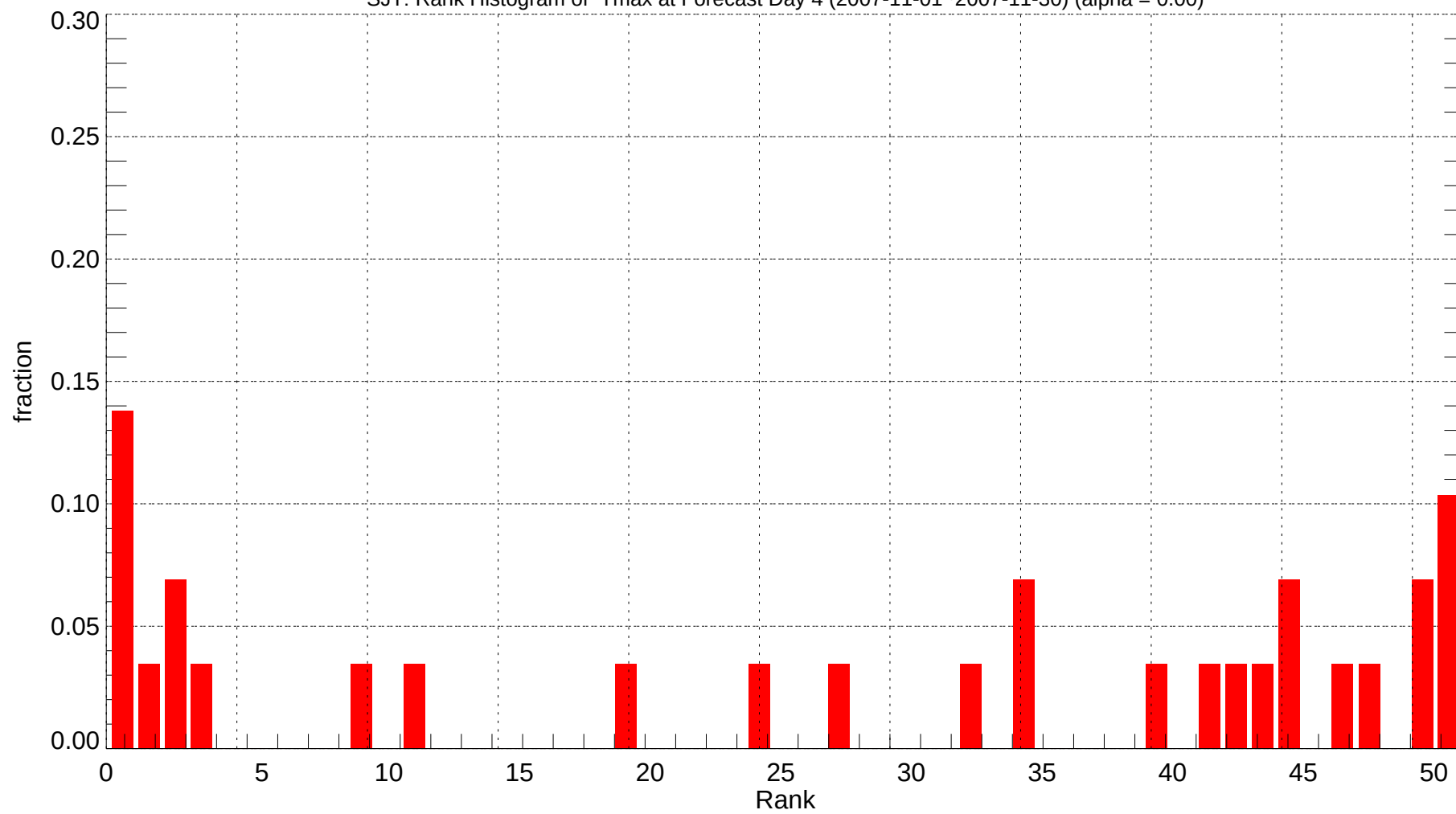
SJT: Rank Histogram of Tmax at Forecast Day 4 (2007-11-01~2007-11-30) (alpha = 0.00)
