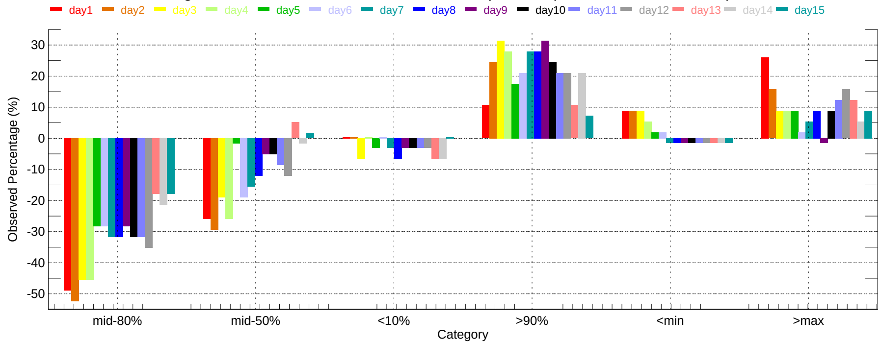
Observed Percentage Deviation of Ensembles - LEX: Max Temperature (2007-11-01~2007-11-30)
