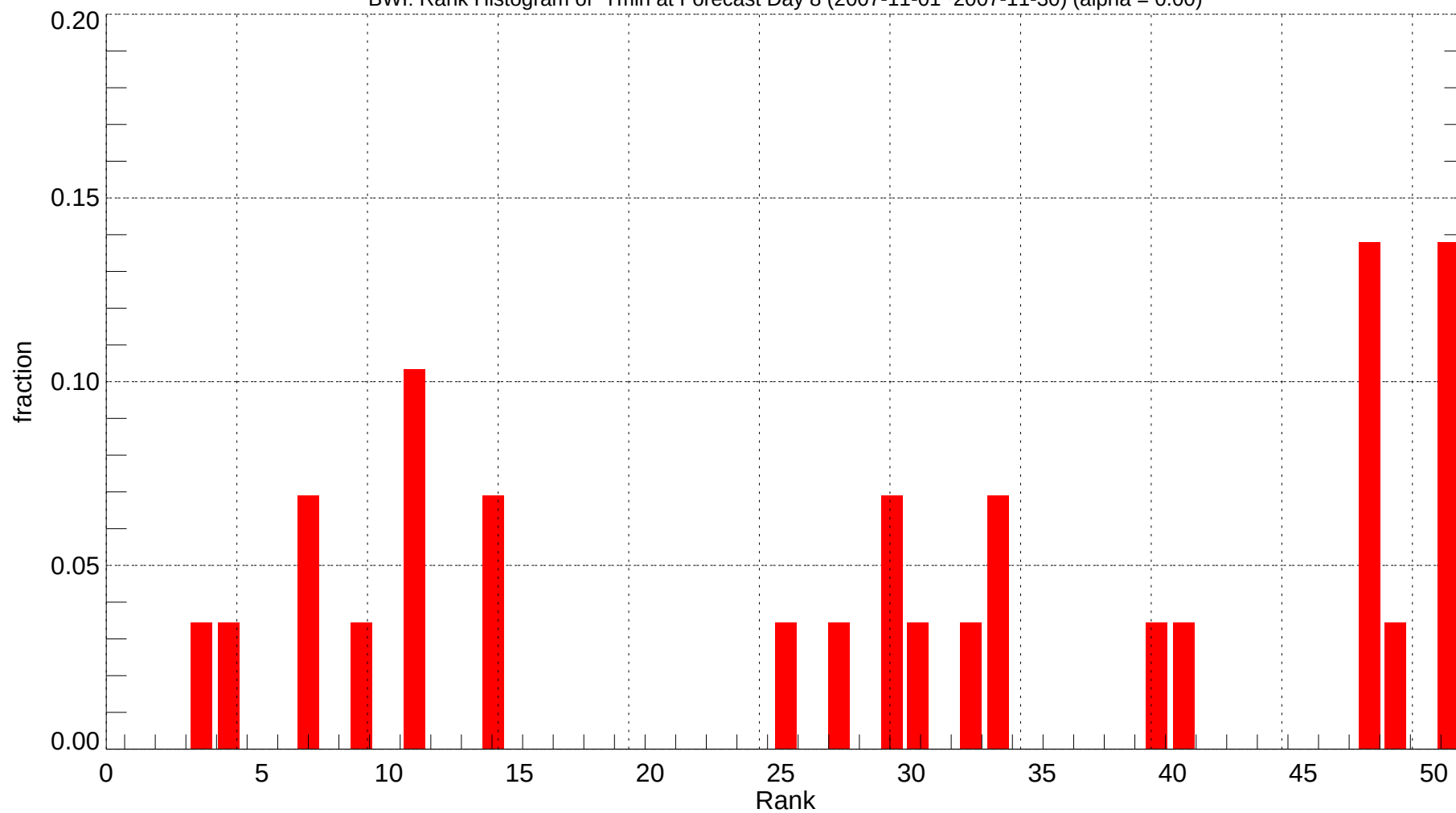
BWI: Rank Histogram of Tmin at Forecast Day 8 (2007-11-01~2007-11-30) (alpha = 0.00)
