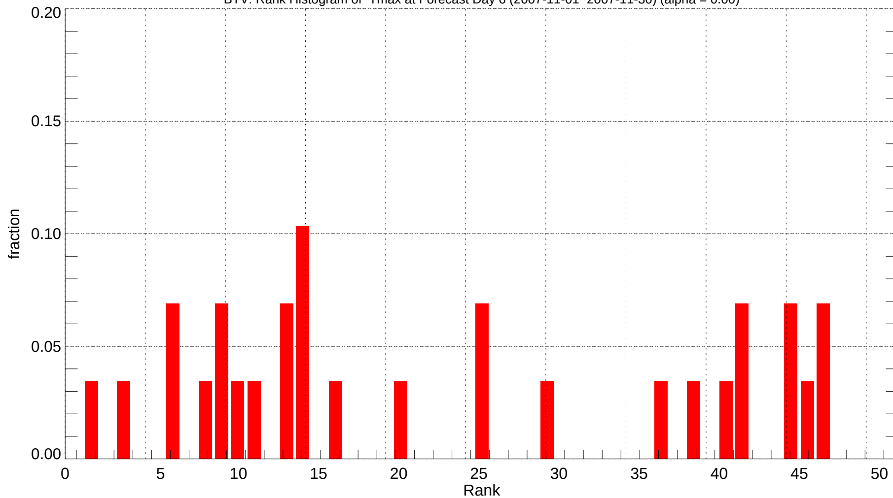
BTV: Rank Histogram of Tmax at Forecast Day 6 (2007-11-01~2007-11-30) (alpha = 0.00)
