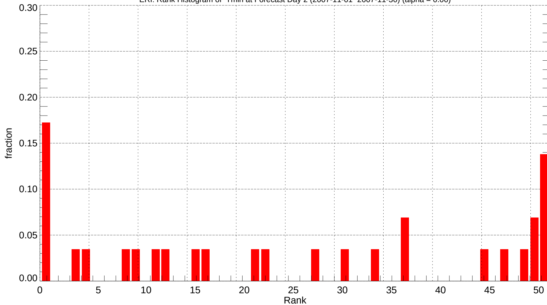
ERI: Rank Histogram of Tmin at Forecast Day 2 (2007-11-01~2007-11-30) (alpha = 0.00)
