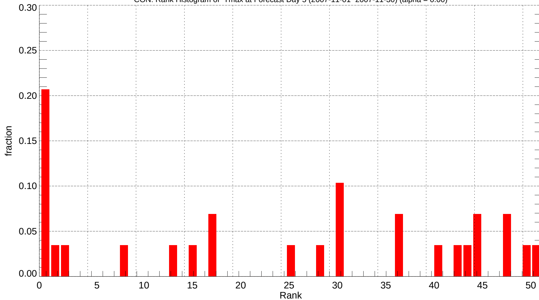
CON: Rank Histogram of Tmax at Forecast Day 5 (2007-11-01~2007-11-30) (alpha = 0.00)
