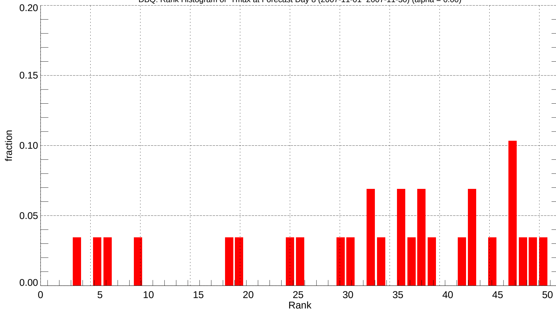
DBQ: Rank Histogram of Tmax at Forecast Day 8 (2007-11-01~2007-11-30) (alpha = 0.00)
