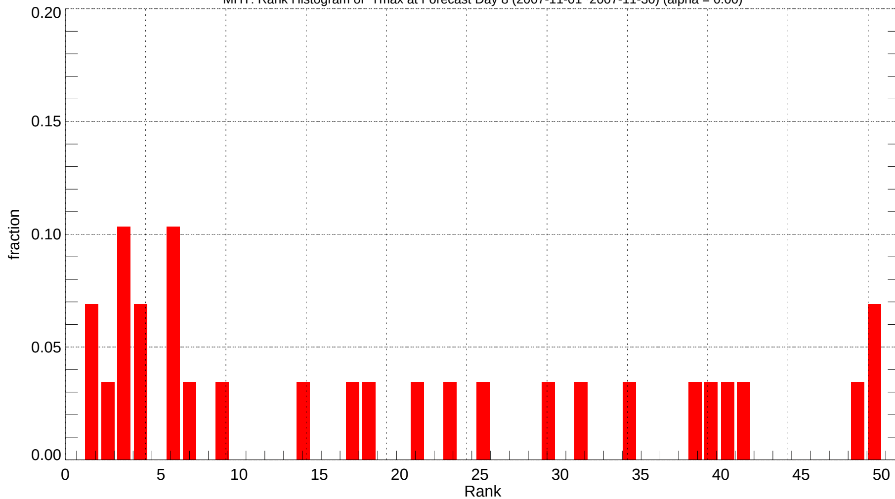
MHT: Rank Histogram of Tmax at Forecast Day 8 (2007-11-01~2007-11-30) (alpha = 0.00)
