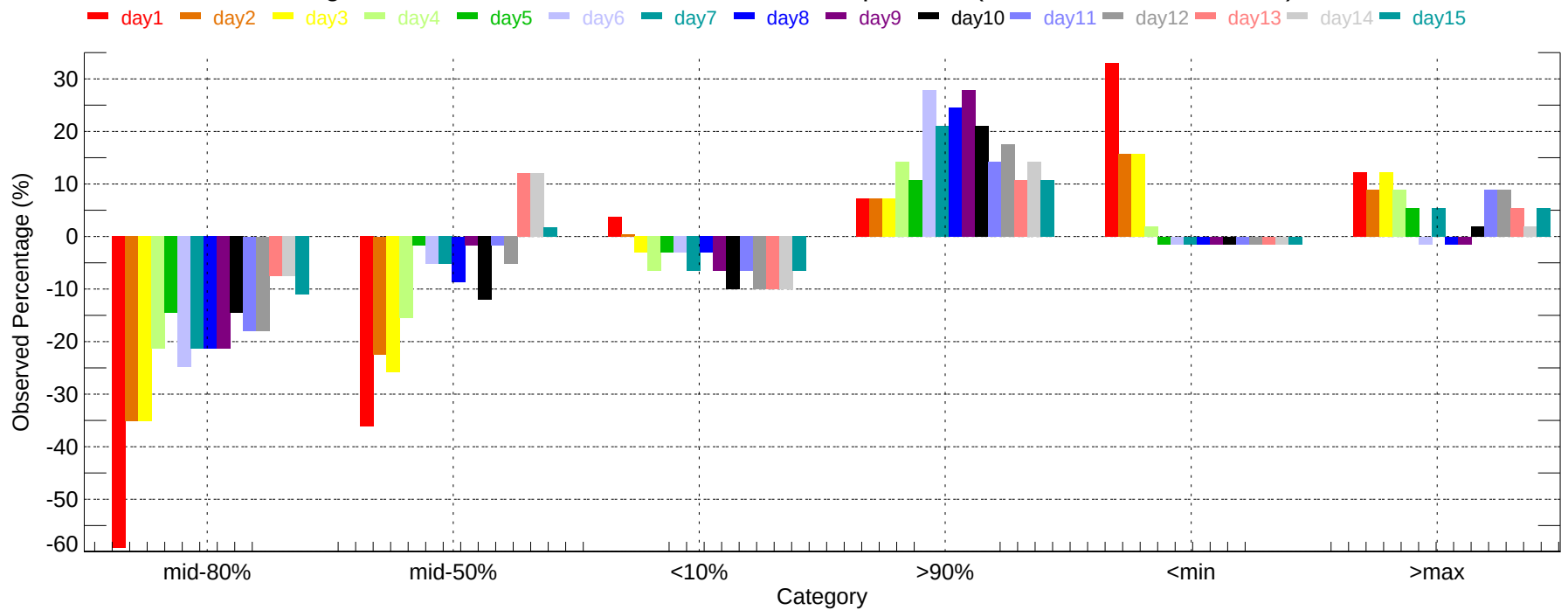
Observed Percentage Deviation of Ensembles - IND: Max Temperature (2007-11-01~2007-11-30)
