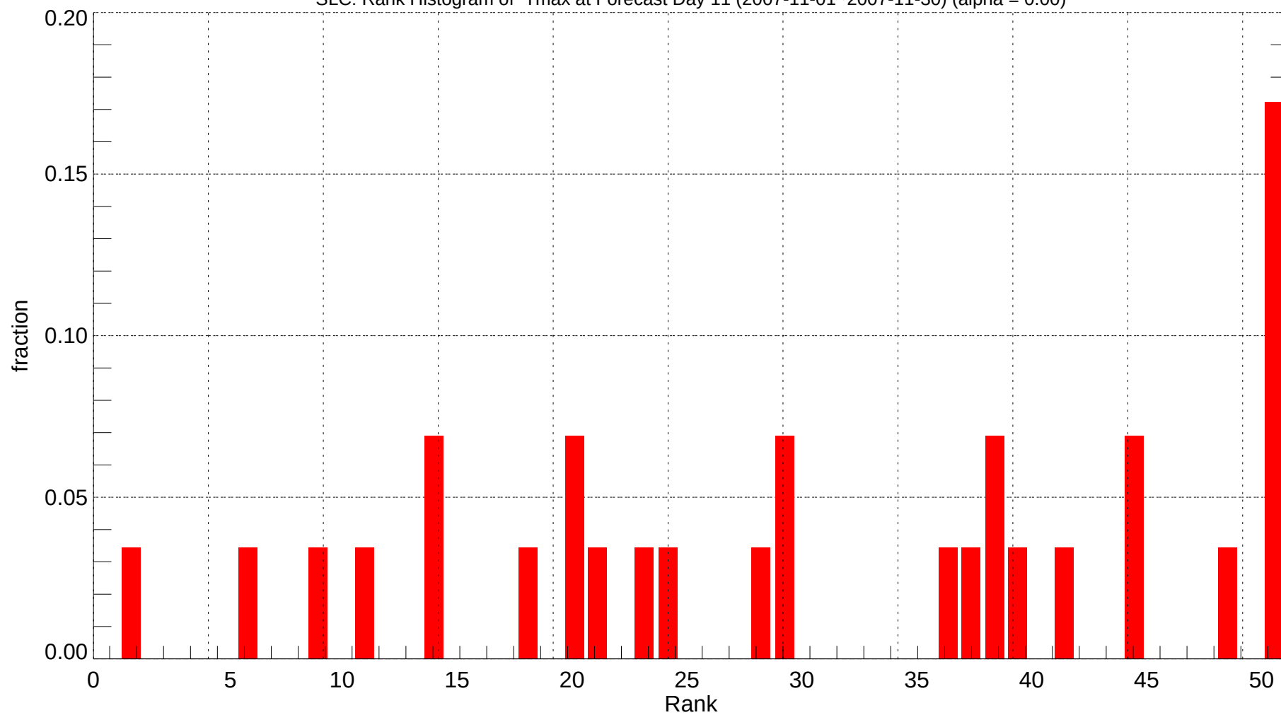
SLC: Rank Histogram of Tmax at Forecast Day 11 (2007-11-01~2007-11-30) (alpha = 0.00)
