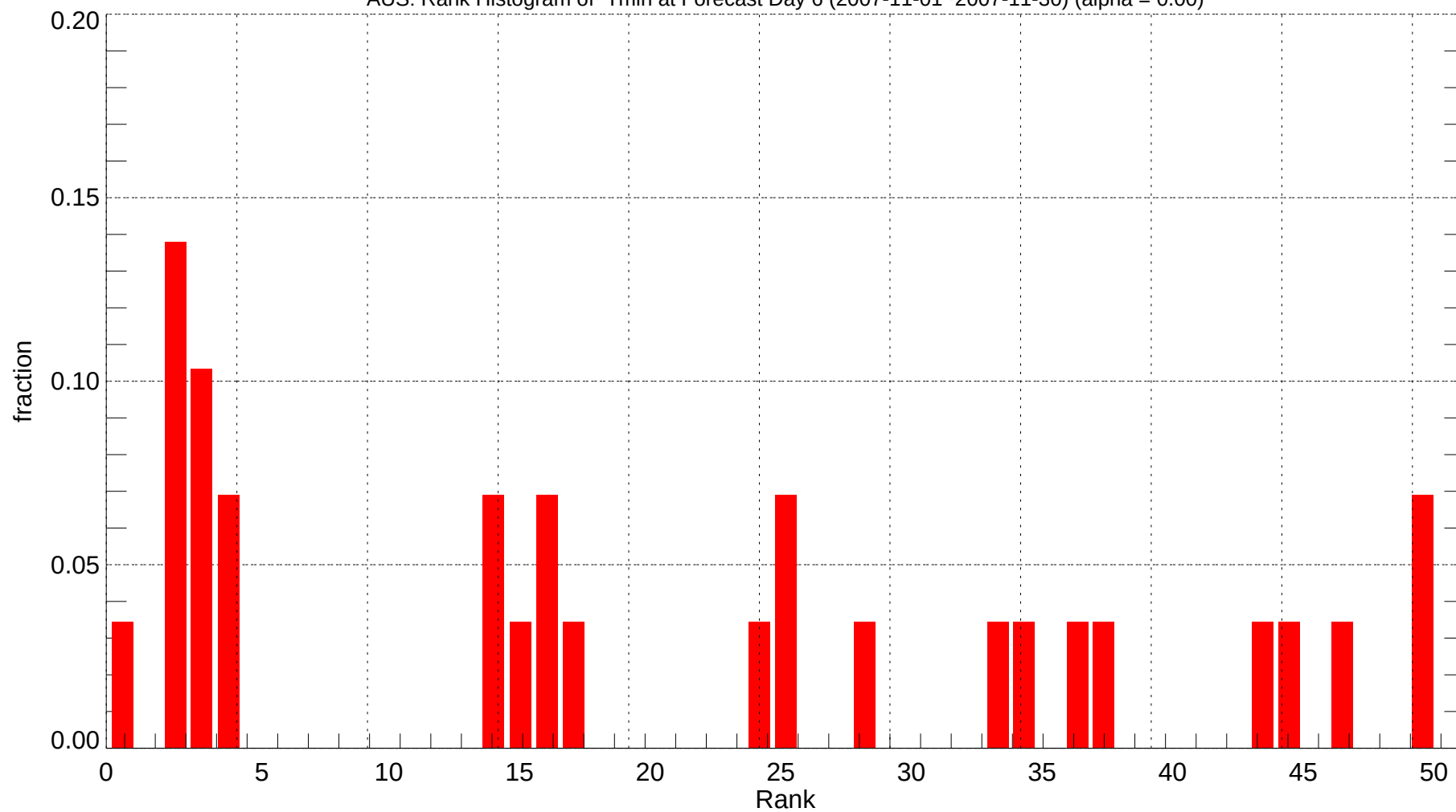
AUS: Rank Histogram of Tmin at Forecast Day 6 (2007-11-01~2007-11-30) (alpha = 0.00)
