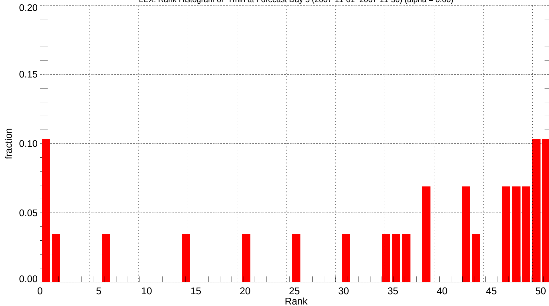
LEX: Rank Histogram of Tmin at Forecast Day 3 (2007-11-01~2007-11-30) (alpha = 0.00)
