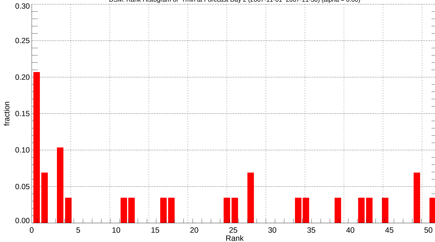
DSM: Rank Histogram of Tmin at Forecast Day 2 (2007-11-01~2007-11-30) (alpha = 0.00)
