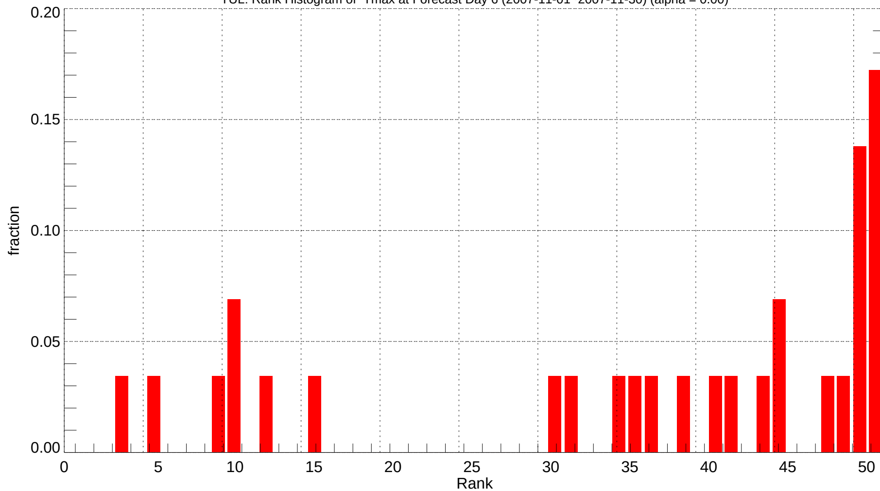
TUL: Rank Histogram of Tmax at Forecast Day 6 (2007-11-01~2007-11-30) (alpha = 0.00)
