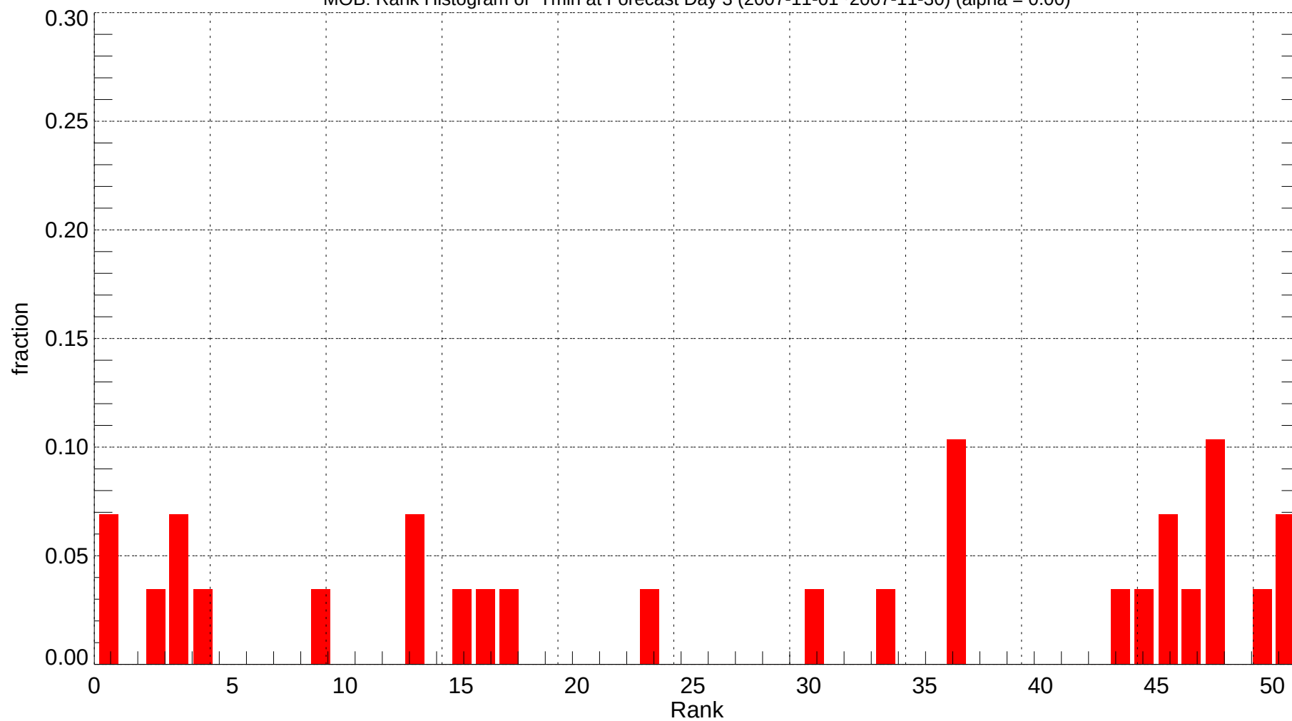
MOB: Rank Histogram of Tmin at Forecast Day 3 (2007-11-01~2007-11-30) (alpha = 0.00)
