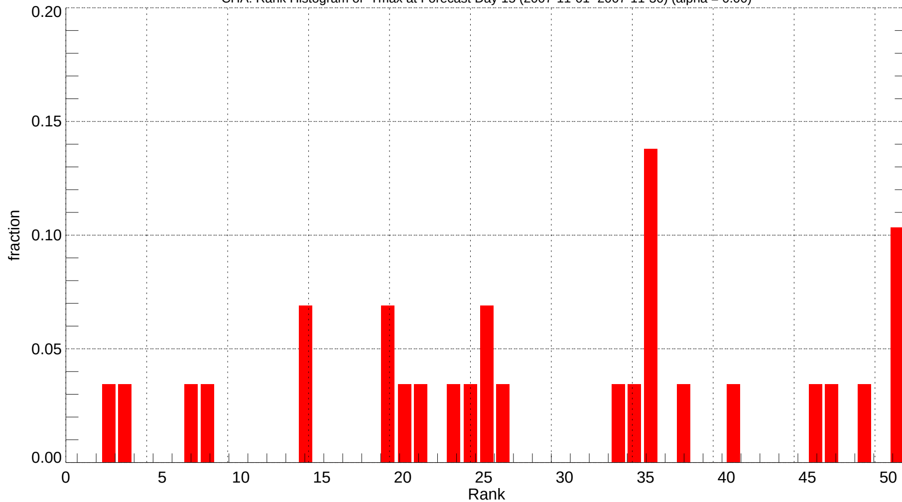
CHA: Rank Histogram of Tmax at Forecast Day 15 (2007-11-01~2007-11-30) (alpha = 0.00)
