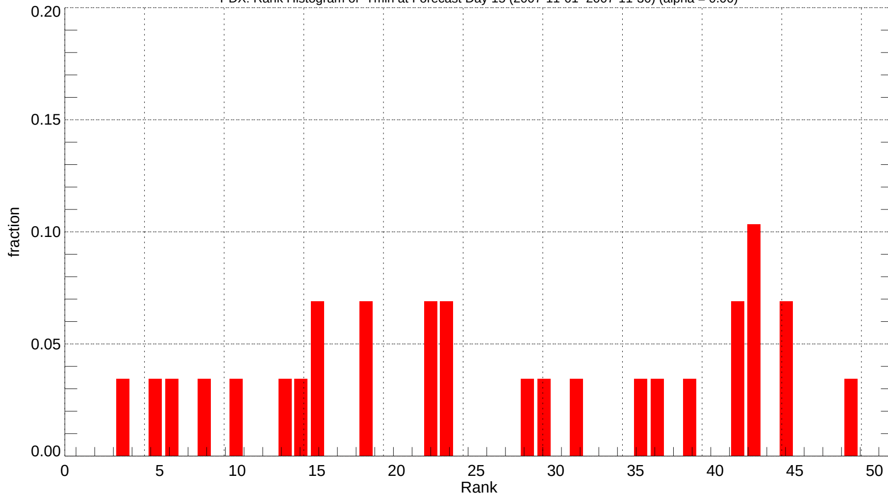
PDX: Rank Histogram of Tmin at Forecast Day 15 (2007-11-01~2007-11-30) (alpha = 0.00)
