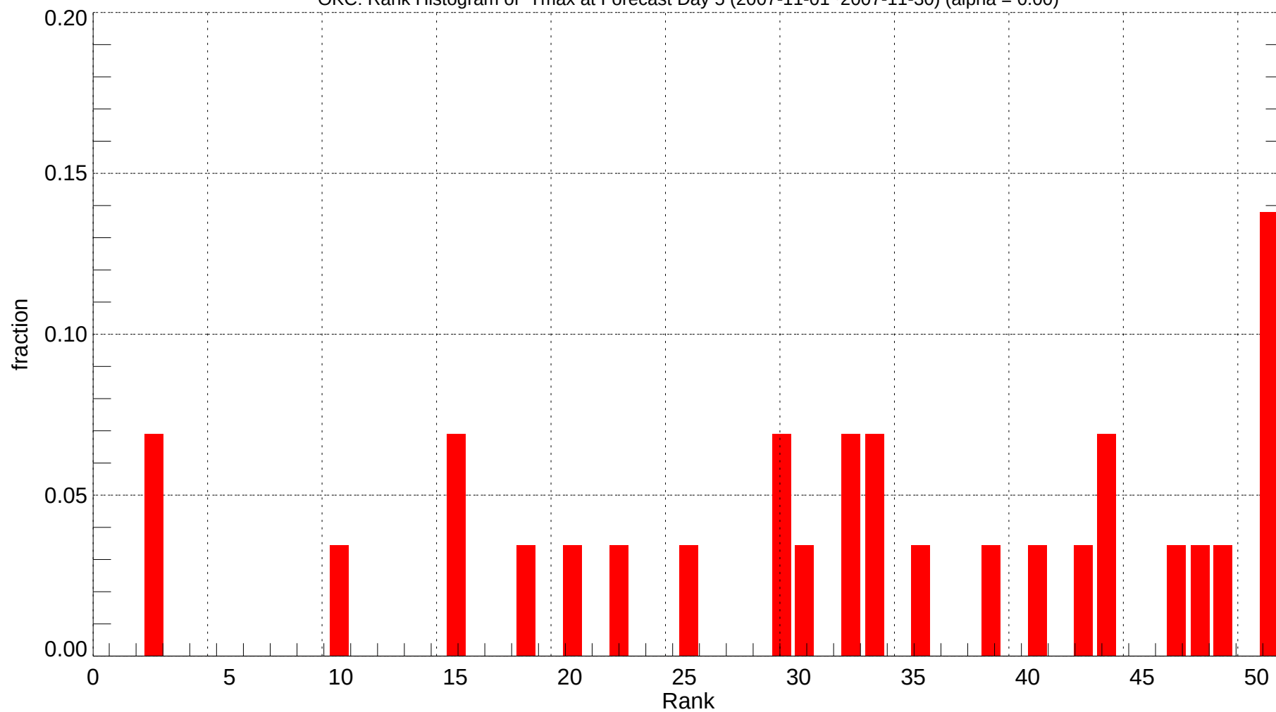
OKC: Rank Histogram of Tmax at Forecast Day 5 (2007-11-01~2007-11-30) (alpha = 0.00)
