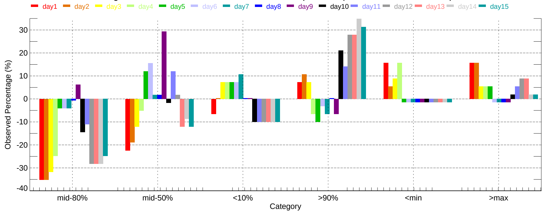
Observed Percentage Deviation of Ensembles - WJF: Max Temperature (2007-11-01~2007-11-30)
