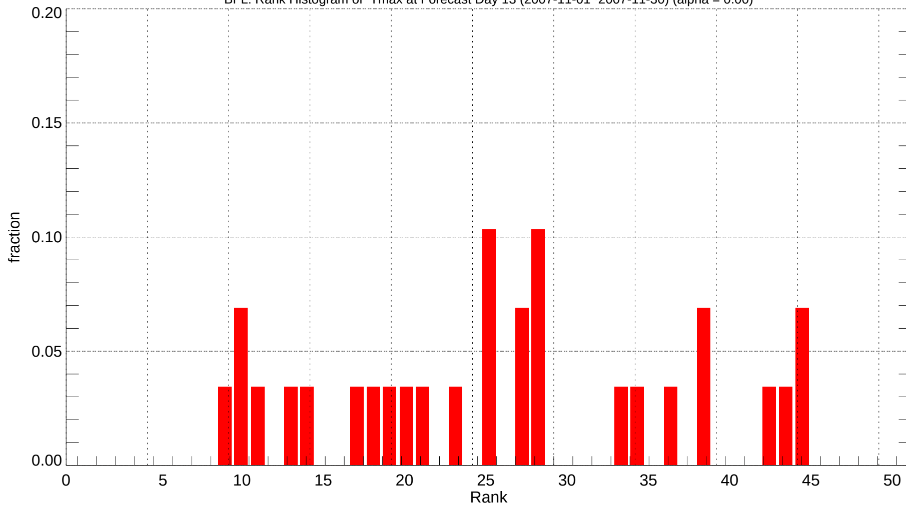
BFL: Rank Histogram of Tmax at Forecast Day 13 (2007-11-01~2007-11-30) (alpha = 0.00)
