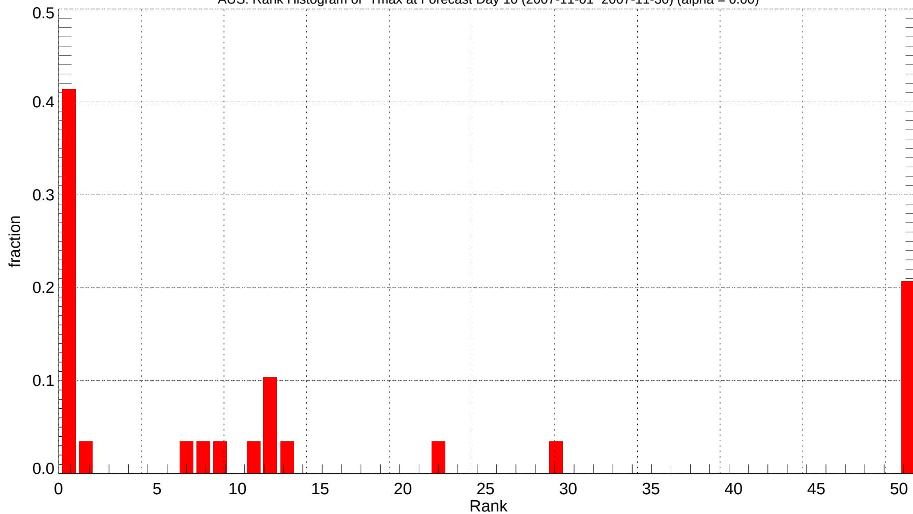
AUS: Rank Histogram of Tmax at Forecast Day 10 (2007-11-01~2007-11-30) (alpha = 0.00)
