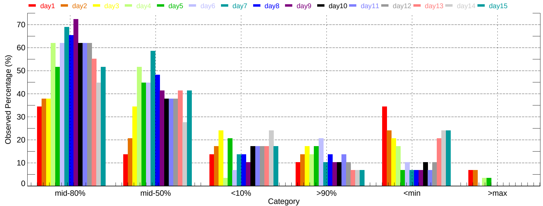
Observed Percentage of Ensembles - AUG: Min Temperature (2007-11-01~2007-11-30)
