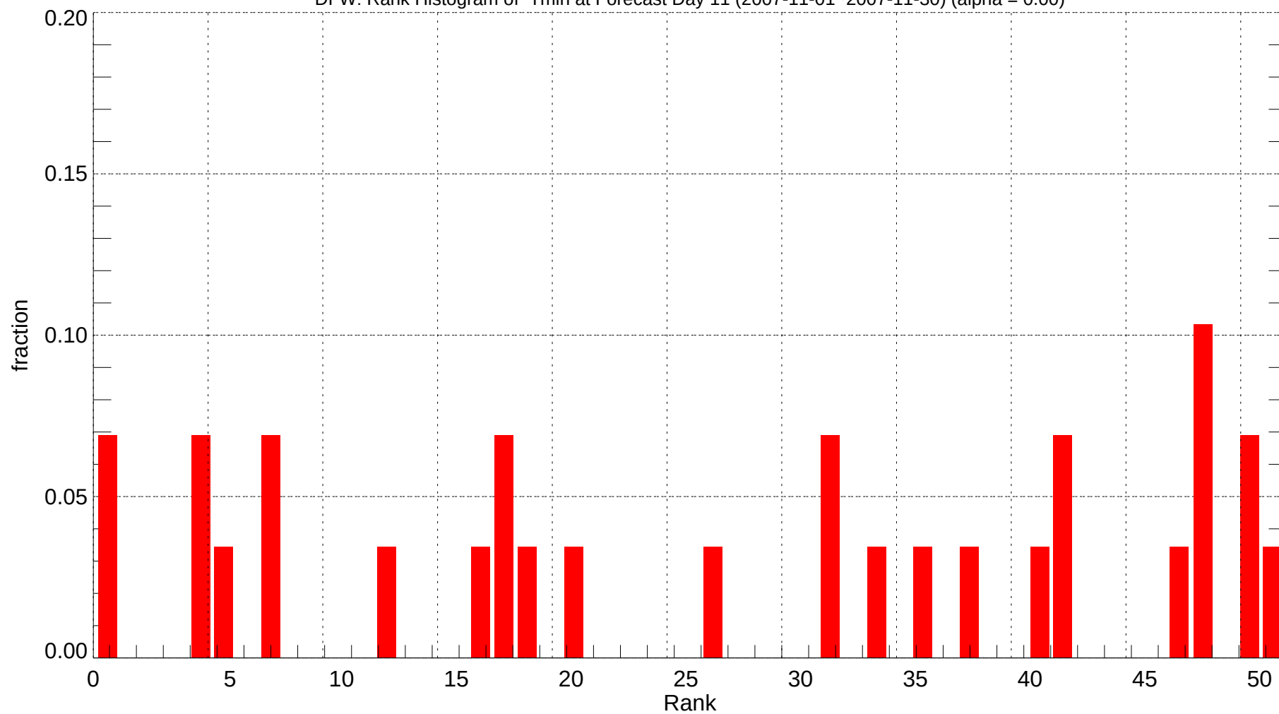
DFW: Rank Histogram of Tmin at Forecast Day 11 (2007-11-01~2007-11-30) (alpha = 0.00)
