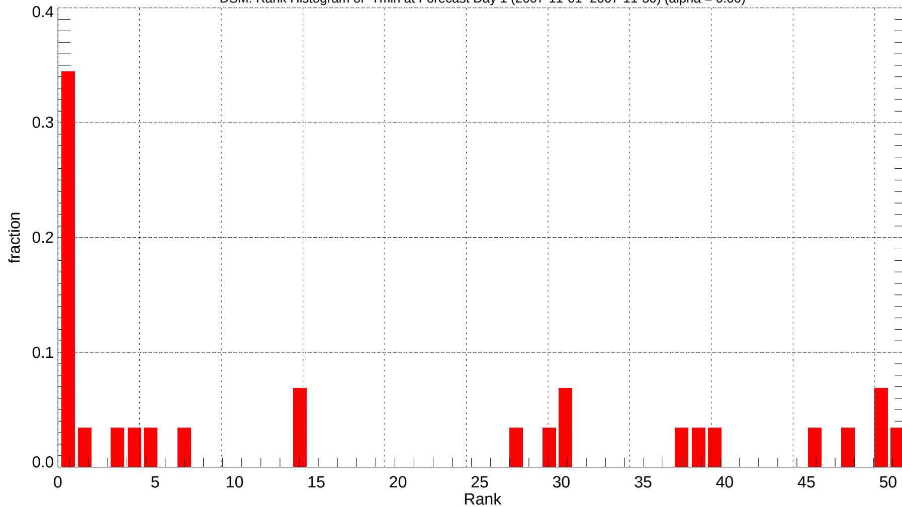
DSM: Rank Histogram of Tmin at Forecast Day 1 (2007-11-01~2007-11-30) (alpha = 0.00)
