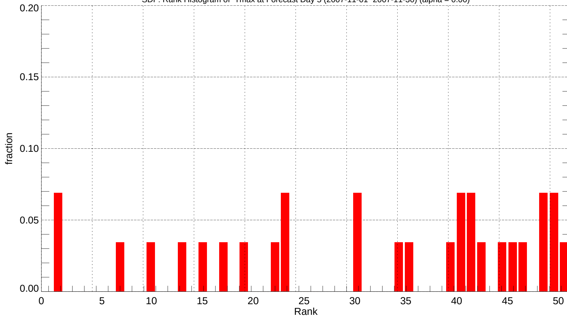
SDF: Rank Histogram of Tmax at Forecast Day 5 (2007-11-01~2007-11-30) (alpha = 0.00)
