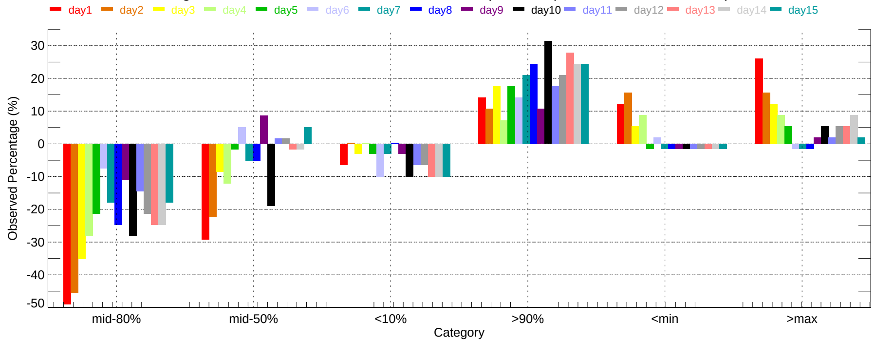
Observed Percentage Deviation of Ensembles - TRM: Max Temperature (2007-11-01~2007-11-30)
