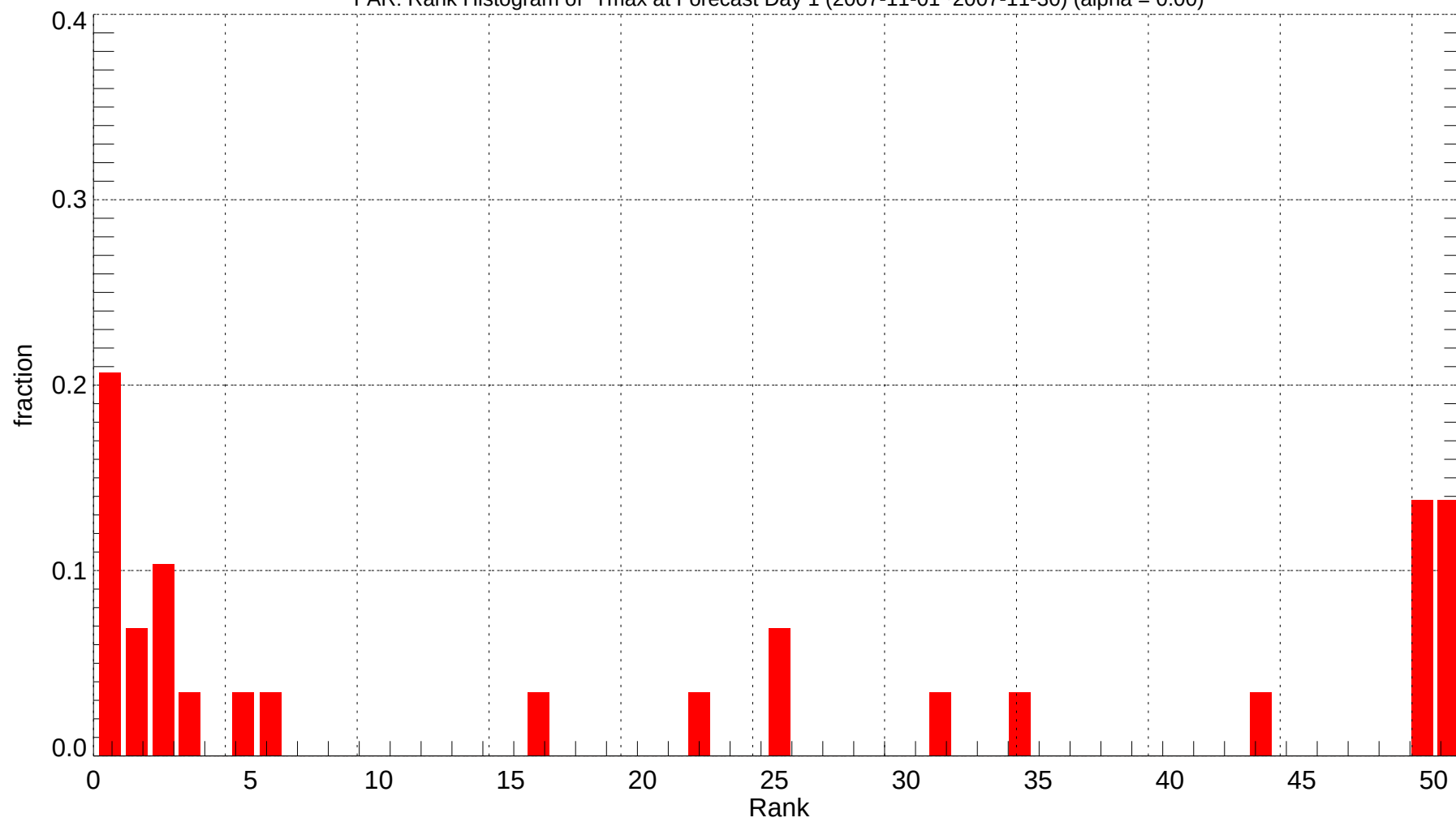
FAR: Rank Histogram of Tmax at Forecast Day 1 (2007-11-01~2007-11-30) (alpha = 0.00)
