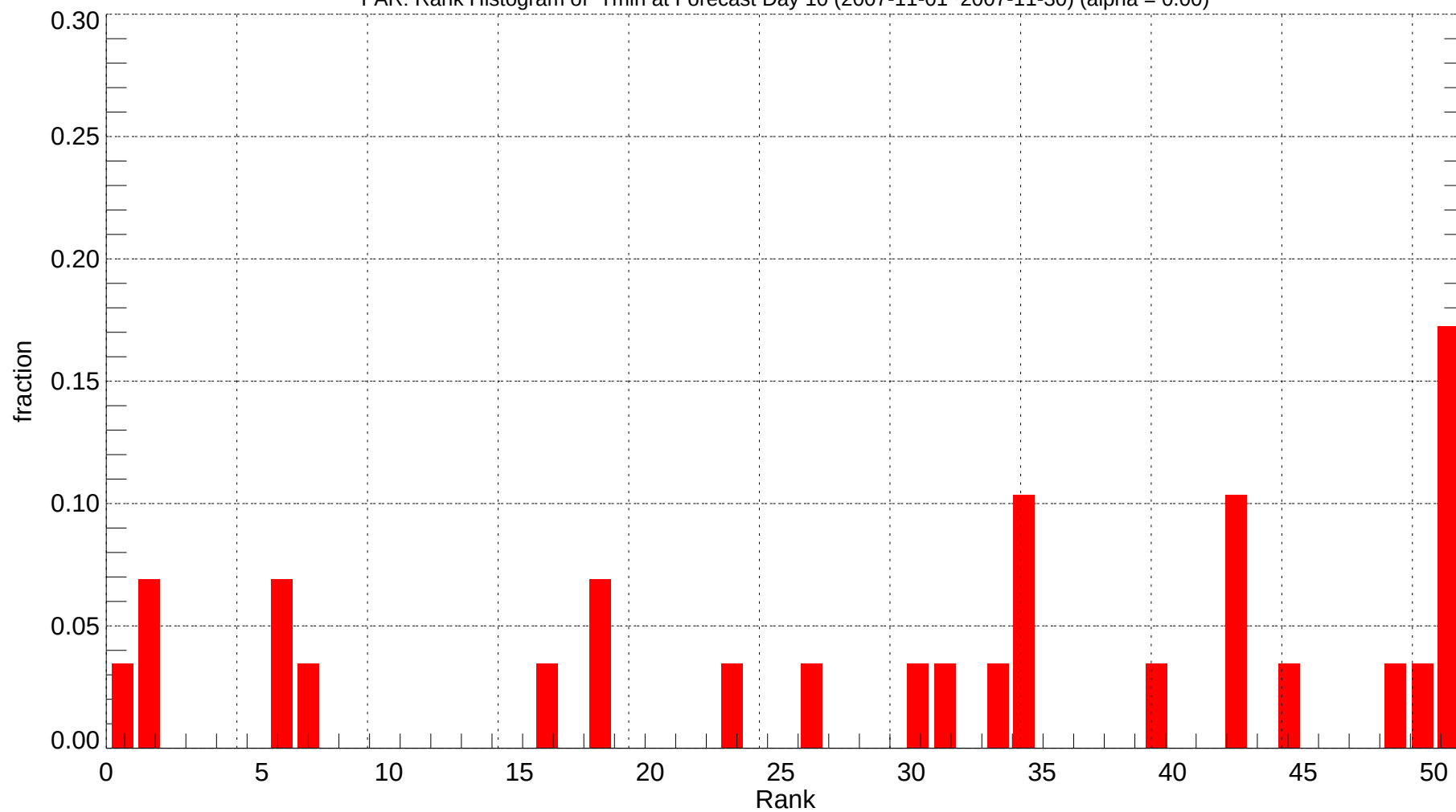
FAR: Rank Histogram of Tmin at Forecast Day 10 (2007-11-01~2007-11-30) (alpha = 0.00)
