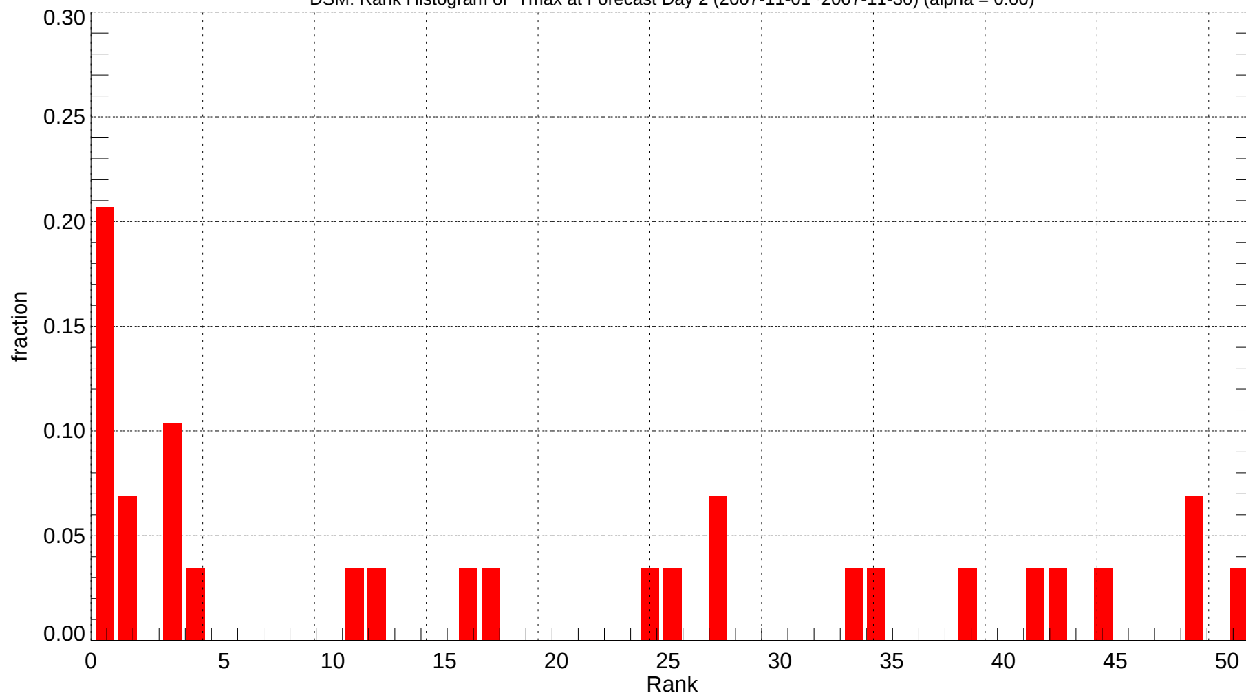
DSM: Rank Histogram of Tmax at Forecast Day 2 (2007-11-01~2007-11-30) (alpha = 0.00)
