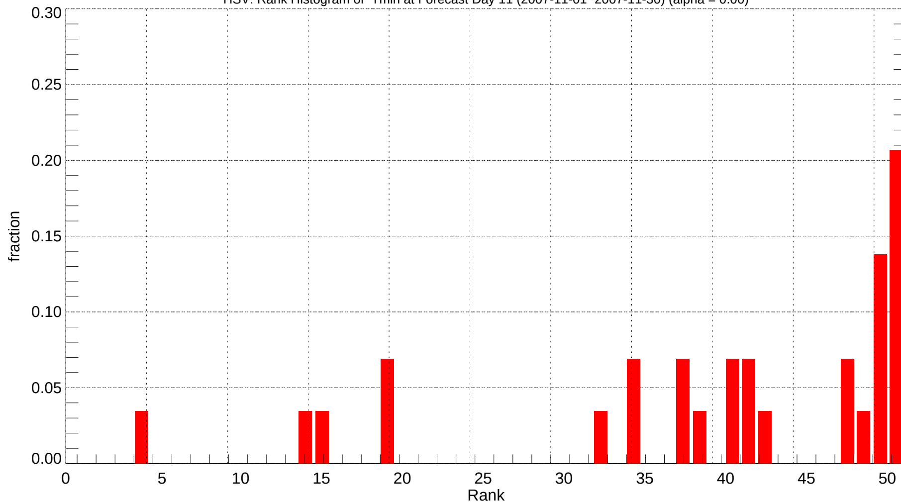
HSV: Rank Histogram of Tmin at Forecast Day 11 (2007-11-01~2007-11-30) (alpha = 0.00)
