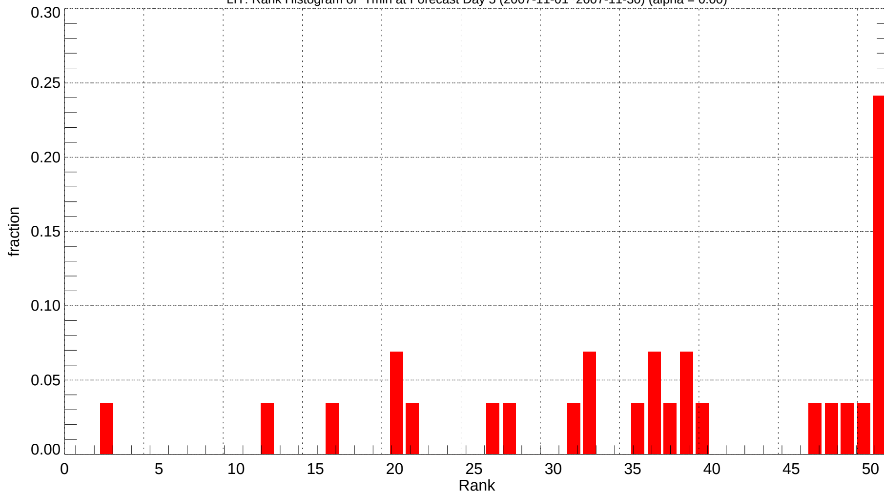
LIT: Rank Histogram of Tmin at Forecast Day 5 (2007-11-01~2007-11-30) (alpha = 0.00)
