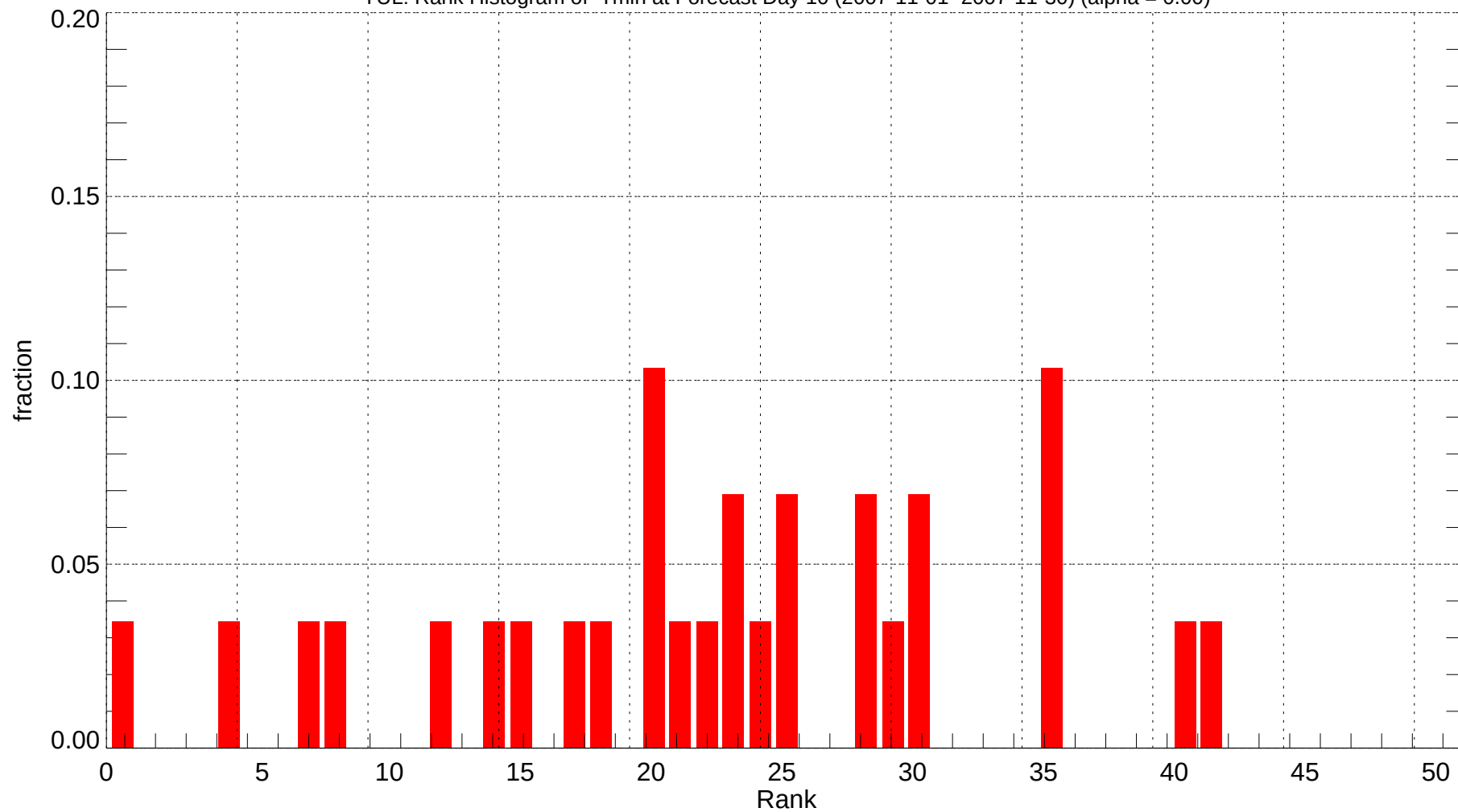
YUL: Rank Histogram of Tmin at Forecast Day 10 (2007-11-01~2007-11-30) (alpha = 0.00)
