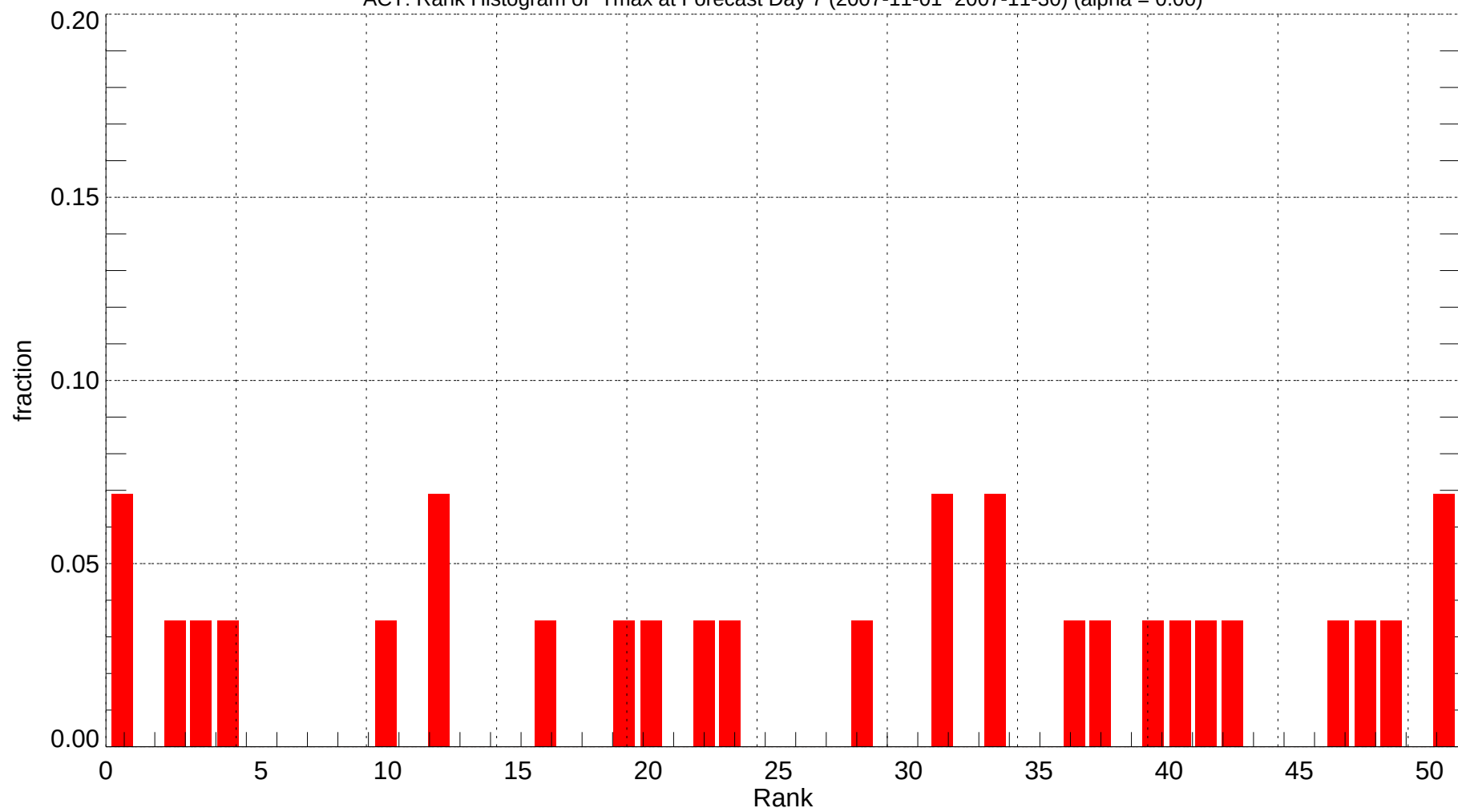
ACT: Rank Histogram of Tmax at Forecast Day 7 (2007-11-01~2007-11-30) (alpha = 0.00)
