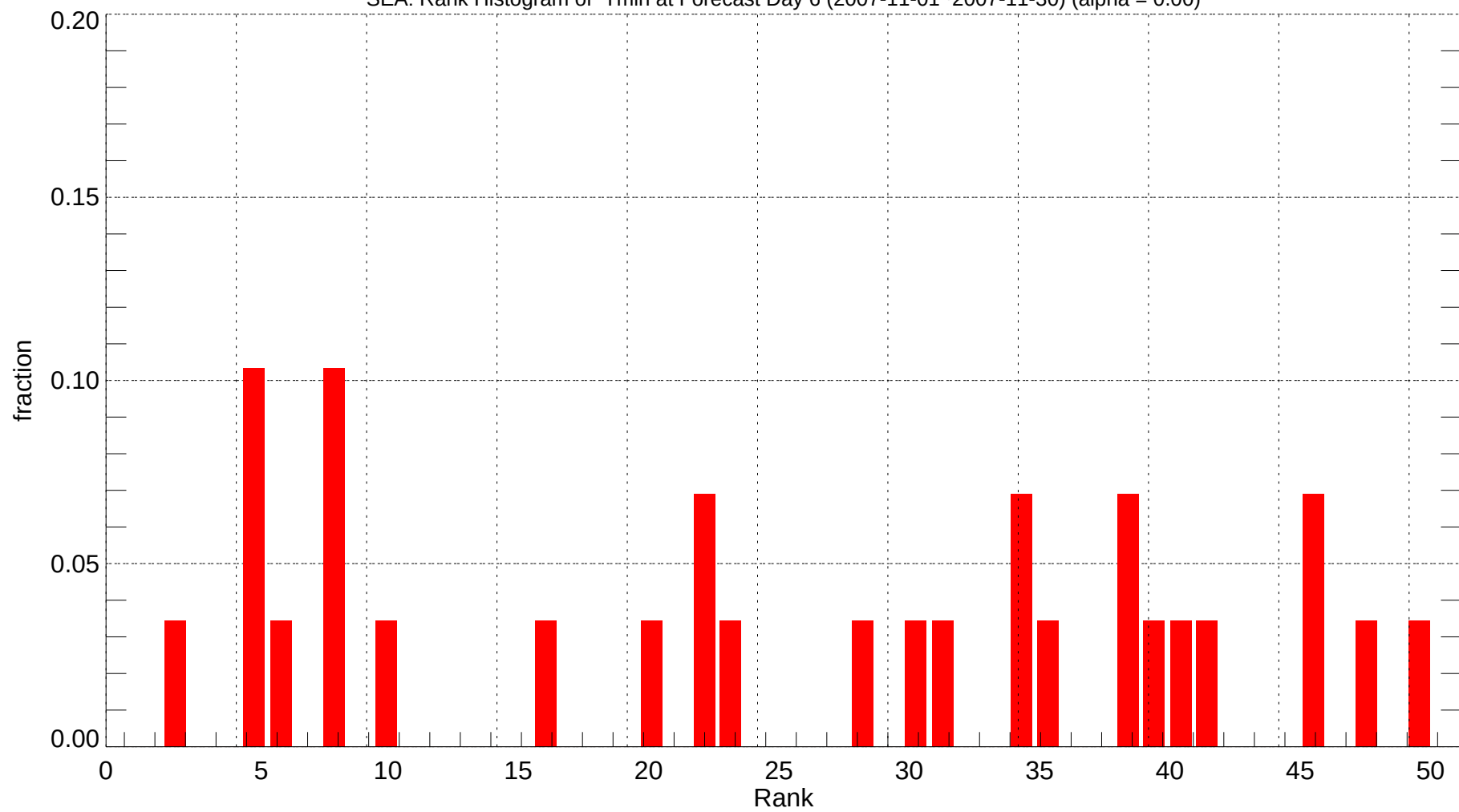
SEA: Rank Histogram of Tmin at Forecast Day 6 (2007-11-01~2007-11-30) (alpha = 0.00)
