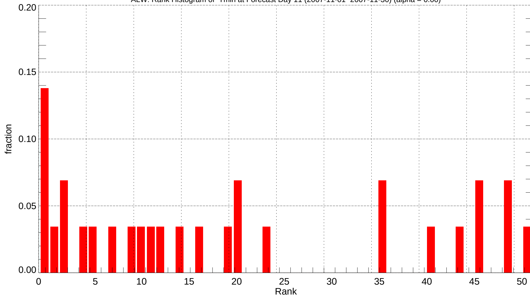
ALW: Rank Histogram of Tmin at Forecast Day 11 (2007-11-01~2007-11-30) (alpha = 0.00)
