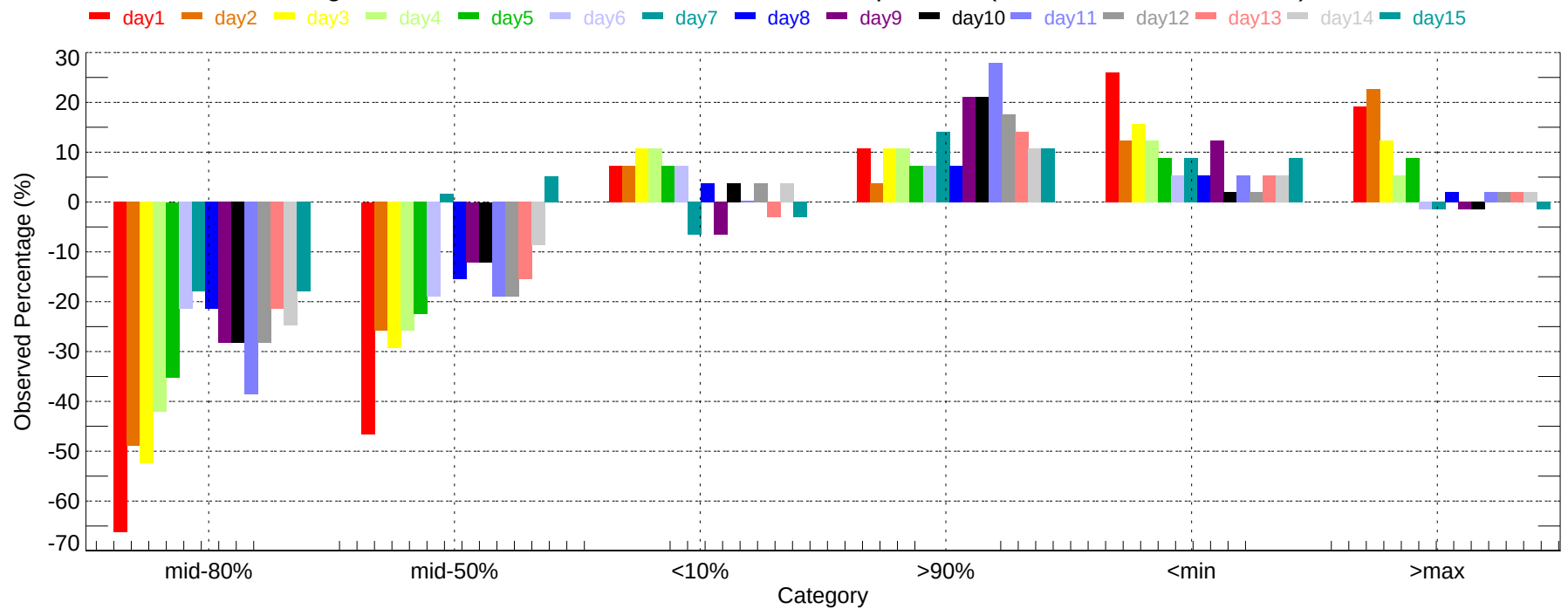
Observed Percentage Deviation of Ensembles - BRO: Max Temperature (2007-11-01~2007-11-30)
