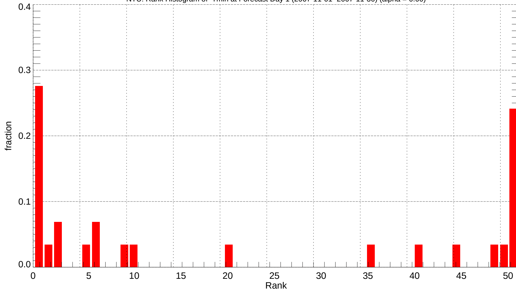
NTU: Rank Histogram of Tmin at Forecast Day 1 (2007-11-01~2007-11-30) (alpha = 0.00)
