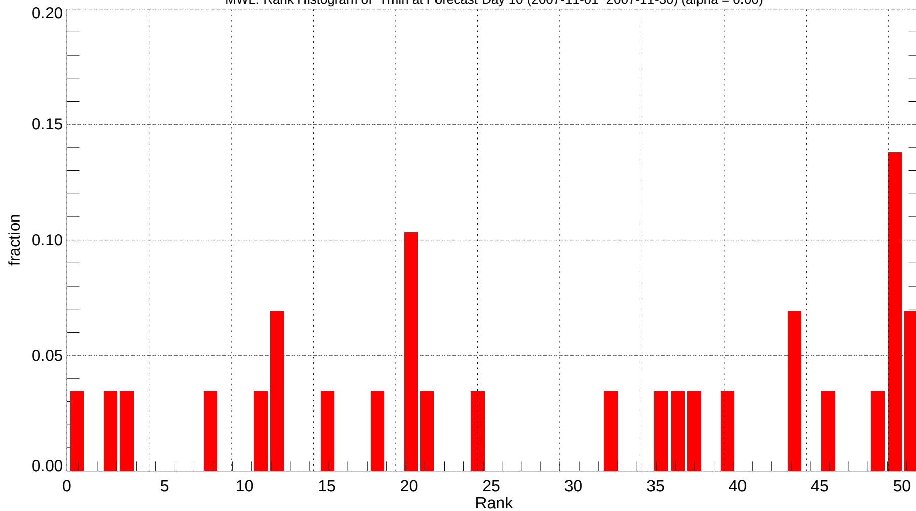
MWL: Rank Histogram of Tmin at Forecast Day 10 (2007-11-01~2007-11-30) (alpha = 0.00)
