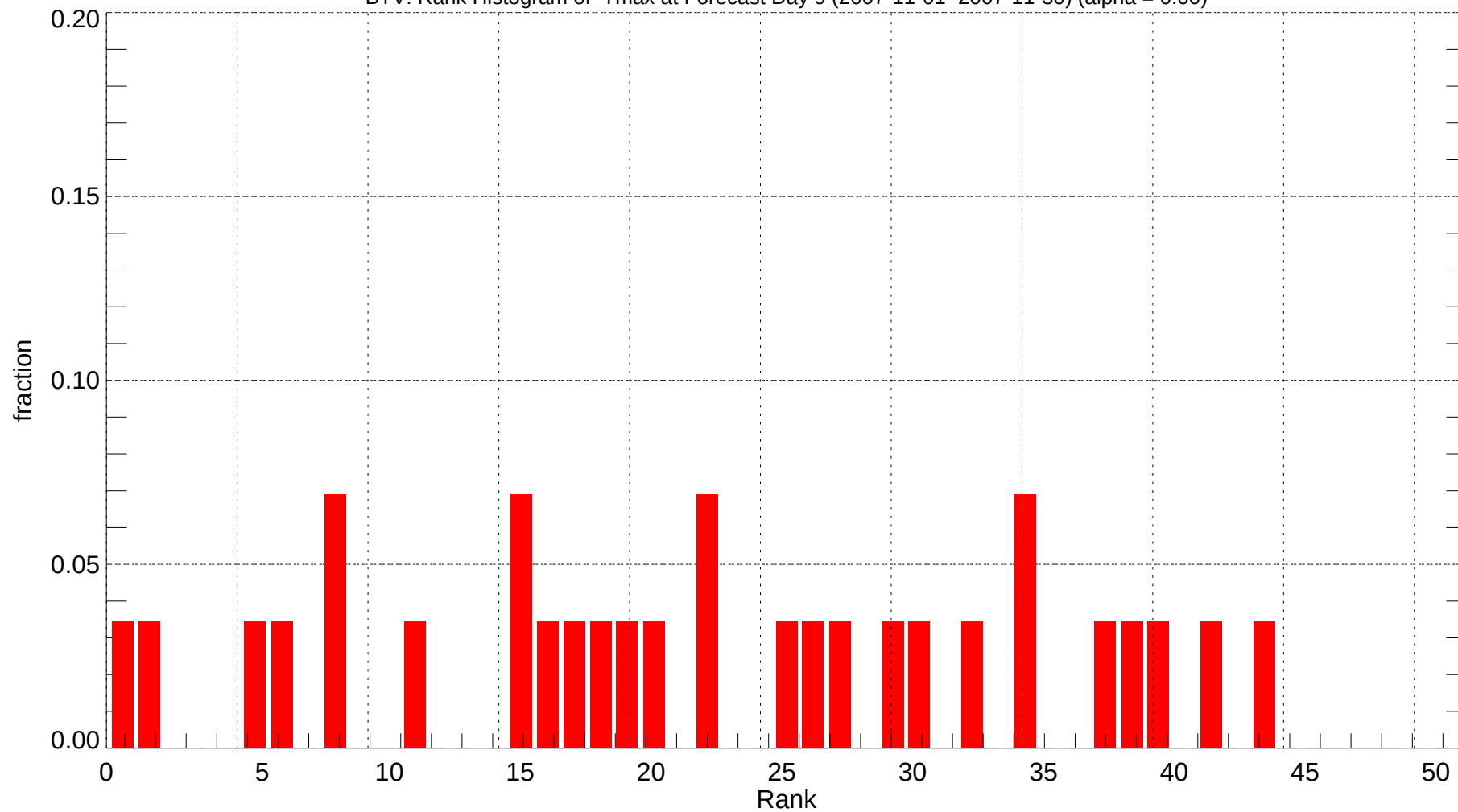
BTV: Rank Histogram of Tmax at Forecast Day 9 (2007-11-01~2007-11-30) (alpha = 0.00)
