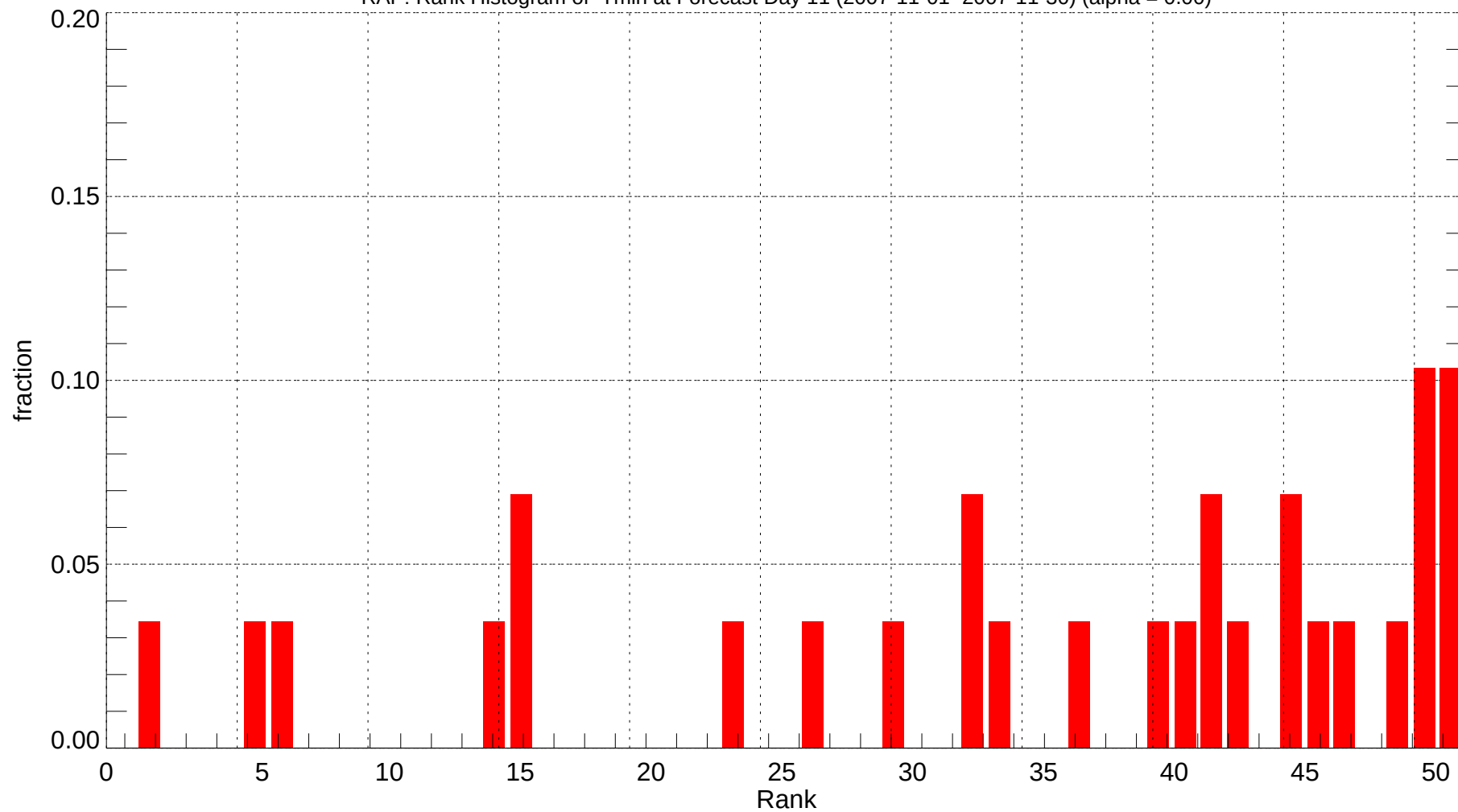
RAP: Rank Histogram of Tmin at Forecast Day 11 (2007-11-01~2007-11-30) (alpha = 0.00)
