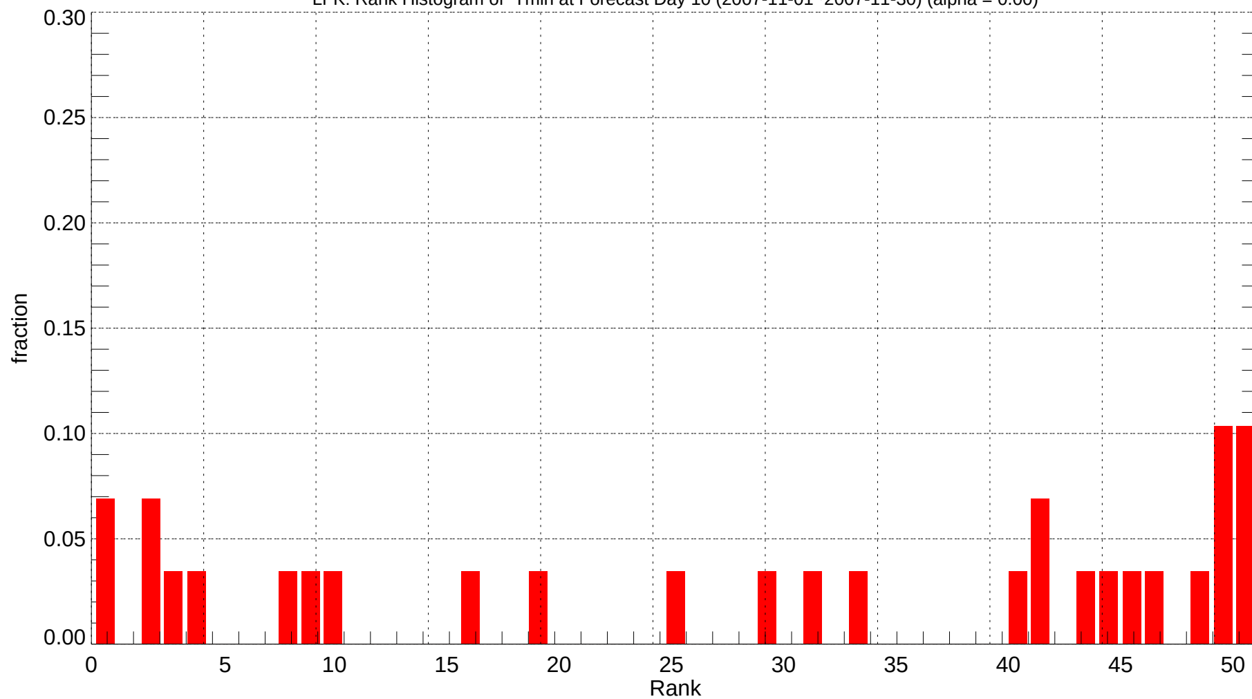
LFK: Rank Histogram of Tmin at Forecast Day 10 (2007-11-01~2007-11-30) (alpha = 0.00)
