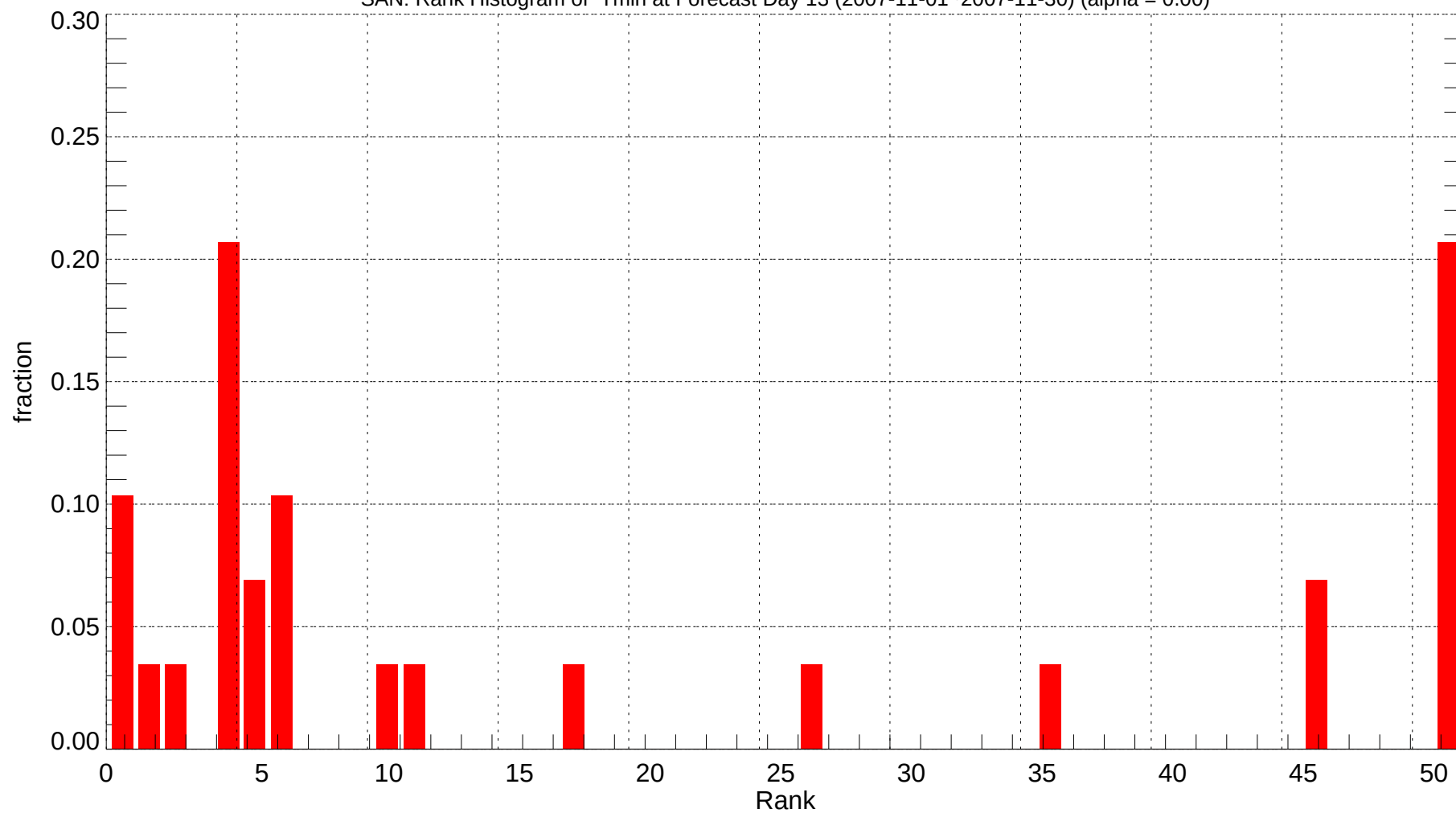
SAN: Rank Histogram of Tmin at Forecast Day 13 (2007-11-01~2007-11-30) (alpha = 0.00)
