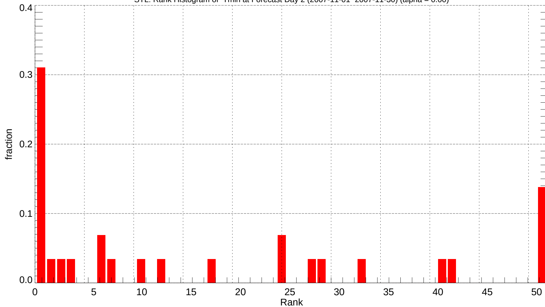
STL: Rank Histogram of Tmin at Forecast Day 2 (2007-11-01~2007-11-30) (alpha = 0.00)
