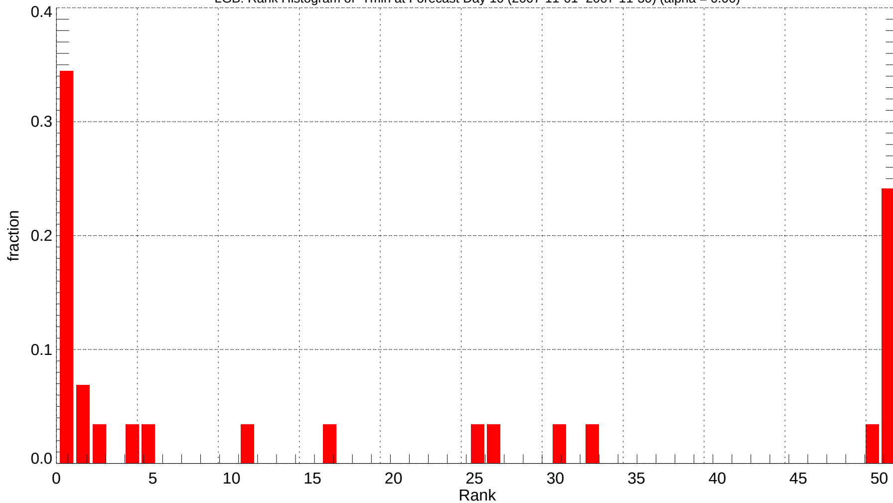
LGB: Rank Histogram of Tmin at Forecast Day 10 (2007-11-01~2007-11-30) (alpha = 0.00)
