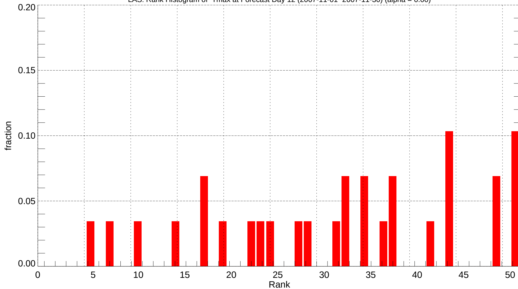
LAS: Rank Histogram of Tmax at Forecast Day 12 (2007-11-01~2007-11-30) (alpha = 0.00)
