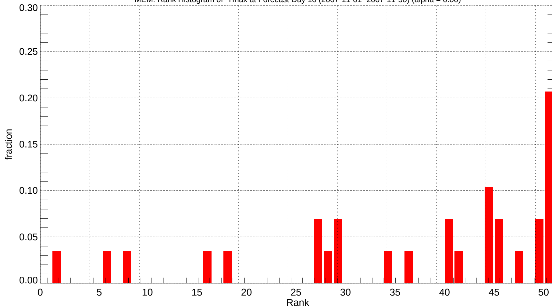
MEM: Rank Histogram of Tmax at Forecast Day 10 (2007-11-01~2007-11-30) (alpha = 0.00)
