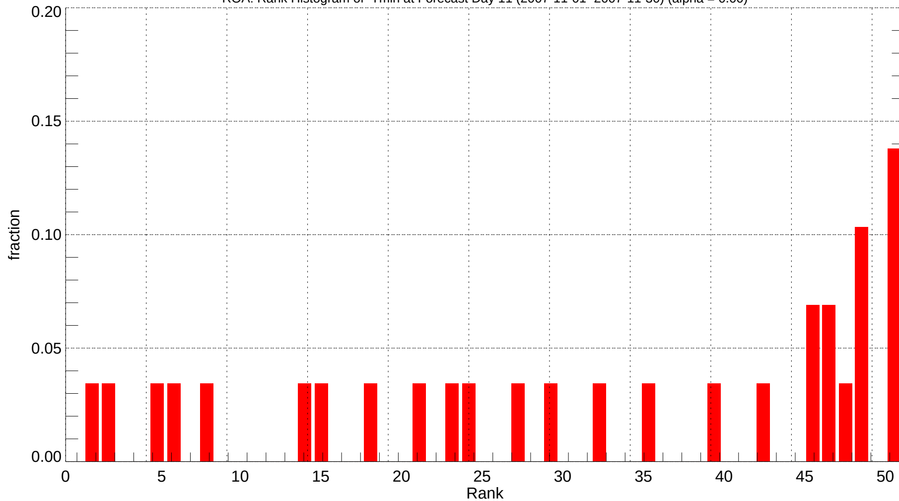
ROA: Rank Histogram of Tmin at Forecast Day 11 (2007-11-01~2007-11-30) (alpha = 0.00)
