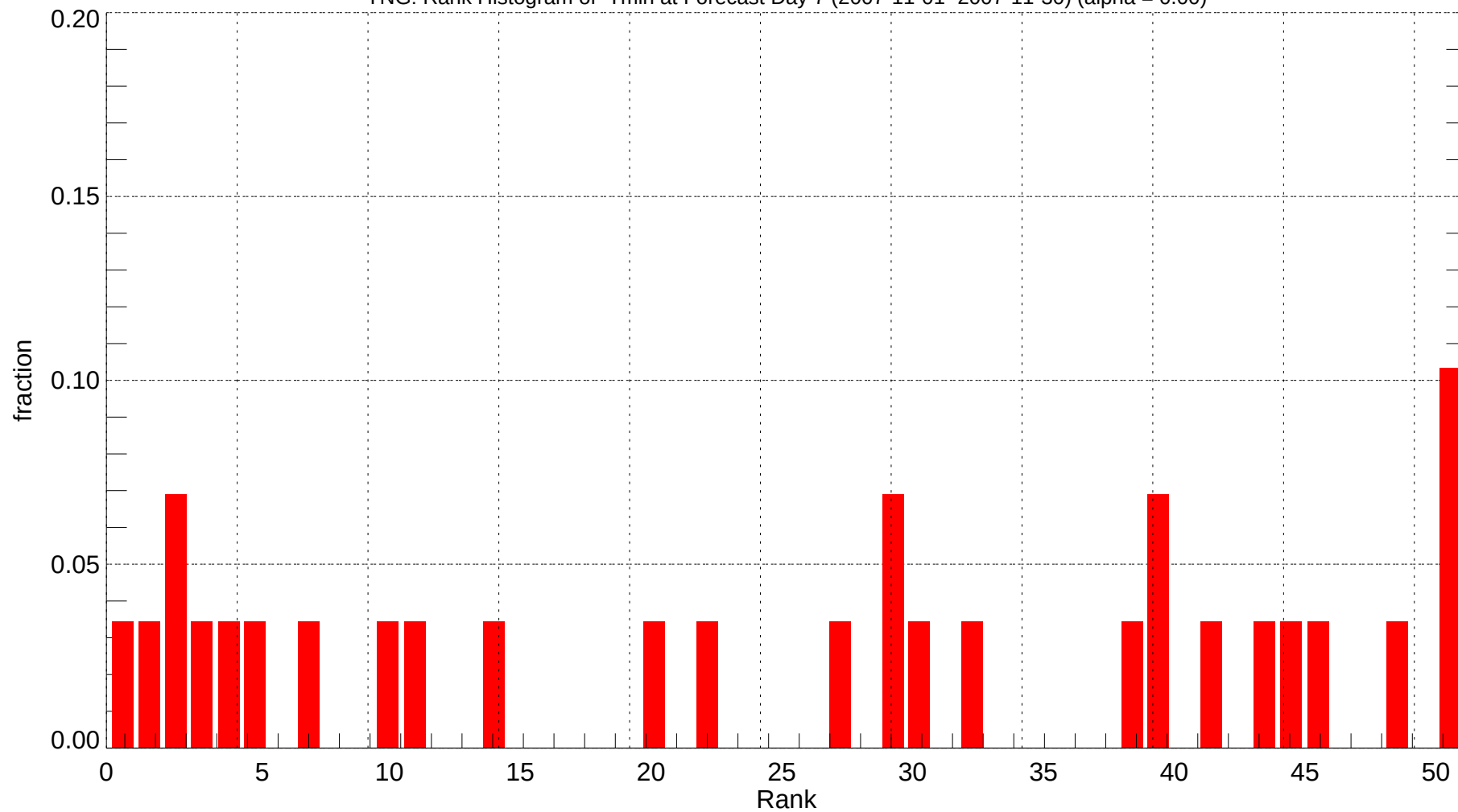
YNG: Rank Histogram of Tmin at Forecast Day 7 (2007-11-01~2007-11-30) (alpha = 0.00)
