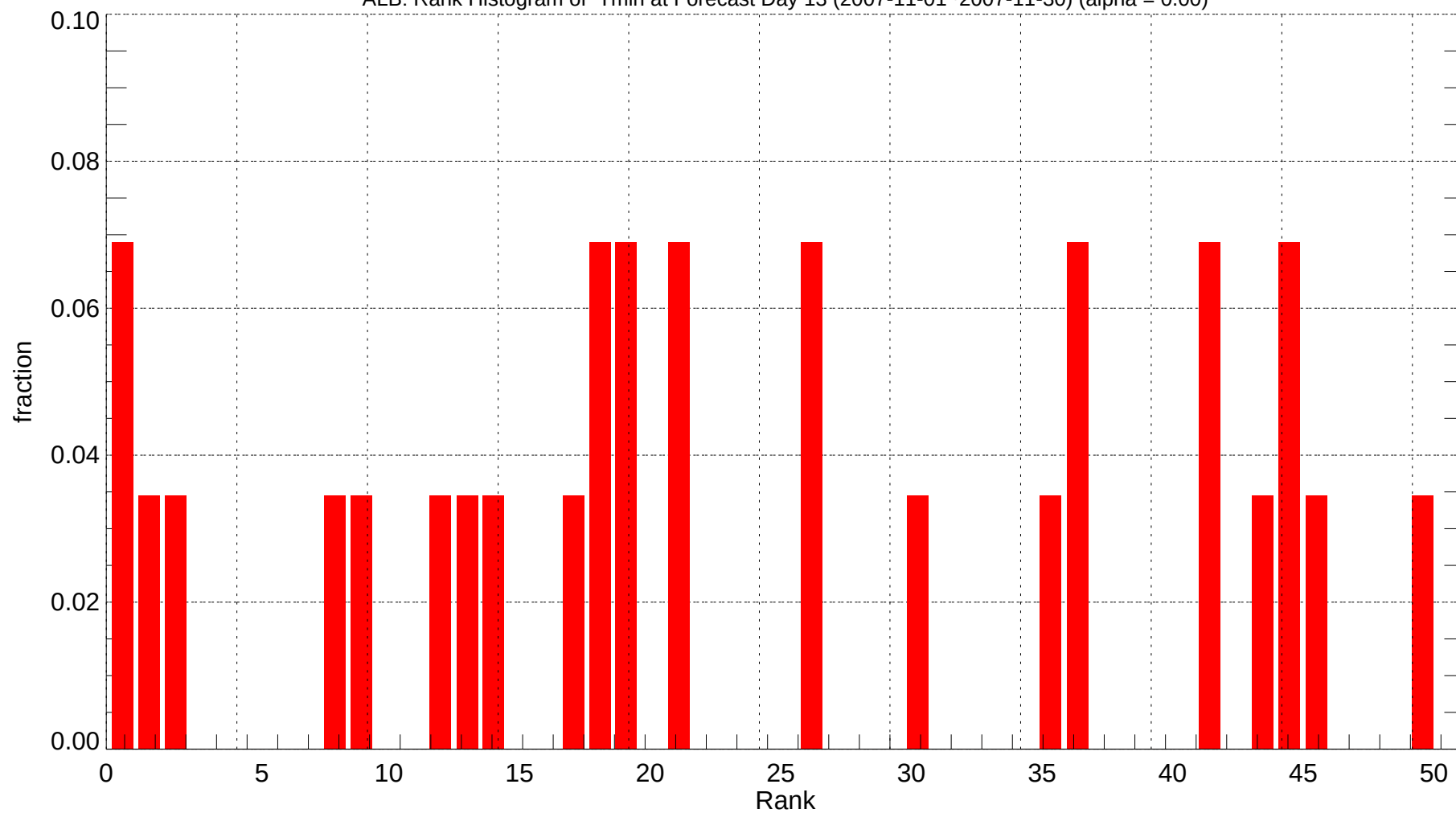
ALB: Rank Histogram of Tmin at Forecast Day 13 (2007-11-01~2007-11-30) (alpha = 0.00)
