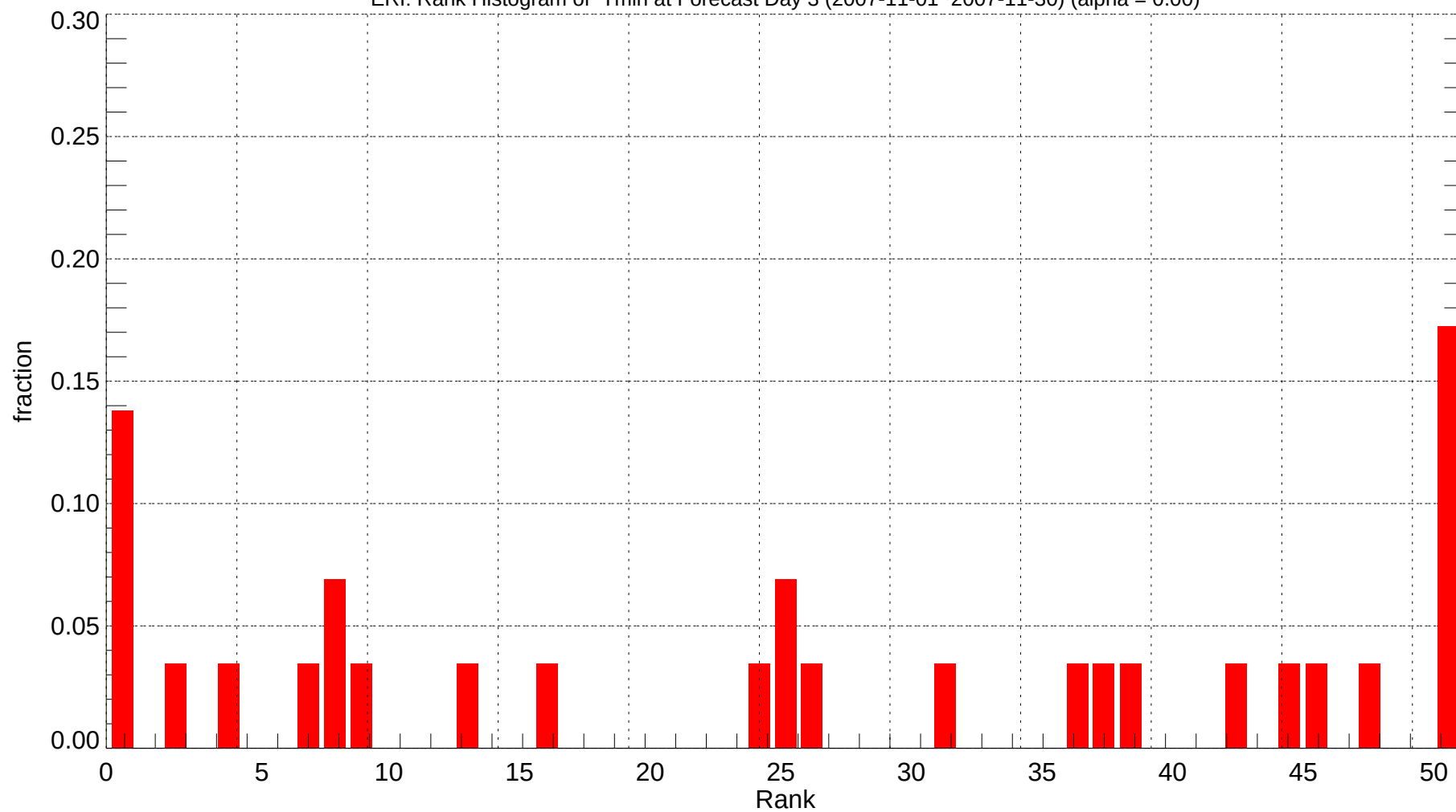
ERI: Rank Histogram of Tmin at Forecast Day 3 (2007-11-01~2007-11-30) (alpha = 0.00)
