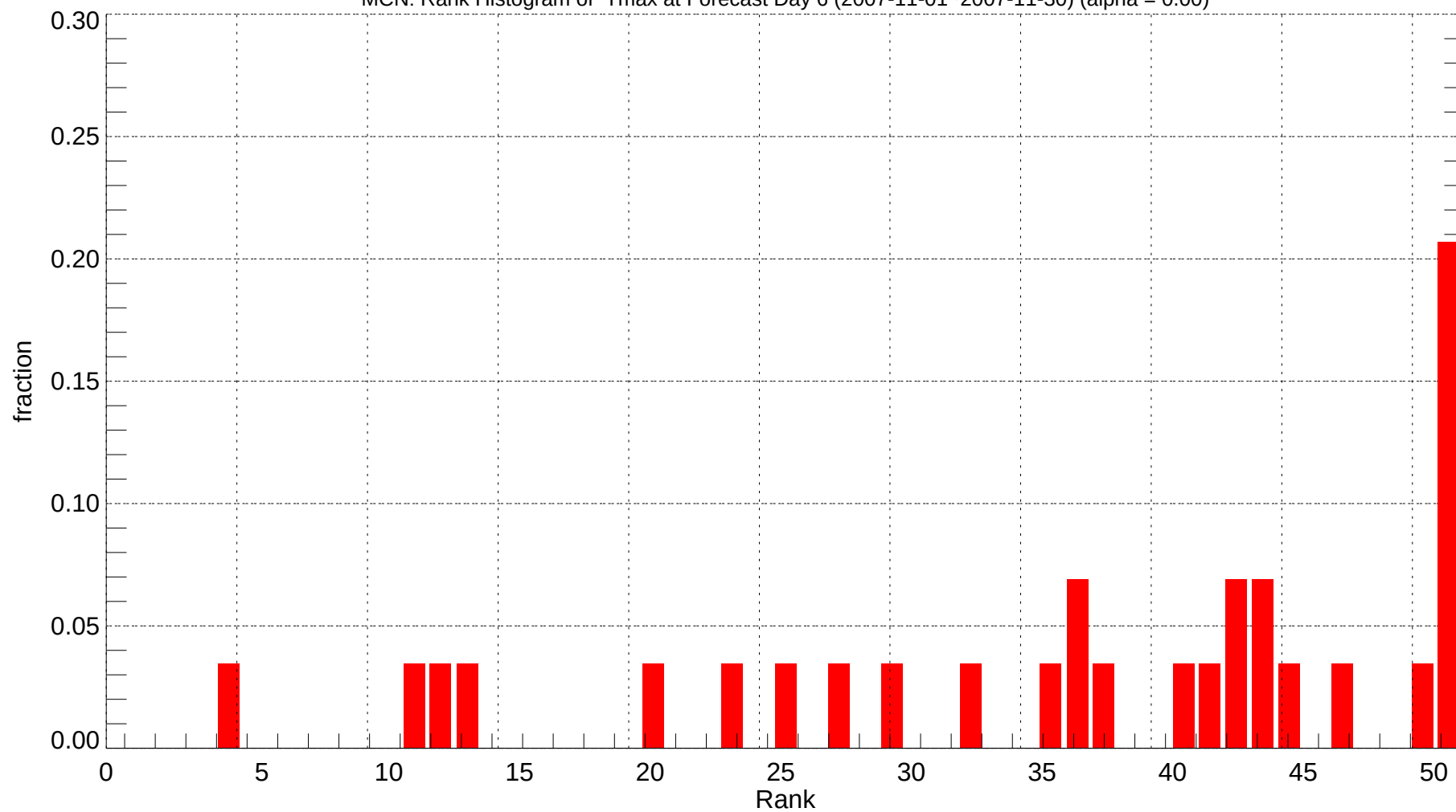
MCN: Rank Histogram of Tmax at Forecast Day 6 (2007-11-01~2007-11-30) (alpha = 0.00)
