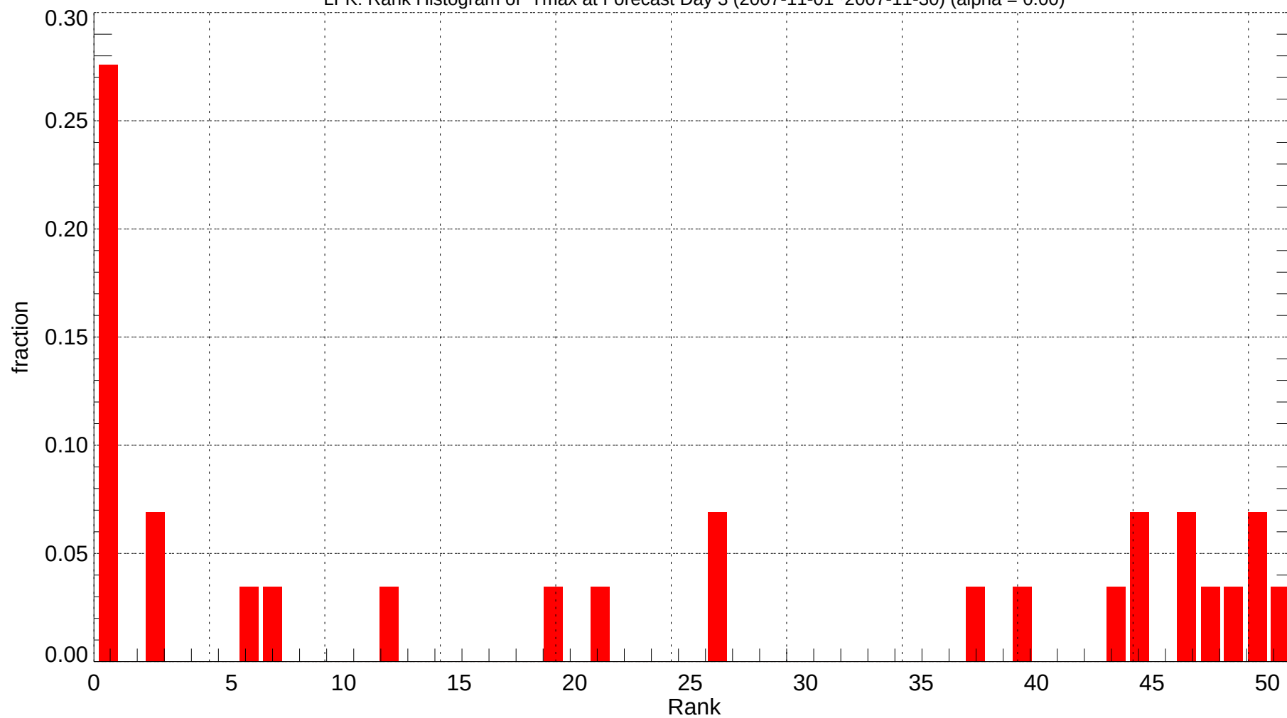
LFK: Rank Histogram of Tmax at Forecast Day 3 (2007-11-01~2007-11-30) (alpha = 0.00)
