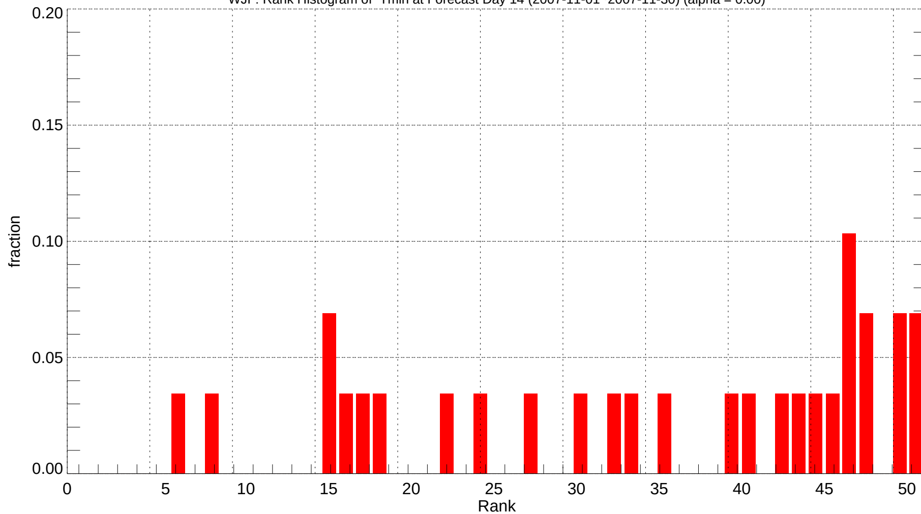
WJF: Rank Histogram of Tmin at Forecast Day 14 (2007-11-01~2007-11-30) (alpha = 0.00)
