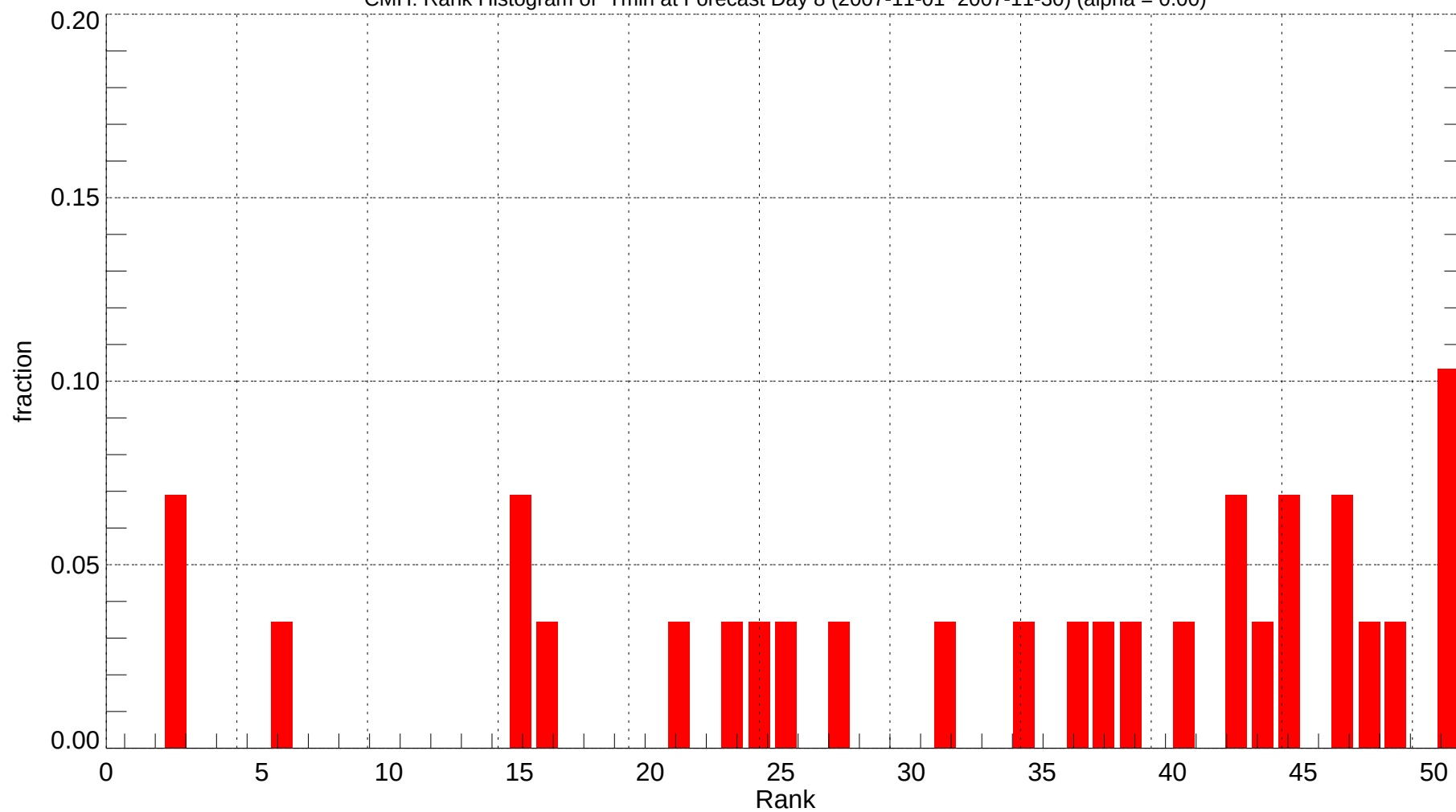
CMH: Rank Histogram of Tmin at Forecast Day 8 (2007-11-01~2007-11-30) (alpha = 0.00)
