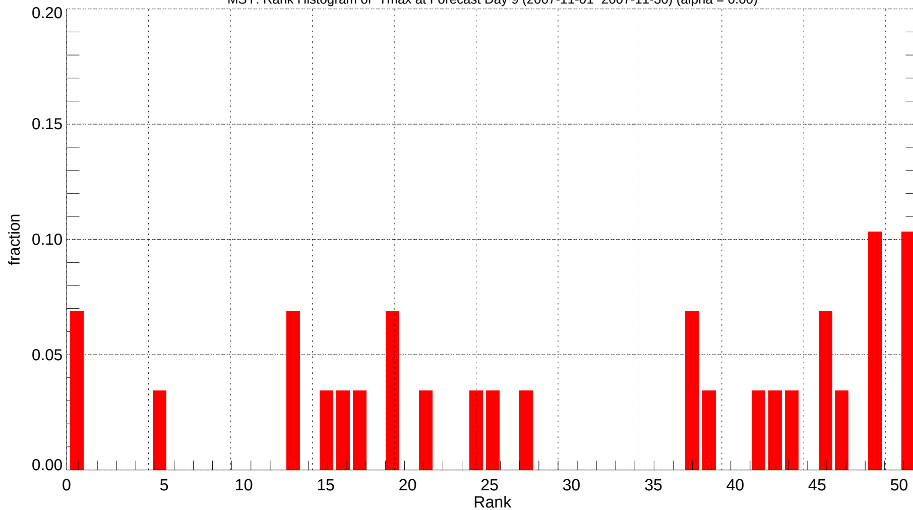
MSY: Rank Histogram of Tmax at Forecast Day 9 (2007-11-01~2007-11-30) (alpha = 0.00)
