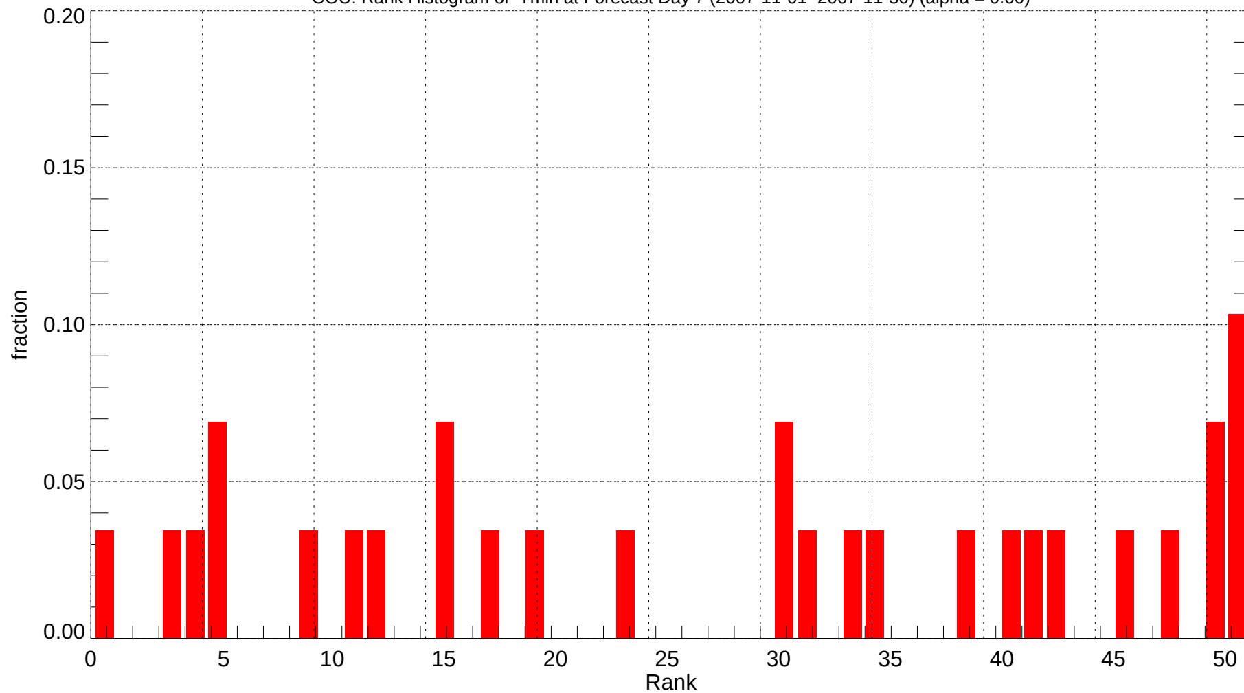
COU: Rank Histogram of Tmin at Forecast Day 7 (2007-11-01~2007-11-30) (alpha = 0.00)
