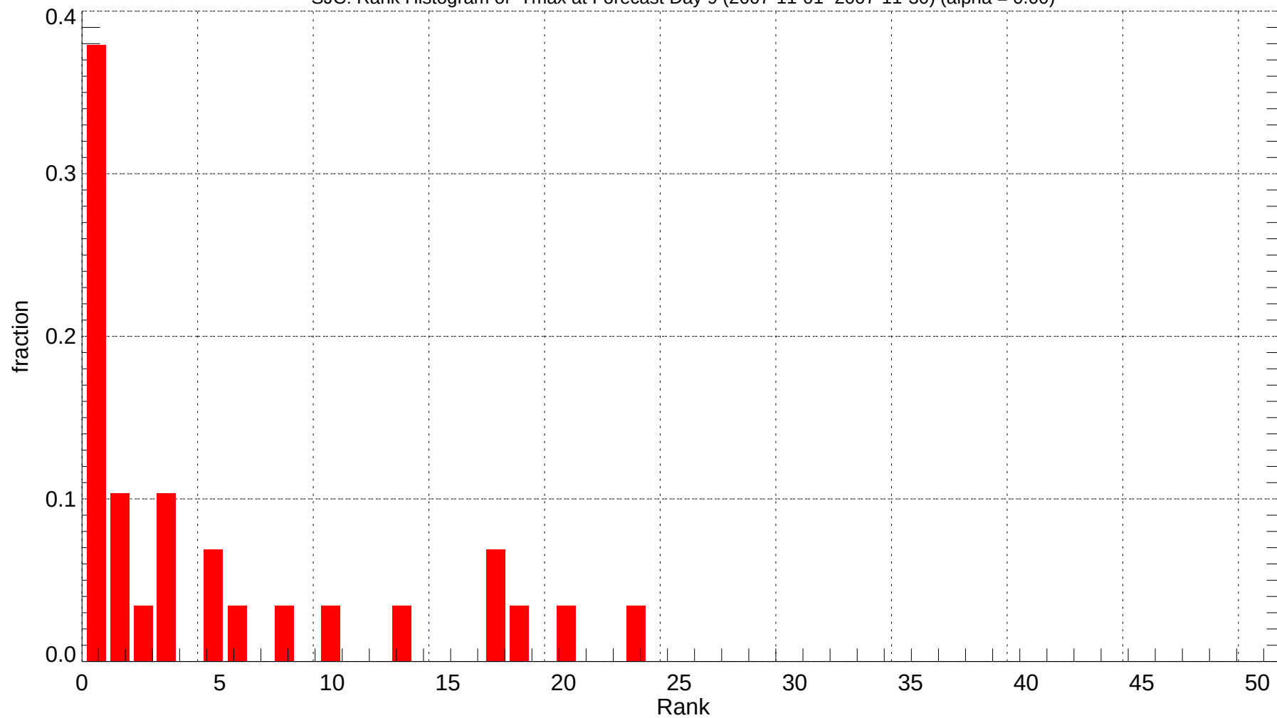
SJC: Rank Histogram of Tmax at Forecast Day 9 (2007-11-01~2007-11-30) (alpha = 0.00)
