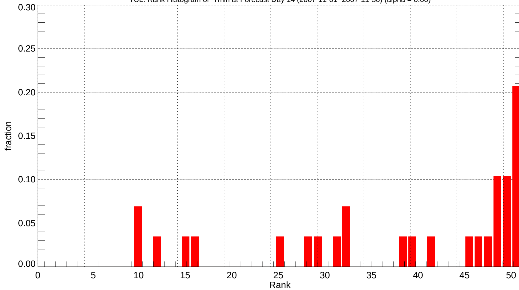
TUL: Rank Histogram of Tmin at Forecast Day 14 (2007-11-01~2007-11-30) (alpha = 0.00)
