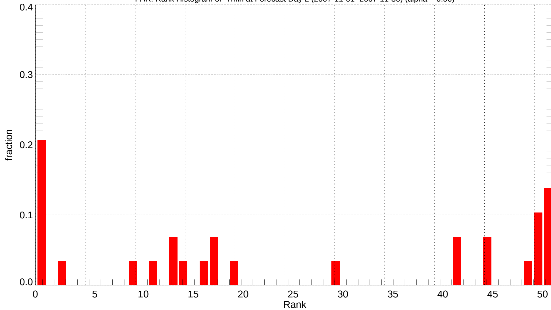
FAR: Rank Histogram of Tmin at Forecast Day 2 (2007-11-01~2007-11-30) (alpha = 0.00)
