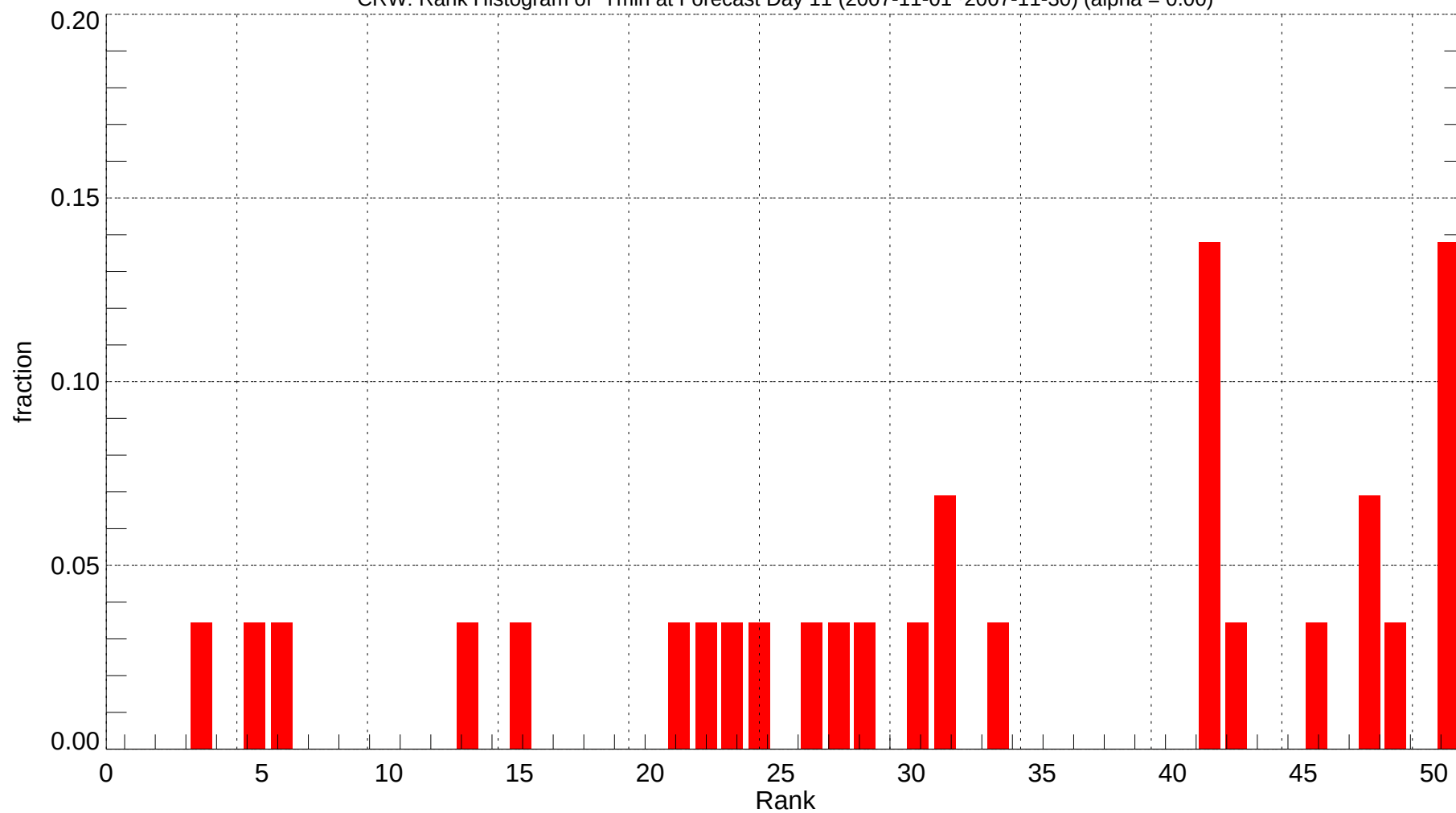
CRW: Rank Histogram of Tmin at Forecast Day 11 (2007-11-01~2007-11-30) (alpha = 0.00)
