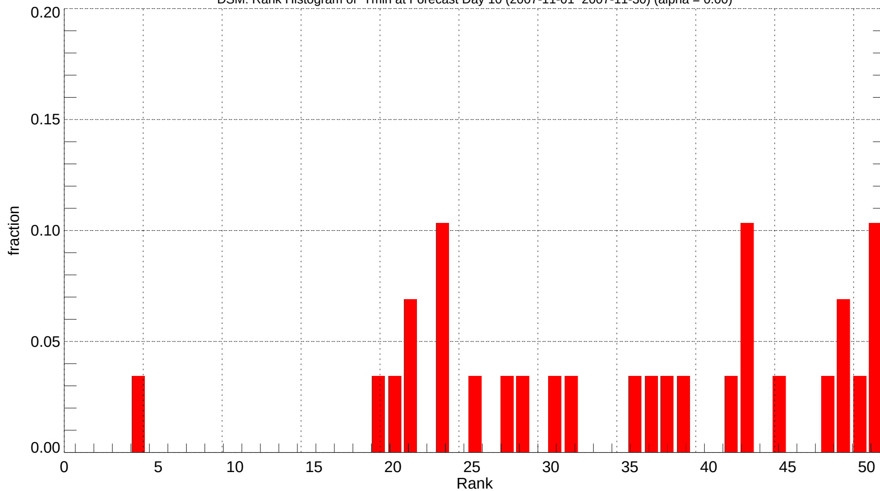
DSM: Rank Histogram of Tmin at Forecast Day 10 (2007-11-01~2007-11-30) (alpha = 0.00)
