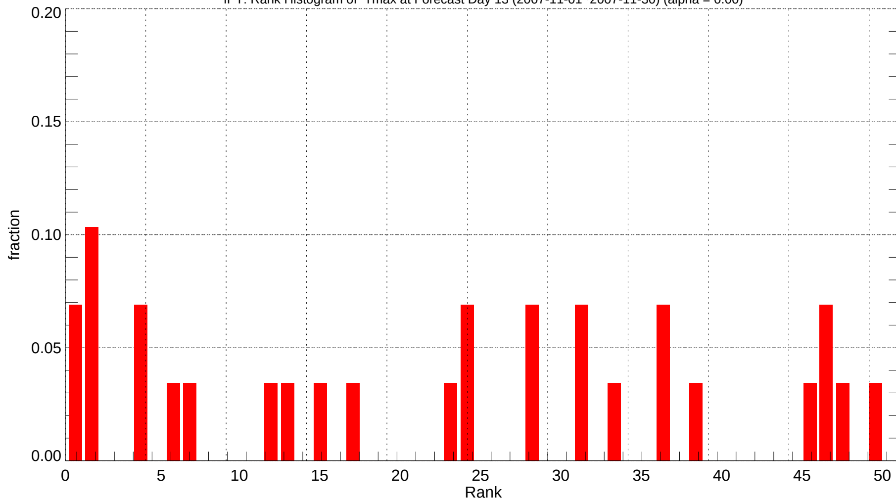
IPT: Rank Histogram of Tmax at Forecast Day 13 (2007-11-01~2007-11-30) (alpha = 0.00)
