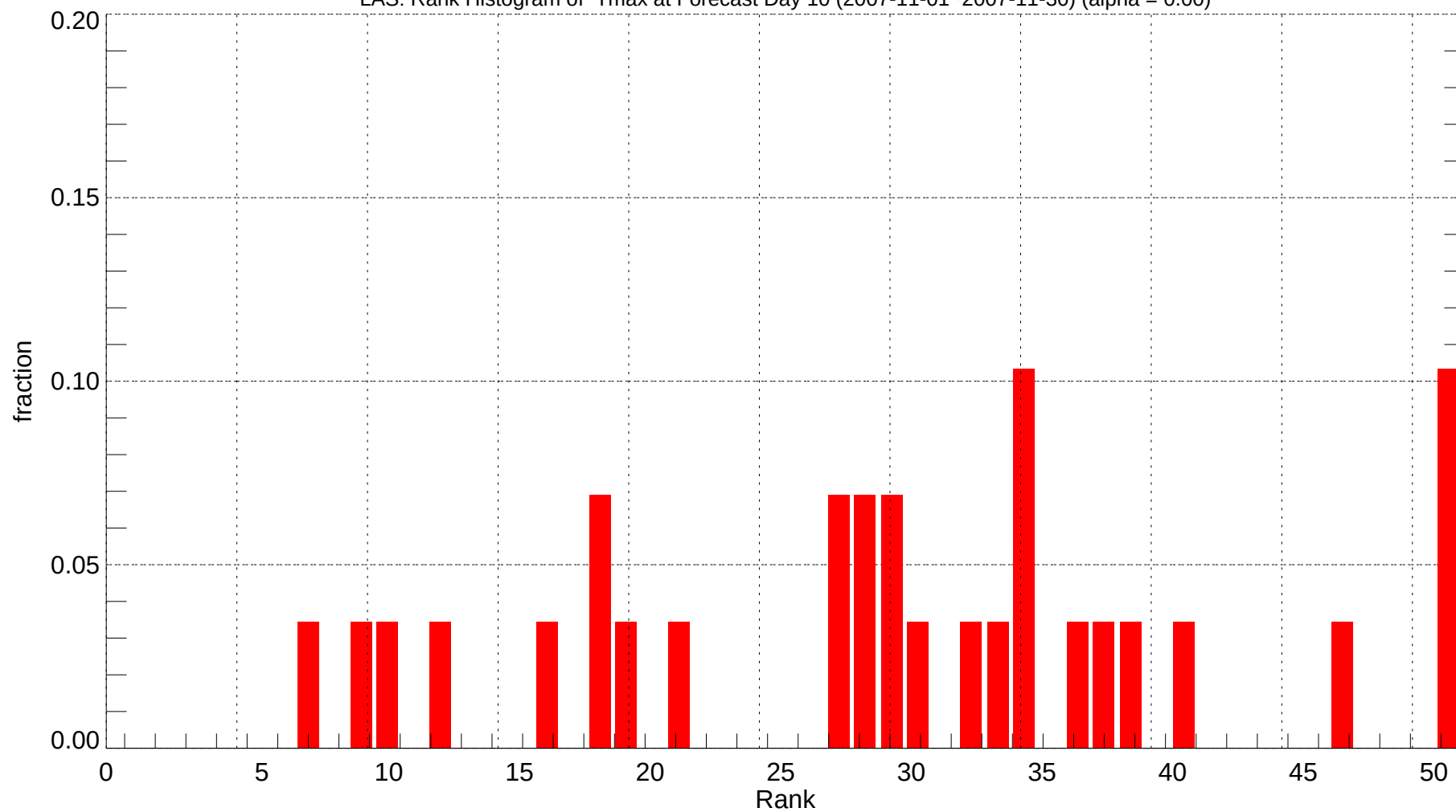
LAS: Rank Histogram of Tmax at Forecast Day 10 (2007-11-01~2007-11-30) (alpha = 0.00)
