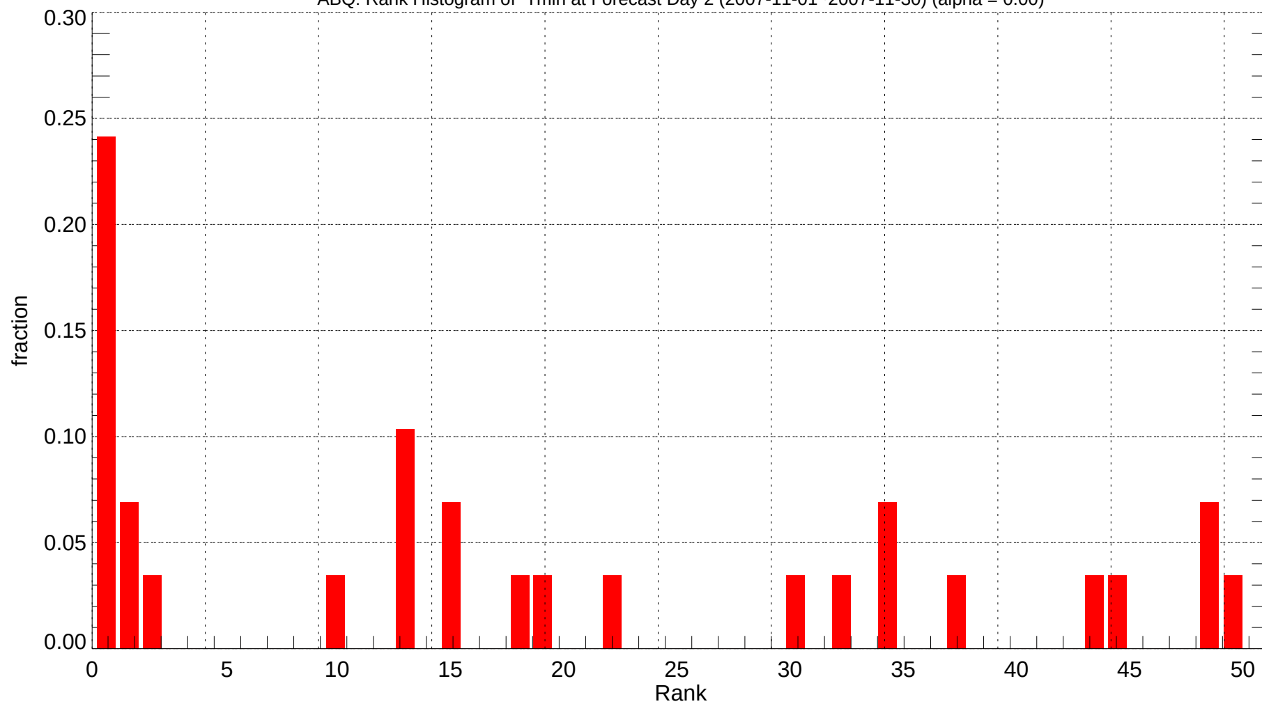
ABQ: Rank Histogram of Tmin at Forecast Day 2 (2007-11-01~2007-11-30) (alpha = 0.00)
