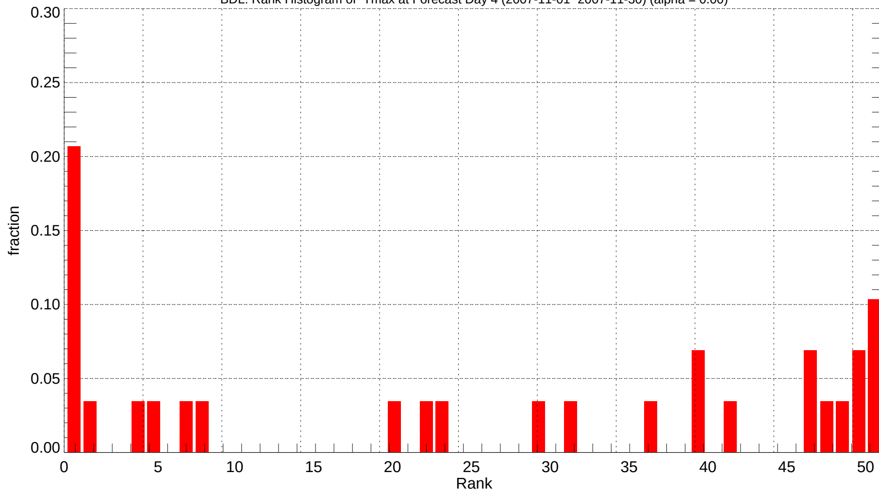
BDL: Rank Histogram of Tmax at Forecast Day 4 (2007-11-01~2007-11-30) (alpha = 0.00)
