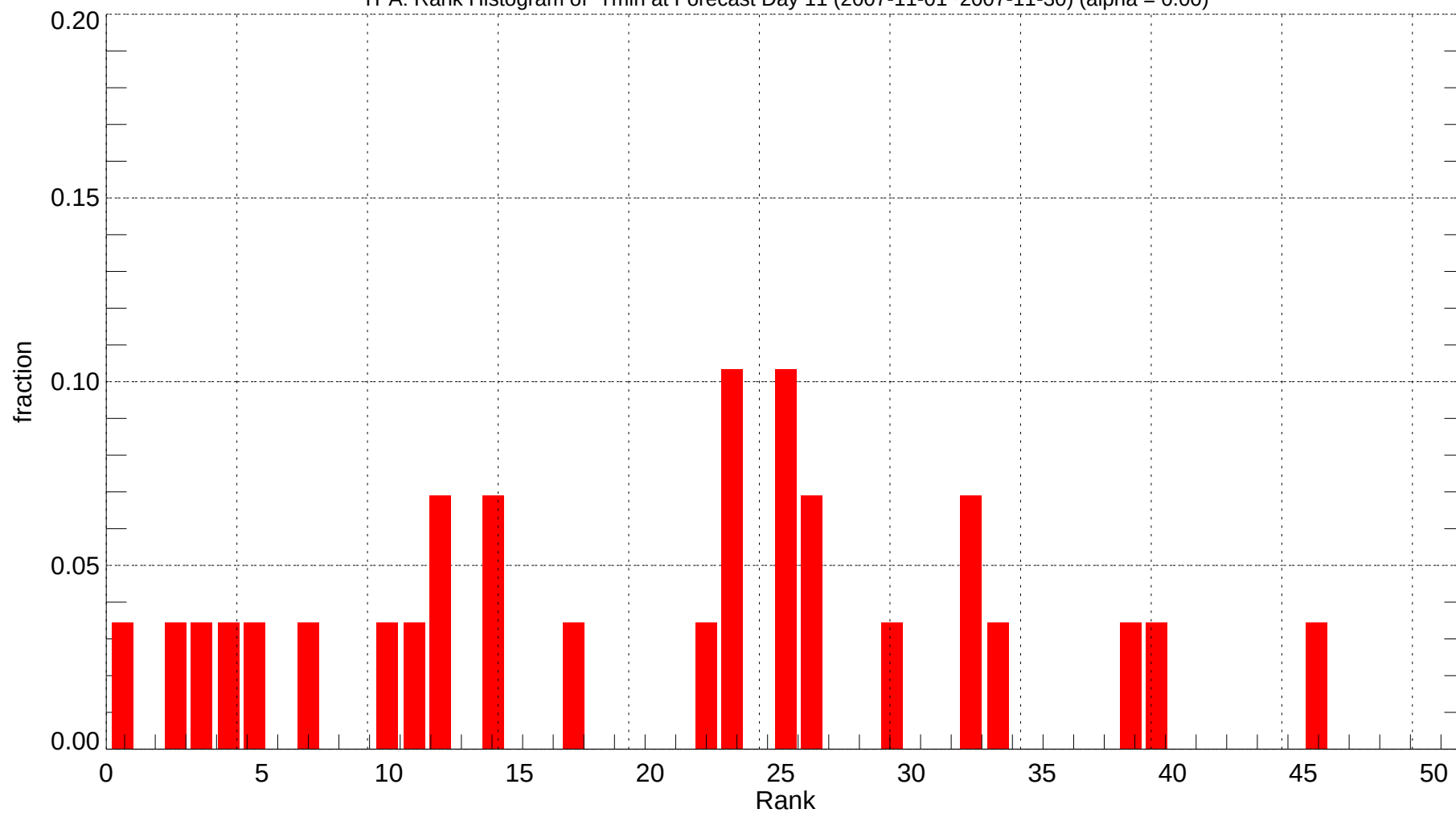
TPA: Rank Histogram of Tmin at Forecast Day 11 (2007-11-01~2007-11-30) (alpha = 0.00)
