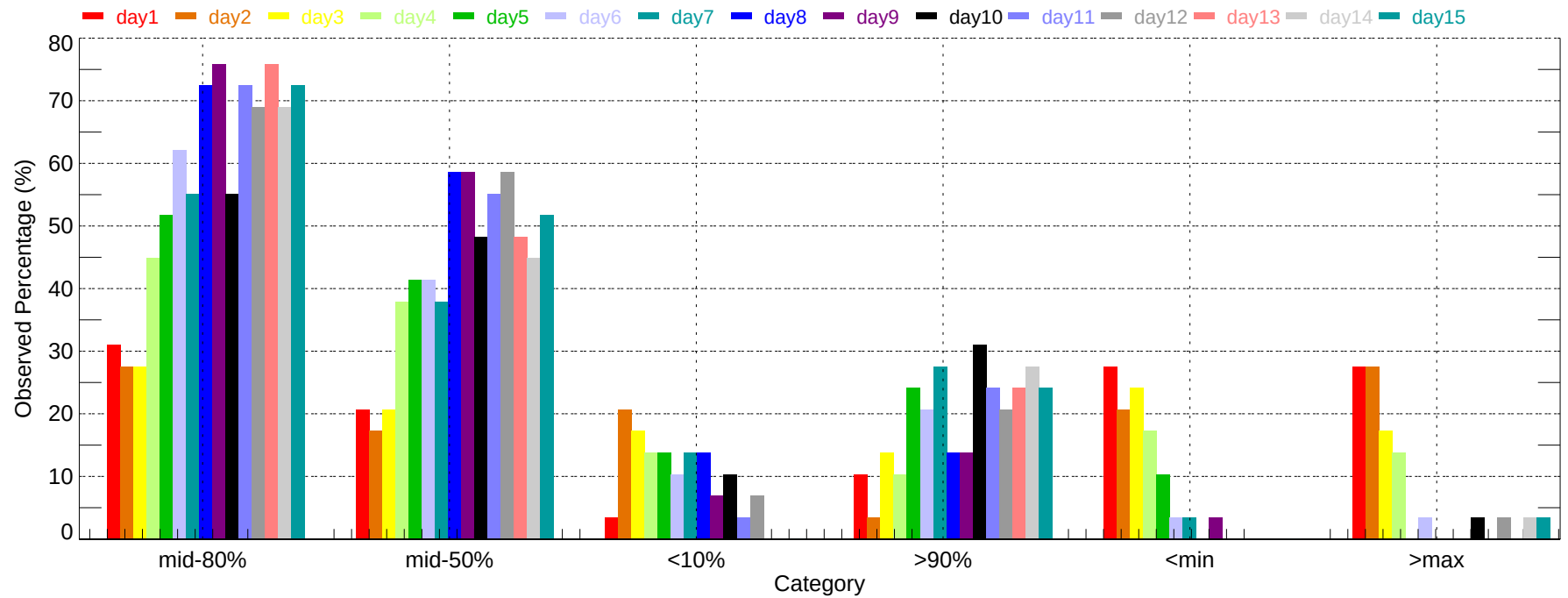
Observed Percentage of Ensembles - RNO: Max Temperature (2007-11-01~2007-11-30)
