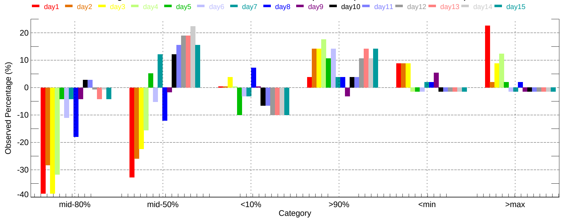
Observed Percentage Deviation of Ensembles - SEA: Max Temperature (2007-11-01~2007-11-30)
