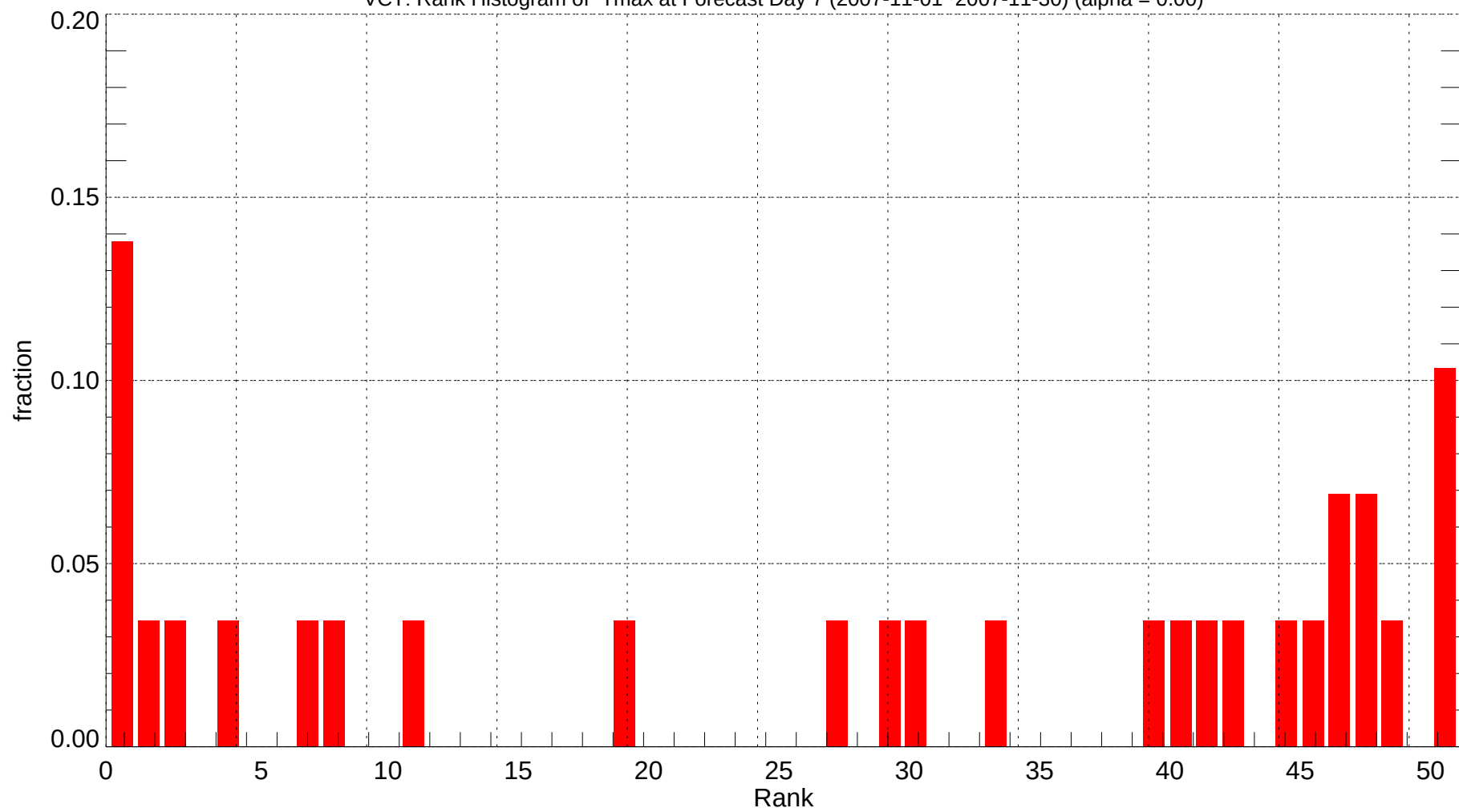
VCT: Rank Histogram of Tmax at Forecast Day 7 (2007-11-01~2007-11-30) (alpha = 0.00)
