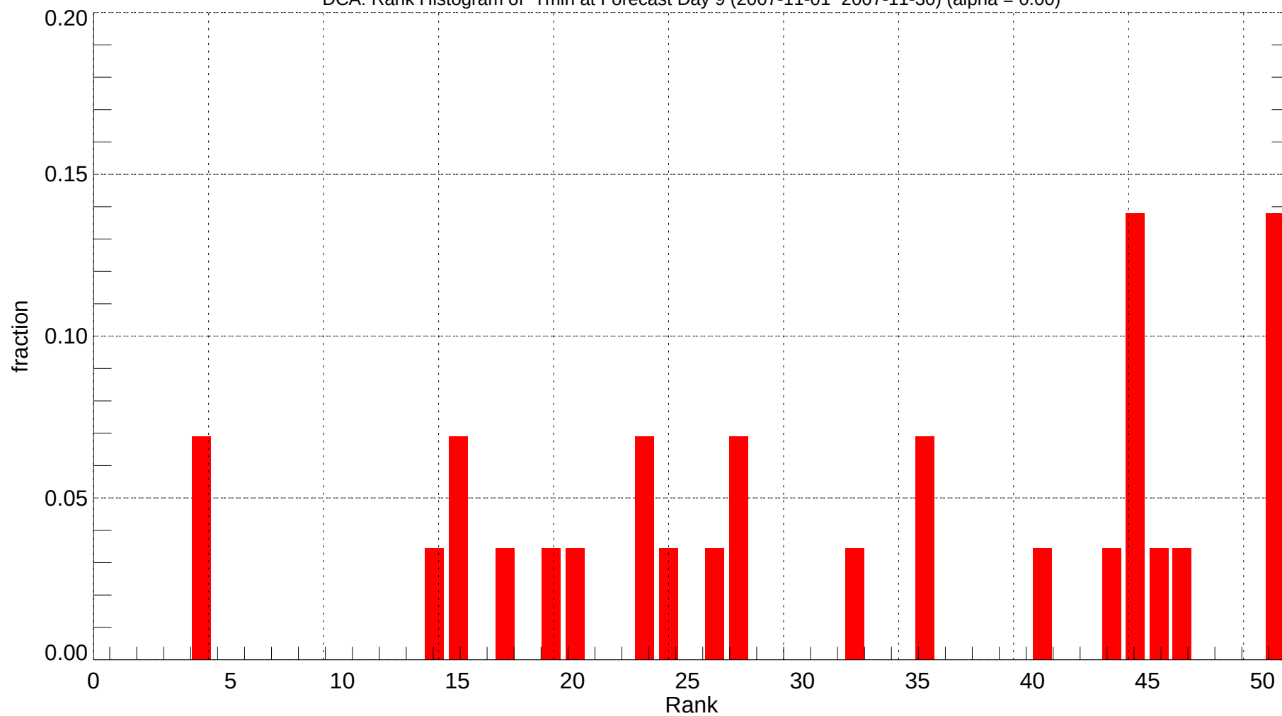
DCA: Rank Histogram of Tmin at Forecast Day 9 (2007-11-01~2007-11-30) (alpha = 0.00)
