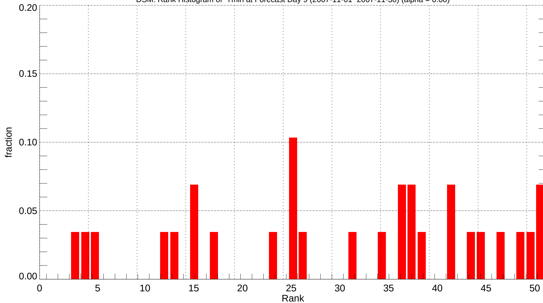
DSM: Rank Histogram of Tmin at Forecast Day 9 (2007-11-01~2007-11-30) (alpha = 0.00)
