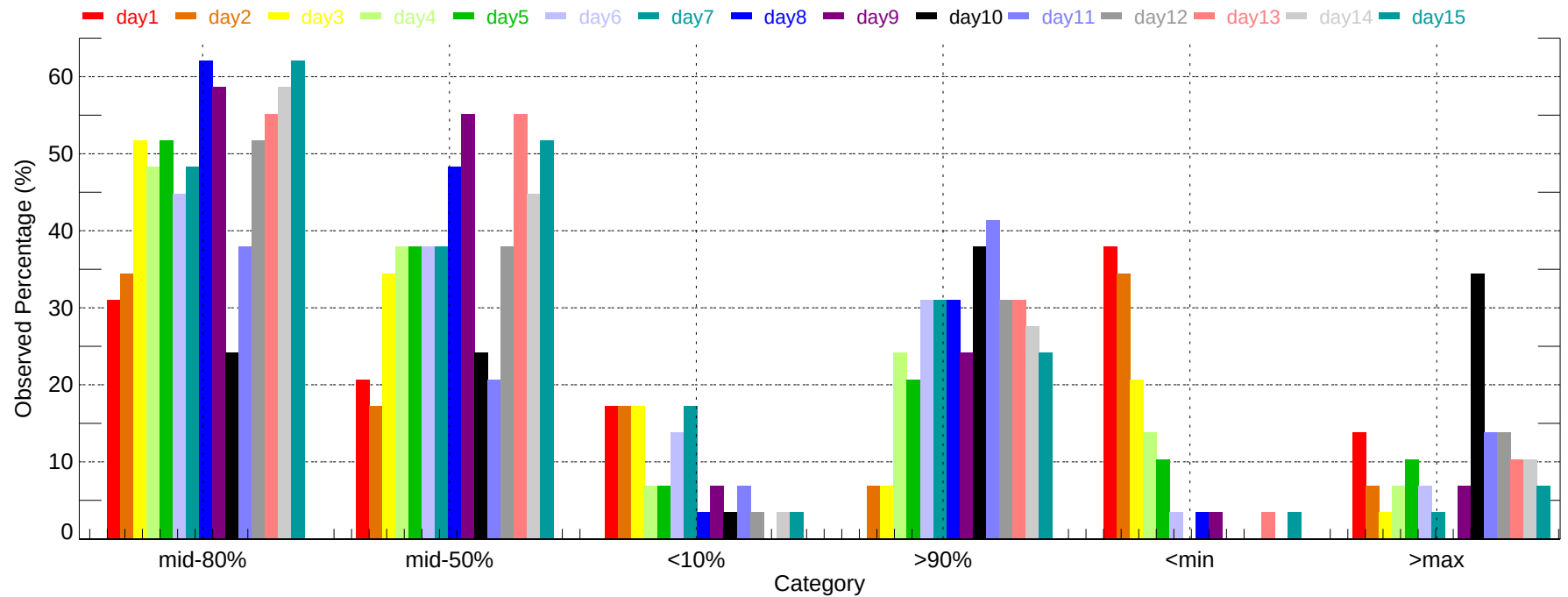
Observed Percentage of Ensembles - OMA: Max Temperature (2007-11-01~2007-11-30)
