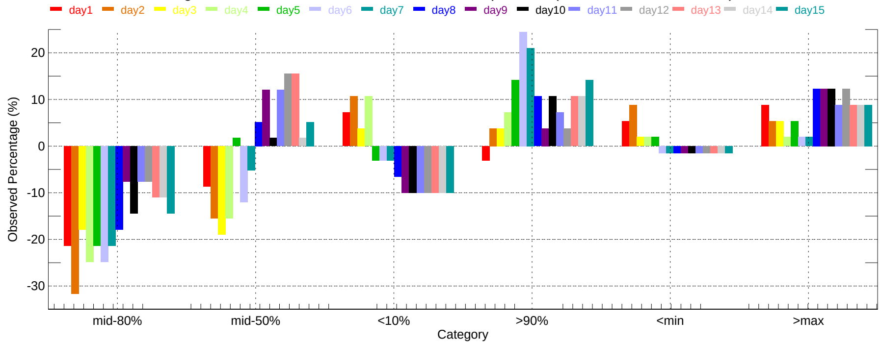
Observed Percentage Deviation of Ensembles - PHX: Max Temperature (2007-11-01~2007-11-30)
