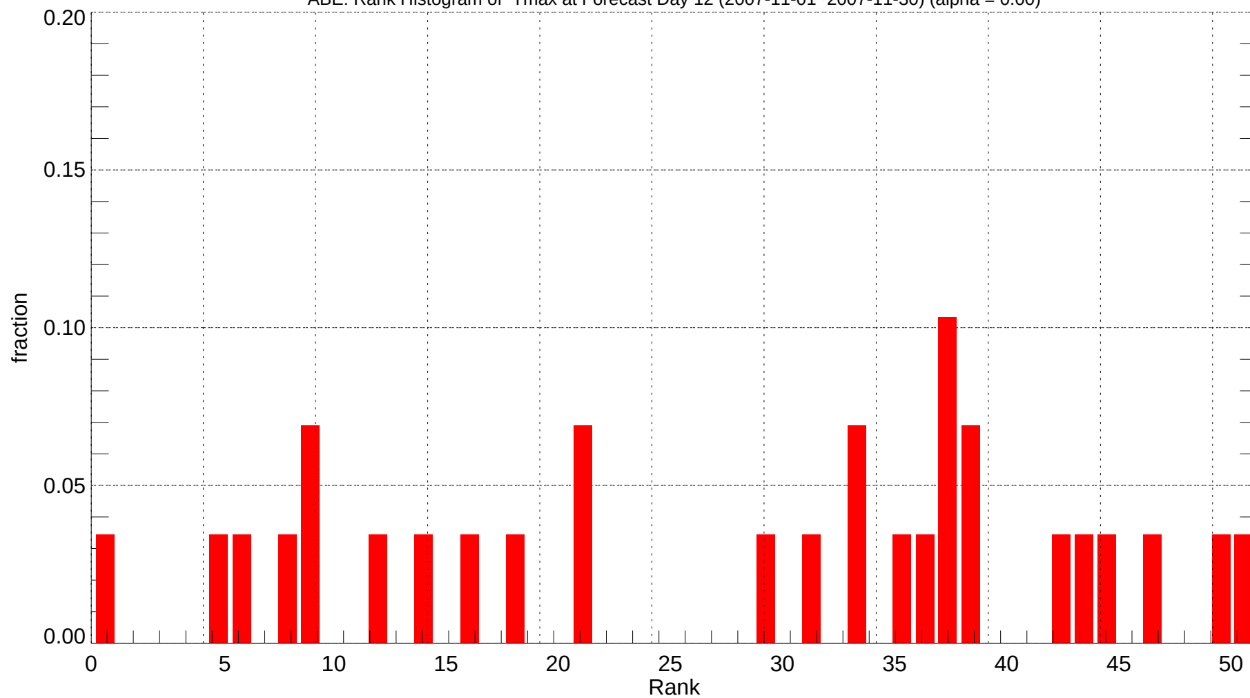
ABE: Rank Histogram of Tmax at Forecast Day 12 (2007-11-01~2007-11-30) (alpha = 0.00)
