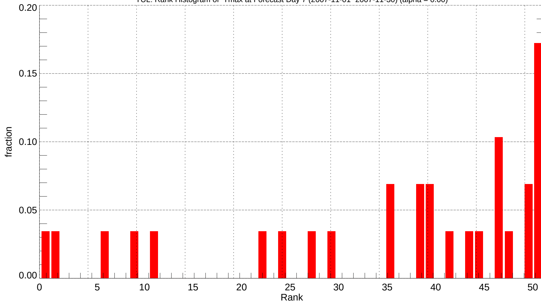
TUL: Rank Histogram of Tmax at Forecast Day 7 (2007-11-01~2007-11-30) (alpha = 0.00)
