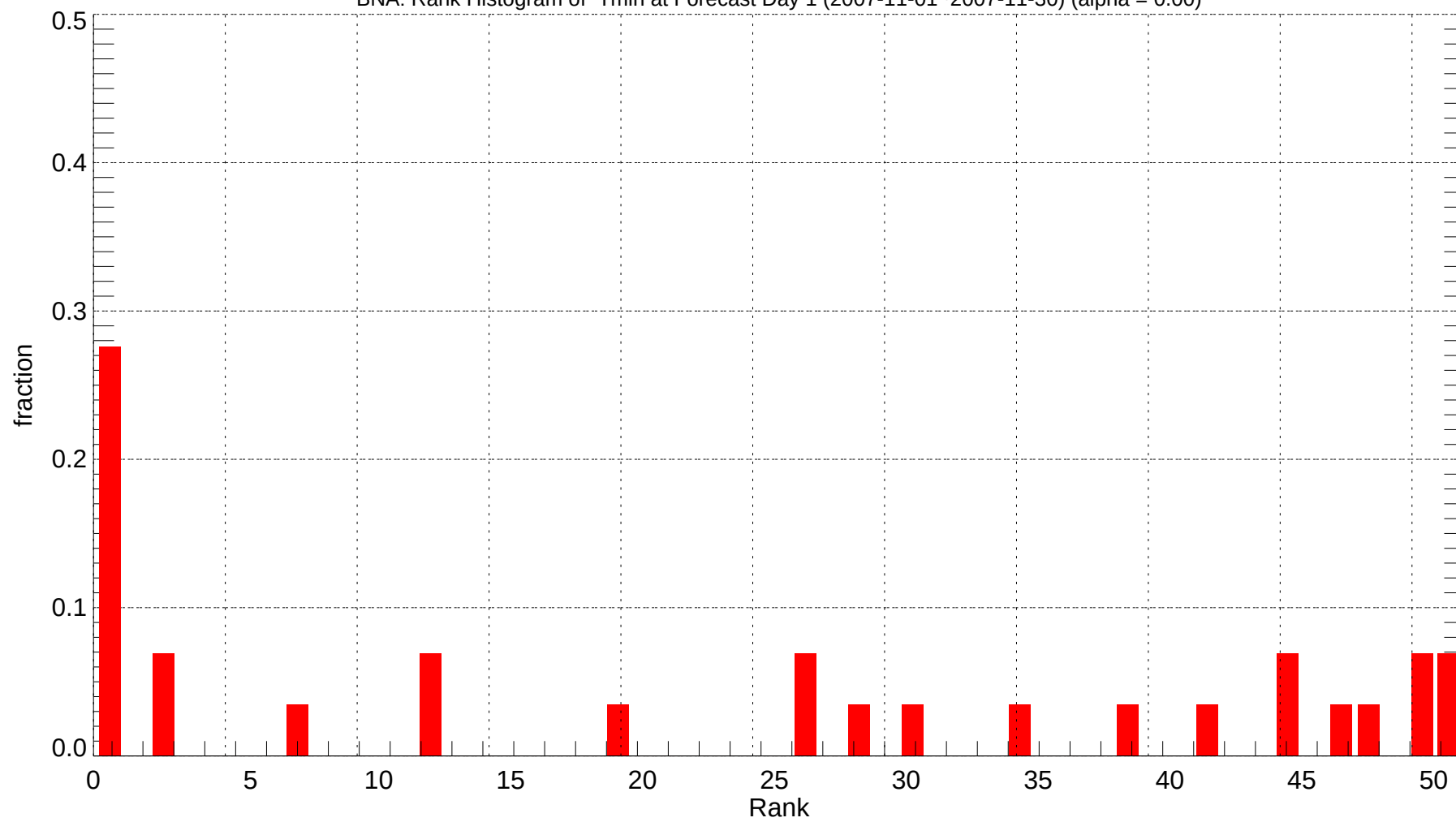
BNA: Rank Histogram of Tmin at Forecast Day 1 (2007-11-01~2007-11-30) (alpha = 0.00)
