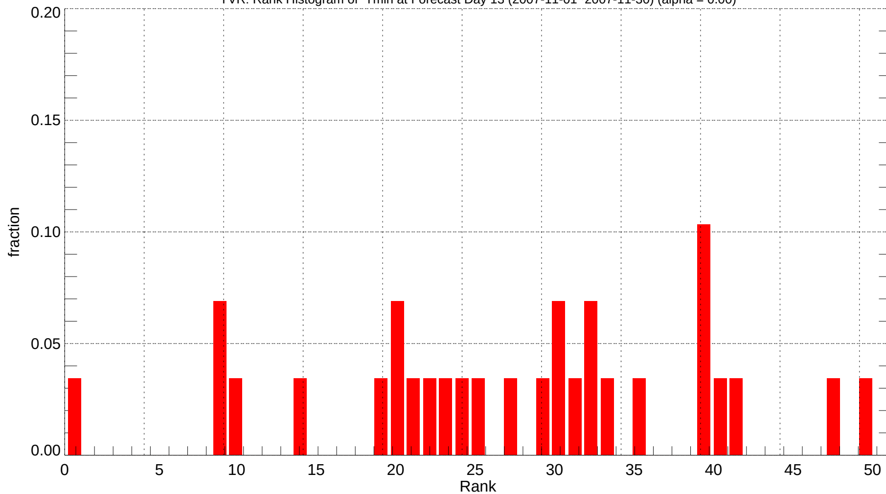
YVR: Rank Histogram of Tmin at Forecast Day 13 (2007-11-01~2007-11-30) (alpha = 0.00)
