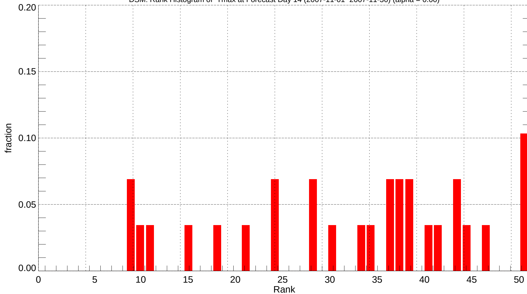
DSM: Rank Histogram of Tmax at Forecast Day 14 (2007-11-01~2007-11-30) (alpha = 0.00)
