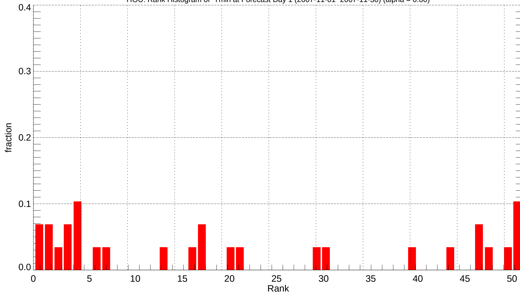
HOU: Rank Histogram of Tmin at Forecast Day 1 (2007-11-01~2007-11-30) (alpha = 0.00)
