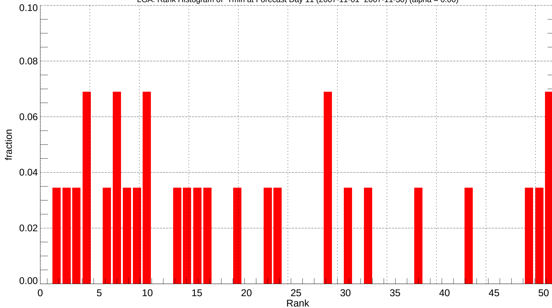
LGA: Rank Histogram of Tmin at Forecast Day 11 (2007-11-01~2007-11-30) (alpha = 0.00)
