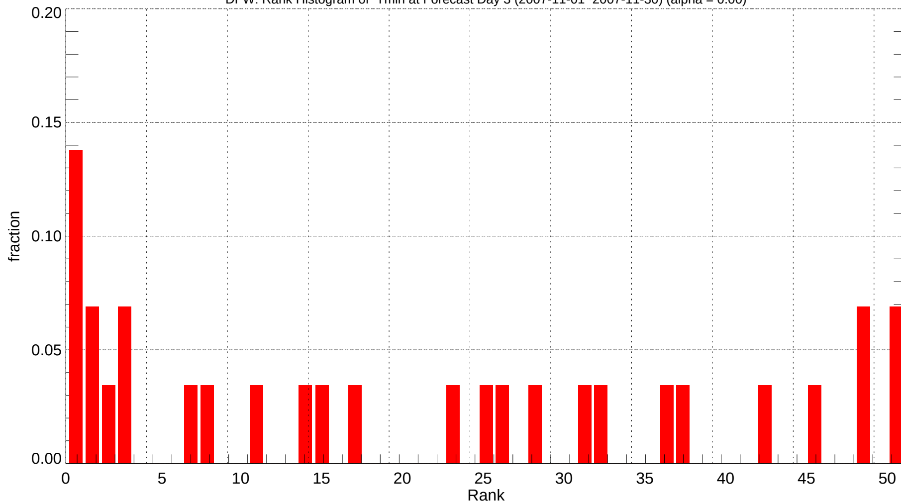
DFW: Rank Histogram of Tmin at Forecast Day 3 (2007-11-01~2007-11-30) (alpha = 0.00)
