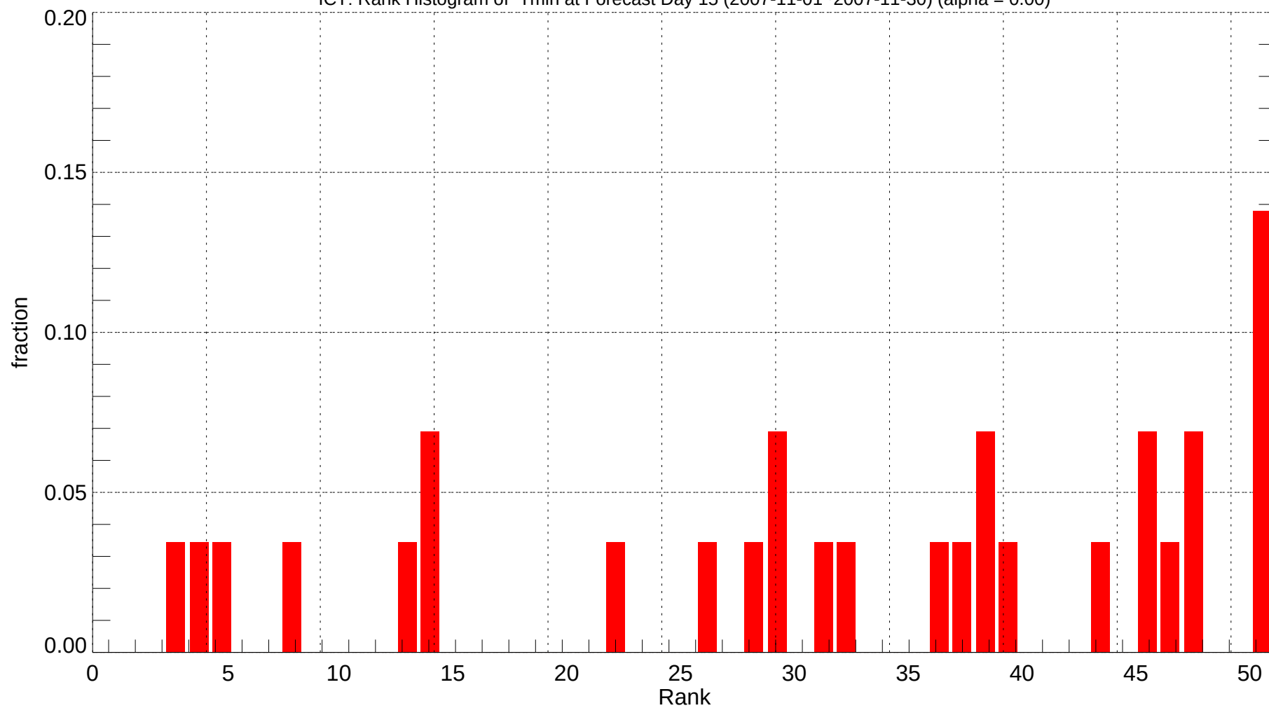
ICT: Rank Histogram of Tmin at Forecast Day 15 (2007-11-01~2007-11-30) (alpha = 0.00)
