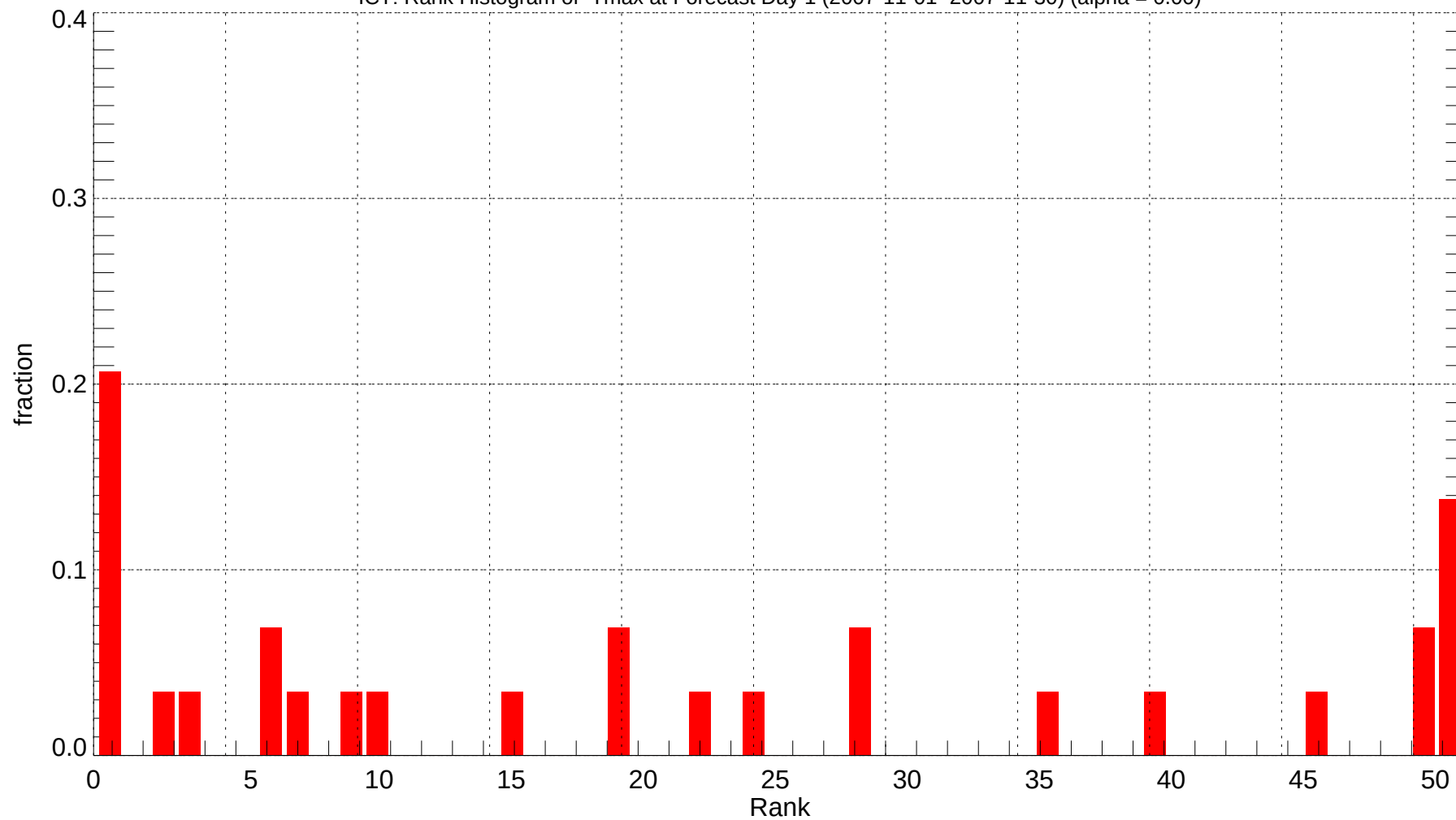
ICT: Rank Histogram of Tmax at Forecast Day 1 (2007-11-01~2007-11-30) (alpha = 0.00)
