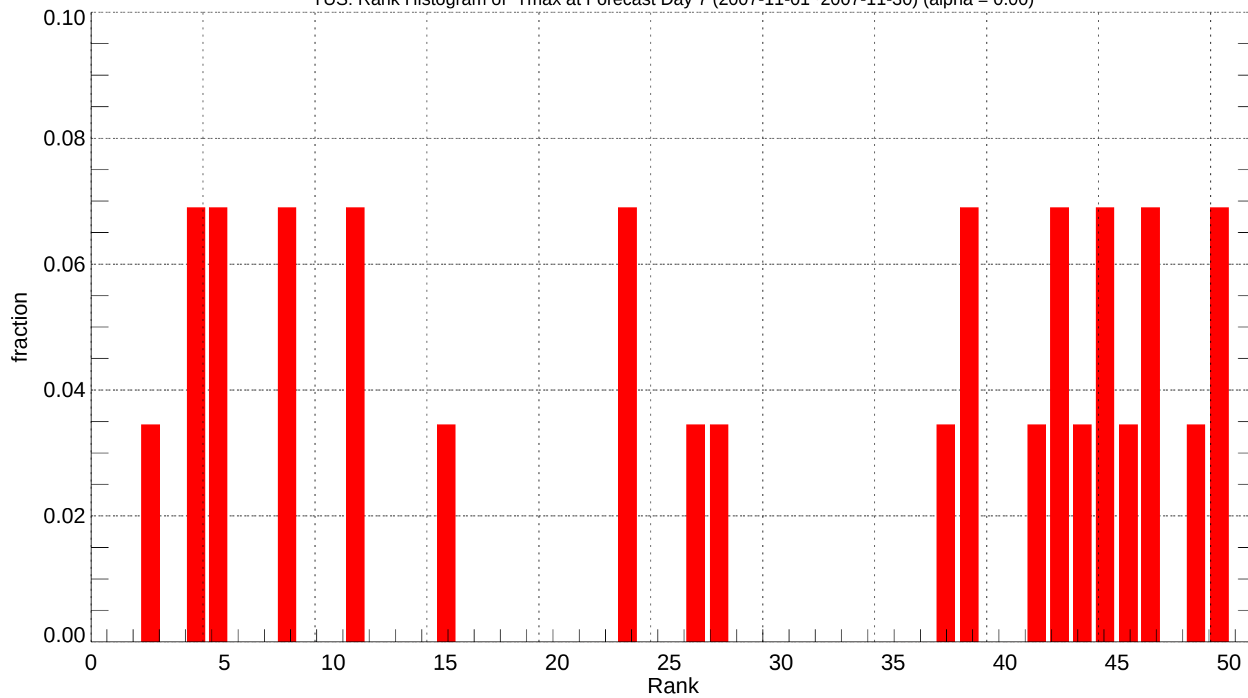
TUS: Rank Histogram of Tmax at Forecast Day 7 (2007-11-01~2007-11-30) (alpha = 0.00)
