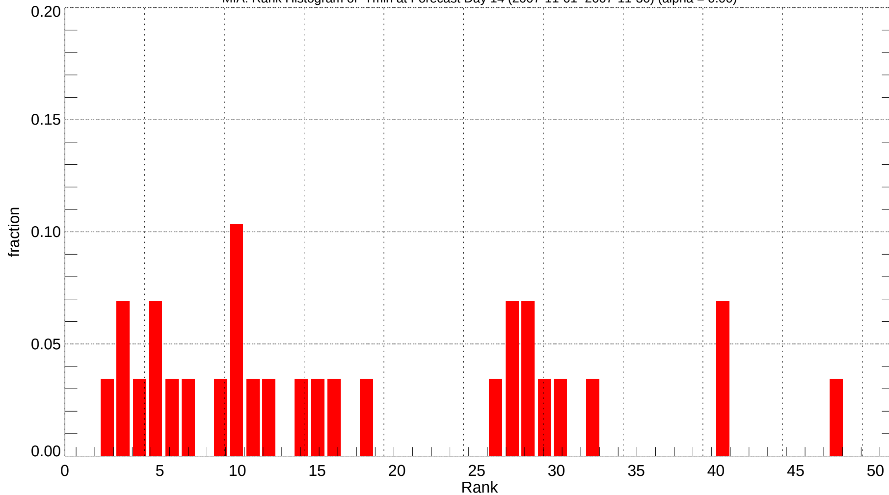
MIA: Rank Histogram of Tmin at Forecast Day 14 (2007-11-01~2007-11-30) (alpha = 0.00)
