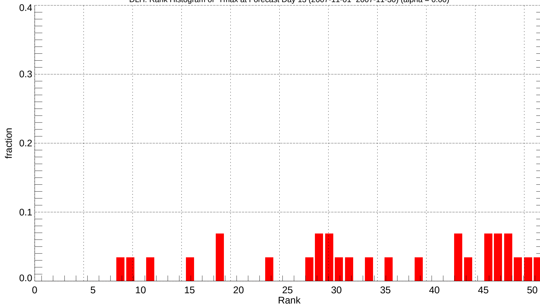
DLH: Rank Histogram of Tmax at Forecast Day 13 (2007-11-01~2007-11-30) (alpha = 0.00)
