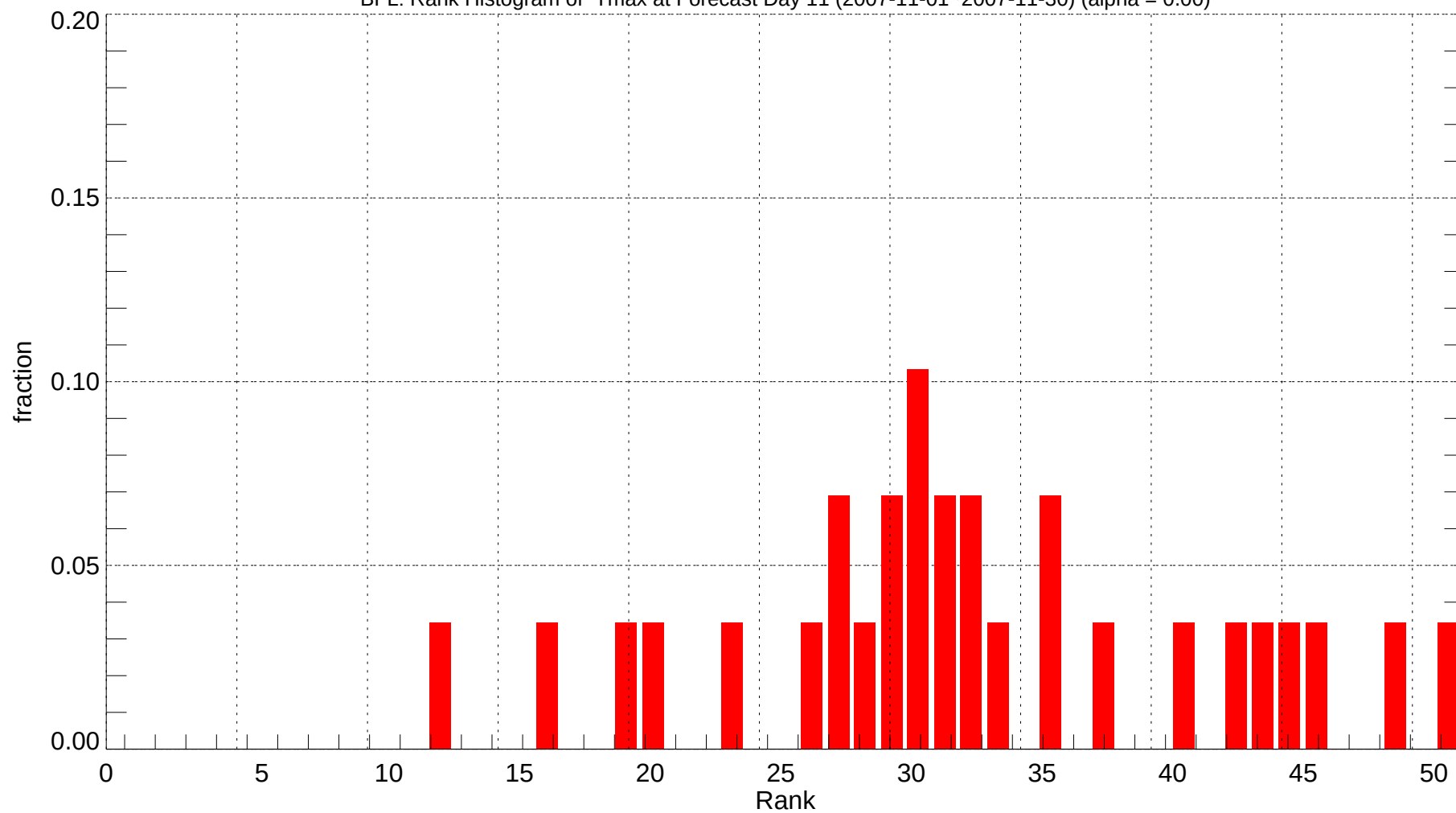
BFL: Rank Histogram of Tmax at Forecast Day 11 (2007-11-01~2007-11-30) (alpha = 0.00)
