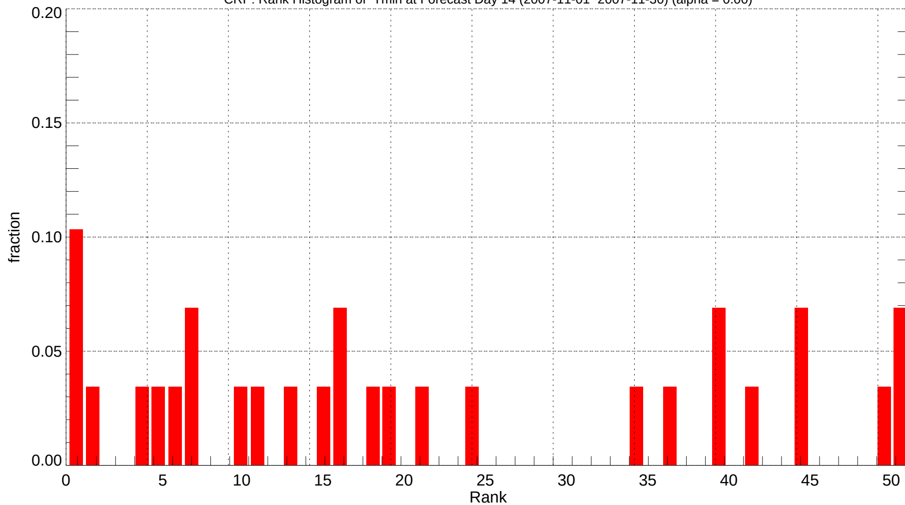
CRP: Rank Histogram of Tmin at Forecast Day 14 (2007-11-01~2007-11-30) (alpha = 0.00)
