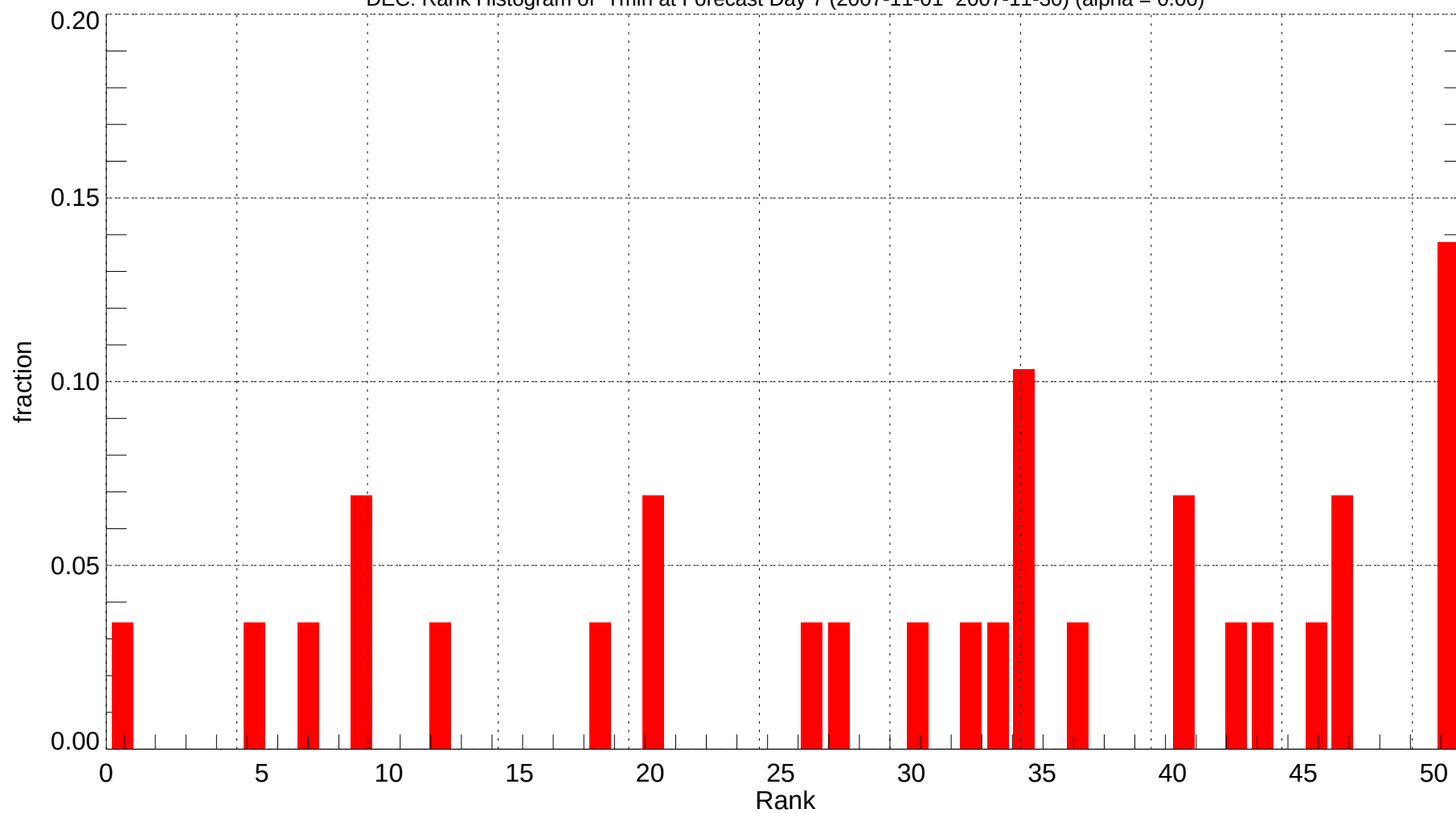
DEC: Rank Histogram of Tmin at Forecast Day 7 (2007-11-01~2007-11-30) (alpha = 0.00)
