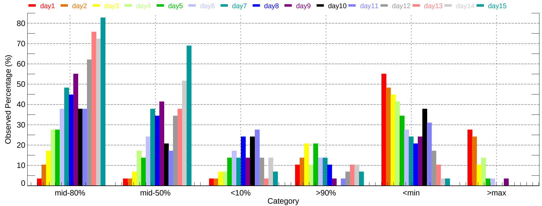
Observed Percentage of Ensembles - EUG: Max Temperature (2007-11-01~2007-11-30)
