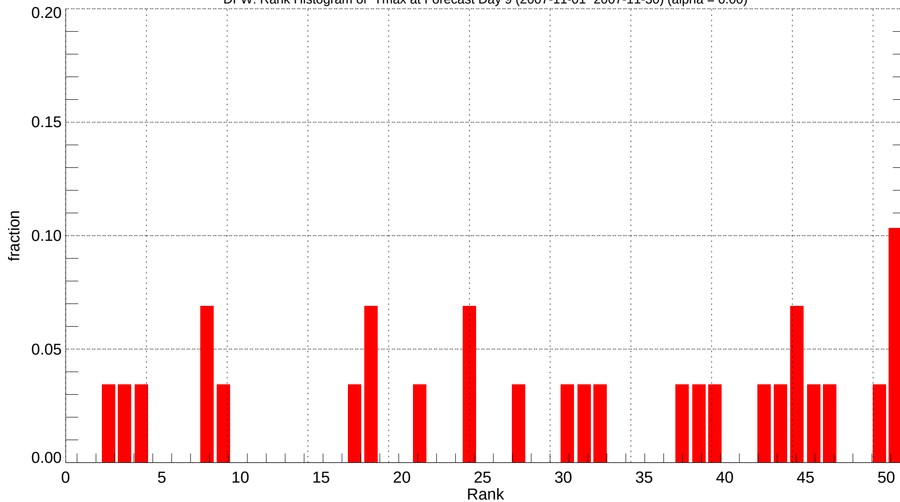
DFW: Rank Histogram of Tmax at Forecast Day 9 (2007-11-01~2007-11-30) (alpha = 0.00)
