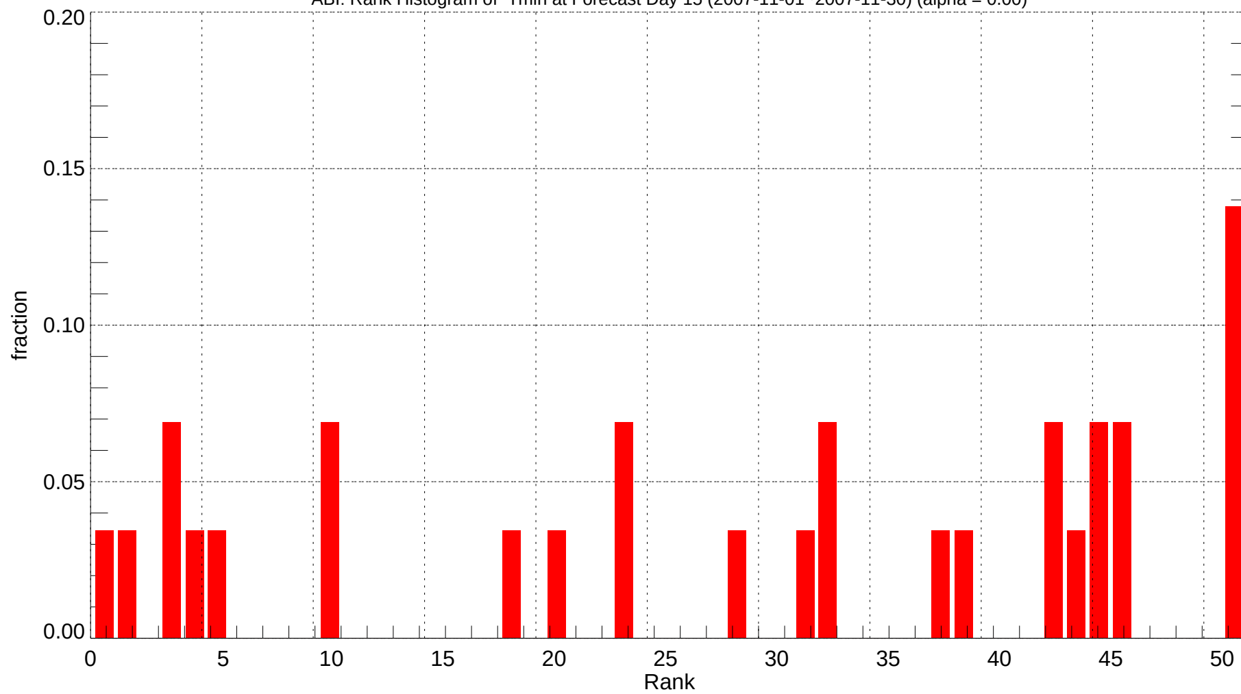
ABI: Rank Histogram of Tmin at Forecast Day 15 (2007-11-01~2007-11-30) (alpha = 0.00)
