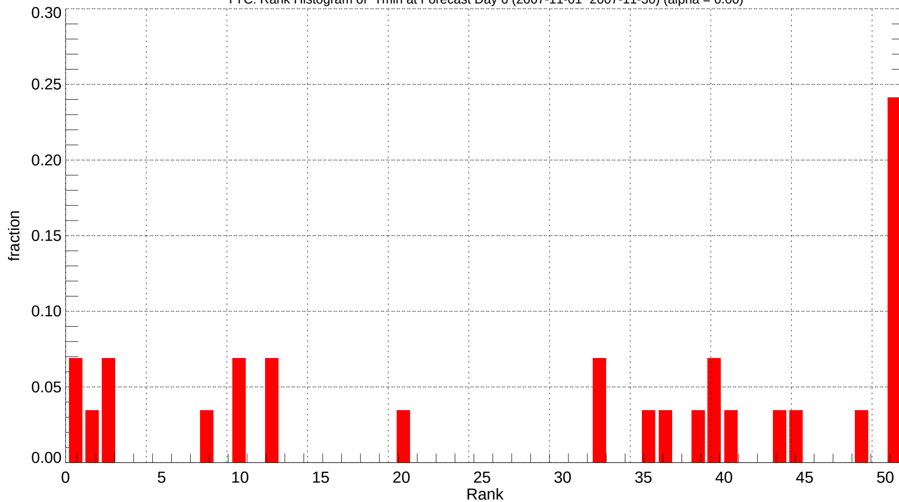
YYC: Rank Histogram of Tmin at Forecast Day 6 (2007-11-01~2007-11-30) (alpha = 0.00)
