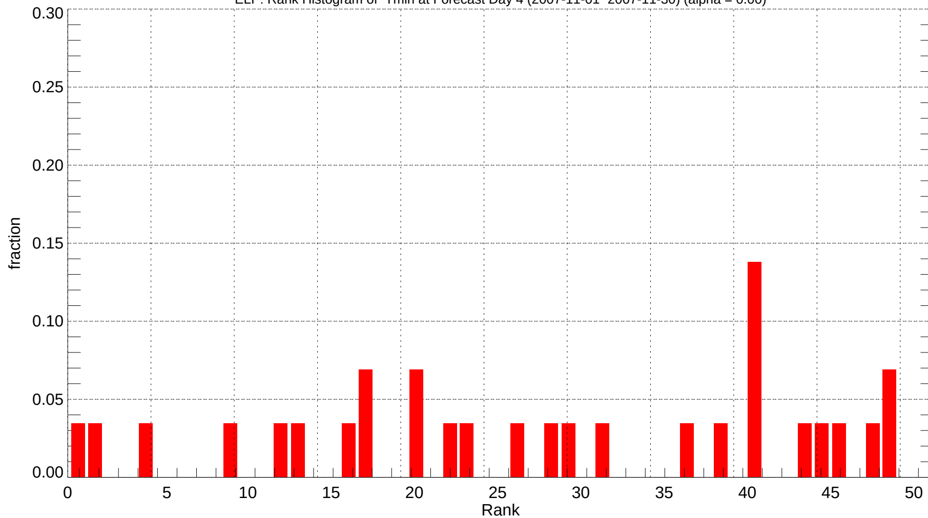
ELP: Rank Histogram of Tmin at Forecast Day 4 (2007-11-01~2007-11-30) (alpha = 0.00)
