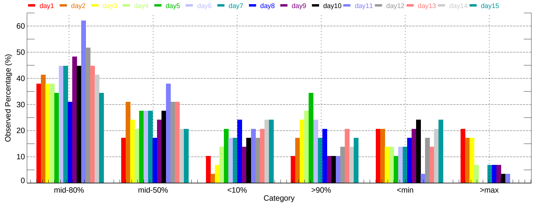
Observed Percentage of Ensembles - BDL: Max Temperature (2007-11-01~2007-11-30)
