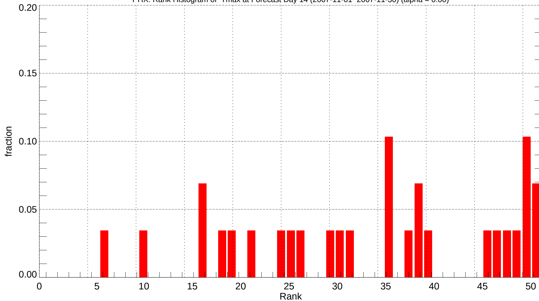
PHX: Rank Histogram of Tmax at Forecast Day 14 (2007-11-01~2007-11-30) (alpha = 0.00)
