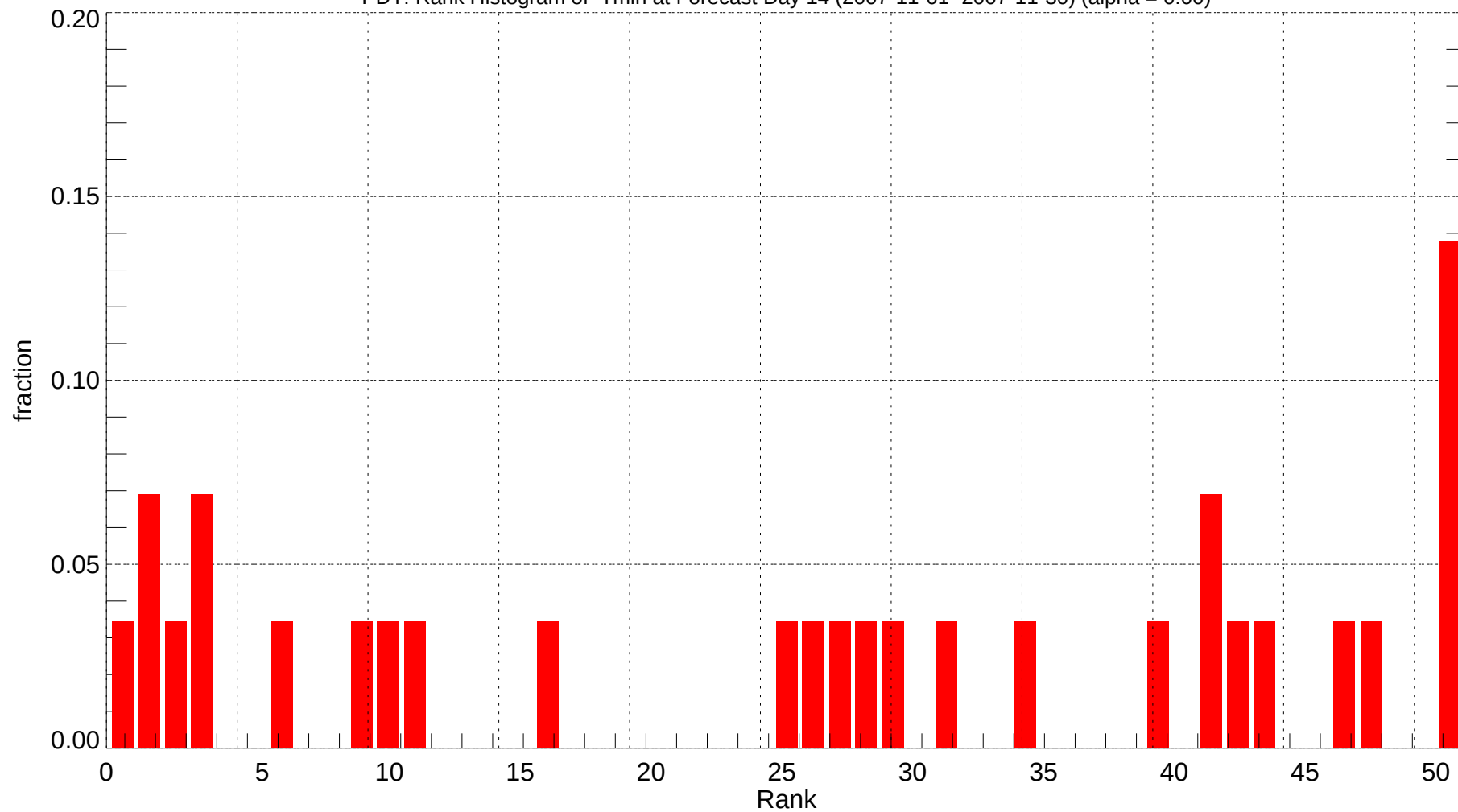
PDT: Rank Histogram of Tmin at Forecast Day 14 (2007-11-01~2007-11-30) (alpha = 0.00)
