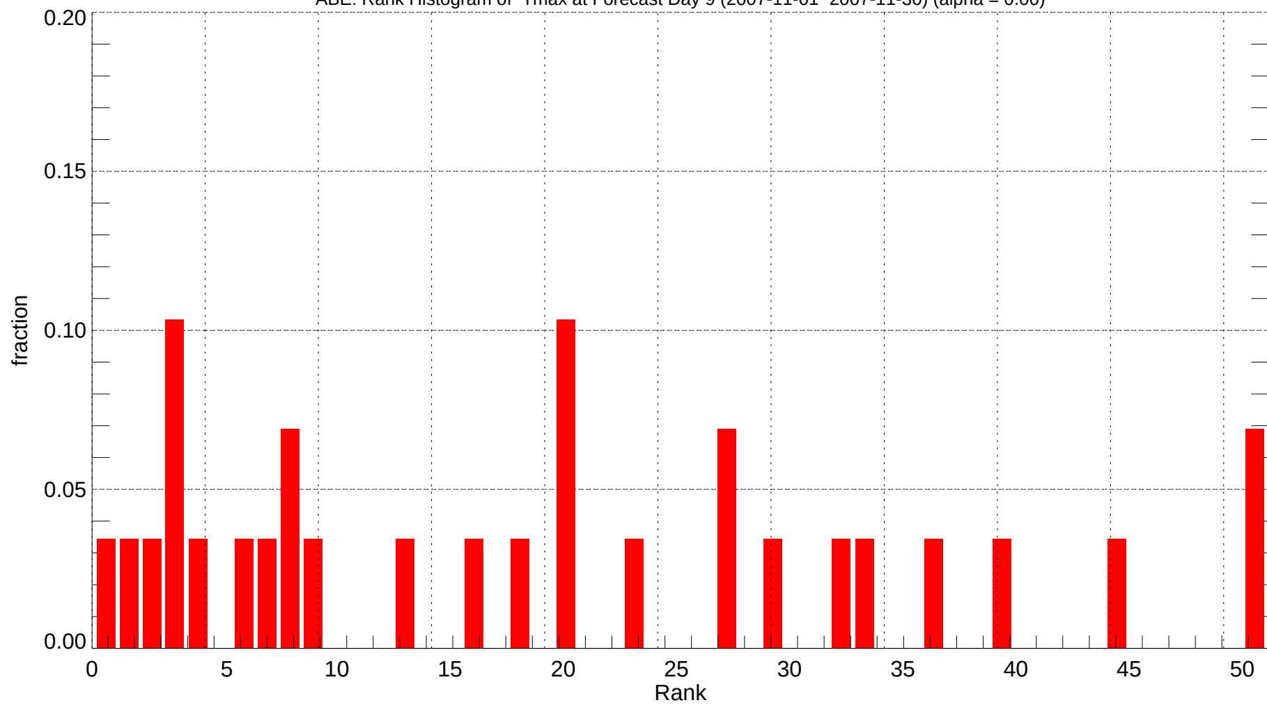
ABE: Rank Histogram of Tmax at Forecast Day 9 (2007-11-01~2007-11-30) (alpha = 0.00)
