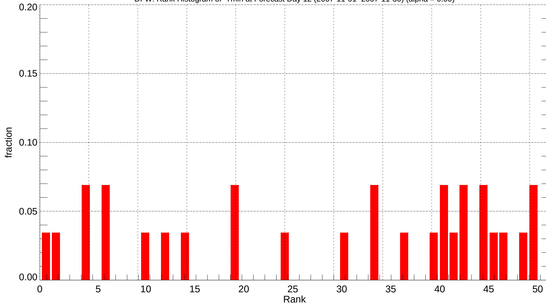
DFW: Rank Histogram of Tmin at Forecast Day 12 (2007-11-01~2007-11-30) (alpha = 0.00)
