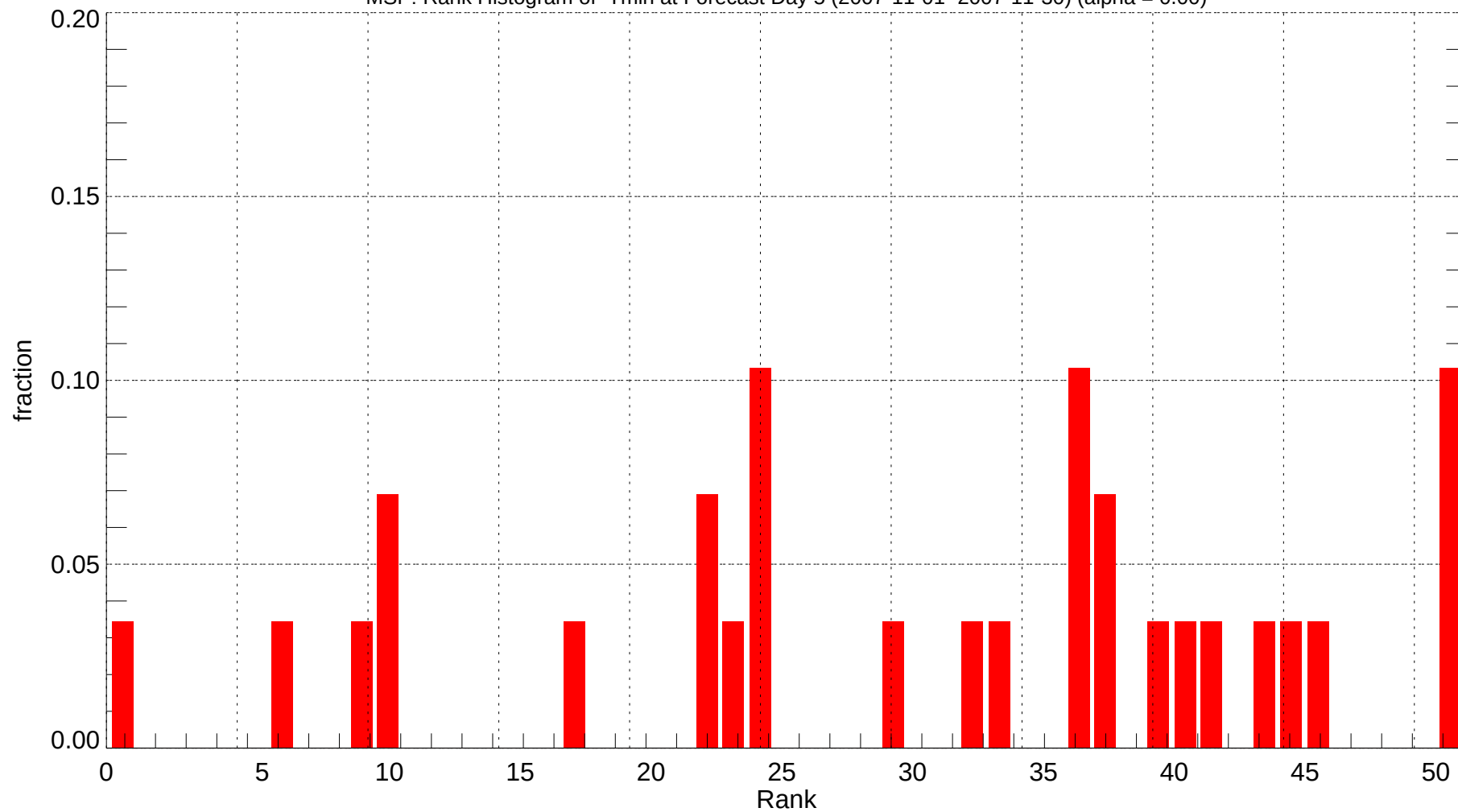
MSP: Rank Histogram of Tmin at Forecast Day 5 (2007-11-01~2007-11-30) (alpha = 0.00)
