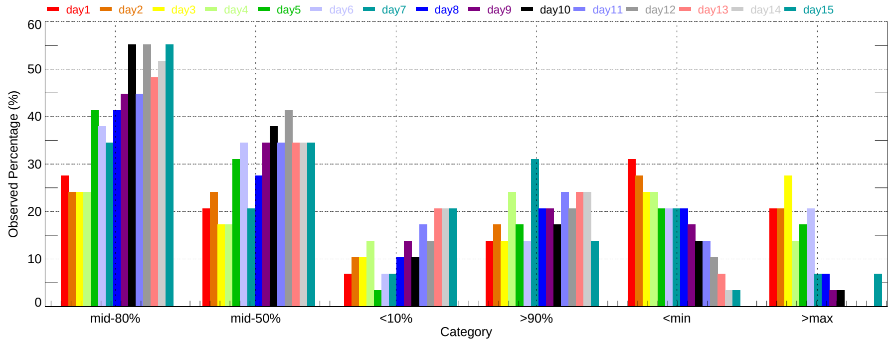
Observed Percentage of Ensembles - ALW: Max Temperature (2007-11-01~2007-11-30)
