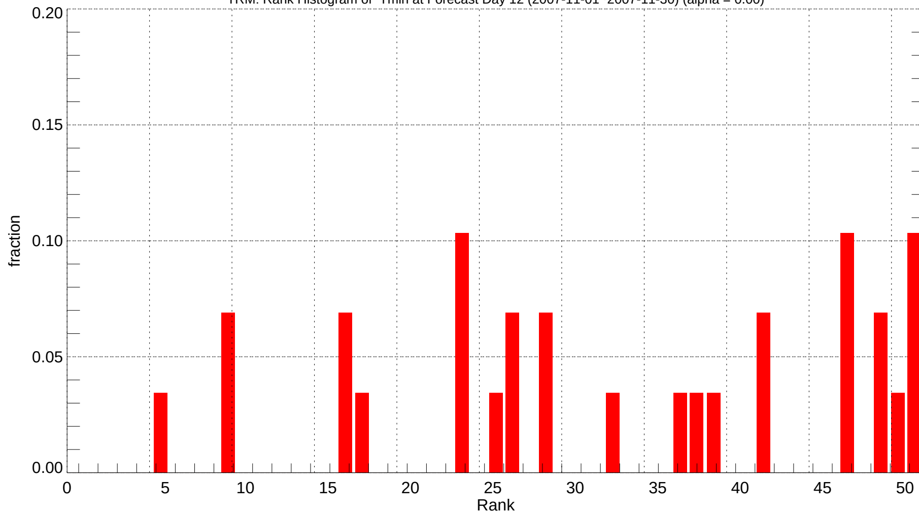
TRM: Rank Histogram of Tmin at Forecast Day 12 (2007-11-01~2007-11-30) (alpha = 0.00)
