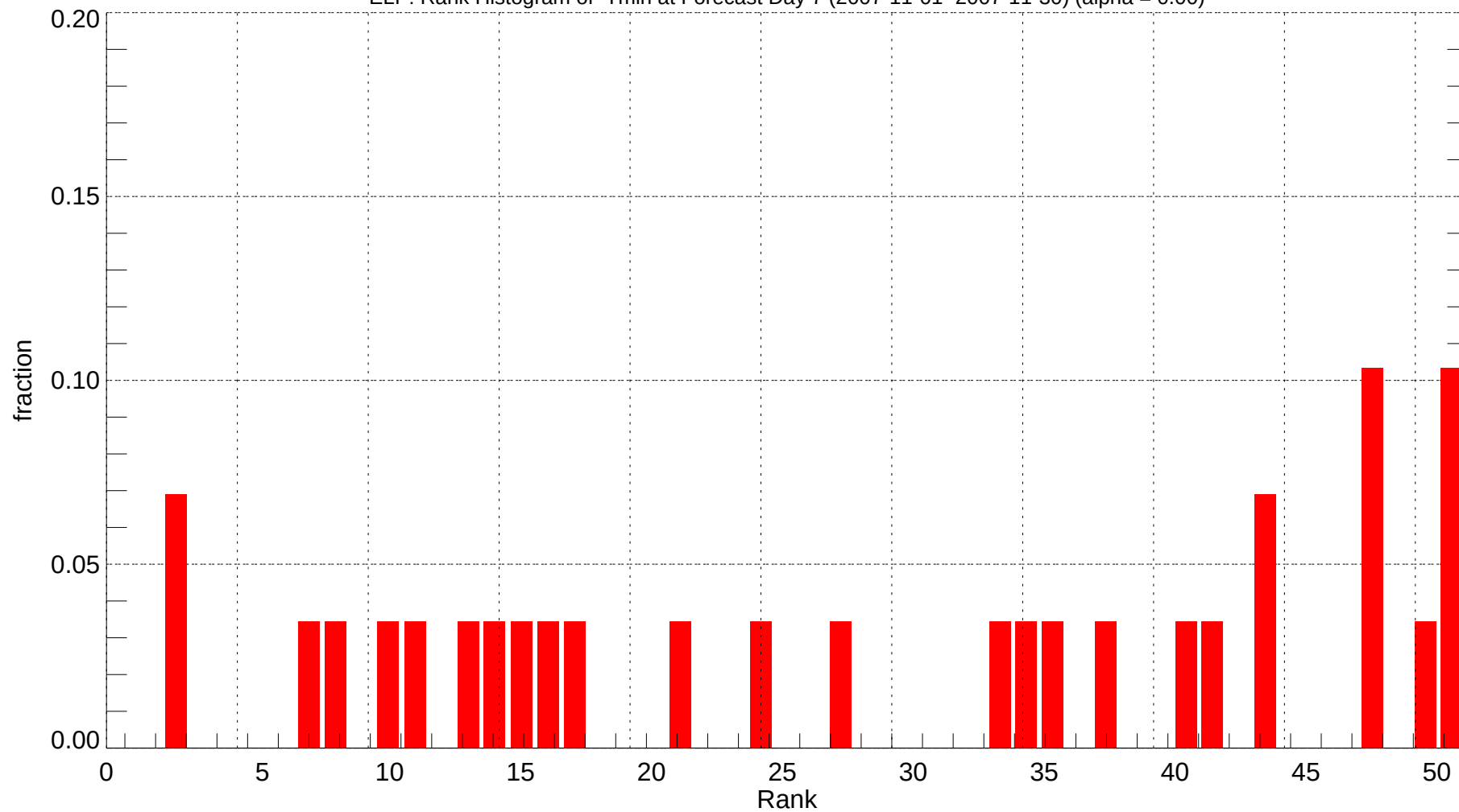
ELP: Rank Histogram of Tmin at Forecast Day 7 (2007-11-01~2007-11-30) (alpha = 0.00)
