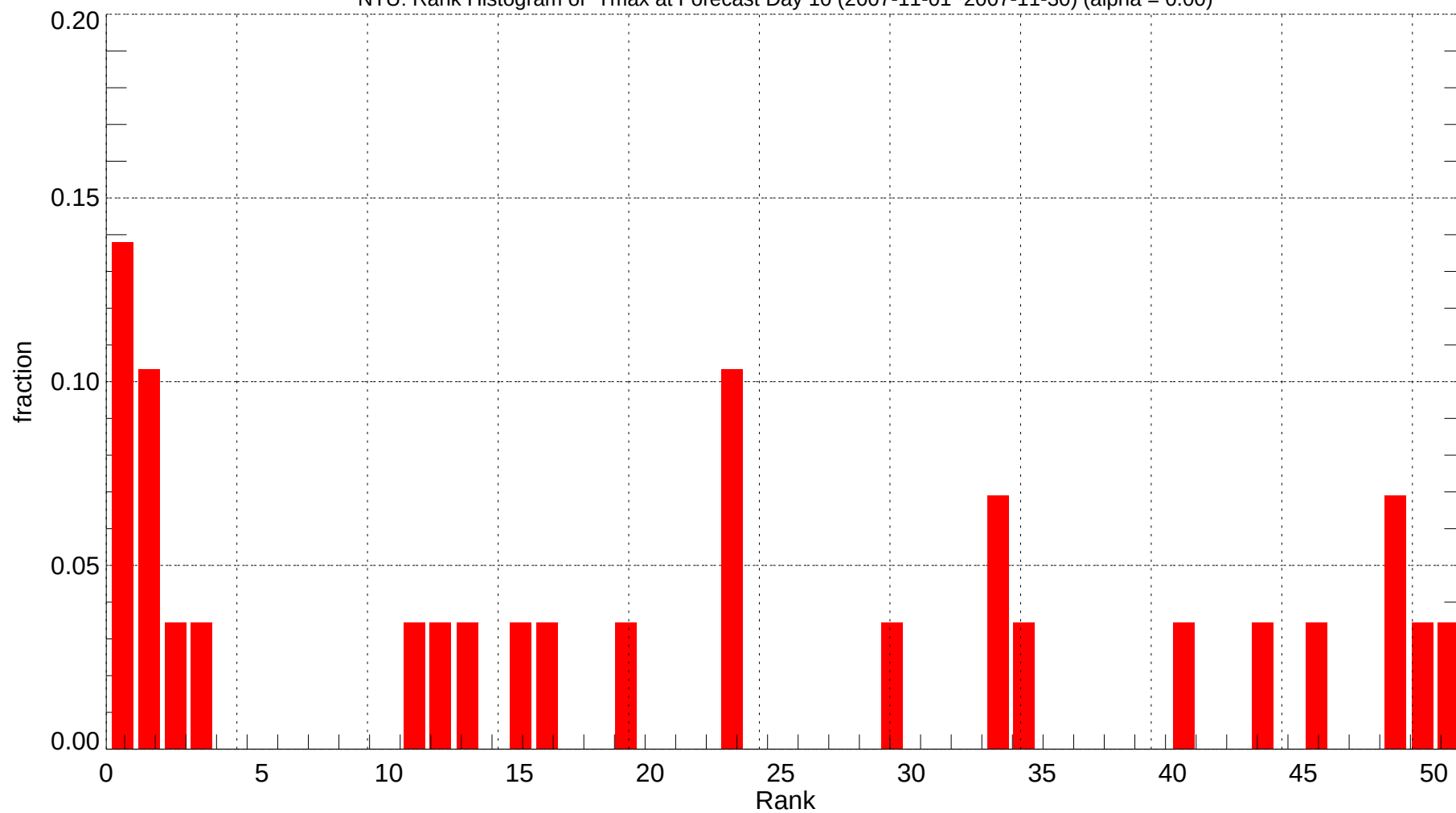
NTU: Rank Histogram of Tmax at Forecast Day 10 (2007-11-01~2007-11-30) (alpha = 0.00)
