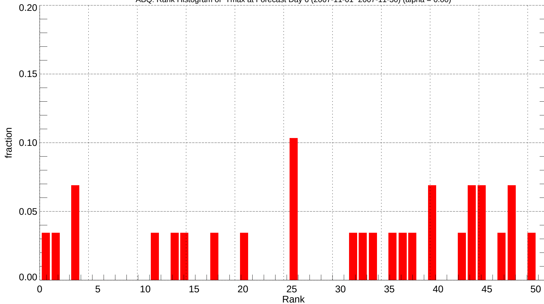
ABQ: Rank Histogram of Tmax at Forecast Day 6 (2007-11-01~2007-11-30) (alpha = 0.00)
