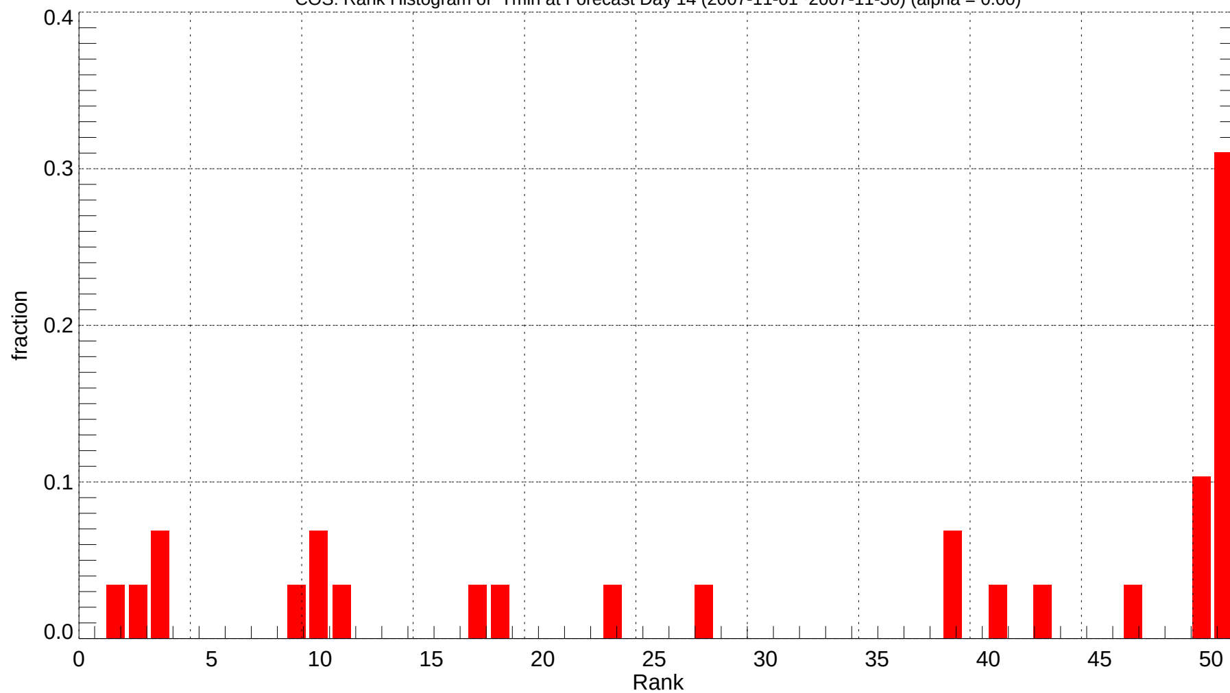
COS: Rank Histogram of Tmin at Forecast Day 14 (2007-11-01~2007-11-30) (alpha = 0.00)
