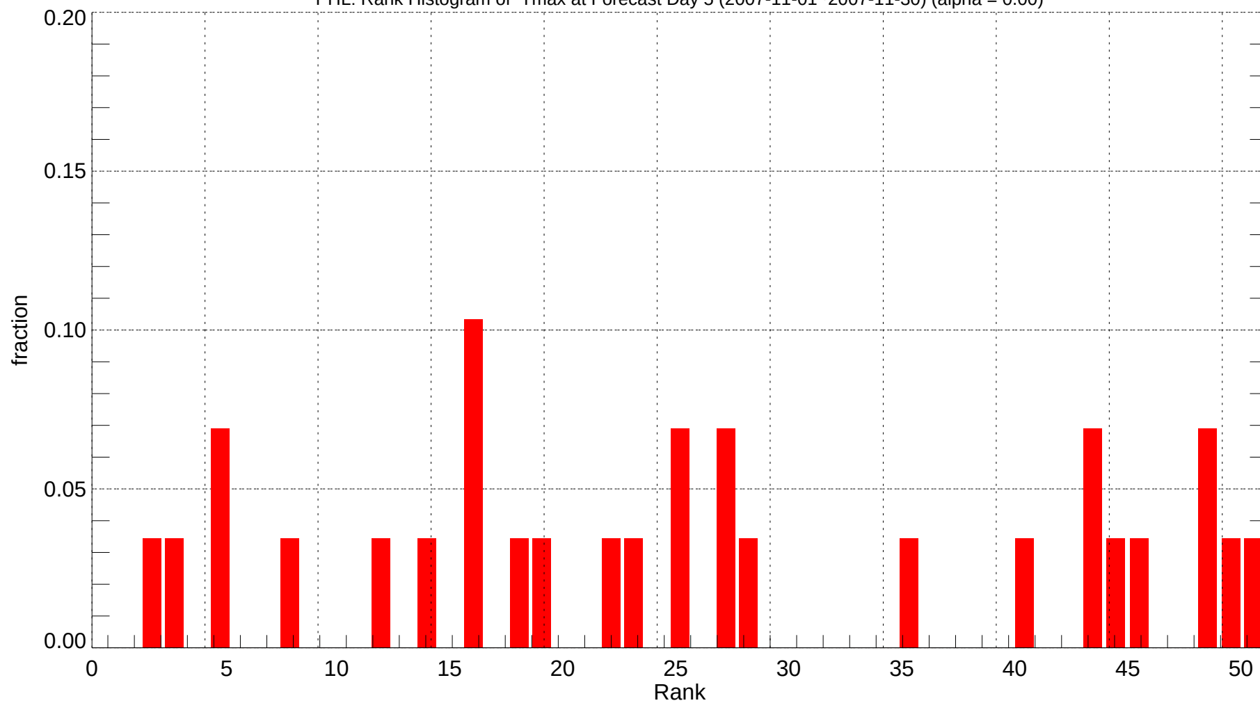
PHL: Rank Histogram of Tmax at Forecast Day 5 (2007-11-01~2007-11-30) (alpha = 0.00)
