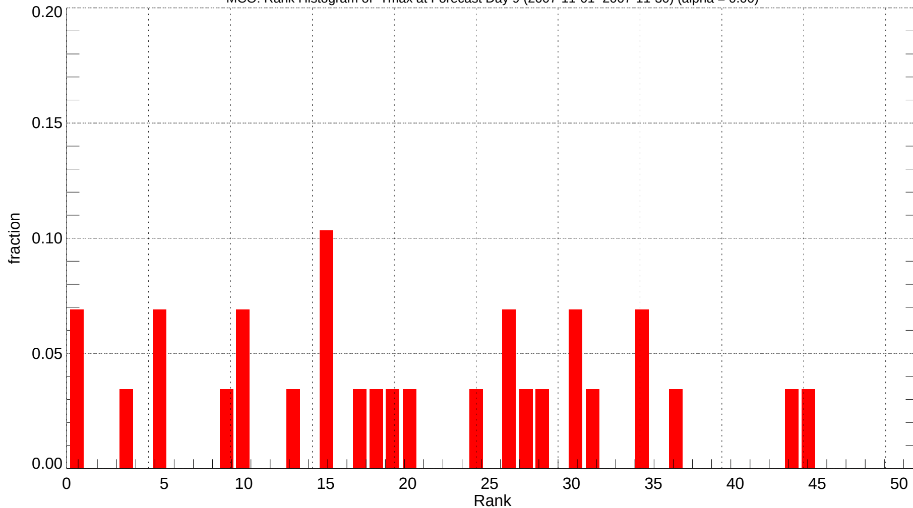
MCO: Rank Histogram of Tmax at Forecast Day 9 (2007-11-01~2007-11-30) (alpha = 0.00)
