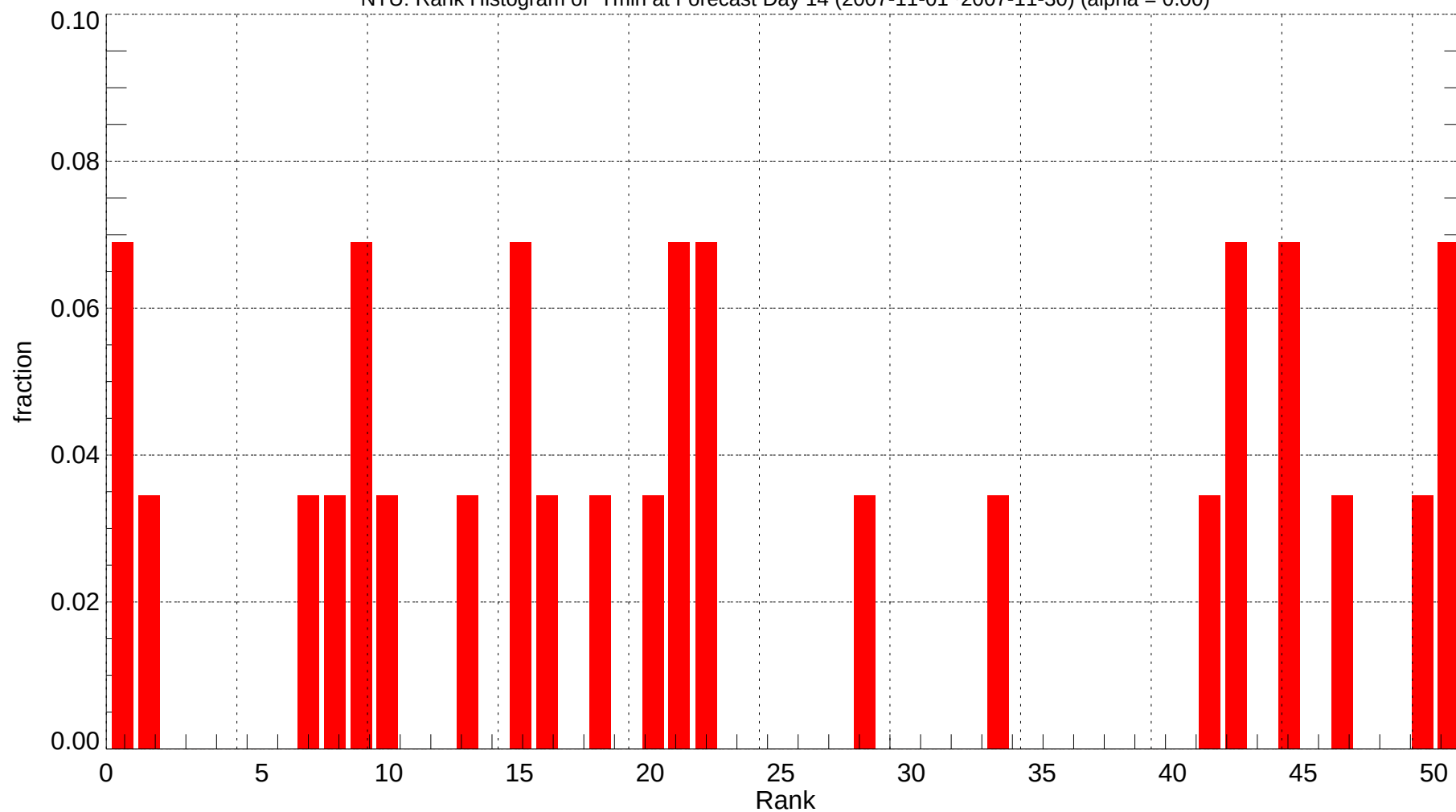
NTU: Rank Histogram of Tmin at Forecast Day 14 (2007-11-01~2007-11-30) (alpha = 0.00)
