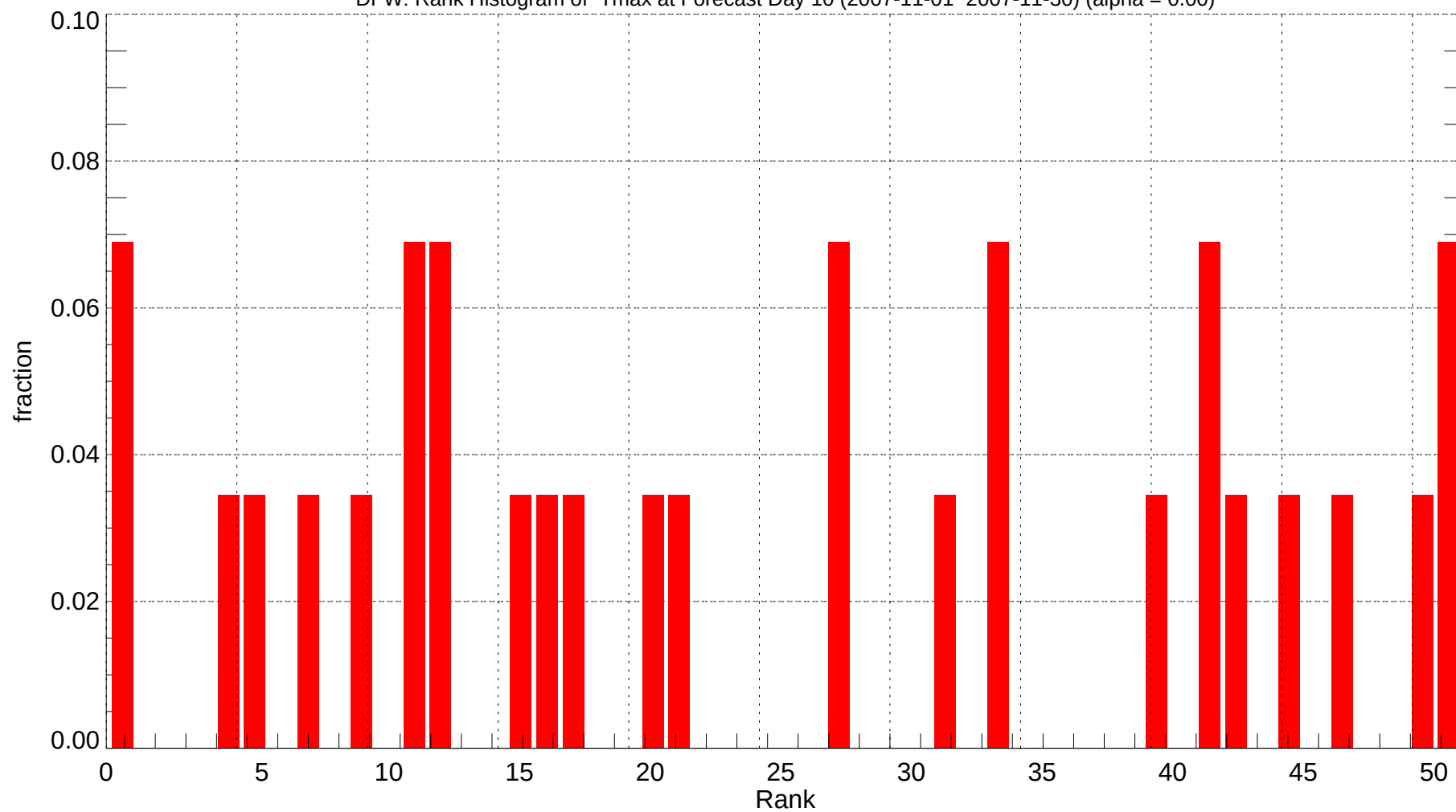
DFW: Rank Histogram of Tmax at Forecast Day 10 (2007-11-01~2007-11-30) (alpha = 0.00)
