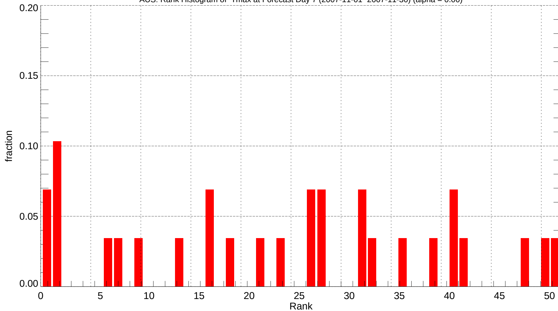
AUS: Rank Histogram of Tmax at Forecast Day 7 (2007-11-01~2007-11-30) (alpha = 0.00)
