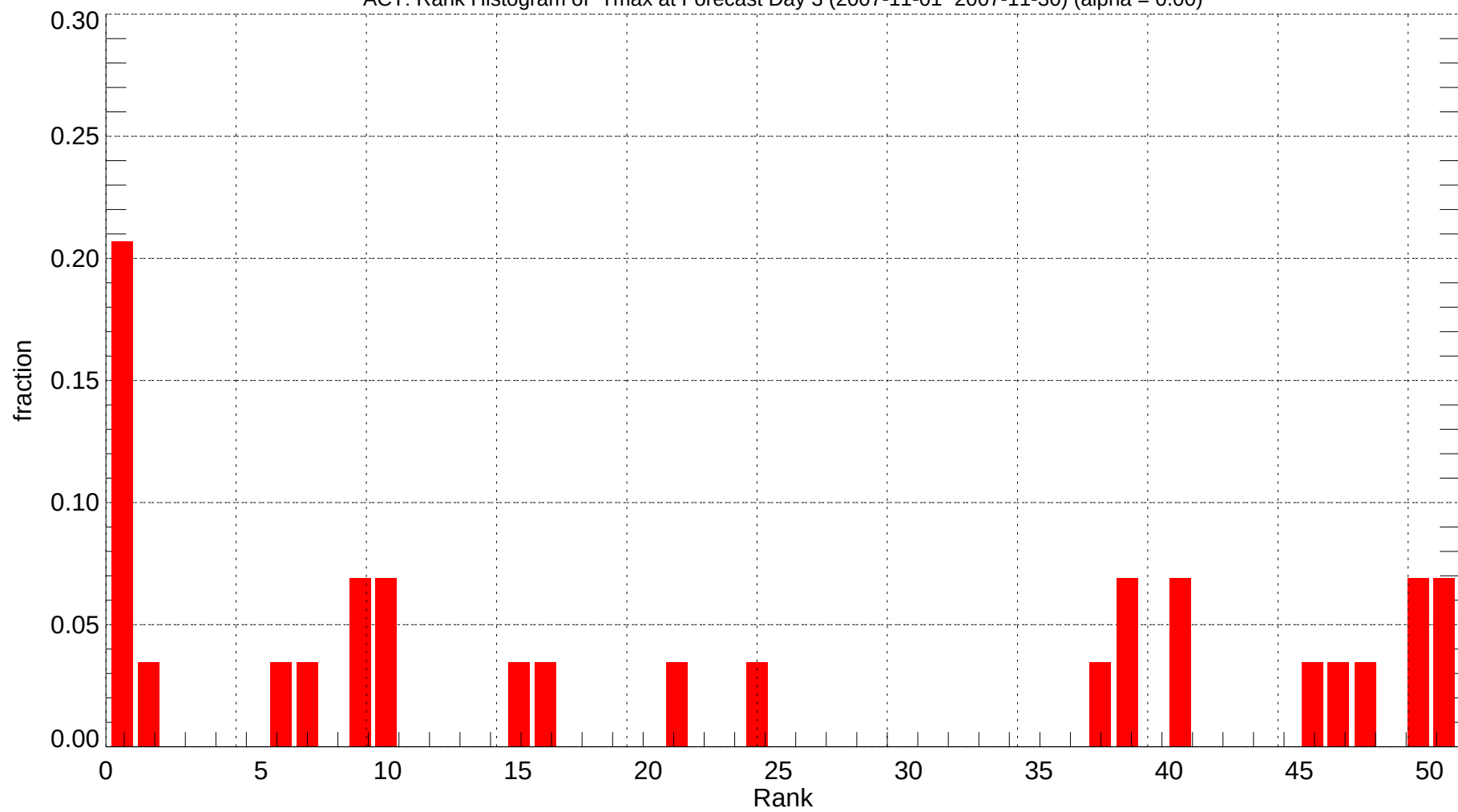
ACT: Rank Histogram of Tmax at Forecast Day 3 (2007-11-01~2007-11-30) (alpha = 0.00)
