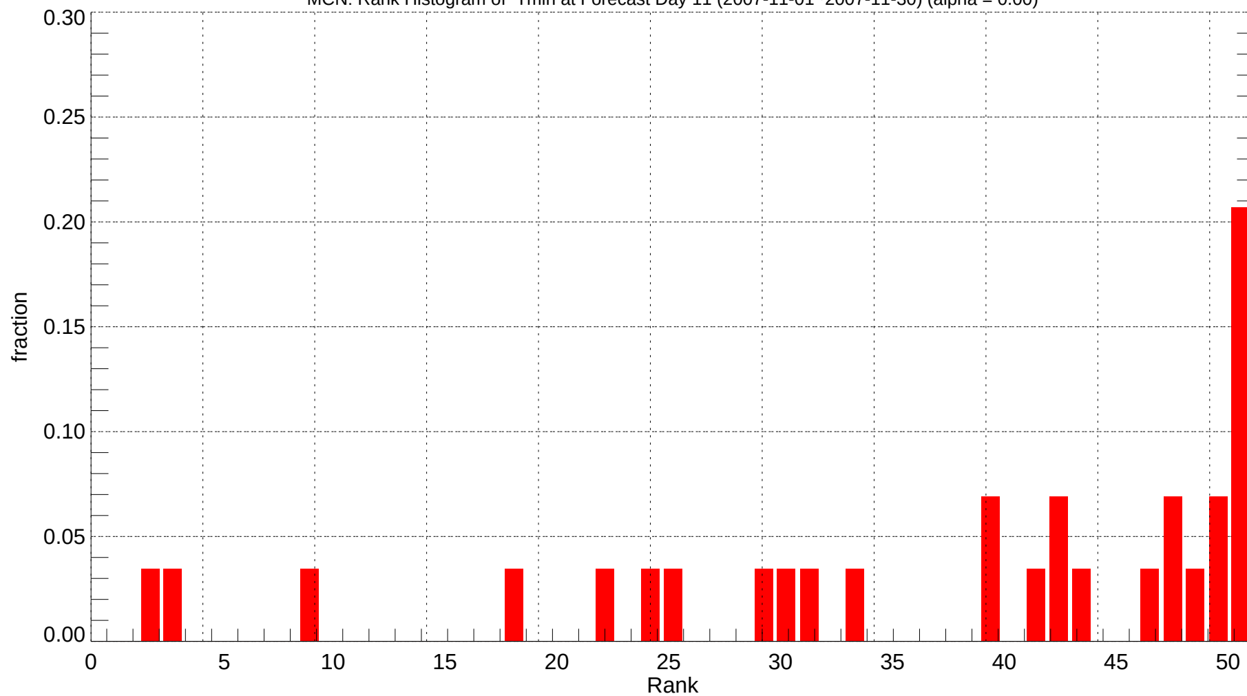
MCN: Rank Histogram of Tmin at Forecast Day 11 (2007-11-01~2007-11-30) (alpha = 0.00)
