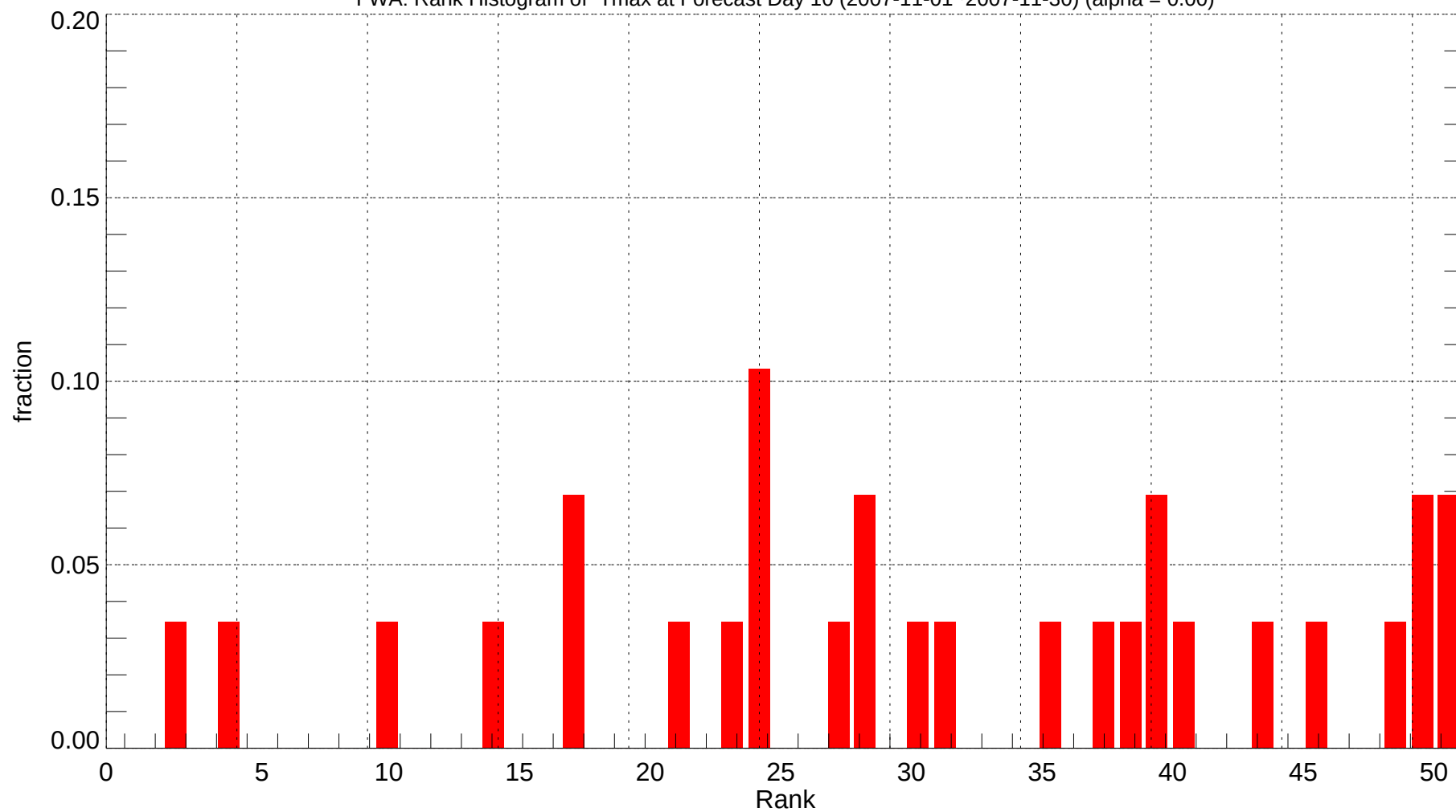
FWA: Rank Histogram of Tmax at Forecast Day 10 (2007-11-01~2007-11-30) (alpha = 0.00)
