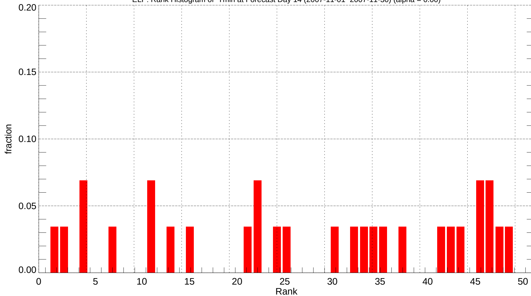
ELP: Rank Histogram of Tmin at Forecast Day 14 (2007-11-01~2007-11-30) (alpha = 0.00)
