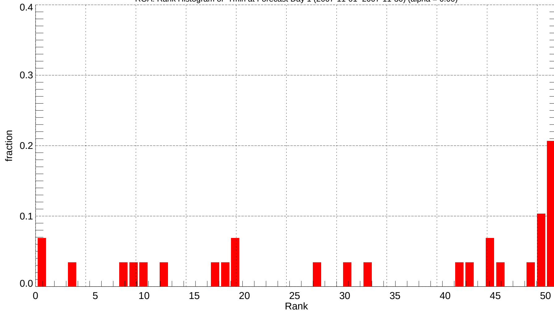
ROA: Rank Histogram of Tmin at Forecast Day 1 (2007-11-01~2007-11-30) (alpha = 0.00)
