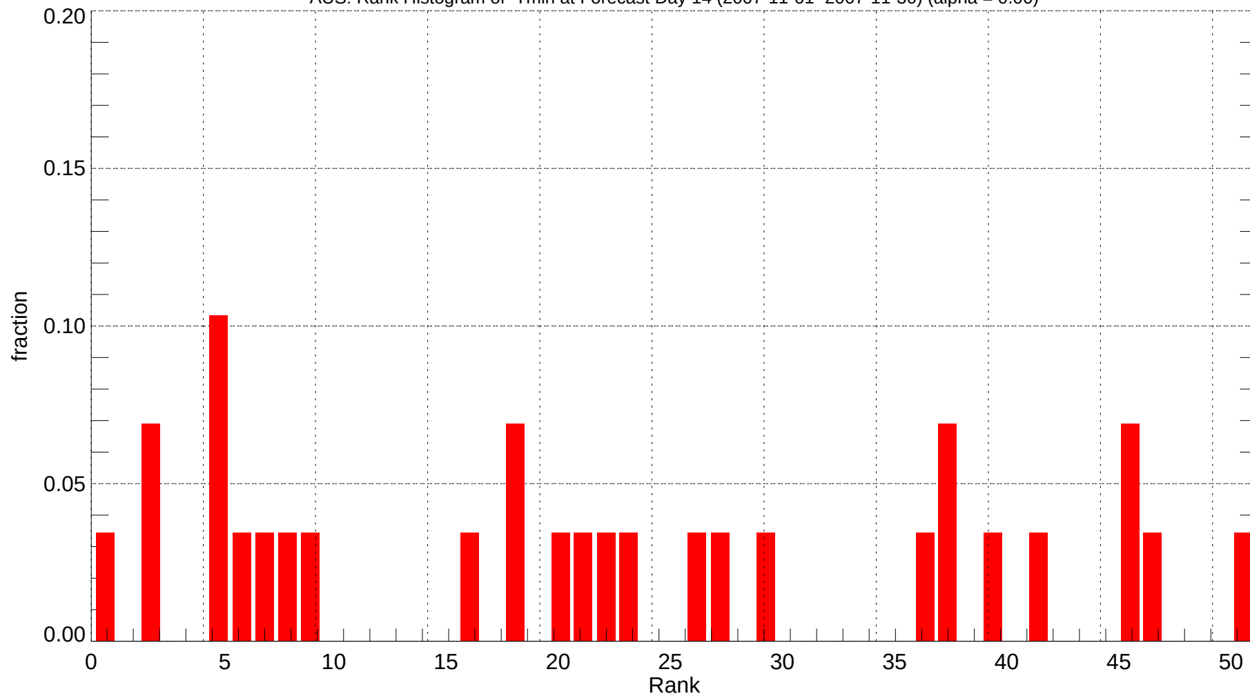
AUS: Rank Histogram of Tmin at Forecast Day 14 (2007-11-01~2007-11-30) (alpha = 0.00)
