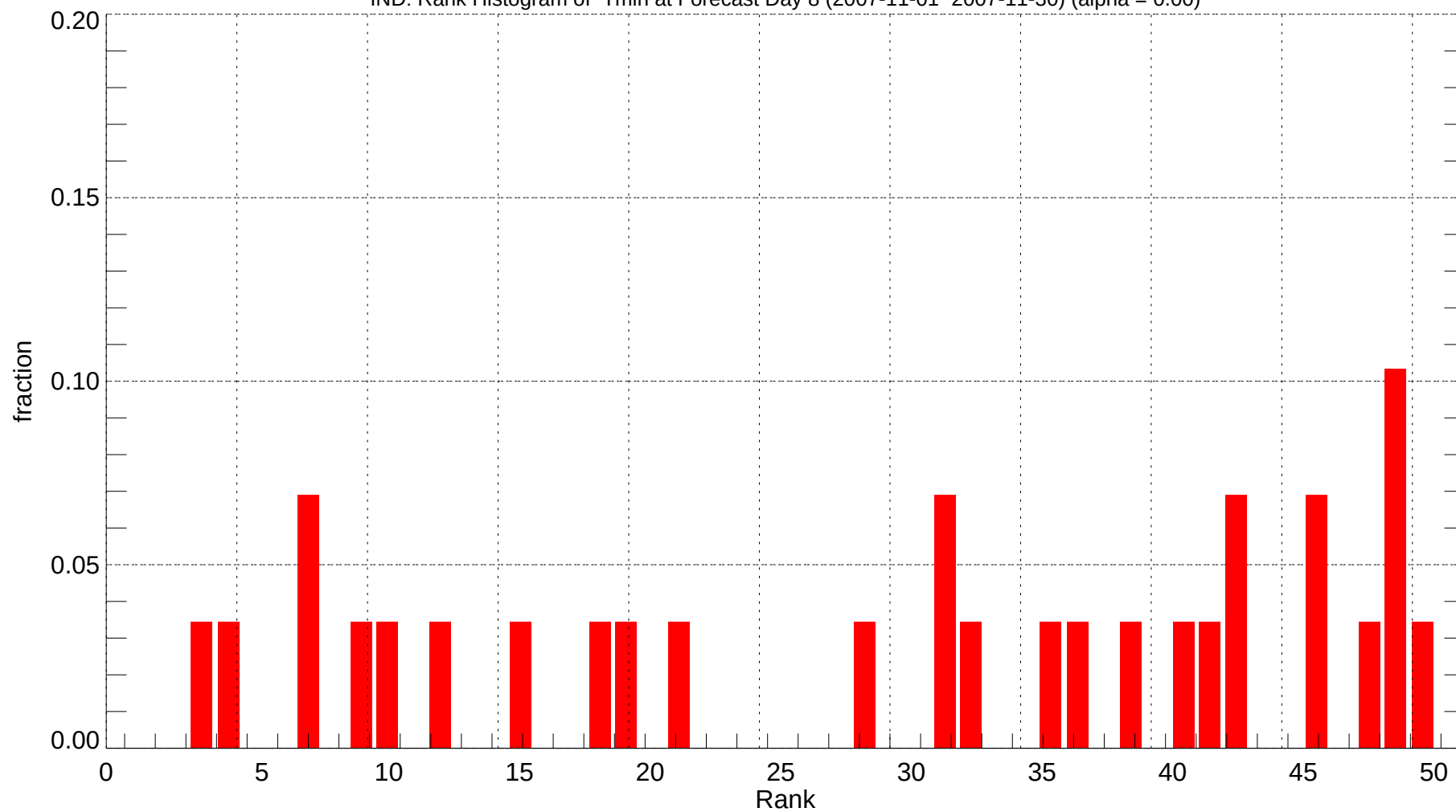
IND: Rank Histogram of Tmin at Forecast Day 8 (2007-11-01~2007-11-30) (alpha = 0.00)
