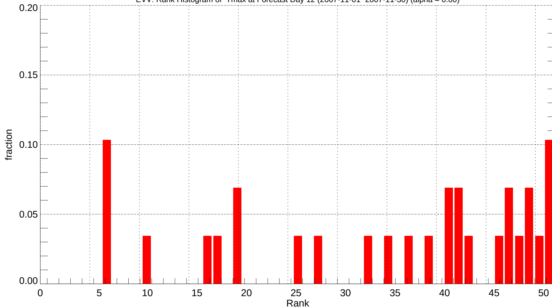
EVV: Rank Histogram of Tmax at Forecast Day 12 (2007-11-01~2007-11-30) (alpha = 0.00)
