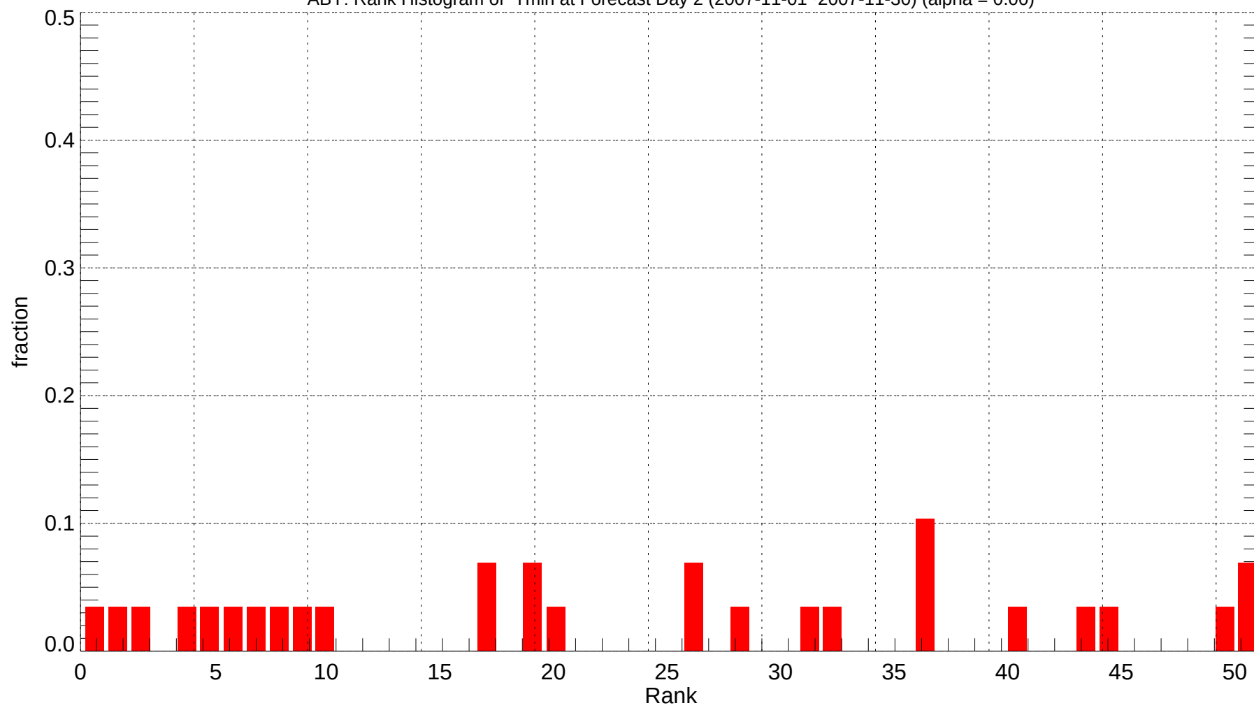
ABY: Rank Histogram of Tmin at Forecast Day 2 (2007-11-01~2007-11-30) (alpha = 0.00)
