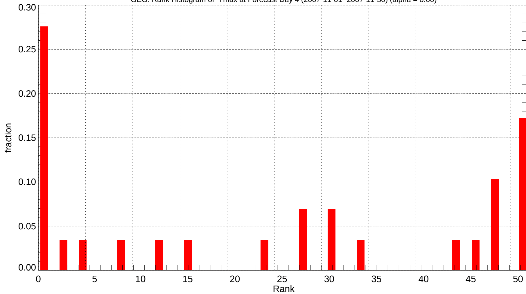
GEG: Rank Histogram of Tmax at Forecast Day 4 (2007-11-01~2007-11-30) (alpha = 0.00)
