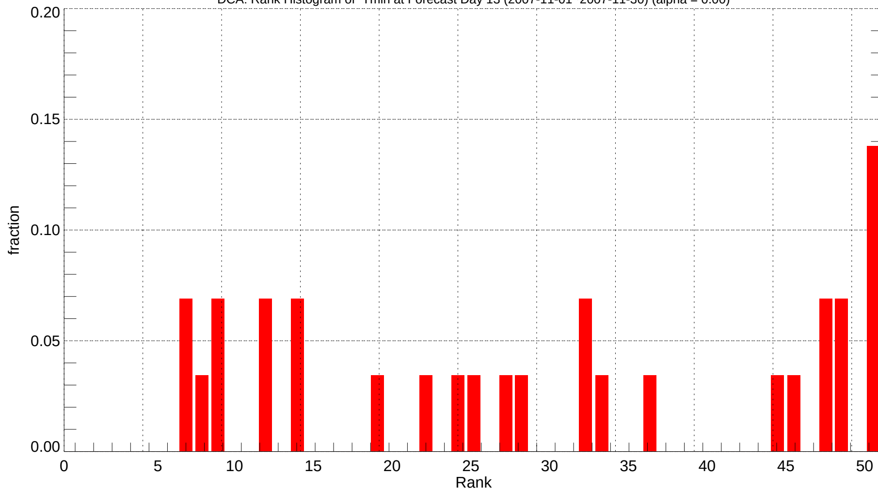
DCA: Rank Histogram of Tmin at Forecast Day 13 (2007-11-01~2007-11-30) (alpha = 0.00)
