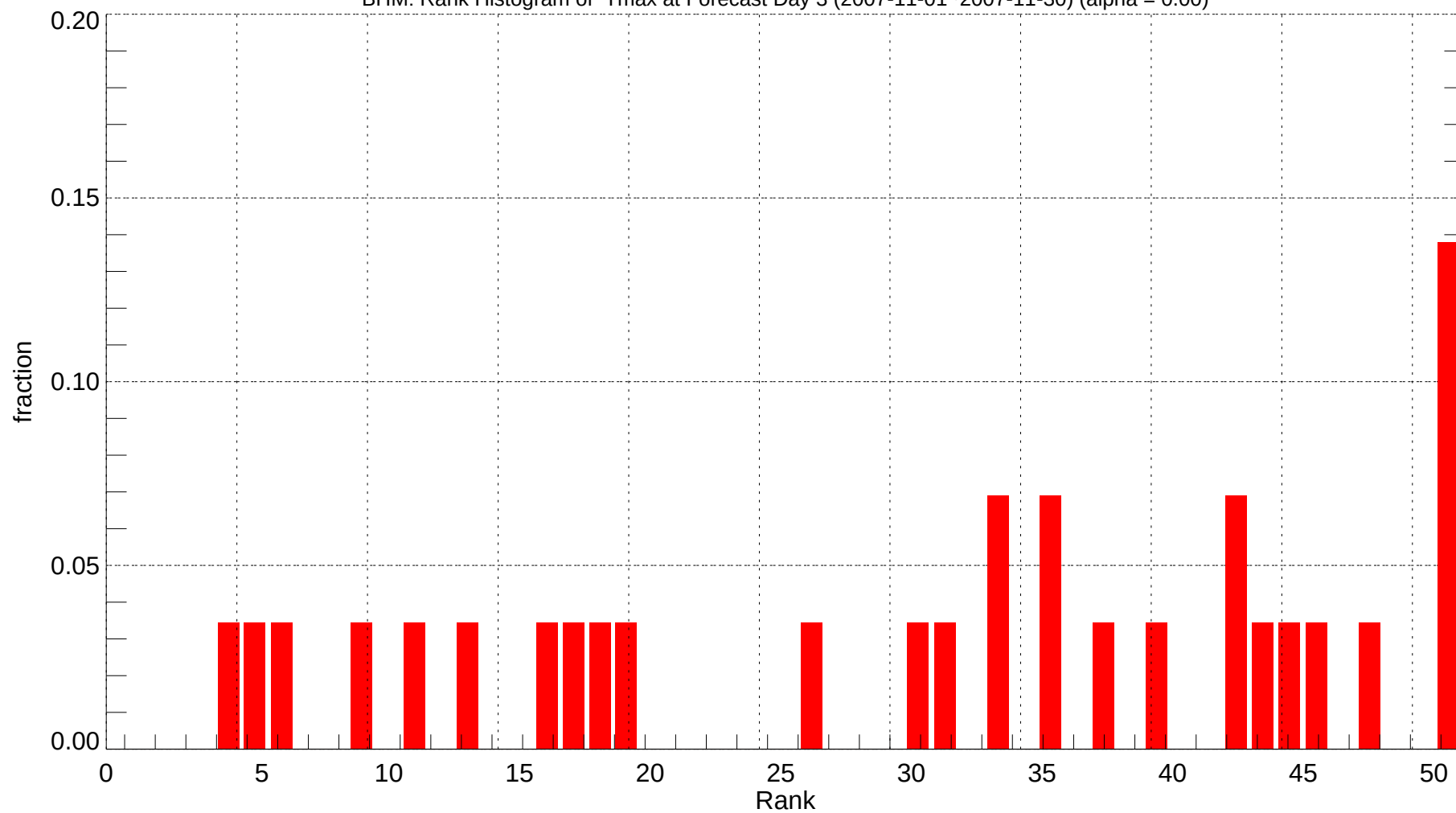
BHM: Rank Histogram of Tmax at Forecast Day 3 (2007-11-01~2007-11-30) (alpha = 0.00)
