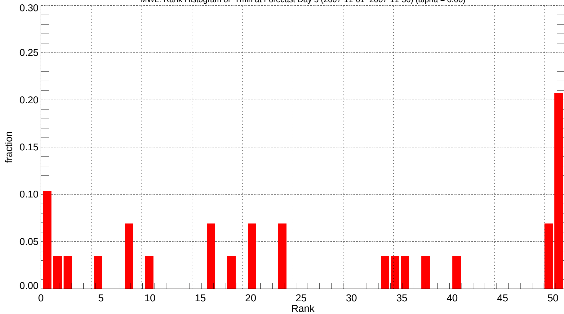
MWL: Rank Histogram of Tmin at Forecast Day 3 (2007-11-01~2007-11-30) (alpha = 0.00)
