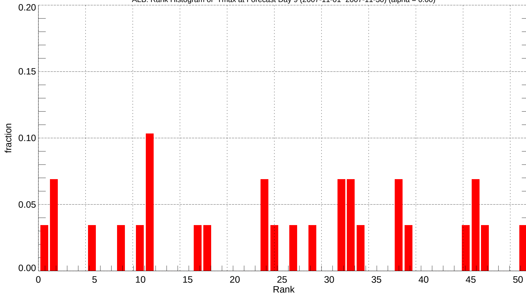
ALB: Rank Histogram of Tmax at Forecast Day 9 (2007-11-01~2007-11-30) (alpha = 0.00)
