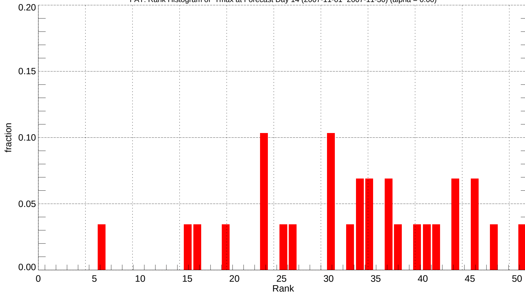
FAT: Rank Histogram of Tmax at Forecast Day 14 (2007-11-01~2007-11-30) (alpha = 0.00)
