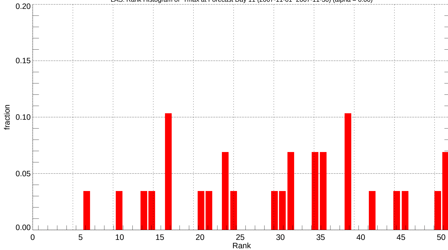
LAS: Rank Histogram of Tmax at Forecast Day 11 (2007-11-01~2007-11-30) (alpha = 0.00)
