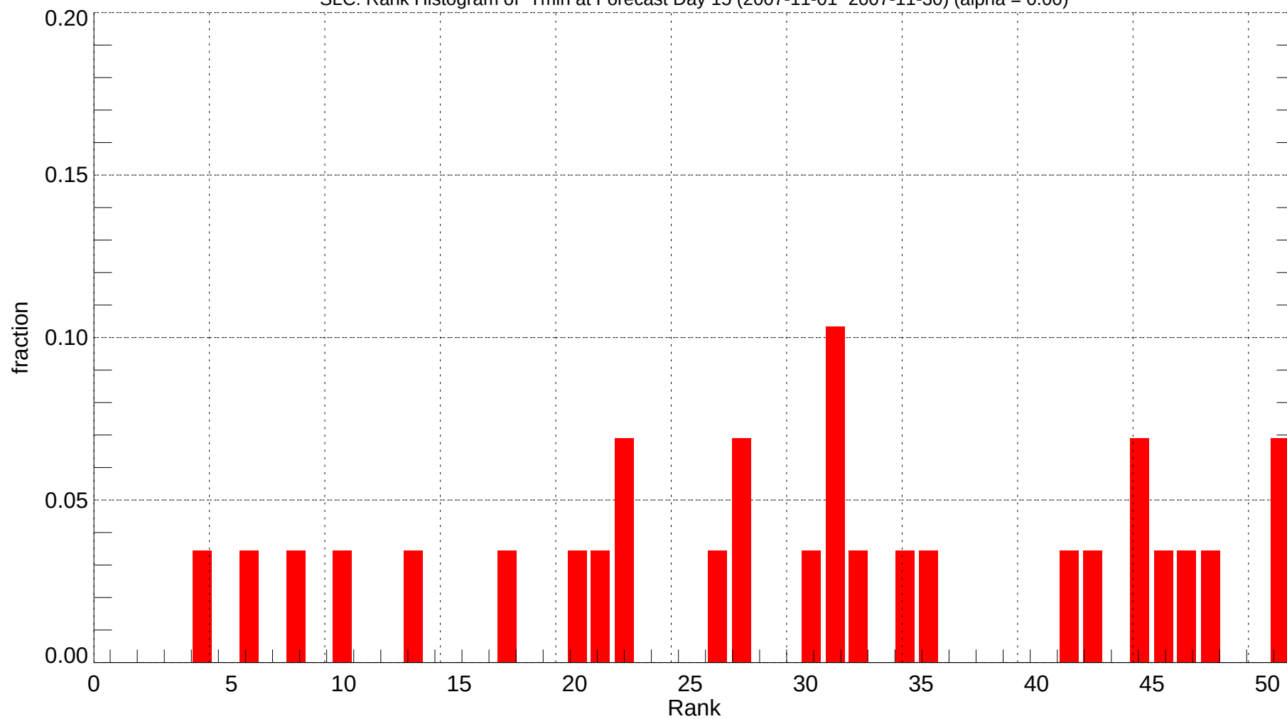
SLC: Rank Histogram of Tmin at Forecast Day 15 (2007-11-01~2007-11-30) (alpha = 0.00)
