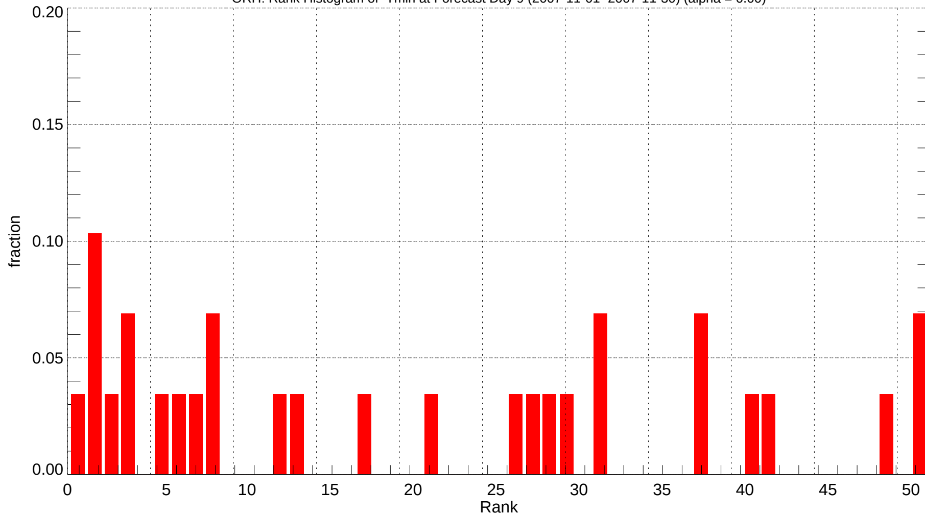
ORH: Rank Histogram of Tmin at Forecast Day 9 (2007-11-01~2007-11-30) (alpha = 0.00)
