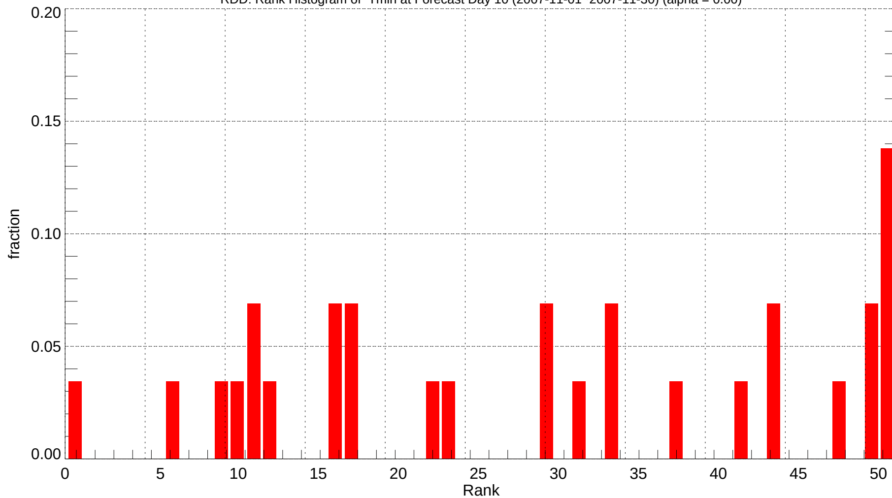
RDD: Rank Histogram of Tmin at Forecast Day 10 (2007-11-01~2007-11-30) (alpha = 0.00)
