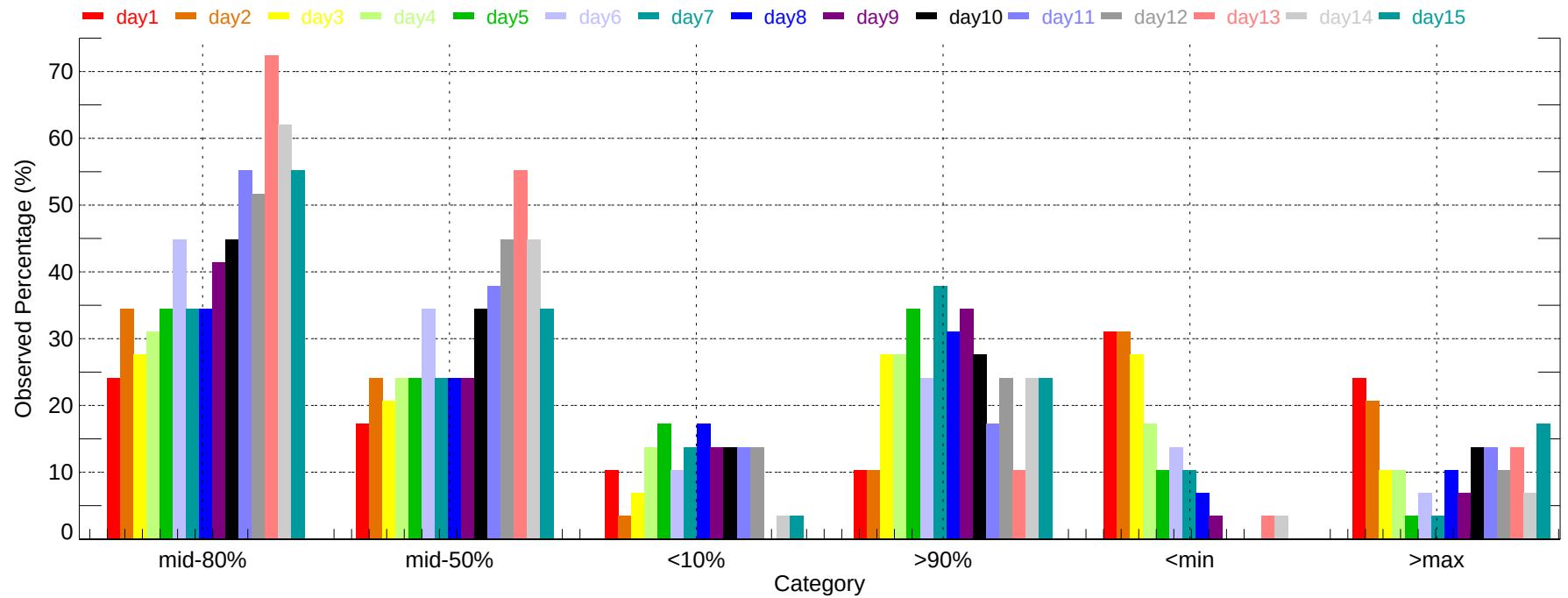
Observed Percentage of Ensembles - SFO: Min Temperature (2007-11-01~2007-11-30)
