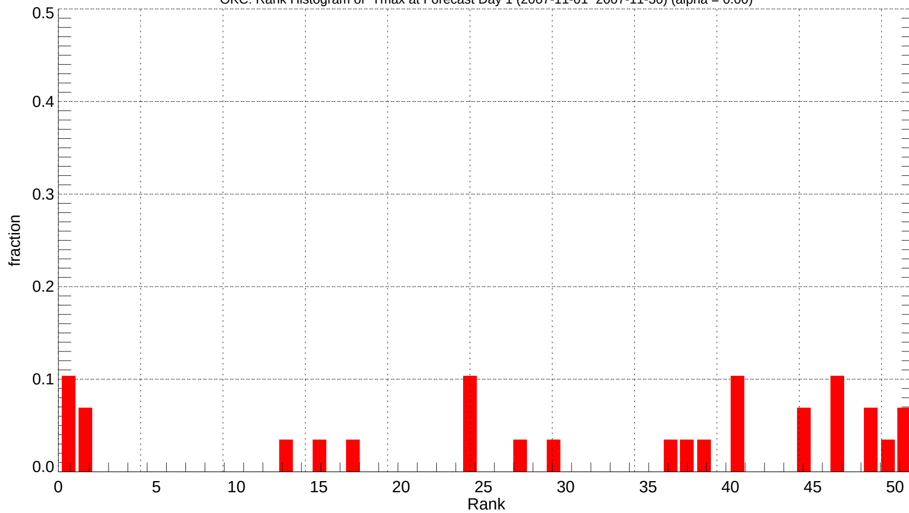
OKC: Rank Histogram of Tmax at Forecast Day 1 (2007-11-01~2007-11-30) (alpha = 0.00)
