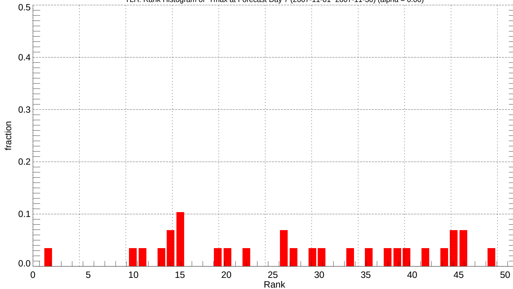
TLH: Rank Histogram of Tmax at Forecast Day 7 (2007-11-01~2007-11-30) (alpha = 0.00)
