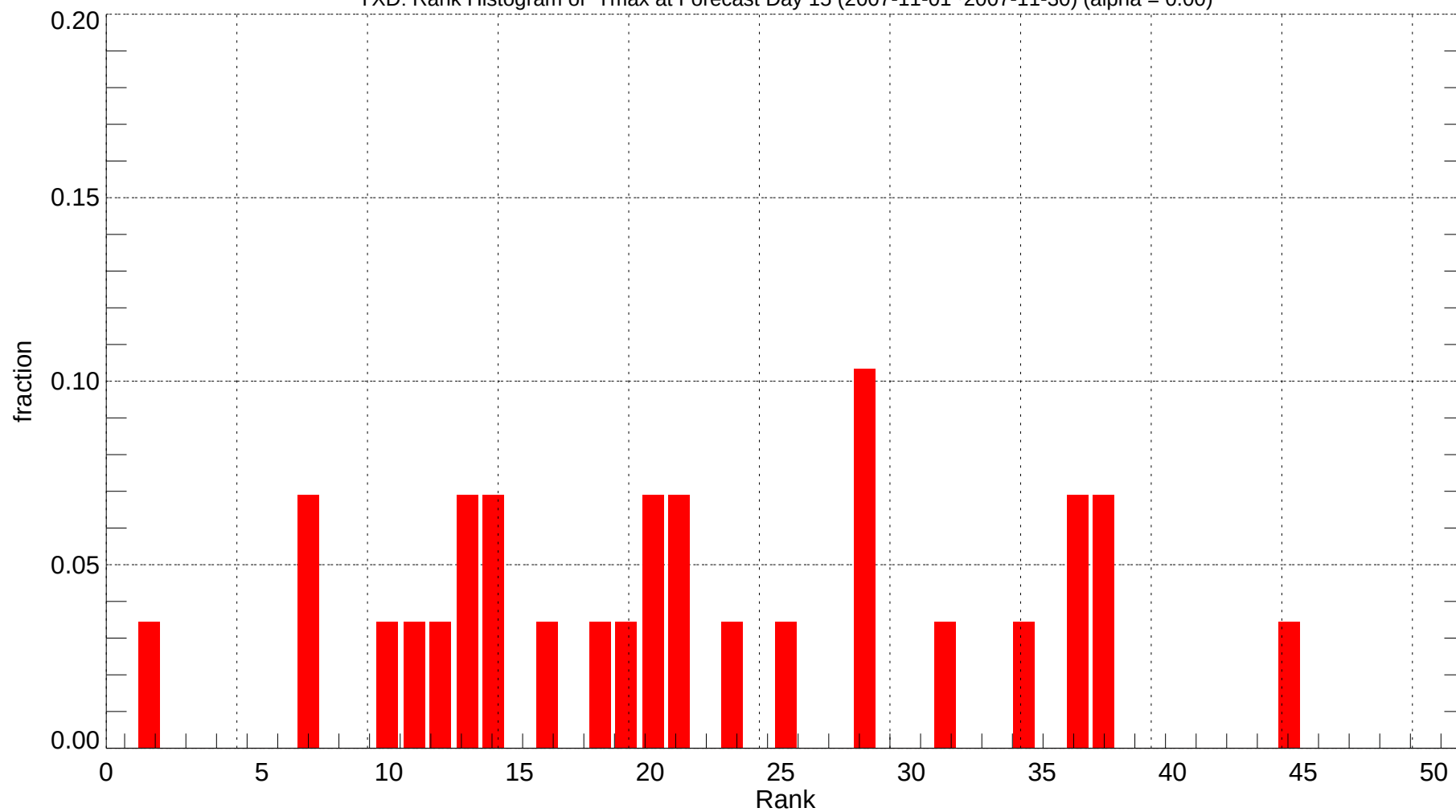
YXD: Rank Histogram of Tmax at Forecast Day 15 (2007-11-01~2007-11-30) (alpha = 0.00)
