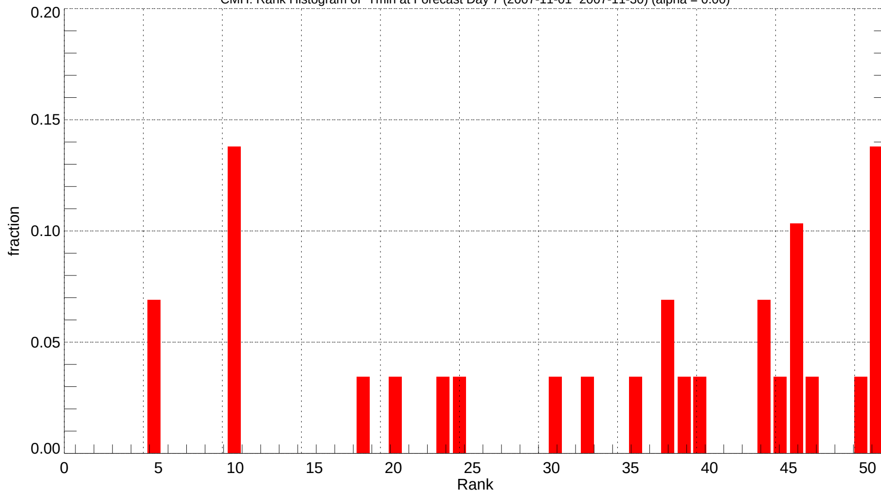
CMH: Rank Histogram of Tmin at Forecast Day 7 (2007-11-01~2007-11-30) (alpha = 0.00)
