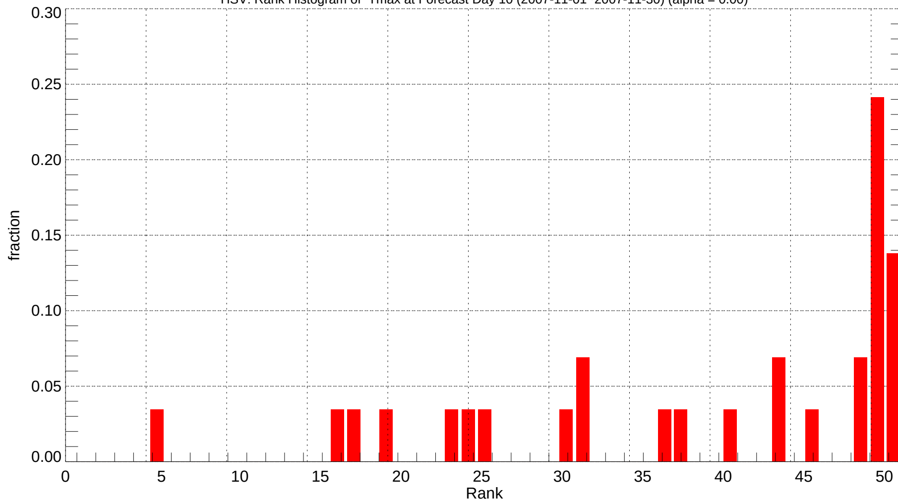
HSV: Rank Histogram of Tmax at Forecast Day 10 (2007-11-01~2007-11-30) (alpha = 0.00)
