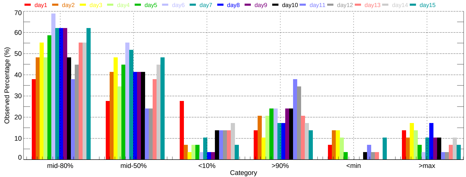
Observed Percentage of Ensembles - HOU: Min Temperature (2007-11-01~2007-11-30)
