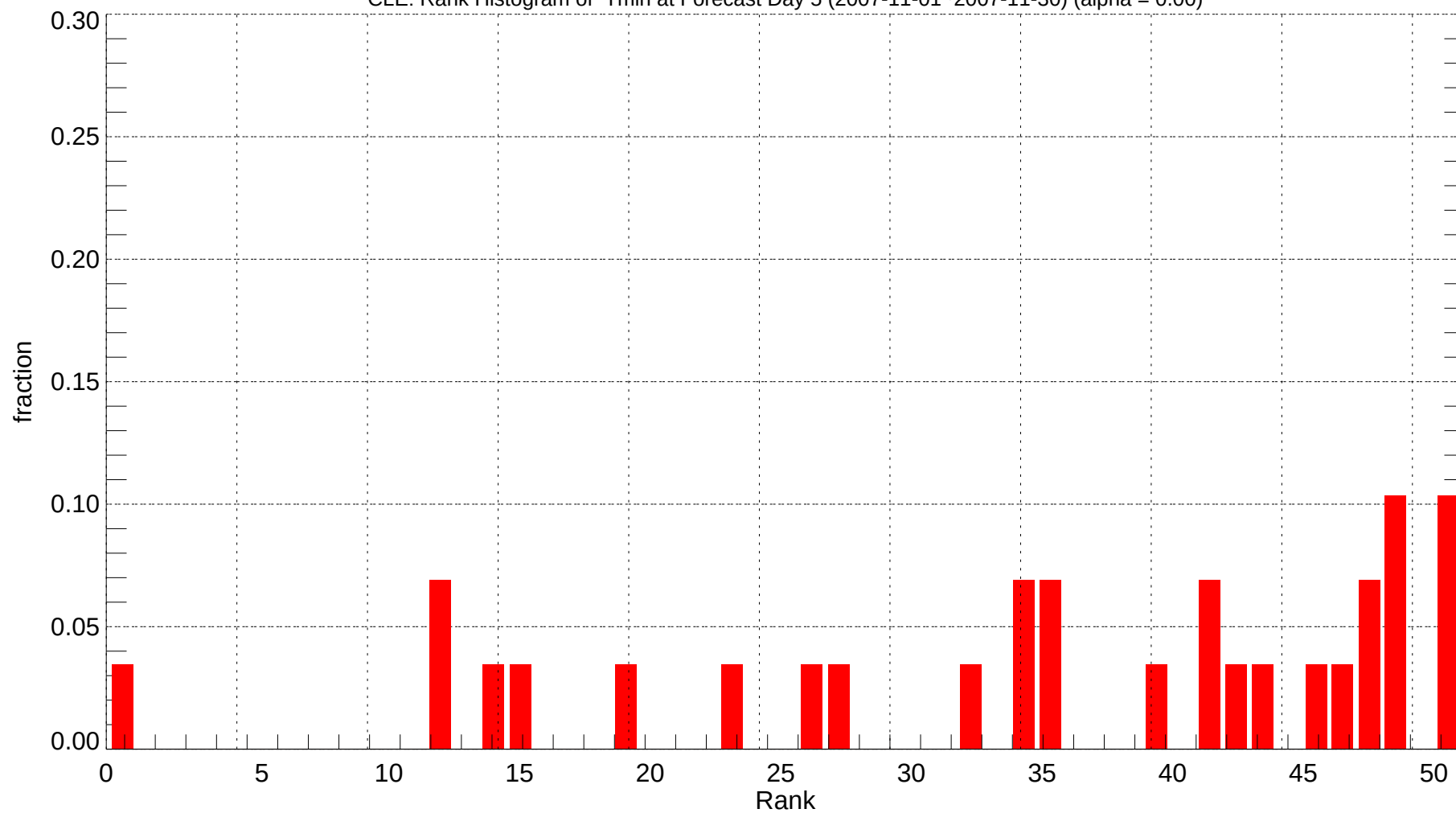
CLE: Rank Histogram of Tmin at Forecast Day 5 (2007-11-01~2007-11-30) (alpha = 0.00)
