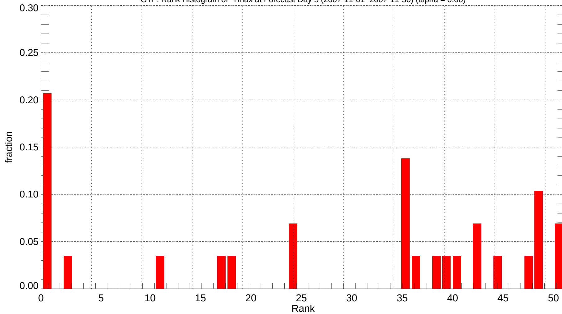
GTF: Rank Histogram of Tmax at Forecast Day 5 (2007-11-01~2007-11-30) (alpha = 0.00)
