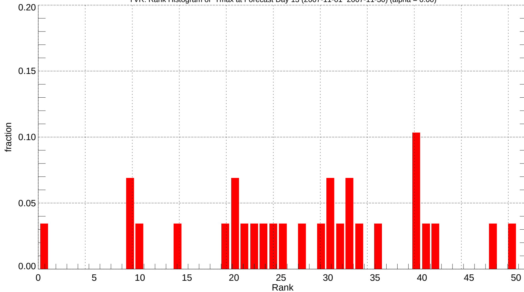
YVR: Rank Histogram of Tmax at Forecast Day 13 (2007-11-01~2007-11-30) (alpha = 0.00)
