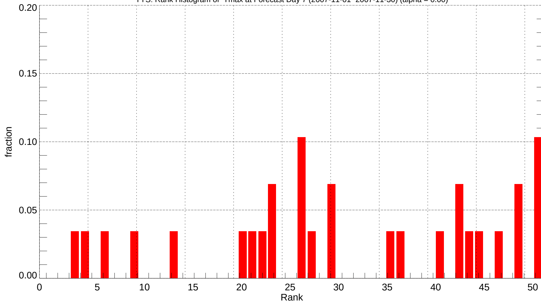
TYS: Rank Histogram of Tmax at Forecast Day 7 (2007-11-01~2007-11-30) (alpha = 0.00)
