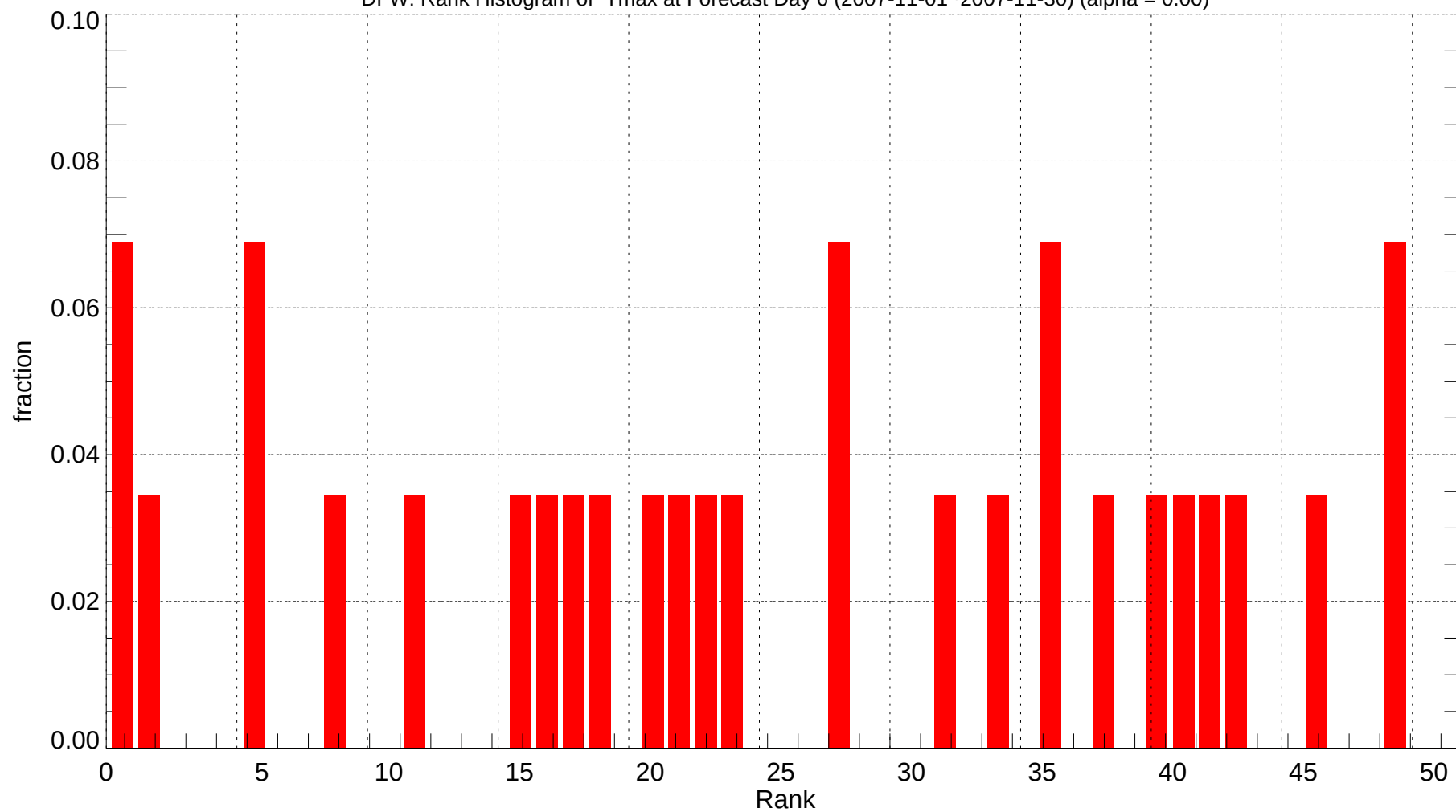
DFW: Rank Histogram of Tmax at Forecast Day 6 (2007-11-01~2007-11-30) (alpha = 0.00)
