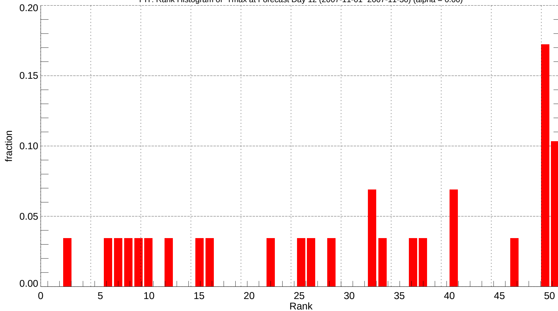
PIT: Rank Histogram of Tmax at Forecast Day 12 (2007-11-01~2007-11-30) (alpha = 0.00)
