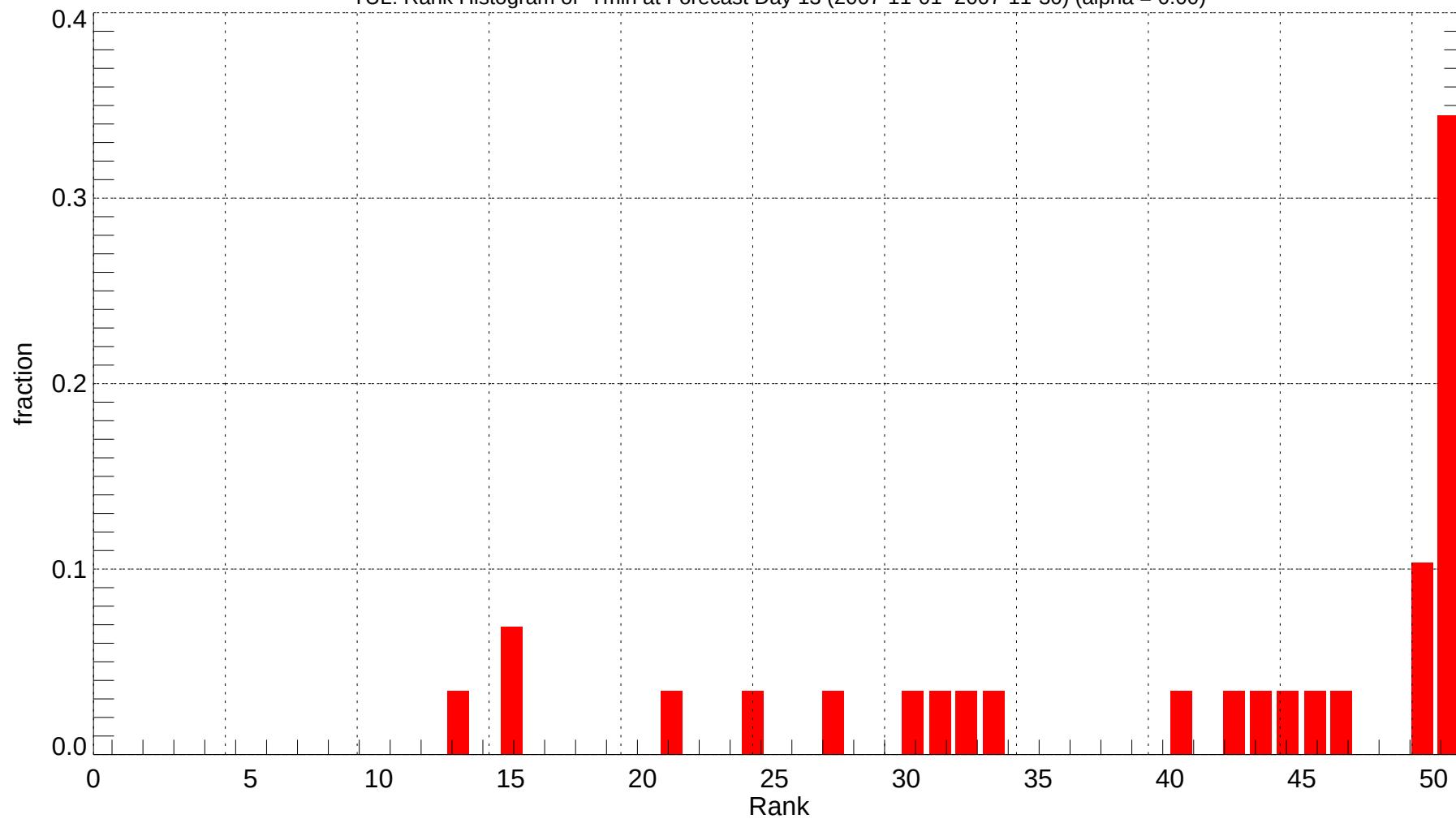
TUL: Rank Histogram of Tmin at Forecast Day 13 (2007-11-01~2007-11-30) (alpha = 0.00)
