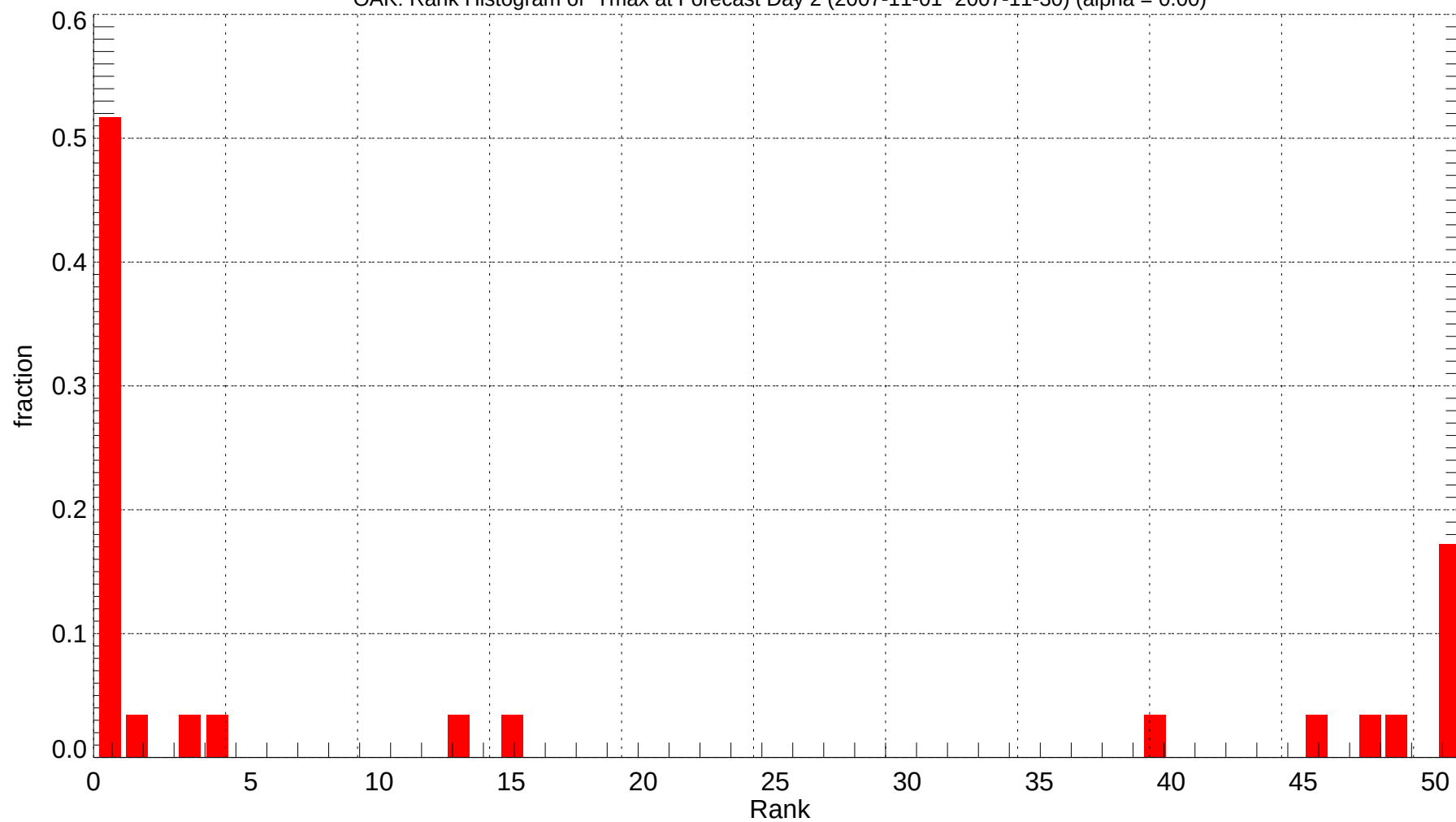
OAK: Rank Histogram of Tmax at Forecast Day 2 (2007-11-01~2007-11-30) (alpha = 0.00)
