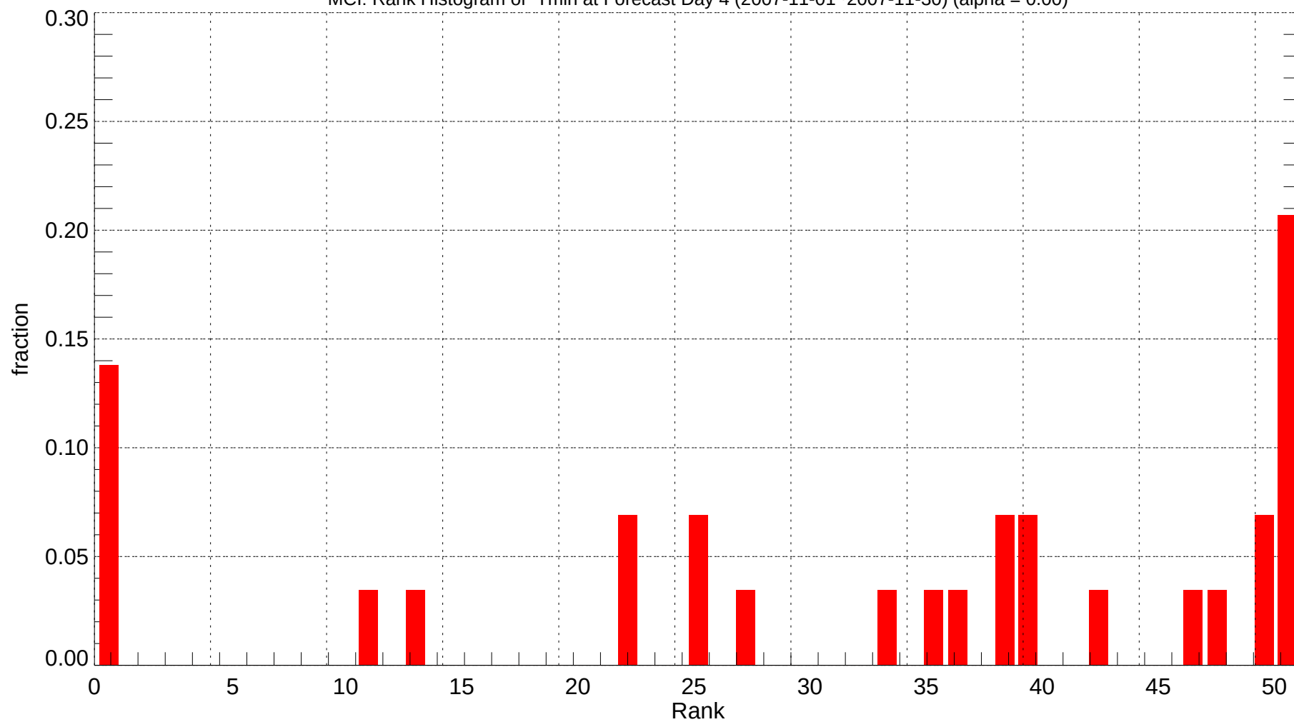
MCI: Rank Histogram of Tmin at Forecast Day 4 (2007-11-01~2007-11-30) (alpha = 0.00)
