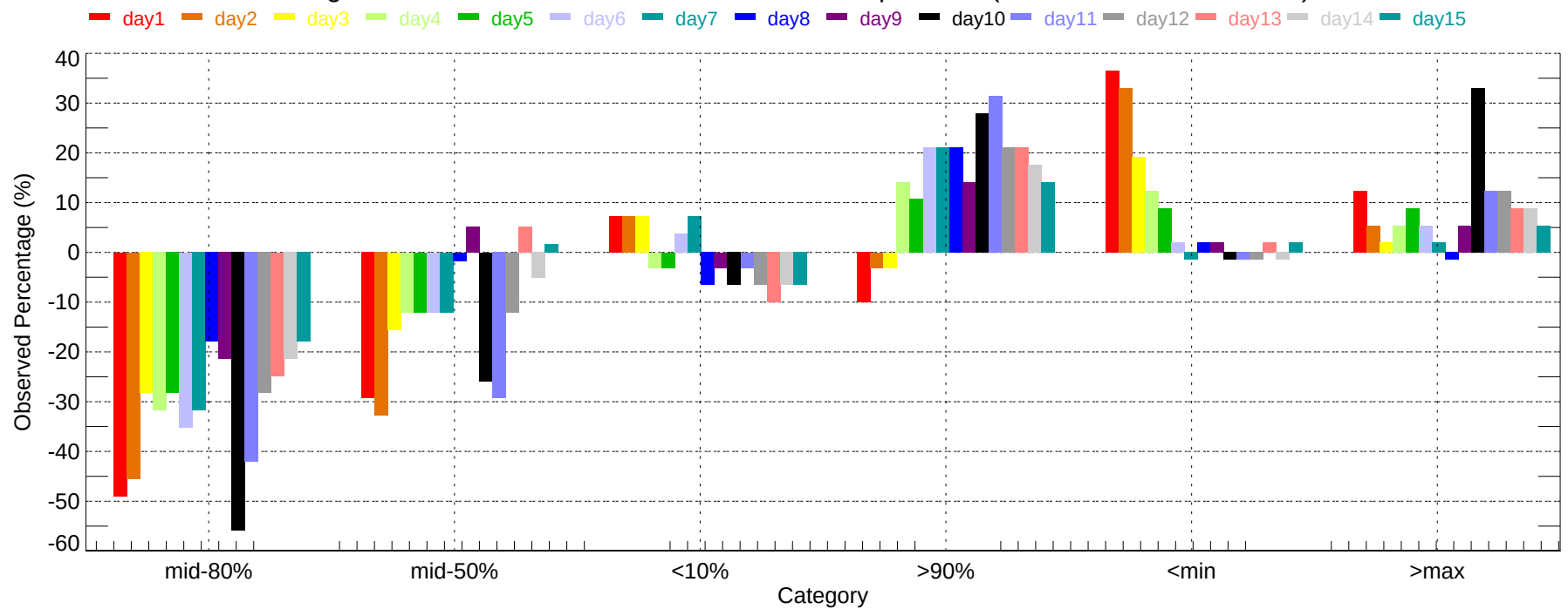
Observed Percentage Deviation of Ensembles - OMA: Max Temperature (2007-11-01~2007-11-30)
