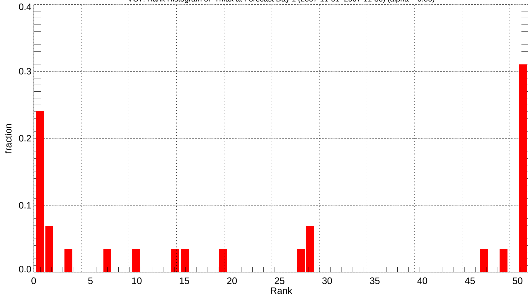
VCT: Rank Histogram of Tmax at Forecast Day 1 (2007-11-01~2007-11-30) (alpha = 0.00)
