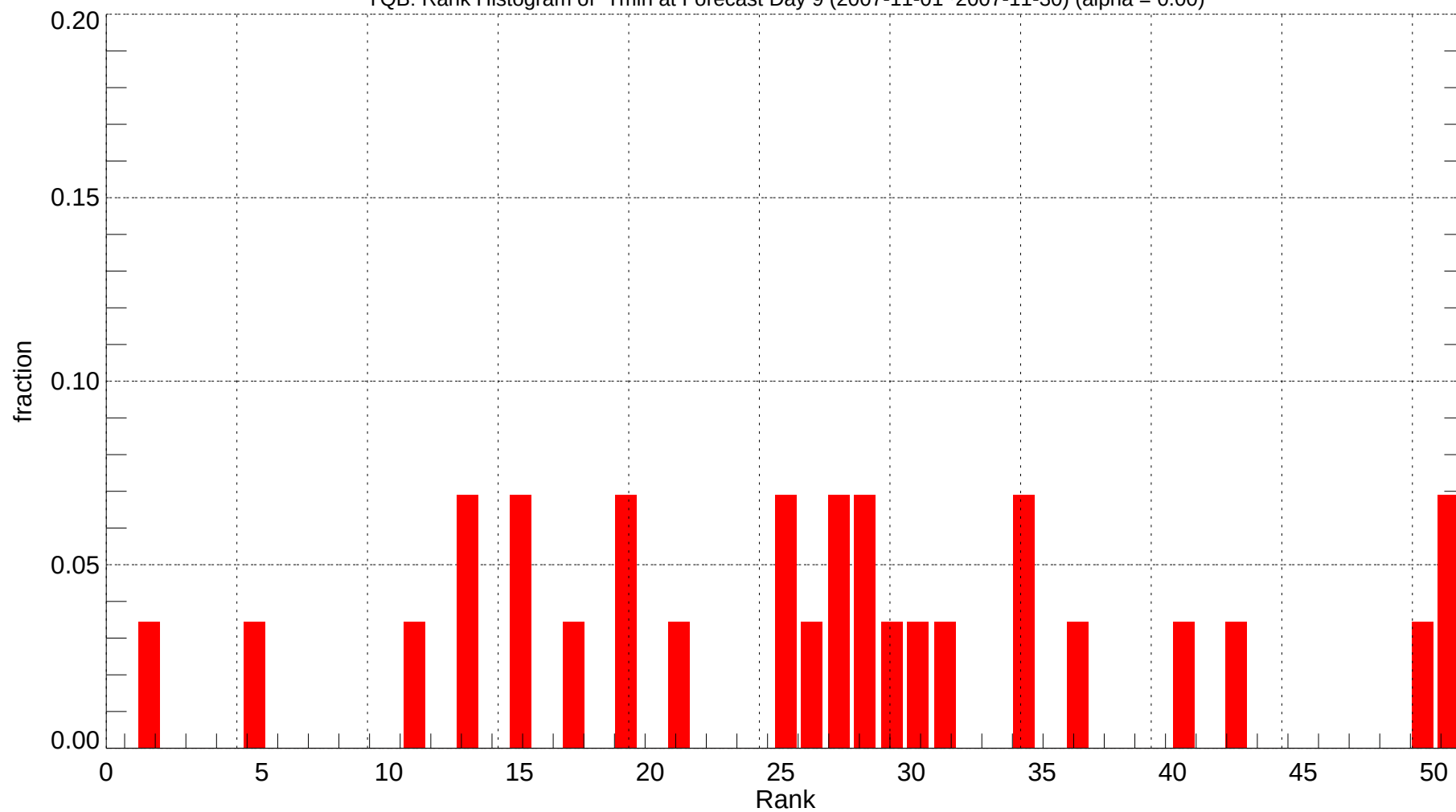
YQB: Rank Histogram of Tmin at Forecast Day 9 (2007-11-01~2007-11-30) (alpha = 0.00)
