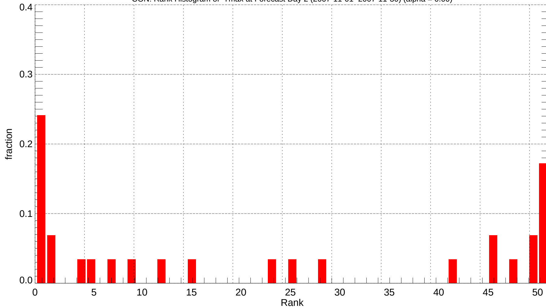
CON: Rank Histogram of Tmax at Forecast Day 2 (2007-11-01~2007-11-30) (alpha = 0.00)
