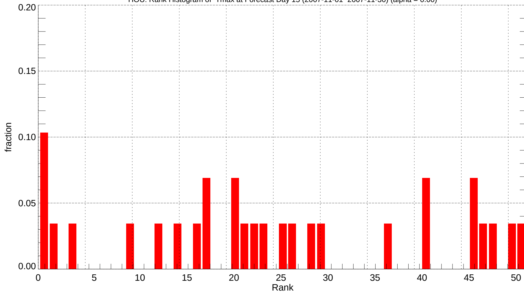
HOU: Rank Histogram of Tmax at Forecast Day 15 (2007-11-01~2007-11-30) (alpha = 0.00)
