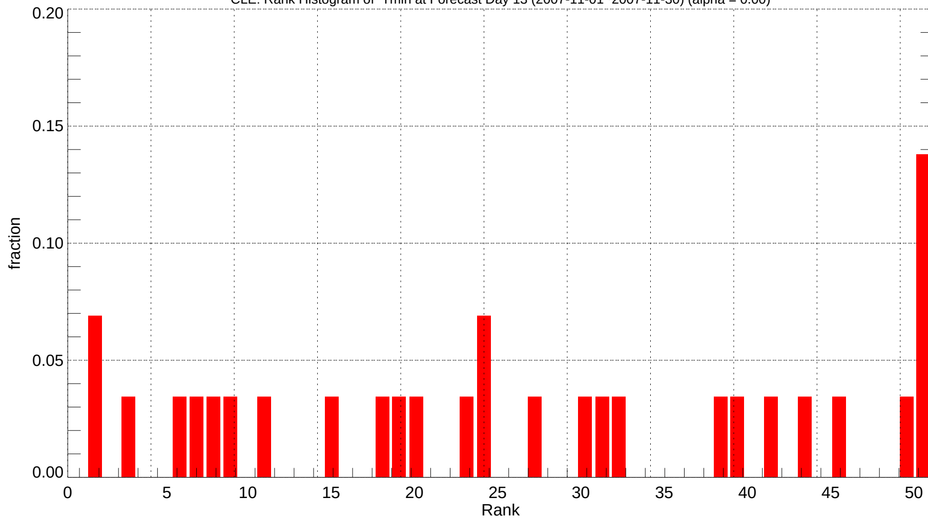
CLE: Rank Histogram of Tmin at Forecast Day 13 (2007-11-01~2007-11-30) (alpha = 0.00)
