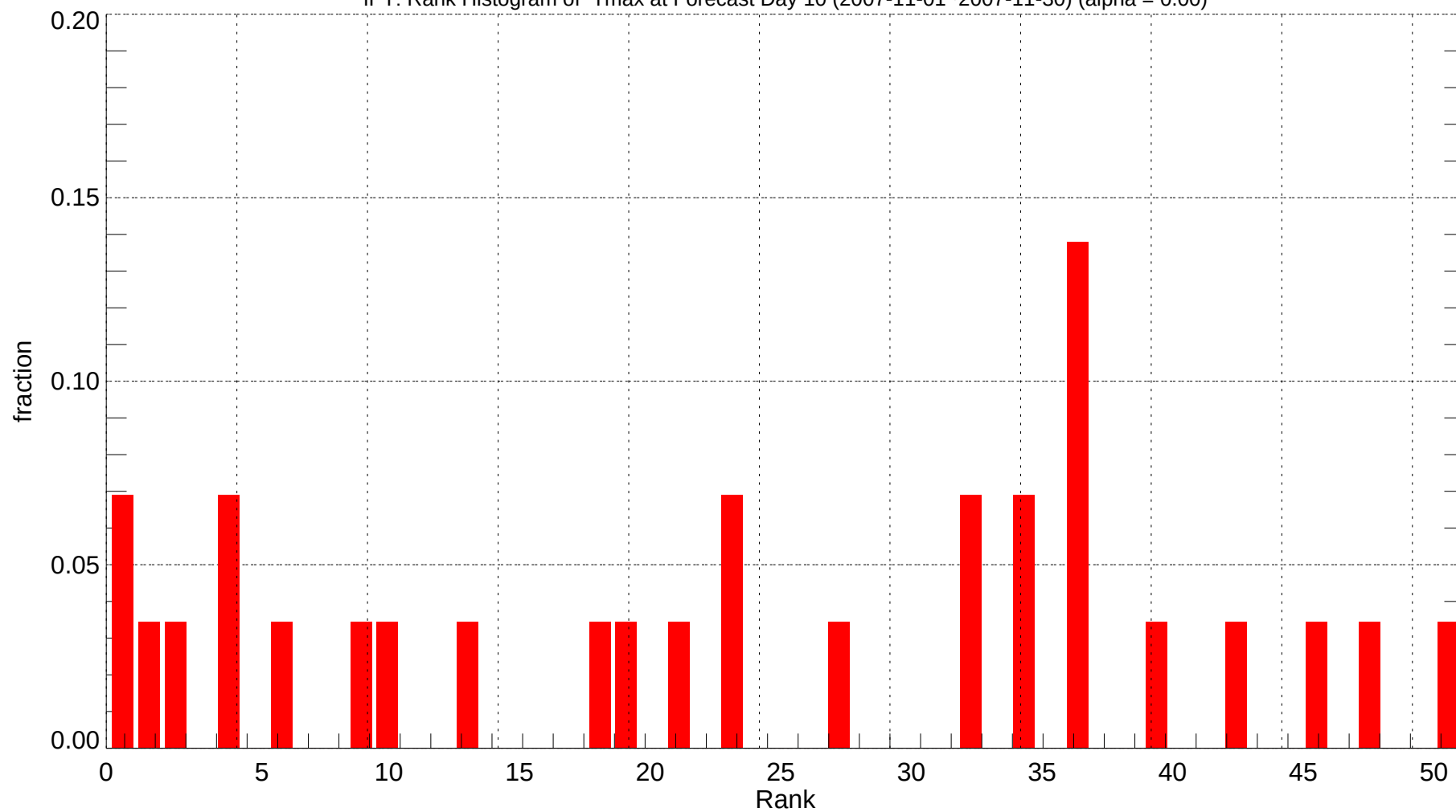
IPT: Rank Histogram of Tmax at Forecast Day 10 (2007-11-01~2007-11-30) (alpha = 0.00)
