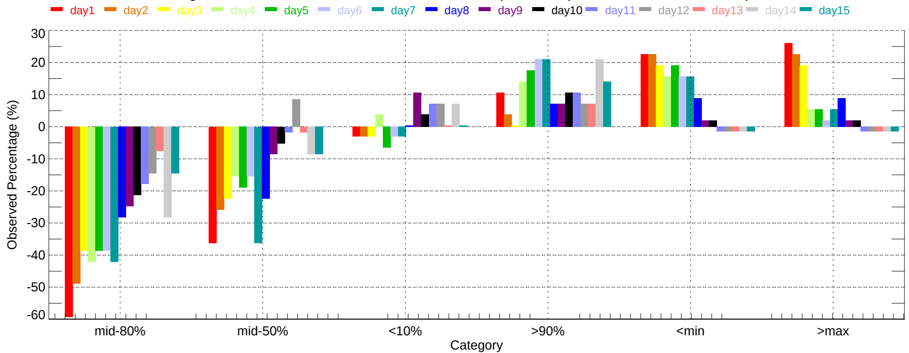
Observed Percentage Deviation of Ensembles - GTF: Min Temperature (2007-11-01~2007-11-30)
