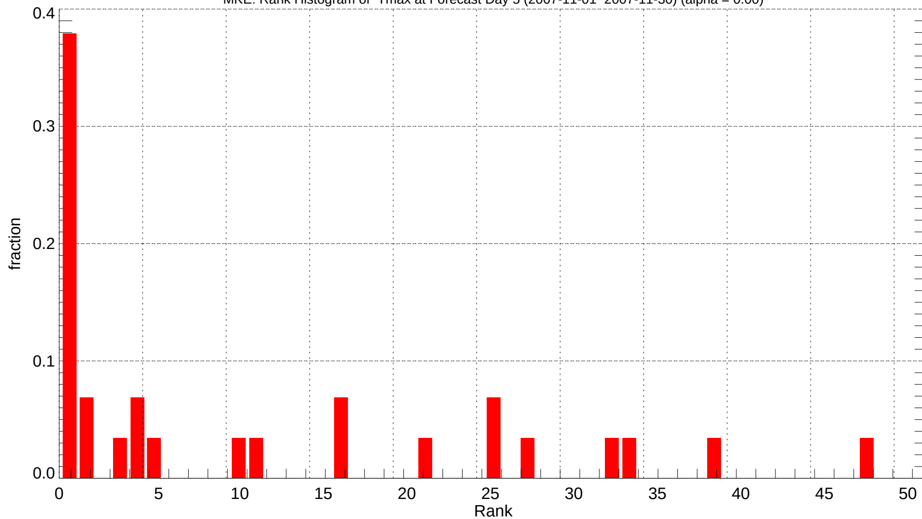
MKE: Rank Histogram of Tmax at Forecast Day 5 (2007-11-01~2007-11-30) (alpha = 0.00)
