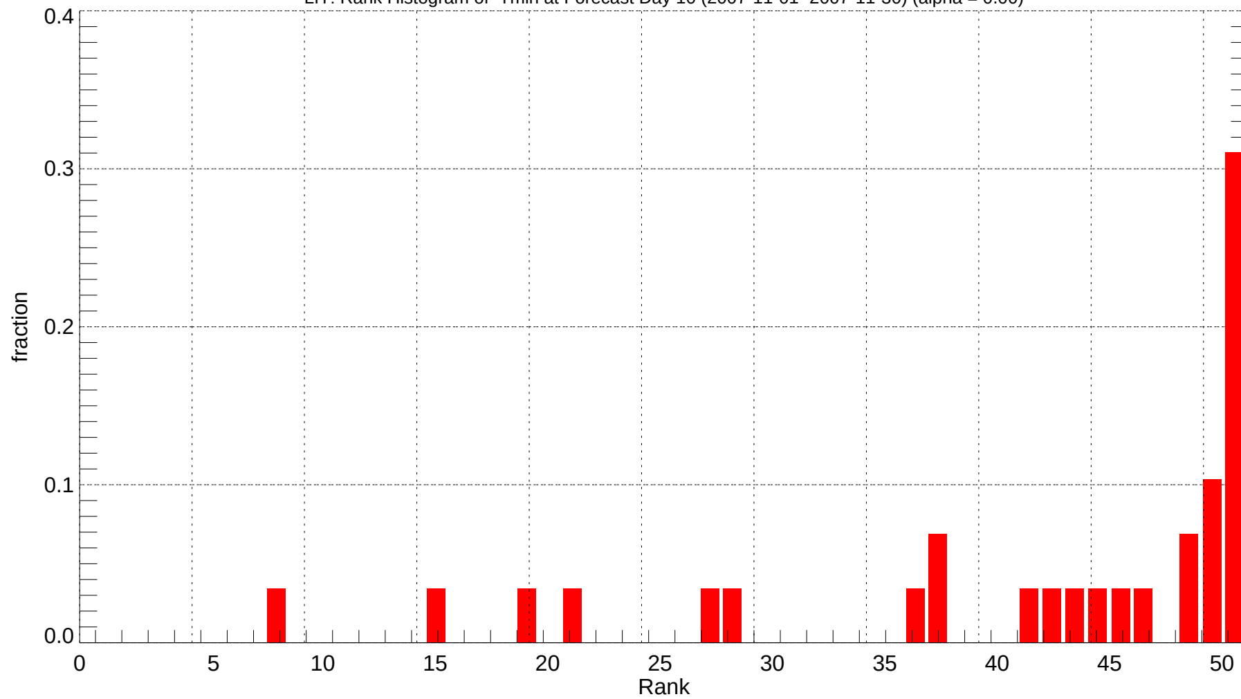
LIT: Rank Histogram of Tmin at Forecast Day 10 (2007-11-01~2007-11-30) (alpha = 0.00)
