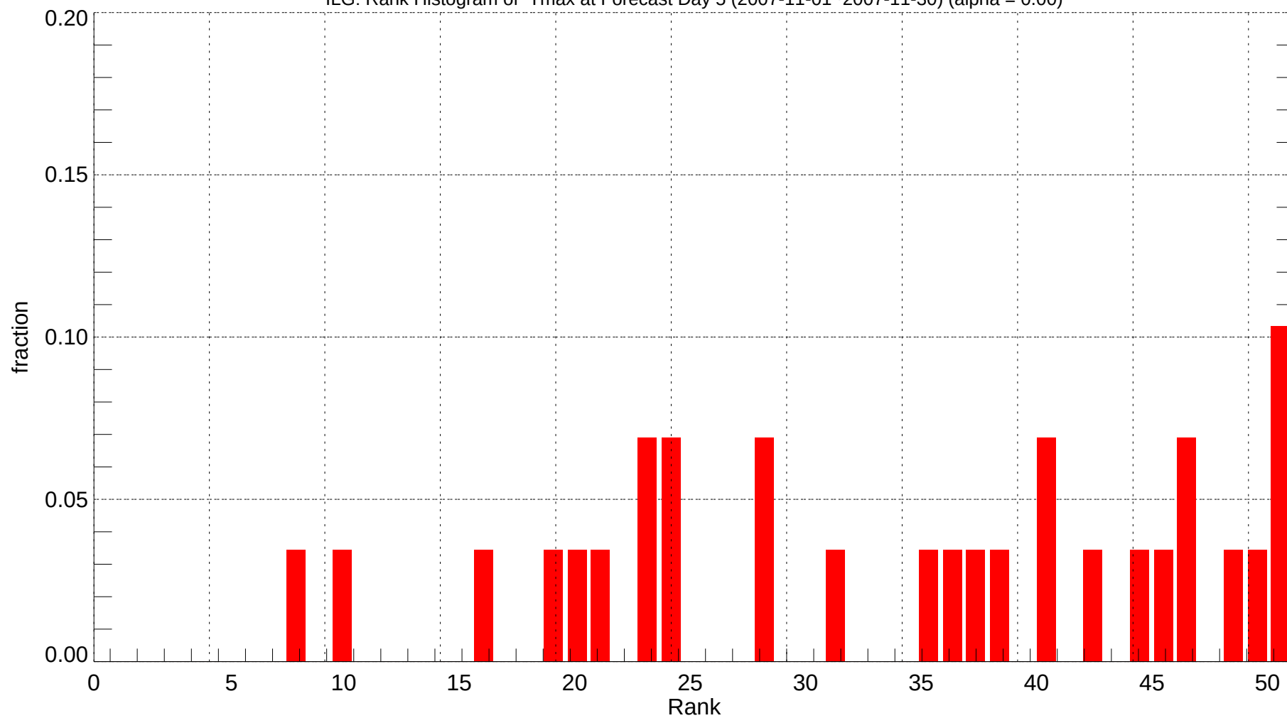
ILG: Rank Histogram of Tmax at Forecast Day 5 (2007-11-01~2007-11-30) (alpha = 0.00)
