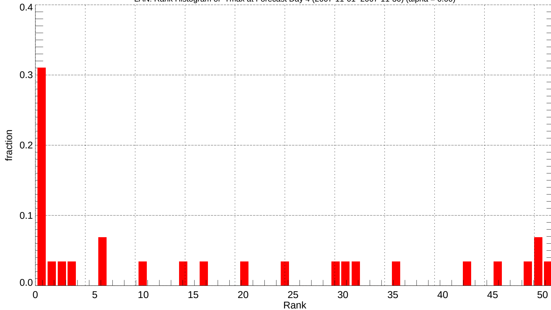
LAN: Rank Histogram of Tmax at Forecast Day 4 (2007-11-01~2007-11-30) (alpha = 0.00)
