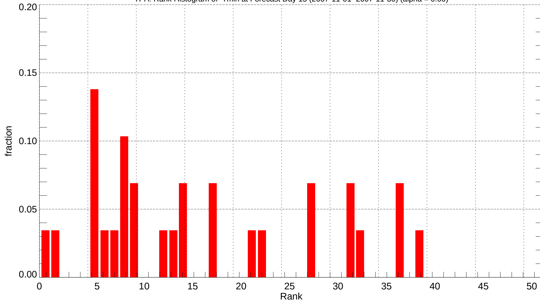
TPA: Rank Histogram of Tmin at Forecast Day 15 (2007-11-01~2007-11-30) (alpha = 0.00)
