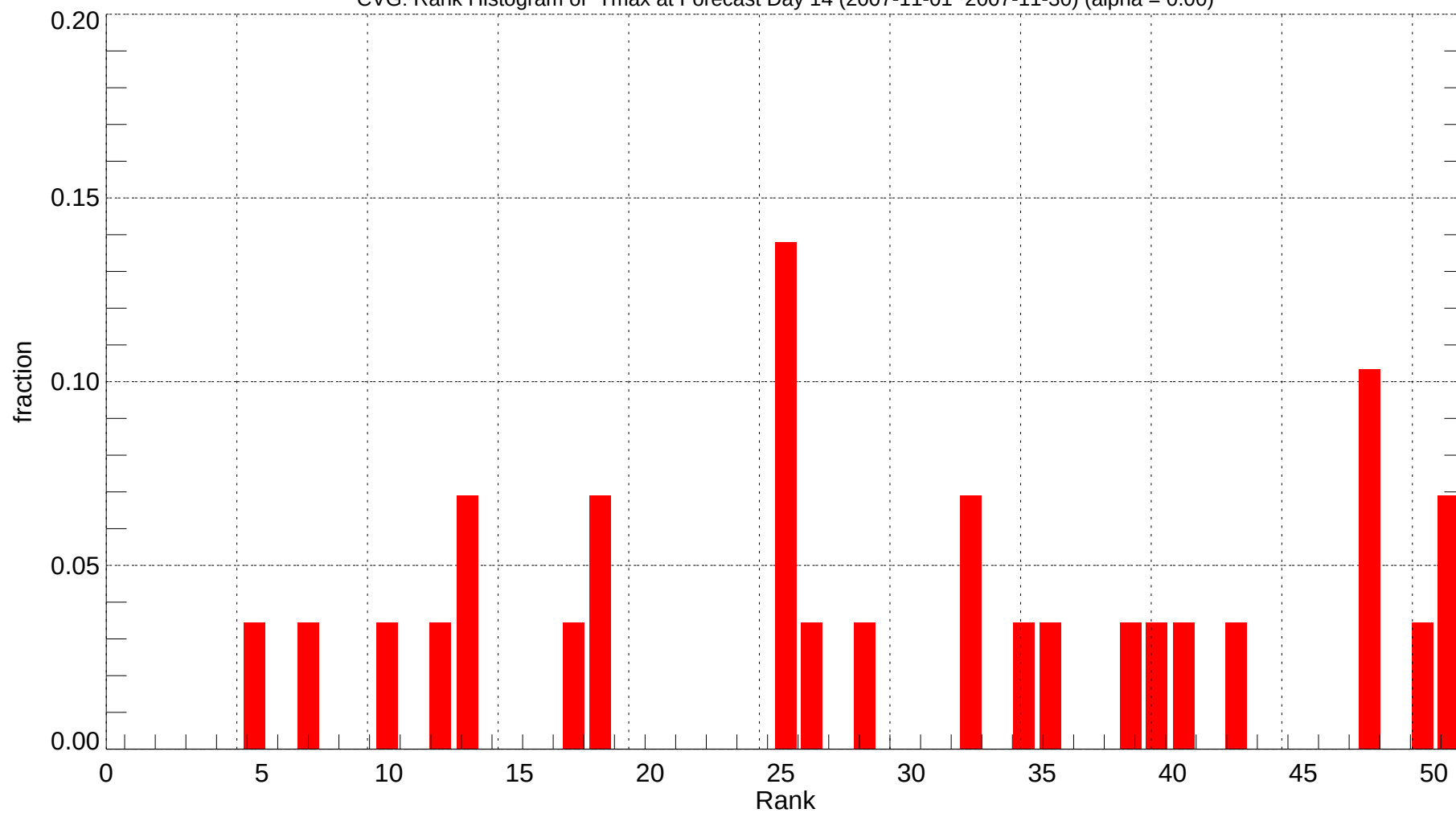
CVG: Rank Histogram of Tmax at Forecast Day 14 (2007-11-01~2007-11-30) (alpha = 0.00)
