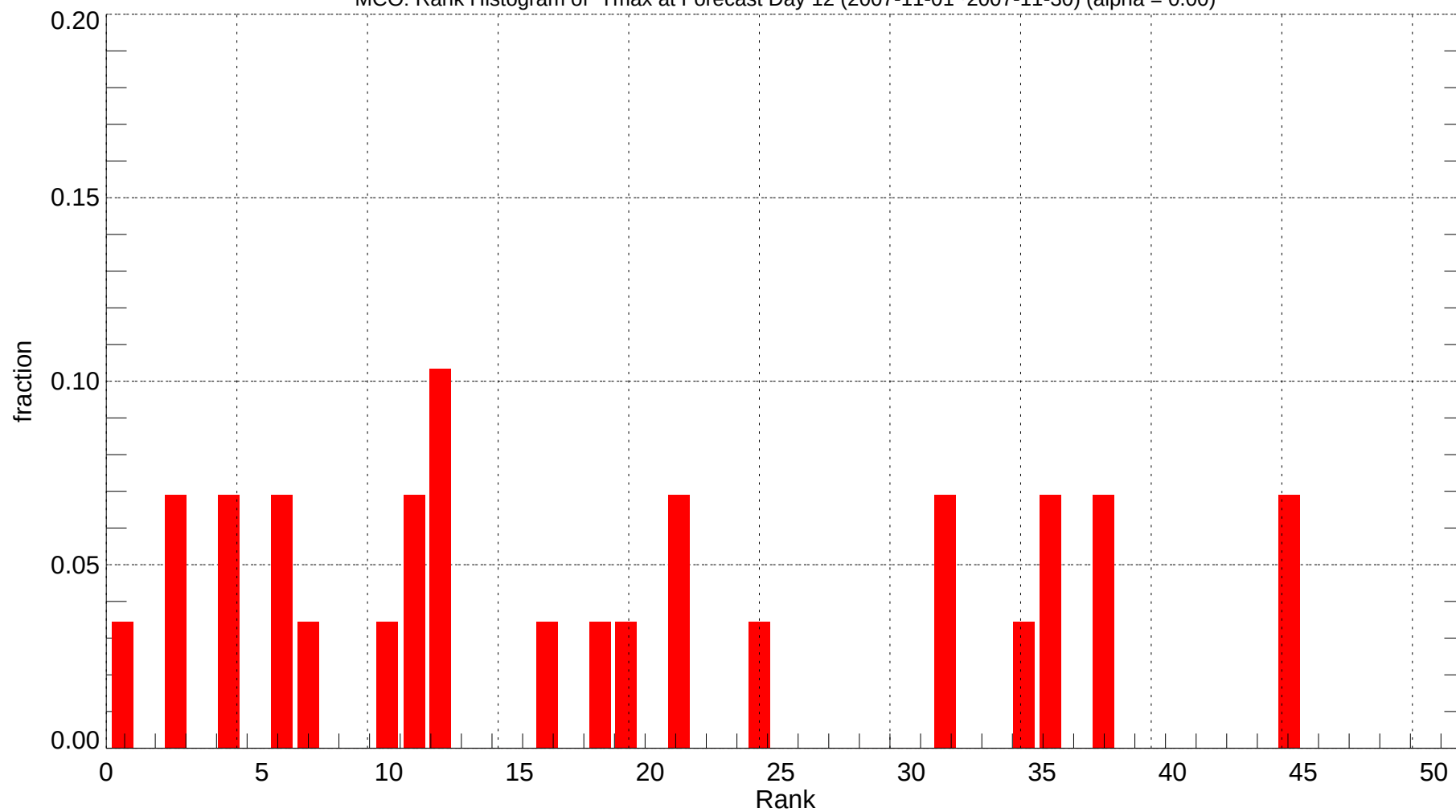
MCO: Rank Histogram of Tmax at Forecast Day 12 (2007-11-01~2007-11-30) (alpha = 0.00)
