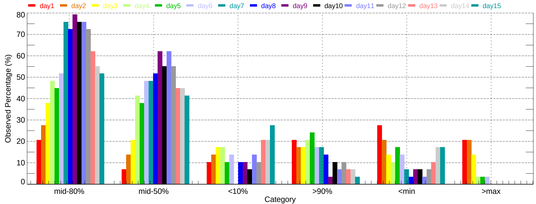
Observed Percentage of Ensembles - CON: Min Temperature (2007-11-01~2007-11-30)
