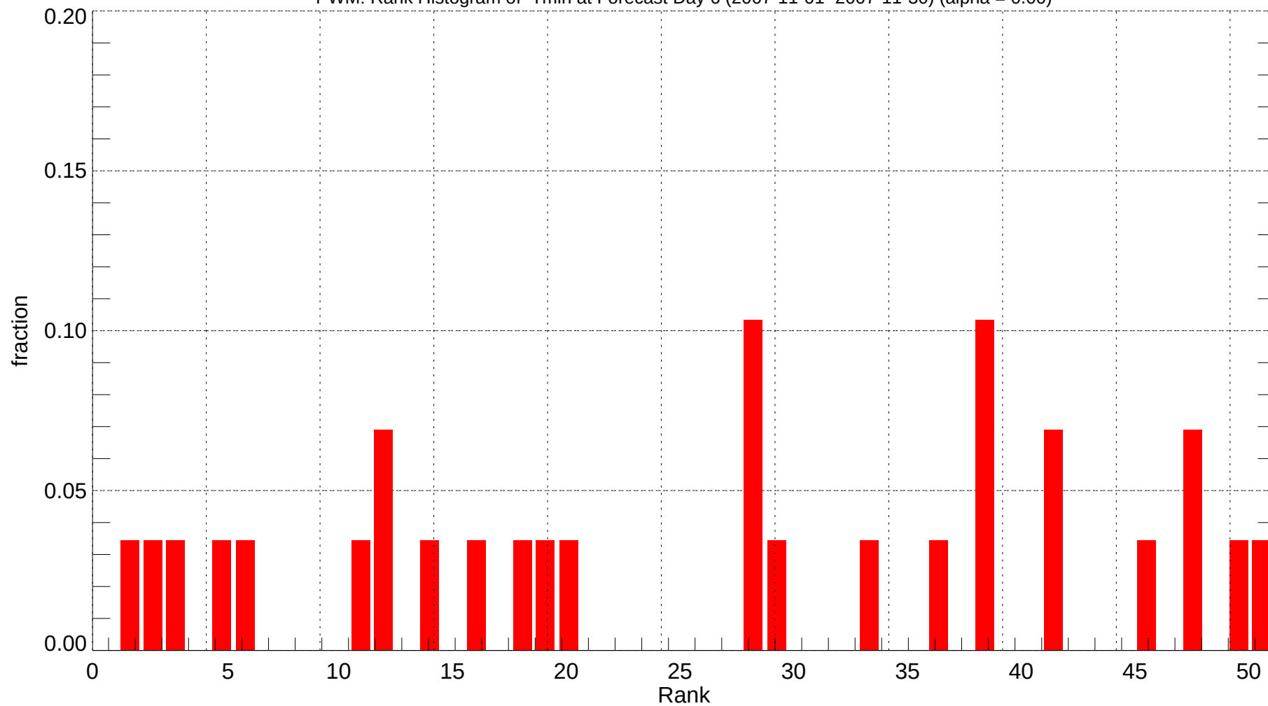
PWM: Rank Histogram of Tmin at Forecast Day 6 (2007-11-01~2007-11-30) (alpha = 0.00)
