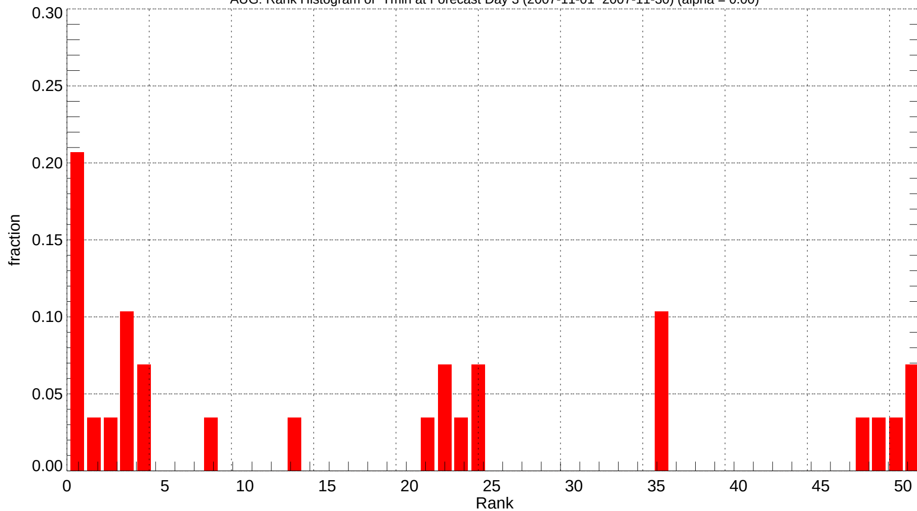
AUG: Rank Histogram of Tmin at Forecast Day 3 (2007-11-01~2007-11-30) (alpha = 0.00)
