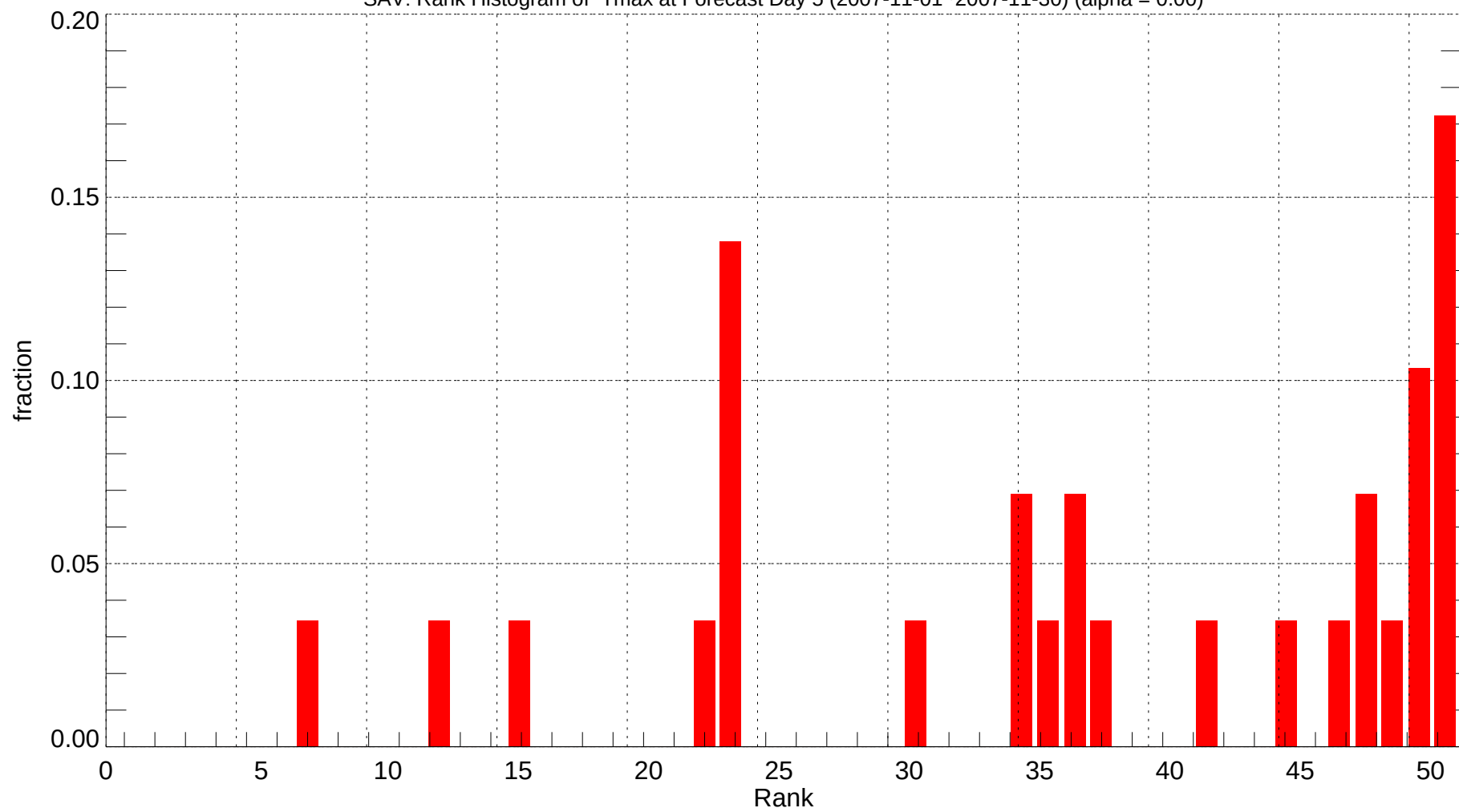
SAV: Rank Histogram of Tmax at Forecast Day 5 (2007-11-01~2007-11-30) (alpha = 0.00)
