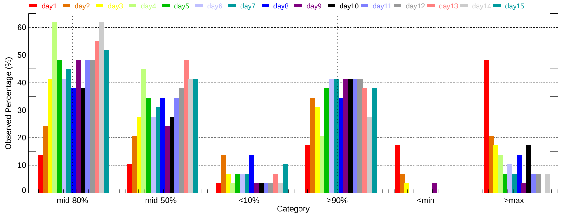
Observed Percentage of Ensembles - RAP: Min Temperature (2007-11-01~2007-11-30)
