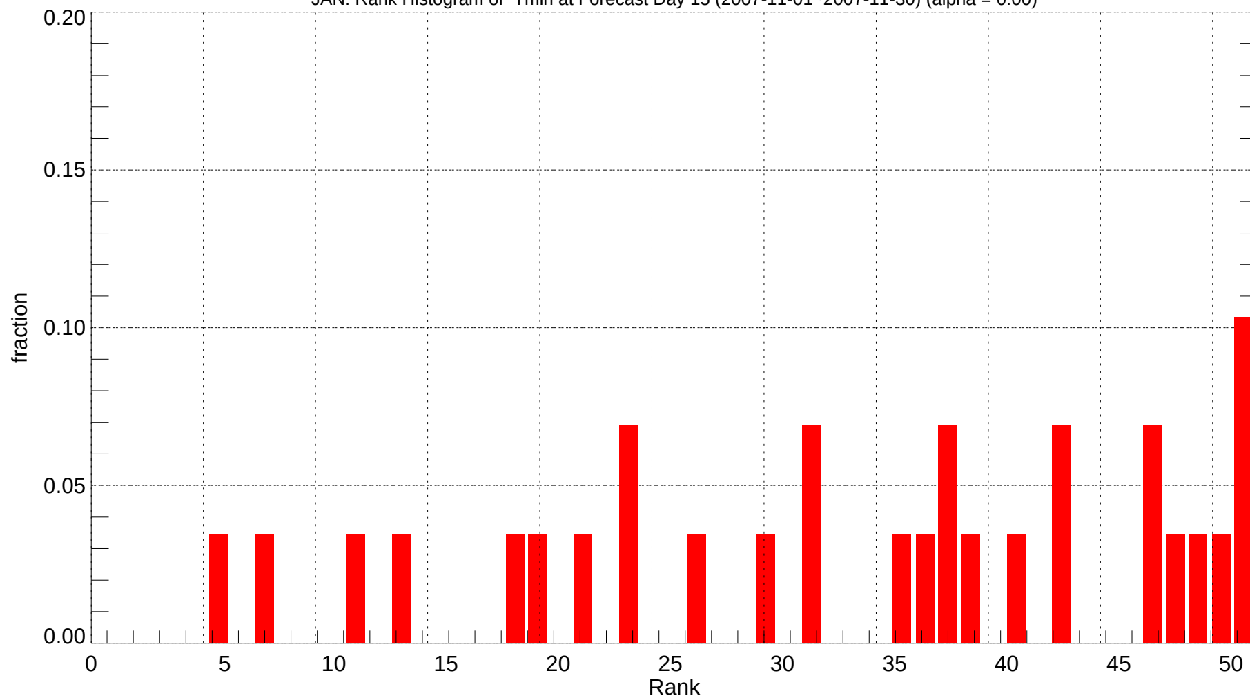
JAN: Rank Histogram of Tmin at Forecast Day 15 (2007-11-01~2007-11-30) (alpha = 0.00)
