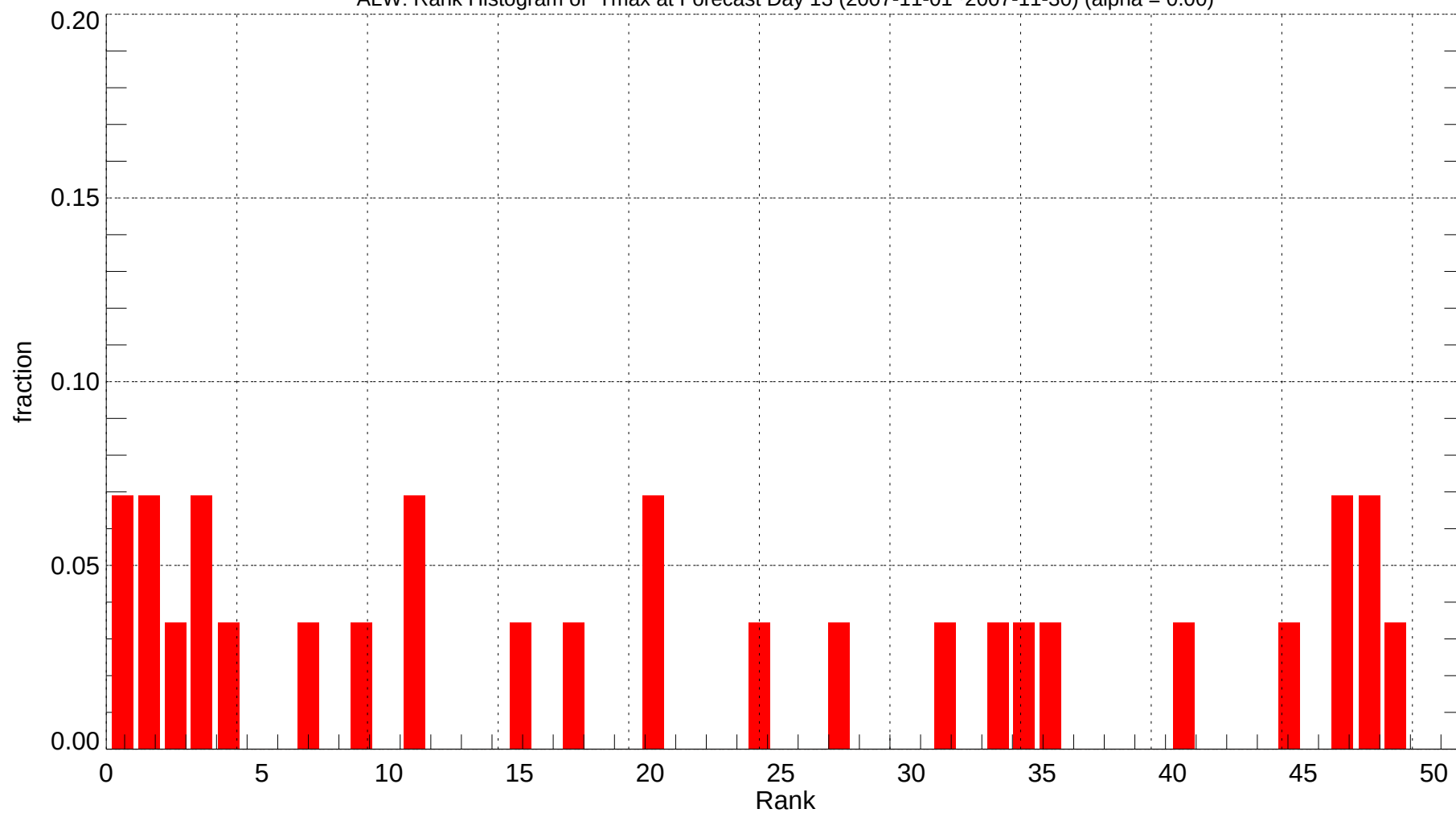
ALW: Rank Histogram of Tmax at Forecast Day 13 (2007-11-01~2007-11-30) (alpha = 0.00)
