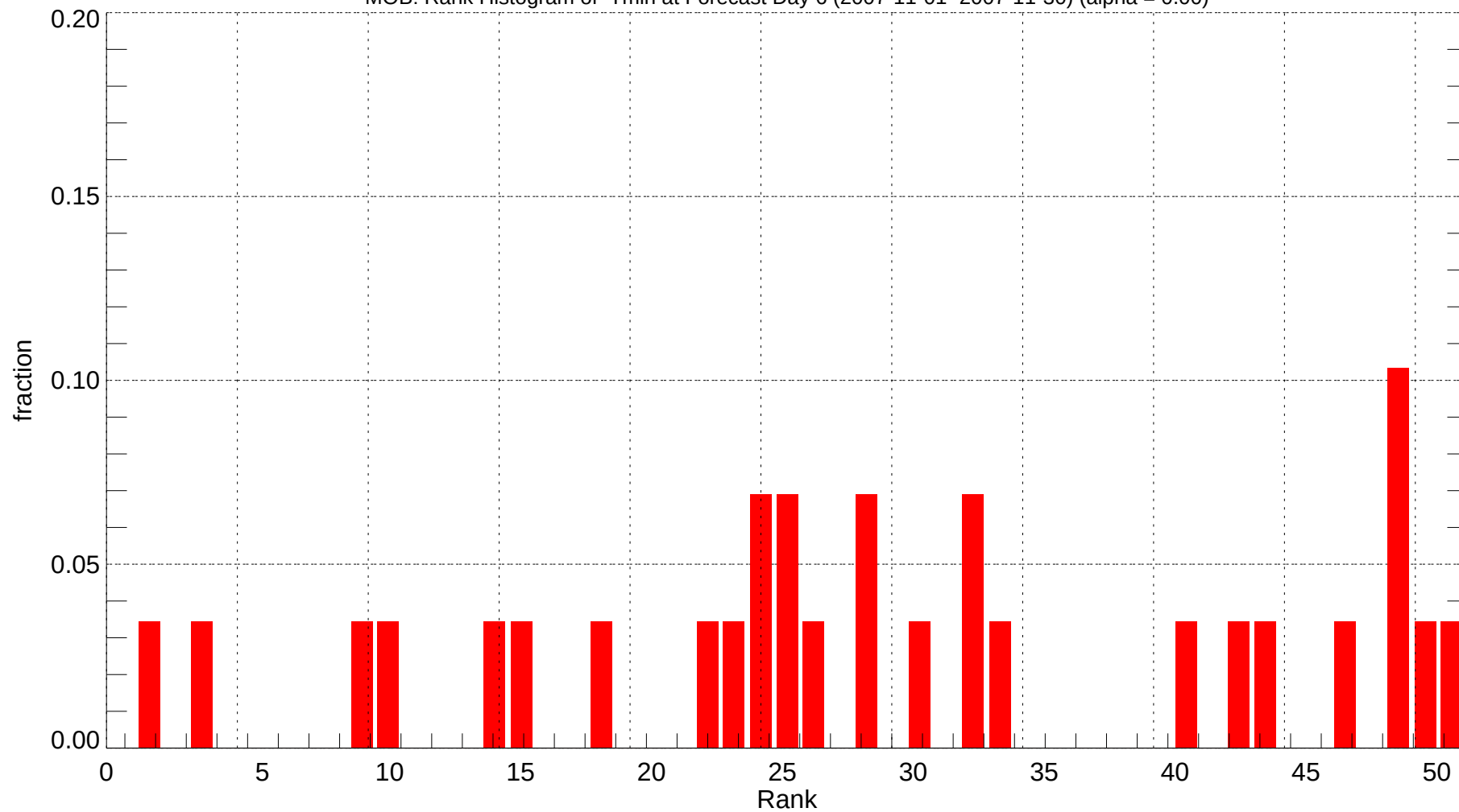
MOB: Rank Histogram of Tmin at Forecast Day 6 (2007-11-01~2007-11-30) (alpha = 0.00)
