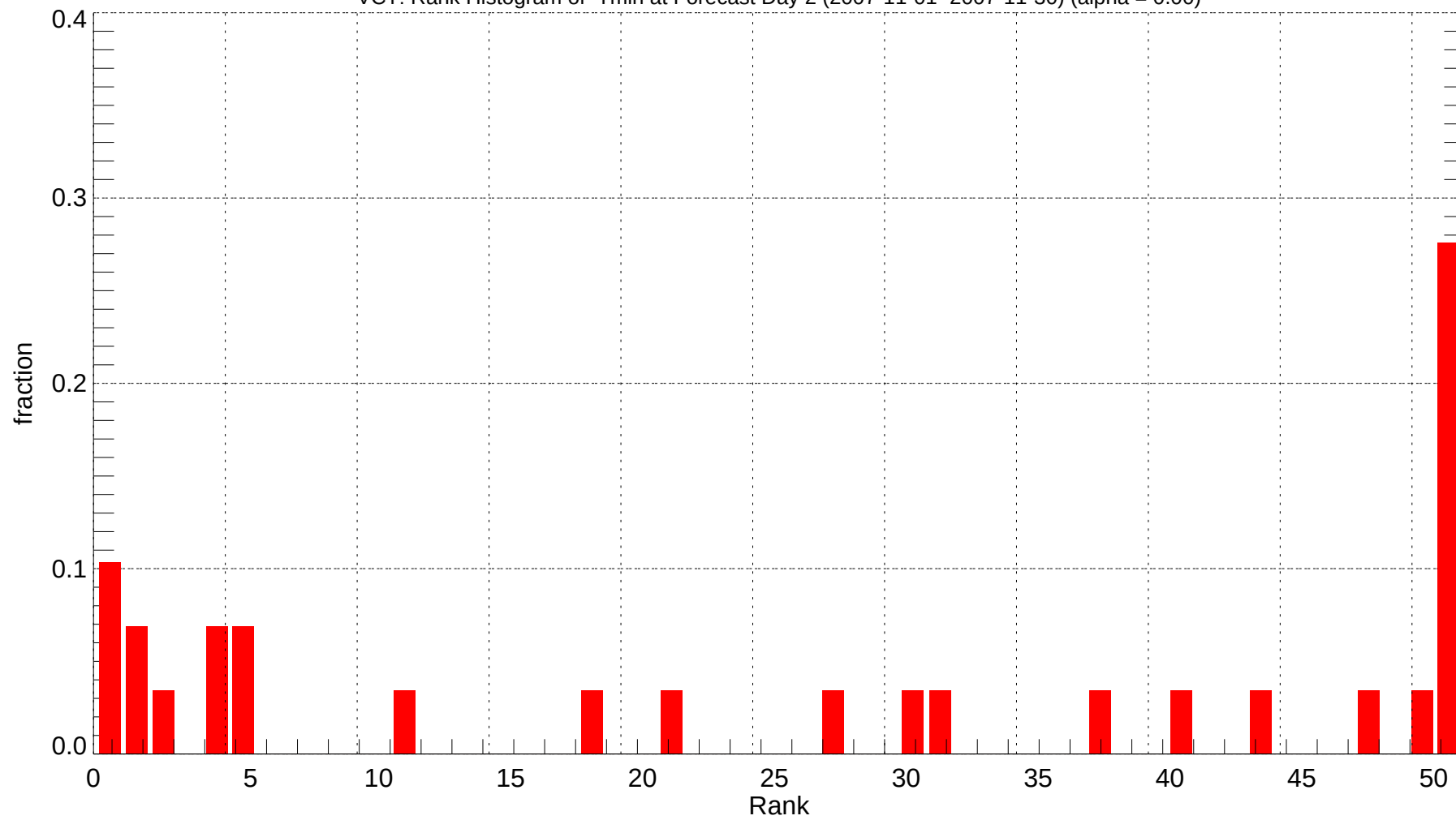
VCT: Rank Histogram of Tmin at Forecast Day 2 (2007-11-01~2007-11-30) (alpha = 0.00)
