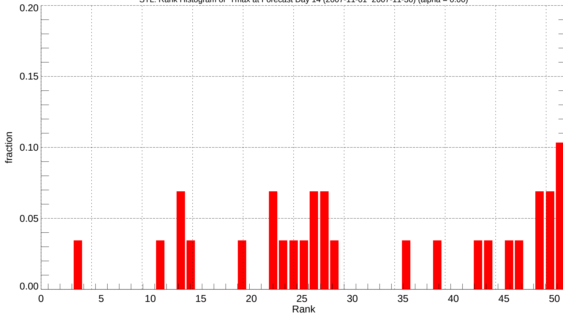
STL: Rank Histogram of Tmax at Forecast Day 14 (2007-11-01~2007-11-30) (alpha = 0.00)
