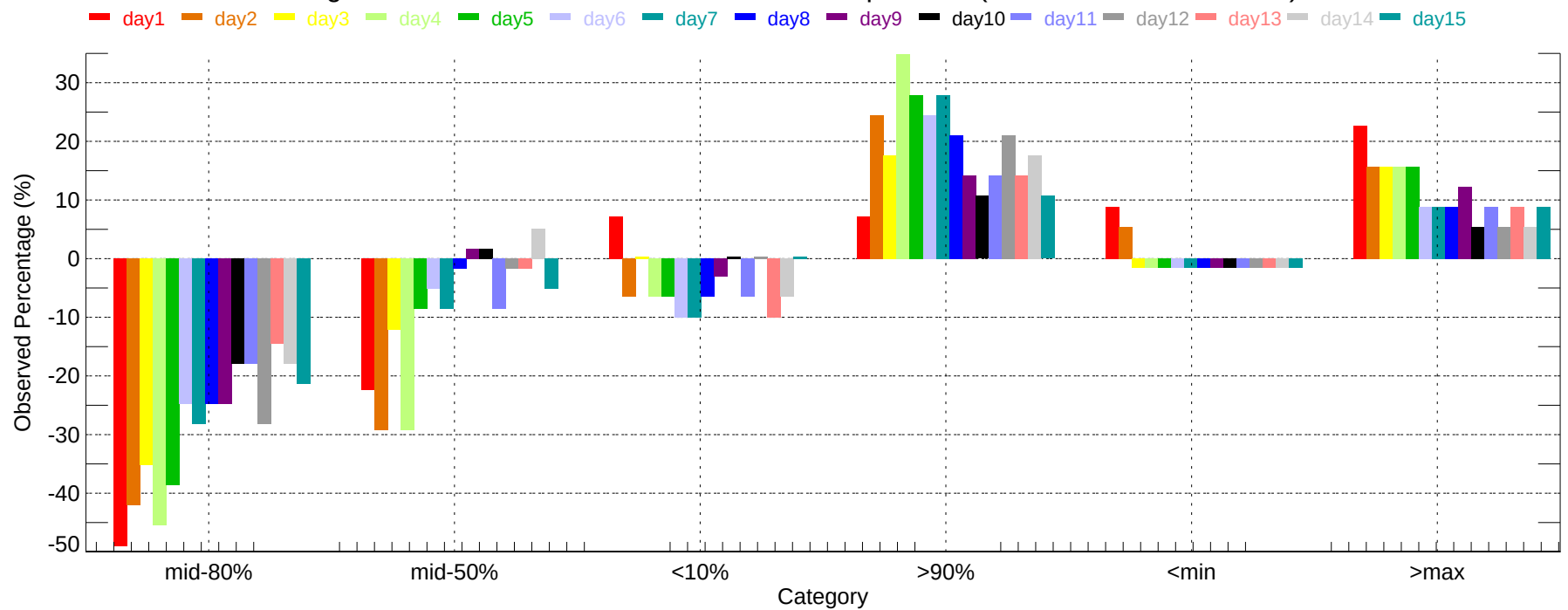
Observed Percentage Deviation of Ensembles - DCA: Min Temperature (2007-11-01~2007-11-30)
