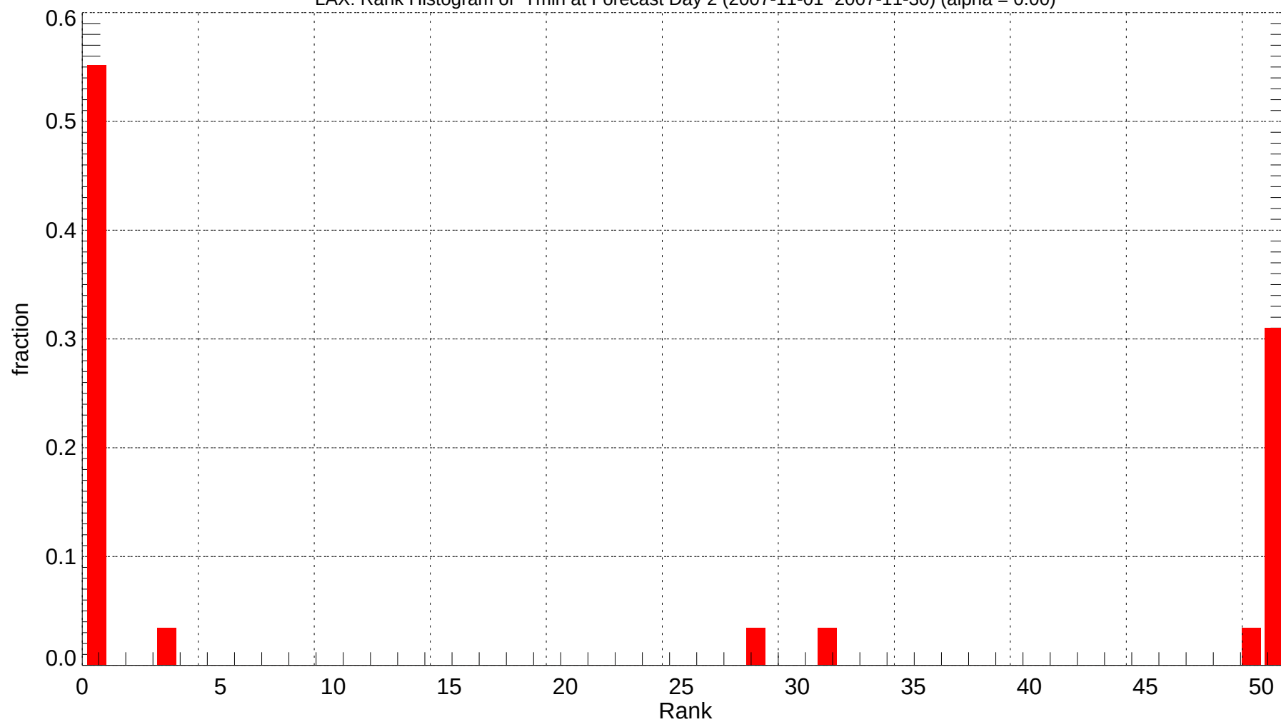
LAX: Rank Histogram of Tmin at Forecast Day 2 (2007-11-01~2007-11-30) (alpha = 0.00)
