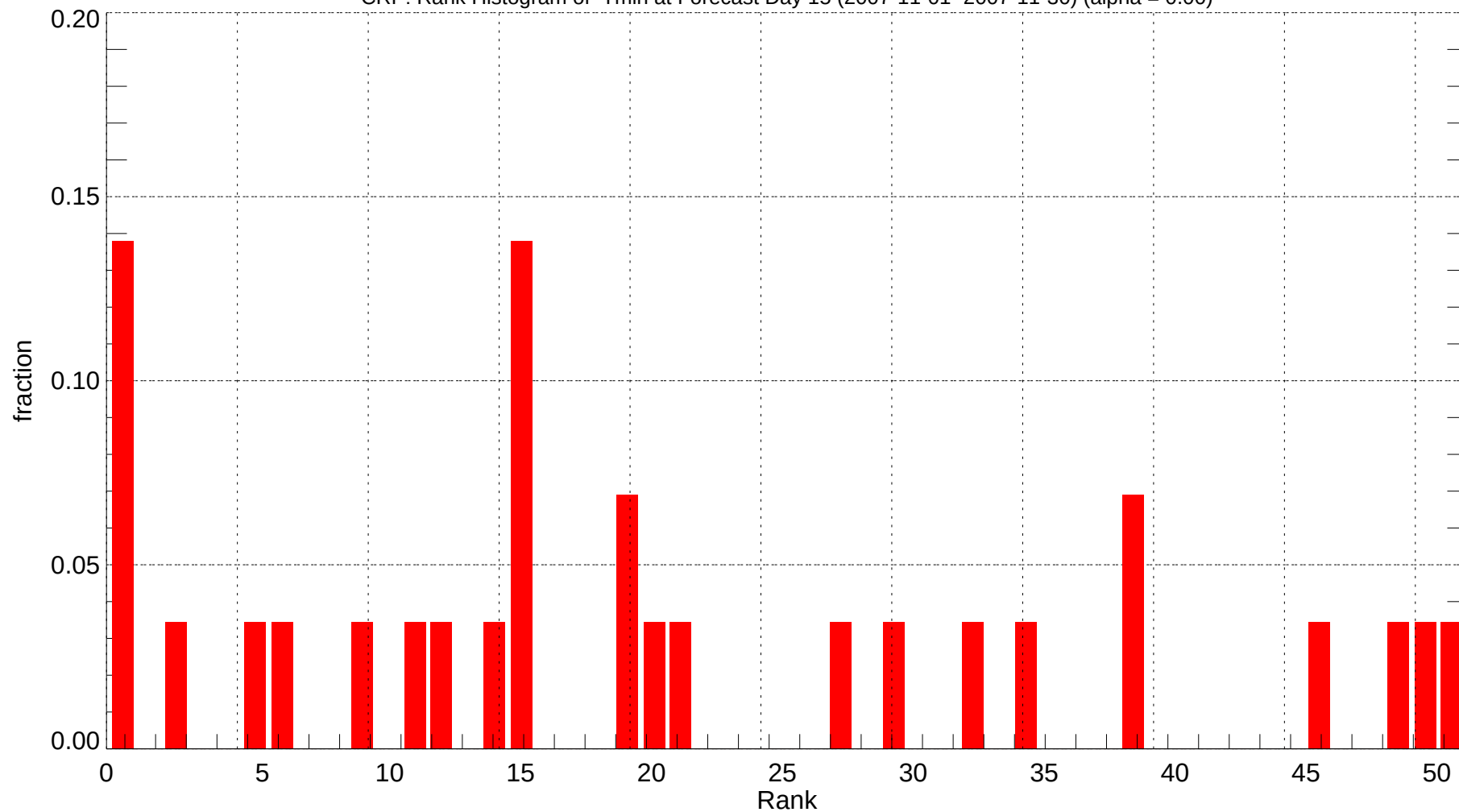
CRP: Rank Histogram of Tmin at Forecast Day 15 (2007-11-01~2007-11-30) (alpha = 0.00)
