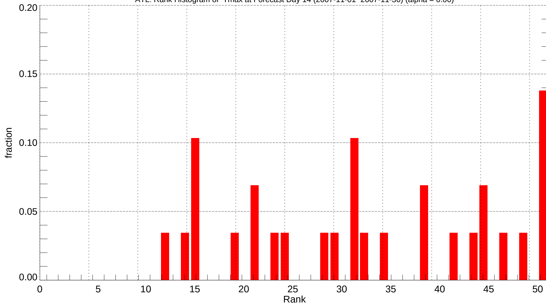
ATL: Rank Histogram of Tmax at Forecast Day 14 (2007-11-01~2007-11-30) (alpha = 0.00)
