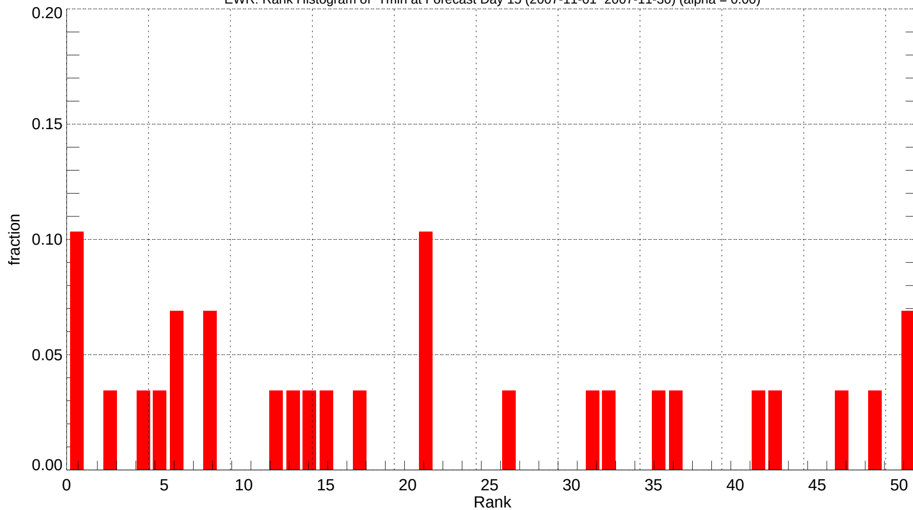
EWR: Rank Histogram of Tmin at Forecast Day 15 (2007-11-01~2007-11-30) (alpha = 0.00)
