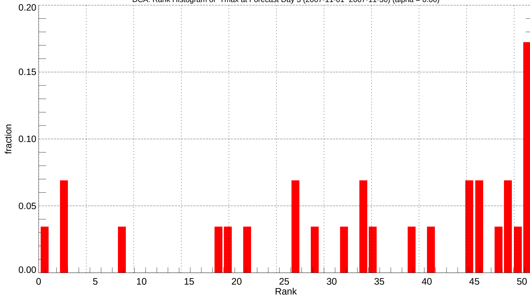
DCA: Rank Histogram of Tmax at Forecast Day 3 (2007-11-01~2007-11-30) (alpha = 0.00)
