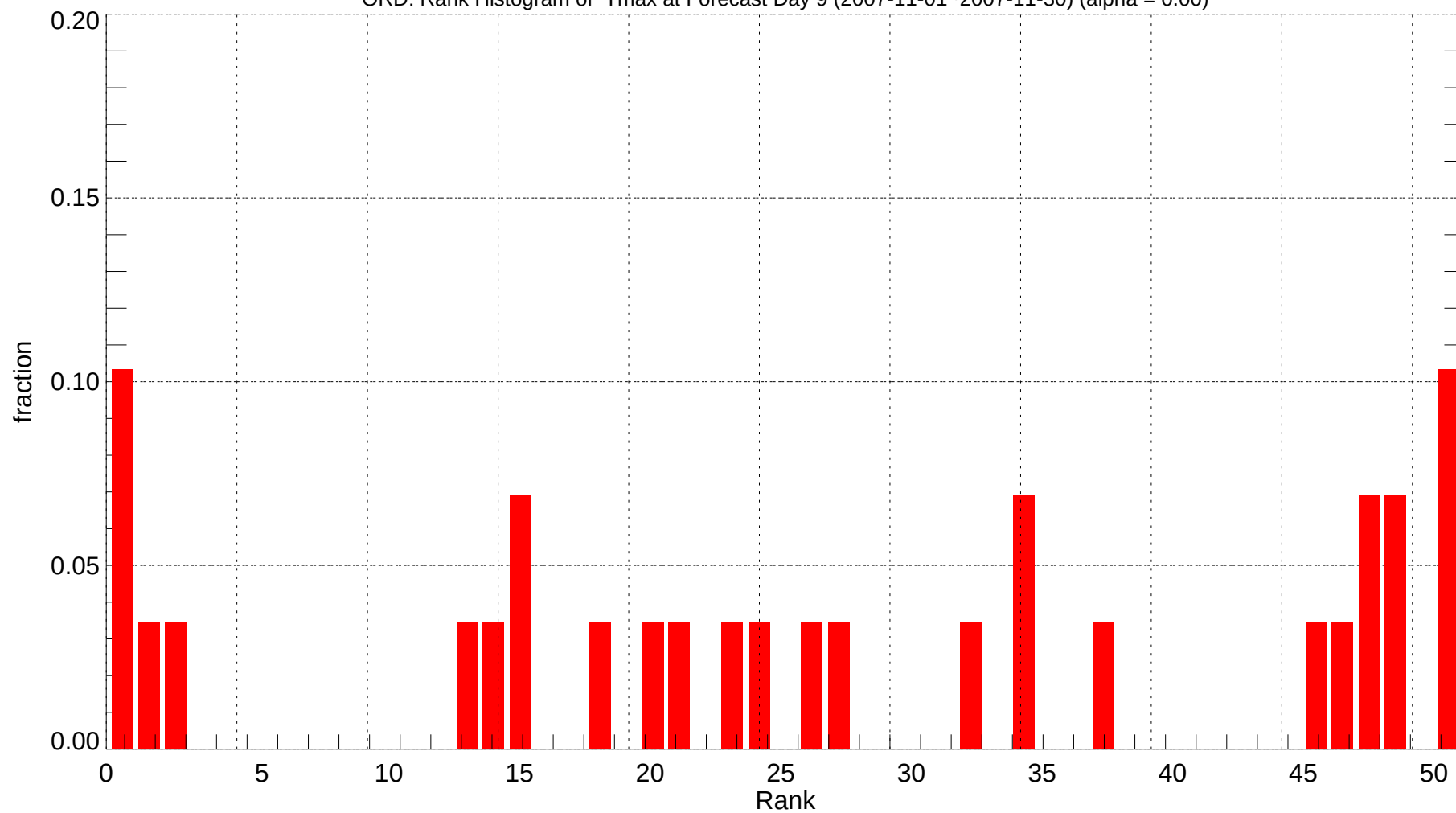
ORD: Rank Histogram of Tmax at Forecast Day 9 (2007-11-01~2007-11-30) (alpha = 0.00)
