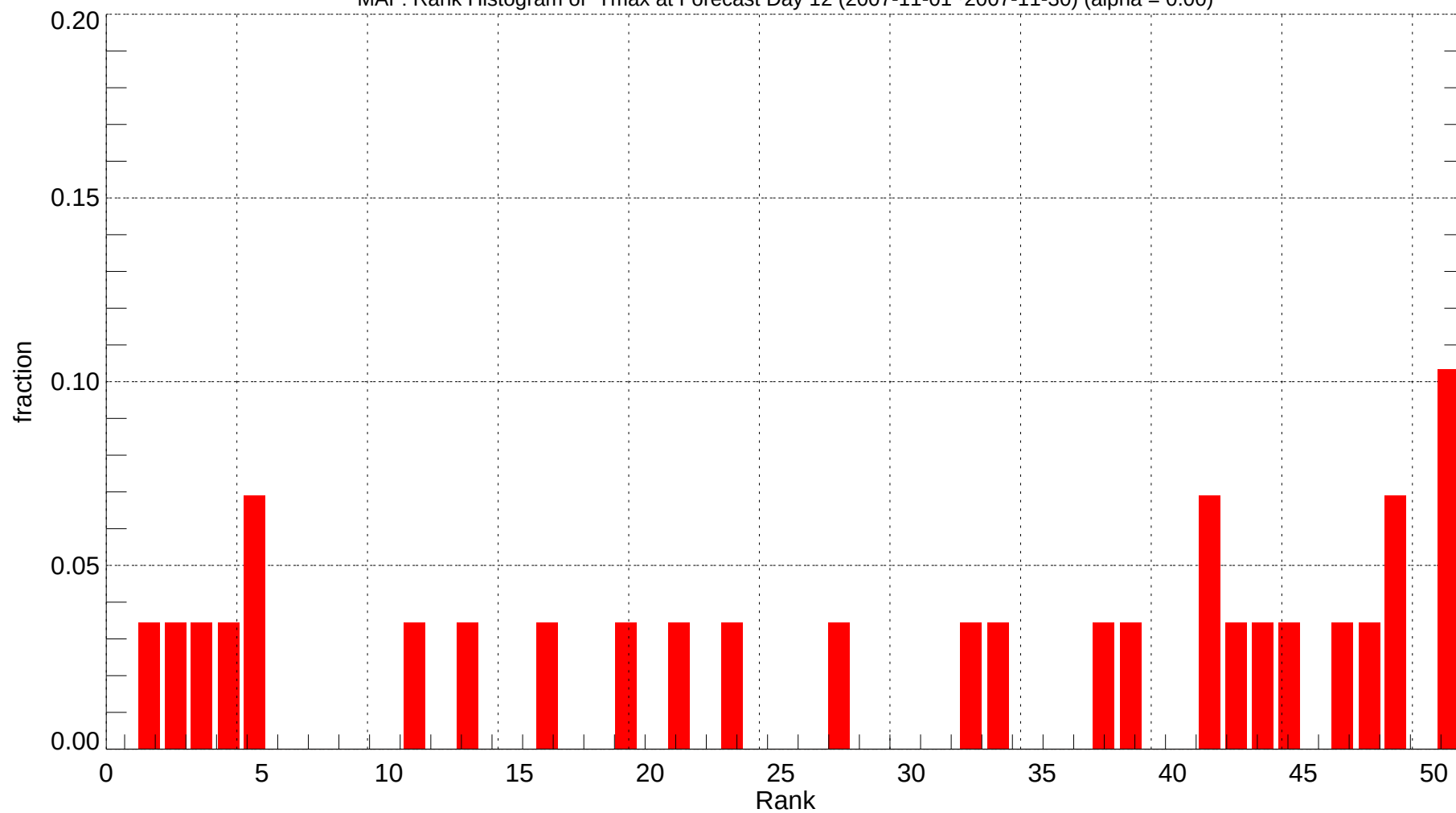
MAF: Rank Histogram of Tmax at Forecast Day 12 (2007-11-01~2007-11-30) (alpha = 0.00)
