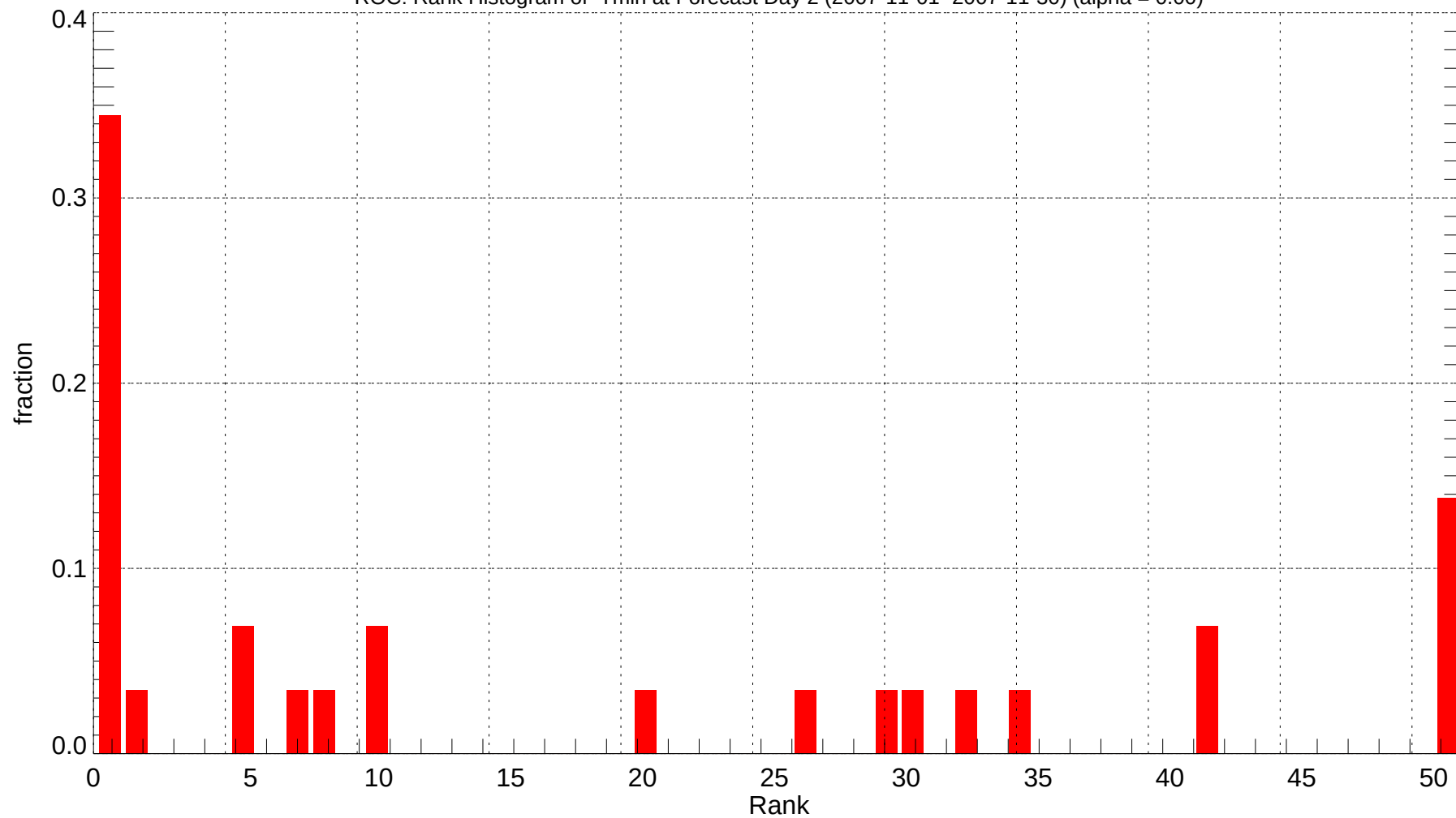
ROC: Rank Histogram of Tmin at Forecast Day 2 (2007-11-01~2007-11-30) (alpha = 0.00)
