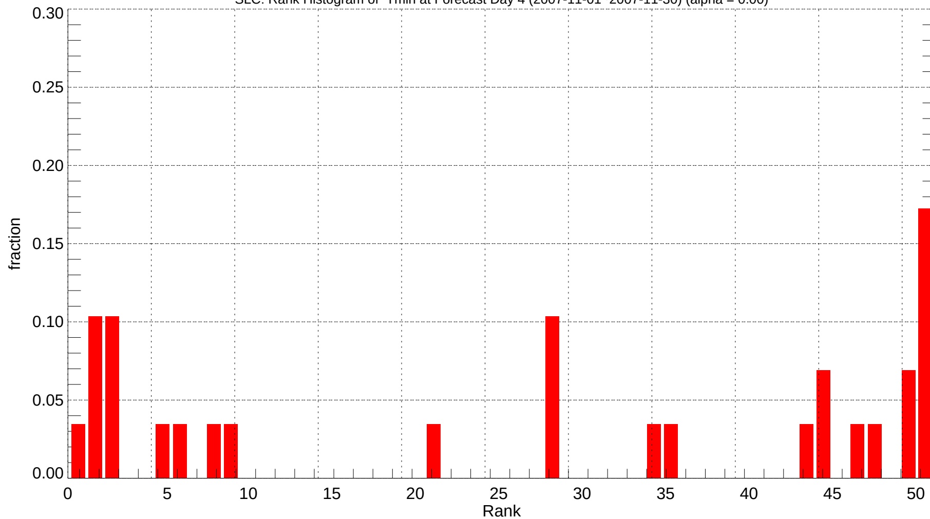
SLC: Rank Histogram of Tmin at Forecast Day 4 (2007-11-01~2007-11-30) (alpha = 0.00)
