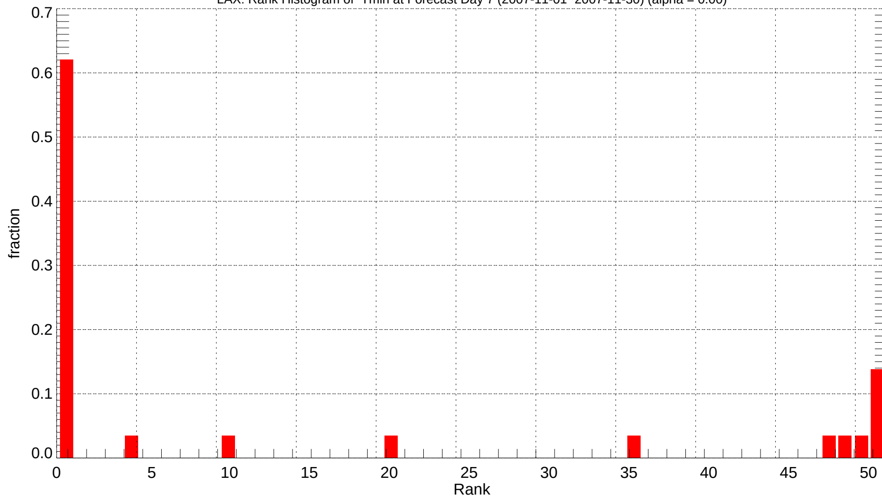
LAX: Rank Histogram of Tmin at Forecast Day 7 (2007-11-01~2007-11-30) (alpha = 0.00)
