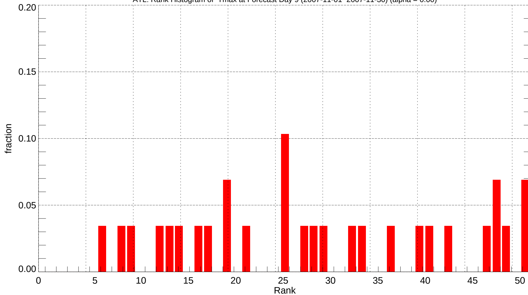
ATL: Rank Histogram of Tmax at Forecast Day 9 (2007-11-01~2007-11-30) (alpha = 0.00)
