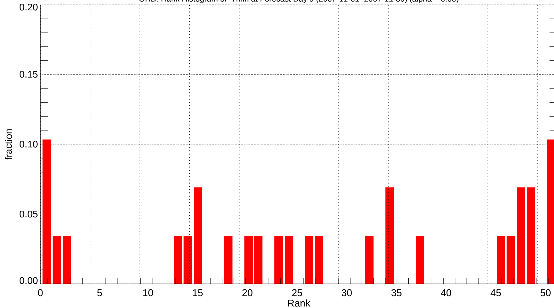
ORD: Rank Histogram of Tmin at Forecast Day 9 (2007-11-01~2007-11-30) (alpha = 0.00)
