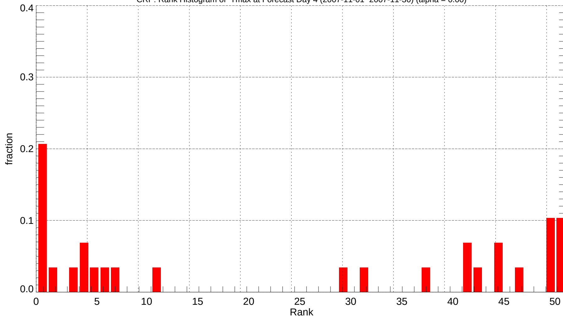
CRP: Rank Histogram of Tmax at Forecast Day 4 (2007-11-01~2007-11-30) (alpha = 0.00)
