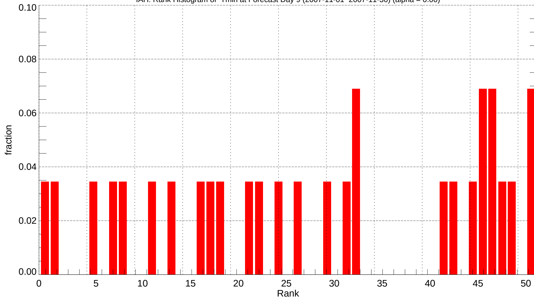
IAH: Rank Histogram of Tmin at Forecast Day 9 (2007-11-01~2007-11-30) (alpha = 0.00)
