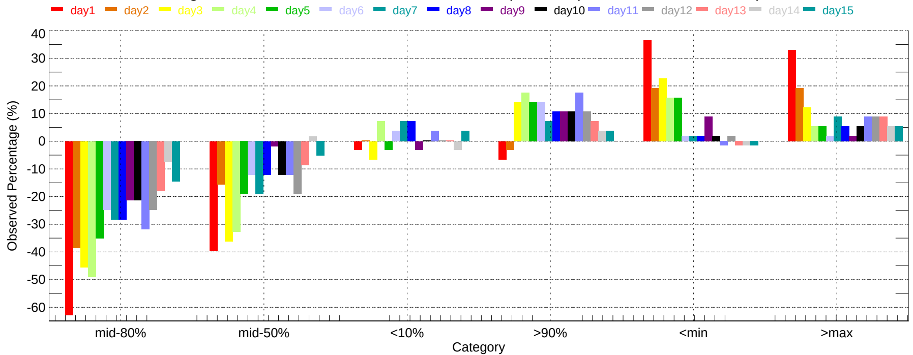
Observed Percentage Deviation of Ensembles - YNG: Max Temperature (2007-11-01~2007-11-30)
