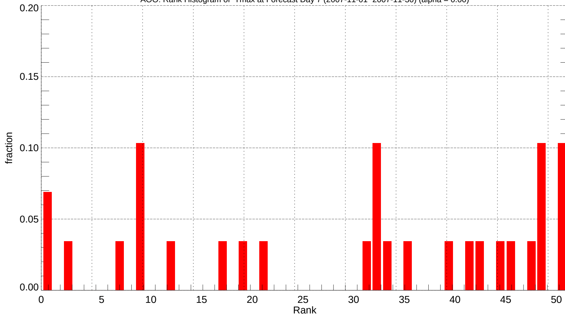
AOO: Rank Histogram of Tmax at Forecast Day 7 (2007-11-01~2007-11-30) (alpha = 0.00)
