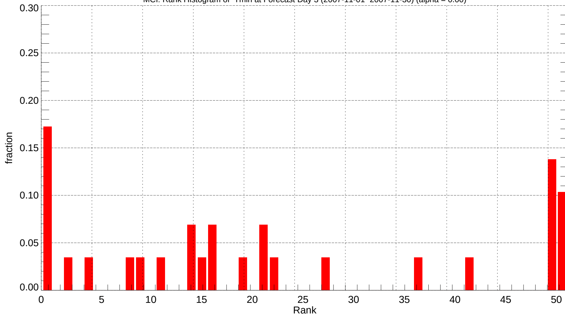
MCI: Rank Histogram of Tmin at Forecast Day 3 (2007-11-01~2007-11-30) (alpha = 0.00)
