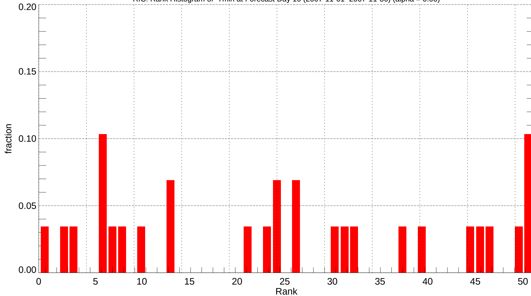
RIC: Rank Histogram of Tmin at Forecast Day 10 (2007-11-01~2007-11-30) (alpha = 0.00)
