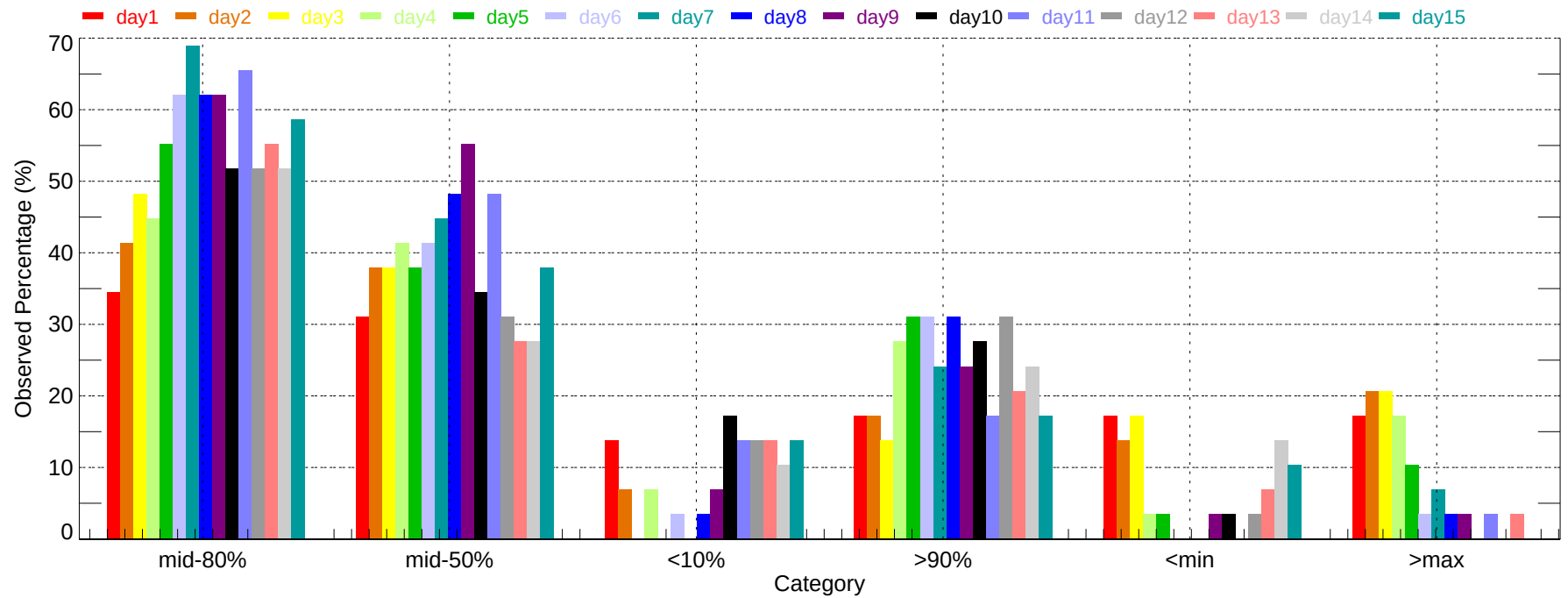
Observed Percentage of Ensembles - MBA: Min Temperature (2007-11-01~2007-11-30)
