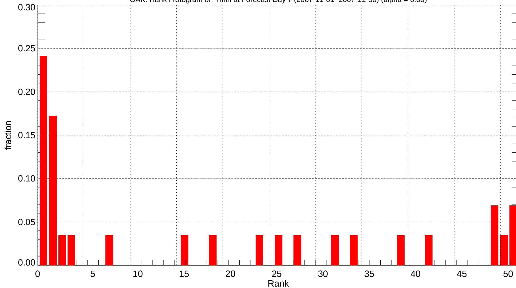
OAK: Rank Histogram of Tmin at Forecast Day 7 (2007-11-01~2007-11-30) (alpha = 0.00)
