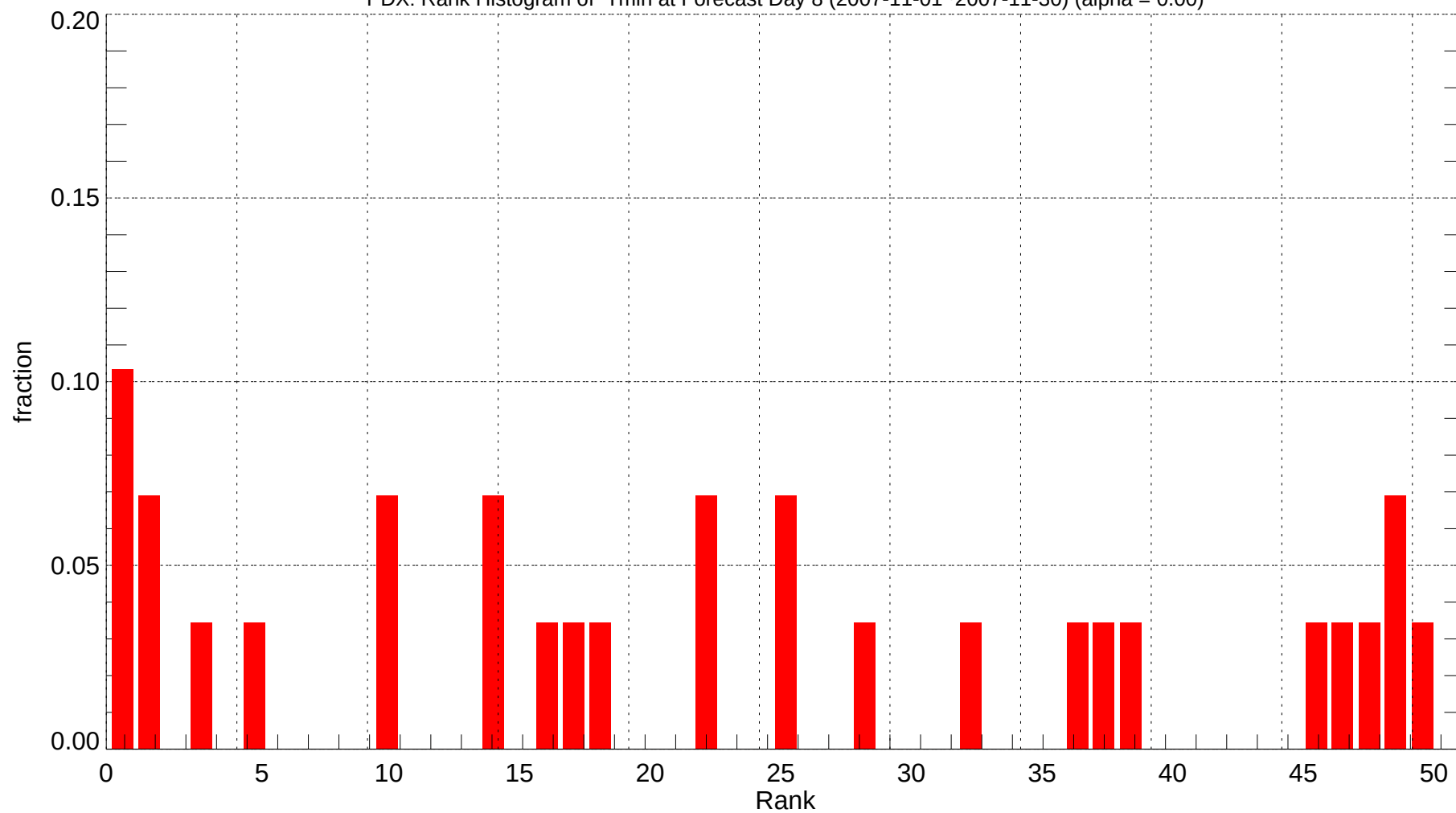
PDX: Rank Histogram of Tmin at Forecast Day 8 (2007-11-01~2007-11-30) (alpha = 0.00)
