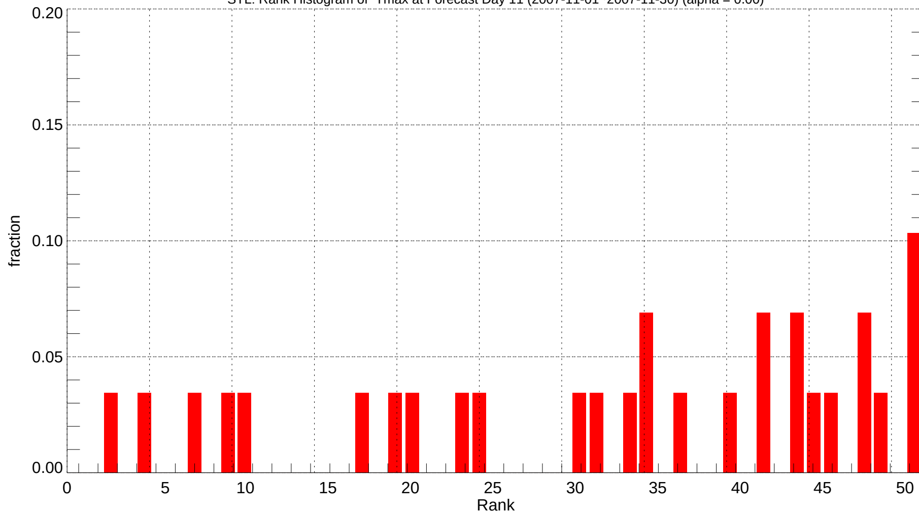
STL: Rank Histogram of Tmax at Forecast Day 11 (2007-11-01~2007-11-30) (alpha = 0.00)
