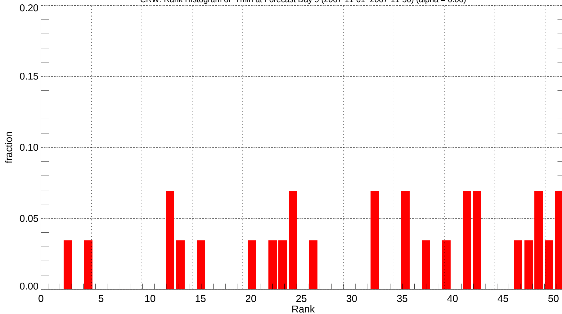
CRW: Rank Histogram of Tmin at Forecast Day 9 (2007-11-01~2007-11-30) (alpha = 0.00)
