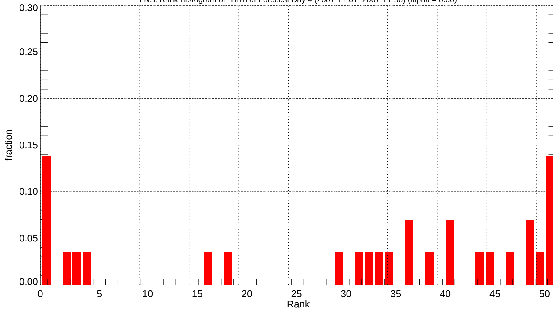
LNS: Rank Histogram of Tmin at Forecast Day 4 (2007-11-01~2007-11-30) (alpha = 0.00)
