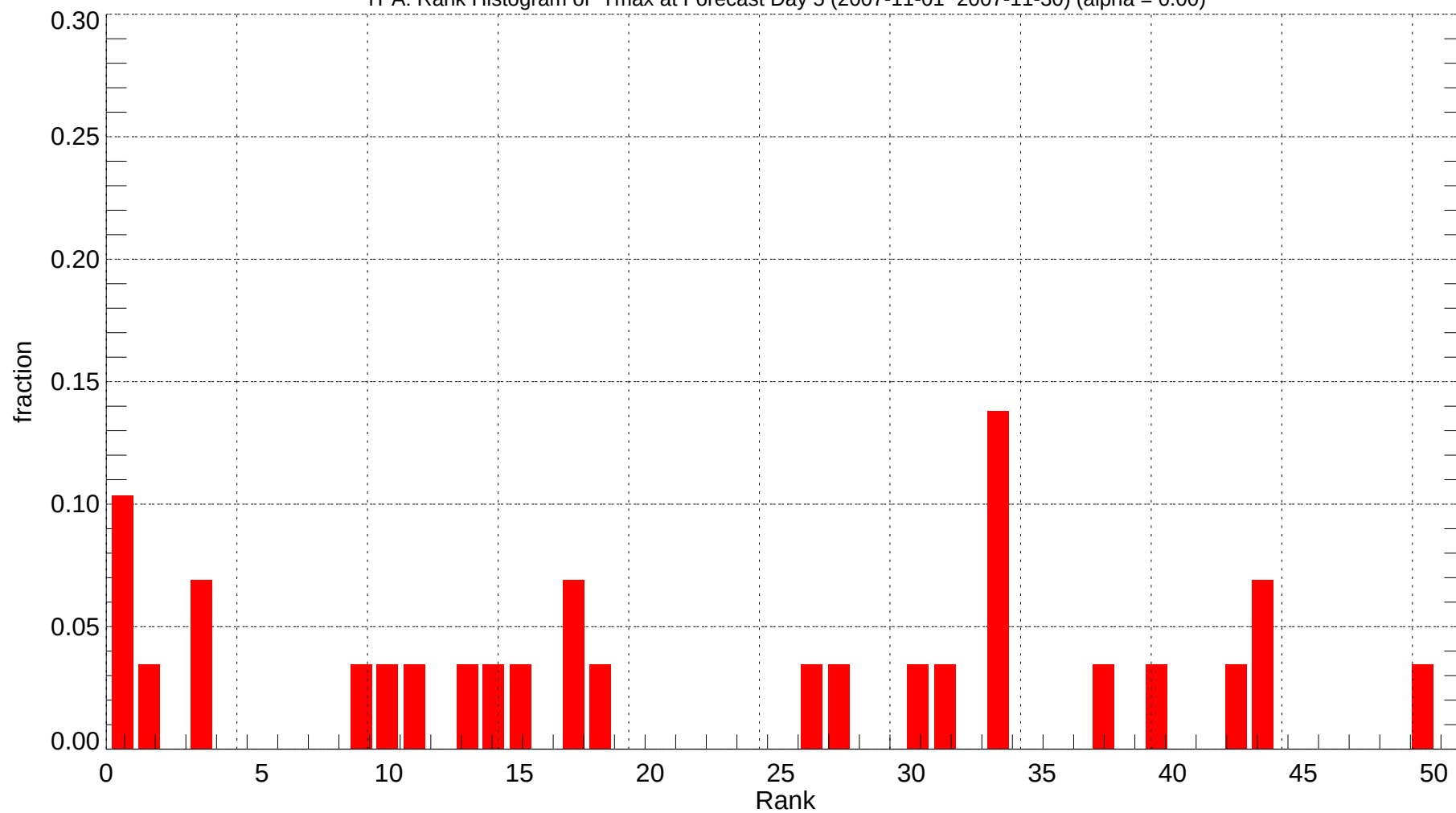
TPA: Rank Histogram of Tmax at Forecast Day 5 (2007-11-01~2007-11-30) (alpha = 0.00)
