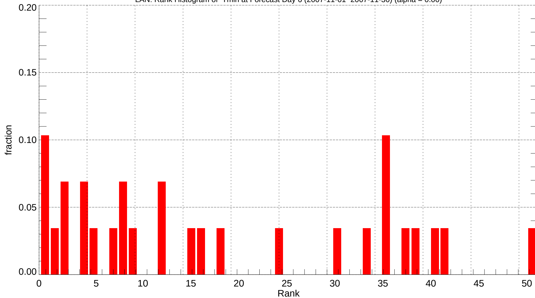
LAN: Rank Histogram of Tmin at Forecast Day 6 (2007-11-01~2007-11-30) (alpha = 0.00)
