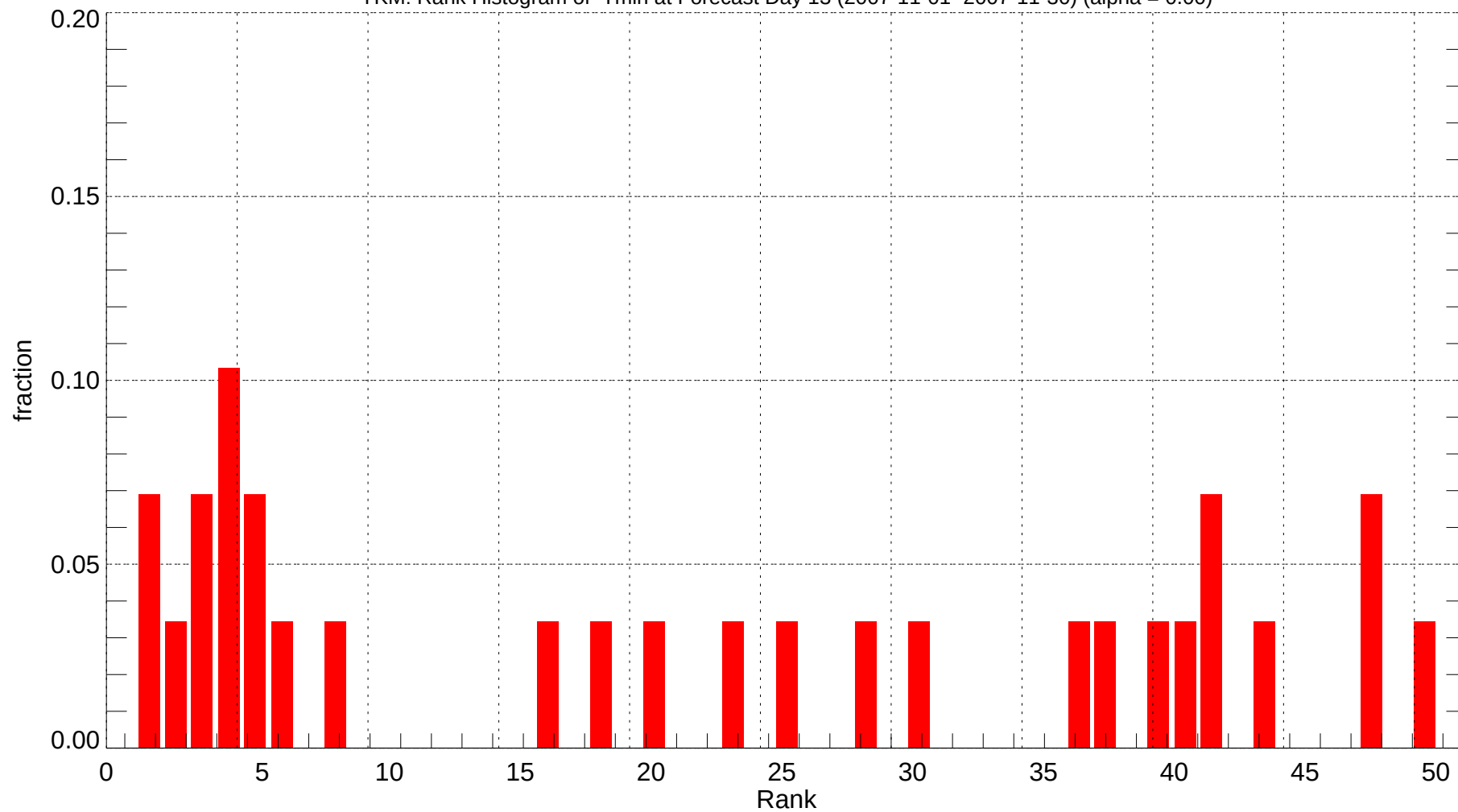
YKM: Rank Histogram of Tmin at Forecast Day 13 (2007-11-01~2007-11-30) (alpha = 0.00)
