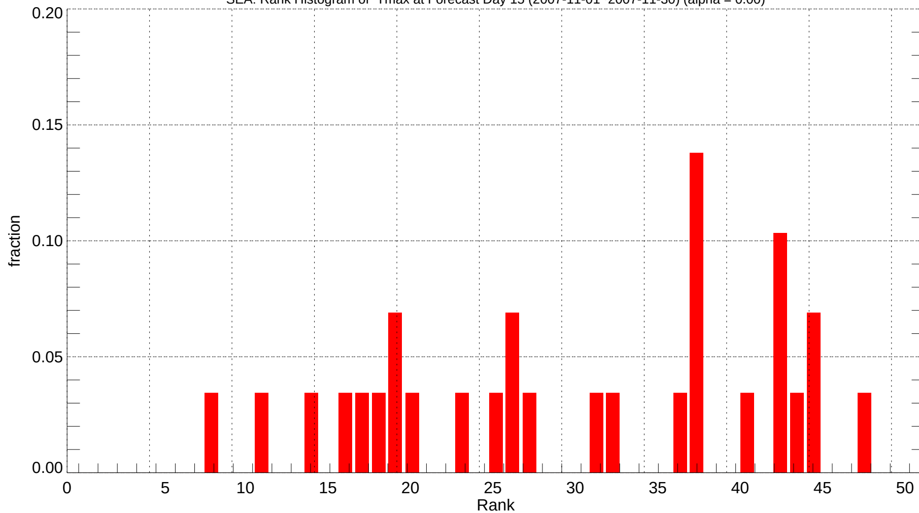
SEA: Rank Histogram of Tmax at Forecast Day 15 (2007-11-01~2007-11-30) (alpha = 0.00)
