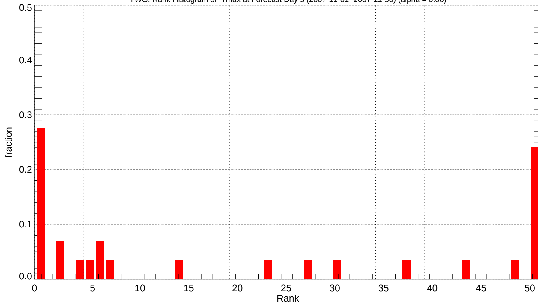
YWG: Rank Histogram of Tmax at Forecast Day 3 (2007-11-01~2007-11-30) (alpha = 0.00)
