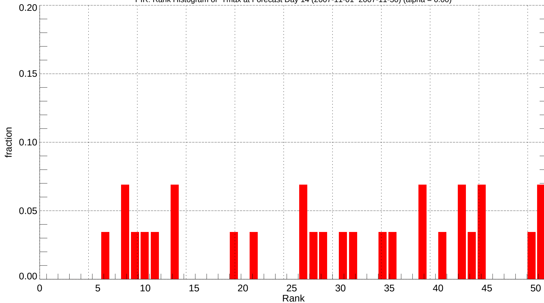
PIR: Rank Histogram of Tmax at Forecast Day 14 (2007-11-01~2007-11-30) (alpha = 0.00)
