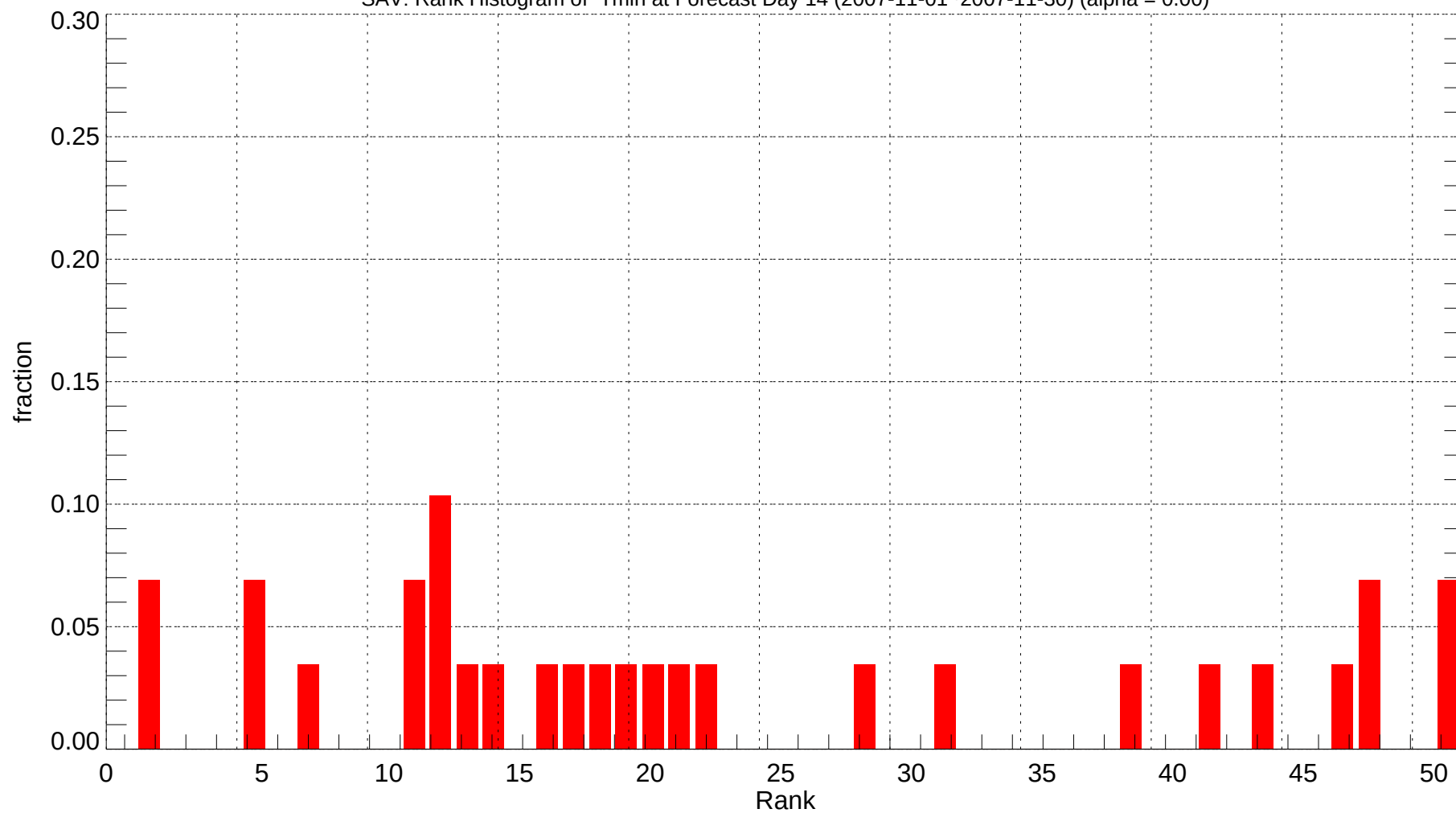
SAV: Rank Histogram of Tmin at Forecast Day 14 (2007-11-01~2007-11-30) (alpha = 0.00)
