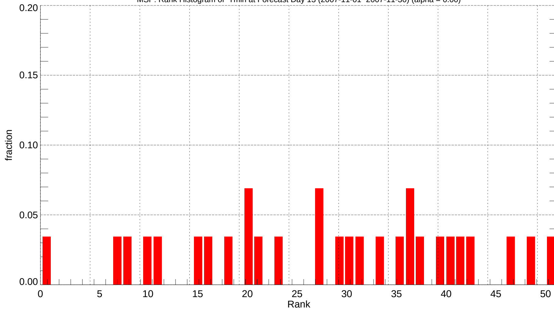
MSP: Rank Histogram of Tmin at Forecast Day 13 (2007-11-01~2007-11-30) (alpha = 0.00)
