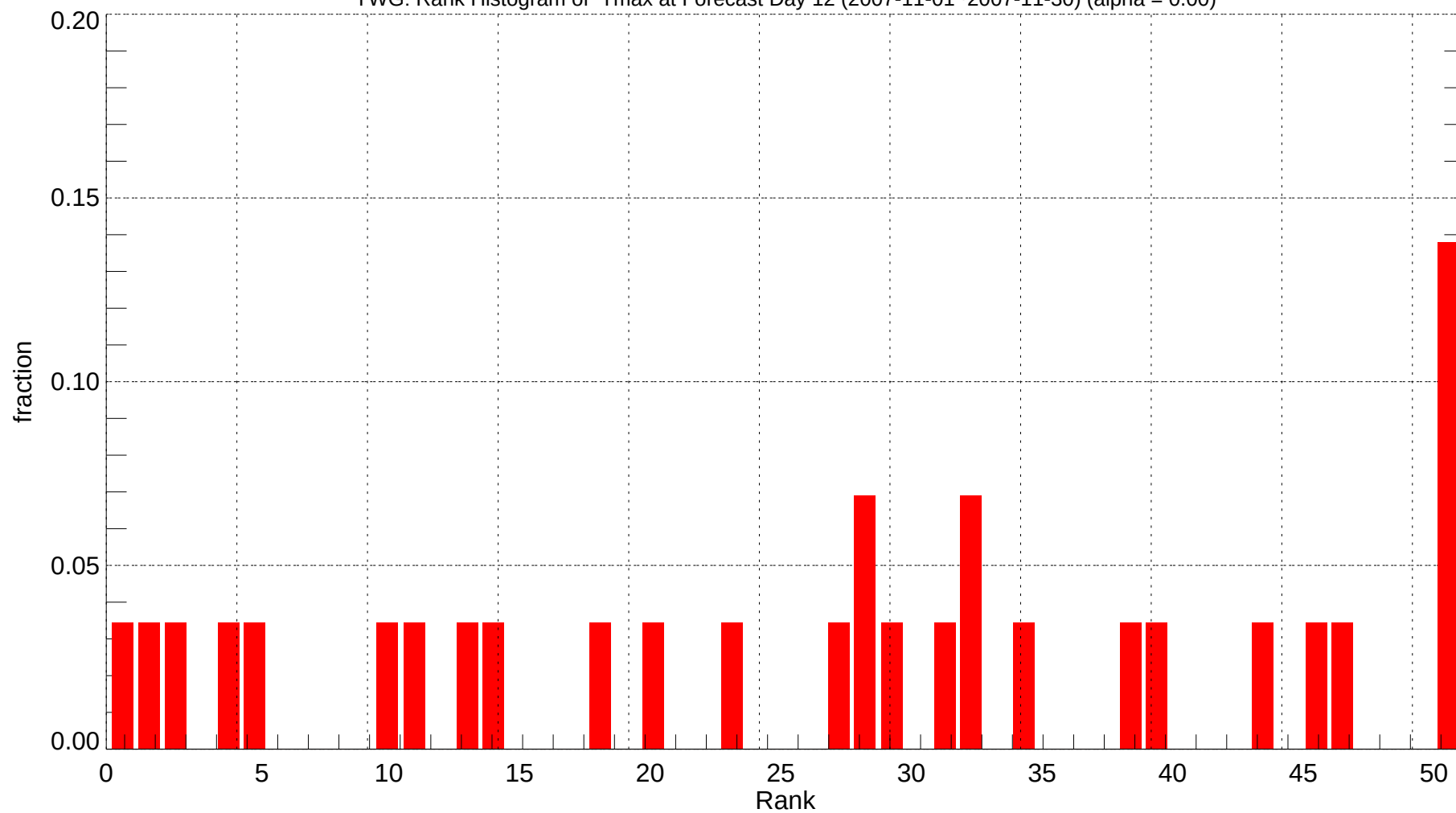
YWG: Rank Histogram of Tmax at Forecast Day 12 (2007-11-01~2007-11-30) (alpha = 0.00)
