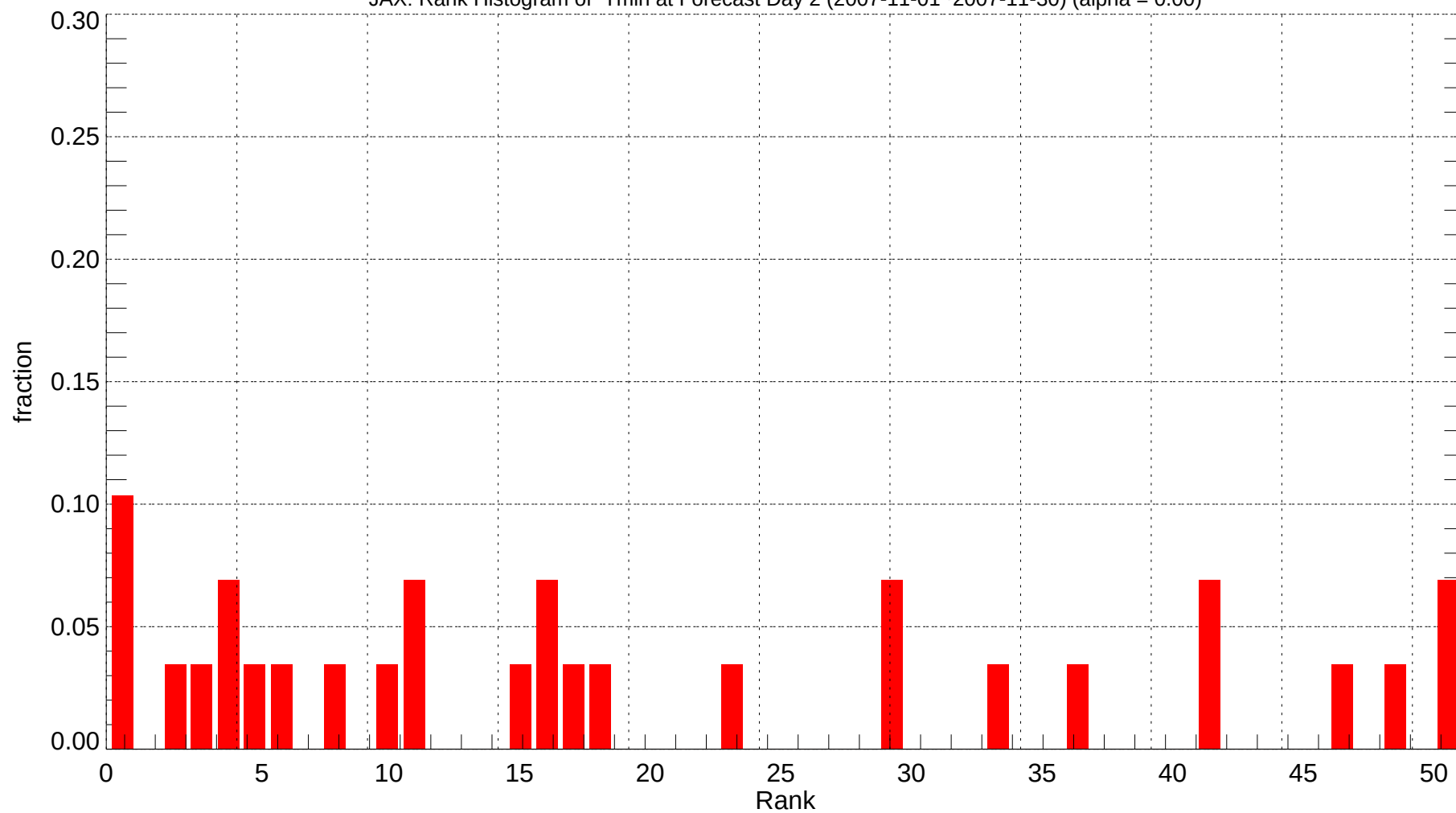
JAX: Rank Histogram of Tmin at Forecast Day 2 (2007-11-01~2007-11-30) (alpha = 0.00)
