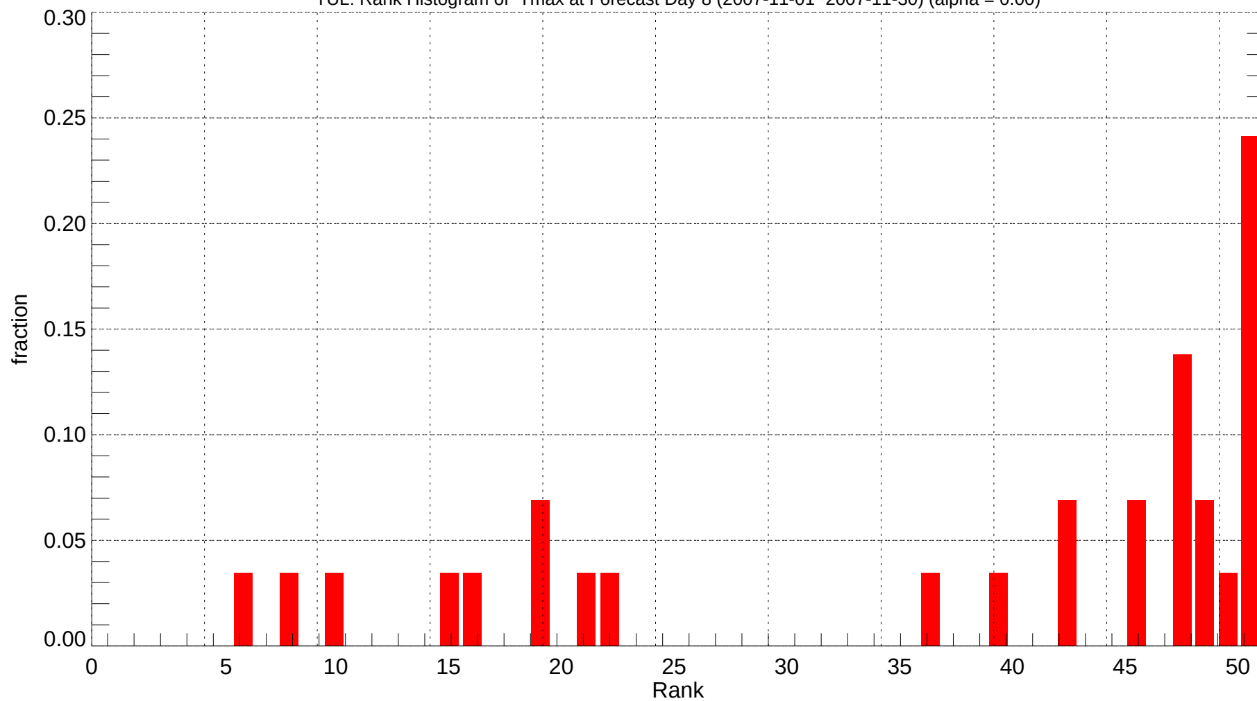
TUL: Rank Histogram of Tmax at Forecast Day 8 (2007-11-01~2007-11-30) (alpha = 0.00)
