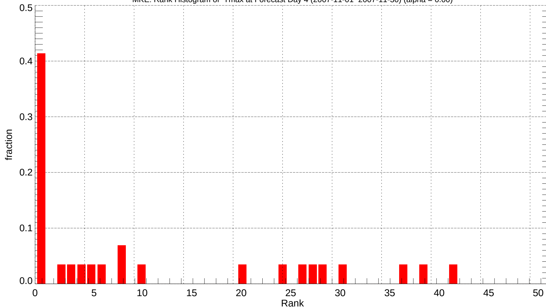
MKE: Rank Histogram of Tmax at Forecast Day 4 (2007-11-01~2007-11-30) (alpha = 0.00)
