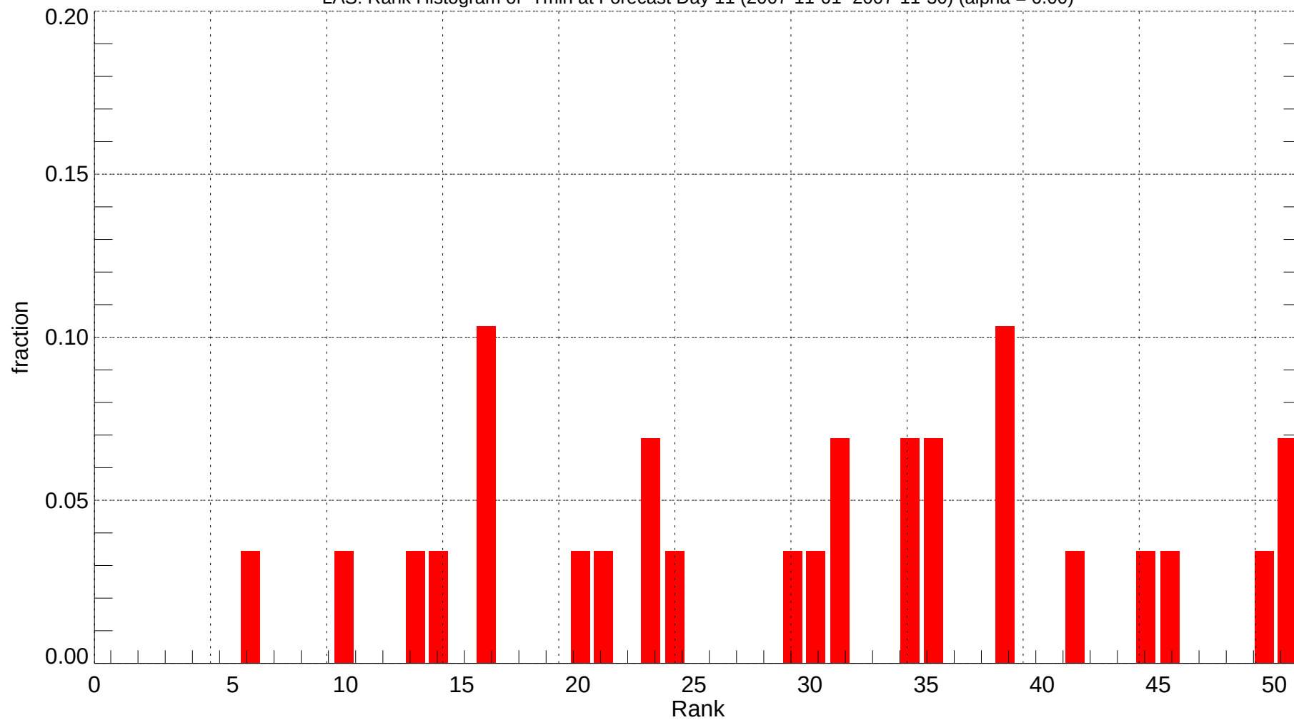
LAS: Rank Histogram of Tmin at Forecast Day 11 (2007-11-01~2007-11-30) (alpha = 0.00)
