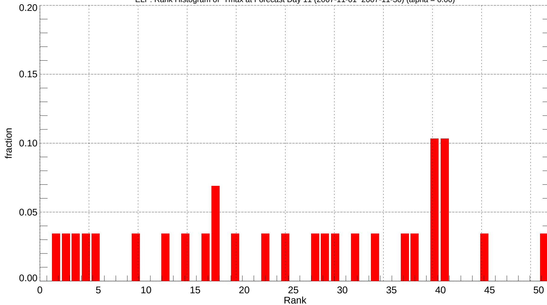
ELP: Rank Histogram of Tmax at Forecast Day 11 (2007-11-01~2007-11-30) (alpha = 0.00)
