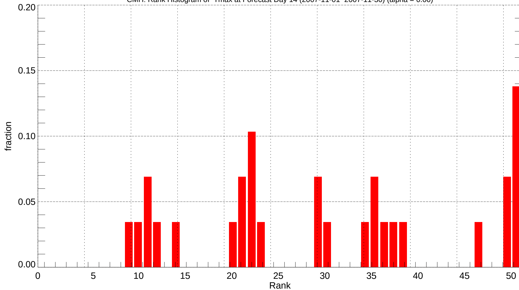
CMH: Rank Histogram of Tmax at Forecast Day 14 (2007-11-01~2007-11-30) (alpha = 0.00)
