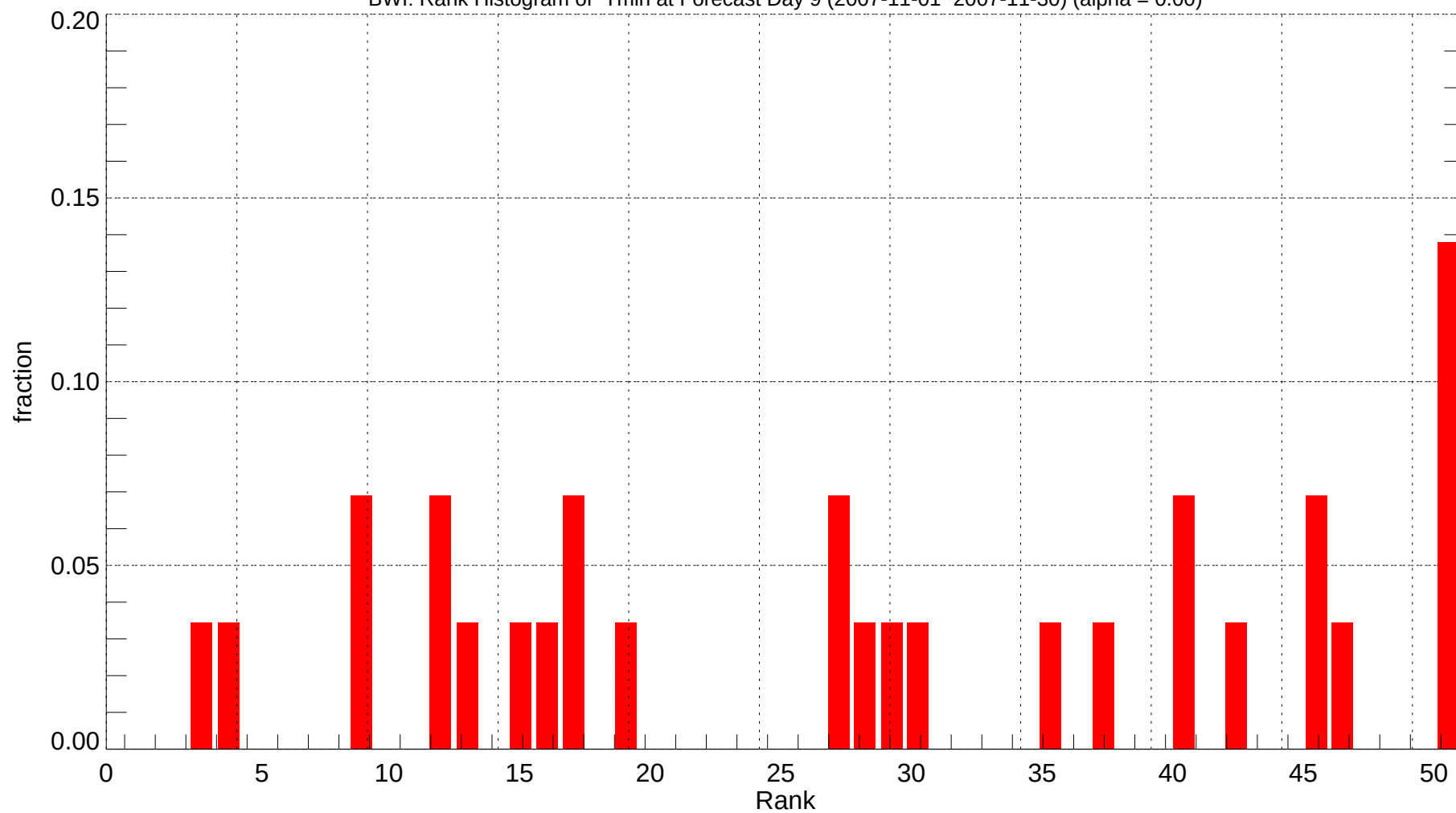
BWI: Rank Histogram of Tmin at Forecast Day 9 (2007-11-01~2007-11-30) (alpha = 0.00)
