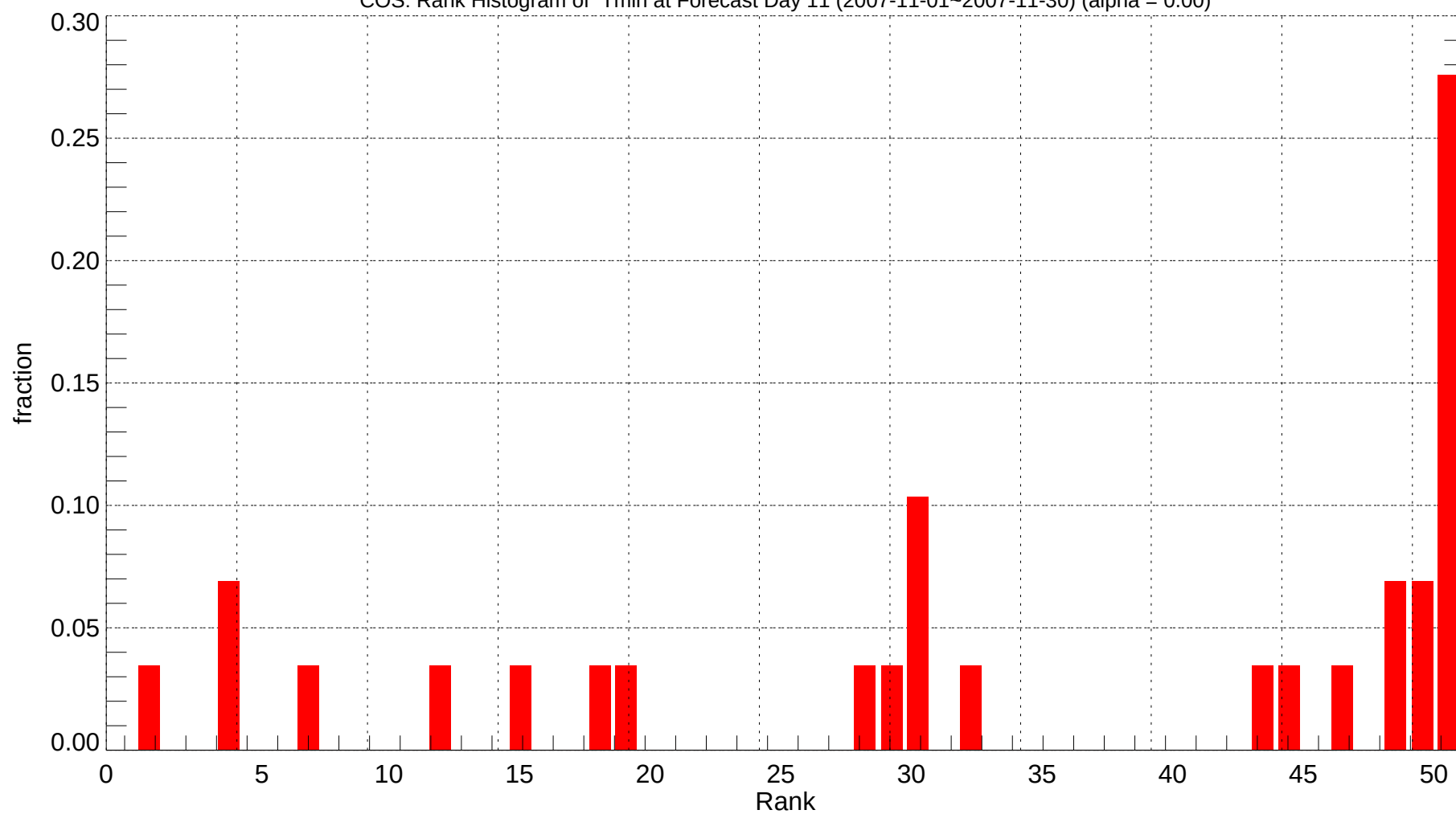
COS: Rank Histogram of Tmin at Forecast Day 11 (2007-11-01~2007-11-30) (alpha = 0.00)
