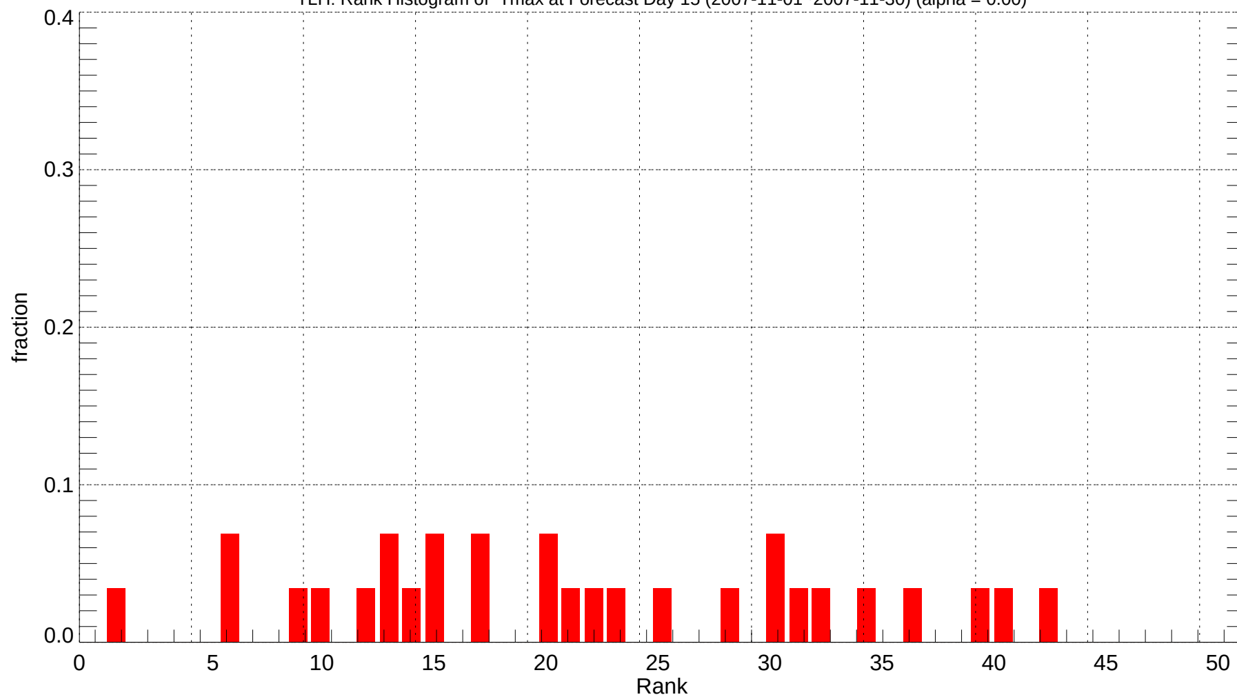
TLH: Rank Histogram of Tmax at Forecast Day 15 (2007-11-01~2007-11-30) (alpha = 0.00)
