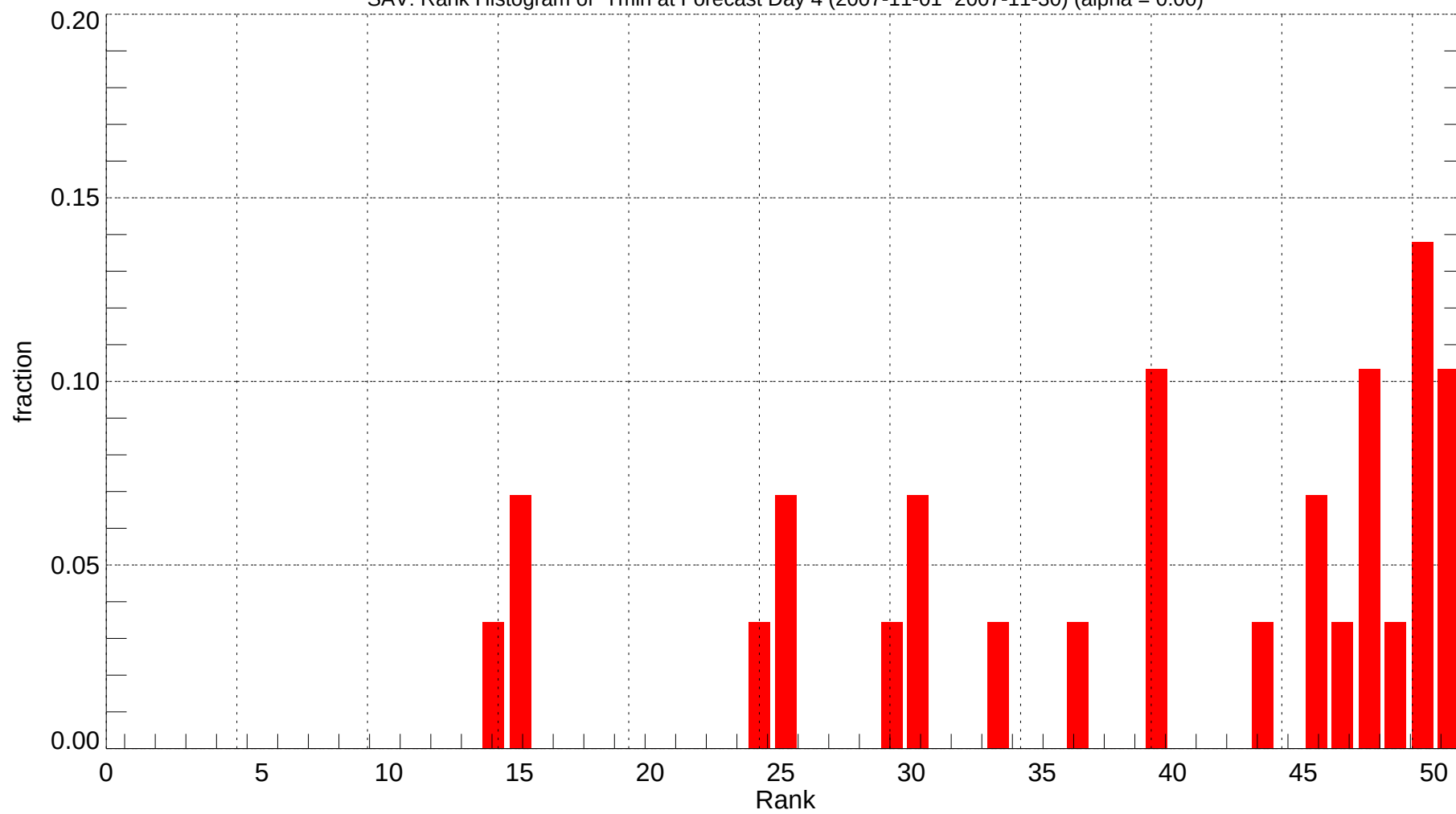
SAV: Rank Histogram of Tmin at Forecast Day 4 (2007-11-01~2007-11-30) (alpha = 0.00)
