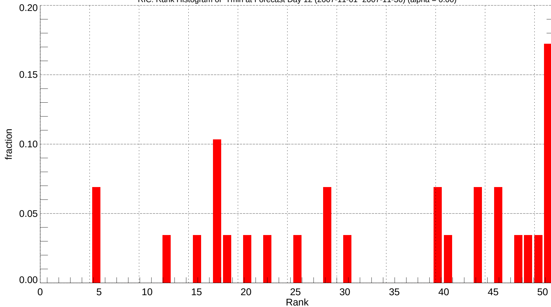
RIC: Rank Histogram of Tmin at Forecast Day 12 (2007-11-01~2007-11-30) (alpha = 0.00)
