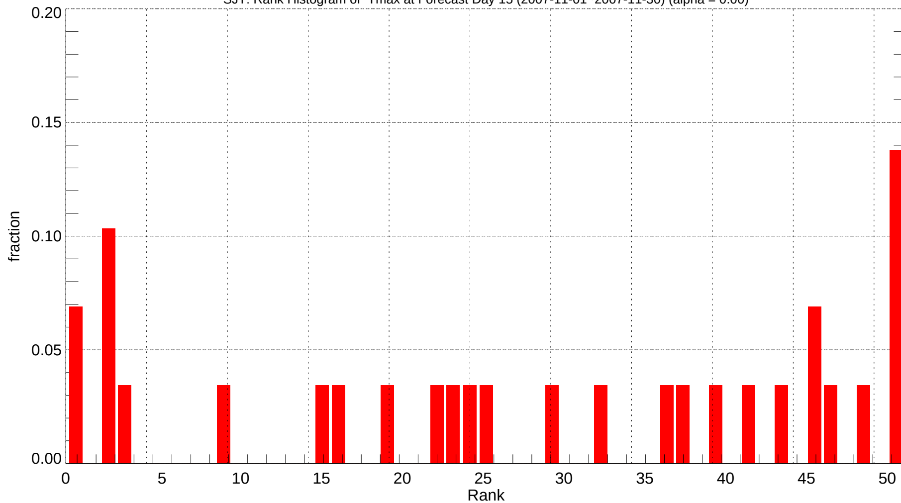
SJT: Rank Histogram of Tmax at Forecast Day 15 (2007-11-01~2007-11-30) (alpha = 0.00)
