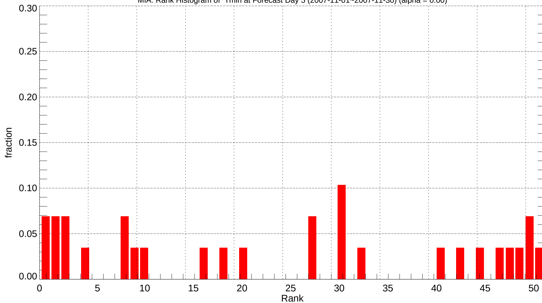
MIA: Rank Histogram of Tmin at Forecast Day 5 (2007-11-01~2007-11-30) (alpha = 0.00)
