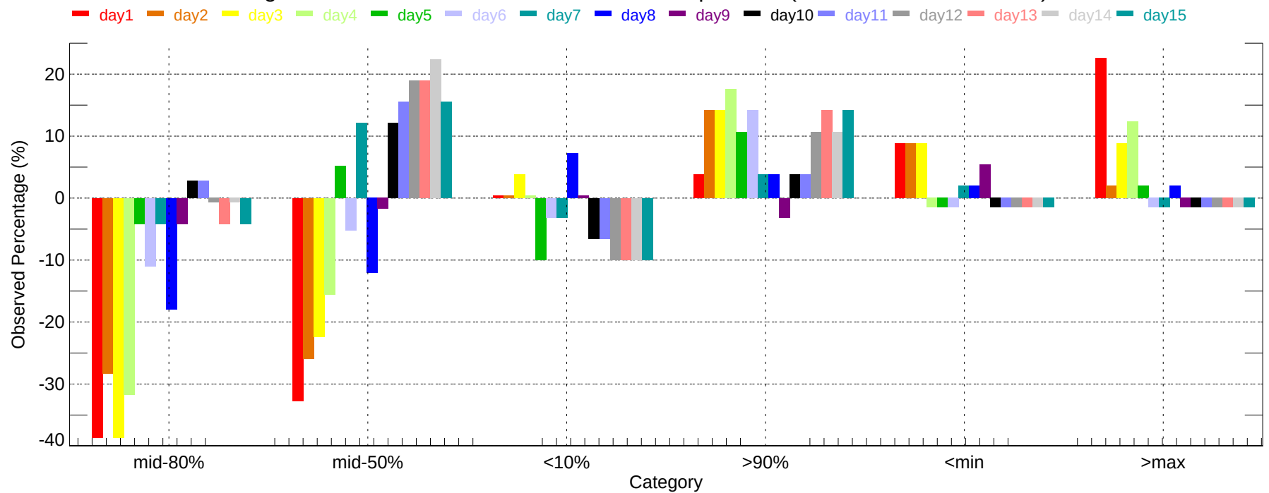
Observed Percentage Deviation of Ensembles - SEA: Min Temperature (2007-11-01~2007-11-30)
