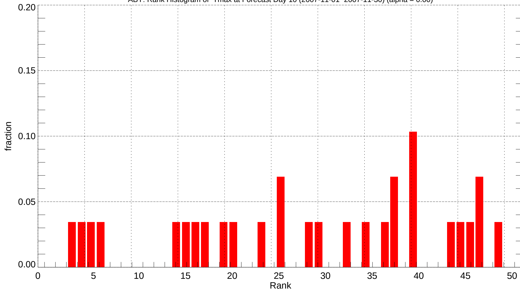
ABY: Rank Histogram of Tmax at Forecast Day 10 (2007-11-01~2007-11-30) (alpha = 0.00)
