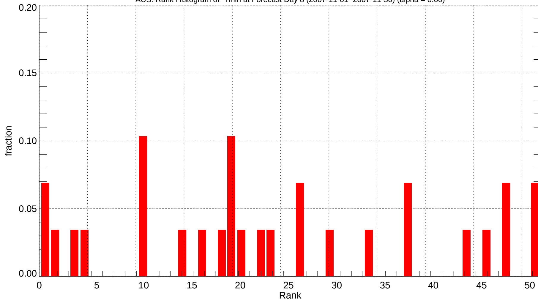
AUS: Rank Histogram of Tmin at Forecast Day 8 (2007-11-01~2007-11-30) (alpha = 0.00)
