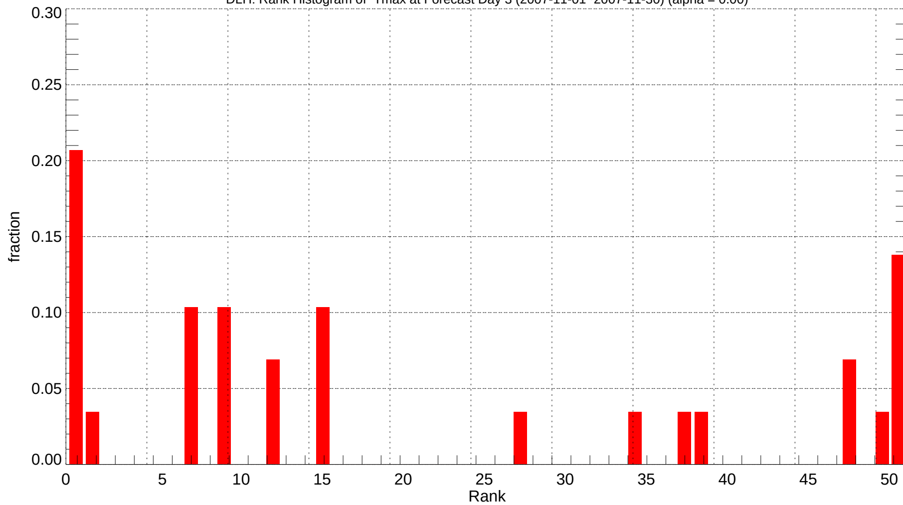
DLH: Rank Histogram of Tmax at Forecast Day 3 (2007-11-01~2007-11-30) (alpha = 0.00)
