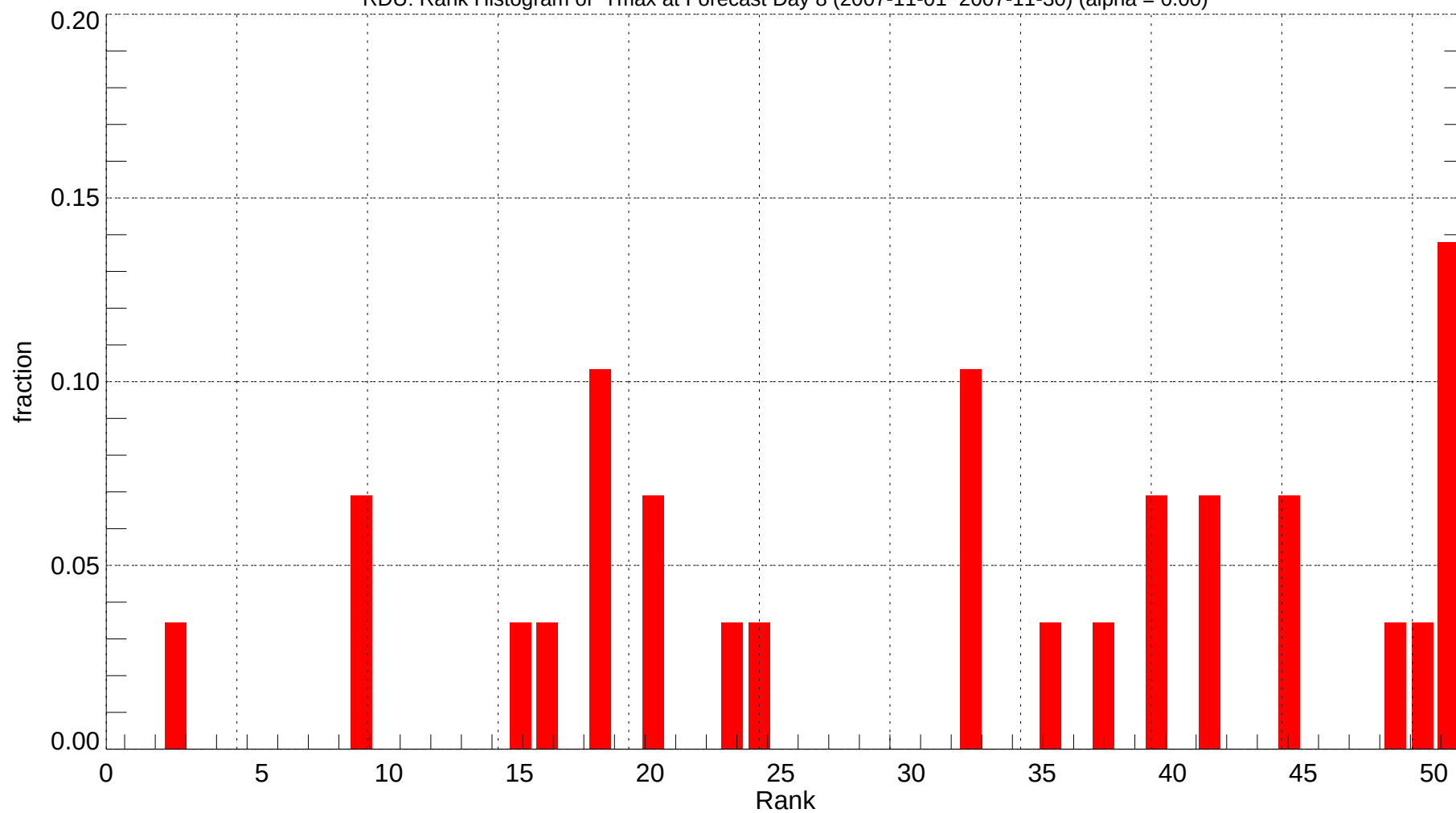
RDU: Rank Histogram of Tmax at Forecast Day 8 (2007-11-01~2007-11-30) (alpha = 0.00)
