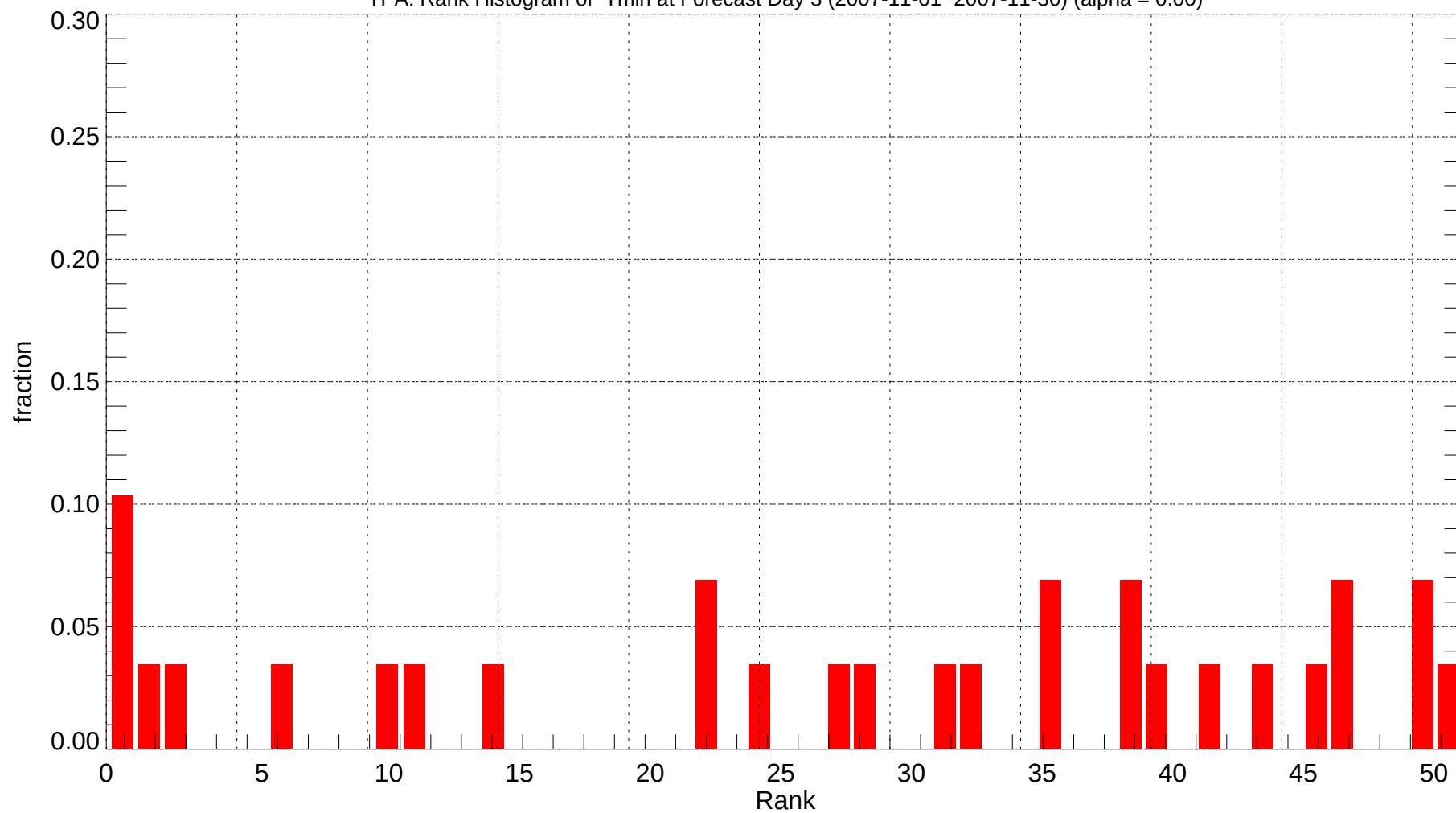
TPA: Rank Histogram of Tmin at Forecast Day 3 (2007-11-01~2007-11-30) (alpha = 0.00)
