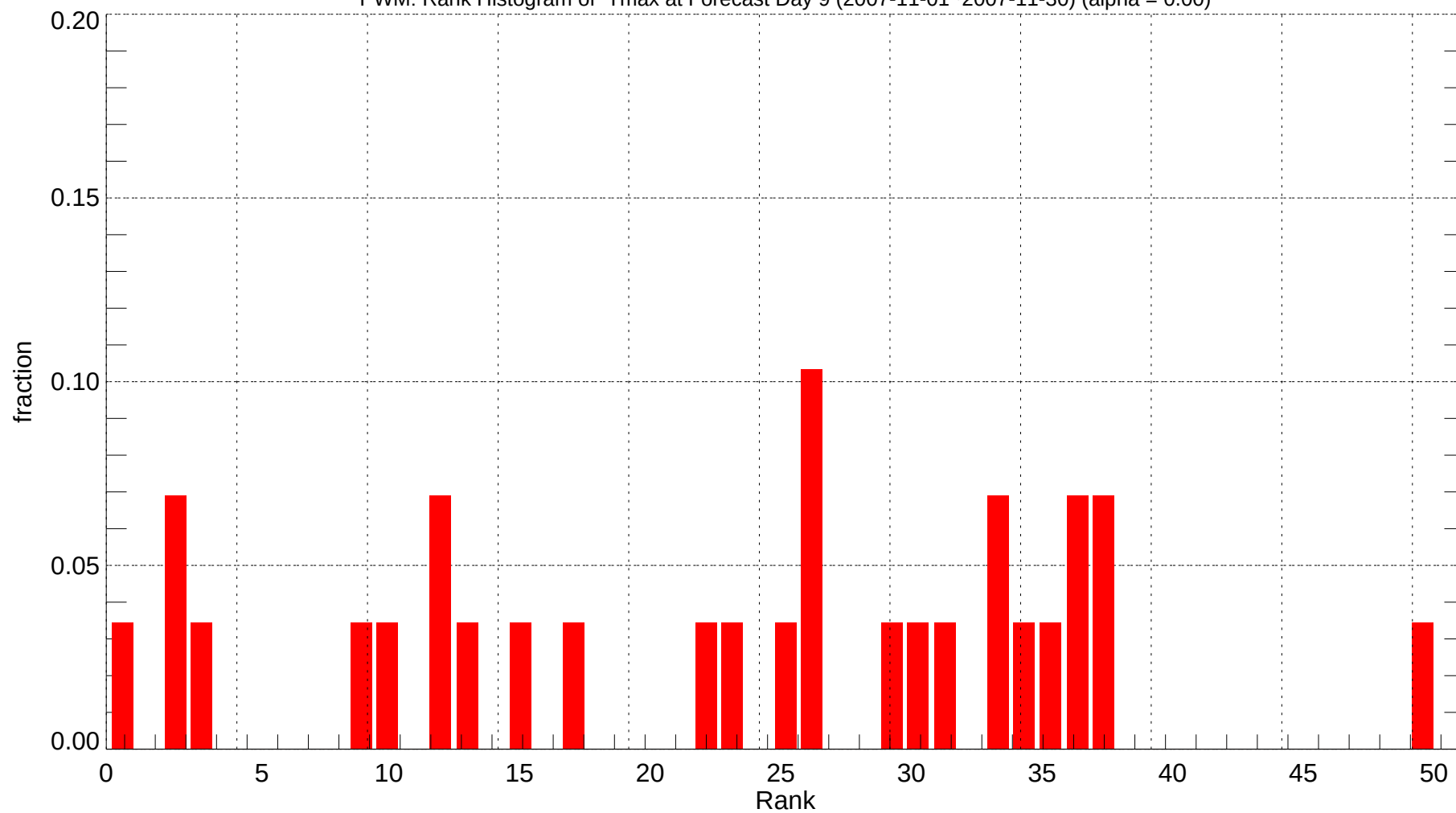
PWM: Rank Histogram of Tmax at Forecast Day 9 (2007-11-01~2007-11-30) (alpha = 0.00)
