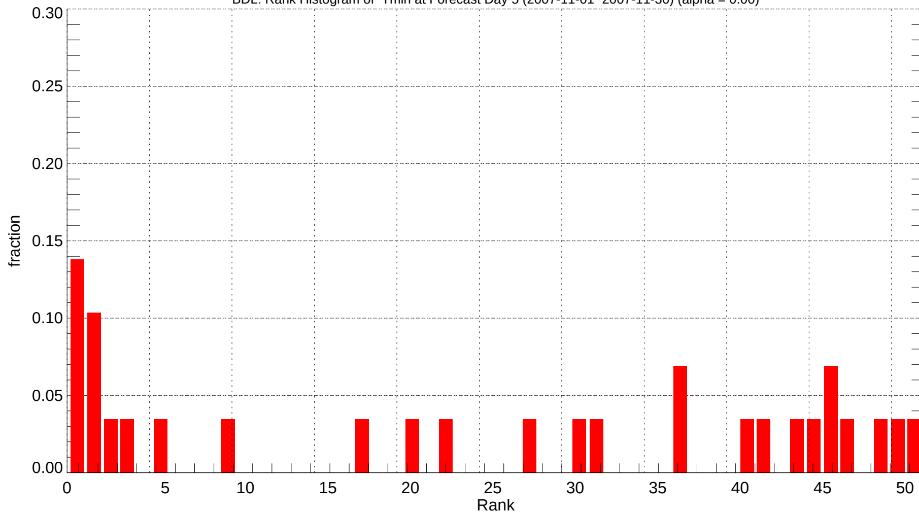
BDL: Rank Histogram of Tmin at Forecast Day 5 (2007-11-01~2007-11-30) (alpha = 0.00)
