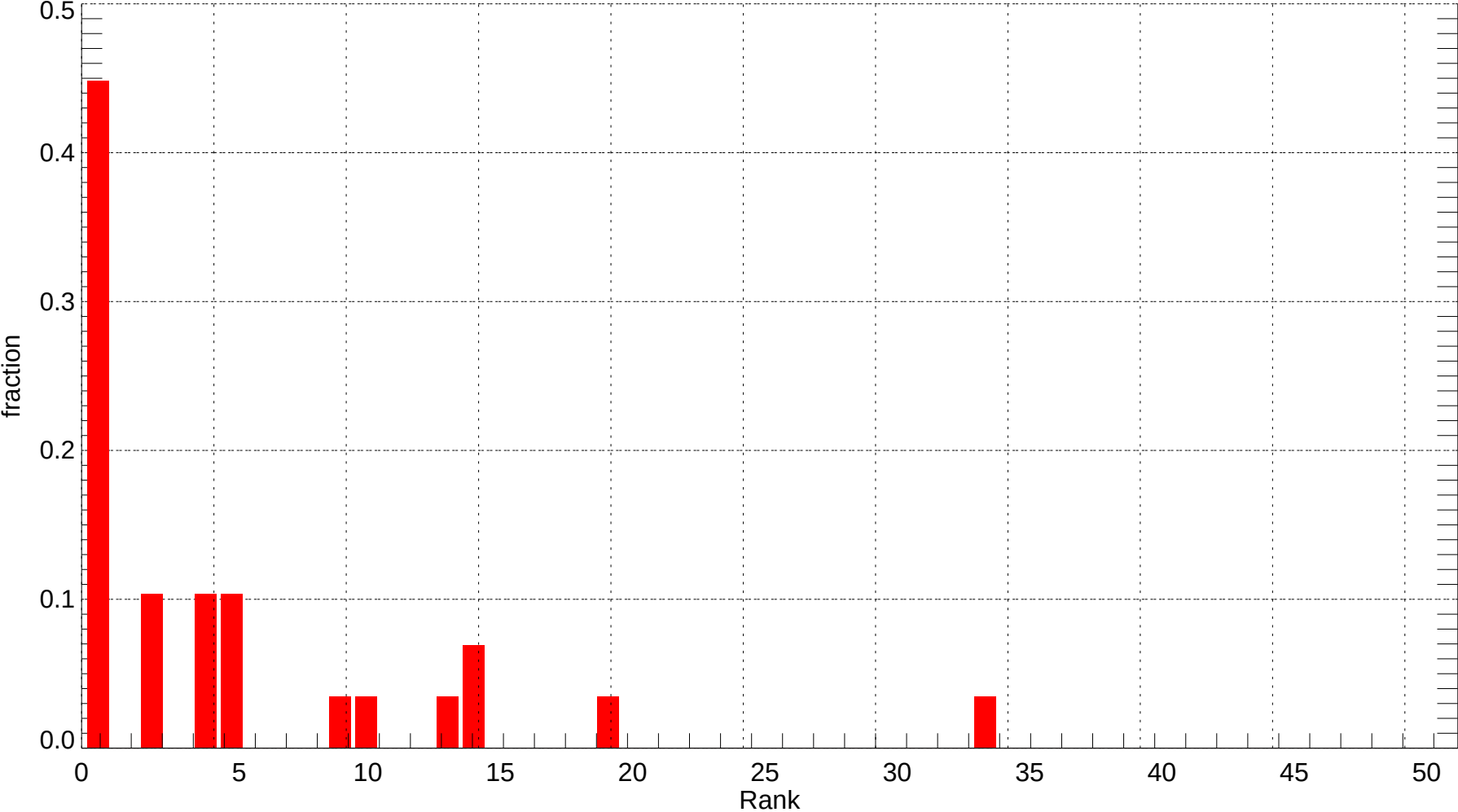
SJC: Rank Histogram of Tmin at Forecast Day 7 (2007-11-01~2007-11-30) (alpha = 0.00)
