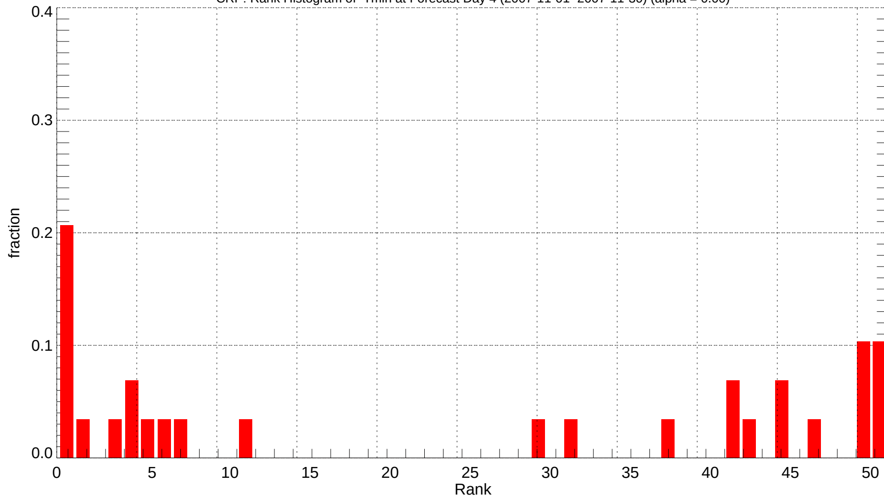
CRP: Rank Histogram of Tmin at Forecast Day 4 (2007-11-01~2007-11-30) (alpha = 0.00)
