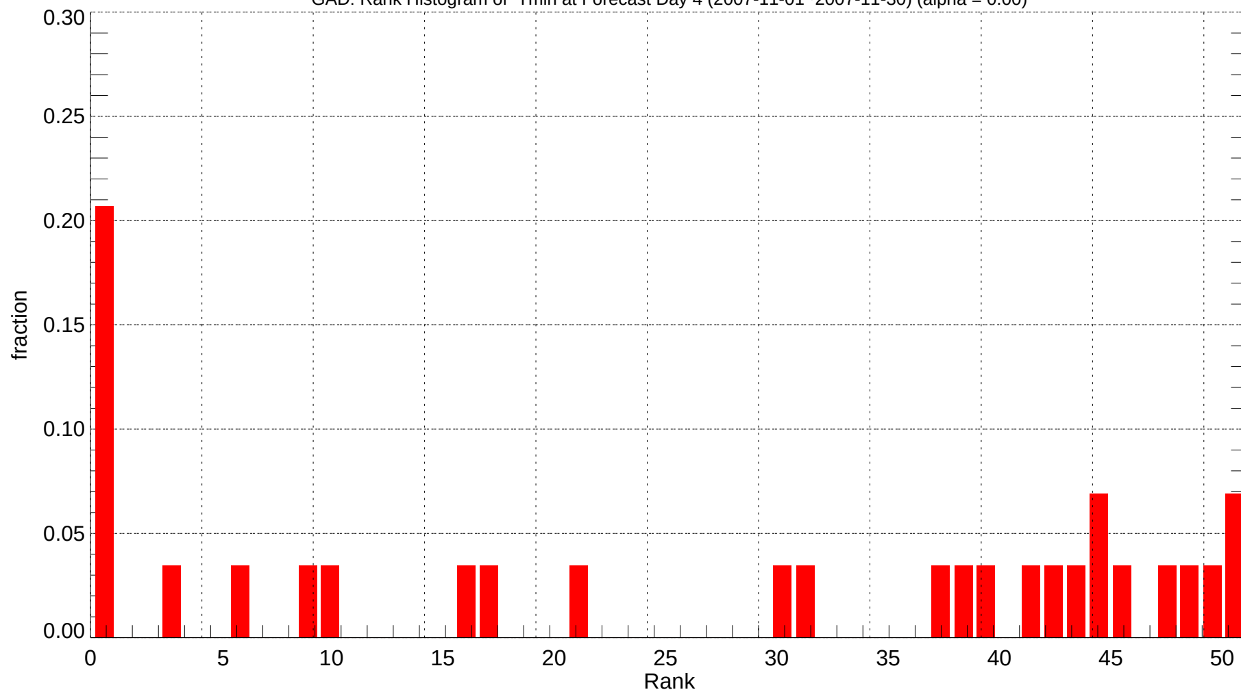
GAD: Rank Histogram of Tmin at Forecast Day 4 (2007-11-01~2007-11-30) (alpha = 0.00)
