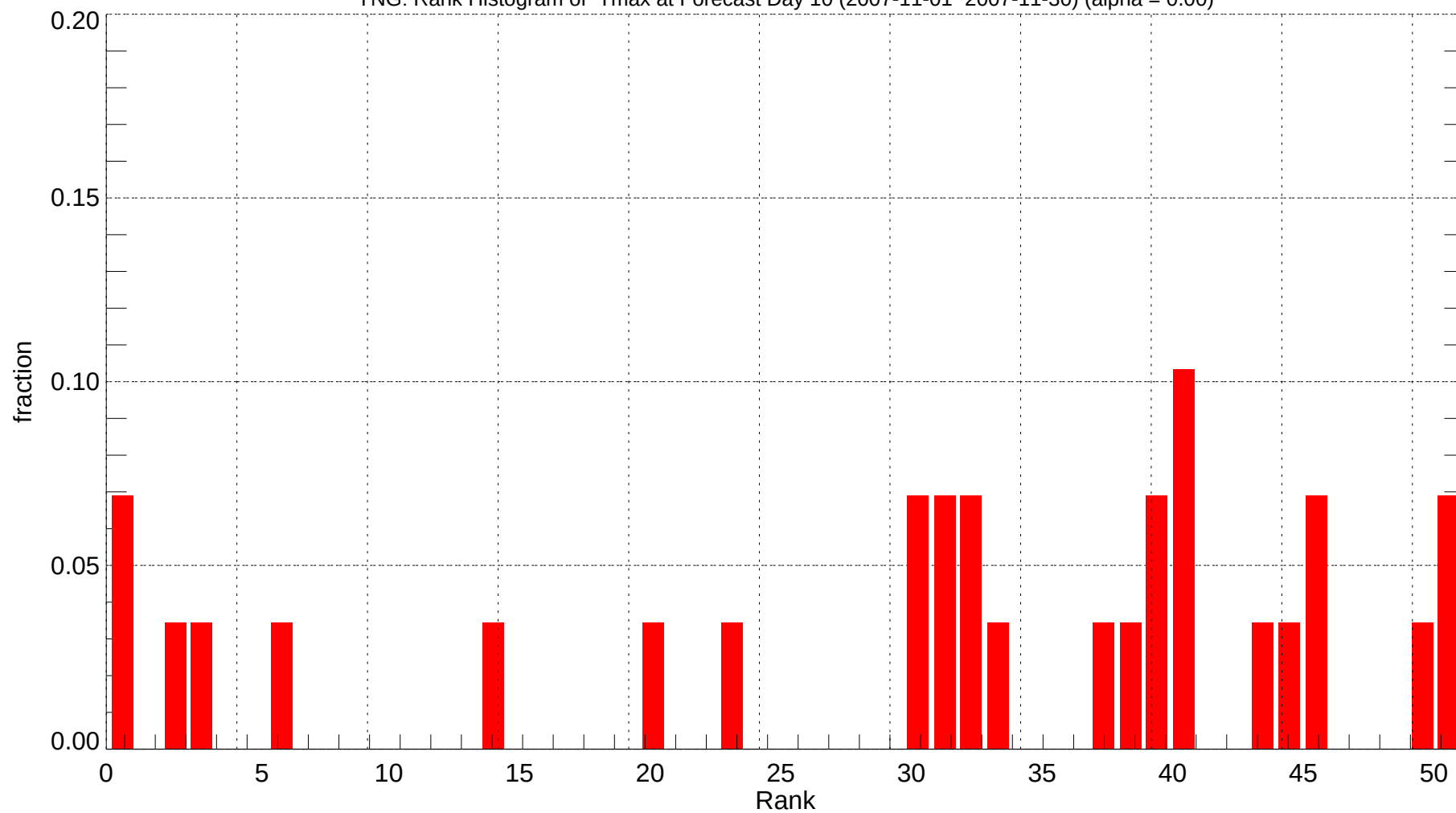
YNG: Rank Histogram of Tmax at Forecast Day 10 (2007-11-01~2007-11-30) (alpha = 0.00)
