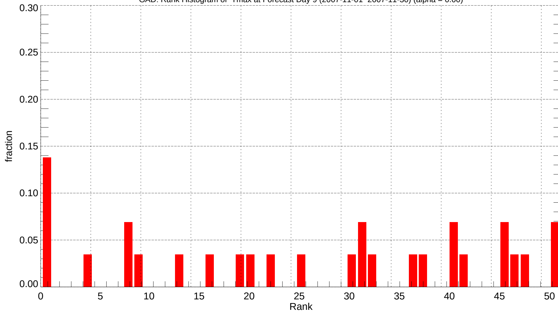
GAD: Rank Histogram of Tmax at Forecast Day 9 (2007-11-01~2007-11-30) (alpha = 0.00)
