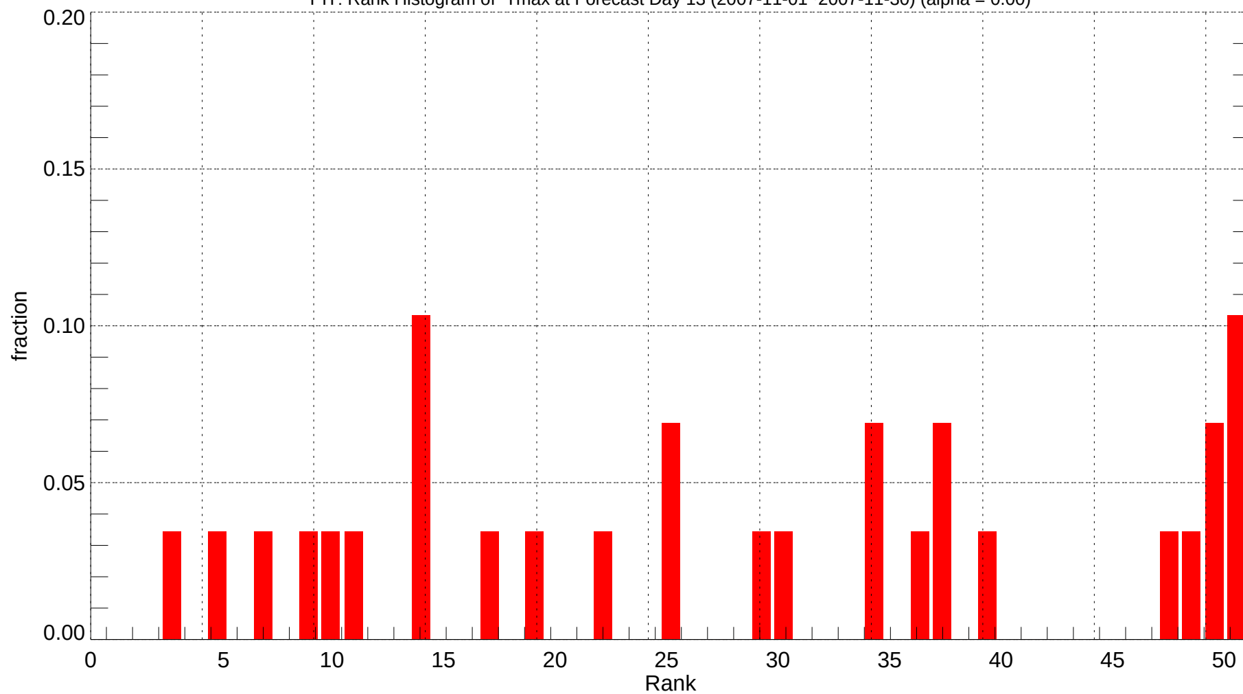
PIT: Rank Histogram of Tmax at Forecast Day 13 (2007-11-01~2007-11-30) (alpha = 0.00)
