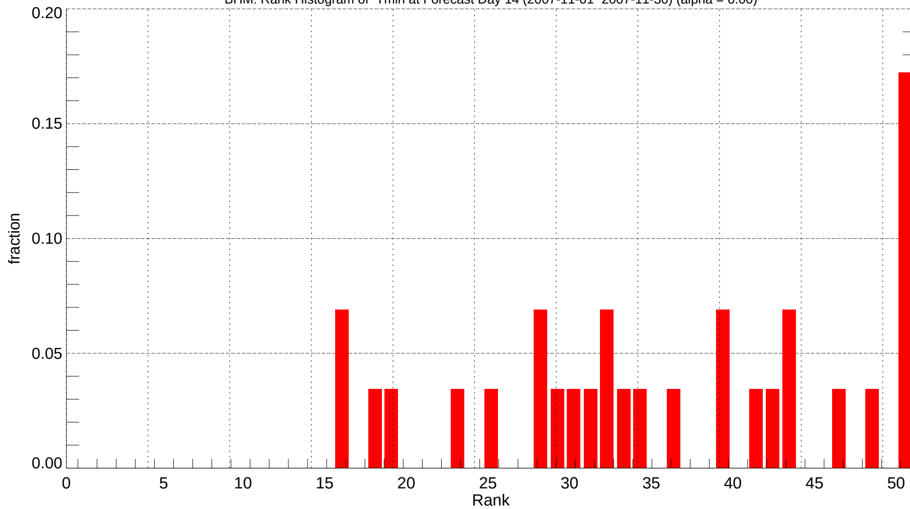
BHM: Rank Histogram of Tmin at Forecast Day 14 (2007-11-01~2007-11-30) (alpha = 0.00)
