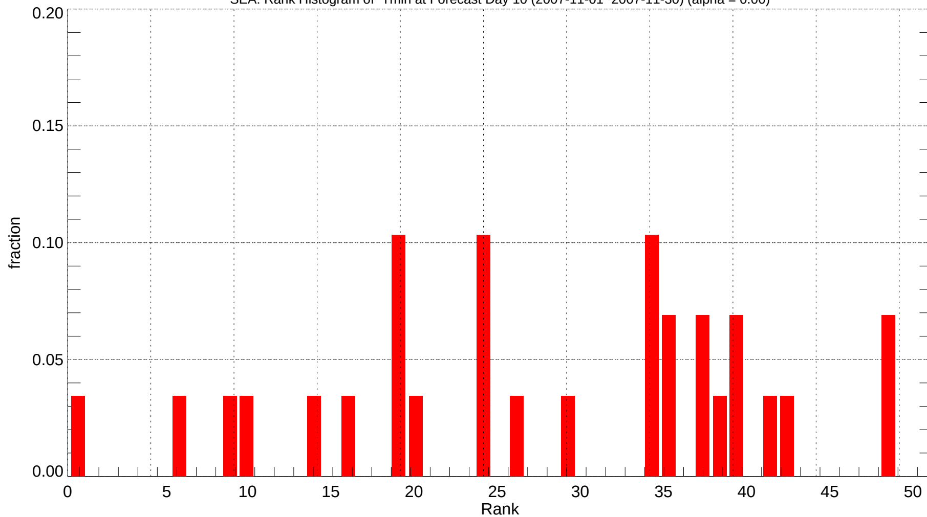
SEA: Rank Histogram of Tmin at Forecast Day 10 (2007-11-01~2007-11-30) (alpha = 0.00)
