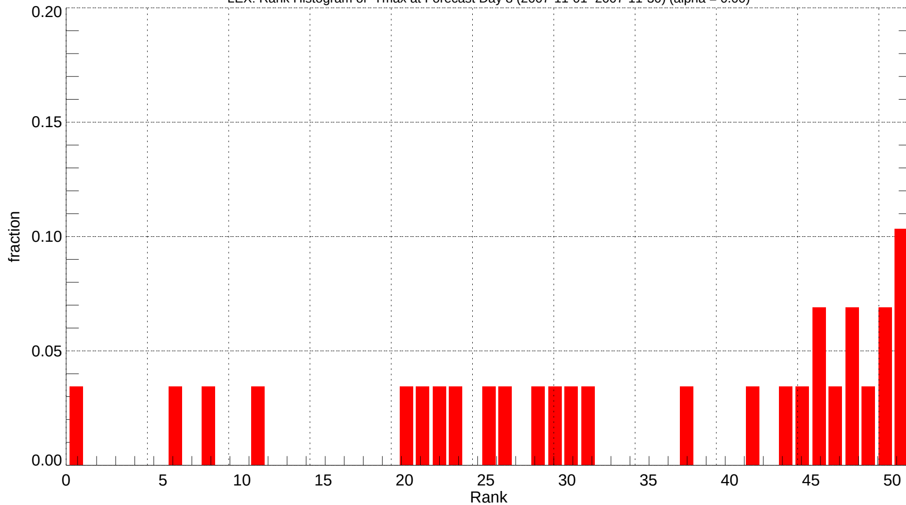
LEX: Rank Histogram of Tmax at Forecast Day 8 (2007-11-01~2007-11-30) (alpha = 0.00)
