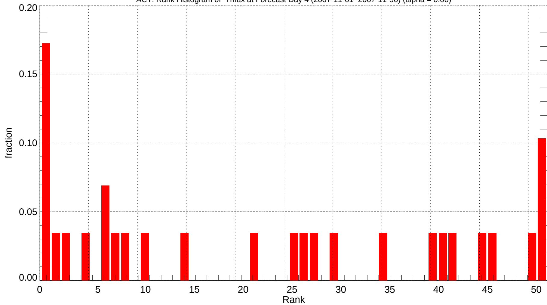
ACT: Rank Histogram of Tmax at Forecast Day 4 (2007-11-01~2007-11-30) (alpha = 0.00)
