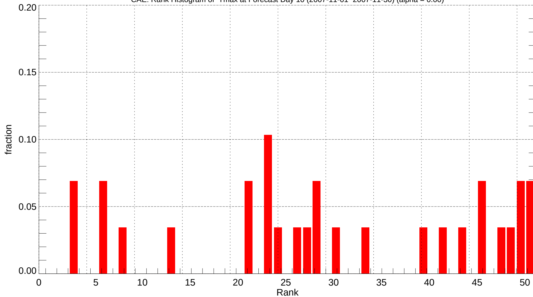
CAE: Rank Histogram of Tmax at Forecast Day 10 (2007-11-01~2007-11-30) (alpha = 0.00)
