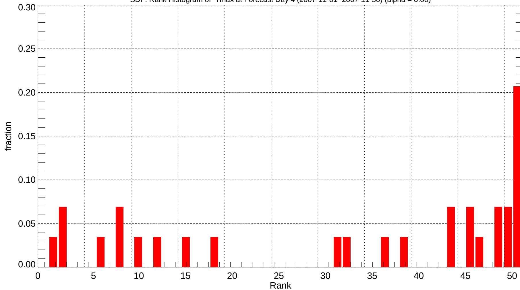
SDF: Rank Histogram of Tmax at Forecast Day 4 (2007-11-01~2007-11-30) (alpha = 0.00)
