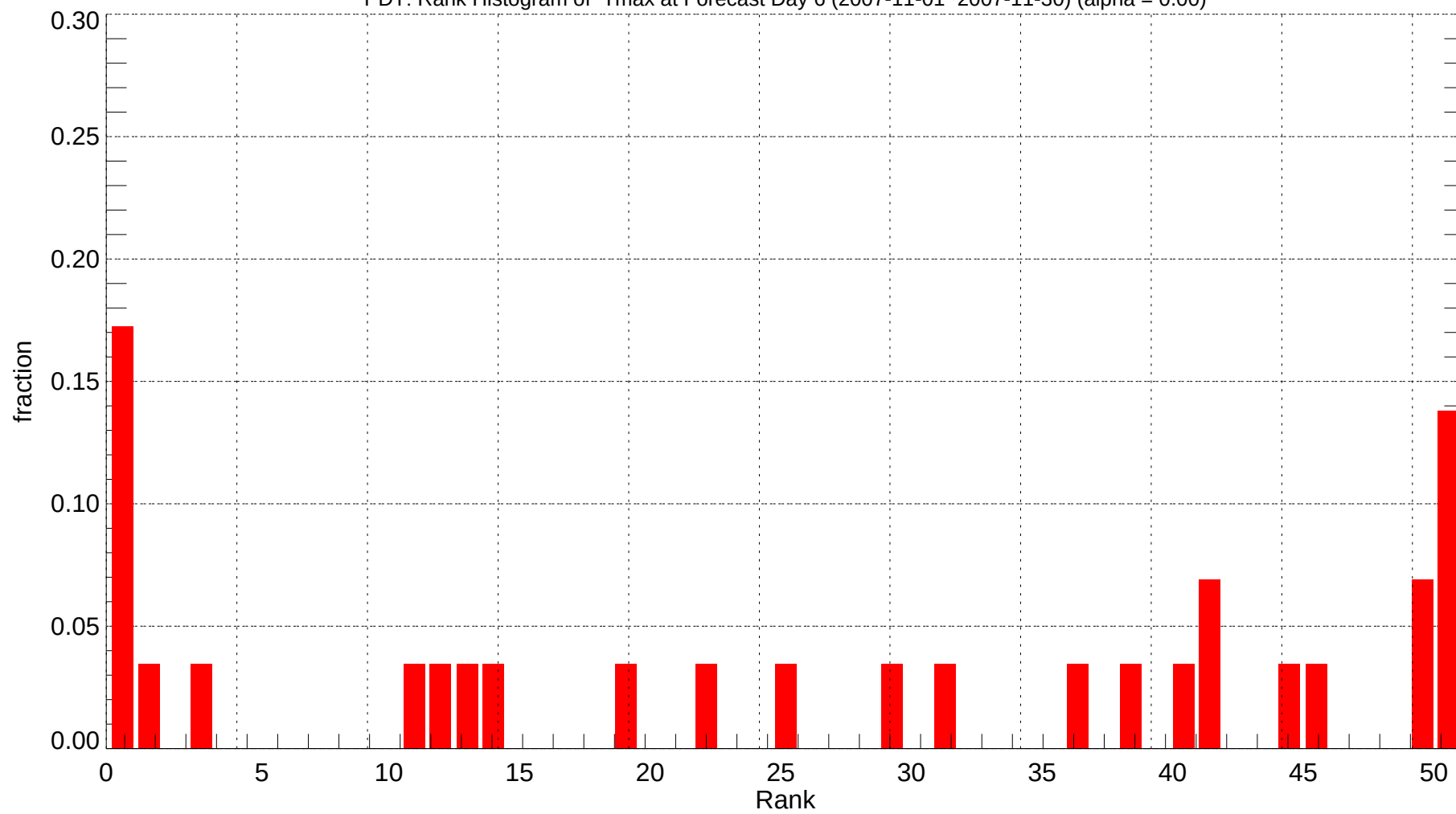
PDT: Rank Histogram of Tmax at Forecast Day 6 (2007-11-01~2007-11-30) (alpha = 0.00)
