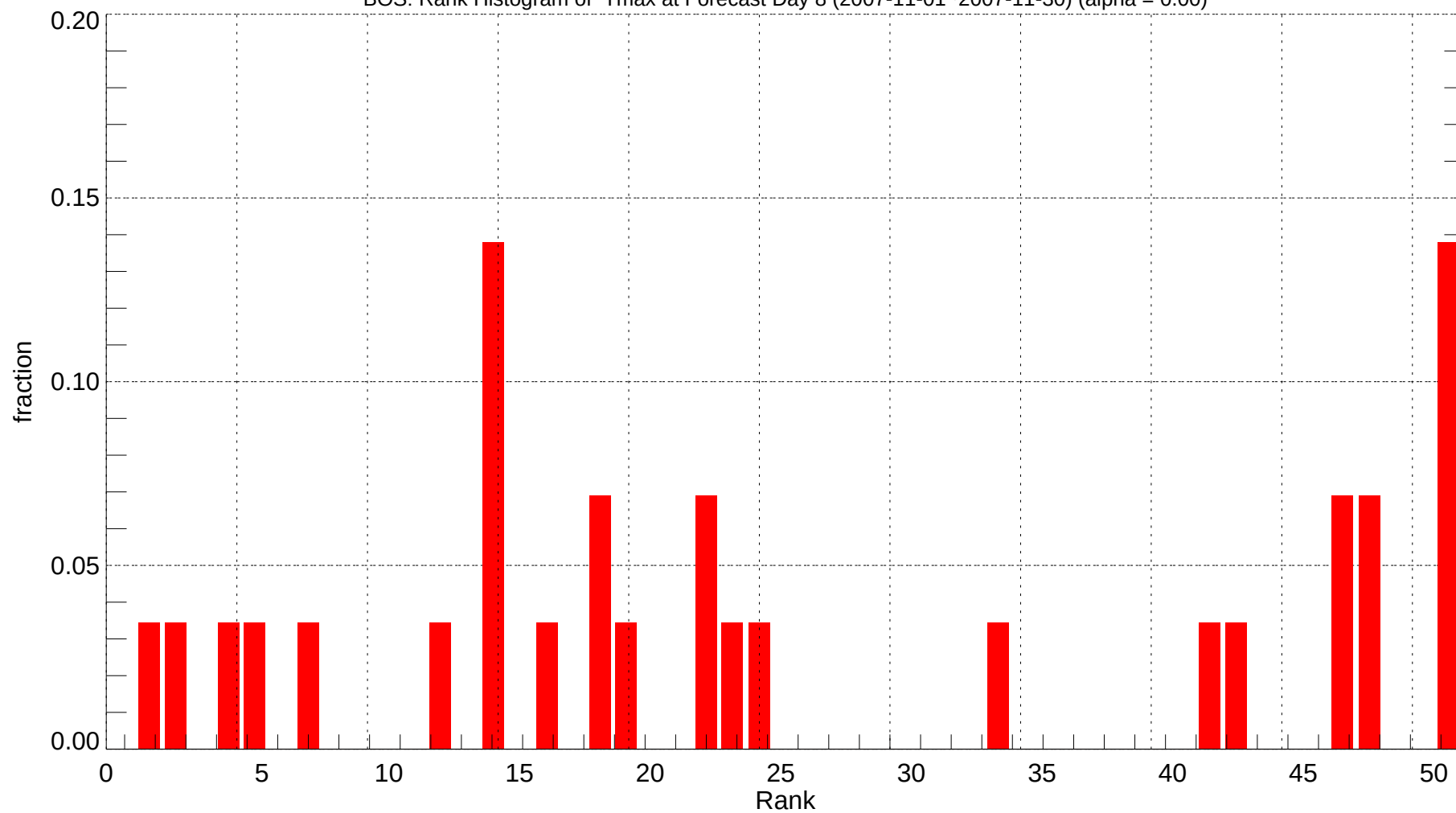
BOS: Rank Histogram of Tmax at Forecast Day 8 (2007-11-01~2007-11-30) (alpha = 0.00)
