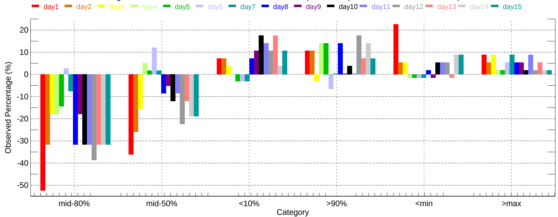
Observed Percentage Deviation of Ensembles - PHL: Min Temperature (2007-11-01~2007-11-30)
