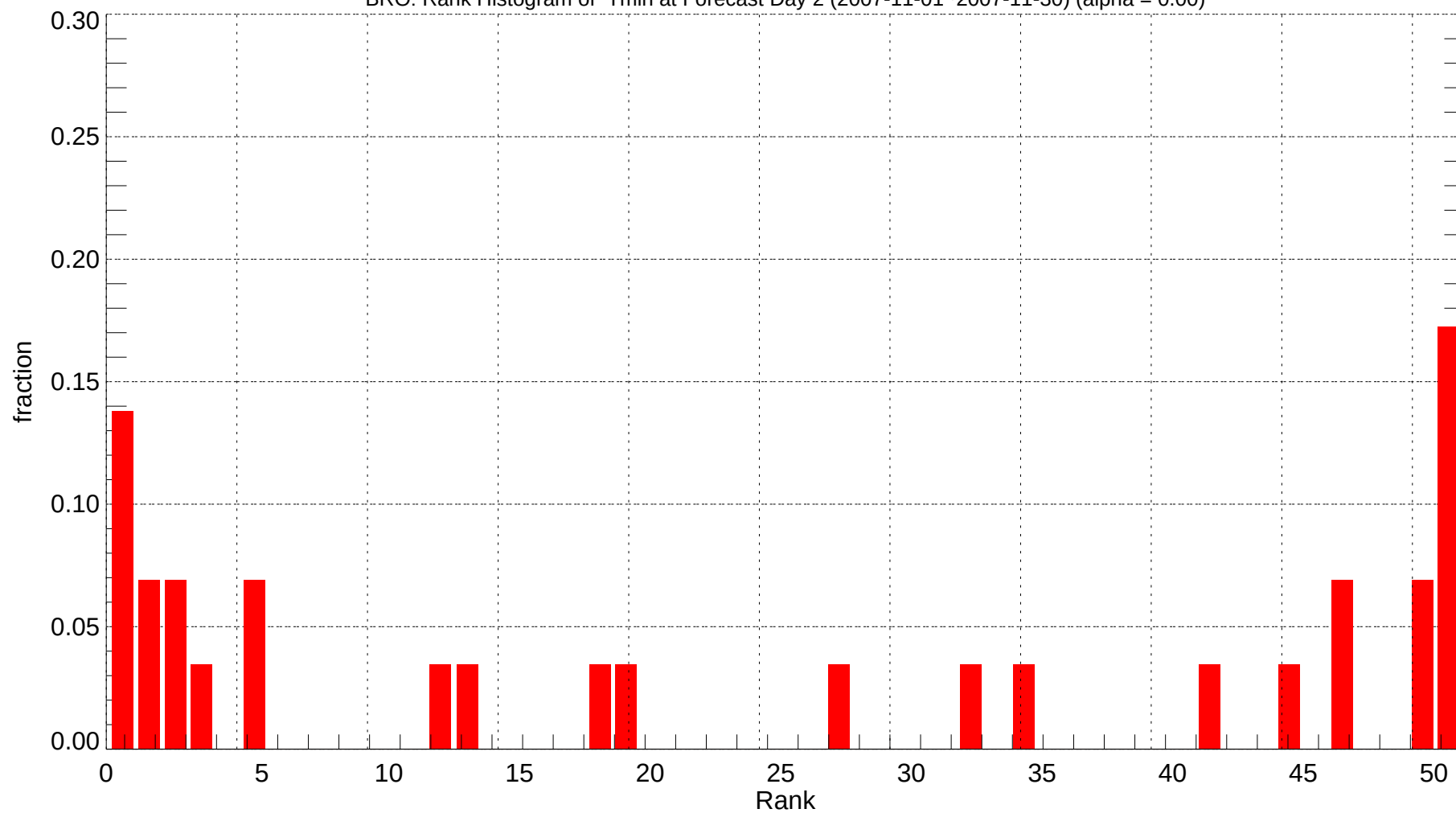
BRO: Rank Histogram of Tmin at Forecast Day 2 (2007-11-01~2007-11-30) (alpha = 0.00)
