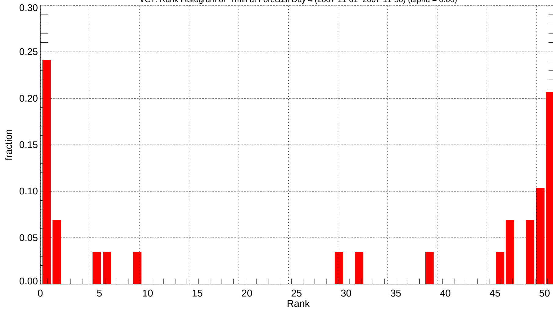
VCT: Rank Histogram of Tmin at Forecast Day 4 (2007-11-01~2007-11-30) (alpha = 0.00)
