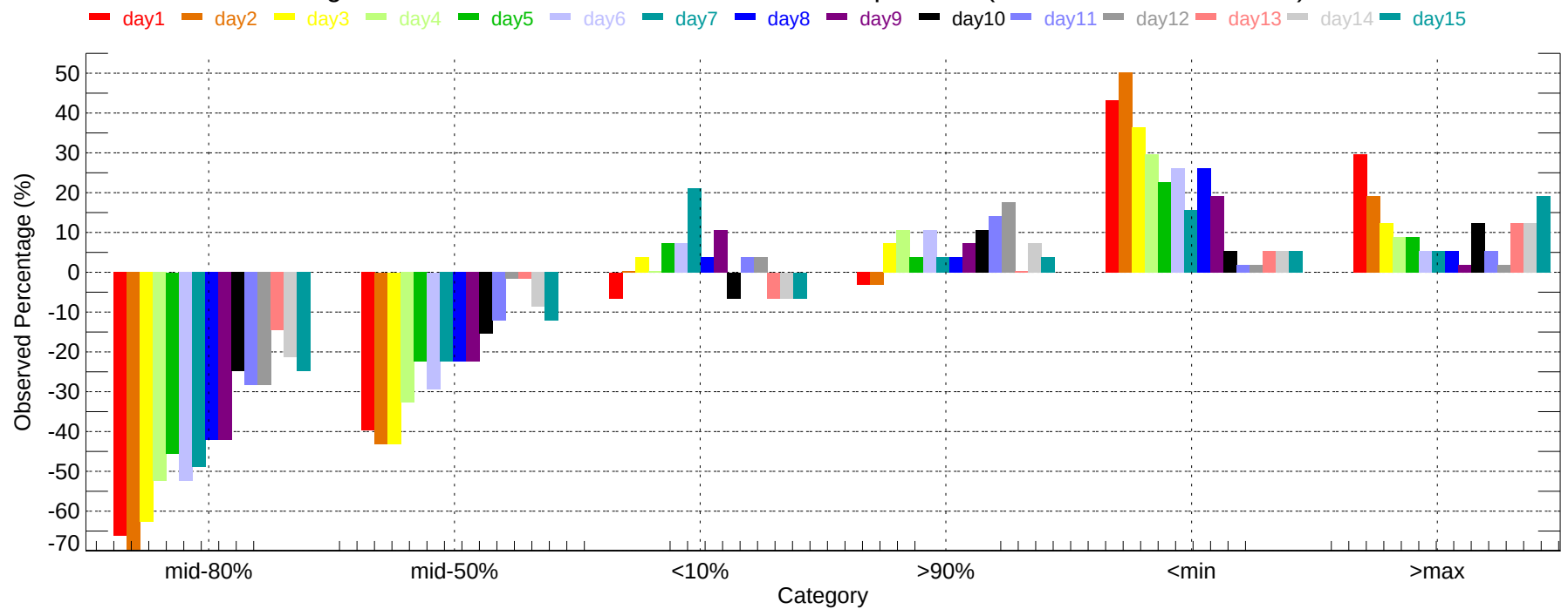
Observed Percentage Deviation of Ensembles - OAK: Max Temperature (2007-11-01~2007-11-30)
