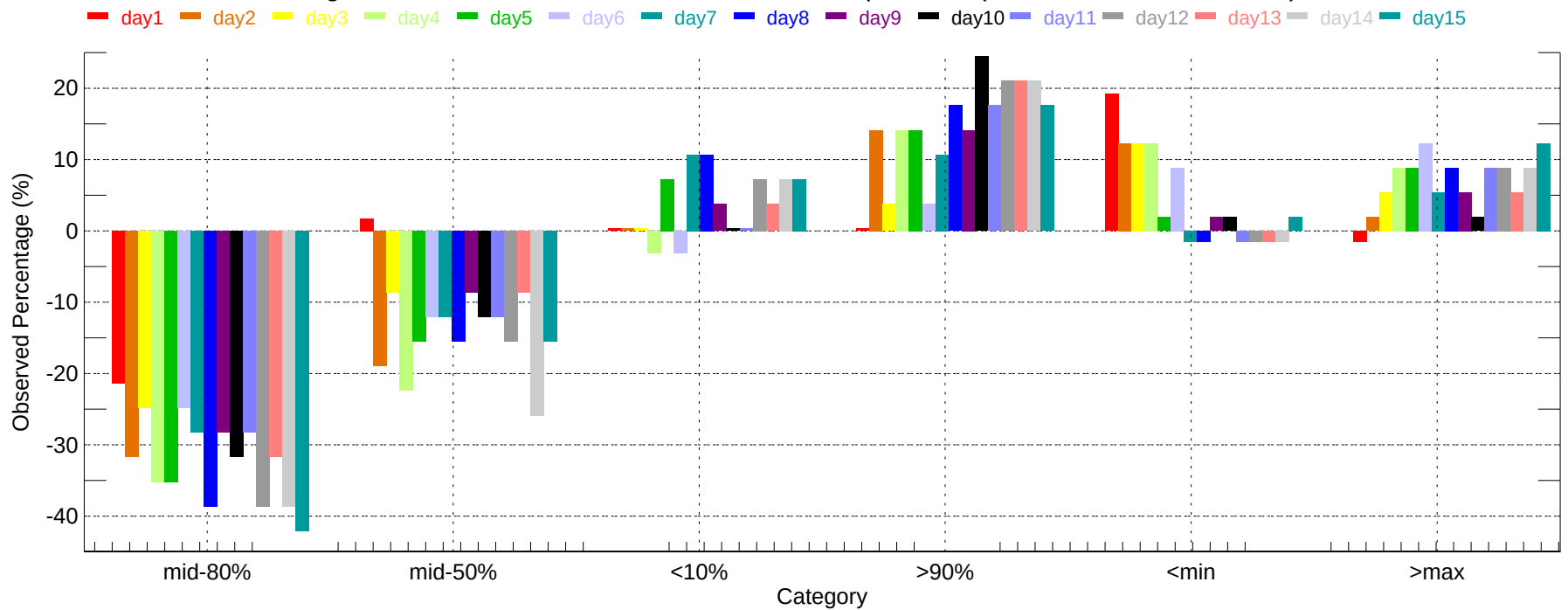
Observed Percentage Deviation of Ensembles - MAF: Min Temperature (2007-11-01~2007-11-30)
