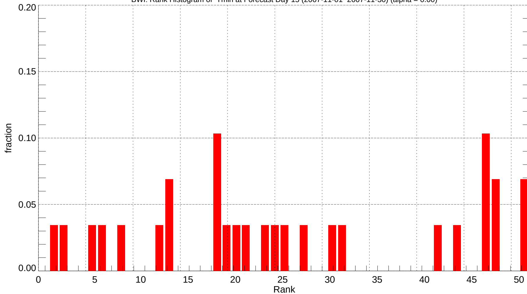
BWl: Rank Histogram of Tmin at Forecast Day 15 (2007-11-01~2007-11-30) (alpha = 0.00)
