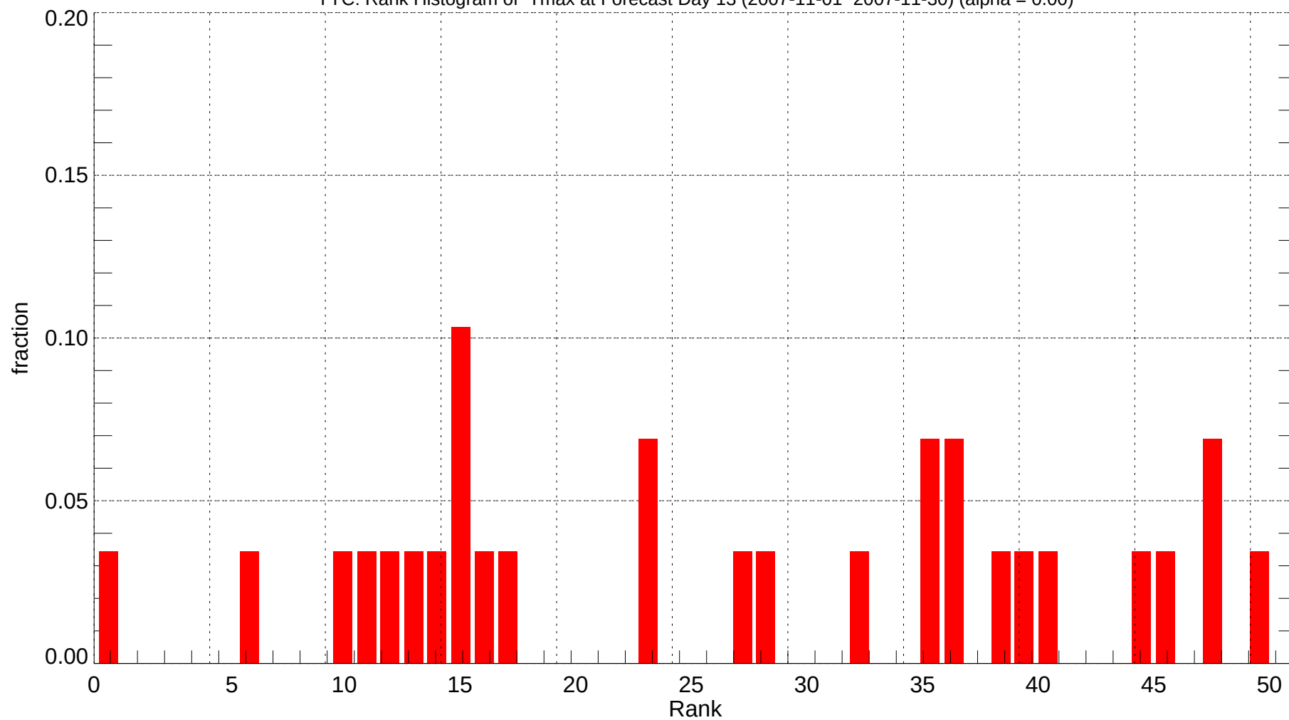
YYC: Rank Histogram of Tmax at Forecast Day 13 (2007-11-01~2007-11-30) (alpha = 0.00)
