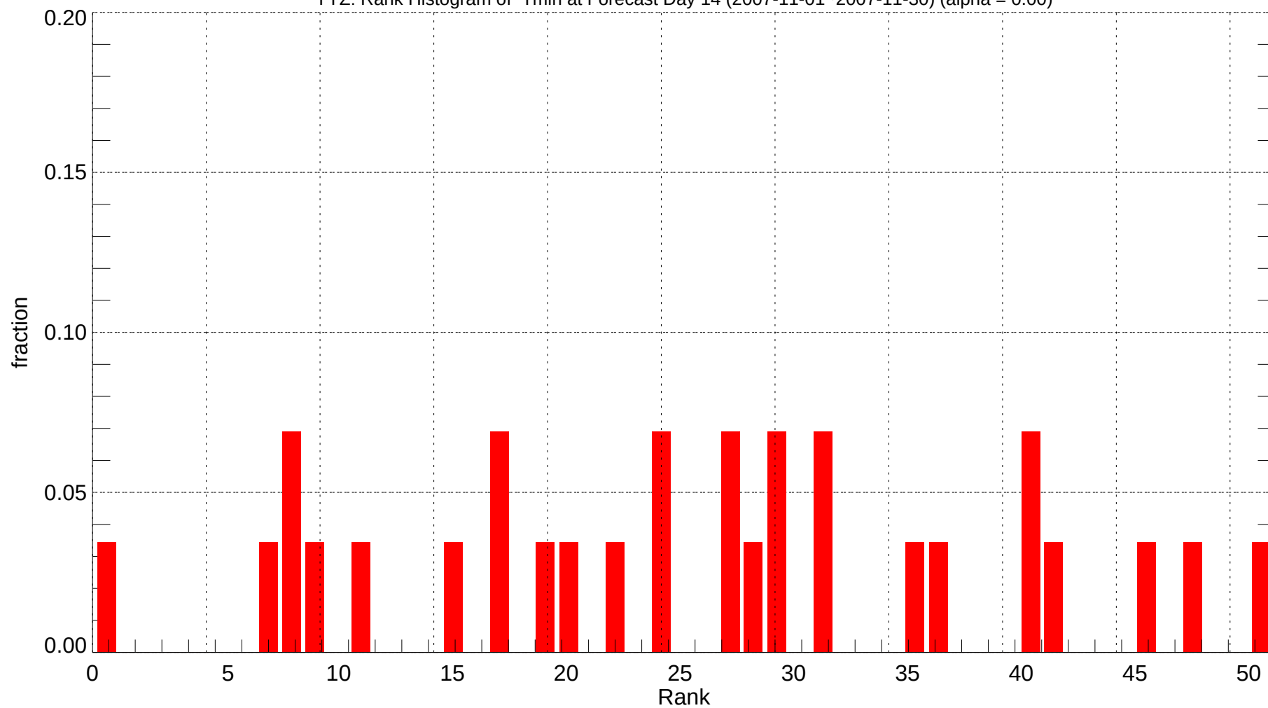
YYZ: Rank Histogram of Tmin at Forecast Day 14 (2007-11-01~2007-11-30) (alpha = 0.00)
