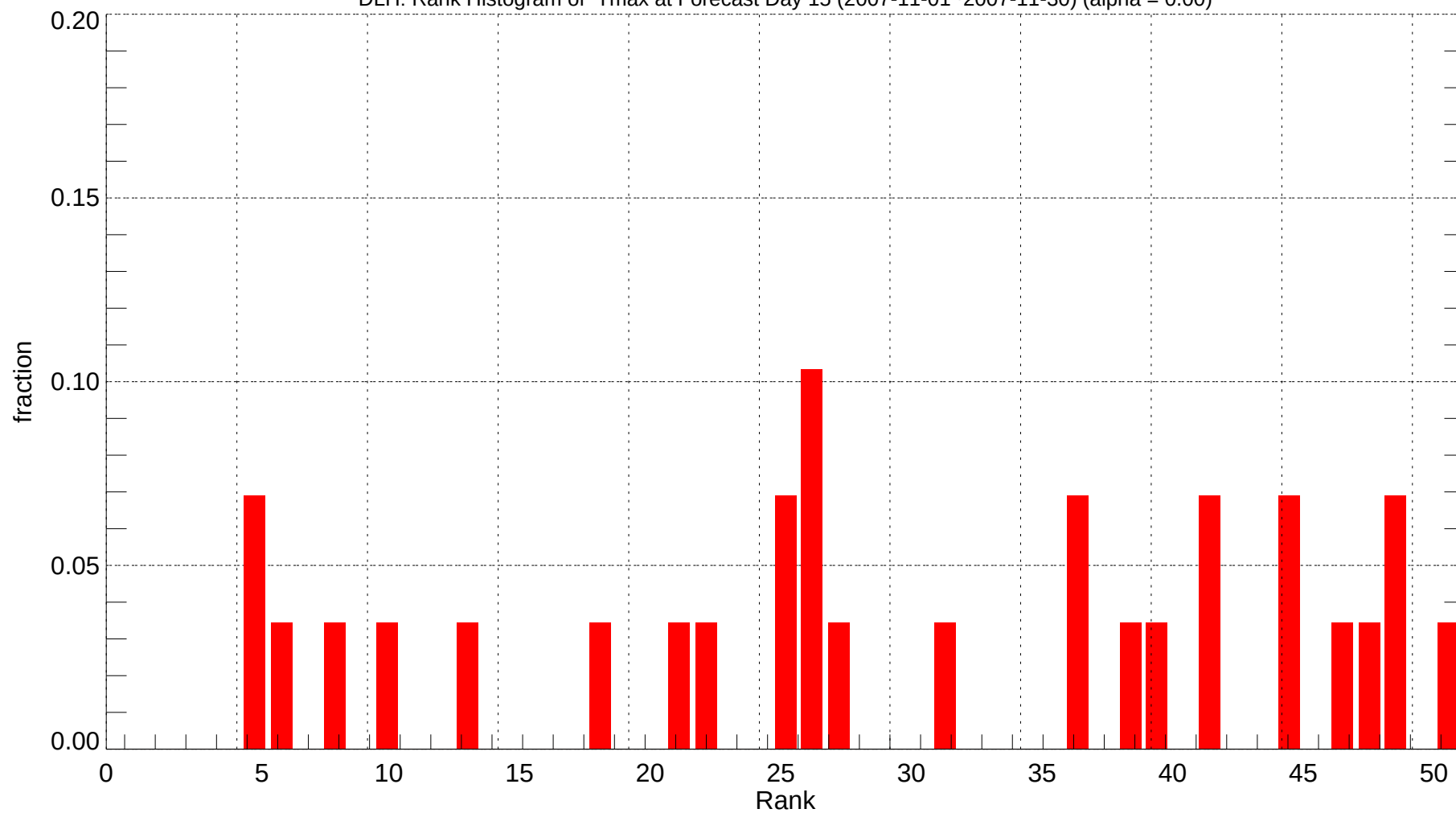
DLH: Rank Histogram of Tmax at Forecast Day 15 (2007-11-01~2007-11-30) (alpha = 0.00)
