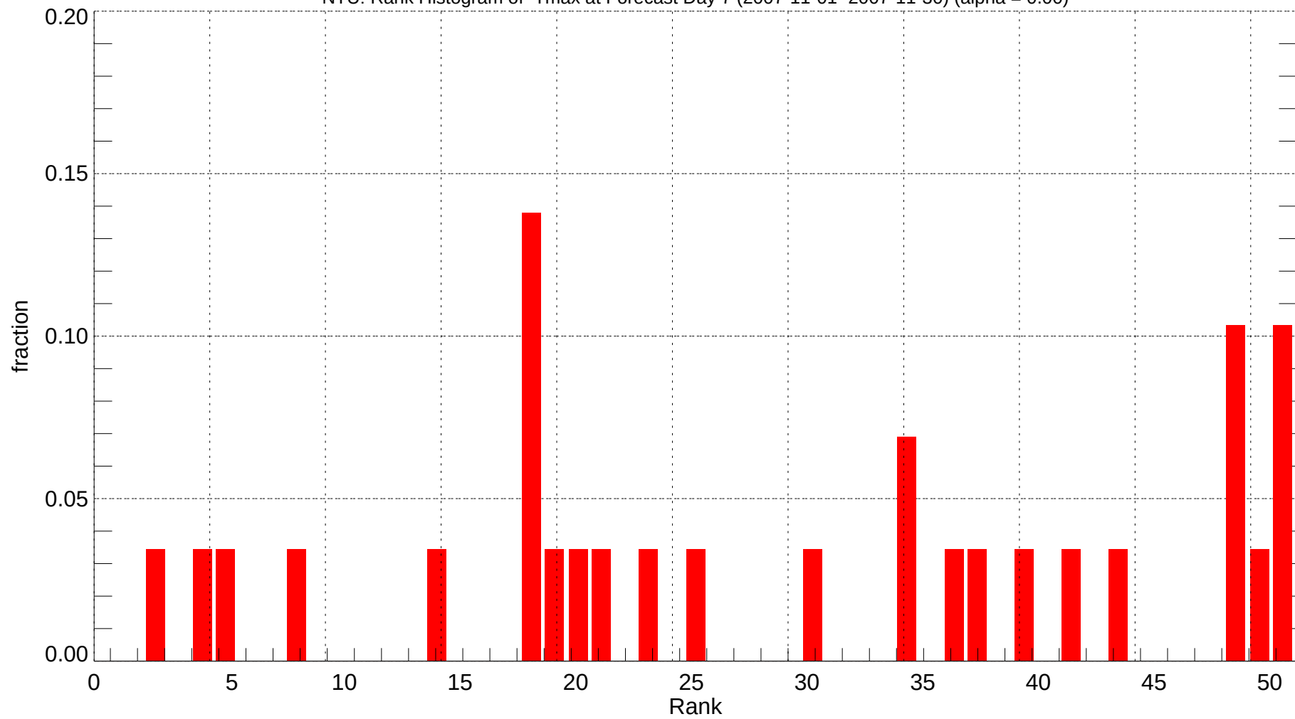
NTU: Rank Histogram of Tmax at Forecast Day 7 (2007-11-01~2007-11-30) (alpha = 0.00)
