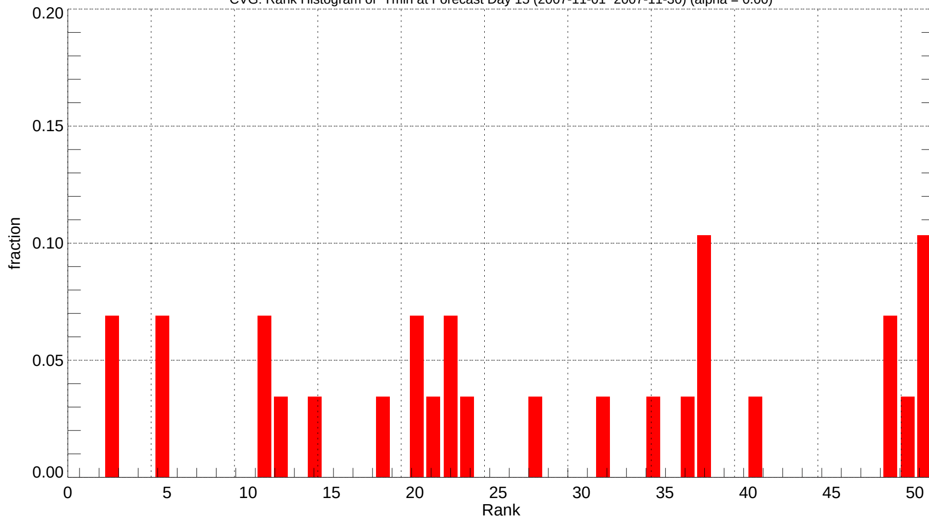
CVG: Rank Histogram of Tmin at Forecast Day 15 (2007-11-01~2007-11-30) (alpha = 0.00)
