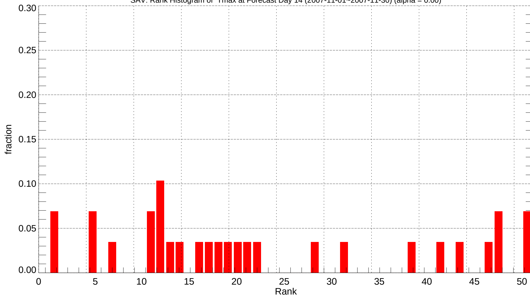
SAV: Rank Histogram of Tmax at Forecast Day 14 (2007-11-01~2007-11-30) (alpha = 0.00)
