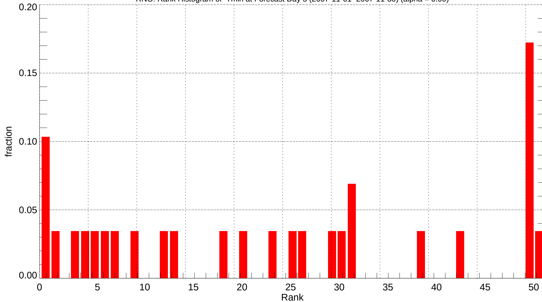
RNO: Rank Histogram of Tmin at Forecast Day 5 (2007-11-01~2007-11-30) (alpha = 0.00)
