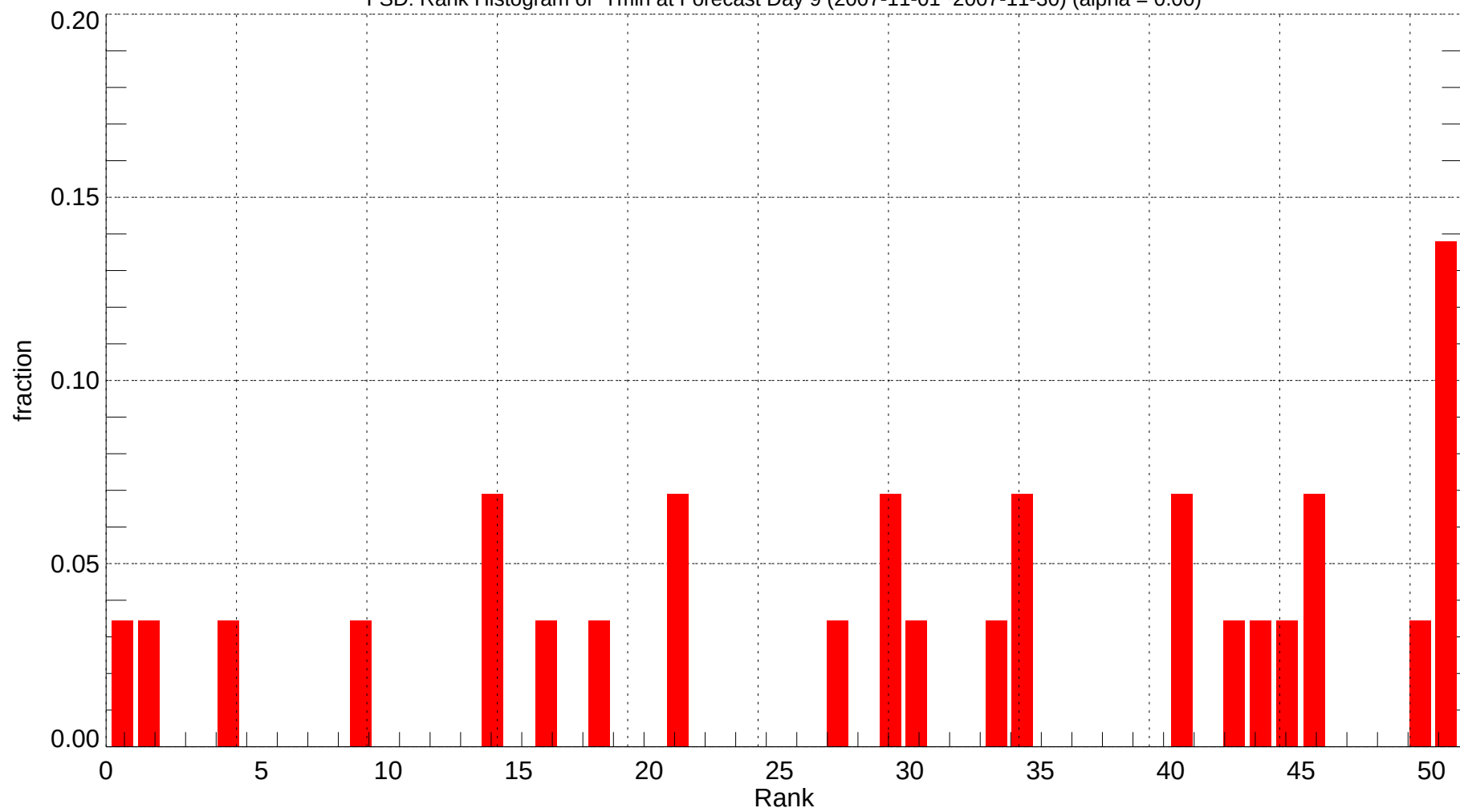
FSD: Rank Histogram of Tmin at Forecast Day 9 (2007-11-01~2007-11-30) (alpha = 0.00)
