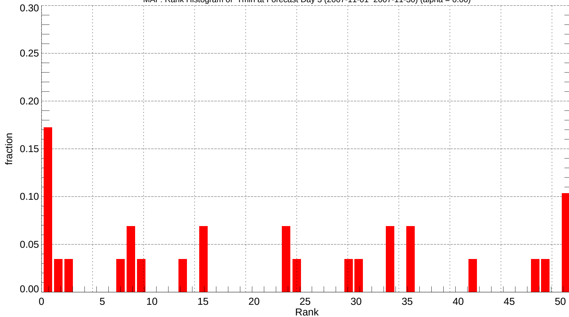
MAF: Rank Histogram of Tmin at Forecast Day 3 (2007-11-01~2007-11-30) (alpha = 0.00)
