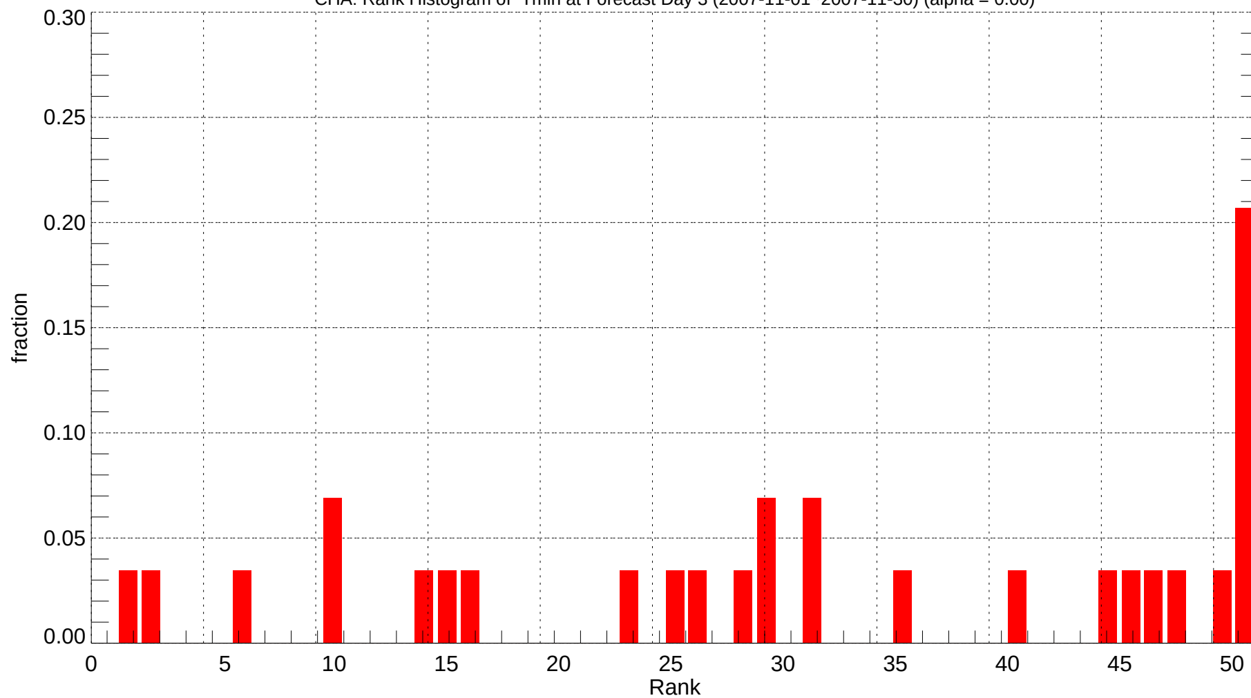
CHA: Rank Histogram of Tmin at Forecast Day 3 (2007-11-01~2007-11-30) (alpha = 0.00)
