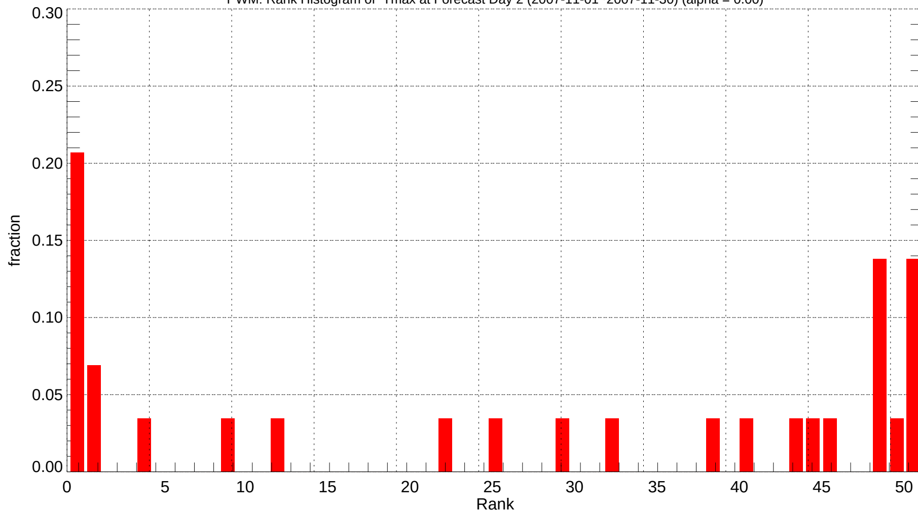
PWM: Rank Histogram of Tmax at Forecast Day 2 (2007-11-01~2007-11-30) (alpha = 0.00)
