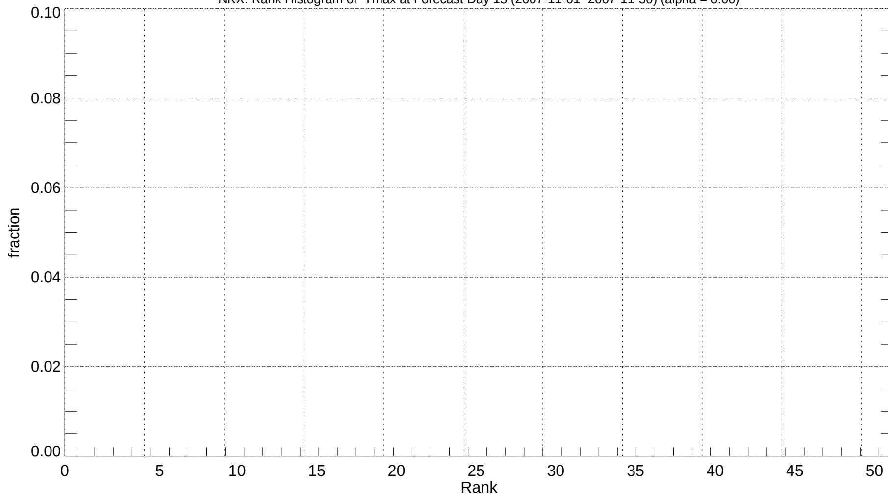
NKX: Rank Histogram of Tmax at Forecast Day 13 (2007-11-01~2007-11-30) (alpha = 0.00)
