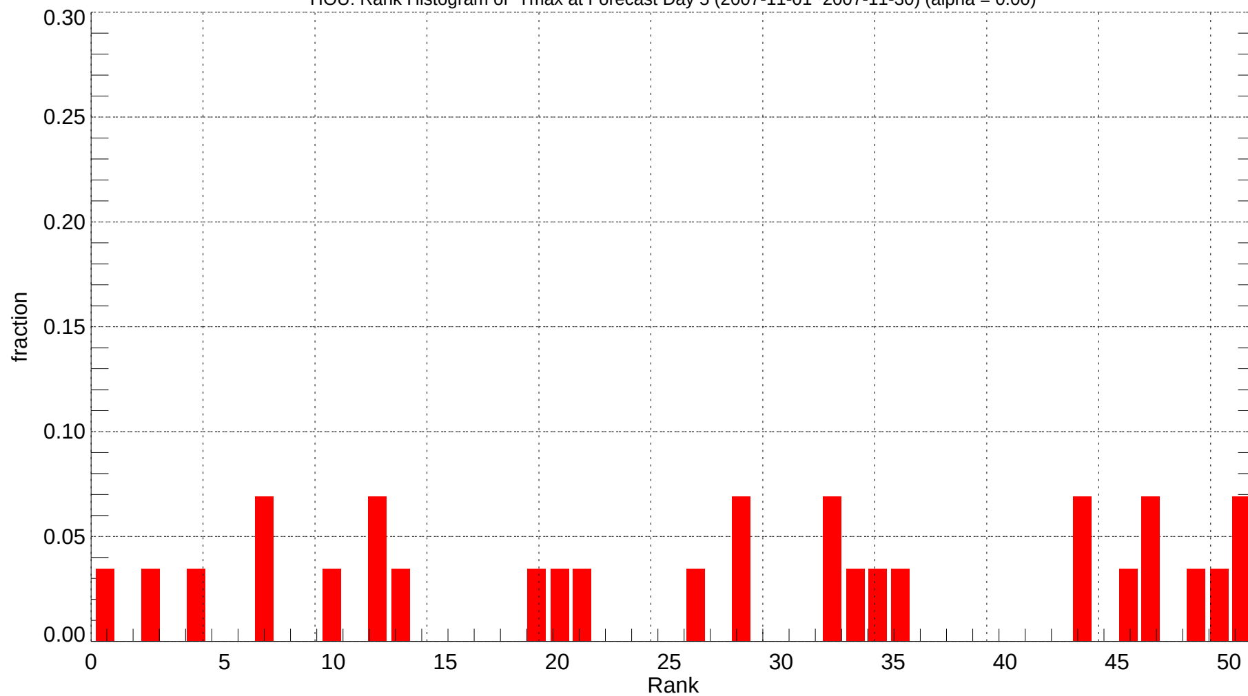
HOU: Rank Histogram of Tmax at Forecast Day 5 (2007-11-01~2007-11-30) (alpha = 0.00)
