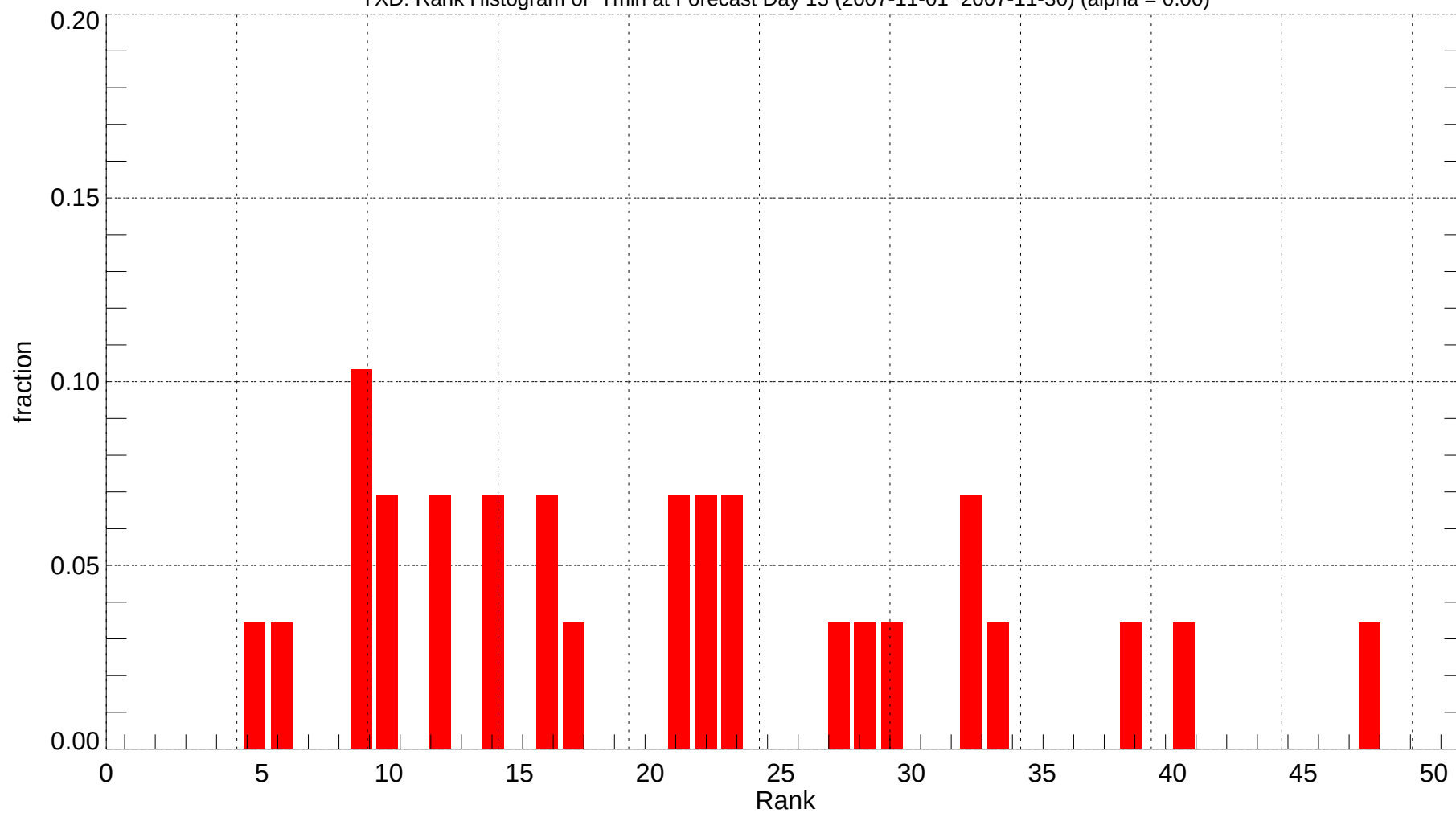
YXD: Rank Histogram of Tmin at Forecast Day 13 (2007-11-01~2007-11-30) (alpha = 0.00)
