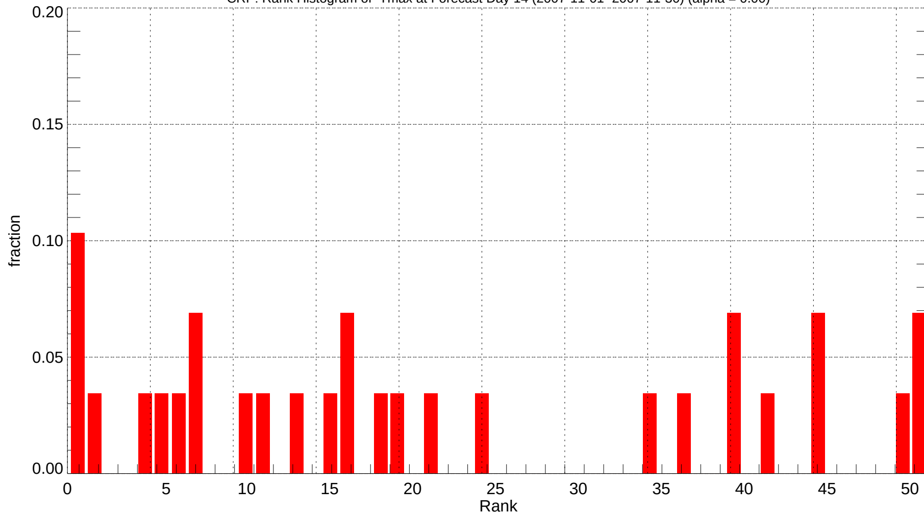
CRP: Rank Histogram of Tmax at Forecast Day 14 (2007-11-01~2007-11-30) (alpha = 0.00)
