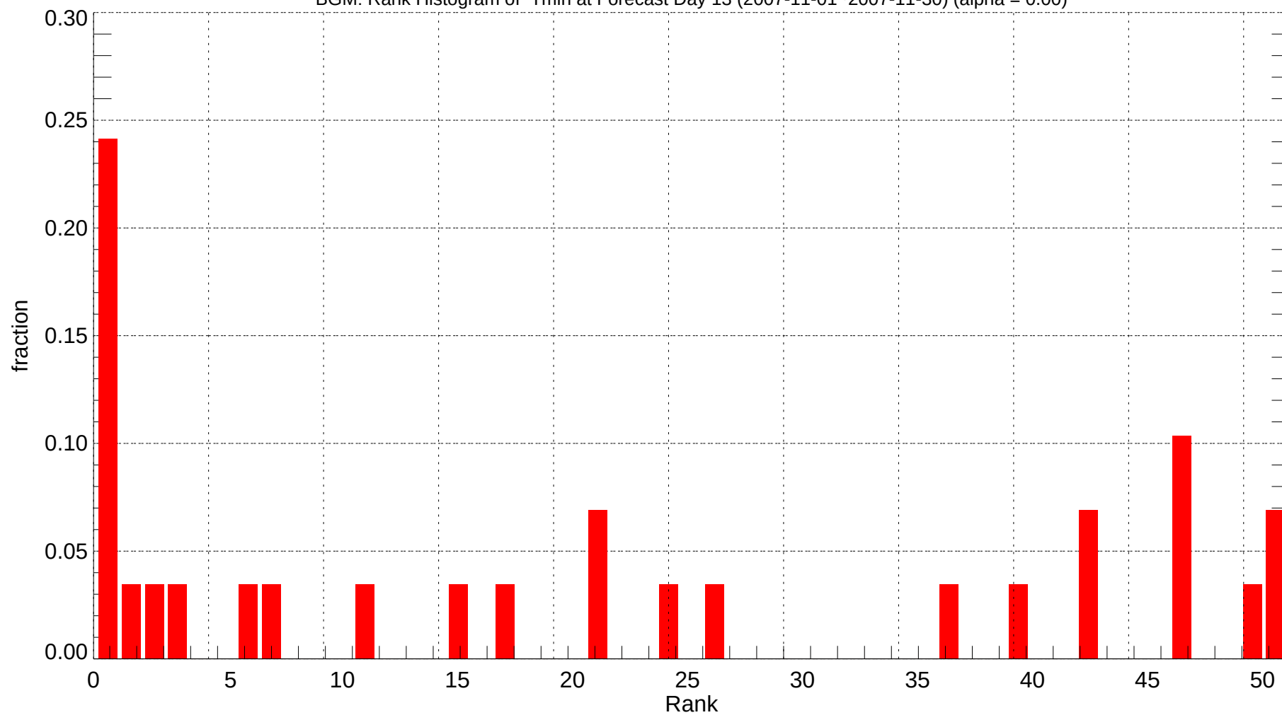
BGM: Rank Histogram of Tmin at Forecast Day 13 (2007-11-01~2007-11-30) (alpha = 0.00)
