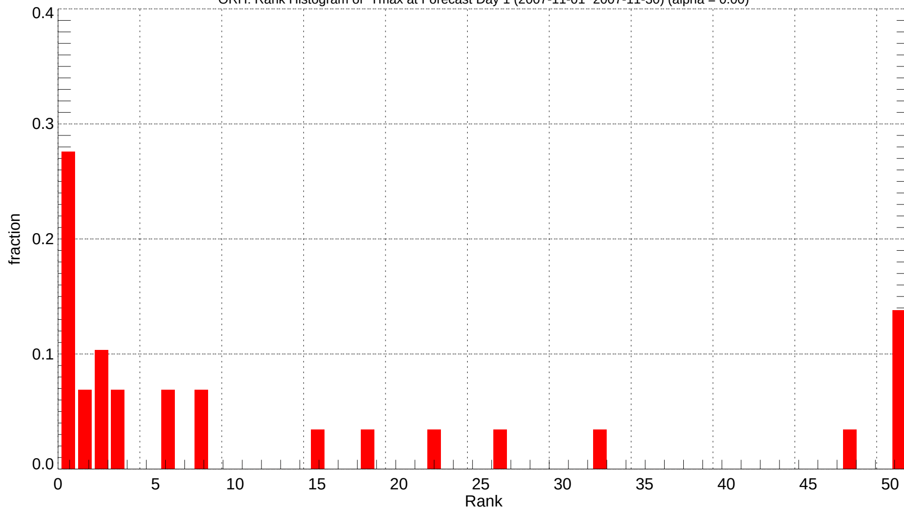
ORH: Rank Histogram of Tmax at Forecast Day 1 (2007-11-01~2007-11-30) (alpha = 0.00)
