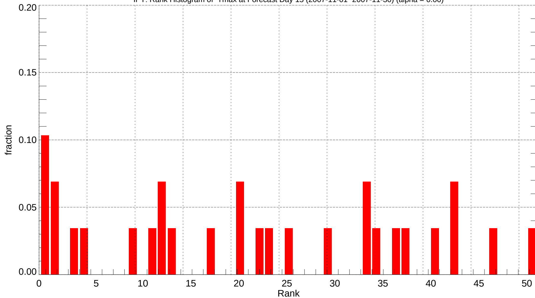
IPT: Rank Histogram of Tmax at Forecast Day 15 (2007-11-01~2007-11-30) (alpha = 0.00)
