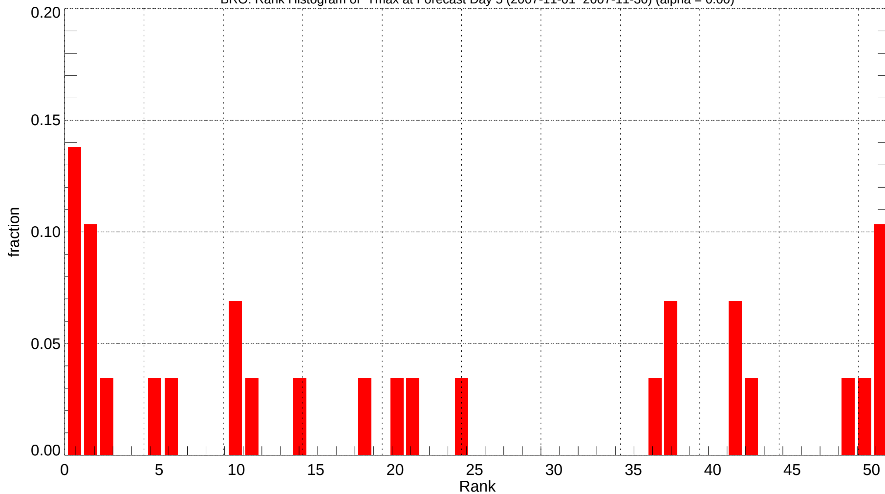
BRO: Rank Histogram of Tmax at Forecast Day 5 (2007-11-01~2007-11-30) (alpha = 0.00)
