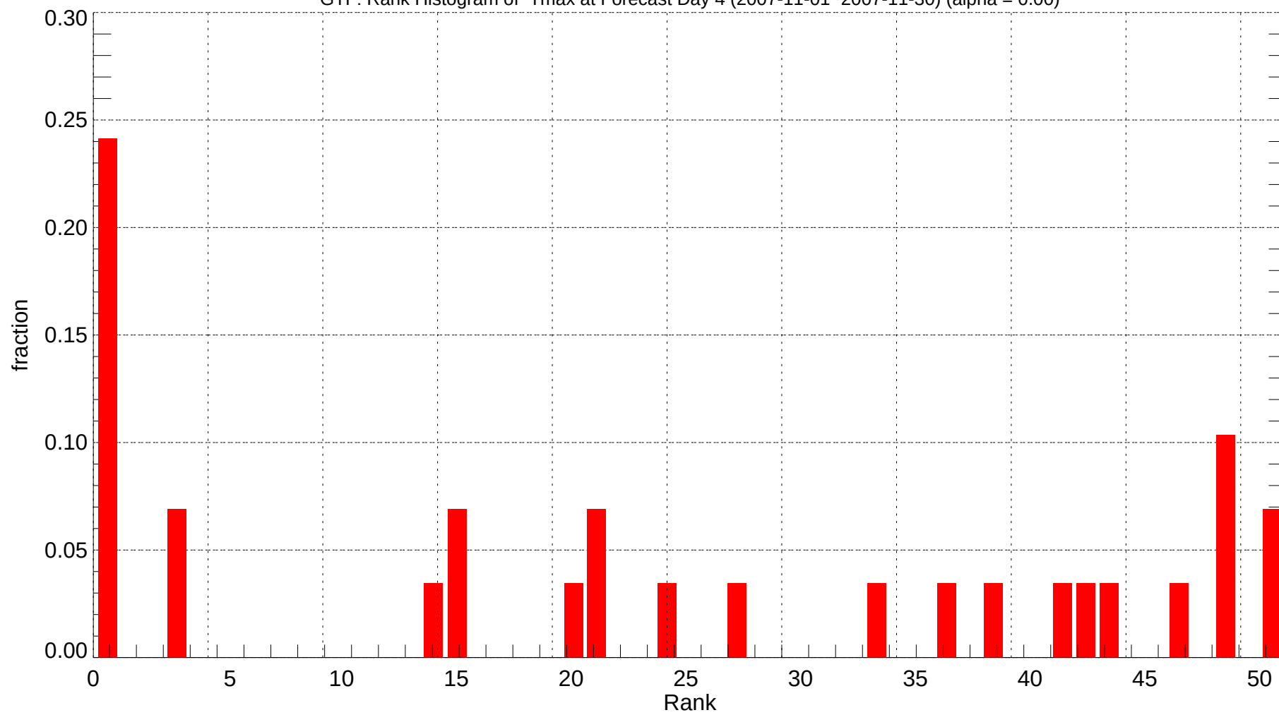
GTF: Rank Histogram of Tmax at Forecast Day 4 (2007-11-01~2007-11-30) (alpha = 0.00)
