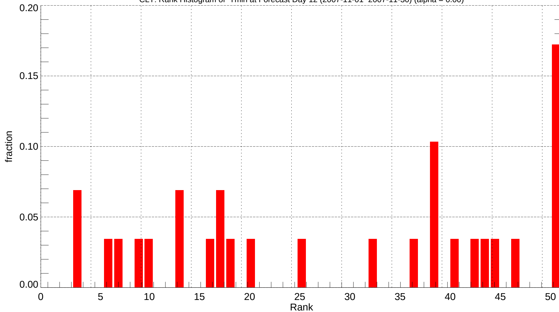
CLT: Rank Histogram of Tmin at Forecast Day 12 (2007-11-01~2007-11-30) (alpha = 0.00)
