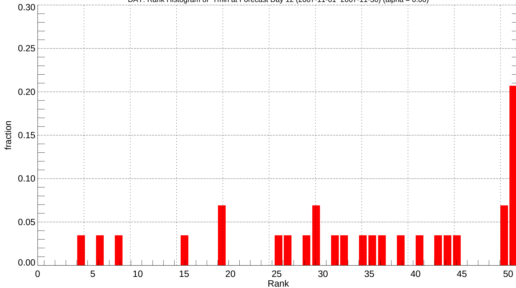
DAY: Rank Histogram of Tmin at Forecast Day 12 (2007-11-01~2007-11-30) (alpha = 0.00)
