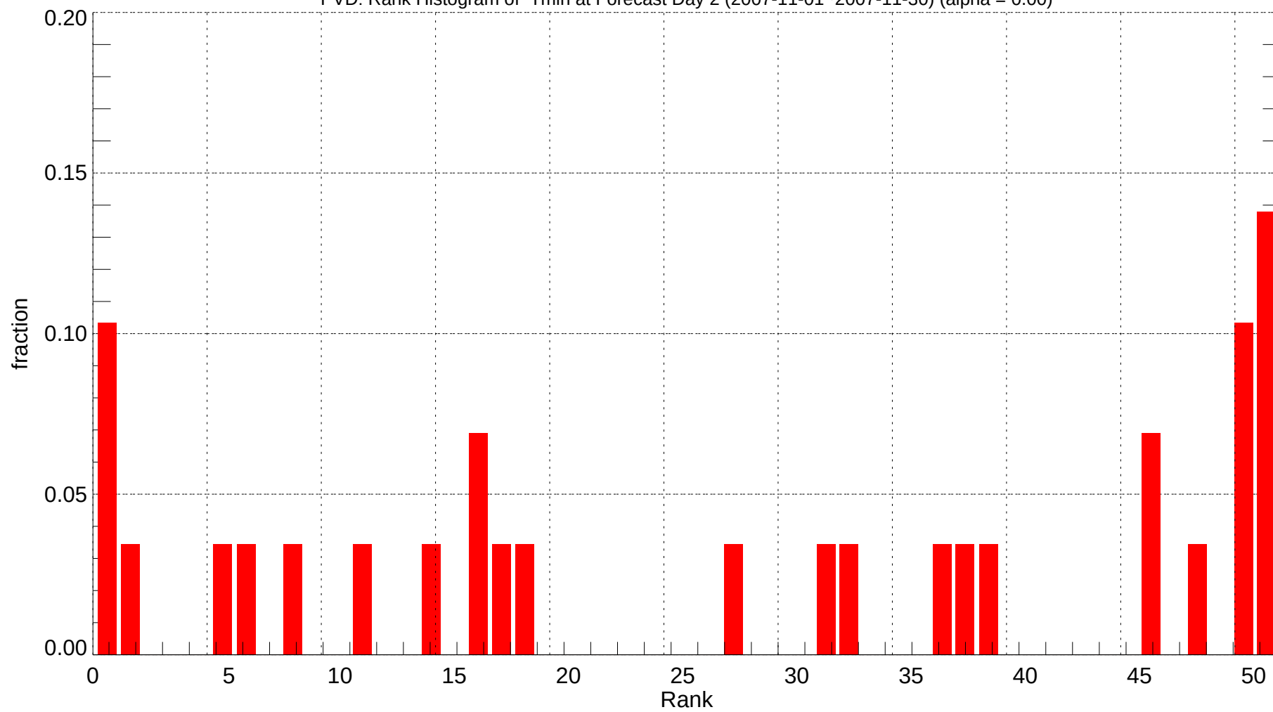
PVD: Rank Histogram of Tmin at Forecast Day 2 (2007-11-01~2007-11-30) (alpha = 0.00)
