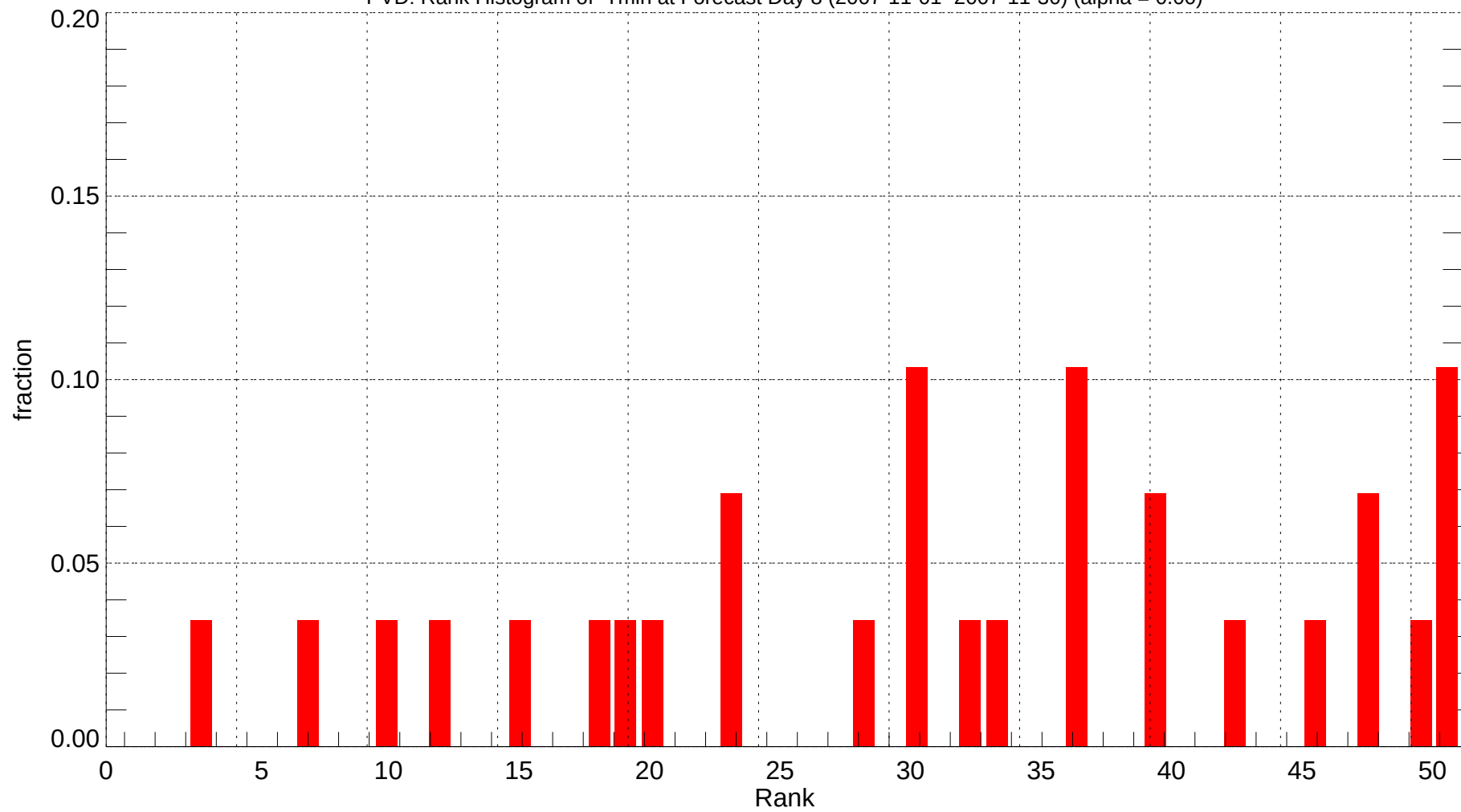
PVD: Rank Histogram of Tmin at Forecast Day 8 (2007-11-01~2007-11-30) (alpha = 0.00)
