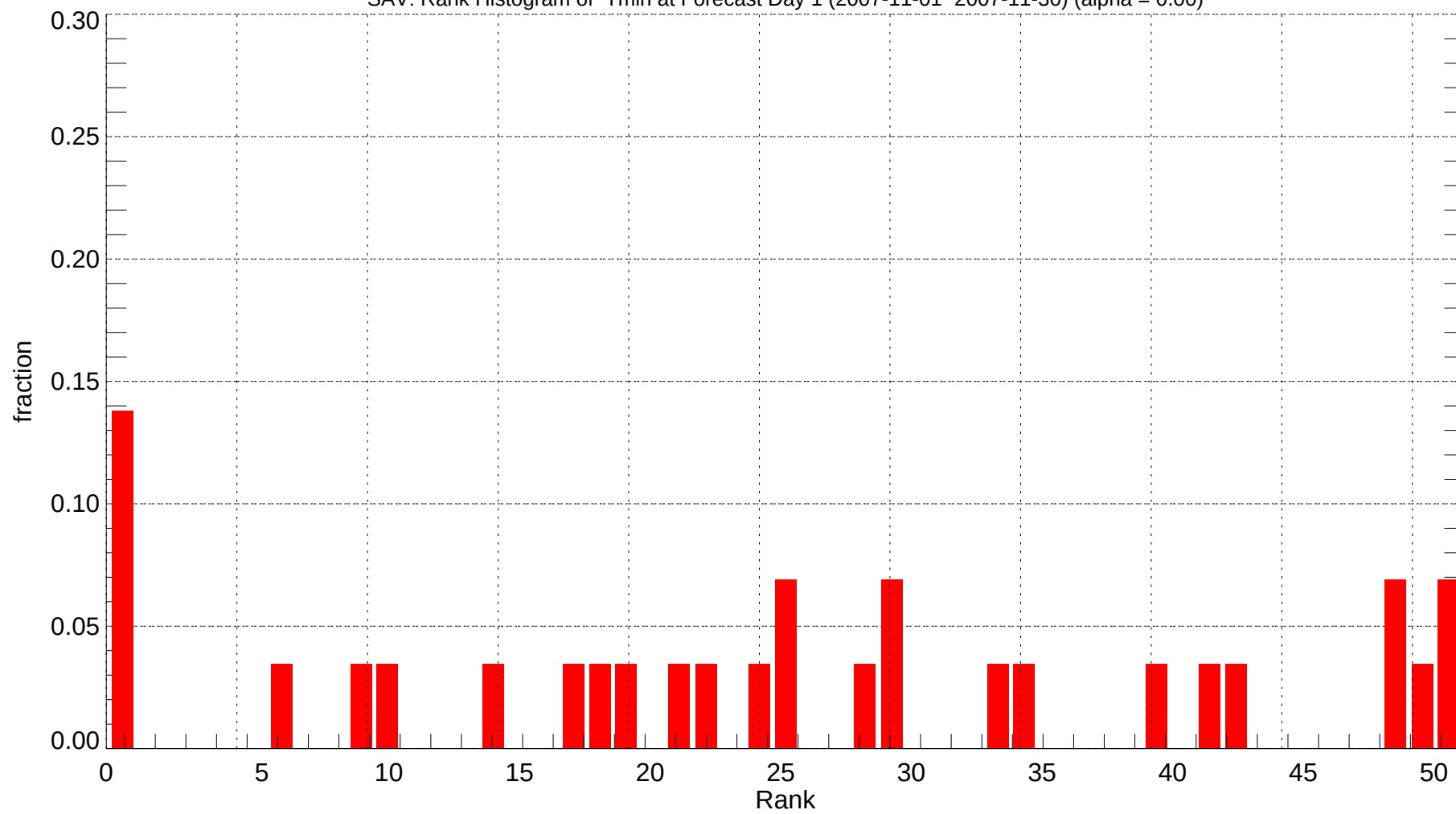
SAV: Rank Histogram of Tmin at Forecast Day 1 (2007-11-01~2007-11-30) (alpha = 0.00)
