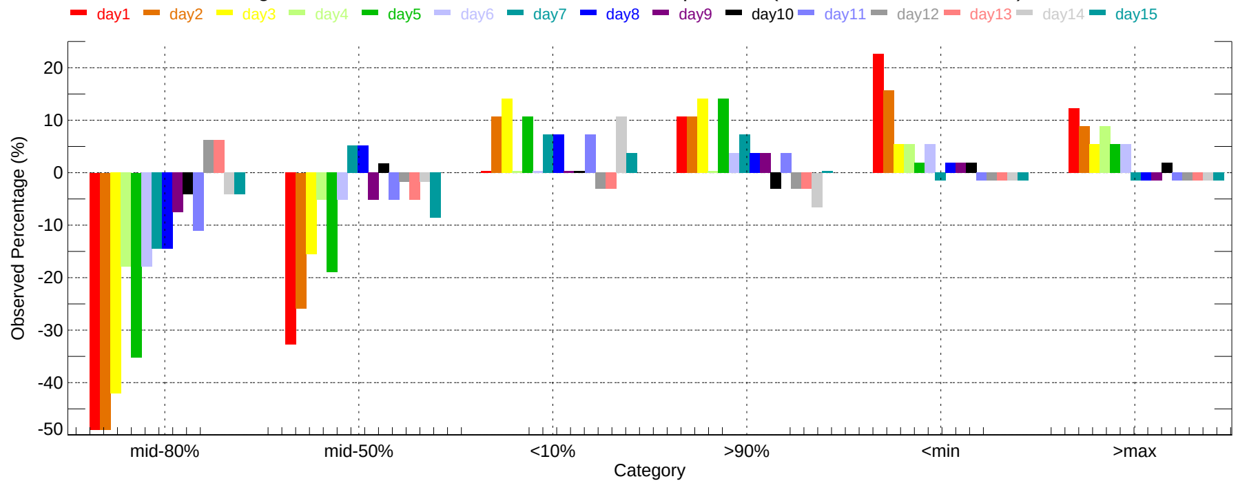
Observed Percentage Deviation of Ensembles - MIA: Max Temperature (2007-11-01~2007-11-30)
