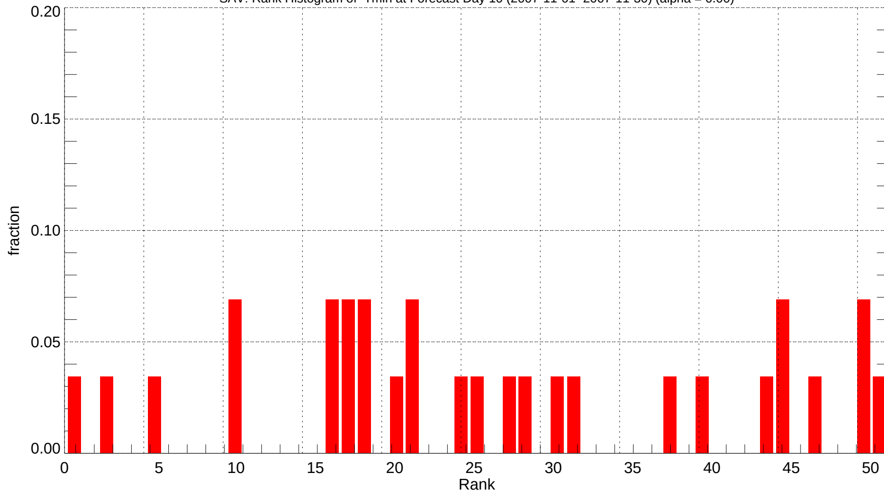
SAV: Rank Histogram of Tmin at Forecast Day 10 (2007-11-01~2007-11-30) (alpha = 0.00)
