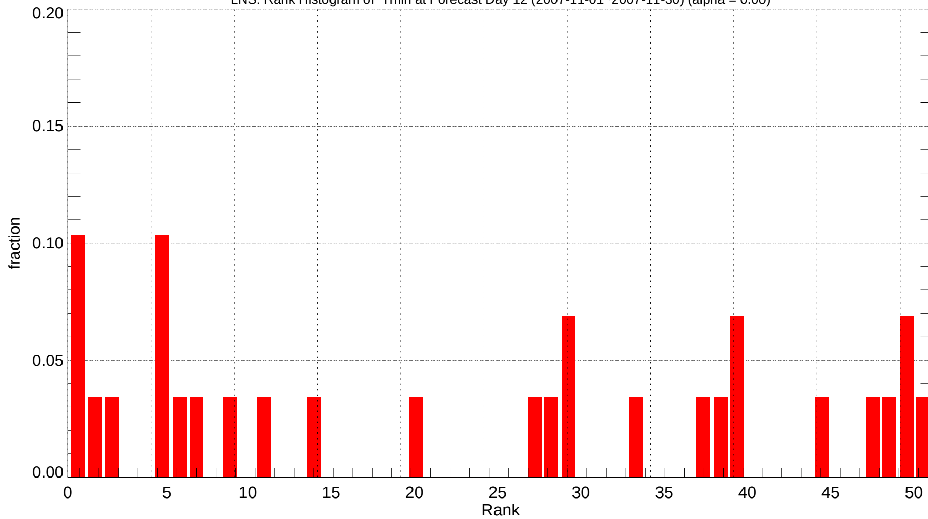
LNS: Rank Histogram of Tmin at Forecast Day 12 (2007-11-01~2007-11-30) (alpha = 0.00)
