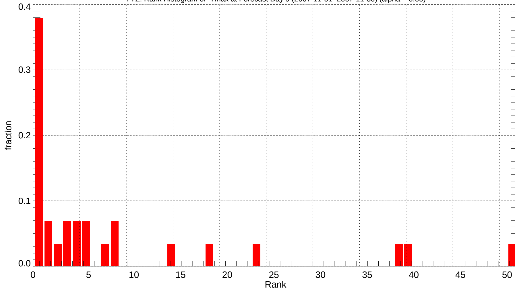
YYZ: Rank Histogram of Tmax at Forecast Day 9 (2007-11-01~2007-11-30) (alpha = 0.00)
