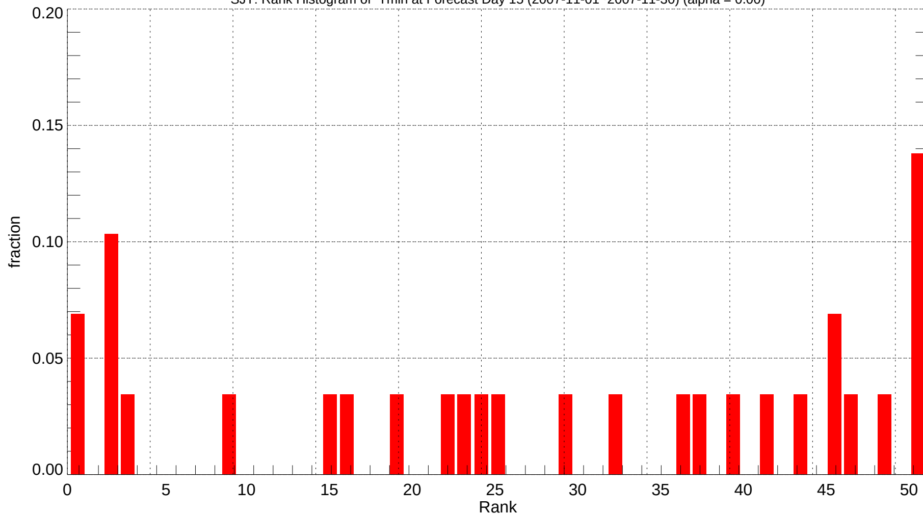
SJT: Rank Histogram of Tmin at Forecast Day 15 (2007-11-01~2007-11-30) (alpha = 0.00)
