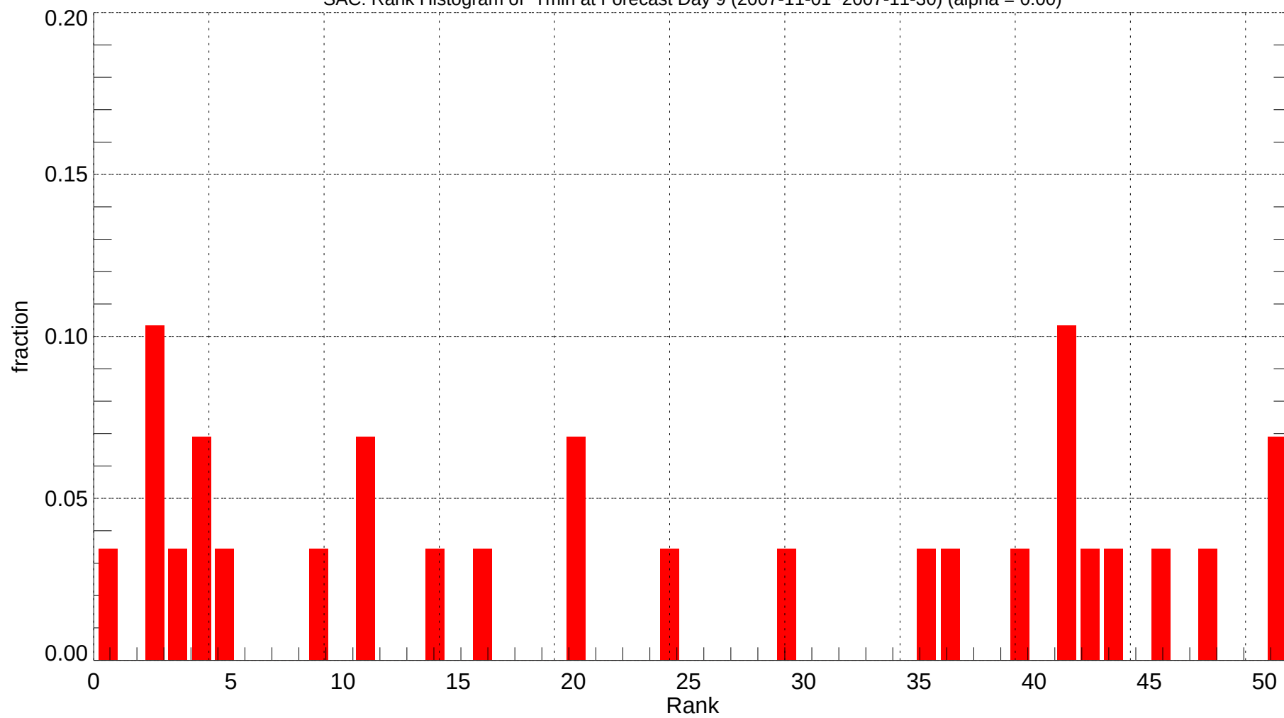
SAC: Rank Histogram of Tmin at Forecast Day 9 (2007-11-01~2007-11-30) (alpha = 0.00)
