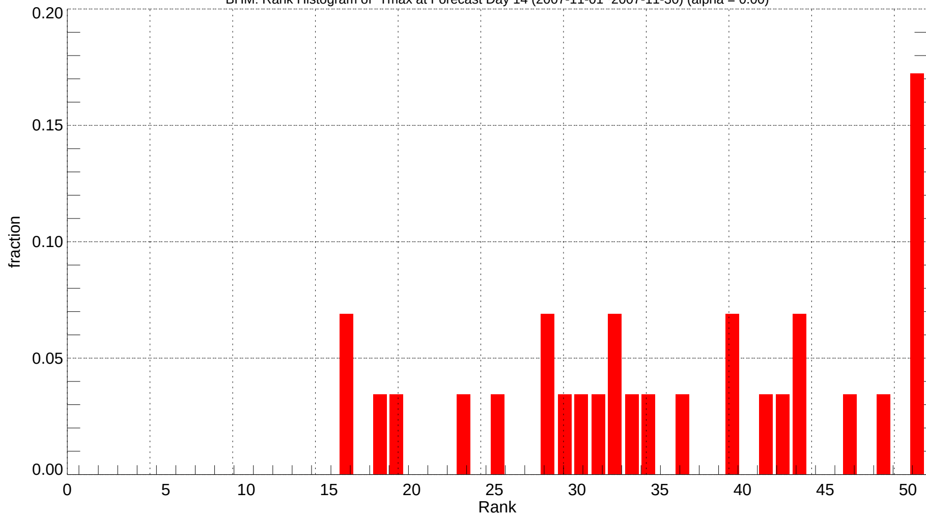
BHM: Rank Histogram of Tmax at Forecast Day 14 (2007-11-01~2007-11-30) (alpha = 0.00)
