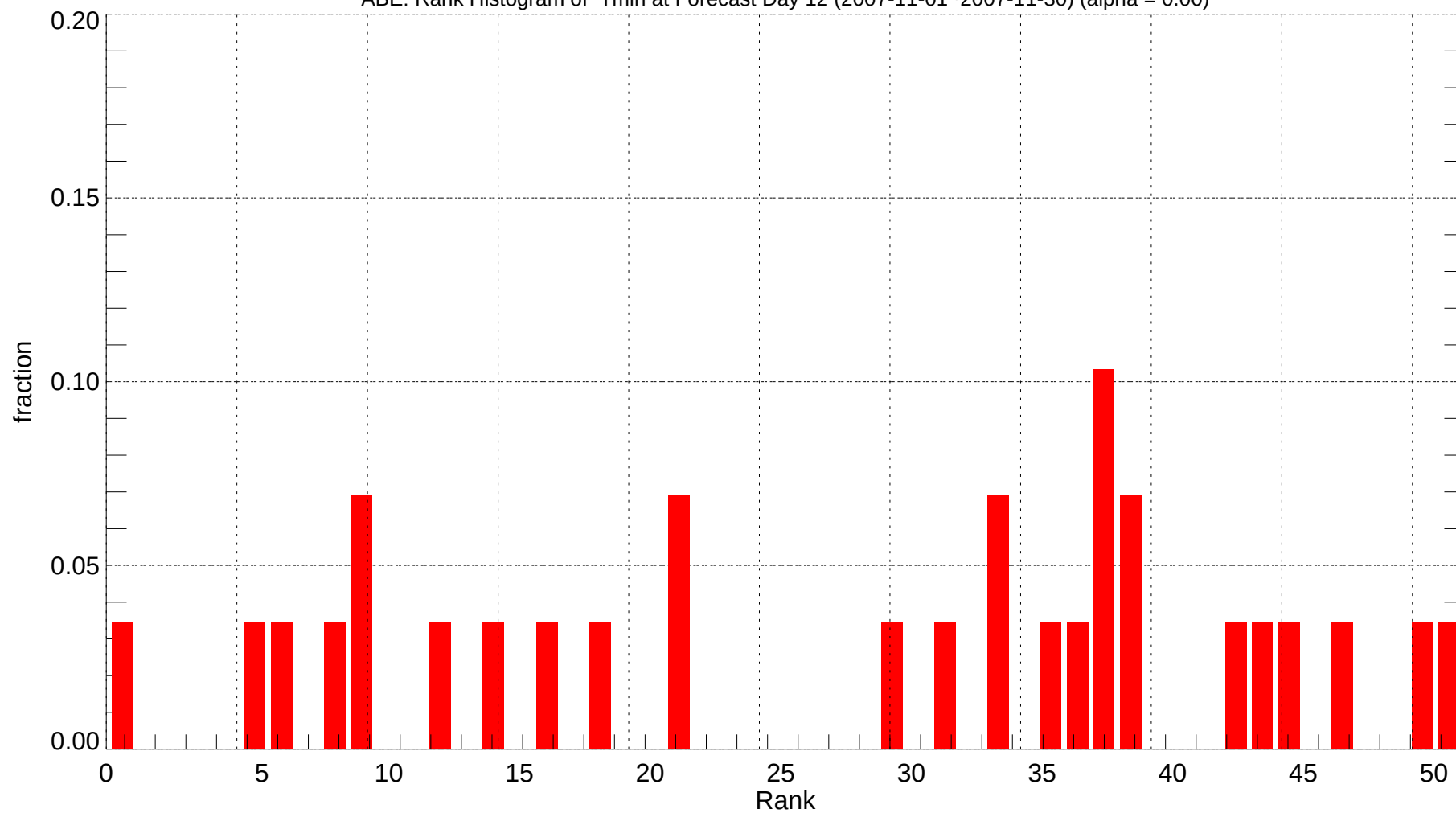
ABE: Rank Histogram of Tmin at Forecast Day 12 (2007-11-01~2007-11-30) (alpha = 0.00)
