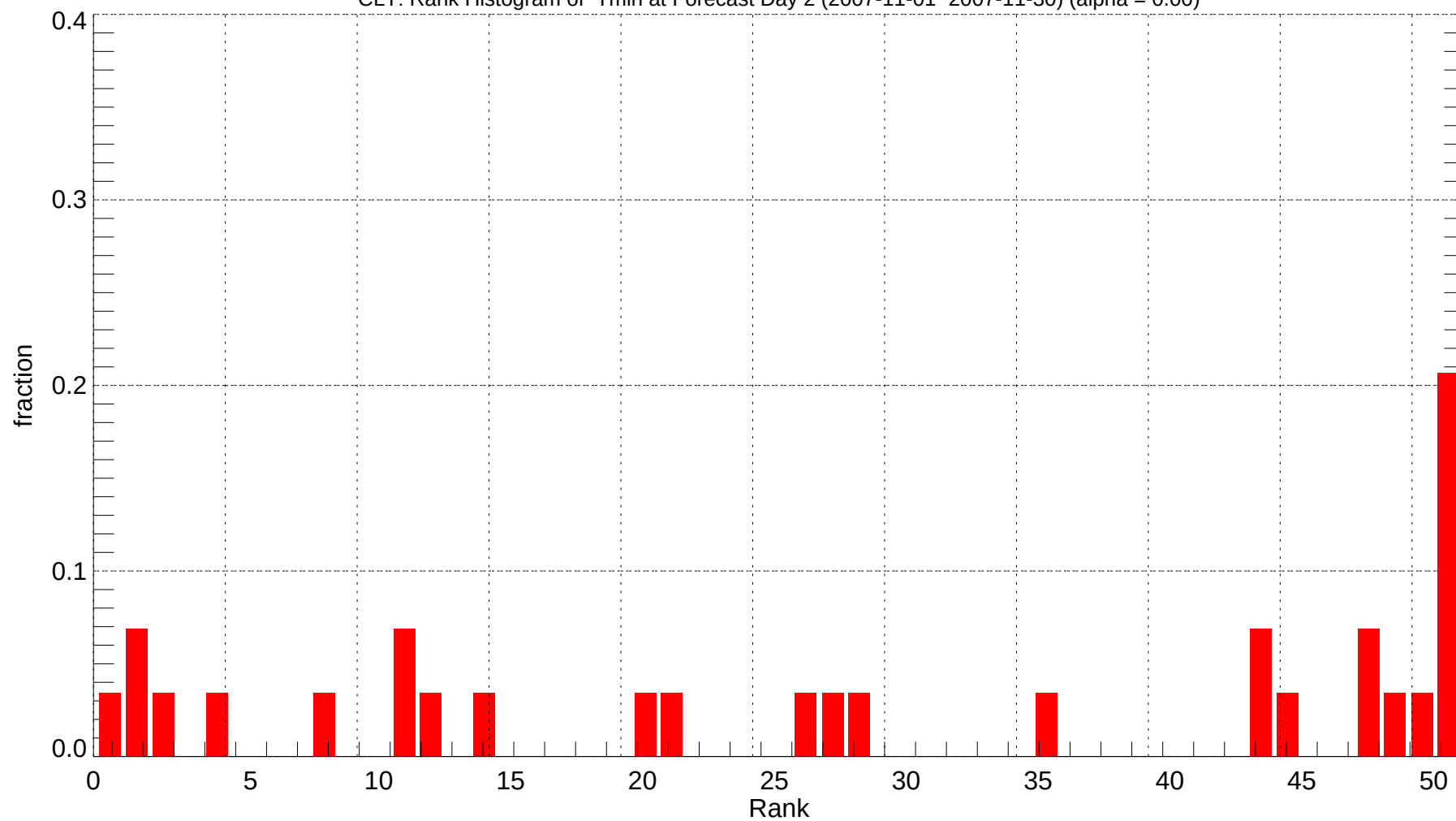
CLT: Rank Histogram of Tmin at Forecast Day 2 (2007-11-01~2007-11-30) (alpha = 0.00)
