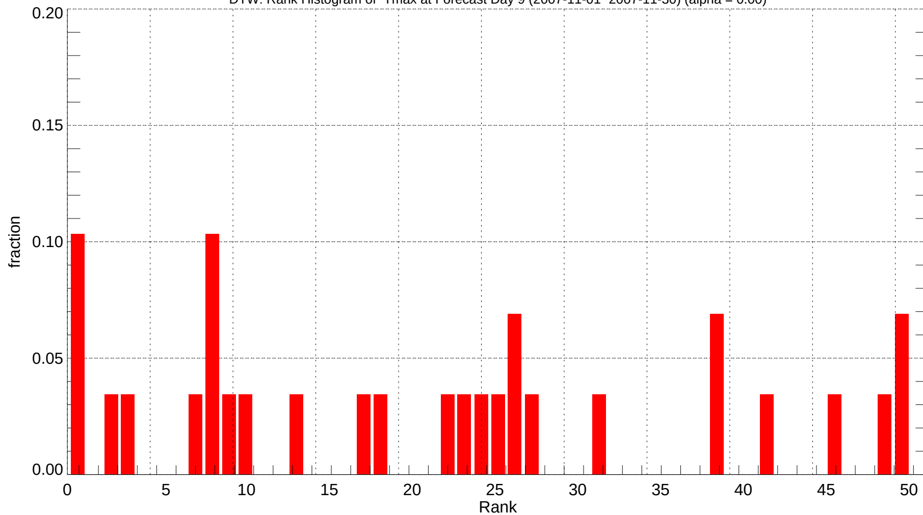
DTW: Rank Histogram of Tmax at Forecast Day 9 (2007-11-01~2007-11-30) (alpha = 0.00)
