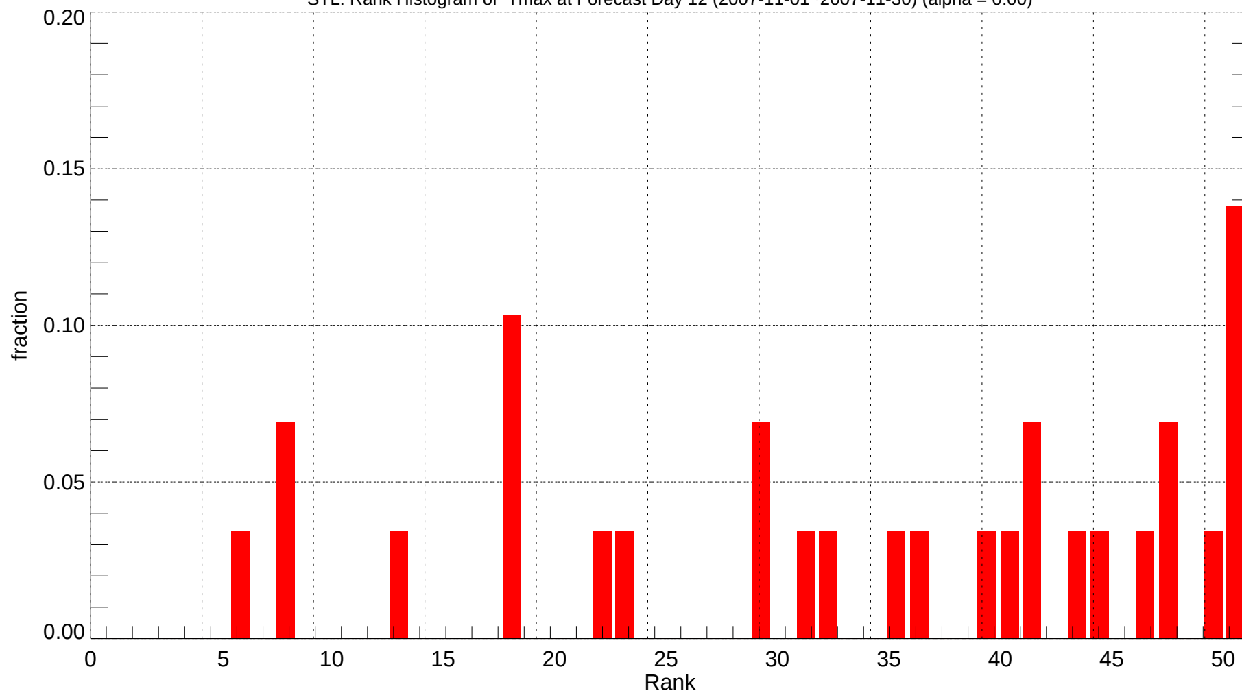
STL: Rank Histogram of Tmax at Forecast Day 12 (2007-11-01~2007-11-30) (alpha = 0.00)
