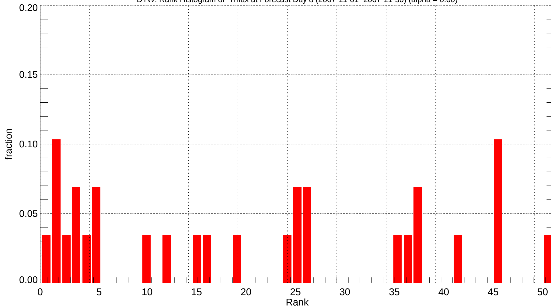
DTW: Rank Histogram of Tmax at Forecast Day 8 (2007-11-01~2007-11-30) (alpha = 0.00)
