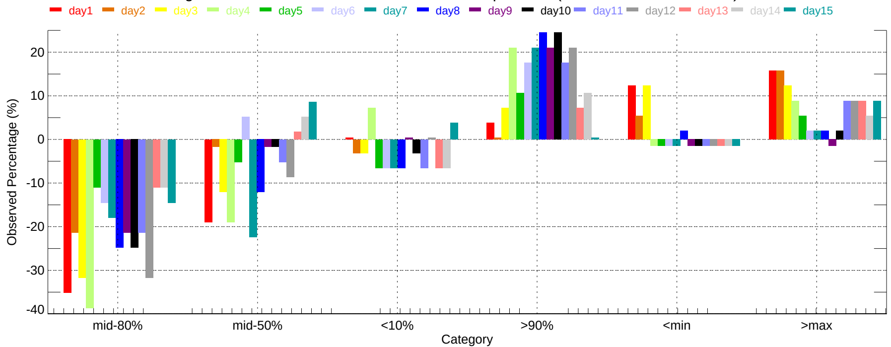
Observed Percentage Deviation of Ensembles - CVG: Min Temperature (2007-11-01~2007-11-30)
