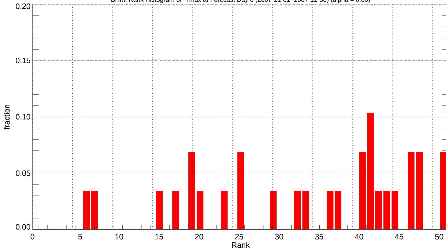
BHM: Rank Histogram of Tmax at Forecast Day 6 (2007-11-01~2007-11-30) (alpha = 0.00)
