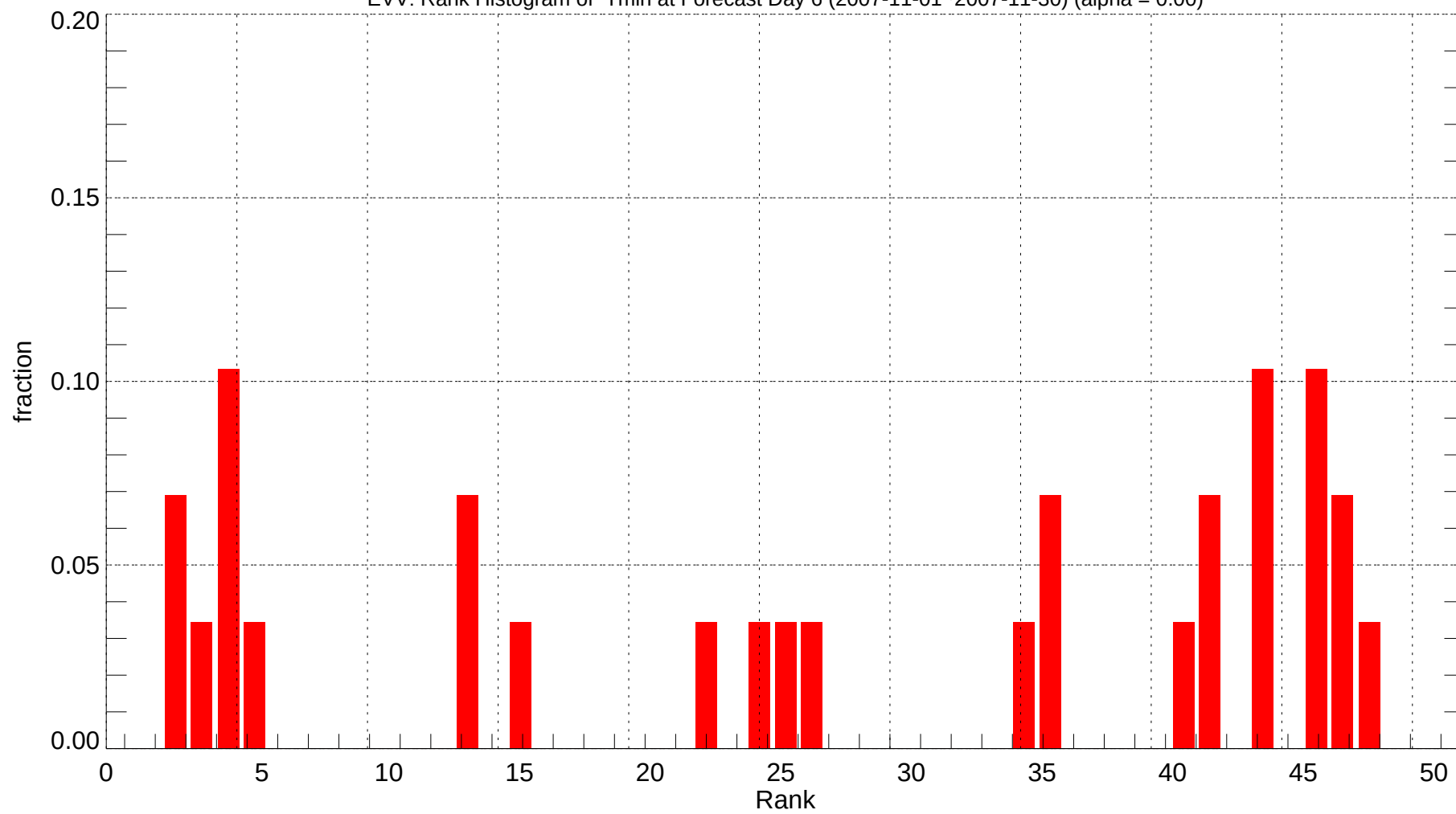
EVV: Rank Histogram of Tmin at Forecast Day 6 (2007-11-01~2007-11-30) (alpha = 0.00)
