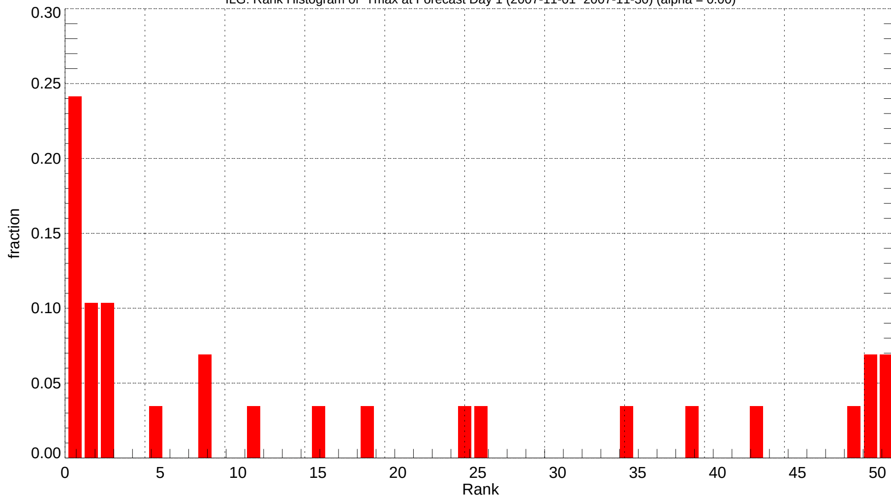
ILG: Rank Histogram of Tmax at Forecast Day 1 (2007-11-01~2007-11-30) (alpha = 0.00)
