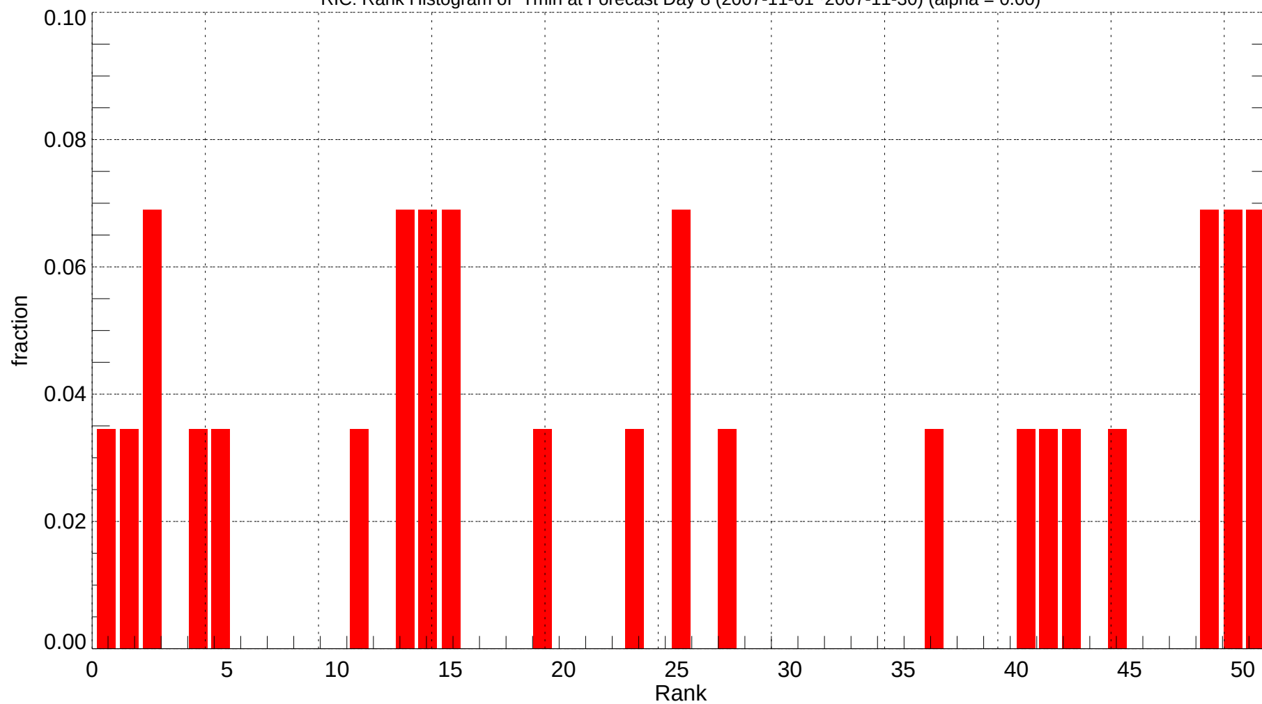
RIC: Rank Histogram of Tmin at Forecast Day 8 (2007-11-01~2007-11-30) (alpha = 0.00)
