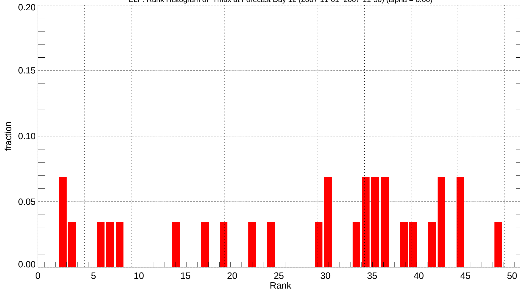
ELP: Rank Histogram of Tmax at Forecast Day 12 (2007-11-01~2007-11-30) (alpha = 0.00)
