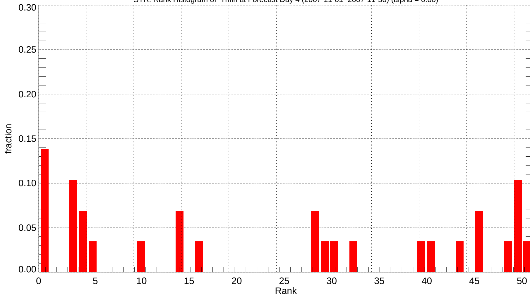
SYR: Rank Histogram of Tmin at Forecast Day 4 (2007-11-01~2007-11-30) (alpha = 0.00)
