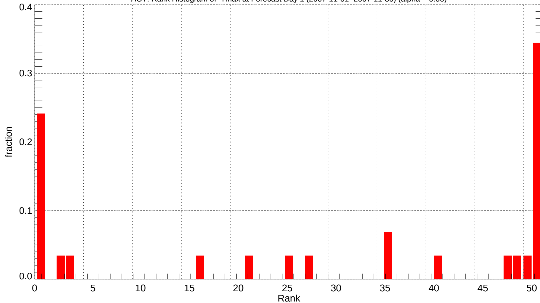
ACY: Rank Histogram of Tmax at Forecast Day 1 (2007-11-01~2007-11-30) (alpha = 0.00)
