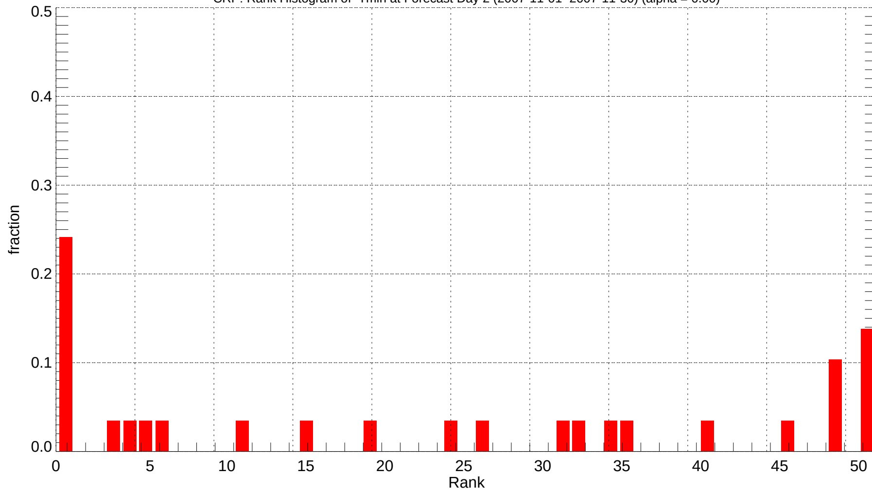
CRP: Rank Histogram of Tmin at Forecast Day 2 (2007-11-01~2007-11-30) (alpha = 0.00)
