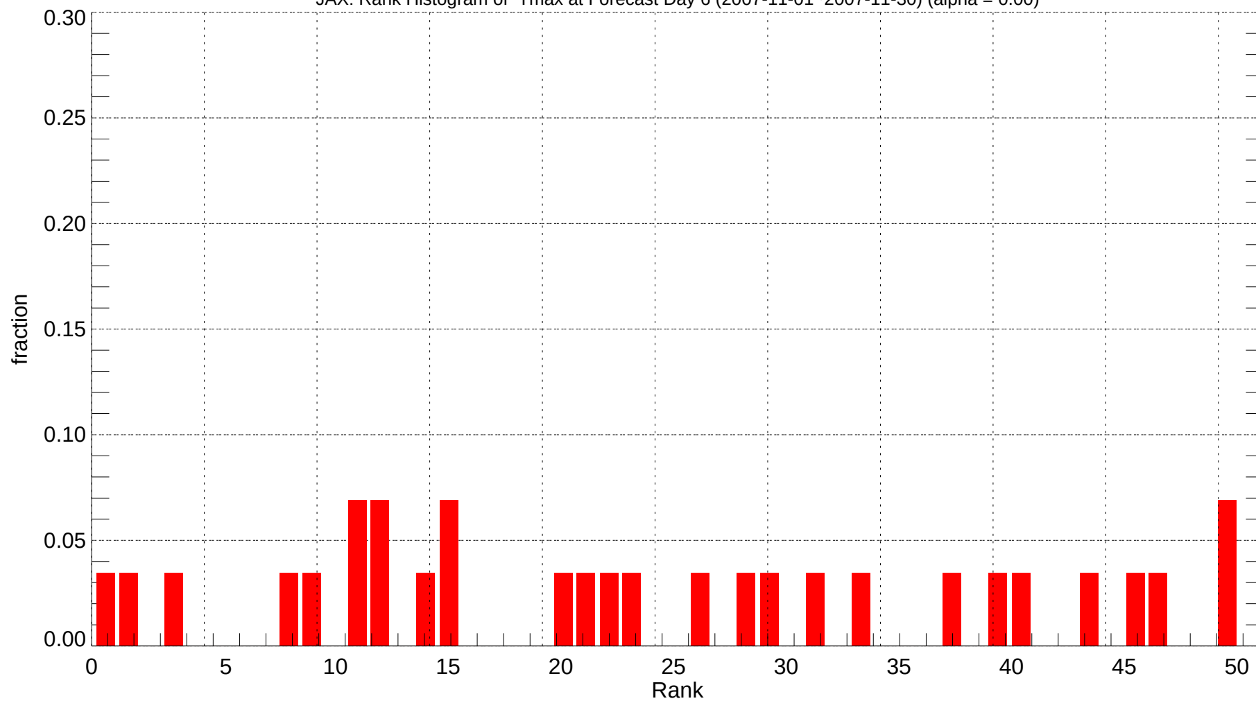
JAX: Rank Histogram of Tmax at Forecast Day 6 (2007-11-01~2007-11-30) (alpha = 0.00)
