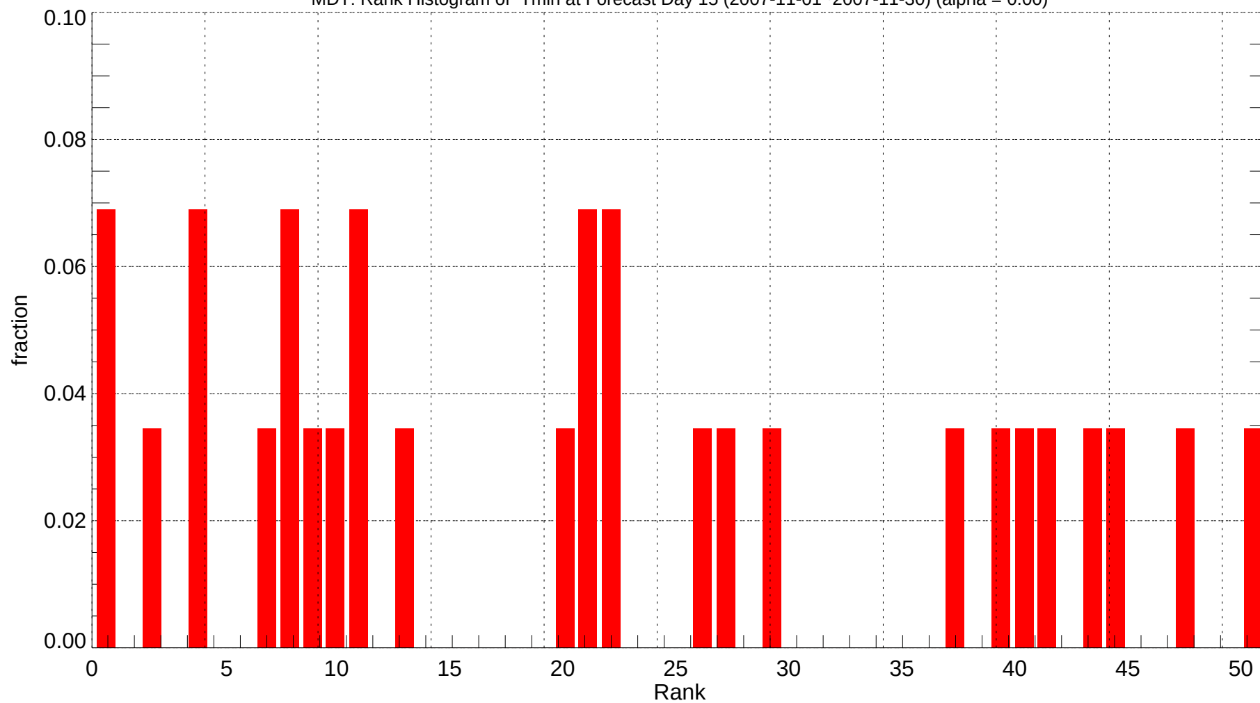
MDT: Rank Histogram of Tmin at Forecast Day 15 (2007-11-01~2007-11-30) (alpha = 0.00)
