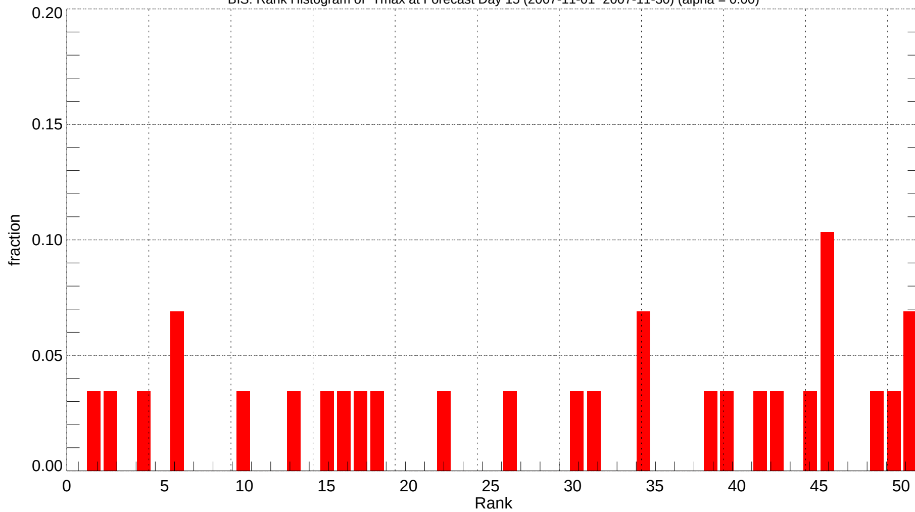
BIS: Rank Histogram of Tmax at Forecast Day 15 (2007-11-01~2007-11-30) (alpha = 0.00)
