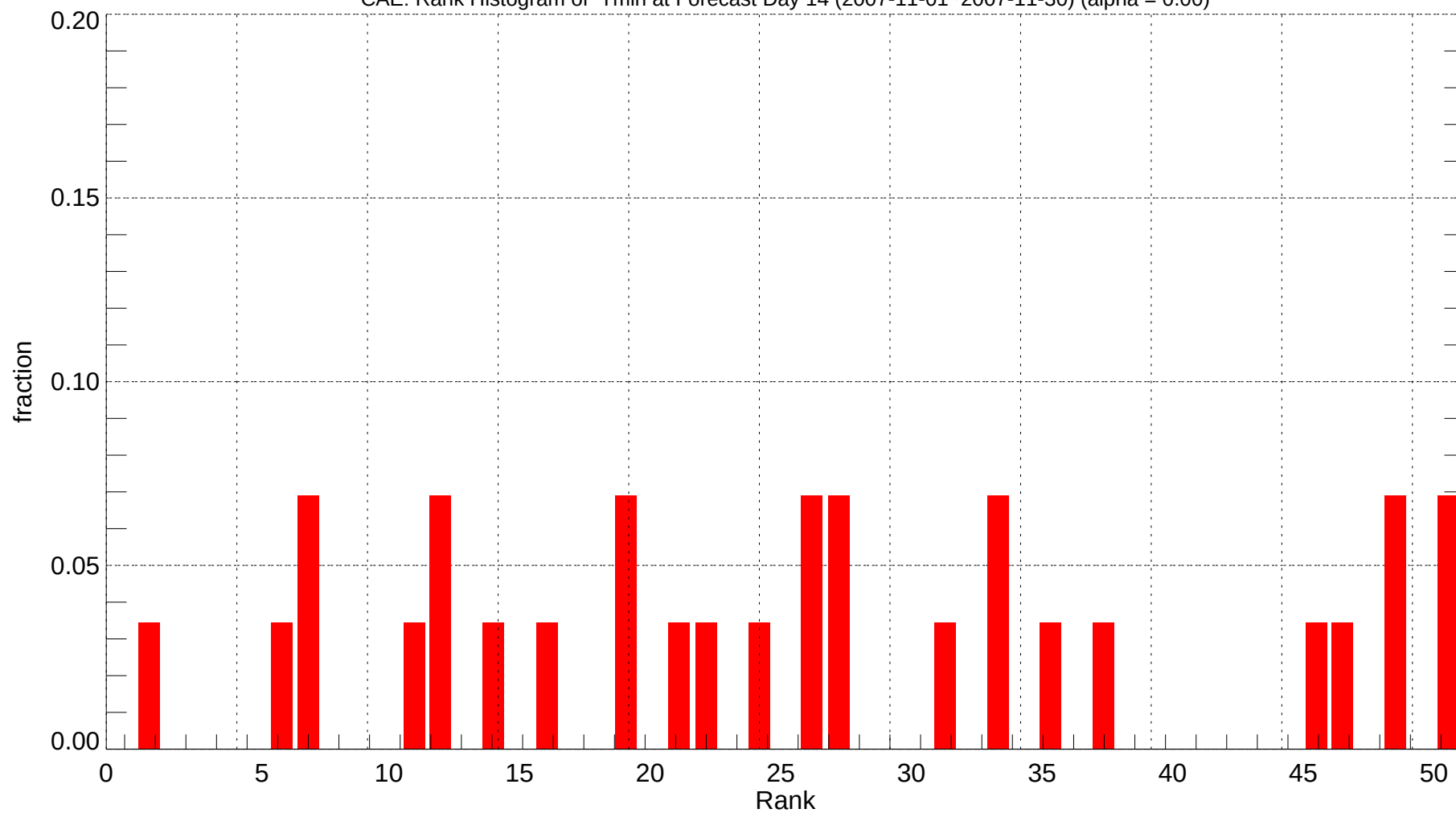
CAE: Rank Histogram of Tmin at Forecast Day 14 (2007-11-01~2007-11-30) (alpha = 0.00)
