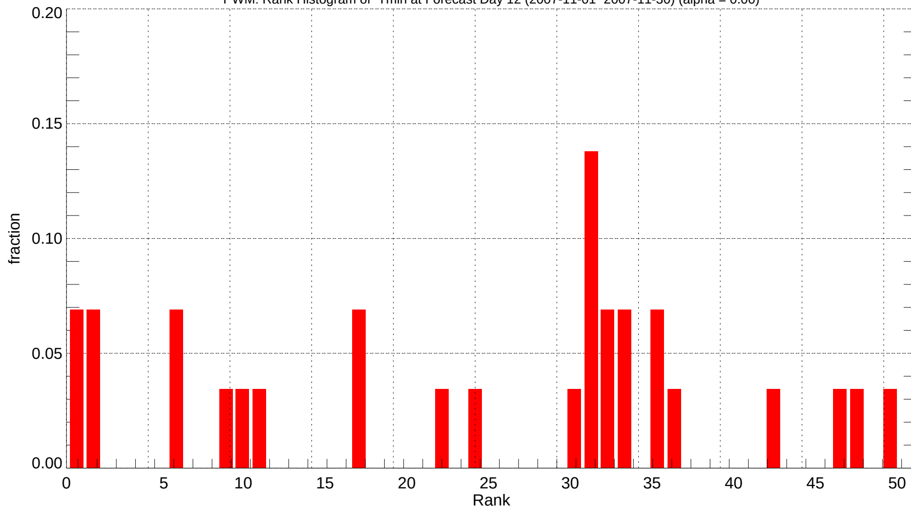
PWM: Rank Histogram of Tmin at Forecast Day 12 (2007-11-01~2007-11-30) (alpha = 0.00)
