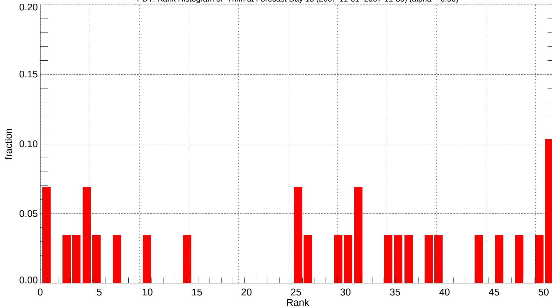
PDT: Rank Histogram of Tmin at Forecast Day 15 (2007-11-01~2007-11-30) (alpha = 0.00)
