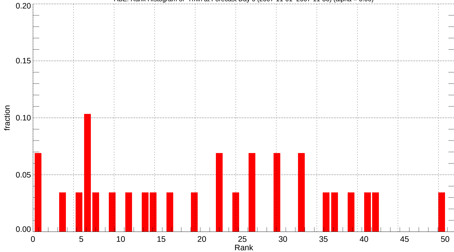
ABE: Rank Histogram of Tmin at Forecast Day 6 (2007-11-01~2007-11-30) (alpha = 0.00)
