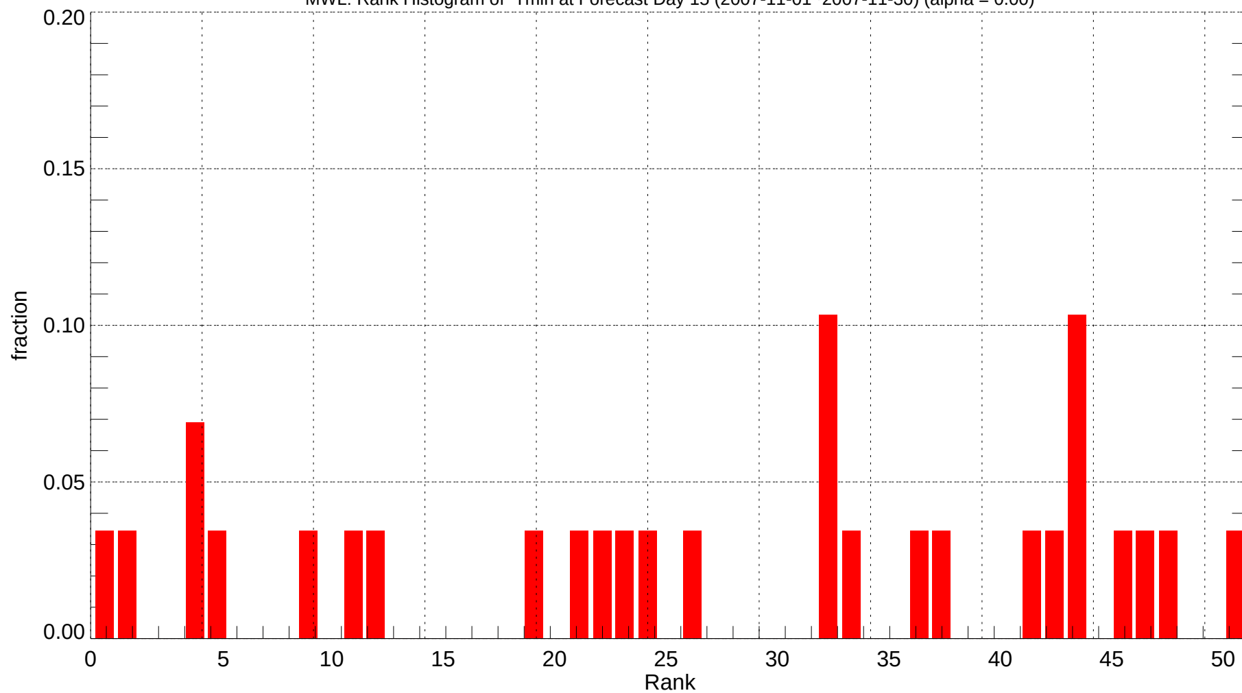
MWL: Rank Histogram of Tmin at Forecast Day 15 (2007-11-01~2007-11-30) (alpha = 0.00)
