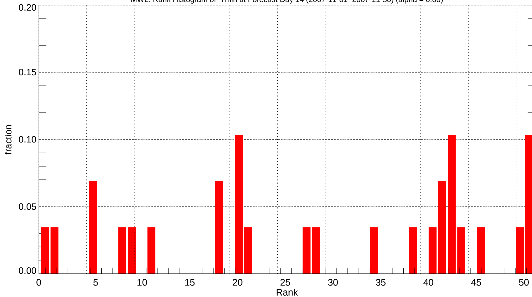
MWL: Rank Histogram of Tmin at Forecast Day 14 (2007-11-01~2007-11-30) (alpha = 0.00)
