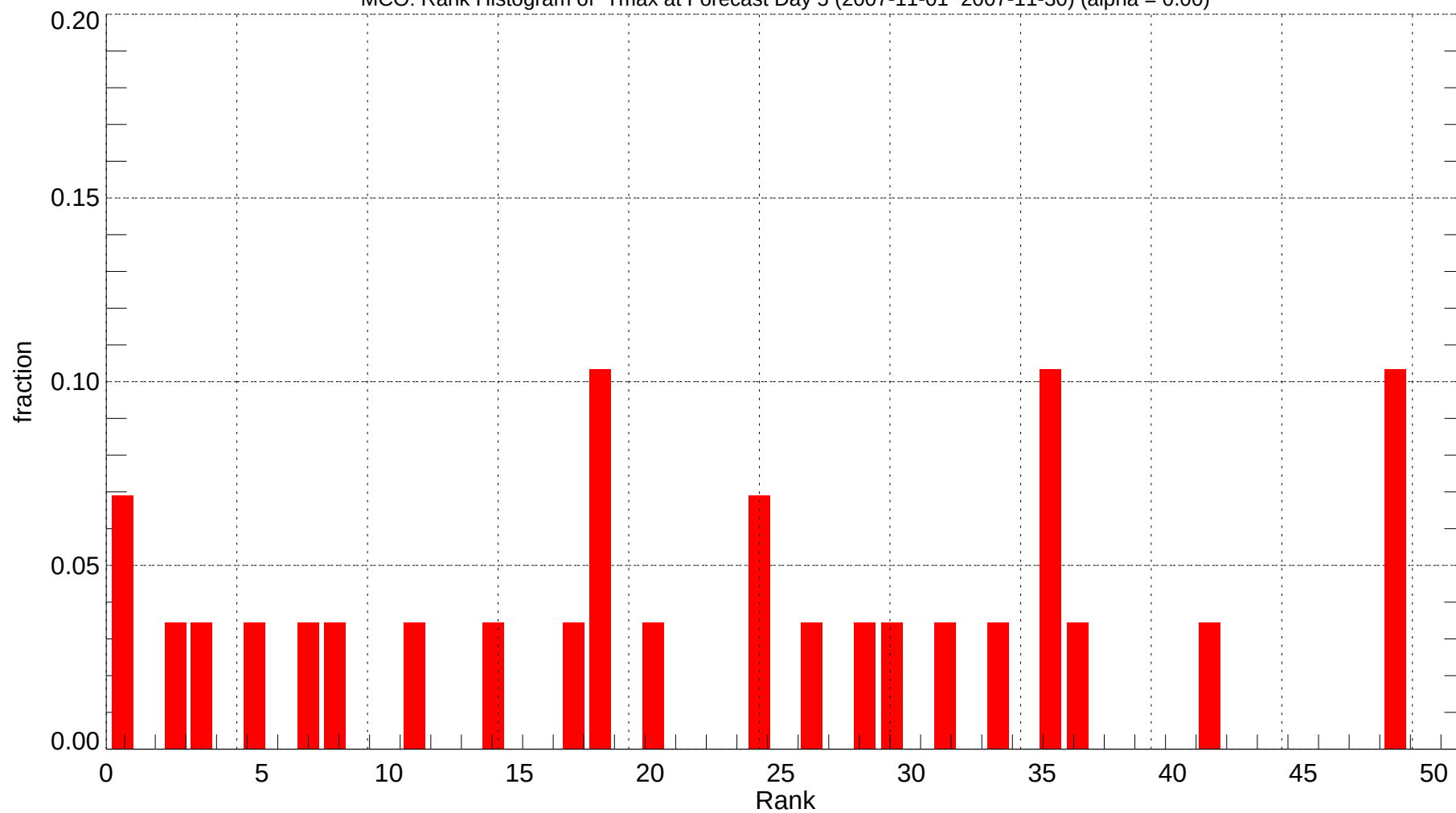
MCO: Rank Histogram of Tmax at Forecast Day 5 (2007-11-01~2007-11-30) (alpha = 0.00)
