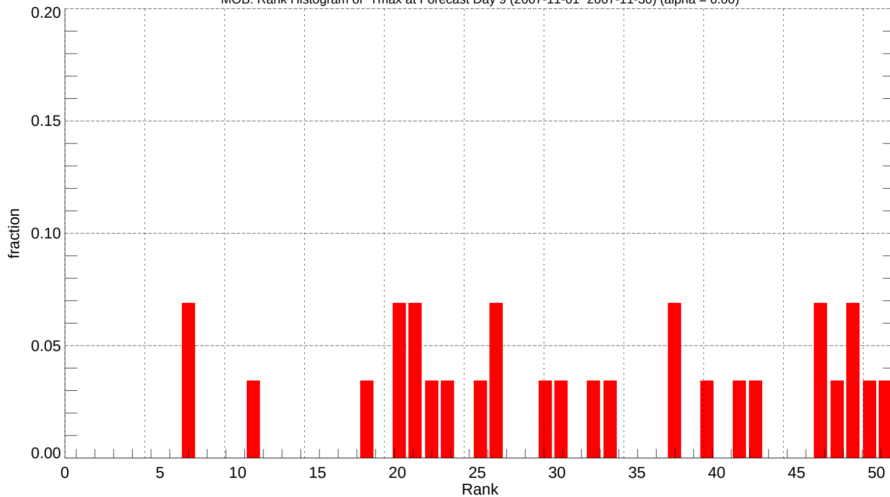
MOB: Rank Histogram of Tmax at Forecast Day 9 (2007-11-01~2007-11-30) (alpha = 0.00)
