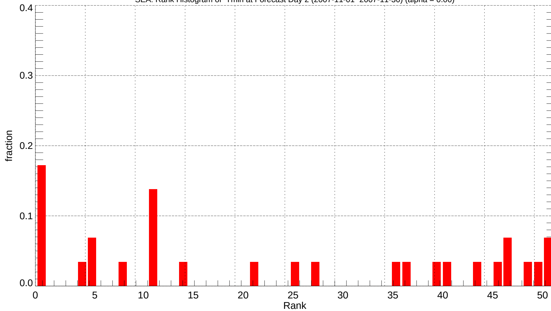
SEA: Rank Histogram of Tmin at Forecast Day 2 (2007-11-01~2007-11-30) (alpha = 0.00)
