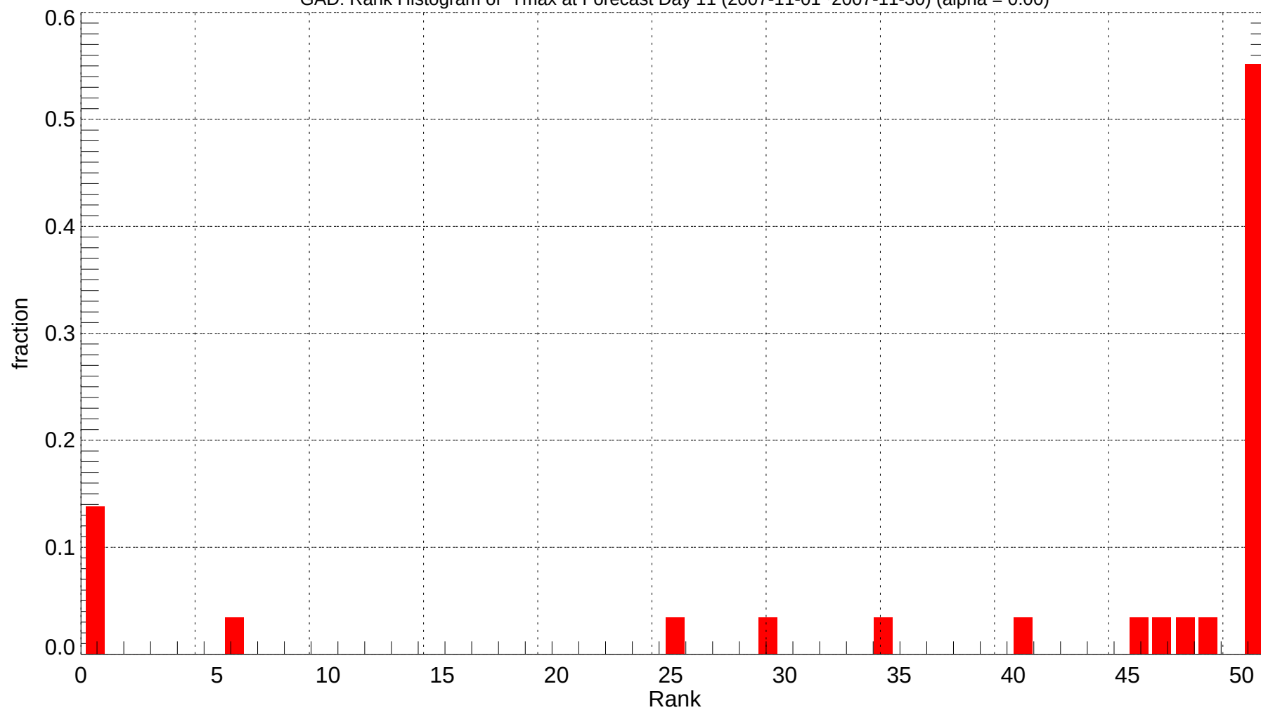
GAD: Rank Histogram of Tmax at Forecast Day 11 (2007-11-01~2007-11-30) (alpha = 0.00)
