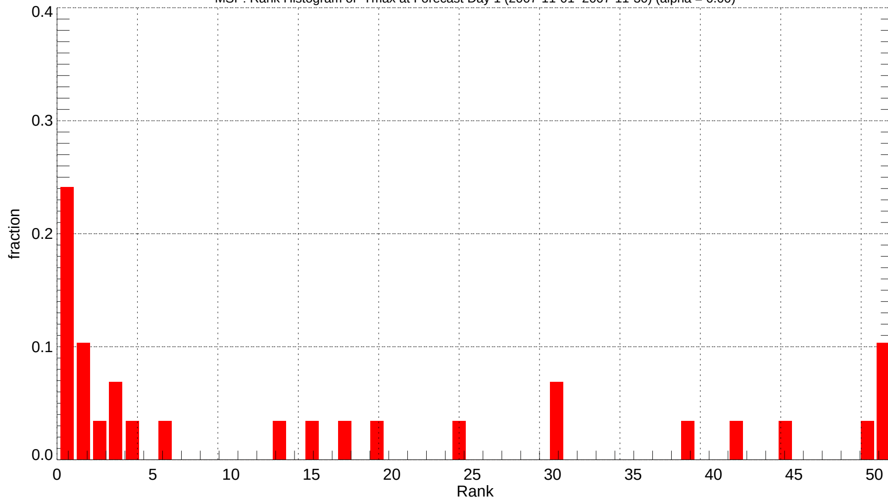
MSP: Rank Histogram of Tmax at Forecast Day 1 (2007-11-01~2007-11-30) (alpha = 0.00)
