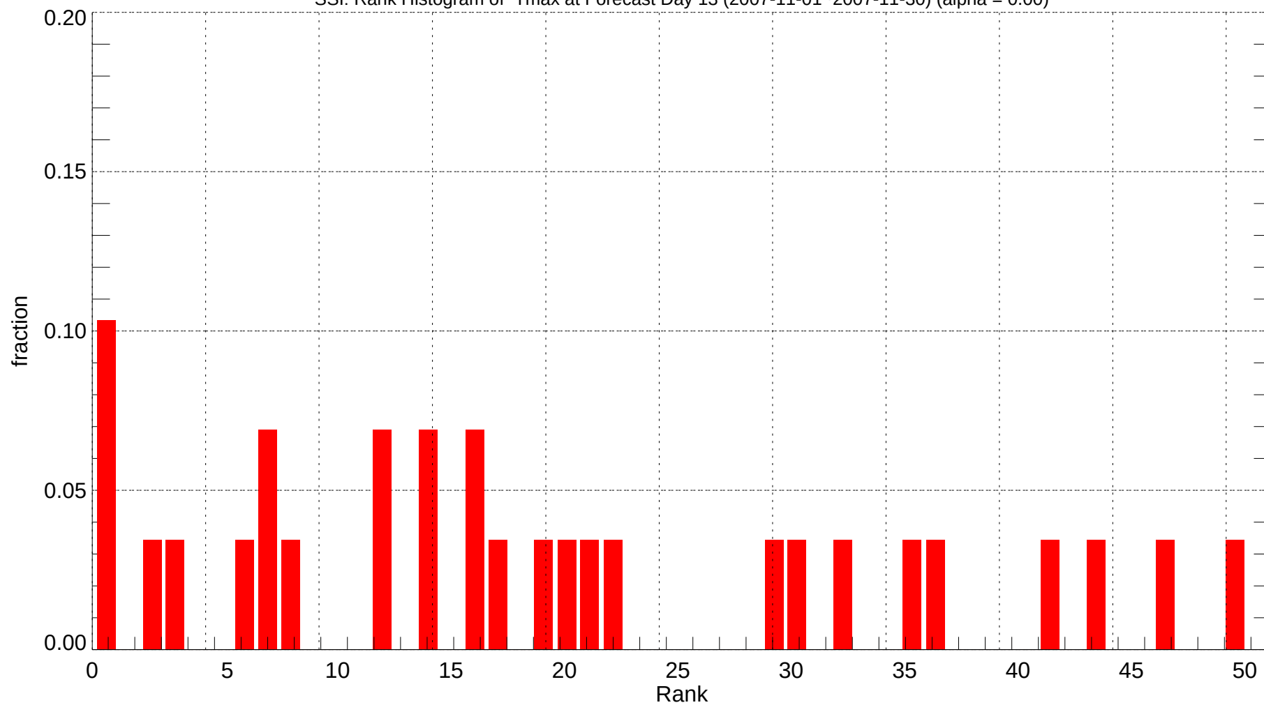
SSI: Rank Histogram of Tmax at Forecast Day 13 (2007-11-01~2007-11-30) (alpha = 0.00)
