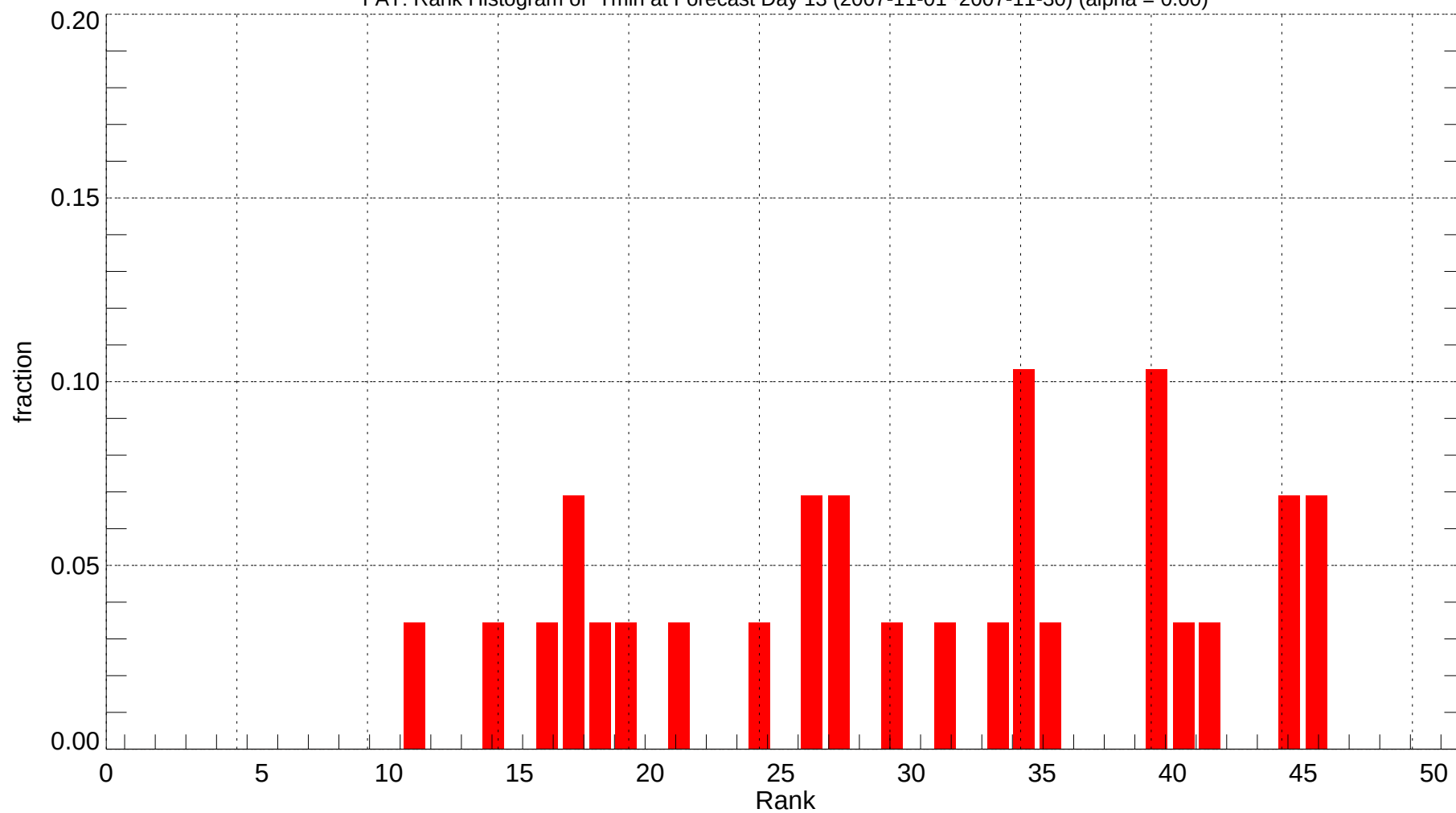
FAT: Rank Histogram of Tmin at Forecast Day 13 (2007-11-01~2007-11-30) (alpha = 0.00)
