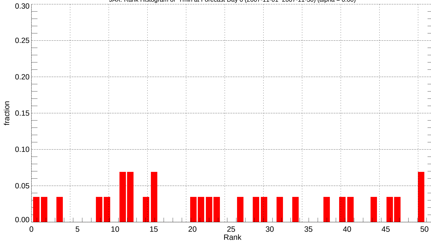
JAX: Rank Histogram of Tmin at Forecast Day 6 (2007-11-01~2007-11-30) (alpha = 0.00)
