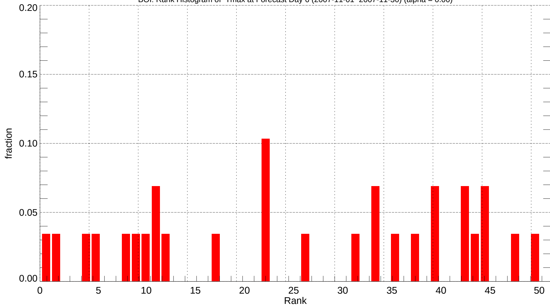
BOI: Rank Histogram of Tmax at Forecast Day 6 (2007-11-01~2007-11-30) (alpha = 0.00)
