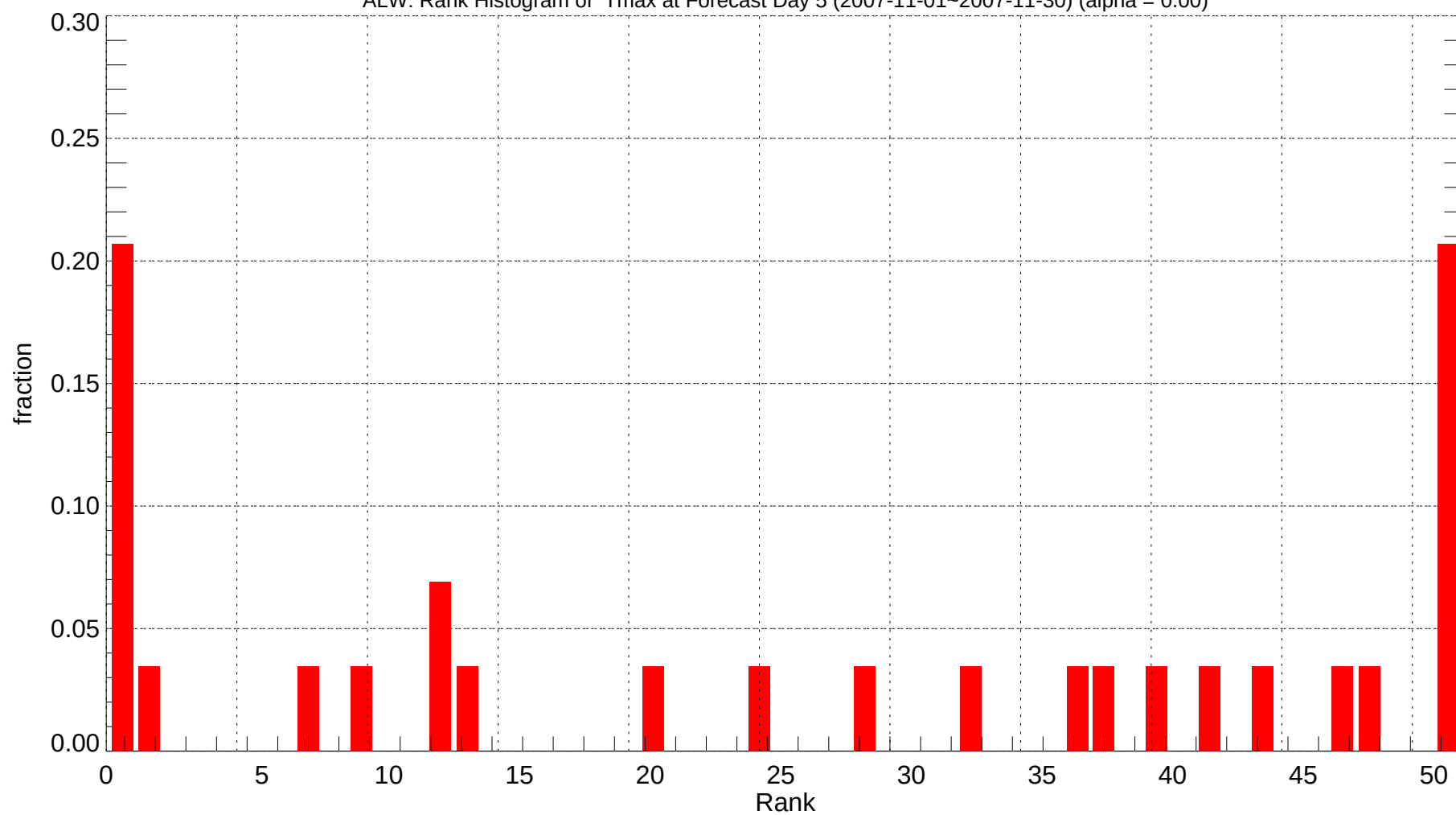
ALW: Rank Histogram of Tmax at Forecast Day 5 (2007-11-01~2007-11-30) (alpha = 0.00)
