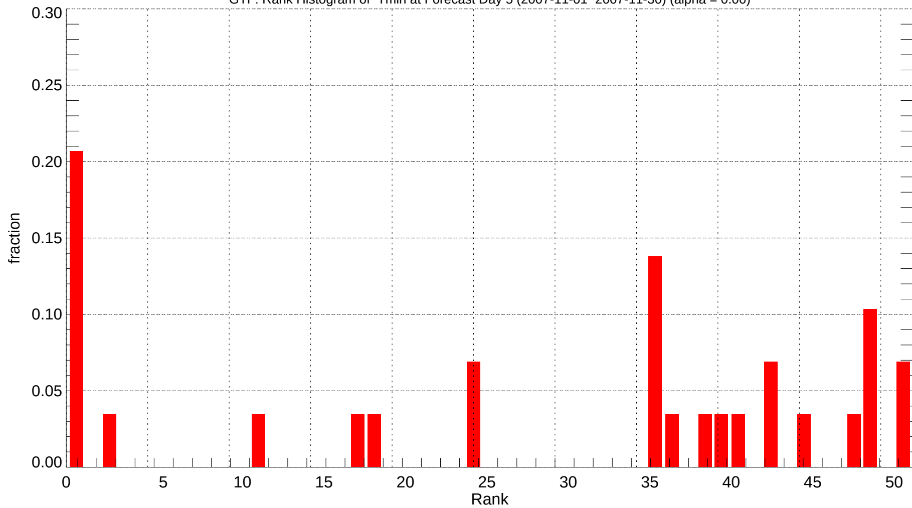
GTF: Rank Histogram of Tmin at Forecast Day 5 (2007-11-01~2007-11-30) (alpha = 0.00)
