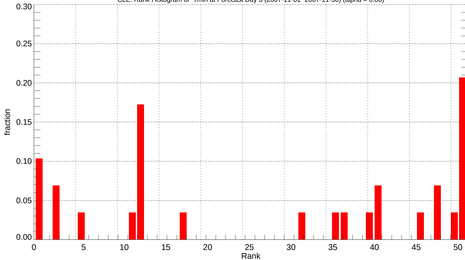
CLE: Rank Histogram of Tmin at Forecast Day 3 (2007-11-01~2007-11-30) (alpha = 0.00)
