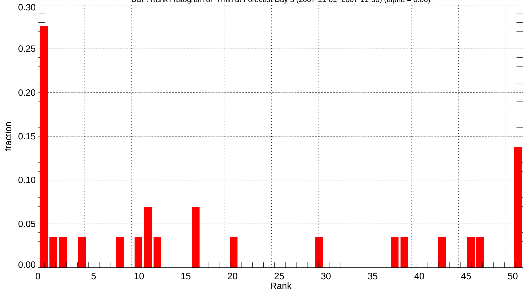
BUF: Rank Histogram of Tmin at Forecast Day 3 (2007-11-01~2007-11-30) (alpha = 0.00)
