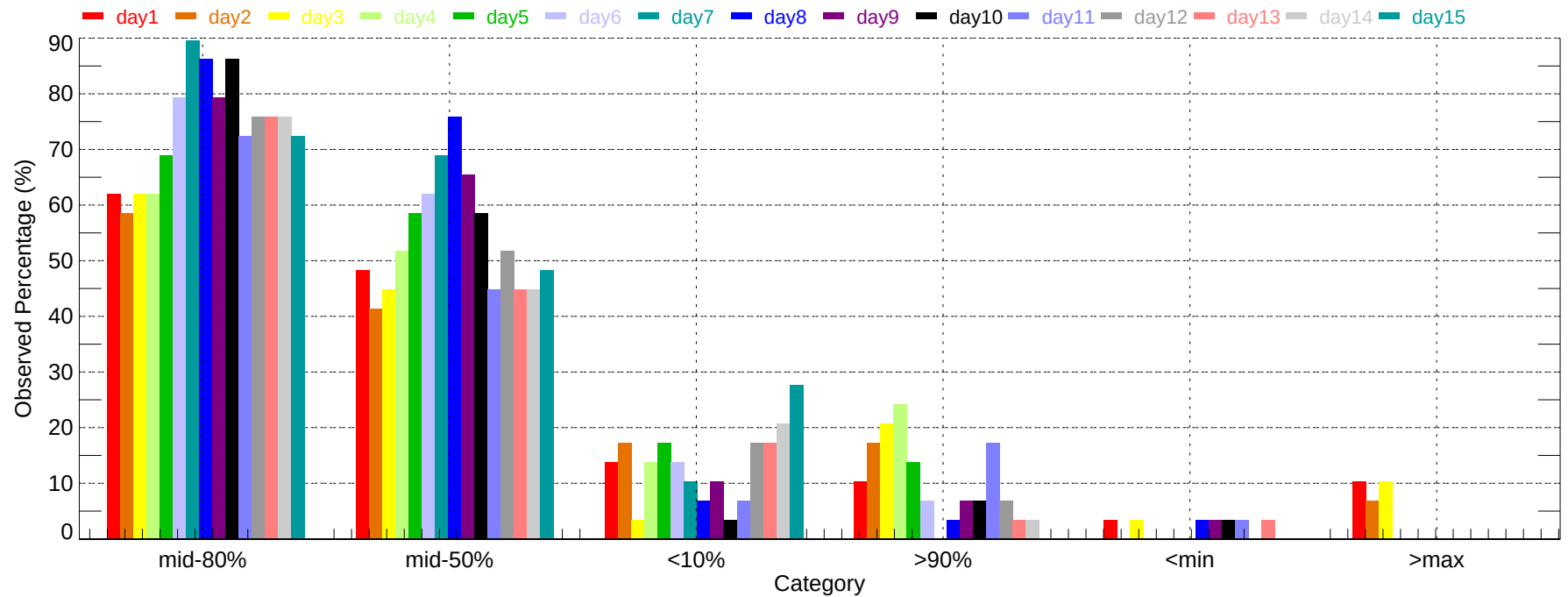
Observed Percentage of Ensembles - MCO: Min Temperature (2007-11-01~2007-11-30)
