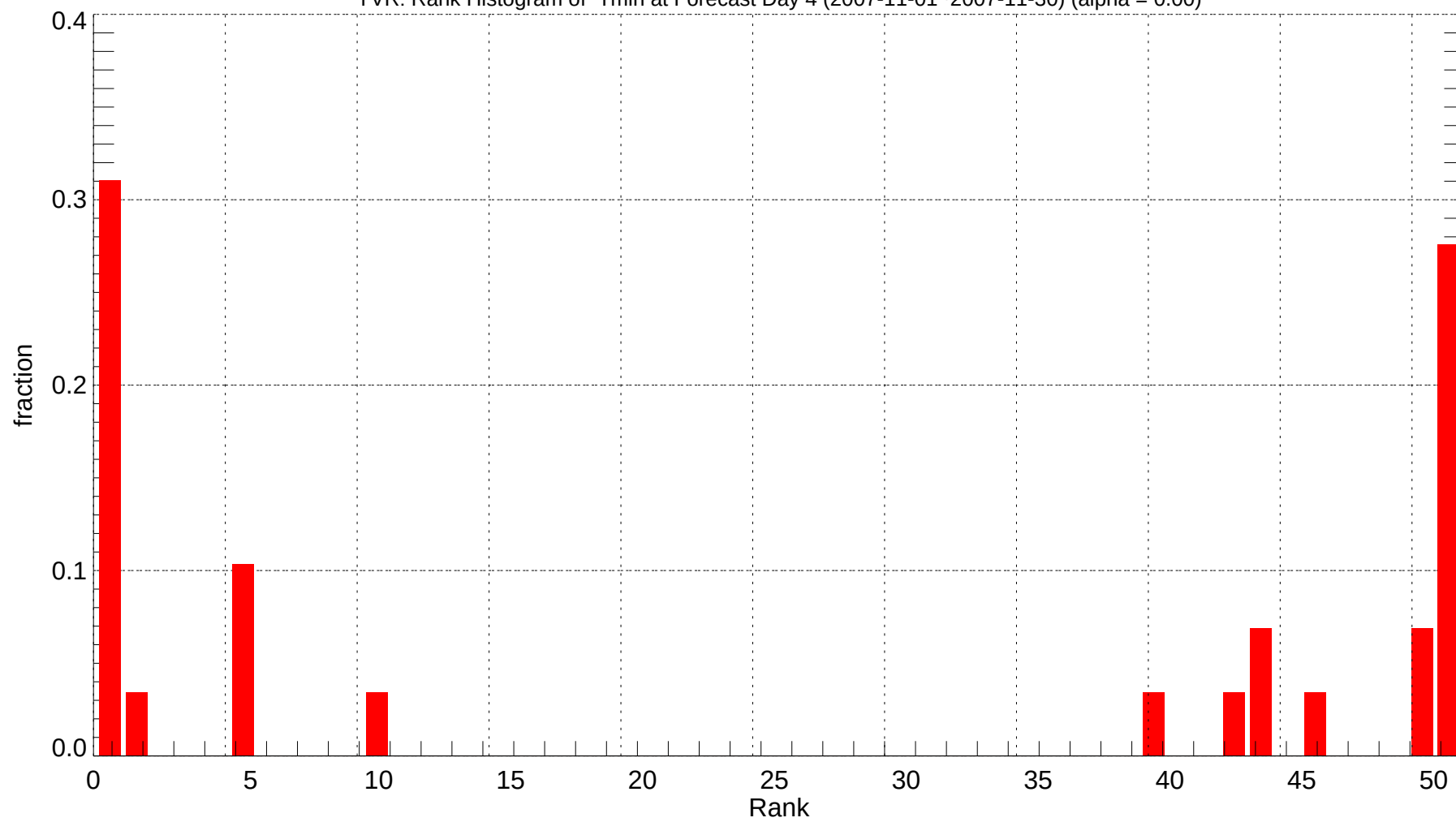
YVR: Rank Histogram of Tmin at Forecast Day 4 (2007-11-01~2007-11-30) (alpha = 0.00)
