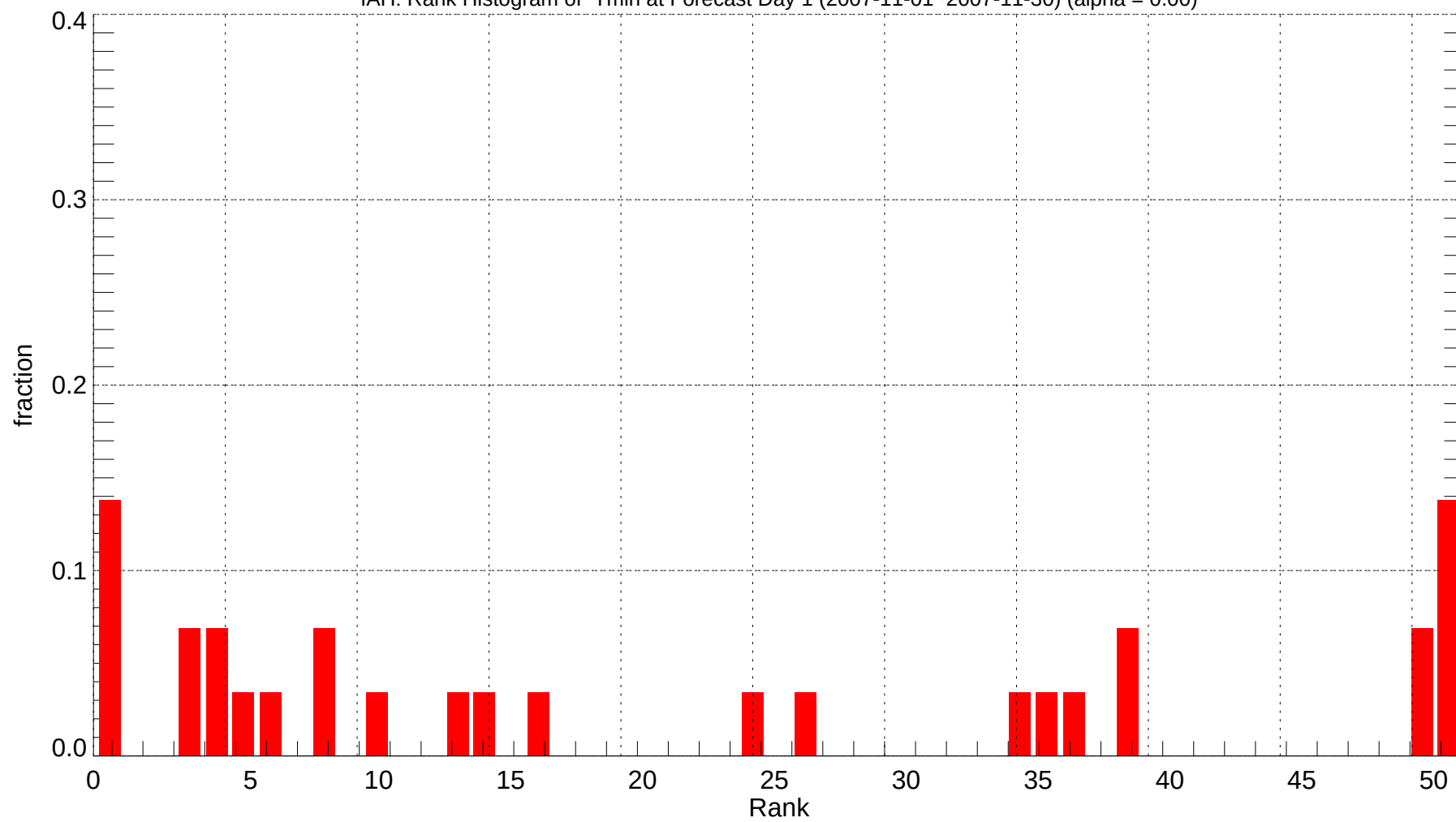
IAH: Rank Histogram of Tmin at Forecast Day 1 (2007-11-01~2007-11-30) (alpha = 0.00)
