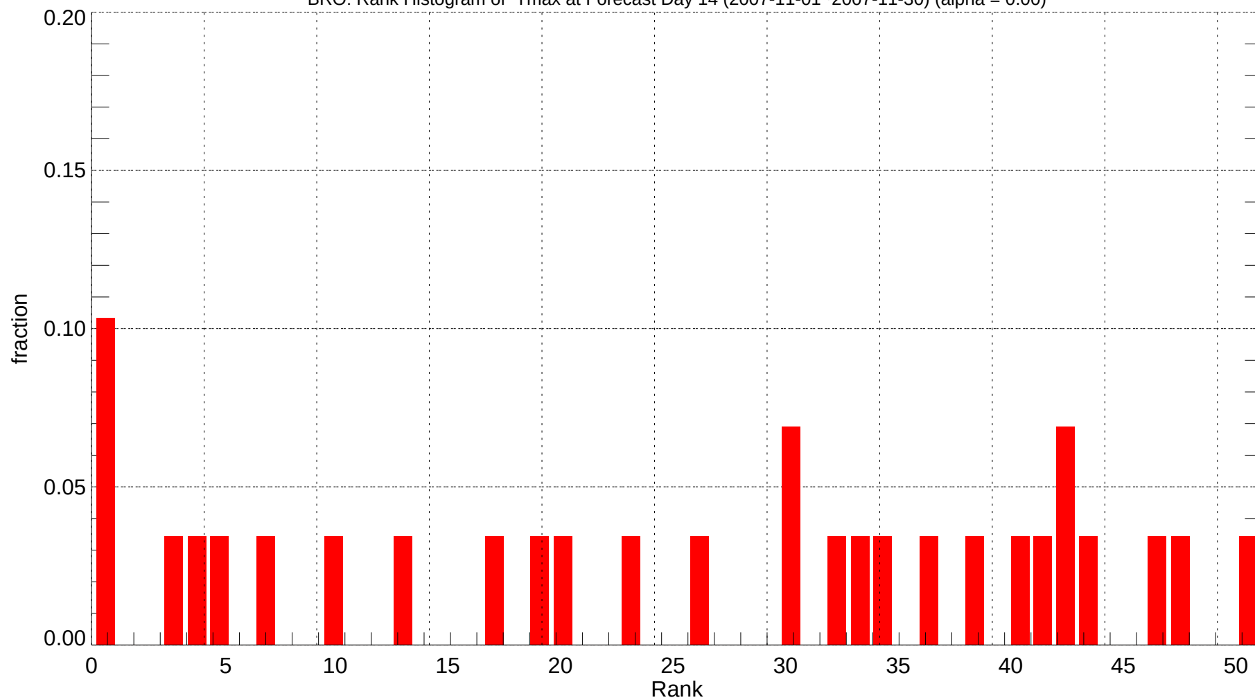
BRO: Rank Histogram of Tmax at Forecast Day 14 (2007-11-01~2007-11-30) (alpha = 0.00)
