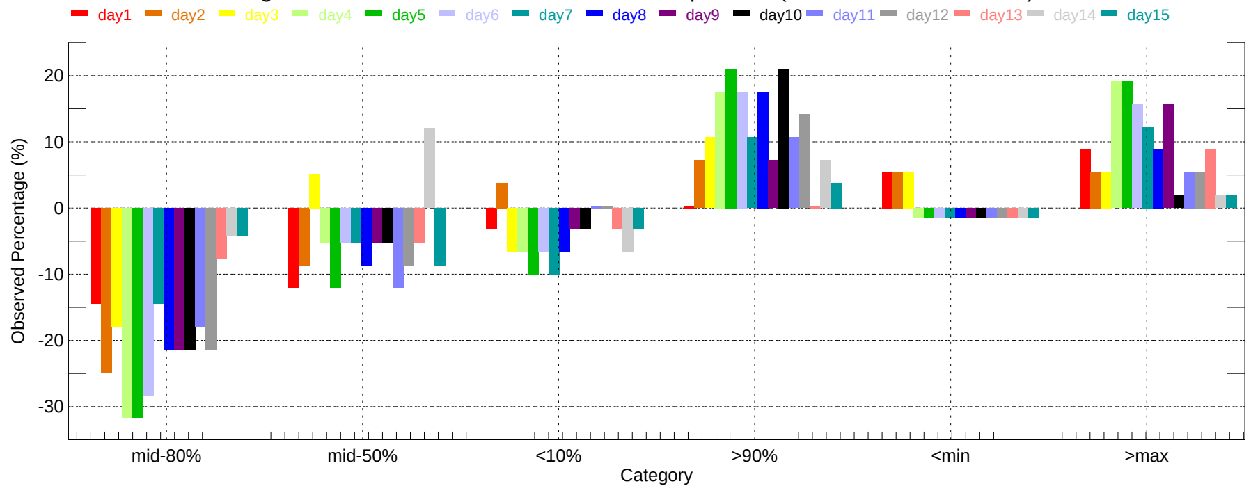
Observed Percentage Deviation of Ensembles - CAE: Min Temperature (2007-11-01~2007-11-30)
