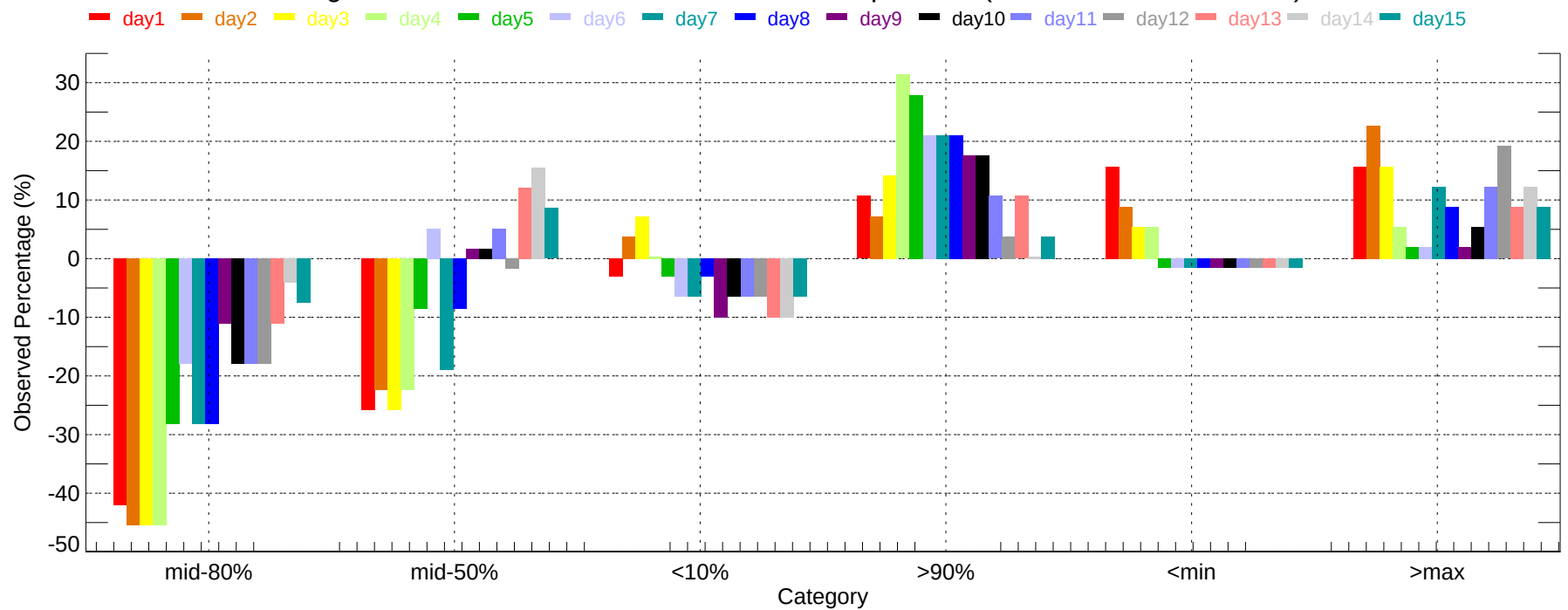
Observed Percentage Deviation of Ensembles - CMH: Min Temperature (2007-11-01~2007-11-30)
