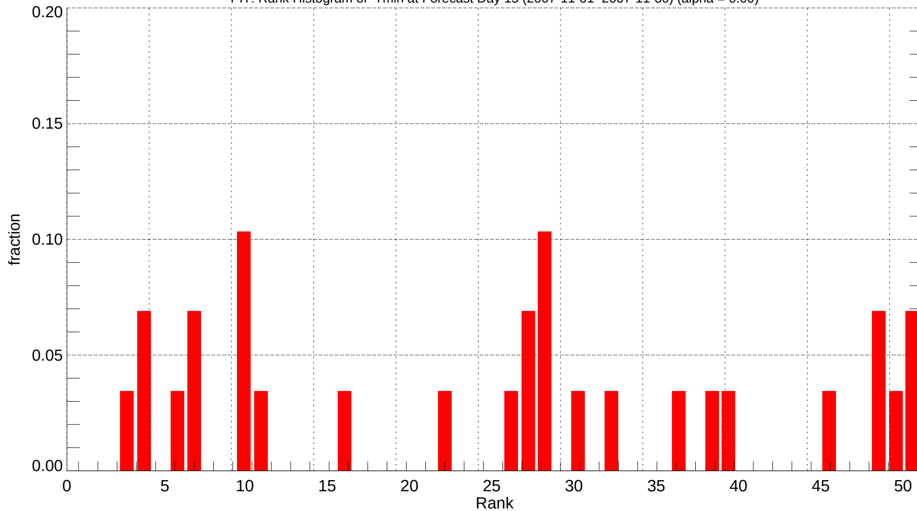
PIT: Rank Histogram of Tmin at Forecast Day 15 (2007-11-01~2007-11-30) (alpha = 0.00)
