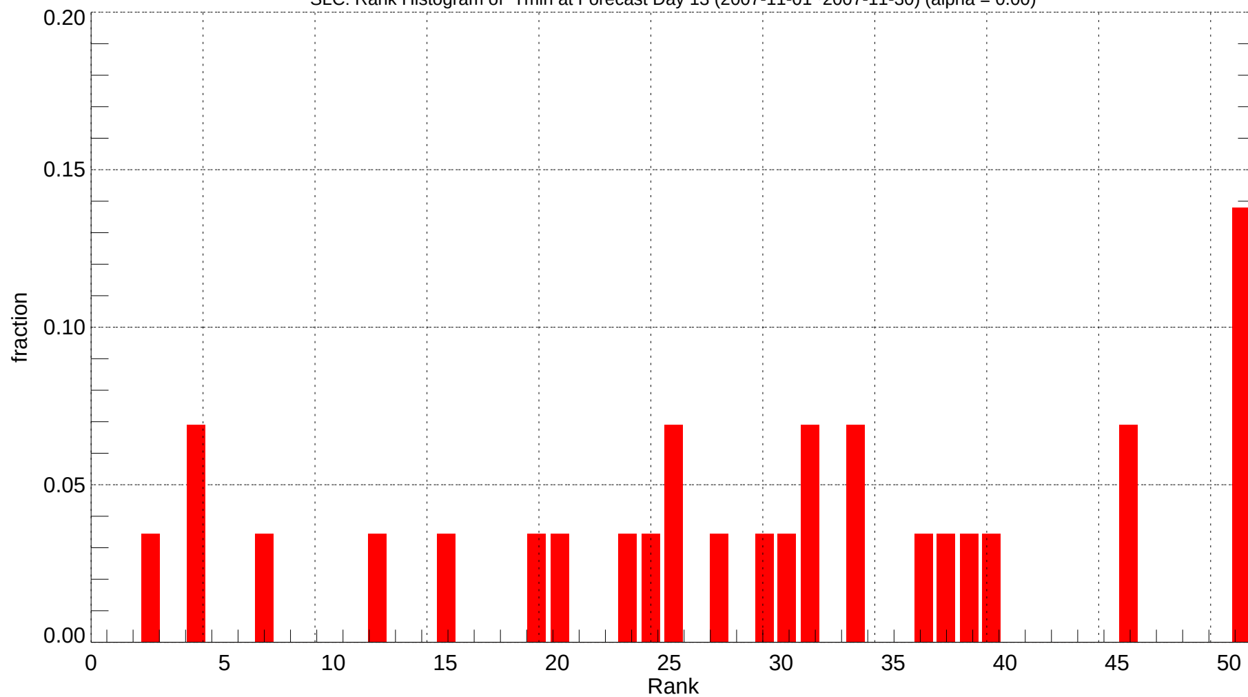
SLC: Rank Histogram of Tmin at Forecast Day 13 (2007-11-01~2007-11-30) (alpha = 0.00)
