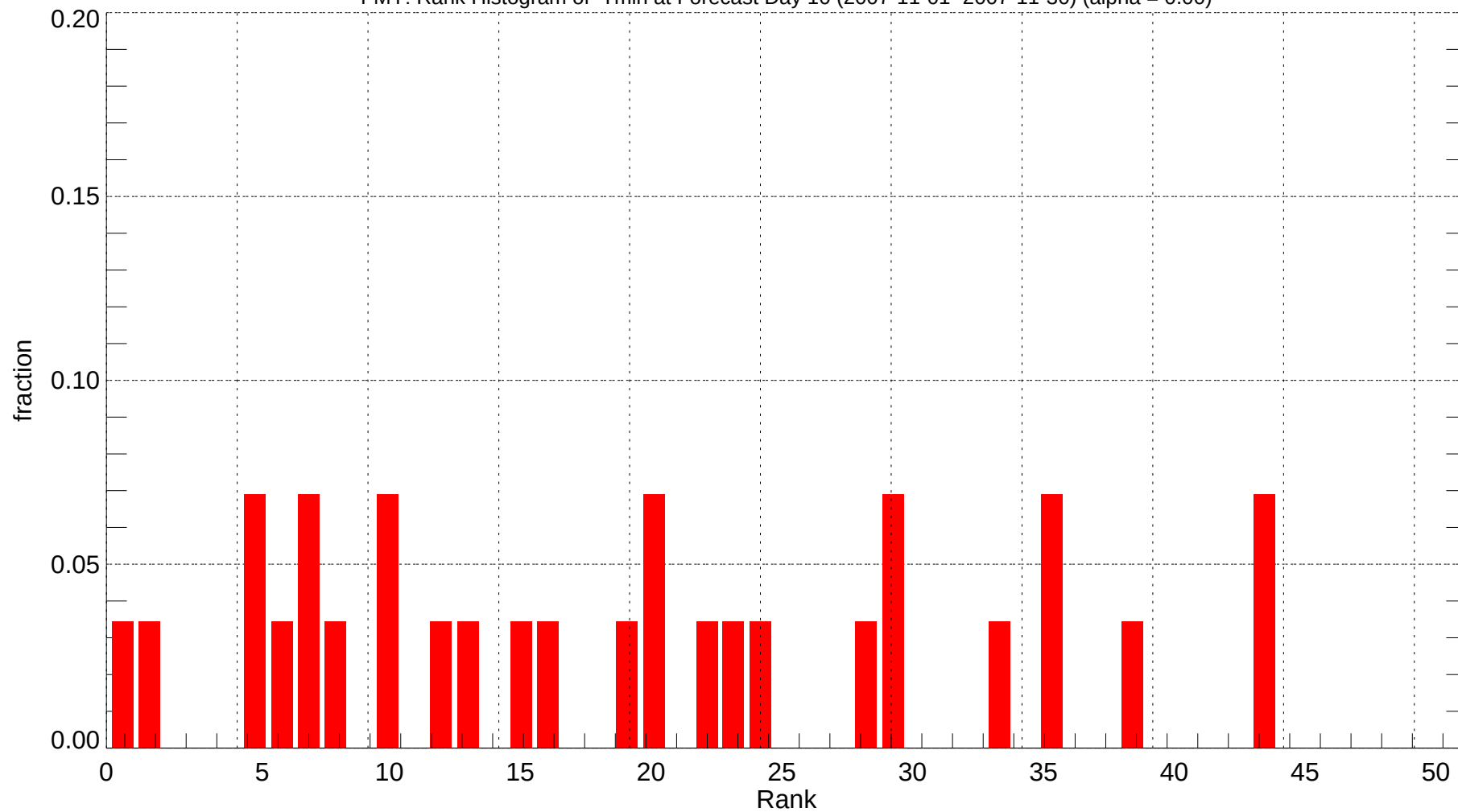
FMY: Rank Histogram of Tmin at Forecast Day 10 (2007-11-01~2007-11-30) (alpha = 0.00)
