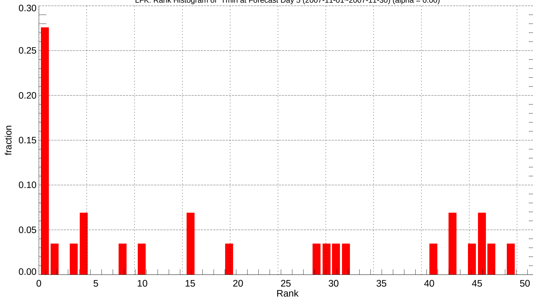
LFK: Rank Histogram of Tmin at Forecast Day 5 (2007-11-01~2007-11-30) (alpha = 0.00)
