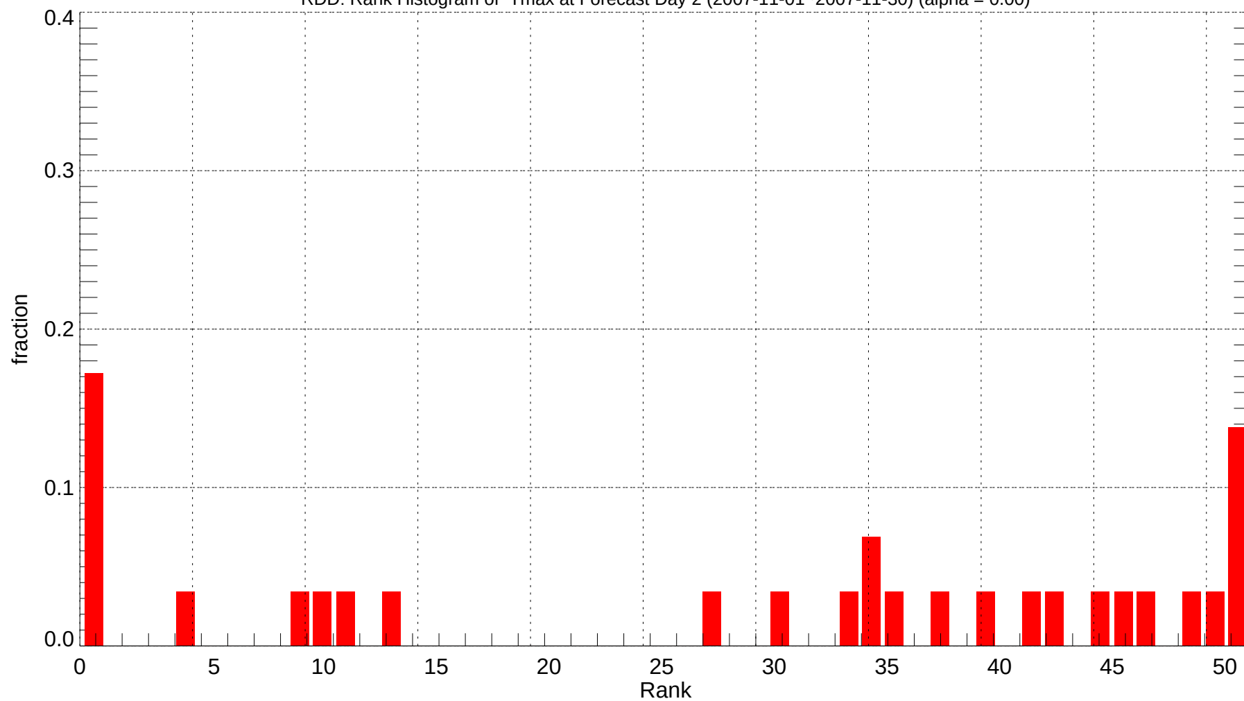
RDD: Rank Histogram of Tmax at Forecast Day 2 (2007-11-01~2007-11-30) (alpha = 0.00)
