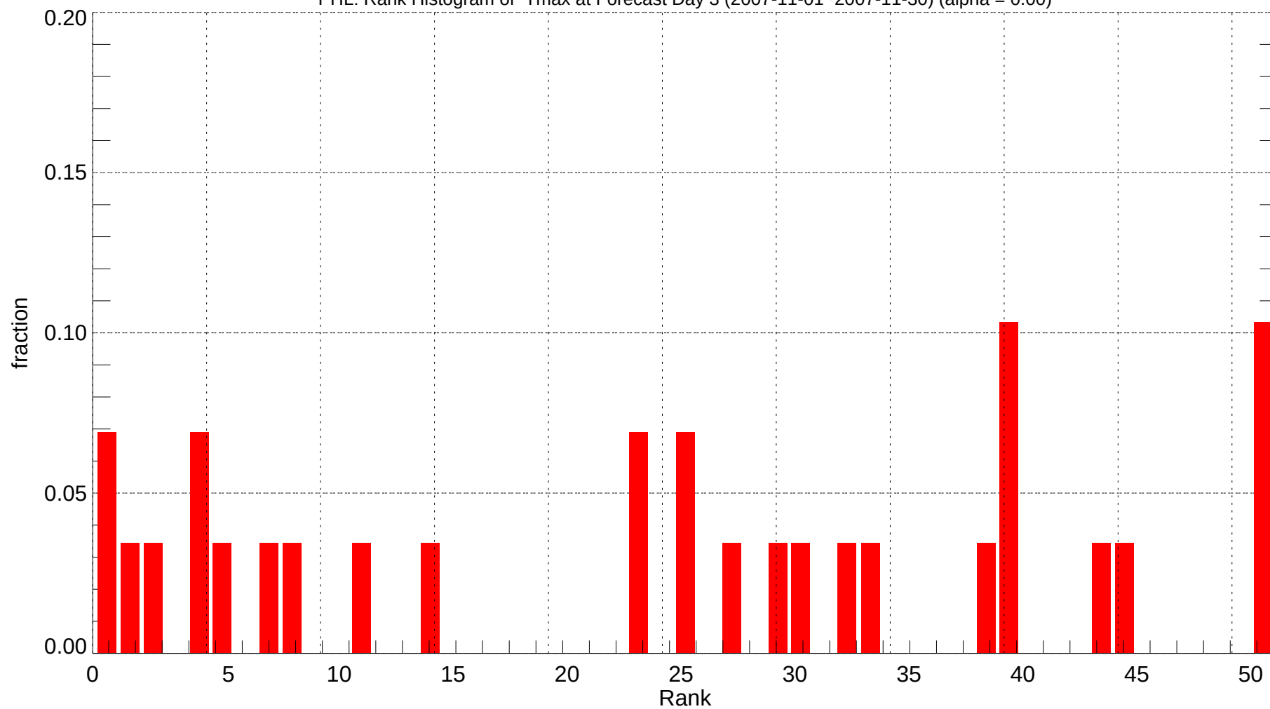
PHL: Rank Histogram of Tmax at Forecast Day 3 (2007-11-01~2007-11-30) (alpha = 0.00)
