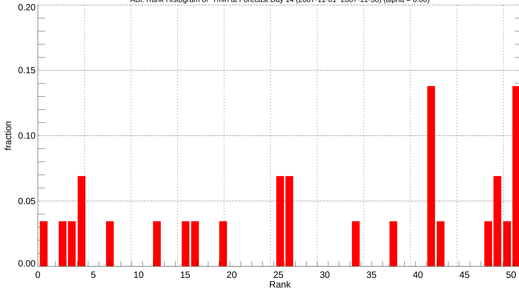
ABI: Rank Histogram of Tmin at Forecast Day 14 (2007-11-01~2007-11-30) (alpha = 0.00)
