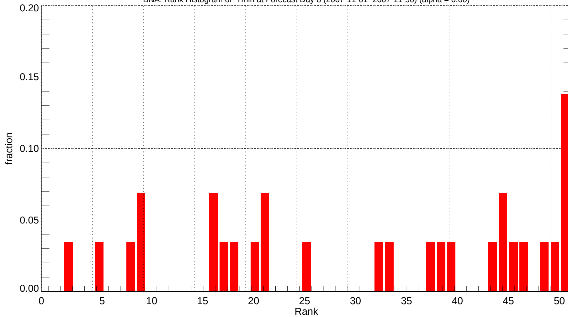
BNA: Rank Histogram of Tmin at Forecast Day 8 (2007-11-01~2007-11-30) (alpha = 0.00)
