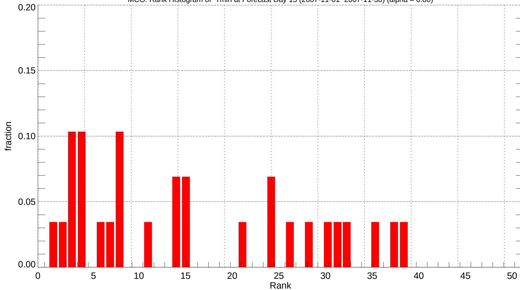
MCO: Rank Histogram of Tmin at Forecast Day 15 (2007-11-01~2007-11-30) (alpha = 0.00)
