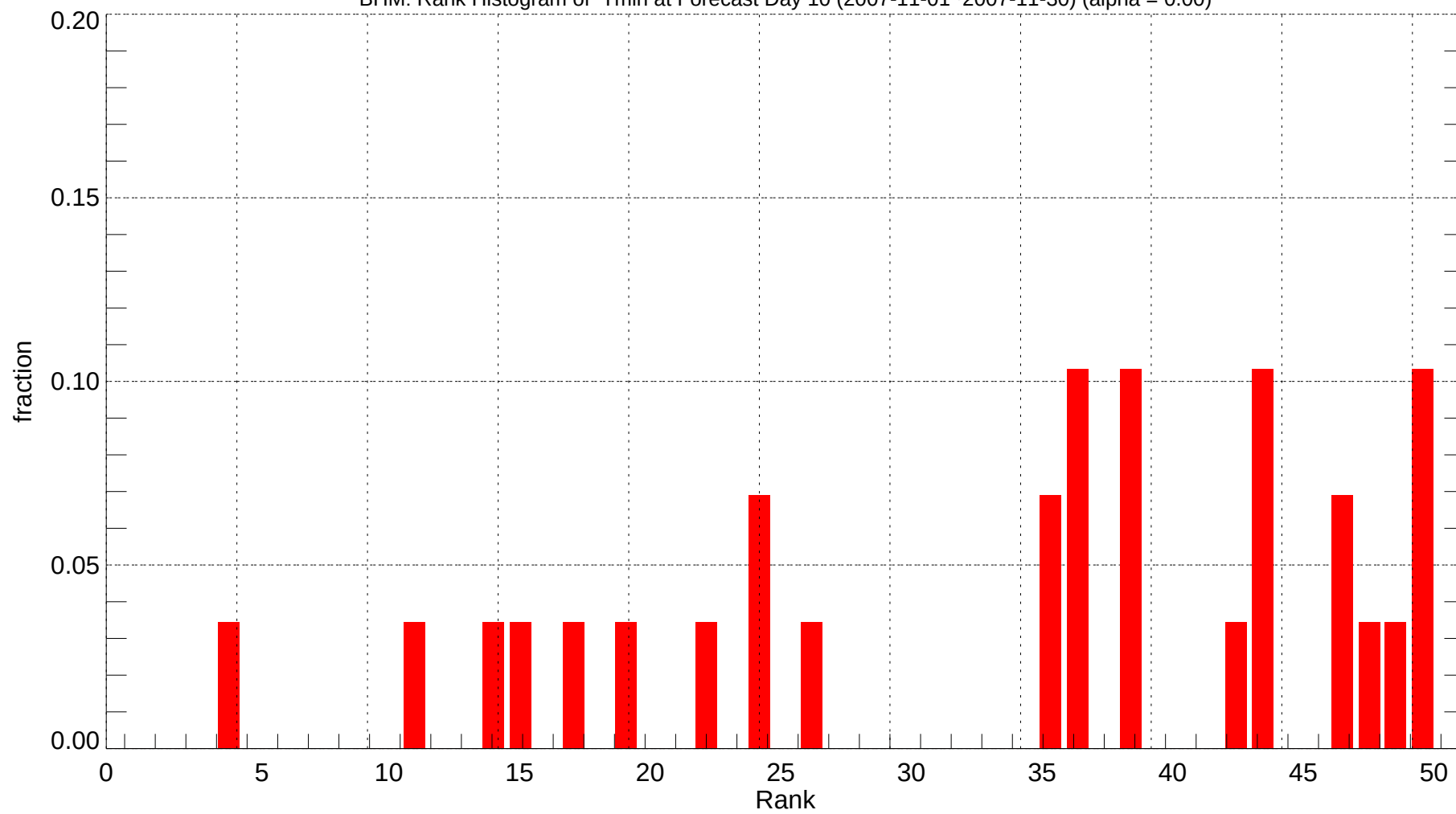
BHM: Rank Histogram of Tmin at Forecast Day 10 (2007-11-01~2007-11-30) (alpha = 0.00)
