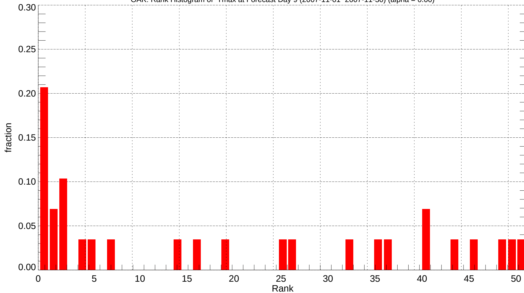
OAK: Rank Histogram of Tmax at Forecast Day 9 (2007-11-01~2007-11-30) (alpha = 0.00)
