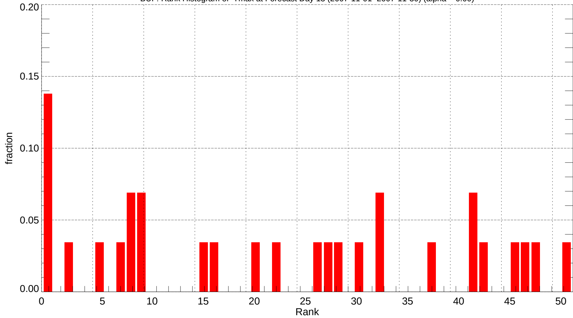
BUF: Rank Histogram of Tmax at Forecast Day 13 (2007-11-01~2007-11-30) (alpha = 0.00)
