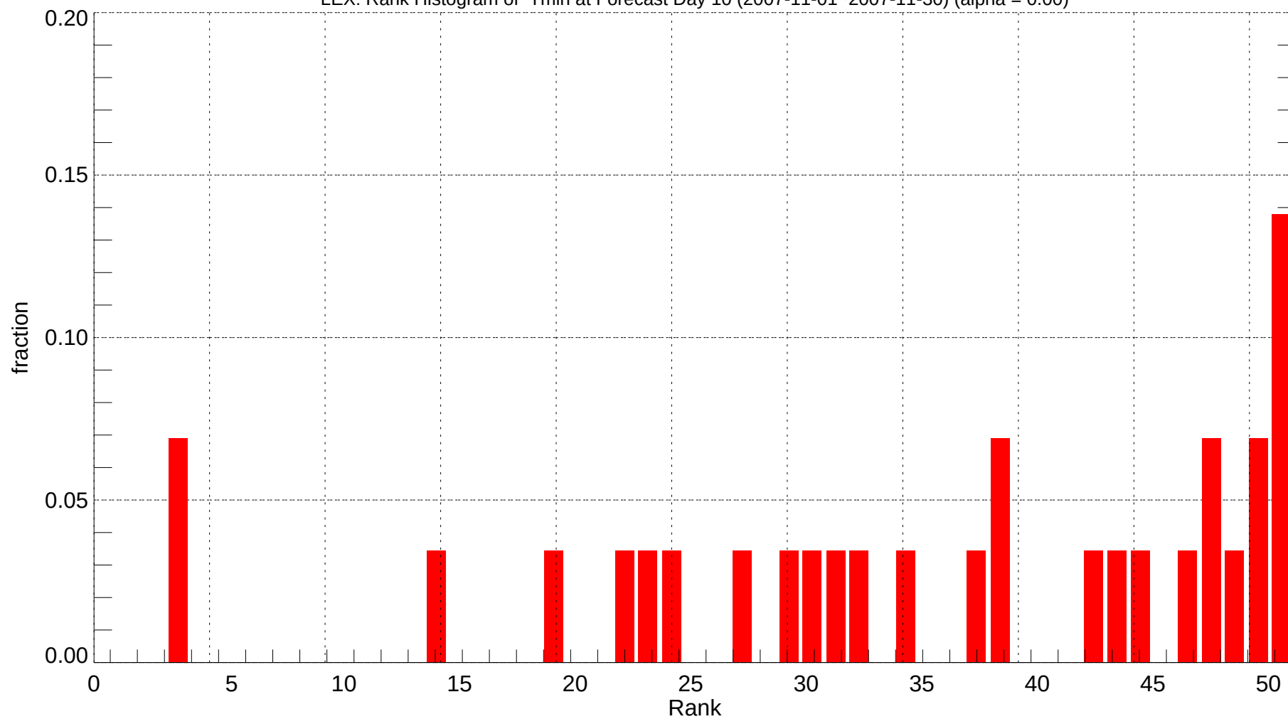
LEX: Rank Histogram of Tmin at Forecast Day 10 (2007-11-01~2007-11-30) (alpha = 0.00)
