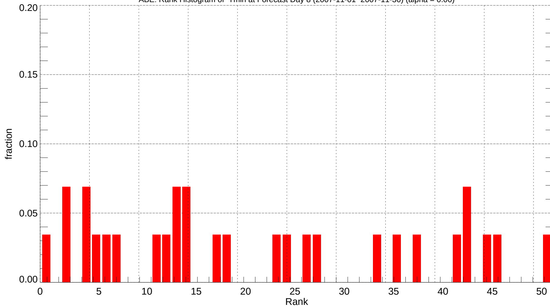
ABE: Rank Histogram of Tmin at Forecast Day 8 (2007-11-01~2007-11-30) (alpha = 0.00)
