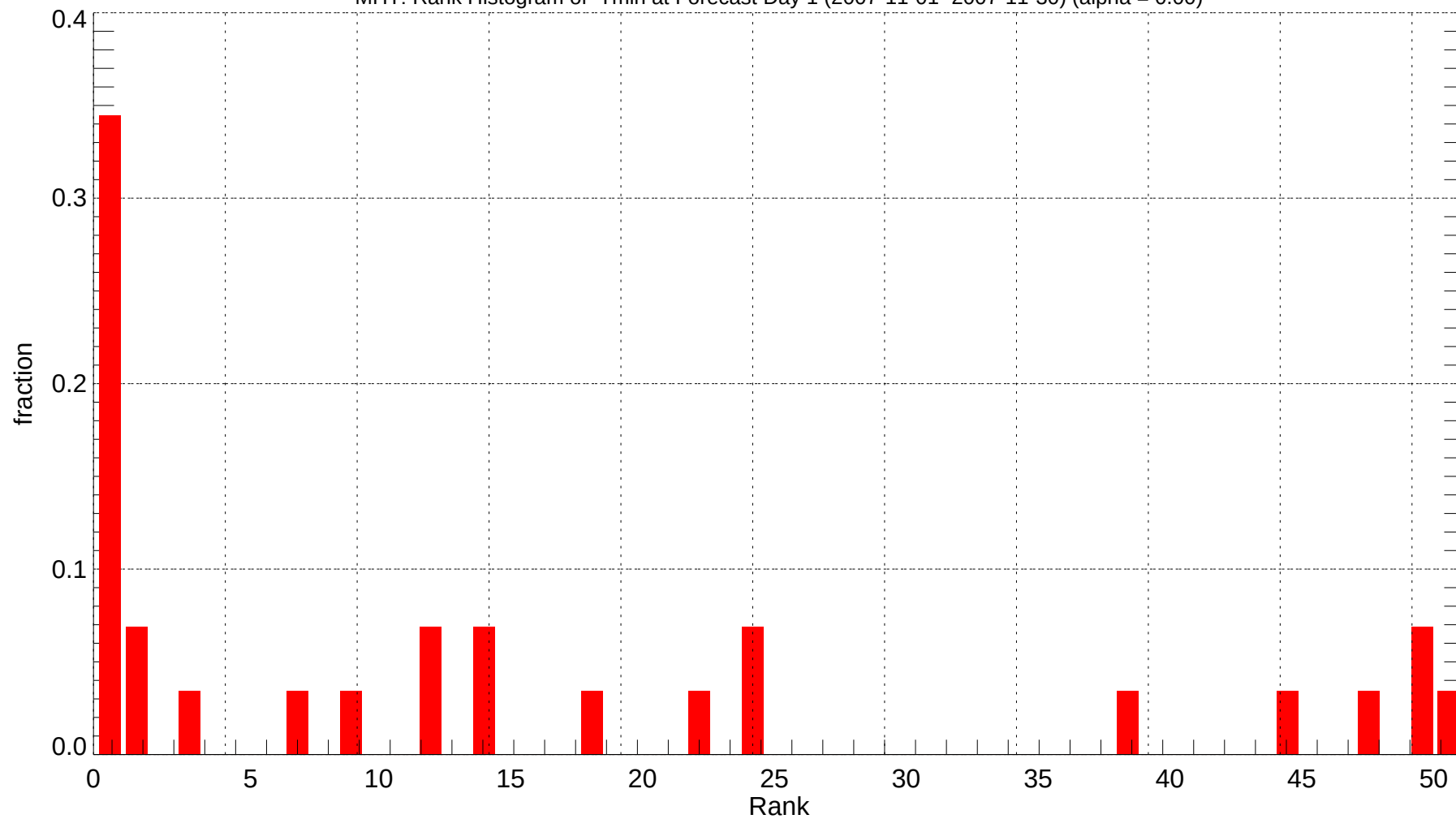
MHT: Rank Histogram of Tmin at Forecast Day 1 (2007-11-01~2007-11-30) (alpha = 0.00)
