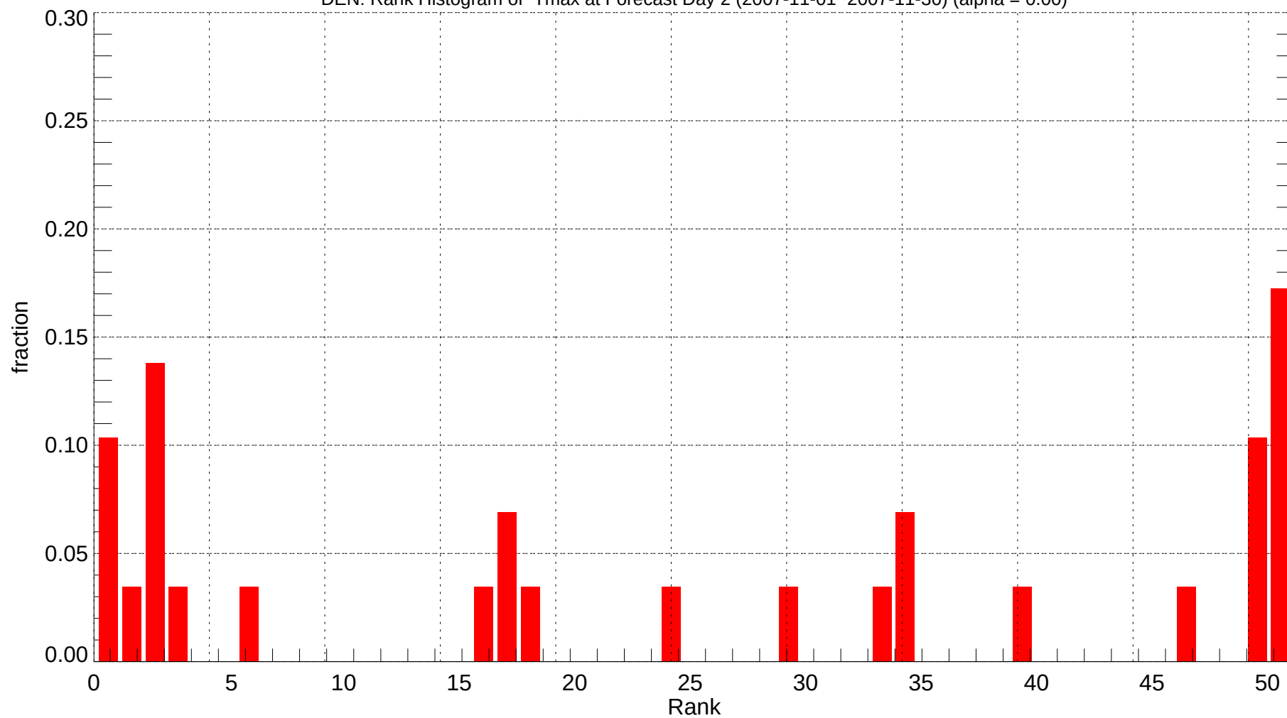
DEN: Rank Histogram of Tmax at Forecast Day 2 (2007-11-01~2007-11-30) (alpha = 0.00)
