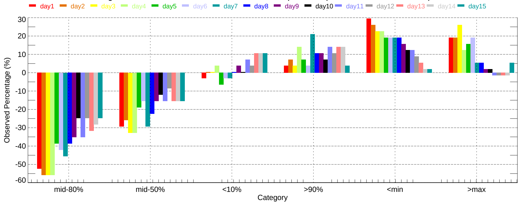
Observed Percentage Deviation of Ensembles - ALW: Min Temperature (2007-11-01~2007-11-30)
