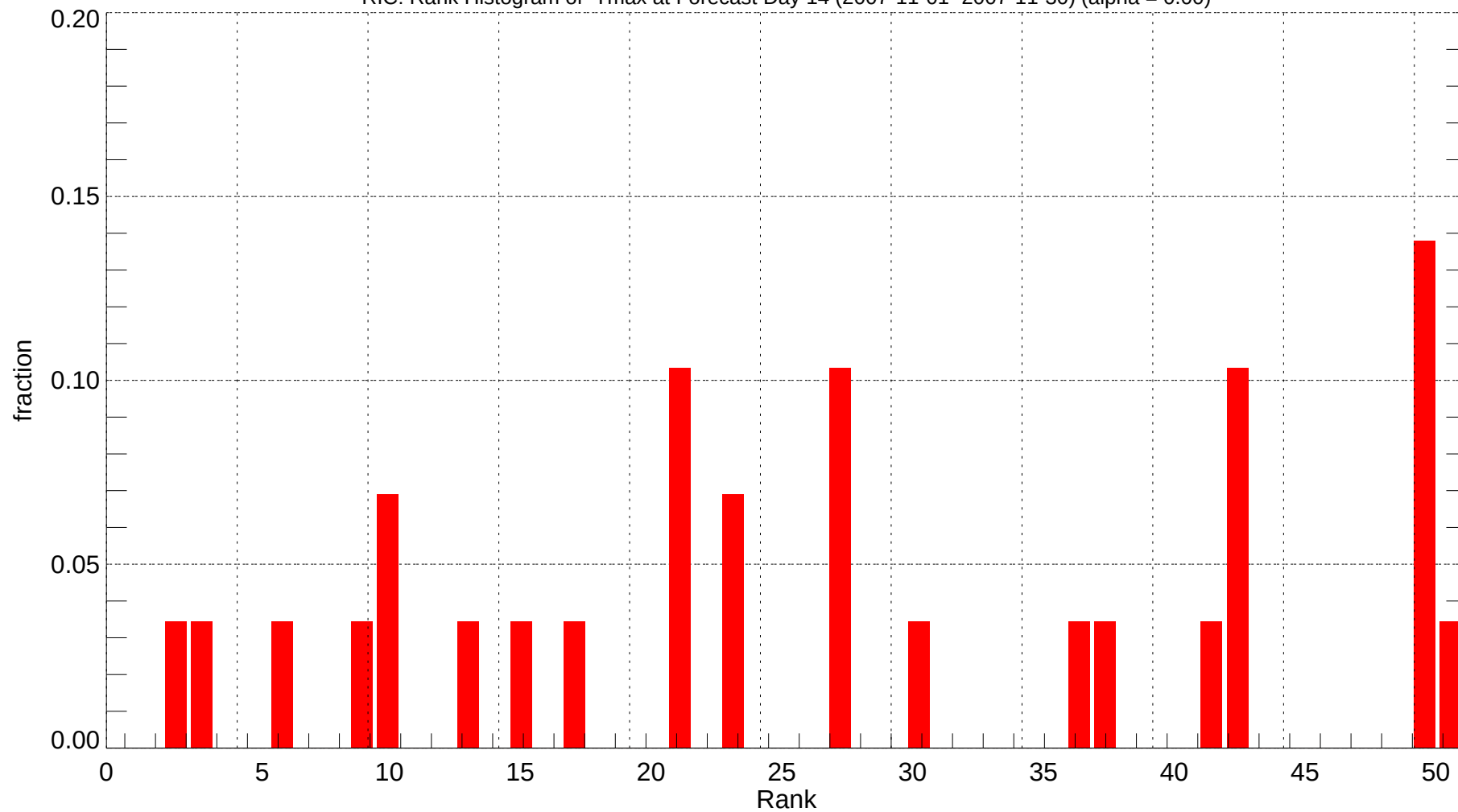
RIC: Rank Histogram of Tmax at Forecast Day 14 (2007-11-01~2007-11-30) (alpha = 0.00)
