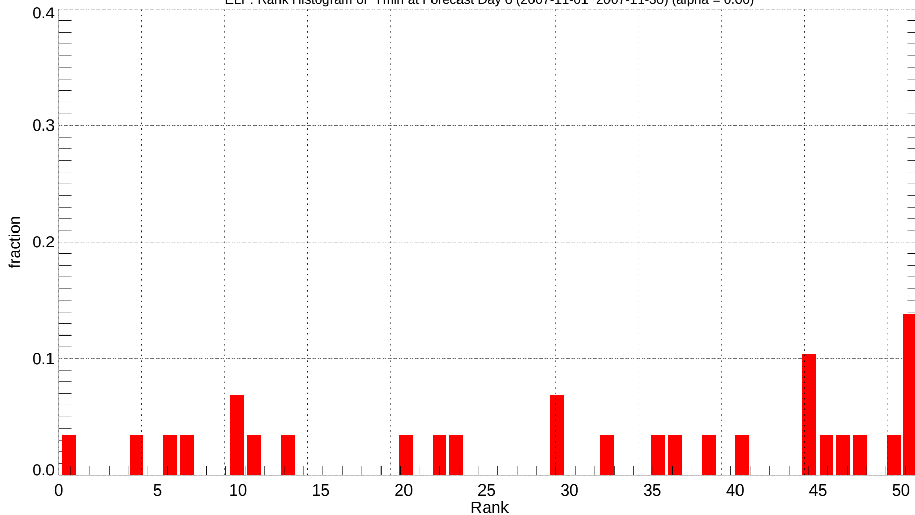
ELP: Rank Histogram of Tmin at Forecast Day 6 (2007-11-01~2007-11-30) (alpha = 0.00)
