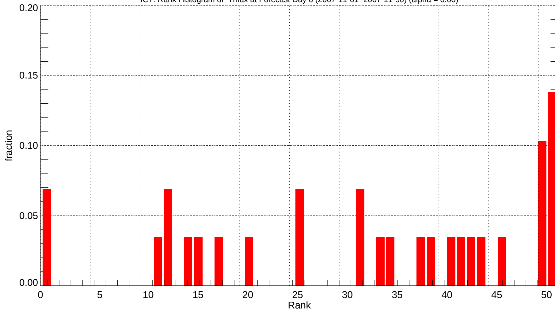
ICT: Rank Histogram of Tmax at Forecast Day 6 (2007-11-01~2007-11-30) (alpha = 0.00)
