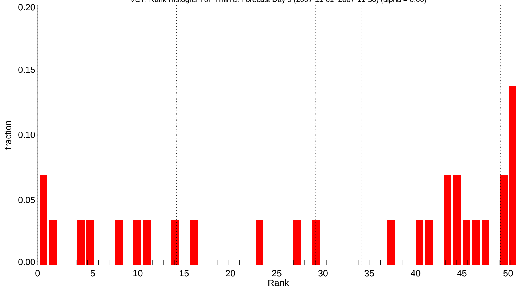
VCT: Rank Histogram of Tmin at Forecast Day 9 (2007-11-01~2007-11-30) (alpha = 0.00)
