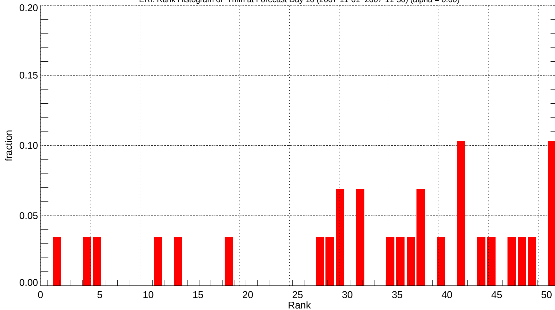
ERI: Rank Histogram of Tmin at Forecast Day 10 (2007-11-01~2007-11-30) (alpha = 0.00)
