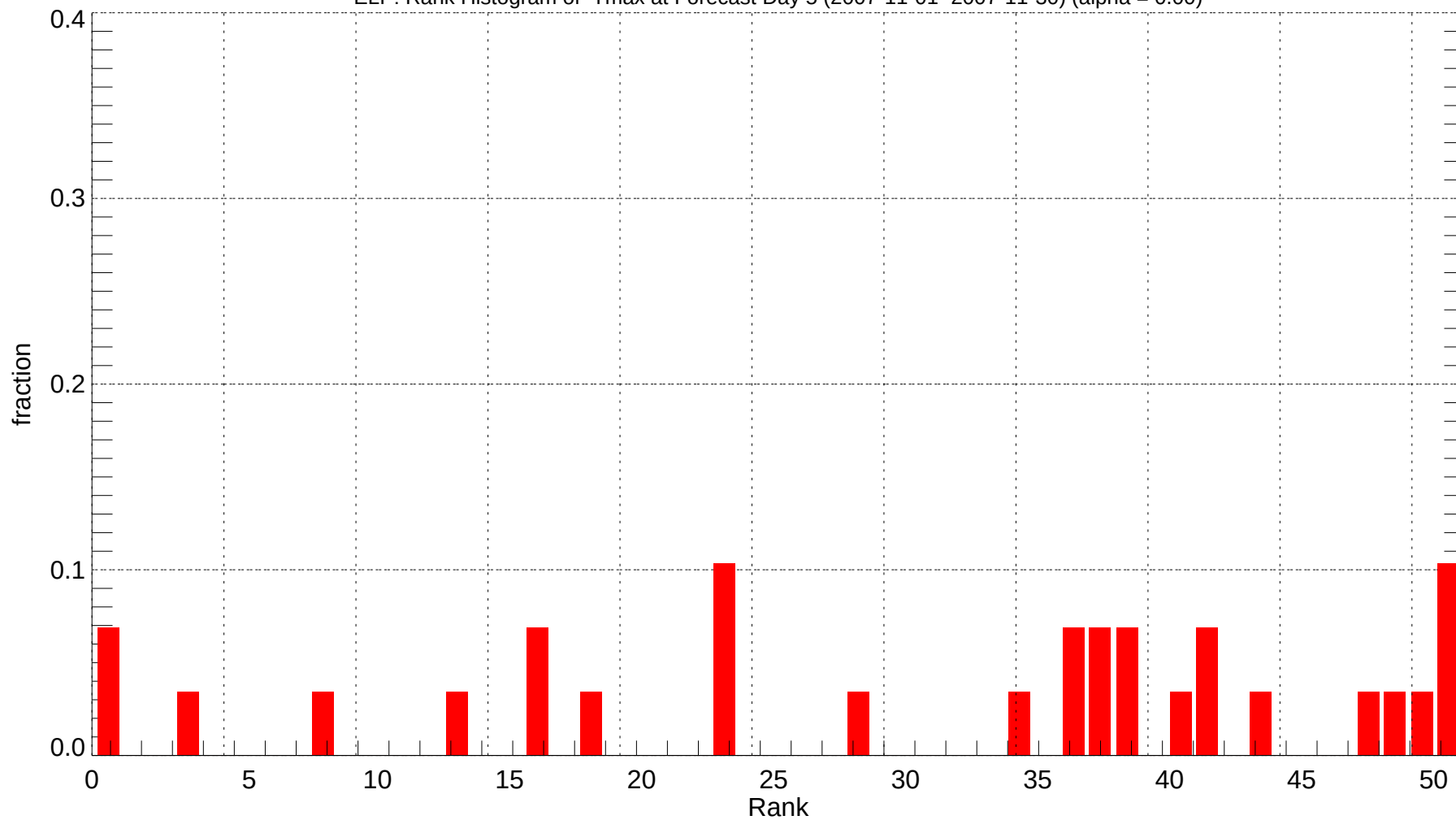
ELP: Rank Histogram of Tmax at Forecast Day 5 (2007-11-01~2007-11-30) (alpha = 0.00)
