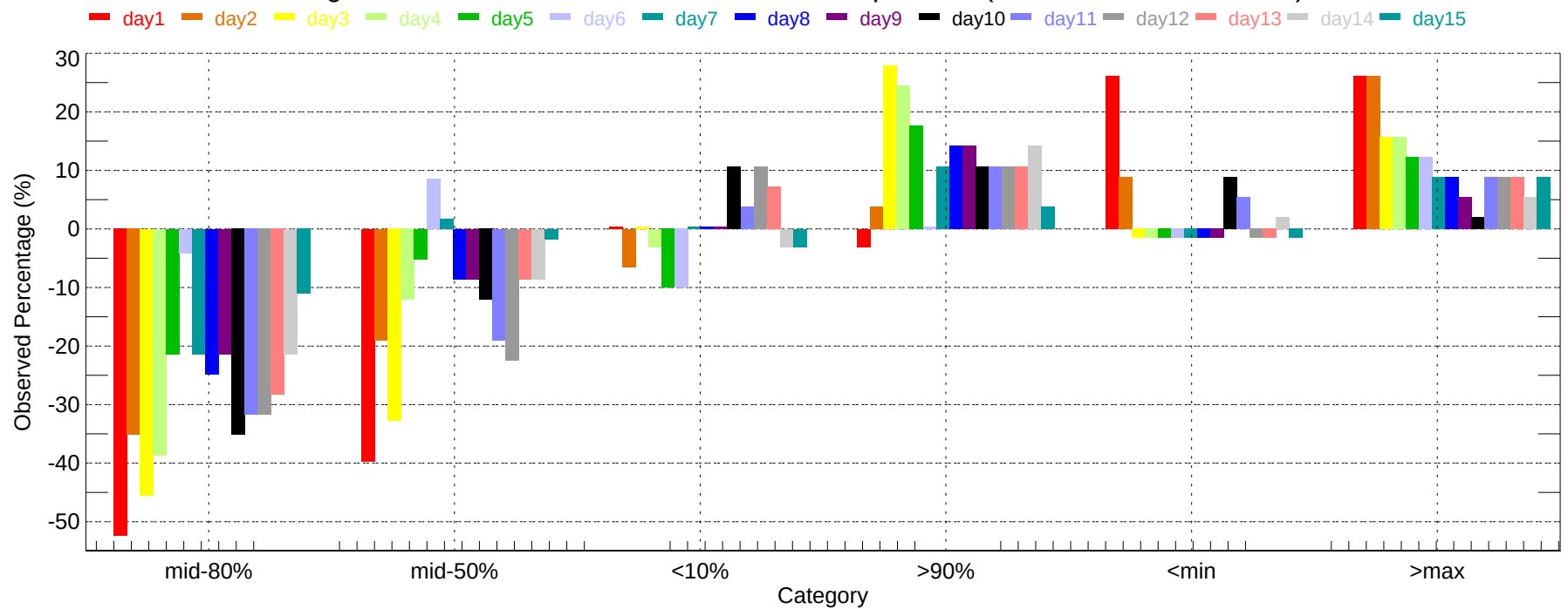
Observed Percentage Deviation of Ensembles - NTU: Max Temperature (2007-11-01~2007-11-30)
