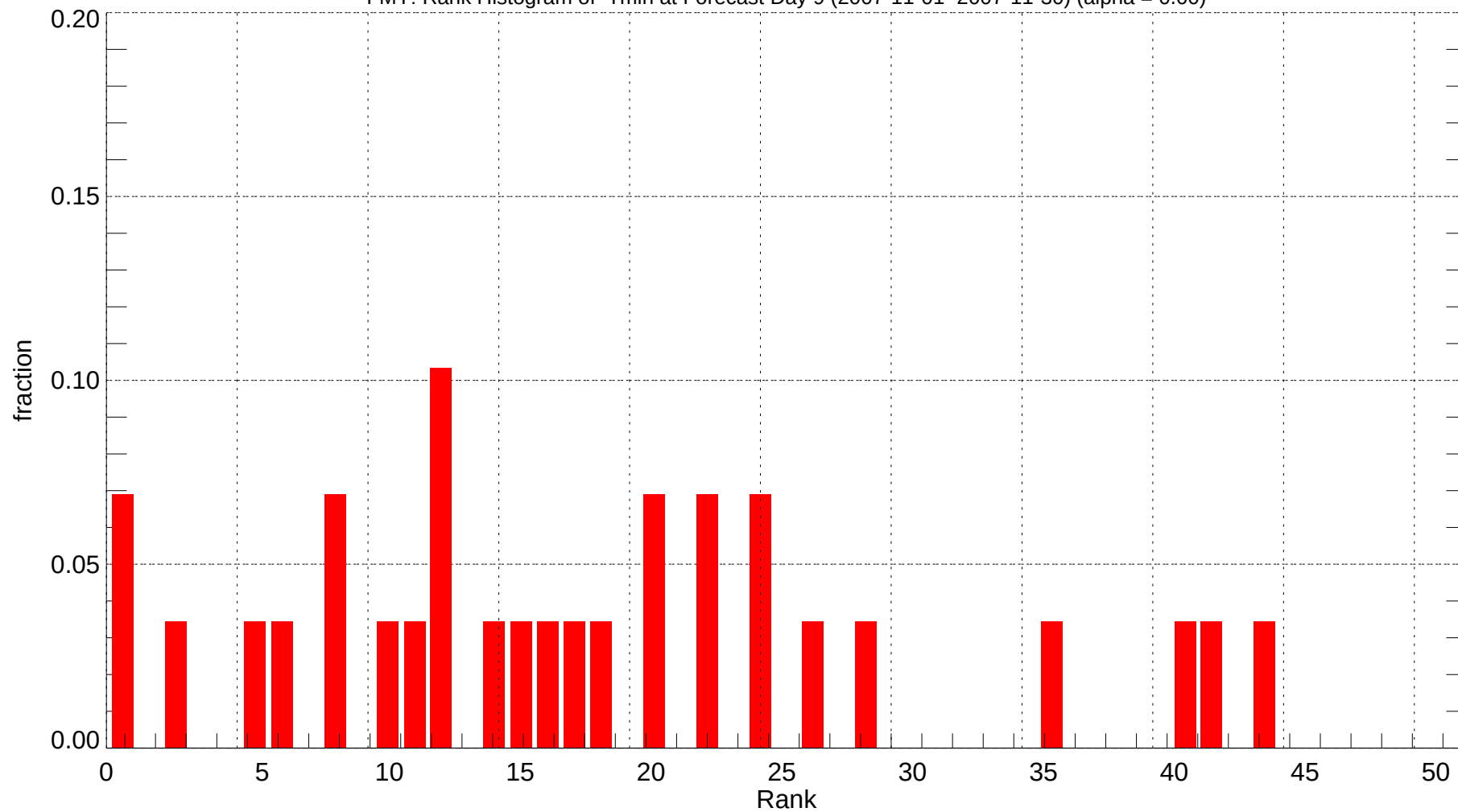
FMY: Rank Histogram of Tmin at Forecast Day 9 (2007-11-01~2007-11-30) (alpha = 0.00)
