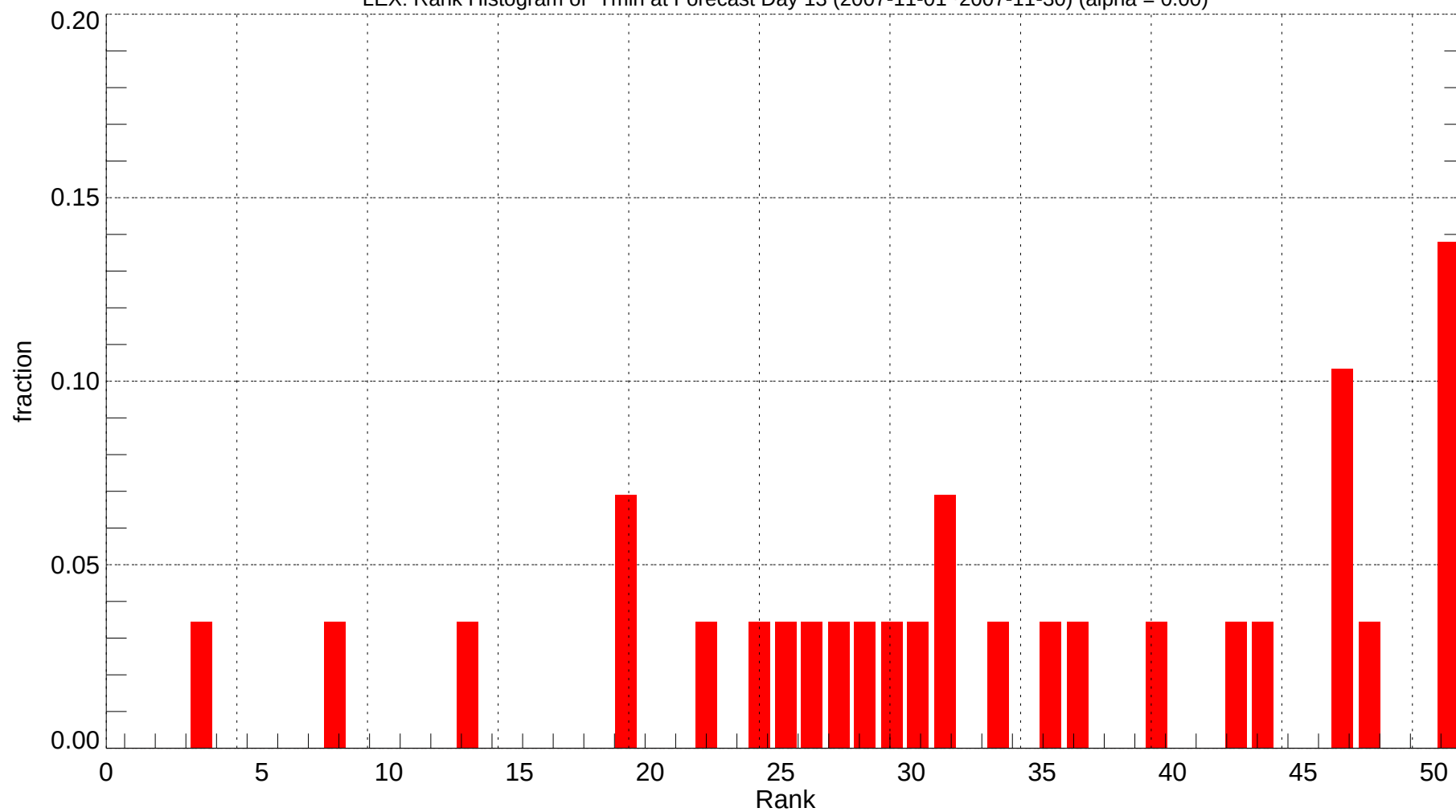
LEX: Rank Histogram of Tmin at Forecast Day 13 (2007-11-01~2007-11-30) (alpha = 0.00)
