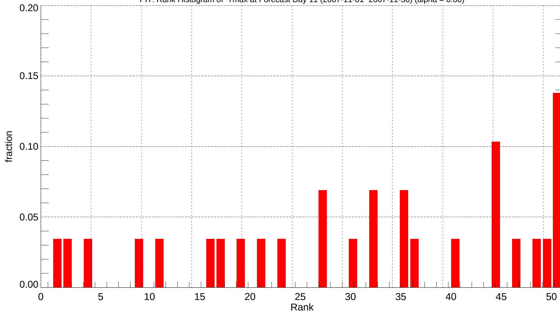
PIT: Rank Histogram of Tmax at Forecast Day 11 (2007-11-01~2007-11-30) (alpha = 0.00)
