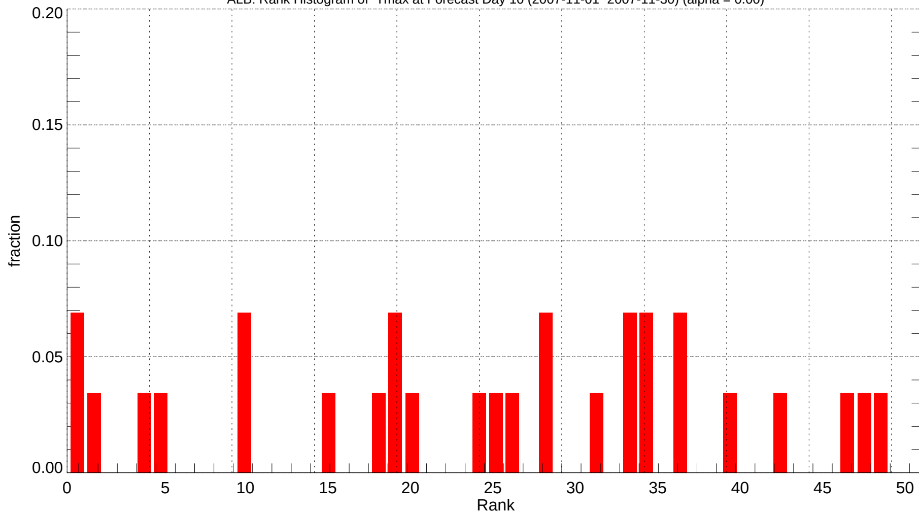
ALB: Rank Histogram of Tmax at Forecast Day 10 (2007-11-01~2007-11-30) (alpha = 0.00)
