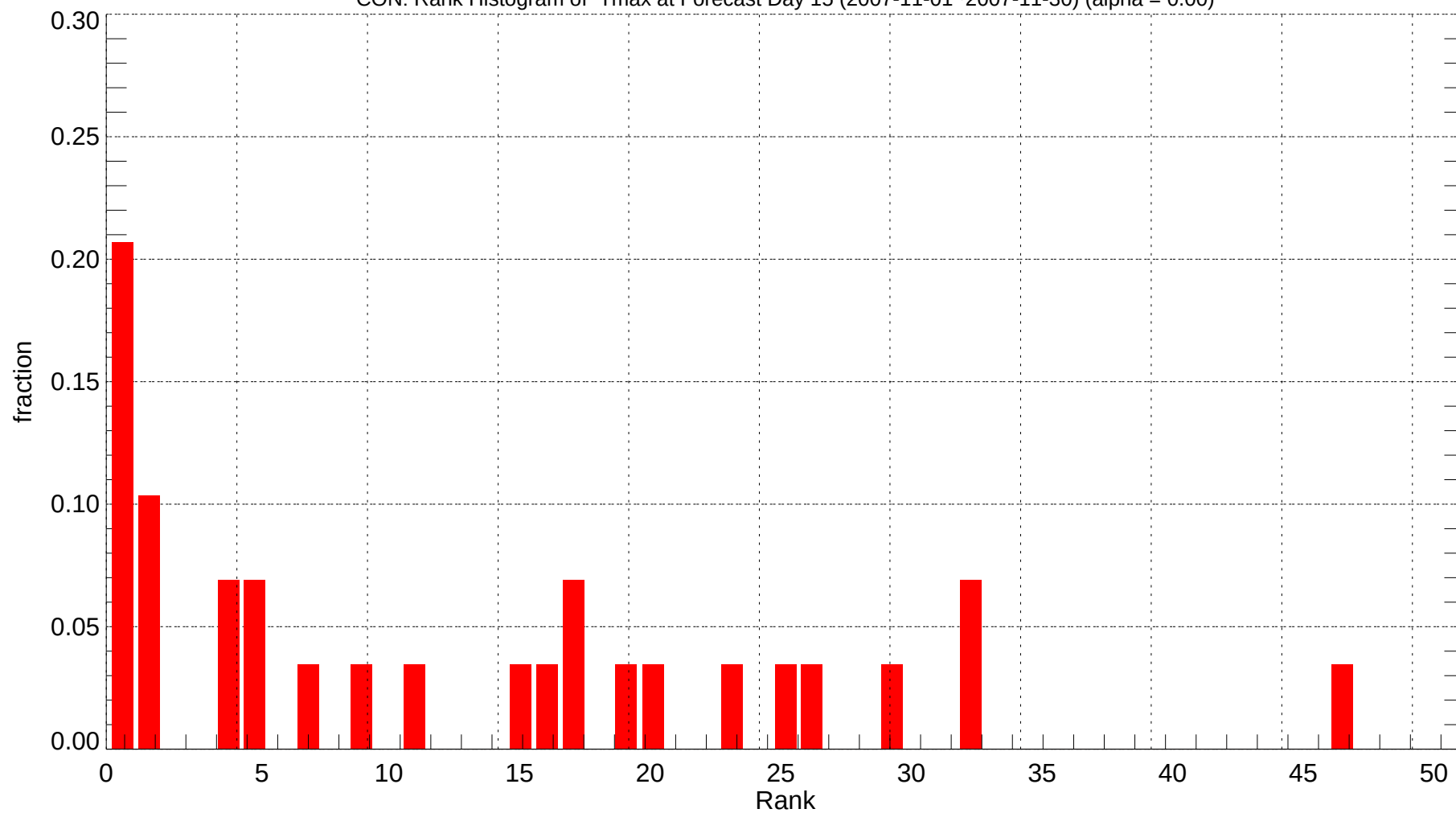
CON: Rank Histogram of Tmax at Forecast Day 15 (2007-11-01~2007-11-30) (alpha = 0.00)
