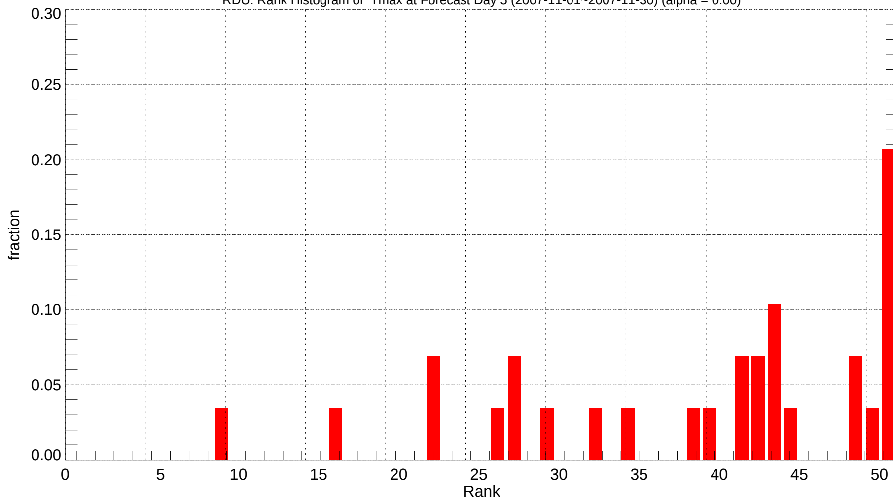
RDU: Rank Histogram of Tmax at Forecast Day 5 (2007-11-01~2007-11-30) (alpha = 0.00)
