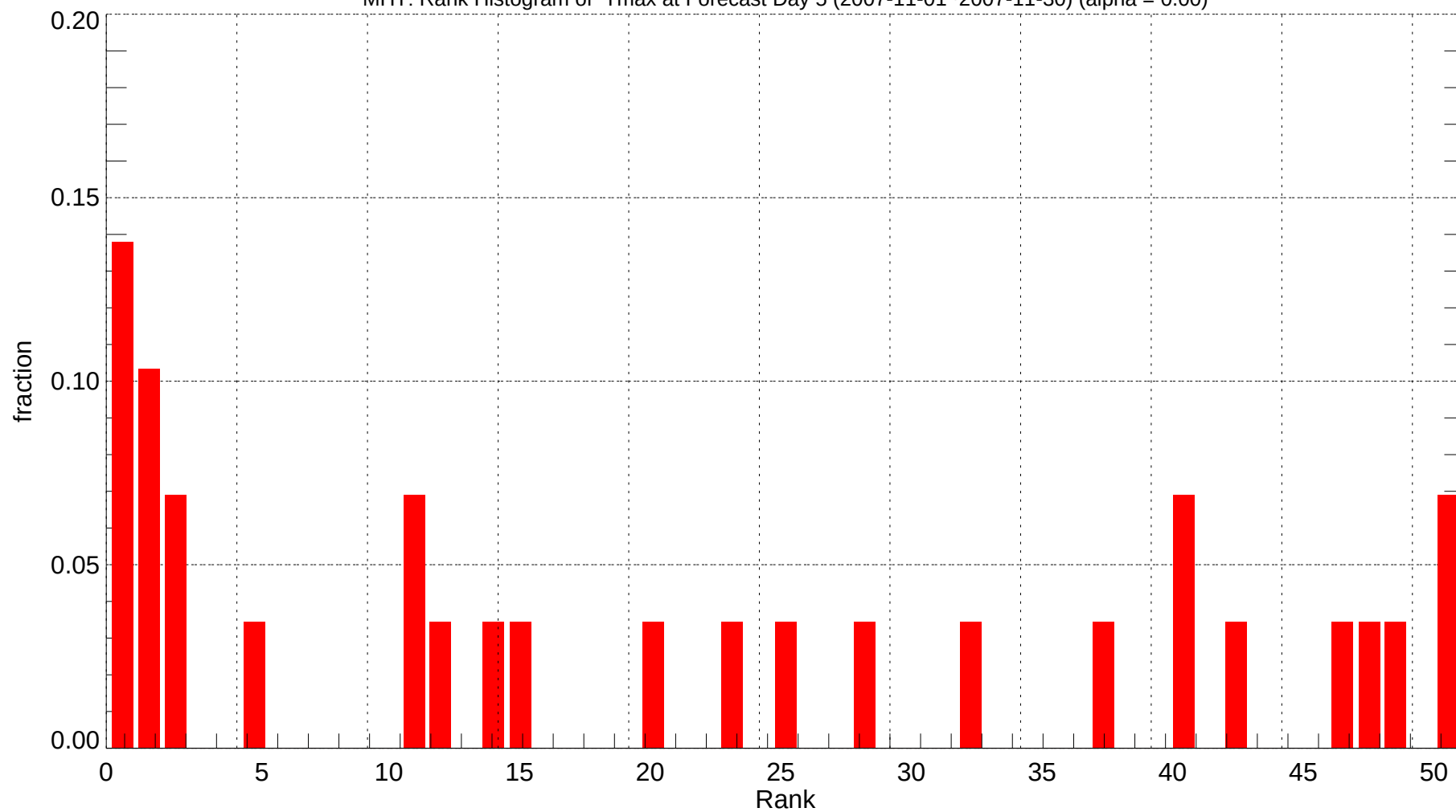
MHT: Rank Histogram of Tmax at Forecast Day 5 (2007-11-01~2007-11-30) (alpha = 0.00)
