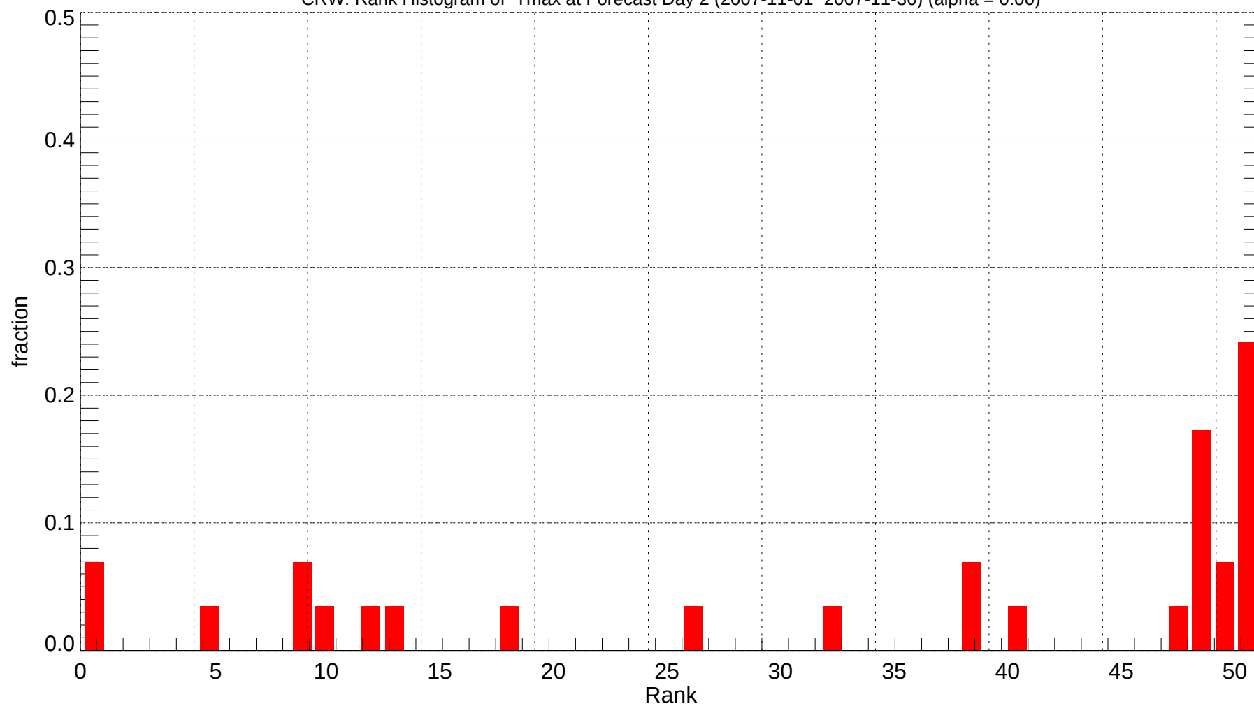
CRW: Rank Histogram of Tmax at Forecast Day 2 (2007-11-01~2007-11-30) (alpha = 0.00)
