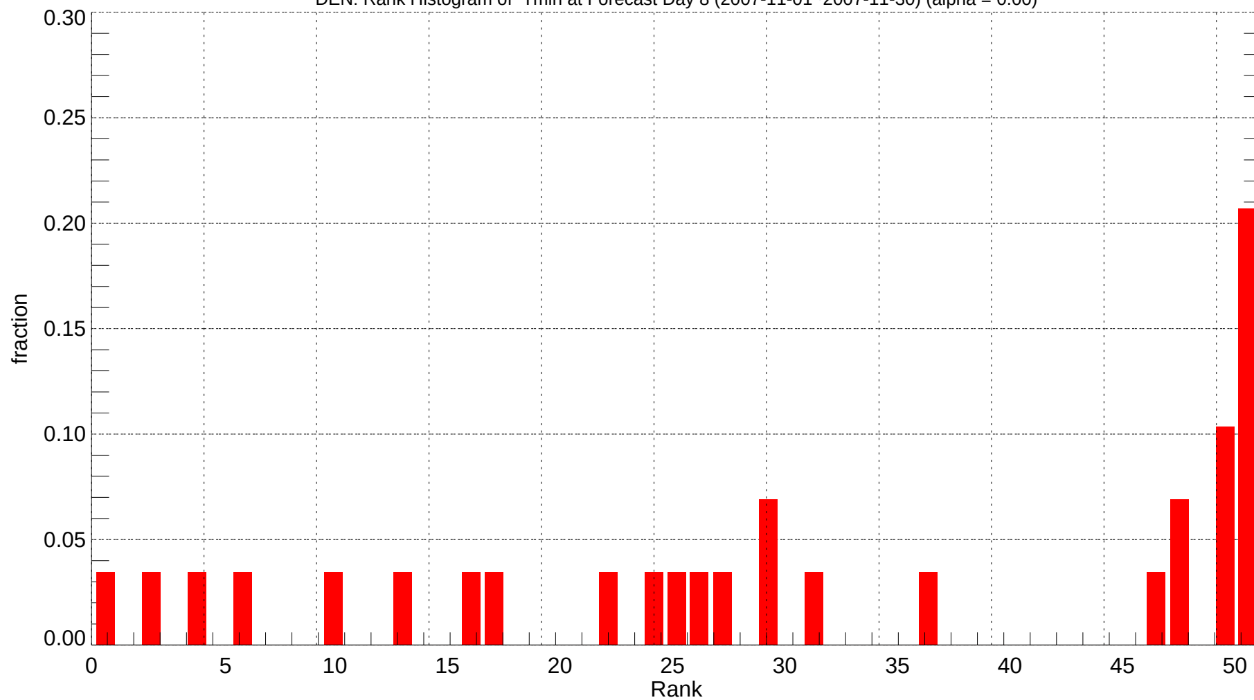
DEN: Rank Histogram of Tmin at Forecast Day 8 (2007-11-01~2007-11-30) (alpha = 0.00)
