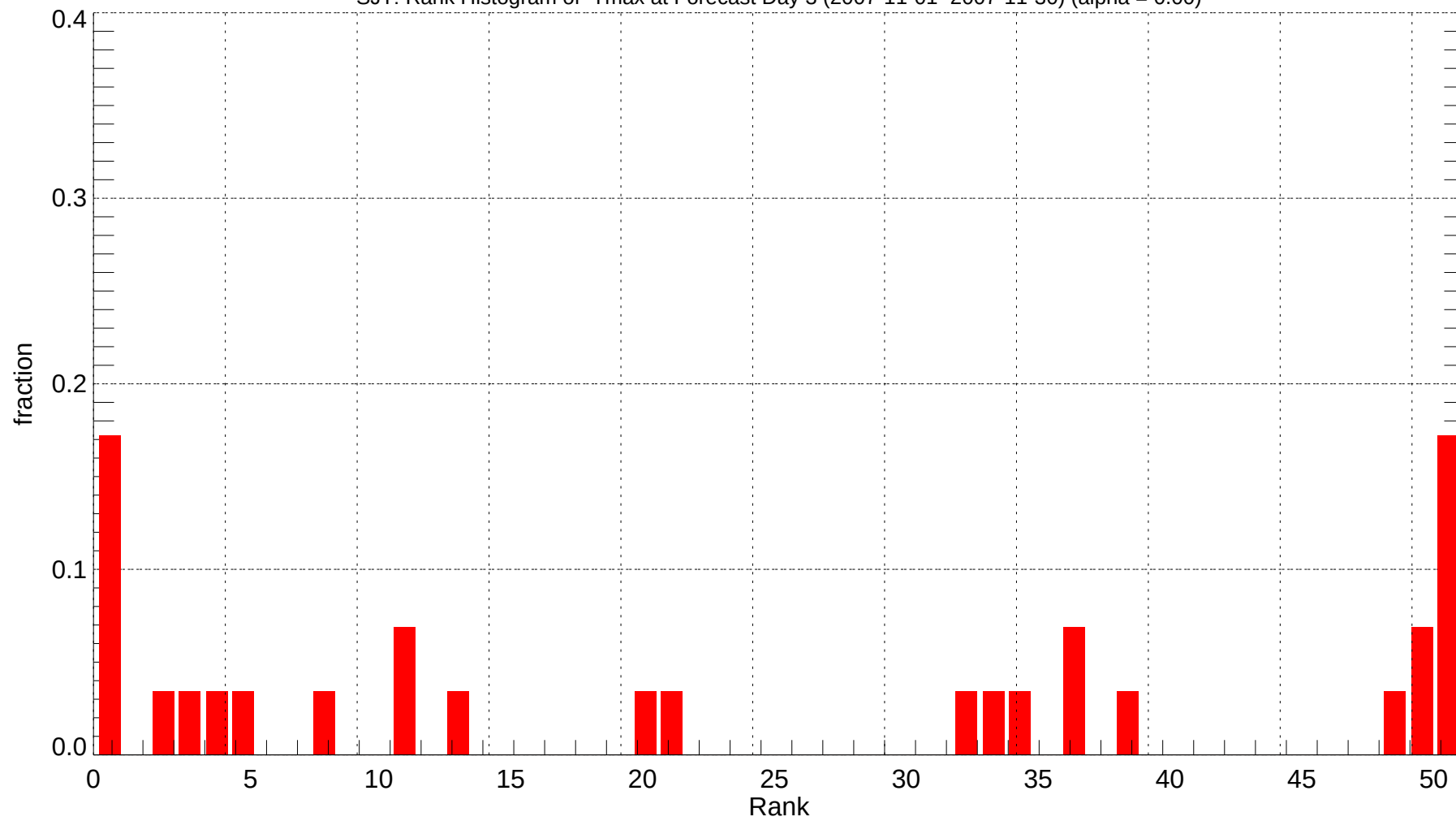
SJT: Rank Histogram of Tmax at Forecast Day 3 (2007-11-01~2007-11-30) (alpha = 0.00)
