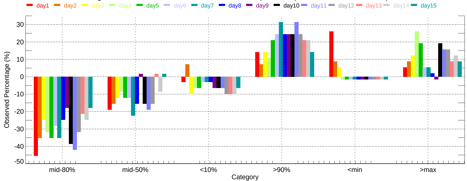
Observed Percentage Deviation of Ensembles - BNA: Max Temperature (2007-11-01~2007-11-30)
