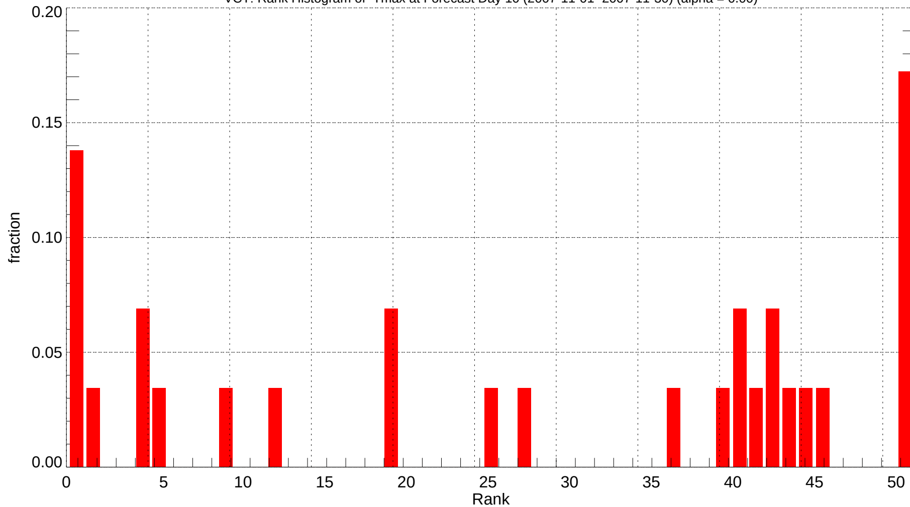
VCT: Rank Histogram of Tmax at Forecast Day 10 (2007-11-01~2007-11-30) (alpha = 0.00)
