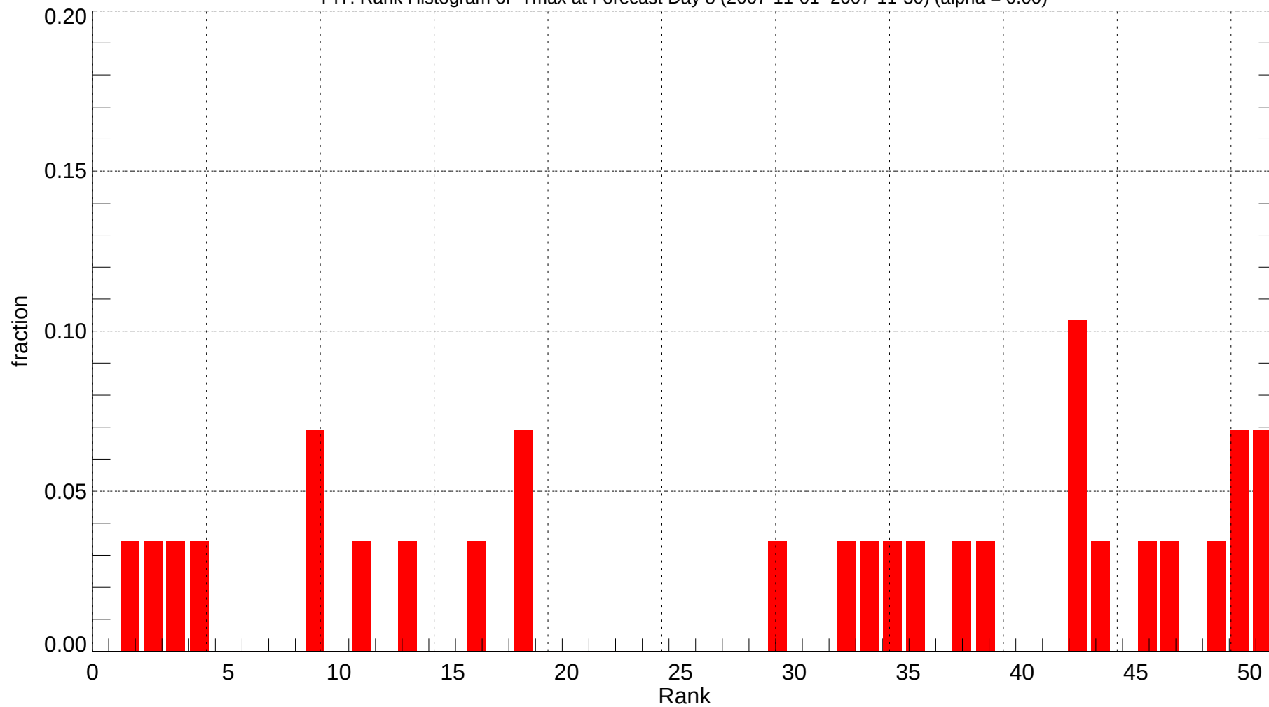
PIT: Rank Histogram of Tmax at Forecast Day 8 (2007-11-01~2007-11-30) (alpha = 0.00)
