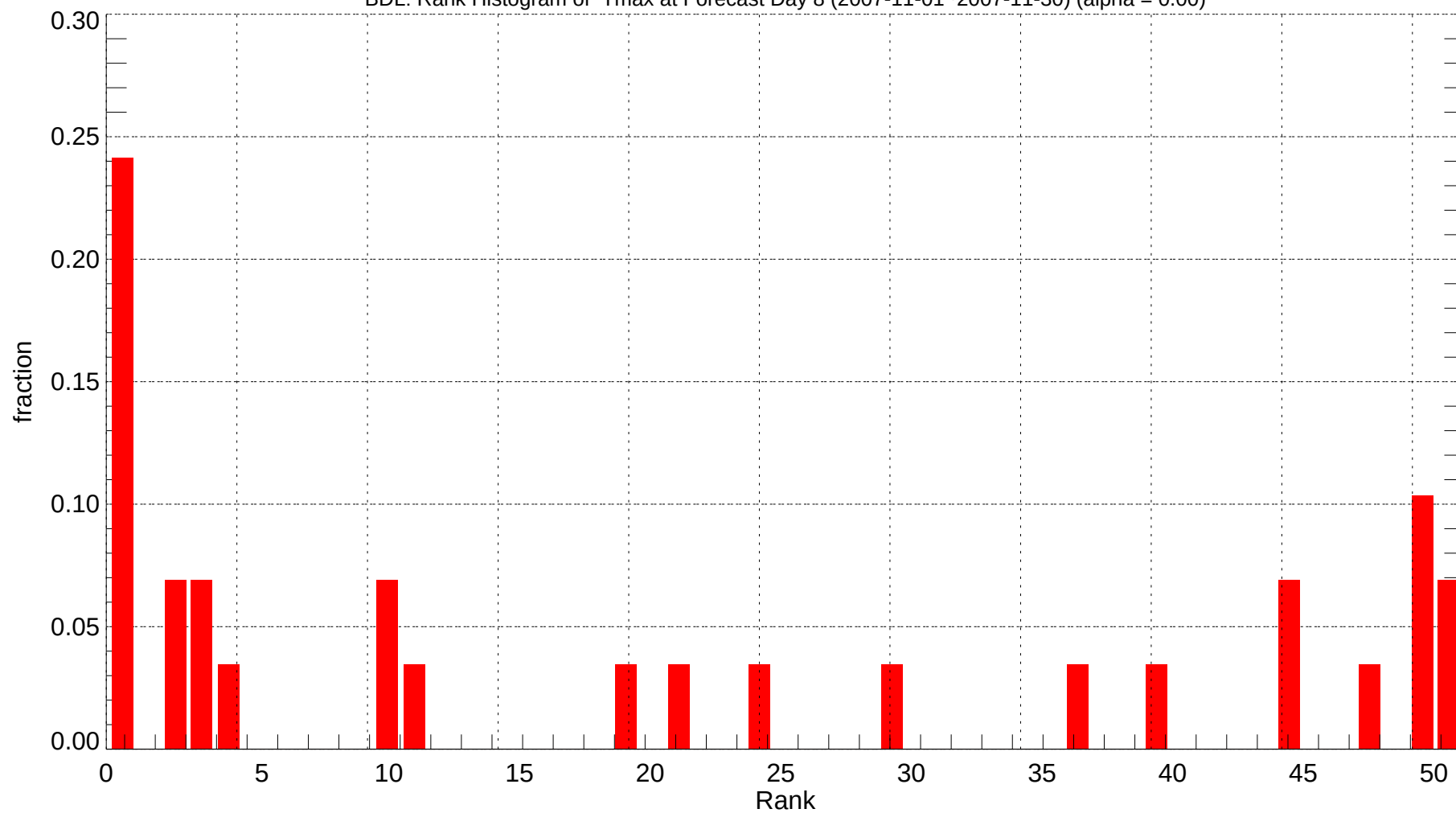
BDL: Rank Histogram of Tmax at Forecast Day 8 (2007-11-01~2007-11-30) (alpha = 0.00)
