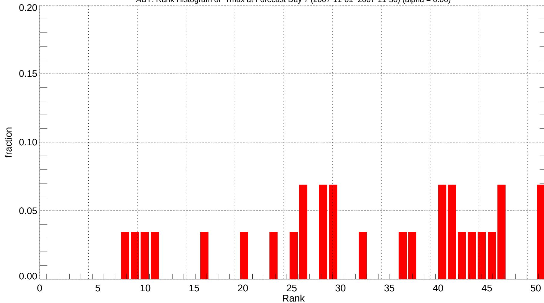
ABY: Rank Histogram of Tmax at Forecast Day 7 (2007-11-01~2007-11-30) (alpha = 0.00)
