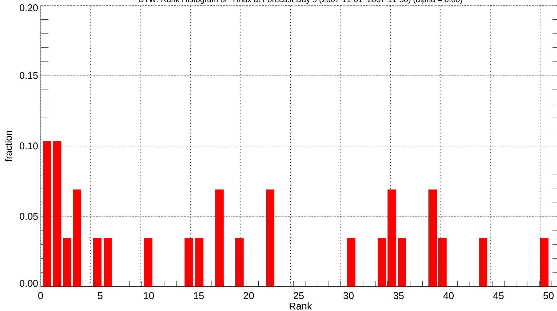
DTW: Rank Histogram of Tmax at Forecast Day 5 (2007-11-01~2007-11-30) (alpha = 0.00)
