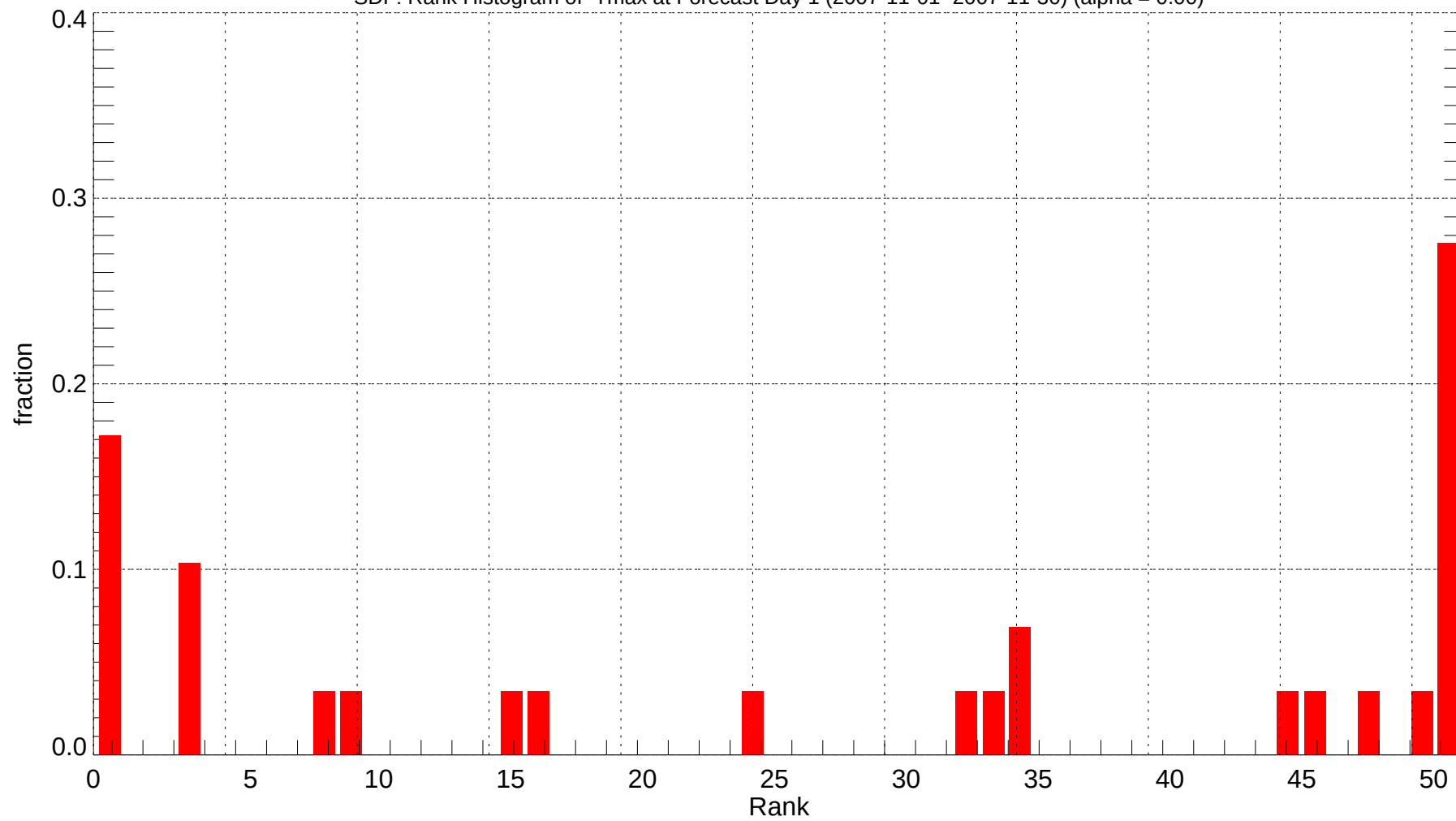
SDF: Rank Histogram of Tmax at Forecast Day 1 (2007-11-01~2007-11-30) (alpha = 0.00)
