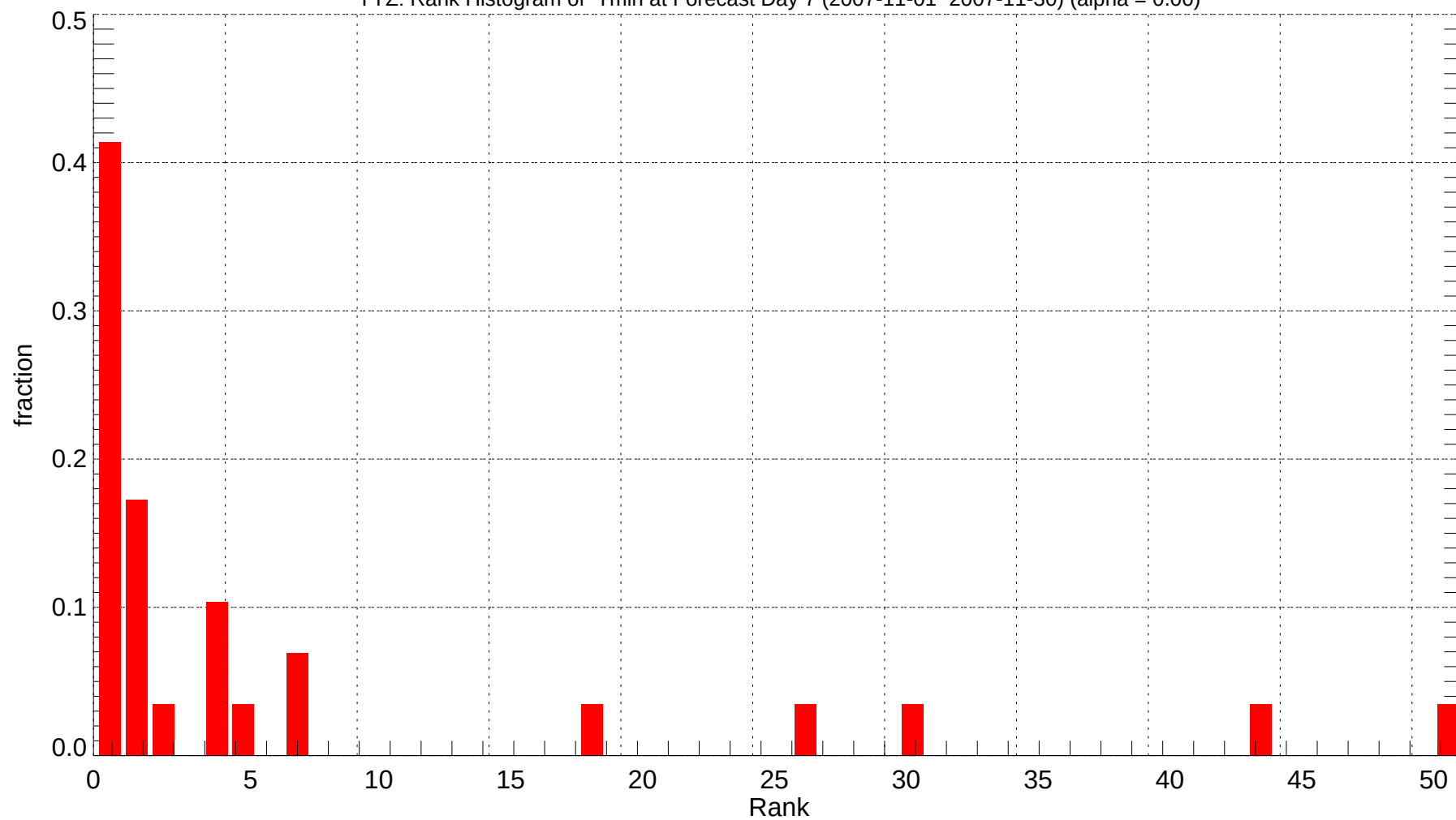
YYZ: Rank Histogram of Tmin at Forecast Day 7 (2007-11-01~2007-11-30) (alpha = 0.00)
