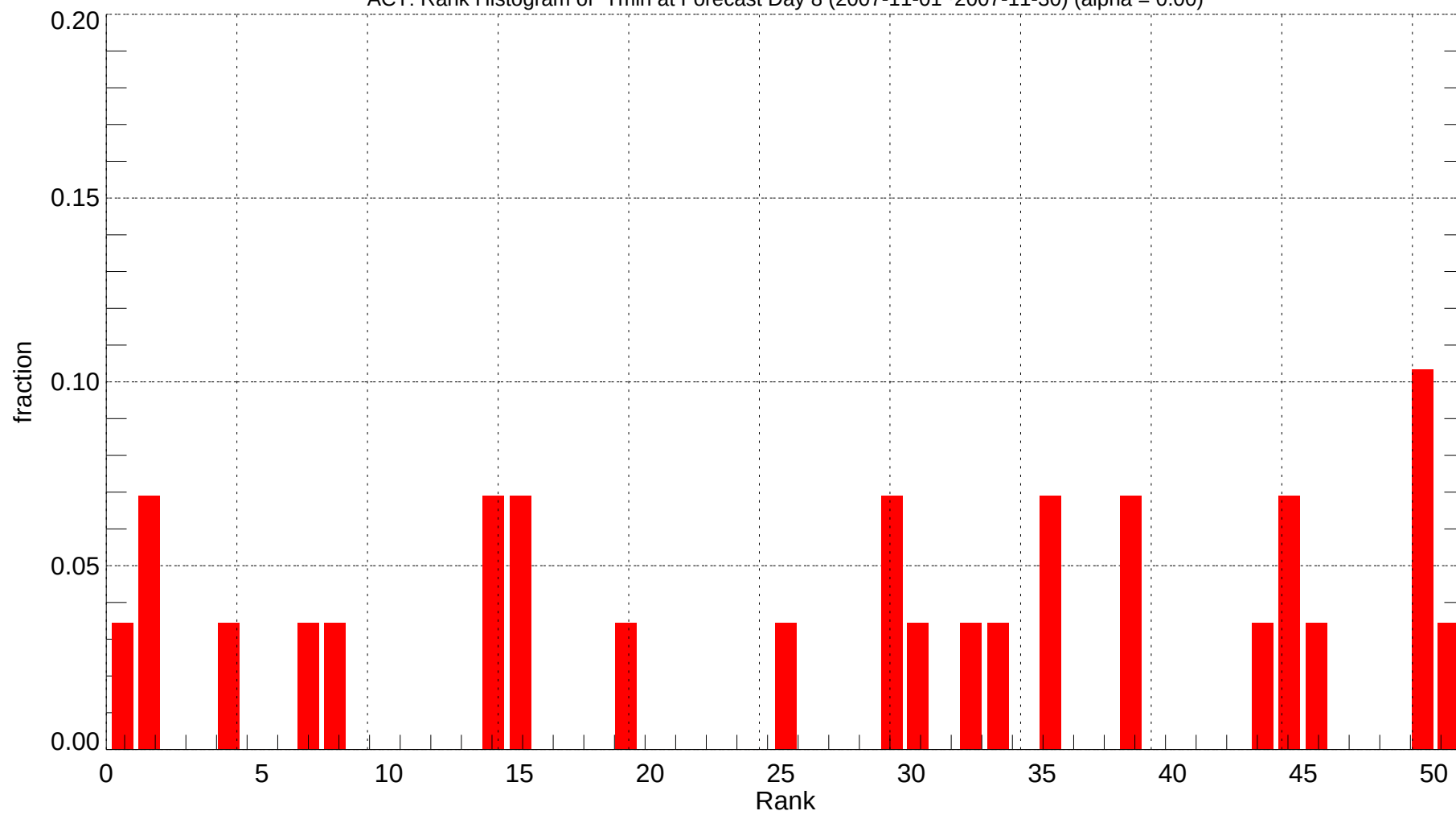
ACT: Rank Histogram of Tmin at Forecast Day 8 (2007-11-01~2007-11-30) (alpha = 0.00)
