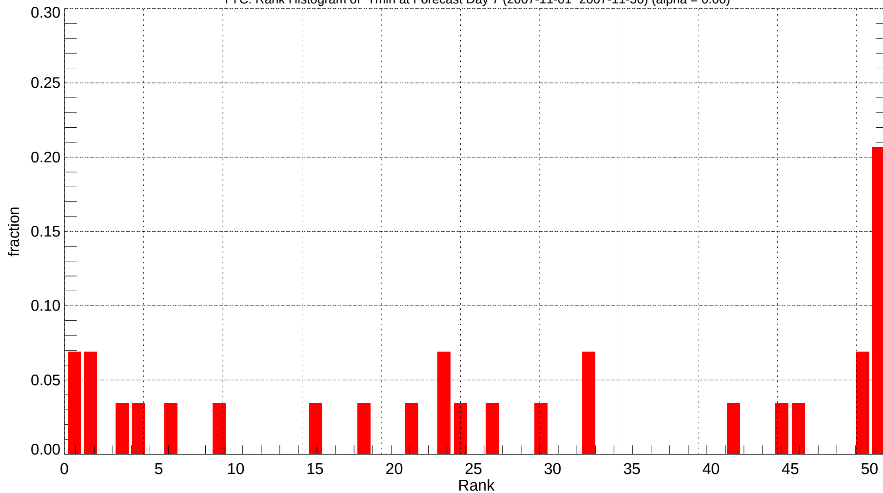
YYC: Rank Histogram of Tmin at Forecast Day 7 (2007-11-01~2007-11-30) (alpha = 0.00)
