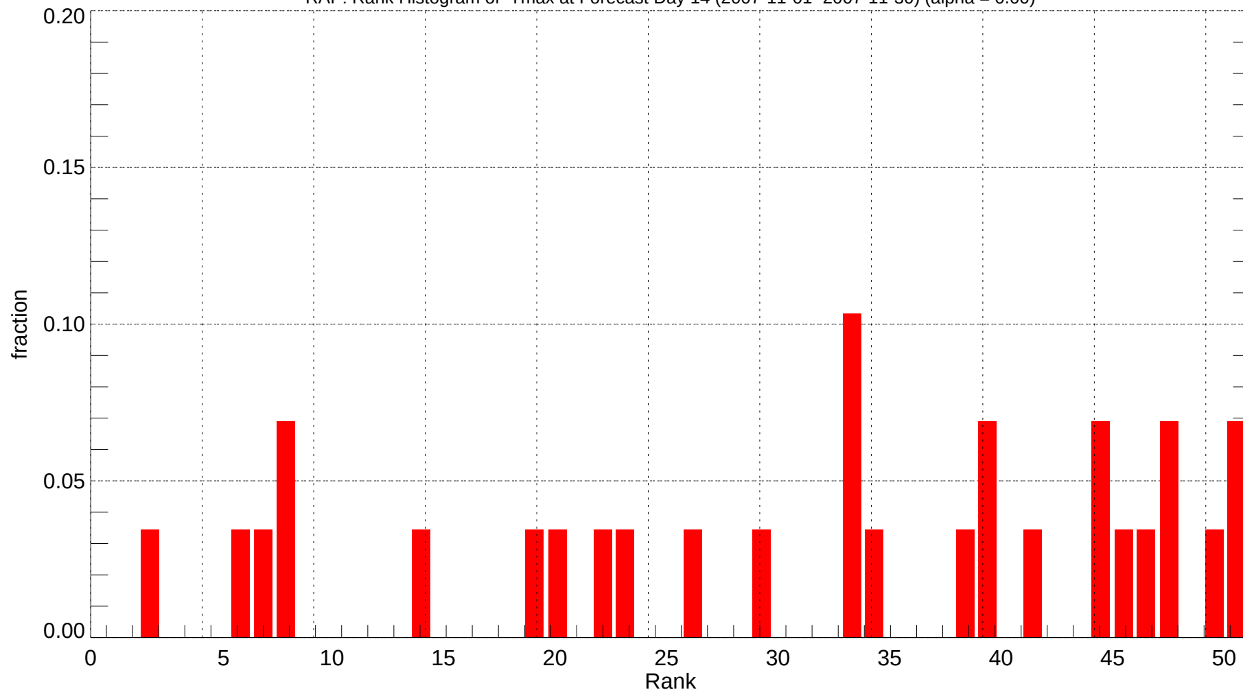
RAP: Rank Histogram of Tmax at Forecast Day 14 (2007-11-01~2007-11-30) (alpha = 0.00)
