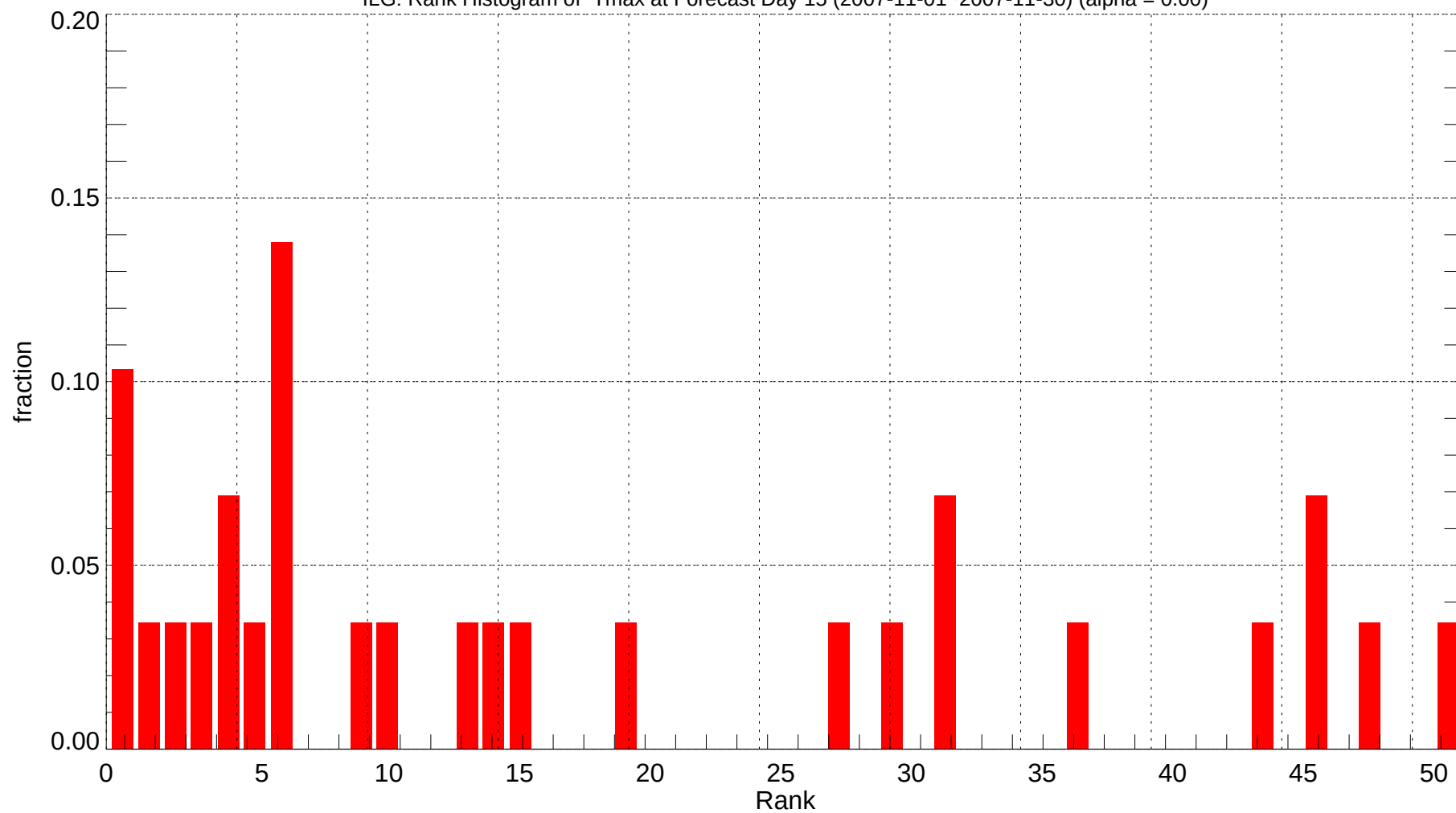
ILG: Rank Histogram of Tmax at Forecast Day 15 (2007-11-01~2007-11-30) (alpha = 0.00)
