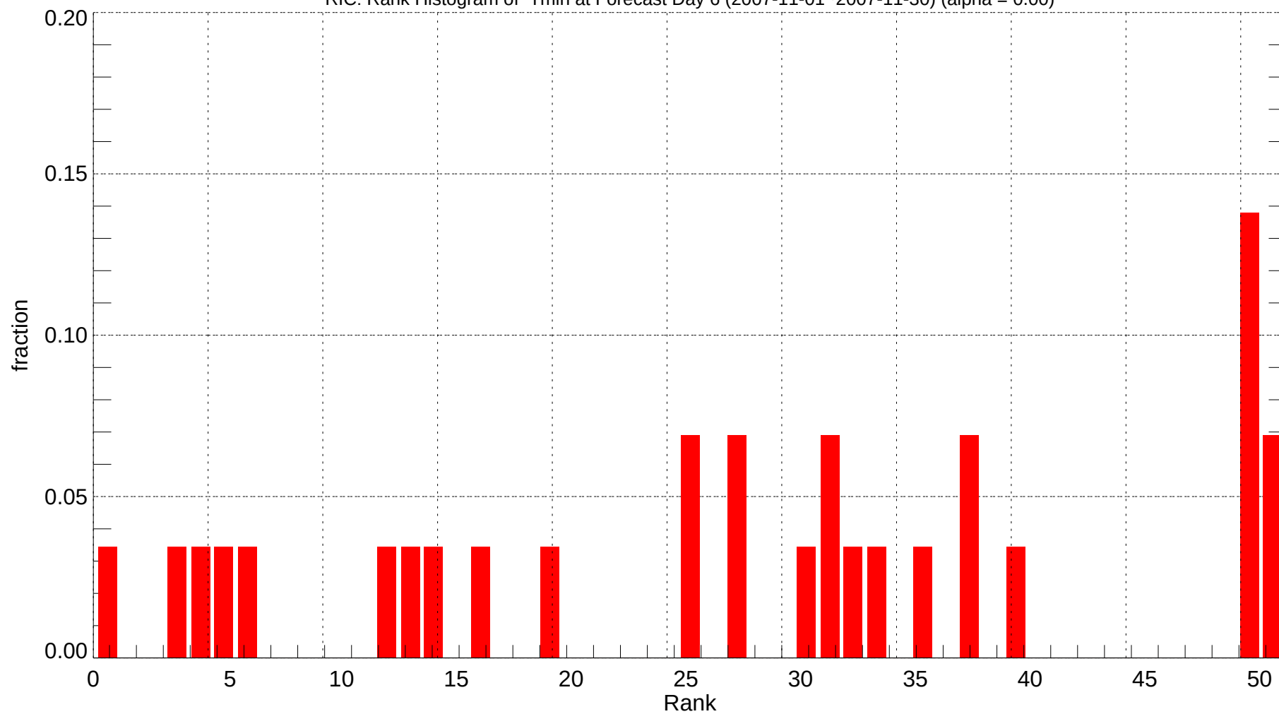
RIC: Rank Histogram of Tmin at Forecast Day 6 (2007-11-01~2007-11-30) (alpha = 0.00)
