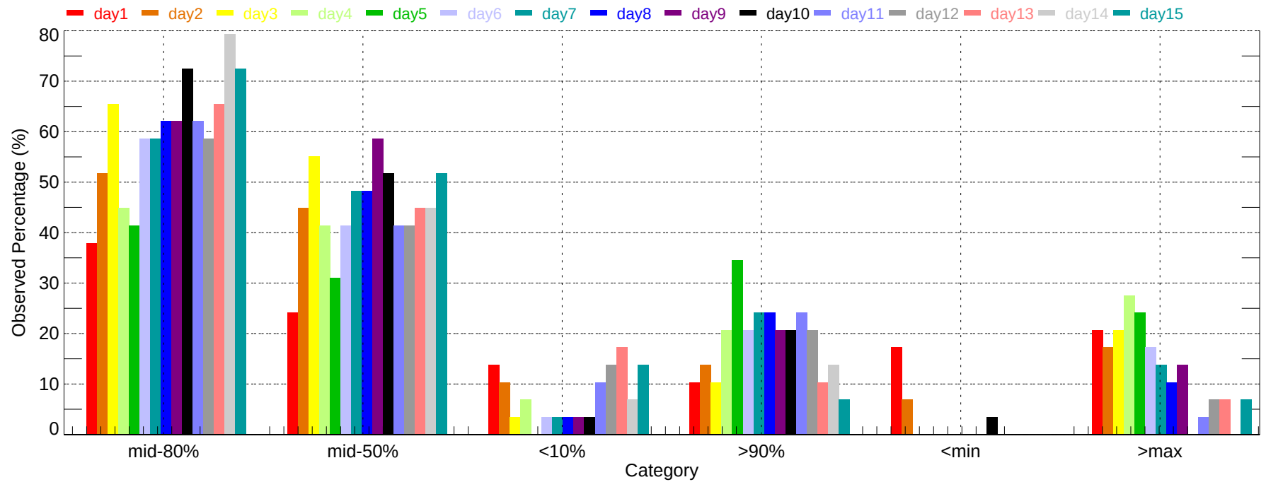
Observed Percentage of Ensembles - RDU: Max Temperature (2007-11-01~2007-11-30)
