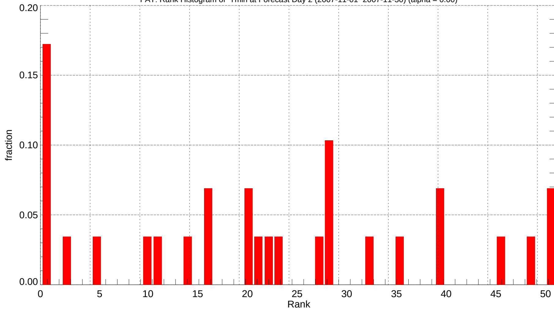
FAT: Rank Histogram of Tmin at Forecast Day 2 (2007-11-01~2007-11-30) (alpha = 0.00)
