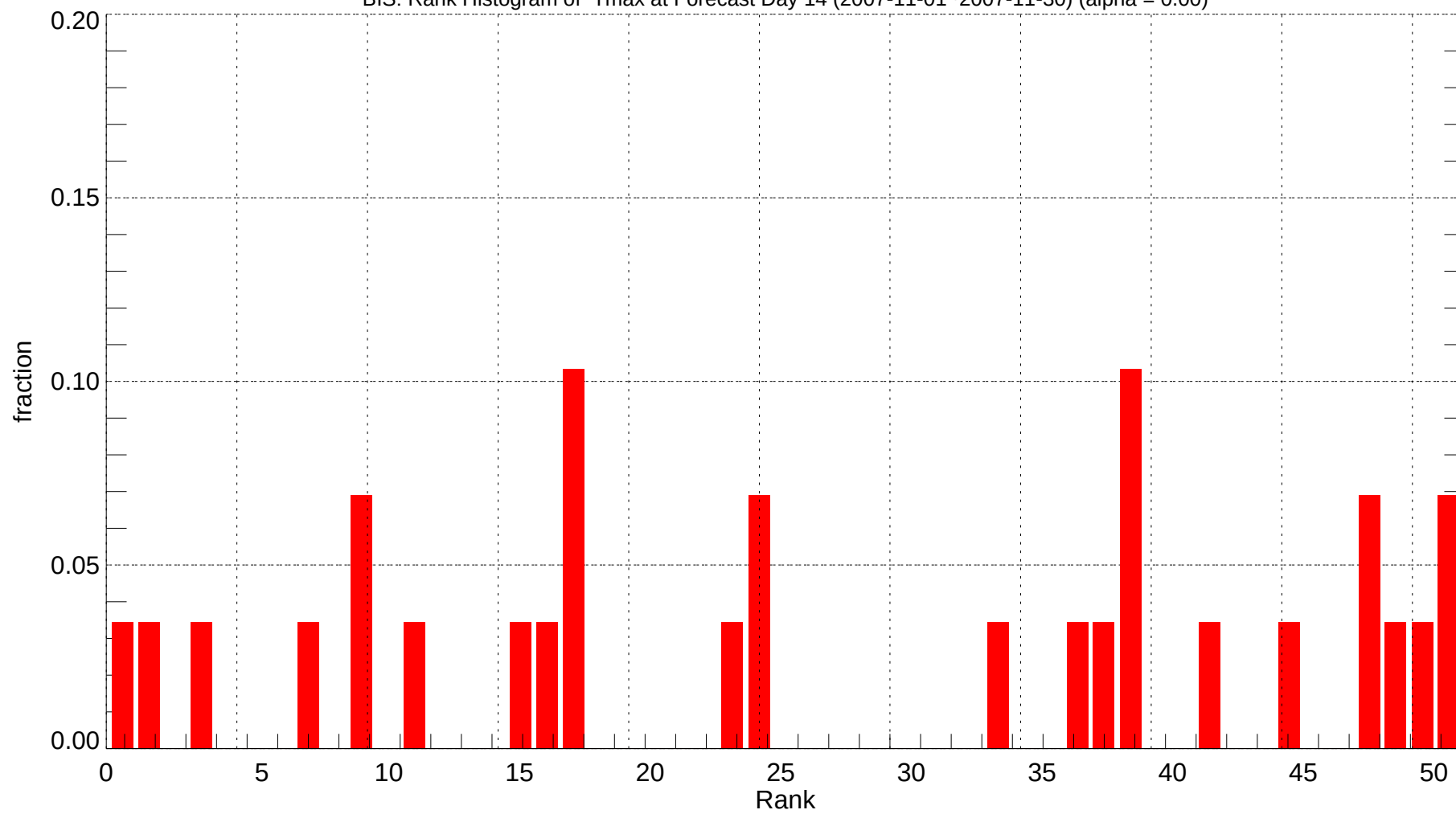
BIS: Rank Histogram of Tmax at Forecast Day 14 (2007-11-01~2007-11-30) (alpha = 0.00)
