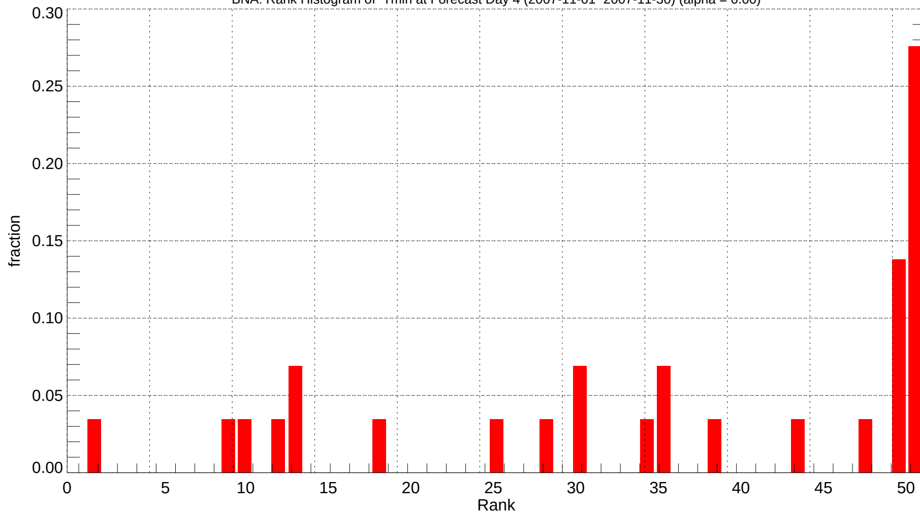
BNA: Rank Histogram of Tmin at Forecast Day 4 (2007-11-01~2007-11-30) (alpha = 0.00)
