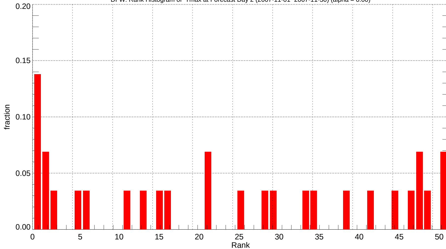
DFW: Rank Histogram of Tmax at Forecast Day 2 (2007-11-01~2007-11-30) (alpha = 0.00)
