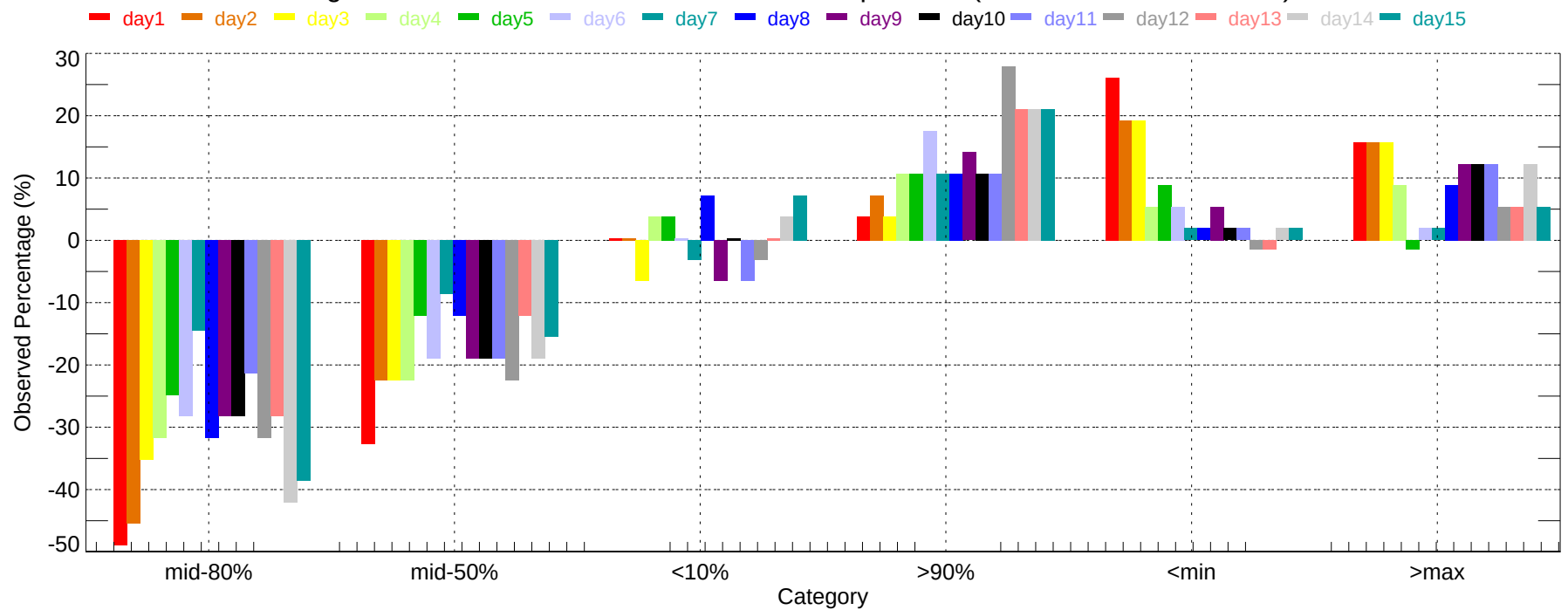
Observed Percentage Deviation of Ensembles - ABI: Max Temperature (2007-11-01~2007-11-30)
