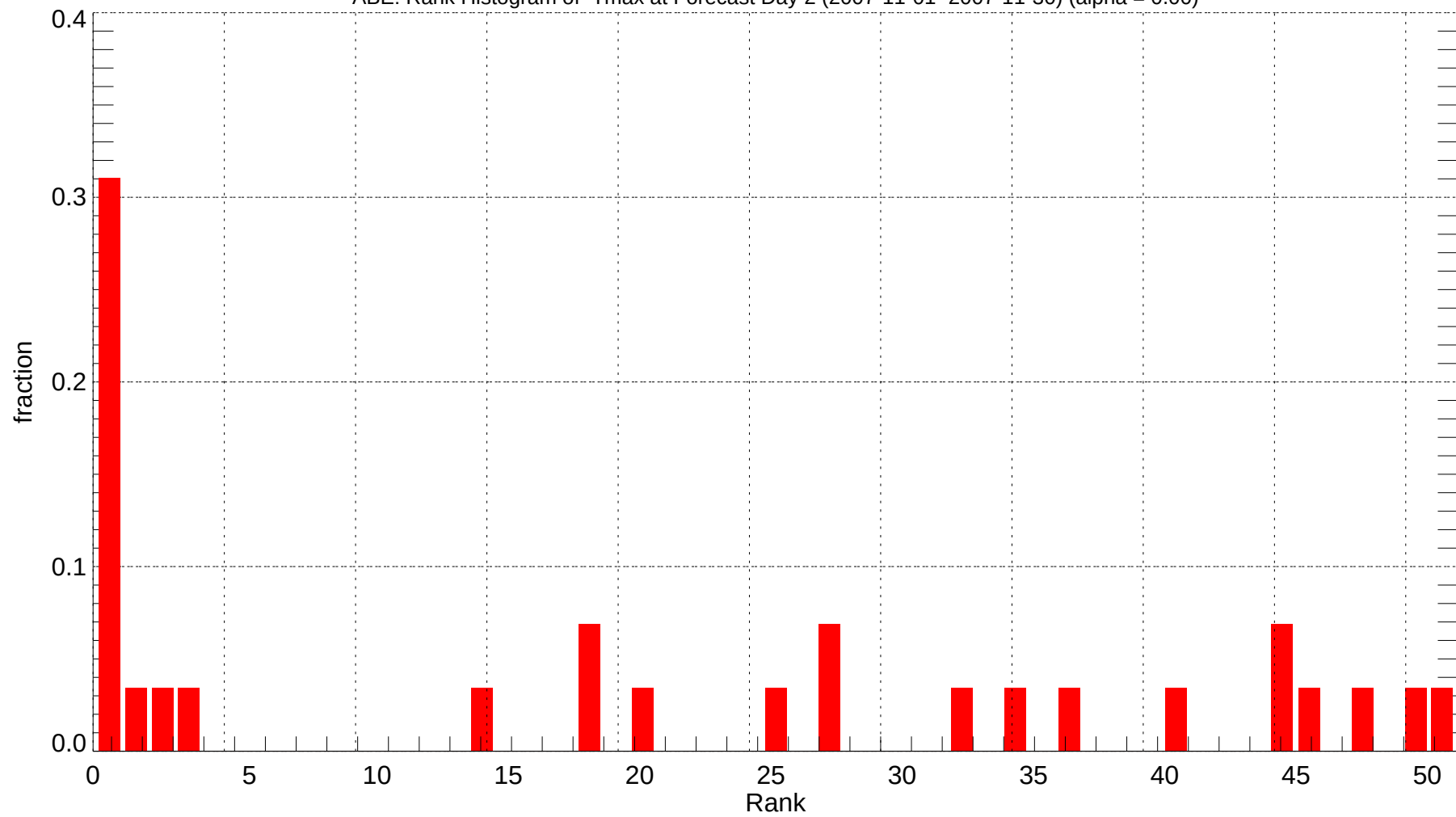
ABE: Rank Histogram of Tmax at Forecast Day 2 (2007-11-01~2007-11-30) (alpha = 0.00)
