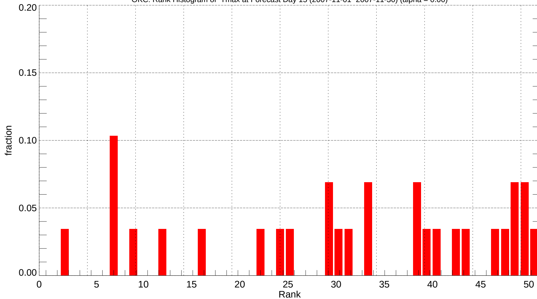
OKC: Rank Histogram of Tmax at Forecast Day 15 (2007-11-01~2007-11-30) (alpha = 0.00)
