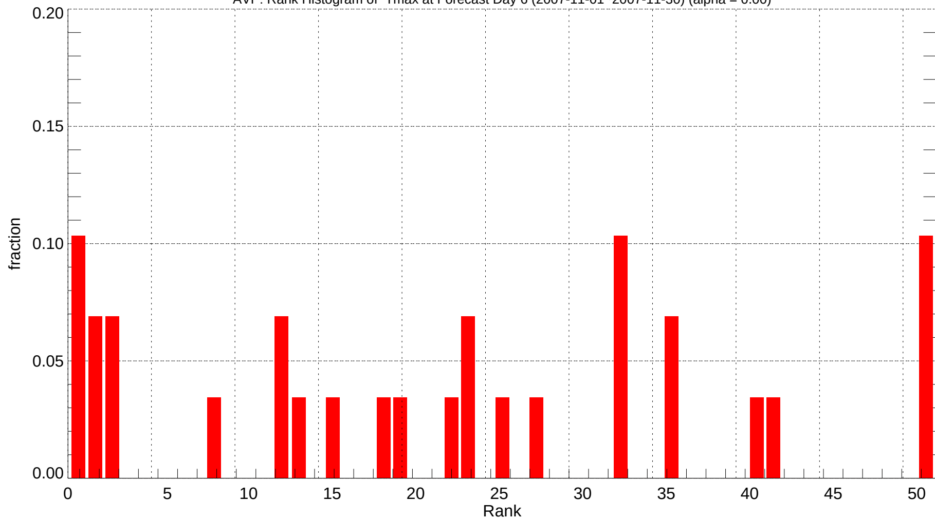
AVP: Rank Histogram of Tmax at Forecast Day 6 (2007-11-01~2007-11-30) (alpha = 0.00)
