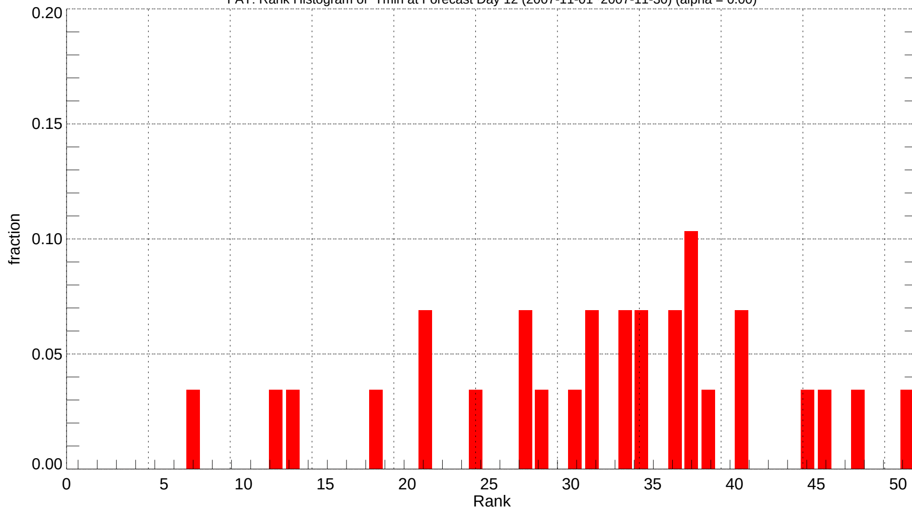
FAT: Rank Histogram of Tmin at Forecast Day 12 (2007-11-01~2007-11-30) (alpha = 0.00)
