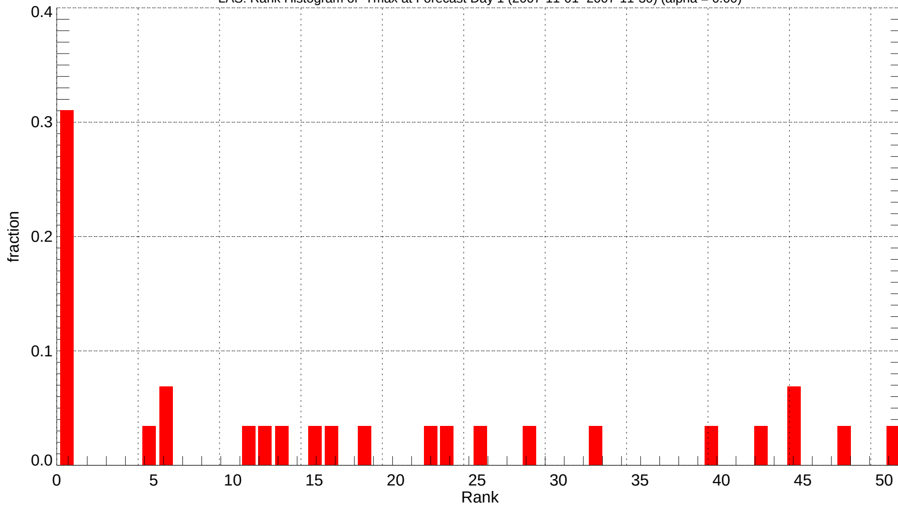
LAS: Rank Histogram of Tmax at Forecast Day 1 (2007-11-01~2007-11-30) (alpha = 0.00)
