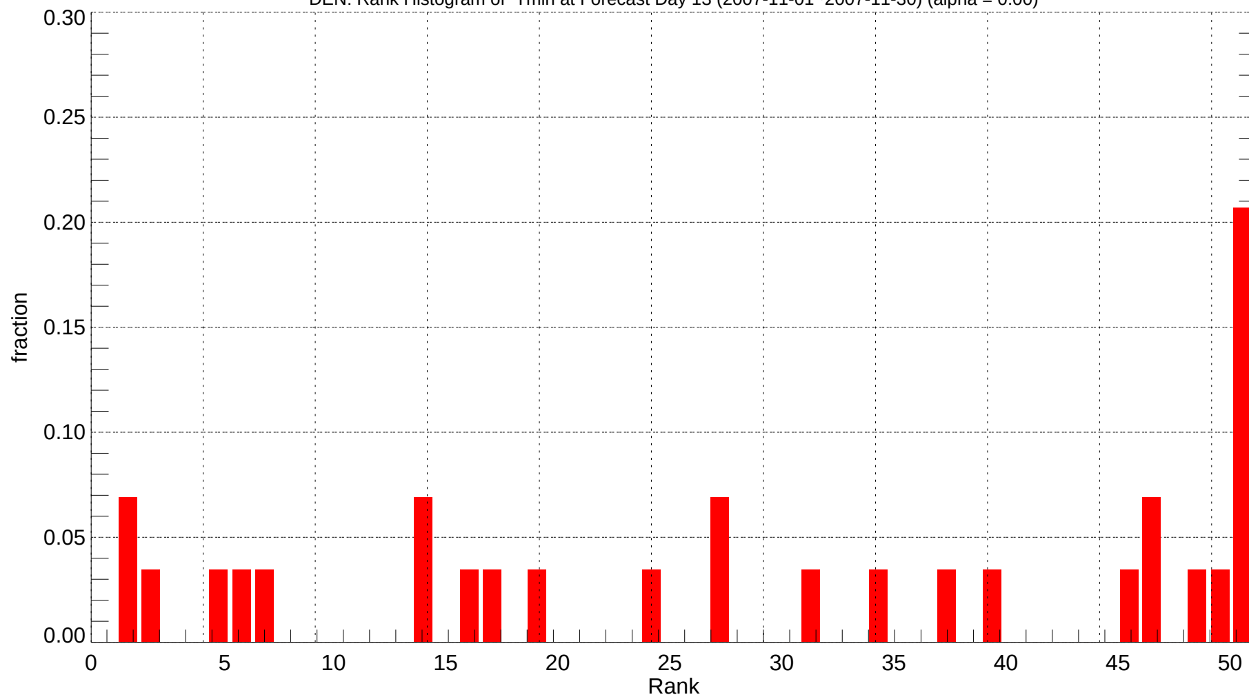
DEN: Rank Histogram of Tmin at Forecast Day 13 (2007-11-01~2007-11-30) (alpha = 0.00)
