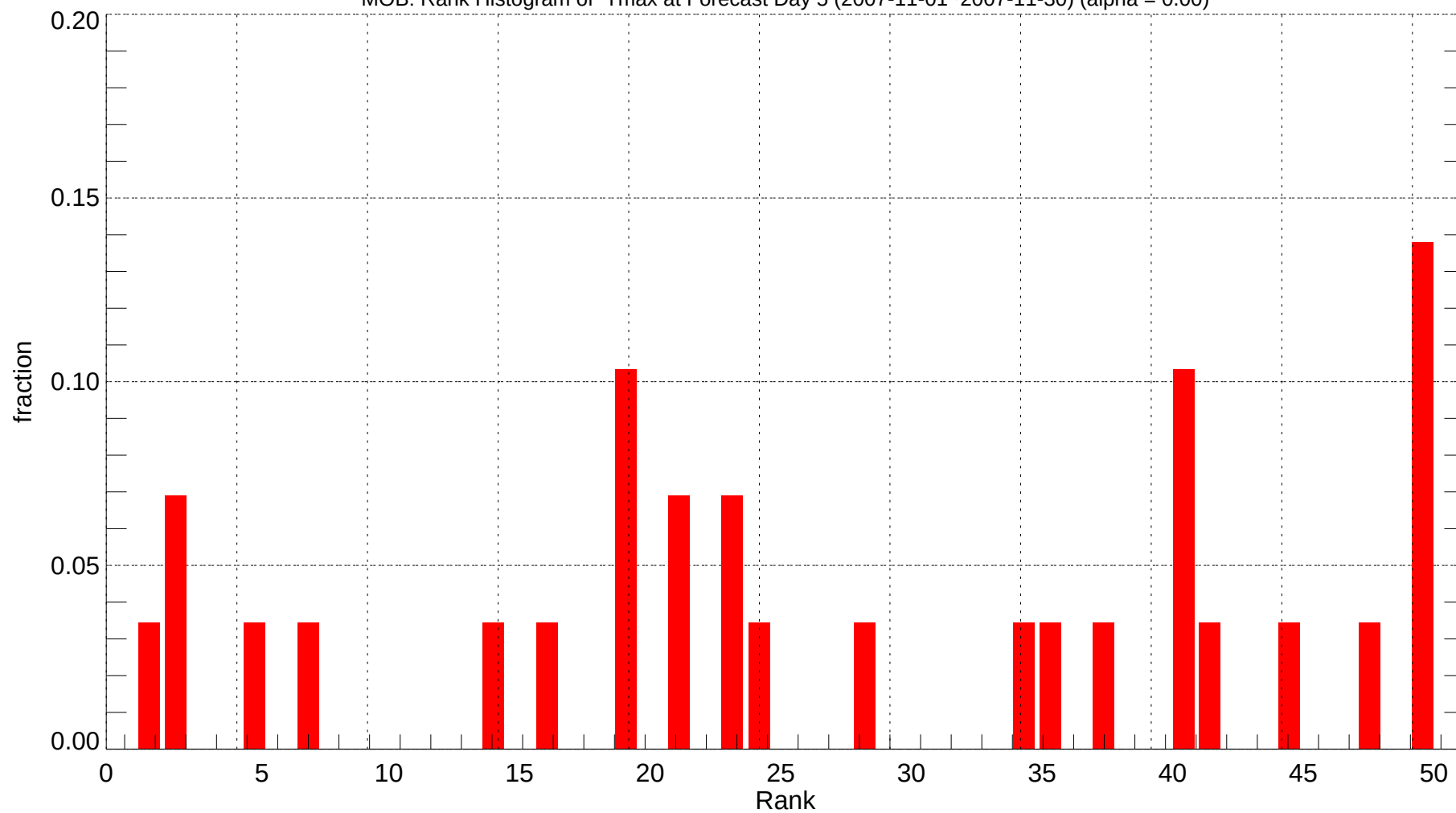
MOB: Rank Histogram of Tmax at Forecast Day 5 (2007-11-01~2007-11-30) (alpha = 0.00)
