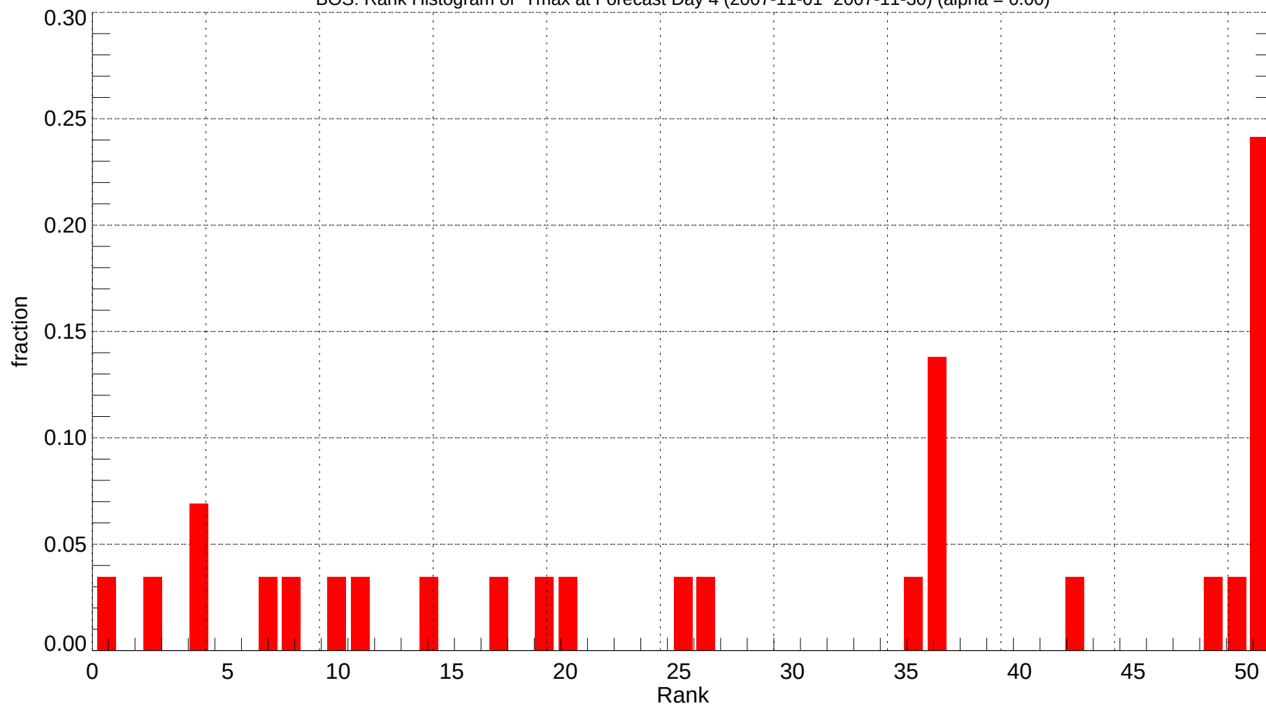
BOS: Rank Histogram of Tmax at Forecast Day 4 (2007-11-01~2007-11-30) (alpha = 0.00)
