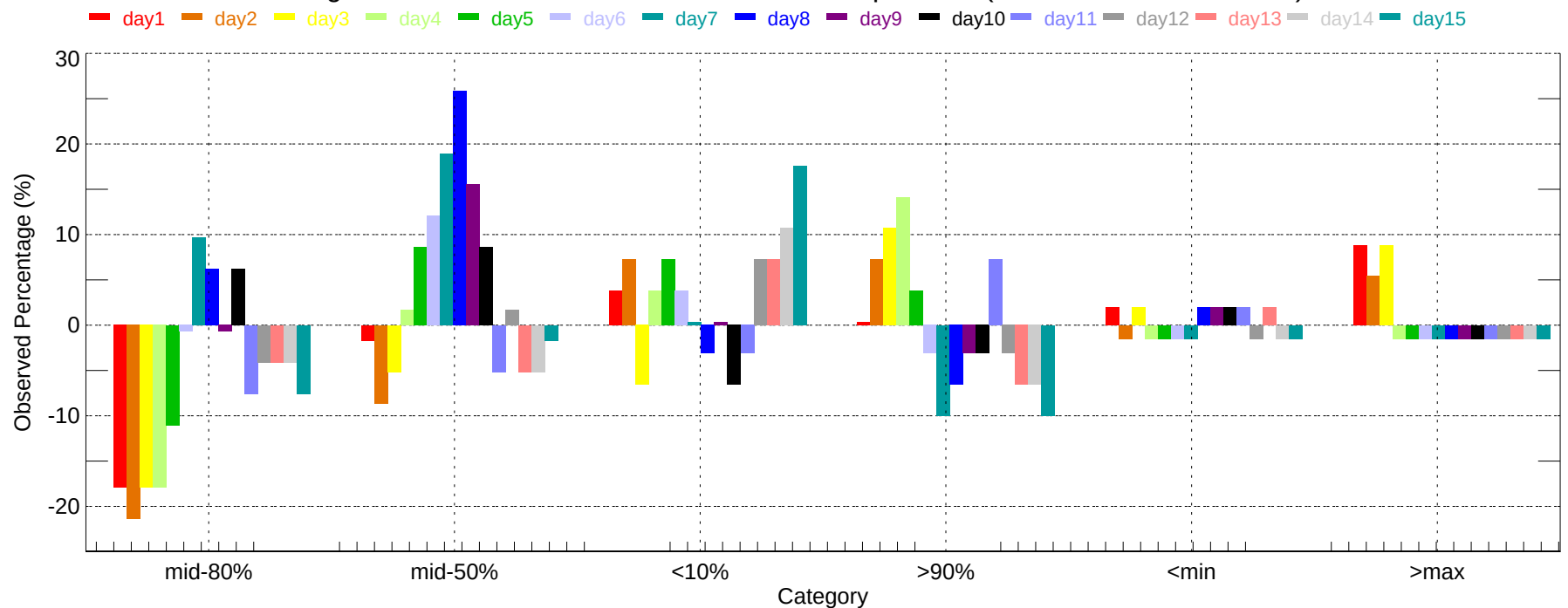
Observed Percentage Deviation of Ensembles - MCO: Min Temperature (2007-11-01~2007-11-30)
