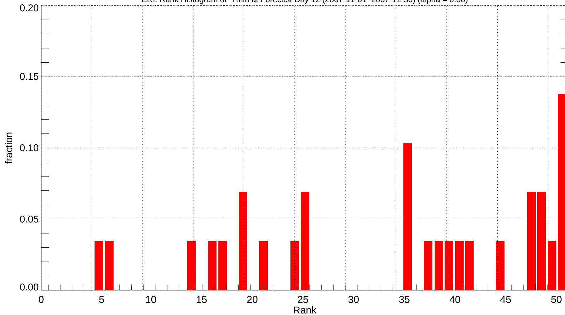
ERI: Rank Histogram of Tmin at Forecast Day 12 (2007-11-01~2007-11-30) (alpha = 0.00)
