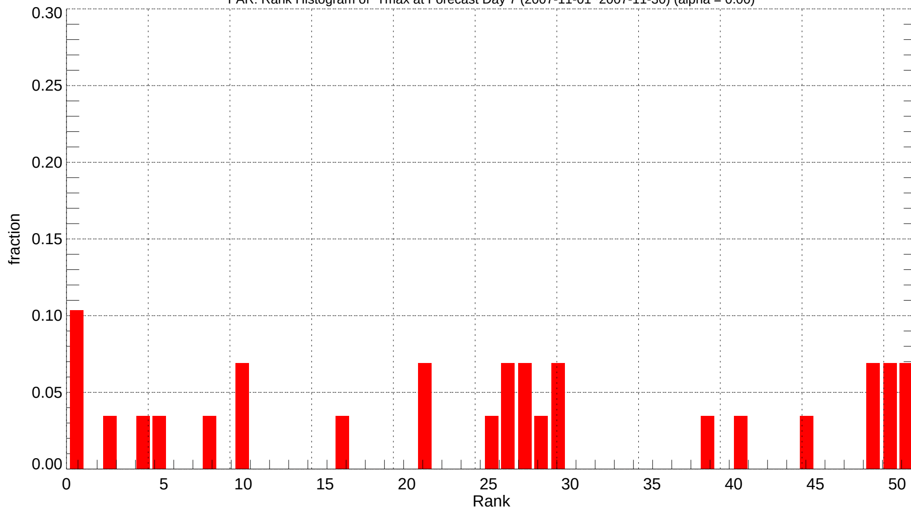
FAR: Rank Histogram of Tmax at Forecast Day 7 (2007-11-01~2007-11-30) (alpha = 0.00)
