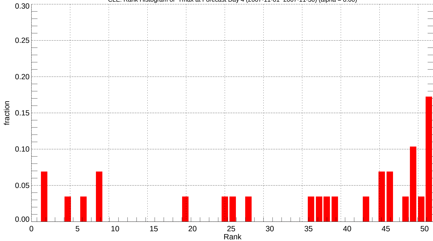
CLE: Rank Histogram of Tmax at Forecast Day 4 (2007-11-01~2007-11-30) (alpha = 0.00)
