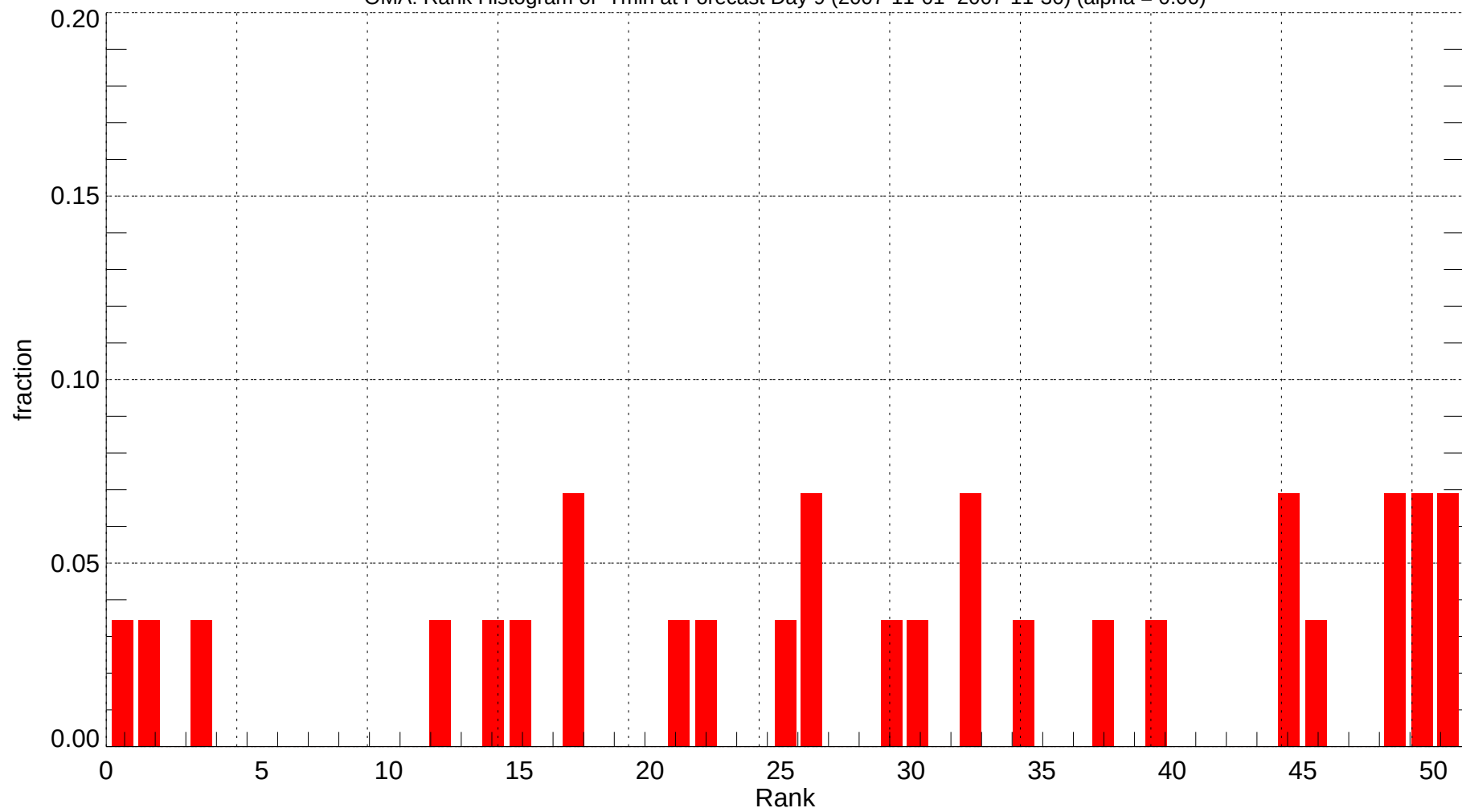
OMA: Rank Histogram of Tmin at Forecast Day 9 (2007-11-01~2007-11-30) (alpha = 0.00)
