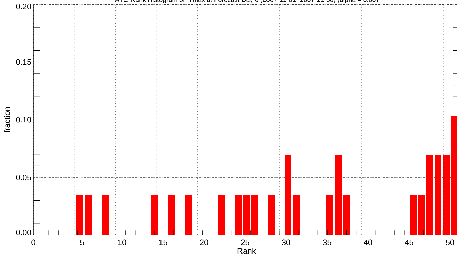
ATL: Rank Histogram of Tmax at Forecast Day 6 (2007-11-01~2007-11-30) (alpha = 0.00)
