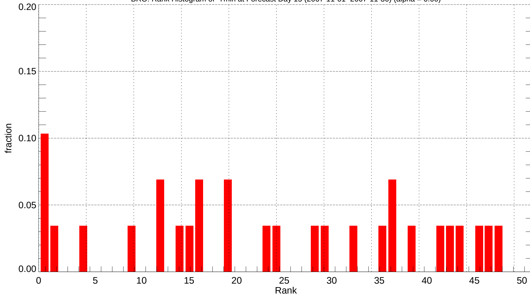
BRO: Rank Histogram of Tmin at Forecast Day 15 (2007-11-01~2007-11-30) (alpha = 0.00)
