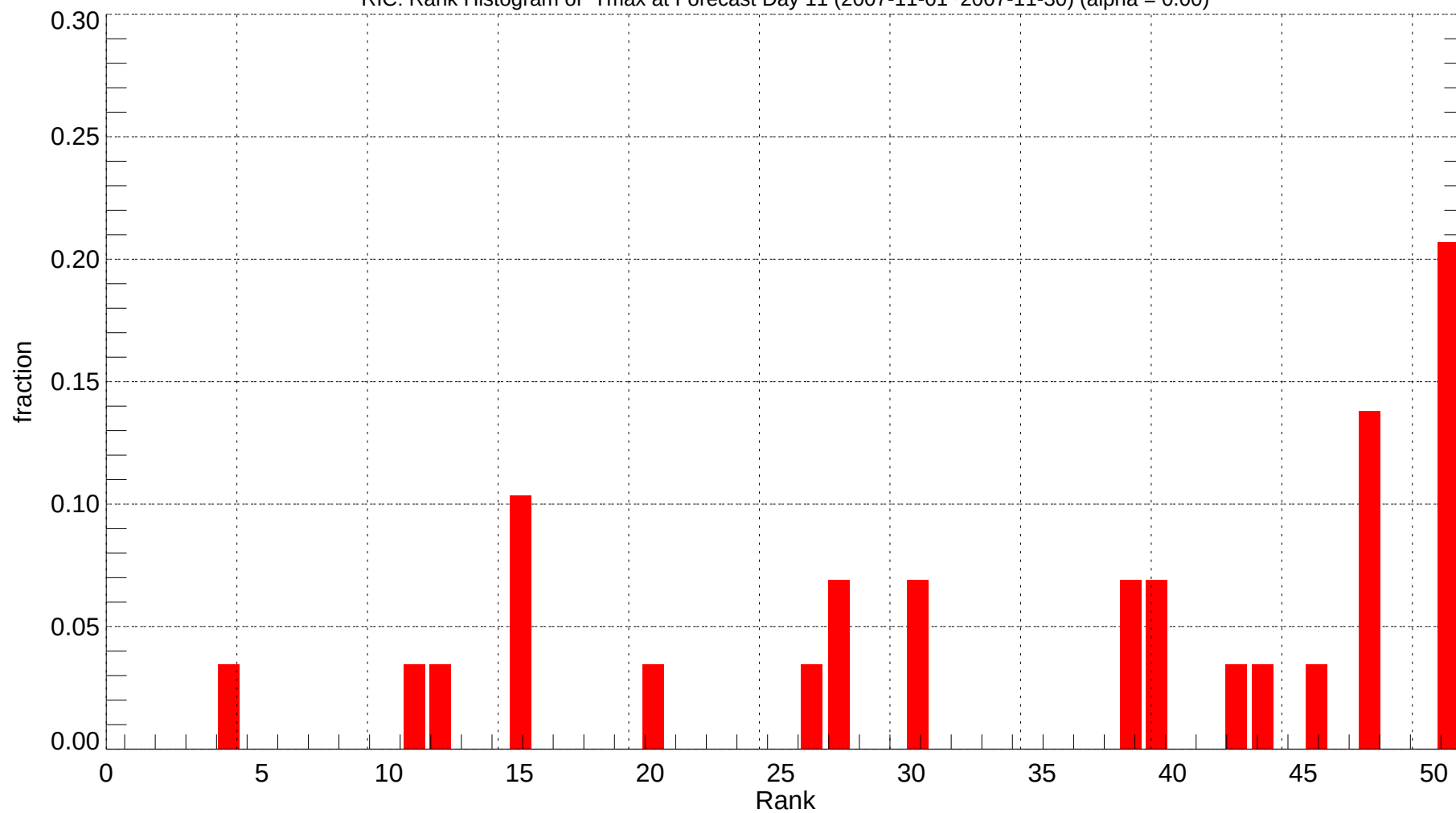
RIC: Rank Histogram of Tmax at Forecast Day 11 (2007-11-01~2007-11-30) (alpha = 0.00)
