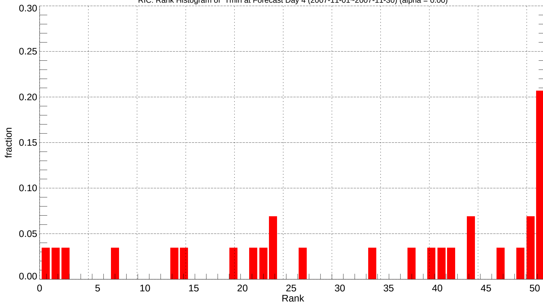
RIC: Rank Histogram of Tmin at Forecast Day 4 (2007-11-01~2007-11-30) (alpha = 0.00)
