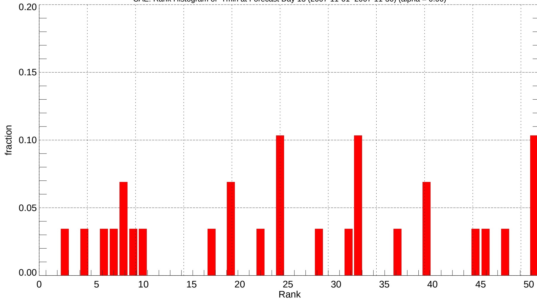
CAE: Rank Histogram of Tmin at Forecast Day 13 (2007-11-01~2007-11-30) (alpha = 0.00)
