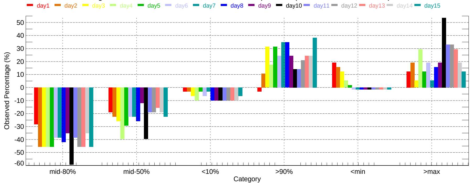
Observed Percentage Deviation of Ensembles - TUL: Max Temperature (2007-11-01~2007-11-30)
