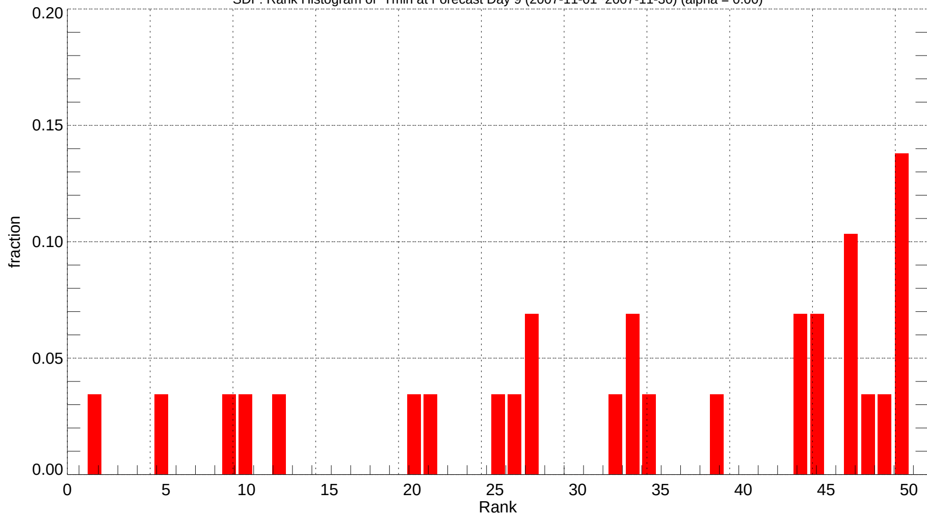
SDF: Rank Histogram of Tmin at Forecast Day 9 (2007-11-01~2007-11-30) (alpha = 0.00)
