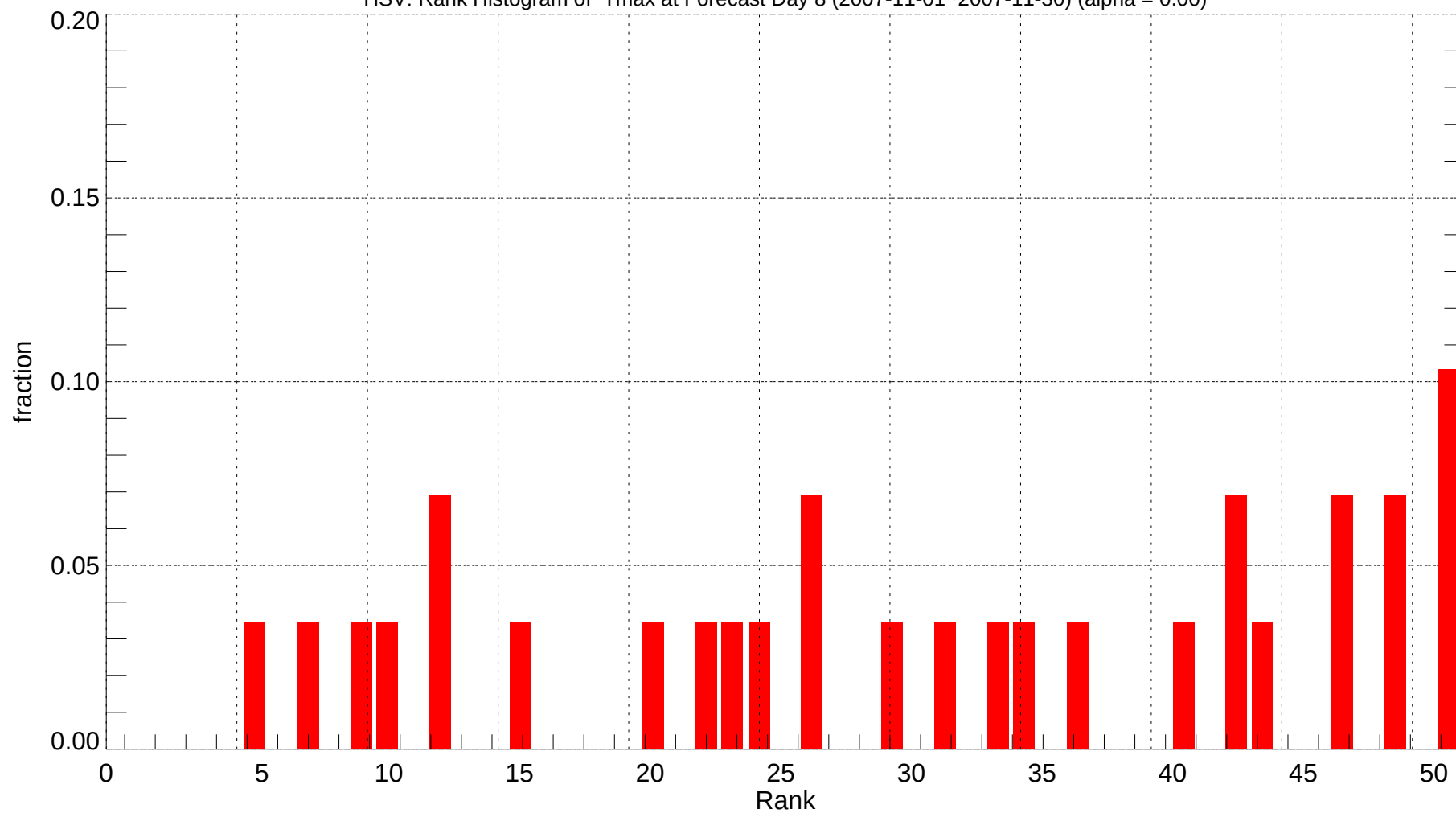
HSV: Rank Histogram of Tmax at Forecast Day 8 (2007-11-01~2007-11-30) (alpha = 0.00)
