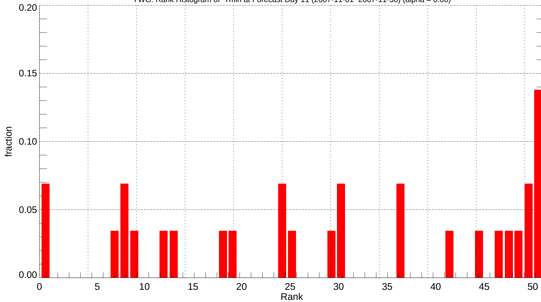
YWG: Rank Histogram of Tmin at Forecast Day 11 (2007-11-01~2007-11-30) (alpha = 0.00)
