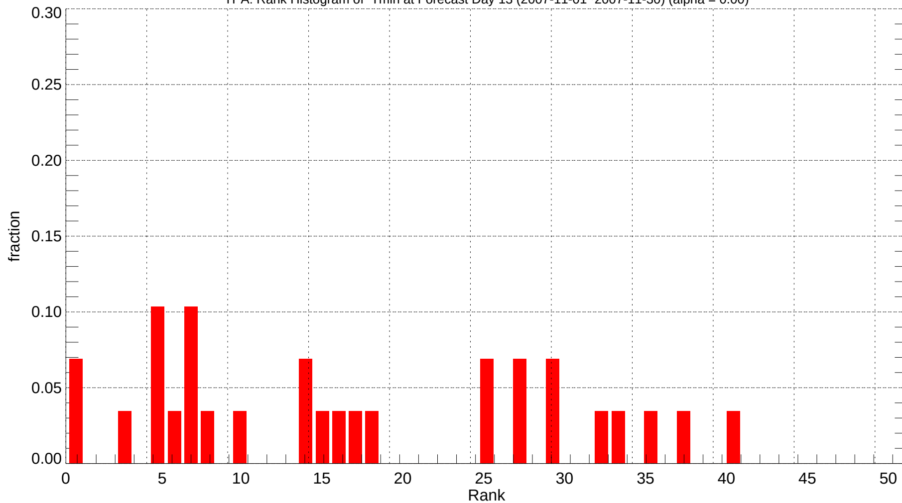
TPA: Rank Histogram of Tmin at Forecast Day 13 (2007-11-01~2007-11-30) (alpha = 0.00)
