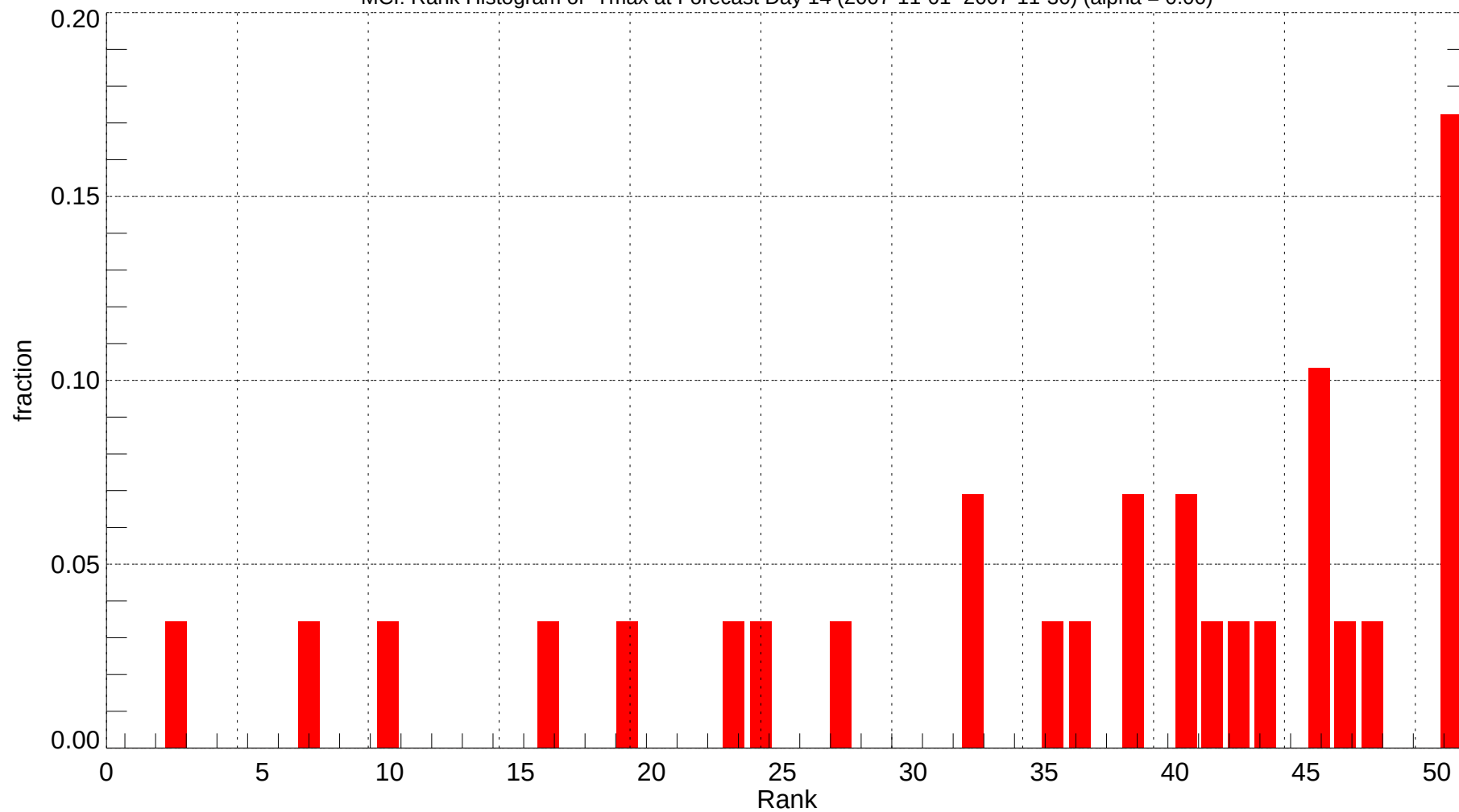
MCI: Rank Histogram of Tmax at Forecast Day 14 (2007-11-01~2007-11-30) (alpha = 0.00)
