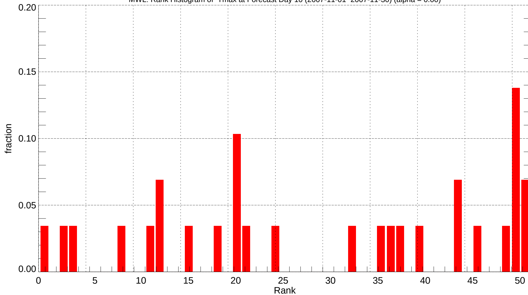
MWL: Rank Histogram of Tmax at Forecast Day 10 (2007-11-01~2007-11-30) (alpha = 0.00)
