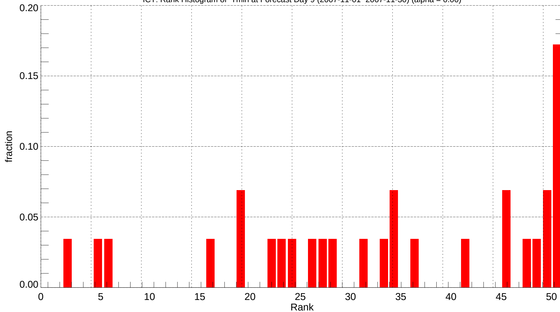
ICT: Rank Histogram of Tmin at Forecast Day 9 (2007-11-01~2007-11-30) (alpha = 0.00)
