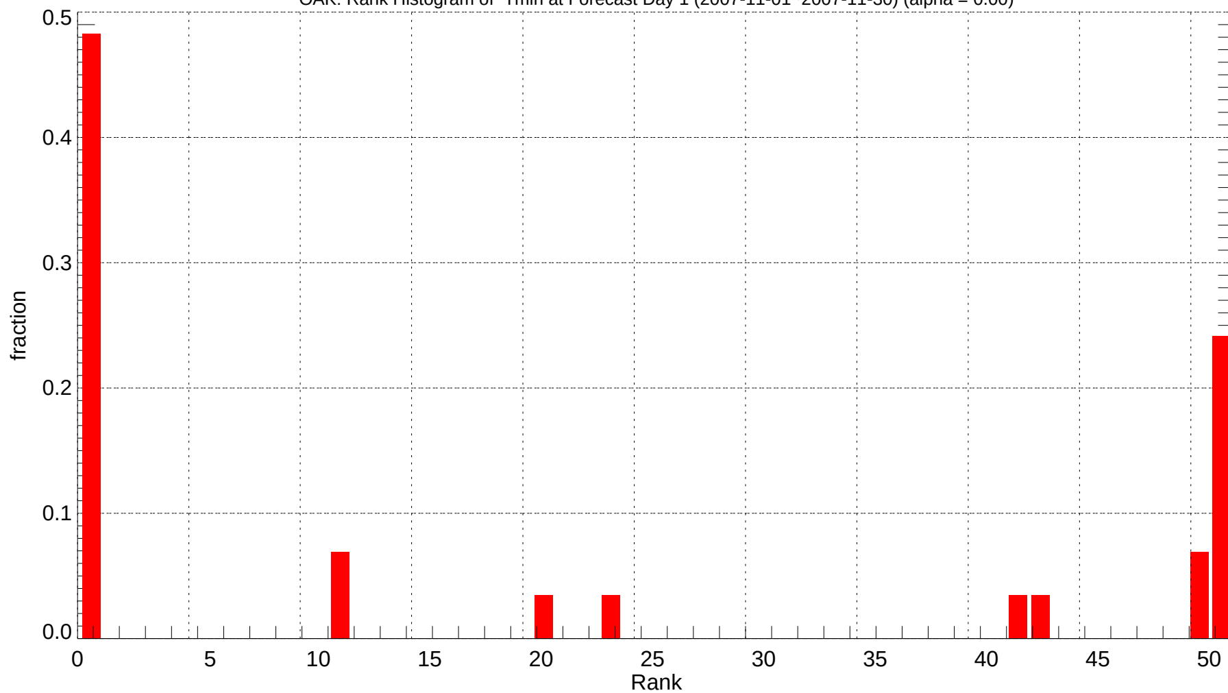
OAK: Rank Histogram of Tmin at Forecast Day 1 (2007-11-01~2007-11-30) (alpha = 0.00)
