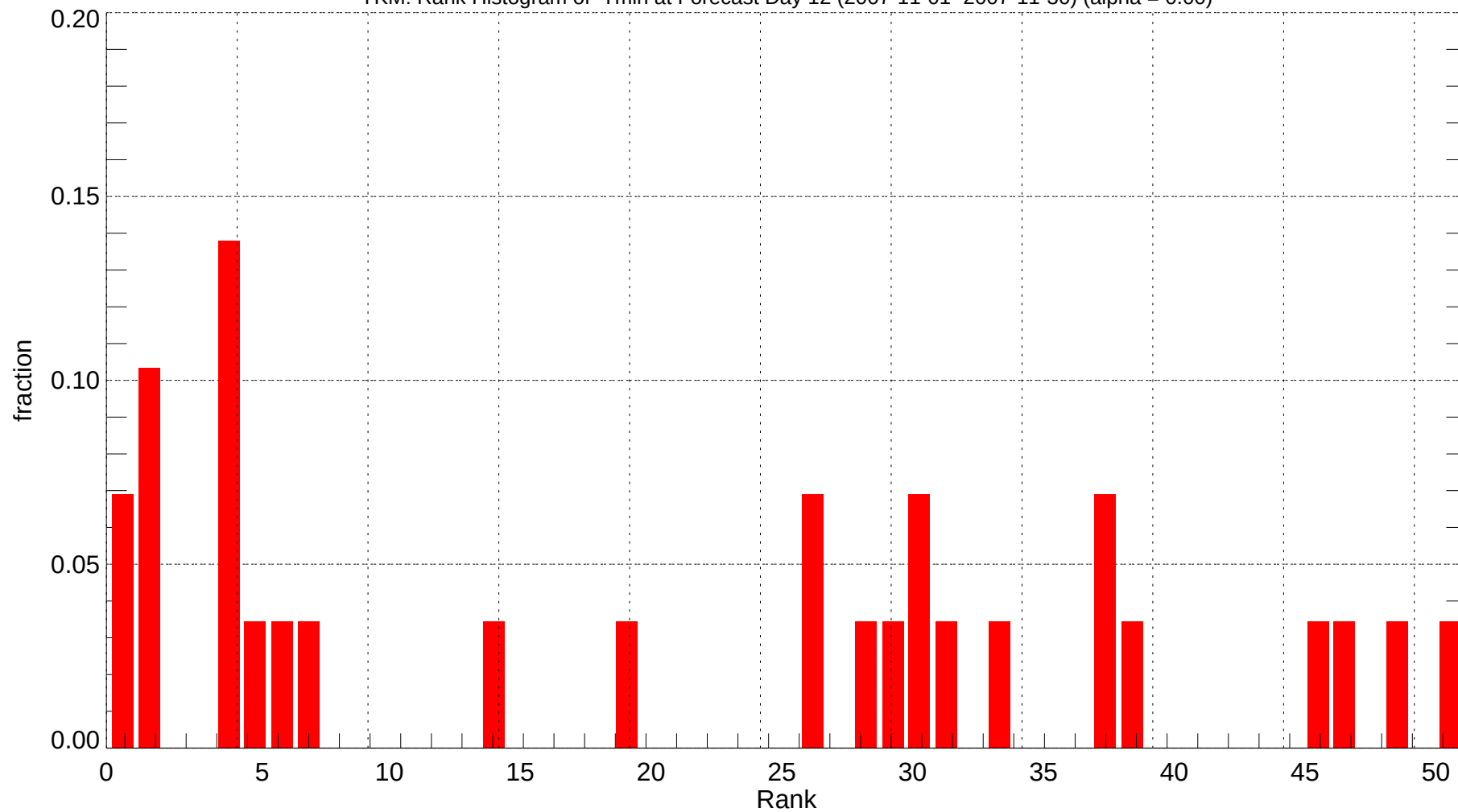
YKM: Rank Histogram of Tmin at Forecast Day 12 (2007-11-01~2007-11-30) (alpha = 0.00)
