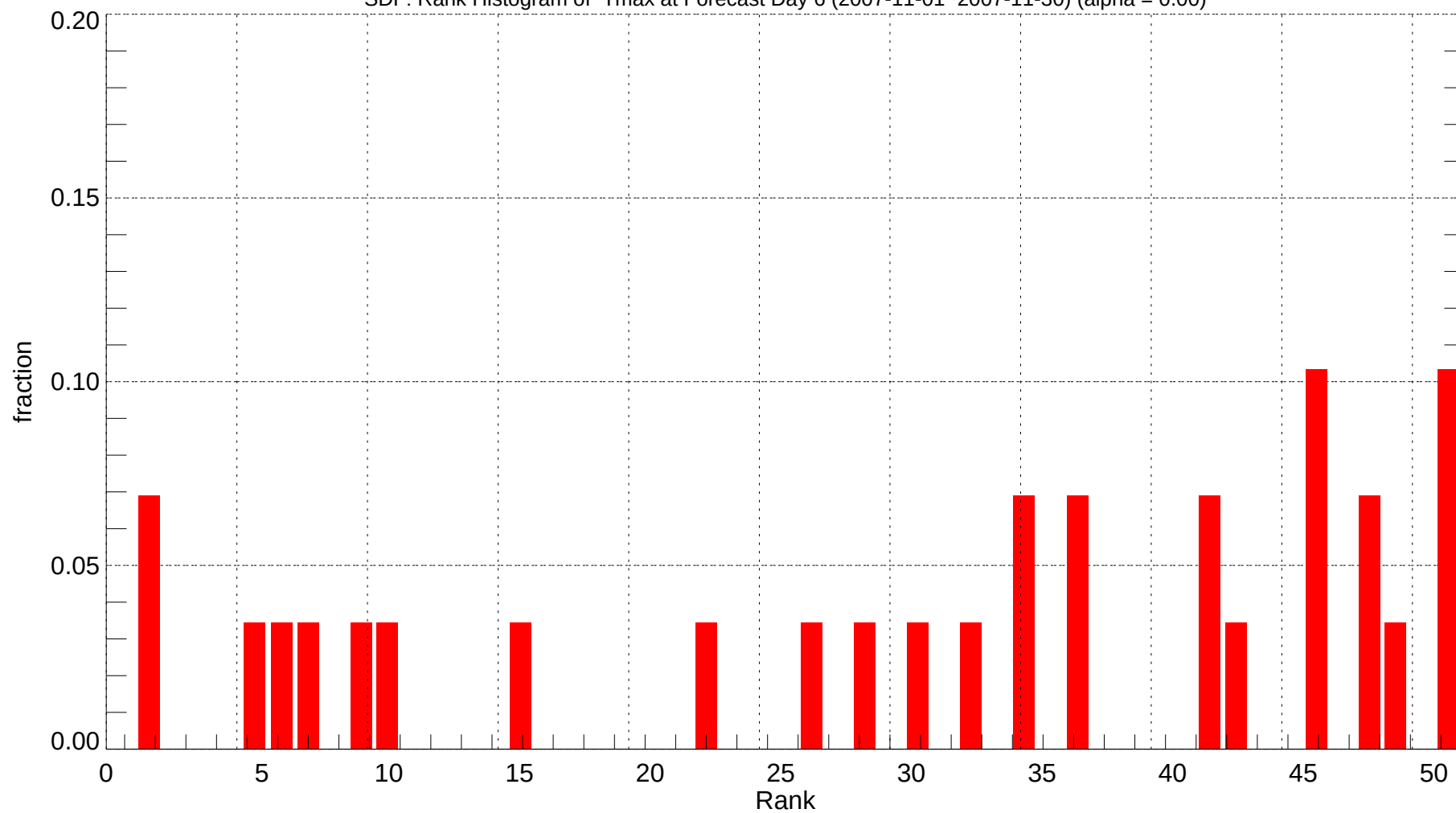
SDF: Rank Histogram of Tmax at Forecast Day 6 (2007-11-01~2007-11-30) (alpha = 0.00)
