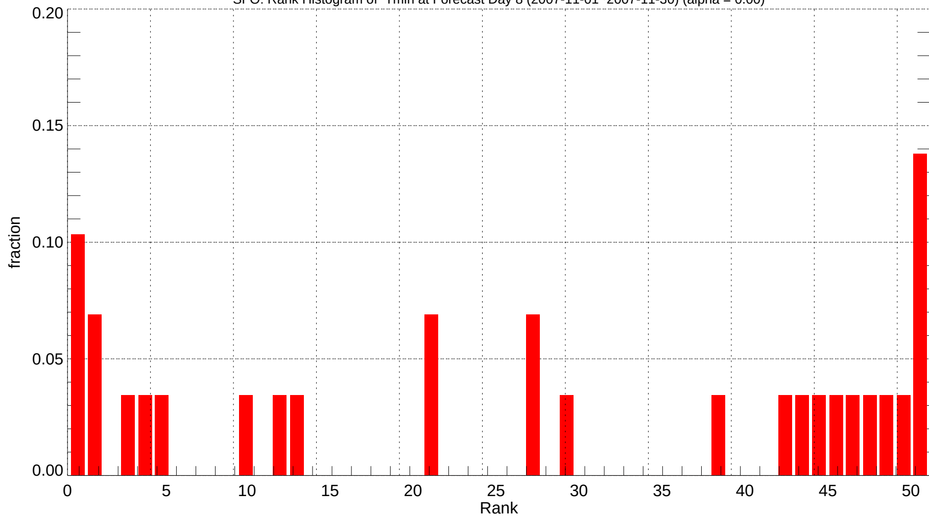
SFO: Rank Histogram of Tmin at Forecast Day 8 (2007-11-01~2007-11-30) (alpha = 0.00)
