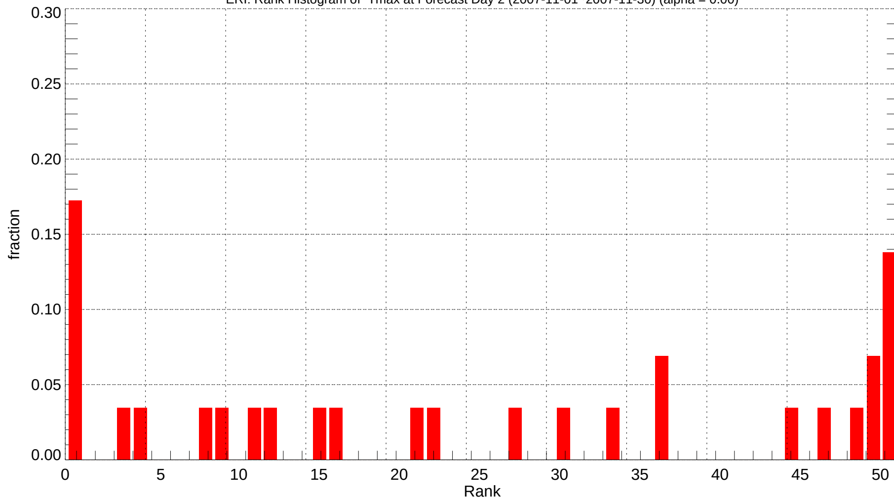
ERI: Rank Histogram of Tmax at Forecast Day 2 (2007-11-01~2007-11-30) (alpha = 0.00)
