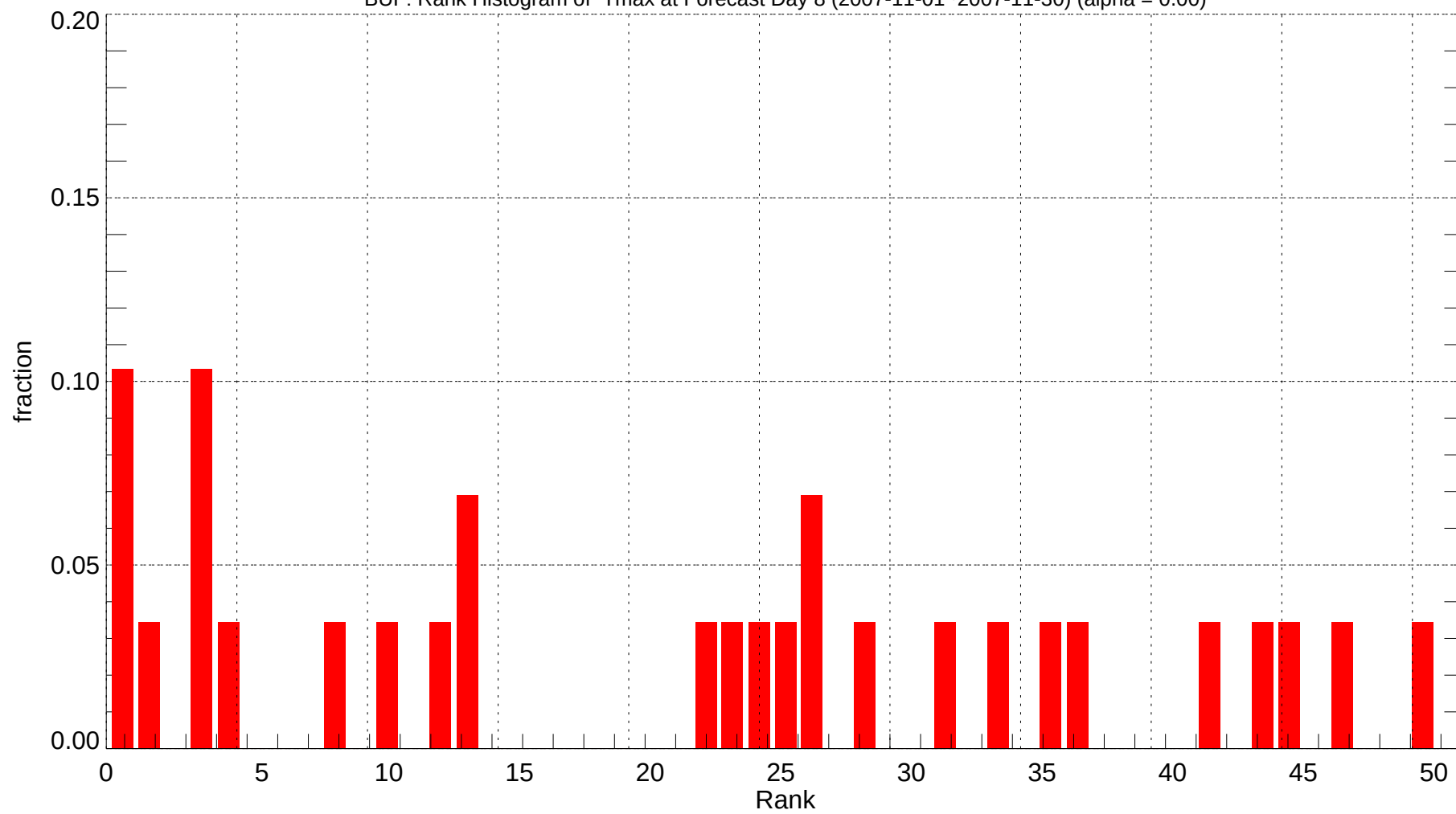
BUF: Rank Histogram of Tmax at Forecast Day 8 (2007-11-01~2007-11-30) (alpha = 0.00)
