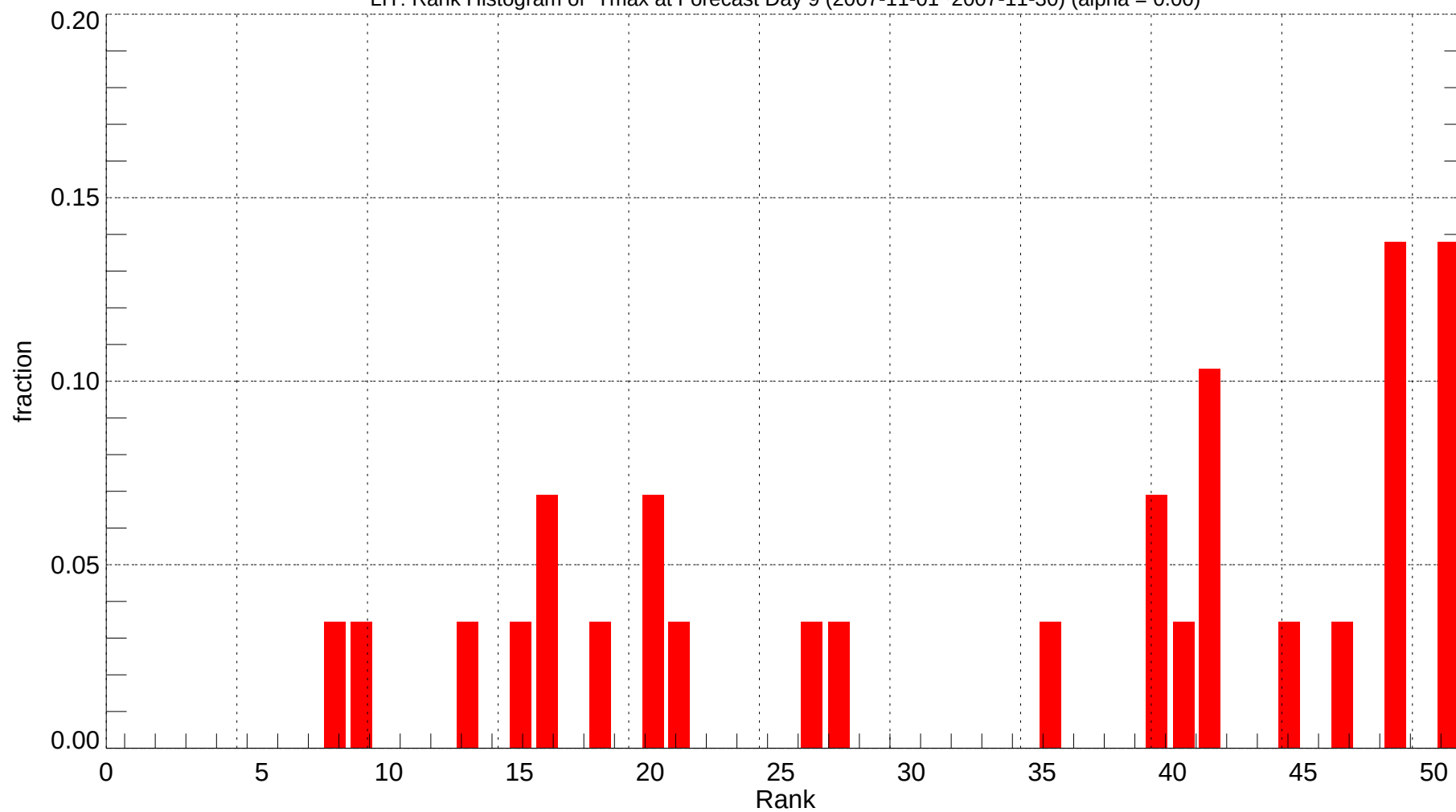
LIT: Rank Histogram of Tmax at Forecast Day 9 (2007-11-01~2007-11-30) (alpha = 0.00)
