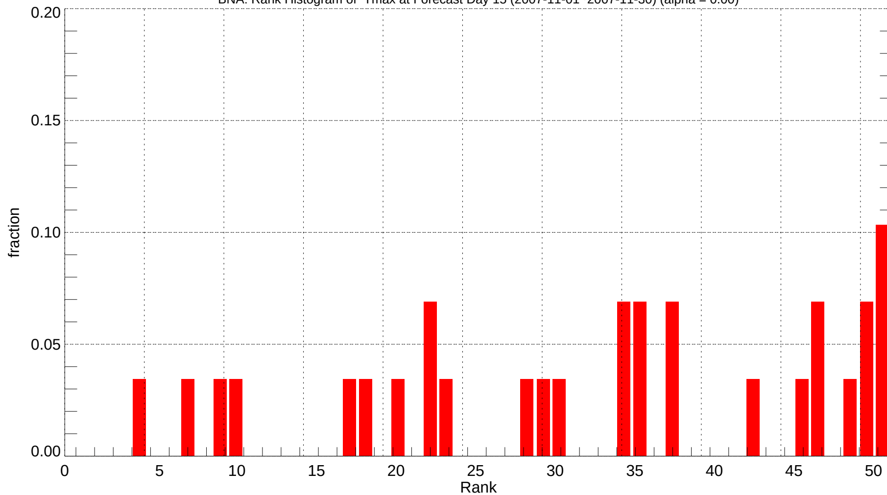
BNA: Rank Histogram of Tmax at Forecast Day 15 (2007-11-01~2007-11-30) (alpha = 0.00)
