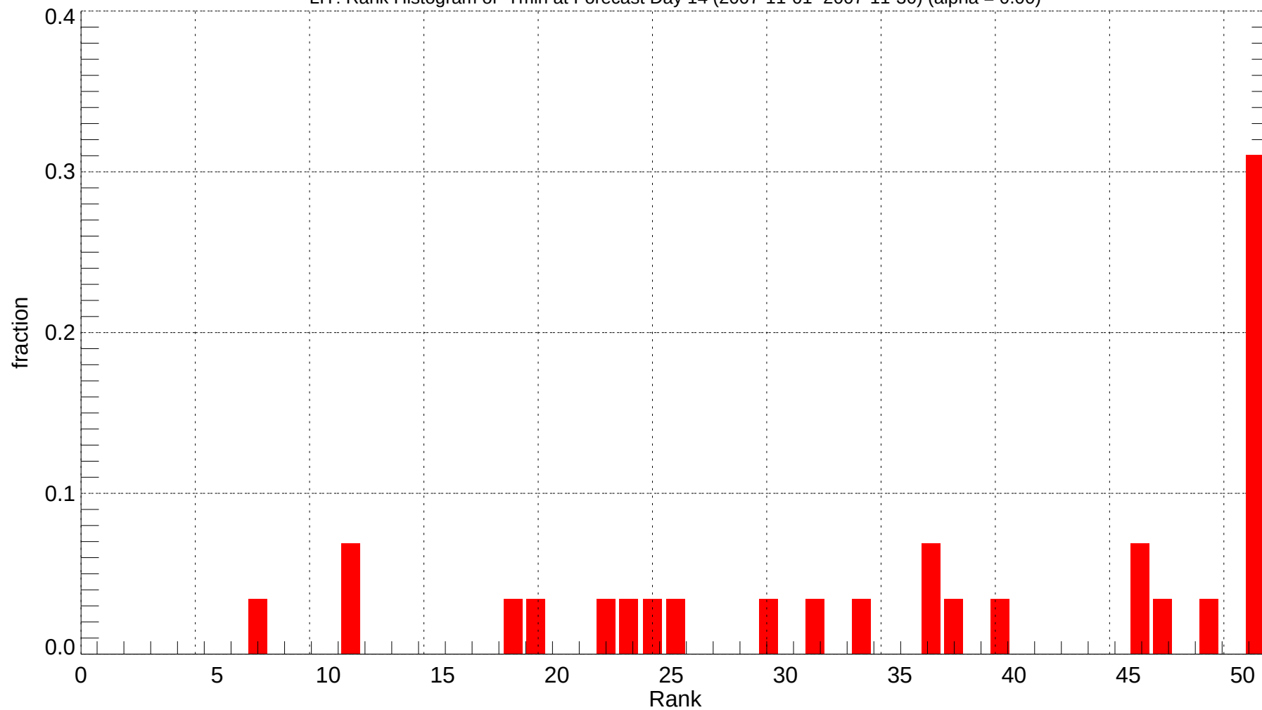
LIT: Rank Histogram of Tmin at Forecast Day 14 (2007-11-01~2007-11-30) (alpha = 0.00)
