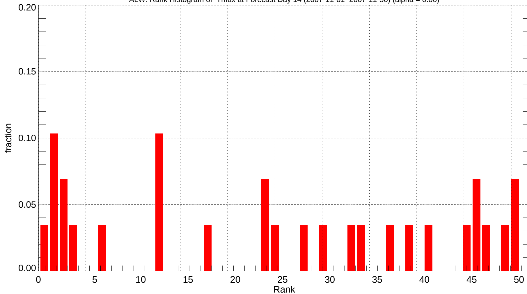
ALW: Rank Histogram of Tmax at Forecast Day 14 (2007-11-01~2007-11-30) (alpha = 0.00)
