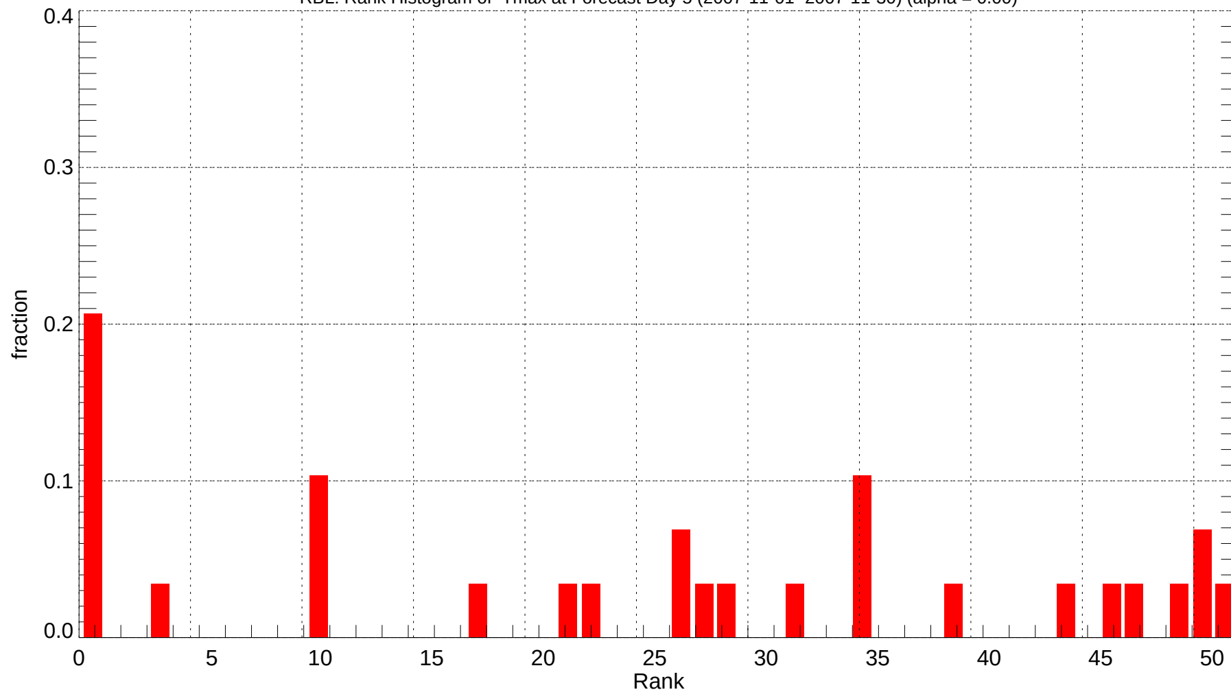
RBL: Rank Histogram of Tmax at Forecast Day 5 (2007-11-01~2007-11-30) (alpha = 0.00)
