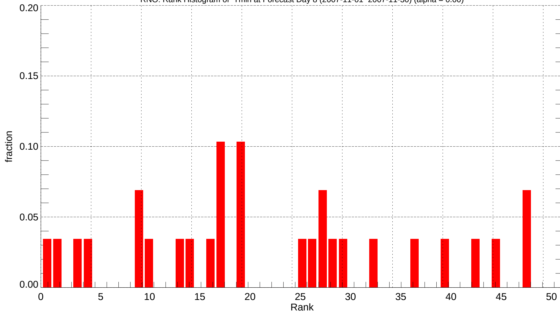
RNO: Rank Histogram of Tmin at Forecast Day 8 (2007-11-01~2007-11-30) (alpha = 0.00)
