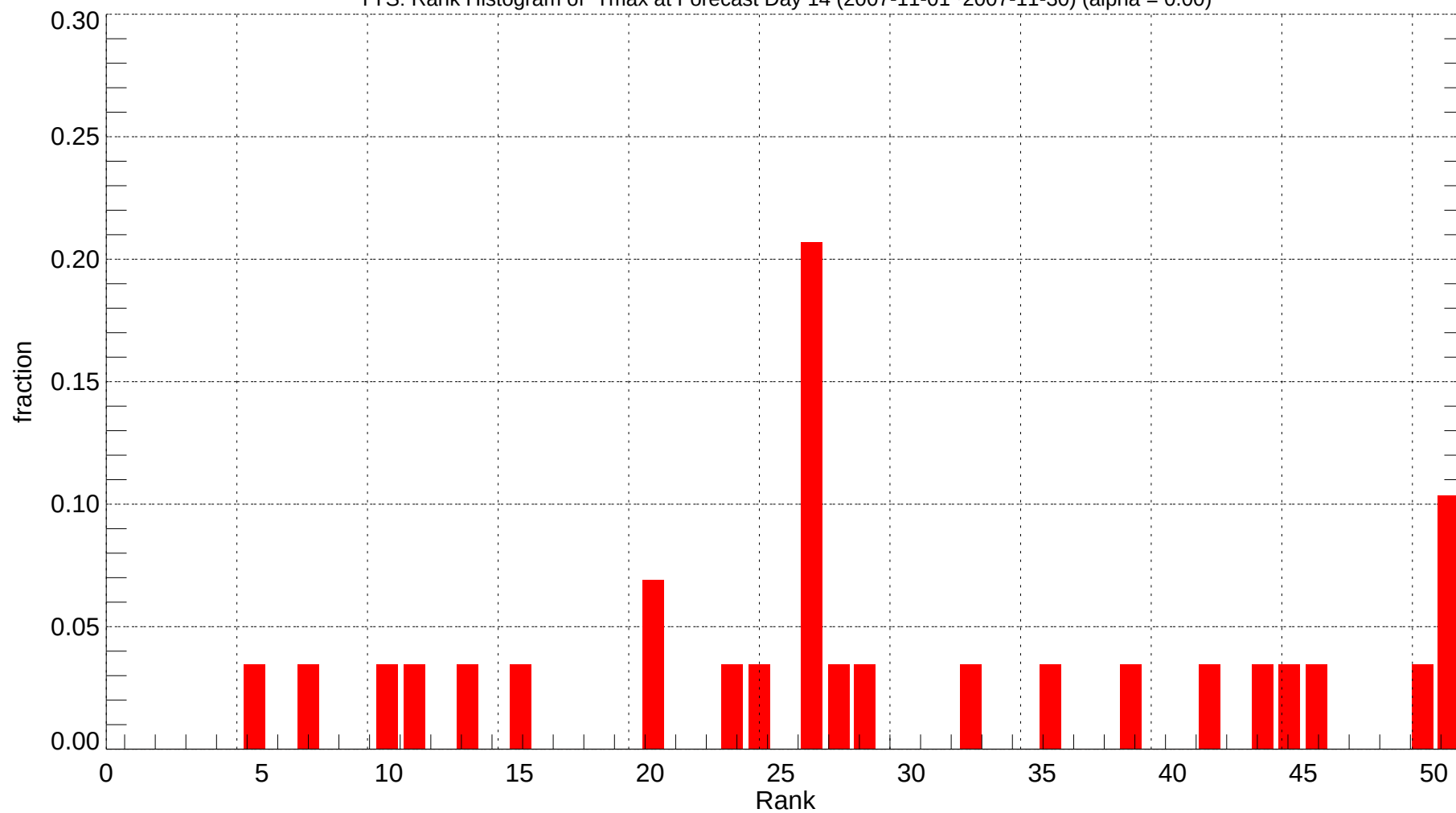
TYS: Rank Histogram of Tmax at Forecast Day 14 (2007-11-01~2007-11-30) (alpha = 0.00)
