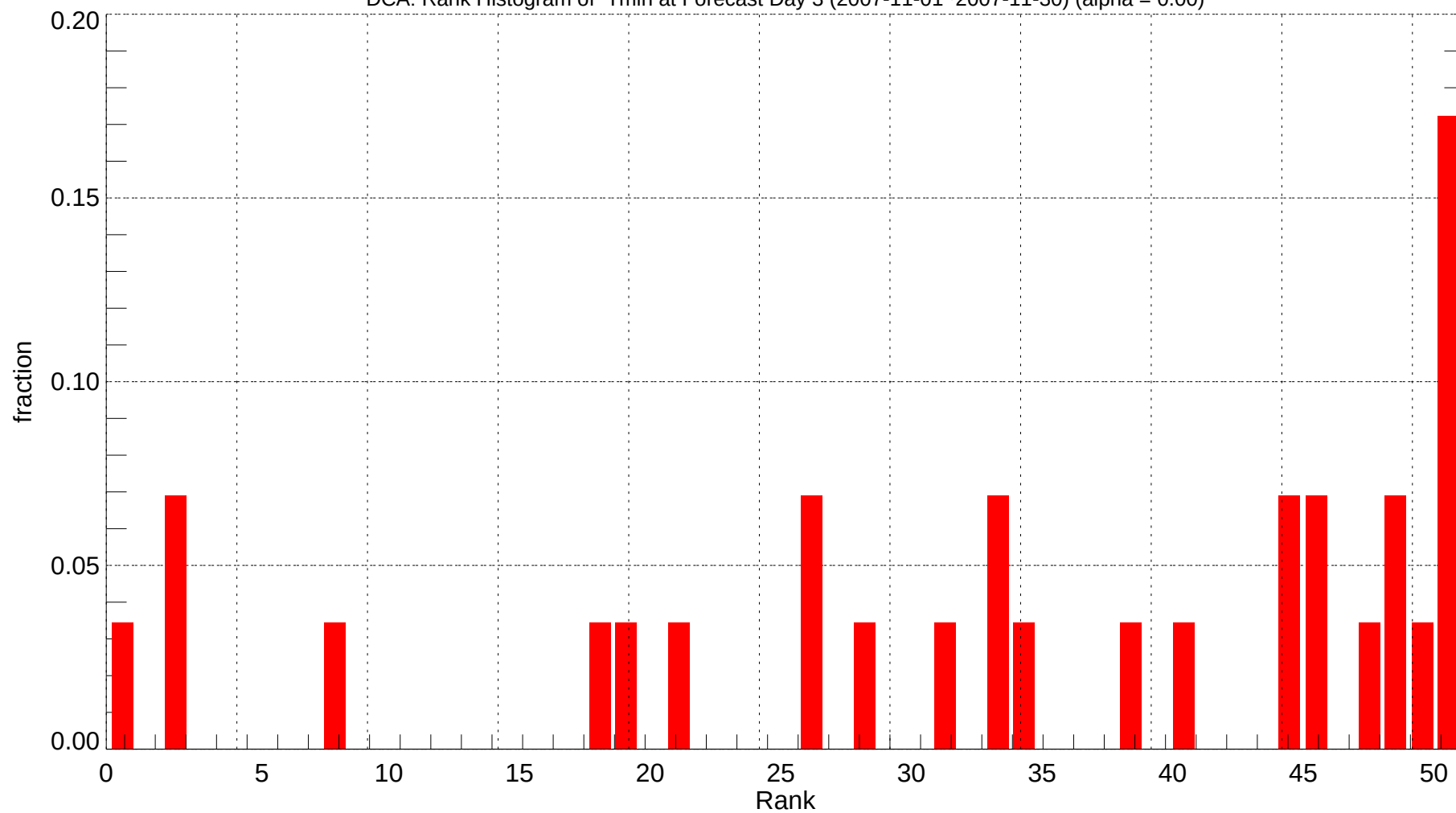
DCA: Rank Histogram of Tmin at Forecast Day 3 (2007-11-01~2007-11-30) (alpha = 0.00)
