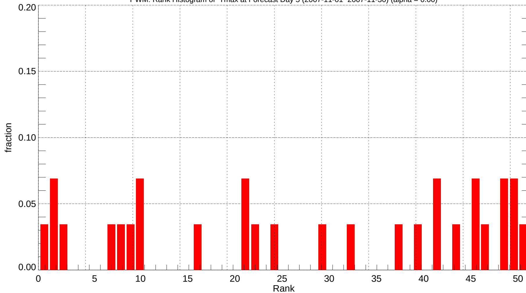
PWM: Rank Histogram of Tmax at Forecast Day 5 (2007-11-01~2007-11-30) (alpha = 0.00)
