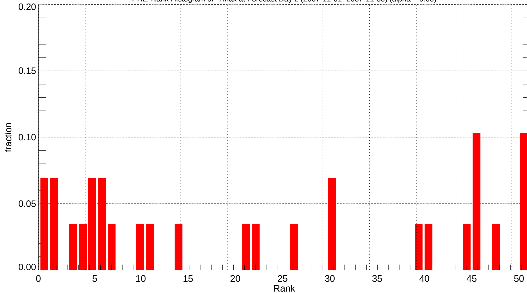
PHL: Rank Histogram of Tmax at Forecast Day 2 (2007-11-01~2007-11-30) (alpha = 0.00)
