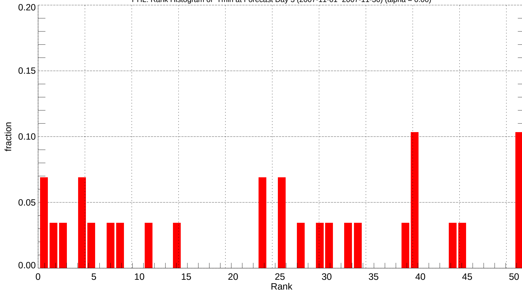
PHL: Rank Histogram of Tmin at Forecast Day 3 (2007-11-01~2007-11-30) (alpha = 0.00)
