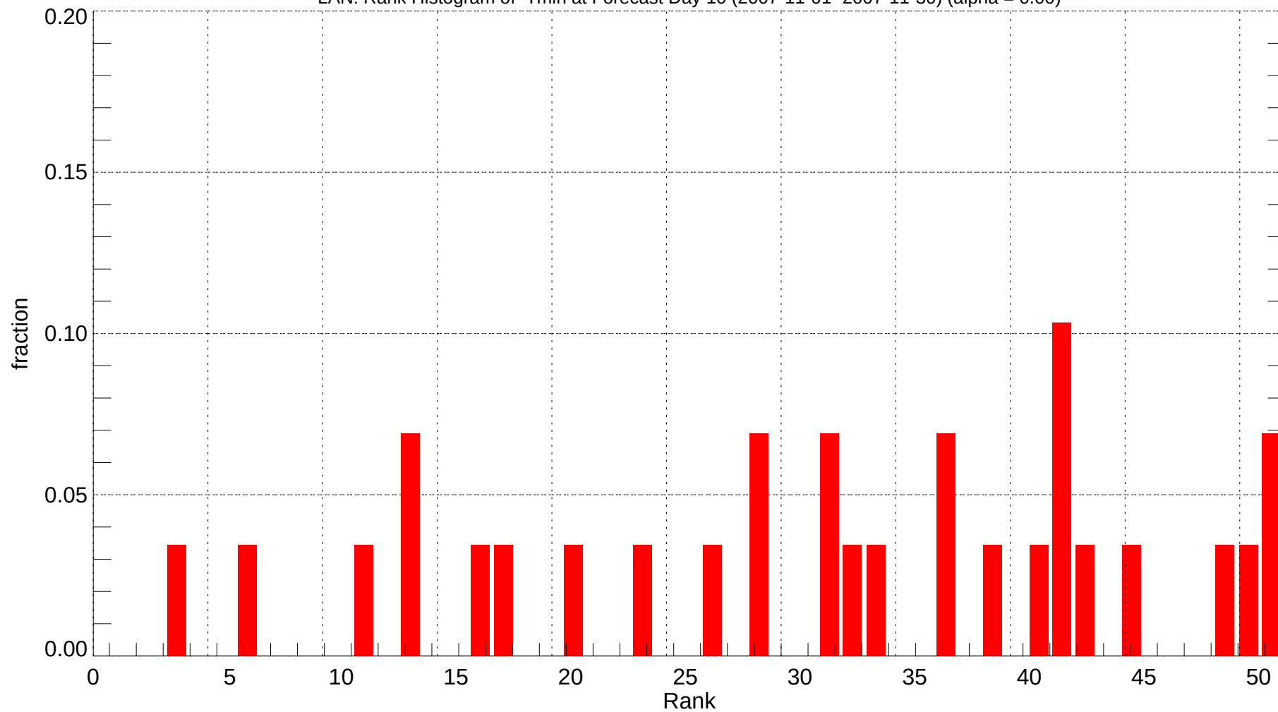
LAN: Rank Histogram of Tmin at Forecast Day 10 (2007-11-01~2007-11-30) (alpha = 0.00)
