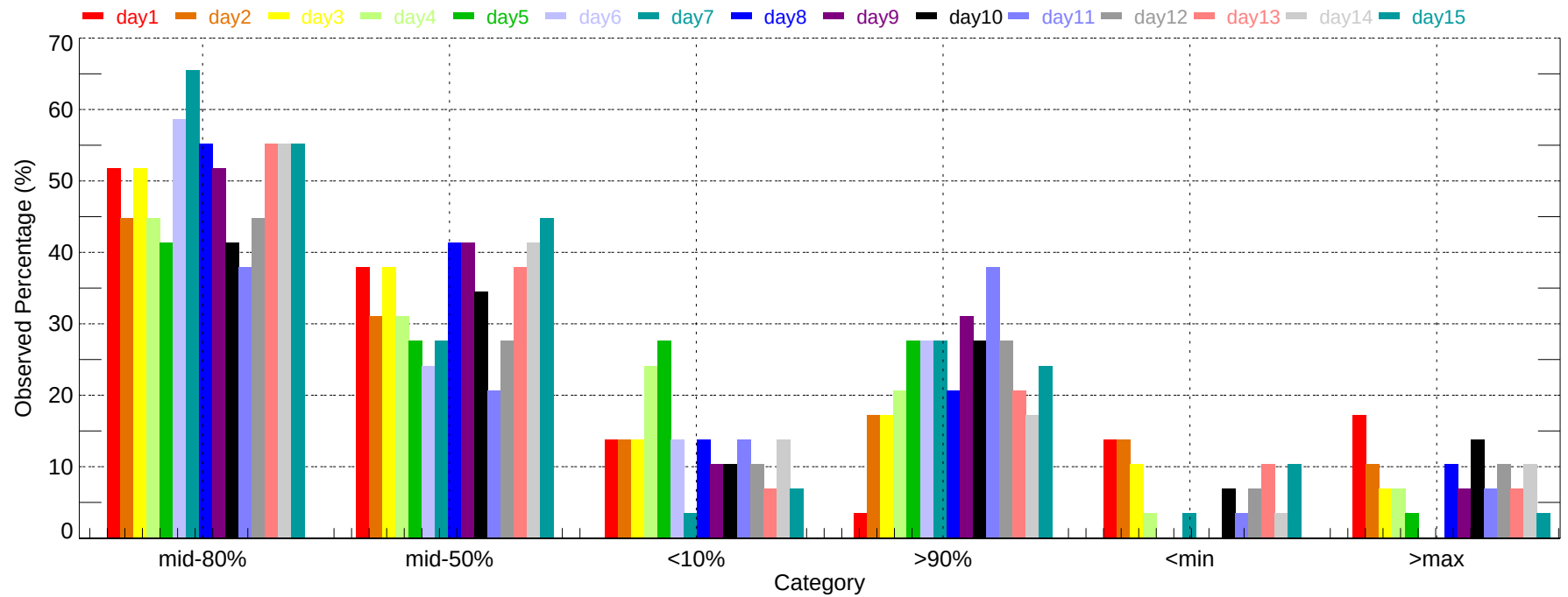
Observed Percentage of Ensembles - IAH: Max Temperature (2007-11-01~2007-11-30)
