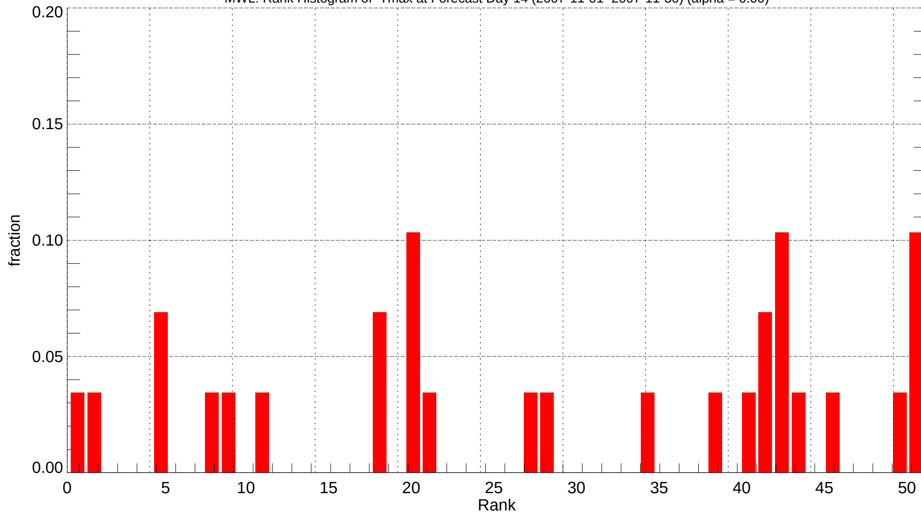
MWL: Rank Histogram of Tmax at Forecast Day 14 (2007-11-01~2007-11-30) (alpha = 0.00)
