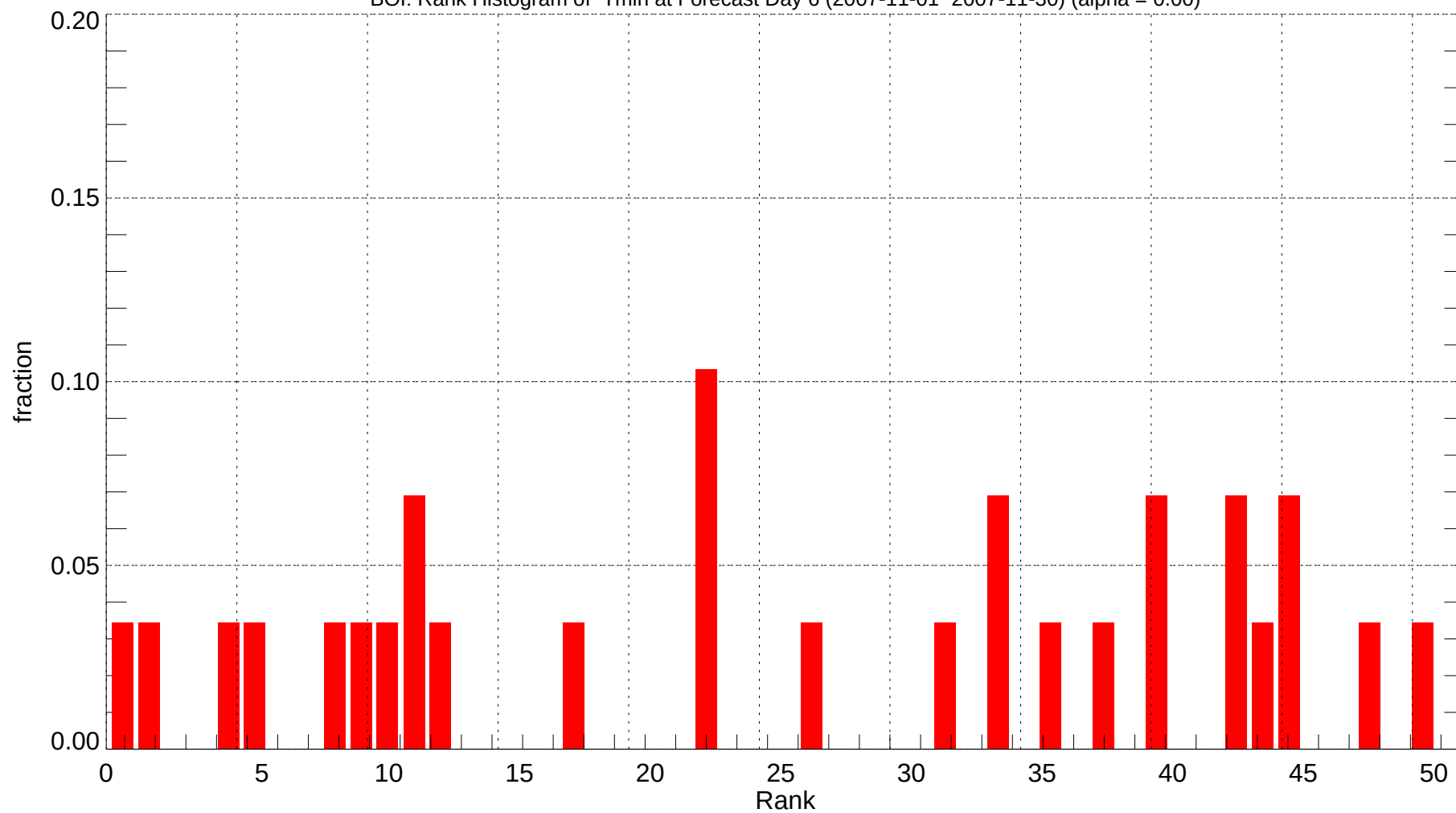
BOI: Rank Histogram of Tmin at Forecast Day 6 (2007-11-01~2007-11-30) (alpha = 0.00)
