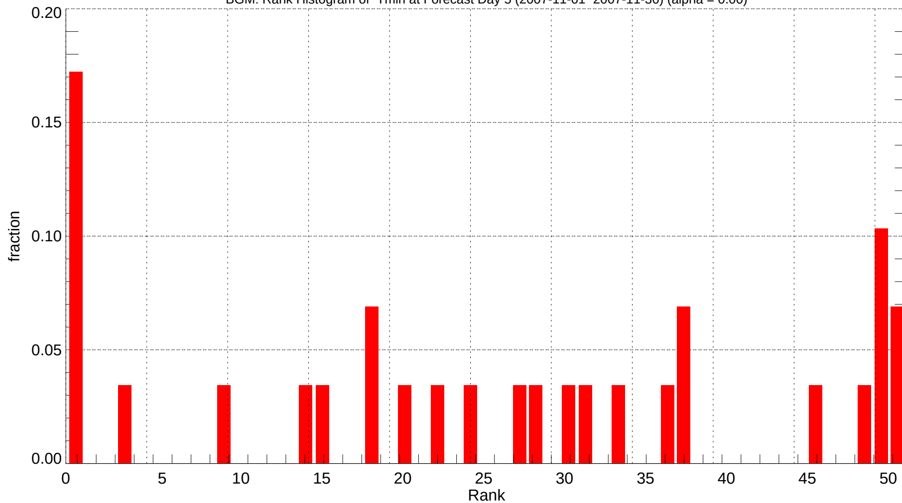
BGM: Rank Histogram of Tmin at Forecast Day 5 (2007-11-01~2007-11-30) (alpha = 0.00)
