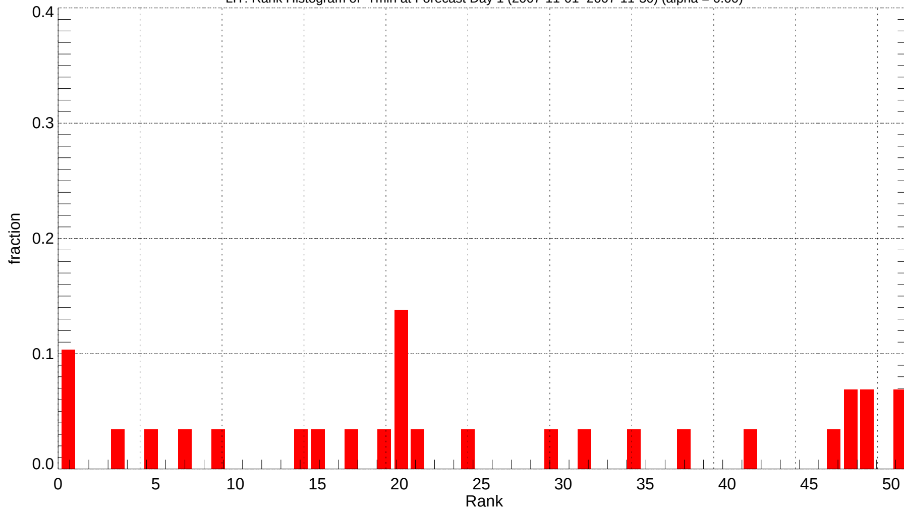
LIT: Rank Histogram of Tmin at Forecast Day 1 (2007-11-01~2007-11-30) (alpha = 0.00)
