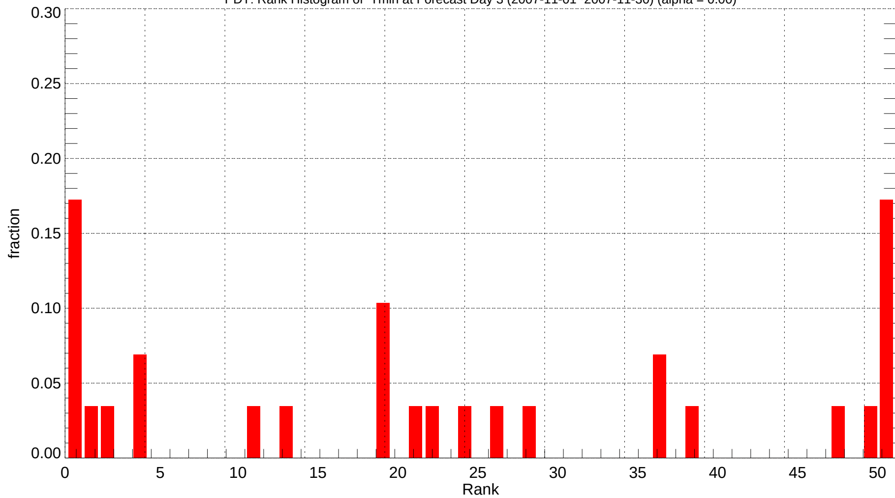
PDT: Rank Histogram of Tmin at Forecast Day 3 (2007-11-01~2007-11-30) (alpha = 0.00)
