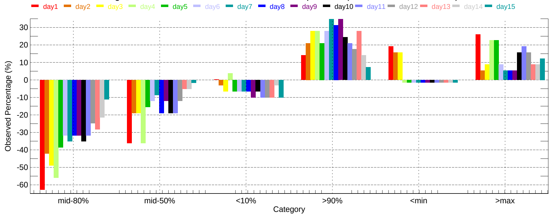
Observed Percentage Deviation of Ensembles - MEM: Min Temperature (2007-11-01~2007-11-30)
