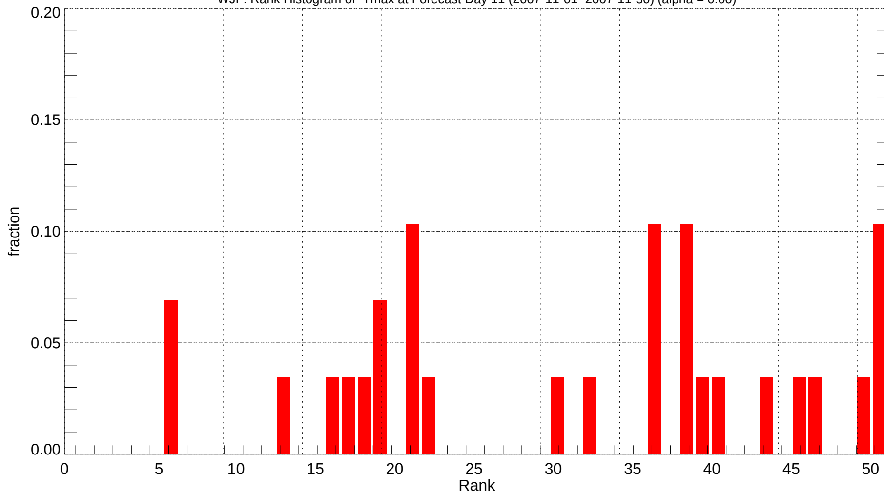
WJF: Rank Histogram of Tmax at Forecast Day 11 (2007-11-01~2007-11-30) (alpha = 0.00)
