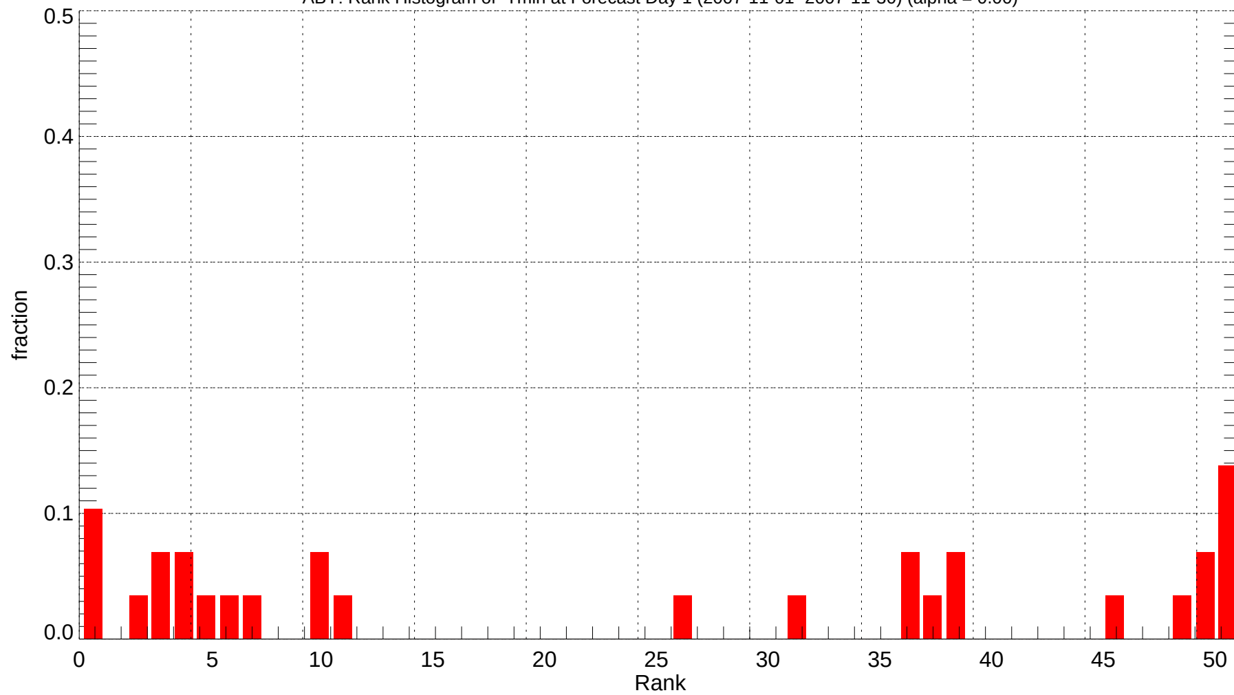
ABY: Rank Histogram of Tmin at Forecast Day 1 (2007-11-01~2007-11-30) (alpha = 0.00)
