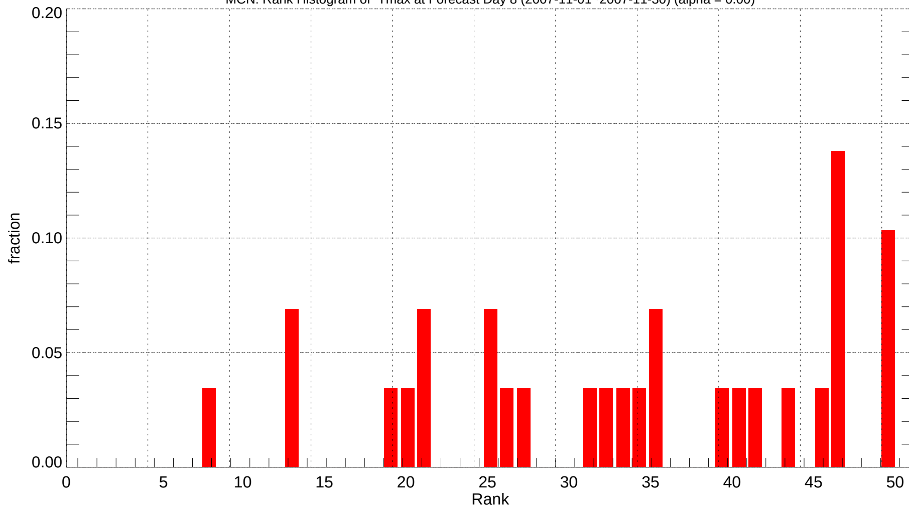
MCN: Rank Histogram of Tmax at Forecast Day 8 (2007-11-01~2007-11-30) (alpha = 0.00)
