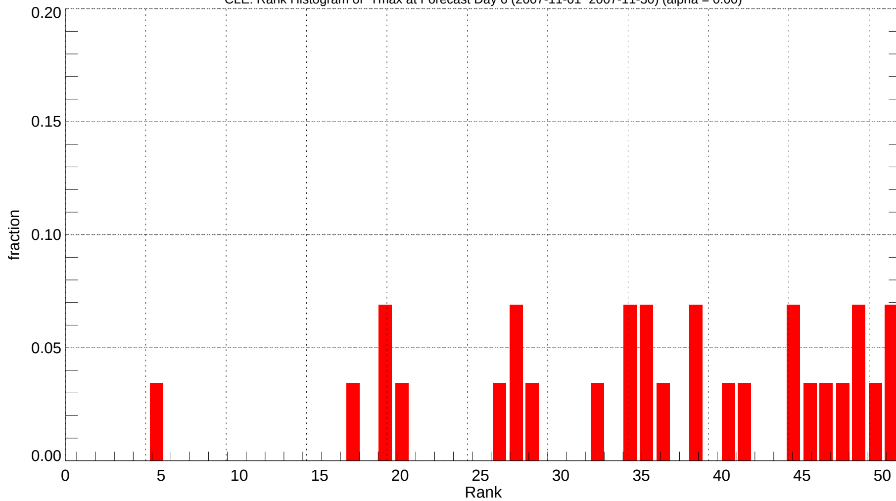
CLE: Rank Histogram of Tmax at Forecast Day 6 (2007-11-01~2007-11-30) (alpha = 0.00)
