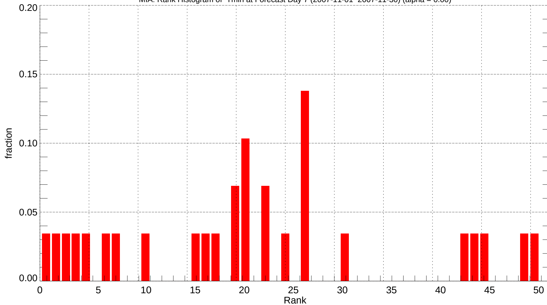
MIA: Rank Histogram of Tmin at Forecast Day 7 (2007-11-01~2007-11-30) (alpha = 0.00)
