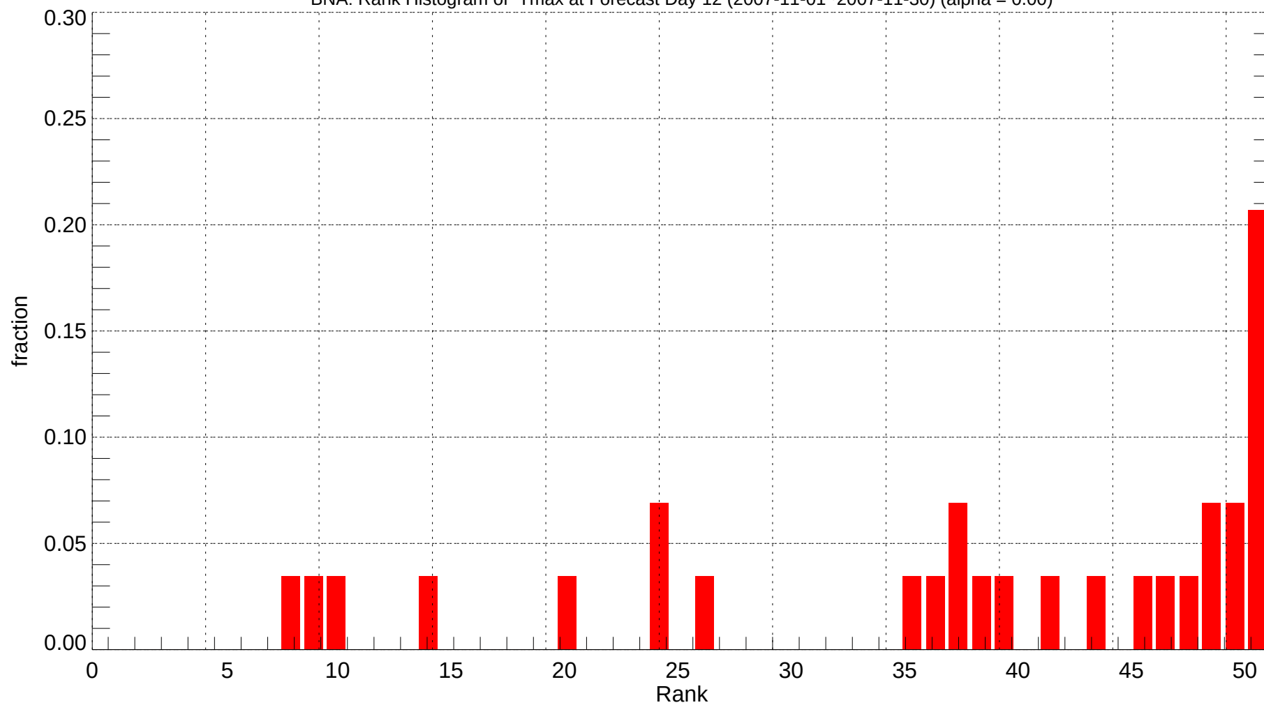
BNA: Rank Histogram of Tmax at Forecast Day 12 (2007-11-01~2007-11-30) (alpha = 0.00)
