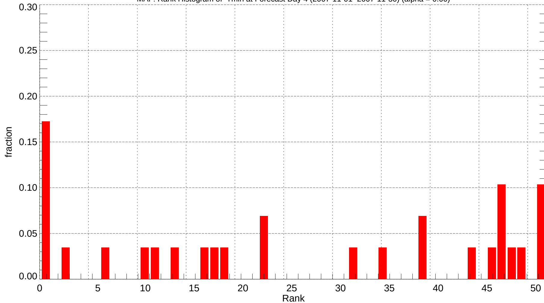
MAF: Rank Histogram of Tmin at Forecast Day 4 (2007-11-01~2007-11-30) (alpha = 0.00)
