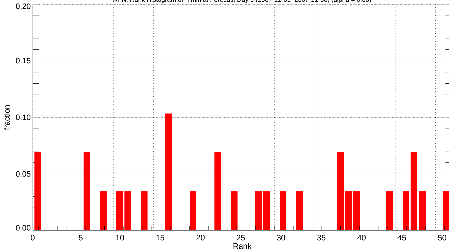
APN: Rank Histogram of Tmin at Forecast Day 9 (2007-11-01~2007-11-30) (alpha = 0.00)
