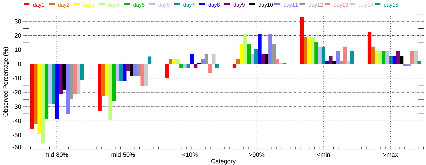
Observed Percentage Deviation of Ensembles - CRP: Min Temperature (2007-11-01~2007-11-30)
