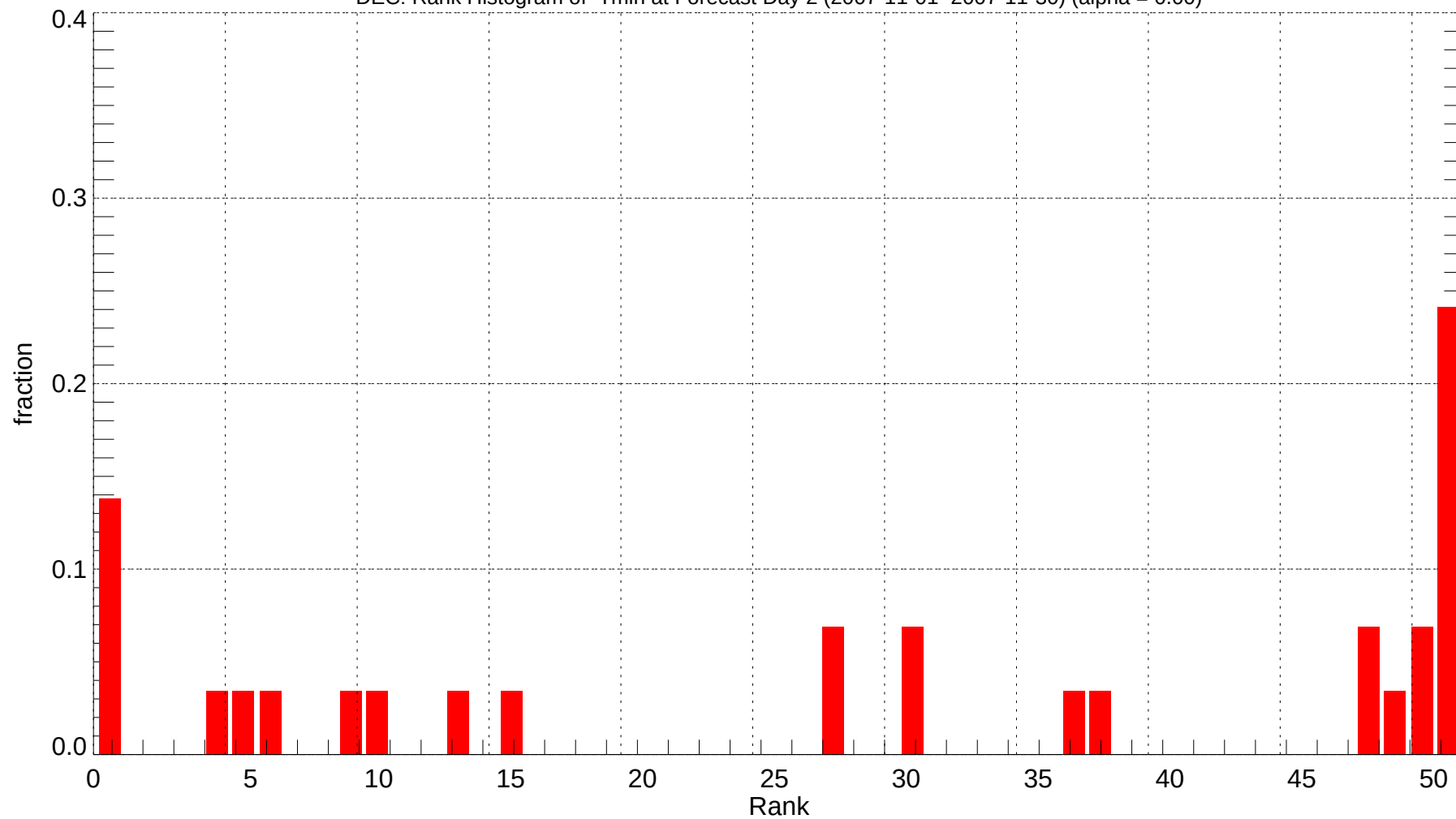
DEC: Rank Histogram of Tmin at Forecast Day 2 (2007-11-01~2007-11-30) (alpha = 0.00)
