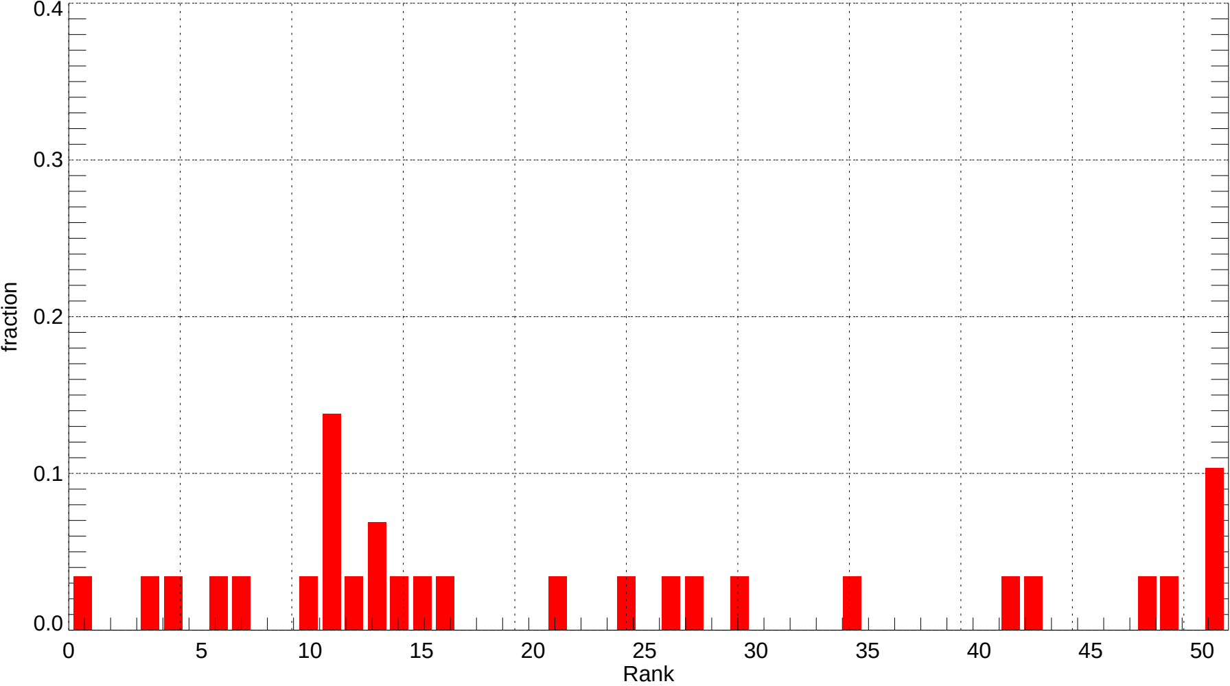
ATL: Rank Histogram of Tmin at Forecast Day 1 (2007-11-01~2007-11-30) (alpha = 0.00)
