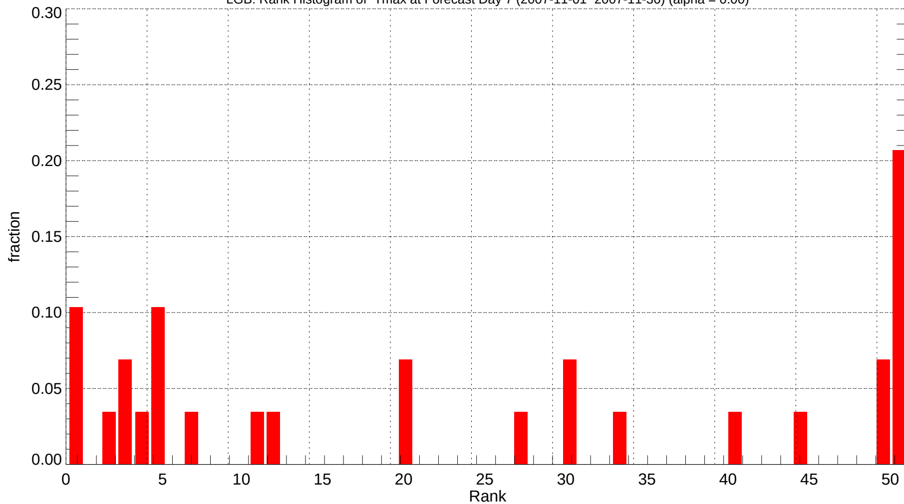
LGB: Rank Histogram of Tmax at Forecast Day 7 (2007-11-01~2007-11-30) (alpha = 0.00)
