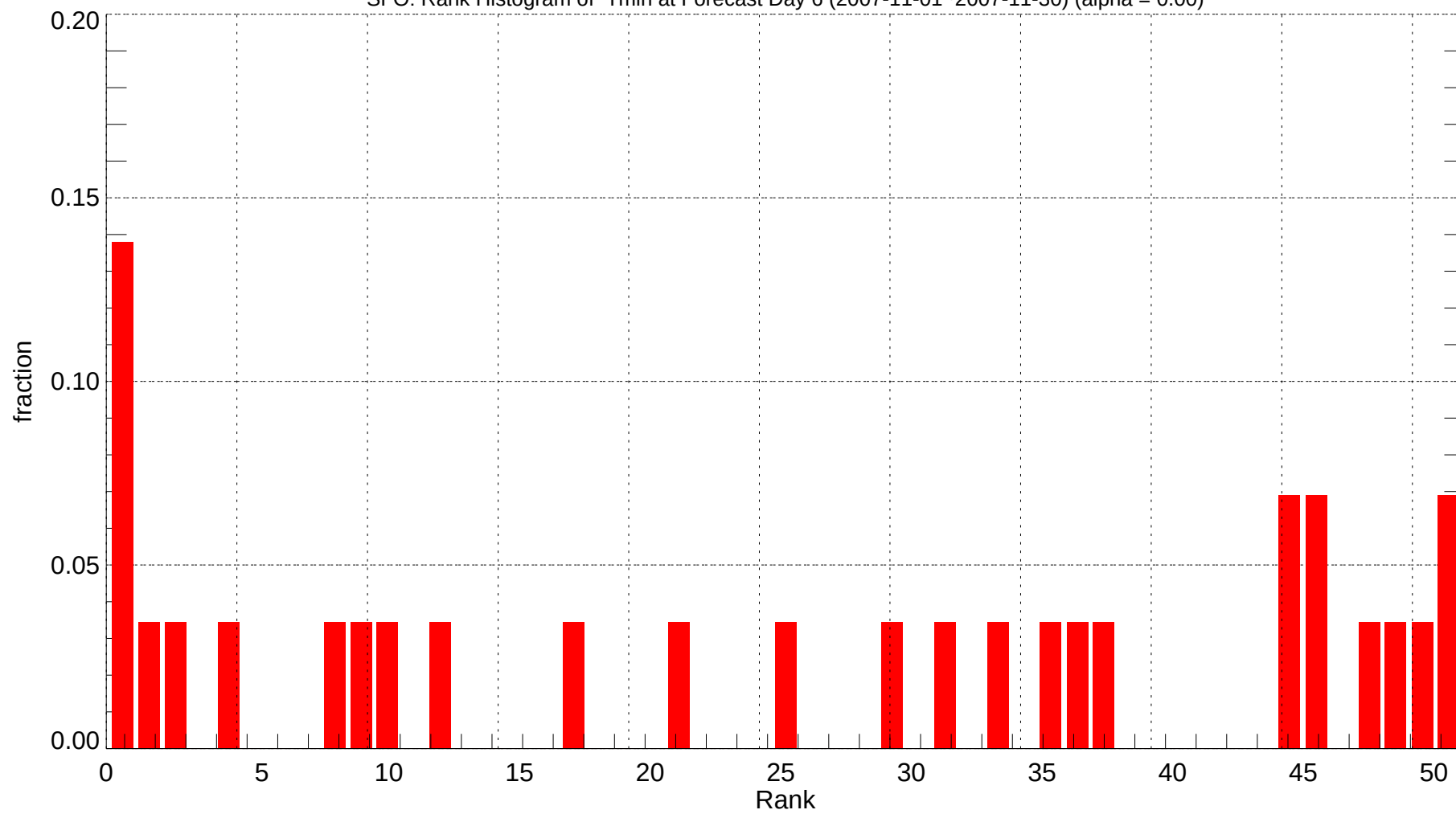
SFO: Rank Histogram of Tmin at Forecast Day 6 (2007-11-01~2007-11-30) (alpha = 0.00)
