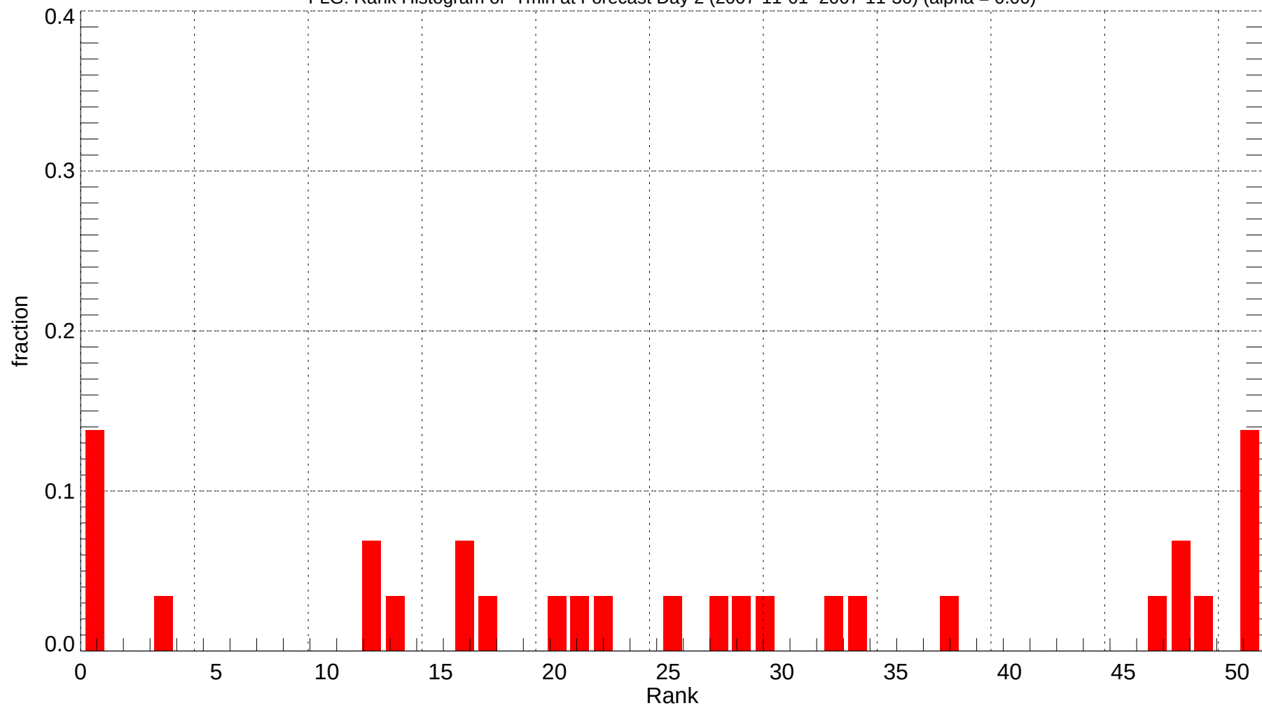
FLG: Rank Histogram of Tmin at Forecast Day 2 (2007-11-01~2007-11-30) (alpha = 0.00)
