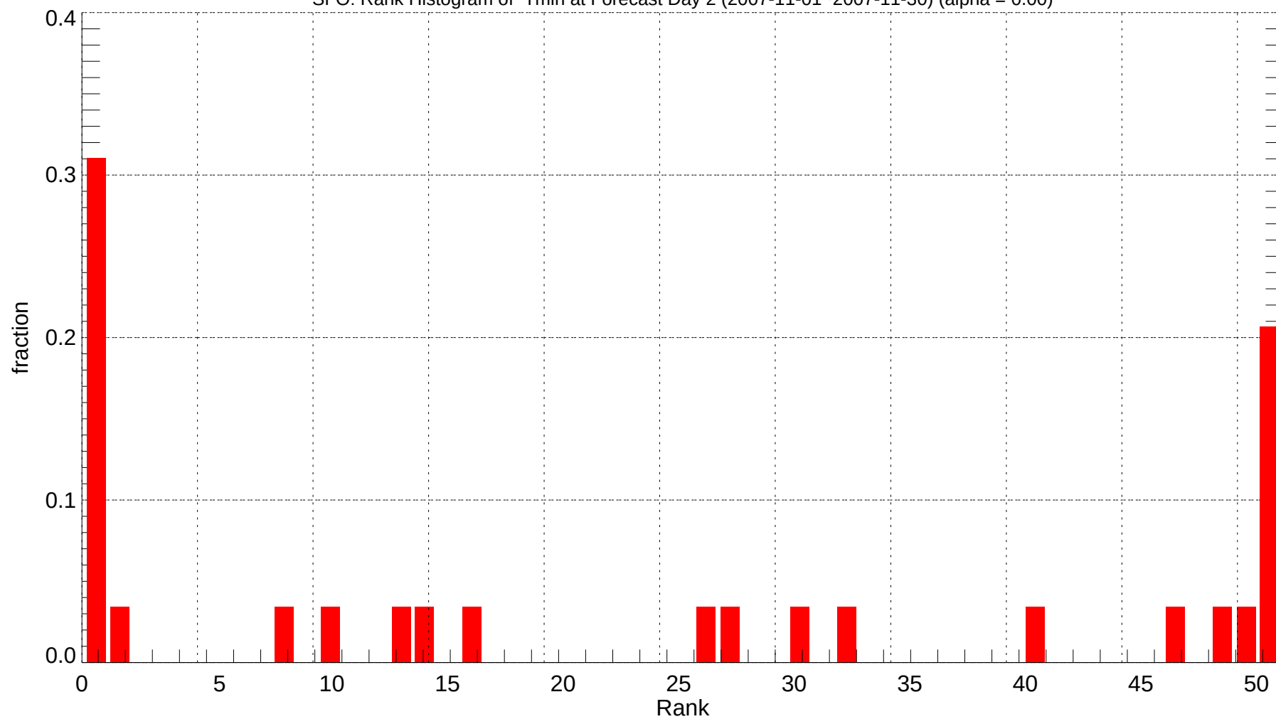
SFO: Rank Histogram of Tmin at Forecast Day 2 (2007-11-01~2007-11-30) (alpha = 0.00)
