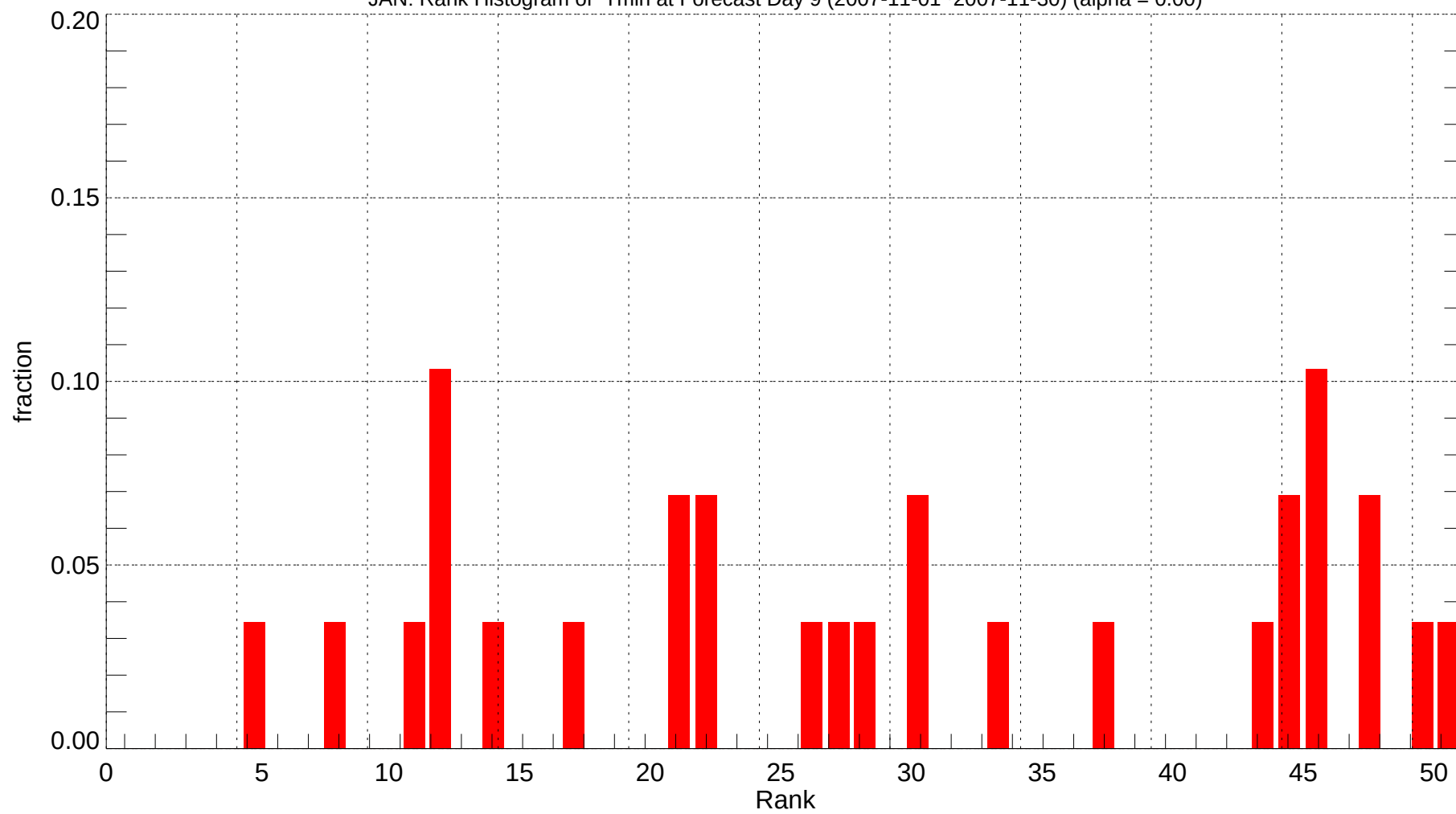
JAN: Rank Histogram of Tmin at Forecast Day 9 (2007-11-01~2007-11-30) (alpha = 0.00)
