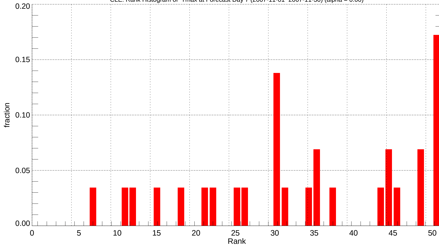
CLE: Rank Histogram of Tmax at Forecast Day 7 (2007-11-01~2007-11-30) (alpha = 0.00)
