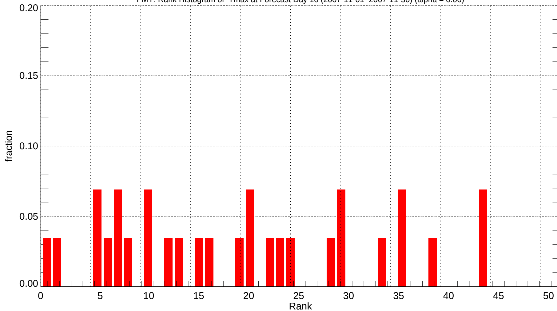
FMY: Rank Histogram of Tmax at Forecast Day 10 (2007-11-01~2007-11-30) (alpha = 0.00)
