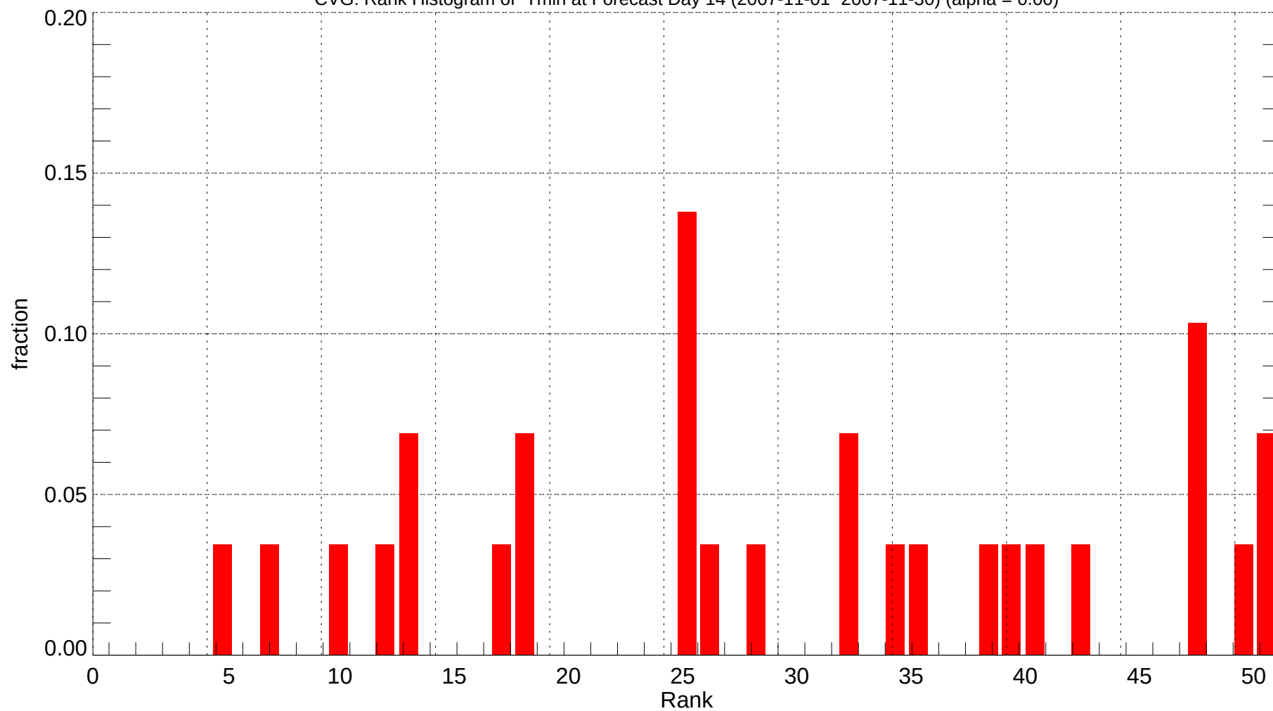
CVG: Rank Histogram of Tmin at Forecast Day 14 (2007-11-01~2007-11-30) (alpha = 0.00)
