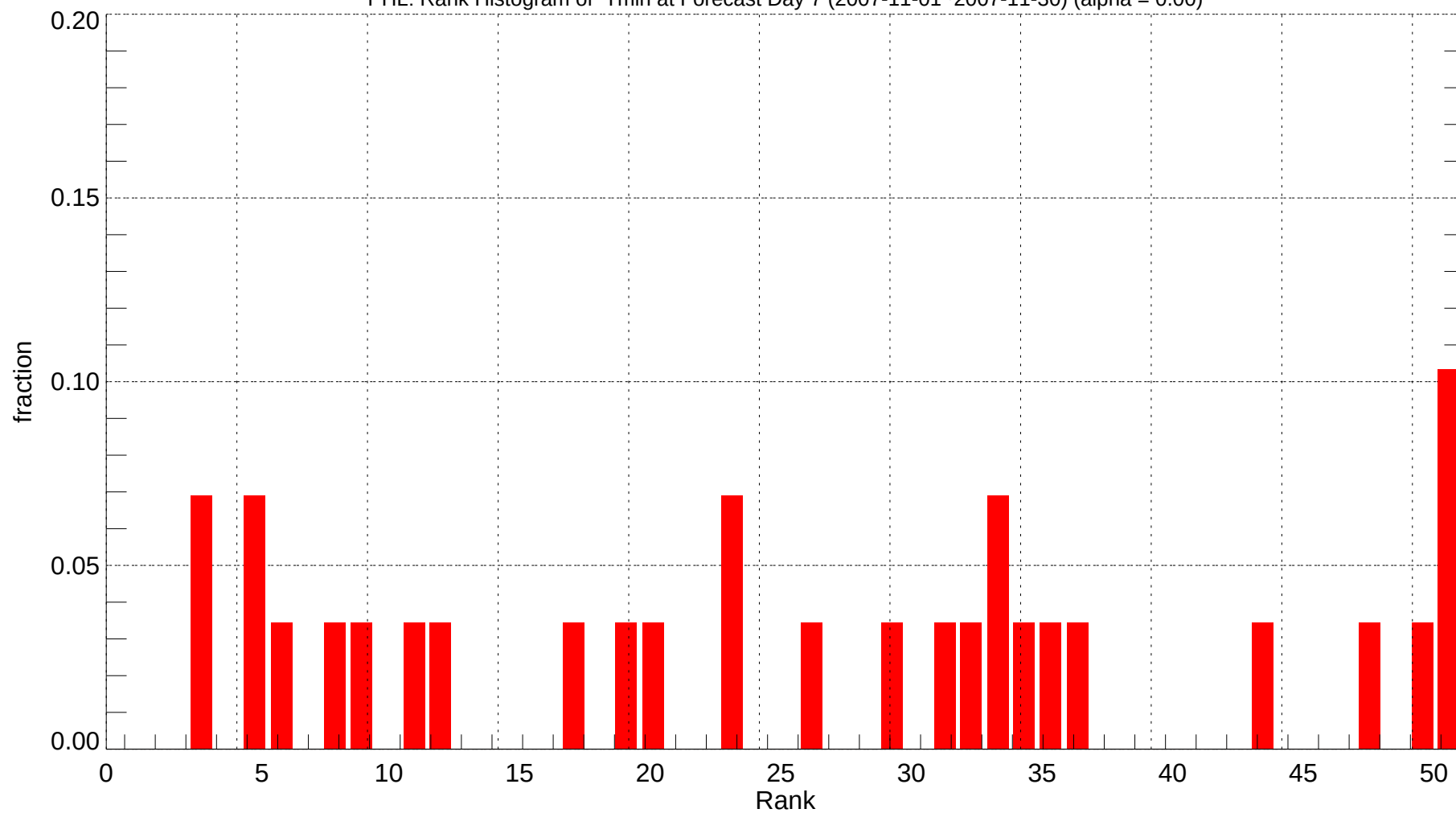
PHL: Rank Histogram of Tmin at Forecast Day 7 (2007-11-01~2007-11-30) (alpha = 0.00)
