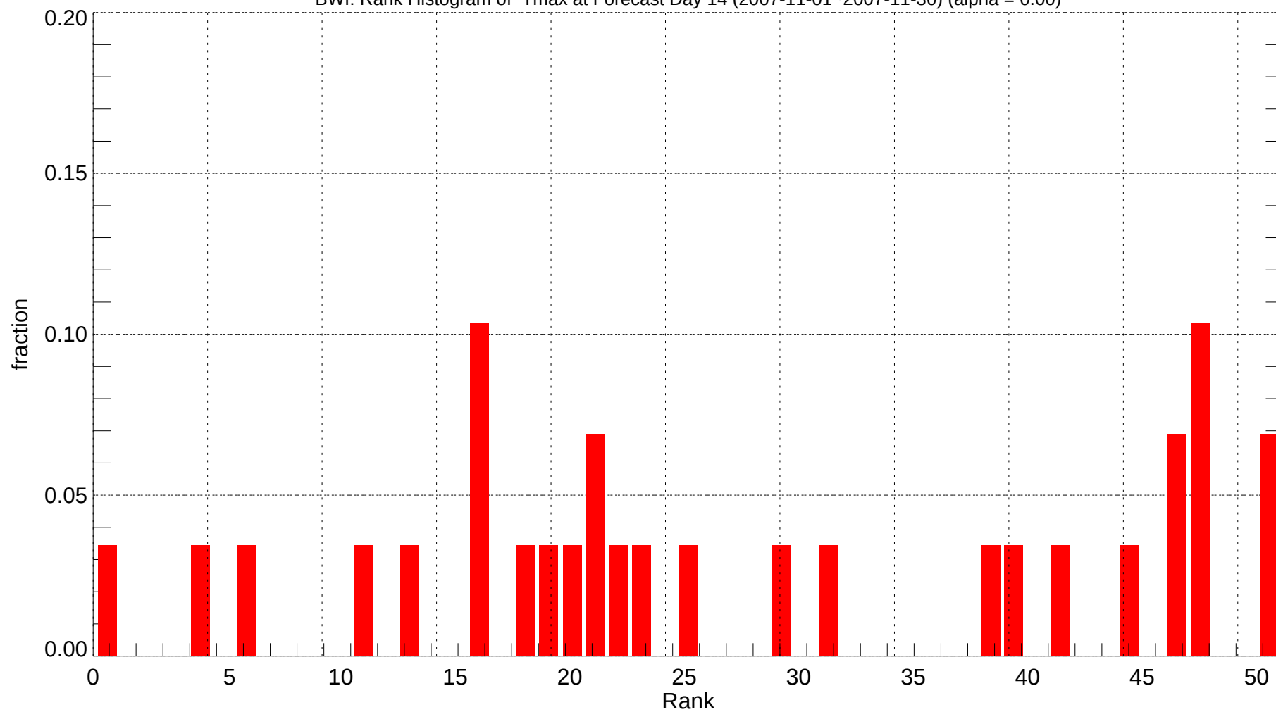
BWI: Rank Histogram of Tmax at Forecast Day 14 (2007-11-01~2007-11-30) (alpha = 0.00)
