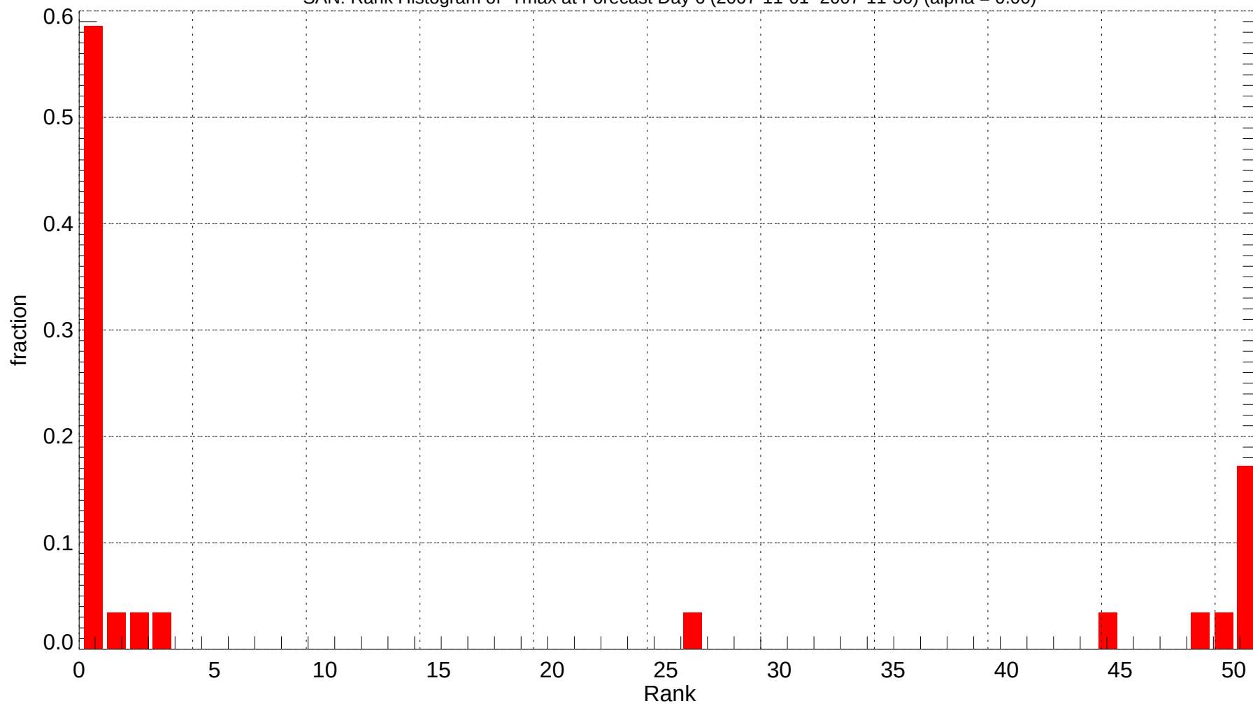
SAN: Rank Histogram of Tmax at Forecast Day 6 (2007-11-01~2007-11-30) (alpha = 0.00)
