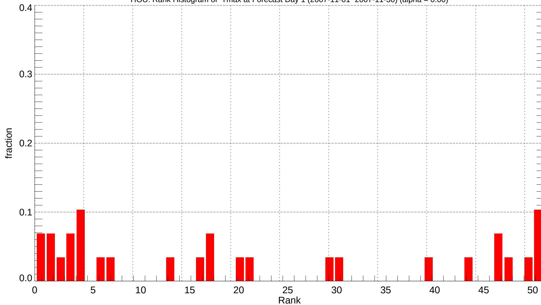
HOU: Rank Histogram of Tmax at Forecast Day 1 (2007-11-01~2007-11-30) (alpha = 0.00)
