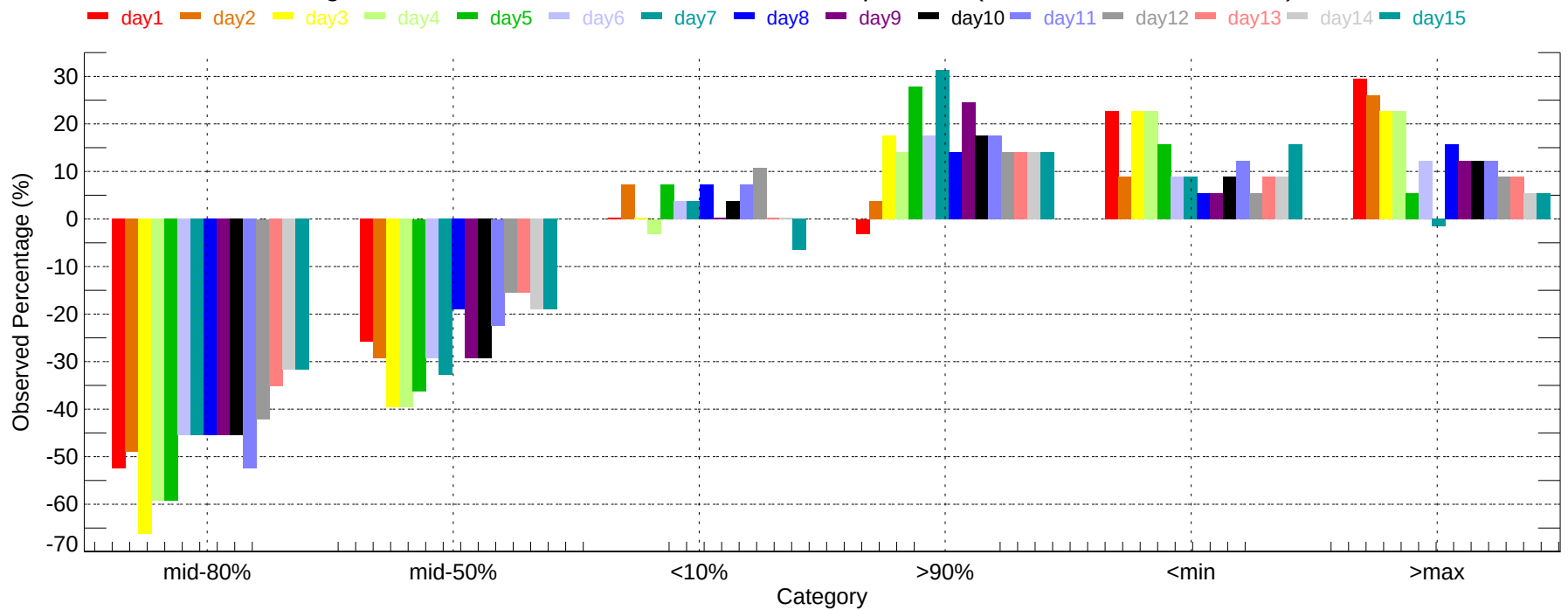
Observed Percentage Deviation of Ensembles - VCT: Min Temperature (2007-11-01~2007-11-30)
