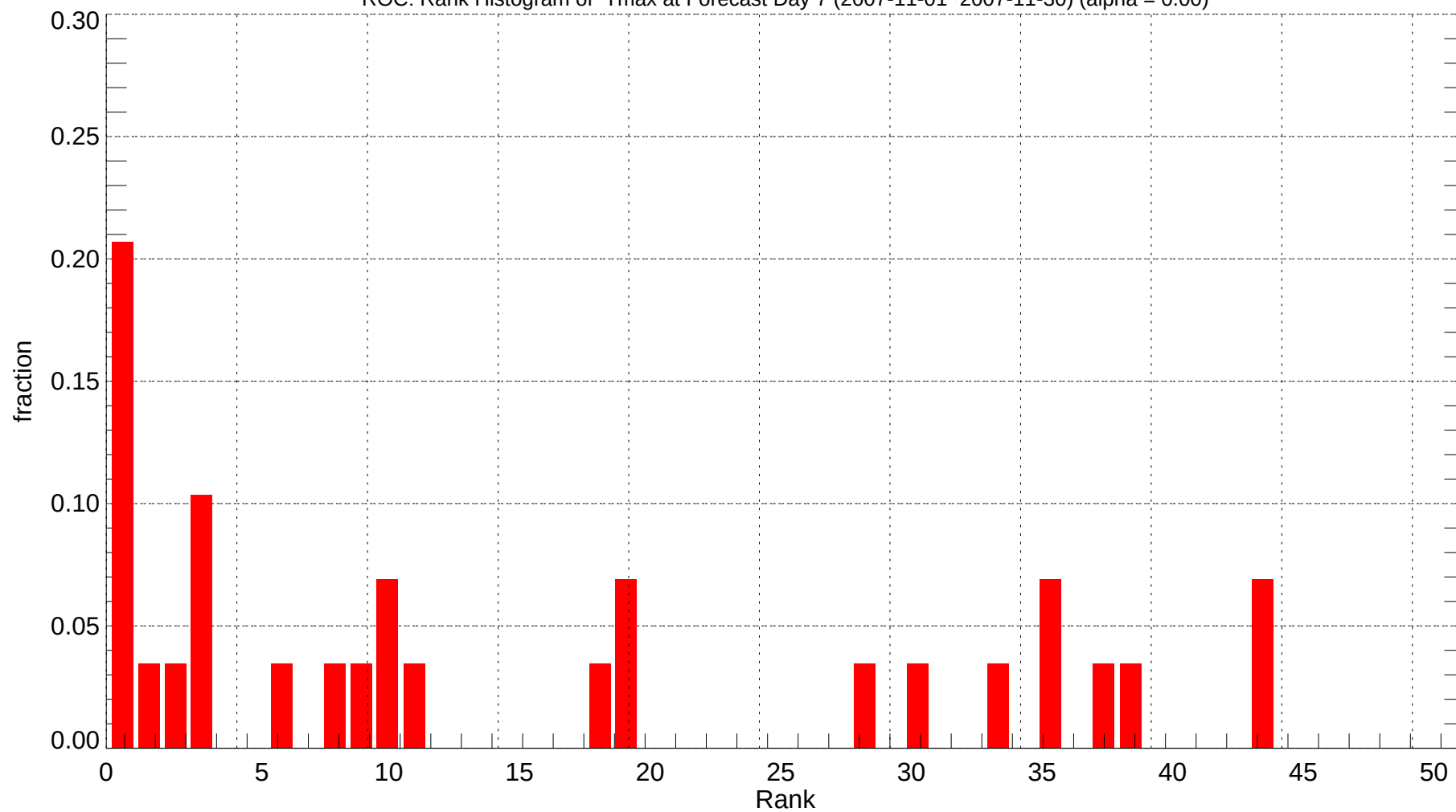
ROC: Rank Histogram of Tmax at Forecast Day 7 (2007-11-01~2007-11-30) (alpha = 0.00)
