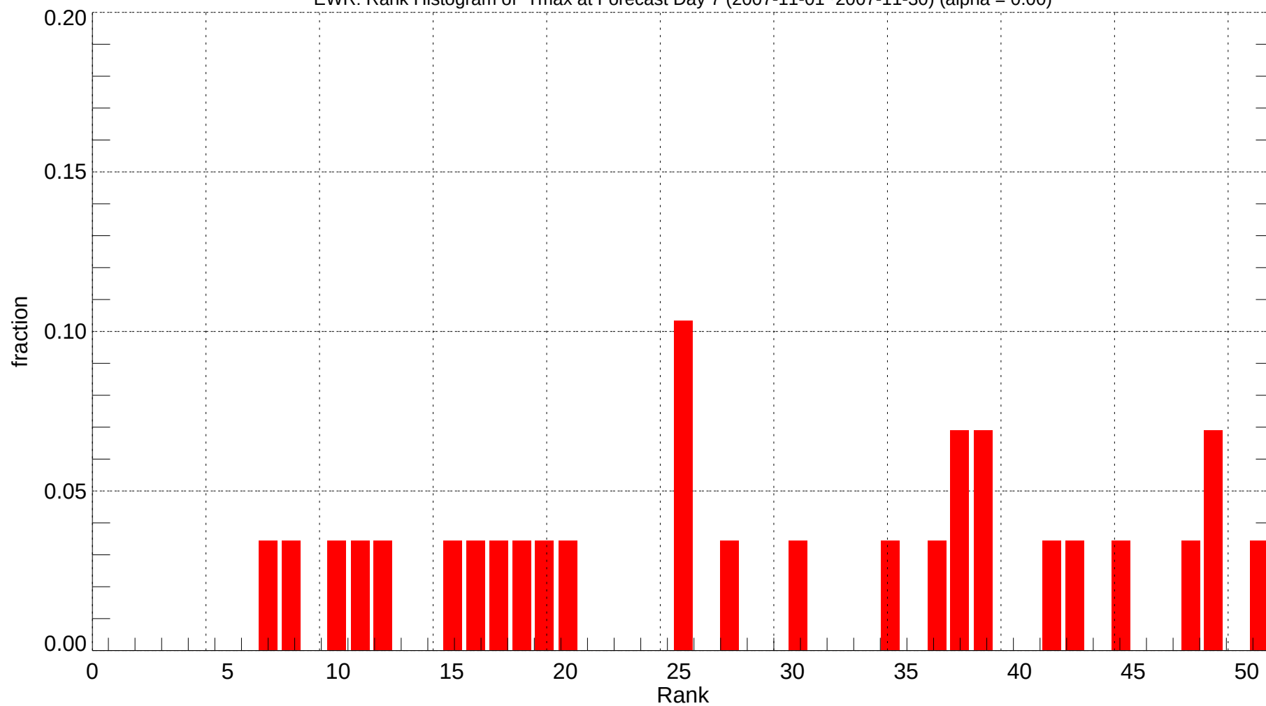
EWR: Rank Histogram of Tmax at Forecast Day 7 (2007-11-01~2007-11-30) (alpha = 0.00)
