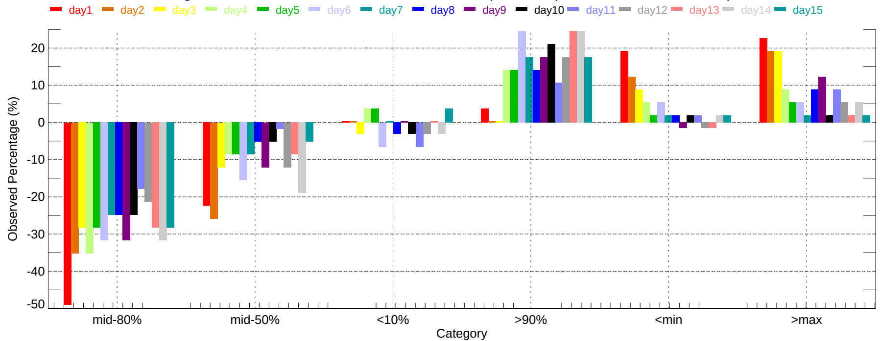
Observed Percentage Deviation of Ensembles - MWL: Min Temperature (2007-11-01~2007-11-30)
