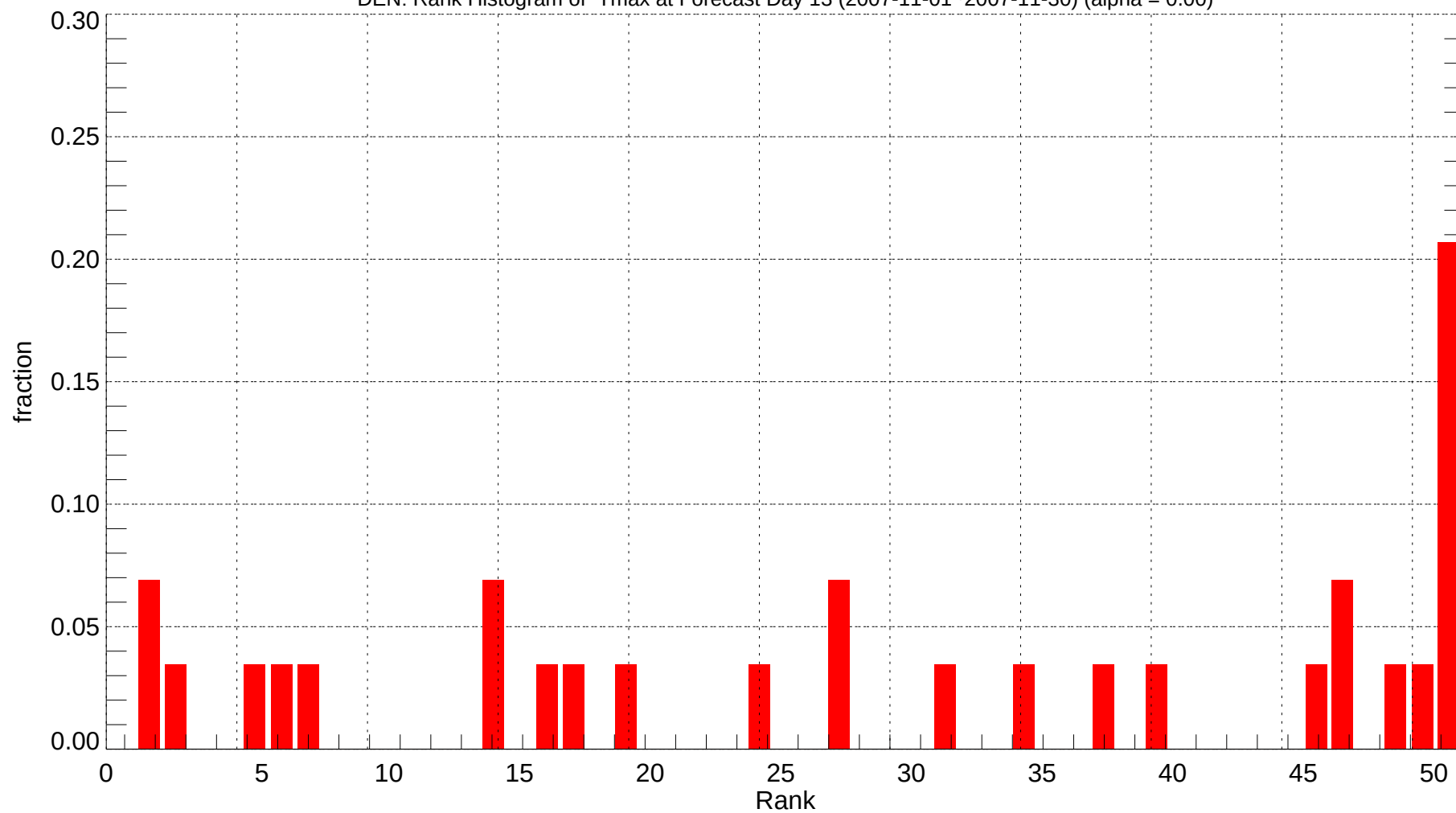
DEN: Rank Histogram of Tmax at Forecast Day 13 (2007-11-01~2007-11-30) (alpha = 0.00)
