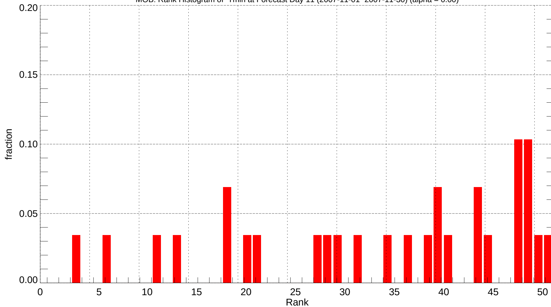
MOB: Rank Histogram of Tmin at Forecast Day 11 (2007-11-01~2007-11-30) (alpha = 0.00)
