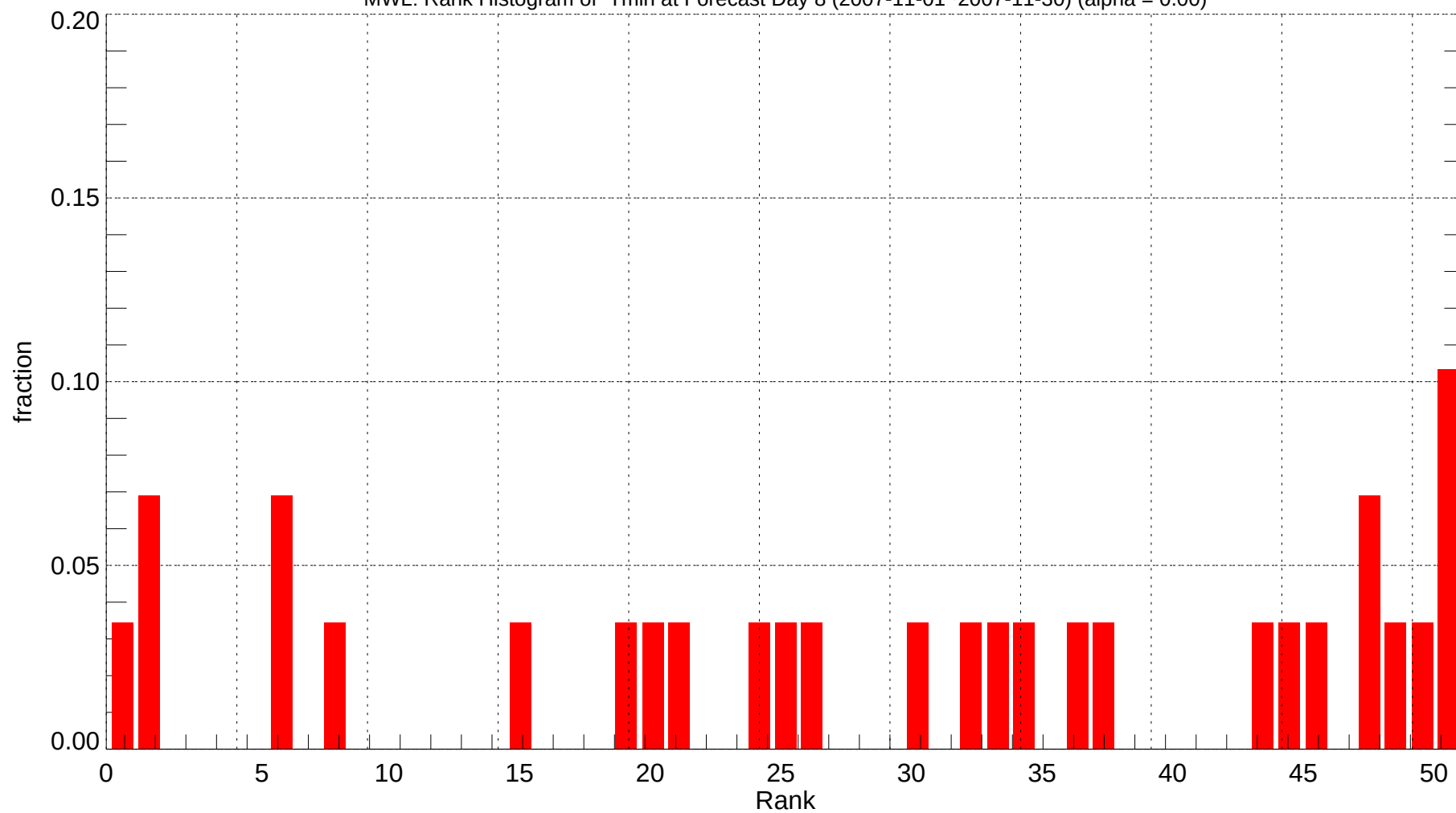
MWL: Rank Histogram of Tmin at Forecast Day 8 (2007-11-01~2007-11-30) (alpha = 0.00)
