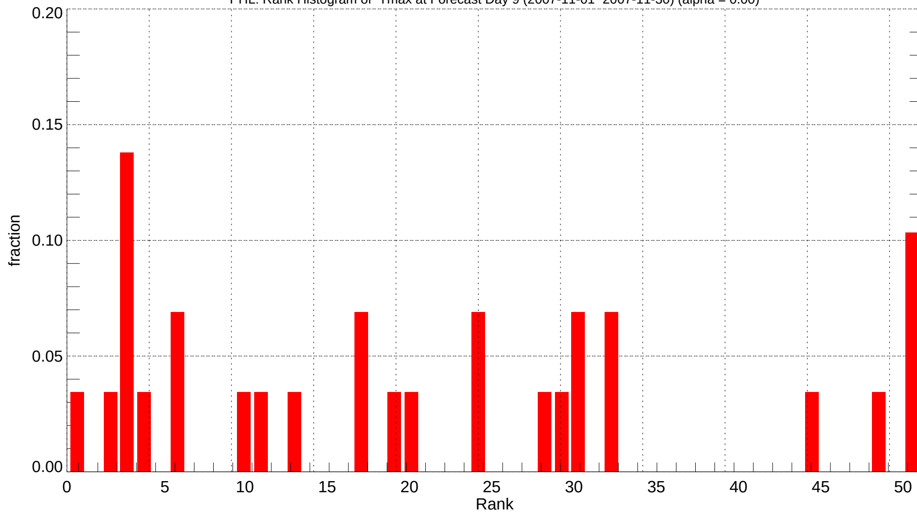
PHL: Rank Histogram of Tmax at Forecast Day 9 (2007-11-01~2007-11-30) (alpha = 0.00)
