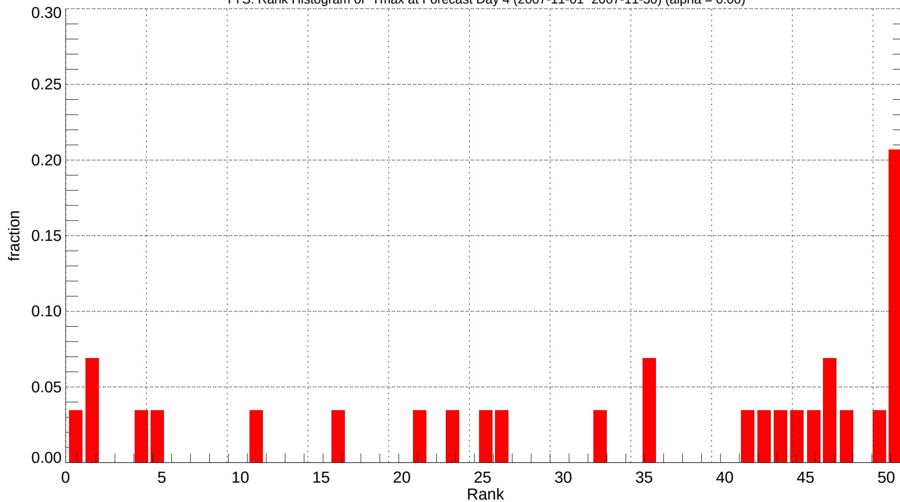
TYS: Rank Histogram of Tmax at Forecast Day 4 (2007-11-01~2007-11-30) (alpha = 0.00)
