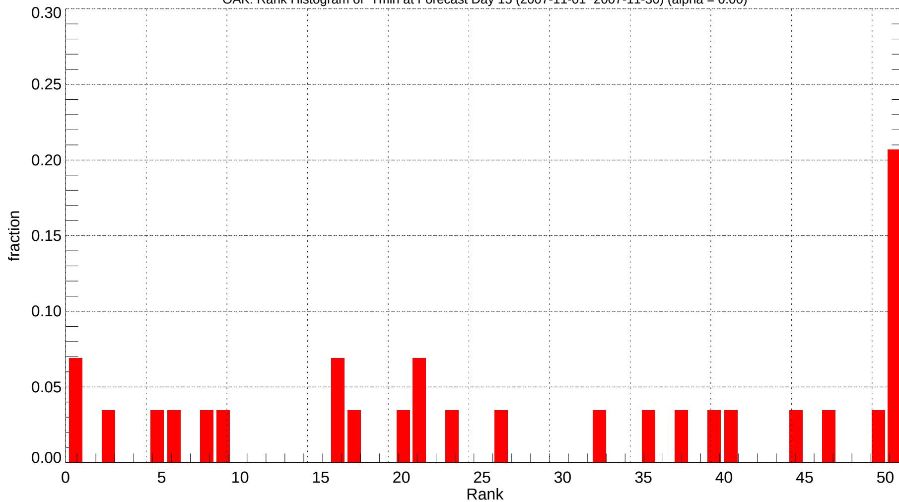
OAK: Rank Histogram of Tmin at Forecast Day 15 (2007-11-01~2007-11-30) (alpha = 0.00)
