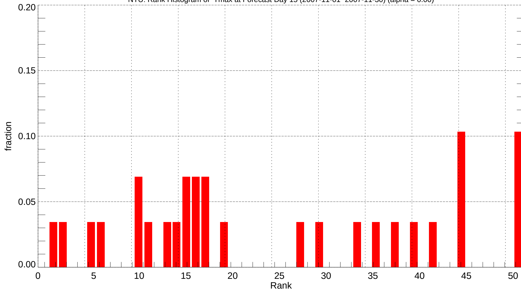
NTU: Rank Histogram of Tmax at Forecast Day 15 (2007-11-01~2007-11-30) (alpha = 0.00)
