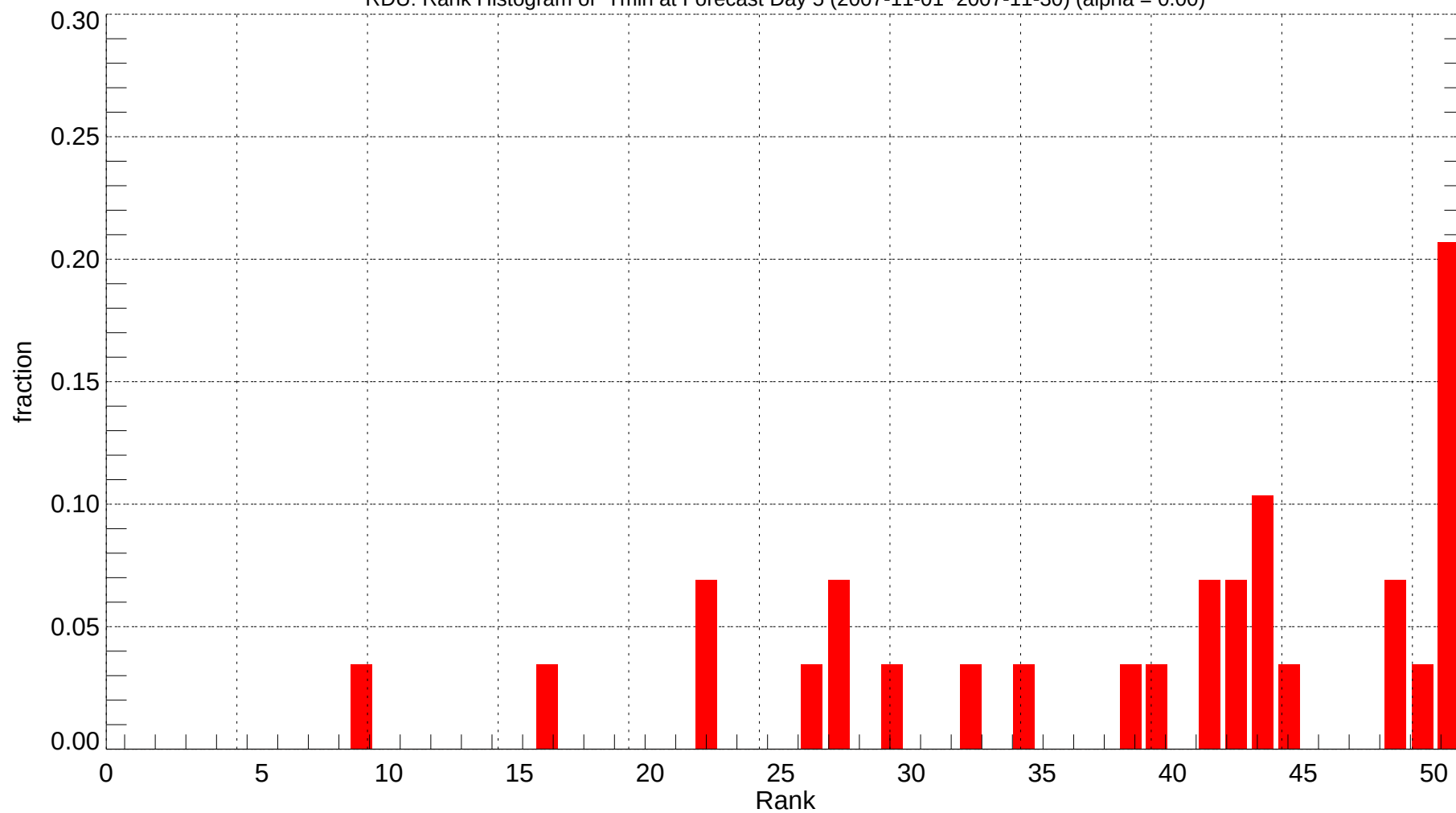
RDU: Rank Histogram of Tmin at Forecast Day 5 (2007-11-01~2007-11-30) (alpha = 0.00)
