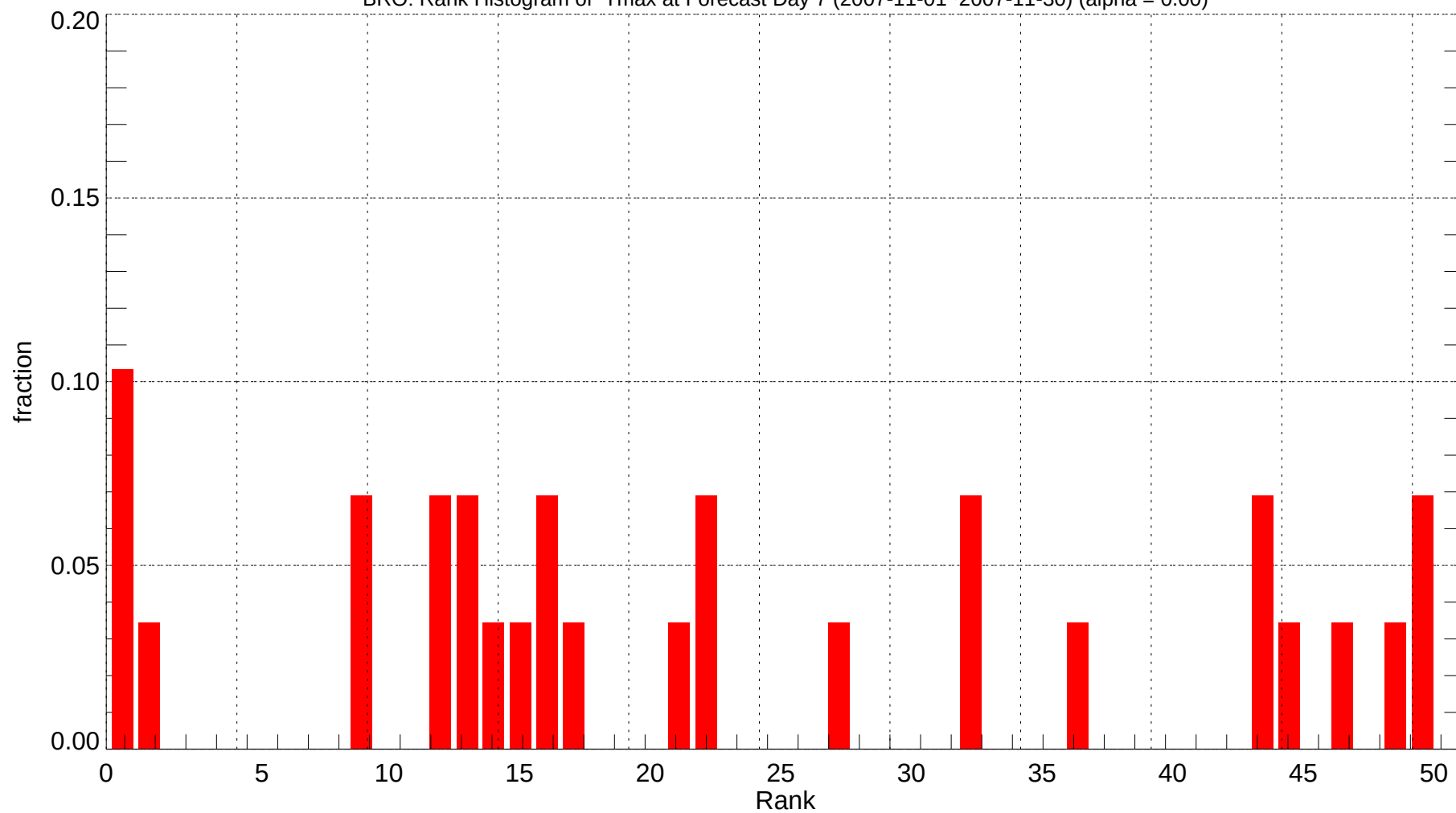
BRO: Rank Histogram of Tmax at Forecast Day 7 (2007-11-01~2007-11-30) (alpha = 0.00)
