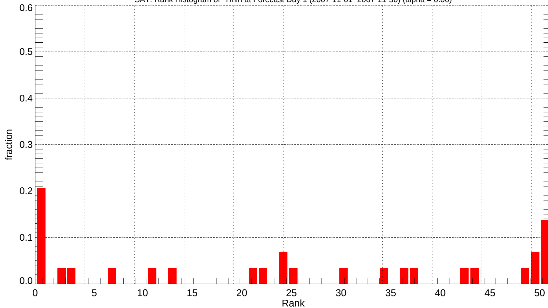
SAT: Rank Histogram of Tmin at Forecast Day 1 (2007-11-01~2007-11-30) (alpha = 0.00)
