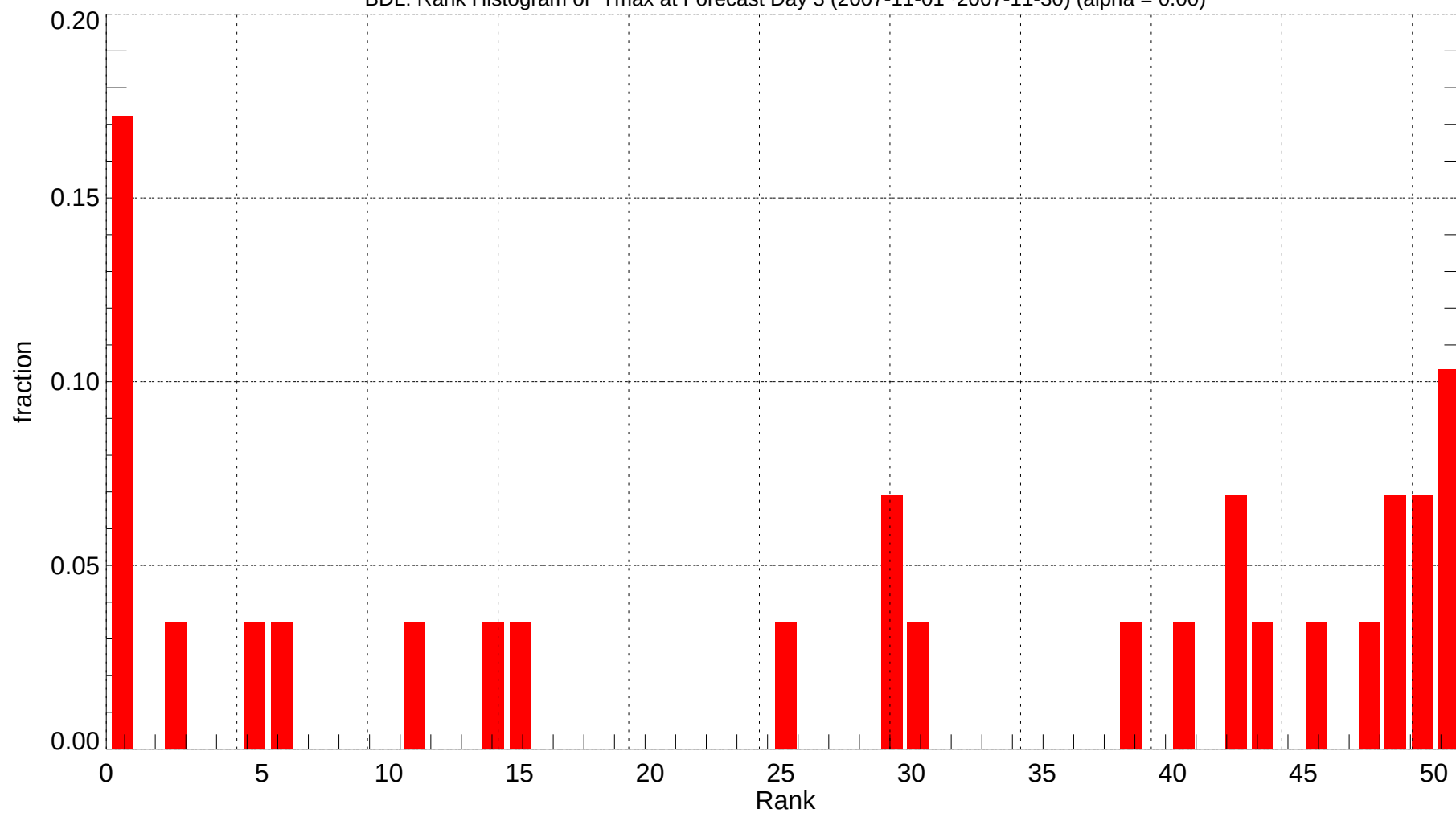
BDL: Rank Histogram of Tmax at Forecast Day 3 (2007-11-01~2007-11-30) (alpha = 0.00)
