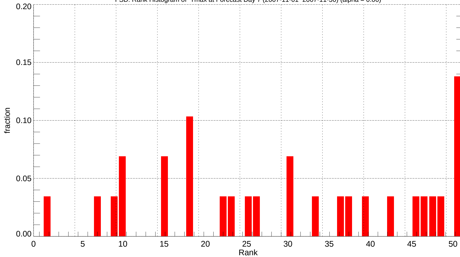
FSD: Rank Histogram of Tmax at Forecast Day 7 (2007-11-01~2007-11-30) (alpha = 0.00)
