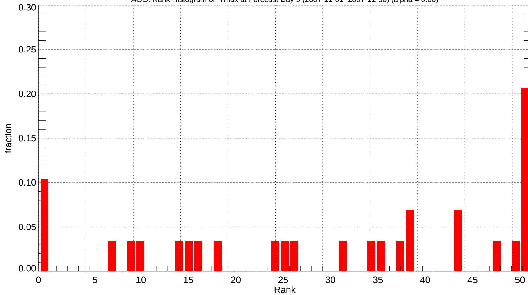
AOO: Rank Histogram of Tmax at Forecast Day 5 (2007-11-01~2007-11-30) (alpha = 0.00)
