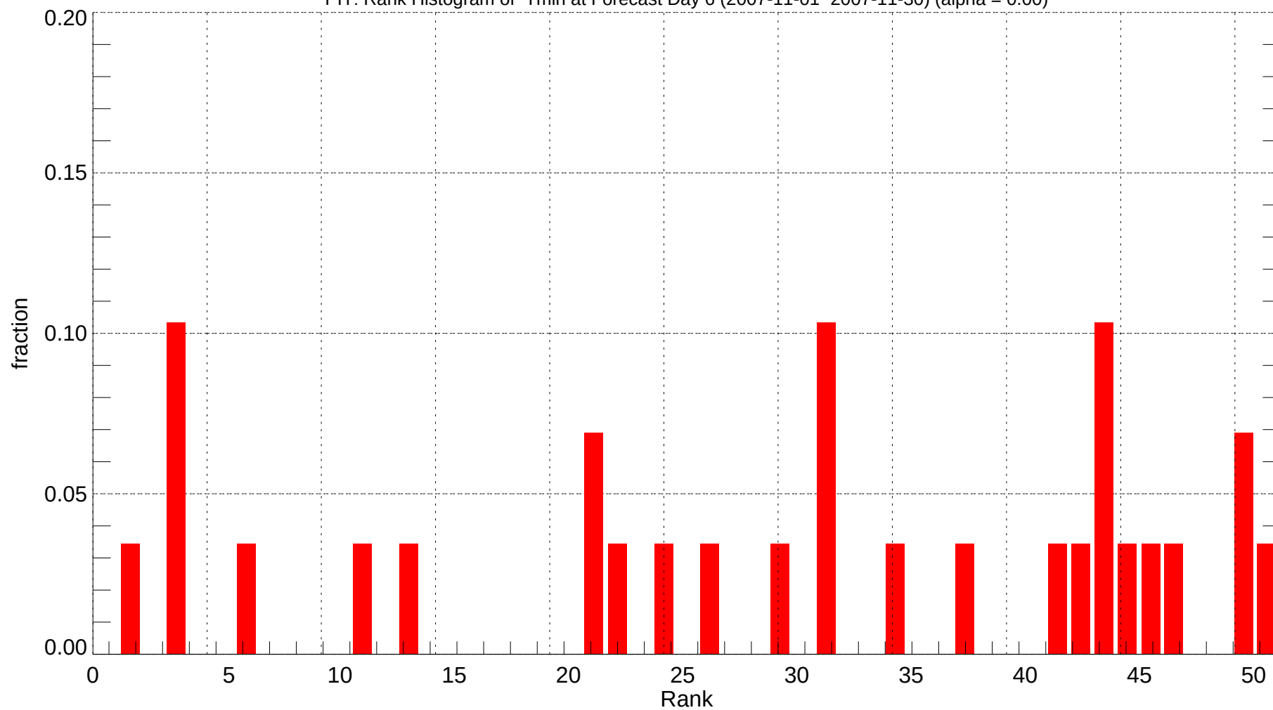
PIT: Rank Histogram of Tmin at Forecast Day 6 (2007-11-01~2007-11-30) (alpha = 0.00)
