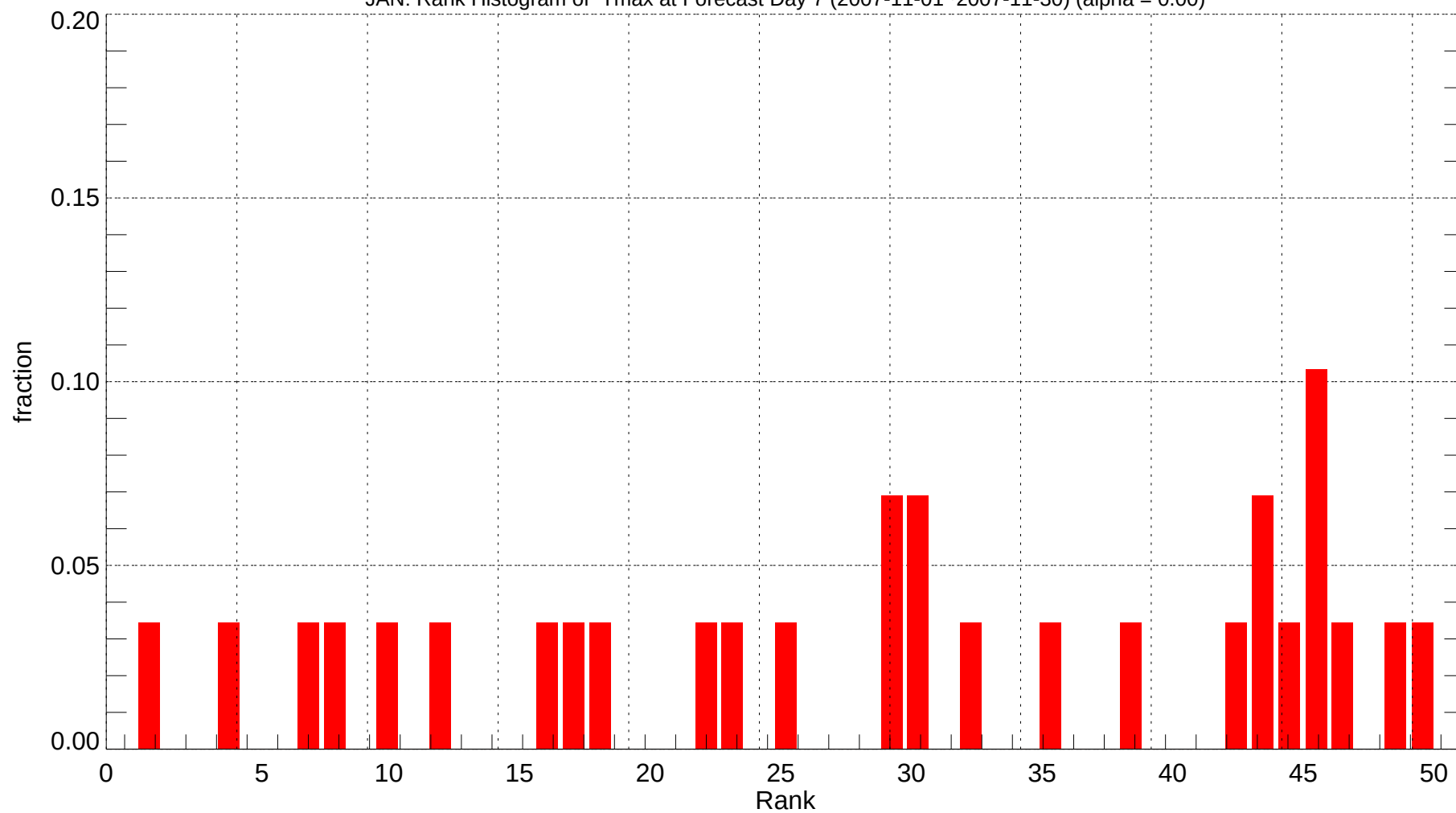
JAN: Rank Histogram of Tmax at Forecast Day 7 (2007-11-01~2007-11-30) (alpha = 0.00)
