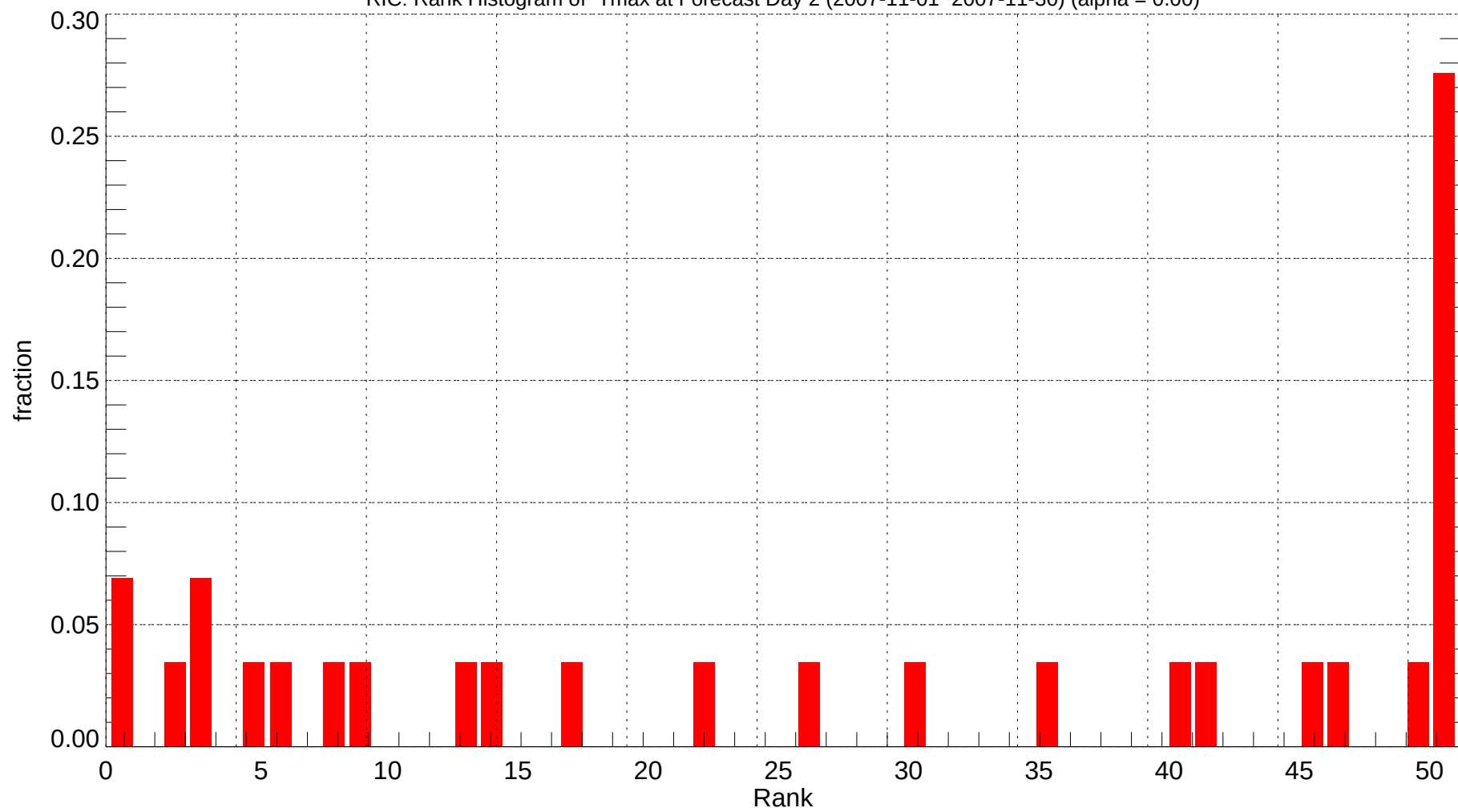
RIC: Rank Histogram of Tmax at Forecast Day 2 (2007-11-01~2007-11-30) (alpha = 0.00)
