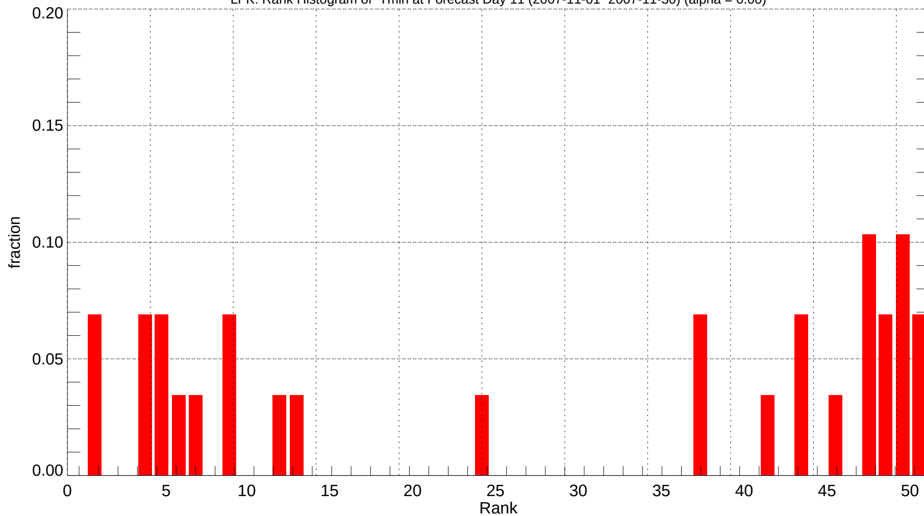
LFK: Rank Histogram of Tmin at Forecast Day 11 (2007-11-01~2007-11-30) (alpha = 0.00)
