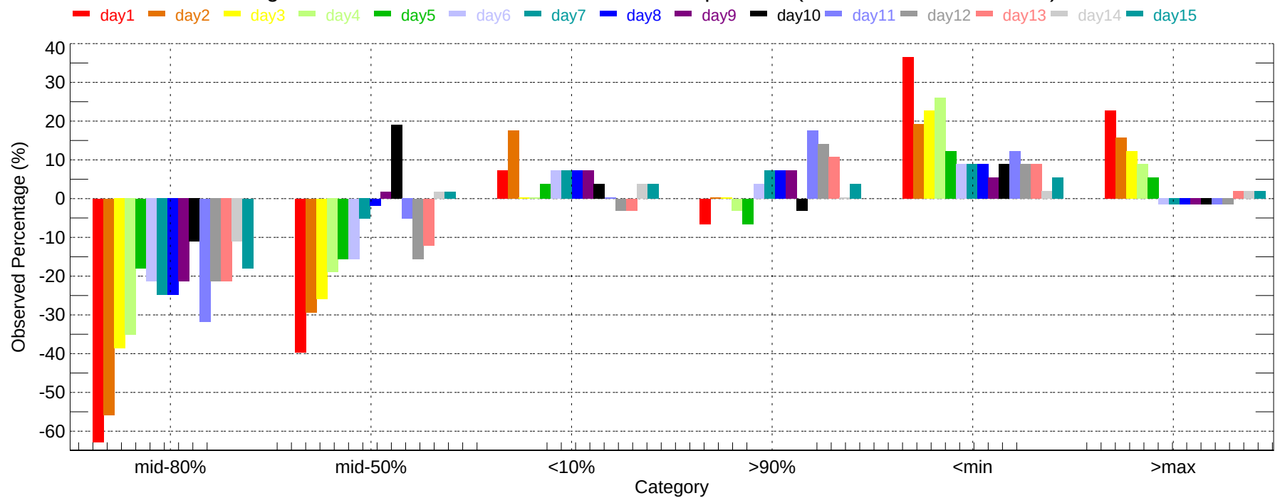
Observed Percentage Deviation of Ensembles - BUF: Min Temperature (2007-11-01~2007-11-30)
