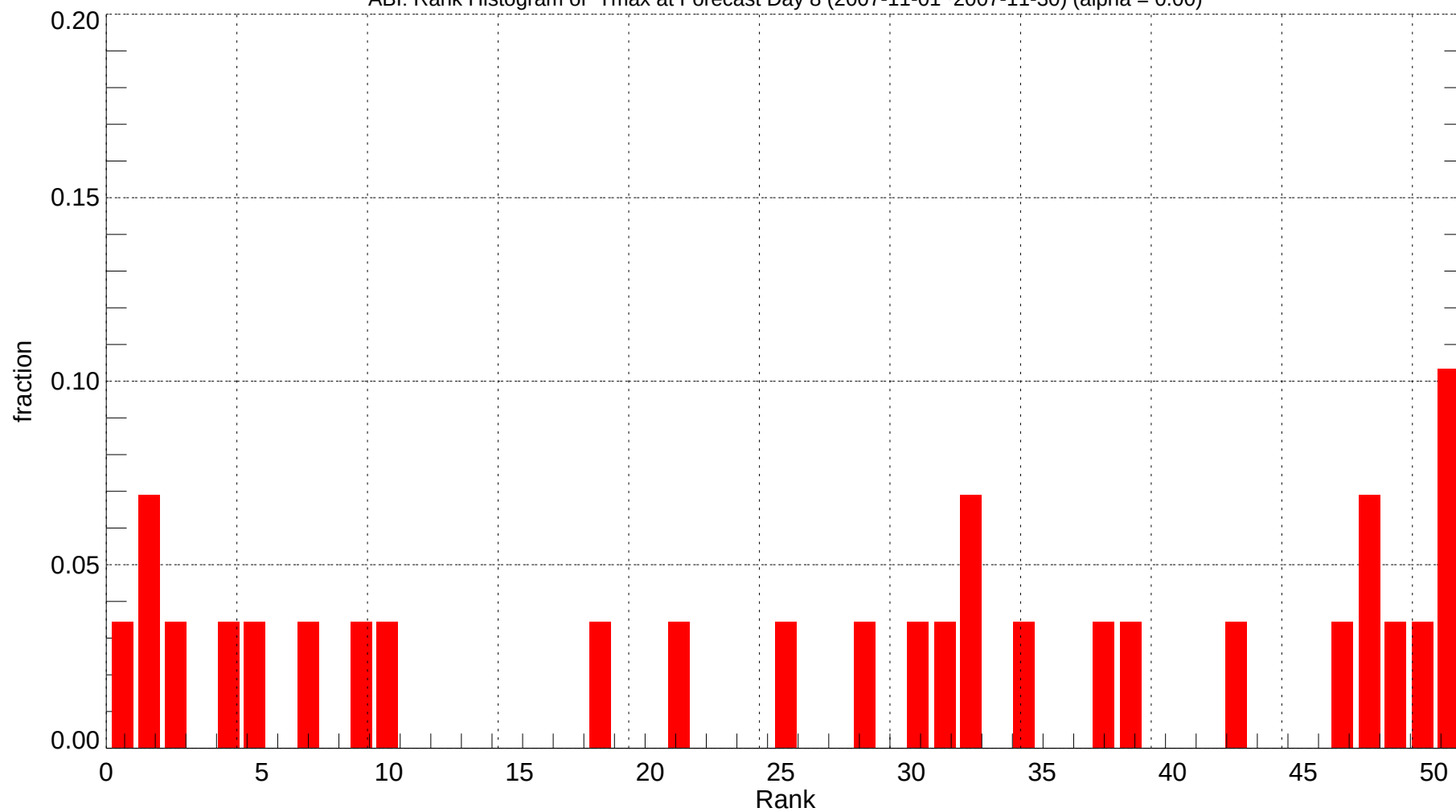
ABI: Rank Histogram of Tmax at Forecast Day 8 (2007-11-01~2007-11-30) (alpha = 0.00)
