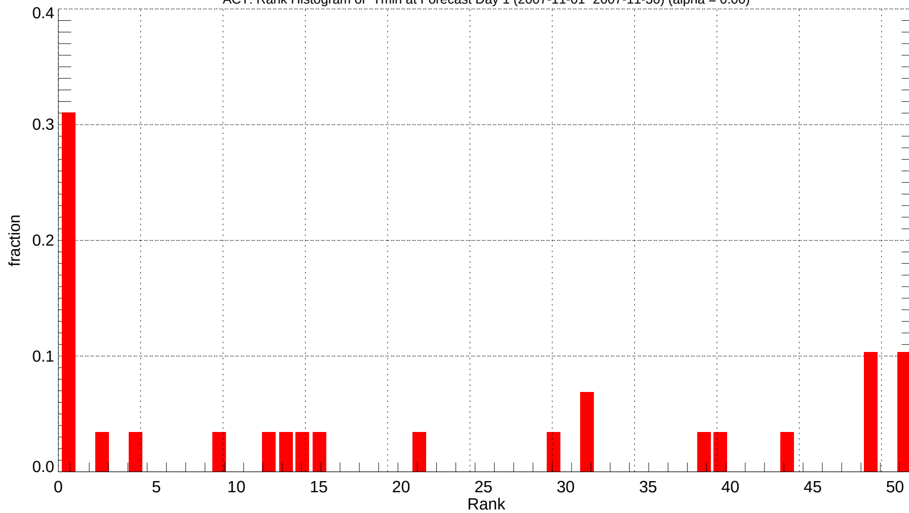
ACT: Rank Histogram of Tmin at Forecast Day 1 (2007-11-01~2007-11-30) (alpha = 0.00)
