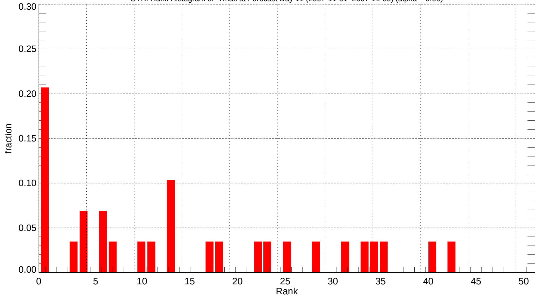
SYR: Rank Histogram of Tmax at Forecast Day 11 (2007-11-01~2007-11-30) (alpha = 0.00)
