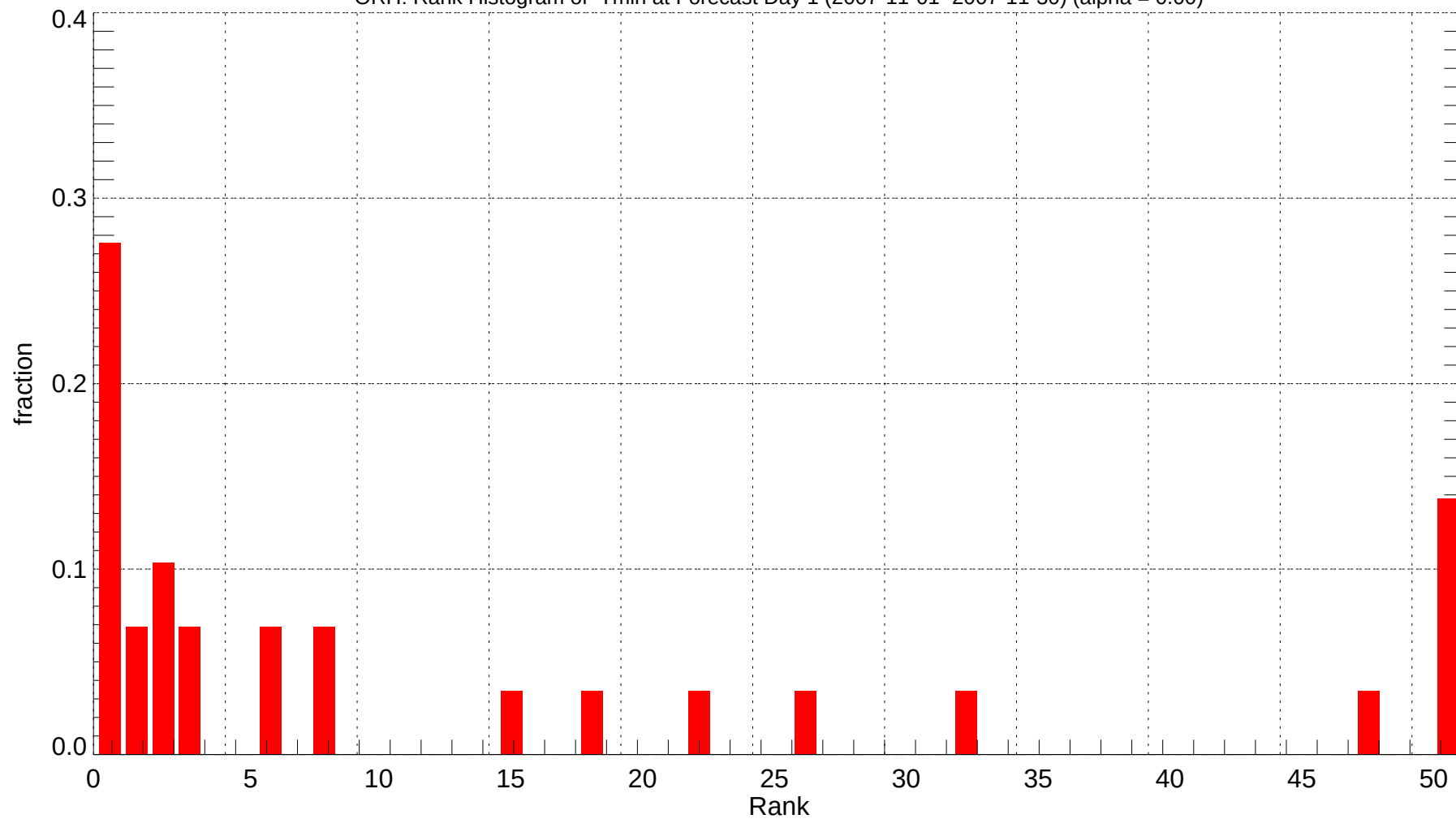
ORH: Rank Histogram of Tmin at Forecast Day 1 (2007-11-01~2007-11-30) (alpha = 0.00)
