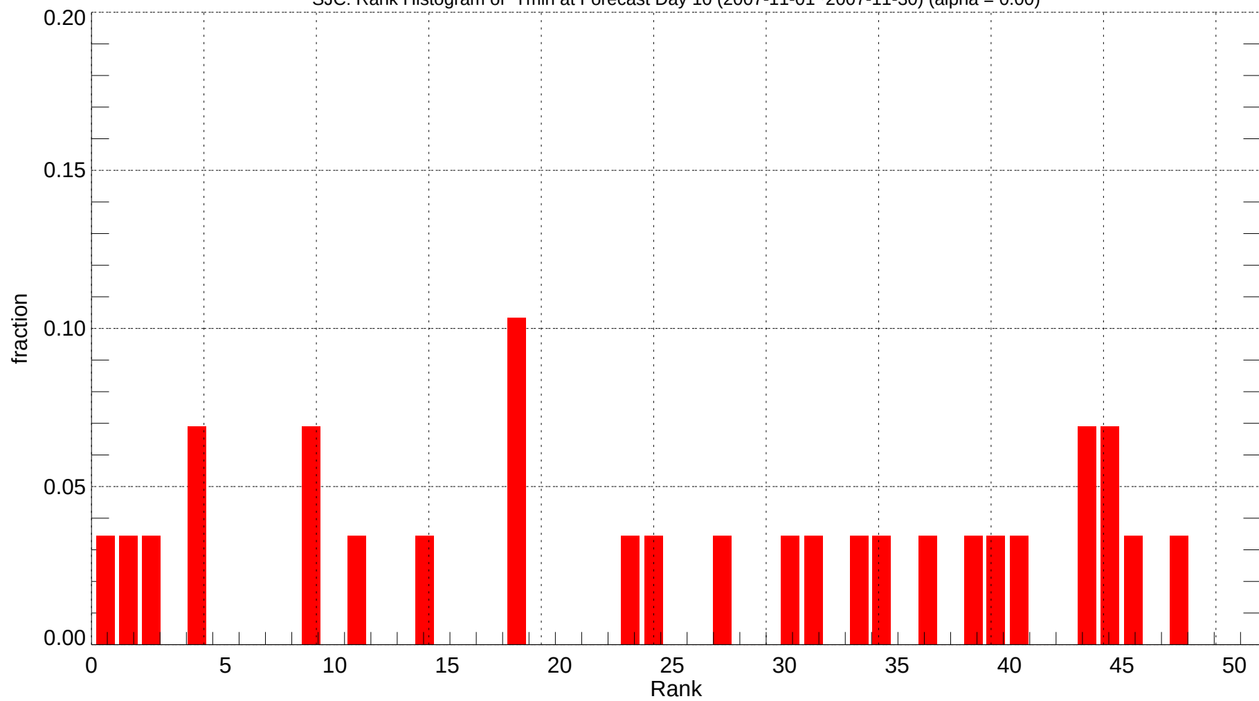
SJC: Rank Histogram of Tmin at Forecast Day 10 (2007-11-01~2007-11-30) (alpha = 0.00)
