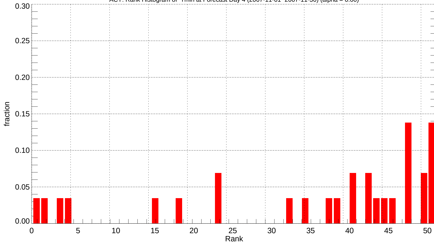
ACY: Rank Histogram of Tmin at Forecast Day 4 (2007-11-01~2007-11-30) (alpha = 0.00)
