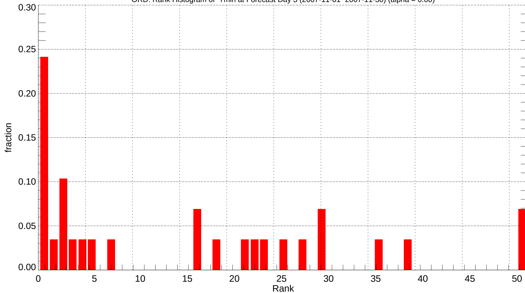
ORD: Rank Histogram of Tmin at Forecast Day 3 (2007-11-01~2007-11-30) (alpha = 0.00)
