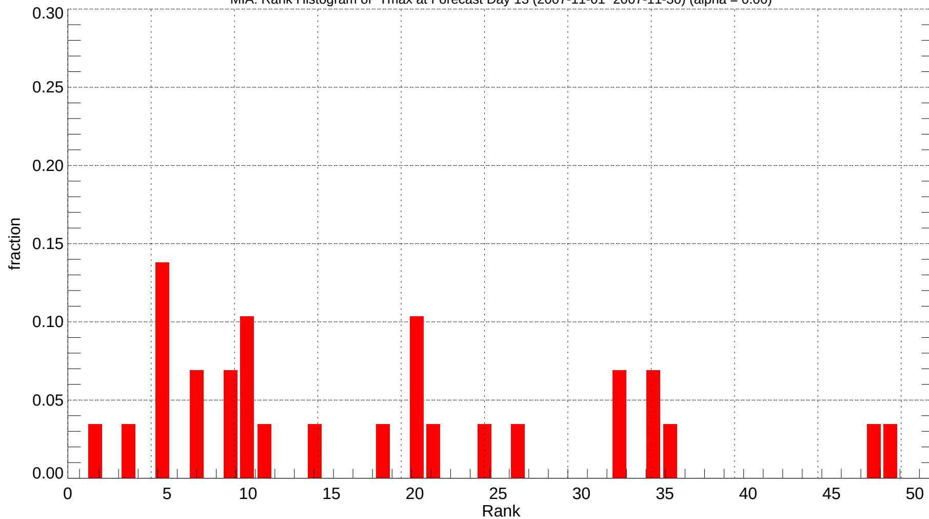
MIA: Rank Histogram of Tmax at Forecast Day 13 (2007-11-01~2007-11-30) (alpha = 0.00)
