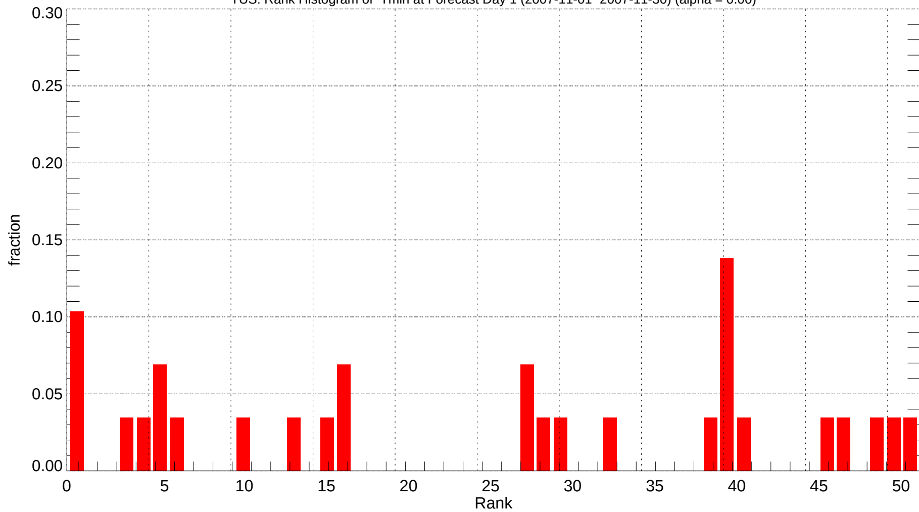
TUS: Rank Histogram of Tmin at Forecast Day 1 (2007-11-01~2007-11-30) (alpha = 0.00)
