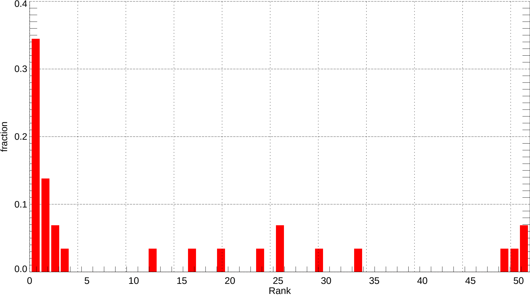
STL: Rank Histogram of Tmin at Forecast Day 1 (2007-11-01~2007-11-30) (alpha = 0.00)
