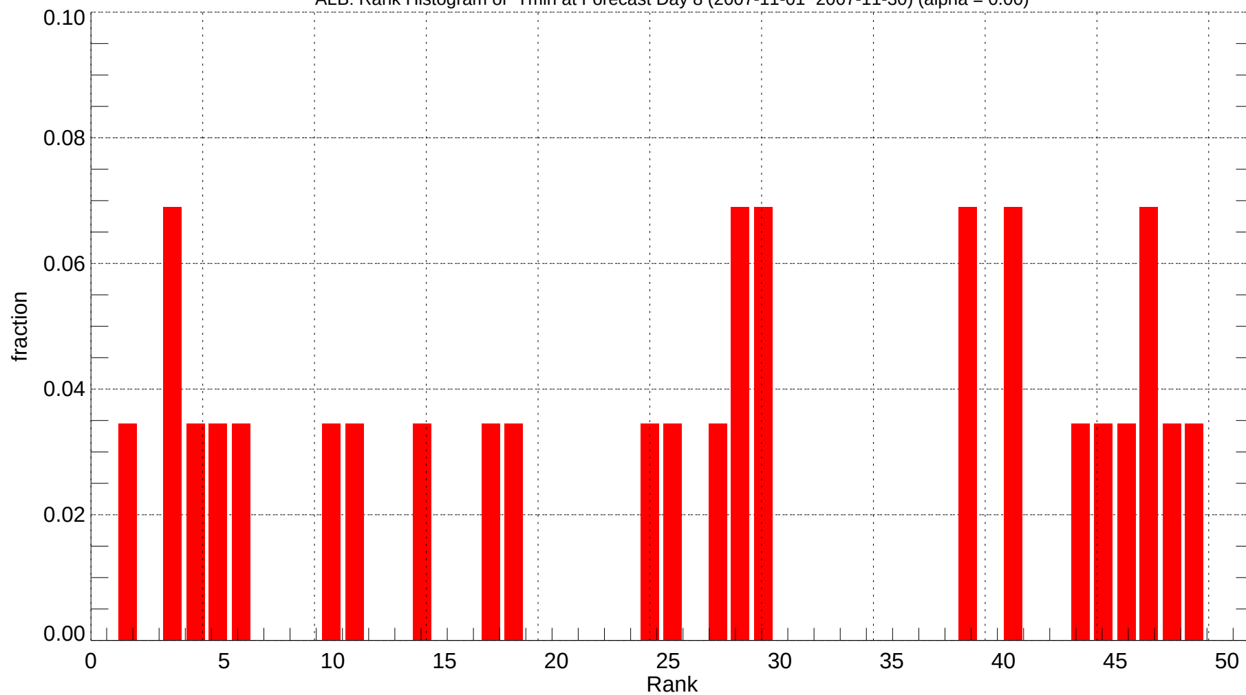
ALB: Rank Histogram of Tmin at Forecast Day 8 (2007-11-01~2007-11-30) (alpha = 0.00)
