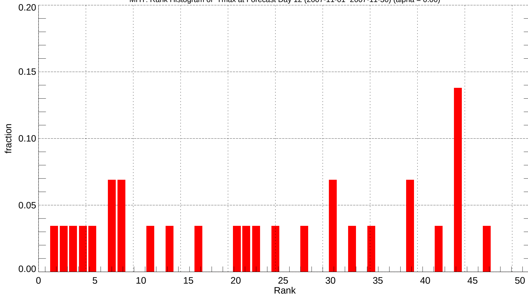
MHT: Rank Histogram of Tmax at Forecast Day 12 (2007-11-01~2007-11-30) (alpha = 0.00)
