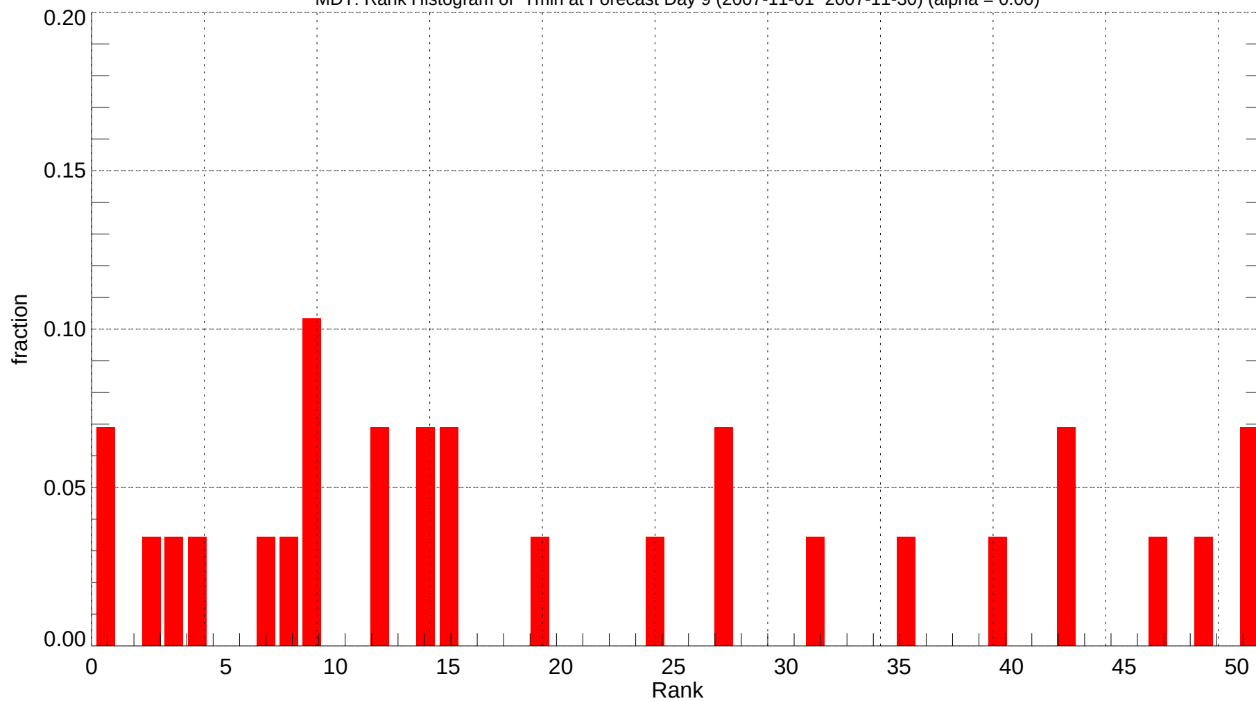
MDT: Rank Histogram of Tmin at Forecast Day 9 (2007-11-01~2007-11-30) (alpha = 0.00)
