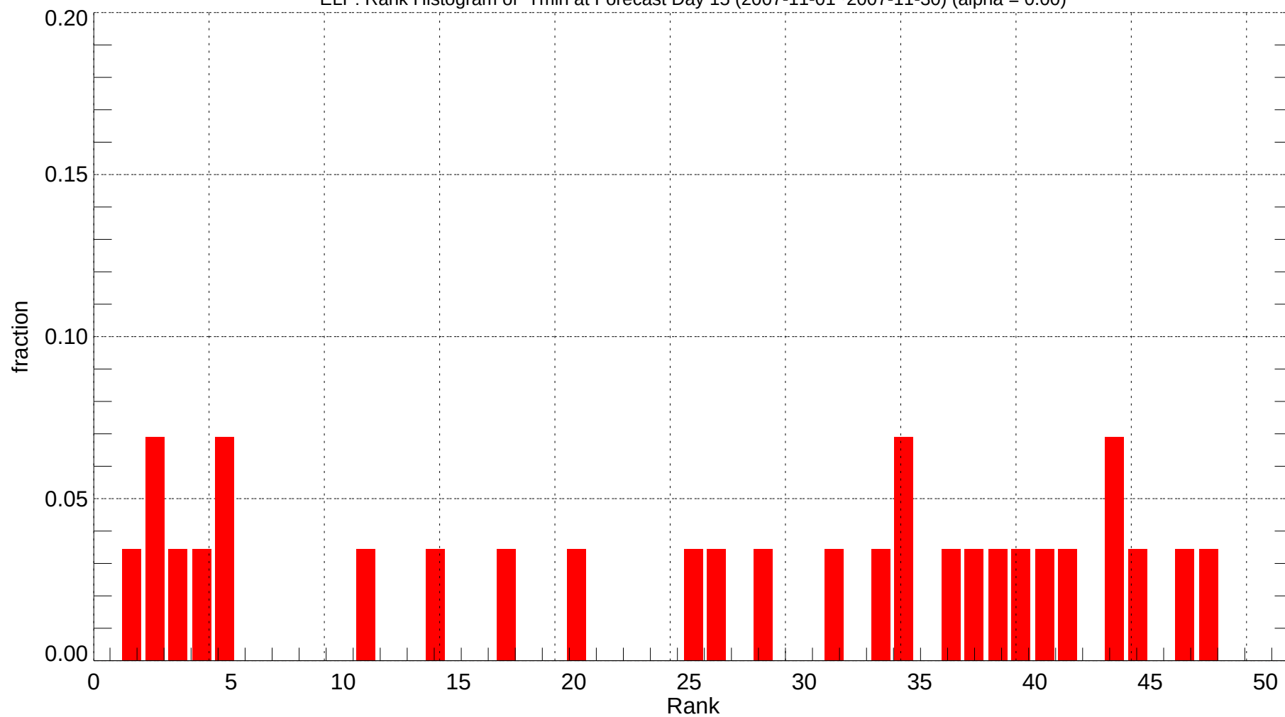
ELP: Rank Histogram of Tmin at Forecast Day 15 (2007-11-01~2007-11-30) (alpha = 0.00)
