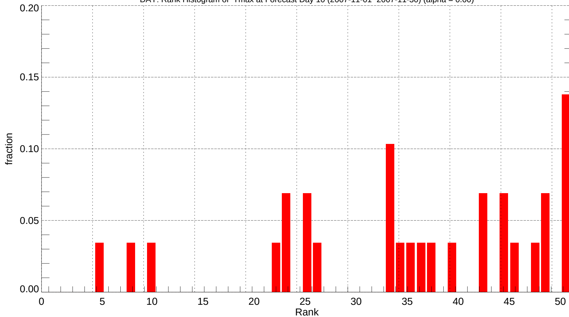
DAY: Rank Histogram of Tmax at Forecast Day 10 (2007-11-01~2007-11-30) (alpha = 0.00)
