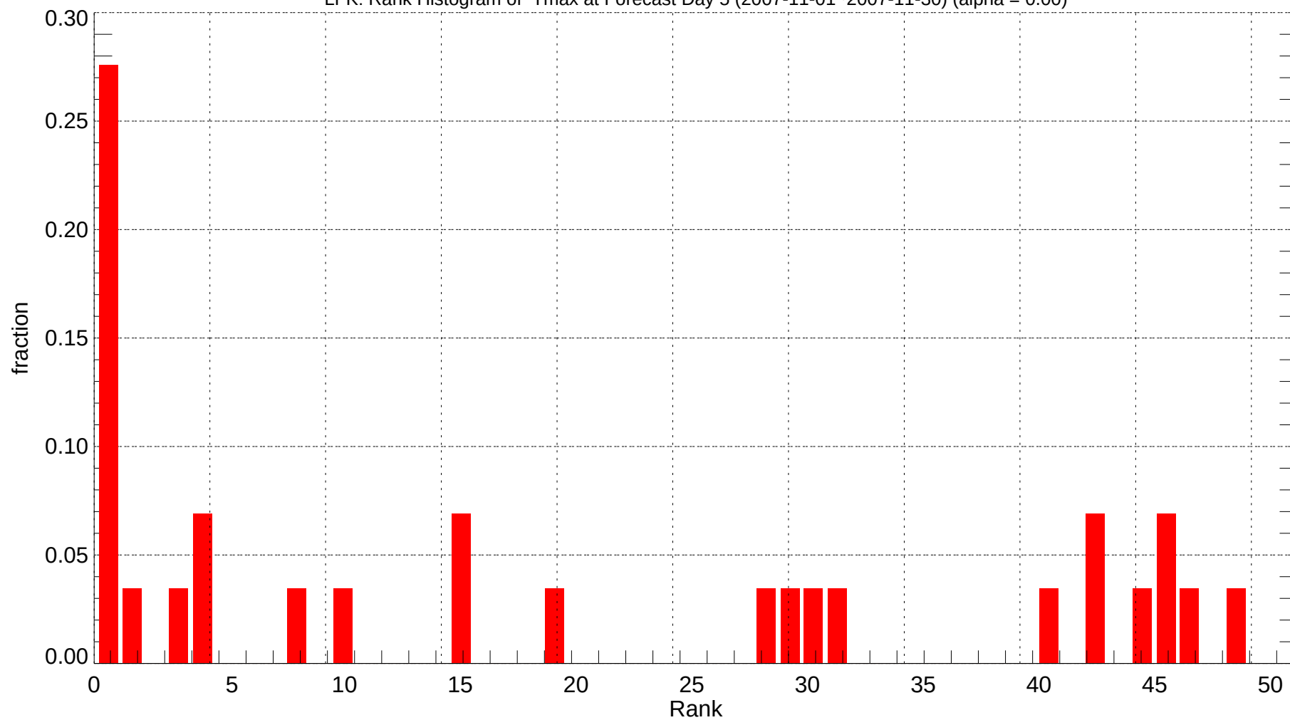
LFK: Rank Histogram of Tmax at Forecast Day 5 (2007-11-01~2007-11-30) (alpha = 0.00)
