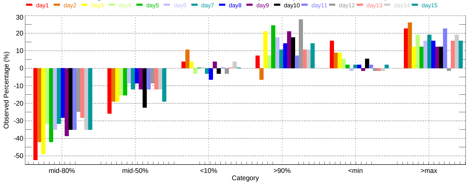
Observed Percentage Deviation of Ensembles - DEN: Min Temperature (2007-11-01~2007-11-30)
