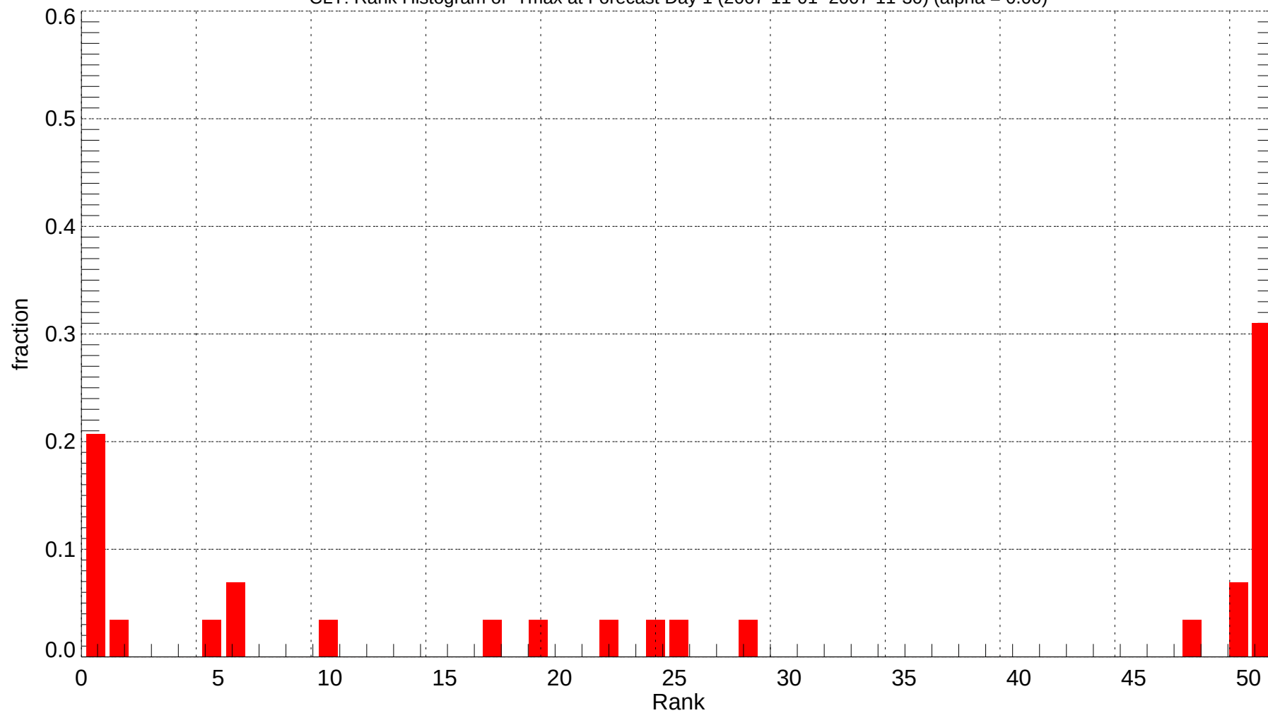
CLT: Rank Histogram of Tmax at Forecast Day 1 (2007-11-01~2007-11-30) (alpha = 0.00)
