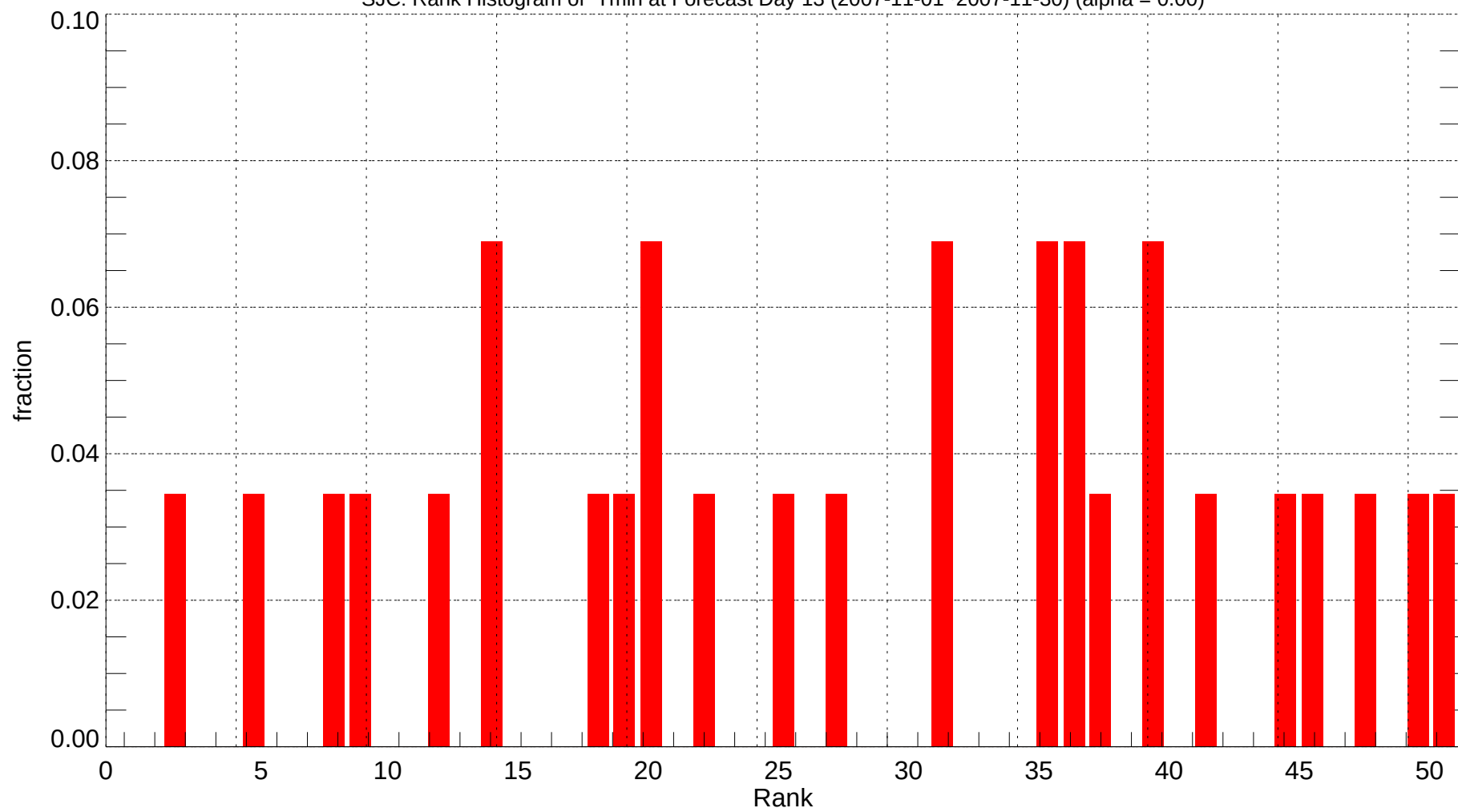
SJC: Rank Histogram of Tmin at Forecast Day 13 (2007-11-01~2007-11-30) (alpha = 0.00)
