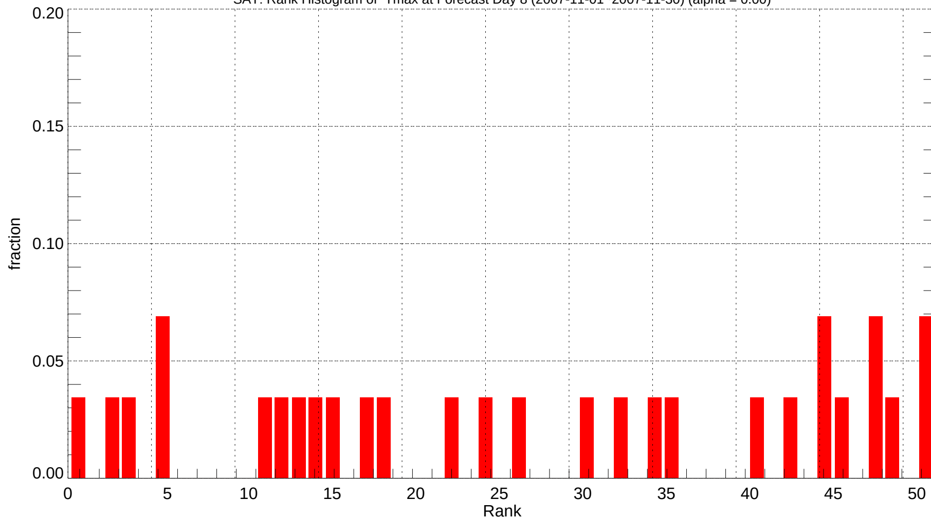
SAT: Rank Histogram of Tmax at Forecast Day 8 (2007-11-01~2007-11-30) (alpha = 0.00)
