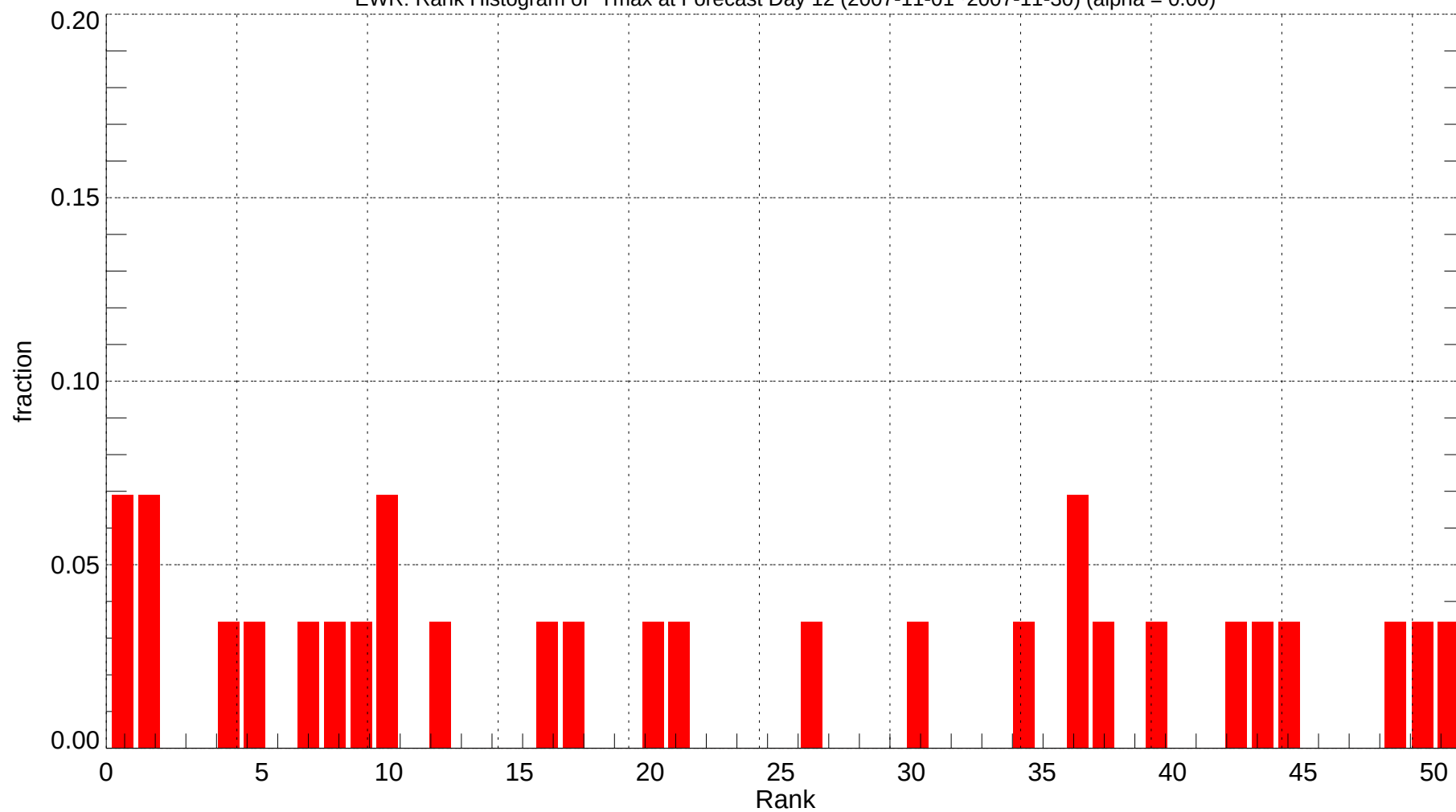
EWR: Rank Histogram of Tmax at Forecast Day 12 (2007-11-01~2007-11-30) (alpha = 0.00)
