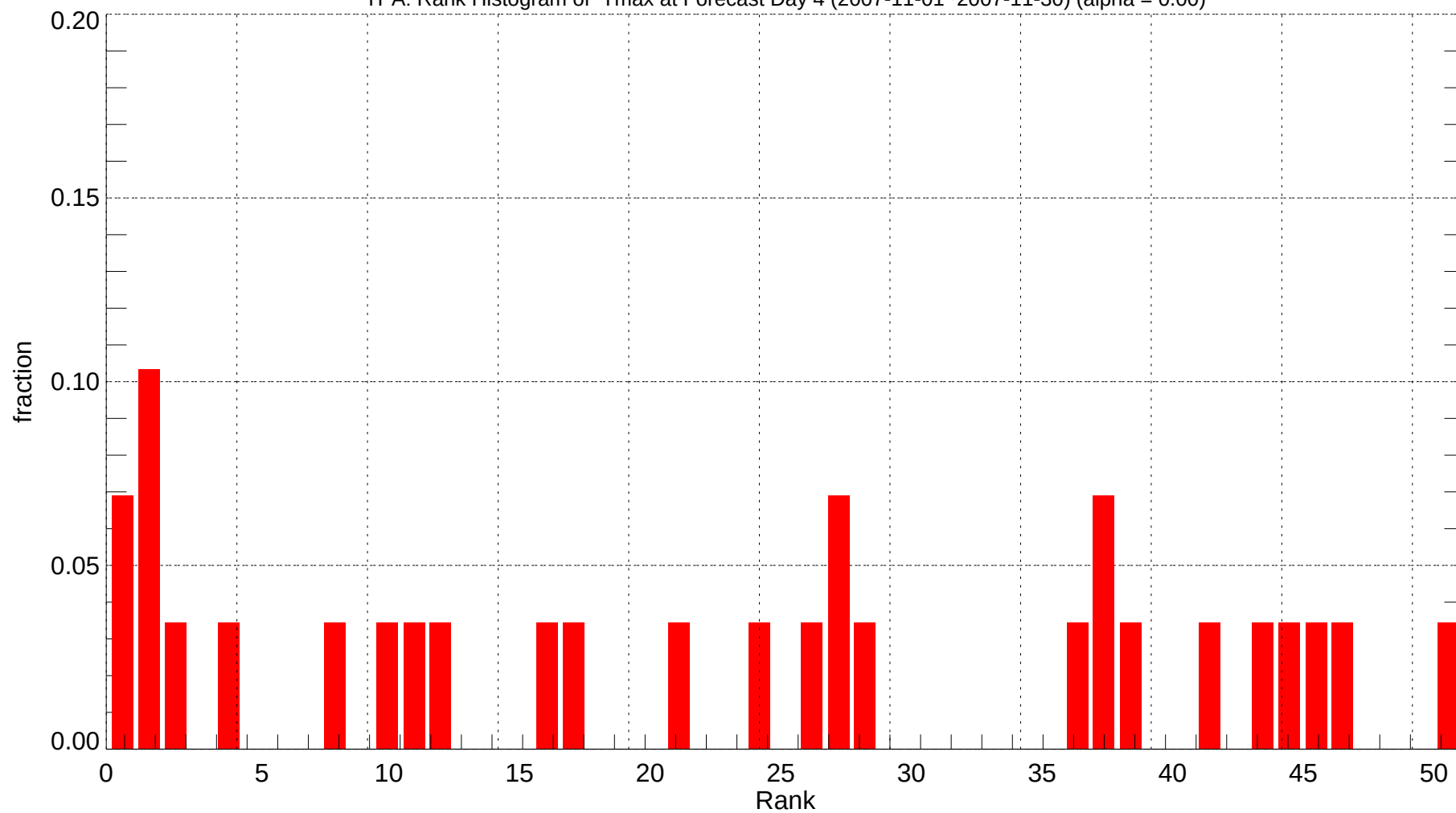
TPA: Rank Histogram of Tmax at Forecast Day 4 (2007-11-01~2007-11-30) (alpha = 0.00)
