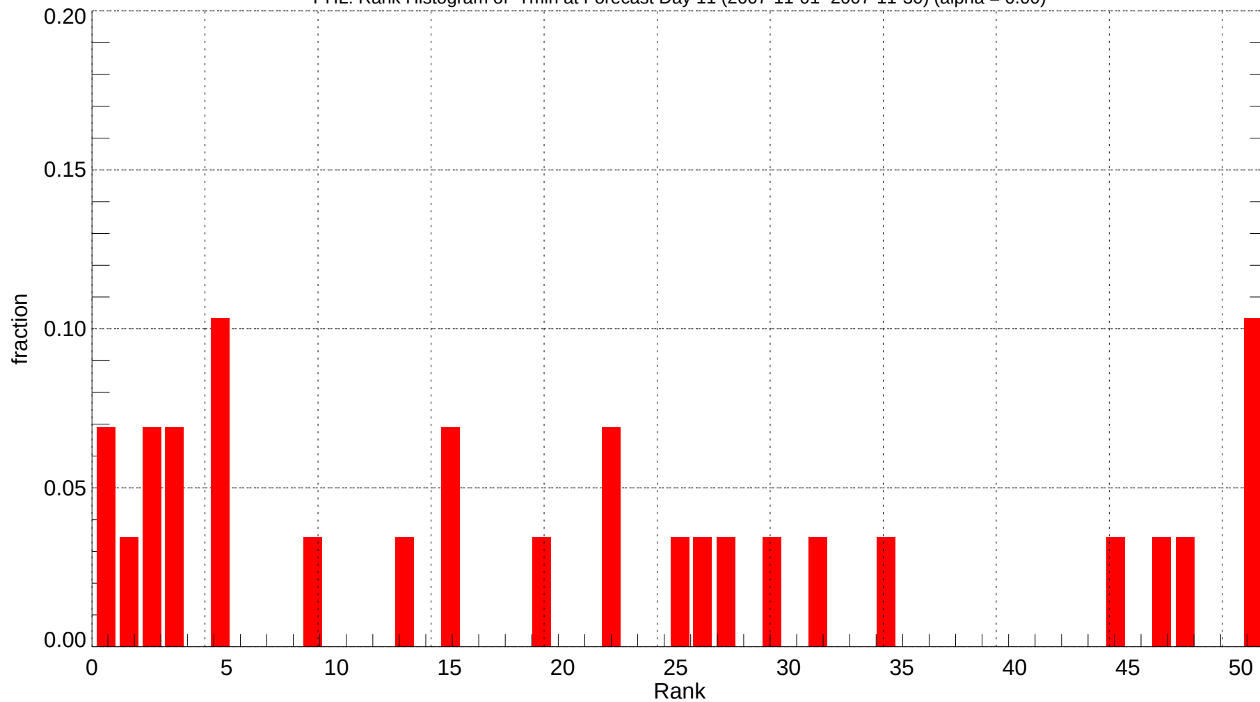
PHL: Rank Histogram of Tmin at Forecast Day 11 (2007-11-01~2007-11-30) (alpha = 0.00)
