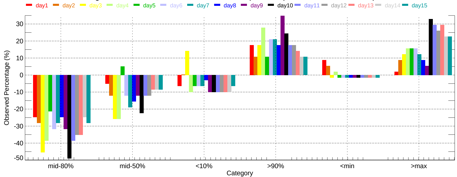
Observed Percentage Deviation of Ensembles - LIT: Max Temperature (2007-11-01~2007-11-30)
