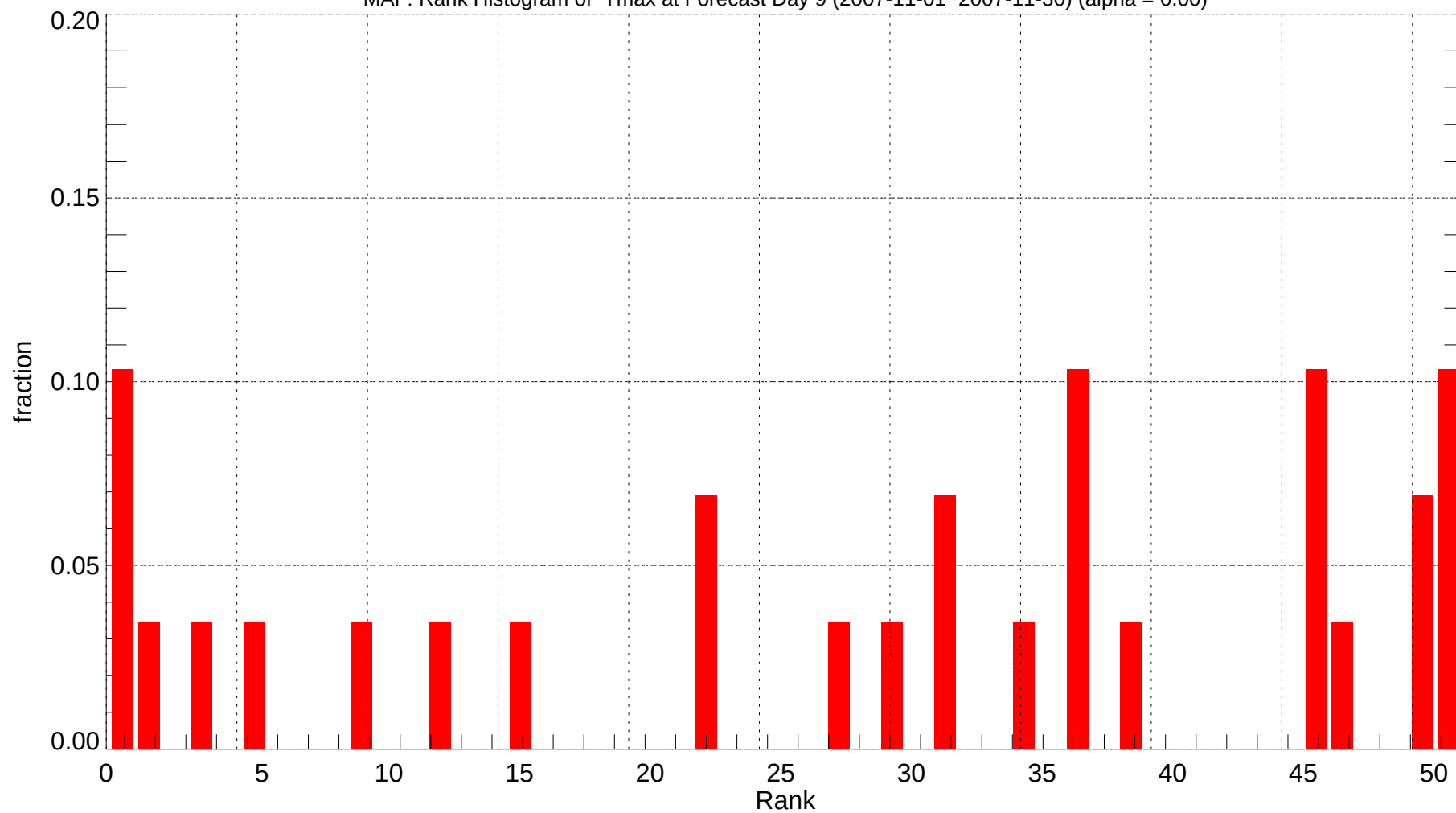
MAF: Rank Histogram of Tmax at Forecast Day 9 (2007-11-01~2007-11-30) (alpha = 0.00)
