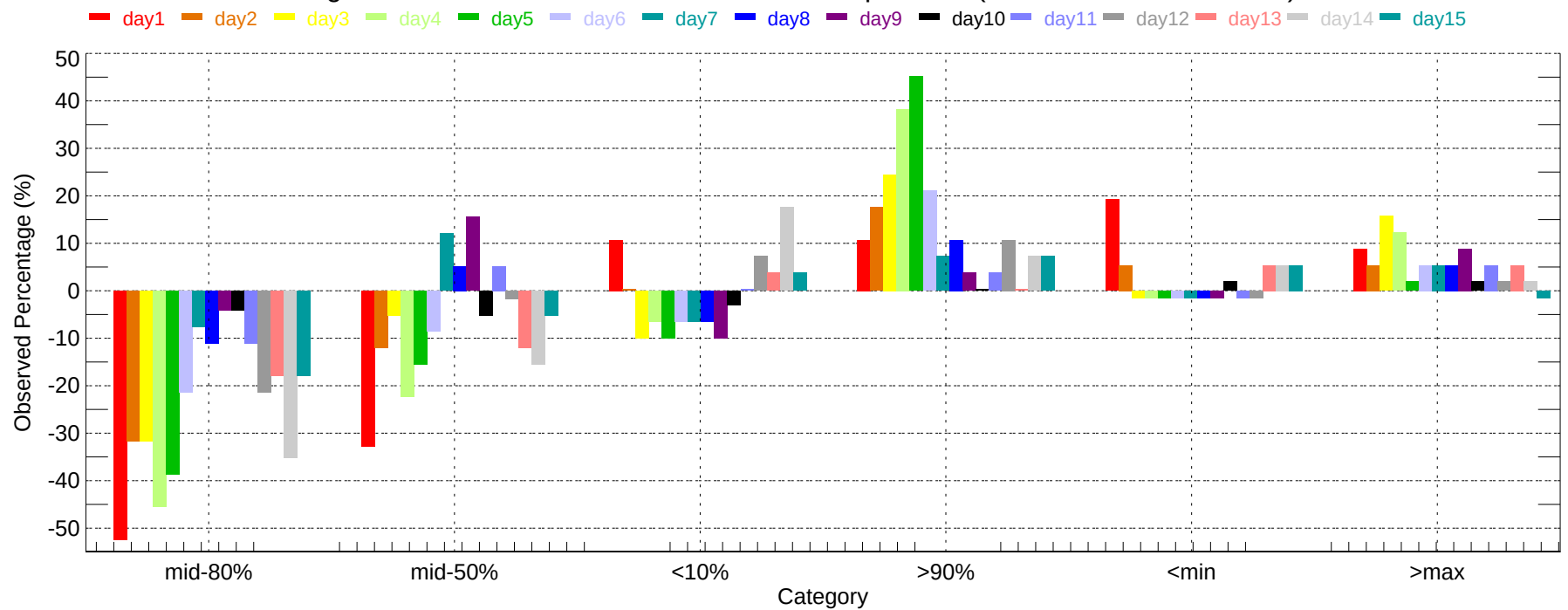
Observed Percentage Deviation of Ensembles - PVD: Min Temperature (2007-11-01~2007-11-30)
