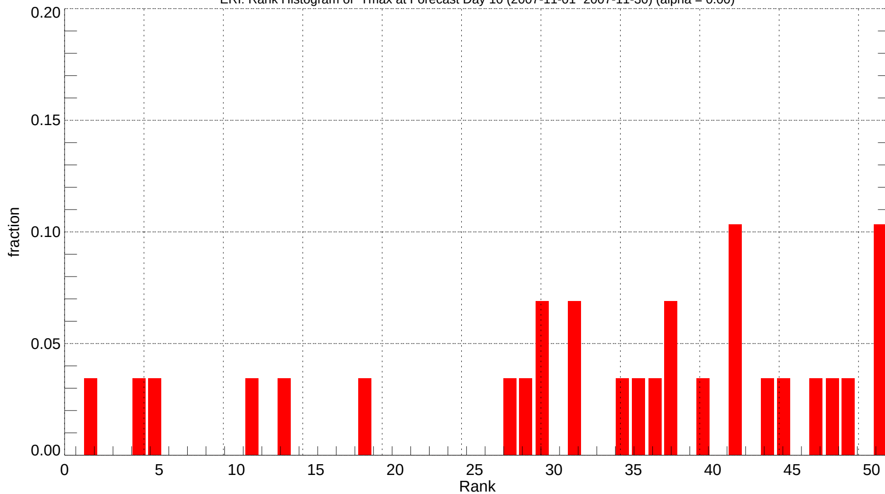
ERI: Rank Histogram of Tmax at Forecast Day 10 (2007-11-01~2007-11-30) (alpha = 0.00)
