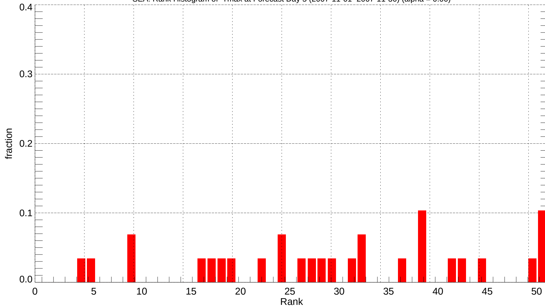
SEA: Rank Histogram of Tmax at Forecast Day 5 (2007-11-01~2007-11-30) (alpha = 0.00)
