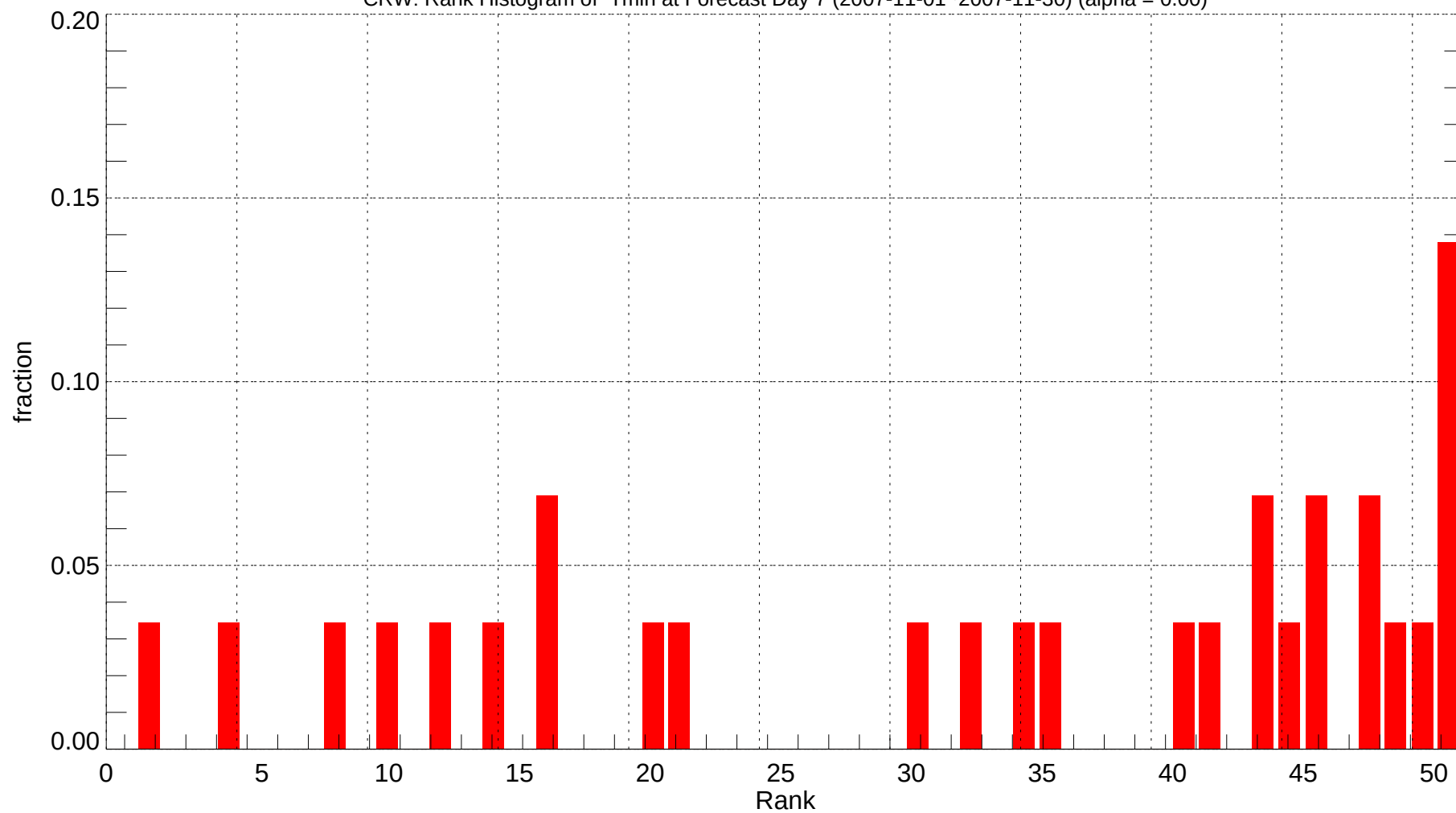
CRW: Rank Histogram of Tmin at Forecast Day 7 (2007-11-01~2007-11-30) (alpha = 0.00)
