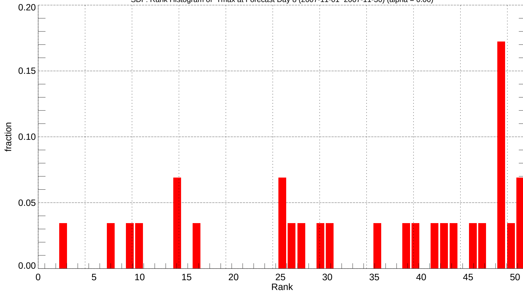
SDF: Rank Histogram of Tmax at Forecast Day 8 (2007-11-01~2007-11-30) (alpha = 0.00)
