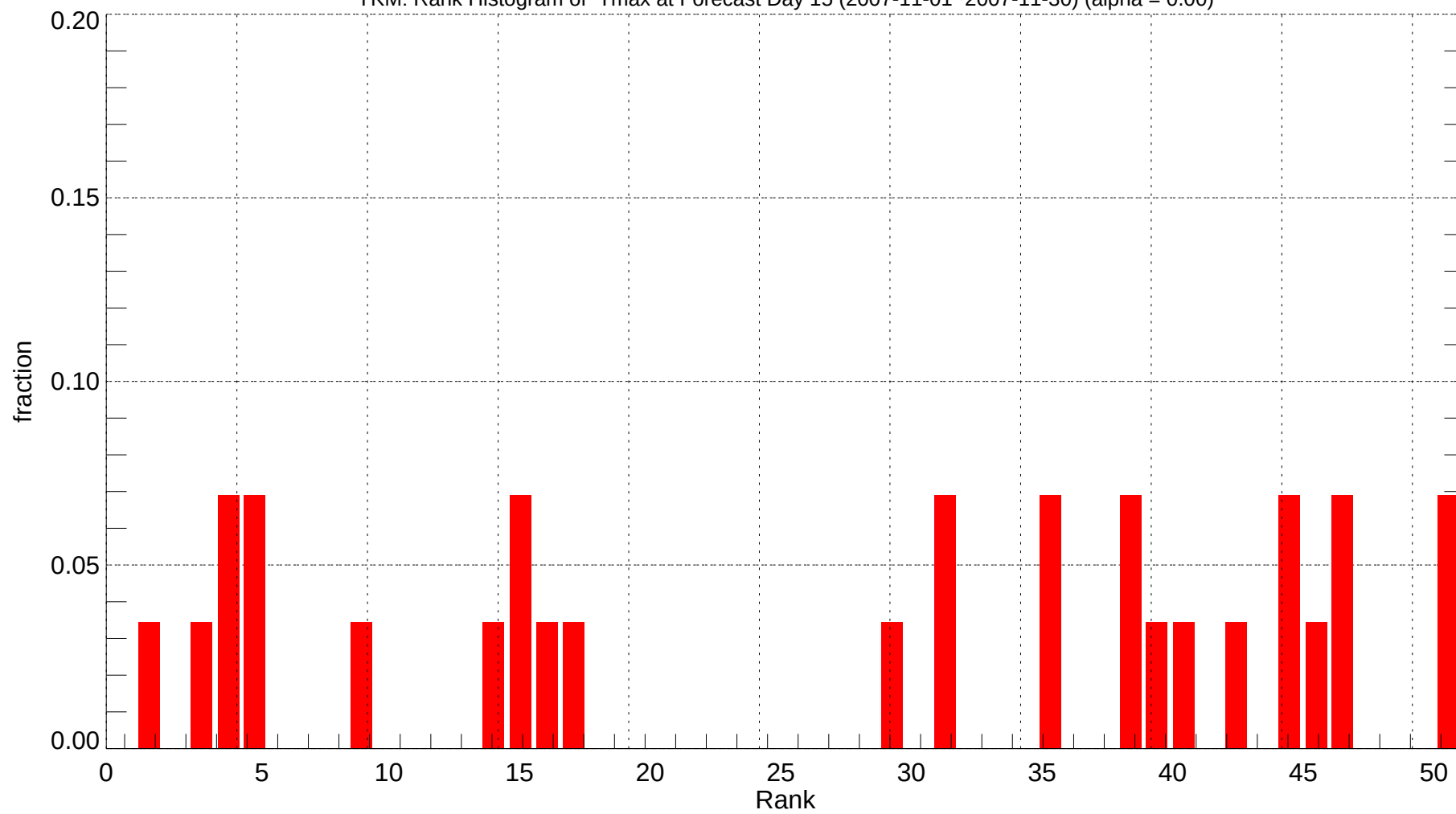
YKM: Rank Histogram of Tmax at Forecast Day 15 (2007-11-01~2007-11-30) (alpha = 0.00)
