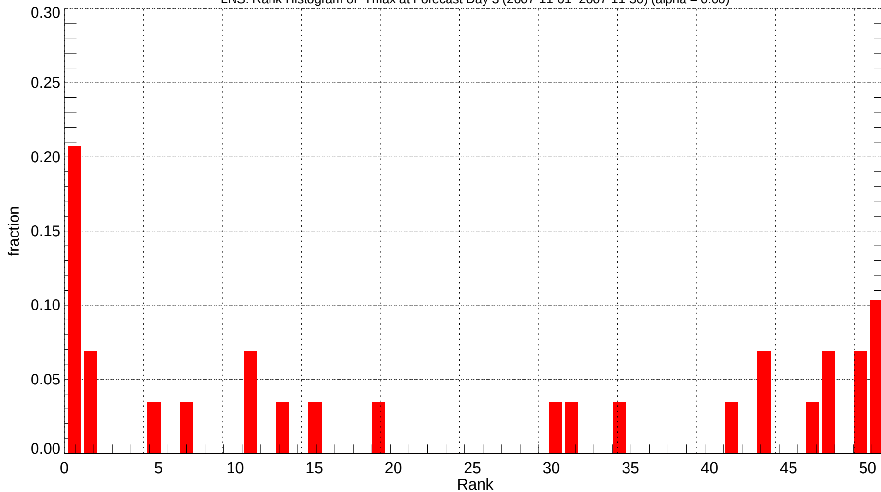
LNS: Rank Histogram of Tmax at Forecast Day 3 (2007-11-01~2007-11-30) (alpha = 0.00)
