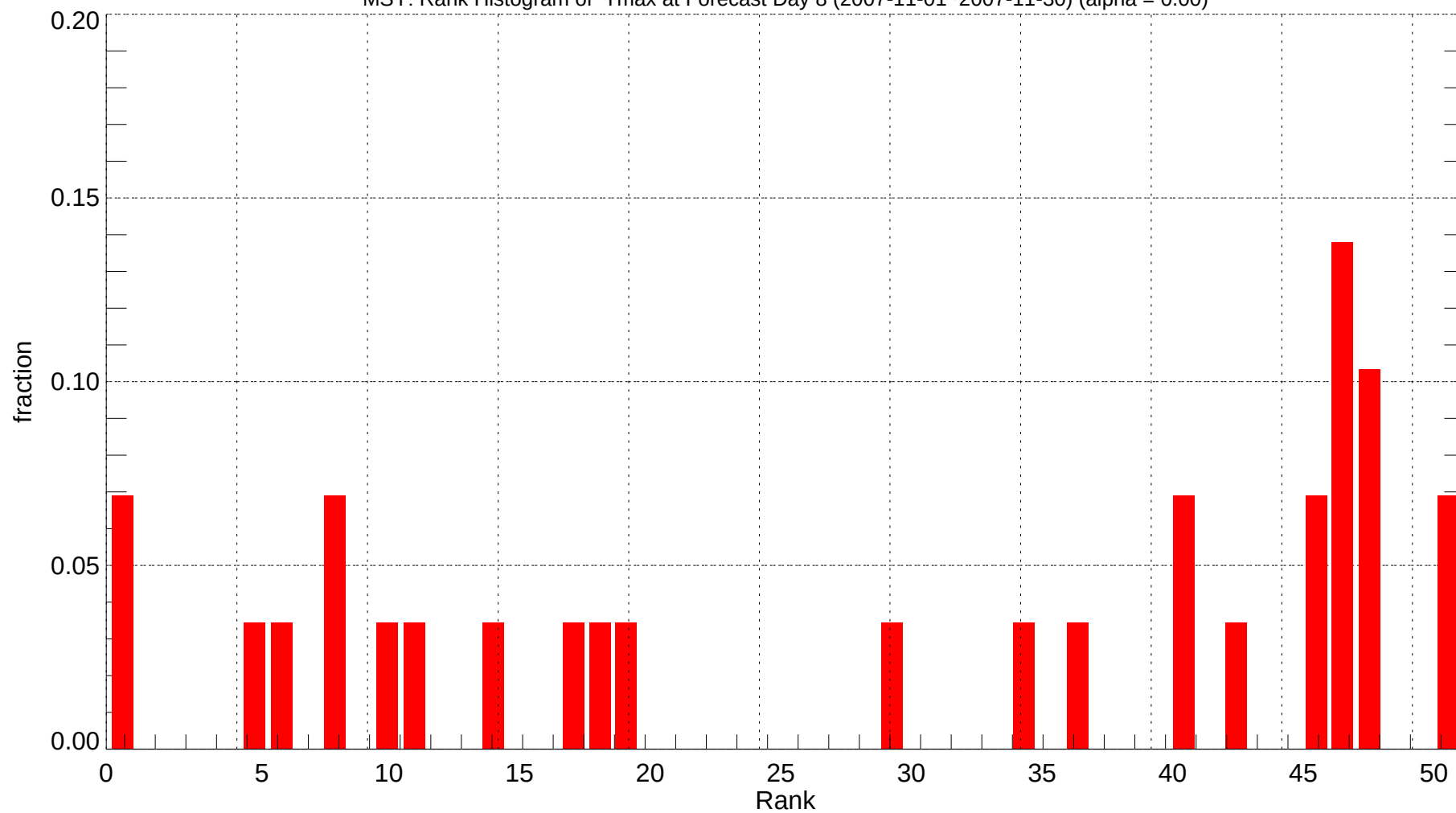
MSY: Rank Histogram of Tmax at Forecast Day 8 (2007-11-01~2007-11-30) (alpha = 0.00)
