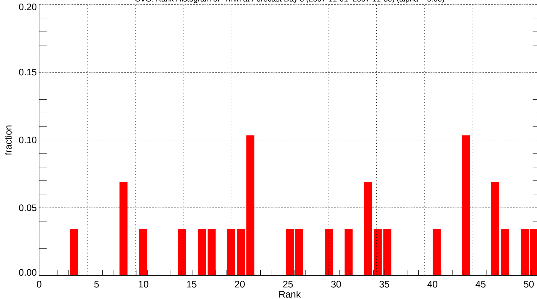
CVG: Rank Histogram of Tmin at Forecast Day 6 (2007-11-01~2007-11-30) (alpha = 0.00)
