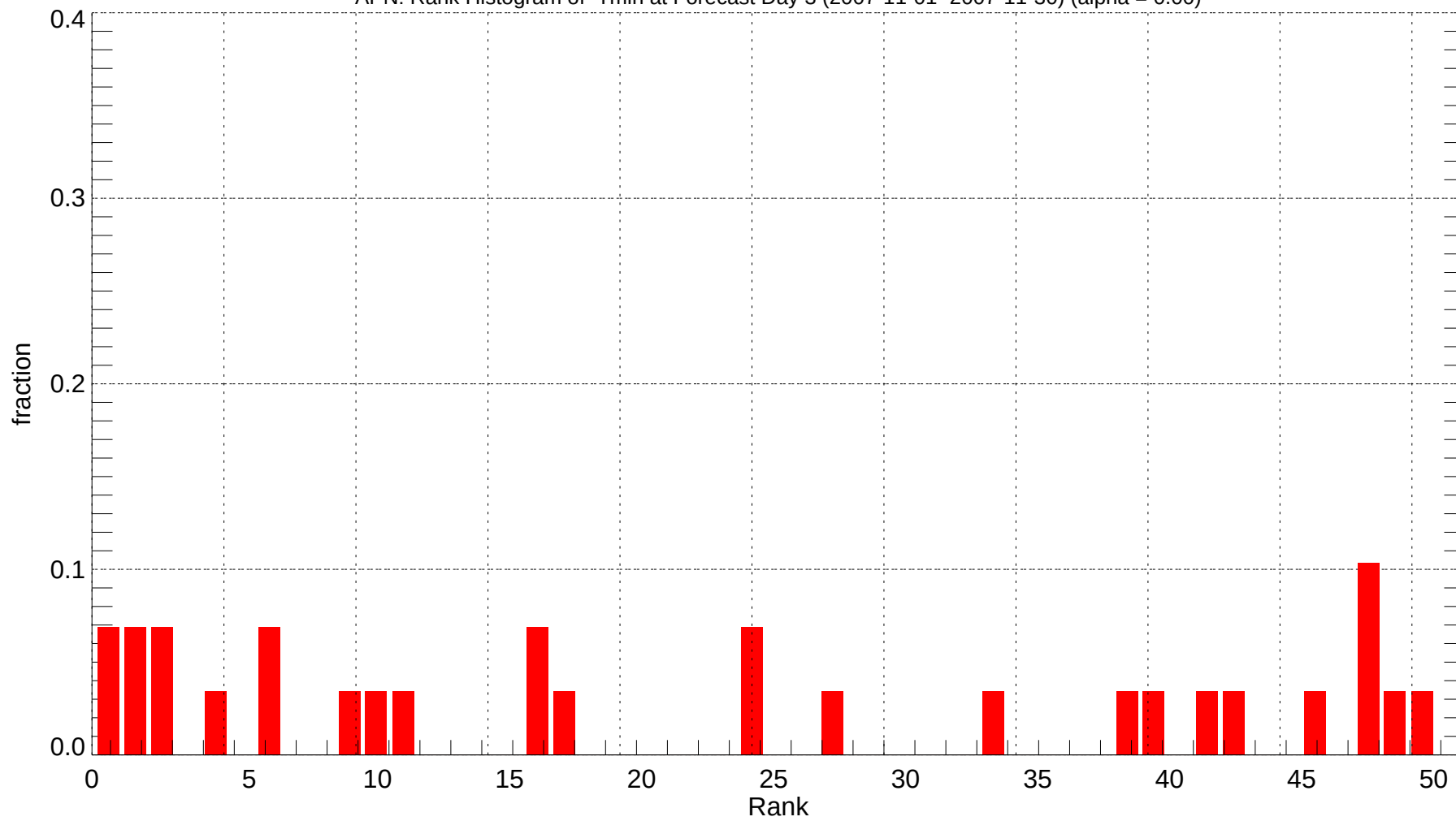
APN: Rank Histogram of Tmin at Forecast Day 3 (2007-11-01~2007-11-30) (alpha = 0.00)
