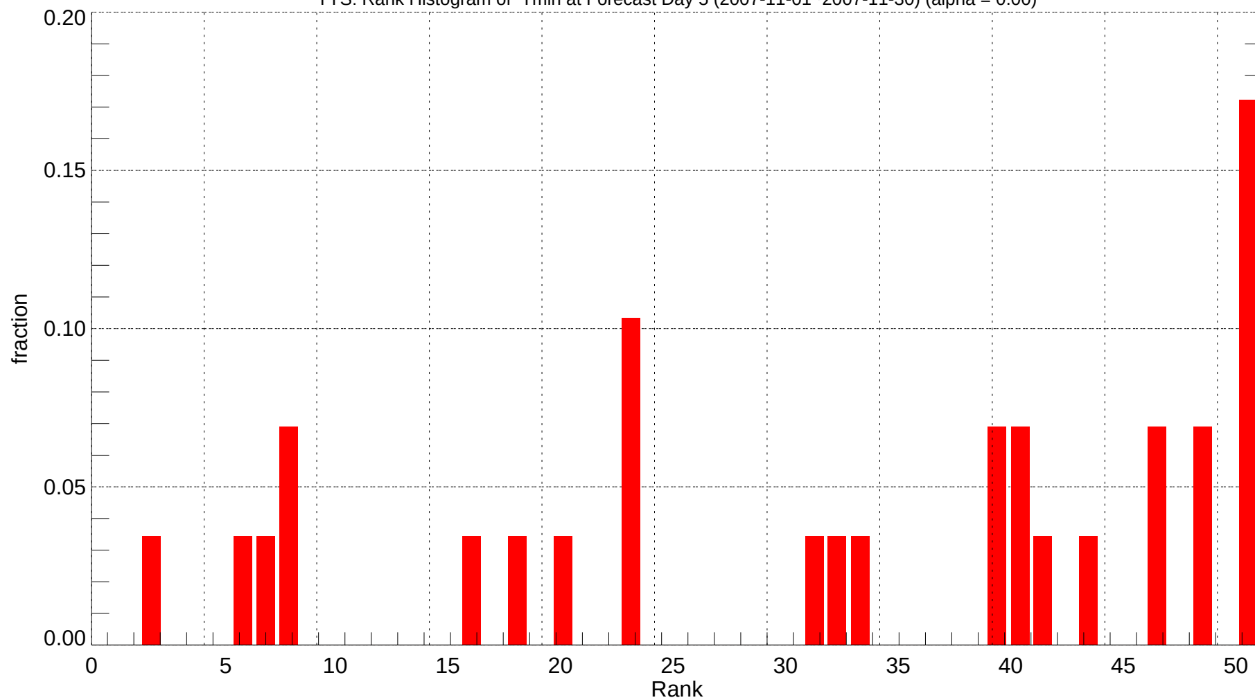
TYS: Rank Histogram of Tmin at Forecast Day 5 (2007-11-01~2007-11-30) (alpha = 0.00)
