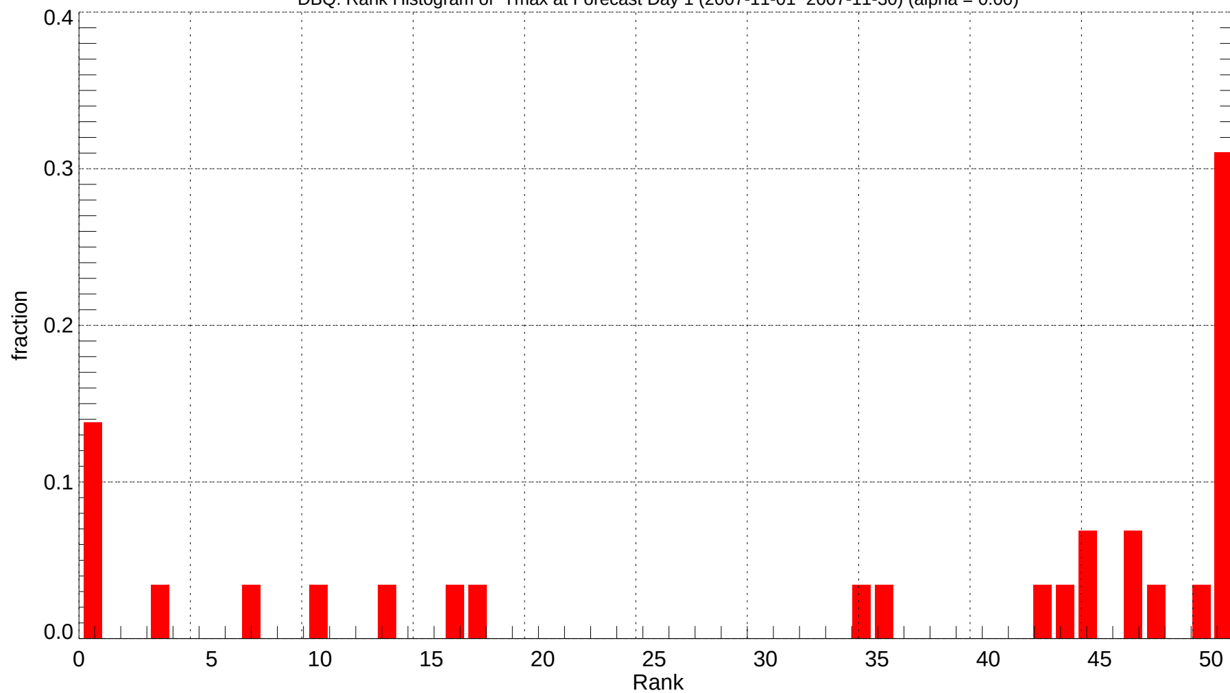
DBQ: Rank Histogram of Tmax at Forecast Day 1 (2007-11-01~2007-11-30) (alpha = 0.00)
