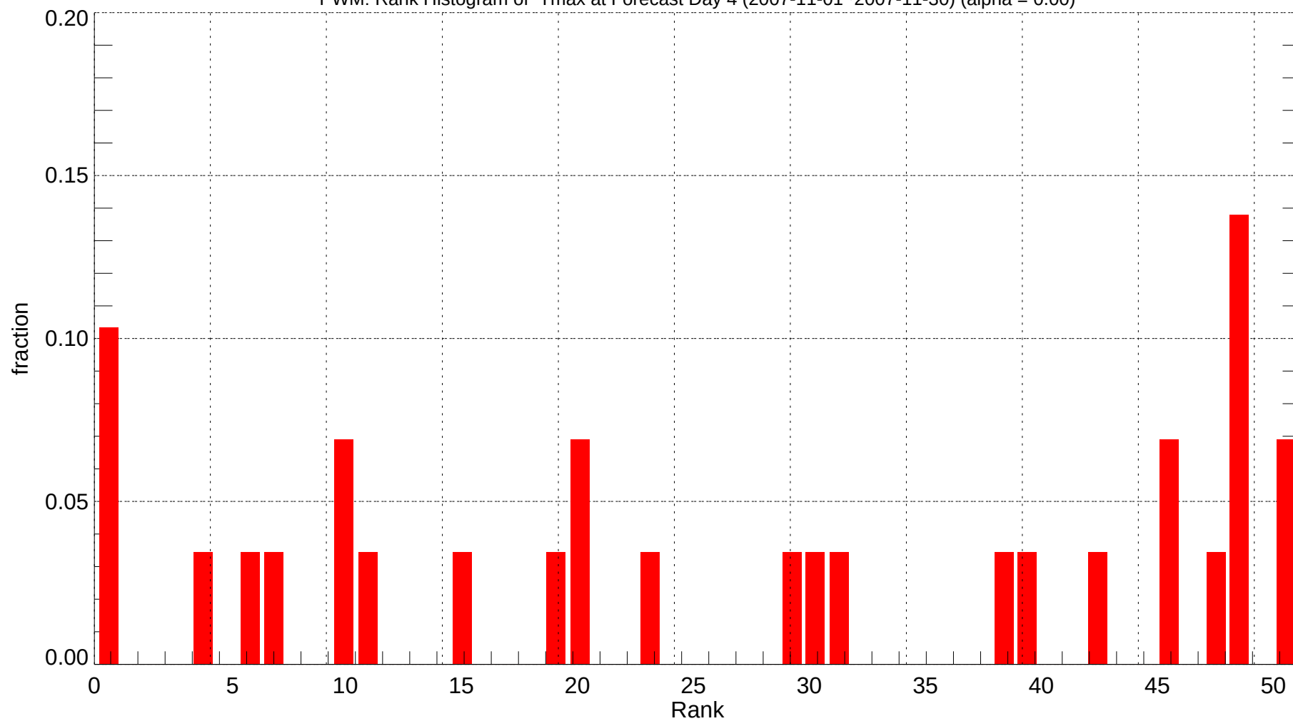
PWM: Rank Histogram of Tmax at Forecast Day 4 (2007-11-01~2007-11-30) (alpha = 0.00)
