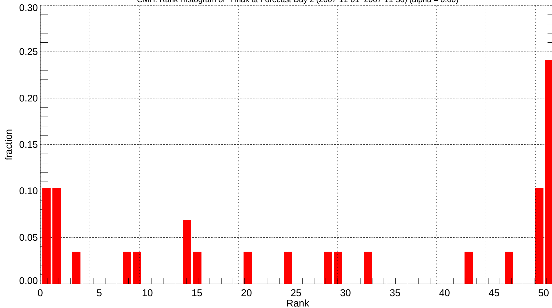
CMH: Rank Histogram of Tmax at Forecast Day 2 (2007-11-01~2007-11-30) (alpha = 0.00)
