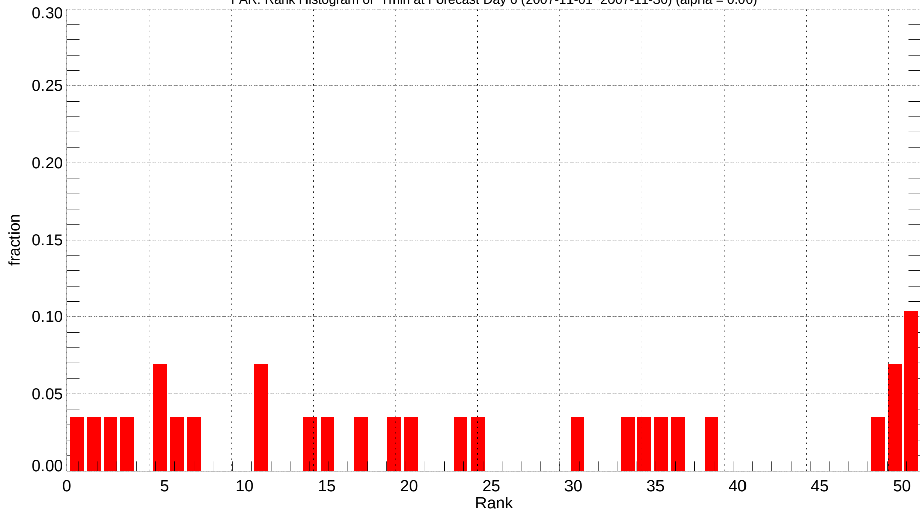
FAR: Rank Histogram of Tmin at Forecast Day 6 (2007-11-01~2007-11-30) (alpha = 0.00)
