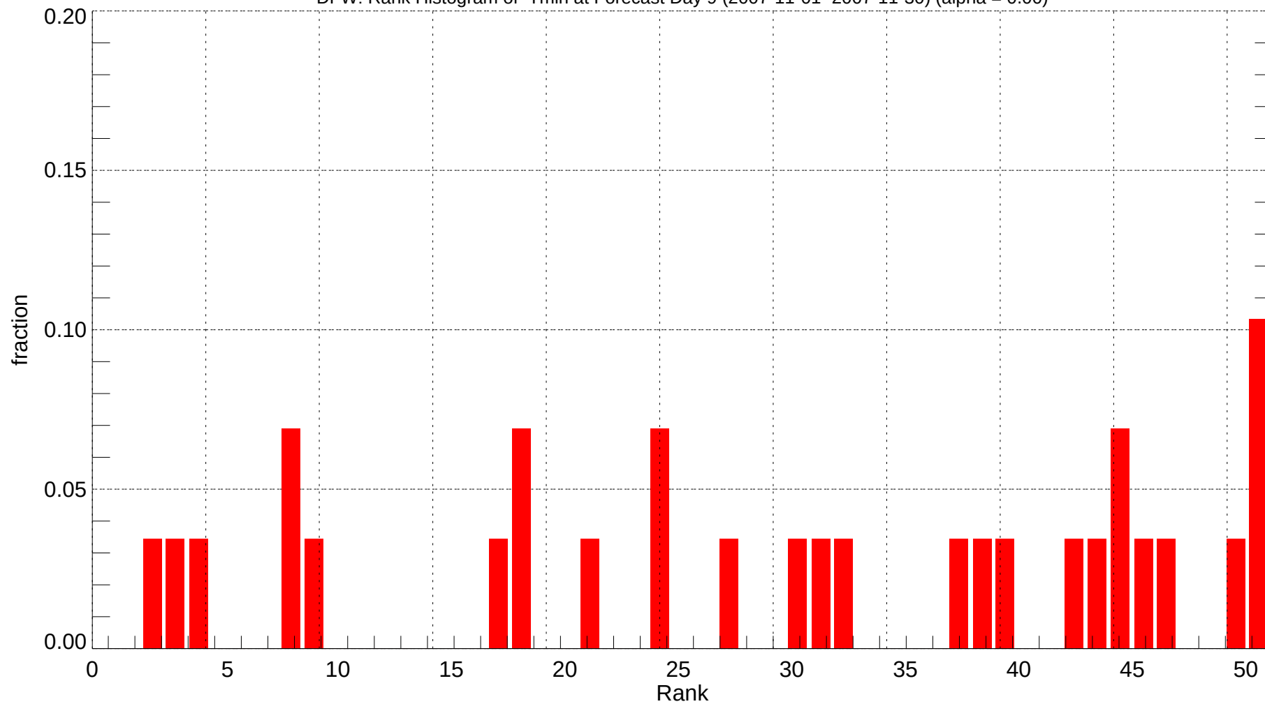
DFW: Rank Histogram of Tmin at Forecast Day 9 (2007-11-01~2007-11-30) (alpha = 0.00)
