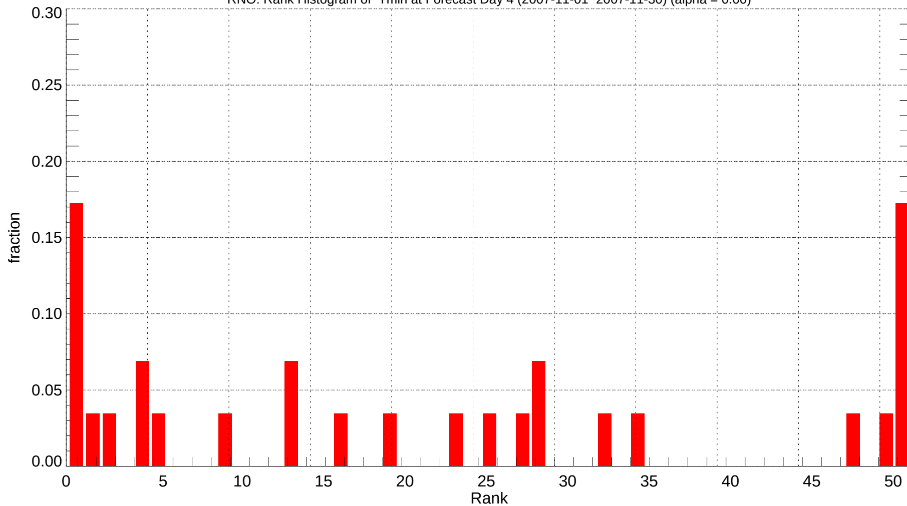
RNO: Rank Histogram of Tmin at Forecast Day 4 (2007-11-01~2007-11-30) (alpha = 0.00)
