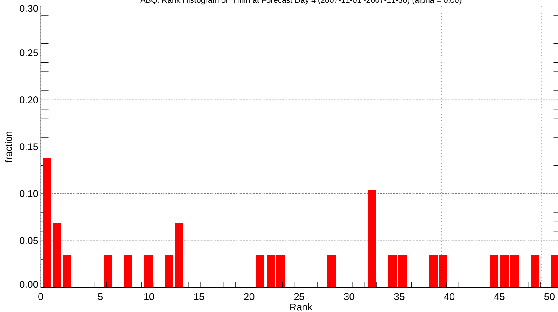
ABQ: Rank Histogram of Tmin at Forecast Day 4 (2007-11-01~2007-11-30) (alpha = 0.00)
