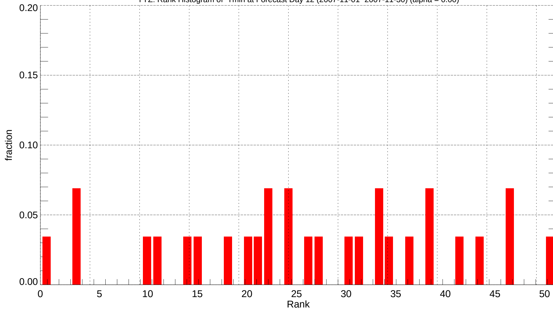
YYZ: Rank Histogram of Tmin at Forecast Day 12 (2007-11-01~2007-11-30) (alpha = 0.00)
