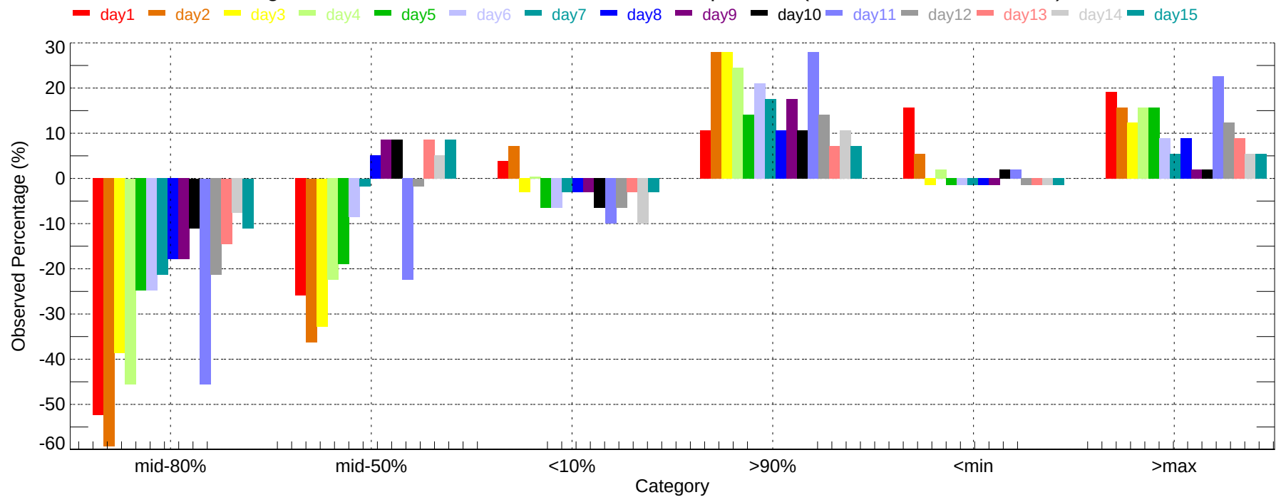
Observed Percentage Deviation of Ensembles - TYS: Max Temperature (2007-11-01~2007-11-30)
