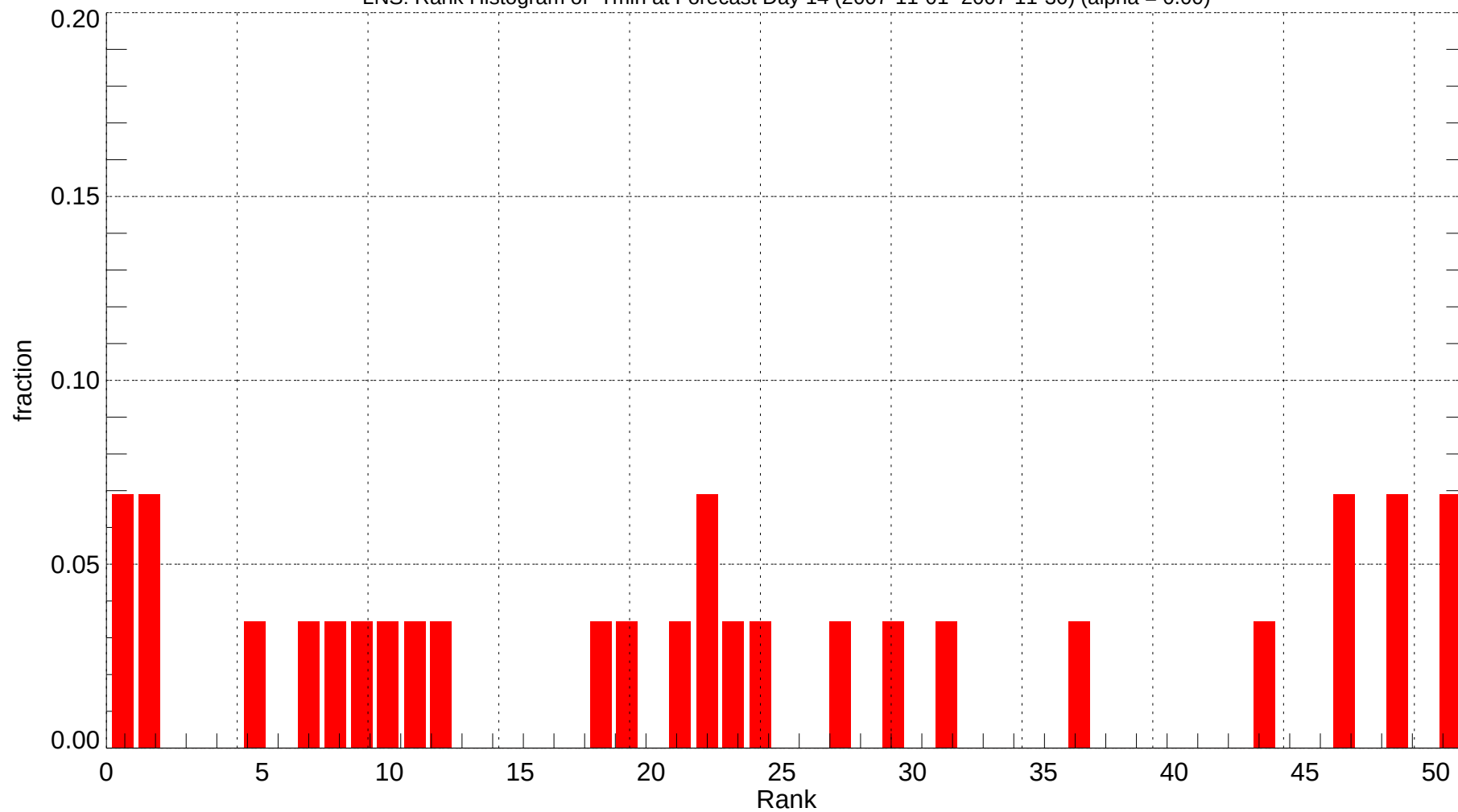
LNS: Rank Histogram of Tmin at Forecast Day 14 (2007-11-01~2007-11-30) (alpha = 0.00)
