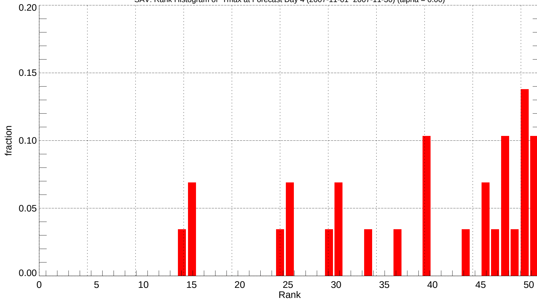
SAV: Rank Histogram of Tmax at Forecast Day 4 (2007-11-01~2007-11-30) (alpha = 0.00)
