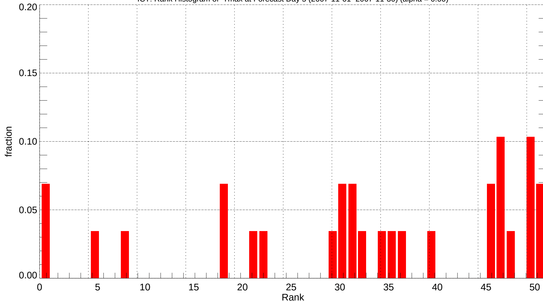
ICT: Rank Histogram of Tmax at Forecast Day 5 (2007-11-01~2007-11-30) (alpha = 0.00)
