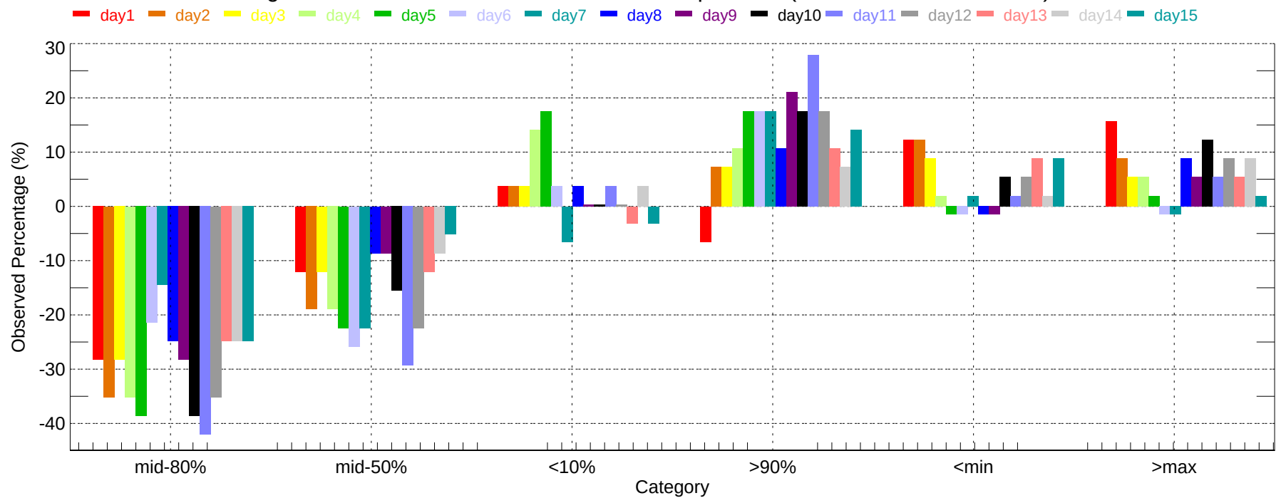
Observed Percentage Deviation of Ensembles - IAH: Min Temperature (2007-11-01~2007-11-30)
