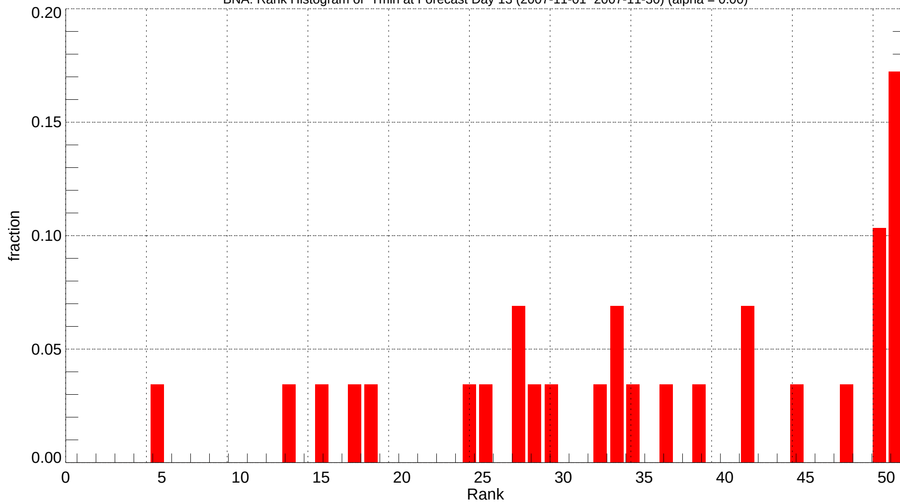
BNA: Rank Histogram of Tmin at Forecast Day 13 (2007-11-01~2007-11-30) (alpha = 0.00)
