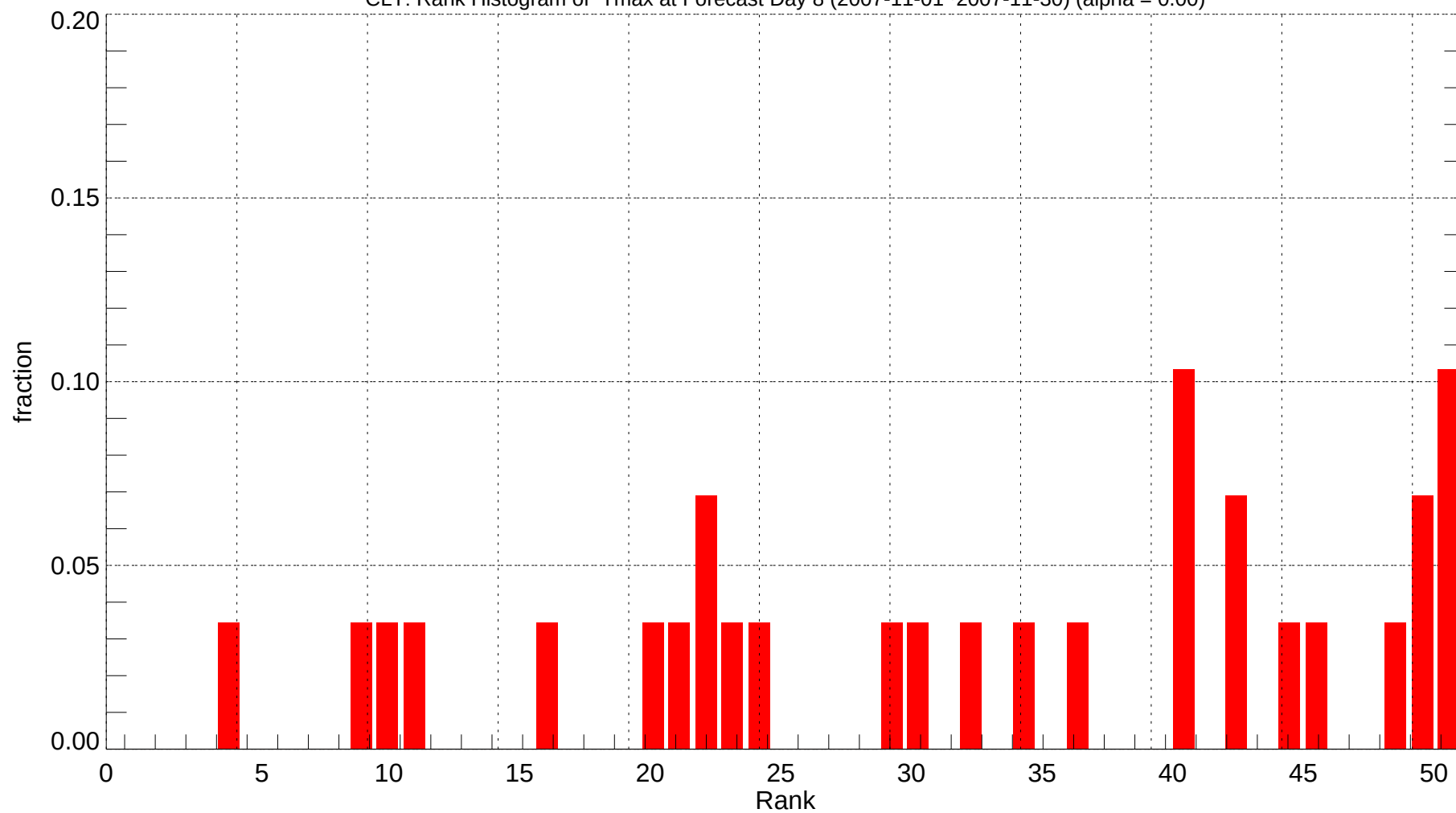
CLT: Rank Histogram of Tmax at Forecast Day 8 (2007-11-01~2007-11-30) (alpha = 0.00)
