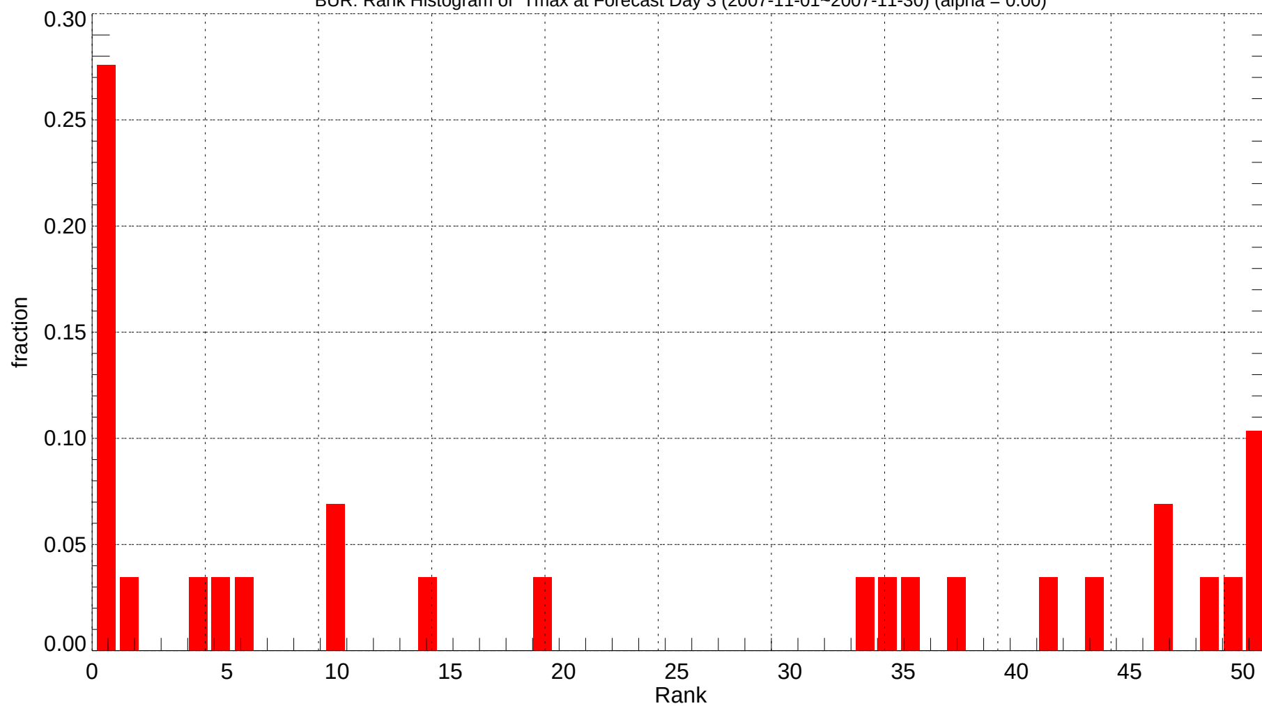
BUR: Rank Histogram of Tmax at Forecast Day 3 (2007-11-01~2007-11-30) (alpha = 0.00)
