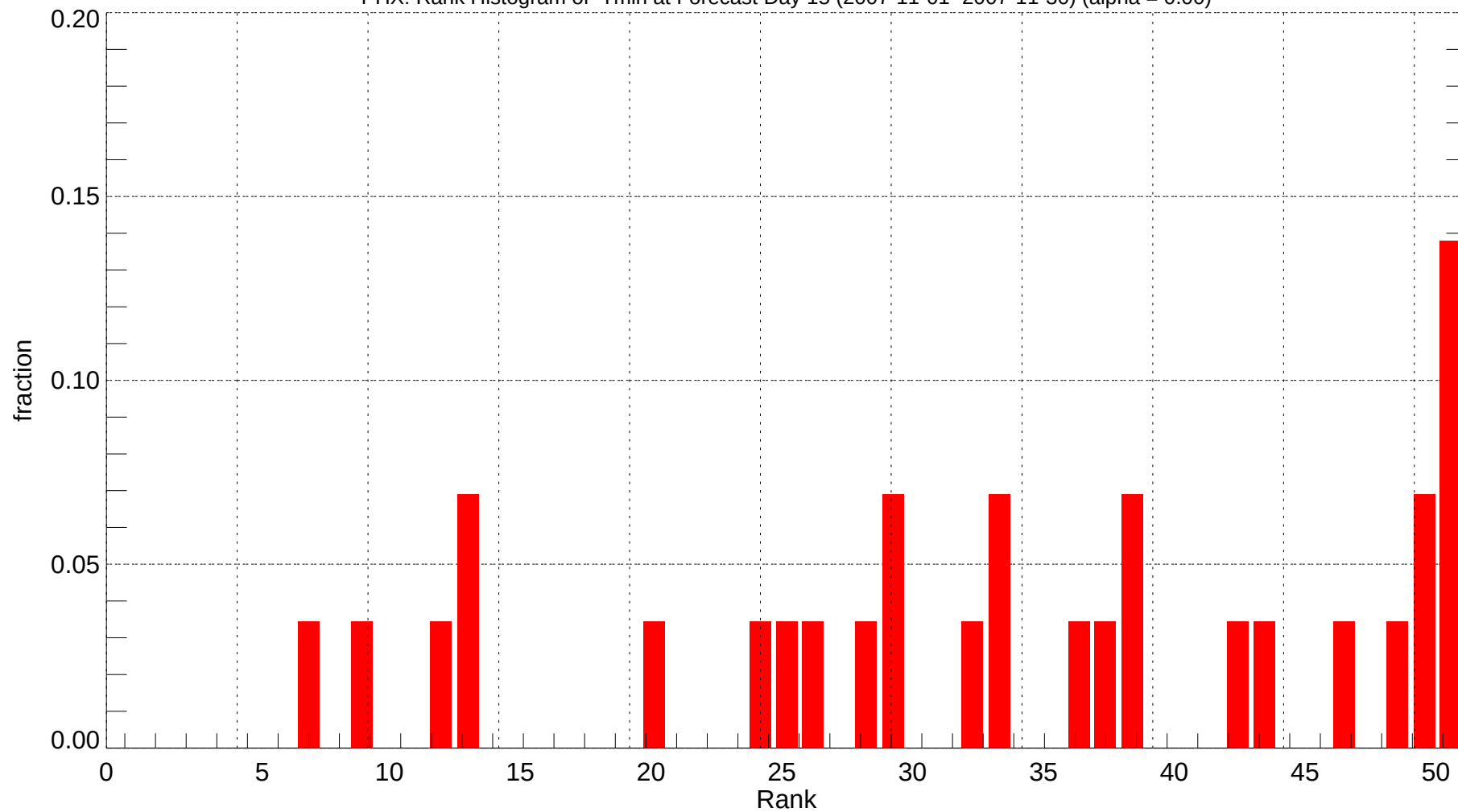
PHX: Rank Histogram of Tmin at Forecast Day 15 (2007-11-01~2007-11-30) (alpha = 0.00)
