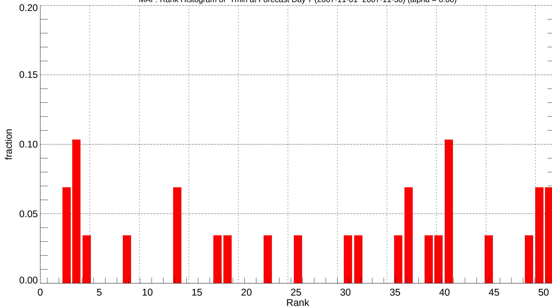
MAF: Rank Histogram of Tmin at Forecast Day 7 (2007-11-01~2007-11-30) (alpha = 0.00)
