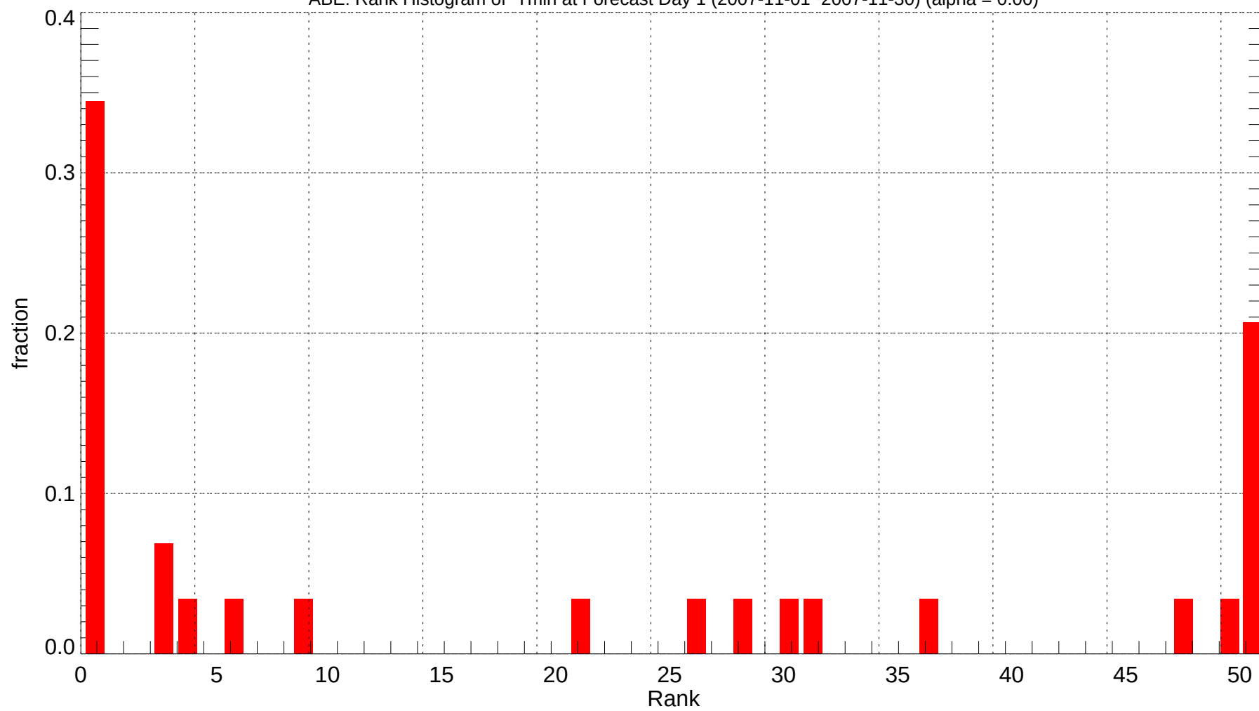
ABE: Rank Histogram of Tmin at Forecast Day 1 (2007-11-01~2007-11-30) (alpha = 0.00)
