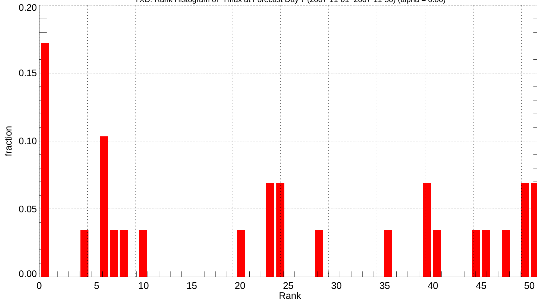
YXD: Rank Histogram of Tmax at Forecast Day 7 (2007-11-01~2007-11-30) (alpha = 0.00)
