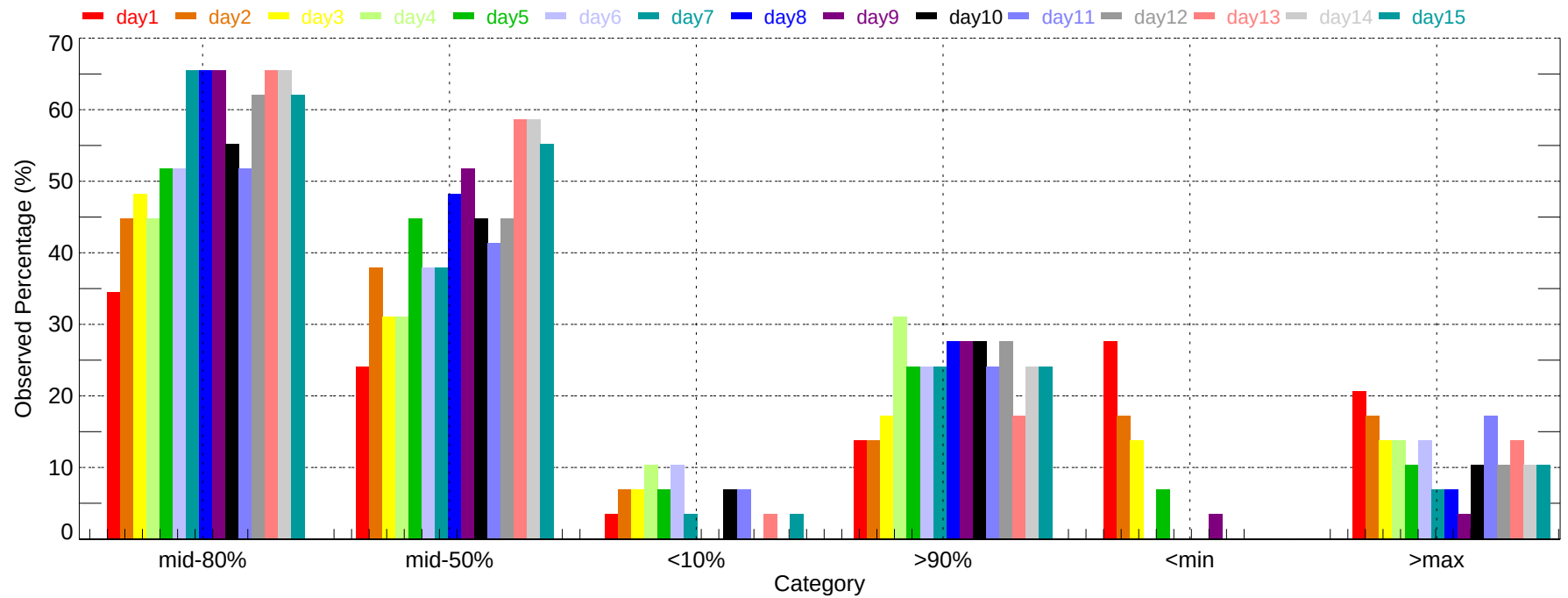
Observed Percentage of Ensembles - ERI: Max Temperature (2007-11-01~2007-11-30)
