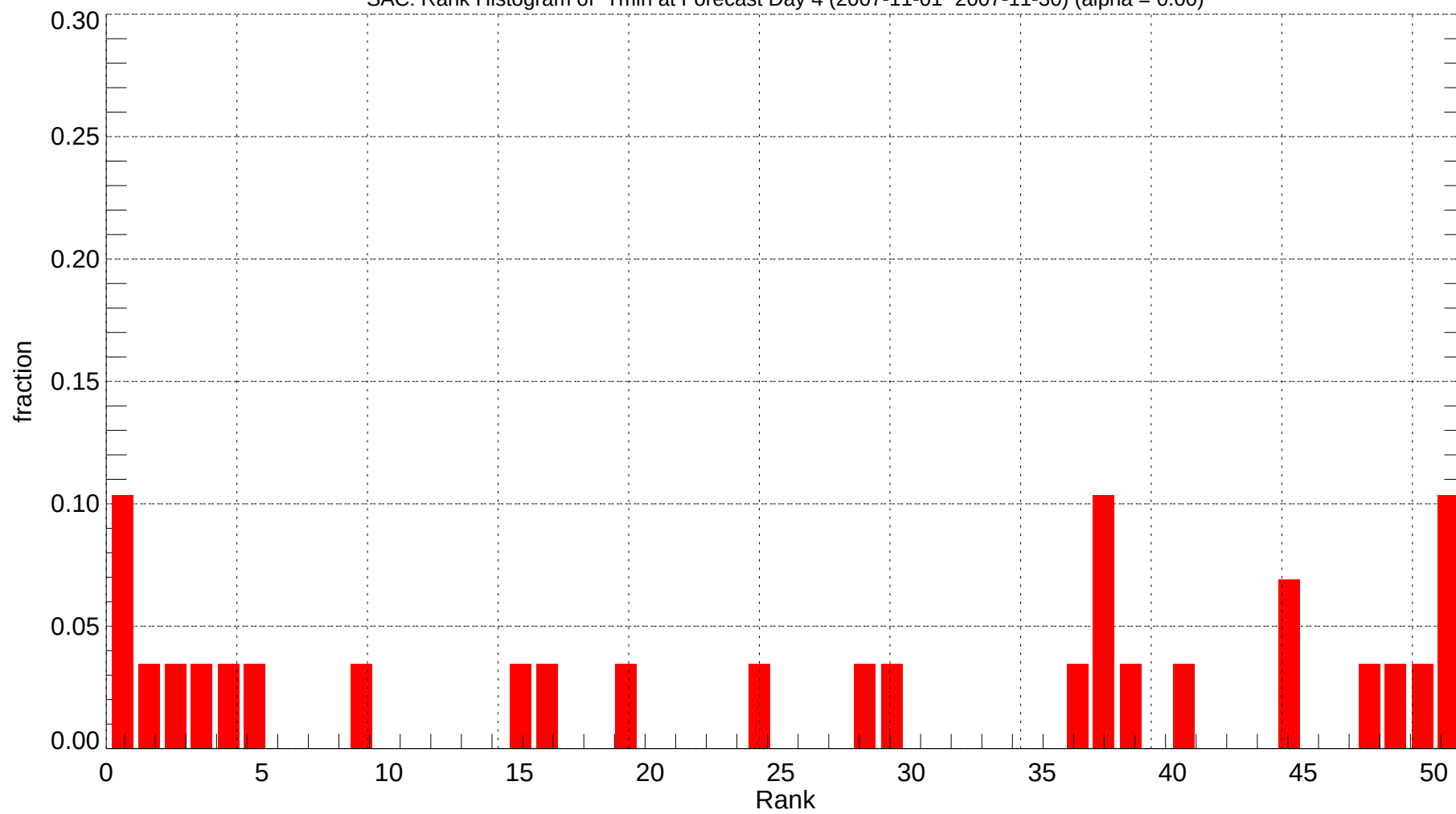
SAC: Rank Histogram of Tmin at Forecast Day 4 (2007-11-01~2007-11-30) (alpha = 0.00)
