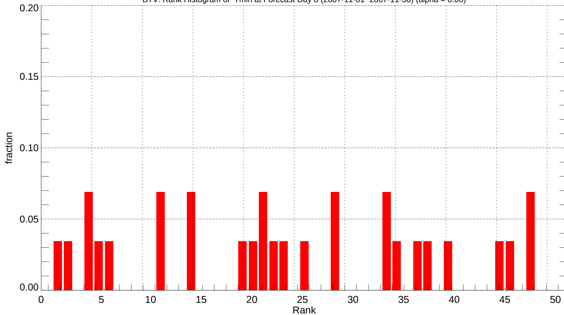
BTV: Rank Histogram of Tmin at Forecast Day 8 (2007-11-01~2007-11-30) (alpha = 0.00)
