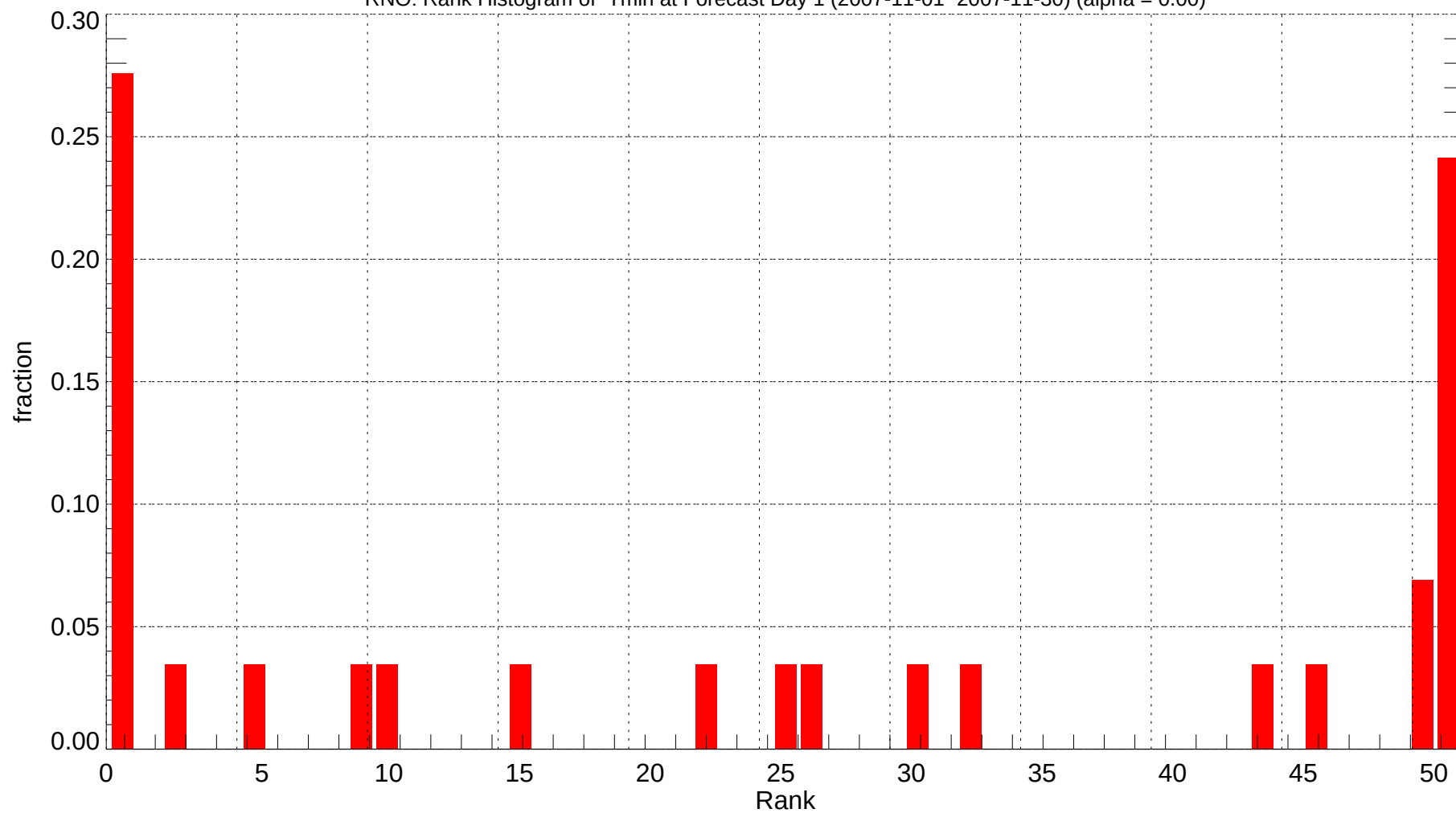
RNO: Rank Histogram of Tmin at Forecast Day 1 (2007-11-01~2007-11-30) (alpha = 0.00)
