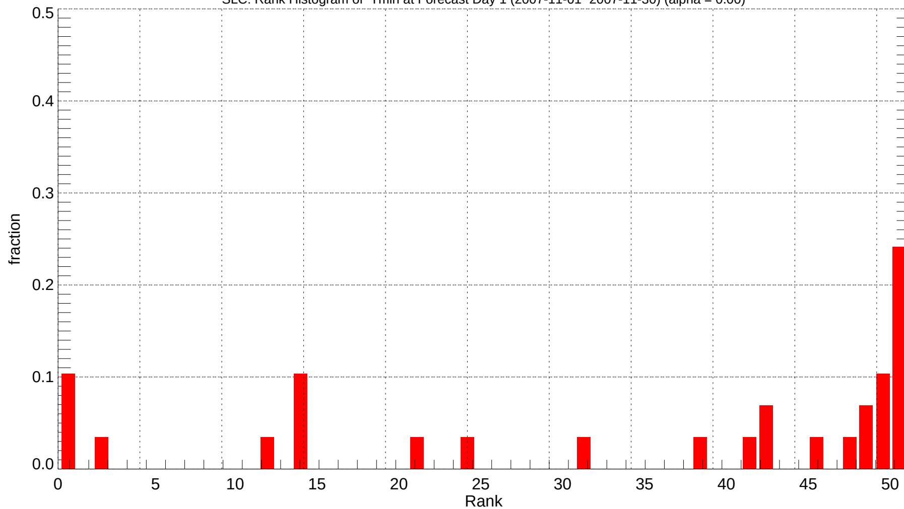
SLC: Rank Histogram of Tmin at Forecast Day 1 (2007-11-01~2007-11-30) (alpha = 0.00)
