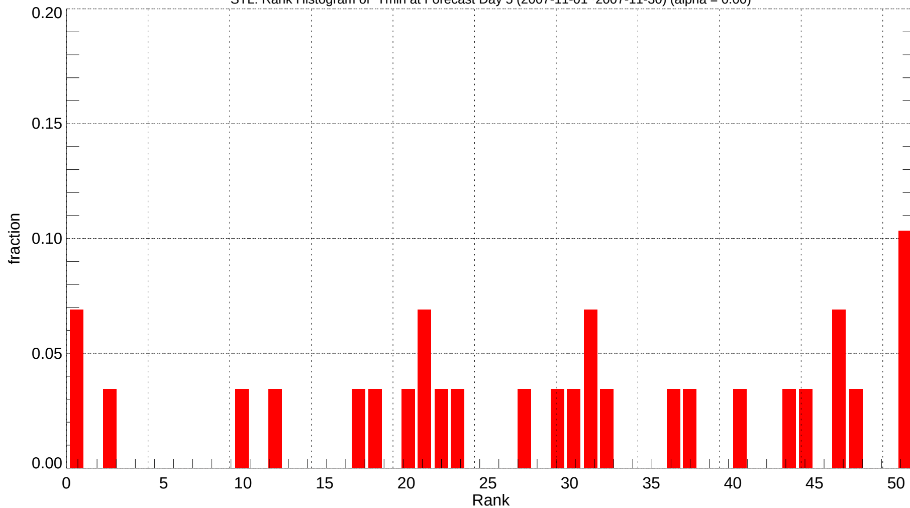
STL: Rank Histogram of Tmin at Forecast Day 5 (2007-11-01~2007-11-30) (alpha = 0.00)
