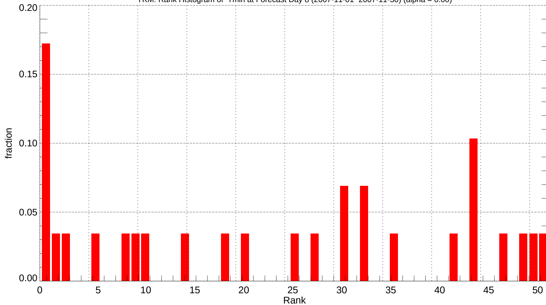
YKM: Rank Histogram of Tmin at Forecast Day 8 (2007-11-01~2007-11-30) (alpha = 0.00)
