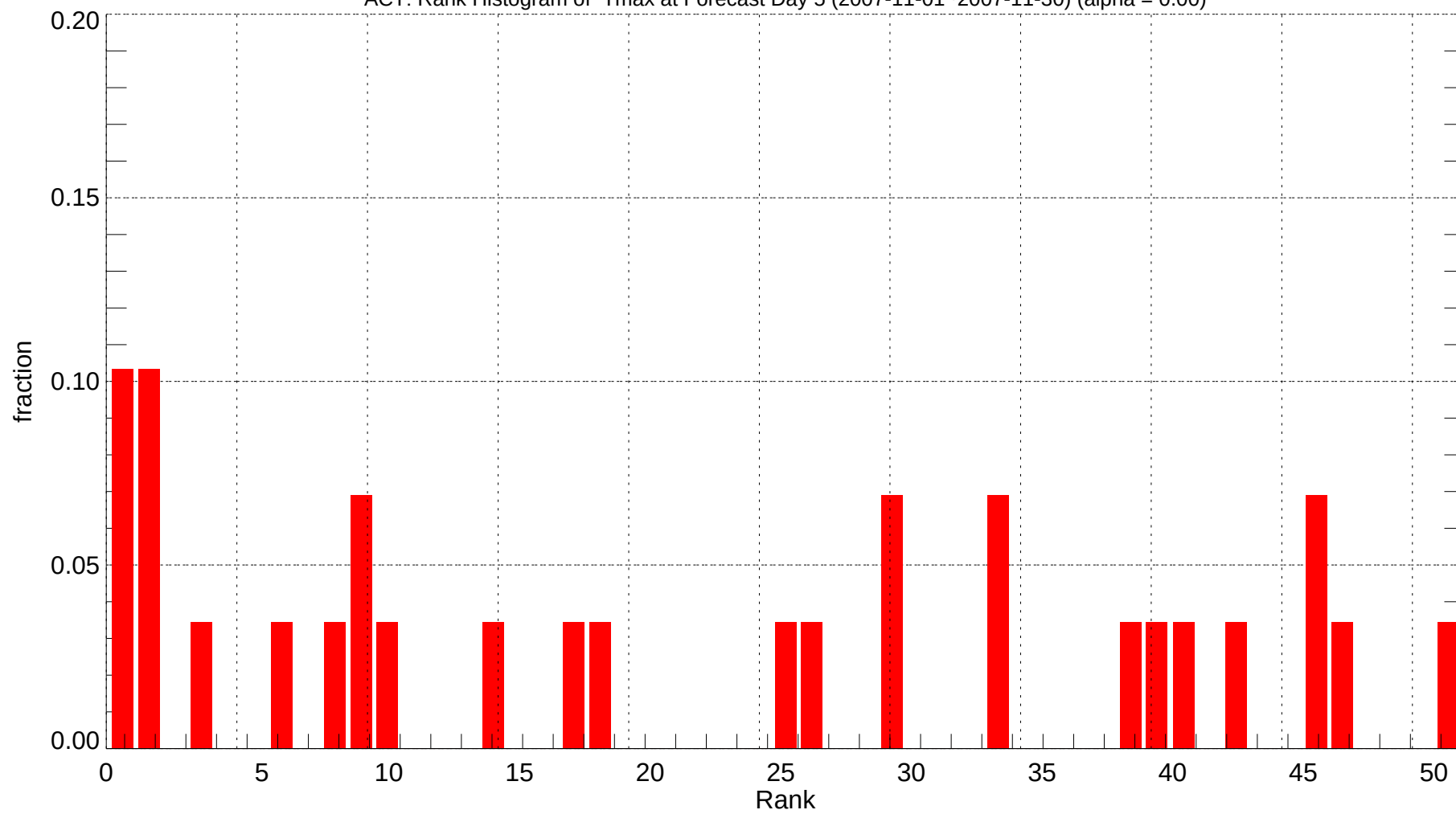
ACT: Rank Histogram of Tmax at Forecast Day 5 (2007-11-01~2007-11-30) (alpha = 0.00)
