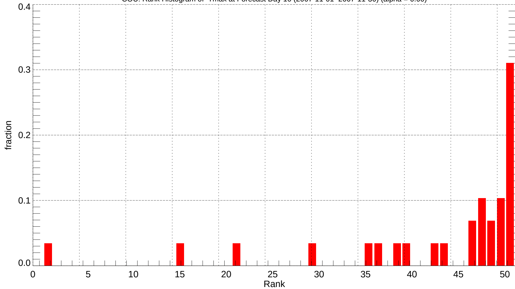
COU: Rank Histogram of Tmax at Forecast Day 10 (2007-11-01~2007-11-30) (alpha = 0.00)
