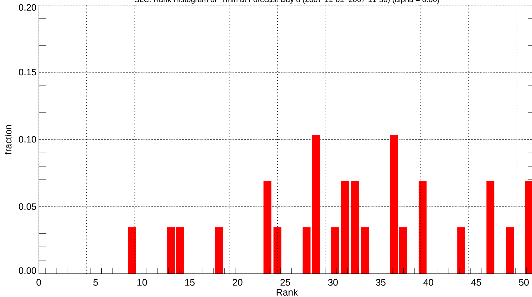
SLC: Rank Histogram of Tmin at Forecast Day 8 (2007-11-01~2007-11-30) (alpha = 0.00)
