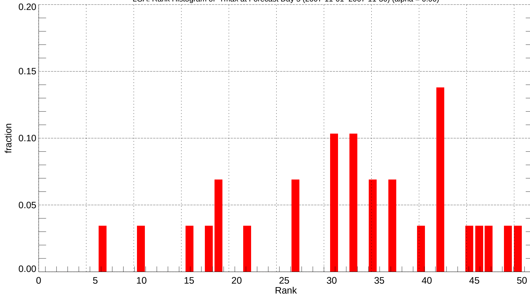
LGA: Rank Histogram of Tmax at Forecast Day 5 (2007-11-01~2007-11-30) (alpha = 0.00)
