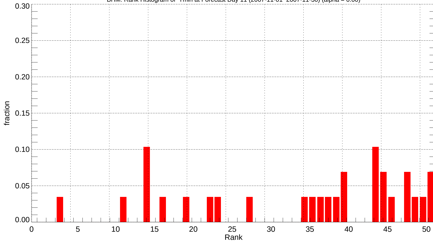
BHM: Rank Histogram of Tmin at Forecast Day 11 (2007-11-01~2007-11-30) (alpha = 0.00)
