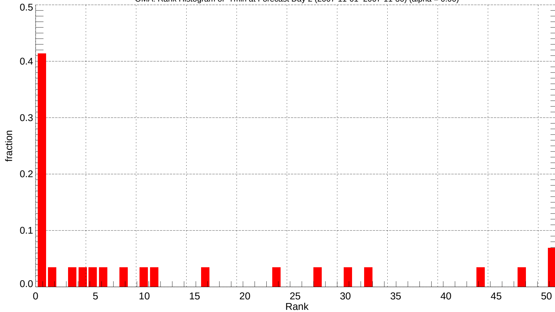
OMA: Rank Histogram of Tmin at Forecast Day 2 (2007-11-01~2007-11-30) (alpha = 0.00)
