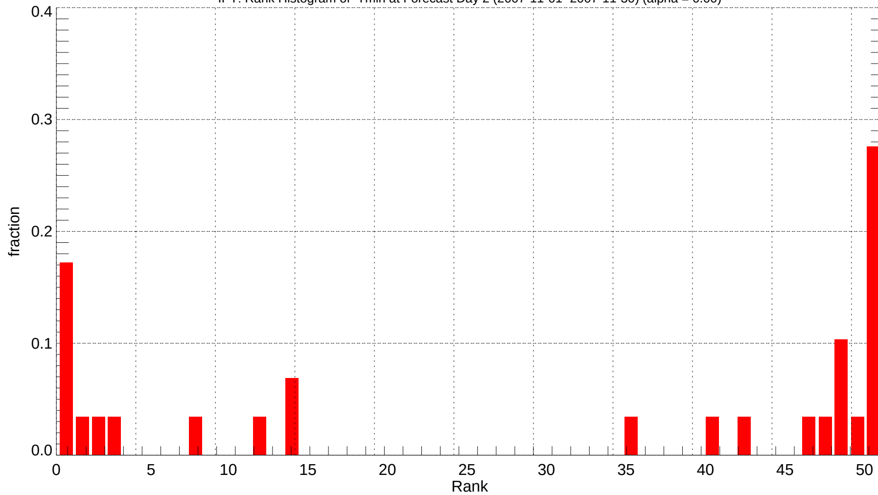
IPT: Rank Histogram of Tmin at Forecast Day 2 (2007-11-01~2007-11-30) (alpha = 0.00)
