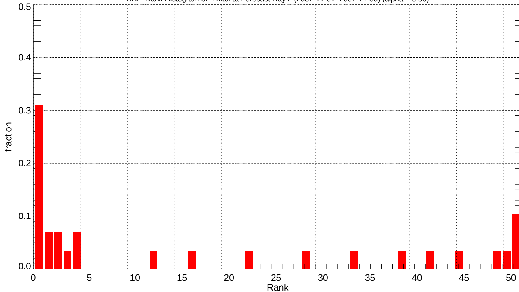
RBL: Rank Histogram of Tmax at Forecast Day 2 (2007-11-01~2007-11-30) (alpha = 0.00)
