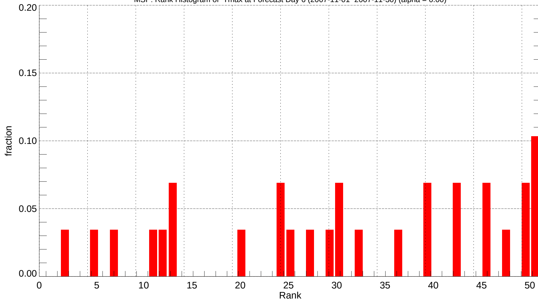
MSP: Rank Histogram of Tmax at Forecast Day 6 (2007-11-01~2007-11-30) (alpha = 0.00)
