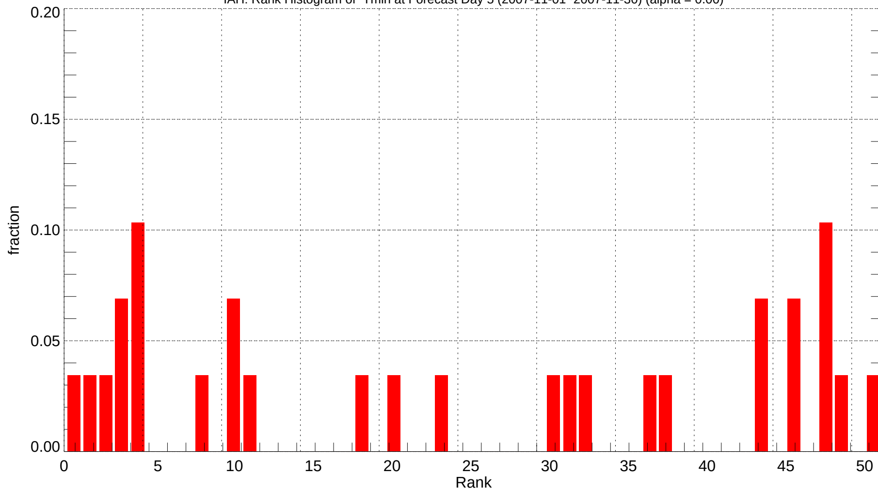
IAH: Rank Histogram of Tmin at Forecast Day 5 (2007-11-01~2007-11-30) (alpha = 0.00)
