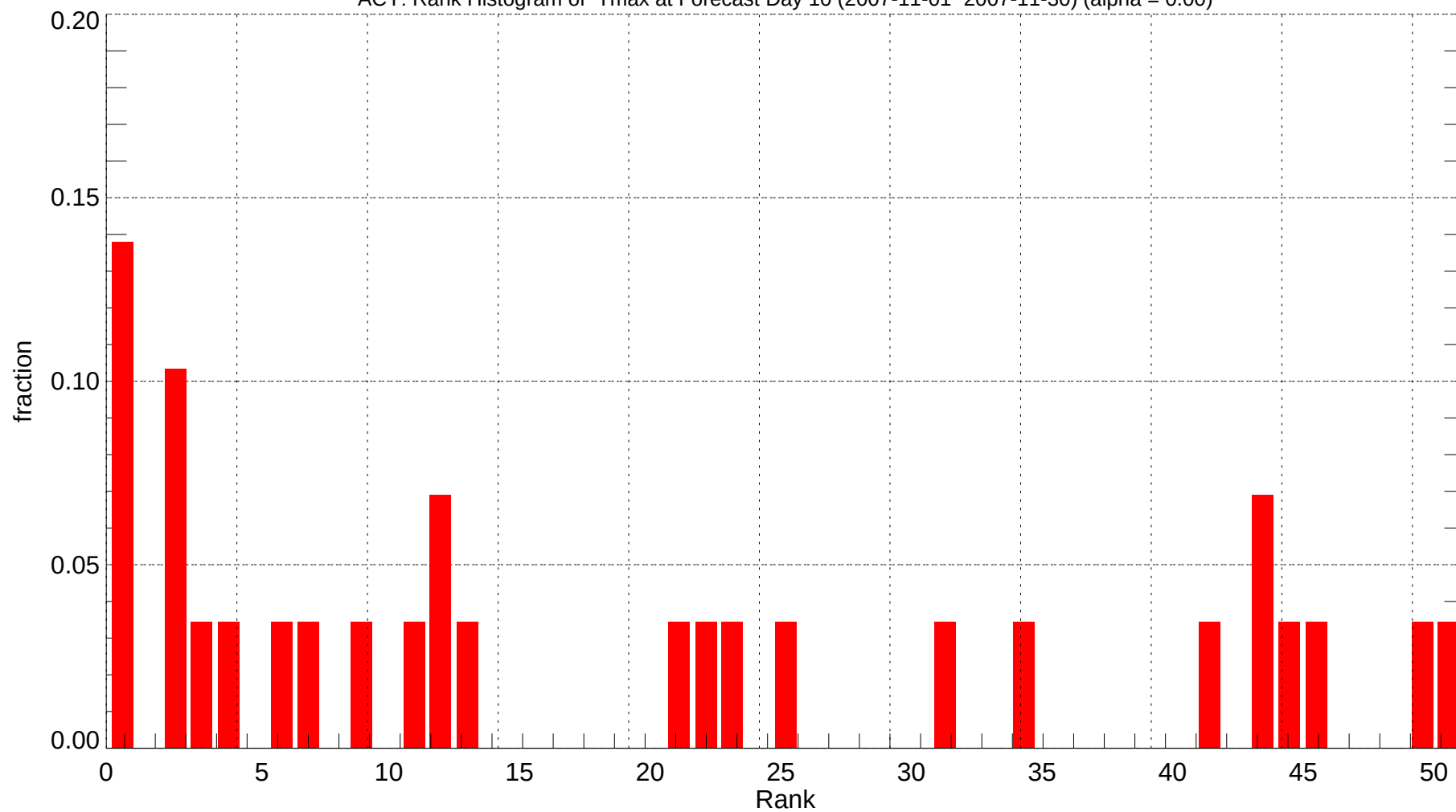
ACY: Rank Histogram of Tmax at Forecast Day 10 (2007-11-01~2007-11-30) (alpha = 0.00)
