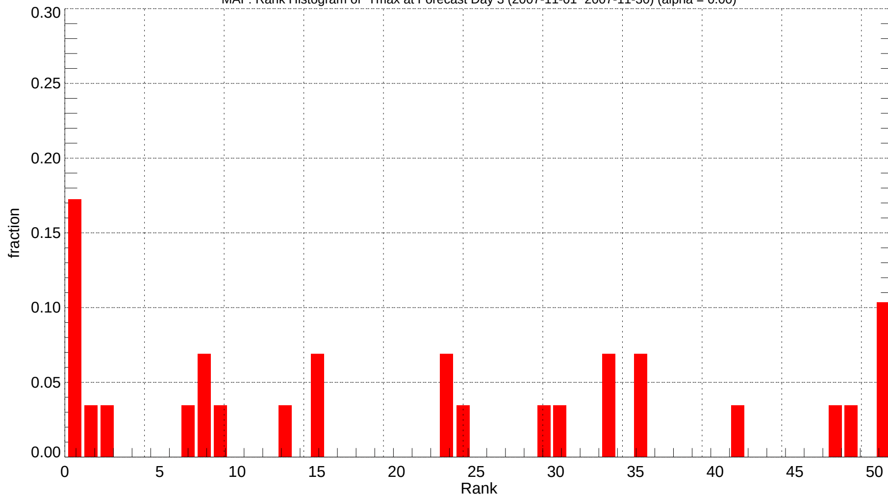
MAF: Rank Histogram of Tmax at Forecast Day 3 (2007-11-01~2007-11-30) (alpha = 0.00)
