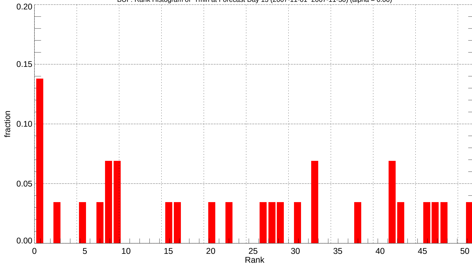
BUF: Rank Histogram of Tmin at Forecast Day 13 (2007-11-01~2007-11-30) (alpha = 0.00)
