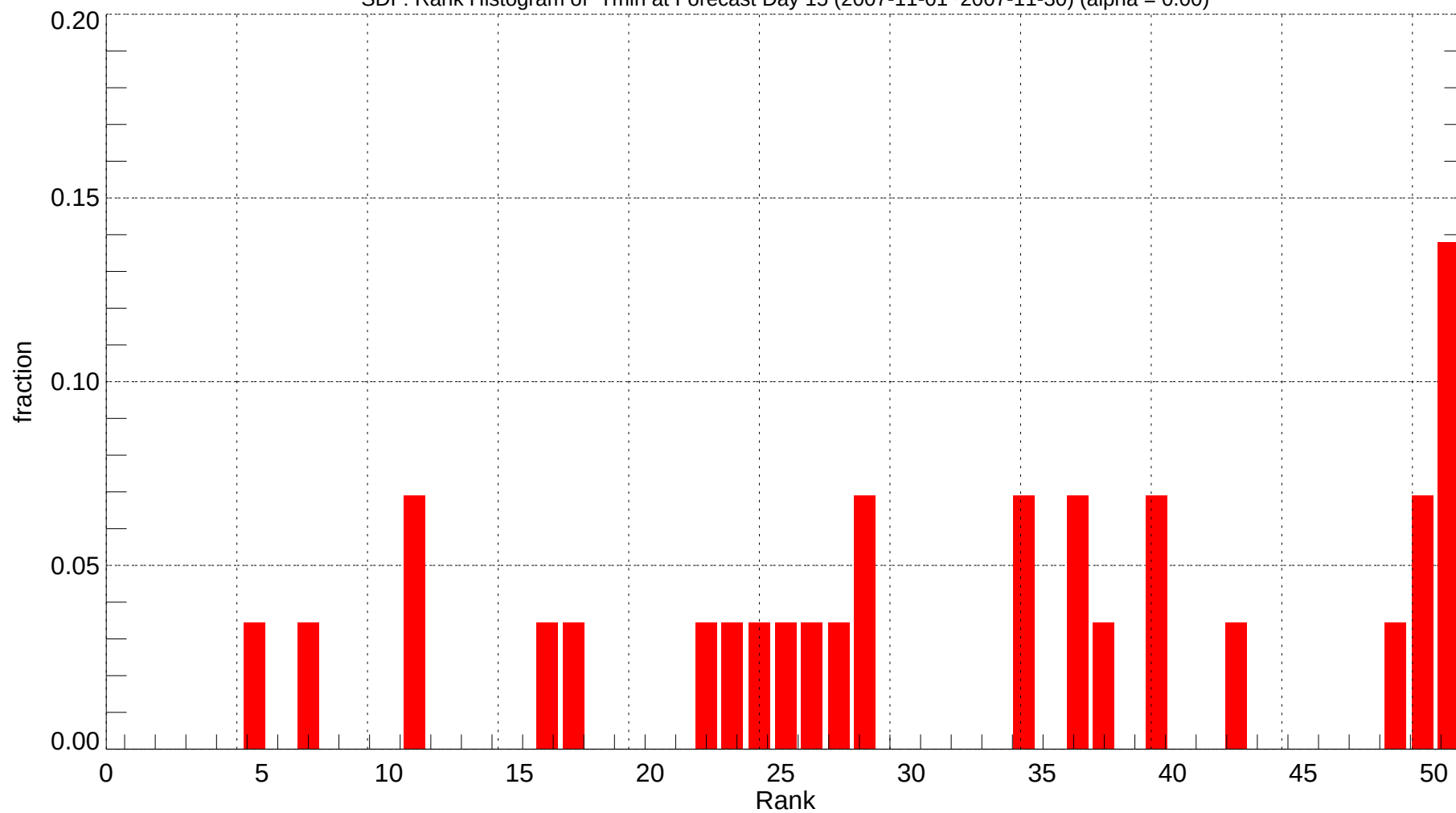
SDF: Rank Histogram of Tmin at Forecast Day 15 (2007-11-01~2007-11-30) (alpha = 0.00)
