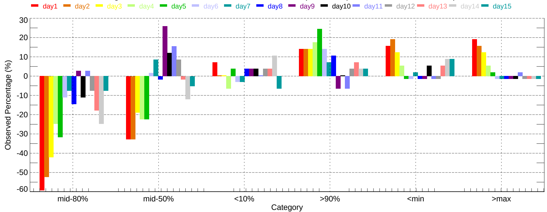
Observed Percentage Deviation of Ensembles - PWM: Min Temperature (2007-11-01~2007-11-30)
