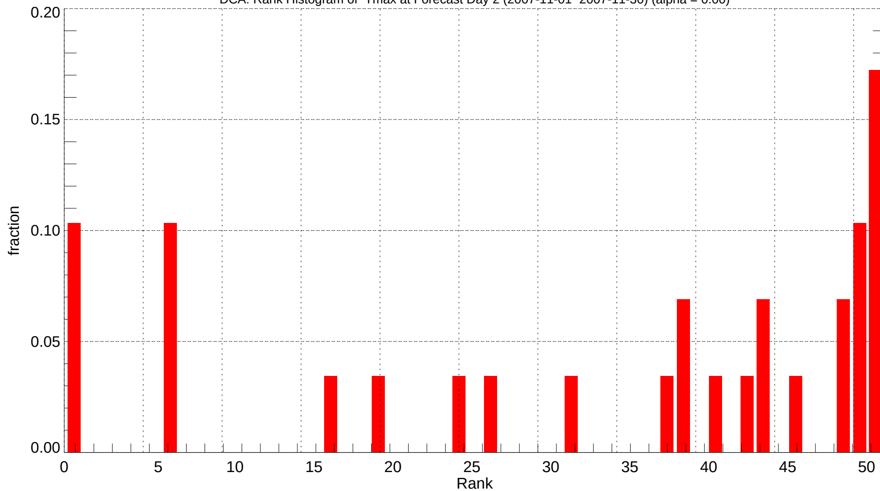
DCA: Rank Histogram of Tmax at Forecast Day 2 (2007-11-01~2007-11-30) (alpha = 0.00)
