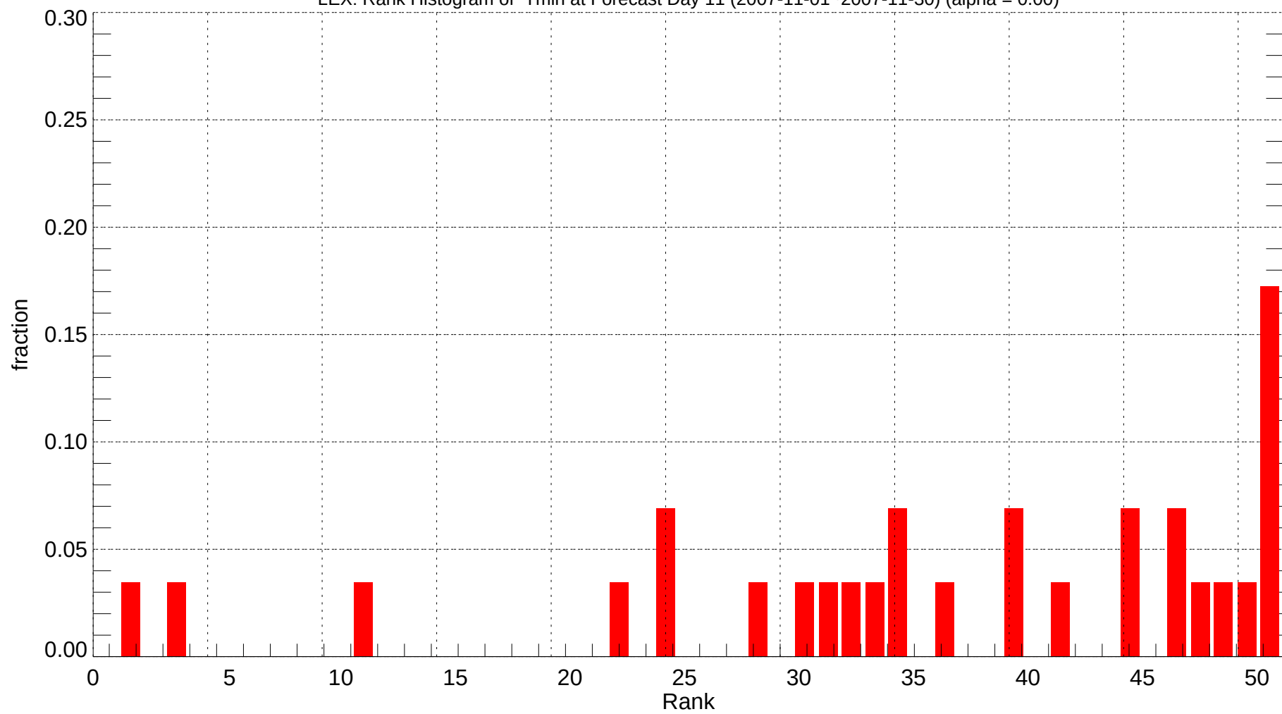
LEX: Rank Histogram of Tmin at Forecast Day 11 (2007-11-01~2007-11-30) (alpha = 0.00)
