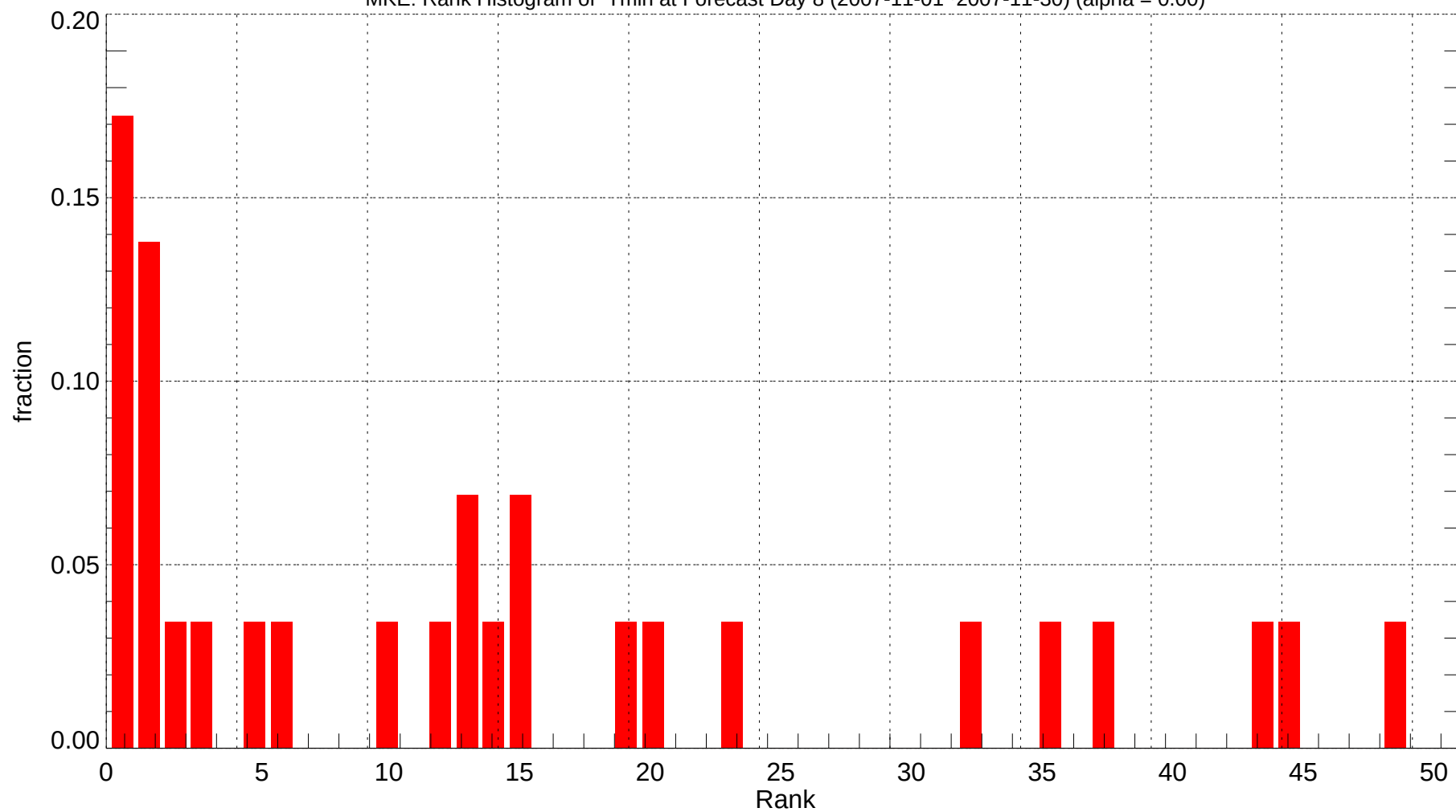
MKE: Rank Histogram of Tmin at Forecast Day 8 (2007-11-01~2007-11-30) (alpha = 0.00)
