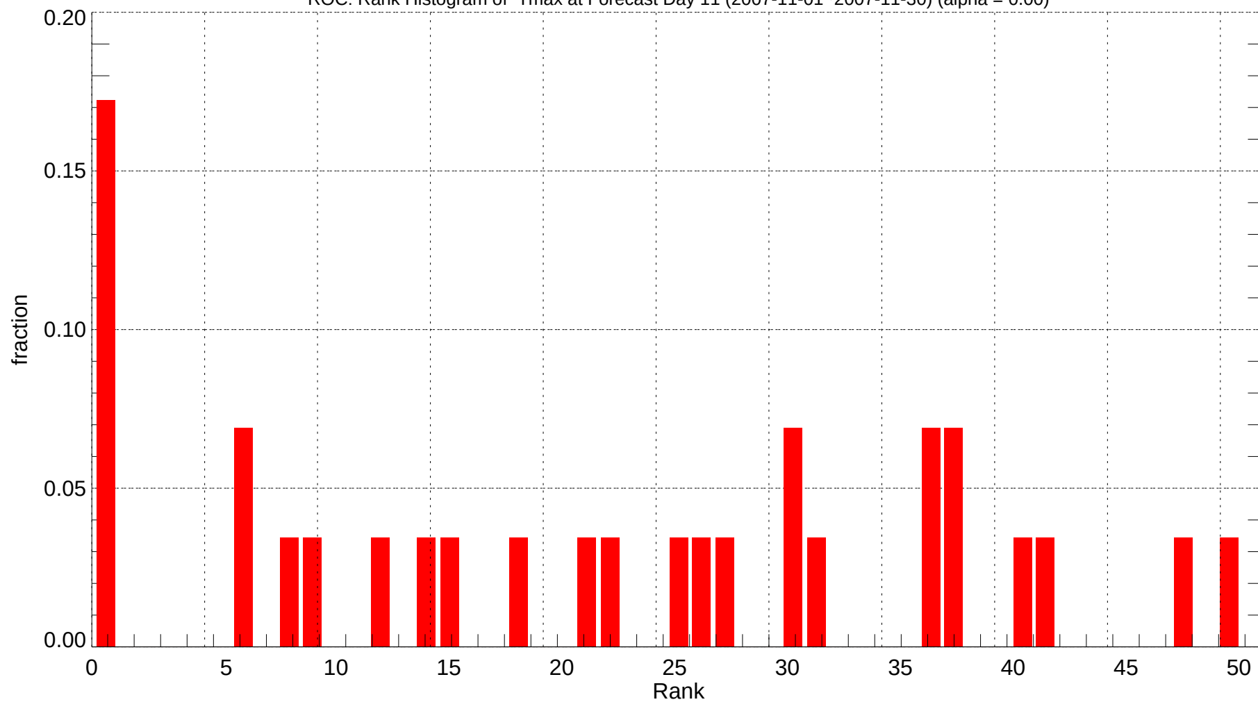
ROC: Rank Histogram of Tmax at Forecast Day 11 (2007-11-01~2007-11-30) (alpha = 0.00)
