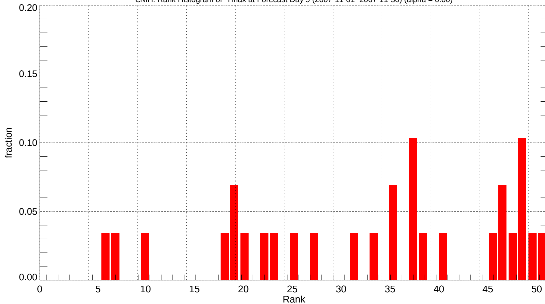
CMH: Rank Histogram of Tmax at Forecast Day 9 (2007-11-01~2007-11-30) (alpha = 0.00)
