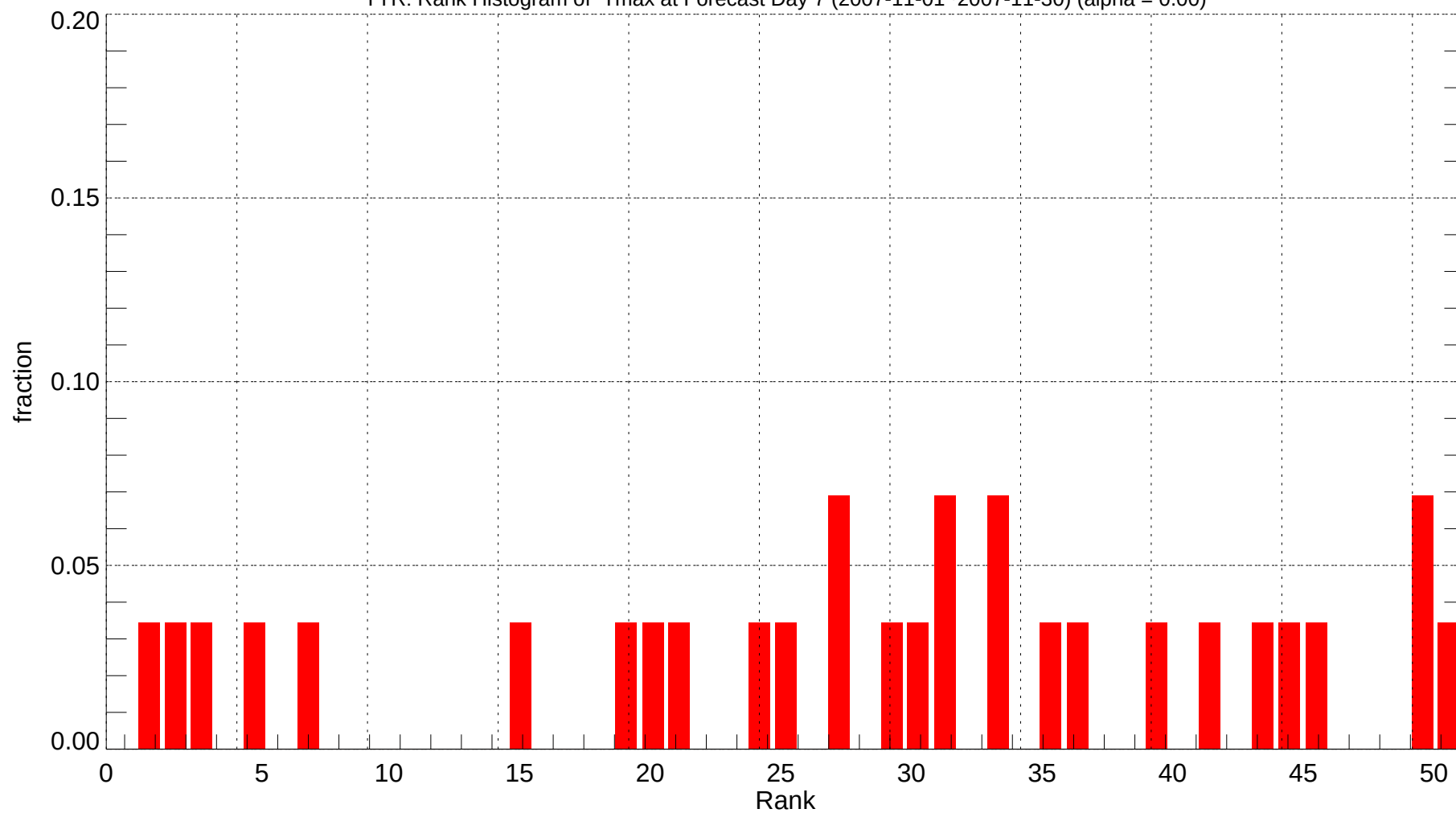
TYR: Rank Histogram of Tmax at Forecast Day 7 (2007-11-01~2007-11-30) (alpha = 0.00)
