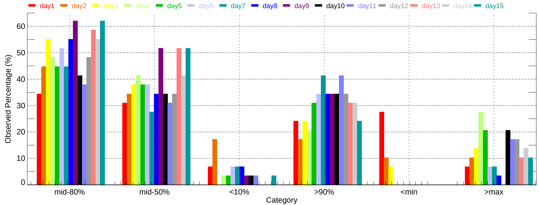
Observed Percentage of Ensembles - BNA: Min Temperature (2007-11-01~2007-11-30)
