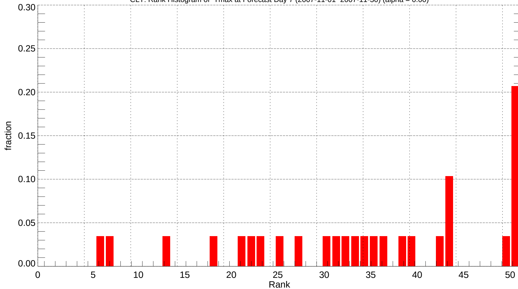
CLT: Rank Histogram of Tmax at Forecast Day 7 (2007-11-01~2007-11-30) (alpha = 0.00)
