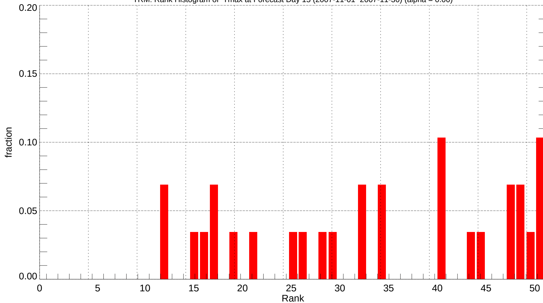
TRM: Rank Histogram of Tmax at Forecast Day 15 (2007-11-01~2007-11-30) (alpha = 0.00)
