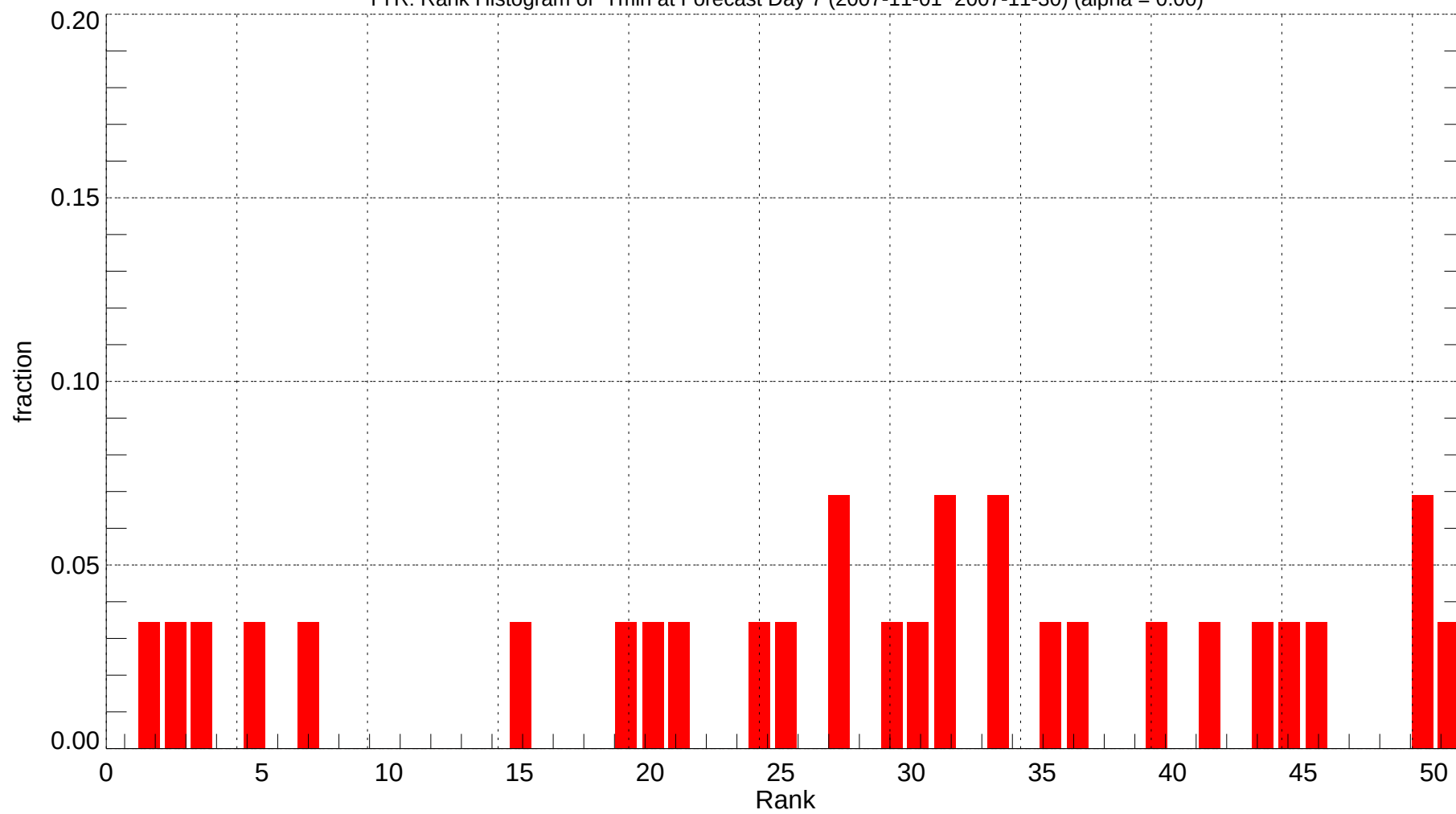
TYR: Rank Histogram of Tmin at Forecast Day 7 (2007-11-01~2007-11-30) (alpha = 0.00)
