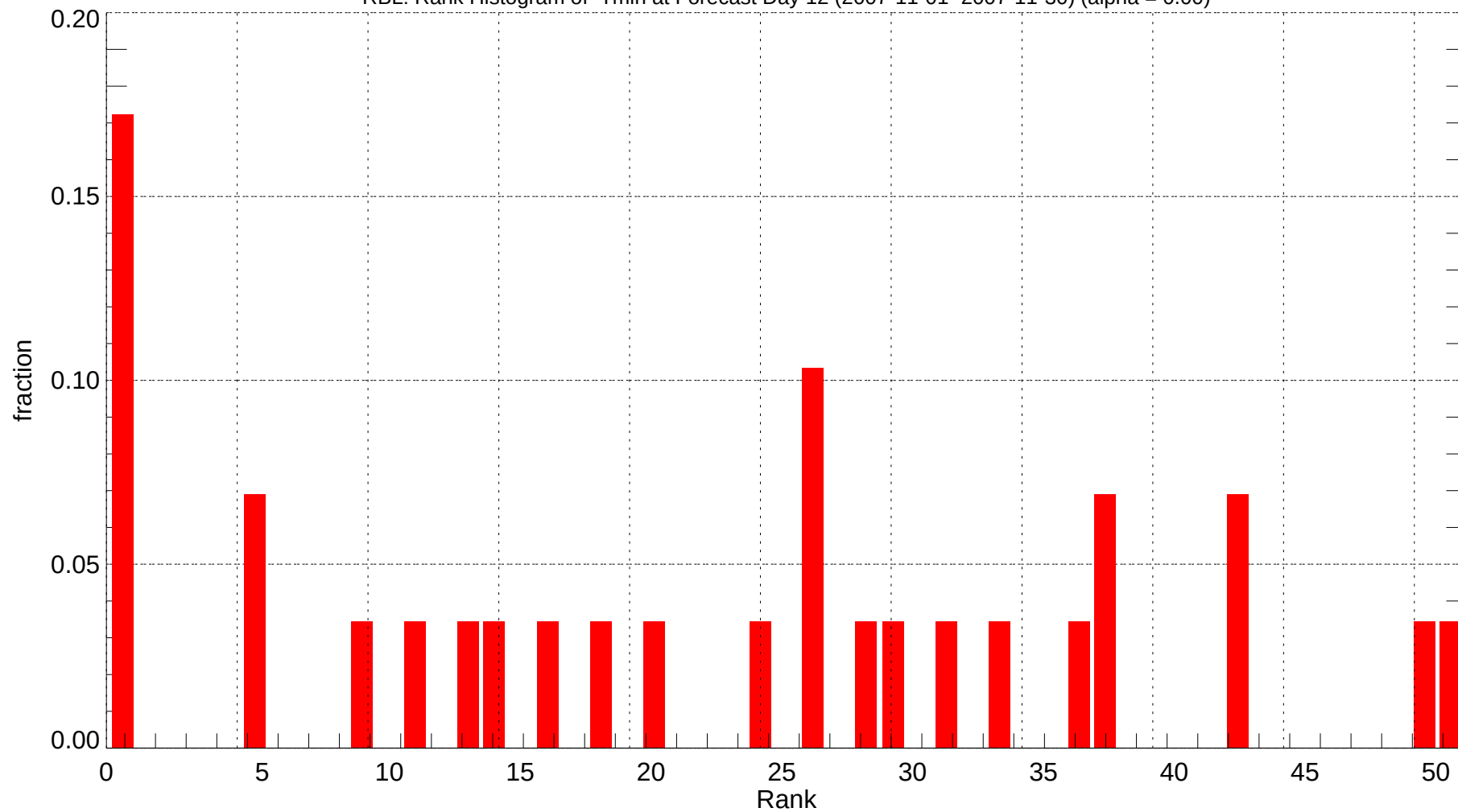
RBL: Rank Histogram of Tmin at Forecast Day 12 (2007-11-01~2007-11-30) (alpha = 0.00)
