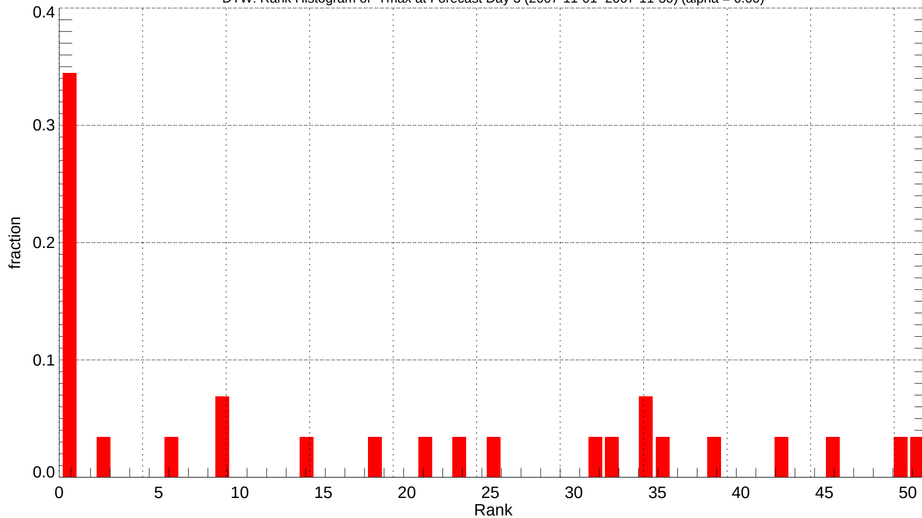
DTW: Rank Histogram of Tmax at Forecast Day 3 (2007-11-01~2007-11-30) (alpha = 0.00)
