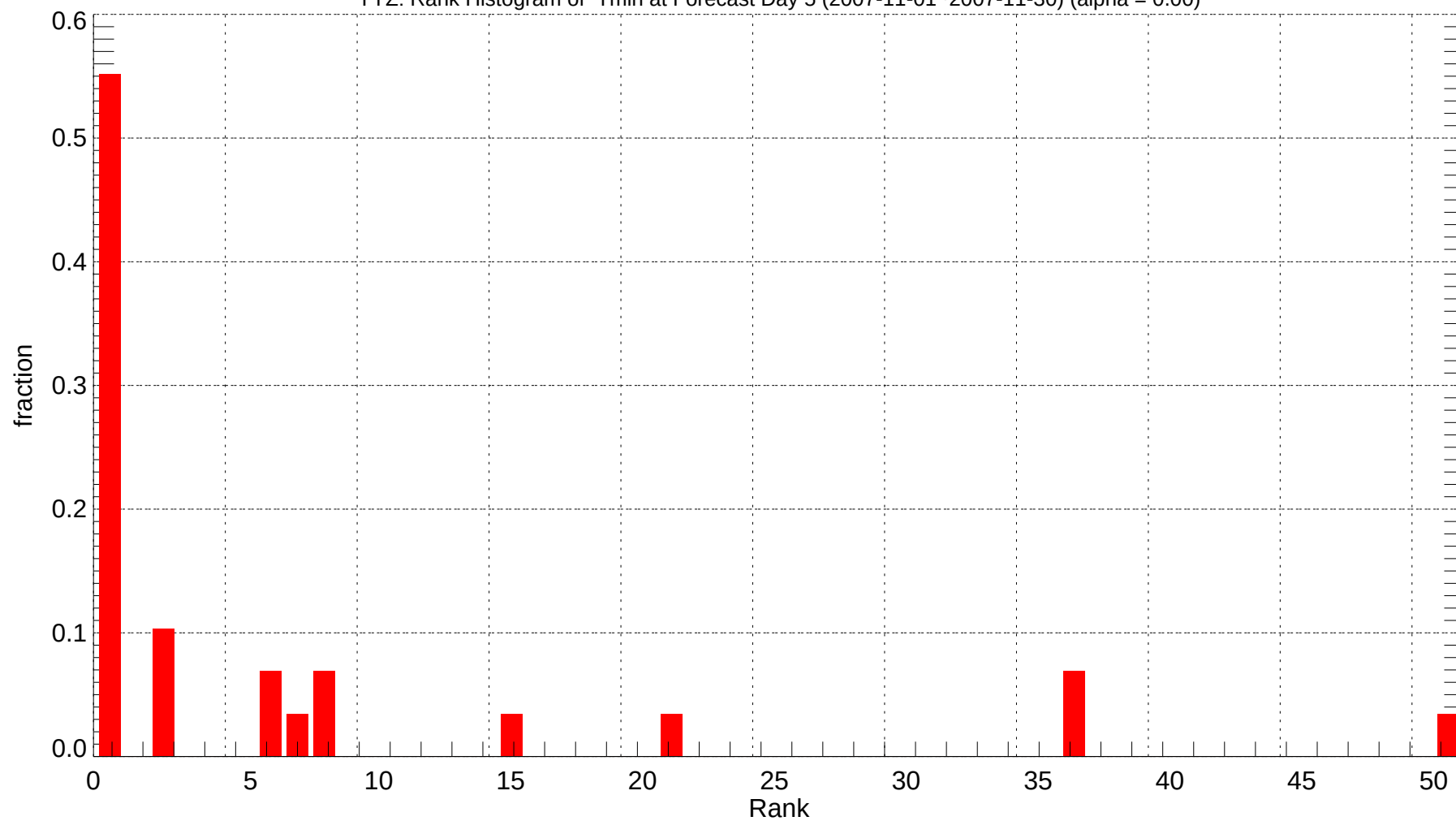
YYZ: Rank Histogram of Tmin at Forecast Day 5 (2007-11-01~2007-11-30) (alpha = 0.00)
