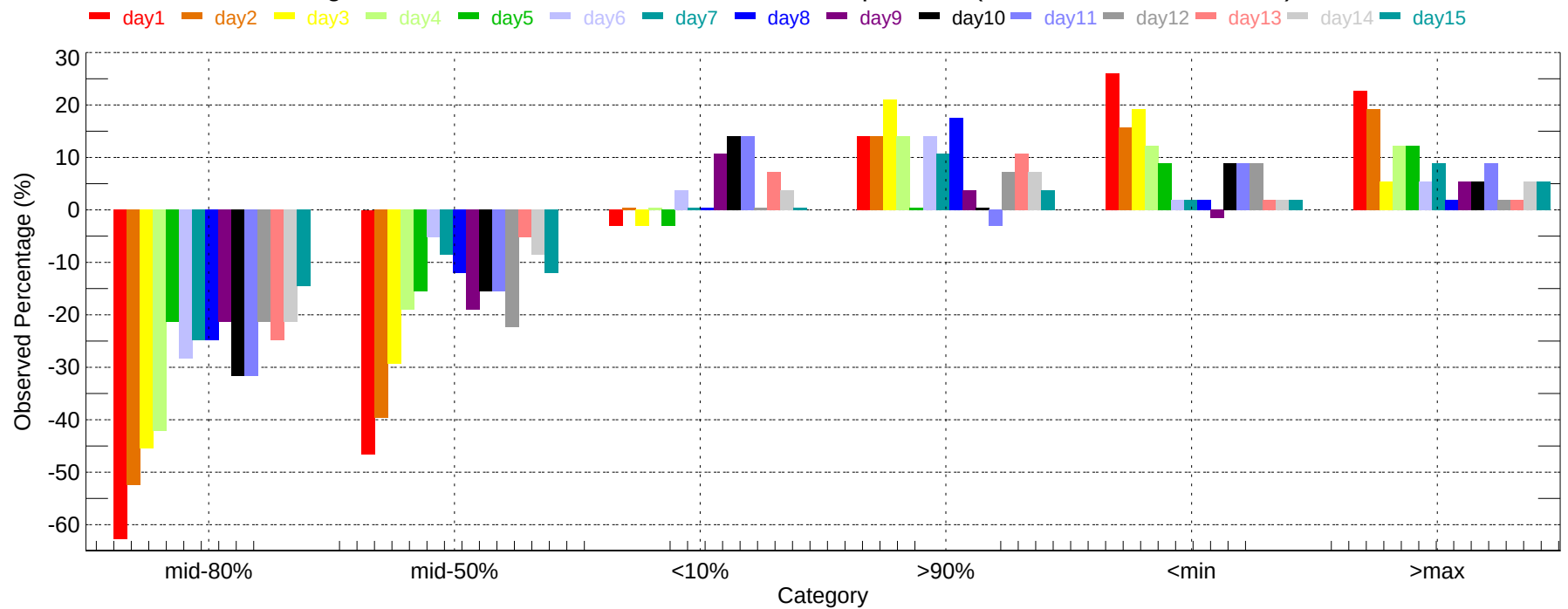
Observed Percentage Deviation of Ensembles - LNS: Min Temperature (2007-11-01~2007-11-30)
