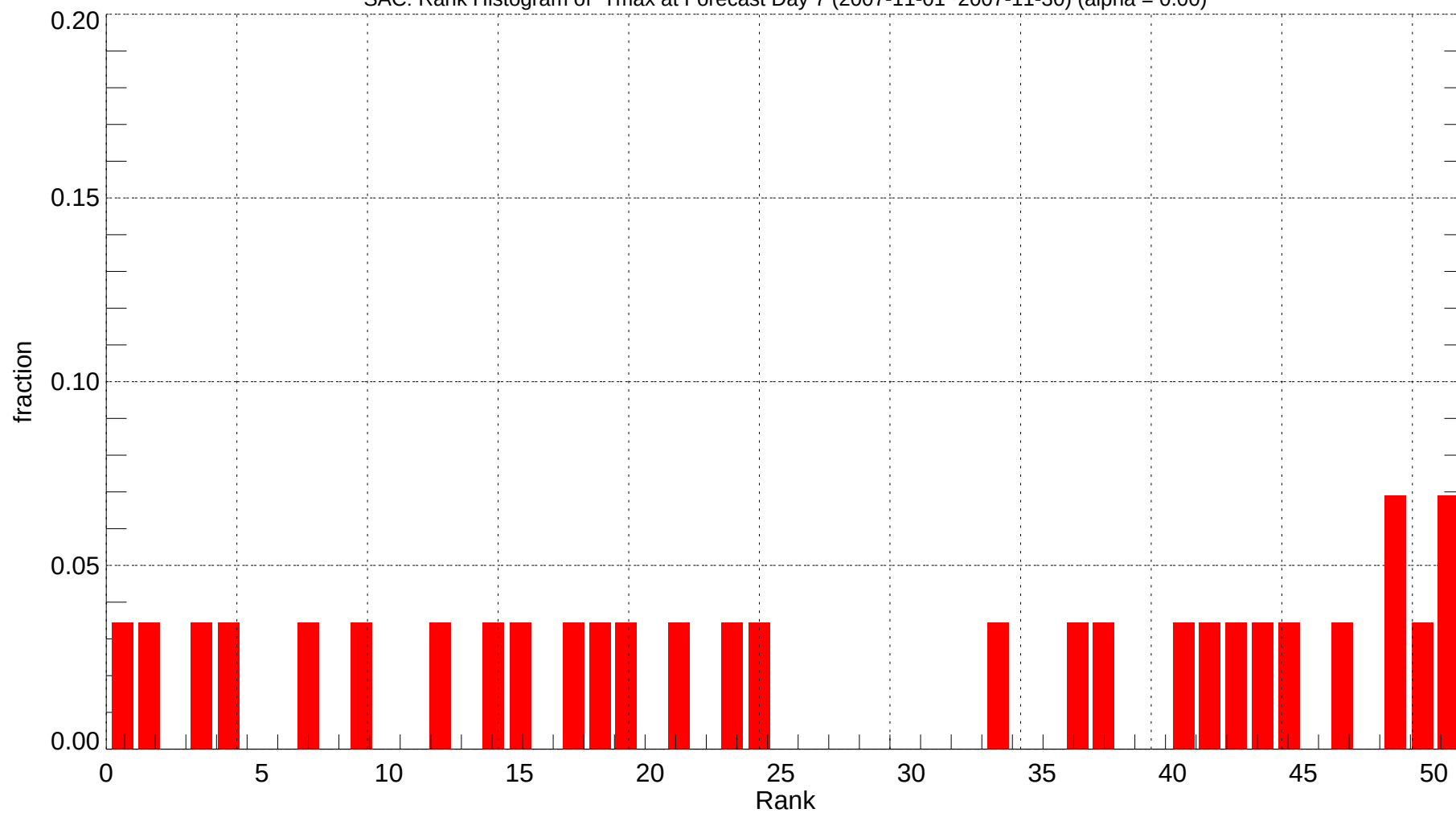
SAC: Rank Histogram of Tmax at Forecast Day 7 (2007-11-01~2007-11-30) (alpha = 0.00)
