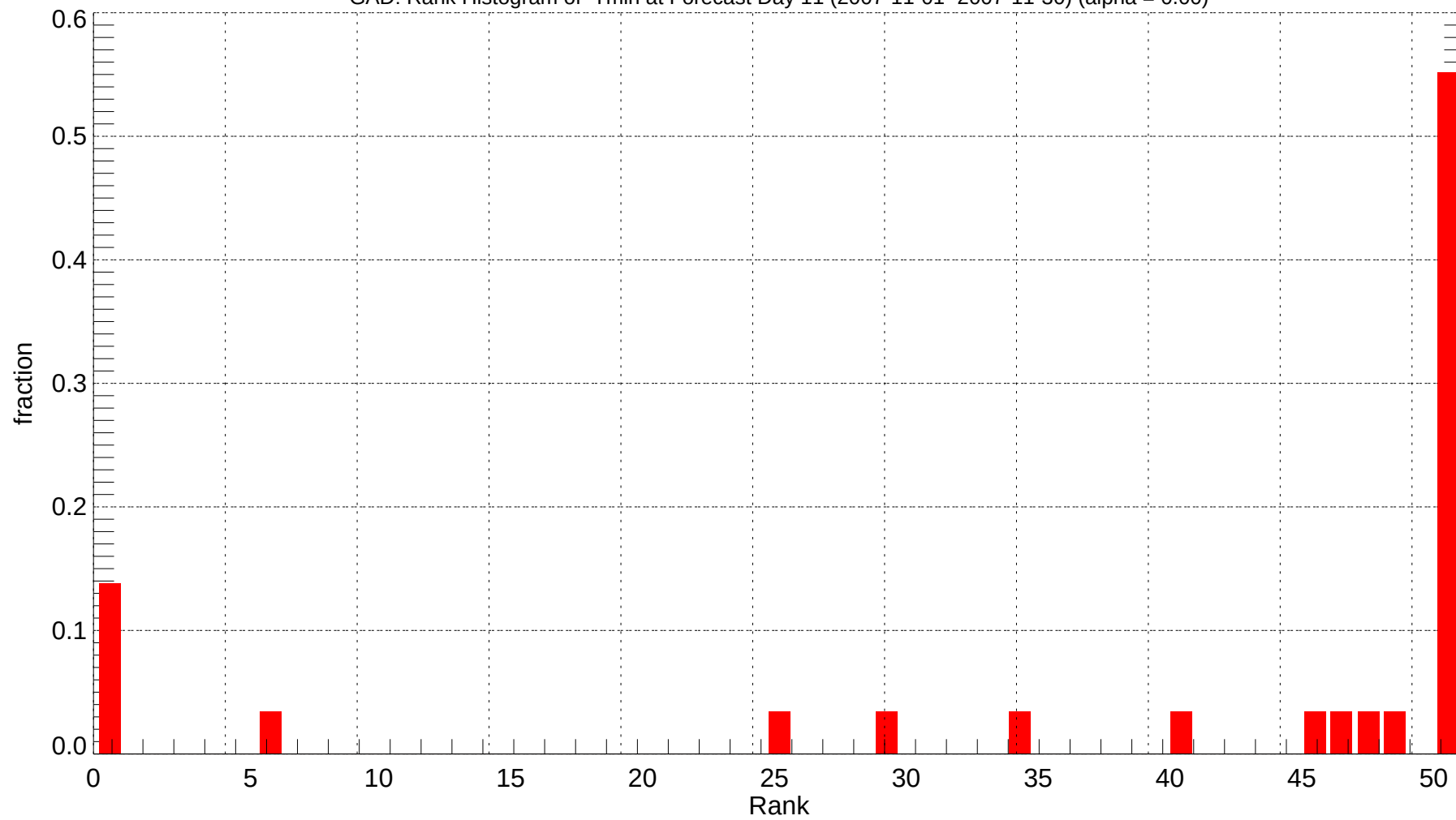
GAD: Rank Histogram of Tmin at Forecast Day 11 (2007-11-01~2007-11-30) (alpha = 0.00)
