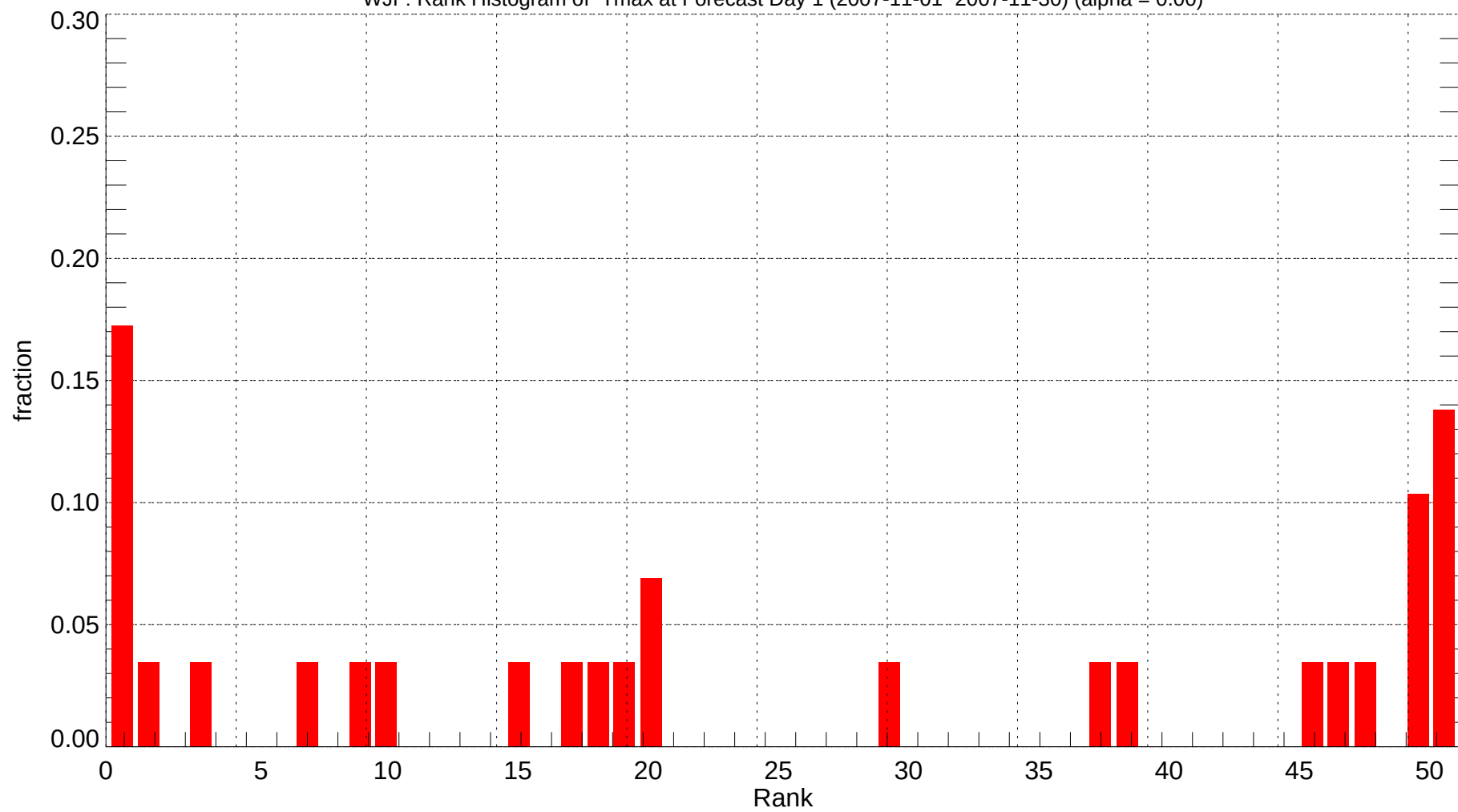
WJF: Rank Histogram of Tmax at Forecast Day 1 (2007-11-01~2007-11-30) (alpha = 0.00)
