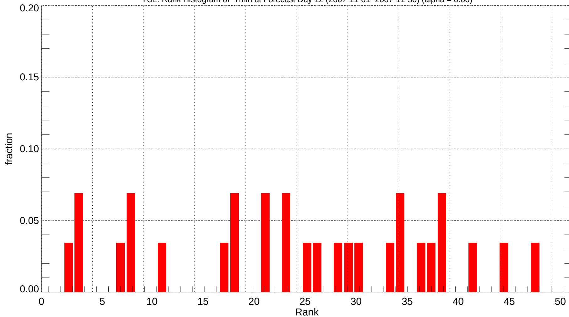
YUL: Rank Histogram of Tmin at Forecast Day 12 (2007-11-01~2007-11-30) (alpha = 0.00)
