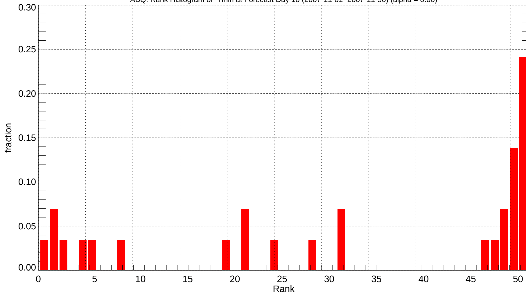
ABQ: Rank Histogram of Tmin at Forecast Day 10 (2007-11-01~2007-11-30) (alpha = 0.00)
