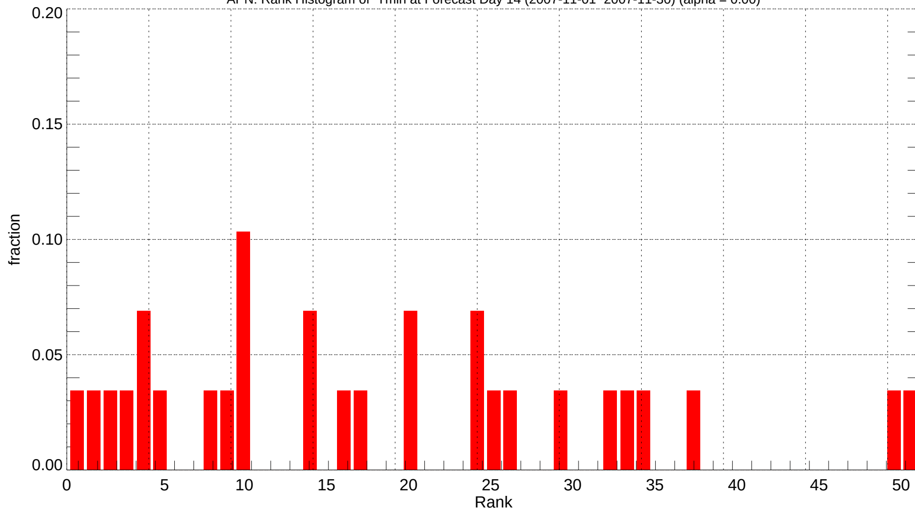
APN: Rank Histogram of Tmin at Forecast Day 14 (2007-11-01~2007-11-30) (alpha = 0.00)
