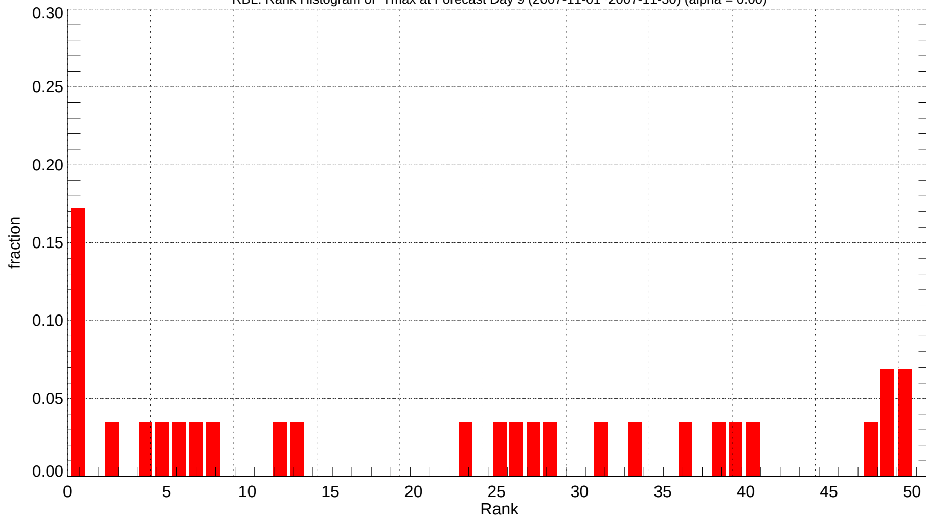
RBL: Rank Histogram of Tmax at Forecast Day 9 (2007-11-01~2007-11-30) (alpha = 0.00)
