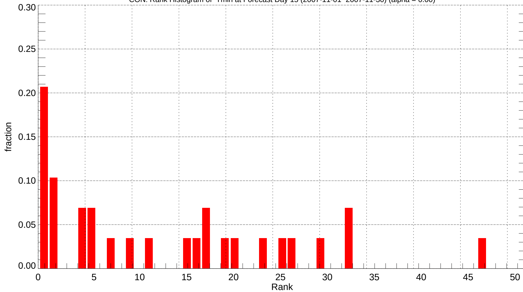
CON: Rank Histogram of Tmin at Forecast Day 15 (2007-11-01~2007-11-30) (alpha = 0.00)
