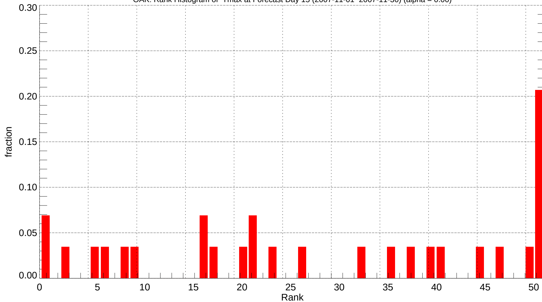
OAK: Rank Histogram of Tmax at Forecast Day 15 (2007-11-01~2007-11-30) (alpha = 0.00)
