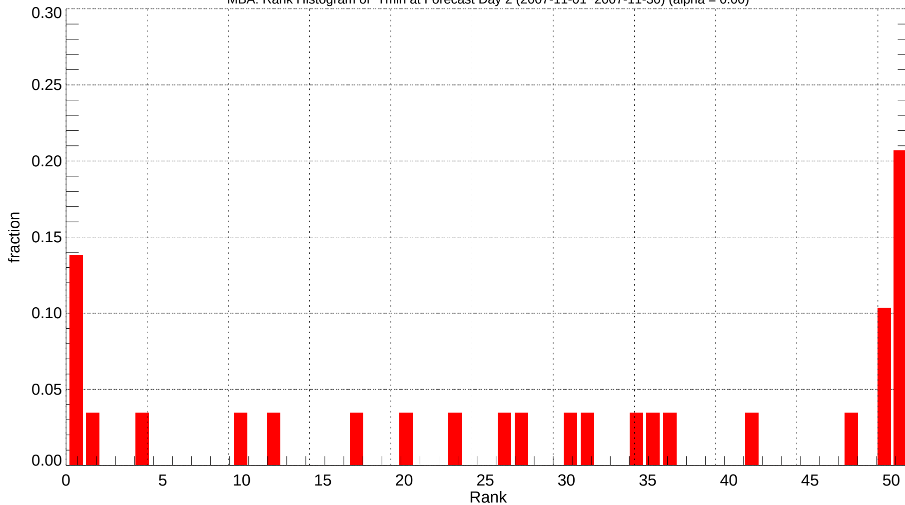
MBA: Rank Histogram of Tmin at Forecast Day 2 (2007-11-01~2007-11-30) (alpha = 0.00)
