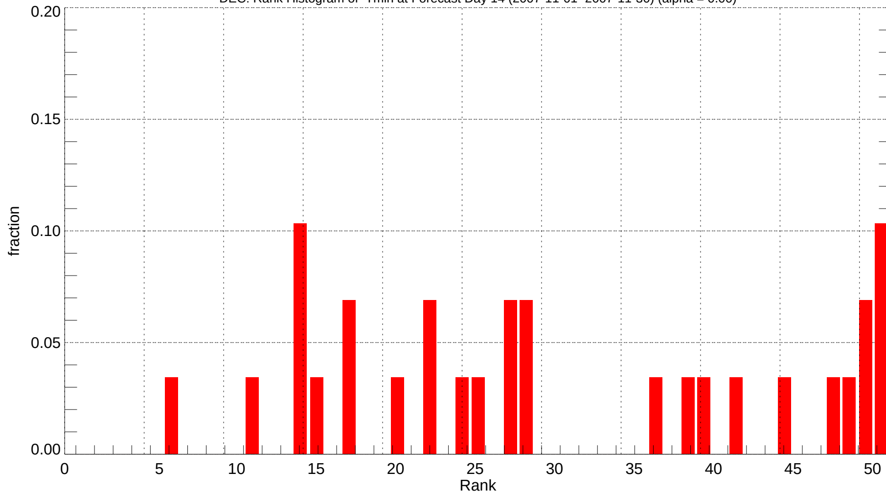
DEC: Rank Histogram of Tmin at Forecast Day 14 (2007-11-01~2007-11-30) (alpha = 0.00)
