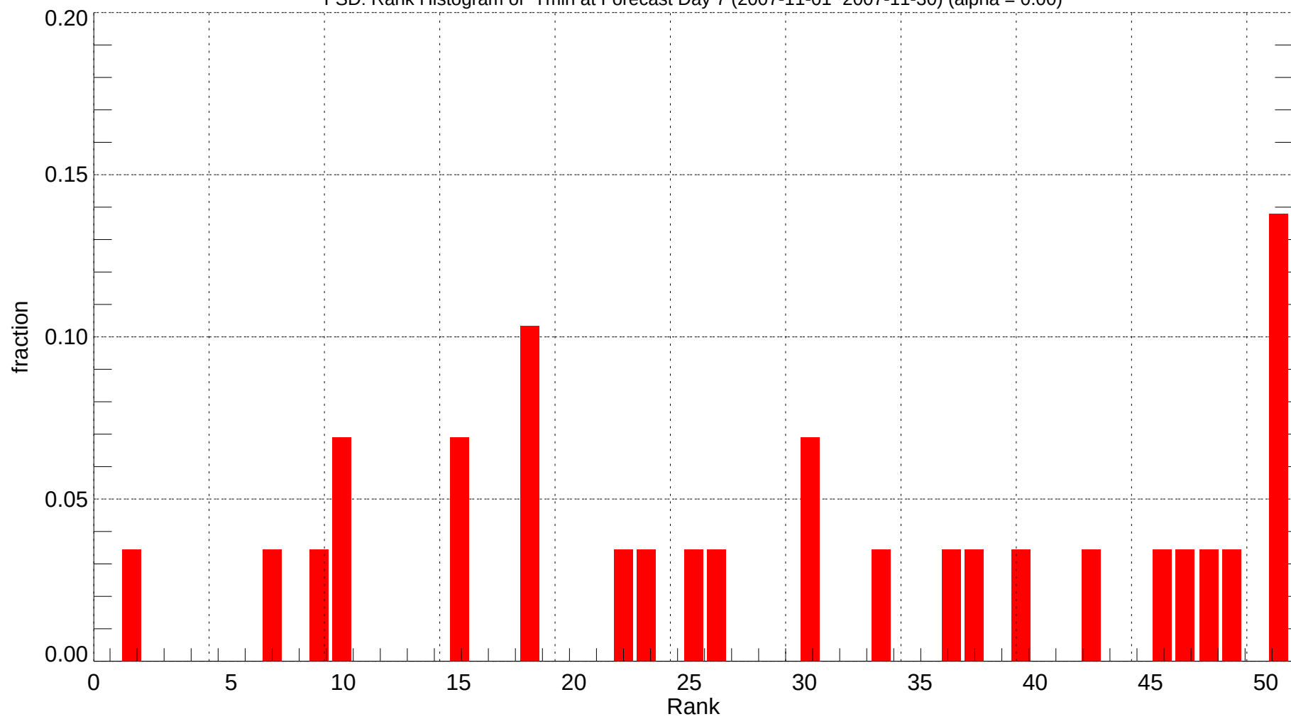
FSD: Rank Histogram of Tmin at Forecast Day 7 (2007-11-01~2007-11-30) (alpha = 0.00)
