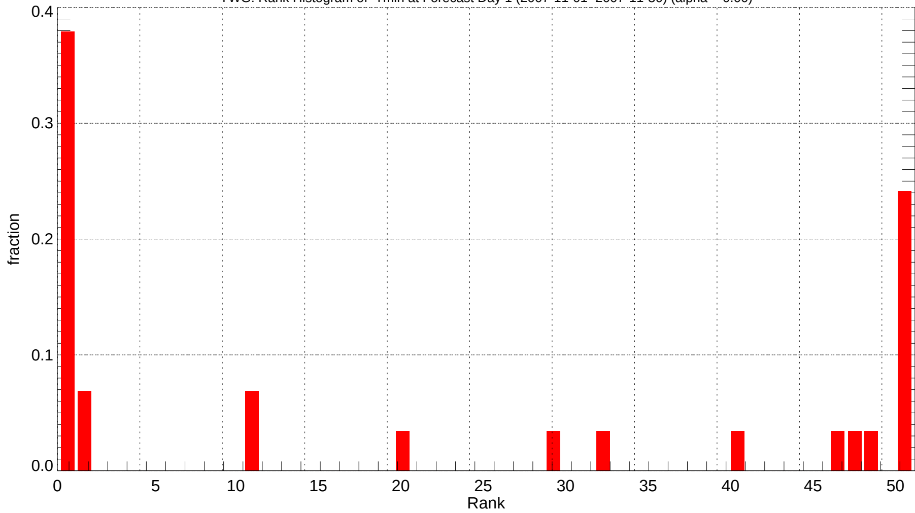
YWG: Rank Histogram of Tmin at Forecast Day 1 (2007-11-01~2007-11-30) (alpha = 0.00)
