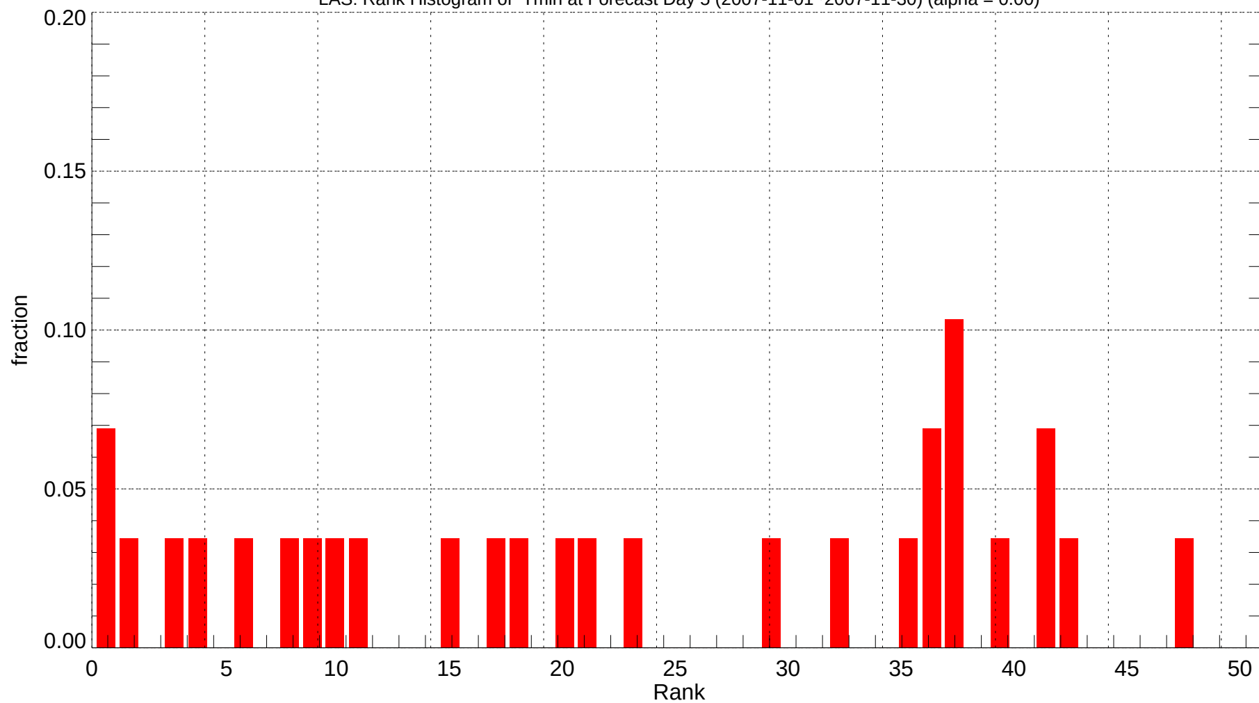
LAS: Rank Histogram of Tmin at Forecast Day 5 (2007-11-01~2007-11-30) (alpha = 0.00)
