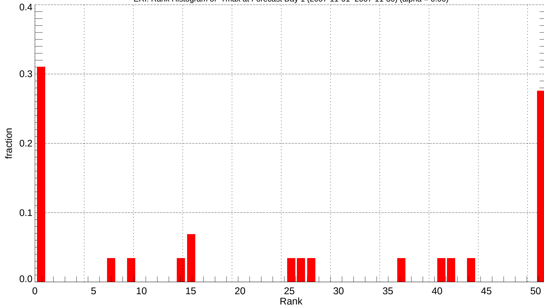
ERI: Rank Histogram of Tmax at Forecast Day 1 (2007-11-01~2007-11-30) (alpha = 0.00)
