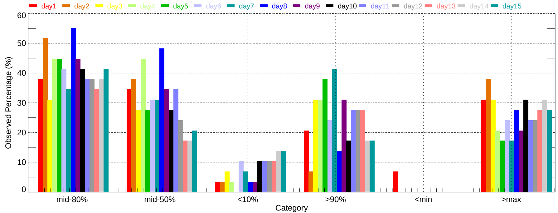
Observed Percentage of Ensembles - COS: Min Temperature (2007-11-01~2007-11-30)
