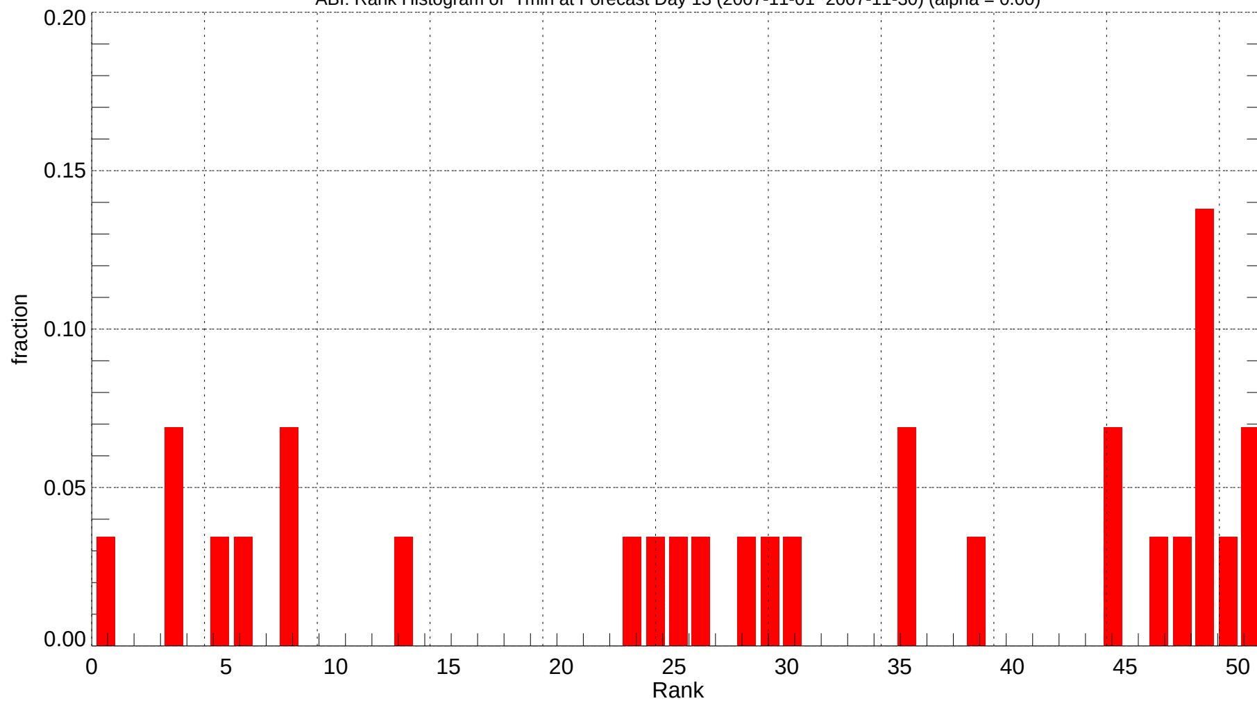
ABI: Rank Histogram of Tmin at Forecast Day 13 (2007-11-01~2007-11-30) (alpha = 0.00)
