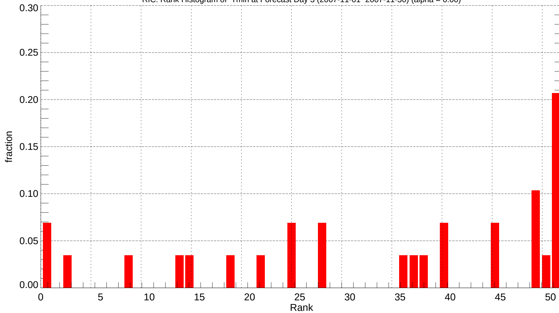
RIC: Rank Histogram of Tmin at Forecast Day 3 (2007-11-01~2007-11-30) (alpha = 0.00)
