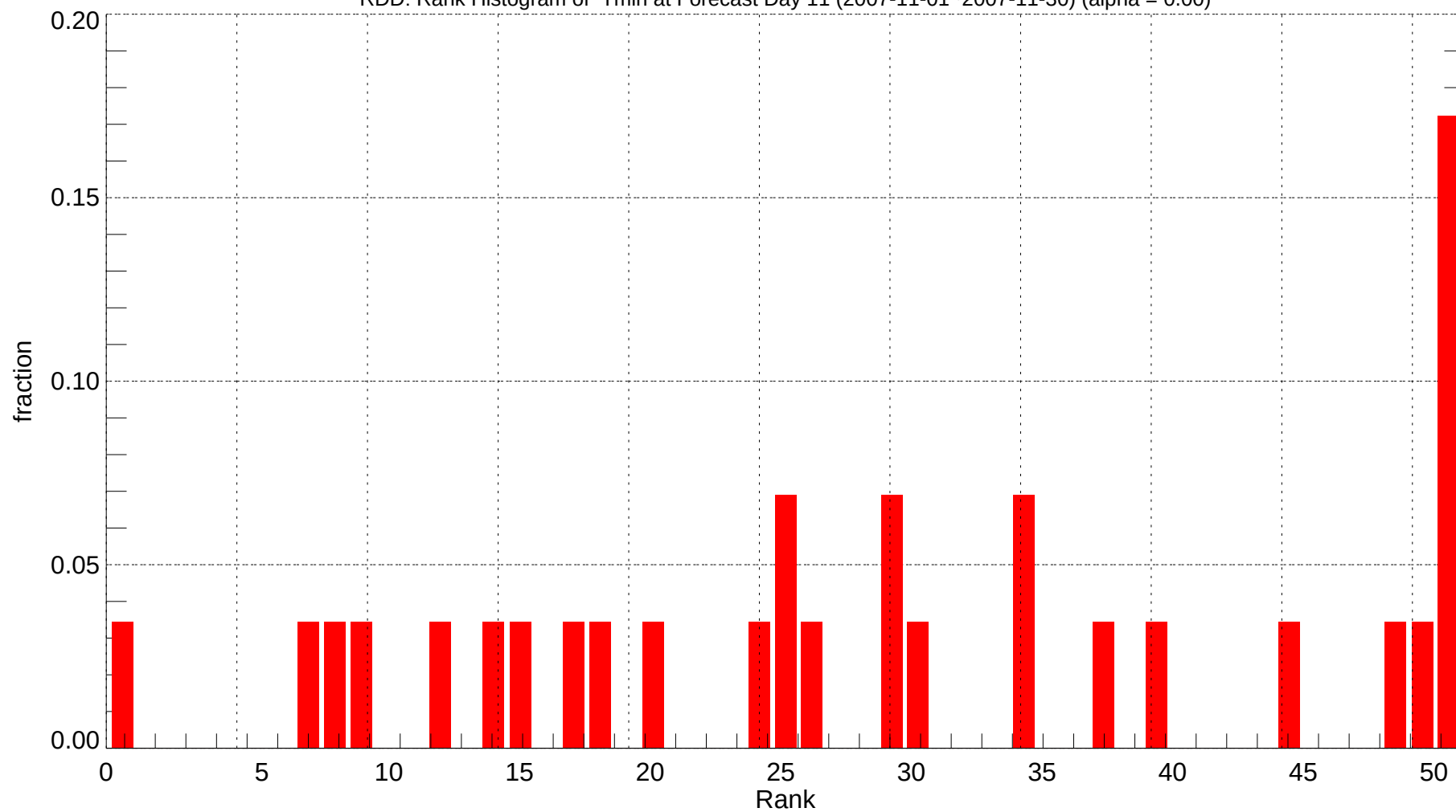
RDD: Rank Histogram of Tmin at Forecast Day 11 (2007-11-01~2007-11-30) (alpha = 0.00)
