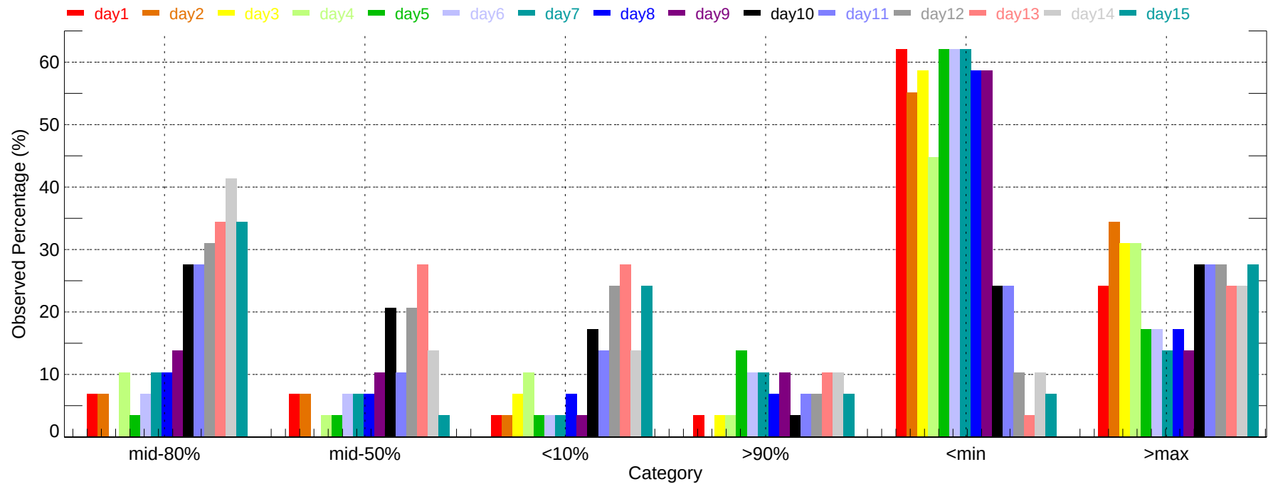
Observed Percentage of Ensembles - LAX: Max Temperature (2007-11-01~2007-11-30)
