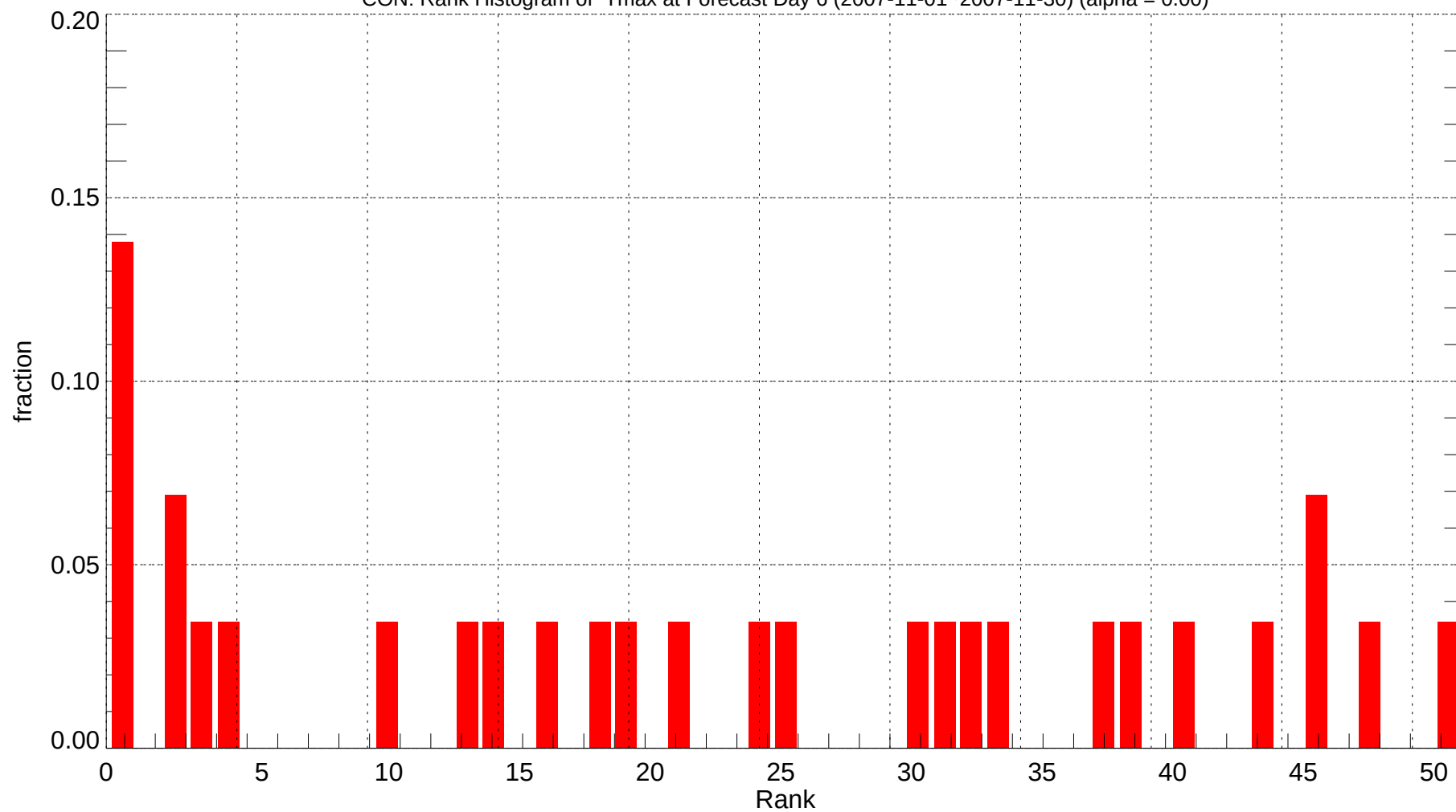
CON: Rank Histogram of Tmax at Forecast Day 6 (2007-11-01~2007-11-30) (alpha = 0.00)
