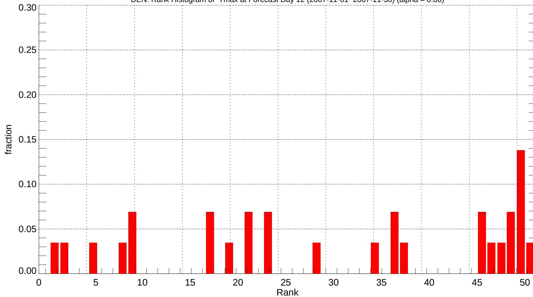
DEN: Rank Histogram of Tmax at Forecast Day 12 (2007-11-01~2007-11-30) (alpha = 0.00)
