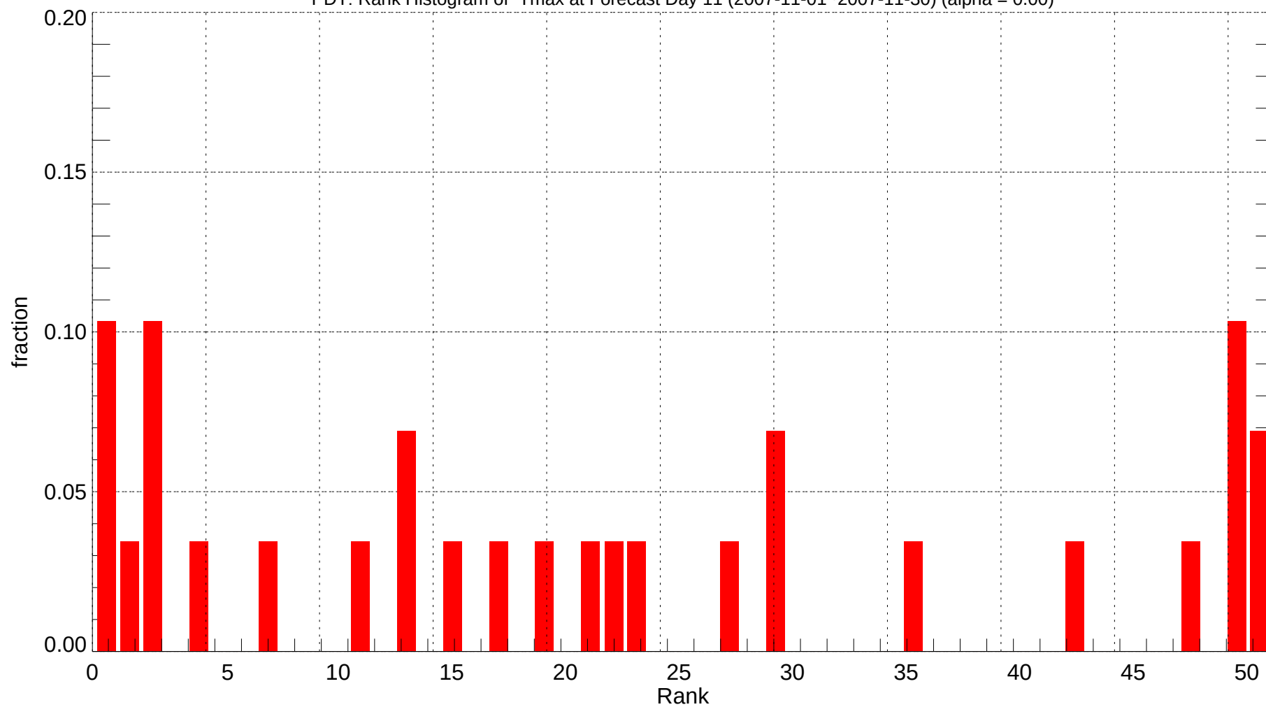
PDT: Rank Histogram of Tmax at Forecast Day 11 (2007-11-01~2007-11-30) (alpha = 0.00)
