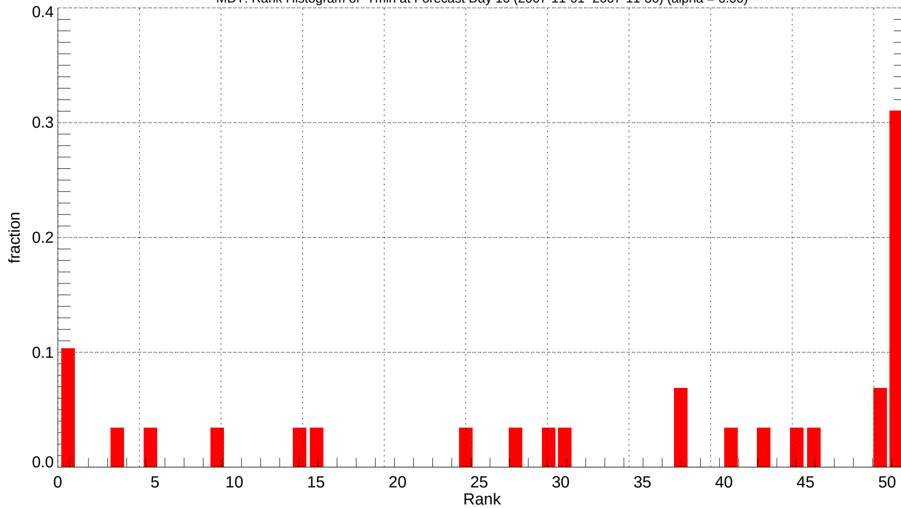
MDT: Rank Histogram of Tmin at Forecast Day 10 (2007-11-01~2007-11-30) (alpha = 0.00)
