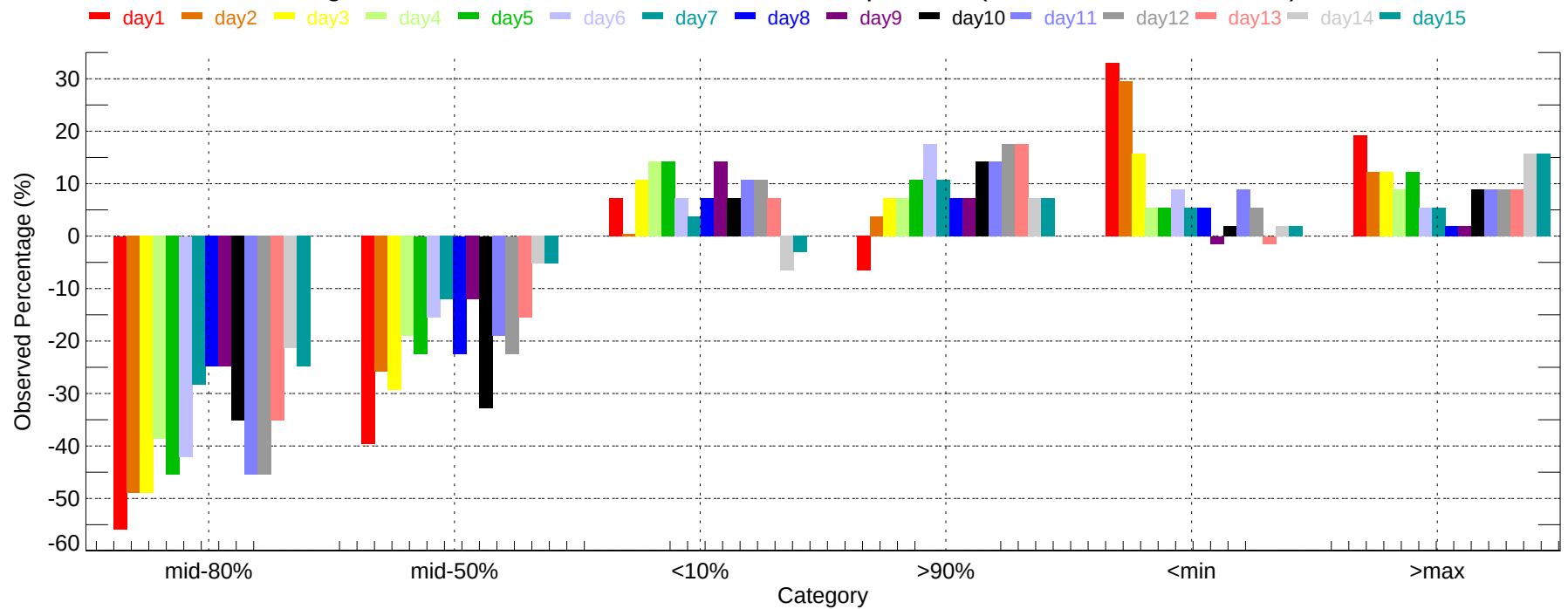
Observed Percentage Deviation of Ensembles - BUR: Min Temperature (2007-11-01~2007-11-30)
