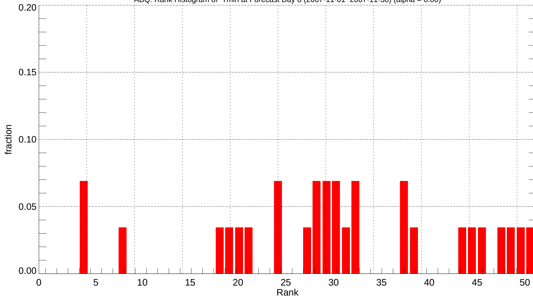
ABQ: Rank Histogram of Tmin at Forecast Day 8 (2007-11-01~2007-11-30) (alpha = 0.00)
