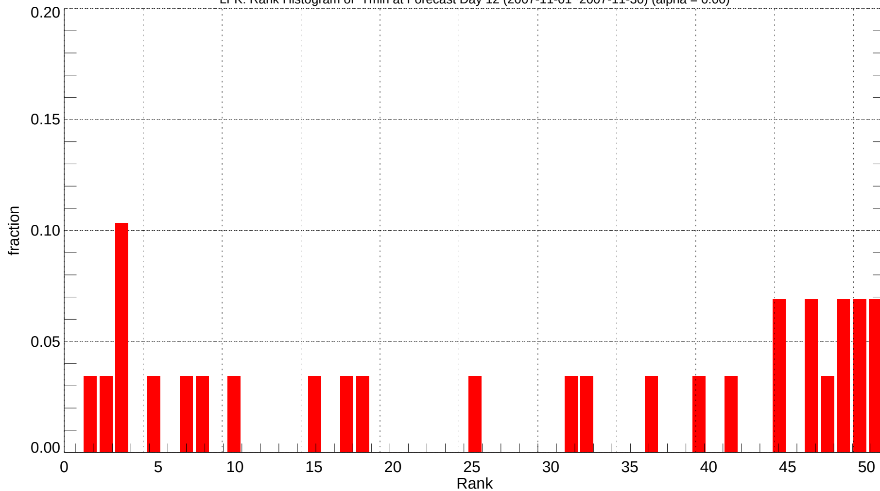
LFK: Rank Histogram of Tmin at Forecast Day 12 (2007-11-01~2007-11-30) (alpha = 0.00)
