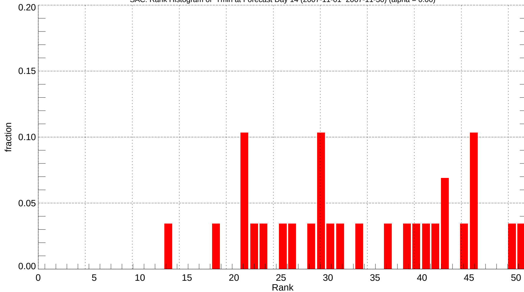
SAC: Rank Histogram of Tmin at Forecast Day 14 (2007-11-01~2007-11-30) (alpha = 0.00)
