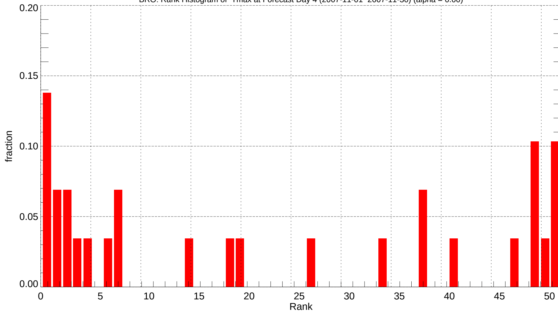
BRO: Rank Histogram of Tmax at Forecast Day 4 (2007-11-01~2007-11-30) (alpha = 0.00)
