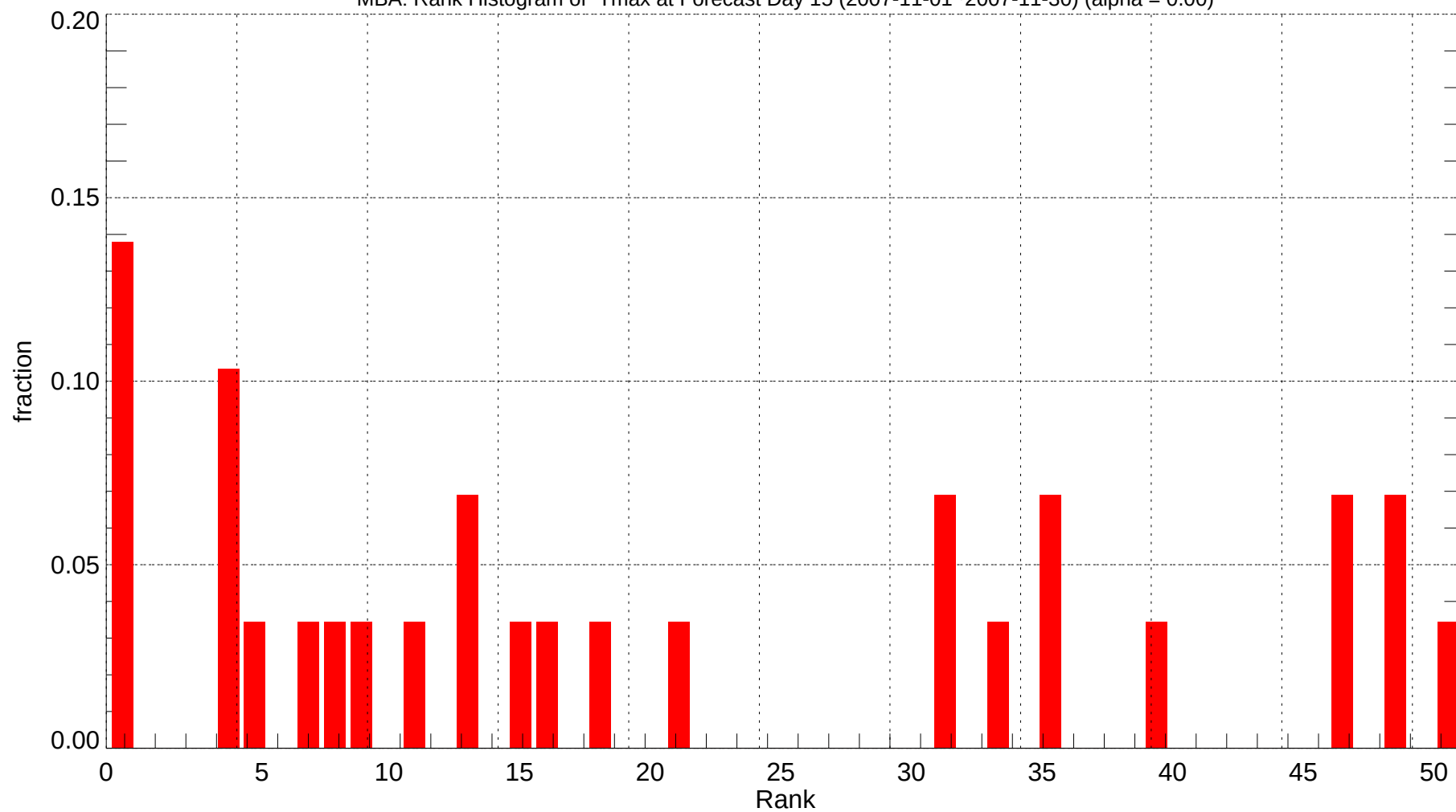
MBA: Rank Histogram of Tmax at Forecast Day 15 (2007-11-01~2007-11-30) (alpha = 0.00)
