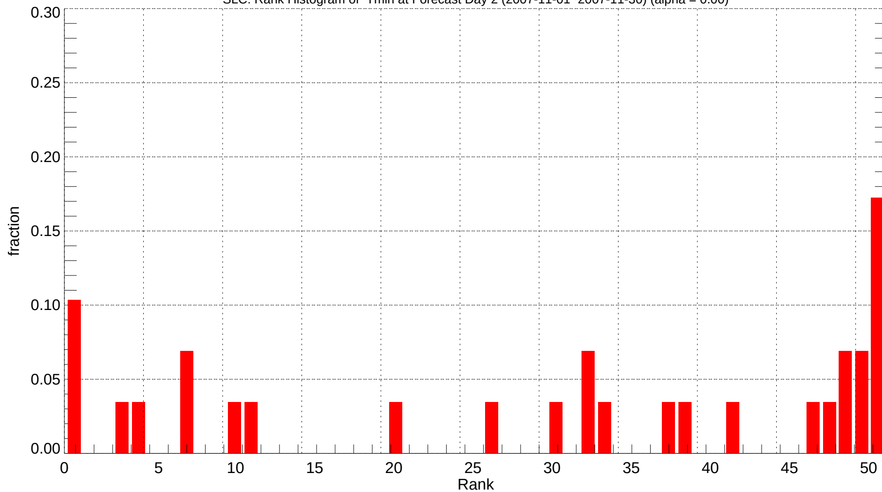
SLC: Rank Histogram of Tmin at Forecast Day 2 (2007-11-01~2007-11-30) (alpha = 0.00)
