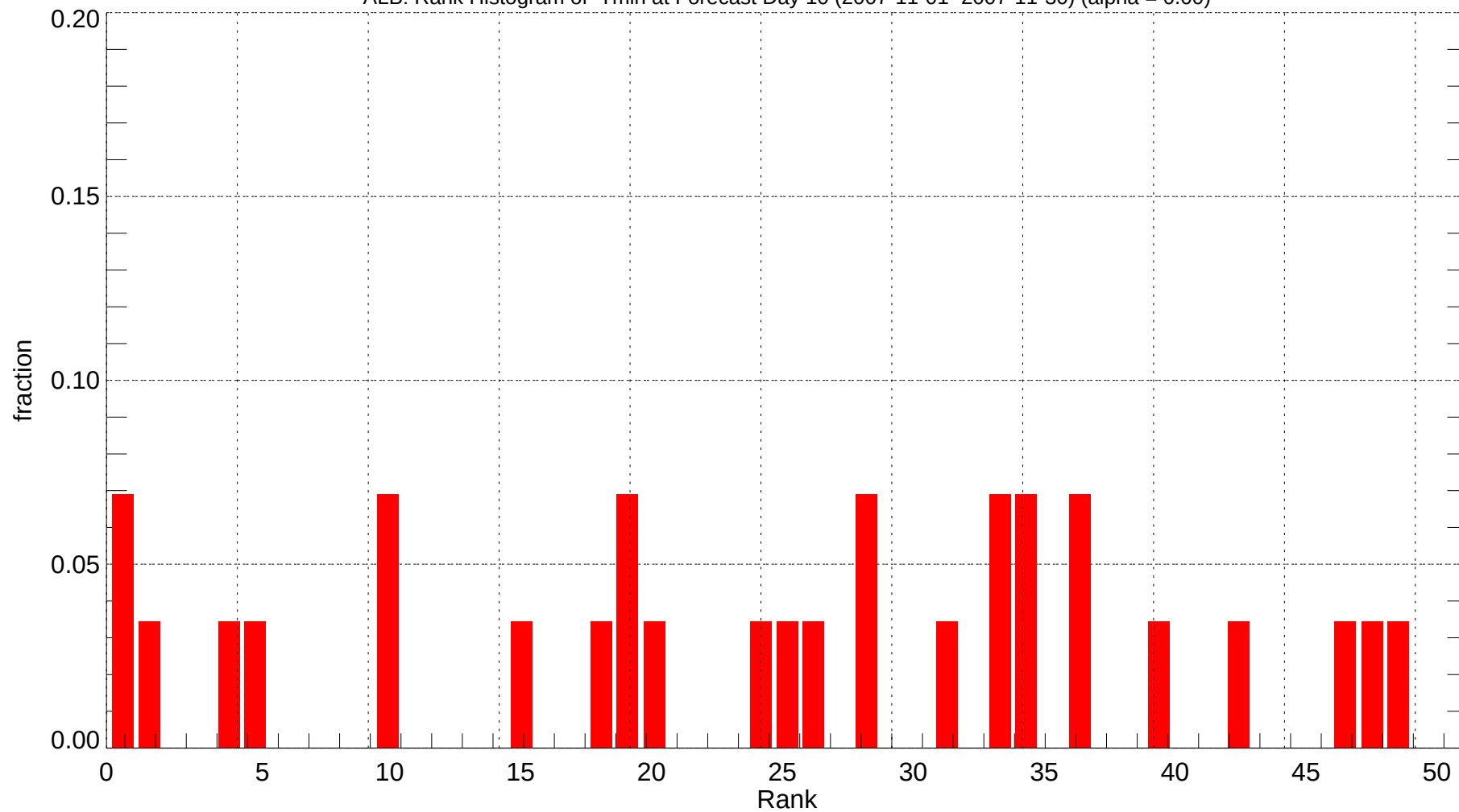
ALB: Rank Histogram of Tmin at Forecast Day 10 (2007-11-01~2007-11-30) (alpha = 0.00)
