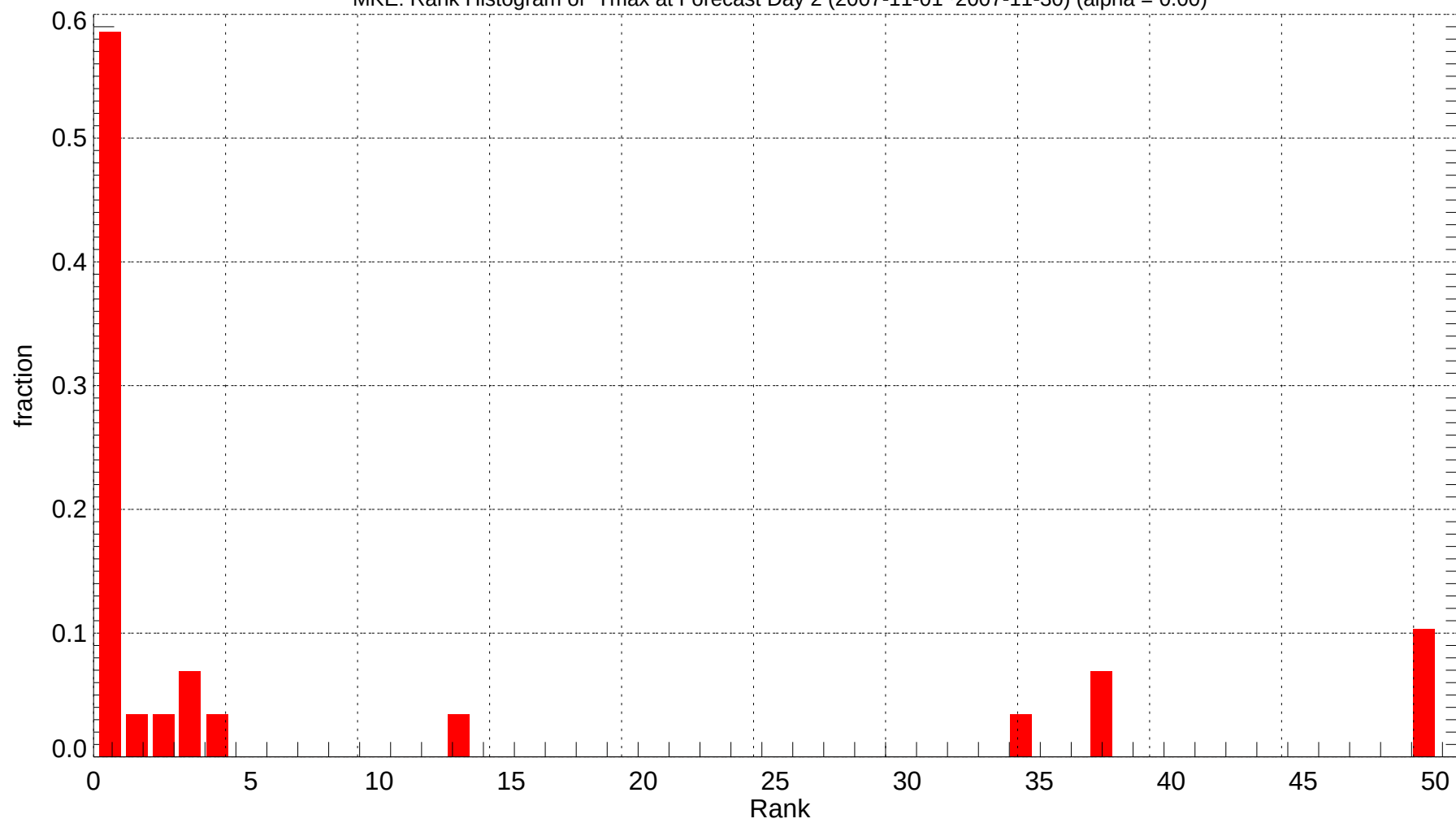
MKE: Rank Histogram of Tmax at Forecast Day 2 (2007-11-01~2007-11-30) (alpha = 0.00)
