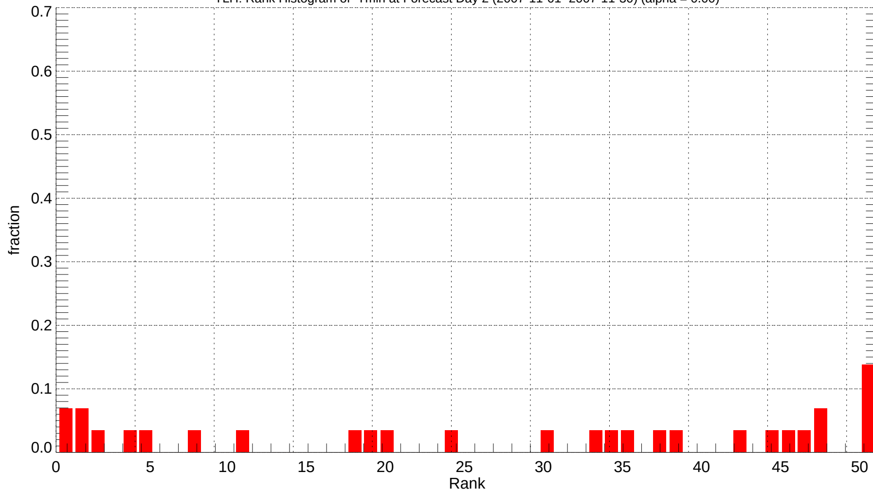
TLH: Rank Histogram of Tmin at Forecast Day 2 (2007-11-01~2007-11-30) (alpha = 0.00)
