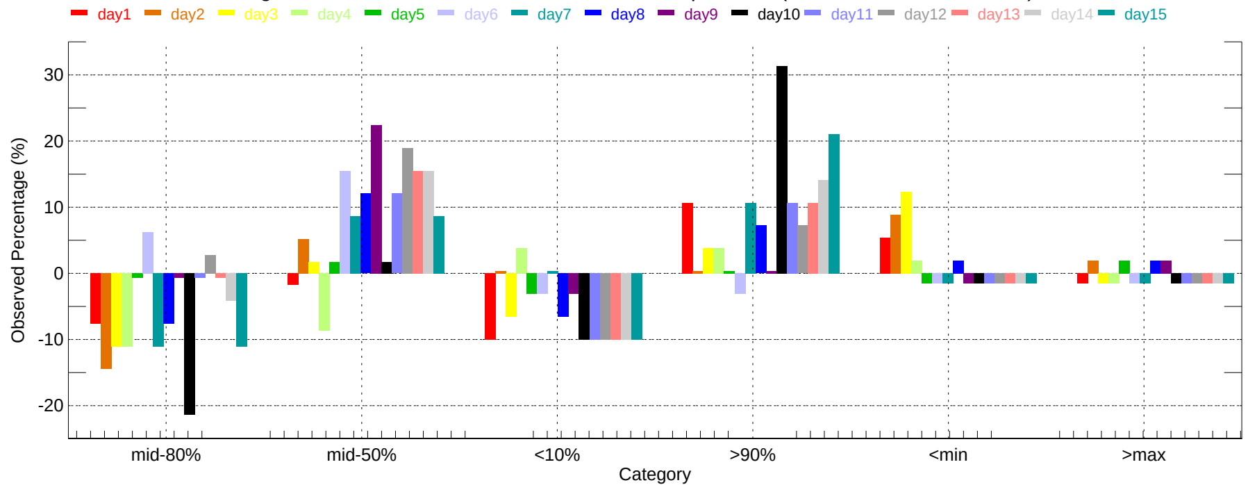
Observed Percentage Deviation of Ensembles - FAT: Max Temperature (2007-11-01~2007-11-30)
