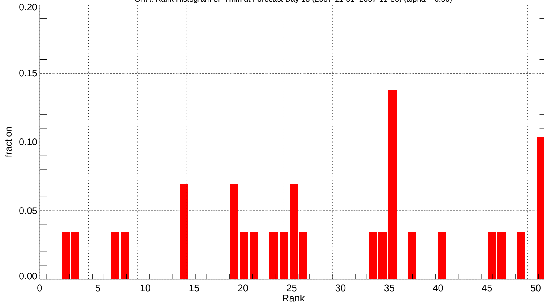
CHA: Rank Histogram of Tmin at Forecast Day 15 (2007-11-01~2007-11-30) (alpha = 0.00)
