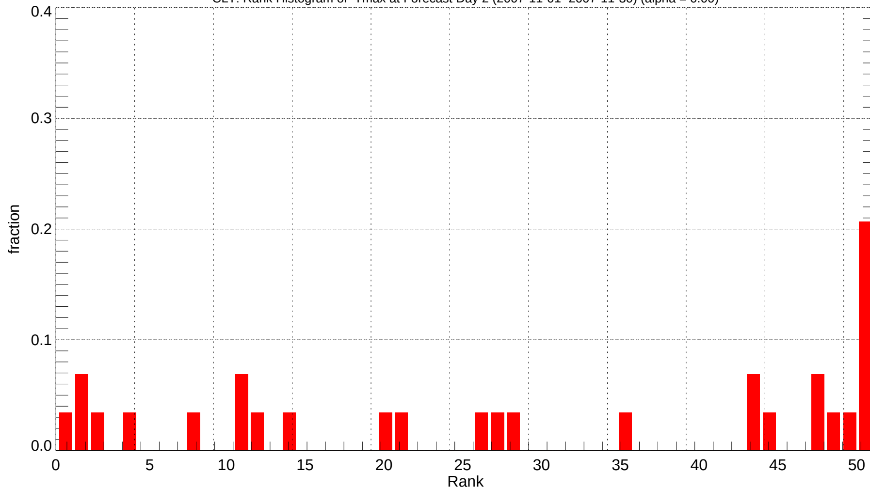
CLT: Rank Histogram of Tmax at Forecast Day 2 (2007-11-01~2007-11-30) (alpha = 0.00)
