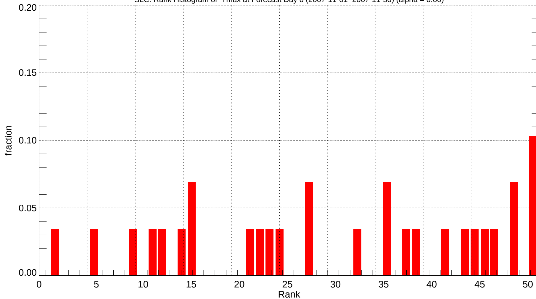
SLC: Rank Histogram of Tmax at Forecast Day 6 (2007-11-01~2007-11-30) (alpha = 0.00)
