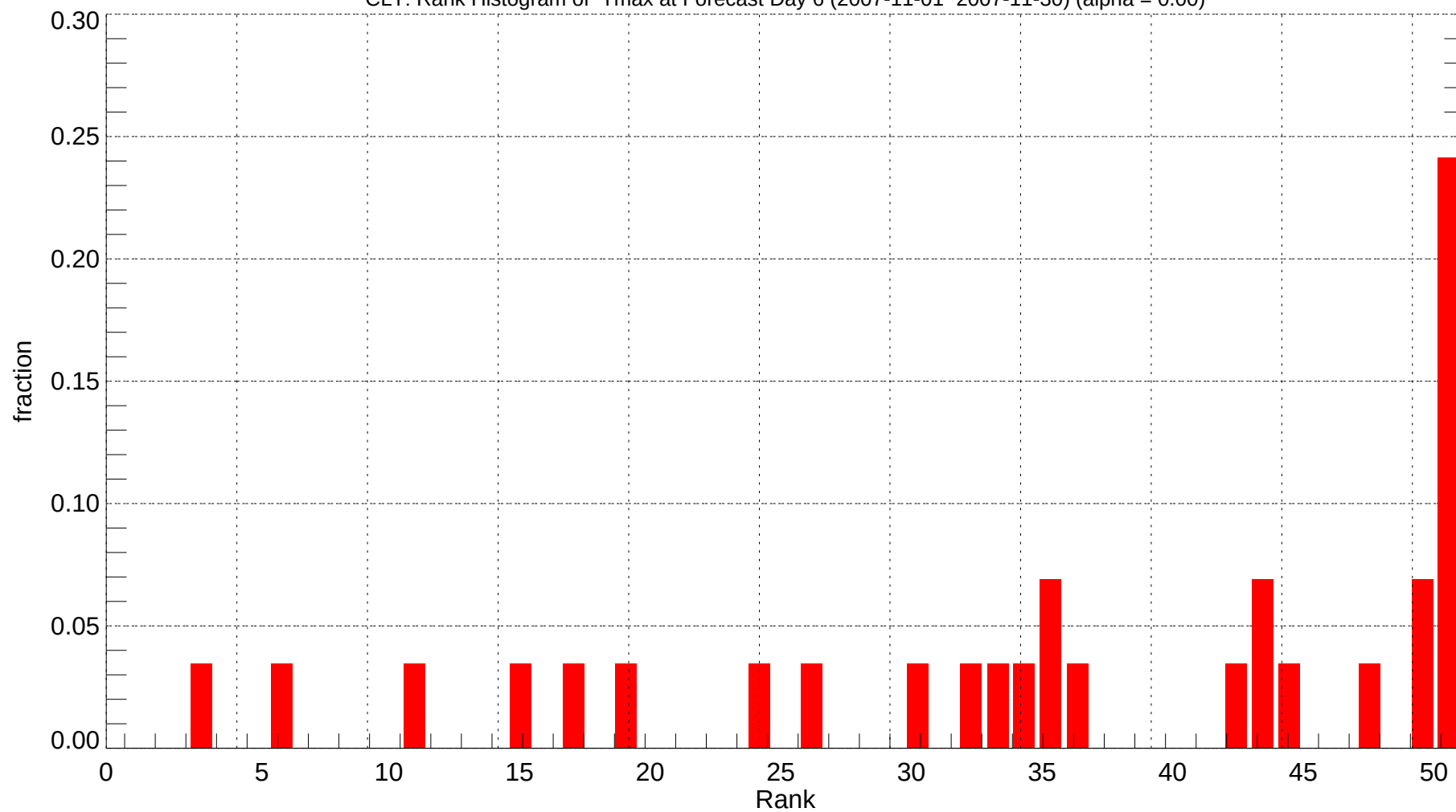
CLT: Rank Histogram of Tmax at Forecast Day 6 (2007-11-01~2007-11-30) (alpha = 0.00)
