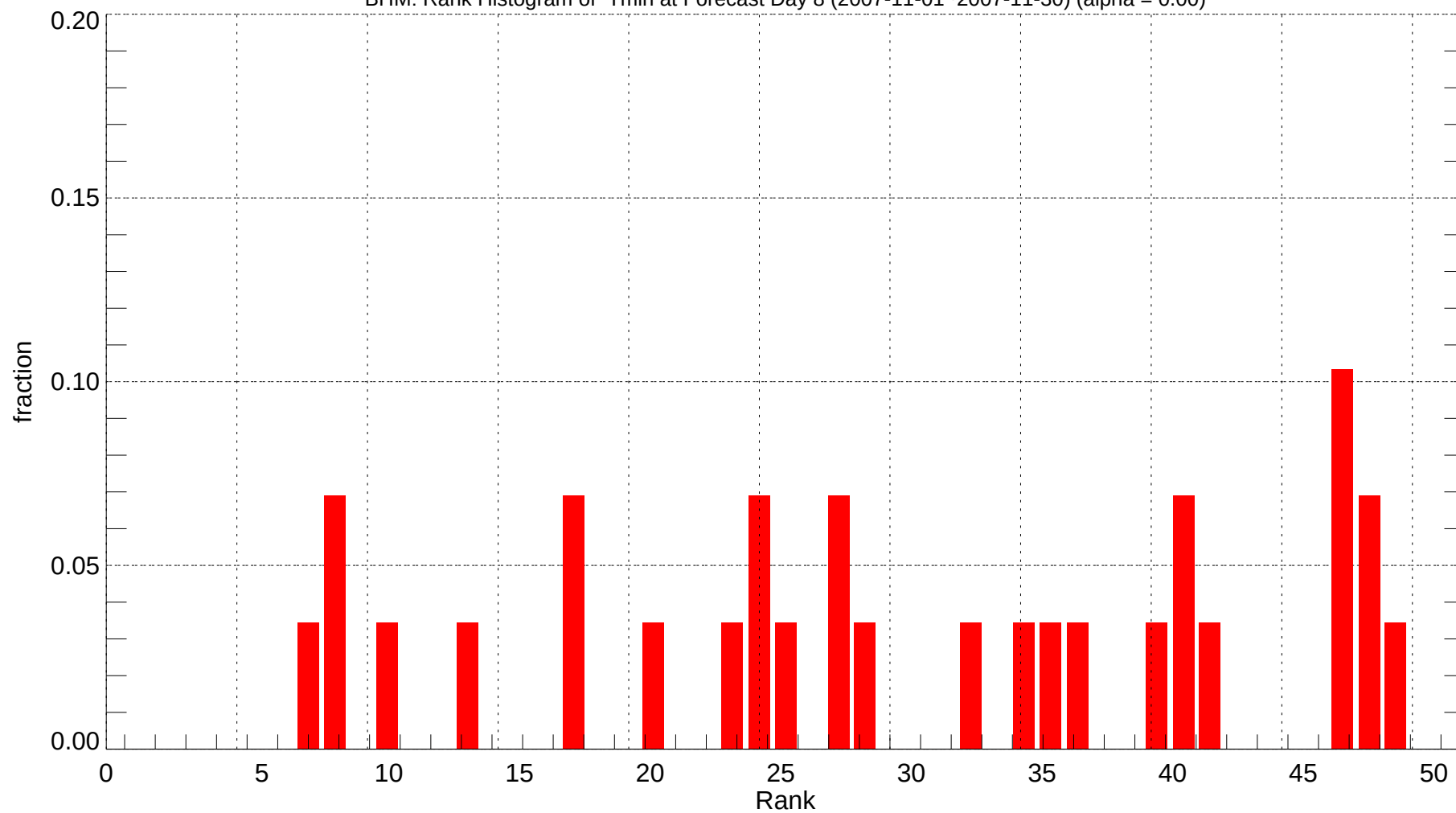
BHM: Rank Histogram of Tmin at Forecast Day 8 (2007-11-01~2007-11-30) (alpha = 0.00)
