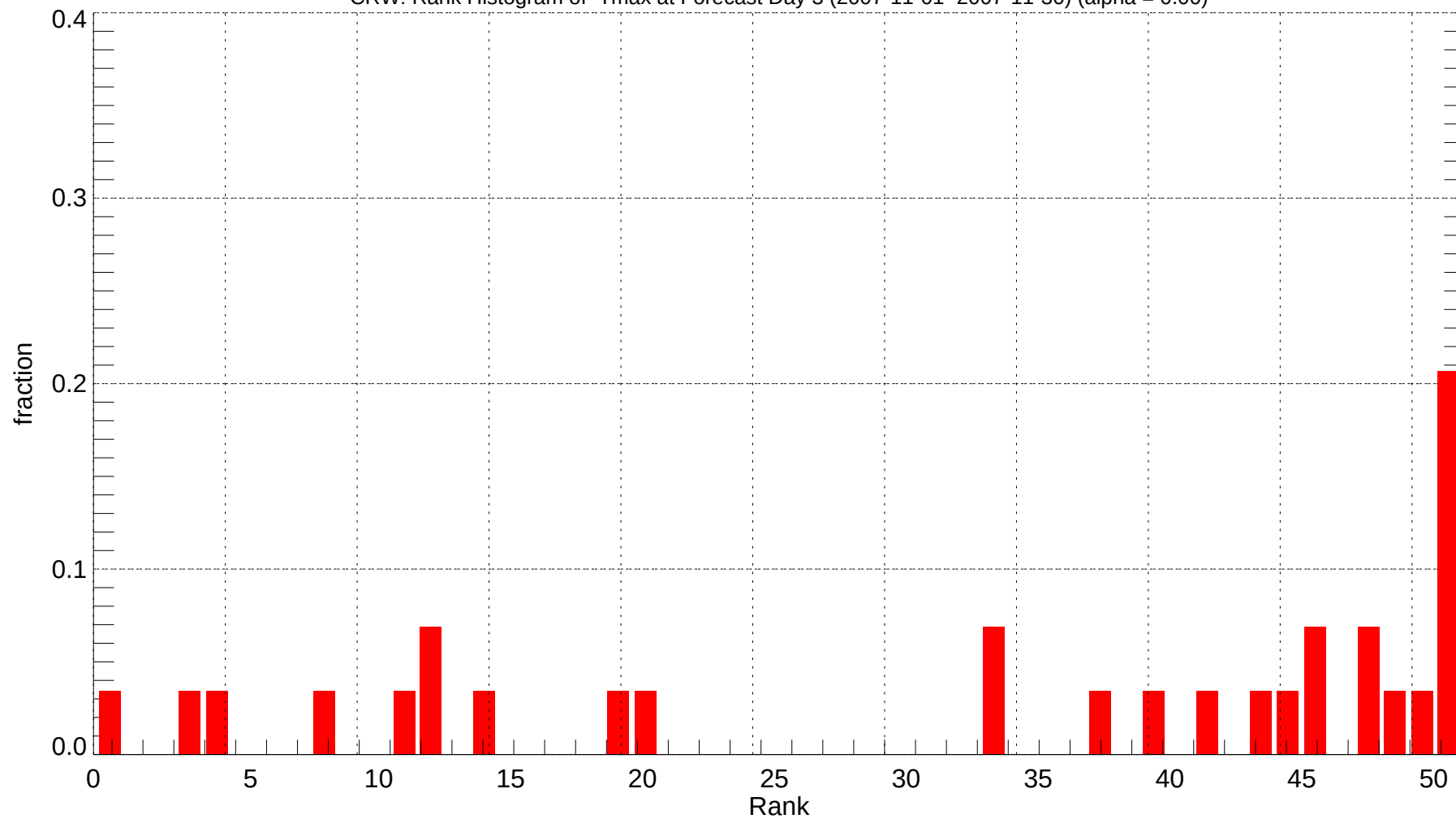
CRW: Rank Histogram of Tmax at Forecast Day 3 (2007-11-01~2007-11-30) (alpha = 0.00)
