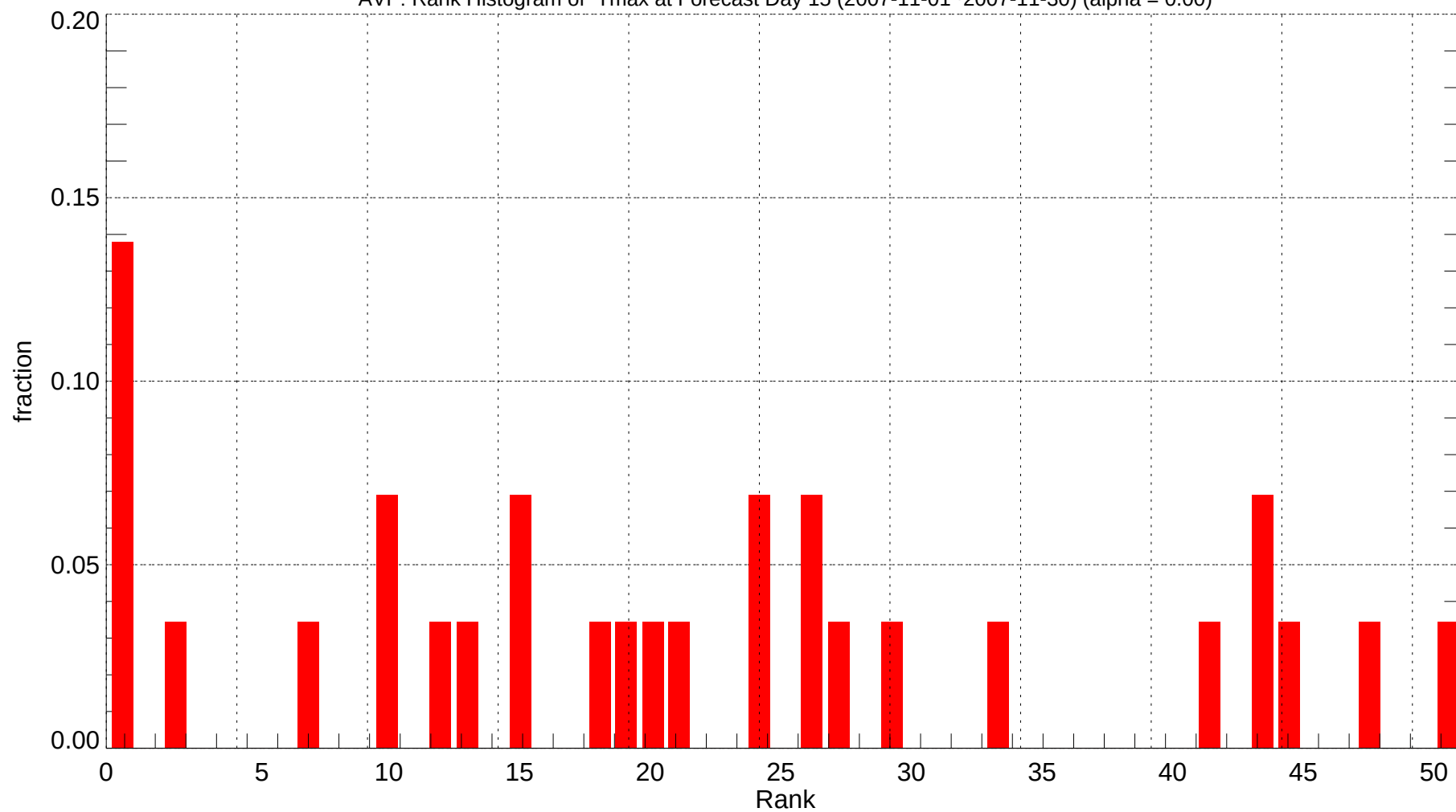
AVP: Rank Histogram of Tmax at Forecast Day 15 (2007-11-01~2007-11-30) (alpha = 0.00)
