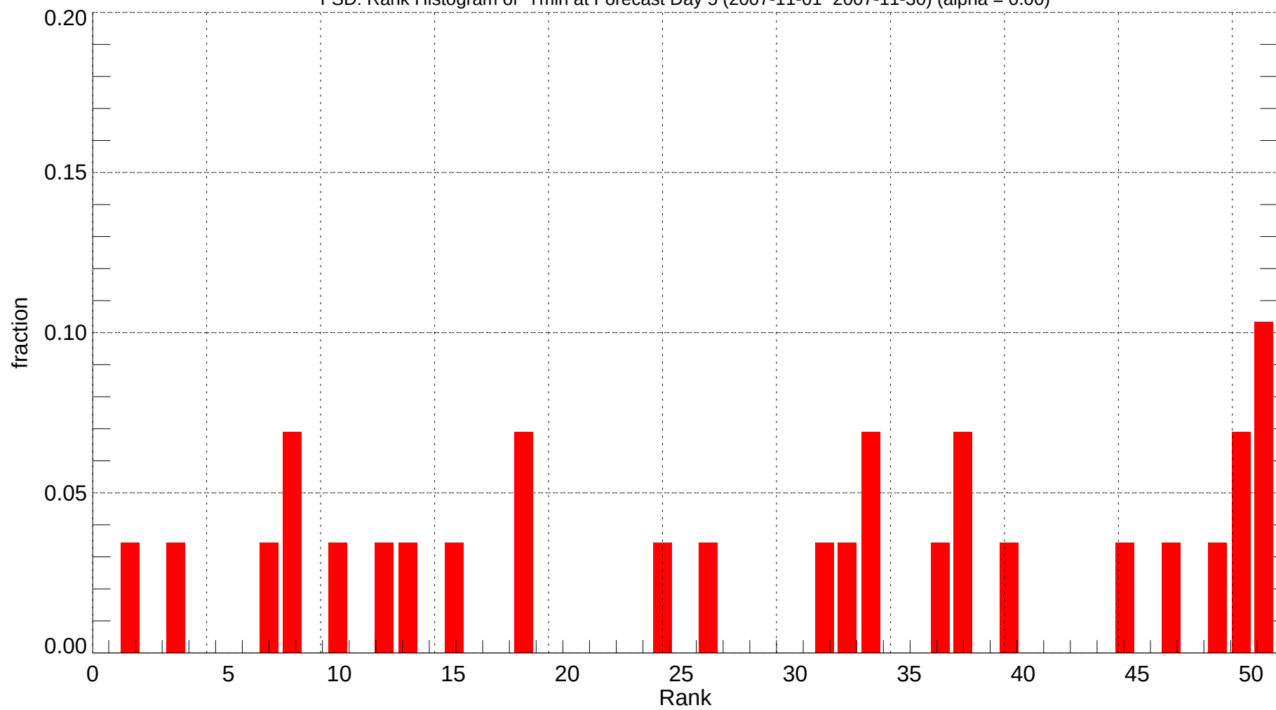
FSD: Rank Histogram of Tmin at Forecast Day 5 (2007-11-01~2007-11-30) (alpha = 0.00)
