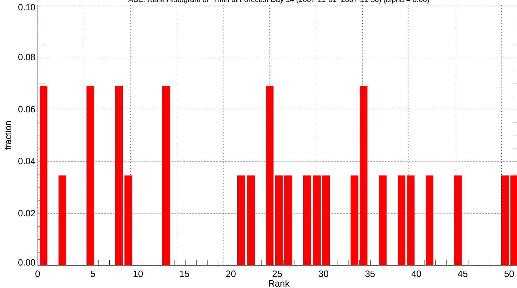
ABE: Rank Histogram of Tmin at Forecast Day 14 (2007-11-01~2007-11-30) (alpha = 0.00)
