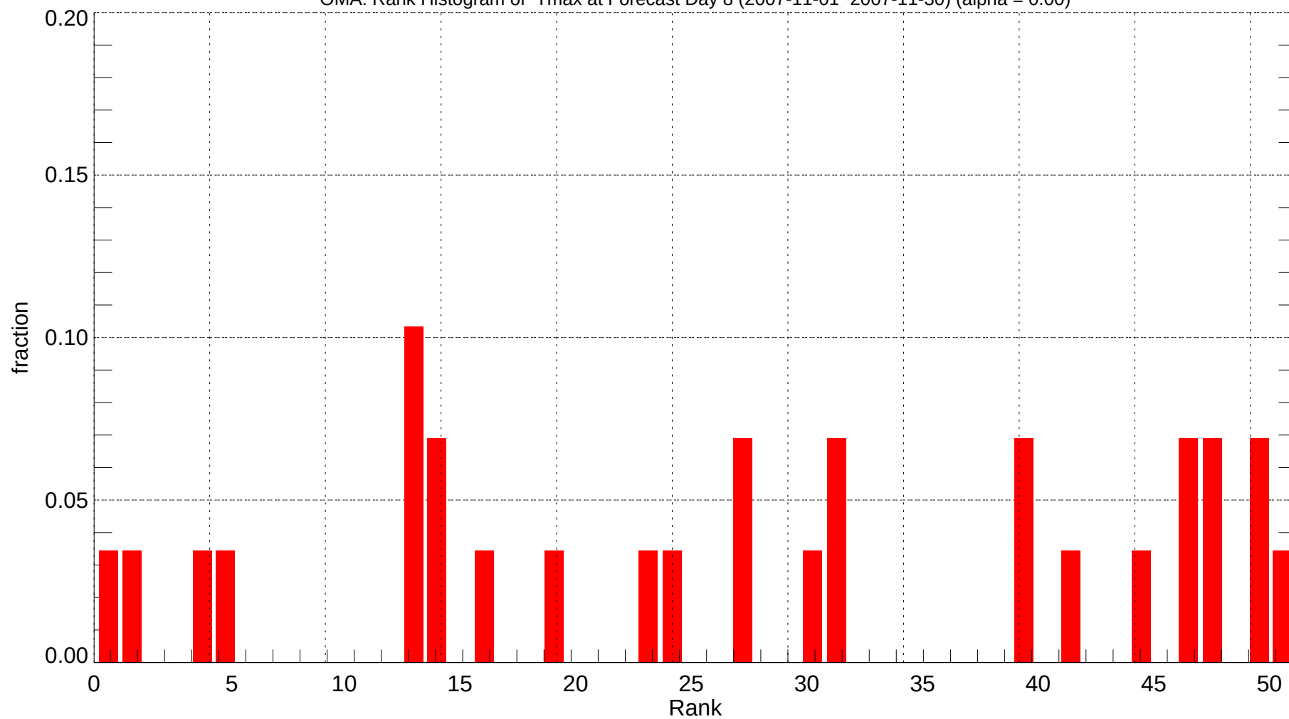
OMA: Rank Histogram of Tmax at Forecast Day 8 (2007-11-01~2007-11-30) (alpha = 0.00)
