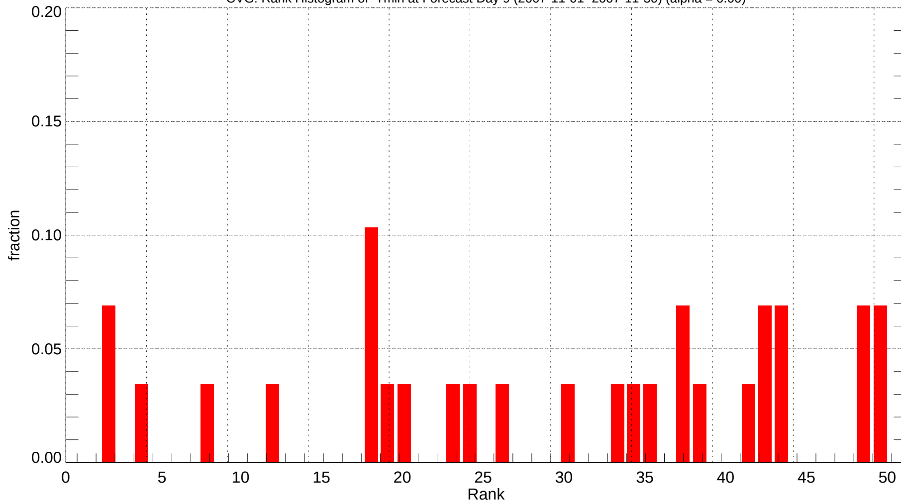
CVG: Rank Histogram of Tmin at Forecast Day 9 (2007-11-01~2007-11-30) (alpha = 0.00)
