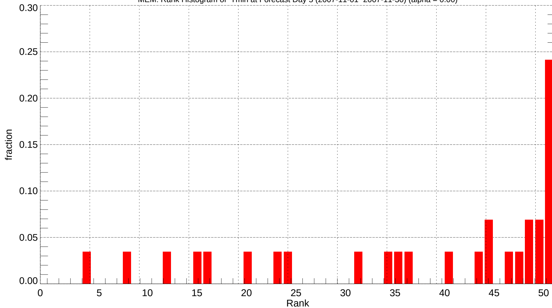
MEM: Rank Histogram of Tmin at Forecast Day 5 (2007-11-01~2007-11-30) (alpha = 0.00)
