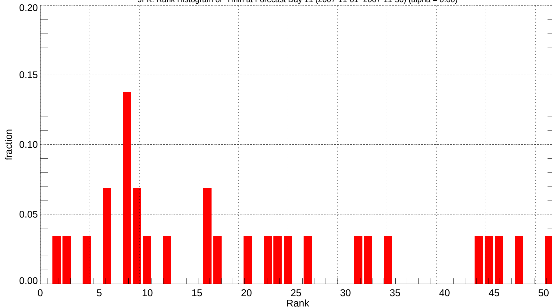
JFK: Rank Histogram of Tmin at Forecast Day 11 (2007-11-01~2007-11-30) (alpha = 0.00)
