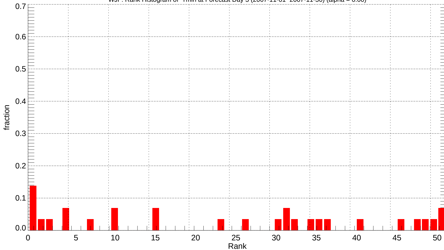
WJF: Rank Histogram of Tmin at Forecast Day 3 (2007-11-01~2007-11-30) (alpha = 0.00)
