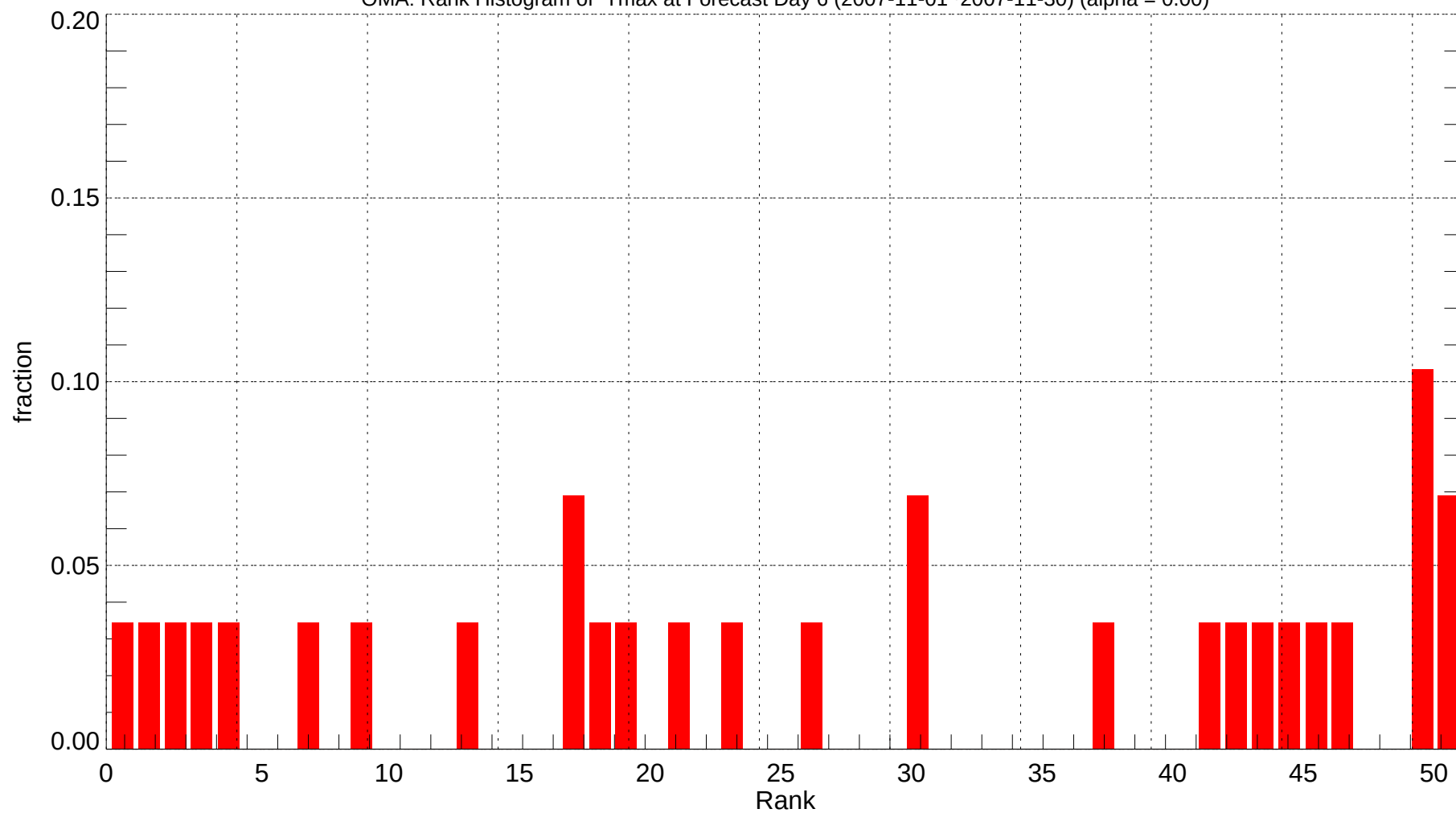
OMA: Rank Histogram of Tmax at Forecast Day 6 (2007-11-01~2007-11-30) (alpha = 0.00)
