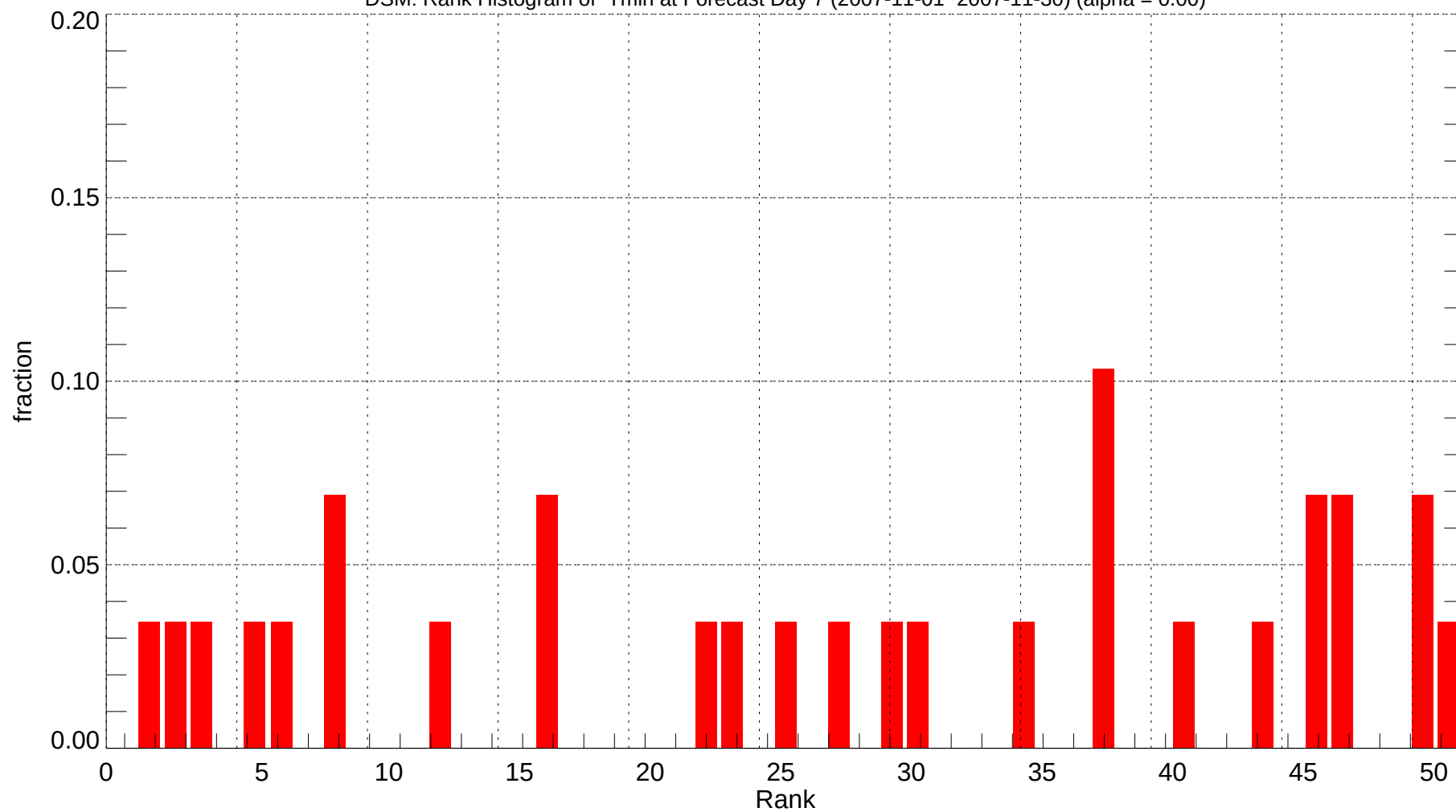
DSM: Rank Histogram of Tmin at Forecast Day 7 (2007-11-01~2007-11-30) (alpha = 0.00)
