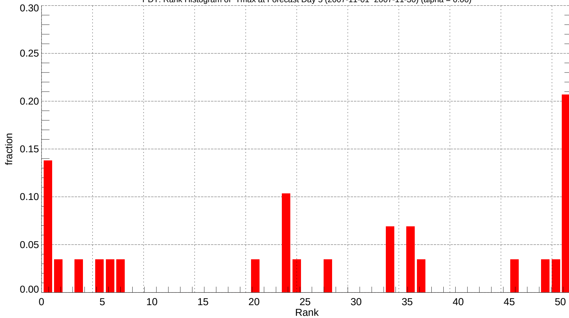
PDT: Rank Histogram of Tmax at Forecast Day 5 (2007-11-01~2007-11-30) (alpha = 0.00)
