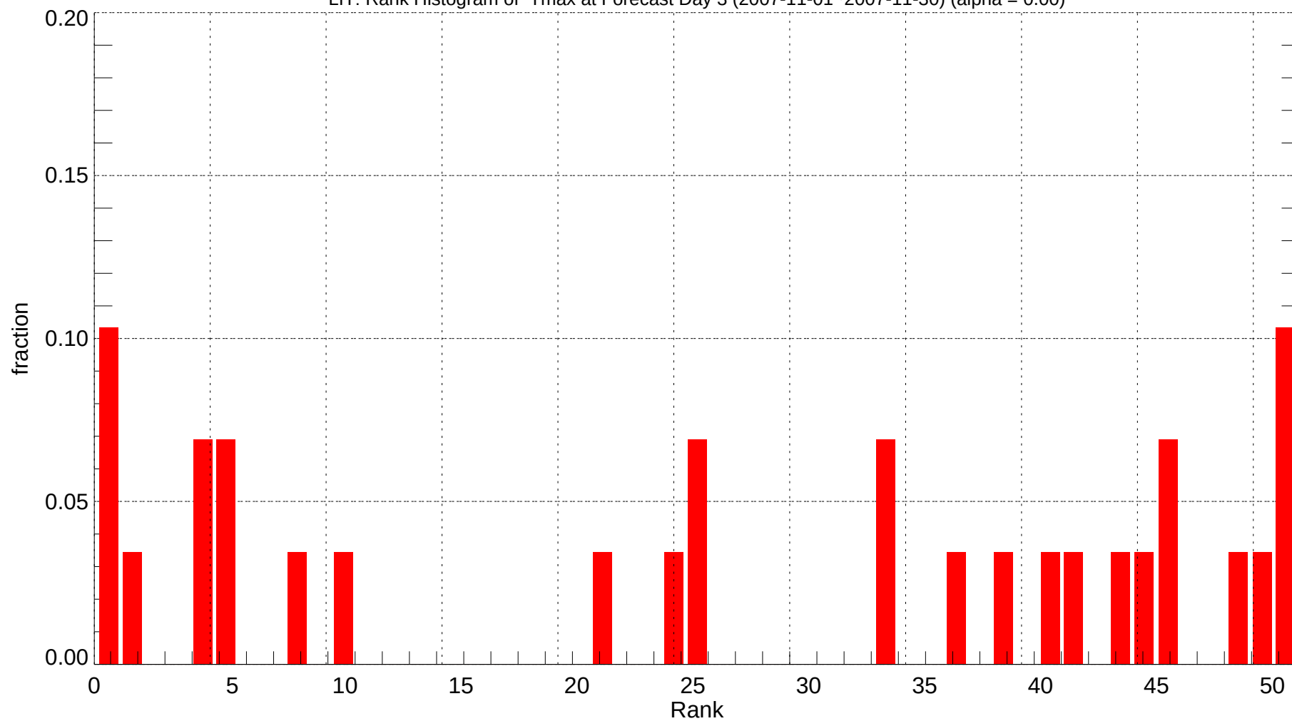
LIT: Rank Histogram of Tmax at Forecast Day 3 (2007-11-01~2007-11-30) (alpha = 0.00)
