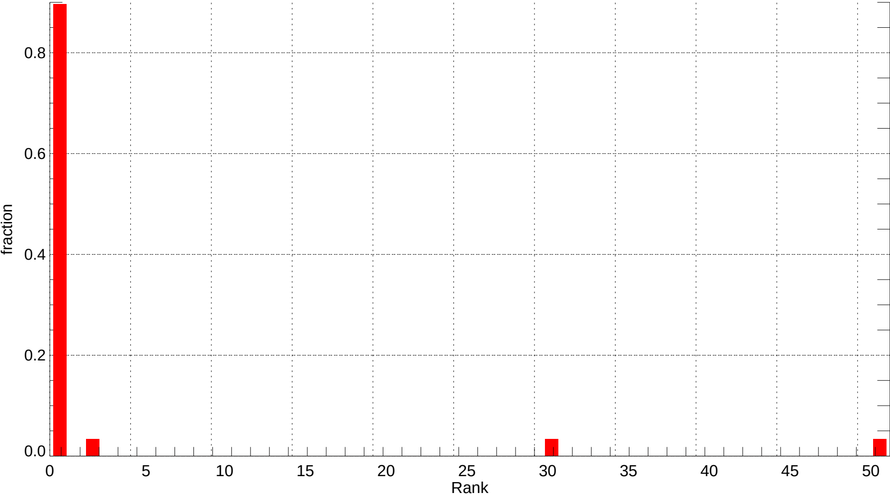
YYZ: Rank Histogram of Tmin at Forecast Day 3 (2007-11-01~2007-11-30) (alpha = 0.00)
