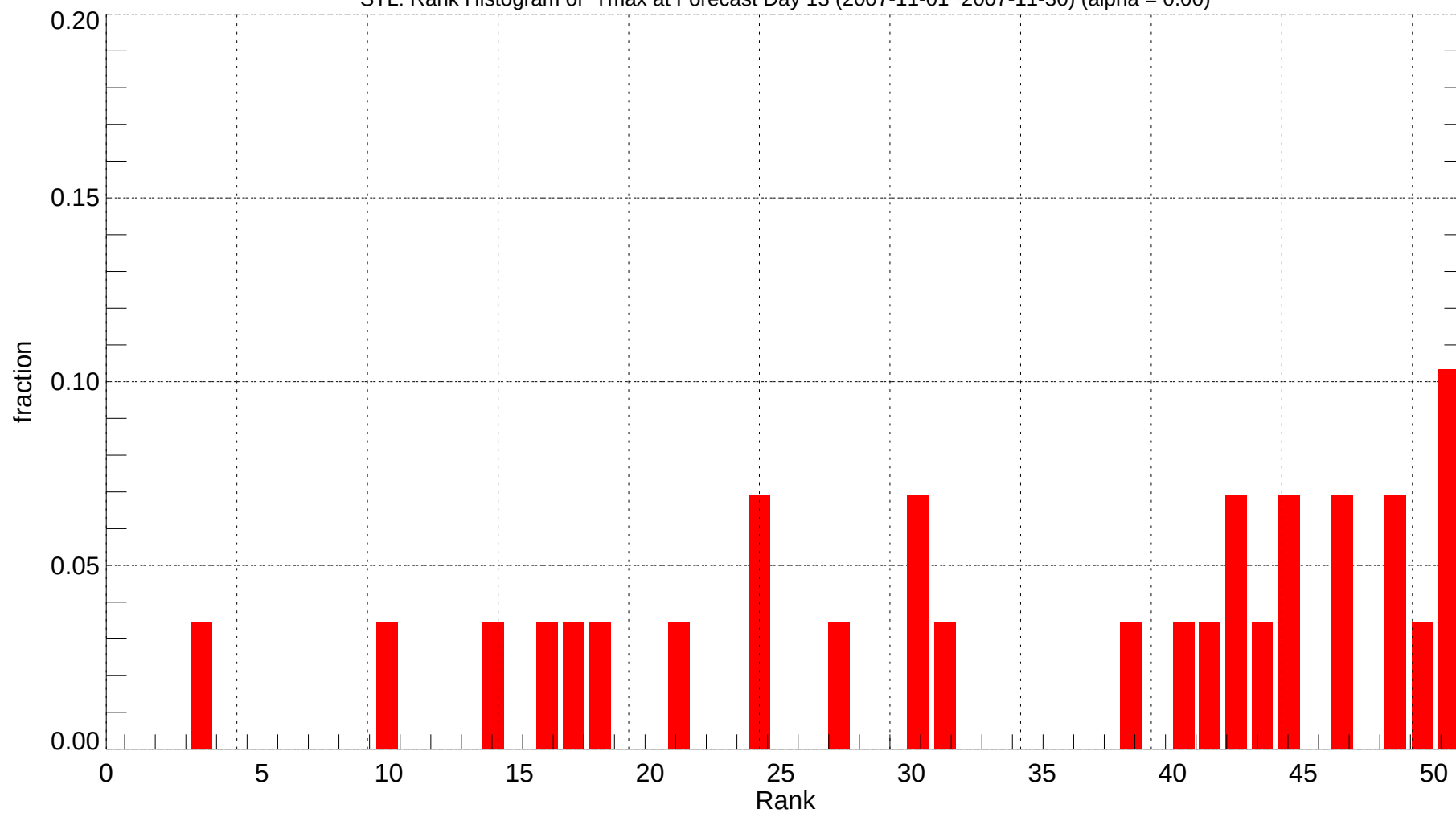
STL: Rank Histogram of Tmax at Forecast Day 13 (2007-11-01~2007-11-30) (alpha = 0.00)
