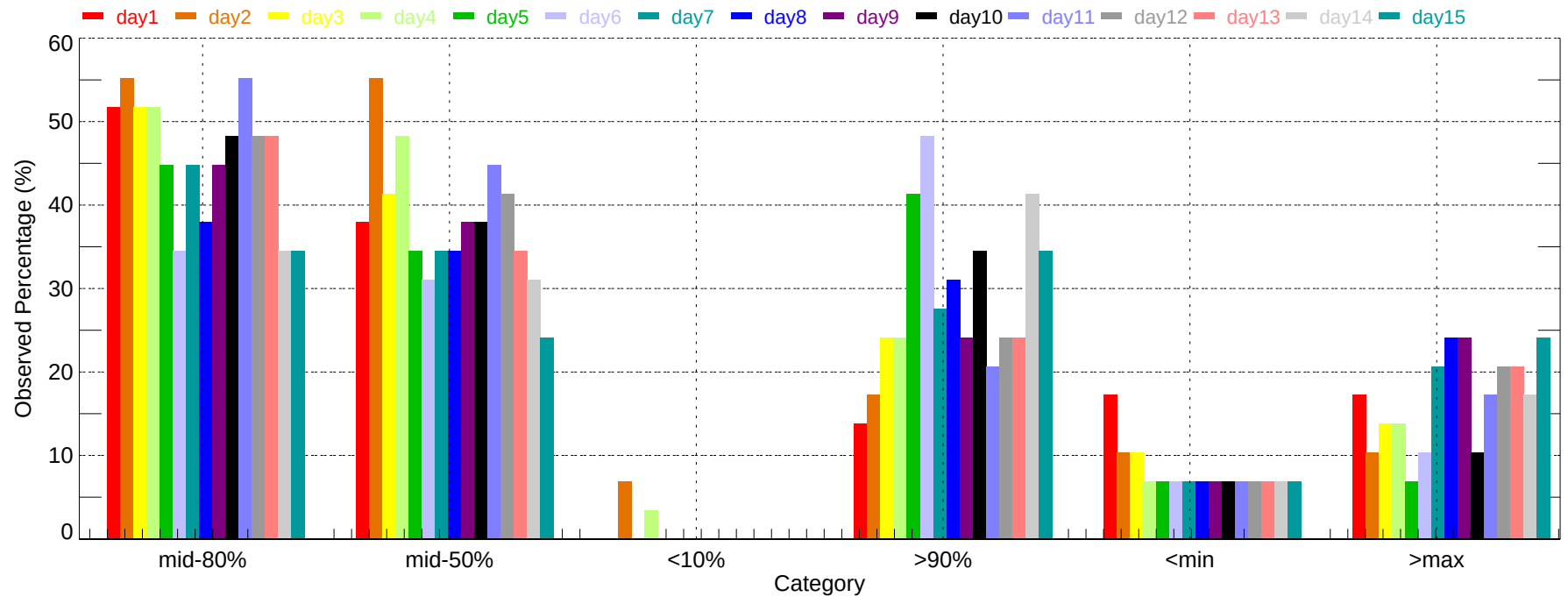
Observed Percentage of Ensembles - FLG: Max Temperature (2007-11-01~2007-11-30)
