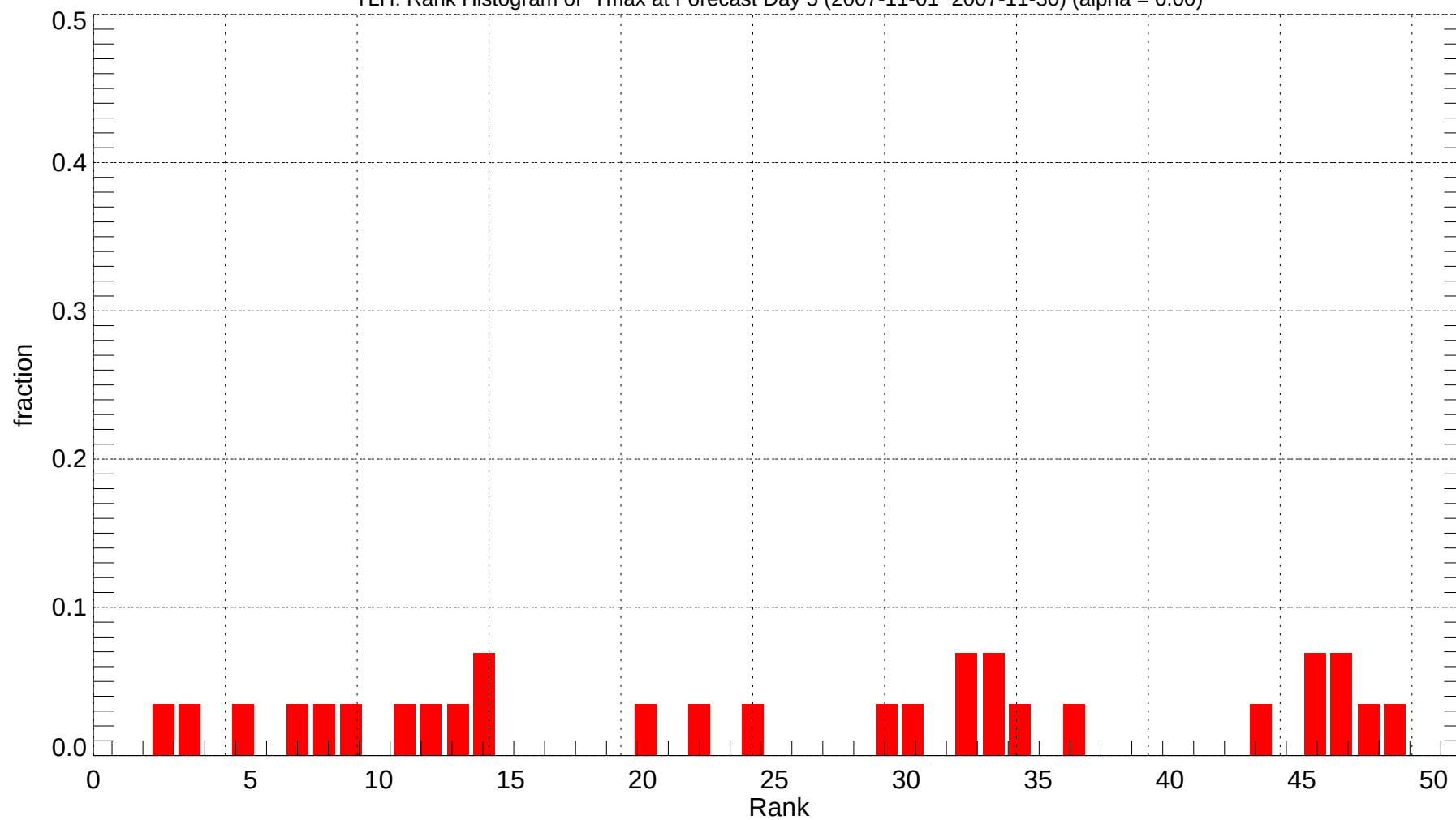
TLH: Rank Histogram of Tmax at Forecast Day 5 (2007-11-01~2007-11-30) (alpha = 0.00)
