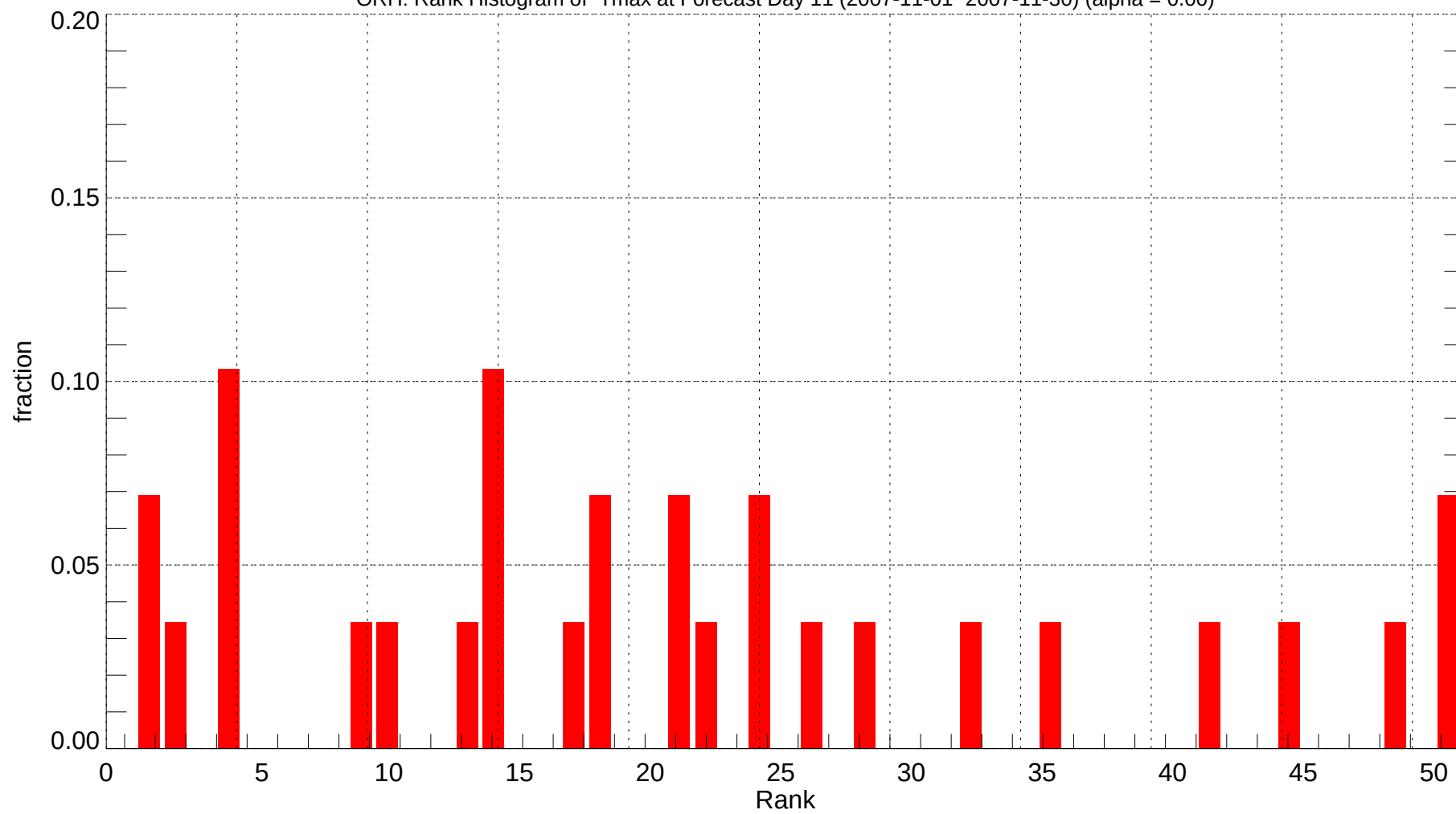
ORH: Rank Histogram of Tmax at Forecast Day 11 (2007-11-01~2007-11-30) (alpha = 0.00)
