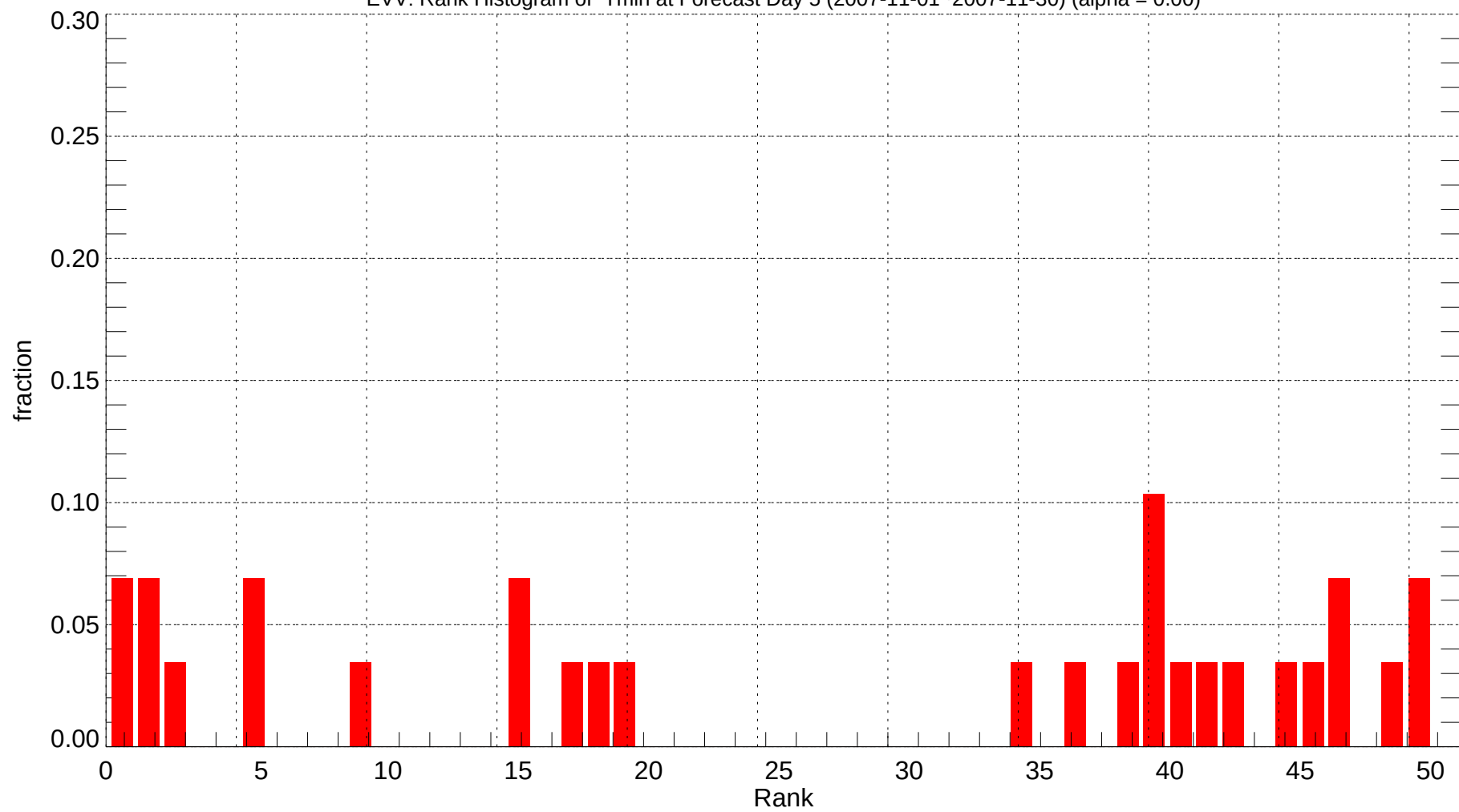
EVV: Rank Histogram of Tmin at Forecast Day 5 (2007-11-01~2007-11-30) (alpha = 0.00)
