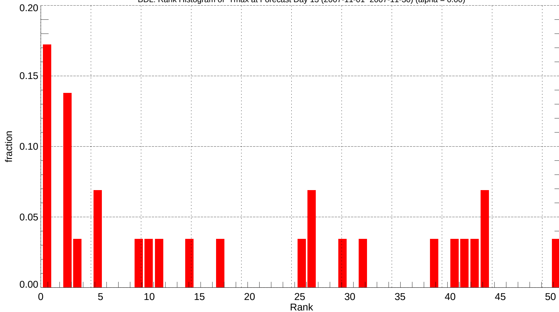
BDL: Rank Histogram of Tmax at Forecast Day 13 (2007-11-01~2007-11-30) (alpha = 0.00)
