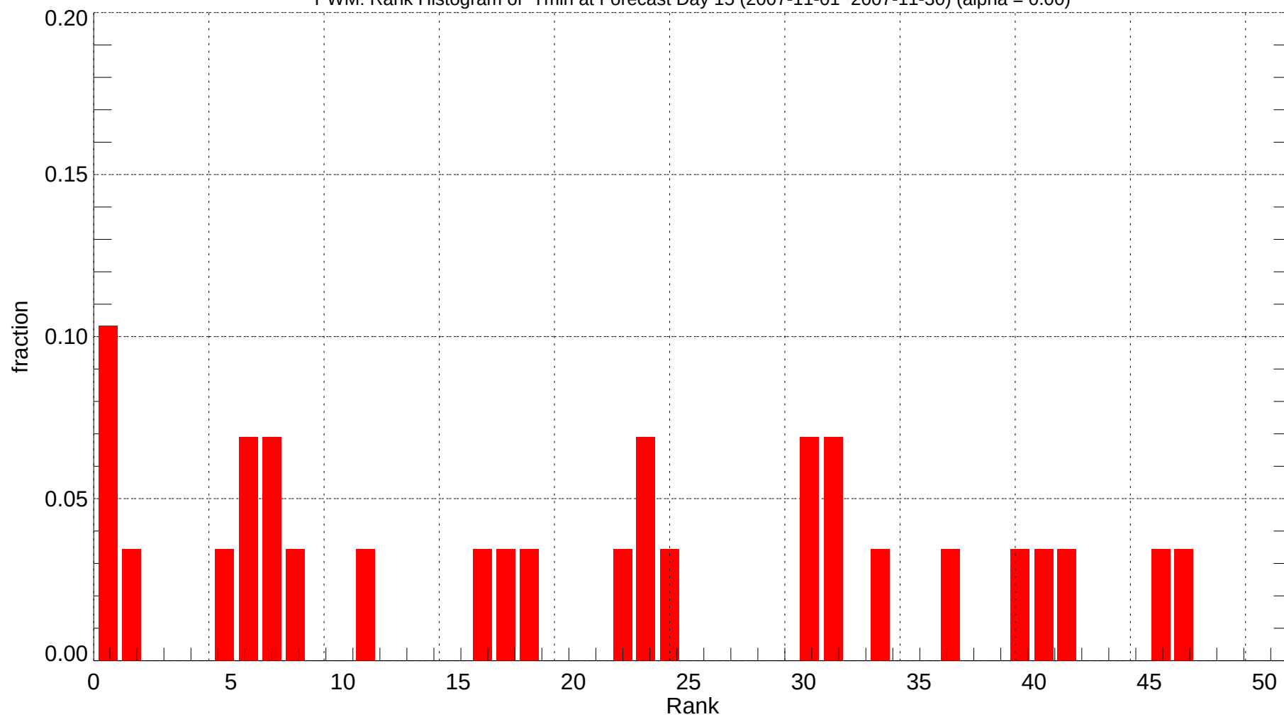
PWM: Rank Histogram of Tmin at Forecast Day 15 (2007-11-01~2007-11-30) (alpha = 0.00)
