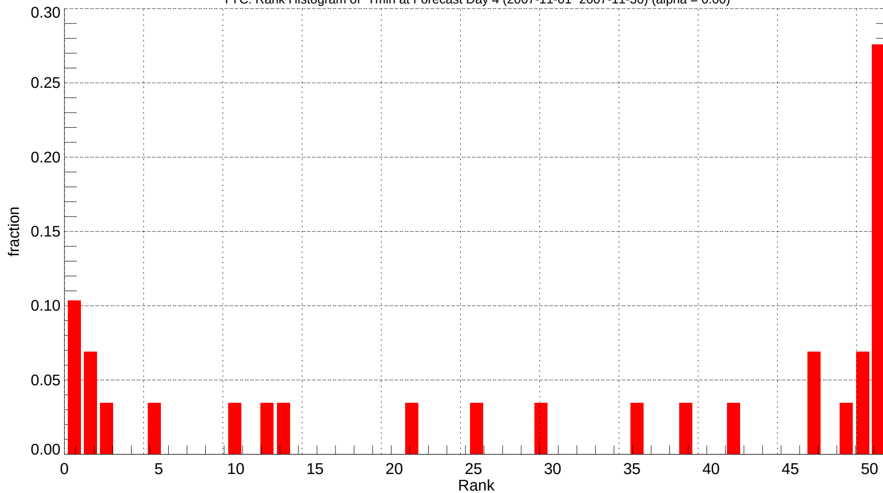
YYC: Rank Histogram of Tmin at Forecast Day 4 (2007-11-01~2007-11-30) (alpha = 0.00)
