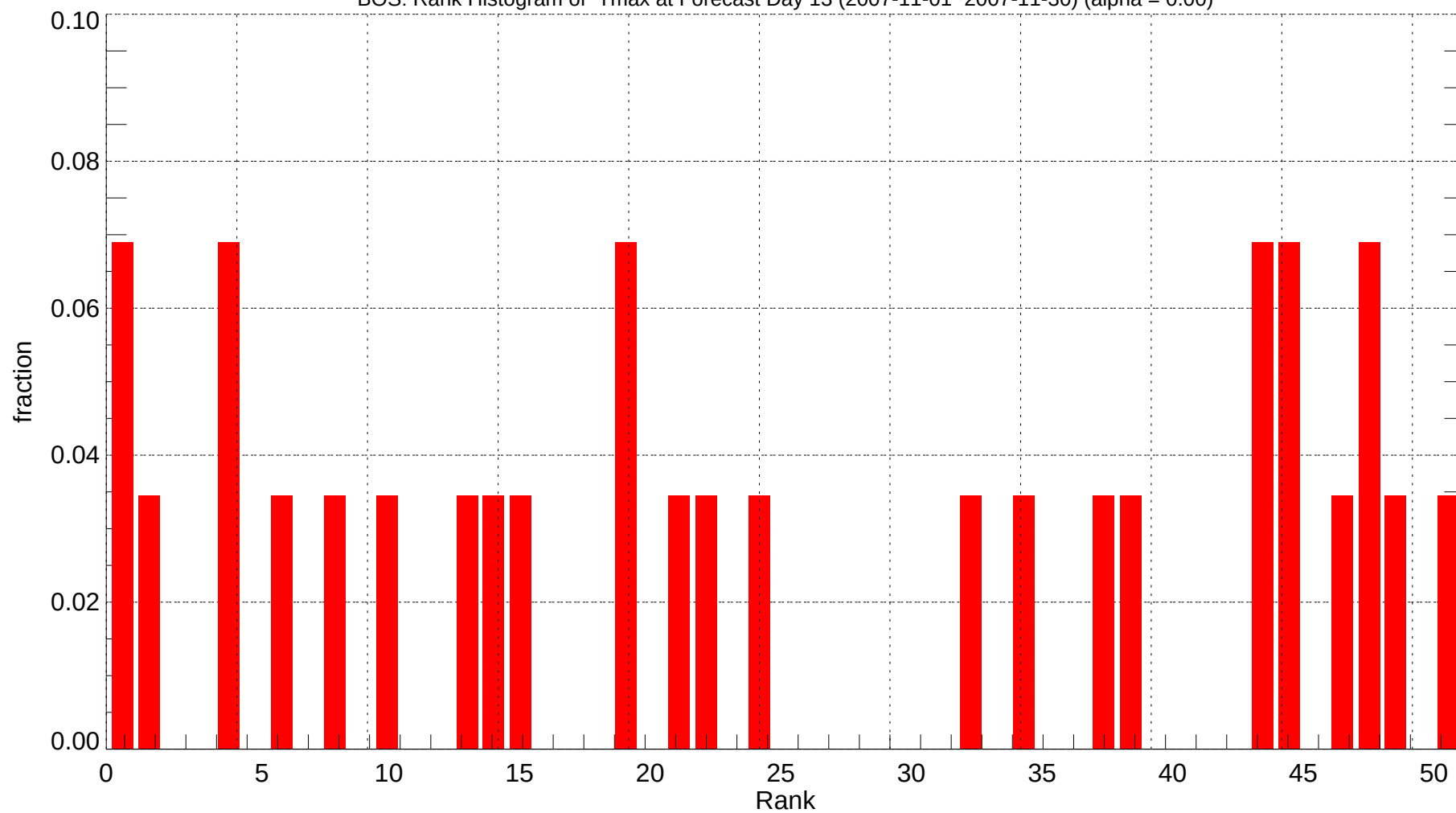
BOS: Rank Histogram of Tmax at Forecast Day 13 (2007-11-01~2007-11-30) (alpha = 0.00)
