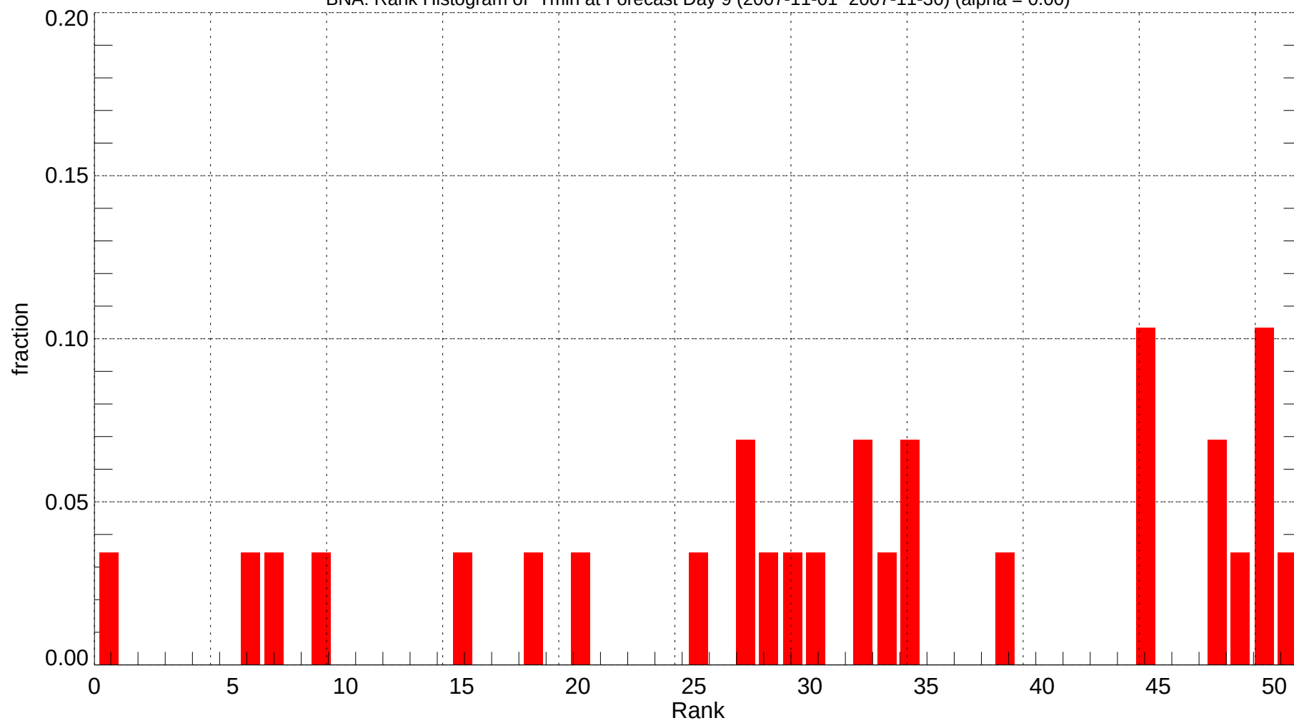
BNA: Rank Histogram of Tmin at Forecast Day 9 (2007-11-01~2007-11-30) (alpha = 0.00)
