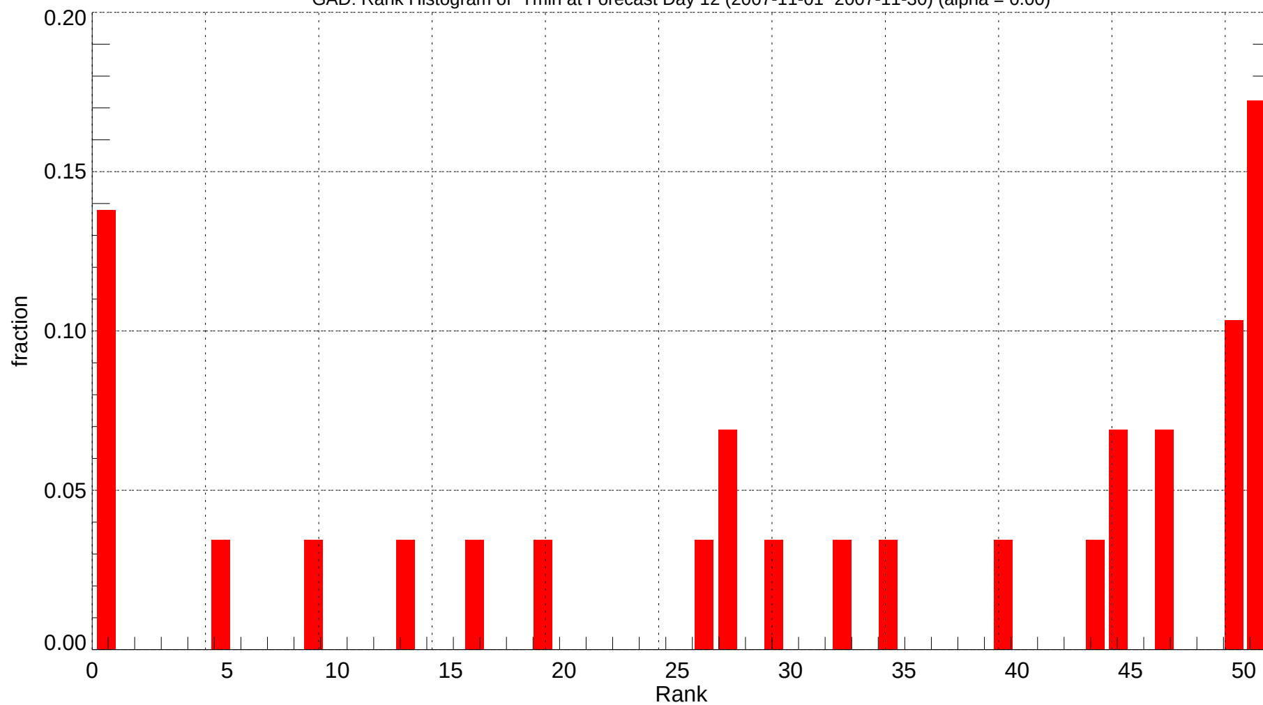
GAD: Rank Histogram of Tmin at Forecast Day 12 (2007-11-01~2007-11-30) (alpha = 0.00)
