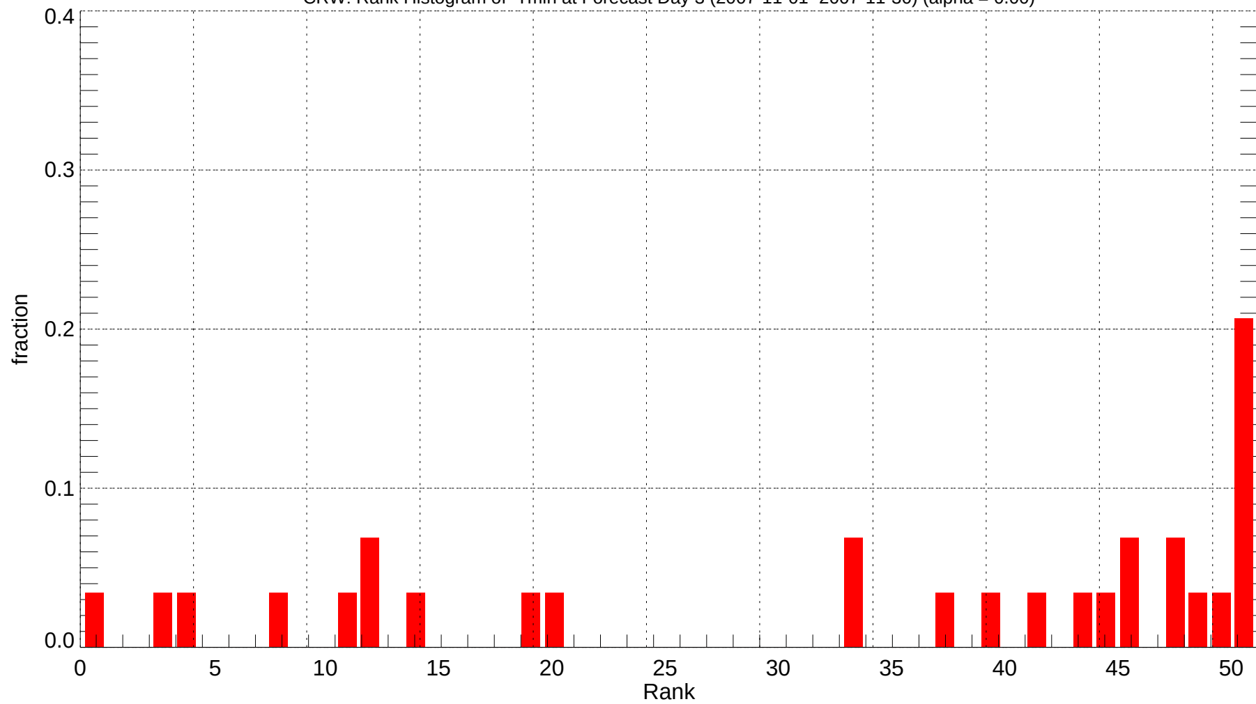
CRW: Rank Histogram of Tmin at Forecast Day 3 (2007-11-01~2007-11-30) (alpha = 0.00)
