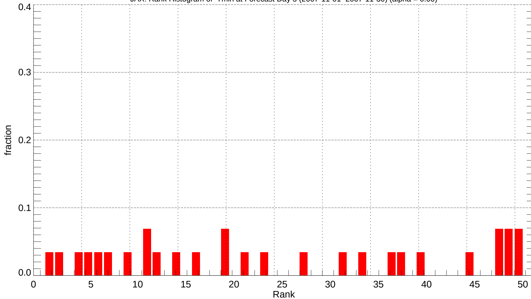
JAX: Rank Histogram of Tmin at Forecast Day 5 (2007-11-01~2007-11-30) (alpha = 0.00)
