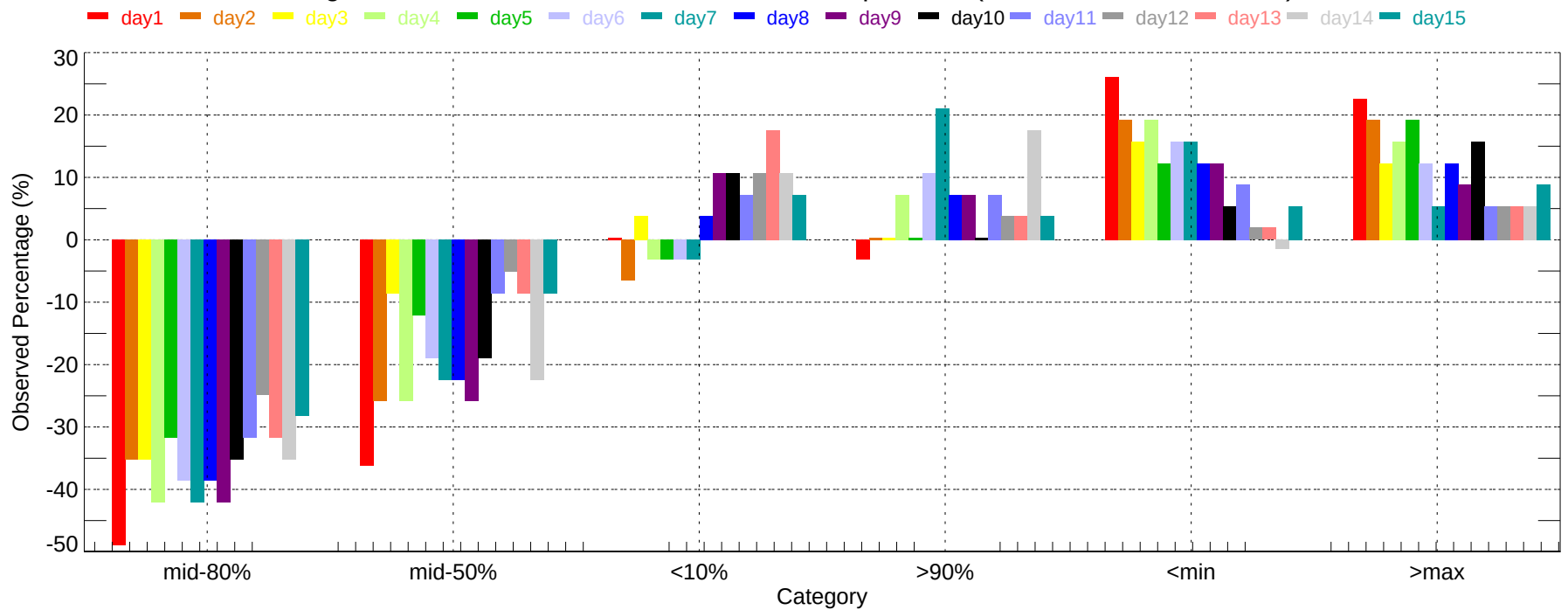
Observed Percentage Deviation of Ensembles - PDT: Min Temperature (2007-11-01~2007-11-30)
