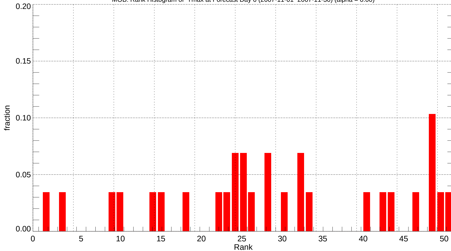
MOB: Rank Histogram of Tmax at Forecast Day 6 (2007-11-01~2007-11-30) (alpha = 0.00)
