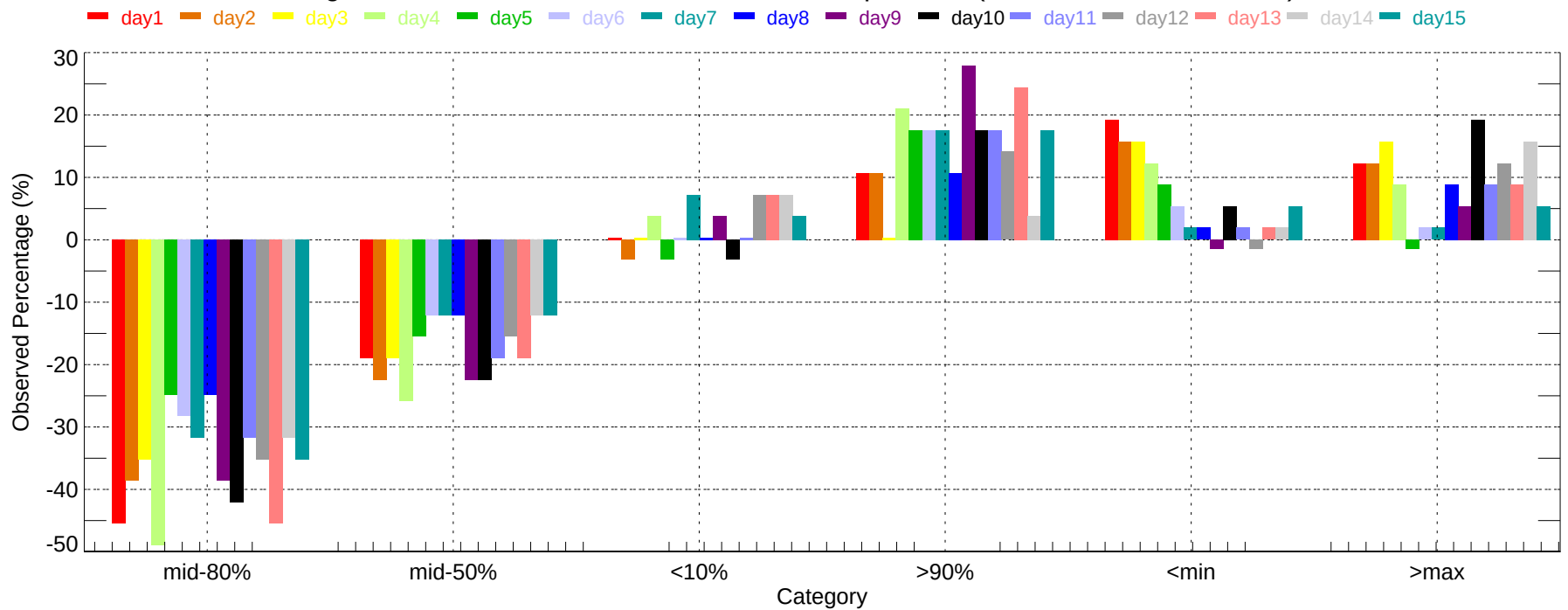
Observed Percentage Deviation of Ensembles - SJT: Max Temperature (2007-11-01~2007-11-30)
