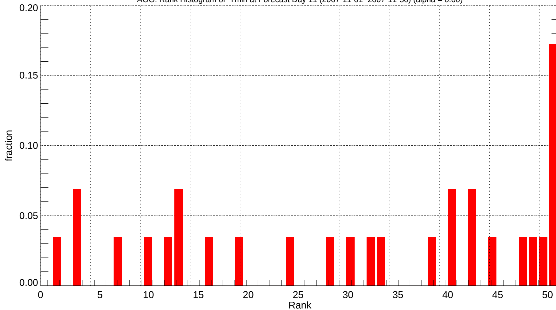
AOO: Rank Histogram of Tmin at Forecast Day 11 (2007-11-01~2007-11-30) (alpha = 0.00)
