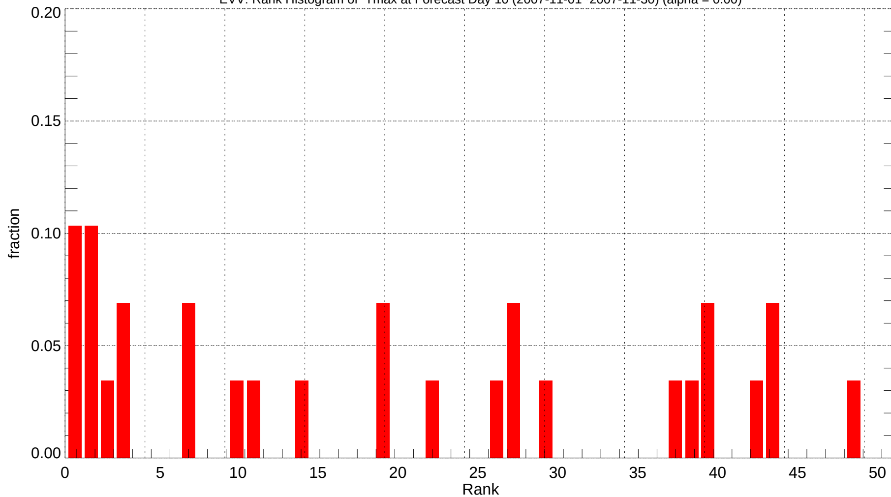
EVV: Rank Histogram of Tmax at Forecast Day 10 (2007-11-01~2007-11-30) (alpha = 0.00)
