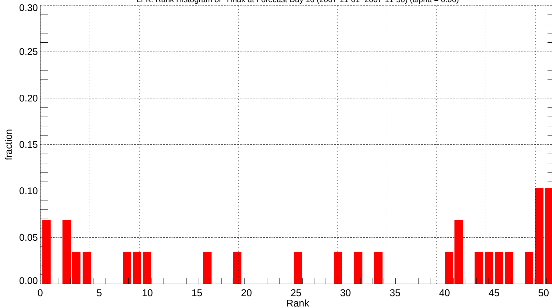
LFK: Rank Histogram of Tmax at Forecast Day 10 (2007-11-01~2007-11-30) (alpha = 0.00)
