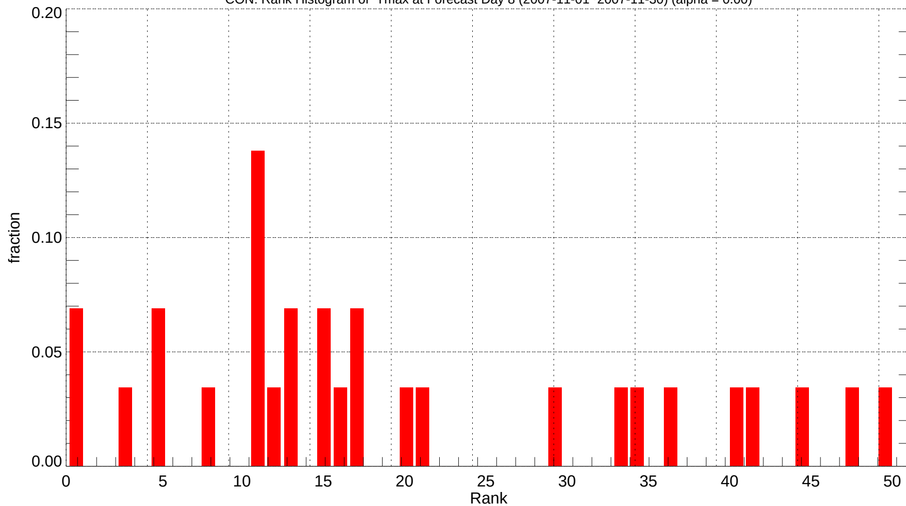
CON: Rank Histogram of Tmax at Forecast Day 8 (2007-11-01~2007-11-30) (alpha = 0.00)
