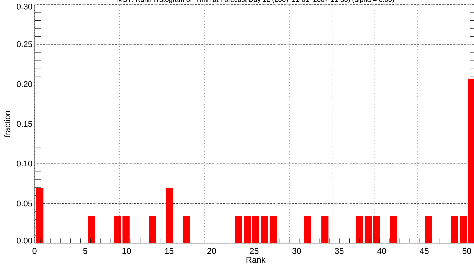
MSY: Rank Histogram of Tmin at Forecast Day 12 (2007-11-01~2007-11-30) (alpha = 0.00)
