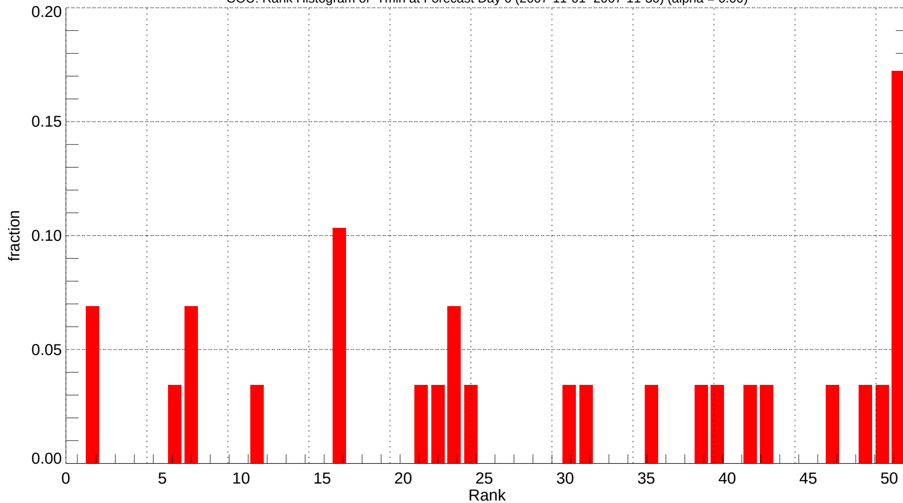
COU: Rank Histogram of Tmin at Forecast Day 6 (2007-11-01~2007-11-30) (alpha = 0.00)
