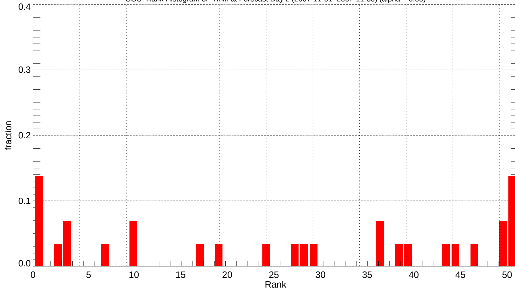
COU: Rank Histogram of Tmin at Forecast Day 2 (2007-11-01~2007-11-30) (alpha = 0.00)
