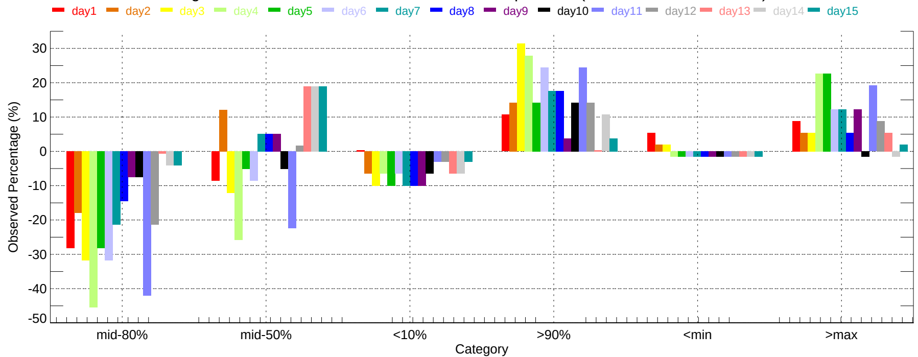
Observed Percentage Deviation of Ensembles - MCN: Max Temperature (2007-11-01~2007-11-30)
