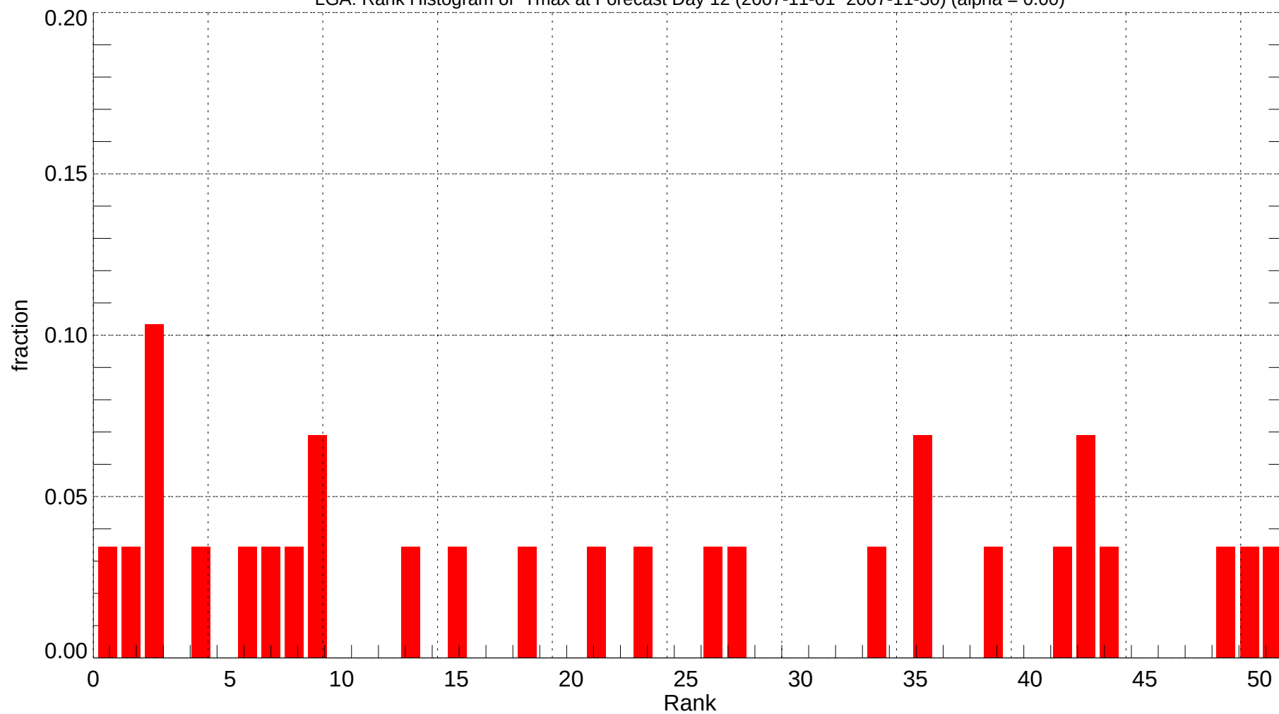
LGA: Rank Histogram of Tmax at Forecast Day 12 (2007-11-01~2007-11-30) (alpha = 0.00)
