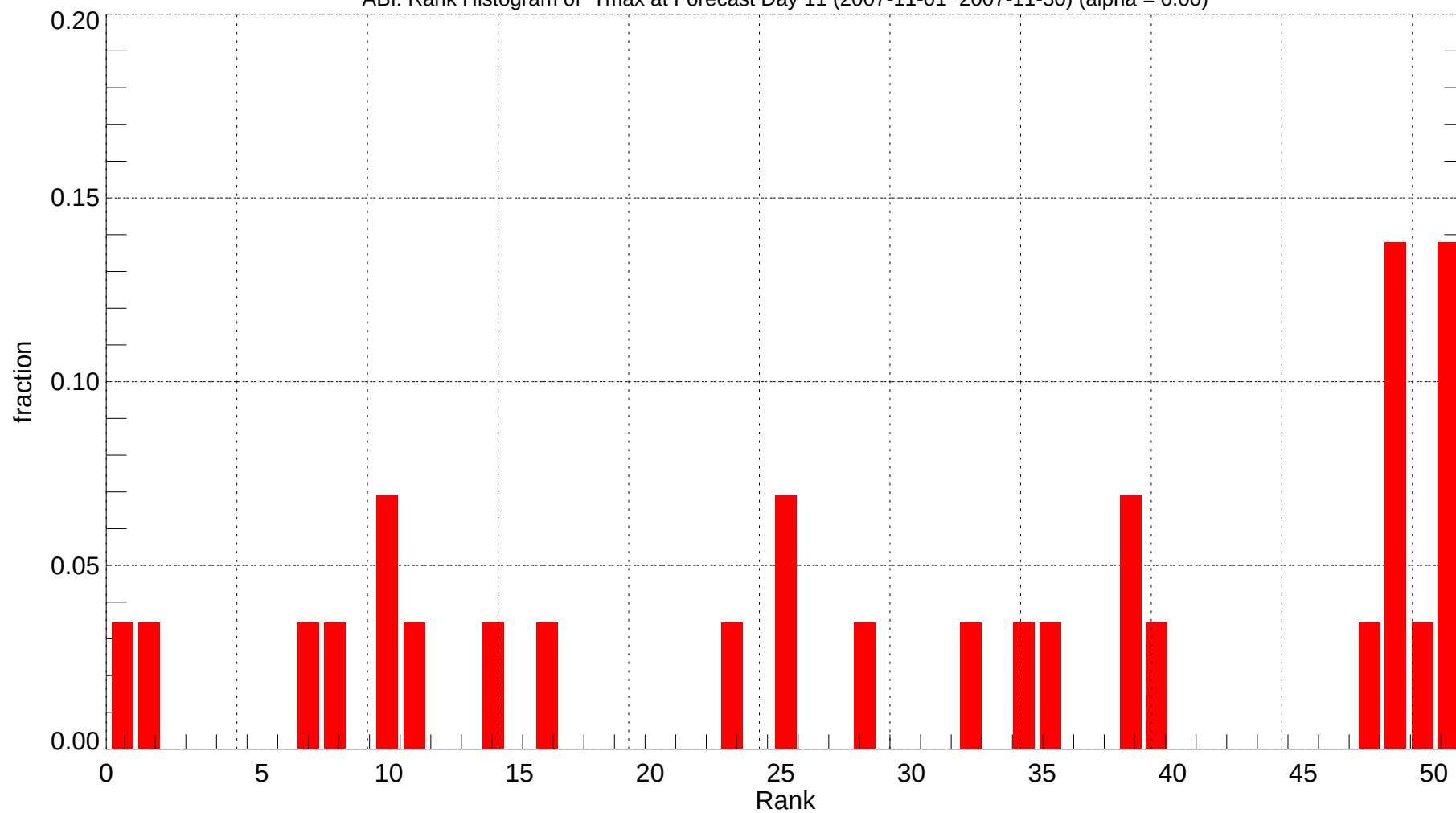
ABI: Rank Histogram of Tmax at Forecast Day 11 (2007-11-01~2007-11-30) (alpha = 0.00)
