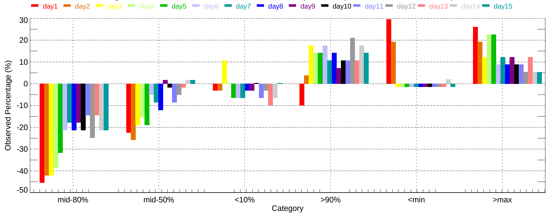
Observed Percentage Deviation of Ensembles - BWI: Max Temperature (2007-11-01~2007-11-30)
