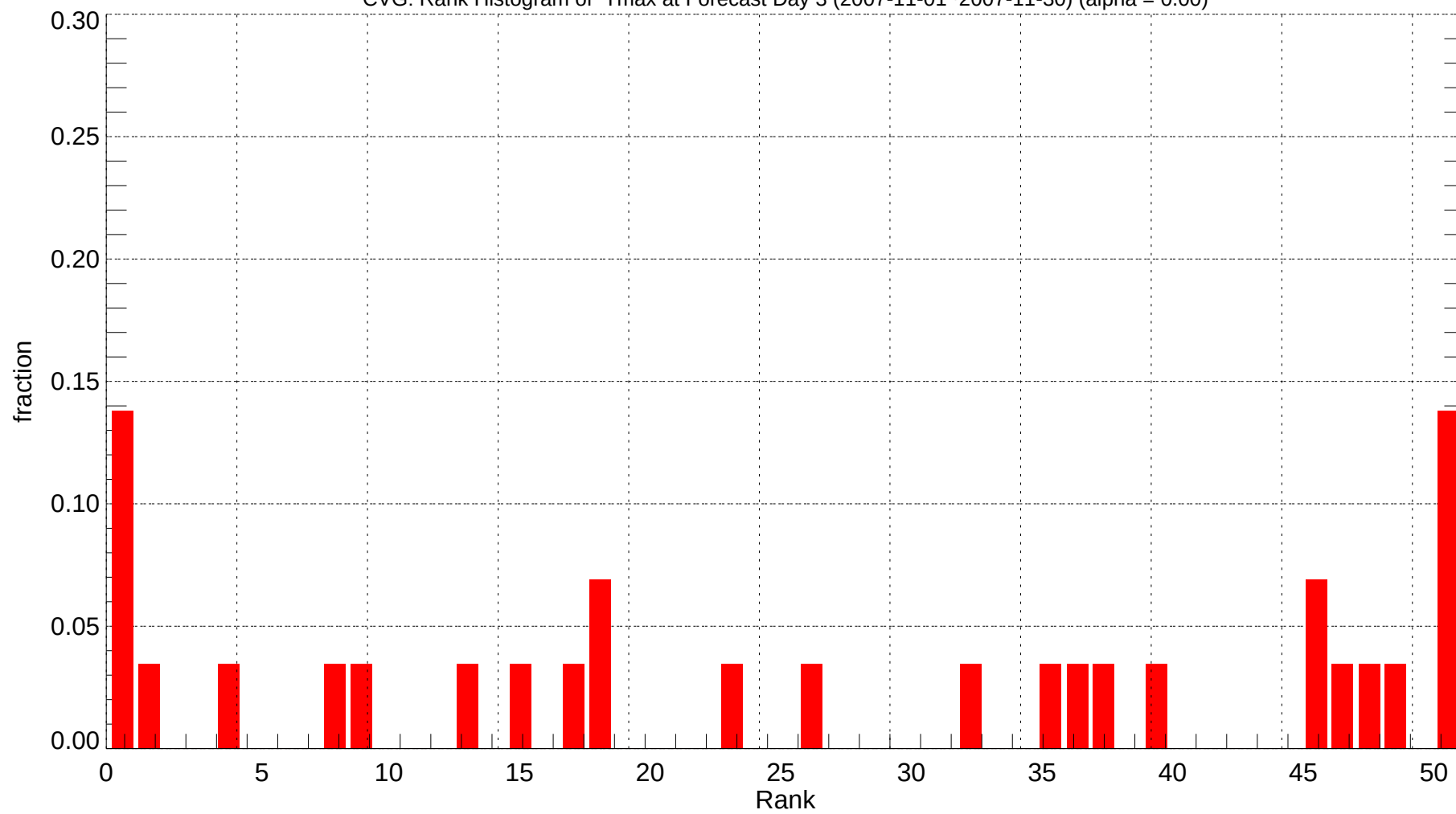
CVG: Rank Histogram of Tmax at Forecast Day 3 (2007-11-01~2007-11-30) (alpha = 0.00)
