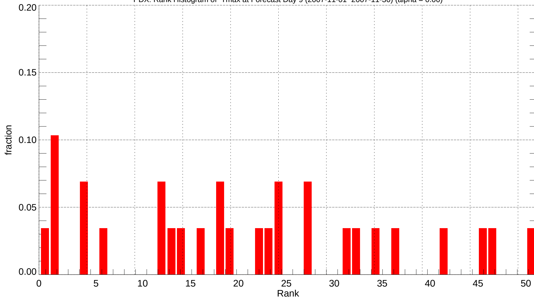
PDX: Rank Histogram of Tmax at Forecast Day 9 (2007-11-01~2007-11-30) (alpha = 0.00)
