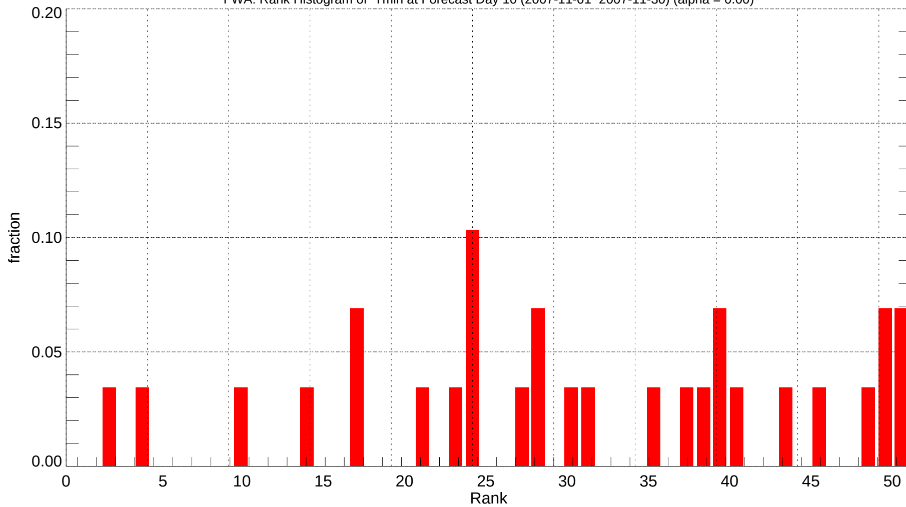
FWA: Rank Histogram of Tmin at Forecast Day 10 (2007-11-01~2007-11-30) (alpha = 0.00)
