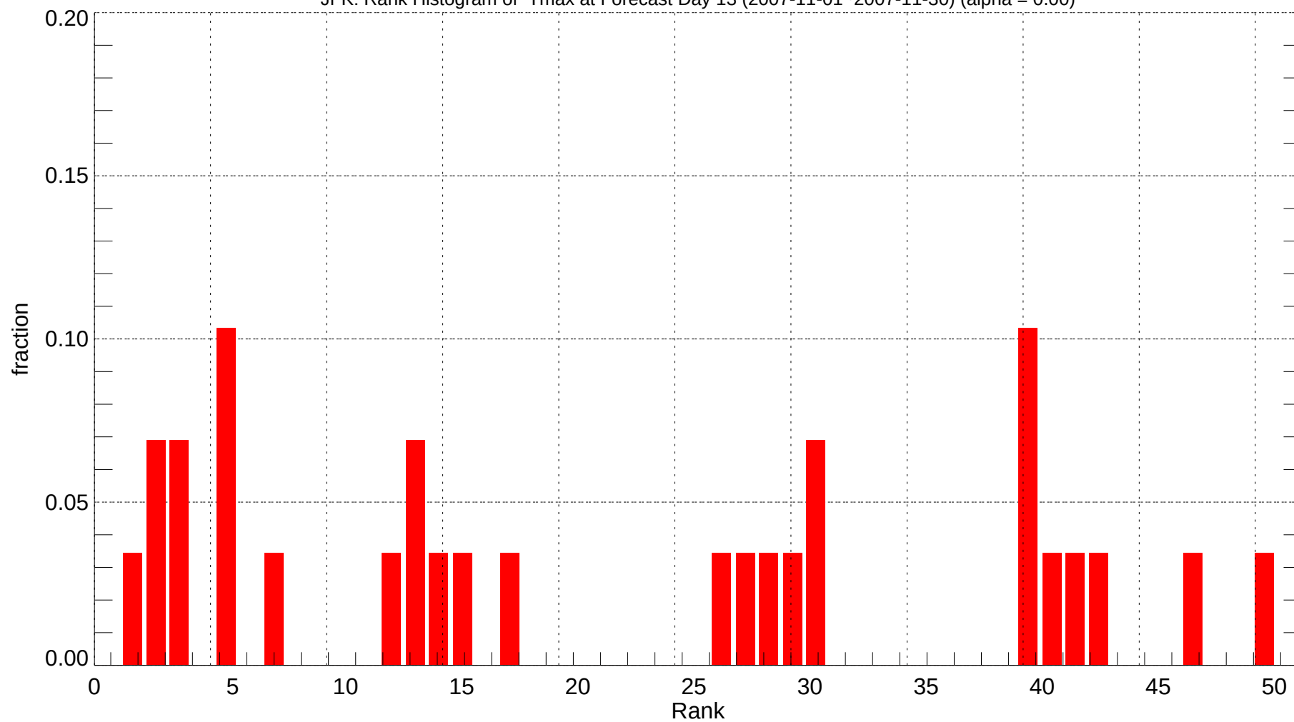
JFK: Rank Histogram of Tmax at Forecast Day 13 (2007-11-01~2007-11-30) (alpha = 0.00)
