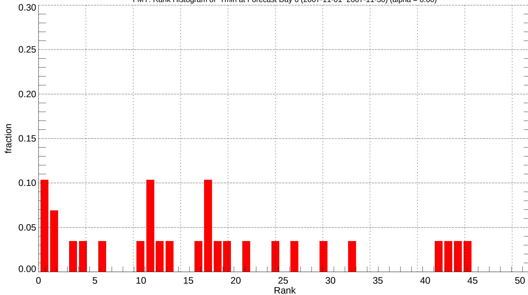
FMY: Rank Histogram of Tmin at Forecast Day 6 (2007-11-01~2007-11-30) (alpha = 0.00)
