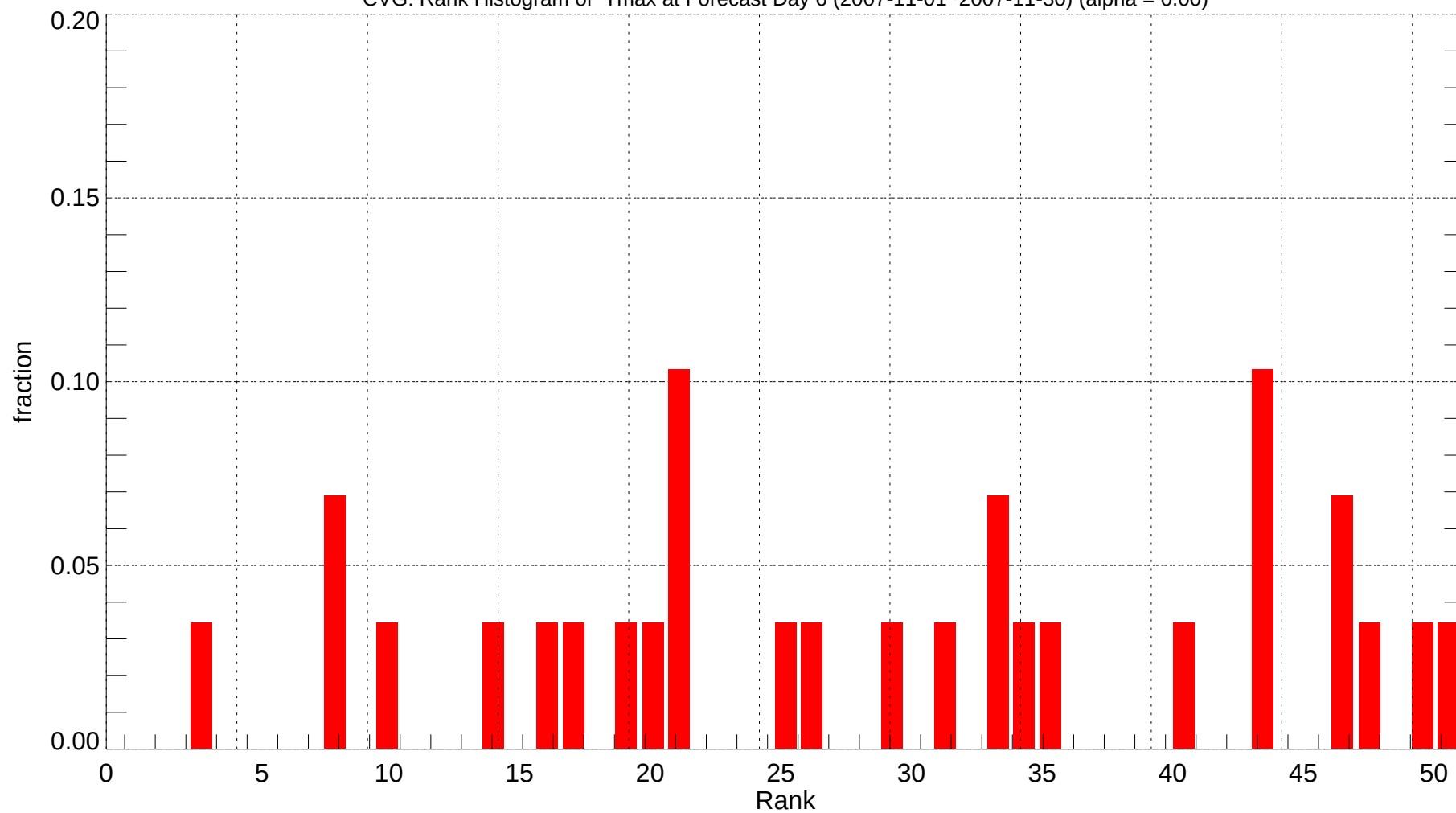
CVG: Rank Histogram of Tmax at Forecast Day 6 (2007-11-01~2007-11-30) (alpha = 0.00)
