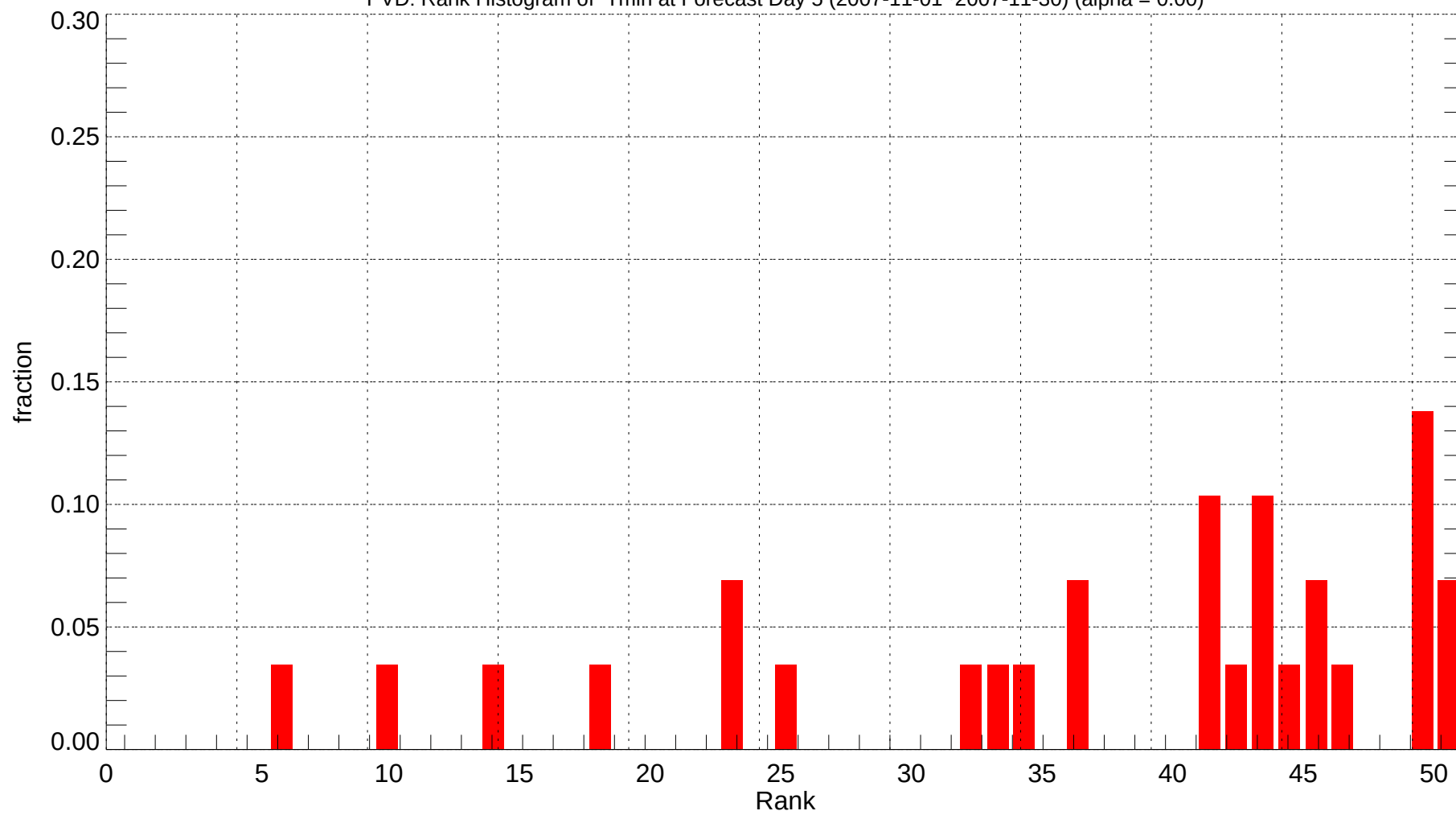
PVD: Rank Histogram of Tmin at Forecast Day 5 (2007-11-01~2007-11-30) (alpha = 0.00)
