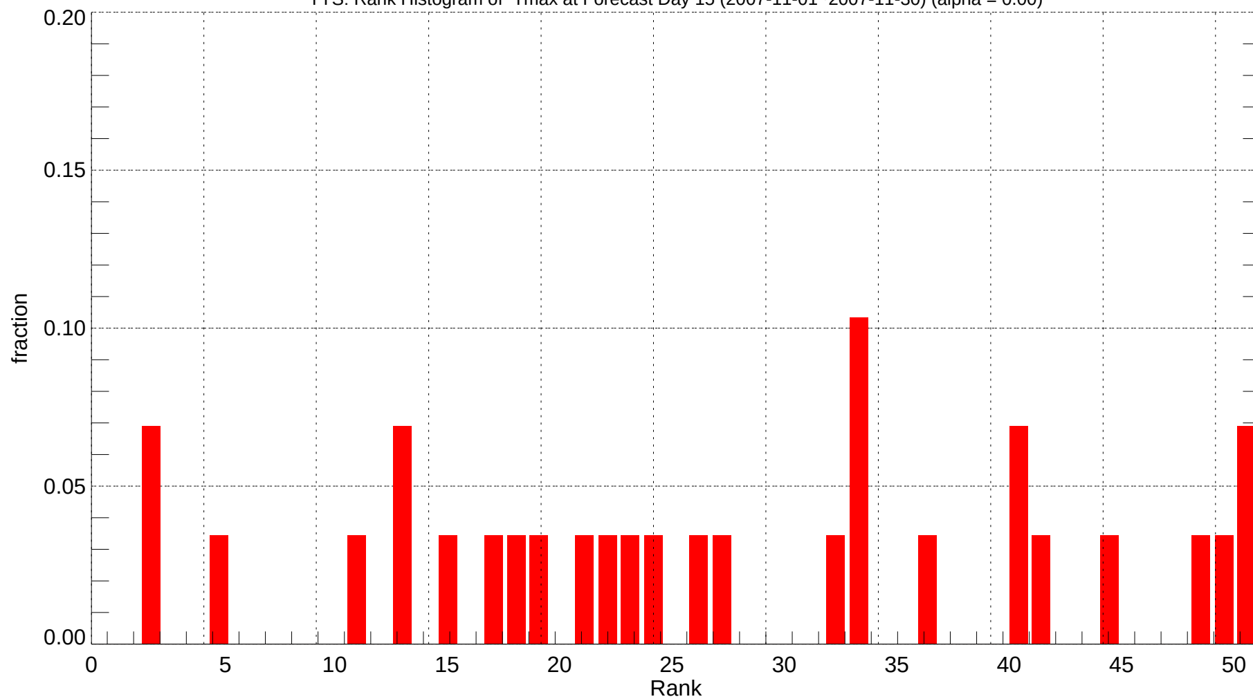
TYS: Rank Histogram of Tmax at Forecast Day 15 (2007-11-01~2007-11-30) (alpha = 0.00)
