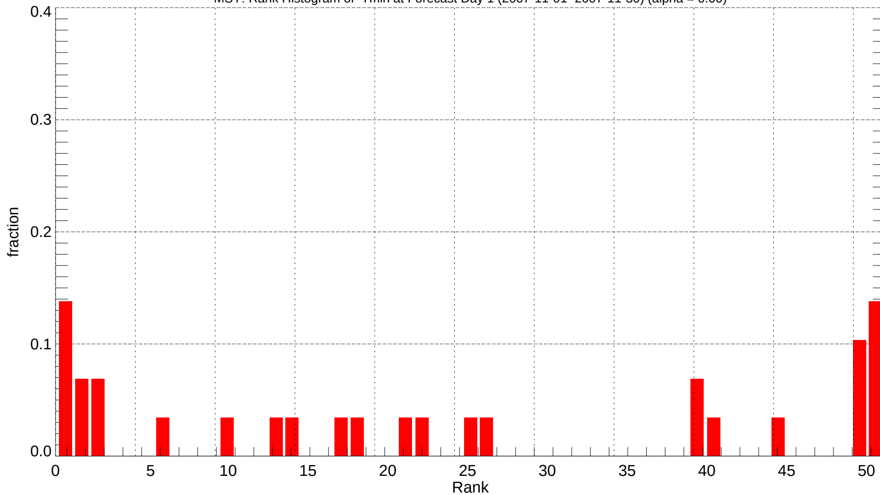
MSY: Rank Histogram of Tmin at Forecast Day 1 (2007-11-01~2007-11-30) (alpha = 0.00)
