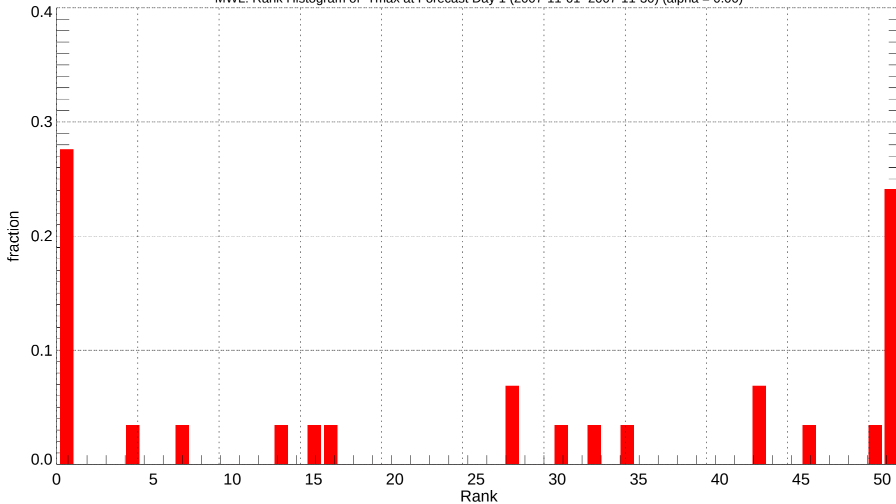
MWL: Rank Histogram of Tmax at Forecast Day 1 (2007-11-01~2007-11-30) (alpha = 0.00)
