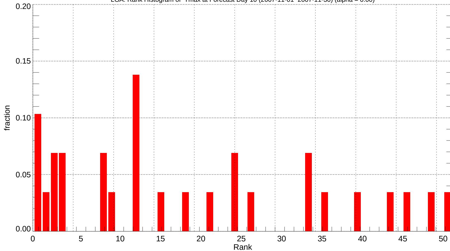
LGA: Rank Histogram of Tmax at Forecast Day 10 (2007-11-01~2007-11-30) (alpha = 0.00)
