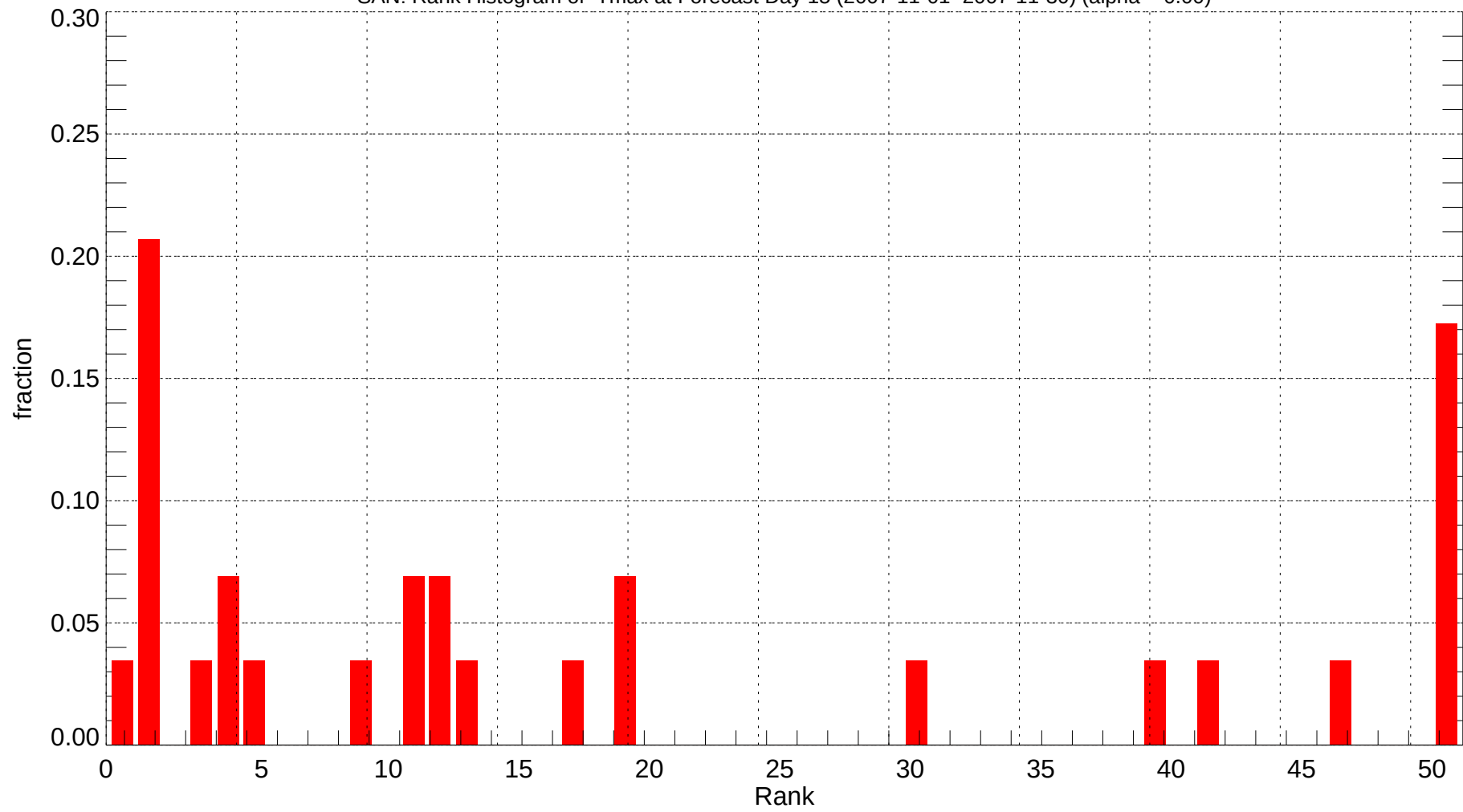
SAN: Rank Histogram of Tmax at Forecast Day 15 (2007-11-01~2007-11-30) (alpha = 0.00)
