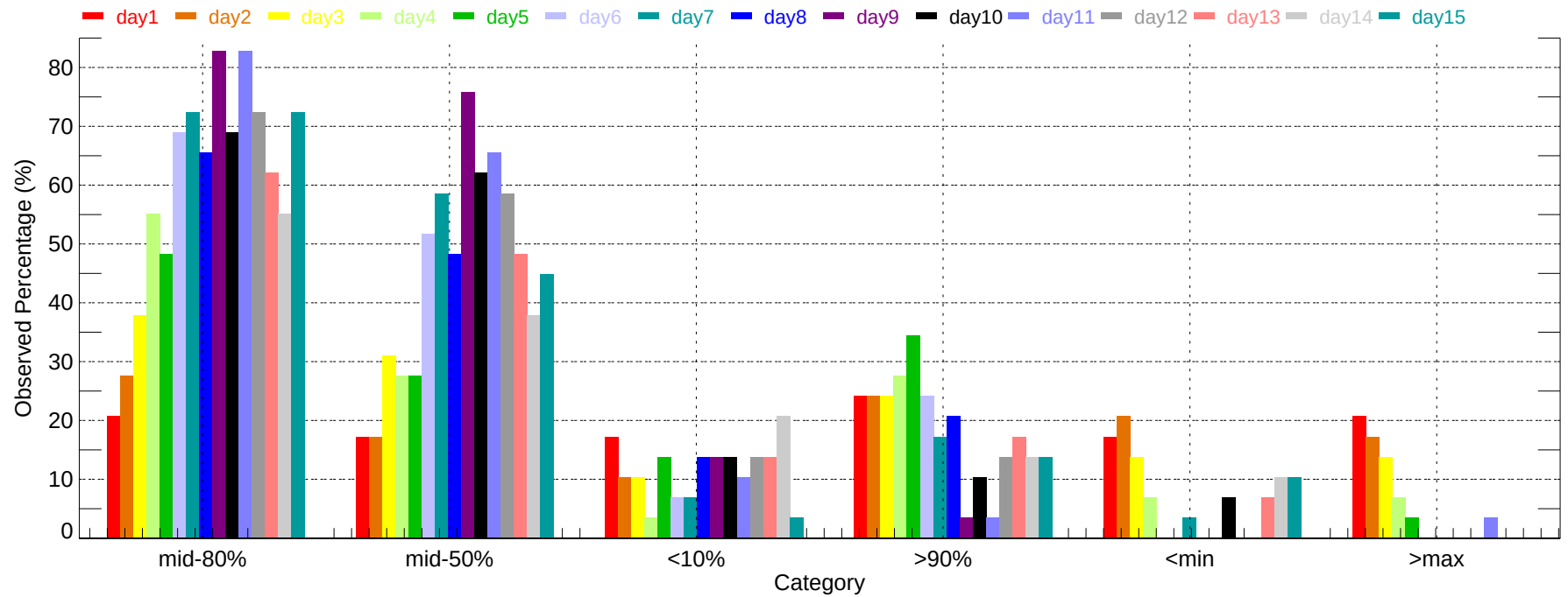
Observed Percentage of Ensembles - PWM: Max Temperature (2007-11-01~2007-11-30)
