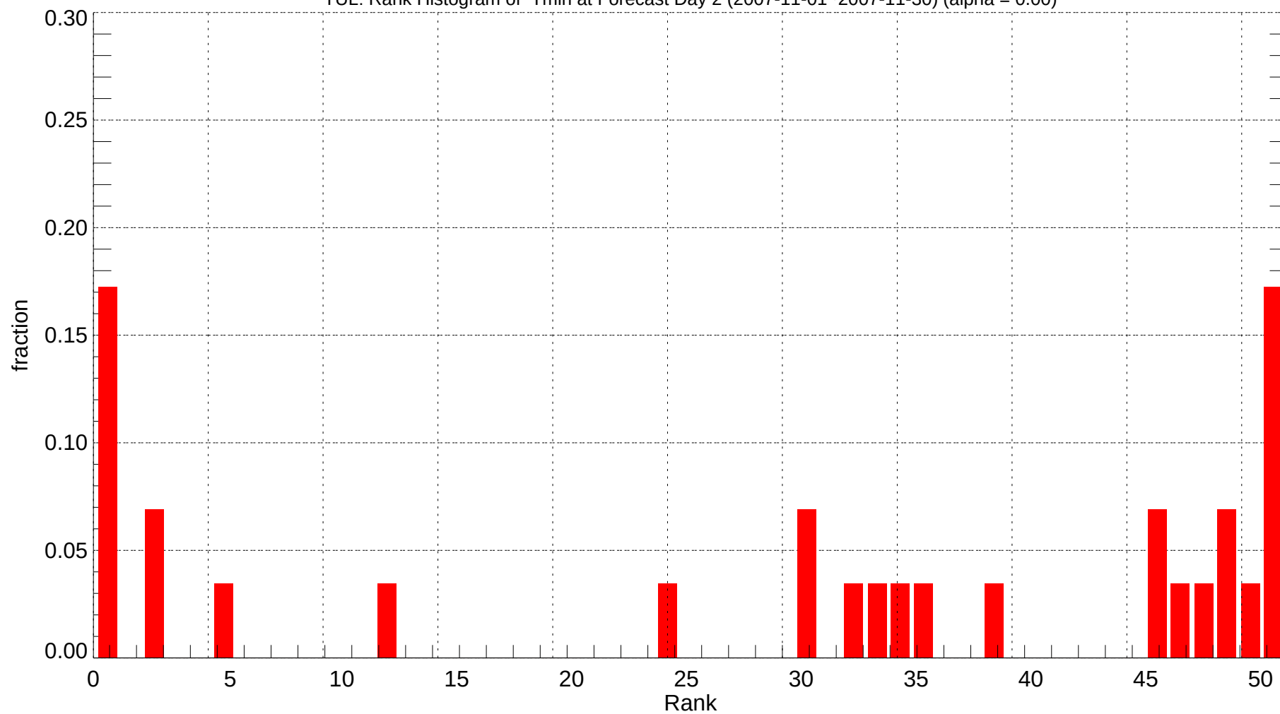
TUL: Rank Histogram of Tmin at Forecast Day 2 (2007-11-01~2007-11-30) (alpha = 0.00)
