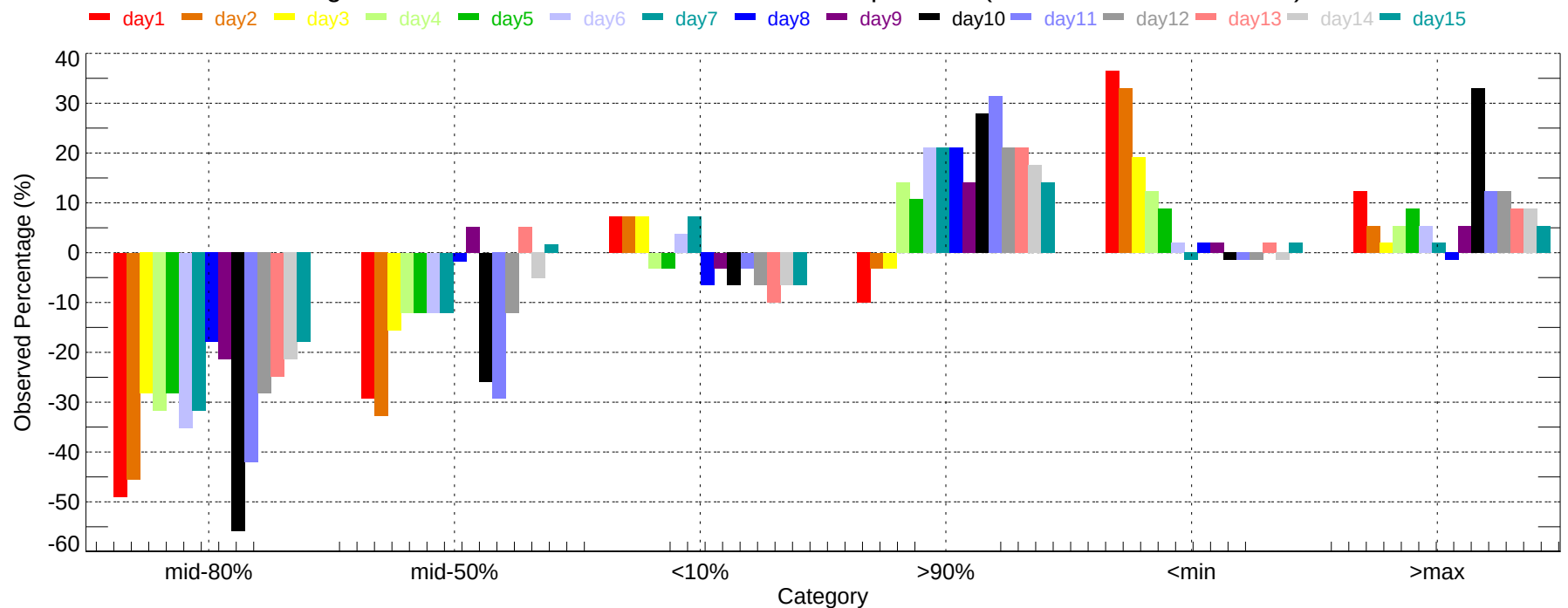
Observed Percentage Deviation of Ensembles - OMA: Min Temperature (2007-11-01~2007-11-30)
