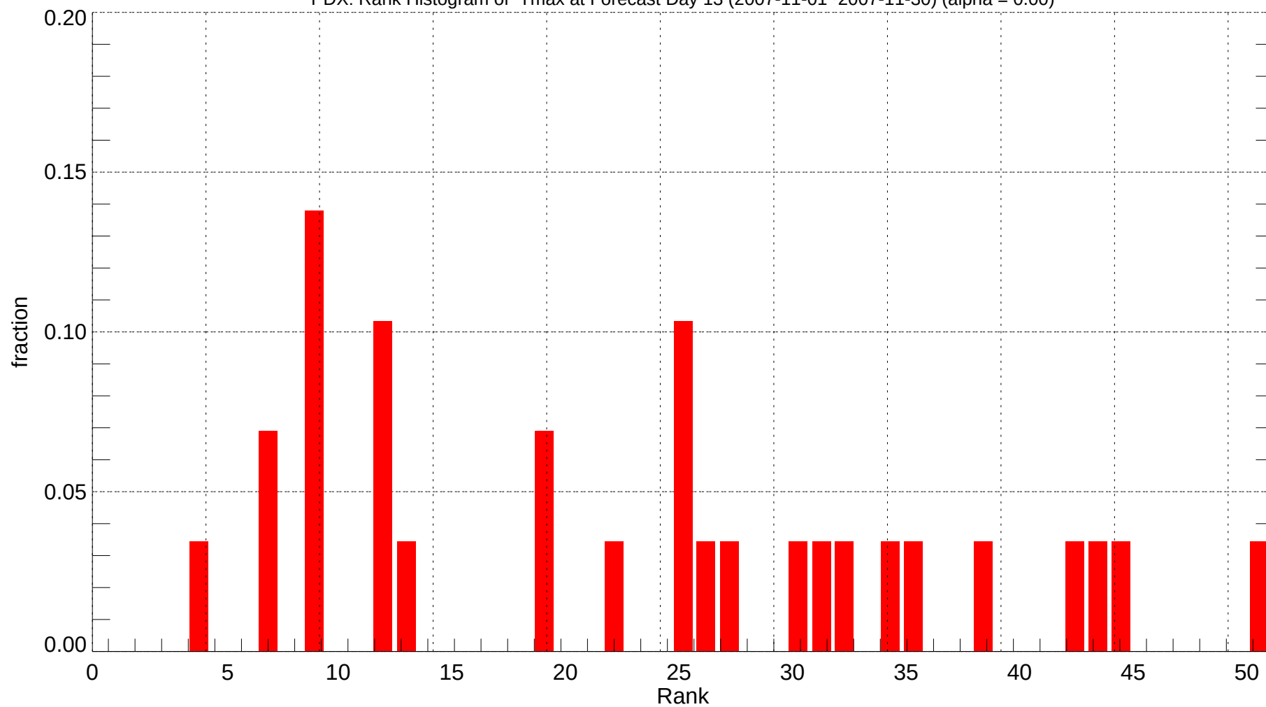
PDX: Rank Histogram of Tmax at Forecast Day 13 (2007-11-01~2007-11-30) (alpha = 0.00)
