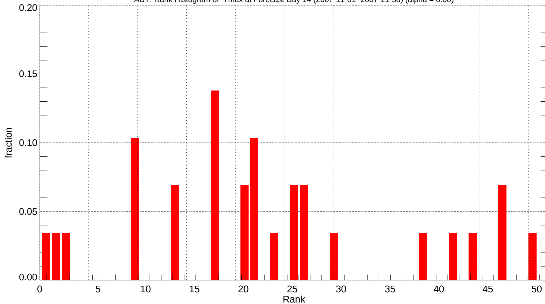
ABY: Rank Histogram of Tmax at Forecast Day 14 (2007-11-01~2007-11-30) (alpha = 0.00)
