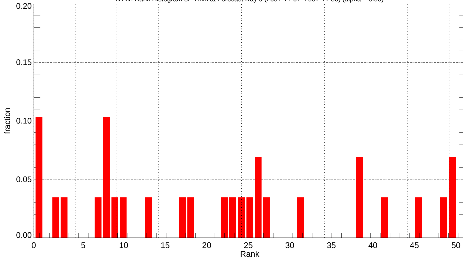
DTW: Rank Histogram of Tmin at Forecast Day 9 (2007-11-01~2007-11-30) (alpha = 0.00)
