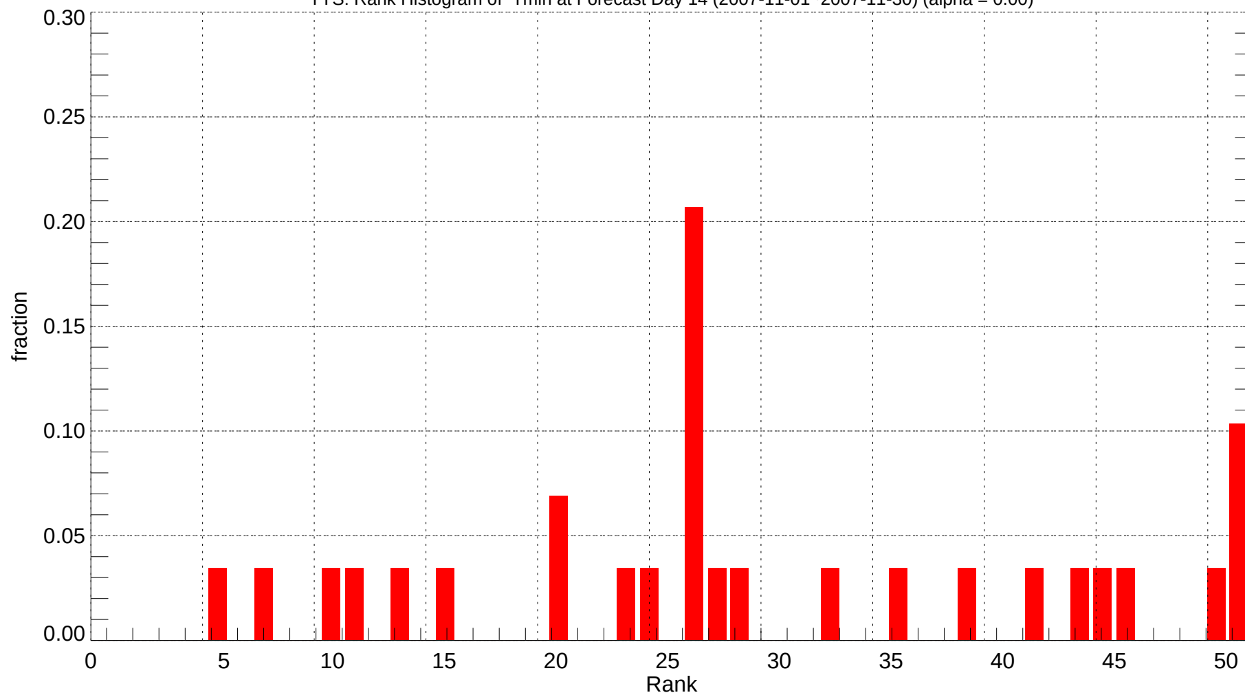
TYS: Rank Histogram of Tmin at Forecast Day 14 (2007-11-01~2007-11-30) (alpha = 0.00)
