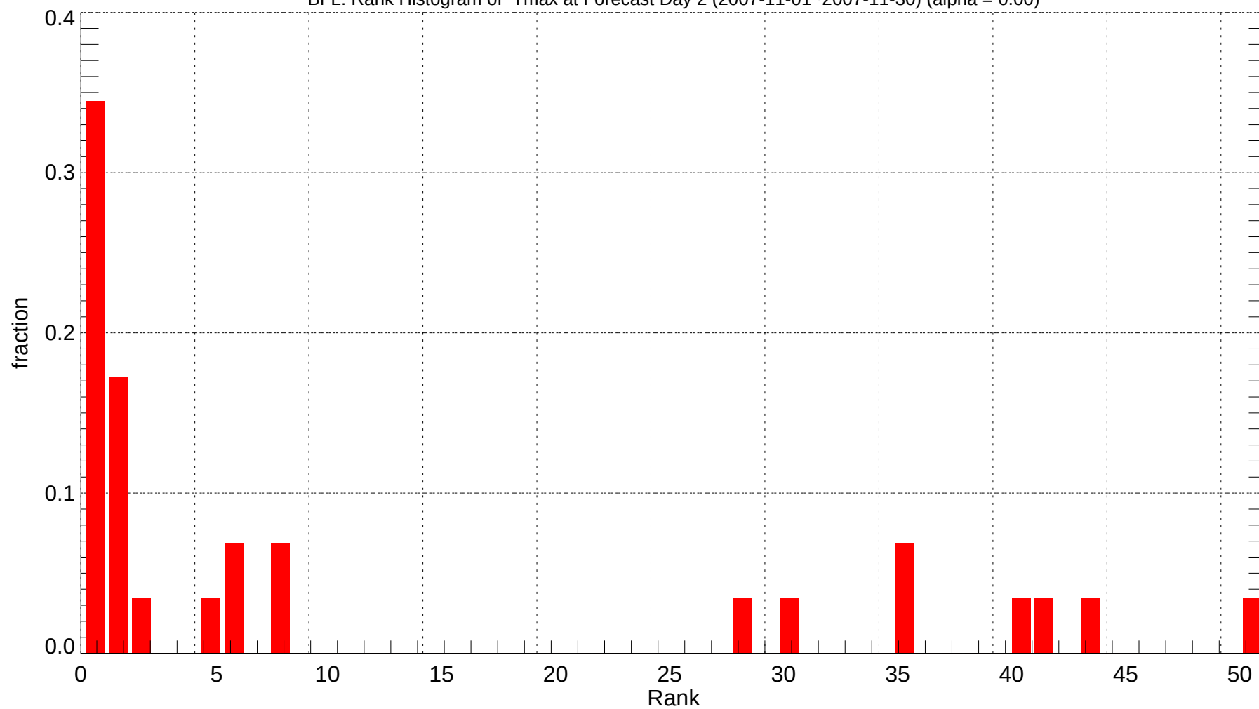
BFL: Rank Histogram of Tmax at Forecast Day 2 (2007-11-01~2007-11-30) (alpha = 0.00)
