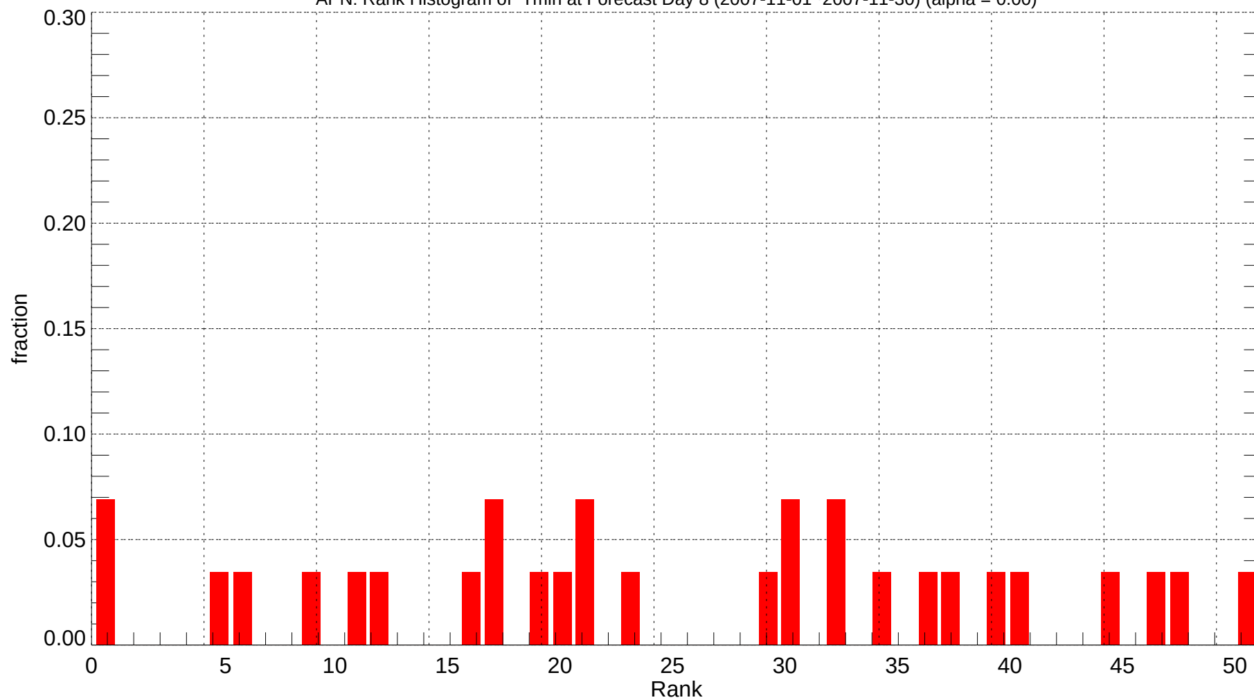
APN: Rank Histogram of Tmin at Forecast Day 8 (2007-11-01~2007-11-30) (alpha = 0.00)
