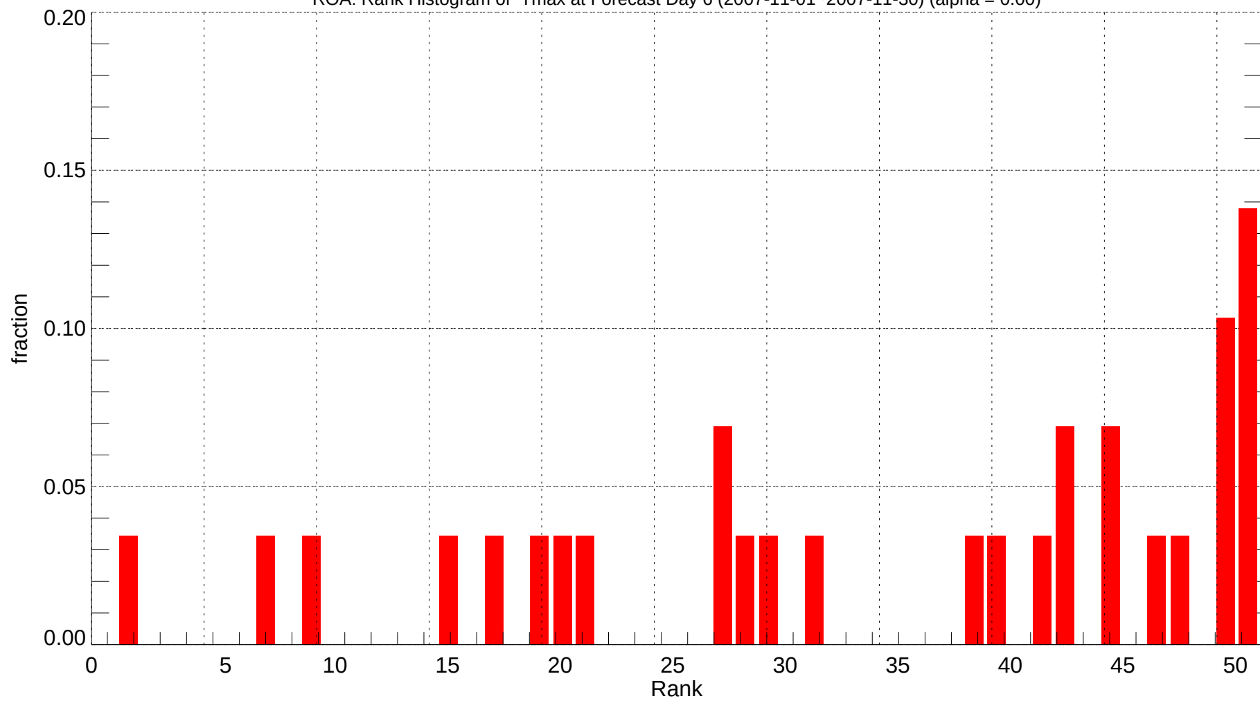
ROA: Rank Histogram of Tmax at Forecast Day 6 (2007-11-01~2007-11-30) (alpha = 0.00)
