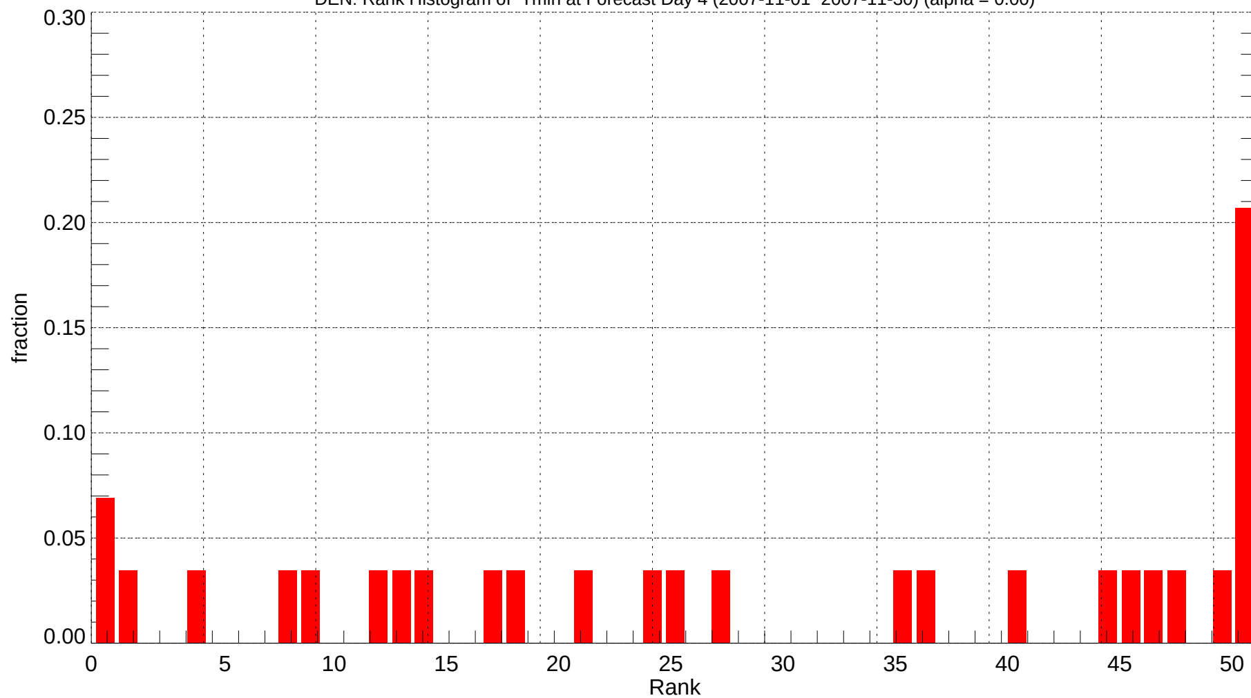
DEN: Rank Histogram of Tmin at Forecast Day 4 (2007-11-01~2007-11-30) (alpha = 0.00)
