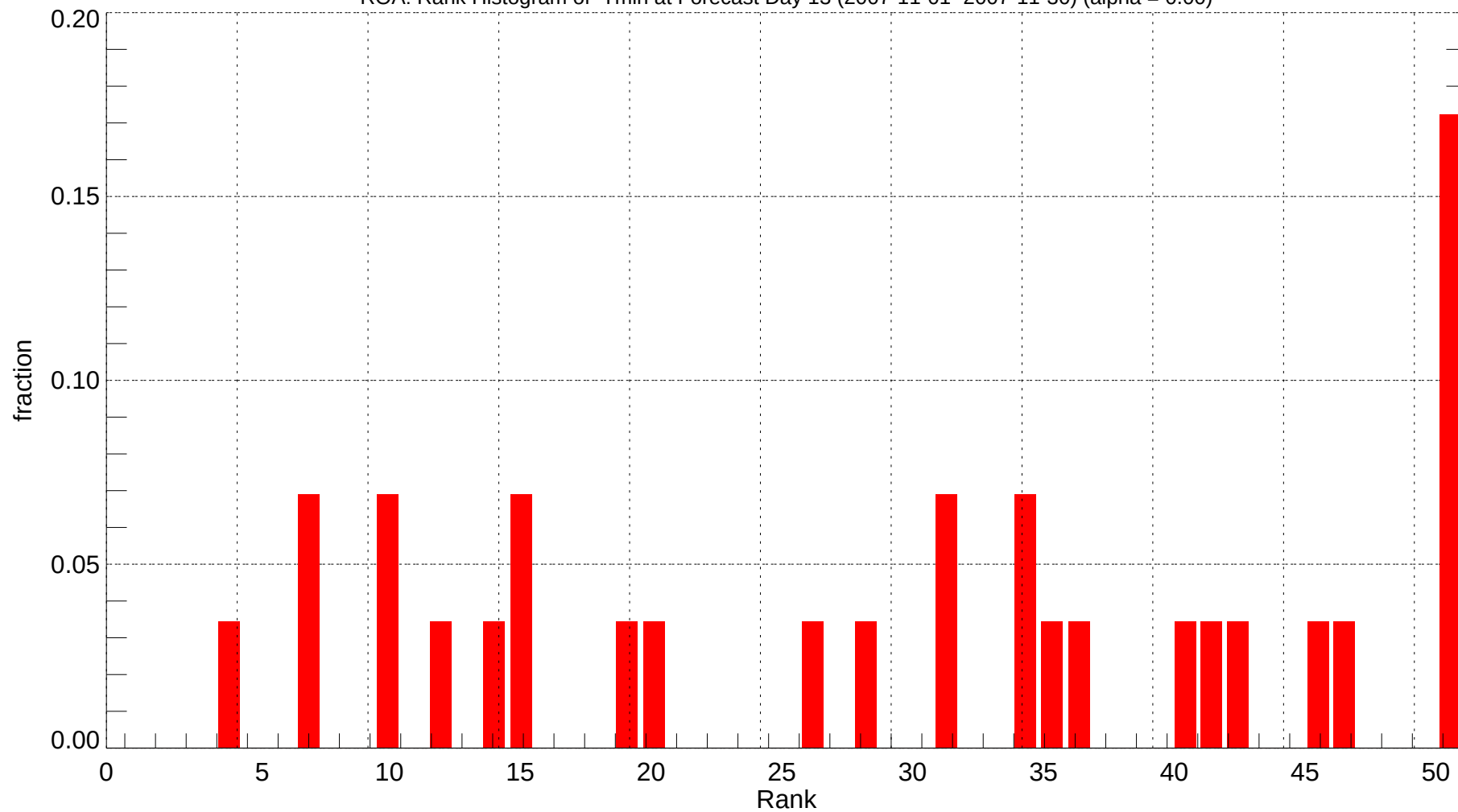
ROA: Rank Histogram of Tmin at Forecast Day 13 (2007-11-01~2007-11-30) (alpha = 0.00)
