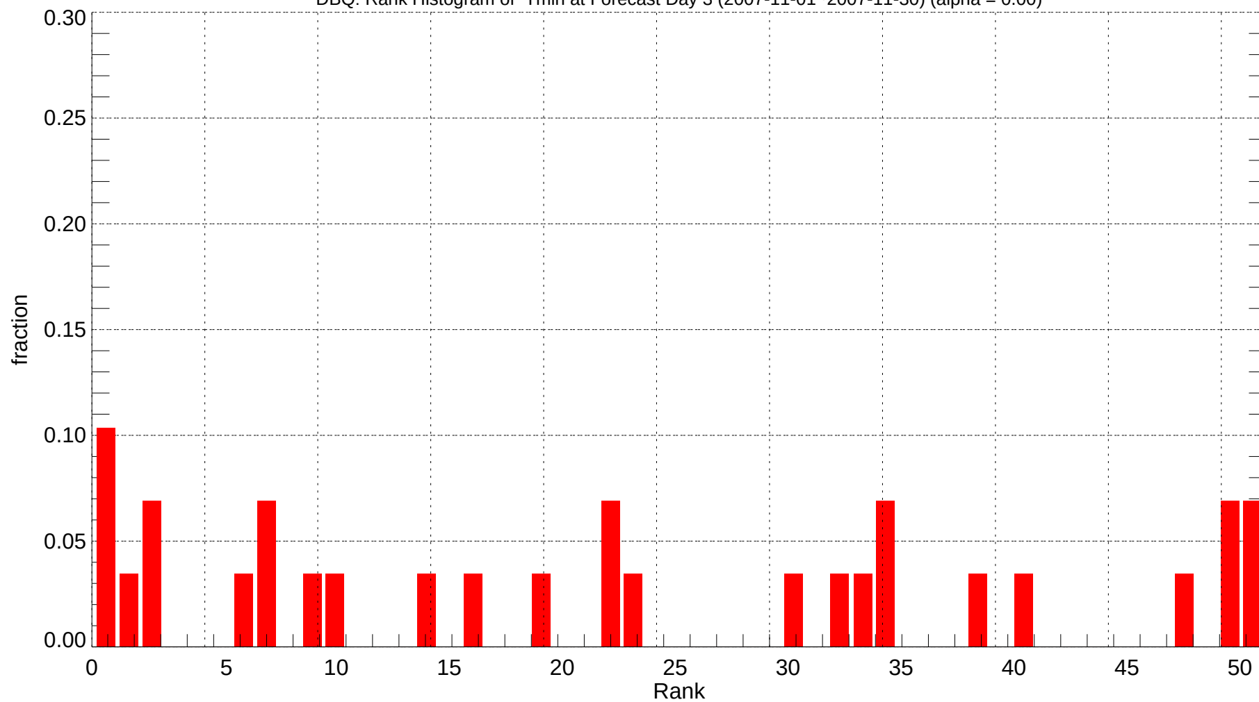
DBQ: Rank Histogram of Tmin at Forecast Day 3 (2007-11-01~2007-11-30) (alpha = 0.00)
