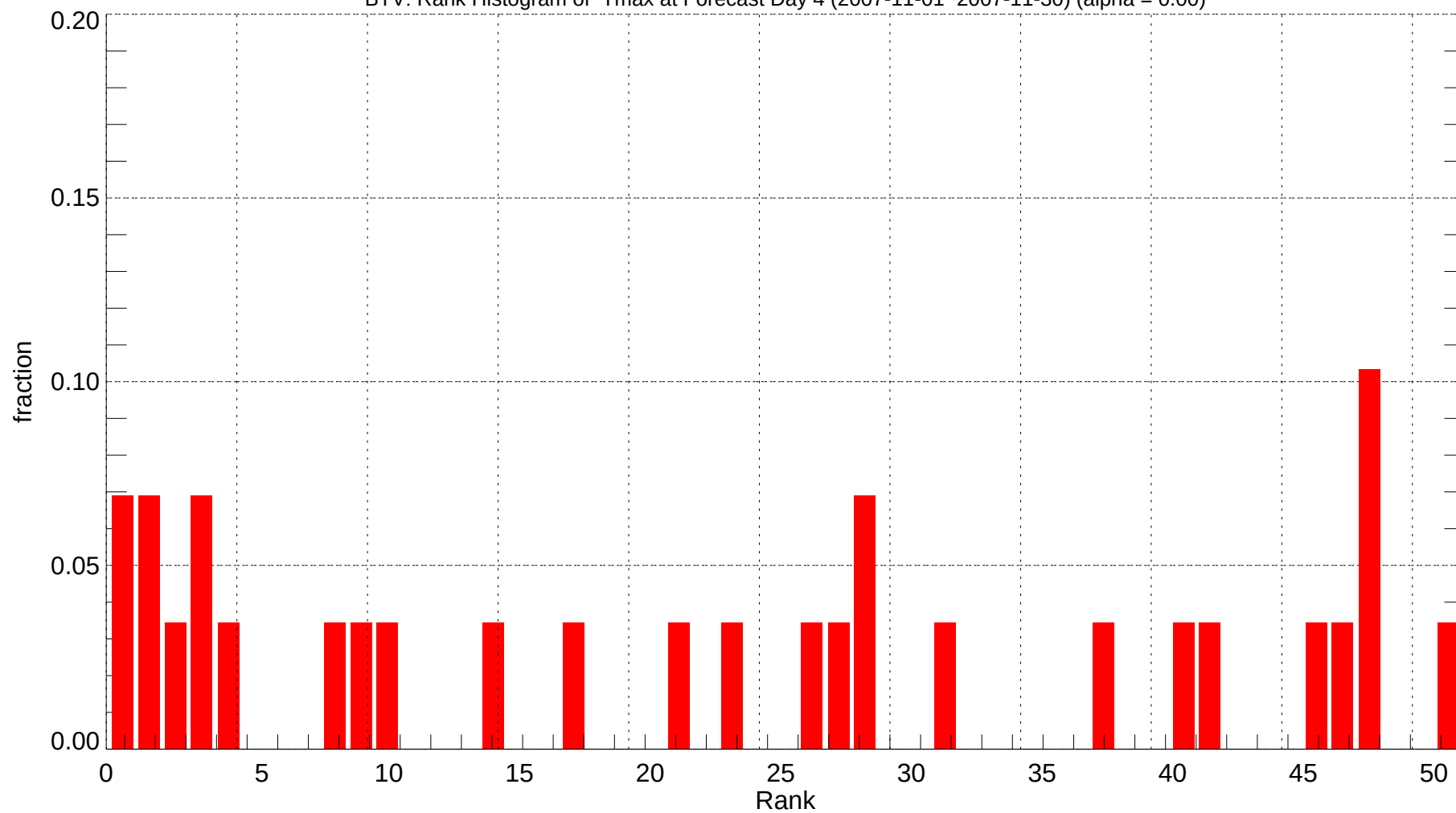
BTV: Rank Histogram of Tmax at Forecast Day 4 (2007-11-01~2007-11-30) (alpha = 0.00)
