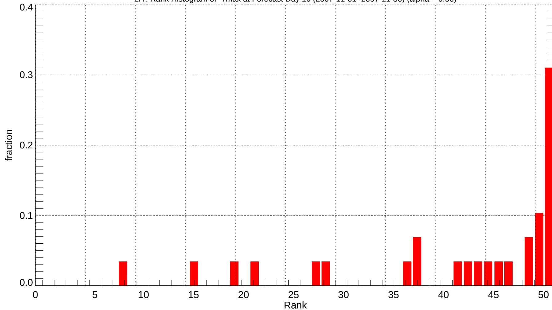
LIT: Rank Histogram of Tmax at Forecast Day 10 (2007-11-01~2007-11-30) (alpha = 0.00)
