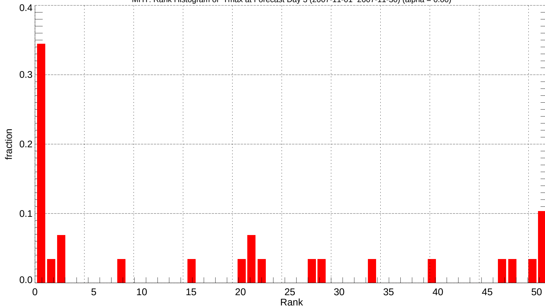
MHT: Rank Histogram of Tmax at Forecast Day 3 (2007-11-01~2007-11-30) (alpha = 0.00)
