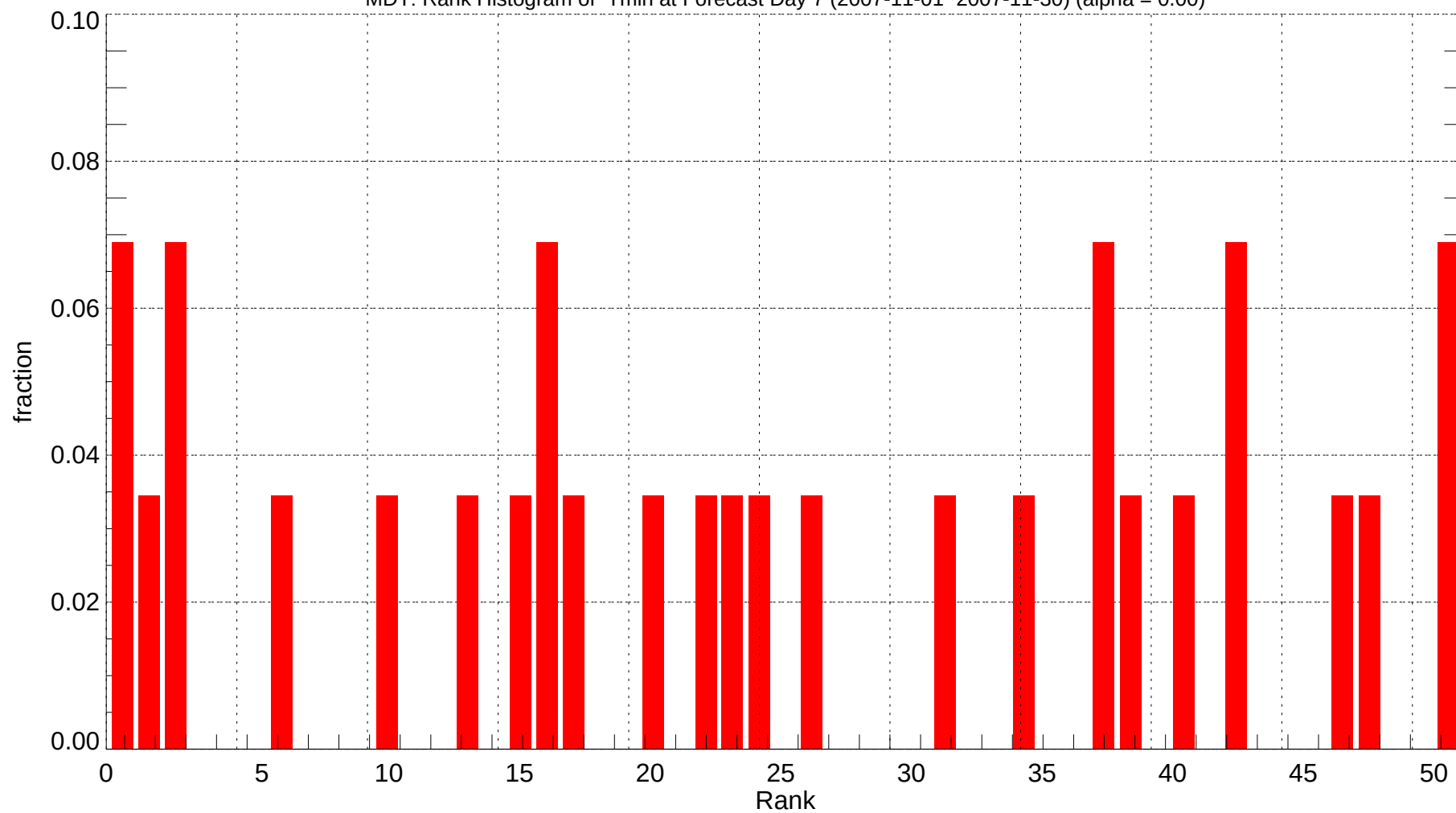
MDT: Rank Histogram of Tmin at Forecast Day 7 (2007-11-01~2007-11-30) (alpha = 0.00)
