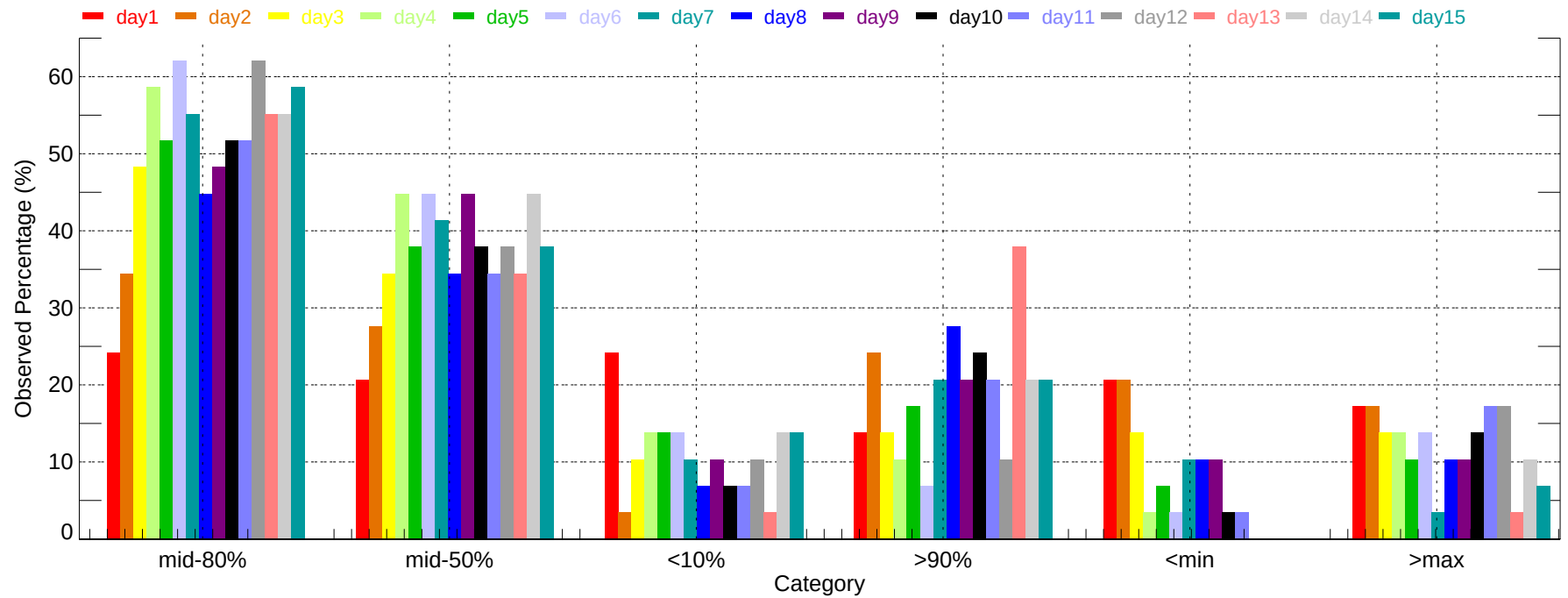
Observed Percentage of Ensembles - FAR: Max Temperature (2007-11-01~2007-11-30)
