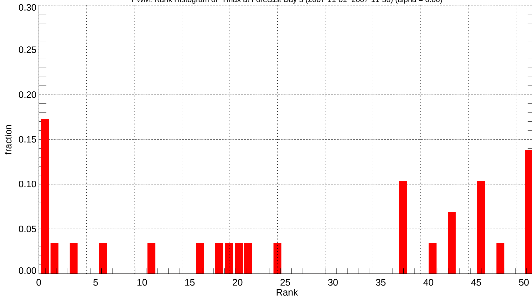
PWM: Rank Histogram of Tmax at Forecast Day 3 (2007-11-01~2007-11-30) (alpha = 0.00)
