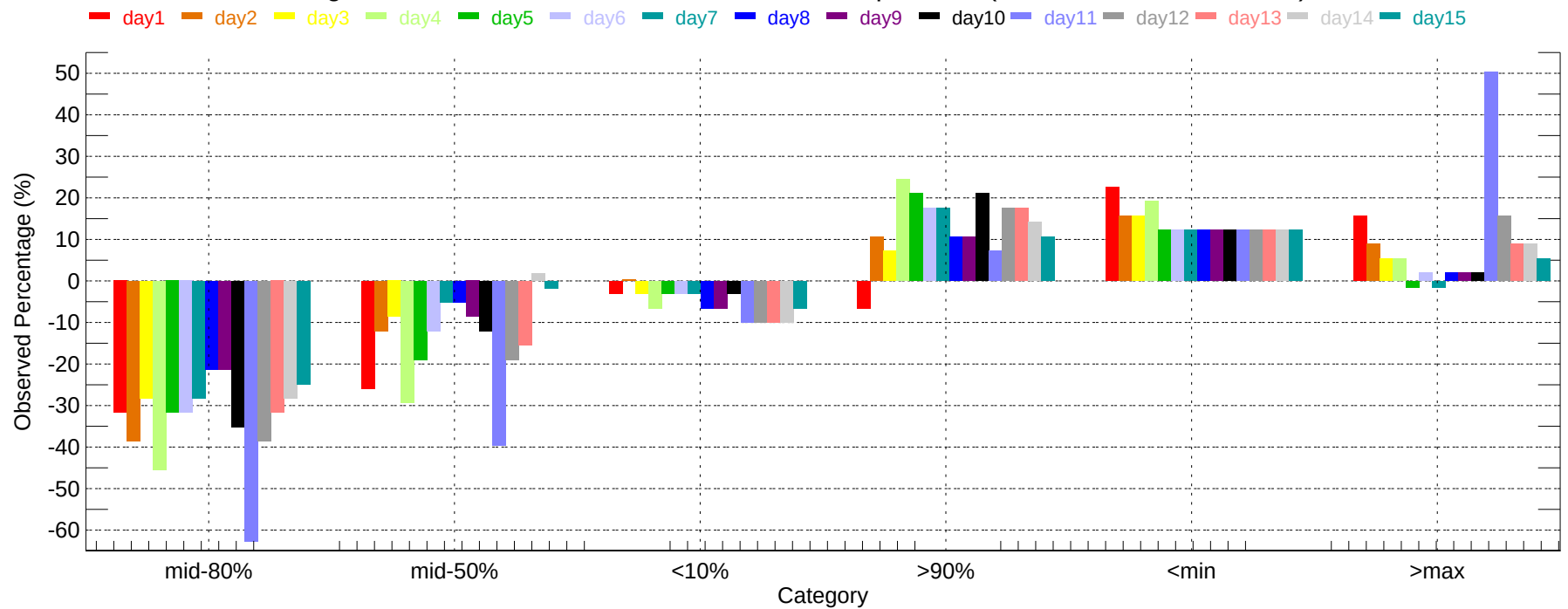
Observed Percentage Deviation of Ensembles - GAD: Max Temperature (2007-11-01~2007-11-30)
