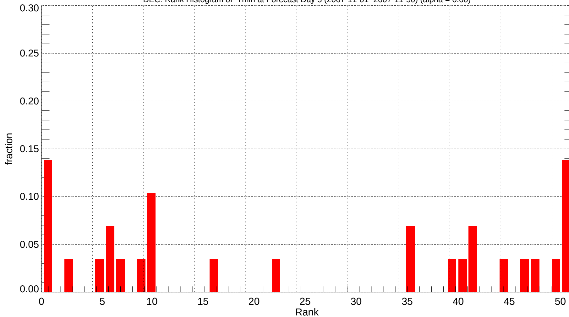
DEC: Rank Histogram of Tmin at Forecast Day 3 (2007-11-01~2007-11-30) (alpha = 0.00)
