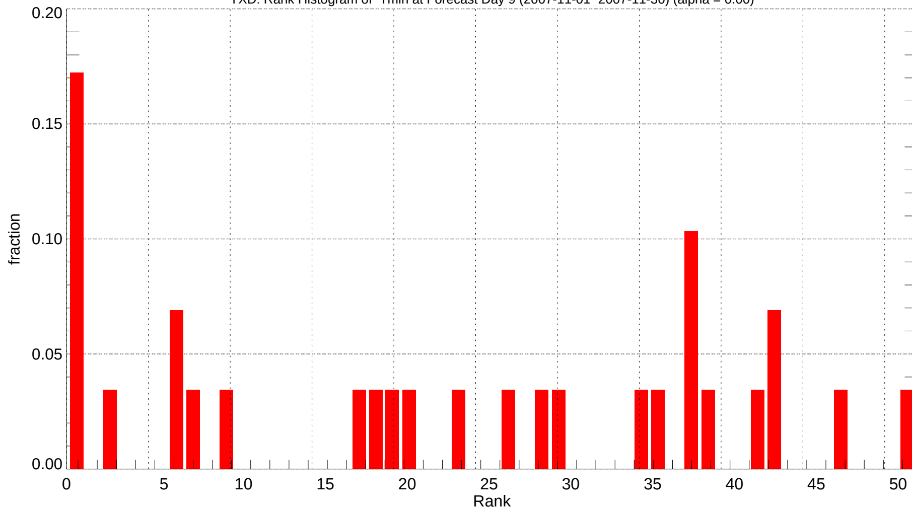
YXD: Rank Histogram of Tmin at Forecast Day 9 (2007-11-01~2007-11-30) (alpha = 0.00)
