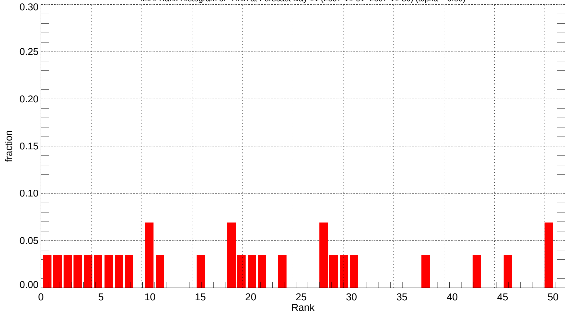
MIA: Rank Histogram of Tmin at Forecast Day 11 (2007-11-01~2007-11-30) (alpha = 0.00)
