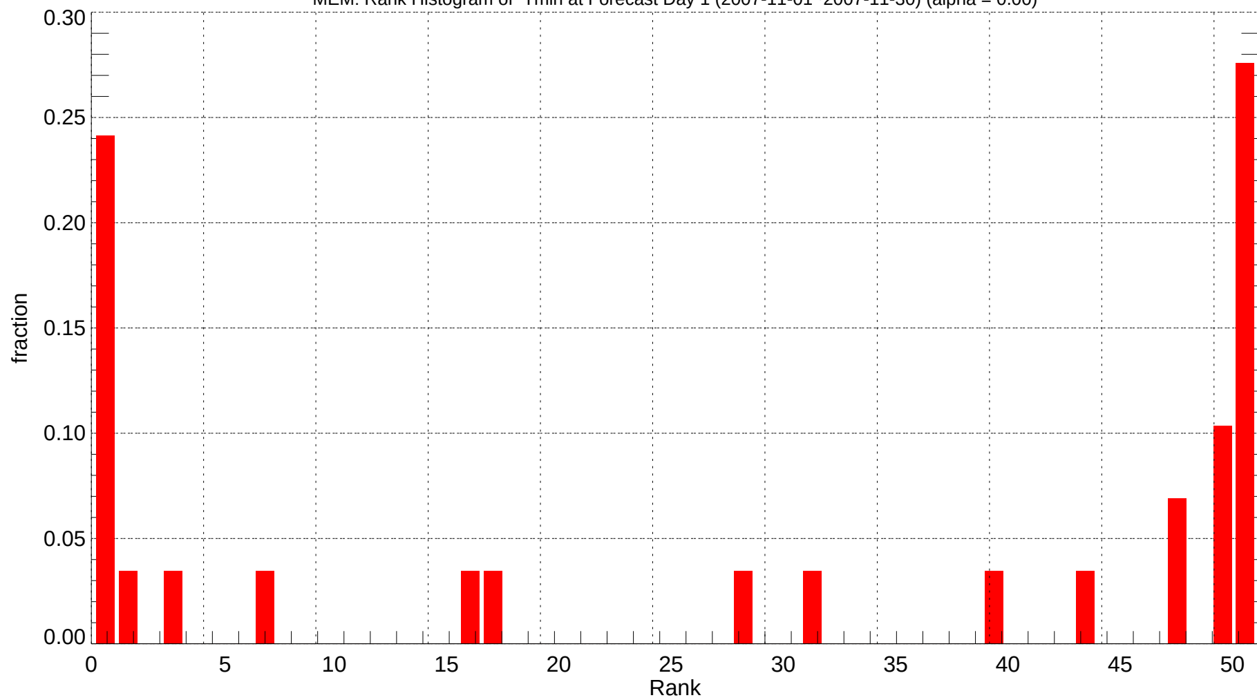
MEM: Rank Histogram of Tmin at Forecast Day 1 (2007-11-01~2007-11-30) (alpha = 0.00)
