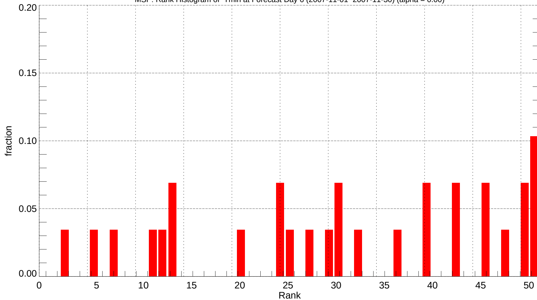
MSP: Rank Histogram of Tmin at Forecast Day 6 (2007-11-01~2007-11-30) (alpha = 0.00)
