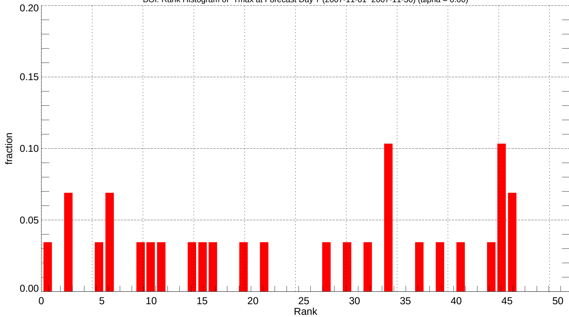
BOI: Rank Histogram of Tmax at Forecast Day 7 (2007-11-01~2007-11-30) (alpha = 0.00)
