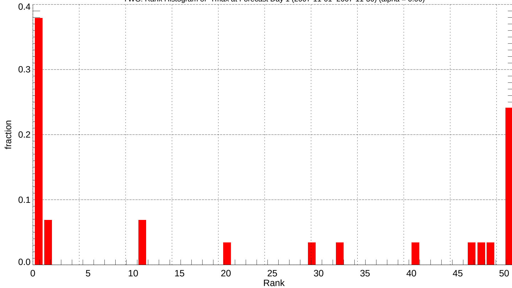
YWG: Rank Histogram of Tmax at Forecast Day 1 (2007-11-01~2007-11-30) (alpha = 0.00)
