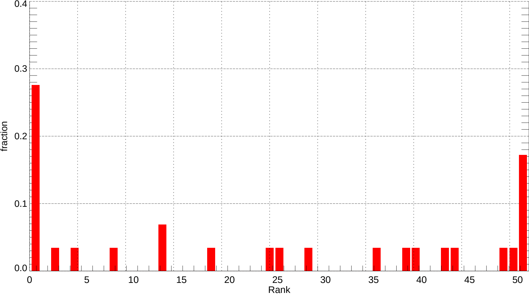
SSI: Rank Histogram of Tmax at Forecast Day 1 (2007-11-01~2007-11-30) (alpha = 0.00)
