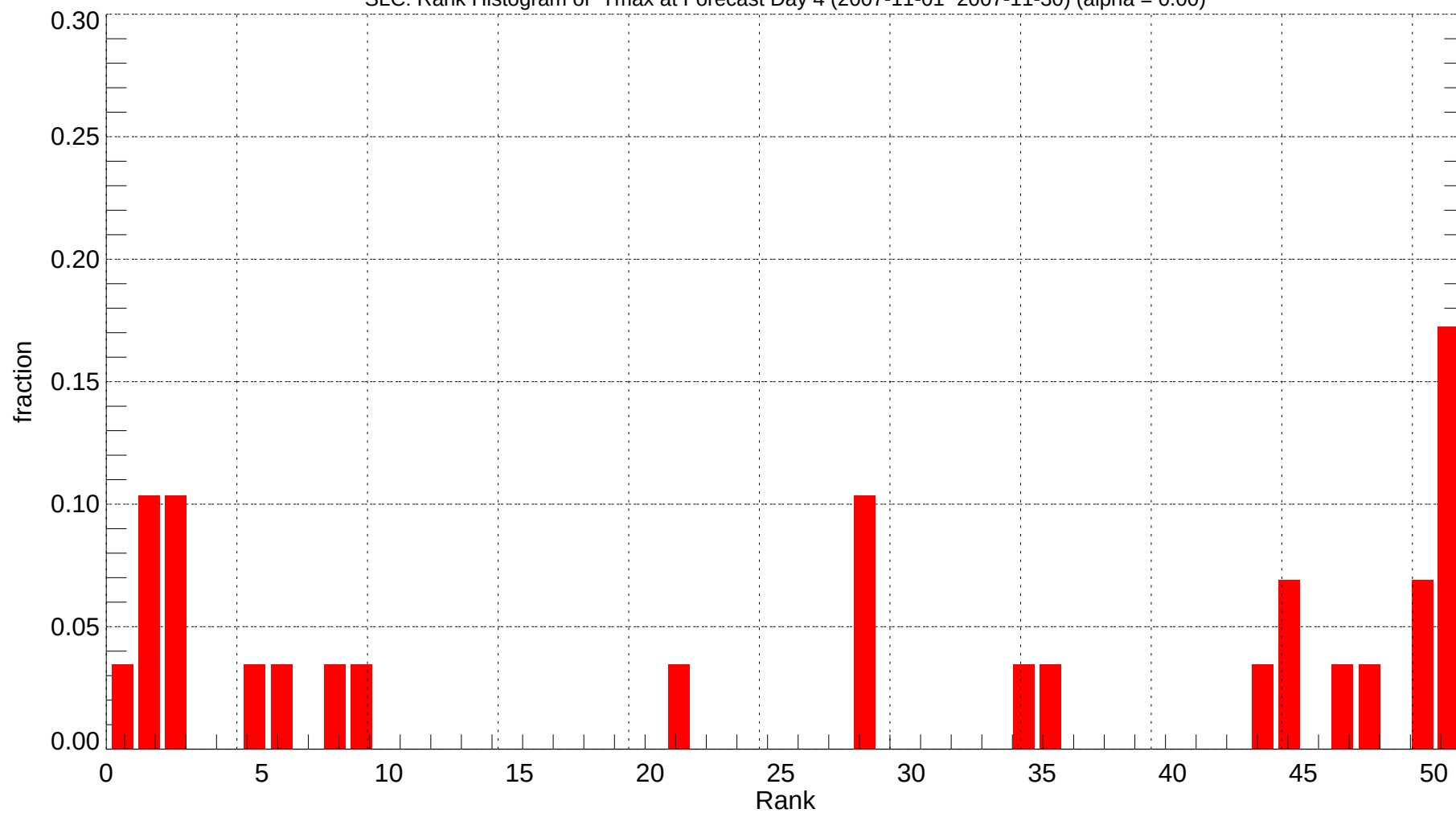
SLC: Rank Histogram of Tmax at Forecast Day 4 (2007-11-01~2007-11-30) (alpha = 0.00)
