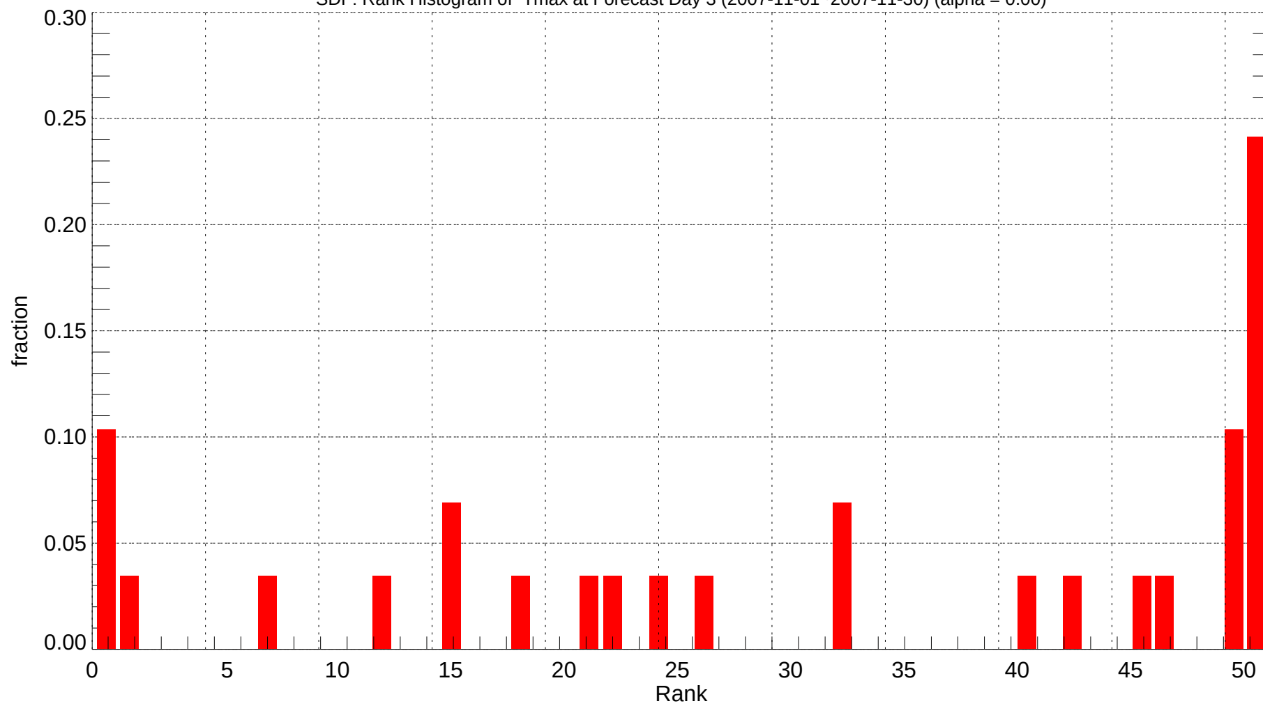
SDF: Rank Histogram of Tmax at Forecast Day 3 (2007-11-01~2007-11-30) (alpha = 0.00)
