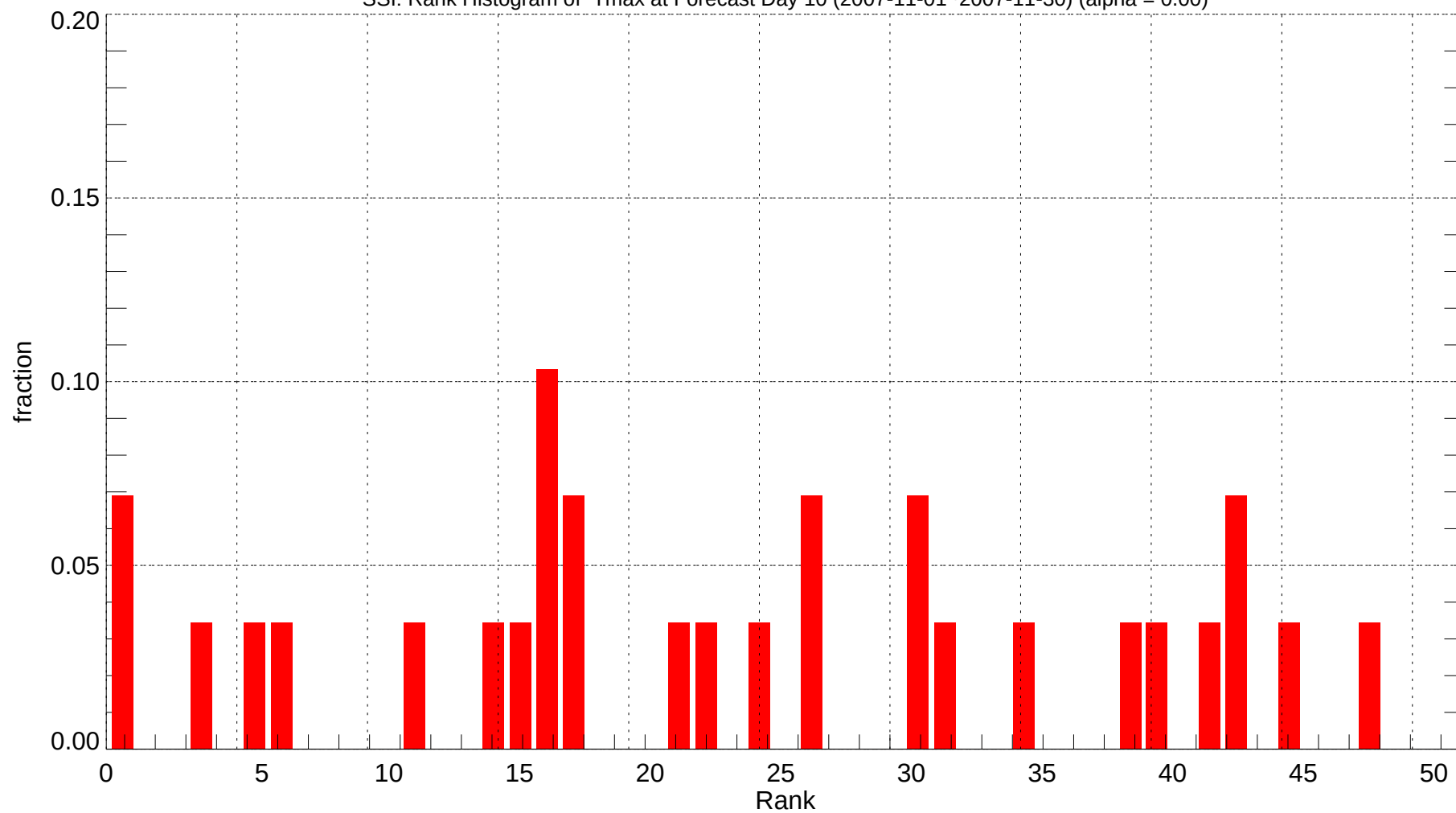
SSI: Rank Histogram of Tmax at Forecast Day 10 (2007-11-01~2007-11-30) (alpha = 0.00)
