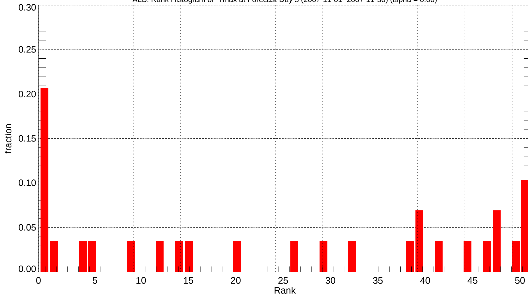
ALB: Rank Histogram of Tmax at Forecast Day 3 (2007-11-01~2007-11-30) (alpha = 0.00)
