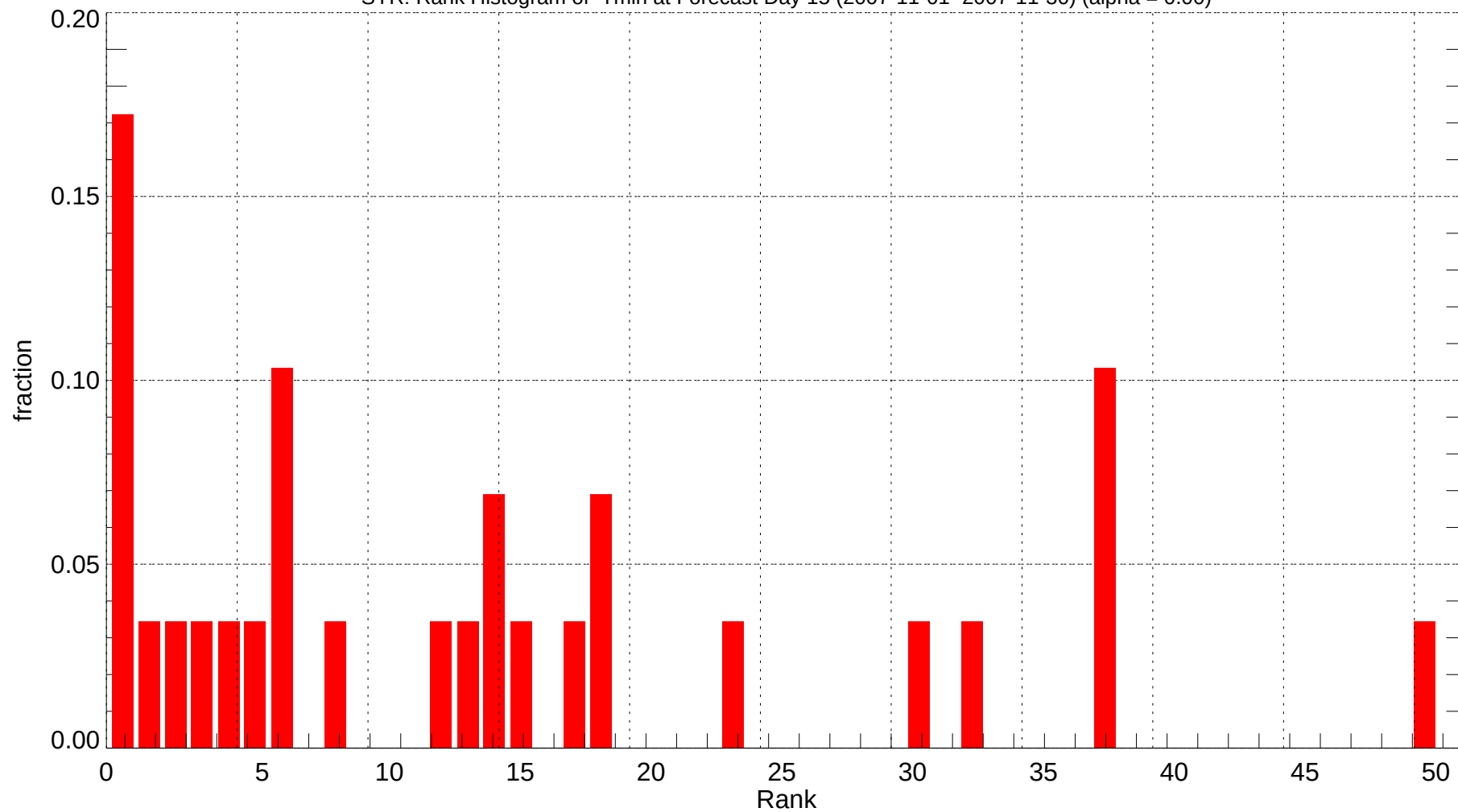
SYR: Rank Histogram of Tmin at Forecast Day 15 (2007-11-01~2007-11-30) (alpha = 0.00)
