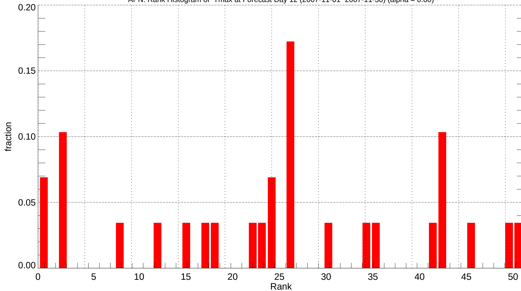
APN: Rank Histogram of Tmax at Forecast Day 12 (2007-11-01~2007-11-30) (alpha = 0.00)
