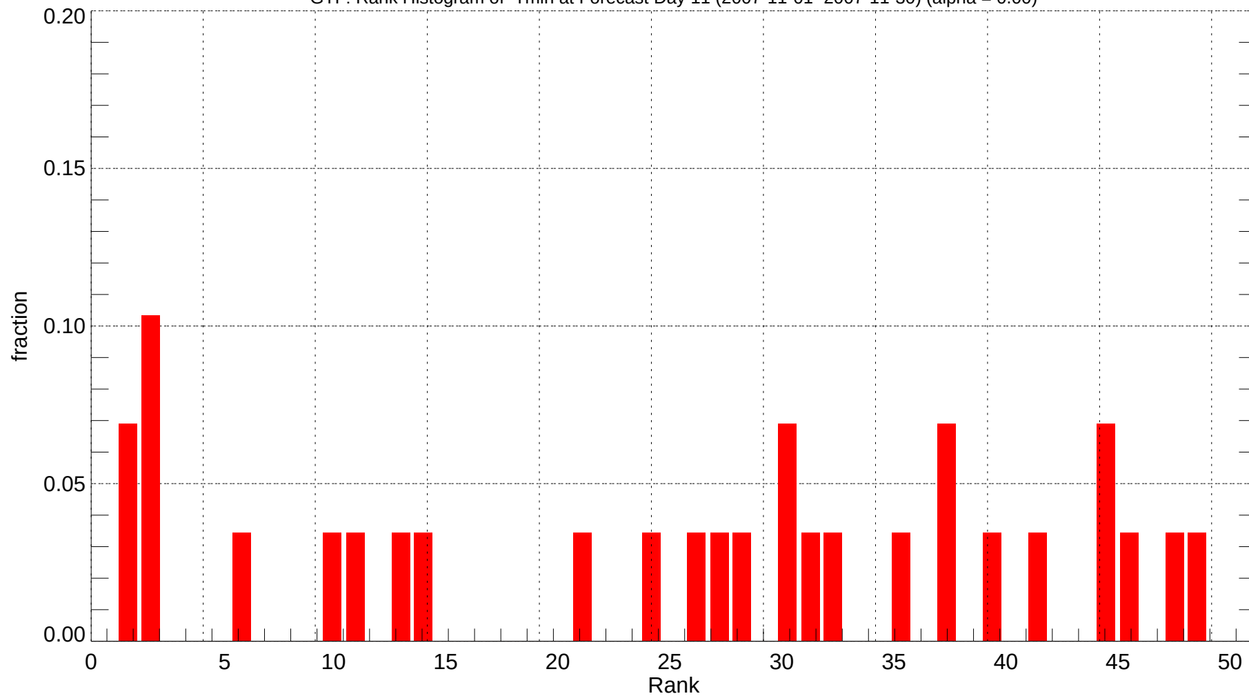
GTF: Rank Histogram of Tmin at Forecast Day 11 (2007-11-01~2007-11-30) (alpha = 0.00)
