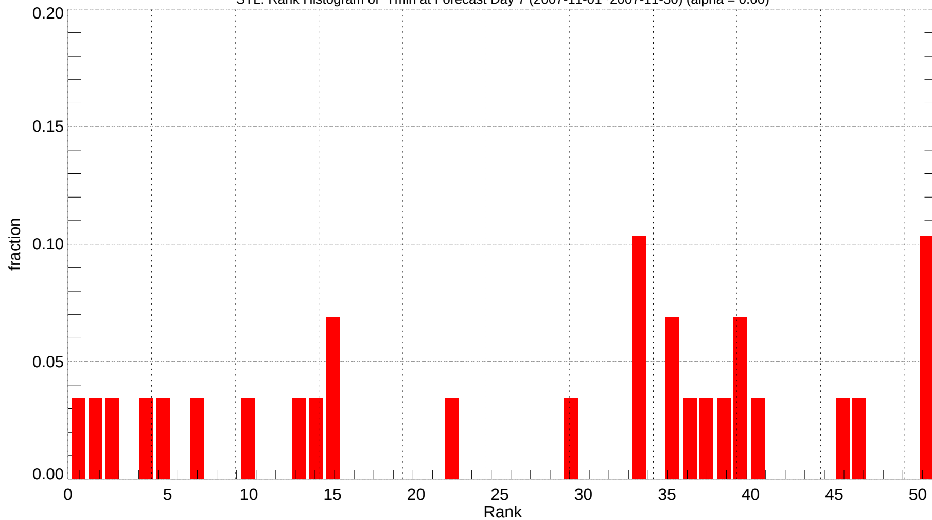
STL: Rank Histogram of Tmin at Forecast Day 7 (2007-11-01~2007-11-30) (alpha = 0.00)
