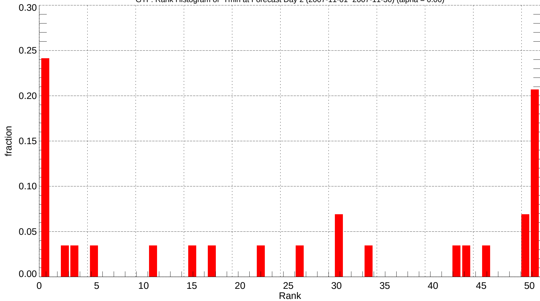
GTF: Rank Histogram of Tmin at Forecast Day 2 (2007-11-01~2007-11-30) (alpha = 0.00)
