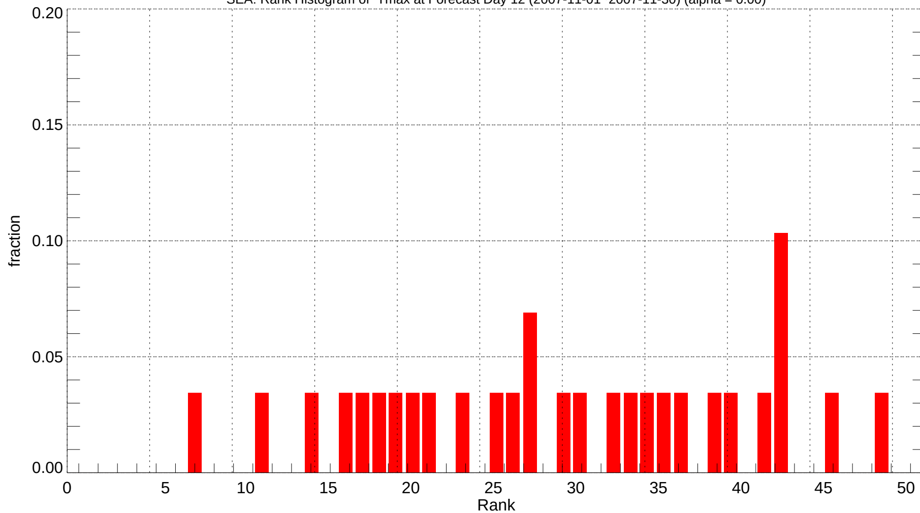
SEA: Rank Histogram of Tmax at Forecast Day 12 (2007-11-01~2007-11-30) (alpha = 0.00)
