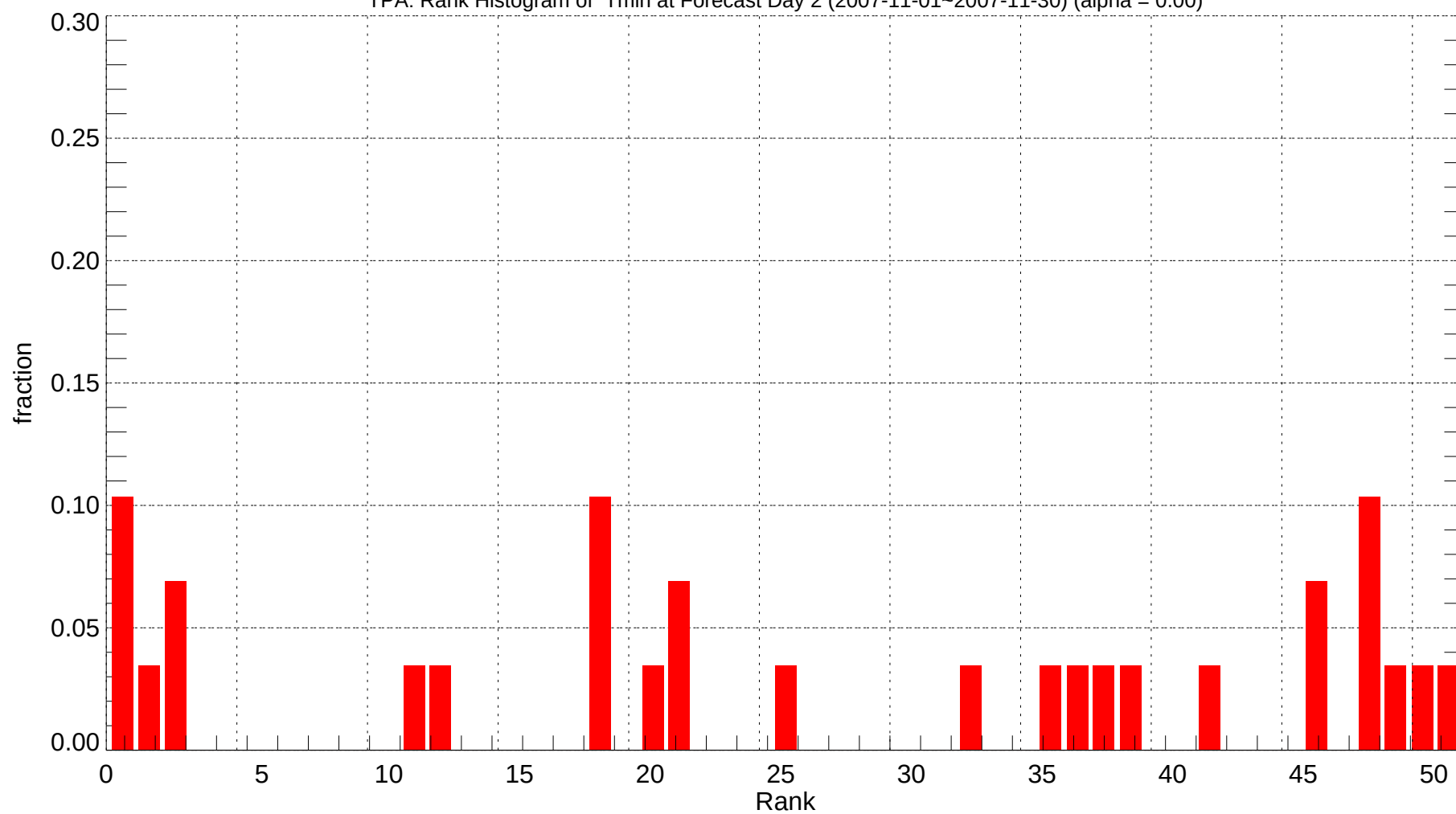
TPA: Rank Histogram of Tmin at Forecast Day 2 (2007-11-01~2007-11-30) (alpha = 0.00)
