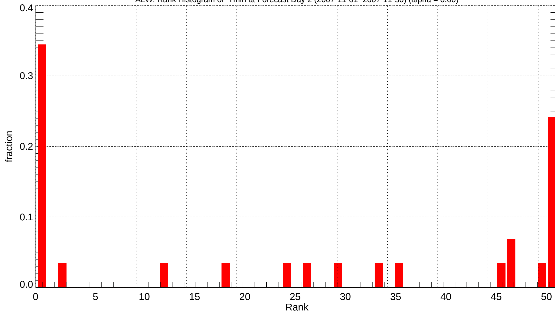
ALW: Rank Histogram of Tmin at Forecast Day 2 (2007-11-01~2007-11-30) (alpha = 0.00)
