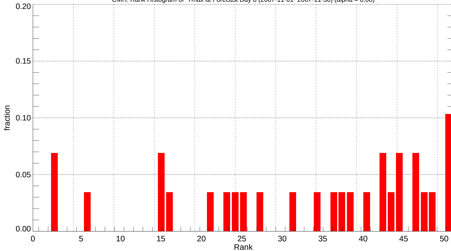
CMH: Rank Histogram of Tmax at Forecast Day 8 (2007-11-01~2007-11-30) (alpha = 0.00)
