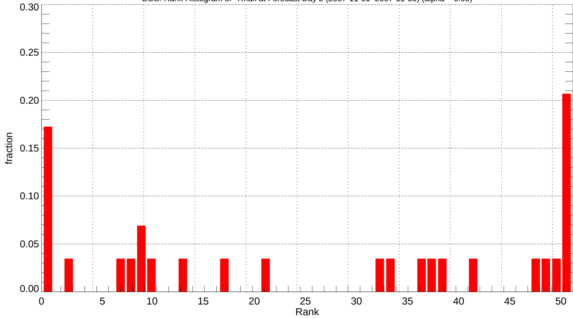
BOS: Rank Histogram of Tmax at Forecast Day 2 (2007-11-01~2007-11-30) (alpha = 0.00)
