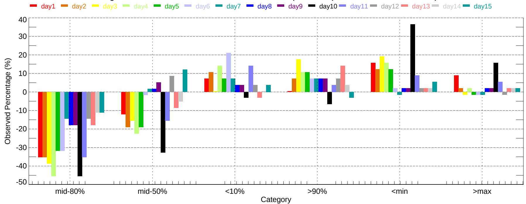
Observed Percentage Deviation of Ensembles - AUS: Max Temperature (2007-11-01~2007-11-30)
