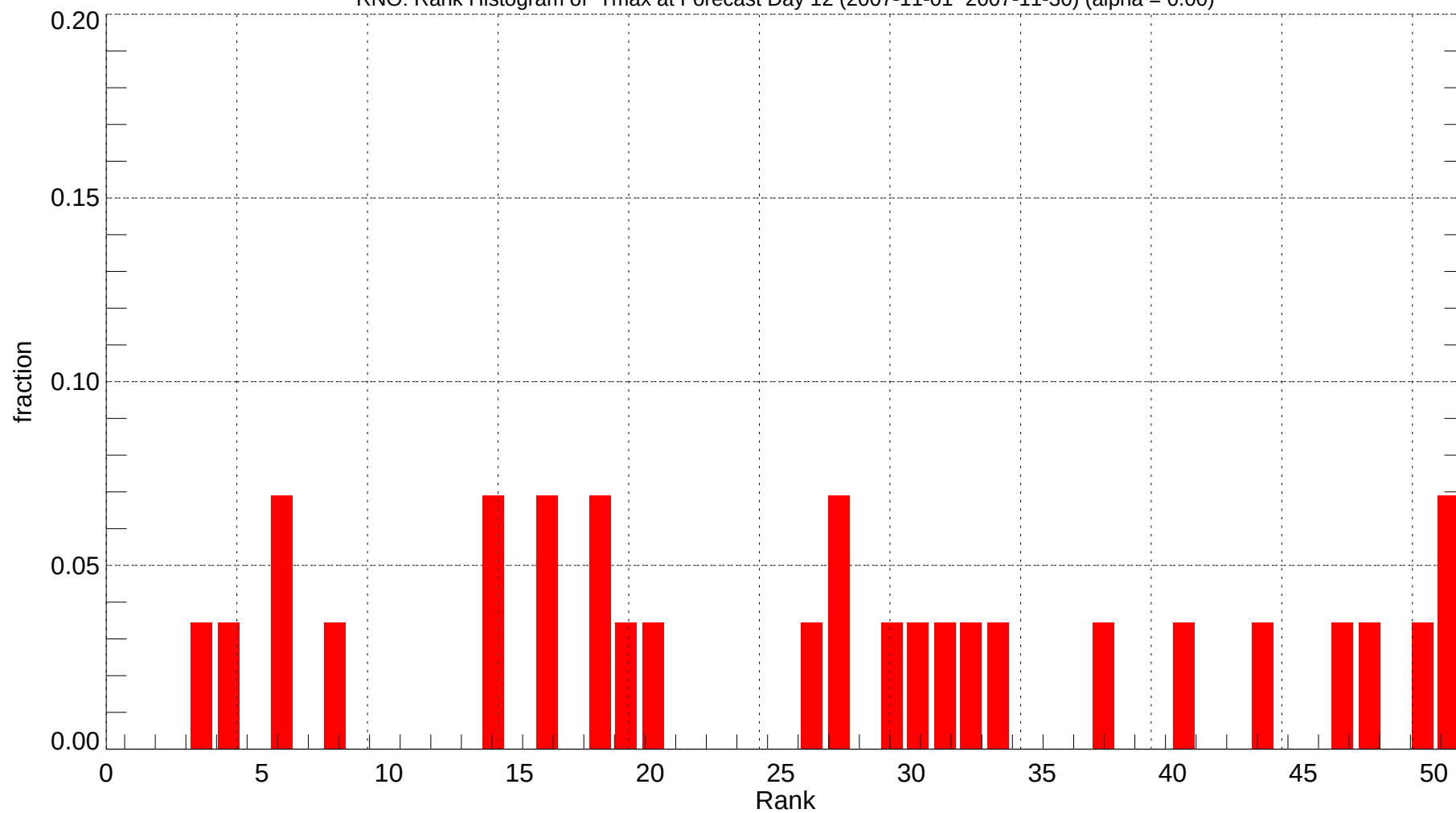
RNO: Rank Histogram of Tmax at Forecast Day 12 (2007-11-01~2007-11-30) (alpha = 0.00)
