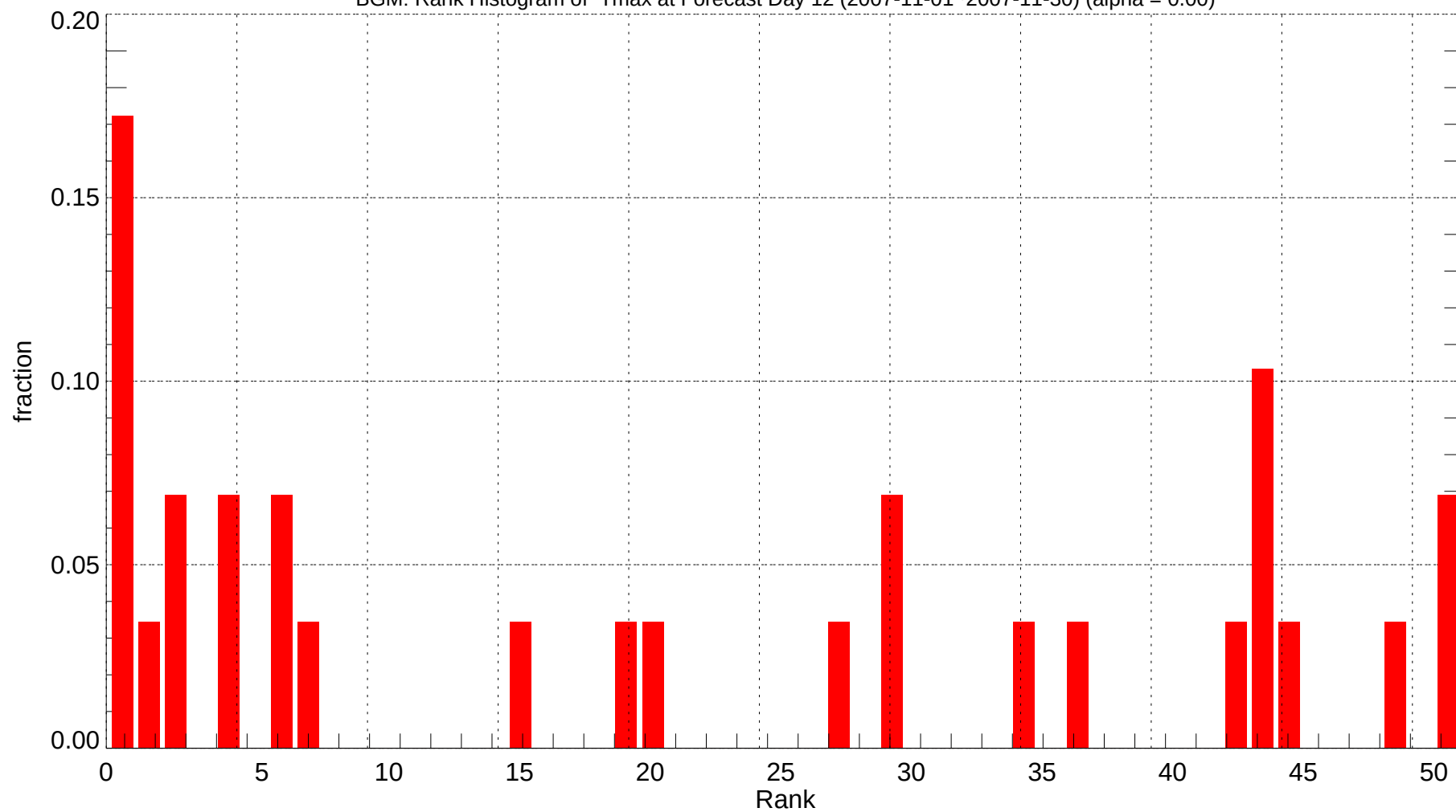
BGM: Rank Histogram of Tmax at Forecast Day 12 (2007-11-01~2007-11-30) (alpha = 0.00)
