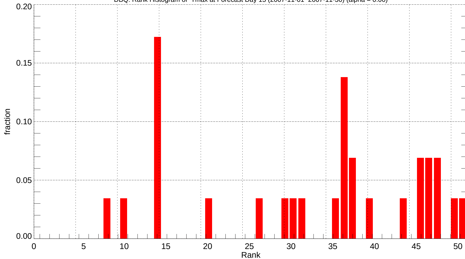
DBQ: Rank Histogram of Tmax at Forecast Day 15 (2007-11-01~2007-11-30) (alpha = 0.00)
