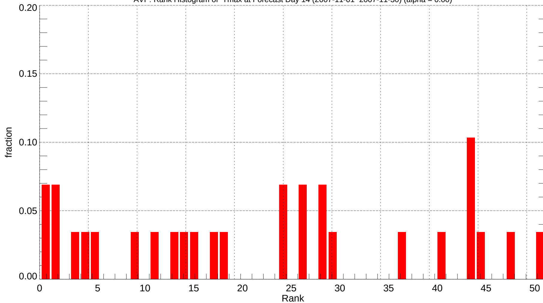
AVP: Rank Histogram of Tmax at Forecast Day 14 (2007-11-01~2007-11-30) (alpha = 0.00)
