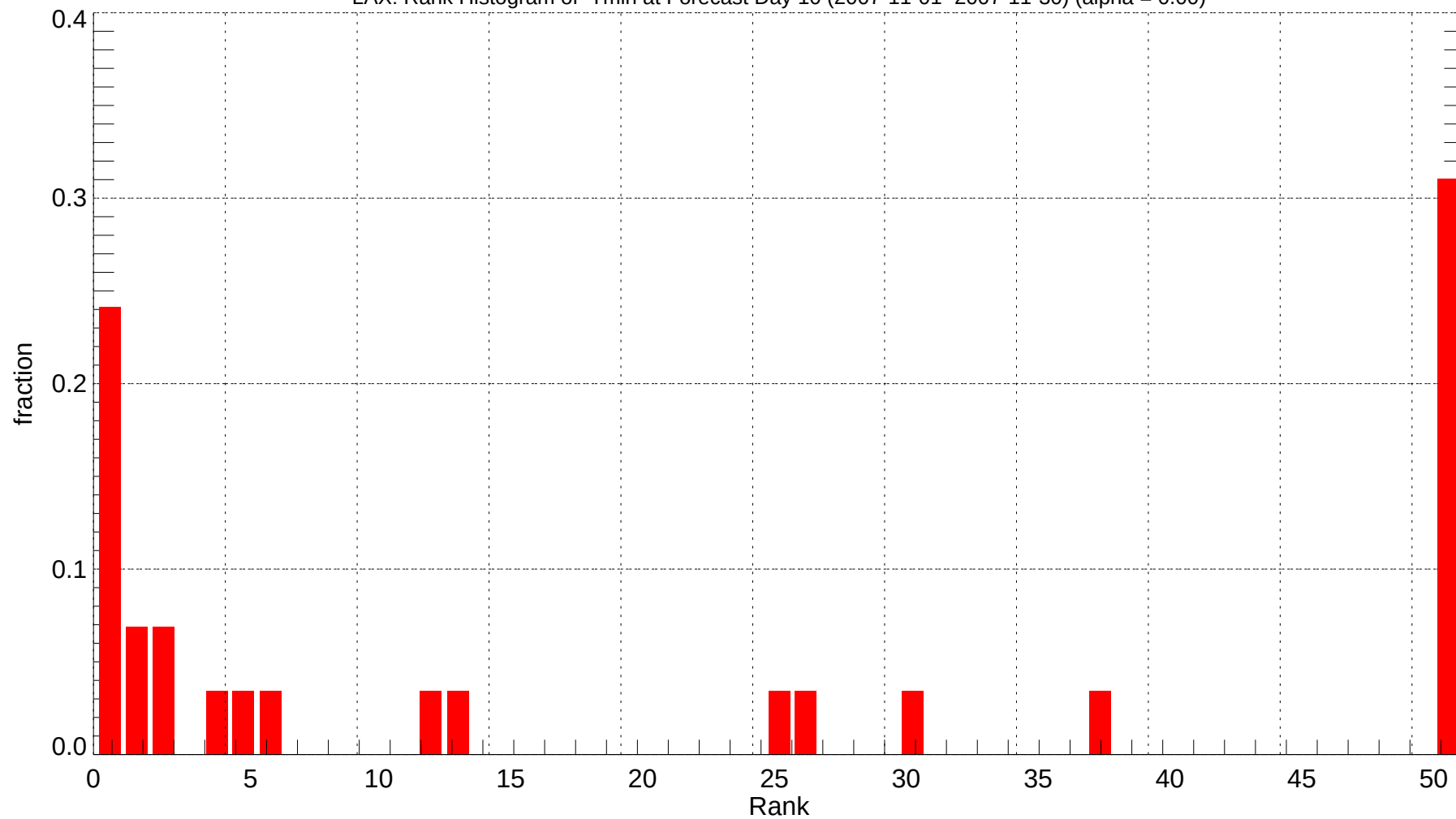
LAX: Rank Histogram of Tmin at Forecast Day 10 (2007-11-01~2007-11-30) (alpha = 0.00)
