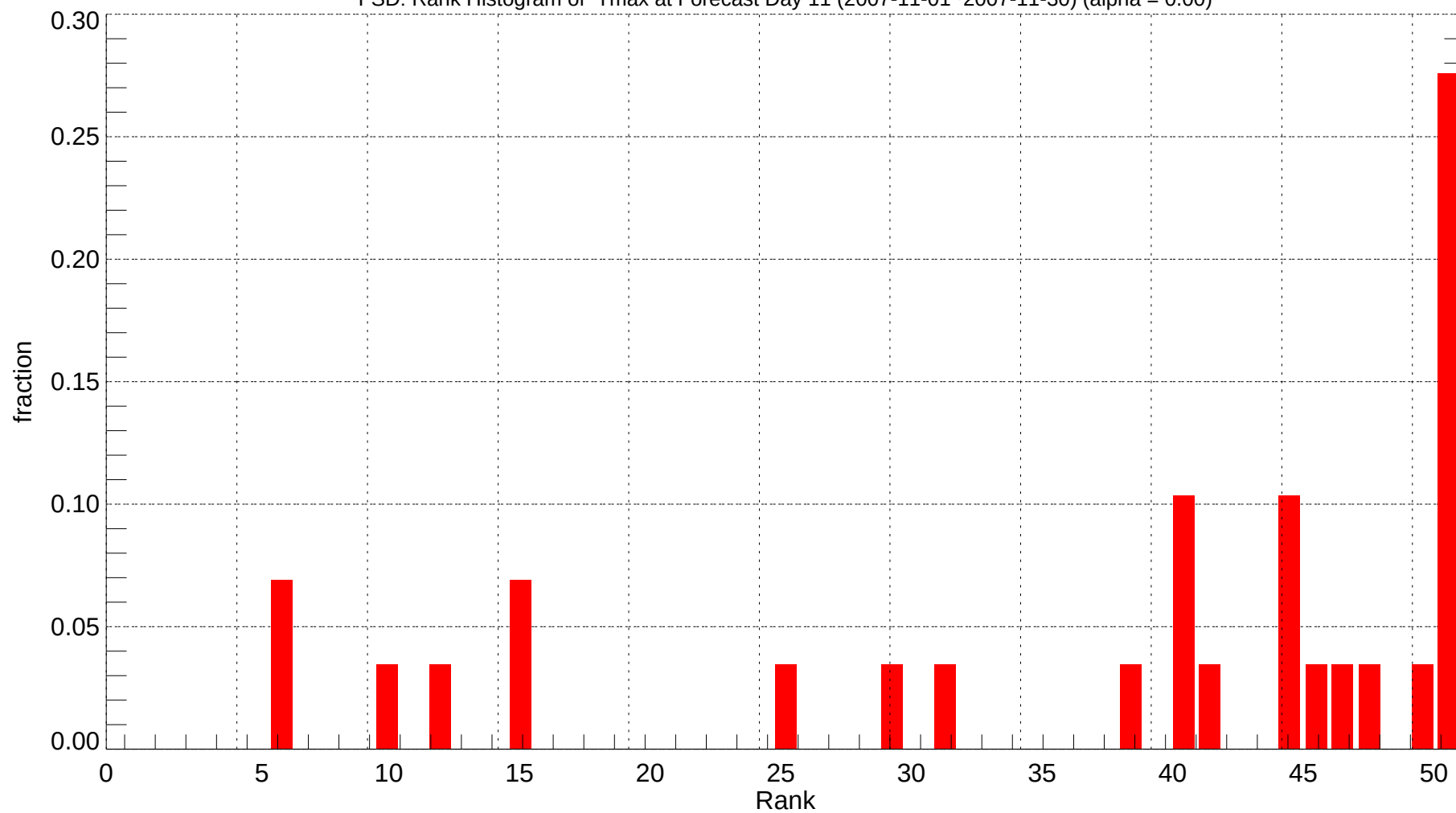
FSD: Rank Histogram of Tmax at Forecast Day 11 (2007-11-01~2007-11-30) (alpha = 0.00)
