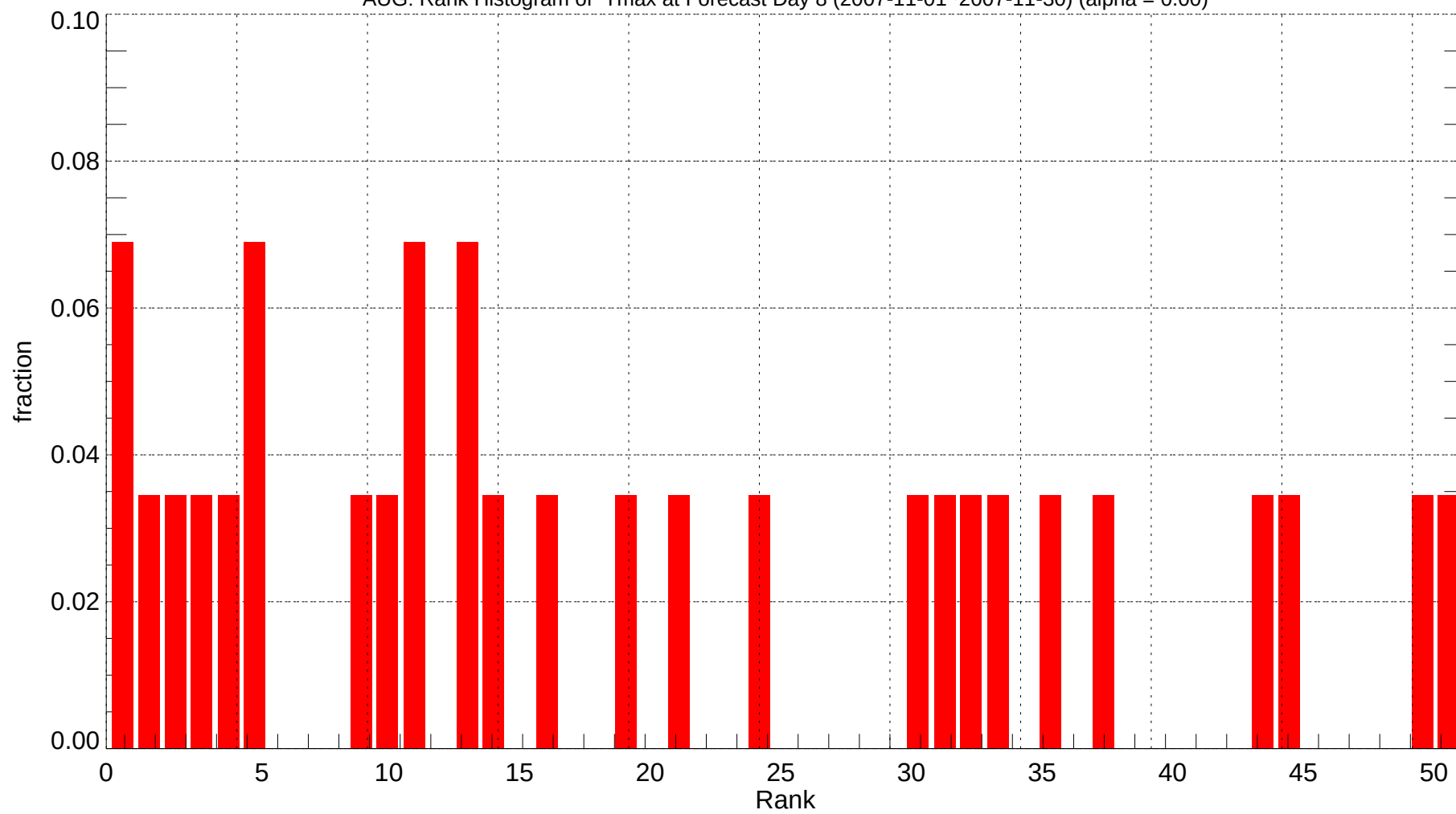
AUG: Rank Histogram of Tmax at Forecast Day 8 (2007-11-01~2007-11-30) (alpha = 0.00)
