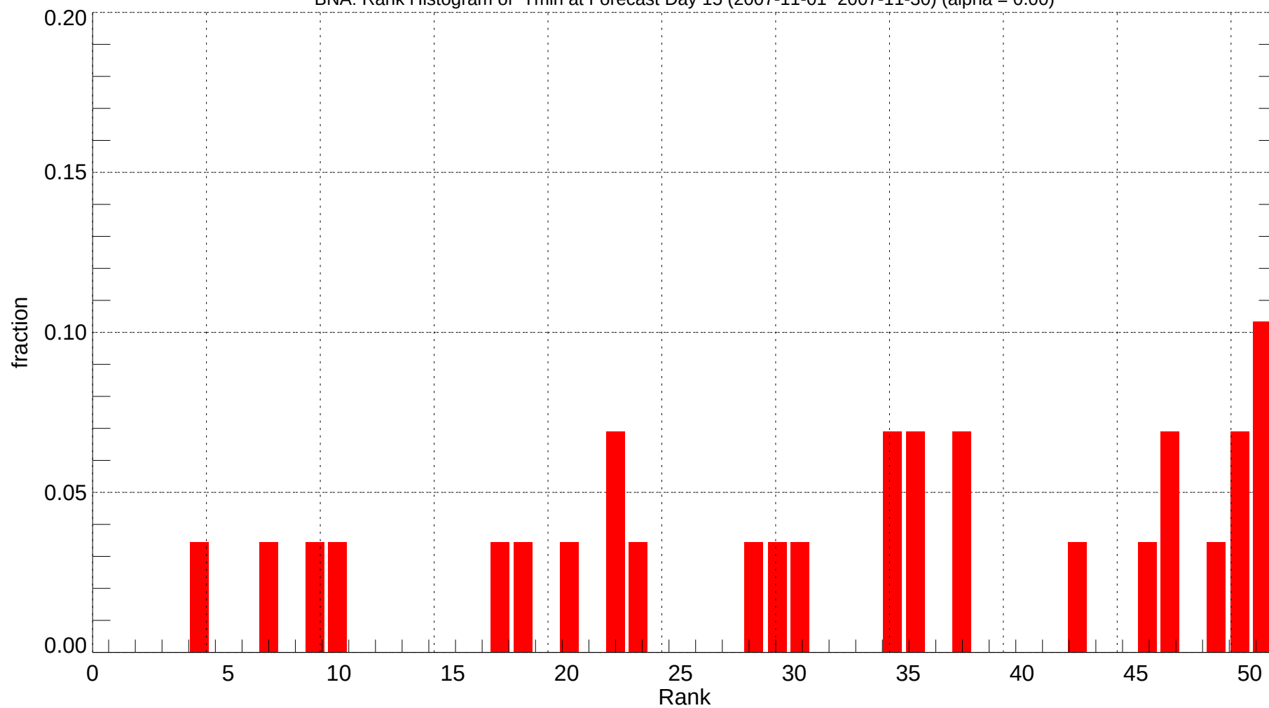
BNA: Rank Histogram of Tmin at Forecast Day 15 (2007-11-01~2007-11-30) (alpha = 0.00)
