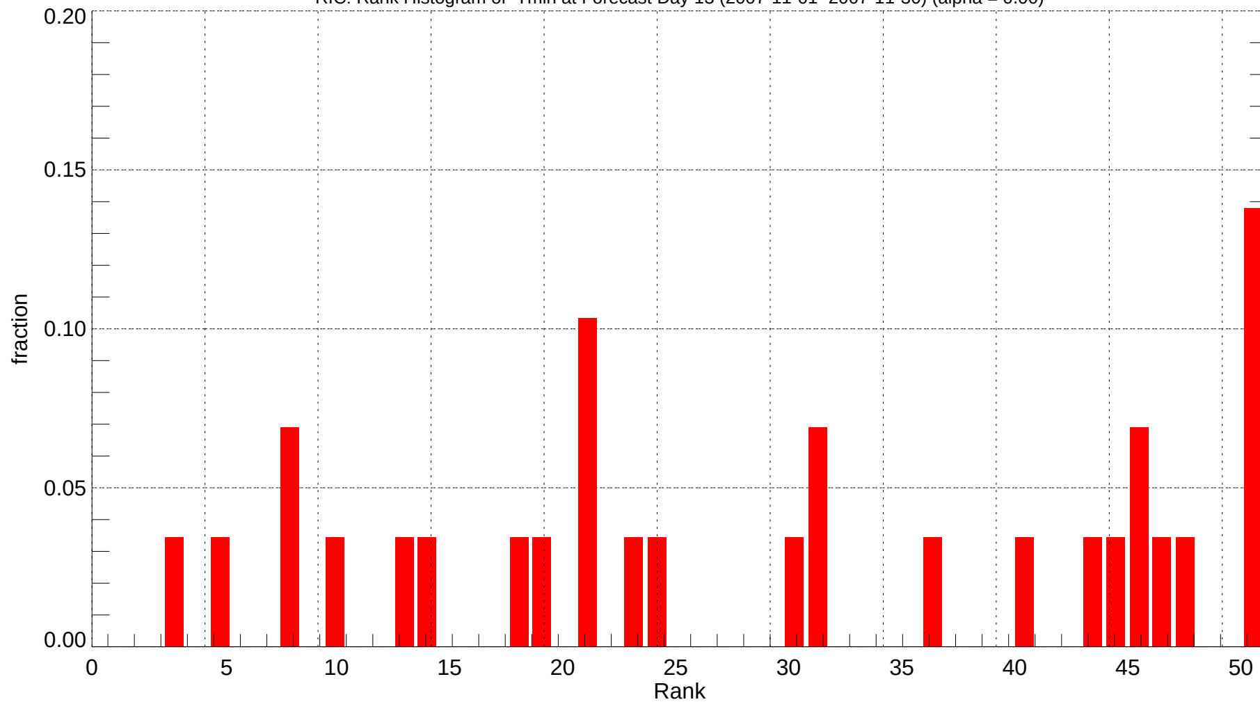
RIC: Rank Histogram of Tmin at Forecast Day 13 (2007-11-01~2007-11-30) (alpha = 0.00)
