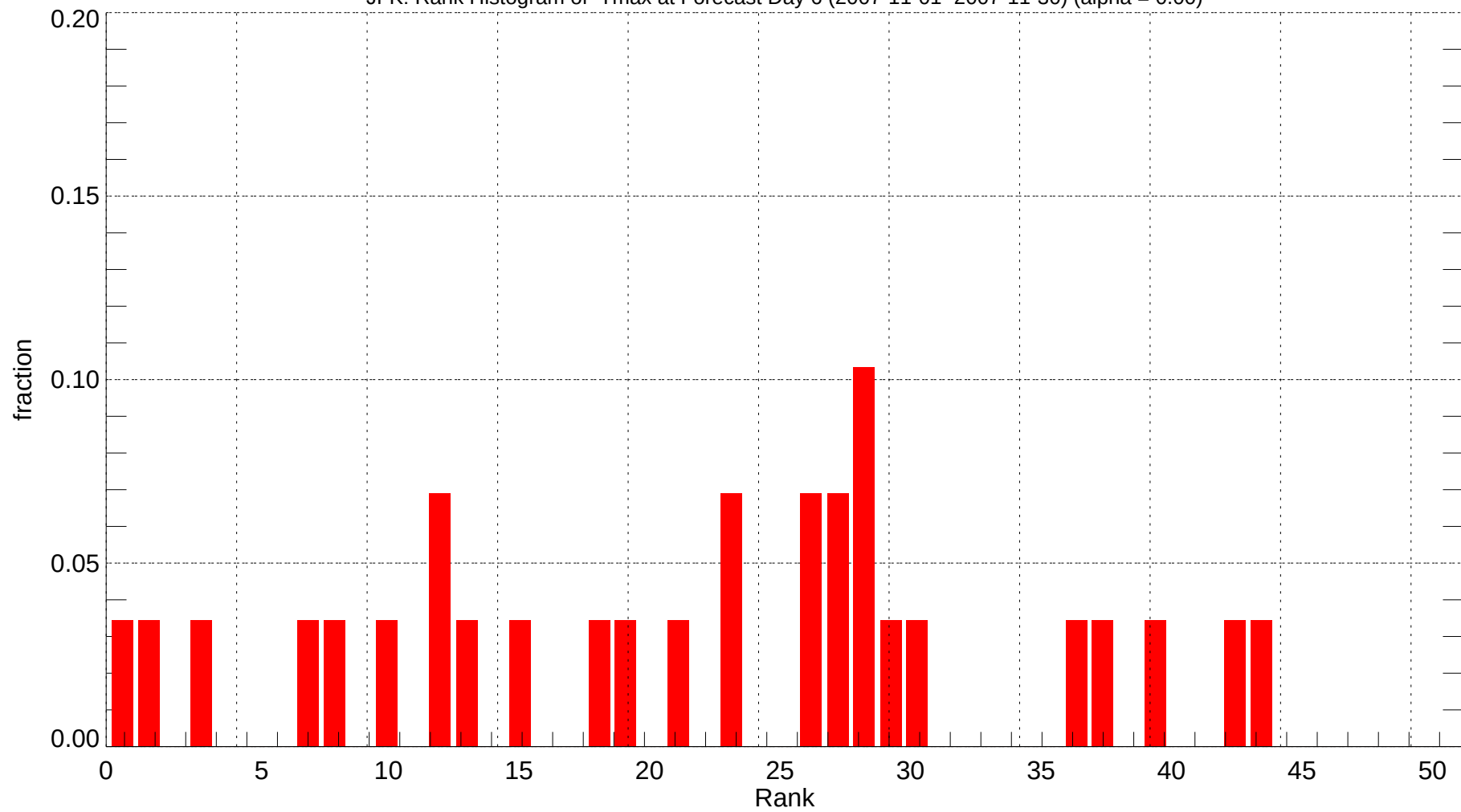
JFK: Rank Histogram of Tmax at Forecast Day 6 (2007-11-01~2007-11-30) (alpha = 0.00)
