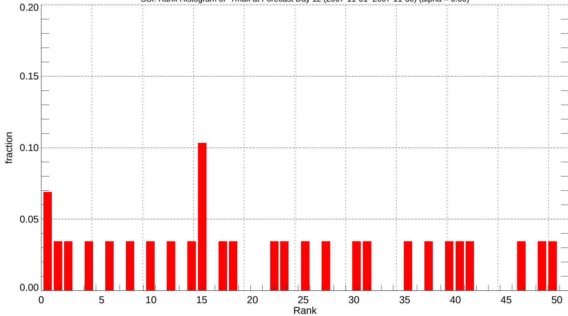
SSI: Rank Histogram of Tmax at Forecast Day 12 (2007-11-01~2007-11-30) (alpha = 0.00)
