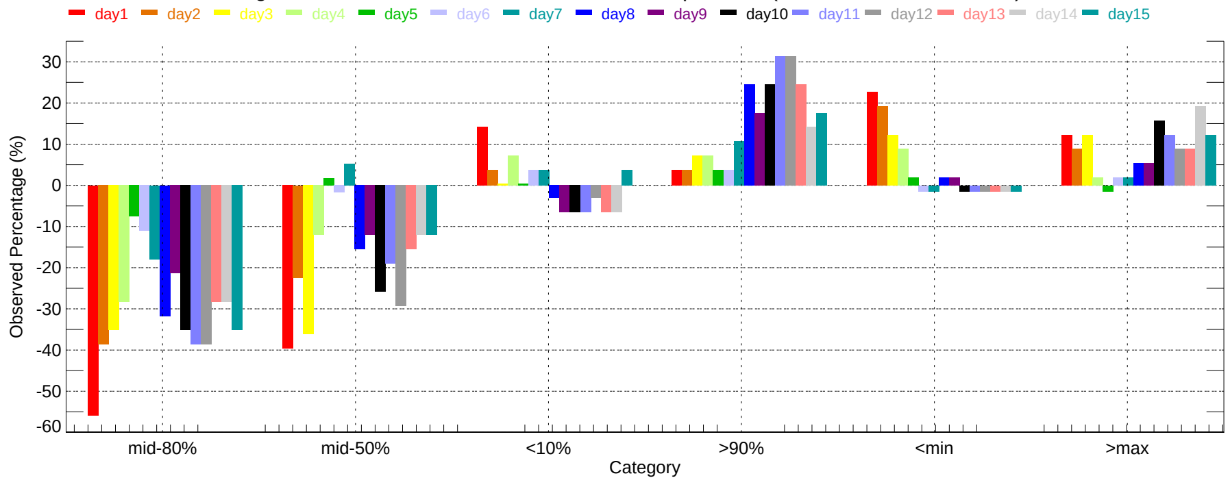
Observed Percentage Deviation of Ensembles - TYR: Max Temperature (2007-11-01~2007-11-30)
