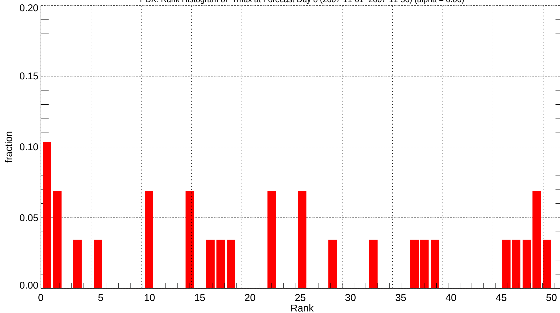
PDX: Rank Histogram of Tmax at Forecast Day 8 (2007-11-01~2007-11-30) (alpha = 0.00)
