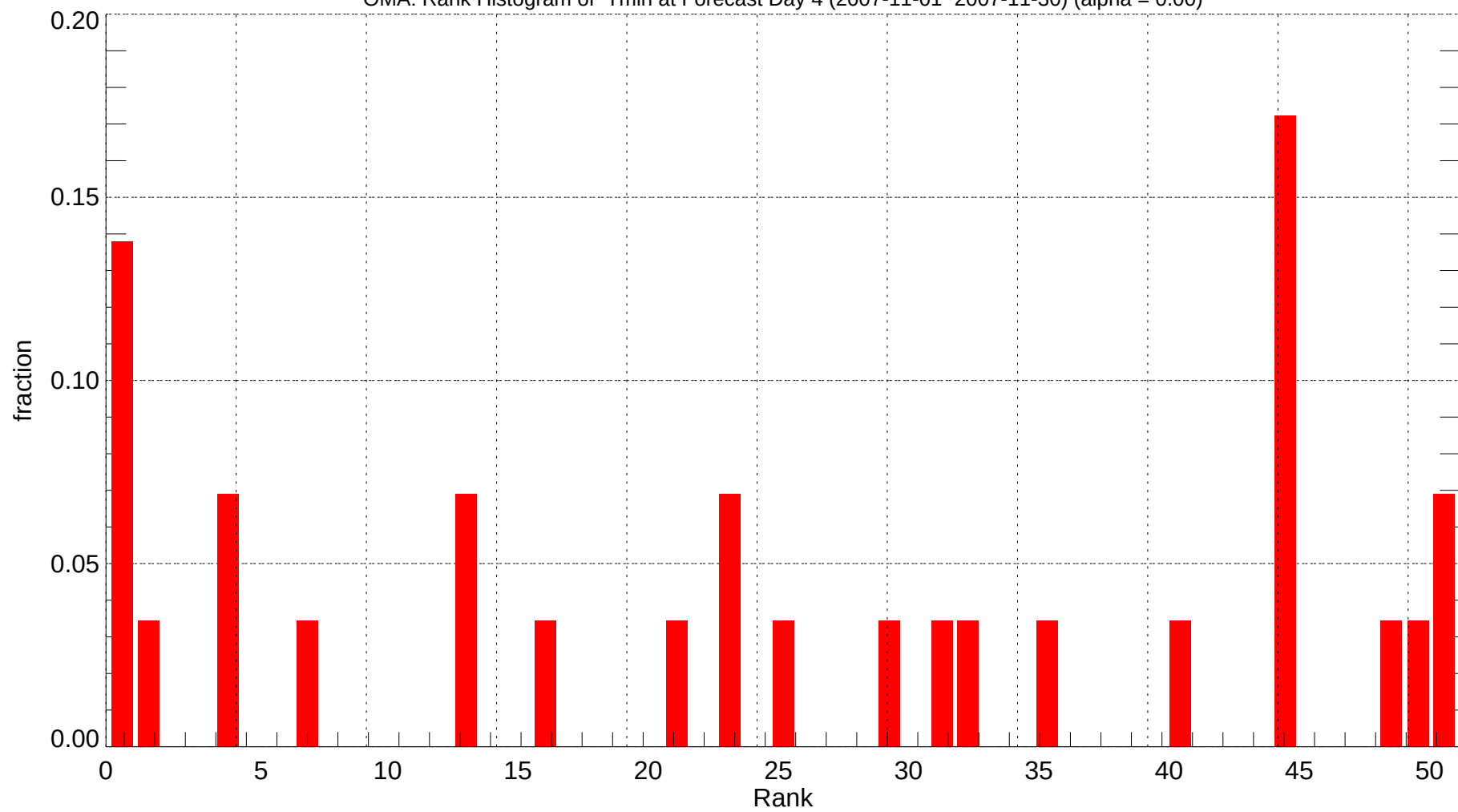
OMA: Rank Histogram of Tmin at Forecast Day 4 (2007-11-01~2007-11-30) (alpha = 0.00)
