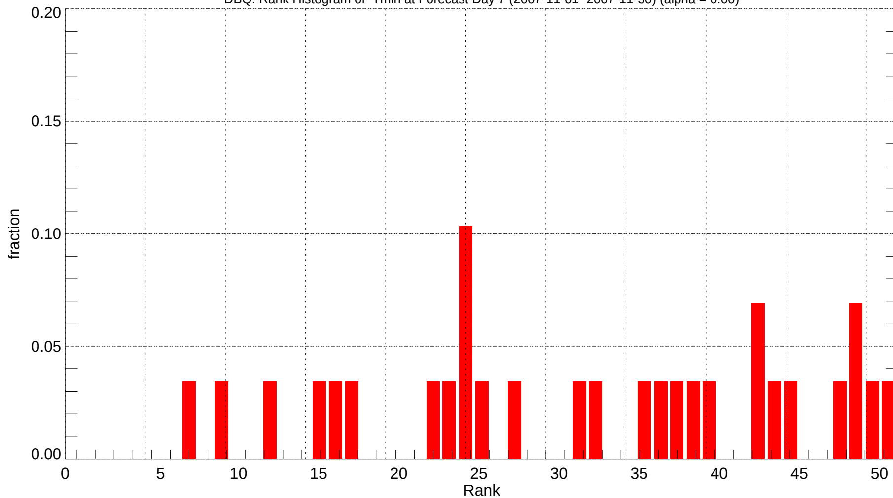
DBQ: Rank Histogram of Tmin at Forecast Day 7 (2007-11-01~2007-11-30) (alpha = 0.00)
