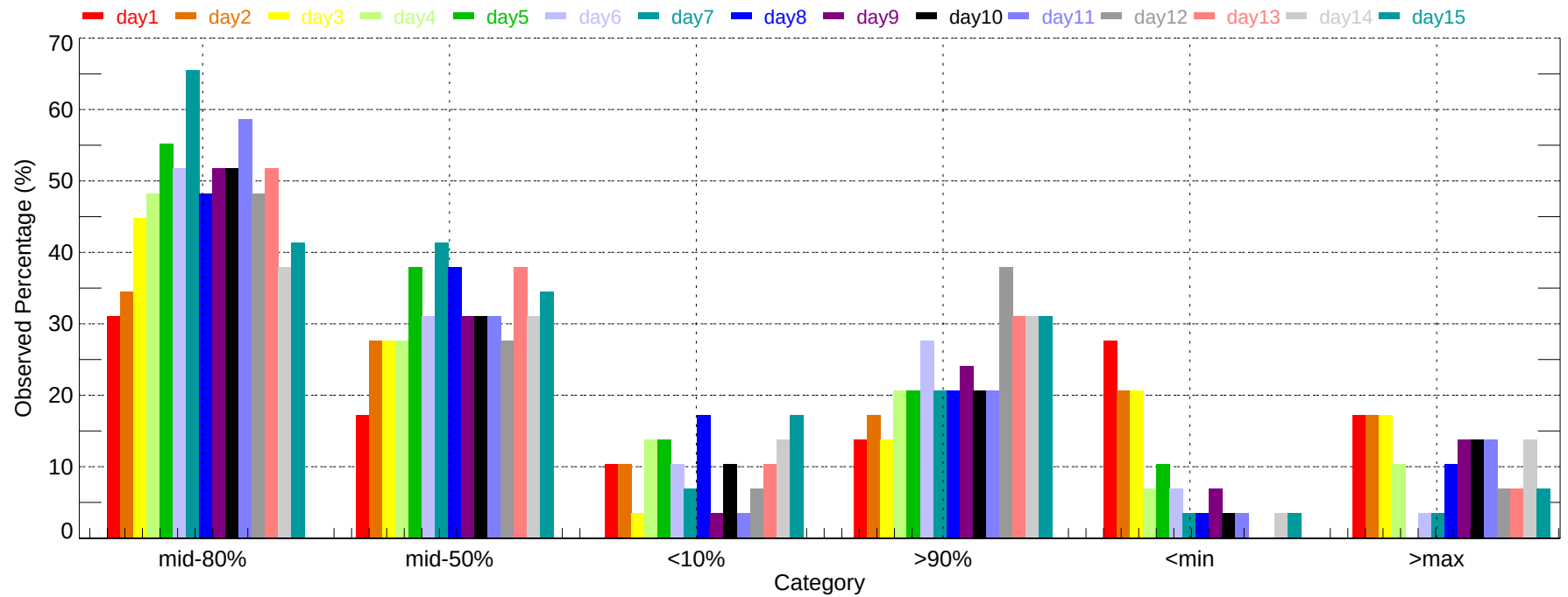
Observed Percentage of Ensembles - ABI: Max Temperature (2007-11-01~2007-11-30)
