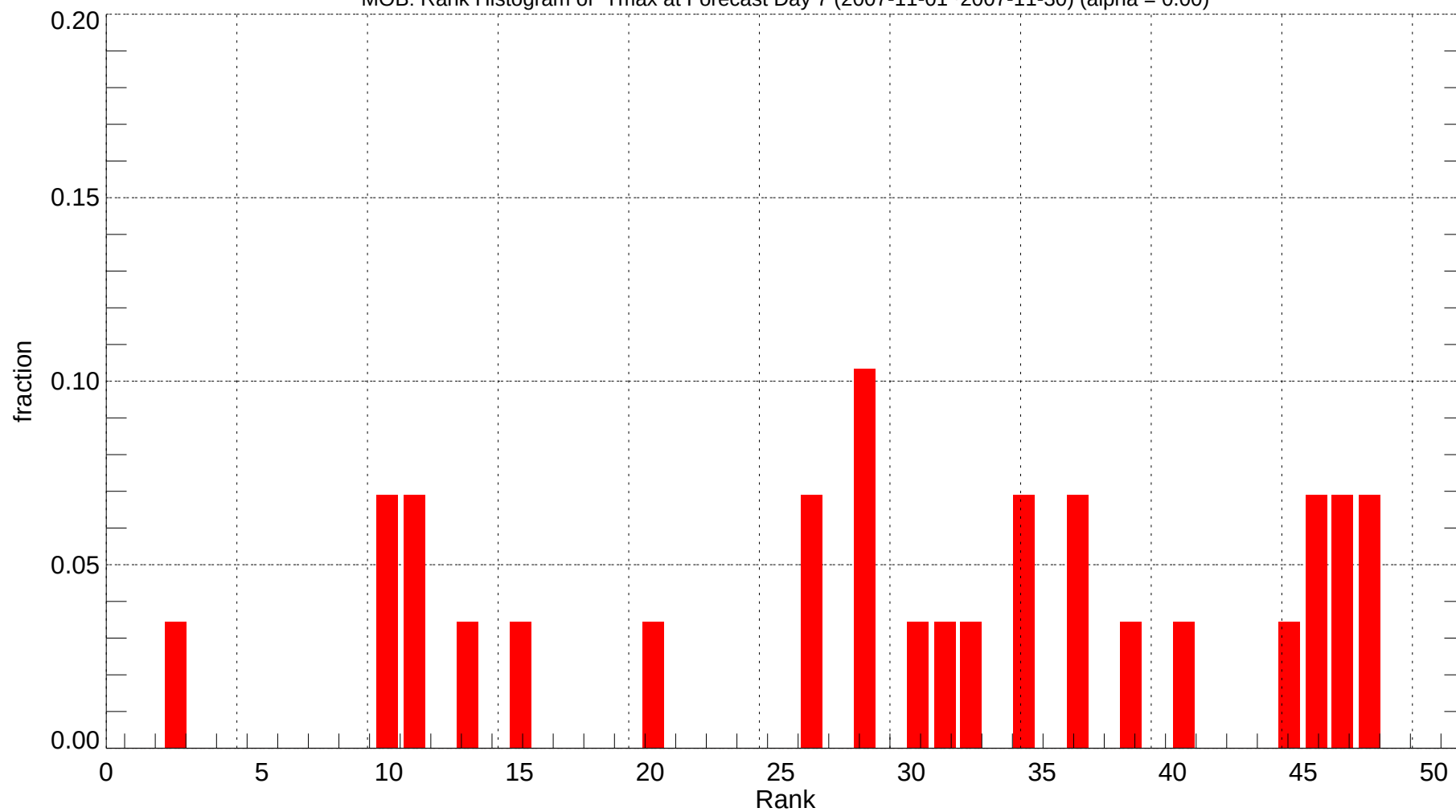
MOB: Rank Histogram of Tmax at Forecast Day 7 (2007-11-01~2007-11-30) (alpha = 0.00)
