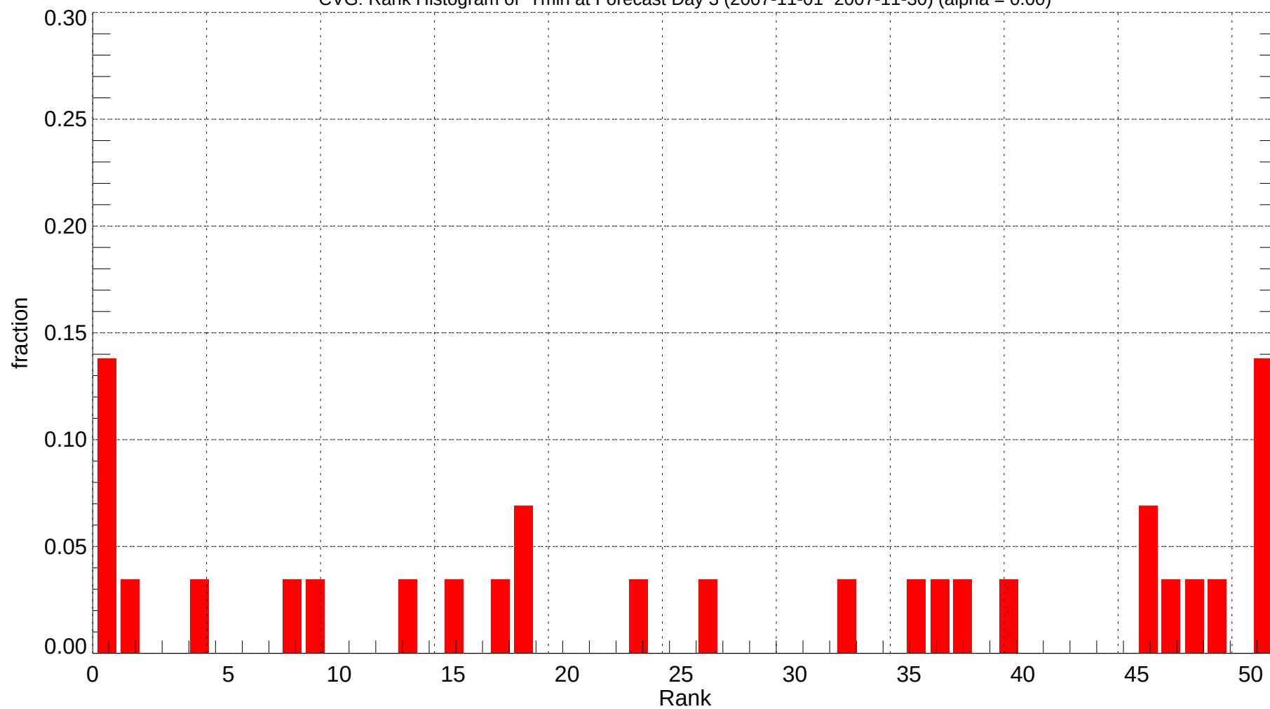
CVG: Rank Histogram of Tmin at Forecast Day 3 (2007-11-01~2007-11-30) (alpha = 0.00)
