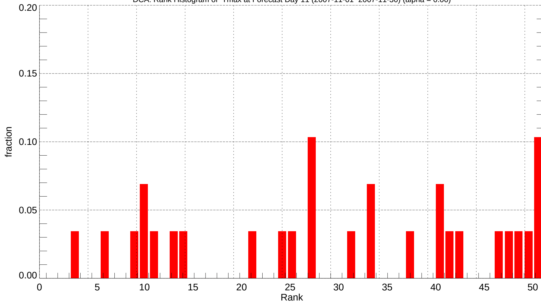
DCA: Rank Histogram of Tmax at Forecast Day 11 (2007-11-01~2007-11-30) (alpha = 0.00)
