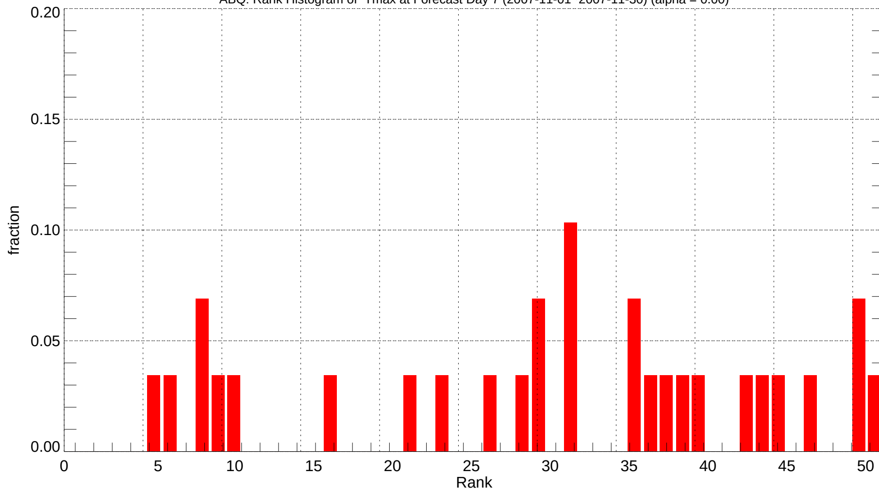
ABQ: Rank Histogram of Tmax at Forecast Day 7 (2007-11-01~2007-11-30) (alpha = 0.00)
