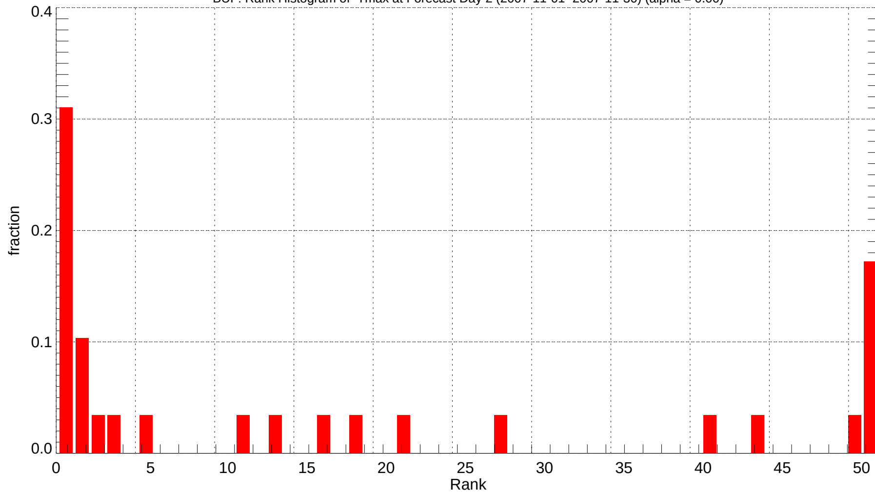
BUF: Rank Histogram of Tmax at Forecast Day 2 (2007-11-01~2007-11-30) (alpha = 0.00)
