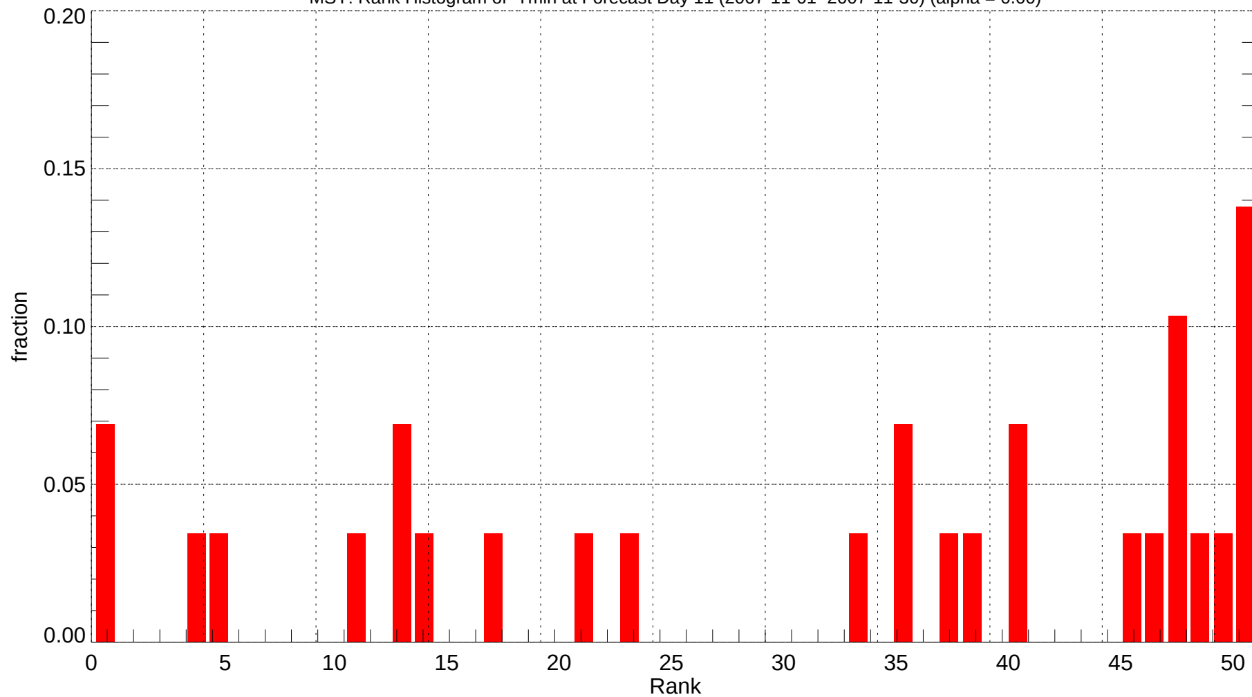
MSY: Rank Histogram of Tmin at Forecast Day 11 (2007-11-01~2007-11-30) (alpha = 0.00)
