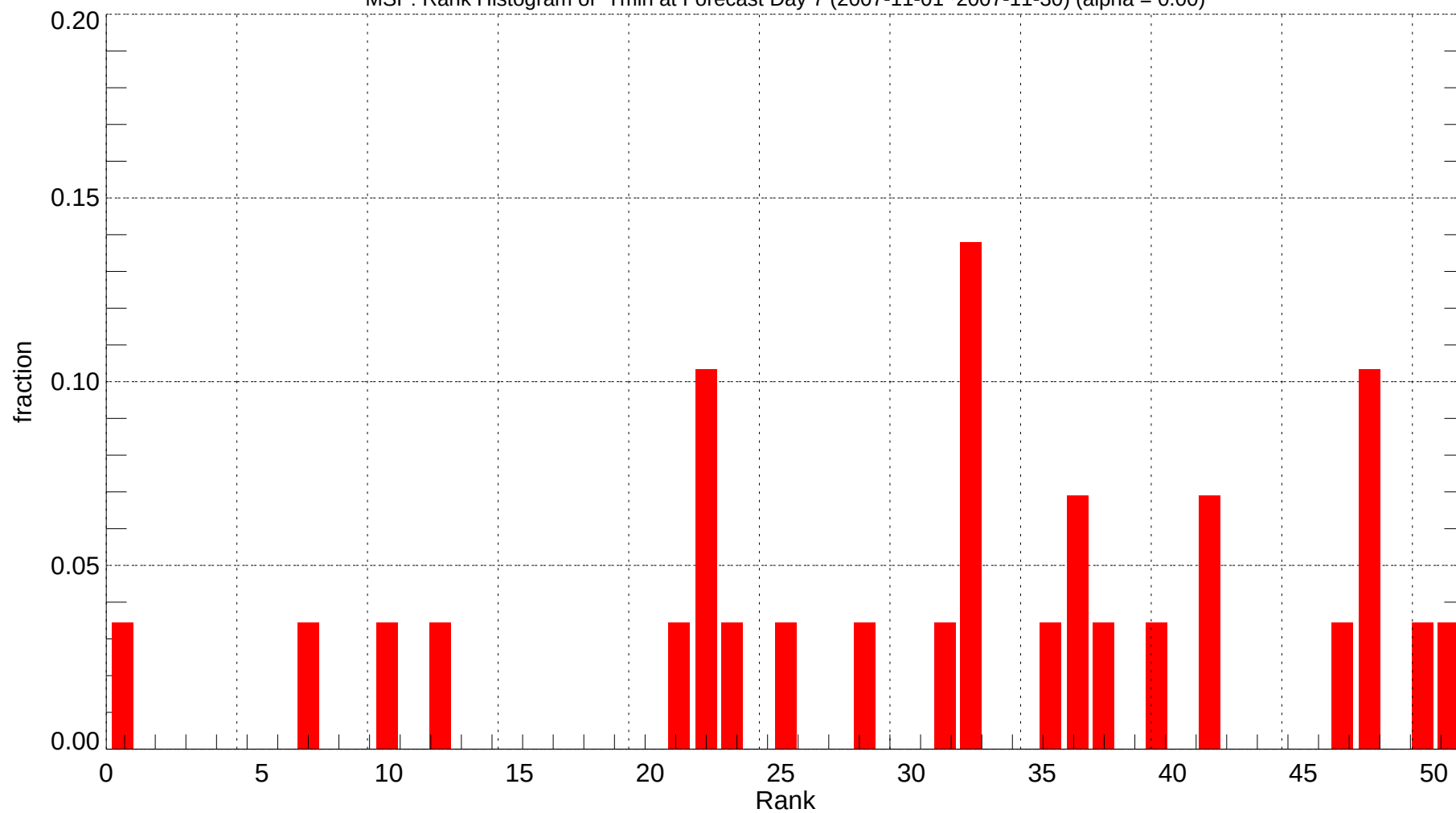
MSP: Rank Histogram of Tmin at Forecast Day 7 (2007-11-01~2007-11-30) (alpha = 0.00)
