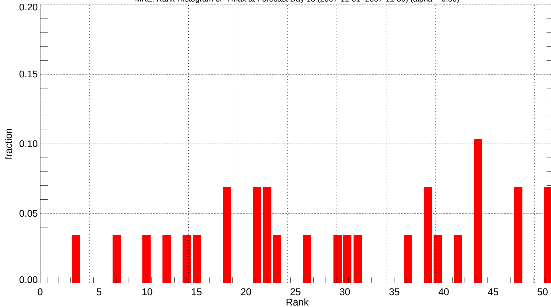
MKE: Rank Histogram of Tmax at Forecast Day 13 (2007-11-01~2007-11-30) (alpha = 0.00)
