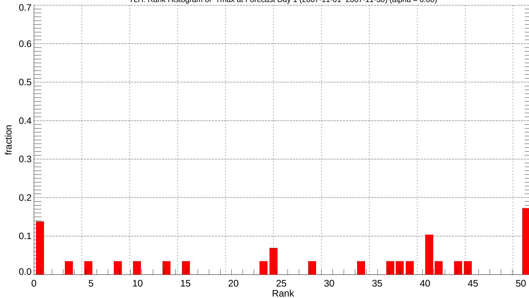
TLH: Rank Histogram of Tmax at Forecast Day 1 (2007-11-01~2007-11-30) (alpha = 0.00)
