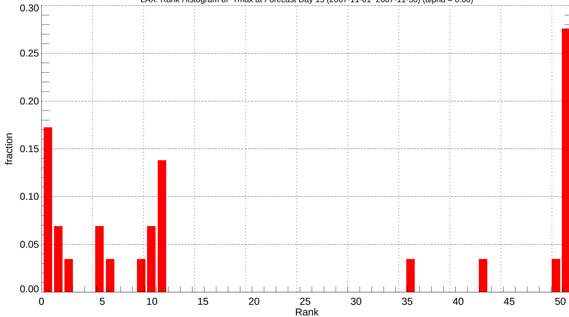
LAX: Rank Histogram of Tmax at Forecast Day 15 (2007-11-01~2007-11-30) (alpha = 0.00)
