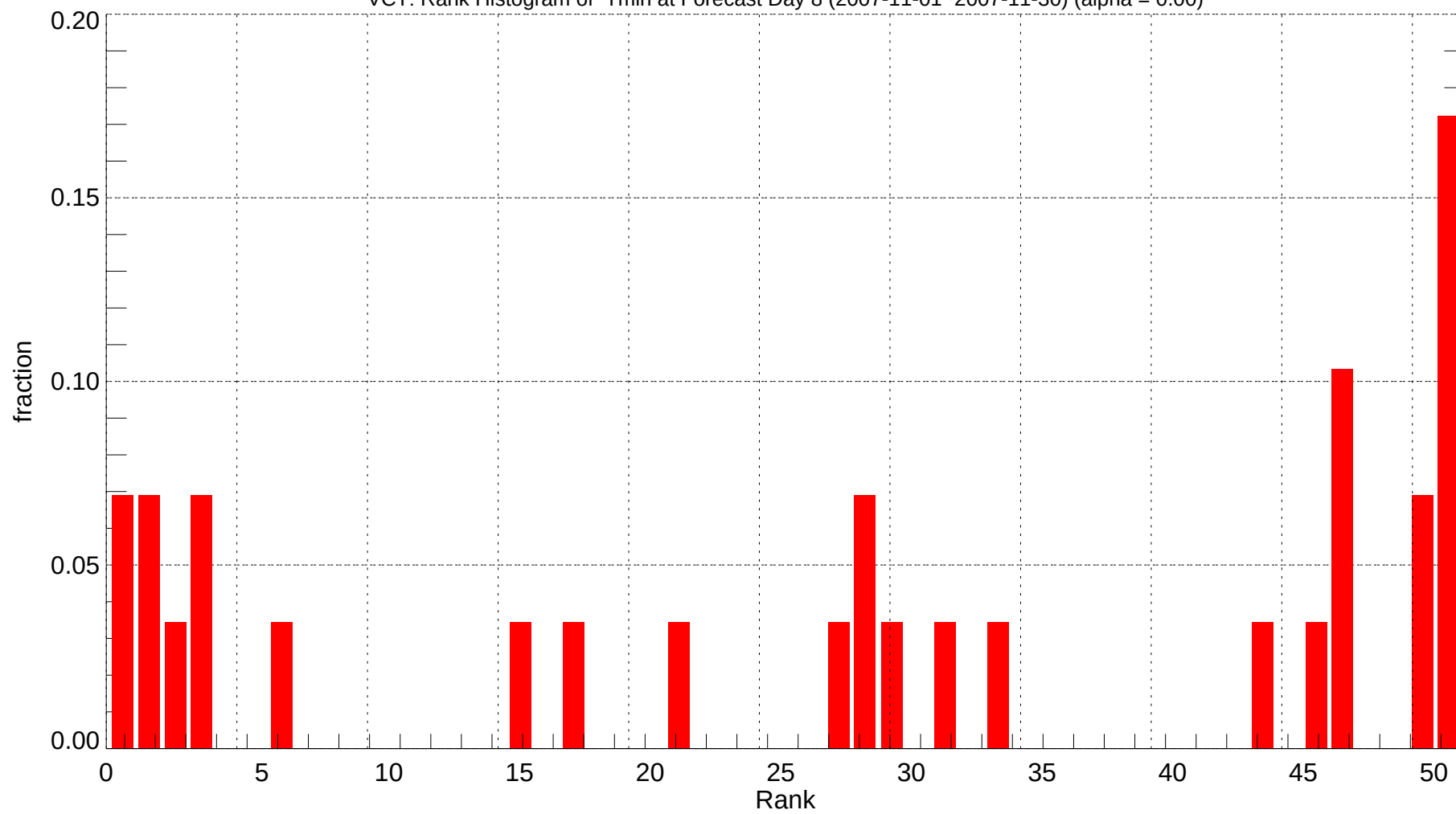
VCT: Rank Histogram of Tmin at Forecast Day 8 (2007-11-01~2007-11-30) (alpha = 0.00)
