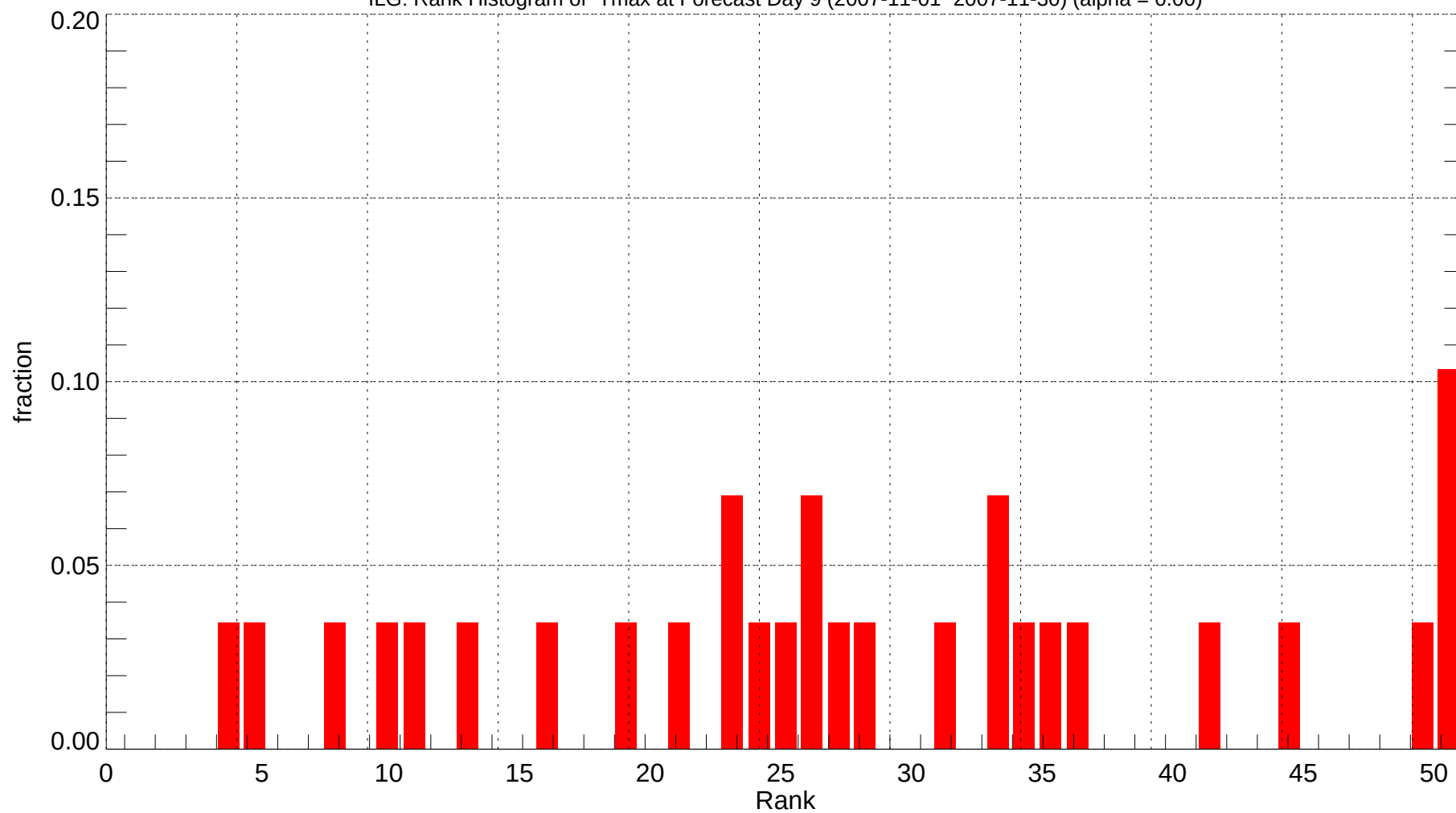
ILG: Rank Histogram of Tmax at Forecast Day 9 (2007-11-01~2007-11-30) (alpha = 0.00)
