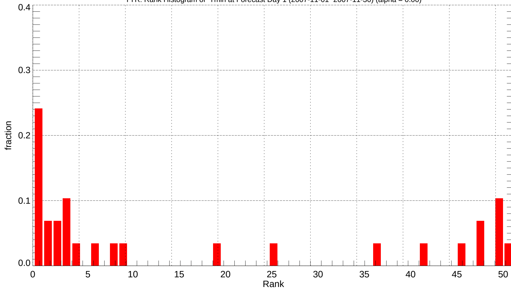
TYR: Rank Histogram of Tmin at Forecast Day 1 (2007-11-01~2007-11-30) (alpha = 0.00)
