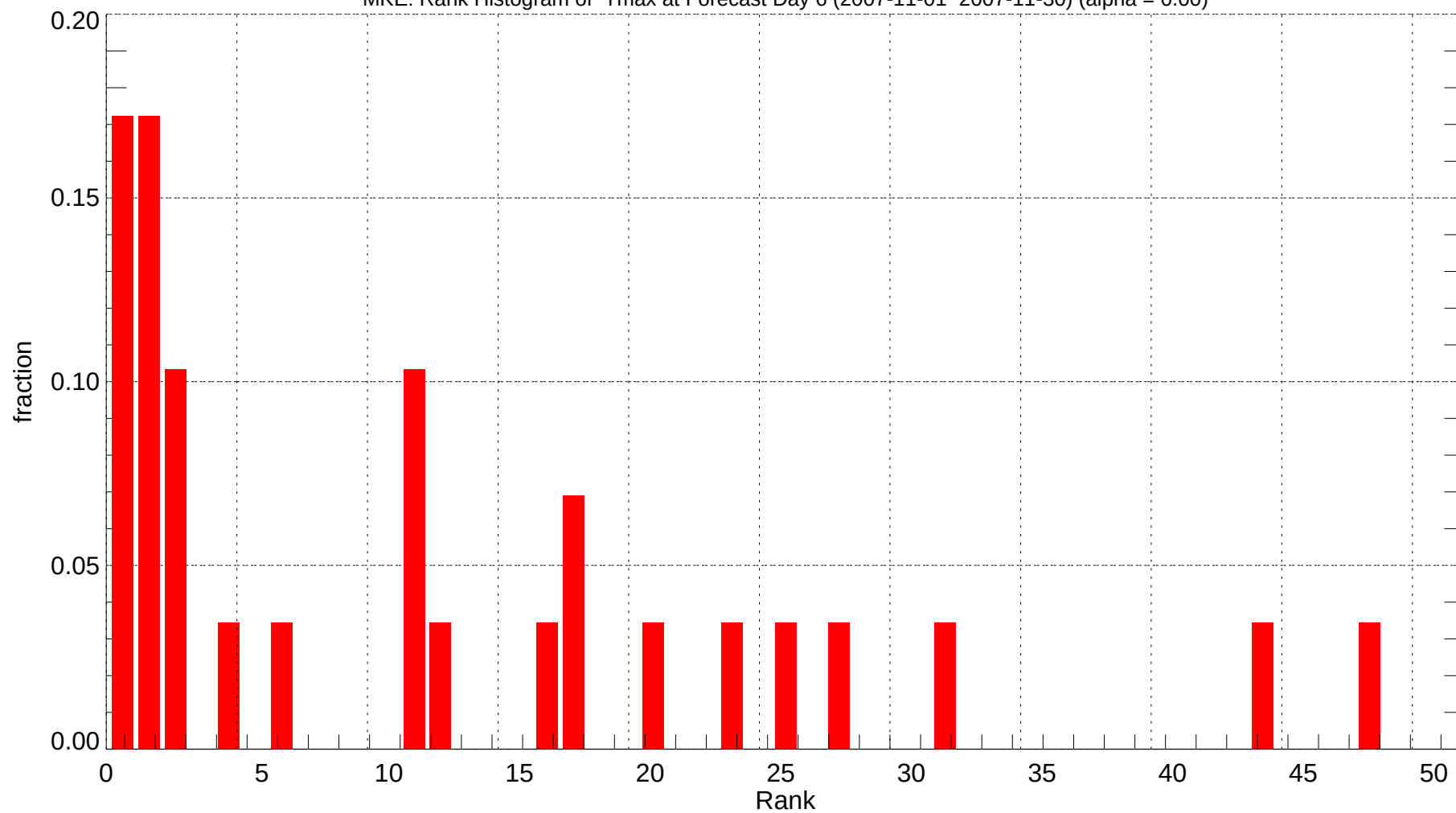
MKE: Rank Histogram of Tmax at Forecast Day 6 (2007-11-01~2007-11-30) (alpha = 0.00)
