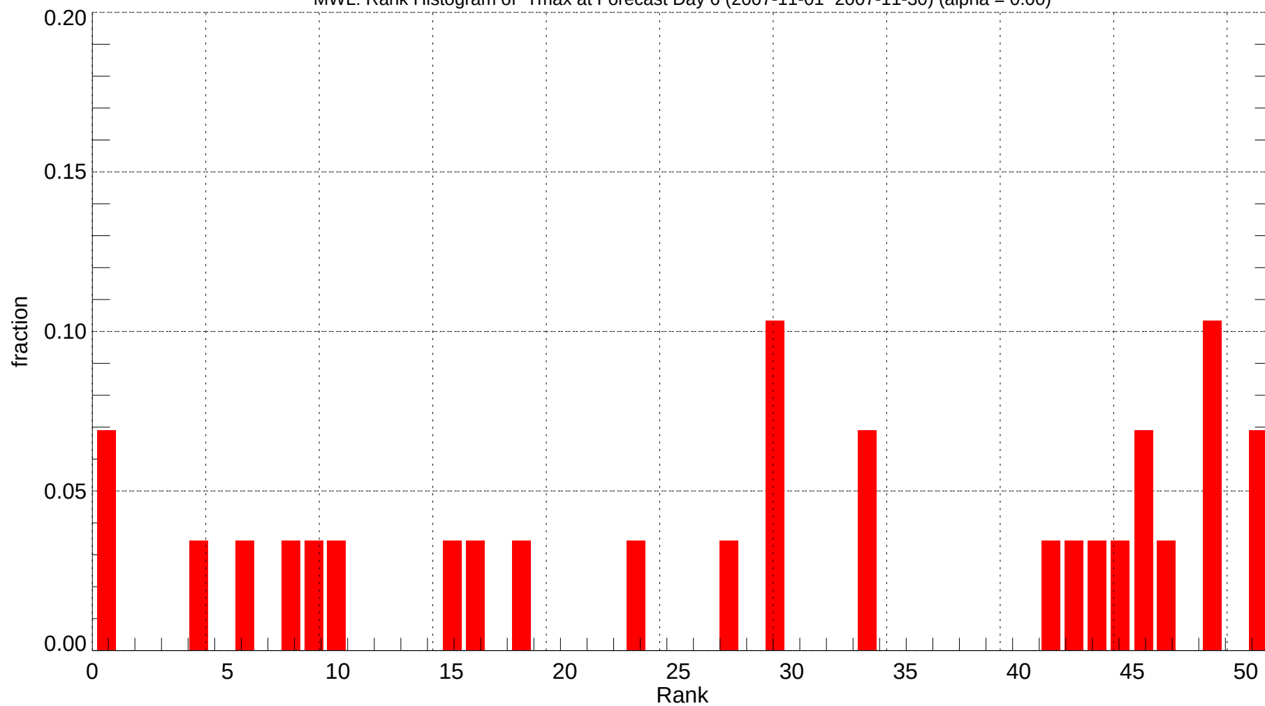
MWL: Rank Histogram of Tmax at Forecast Day 6 (2007-11-01~2007-11-30) (alpha = 0.00)
