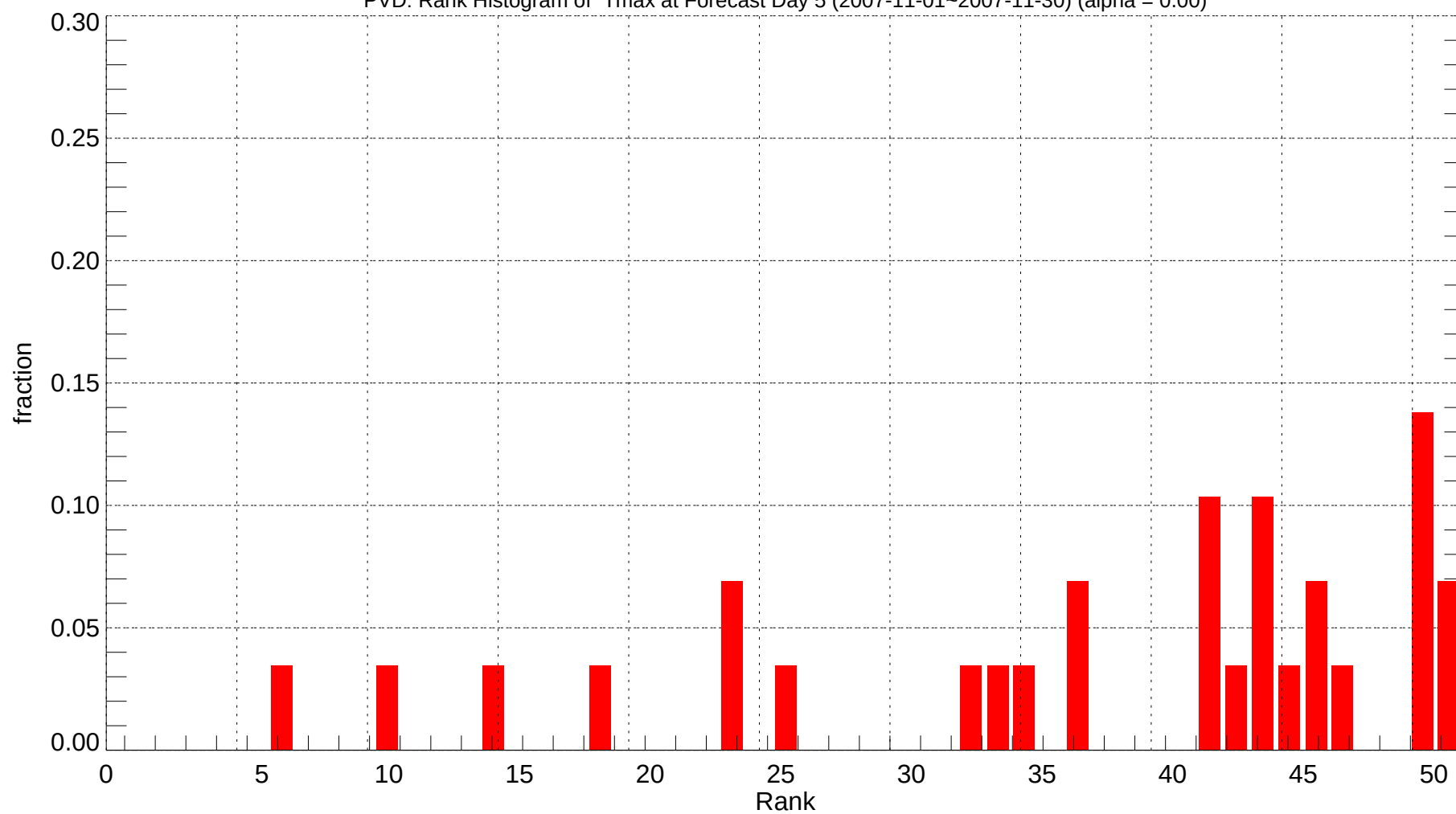
PVD: Rank Histogram of Tmax at Forecast Day 5 (2007-11-01~2007-11-30) (alpha = 0.00)
