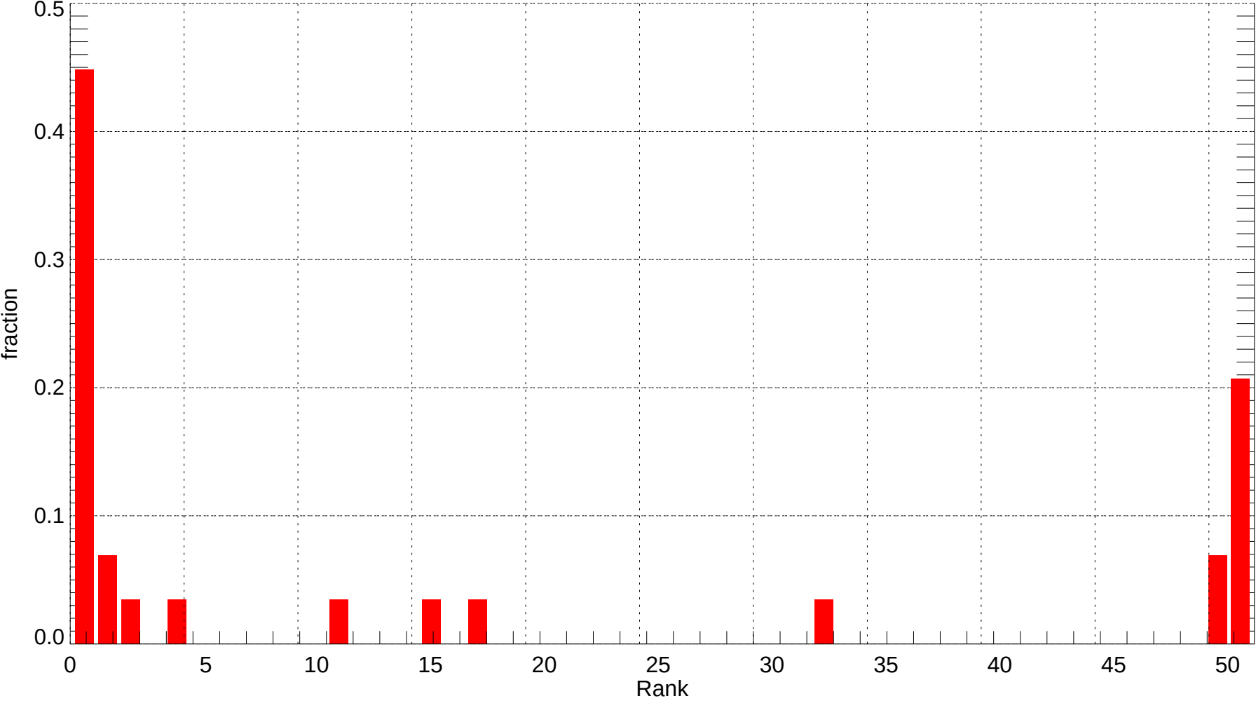
BUF: Rank Histogram of Tmin at Forecast Day 1 (2007-11-01~2007-11-30) (alpha = 0.00)
