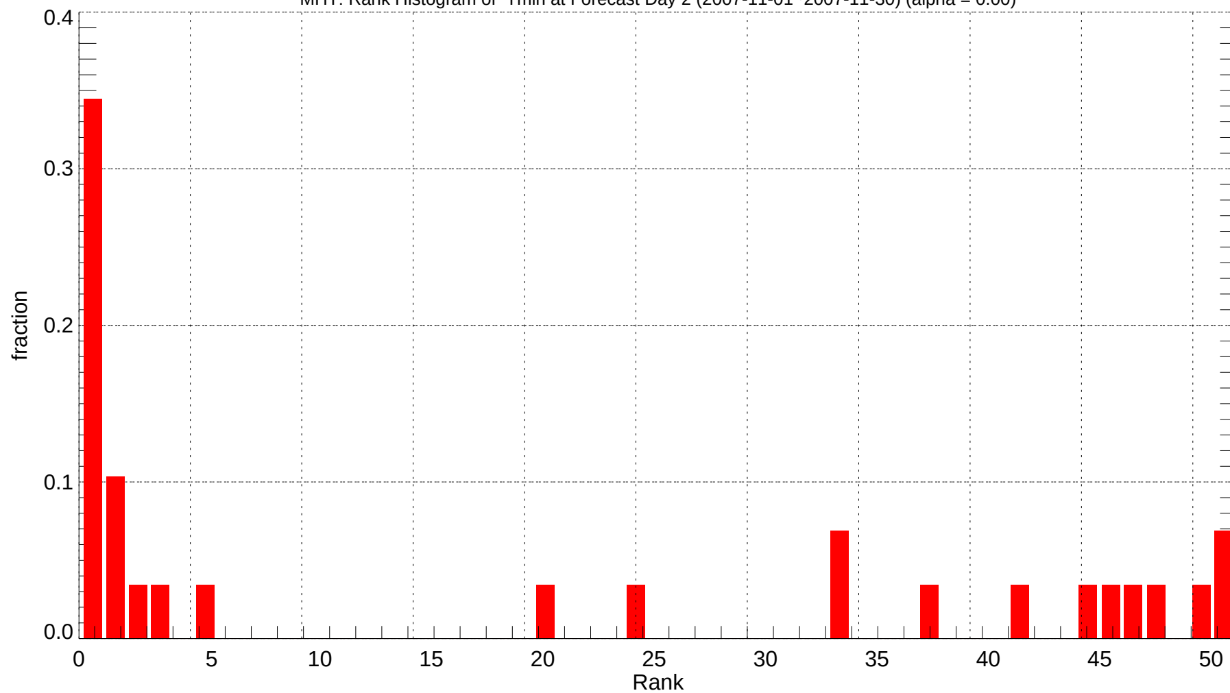
MHT: Rank Histogram of Tmin at Forecast Day 2 (2007-11-01~2007-11-30) (alpha = 0.00)
