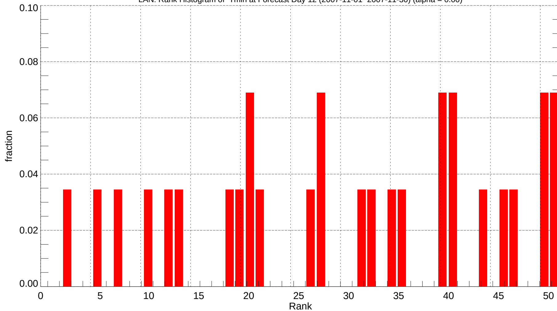
LAN: Rank Histogram of Tmin at Forecast Day 12 (2007-11-01~2007-11-30) (alpha = 0.00)
