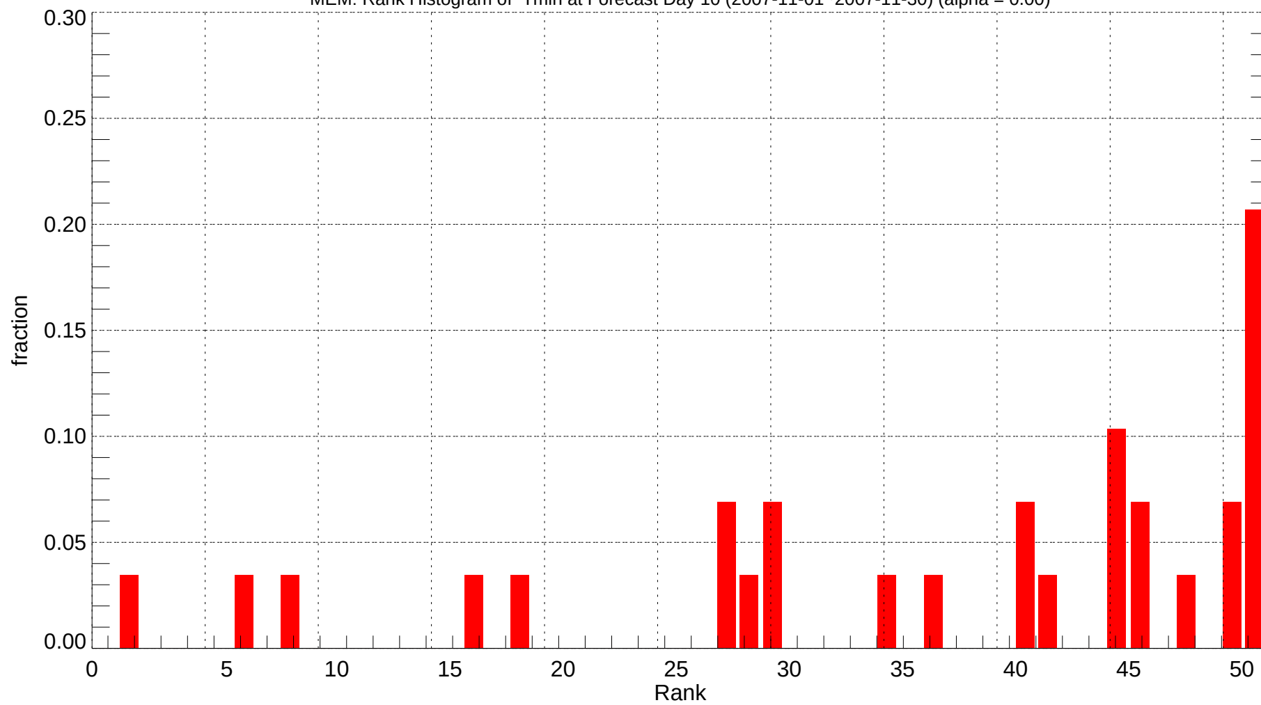
MEM: Rank Histogram of Tmin at Forecast Day 10 (2007-11-01~2007-11-30) (alpha = 0.00)
