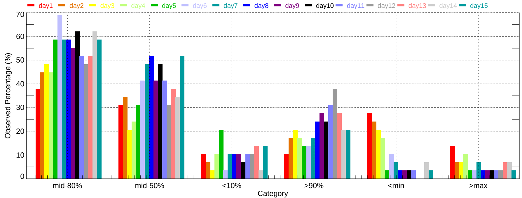
Observed Percentage of Ensembles - ACT: Max Temperature (2007-11-01~2007-11-30)
