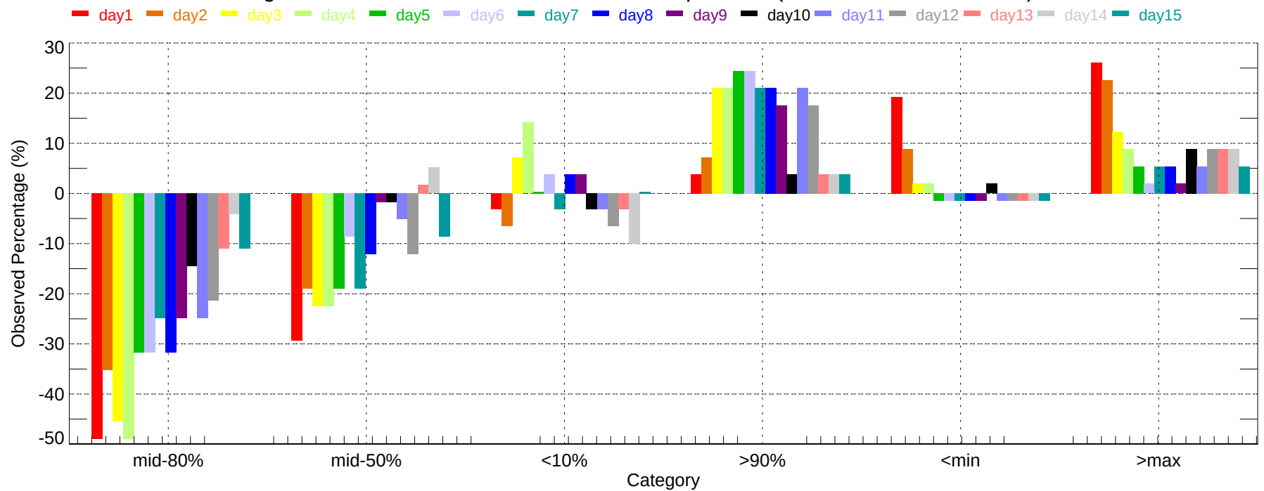
Observed Percentage Deviation of Ensembles - PIT: Min Temperature (2007-11-01~2007-11-30)
