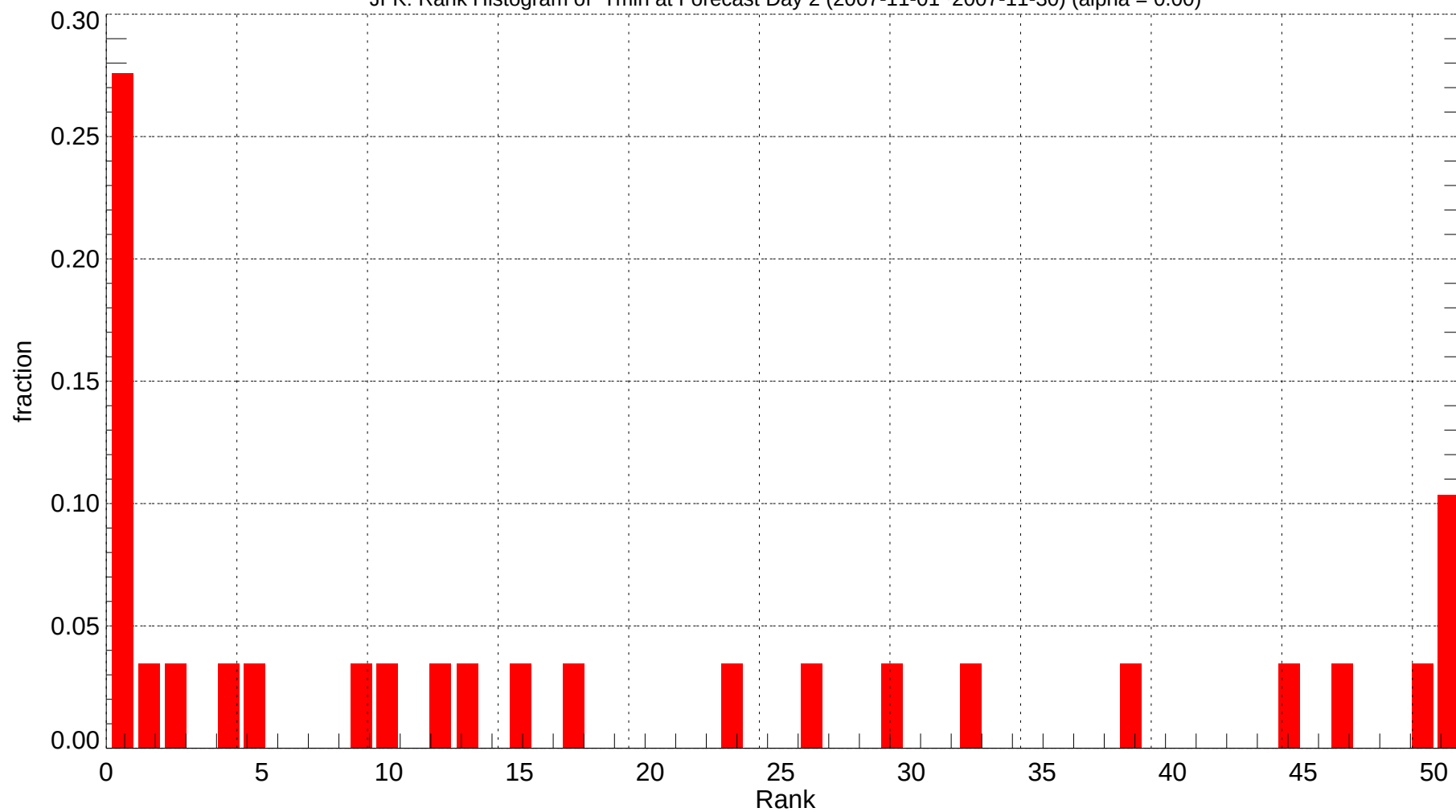
JFK: Rank Histogram of Tmin at Forecast Day 2 (2007-11-01~2007-11-30) (alpha = 0.00)
