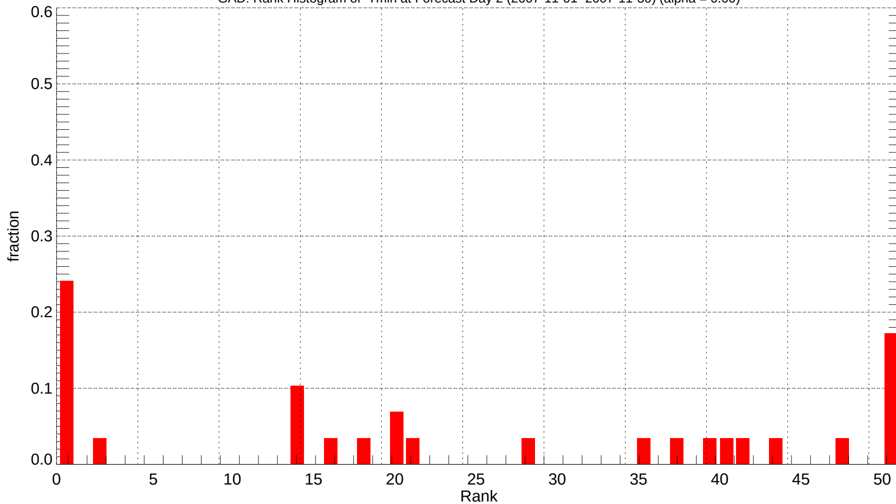
GAD: Rank Histogram of Tmin at Forecast Day 2 (2007-11-01~2007-11-30) (alpha = 0.00)
