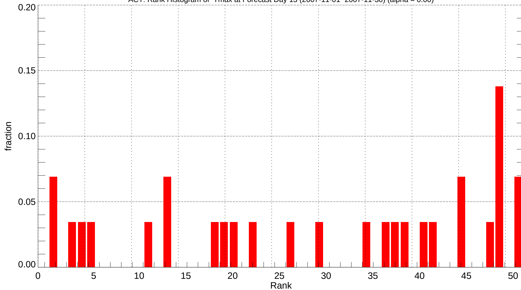
ACT: Rank Histogram of Tmax at Forecast Day 13 (2007-11-01~2007-11-30) (alpha = 0.00)
