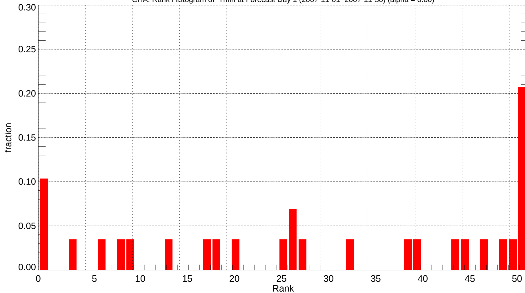
CHA: Rank Histogram of Tmin at Forecast Day 1 (2007-11-01~2007-11-30) (alpha = 0.00)
