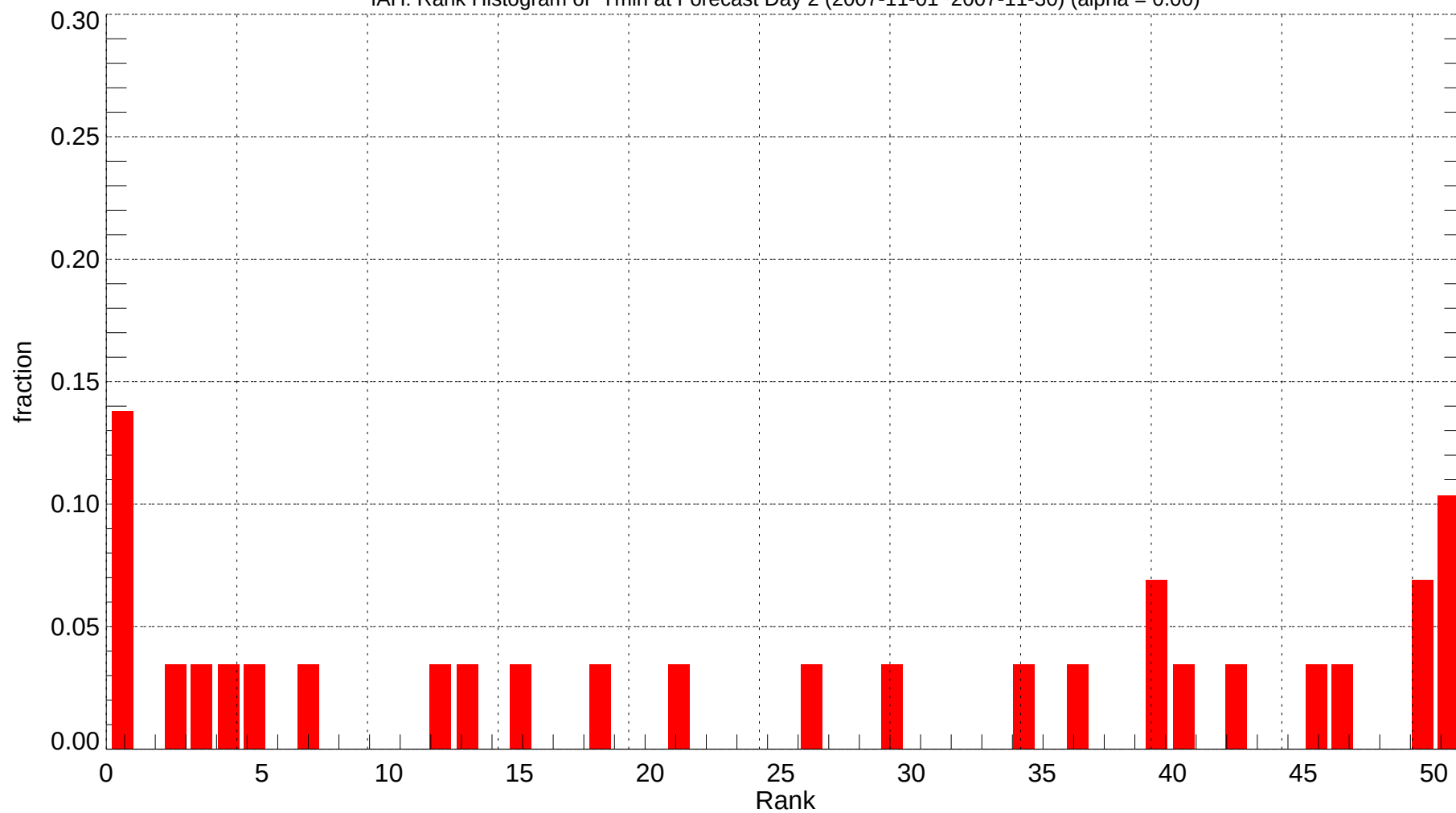
IAH: Rank Histogram of Tmin at Forecast Day 2 (2007-11-01~2007-11-30) (alpha = 0.00)
