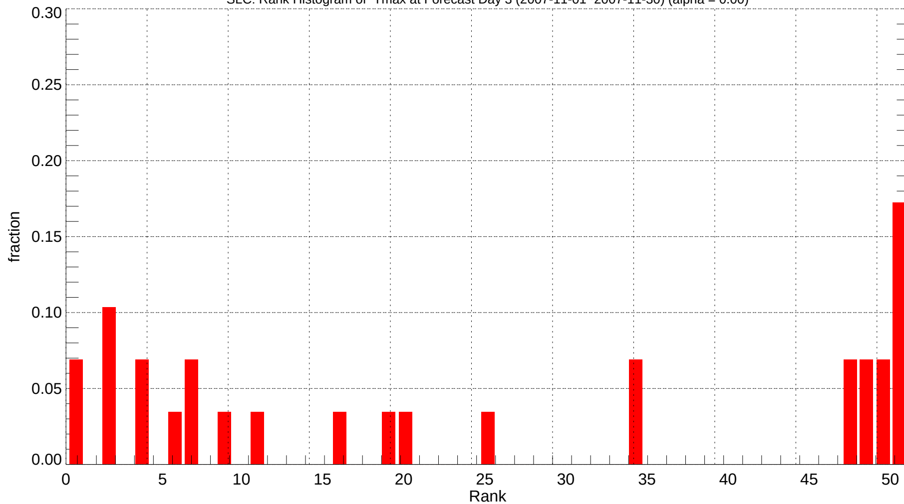
SLC: Rank Histogram of Tmax at Forecast Day 3 (2007-11-01~2007-11-30) (alpha = 0.00)
