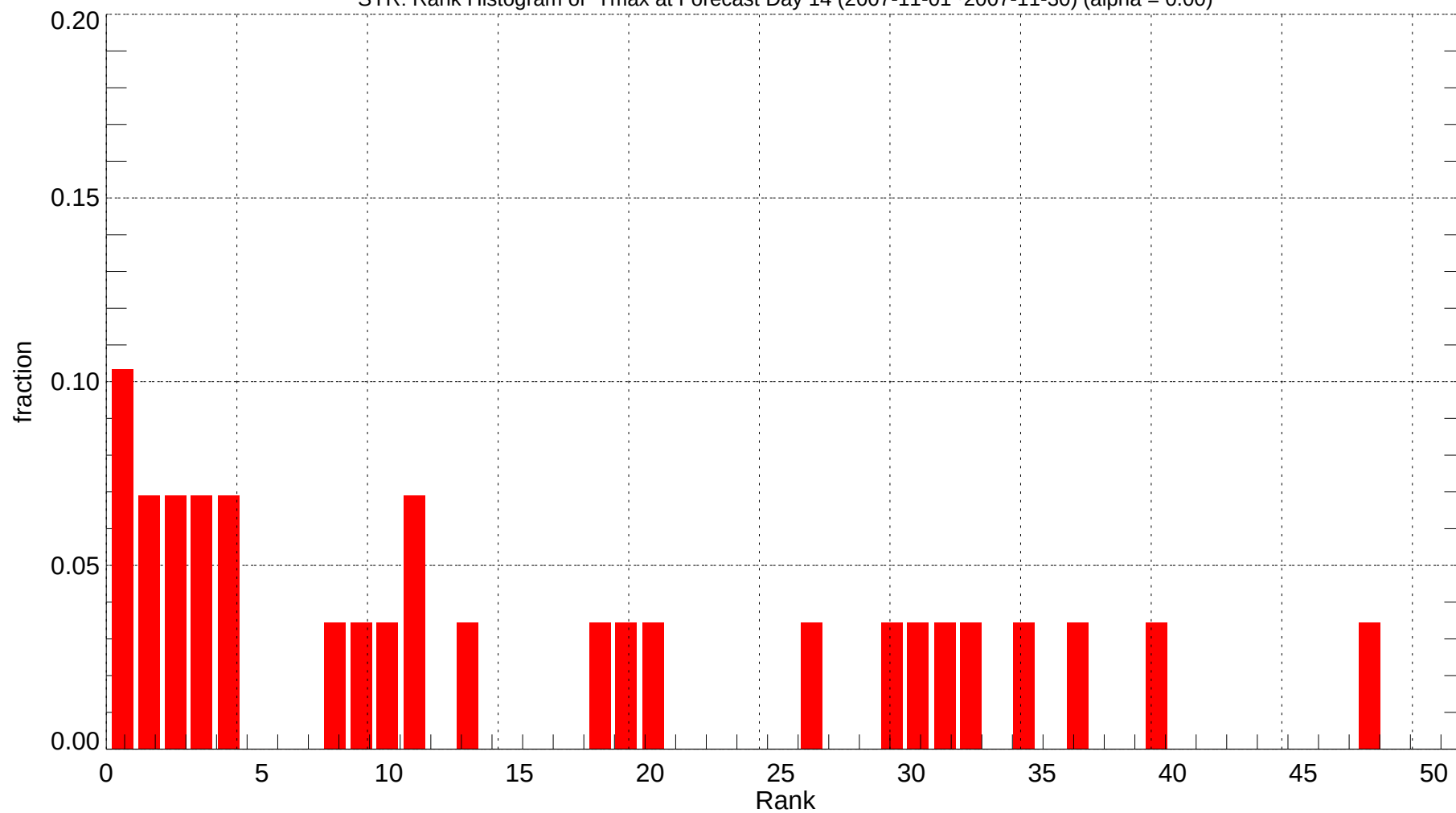
SYR: Rank Histogram of Tmax at Forecast Day 14 (2007-11-01~2007-11-30) (alpha = 0.00)
