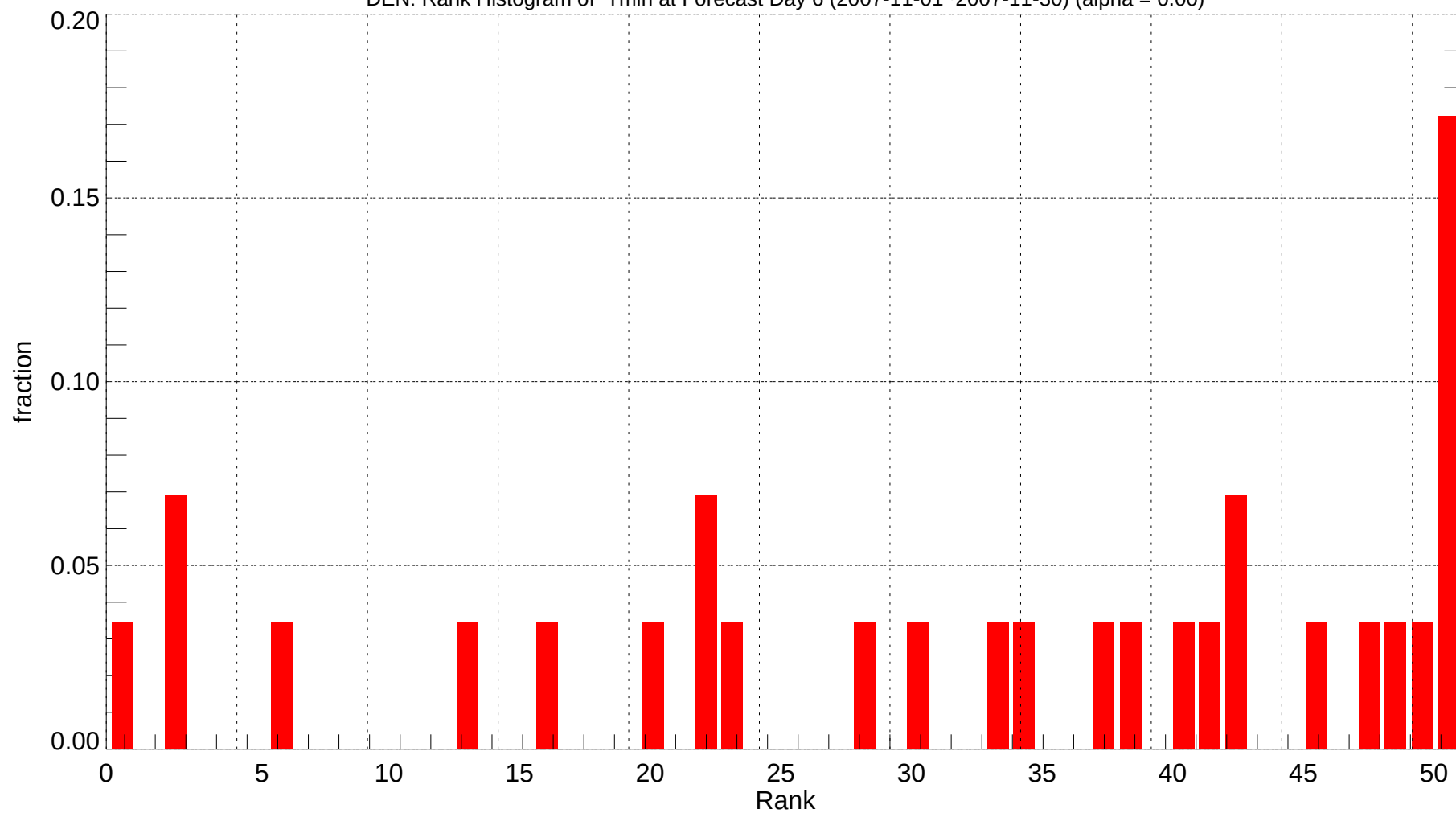
DEN: Rank Histogram of Tmin at Forecast Day 6 (2007-11-01~2007-11-30) (alpha = 0.00)
