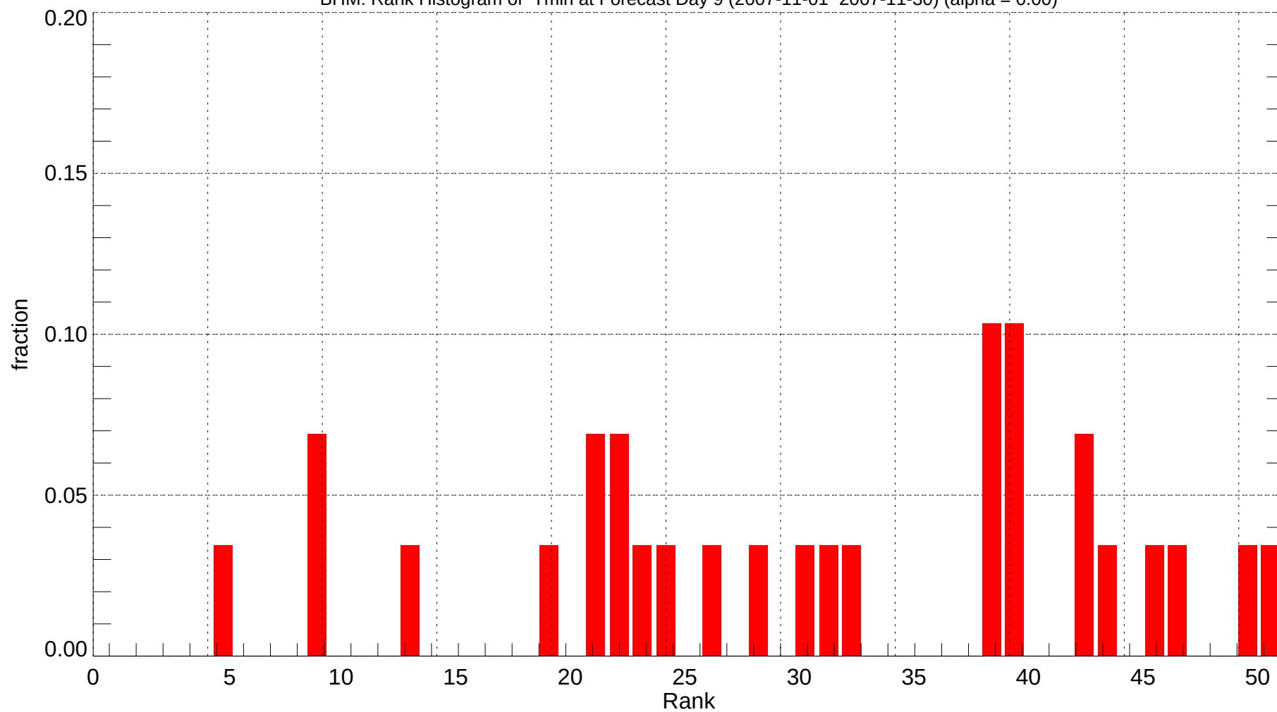
BHM: Rank Histogram of Tmin at Forecast Day 9 (2007-11-01~2007-11-30) (alpha = 0.00)
