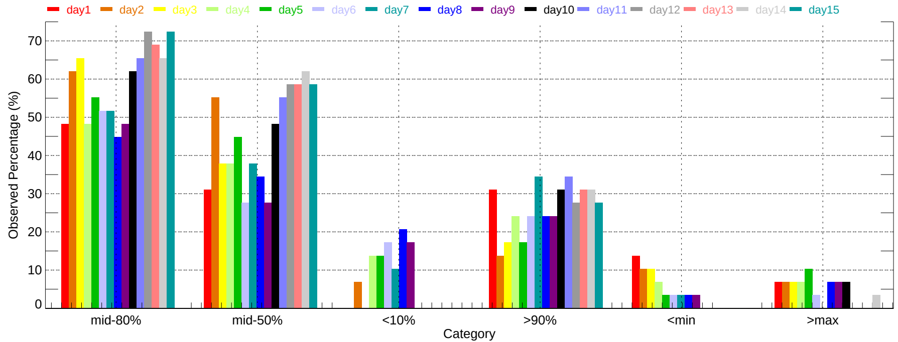
Observed Percentage of Ensembles - SAC: Min Temperature (2007-11-01~2007-11-30)
