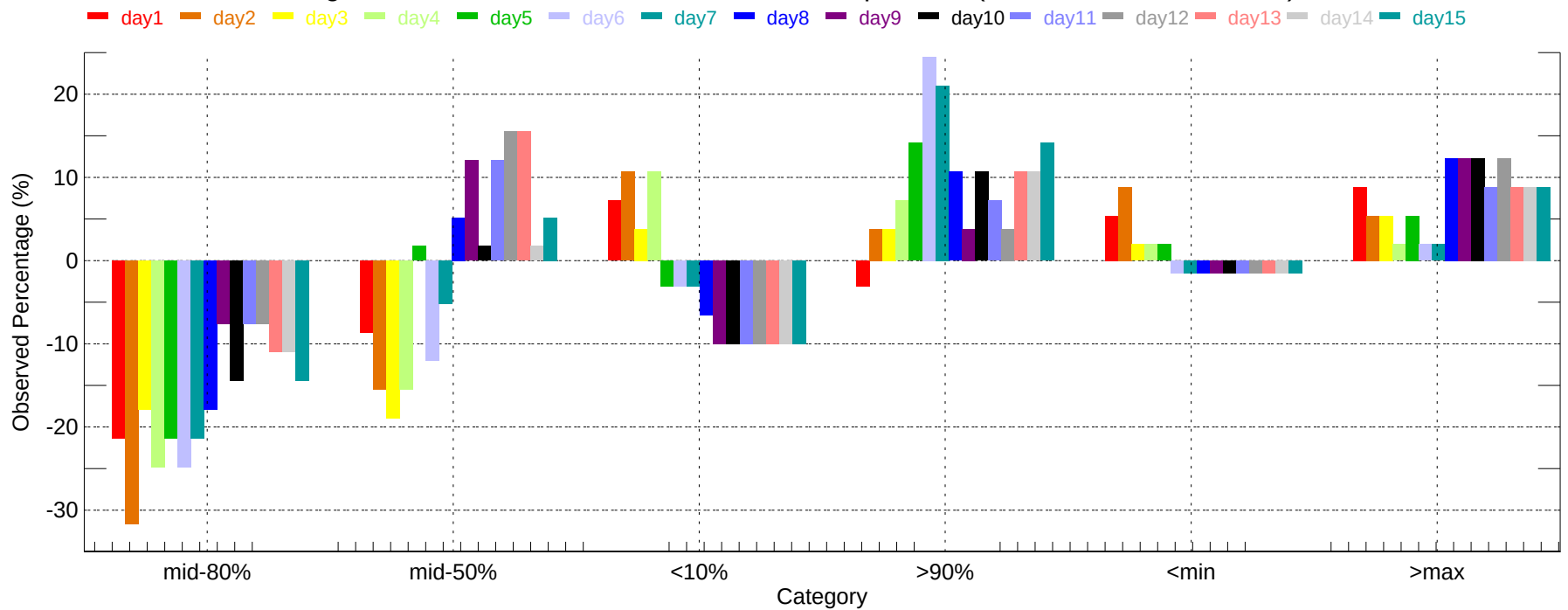
Observed Percentage Deviation of Ensembles - PHX: Min Temperature (2007-11-01~2007-11-30)
