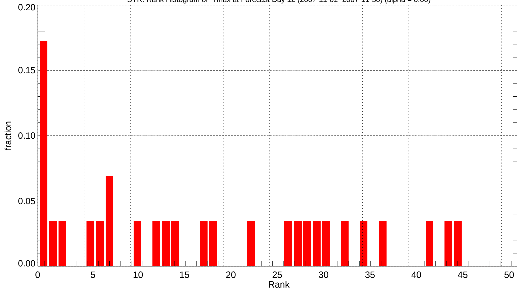
SYR: Rank Histogram of Tmax at Forecast Day 12 (2007-11-01~2007-11-30) (alpha = 0.00)
