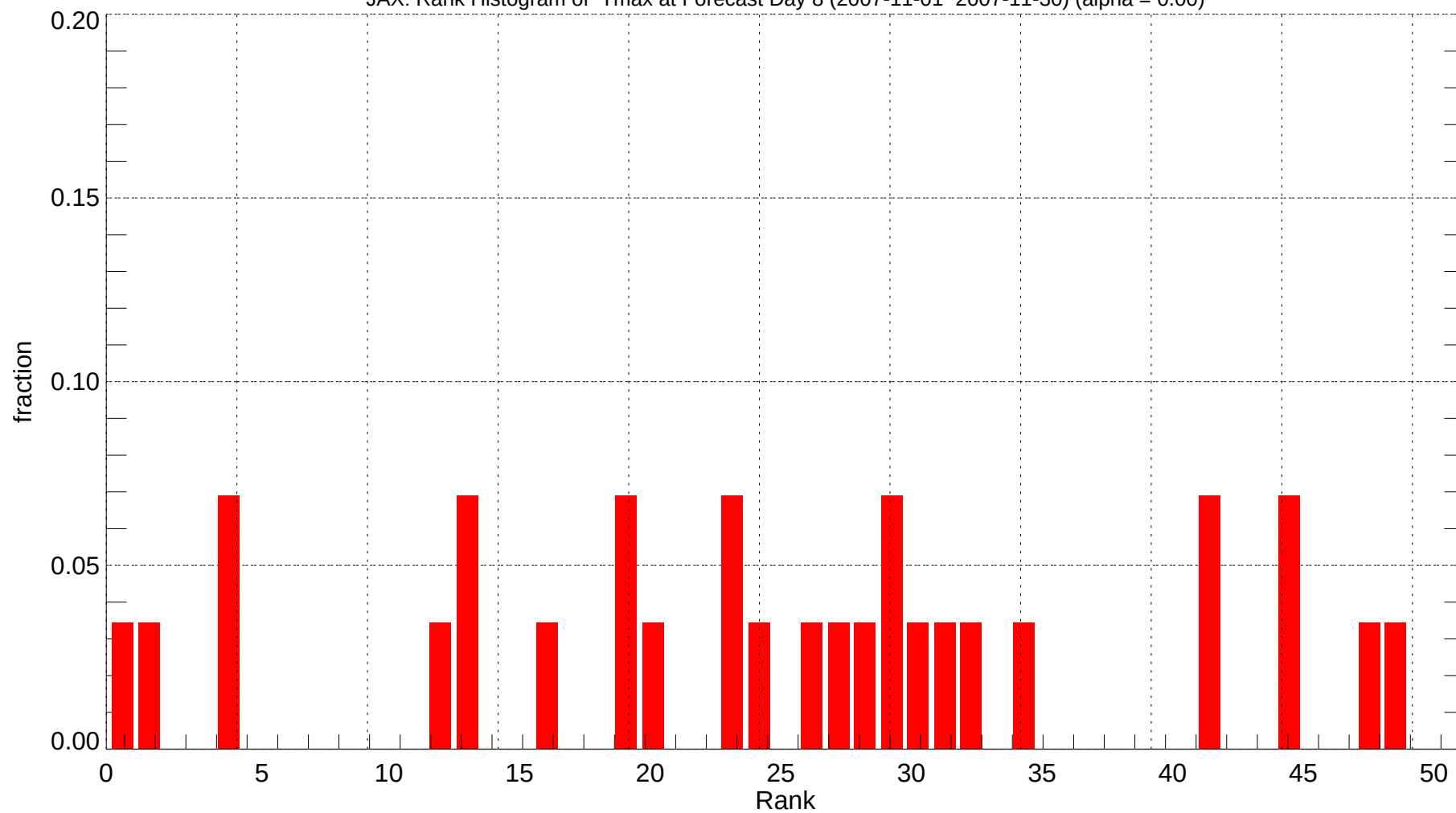
JAX: Rank Histogram of Tmax at Forecast Day 8 (2007-11-01~2007-11-30) (alpha = 0.00)
