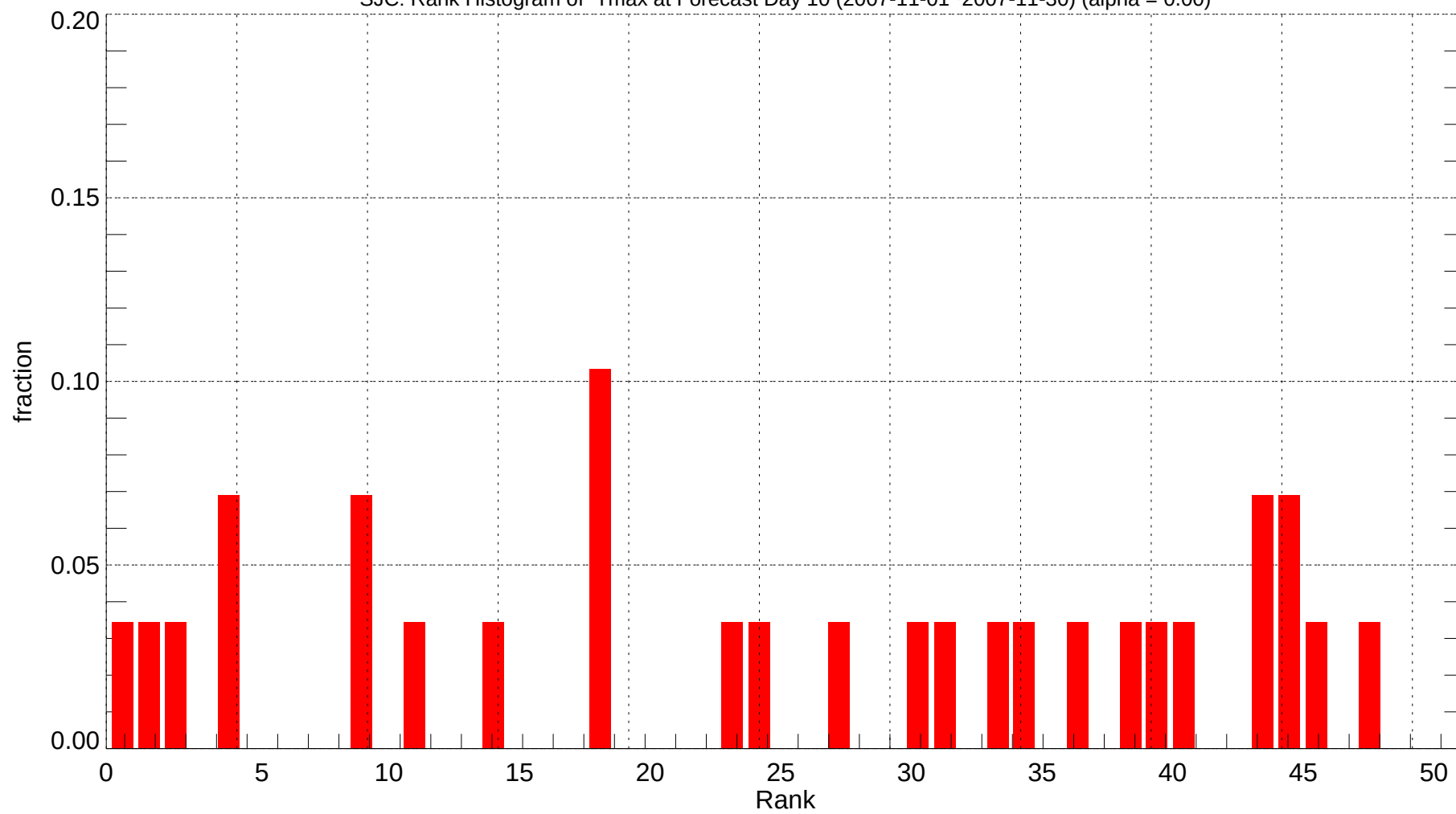
SJC: Rank Histogram of Tmax at Forecast Day 10 (2007-11-01~2007-11-30) (alpha = 0.00)
