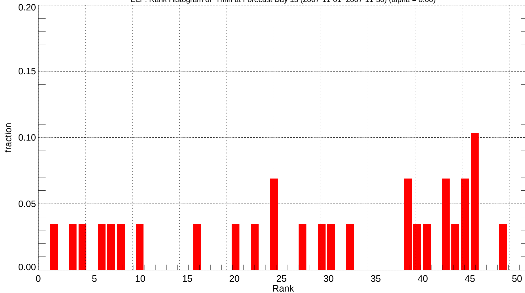
ELP: Rank Histogram of Tmin at Forecast Day 13 (2007-11-01~2007-11-30) (alpha = 0.00)
