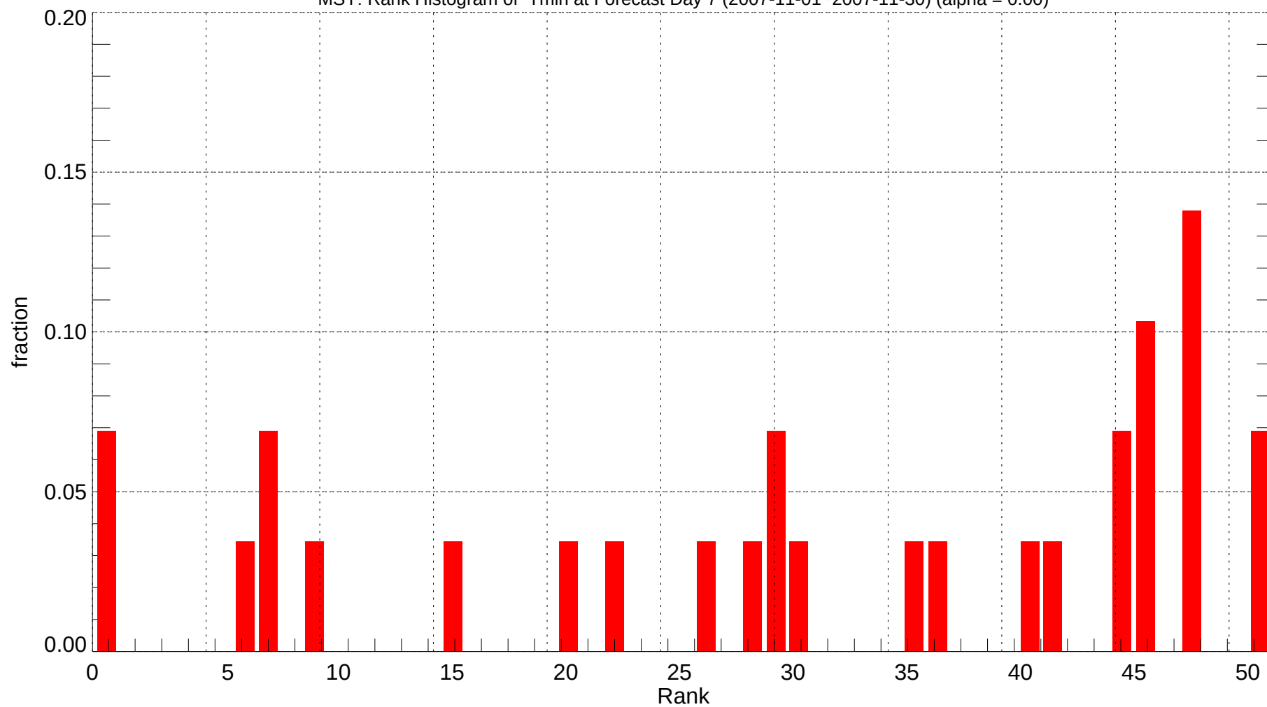
MSY: Rank Histogram of Tmin at Forecast Day 7 (2007-11-01~2007-11-30) (alpha = 0.00)
