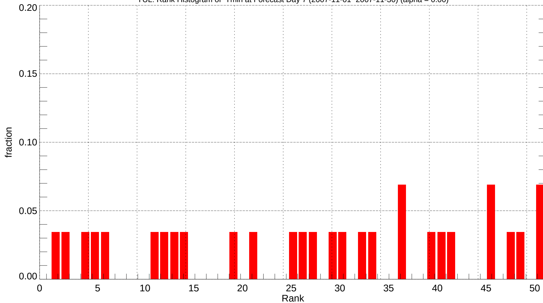
YUL: Rank Histogram of Tmin at Forecast Day 7 (2007-11-01~2007-11-30) (alpha = 0.00)
