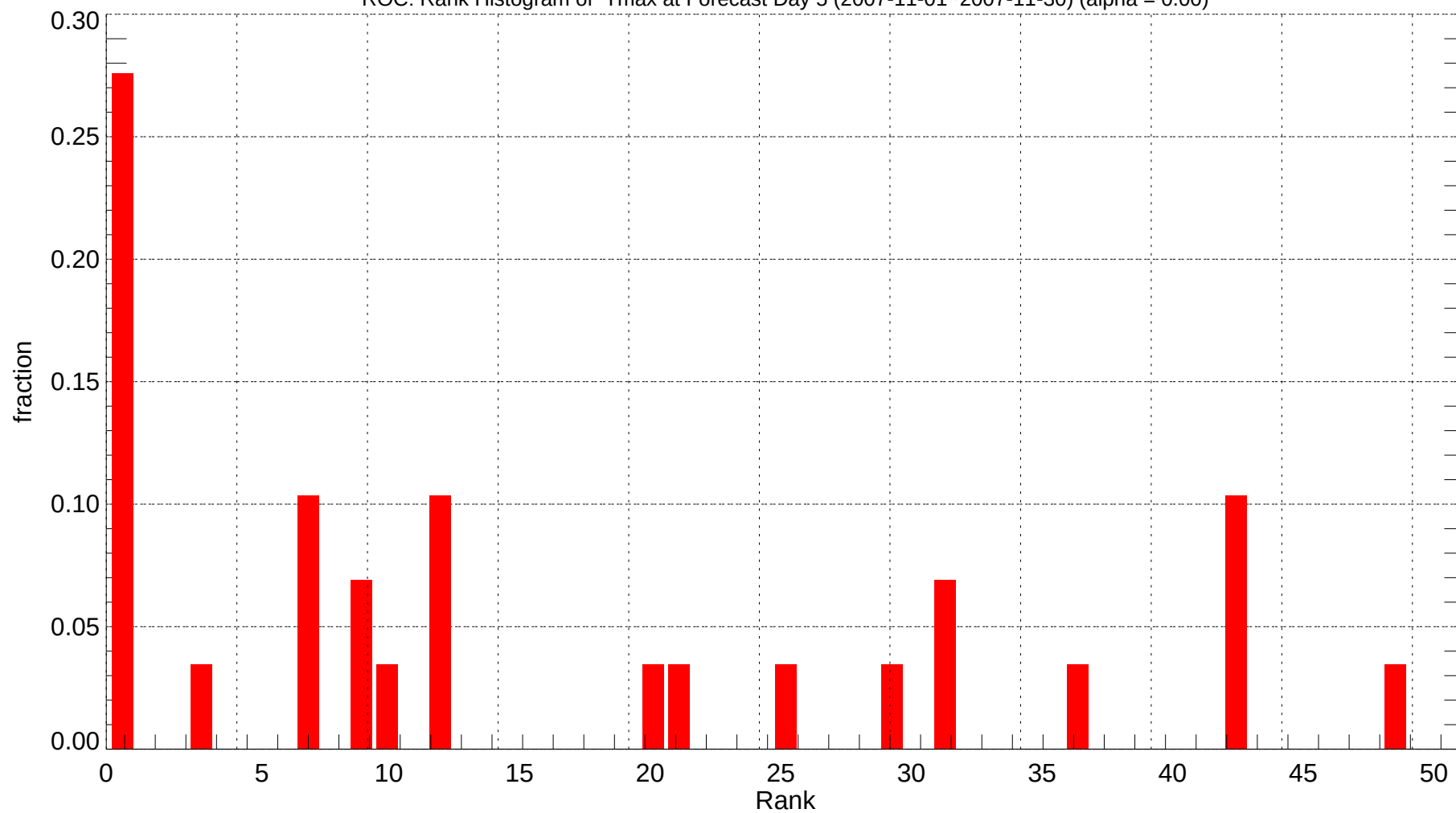
ROC: Rank Histogram of Tmax at Forecast Day 5 (2007-11-01~2007-11-30) (alpha = 0.00)
