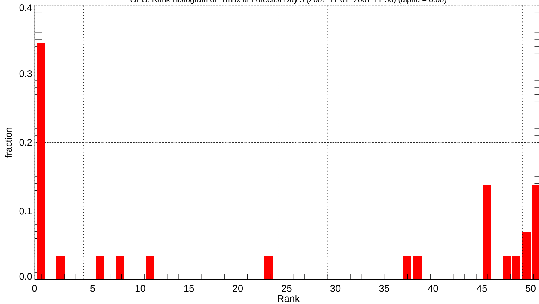
GEG: Rank Histogram of Tmax at Forecast Day 3 (2007-11-01~2007-11-30) (alpha = 0.00)
