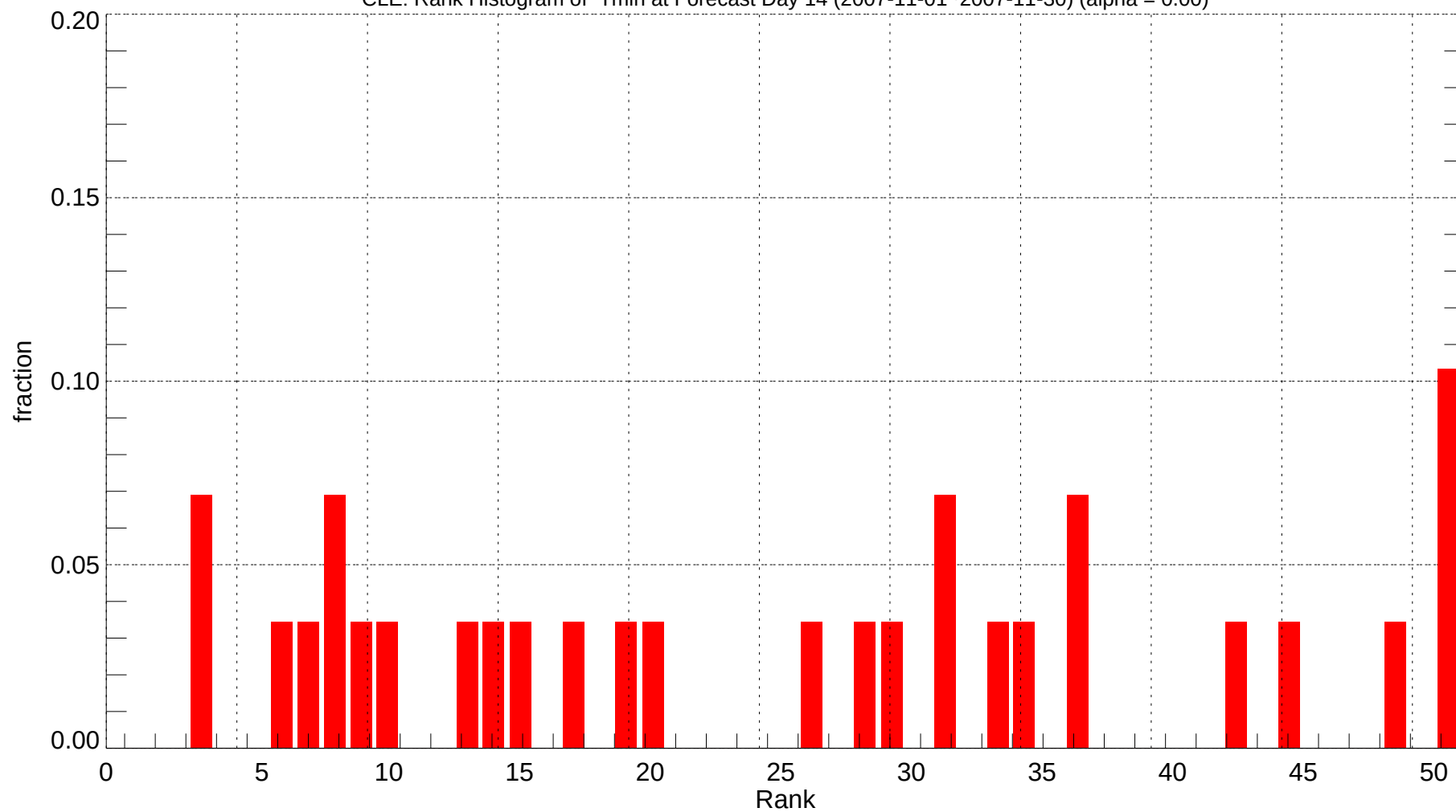
CLE: Rank Histogram of Tmin at Forecast Day 14 (2007-11-01~2007-11-30) (alpha = 0.00)
