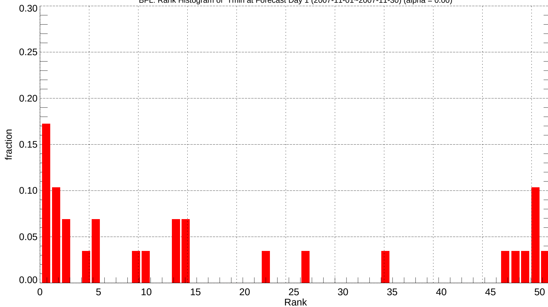
BFL: Rank Histogram of Tmin at Forecast Day 1 (2007-11-01~2007-11-30) (alpha = 0.00)
