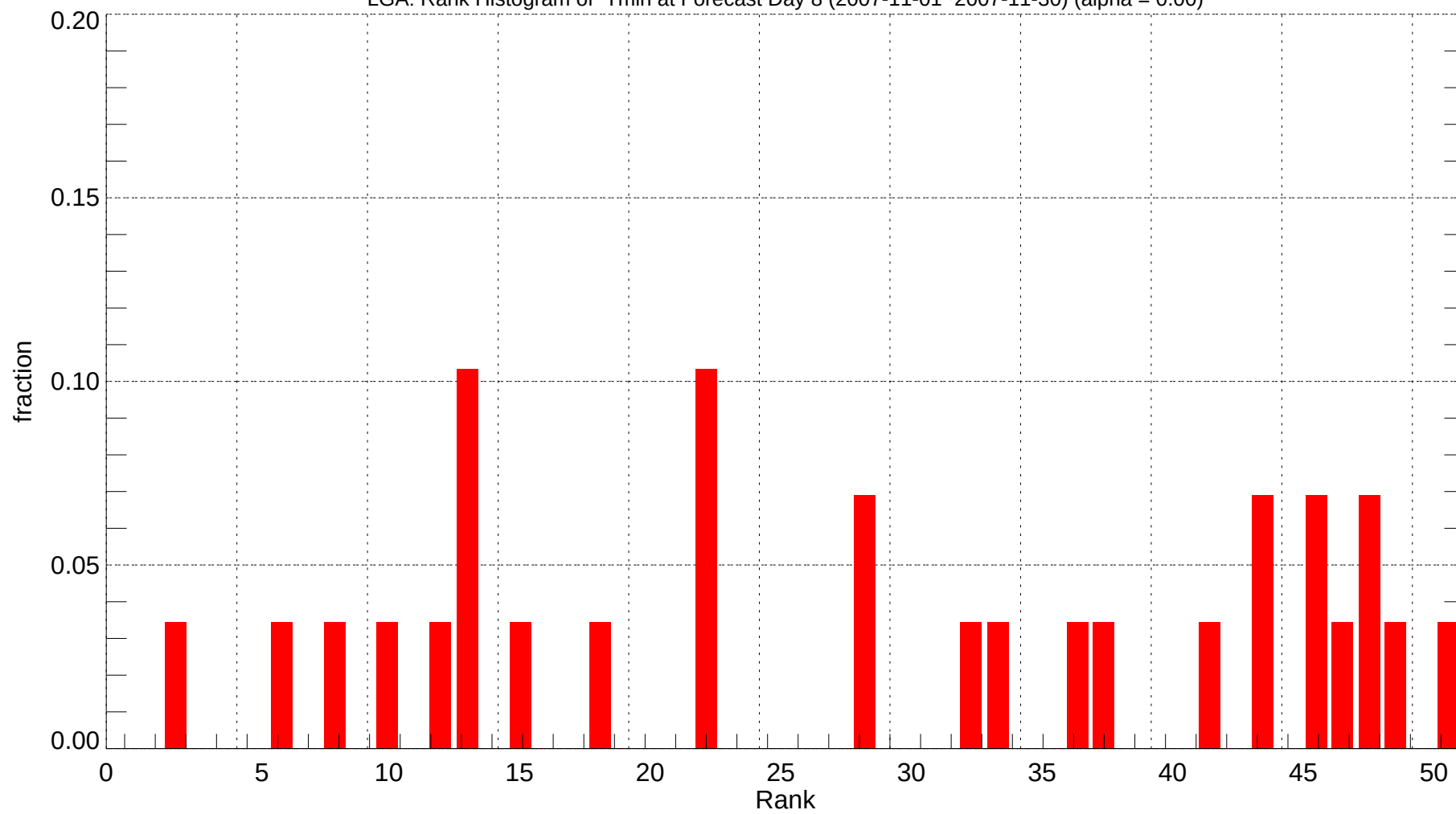
LGA: Rank Histogram of Tmin at Forecast Day 8 (2007-11-01~2007-11-30) (alpha = 0.00)
