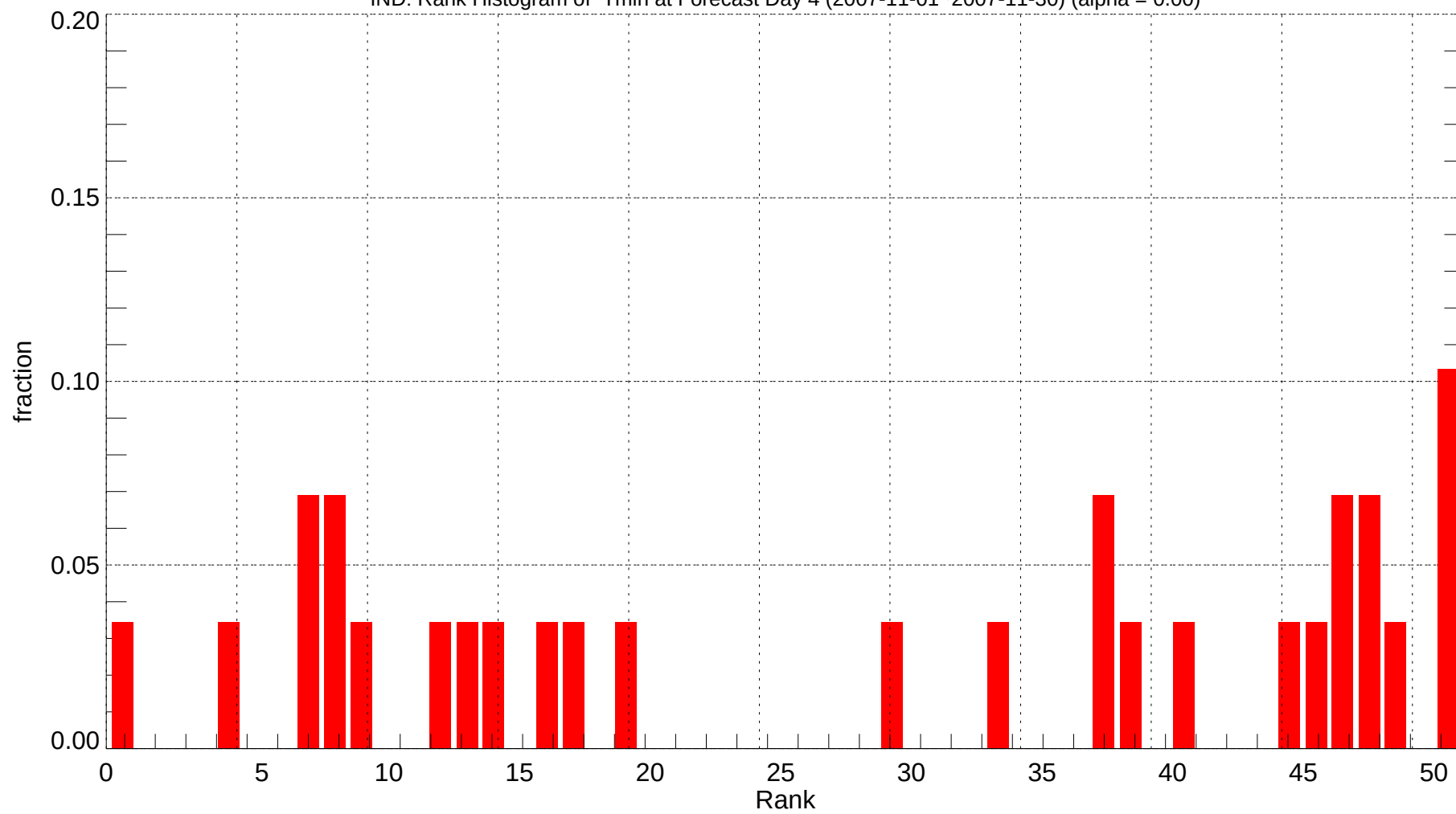
IND: Rank Histogram of Tmin at Forecast Day 4 (2007-11-01~2007-11-30) (alpha = 0.00)
