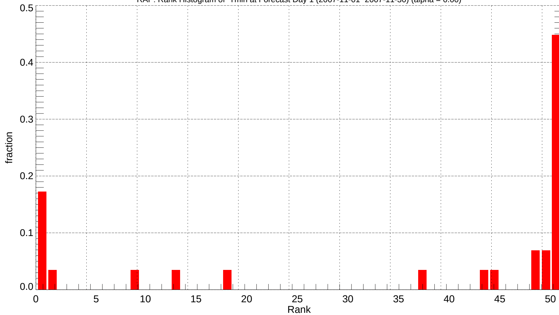
RAP: Rank Histogram of Tmin at Forecast Day 1 (2007-11-01~2007-11-30) (alpha = 0.00)
