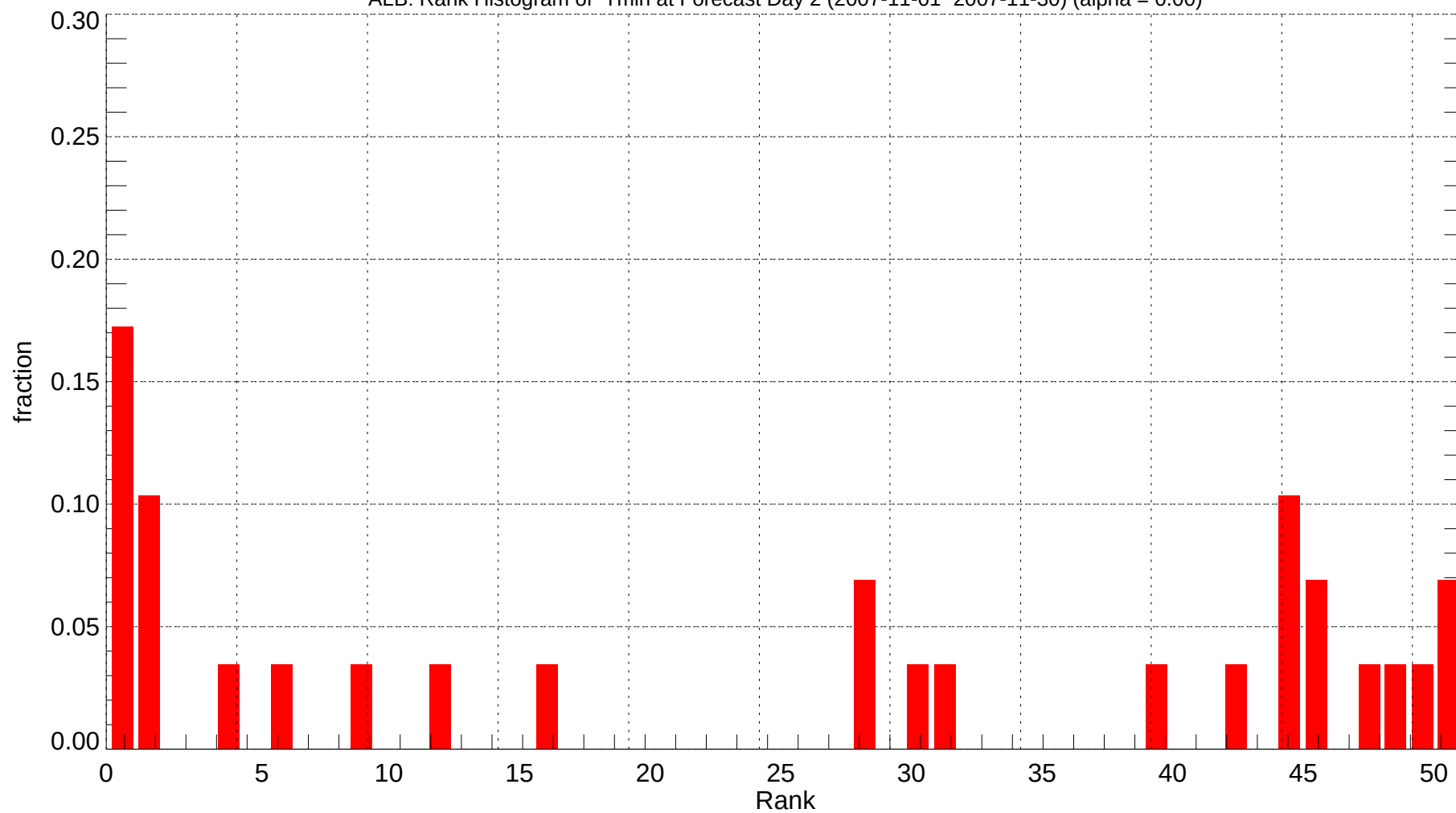
ALB: Rank Histogram of Tmin at Forecast Day 2 (2007-11-01~2007-11-30) (alpha = 0.00)
