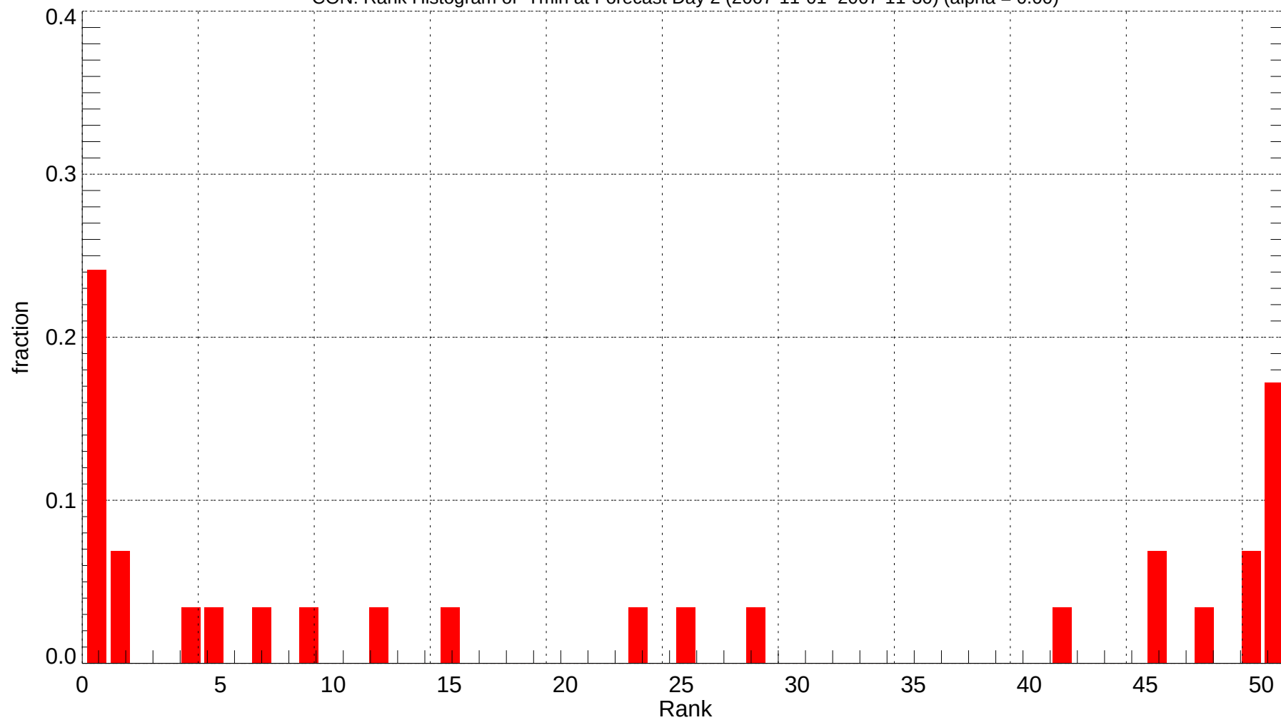
CON: Rank Histogram of Tmin at Forecast Day 2 (2007-11-01~2007-11-30) (alpha = 0.00)
