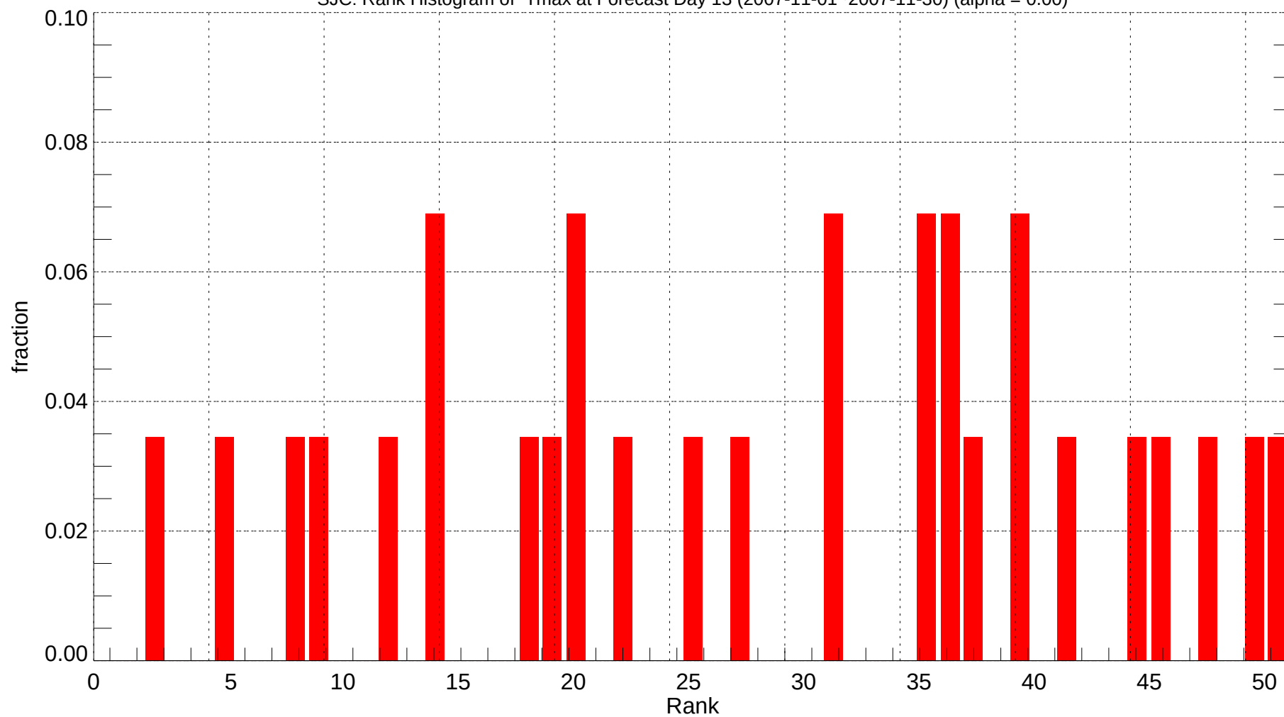
SJC: Rank Histogram of Tmax at Forecast Day 13 (2007-11-01~2007-11-30) (alpha = 0.00)
