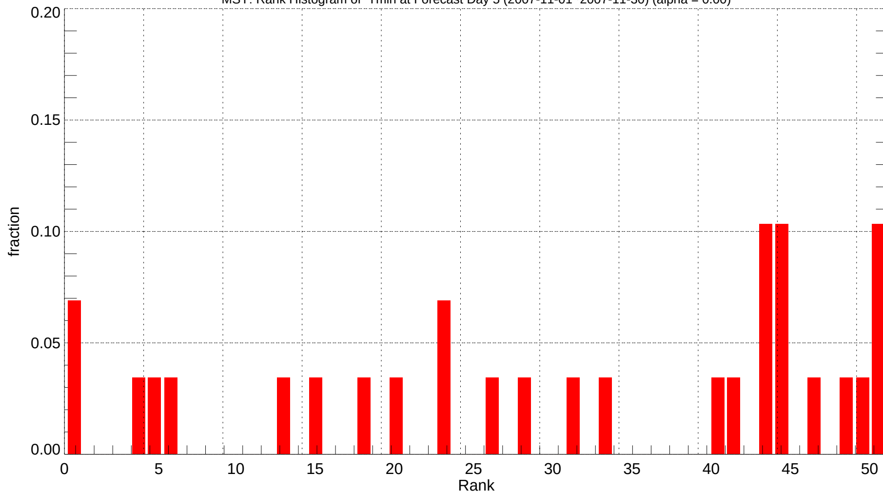
MSY: Rank Histogram of Tmin at Forecast Day 5 (2007-11-01~2007-11-30) (alpha = 0.00)
