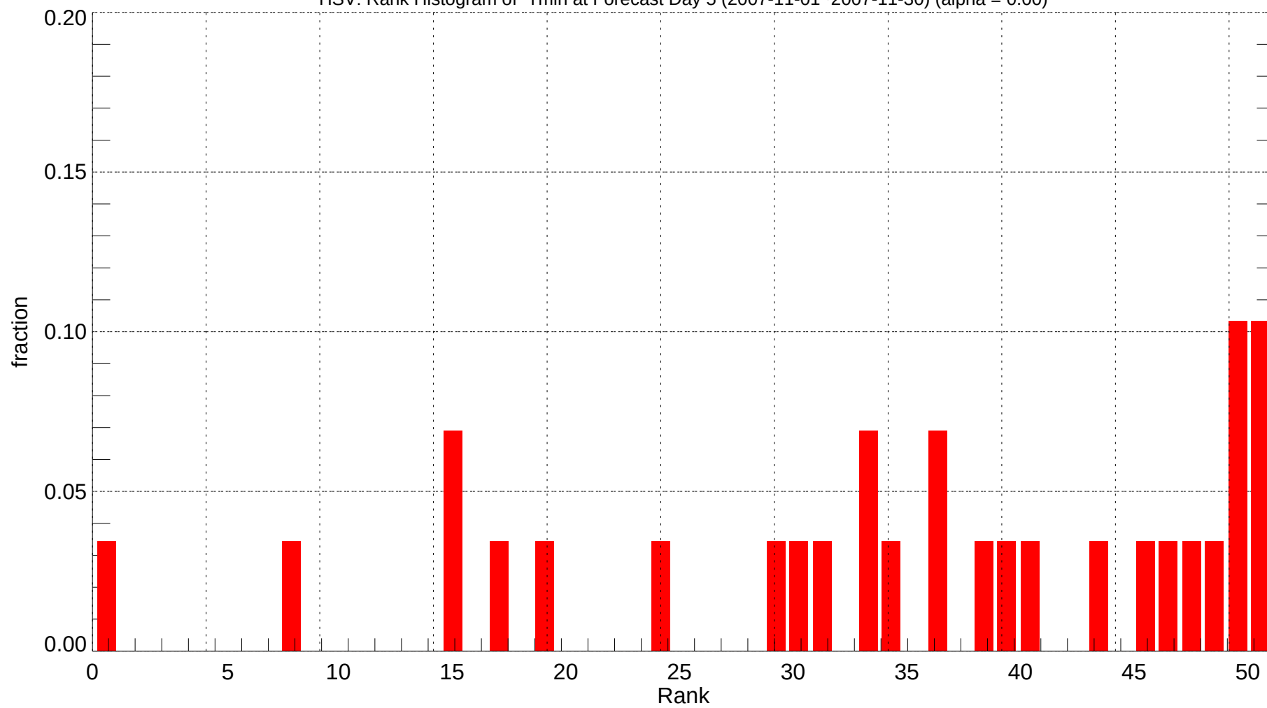
HSV: Rank Histogram of Tmin at Forecast Day 5 (2007-11-01~2007-11-30) (alpha = 0.00)
