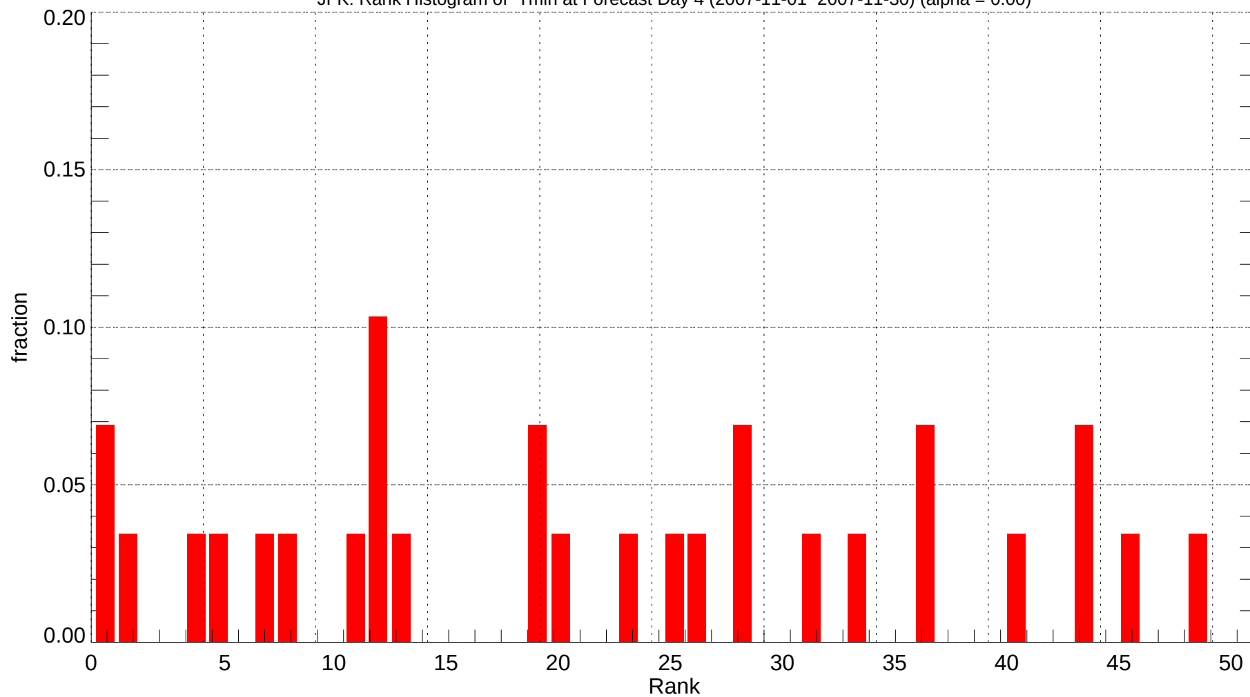
JFK: Rank Histogram of Tmin at Forecast Day 4 (2007-11-01~2007-11-30) (alpha = 0.00)
