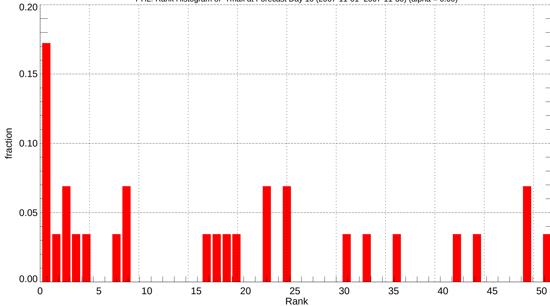
PHL: Rank Histogram of Tmax at Forecast Day 10 (2007-11-01~2007-11-30) (alpha = 0.00)
