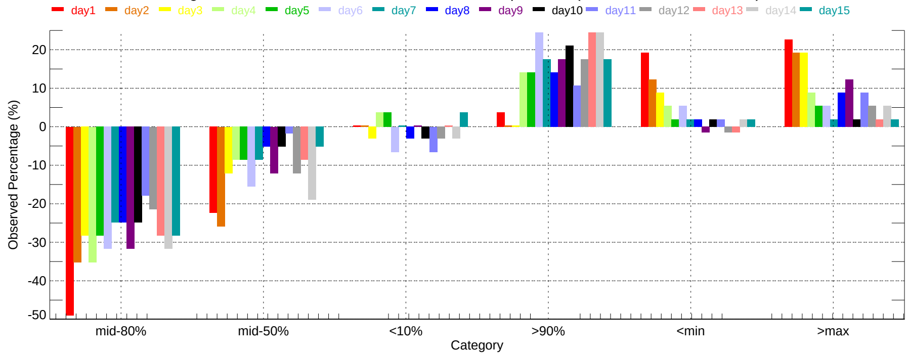
Observed Percentage Deviation of Ensembles - MWL: Max Temperature (2007-11-01~2007-11-30)
