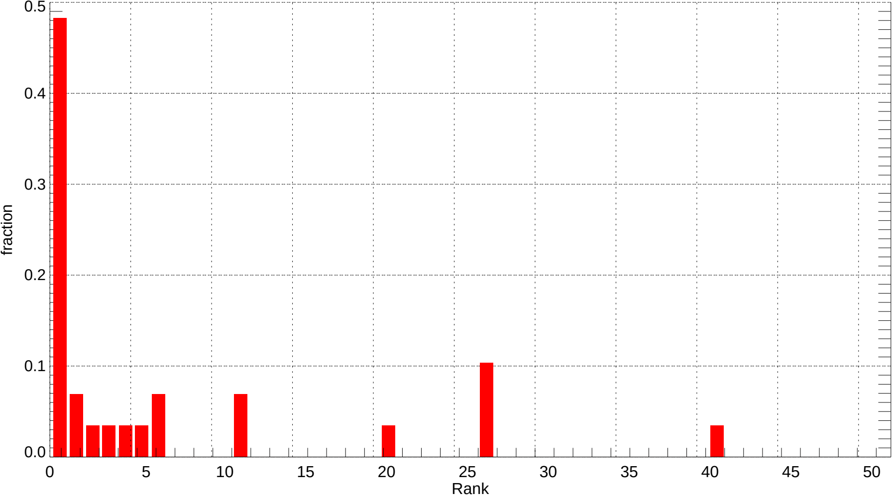
SJC: Rank Histogram of Tmin at Forecast Day 4 (2007-11-01~2007-11-30) (alpha = 0.00)
