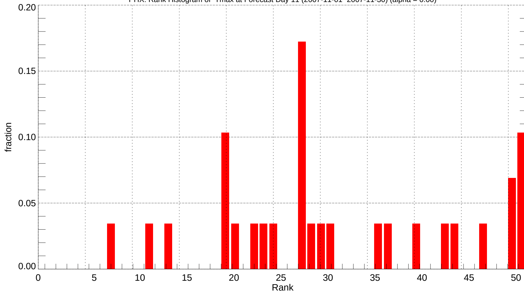
PHX: Rank Histogram of Tmax at Forecast Day 11 (2007-11-01~2007-11-30) (alpha = 0.00)
