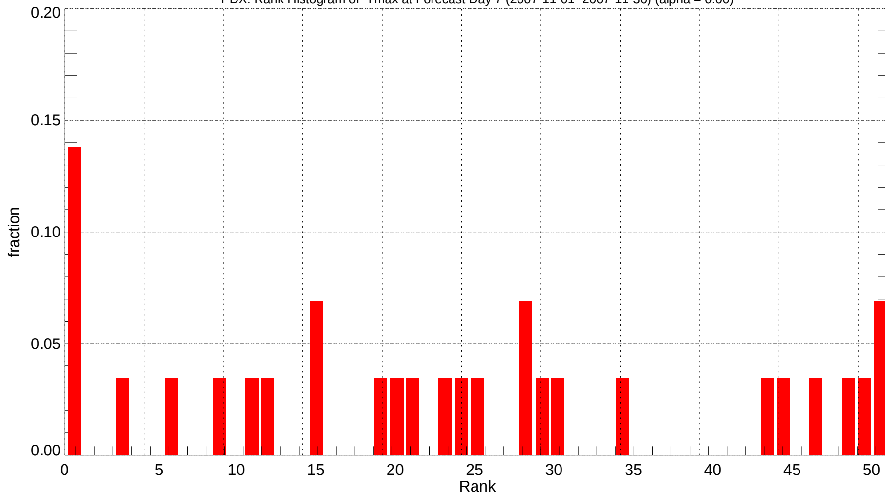
PDX: Rank Histogram of Tmax at Forecast Day 7 (2007-11-01~2007-11-30) (alpha = 0.00)
