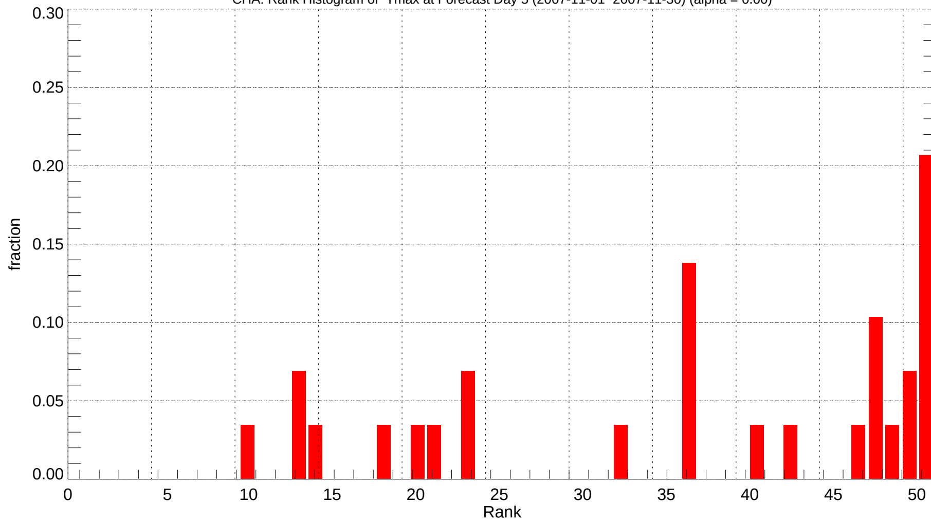
CHA: Rank Histogram of Tmax at Forecast Day 5 (2007-11-01~2007-11-30) (alpha = 0.00)
