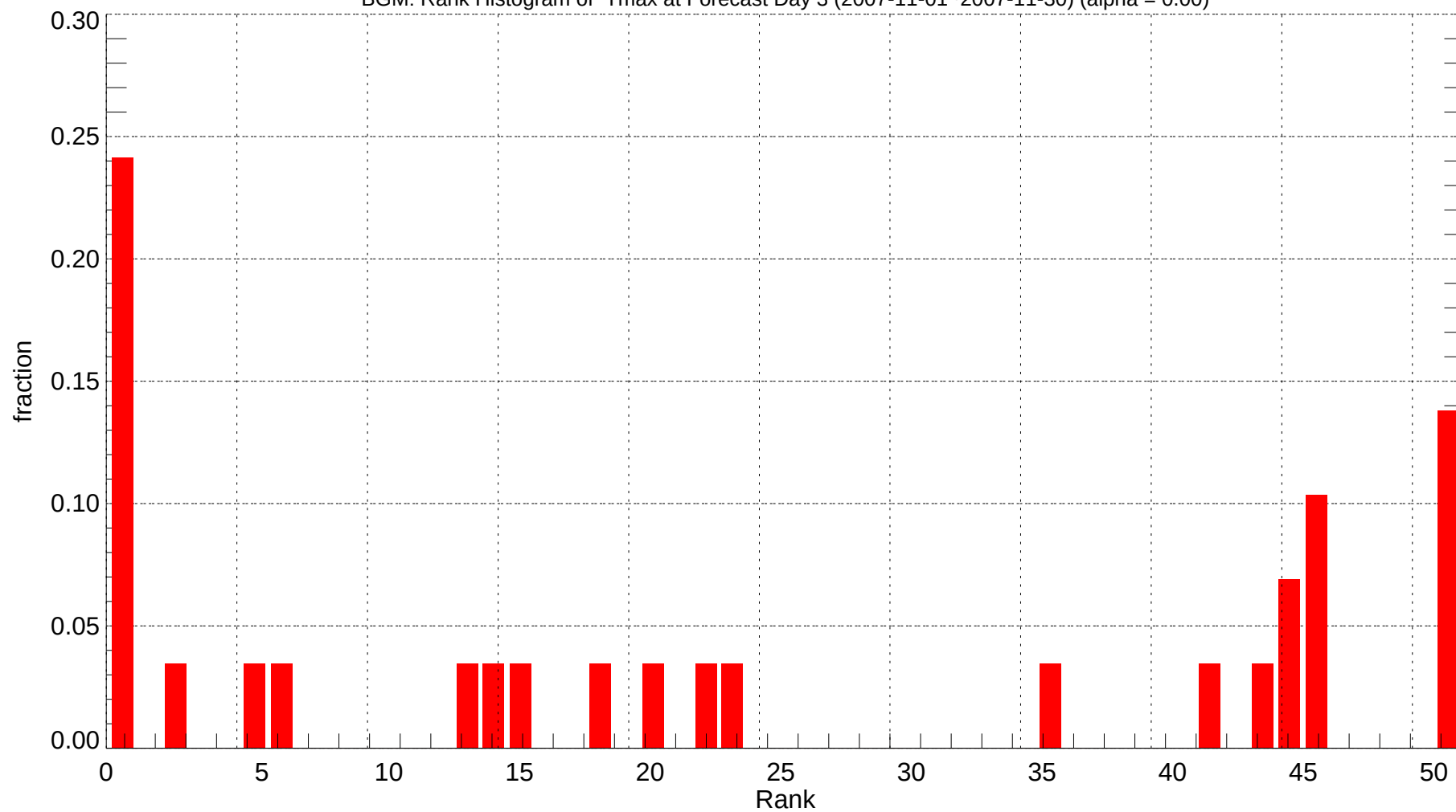
BGM: Rank Histogram of Tmax at Forecast Day 3 (2007-11-01~2007-11-30) (alpha = 0.00)
