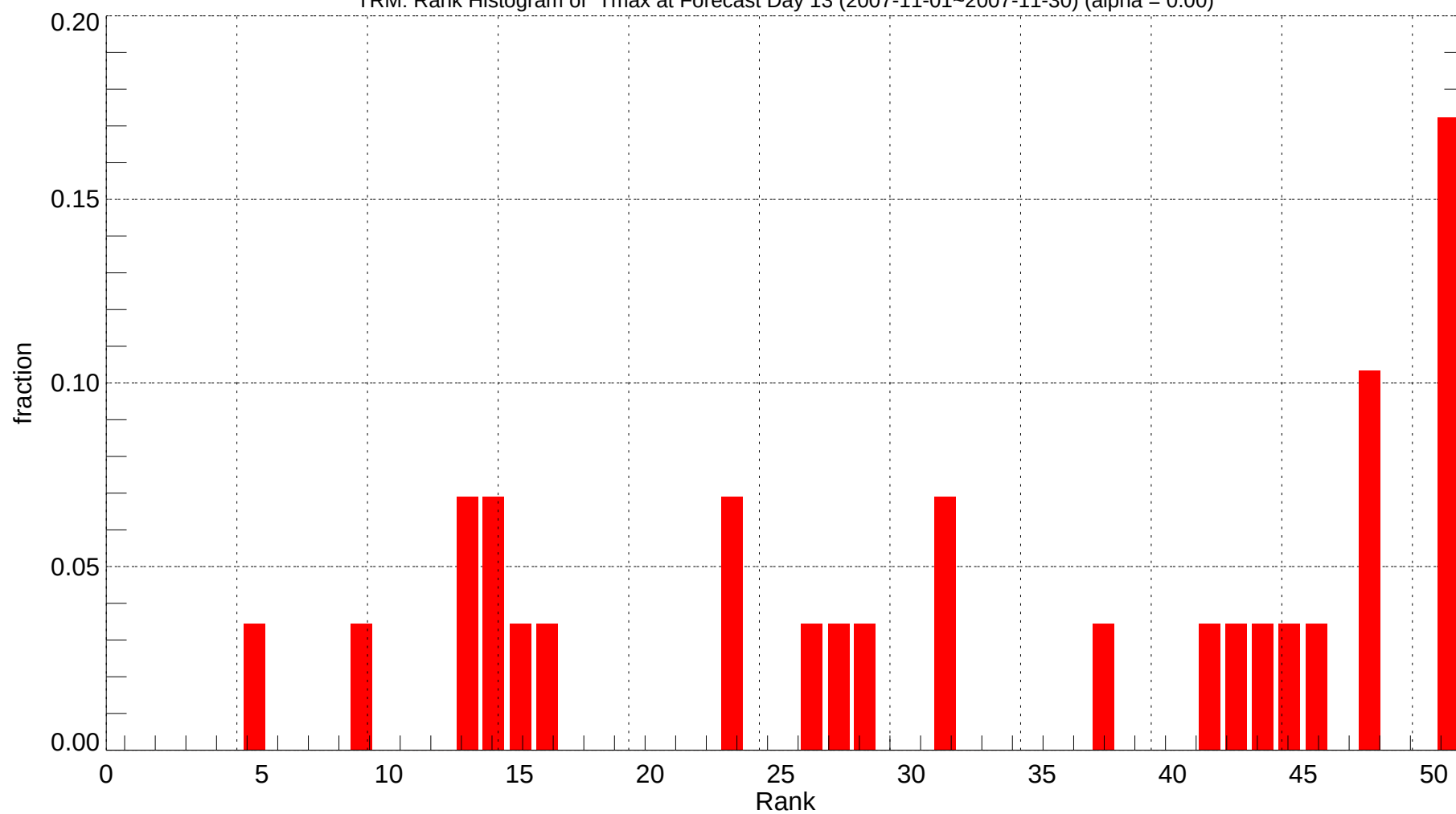
TRM: Rank Histogram of Tmax at Forecast Day 13 (2007-11-01~2007-11-30) (alpha = 0.00)
