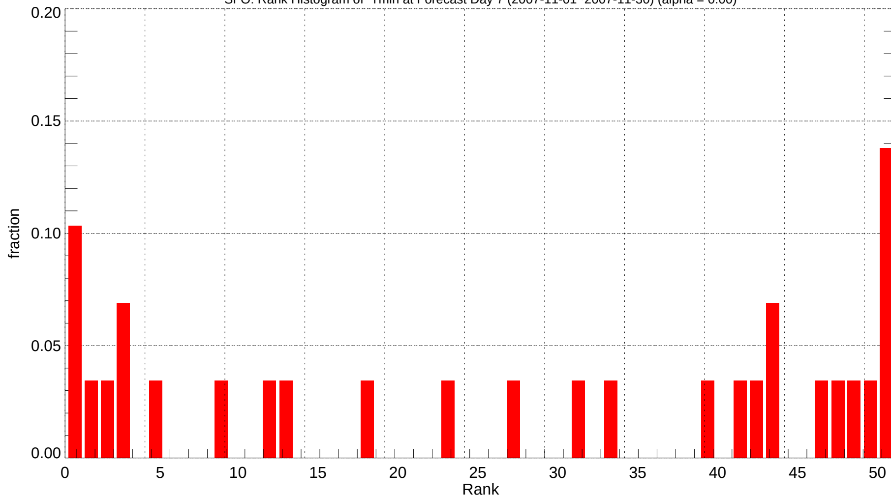
SFO: Rank Histogram of Tmin at Forecast Day 7 (2007-11-01~2007-11-30) (alpha = 0.00)
