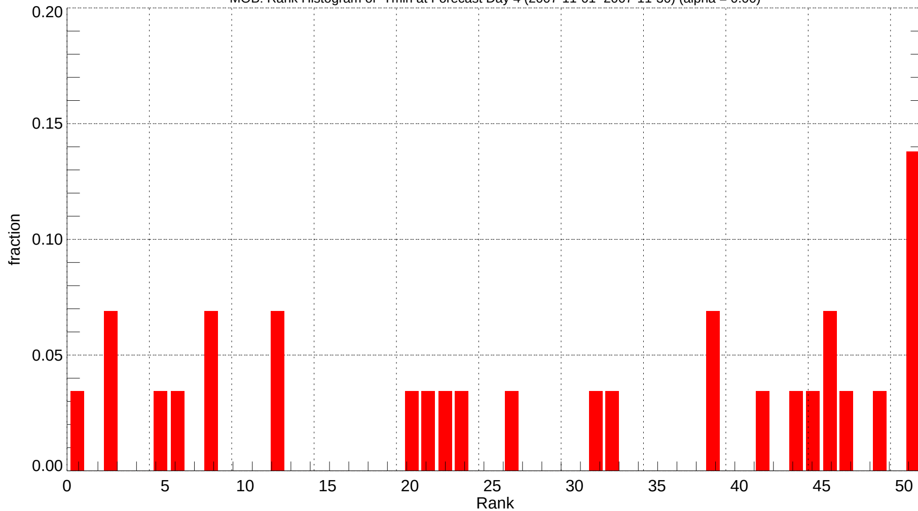
MOB: Rank Histogram of Tmin at Forecast Day 4 (2007-11-01~2007-11-30) (alpha = 0.00)
