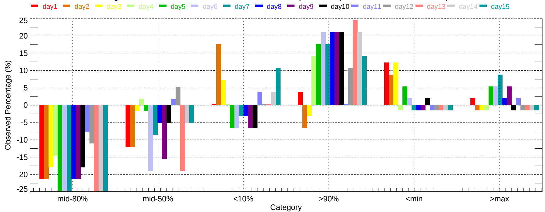
Observed Percentage Deviation of Ensembles - ELP: Min Temperature (2007-11-01~2007-11-30)
