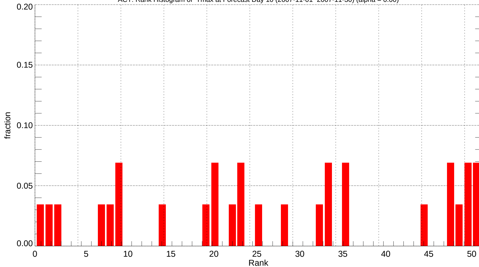
ACT: Rank Histogram of Tmax at Forecast Day 10 (2007-11-01~2007-11-30) (alpha = 0.00)
