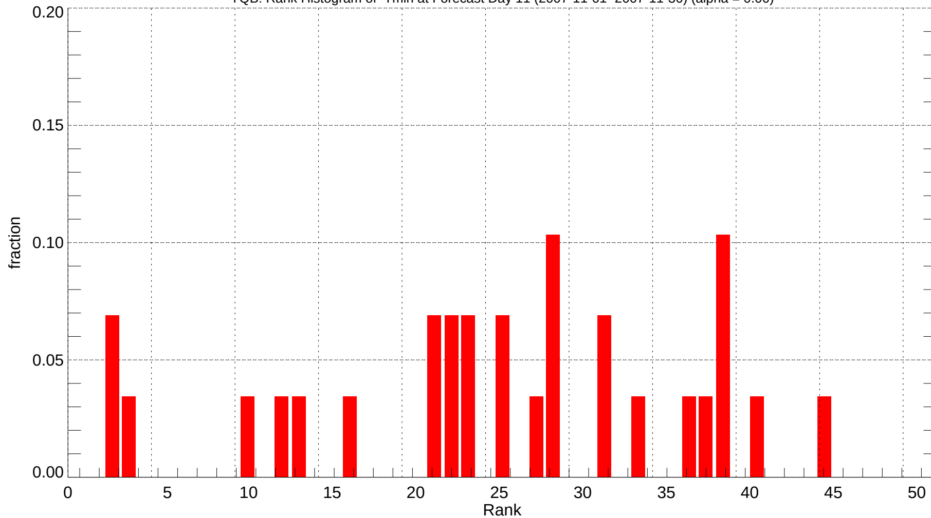
YQB: Rank Histogram of Tmin at Forecast Day 11 (2007-11-01~2007-11-30) (alpha = 0.00)
