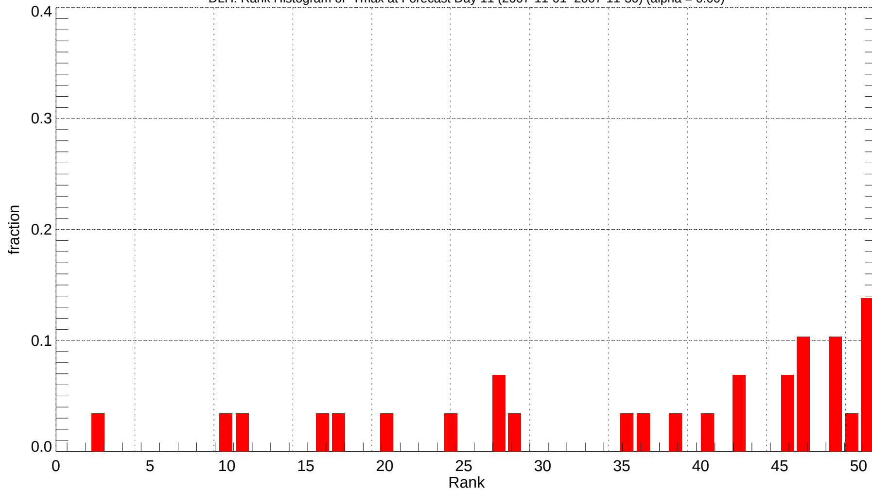
DLH: Rank Histogram of Tmax at Forecast Day 11 (2007-11-01~2007-11-30) (alpha = 0.00)
