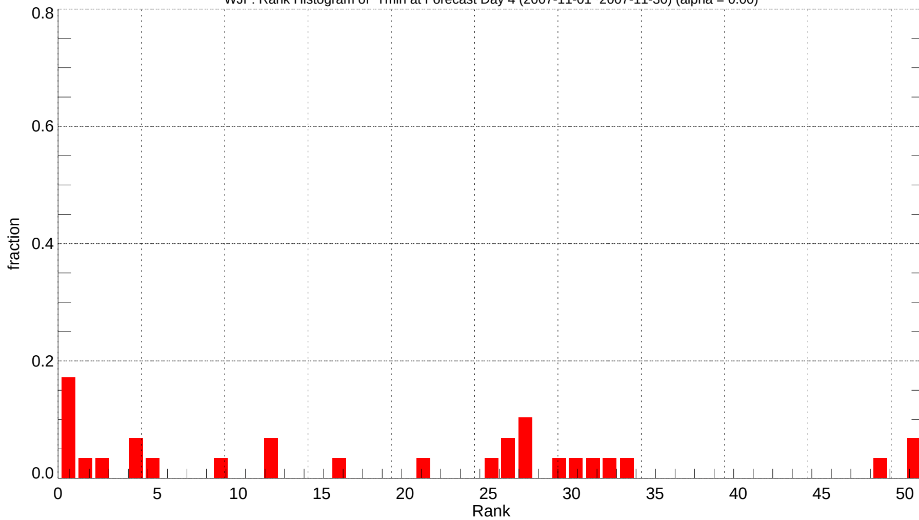
WJF: Rank Histogram of Tmin at Forecast Day 4 (2007-11-01~2007-11-30) (alpha = 0.00)
