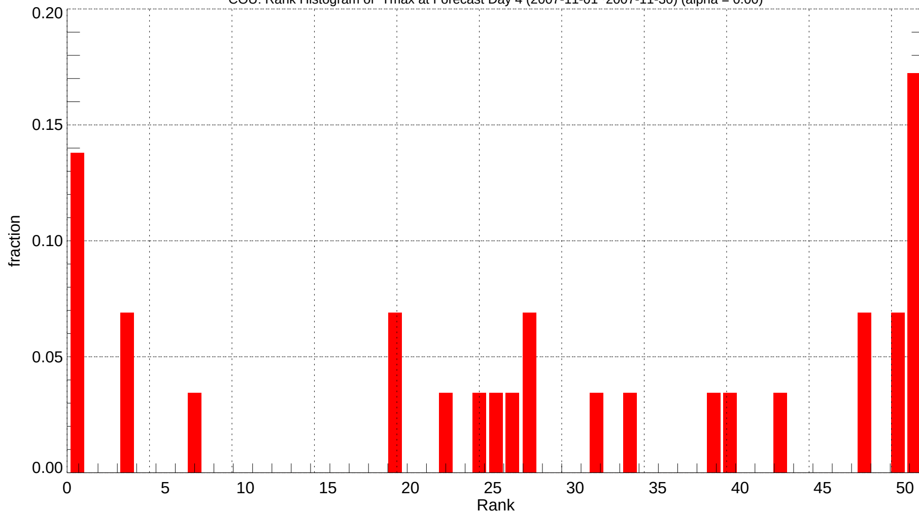
COU: Rank Histogram of Tmax at Forecast Day 4 (2007-11-01~2007-11-30) (alpha = 0.00)
