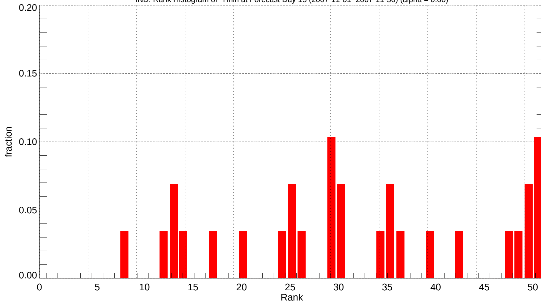
IND: Rank Histogram of Tmin at Forecast Day 13 (2007-11-01~2007-11-30) (alpha = 0.00)
