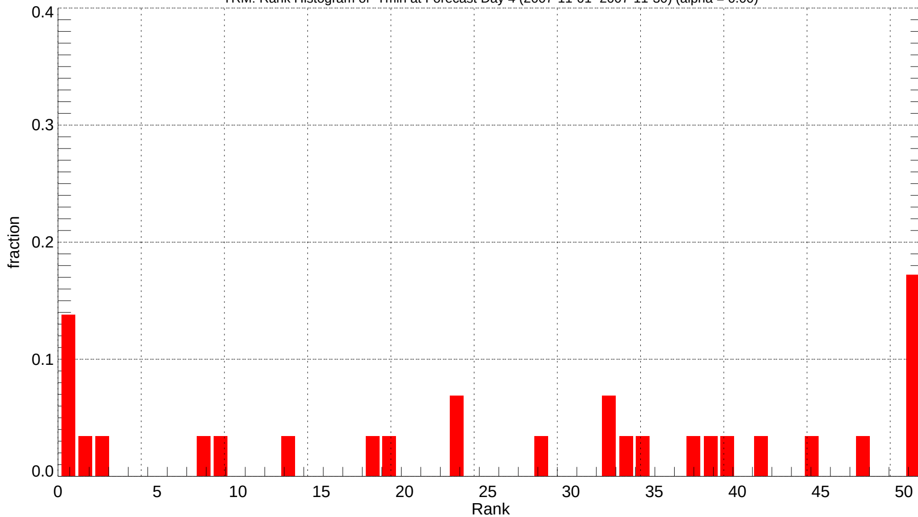
TRM: Rank Histogram of Tmin at Forecast Day 4 (2007-11-01~2007-11-30) (alpha = 0.00)
