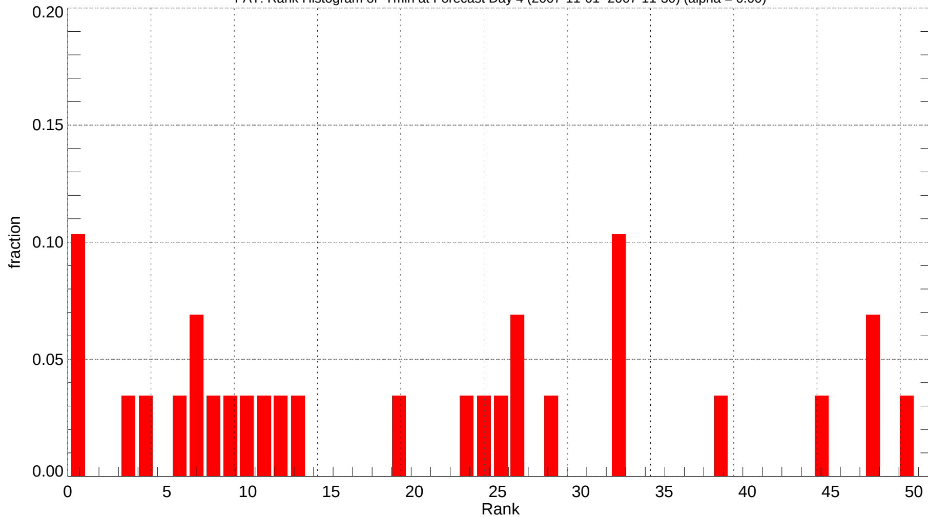
FAT: Rank Histogram of Tmin at Forecast Day 4 (2007-11-01~2007-11-30) (alpha = 0.00)
