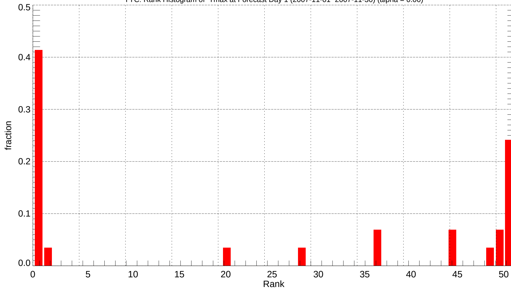
YYC: Rank Histogram of Tmax at Forecast Day 1 (2007-11-01~2007-11-30) (alpha = 0.00)
