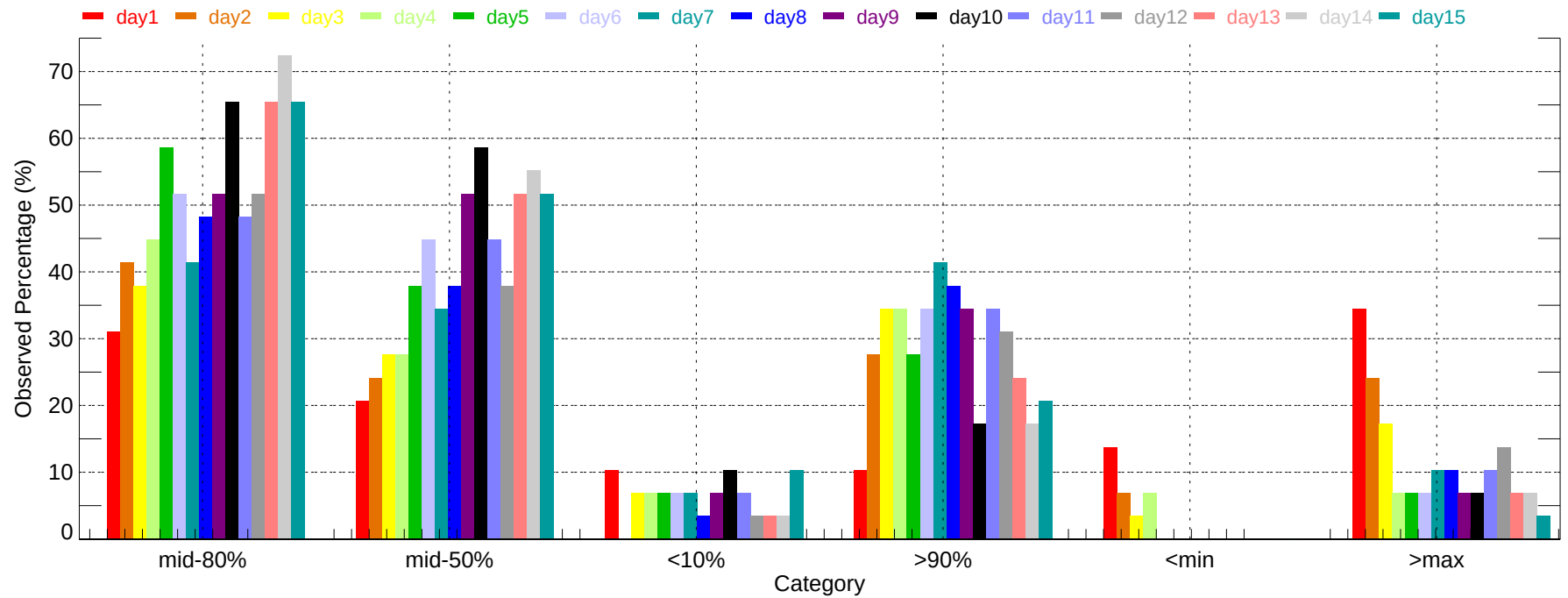
Observed Percentage of Ensembles - CRW: Max Temperature (2007-11-01~2007-11-30)
