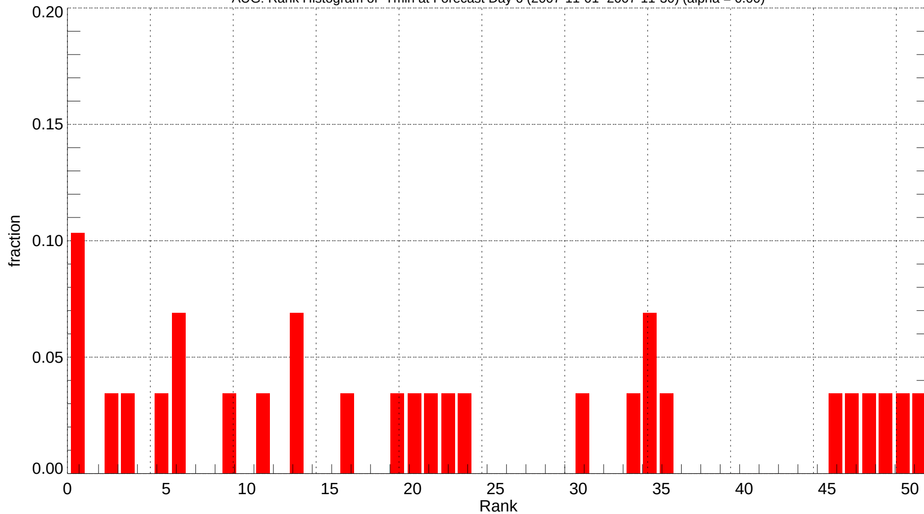
AUG: Rank Histogram of Tmin at Forecast Day 6 (2007-11-01~2007-11-30) (alpha = 0.00)
