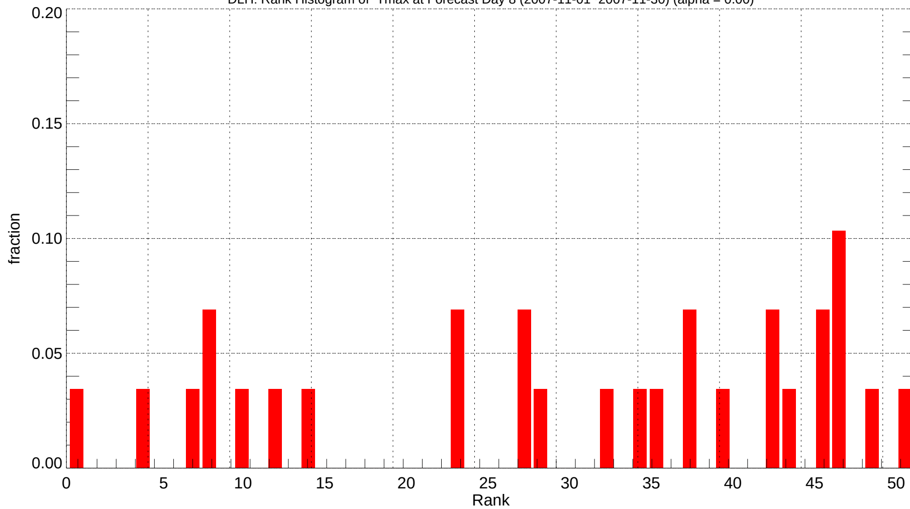
DLH: Rank Histogram of Tmax at Forecast Day 8 (2007-11-01~2007-11-30) (alpha = 0.00)
