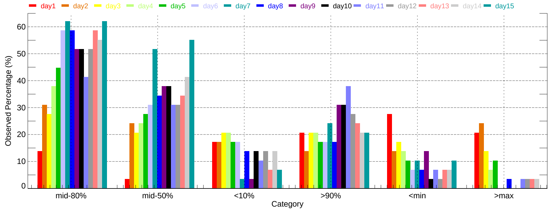
Observed Percentage of Ensembles - BRO: Min Temperature (2007-11-01~2007-11-30)
