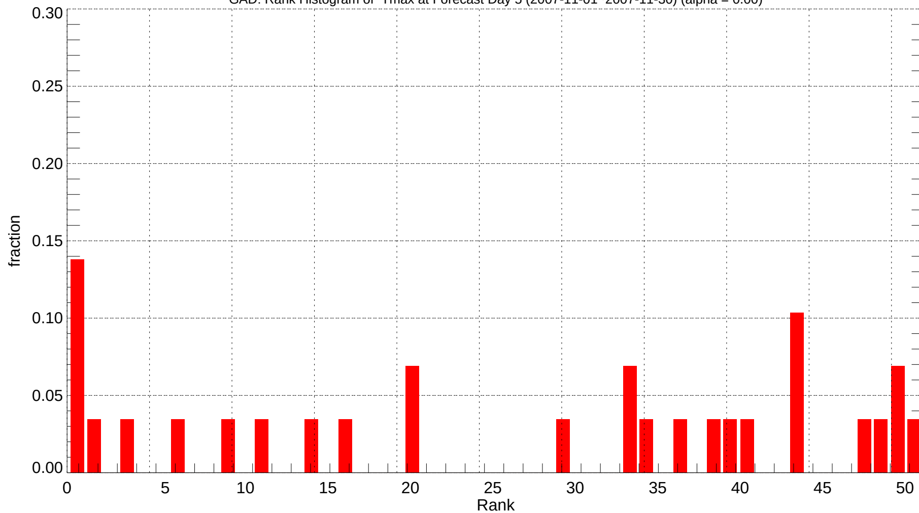
GAD: Rank Histogram of Tmax at Forecast Day 5 (2007-11-01~2007-11-30) (alpha = 0.00)
