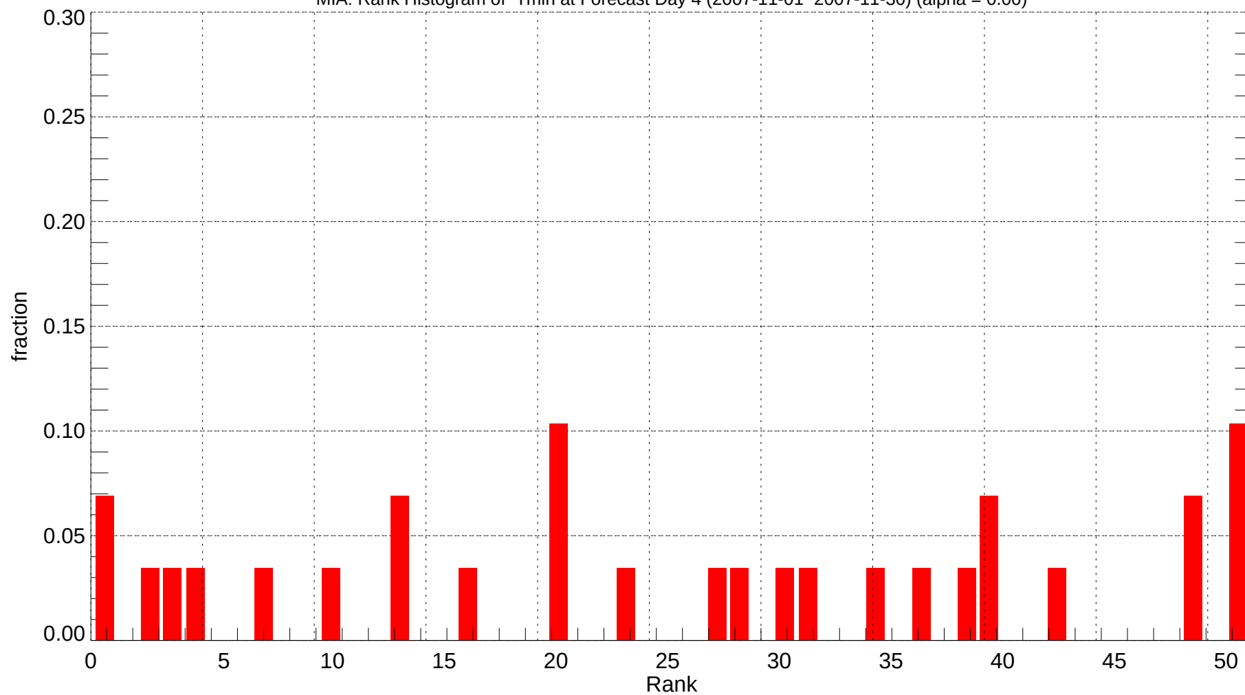
MIA: Rank Histogram of Tmin at Forecast Day 4 (2007-11-01~2007-11-30) (alpha = 0.00)
