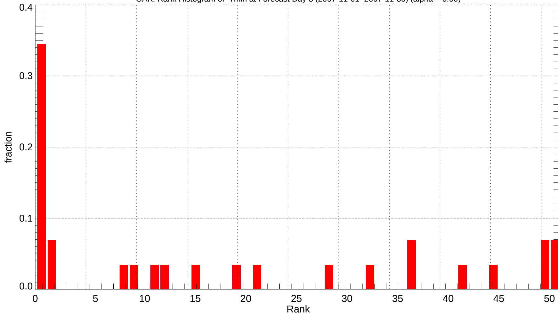
OAK: Rank Histogram of Tmin at Forecast Day 8 (2007-11-01~2007-11-30) (alpha = 0.00)
