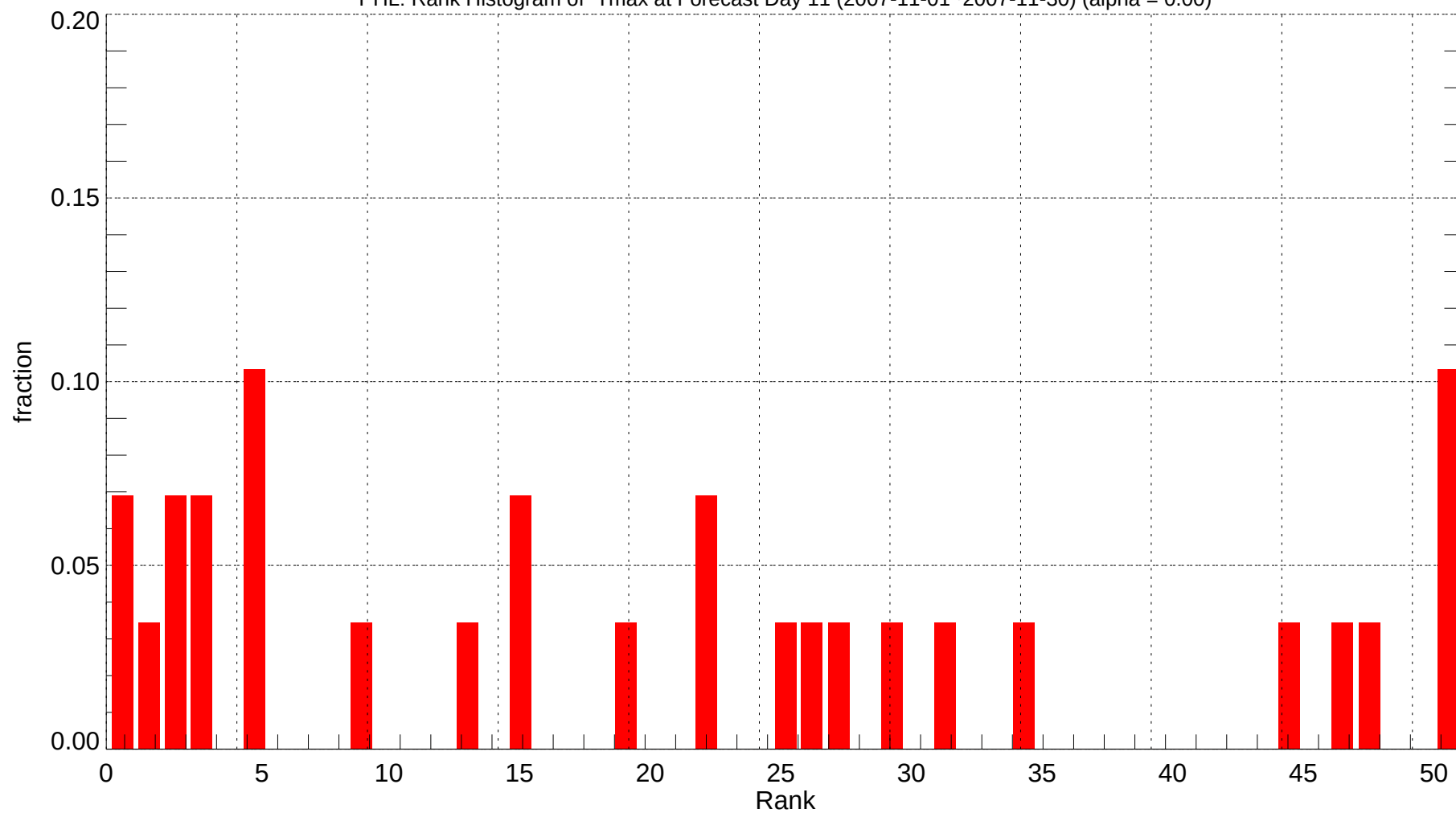
PHL: Rank Histogram of Tmax at Forecast Day 11 (2007-11-01~2007-11-30) (alpha = 0.00)
