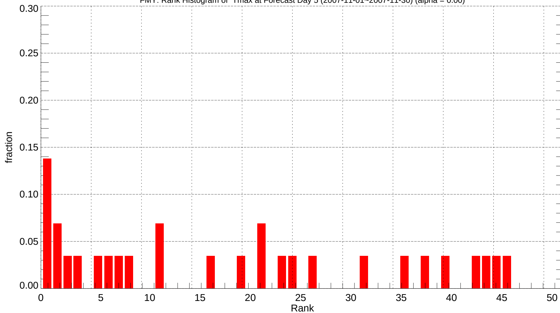
FMY: Rank Histogram of Tmax at Forecast Day 5 (2007-11-01~2007-11-30) (alpha = 0.00)
