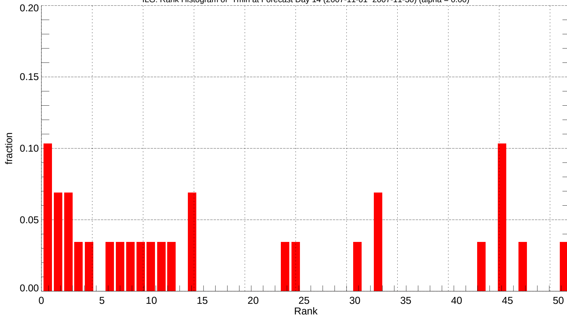
ILG: Rank Histogram of Tmin at Forecast Day 14 (2007-11-01~2007-11-30) (alpha = 0.00)
