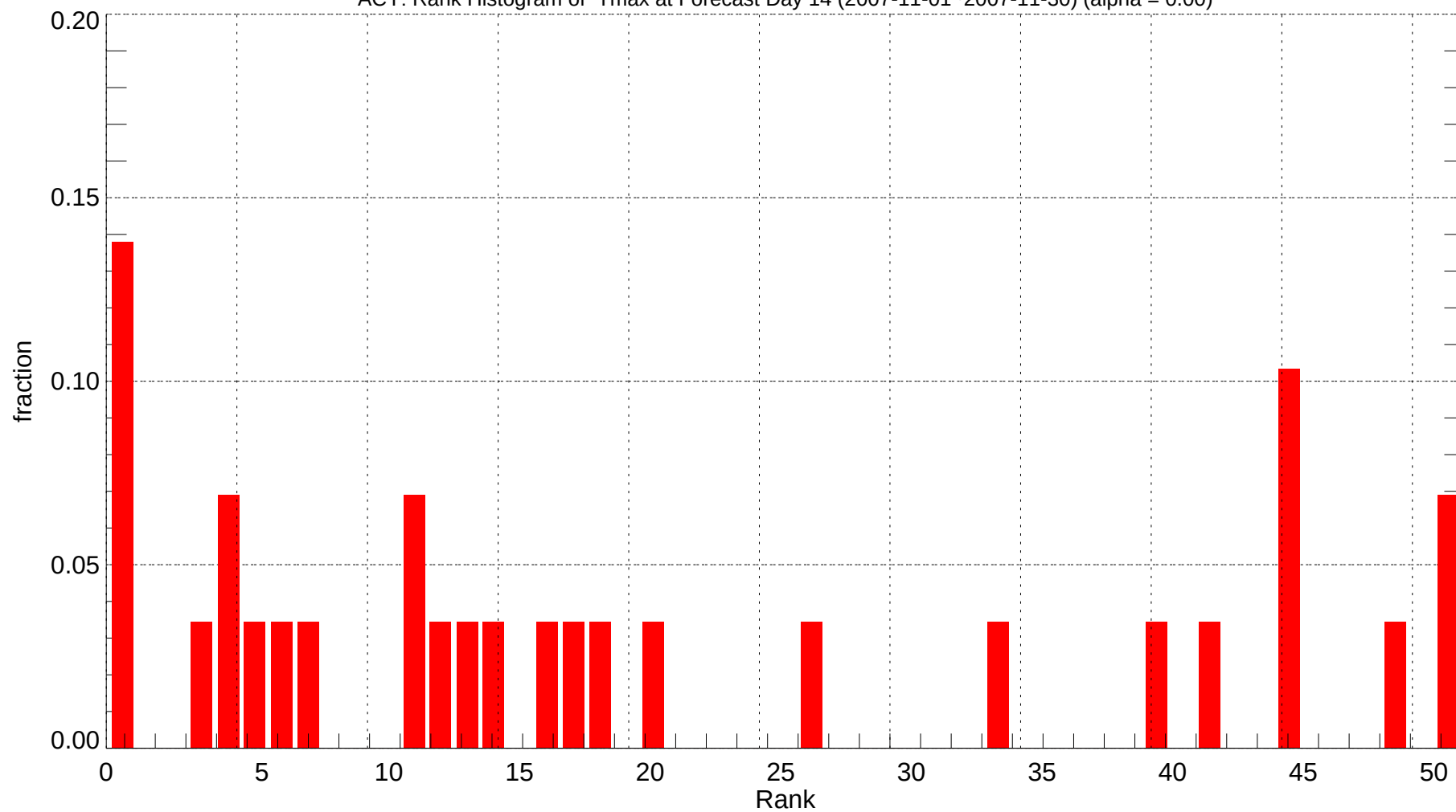
ACY: Rank Histogram of Tmax at Forecast Day 14 (2007-11-01~2007-11-30) (alpha = 0.00)
