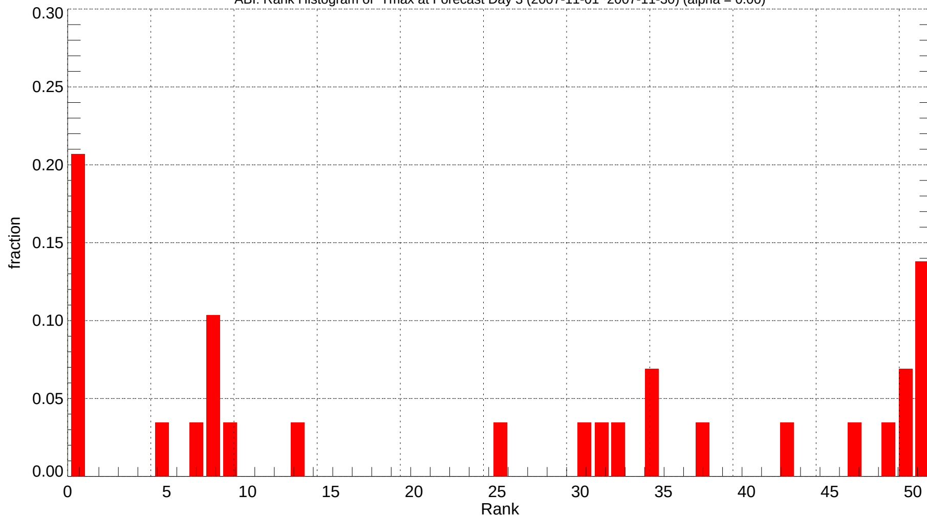
ABI: Rank Histogram of Tmax at Forecast Day 3 (2007-11-01~2007-11-30) (alpha = 0.00)
