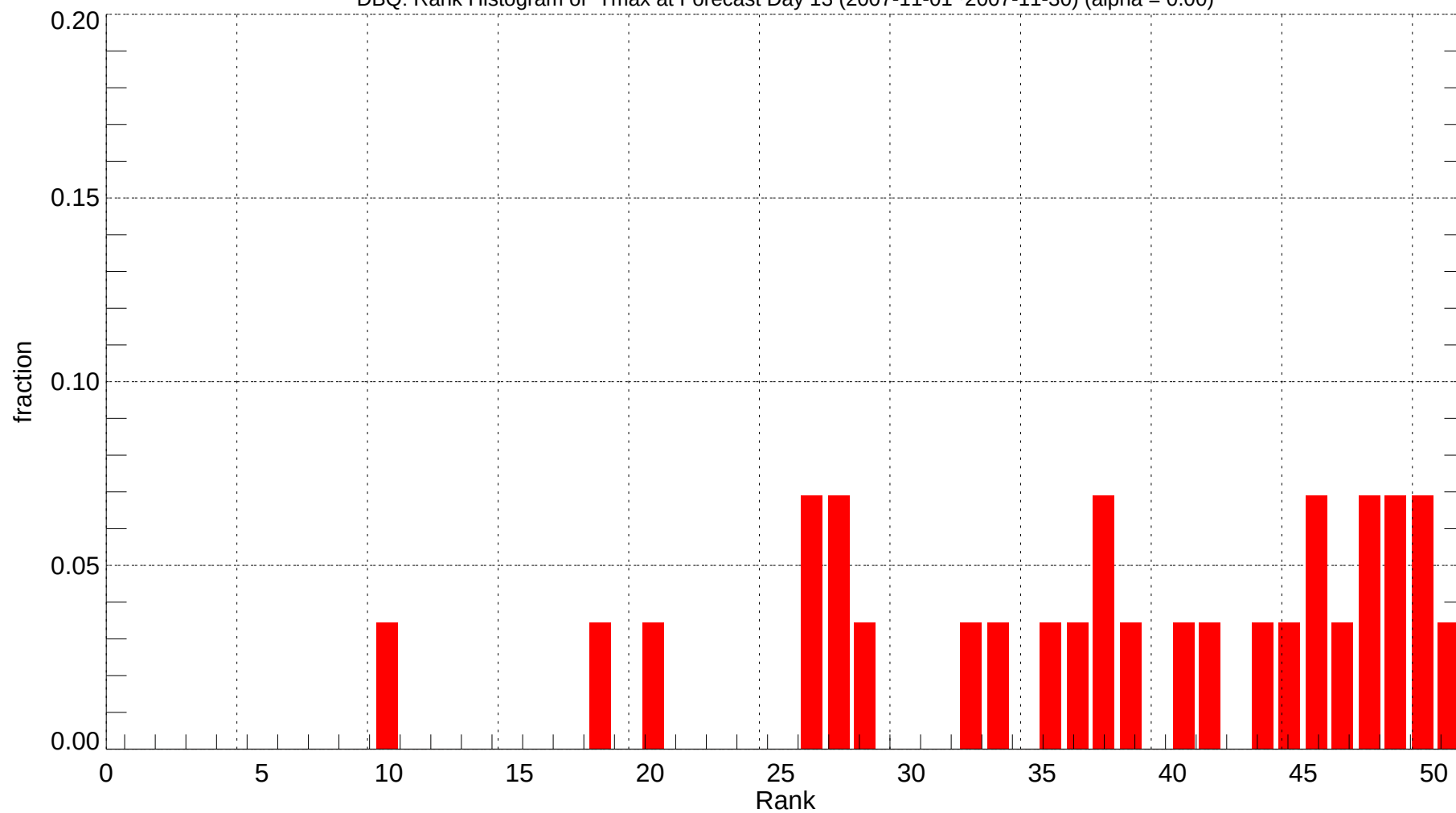
DBQ: Rank Histogram of Tmax at Forecast Day 13 (2007-11-01~2007-11-30) (alpha = 0.00)
