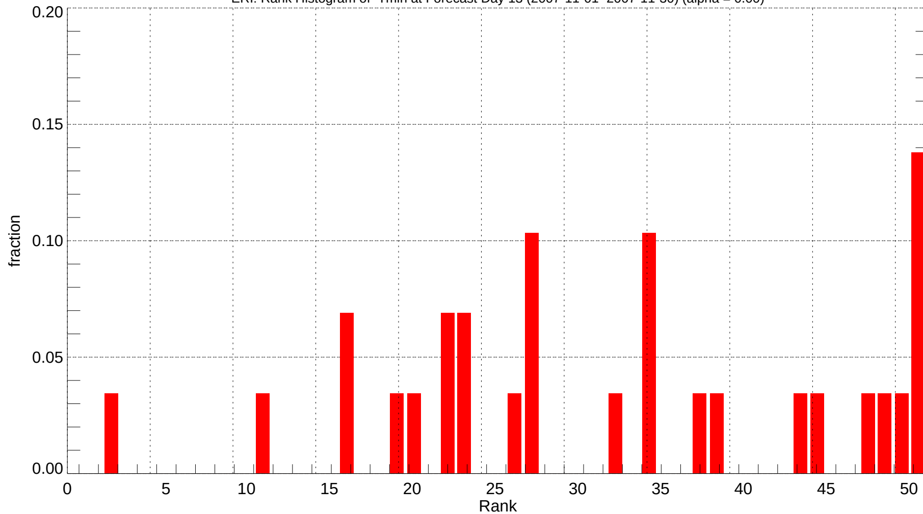
ERI: Rank Histogram of Tmin at Forecast Day 13 (2007-11-01~2007-11-30) (alpha = 0.00)
