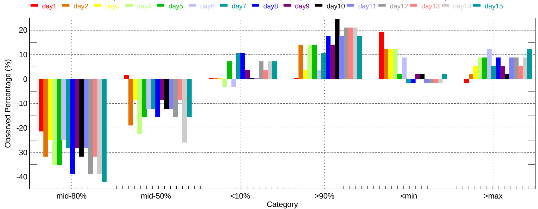
Observed Percentage Deviation of Ensembles - MAF: Max Temperature (2007-11-01~2007-11-30)
