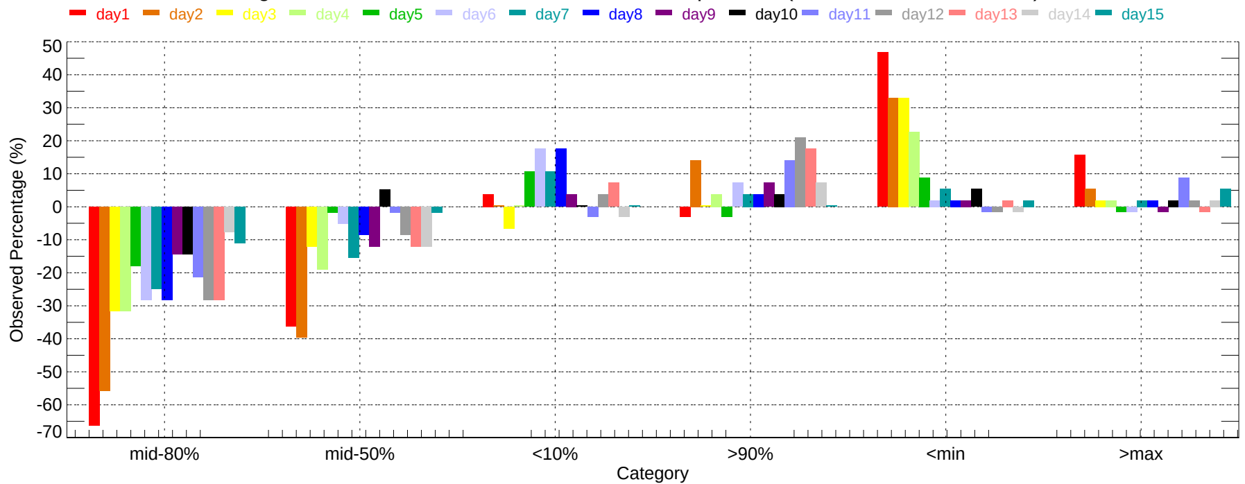
Observed Percentage Deviation of Ensembles - DTW: Max Temperature (2007-11-01~2007-11-30)
