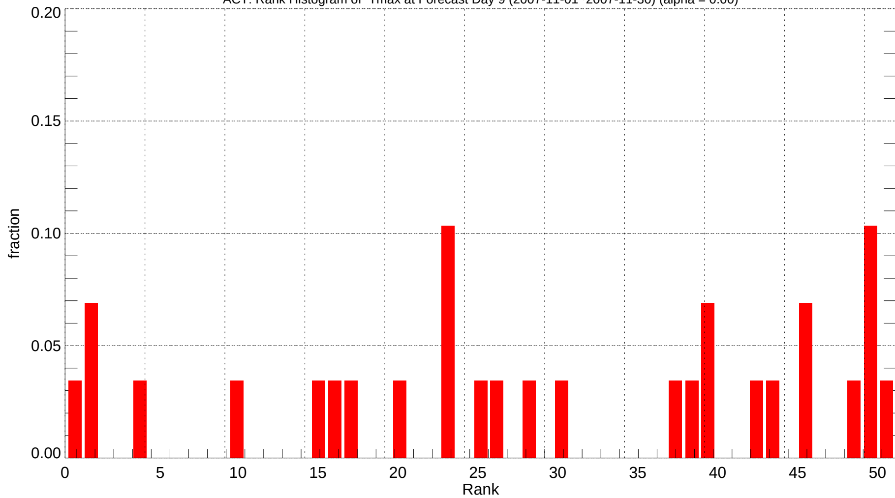
ACT: Rank Histogram of Tmax at Forecast Day 9 (2007-11-01~2007-11-30) (alpha = 0.00)
