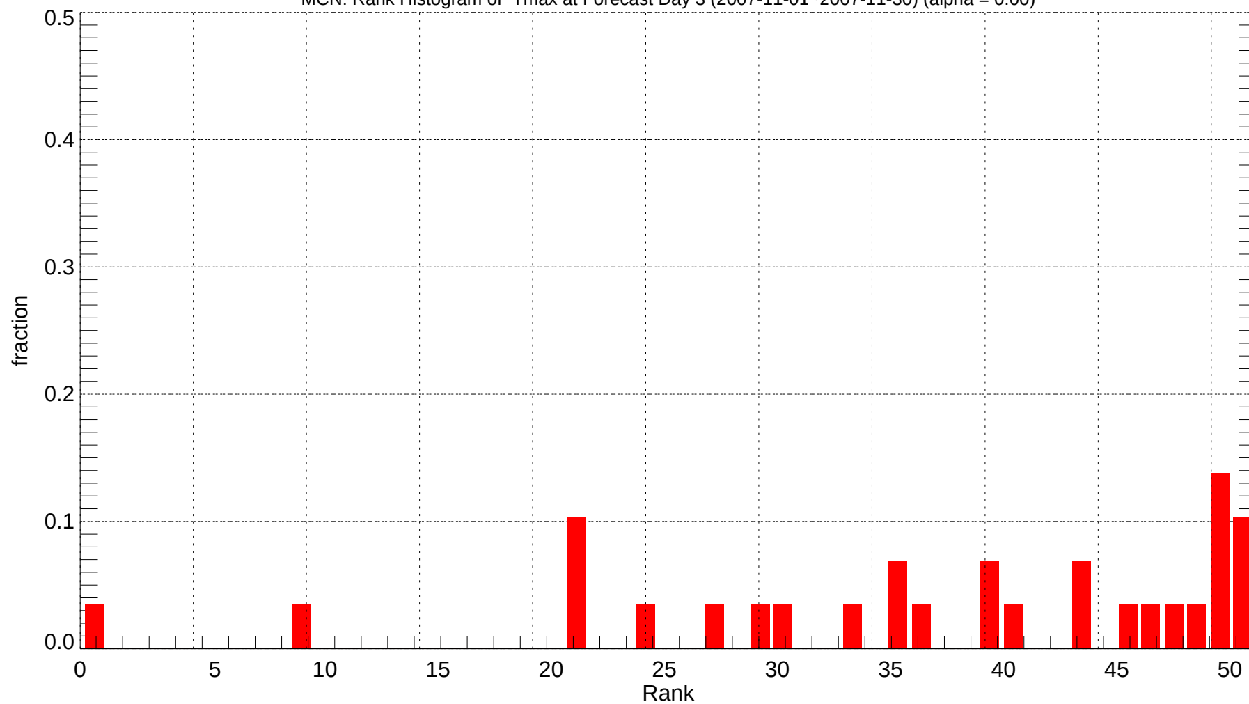
MCN: Rank Histogram of Tmax at Forecast Day 3 (2007-11-01~2007-11-30) (alpha = 0.00)
