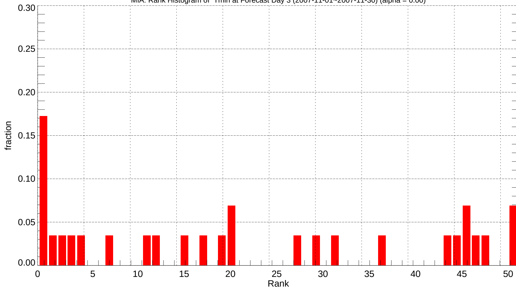
MIA: Rank Histogram of Tmin at Forecast Day 3 (2007-11-01~2007-11-30) (alpha = 0.00)
