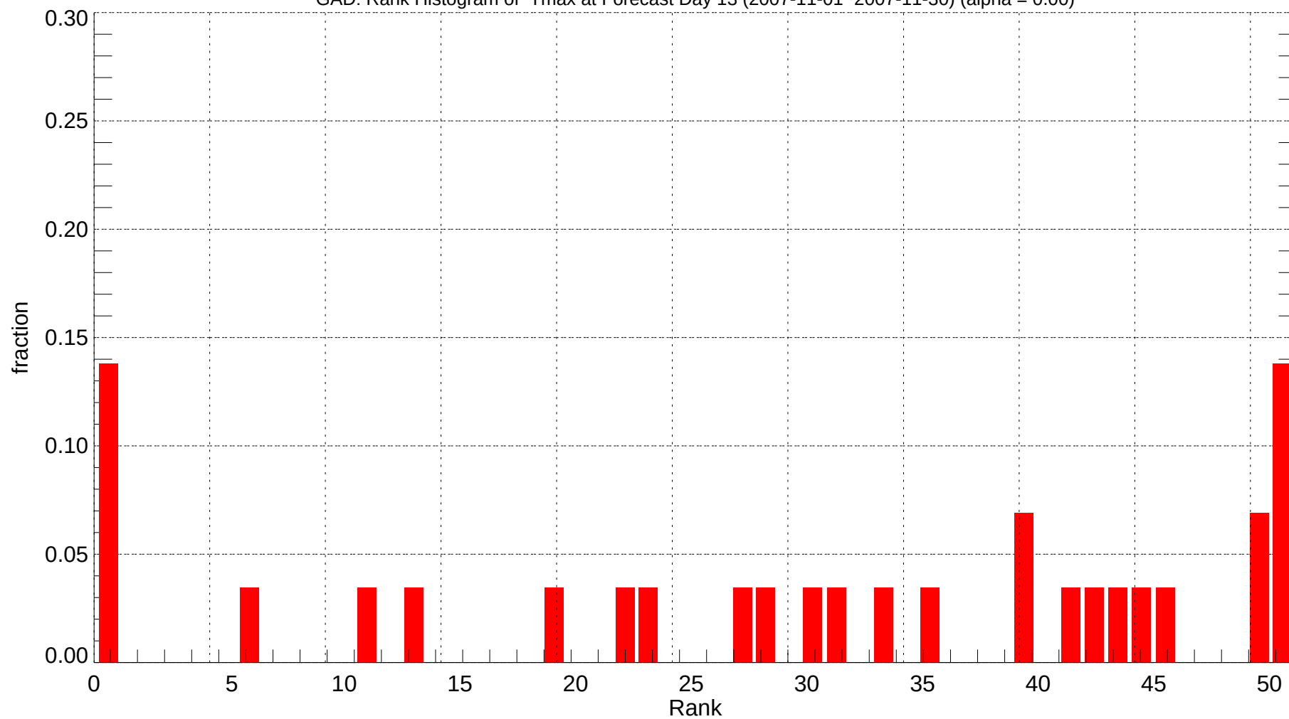
GAD: Rank Histogram of Tmax at Forecast Day 13 (2007-11-01~2007-11-30) (alpha = 0.00)
