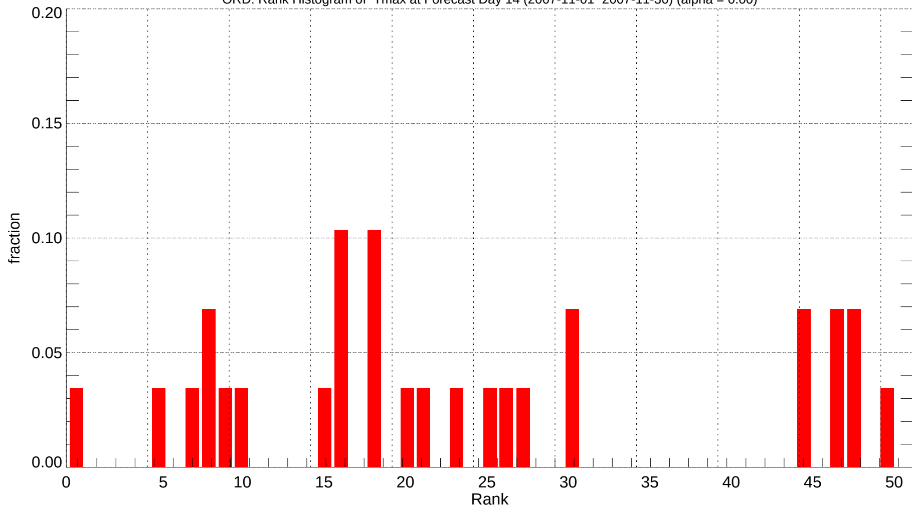
ORD: Rank Histogram of Tmax at Forecast Day 14 (2007-11-01~2007-11-30) (alpha = 0.00)
