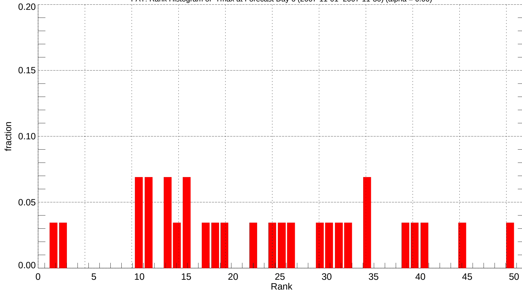
FAT: Rank Histogram of Tmax at Forecast Day 6 (2007-11-01~2007-11-30) (alpha = 0.00)
