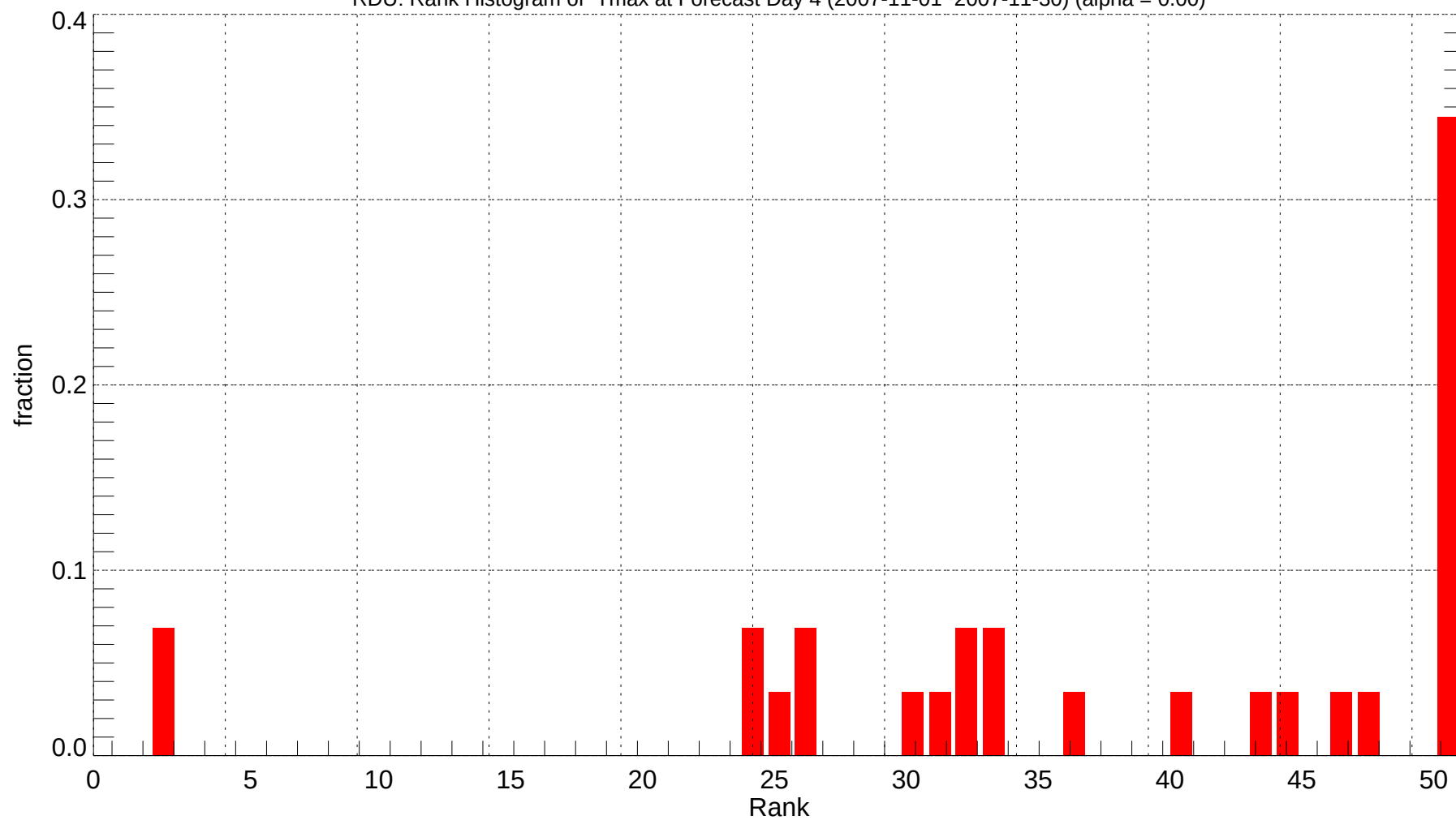
RDU: Rank Histogram of Tmax at Forecast Day 4 (2007-11-01~2007-11-30) (alpha = 0.00)
