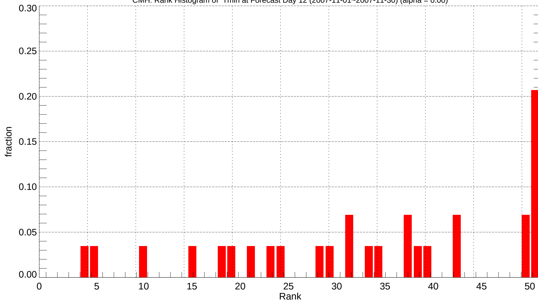
CMH: Rank Histogram of Tmin at Forecast Day 12 (2007-11-01~2007-11-30) (alpha = 0.00)
