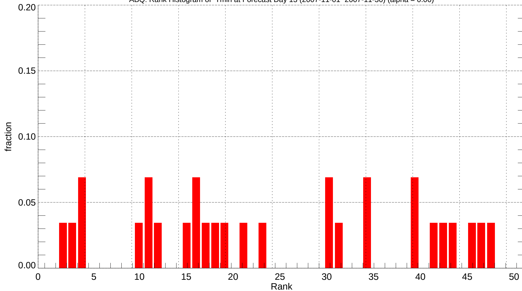
ABQ: Rank Histogram of Tmin at Forecast Day 13 (2007-11-01~2007-11-30) (alpha = 0.00)
