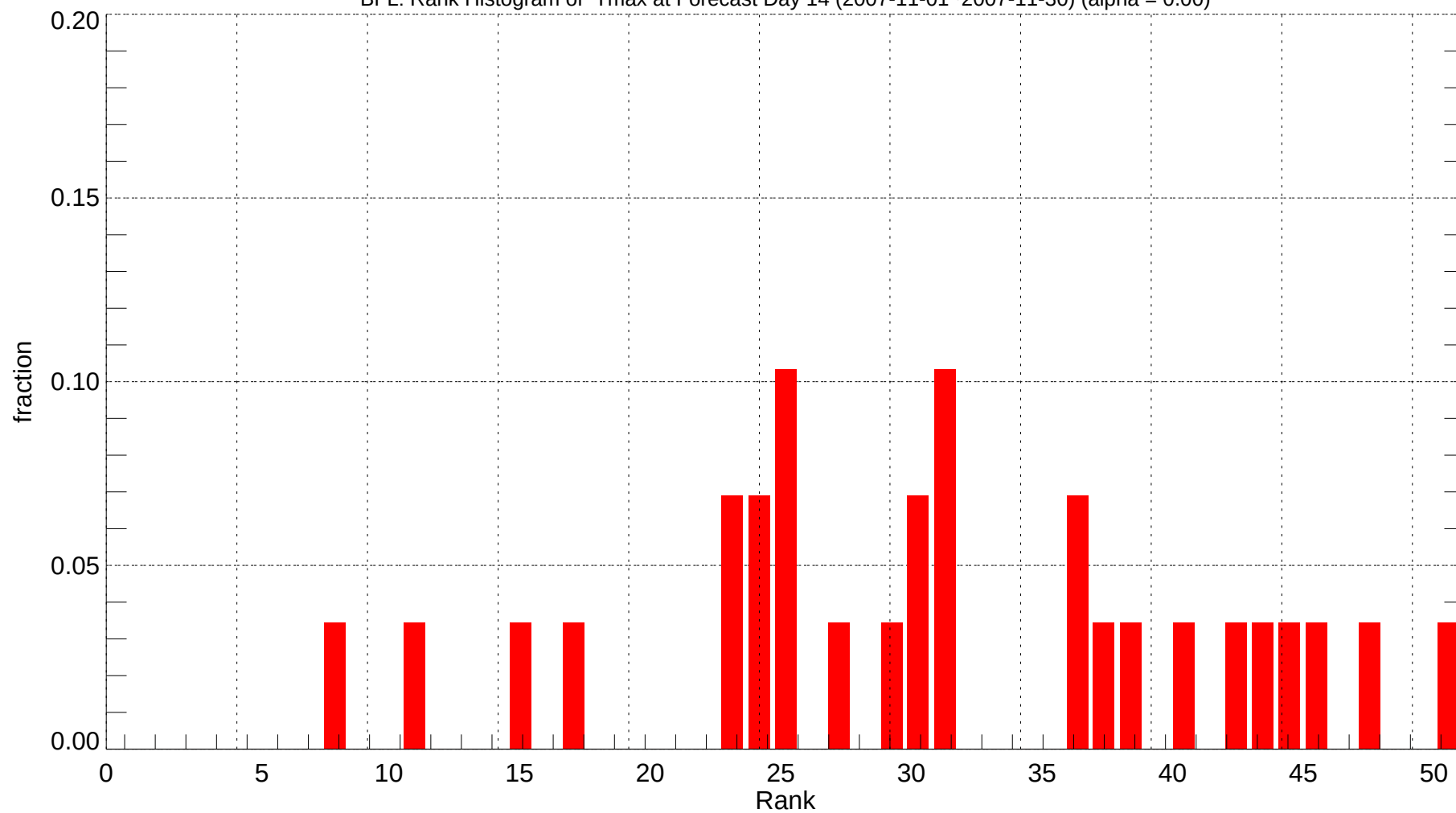
BFL: Rank Histogram of Tmax at Forecast Day 14 (2007-11-01~2007-11-30) (alpha = 0.00)
