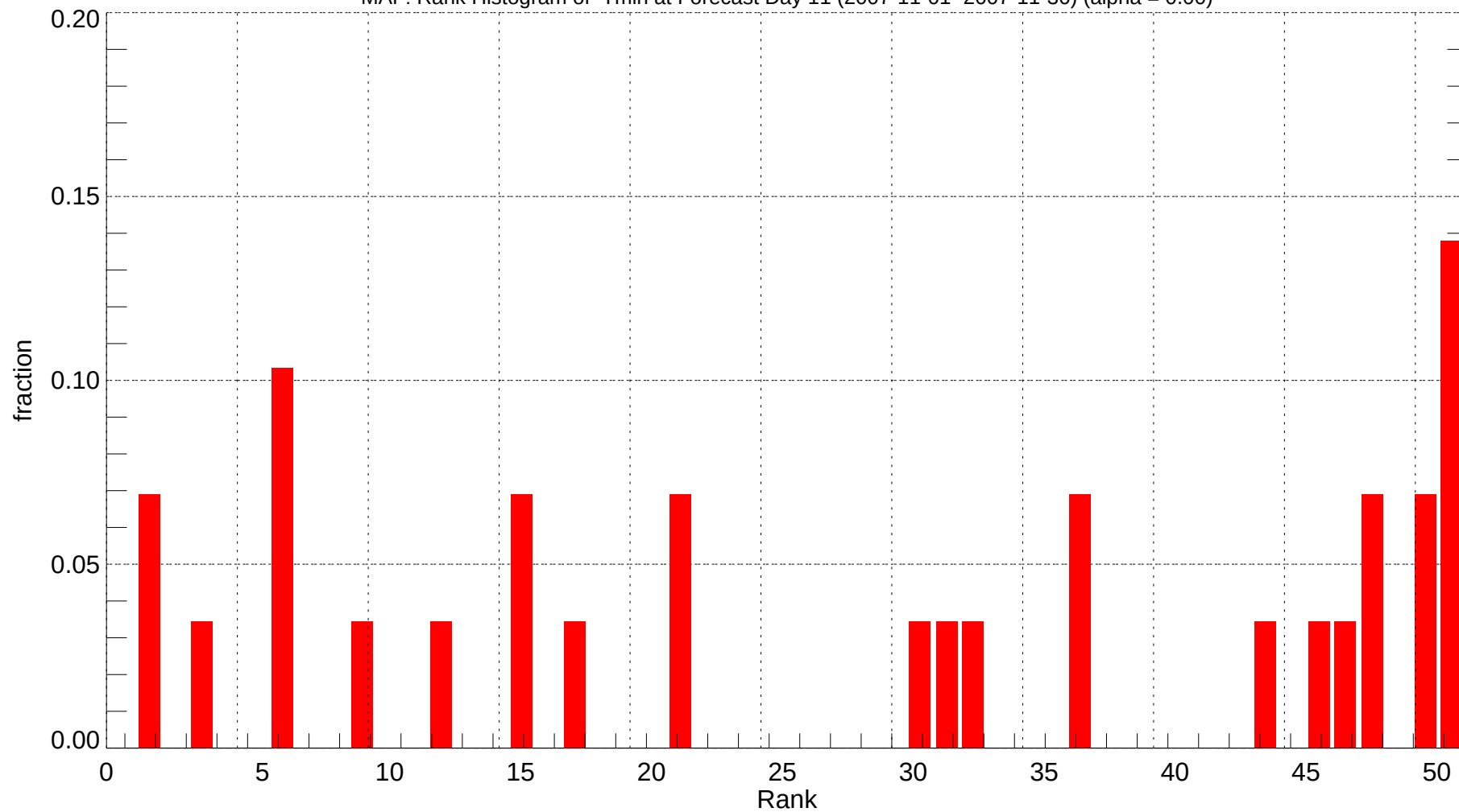
MAF: Rank Histogram of Tmin at Forecast Day 11 (2007-11-01~2007-11-30) (alpha = 0.00)
