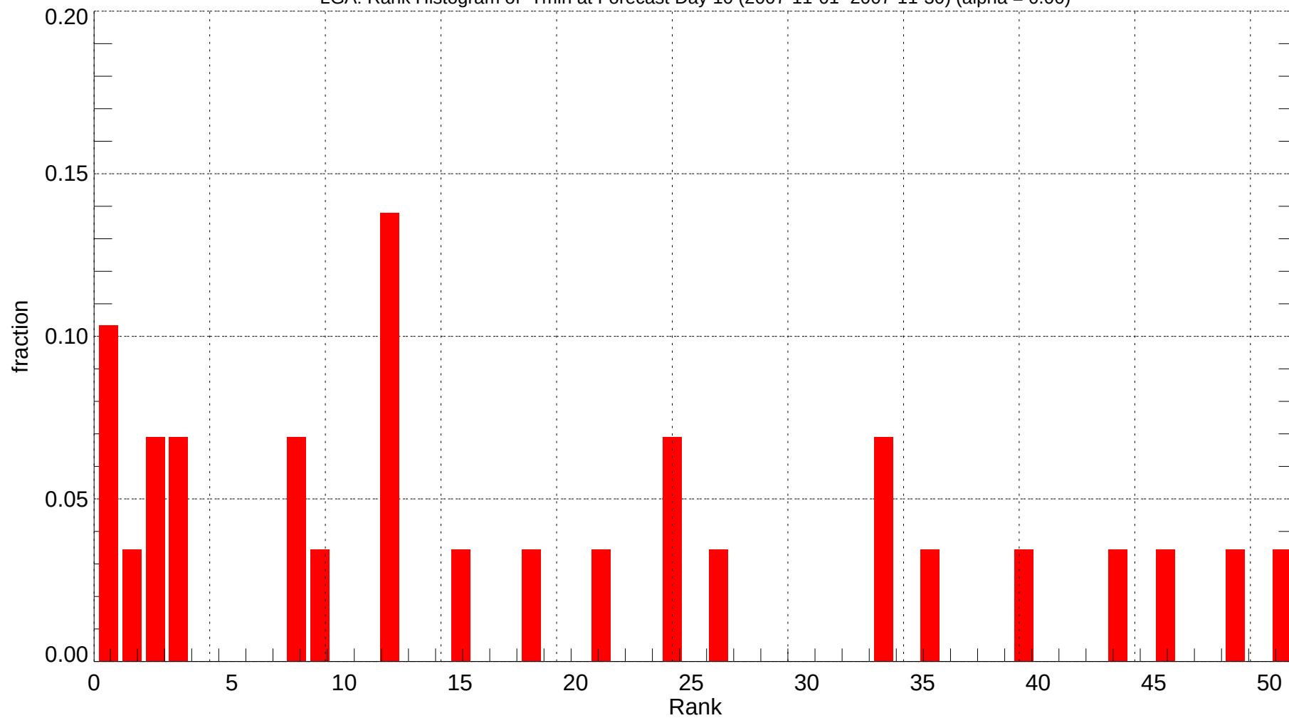
LGA: Rank Histogram of Tmin at Forecast Day 10 (2007-11-01~2007-11-30) (alpha = 0.00)
