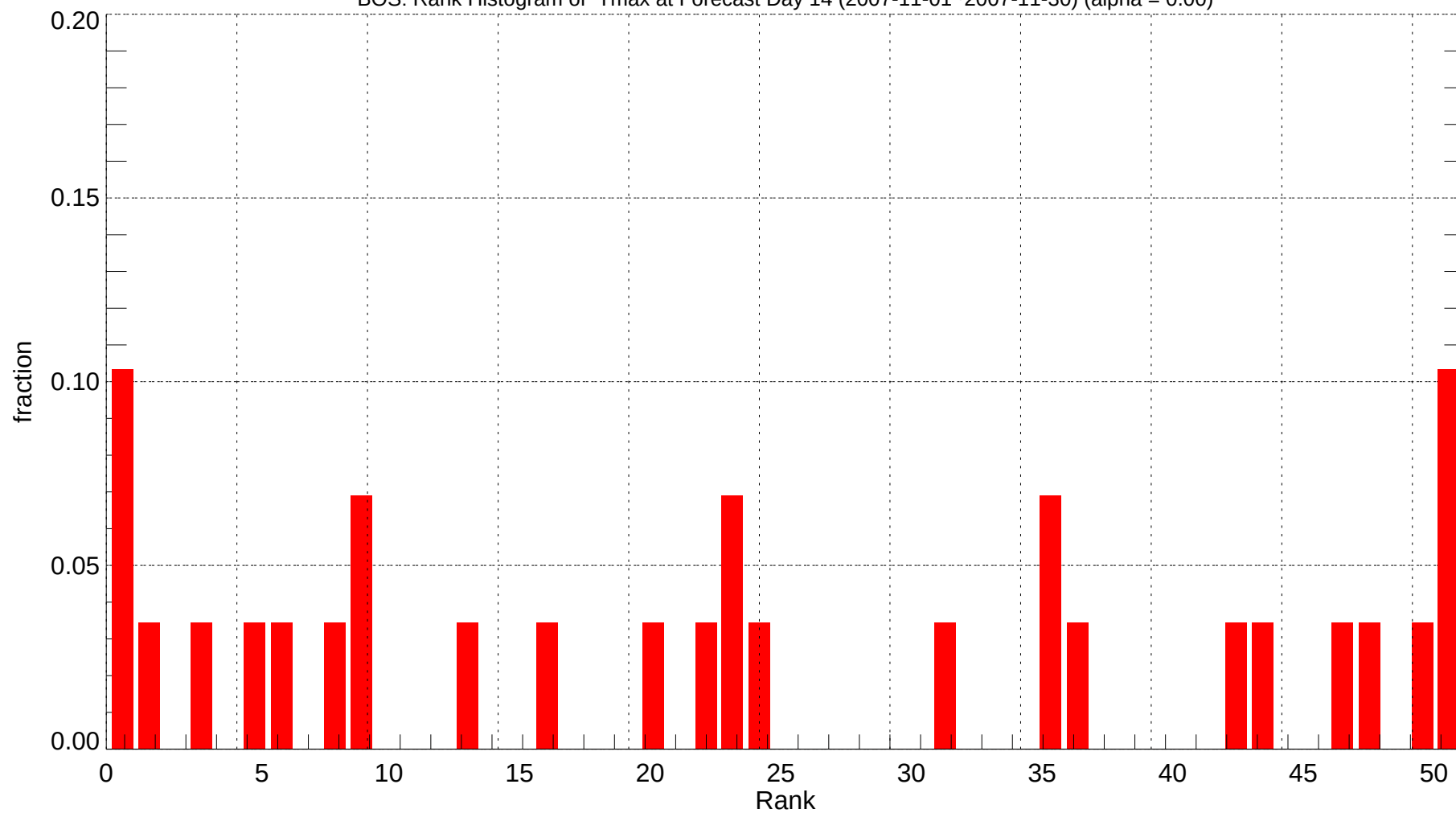
BOS: Rank Histogram of Tmax at Forecast Day 14 (2007-11-01~2007-11-30) (alpha = 0.00)
