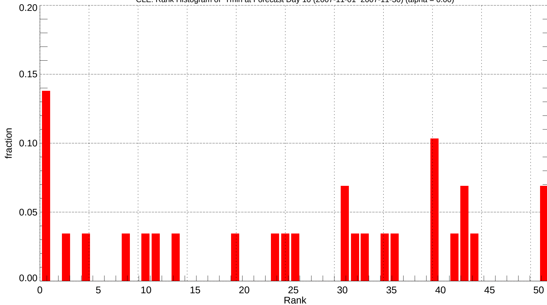
CLE: Rank Histogram of Tmin at Forecast Day 10 (2007-11-01~2007-11-30) (alpha = 0.00)
