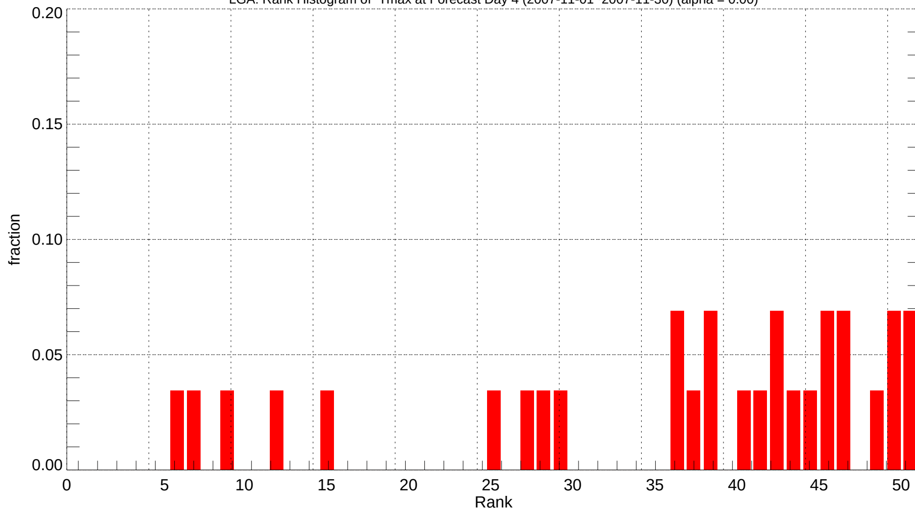
LGA: Rank Histogram of Tmax at Forecast Day 4 (2007-11-01~2007-11-30) (alpha = 0.00)
