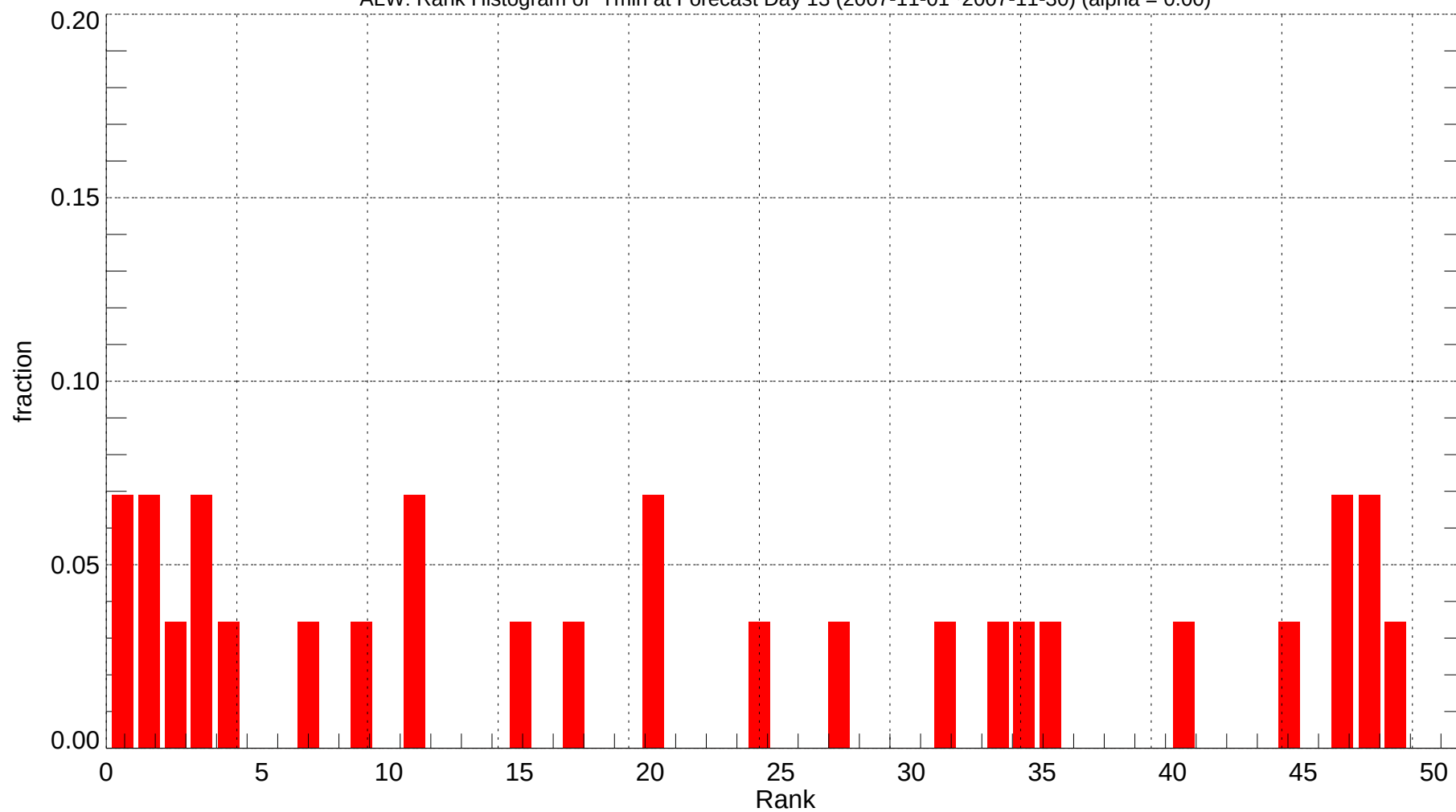
ALW: Rank Histogram of Tmin at Forecast Day 13 (2007-11-01~2007-11-30) (alpha = 0.00)
