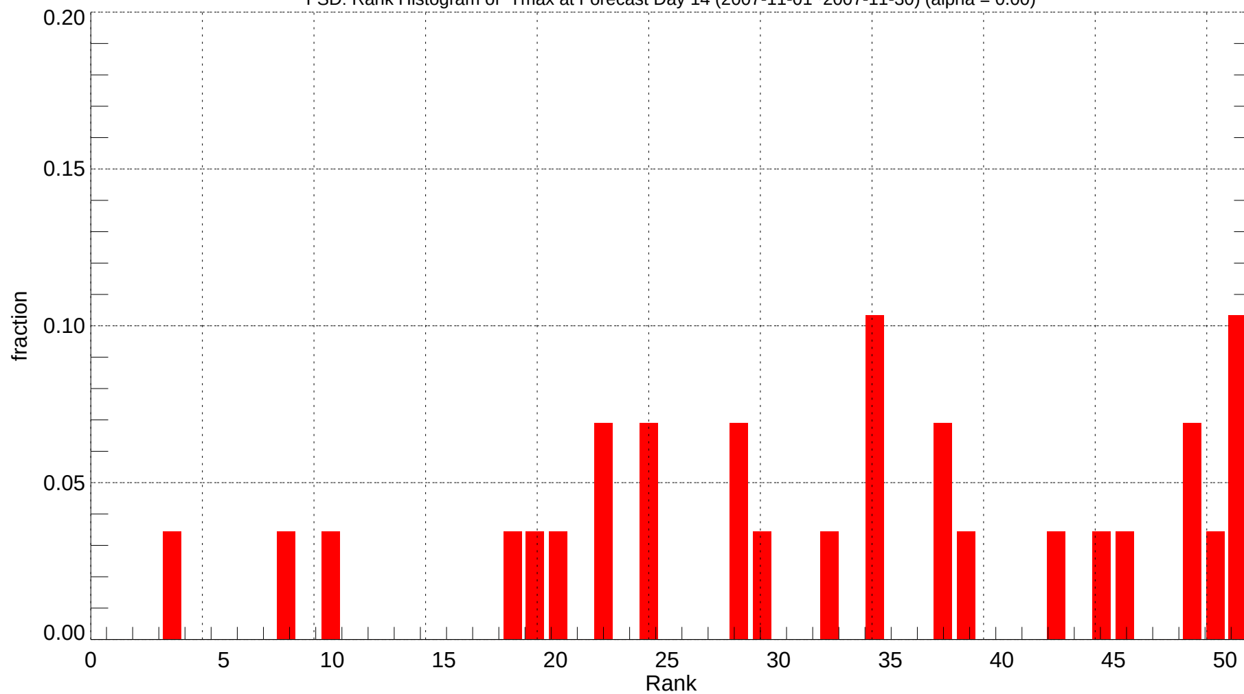
FSD: Rank Histogram of Tmax at Forecast Day 14 (2007-11-01~2007-11-30) (alpha = 0.00)
