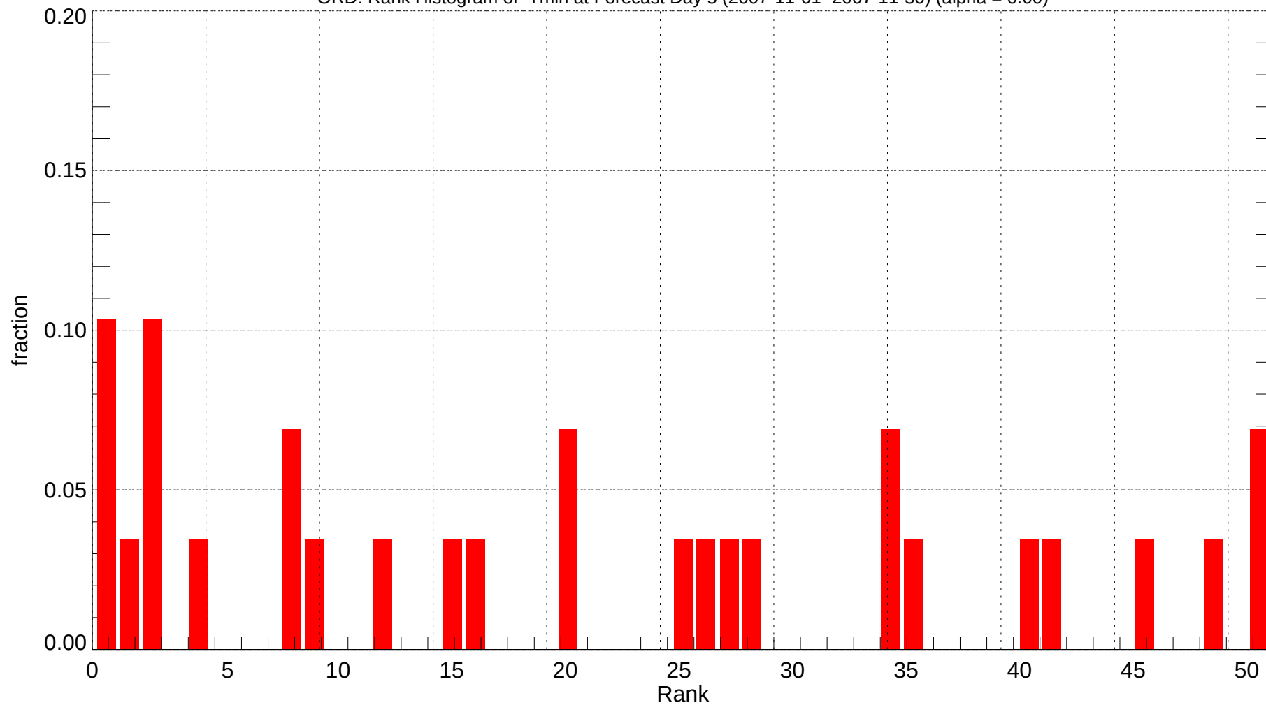
ORD: Rank Histogram of Tmin at Forecast Day 5 (2007-11-01~2007-11-30) (alpha = 0.00)
