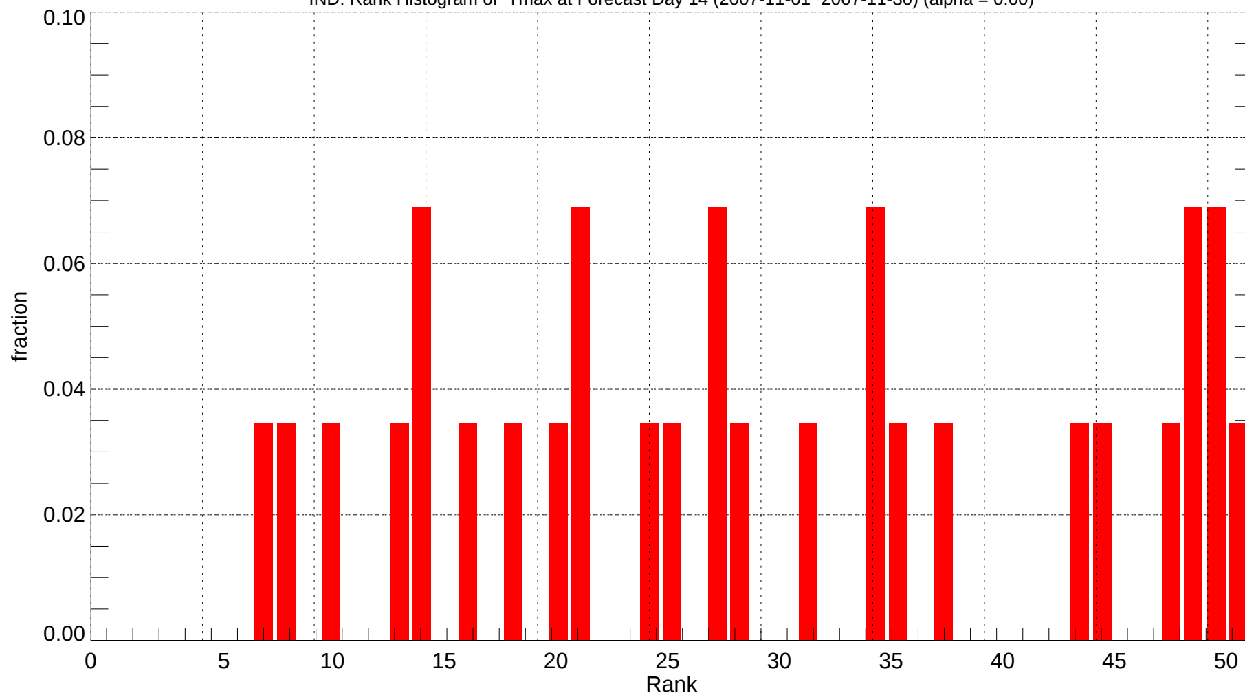
IND: Rank Histogram of Tmax at Forecast Day 14 (2007-11-01~2007-11-30) (alpha = 0.00)
