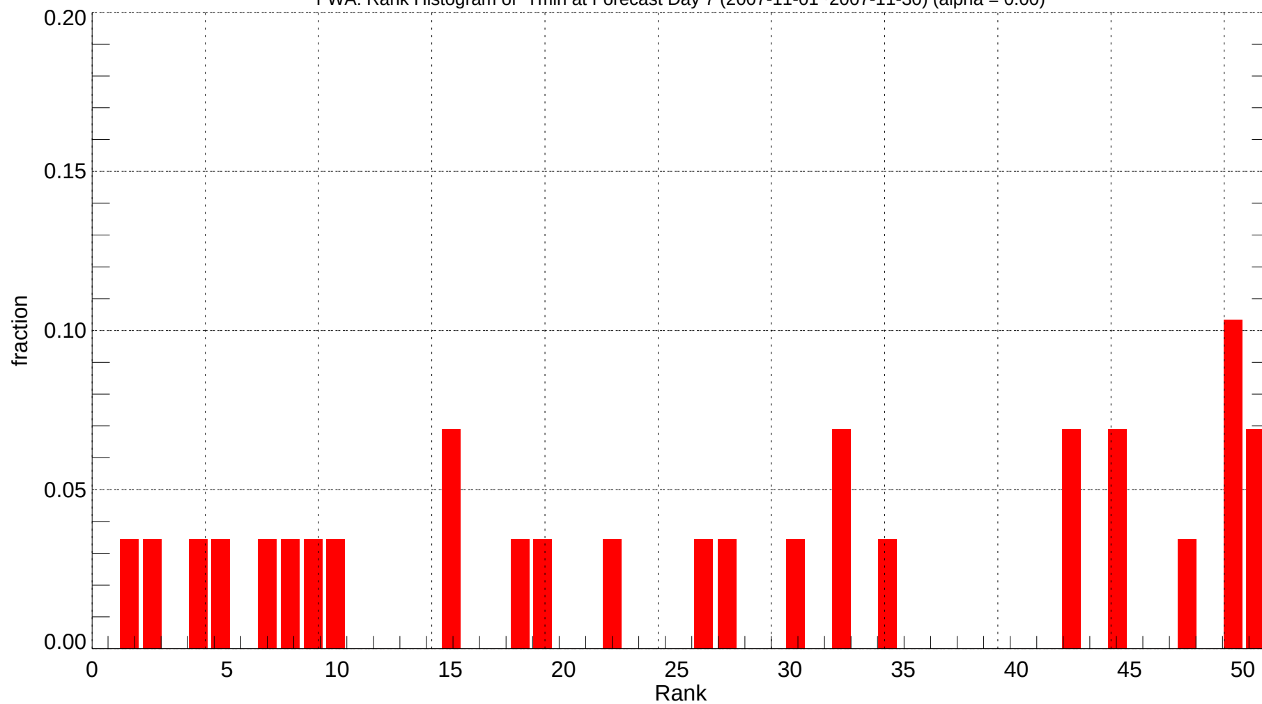
FWA: Rank Histogram of Tmin at Forecast Day 7 (2007-11-01~2007-11-30) (alpha = 0.00)
