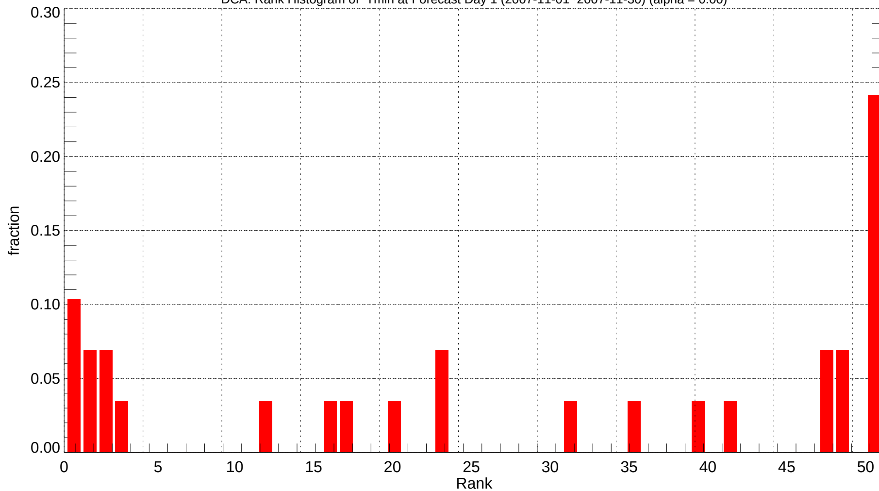
DCA: Rank Histogram of Tmin at Forecast Day 1 (2007-11-01~2007-11-30) (alpha = 0.00)
