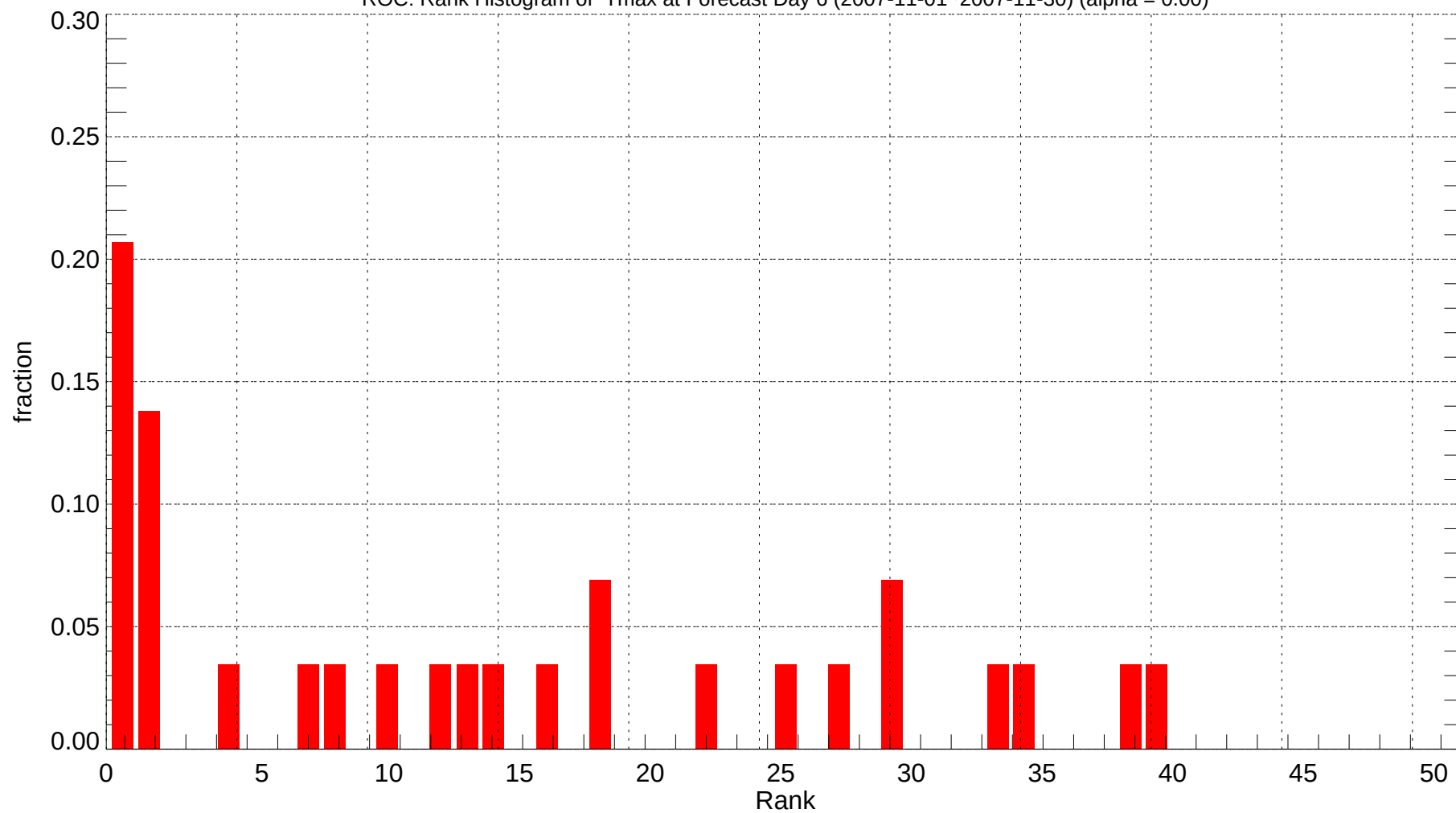
ROC: Rank Histogram of Tmax at Forecast Day 6 (2007-11-01~2007-11-30) (alpha = 0.00)
