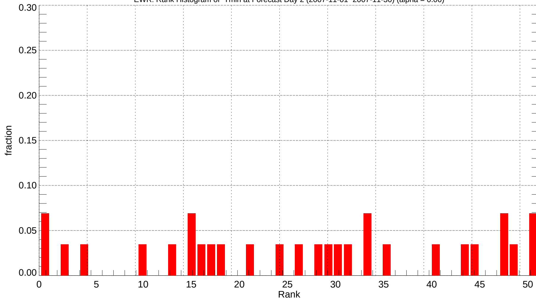
EWR: Rank Histogram of Tmin at Forecast Day 2 (2007-11-01~2007-11-30) (alpha = 0.00)
