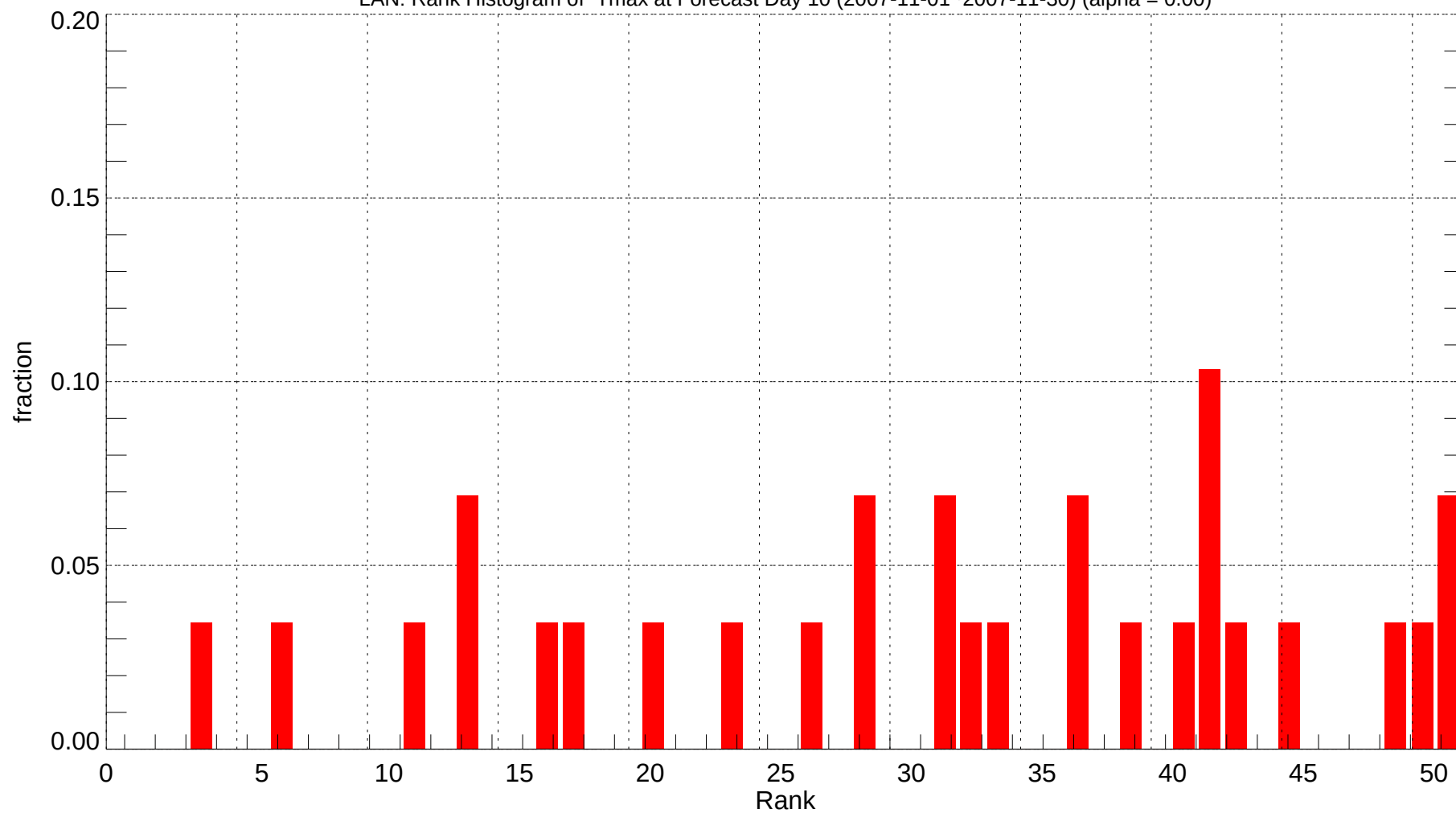
LAN: Rank Histogram of Tmax at Forecast Day 10 (2007-11-01~2007-11-30) (alpha = 0.00)
