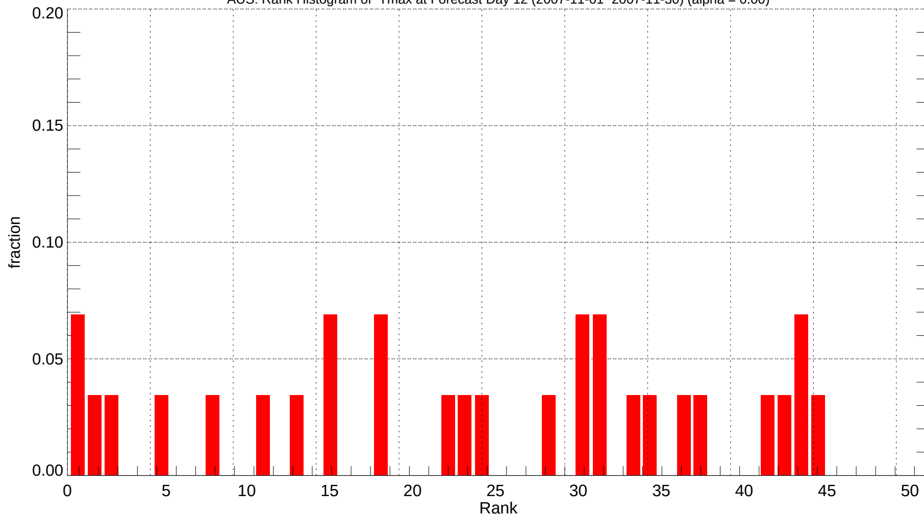
AUS: Rank Histogram of Tmax at Forecast Day 12 (2007-11-01~2007-11-30) (alpha = 0.00)
