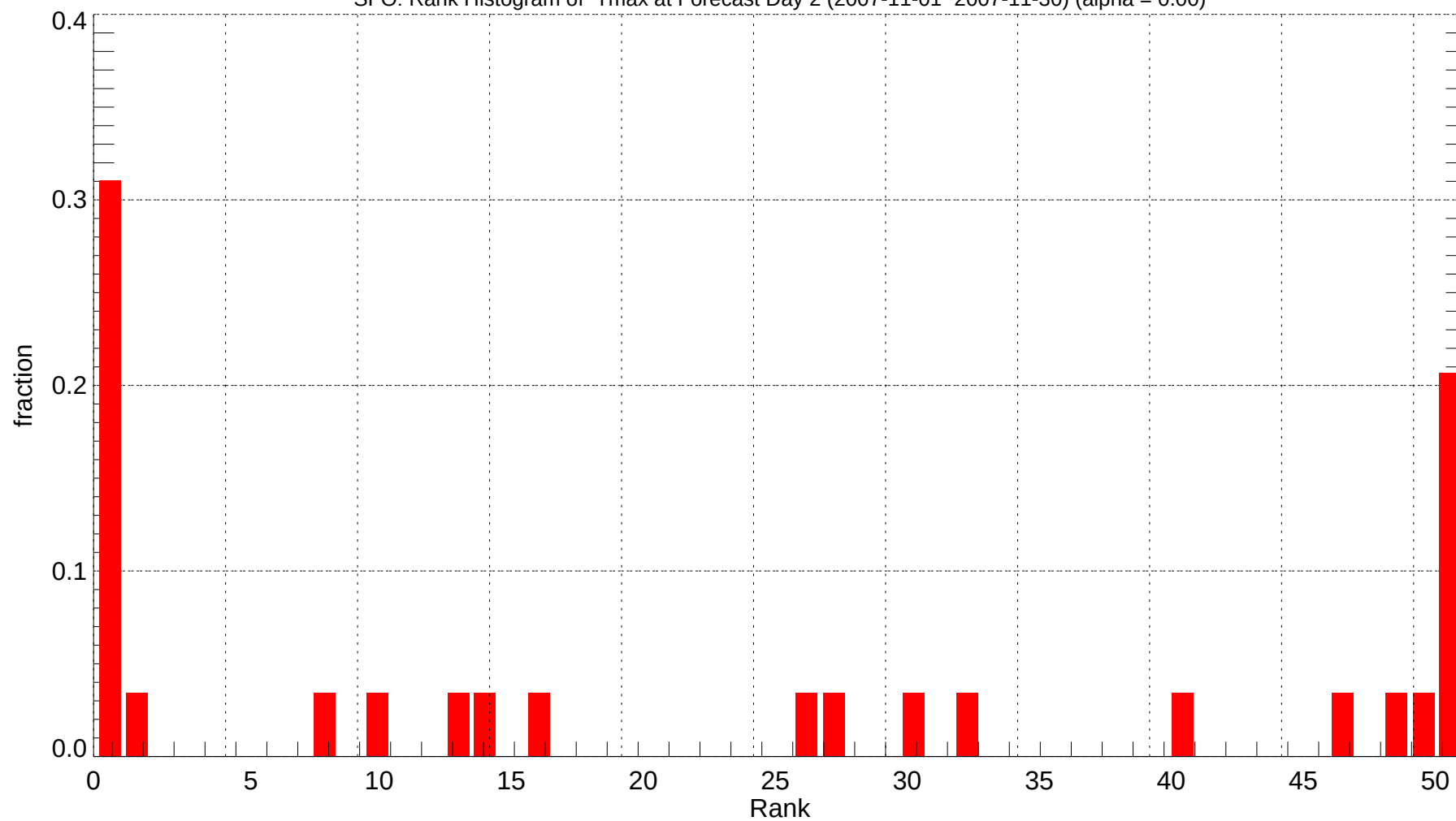
SFO: Rank Histogram of Tmax at Forecast Day 2 (2007-11-01~2007-11-30) (alpha = 0.00)
