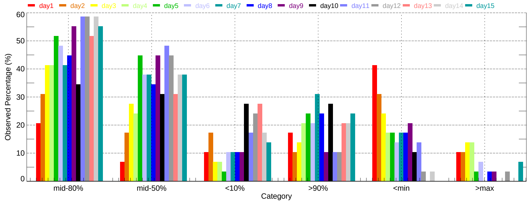
Observed Percentage of Ensembles - YKM: Max Temperature (2007-11-01~2007-11-30)
