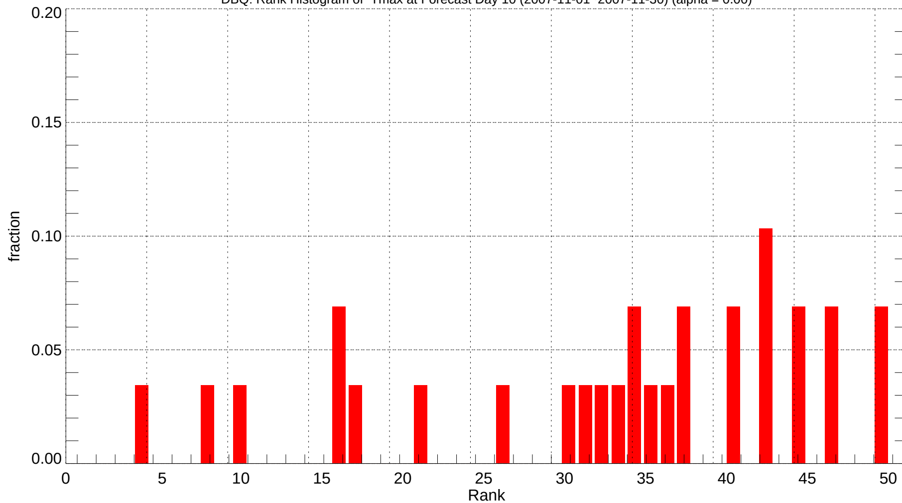
DBQ: Rank Histogram of Tmax at Forecast Day 10 (2007-11-01~2007-11-30) (alpha = 0.00)
