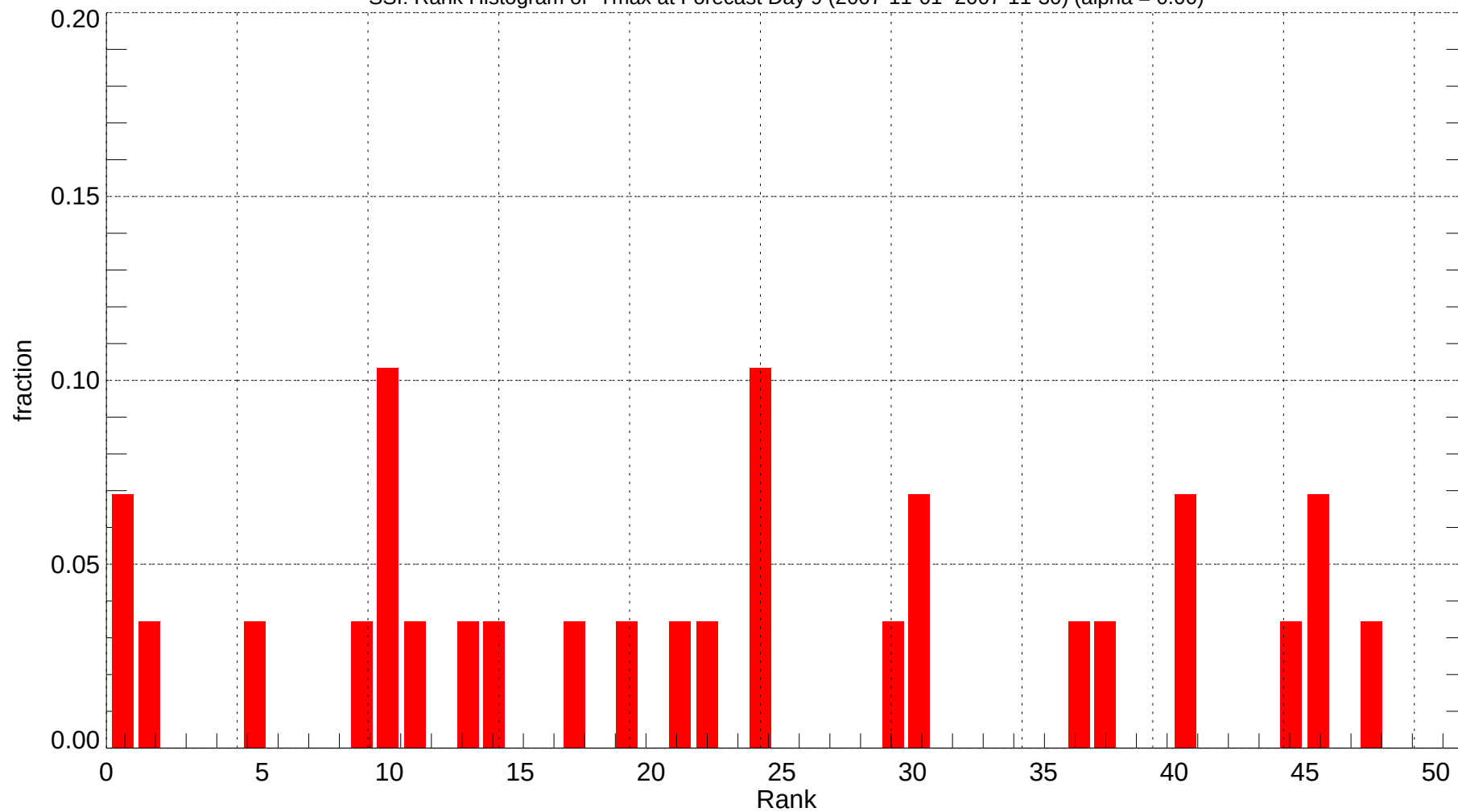
SSI: Rank Histogram of Tmax at Forecast Day 9 (2007-11-01~2007-11-30) (alpha = 0.00)
