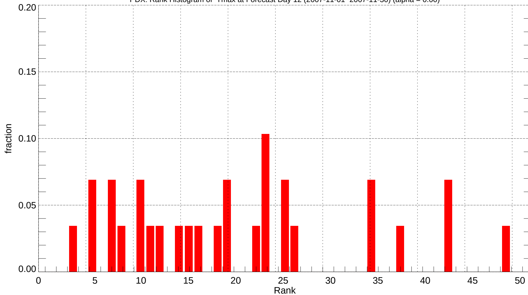
PDX: Rank Histogram of Tmax at Forecast Day 12 (2007-11-01~2007-11-30) (alpha = 0.00)
