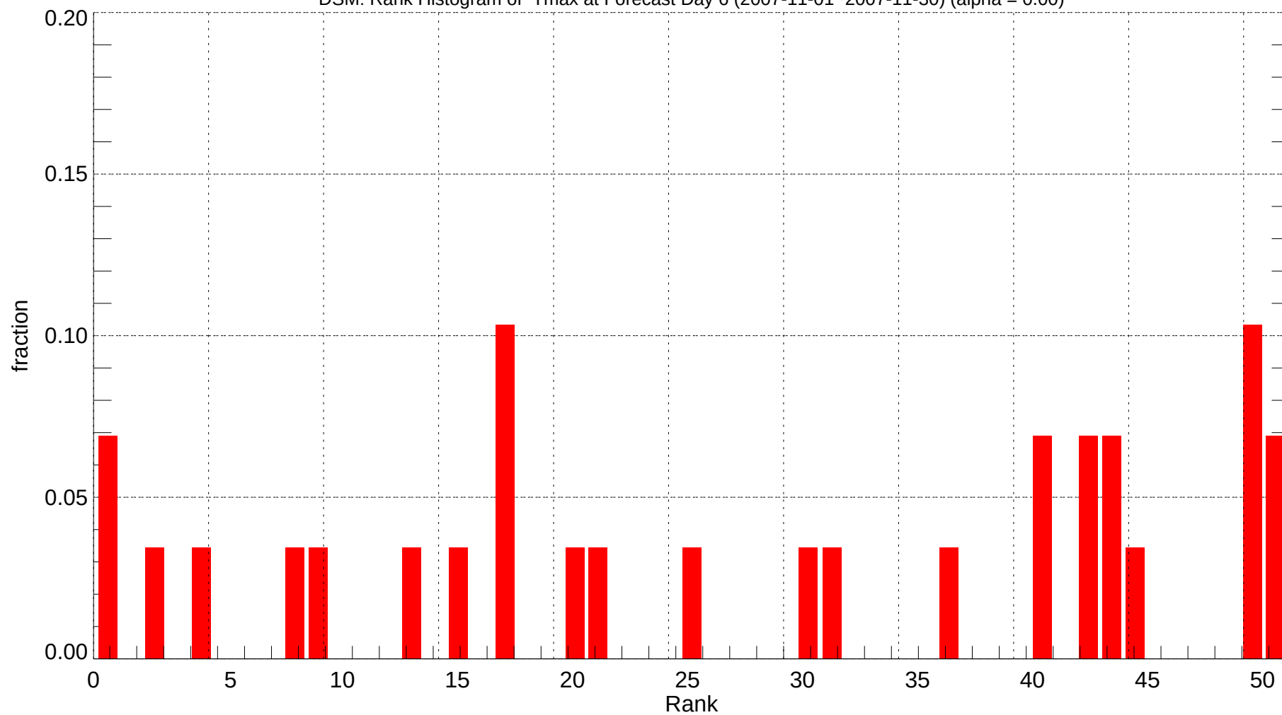
DSM: Rank Histogram of Tmax at Forecast Day 6 (2007-11-01~2007-11-30) (alpha = 0.00)
