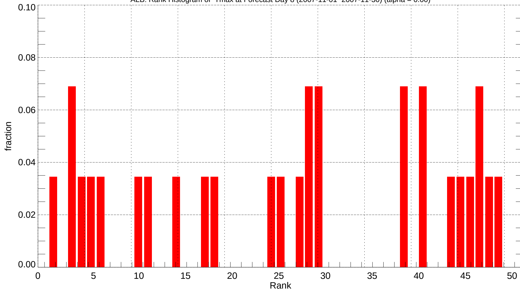
ALB: Rank Histogram of Tmax at Forecast Day 8 (2007-11-01~2007-11-30) (alpha = 0.00)
