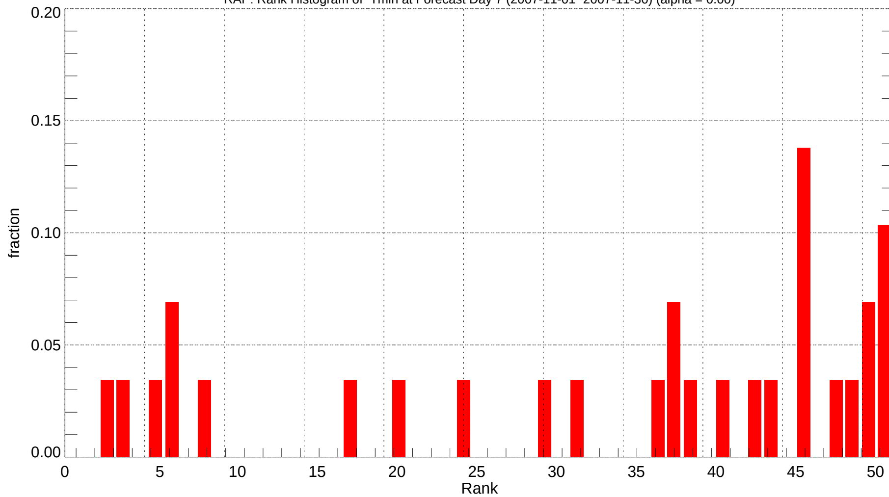
RAP: Rank Histogram of Tmin at Forecast Day 7 (2007-11-01~2007-11-30) (alpha = 0.00)
