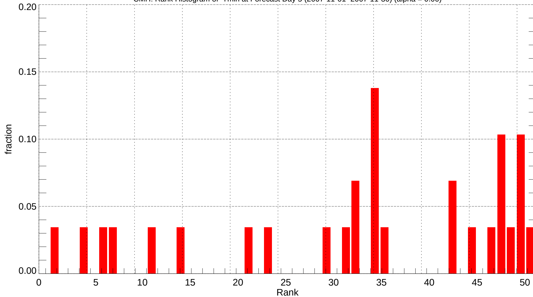
CMH: Rank Histogram of Tmin at Forecast Day 5 (2007-11-01~2007-11-30) (alpha = 0.00)
