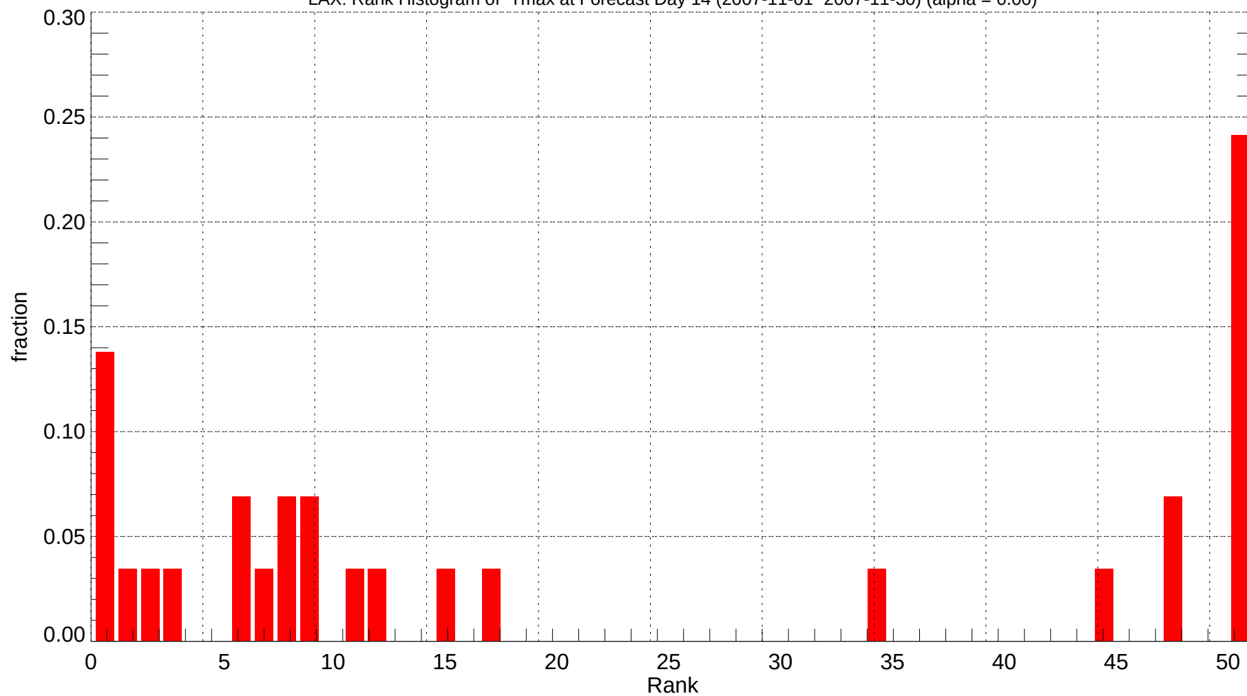
LAX: Rank Histogram of Tmax at Forecast Day 14 (2007-11-01~2007-11-30) (alpha = 0.00)
