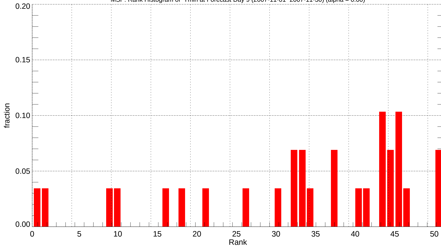
MSP: Rank Histogram of Tmin at Forecast Day 9 (2007-11-01~2007-11-30) (alpha = 0.00)
