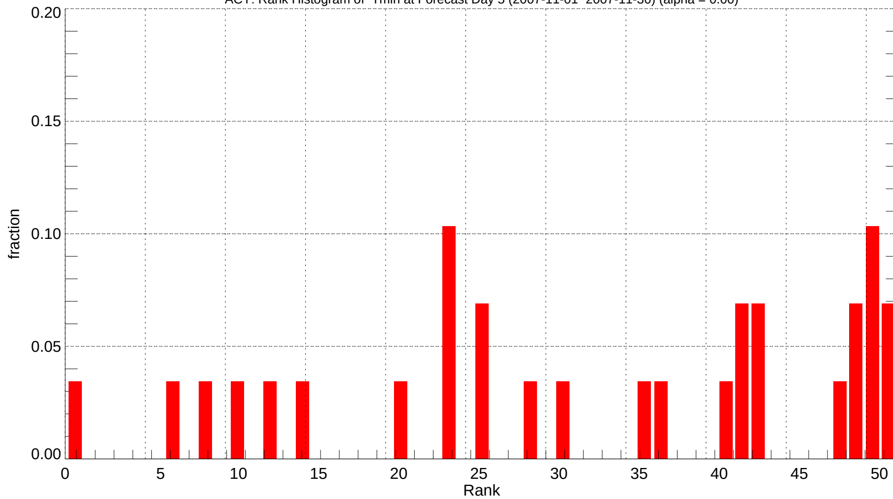
ACY: Rank Histogram of Tmin at Forecast Day 5 (2007-11-01~2007-11-30) (alpha = 0.00)
