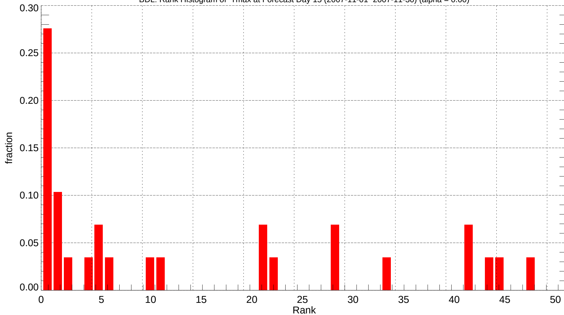
BDL: Rank Histogram of Tmax at Forecast Day 15 (2007-11-01~2007-11-30) (alpha = 0.00)
