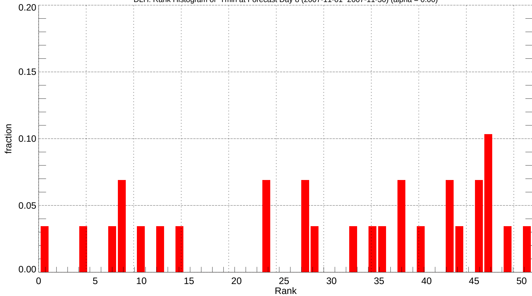
DLH: Rank Histogram of Tmin at Forecast Day 8 (2007-11-01~2007-11-30) (alpha = 0.00)
