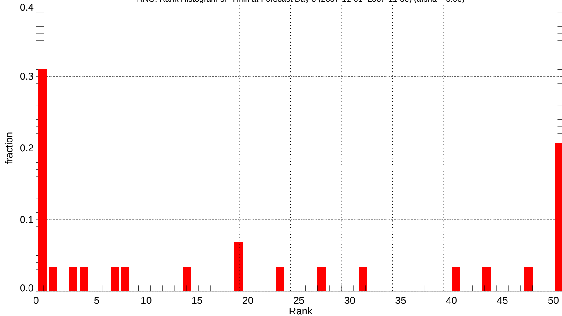
RNO: Rank Histogram of Tmin at Forecast Day 3 (2007-11-01~2007-11-30) (alpha = 0.00)
