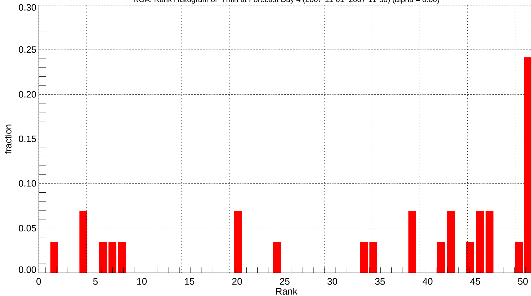
ROA: Rank Histogram of Tmin at Forecast Day 4 (2007-11-01~2007-11-30) (alpha = 0.00)
