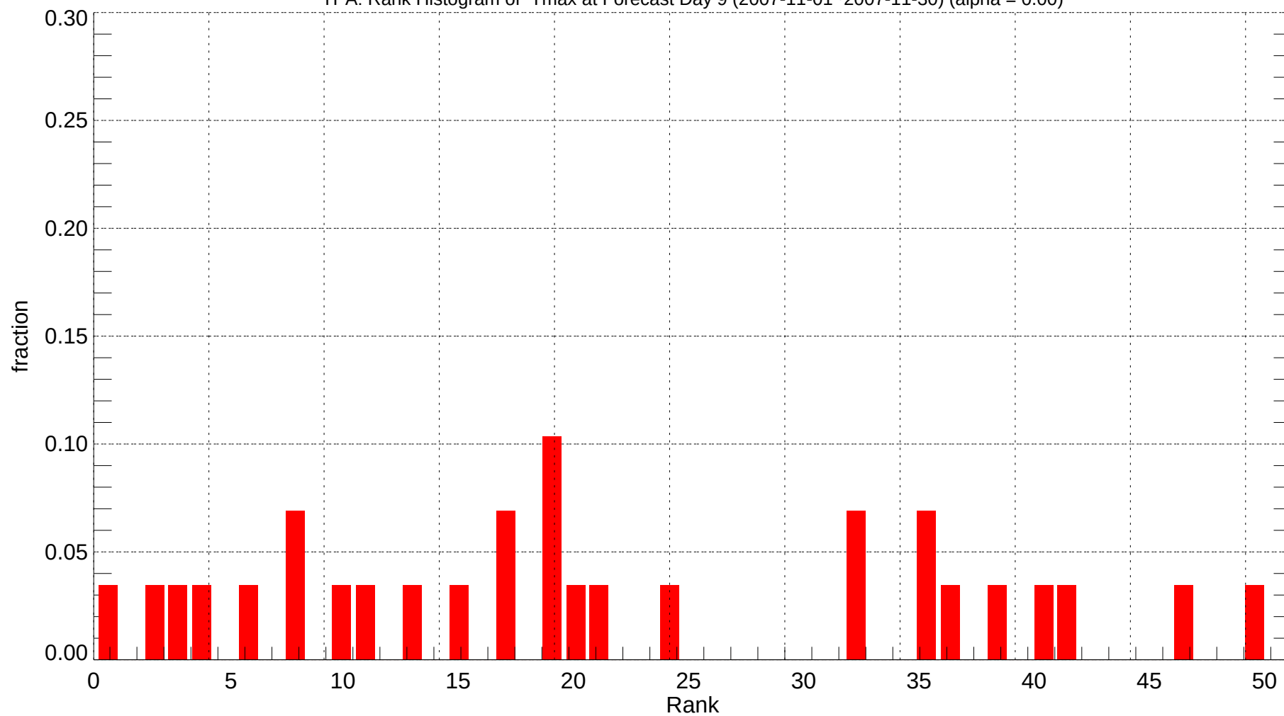
TPA: Rank Histogram of Tmax at Forecast Day 9 (2007-11-01~2007-11-30) (alpha = 0.00)
