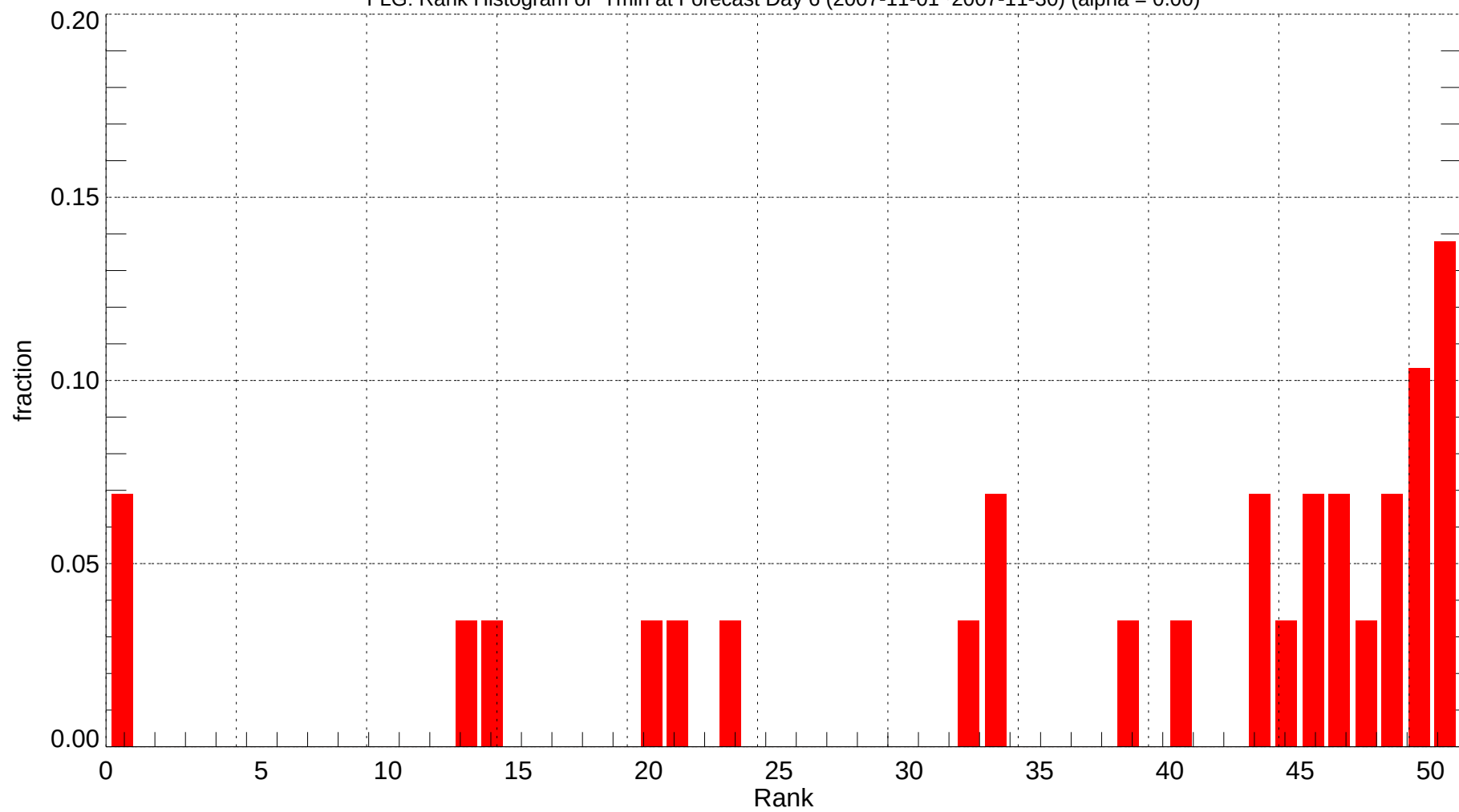
FLG: Rank Histogram of Tmin at Forecast Day 6 (2007-11-01~2007-11-30) (alpha = 0.00)
