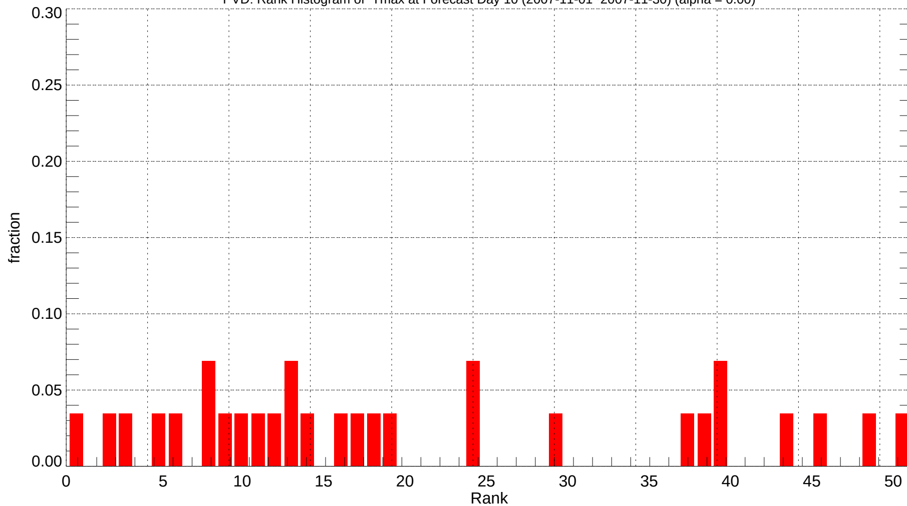
PVD: Rank Histogram of Tmax at Forecast Day 10 (2007-11-01~2007-11-30) (alpha = 0.00)
