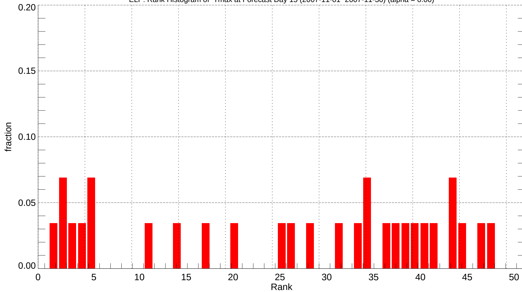
ELP: Rank Histogram of Tmax at Forecast Day 15 (2007-11-01~2007-11-30) (alpha = 0.00)
