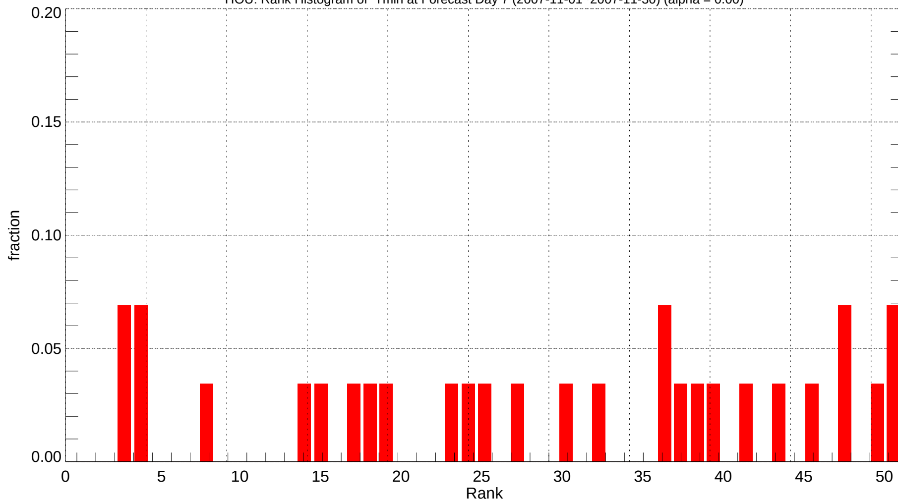
HOU: Rank Histogram of Tmin at Forecast Day 7 (2007-11-01~2007-11-30) (alpha = 0.00)
