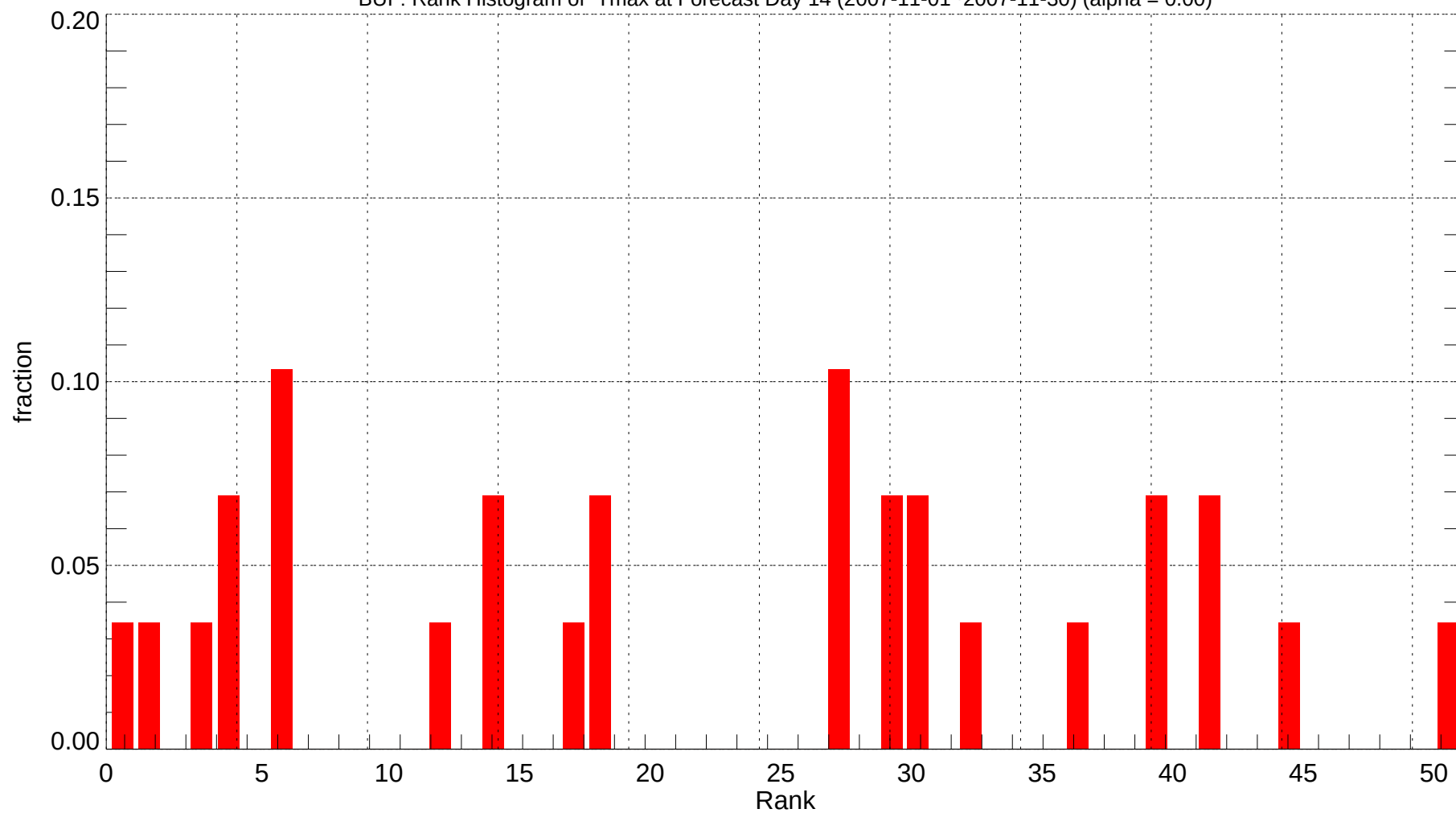
BUF: Rank Histogram of Tmax at Forecast Day 14 (2007-11-01~2007-11-30) (alpha = 0.00)
