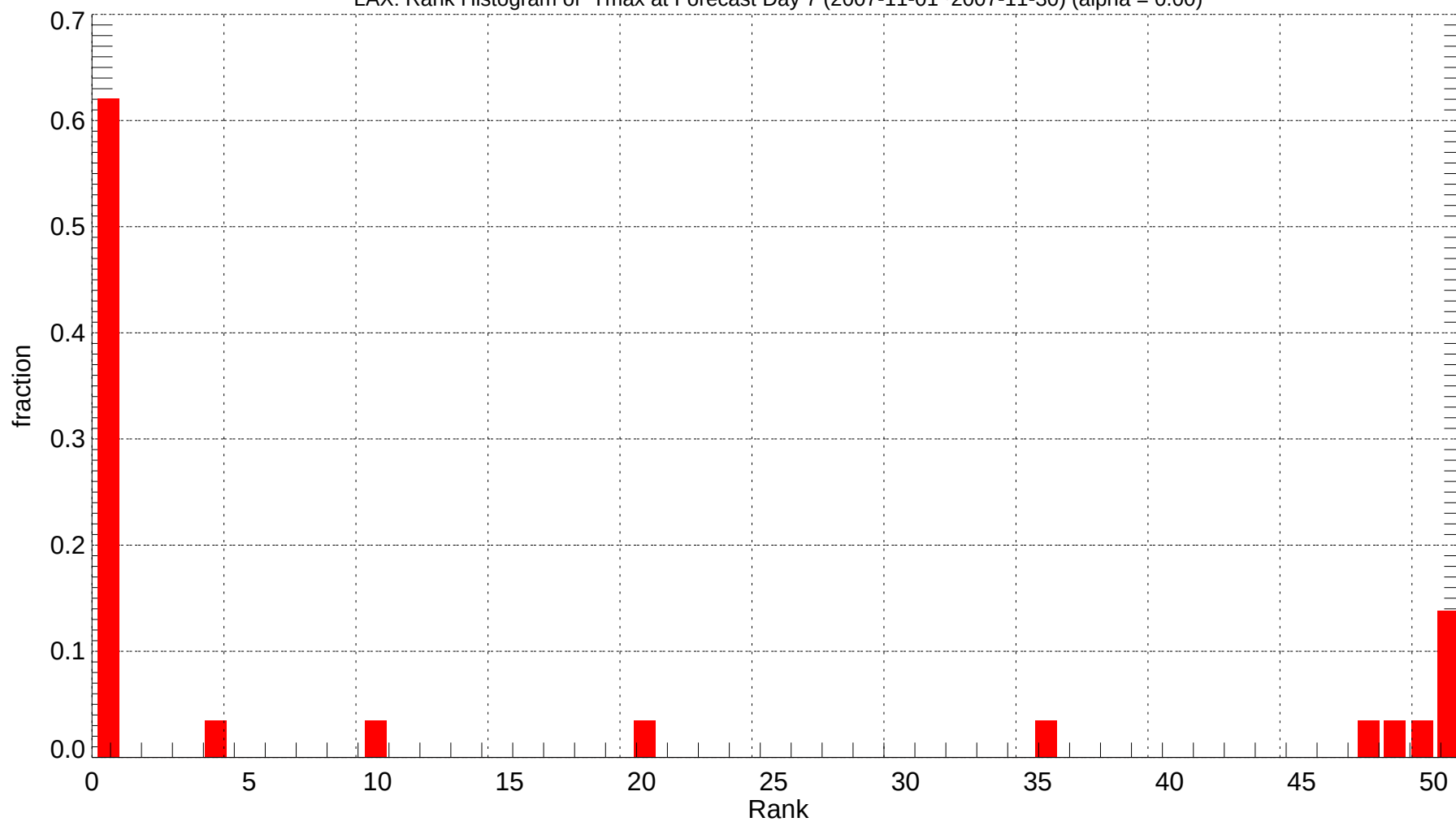
LAX: Rank Histogram of Tmax at Forecast Day 7 (2007-11-01~2007-11-30) (alpha = 0.00)
