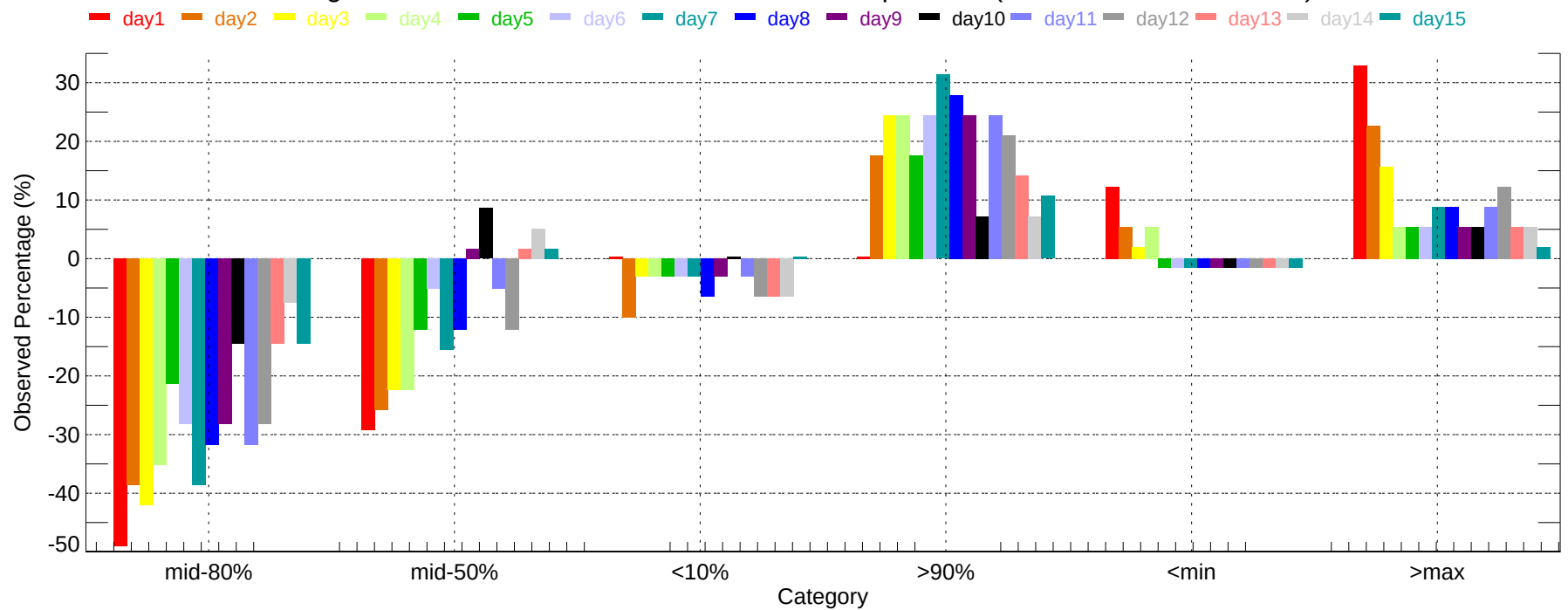
Observed Percentage Deviation of Ensembles - CRW: Max Temperature (2007-11-01~2007-11-30)
