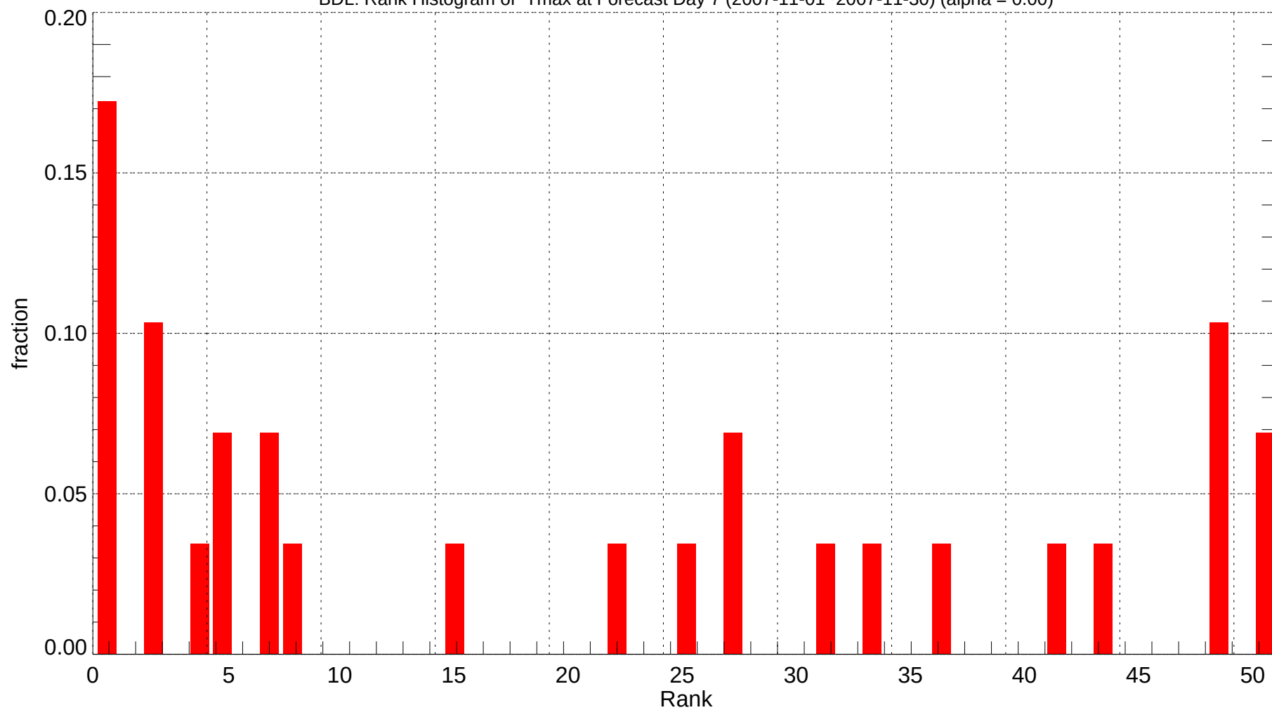
BDL: Rank Histogram of Tmax at Forecast Day 7 (2007-11-01~2007-11-30) (alpha = 0.00)
