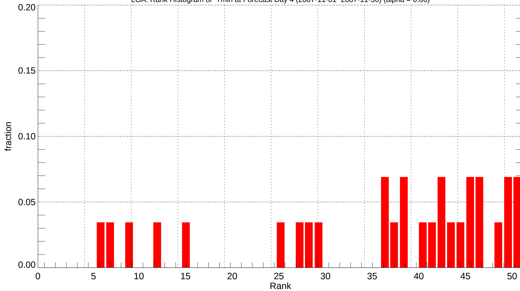
LGA: Rank Histogram of Tmin at Forecast Day 4 (2007-11-01~2007-11-30) (alpha = 0.00)
