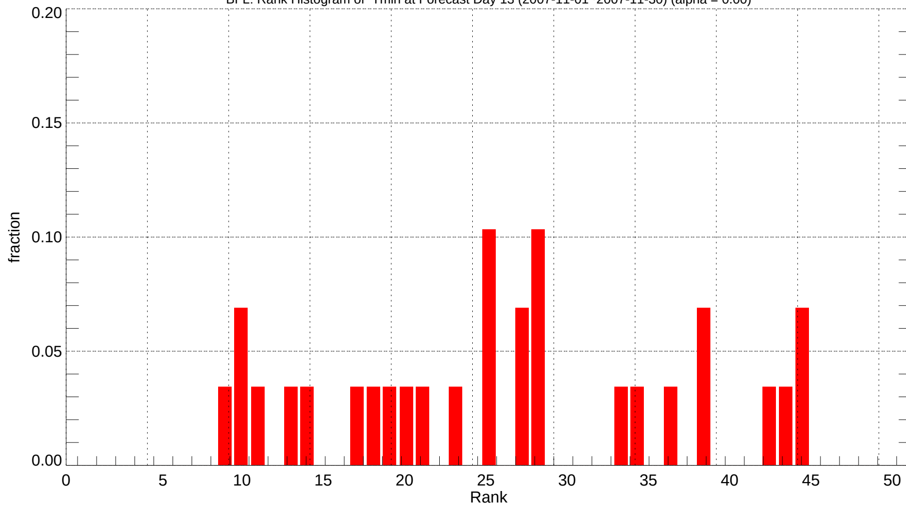
BFL: Rank Histogram of Tmin at Forecast Day 13 (2007-11-01~2007-11-30) (alpha = 0.00)
