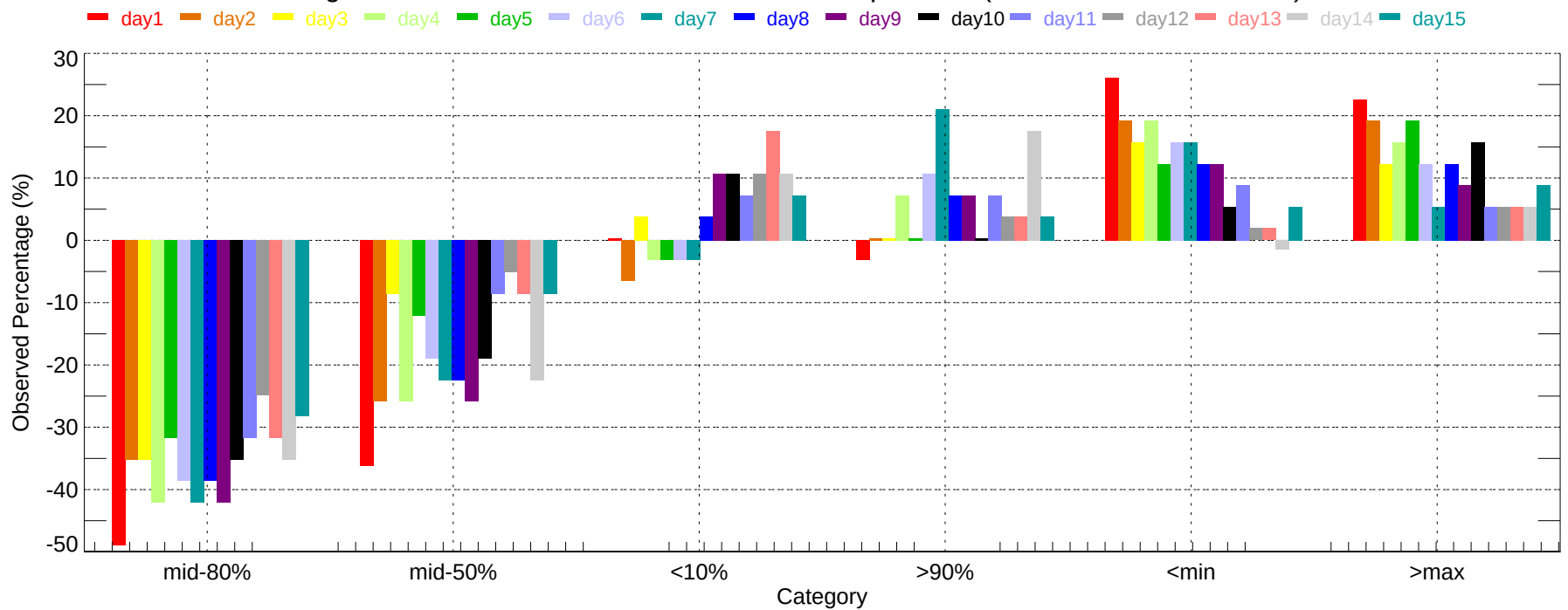
Observed Percentage Deviation of Ensembles - PDT: Max Temperature (2007-11-01~2007-11-30)
