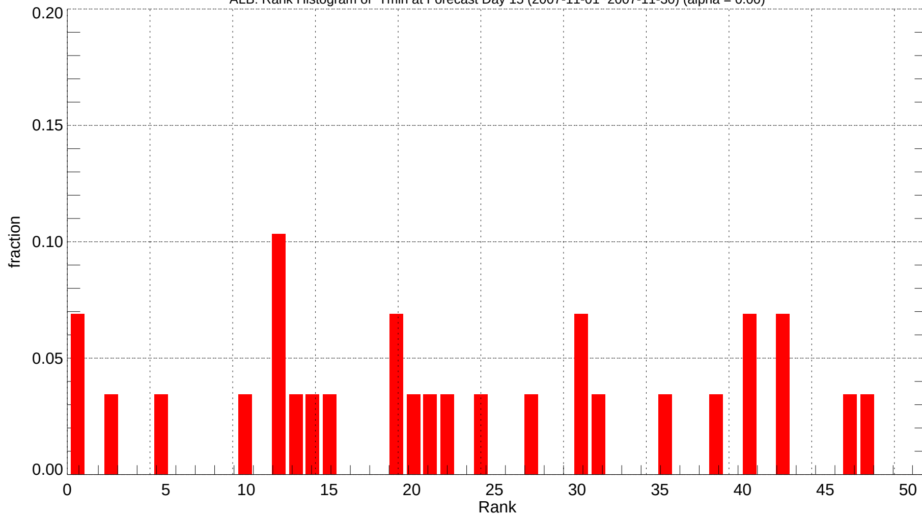
ALB: Rank Histogram of Tmin at Forecast Day 15 (2007-11-01~2007-11-30) (alpha = 0.00)
