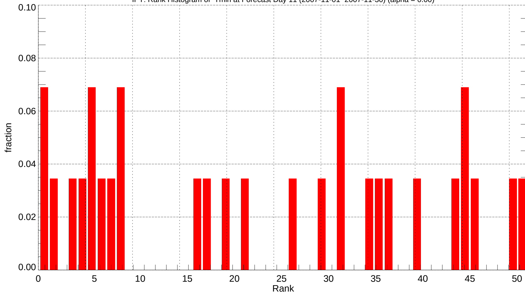
IPT: Rank Histogram of Tmin at Forecast Day 11 (2007-11-01~2007-11-30) (alpha = 0.00)
