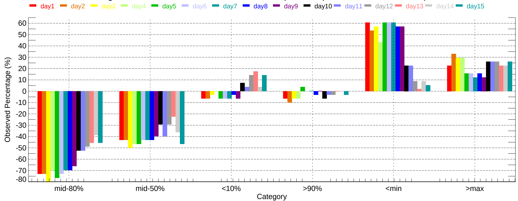
Observed Percentage Deviation of Ensembles - LAX: Min Temperature (2007-11-01~2007-11-30)
