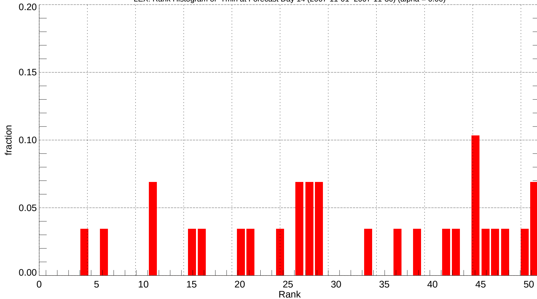
LEX: Rank Histogram of Tmin at Forecast Day 14 (2007-11-01~2007-11-30) (alpha = 0.00)
