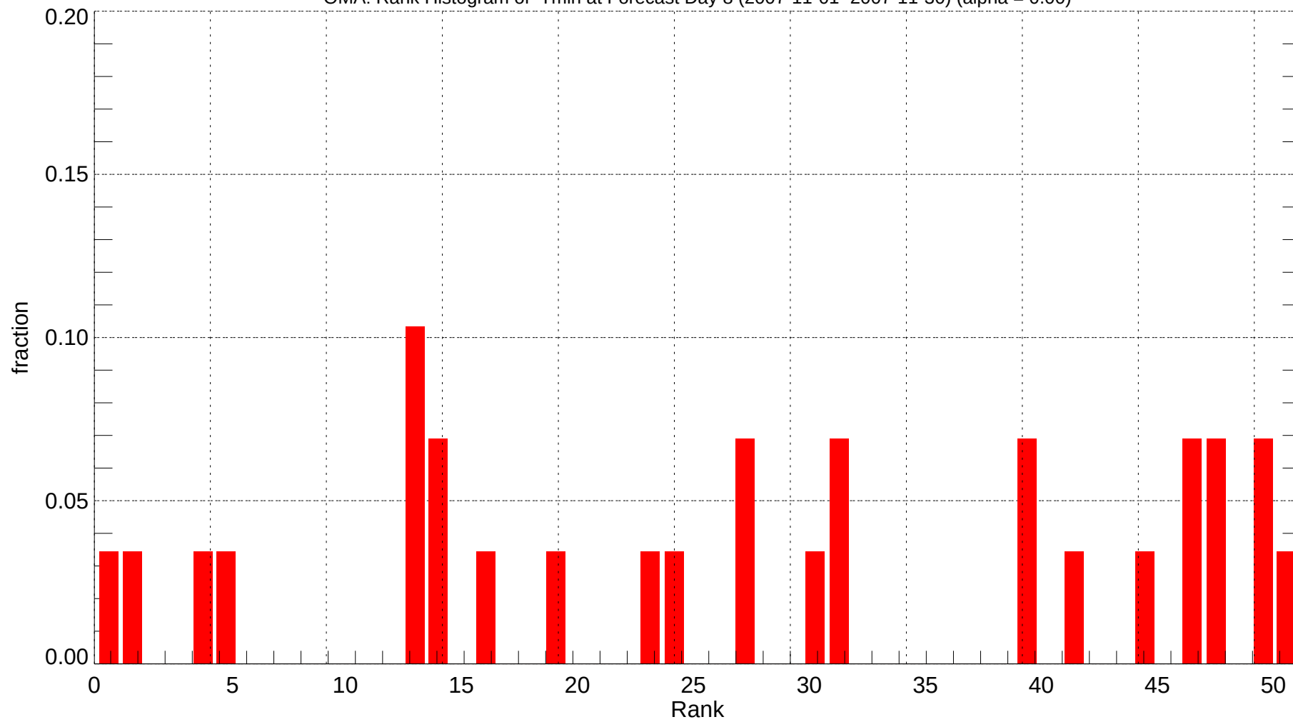
OMA: Rank Histogram of Tmin at Forecast Day 8 (2007-11-01~2007-11-30) (alpha = 0.00)
