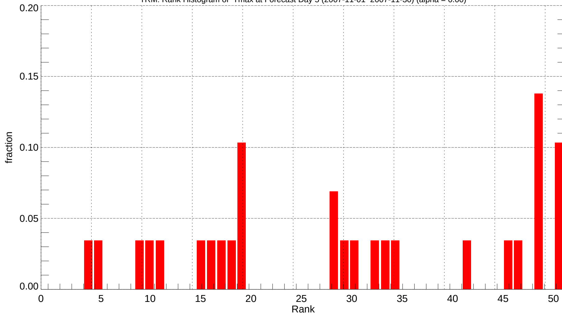
TRM: Rank Histogram of Tmax at Forecast Day 5 (2007-11-01~2007-11-30) (alpha = 0.00)
