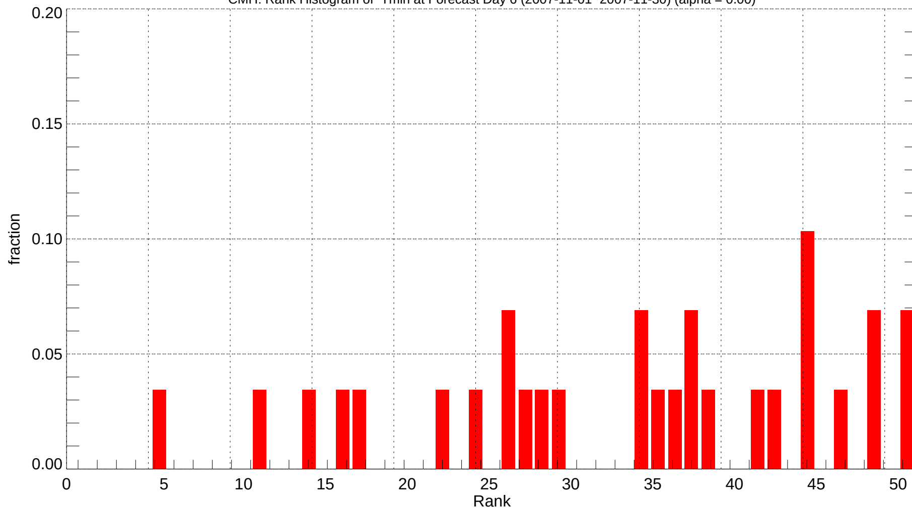
CMH: Rank Histogram of Tmin at Forecast Day 6 (2007-11-01~2007-11-30) (alpha = 0.00)
