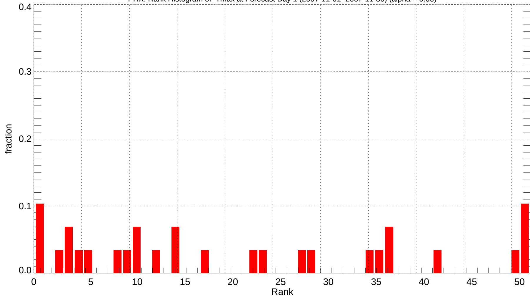
PHX: Rank Histogram of Tmax at Forecast Day 1 (2007-11-01~2007-11-30) (alpha = 0.00)
