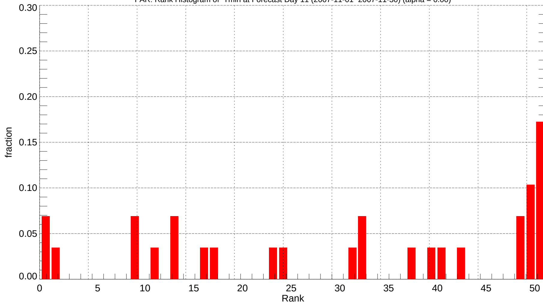
FAR: Rank Histogram of Tmin at Forecast Day 11 (2007-11-01~2007-11-30) (alpha = 0.00)
