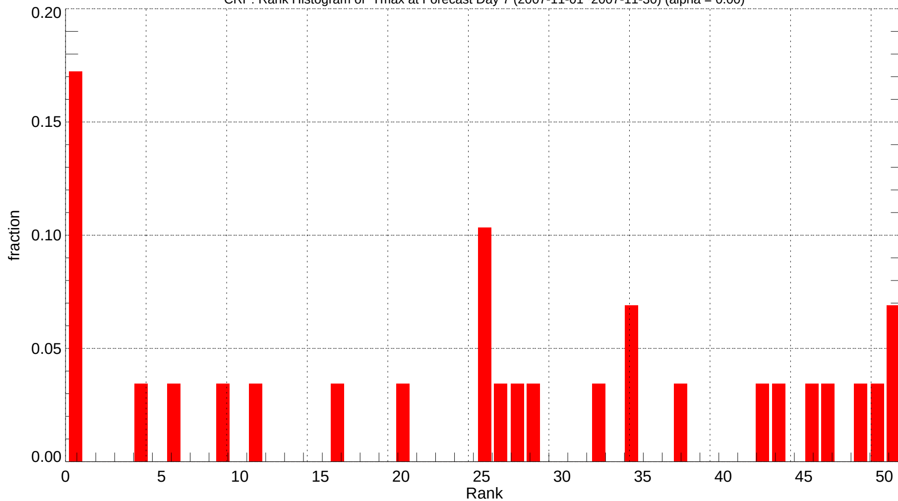
CRP: Rank Histogram of Tmax at Forecast Day 7 (2007-11-01~2007-11-30) (alpha = 0.00)
