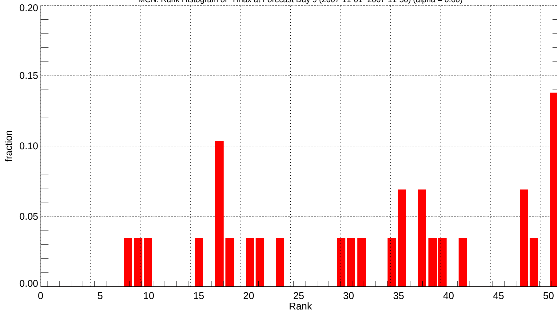
MCN: Rank Histogram of Tmax at Forecast Day 9 (2007-11-01~2007-11-30) (alpha = 0.00)
