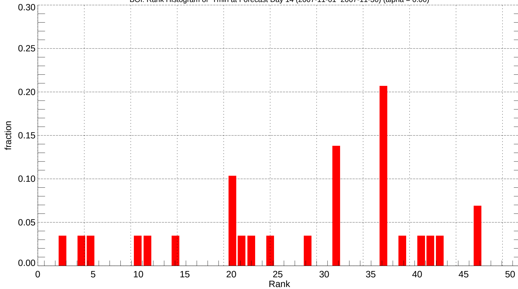
BOI: Rank Histogram of Tmin at Forecast Day 14 (2007-11-01~2007-11-30) (alpha = 0.00)
