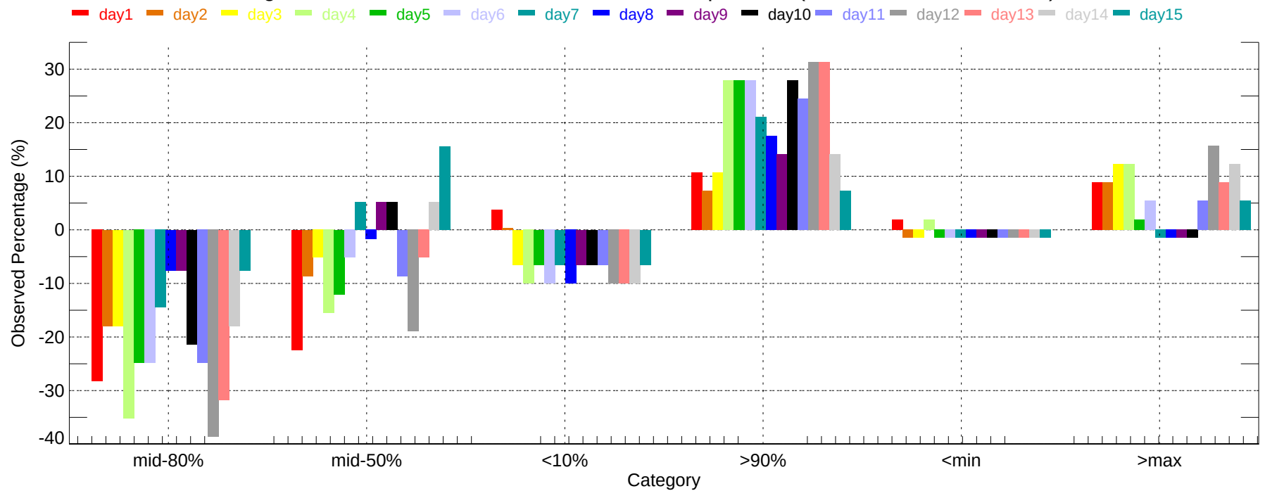
Observed Percentage Deviation of Ensembles - BHM: Max Temperature (2007-11-01~2007-11-30)
