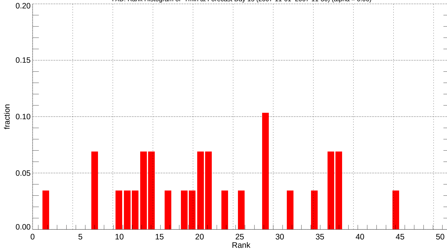
YXD: Rank Histogram of Tmin at Forecast Day 15 (2007-11-01~2007-11-30) (alpha = 0.00)
