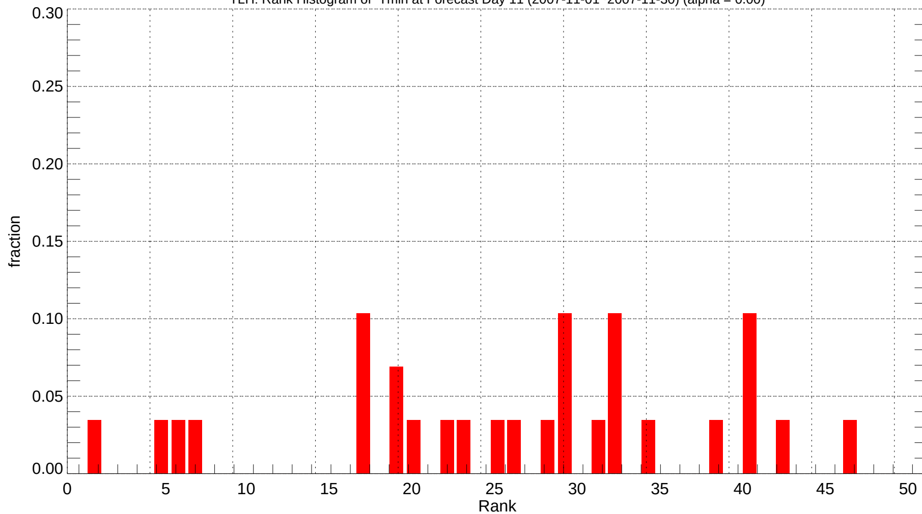
TLH: Rank Histogram of Tmin at Forecast Day 11 (2007-11-01~2007-11-30) (alpha = 0.00)
