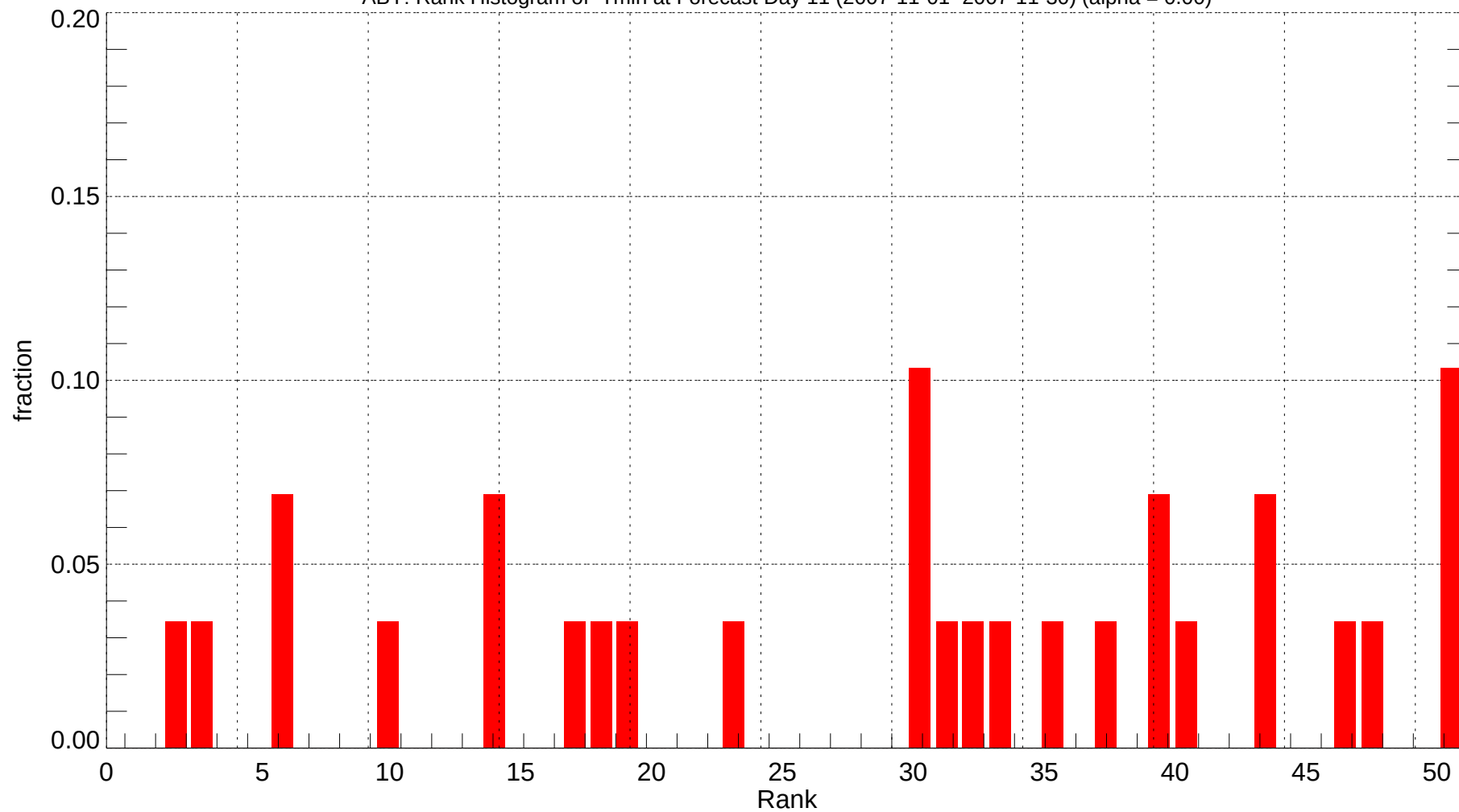
ABY: Rank Histogram of Tmin at Forecast Day 11 (2007-11-01~2007-11-30) (alpha = 0.00)
