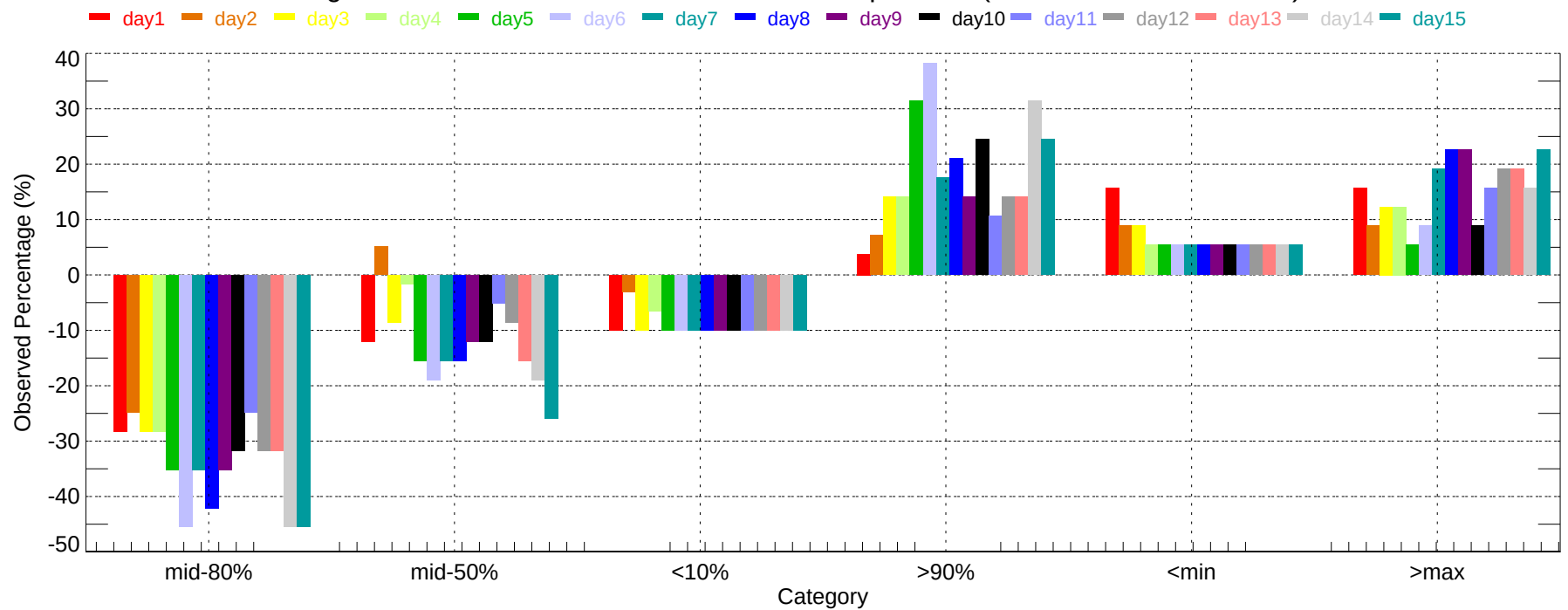
Observed Percentage Deviation of Ensembles - FLG: Max Temperature (2007-11-01~2007-11-30)
