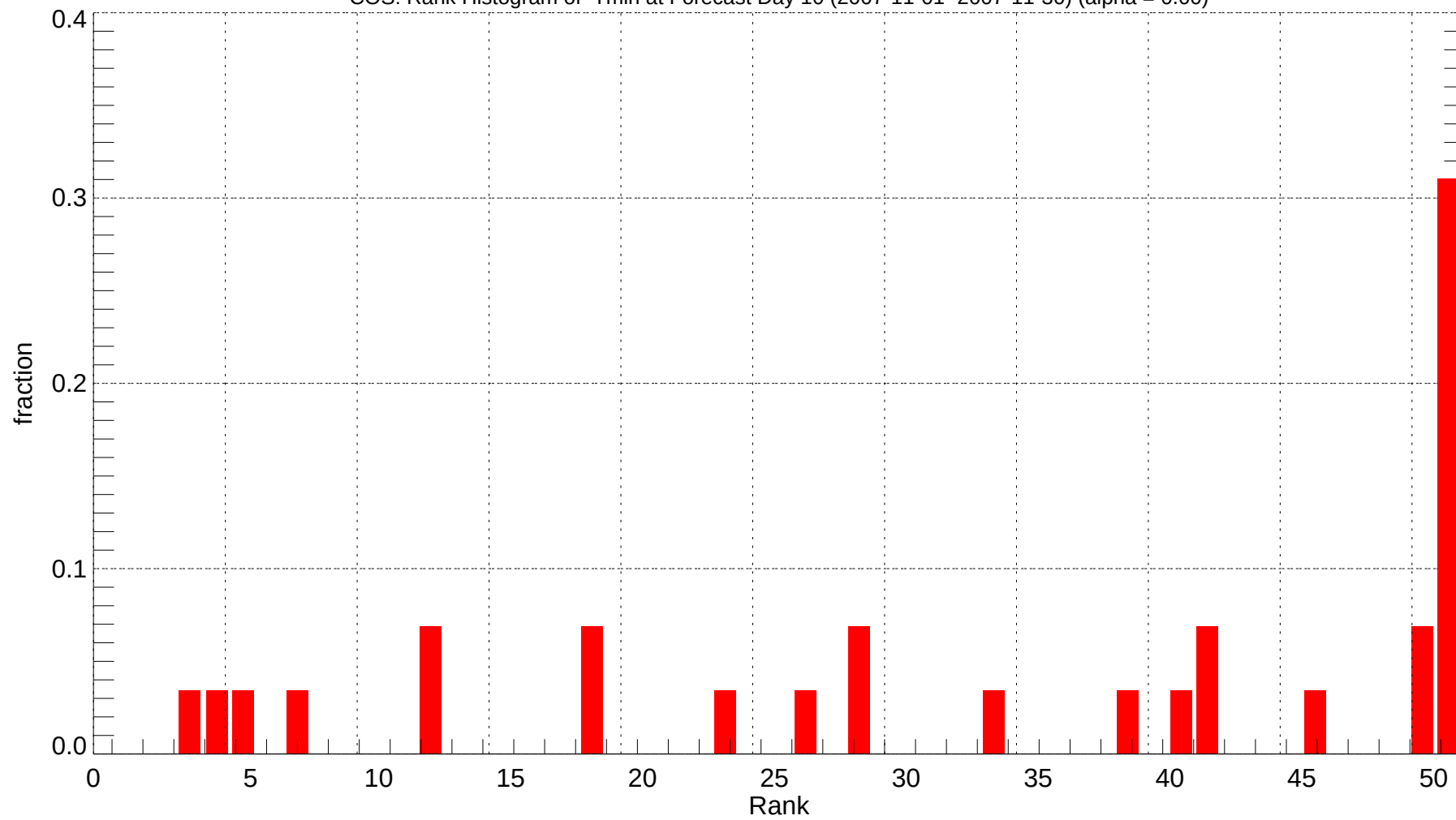
COS: Rank Histogram of Tmin at Forecast Day 10 (2007-11-01~2007-11-30) (alpha = 0.00)
