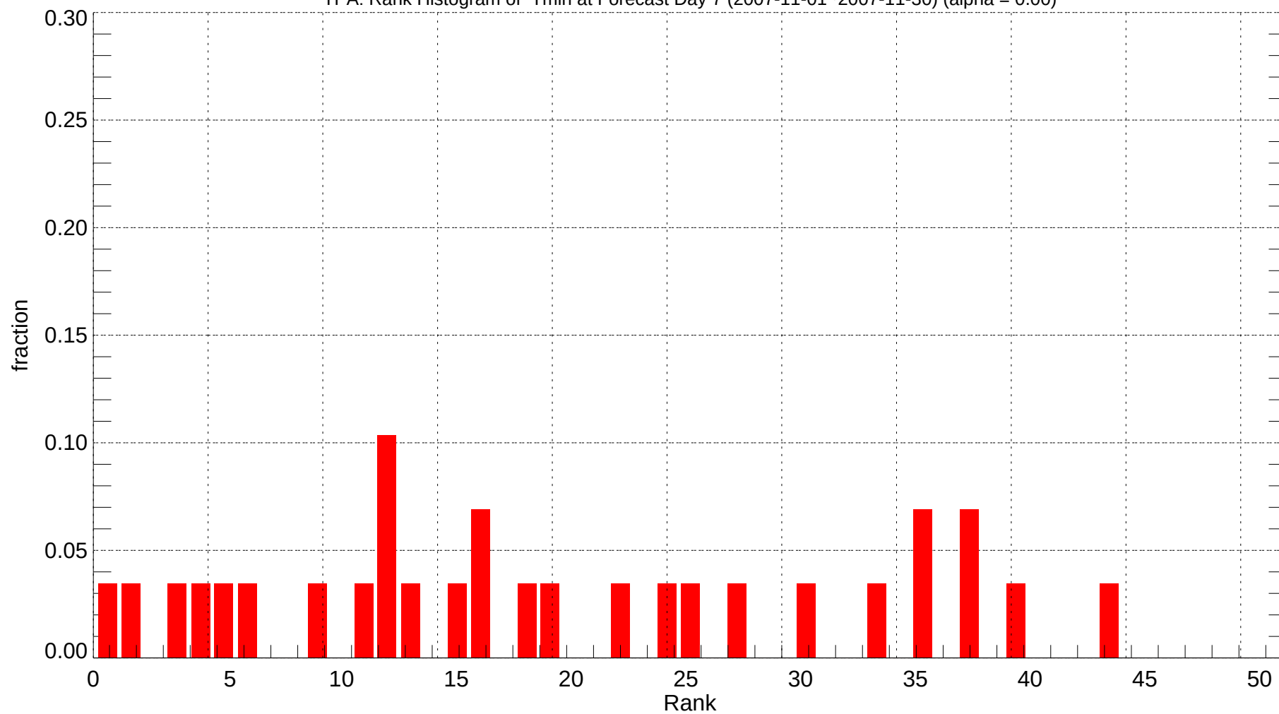
TPA: Rank Histogram of Tmin at Forecast Day 7 (2007-11-01~2007-11-30) (alpha = 0.00)
