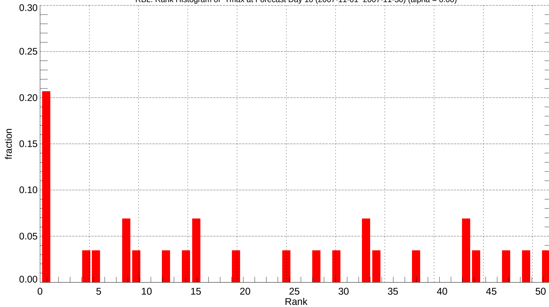
RBL: Rank Histogram of Tmax at Forecast Day 10 (2007-11-01~2007-11-30) (alpha = 0.00)
