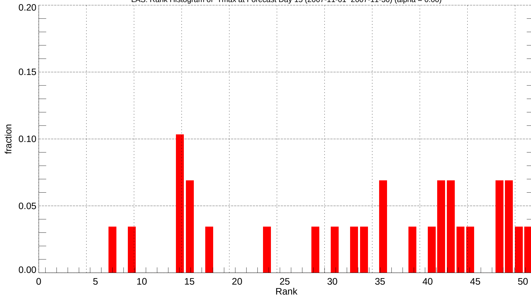
LAS: Rank Histogram of Tmax at Forecast Day 15 (2007-11-01~2007-11-30) (alpha = 0.00)
