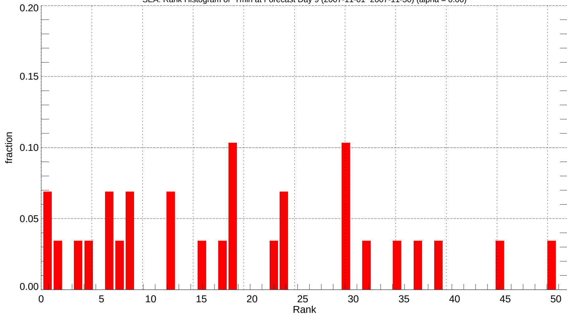
SEA: Rank Histogram of Tmin at Forecast Day 9 (2007-11-01~2007-11-30) (alpha = 0.00)
