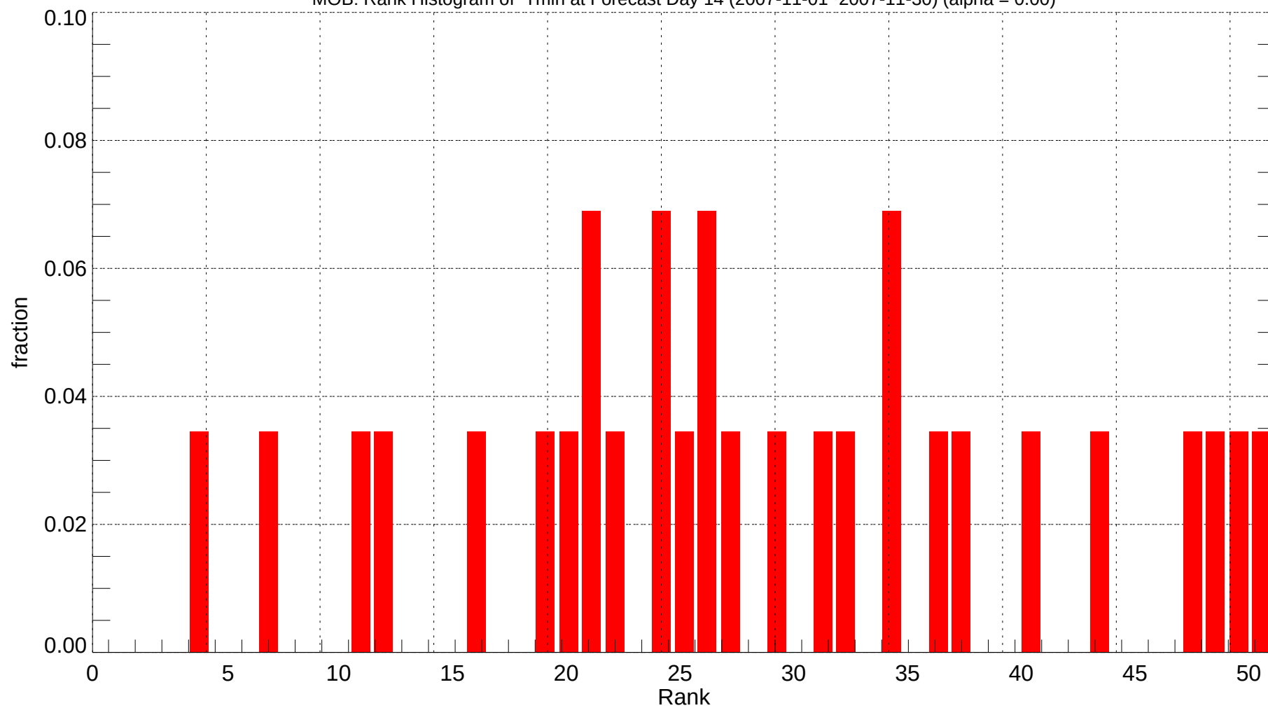
MOB: Rank Histogram of Tmin at Forecast Day 14 (2007-11-01~2007-11-30) (alpha = 0.00)
