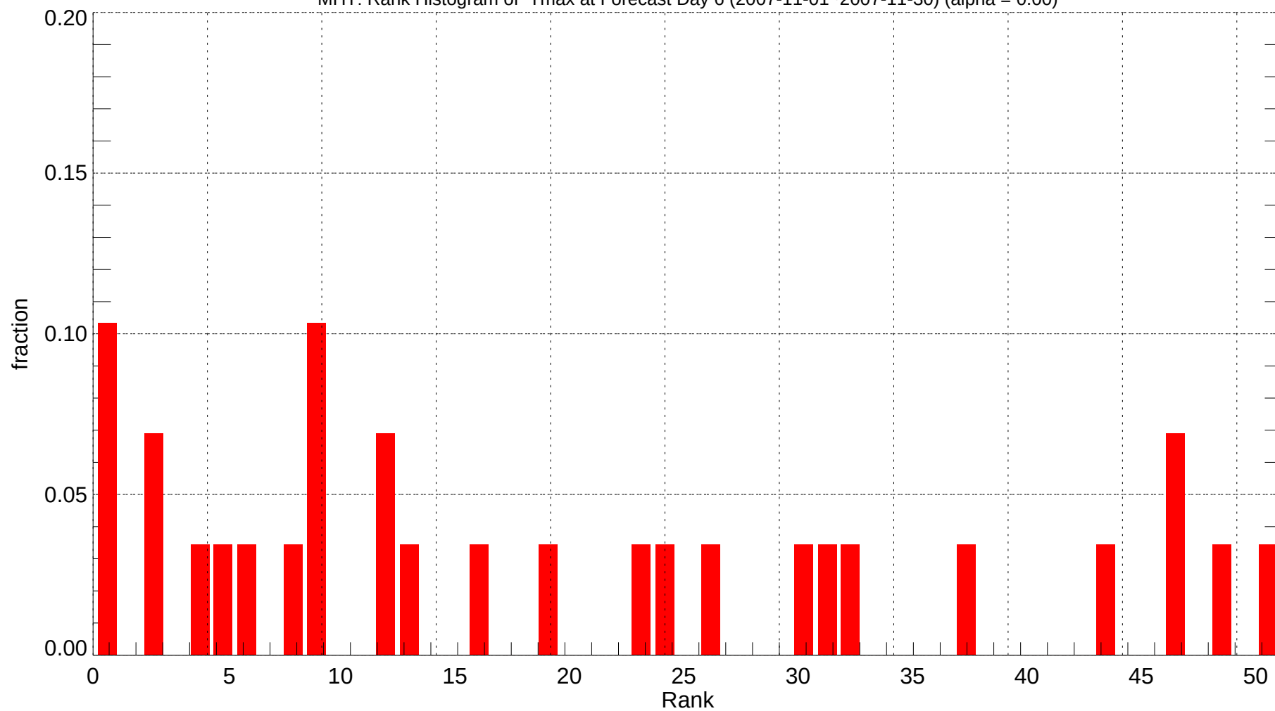
MHT: Rank Histogram of Tmax at Forecast Day 6 (2007-11-01~2007-11-30) (alpha = 0.00)
