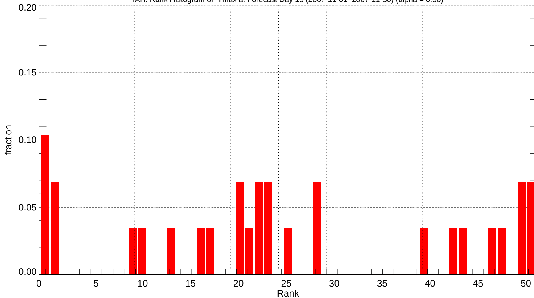
IAH: Rank Histogram of Tmax at Forecast Day 15 (2007-11-01~2007-11-30) (alpha = 0.00)
