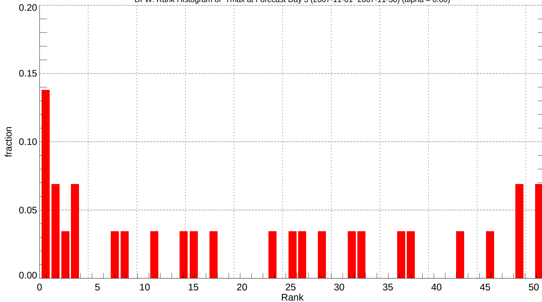
DFW: Rank Histogram of Tmax at Forecast Day 3 (2007-11-01~2007-11-30) (alpha = 0.00)
