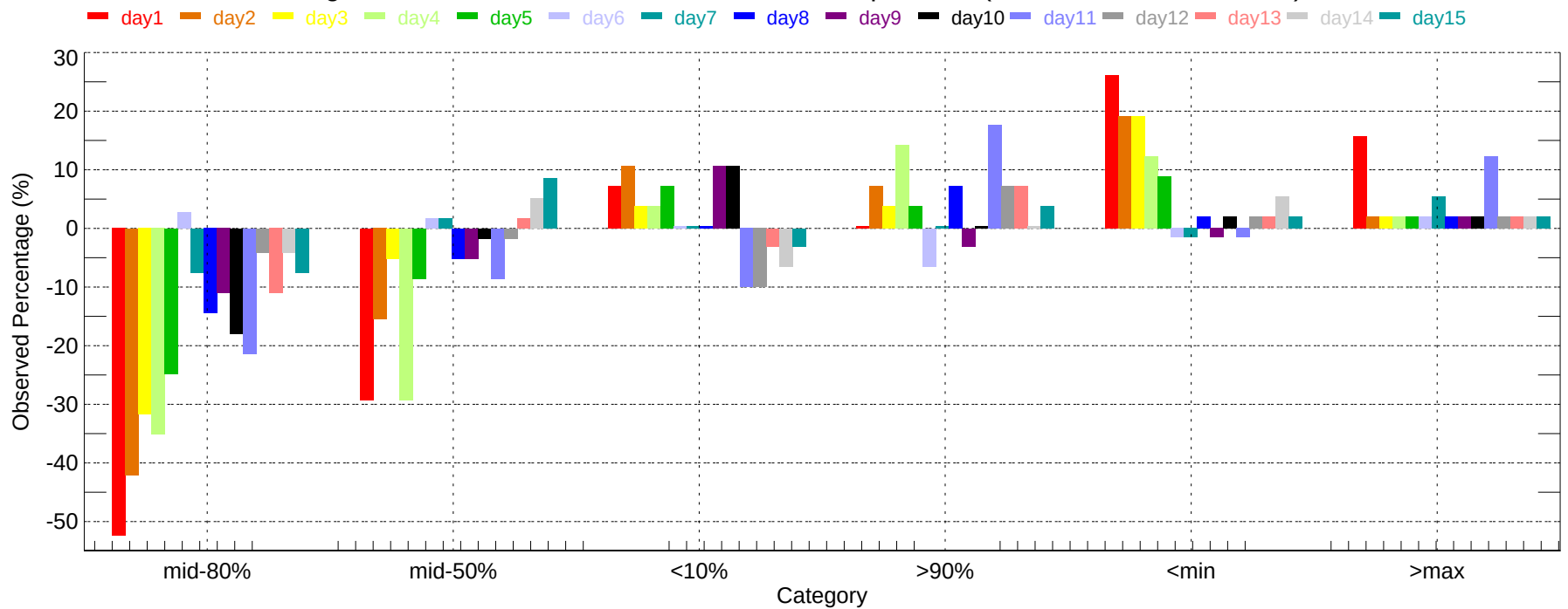
Observed Percentage Deviation of Ensembles - ABE: Max Temperature (2007-11-01~2007-11-30)
