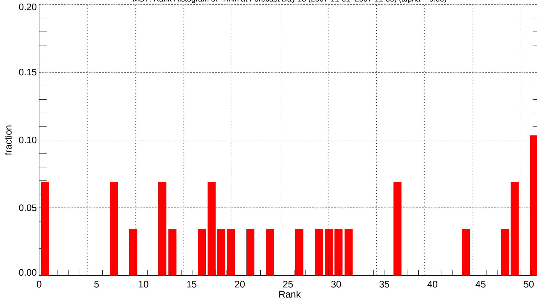
MSY: Rank Histogram of Tmin at Forecast Day 15 (2007-11-01~2007-11-30) (alpha = 0.00)
