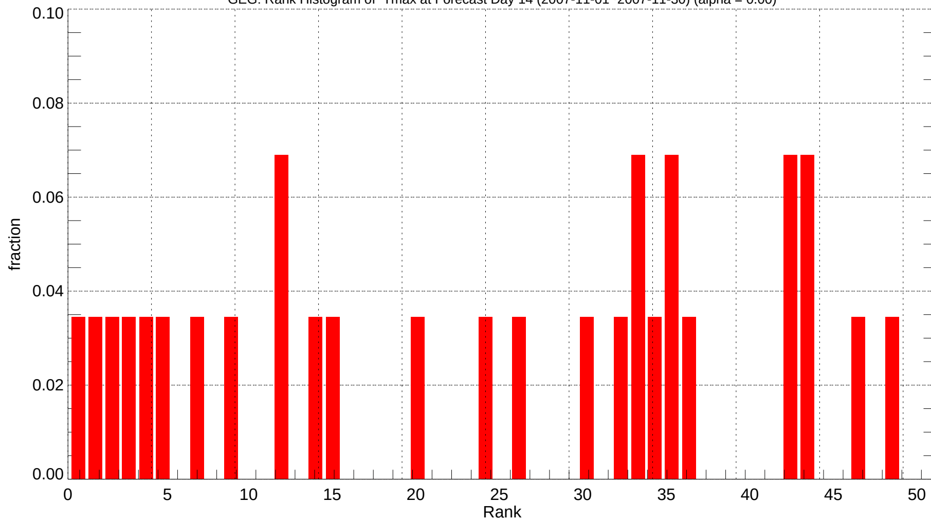
GEG: Rank Histogram of Tmax at Forecast Day 14 (2007-11-01~2007-11-30) (alpha = 0.00)
