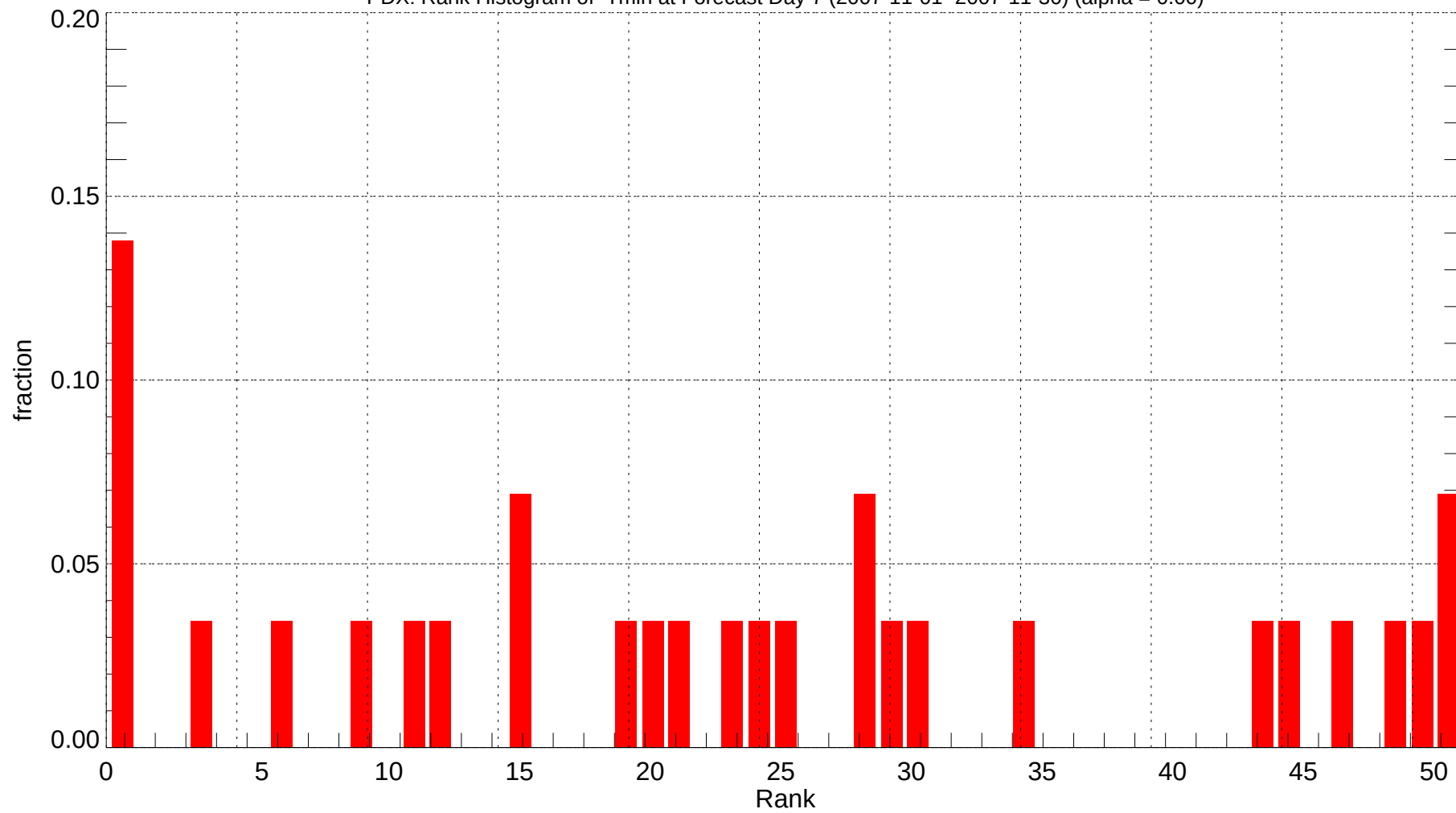
PDX: Rank Histogram of Tmin at Forecast Day 7 (2007-11-01~2007-11-30) (alpha = 0.00)
