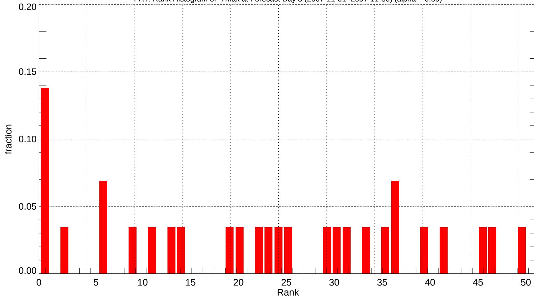
FAT: Rank Histogram of Tmax at Forecast Day 3 (2007-11-01~2007-11-30) (alpha = 0.00)
