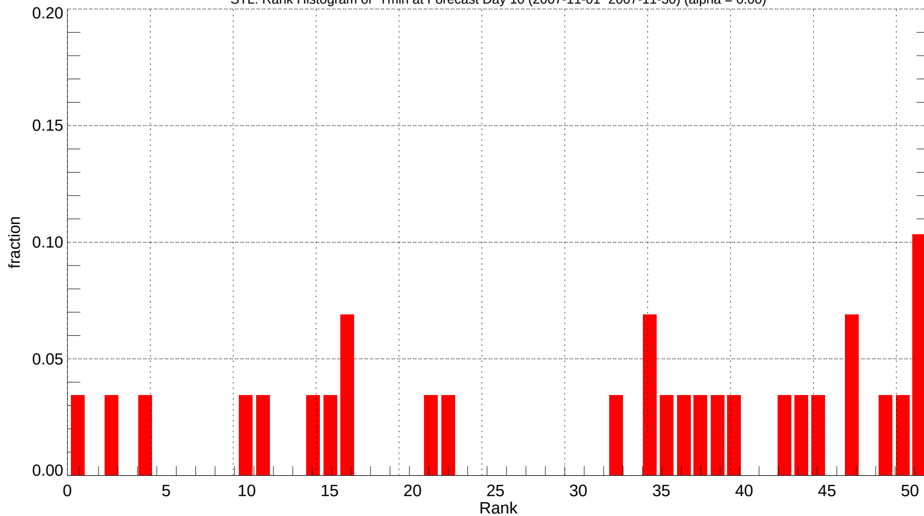
STL: Rank Histogram of Tmin at Forecast Day 10 (2007-11-01~2007-11-30) (alpha = 0.00)
