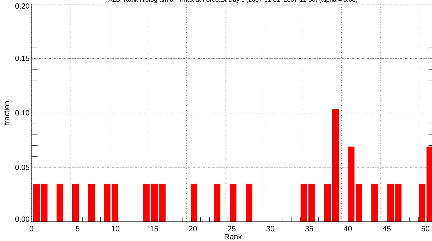
ALB: Rank Histogram of Tmax at Forecast Day 5 (2007-11-01~2007-11-30) (alpha = 0.00)
