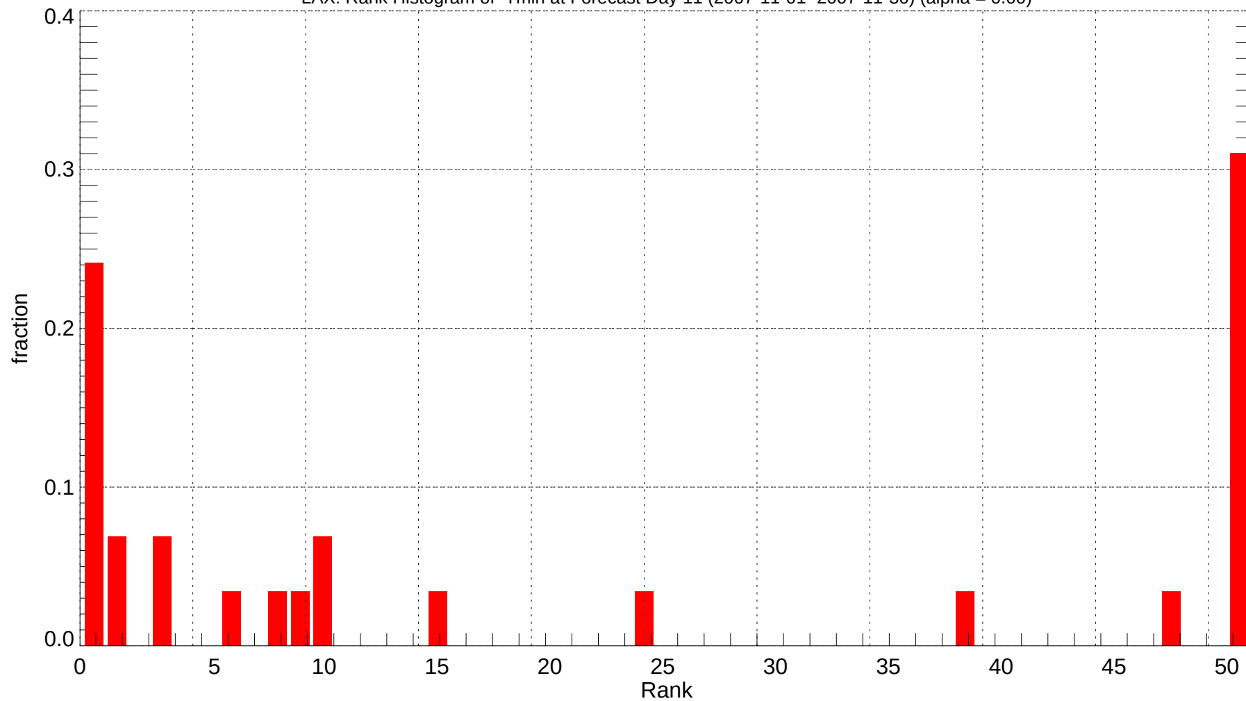
LAX: Rank Histogram of Tmin at Forecast Day 11 (2007-11-01~2007-11-30) (alpha = 0.00)
