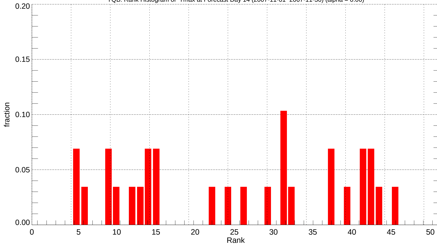
YQB: Rank Histogram of Tmax at Forecast Day 14 (2007-11-01~2007-11-30) (alpha = 0.00)
