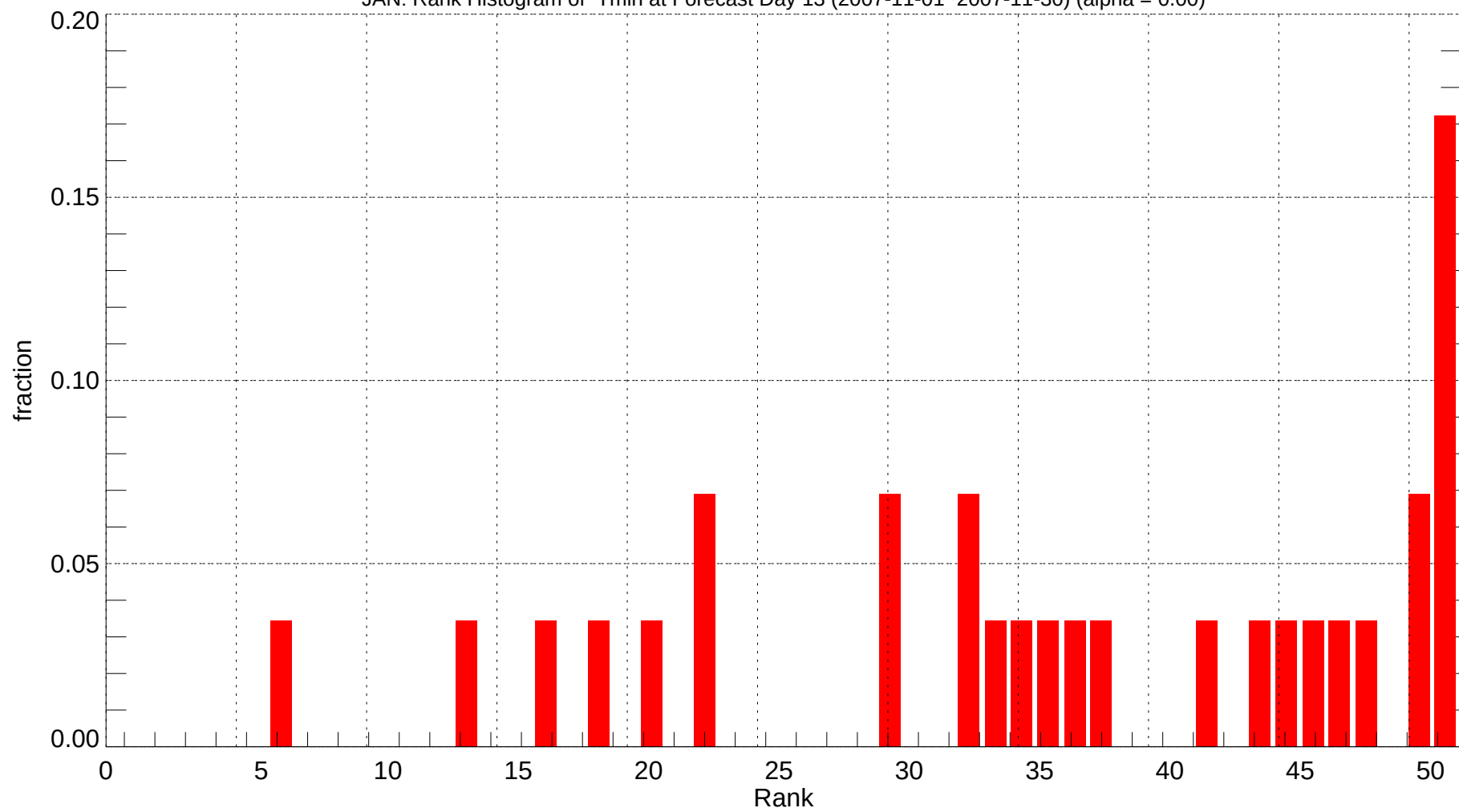
JAN: Rank Histogram of Tmin at Forecast Day 13 (2007-11-01~2007-11-30) (alpha = 0.00)
