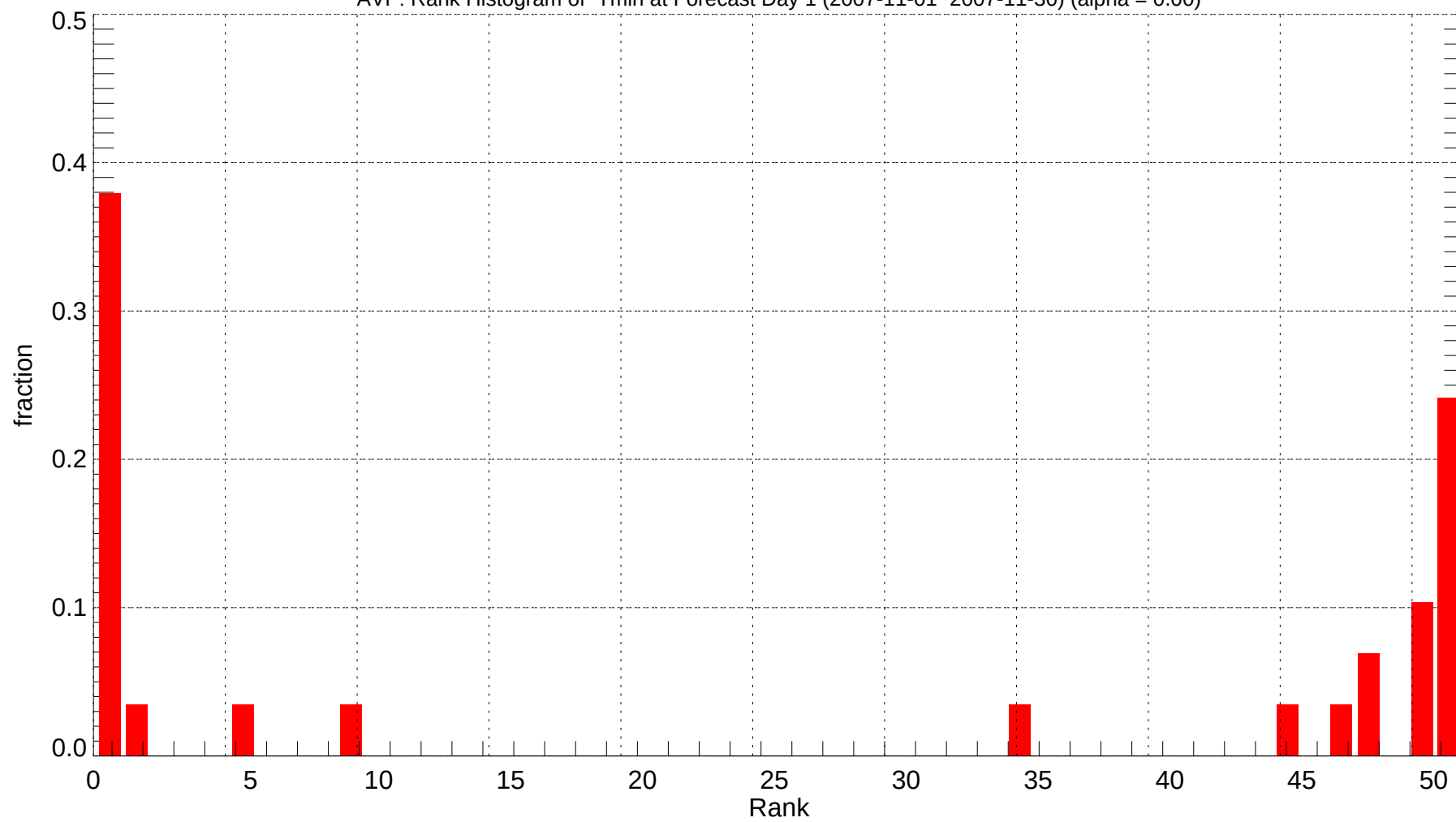
AVP: Rank Histogram of Tmin at Forecast Day 1 (2007-11-01~2007-11-30) (alpha = 0.00)
