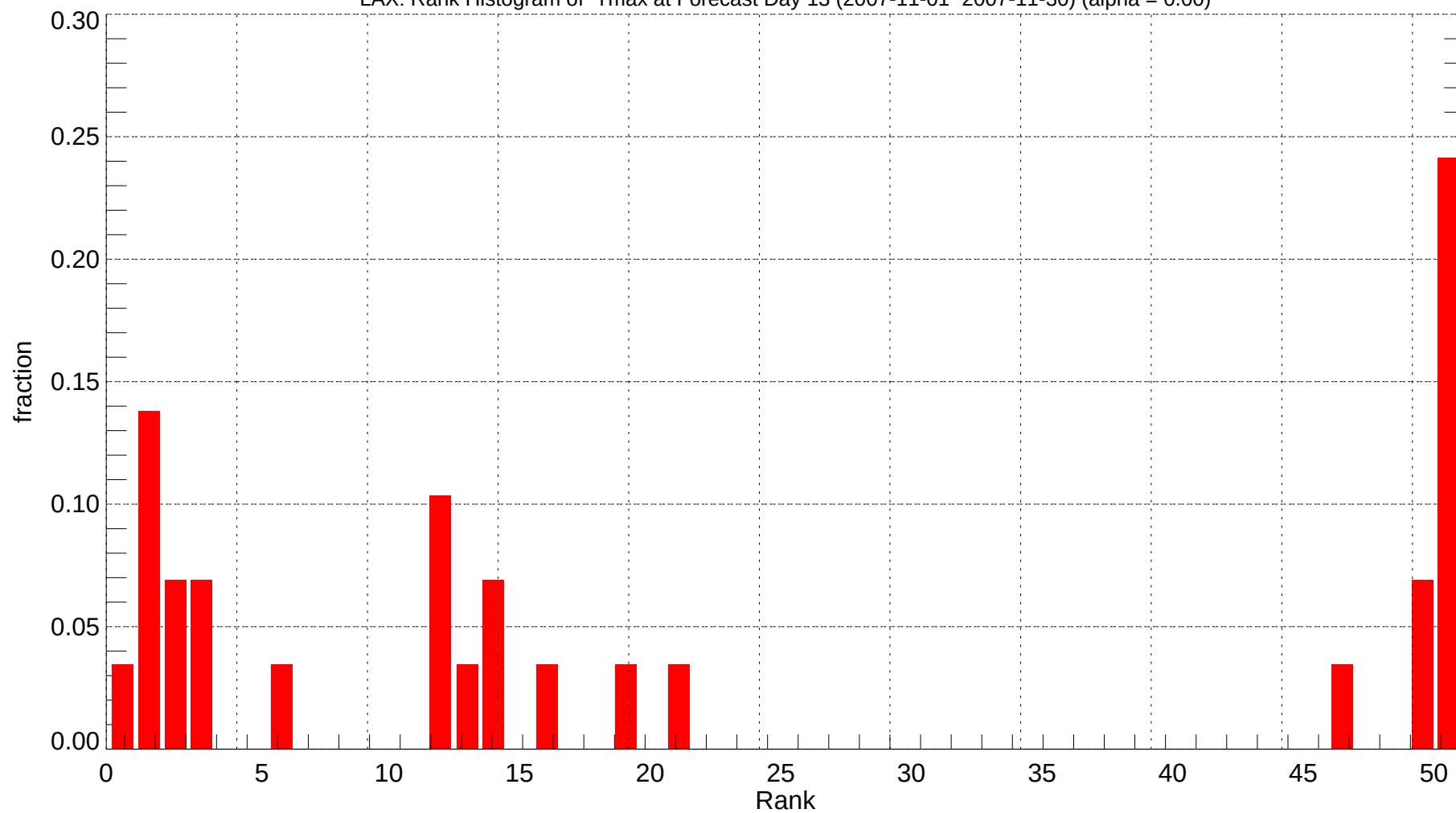
LAX: Rank Histogram of Tmax at Forecast Day 13 (2007-11-01~2007-11-30) (alpha = 0.00)
