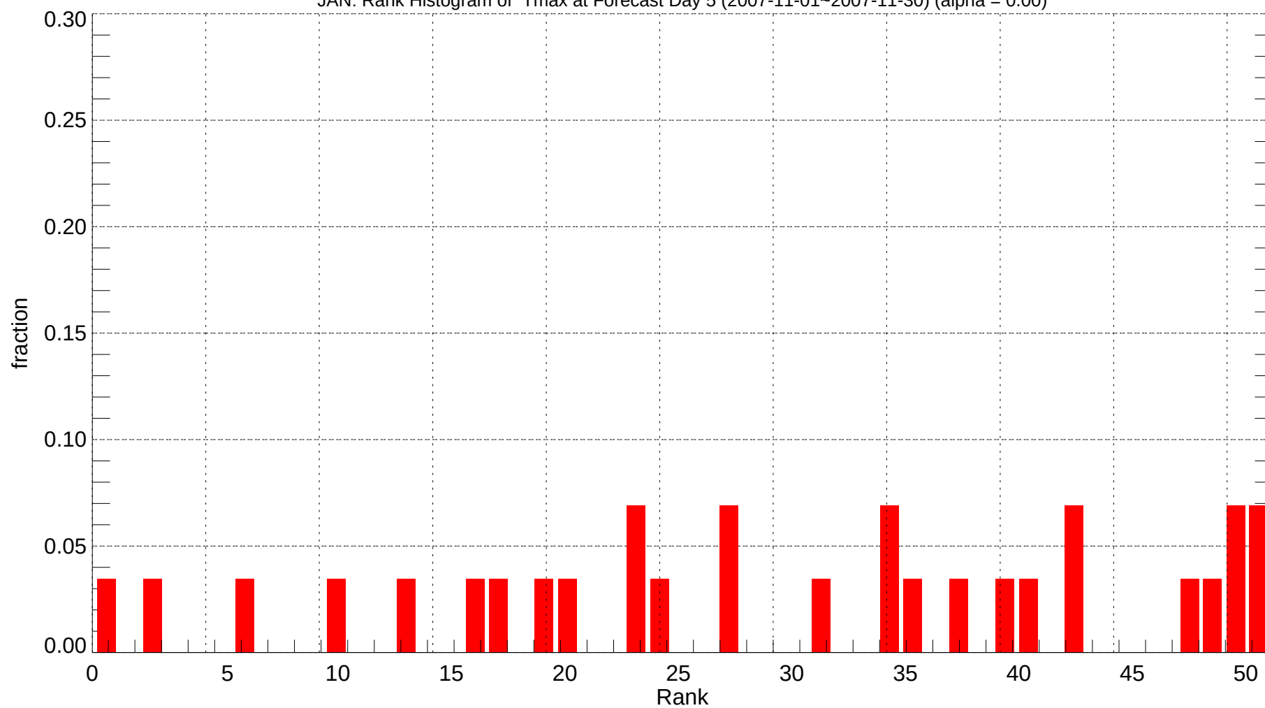
JAN: Rank Histogram of Tmax at Forecast Day 5 (2007-11-01~2007-11-30) (alpha = 0.00)
