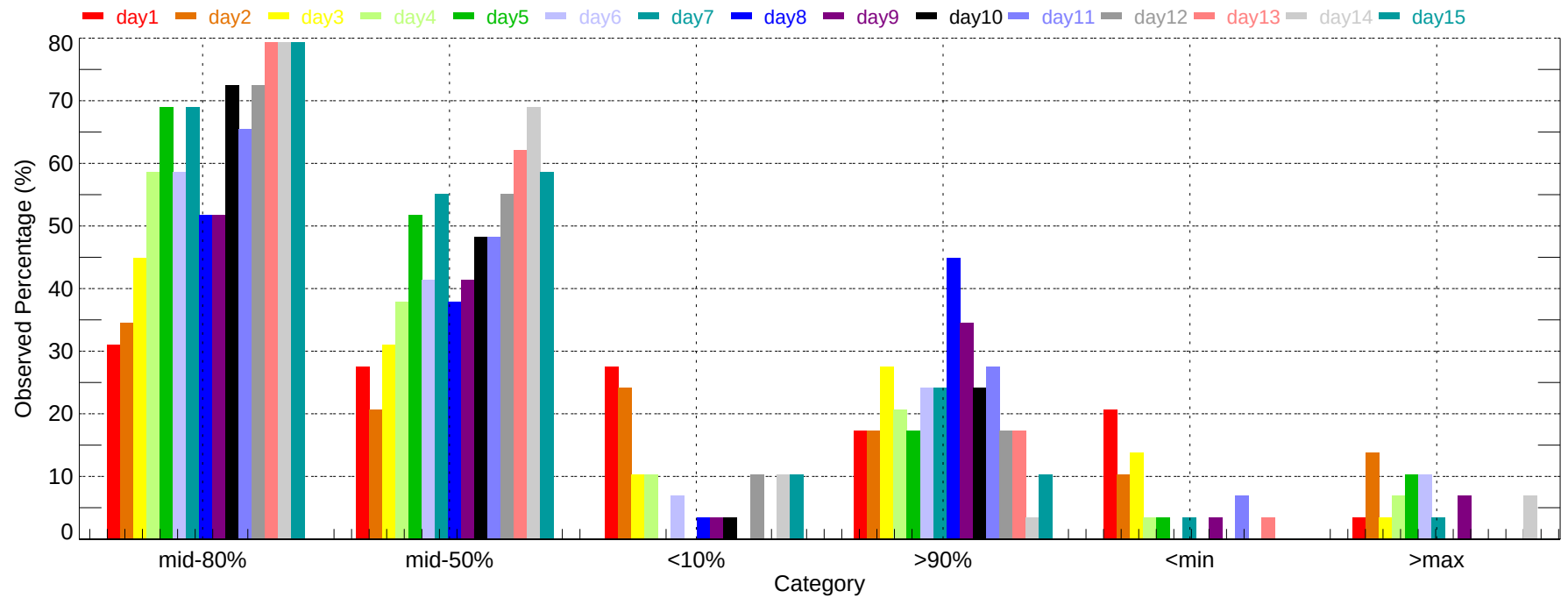
Observed Percentage of Ensembles - MSP: Max Temperature (2007-11-01~2007-11-30)
