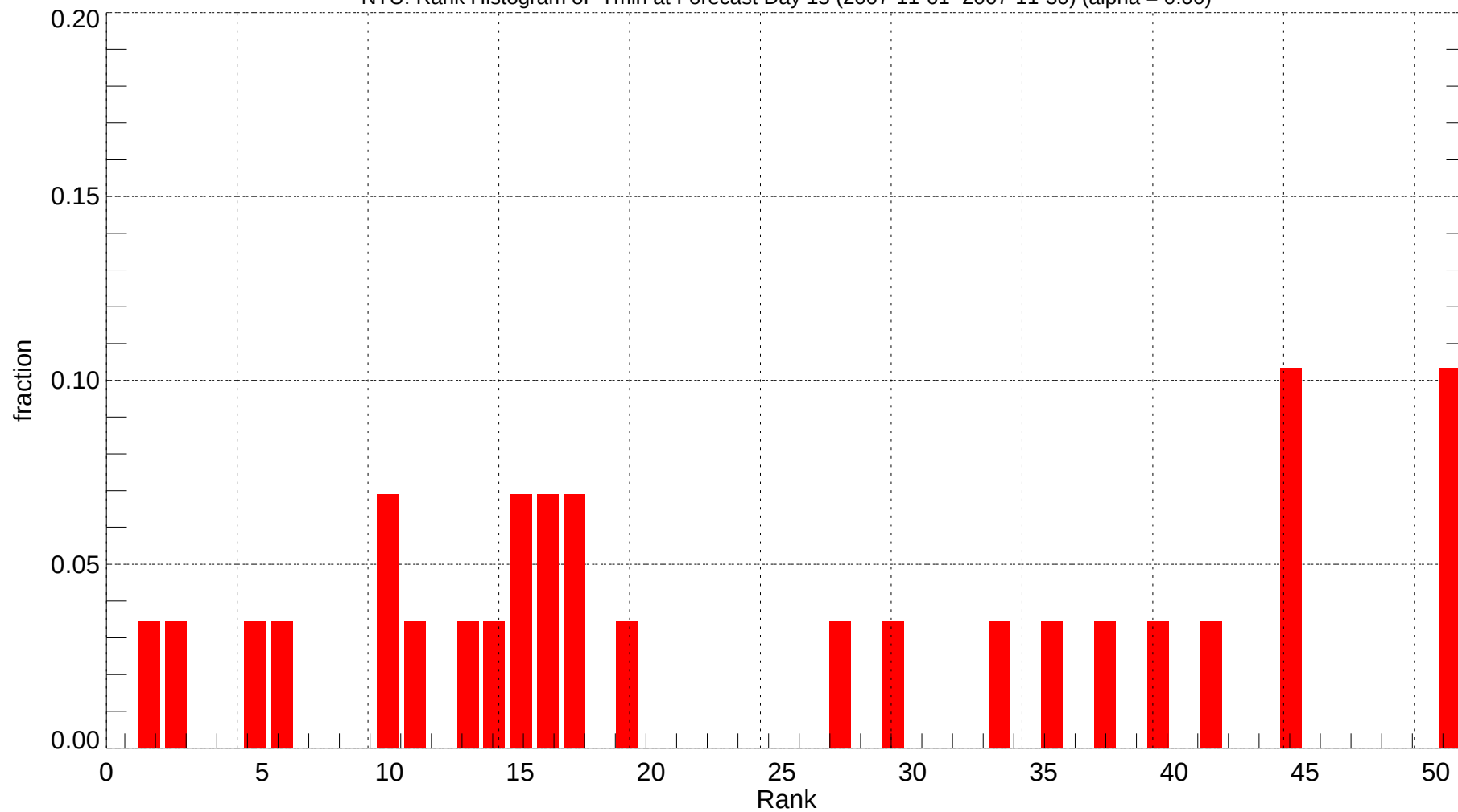
NTU: Rank Histogram of Tmin at Forecast Day 15 (2007-11-01~2007-11-30) (alpha = 0.00)
