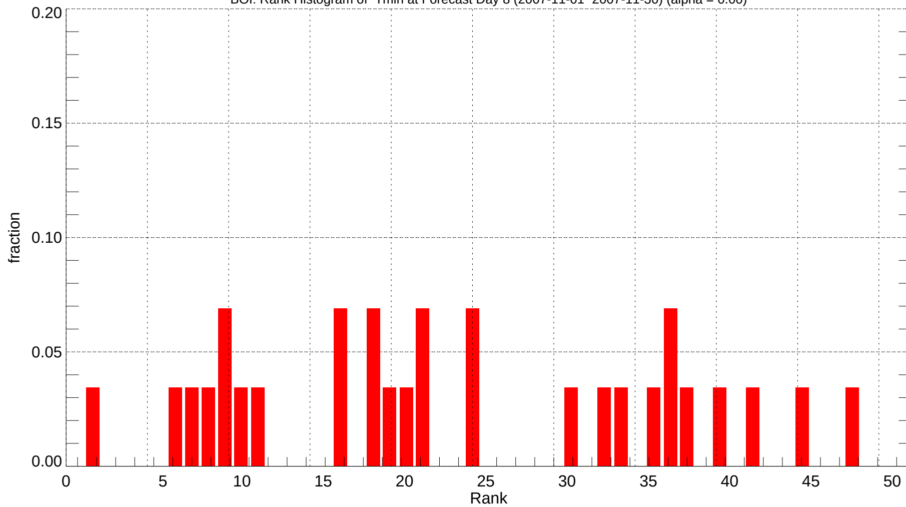
BOI: Rank Histogram of Tmin at Forecast Day 8 (2007-11-01~2007-11-30) (alpha = 0.00)
