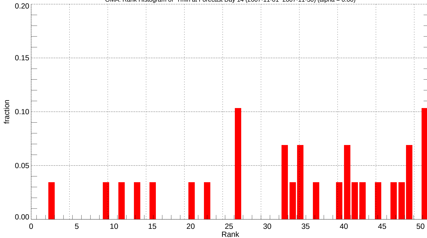
OMA: Rank Histogram of Tmin at Forecast Day 14 (2007-11-01~2007-11-30) (alpha = 0.00)
