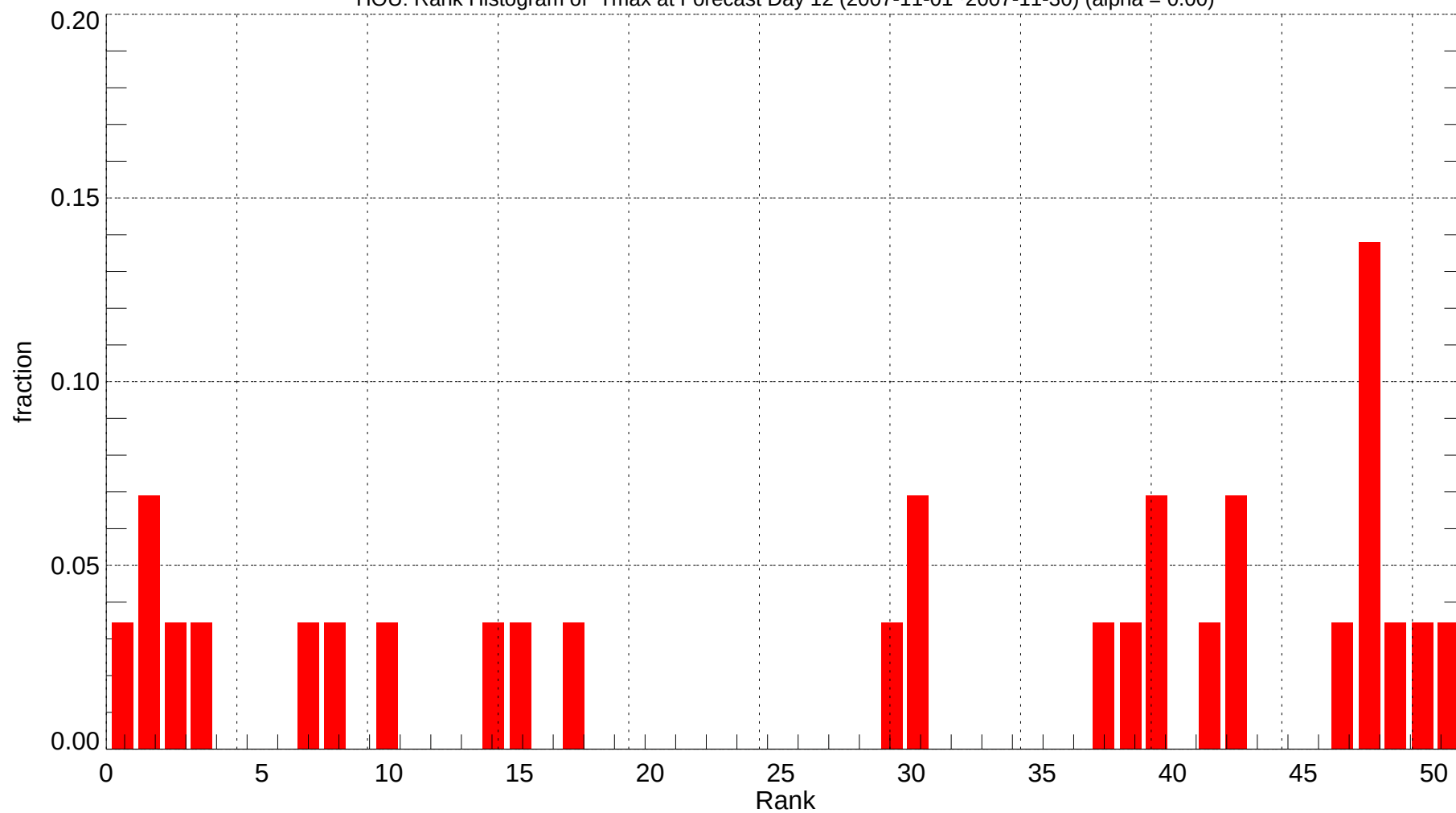
HOU: Rank Histogram of Tmax at Forecast Day 12 (2007-11-01~2007-11-30) (alpha = 0.00)
