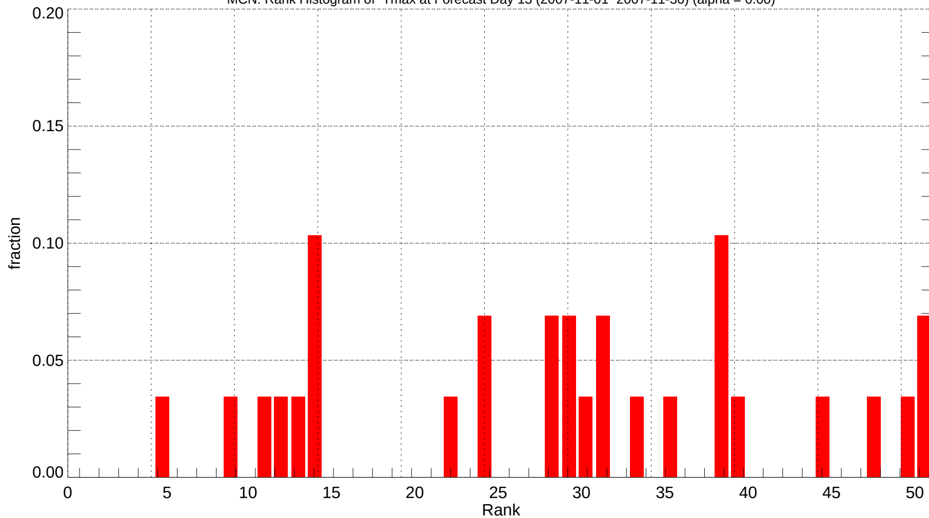
MCN: Rank Histogram of Tmax at Forecast Day 13 (2007-11-01~2007-11-30) (alpha = 0.00)
