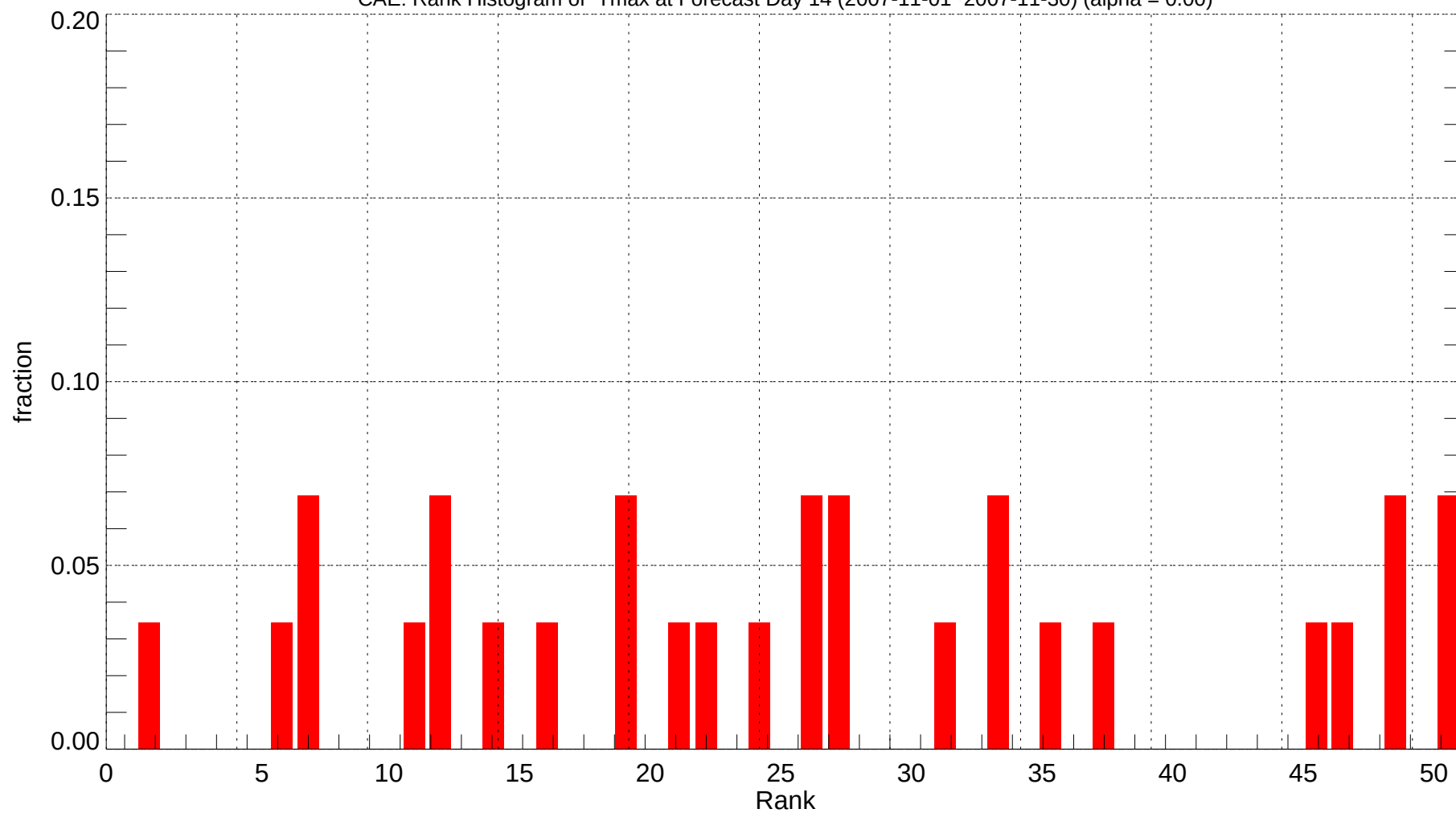
CAE: Rank Histogram of Tmax at Forecast Day 14 (2007-11-01~2007-11-30) (alpha = 0.00)
