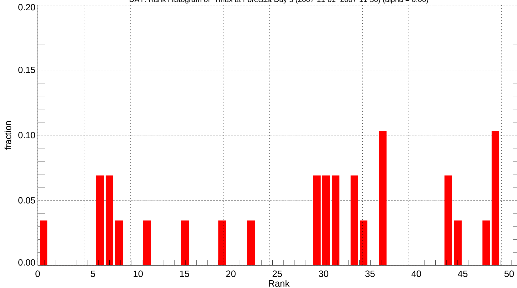
DAY: Rank Histogram of Tmax at Forecast Day 5 (2007-11-01~2007-11-30) (alpha = 0.00)
