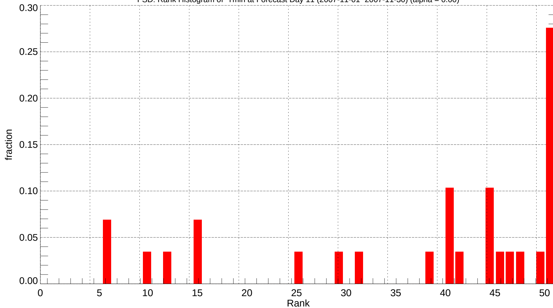
FSD: Rank Histogram of Tmin at Forecast Day 11 (2007-11-01~2007-11-30) (alpha = 0.00)
