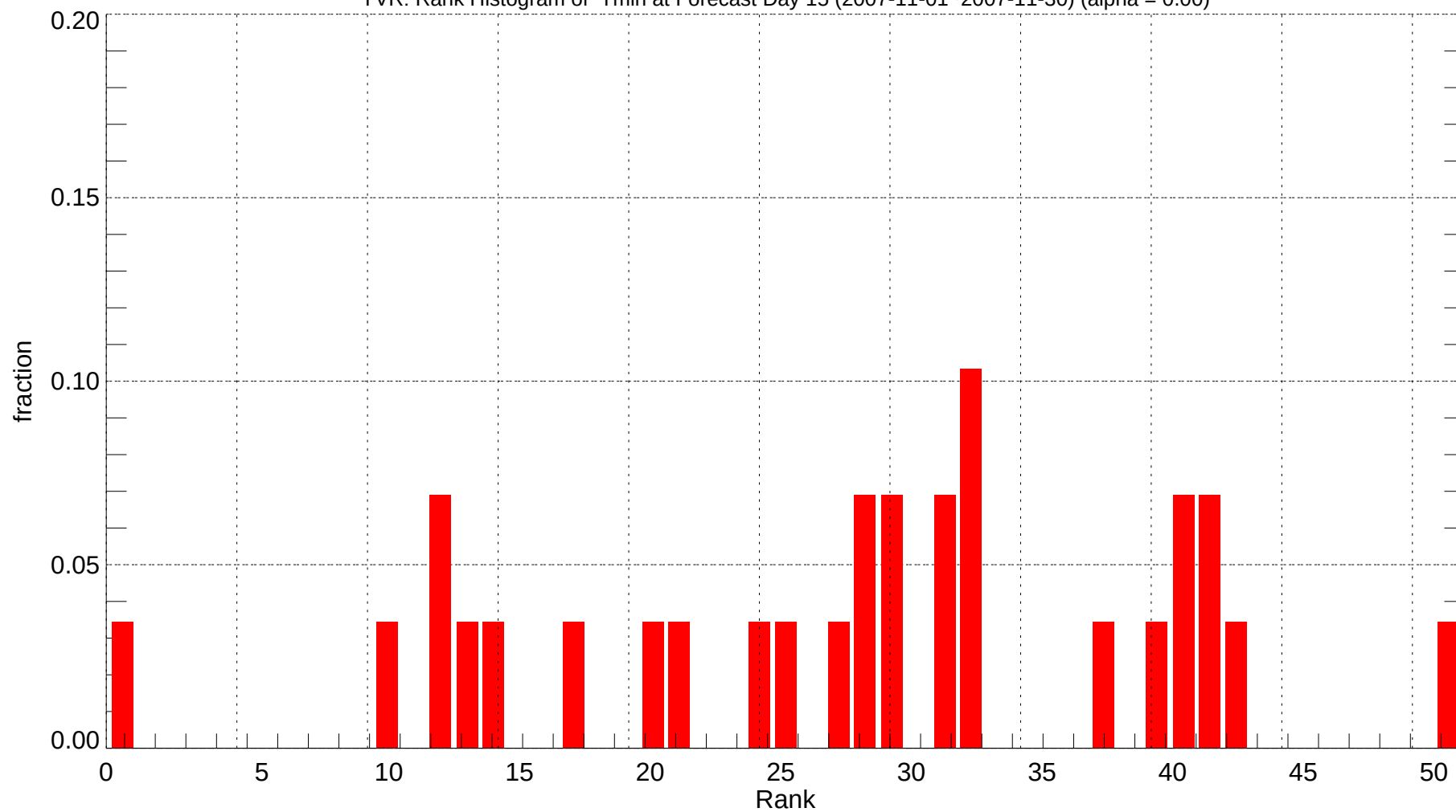
YVR: Rank Histogram of Tmin at Forecast Day 15 (2007-11-01~2007-11-30) (alpha = 0.00)
