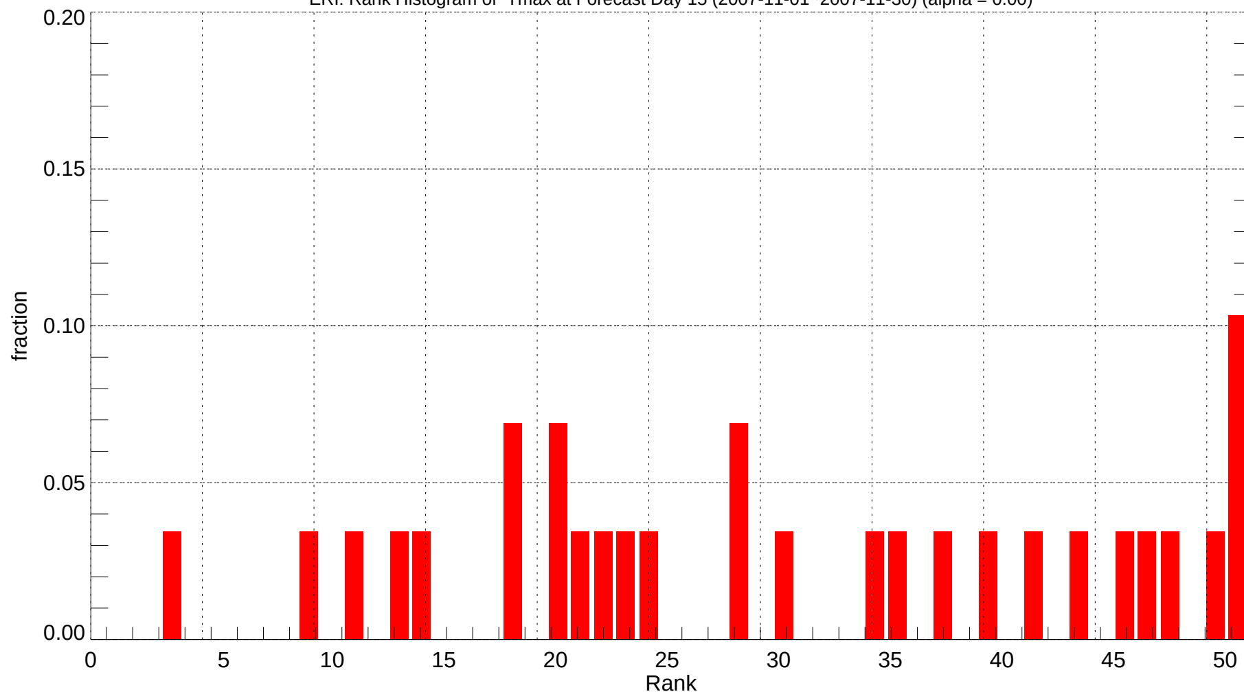
ERI: Rank Histogram of Tmax at Forecast Day 15 (2007-11-01~2007-11-30) (alpha = 0.00)
