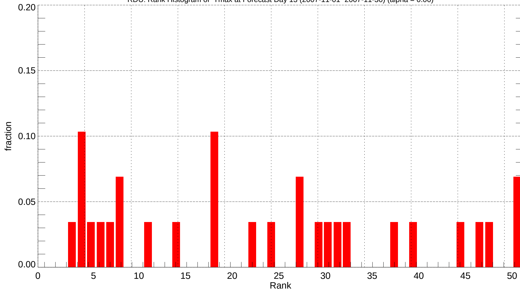
RDU: Rank Histogram of Tmax at Forecast Day 13 (2007-11-01~2007-11-30) (alpha = 0.00)
