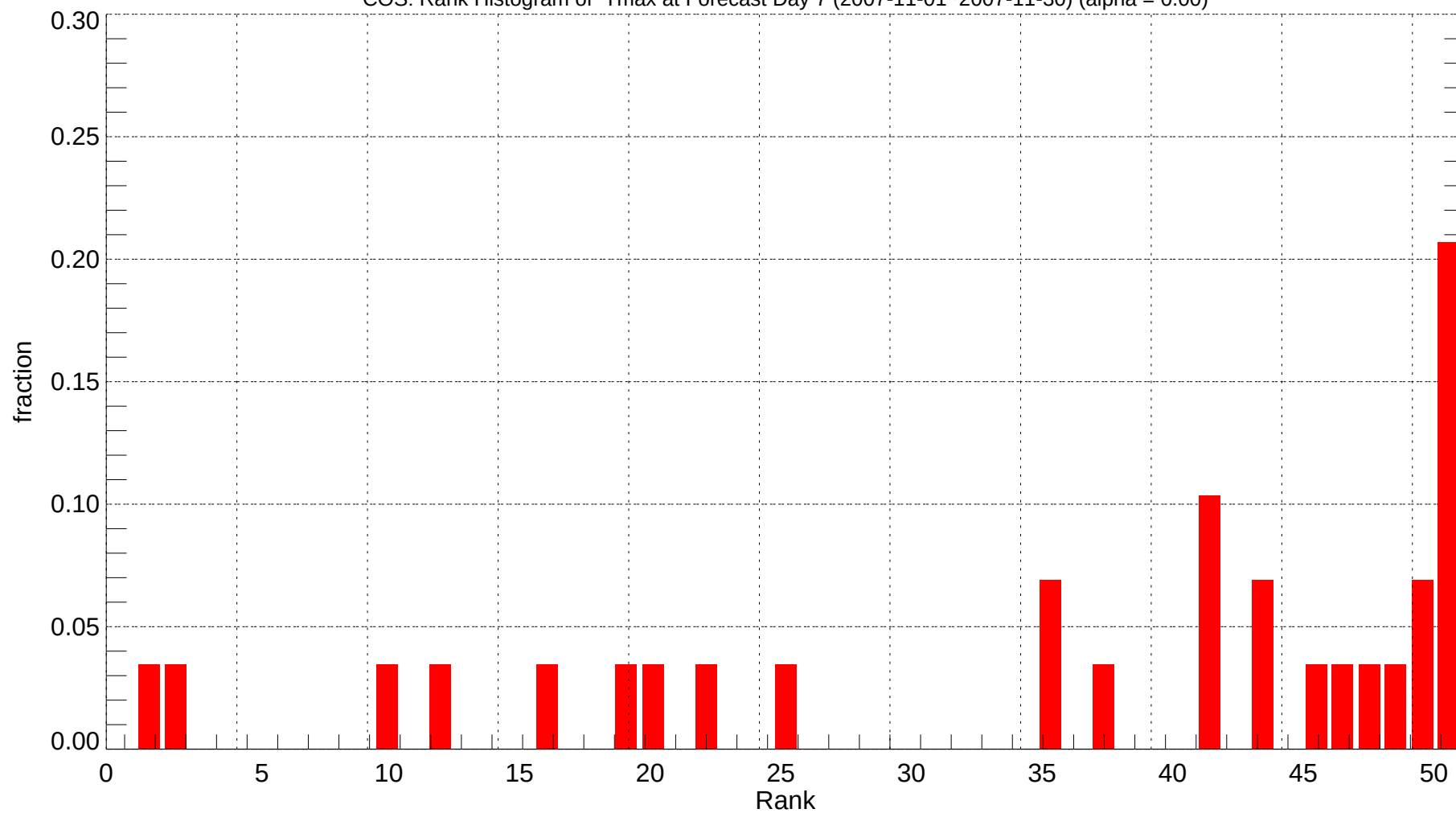
COS: Rank Histogram of Tmax at Forecast Day 7 (2007-11-01~2007-11-30) (alpha = 0.00)
