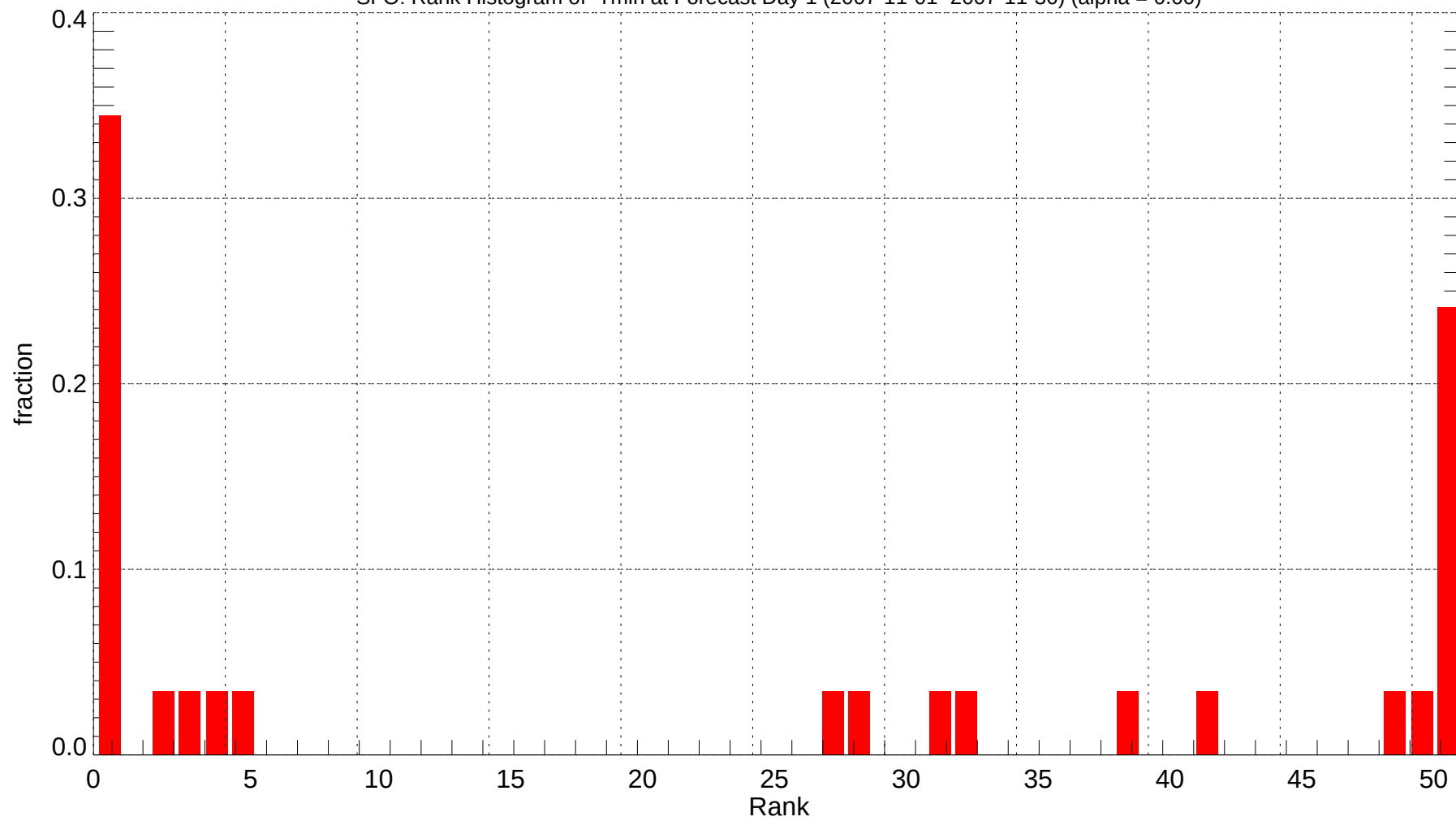
SFO: Rank Histogram of Tmin at Forecast Day 1 (2007-11-01~2007-11-30) (alpha = 0.00)
