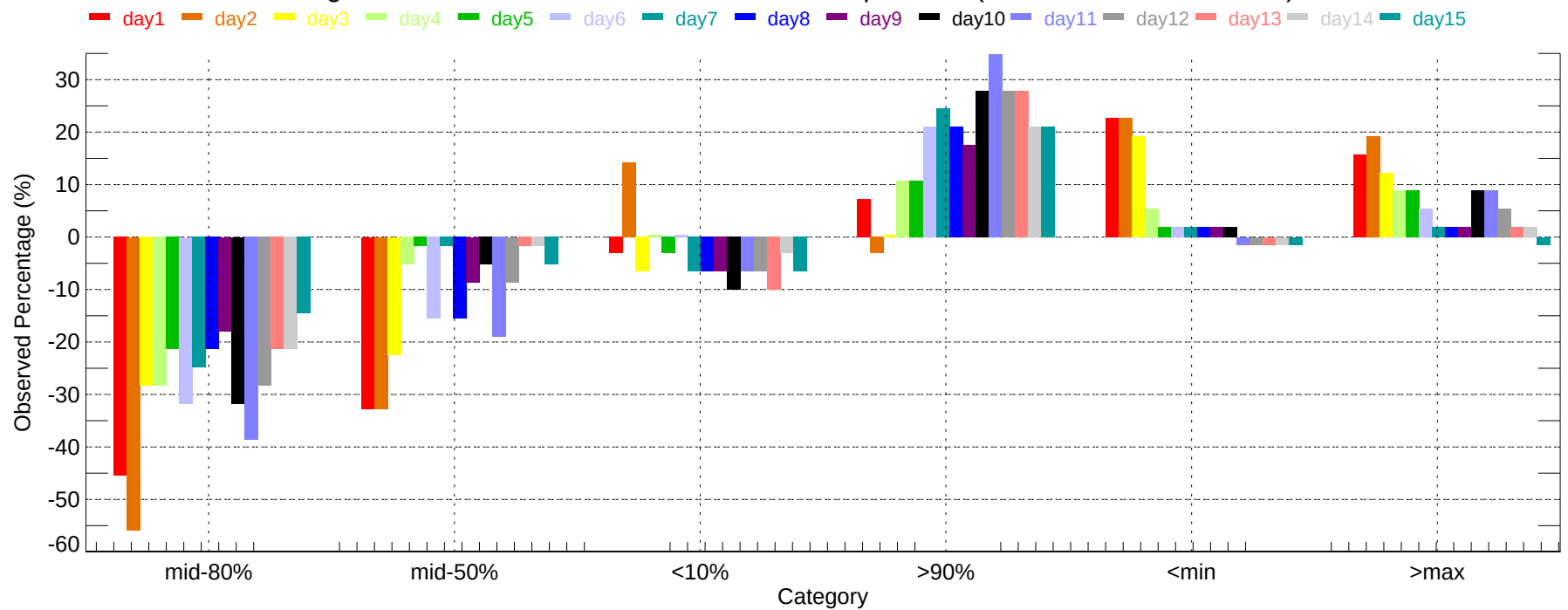
Observed Percentage Deviation of Ensembles - DLH: Min Temperature (2007-11-01~2007-11-30)
