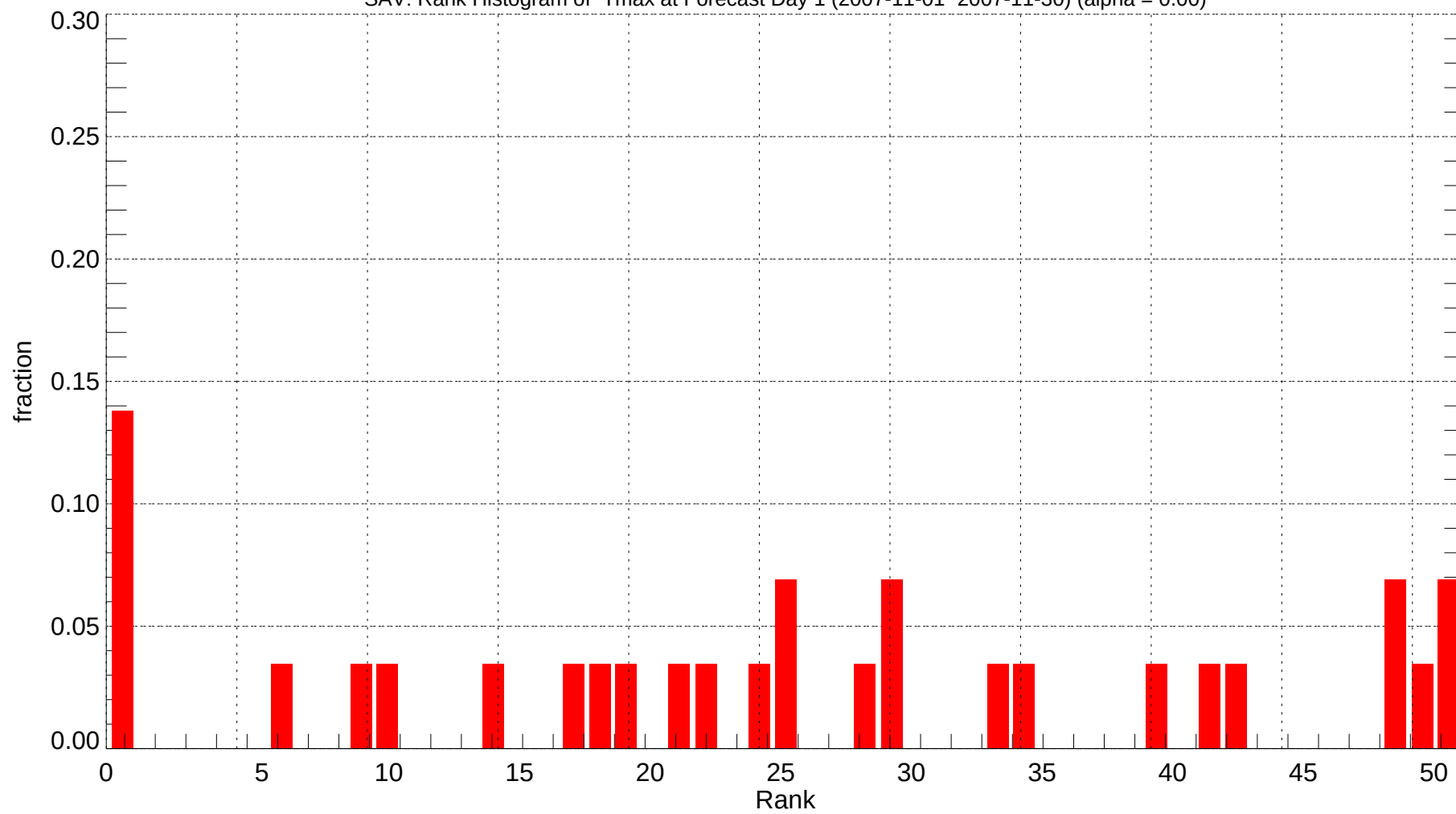
SAV: Rank Histogram of Tmax at Forecast Day 1 (2007-11-01~2007-11-30) (alpha = 0.00)
