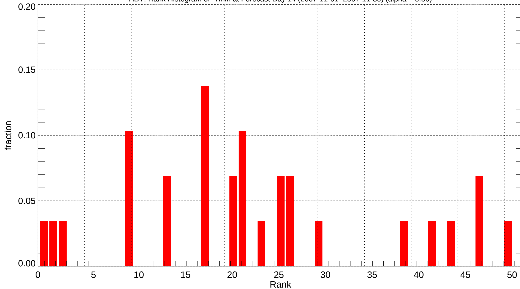
ABY: Rank Histogram of Tmin at Forecast Day 14 (2007-11-01~2007-11-30) (alpha = 0.00)
