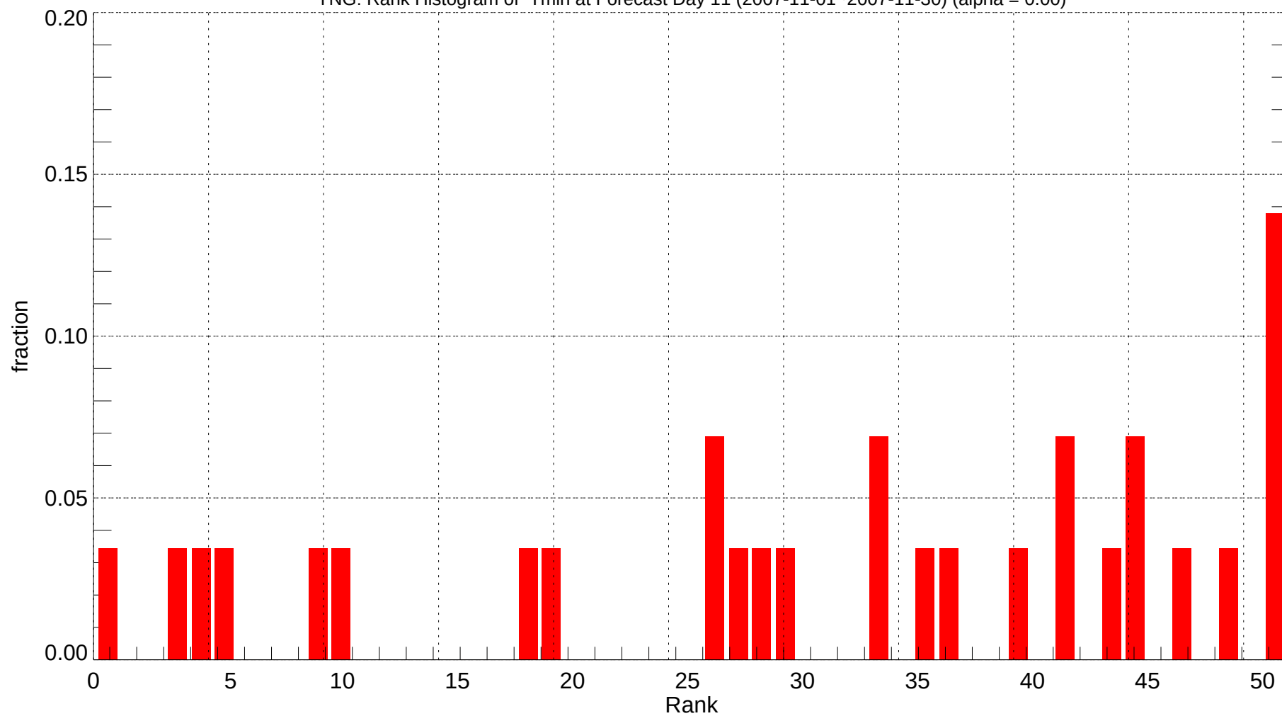
YNG: Rank Histogram of Tmin at Forecast Day 11 (2007-11-01~2007-11-30) (alpha = 0.00)
