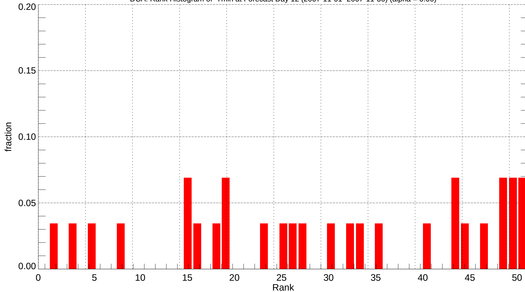
DCA: Rank Histogram of Tmin at Forecast Day 12 (2007-11-01~2007-11-30) (alpha = 0.00)
