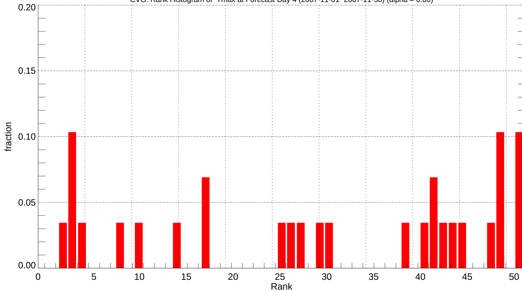
CVG: Rank Histogram of Tmax at Forecast Day 4 (2007-11-01~2007-11-30) (alpha = 0.00)
