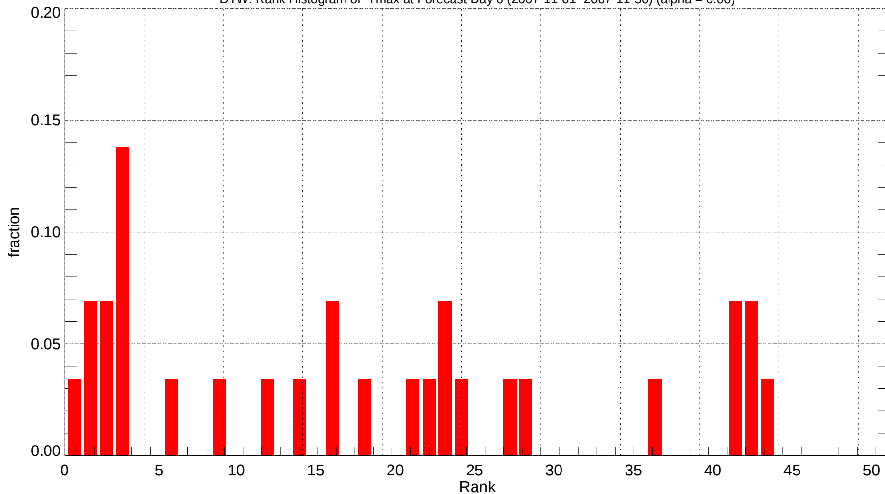
DTW: Rank Histogram of Tmax at Forecast Day 6 (2007-11-01~2007-11-30) (alpha = 0.00)
