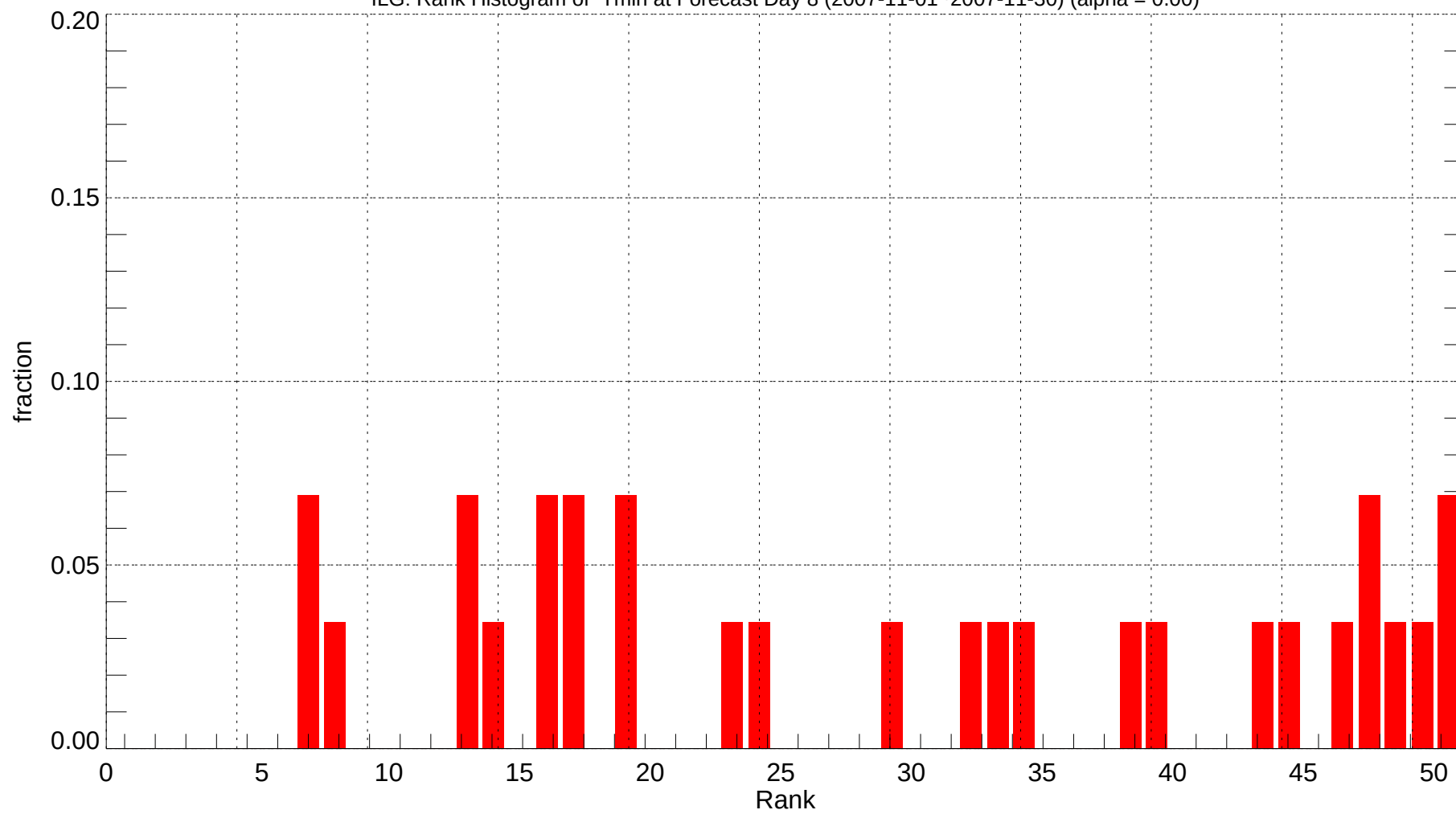
ILG: Rank Histogram of Tmin at Forecast Day 8 (2007-11-01~2007-11-30) (alpha = 0.00)
