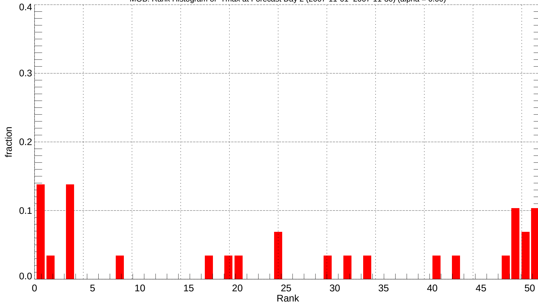
MOB: Rank Histogram of Tmax at Forecast Day 2 (2007-11-01~2007-11-30) (alpha = 0.00)
