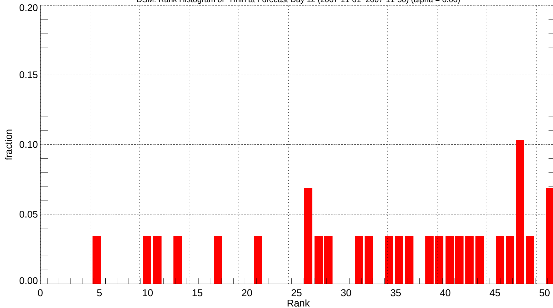
DSM: Rank Histogram of Tmin at Forecast Day 12 (2007-11-01~2007-11-30) (alpha = 0.00)
