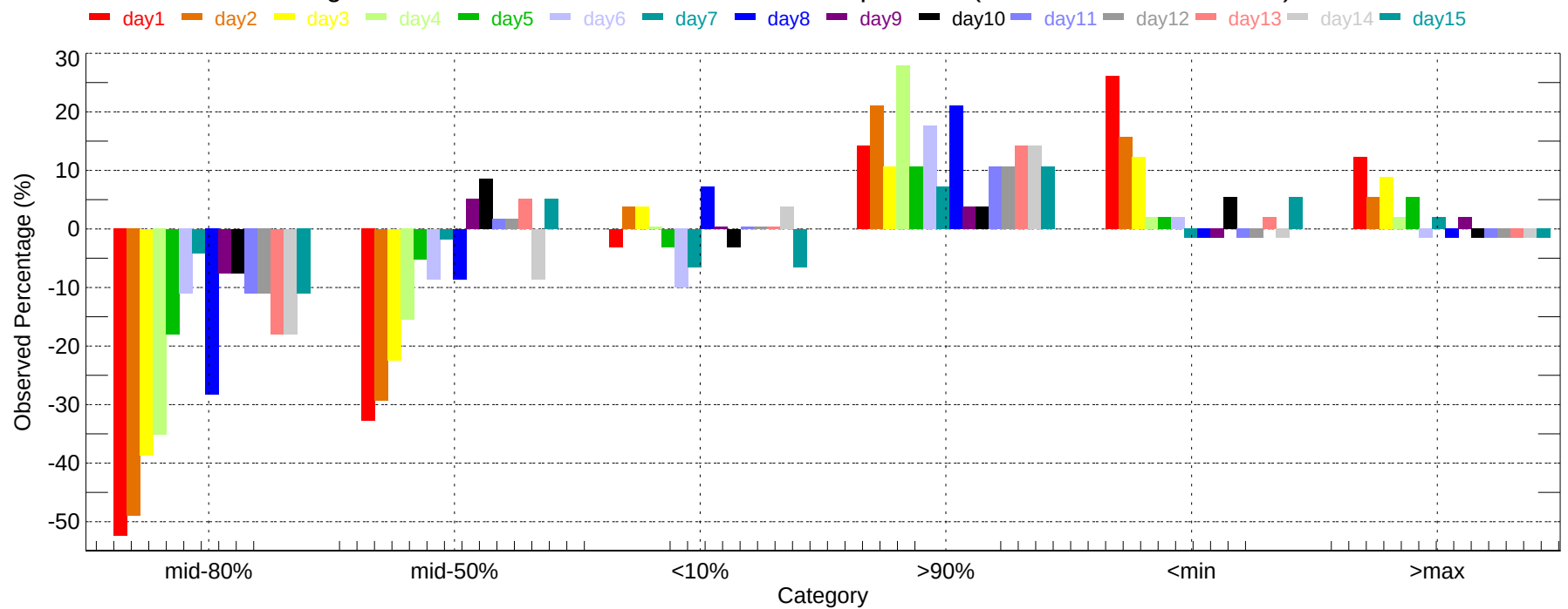
Observed Percentage Deviation of Ensembles - ALB: Min Temperature (2007-11-01~2007-11-30)
