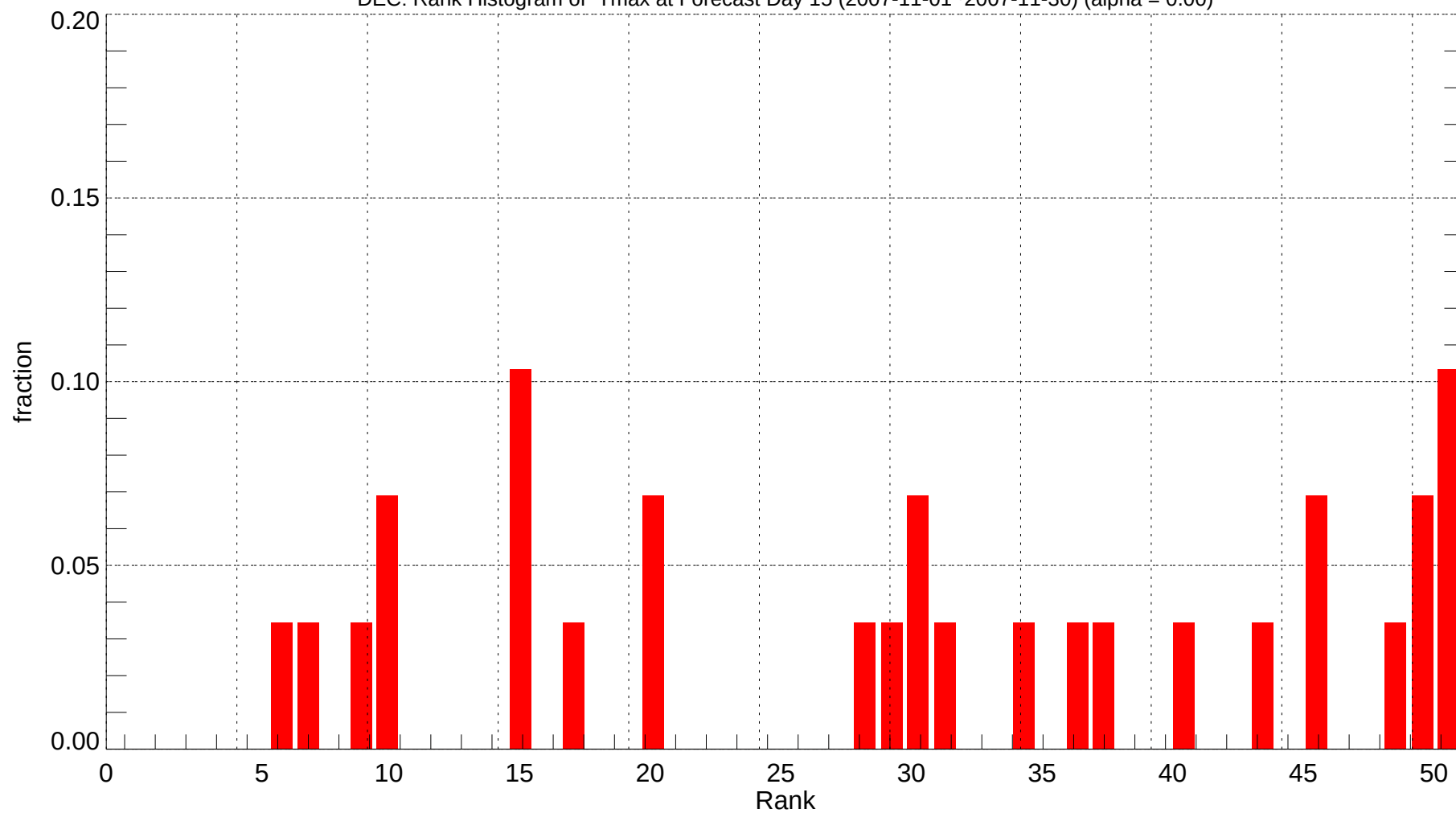
DEC: Rank Histogram of Tmax at Forecast Day 15 (2007-11-01~2007-11-30) (alpha = 0.00)
