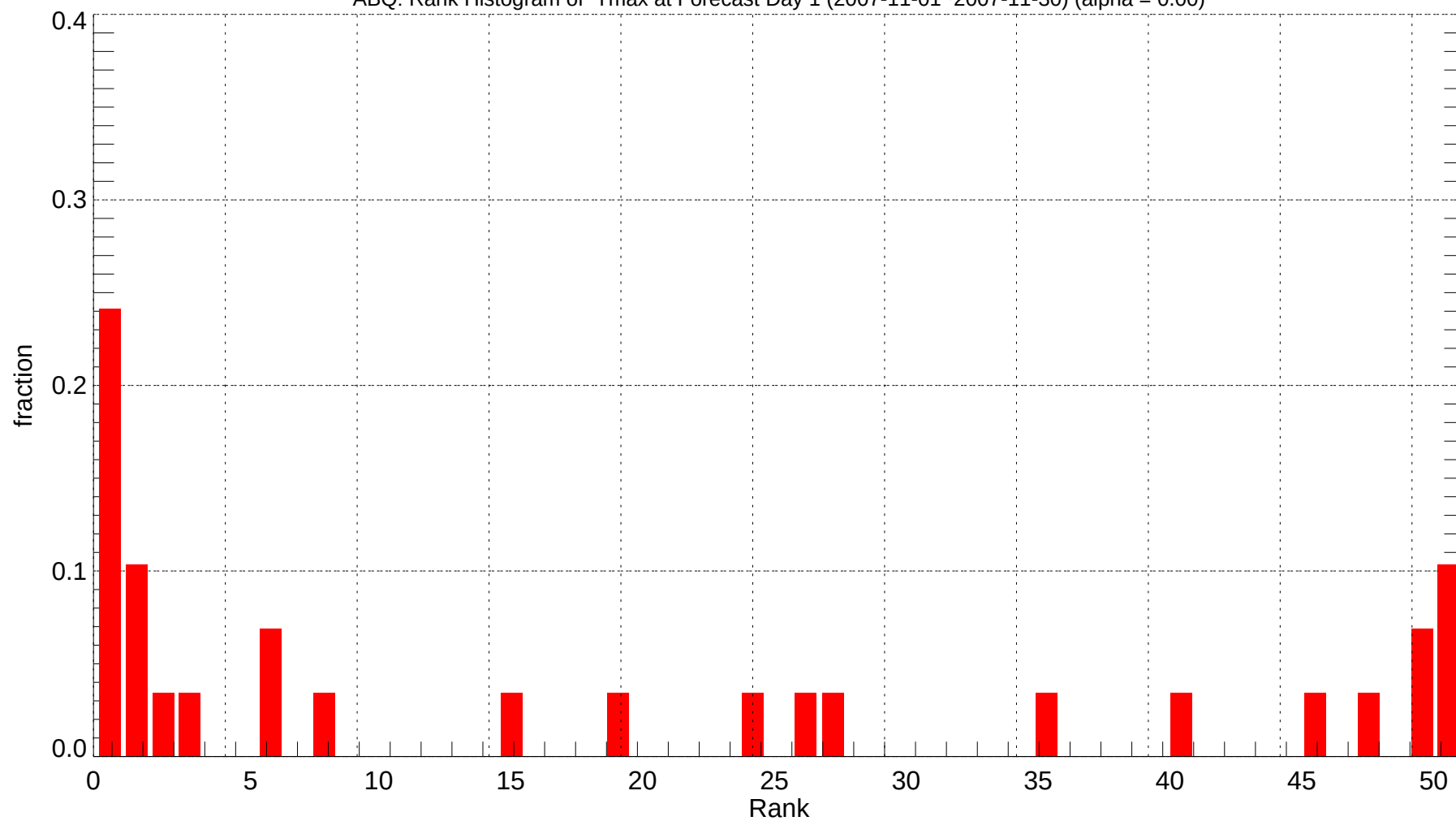
ABQ: Rank Histogram of Tmax at Forecast Day 1 (2007-11-01~2007-11-30) (alpha = 0.00)
