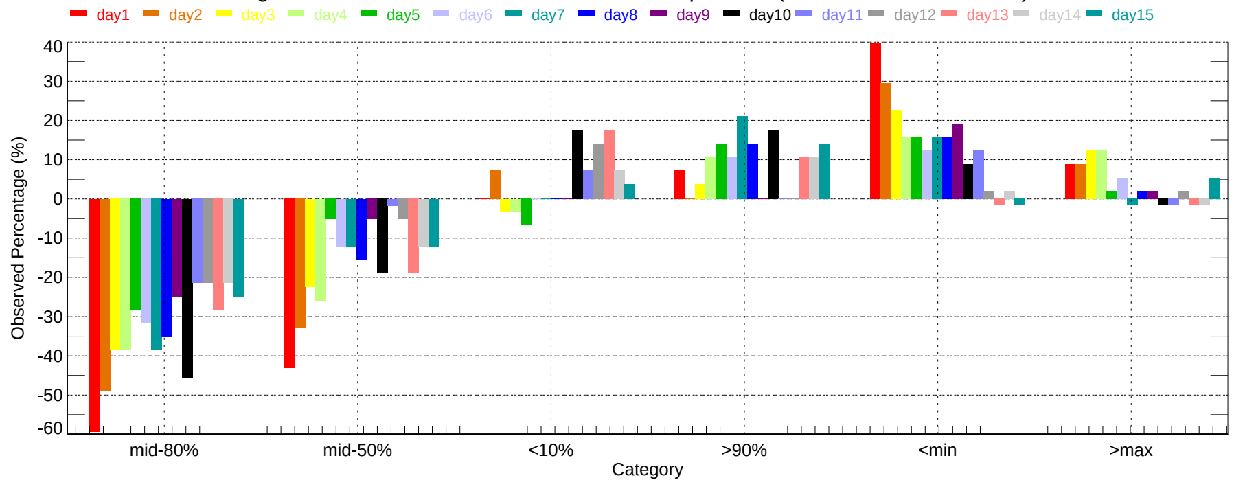
Observed Percentage Deviation of Ensembles - YKM: Max Temperature (2007-11-01~2007-11-30)
