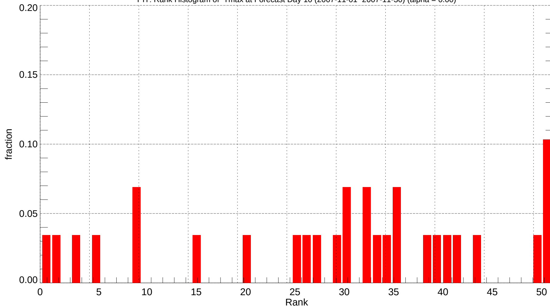
PIT: Rank Histogram of Tmax at Forecast Day 10 (2007-11-01~2007-11-30) (alpha = 0.00)
