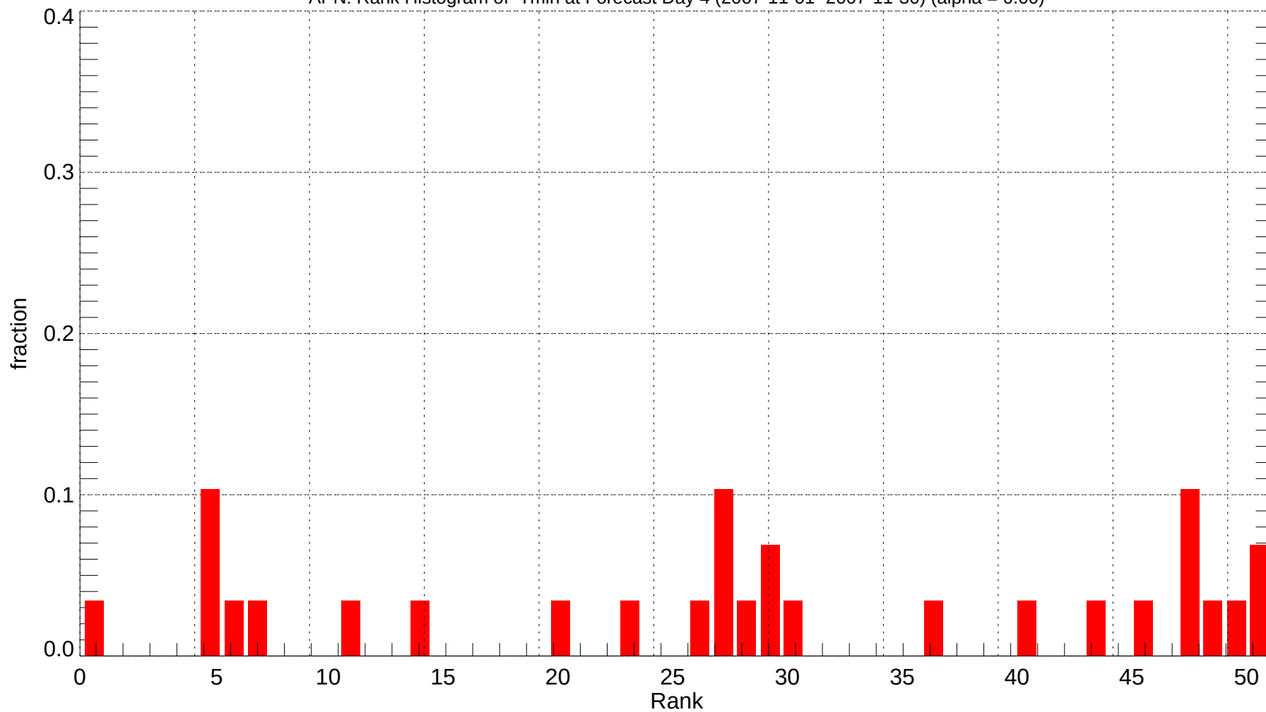
APN: Rank Histogram of Tmin at Forecast Day 4 (2007-11-01~2007-11-30) (alpha = 0.00)
