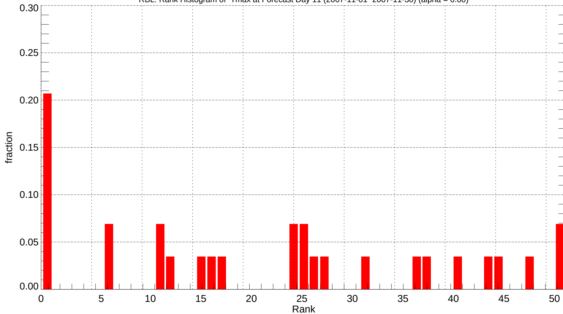
RBL: Rank Histogram of Tmax at Forecast Day 11 (2007-11-01~2007-11-30) (alpha = 0.00)
