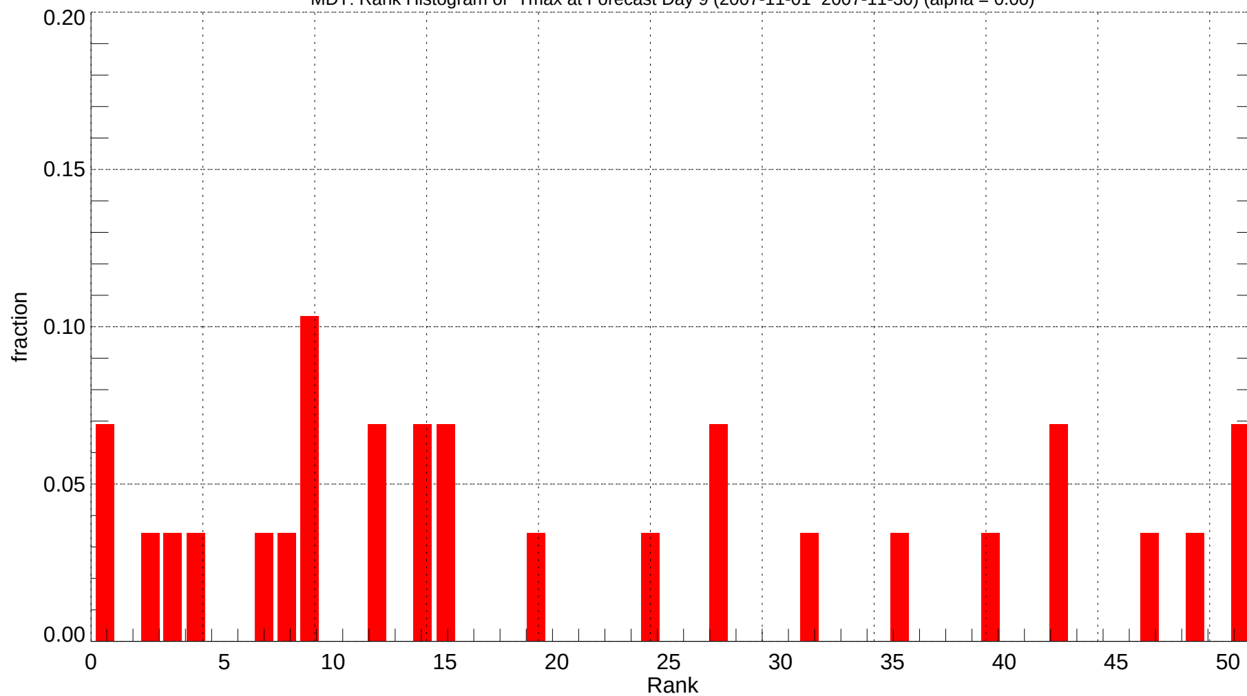
MDT: Rank Histogram of Tmax at Forecast Day 9 (2007-11-01~2007-11-30) (alpha = 0.00)
