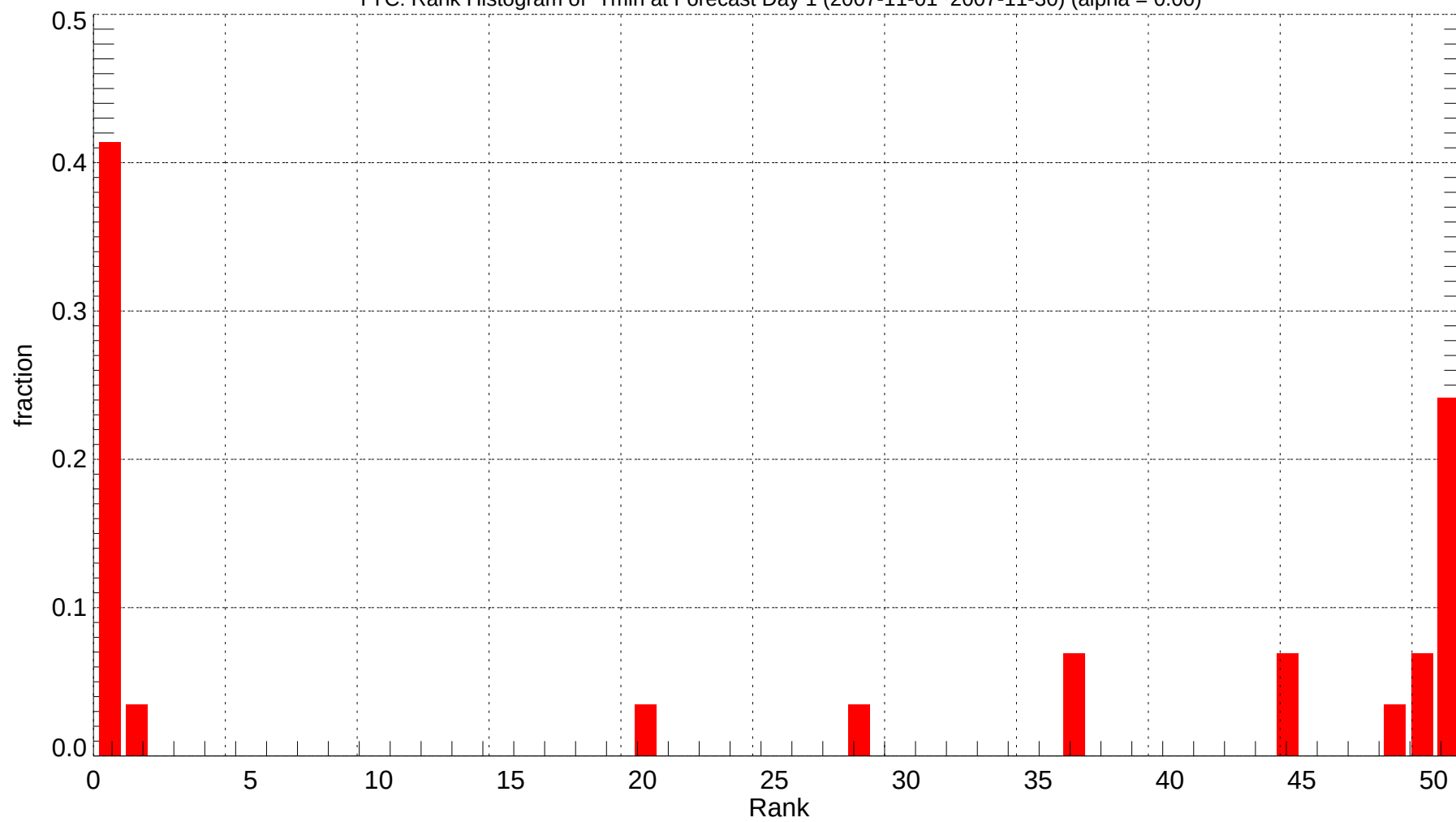
YYC: Rank Histogram of Tmin at Forecast Day 1 (2007-11-01~2007-11-30) (alpha = 0.00)
