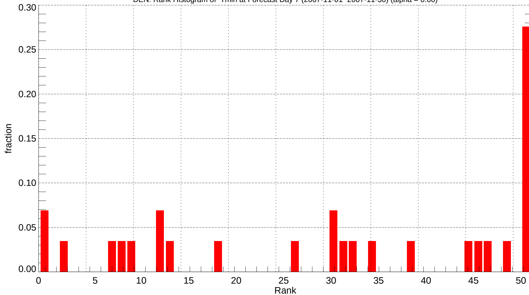
DEN: Rank Histogram of Tmin at Forecast Day 7 (2007-11-01~2007-11-30) (alpha = 0.00)
