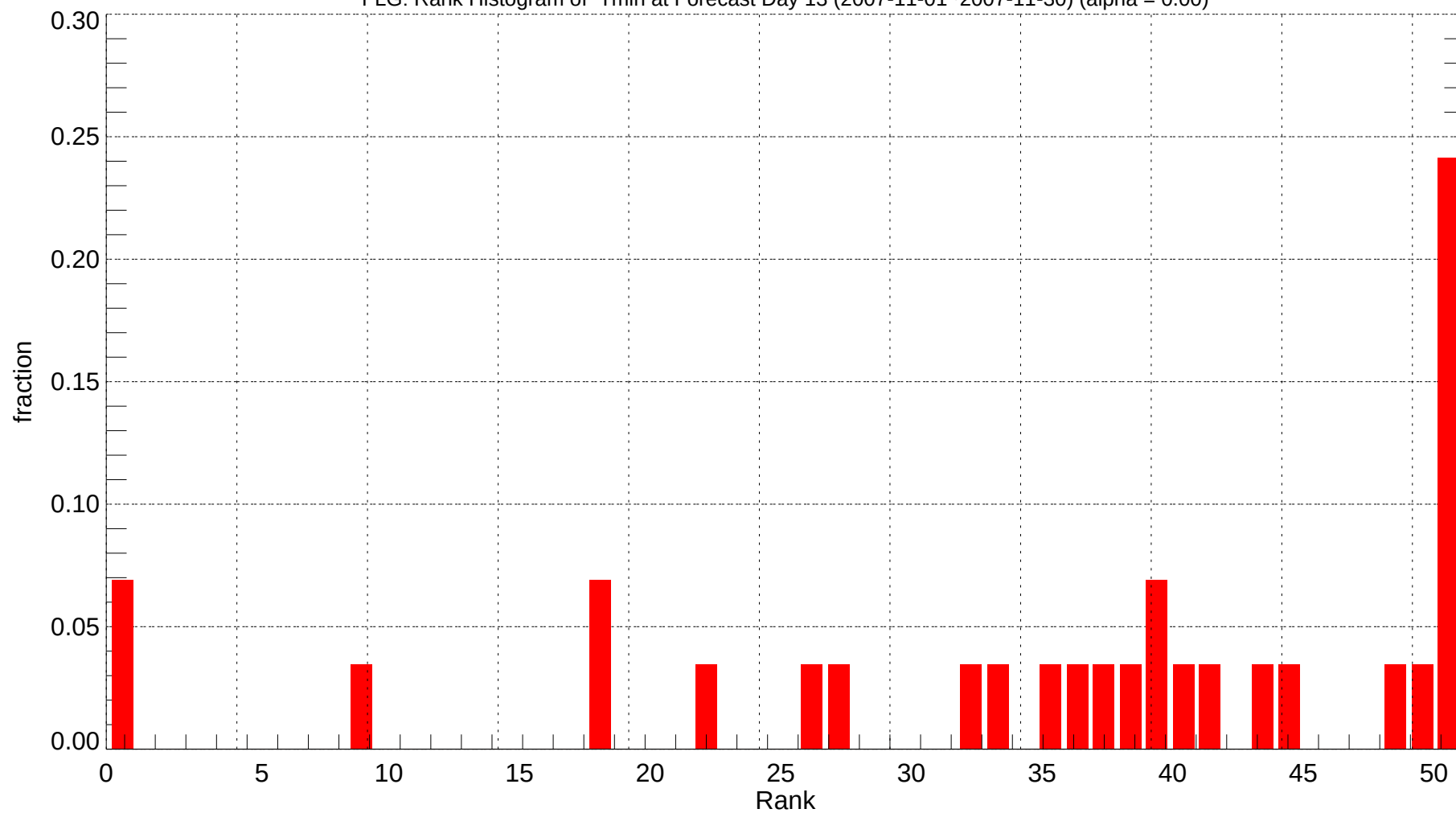
FLG: Rank Histogram of Tmin at Forecast Day 13 (2007-11-01~2007-11-30) (alpha = 0.00)
