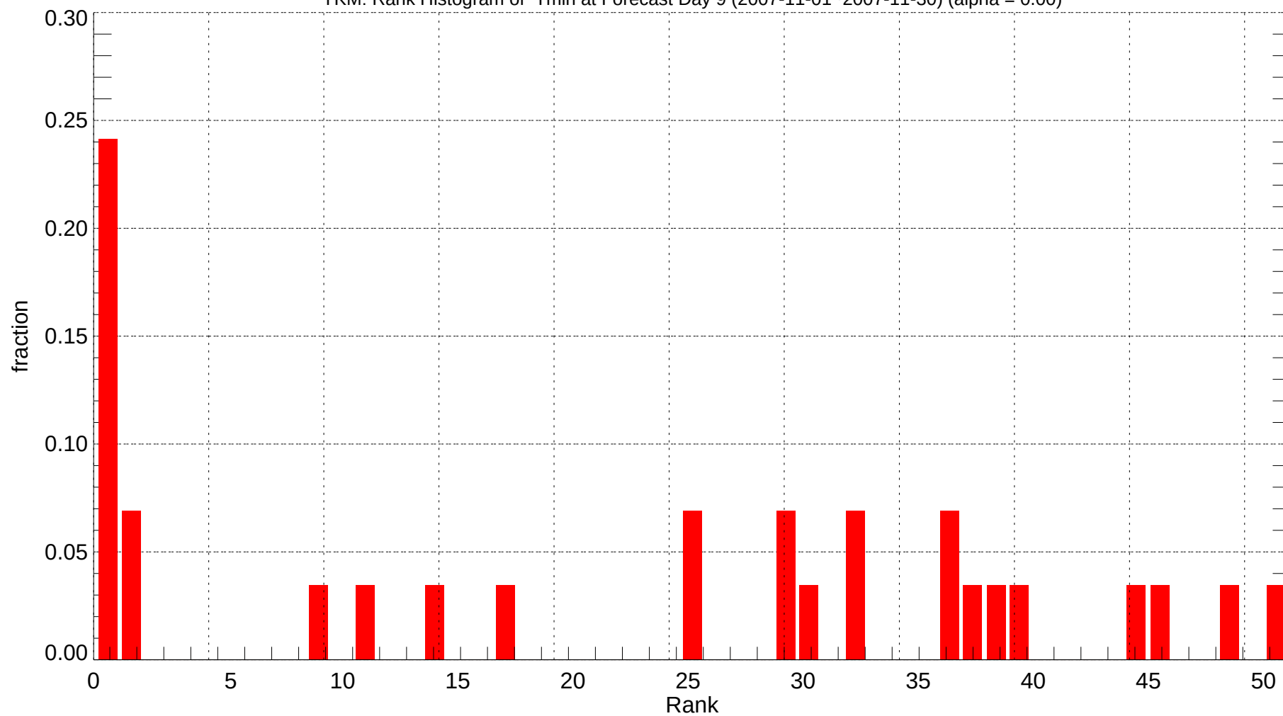
YKM: Rank Histogram of Tmin at Forecast Day 9 (2007-11-01~2007-11-30) (alpha = 0.00)
