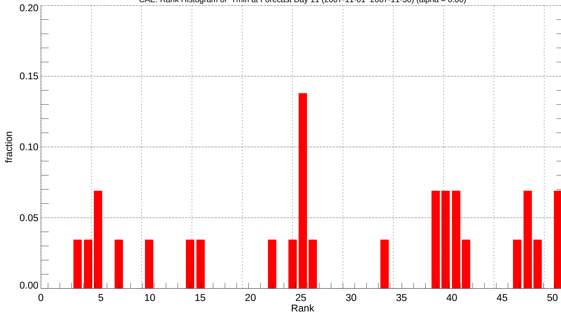
CAE: Rank Histogram of Tmin at Forecast Day 11 (2007-11-01~2007-11-30) (alpha = 0.00)
