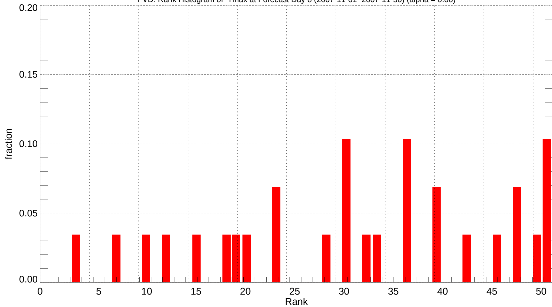
PVD: Rank Histogram of Tmax at Forecast Day 8 (2007-11-01~2007-11-30) (alpha = 0.00)
