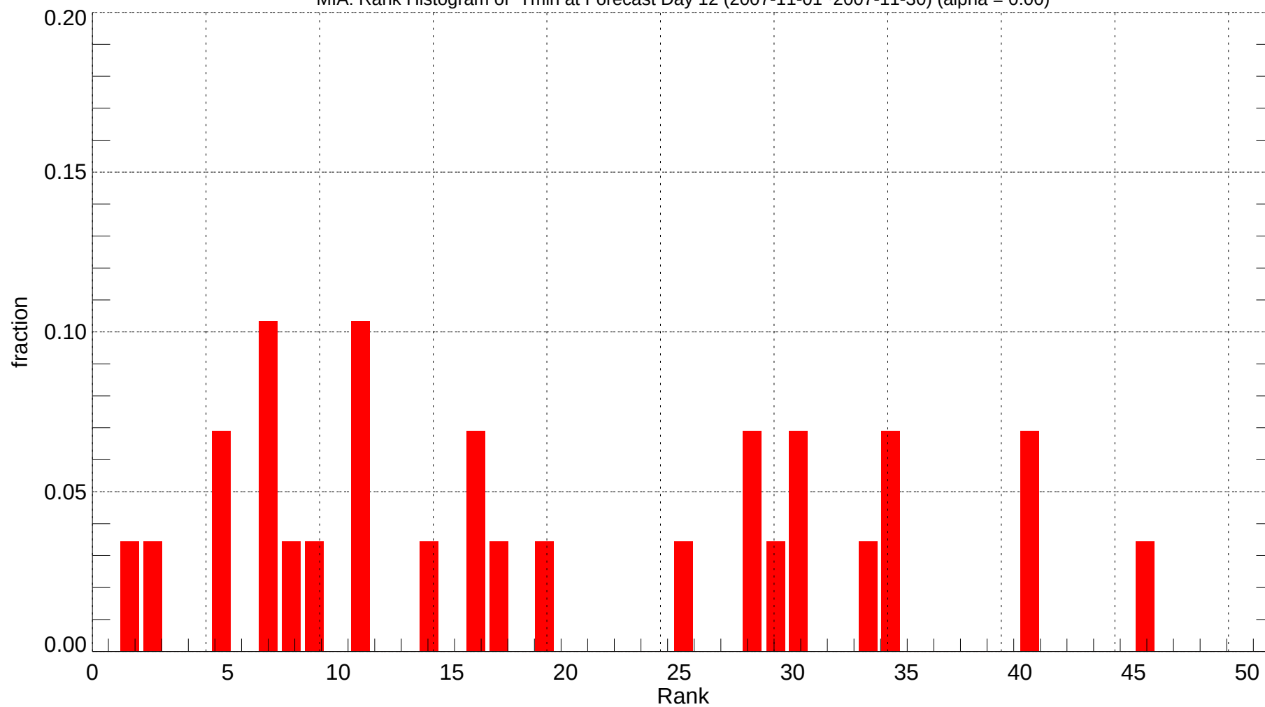
MIA: Rank Histogram of Tmin at Forecast Day 12 (2007-11-01~2007-11-30) (alpha = 0.00)
