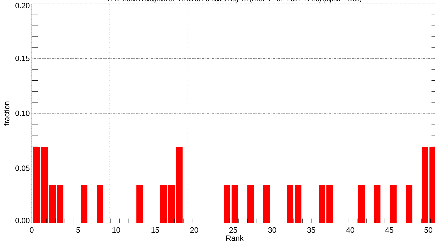
LFK: Rank Histogram of Tmax at Forecast Day 15 (2007-11-01~2007-11-30) (alpha = 0.00)
