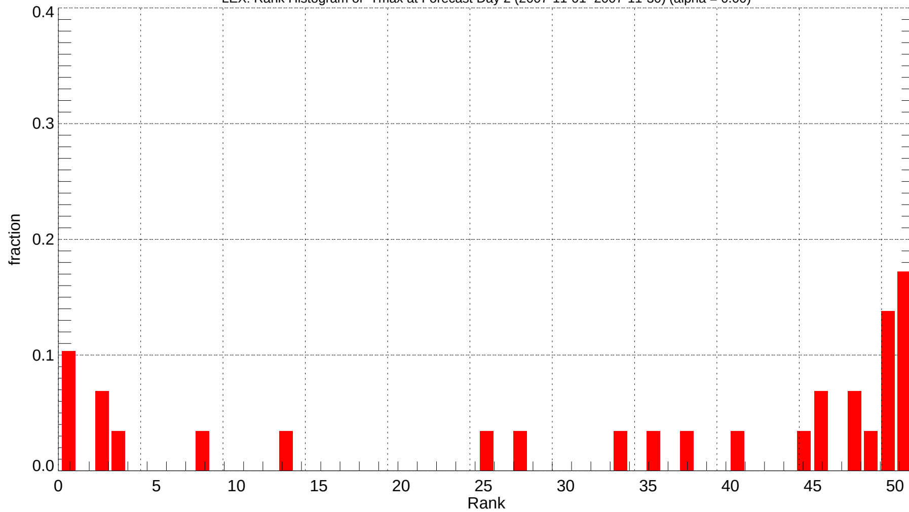
LEX: Rank Histogram of Tmax at Forecast Day 2 (2007-11-01~2007-11-30) (alpha = 0.00)
