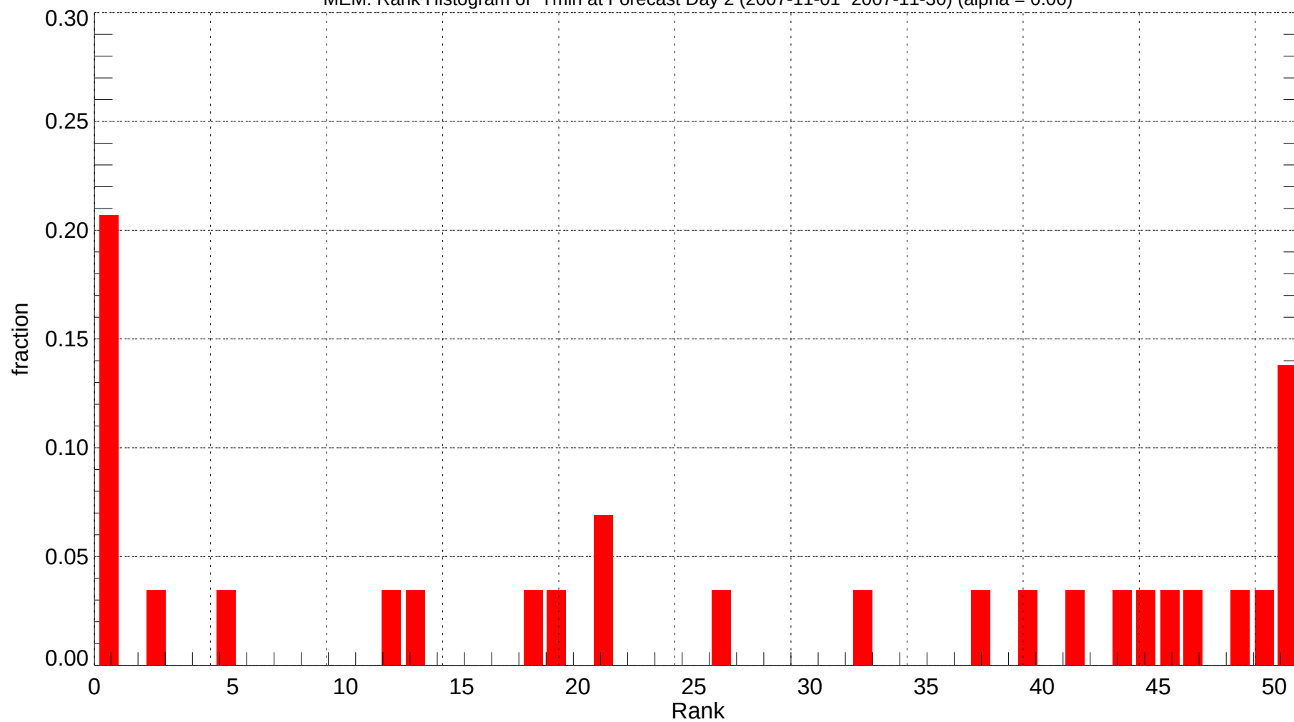
MEM: Rank Histogram of Tmin at Forecast Day 2 (2007-11-01~2007-11-30) (alpha = 0.00)
