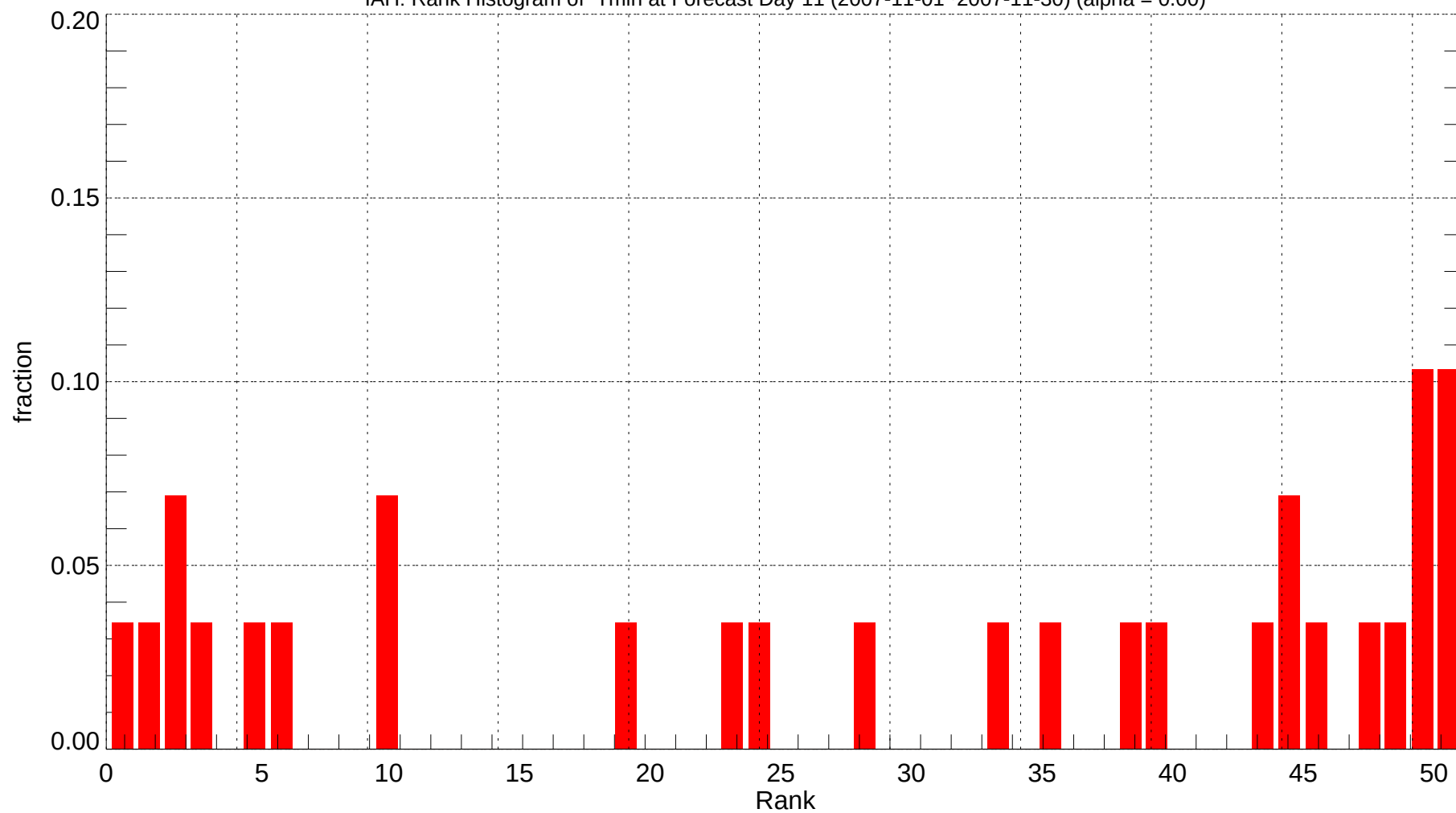
IAH: Rank Histogram of Tmin at Forecast Day 11 (2007-11-01~2007-11-30) (alpha = 0.00)
