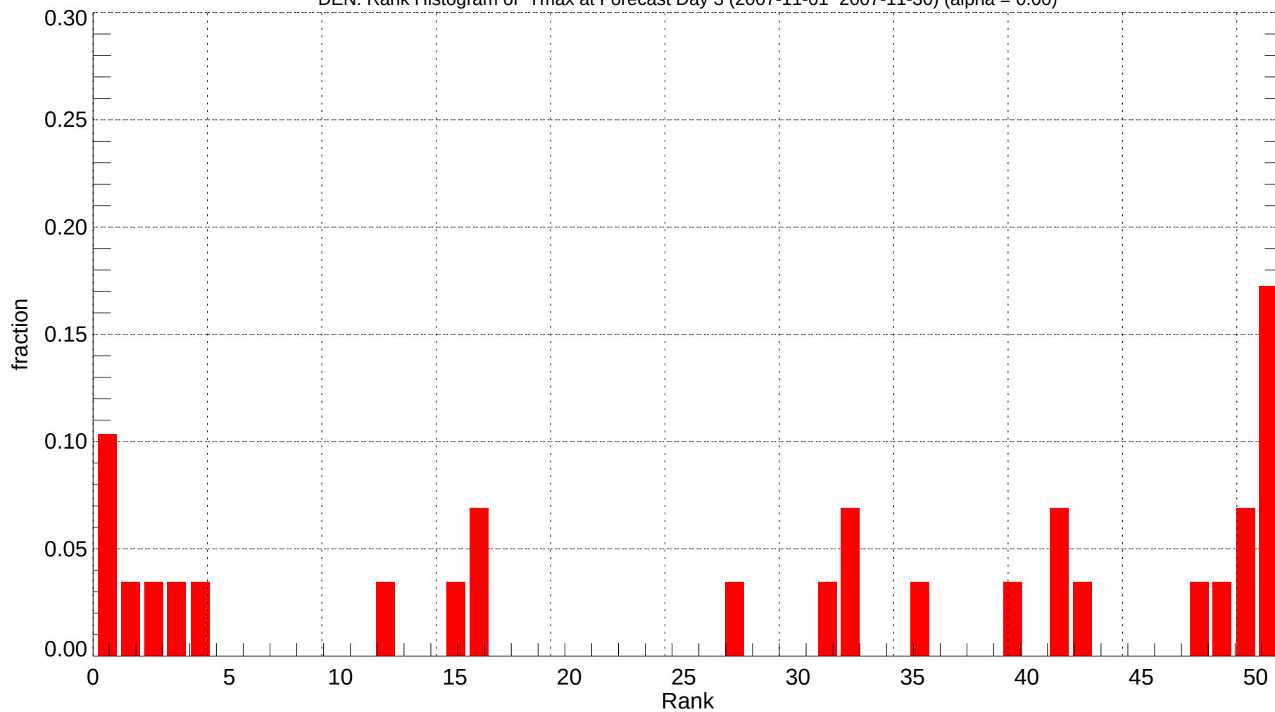
DEN: Rank Histogram of Tmax at Forecast Day 3 (2007-11-01~2007-11-30) (alpha = 0.00)
