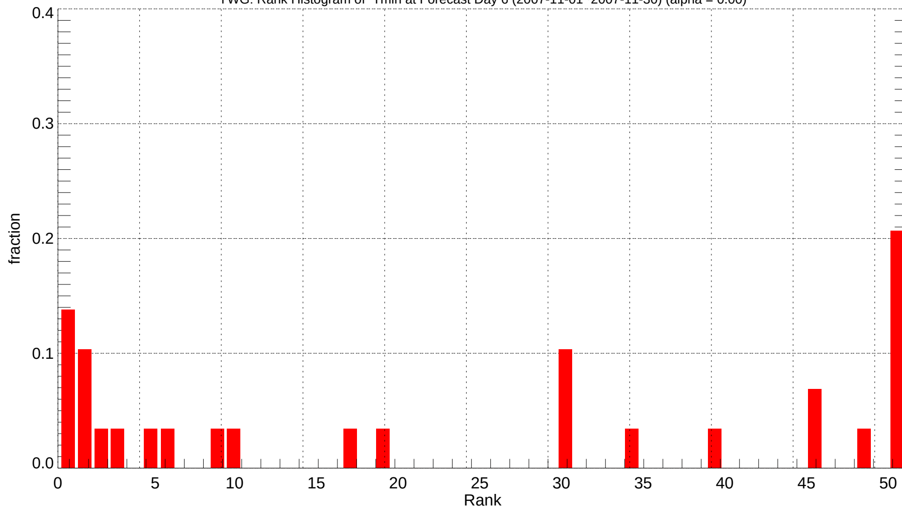
YWG: Rank Histogram of Tmin at Forecast Day 6 (2007-11-01~2007-11-30) (alpha = 0.00)
