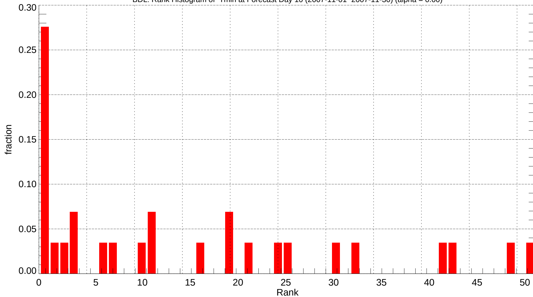
BDL: Rank Histogram of Tmin at Forecast Day 10 (2007-11-01~2007-11-30) (alpha = 0.00)
