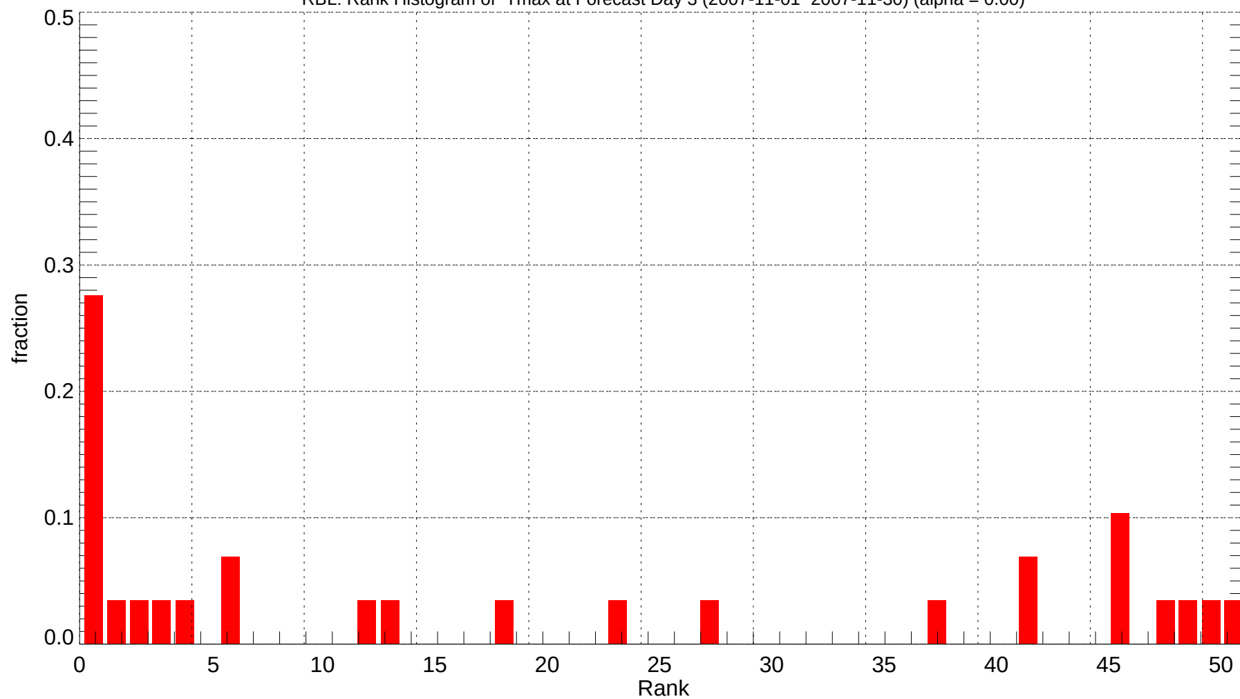
RBL: Rank Histogram of Tmax at Forecast Day 3 (2007-11-01~2007-11-30) (alpha = 0.00)
