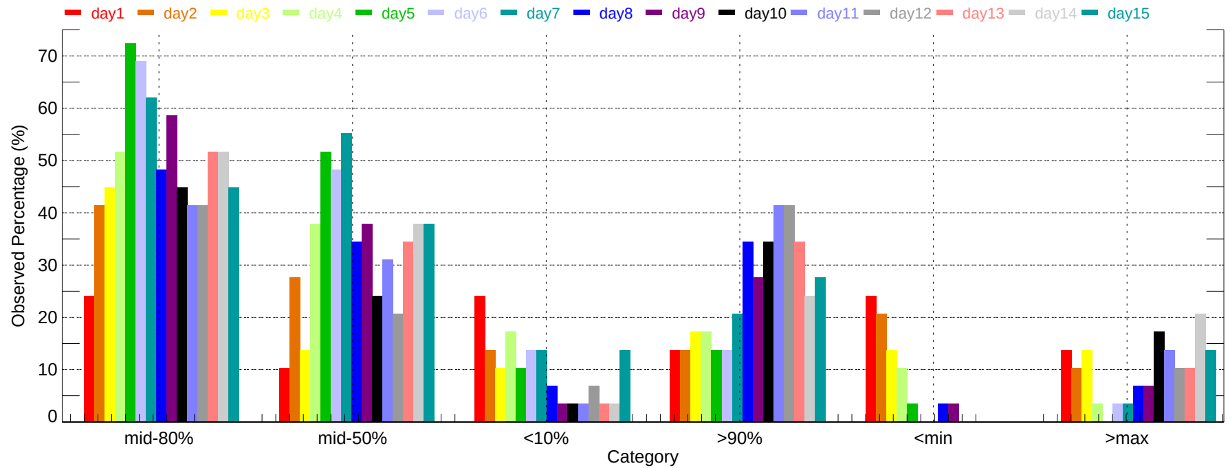
Observed Percentage of Ensembles - TYR: Max Temperature (2007-11-01~2007-11-30)
