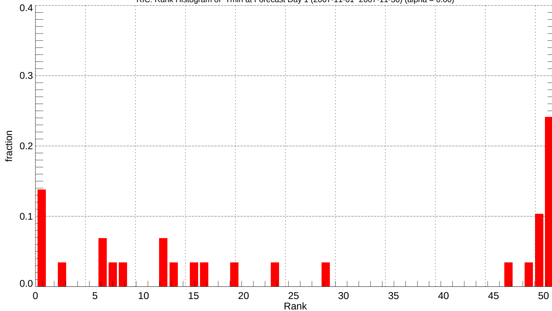
RIC: Rank Histogram of Tmin at Forecast Day 1 (2007-11-01~2007-11-30) (alpha = 0.00)
