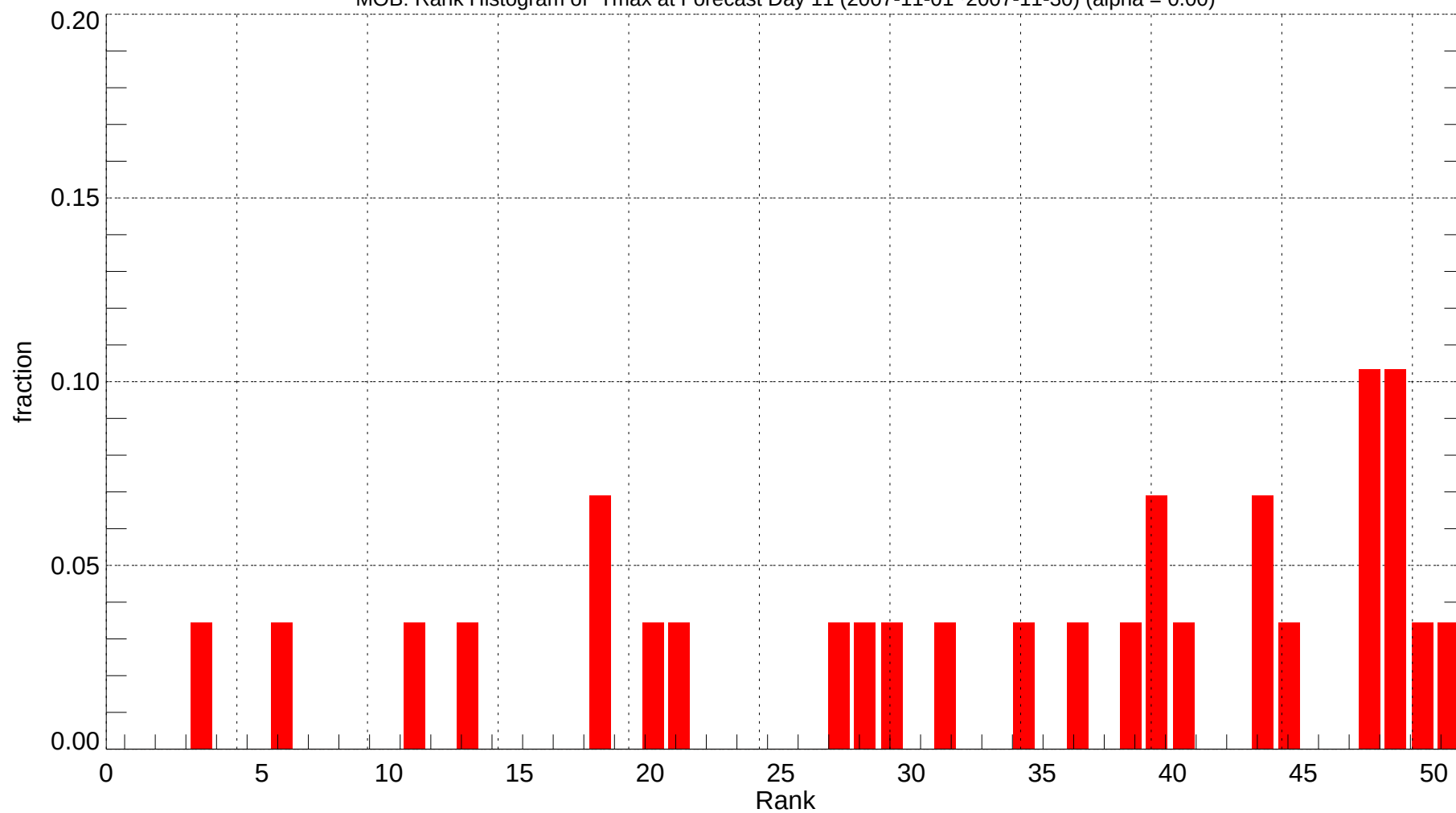
MOB: Rank Histogram of Tmax at Forecast Day 11 (2007-11-01~2007-11-30) (alpha = 0.00)
