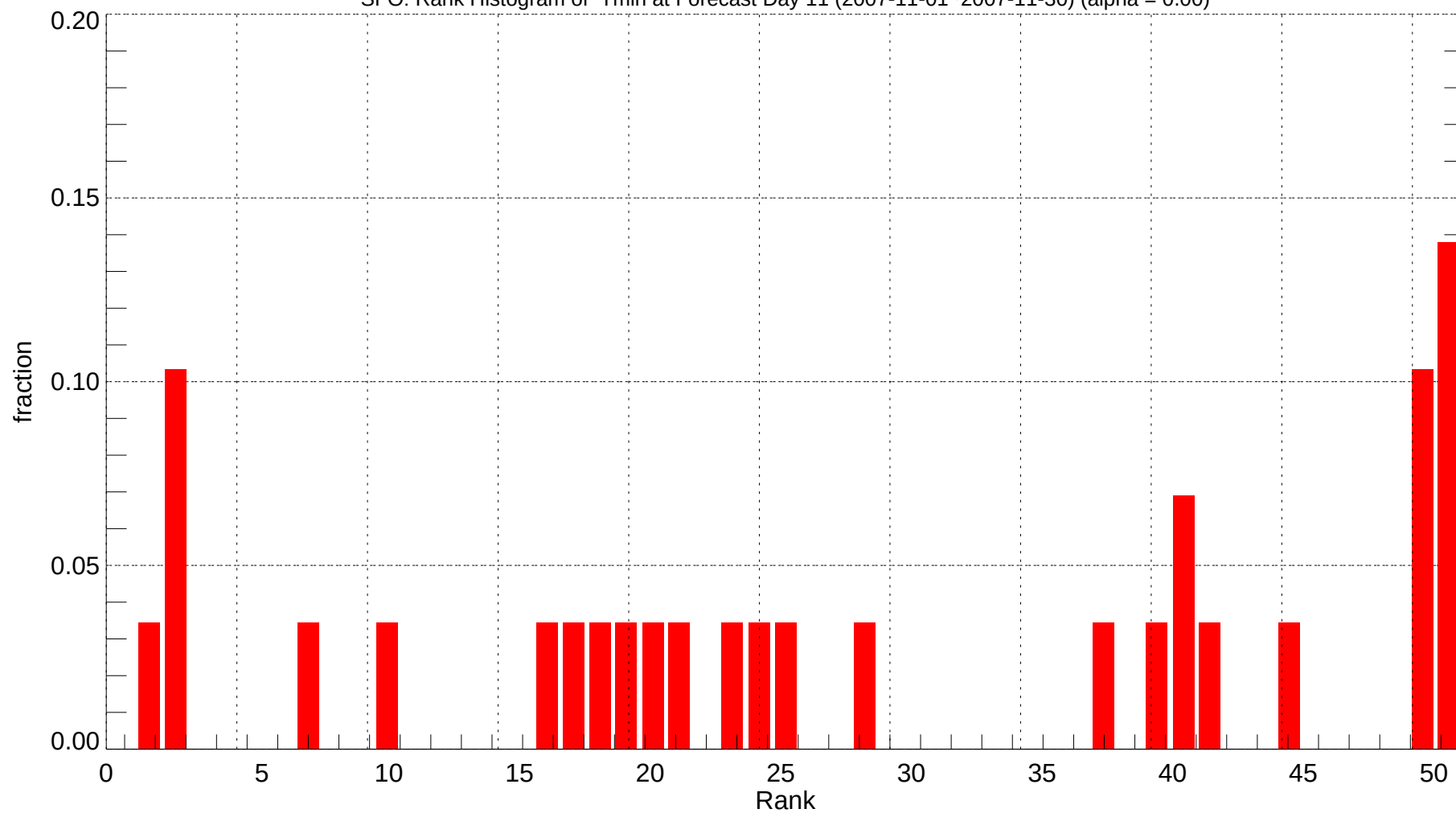
SFO: Rank Histogram of Tmin at Forecast Day 11 (2007-11-01~2007-11-30) (alpha = 0.00)
