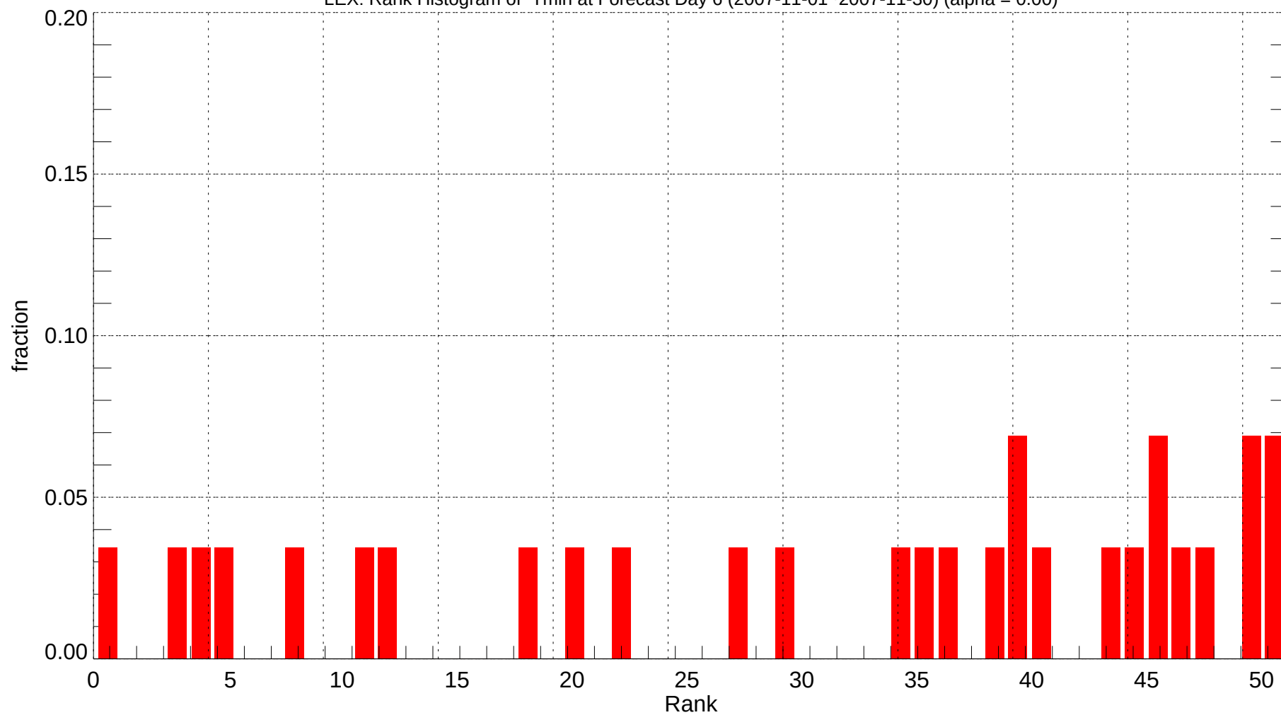
LEX: Rank Histogram of Tmin at Forecast Day 6 (2007-11-01~2007-11-30) (alpha = 0.00)
