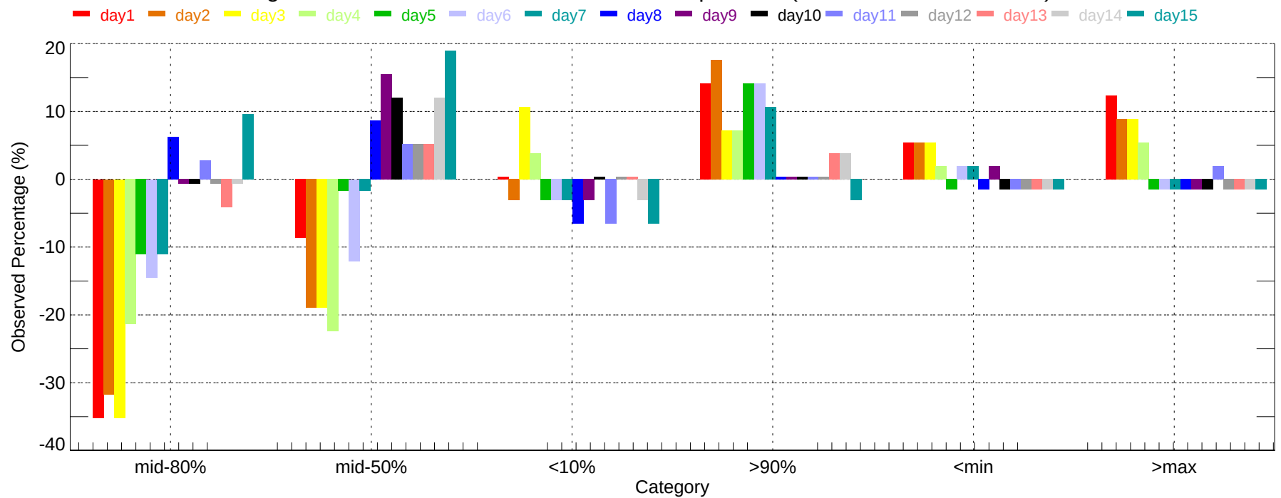
Observed Percentage Deviation of Ensembles - BOI: Min Temperature (2007-11-01~2007-11-30)
