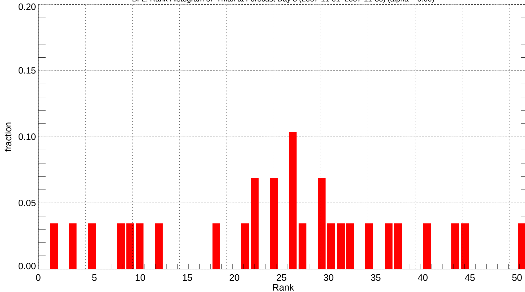
BFL: Rank Histogram of Tmax at Forecast Day 5 (2007-11-01~2007-11-30) (alpha = 0.00)
