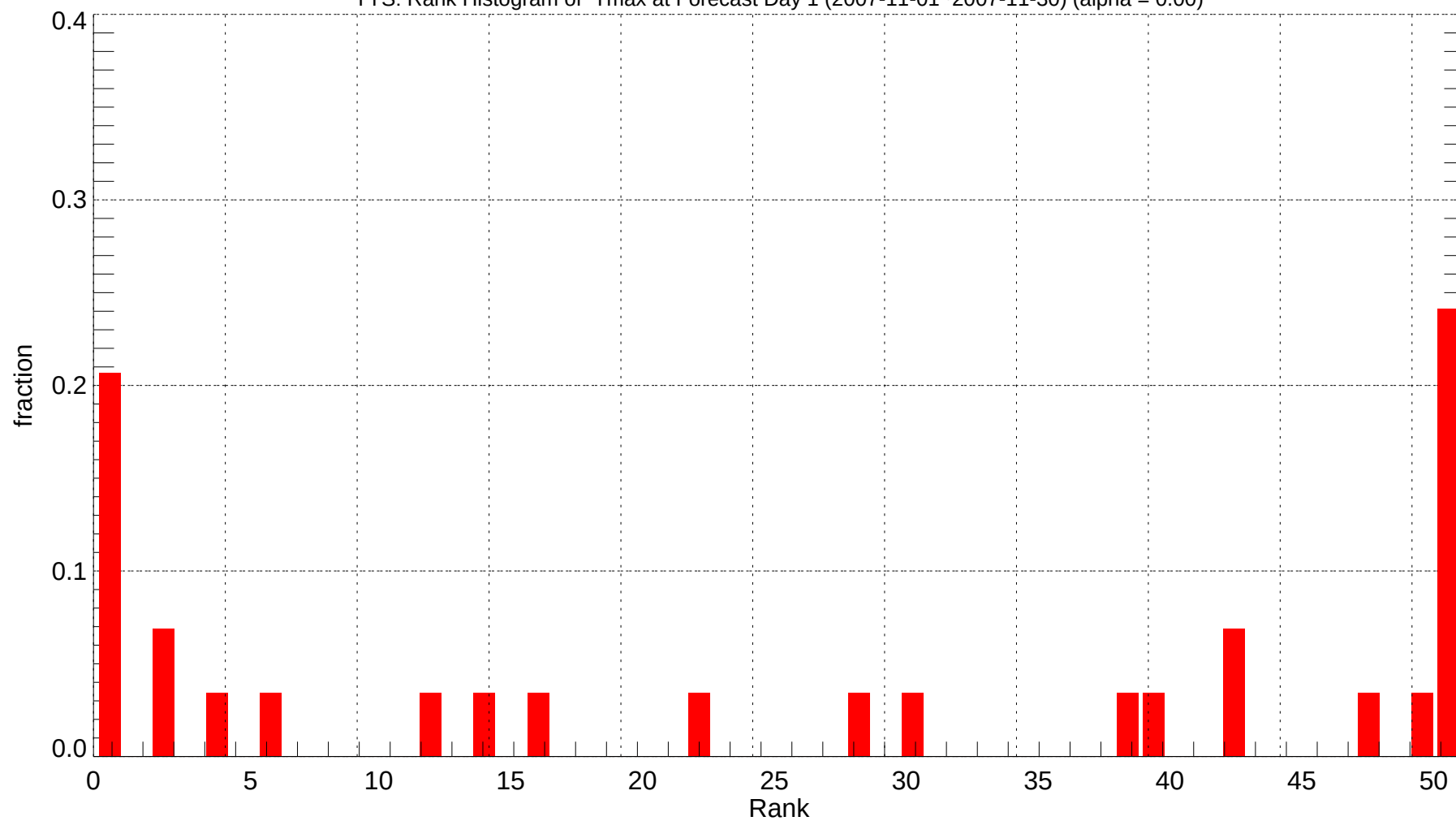
TYS: Rank Histogram of Tmax at Forecast Day 1 (2007-11-01~2007-11-30) (alpha = 0.00)
