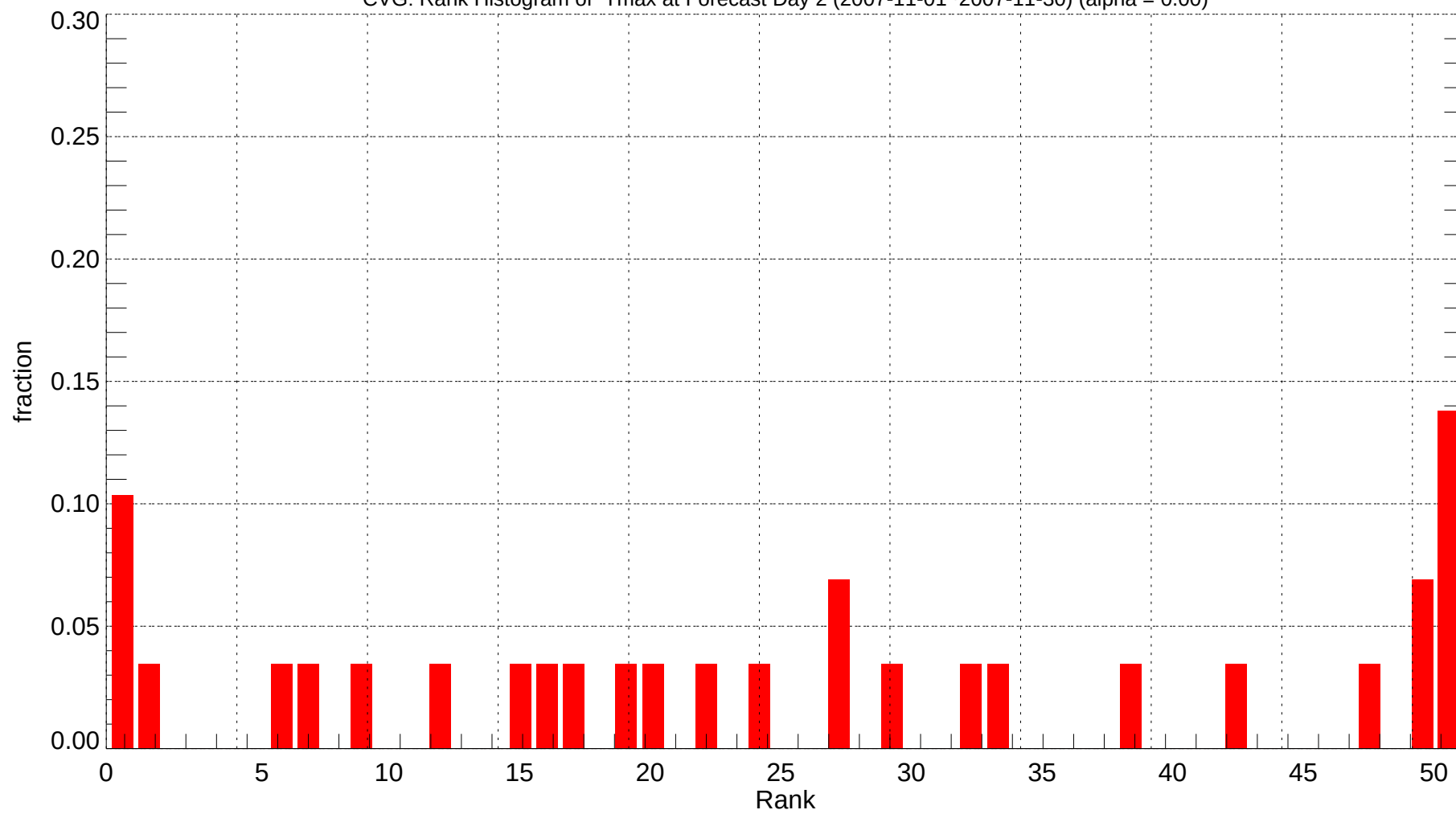
CVG: Rank Histogram of Tmax at Forecast Day 2 (2007-11-01~2007-11-30) (alpha = 0.00)
