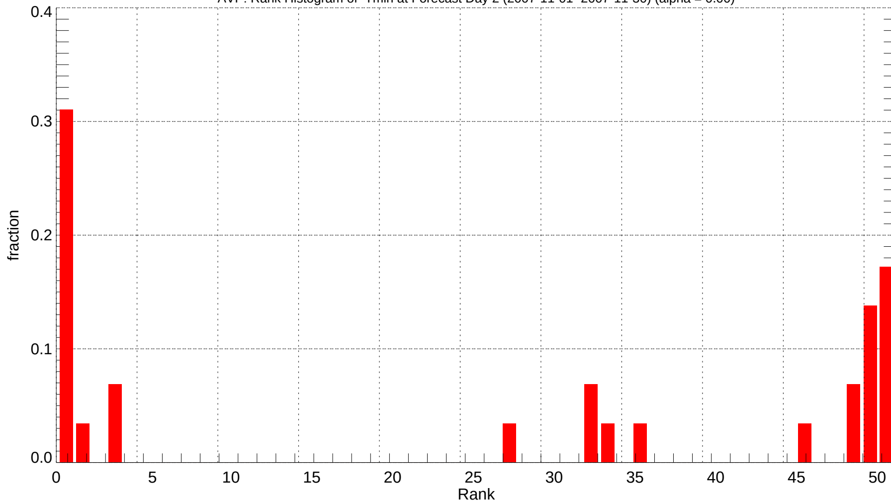
AVP: Rank Histogram of Tmin at Forecast Day 2 (2007-11-01~2007-11-30) (alpha = 0.00)
