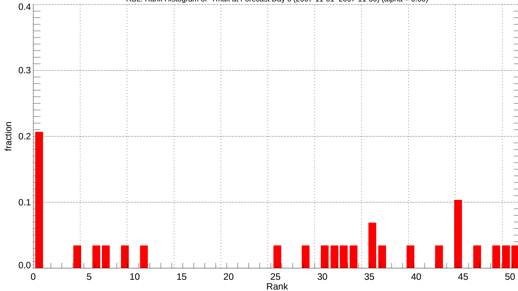
RBL: Rank Histogram of Tmax at Forecast Day 6 (2007-11-01~2007-11-30) (alpha = 0.00)
