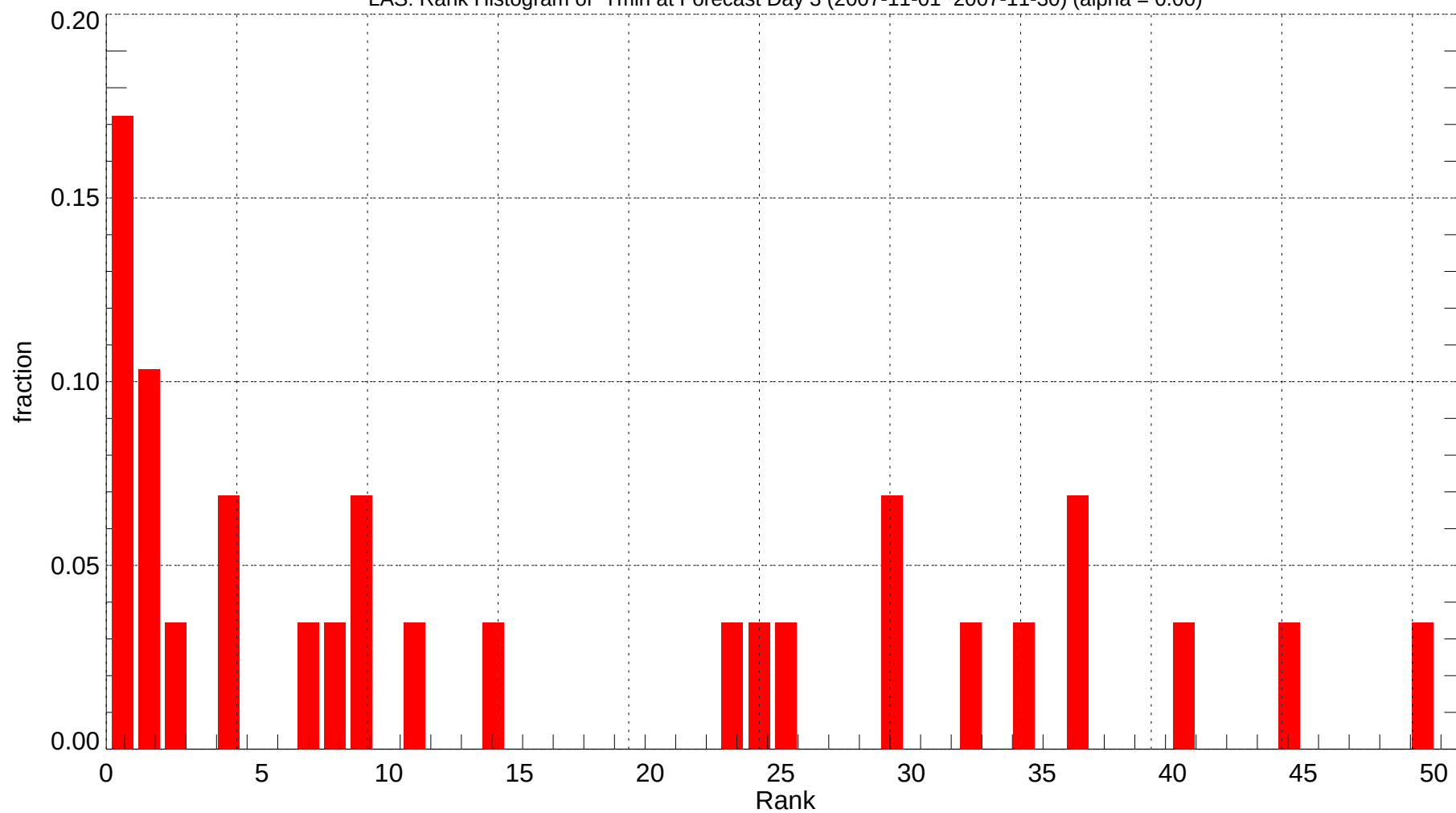
LAS: Rank Histogram of Tmin at Forecast Day 3 (2007-11-01~2007-11-30) (alpha = 0.00)
