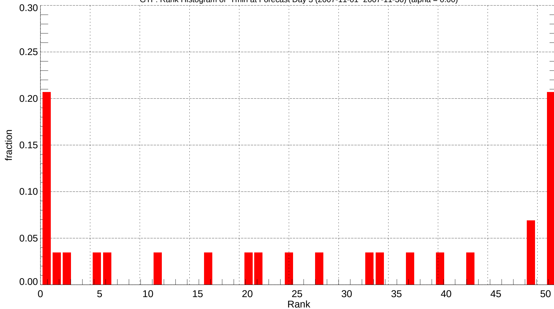
GTF: Rank Histogram of Tmin at Forecast Day 3 (2007-11-01~2007-11-30) (alpha = 0.00)
