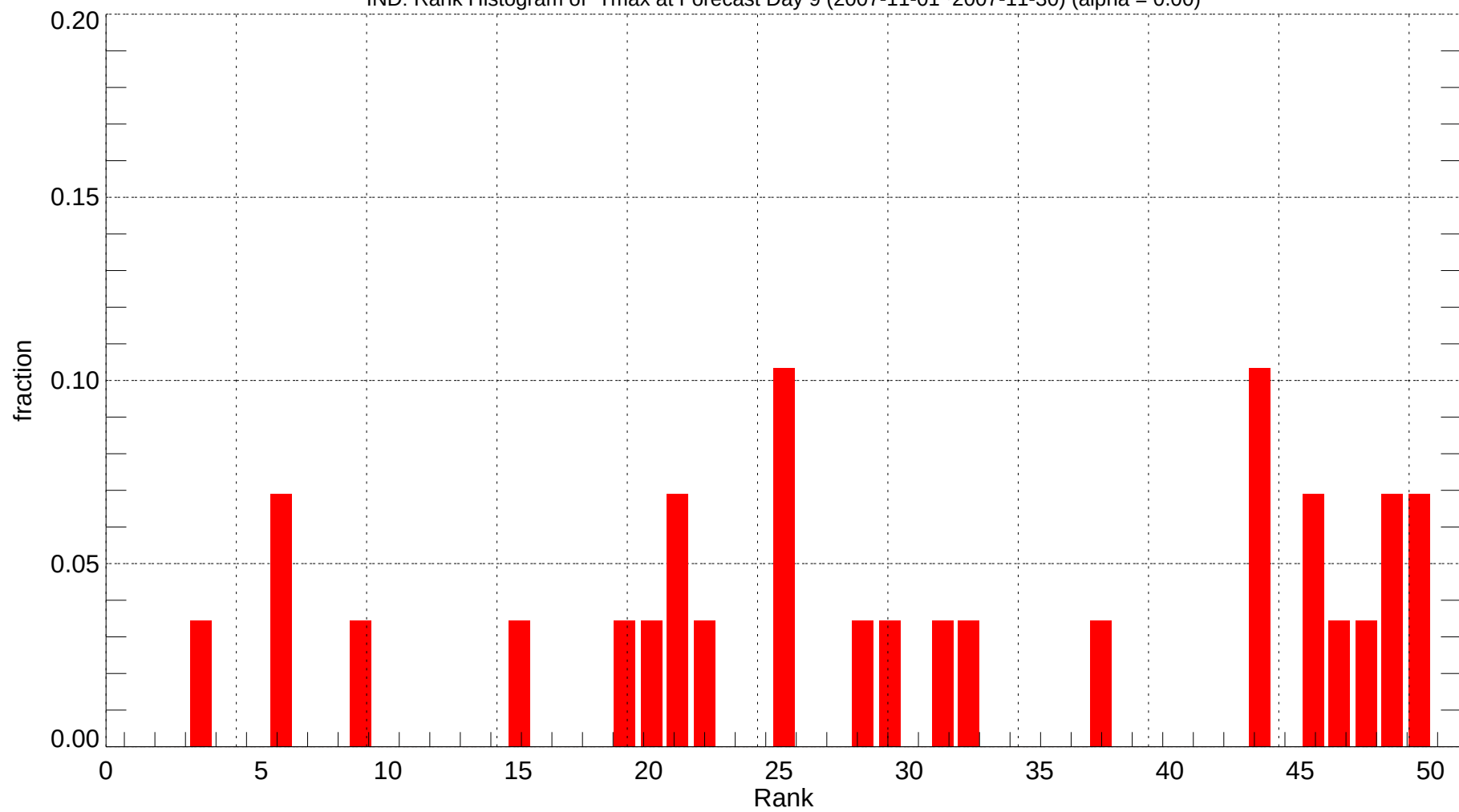
IND: Rank Histogram of Tmax at Forecast Day 9 (2007-11-01~2007-11-30) (alpha = 0.00)
