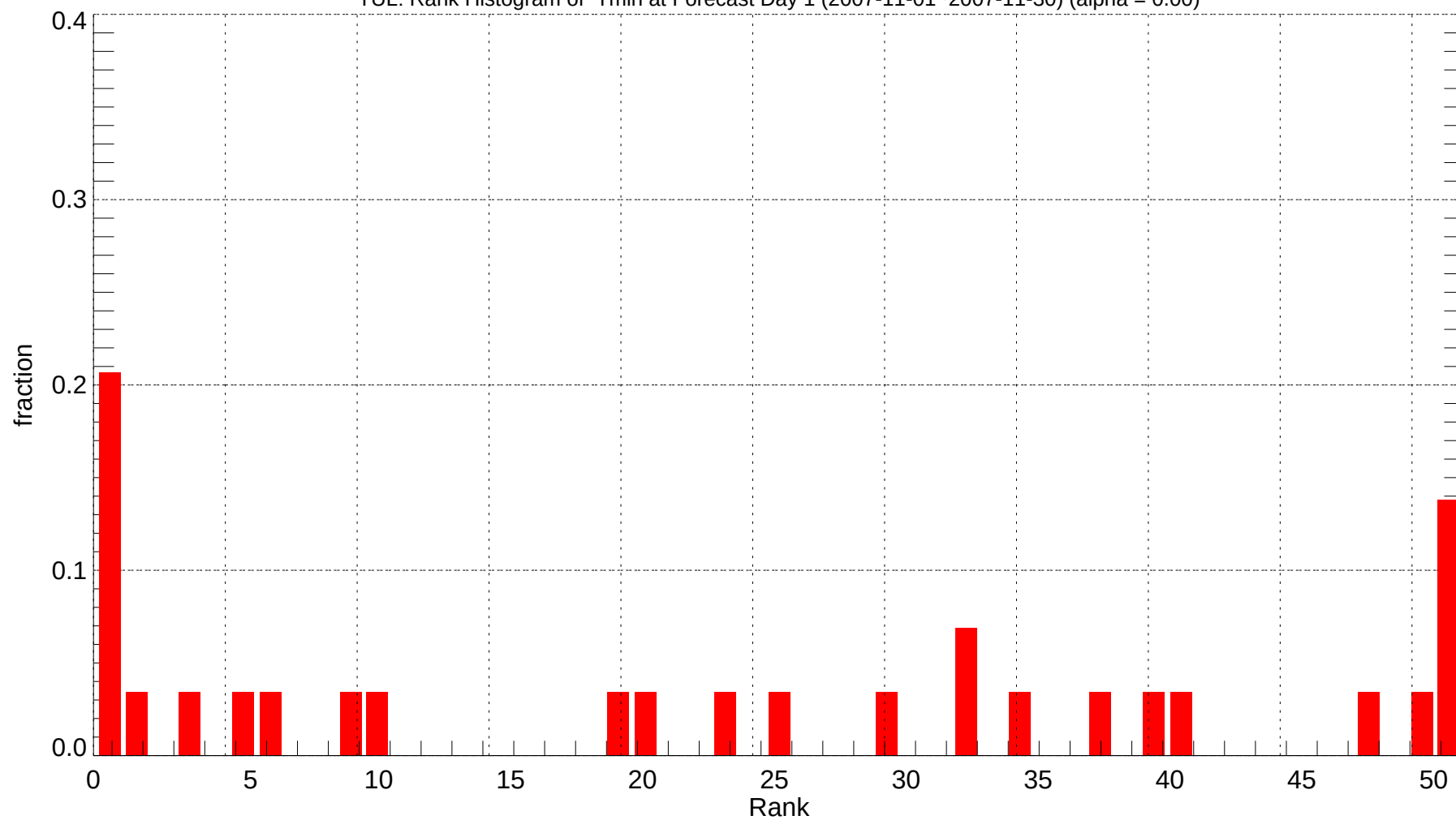
TUL: Rank Histogram of Tmin at Forecast Day 1 (2007-11-01~2007-11-30) (alpha = 0.00)
