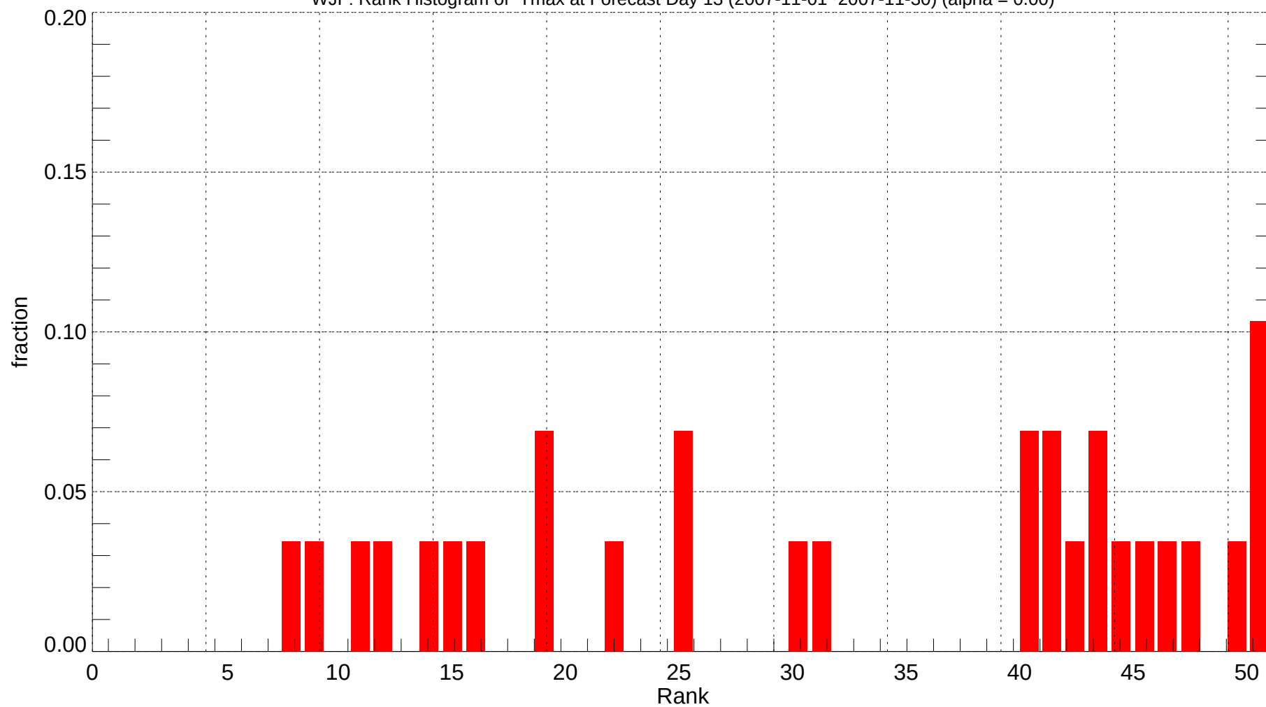
WJF: Rank Histogram of Tmax at Forecast Day 13 (2007-11-01~2007-11-30) (alpha = 0.00)
