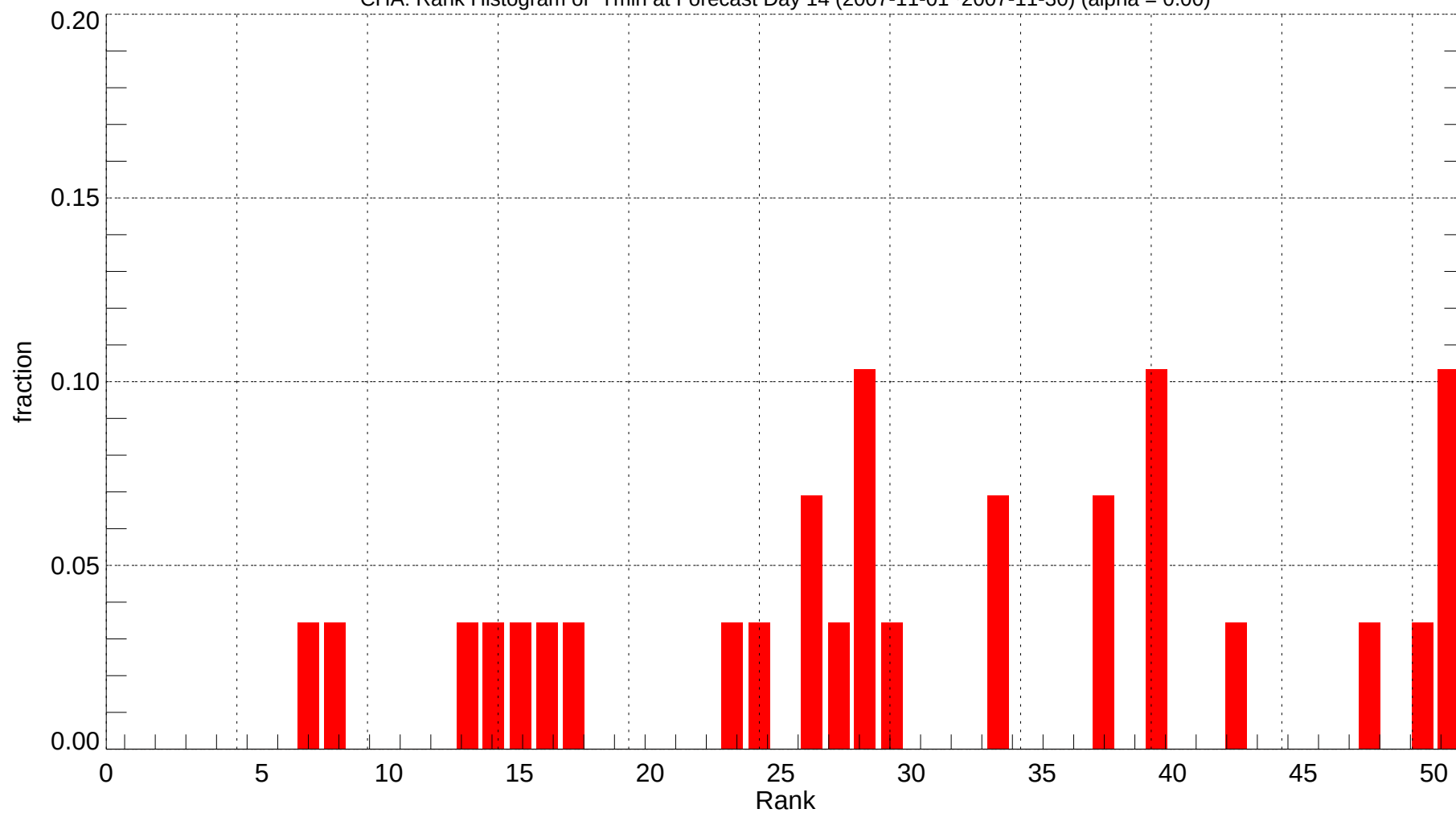
CHA: Rank Histogram of Tmin at Forecast Day 14 (2007-11-01~2007-11-30) (alpha = 0.00)
