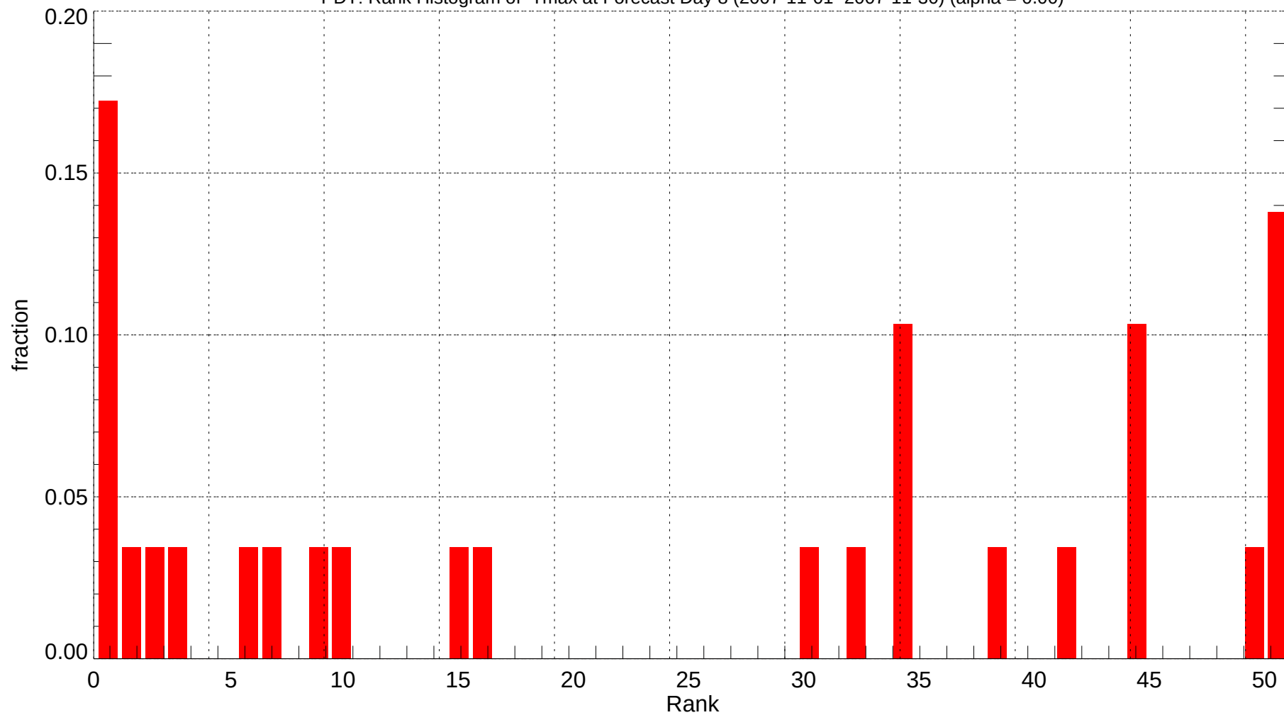
PDT: Rank Histogram of Tmax at Forecast Day 8 (2007-11-01~2007-11-30) (alpha = 0.00)
