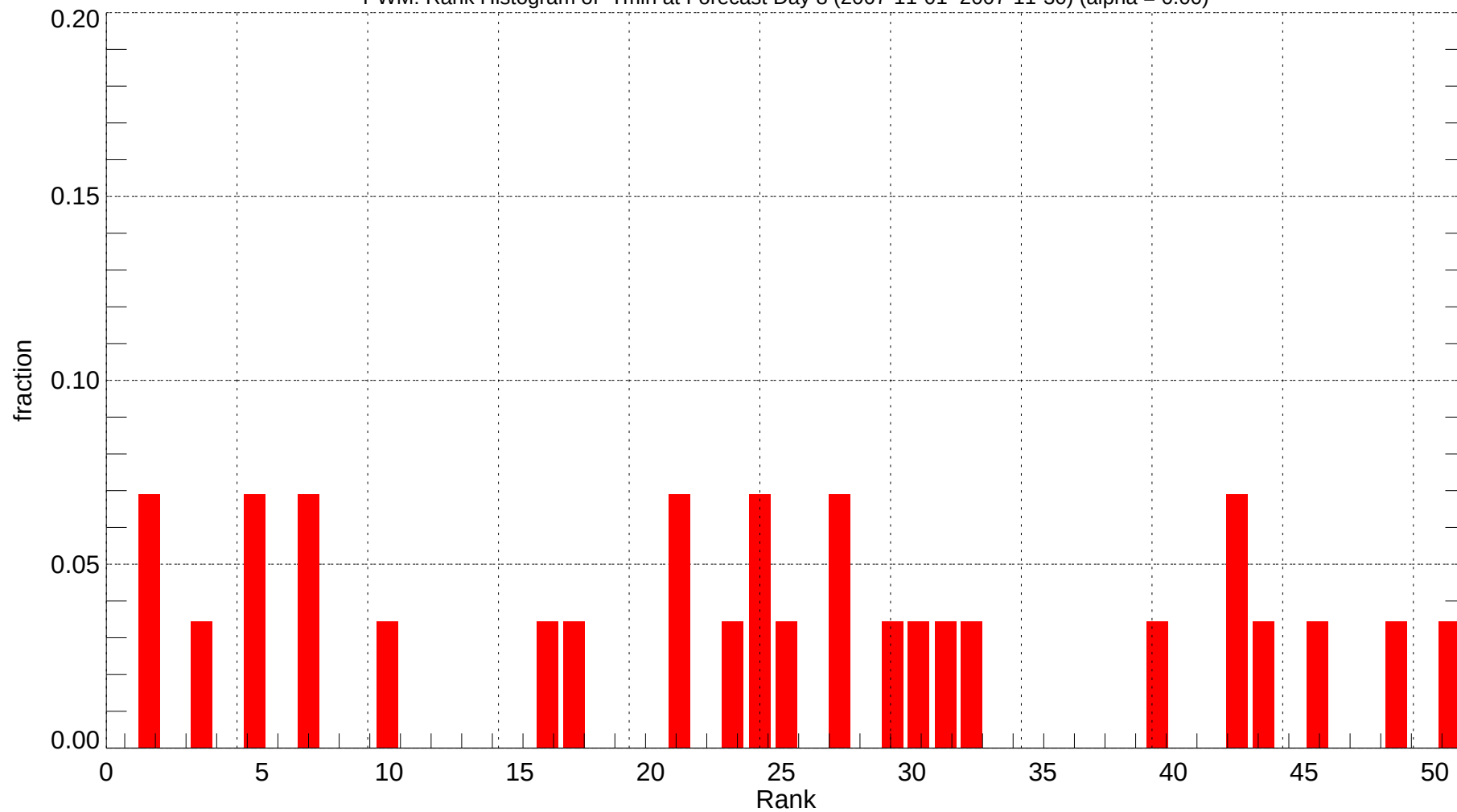
PWM: Rank Histogram of Tmin at Forecast Day 8 (2007-11-01~2007-11-30) (alpha = 0.00)
