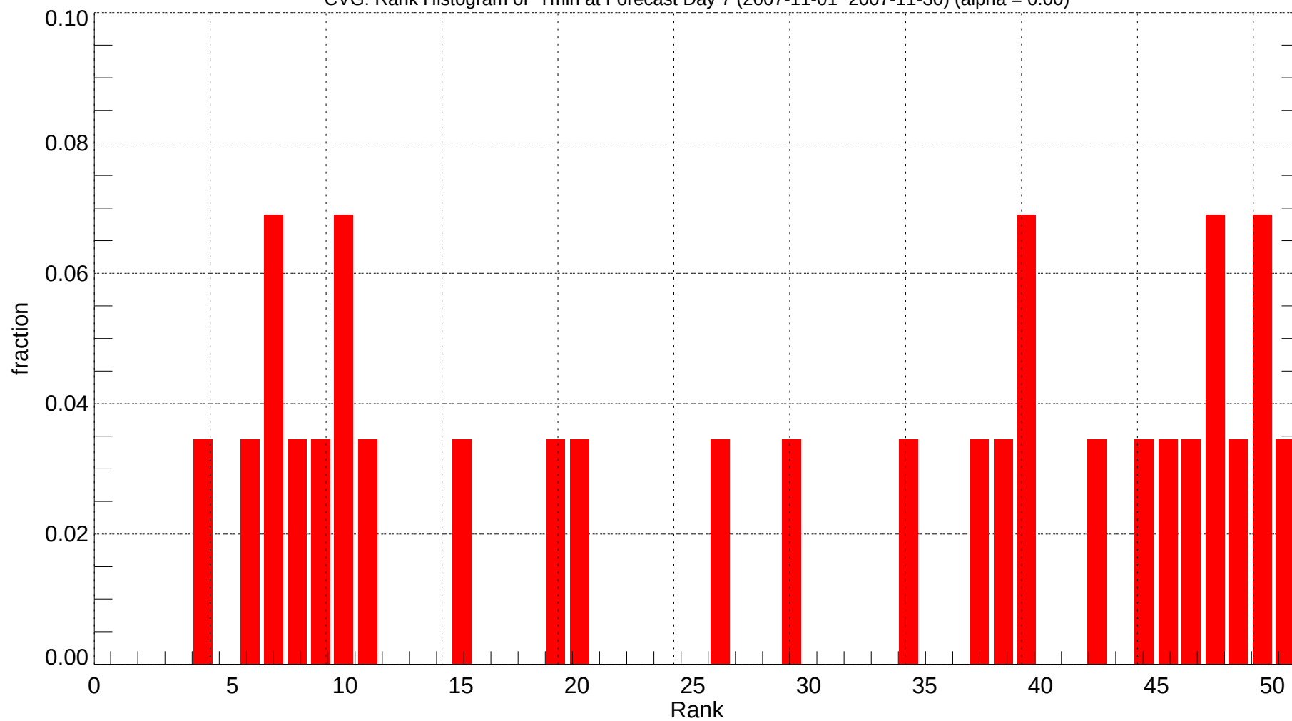
CVG: Rank Histogram of Tmin at Forecast Day 7 (2007-11-01~2007-11-30) (alpha = 0.00)
