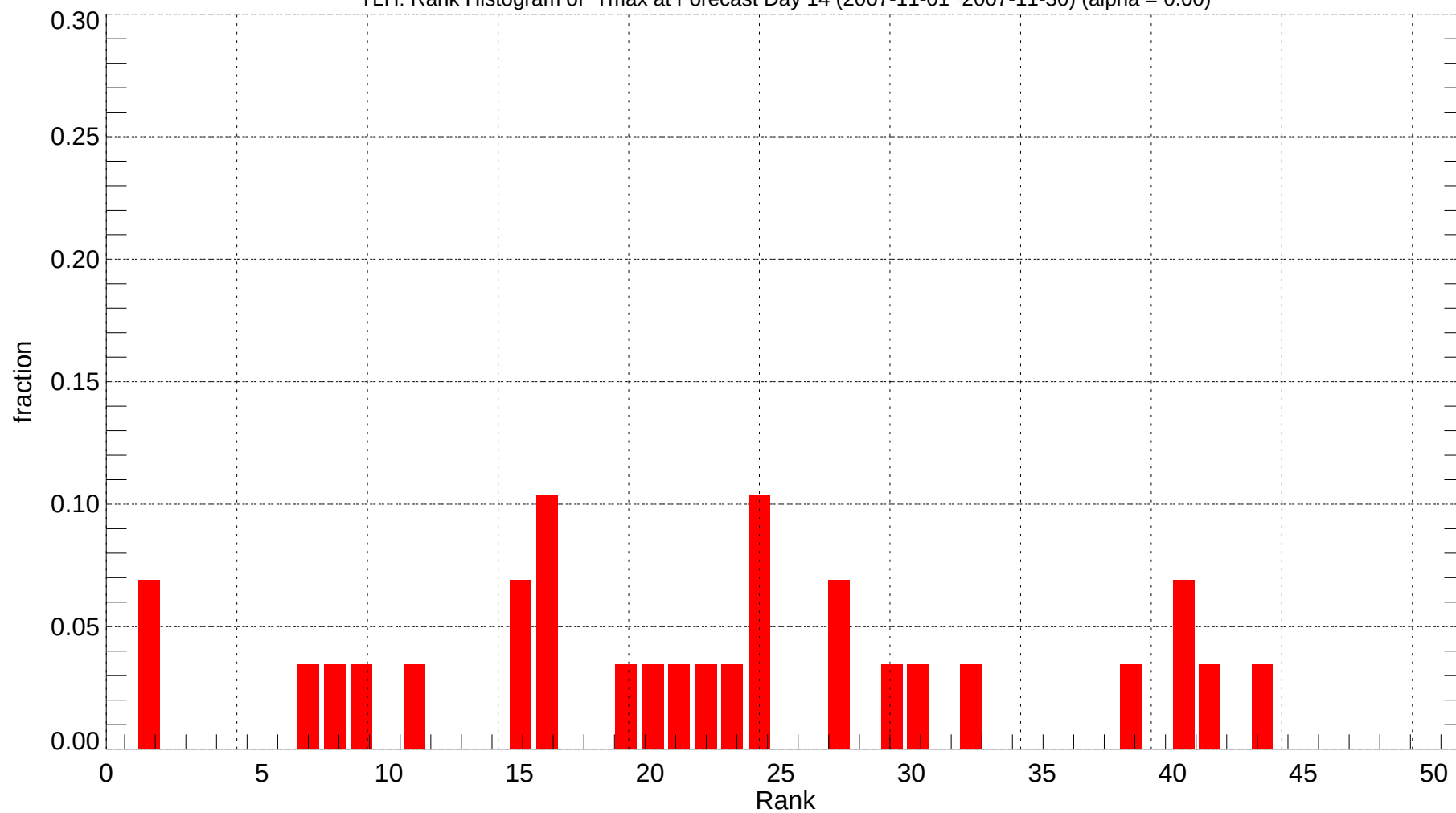
TLH: Rank Histogram of Tmax at Forecast Day 14 (2007-11-01~2007-11-30) (alpha = 0.00)
