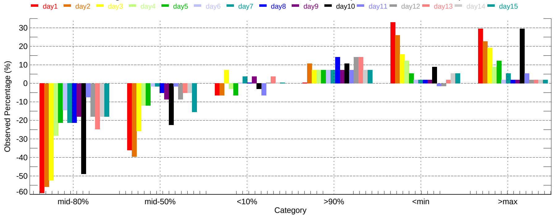
Observed Percentage Deviation of Ensembles - MDT: Max Temperature (2007-11-01~2007-11-30)
