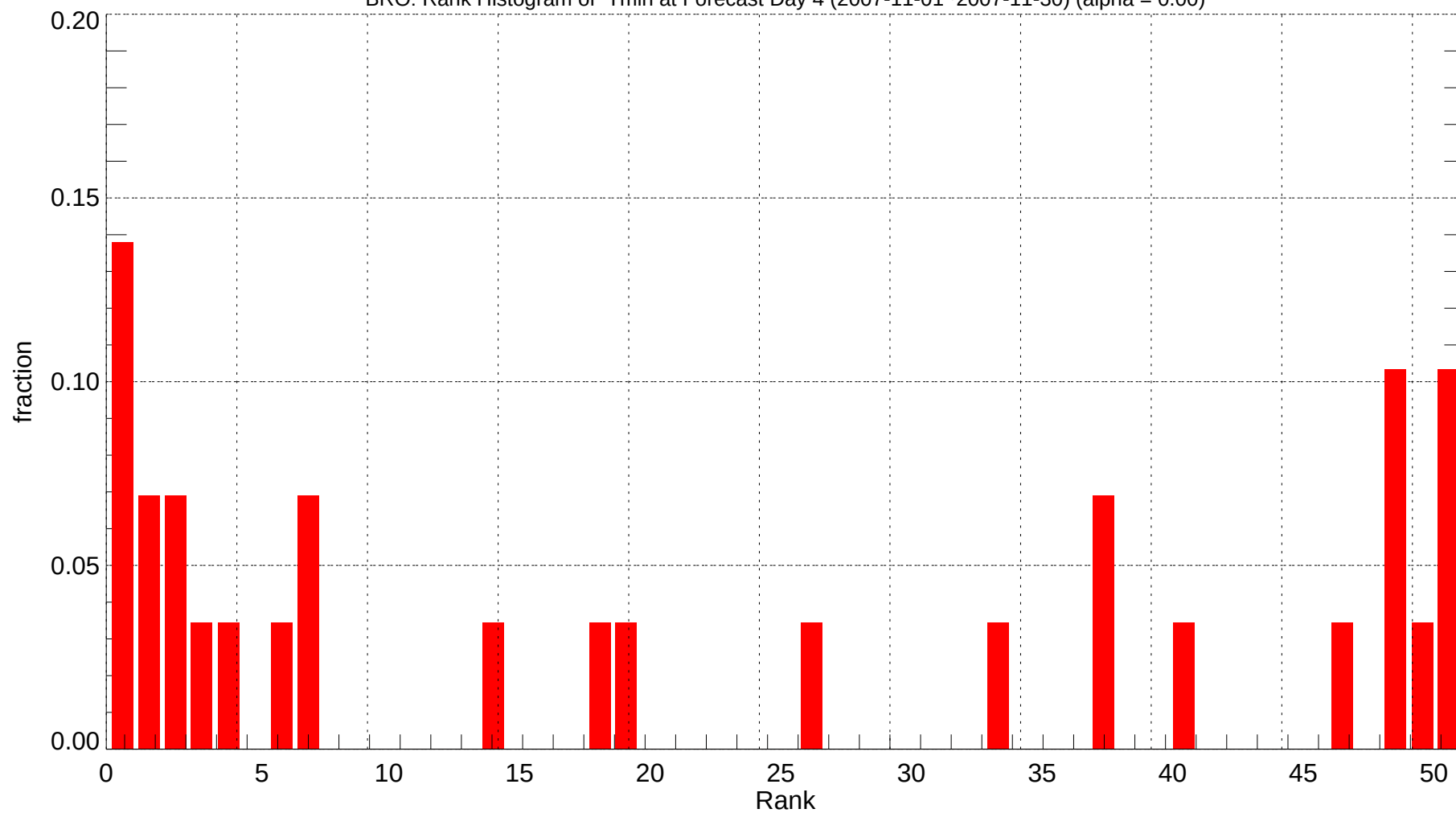
BRO: Rank Histogram of Tmin at Forecast Day 4 (2007-11-01~2007-11-30) (alpha = 0.00)
