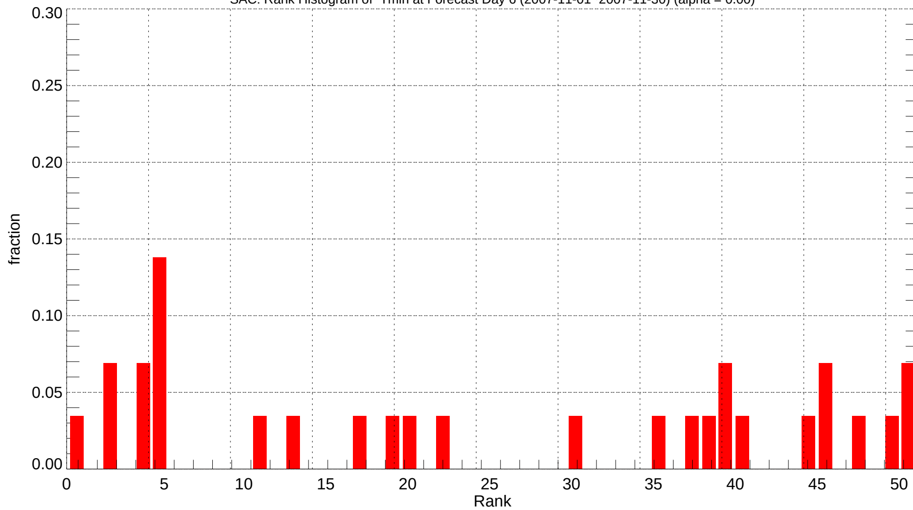
SAC: Rank Histogram of Tmin at Forecast Day 6 (2007-11-01~2007-11-30) (alpha = 0.00)
