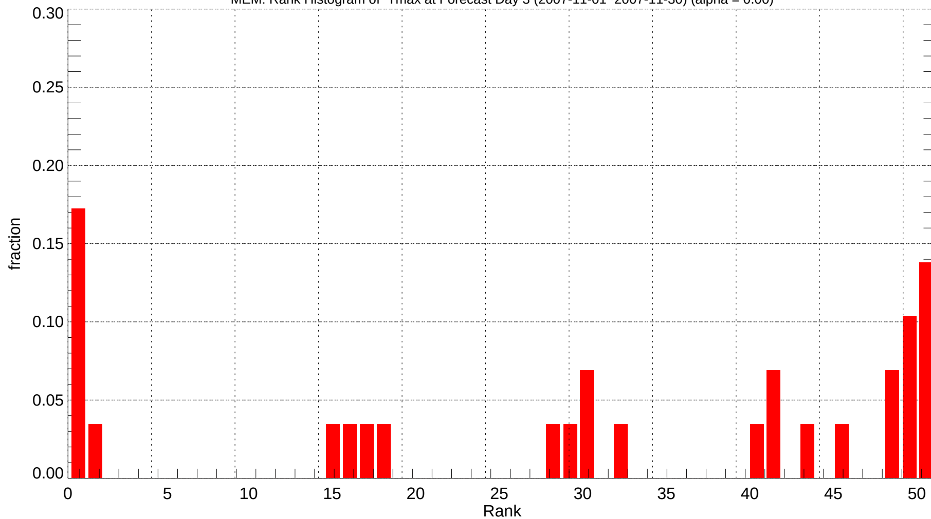
MEM: Rank Histogram of Tmax at Forecast Day 3 (2007-11-01~2007-11-30) (alpha = 0.00)
