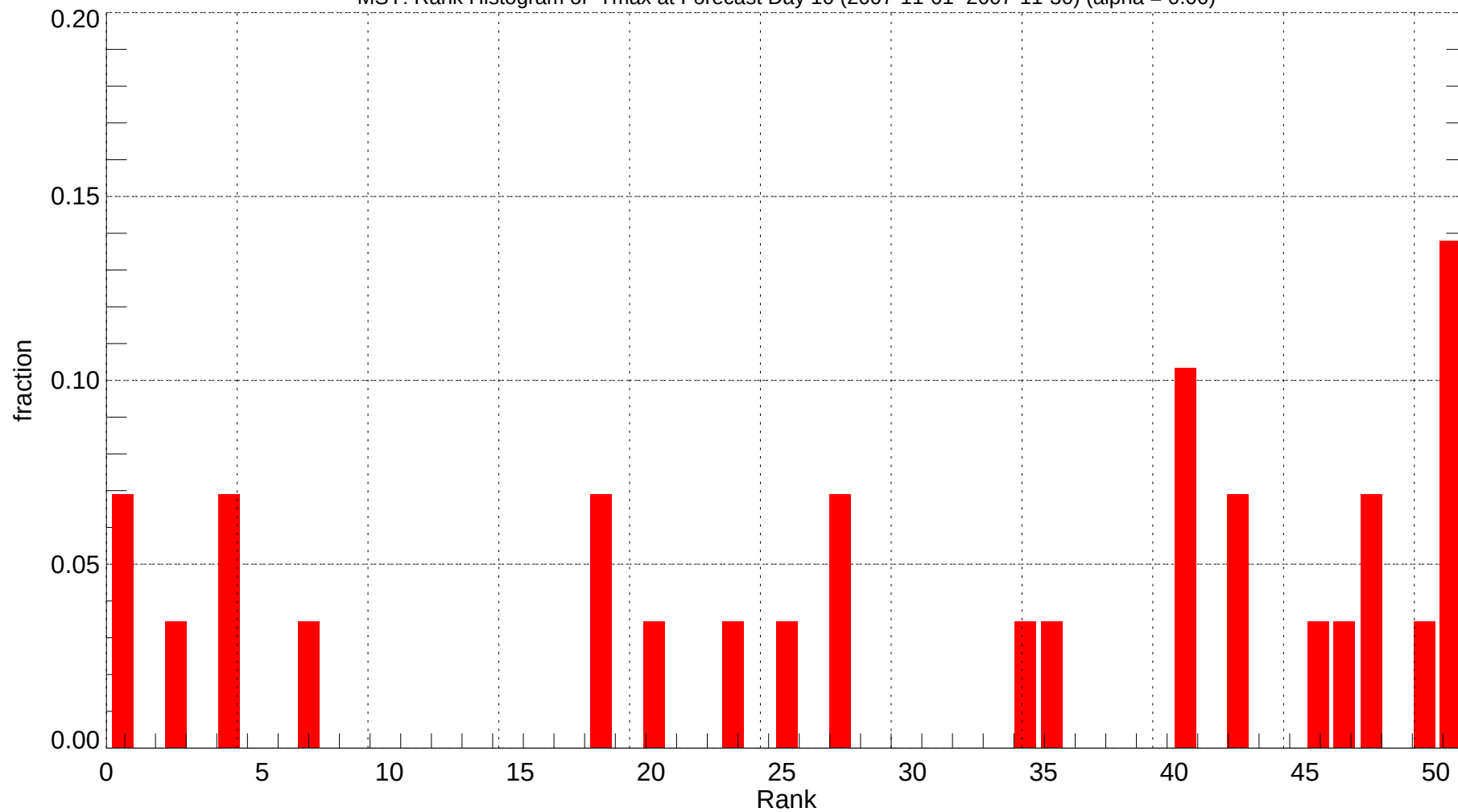
MSY: Rank Histogram of Tmax at Forecast Day 10 (2007-11-01~2007-11-30) (alpha = 0.00)
