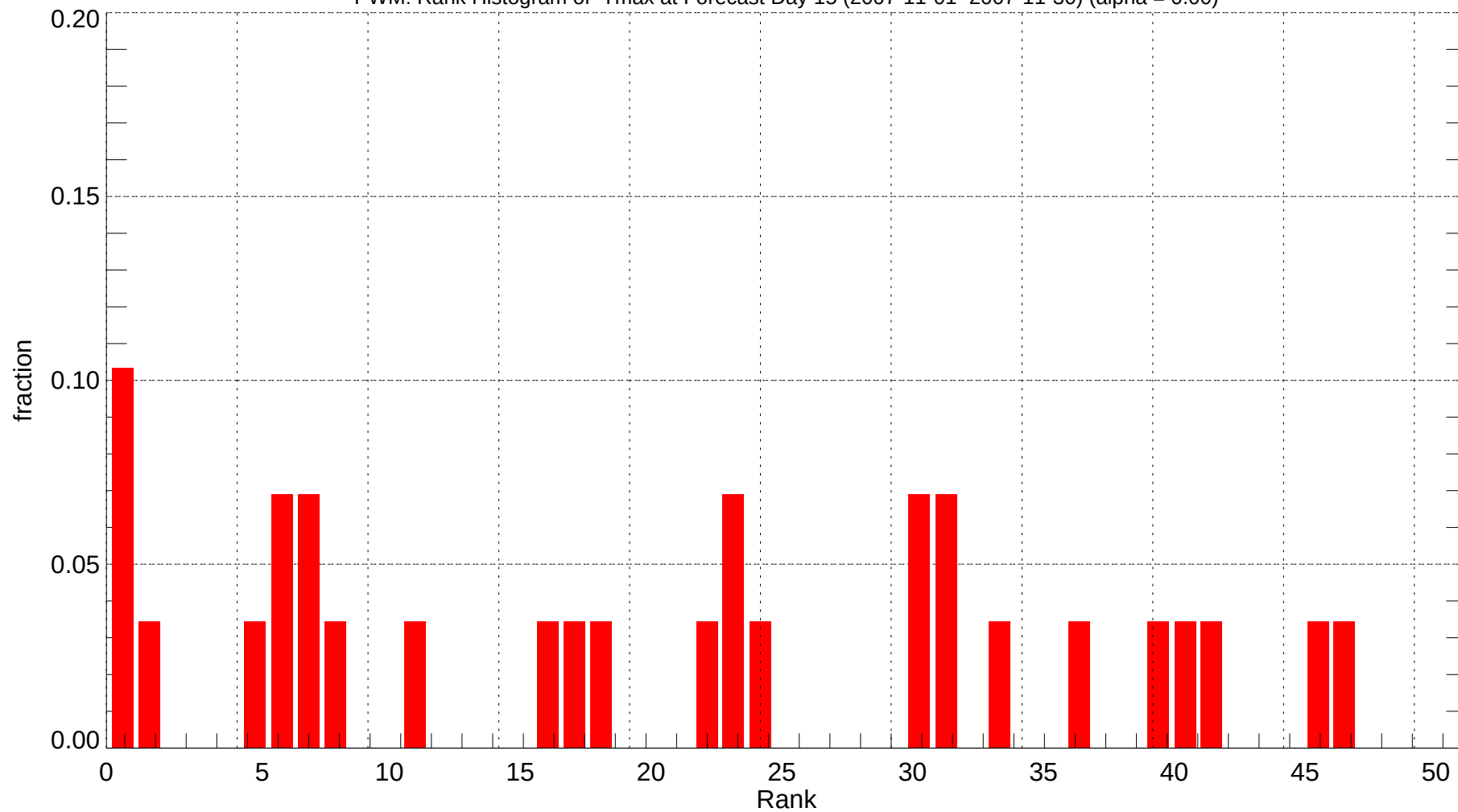
PWM: Rank Histogram of Tmax at Forecast Day 15 (2007-11-01~2007-11-30) (alpha = 0.00)
