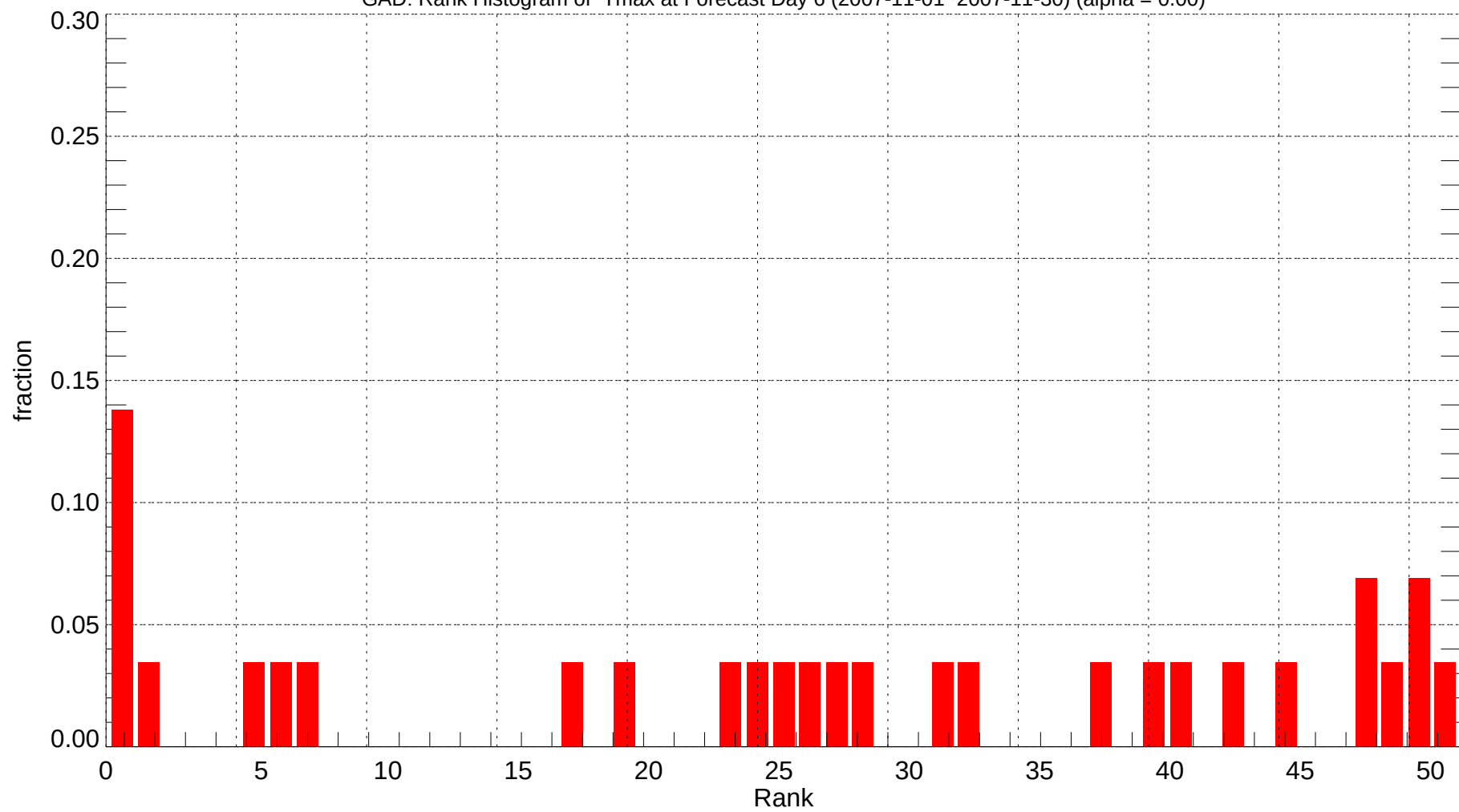
GAD: Rank Histogram of Tmax at Forecast Day 6 (2007-11-01~2007-11-30) (alpha = 0.00)
