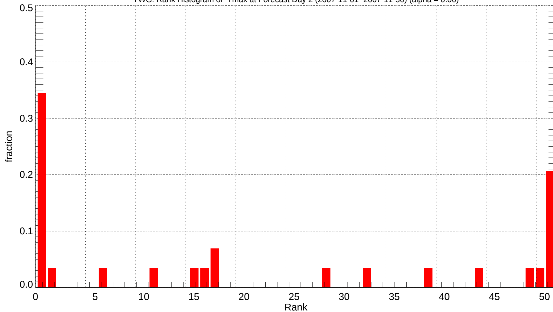
YWG: Rank Histogram of Tmax at Forecast Day 2 (2007-11-01~2007-11-30) (alpha = 0.00)
