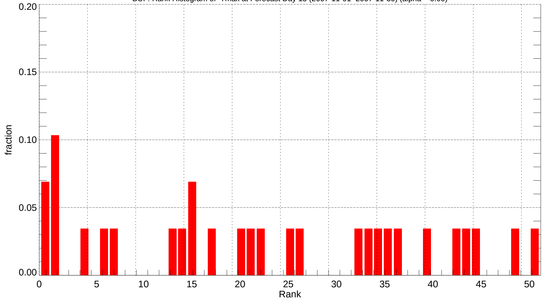
BUF: Rank Histogram of Tmax at Forecast Day 15 (2007-11-01~2007-11-30) (alpha = 0.00)
