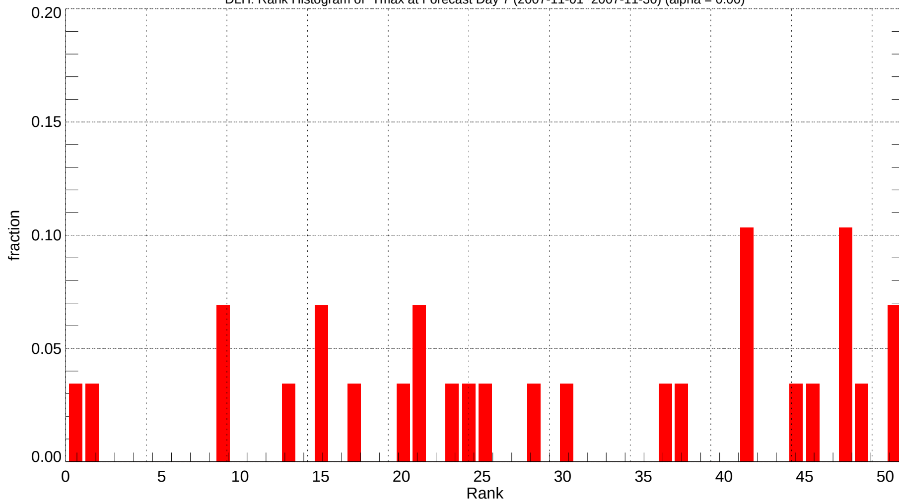
DLH: Rank Histogram of Tmax at Forecast Day 7 (2007-11-01~2007-11-30) (alpha = 0.00)
