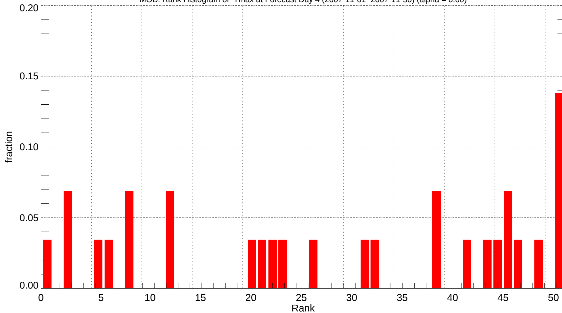
MOB: Rank Histogram of Tmax at Forecast Day 4 (2007-11-01~2007-11-30) (alpha = 0.00)
