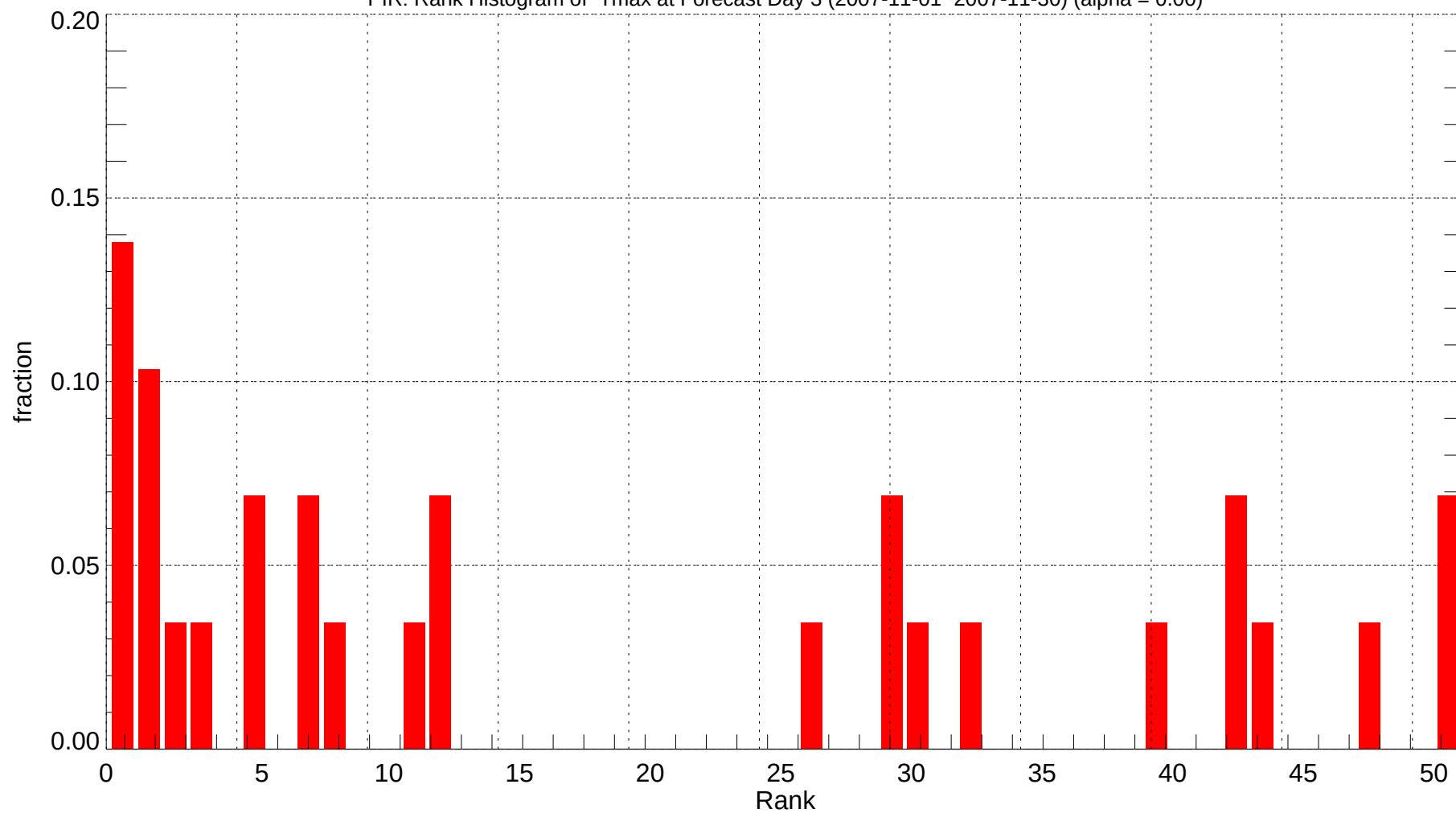
PIR: Rank Histogram of Tmax at Forecast Day 3 (2007-11-01~2007-11-30) (alpha = 0.00)
