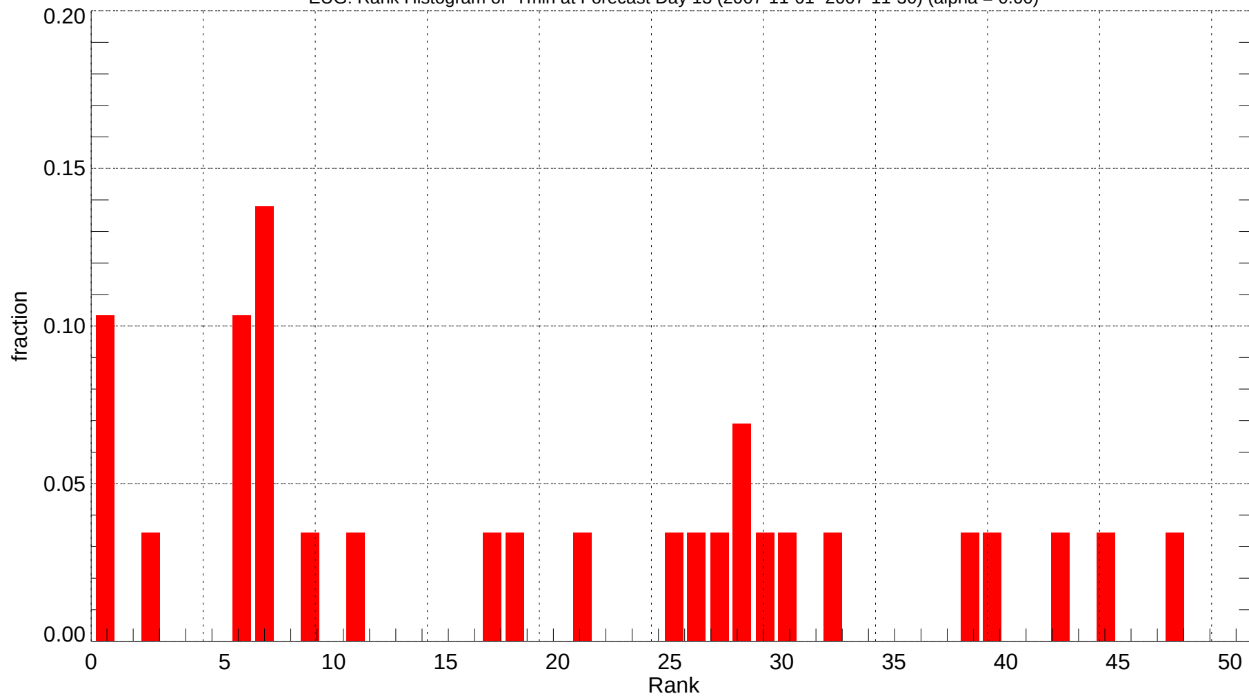
EUG: Rank Histogram of Tmin at Forecast Day 13 (2007-11-01~2007-11-30) (alpha = 0.00)
