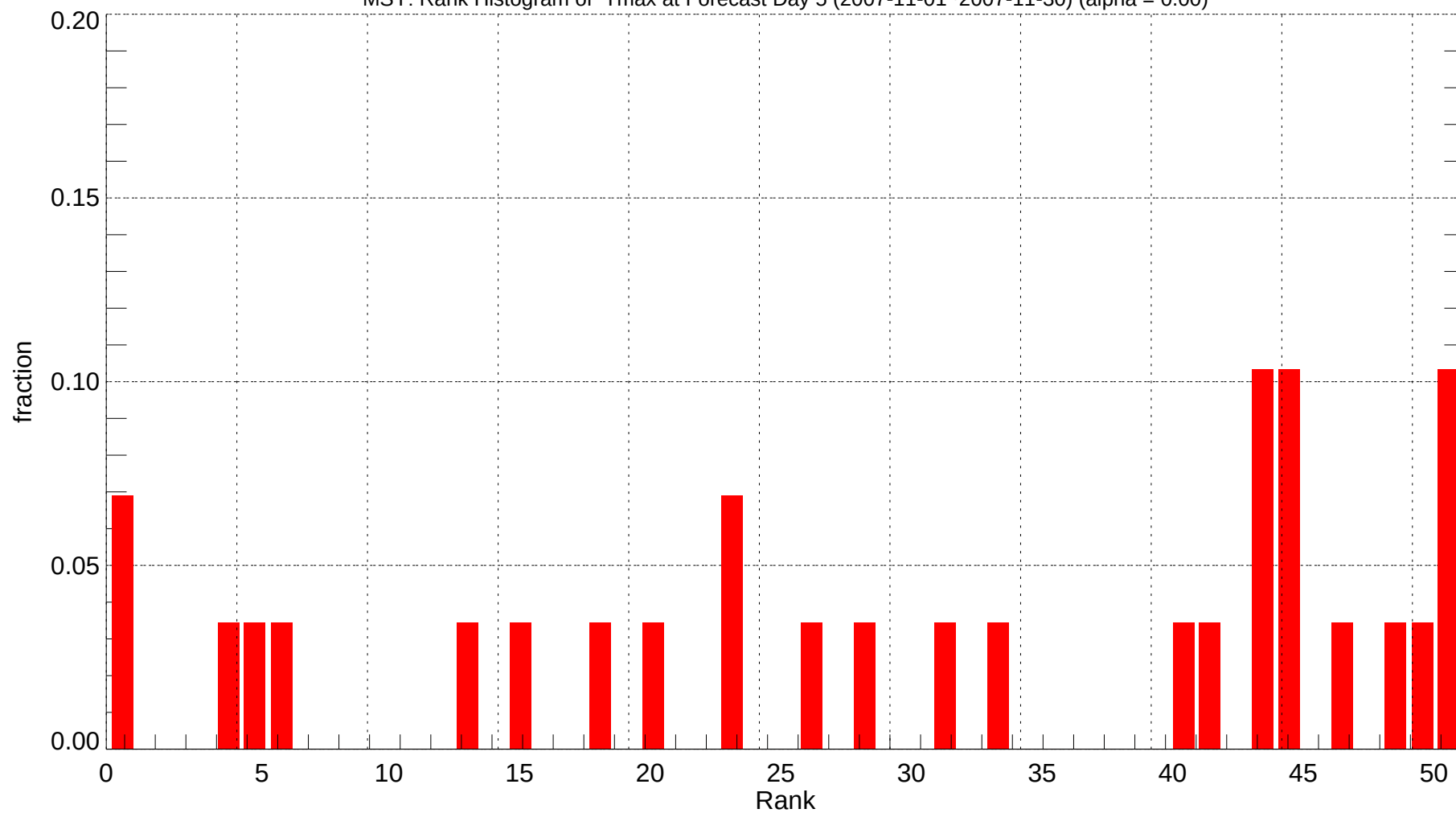
MSY: Rank Histogram of Tmax at Forecast Day 5 (2007-11-01~2007-11-30) (alpha = 0.00)
