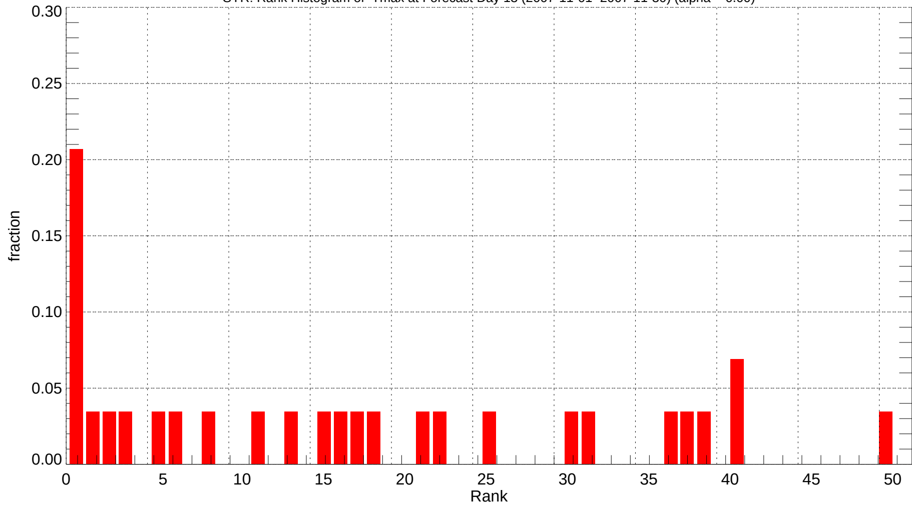
SYR: Rank Histogram of Tmax at Forecast Day 13 (2007-11-01~2007-11-30) (alpha = 0.00)
