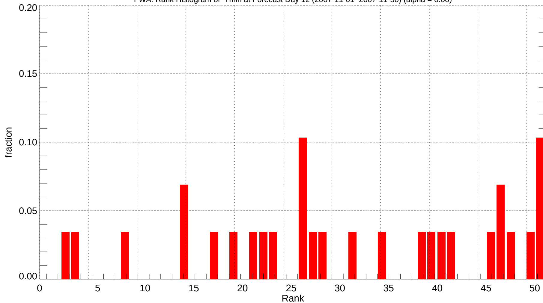
FWA: Rank Histogram of Tmin at Forecast Day 12 (2007-11-01~2007-11-30) (alpha = 0.00)
