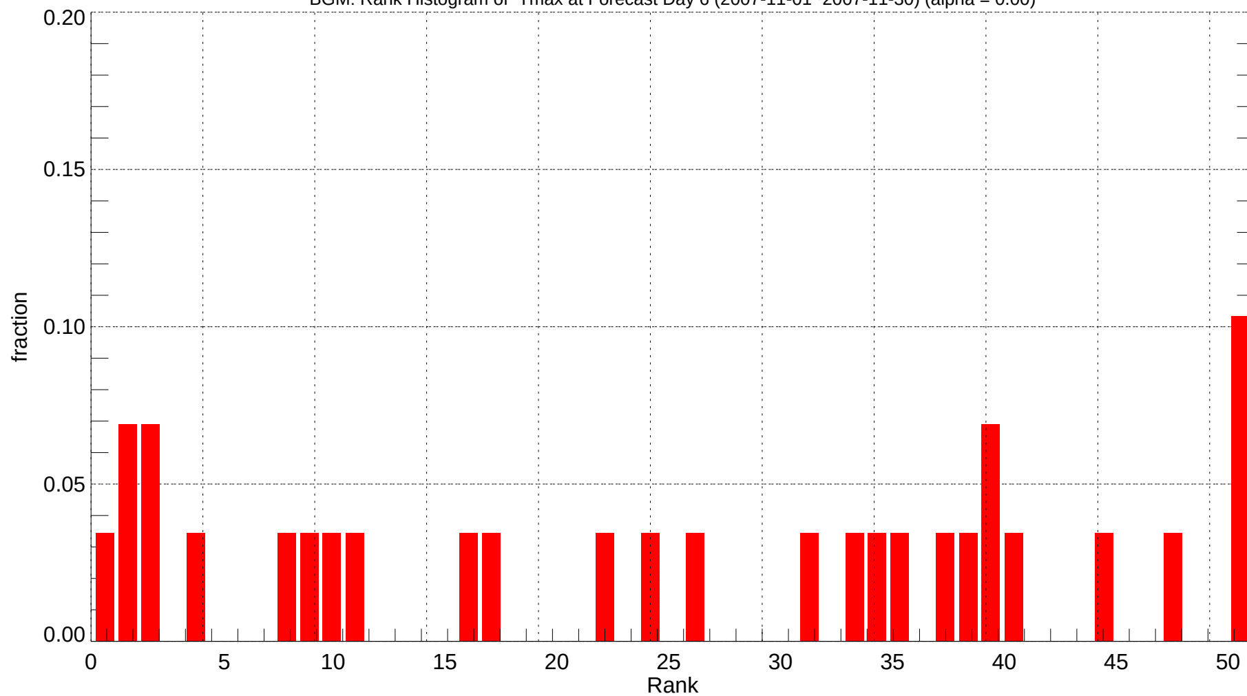
BGM: Rank Histogram of Tmax at Forecast Day 6 (2007-11-01~2007-11-30) (alpha = 0.00)
