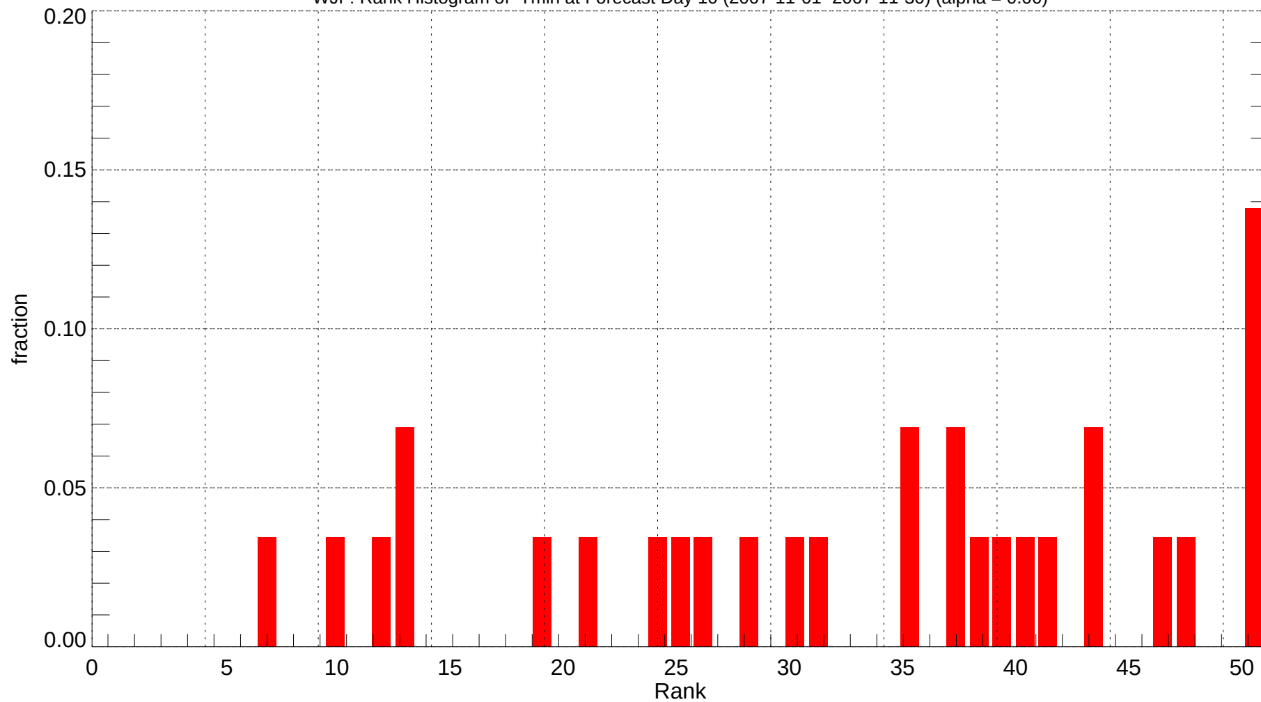
WJF: Rank Histogram of Tmin at Forecast Day 10 (2007-11-01~2007-11-30) (alpha = 0.00)
