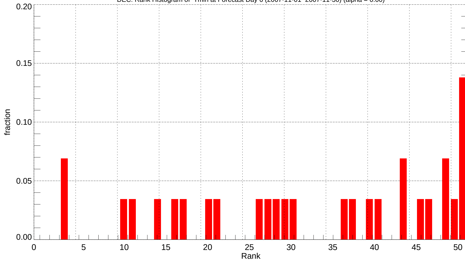
DEC: Rank Histogram of Tmin at Forecast Day 6 (2007-11-01~2007-11-30) (alpha = 0.00)
