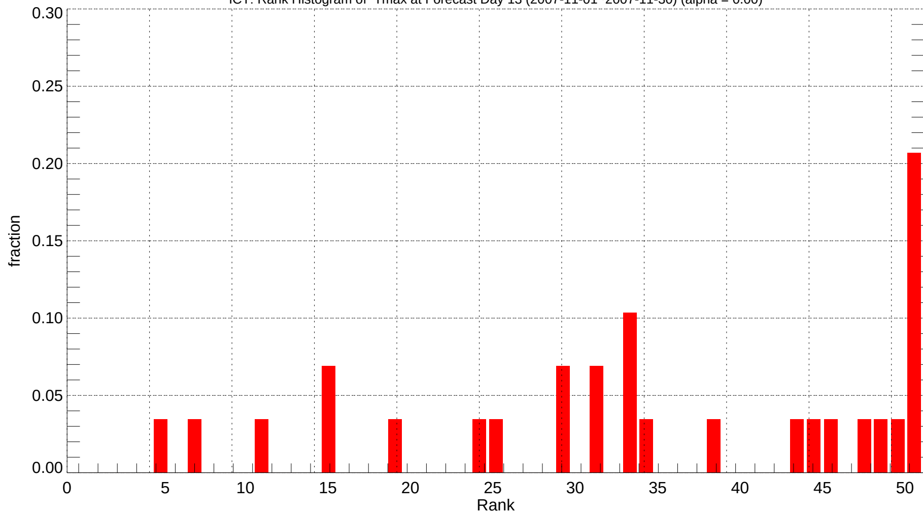
ICT: Rank Histogram of Tmax at Forecast Day 13 (2007-11-01~2007-11-30) (alpha = 0.00)
