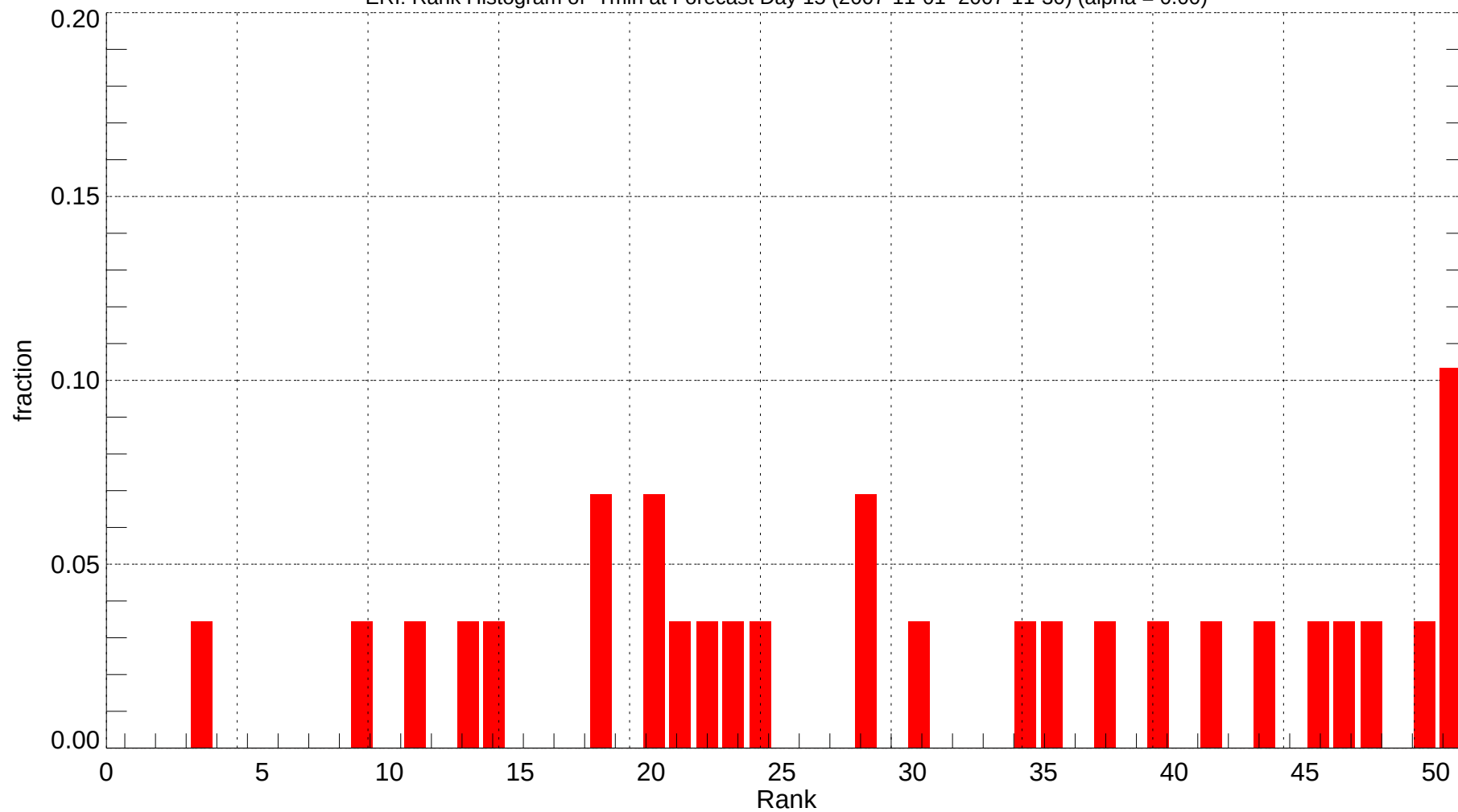
ERI: Rank Histogram of Tmin at Forecast Day 15 (2007-11-01~2007-11-30) (alpha = 0.00)
