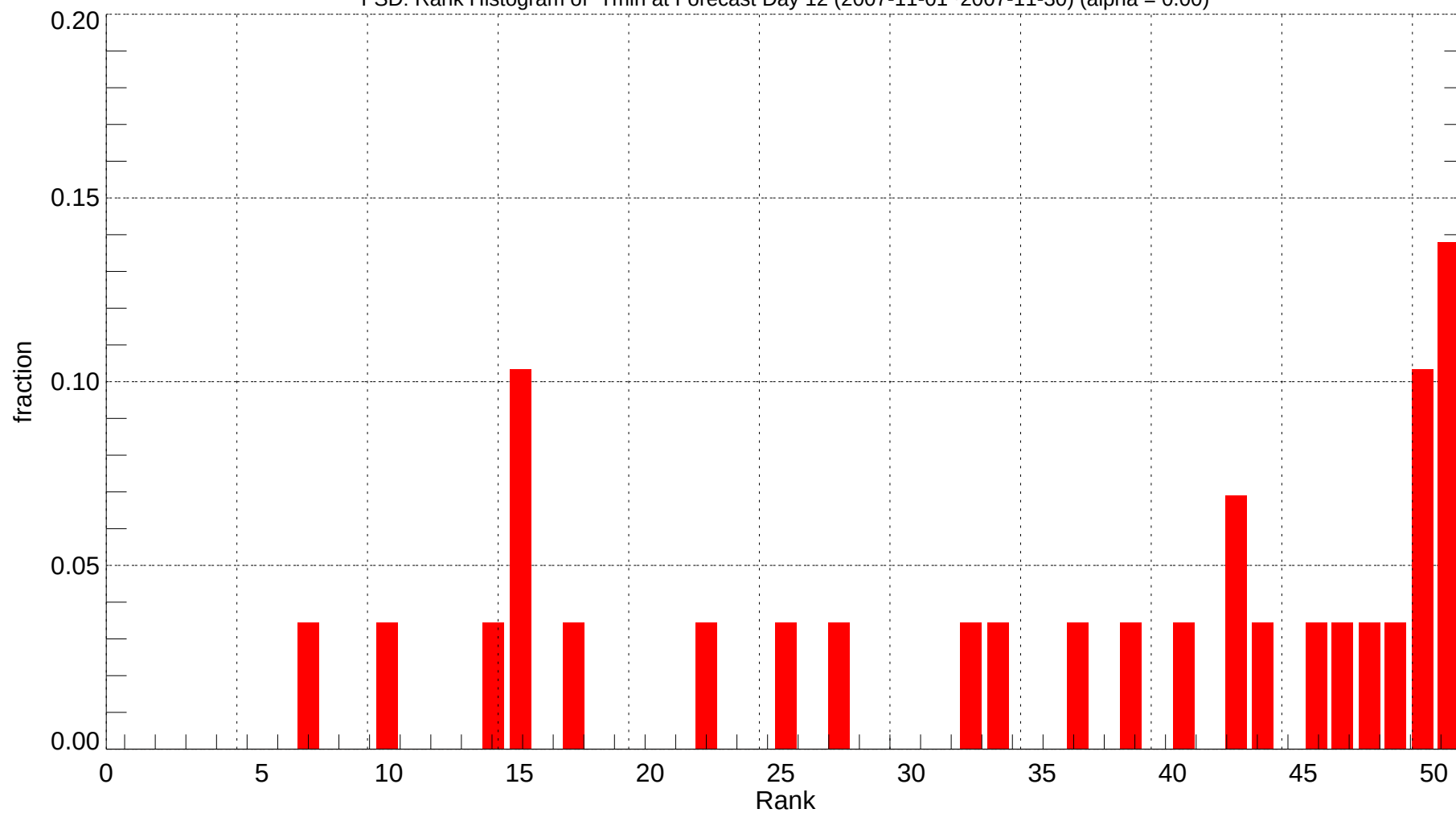
FSD: Rank Histogram of Tmin at Forecast Day 12 (2007-11-01~2007-11-30) (alpha = 0.00)
