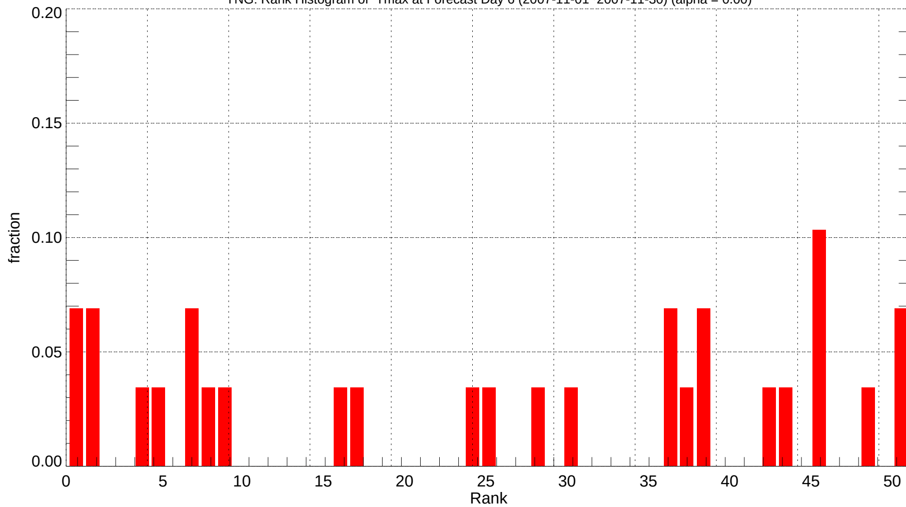
YNG: Rank Histogram of Tmax at Forecast Day 6 (2007-11-01~2007-11-30) (alpha = 0.00)
