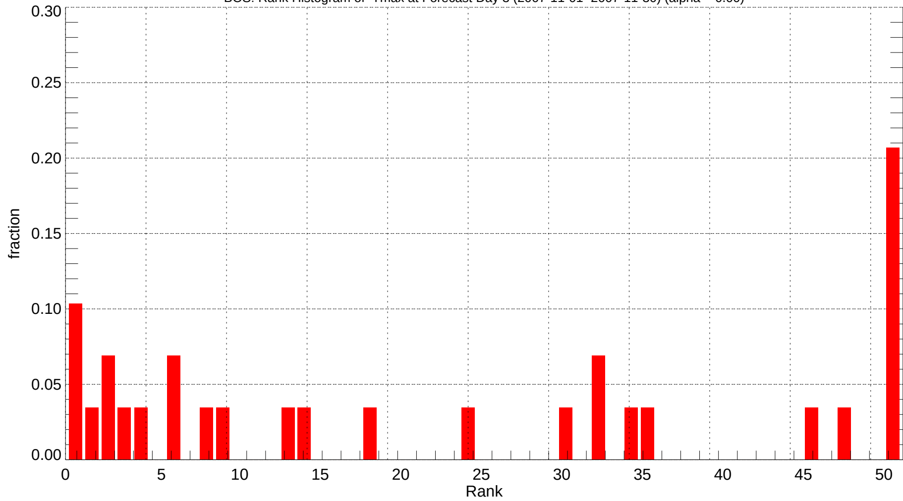
BOS: Rank Histogram of Tmax at Forecast Day 3 (2007-11-01~2007-11-30) (alpha = 0.00)
