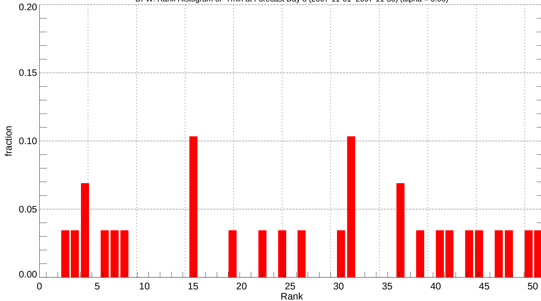
DFW: Rank Histogram of Tmin at Forecast Day 8 (2007-11-01~2007-11-30) (alpha = 0.00)
