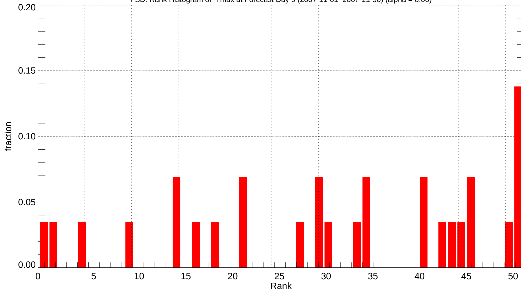
FSD: Rank Histogram of Tmax at Forecast Day 9 (2007-11-01~2007-11-30) (alpha = 0.00)
