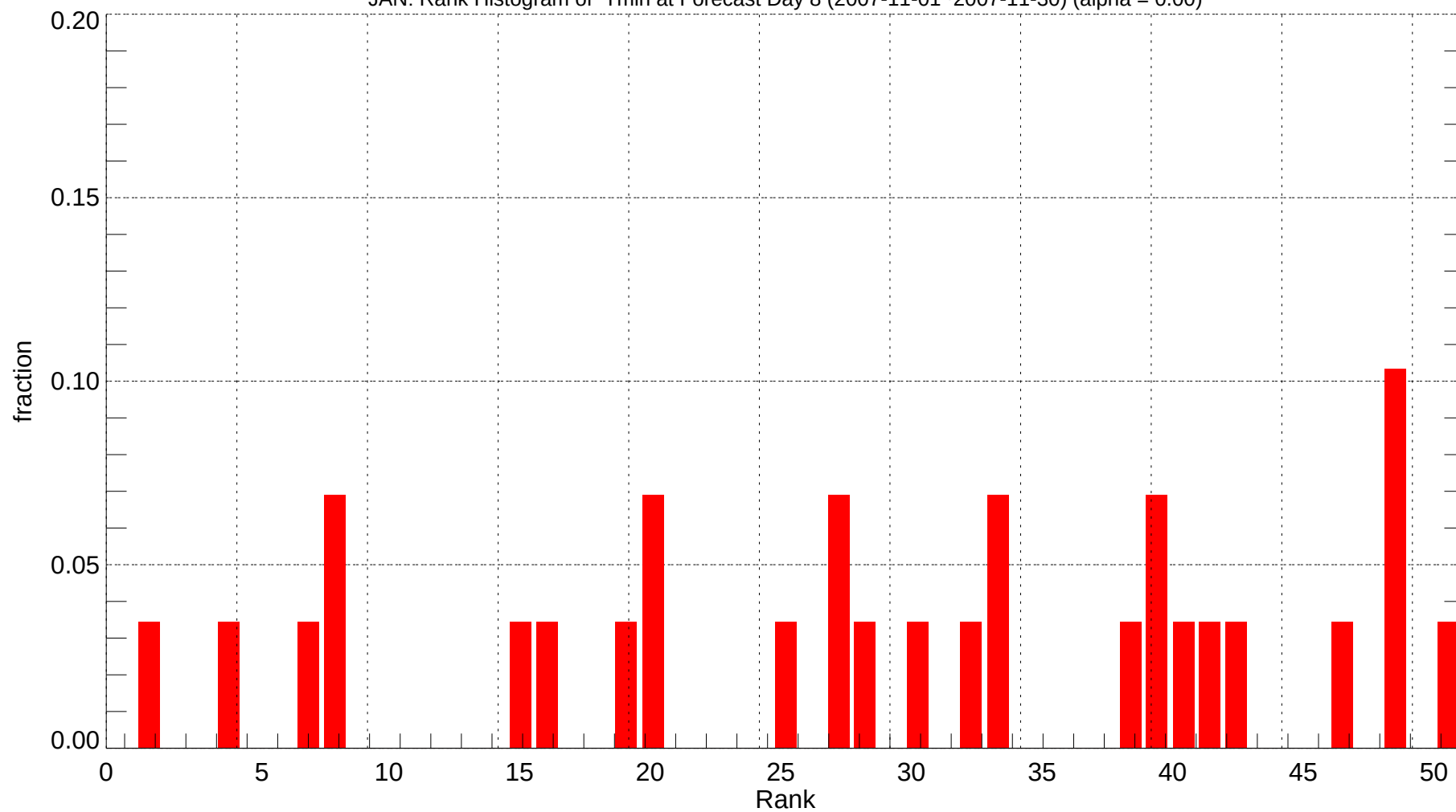
JAN: Rank Histogram of Tmin at Forecast Day 8 (2007-11-01~2007-11-30) (alpha = 0.00)
