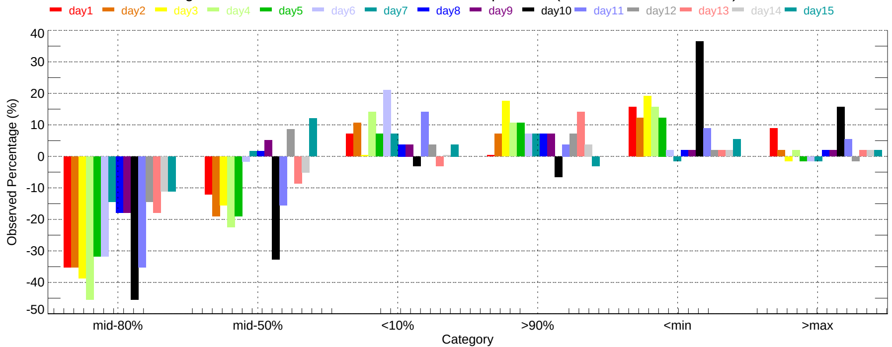
Observed Percentage Deviation of Ensembles - AUS: Min Temperature (2007-11-01~2007-11-30)
