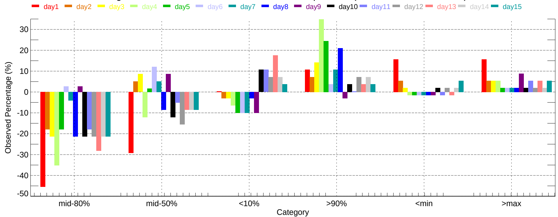
Observed Percentage Deviation of Ensembles - EWR: Max Temperature (2007-11-01~2007-11-30)
