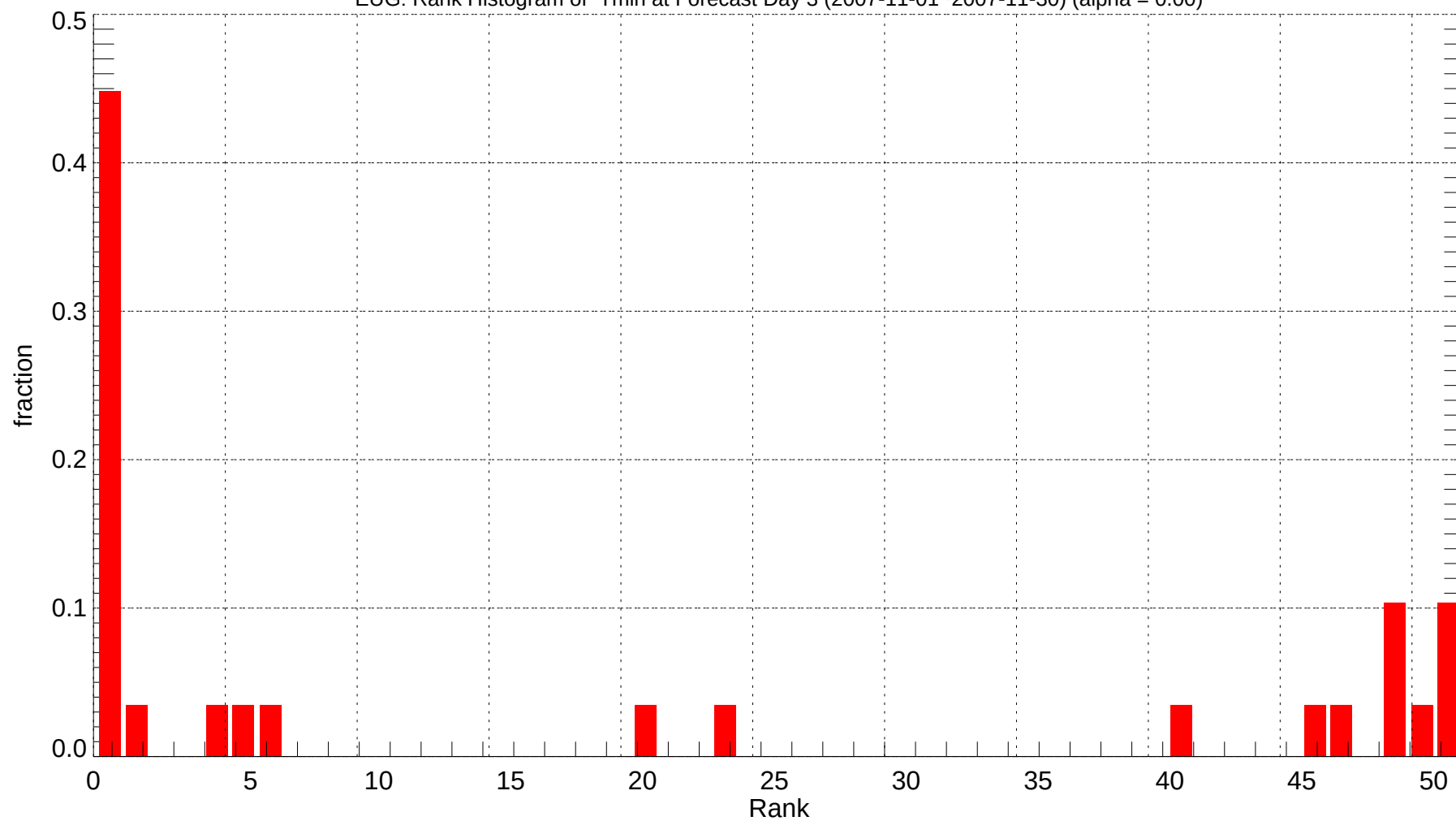
EUG: Rank Histogram of Tmin at Forecast Day 3 (2007-11-01~2007-11-30) (alpha = 0.00)
