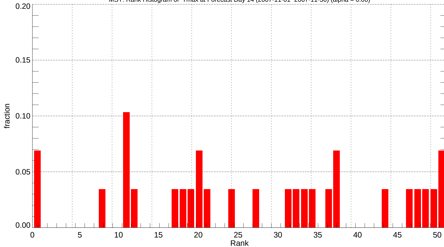
MSY: Rank Histogram of Tmax at Forecast Day 14 (2007-11-01~2007-11-30) (alpha = 0.00)
