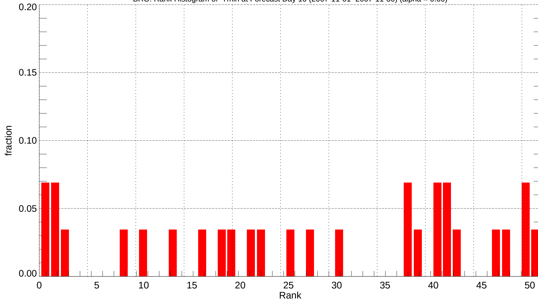
BRO: Rank Histogram of Tmin at Forecast Day 10 (2007-11-01~2007-11-30) (alpha = 0.00)
