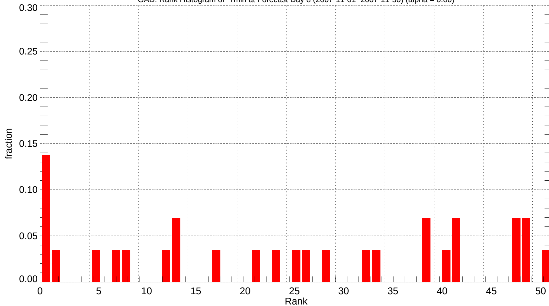
GAD: Rank Histogram of Tmin at Forecast Day 8 (2007-11-01~2007-11-30) (alpha = 0.00)
