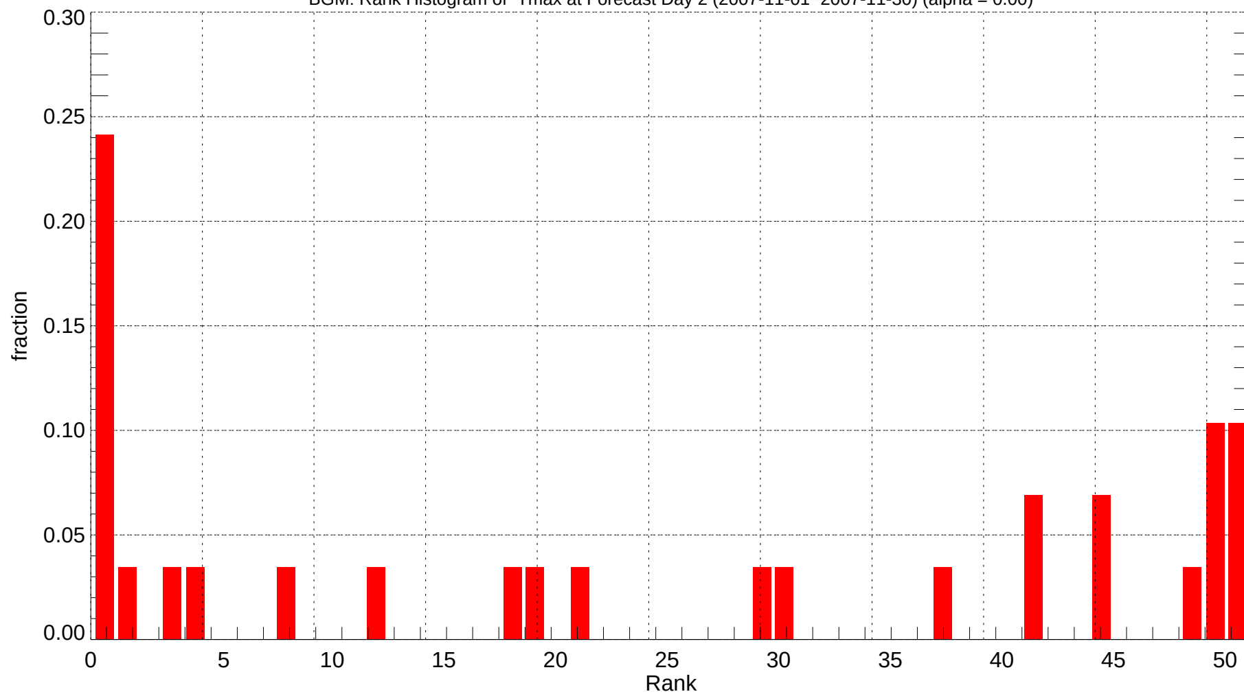
BGM: Rank Histogram of Tmax at Forecast Day 2 (2007-11-01~2007-11-30) (alpha = 0.00)
