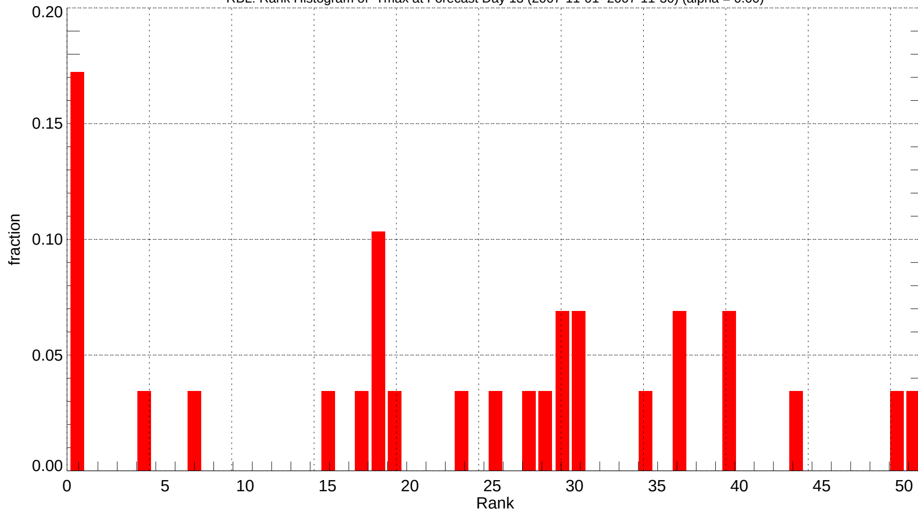
RBL: Rank Histogram of Tmax at Forecast Day 13 (2007-11-01~2007-11-30) (alpha = 0.00)
