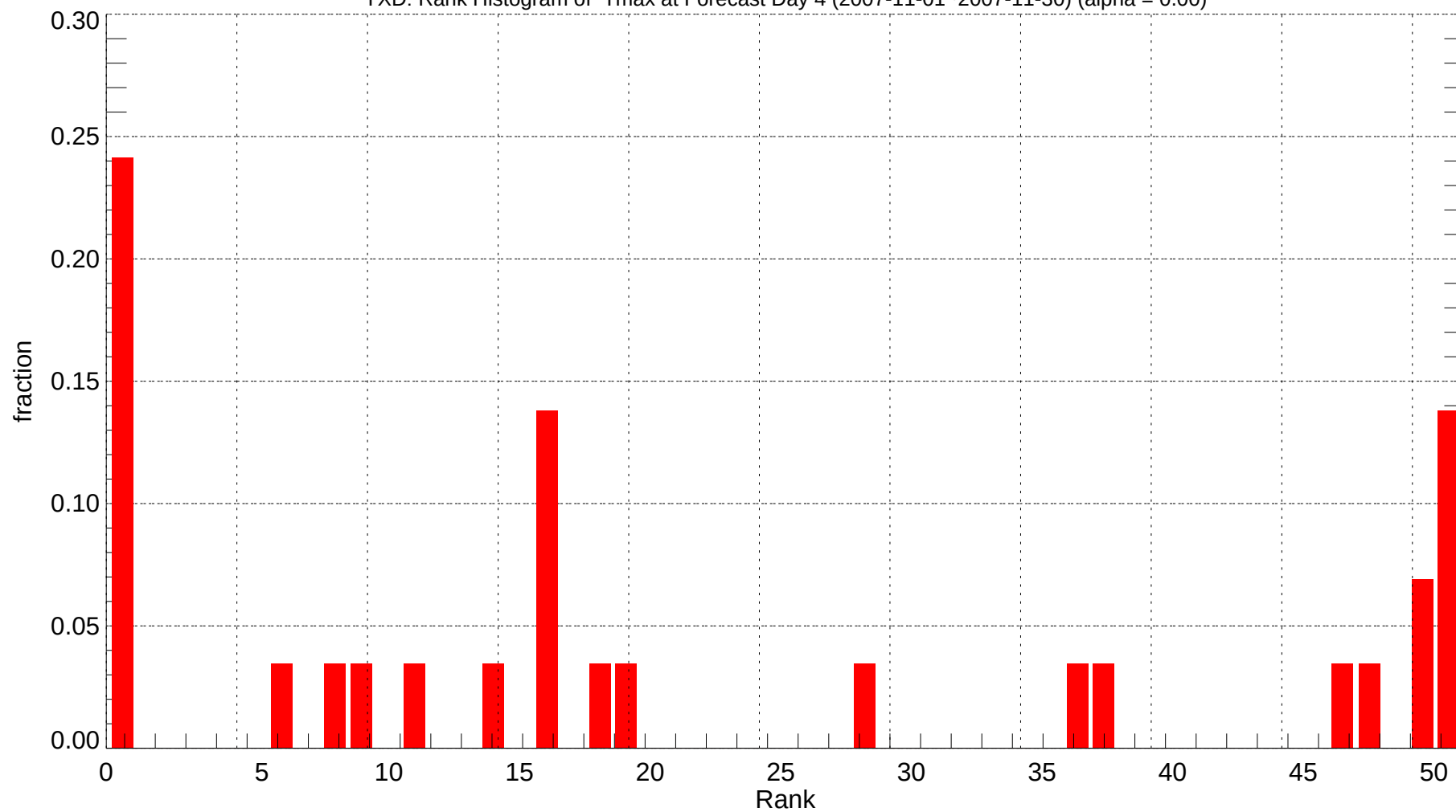
YXD: Rank Histogram of Tmax at Forecast Day 4 (2007-11-01~2007-11-30) (alpha = 0.00)
