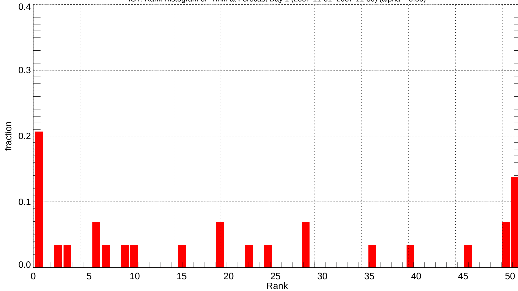
ICT: Rank Histogram of Tmin at Forecast Day 1 (2007-11-01~2007-11-30) (alpha = 0.00)
