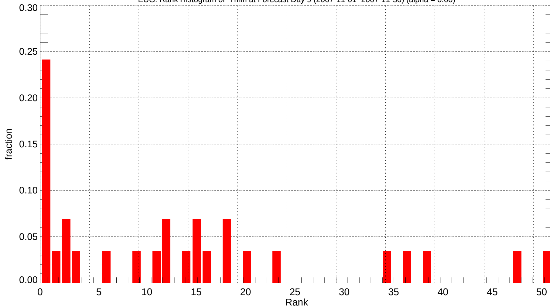
EUG: Rank Histogram of Tmin at Forecast Day 9 (2007-11-01~2007-11-30) (alpha = 0.00)
