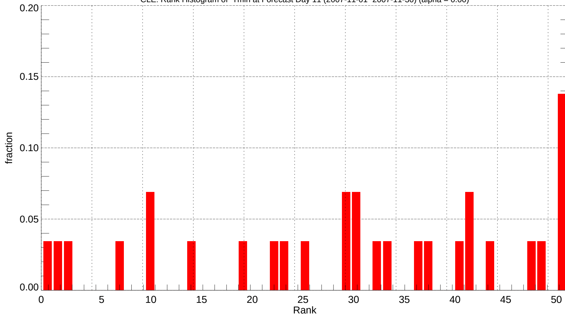
CLE: Rank Histogram of Tmin at Forecast Day 11 (2007-11-01~2007-11-30) (alpha = 0.00)
