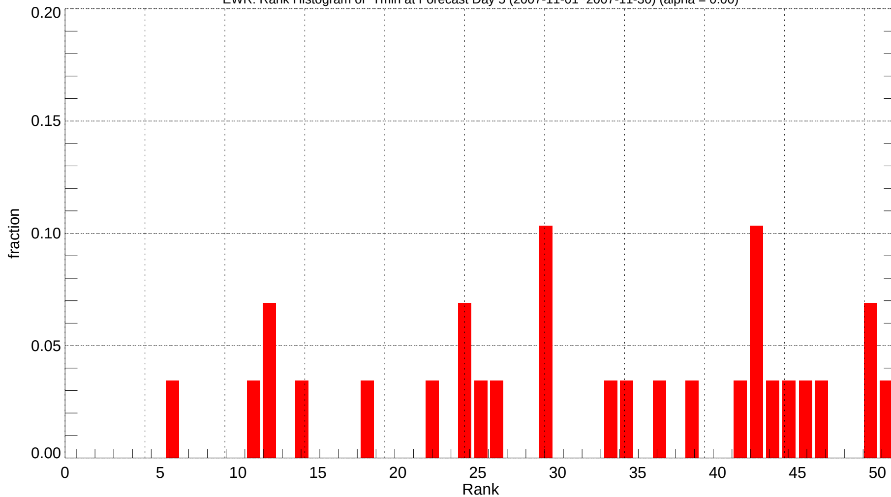
EWR: Rank Histogram of Tmin at Forecast Day 5 (2007-11-01~2007-11-30) (alpha = 0.00)
