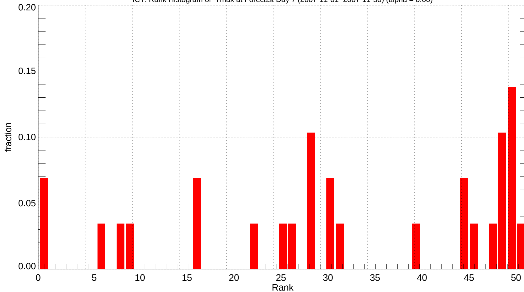
ICT: Rank Histogram of Tmax at Forecast Day 7 (2007-11-01~2007-11-30) (alpha = 0.00)
