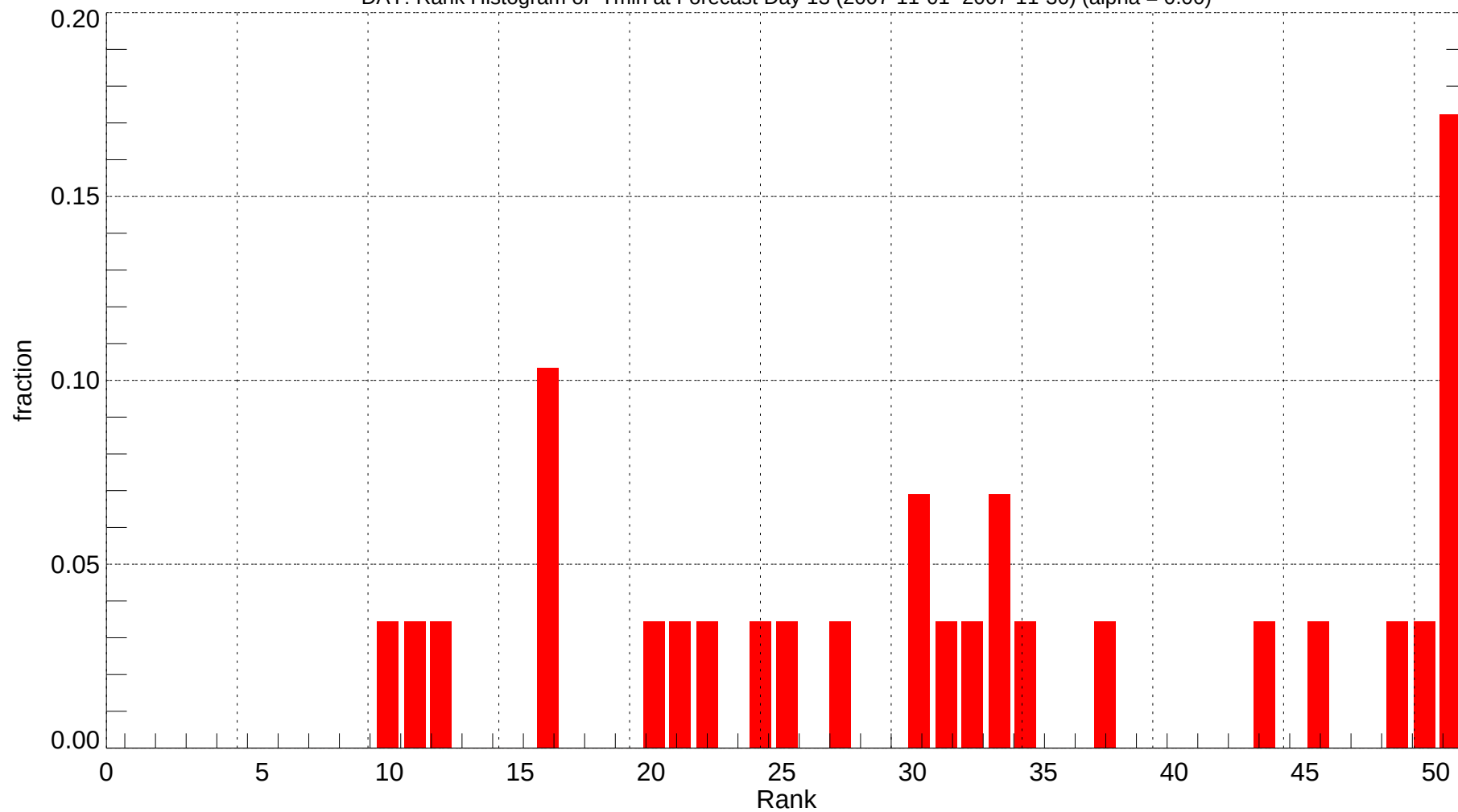
DAY: Rank Histogram of Tmin at Forecast Day 13 (2007-11-01~2007-11-30) (alpha = 0.00)
