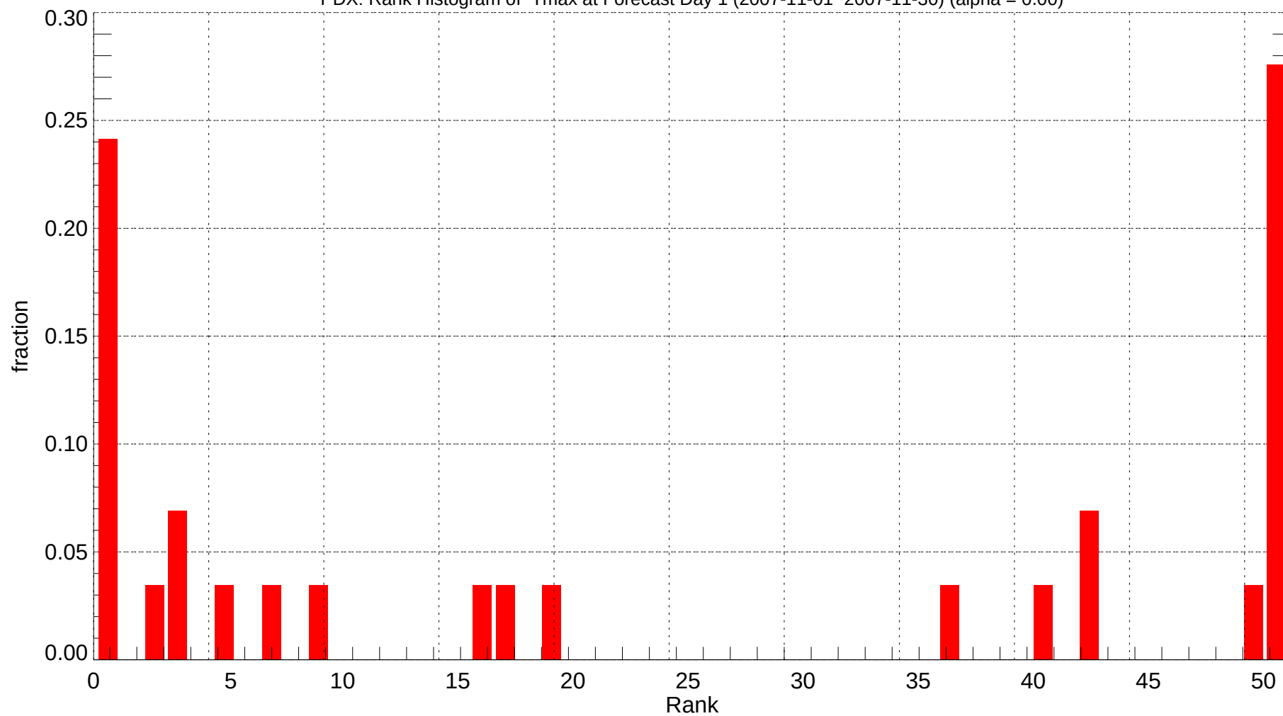
PDX: Rank Histogram of Tmax at Forecast Day 1 (2007-11-01~2007-11-30) (alpha = 0.00)
