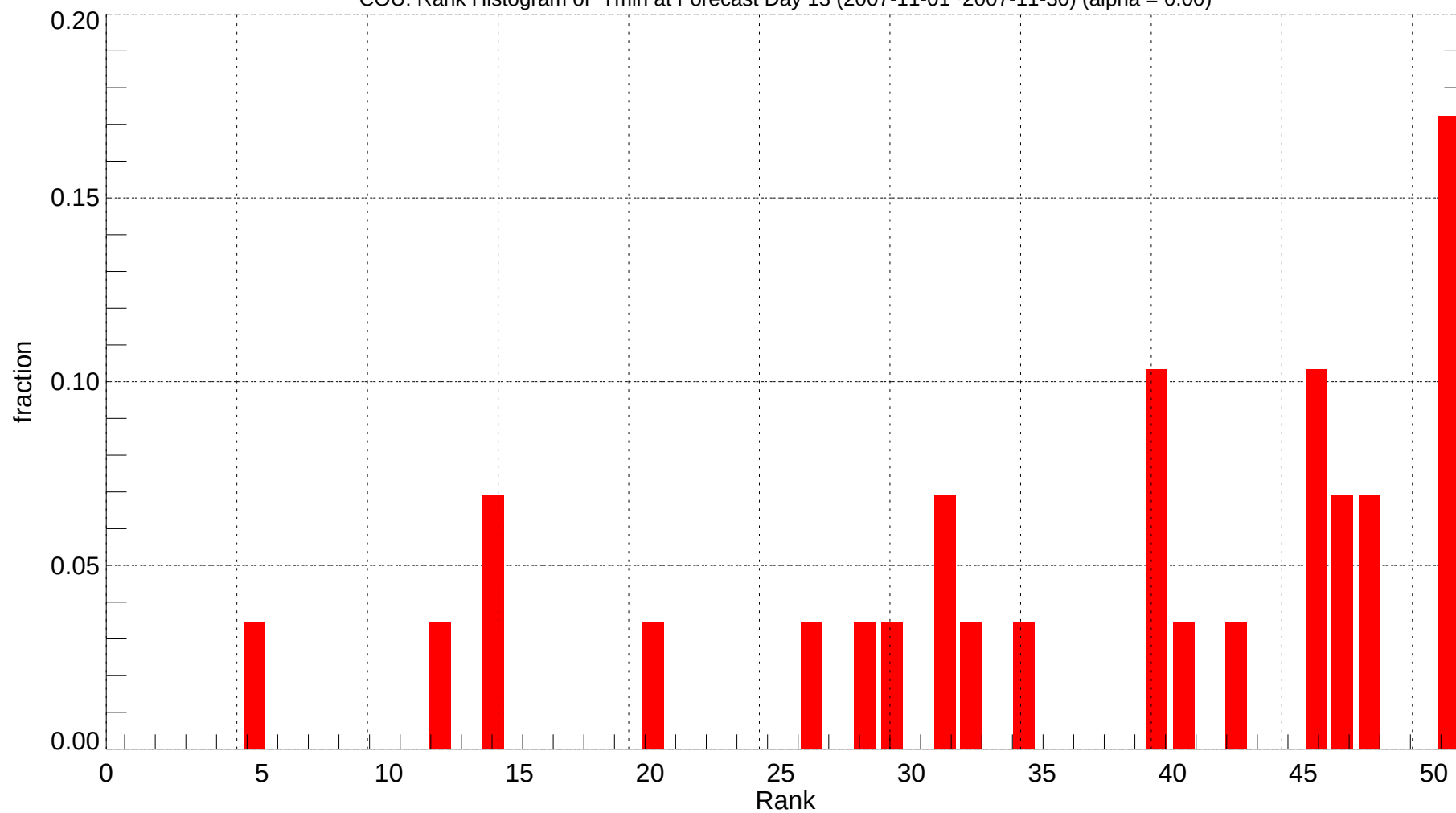
COU: Rank Histogram of Tmin at Forecast Day 13 (2007-11-01~2007-11-30) (alpha = 0.00)
