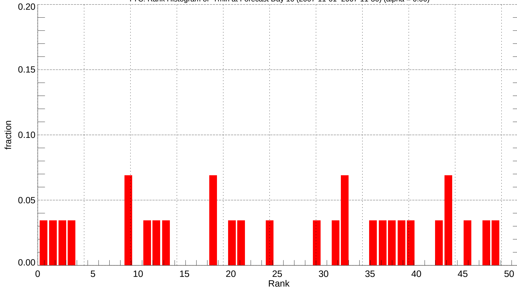
YYC: Rank Histogram of Tmin at Forecast Day 10 (2007-11-01~2007-11-30) (alpha = 0.00)
