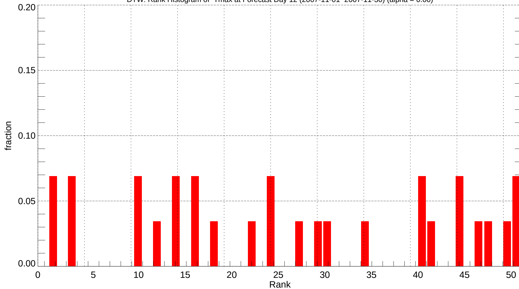
DTW: Rank Histogram of Tmax at Forecast Day 12 (2007-11-01~2007-11-30) (alpha = 0.00)
