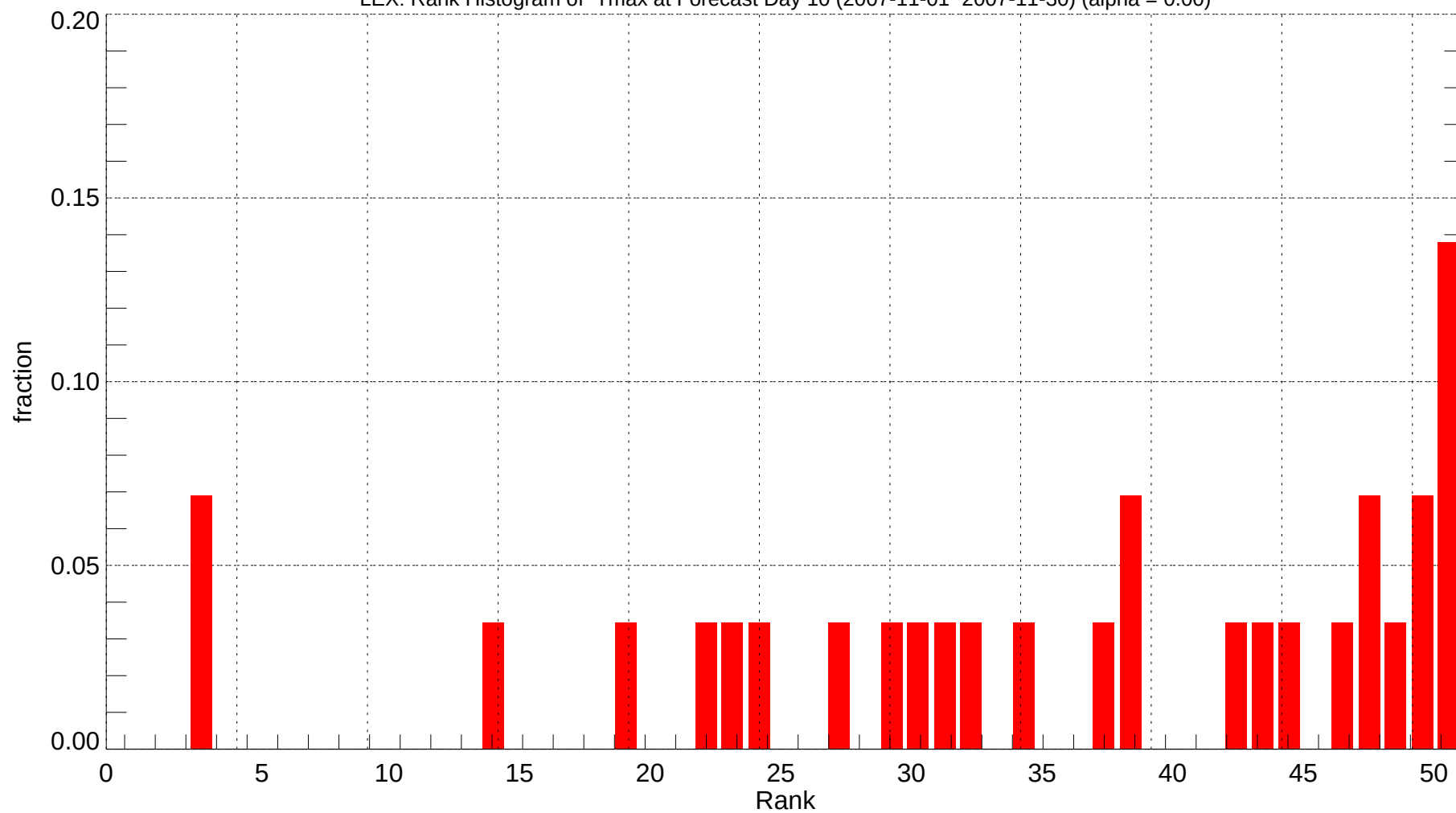
LEX: Rank Histogram of Tmax at Forecast Day 10 (2007-11-01~2007-11-30) (alpha = 0.00)
