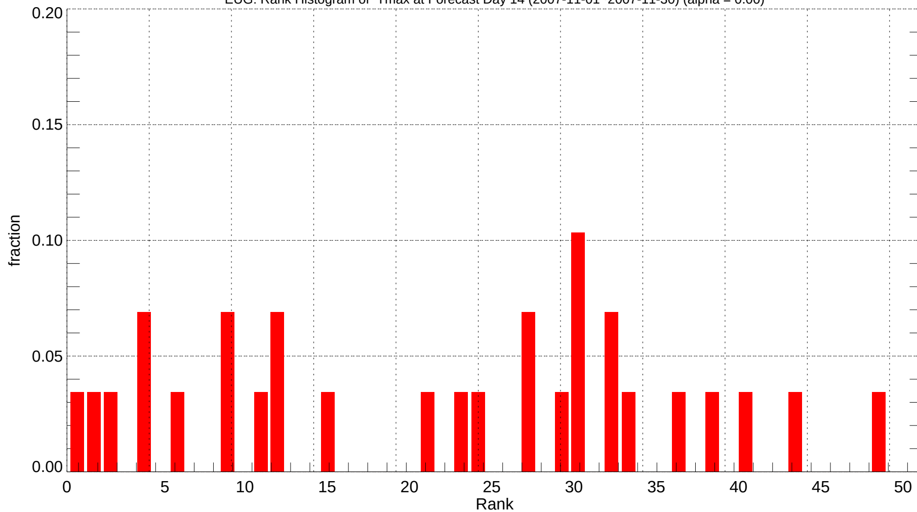
EUG: Rank Histogram of Tmax at Forecast Day 14 (2007-11-01~2007-11-30) (alpha = 0.00)
