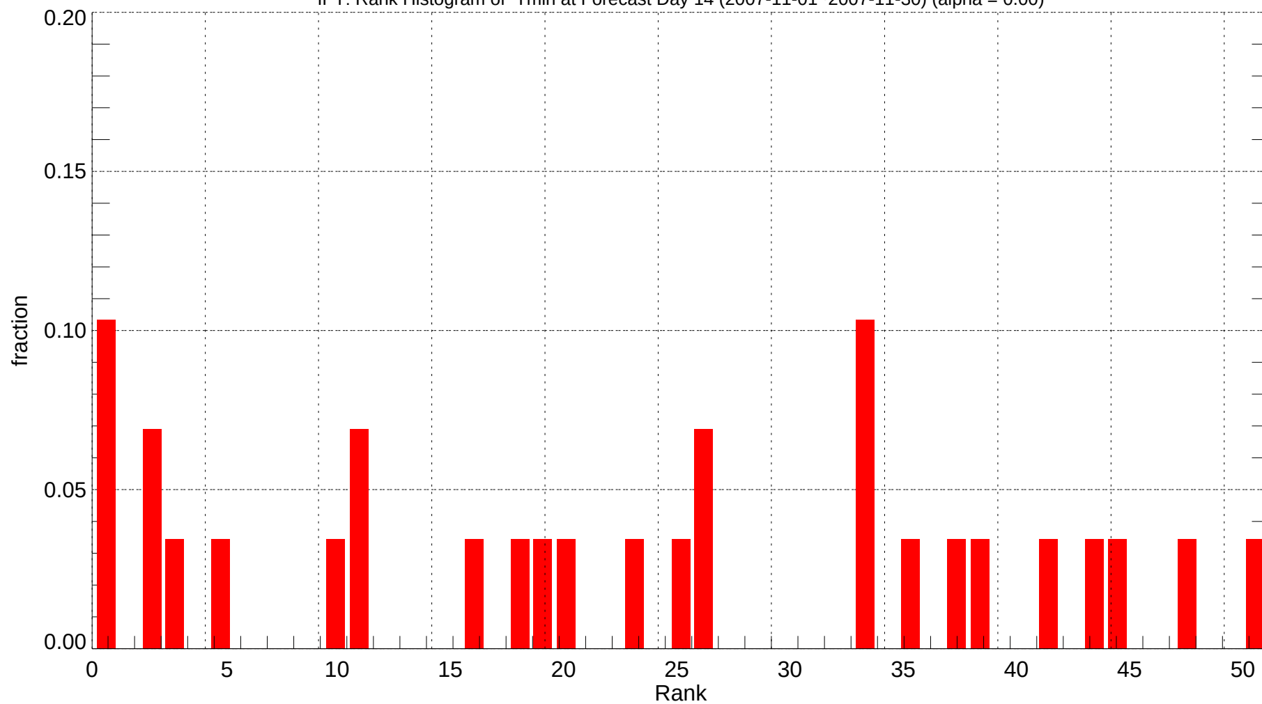
IPT: Rank Histogram of Tmin at Forecast Day 14 (2007-11-01~2007-11-30) (alpha = 0.00)
