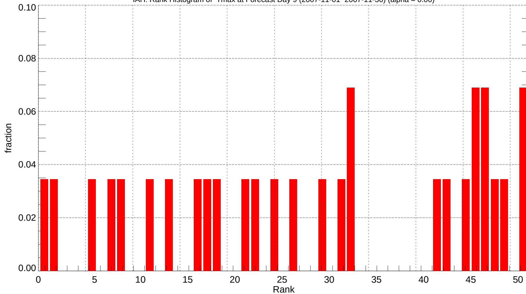
IAH: Rank Histogram of Tmax at Forecast Day 9 (2007-11-01~2007-11-30) (alpha = 0.00)
