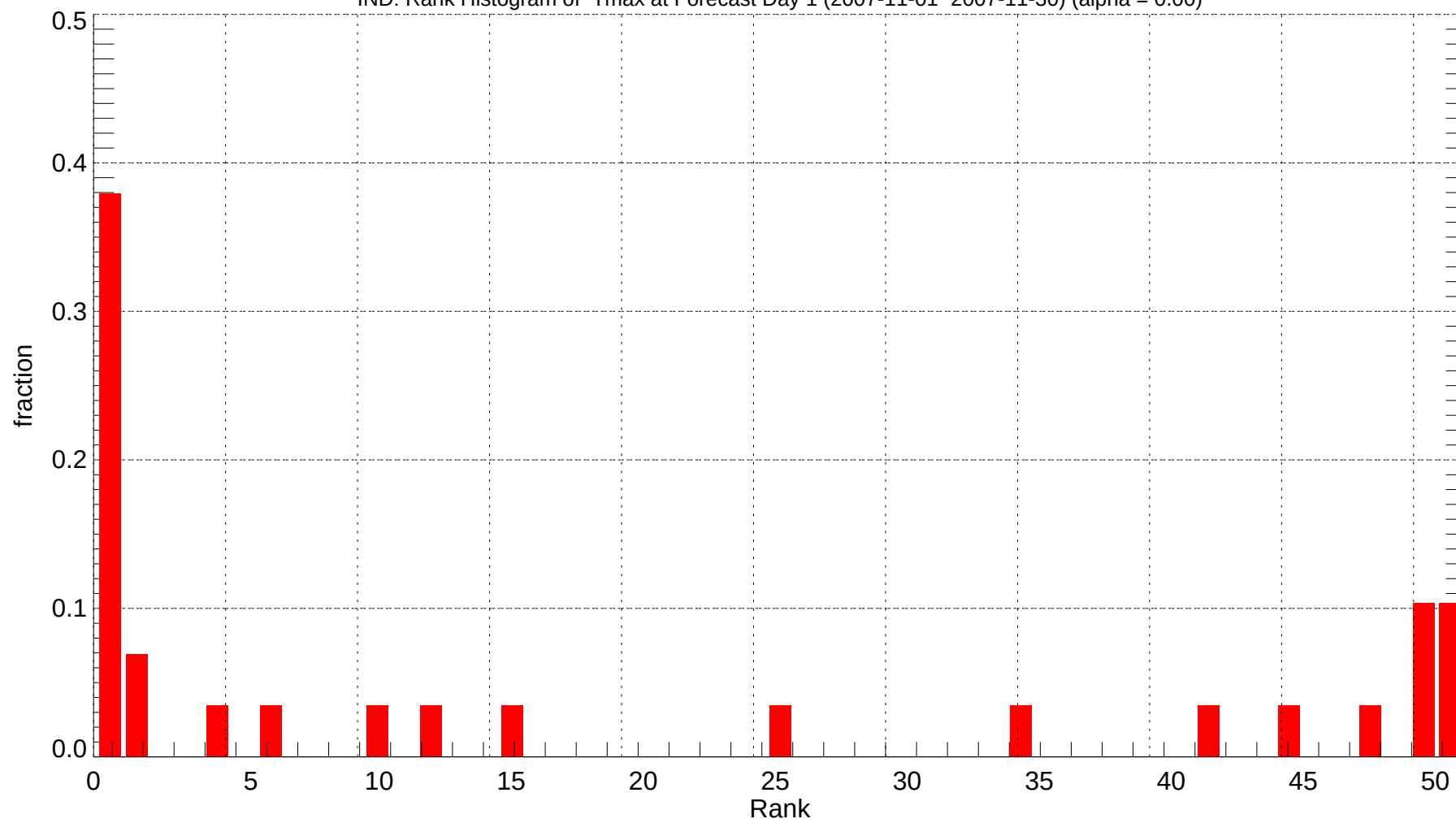
IND: Rank Histogram of Tmax at Forecast Day 1 (2007-11-01~2007-11-30) (alpha = 0.00)
