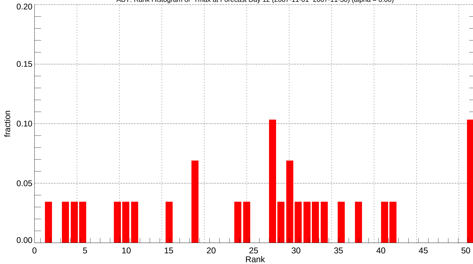
ABY: Rank Histogram of Tmax at Forecast Day 12 (2007-11-01~2007-11-30) (alpha = 0.00)
