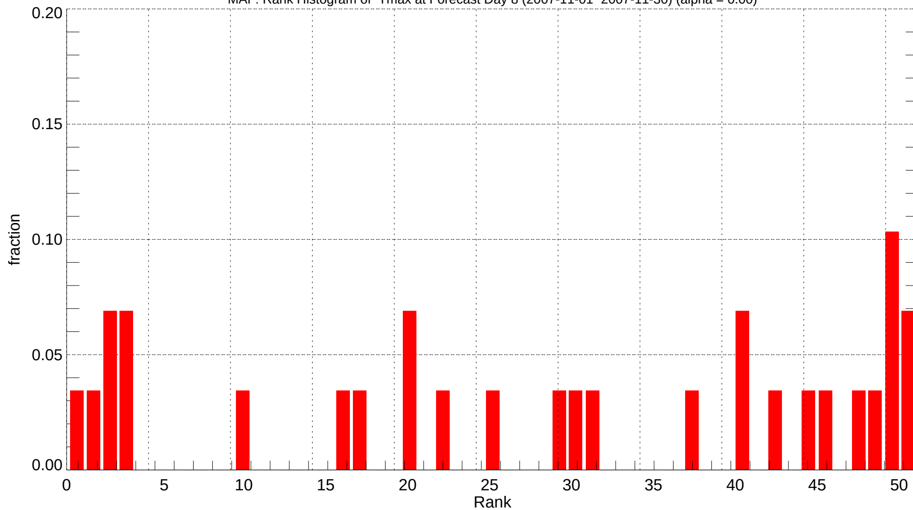
MAF: Rank Histogram of Tmax at Forecast Day 8 (2007-11-01~2007-11-30) (alpha = 0.00)
