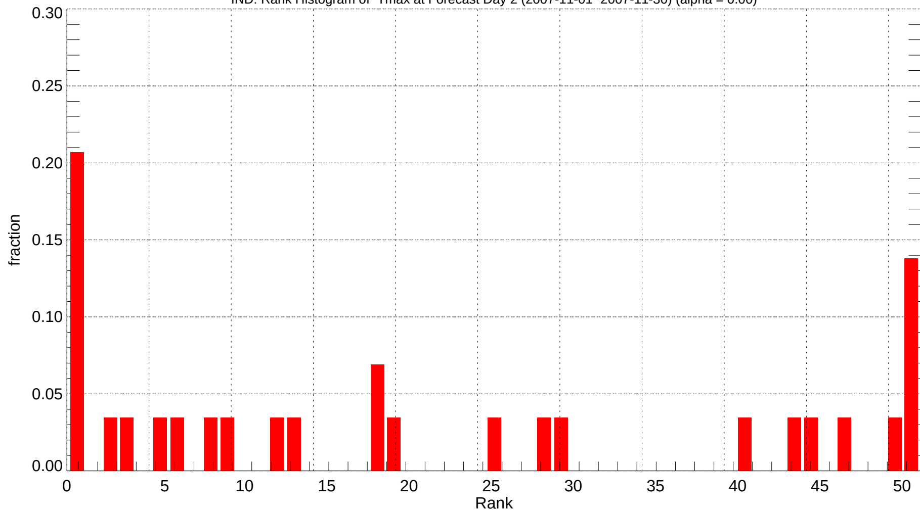
IND: Rank Histogram of Tmax at Forecast Day 2 (2007-11-01~2007-11-30) (alpha = 0.00)
