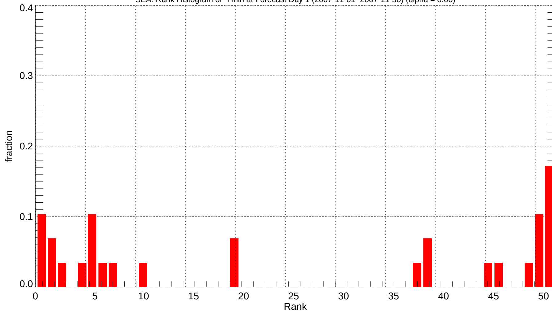
SEA: Rank Histogram of Tmin at Forecast Day 1 (2007-11-01~2007-11-30) (alpha = 0.00)
