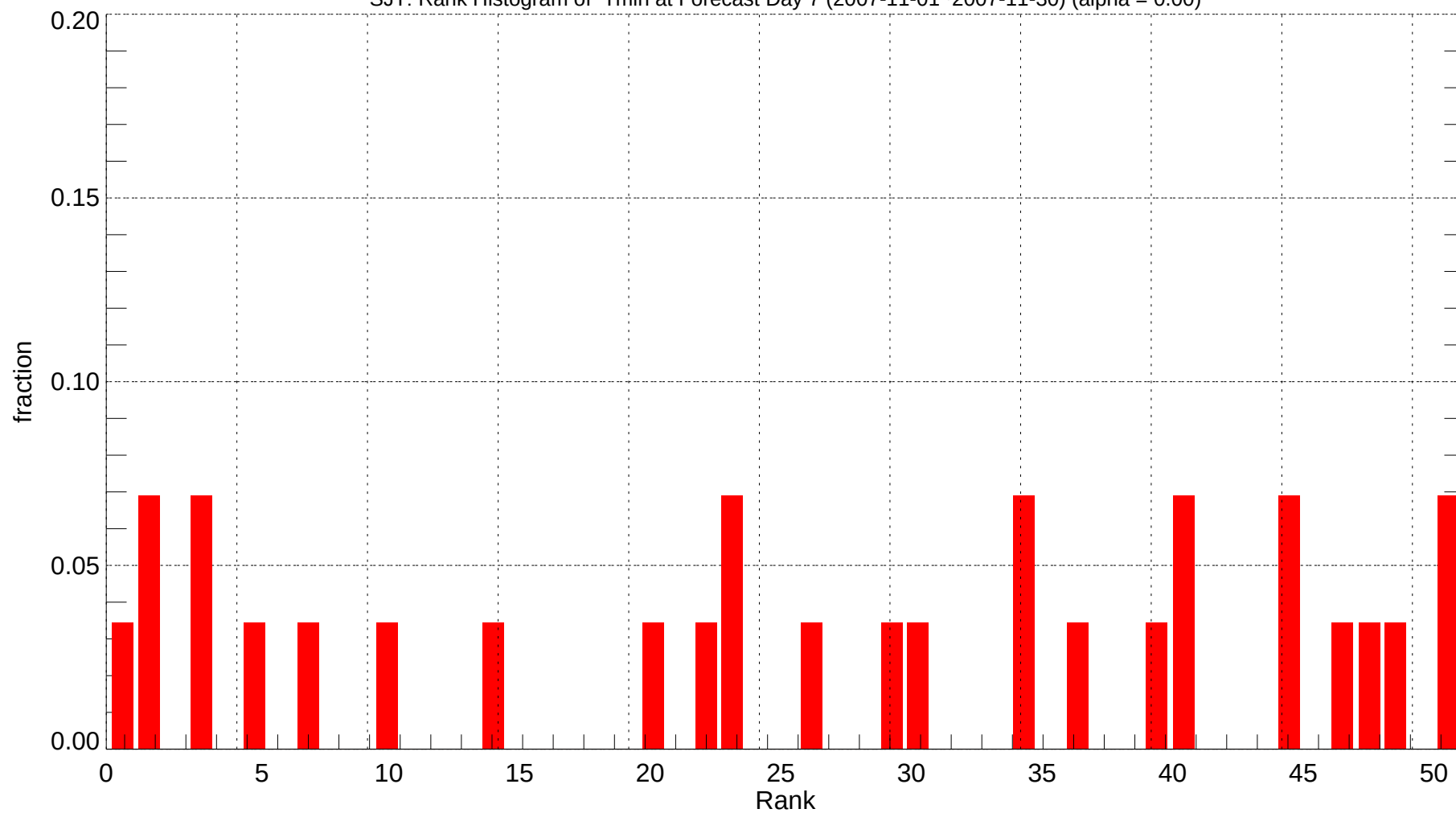
SJT: Rank Histogram of Tmin at Forecast Day 7 (2007-11-01~2007-11-30) (alpha = 0.00)
