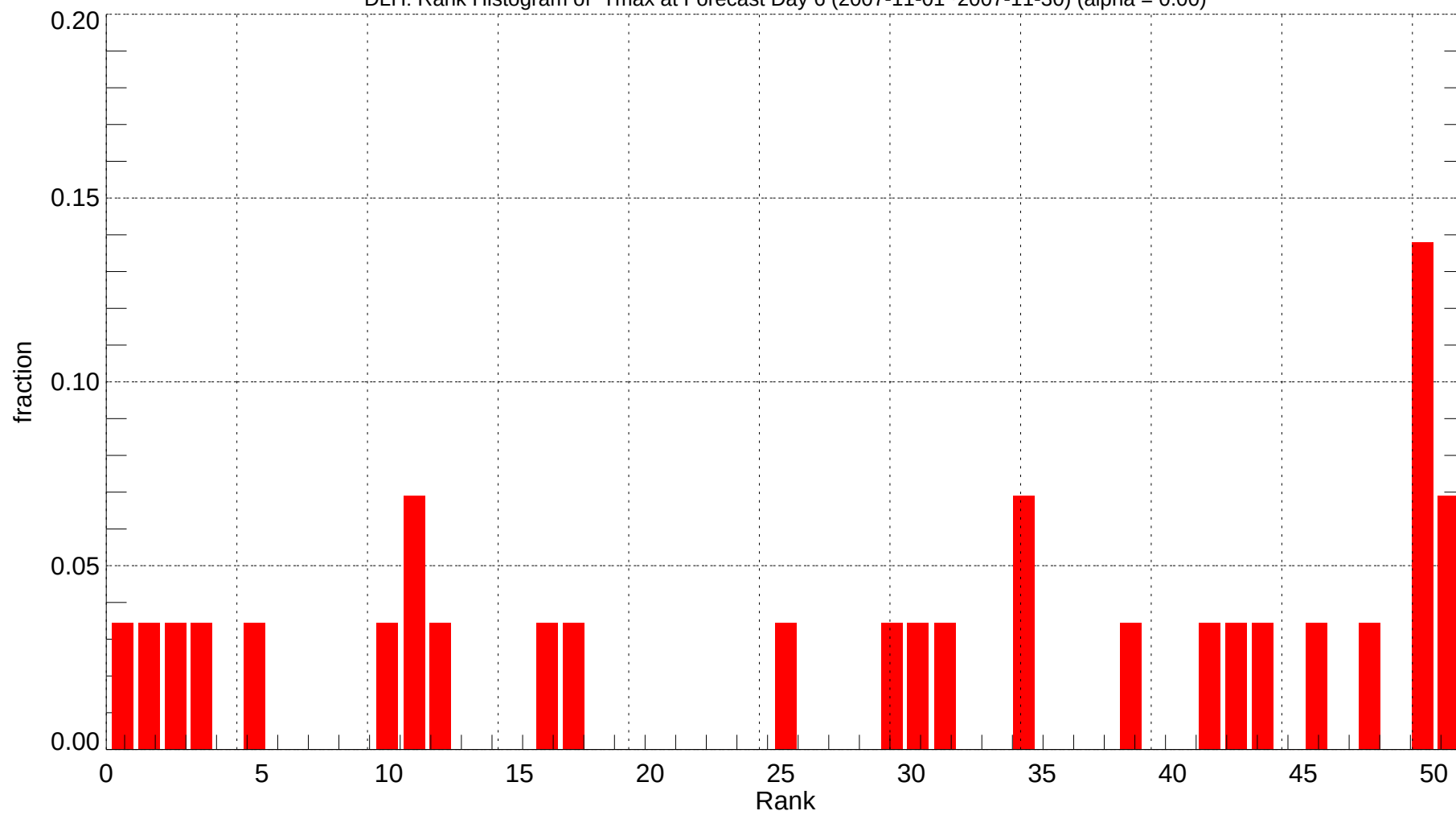
DLH: Rank Histogram of Tmax at Forecast Day 6 (2007-11-01~2007-11-30) (alpha = 0.00)
