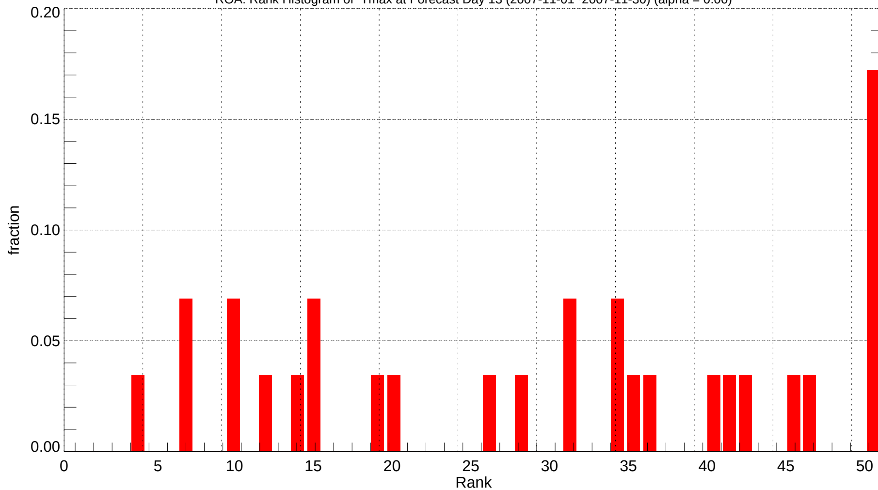
ROA: Rank Histogram of Tmax at Forecast Day 13 (2007-11-01~2007-11-30) (alpha = 0.00)
