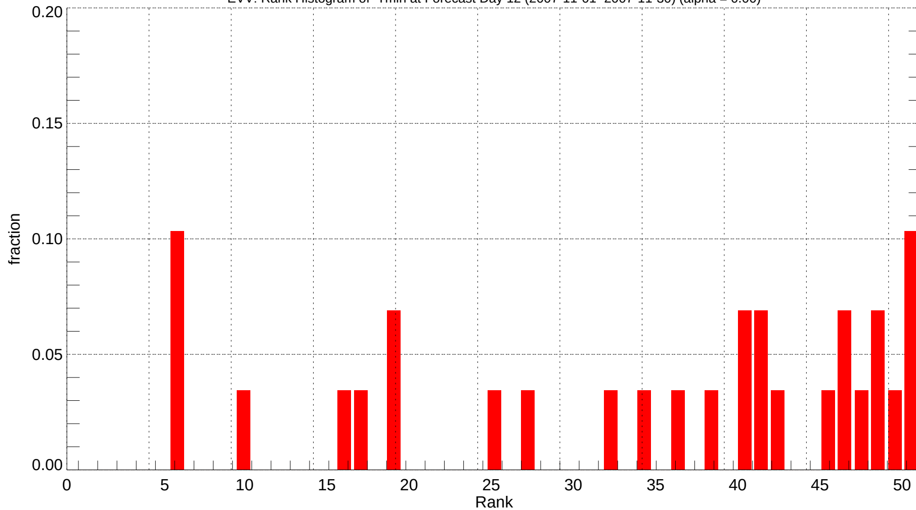
EVV: Rank Histogram of Tmin at Forecast Day 12 (2007-11-01~2007-11-30) (alpha = 0.00)
