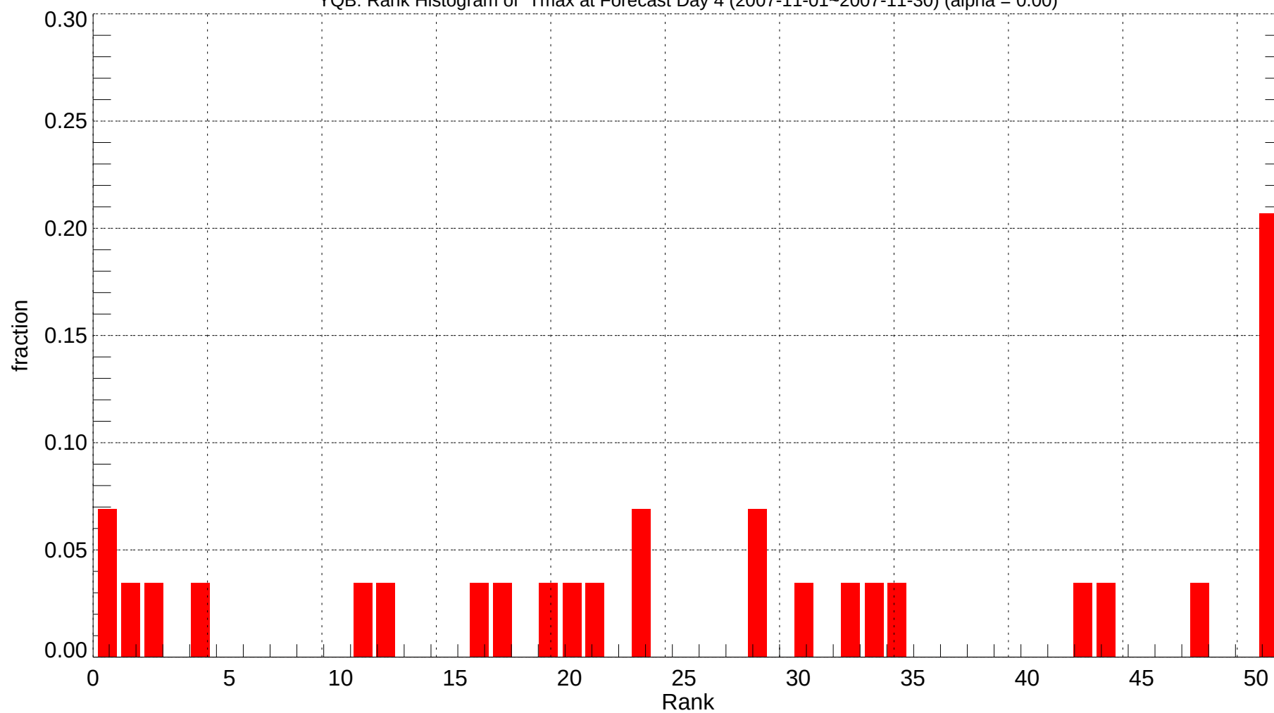
YQB: Rank Histogram of Tmax at Forecast Day 4 (2007-11-01~2007-11-30) (alpha = 0.00)
