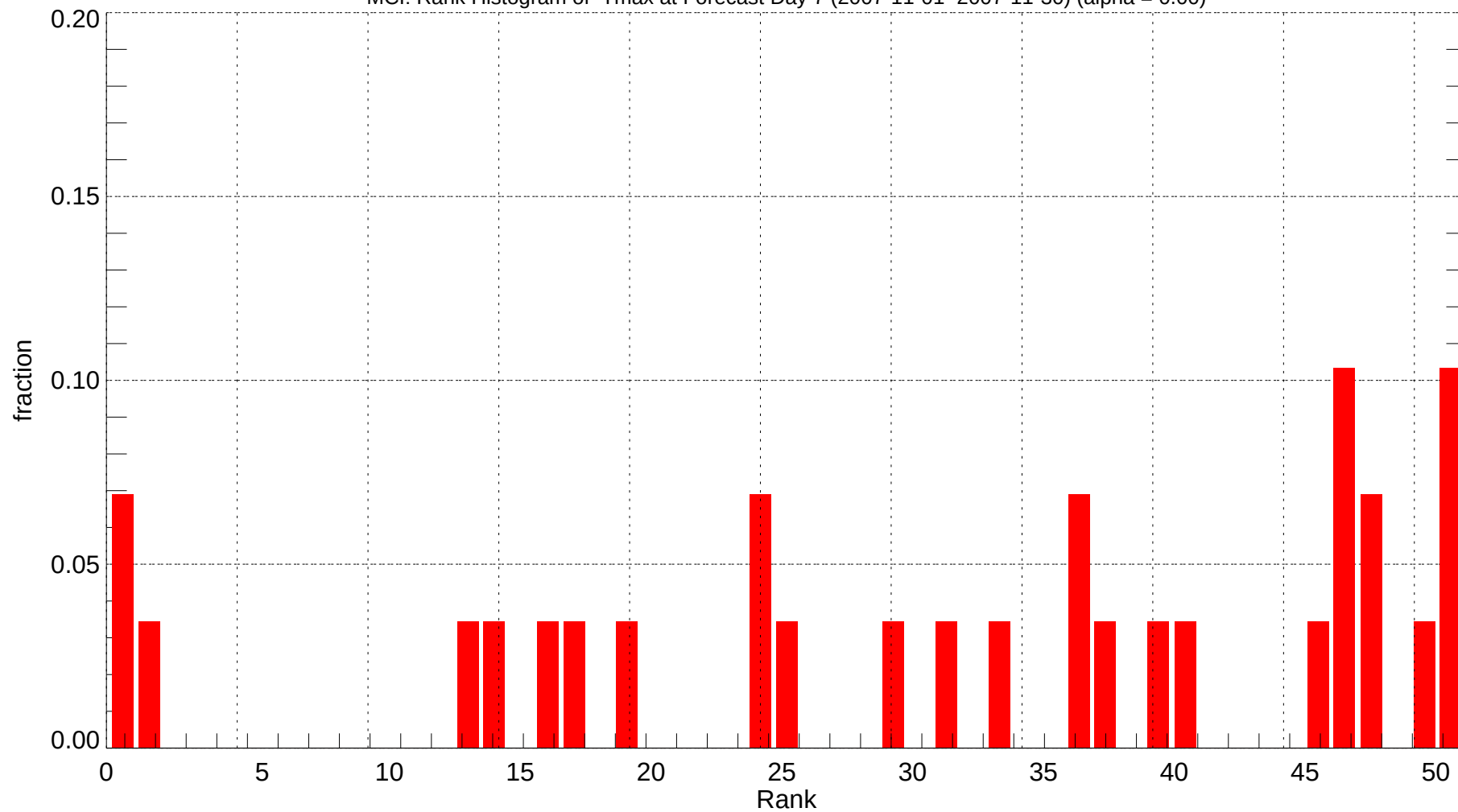
MCI: Rank Histogram of Tmax at Forecast Day 7 (2007-11-01~2007-11-30) (alpha = 0.00)
