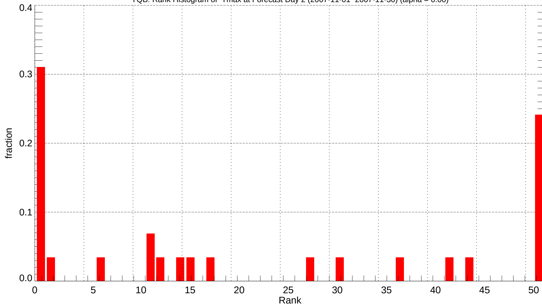
YQB: Rank Histogram of Tmax at Forecast Day 2 (2007-11-01~2007-11-30) (alpha = 0.00)
