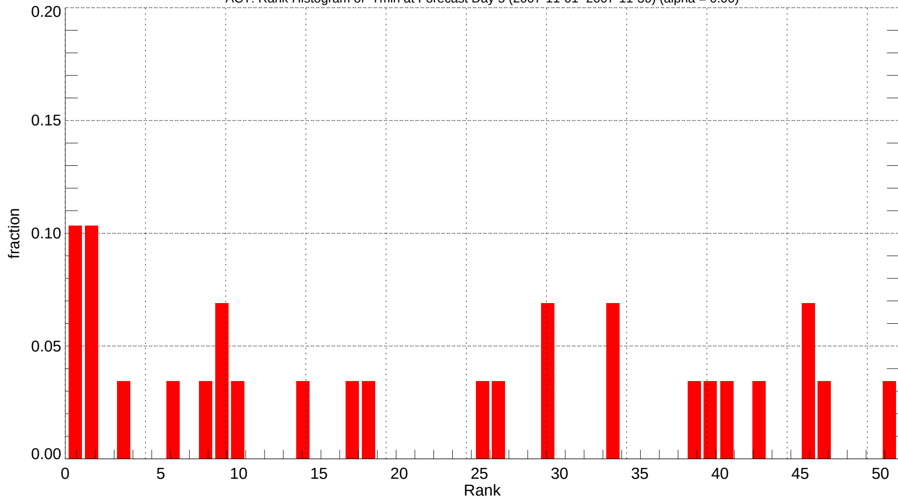
ACT: Rank Histogram of Tmin at Forecast Day 5 (2007-11-01~2007-11-30) (alpha = 0.00)
