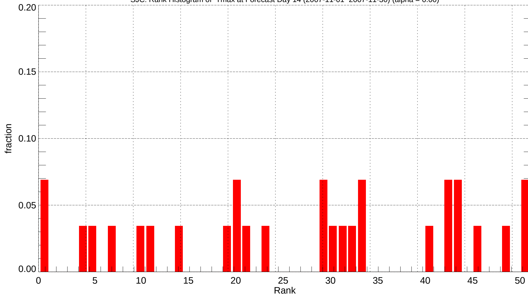
SJC: Rank Histogram of Tmax at Forecast Day 14 (2007-11-01~2007-11-30) (alpha = 0.00)
