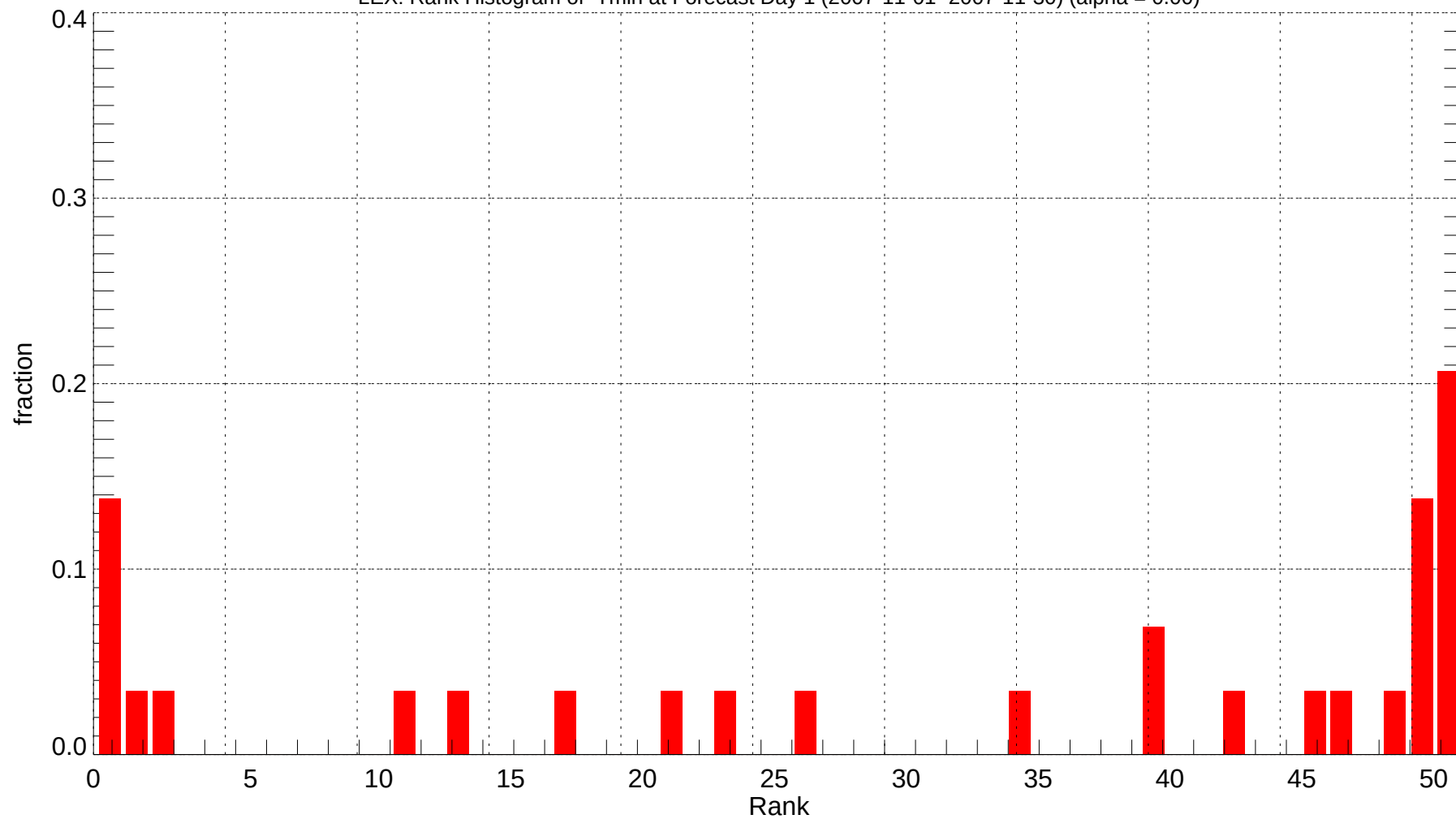
LEX: Rank Histogram of Tmin at Forecast Day 1 (2007-11-01~2007-11-30) (alpha = 0.00)
