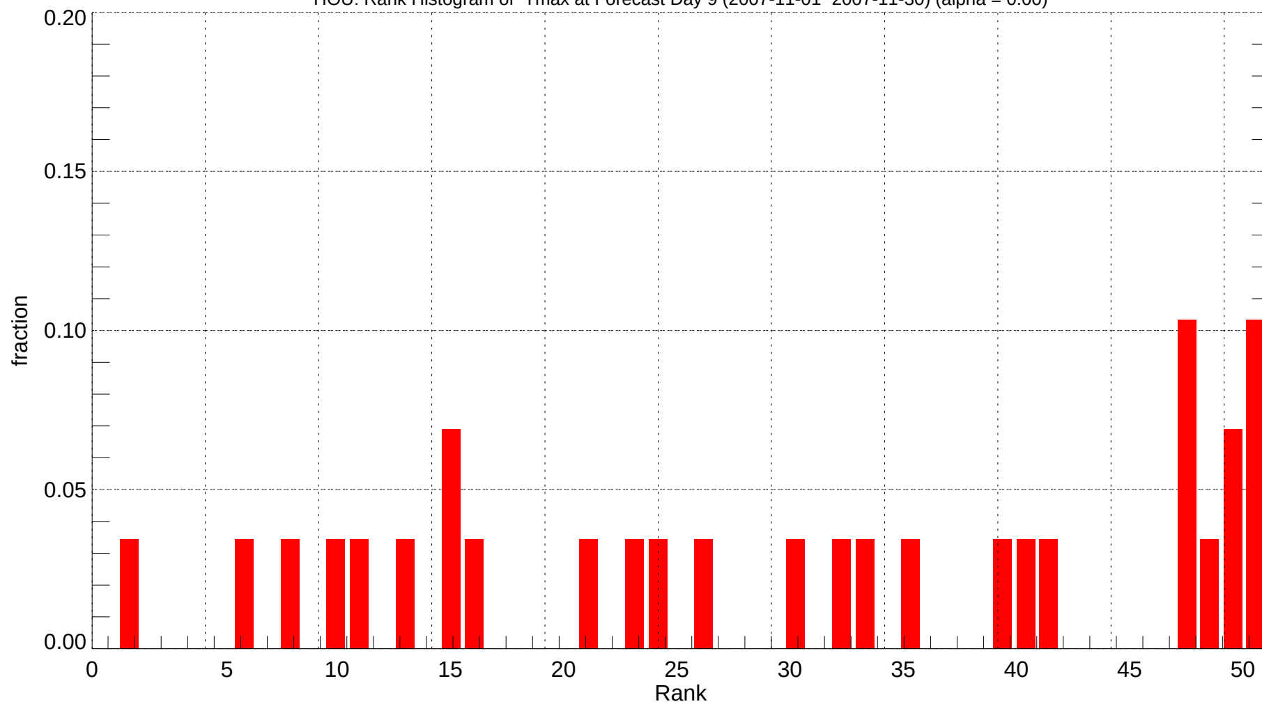
HOU: Rank Histogram of Tmax at Forecast Day 9 (2007-11-01~2007-11-30) (alpha = 0.00)
