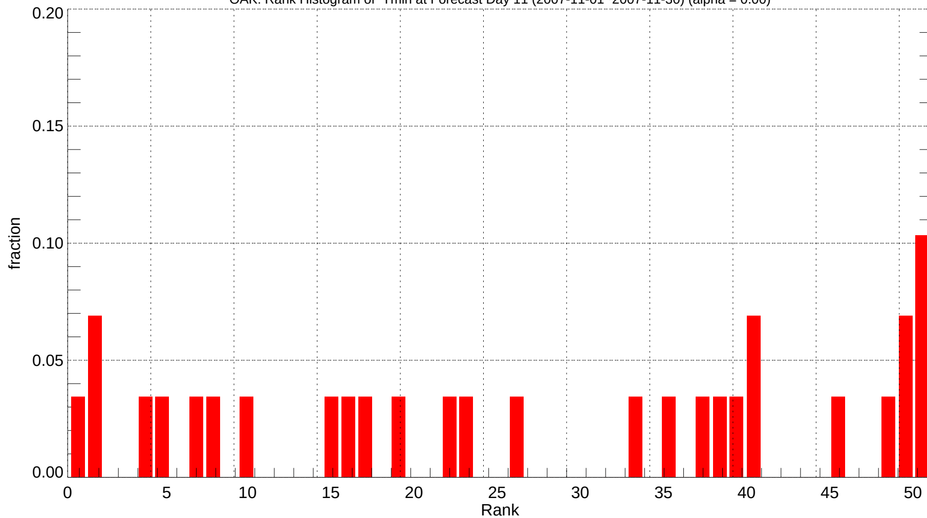
OAK: Rank Histogram of Tmin at Forecast Day 11 (2007-11-01~2007-11-30) (alpha = 0.00)
