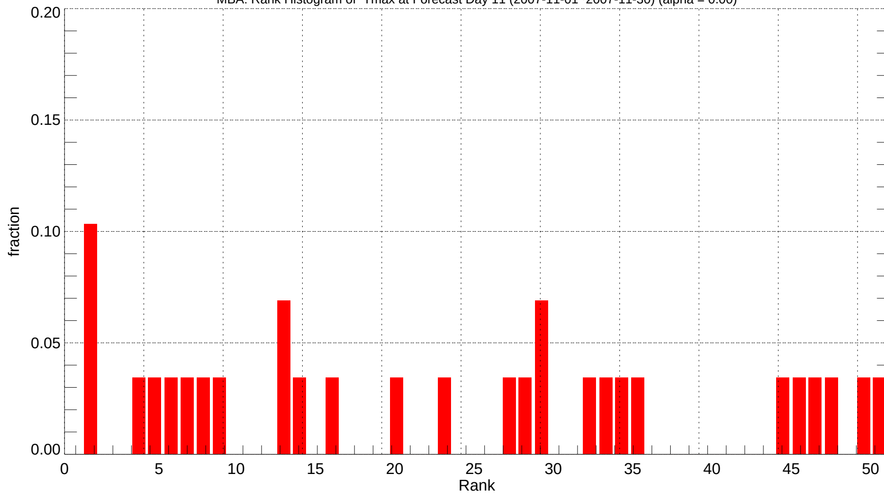
MBA: Rank Histogram of Tmax at Forecast Day 11 (2007-11-01~2007-11-30) (alpha = 0.00)
