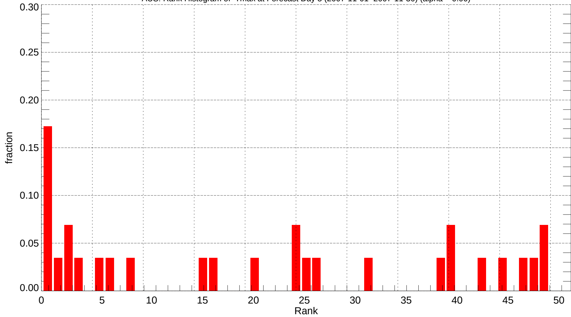
AUS: Rank Histogram of Tmax at Forecast Day 5 (2007-11-01~2007-11-30) (alpha = 0.00)
