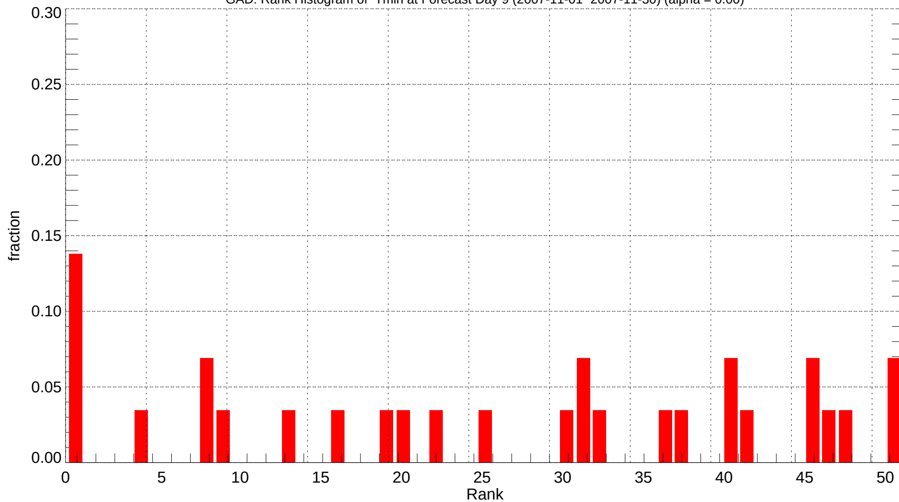
GAD: Rank Histogram of Tmin at Forecast Day 9 (2007-11-01~2007-11-30) (alpha = 0.00)
