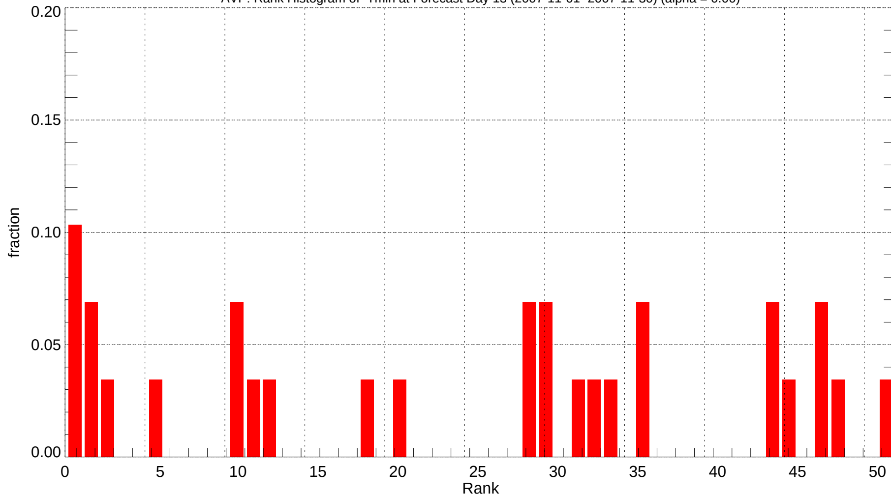
AVP: Rank Histogram of Tmin at Forecast Day 13 (2007-11-01~2007-11-30) (alpha = 0.00)
