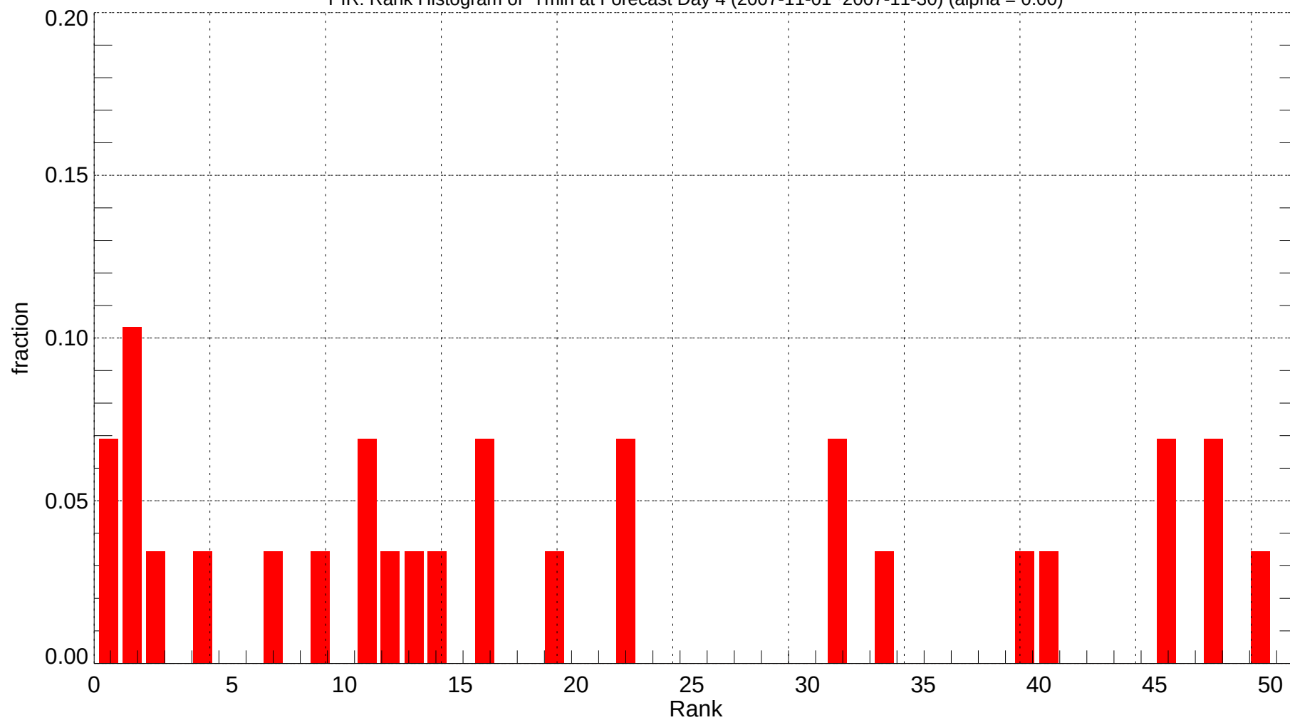
PIR: Rank Histogram of Tmin at Forecast Day 4 (2007-11-01~2007-11-30) (alpha = 0.00)
