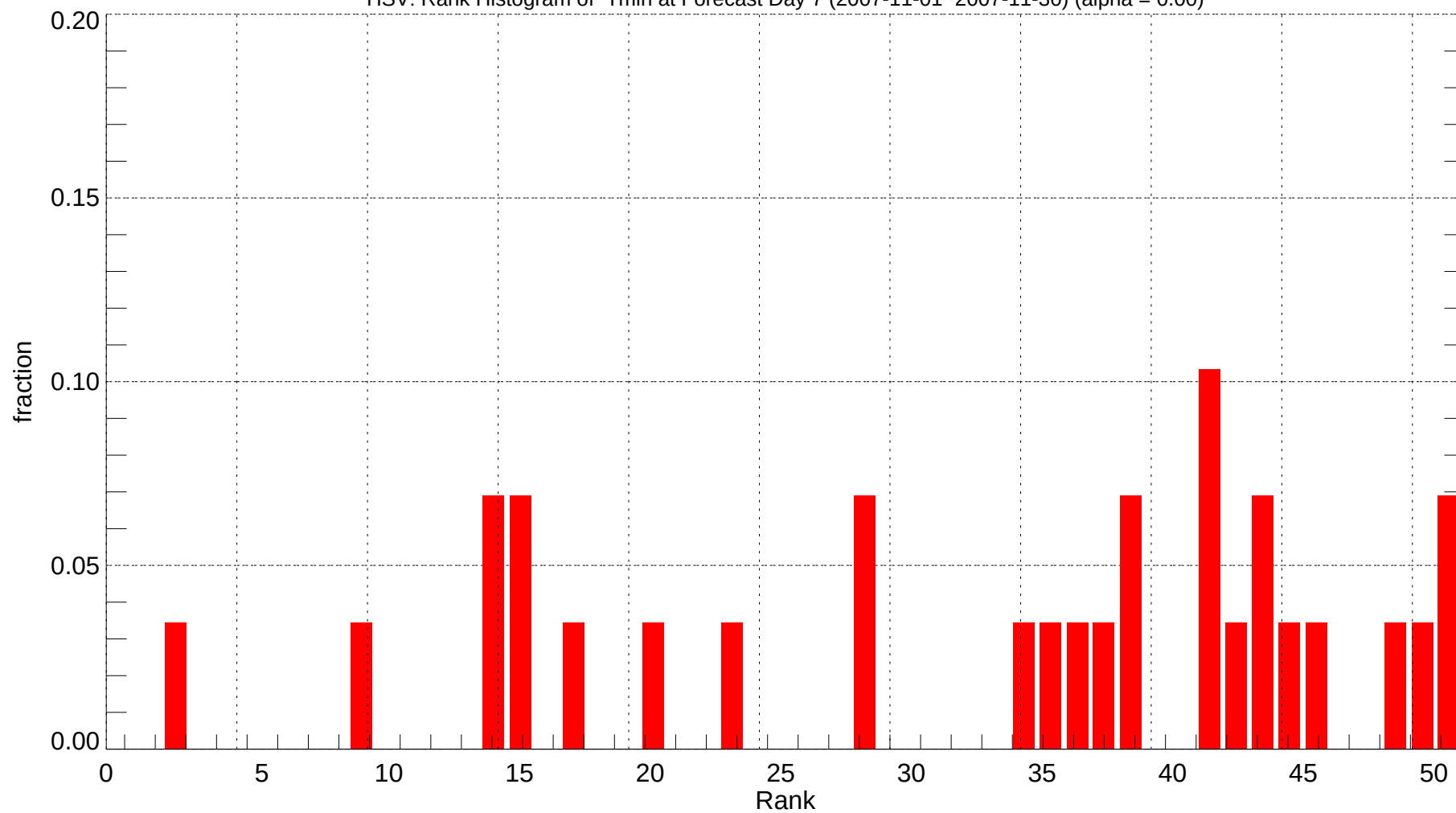
HSV: Rank Histogram of Tmin at Forecast Day 7 (2007-11-01~2007-11-30) (alpha = 0.00)
