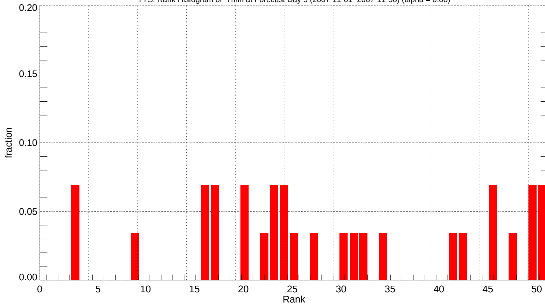
TYS: Rank Histogram of Tmin at Forecast Day 9 (2007-11-01~2007-11-30) (alpha = 0.00)
