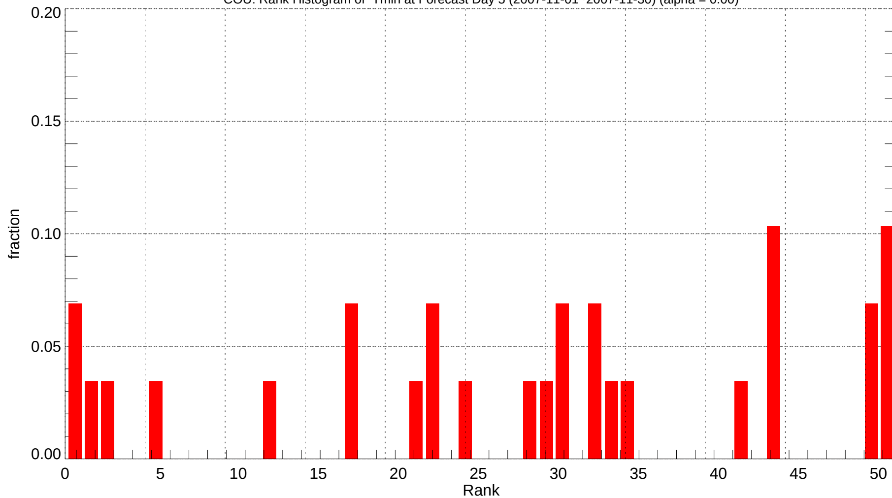
COU: Rank Histogram of Tmin at Forecast Day 5 (2007-11-01~2007-11-30) (alpha = 0.00)
