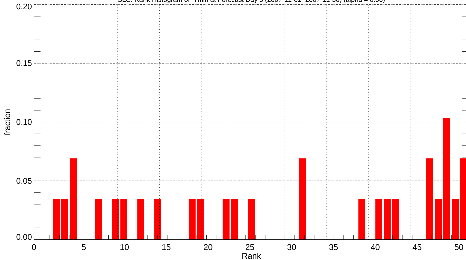
SLC: Rank Histogram of Tmin at Forecast Day 5 (2007-11-01~2007-11-30) (alpha = 0.00)
