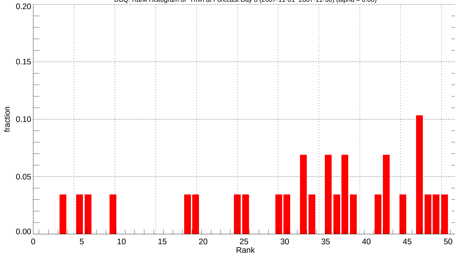
DBQ: Rank Histogram of Tmin at Forecast Day 8 (2007-11-01~2007-11-30) (alpha = 0.00)
