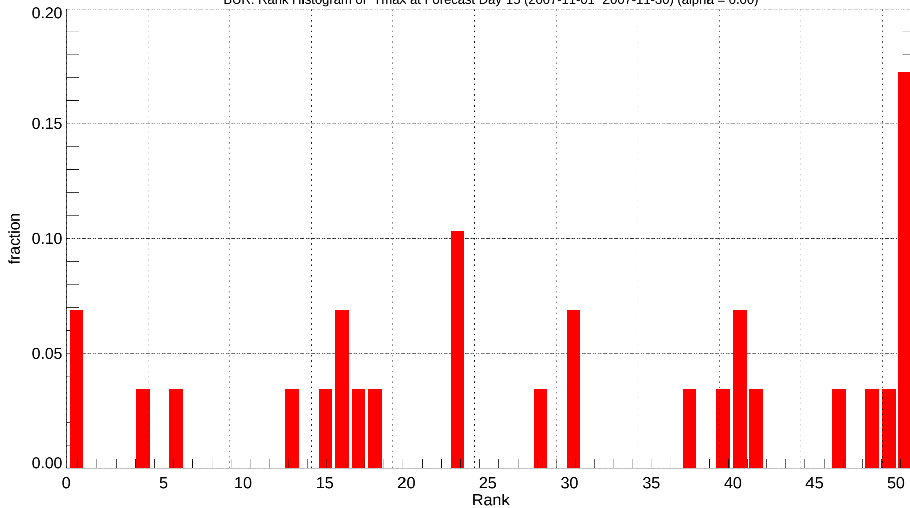
BUR: Rank Histogram of Tmax at Forecast Day 15 (2007-11-01~2007-11-30) (alpha = 0.00)
