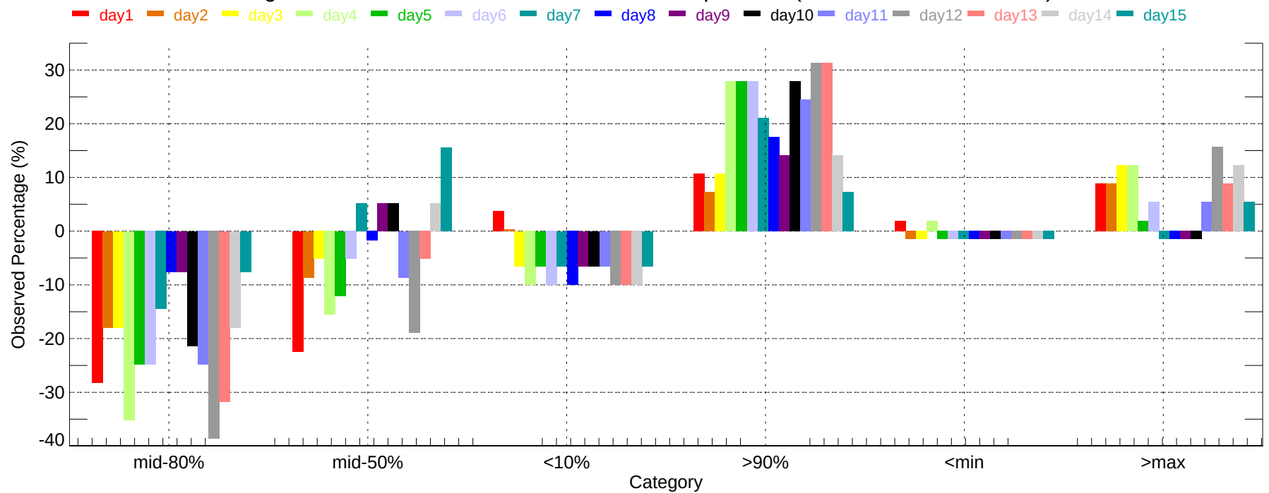
Observed Percentage Deviation of Ensembles - BHM: Min Temperature (2007-11-01~2007-11-30)
