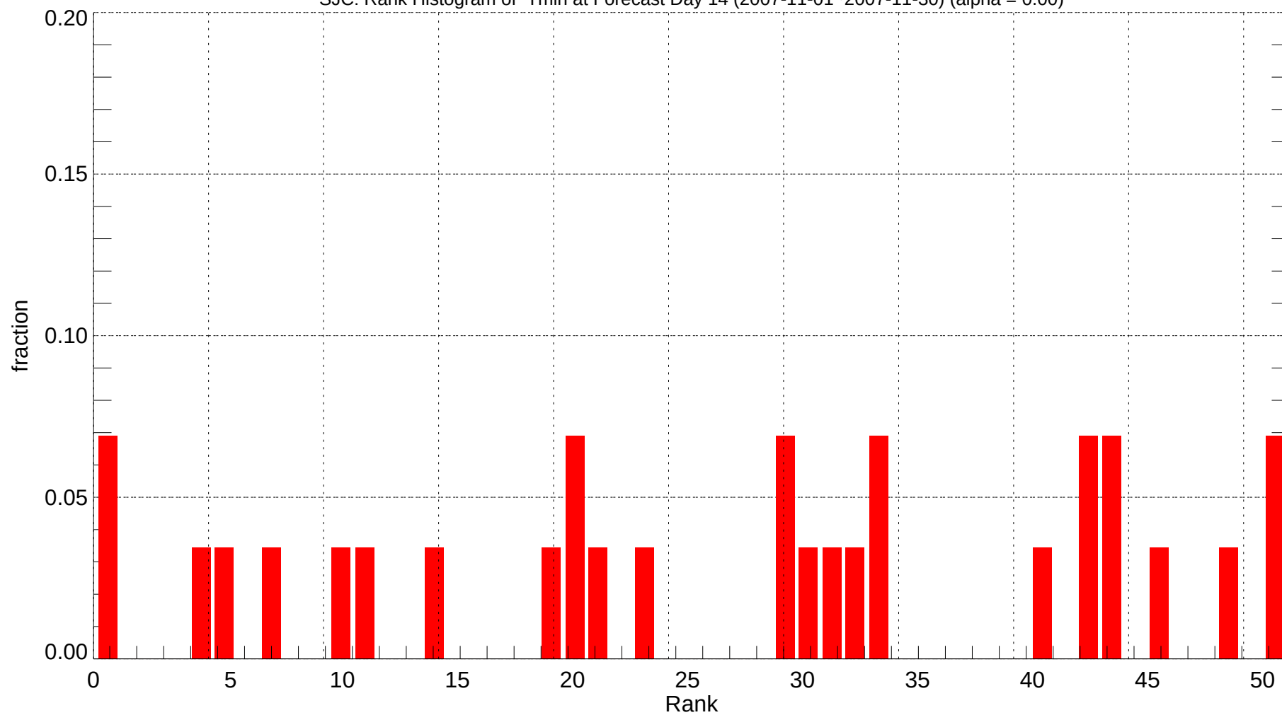
SJC: Rank Histogram of Tmin at Forecast Day 14 (2007-11-01~2007-11-30) (alpha = 0.00)
