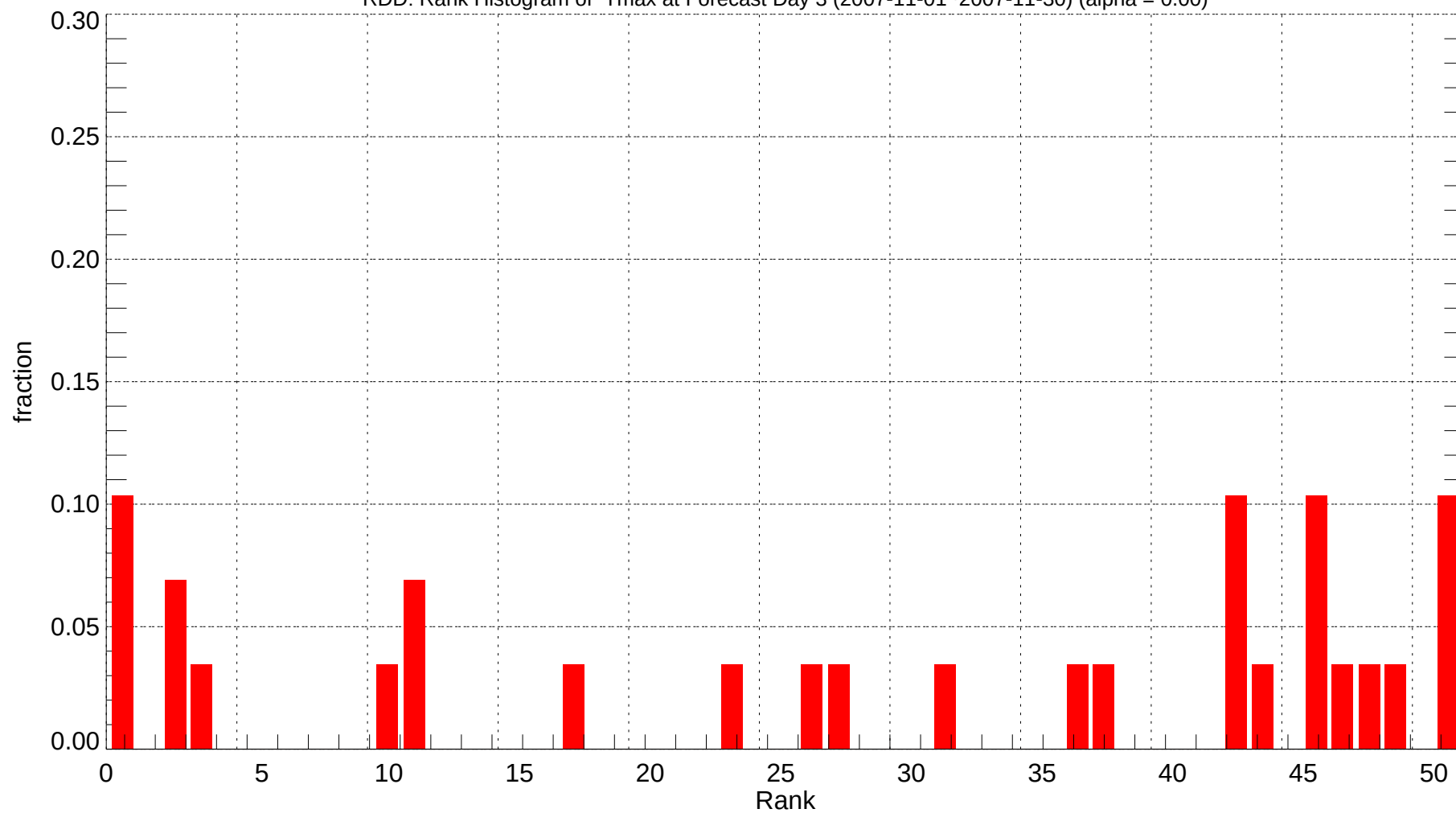
RDD: Rank Histogram of Tmax at Forecast Day 3 (2007-11-01~2007-11-30) (alpha = 0.00)
