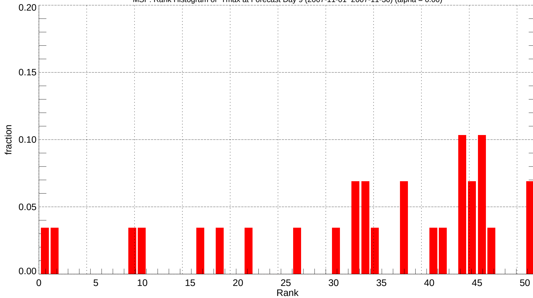
MSP: Rank Histogram of Tmax at Forecast Day 9 (2007-11-01~2007-11-30) (alpha = 0.00)
