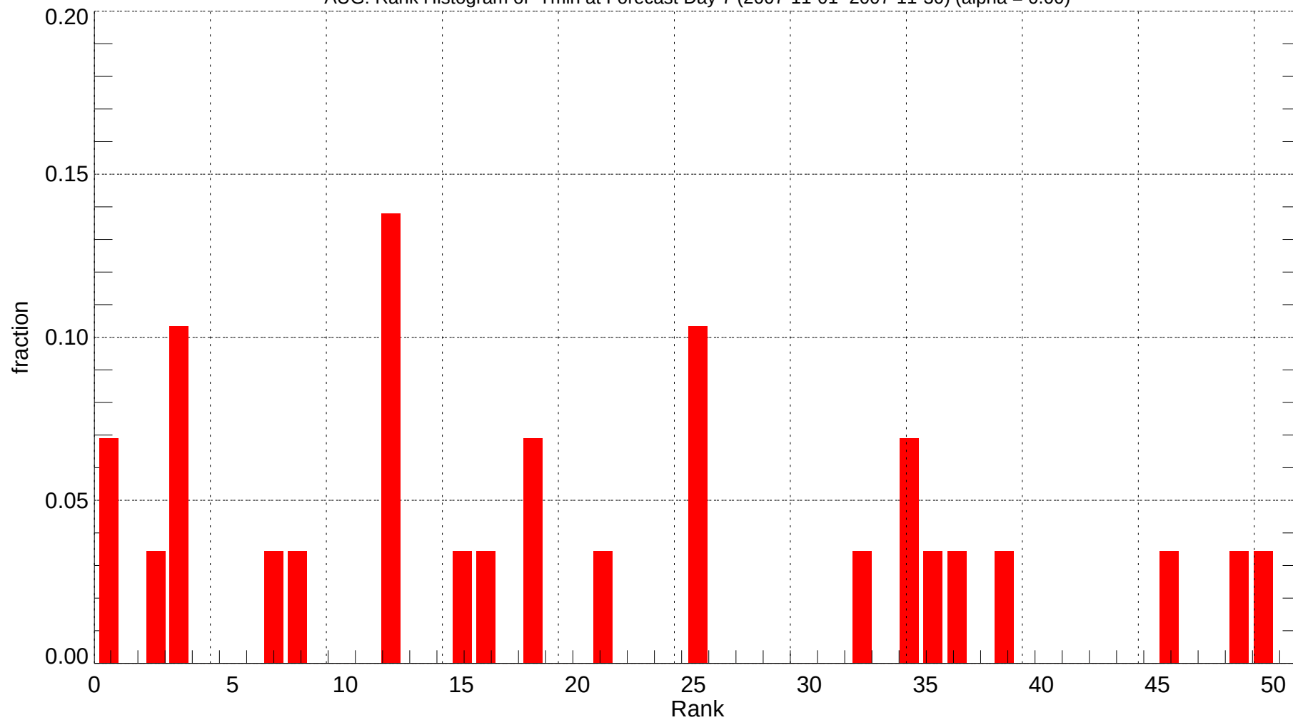
AUG: Rank Histogram of Tmin at Forecast Day 7 (2007-11-01~2007-11-30) (alpha = 0.00)
