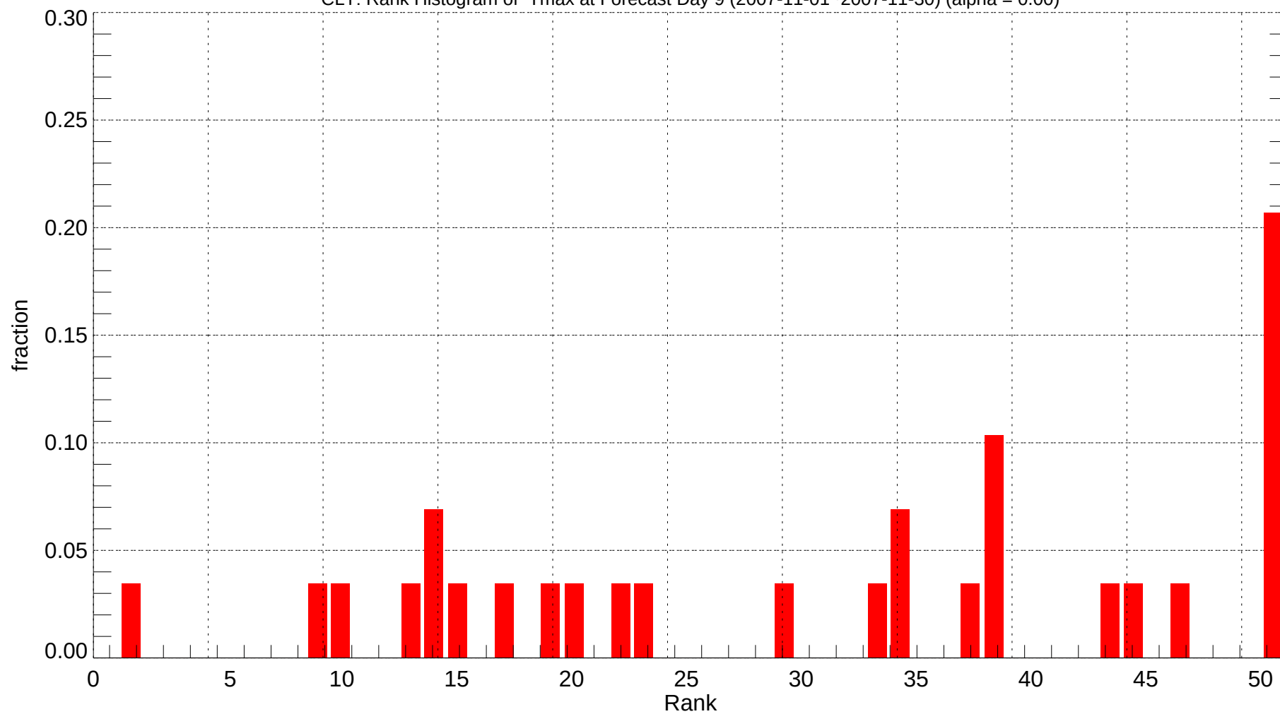
CLT: Rank Histogram of Tmax at Forecast Day 9 (2007-11-01~2007-11-30) (alpha = 0.00)
