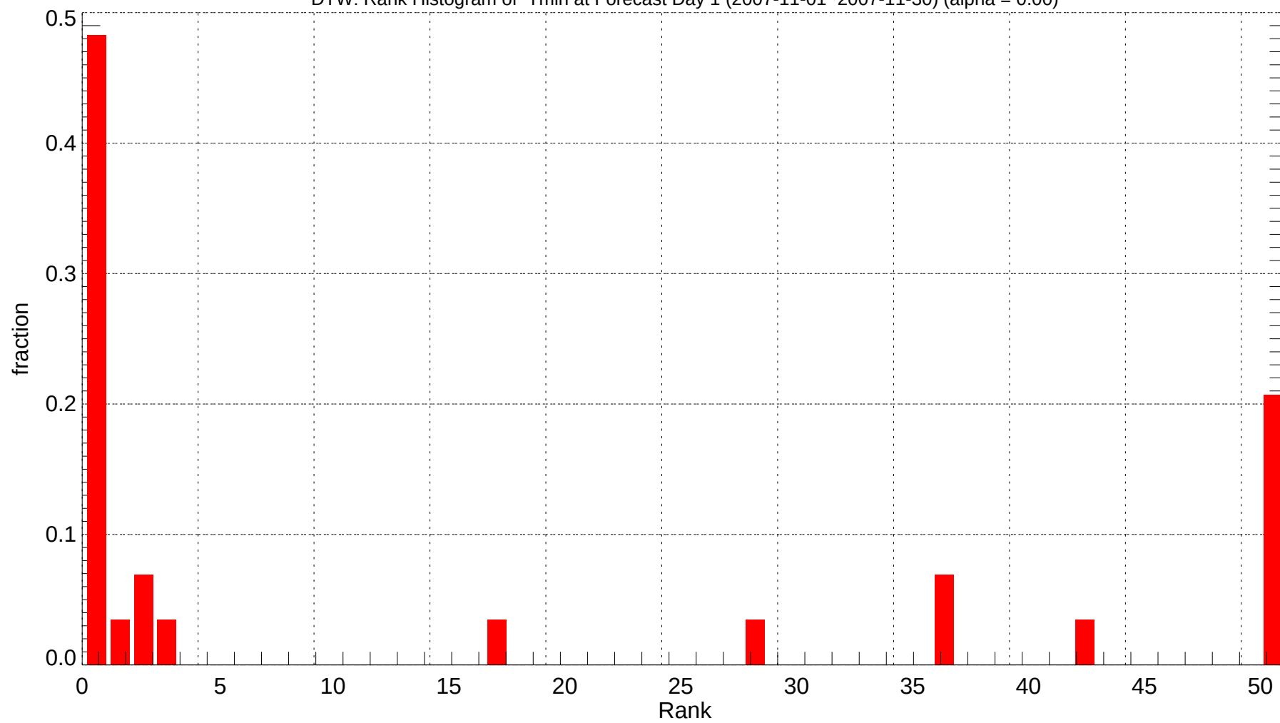
DTW: Rank Histogram of Tmin at Forecast Day 1 (2007-11-01~2007-11-30) (alpha = 0.00)
