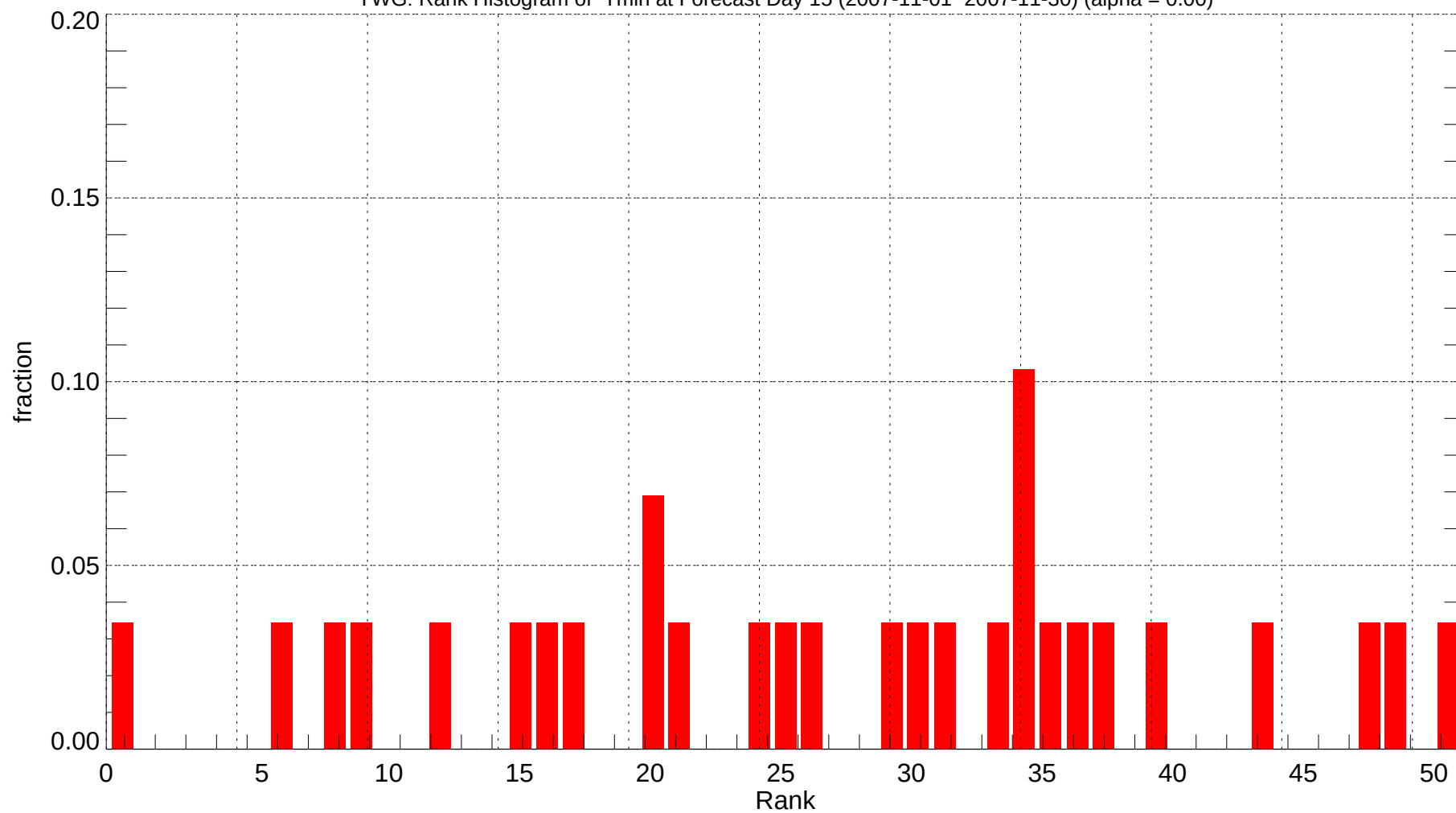
YWG: Rank Histogram of Tmin at Forecast Day 15 (2007-11-01~2007-11-30) (alpha = 0.00)
