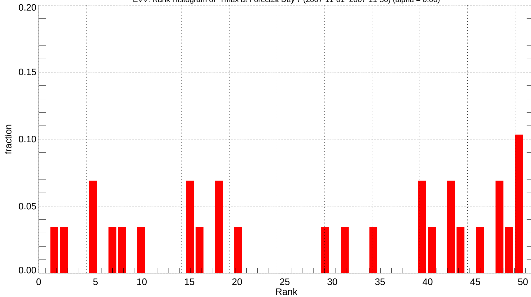
EVV: Rank Histogram of Tmax at Forecast Day 7 (2007-11-01~2007-11-30) (alpha = 0.00)
