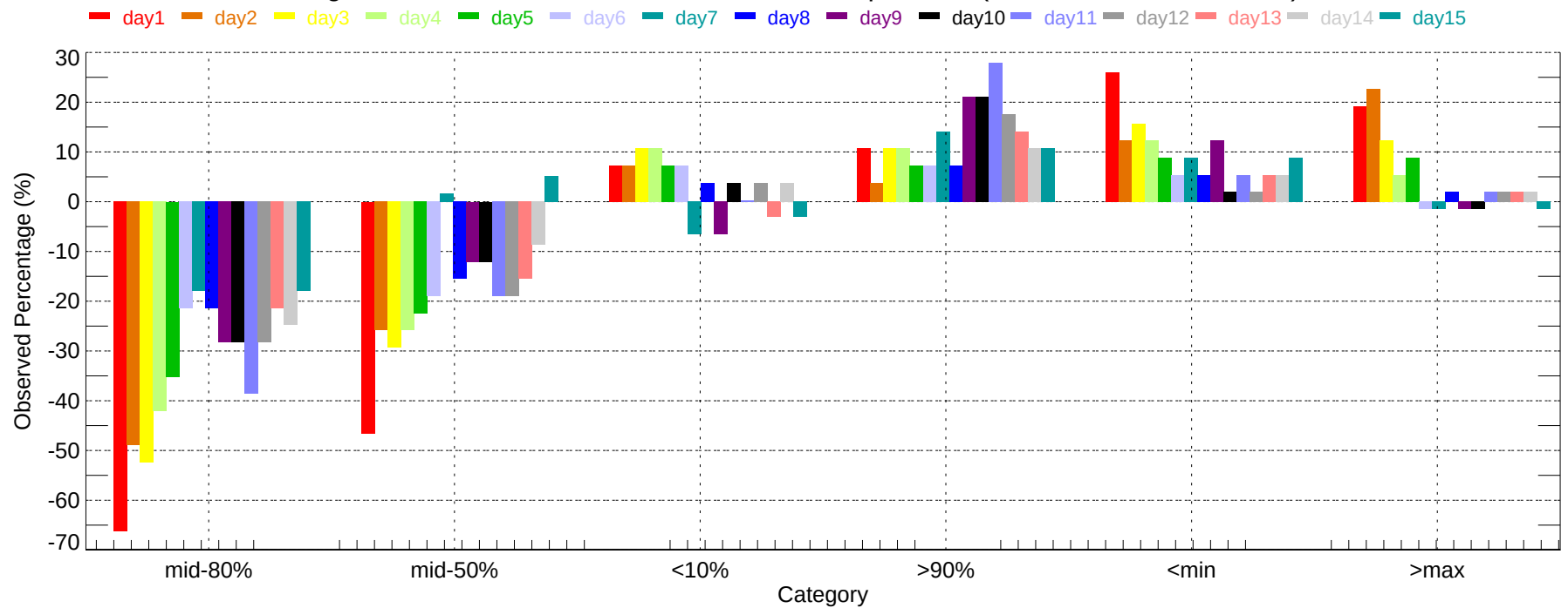
Observed Percentage Deviation of Ensembles - BRO: Min Temperature (2007-11-01~2007-11-30)
