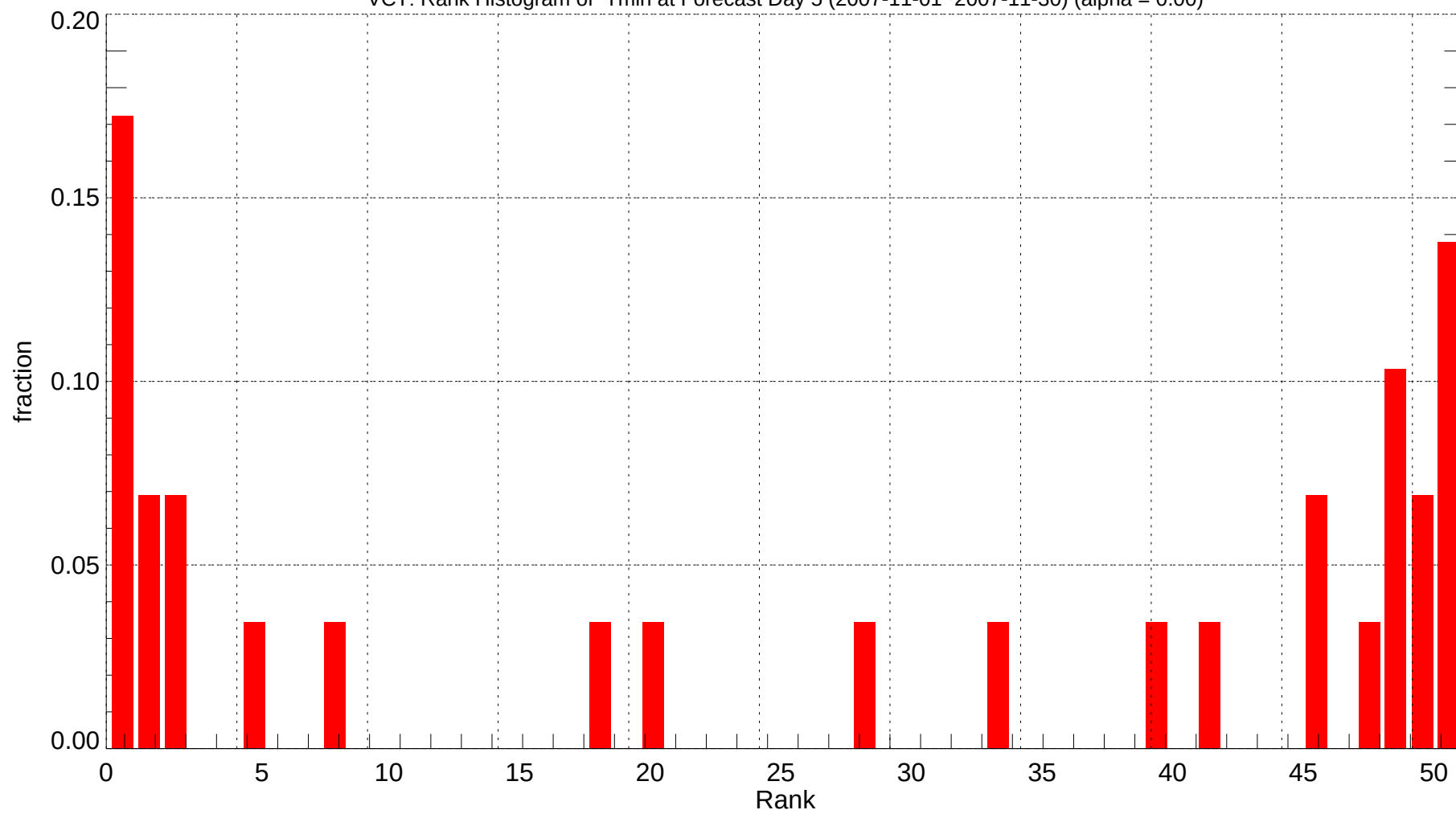
VCT: Rank Histogram of Tmin at Forecast Day 5 (2007-11-01~2007-11-30) (alpha = 0.00)
