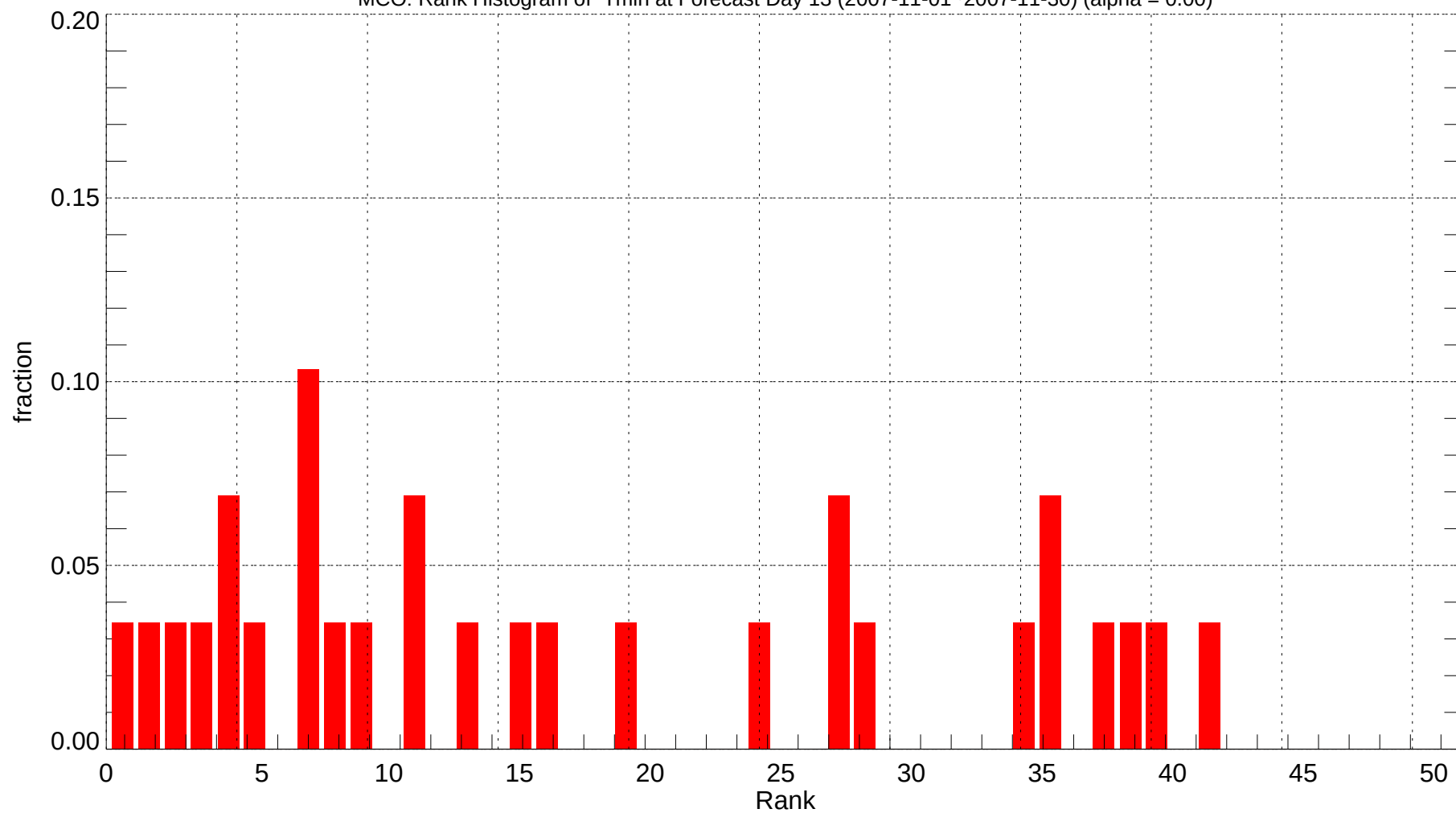
MCO: Rank Histogram of Tmin at Forecast Day 13 (2007-11-01~2007-11-30) (alpha = 0.00)
