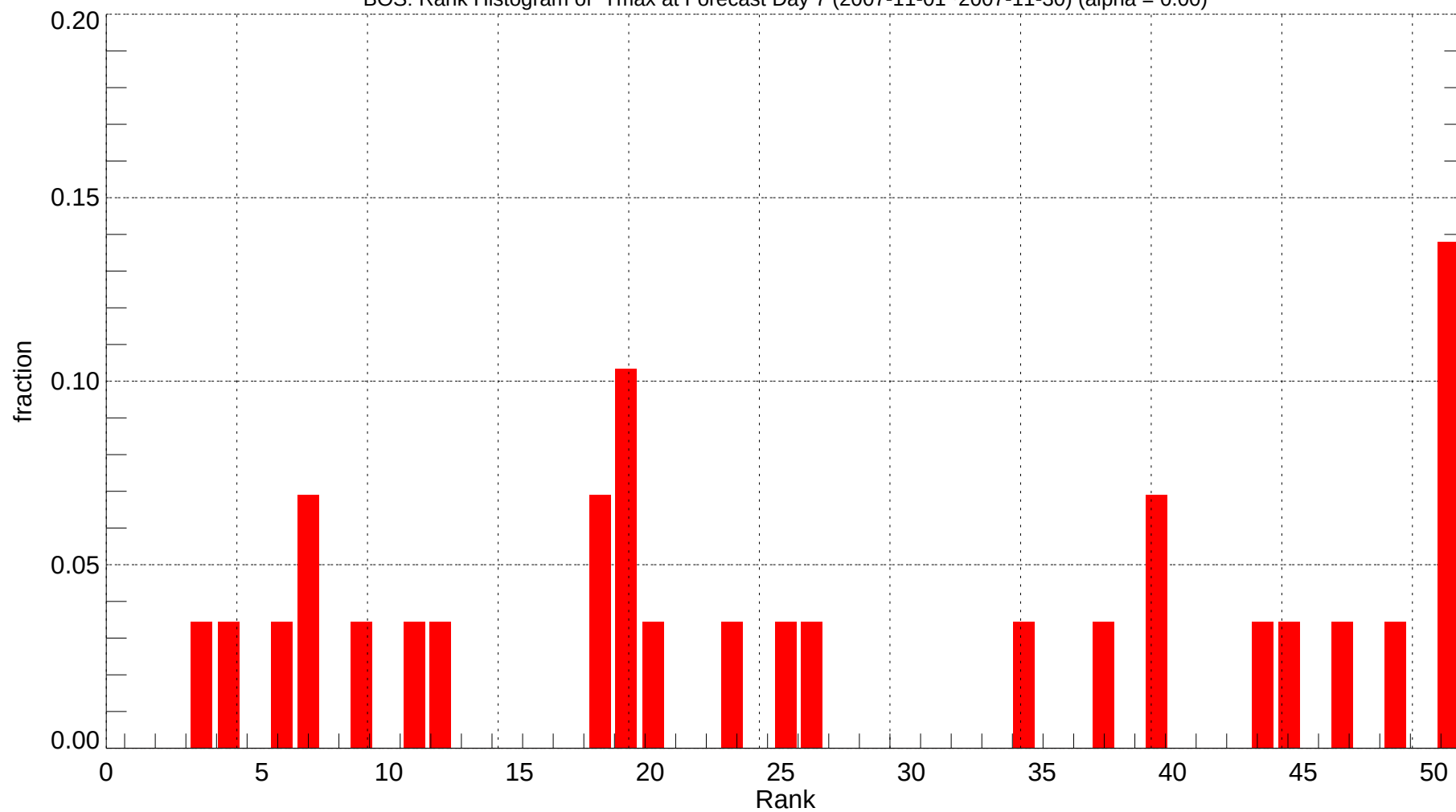
BOS: Rank Histogram of Tmax at Forecast Day 7 (2007-11-01~2007-11-30) (alpha = 0.00)
