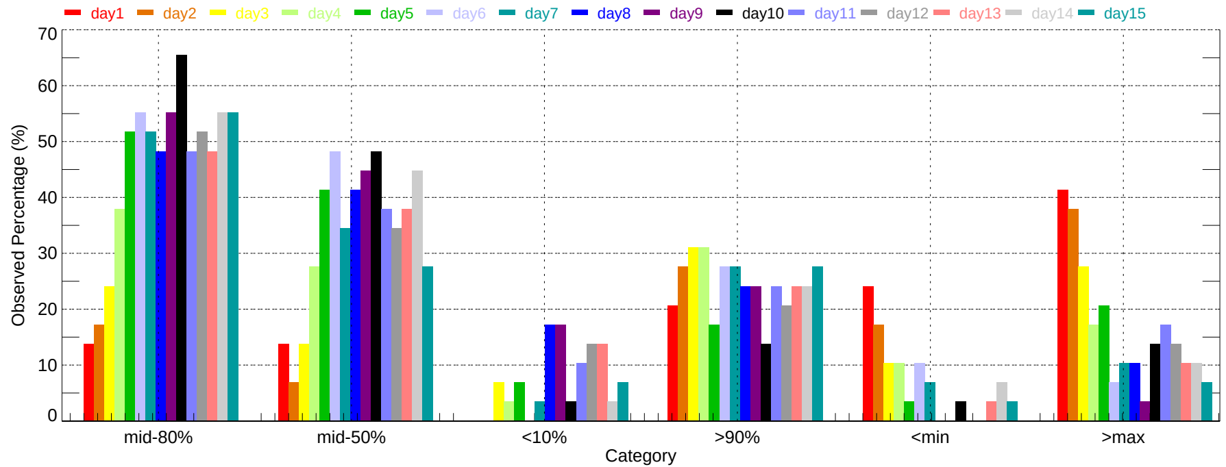
Observed Percentage of Ensembles - AOO: Min Temperature (2007-11-01~2007-11-30)
