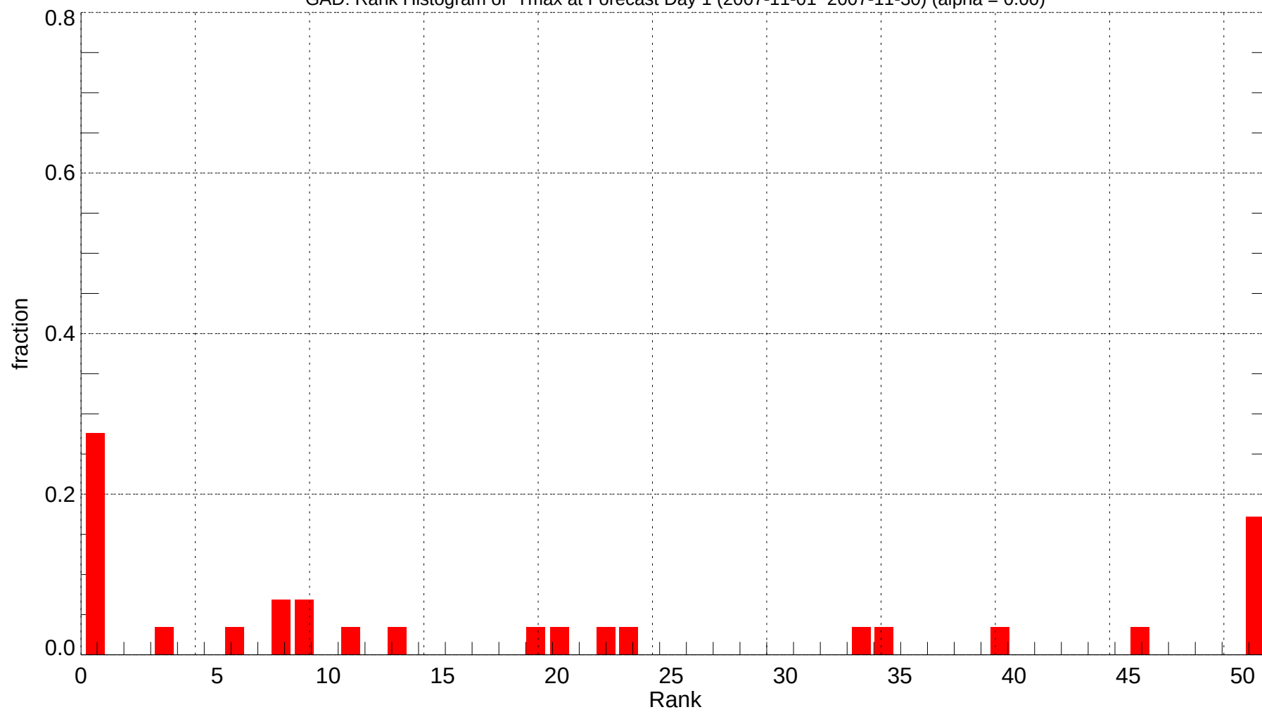
GAD: Rank Histogram of Tmax at Forecast Day 1 (2007-11-01~2007-11-30) (alpha = 0.00)
