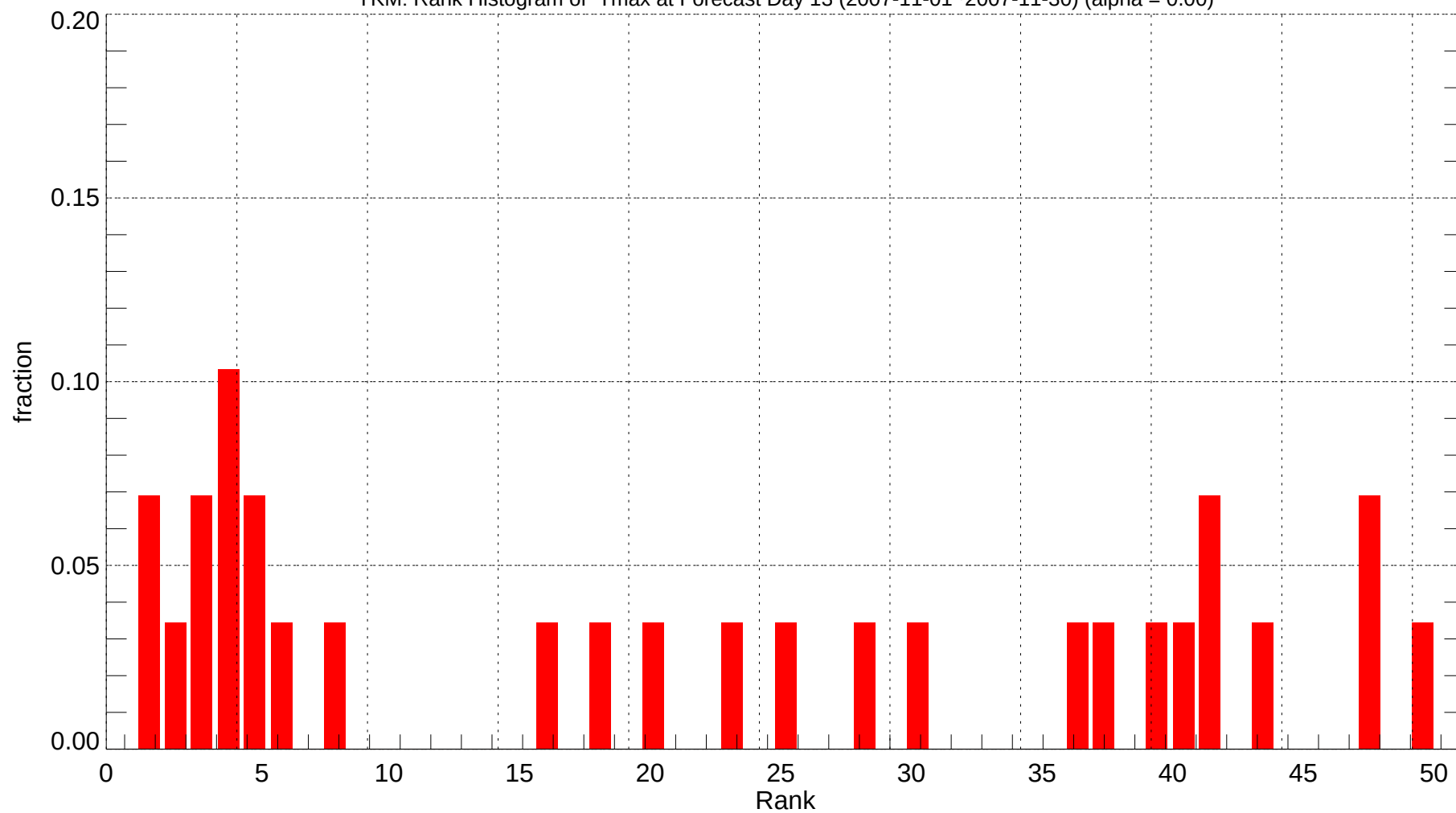
YKM: Rank Histogram of Tmax at Forecast Day 13 (2007-11-01~2007-11-30) (alpha = 0.00)
