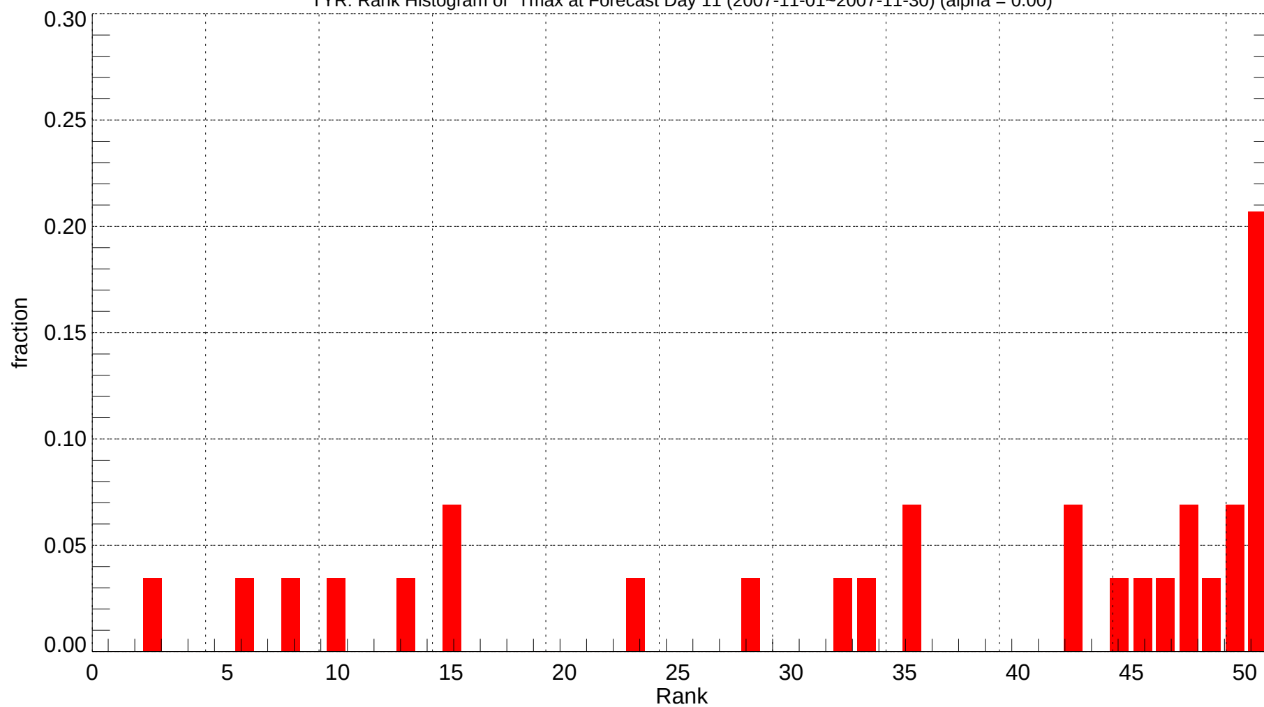
TYR: Rank Histogram of Tmax at Forecast Day 11 (2007-11-01~2007-11-30) (alpha = 0.00)
