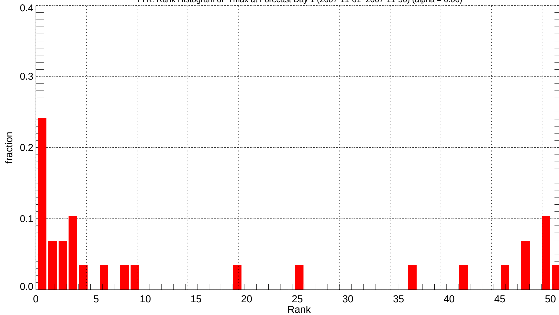
TYR: Rank Histogram of Tmax at Forecast Day 1 (2007-11-01~2007-11-30) (alpha = 0.00)
