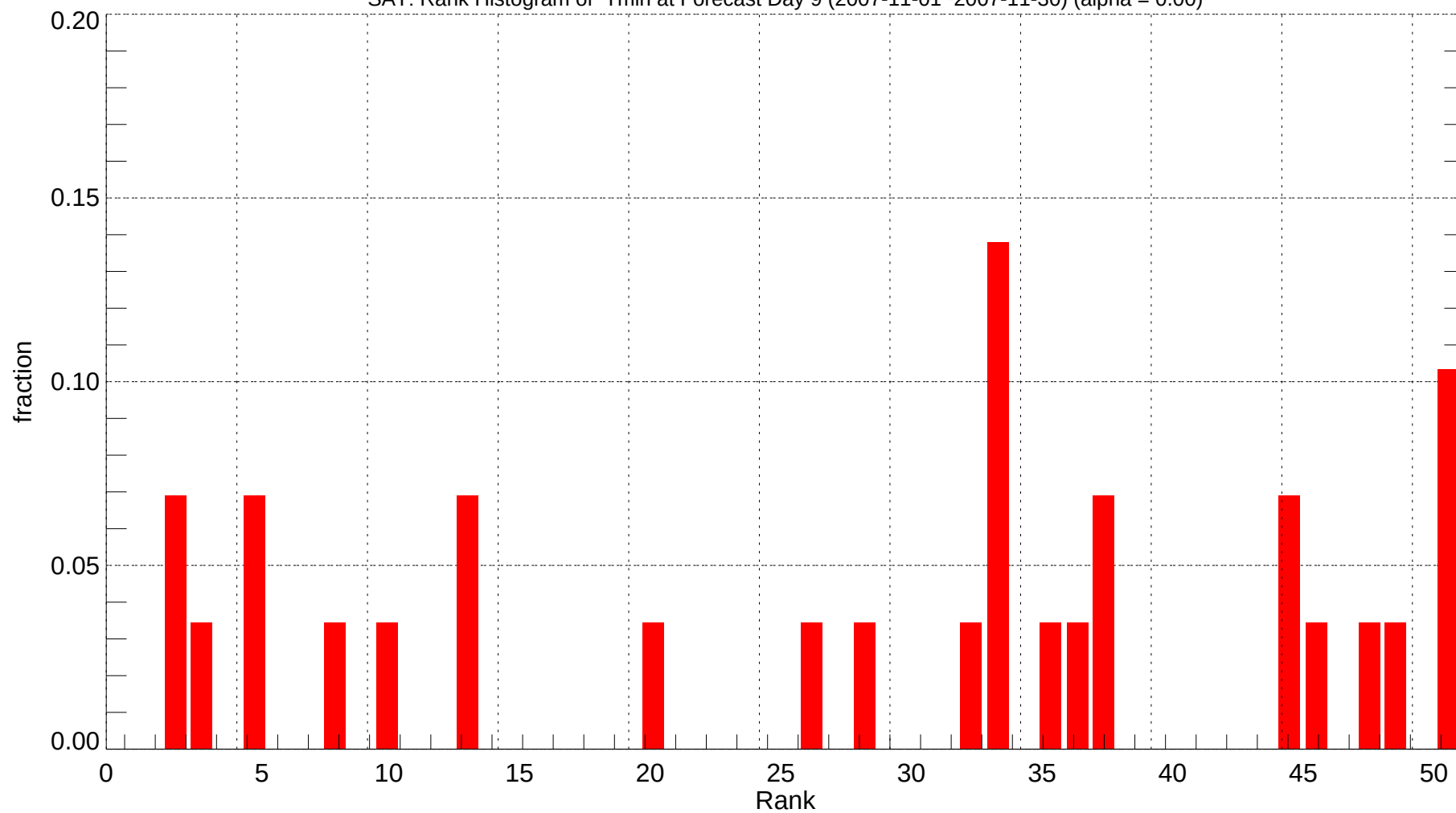
SAT: Rank Histogram of Tmin at Forecast Day 9 (2007-11-01~2007-11-30) (alpha = 0.00)
