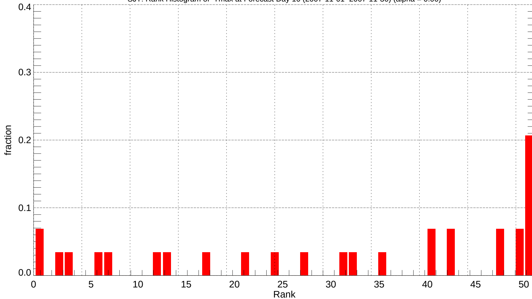
SJT: Rank Histogram of Tmax at Forecast Day 10 (2007-11-01~2007-11-30) (alpha = 0.00)
