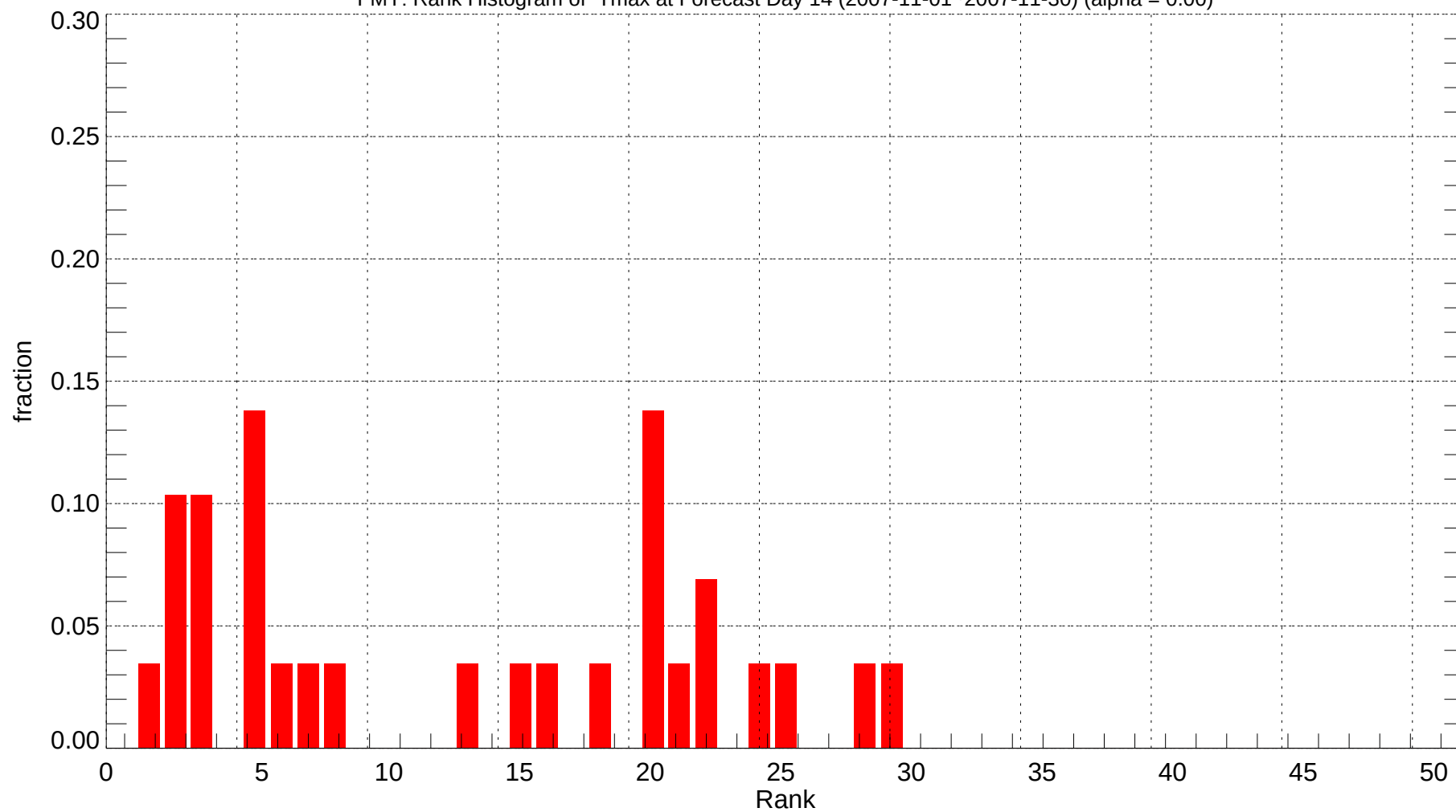
FMY: Rank Histogram of Tmax at Forecast Day 14 (2007-11-01~2007-11-30) (alpha = 0.00)
