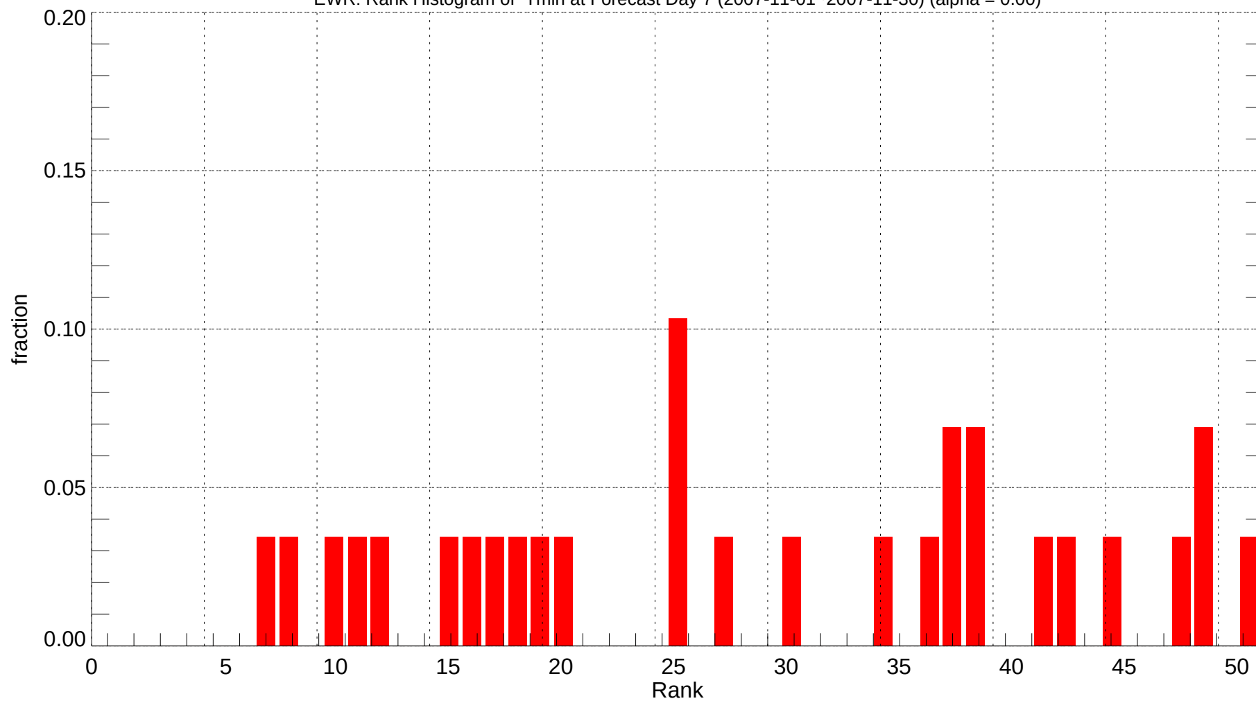
EWR: Rank Histogram of Tmin at Forecast Day 7 (2007-11-01~2007-11-30) (alpha = 0.00)
