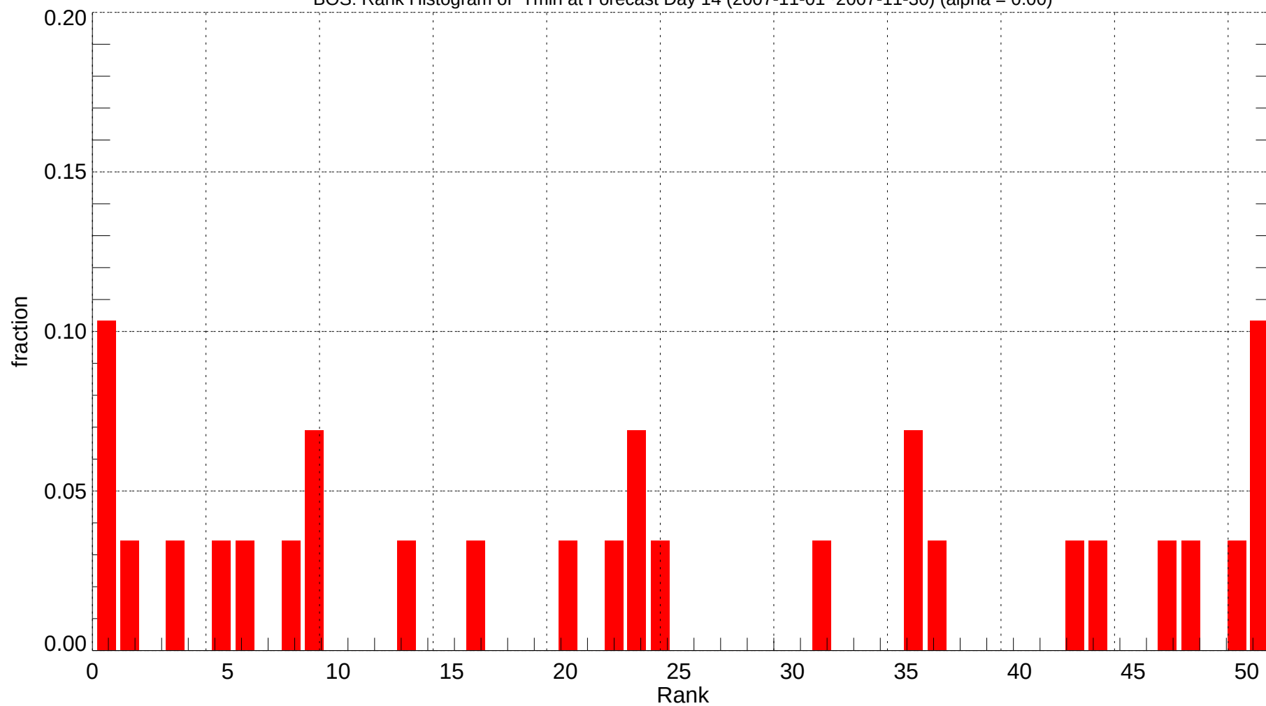
BOS: Rank Histogram of Tmin at Forecast Day 14 (2007-11-01~2007-11-30) (alpha = 0.00)
