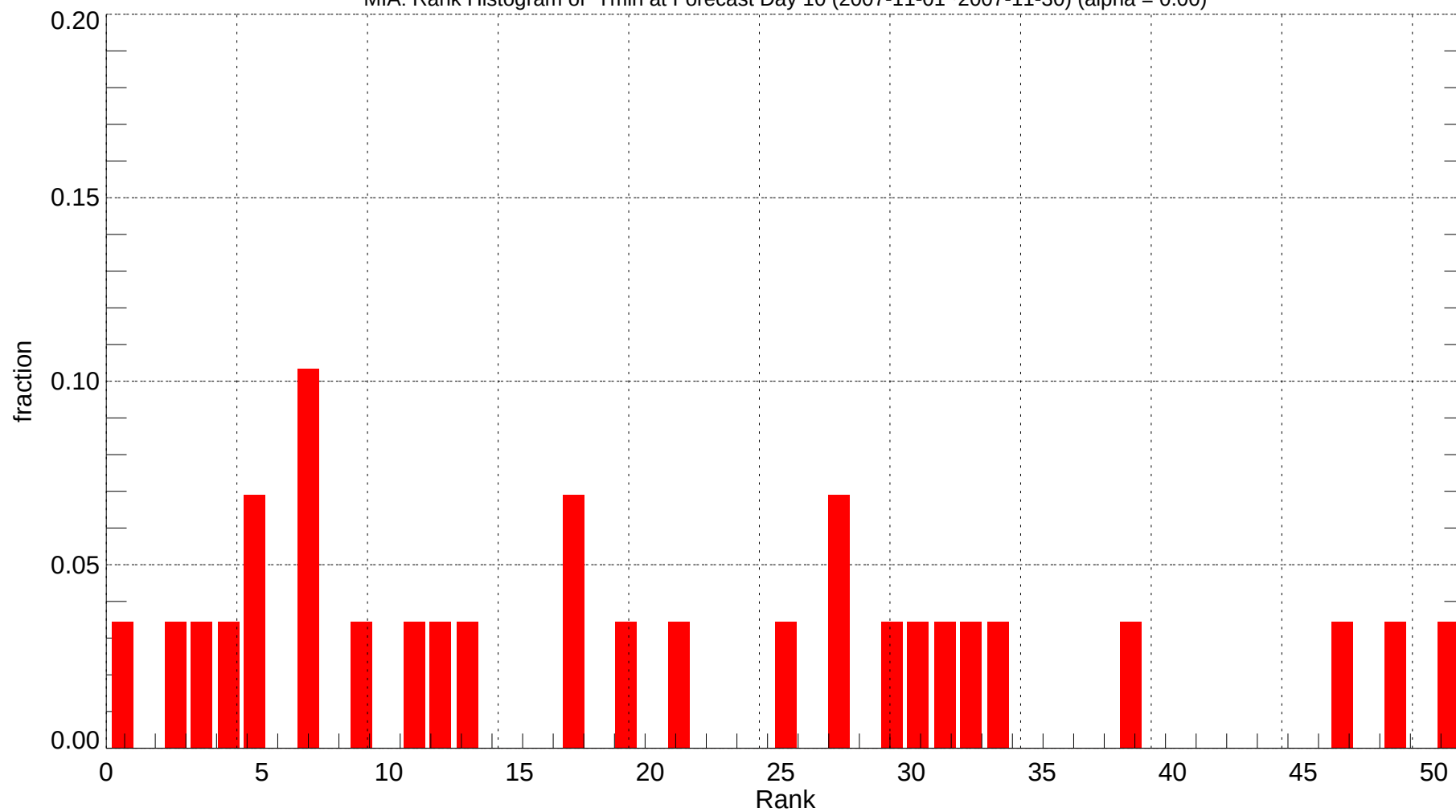
MIA: Rank Histogram of Tmin at Forecast Day 10 (2007-11-01~2007-11-30) (alpha = 0.00)
