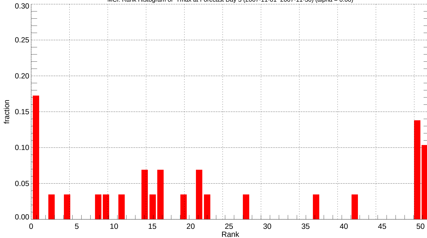
MCI: Rank Histogram of Tmax at Forecast Day 3 (2007-11-01~2007-11-30) (alpha = 0.00)
