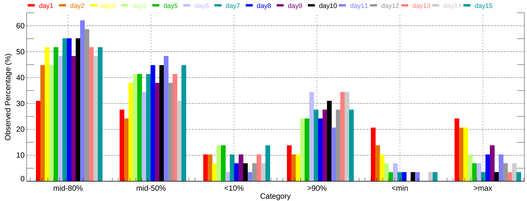
Observed Percentage of Ensembles - MWL: Min Temperature (2007-11-01~2007-11-30)
