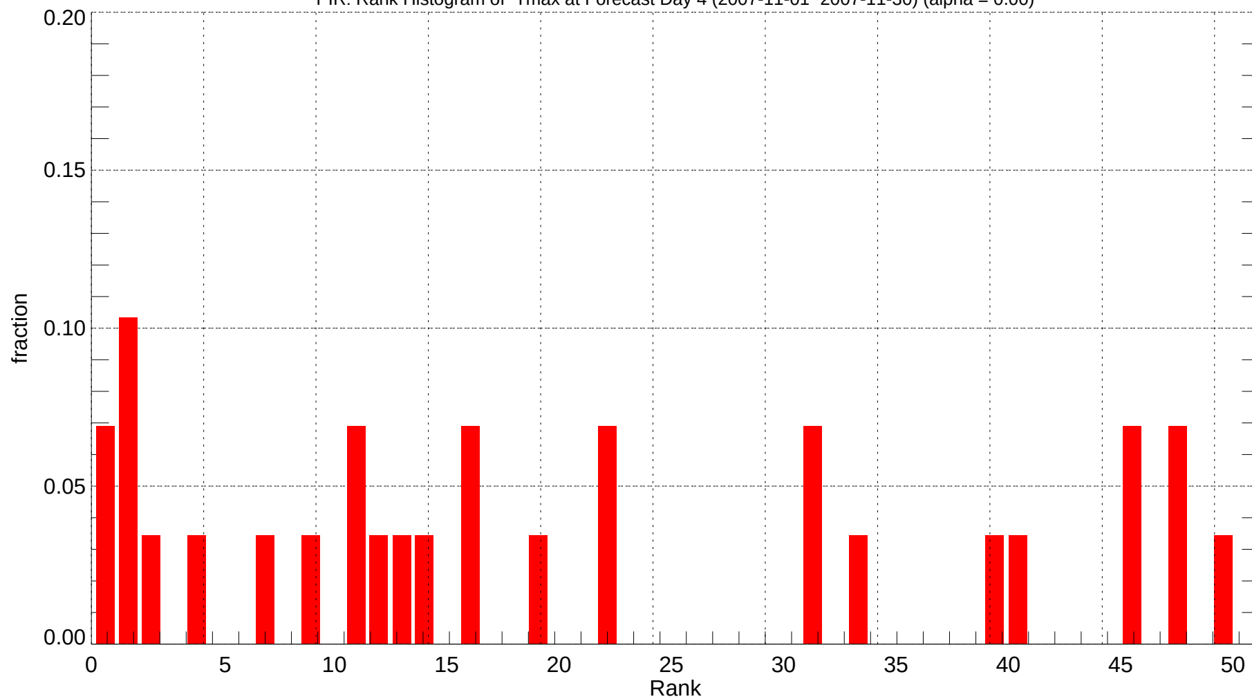
PIR: Rank Histogram of Tmax at Forecast Day 4 (2007-11-01~2007-11-30) (alpha = 0.00)
