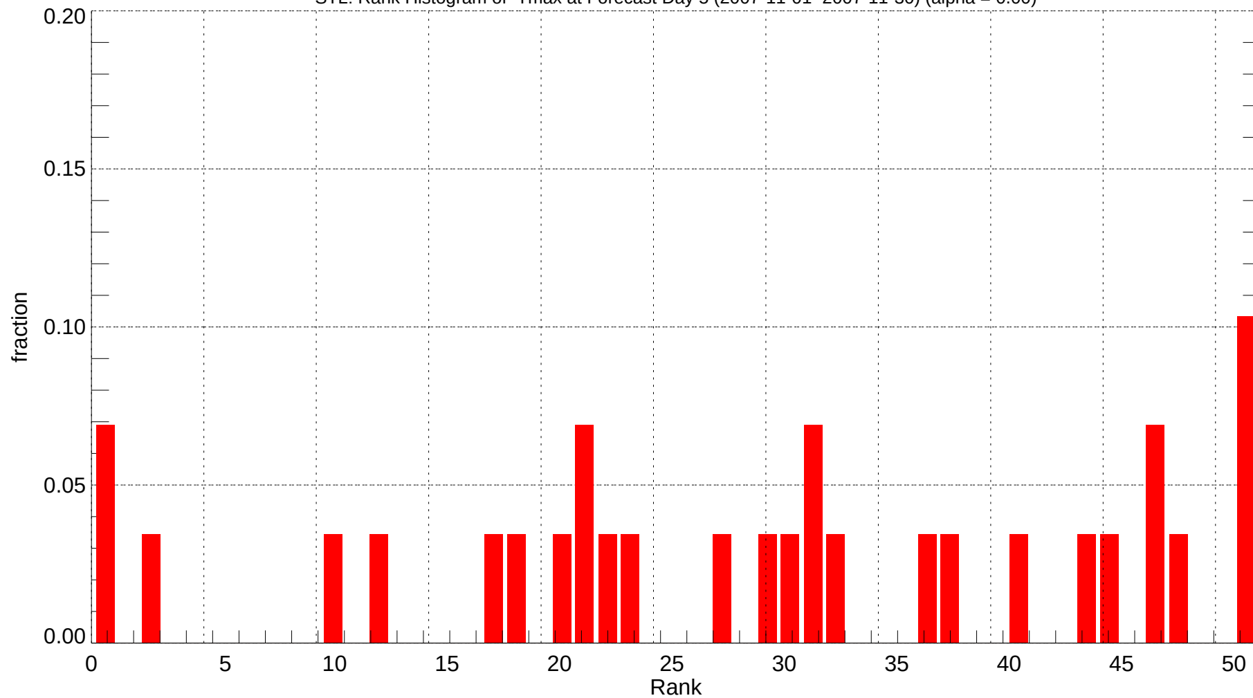
STL: Rank Histogram of Tmax at Forecast Day 5 (2007-11-01~2007-11-30) (alpha = 0.00)
