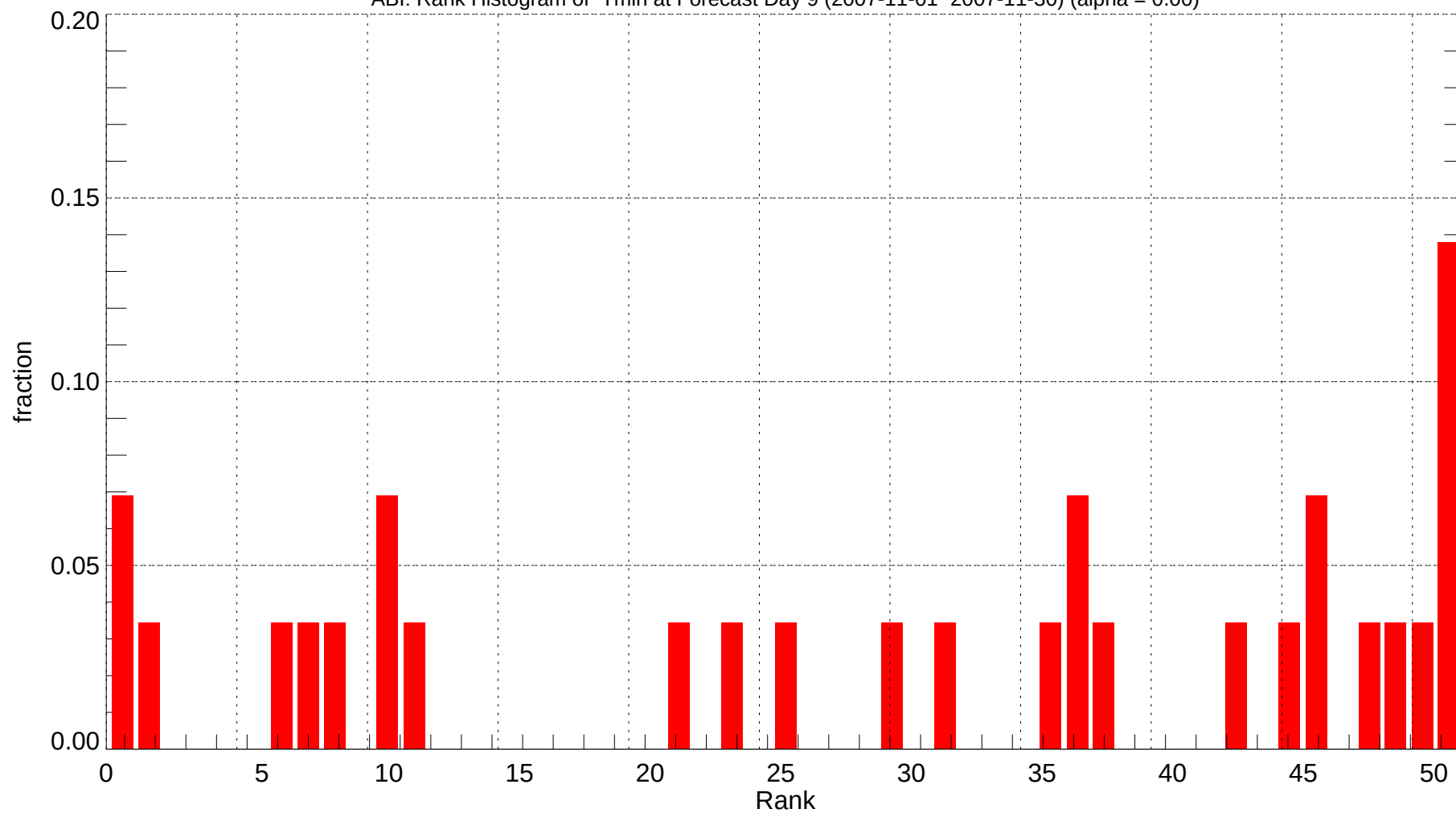
ABI: Rank Histogram of Tmin at Forecast Day 9 (2007-11-01~2007-11-30) (alpha = 0.00)
