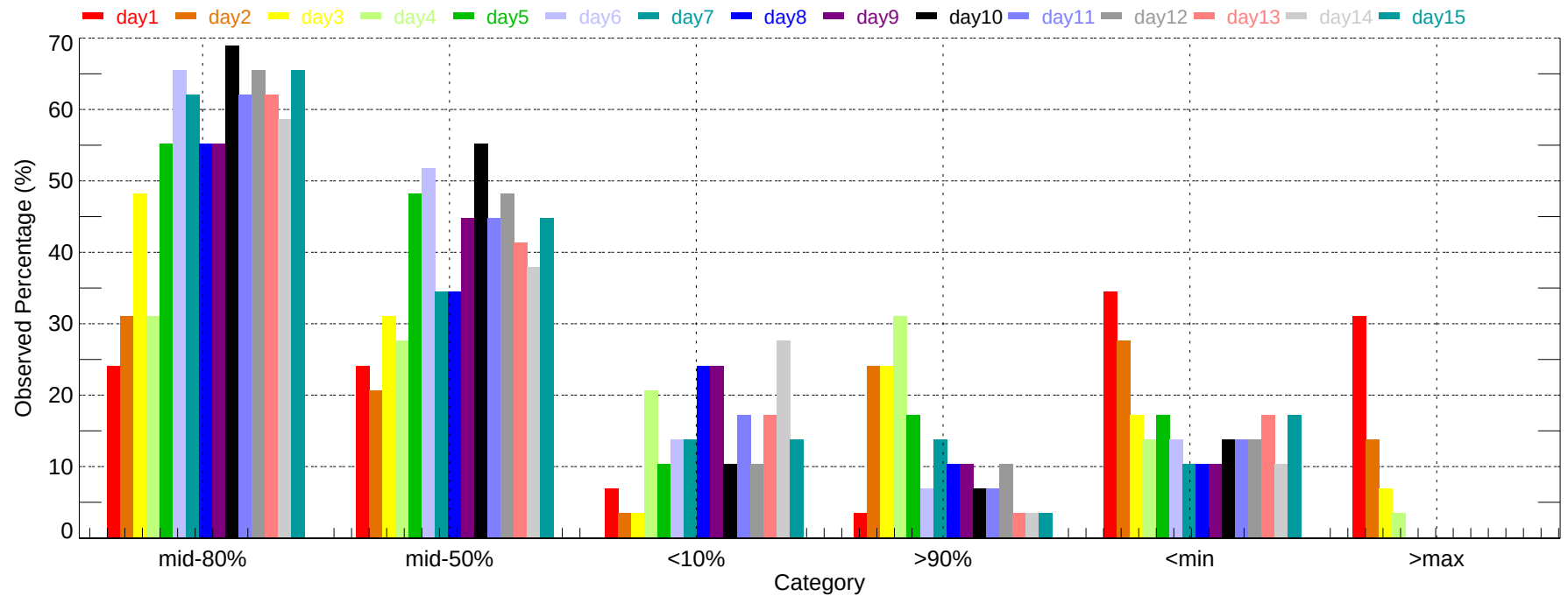
Observed Percentage of Ensembles - SYR: Min Temperature (2007-11-01~2007-11-30)
