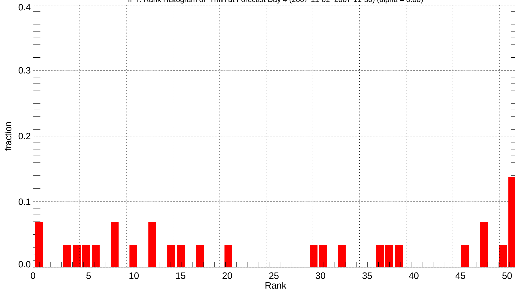
IPT: Rank Histogram of Tmin at Forecast Day 4 (2007-11-01~2007-11-30) (alpha = 0.00)
