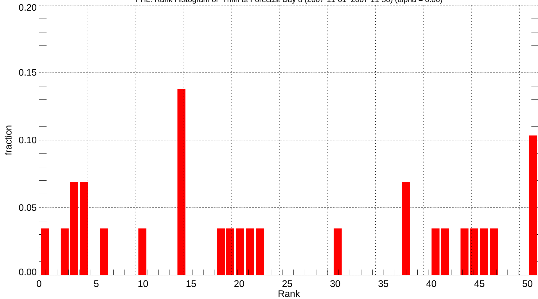
PHL: Rank Histogram of Tmin at Forecast Day 8 (2007-11-01~2007-11-30) (alpha = 0.00)
