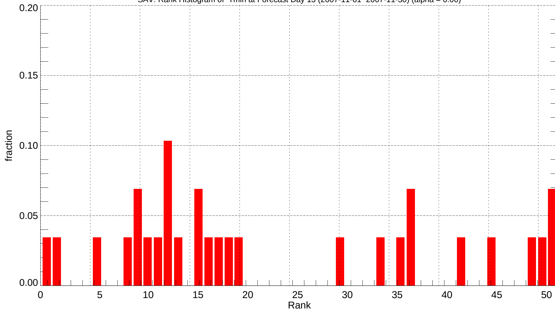
SAV: Rank Histogram of Tmin at Forecast Day 13 (2007-11-01~2007-11-30) (alpha = 0.00)
