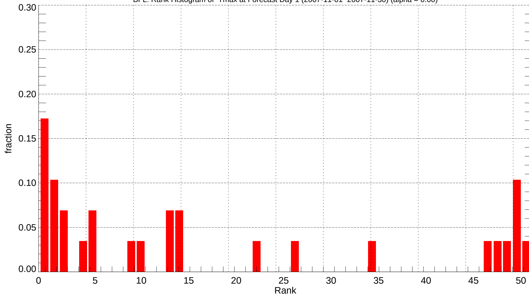
BFL: Rank Histogram of Tmax at Forecast Day 1 (2007-11-01~2007-11-30) (alpha = 0.00)
