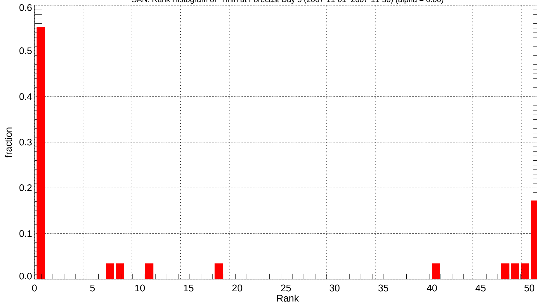
SAN: Rank Histogram of Tmin at Forecast Day 3 (2007-11-01~2007-11-30) (alpha = 0.00)
