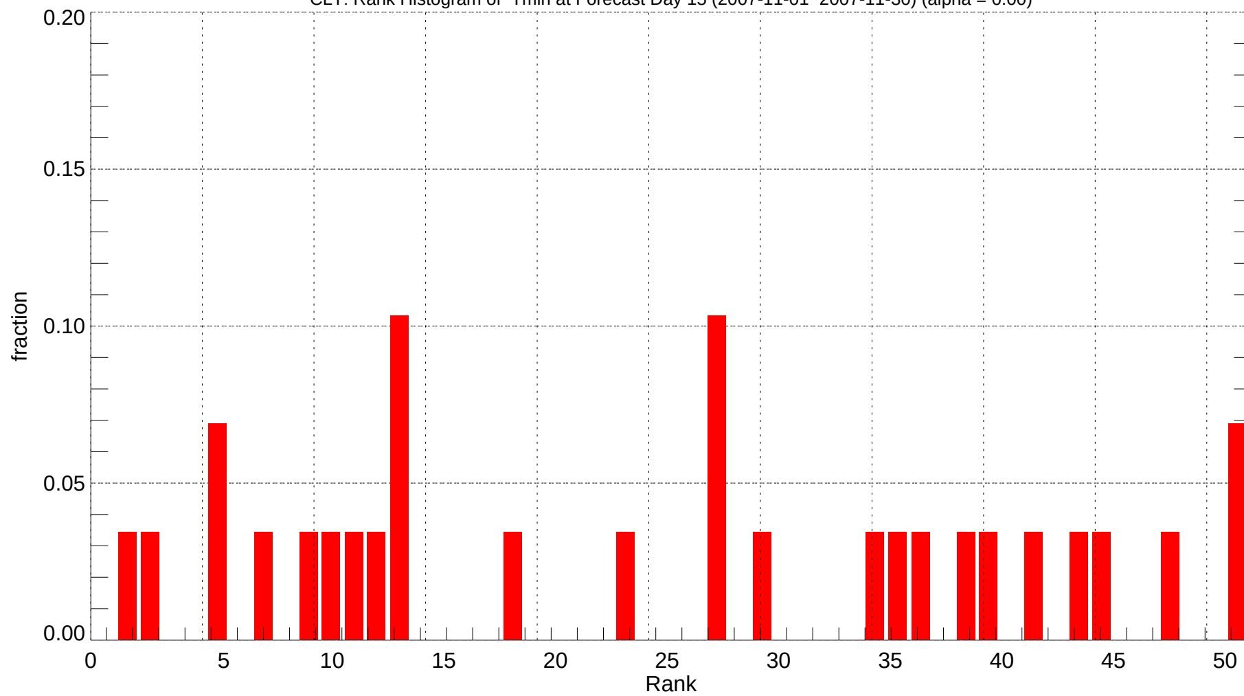
CLT: Rank Histogram of Tmin at Forecast Day 15 (2007-11-01~2007-11-30) (alpha = 0.00)
