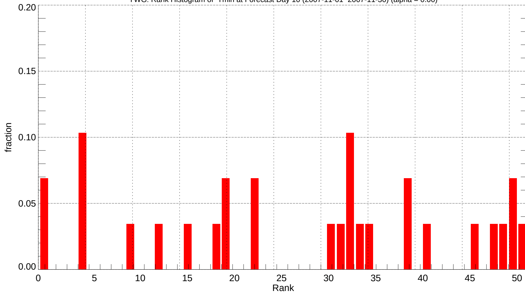
YWG: Rank Histogram of Tmin at Forecast Day 10 (2007-11-01~2007-11-30) (alpha = 0.00)
