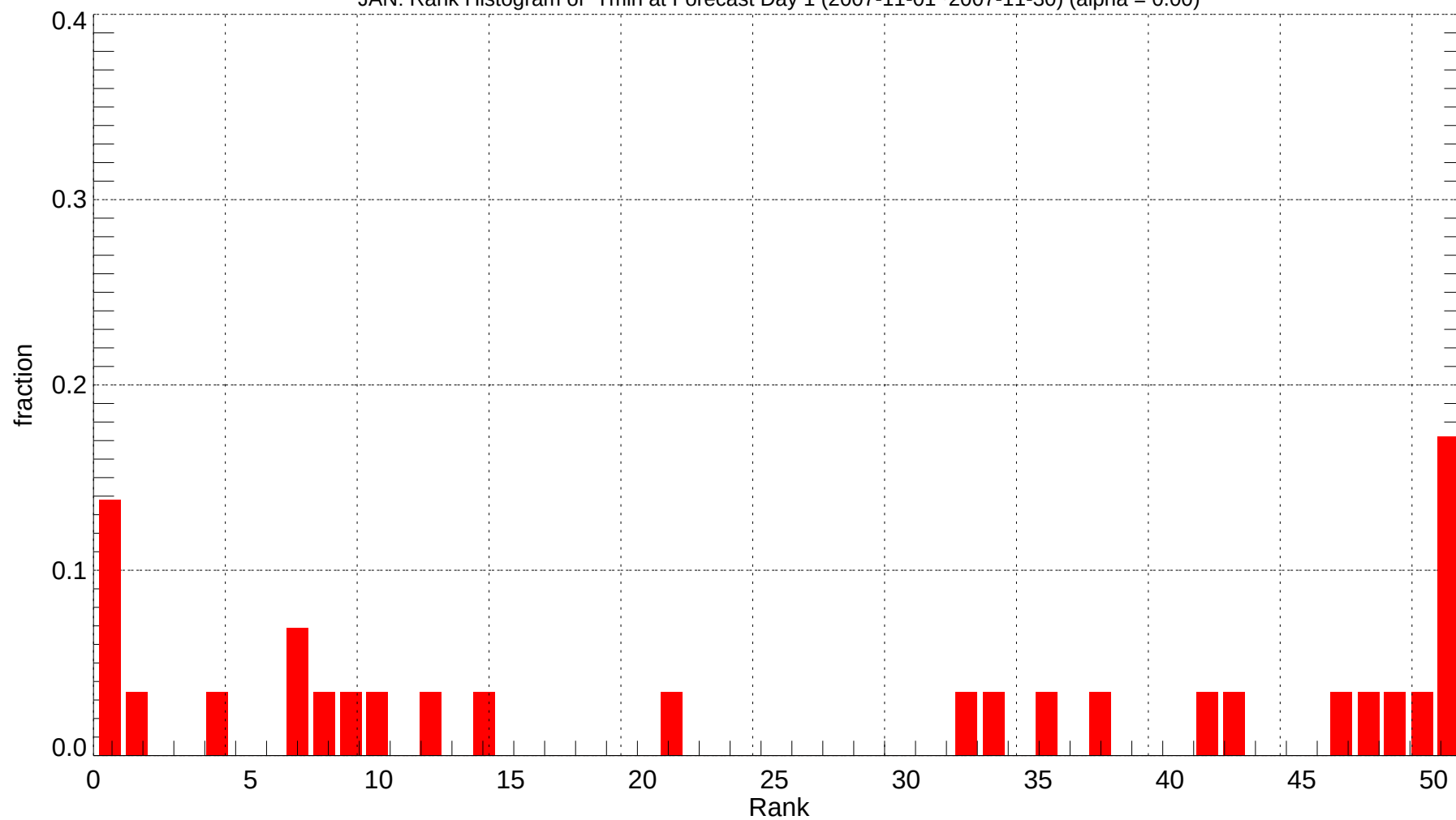
JAN: Rank Histogram of Tmin at Forecast Day 1 (2007-11-01~2007-11-30) (alpha = 0.00)
