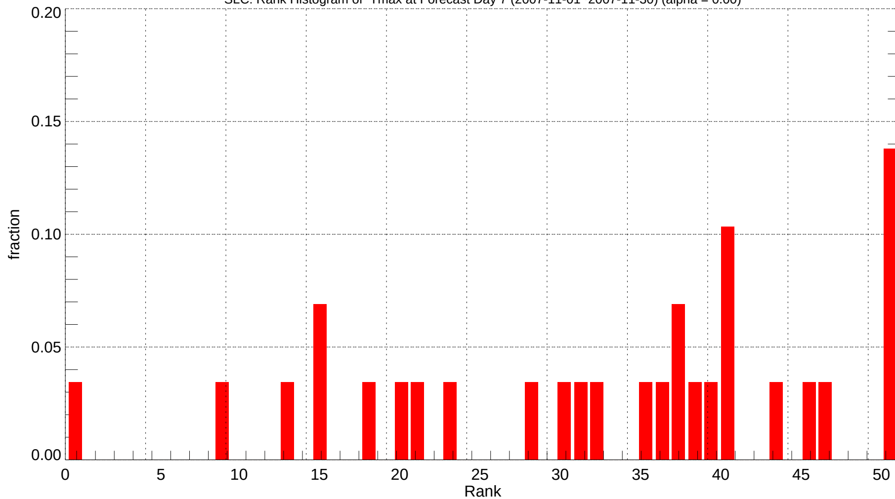
SLC: Rank Histogram of Tmax at Forecast Day 7 (2007-11-01~2007-11-30) (alpha = 0.00)
