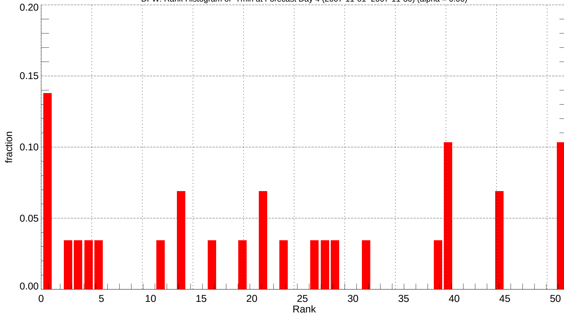
DFW: Rank Histogram of Tmin at Forecast Day 4 (2007-11-01~2007-11-30) (alpha = 0.00)
