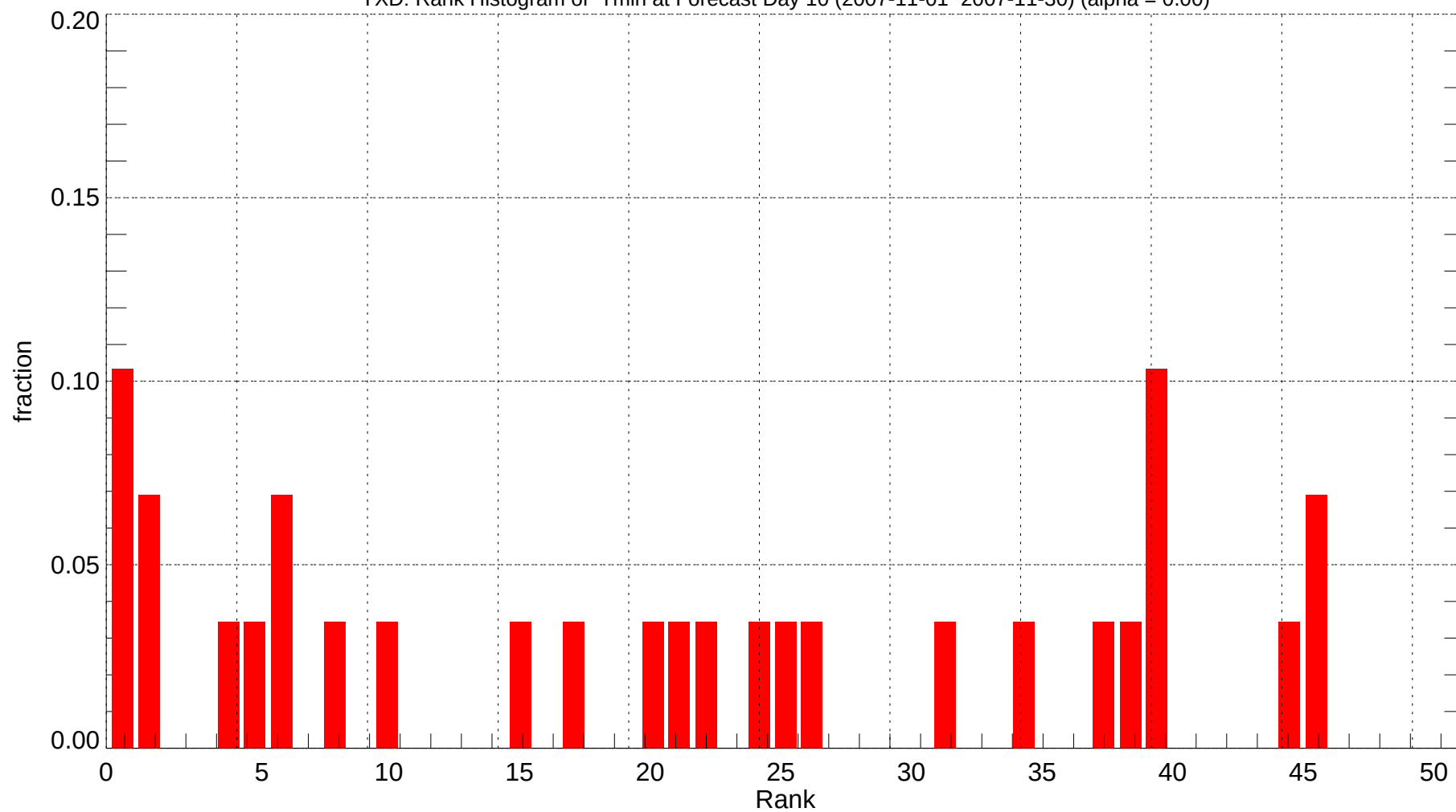
YXD: Rank Histogram of Tmin at Forecast Day 10 (2007-11-01~2007-11-30) (alpha = 0.00)
