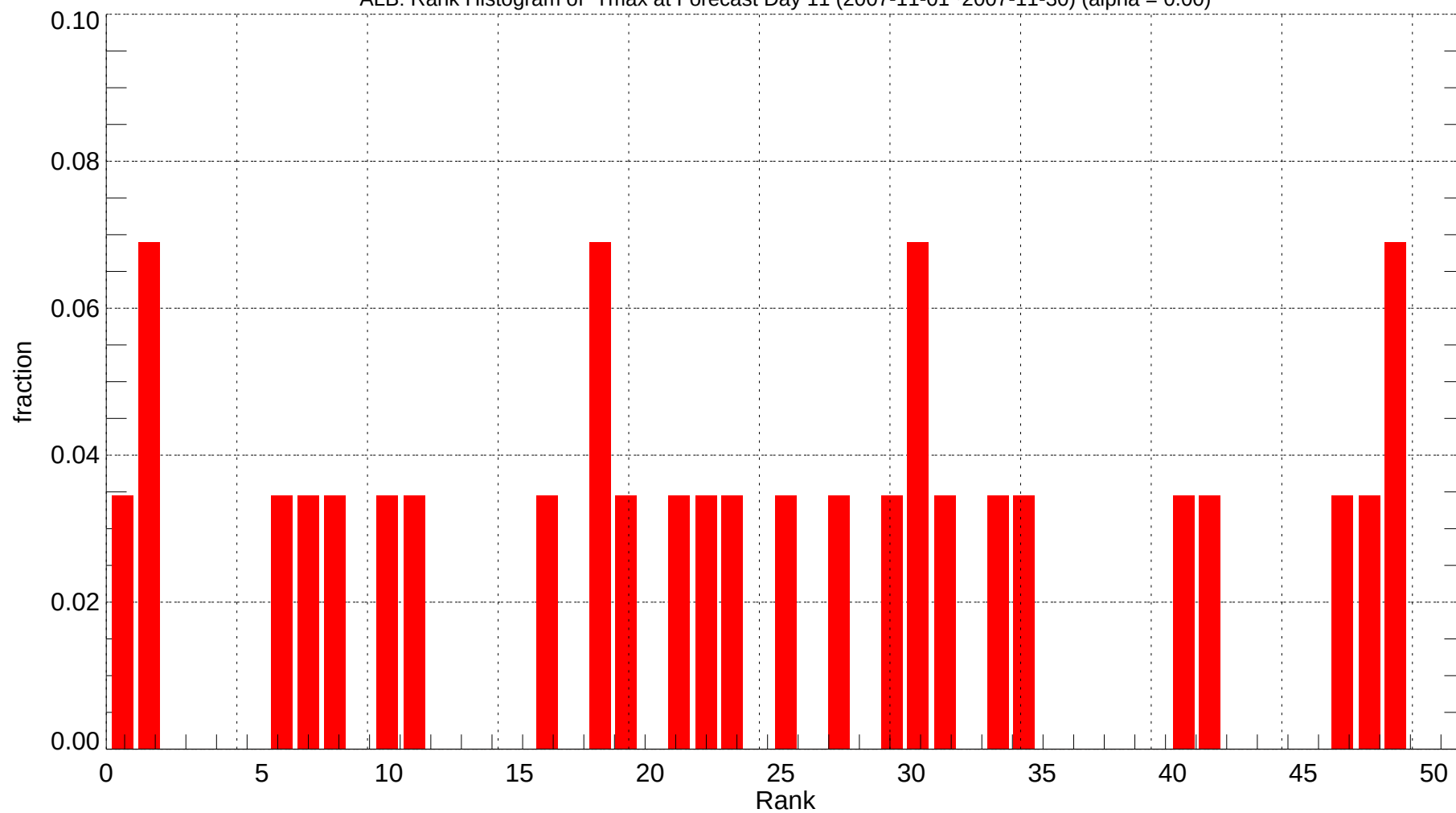
ALB: Rank Histogram of Tmax at Forecast Day 11 (2007-11-01~2007-11-30) (alpha = 0.00)
