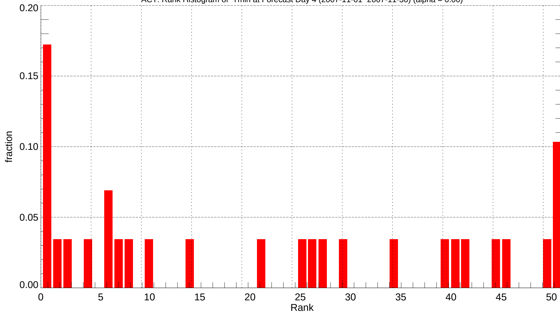
ACT: Rank Histogram of Tmin at Forecast Day 4 (2007-11-01~2007-11-30) (alpha = 0.00)
