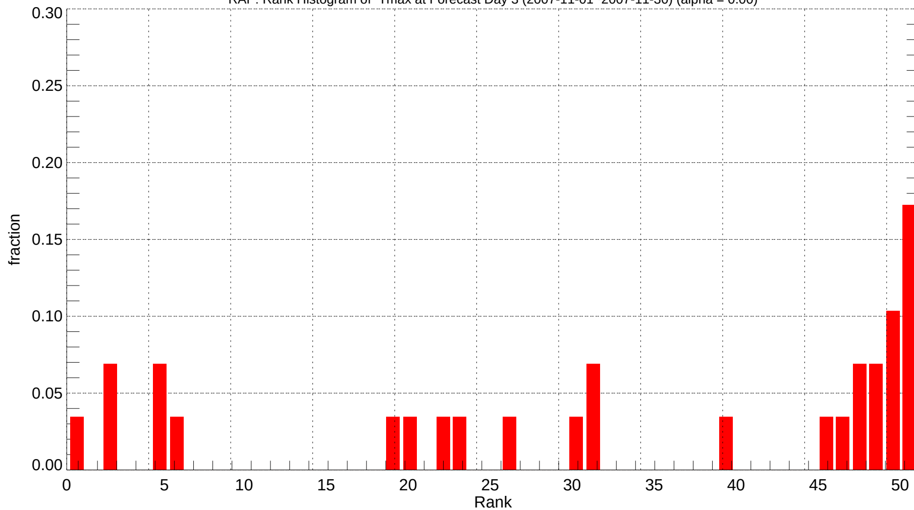
RAP: Rank Histogram of Tmax at Forecast Day 3 (2007-11-01~2007-11-30) (alpha = 0.00)
