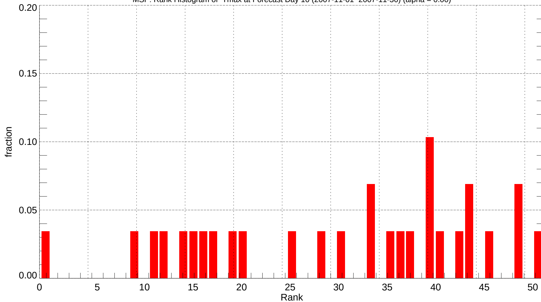
MSP: Rank Histogram of Tmax at Forecast Day 10 (2007-11-01~2007-11-30) (alpha = 0.00)
