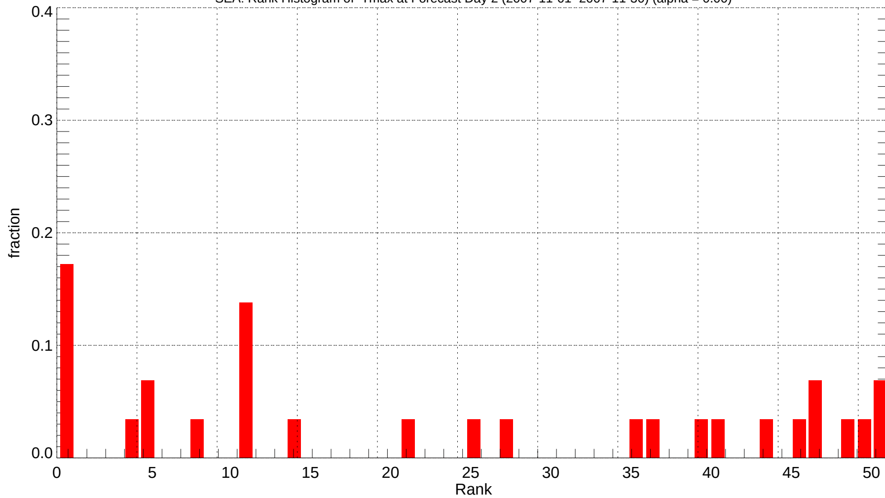
SEA: Rank Histogram of Tmax at Forecast Day 2 (2007-11-01~2007-11-30) (alpha = 0.00)
