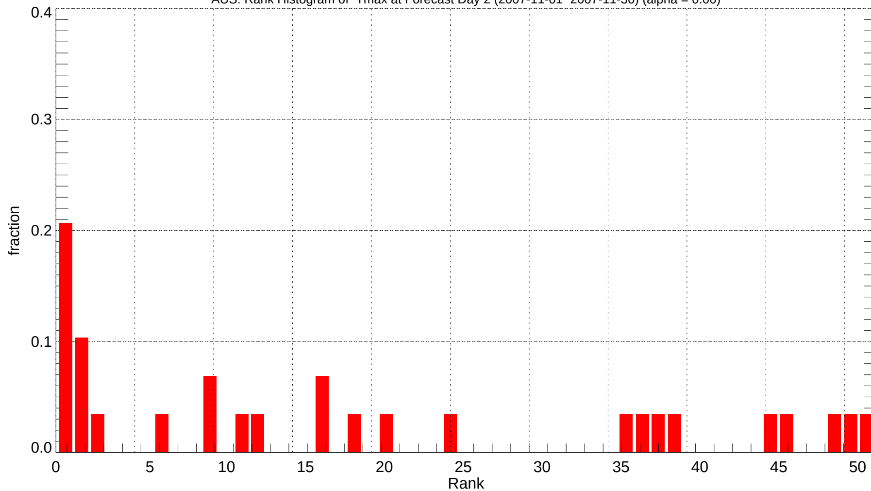
AUS: Rank Histogram of Tmax at Forecast Day 2 (2007-11-01~2007-11-30) (alpha = 0.00)
