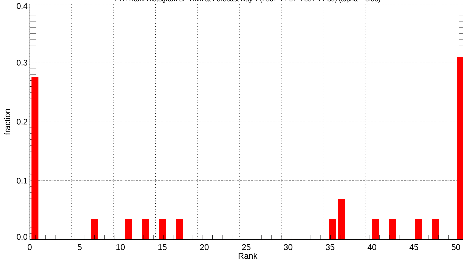
PIT: Rank Histogram of Tmin at Forecast Day 1 (2007-11-01~2007-11-30) (alpha = 0.00)
