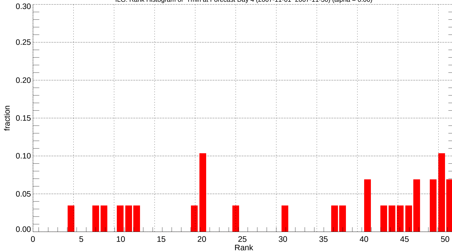
ILG: Rank Histogram of Tmin at Forecast Day 4 (2007-11-01~2007-11-30) (alpha = 0.00)
