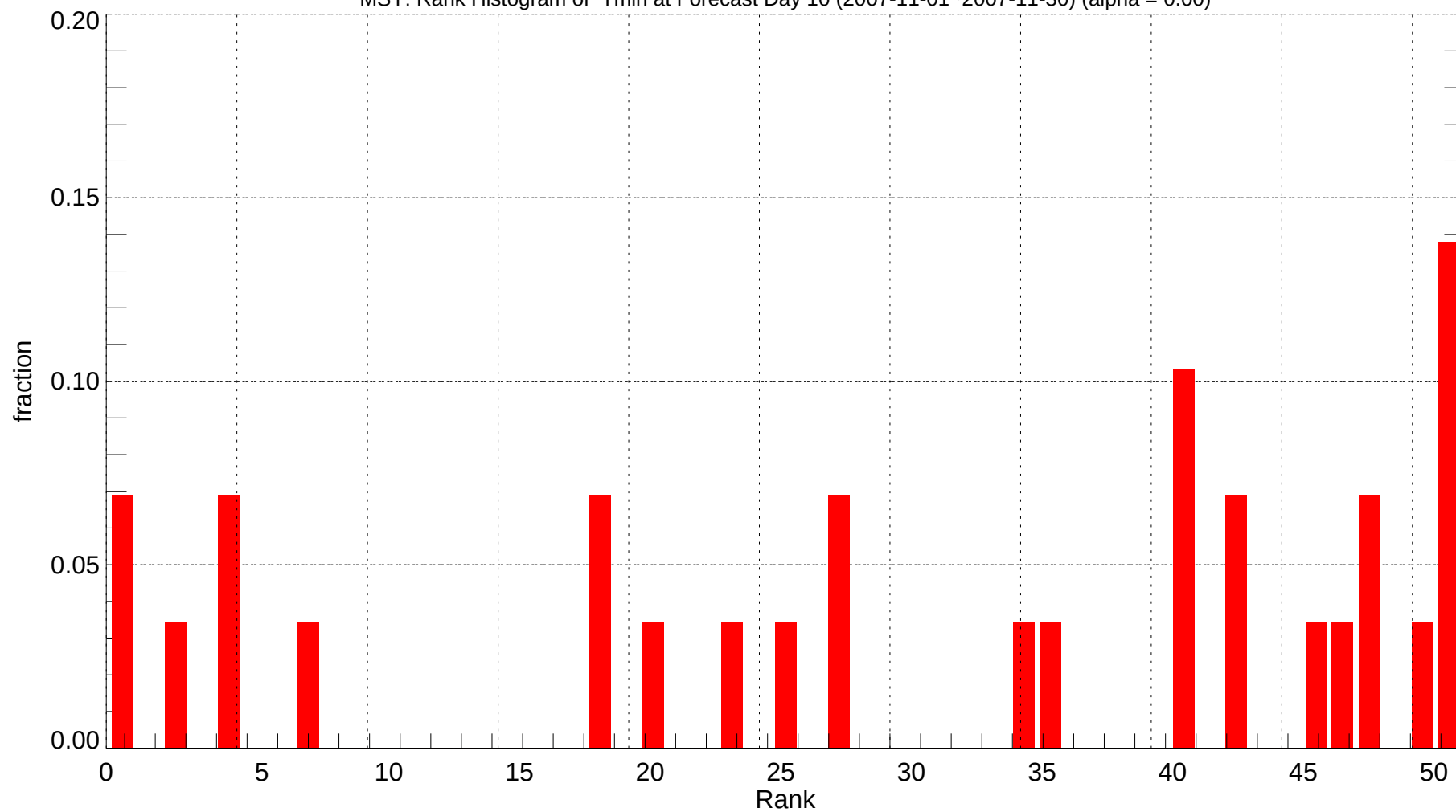
MSY: Rank Histogram of Tmin at Forecast Day 10 (2007-11-01~2007-11-30) (alpha = 0.00)
