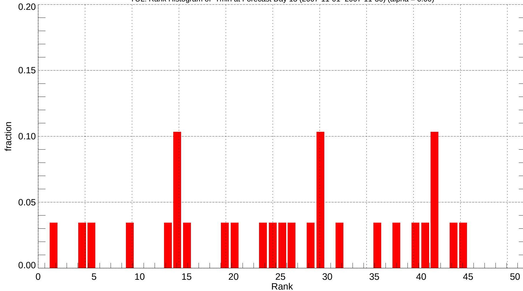
YUL: Rank Histogram of Tmin at Forecast Day 13 (2007-11-01~2007-11-30) (alpha = 0.00)
