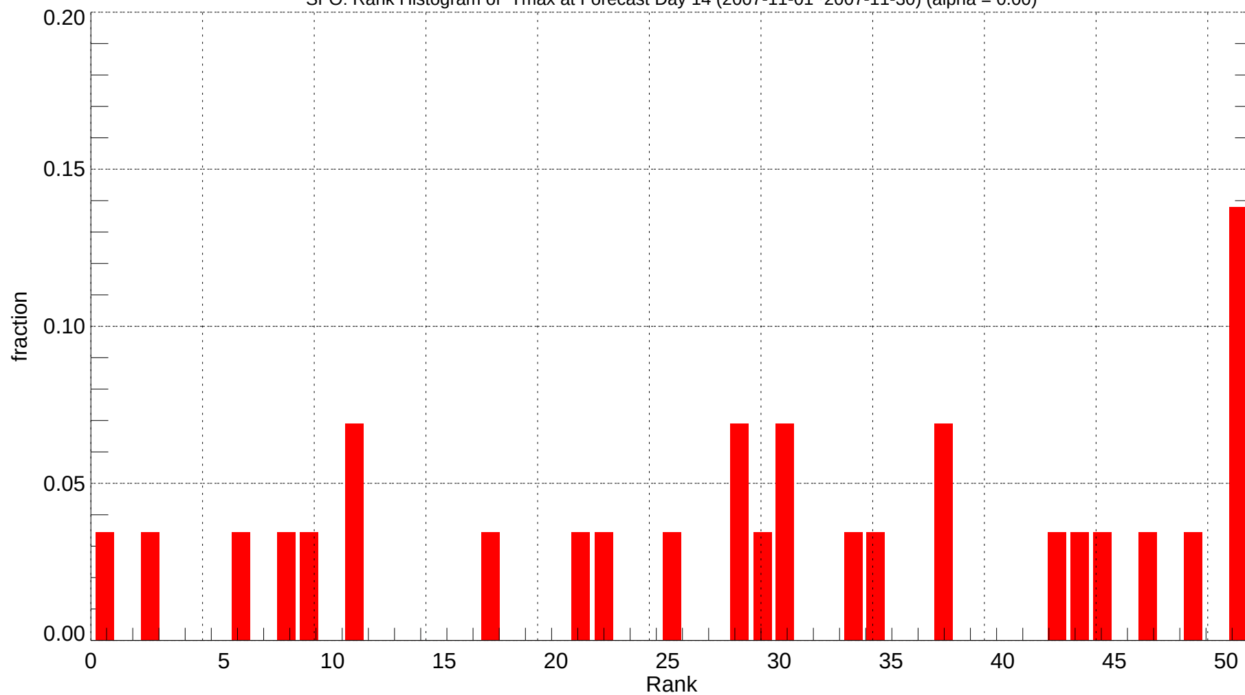
SFO: Rank Histogram of Tmax at Forecast Day 14 (2007-11-01~2007-11-30) (alpha = 0.00)
