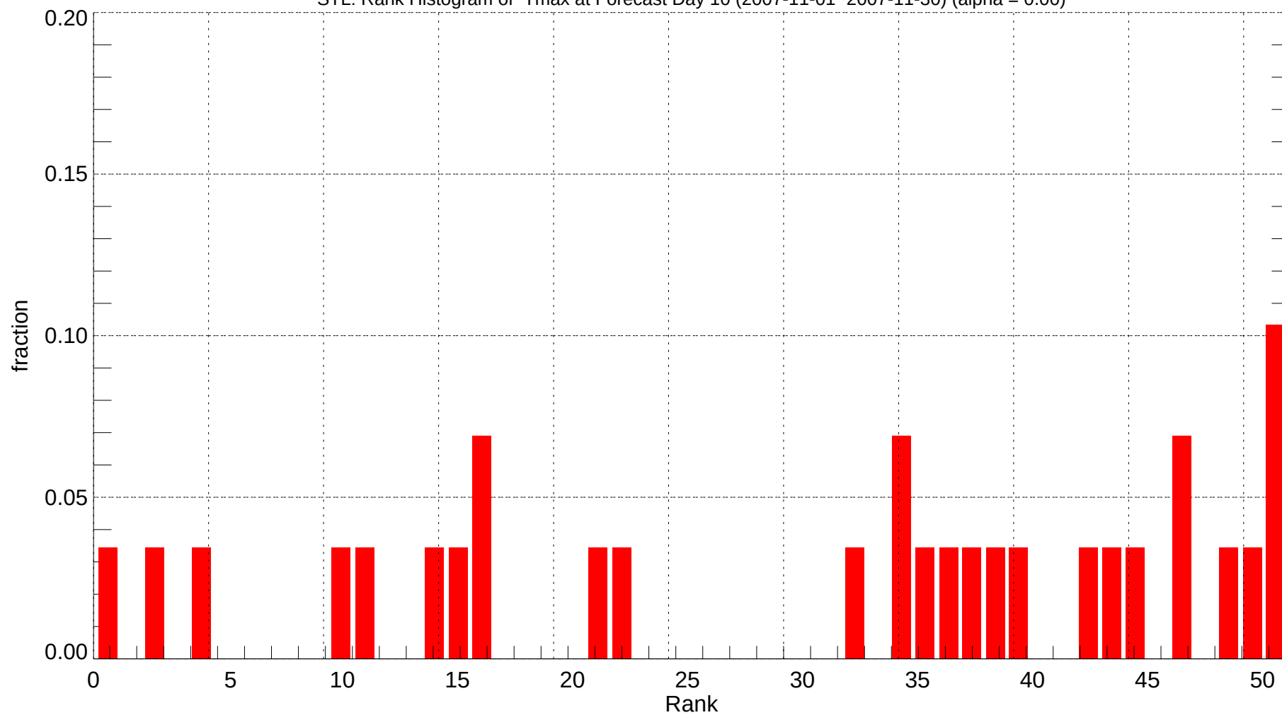
STL: Rank Histogram of Tmax at Forecast Day 10 (2007-11-01~2007-11-30) (alpha = 0.00)
