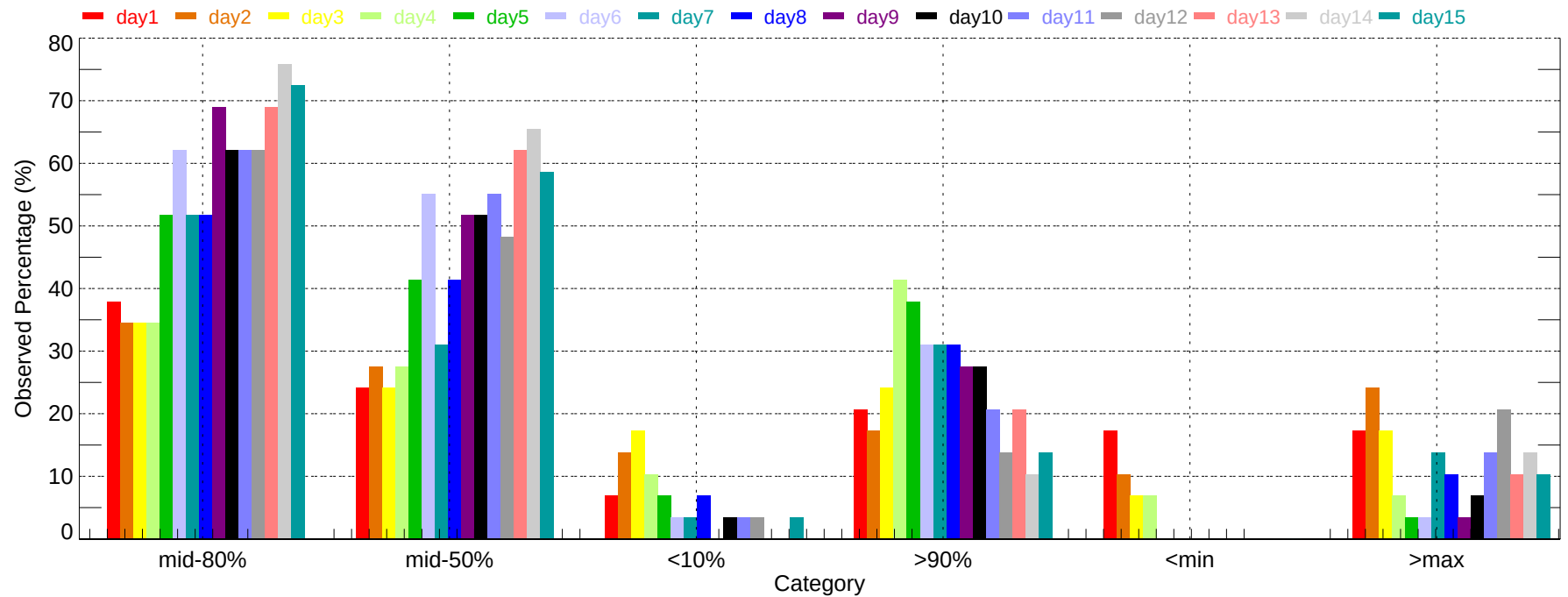
Observed Percentage of Ensembles - CMH: Max Temperature (2007-11-01~2007-11-30)
