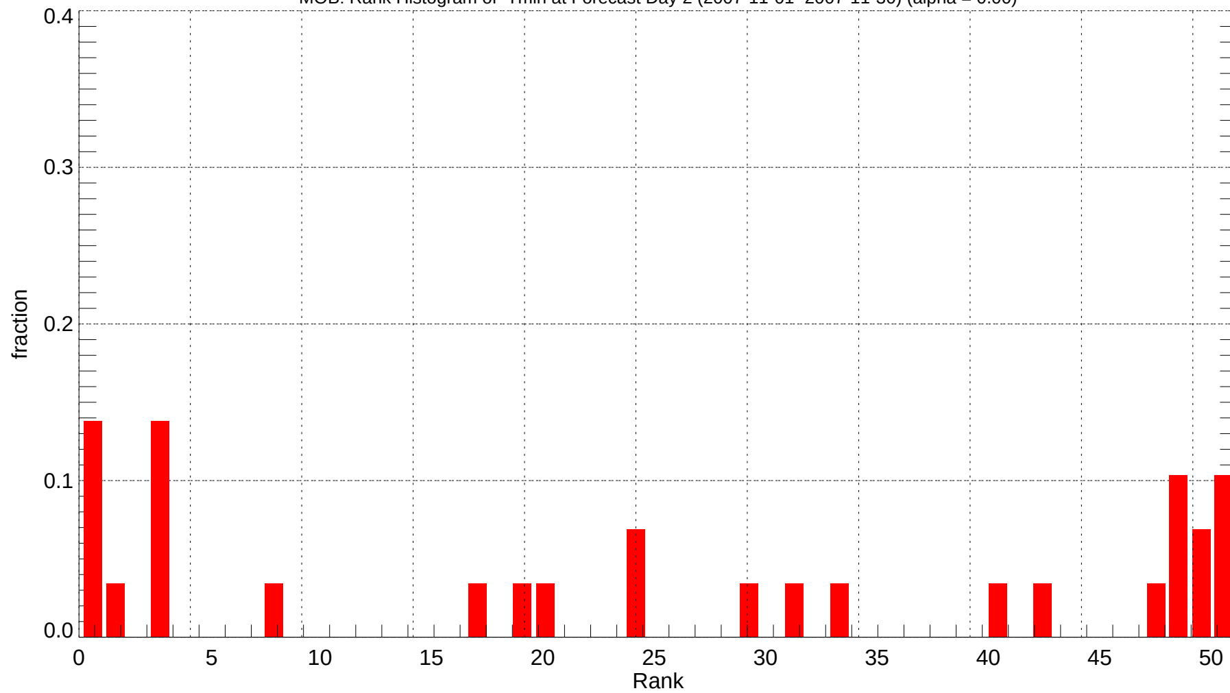
MOB: Rank Histogram of Tmin at Forecast Day 2 (2007-11-01~2007-11-30) (alpha = 0.00)
