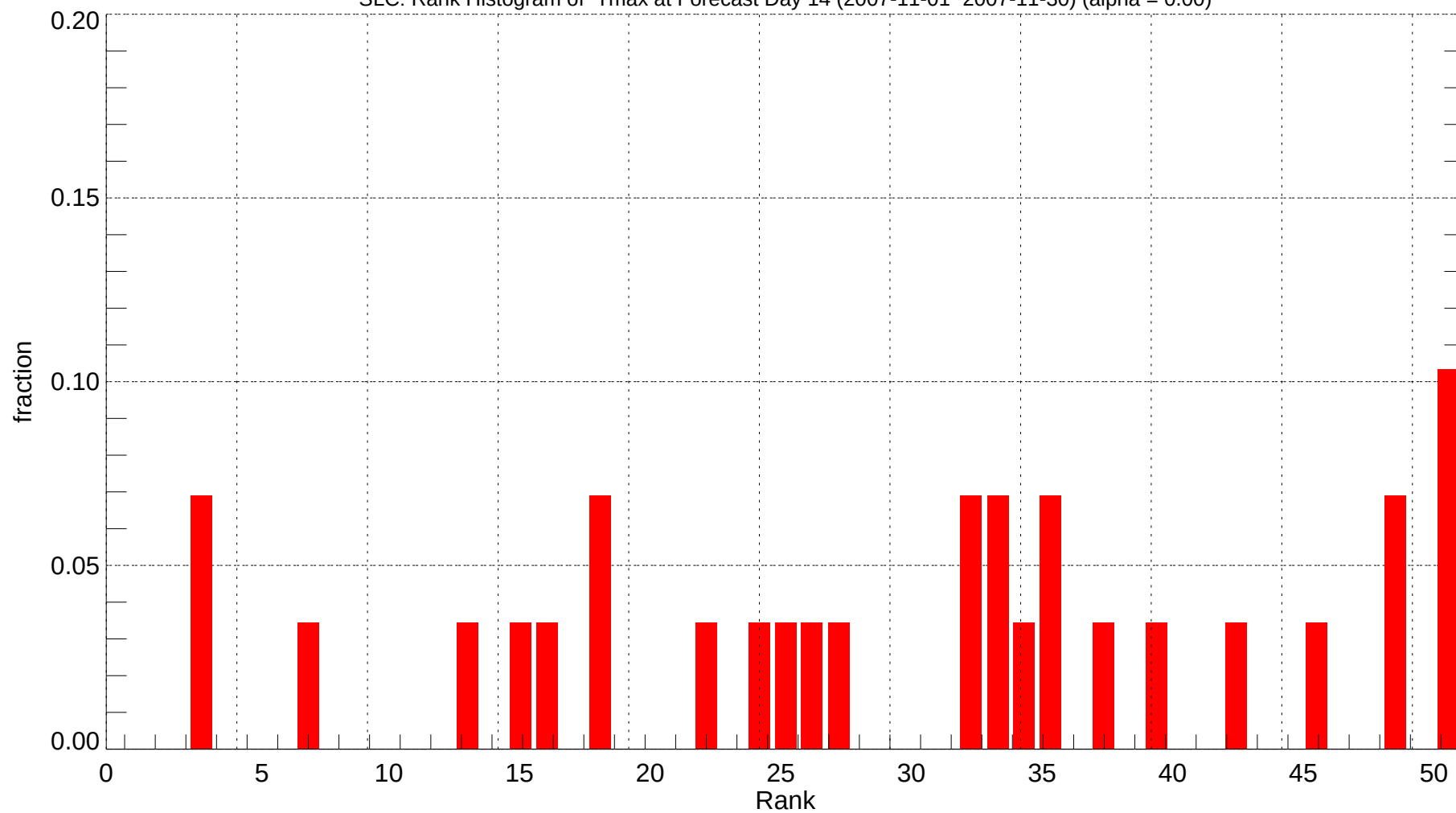
SLC: Rank Histogram of Tmax at Forecast Day 14 (2007-11-01~2007-11-30) (alpha = 0.00)
