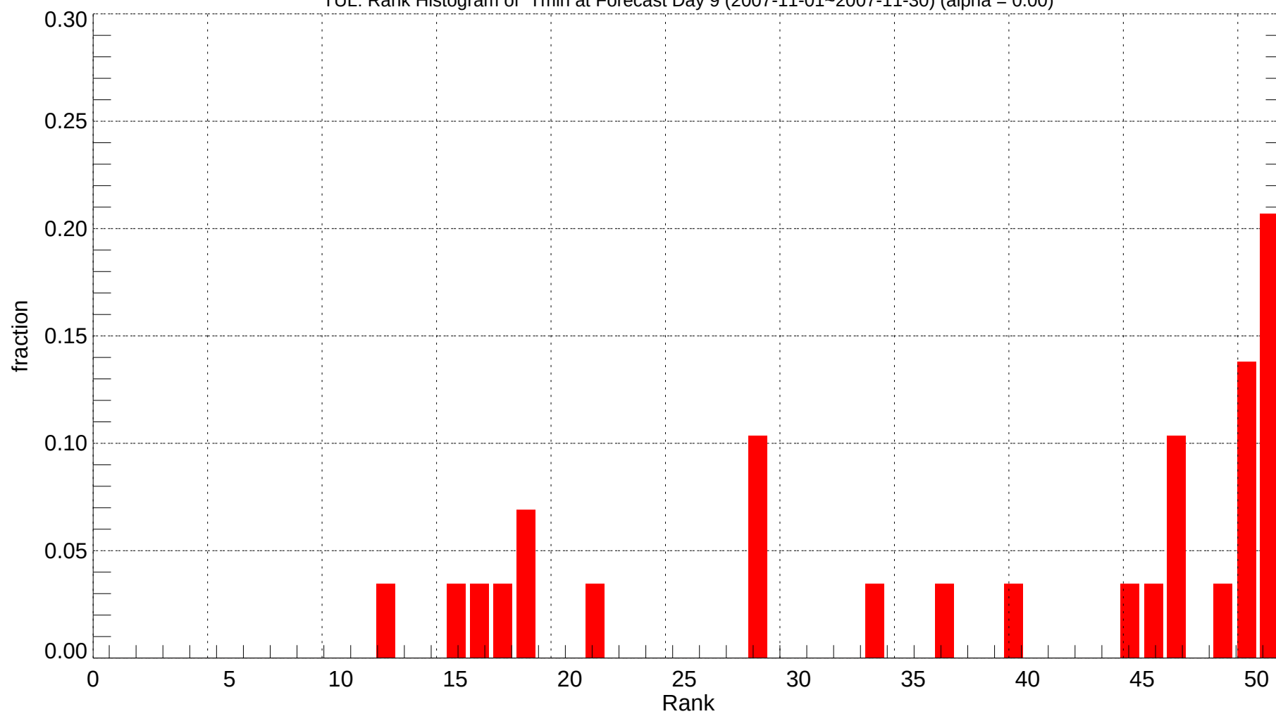
TUL: Rank Histogram of Tmin at Forecast Day 9 (2007-11-01~2007-11-30) (alpha = 0.00)
