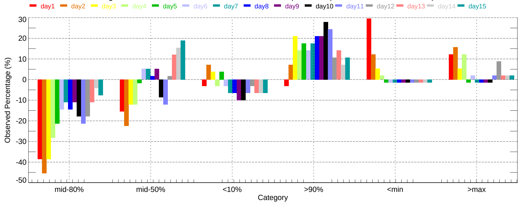
Observed Percentage Deviation of Ensembles - MOB: Max Temperature (2007-11-01~2007-11-30)
