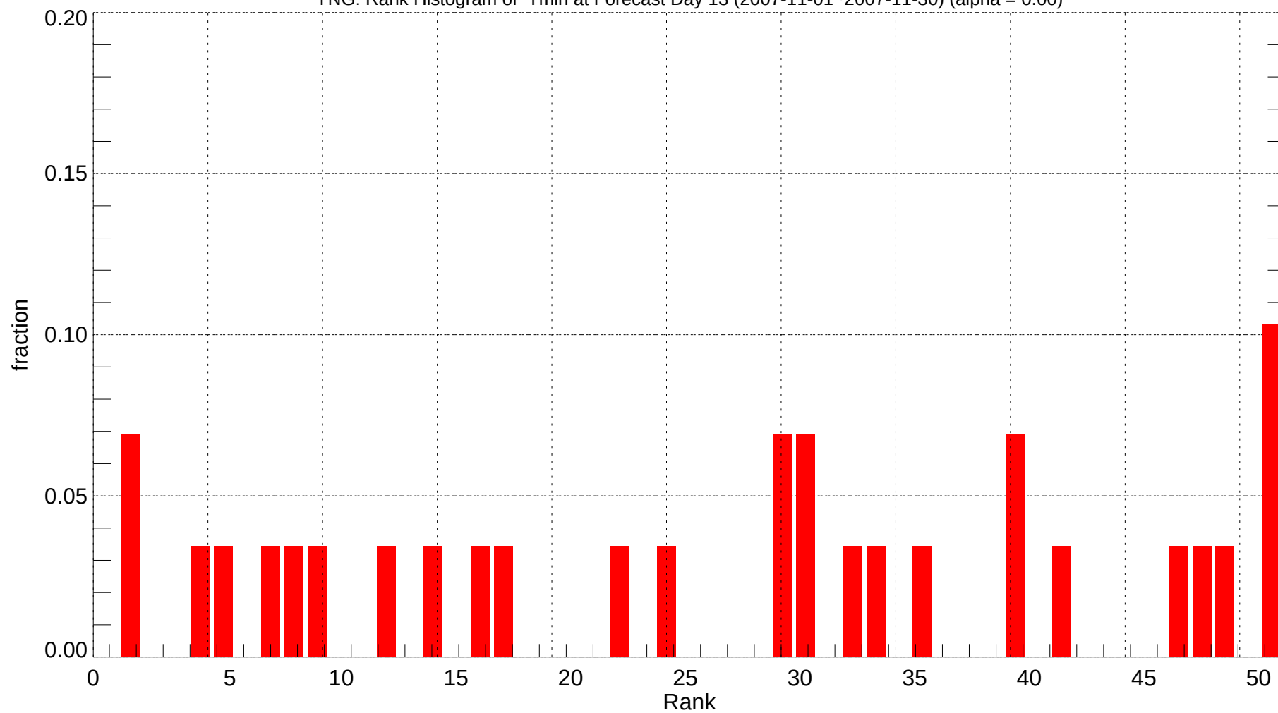
YNG: Rank Histogram of Tmin at Forecast Day 13 (2007-11-01~2007-11-30) (alpha = 0.00)
