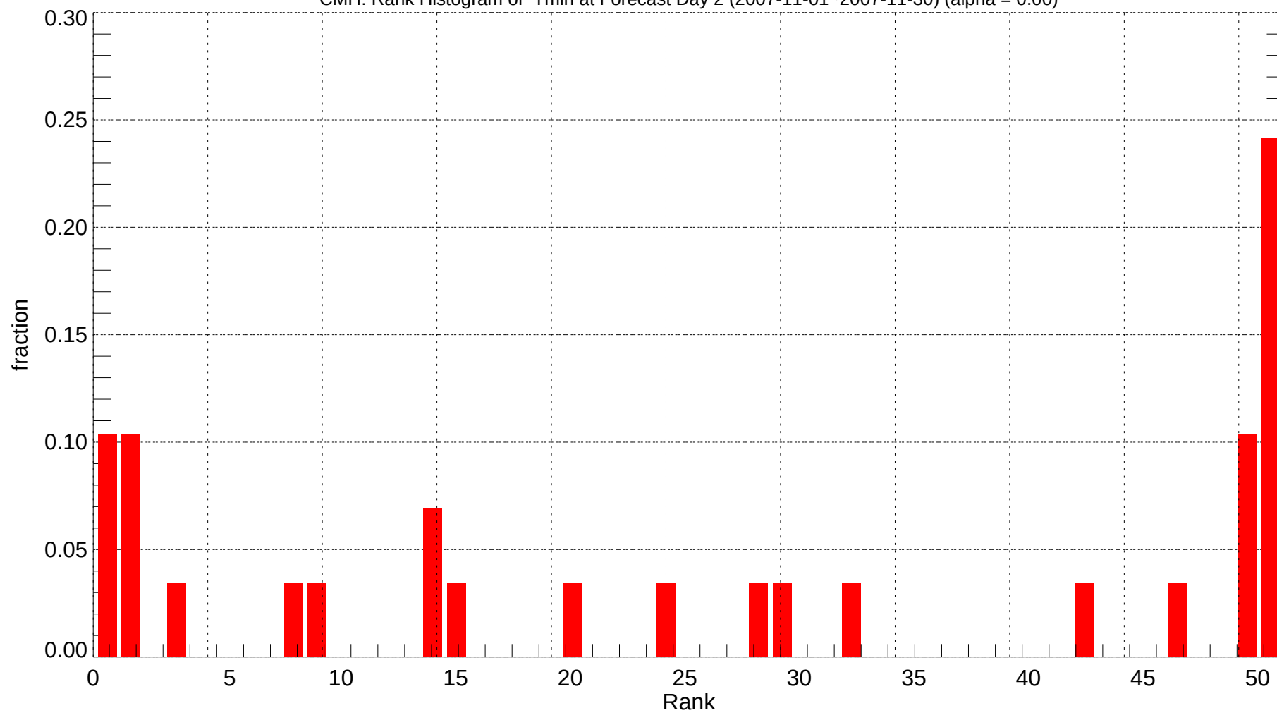
CMH: Rank Histogram of Tmin at Forecast Day 2 (2007-11-01~2007-11-30) (alpha = 0.00)
