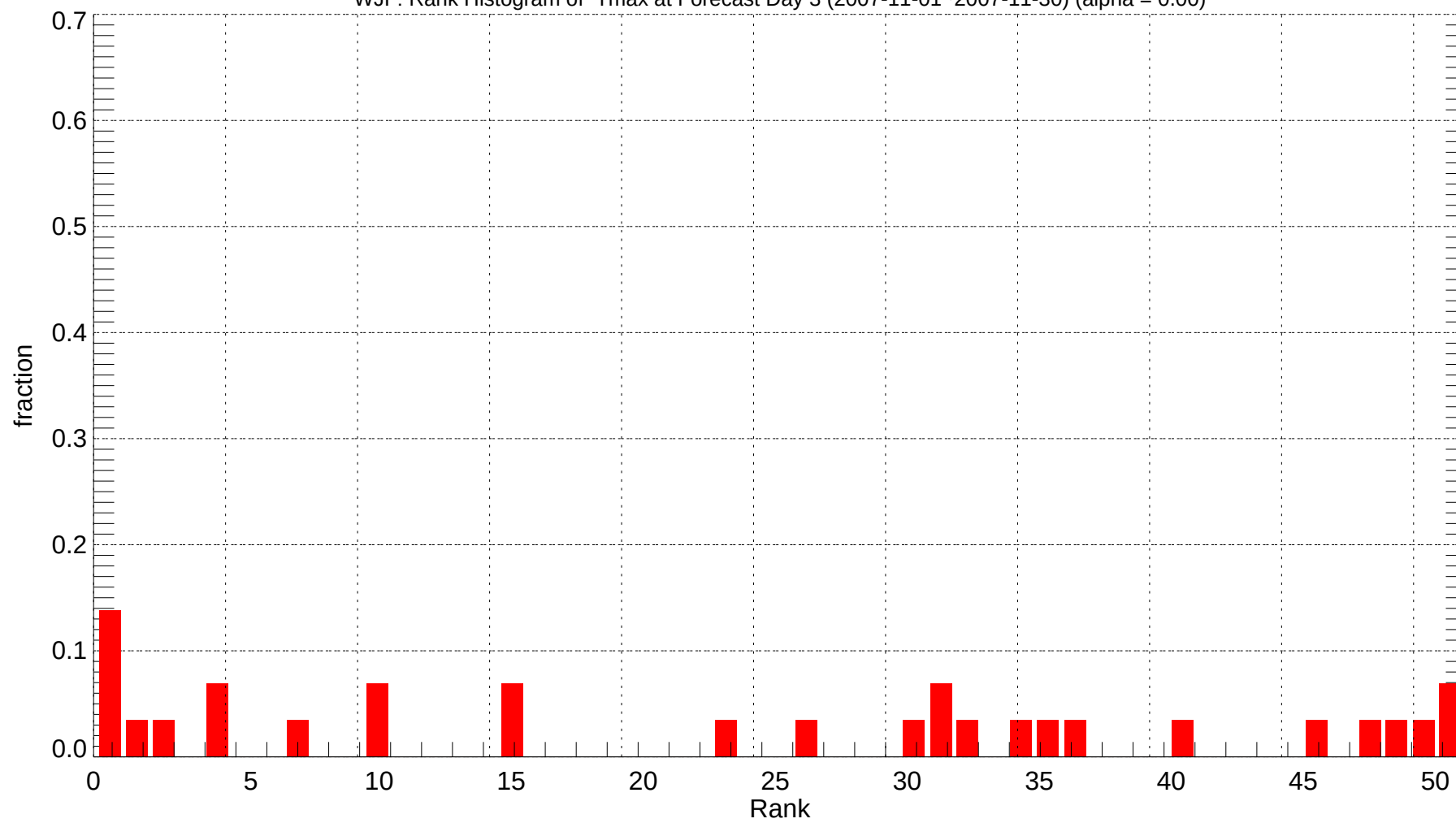
WJF: Rank Histogram of Tmax at Forecast Day 3 (2007-11-01~2007-11-30) (alpha = 0.00)
