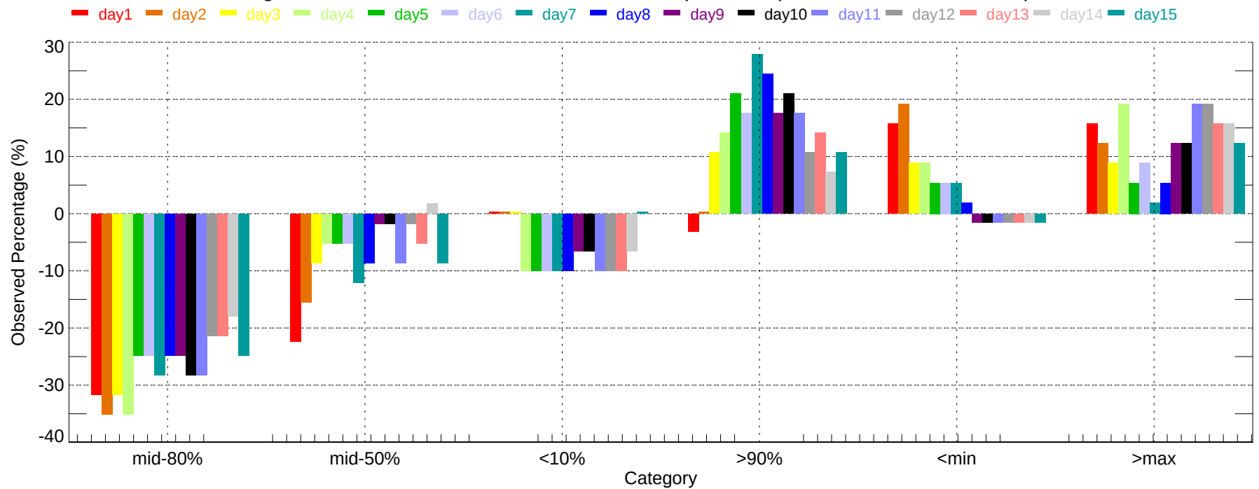
Observed Percentage Deviation of Ensembles - ICT: Min Temperature (2007-11-01~2007-11-30)
