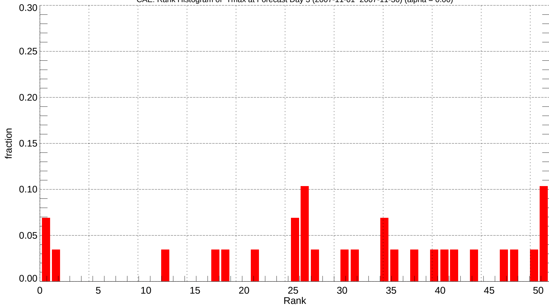
CAE: Rank Histogram of Tmax at Forecast Day 3 (2007-11-01~2007-11-30) (alpha = 0.00)
