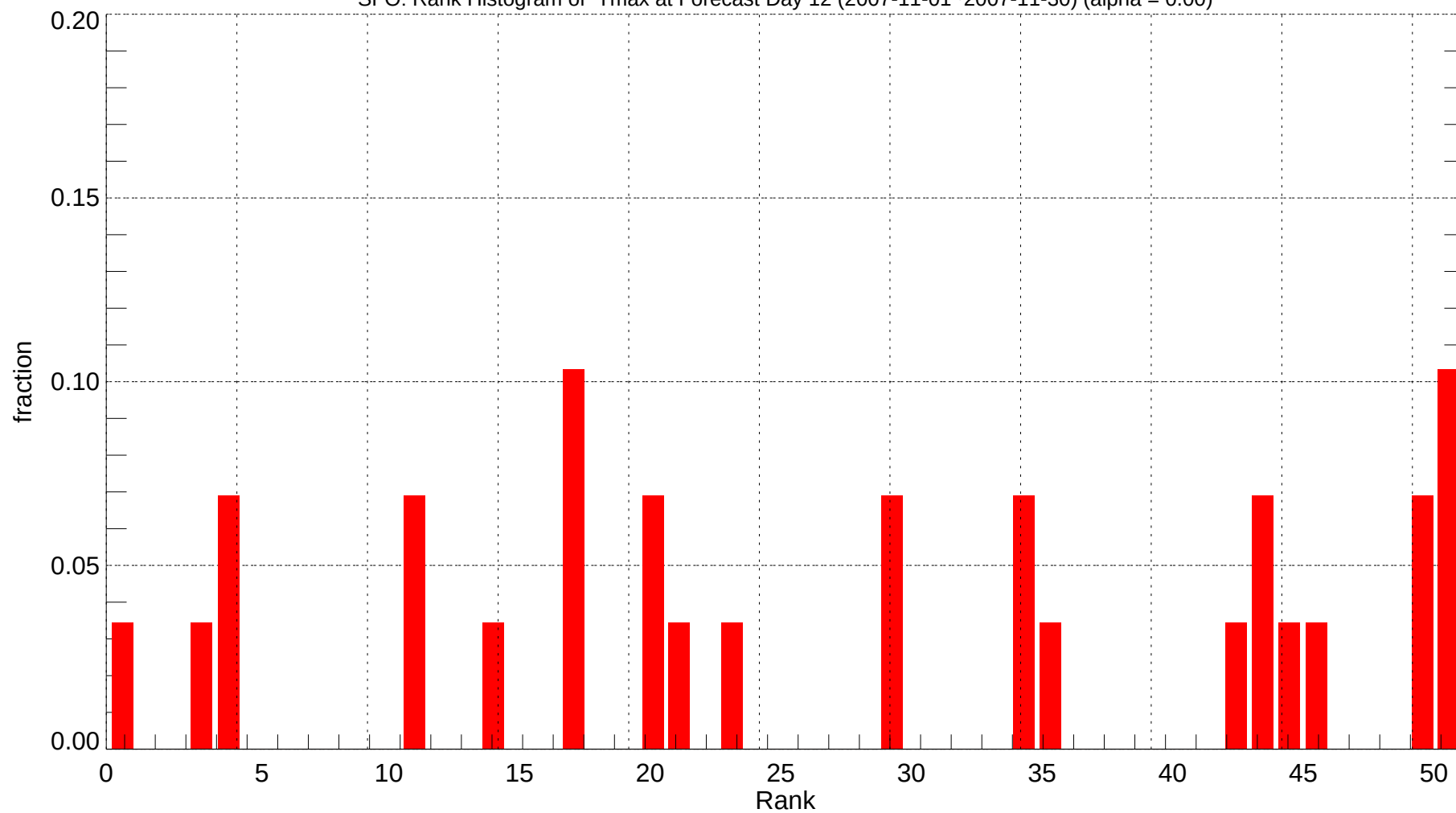
SFO: Rank Histogram of Tmax at Forecast Day 12 (2007-11-01~2007-11-30) (alpha = 0.00)
