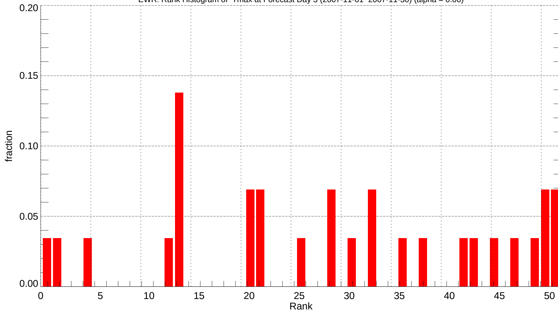
EWR: Rank Histogram of Tmax at Forecast Day 3 (2007-11-01~2007-11-30) (alpha = 0.00)
