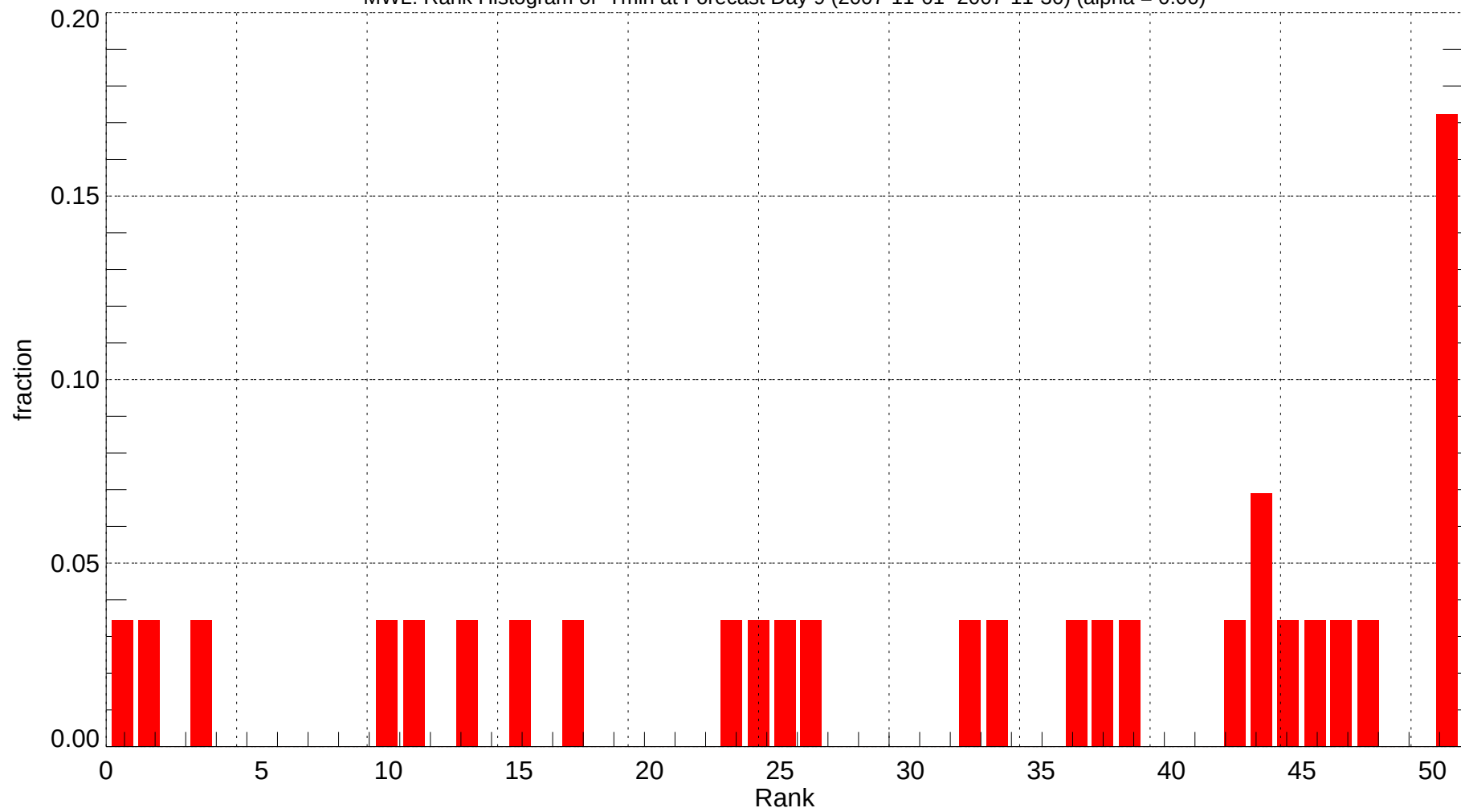
MWL: Rank Histogram of Tmin at Forecast Day 9 (2007-11-01~2007-11-30) (alpha = 0.00)
