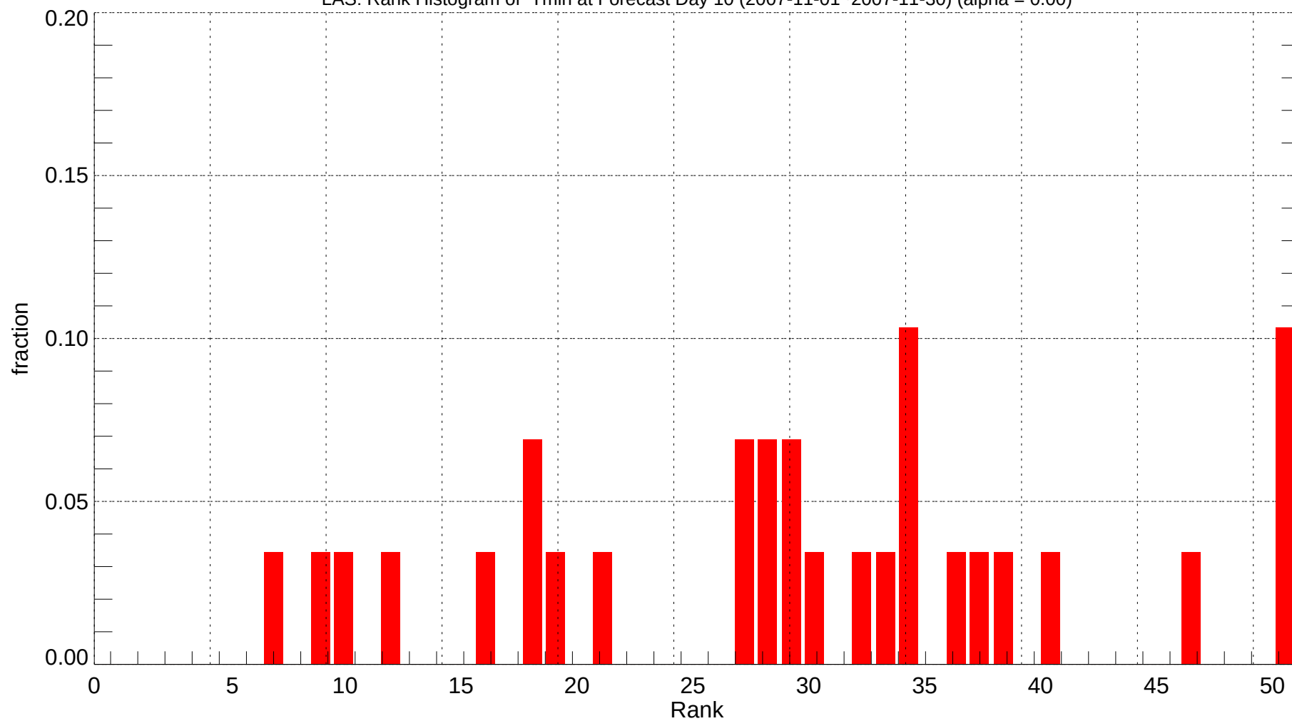
LAS: Rank Histogram of Tmin at Forecast Day 10 (2007-11-01~2007-11-30) (alpha = 0.00)
