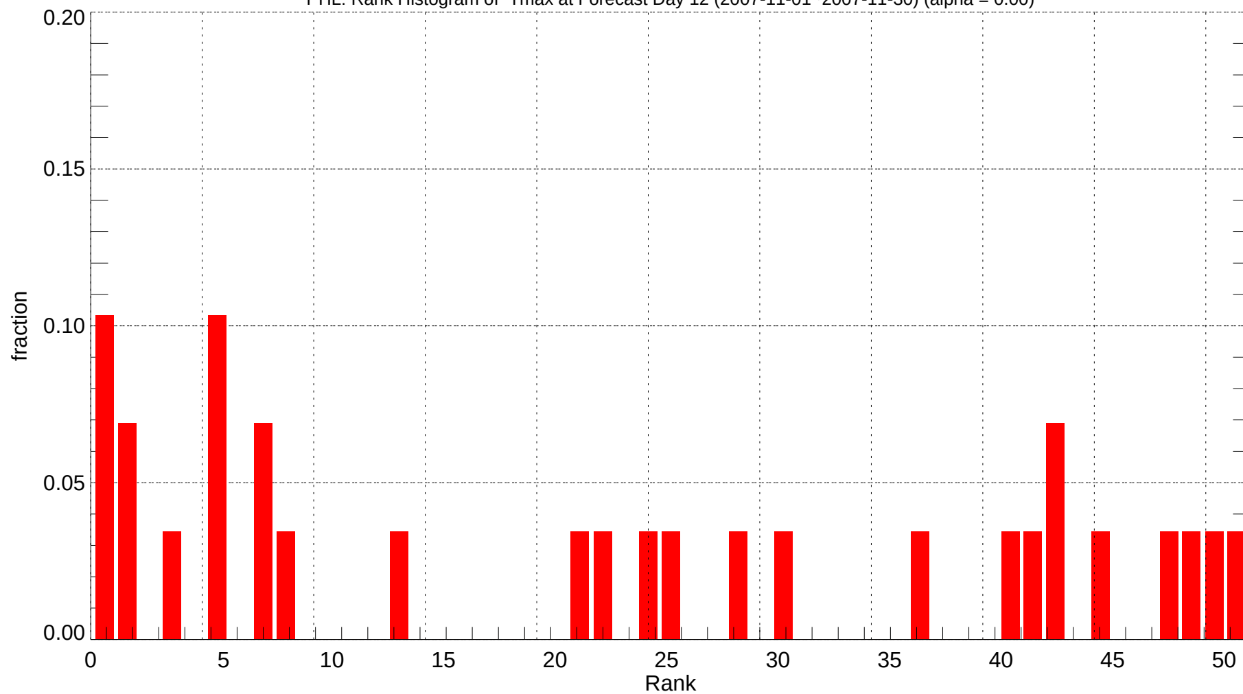
PHL: Rank Histogram of Tmax at Forecast Day 12 (2007-11-01~2007-11-30) (alpha = 0.00)
