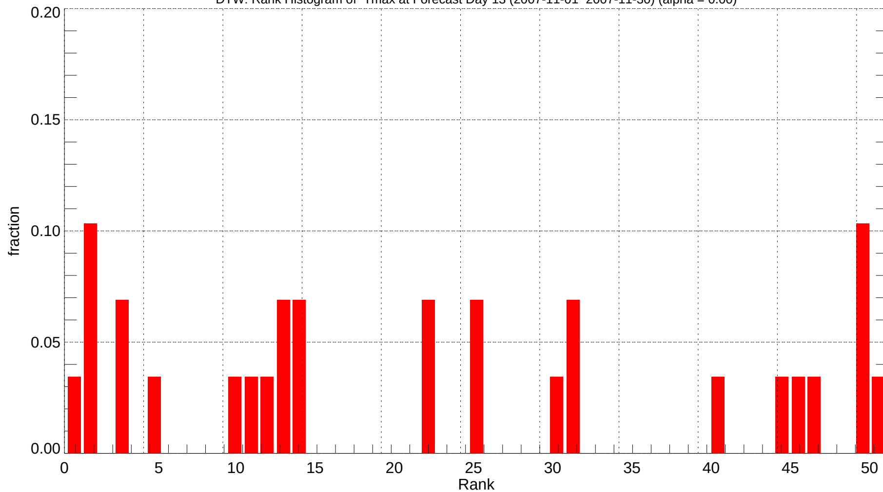
DTW: Rank Histogram of Tmax at Forecast Day 13 (2007-11-01~2007-11-30) (alpha = 0.00)
