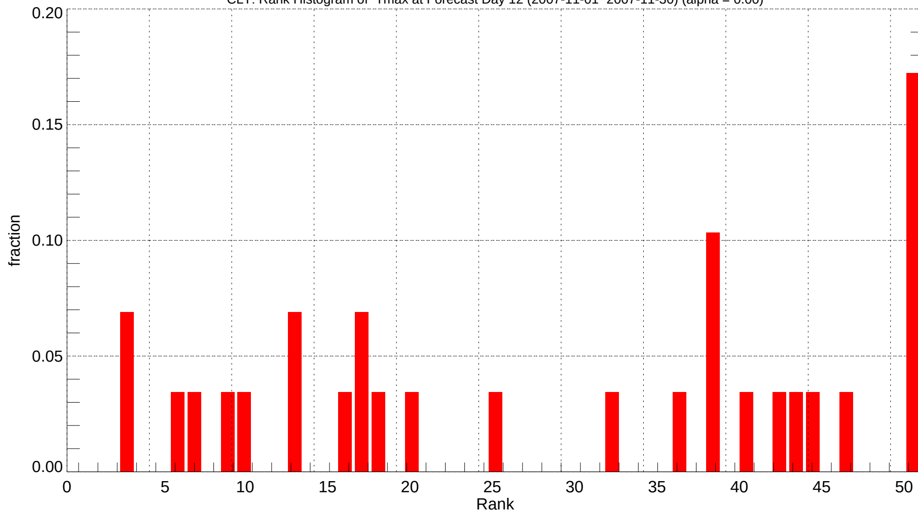
CLT: Rank Histogram of Tmax at Forecast Day 12 (2007-11-01~2007-11-30) (alpha = 0.00)
