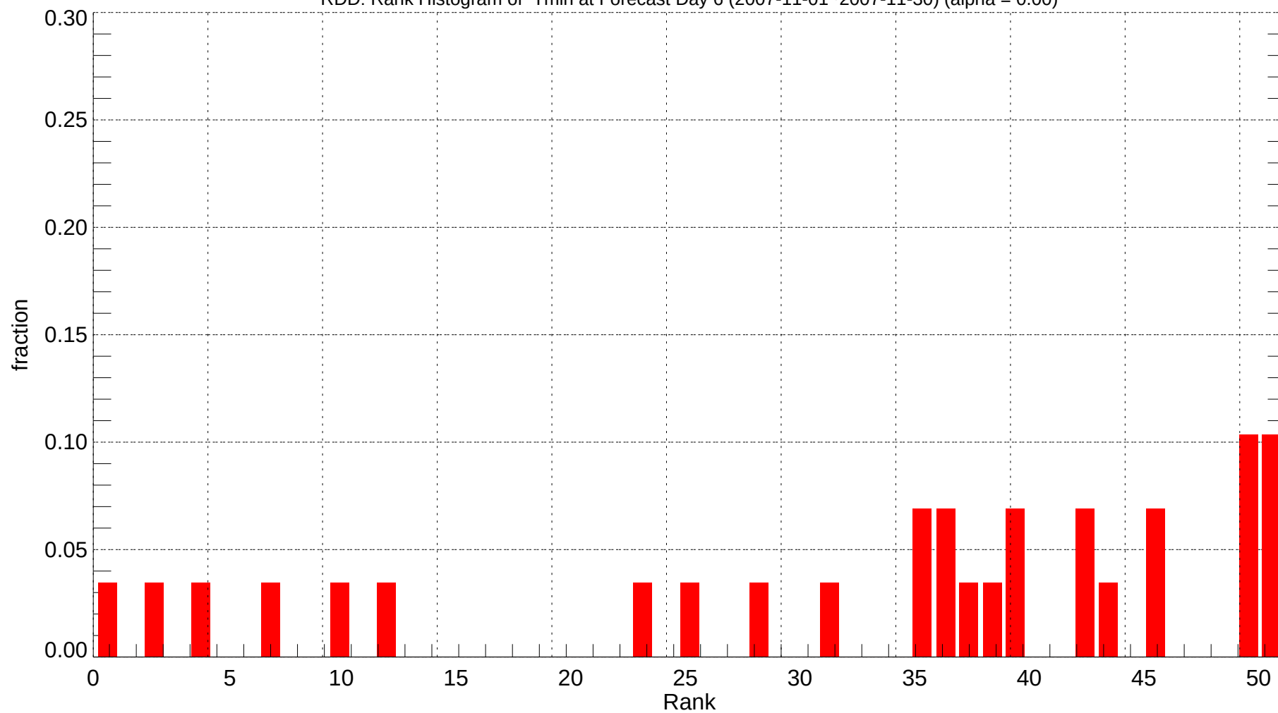
RDD: Rank Histogram of Tmin at Forecast Day 6 (2007-11-01~2007-11-30) (alpha = 0.00)
