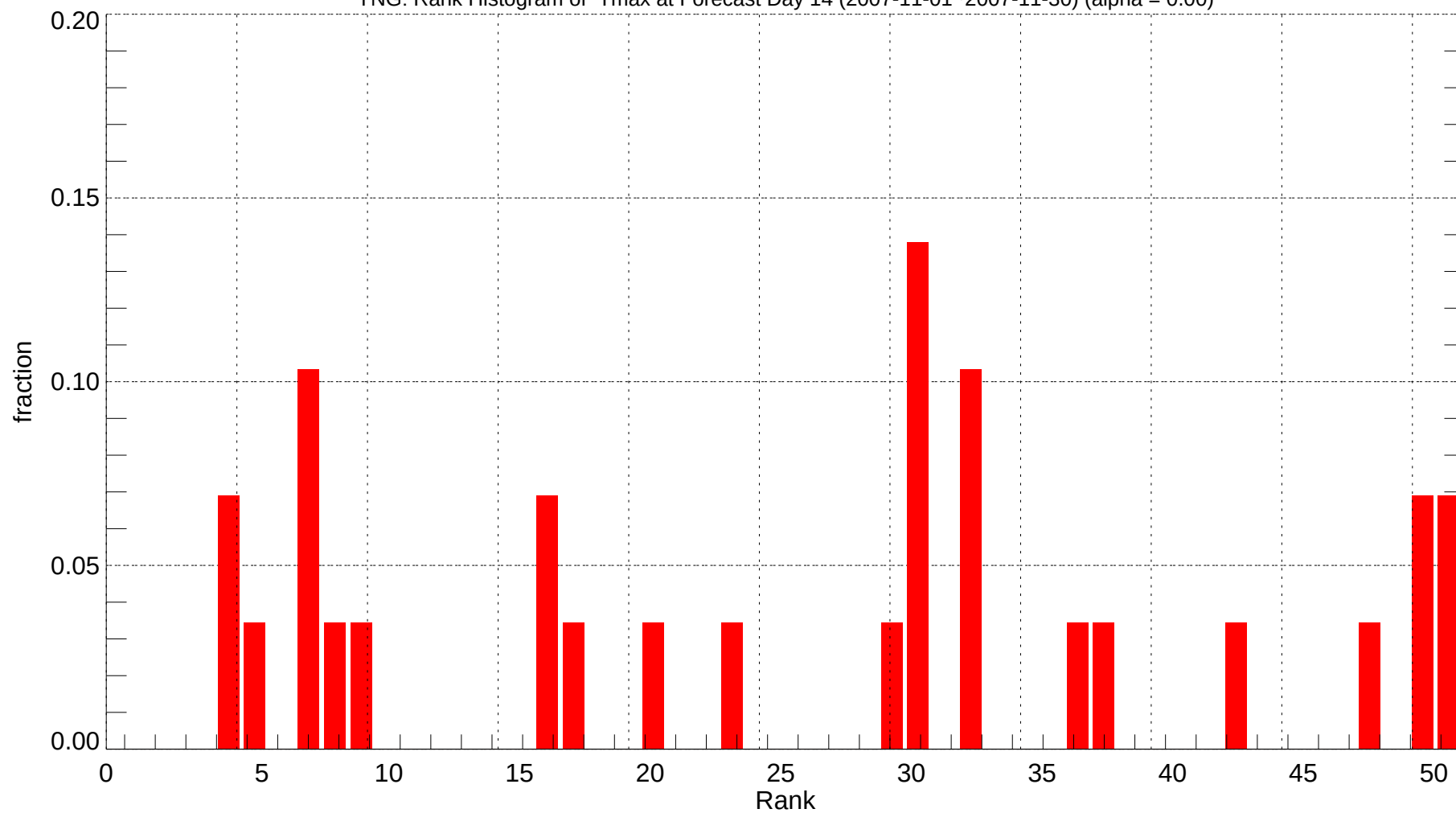
YNG: Rank Histogram of Tmax at Forecast Day 14 (2007-11-01~2007-11-30) (alpha = 0.00)
