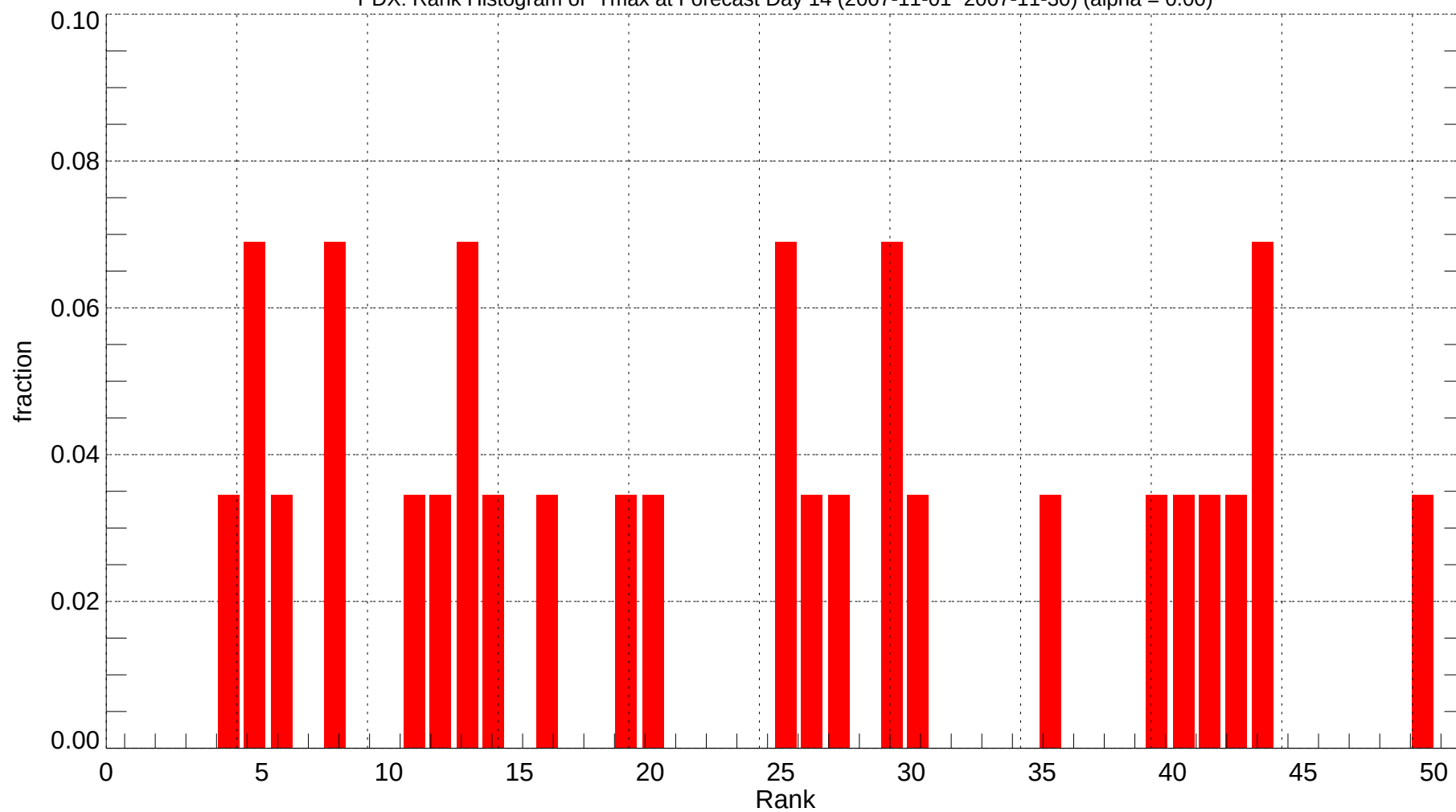
PDX: Rank Histogram of Tmax at Forecast Day 14 (2007-11-01~2007-11-30) (alpha = 0.00)
