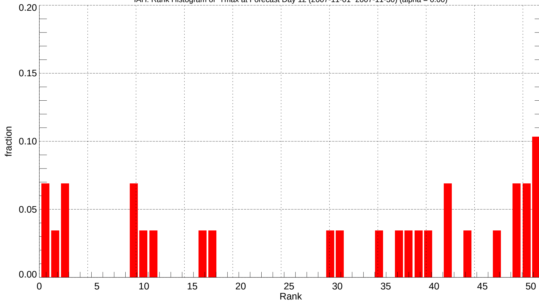
IAH: Rank Histogram of Tmax at Forecast Day 12 (2007-11-01~2007-11-30) (alpha = 0.00)
