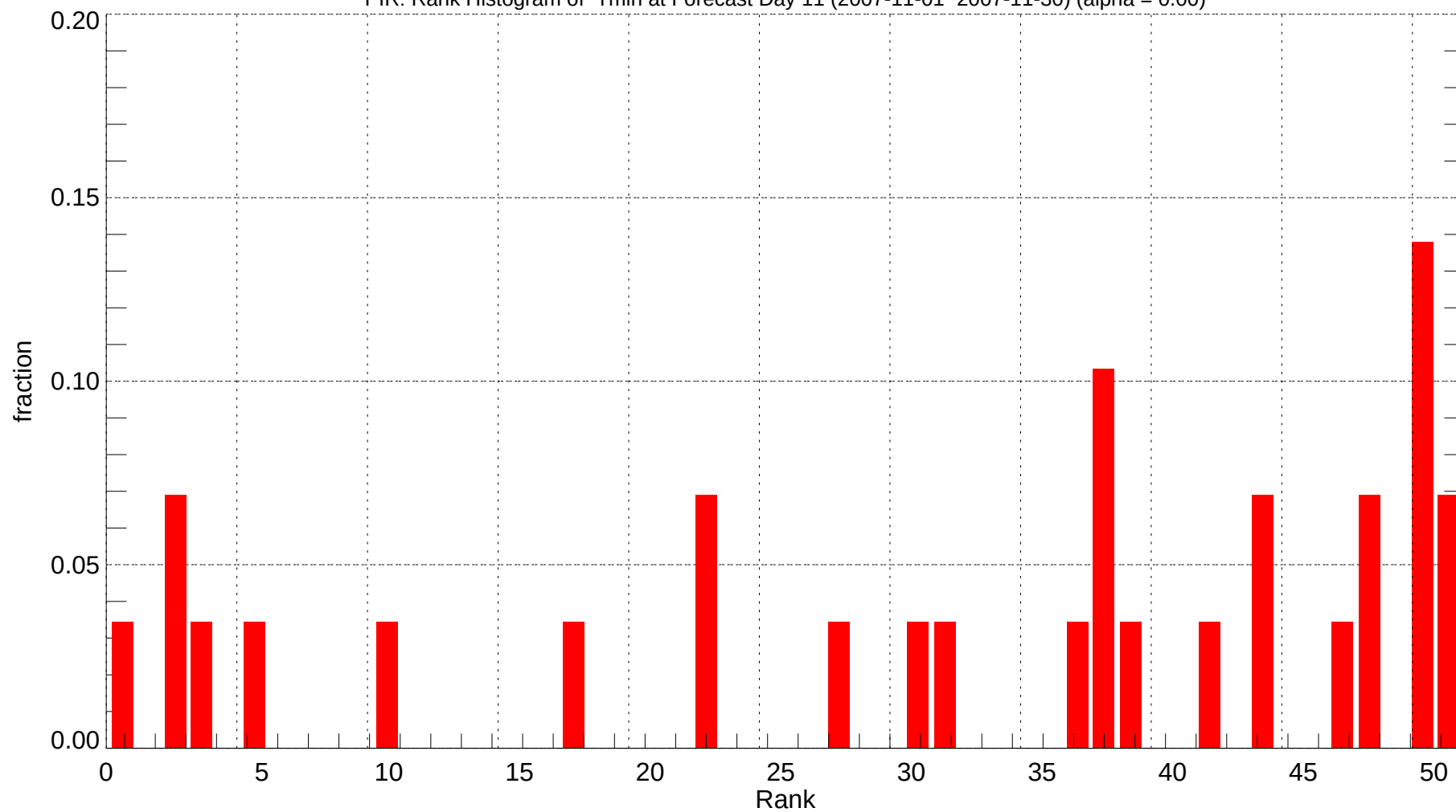
PIR: Rank Histogram of Tmin at Forecast Day 11 (2007-11-01~2007-11-30) (alpha = 0.00)
