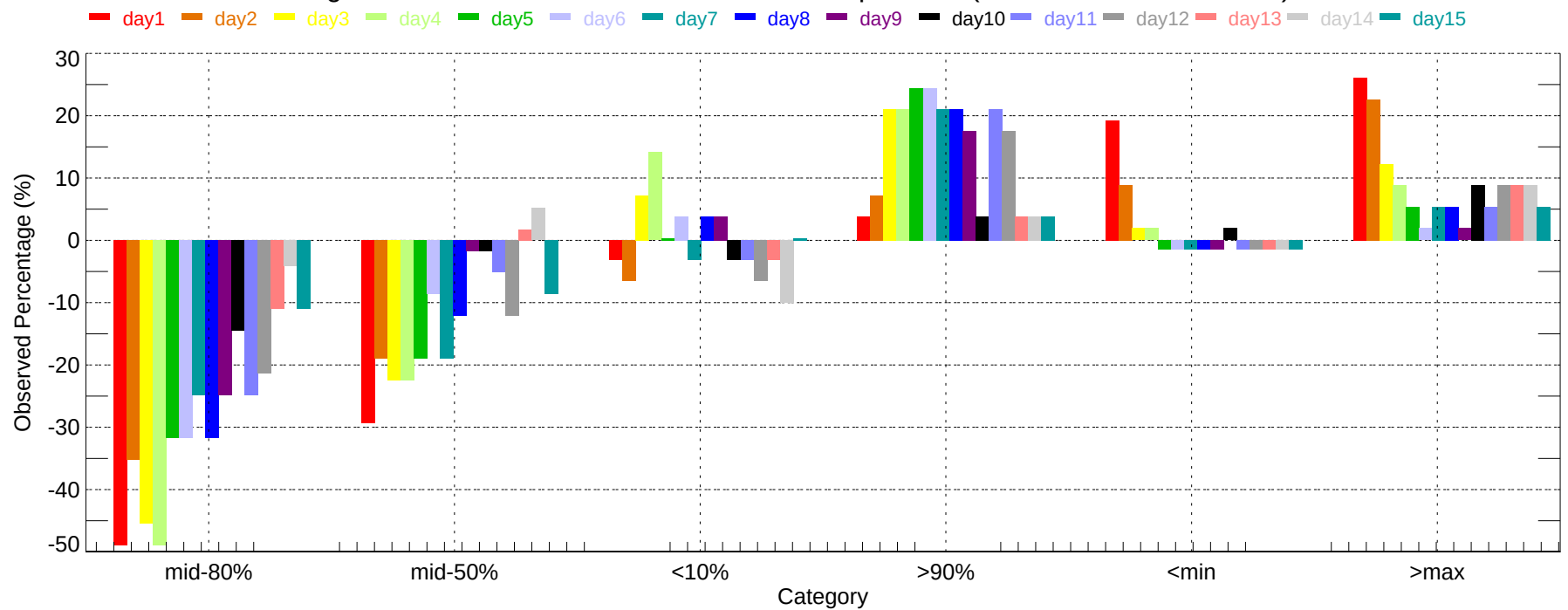
Observed Percentage Deviation of Ensembles - PIT: Max Temperature (2007-11-01~2007-11-30)
