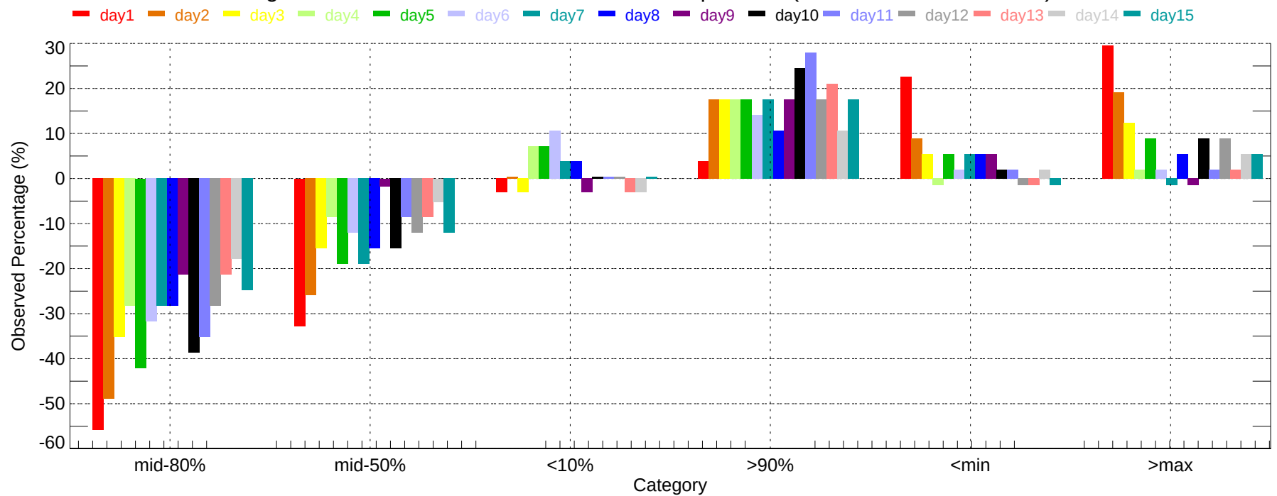
Observed Percentage Deviation of Ensembles - BIS: Max Temperature (2007-11-01~2007-11-30)
