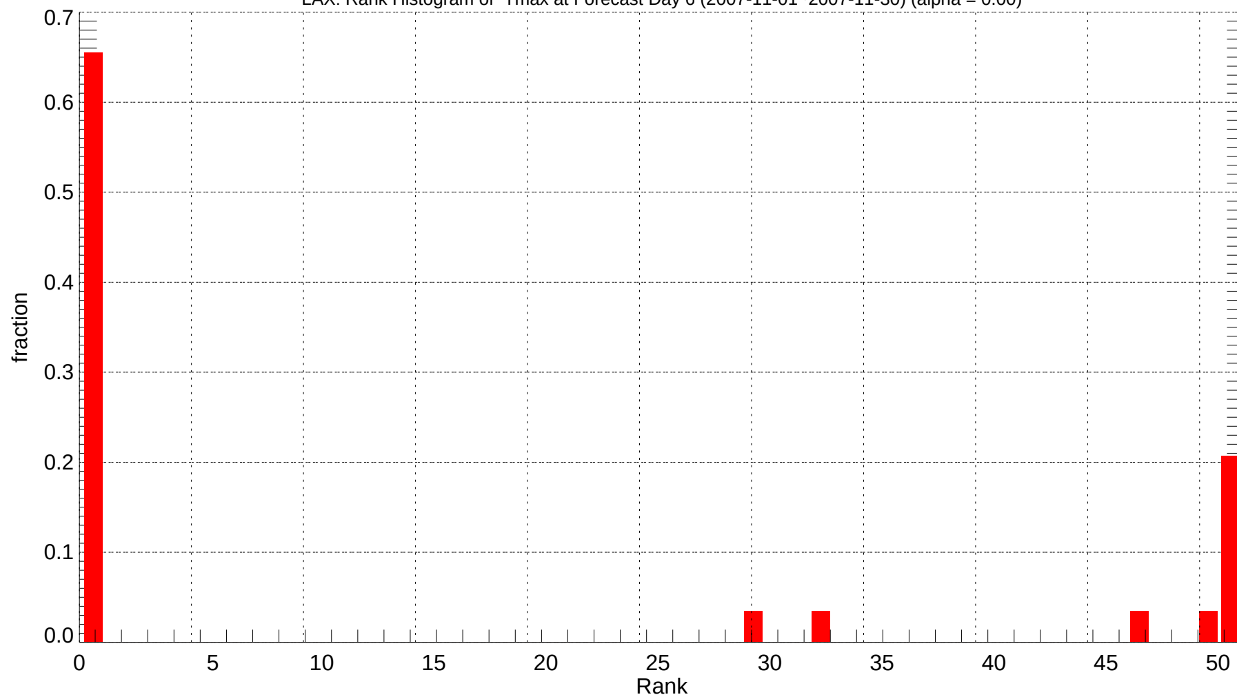
LAX: Rank Histogram of Tmax at Forecast Day 6 (2007-11-01~2007-11-30) (alpha = 0.00)
