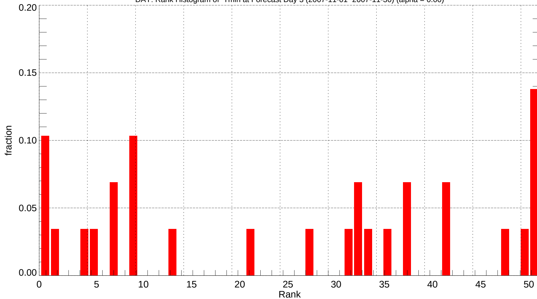
DAY: Rank Histogram of Tmin at Forecast Day 3 (2007-11-01~2007-11-30) (alpha = 0.00)
