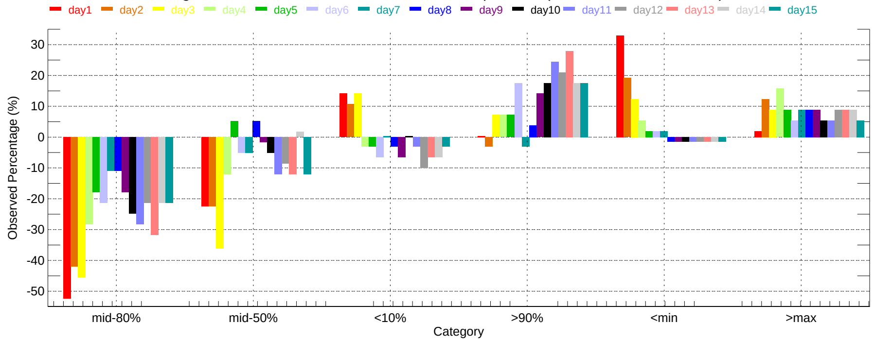
Observed Percentage Deviation of Ensembles - STL: Max Temperature (2007-11-01~2007-11-30)
