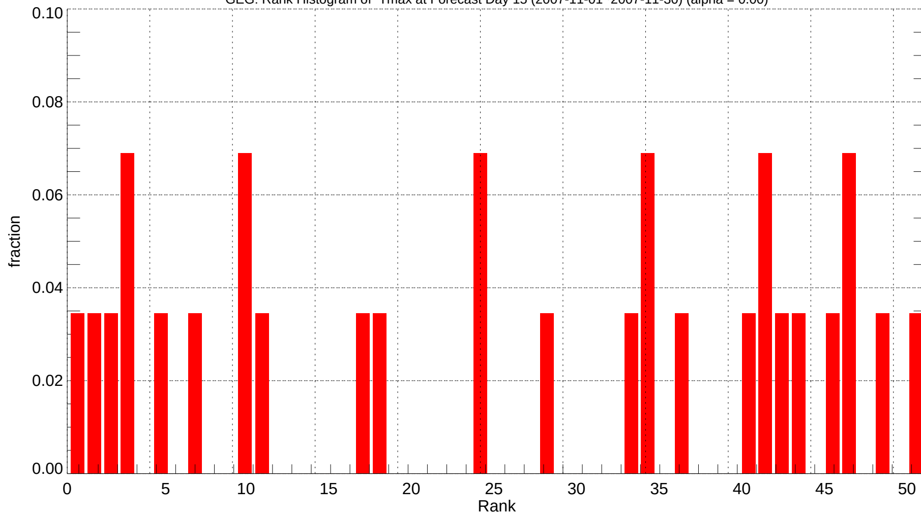
GEG: Rank Histogram of Tmax at Forecast Day 15 (2007-11-01~2007-11-30) (alpha = 0.00)
