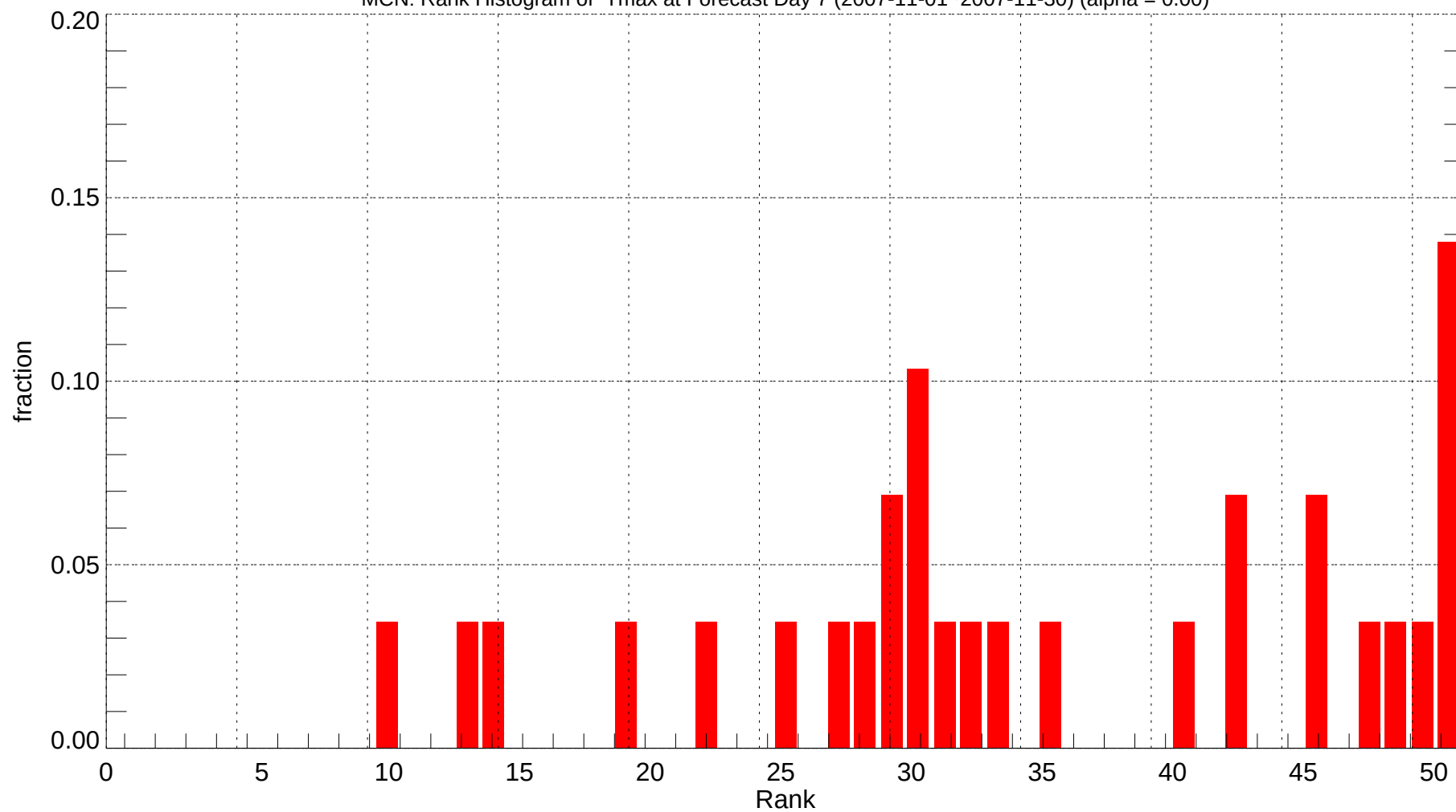
MCN: Rank Histogram of Tmax at Forecast Day 7 (2007-11-01~2007-11-30) (alpha = 0.00)
