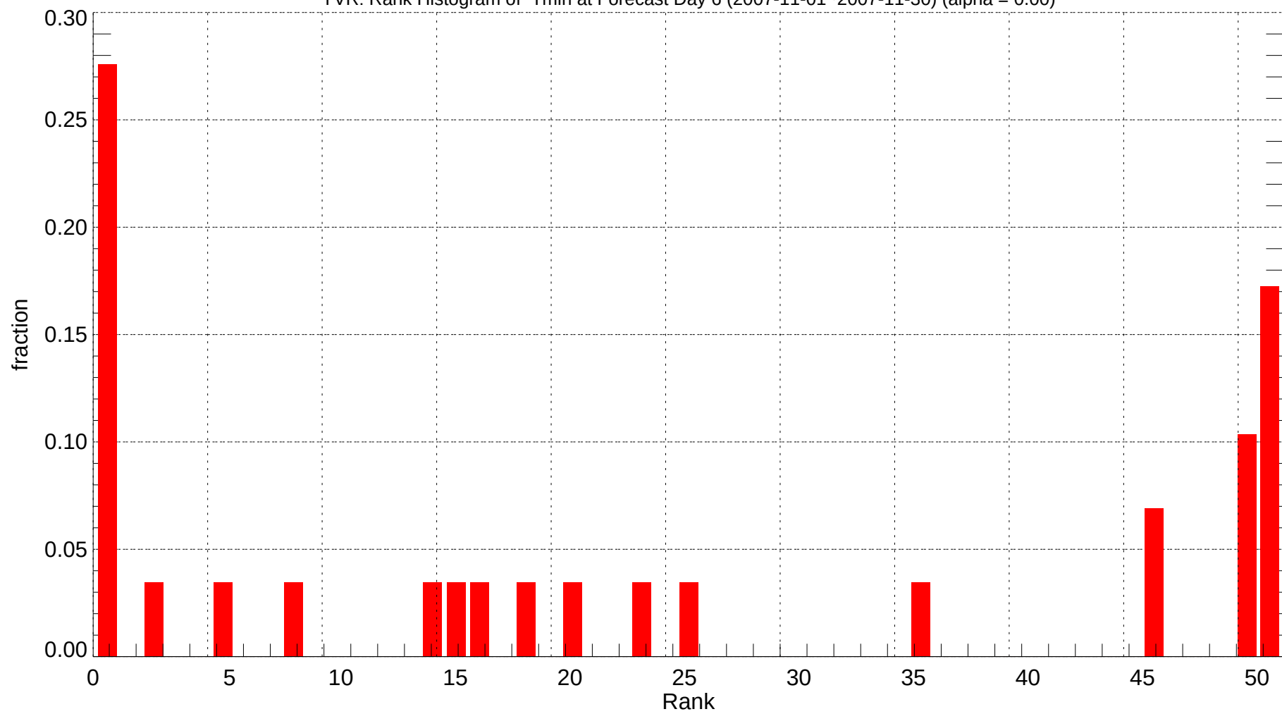
YVR: Rank Histogram of Tmin at Forecast Day 6 (2007-11-01~2007-11-30) (alpha = 0.00)
