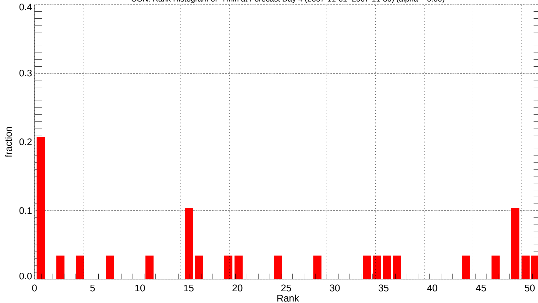
CON: Rank Histogram of Tmin at Forecast Day 4 (2007-11-01~2007-11-30) (alpha = 0.00)
