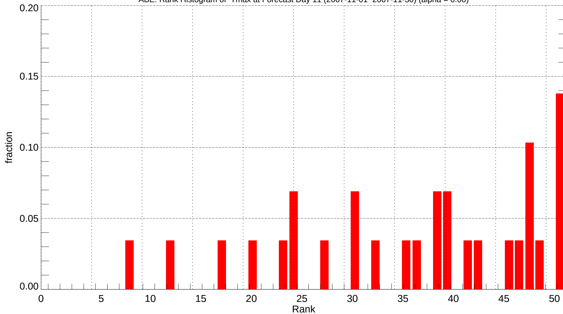
ABE: Rank Histogram of Tmax at Forecast Day 11 (2007-11-01~2007-11-30) (alpha = 0.00)
