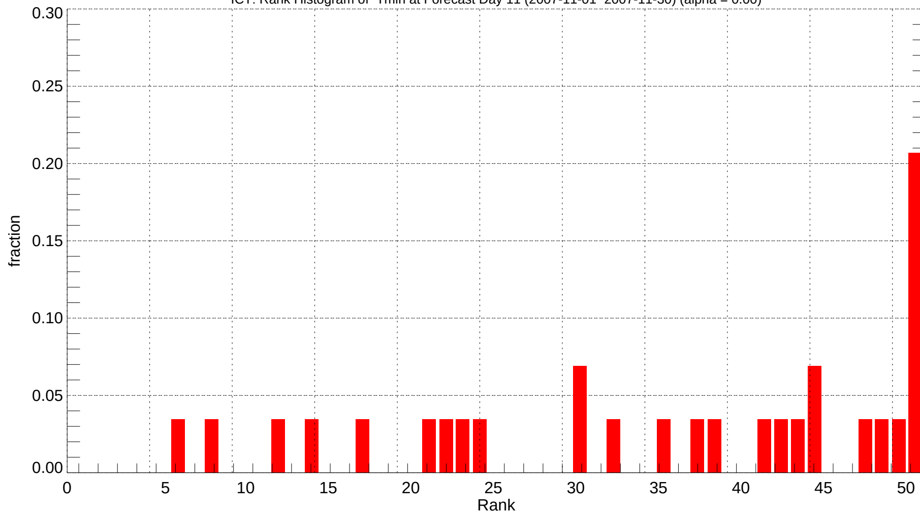
ICT: Rank Histogram of Tmin at Forecast Day 11 (2007-11-01~2007-11-30) (alpha = 0.00)
