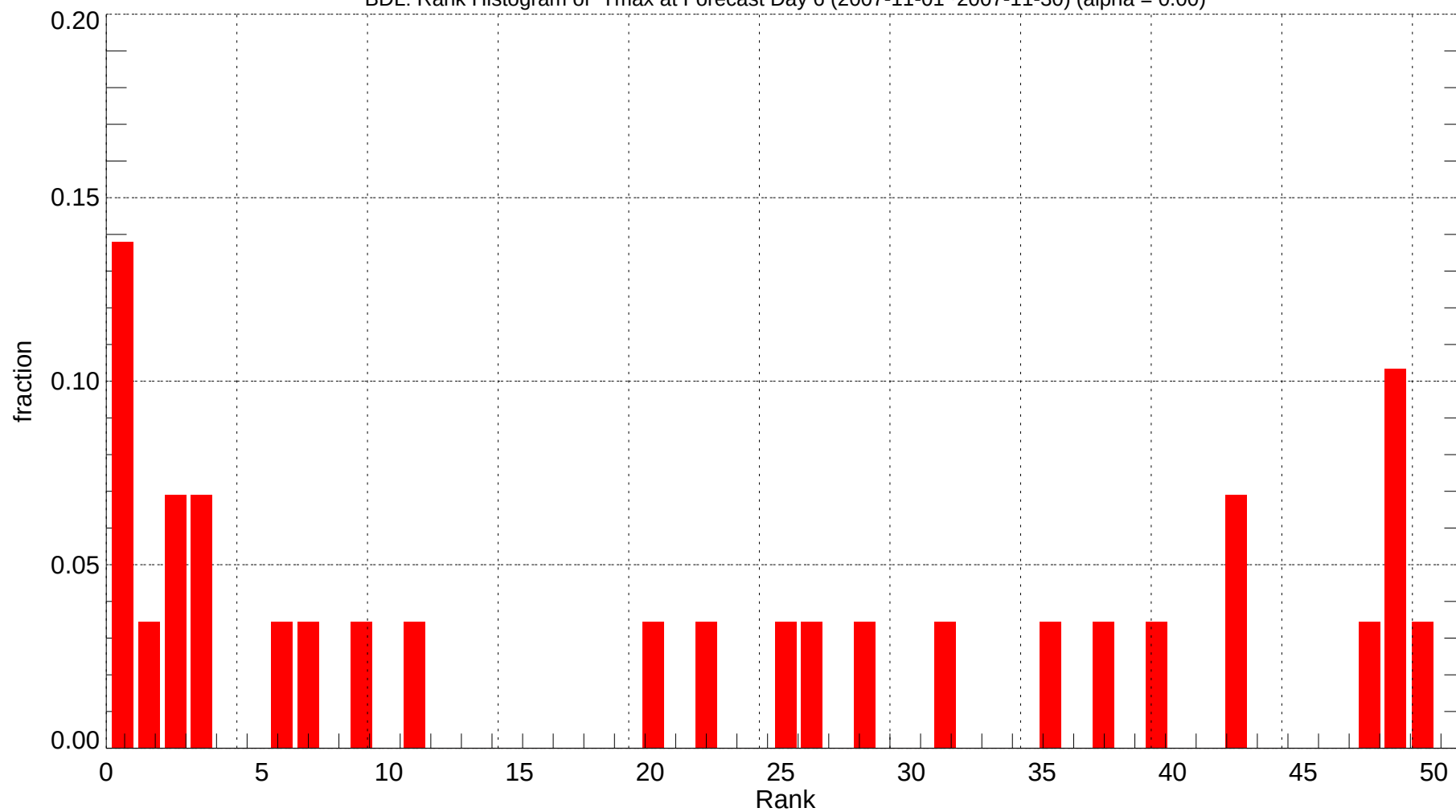
BDL: Rank Histogram of Tmax at Forecast Day 6 (2007-11-01~2007-11-30) (alpha = 0.00)
