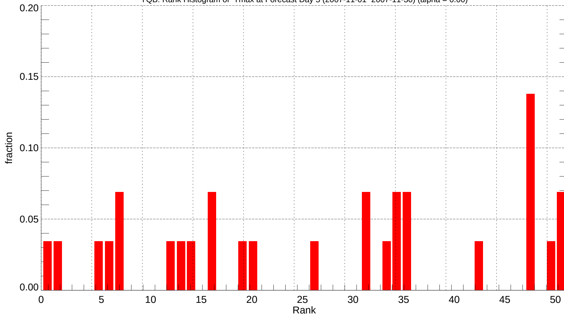
YQB: Rank Histogram of Tmax at Forecast Day 5 (2007-11-01~2007-11-30) (alpha = 0.00)
