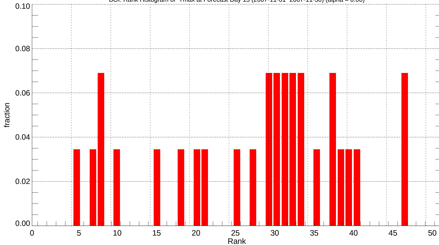
BOI: Rank Histogram of Tmax at Forecast Day 15 (2007-11-01~2007-11-30) (alpha = 0.00)
