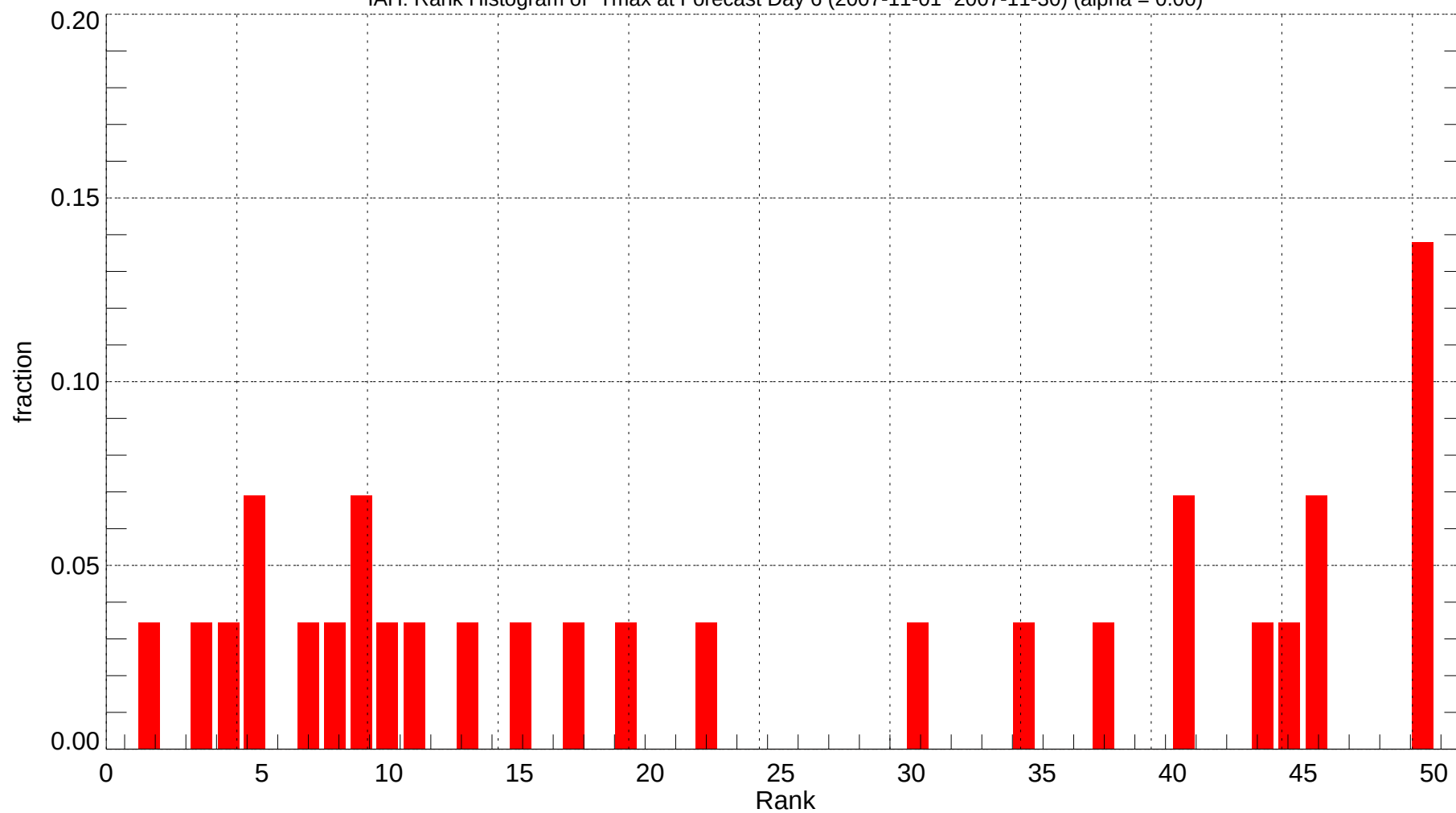
IAH: Rank Histogram of Tmax at Forecast Day 6 (2007-11-01~2007-11-30) (alpha = 0.00)
