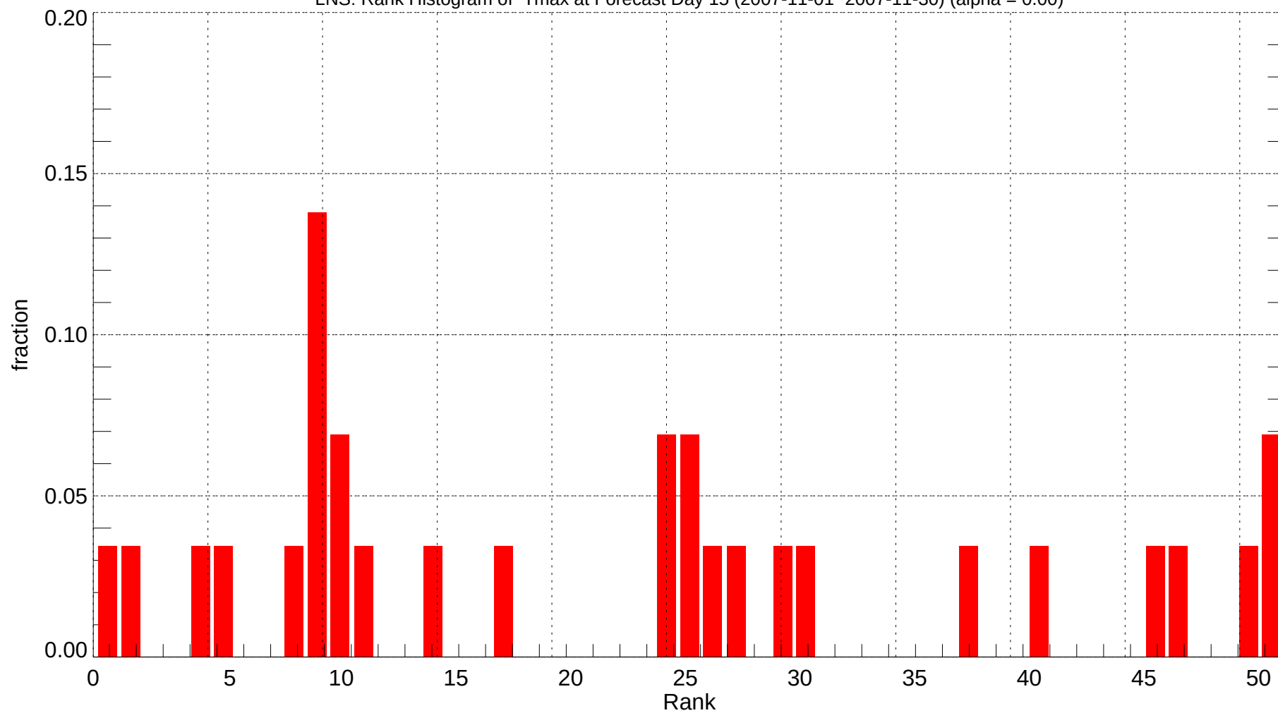
LNS: Rank Histogram of Tmax at Forecast Day 15 (2007-11-01~2007-11-30) (alpha = 0.00)
