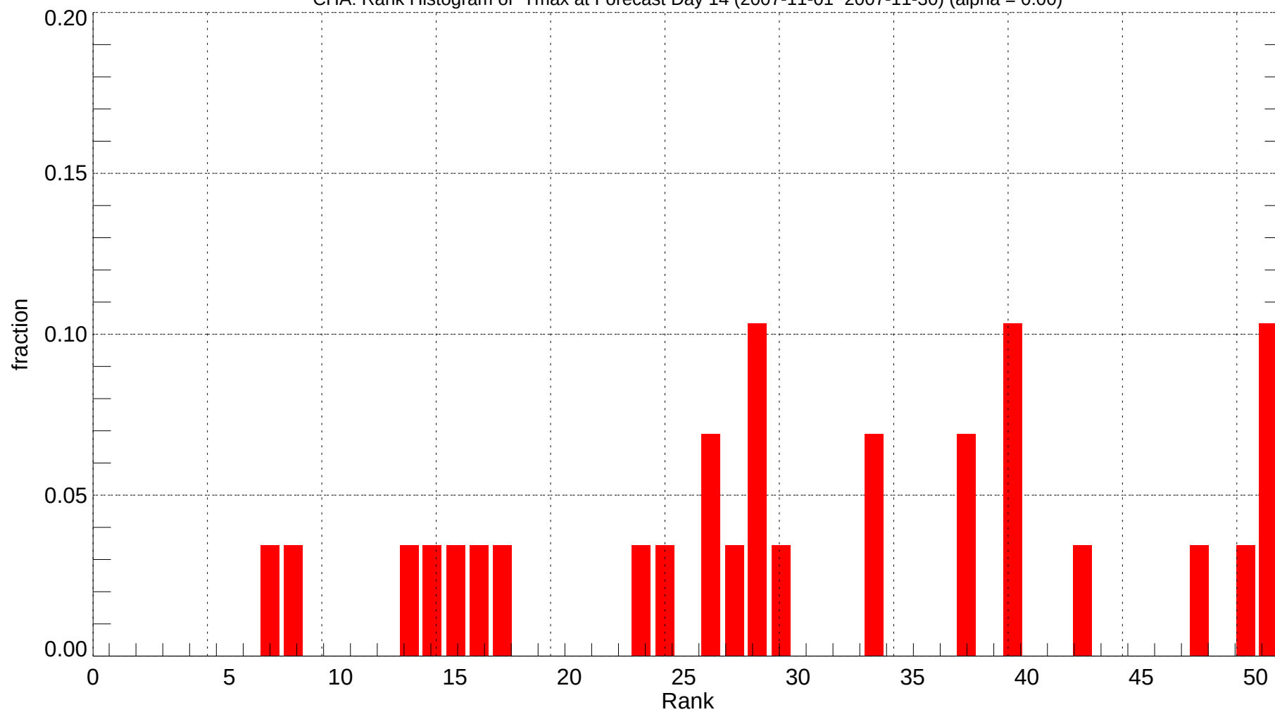
CHA: Rank Histogram of Tmax at Forecast Day 14 (2007-11-01~2007-11-30) (alpha = 0.00)
