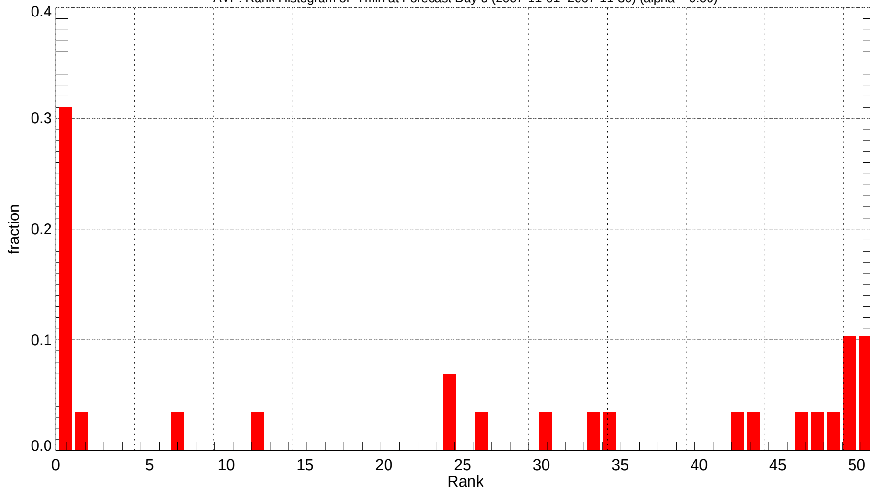
AVP: Rank Histogram of Tmin at Forecast Day 3 (2007-11-01~2007-11-30) (alpha = 0.00)
