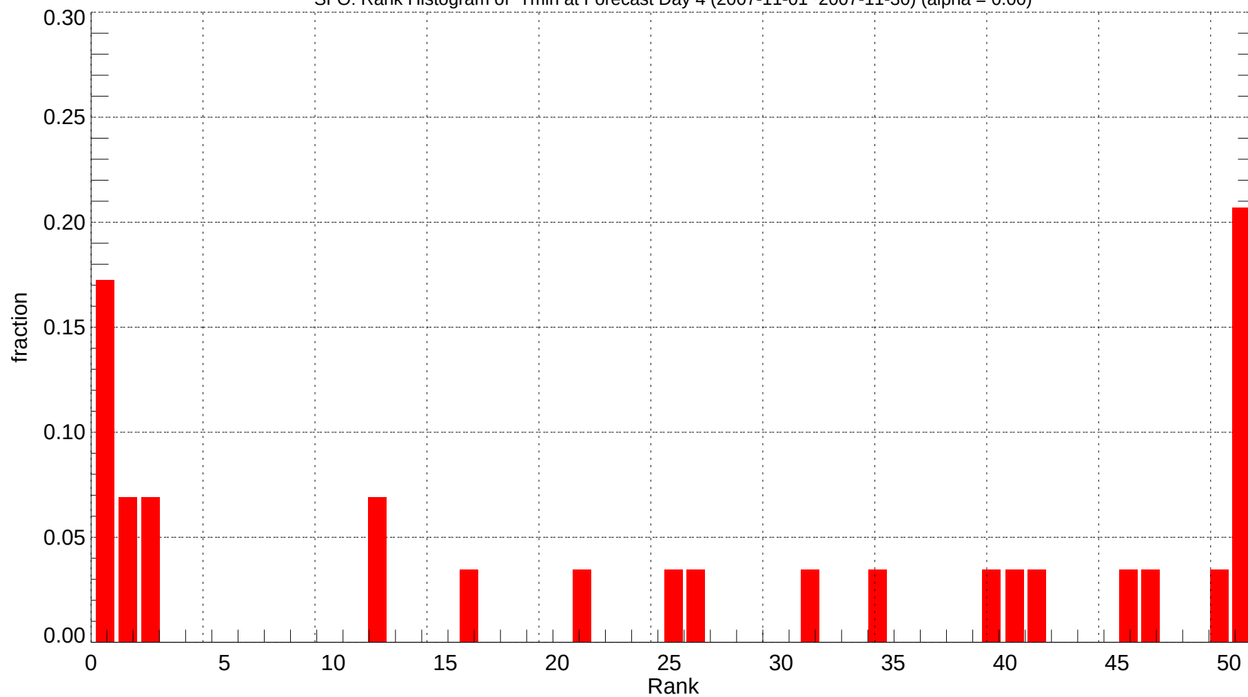
SFO: Rank Histogram of Tmin at Forecast Day 4 (2007-11-01~2007-11-30) (alpha = 0.00)
