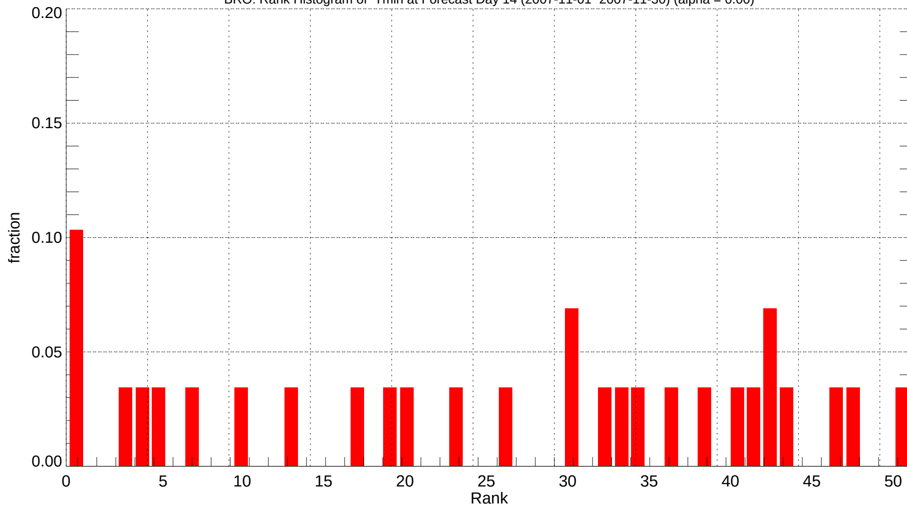
BRO: Rank Histogram of Tmin at Forecast Day 14 (2007-11-01~2007-11-30) (alpha = 0.00)
