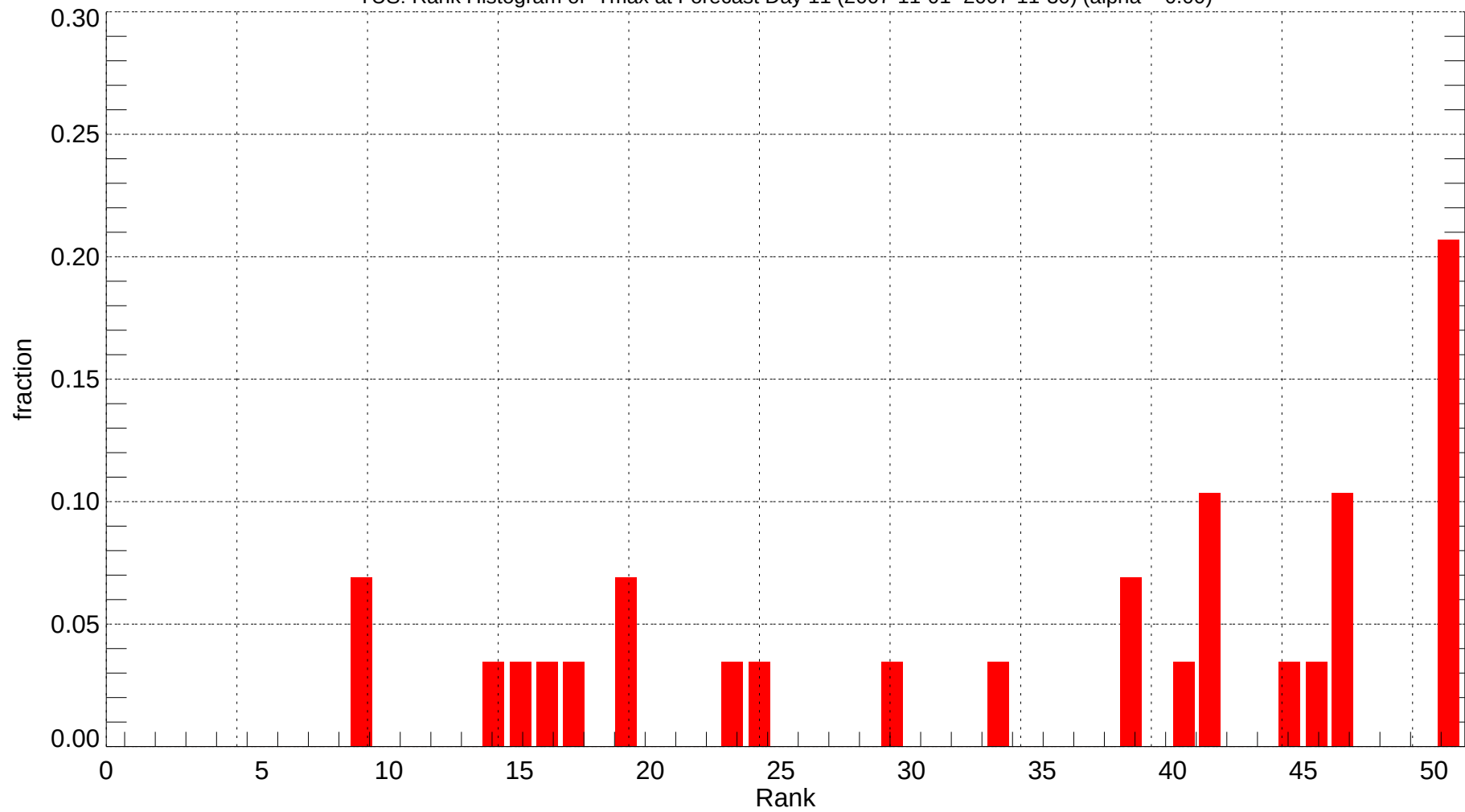
TUS: Rank Histogram of Tmax at Forecast Day 11 (2007-11-01~2007-11-30) (alpha = 0.00)
