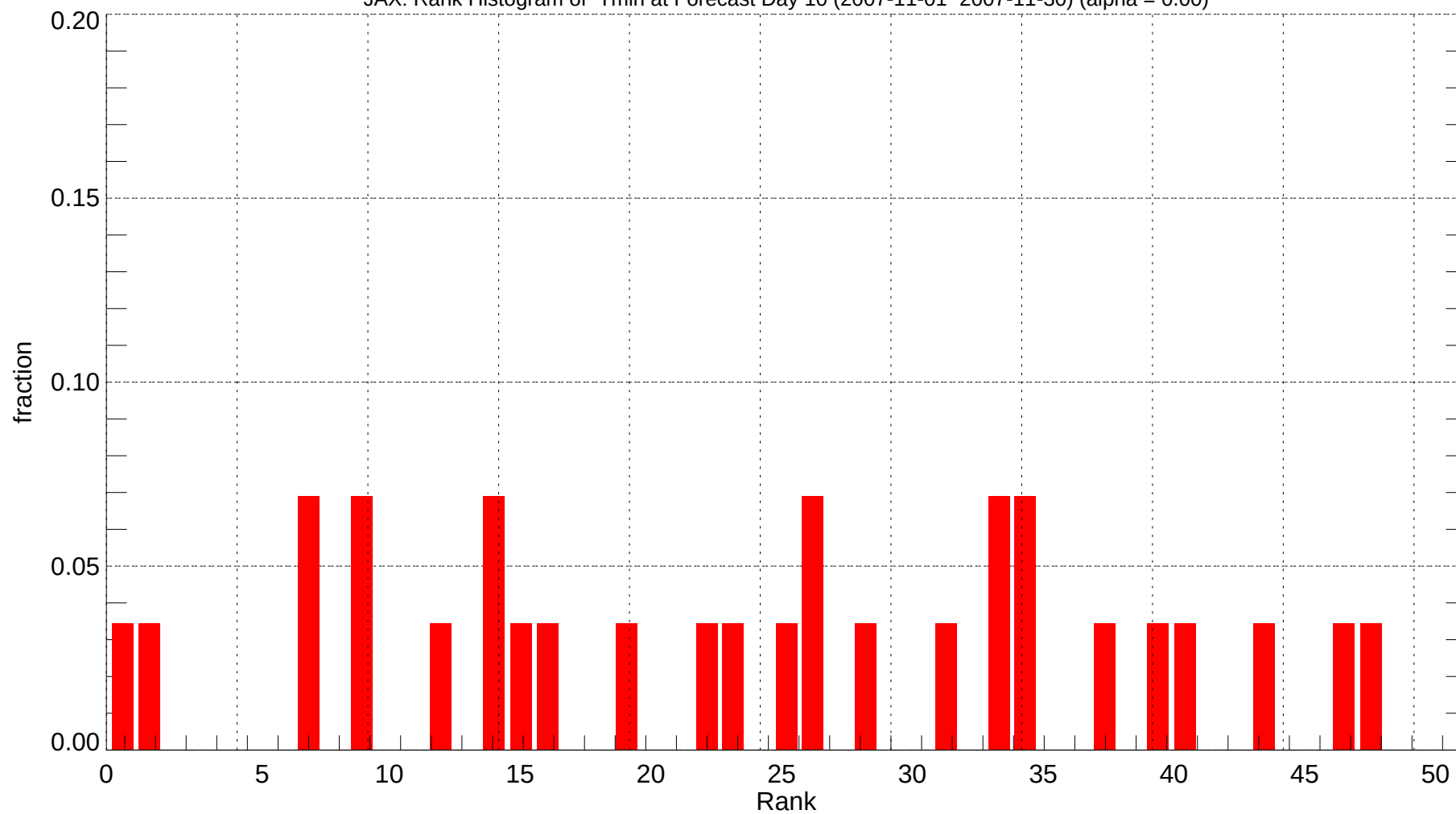
JAX: Rank Histogram of Tmin at Forecast Day 10 (2007-11-01~2007-11-30) (alpha = 0.00)
