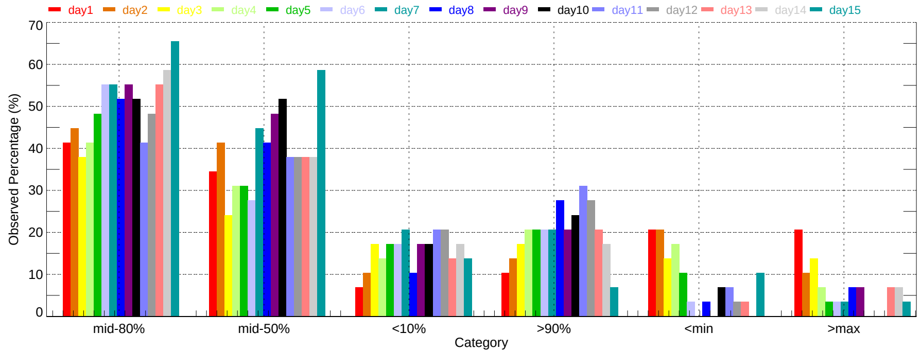
Observed Percentage of Ensembles - SAT: Max Temperature (2007-11-01~2007-11-30)
