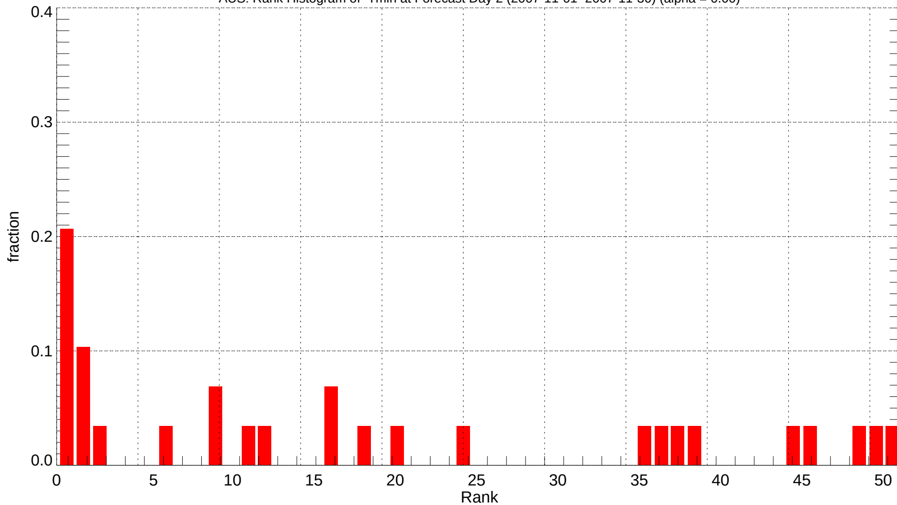
AUS: Rank Histogram of Tmin at Forecast Day 2 (2007-11-01~2007-11-30) (alpha = 0.00)
