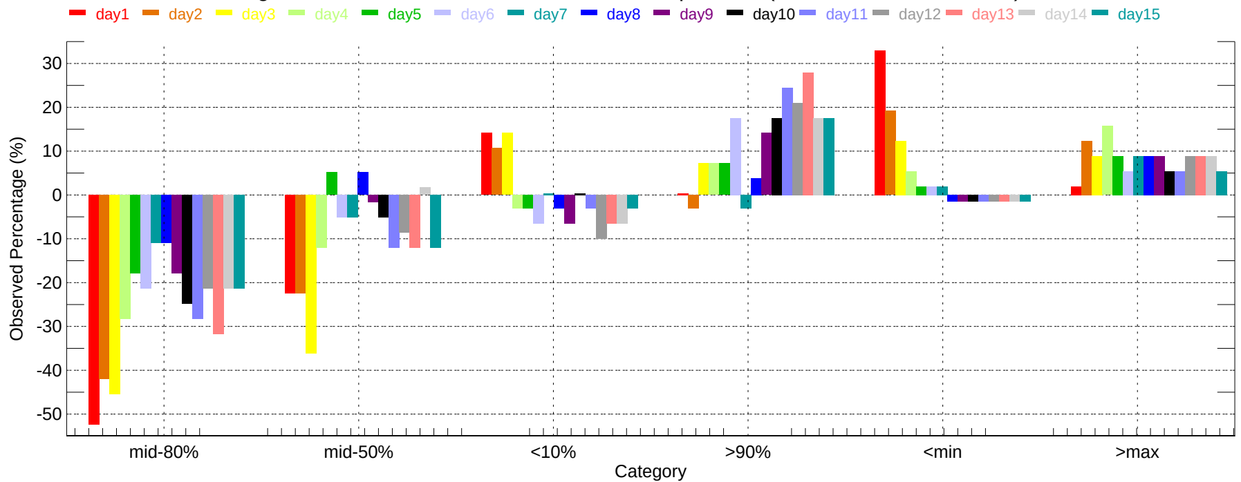
Observed Percentage Deviation of Ensembles - STL: Min Temperature (2007-11-01~2007-11-30)
