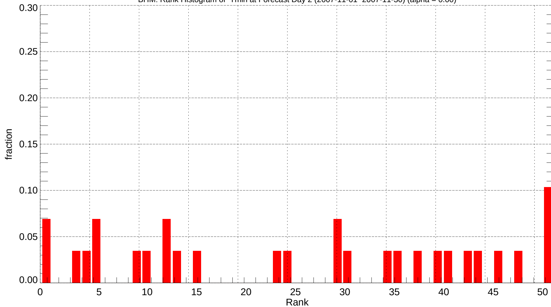
BHM: Rank Histogram of Tmin at Forecast Day 2 (2007-11-01~2007-11-30) (alpha = 0.00)
