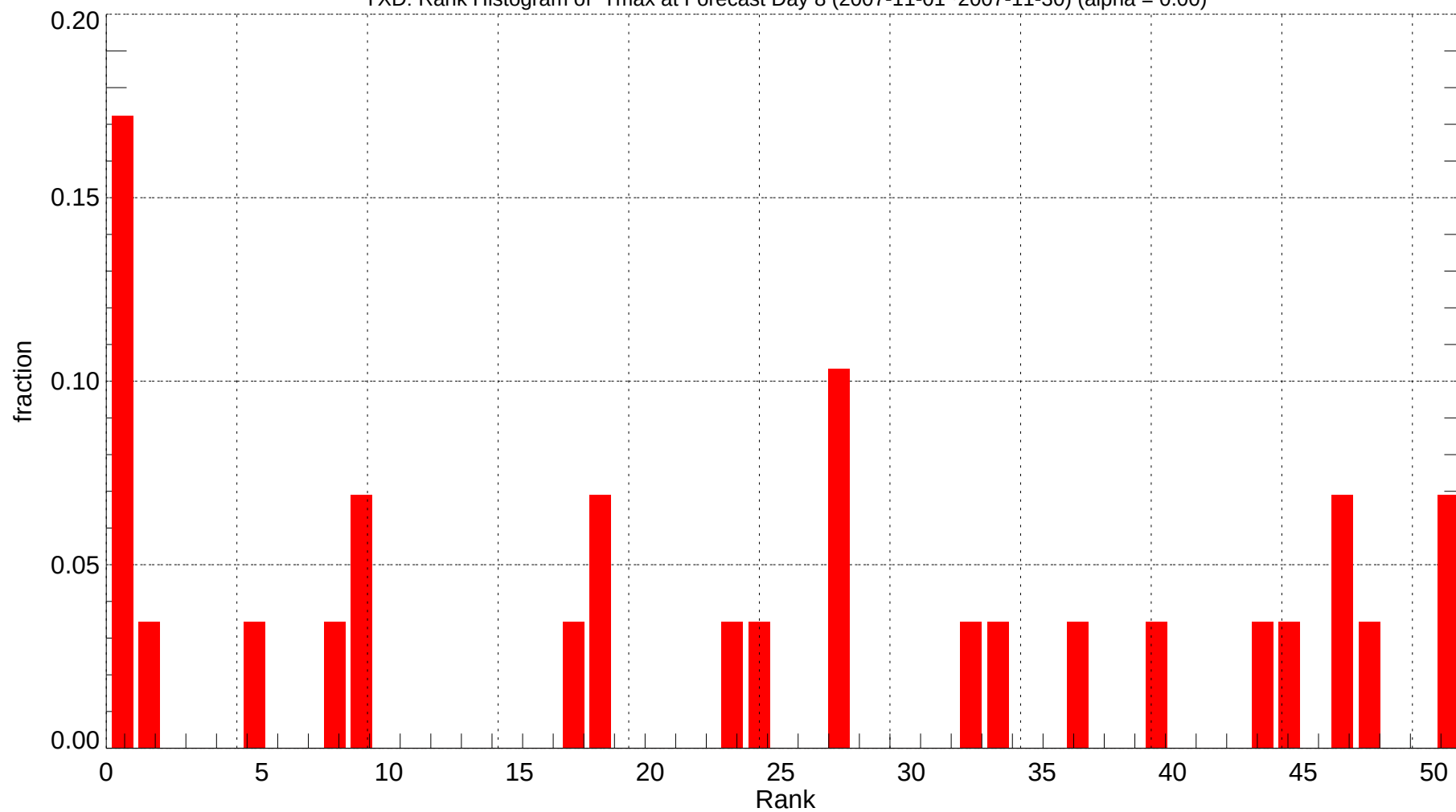
YXD: Rank Histogram of Tmax at Forecast Day 8 (2007-11-01~2007-11-30) (alpha = 0.00)
