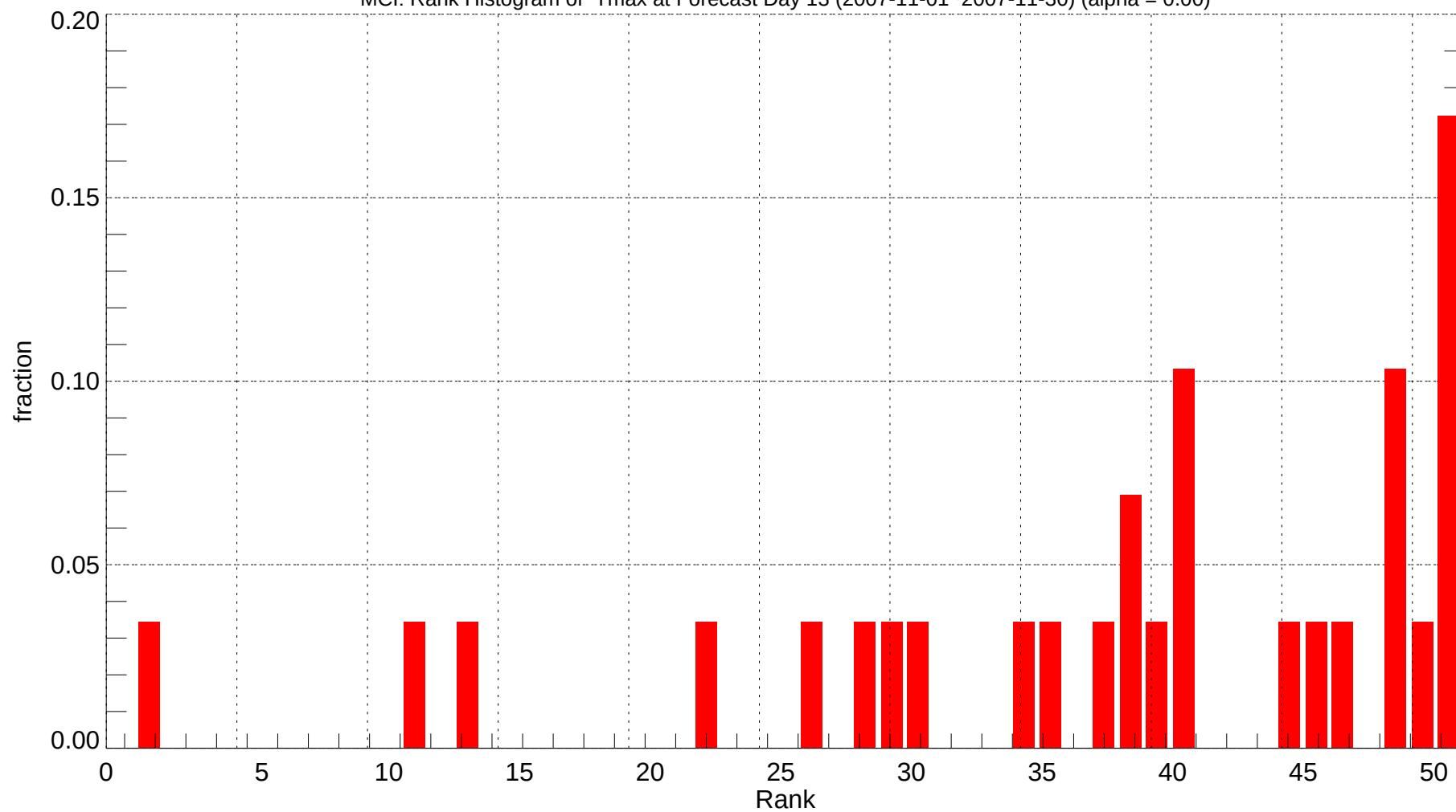
MCI: Rank Histogram of Tmax at Forecast Day 13 (2007-11-01~2007-11-30) (alpha = 0.00)
