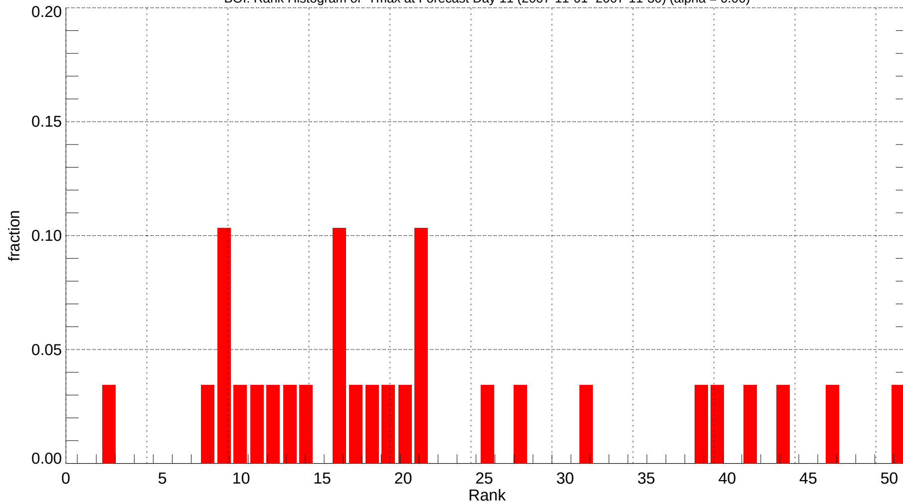
BOI: Rank Histogram of Tmax at Forecast Day 11 (2007-11-01~2007-11-30) (alpha = 0.00)
