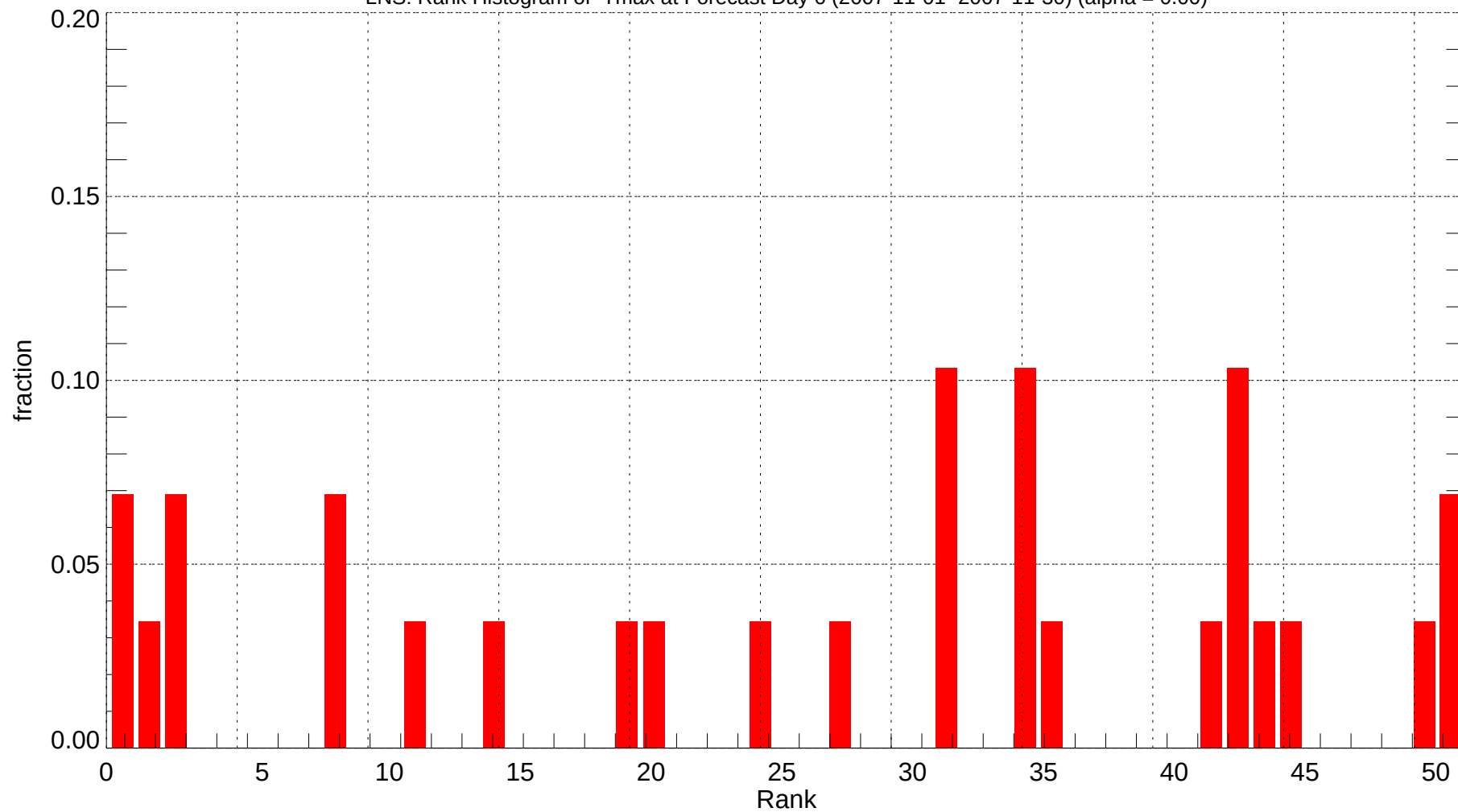
LNS: Rank Histogram of Tmax at Forecast Day 6 (2007-11-01~2007-11-30) (alpha = 0.00)
