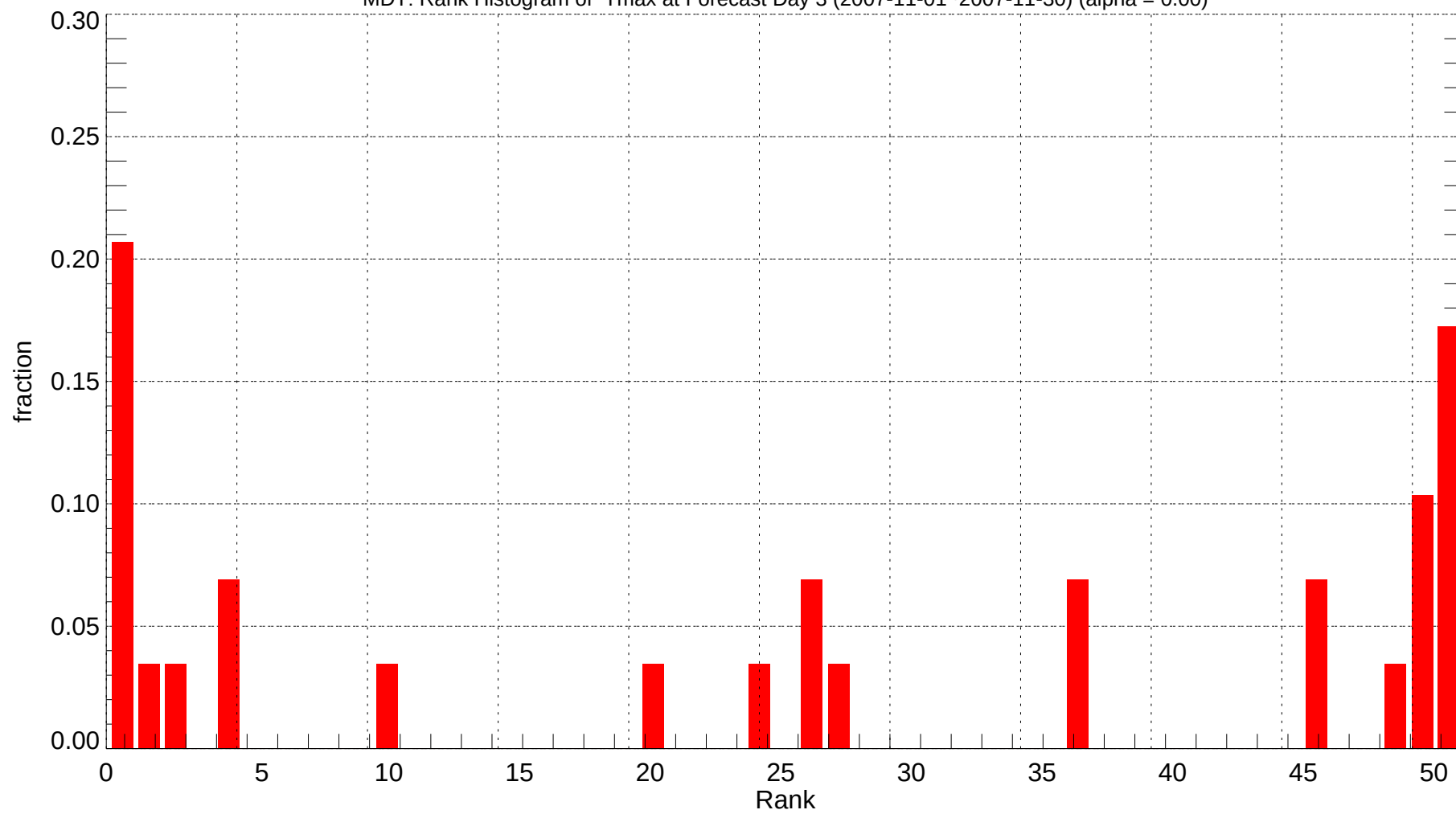
MDT: Rank Histogram of Tmax at Forecast Day 3 (2007-11-01~2007-11-30) (alpha = 0.00)
