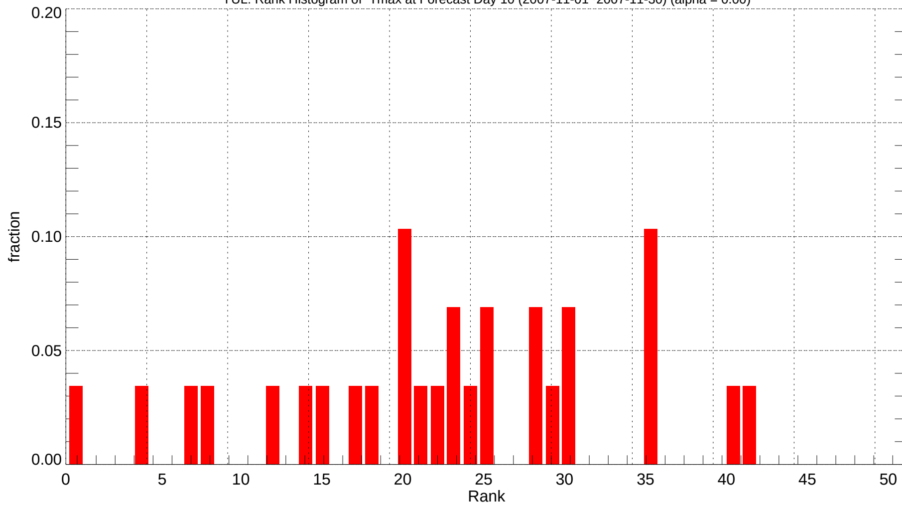
YUL: Rank Histogram of Tmax at Forecast Day 10 (2007-11-01~2007-11-30) (alpha = 0.00)
