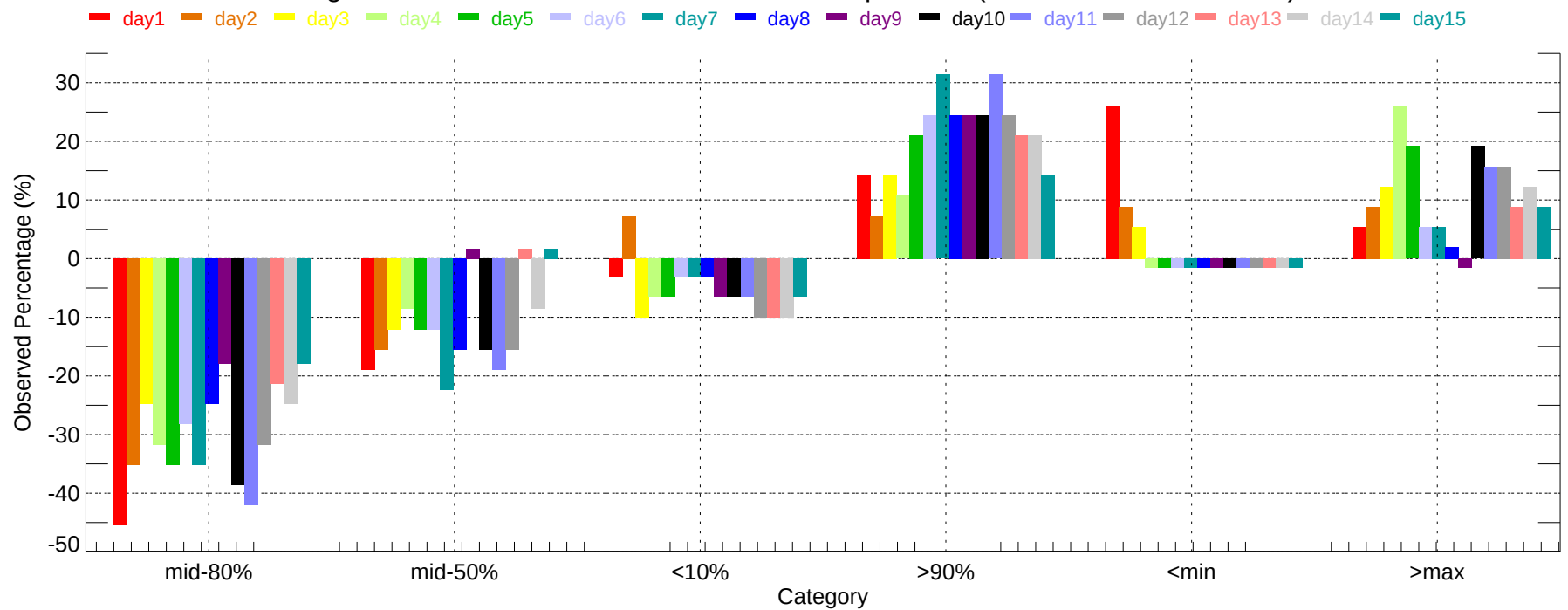
Observed Percentage Deviation of Ensembles - BNA: Min Temperature (2007-11-01~2007-11-30)
