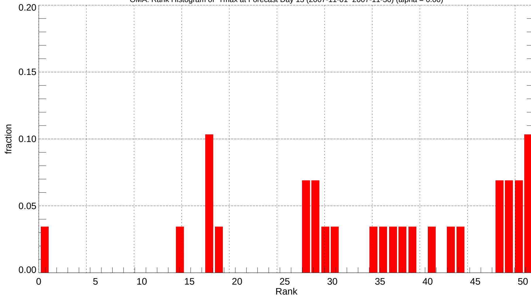
OMA: Rank Histogram of Tmax at Forecast Day 13 (2007-11-01~2007-11-30) (alpha = 0.00)
