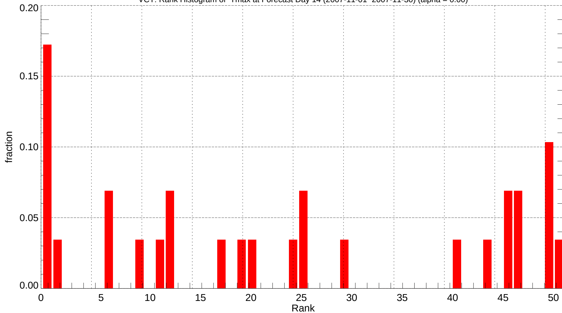
VCT: Rank Histogram of Tmax at Forecast Day 14 (2007-11-01~2007-11-30) (alpha = 0.00)
