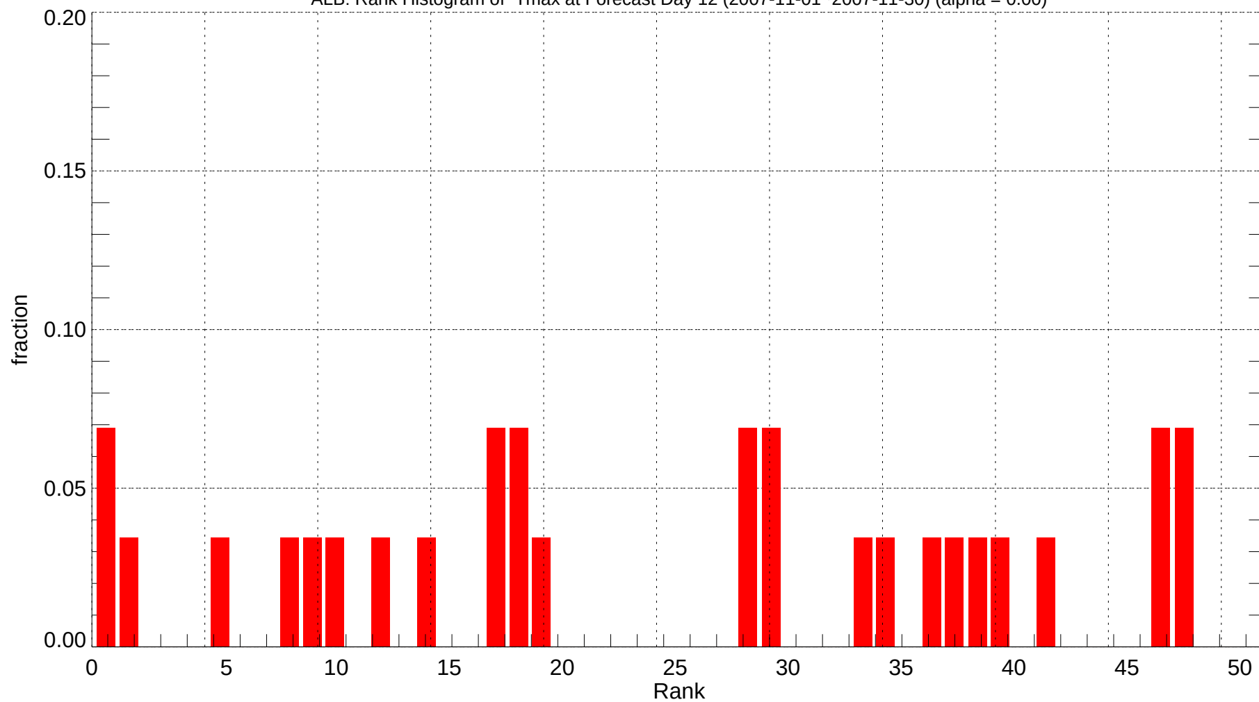
ALB: Rank Histogram of Tmax at Forecast Day 12 (2007-11-01~2007-11-30) (alpha = 0.00)
