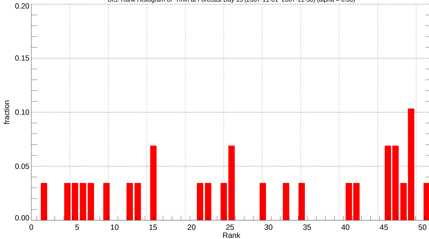
BIS: Rank Histogram of Tmin at Forecast Day 13 (2007-11-01~2007-11-30) (alpha = 0.00)
