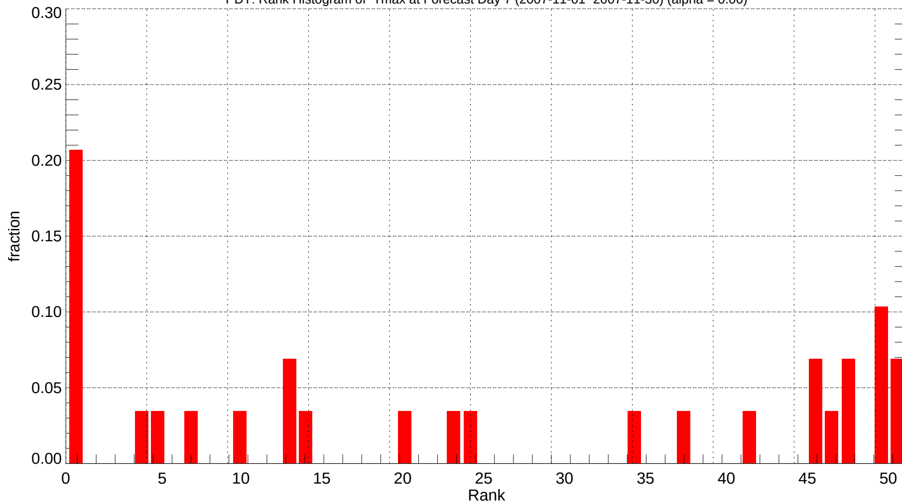
PDT: Rank Histogram of Tmax at Forecast Day 7 (2007-11-01~2007-11-30) (alpha = 0.00)
