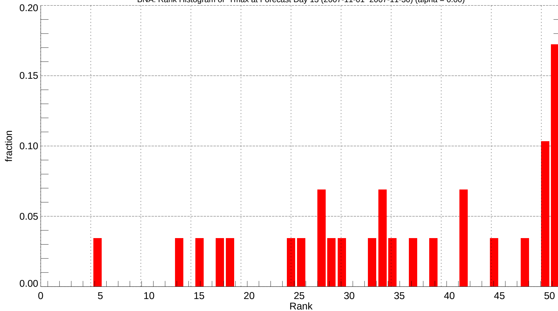
BNA: Rank Histogram of Tmax at Forecast Day 13 (2007-11-01~2007-11-30) (alpha = 0.00)
