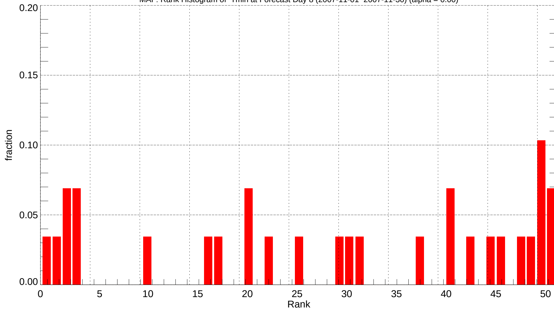
MAF: Rank Histogram of Tmin at Forecast Day 8 (2007-11-01~2007-11-30) (alpha = 0.00)
