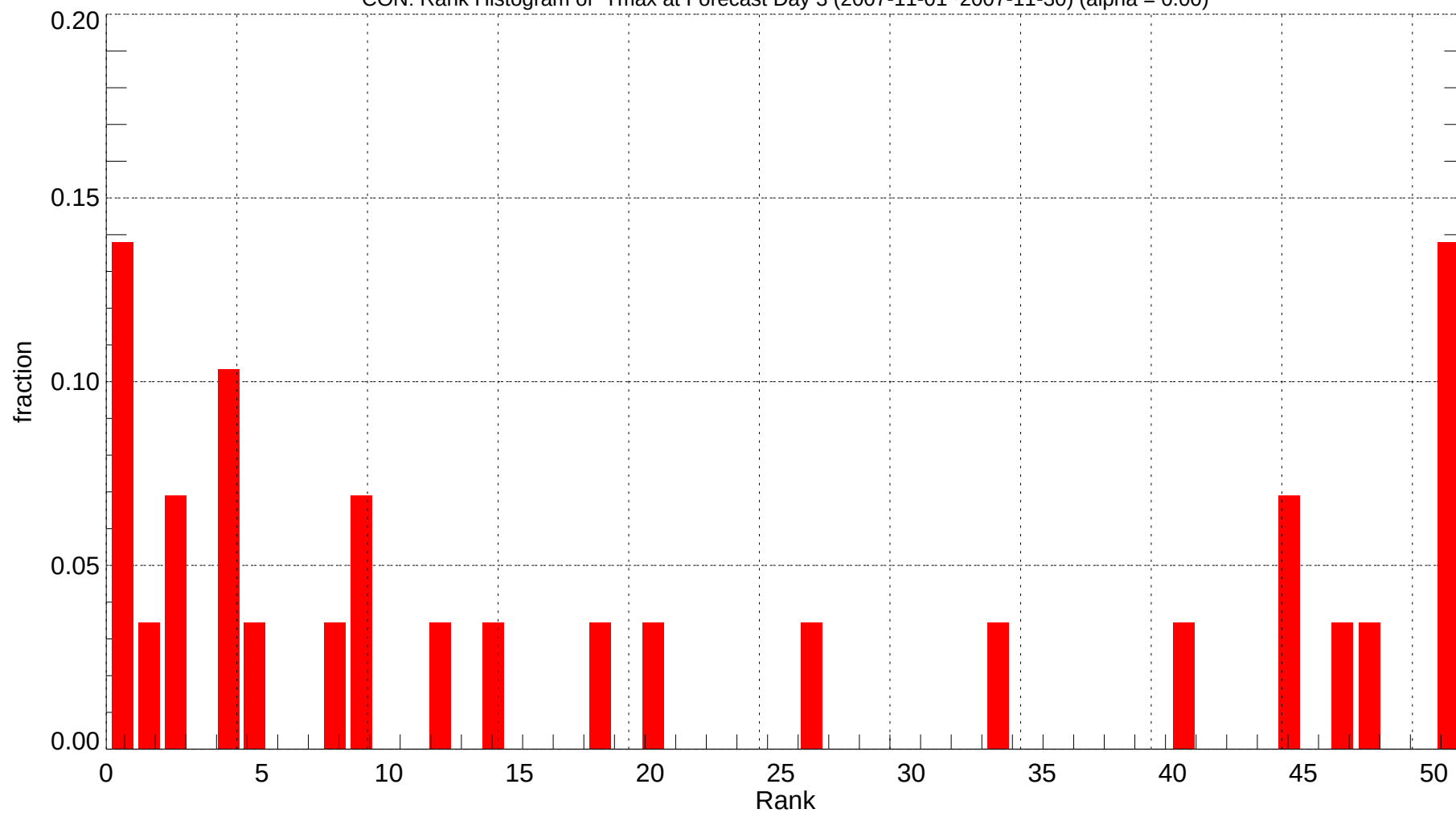
CON: Rank Histogram of Tmax at Forecast Day 3 (2007-11-01~2007-11-30) (alpha = 0.00)
