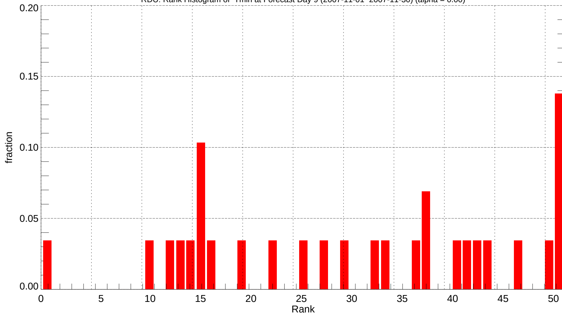
RDU: Rank Histogram of Tmin at Forecast Day 9 (2007-11-01~2007-11-30) (alpha = 0.00)
