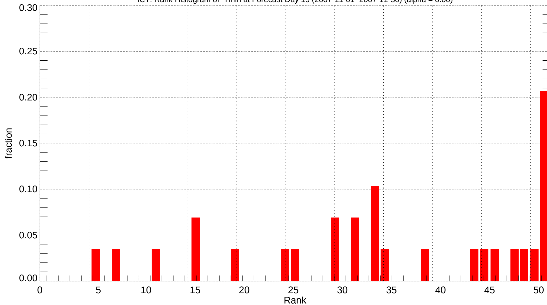
ICT: Rank Histogram of Tmin at Forecast Day 13 (2007-11-01~2007-11-30) (alpha = 0.00)
