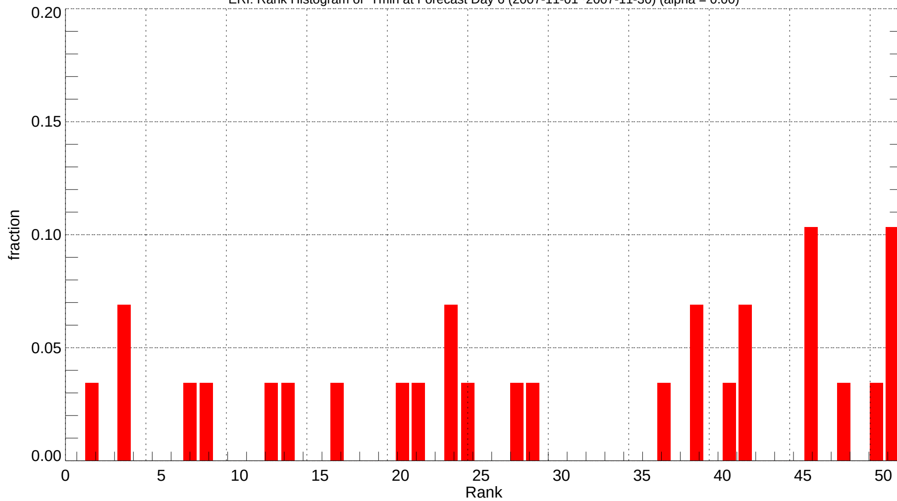
ERI: Rank Histogram of Tmin at Forecast Day 6 (2007-11-01~2007-11-30) (alpha = 0.00)
