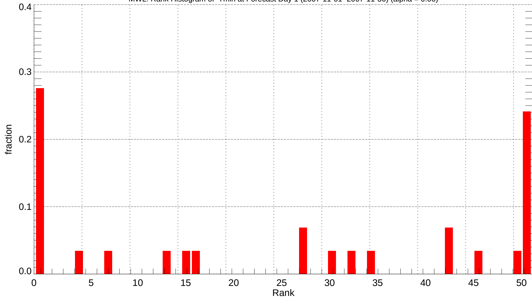
MWL: Rank Histogram of Tmin at Forecast Day 1 (2007-11-01~2007-11-30) (alpha = 0.00)
