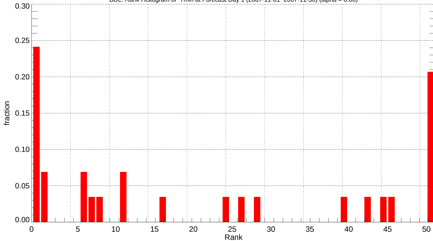
BDL: Rank Histogram of Tmin at Forecast Day 1 (2007-11-01~2007-11-30) (alpha = 0.00)
