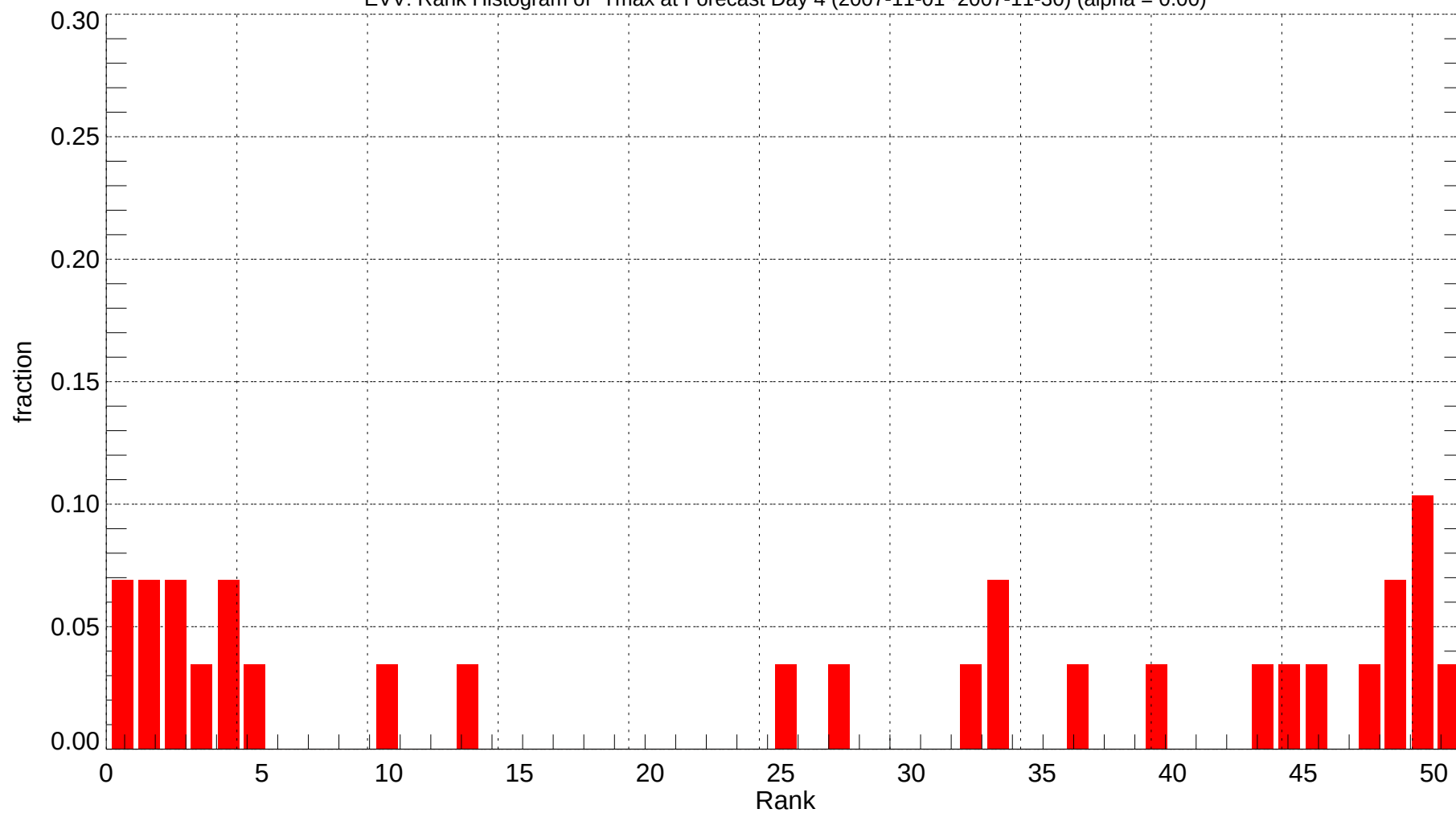
EVV: Rank Histogram of Tmax at Forecast Day 4 (2007-11-01~2007-11-30) (alpha = 0.00)
