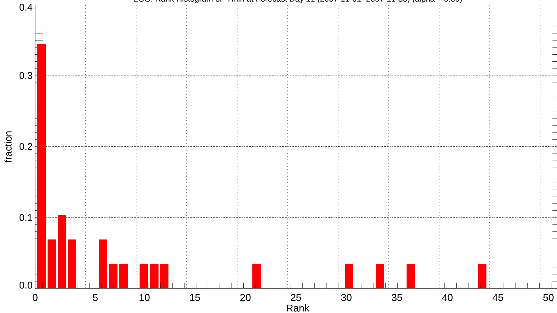
EUG: Rank Histogram of Tmin at Forecast Day 11 (2007-11-01~2007-11-30) (alpha = 0.00)
