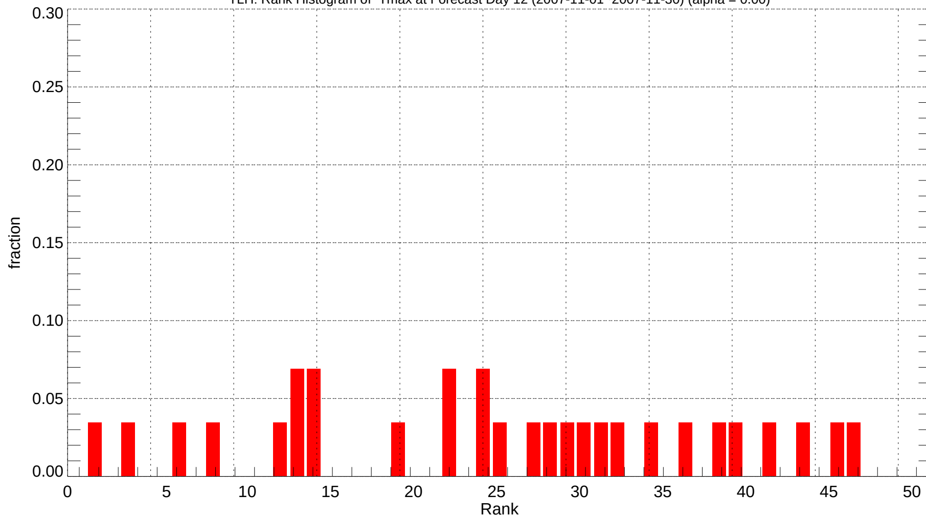
TLH: Rank Histogram of Tmax at Forecast Day 12 (2007-11-01~2007-11-30) (alpha = 0.00)
