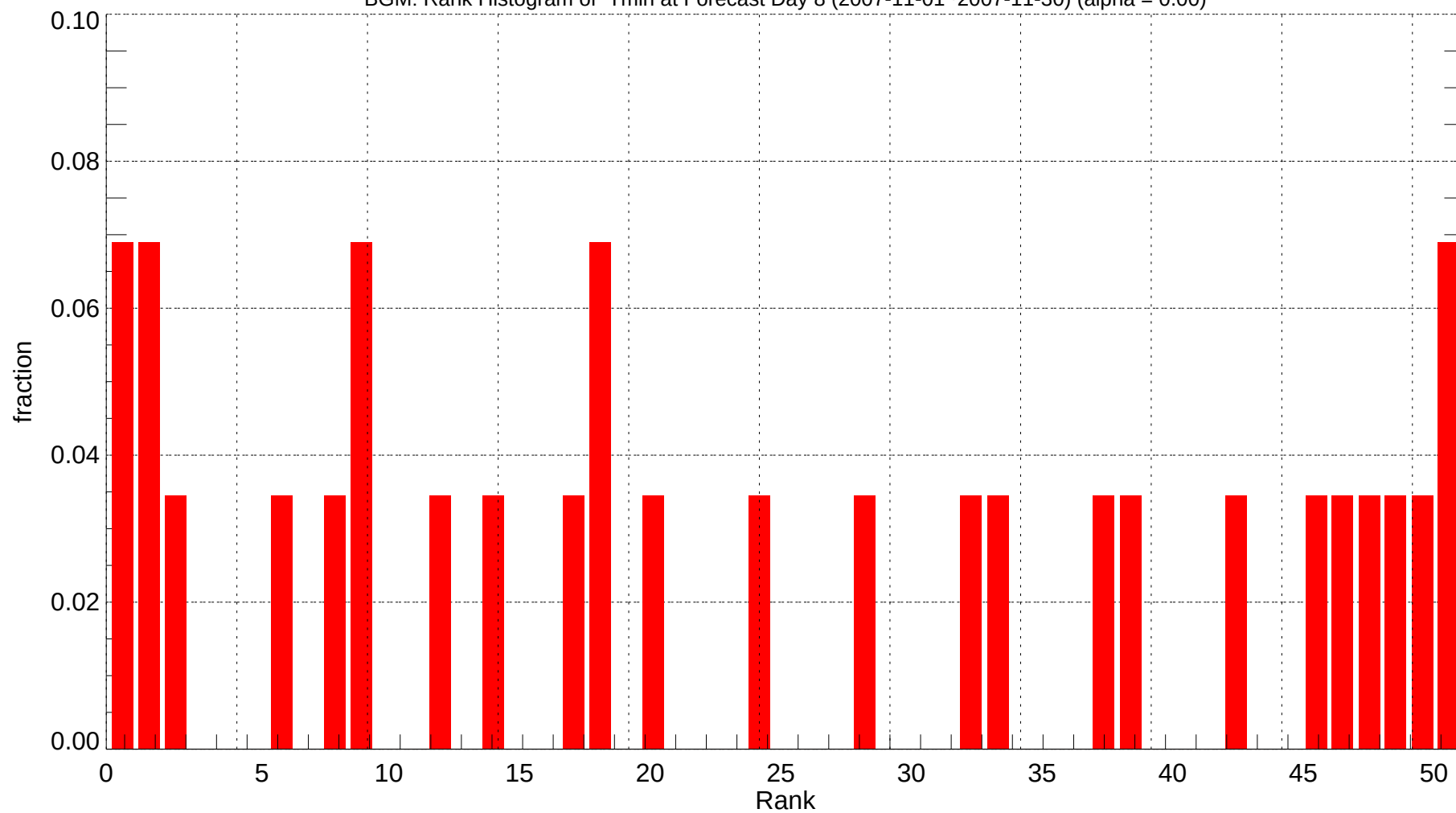
BGM: Rank Histogram of Tmin at Forecast Day 8 (2007-11-01~2007-11-30) (alpha = 0.00)
