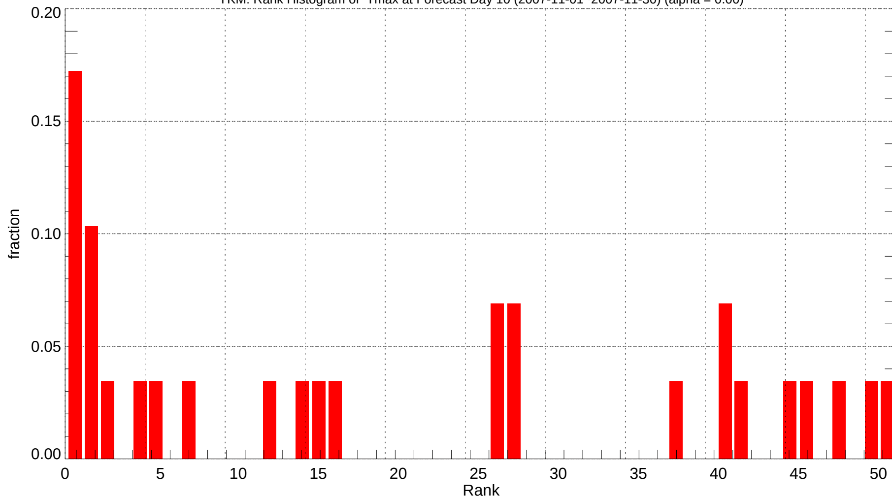
YKM: Rank Histogram of Tmax at Forecast Day 10 (2007-11-01~2007-11-30) (alpha = 0.00)
