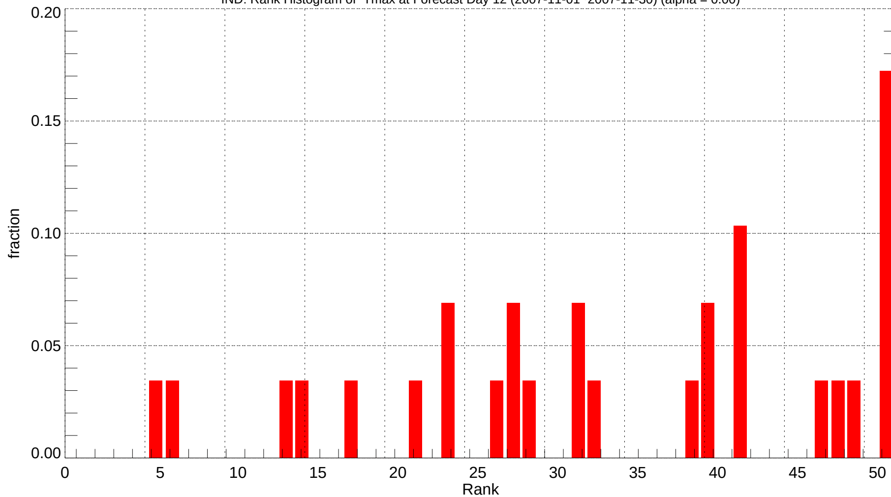
IND: Rank Histogram of Tmax at Forecast Day 12 (2007-11-01~2007-11-30) (alpha = 0.00)
