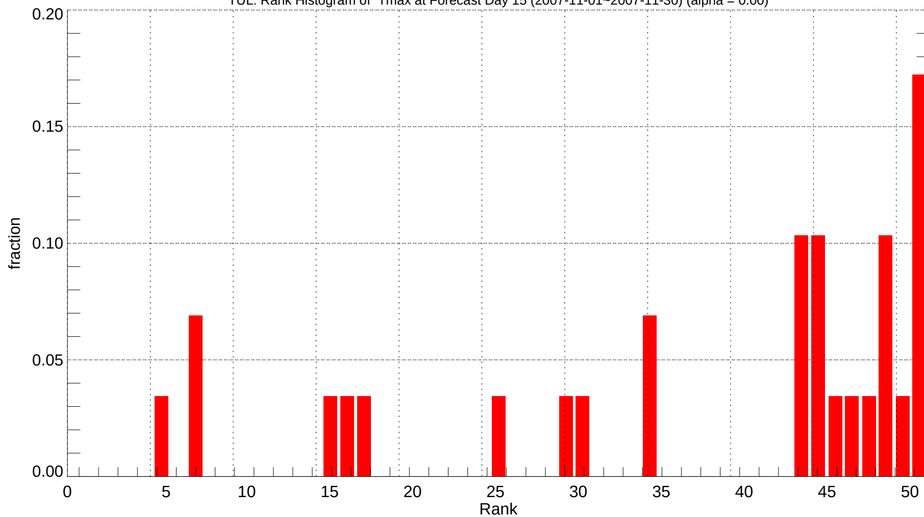
TUL: Rank Histogram of Tmax at Forecast Day 15 (2007-11-01~2007-11-30) (alpha = 0.00)
