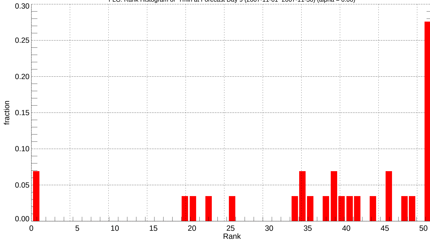
FLG: Rank Histogram of Tmin at Forecast Day 9 (2007-11-01~2007-11-30) (alpha = 0.00)
