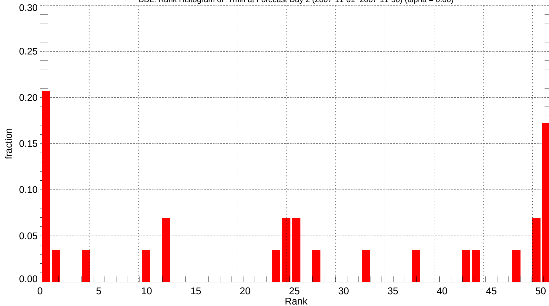
BDL: Rank Histogram of Tmin at Forecast Day 2 (2007-11-01~2007-11-30) (alpha = 0.00)
