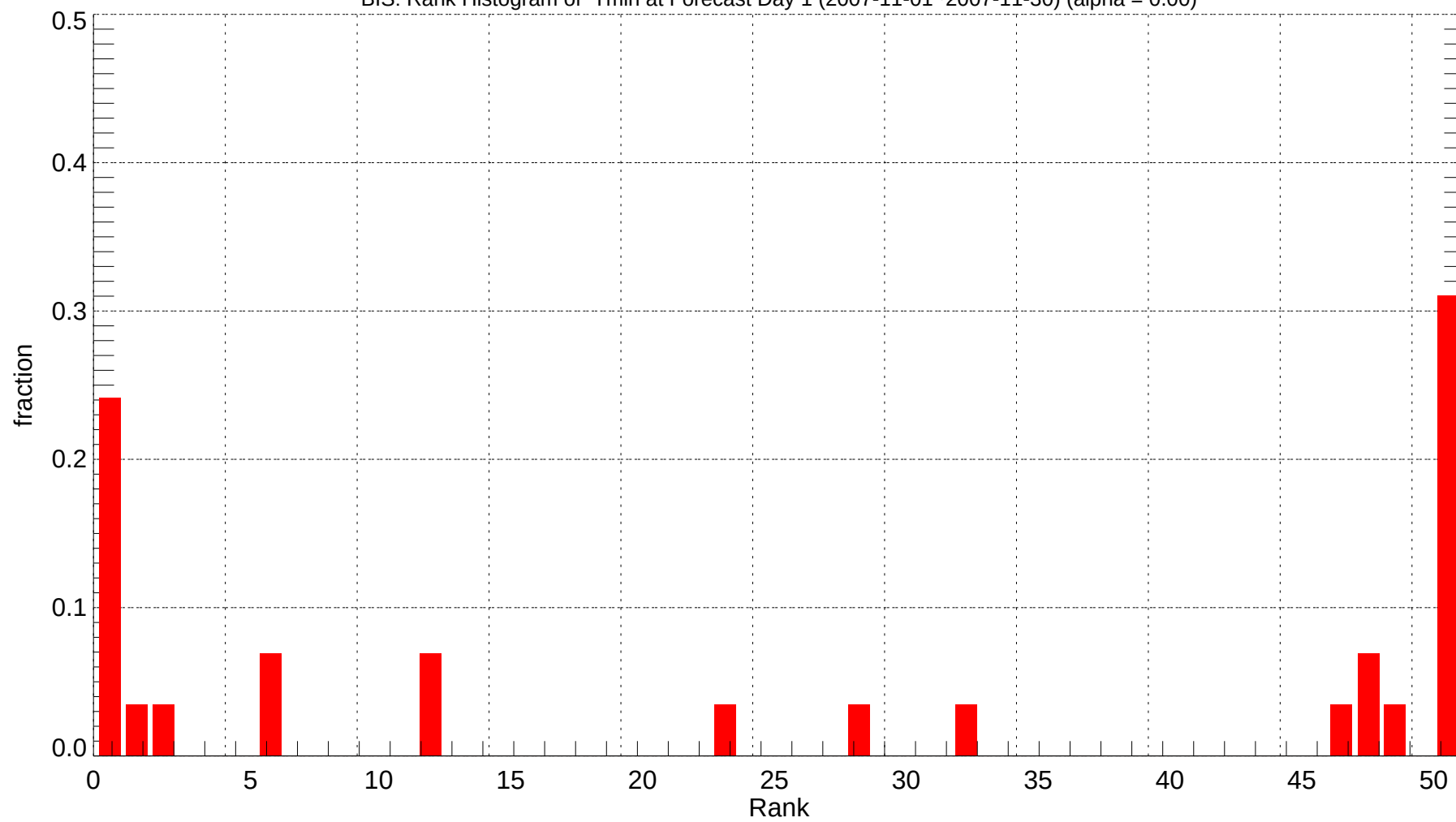
BIS: Rank Histogram of Tmin at Forecast Day 1 (2007-11-01~2007-11-30) (alpha = 0.00)
