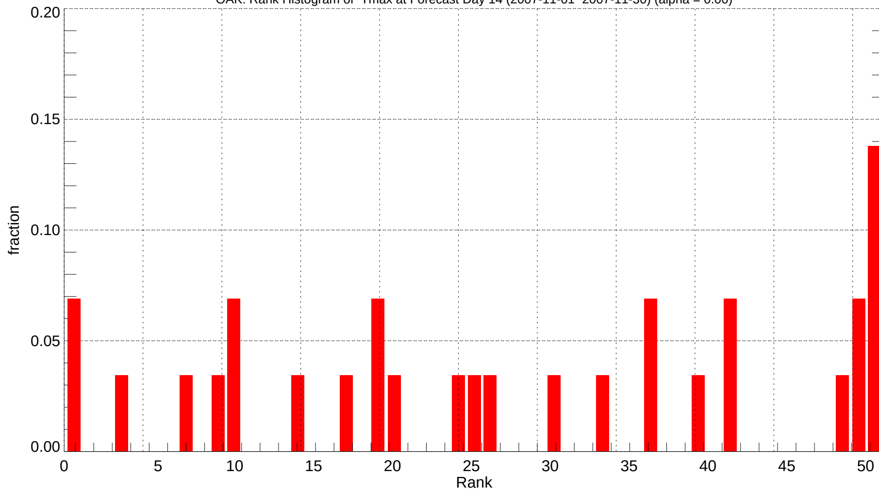
OAK: Rank Histogram of Tmax at Forecast Day 14 (2007-11-01~2007-11-30) (alpha = 0.00)
