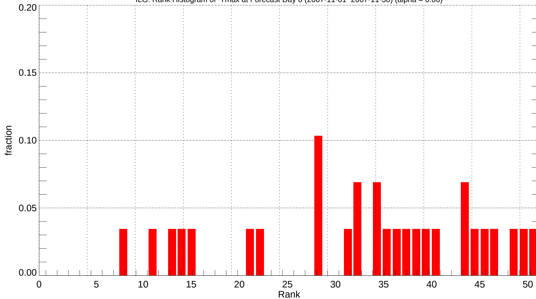
ILG: Rank Histogram of Tmax at Forecast Day 6 (2007-11-01~2007-11-30) (alpha = 0.00)
