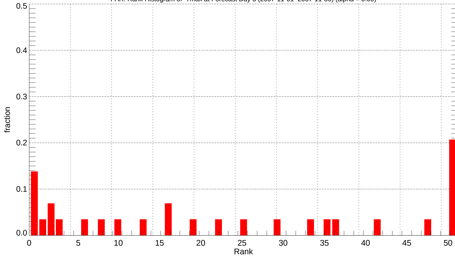
FAR: Rank Histogram of Tmax at Forecast Day 3 (2007-11-01~2007-11-30) (alpha = 0.00)
