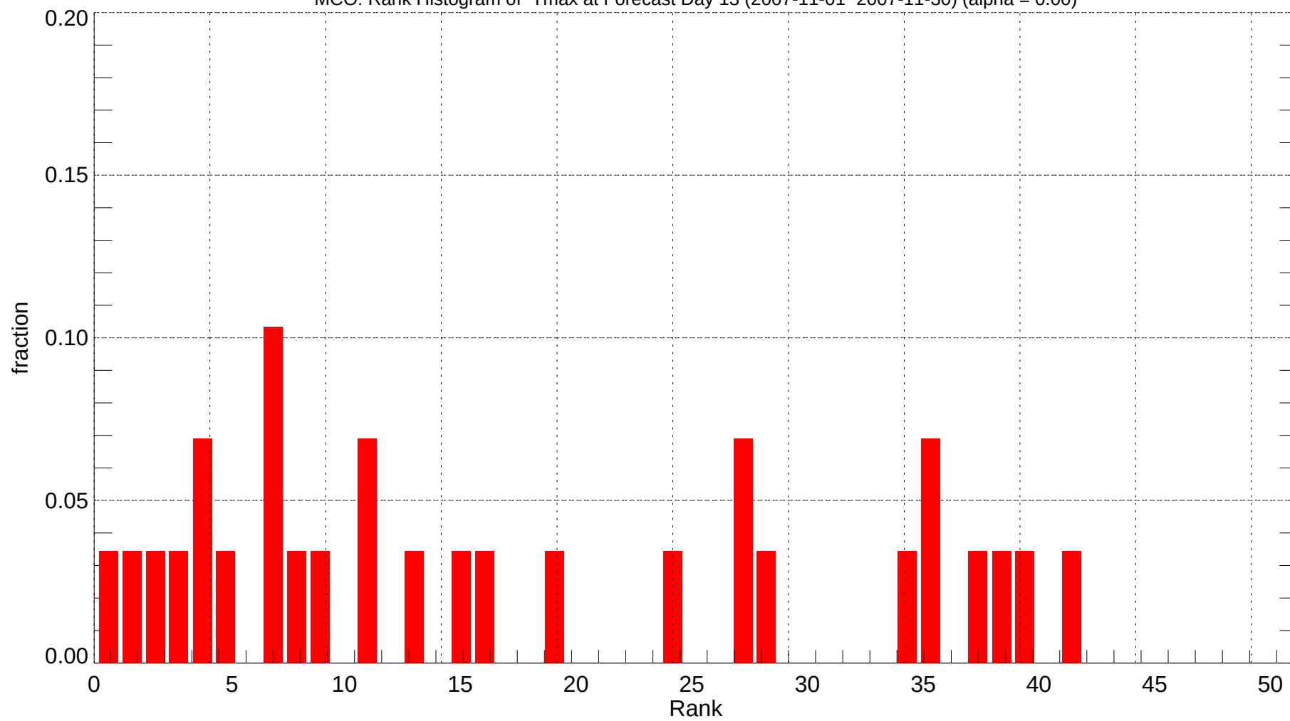
MCO: Rank Histogram of Tmax at Forecast Day 13 (2007-11-01~2007-11-30) (alpha = 0.00)
