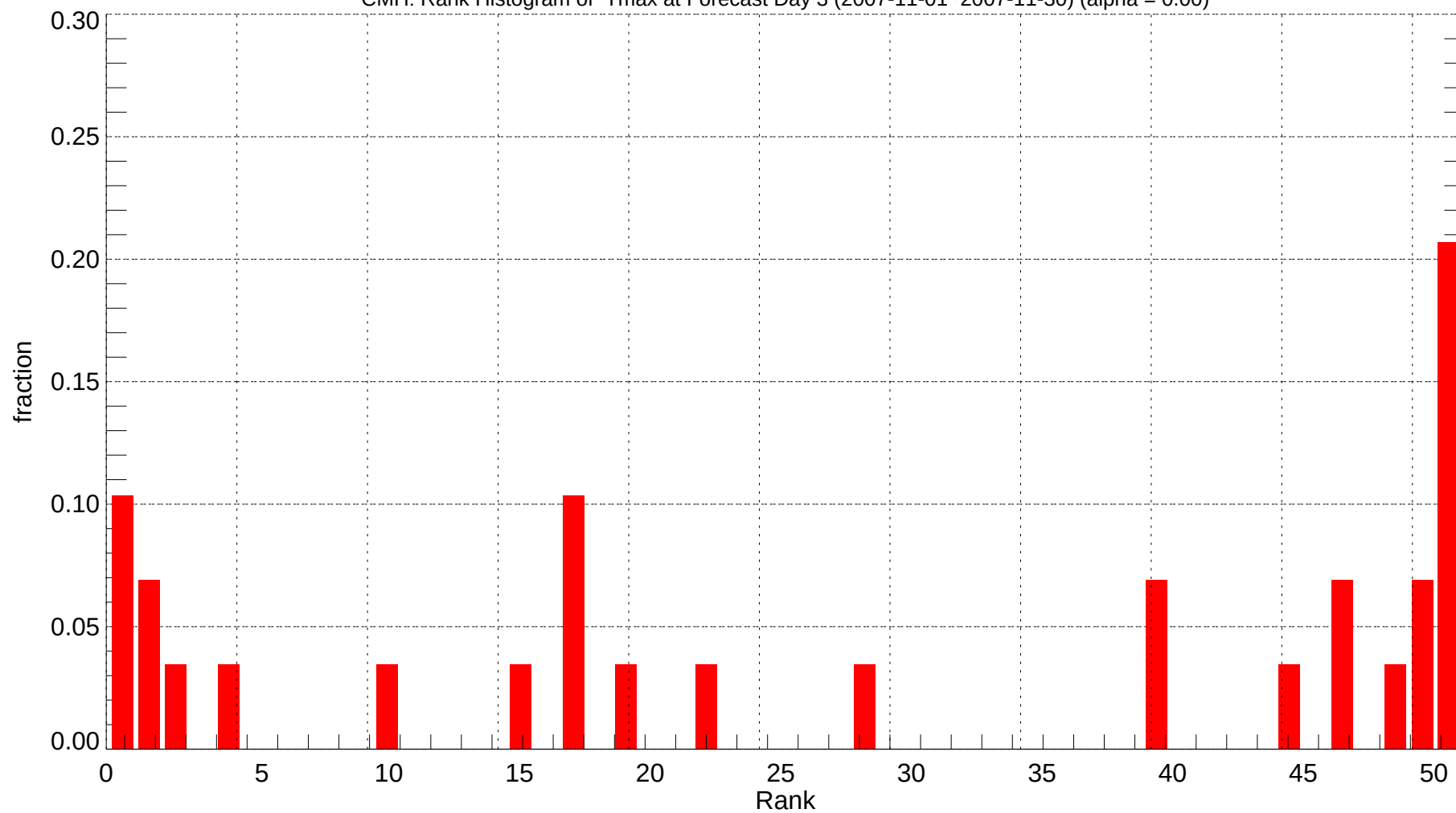
CMH: Rank Histogram of Tmax at Forecast Day 3 (2007-11-01~2007-11-30) (alpha = 0.00)
