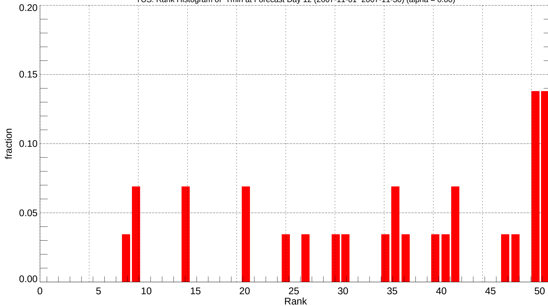
TUS: Rank Histogram of Tmin at Forecast Day 12 (2007-11-01~2007-11-30) (alpha = 0.00)
