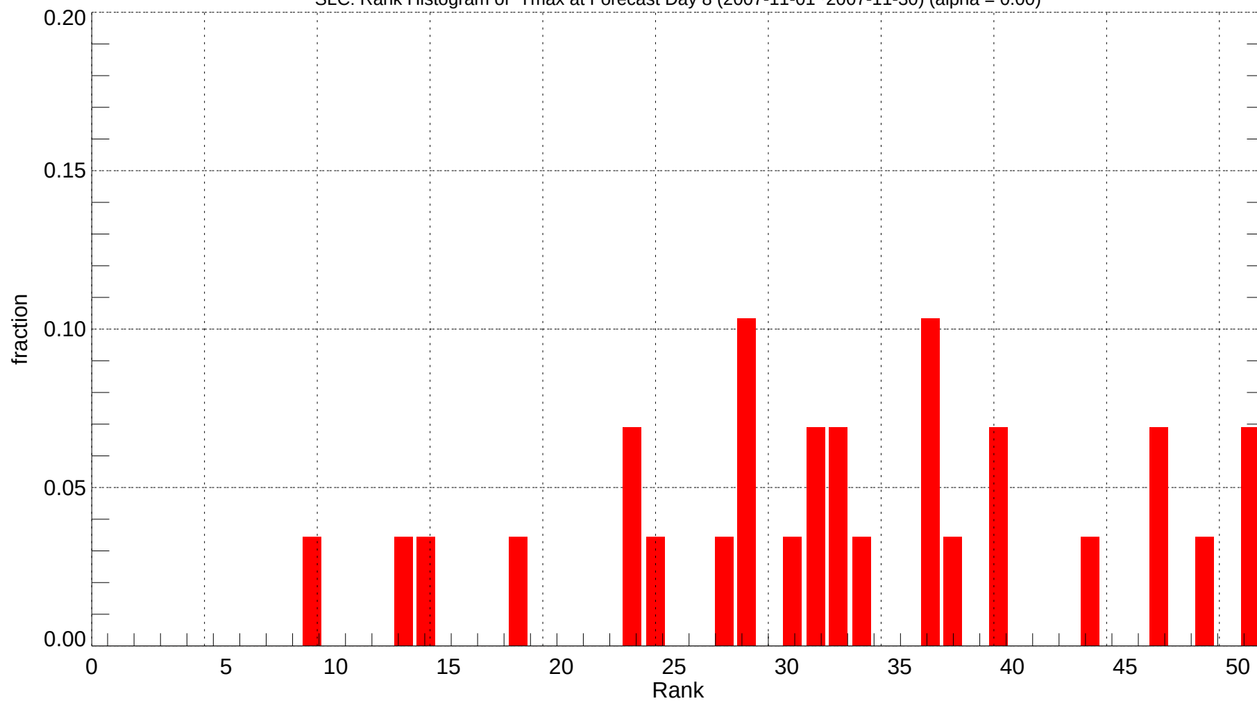
SLC: Rank Histogram of Tmax at Forecast Day 8 (2007-11-01~2007-11-30) (alpha = 0.00)
