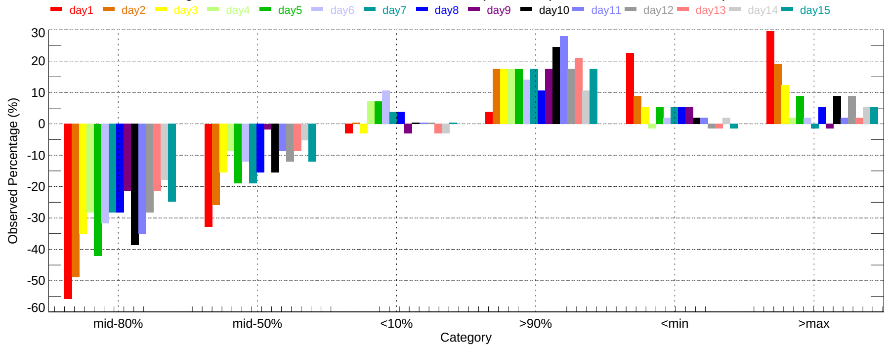
Observed Percentage Deviation of Ensembles - BIS: Min Temperature (2007-11-01~2007-11-30)
