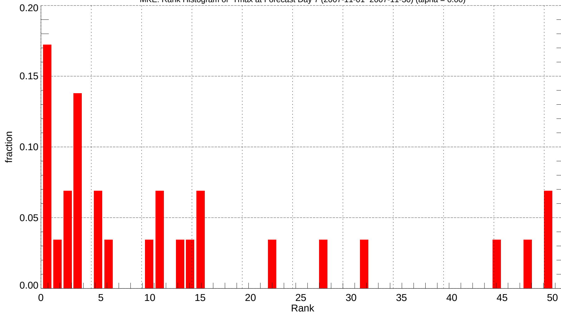
MKE: Rank Histogram of Tmax at Forecast Day 7 (2007-11-01~2007-11-30) (alpha = 0.00)
