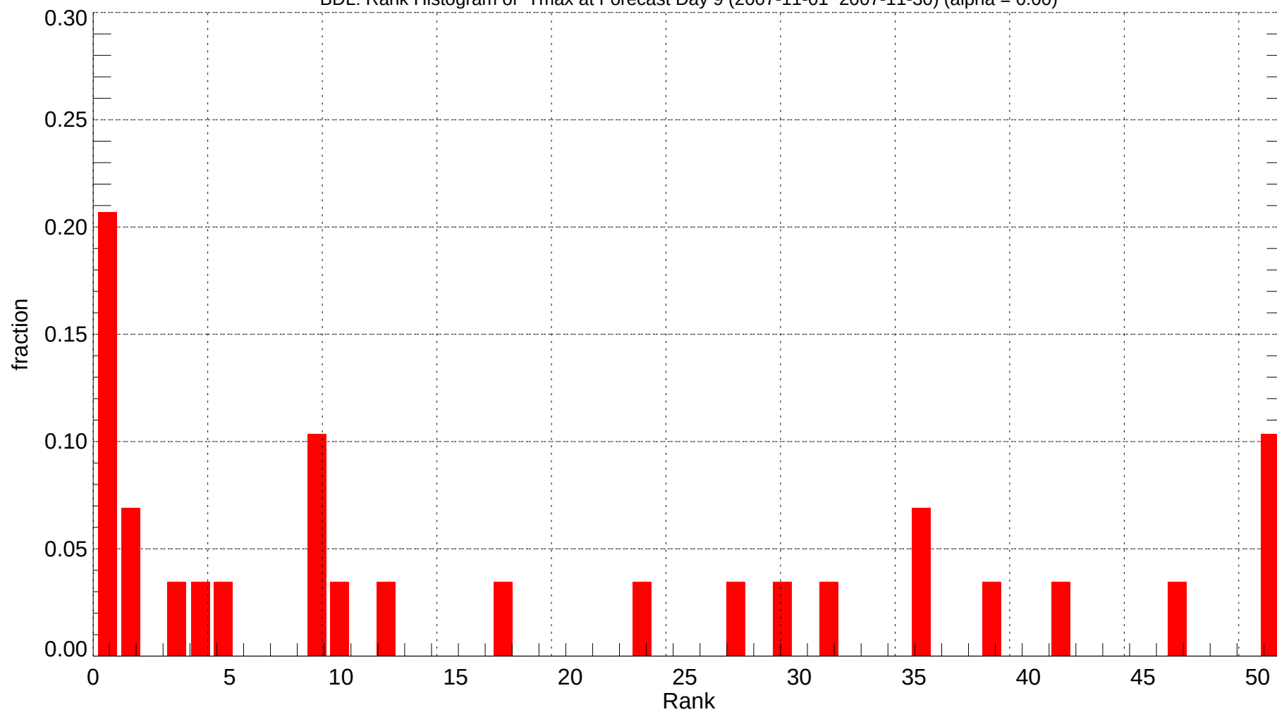
BDL: Rank Histogram of Tmax at Forecast Day 9 (2007-11-01~2007-11-30) (alpha = 0.00)
