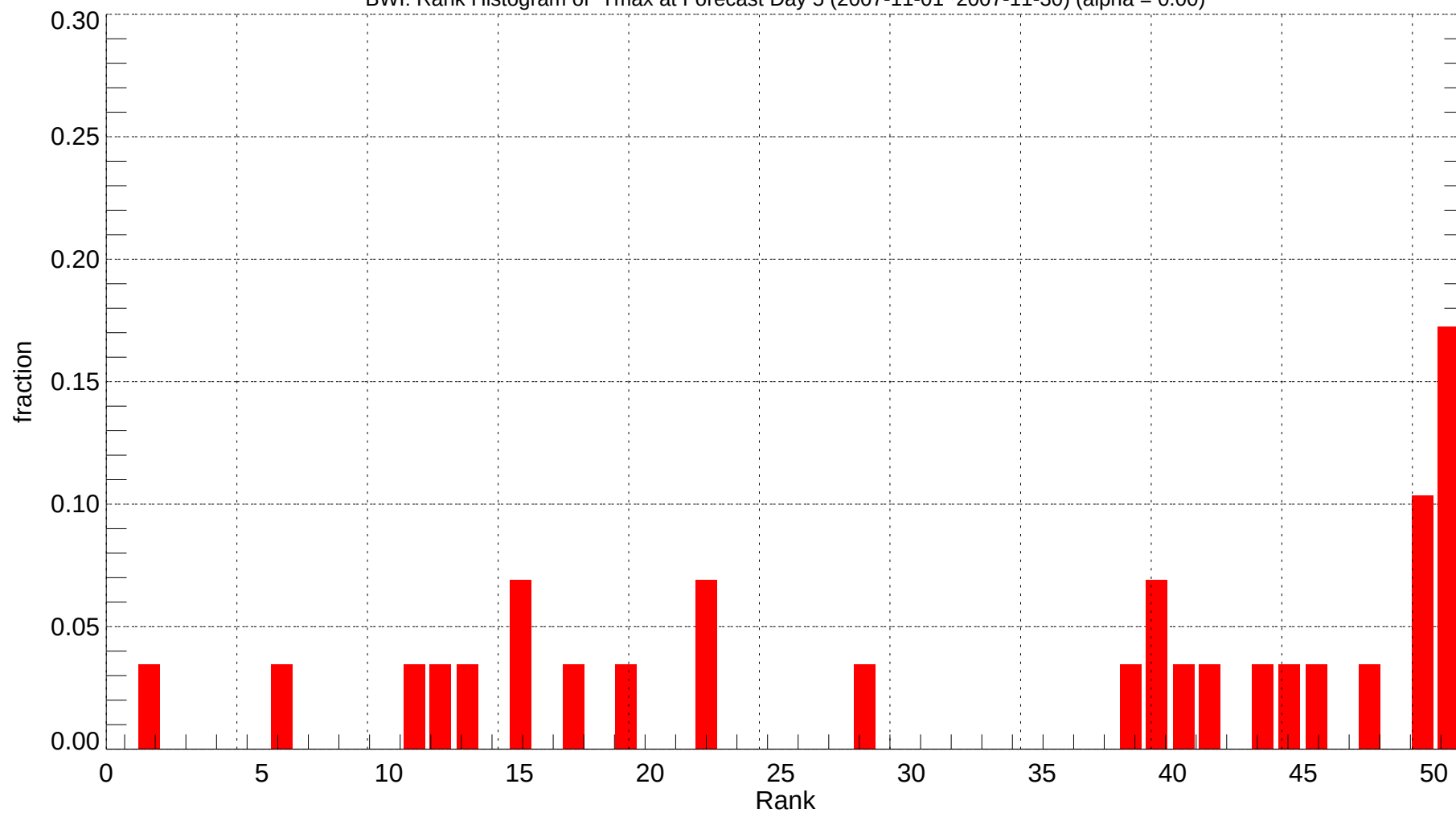
BWI: Rank Histogram of Tmax at Forecast Day 5 (2007-11-01~2007-11-30) (alpha = 0.00)
