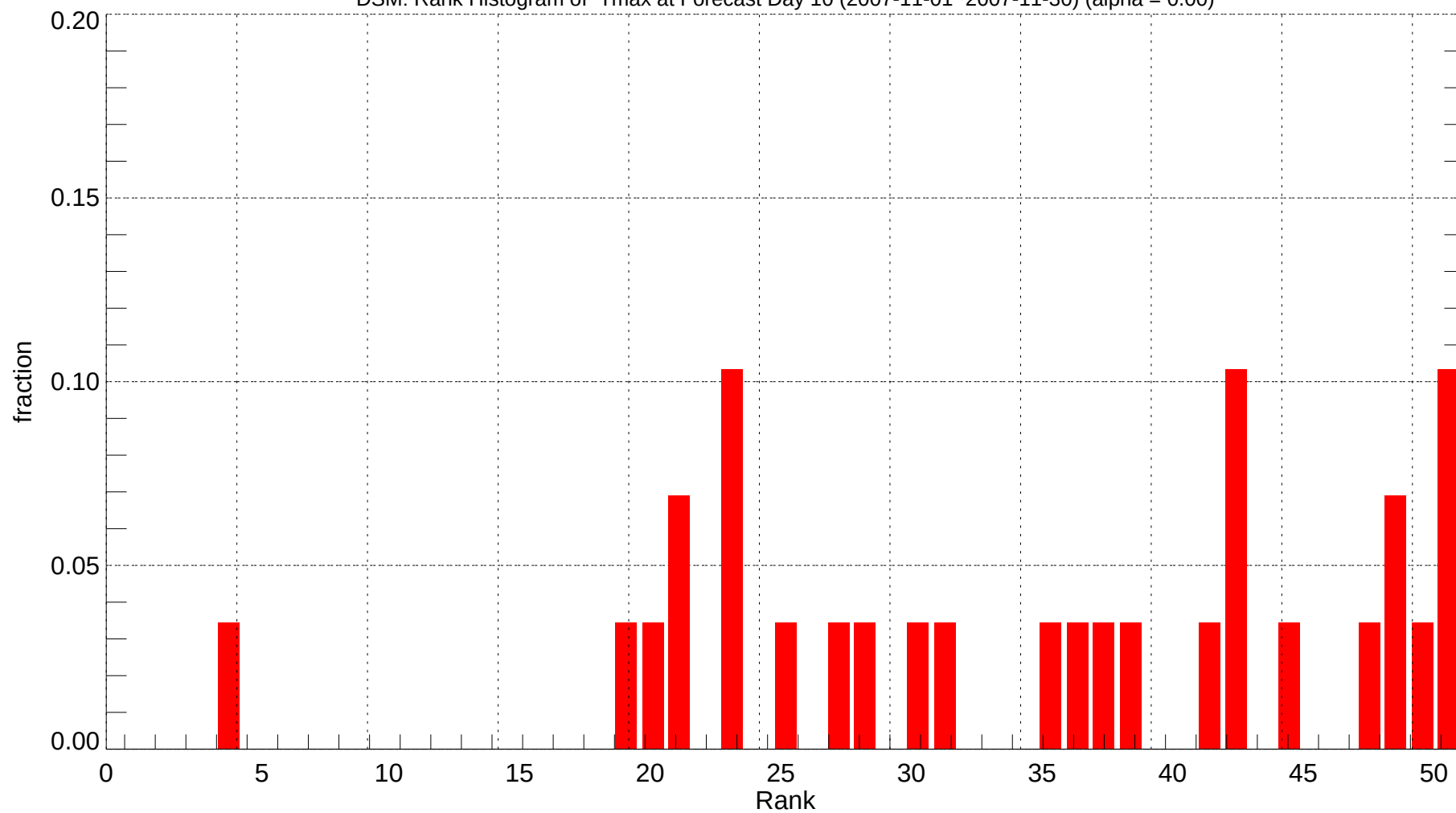
DSM: Rank Histogram of Tmax at Forecast Day 10 (2007-11-01~2007-11-30) (alpha = 0.00)
