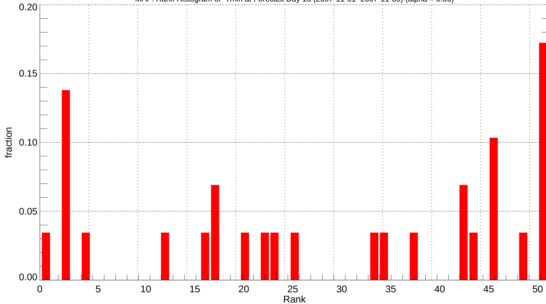
MAF: Rank Histogram of Tmin at Forecast Day 15 (2007-11-01~2007-11-30) (alpha = 0.00)
