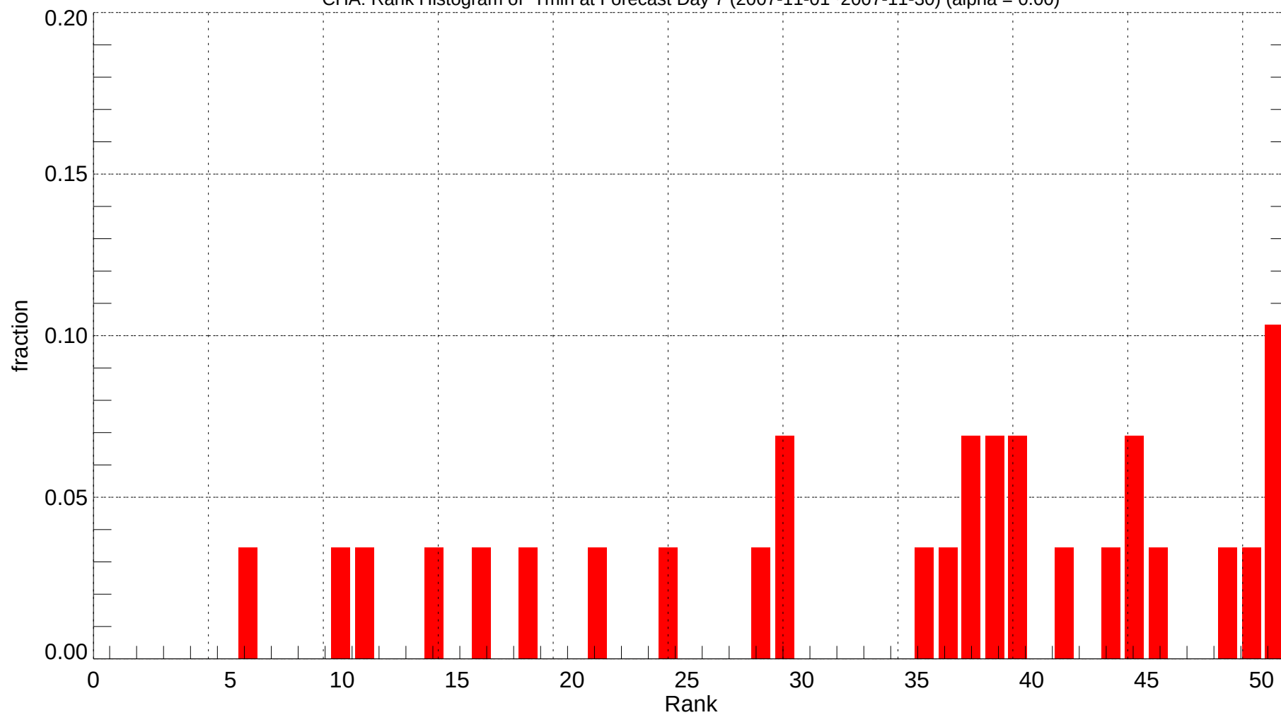
CHA: Rank Histogram of Tmin at Forecast Day 7 (2007-11-01~2007-11-30) (alpha = 0.00)
