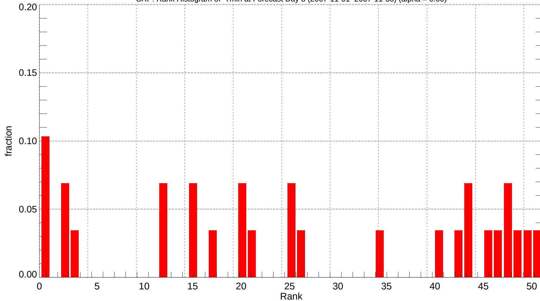
CRP: Rank Histogram of Tmin at Forecast Day 8 (2007-11-01~2007-11-30) (alpha = 0.00)
