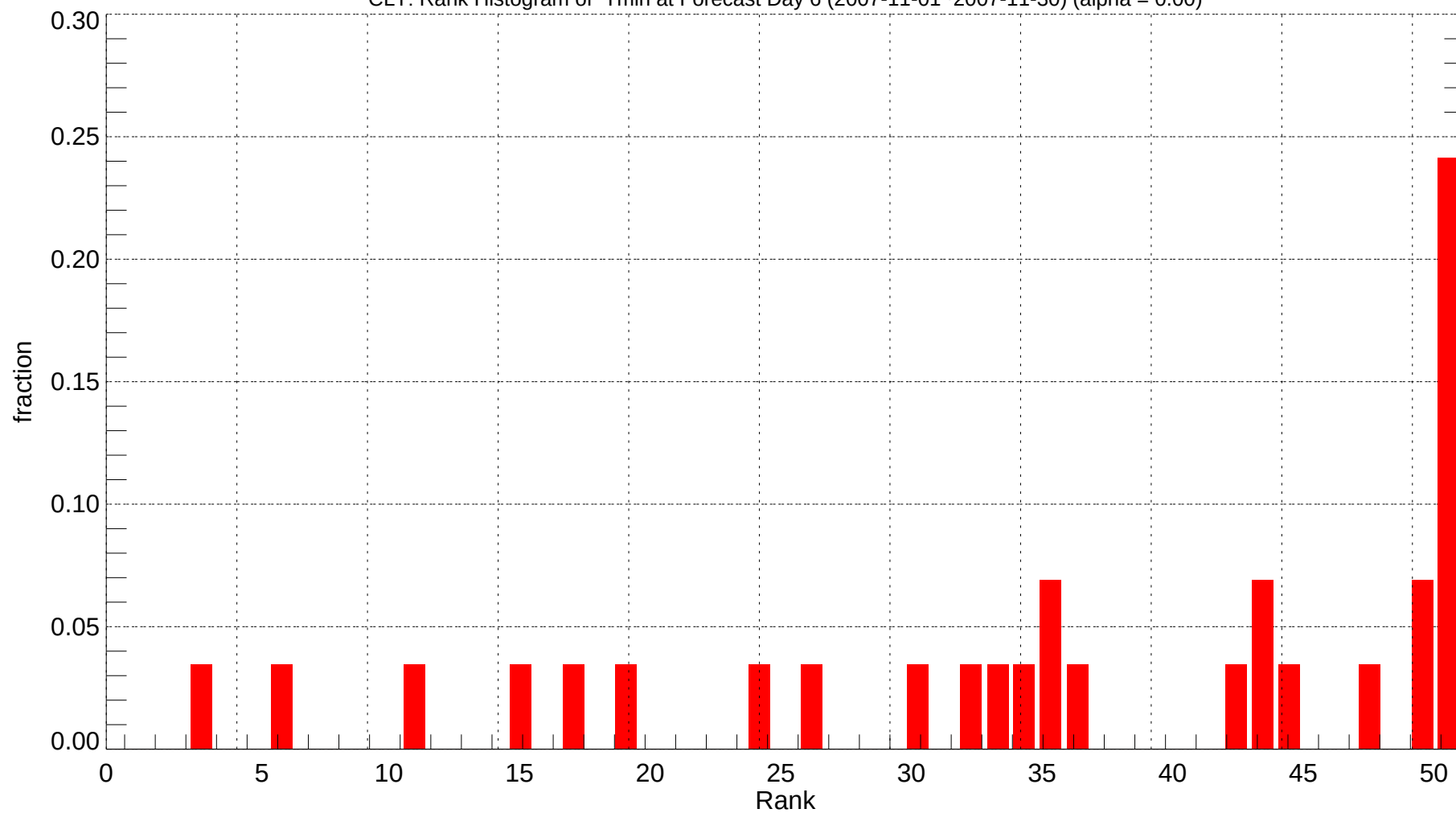
CLT: Rank Histogram of Tmin at Forecast Day 6 (2007-11-01~2007-11-30) (alpha = 0.00)
