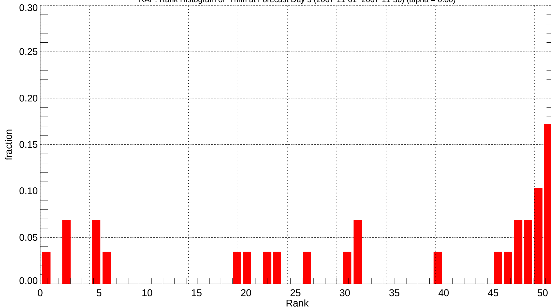
RAP: Rank Histogram of Tmin at Forecast Day 3 (2007-11-01~2007-11-30) (alpha = 0.00)
