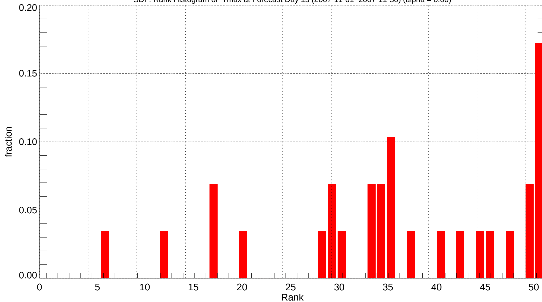
SDF: Rank Histogram of Tmax at Forecast Day 13 (2007-11-01~2007-11-30) (alpha = 0.00)
