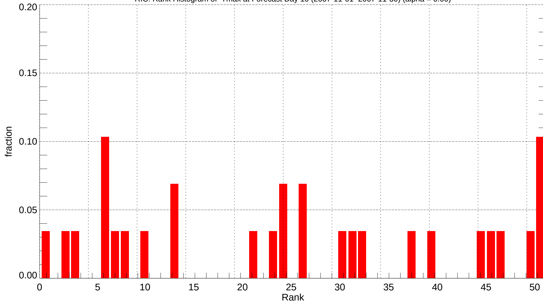
RIC: Rank Histogram of Tmax at Forecast Day 10 (2007-11-01~2007-11-30) (alpha = 0.00)
