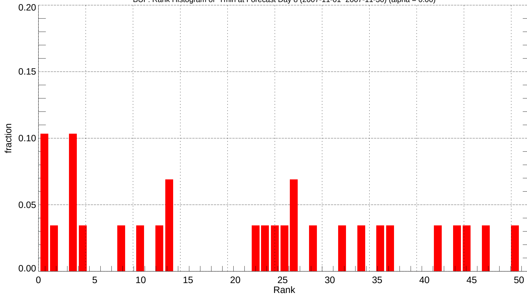
BUF: Rank Histogram of Tmin at Forecast Day 8 (2007-11-01~2007-11-30) (alpha = 0.00)
