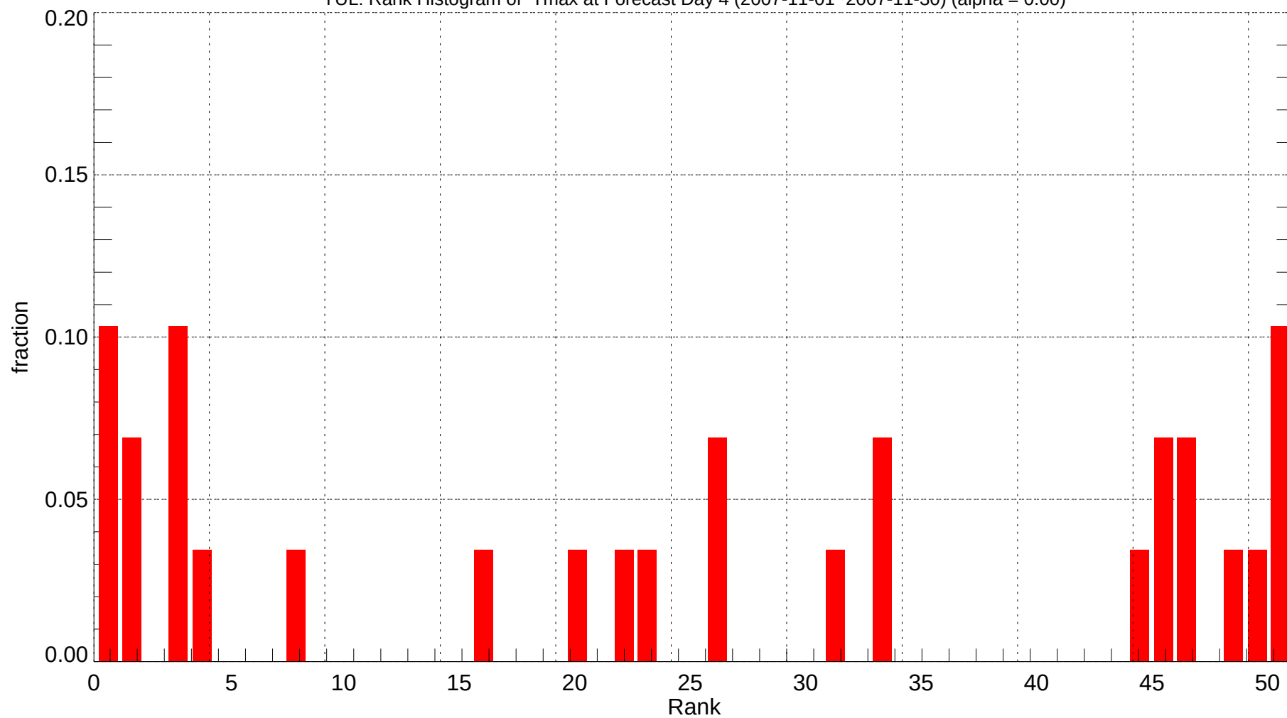
YUL: Rank Histogram of Tmax at Forecast Day 4 (2007-11-01~2007-11-30) (alpha = 0.00)
