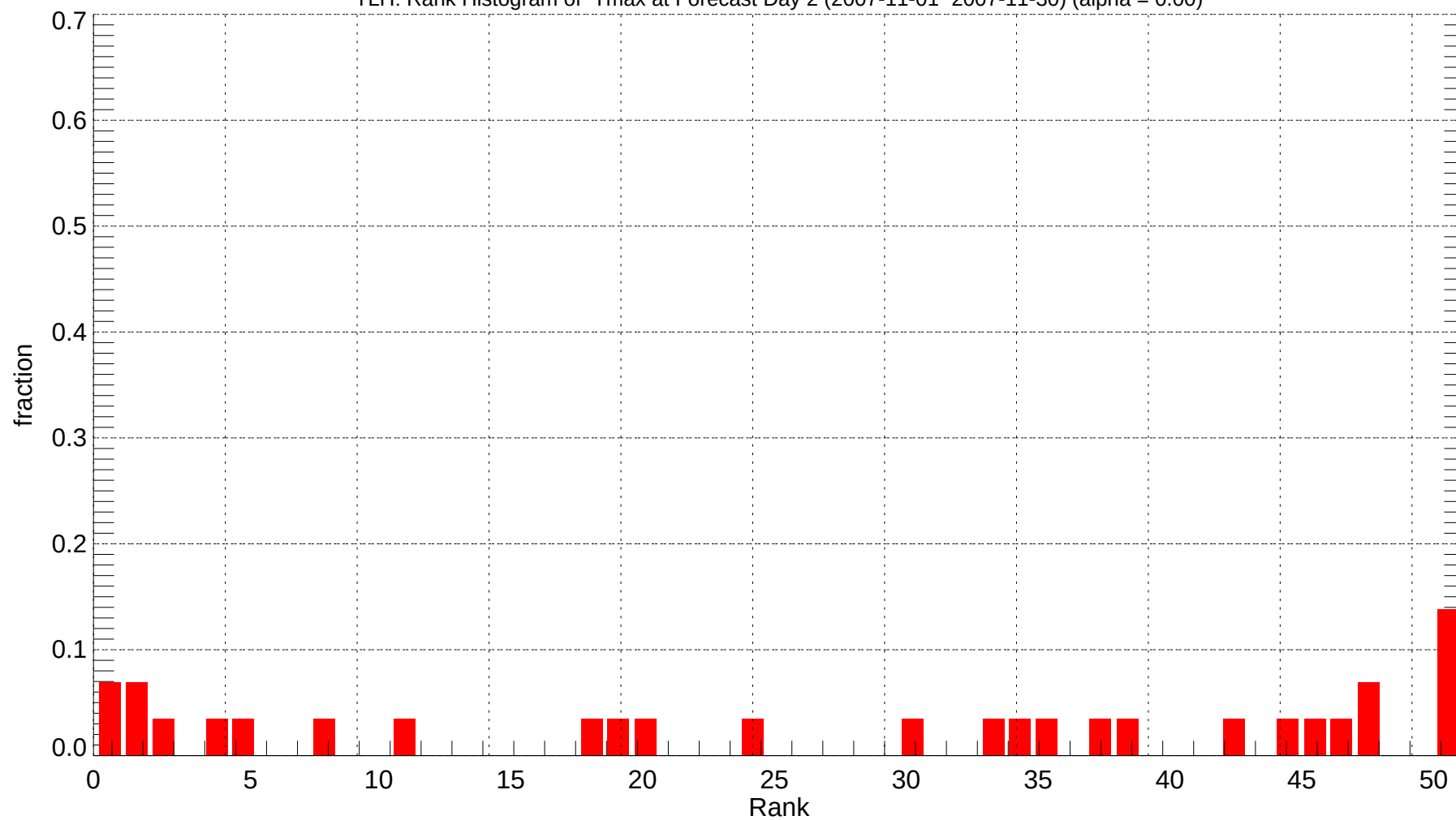
TLH: Rank Histogram of Tmax at Forecast Day 2 (2007-11-01~2007-11-30) (alpha = 0.00)
