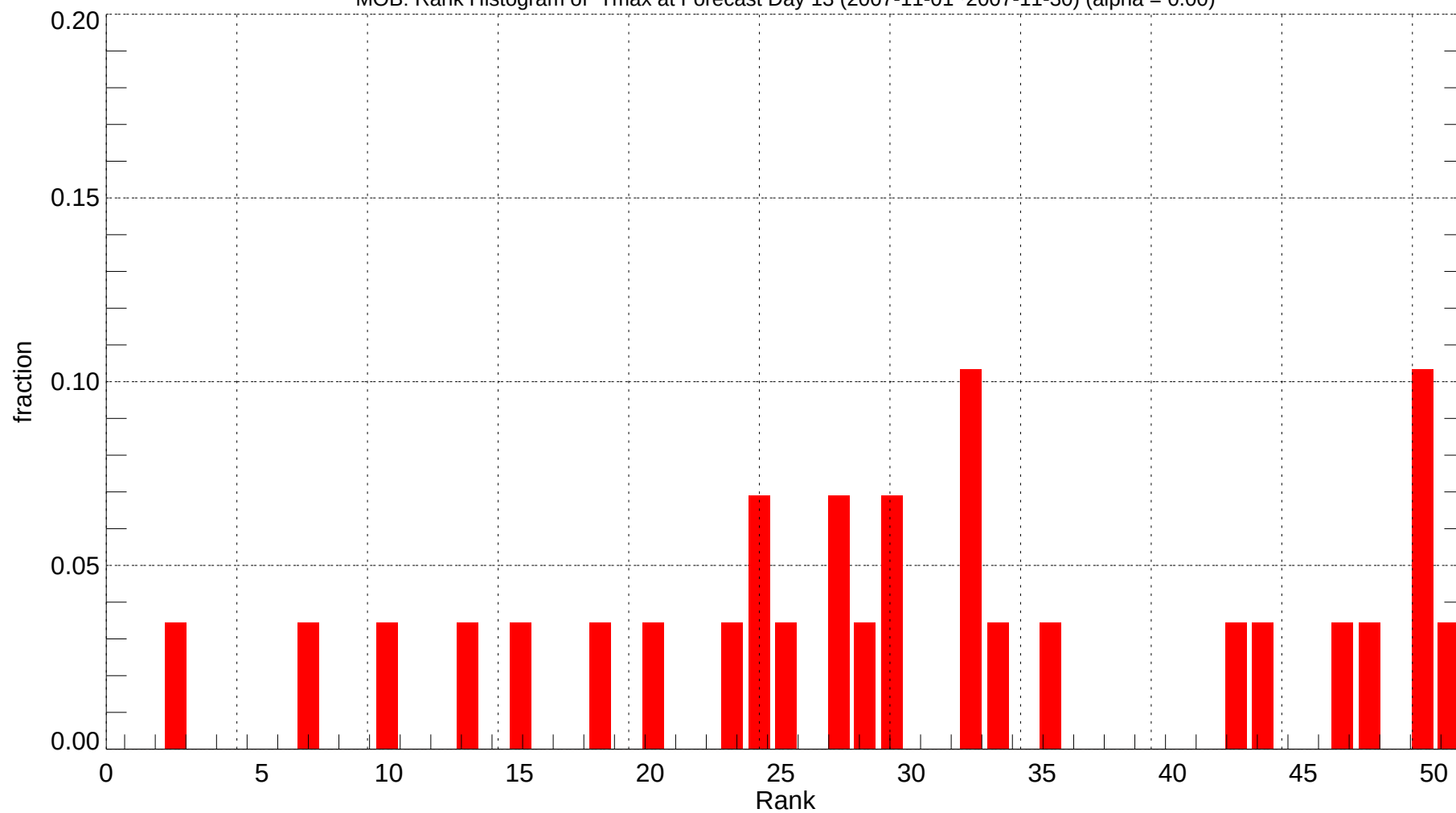
MOB: Rank Histogram of Tmax at Forecast Day 13 (2007-11-01~2007-11-30) (alpha = 0.00)
