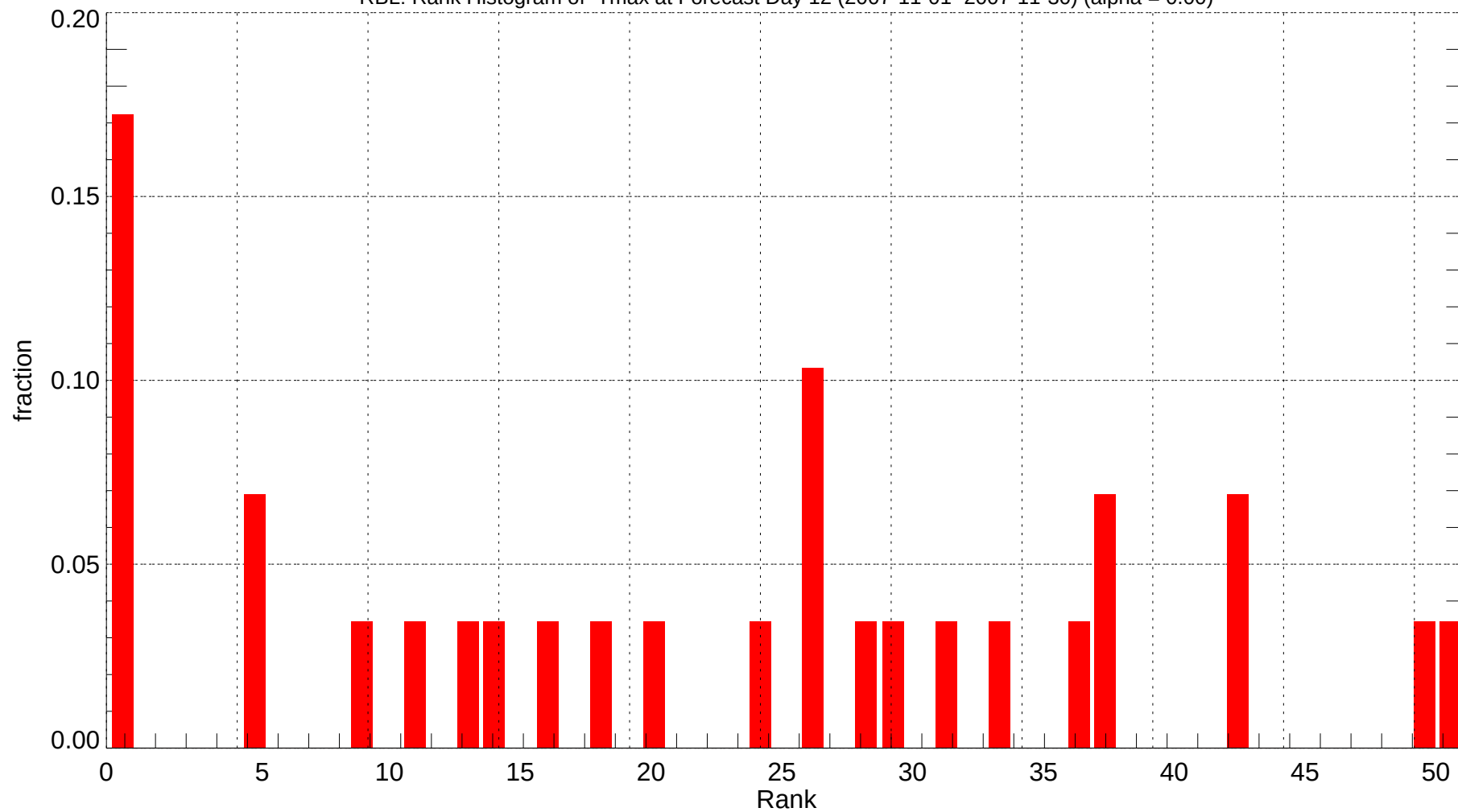
RBL: Rank Histogram of Tmax at Forecast Day 12 (2007-11-01~2007-11-30) (alpha = 0.00)
