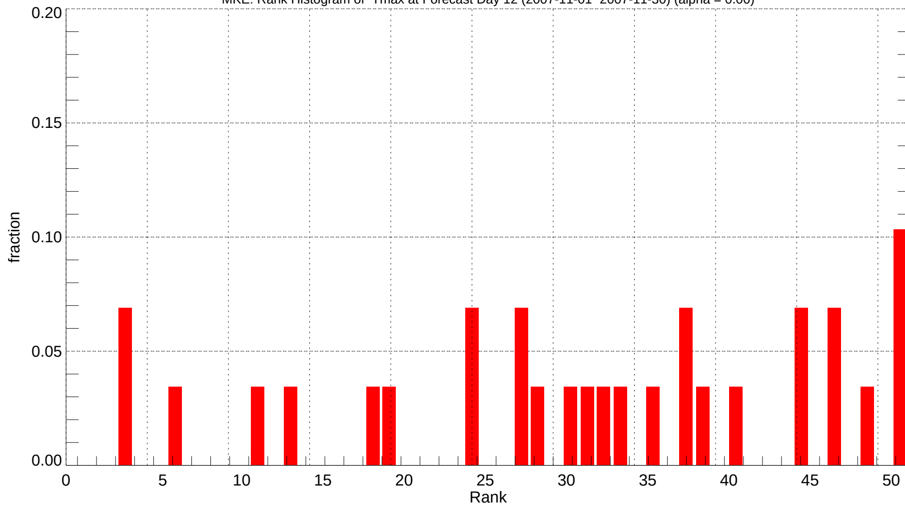
MKE: Rank Histogram of Tmax at Forecast Day 12 (2007-11-01~2007-11-30) (alpha = 0.00)
