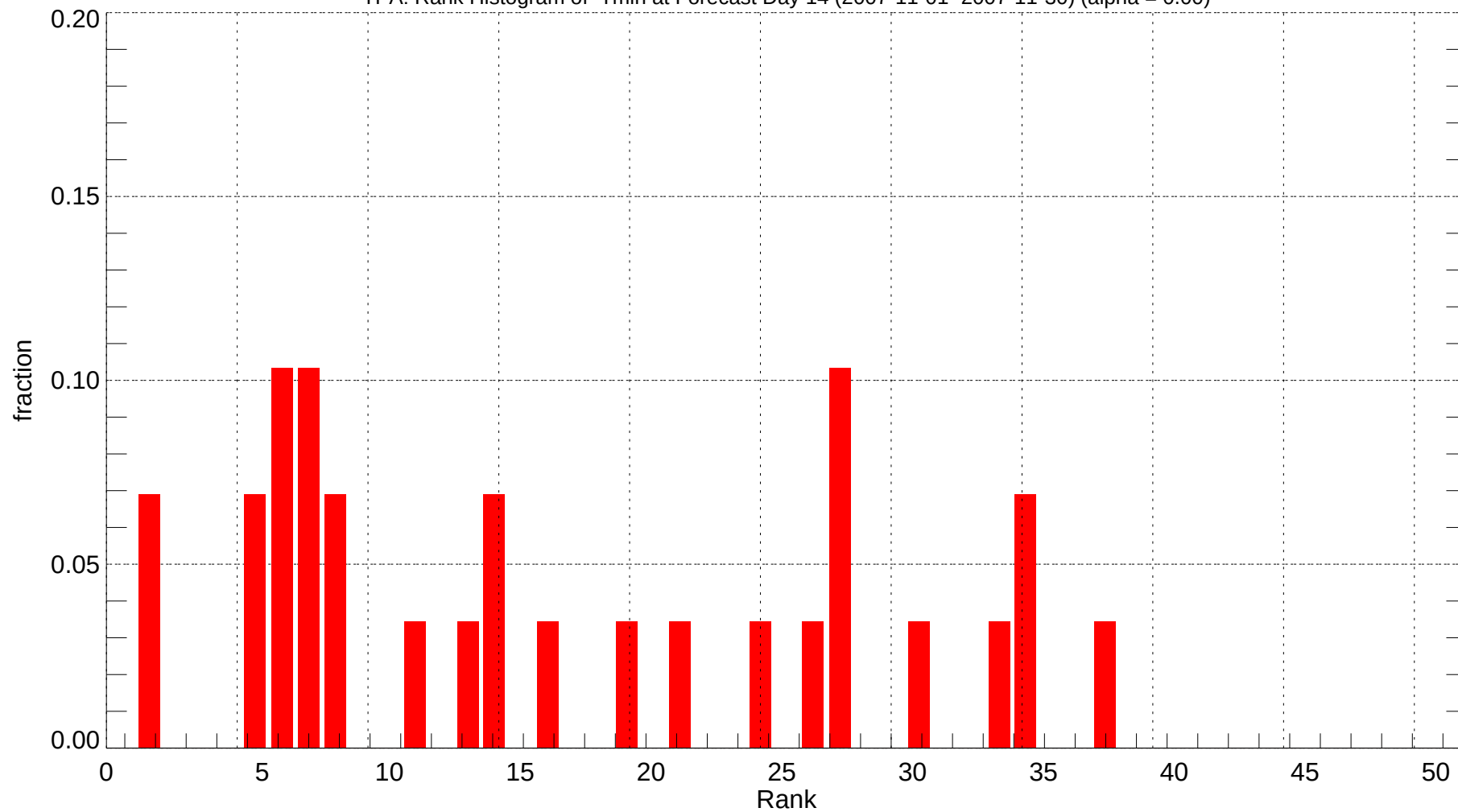
TPA: Rank Histogram of Tmin at Forecast Day 14 (2007-11-01~2007-11-30) (alpha = 0.00)
