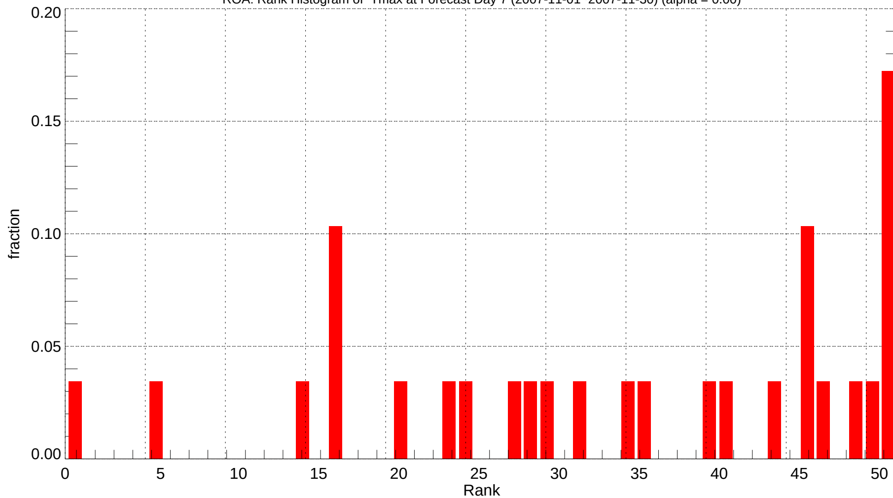
ROA: Rank Histogram of Tmax at Forecast Day 7 (2007-11-01~2007-11-30) (alpha = 0.00)
