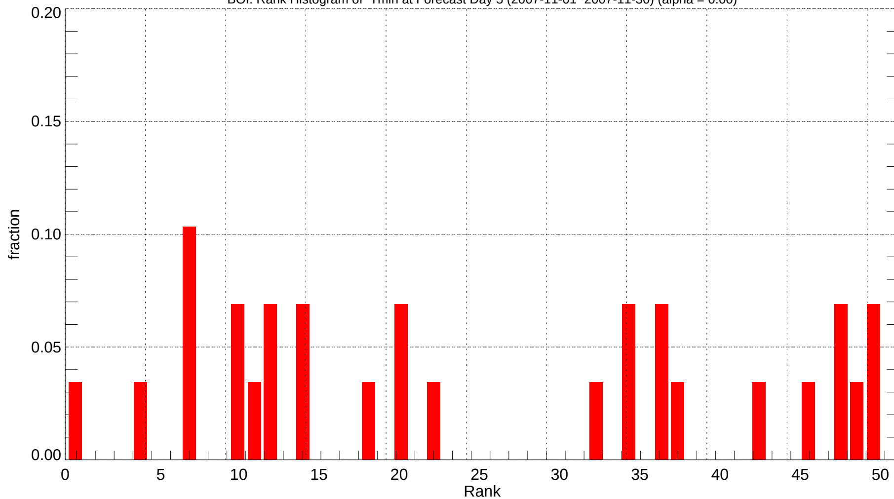
BOI: Rank Histogram of Tmin at Forecast Day 5 (2007-11-01~2007-11-30) (alpha = 0.00)
