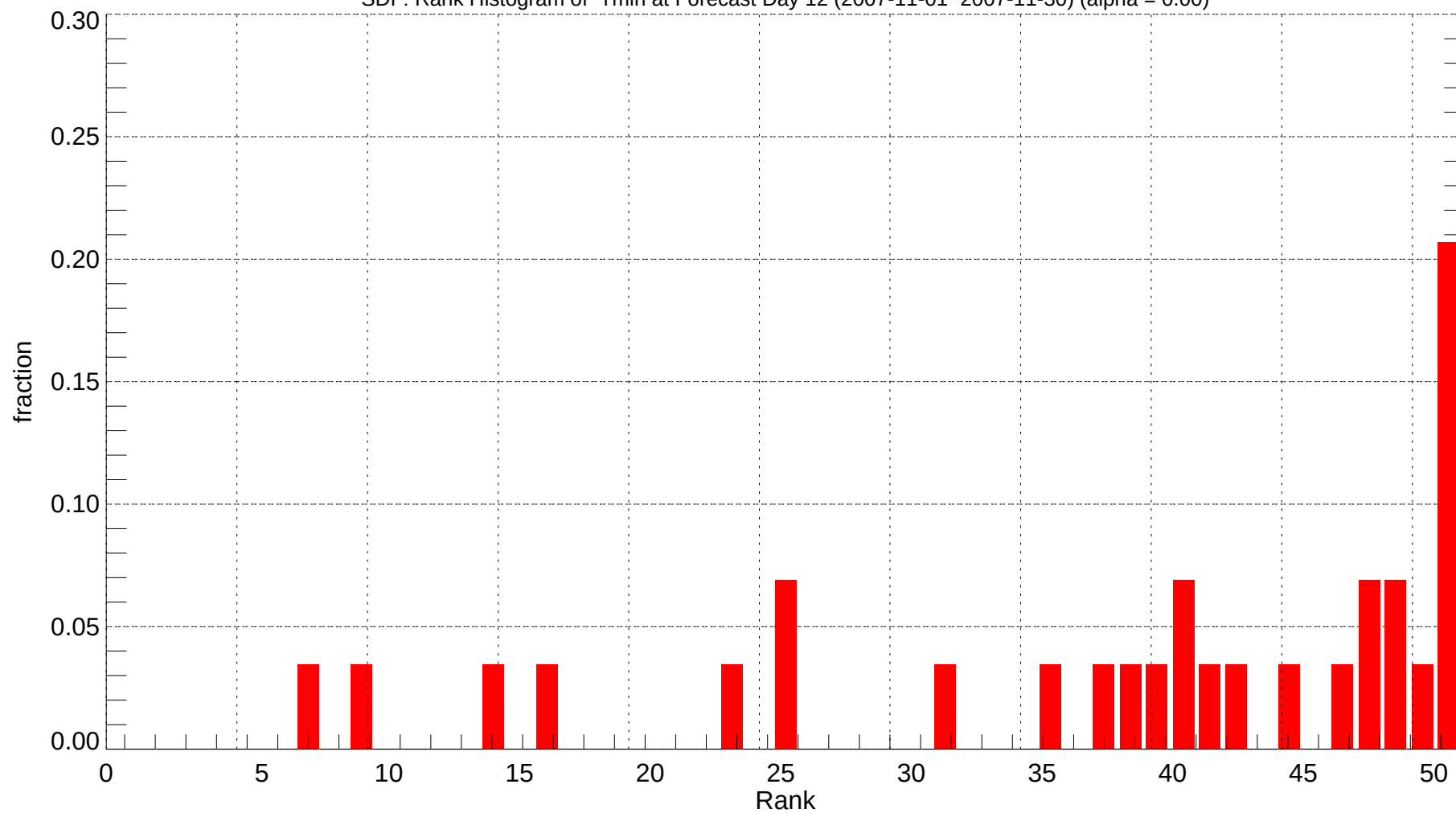
SDF: Rank Histogram of Tmin at Forecast Day 12 (2007-11-01~2007-11-30) (alpha = 0.00)
