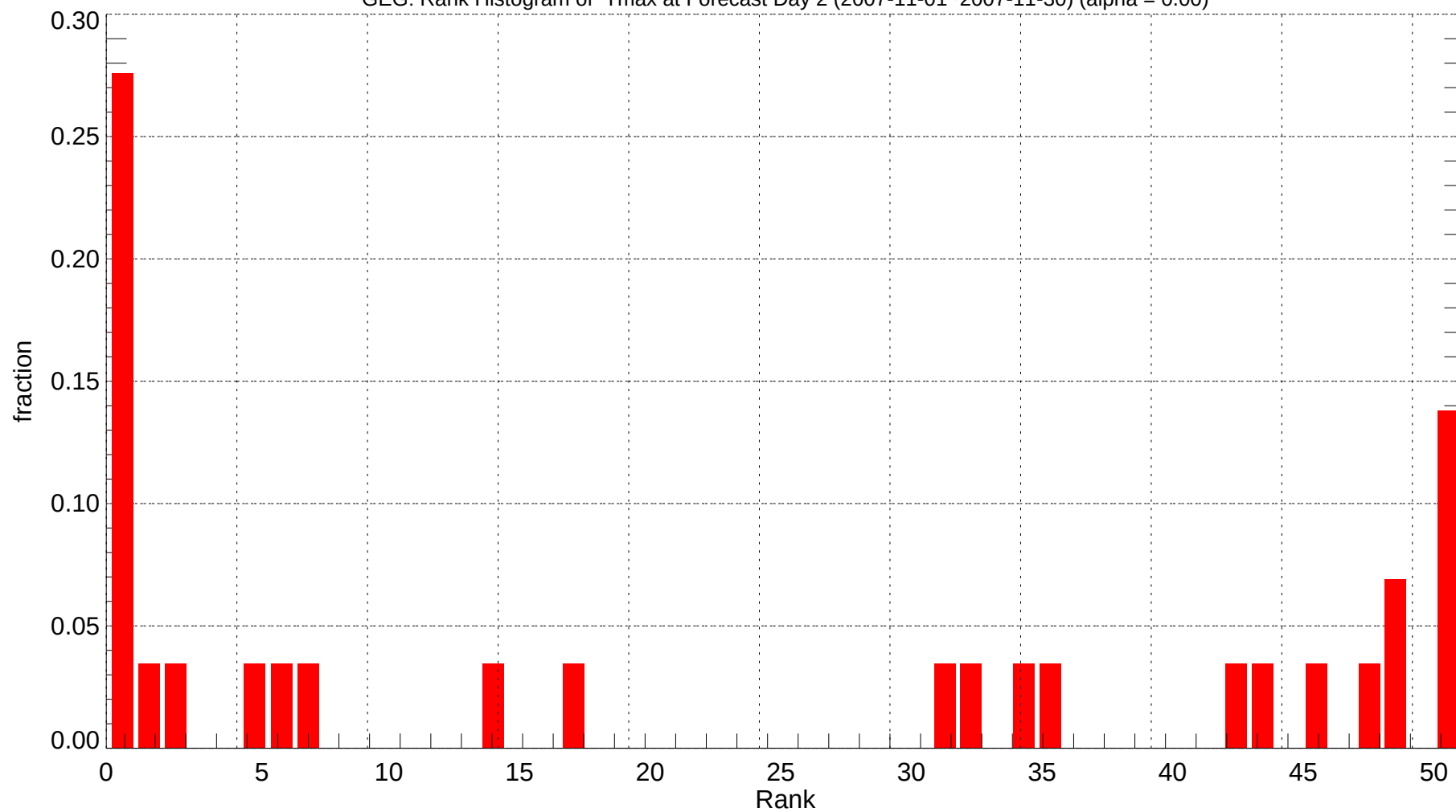
GEG: Rank Histogram of Tmax at Forecast Day 2 (2007-11-01~2007-11-30) (alpha = 0.00)
