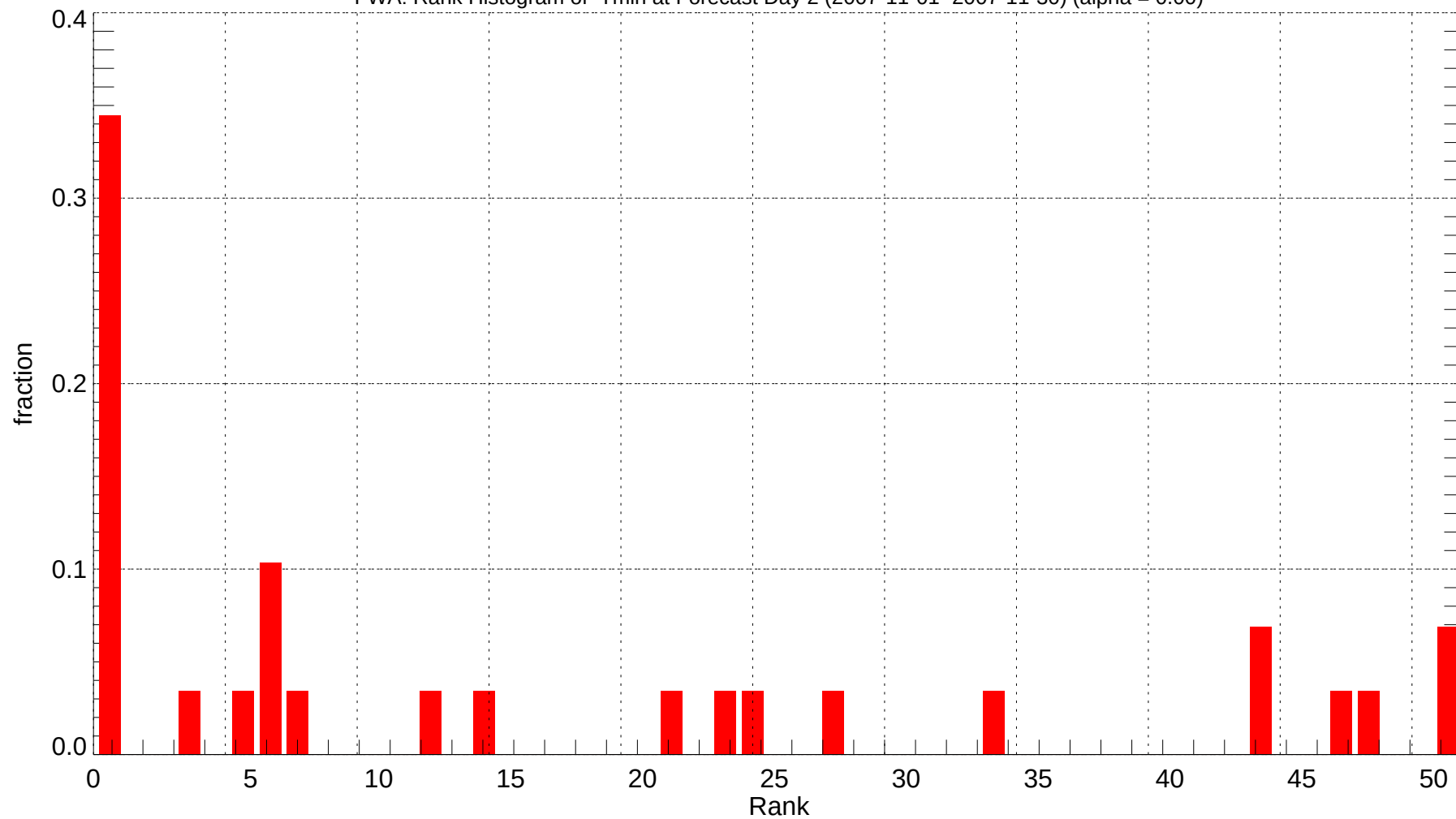
FWA: Rank Histogram of Tmin at Forecast Day 2 (2007-11-01~2007-11-30) (alpha = 0.00)
