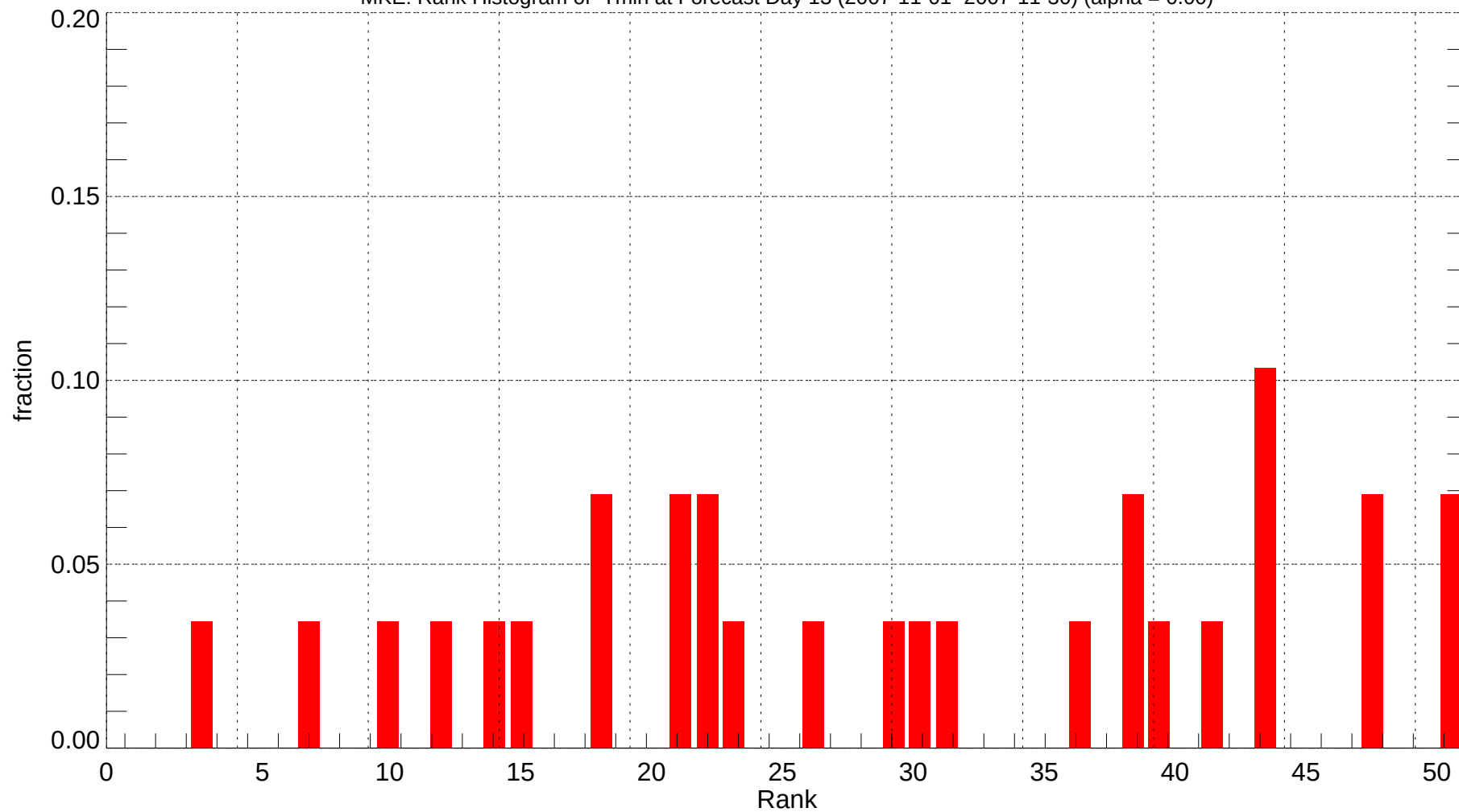
MKE: Rank Histogram of Tmin at Forecast Day 13 (2007-11-01~2007-11-30) (alpha = 0.00)
