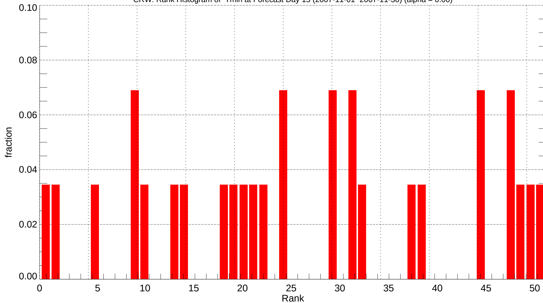
CRW: Rank Histogram of Tmin at Forecast Day 15 (2007-11-01~2007-11-30) (alpha = 0.00)
