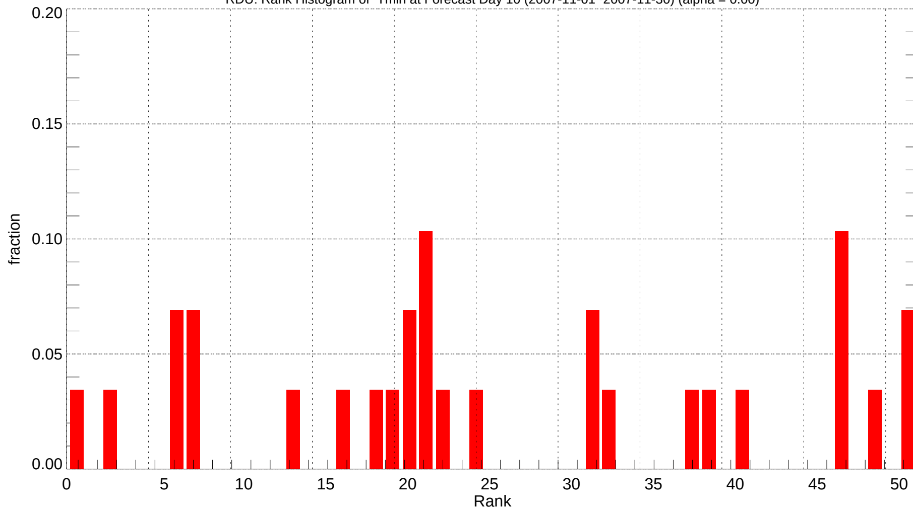
RDU: Rank Histogram of Tmin at Forecast Day 10 (2007-11-01~2007-11-30) (alpha = 0.00)
