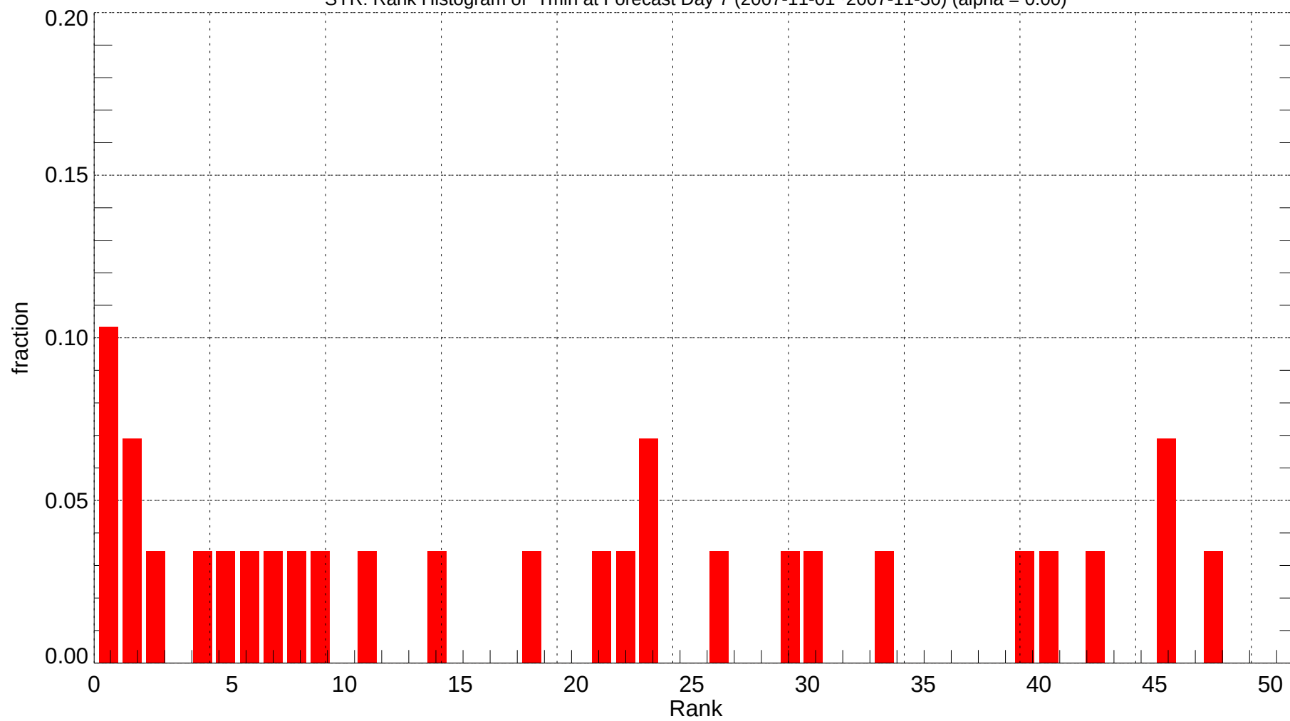
SYR: Rank Histogram of Tmin at Forecast Day 7 (2007-11-01~2007-11-30) (alpha = 0.00)
