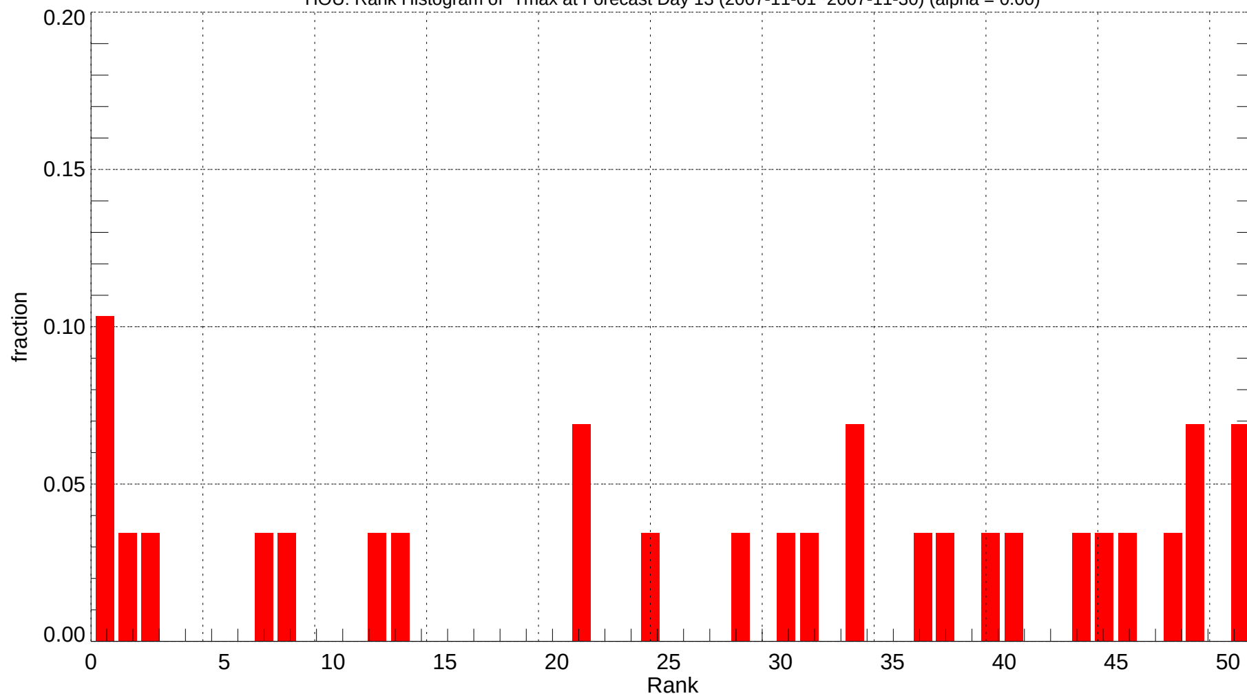
HOU: Rank Histogram of Tmax at Forecast Day 13 (2007-11-01~2007-11-30) (alpha = 0.00)
