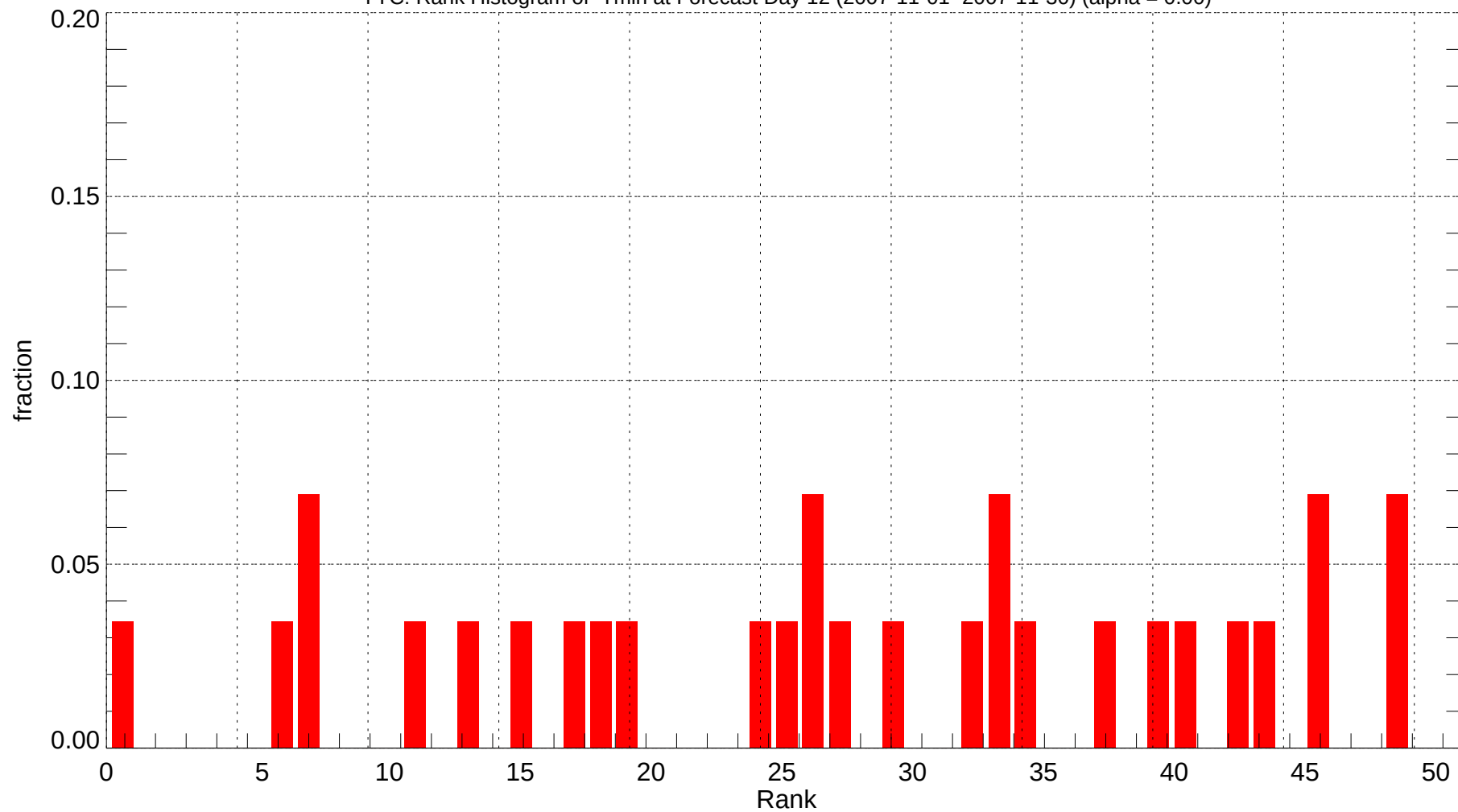
YYC: Rank Histogram of Tmin at Forecast Day 12 (2007-11-01~2007-11-30) (alpha = 0.00)
