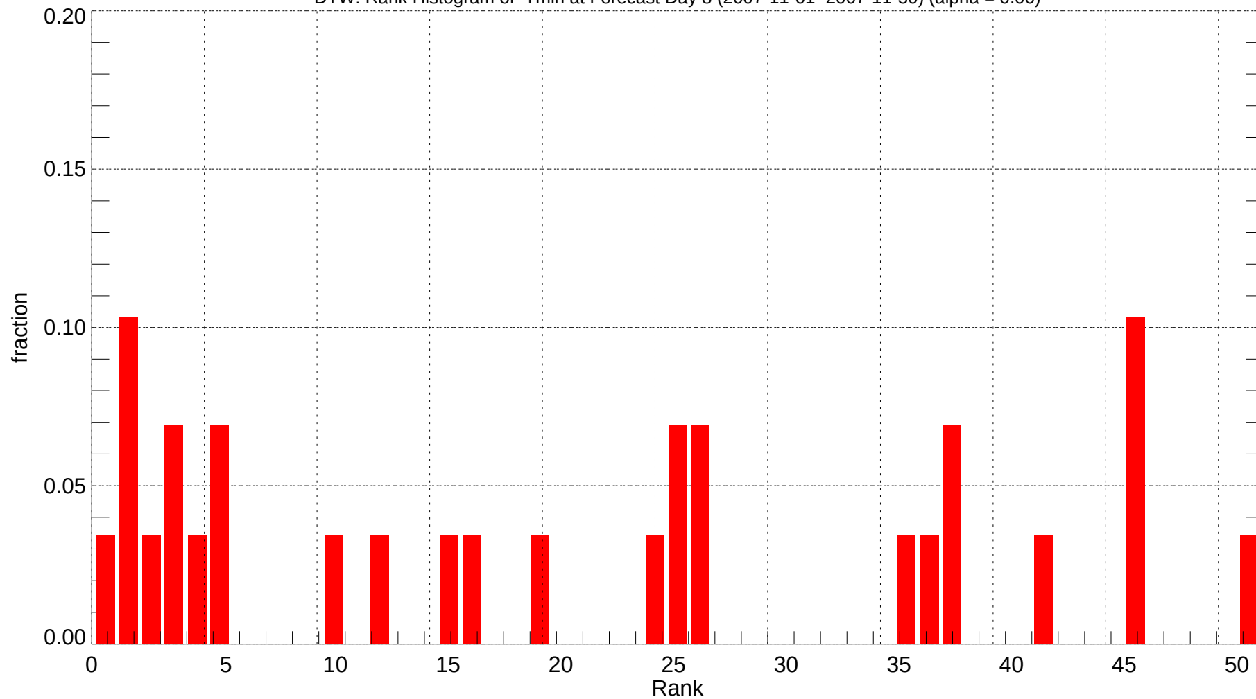
DTW: Rank Histogram of Tmin at Forecast Day 8 (2007-11-01~2007-11-30) (alpha = 0.00)
