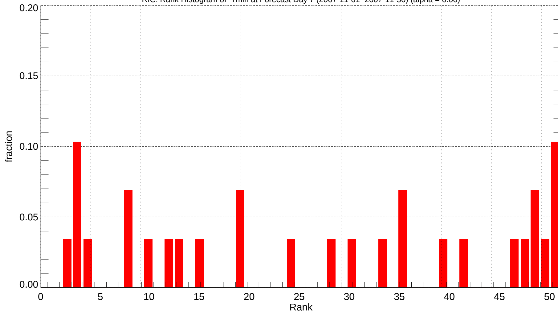
RIC: Rank Histogram of Tmin at Forecast Day 7 (2007-11-01~2007-11-30) (alpha = 0.00)
