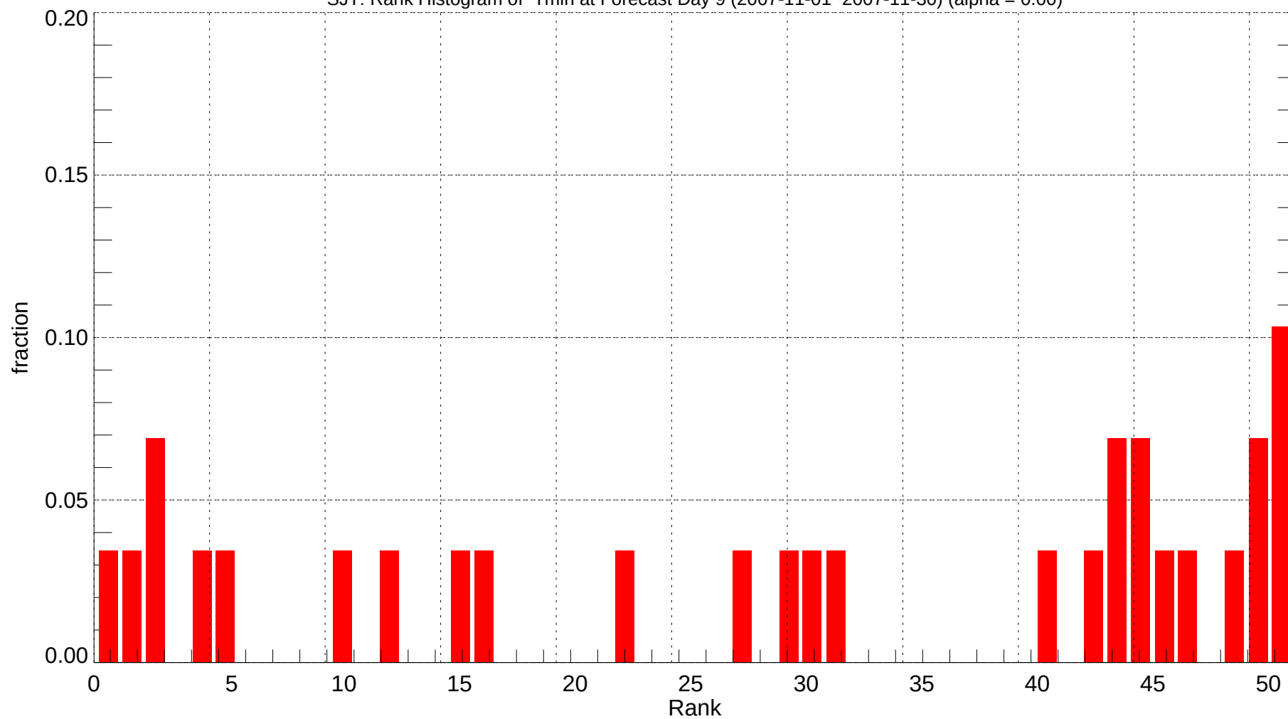
SJT: Rank Histogram of Tmin at Forecast Day 9 (2007-11-01~2007-11-30) (alpha = 0.00)
