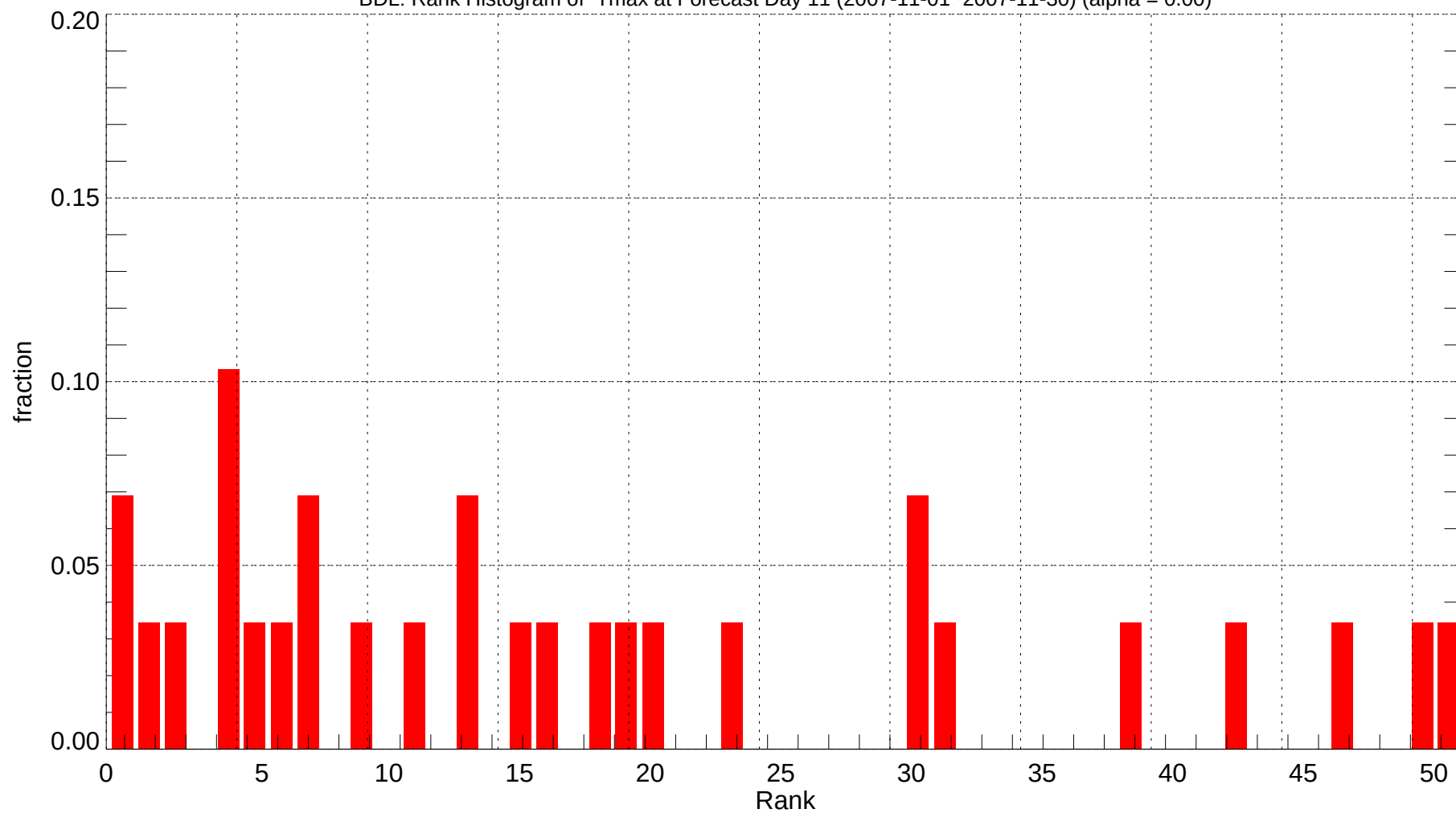
BDL: Rank Histogram of Tmax at Forecast Day 11 (2007-11-01~2007-11-30) (alpha = 0.00)
