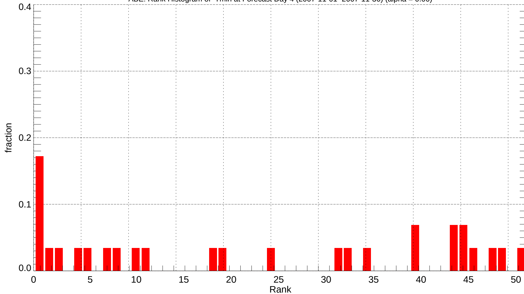
ABE: Rank Histogram of Tmin at Forecast Day 4 (2007-11-01~2007-11-30) (alpha = 0.00)
