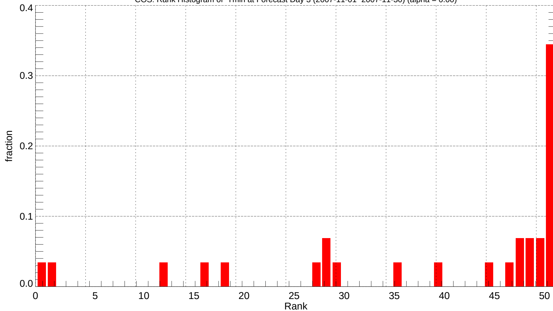
COS: Rank Histogram of Tmin at Forecast Day 3 (2007-11-01~2007-11-30) (alpha = 0.00)
