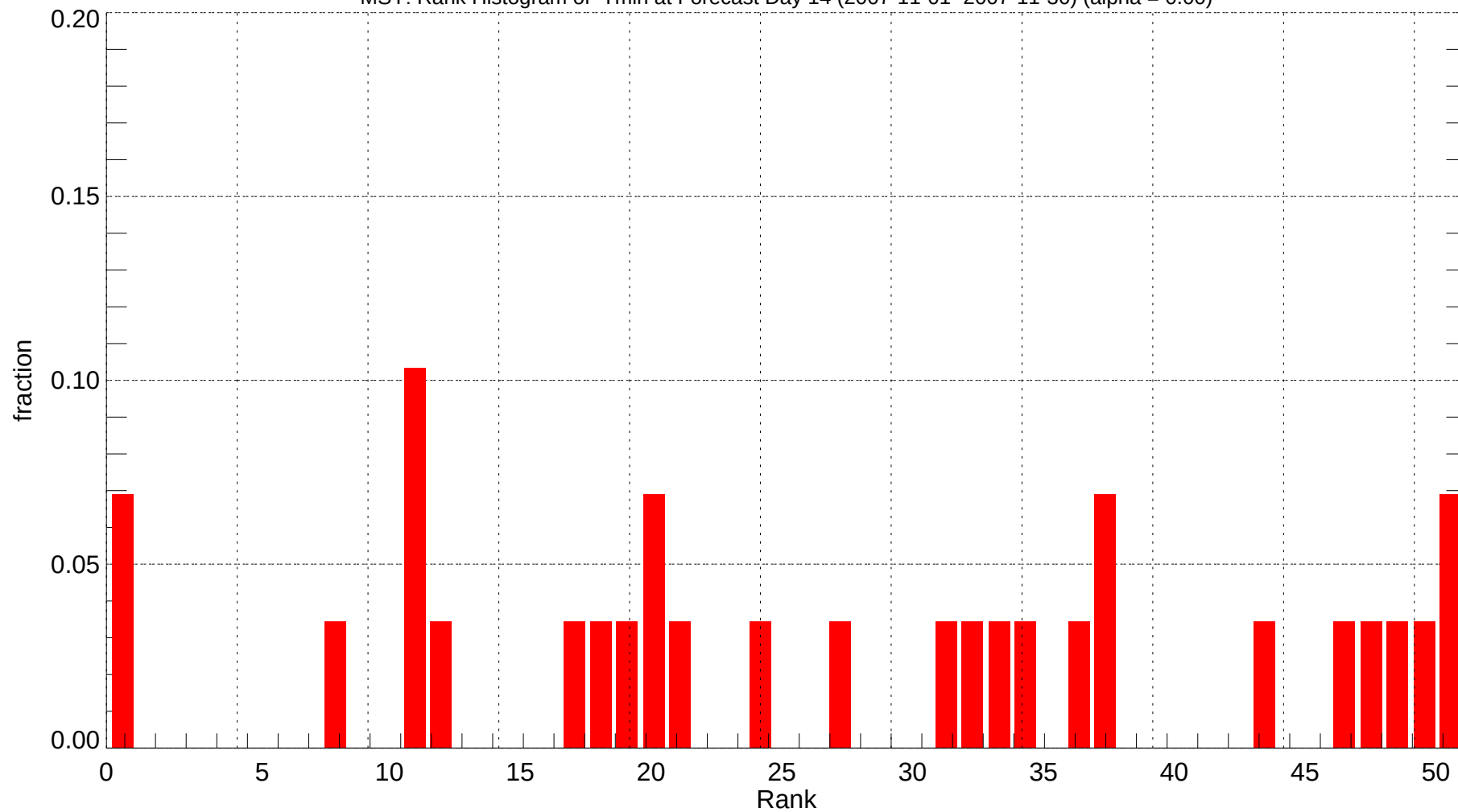
MSY: Rank Histogram of Tmin at Forecast Day 14 (2007-11-01~2007-11-30) (alpha = 0.00)
