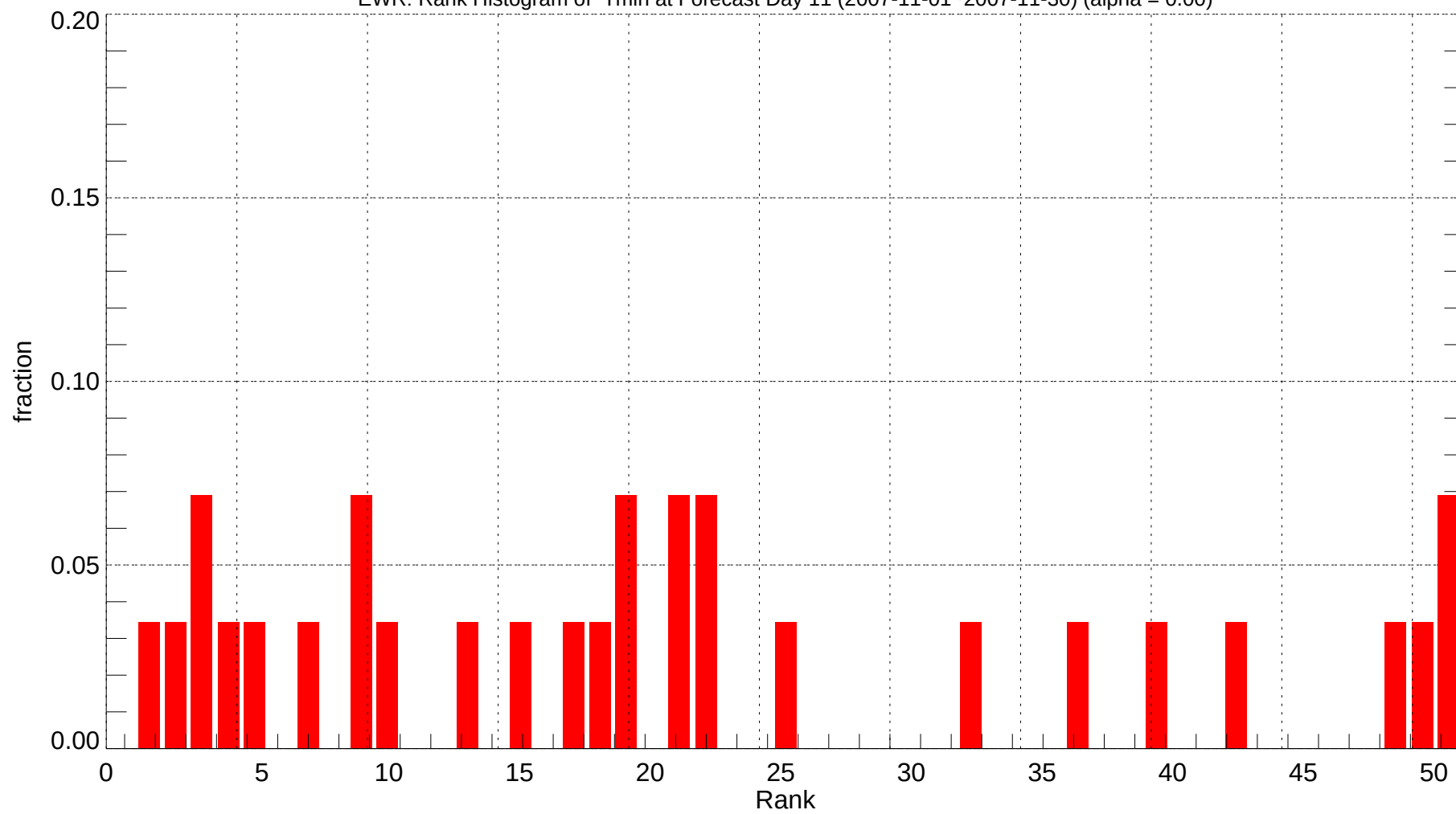
EWR: Rank Histogram of Tmin at Forecast Day 11 (2007-11-01~2007-11-30) (alpha = 0.00)
