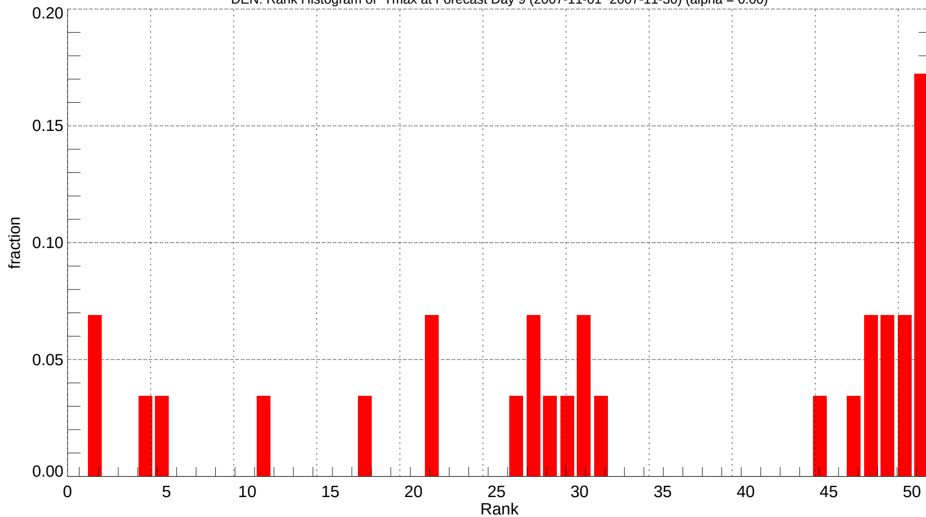
DEN: Rank Histogram of Tmax at Forecast Day 9 (2007-11-01~2007-11-30) (alpha = 0.00)
