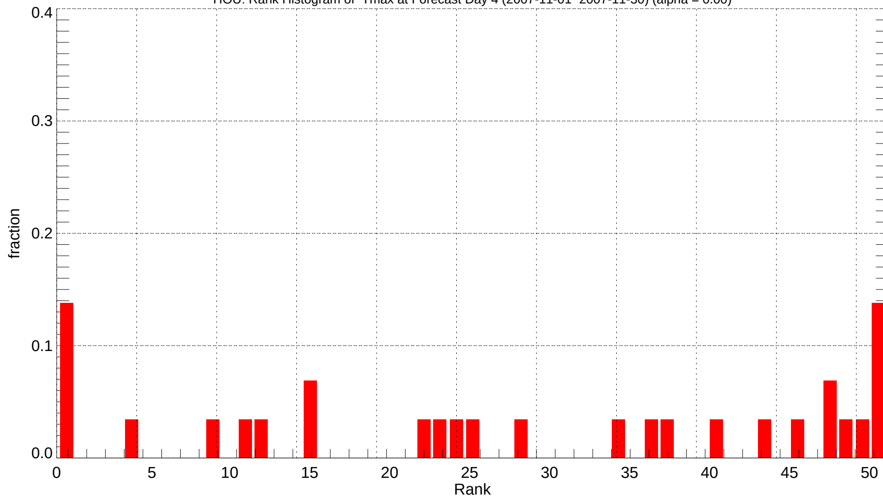
HOU: Rank Histogram of Tmax at Forecast Day 4 (2007-11-01~2007-11-30) (alpha = 0.00)
