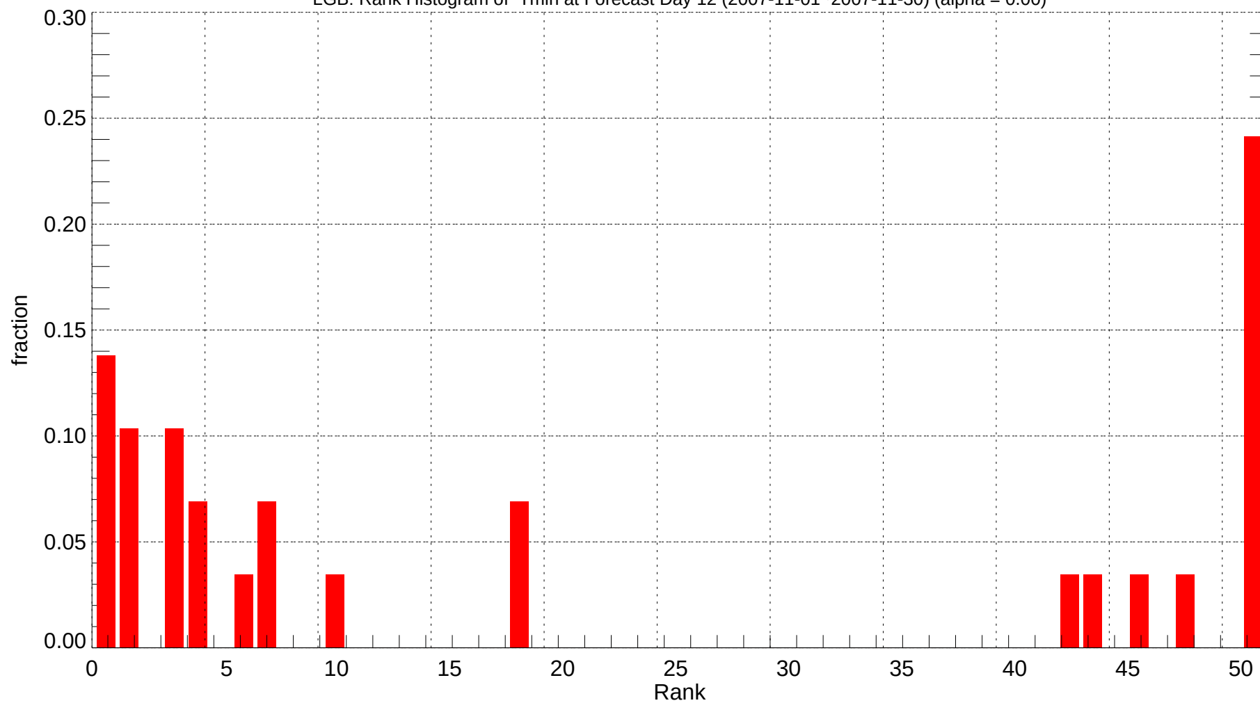
LGB: Rank Histogram of Tmin at Forecast Day 12 (2007-11-01~2007-11-30) (alpha = 0.00)
