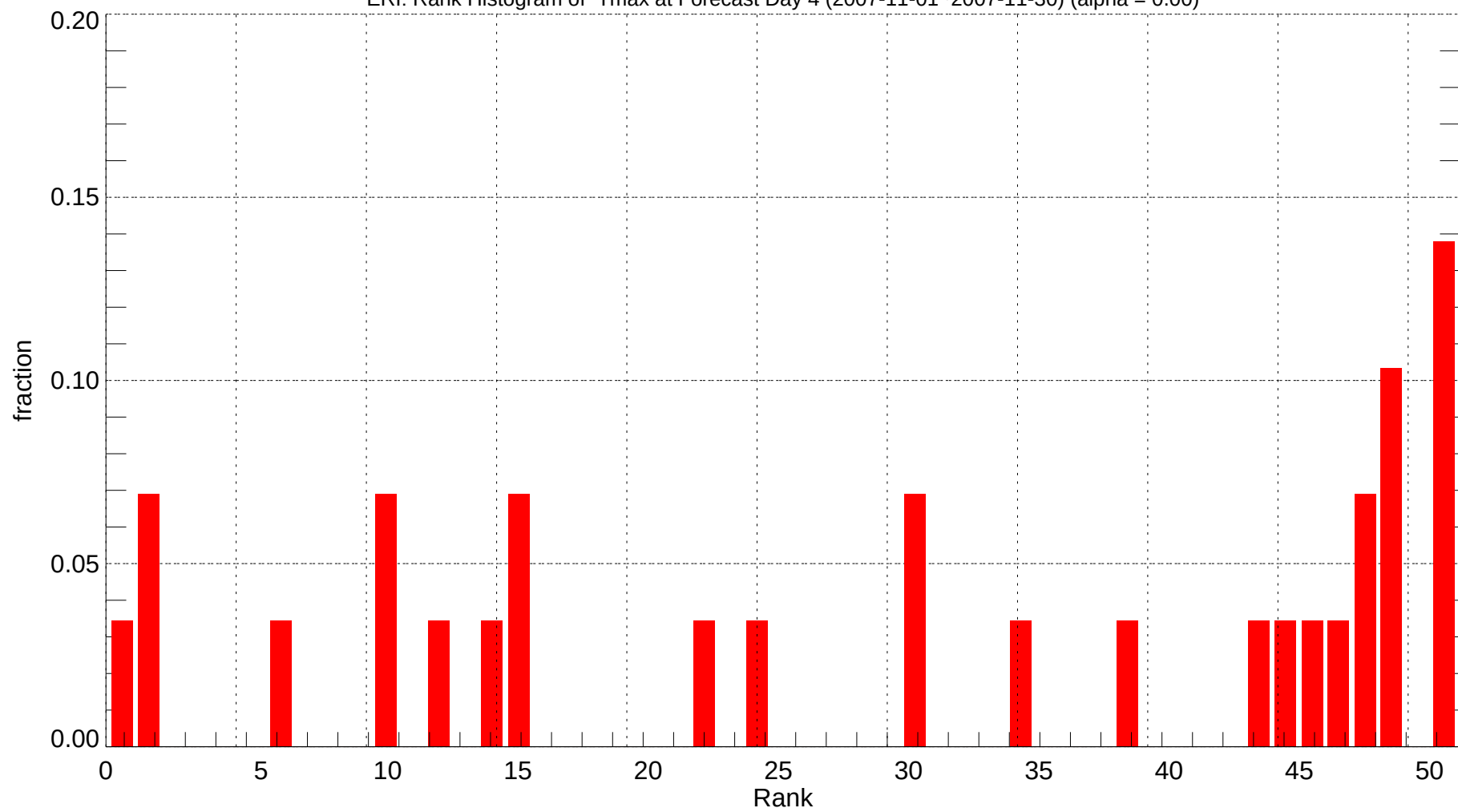
ERI: Rank Histogram of Tmax at Forecast Day 4 (2007-11-01~2007-11-30) (alpha = 0.00)
