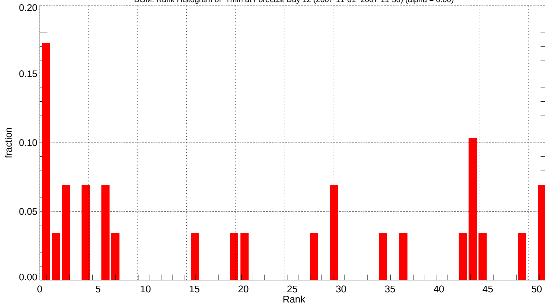
BGM: Rank Histogram of Tmin at Forecast Day 12 (2007-11-01~2007-11-30) (alpha = 0.00)
