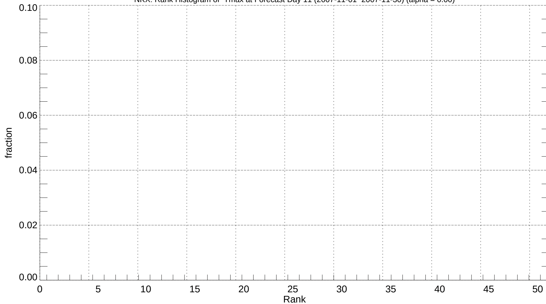
NKX: Rank Histogram of Tmax at Forecast Day 11 (2007-11-01~2007-11-30) (alpha = 0.00)
