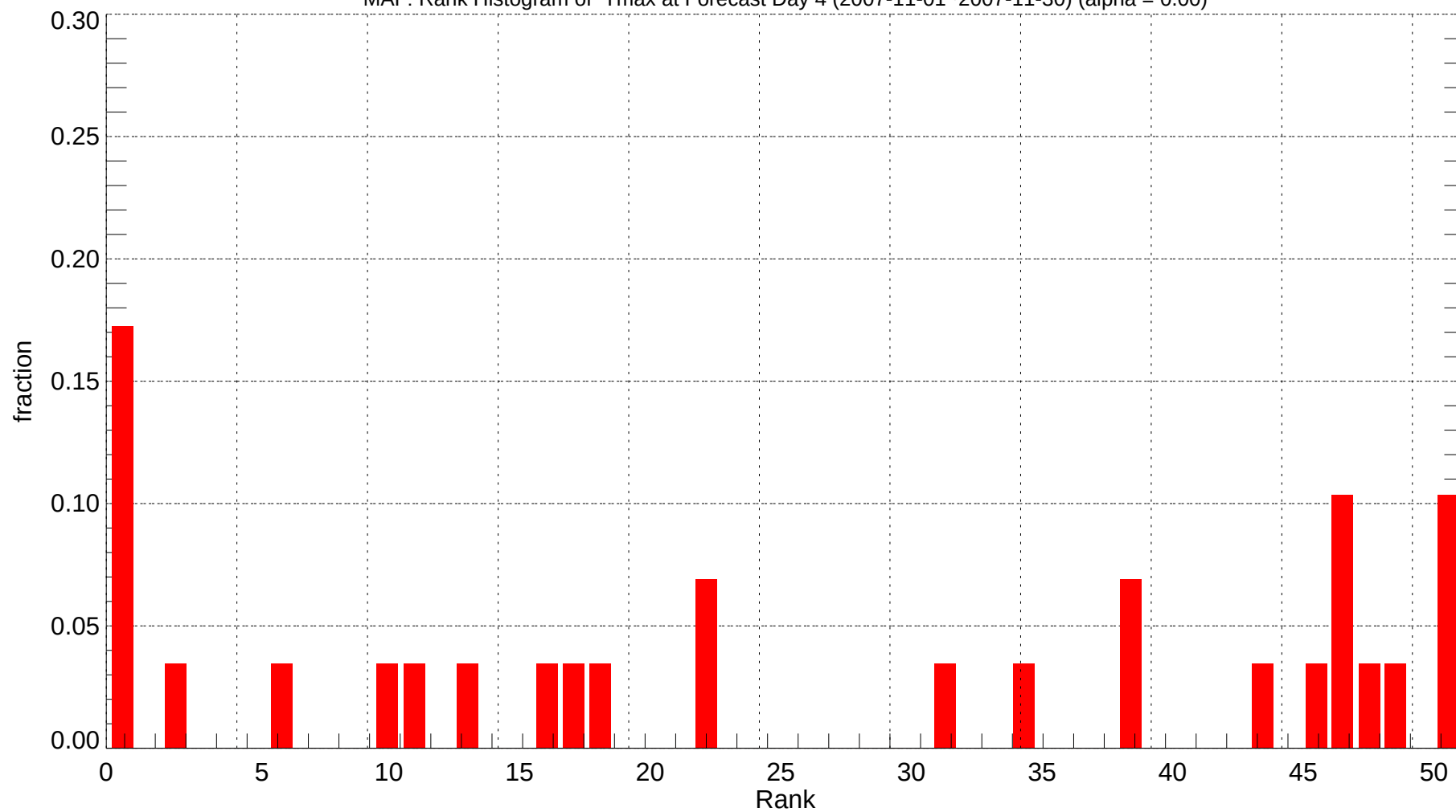
MAF: Rank Histogram of Tmax at Forecast Day 4 (2007-11-01~2007-11-30) (alpha = 0.00)
