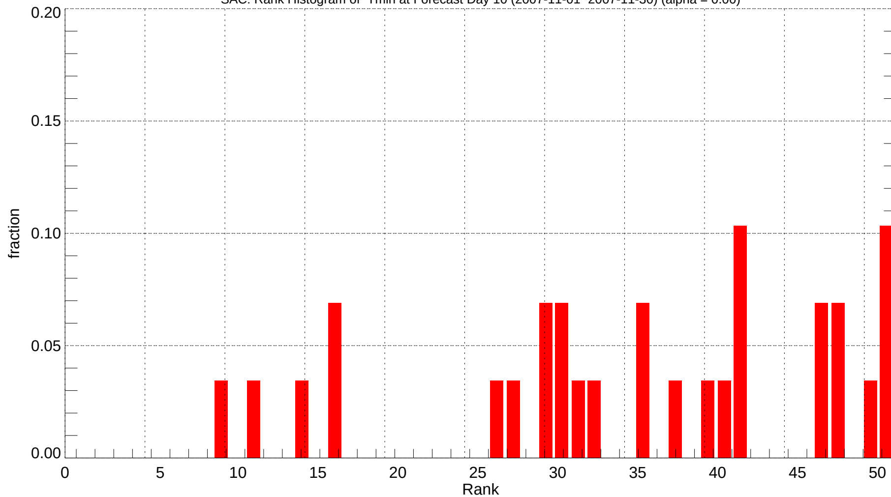
SAC: Rank Histogram of Tmin at Forecast Day 10 (2007-11-01~2007-11-30) (alpha = 0.00)
