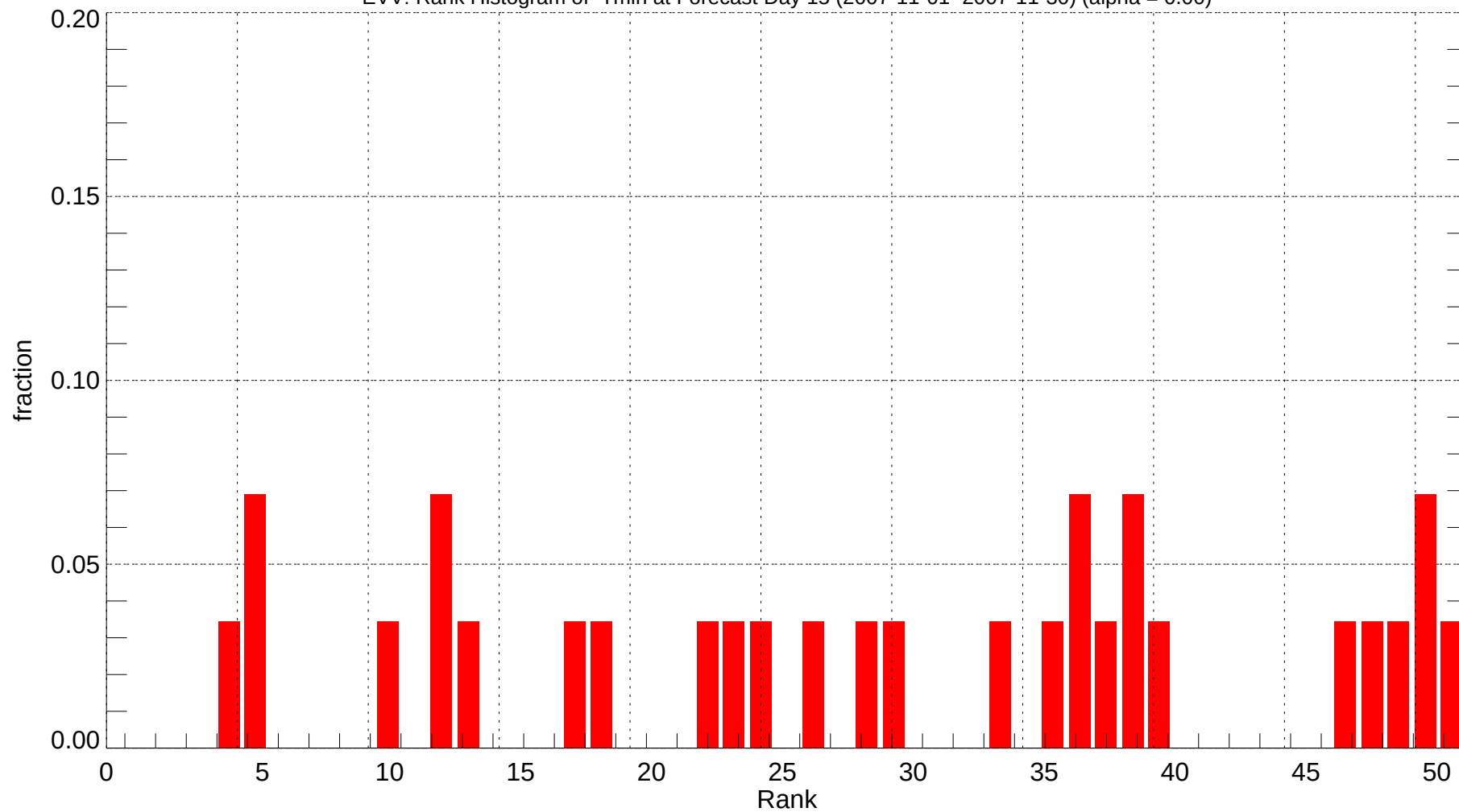
EVV: Rank Histogram of Tmin at Forecast Day 15 (2007-11-01~2007-11-30) (alpha = 0.00)
