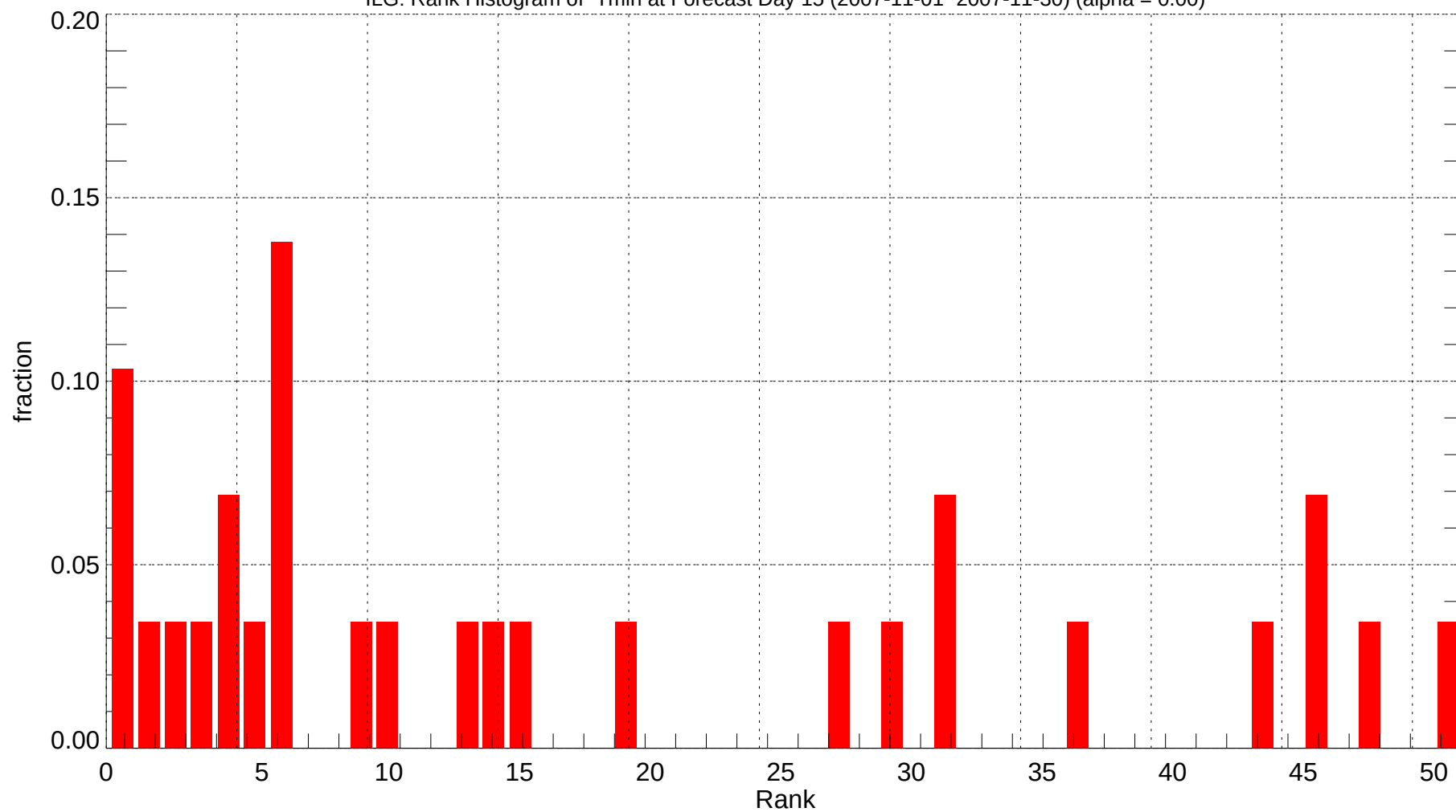
ILG: Rank Histogram of Tmin at Forecast Day 15 (2007-11-01~2007-11-30) (alpha = 0.00)
