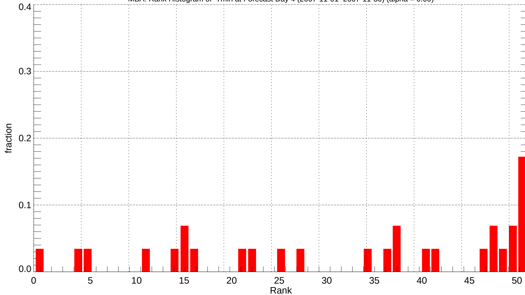
MBA: Rank Histogram of Tmin at Forecast Day 4 (2007-11-01~2007-11-30) (alpha = 0.00)
