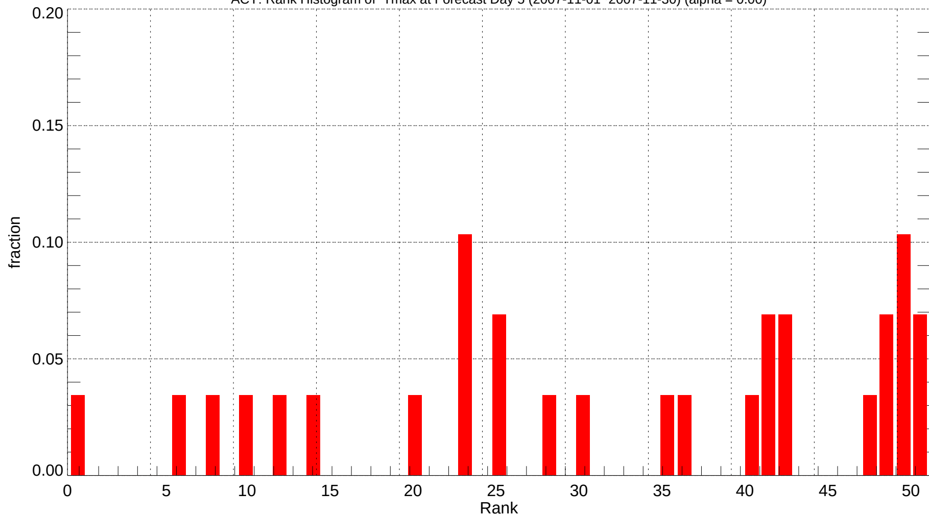
ACY: Rank Histogram of Tmax at Forecast Day 5 (2007-11-01~2007-11-30) (alpha = 0.00)
