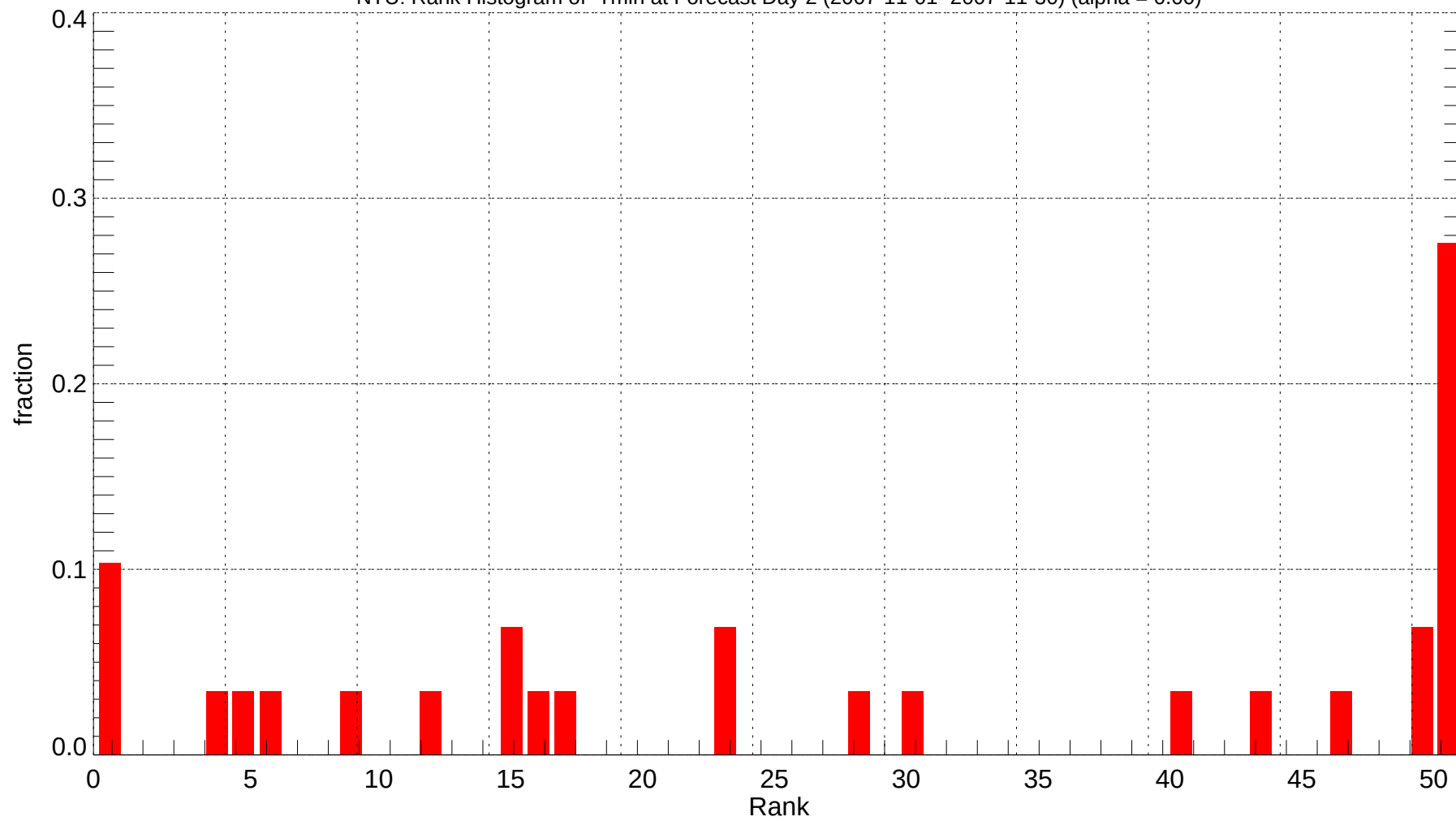
NTU: Rank Histogram of Tmin at Forecast Day 2 (2007-11-01~2007-11-30) (alpha = 0.00)
