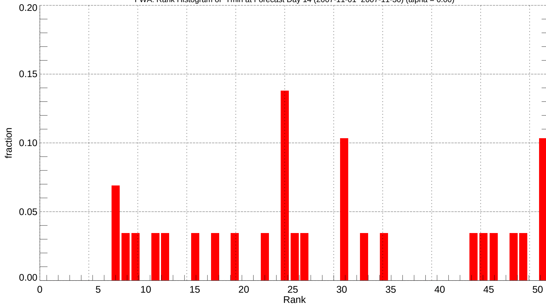
FWA: Rank Histogram of Tmin at Forecast Day 14 (2007-11-01~2007-11-30) (alpha = 0.00)
