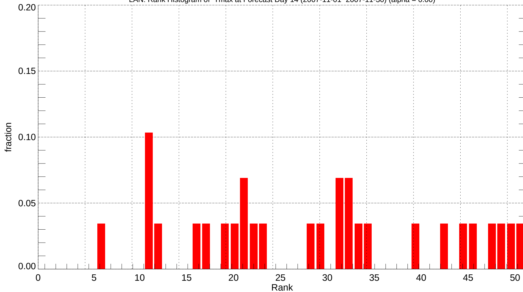
LAN: Rank Histogram of Tmax at Forecast Day 14 (2007-11-01~2007-11-30) (alpha = 0.00)
