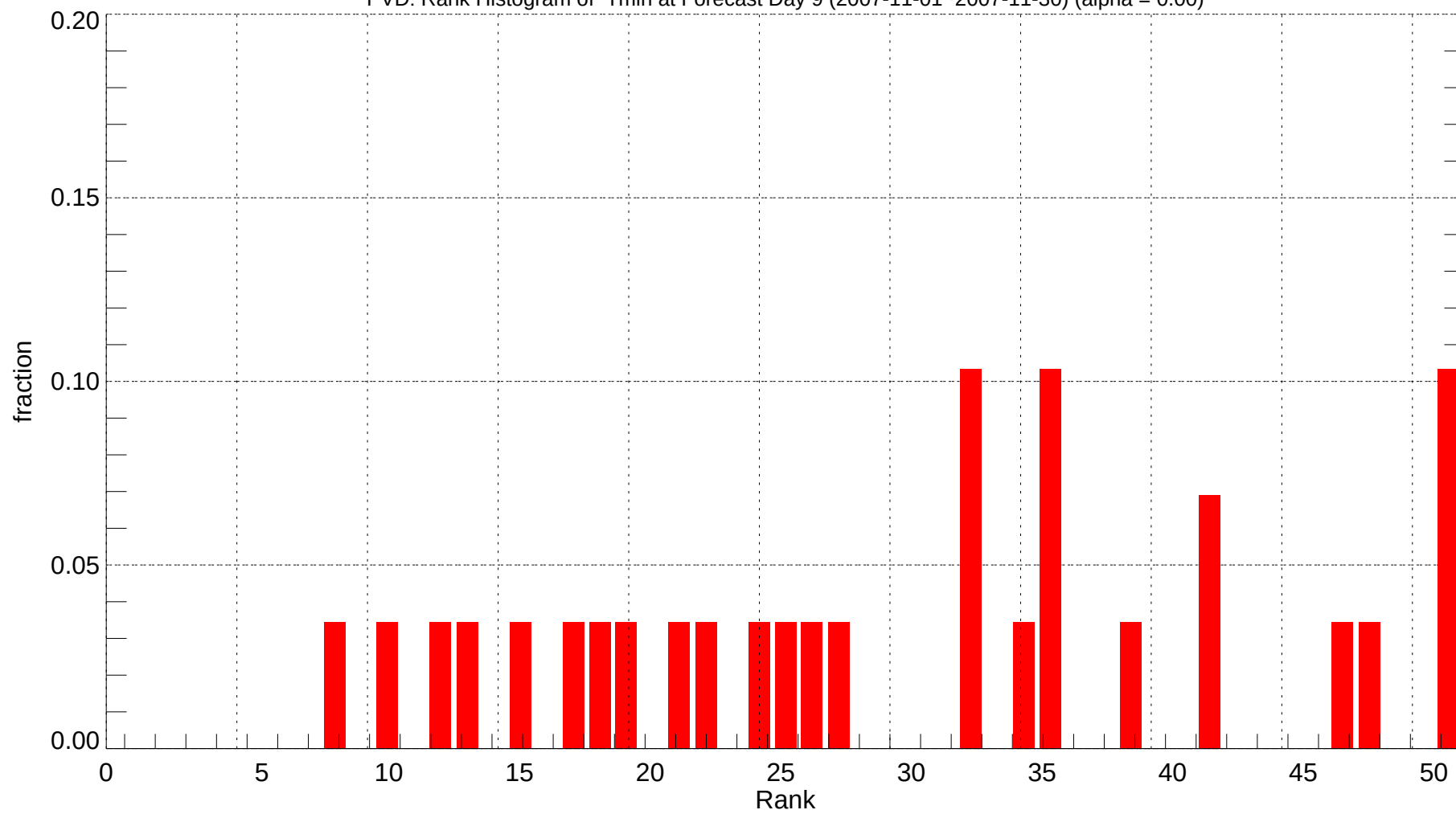
PVD: Rank Histogram of Tmin at Forecast Day 9 (2007-11-01~2007-11-30) (alpha = 0.00)
