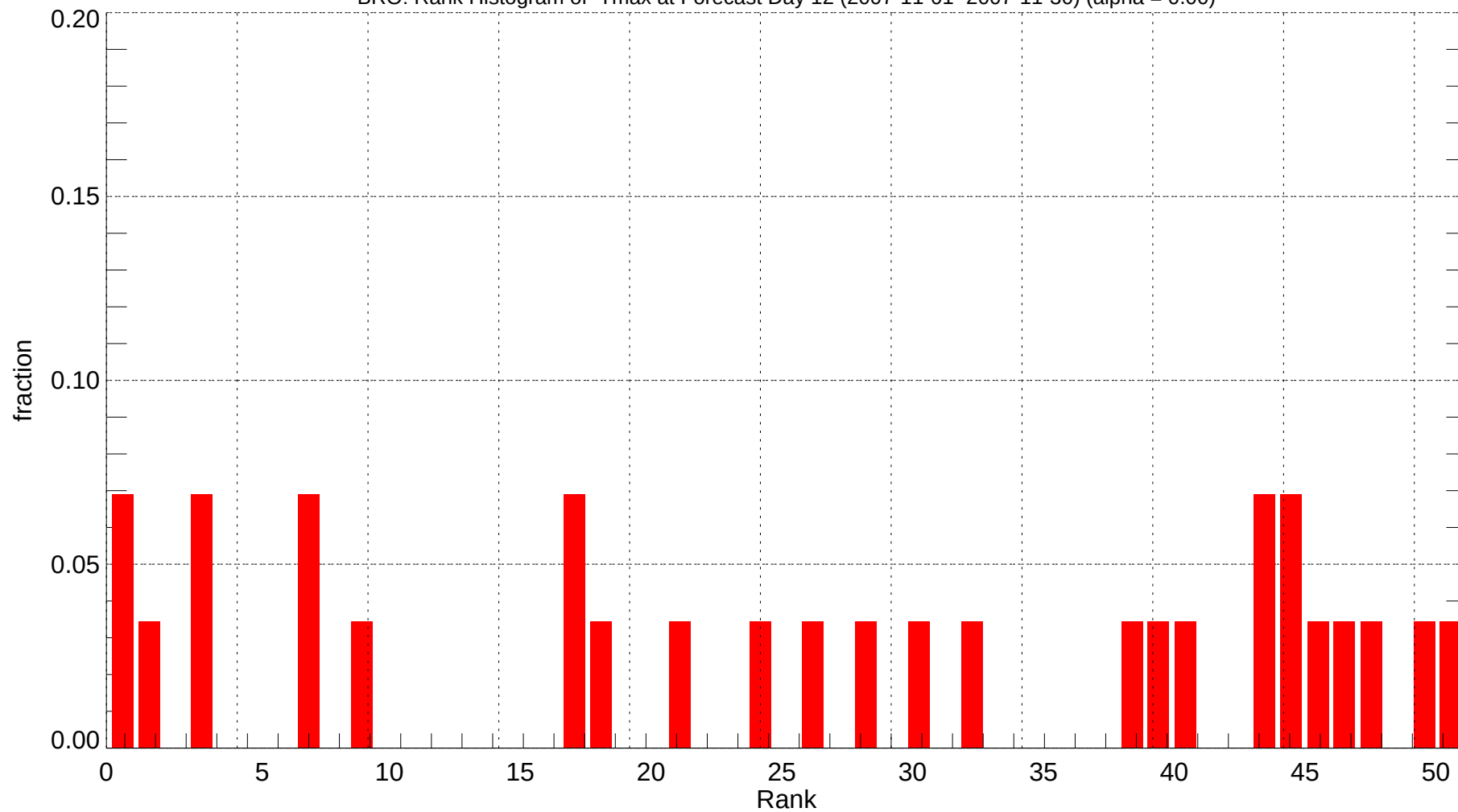
BRO: Rank Histogram of Tmax at Forecast Day 12 (2007-11-01~2007-11-30) (alpha = 0.00)
