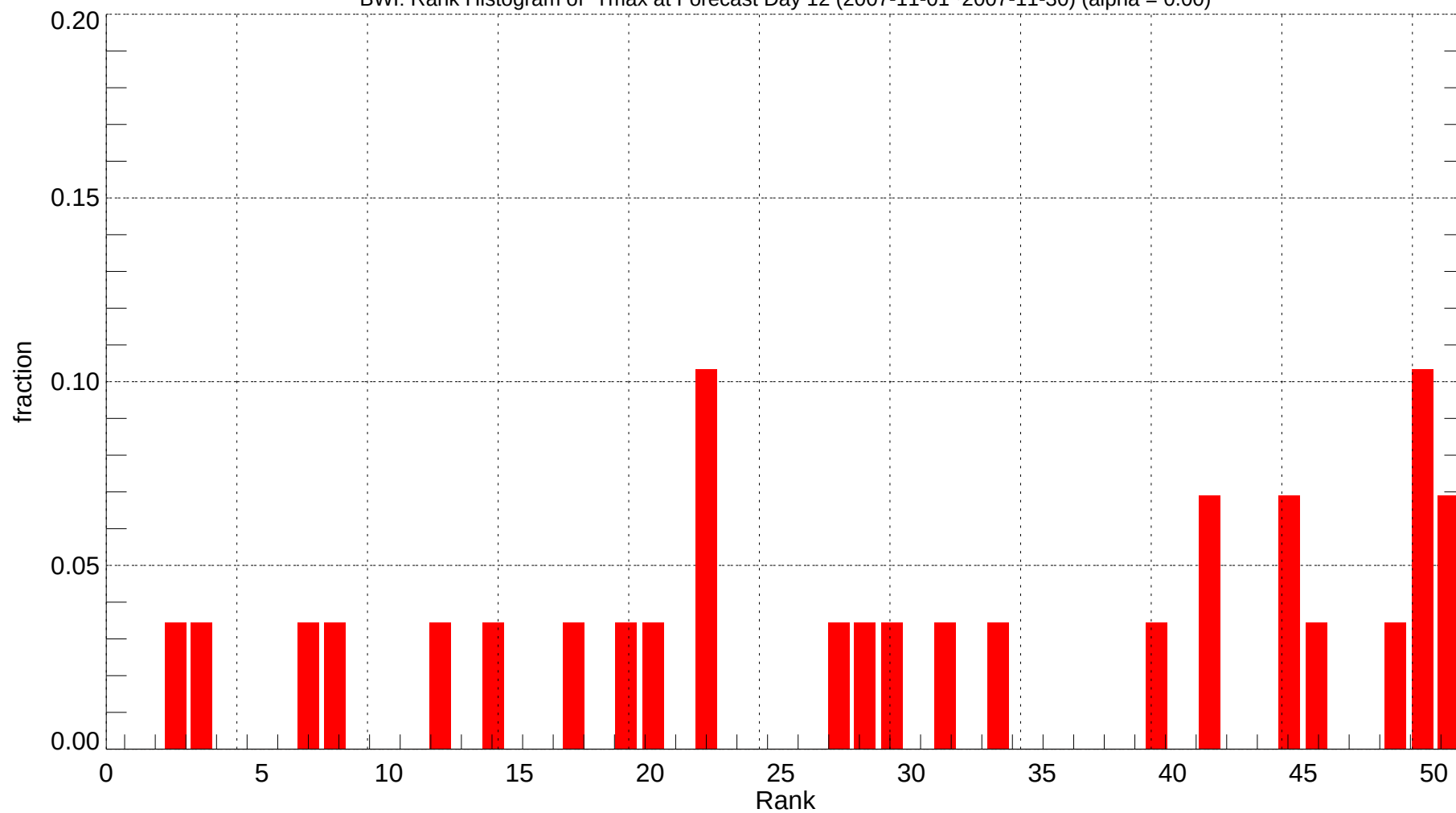
BWI: Rank Histogram of Tmax at Forecast Day 12 (2007-11-01~2007-11-30) (alpha = 0.00)
