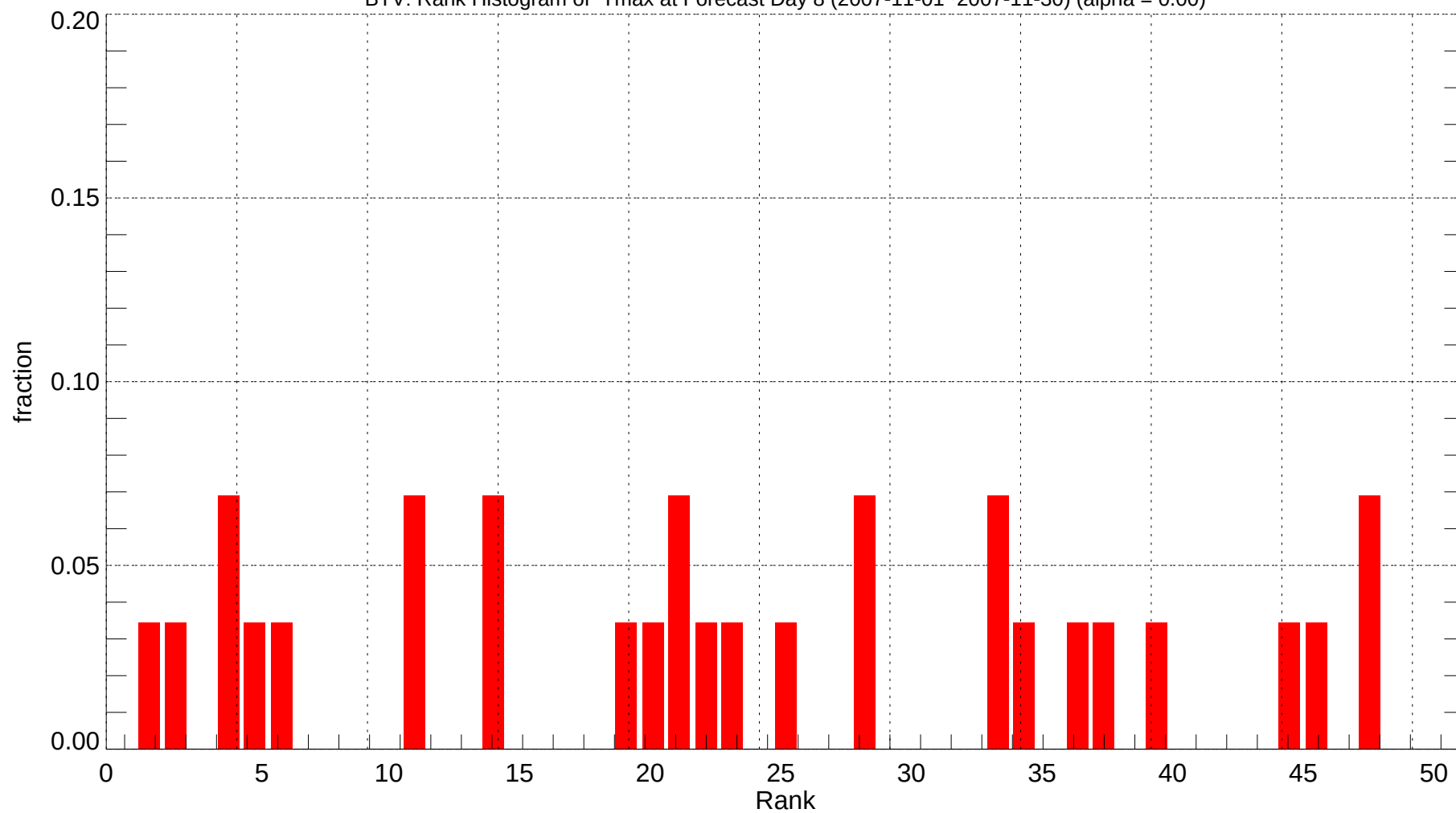
BTV: Rank Histogram of Tmax at Forecast Day 8 (2007-11-01~2007-11-30) (alpha = 0.00)
