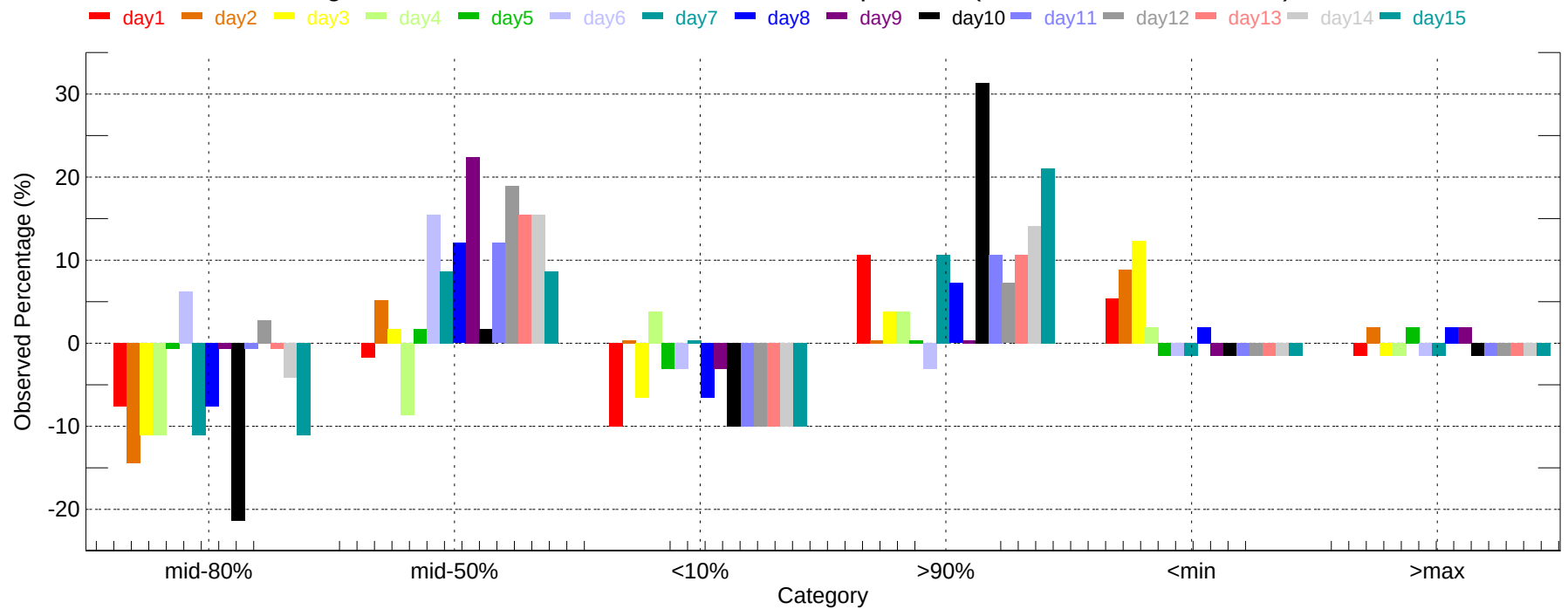
Observed Percentage Deviation of Ensembles - FAT: Min Temperature (2007-11-01~2007-11-30)
