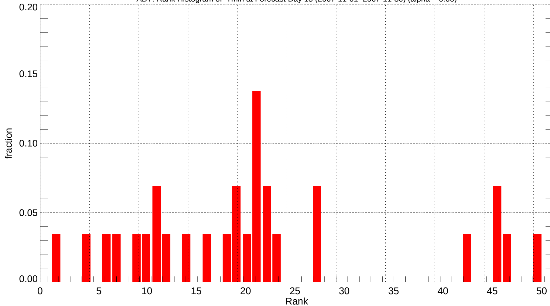
ABY: Rank Histogram of Tmin at Forecast Day 15 (2007-11-01~2007-11-30) (alpha = 0.00)
