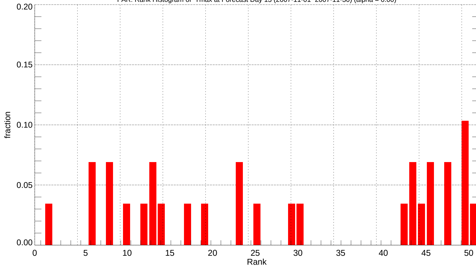
FAR: Rank Histogram of Tmax at Forecast Day 13 (2007-11-01~2007-11-30) (alpha = 0.00)
