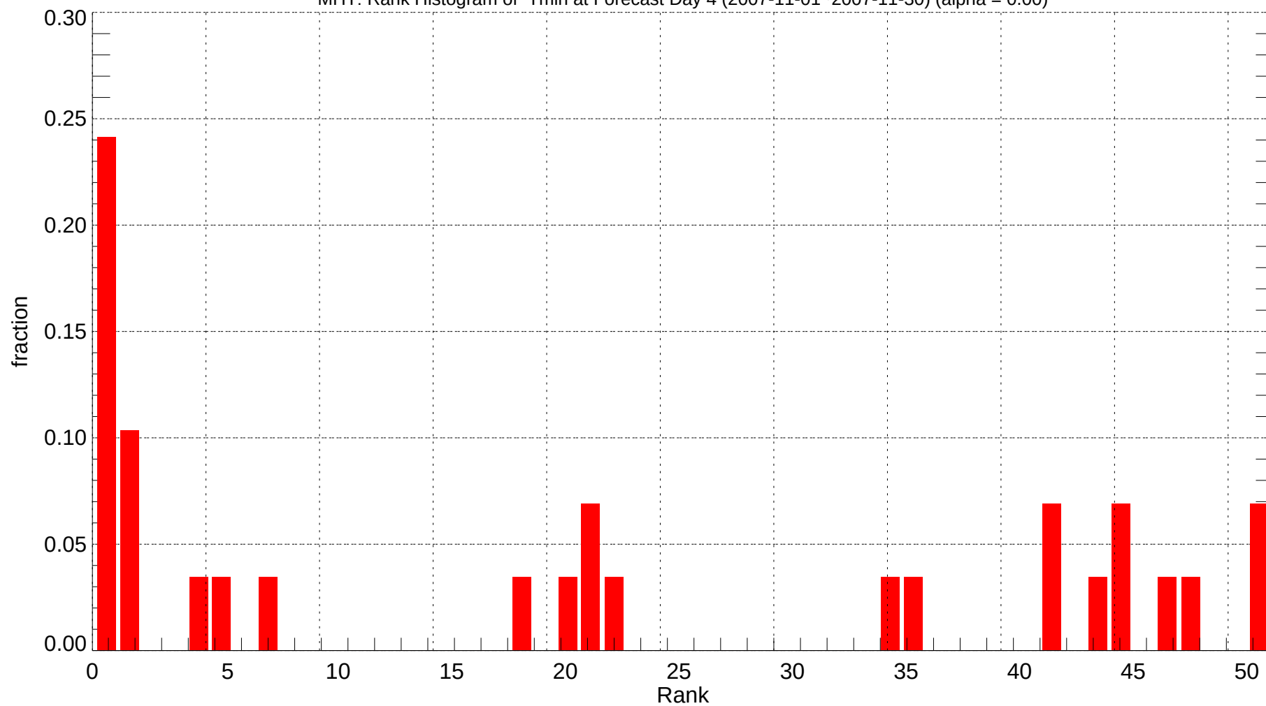
MHT: Rank Histogram of Tmin at Forecast Day 4 (2007-11-01~2007-11-30) (alpha = 0.00)
