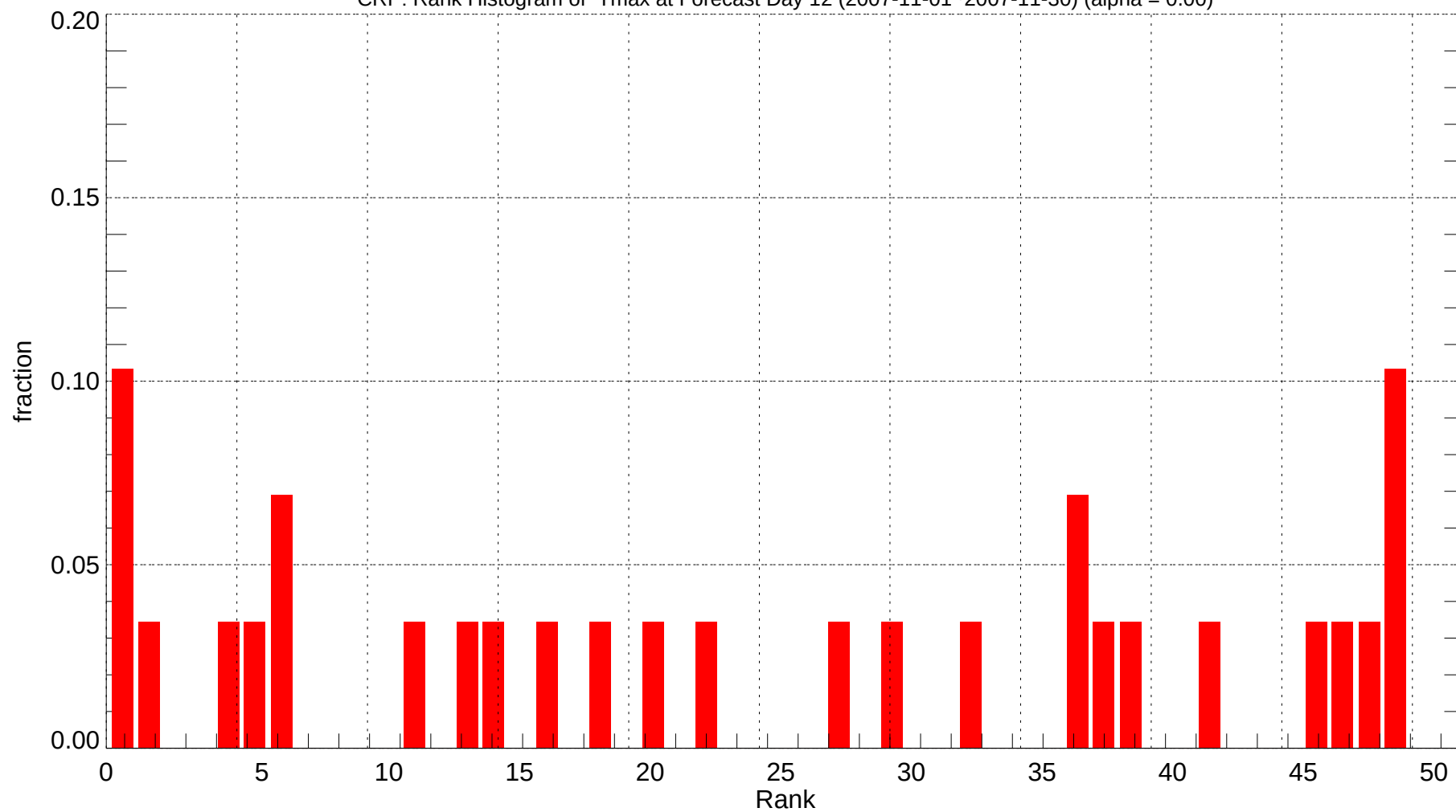
CRP: Rank Histogram of Tmax at Forecast Day 12 (2007-11-01~2007-11-30) (alpha = 0.00)
