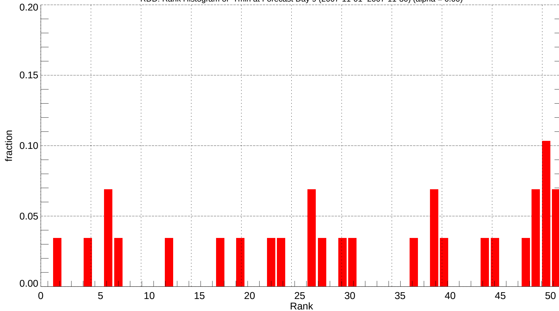
RDD: Rank Histogram of Tmin at Forecast Day 9 (2007-11-01~2007-11-30) (alpha = 0.00)
