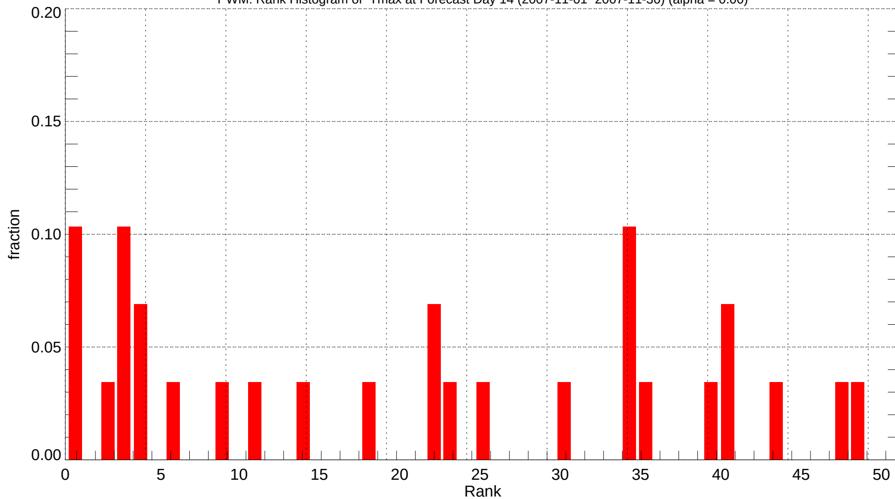
PWM: Rank Histogram of Tmax at Forecast Day 14 (2007-11-01~2007-11-30) (alpha = 0.00)
