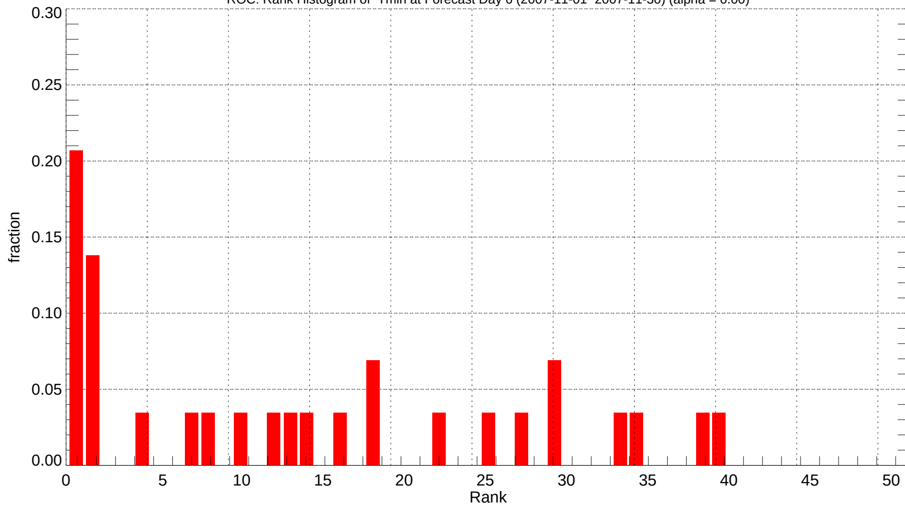
ROC: Rank Histogram of Tmin at Forecast Day 6 (2007-11-01~2007-11-30) (alpha = 0.00)
