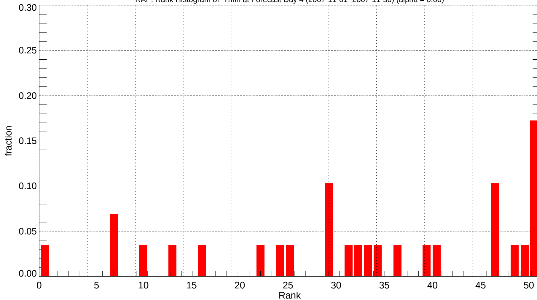
RAP: Rank Histogram of Tmin at Forecast Day 4 (2007-11-01~2007-11-30) (alpha = 0.00)
