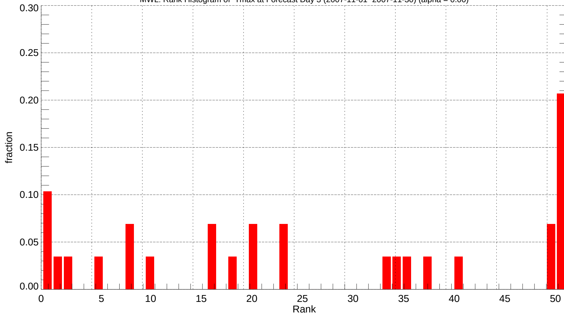
MWL: Rank Histogram of Tmax at Forecast Day 3 (2007-11-01~2007-11-30) (alpha = 0.00)
