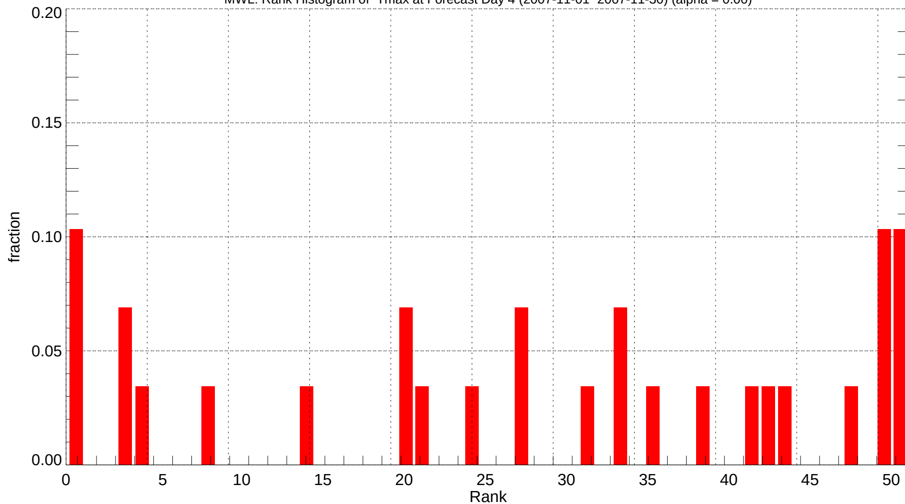
MWL: Rank Histogram of Tmax at Forecast Day 4 (2007-11-01~2007-11-30) (alpha = 0.00)
