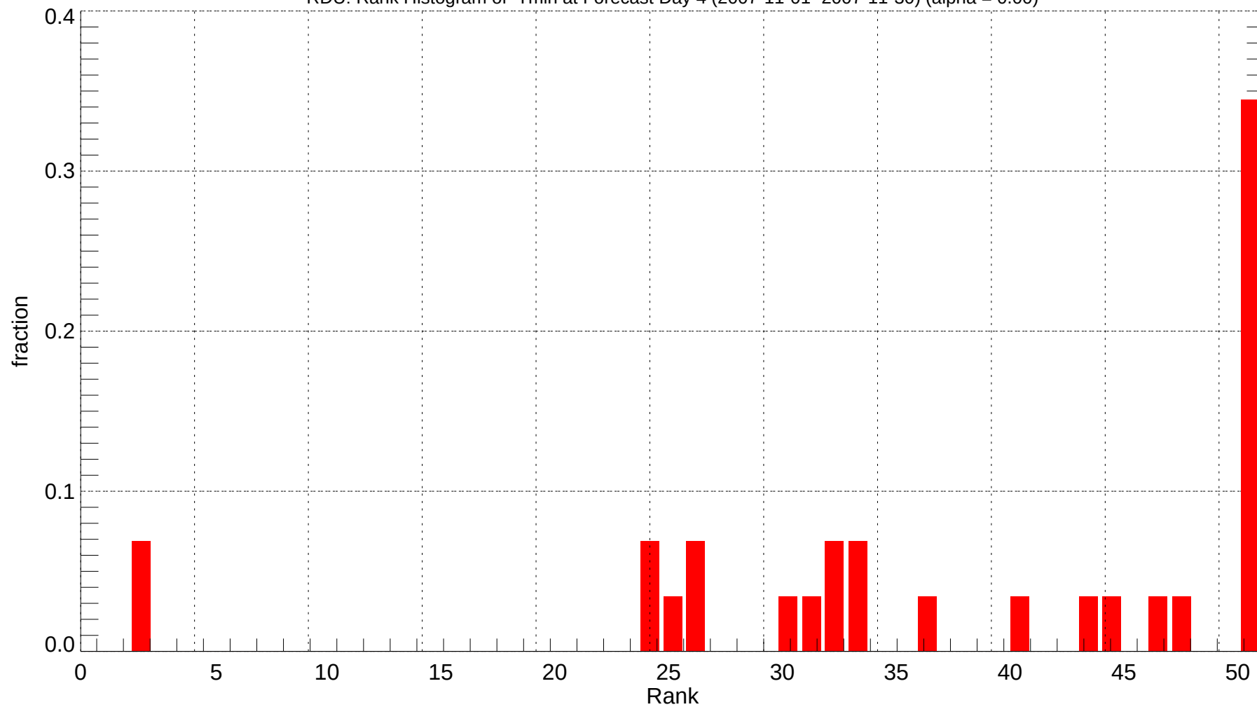
RDU: Rank Histogram of Tmin at Forecast Day 4 (2007-11-01~2007-11-30) (alpha = 0.00)
