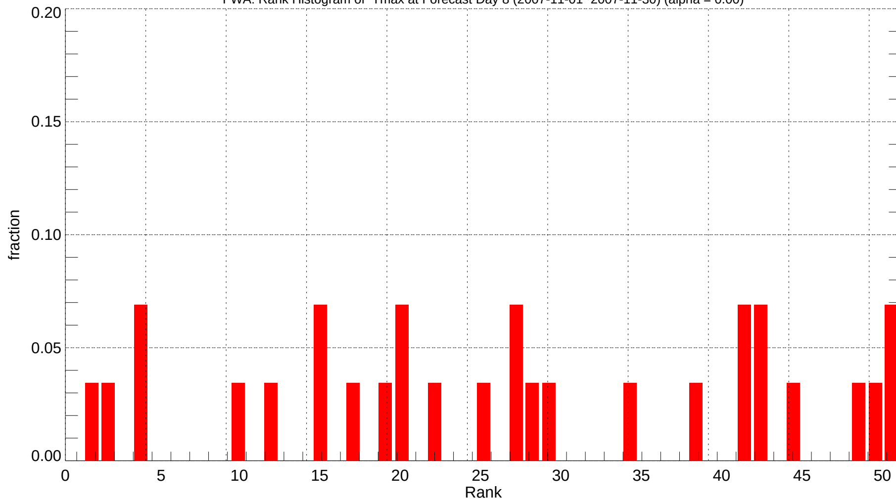
FWA: Rank Histogram of Tmax at Forecast Day 8 (2007-11-01~2007-11-30) (alpha = 0.00)
