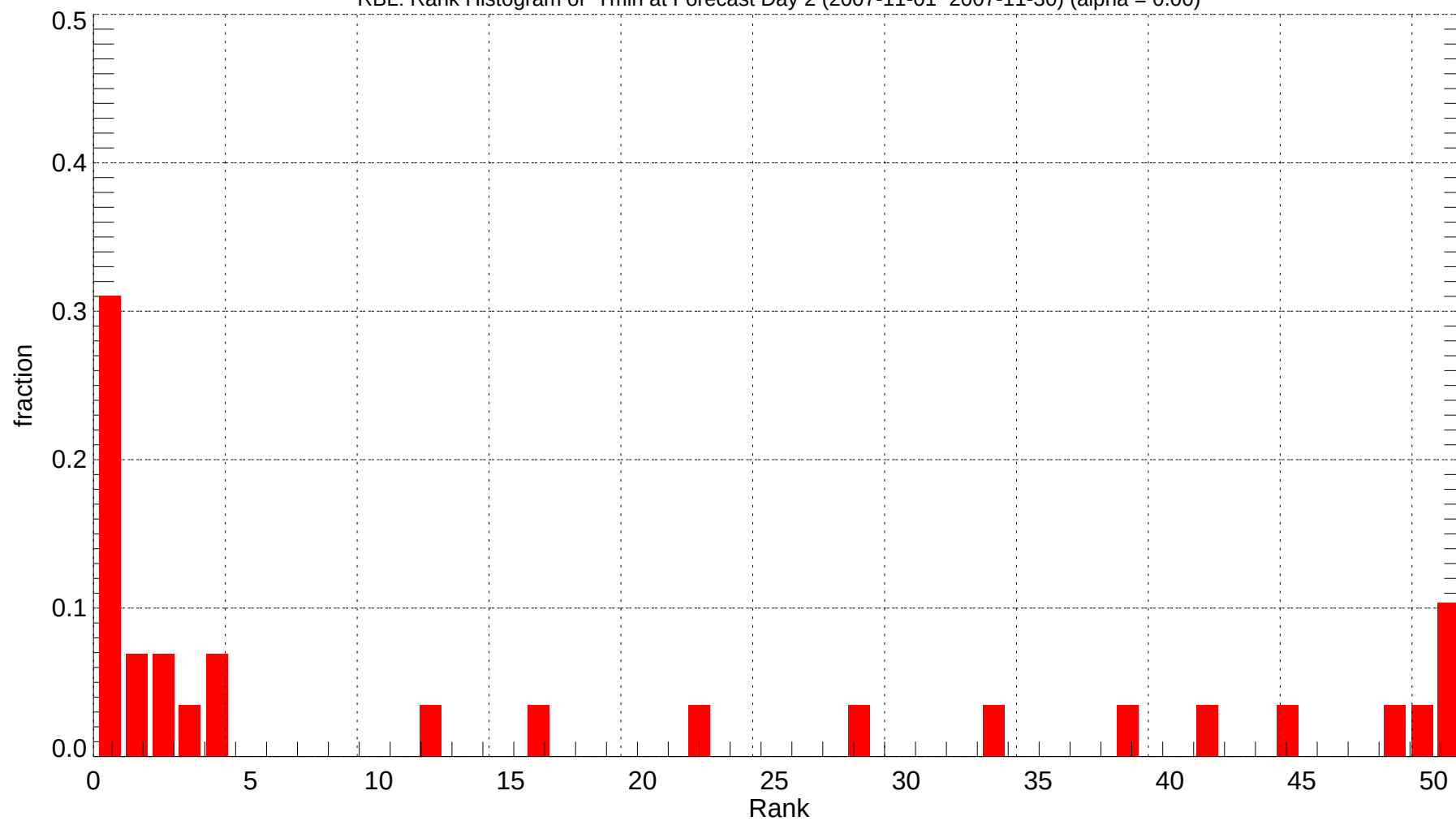
RBL: Rank Histogram of Tmin at Forecast Day 2 (2007-11-01~2007-11-30) (alpha = 0.00)
