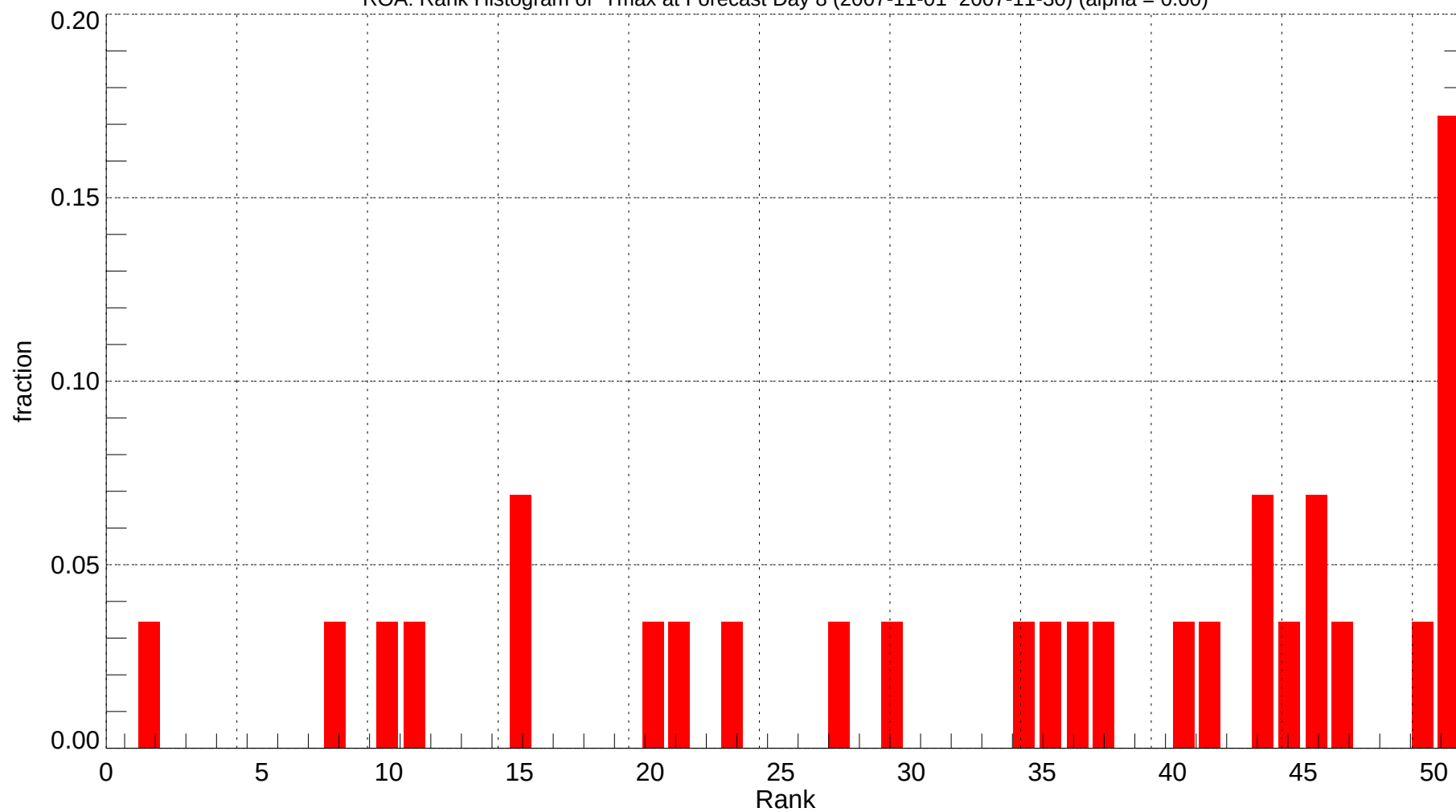
ROA: Rank Histogram of Tmax at Forecast Day 8 (2007-11-01~2007-11-30) (alpha = 0.00)
