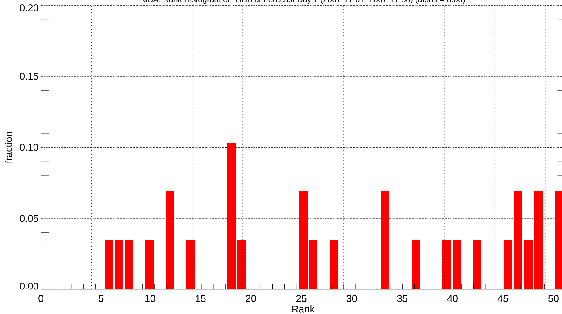
MBA: Rank Histogram of Tmin at Forecast Day 7 (2007-11-01~2007-11-30) (alpha = 0.00)
