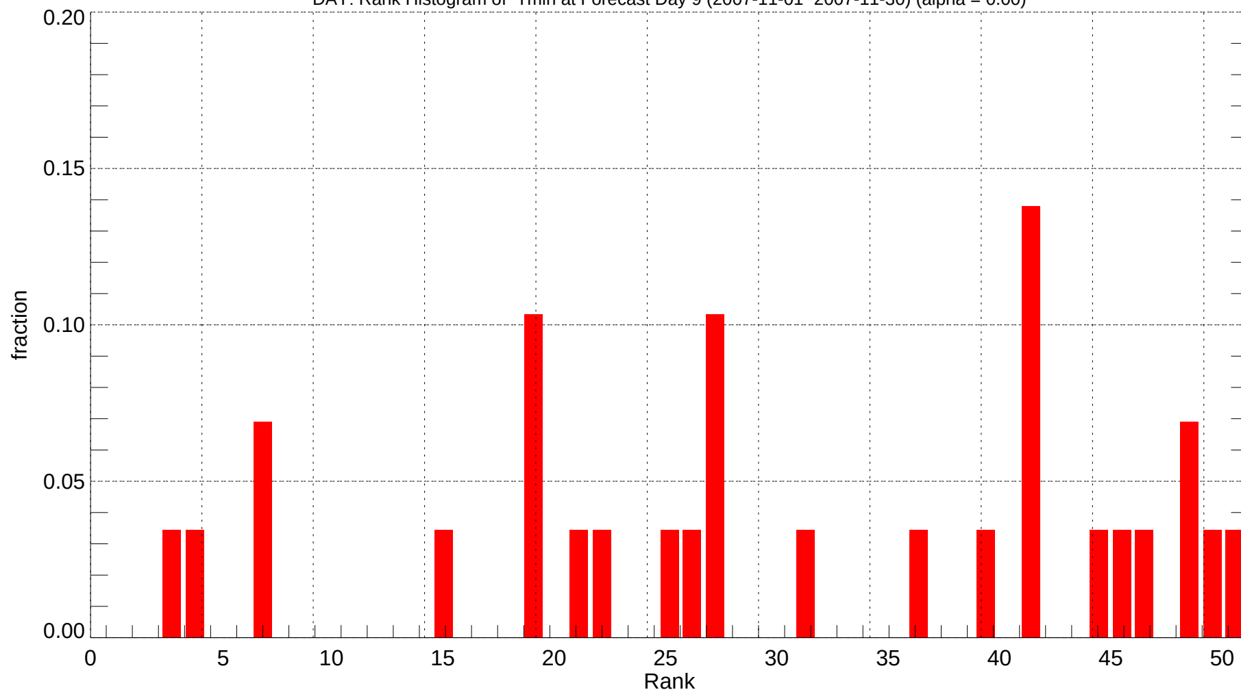
DAY: Rank Histogram of Tmin at Forecast Day 9 (2007-11-01~2007-11-30) (alpha = 0.00)
