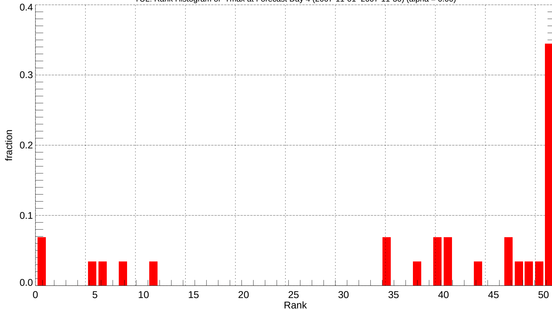
TUL: Rank Histogram of Tmax at Forecast Day 4 (2007-11-01~2007-11-30) (alpha = 0.00)
