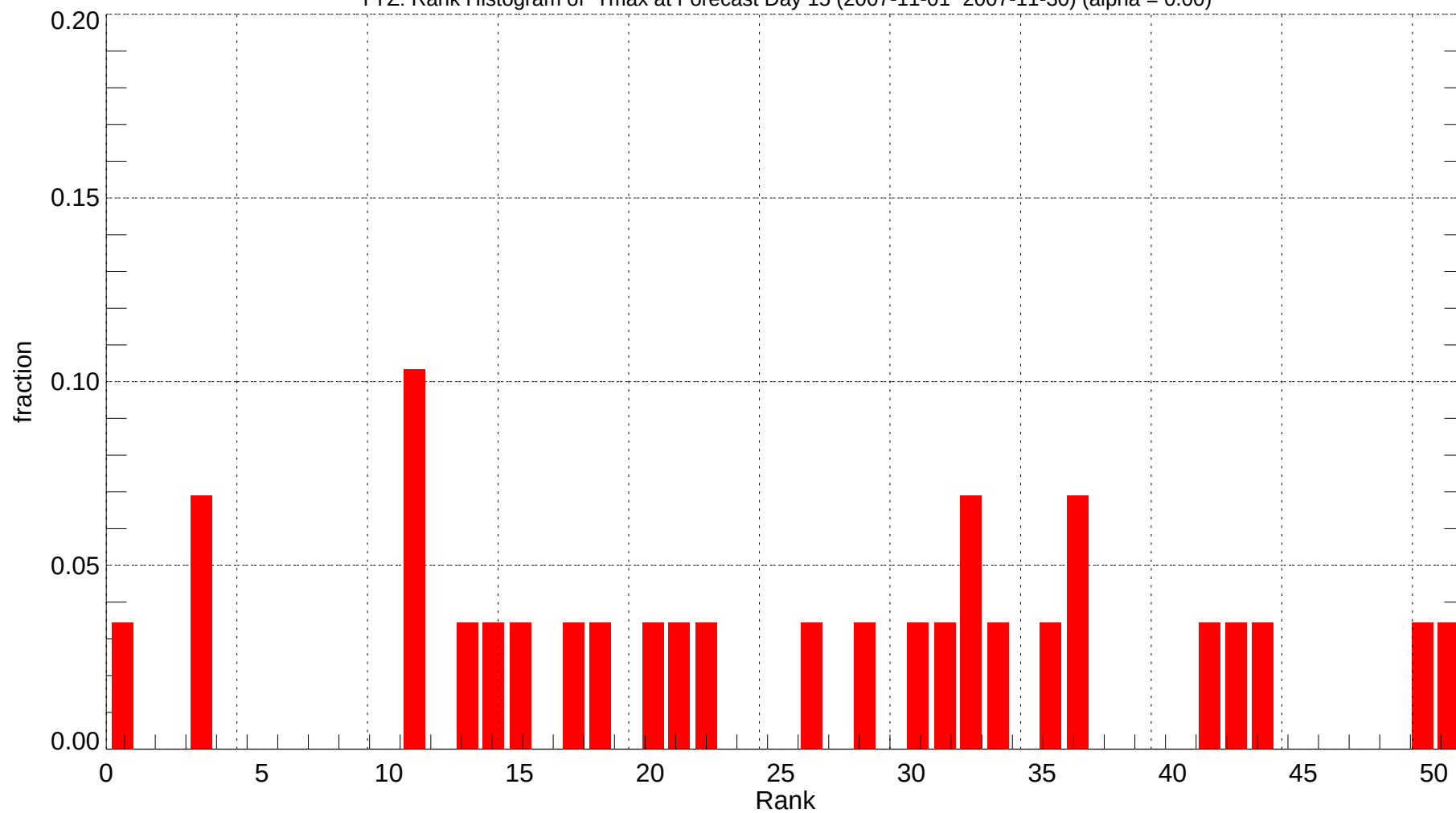
YYZ: Rank Histogram of Tmax at Forecast Day 15 (2007-11-01~2007-11-30) (alpha = 0.00)
