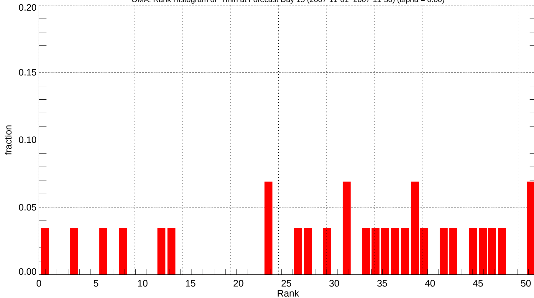
OMA: Rank Histogram of Tmin at Forecast Day 15 (2007-11-01~2007-11-30) (alpha = 0.00)
