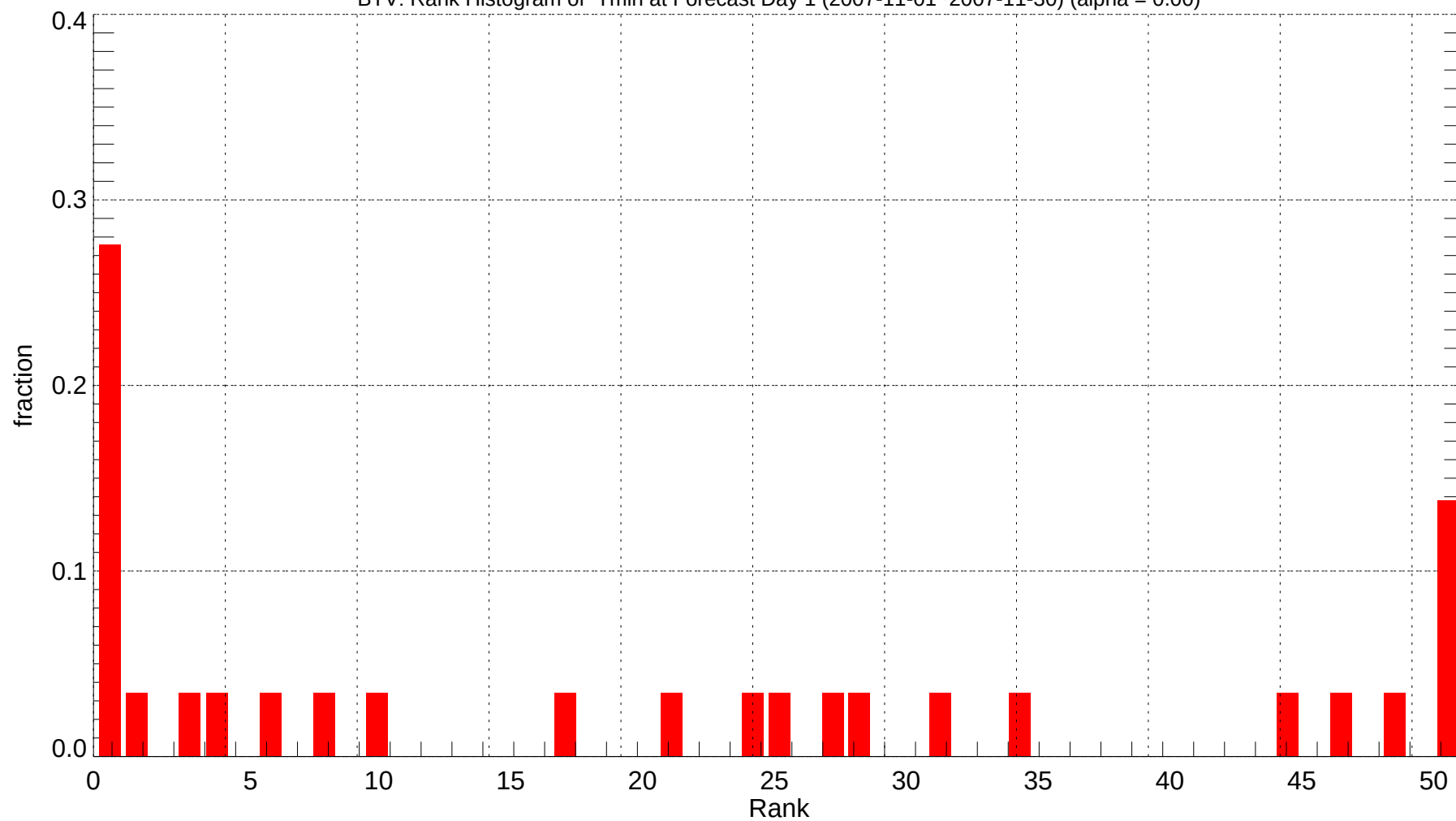
BTV: Rank Histogram of Tmin at Forecast Day 1 (2007-11-01~2007-11-30) (alpha = 0.00)
