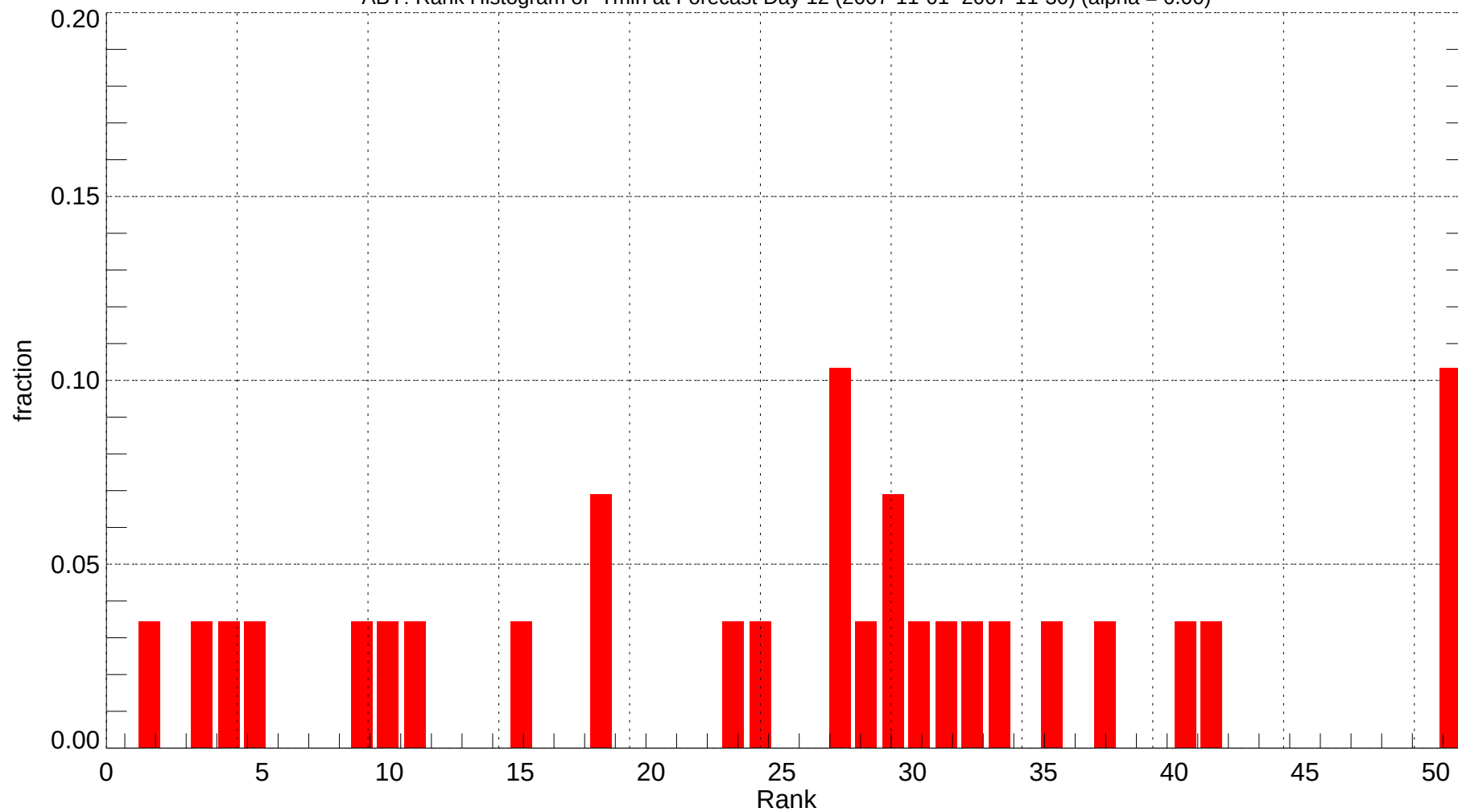
ABY: Rank Histogram of Tmin at Forecast Day 12 (2007-11-01~2007-11-30) (alpha = 0.00)
