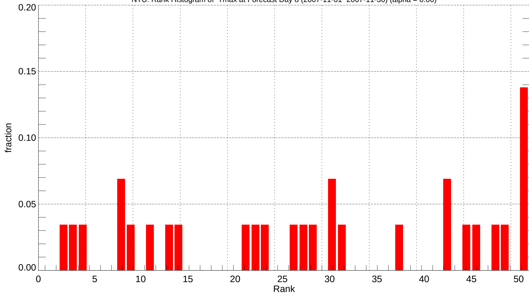
NTU: Rank Histogram of Tmax at Forecast Day 8 (2007-11-01~2007-11-30) (alpha = 0.00)
