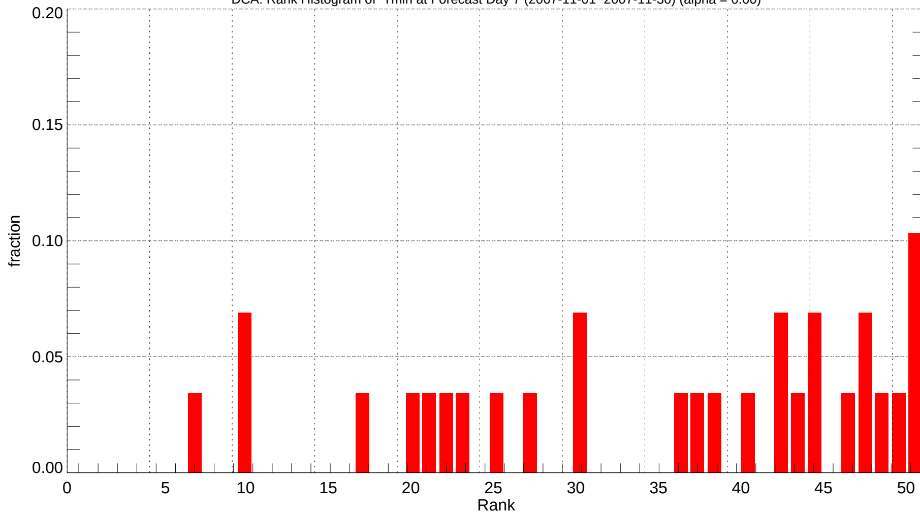
DCA: Rank Histogram of Tmin at Forecast Day 7 (2007-11-01~2007-11-30) (alpha = 0.00)
