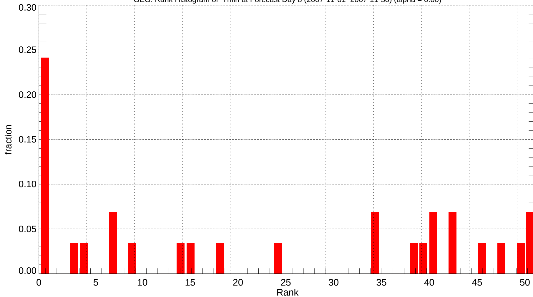
GEG: Rank Histogram of Tmin at Forecast Day 8 (2007-11-01~2007-11-30) (alpha = 0.00)
