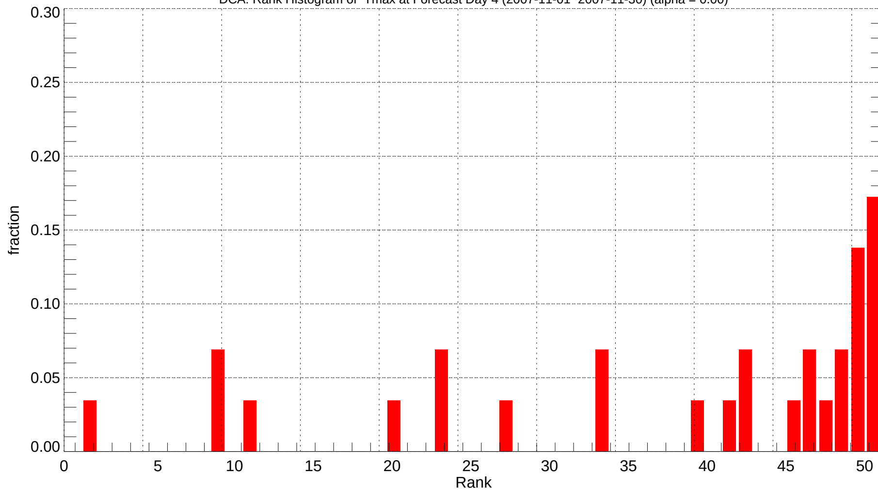
DCA: Rank Histogram of Tmax at Forecast Day 4 (2007-11-01~2007-11-30) (alpha = 0.00)
