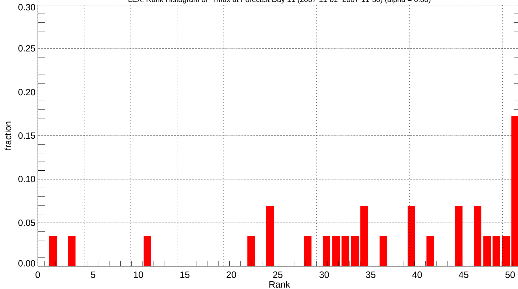
LEX: Rank Histogram of Tmax at Forecast Day 11 (2007-11-01~2007-11-30) (alpha = 0.00)
