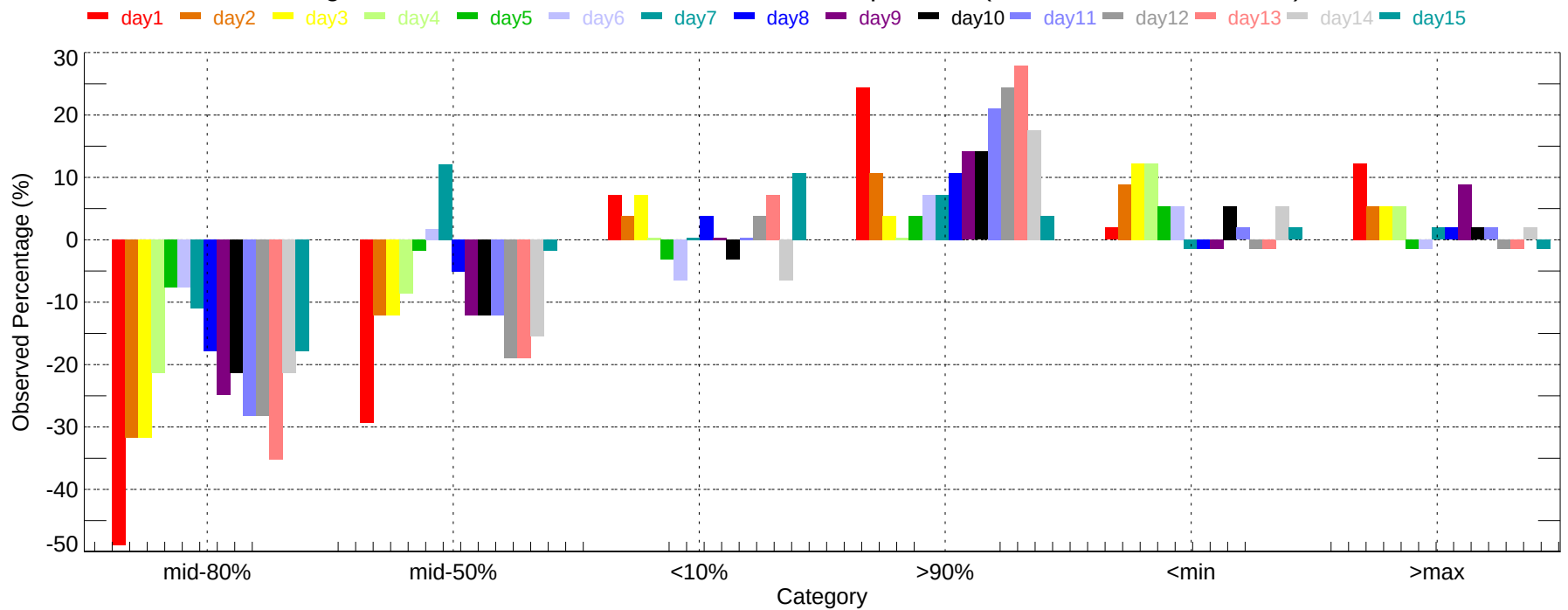
Observed Percentage Deviation of Ensembles - DFW: Min Temperature (2007-11-01~2007-11-30)
