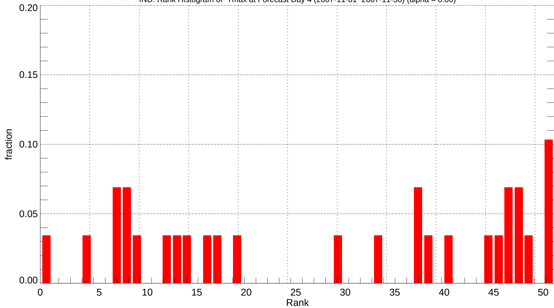
IND: Rank Histogram of Tmax at Forecast Day 4 (2007-11-01~2007-11-30) (alpha = 0.00)
