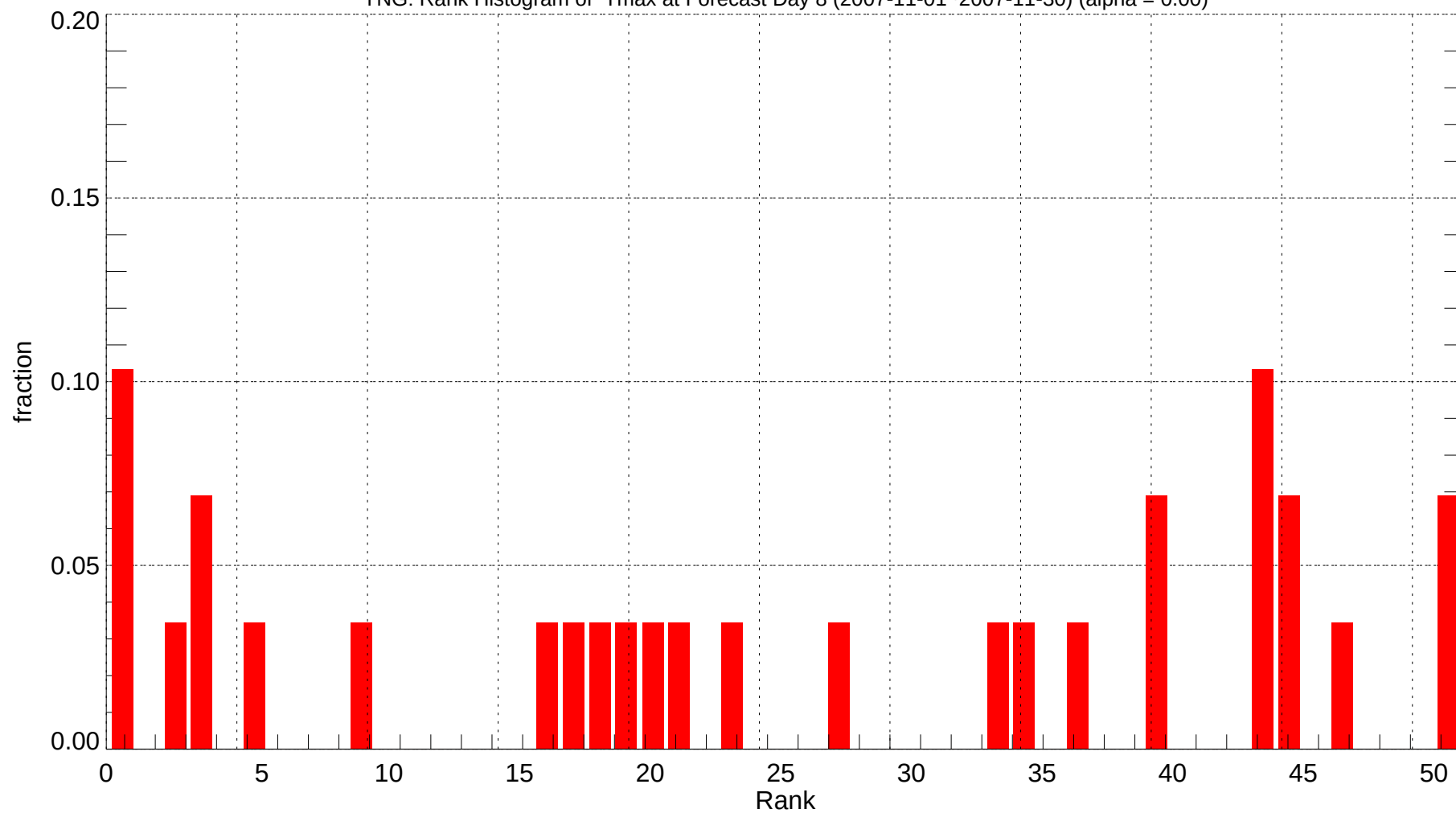
YNG: Rank Histogram of Tmax at Forecast Day 8 (2007-11-01~2007-11-30) (alpha = 0.00)
