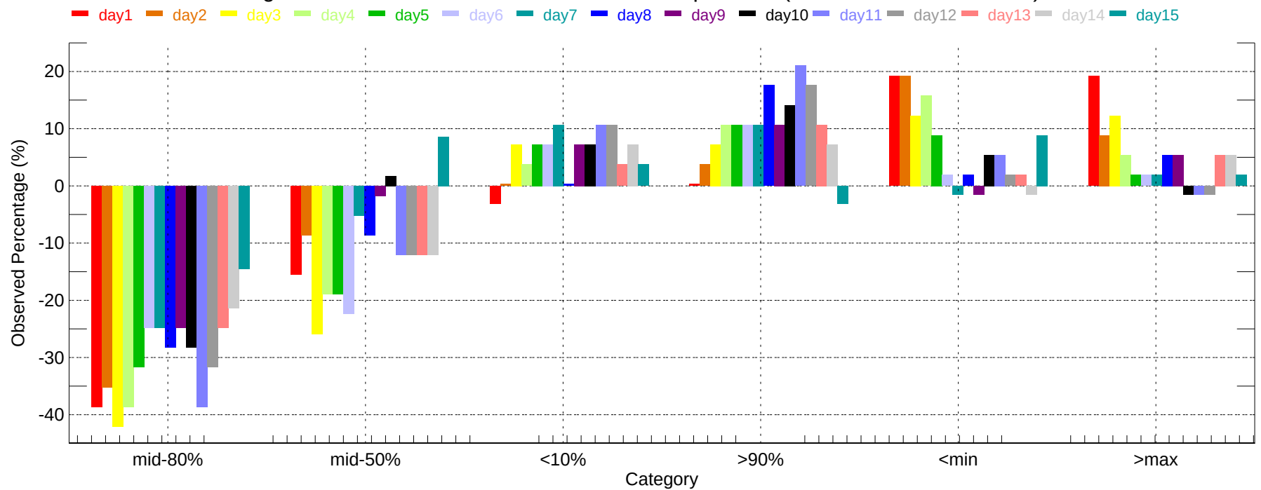
Observed Percentage Deviation of Ensembles - SAT: Min Temperature (2007-11-01~2007-11-30)
