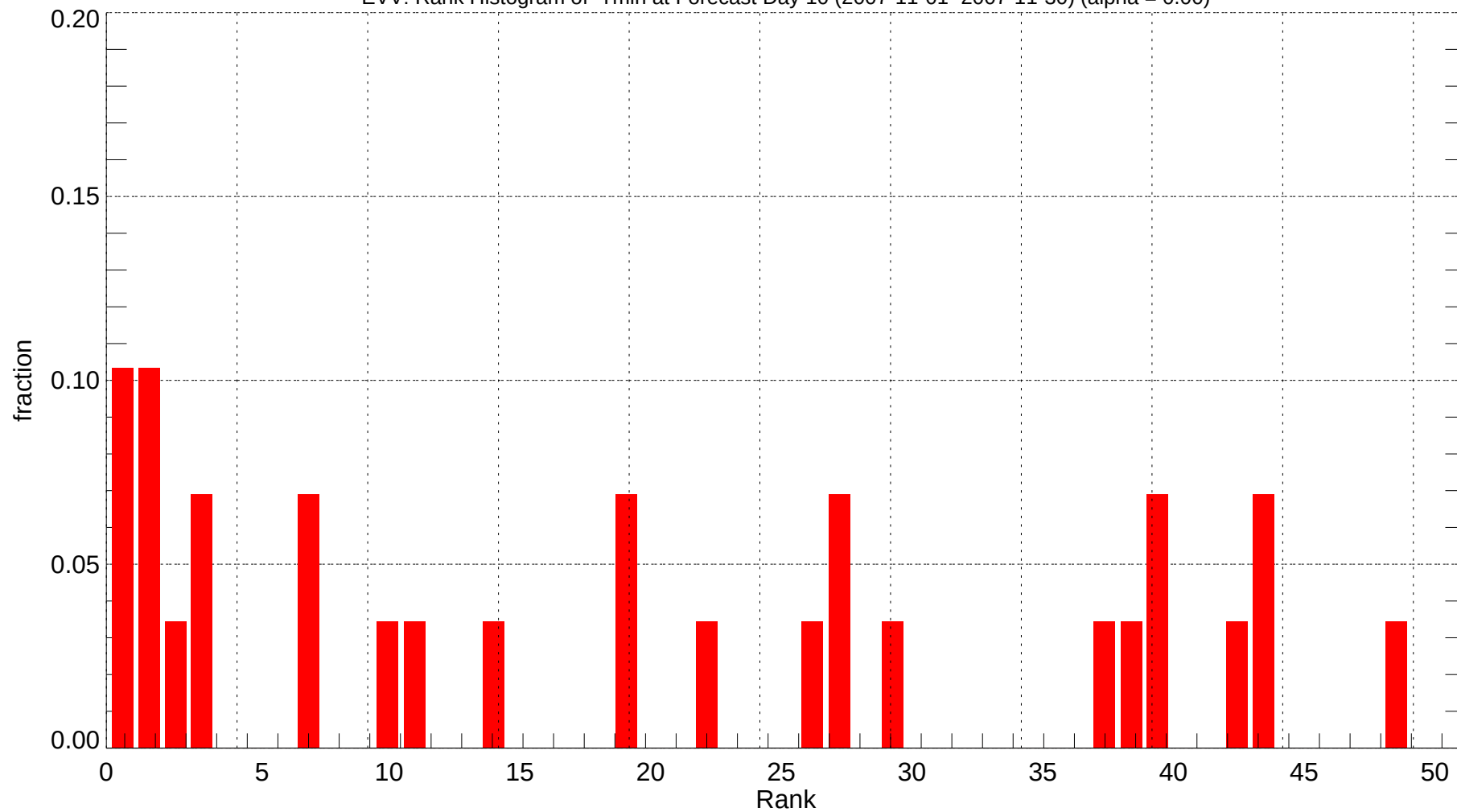
EVV: Rank Histogram of Tmin at Forecast Day 10 (2007-11-01~2007-11-30) (alpha = 0.00)
