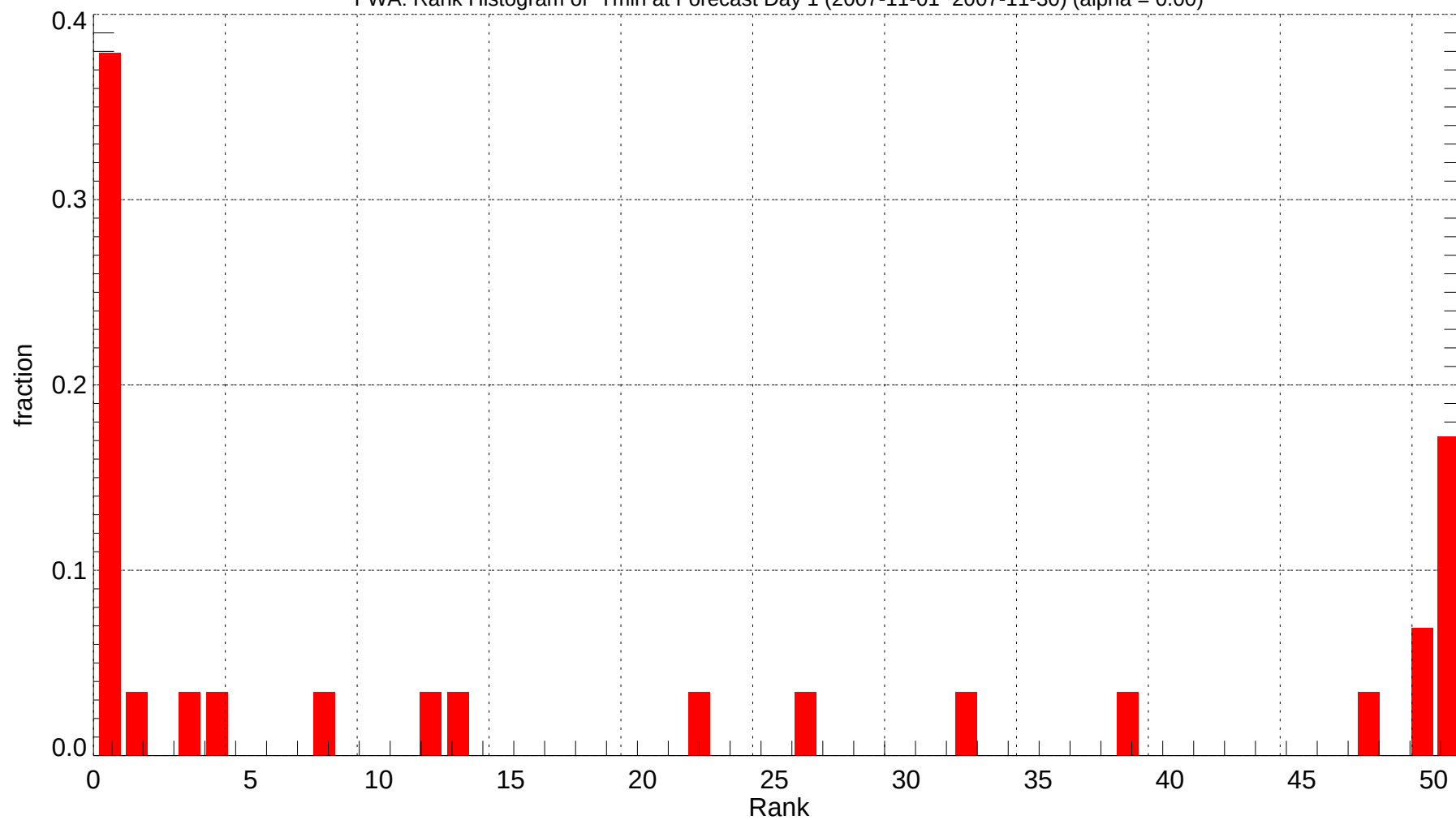
FWA: Rank Histogram of Tmin at Forecast Day 1 (2007-11-01~2007-11-30) (alpha = 0.00)
