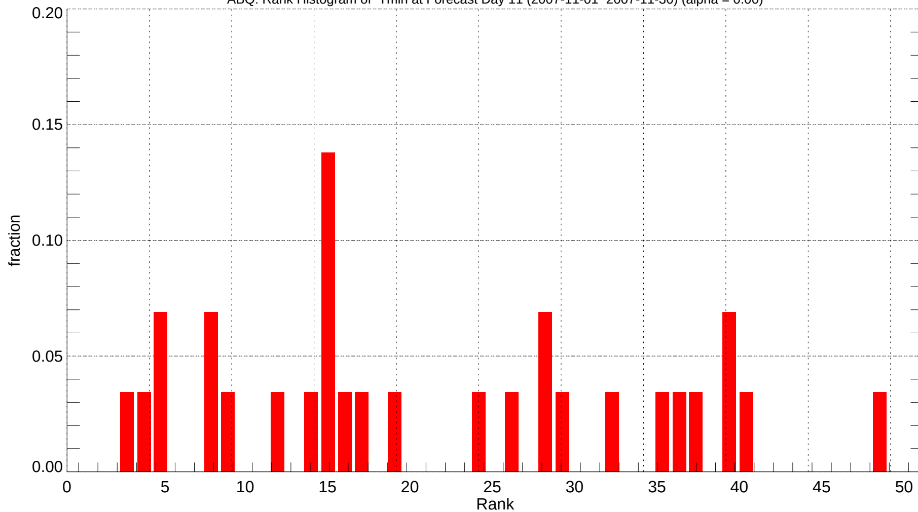
ABQ: Rank Histogram of Tmin at Forecast Day 11 (2007-11-01~2007-11-30) (alpha = 0.00)
