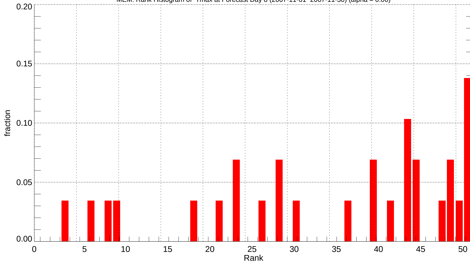
MEM: Rank Histogram of Tmax at Forecast Day 8 (2007-11-01~2007-11-30) (alpha = 0.00)
