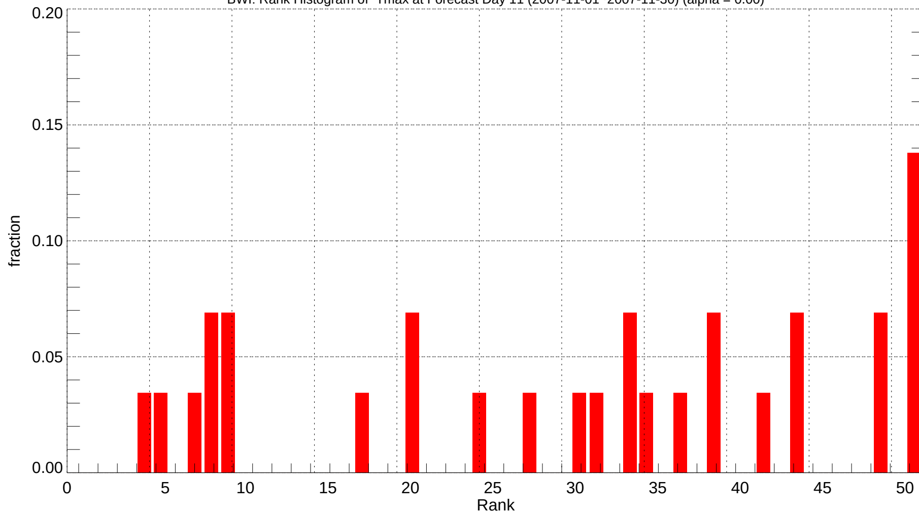
BWI: Rank Histogram of Tmax at Forecast Day 11 (2007-11-01~2007-11-30) (alpha = 0.00)
