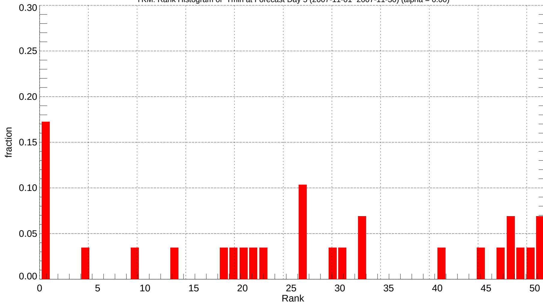
YKM: Rank Histogram of Tmin at Forecast Day 5 (2007-11-01~2007-11-30) (alpha = 0.00)
