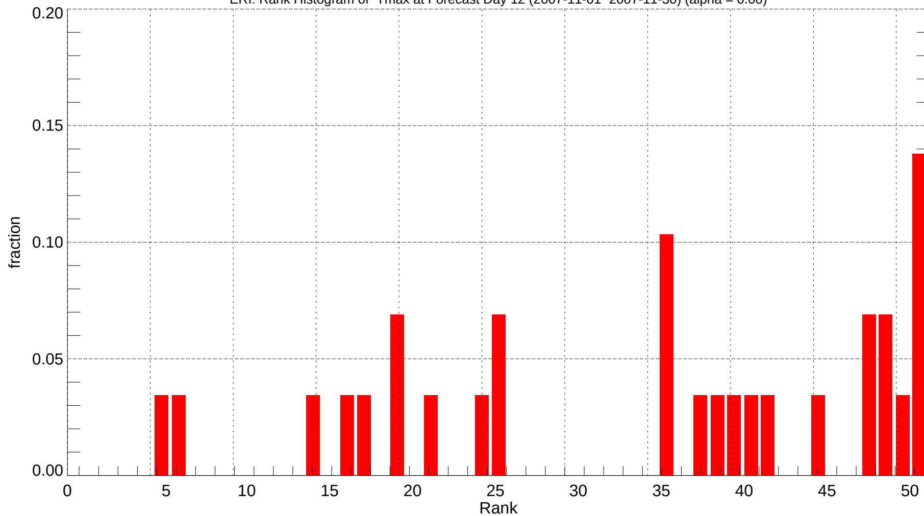
ERI: Rank Histogram of Tmax at Forecast Day 12 (2007-11-01~2007-11-30) (alpha = 0.00)
