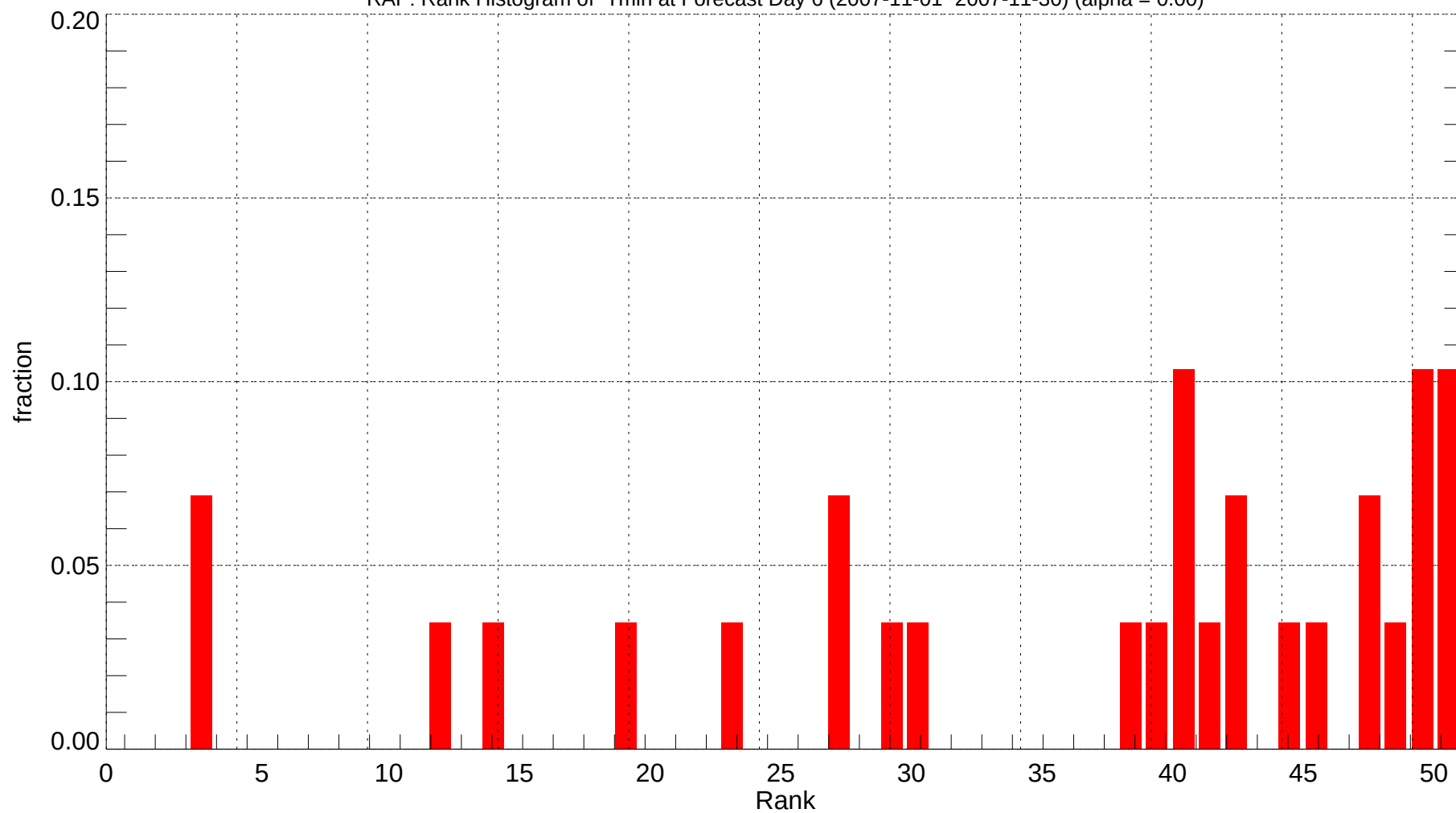
RAP: Rank Histogram of Tmin at Forecast Day 6 (2007-11-01~2007-11-30) (alpha = 0.00)
