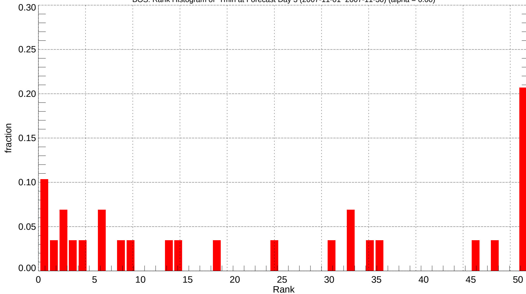
BOS: Rank Histogram of Tmin at Forecast Day 3 (2007-11-01~2007-11-30) (alpha = 0.00)
