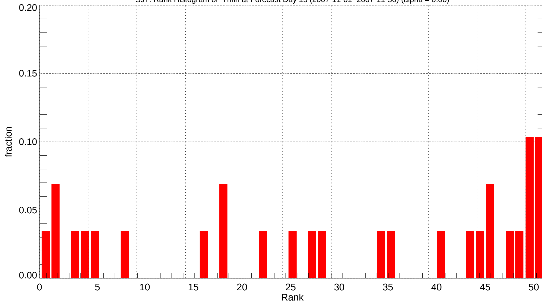
SJT: Rank Histogram of Tmin at Forecast Day 13 (2007-11-01~2007-11-30) (alpha = 0.00)
