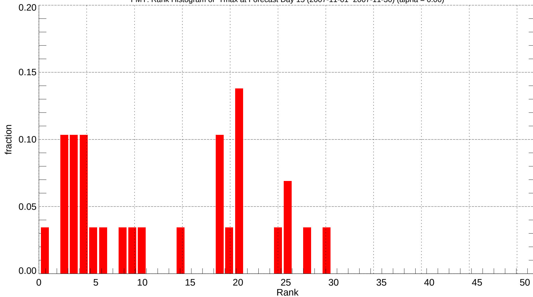
FMY: Rank Histogram of Tmax at Forecast Day 15 (2007-11-01~2007-11-30) (alpha = 0.00)
