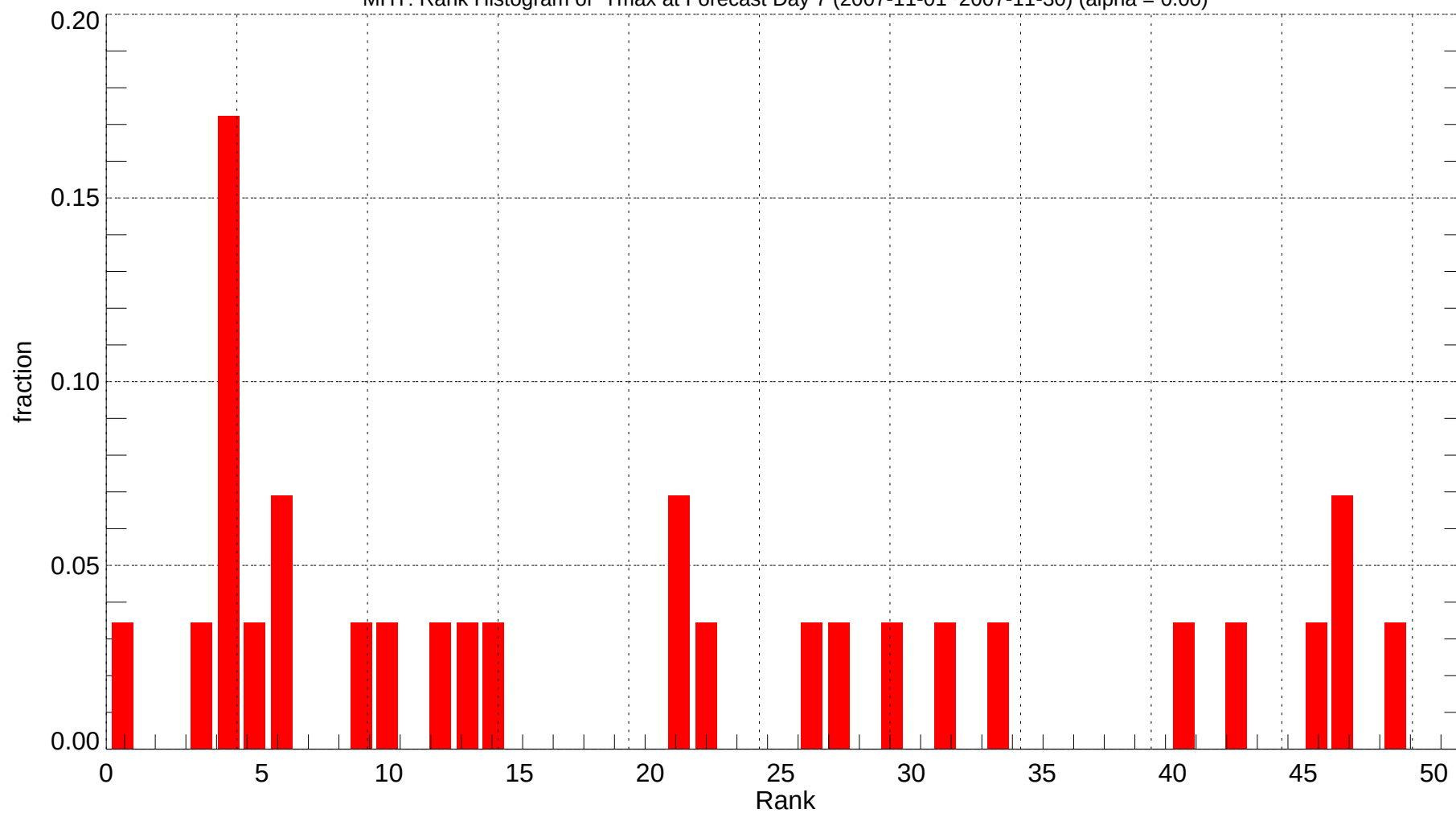
MHT: Rank Histogram of Tmax at Forecast Day 7 (2007-11-01~2007-11-30) (alpha = 0.00)
