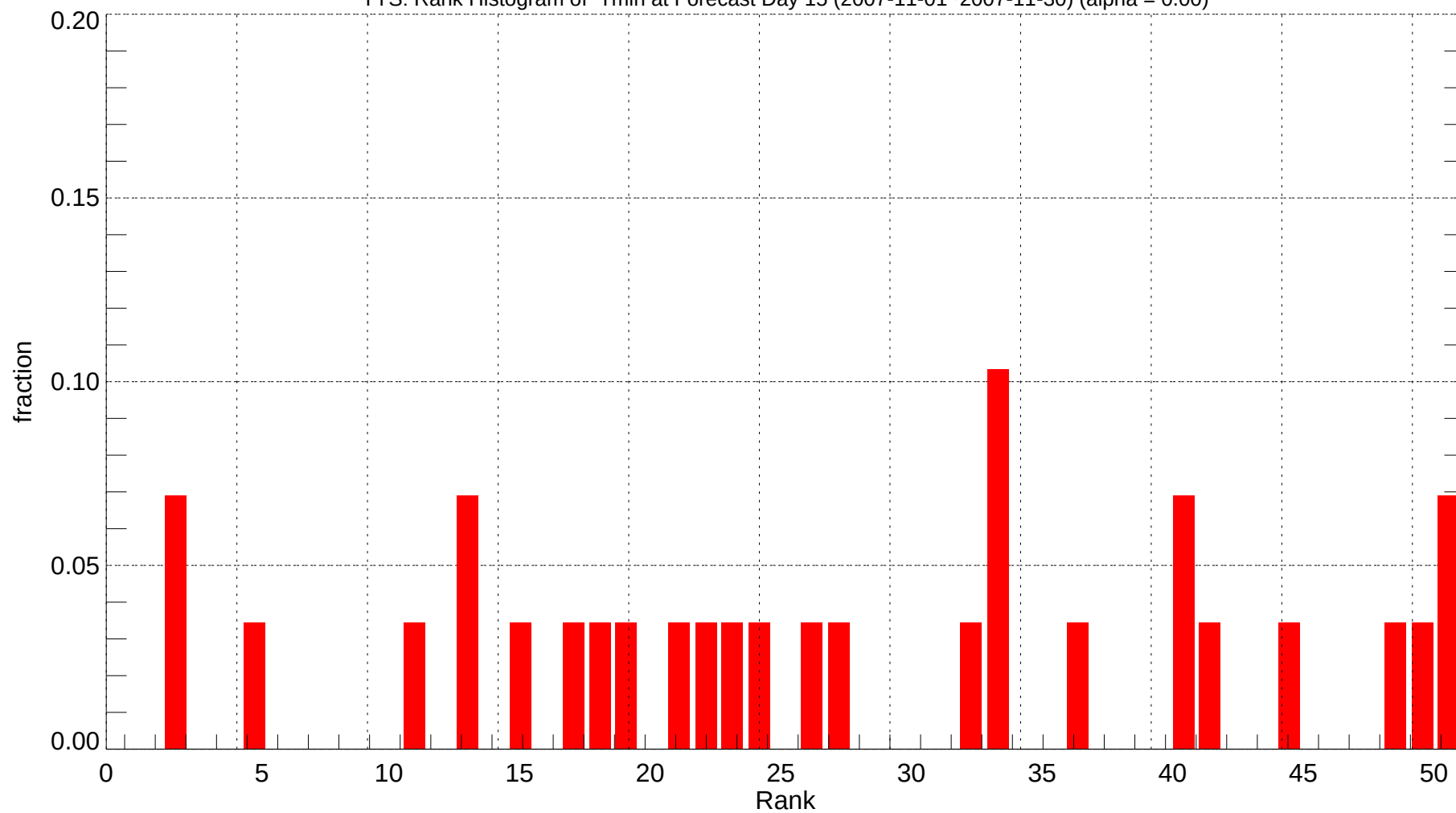
TYS: Rank Histogram of Tmin at Forecast Day 15 (2007-11-01~2007-11-30) (alpha = 0.00)
