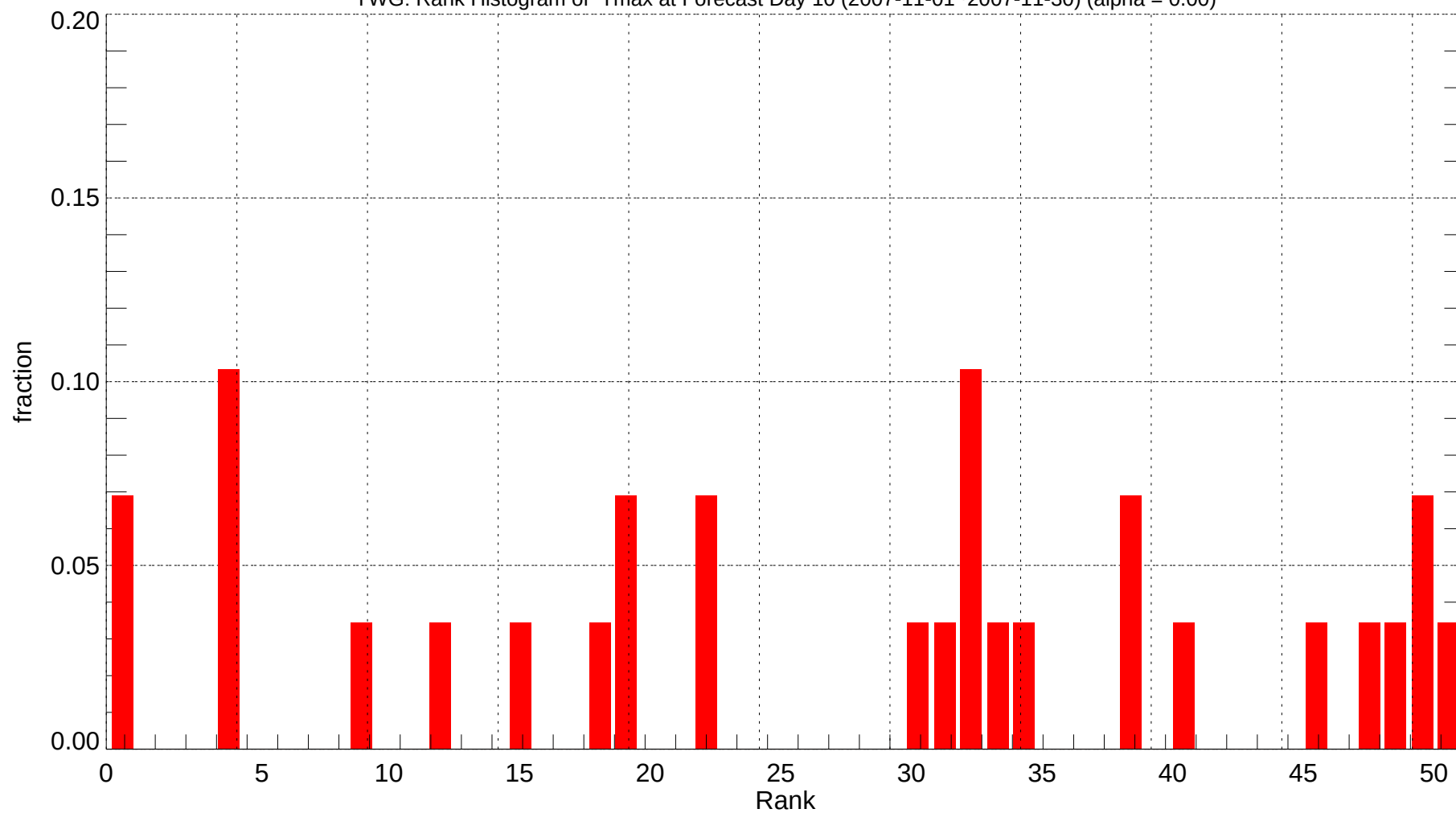
YWG: Rank Histogram of Tmax at Forecast Day 10 (2007-11-01~2007-11-30) (alpha = 0.00)
