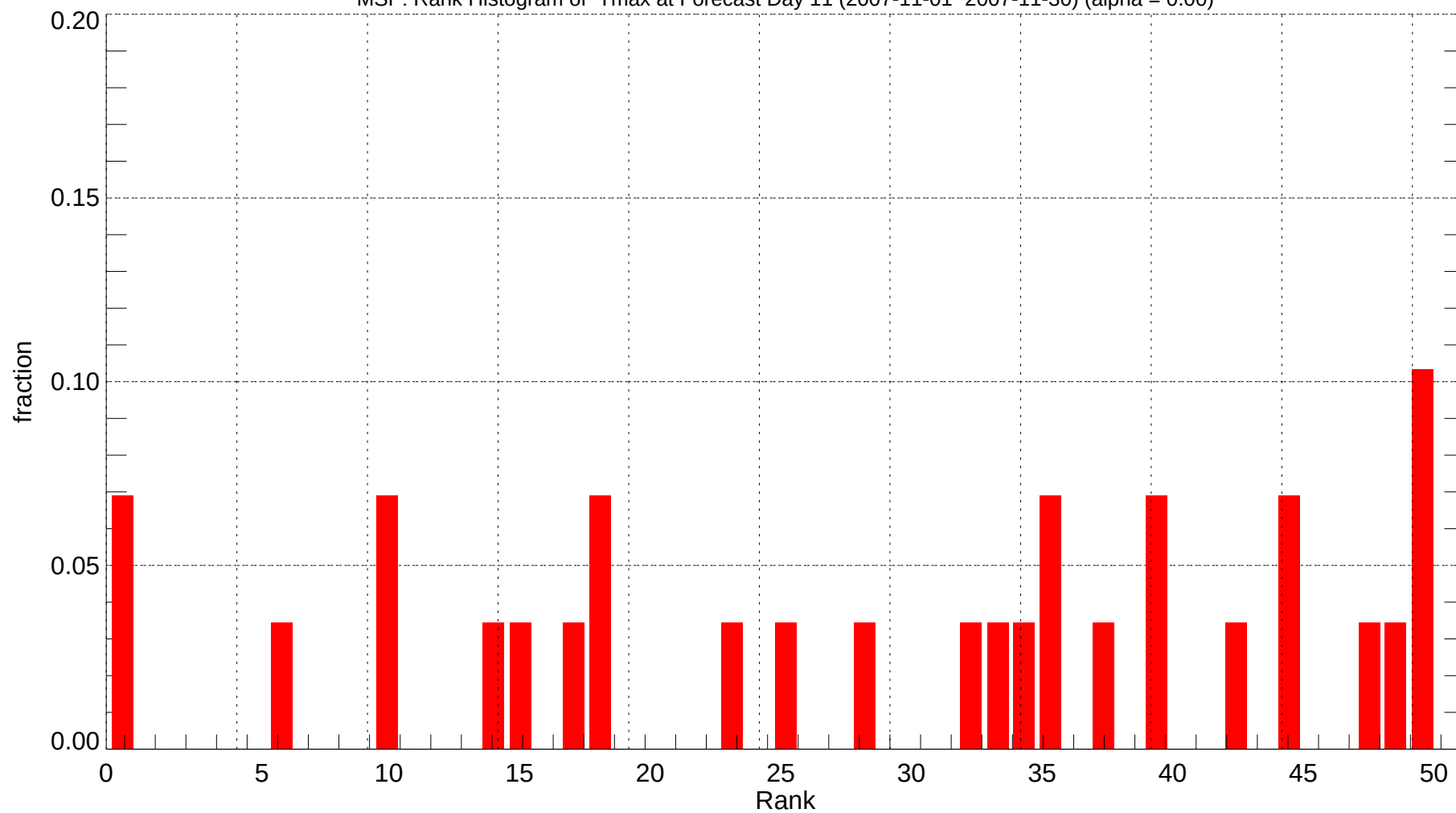
MSP: Rank Histogram of Tmax at Forecast Day 11 (2007-11-01~2007-11-30) (alpha = 0.00)
