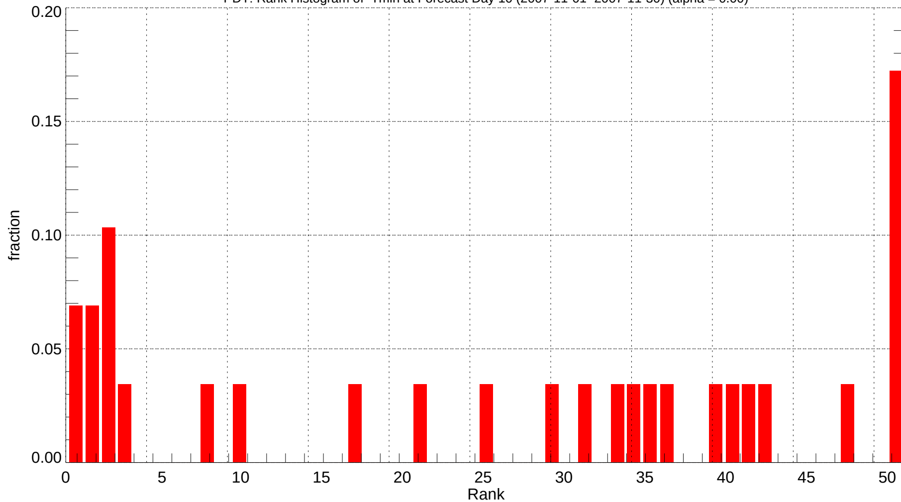
PDT: Rank Histogram of Tmin at Forecast Day 10 (2007-11-01~2007-11-30) (alpha = 0.00)
