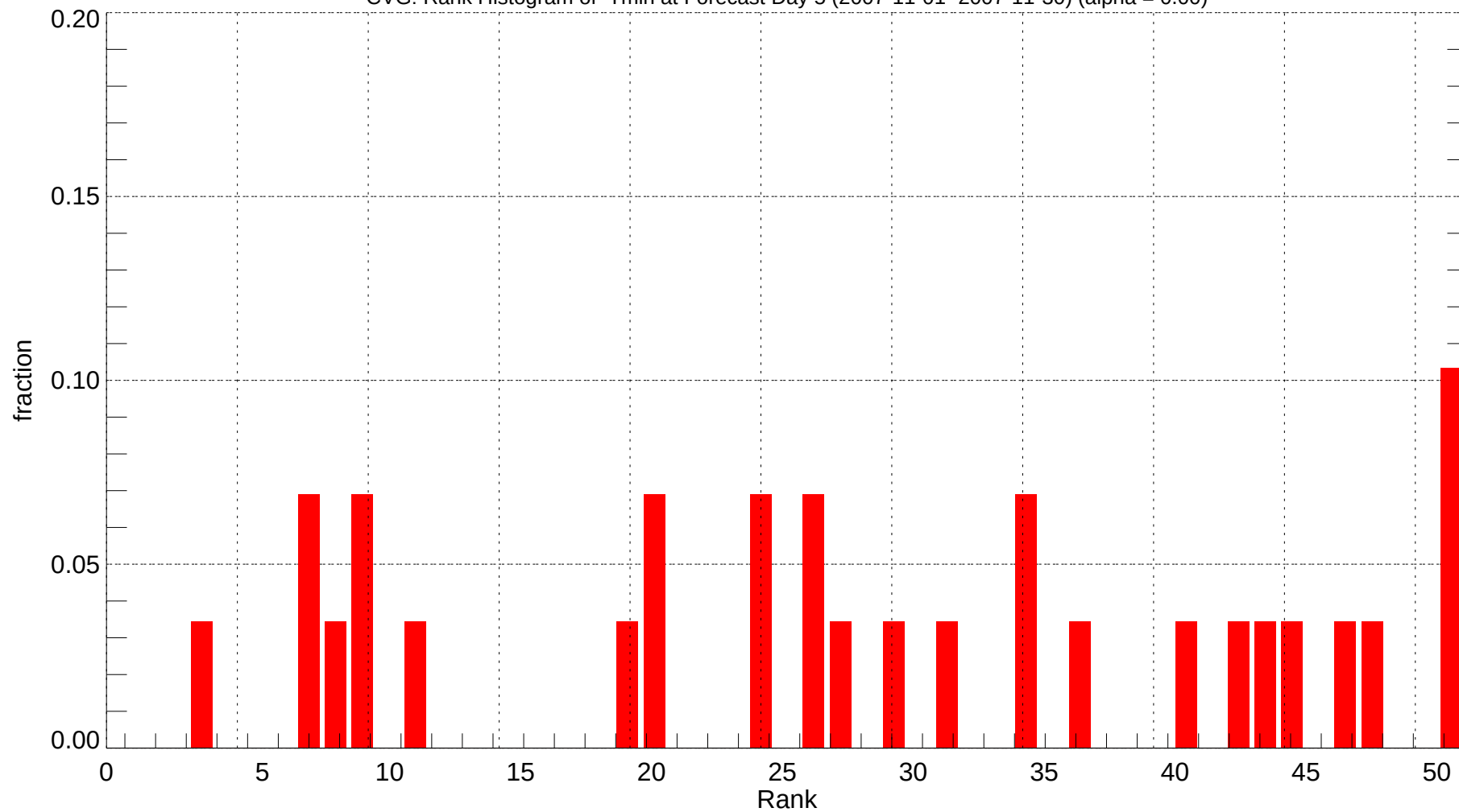
CVG: Rank Histogram of Tmin at Forecast Day 5 (2007-11-01~2007-11-30) (alpha = 0.00)
