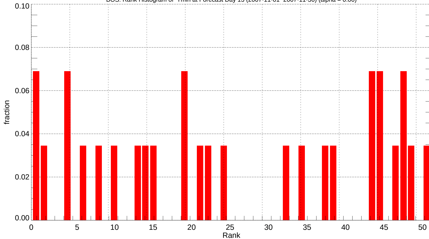
BOS: Rank Histogram of Tmin at Forecast Day 13 (2007-11-01~2007-11-30) (alpha = 0.00)
