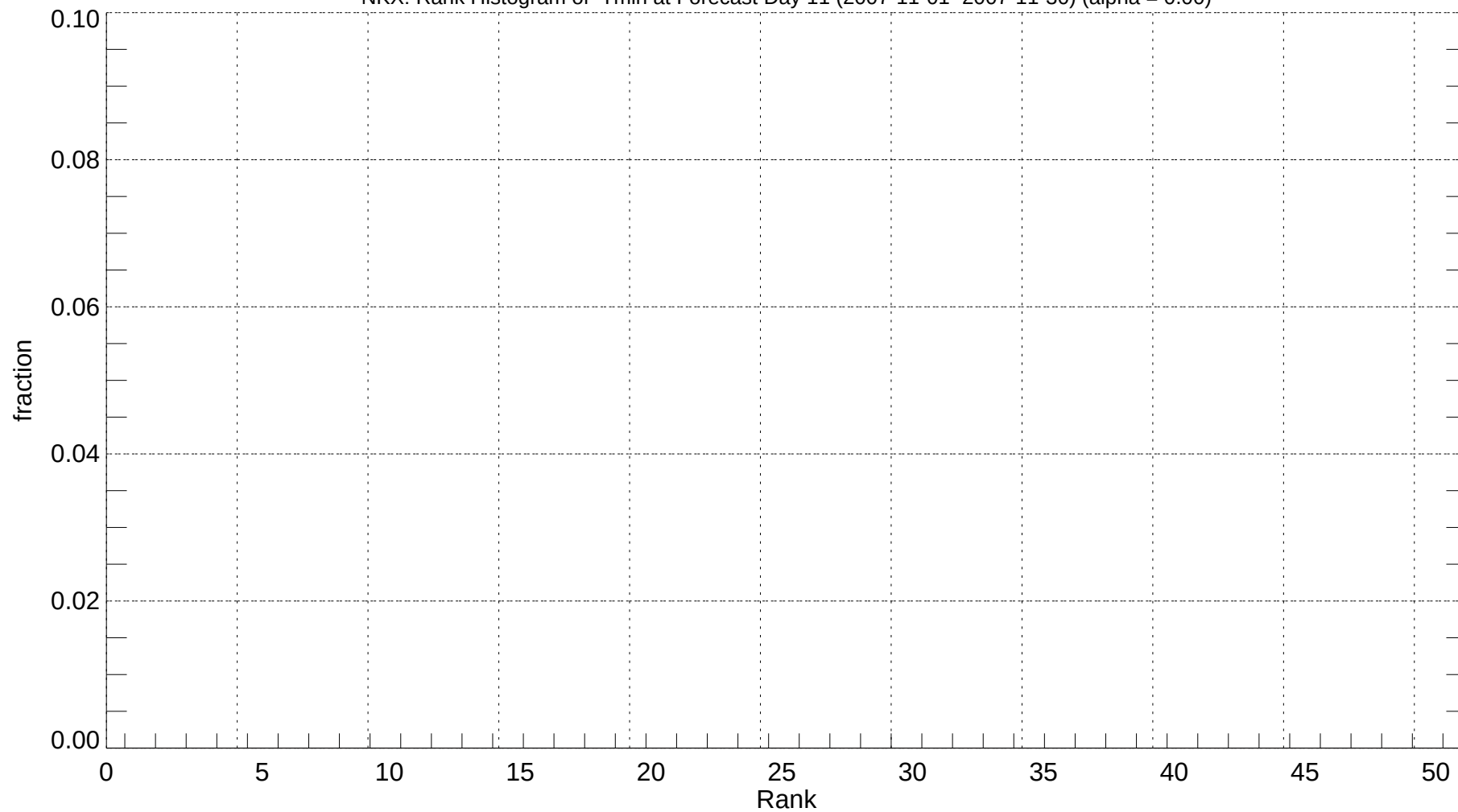
NKX: Rank Histogram of Tmin at Forecast Day 11 (2007-11-01~2007-11-30) (alpha = 0.00)
