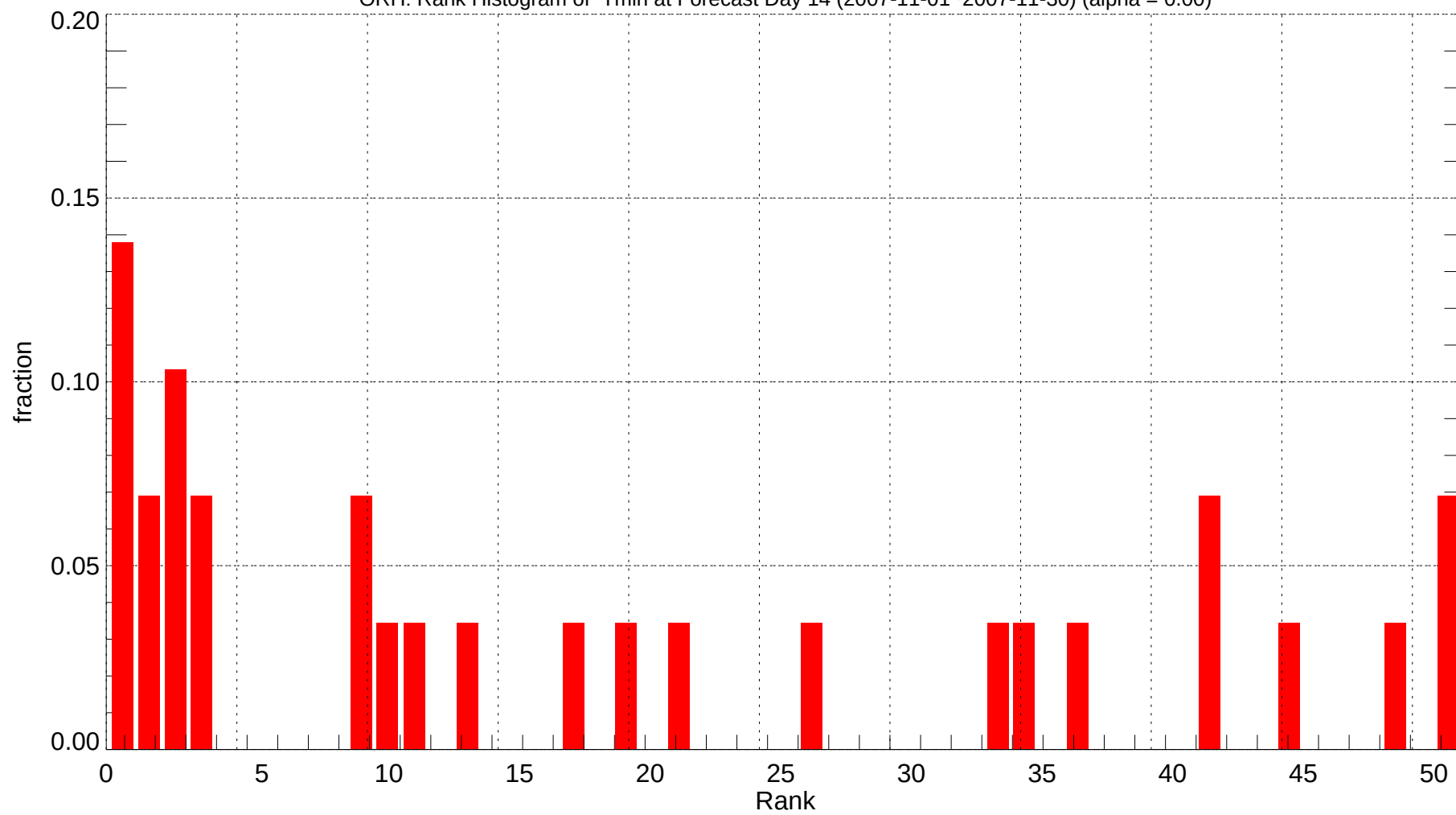
ORH: Rank Histogram of Tmin at Forecast Day 14 (2007-11-01~2007-11-30) (alpha = 0.00)
