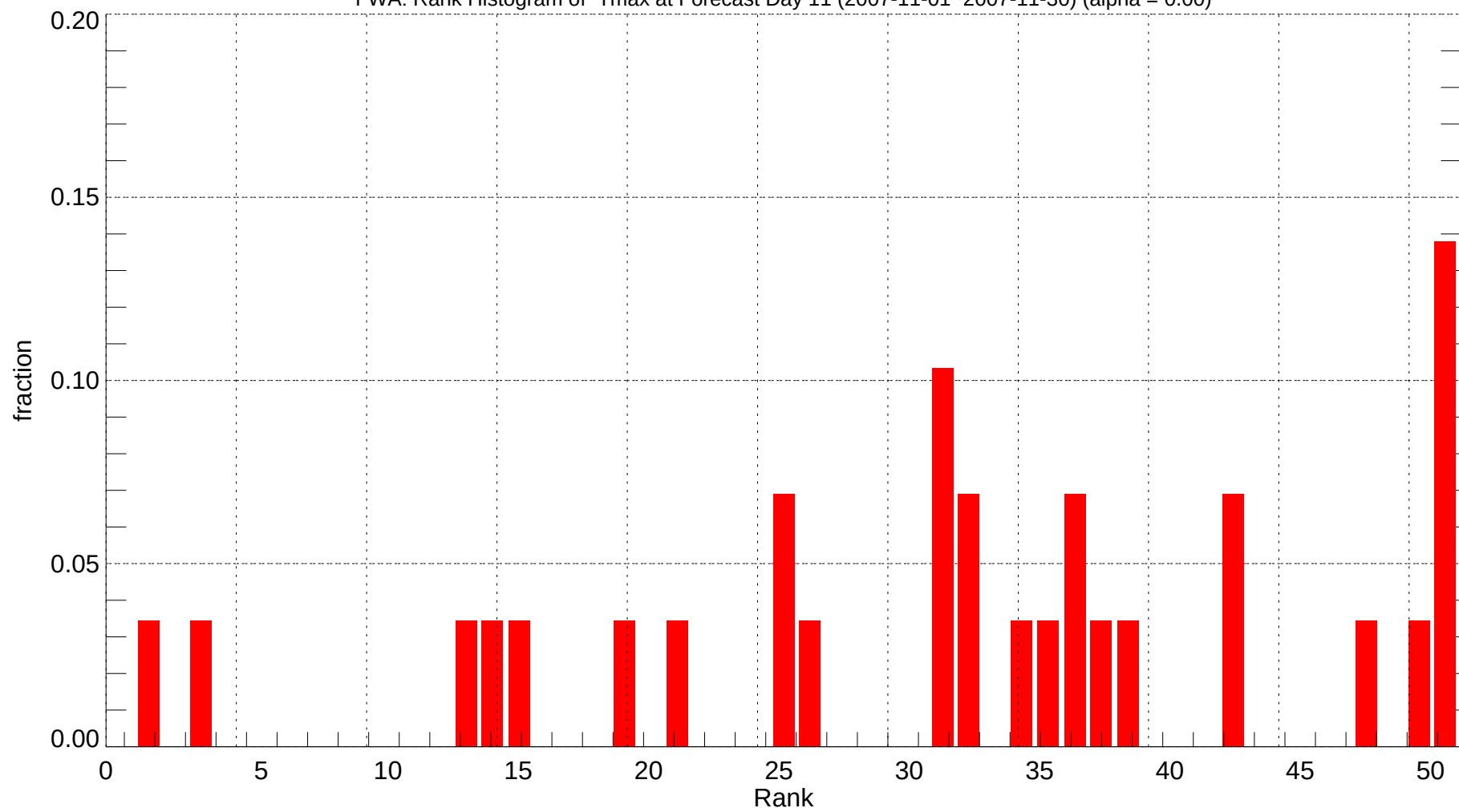
FWA: Rank Histogram of Tmax at Forecast Day 11 (2007-11-01~2007-11-30) (alpha = 0.00)
