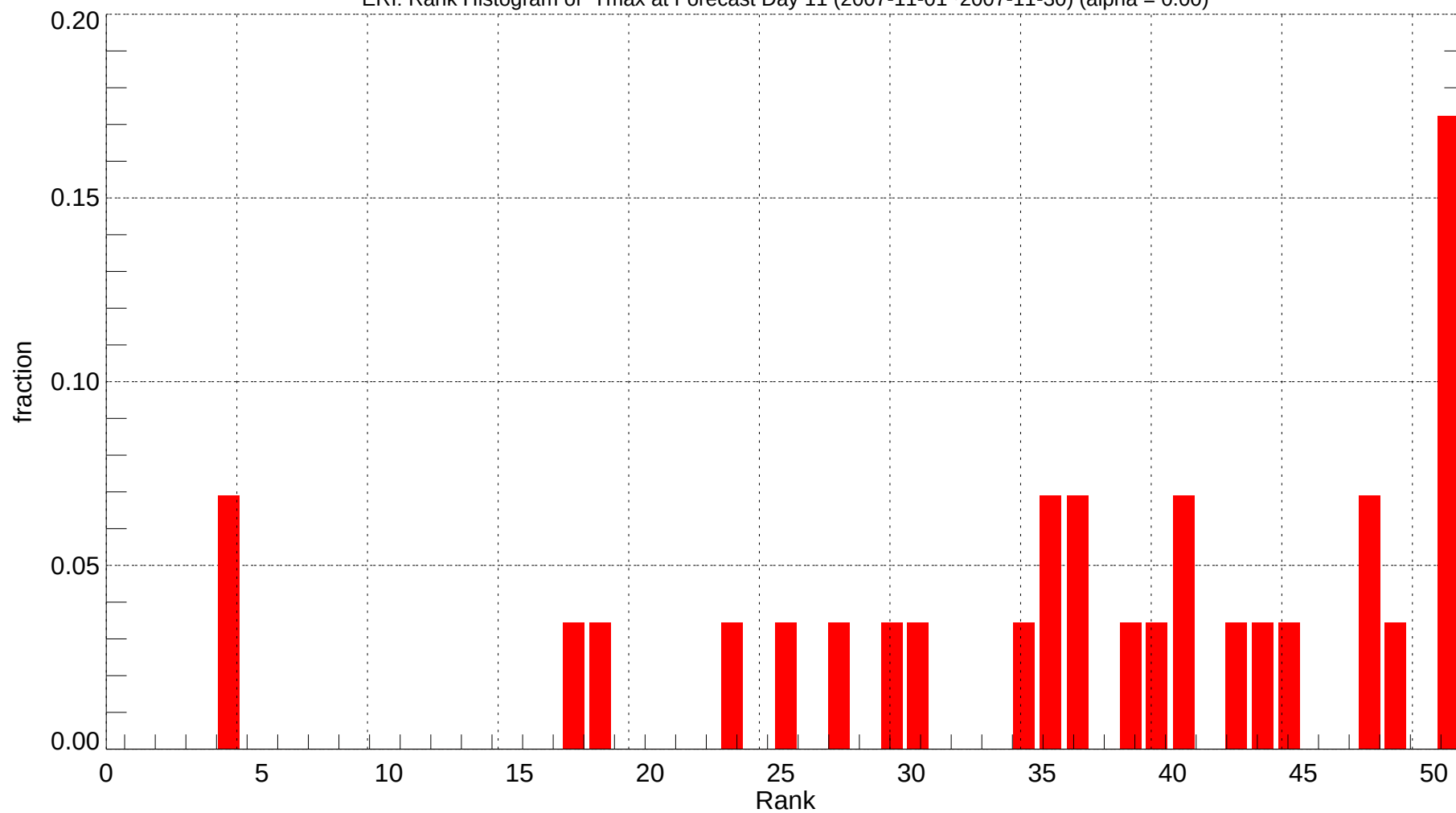
ERI: Rank Histogram of Tmax at Forecast Day 11 (2007-11-01~2007-11-30) (alpha = 0.00)
