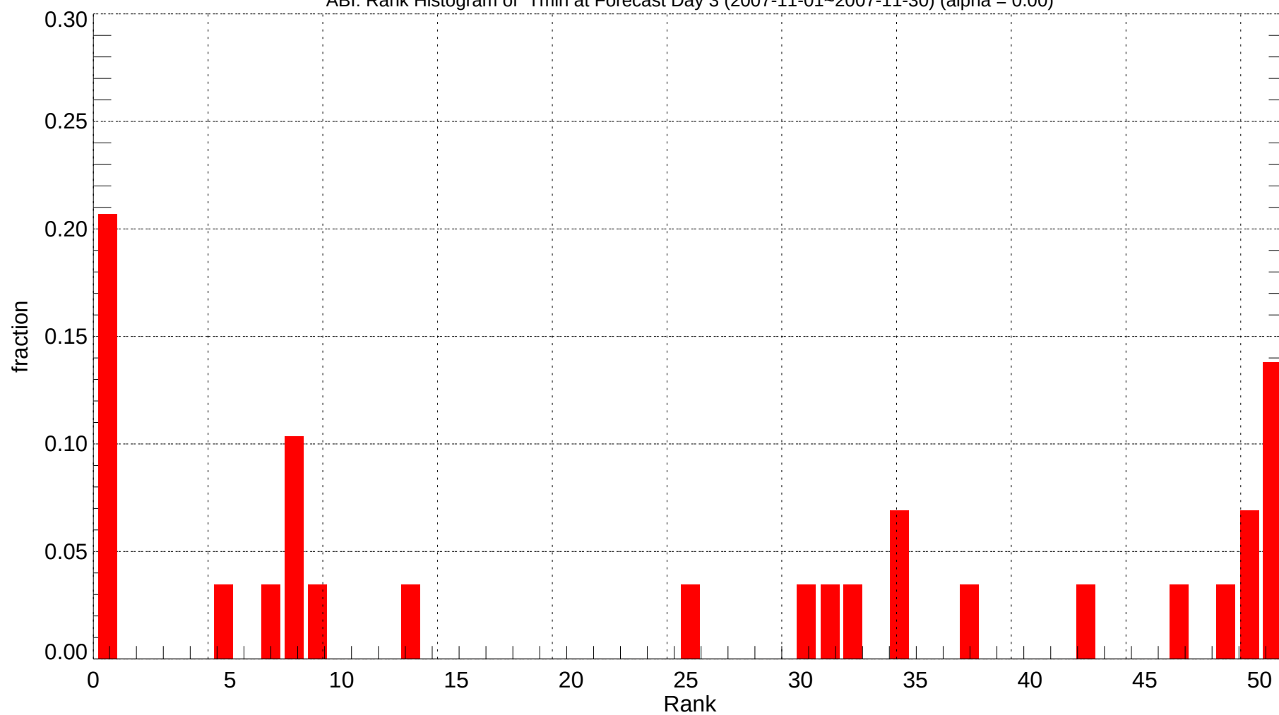
ABI: Rank Histogram of Tmin at Forecast Day 3 (2007-11-01~2007-11-30) (alpha = 0.00)
