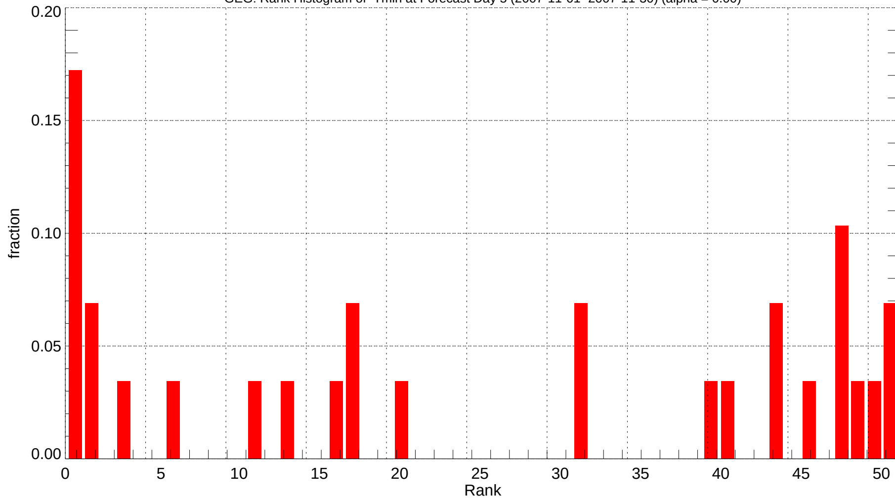
GEG: Rank Histogram of Tmin at Forecast Day 5 (2007-11-01~2007-11-30) (alpha = 0.00)
