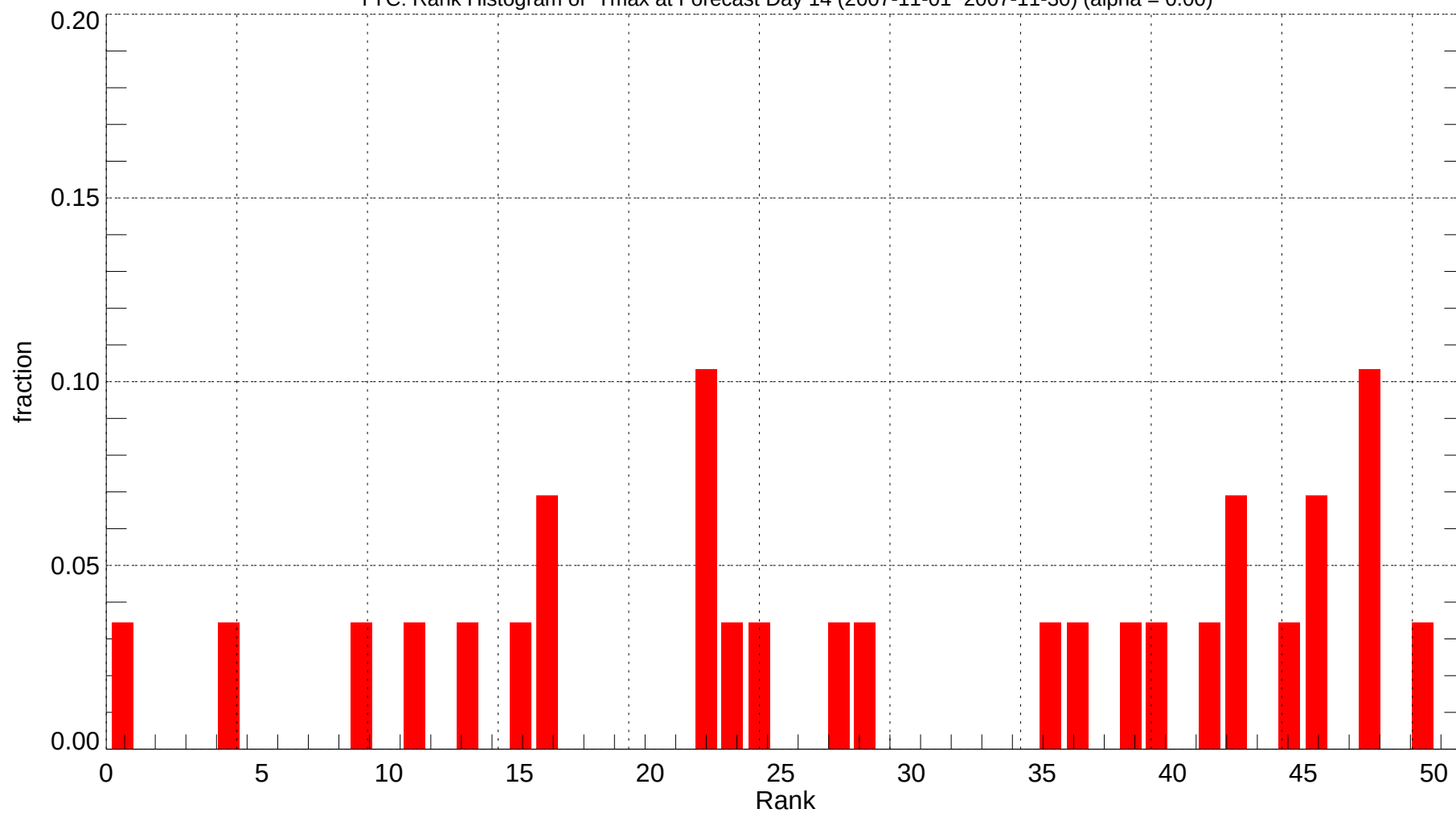
YYC: Rank Histogram of Tmax at Forecast Day 14 (2007-11-01~2007-11-30) (alpha = 0.00)
