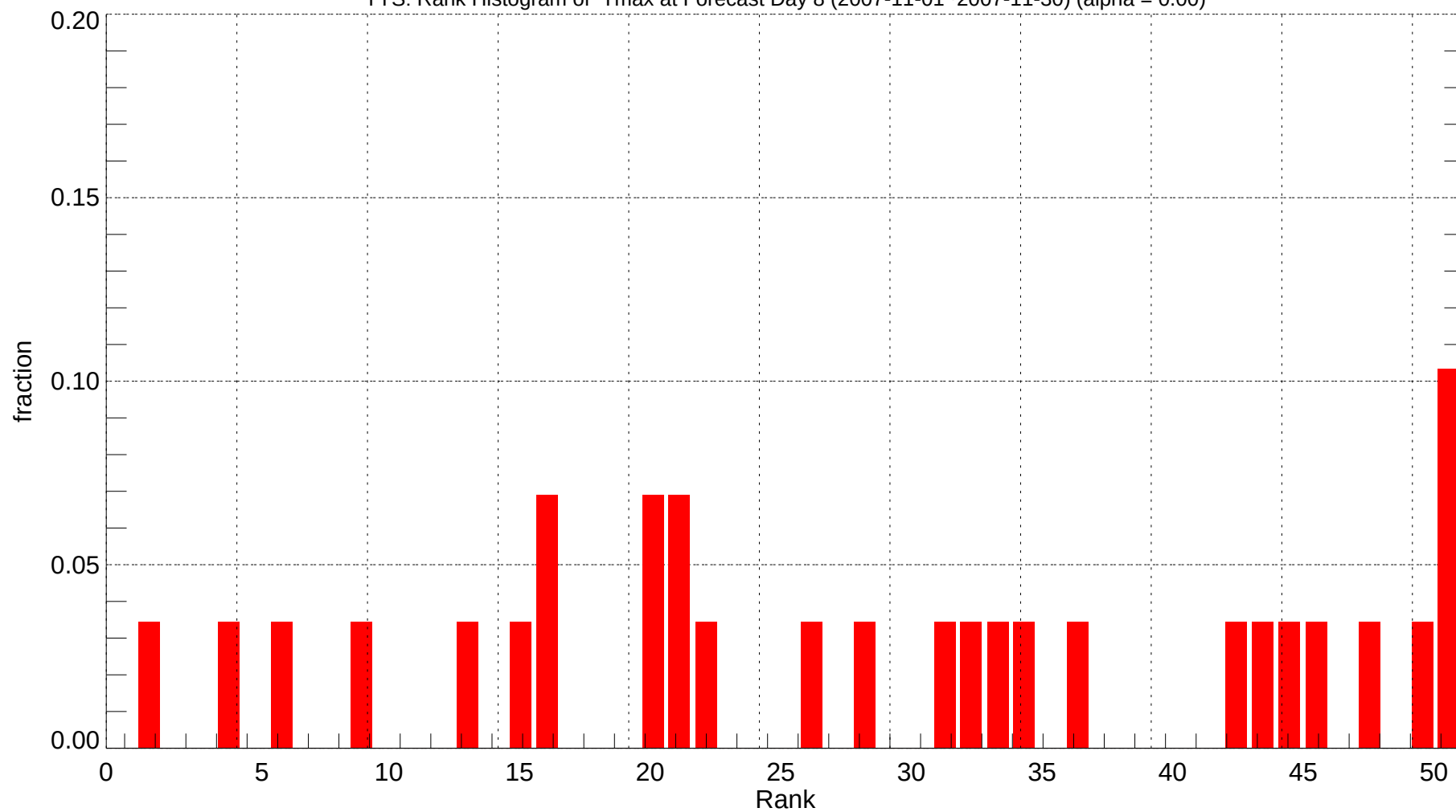
TYS: Rank Histogram of Tmax at Forecast Day 8 (2007-11-01~2007-11-30) (alpha = 0.00)
