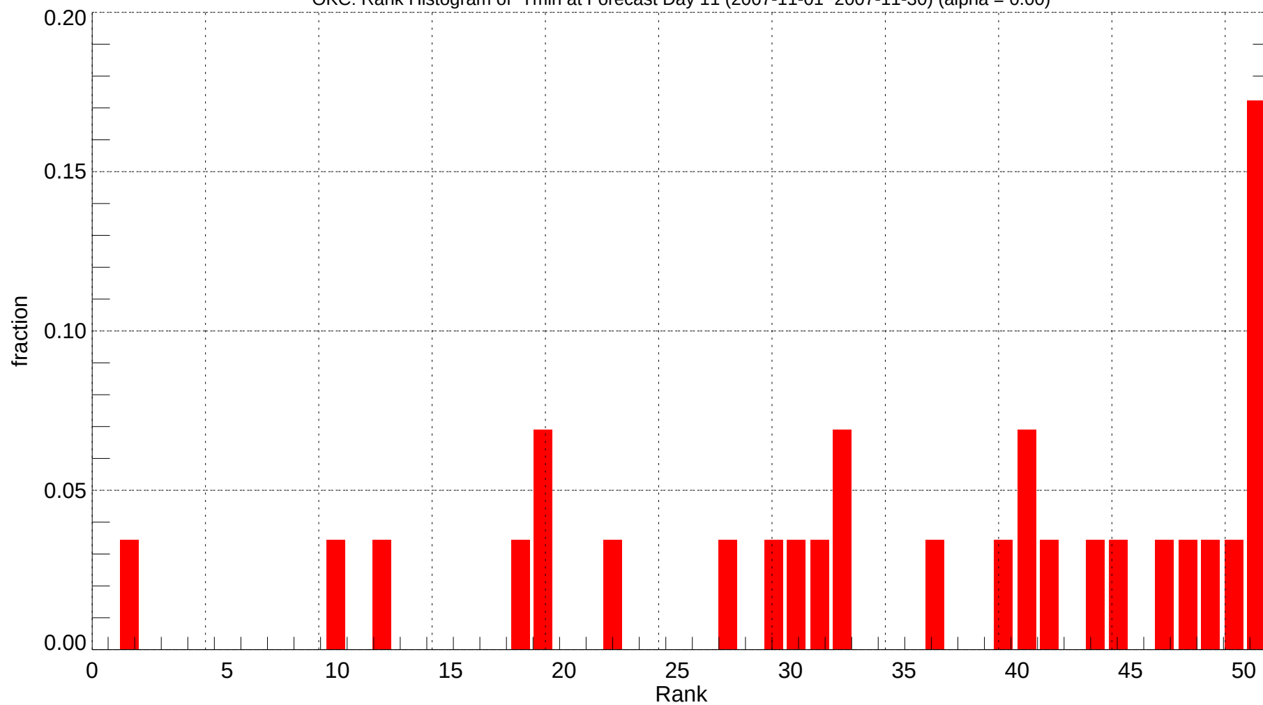
OKC: Rank Histogram of Tmin at Forecast Day 11 (2007-11-01~2007-11-30) (alpha = 0.00)
