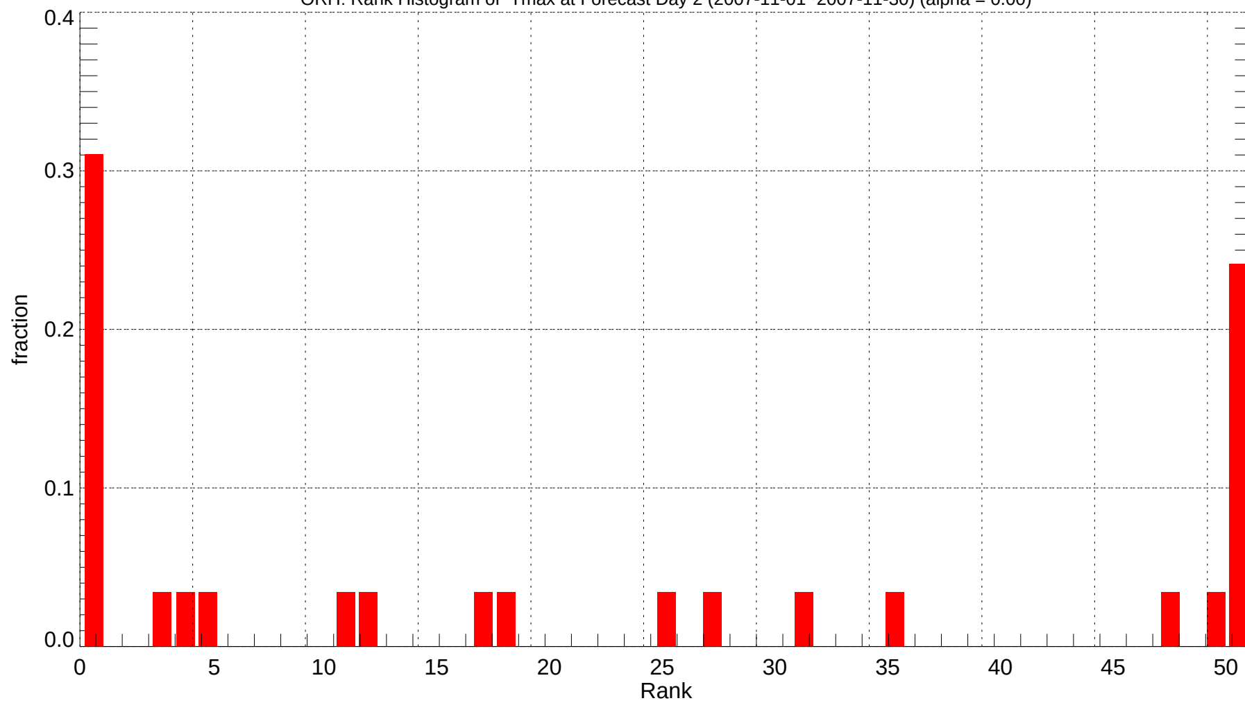
ORH: Rank Histogram of Tmax at Forecast Day 2 (2007-11-01~2007-11-30) (alpha = 0.00)
