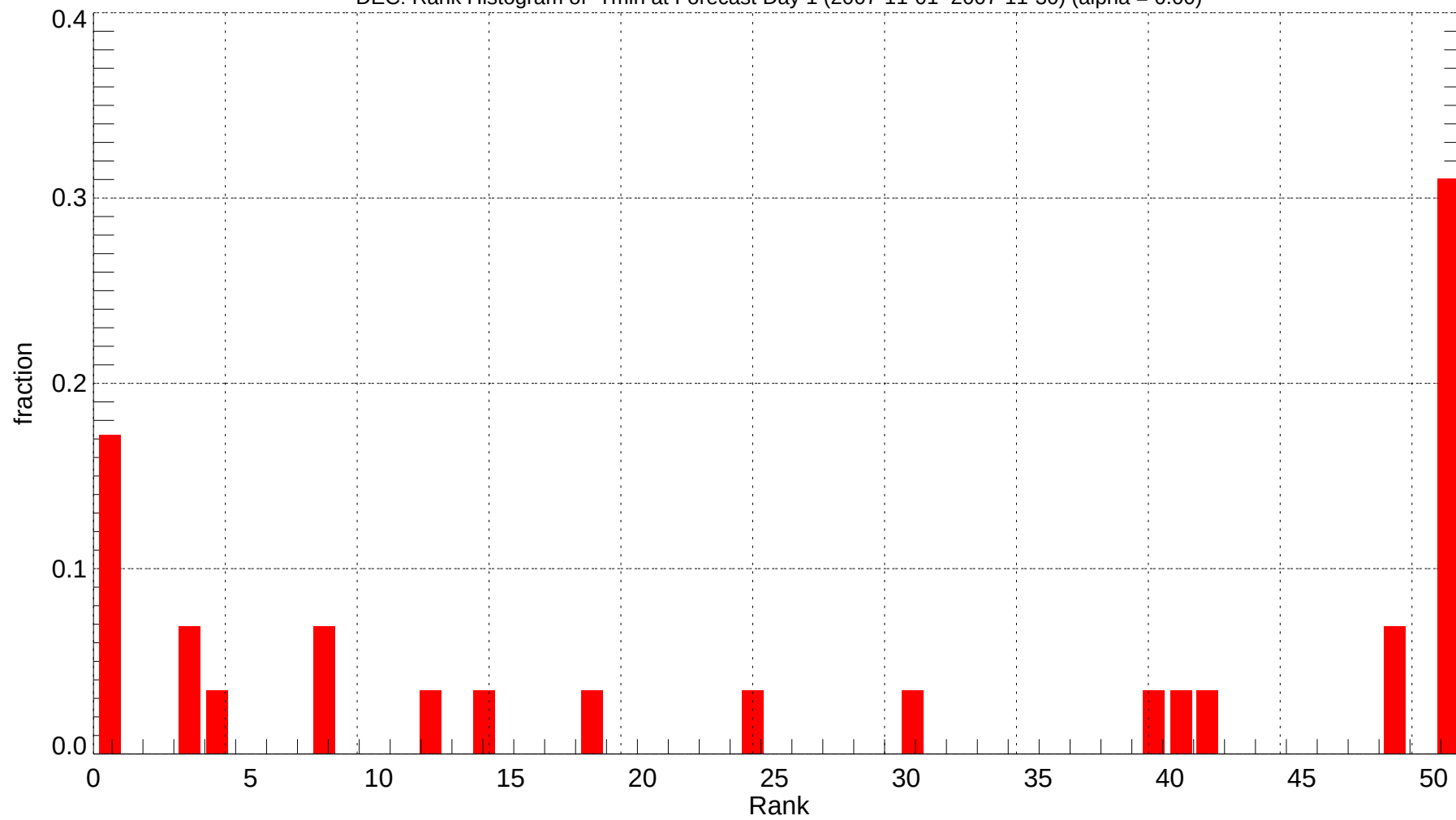
DEC: Rank Histogram of Tmin at Forecast Day 1 (2007-11-01~2007-11-30) (alpha = 0.00)
