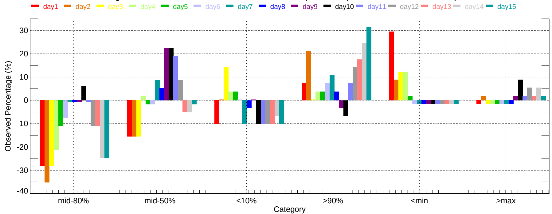
Observed Percentage Deviation of Ensembles - LAS: Max Temperature (2007-11-01~2007-11-30)
