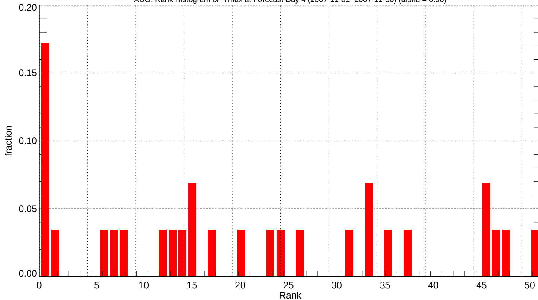
AUG: Rank Histogram of Tmax at Forecast Day 4 (2007-11-01~2007-11-30) (alpha = 0.00)
