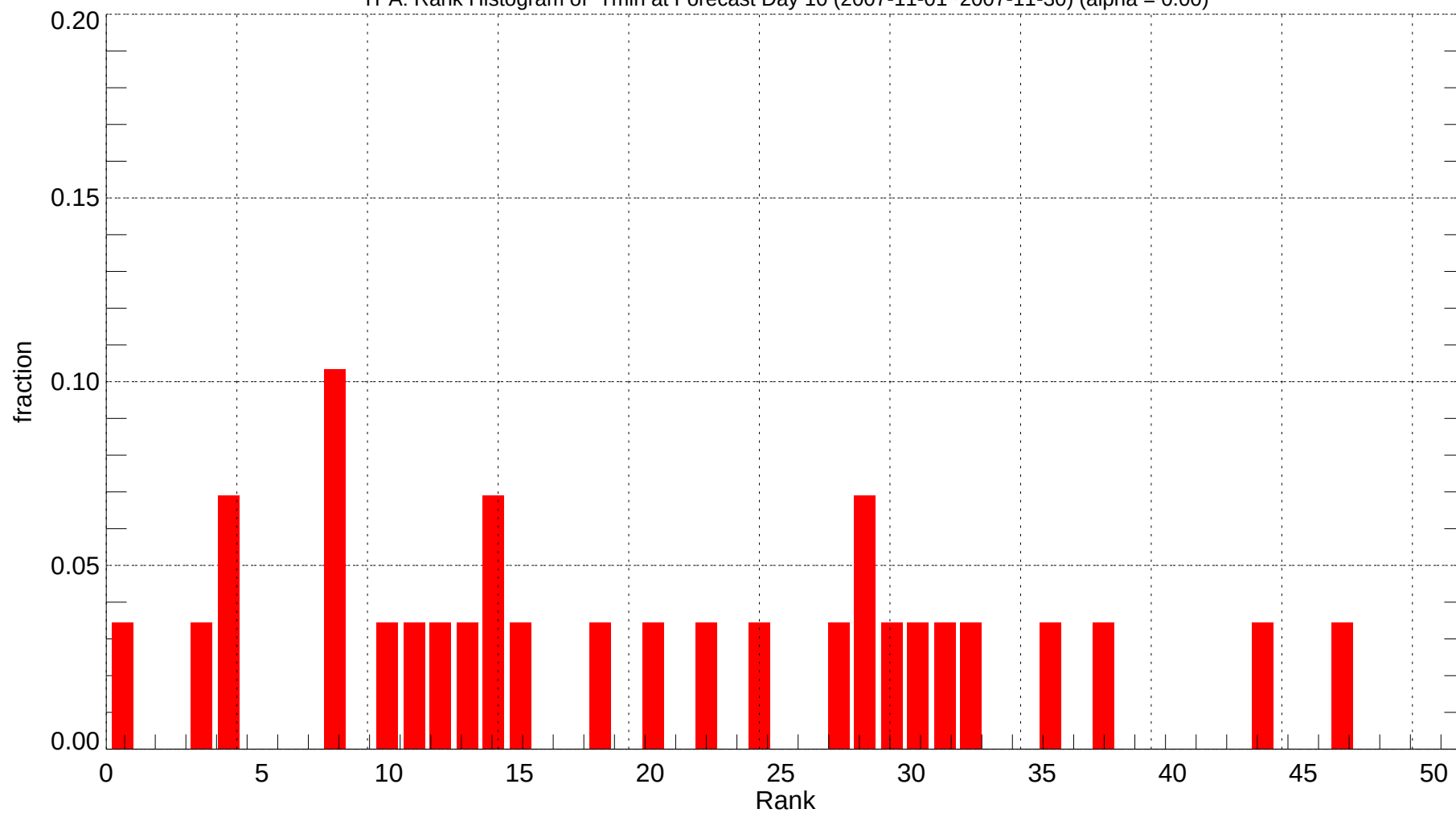
TPA: Rank Histogram of Tmin at Forecast Day 10 (2007-11-01~2007-11-30) (alpha = 0.00)
