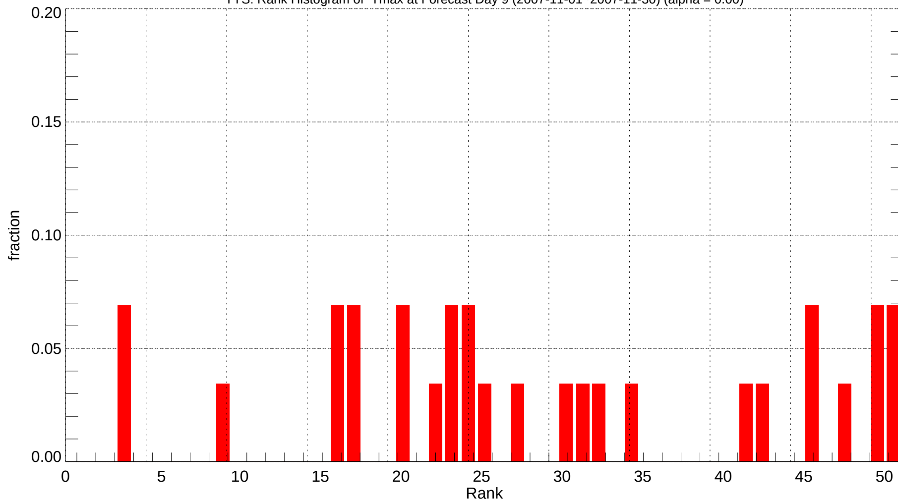
TYS: Rank Histogram of Tmax at Forecast Day 9 (2007-11-01~2007-11-30) (alpha = 0.00)
