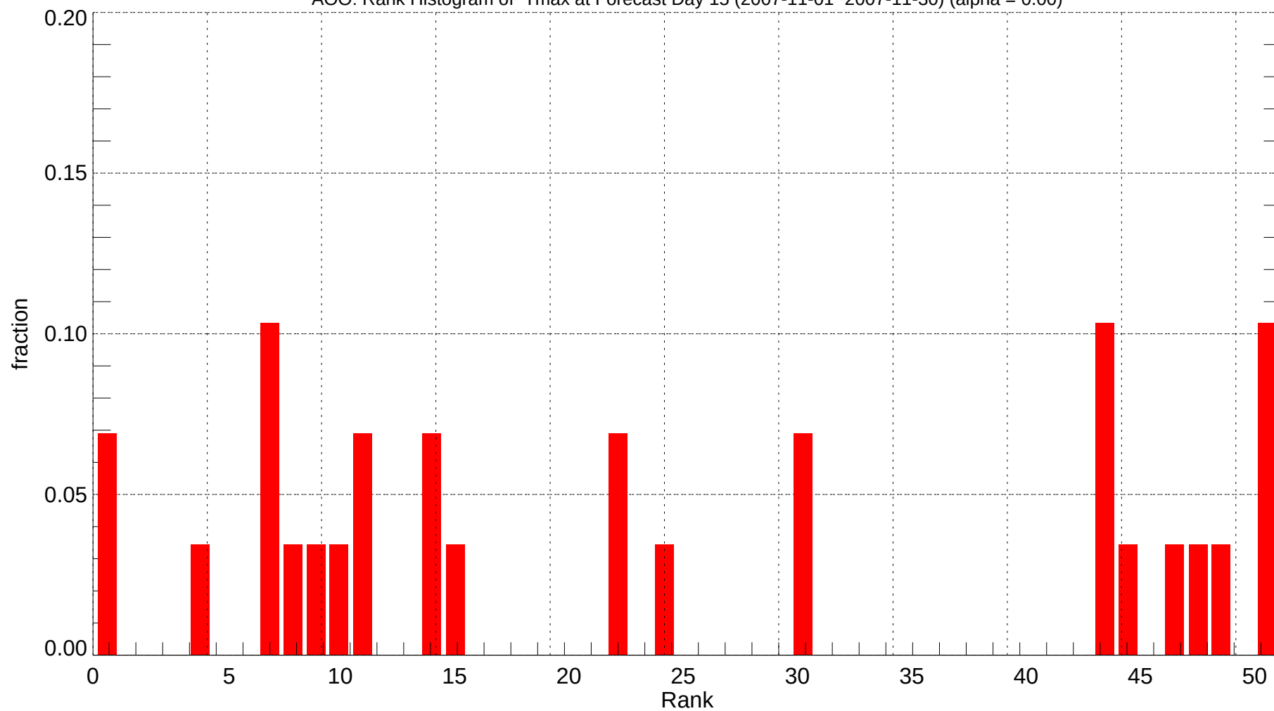
AOO: Rank Histogram of Tmax at Forecast Day 15 (2007-11-01~2007-11-30) (alpha = 0.00)
