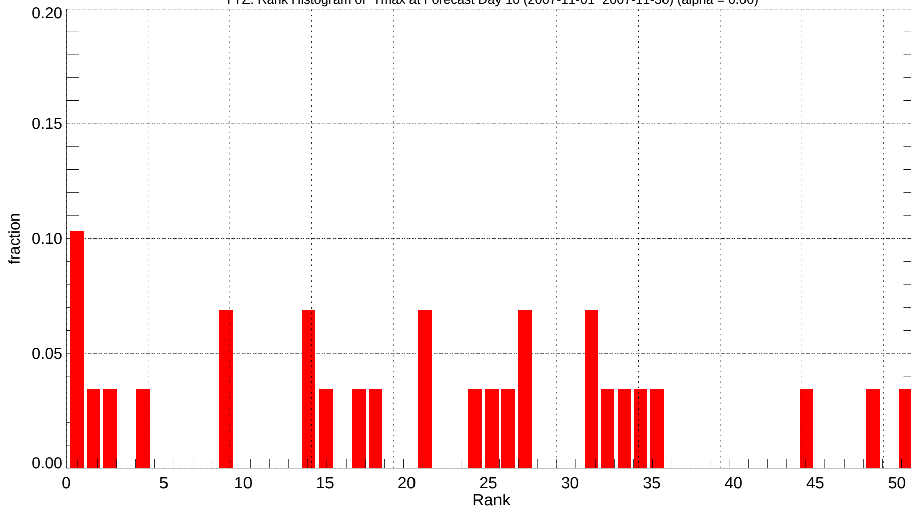
YYZ: Rank Histogram of Tmax at Forecast Day 10 (2007-11-01~2007-11-30) (alpha = 0.00)
