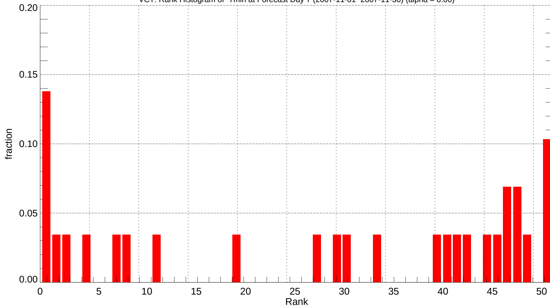
VCT: Rank Histogram of Tmin at Forecast Day 7 (2007-11-01~2007-11-30) (alpha = 0.00)
