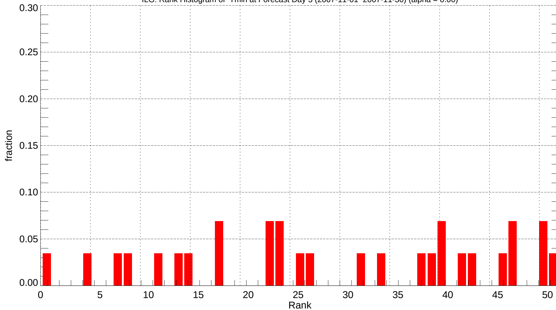
ILG: Rank Histogram of Tmin at Forecast Day 3 (2007-11-01~2007-11-30) (alpha = 0.00)
