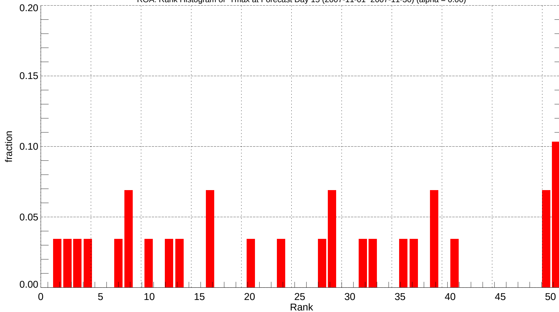
ROA: Rank Histogram of Tmax at Forecast Day 15 (2007-11-01~2007-11-30) (alpha = 0.00)
