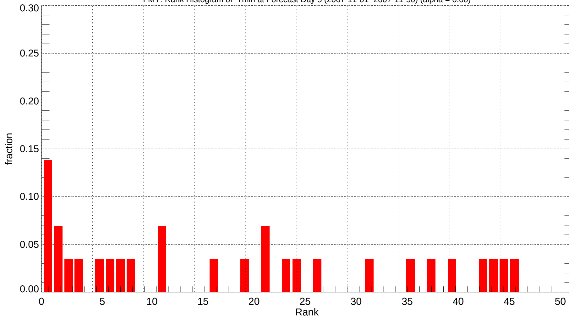
FMY: Rank Histogram of Tmin at Forecast Day 5 (2007-11-01~2007-11-30) (alpha = 0.00)
