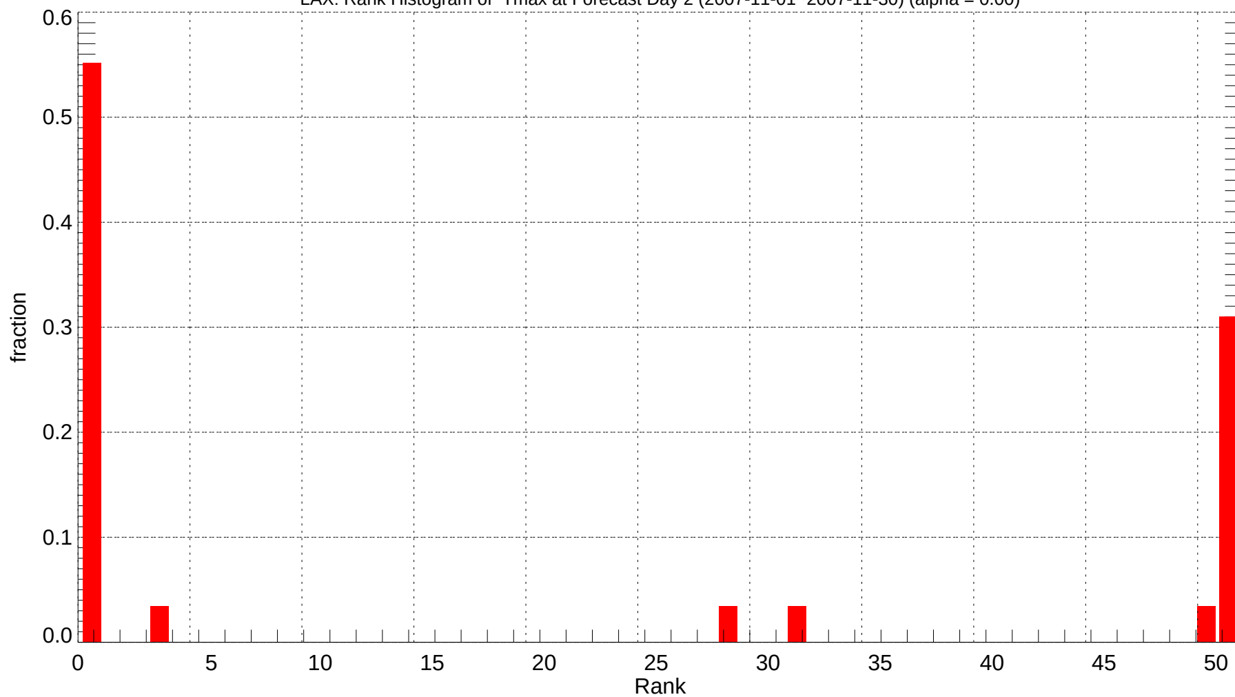
LAX: Rank Histogram of Tmax at Forecast Day 2 (2007-11-01~2007-11-30) (alpha = 0.00)
