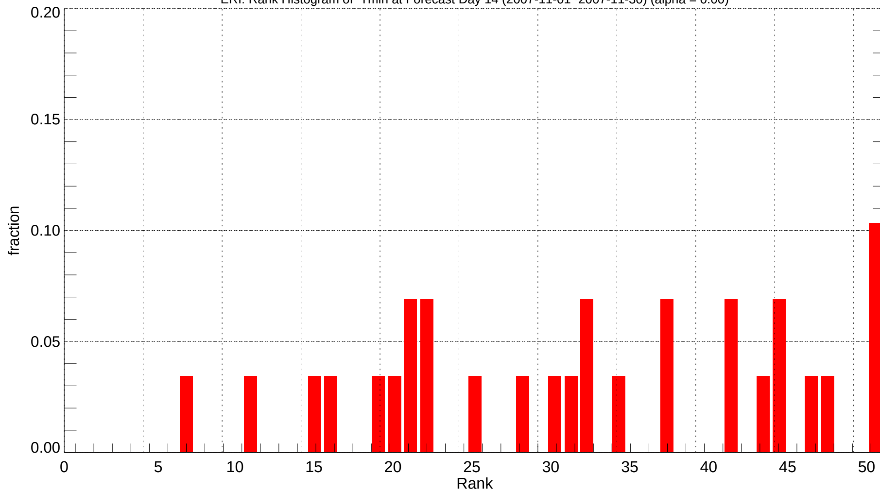
ERI: Rank Histogram of Tmin at Forecast Day 14 (2007-11-01~2007-11-30) (alpha = 0.00)
