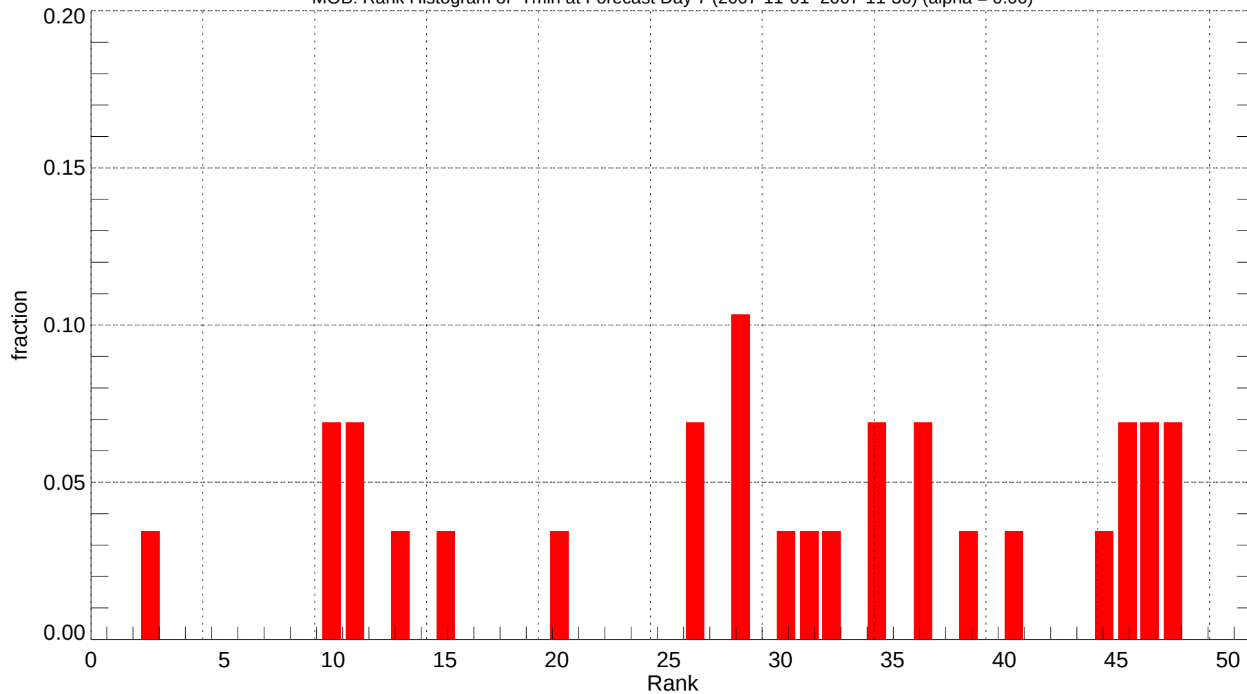
MOB: Rank Histogram of Tmin at Forecast Day 7 (2007-11-01~2007-11-30) (alpha = 0.00)
