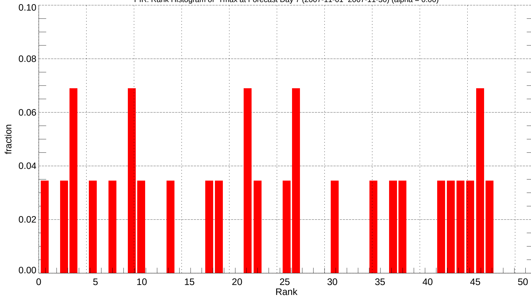
PIR: Rank Histogram of Tmax at Forecast Day 7 (2007-11-01~2007-11-30) (alpha = 0.00)
