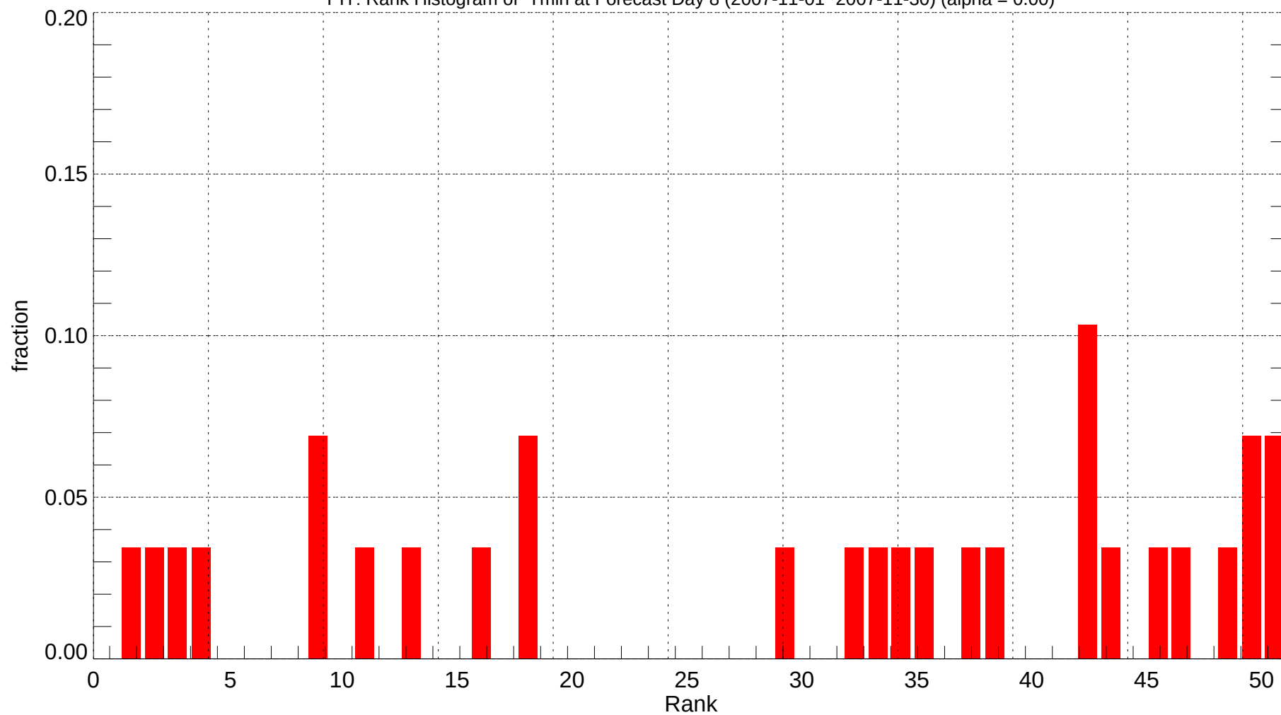
PIT: Rank Histogram of Tmin at Forecast Day 8 (2007-11-01~2007-11-30) (alpha = 0.00)
