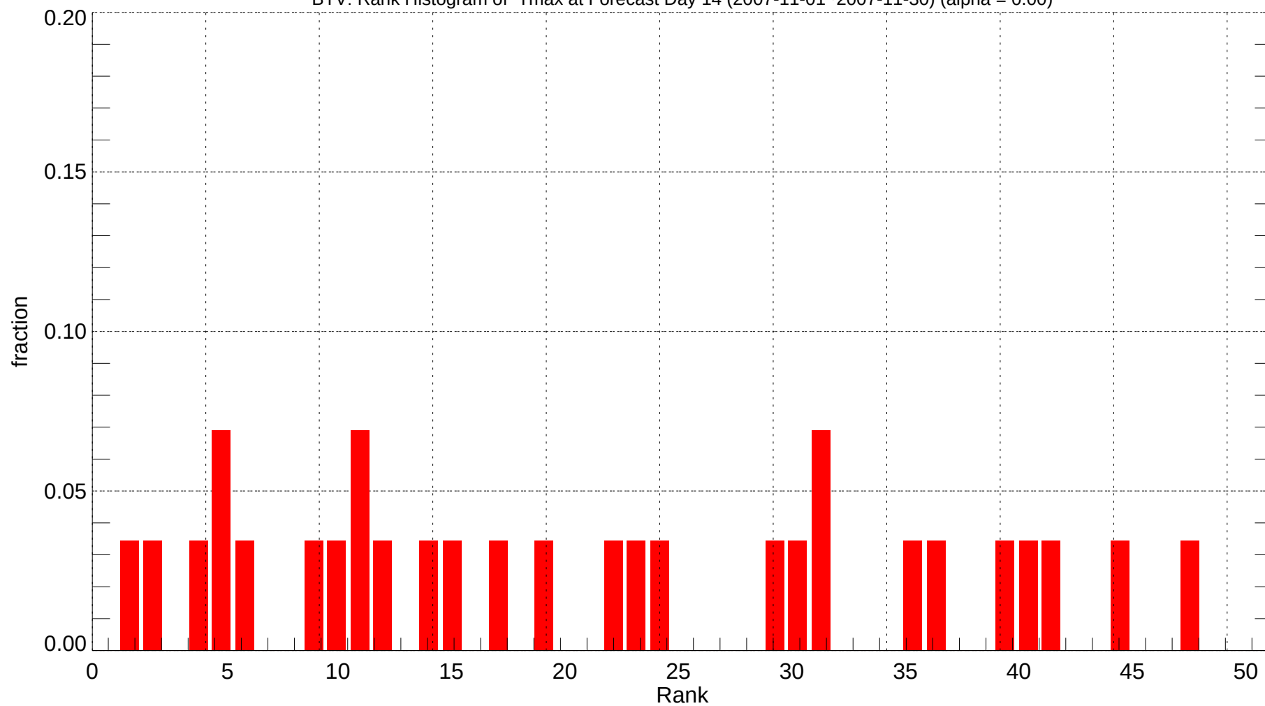
BTV: Rank Histogram of Tmax at Forecast Day 14 (2007-11-01~2007-11-30) (alpha = 0.00)
