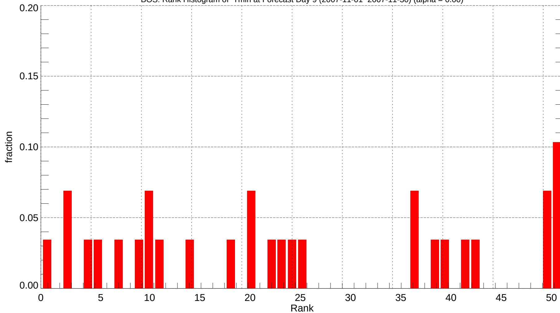
BOS: Rank Histogram of Tmin at Forecast Day 9 (2007-11-01~2007-11-30) (alpha = 0.00)
