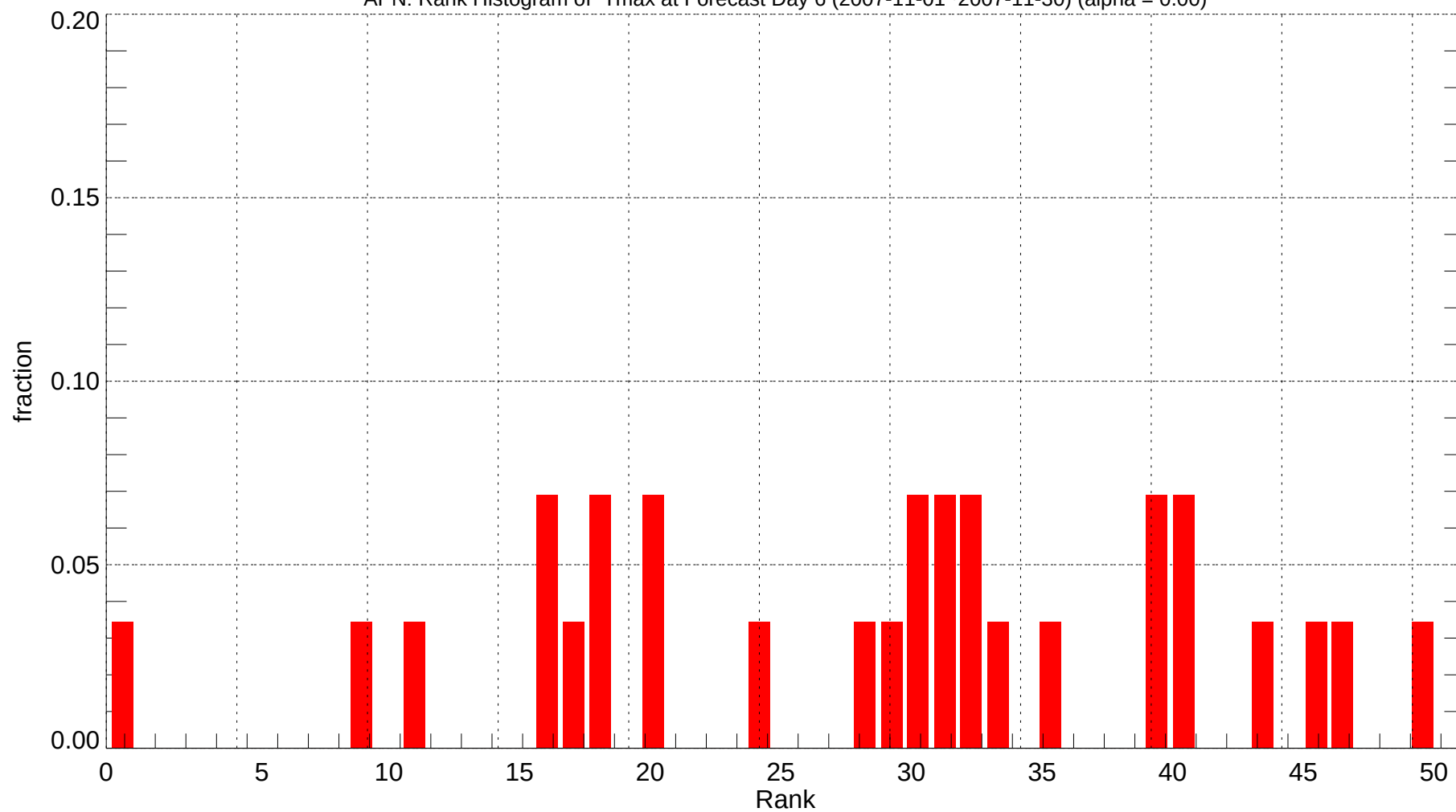
APN: Rank Histogram of Tmax at Forecast Day 6 (2007-11-01~2007-11-30) (alpha = 0.00)
