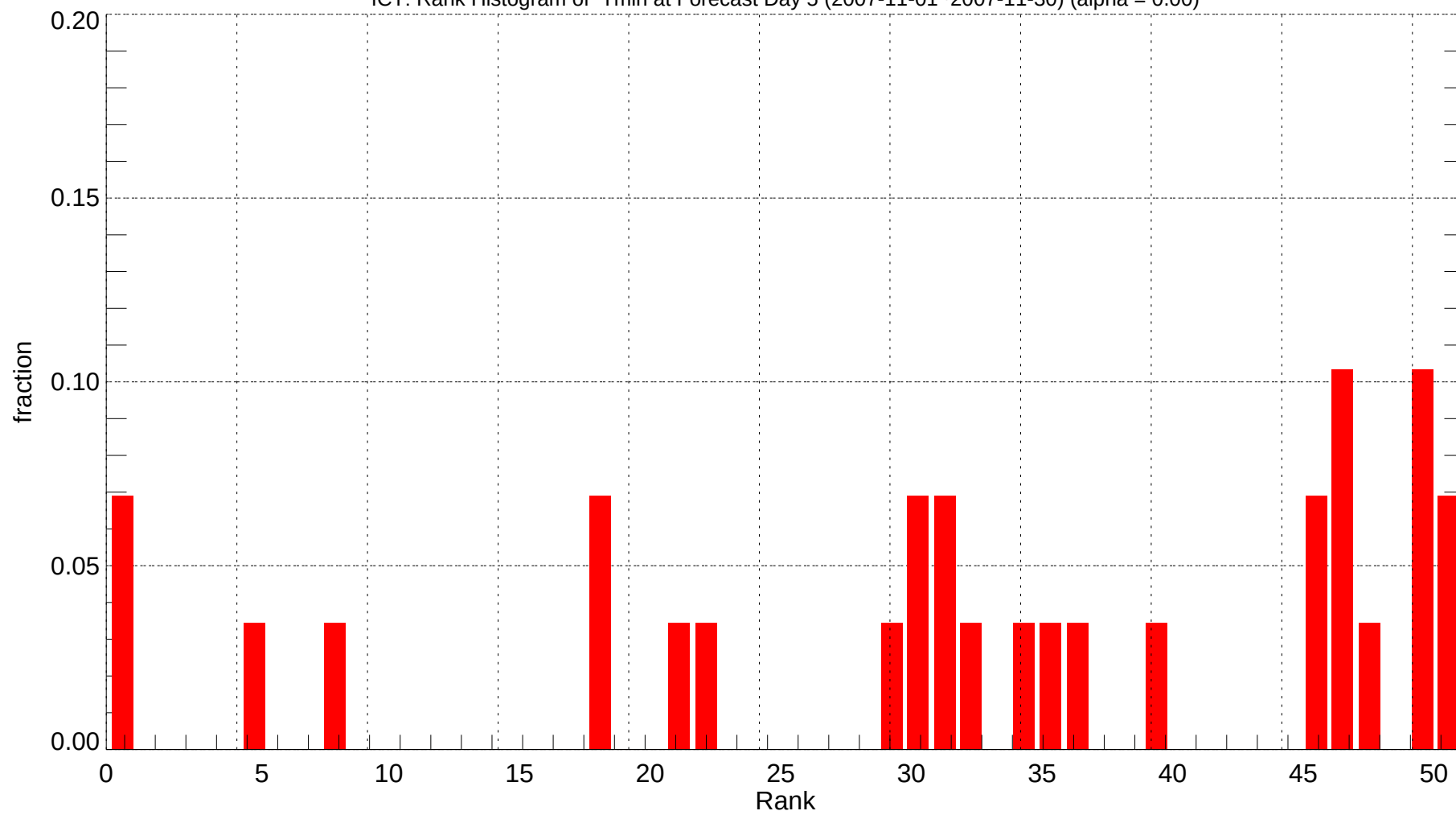
ICT: Rank Histogram of Tmin at Forecast Day 5 (2007-11-01~2007-11-30) (alpha = 0.00)
