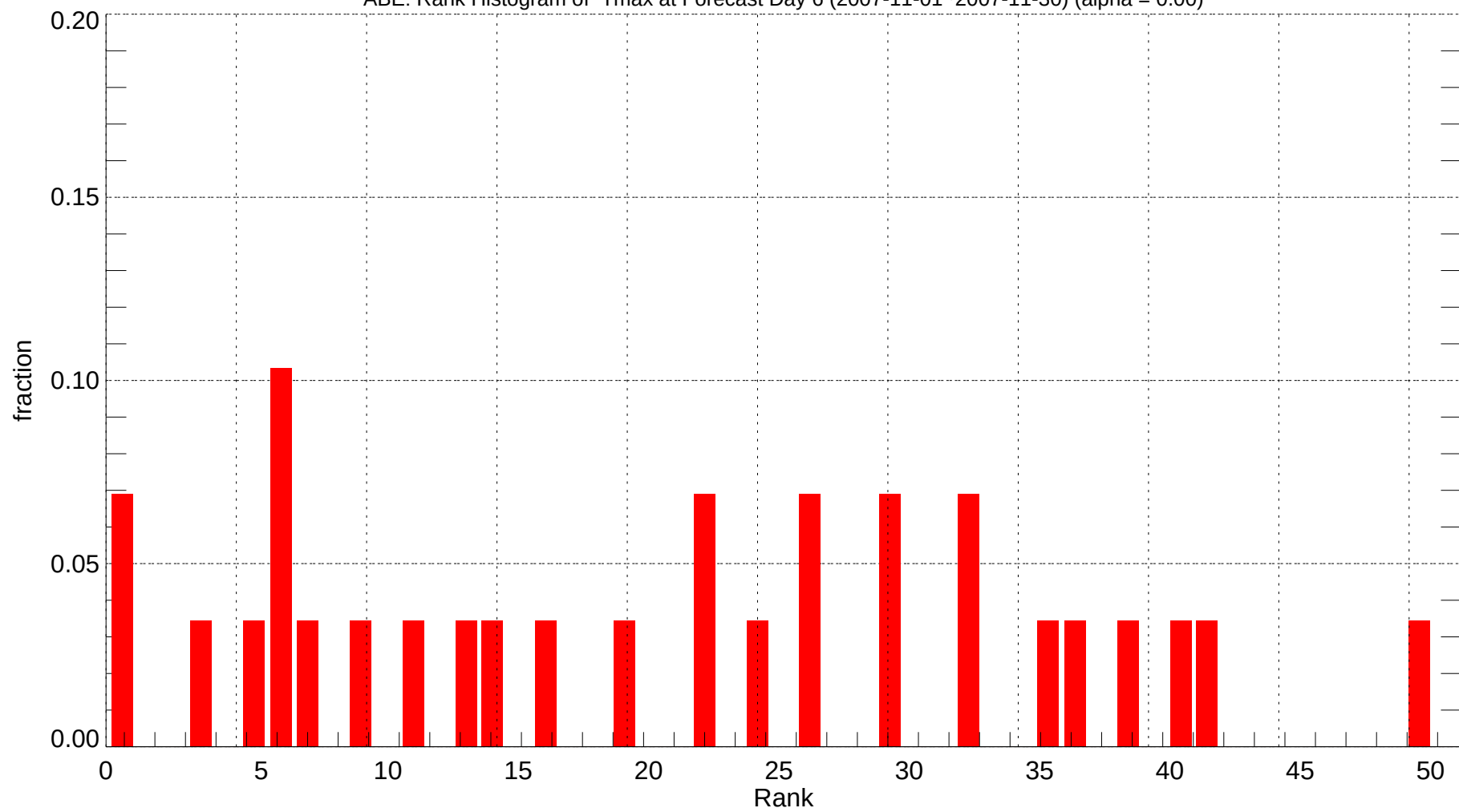
ABE: Rank Histogram of Tmax at Forecast Day 6 (2007-11-01~2007-11-30) (alpha = 0.00)
