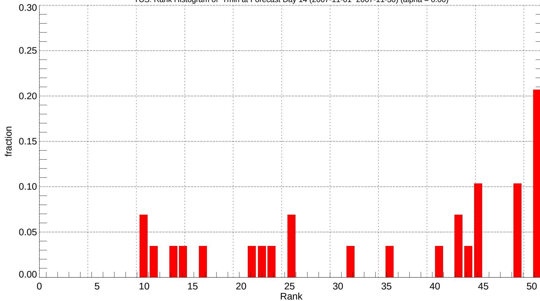
TUS: Rank Histogram of Tmin at Forecast Day 14 (2007-11-01~2007-11-30) (alpha = 0.00)
