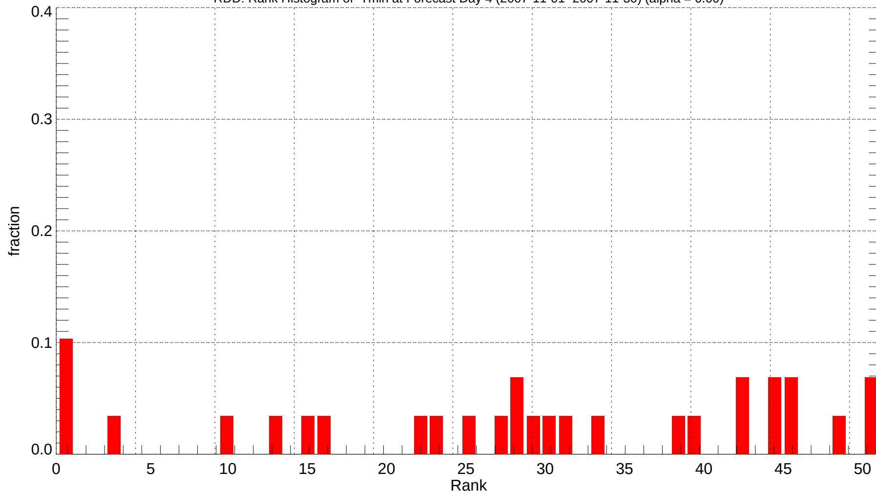
RDD: Rank Histogram of Tmin at Forecast Day 4 (2007-11-01~2007-11-30) (alpha = 0.00)
