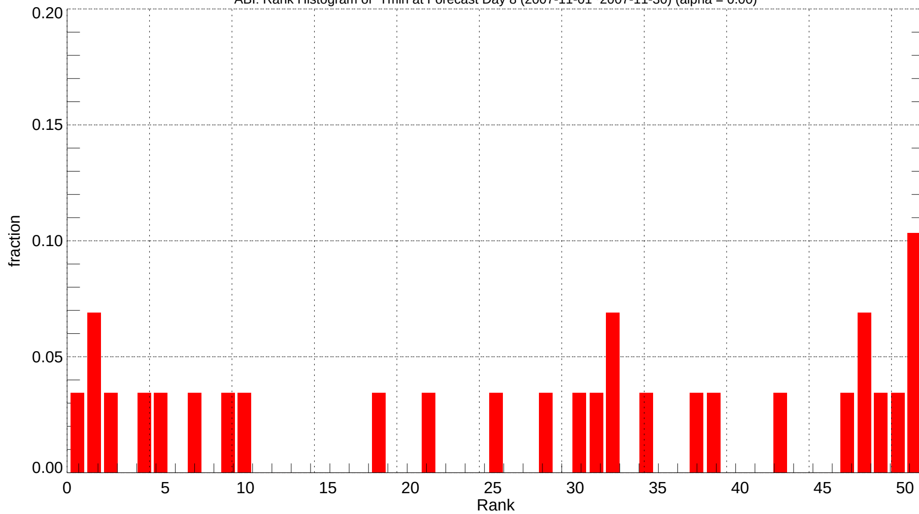
ABI: Rank Histogram of Tmin at Forecast Day 8 (2007-11-01~2007-11-30) (alpha = 0.00)
