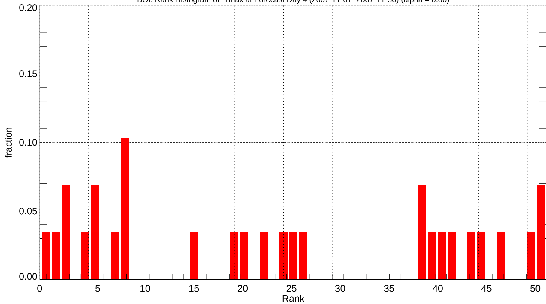
BOI: Rank Histogram of Tmax at Forecast Day 4 (2007-11-01~2007-11-30) (alpha = 0.00)
