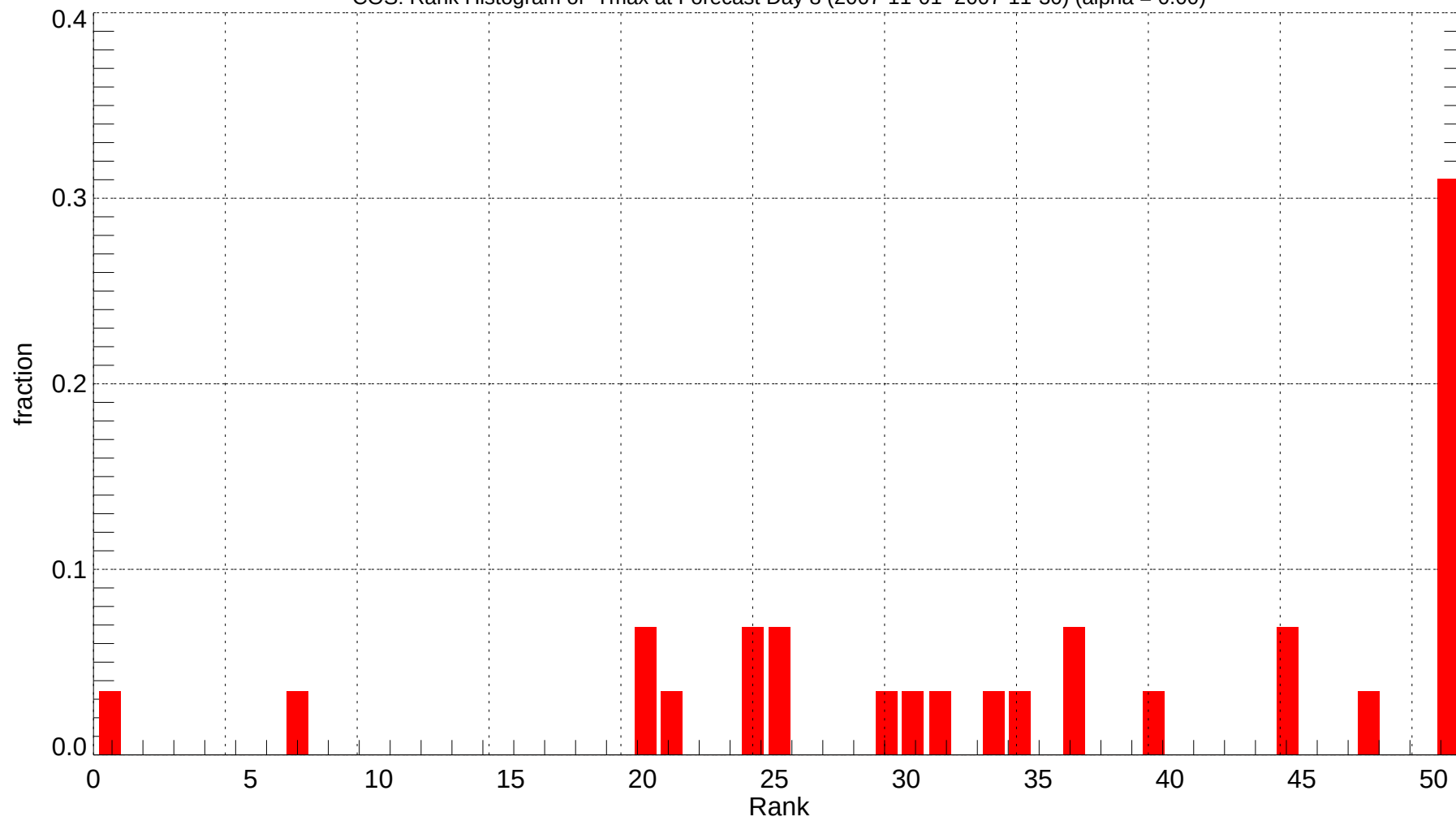
COS: Rank Histogram of Tmax at Forecast Day 8 (2007-11-01~2007-11-30) (alpha = 0.00)
