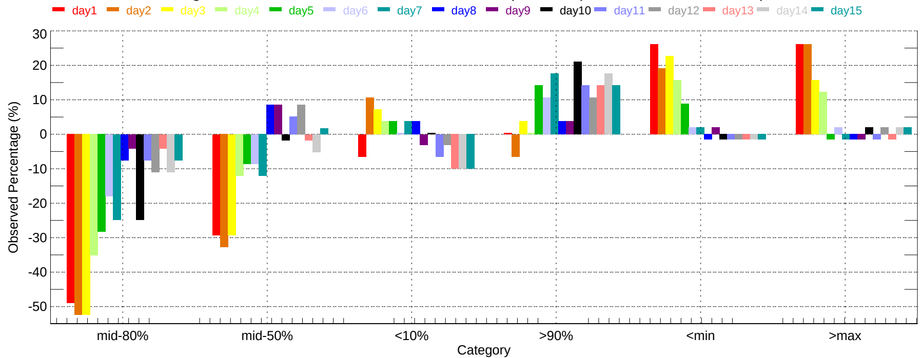
Observed Percentage Deviation of Ensembles - RNO: Min Temperature (2007-11-01~2007-11-30)
