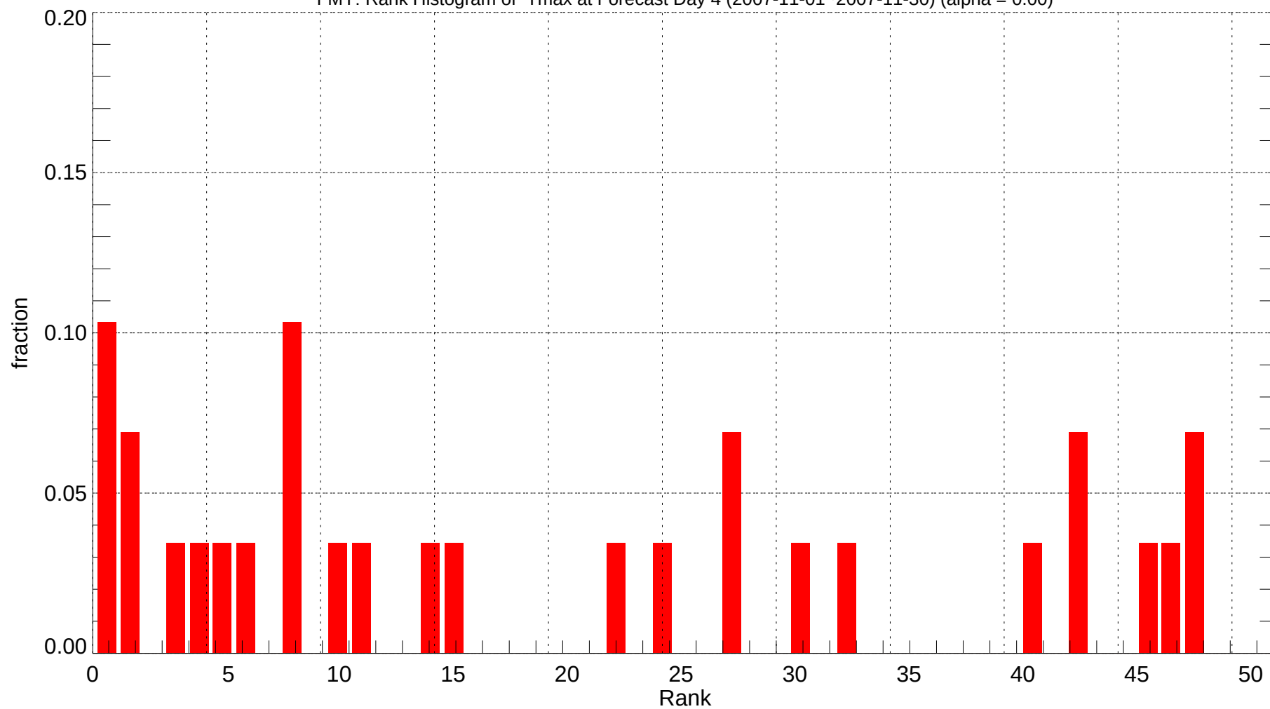
FMY: Rank Histogram of Tmax at Forecast Day 4 (2007-11-01~2007-11-30) (alpha = 0.00)
