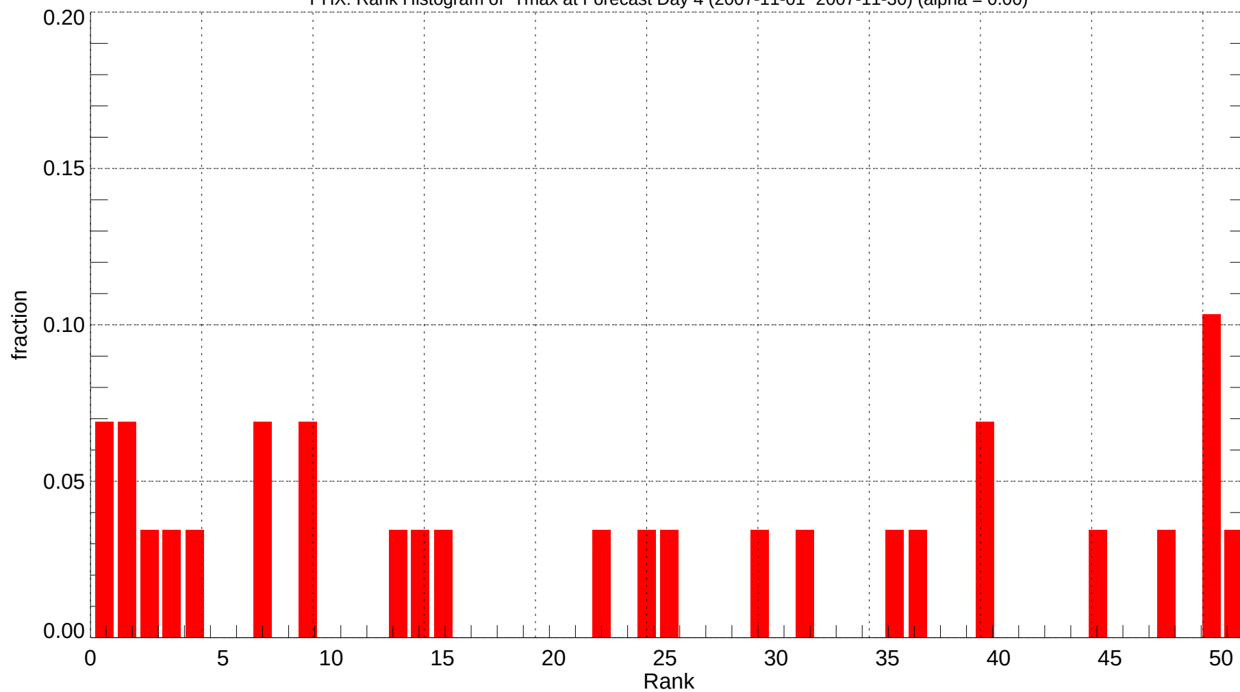
PHX: Rank Histogram of Tmax at Forecast Day 4 (2007-11-01~2007-11-30) (alpha = 0.00)
