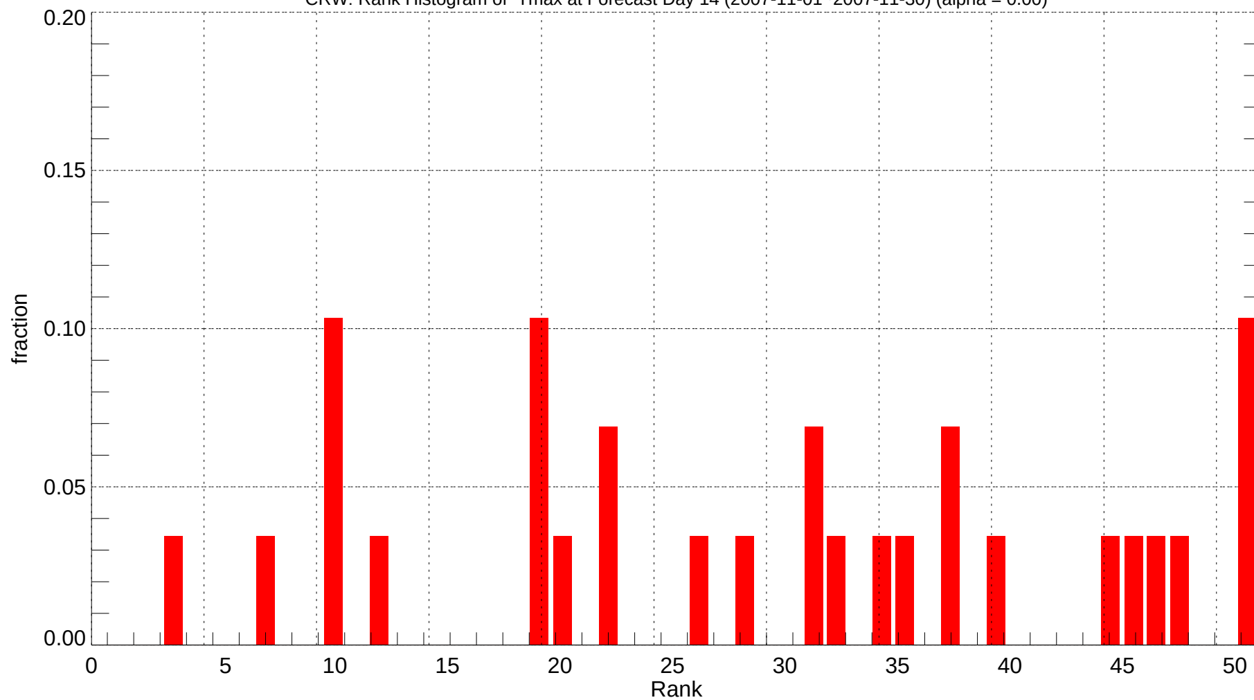
CRW: Rank Histogram of Tmax at Forecast Day 14 (2007-11-01~2007-11-30) (alpha = 0.00)
