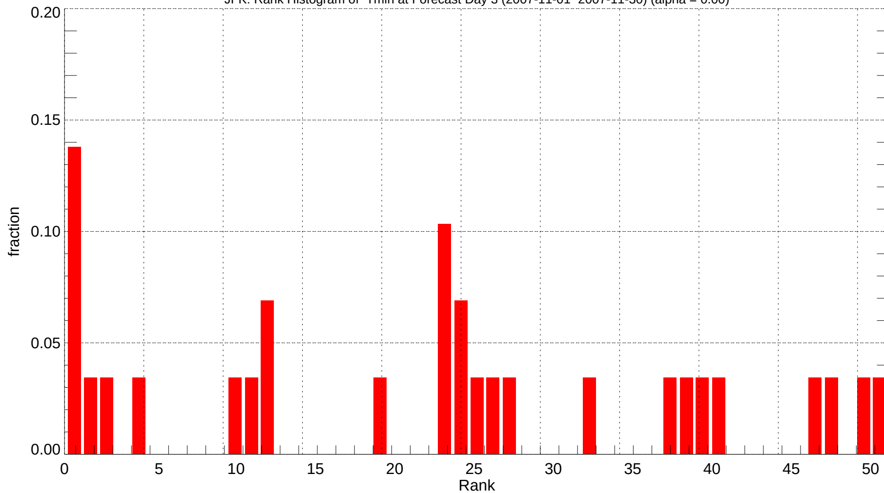
JFK: Rank Histogram of Tmin at Forecast Day 3 (2007-11-01~2007-11-30) (alpha = 0.00)
