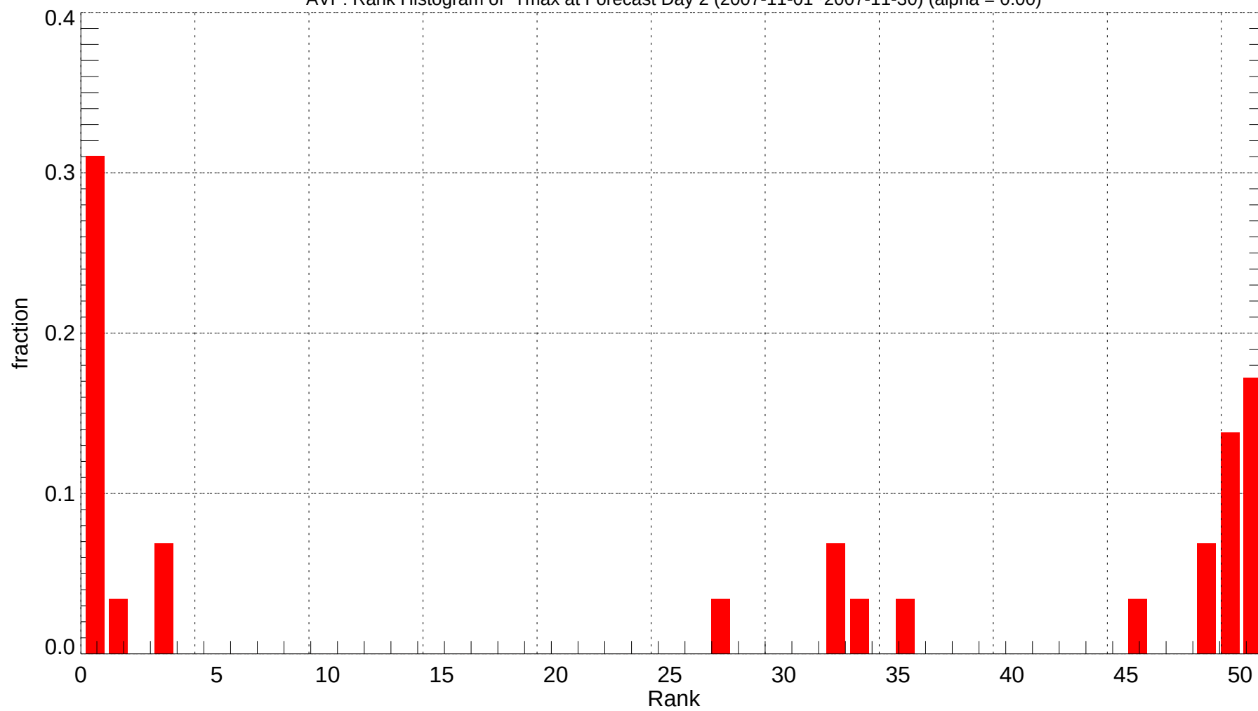
AVP: Rank Histogram of Tmax at Forecast Day 2 (2007-11-01~2007-11-30) (alpha = 0.00)
