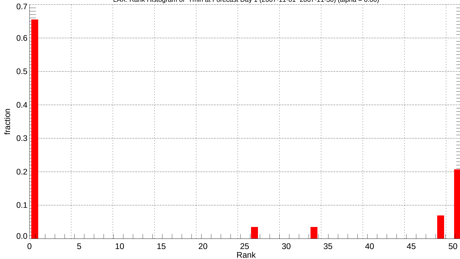
LAX: Rank Histogram of Tmin at Forecast Day 1 (2007-11-01~2007-11-30) (alpha = 0.00)
