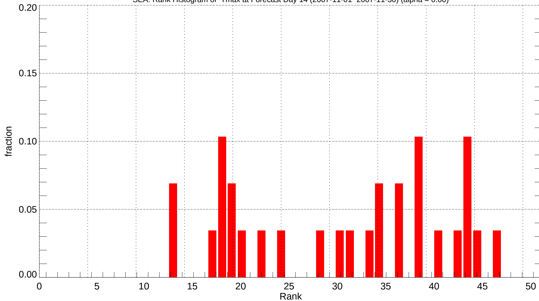
SEA: Rank Histogram of Tmax at Forecast Day 14 (2007-11-01~2007-11-30) (alpha = 0.00)
