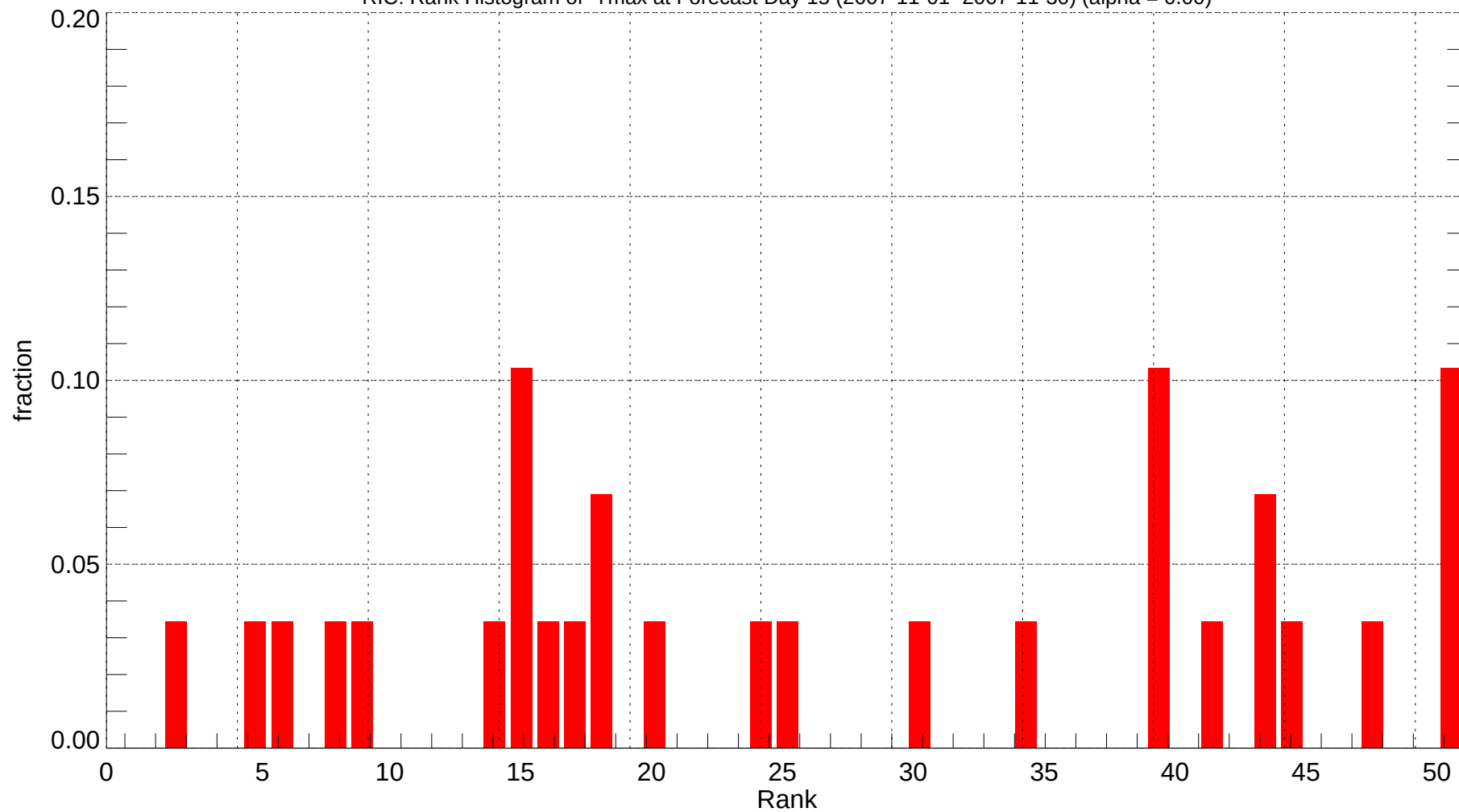
RIC: Rank Histogram of Tmax at Forecast Day 15 (2007-11-01~2007-11-30) (alpha = 0.00)
