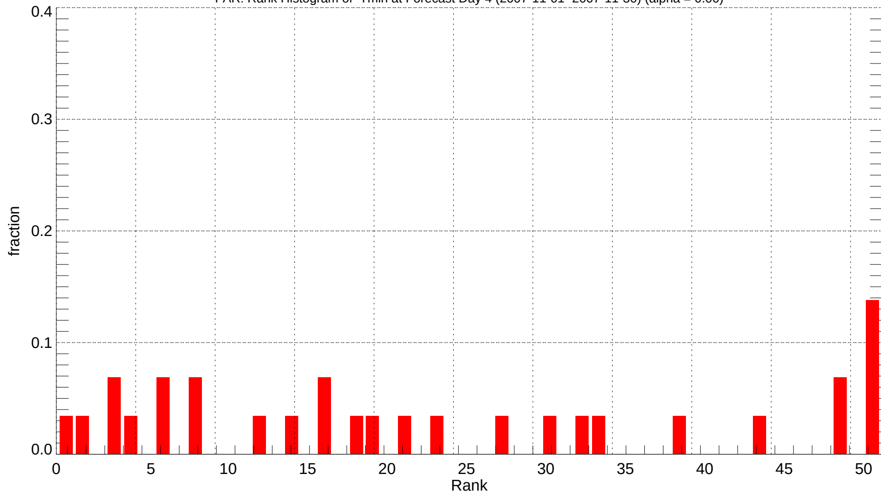
FAR: Rank Histogram of Tmin at Forecast Day 4 (2007-11-01~2007-11-30) (alpha = 0.00)
