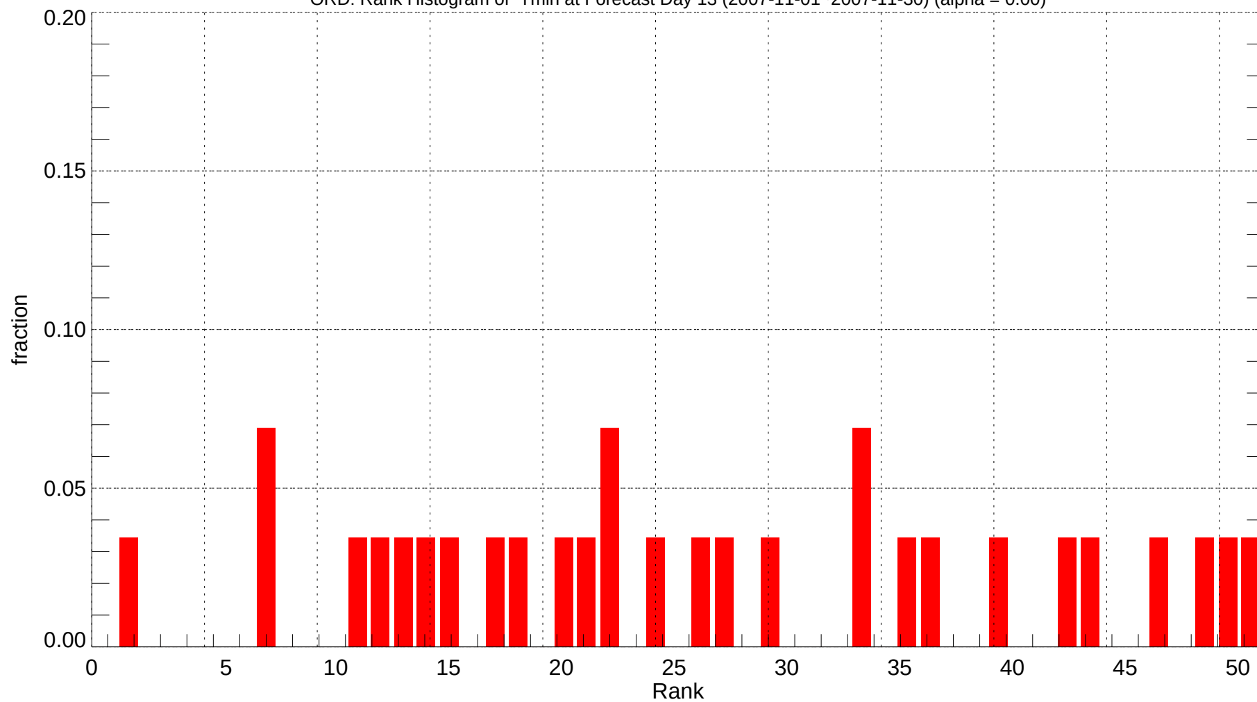
ORD: Rank Histogram of Tmin at Forecast Day 13 (2007-11-01~2007-11-30) (alpha = 0.00)
