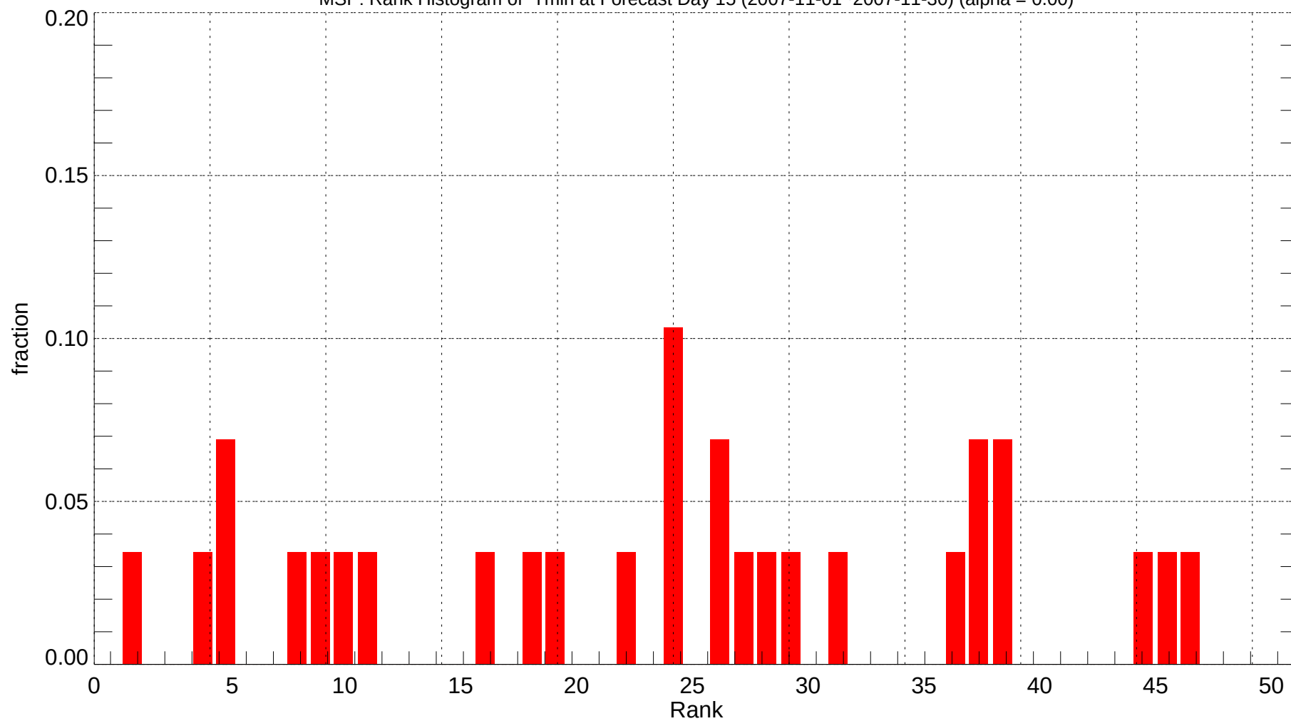
MSP: Rank Histogram of Tmin at Forecast Day 15 (2007-11-01~2007-11-30) (alpha = 0.00)
