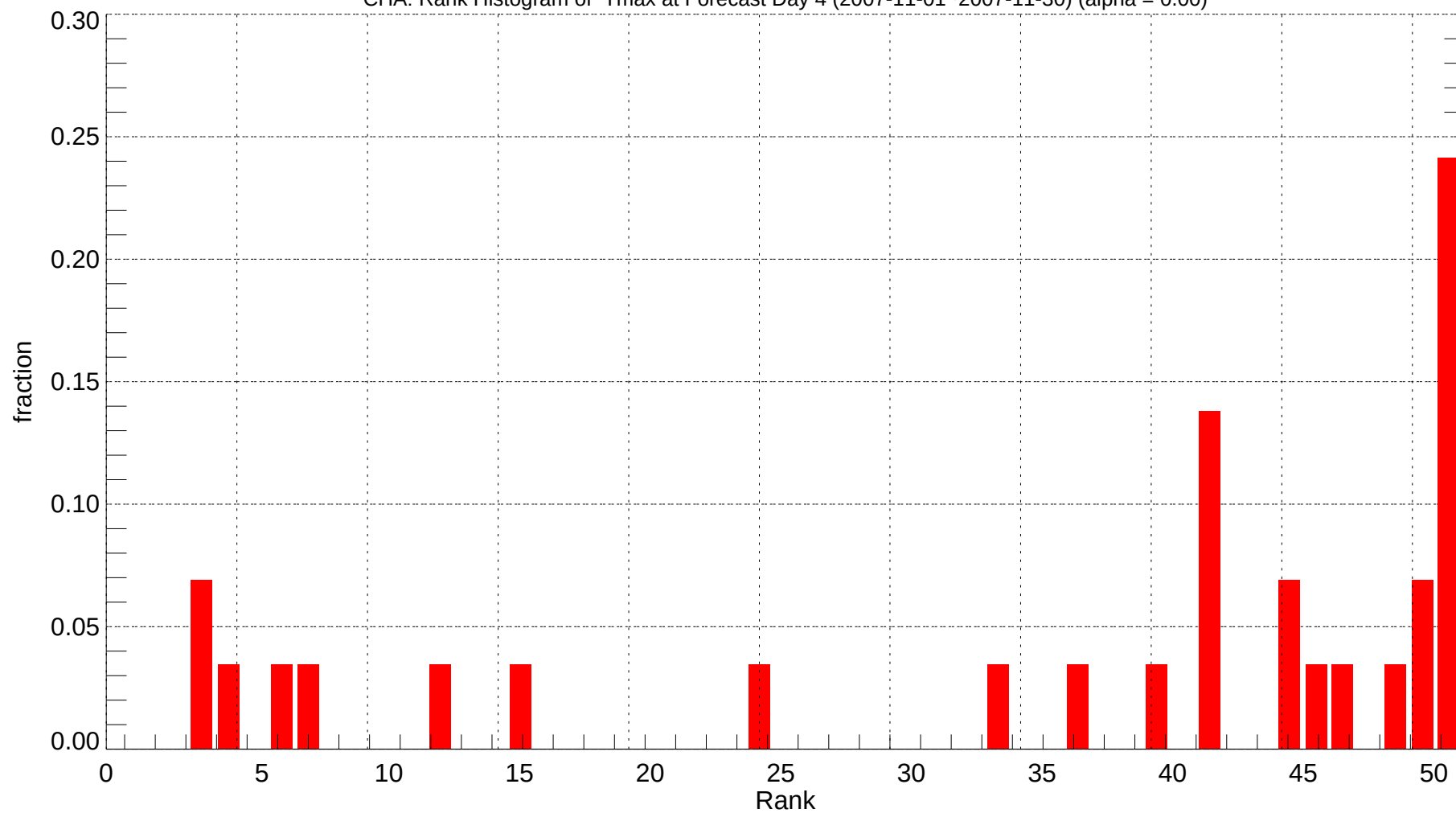
CHA: Rank Histogram of Tmax at Forecast Day 4 (2007-11-01~2007-11-30) (alpha = 0.00)
