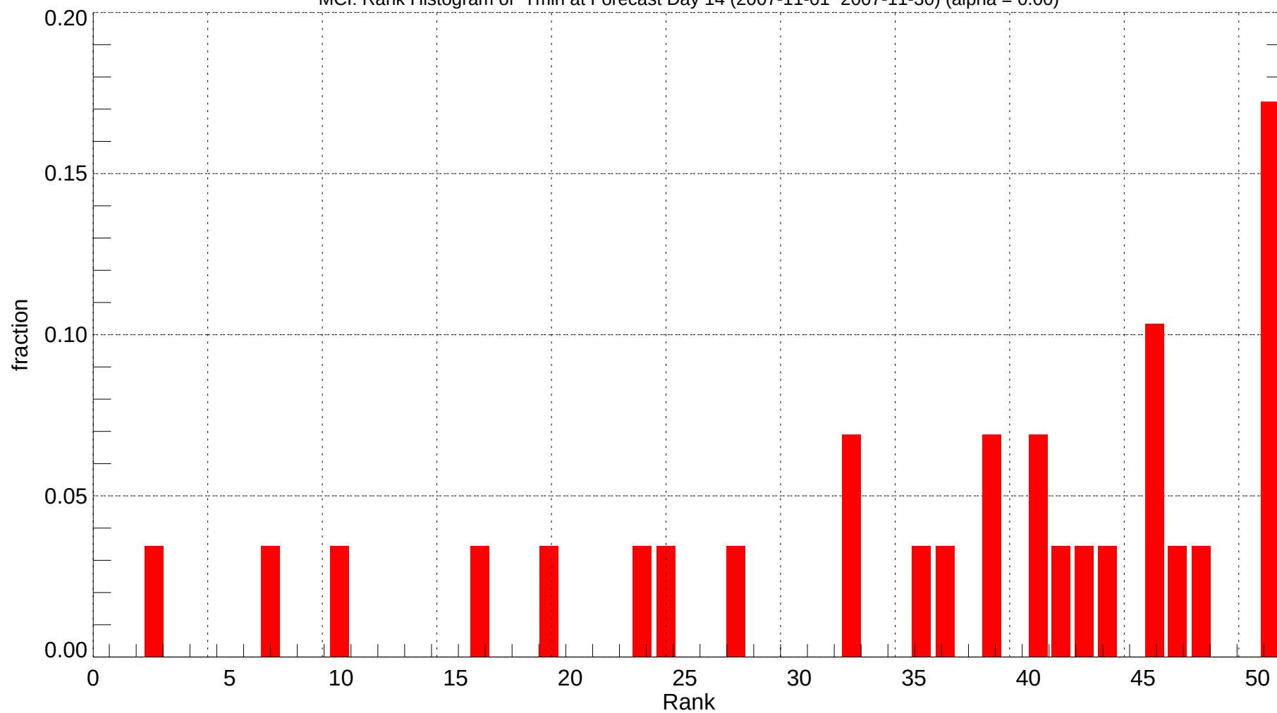
MCI: Rank Histogram of Tmin at Forecast Day 14 (2007-11-01~2007-11-30) (alpha = 0.00)
