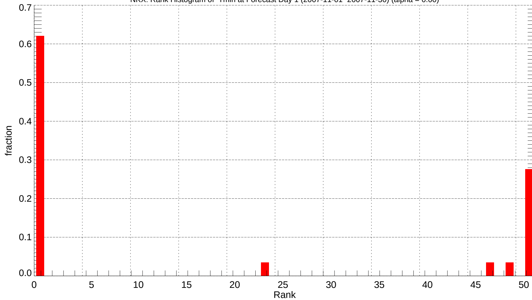
NKX: Rank Histogram of Tmin at Forecast Day 1 (2007-11-01~2007-11-30) (alpha = 0.00)
