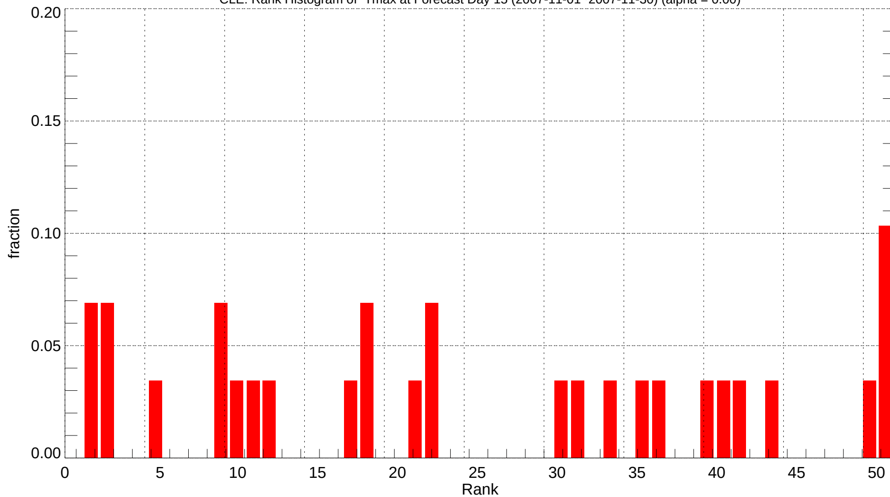
CLE: Rank Histogram of Tmax at Forecast Day 15 (2007-11-01~2007-11-30) (alpha = 0.00)
