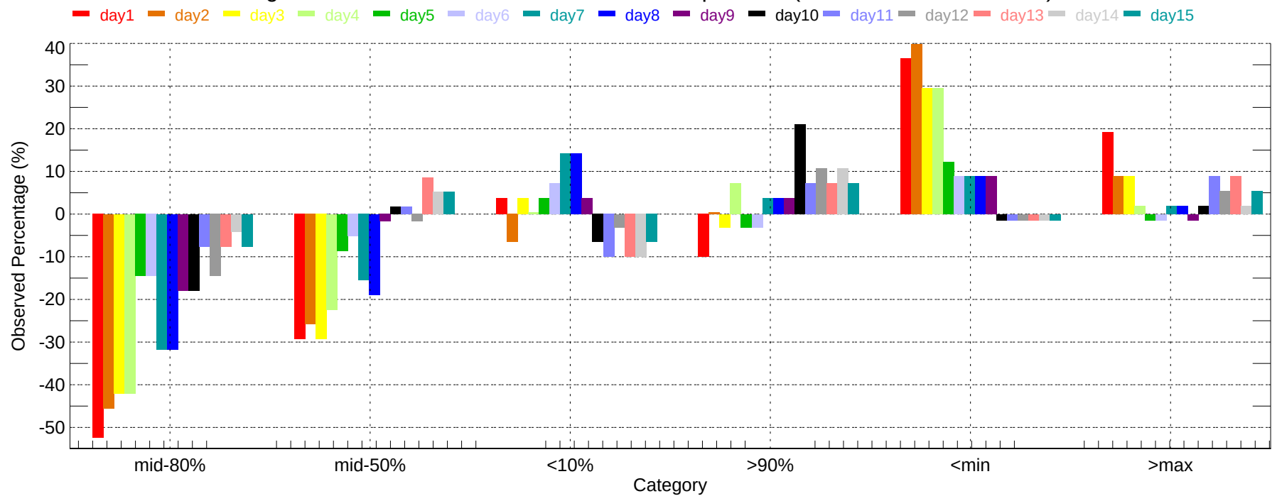
Observed Percentage Deviation of Ensembles - LAN: Min Temperature (2007-11-01~2007-11-30)
