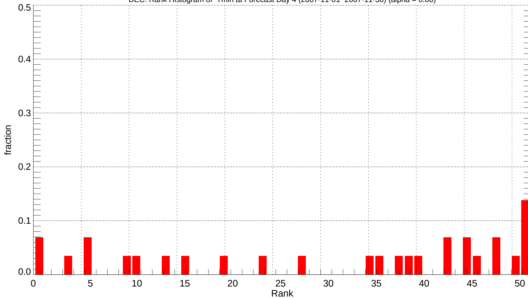
DEC: Rank Histogram of Tmin at Forecast Day 4 (2007-11-01~2007-11-30) (alpha = 0.00)
