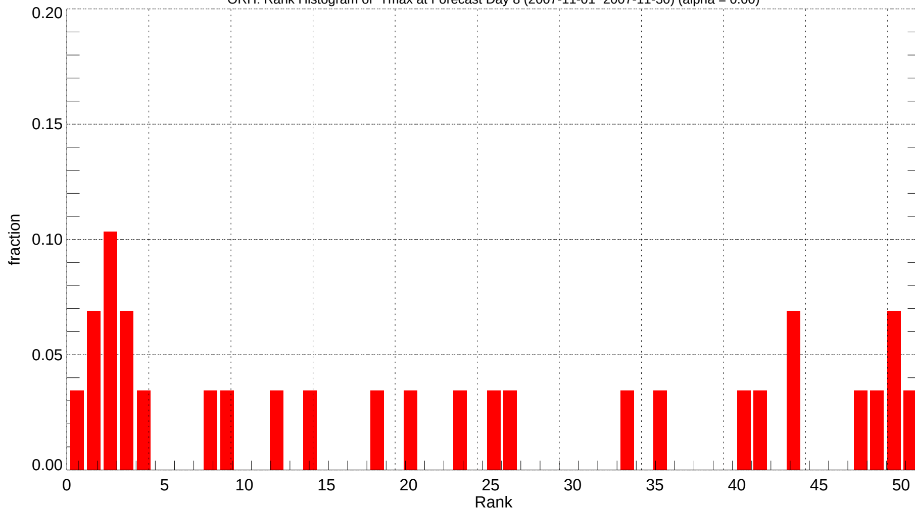
ORH: Rank Histogram of Tmax at Forecast Day 8 (2007-11-01~2007-11-30) (alpha = 0.00)
