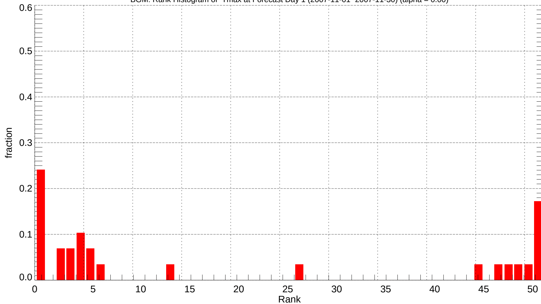
BGM: Rank Histogram of Tmax at Forecast Day 1 (2007-11-01~2007-11-30) (alpha = 0.00)
