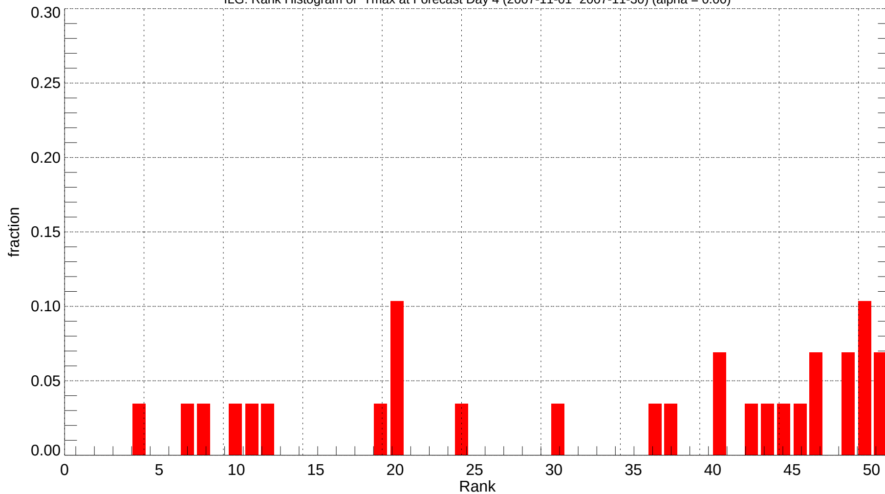
ILG: Rank Histogram of Tmax at Forecast Day 4 (2007-11-01~2007-11-30) (alpha = 0.00)
