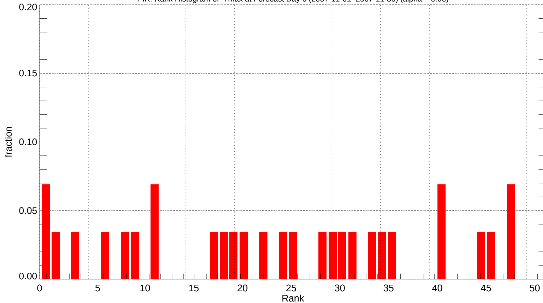
PIR: Rank Histogram of Tmax at Forecast Day 6 (2007-11-01~2007-11-30) (alpha = 0.00)
