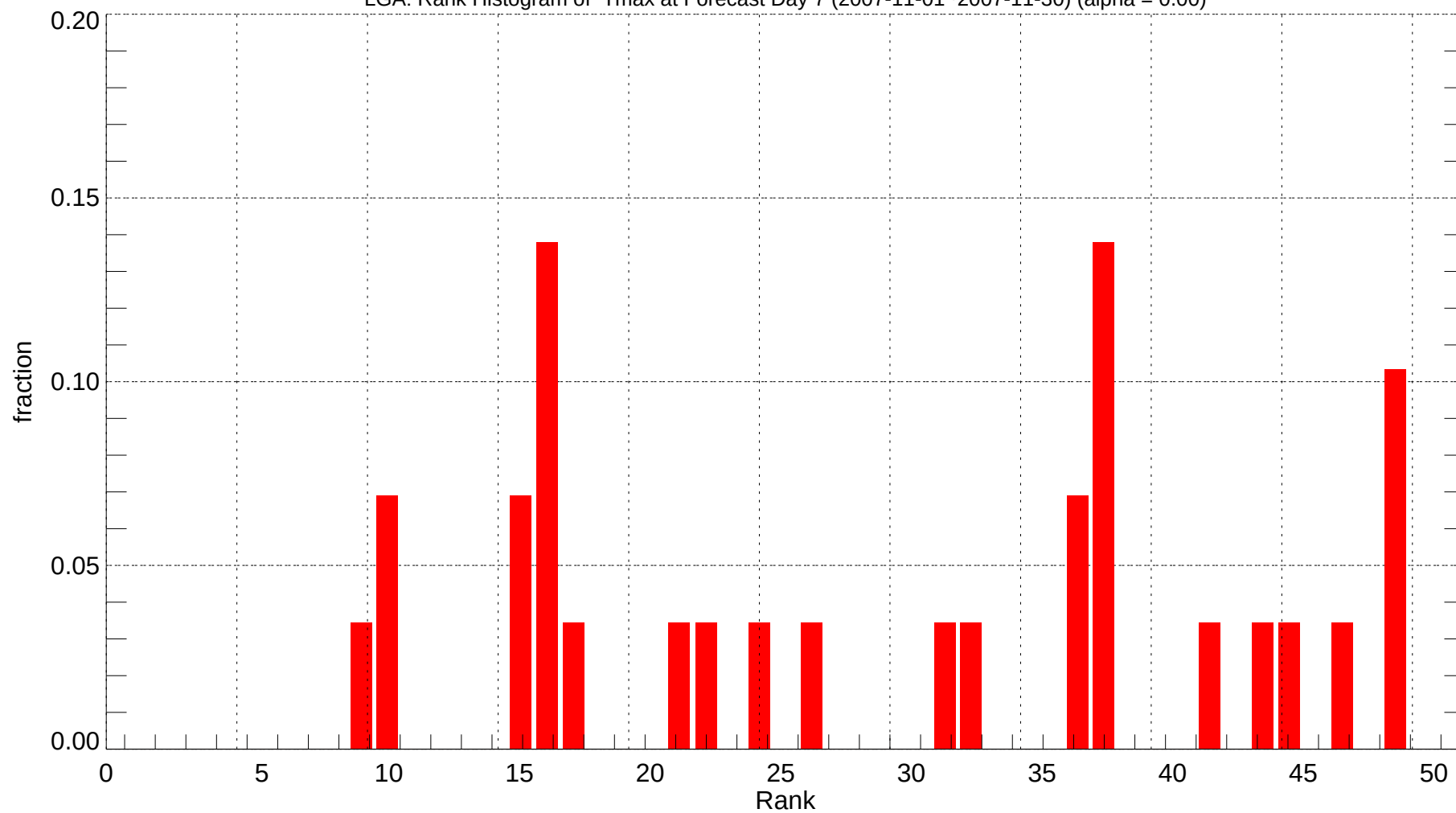
LGA: Rank Histogram of Tmax at Forecast Day 7 (2007-11-01~2007-11-30) (alpha = 0.00)
