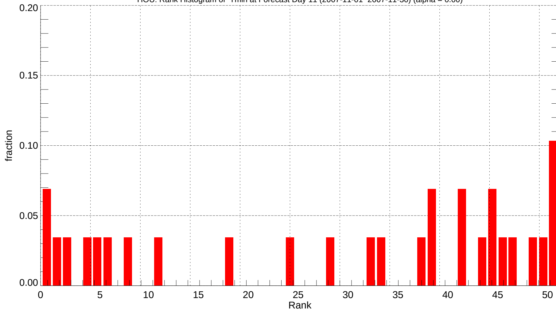
HOU: Rank Histogram of Tmin at Forecast Day 11 (2007-11-01~2007-11-30) (alpha = 0.00)
