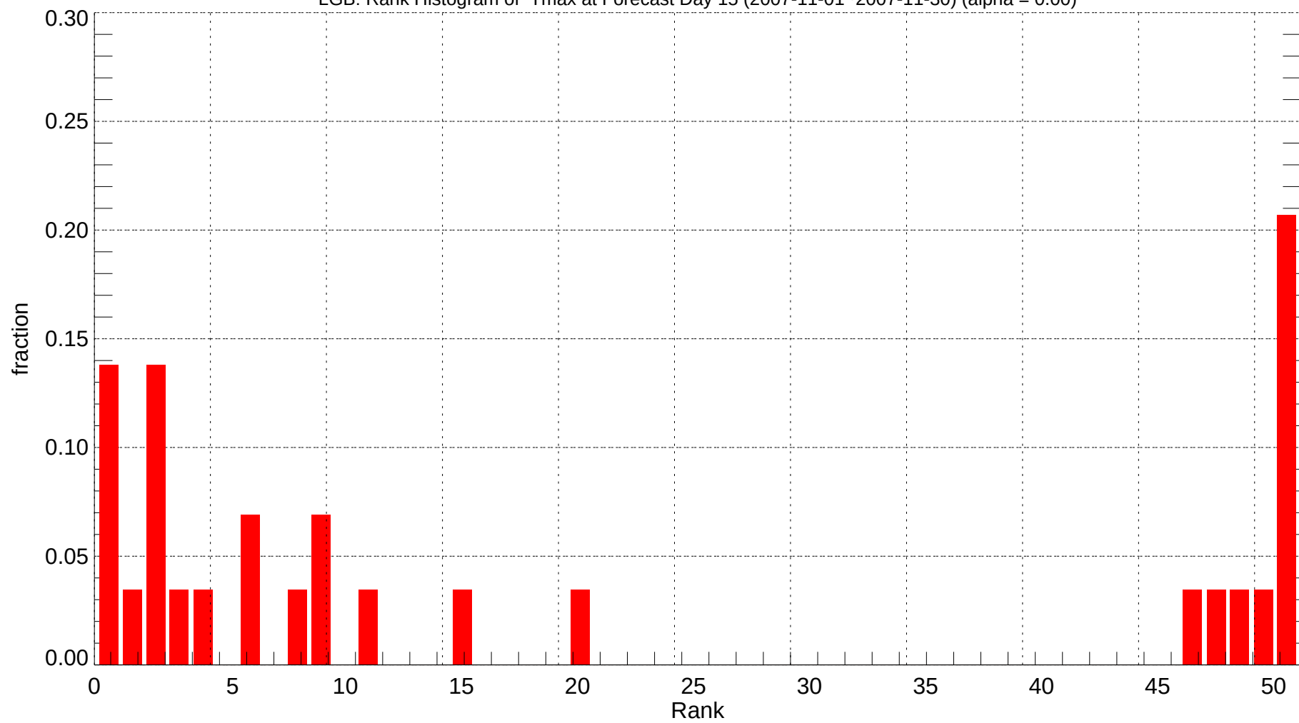
LGB: Rank Histogram of Tmax at Forecast Day 15 (2007-11-01~2007-11-30) (alpha = 0.00)
