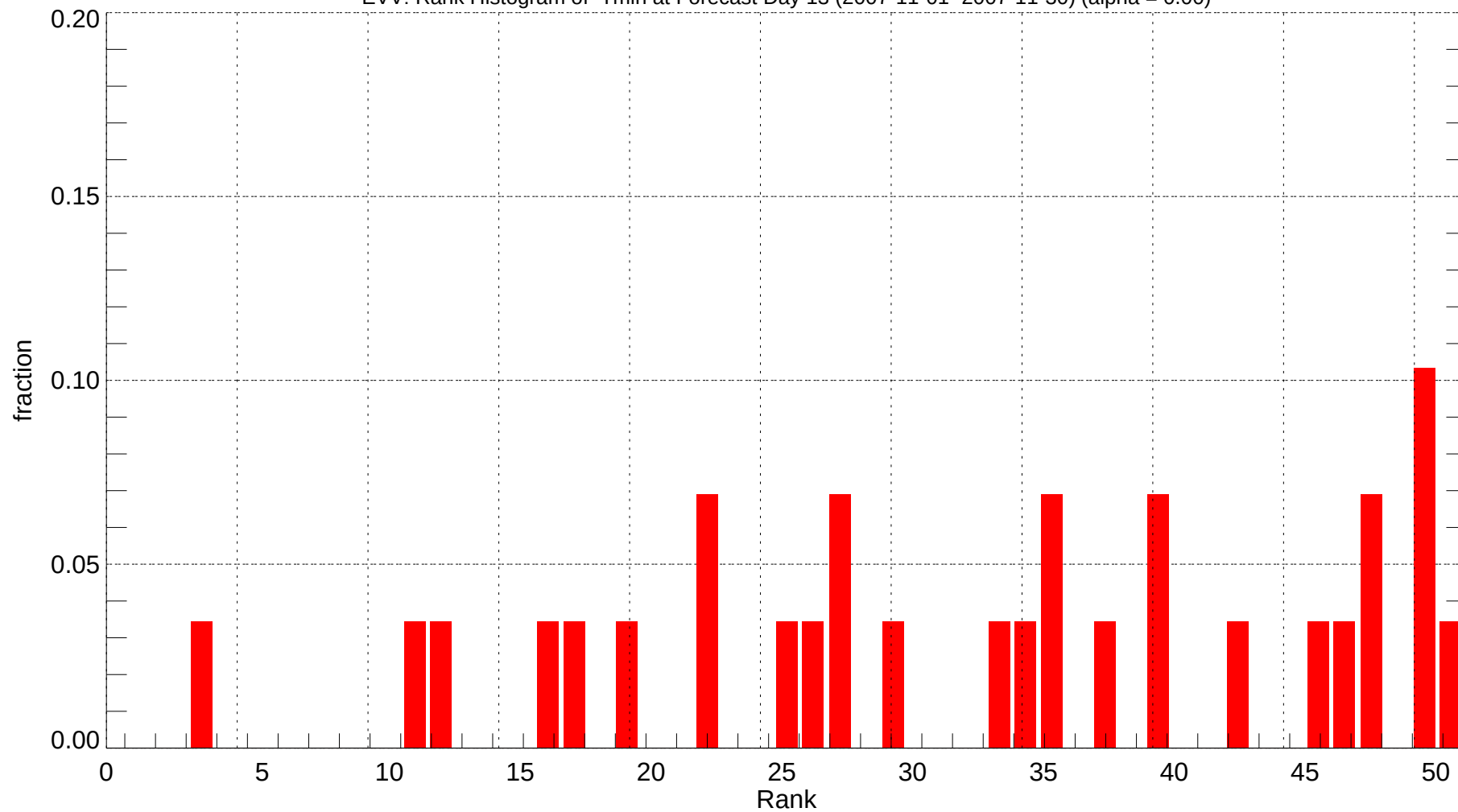
EVV: Rank Histogram of Tmin at Forecast Day 13 (2007-11-01~2007-11-30) (alpha = 0.00)
