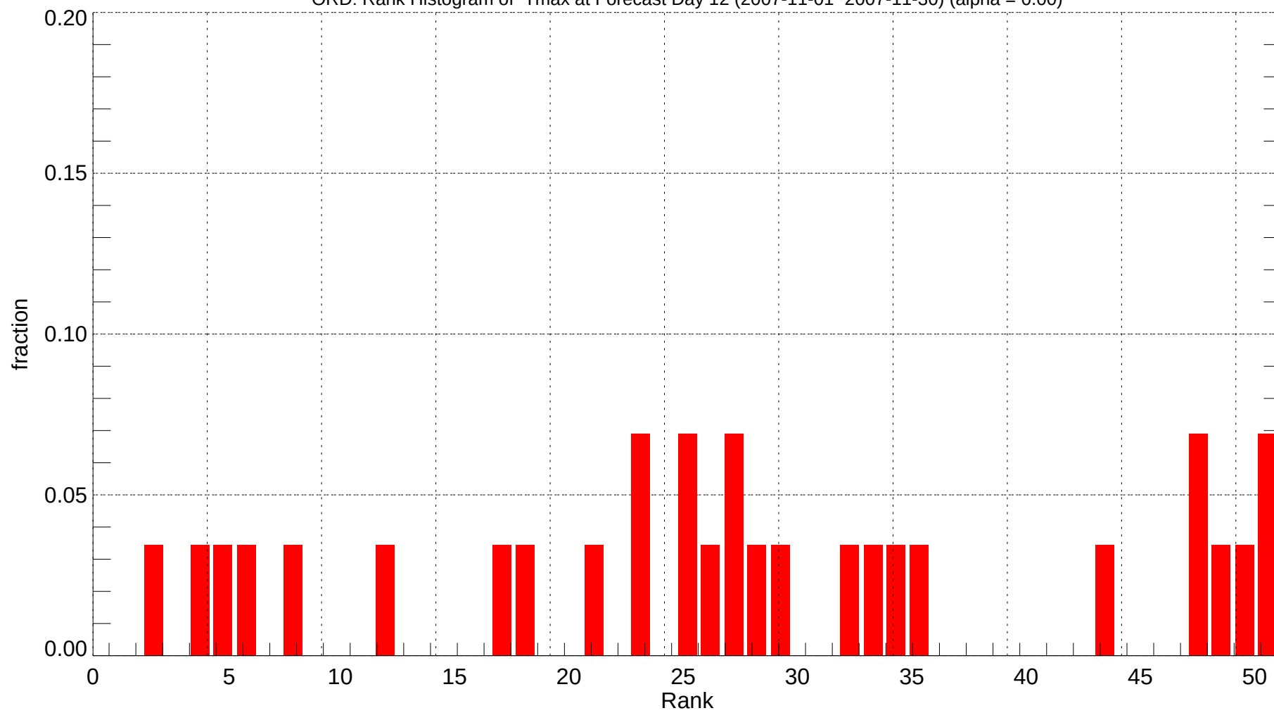
ORD: Rank Histogram of Tmax at Forecast Day 12 (2007-11-01~2007-11-30) (alpha = 0.00)
