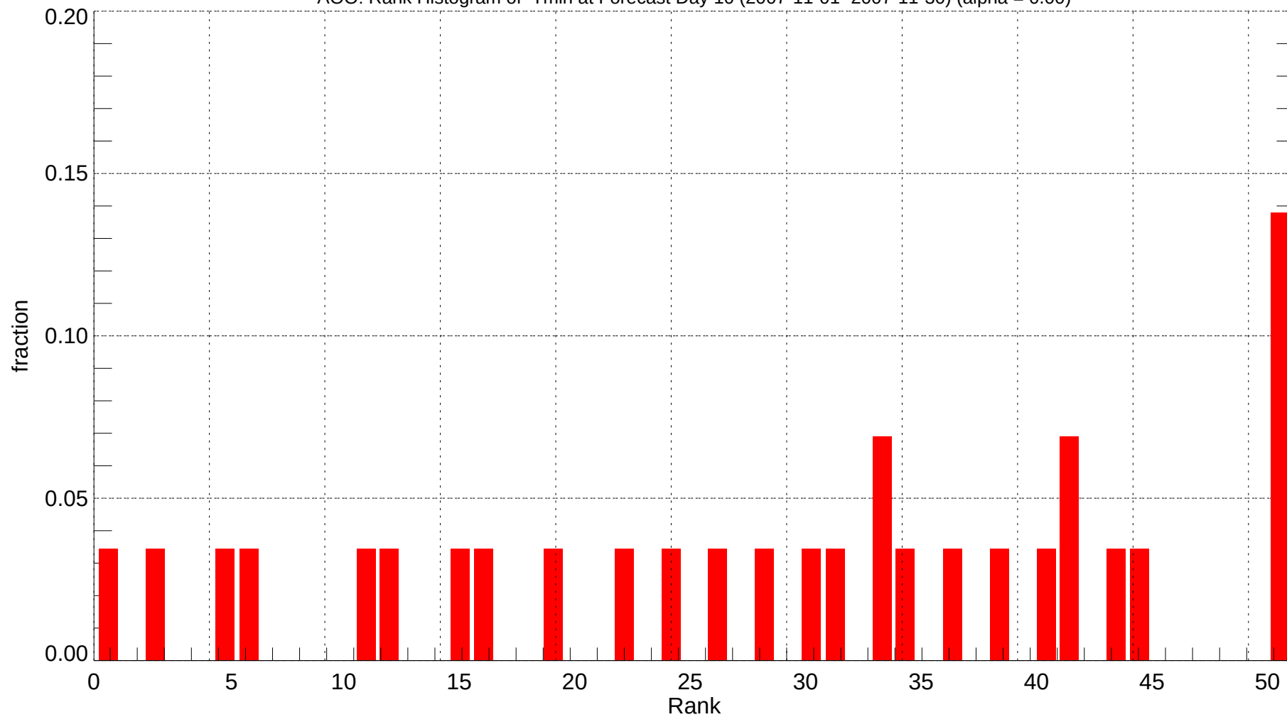
AOO: Rank Histogram of Tmin at Forecast Day 10 (2007-11-01~2007-11-30) (alpha = 0.00)
