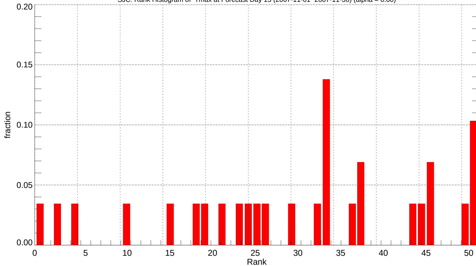
SJC: Rank Histogram of Tmax at Forecast Day 15 (2007-11-01~2007-11-30) (alpha = 0.00)
