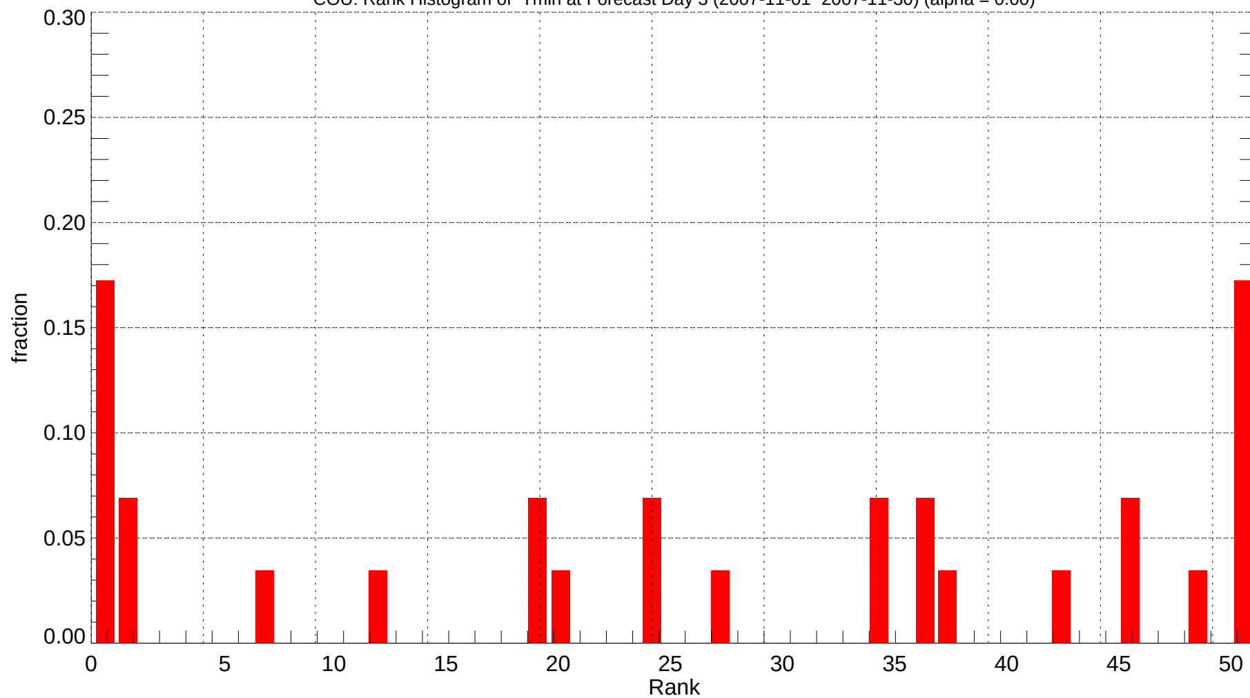
COU: Rank Histogram of Tmin at Forecast Day 3 (2007-11-01~2007-11-30) (alpha = 0.00)
