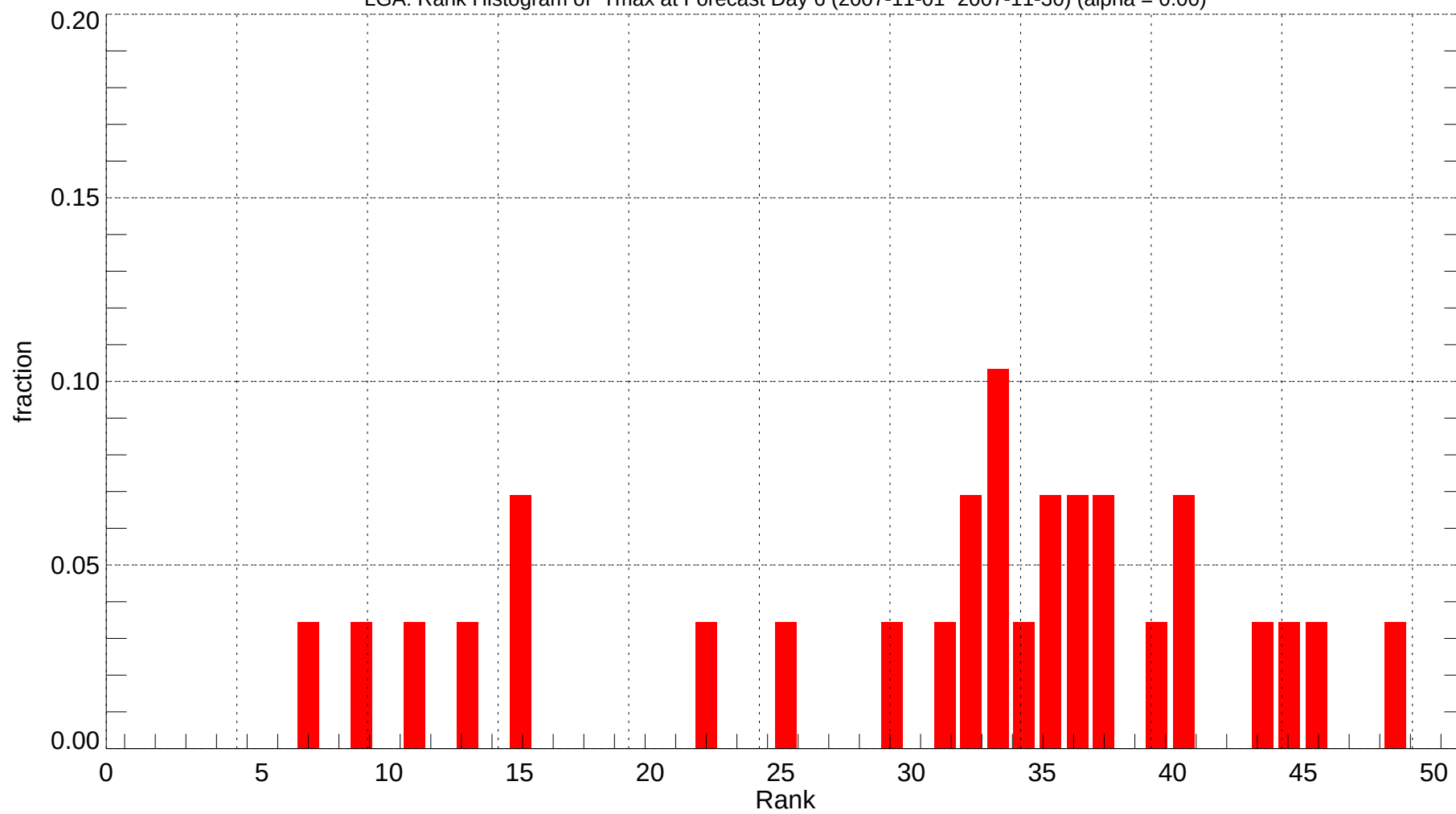
LGA: Rank Histogram of Tmax at Forecast Day 6 (2007-11-01~2007-11-30) (alpha = 0.00)
