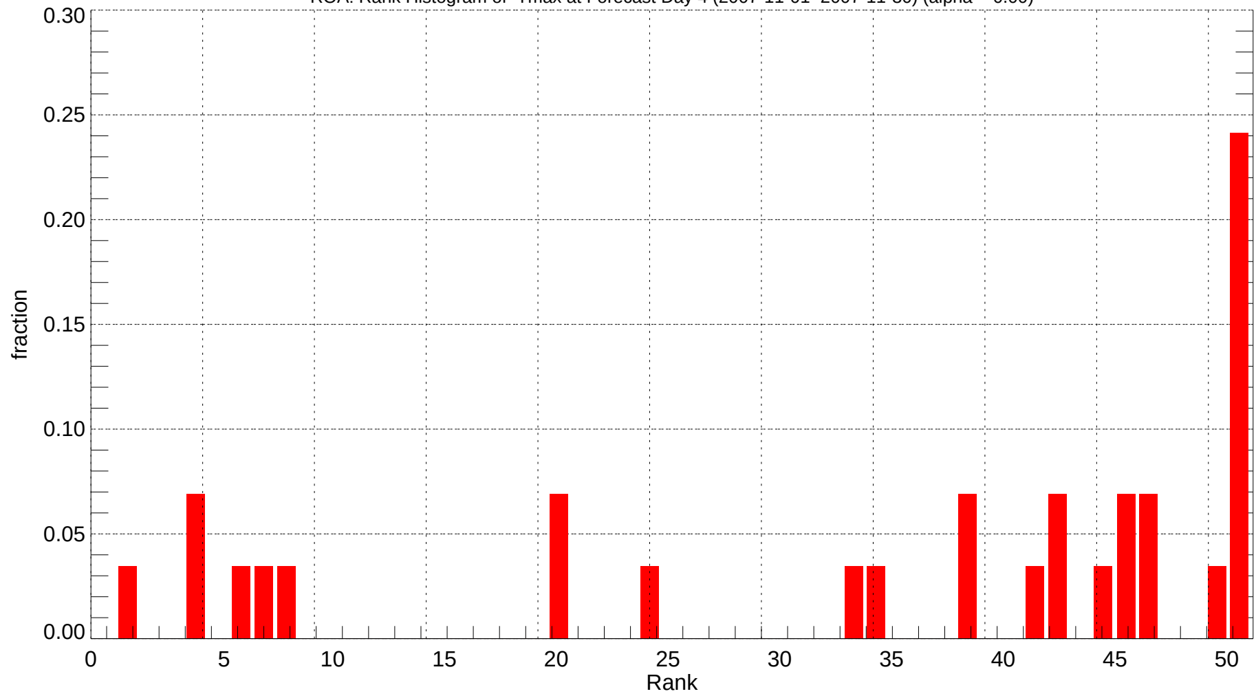
ROA: Rank Histogram of Tmax at Forecast Day 4 (2007-11-01~2007-11-30) (alpha = 0.00)
