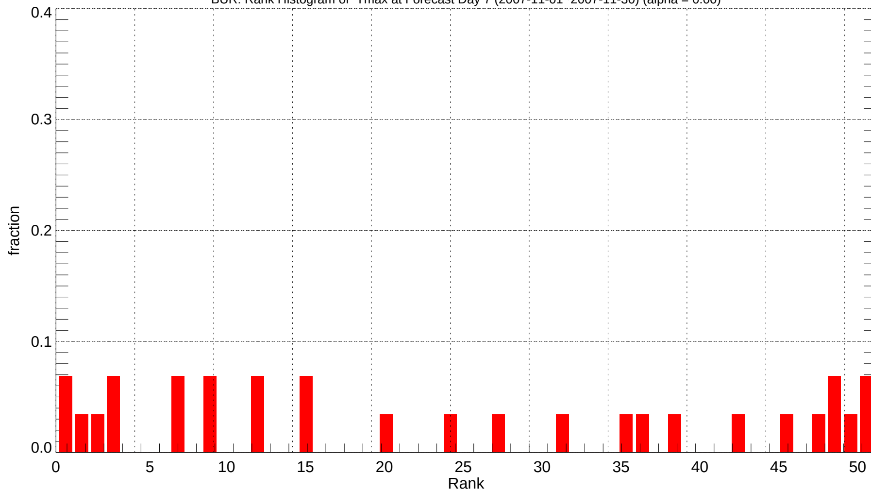
BUR: Rank Histogram of Tmax at Forecast Day 7 (2007-11-01~2007-11-30) (alpha = 0.00)
