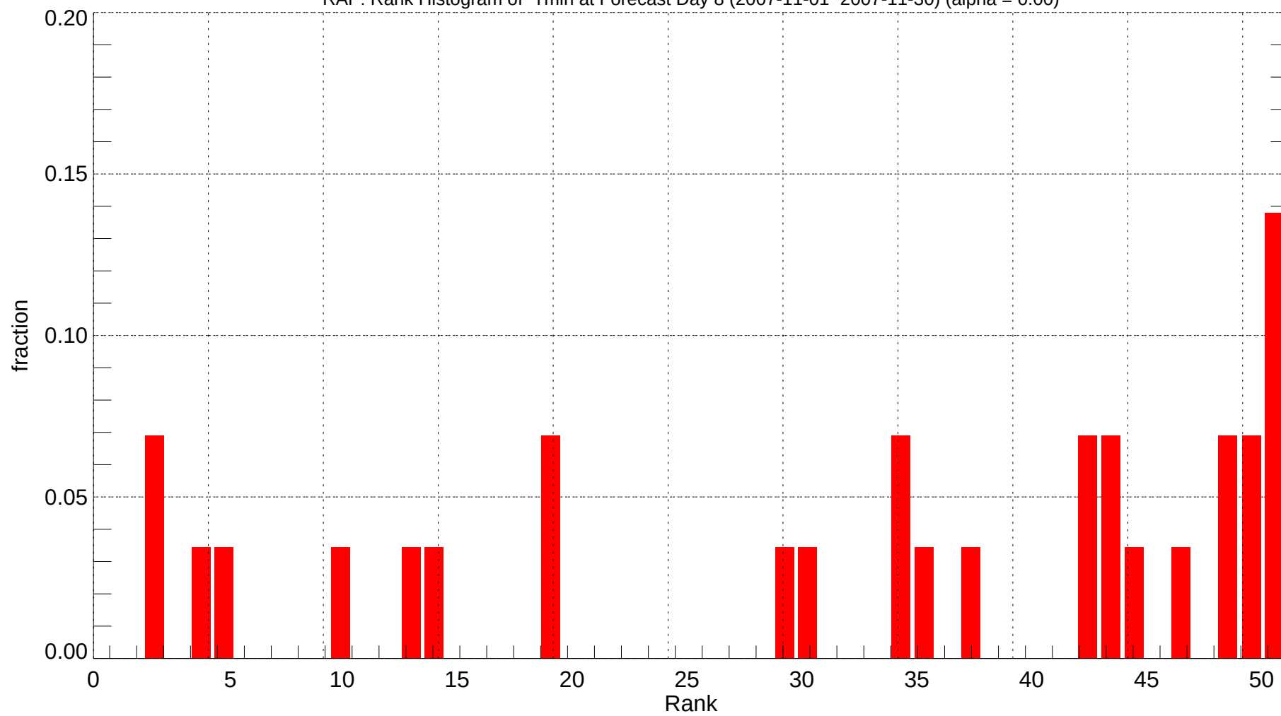
RAP: Rank Histogram of Tmin at Forecast Day 8 (2007-11-01~2007-11-30) (alpha = 0.00)
