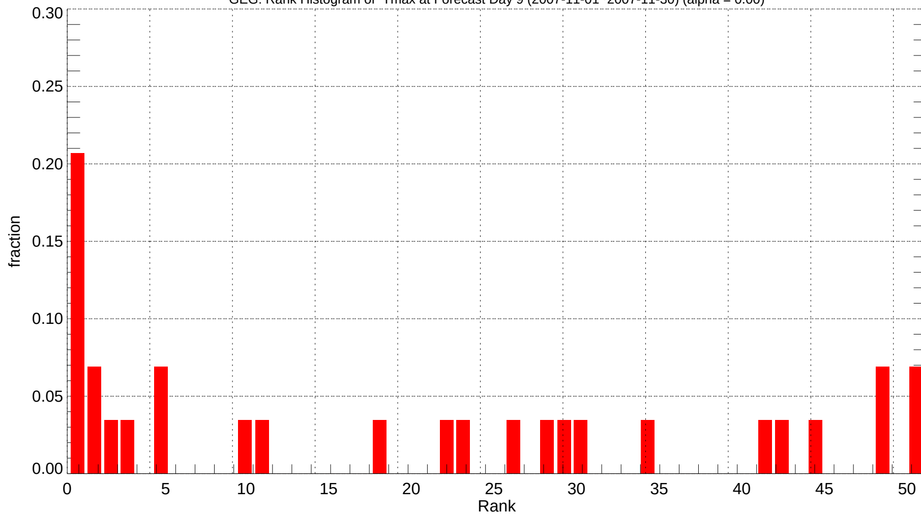
GEG: Rank Histogram of Tmax at Forecast Day 9 (2007-11-01~2007-11-30) (alpha = 0.00)
