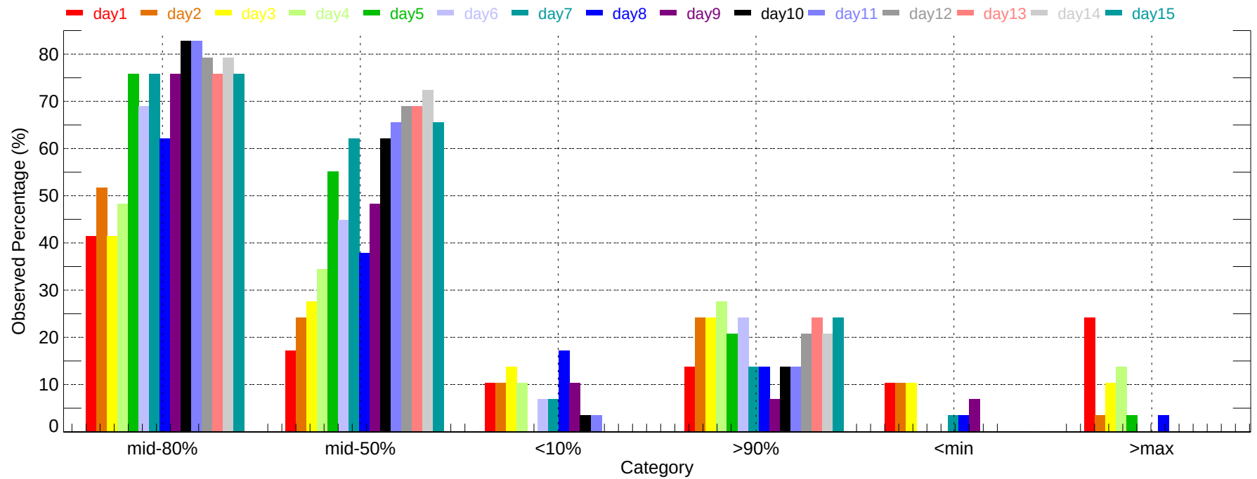
Observed Percentage of Ensembles - SEA: Min Temperature (2007-11-01~2007-11-30)
