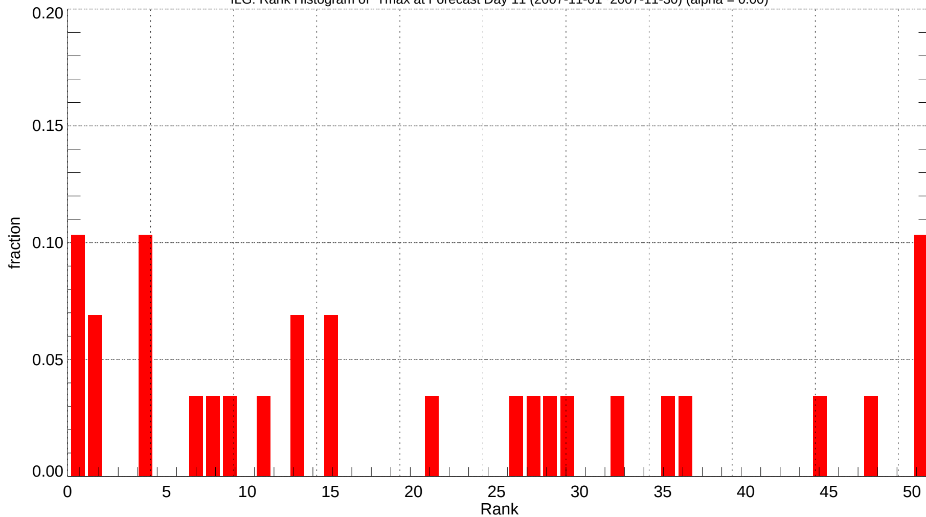
ILG: Rank Histogram of Tmax at Forecast Day 11 (2007-11-01~2007-11-30) (alpha = 0.00)
