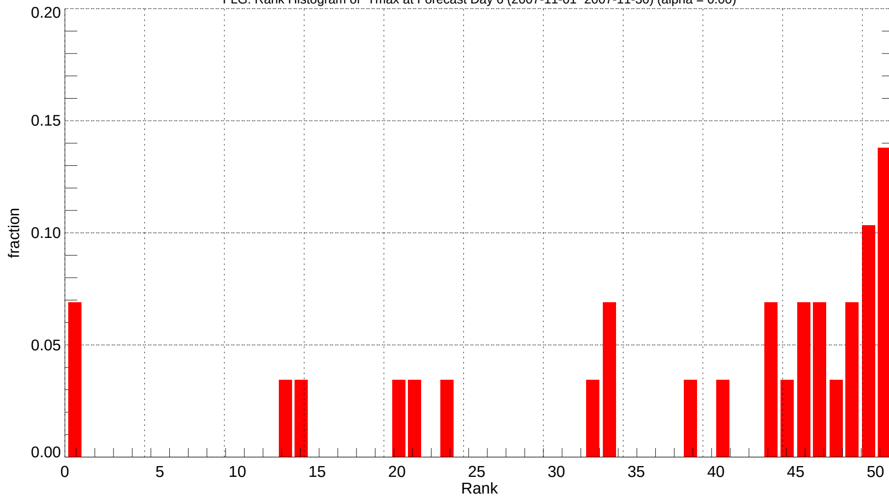
FLG: Rank Histogram of Tmax at Forecast Day 6 (2007-11-01~2007-11-30) (alpha = 0.00)
