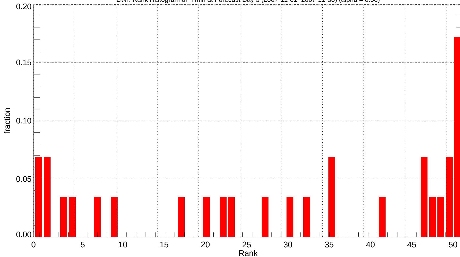
BWI: Rank Histogram of Tmin at Forecast Day 3 (2007-11-01~2007-11-30) (alpha = 0.00)
