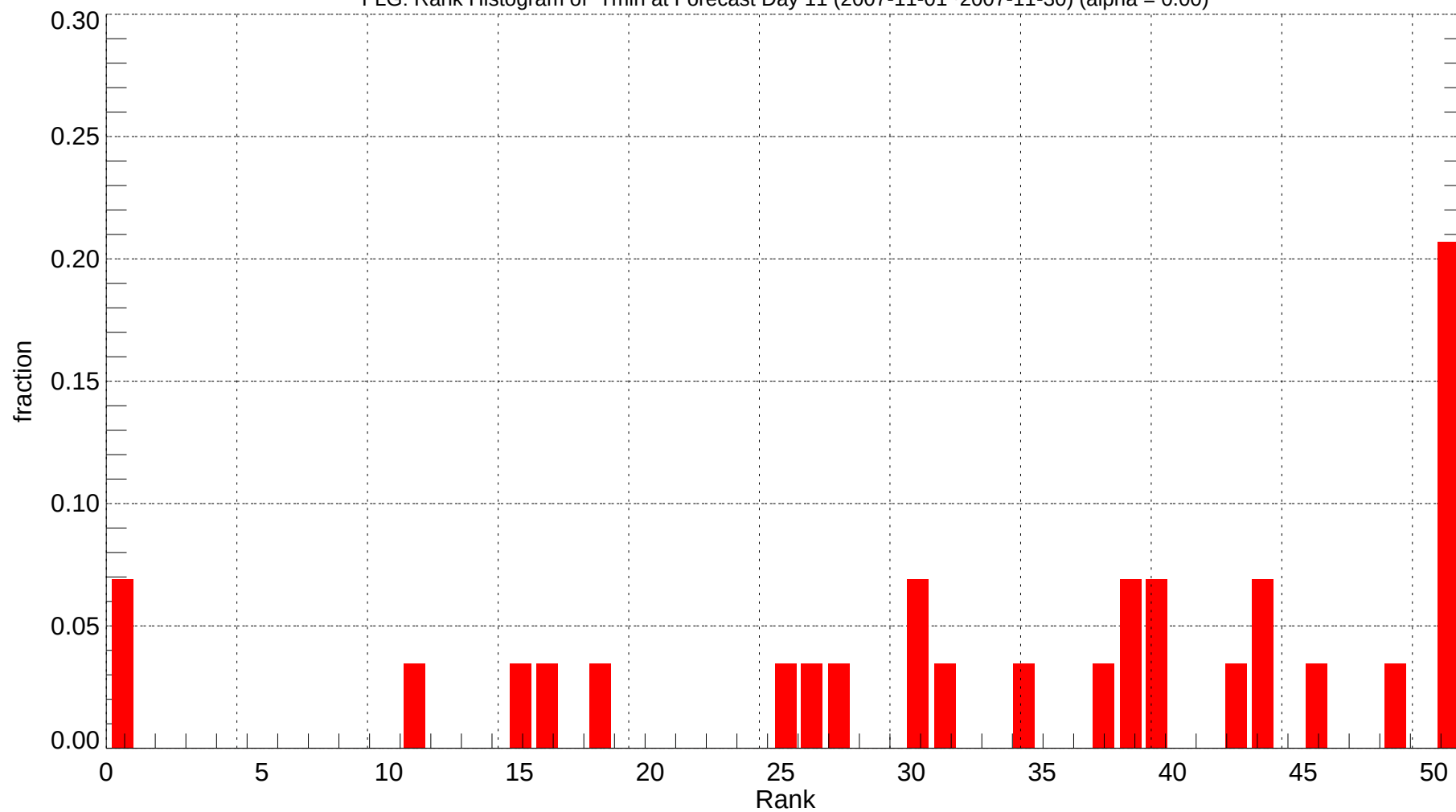
FLG: Rank Histogram of Tmin at Forecast Day 11 (2007-11-01~2007-11-30) (alpha = 0.00)
