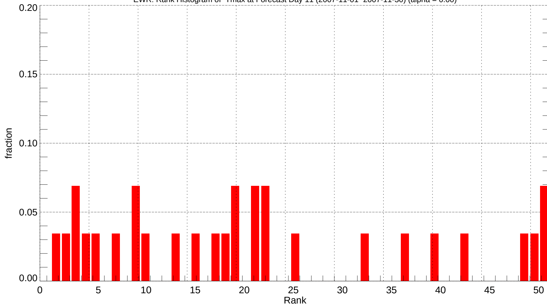
EW: Rank Histogram of Tmax at Forecast Day 11 (2007-11-01~2007-11-30) (alpha = 0.00)
