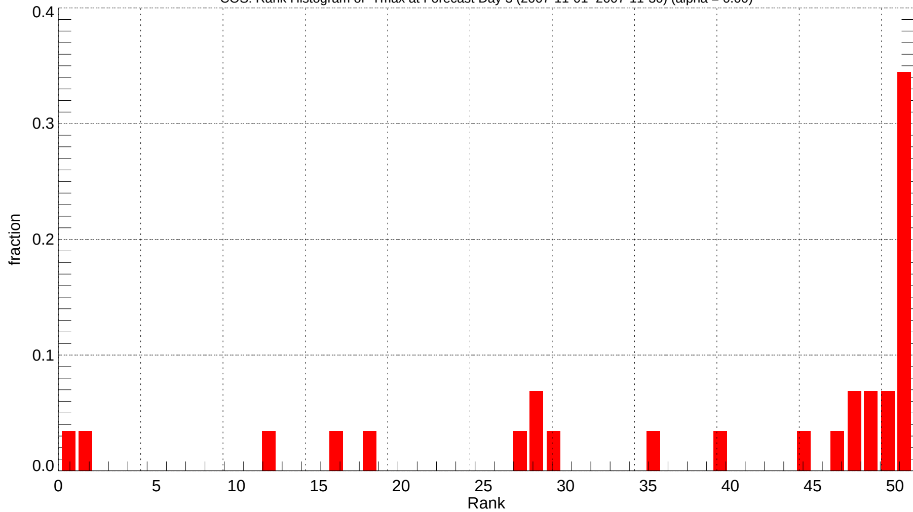
COS: Rank Histogram of Tmax at Forecast Day 3 (2007-11-01~2007-11-30) (alpha = 0.00)
