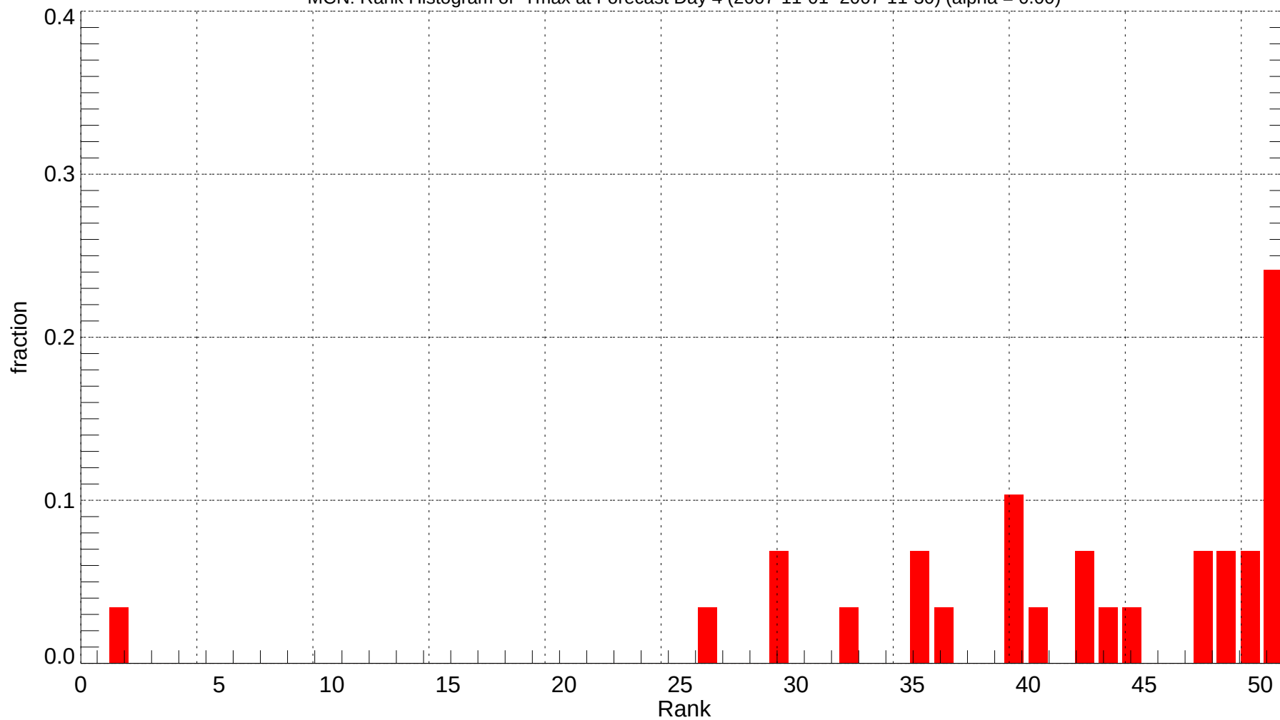
MCN: Rank Histogram of Tmax at Forecast Day 4 (2007-11-01~2007-11-30) (alpha = 0.00)
