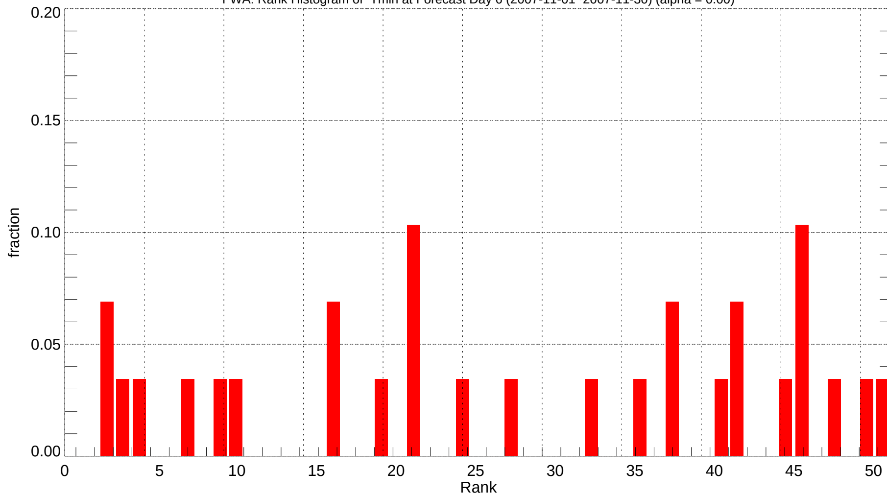
FWA: Rank Histogram of Tmin at Forecast Day 6 (2007-11-01~2007-11-30) (alpha = 0.00)
