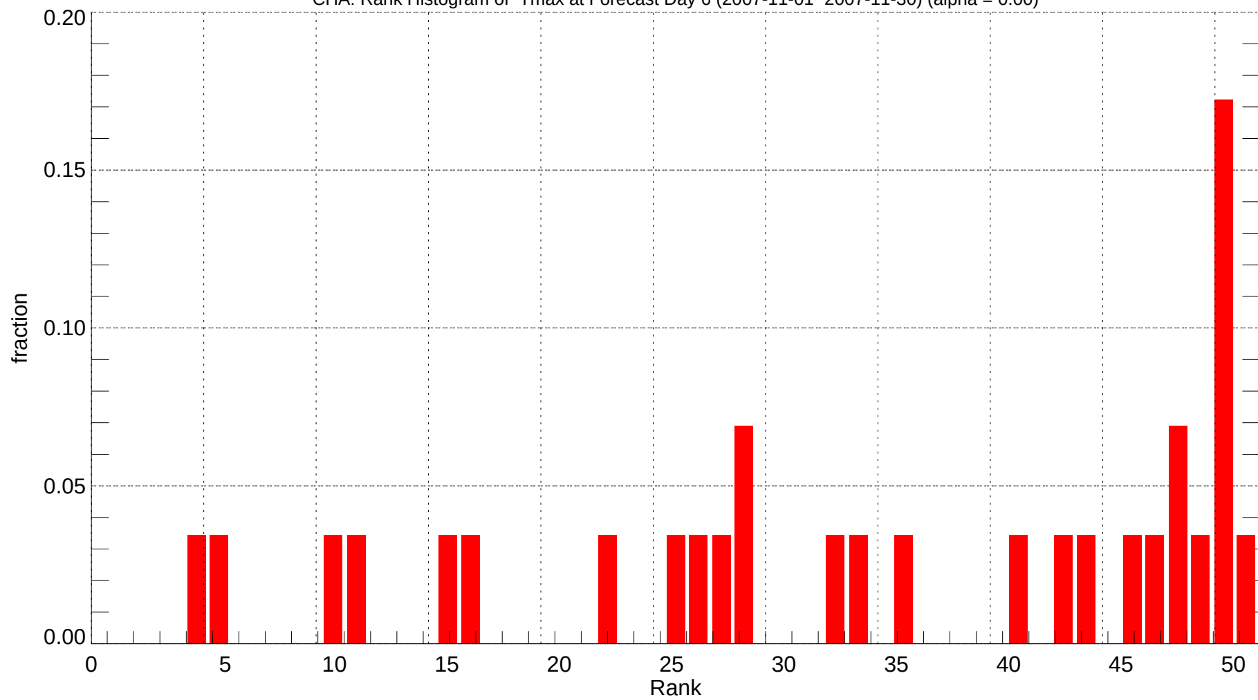
CHA: Rank Histogram of Tmax at Forecast Day 6 (2007-11-01~2007-11-30) (alpha = 0.00)
