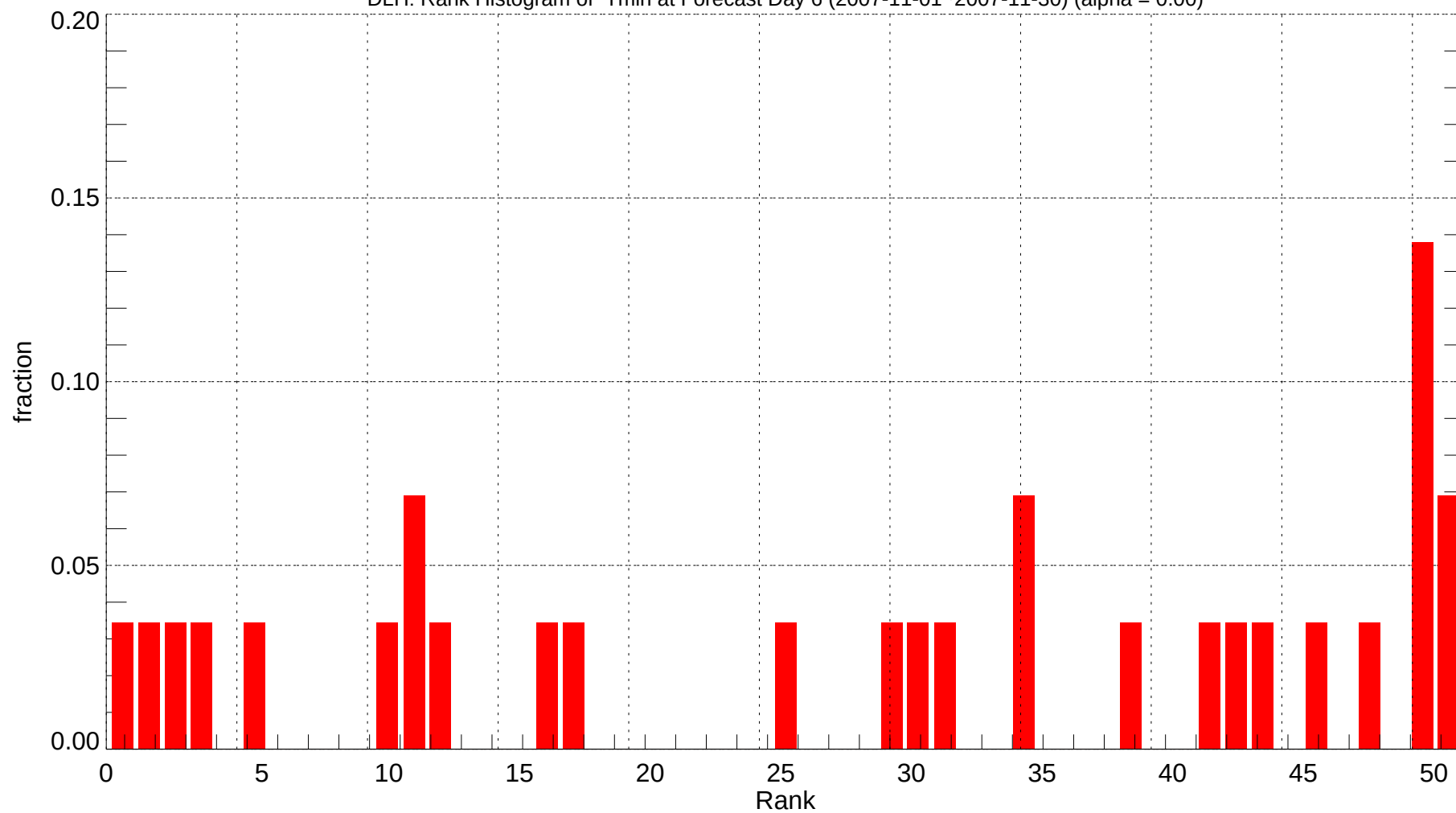
DLH: Rank Histogram of Tmin at Forecast Day 6 (2007-11-01~2007-11-30) (alpha = 0.00)
