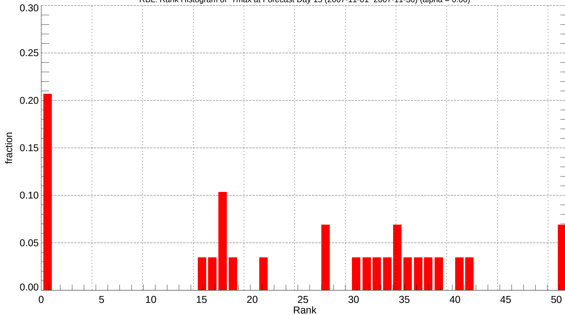
RBL: Rank Histogram of Tmax at Forecast Day 15 (2007-11-01~2007-11-30) (alpha = 0.00)
