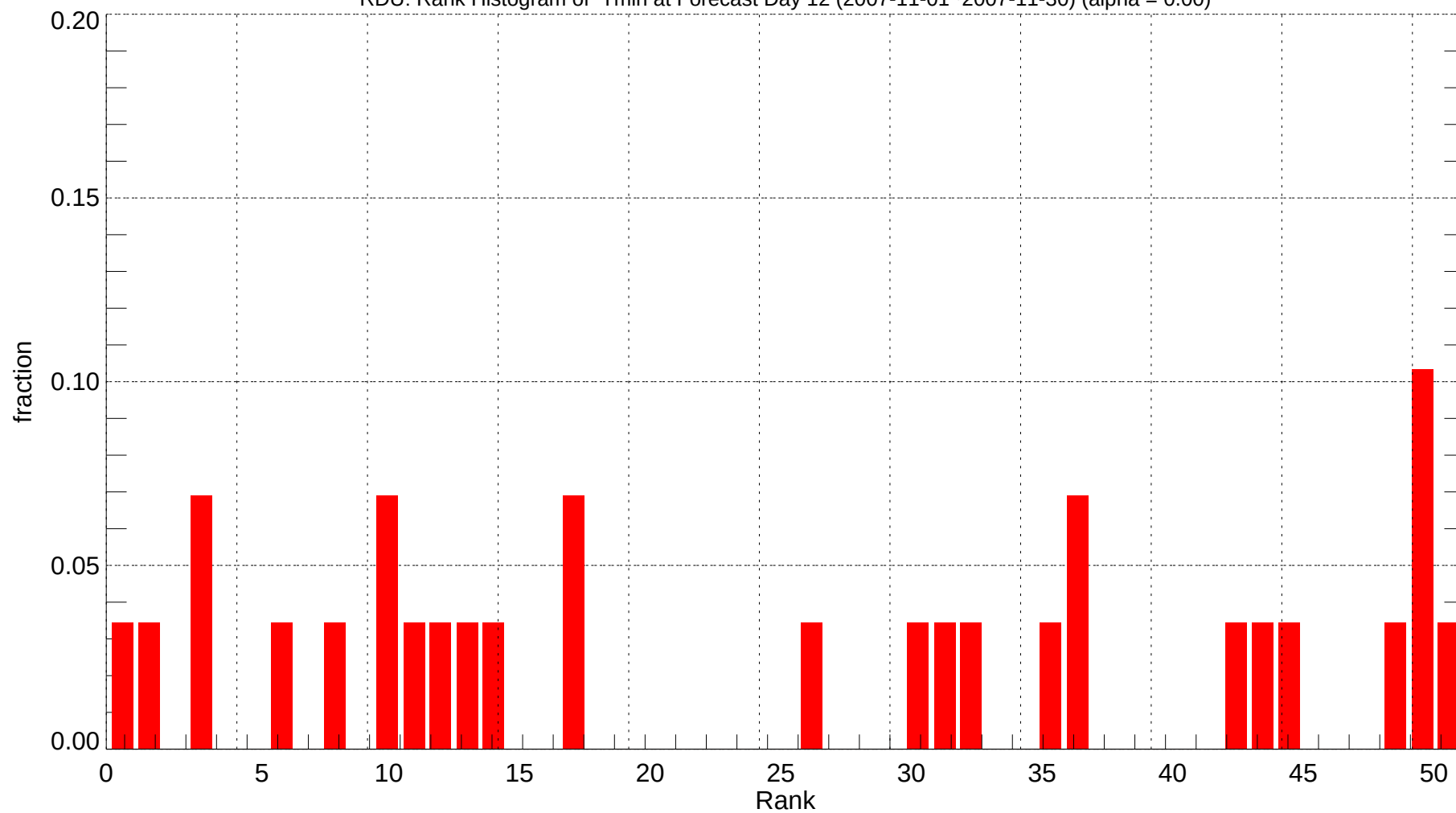
RDU: Rank Histogram of Tmin at Forecast Day 12 (2007-11-01~2007-11-30) (alpha = 0.00)
