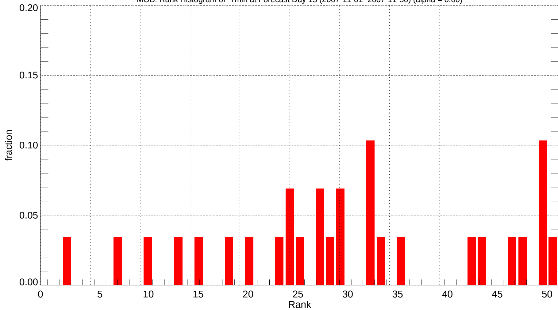
MOB: Rank Histogram of Tmin at Forecast Day 13 (2007-11-01~2007-11-30) (alpha = 0.00)
