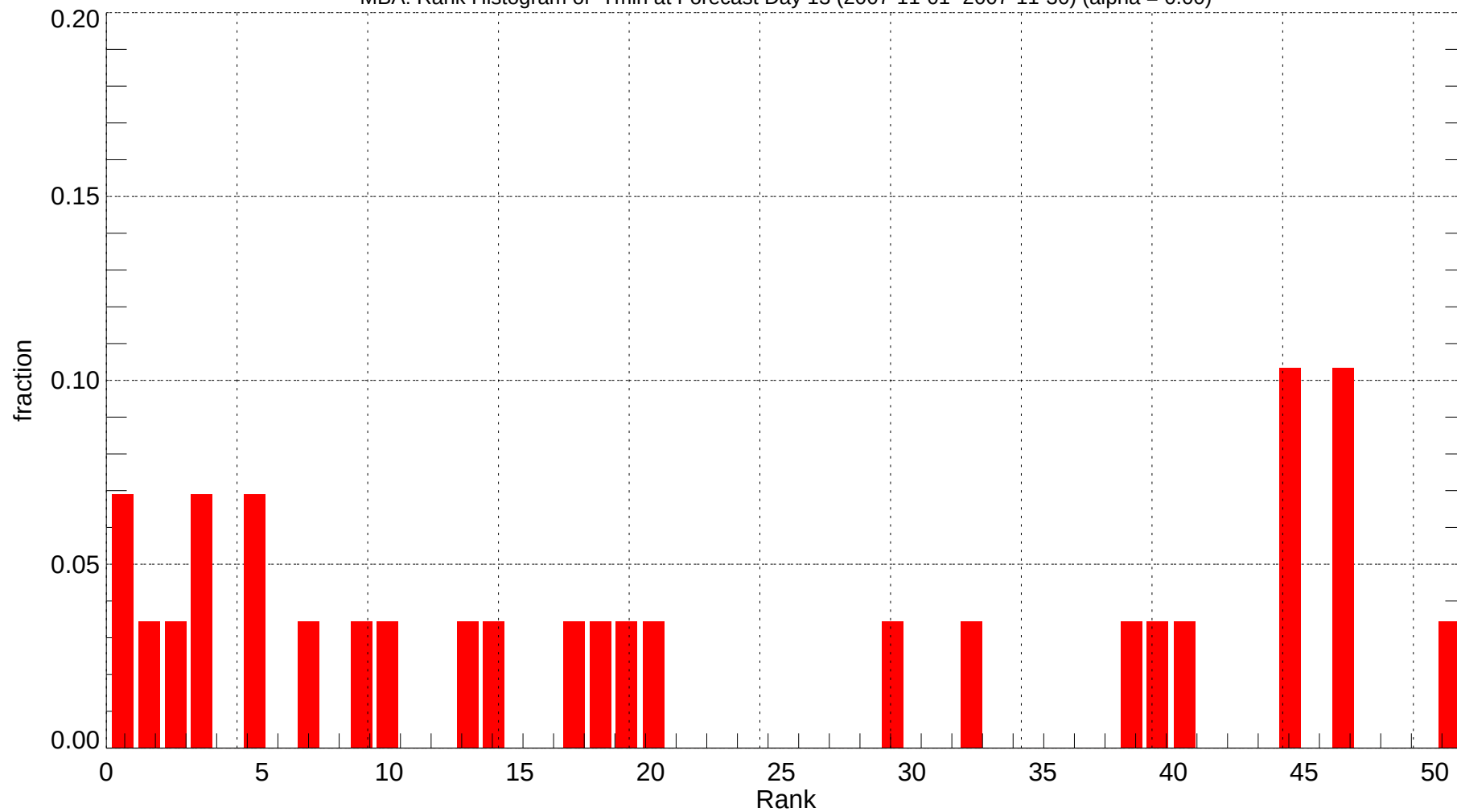
MBA: Rank Histogram of Tmin at Forecast Day 13 (2007-11-01~2007-11-30) (alpha = 0.00)
