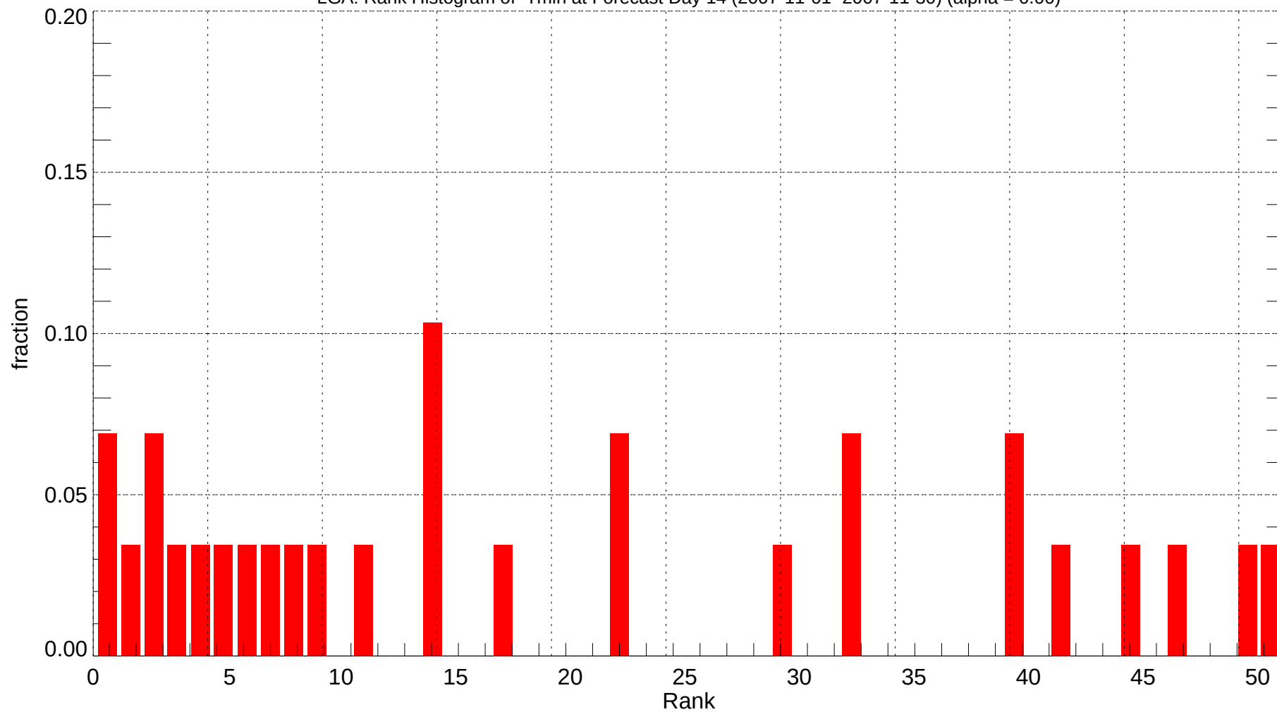
LGA: Rank Histogram of Tmin at Forecast Day 14 (2007-11-01~2007-11-30) (alpha = 0.00)
