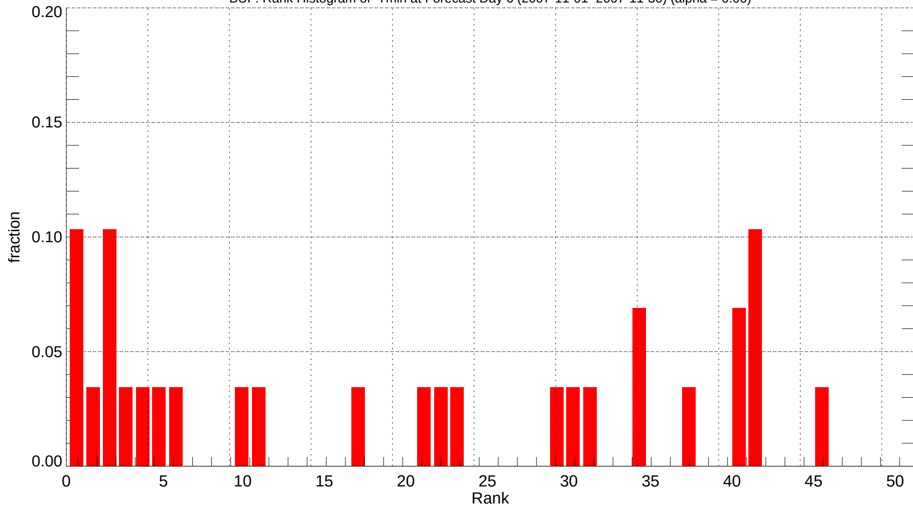
BUF: Rank Histogram of Tmin at Forecast Day 6 (2007-11-01~2007-11-30) (alpha = 0.00)
