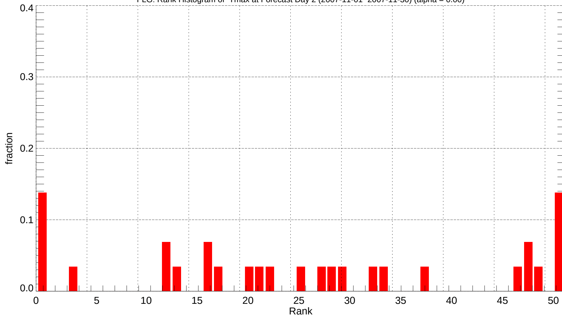
FLG: Rank Histogram of Tmax at Forecast Day 2 (2007-11-01~2007-11-30) (alpha = 0.00)
