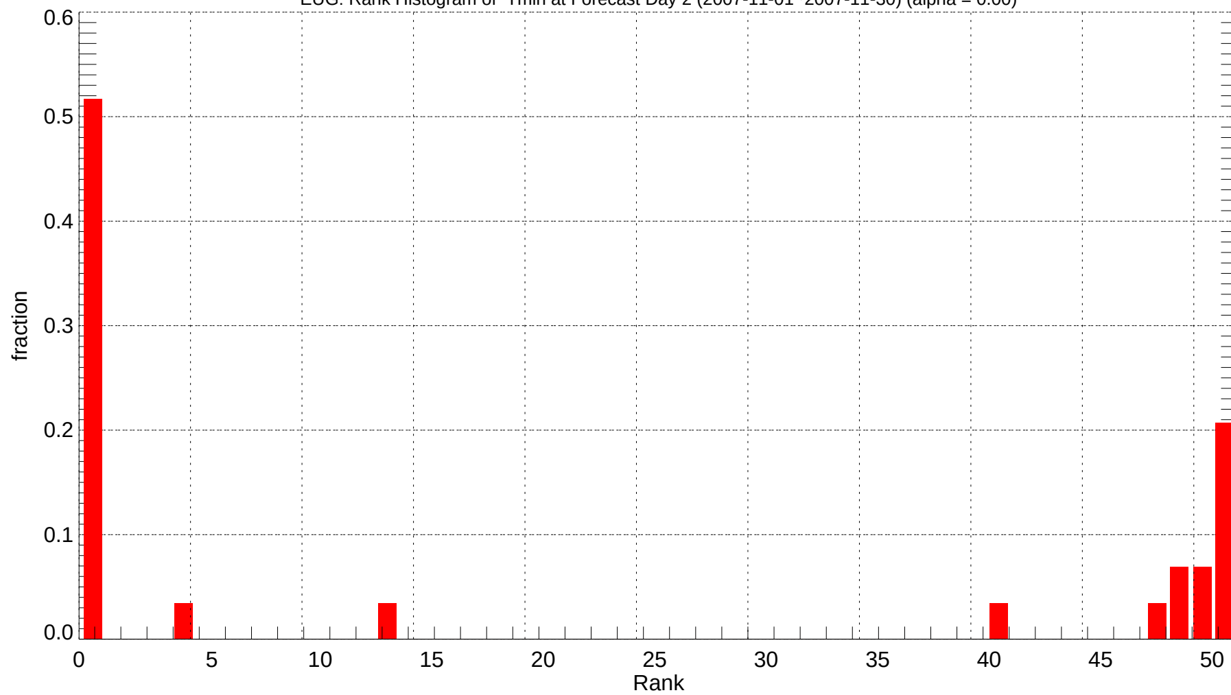
EUG: Rank Histogram of Tmin at Forecast Day 2 (2007-11-01~2007-11-30) (alpha = 0.00)
