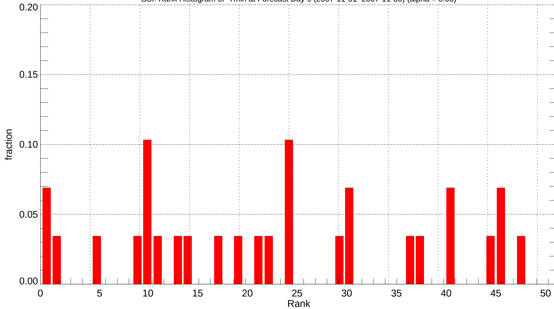
SSI: Rank Histogram of Tmin at Forecast Day 9 (2007-11-01~2007-11-30) (alpha = 0.00)
