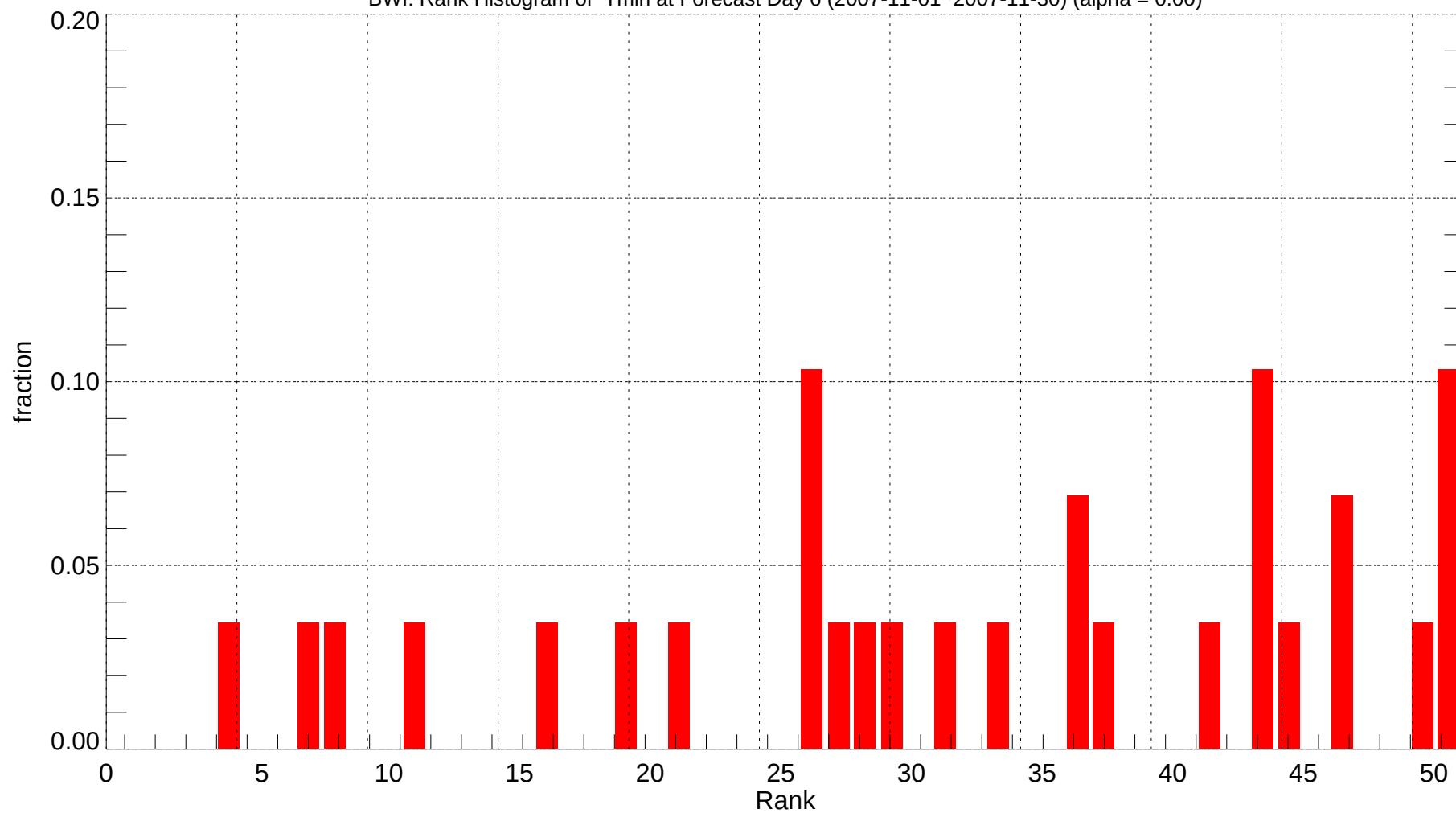
BWI: Rank Histogram of Tmin at Forecast Day 6 (2007-11-01~2007-11-30) (alpha = 0.00)
