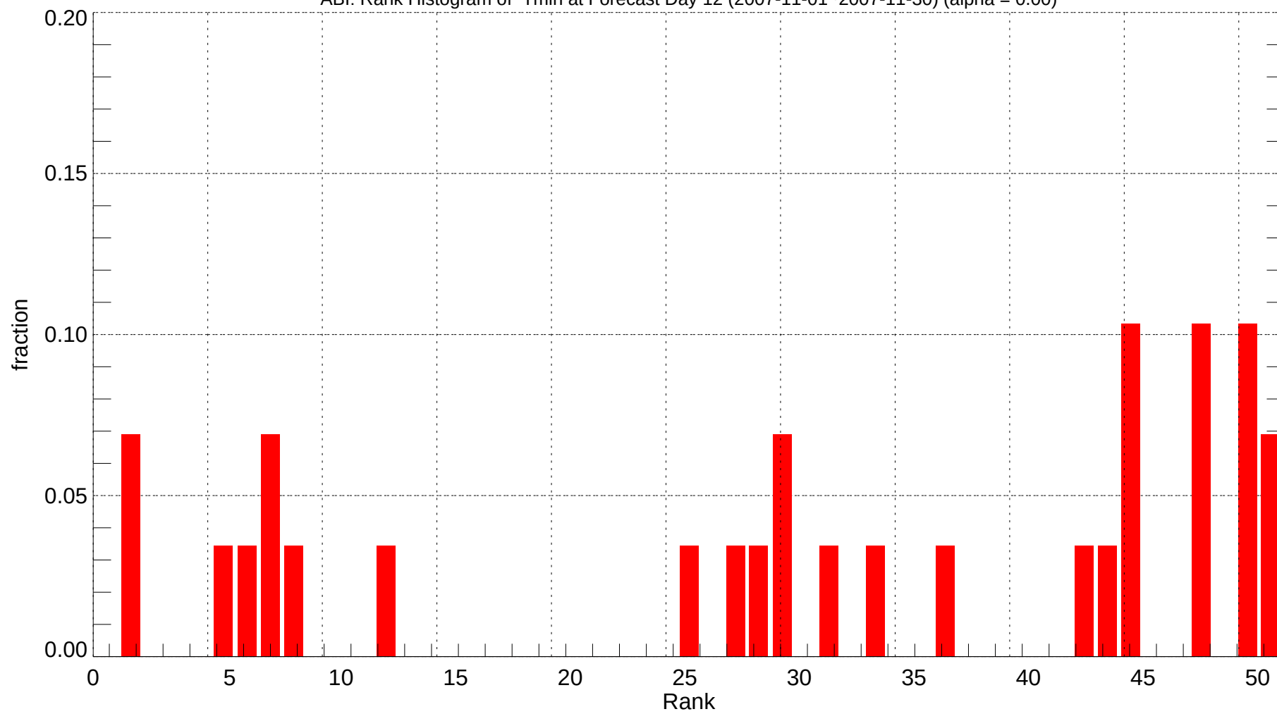
ABI: Rank Histogram of Tmin at Forecast Day 12 (2007-11-01~2007-11-30) (alpha = 0.00)
