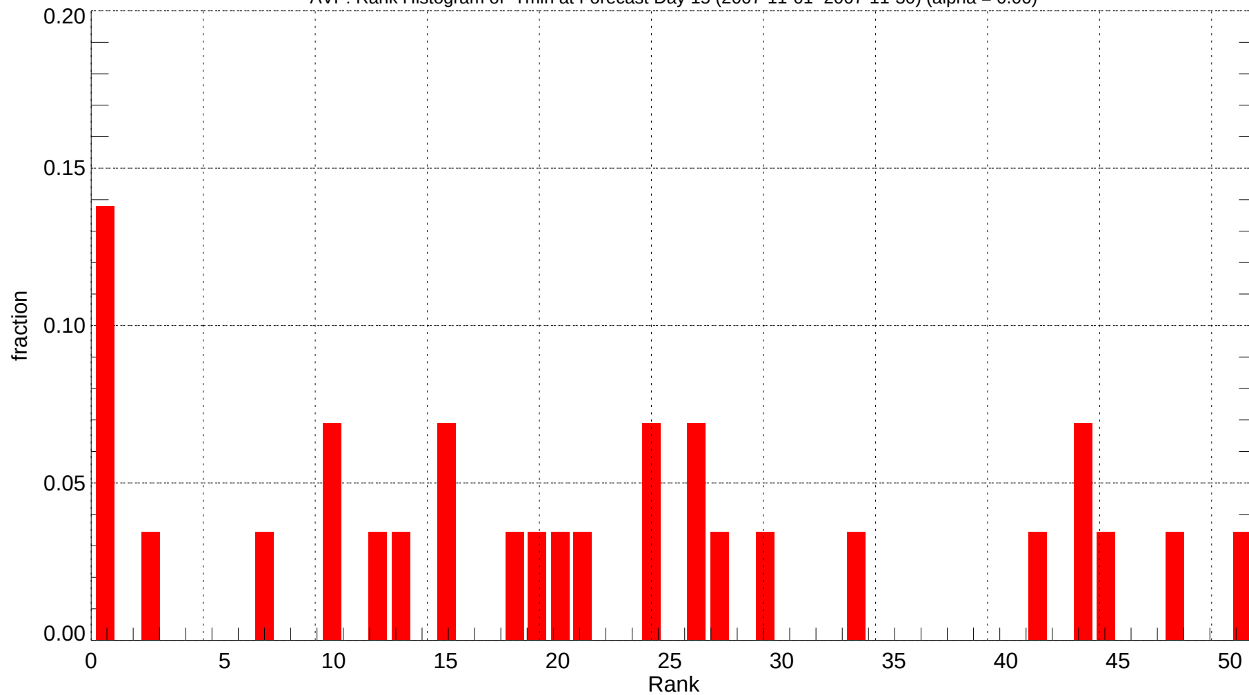
AVP: Rank Histogram of Tmin at Forecast Day 15 (2007-11-01~2007-11-30) (alpha = 0.00)
