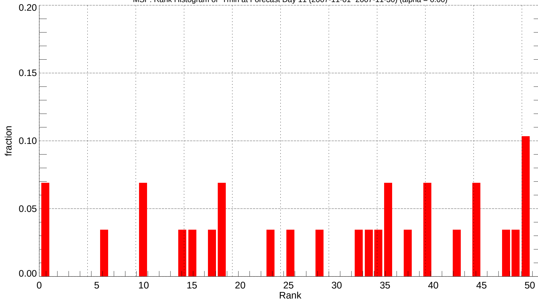
MSP: Rank Histogram of Tmin at Forecast Day 11 (2007-11-01~2007-11-30) (alpha = 0.00)
