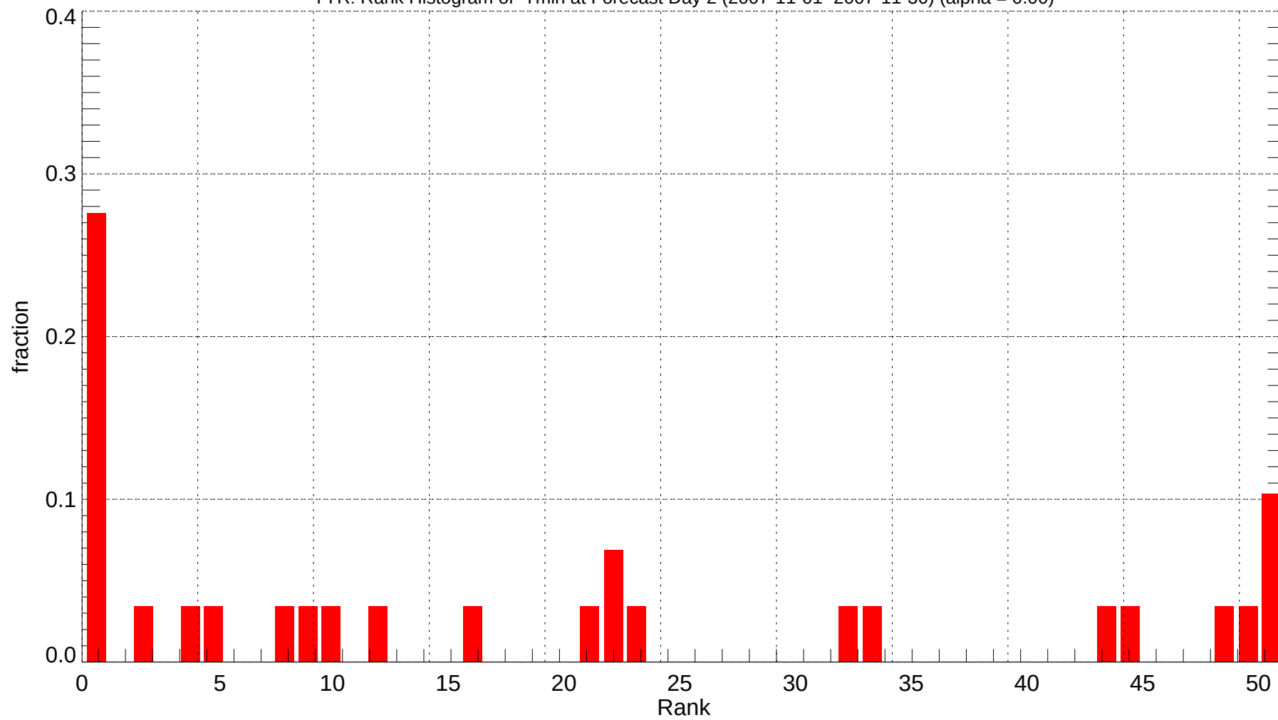
TYR: Rank Histogram of Tmin at Forecast Day 2 (2007-11-01~2007-11-30) (alpha = 0.00)
