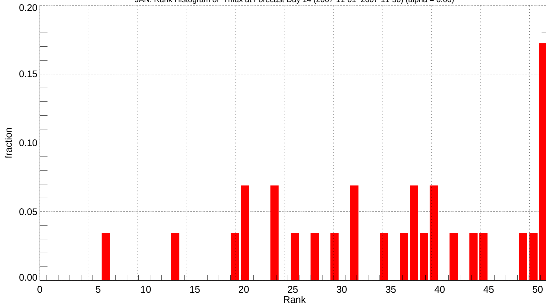
JAN: Rank Histogram of Tmax at Forecast Day 14 (2007-11-01~2007-11-30) (alpha = 0.00)
