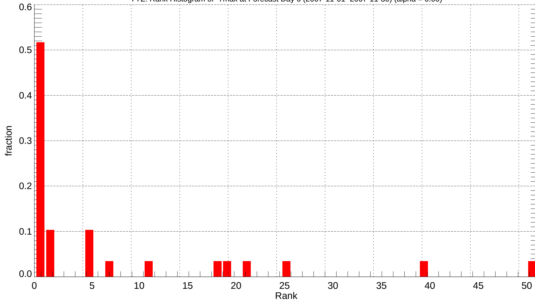
YYZ: Rank Histogram of Tmax at Forecast Day 6 (2007-11-01~2007-11-30) (alpha = 0.00)
