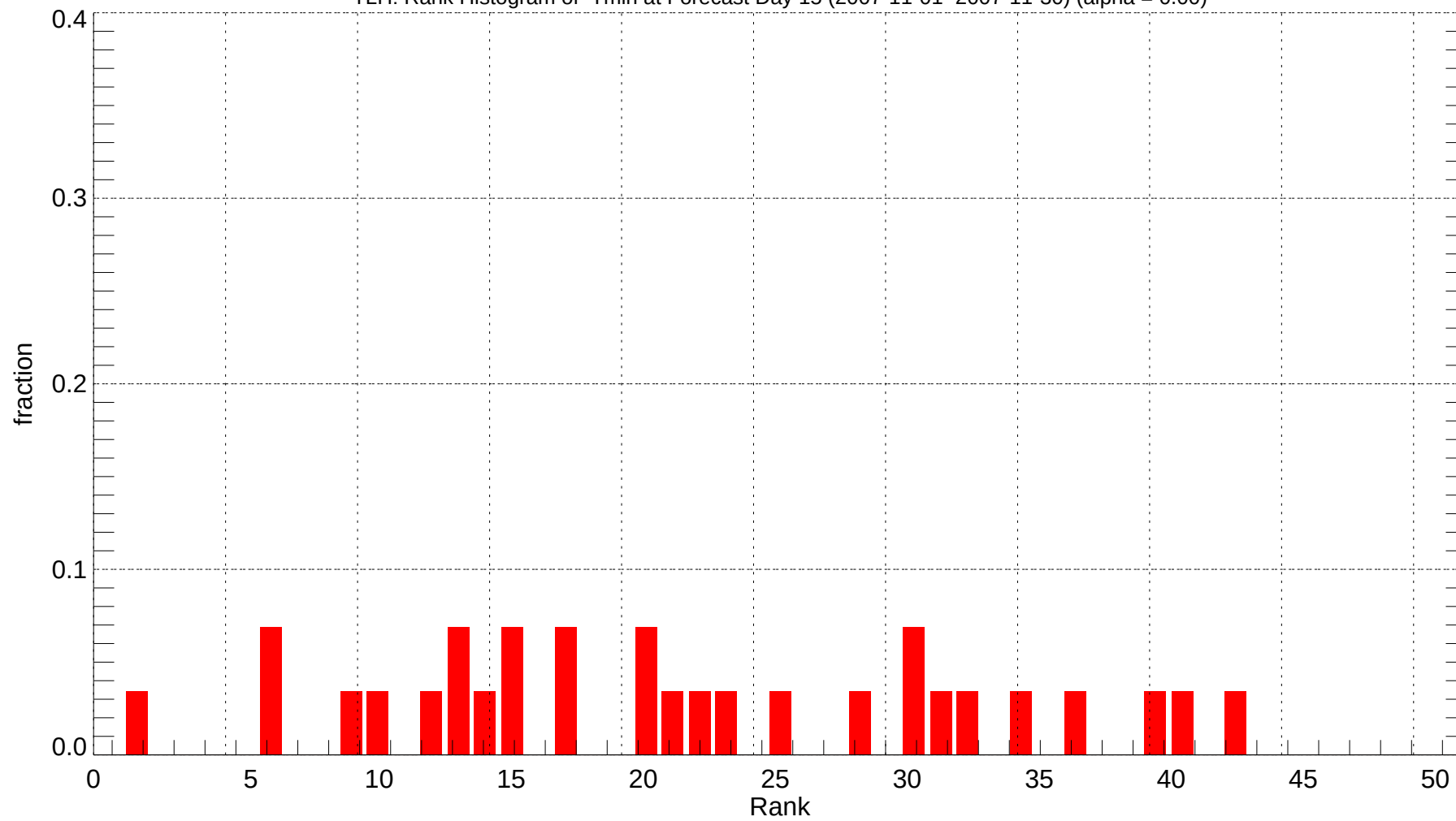
TLH: Rank Histogram of Tmin at Forecast Day 15 (2007-11-01~2007-11-30) (alpha = 0.00)
