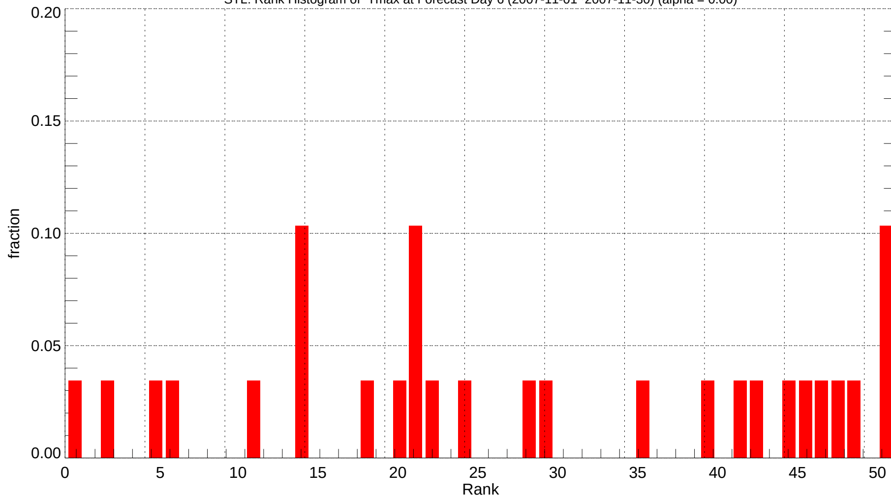
STL: Rank Histogram of Tmax at Forecast Day 6 (2007-11-01~2007-11-30) (alpha = 0.00)
