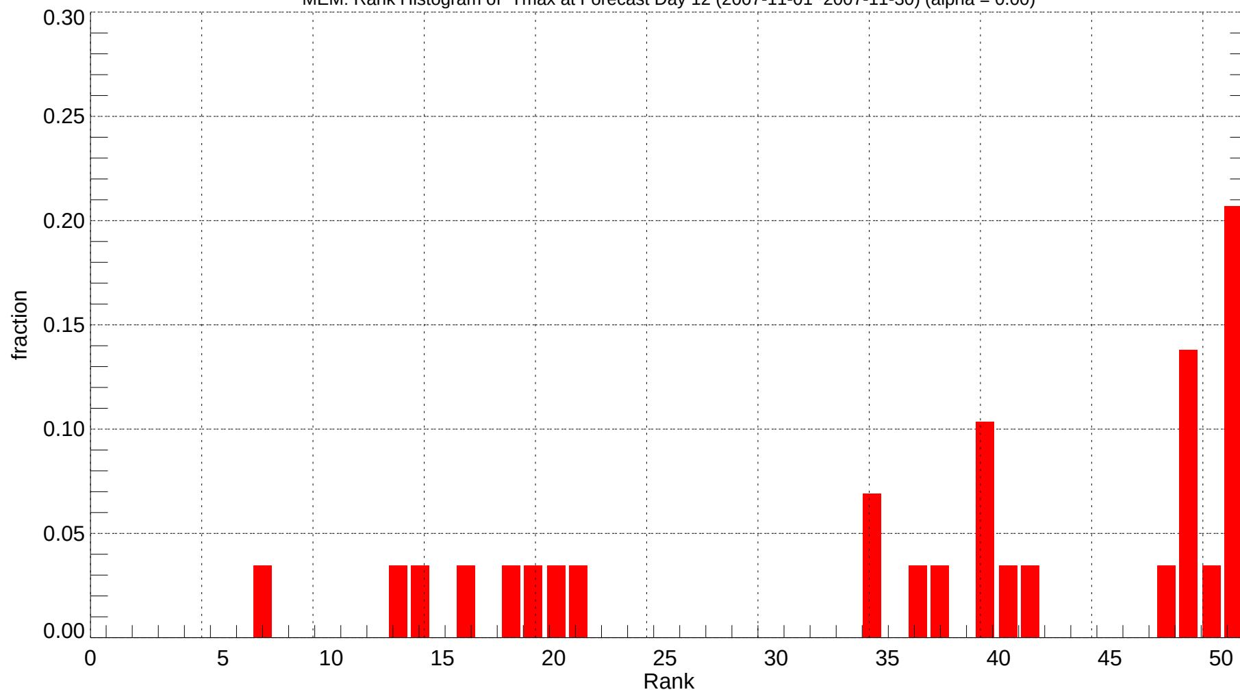
MEM: Rank Histogram of Tmax at Forecast Day 12 (2007-11-01~2007-11-30) (alpha = 0.00)
