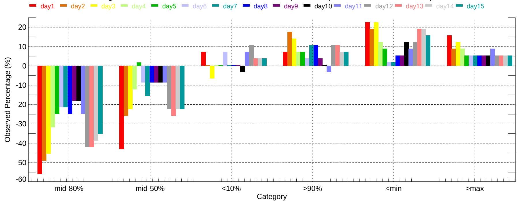
Observed Percentage Deviation of Ensembles - BGM: Max Temperature (2007-11-01~2007-11-30)
