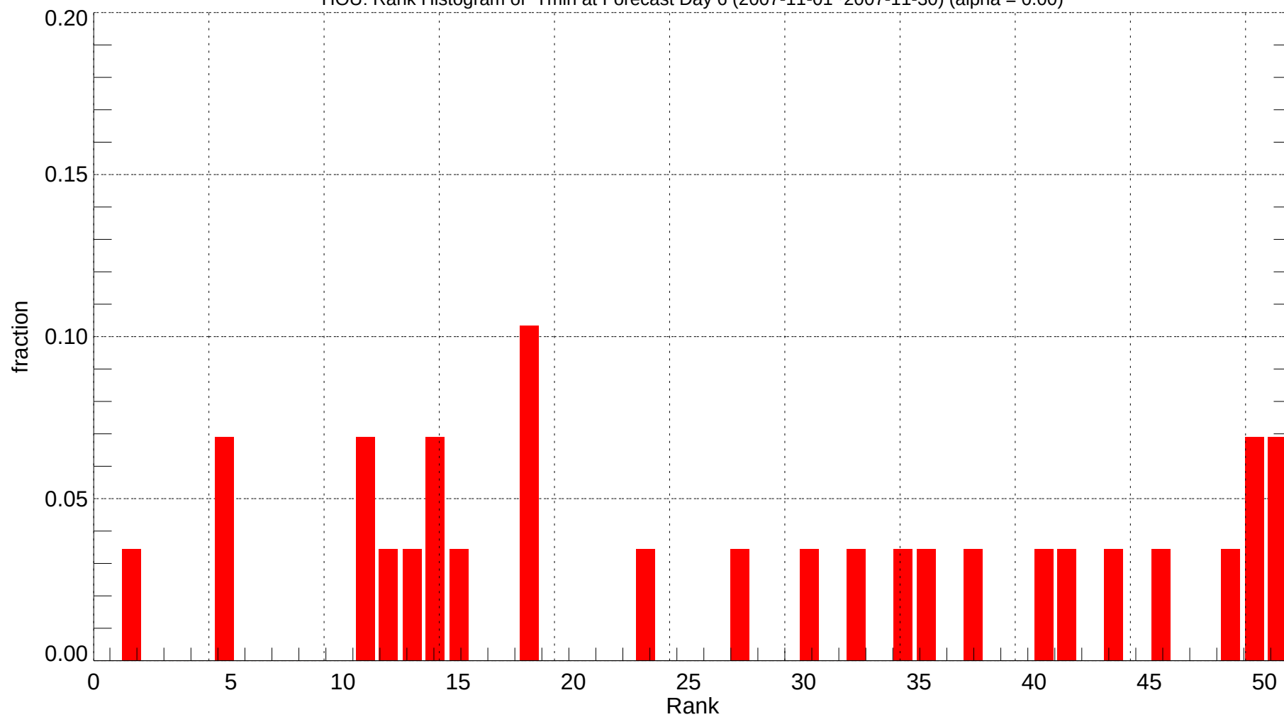
HOU: Rank Histogram of Tmin at Forecast Day 6 (2007-11-01~2007-11-30) (alpha = 0.00)
