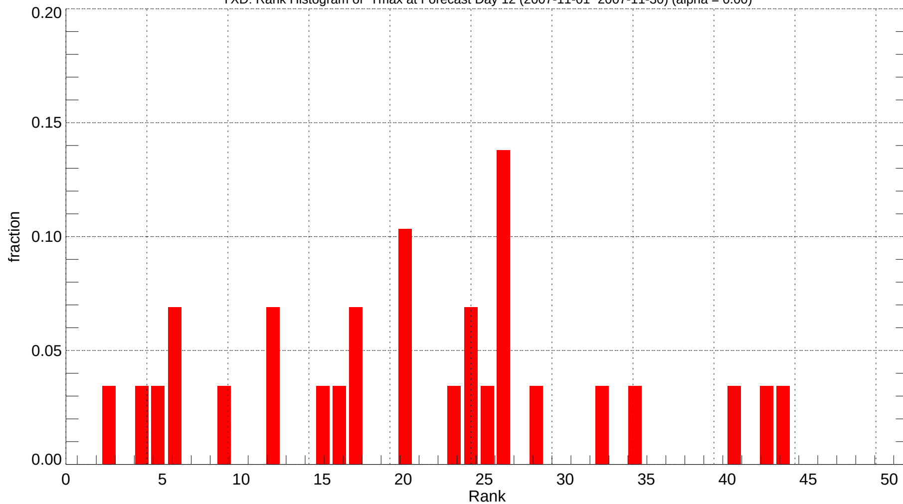
YXD: Rank Histogram of Tmax at Forecast Day 12 (2007-11-01~2007-11-30) (alpha = 0.00)
