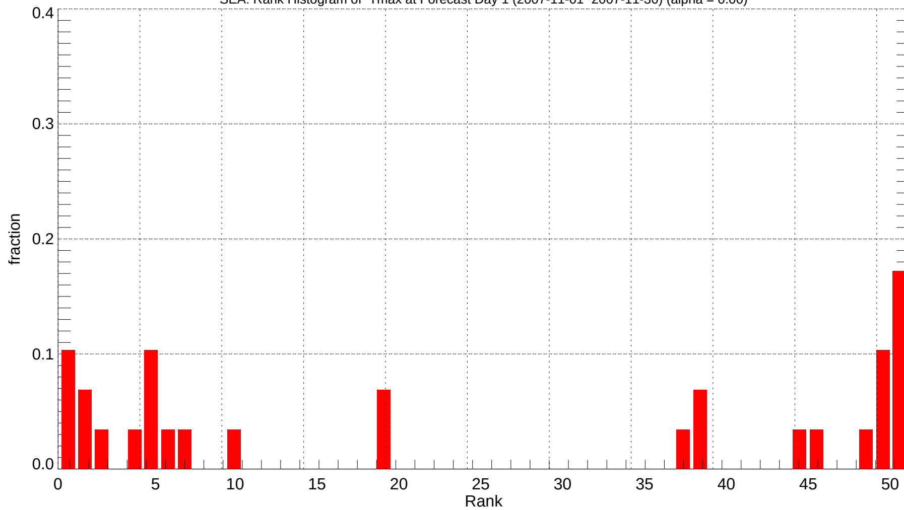
SEA: Rank Histogram of Tmax at Forecast Day 1 (2007-11-01~2007-11-30) (alpha = 0.00)
