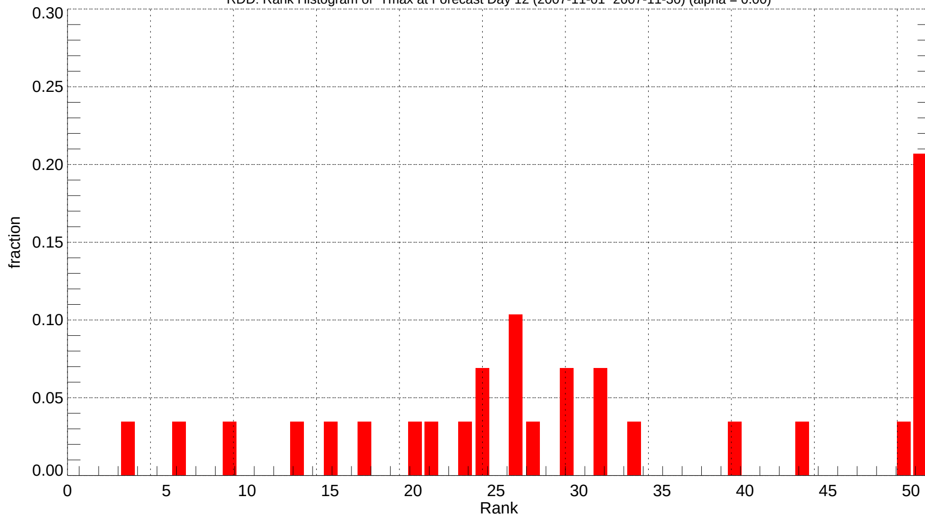
RDD: Rank Histogram of Tmax at Forecast Day 12 (2007-11-01~2007-11-30) (alpha = 0.00)
