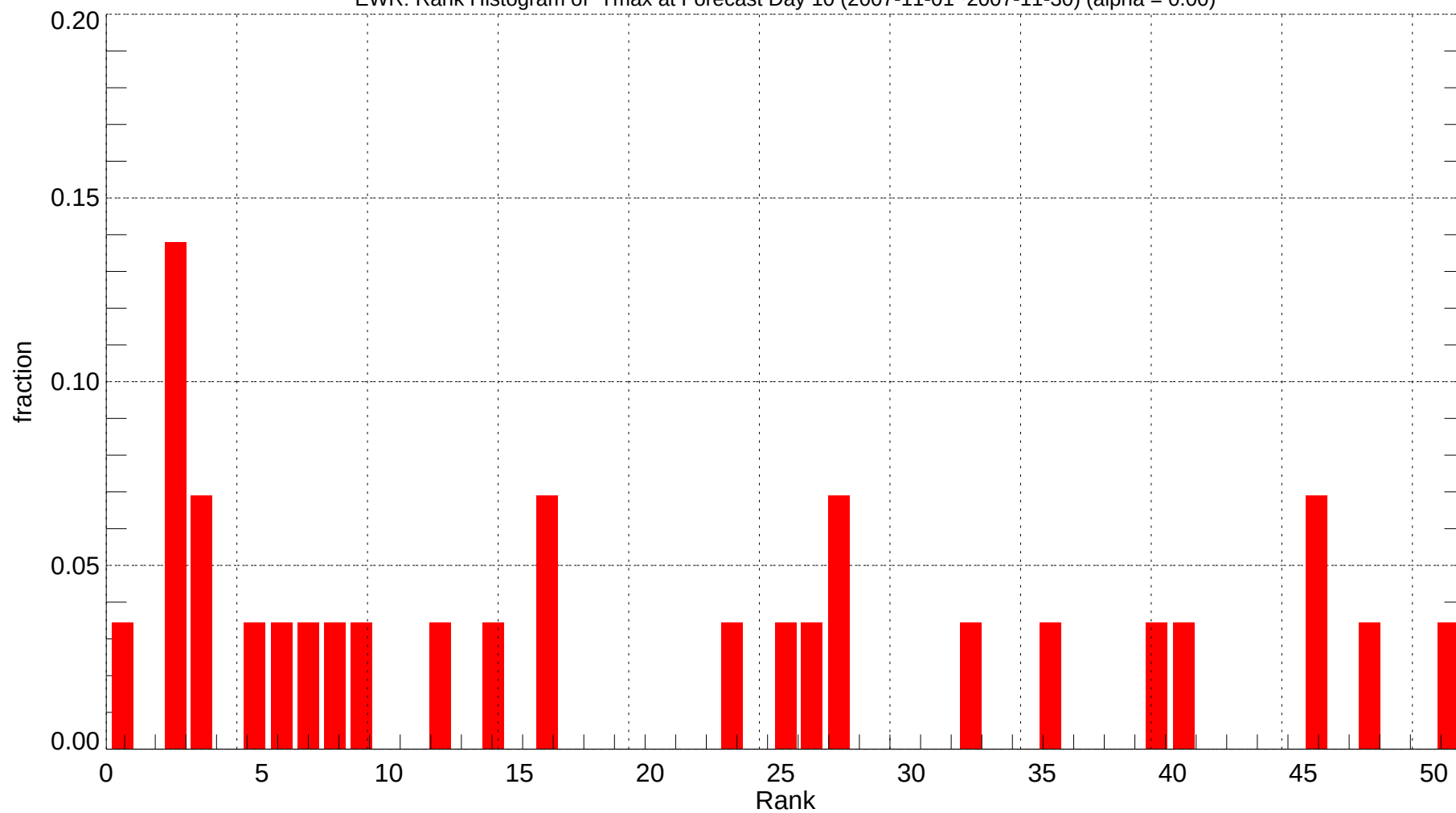
EWR: Rank Histogram of Tmax at Forecast Day 10 (2007-11-01~2007-11-30) (alpha = 0.00)
