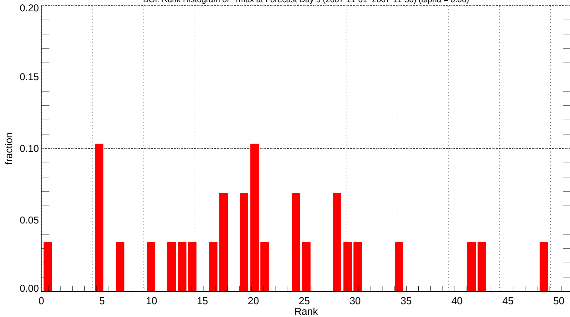
BOI: Rank Histogram of Tmax at Forecast Day 9 (2007-11-01~2007-11-30) (alpha = 0.00)
