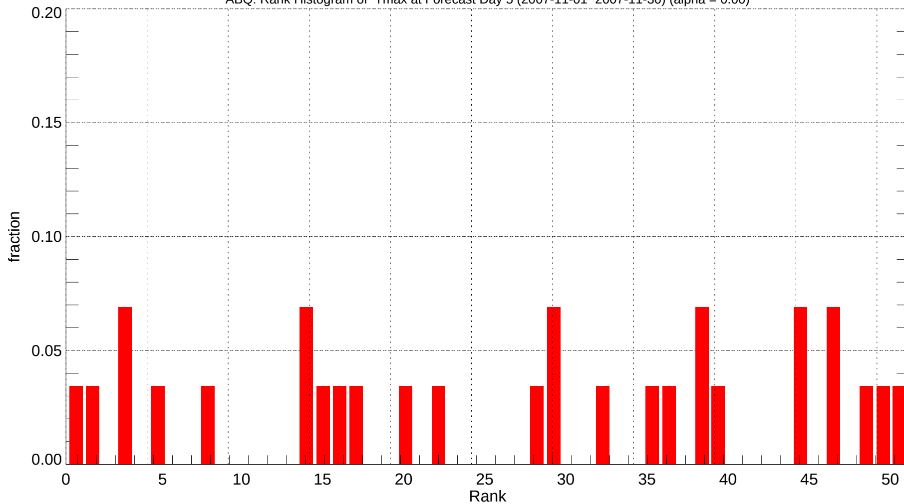
ABQ: Rank Histogram of Tmax at Forecast Day 5 (2007-11-01~2007-11-30) (alpha = 0.00)
