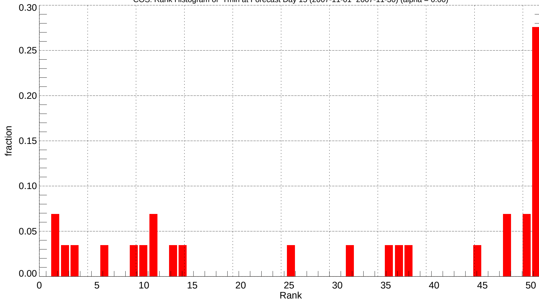
COS: Rank Histogram of Tmin at Forecast Day 15 (2007-11-01~2007-11-30) (alpha = 0.00)
