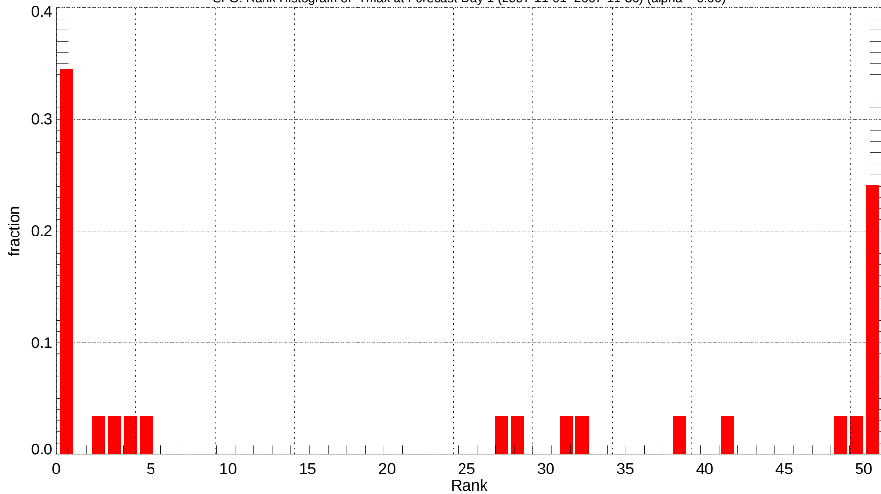
SFO: Rank Histogram of Tmax at Forecast Day 1 (2007-11-01~2007-11-30) (alpha = 0.00)
