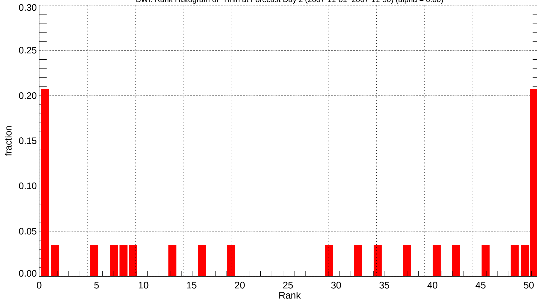
BWI: Rank Histogram of Tmin at Forecast Day 2 (2007-11-01~2007-11-30) (alpha = 0.00)
