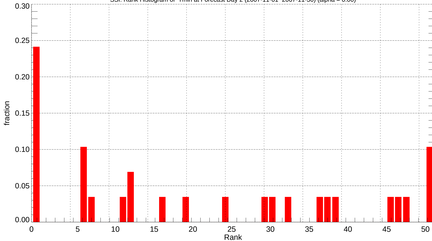
SSI: Rank Histogram of Tmin at Forecast Day 2 (2007-11-01~2007-11-30) (alpha = 0.00)
