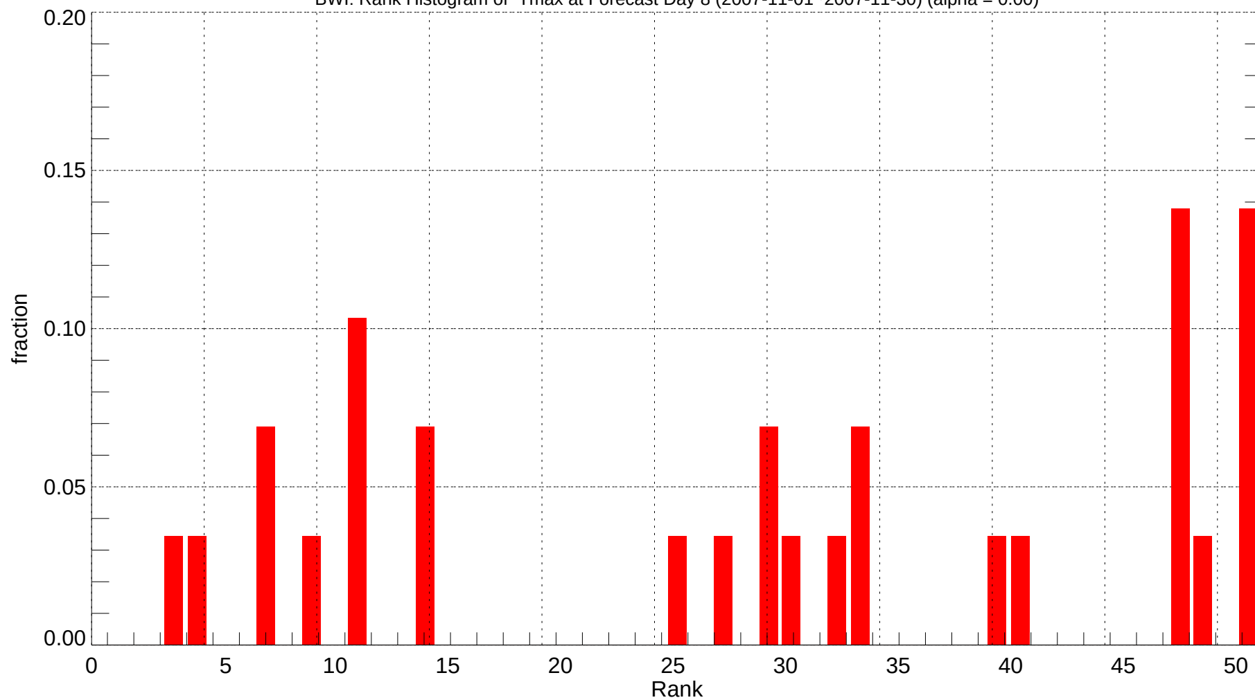
BWI: Rank Histogram of Tmax at Forecast Day 8 (2007-11-01~2007-11-30) (alpha = 0.00)
