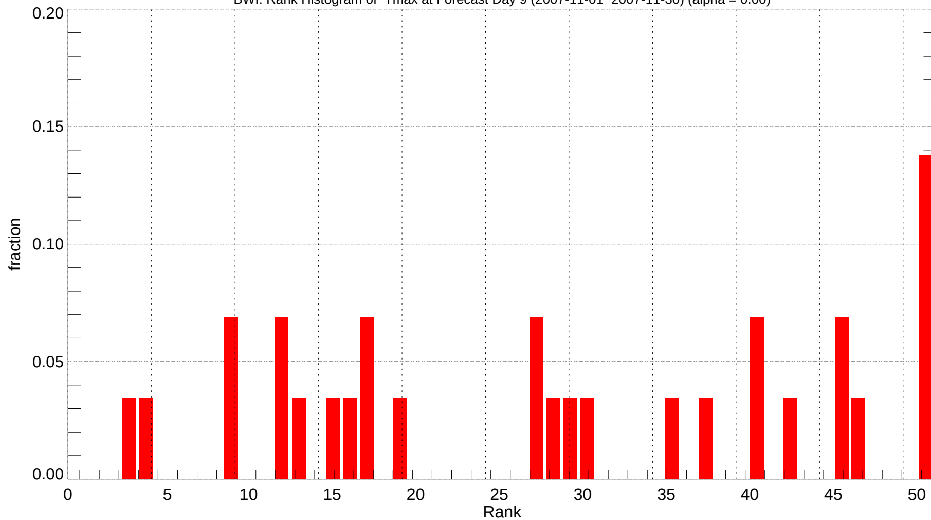
BWI: Rank Histogram of Tmax at Forecast Day 9 (2007-11-01~2007-11-30) (alpha = 0.00)
