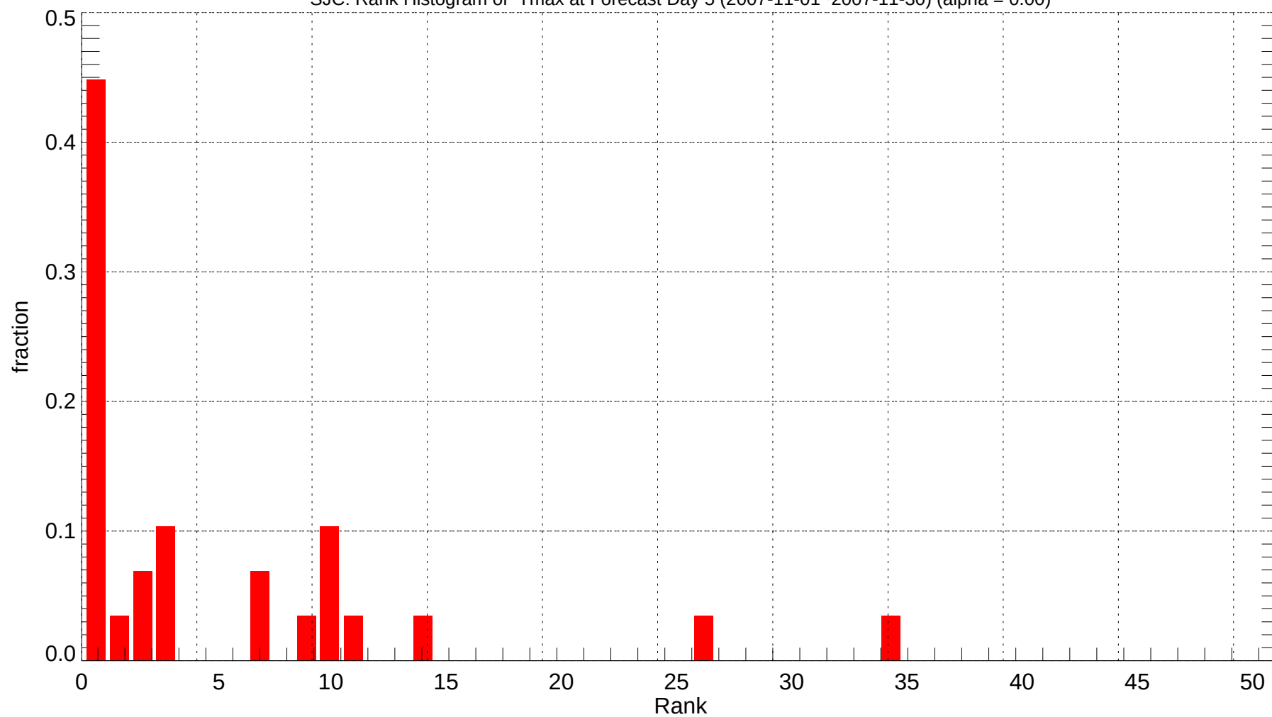
SJC: Rank Histogram of Tmax at Forecast Day 5 (2007-11-01~2007-11-30) (alpha = 0.00)
