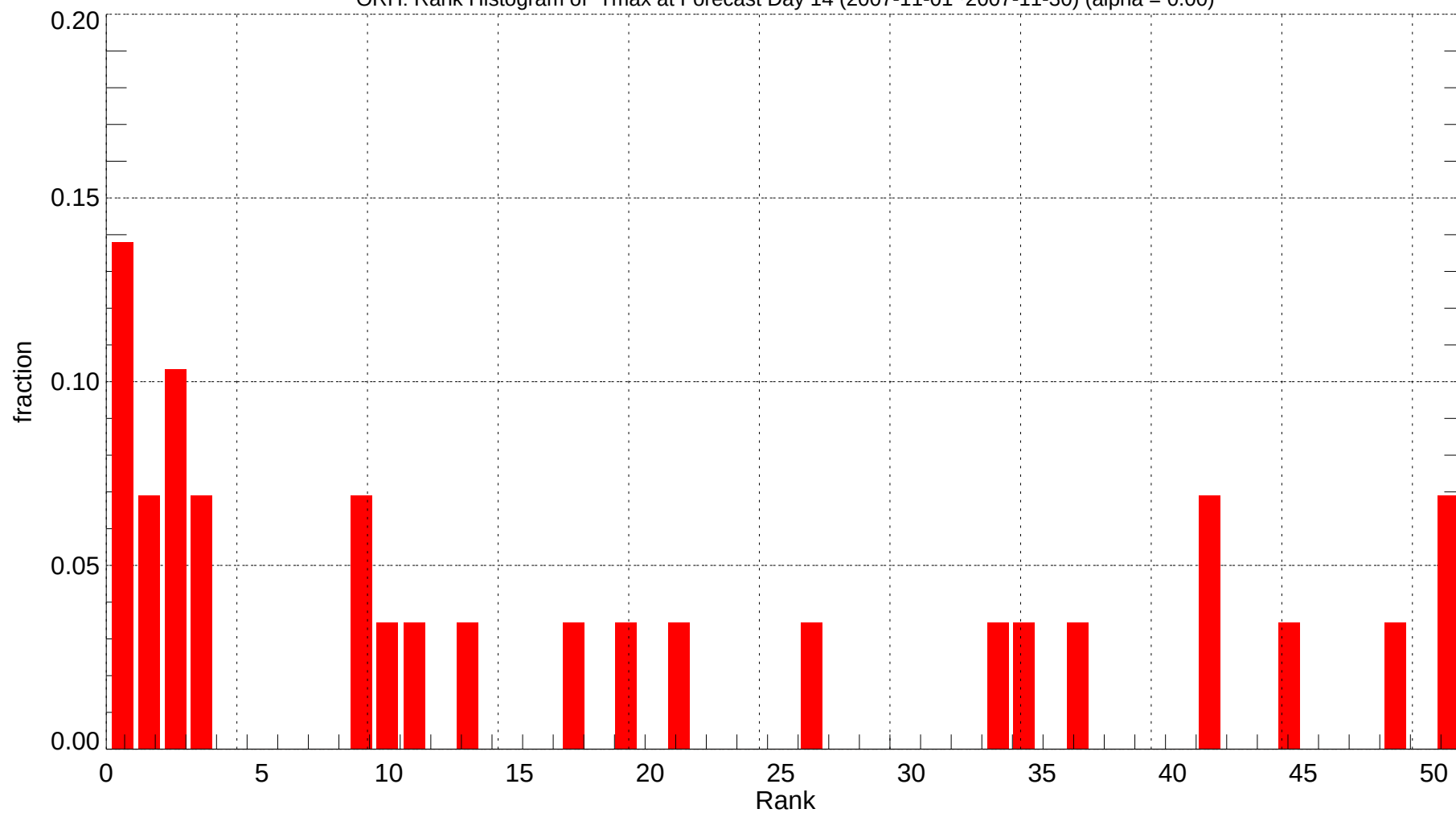
ORH: Rank Histogram of Tmax at Forecast Day 14 (2007-11-01~2007-11-30) (alpha = 0.00)
