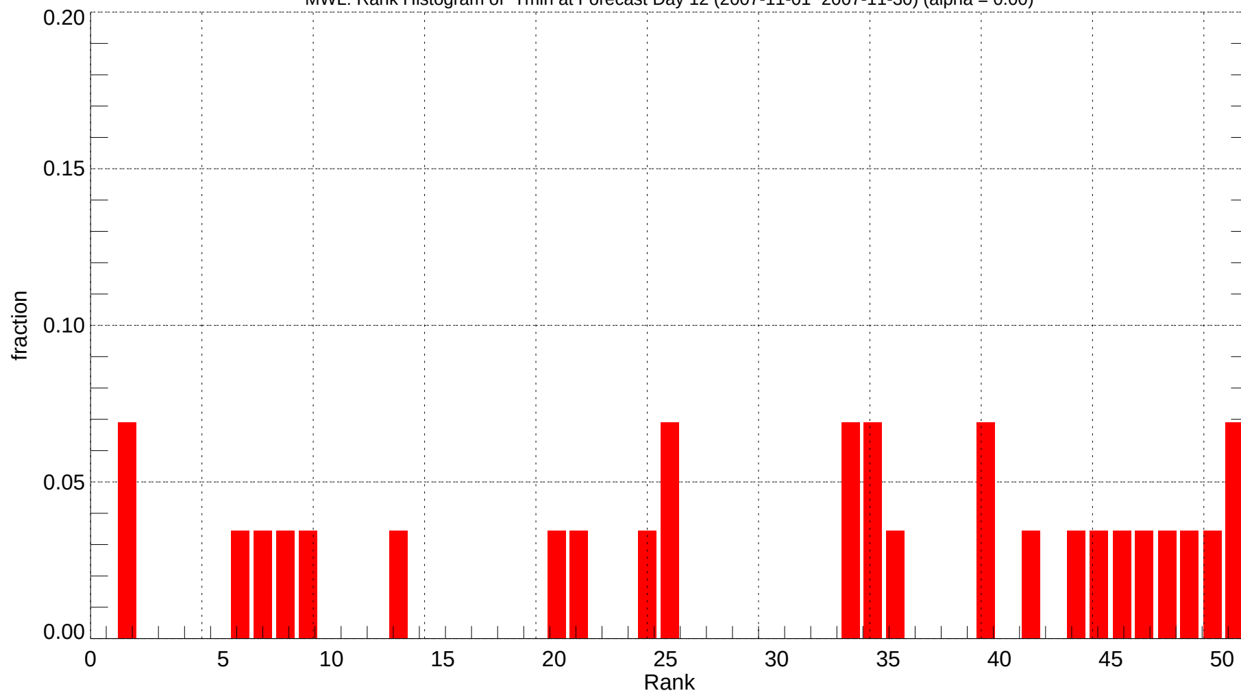
MWL: Rank Histogram of Tmin at Forecast Day 12 (2007-11-01~2007-11-30) (alpha = 0.00)
