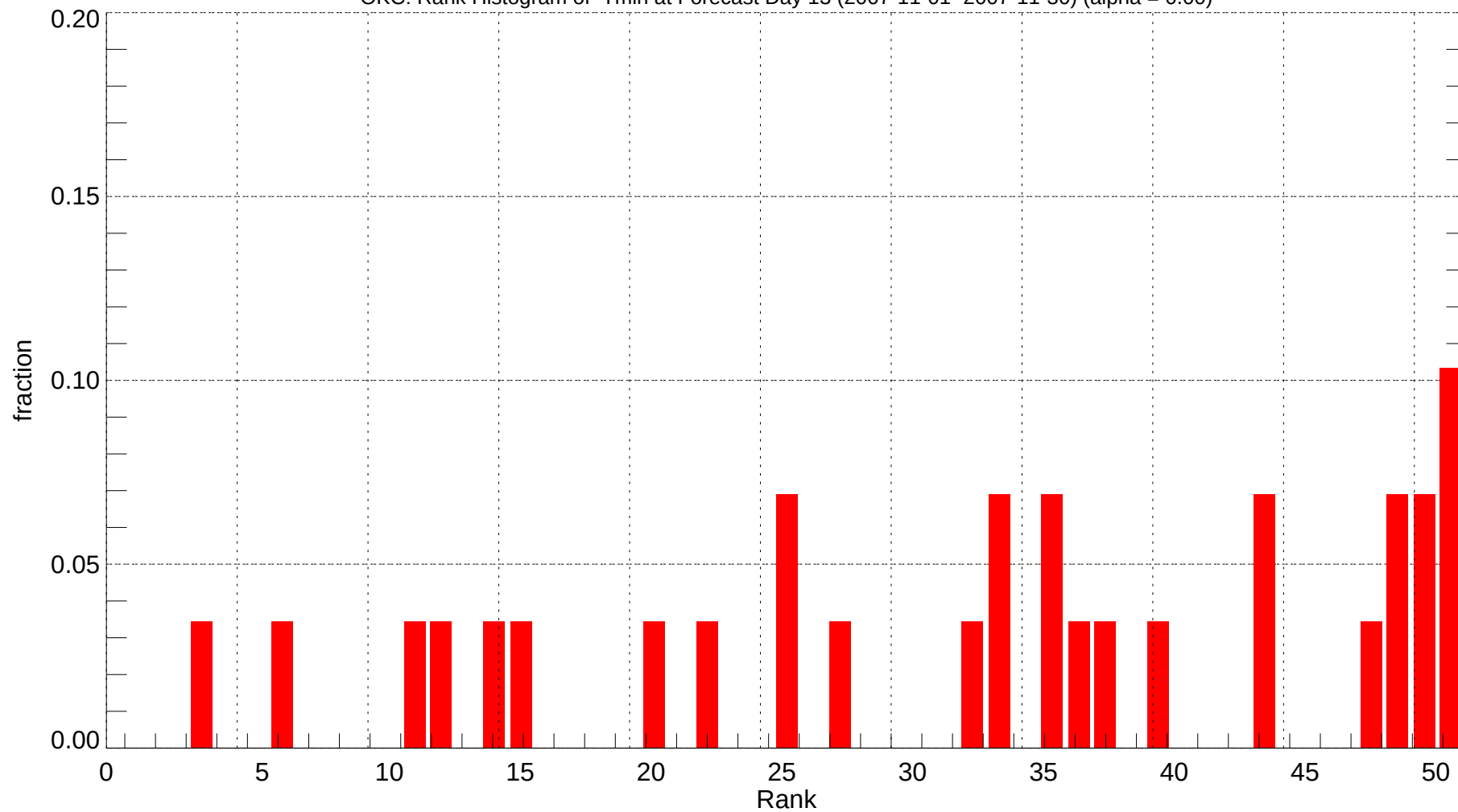
OKC: Rank Histogram of Tmin at Forecast Day 13 (2007-11-01~2007-11-30) (alpha = 0.00)
