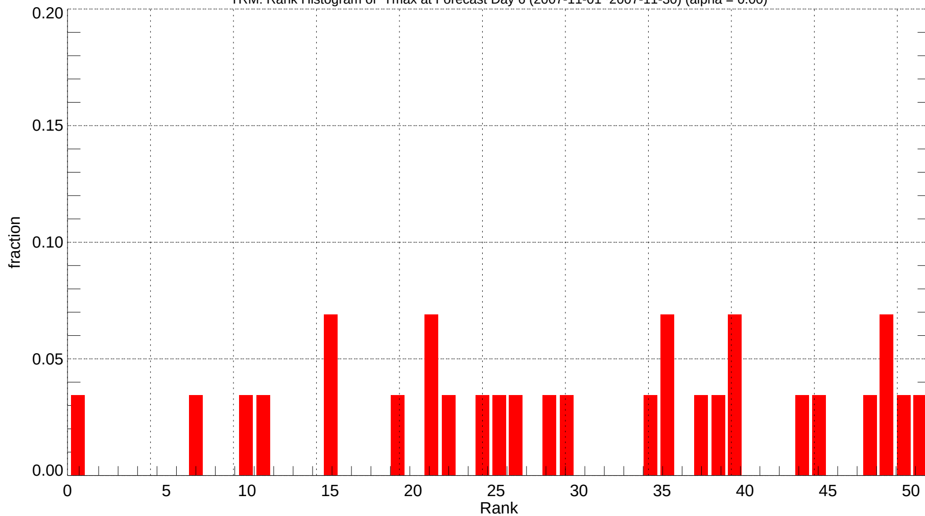
TRM: Rank Histogram of Tmax at Forecast Day 6 (2007-11-01~2007-11-30) (alpha = 0.00)
