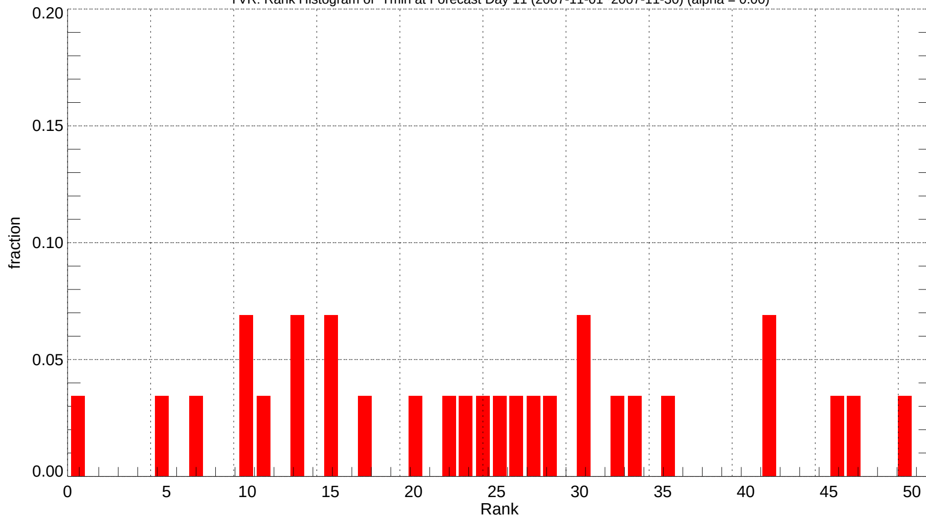
YVR: Rank Histogram of Tmin at Forecast Day 11 (2007-11-01~2007-11-30) (alpha = 0.00)
