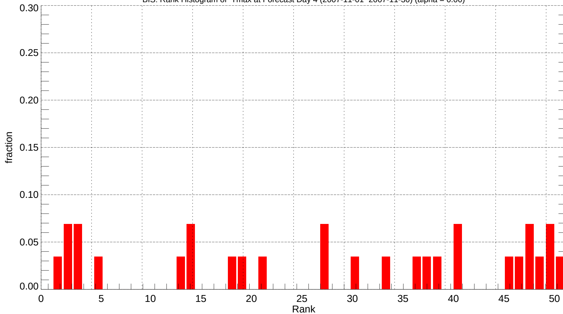
BIS: Rank Histogram of Tmax at Forecast Day 4 (2007-11-01~2007-11-30) (alpha = 0.00)
