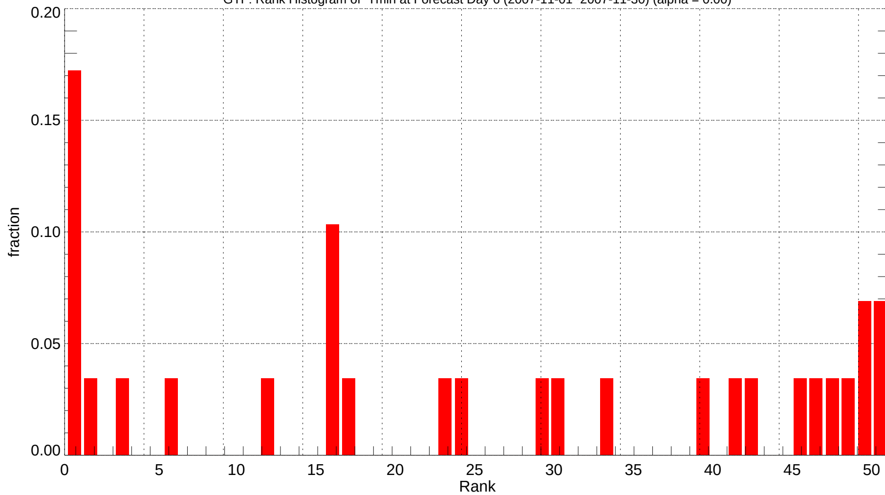
GTF: Rank Histogram of Tmin at Forecast Day 6 (2007-11-01~2007-11-30) (alpha = 0.00)
