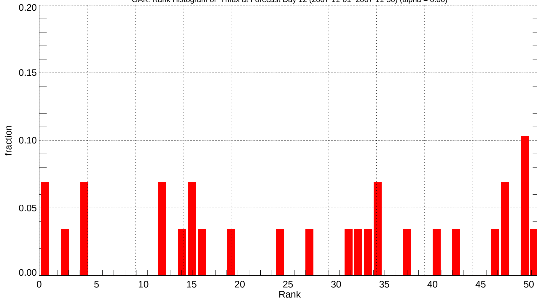
OAK: Rank Histogram of Tmax at Forecast Day 12 (2007-11-01~2007-11-30) (alpha = 0.00)
