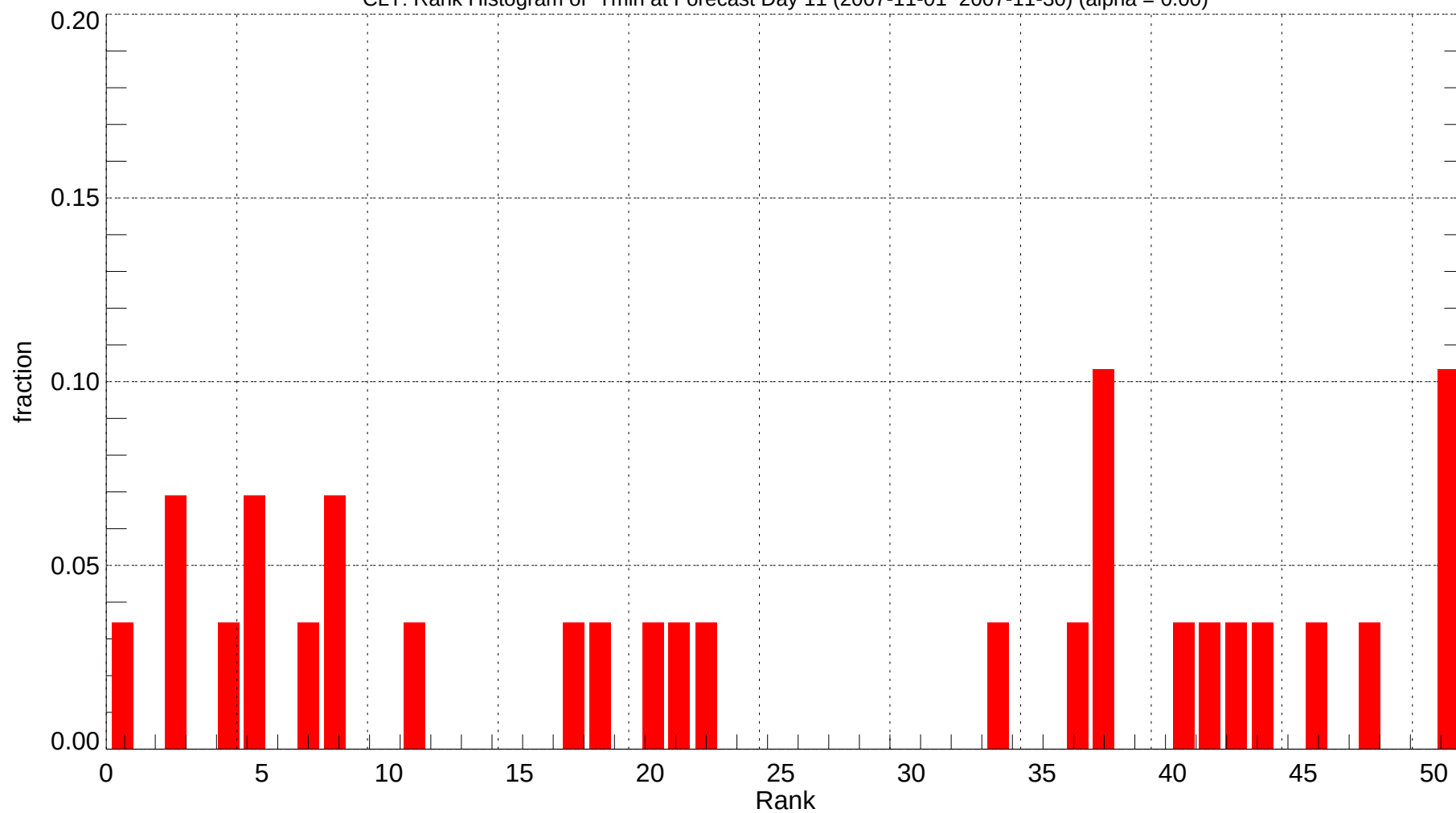
CLT: Rank Histogram of Tmin at Forecast Day 11 (2007-11-01~2007-11-30) (alpha = 0.00)
