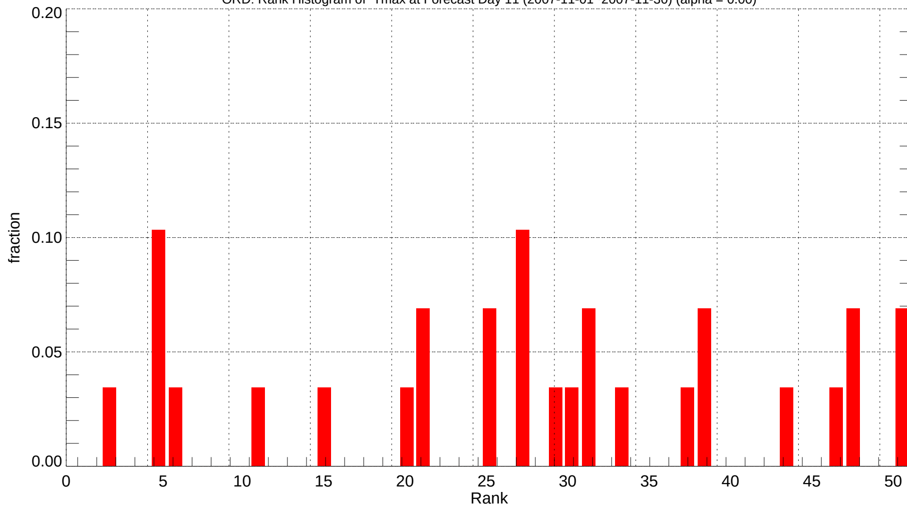
ORD: Rank Histogram of Tmax at Forecast Day 11 (2007-11-01~2007-11-30) (alpha = 0.00)
