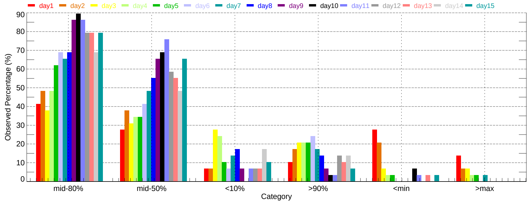
Observed Percentage of Ensembles - BTV: Min Temperature (2007-11-01~2007-11-30)
