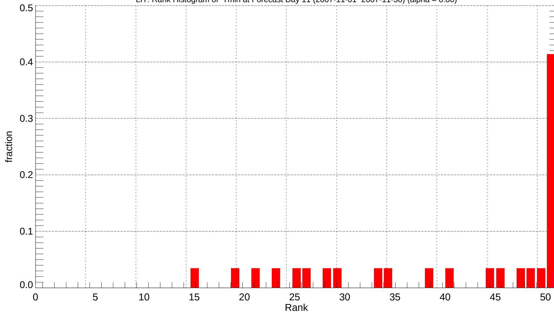
LIT: Rank Histogram of Tmin at Forecast Day 11 (2007-11-01~2007-11-30) (alpha = 0.00)
