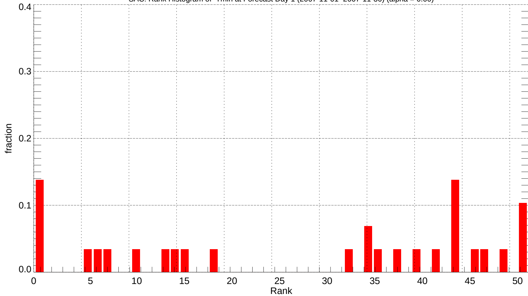
SAC: Rank Histogram of Tmin at Forecast Day 1 (2007-11-01~2007-11-30) (alpha = 0.00)
