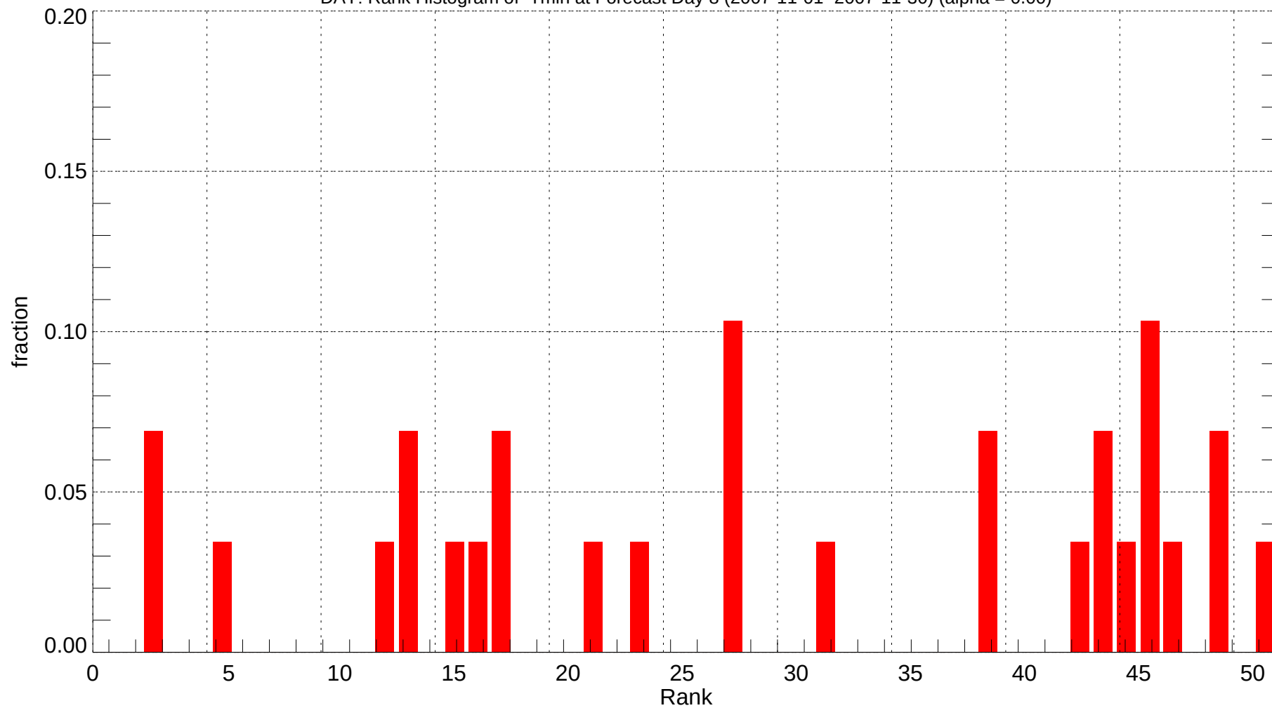
DAY: Rank Histogram of Tmin at Forecast Day 8 (2007-11-01~2007-11-30) (alpha = 0.00)
