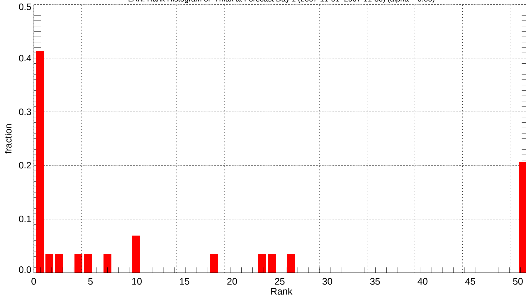
LAN: Rank Histogram of Tmax at Forecast Day 1 (2007-11-01~2007-11-30) (alpha = 0.00)
