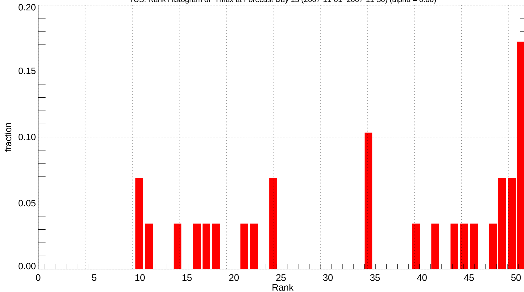
TUS: Rank Histogram of Tmax at Forecast Day 13 (2007-11-01~2007-11-30) (alpha = 0.00)
