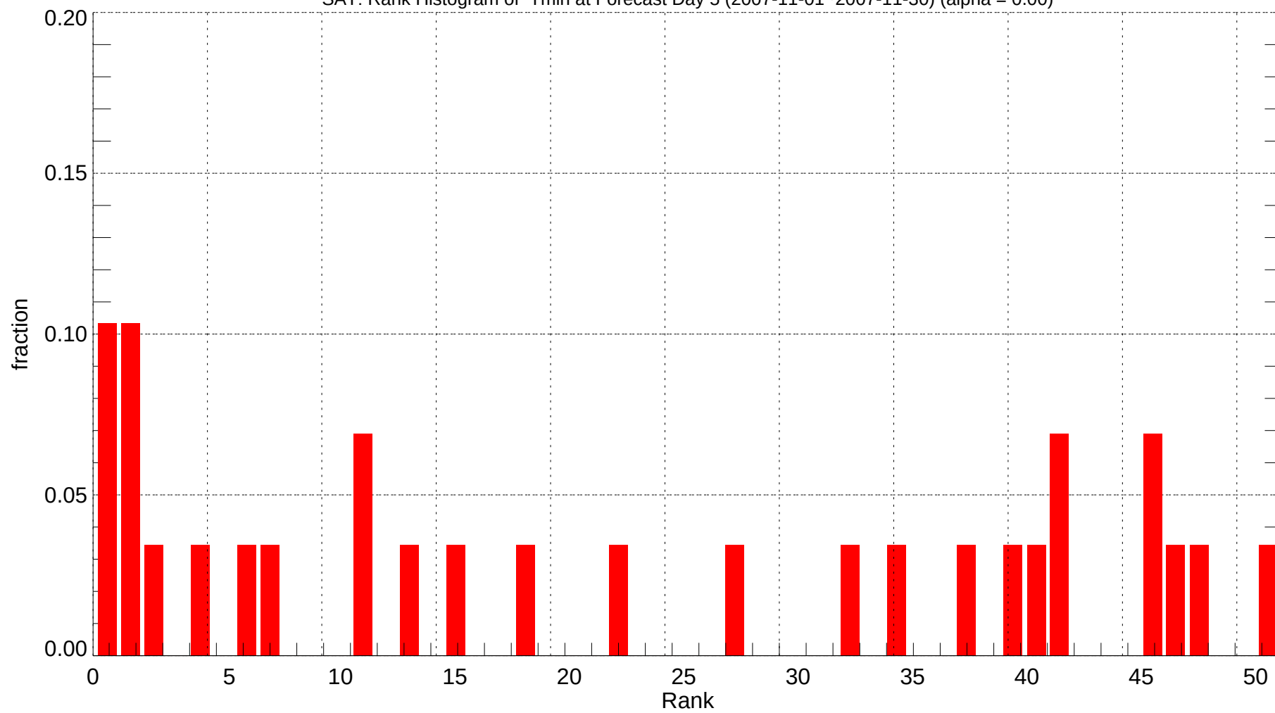
SAT: Rank Histogram of Tmin at Forecast Day 5 (2007-11-01~2007-11-30) (alpha = 0.00)
