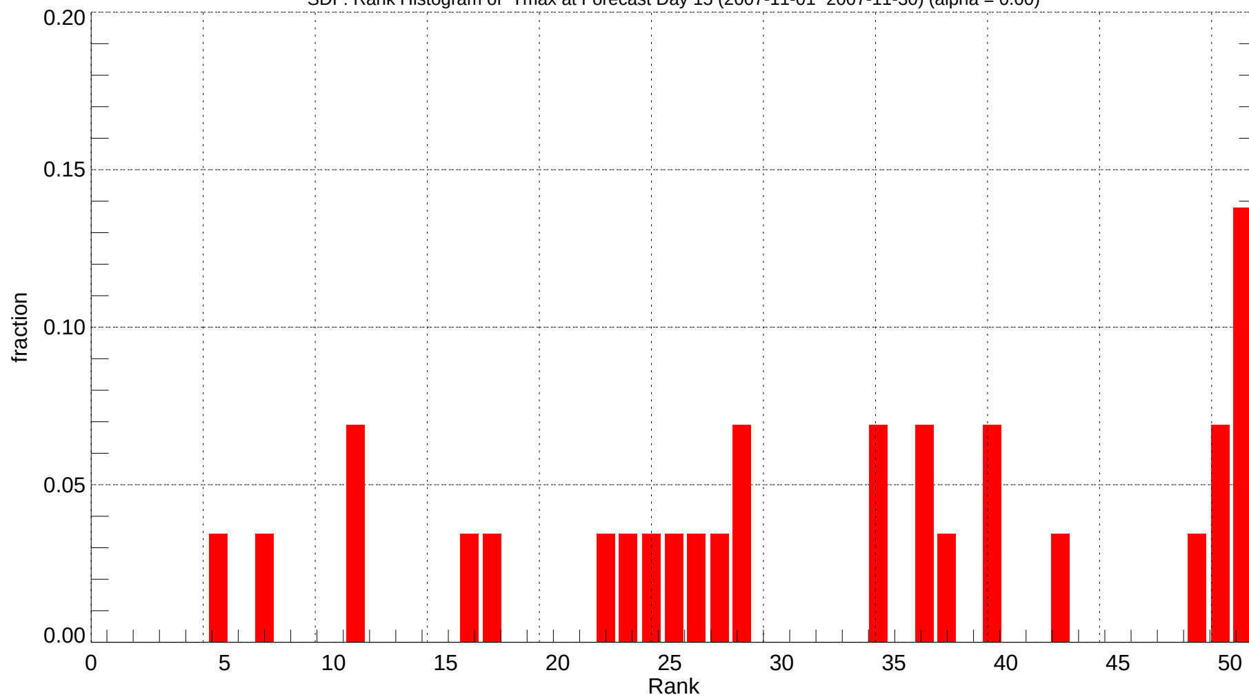
SDF: Rank Histogram of Tmax at Forecast Day 15 (2007-11-01~2007-11-30) (alpha = 0.00)
