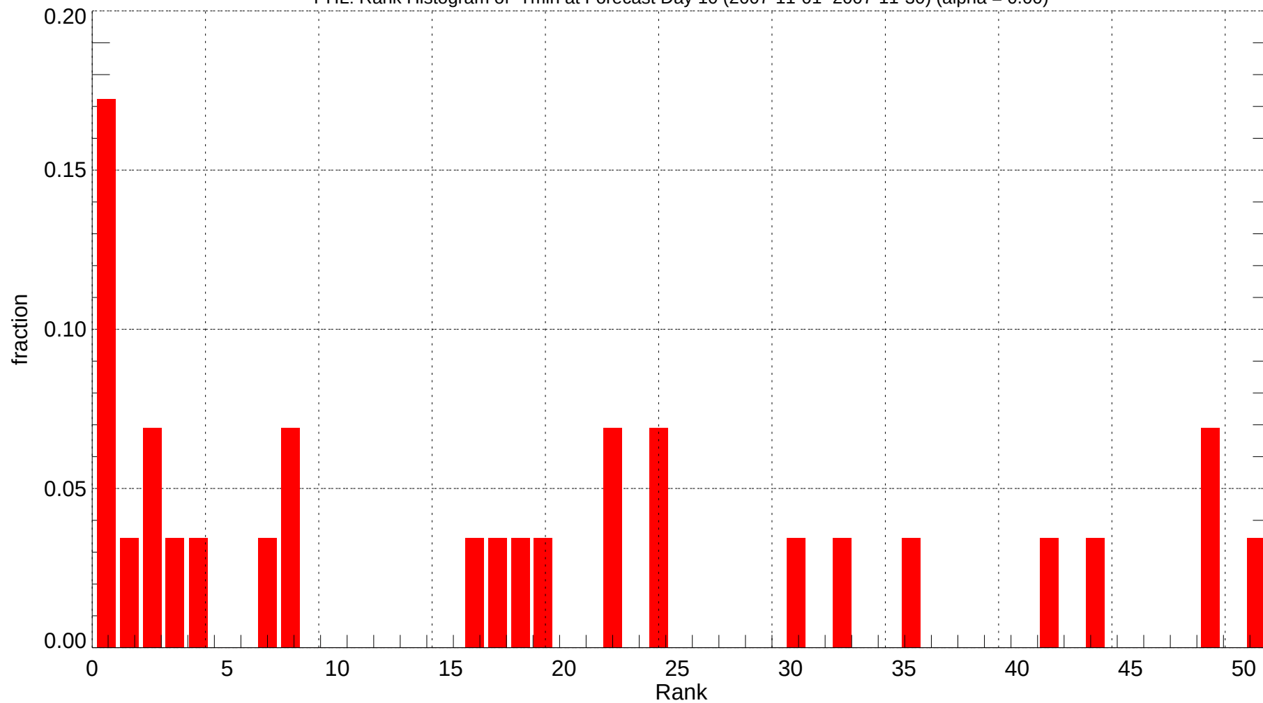
PHL: Rank Histogram of Tmin at Forecast Day 10 (2007-11-01~2007-11-30) (alpha = 0.00)
