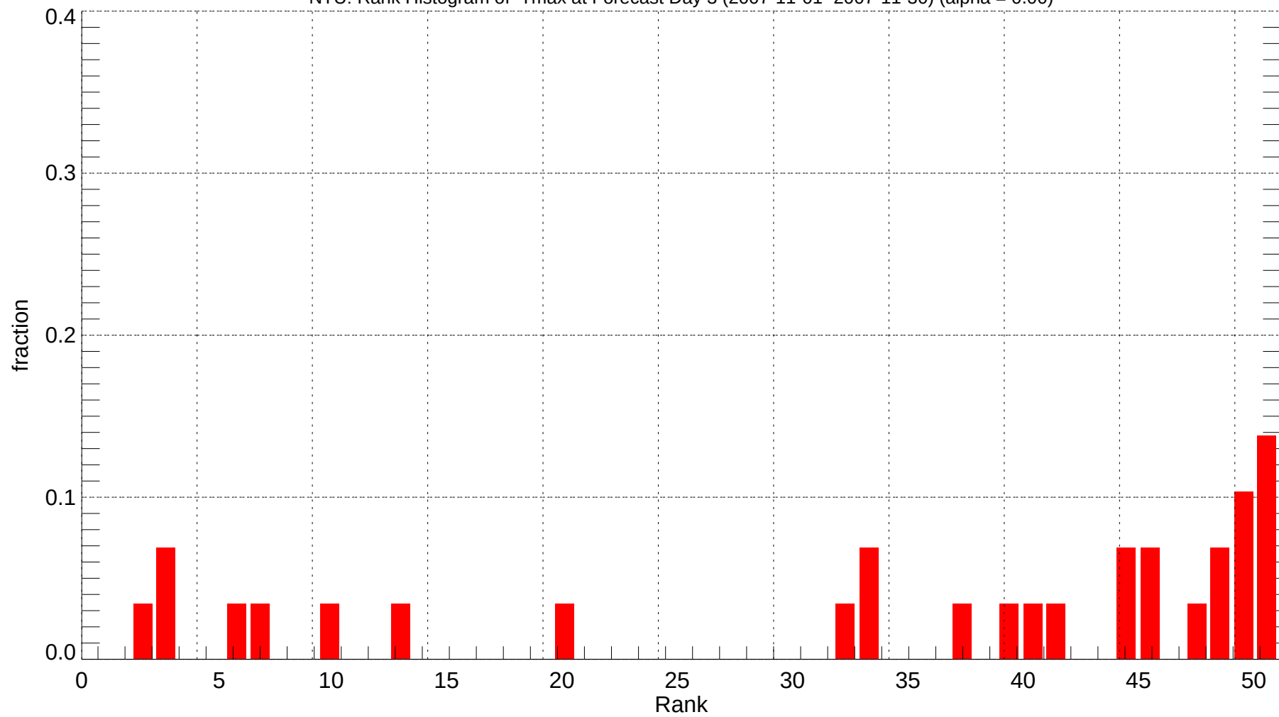
NTU: Rank Histogram of Tmax at Forecast Day 3 (2007-11-01~2007-11-30) (alpha = 0.00)
