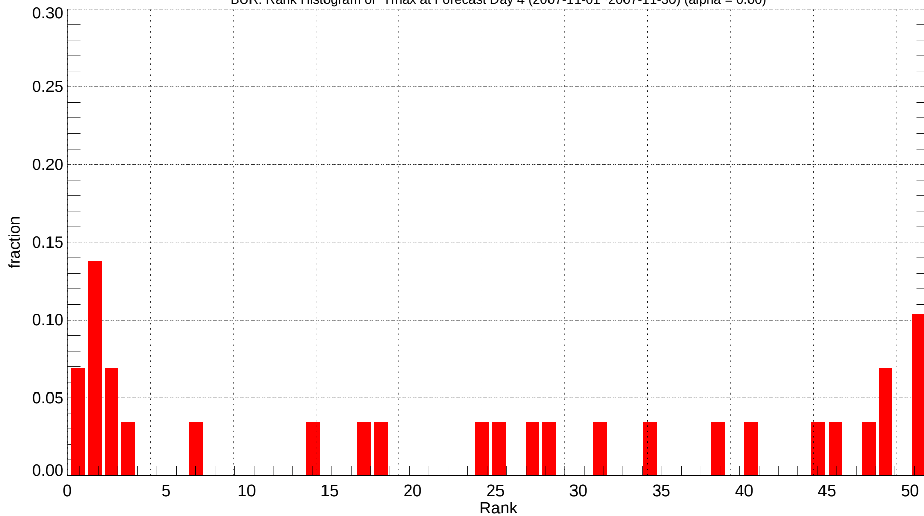
BUR: Rank Histogram of Tmax at Forecast Day 4 (2007-11-01~2007-11-30) (alpha = 0.00)
