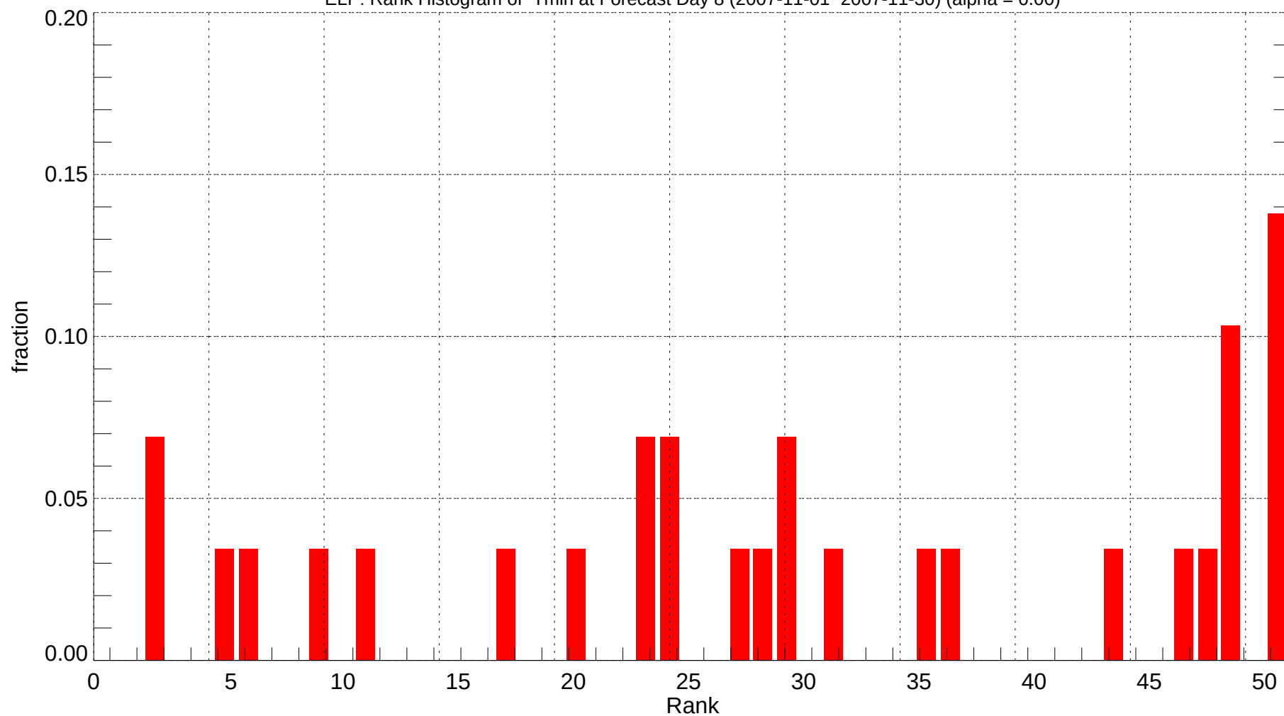
ELP: Rank Histogram of Tmin at Forecast Day 8 (2007-11-01~2007-11-30) (alpha = 0.00)
