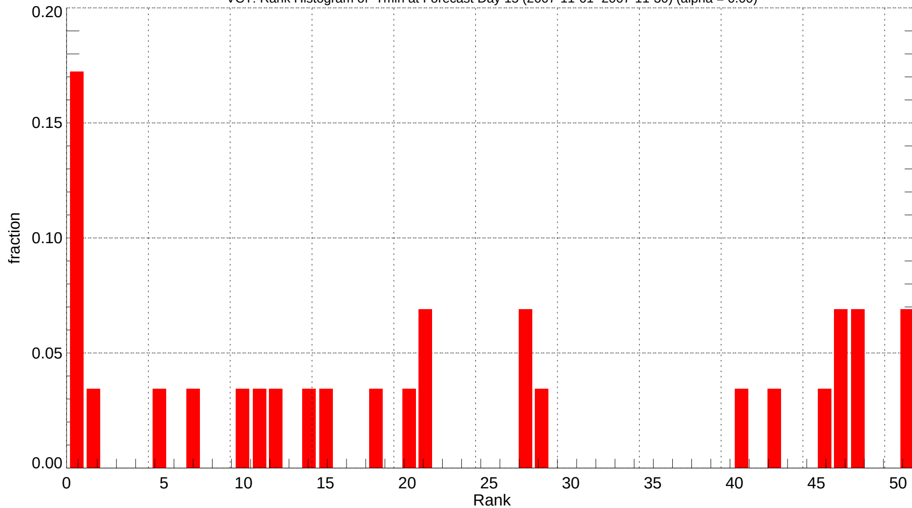
VCT: Rank Histogram of Tmin at Forecast Day 15 (2007-11-01~2007-11-30) (alpha = 0.00)
