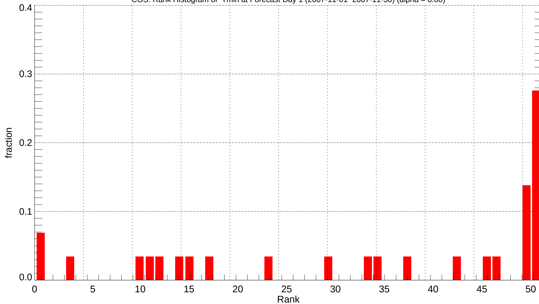
COS: Rank Histogram of Tmin at Forecast Day 1 (2007-11-01~2007-11-30) (alpha = 0.00)
