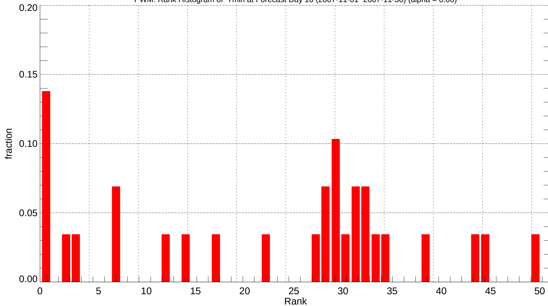
PWM: Rank Histogram of Tmin at Forecast Day 10 (2007-11-01~2007-11-30) (alpha = 0.00)
