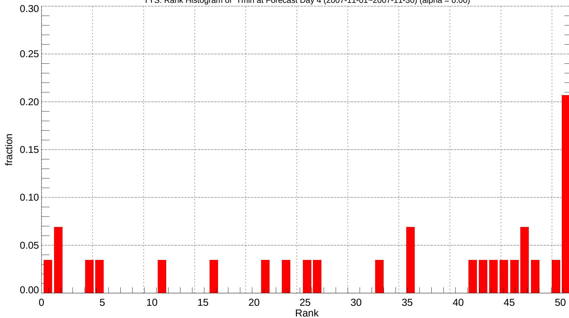
TYS: Rank Histogram of Tmin at Forecast Day 4 (2007-11-01~2007-11-30) (alpha = 0.00)
