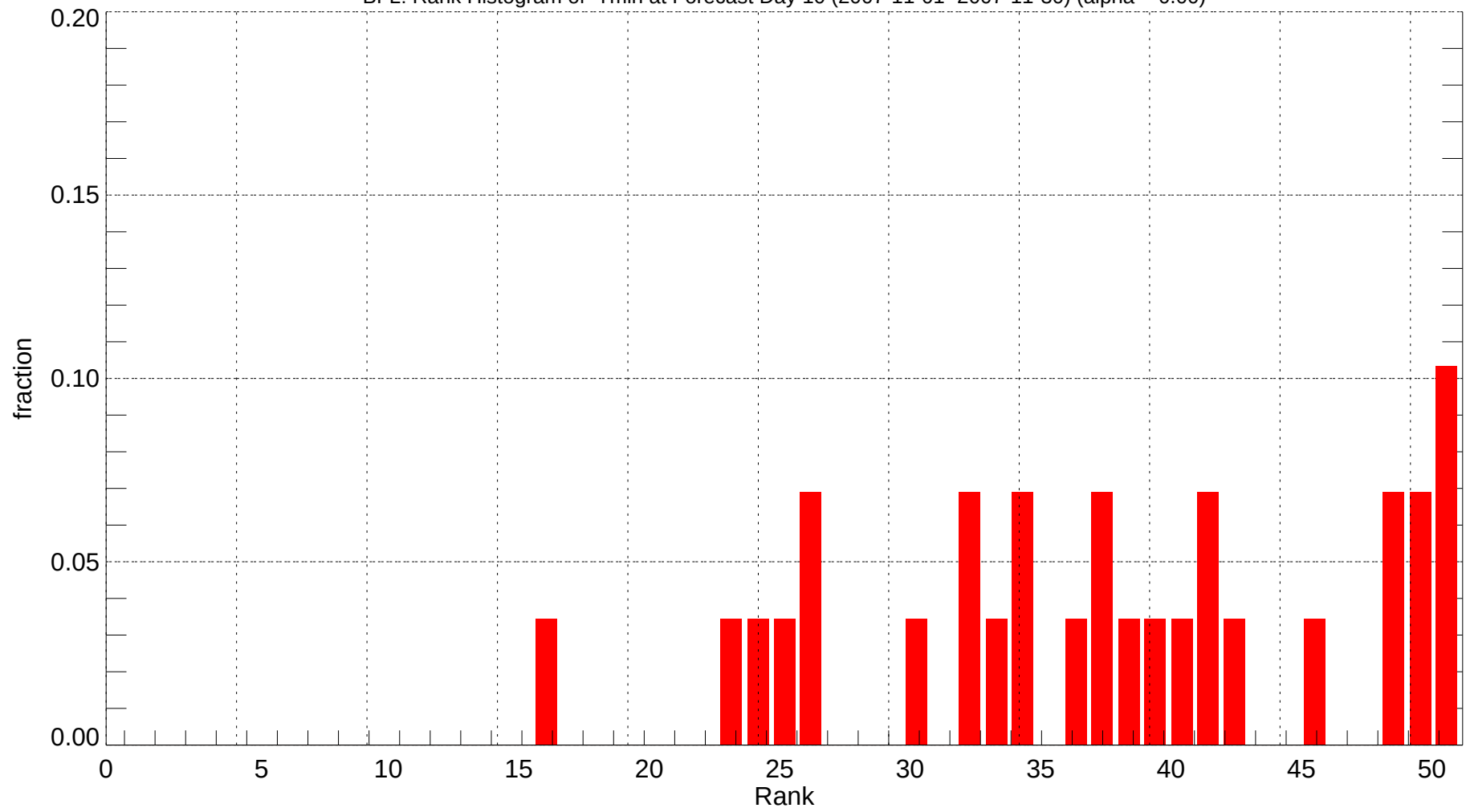
BFL: Rank Histogram of Tmin at Forecast Day 10 (2007-11-01~2007-11-30) (alpha = 0.00)
