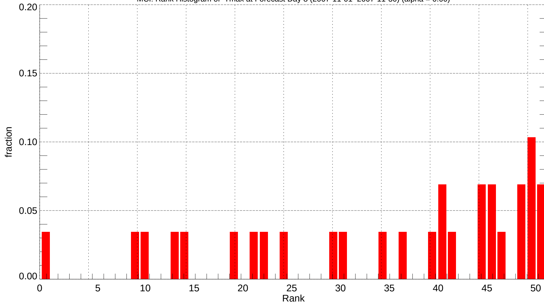
MCI: Rank Histogram of Tmax at Forecast Day 8 (2007-11-01~2007-11-30) (alpha = 0.00)
