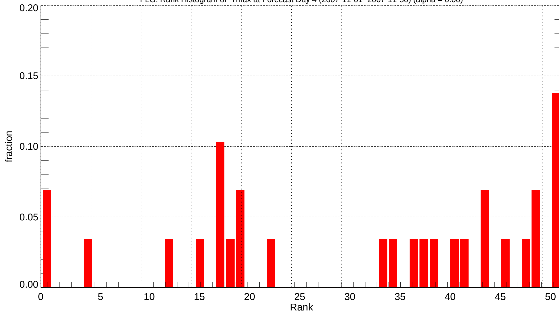
FLG: Rank Histogram of Tmax at Forecast Day 4 (2007-11-01~2007-11-30) (alpha = 0.00)
