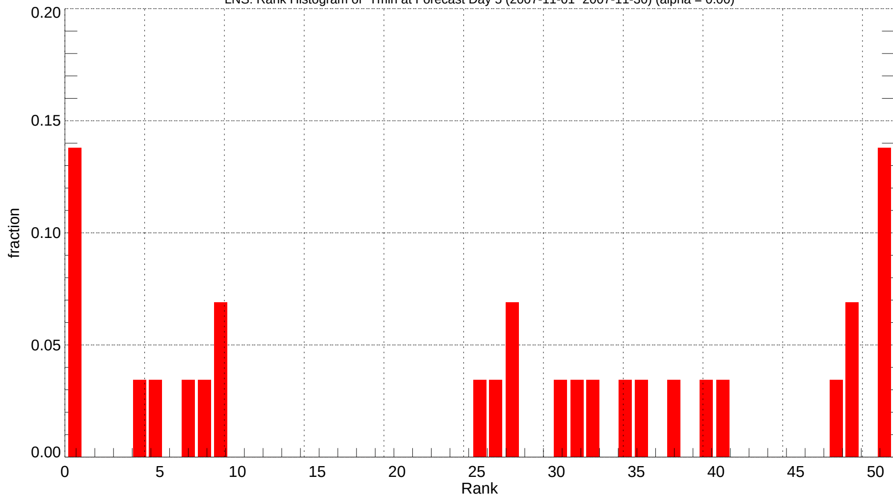
LNS: Rank Histogram of Tmin at Forecast Day 5 (2007-11-01~2007-11-30) (alpha = 0.00)
