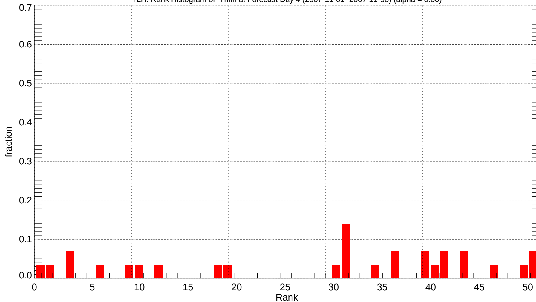
TLH: Rank Histogram of Tmin at Forecast Day 4 (2007-11-01~2007-11-30) (alpha = 0.00)
