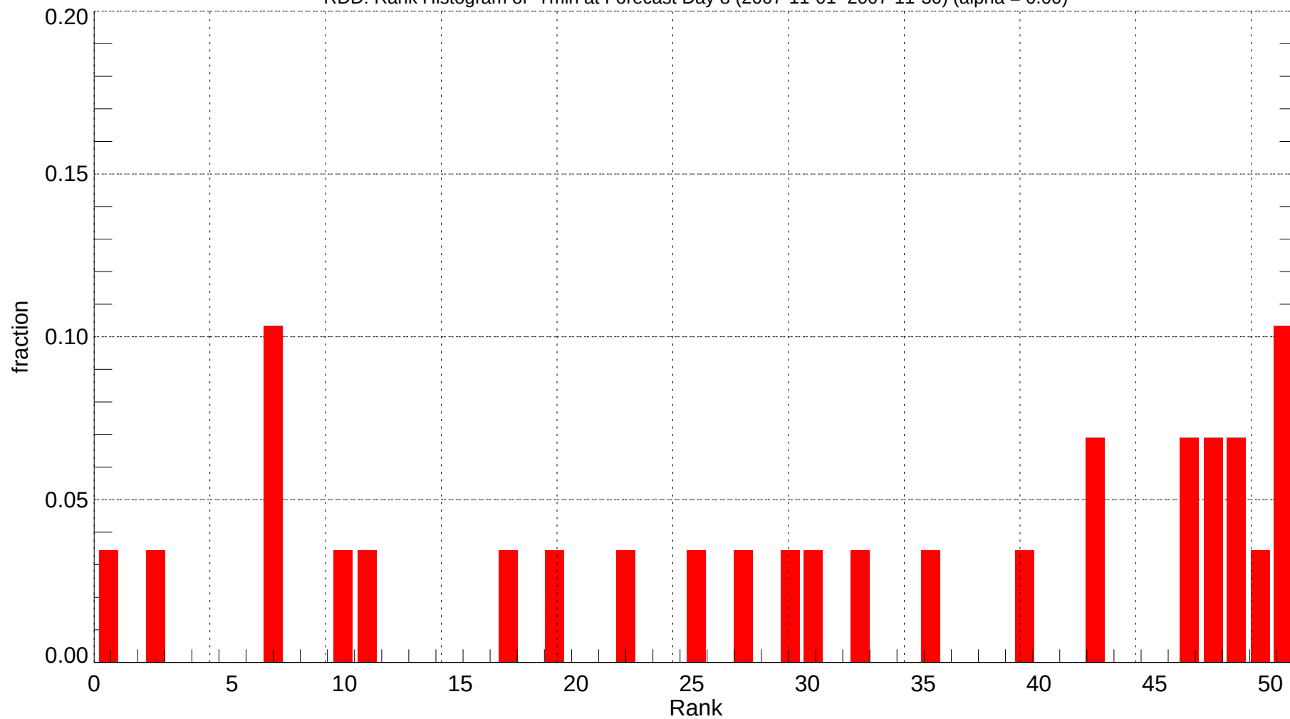
RDD: Rank Histogram of Tmin at Forecast Day 8 (2007-11-01~2007-11-30) (alpha = 0.00)
