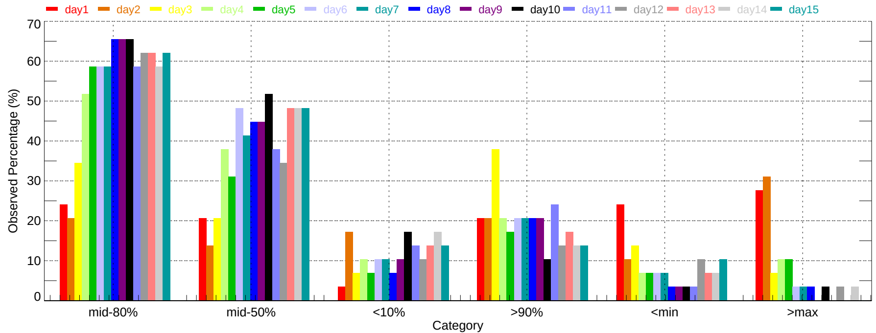
Observed Percentage of Ensembles - IPT: Min Temperature (2007-11-01~2007-11-30)
