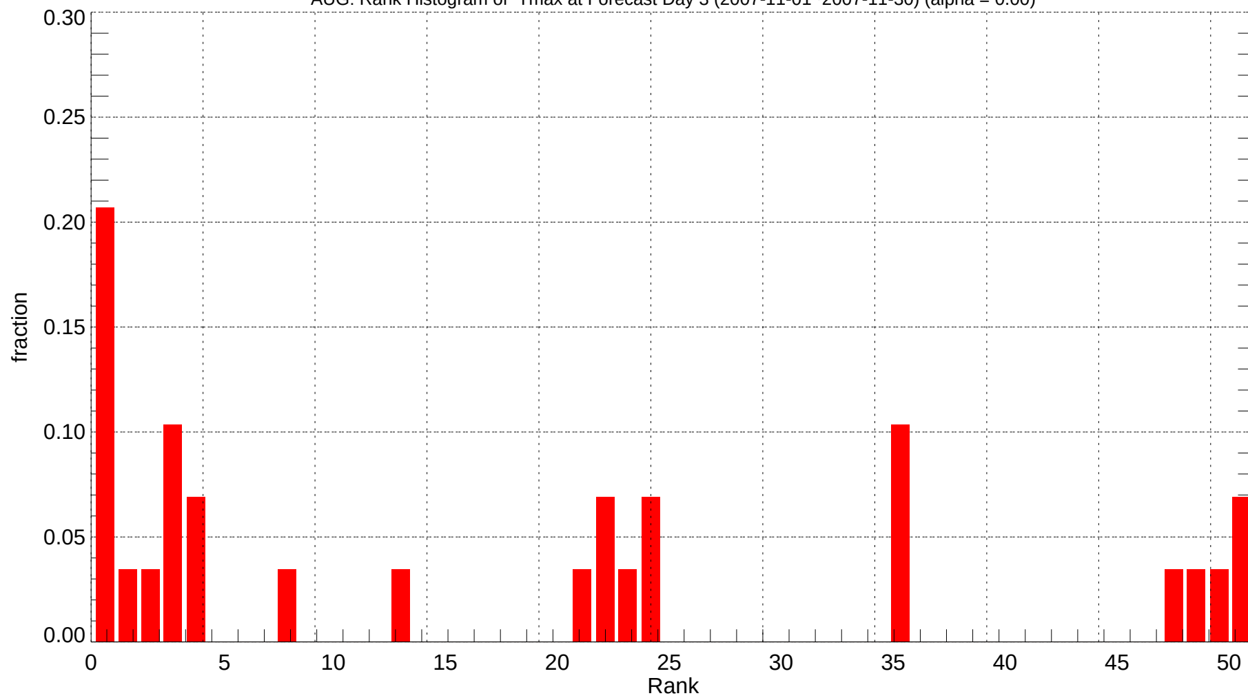
AUG: Rank Histogram of Tmax at Forecast Day 3 (2007-11-01~2007-11-30) (alpha = 0.00)
