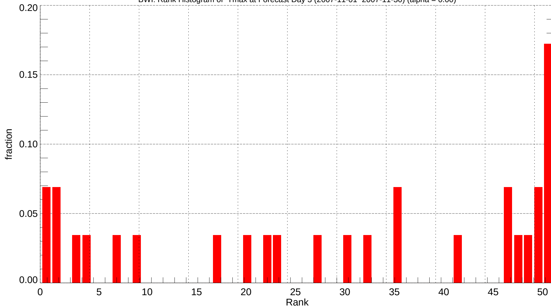
BWI: Rank Histogram of Tmax at Forecast Day 3 (2007-11-01~2007-11-30) (alpha = 0.00)
