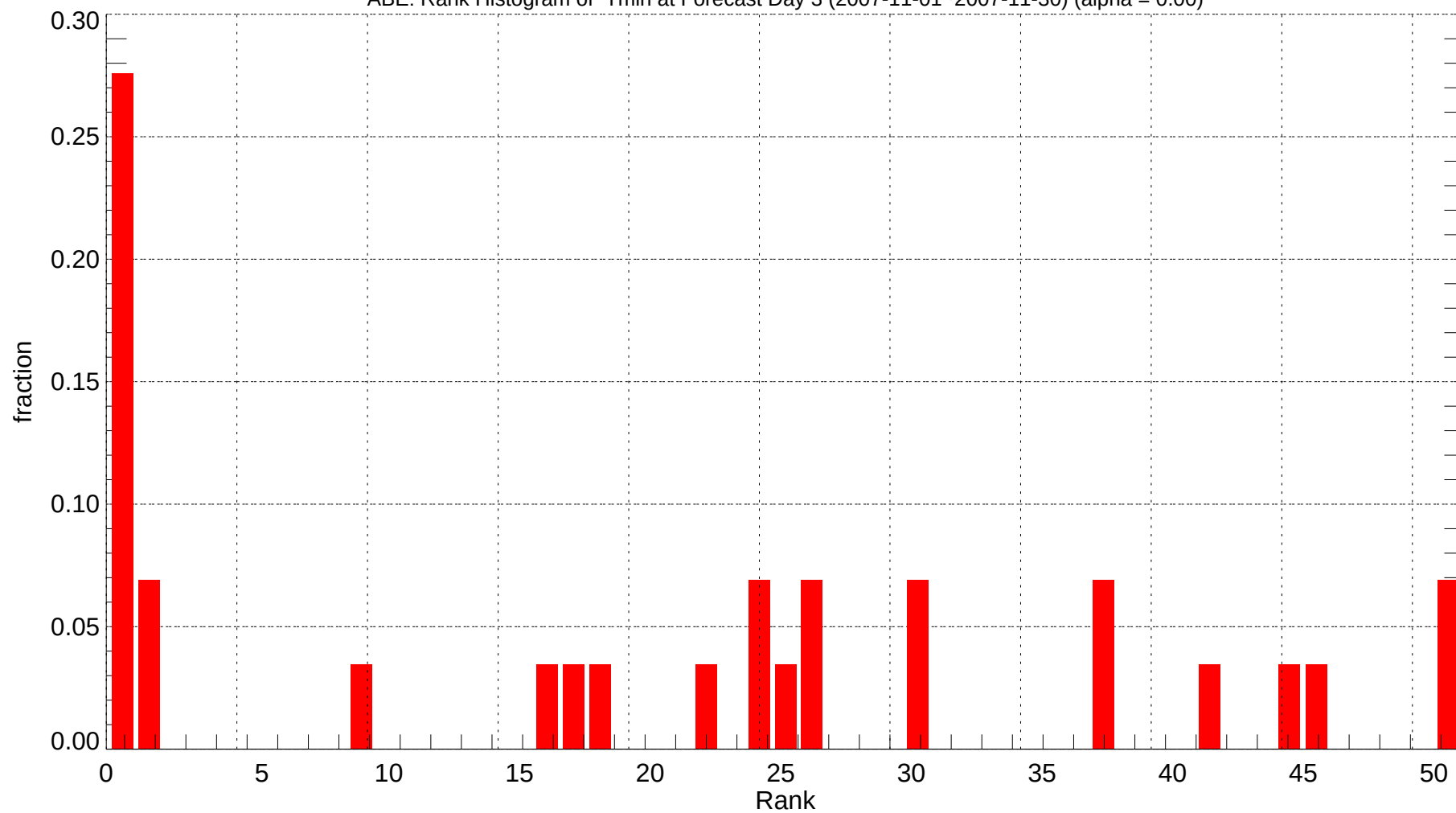
ABE: Rank Histogram of Tmin at Forecast Day 3 (2007-11-01~2007-11-30) (alpha = 0.00)
