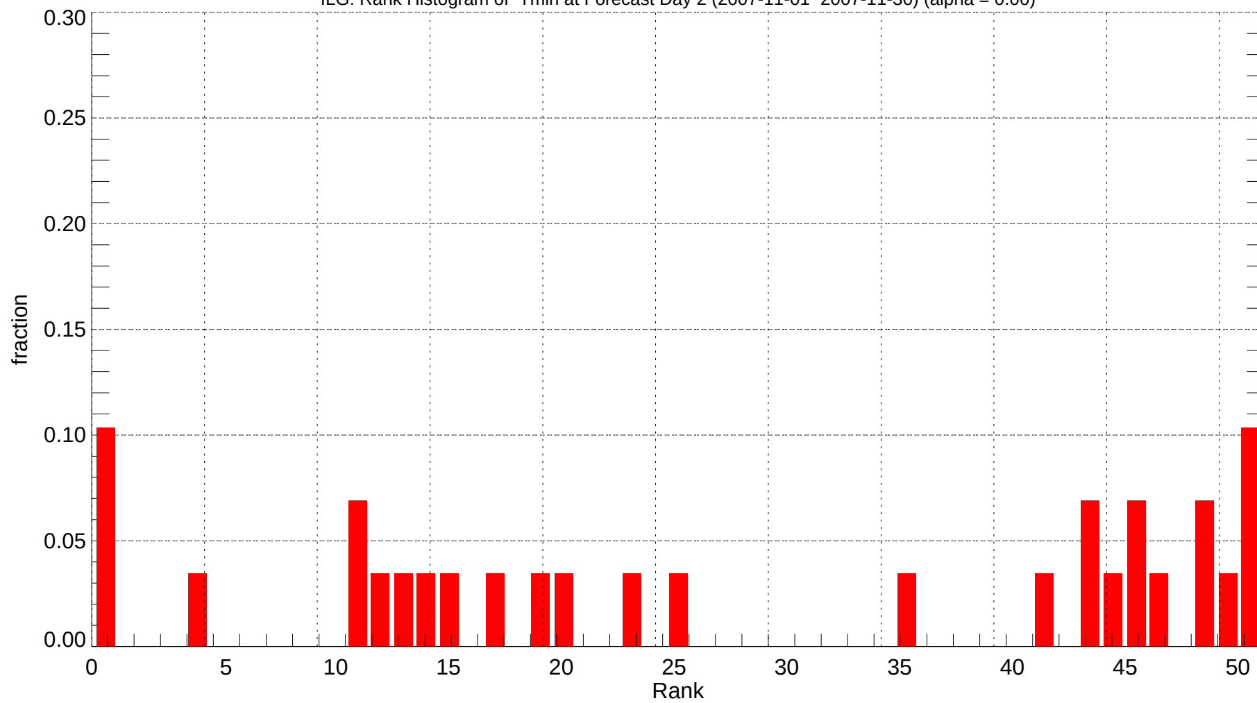
ILG: Rank Histogram of Tmin at Forecast Day 2 (2007-11-01~2007-11-30) (alpha = 0.00)
