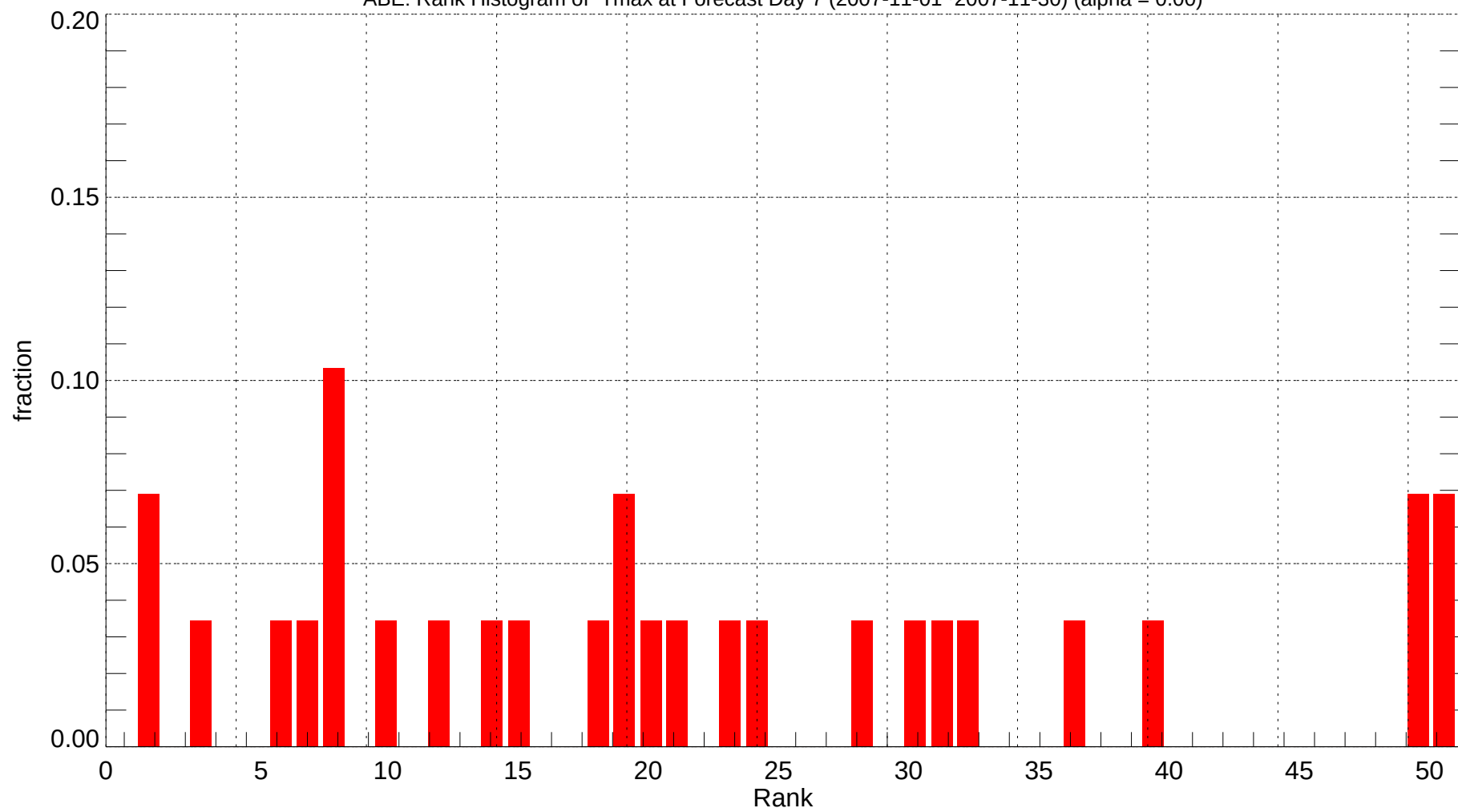
ABE: Rank Histogram of Tmax at Forecast Day 7 (2007-11-01~2007-11-30) (alpha = 0.00)
