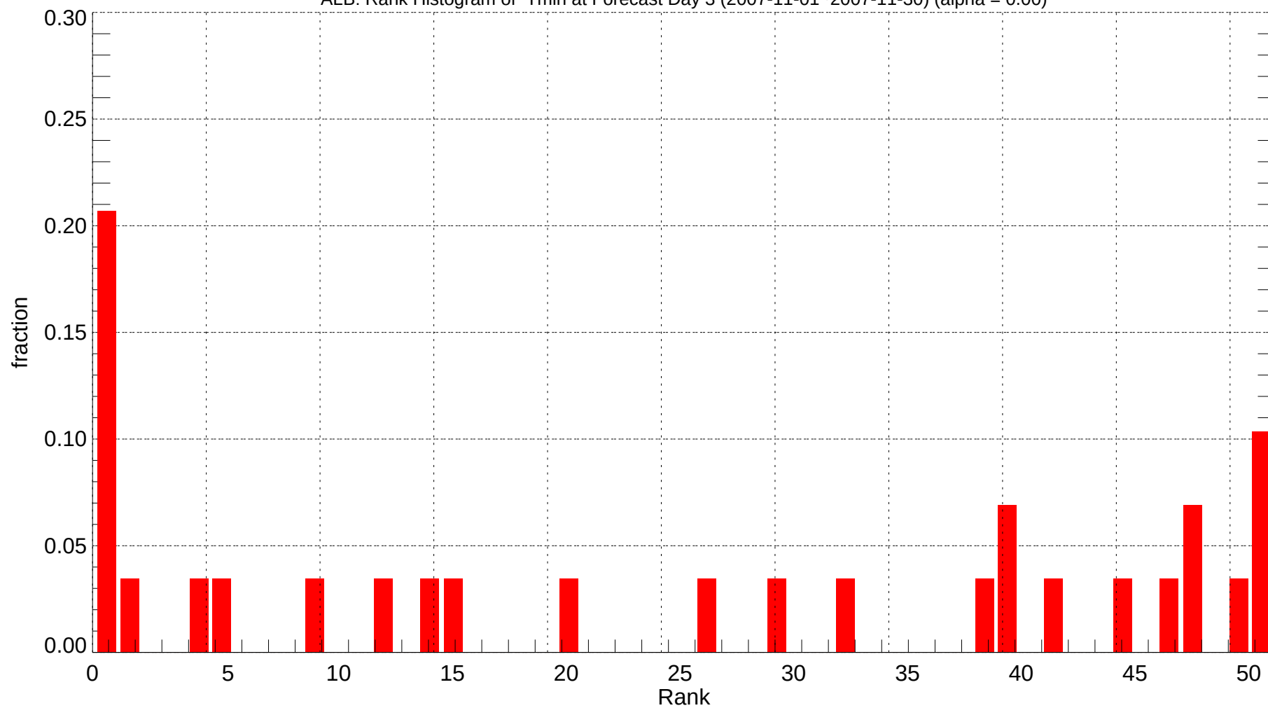
ALB: Rank Histogram of Tmin at Forecast Day 3 (2007-11-01~2007-11-30) (alpha = 0.00)
