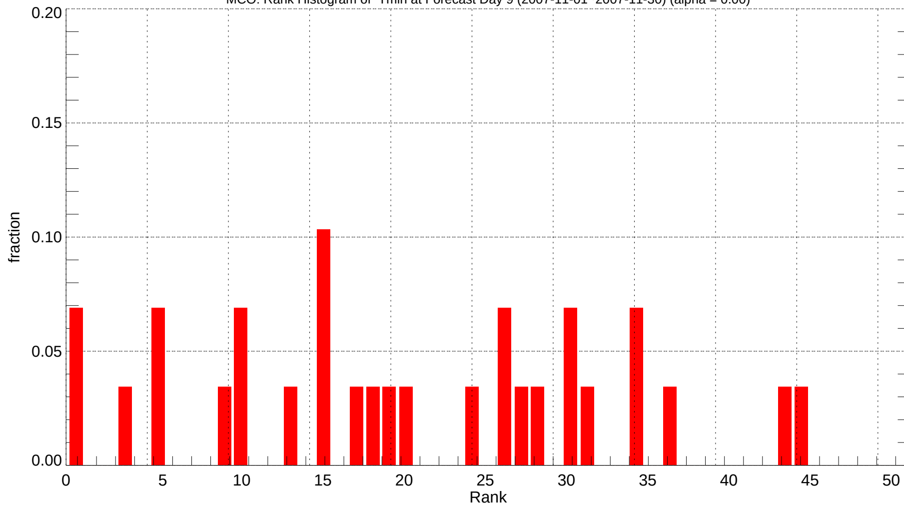
MCO: Rank Histogram of Tmin at Forecast Day 9 (2007-11-01~2007-11-30) (alpha = 0.00)
