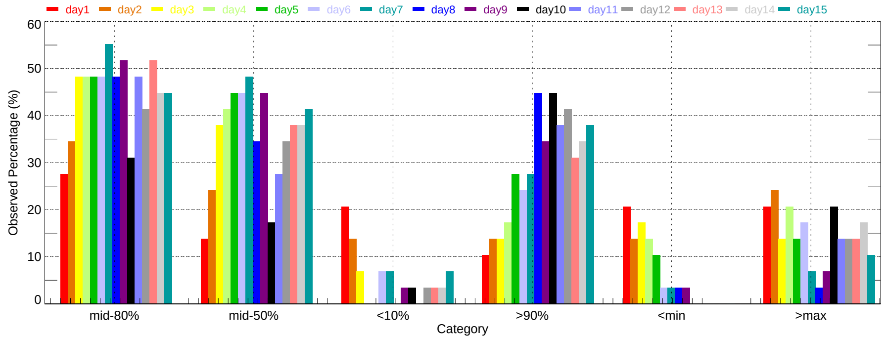
Observed Percentage of Ensembles - MCI: Min Temperature (2007-11-01~2007-11-30)
