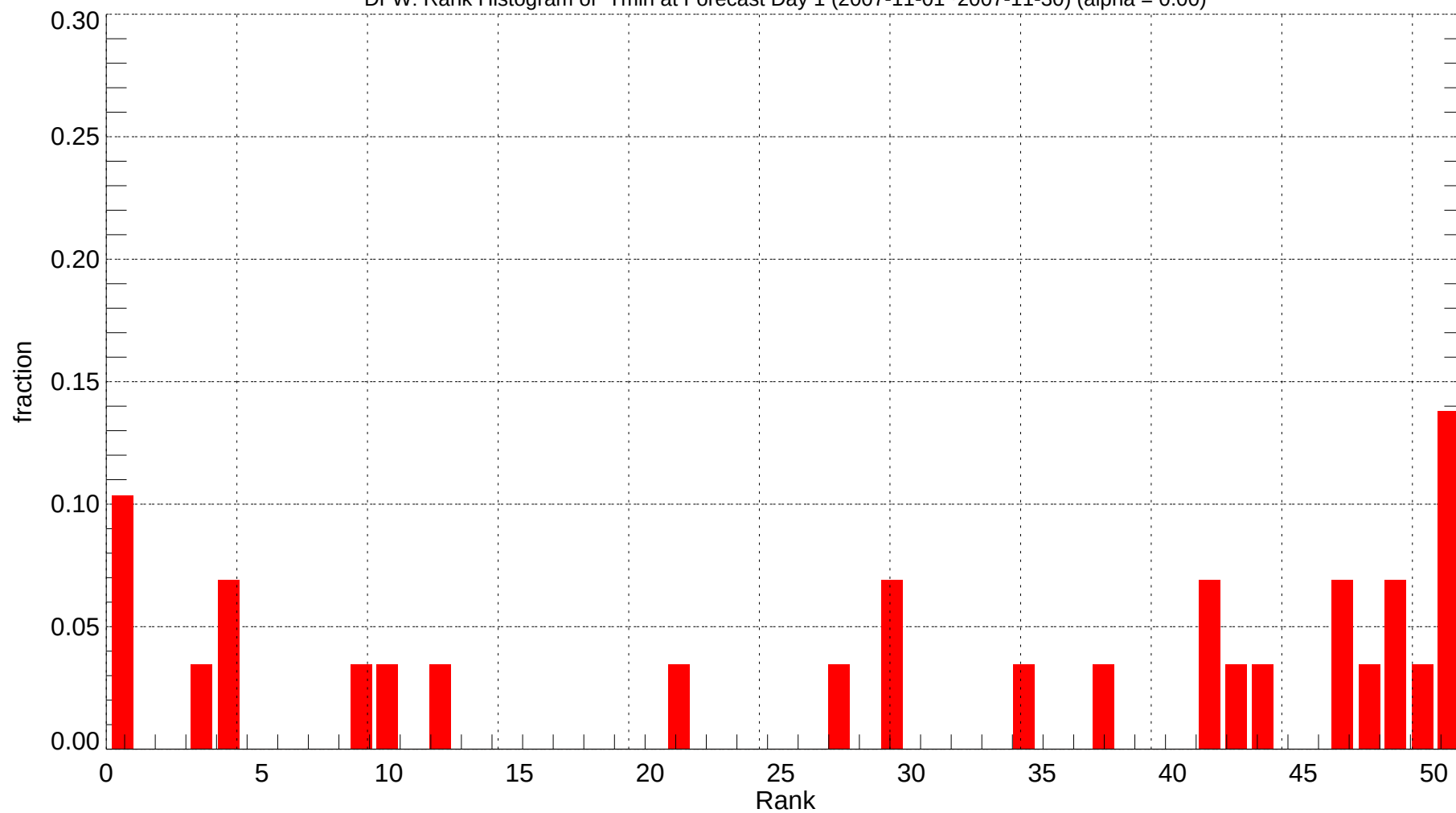
DFW: Rank Histogram of Tmin at Forecast Day 1 (2007-11-01~2007-11-30) (alpha = 0.00)
