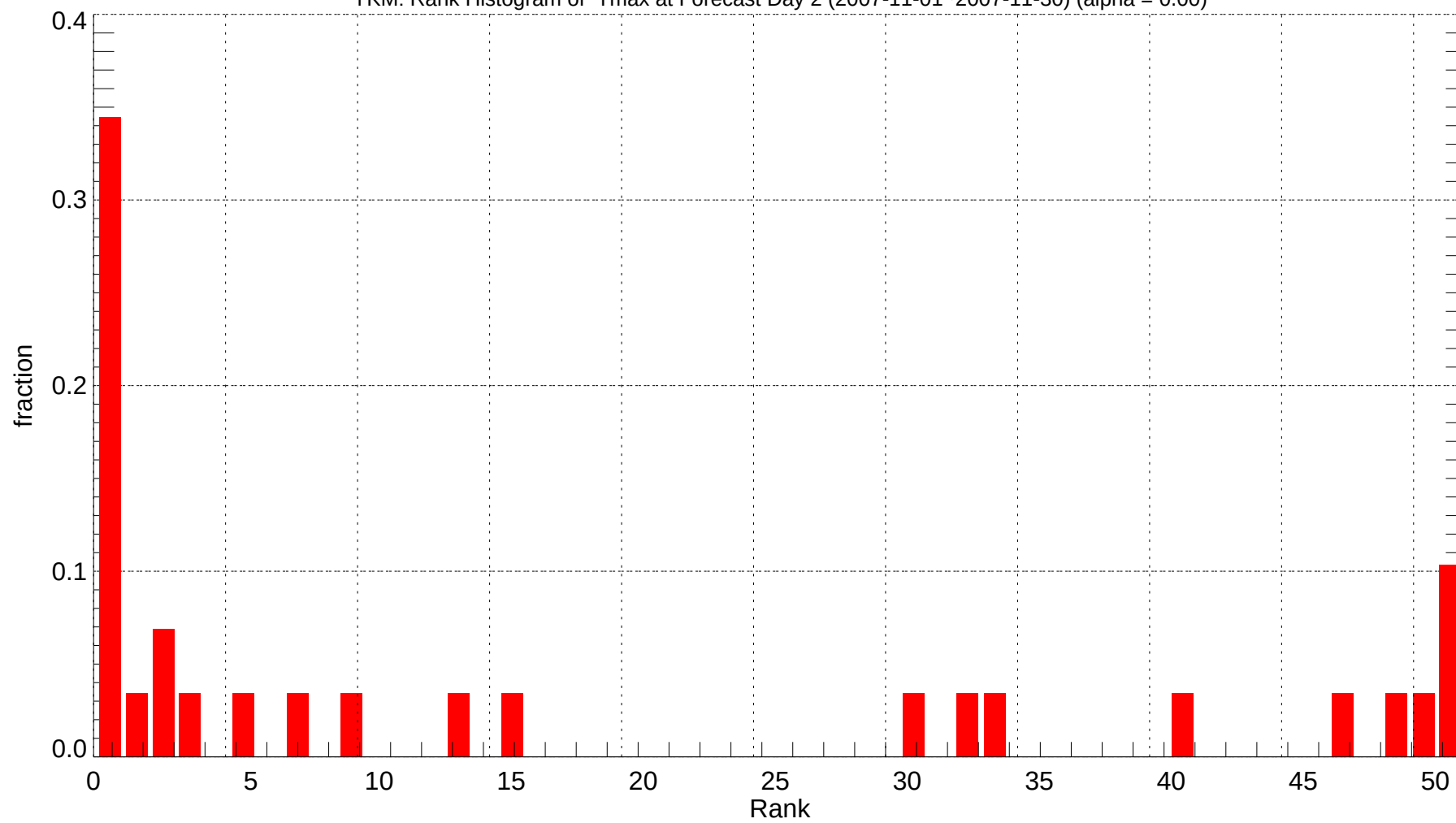
YKM: Rank Histogram of Tmax at Forecast Day 2 (2007-11-01~2007-11-30) (alpha = 0.00)
