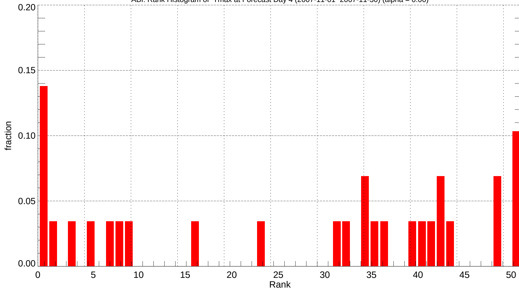
ABI: Rank Histogram of Tmax at Forecast Day 4 (2007-11-01~2007-11-30) (alpha = 0.00)
