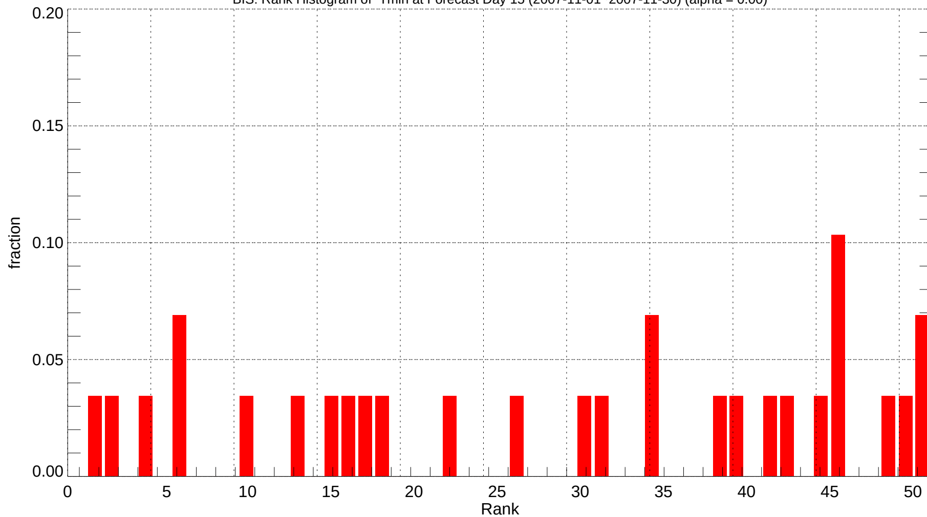
BIS: Rank Histogram of Tmin at Forecast Day 15 (2007-11-01~2007-11-30) (alpha = 0.00)
