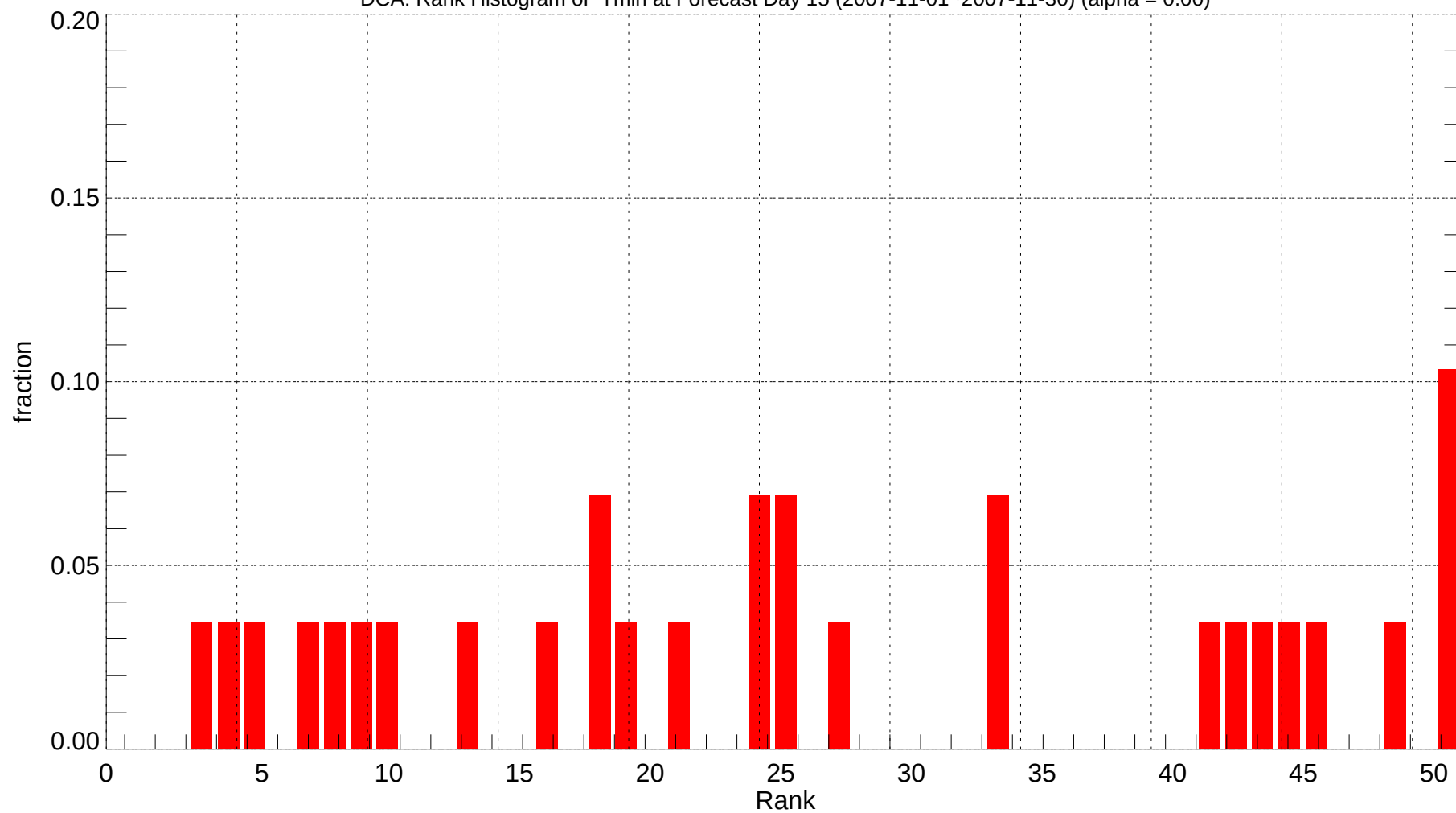
DCA: Rank Histogram of Tmin at Forecast Day 15 (2007-11-01~2007-11-30) (alpha = 0.00)
