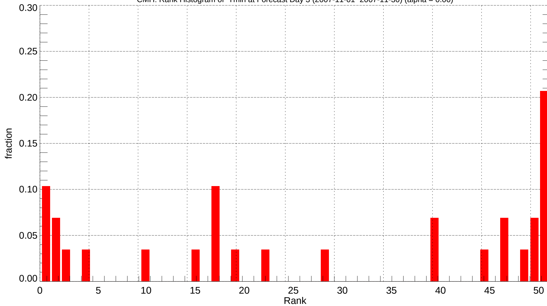
CMH: Rank Histogram of Tmin at Forecast Day 3 (2007-11-01~2007-11-30) (alpha = 0.00)
