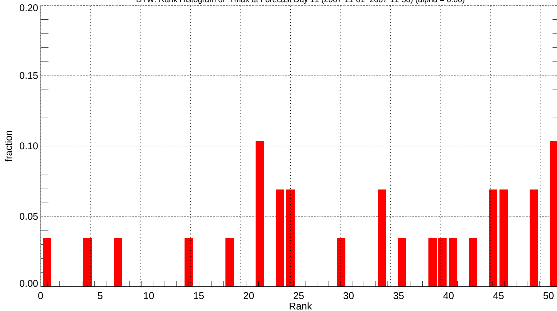
DTW: Rank Histogram of Tmax at Forecast Day 11 (2007-11-01~2007-11-30) (alpha = 0.00)
