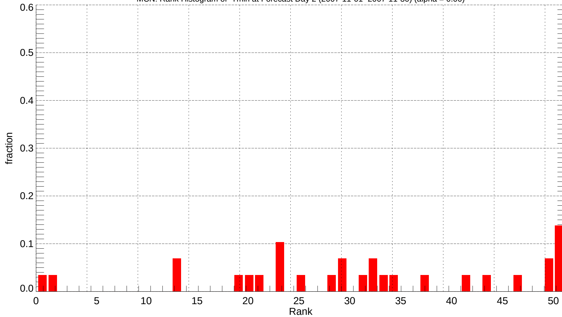
MCN: Rank Histogram of Tmin at Forecast Day 2 (2007-11-01~2007-11-30) (alpha = 0.00)
