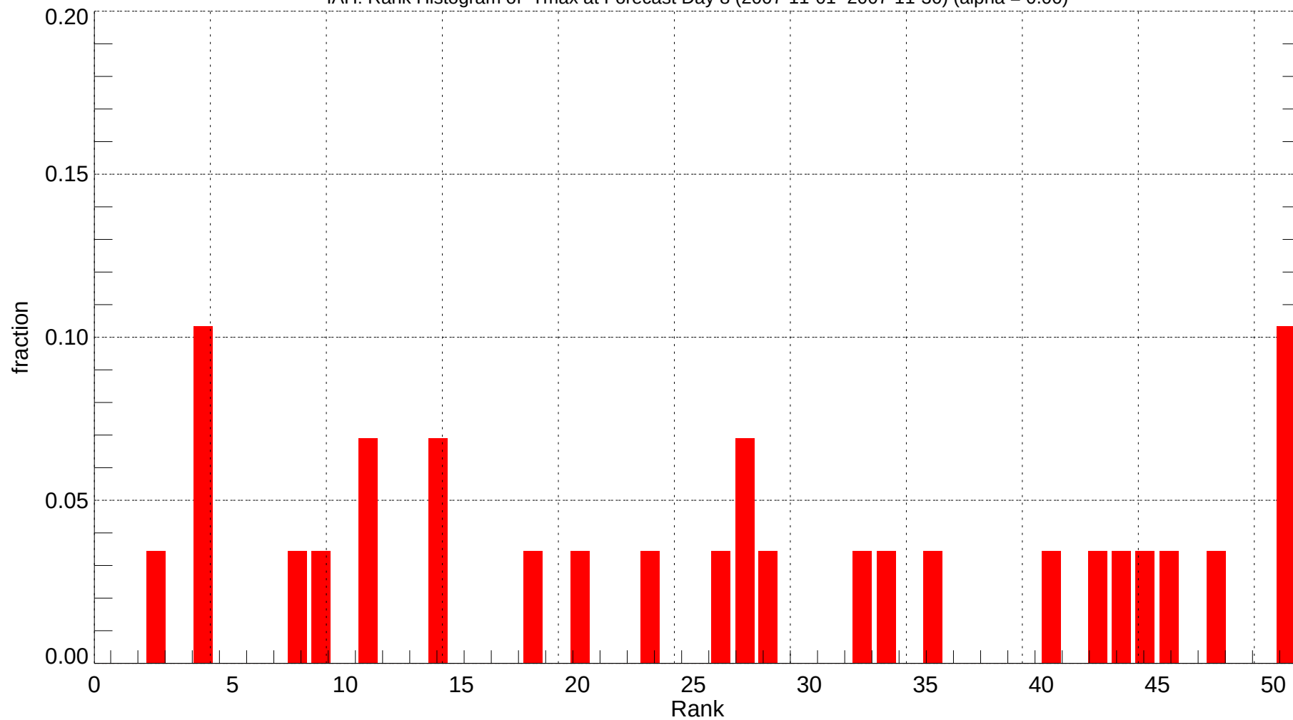
IAH: Rank Histogram of Tmax at Forecast Day 8 (2007-11-01~2007-11-30) (alpha = 0.00)
