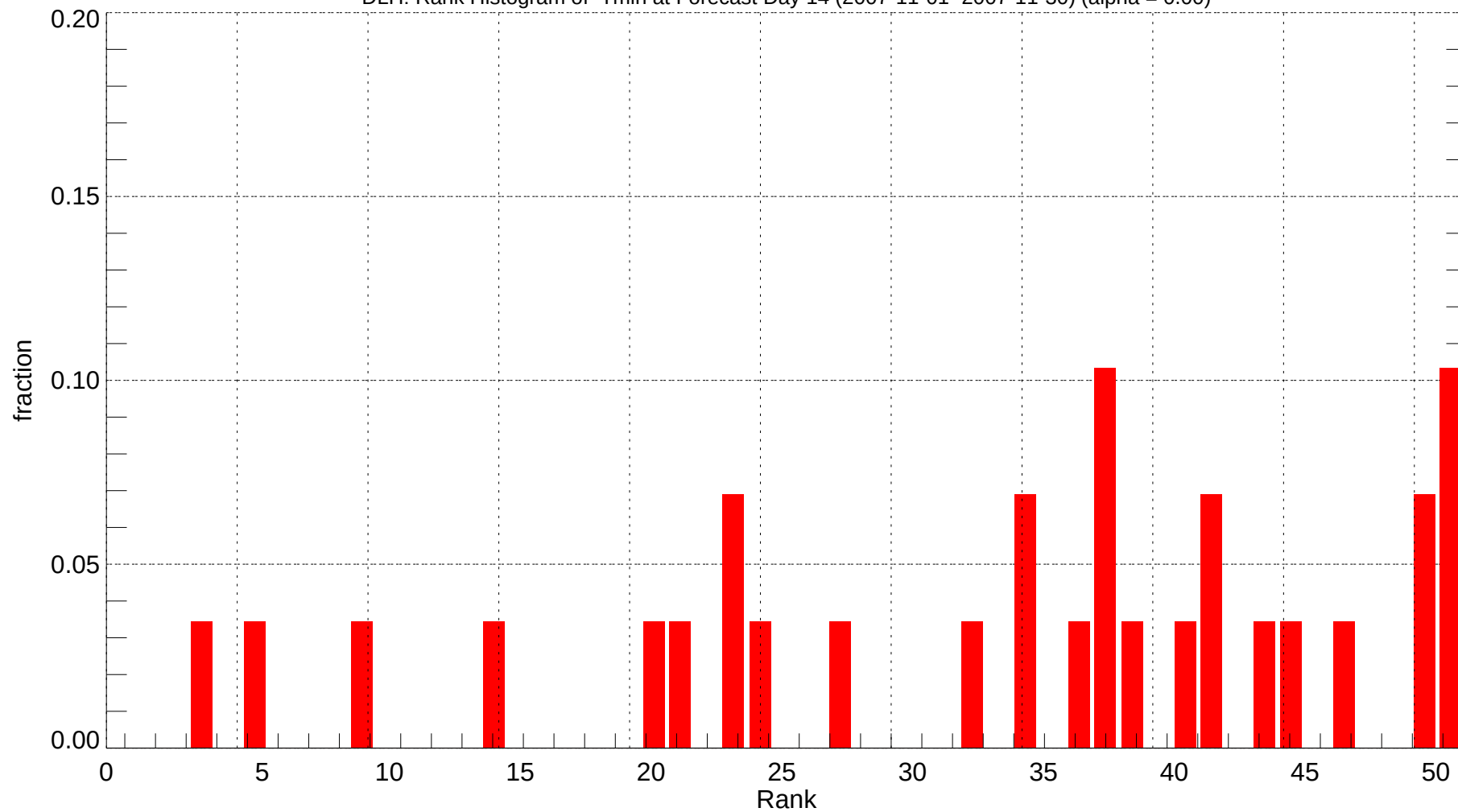
DLH: Rank Histogram of Tmin at Forecast Day 14 (2007-11-01~2007-11-30) (alpha = 0.00)
