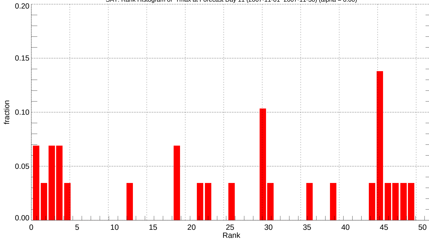
SAT: Rank Histogram of Tmax at Forecast Day 11 (2007-11-01~2007-11-30) (alpha = 0.00)
