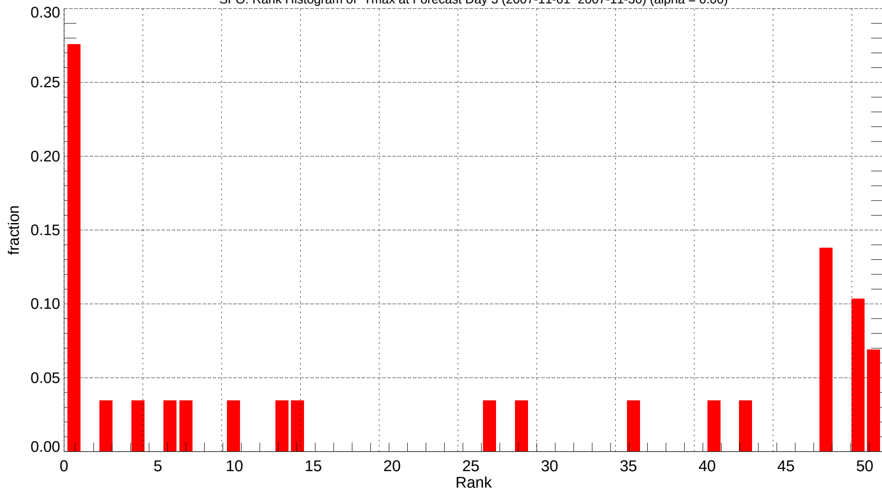
SFO: Rank Histogram of Tmax at Forecast Day 3 (2007-11-01~2007-11-30) (alpha = 0.00)
