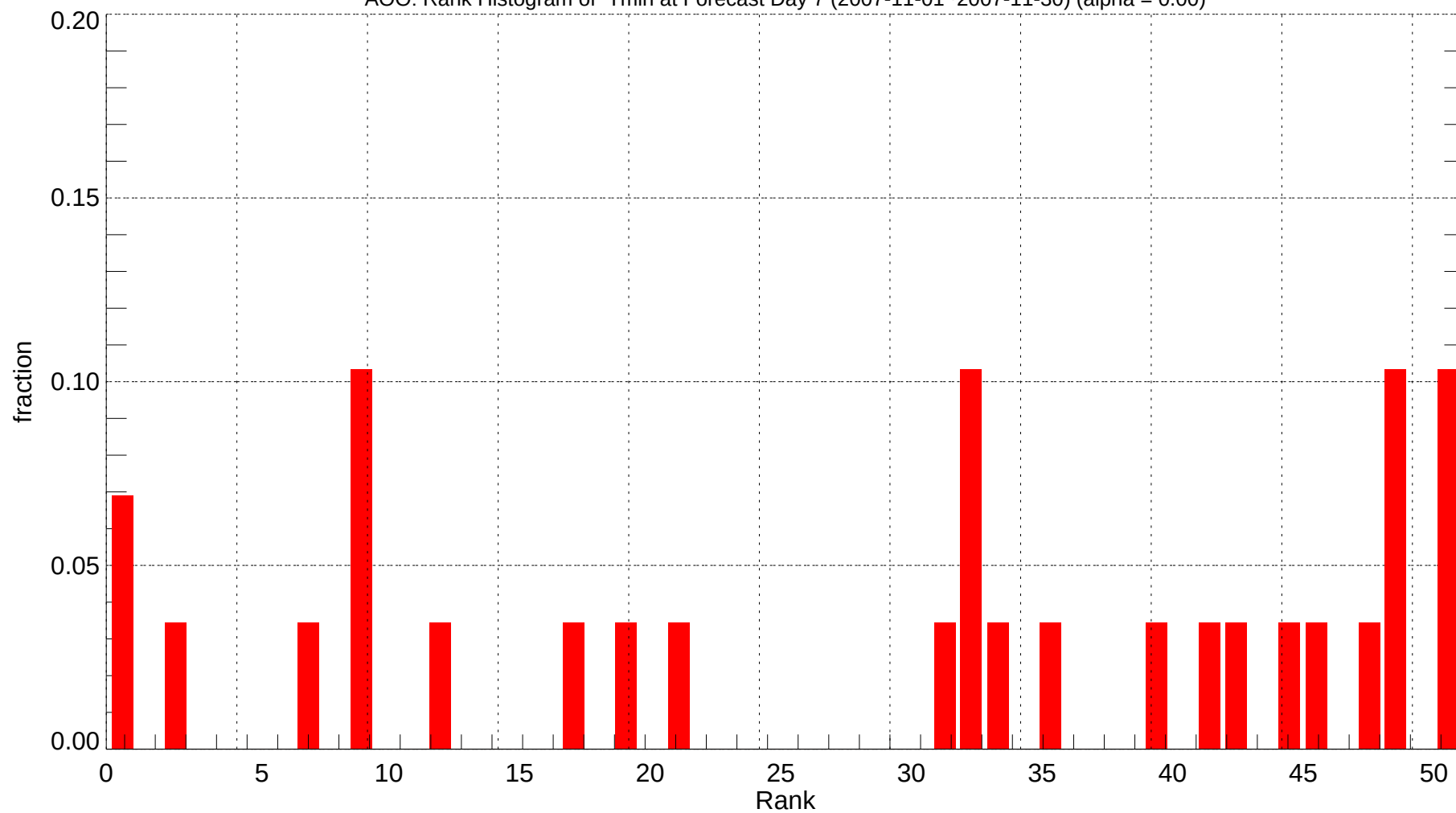
AOO: Rank Histogram of Tmin at Forecast Day 7 (2007-11-01~2007-11-30) (alpha = 0.00)
