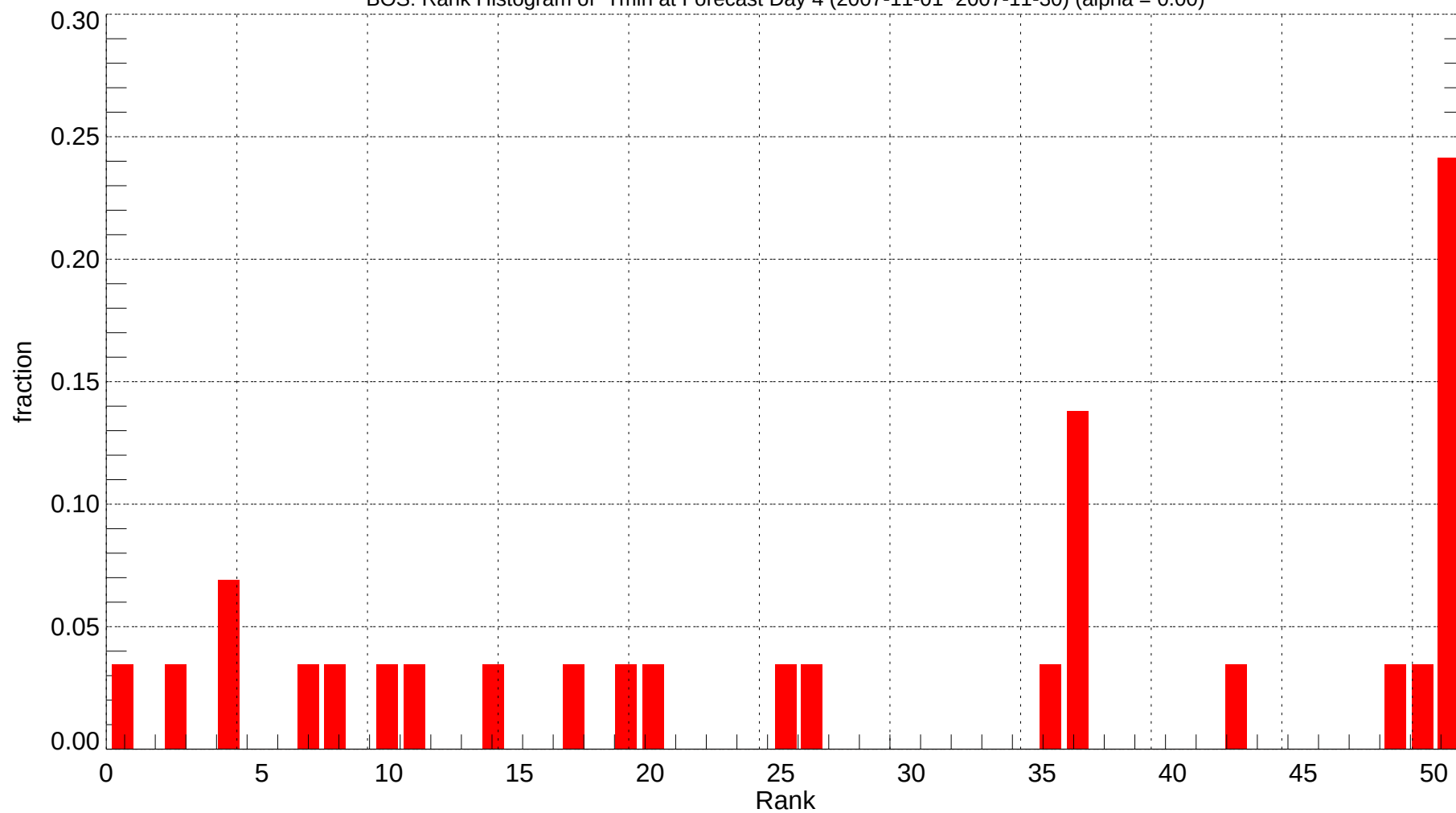
BOS: Rank Histogram of Tmin at Forecast Day 4 (2007-11-01~2007-11-30) (alpha = 0.00)
