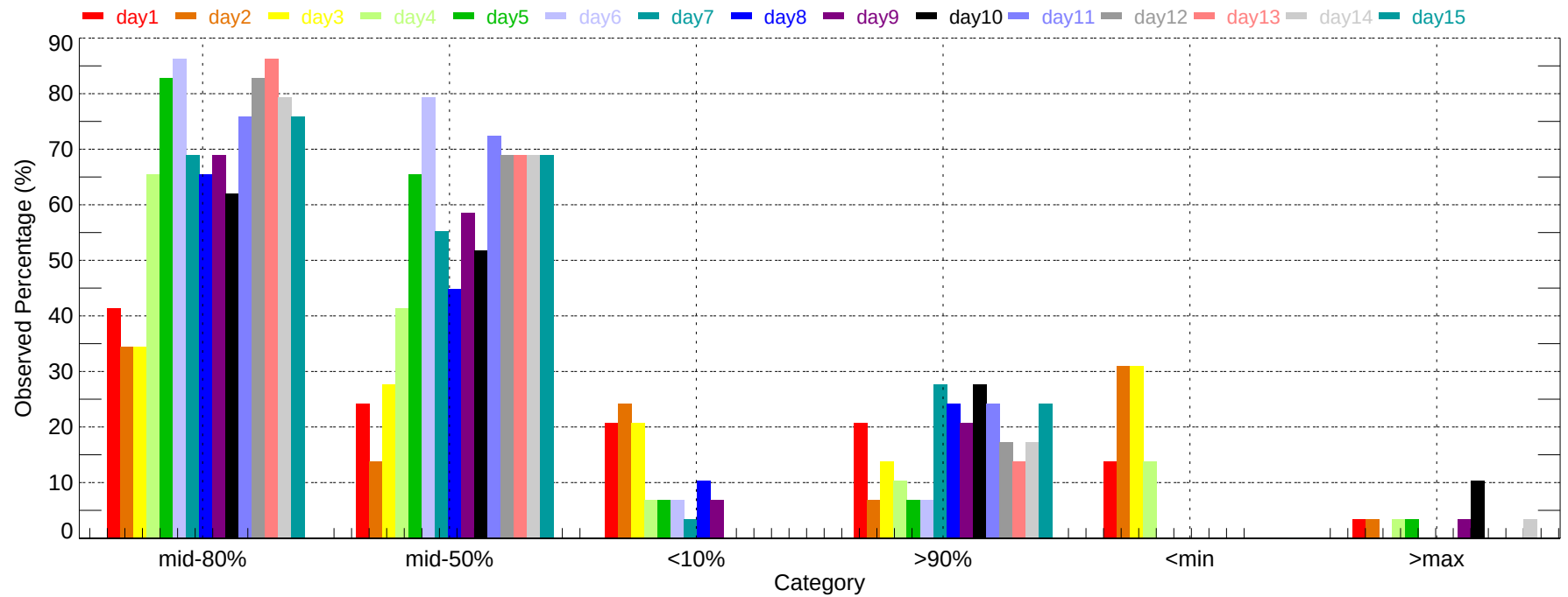
Observed Percentage of Ensembles - BFL: Min Temperature (2007-11-01~2007-11-30)
