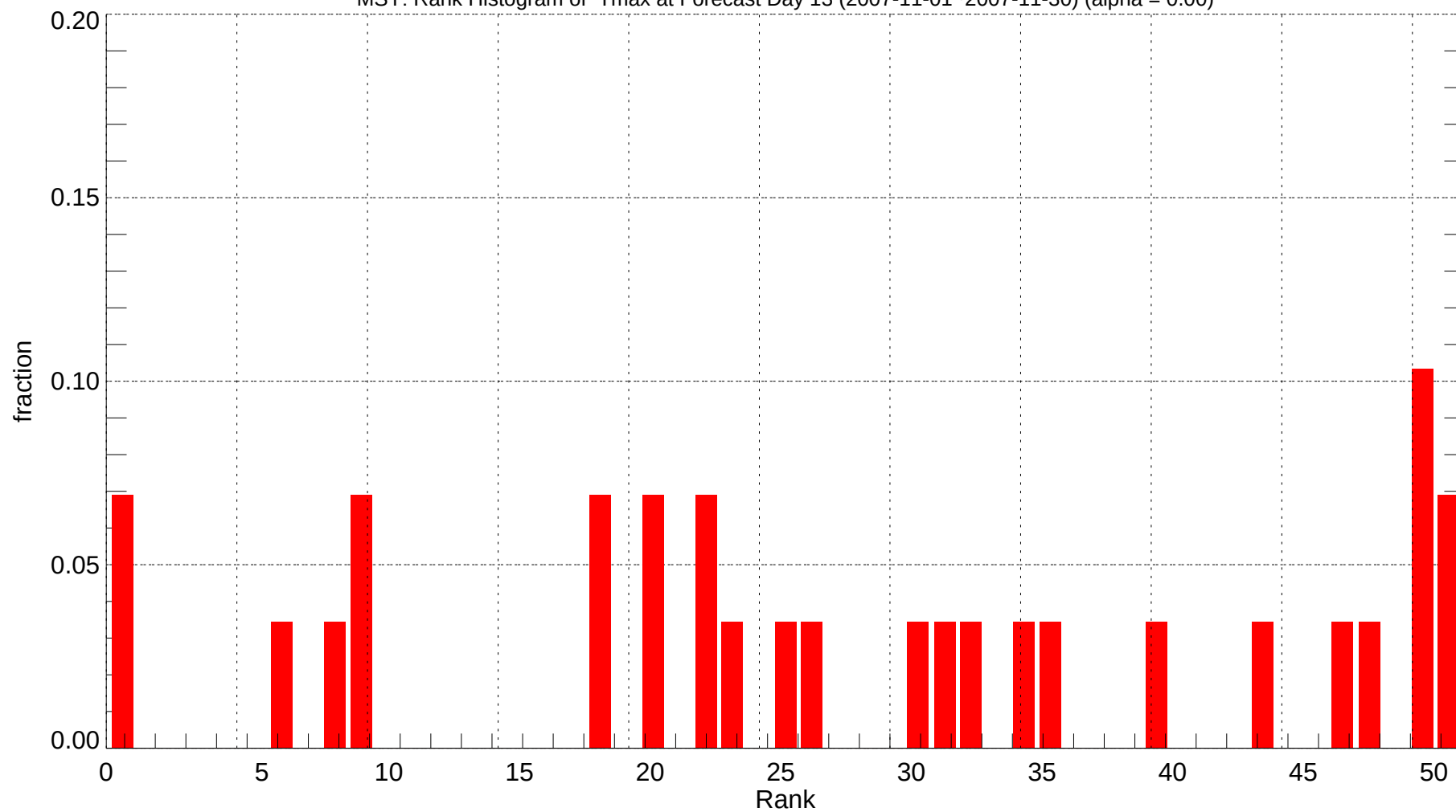
MSY: Rank Histogram of Tmax at Forecast Day 13 (2007-11-01~2007-11-30) (alpha = 0.00)
