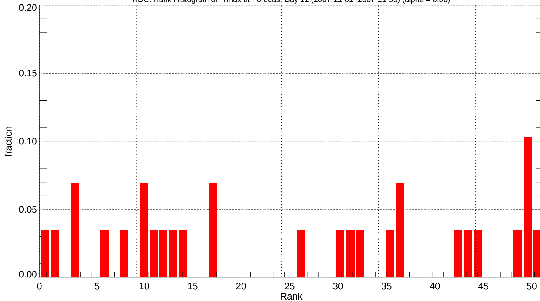
RDU: Rank Histogram of Tmax at Forecast Day 12 (2007-11-01~2007-11-30) (alpha = 0.00)
