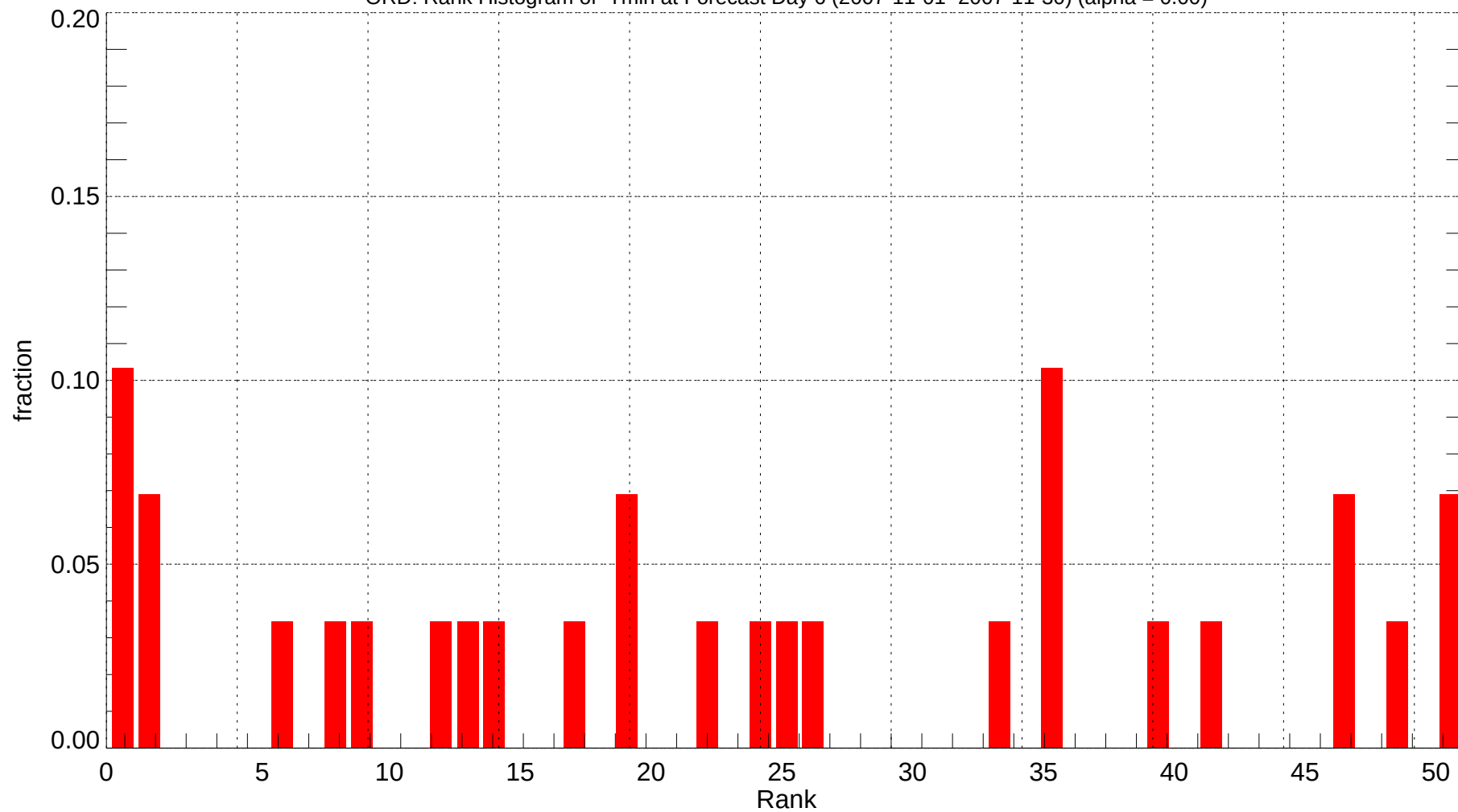
ORD: Rank Histogram of Tmin at Forecast Day 6 (2007-11-01~2007-11-30) (alpha = 0.00)
