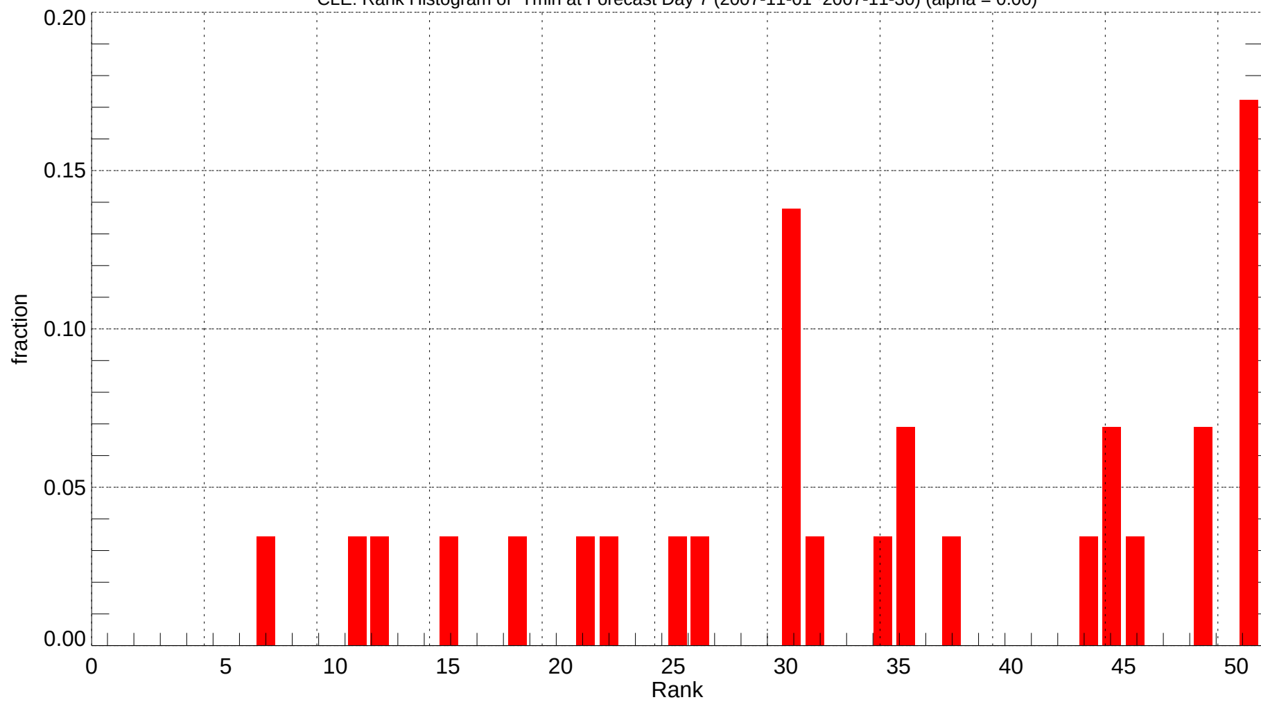
CLE: Rank Histogram of Tmin at Forecast Day 7 (2007-11-01~2007-11-30) (alpha = 0.00)
