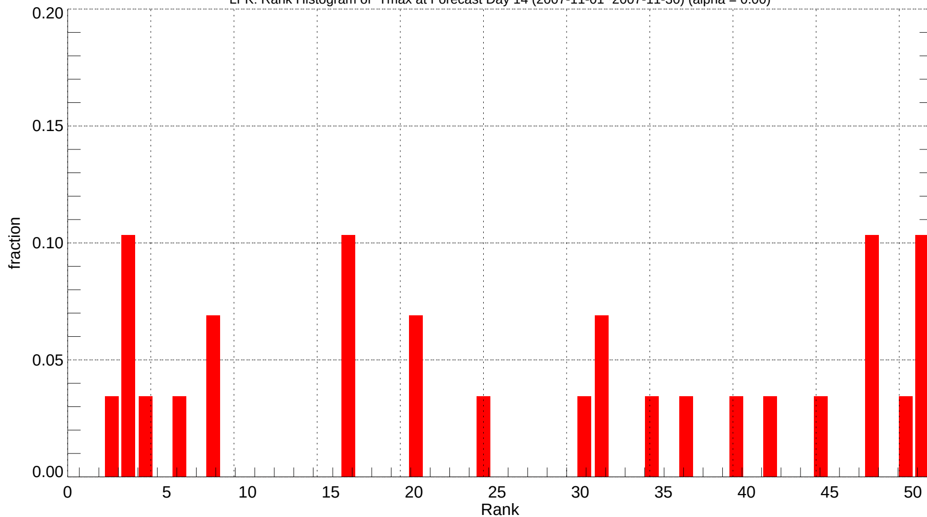
LFK: Rank Histogram of Tmax at Forecast Day 14 (2007-11-01~2007-11-30) (alpha = 0.00)
