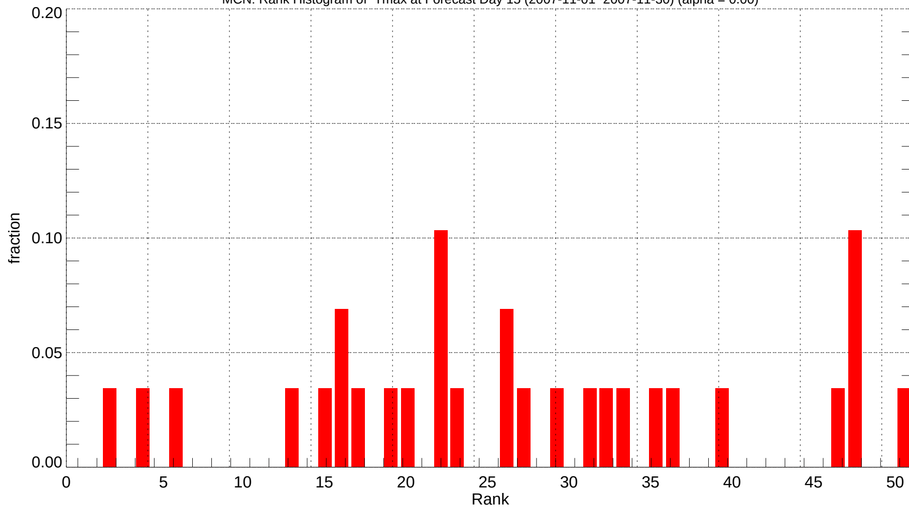
MCN: Rank Histogram of Tmax at Forecast Day 15 (2007-11-01~2007-11-30) (alpha = 0.00)
