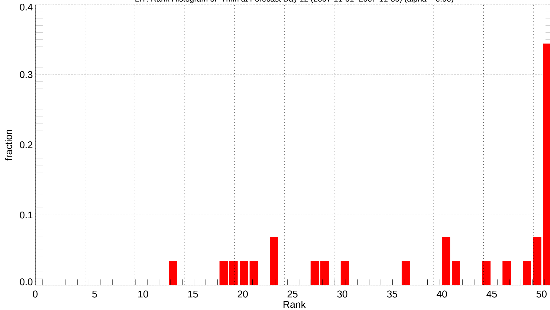
LIT: Rank Histogram of Tmin at Forecast Day 12 (2007-11-01~2007-11-30) (alpha = 0.00)
