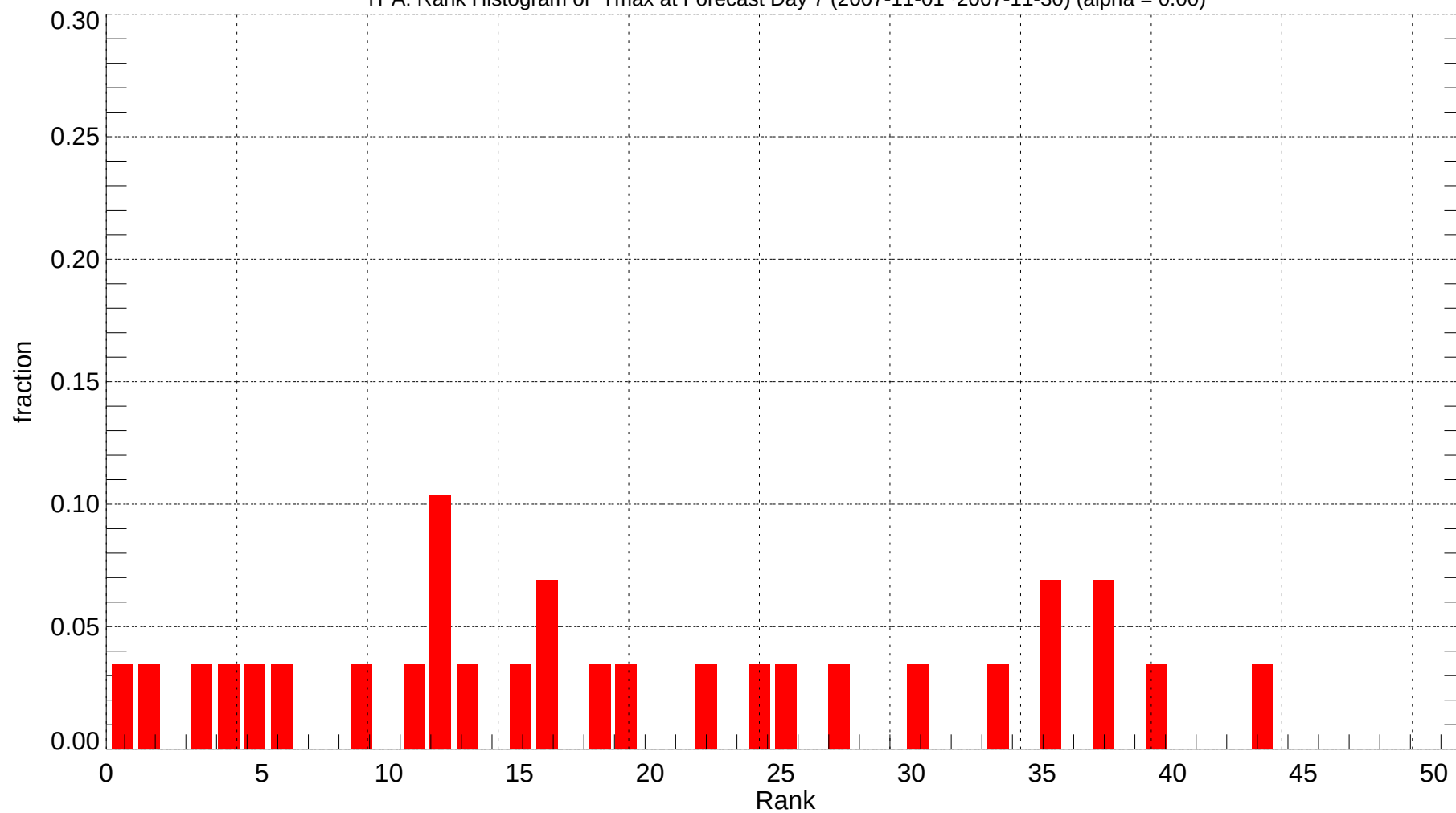
TPA: Rank Histogram of Tmax at Forecast Day 7 (2007-11-01~2007-11-30) (alpha = 0.00)
