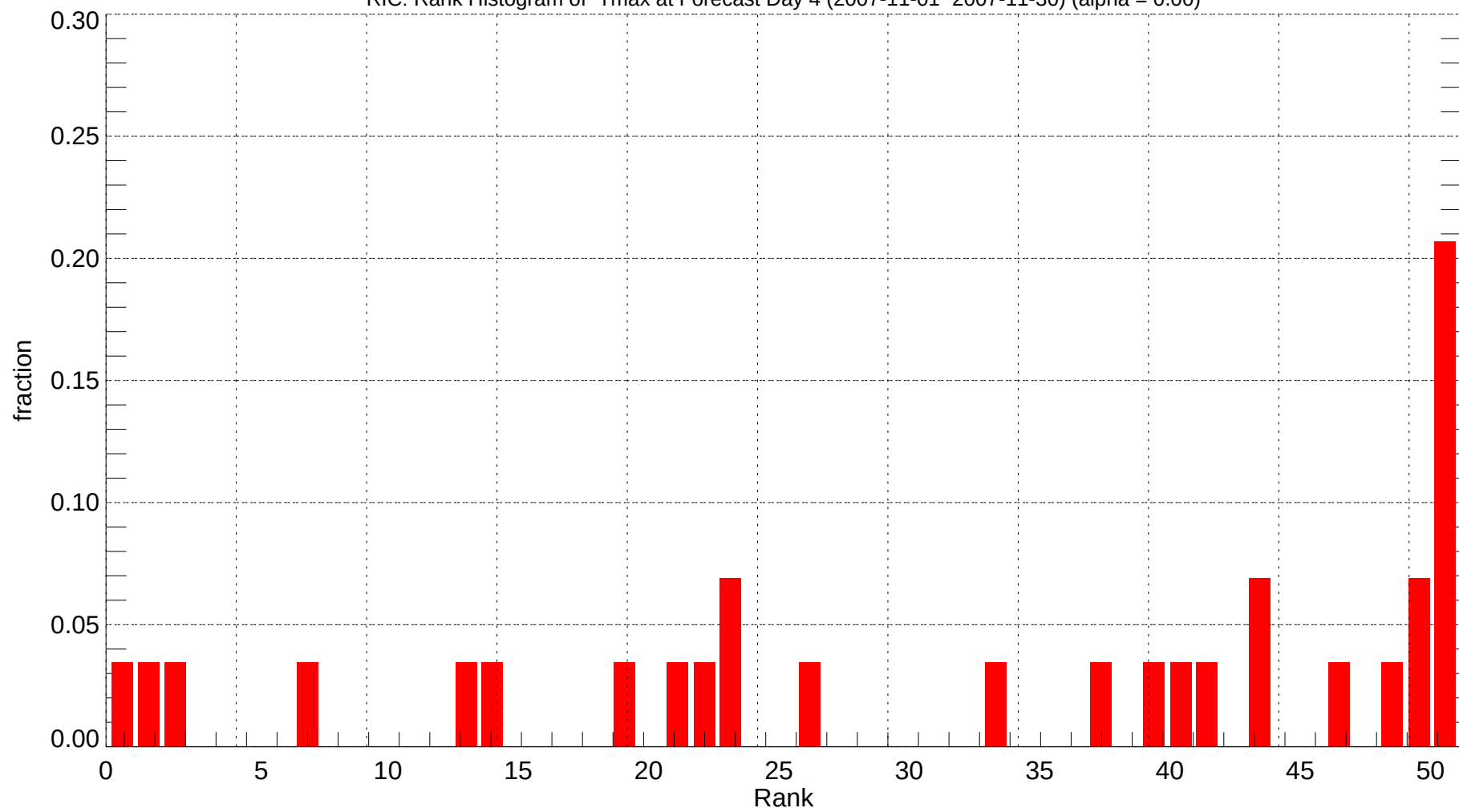
RIC: Rank Histogram of Tmax at Forecast Day 4 (2007-11-01~2007-11-30) (alpha = 0.00)
