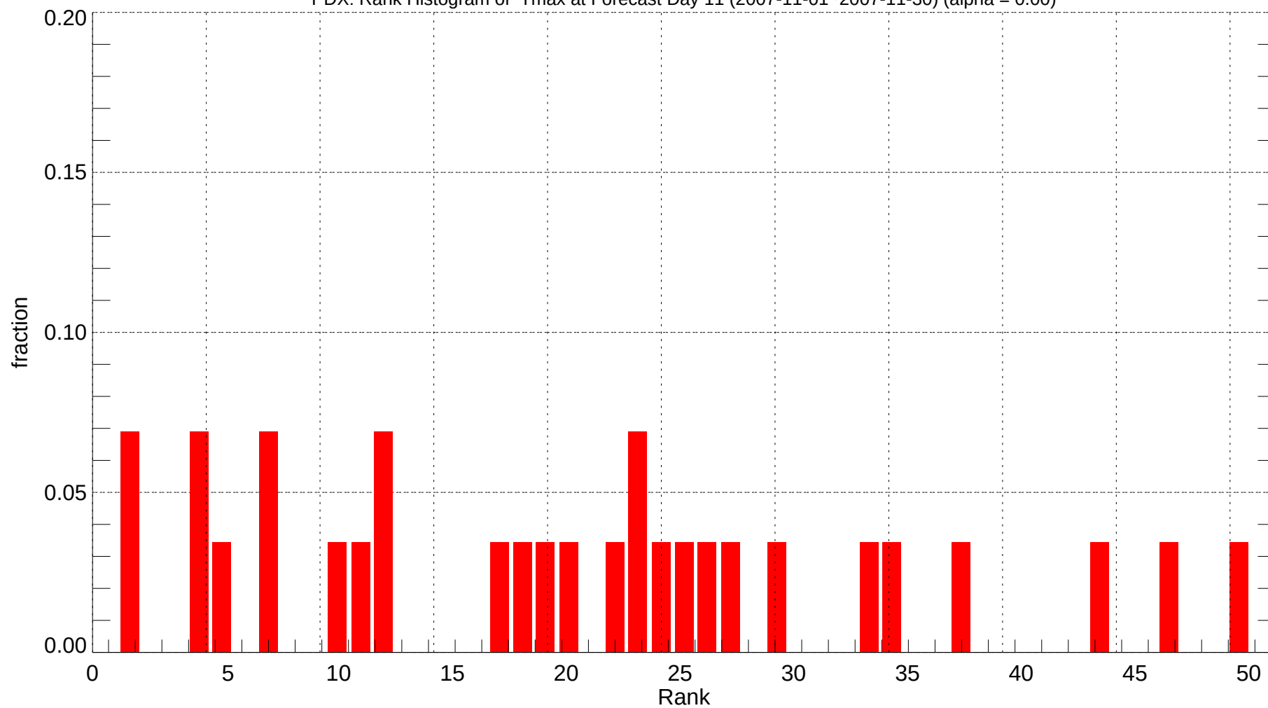
PDX: Rank Histogram of Tmax at Forecast Day 11 (2007-11-01~2007-11-30) (alpha = 0.00)
