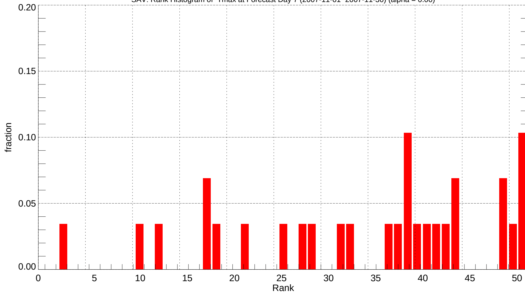
SAV: Rank Histogram of Tmax at Forecast Day 7 (2007-11-01~2007-11-30) (alpha = 0.00)
