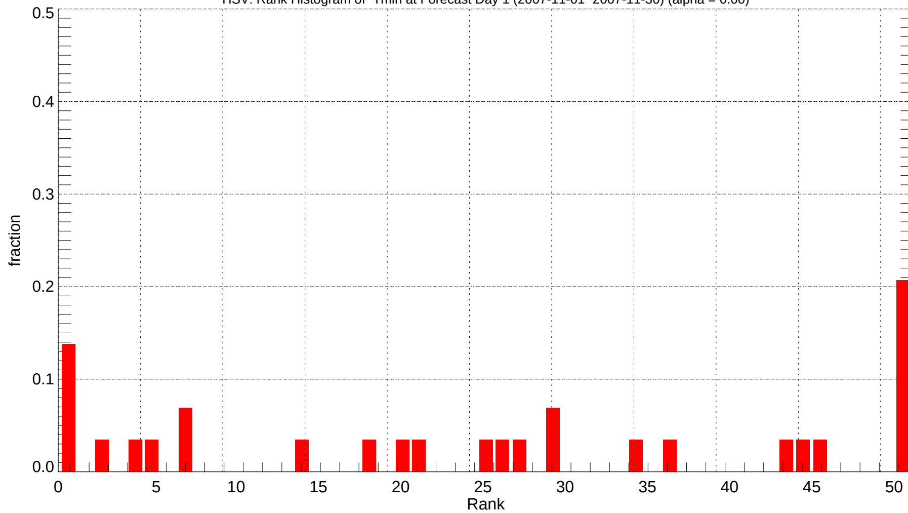
HSV: Rank Histogram of Tmin at Forecast Day 1 (2007-11-01~2007-11-30) (alpha = 0.00)
