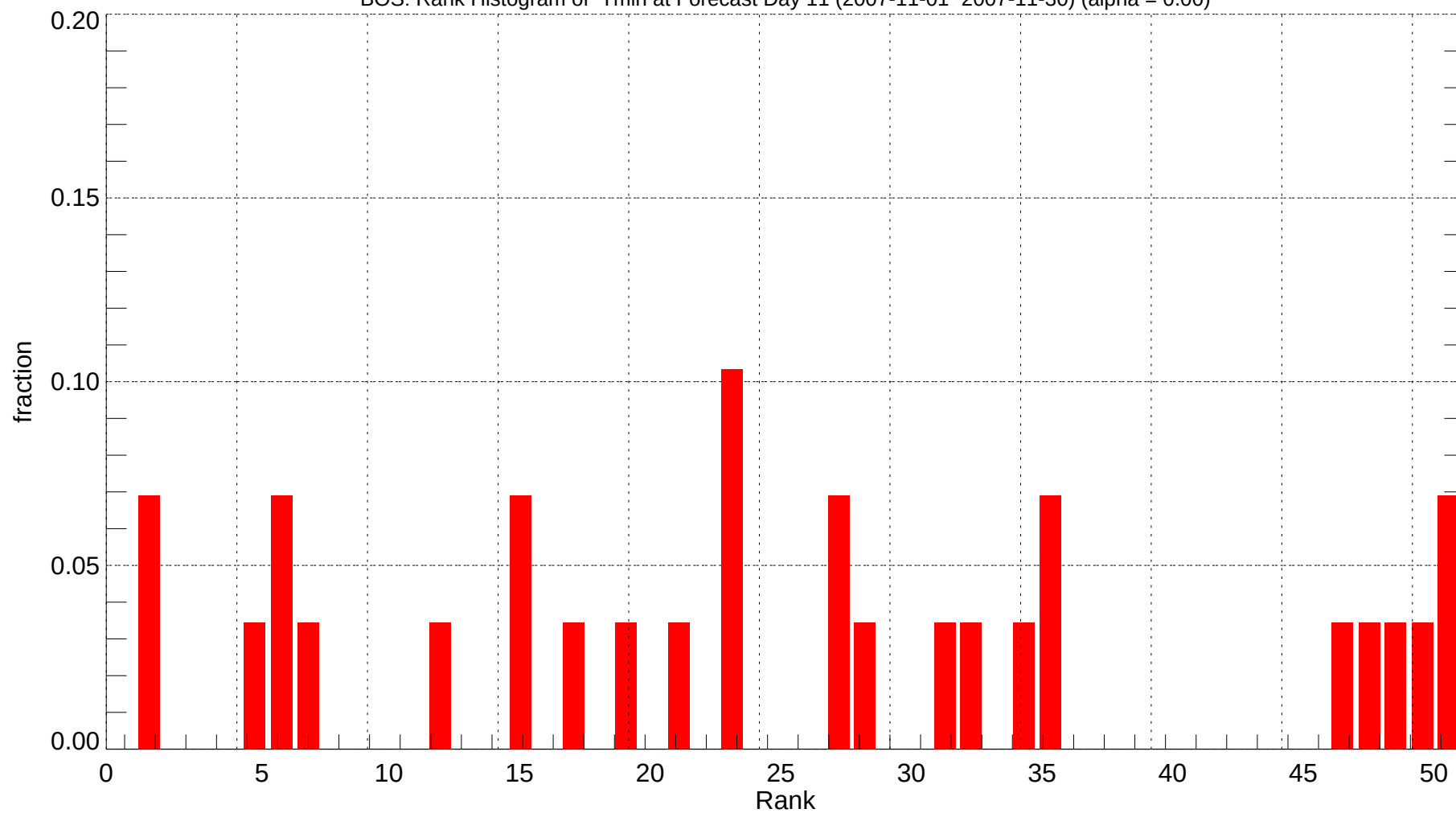
BOS: Rank Histogram of Tmin at Forecast Day 11 (2007-11-01~2007-11-30) (alpha = 0.00)
