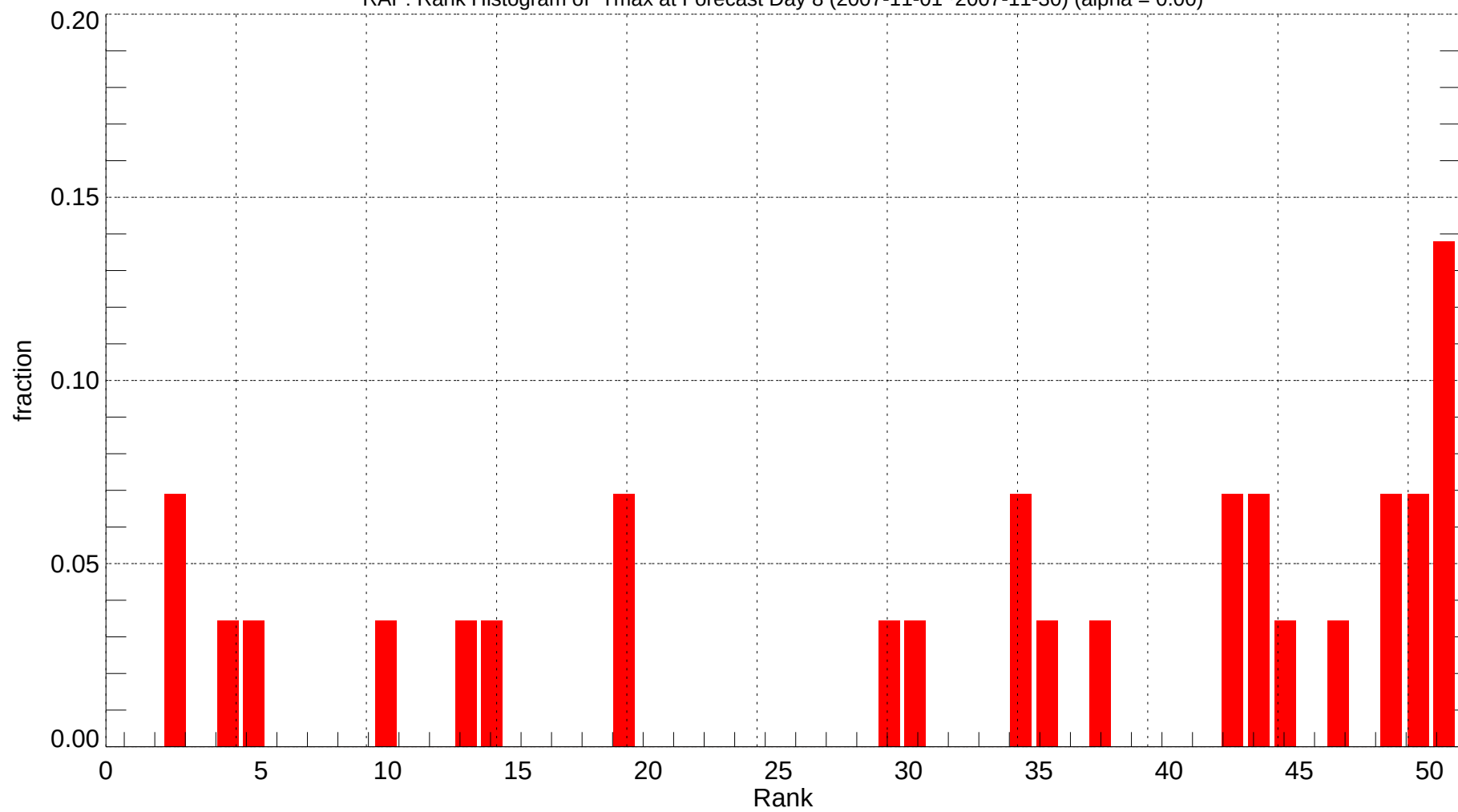
RAP: Rank Histogram of Tmax at Forecast Day 8 (2007-11-01~2007-11-30) (alpha = 0.00)
