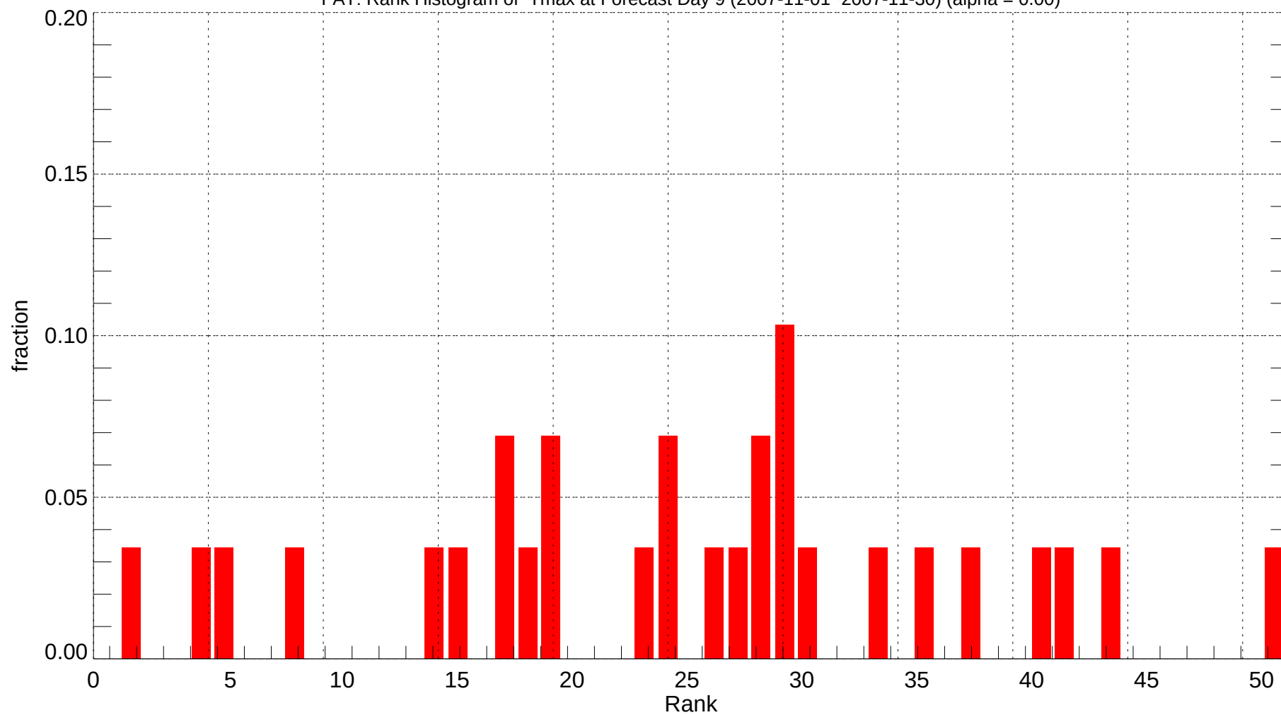
FAT: Rank Histogram of Tmax at Forecast Day 9 (2007-11-01~2007-11-30) (alpha = 0.00)
