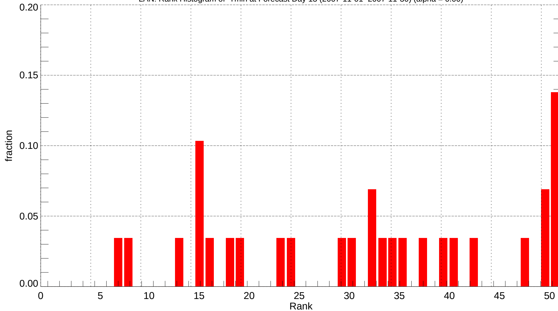
LAN: Rank Histogram of Tmin at Forecast Day 13 (2007-11-01~2007-11-30) (alpha = 0.00)
