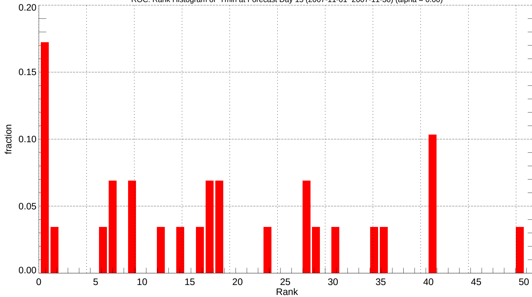
ROC: Rank Histogram of Tmin at Forecast Day 15 (2007-11-01~2007-11-30) (alpha = 0.00)
