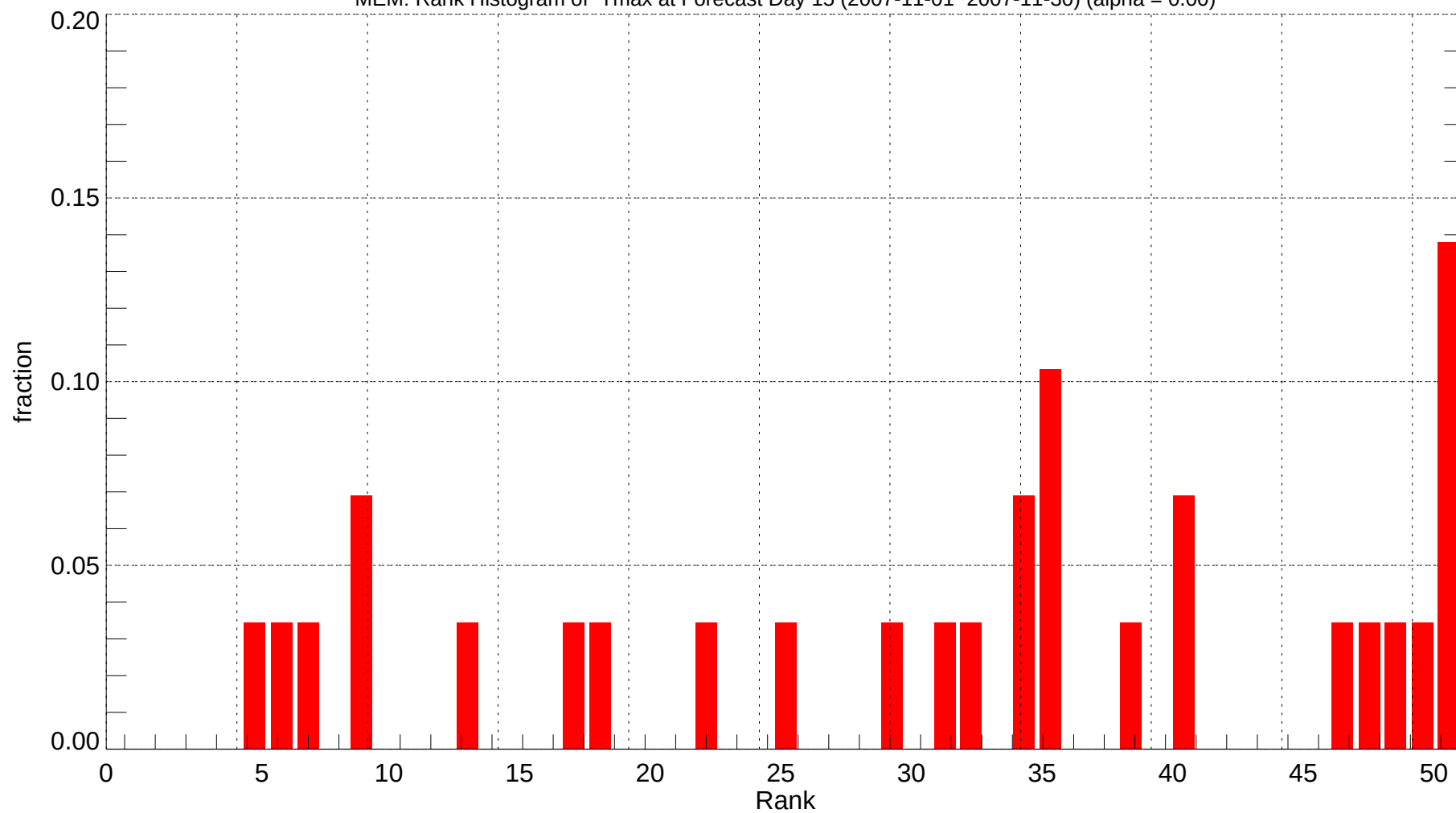
MEM: Rank Histogram of Tmax at Forecast Day 15 (2007-11-01~2007-11-30) (alpha = 0.00)
