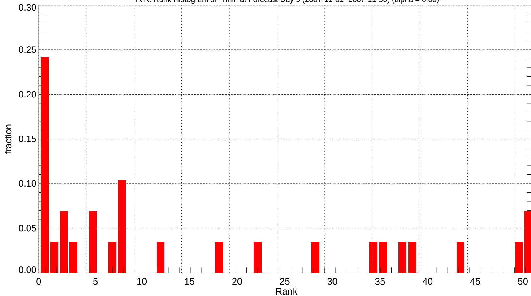
YVR: Rank Histogram of Tmin at Forecast Day 9 (2007-11-01~2007-11-30) (alpha = 0.00)
