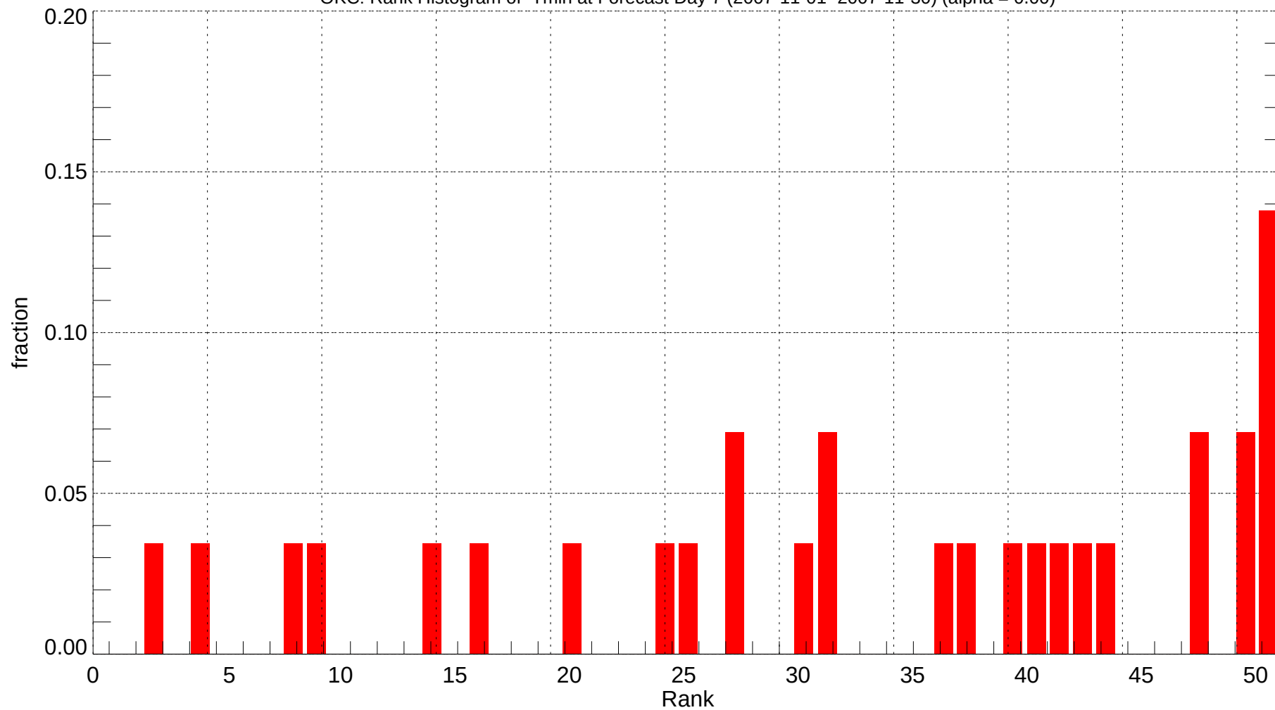
OKC: Rank Histogram of Tmin at Forecast Day 7 (2007-11-01~2007-11-30) (alpha = 0.00)
