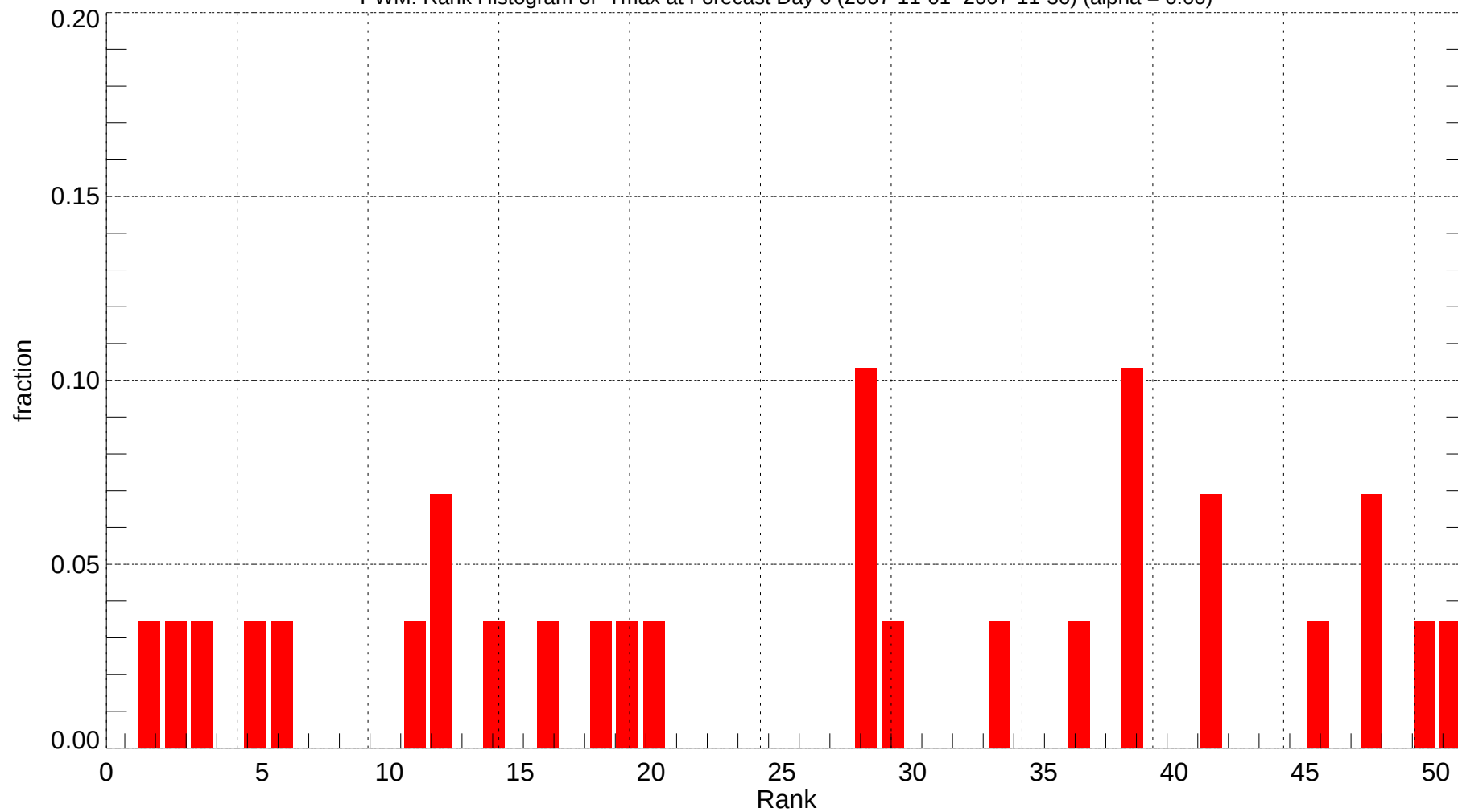
PWM: Rank Histogram of Tmax at Forecast Day 6 (2007-11-01~2007-11-30) (alpha = 0.00)
