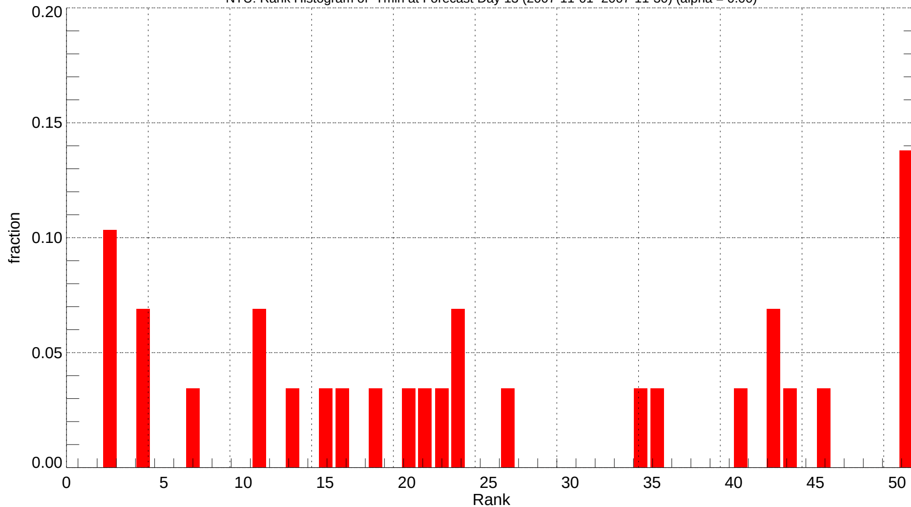
NTU: Rank Histogram of Tmin at Forecast Day 13 (2007-11-01~2007-11-30) (alpha = 0.00)
