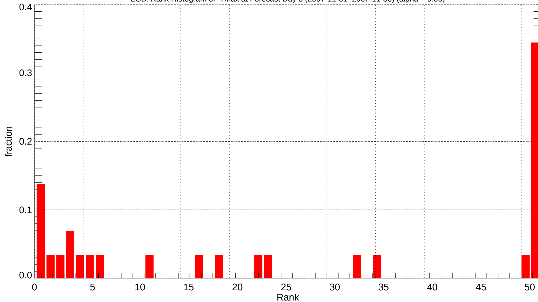
LGB: Rank Histogram of Tmax at Forecast Day 5 (2007-11-01~2007-11-30) (alpha = 0.00)
