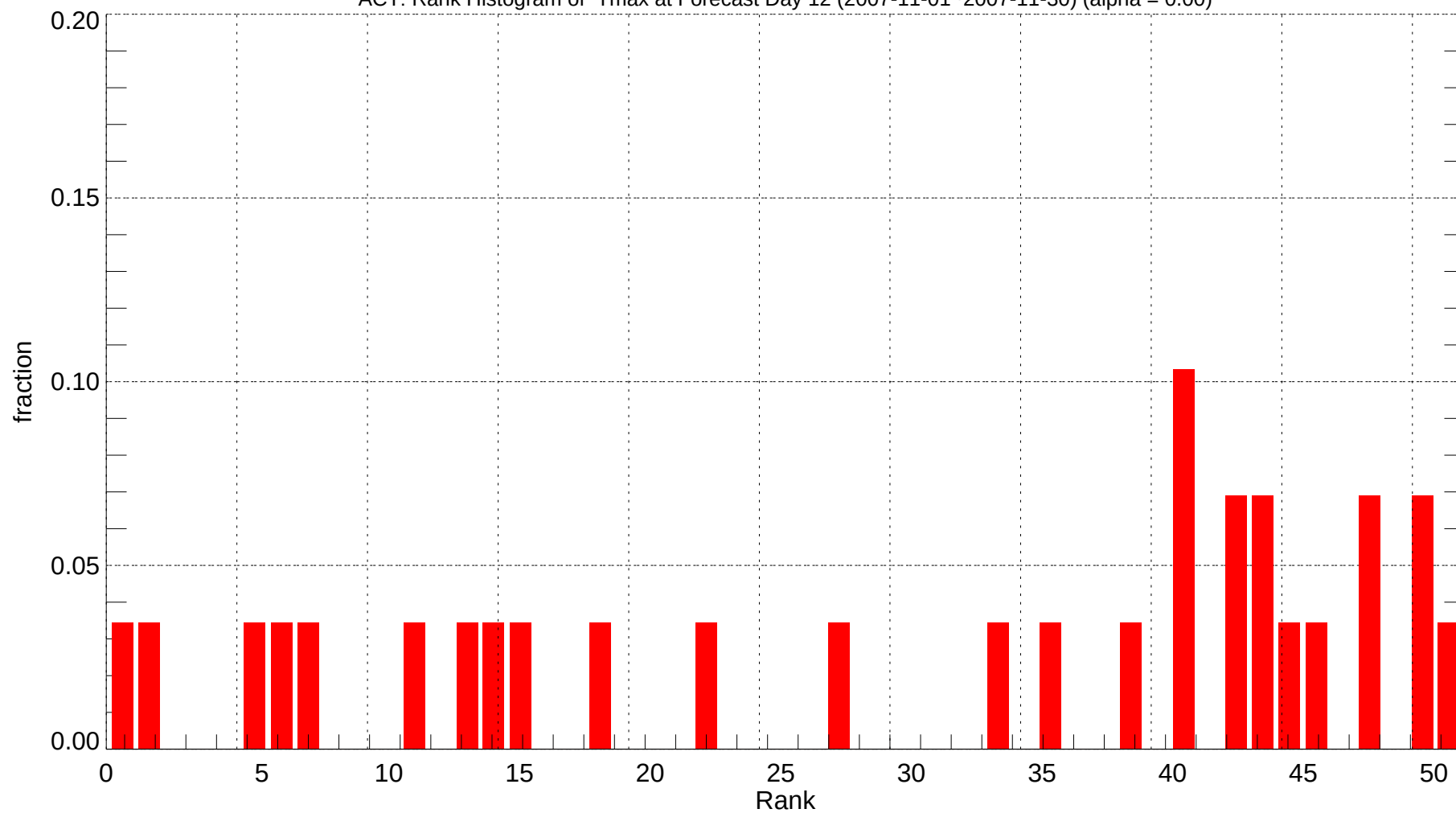
ACT: Rank Histogram of Tmax at Forecast Day 12 (2007-11-01~2007-11-30) (alpha = 0.00)
