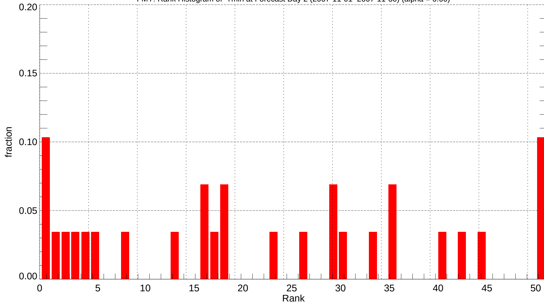
FMY: Rank Histogram of Tmin at Forecast Day 2 (2007-11-01~2007-11-30) (alpha = 0.00)
