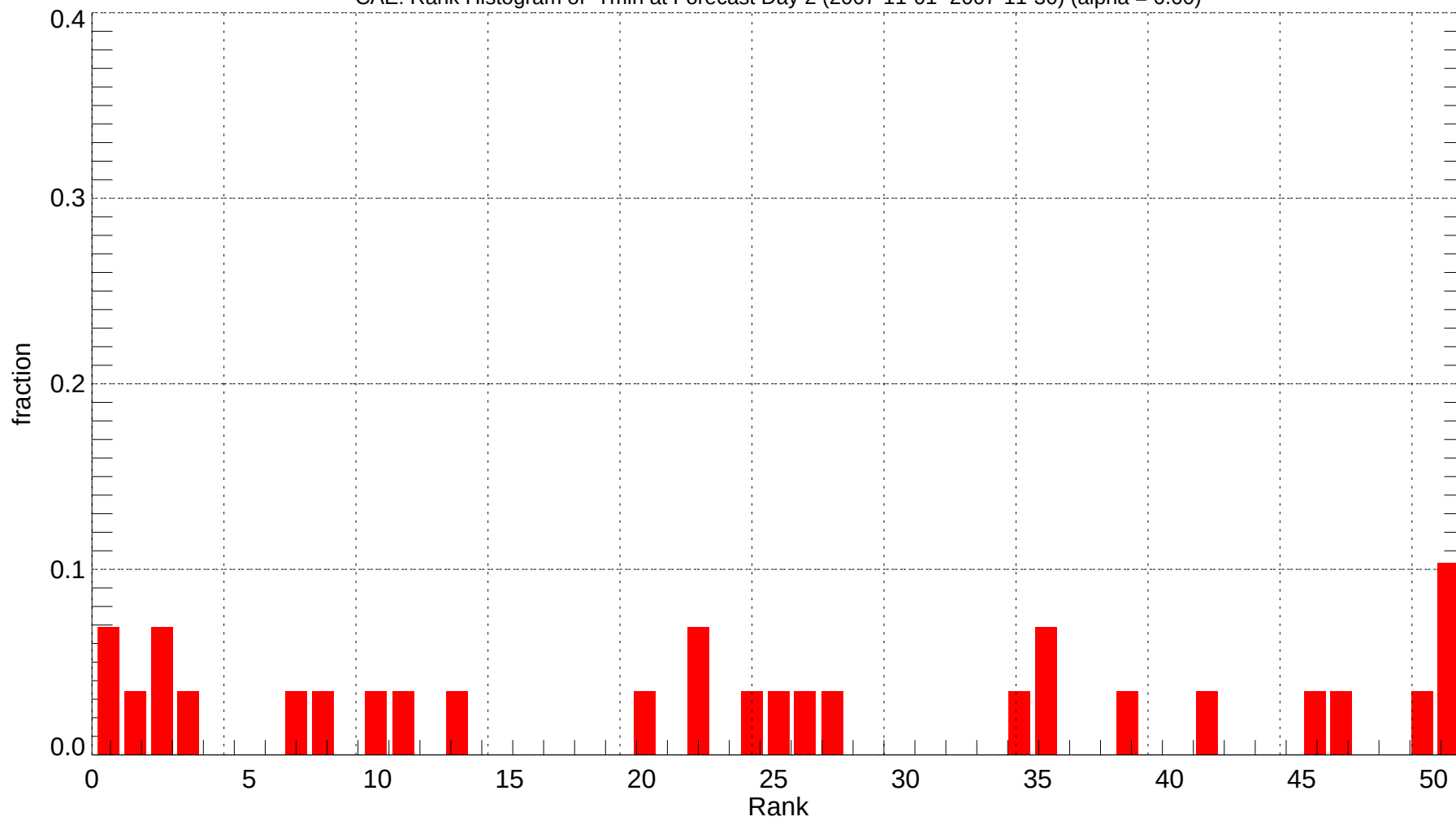
CAE: Rank Histogram of Tmin at Forecast Day 2 (2007-11-01~2007-11-30) (alpha = 0.00)
