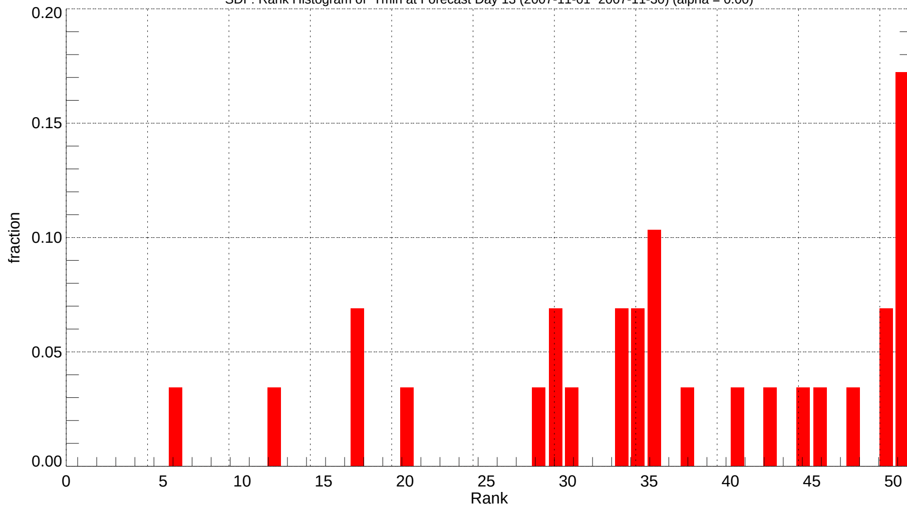
SDF: Rank Histogram of Tmin at Forecast Day 13 (2007-11-01~2007-11-30) (alpha = 0.00)
