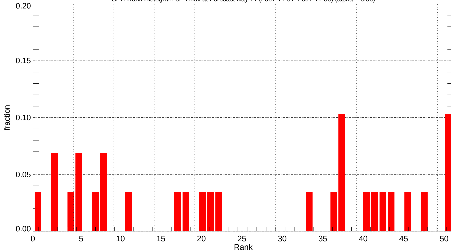
CLT: Rank Histogram of Tmax at Forecast Day 11 (2007-11-01~2007-11-30) (alpha = 0.00)
