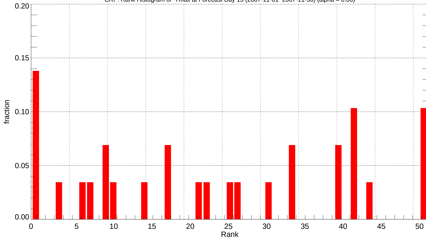
CRP: Rank Histogram of Tmax at Forecast Day 13 (2007-11-01~2007-11-30) (alpha = 0.00)
