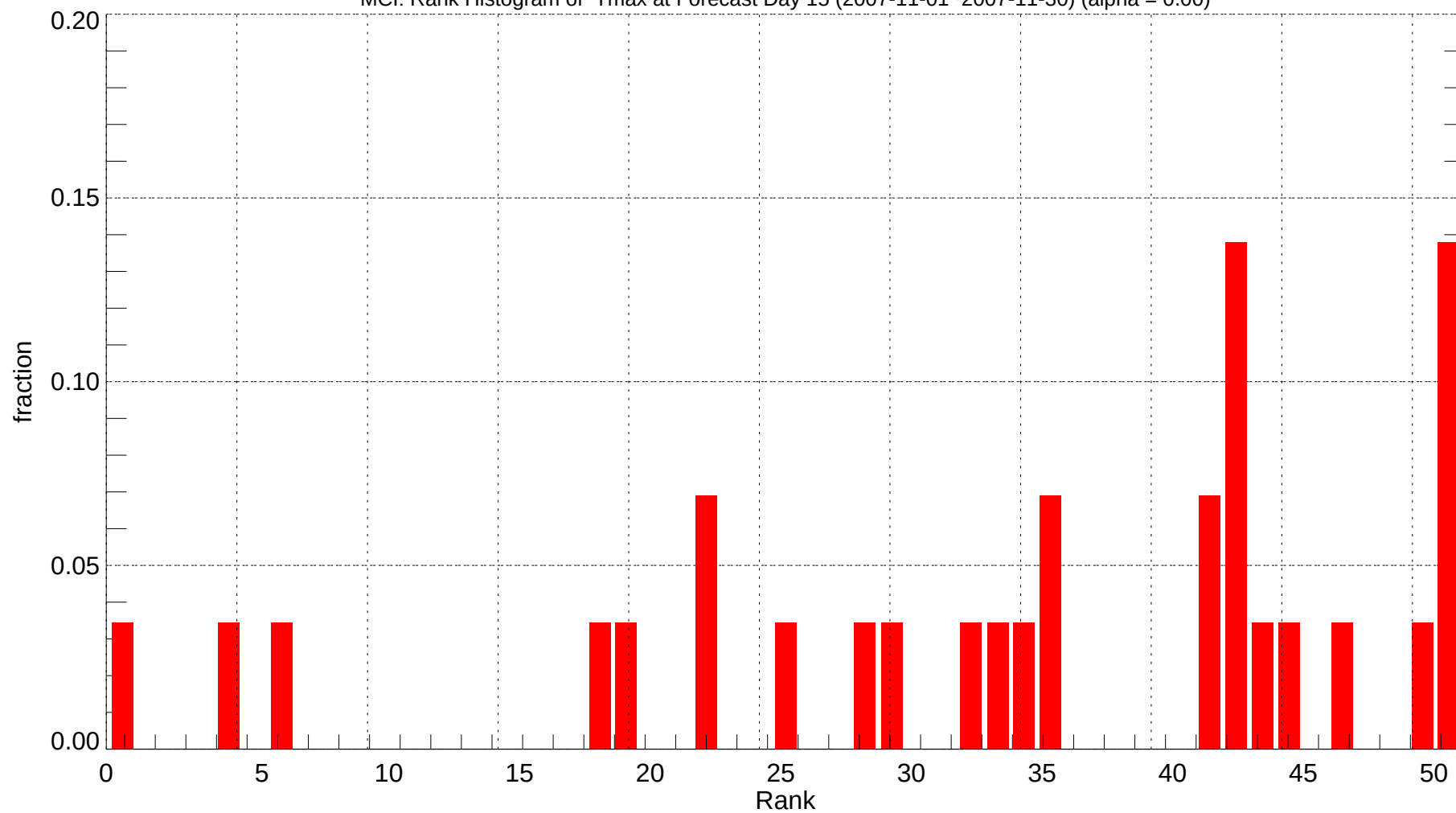
MCI: Rank Histogram of Tmax at Forecast Day 15 (2007-11-01~2007-11-30) (alpha = 0.00)
