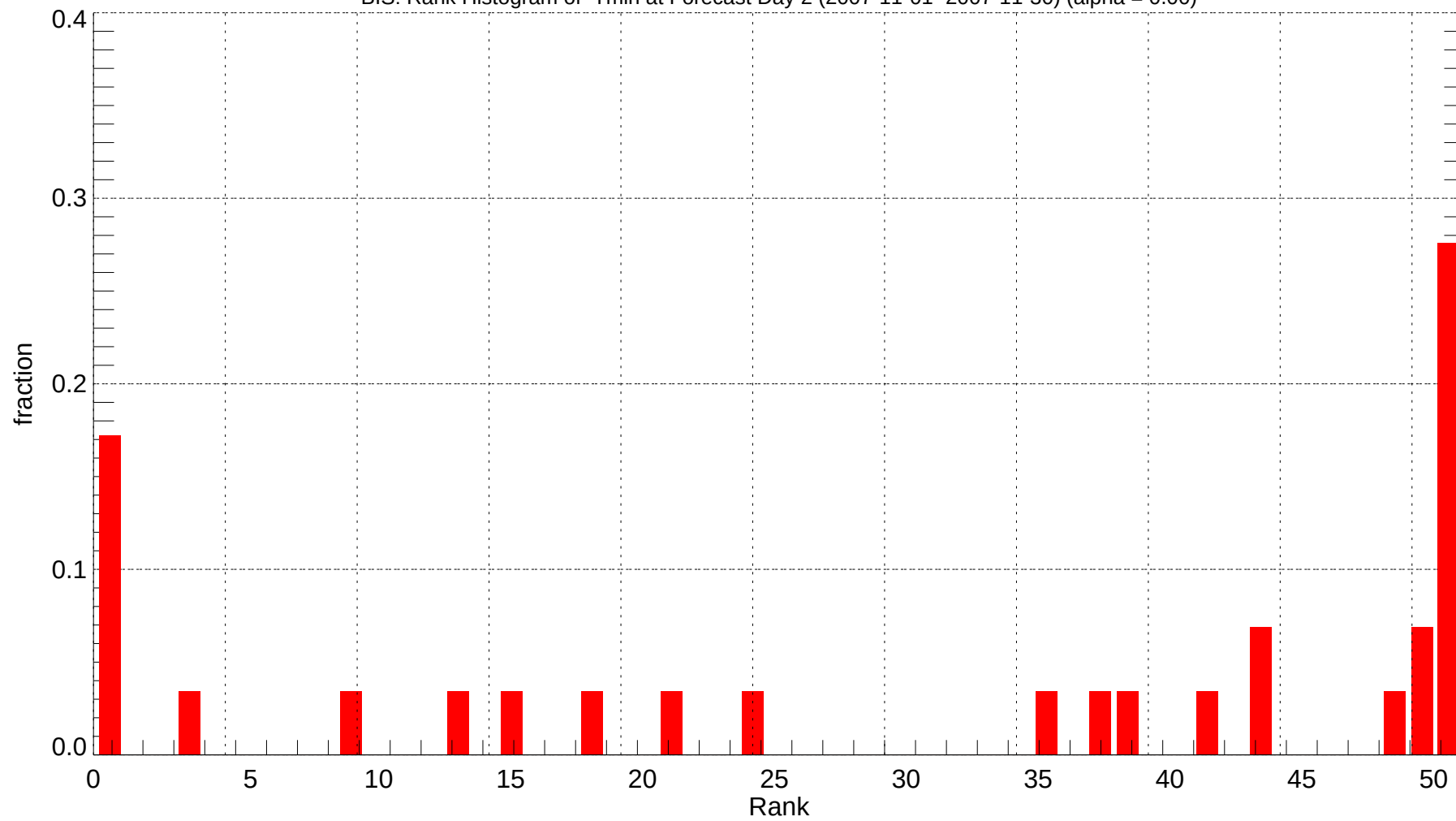
BIS: Rank Histogram of Tmin at Forecast Day 2 (2007-11-01~2007-11-30) (alpha = 0.00)
