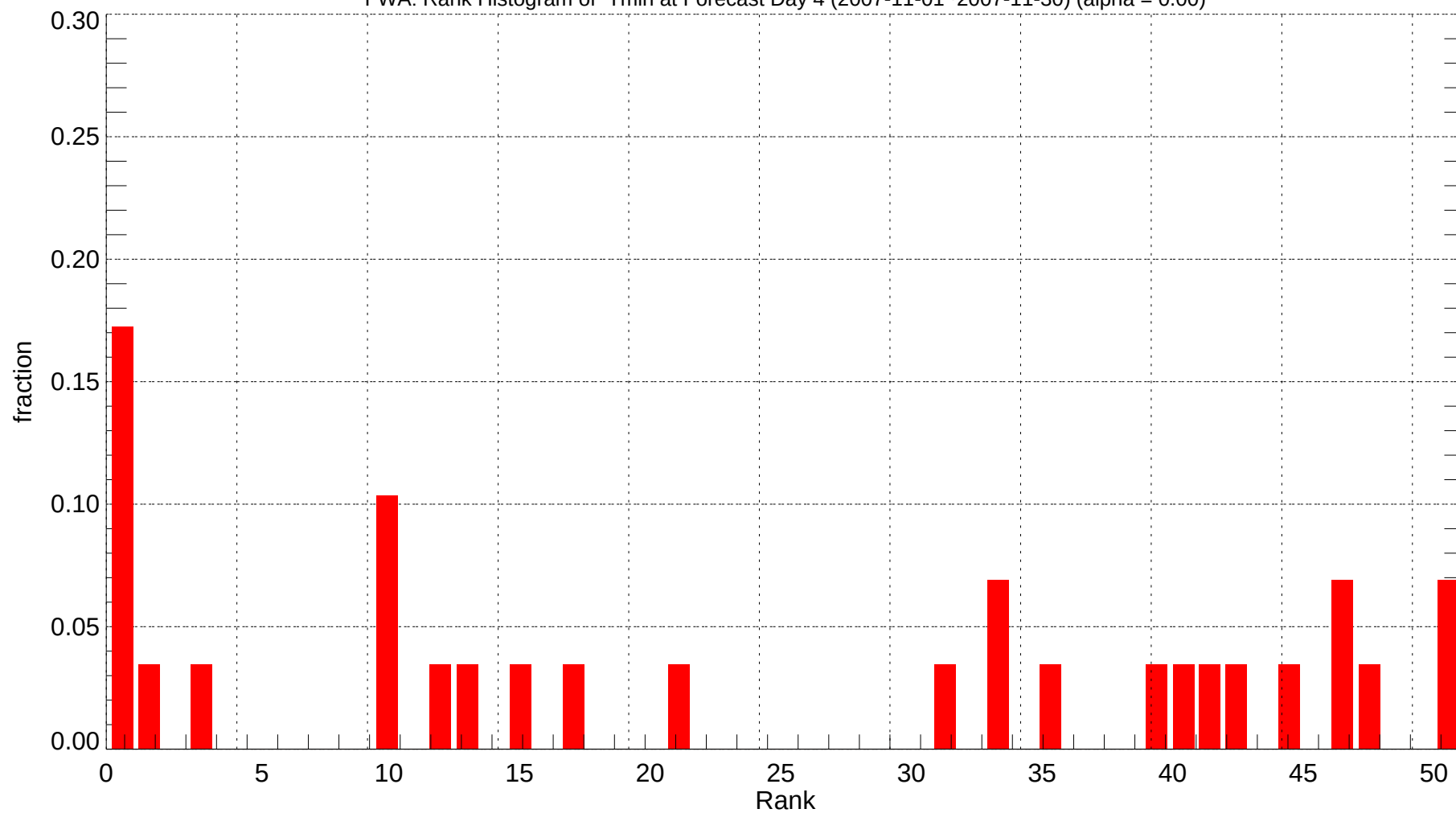
FWA: Rank Histogram of Tmin at Forecast Day 4 (2007-11-01~2007-11-30) (alpha = 0.00)
