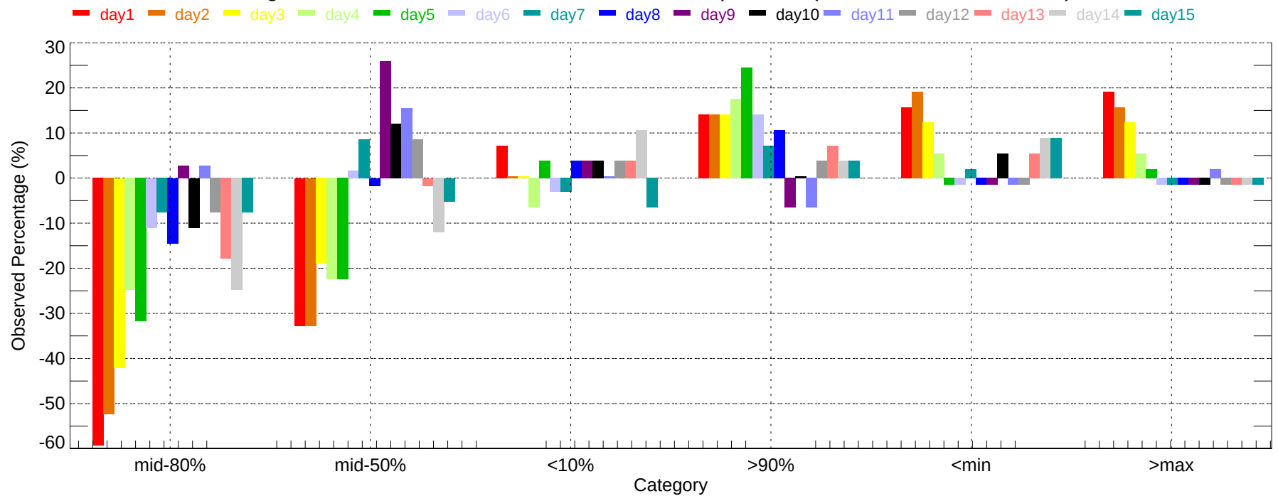
Observed Percentage Deviation of Ensembles - PWM: Max Temperature (2007-11-01~2007-11-30)
