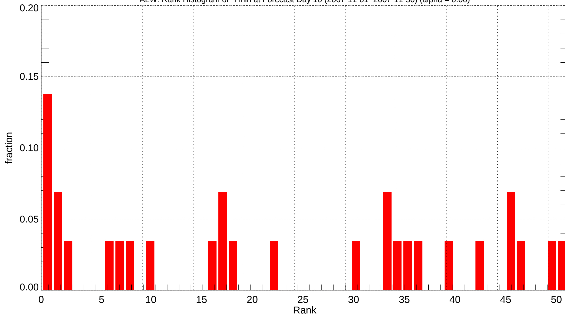
ALW: Rank Histogram of Tmin at Forecast Day 10 (2007-11-01~2007-11-30) (alpha = 0.00)
