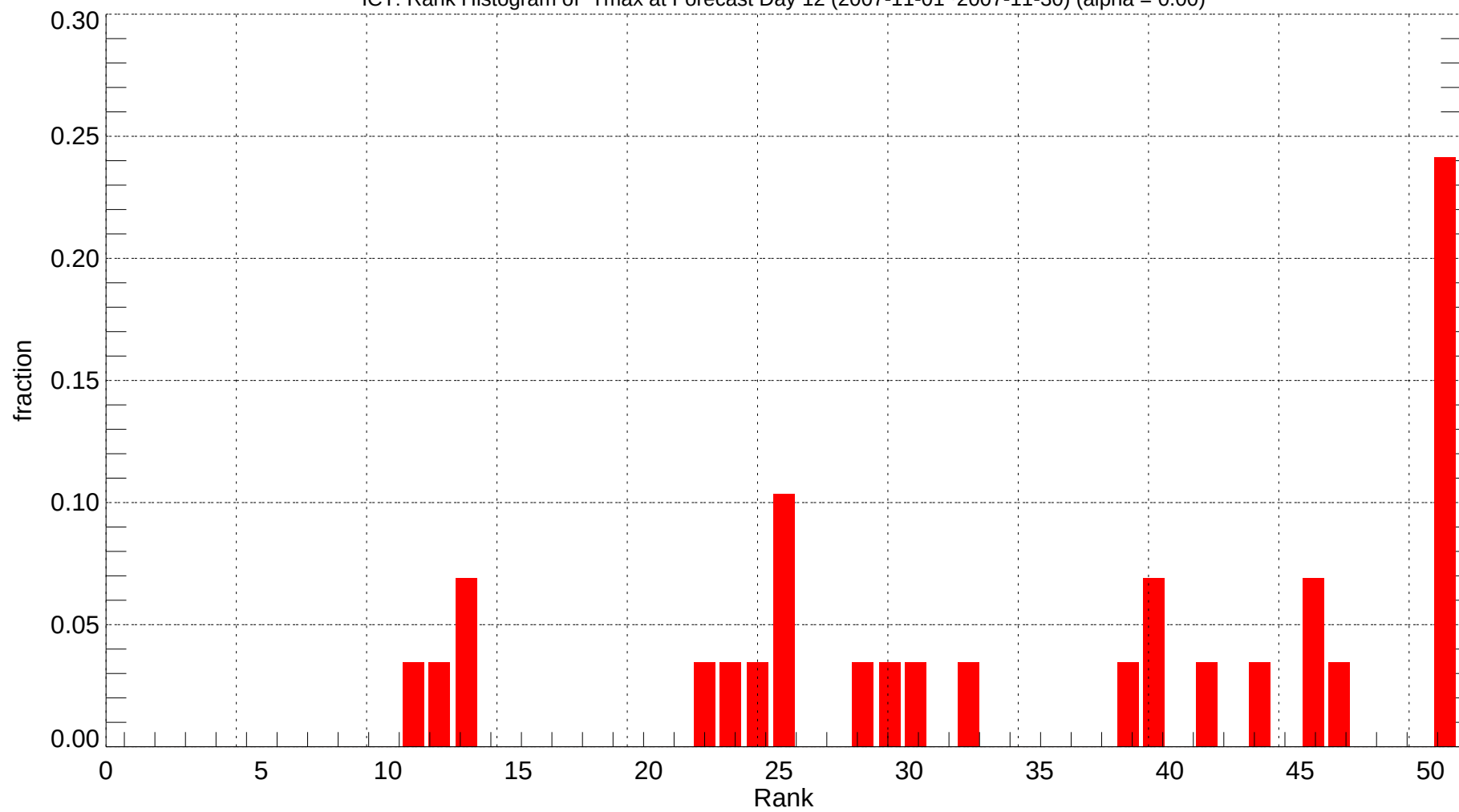
ICT: Rank Histogram of Tmax at Forecast Day 12 (2007-11-01~2007-11-30) (alpha = 0.00)
