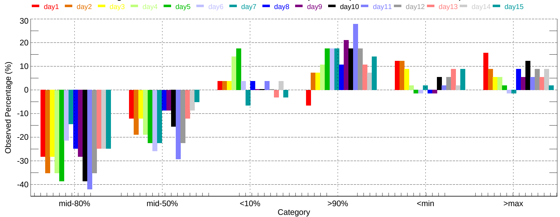
Observed Percentage Deviation of Ensembles - IAH: Max Temperature (2007-11-01~2007-11-30)
