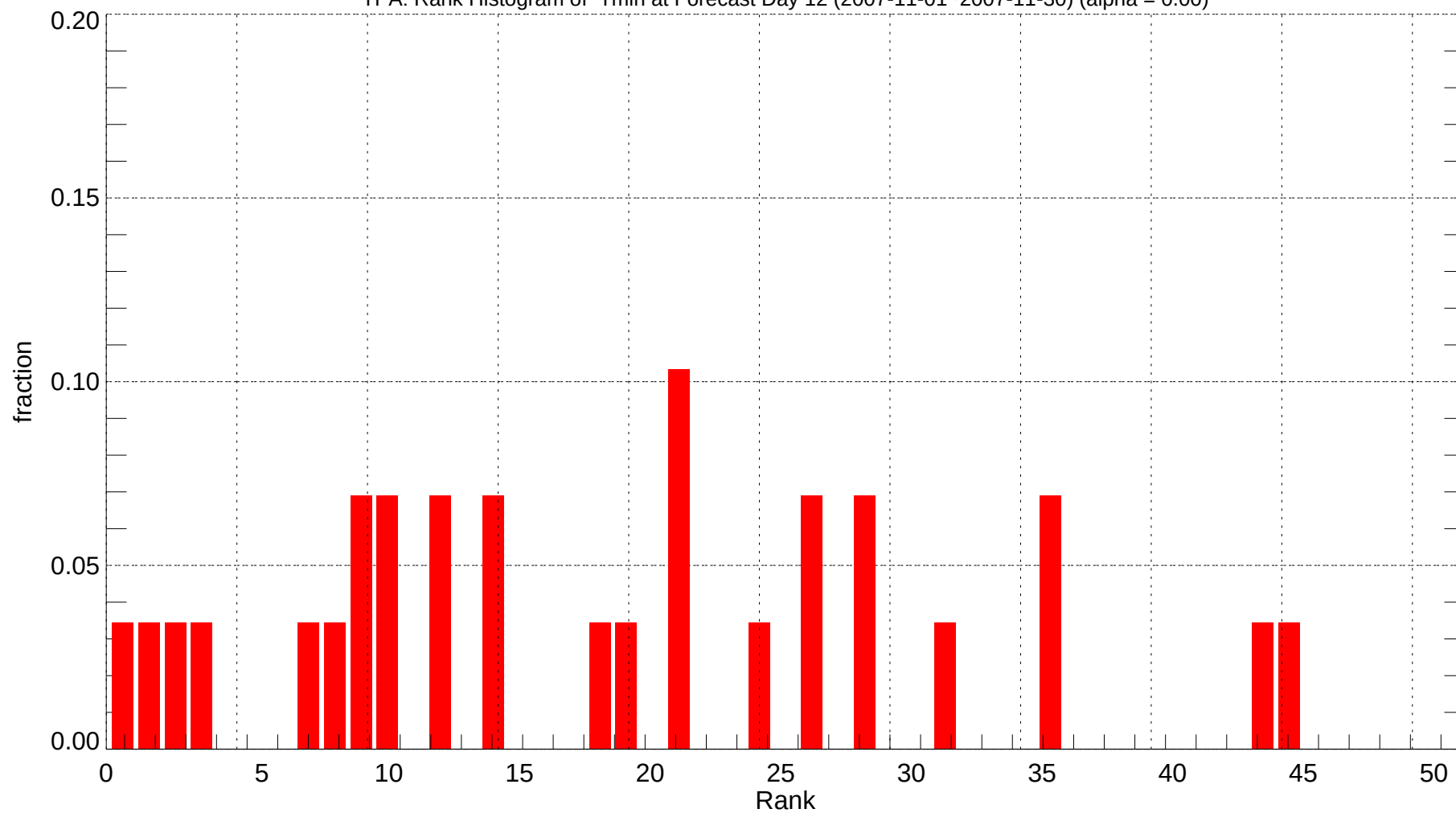
TPA: Rank Histogram of Tmin at Forecast Day 12 (2007-11-01~2007-11-30) (alpha = 0.00)
