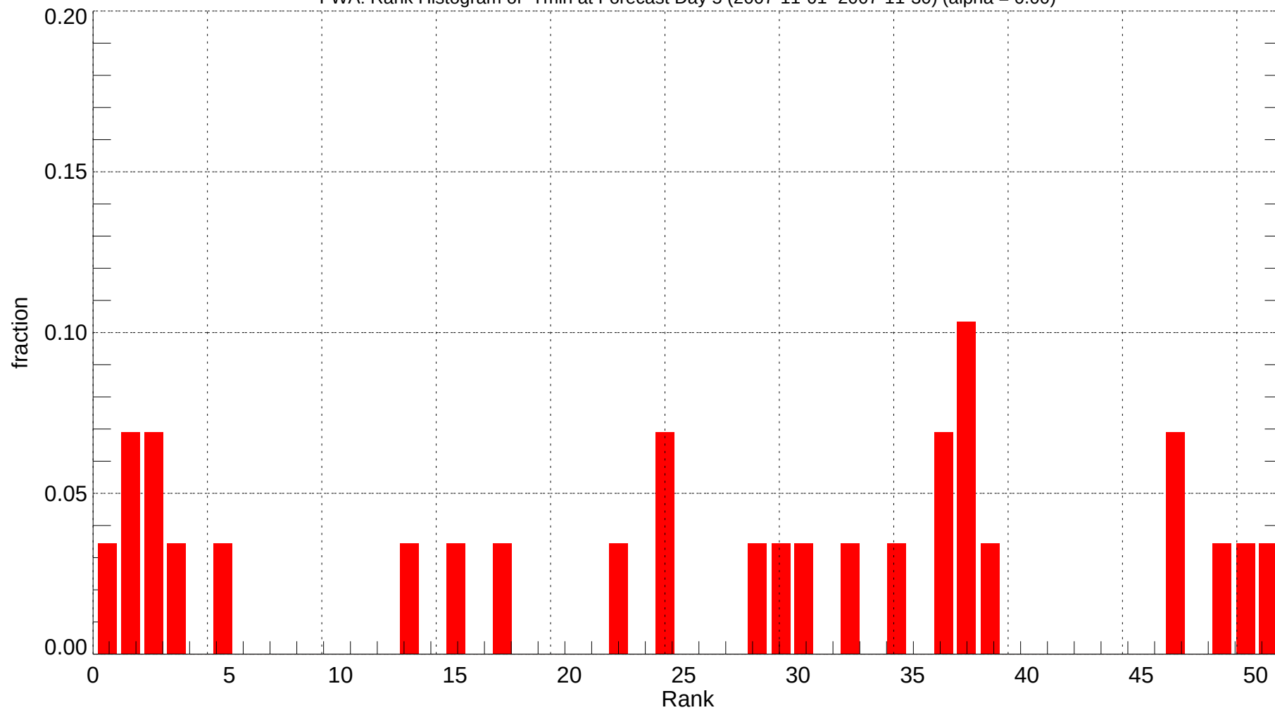
FWA: Rank Histogram of Tmin at Forecast Day 5 (2007-11-01~2007-11-30) (alpha = 0.00)
