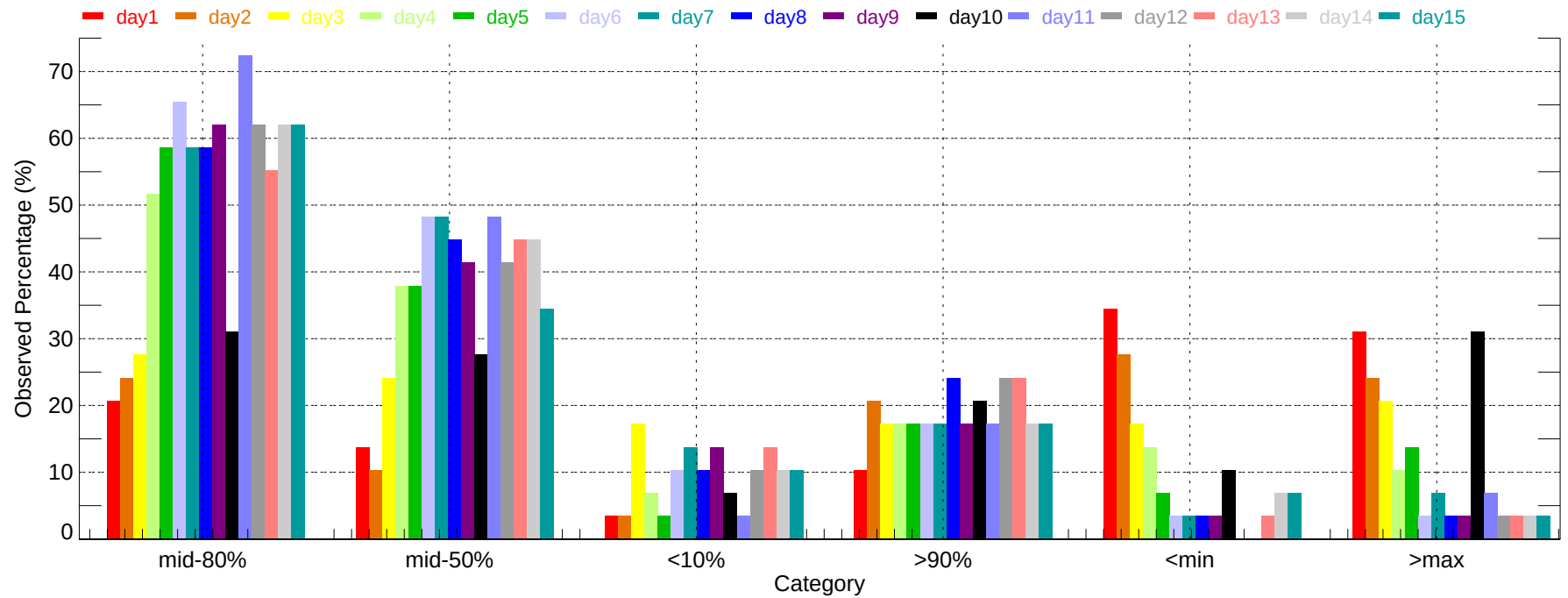
Observed Percentage of Ensembles - MDT: Max Temperature (2007-11-01~2007-11-30)
