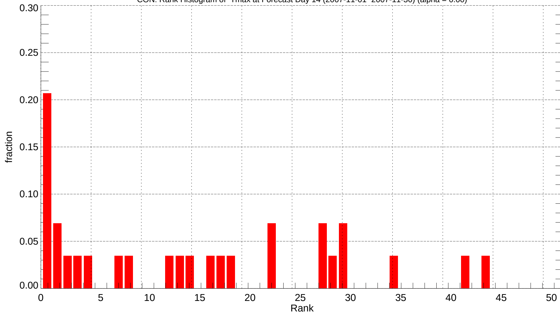
CON: Rank Histogram of Tmax at Forecast Day 14 (2007-11-01~2007-11-30) (alpha = 0.00)
