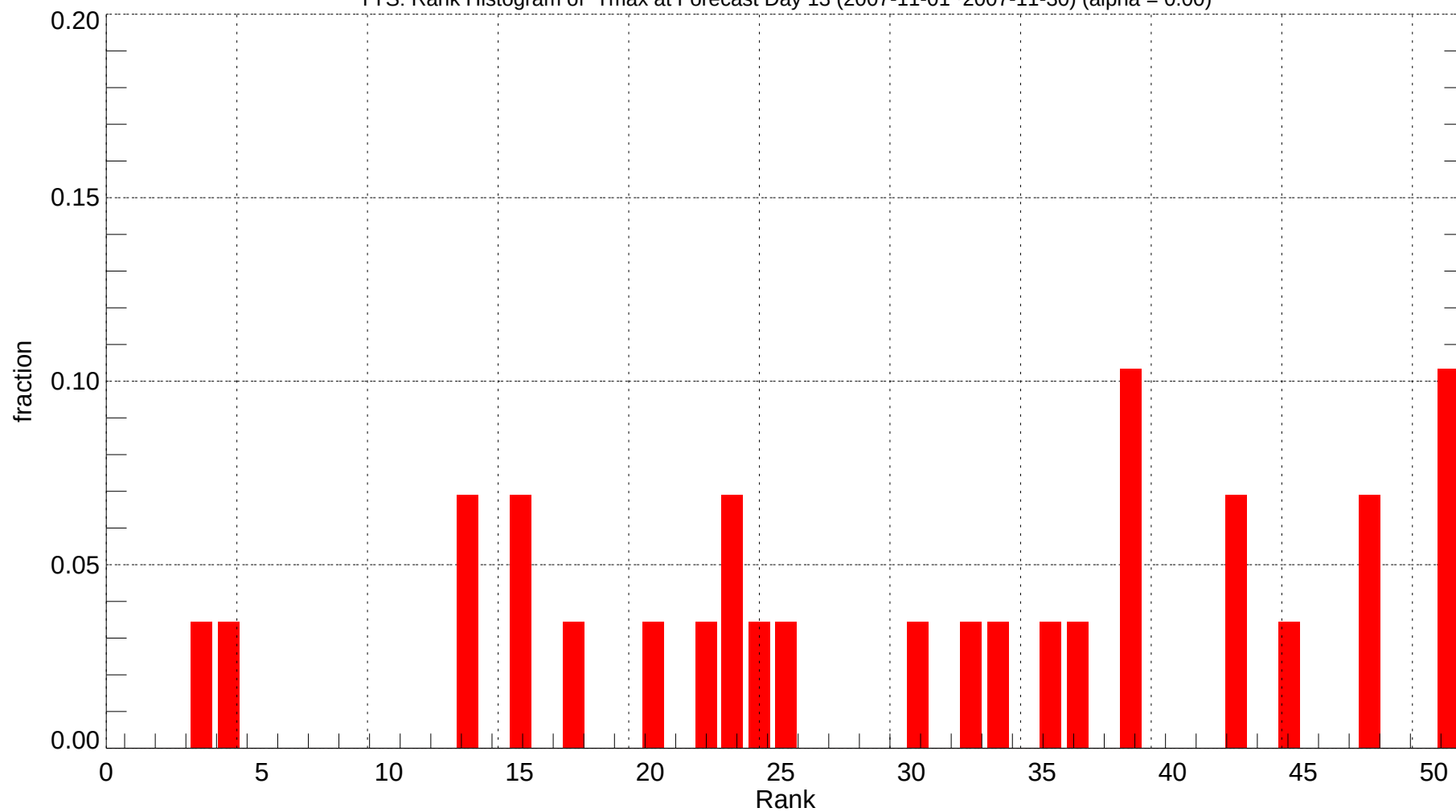
TYS: Rank Histogram of Tmax at Forecast Day 13 (2007-11-01~2007-11-30) (alpha = 0.00)
