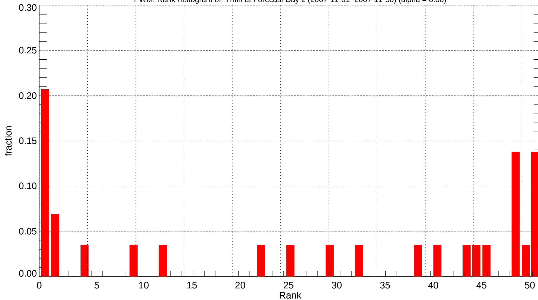
PWM: Rank Histogram of Tmin at Forecast Day 2 (2007-11-01~2007-11-30) (alpha = 0.00)
