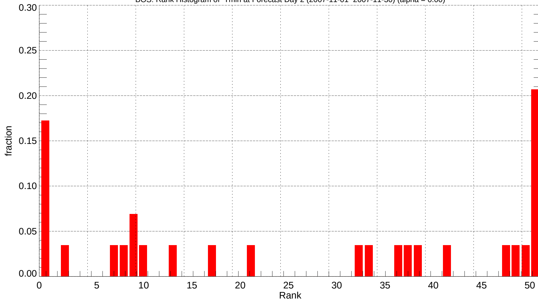
BOS: Rank Histogram of Tmin at Forecast Day 2 (2007-11-01~2007-11-30) (alpha = 0.00)
