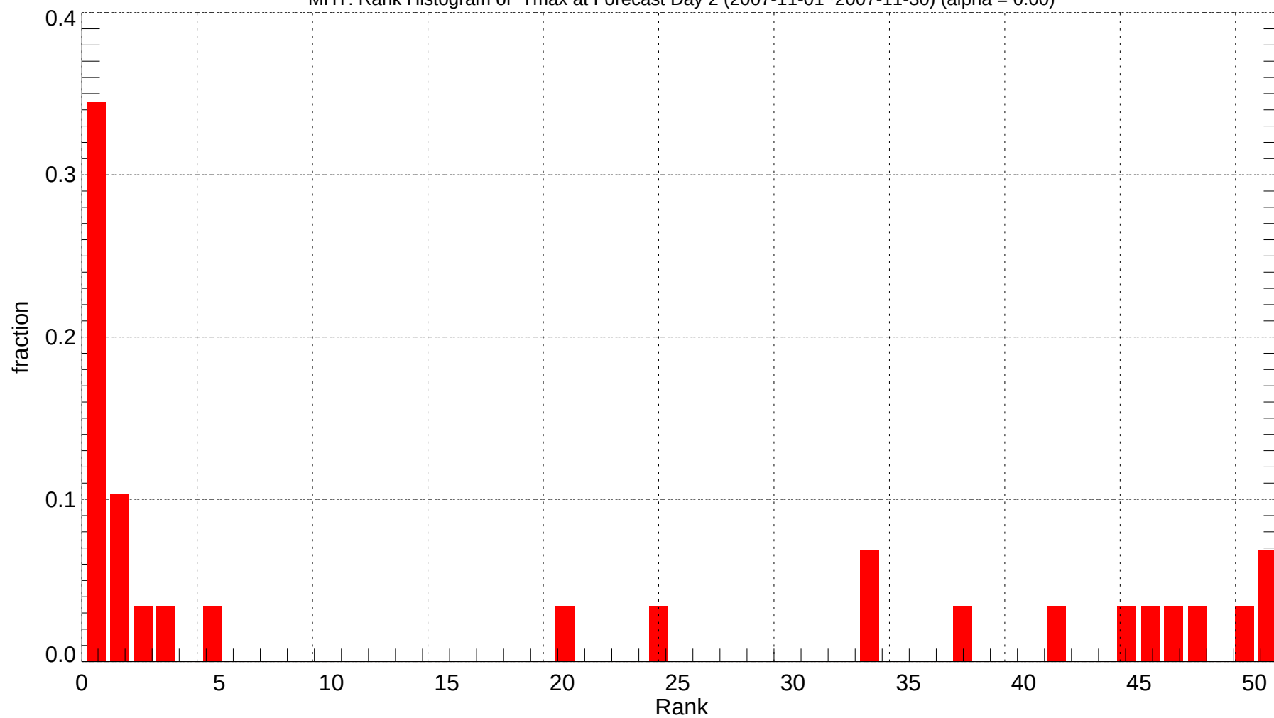
MHT: Rank Histogram of Tmax at Forecast Day 2 (2007-11-01~2007-11-30) (alpha = 0.00)
