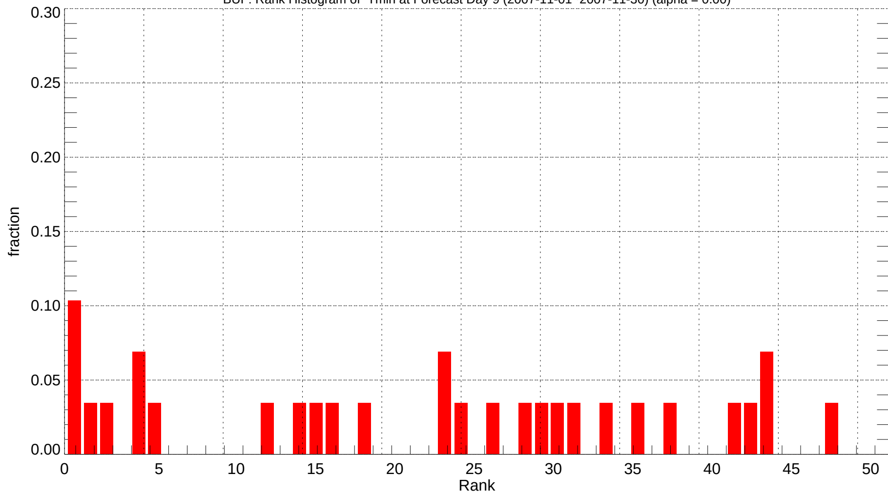
BUF: Rank Histogram of Tmin at Forecast Day 9 (2007-11-01~2007-11-30) (alpha = 0.00)
