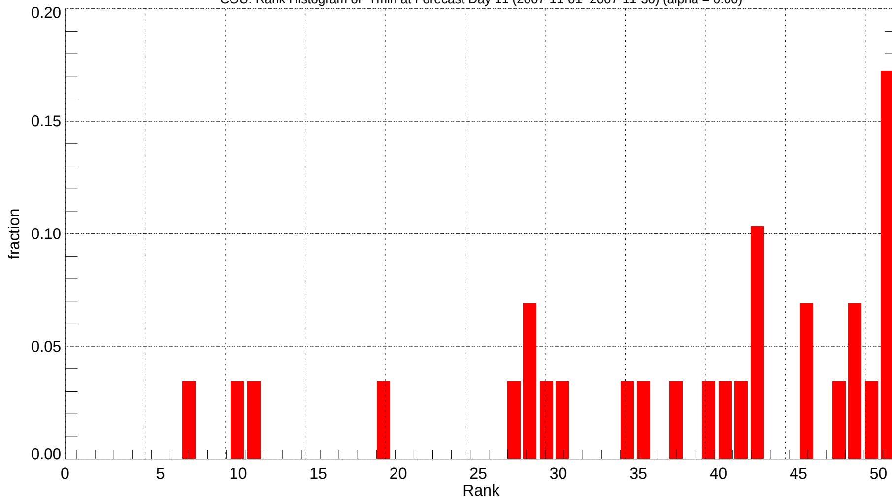
COU: Rank Histogram of Tmin at Forecast Day 11 (2007-11-01~2007-11-30) (alpha = 0.00)
