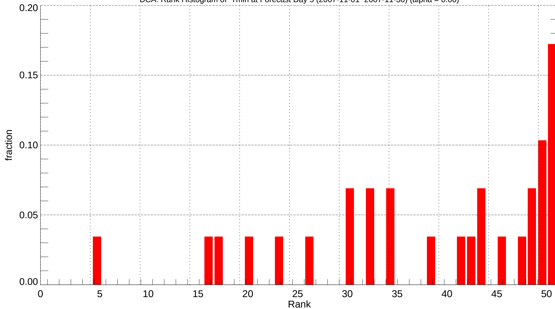
DCA: Rank Histogram of Tmin at Forecast Day 5 (2007-11-01~2007-11-30) (alpha = 0.00)
