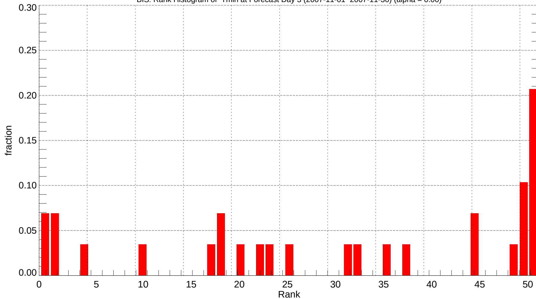
BIS: Rank Histogram of Tmin at Forecast Day 3 (2007-11-01~2007-11-30) (alpha = 0.00)
