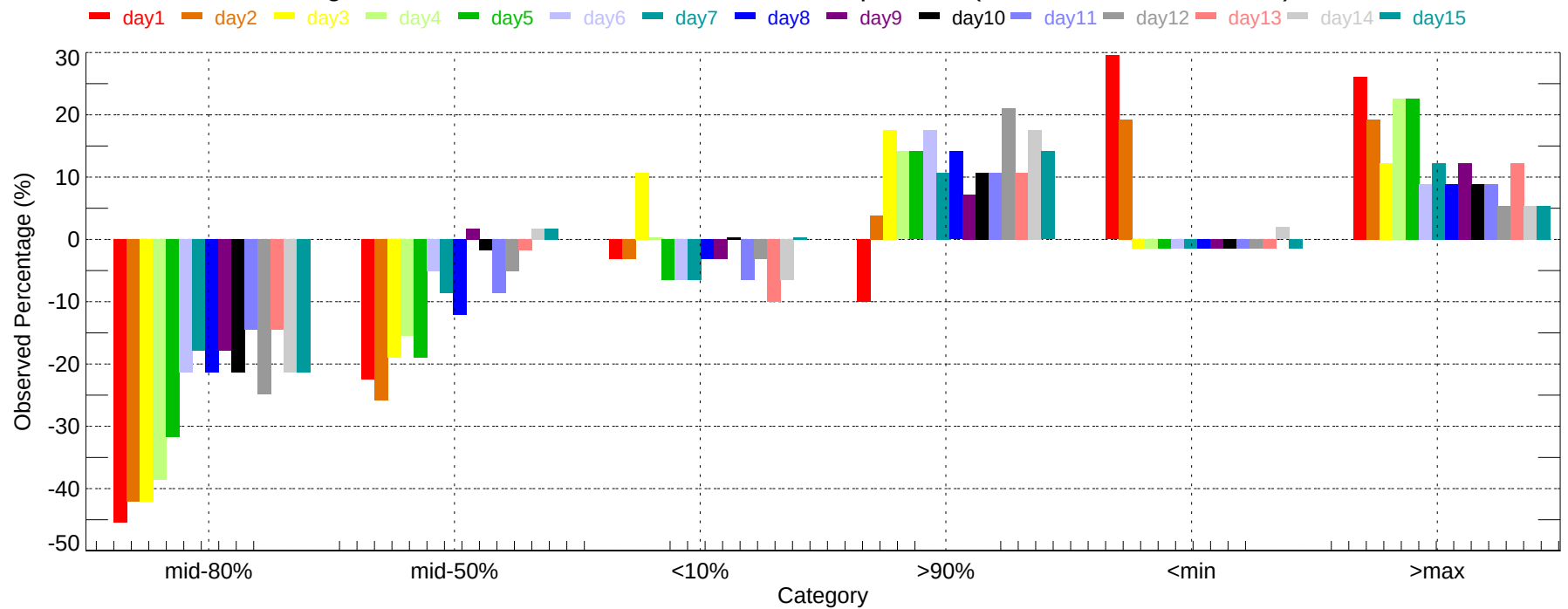
Observed Percentage Deviation of Ensembles - BWI: Min Temperature (2007-11-01~2007-11-30)
