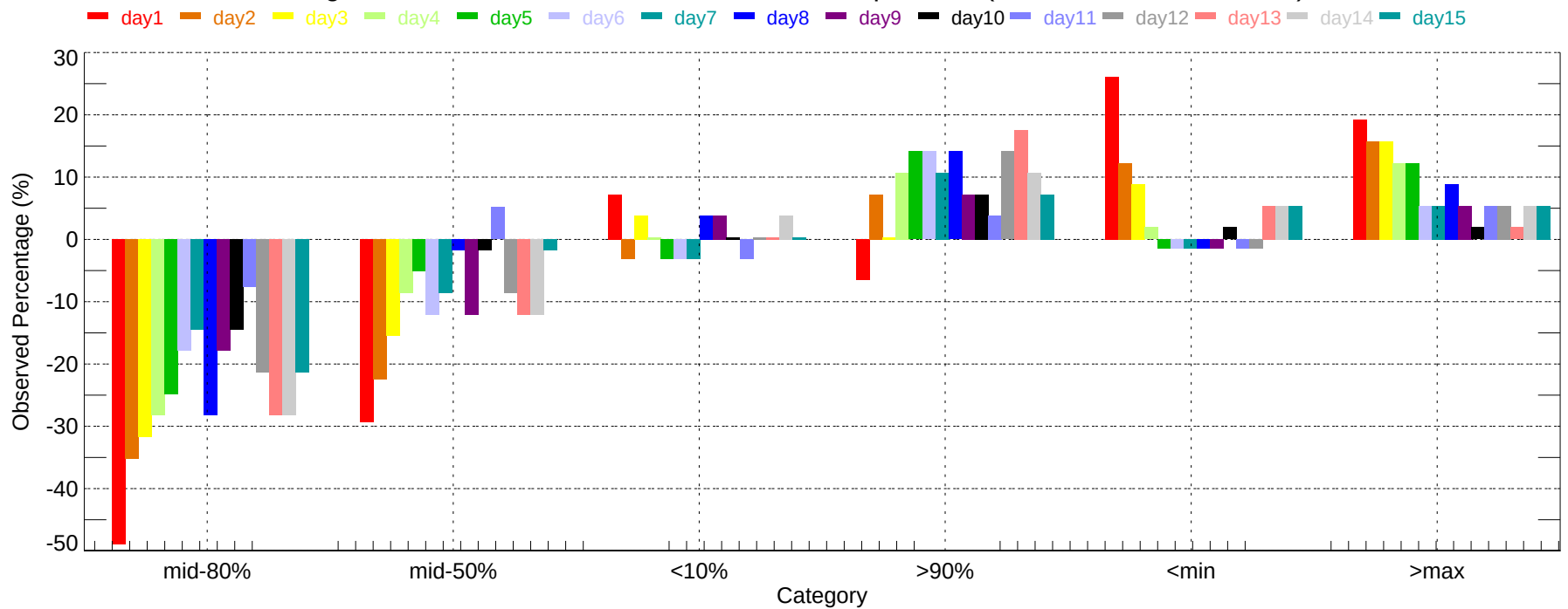
Observed Percentage Deviation of Ensembles - BOS: Max Temperature (2007-11-01~2007-11-30)
