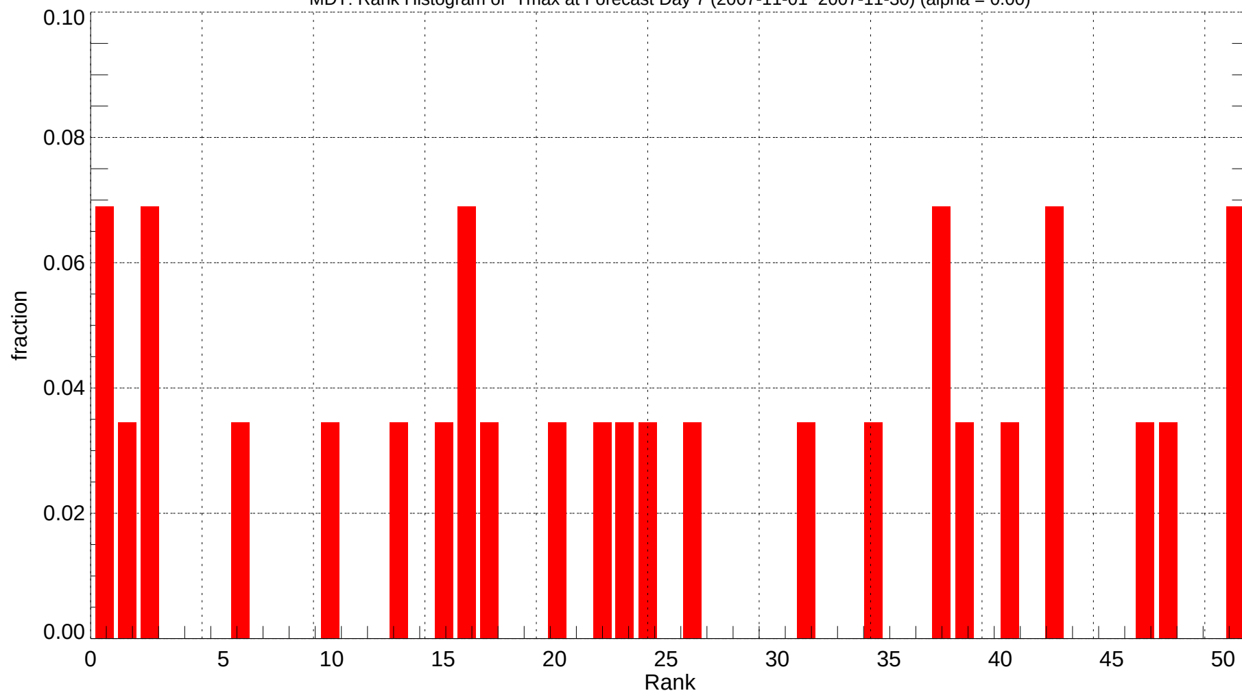
MDT: Rank Histogram of Tmax at Forecast Day 7 (2007-11-01~2007-11-30) (alpha = 0.00)
