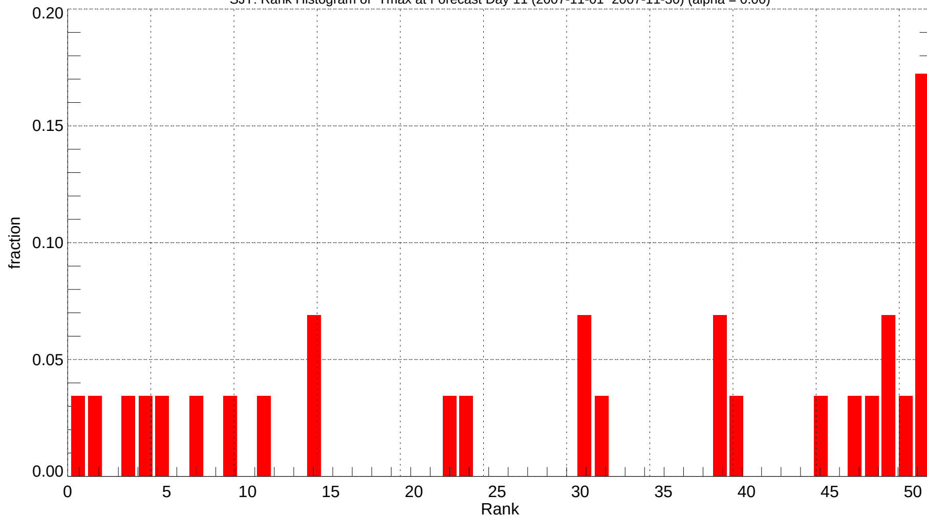
SJT: Rank Histogram of Tmax at Forecast Day 11 (2007-11-01~2007-11-30) (alpha = 0.00)
