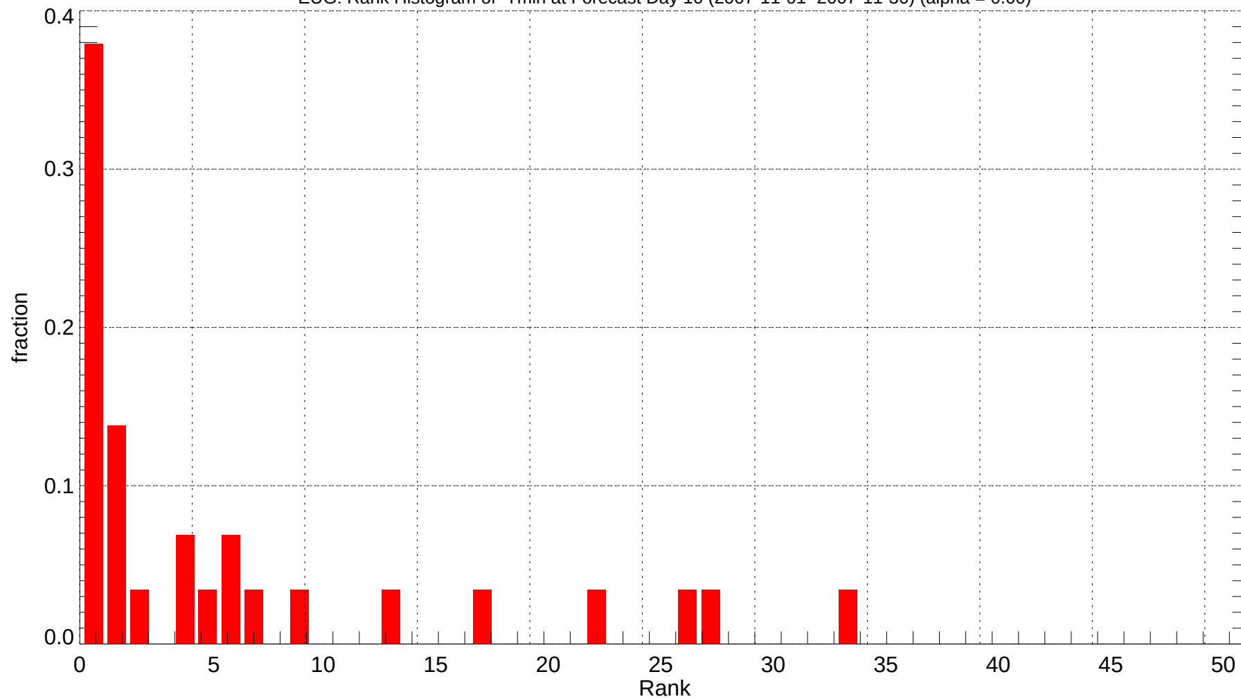
EUG: Rank Histogram of Tmin at Forecast Day 10 (2007-11-01~2007-11-30) (alpha = 0.00)
