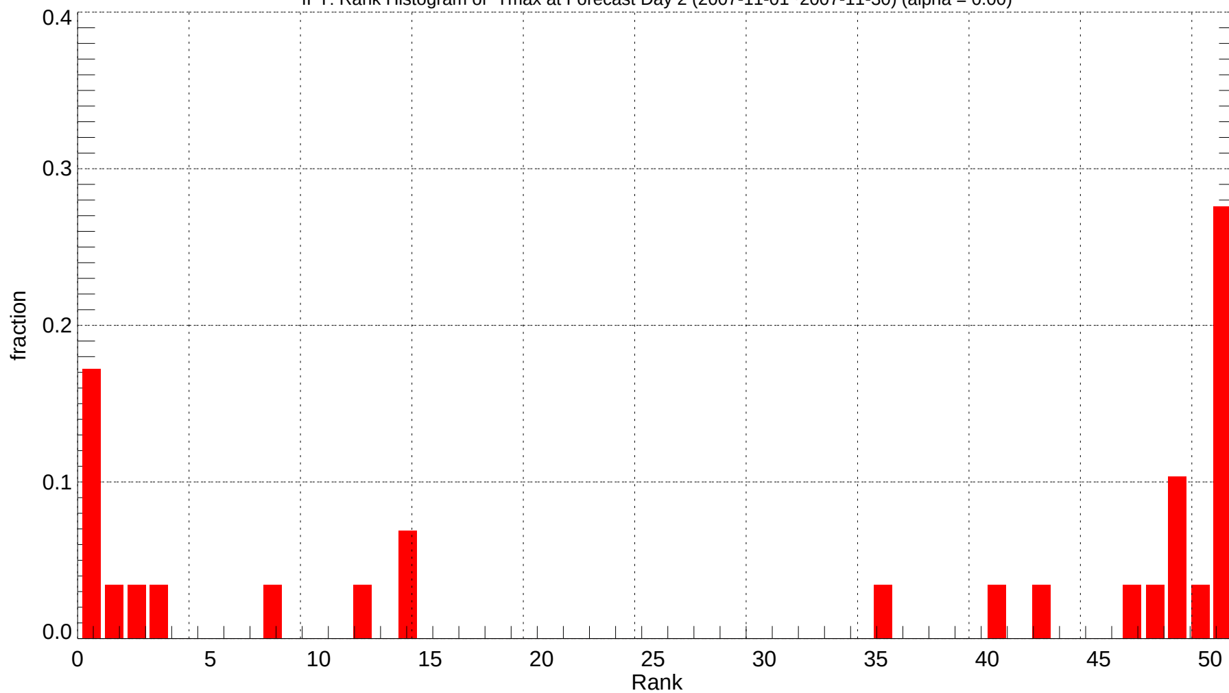
IPT: Rank Histogram of Tmax at Forecast Day 2 (2007-11-01~2007-11-30) (alpha = 0.00)
