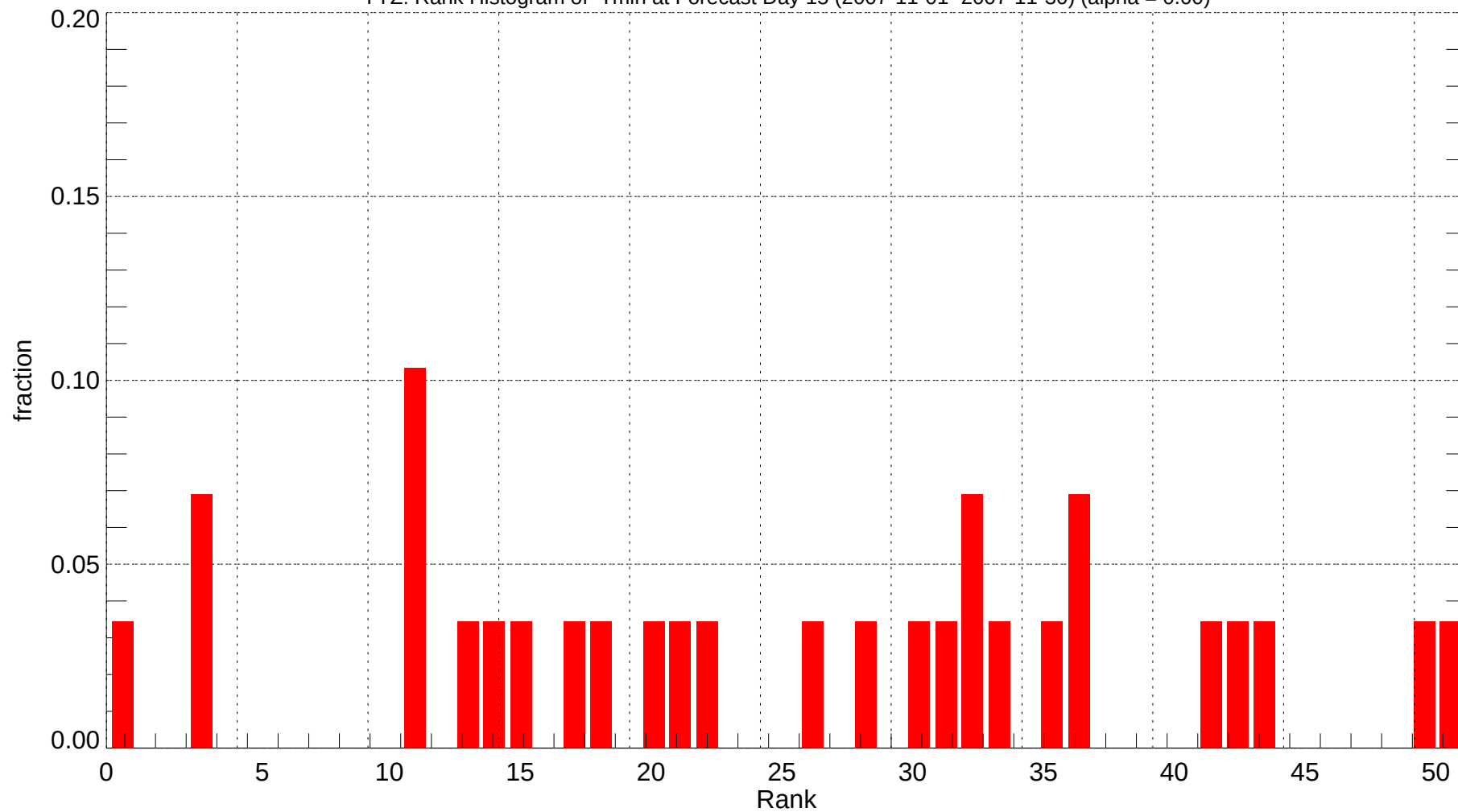
YYZ: Rank Histogram of Tmin at Forecast Day 15 (2007-11-01~2007-11-30) (alpha = 0.00)
