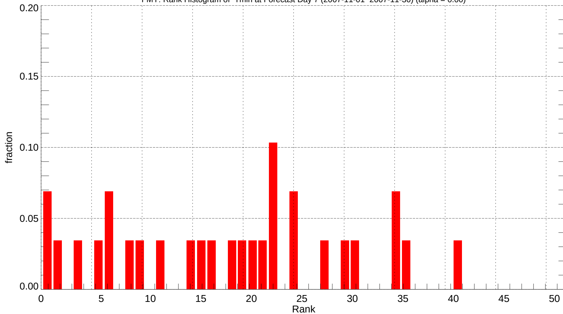
FMY: Rank Histogram of Tmin at Forecast Day 7 (2007-11-01~2007-11-30) (alpha = 0.00)
