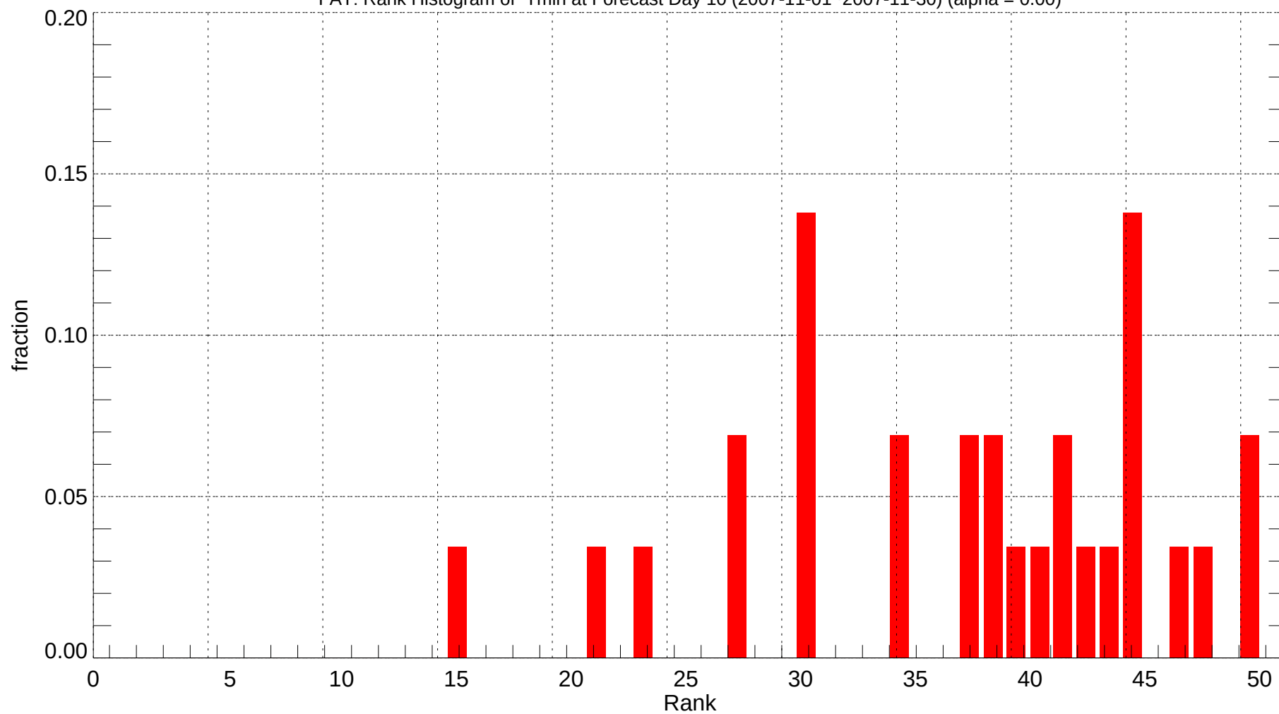
FAT: Rank Histogram of Tmin at Forecast Day 10 (2007-11-01~2007-11-30) (alpha = 0.00)
