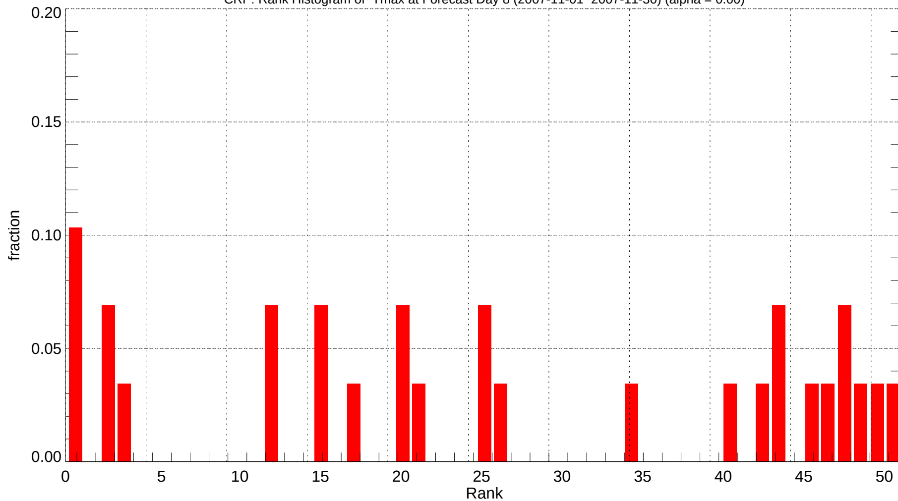
CRP: Rank Histogram of Tmax at Forecast Day 8 (2007-11-01~2007-11-30) (alpha = 0.00)
