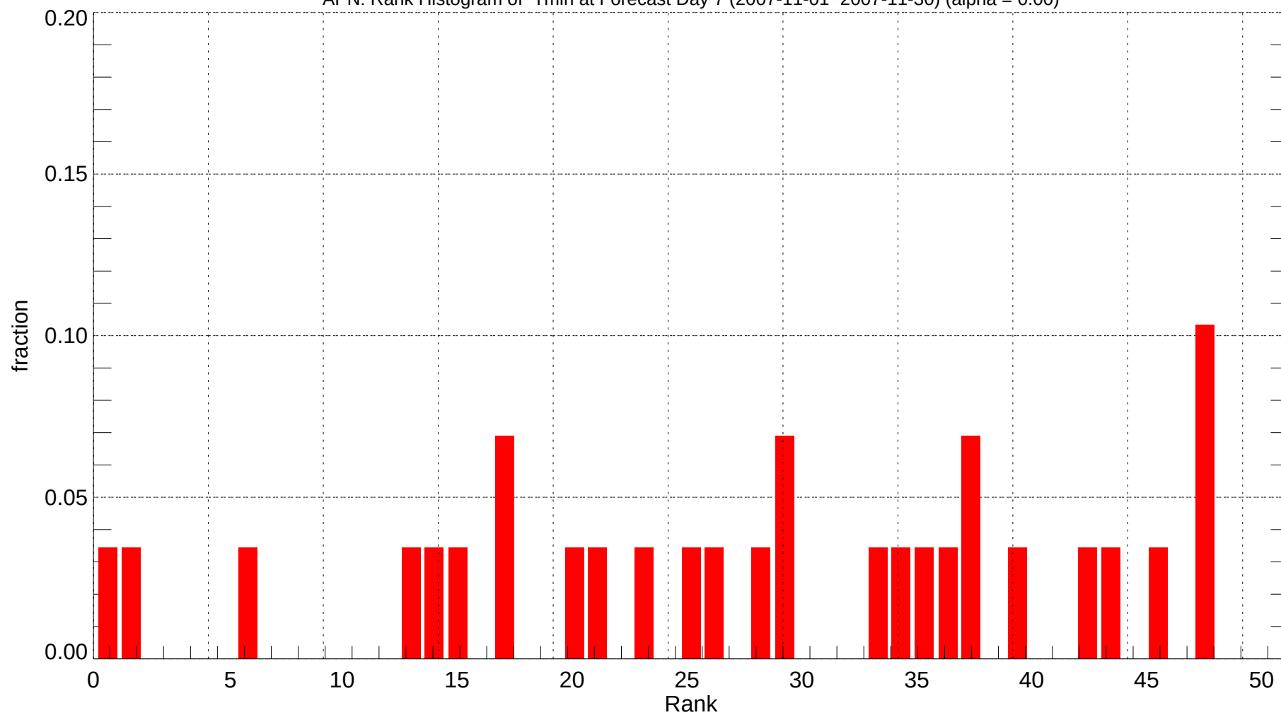
APN: Rank Histogram of Tmin at Forecast Day 7 (2007-11-01~2007-11-30) (alpha = 0.00)
