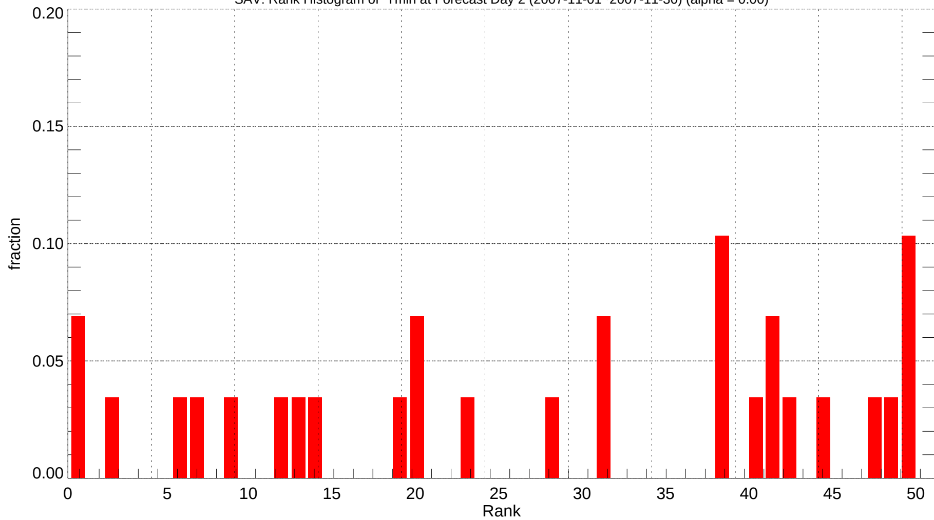
SAV: Rank Histogram of Tmin at Forecast Day 2 (2007-11-01~2007-11-30) (alpha = 0.00)
