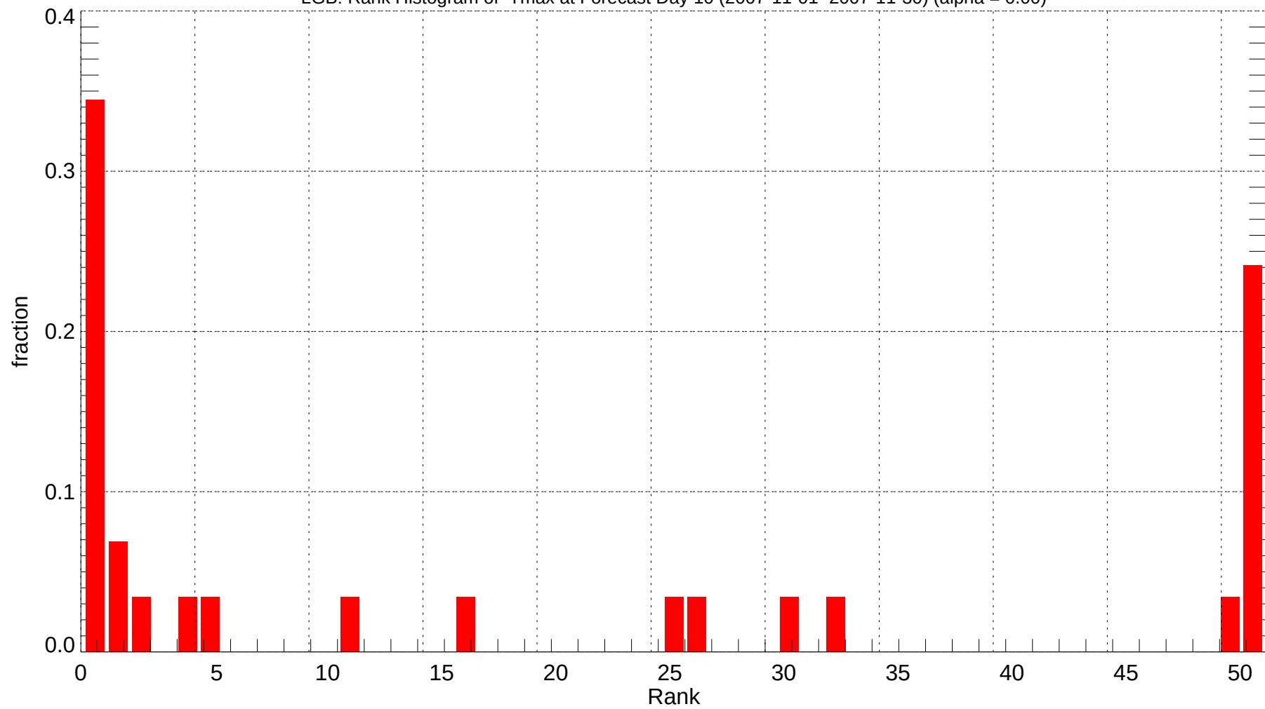
LGB: Rank Histogram of Tmax at Forecast Day 10 (2007-11-01~2007-11-30) (alpha = 0.00)
