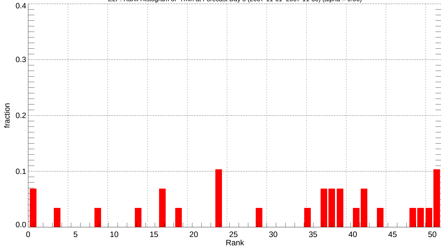
ELP: Rank Histogram of Tmin at Forecast Day 5 (2007-11-01~2007-11-30) (alpha = 0.00)
