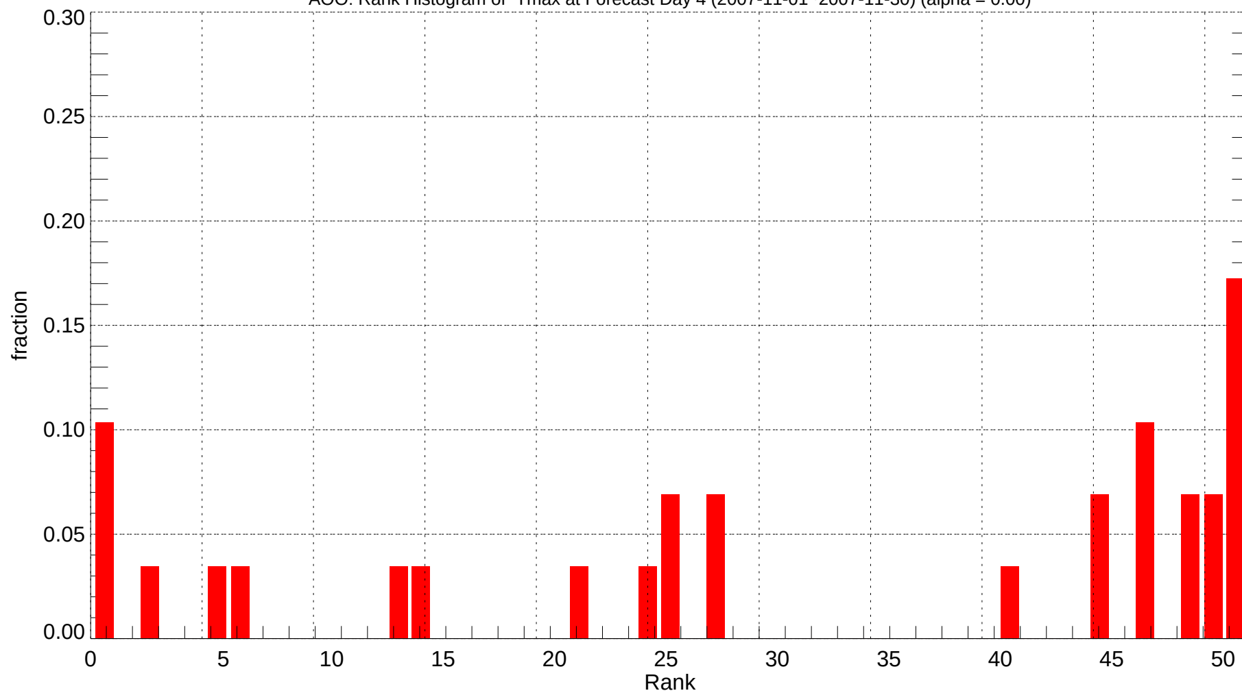
AOO: Rank Histogram of Tmax at Forecast Day 4 (2007-11-01~2007-11-30) (alpha = 0.00)
