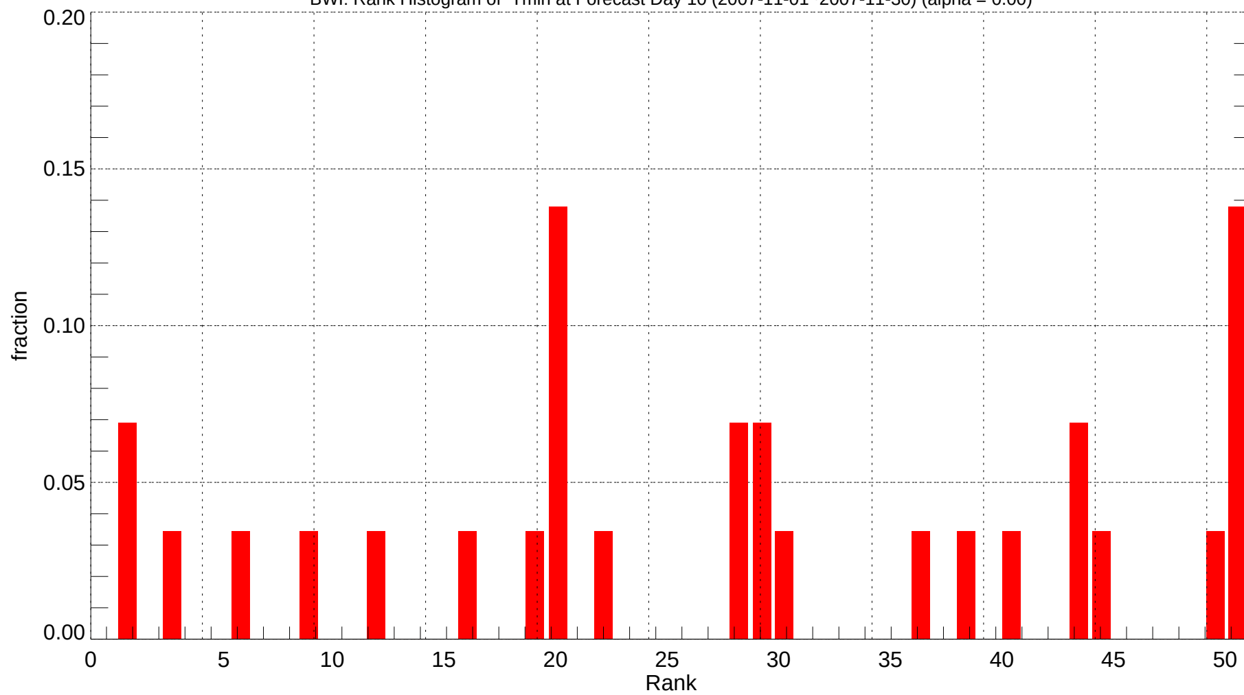
BWI: Rank Histogram of Tmin at Forecast Day 10 (2007-11-01~2007-11-30) (alpha = 0.00)
