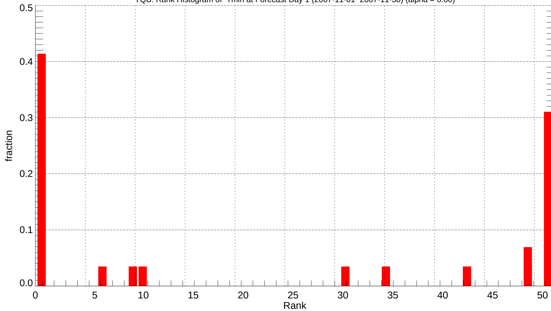
YQB: Rank Histogram of Tmin at Forecast Day 1 (2007-11-01~2007-11-30) (alpha = 0.00)
