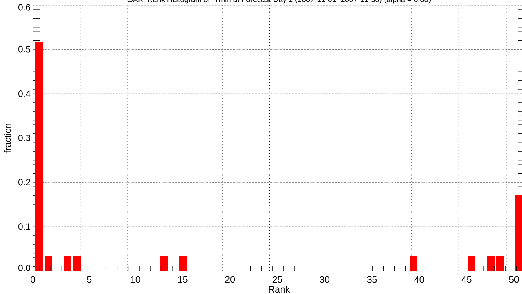
OAK: Rank Histogram of Tmin at Forecast Day 2 (2007-11-01~2007-11-30) (alpha = 0.00)
