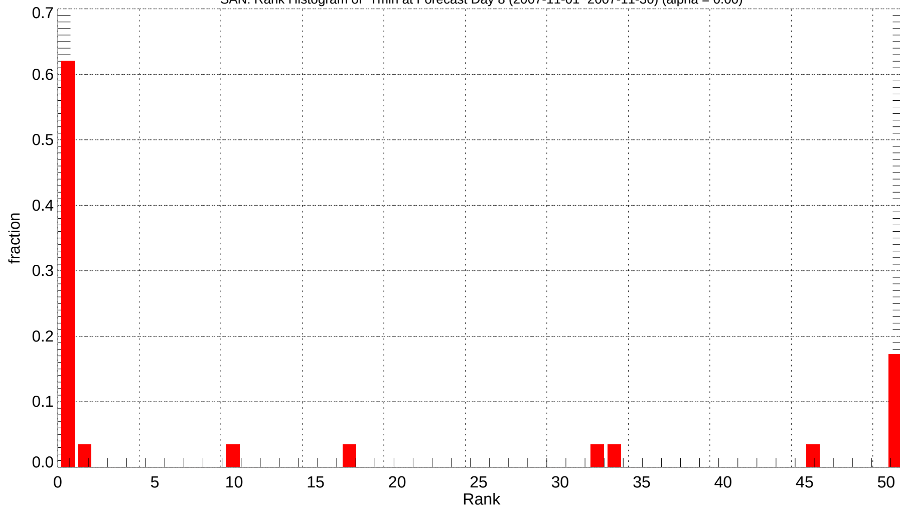
SAN: Rank Histogram of Tmin at Forecast Day 8 (2007-11-01~2007-11-30) (alpha = 0.00)
