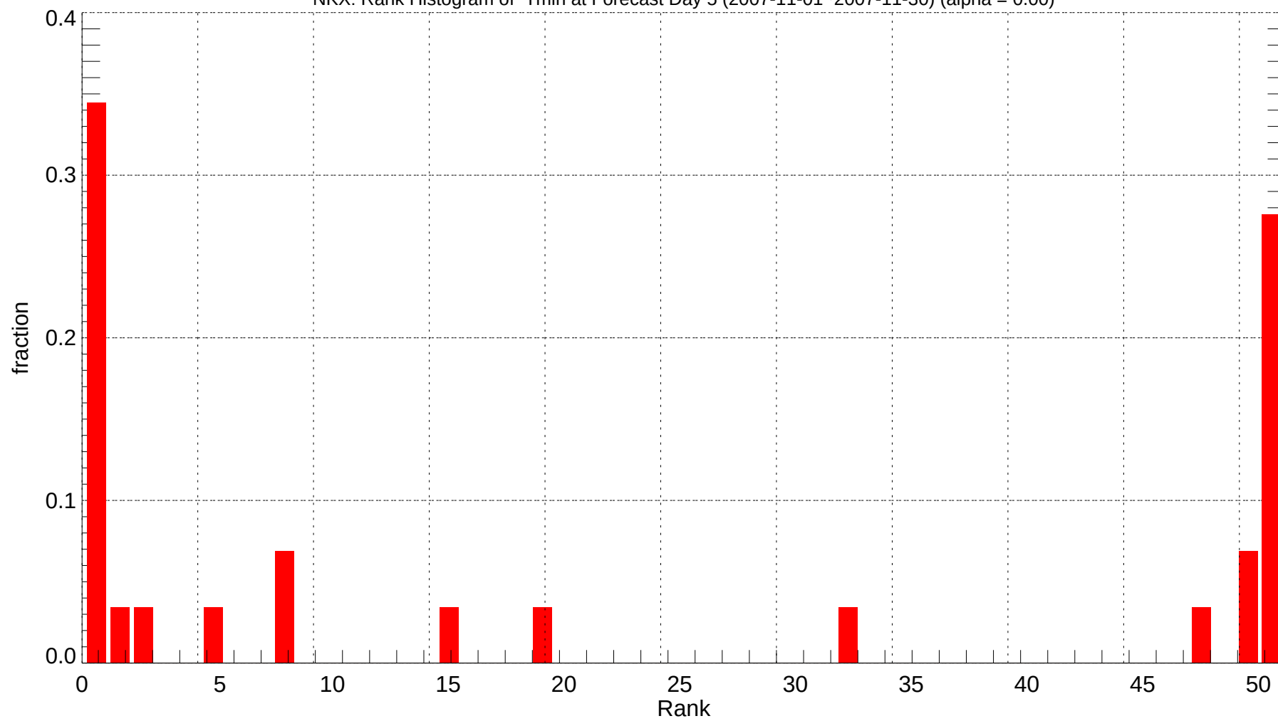
NKX: Rank Histogram of Tmin at Forecast Day 5 (2007-11-01~2007-11-30) (alpha = 0.00)
