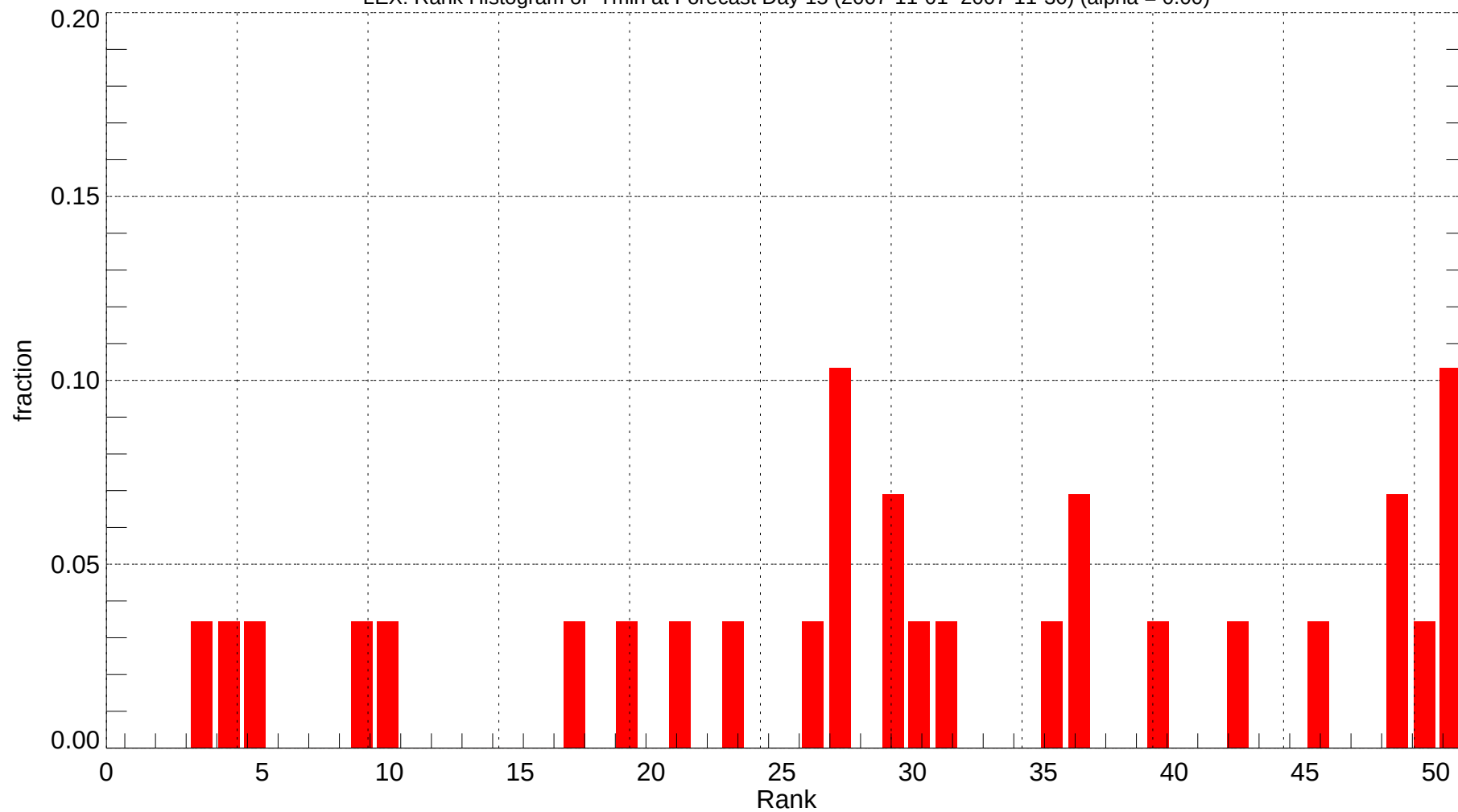
LEX: Rank Histogram of Tmin at Forecast Day 15 (2007-11-01~2007-11-30) (alpha = 0.00)
