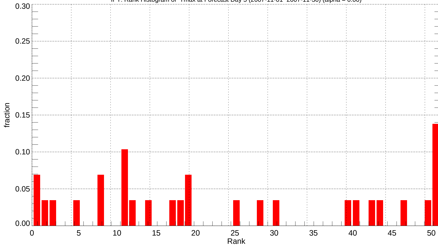
IPT: Rank Histogram of Tmax at Forecast Day 5 (2007-11-01~2007-11-30) (alpha = 0.00)
