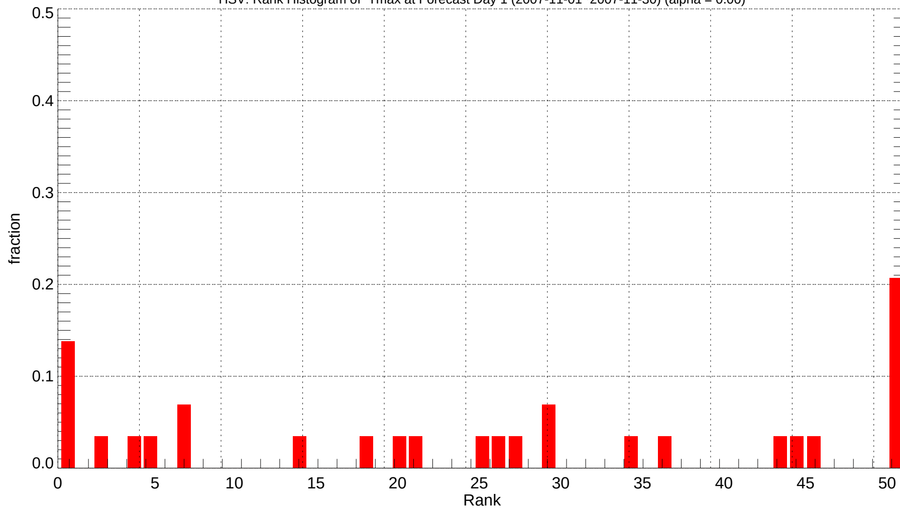
HSV: Rank Histogram of Tmax at Forecast Day 1 (2007-11-01~2007-11-30) (alpha = 0.00)
