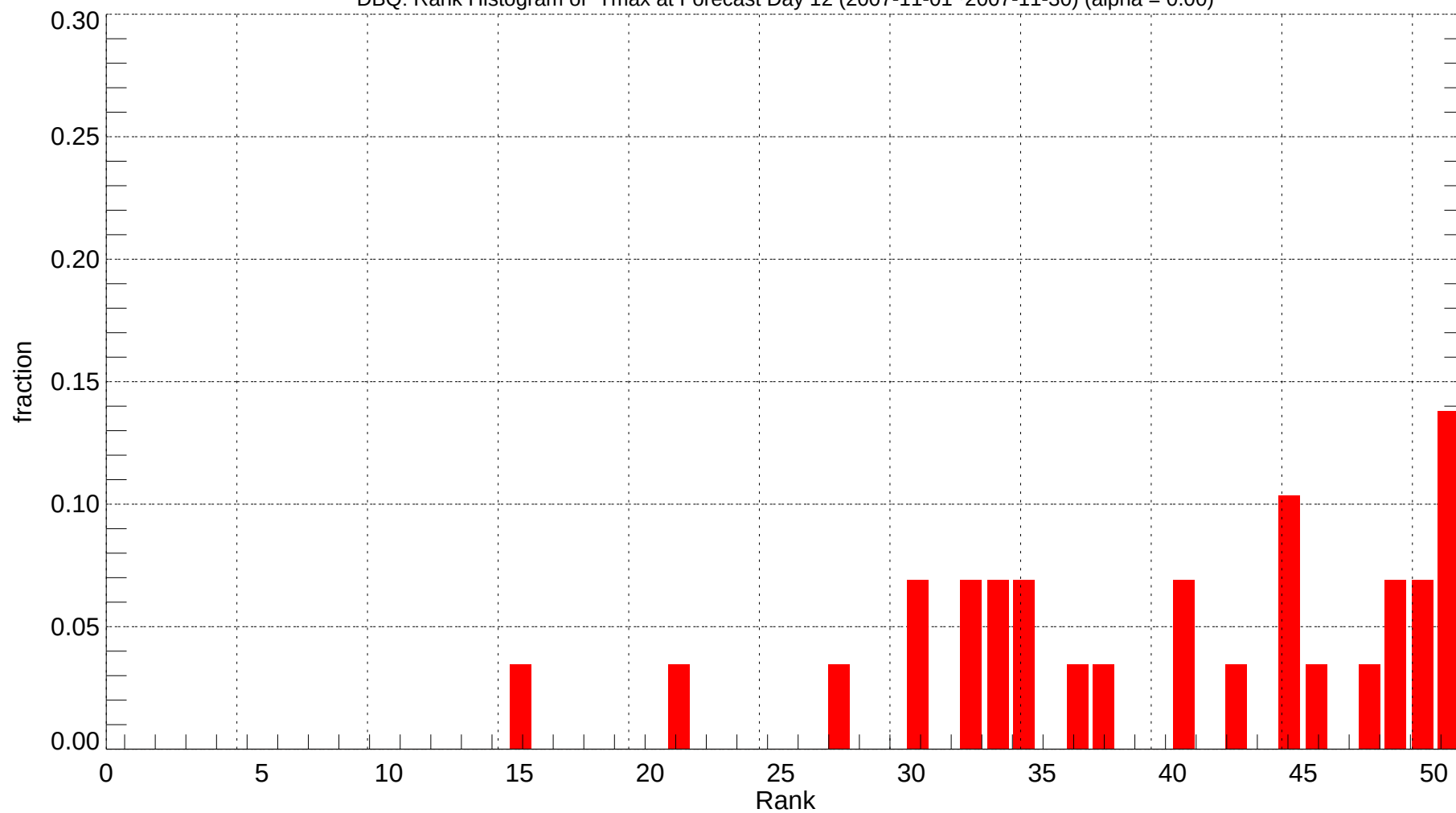
DBQ: Rank Histogram of Tmax at Forecast Day 12 (2007-11-01~2007-11-30) (alpha = 0.00)
