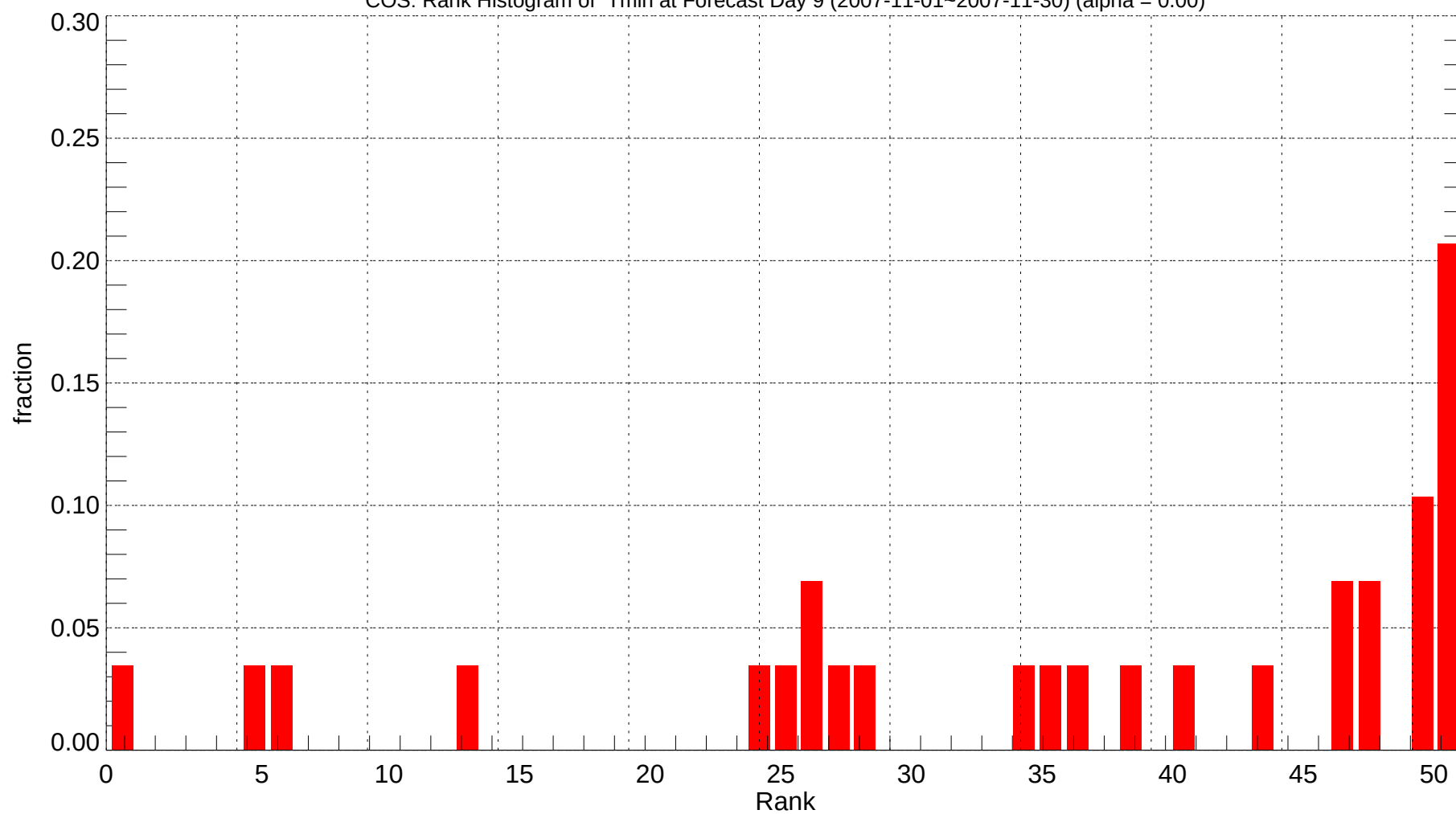
COS: Rank Histogram of Tmin at Forecast Day 9 (2007-11-01~2007-11-30) (alpha = 0.00)
