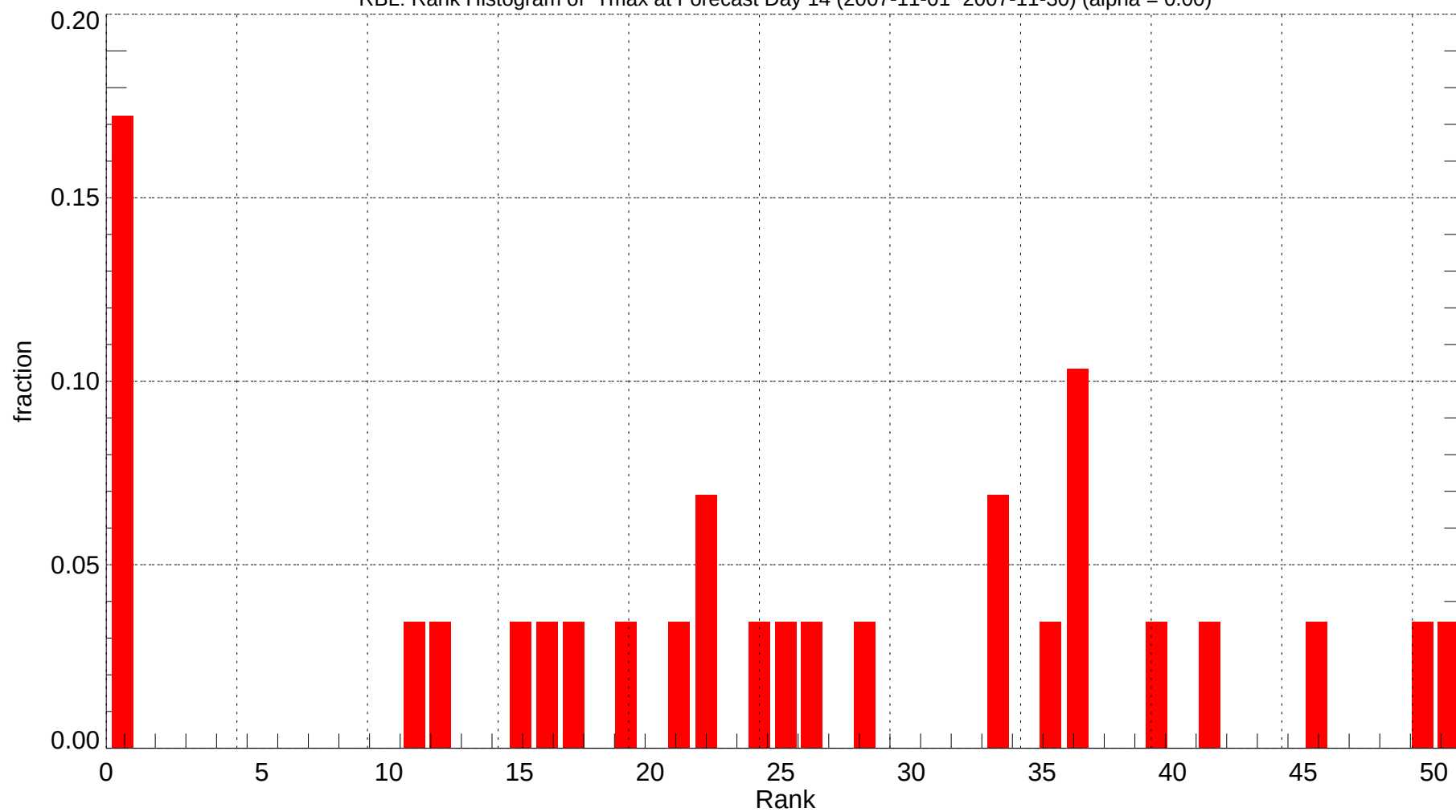
RBL: Rank Histogram of Tmax at Forecast Day 14 (2007-11-01~2007-11-30) (alpha = 0.00)
