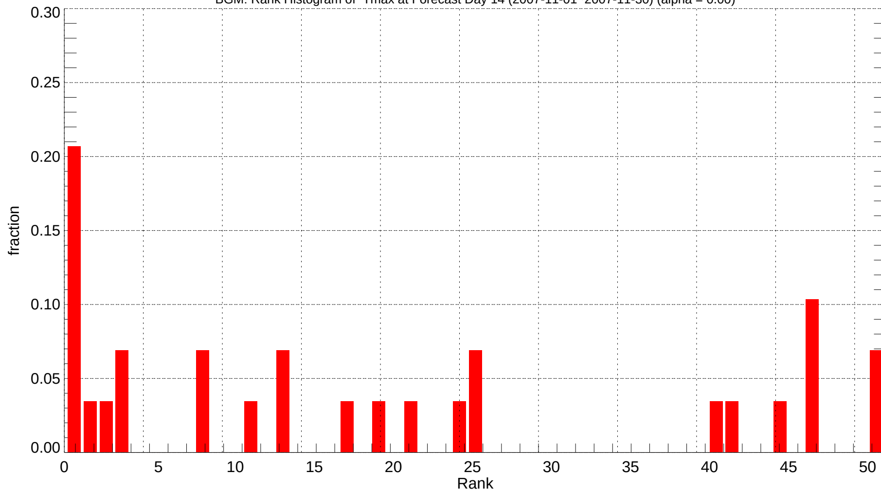
BGM: Rank Histogram of Tmax at Forecast Day 14 (2007-11-01~2007-11-30) (alpha = 0.00)
