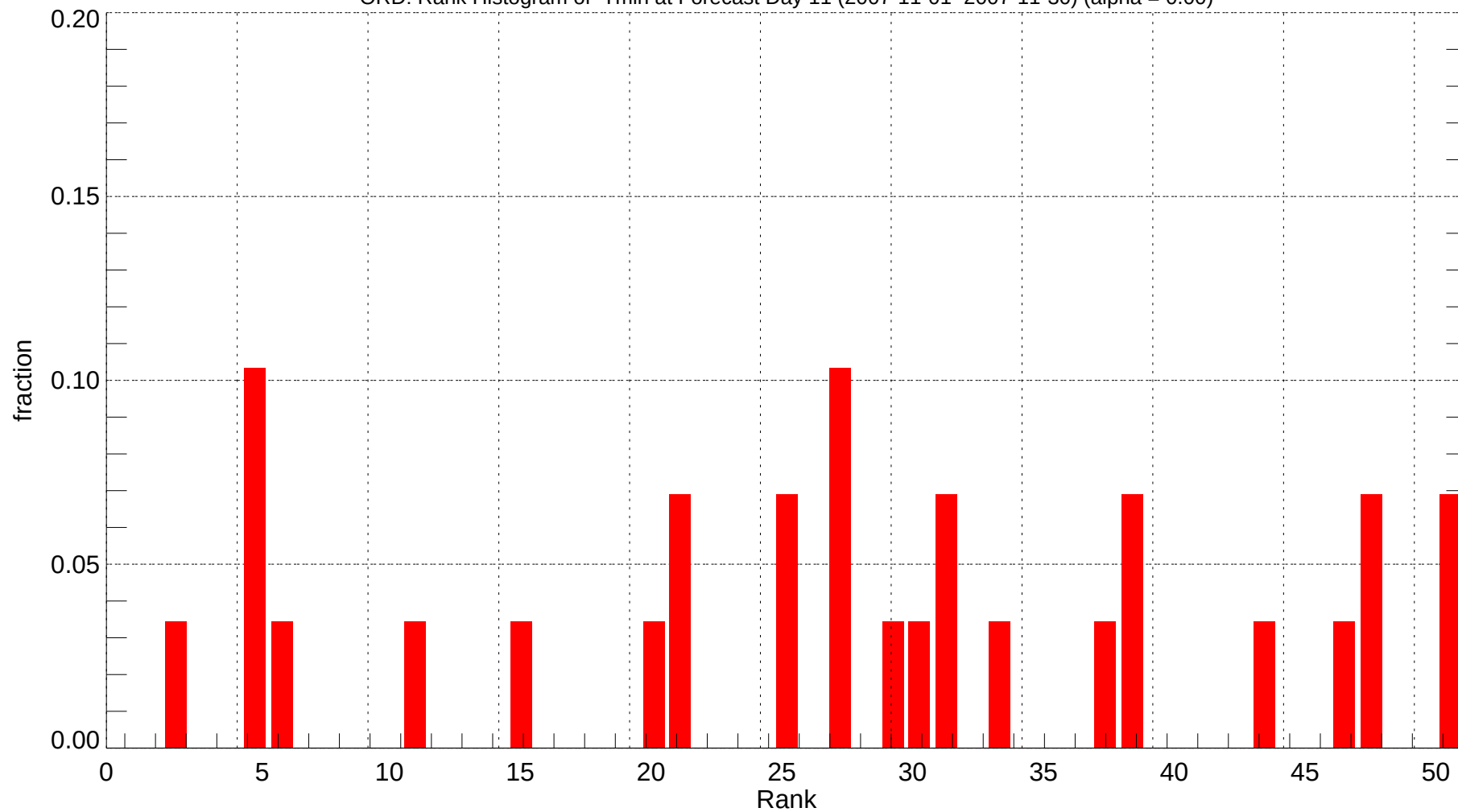
ORD: Rank Histogram of Tmin at Forecast Day 11 (2007-11-01~2007-11-30) (alpha = 0.00)
