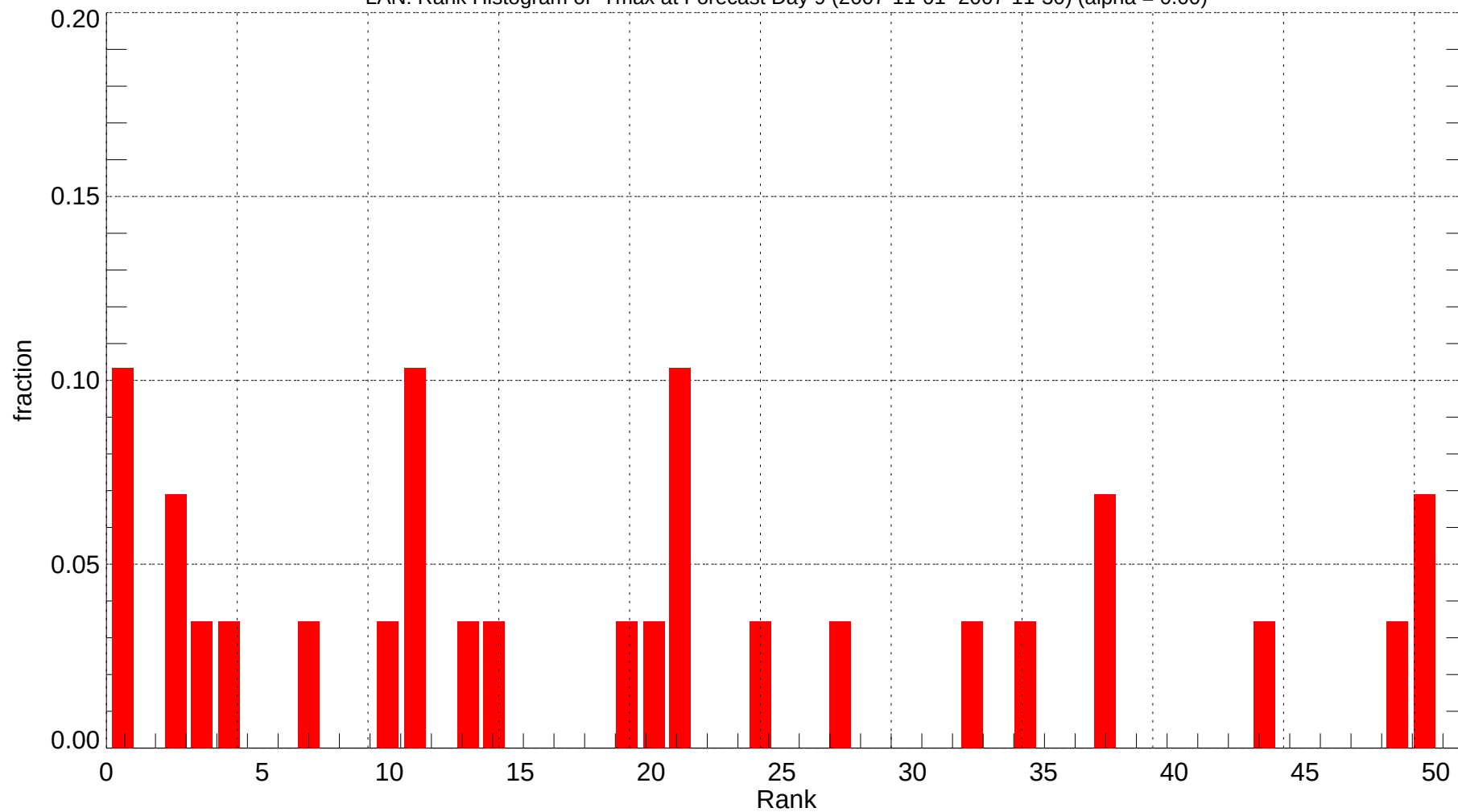
LAN: Rank Histogram of Tmax at Forecast Day 9 (2007-11-01~2007-11-30) (alpha = 0.00)
