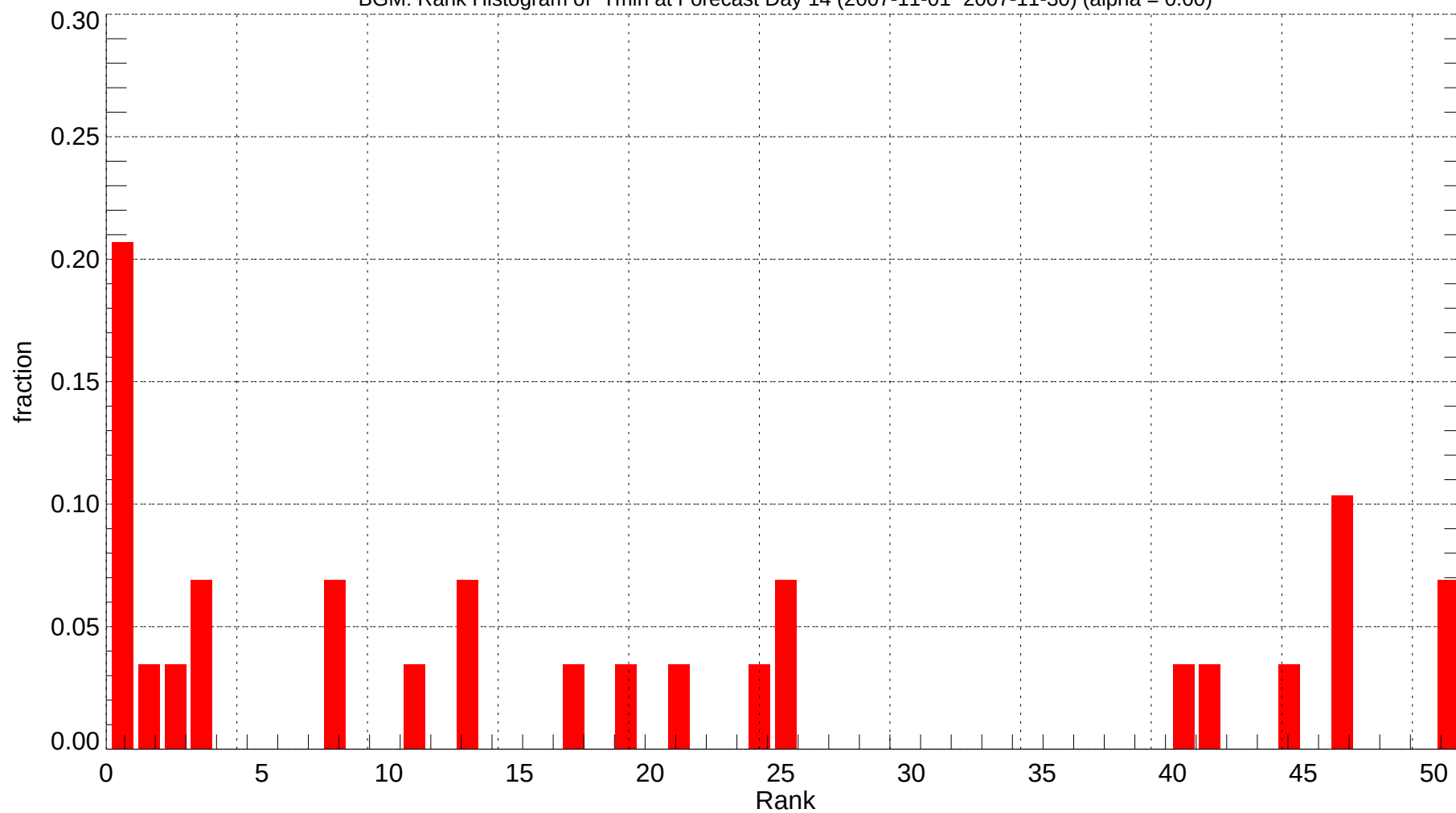
BGM: Rank Histogram of Tmin at Forecast Day 14 (2007-11-01~2007-11-30) (alpha = 0.00)
