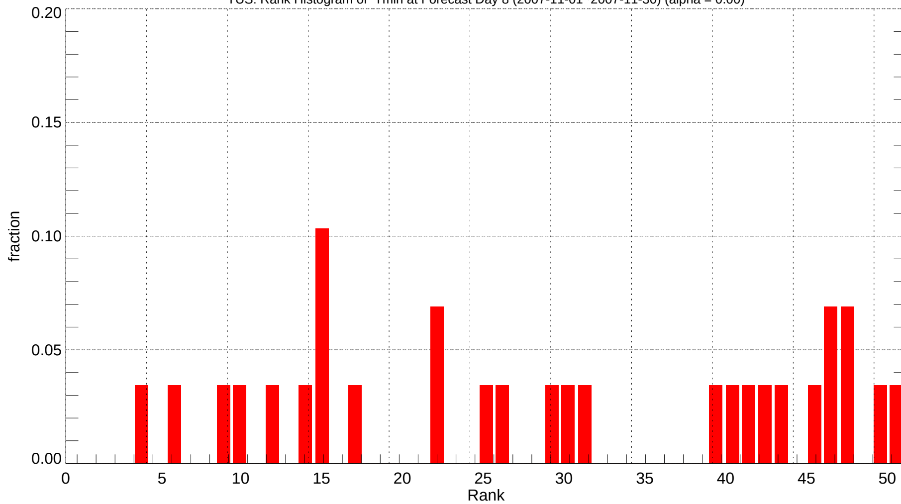
TUS: Rank Histogram of Tmin at Forecast Day 8 (2007-11-01~2007-11-30) (alpha = 0.00)
