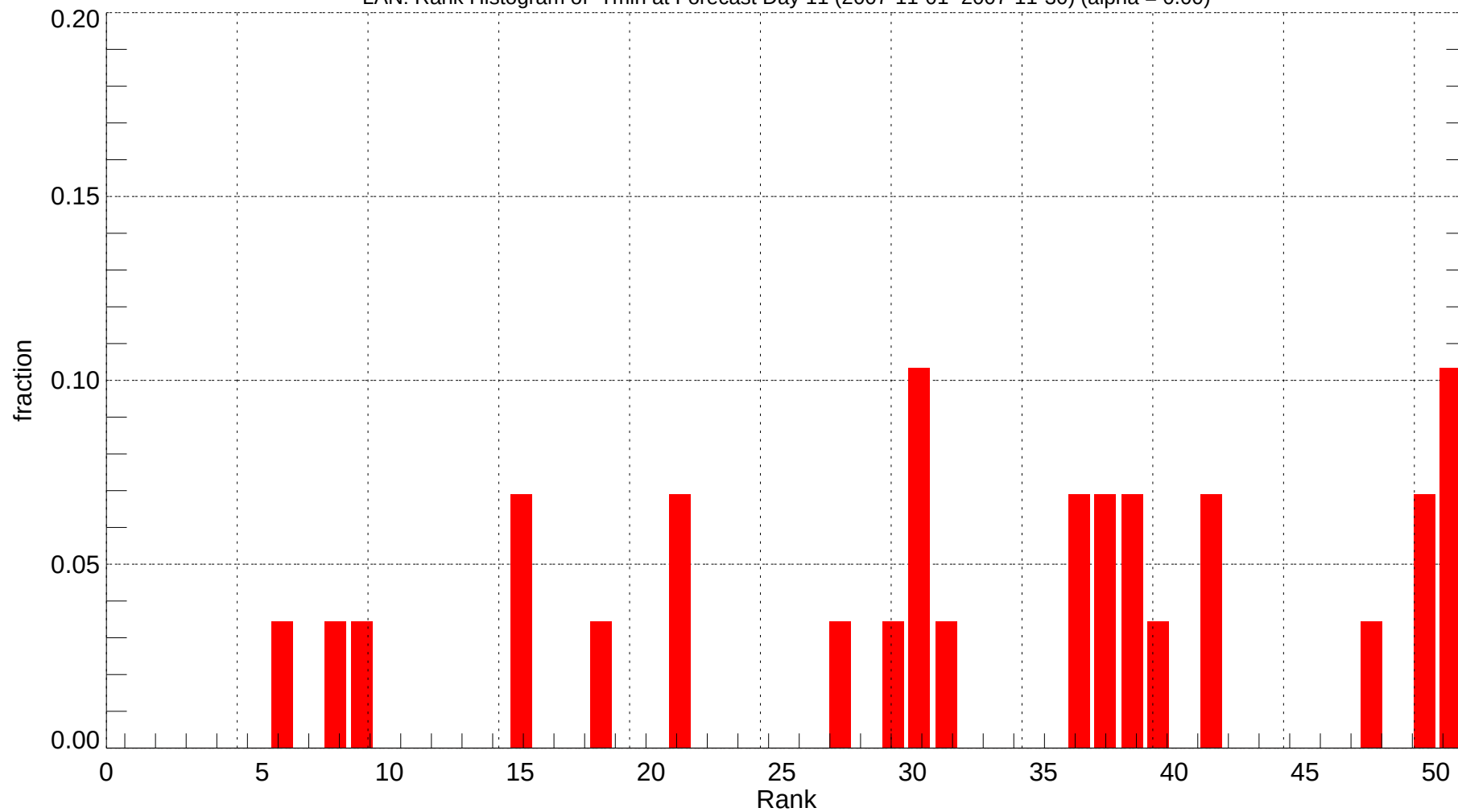
LAN: Rank Histogram of Tmin at Forecast Day 11 (2007-11-01~2007-11-30) (alpha = 0.00)
