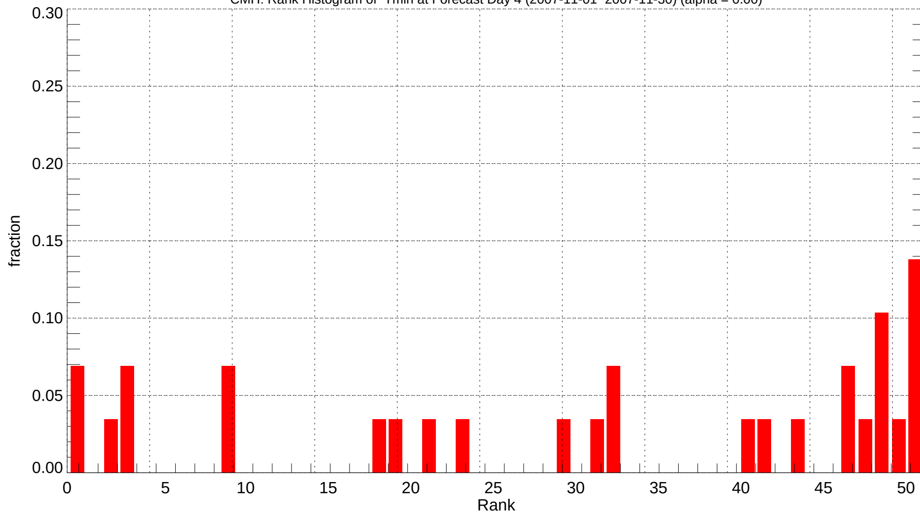
CMH: Rank Histogram of Tmin at Forecast Day 4 (2007-11-01~2007-11-30) (alpha = 0.00)
