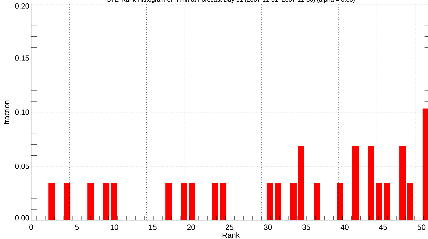
STL: Rank Histogram of Tmin at Forecast Day 11 (2007-11-01~2007-11-30) (alpha = 0.00)
