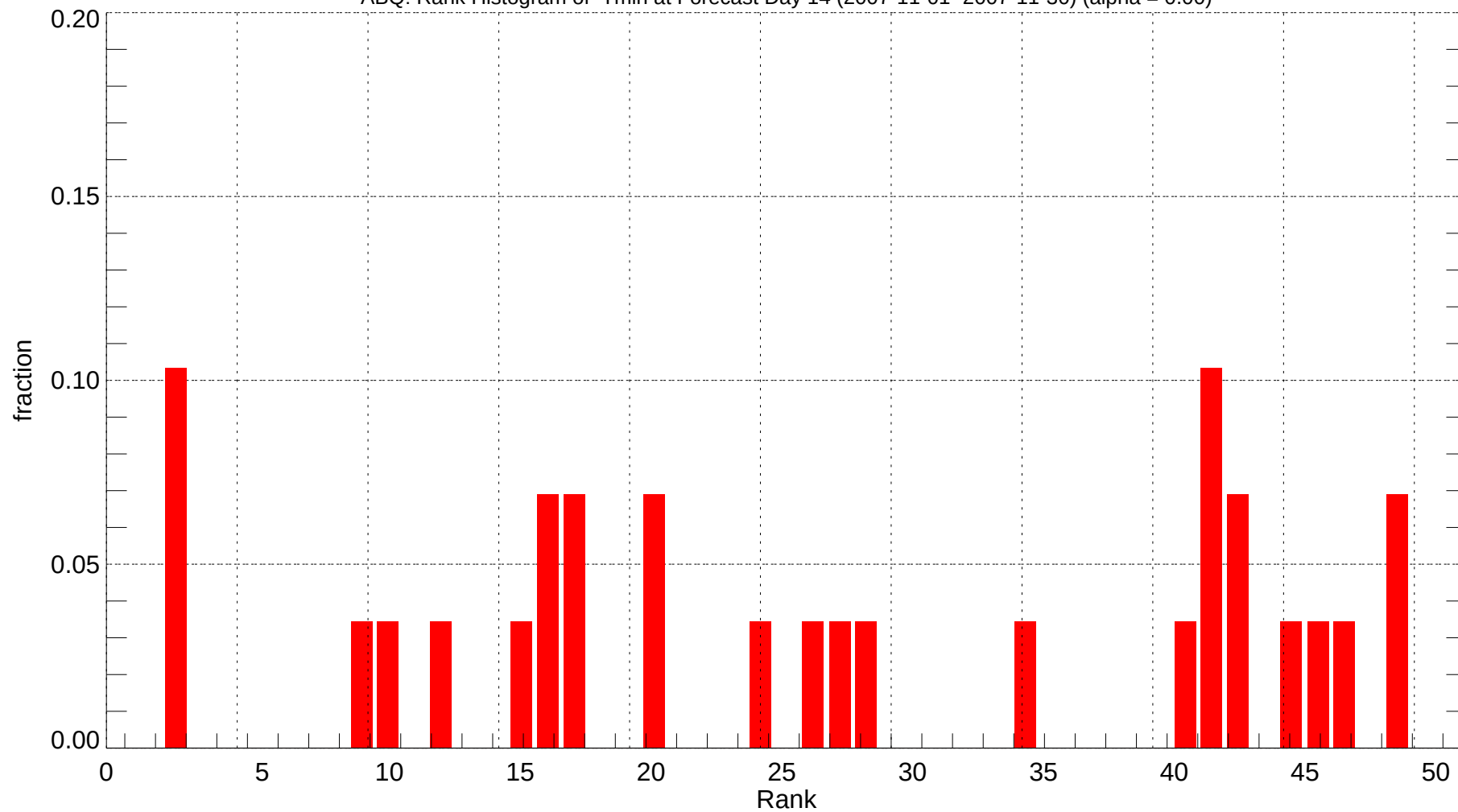
ABQ: Rank Histogram of Tmin at Forecast Day 14 (2007-11-01~2007-11-30) (alpha = 0.00)
