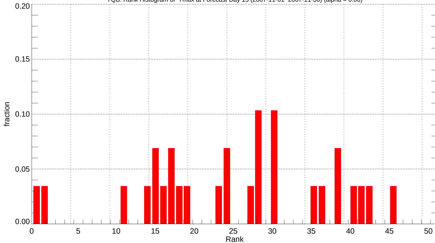
YQB: Rank Histogram of Tmax at Forecast Day 15 (2007-11-01~2007-11-30) (alpha = 0.00)
