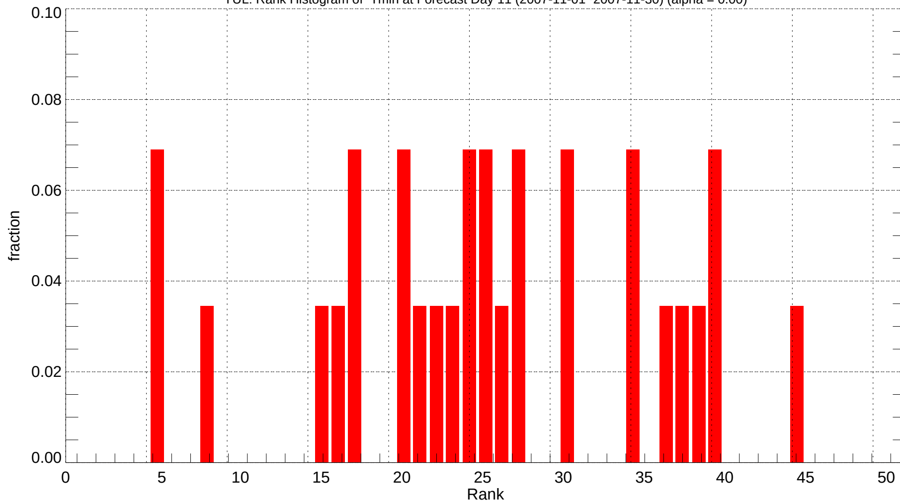
YUL: Rank Histogram of Tmin at Forecast Day 11 (2007-11-01~2007-11-30) (alpha = 0.00)
