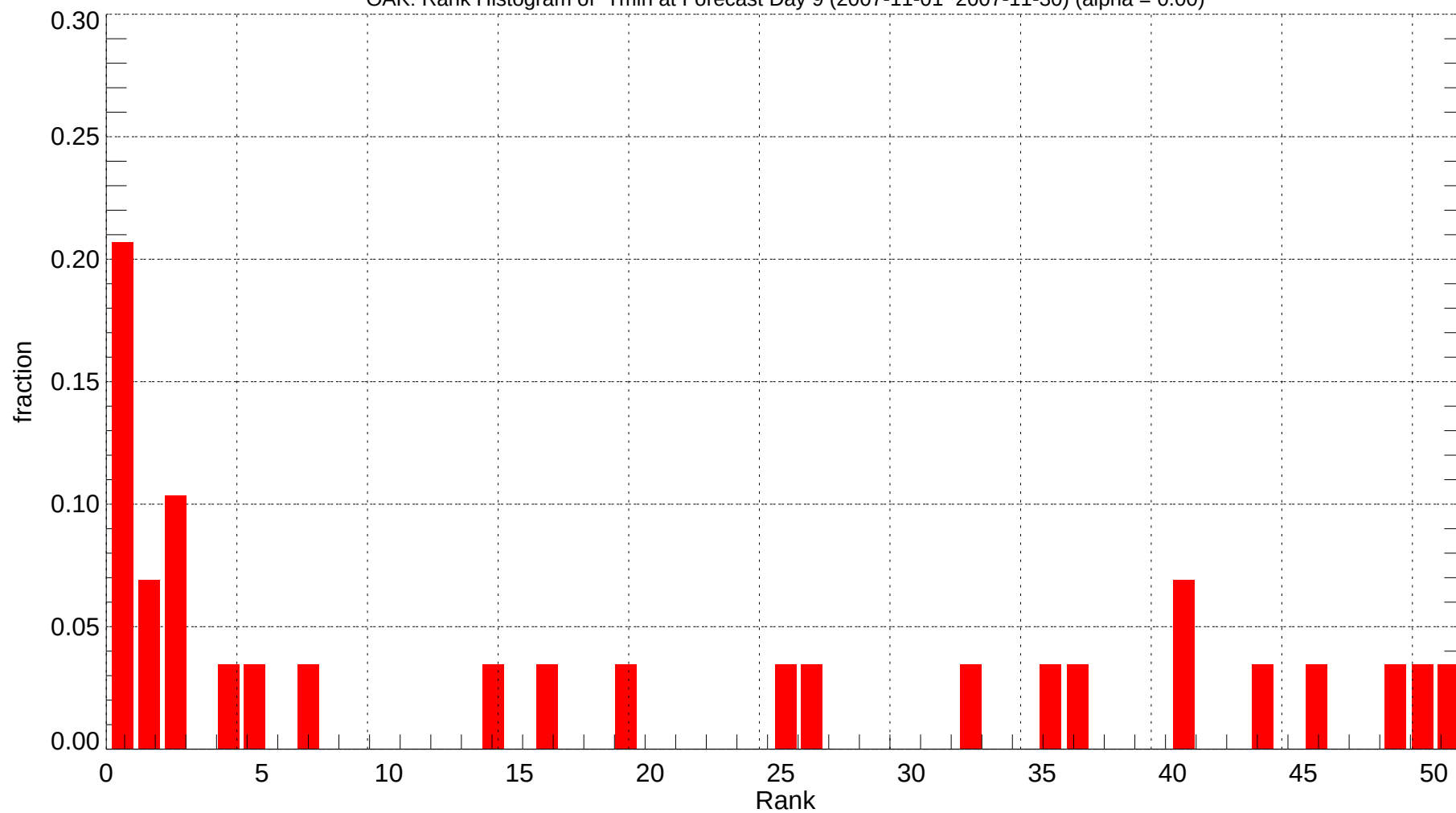
OAK: Rank Histogram of Tmin at Forecast Day 9 (2007-11-01~2007-11-30) (alpha = 0.00)
