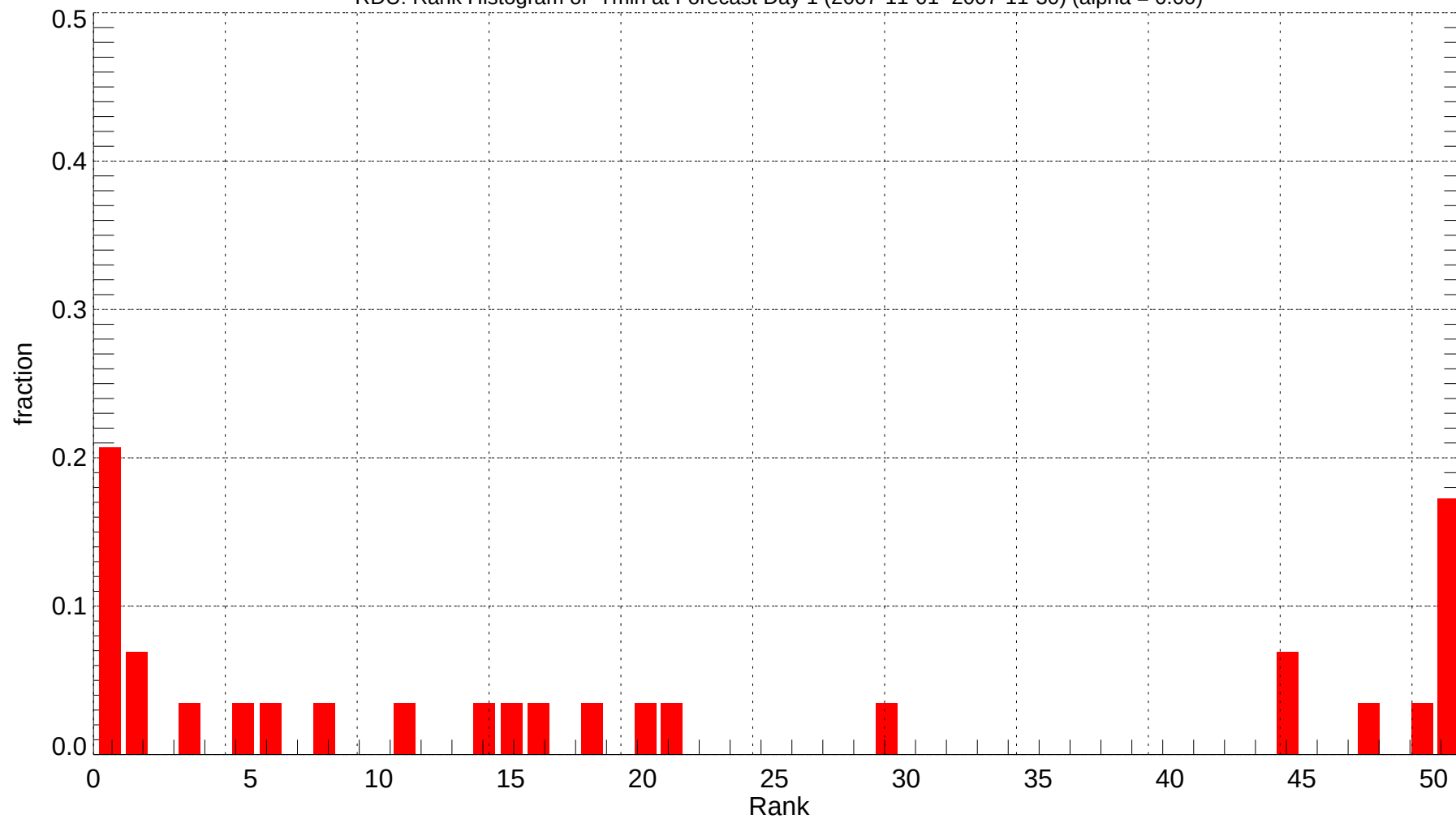
RDU: Rank Histogram of Tmin at Forecast Day 1 (2007-11-01~2007-11-30) (alpha = 0.00)
