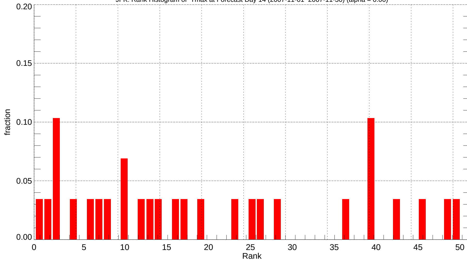
JFK: Rank Histogram of Tmax at Forecast Day 14 (2007-11-01~2007-11-30) (alpha = 0.00)
