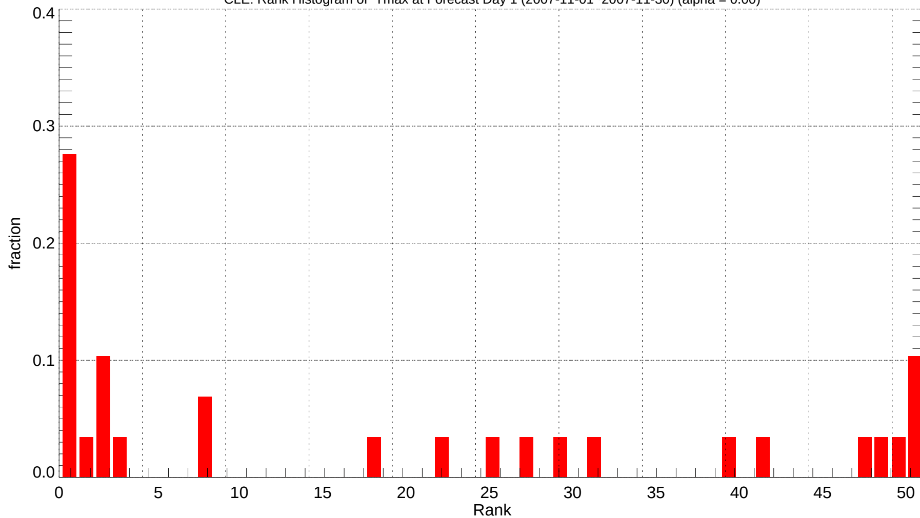
CLE: Rank Histogram of Tmax at Forecast Day 1 (2007-11-01~2007-11-30) (alpha = 0.00)
