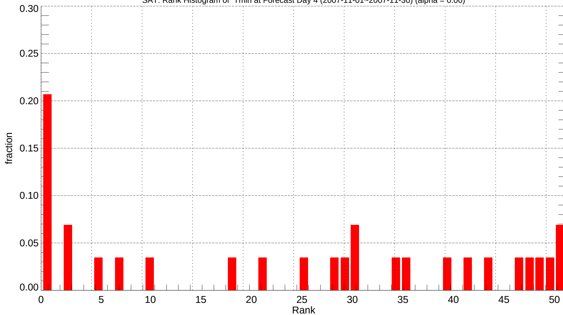
SAT: Rank Histogram of Tmin at Forecast Day 4 (2007-11-01~2007-11-30) (alpha = 0.00)
