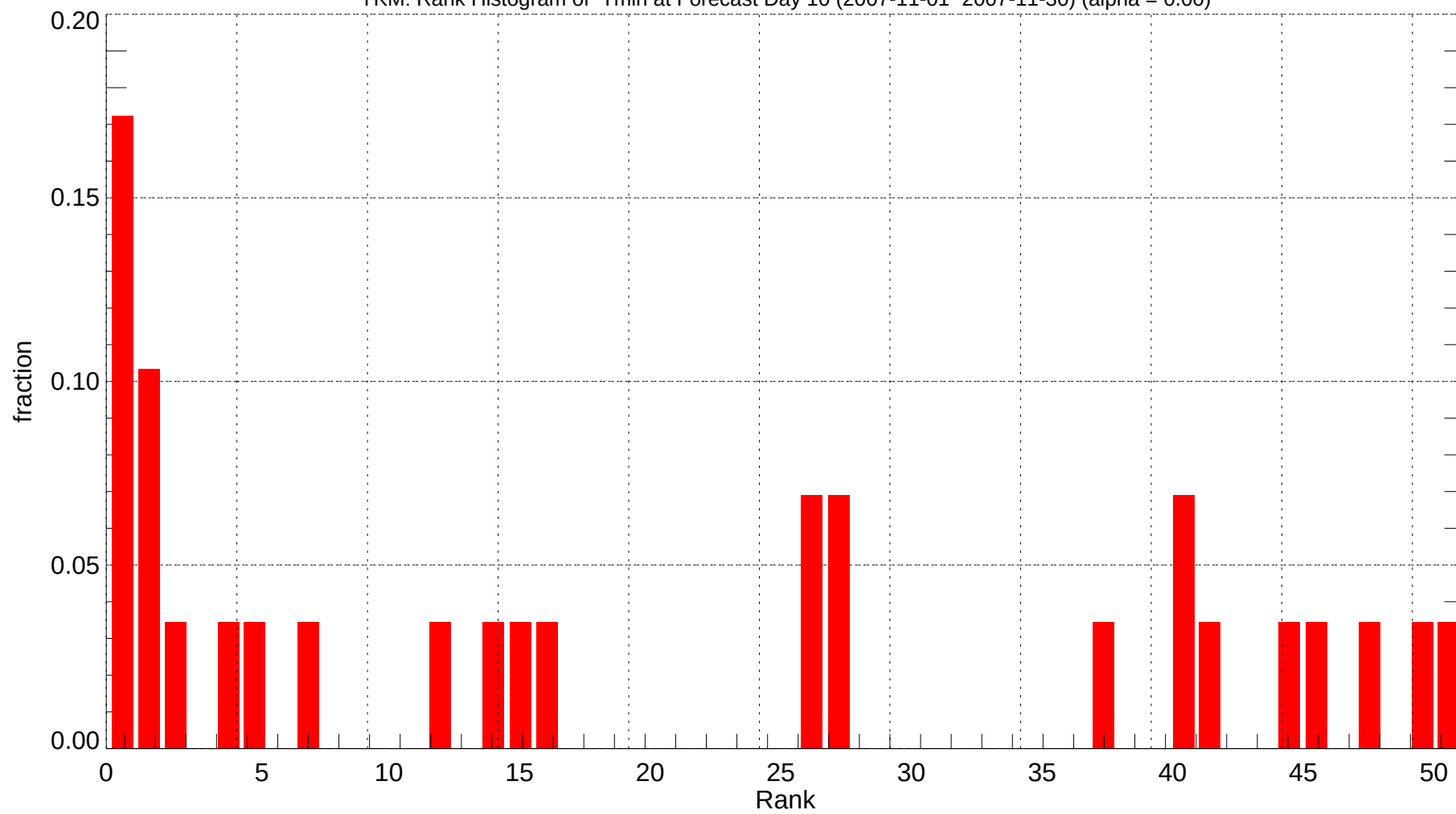
YKM: Rank Histogram of Tmin at Forecast Day 10 (2007-11-01~2007-11-30) (alpha = 0.00)
