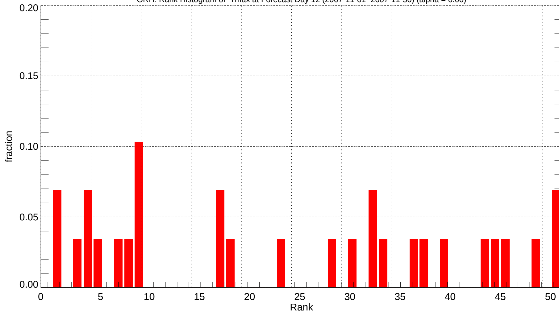
ORH: Rank Histogram of Tmax at Forecast Day 12 (2007-11-01~2007-11-30) (alpha = 0.00)
