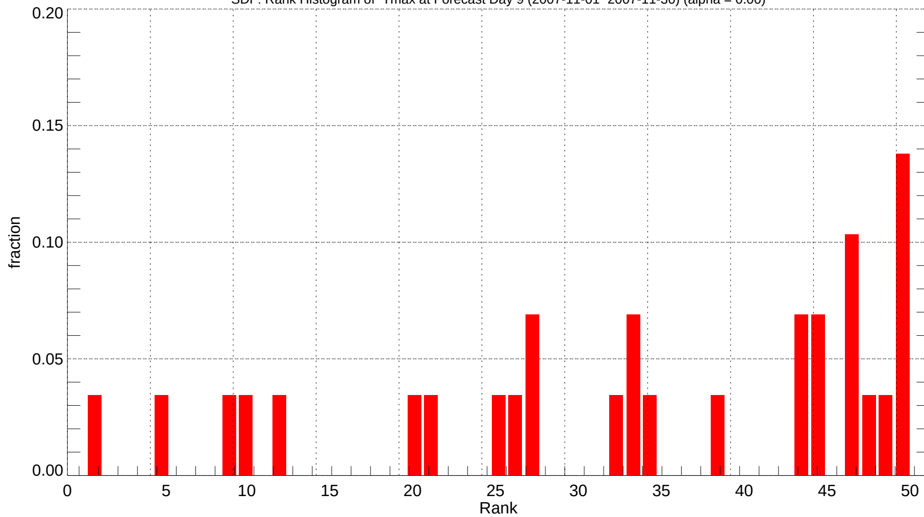
SDF: Rank Histogram of Tmax at Forecast Day 9 (2007-11-01~2007-11-30) (alpha = 0.00)
