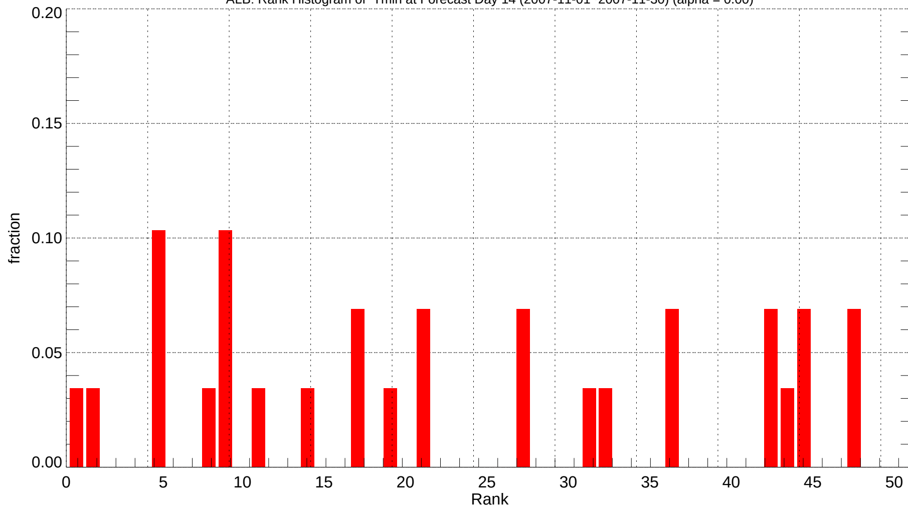
ALB: Rank Histogram of Tmin at Forecast Day 14 (2007-11-01~2007-11-30) (alpha = 0.00)
