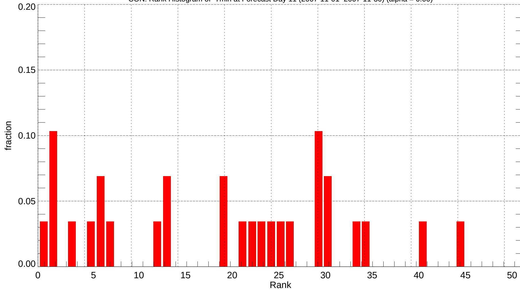
CON: Rank Histogram of Tmin at Forecast Day 11 (2007-11-01~2007-11-30) (alpha = 0.00)
