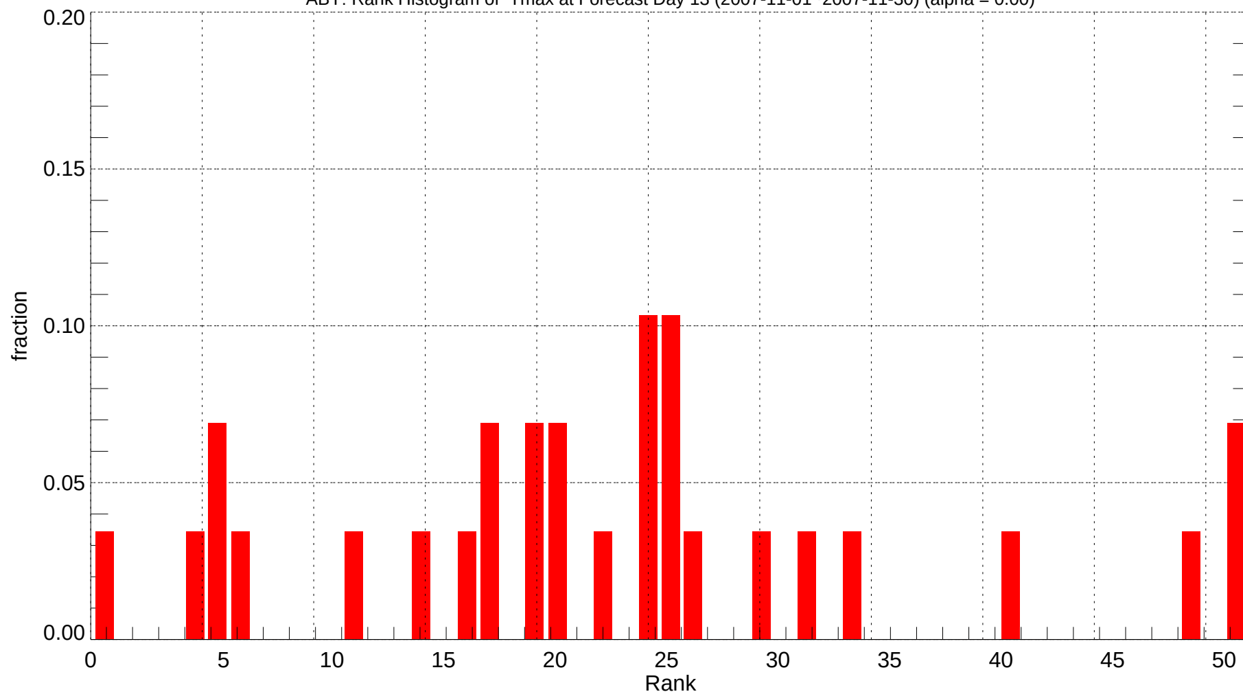
ABY: Rank Histogram of Tmax at Forecast Day 13 (2007-11-01~2007-11-30) (alpha = 0.00)
