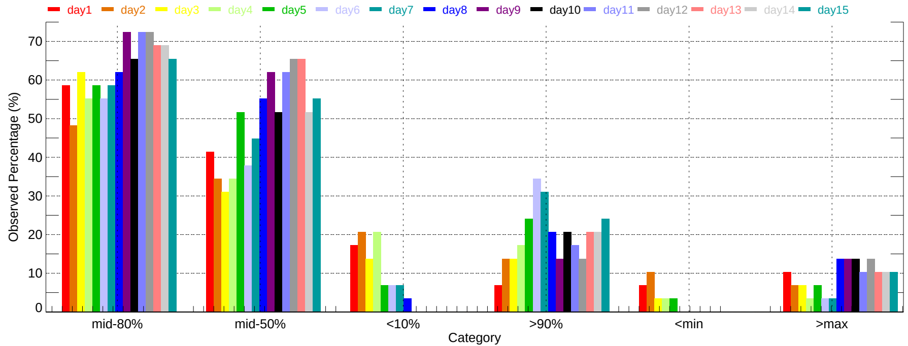
Observed Percentage of Ensembles - PHX: Max Temperature (2007-11-01~2007-11-30)
