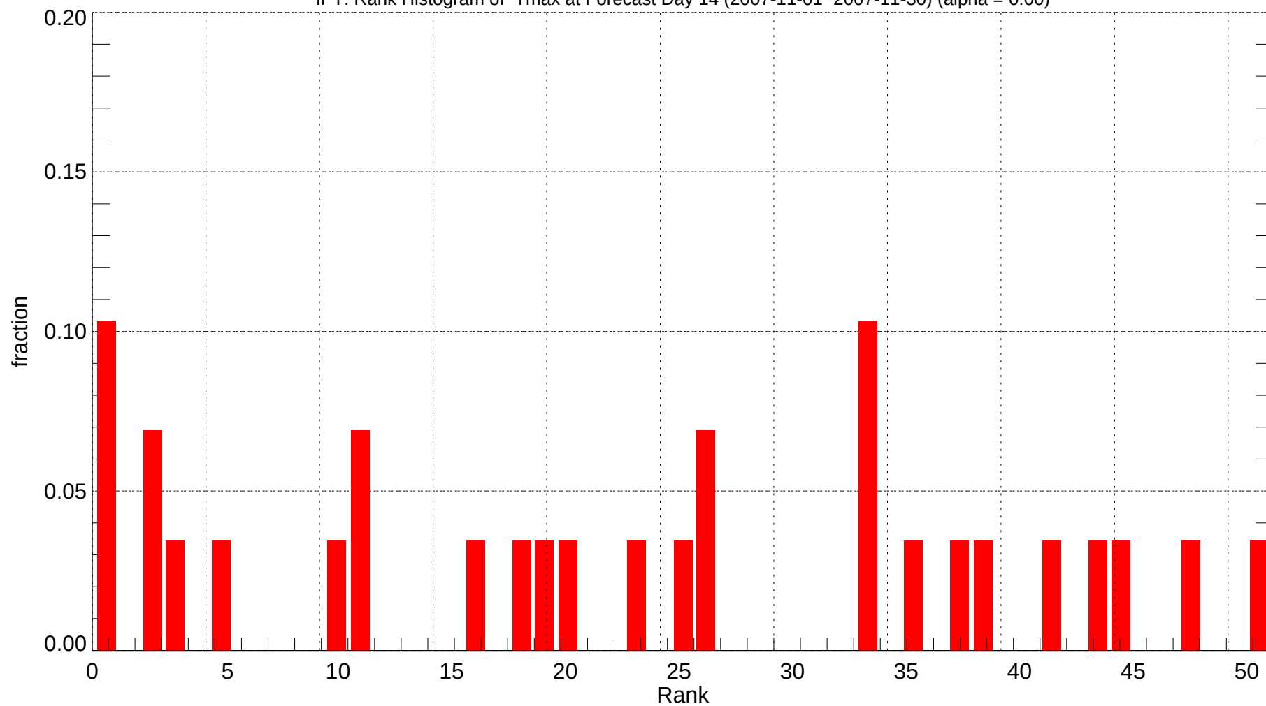
IPT: Rank Histogram of Tmax at Forecast Day 14 (2007-11-01~2007-11-30) (alpha = 0.00)
