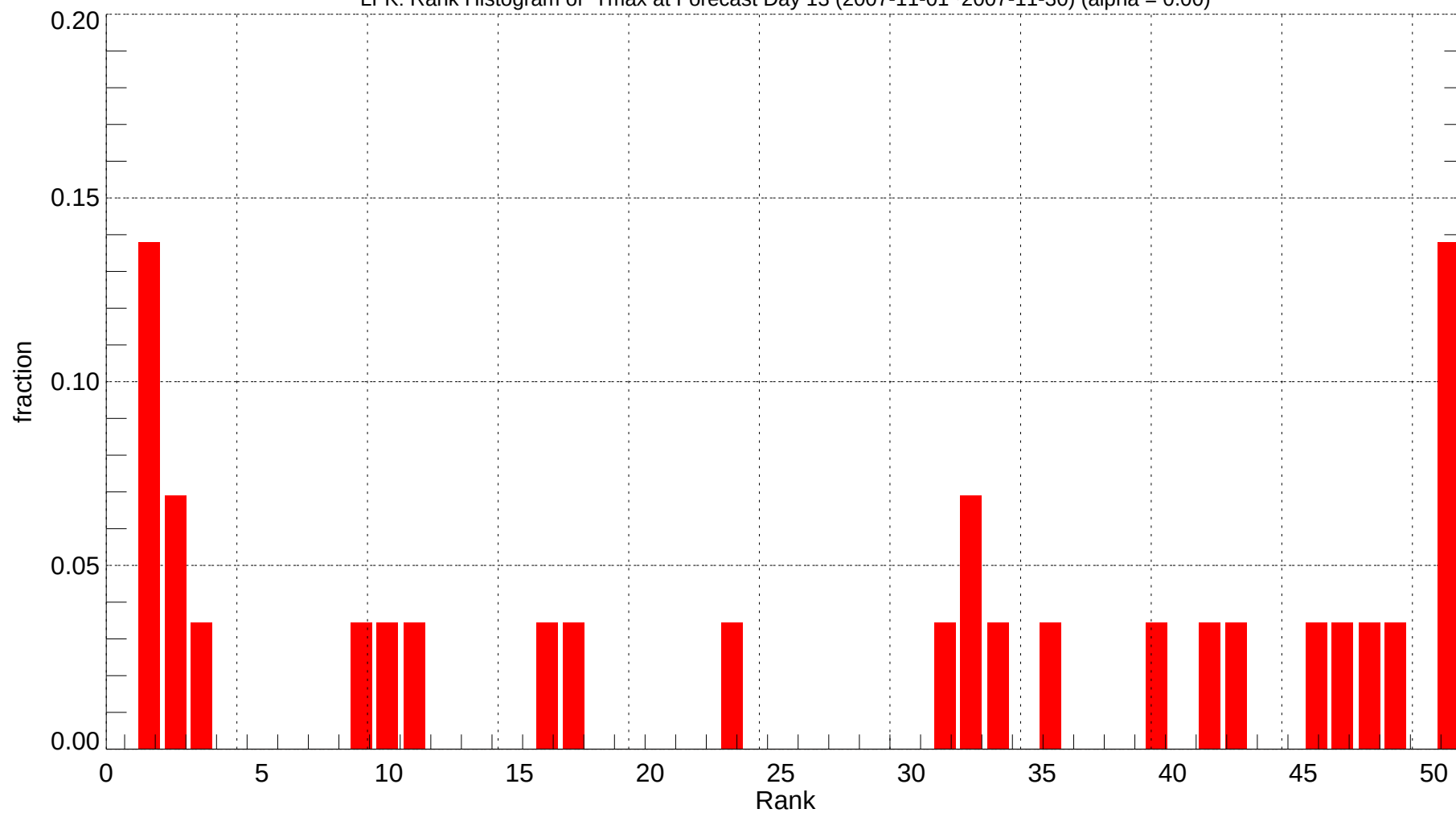
LFK: Rank Histogram of Tmax at Forecast Day 13 (2007-11-01~2007-11-30) (alpha = 0.00)
