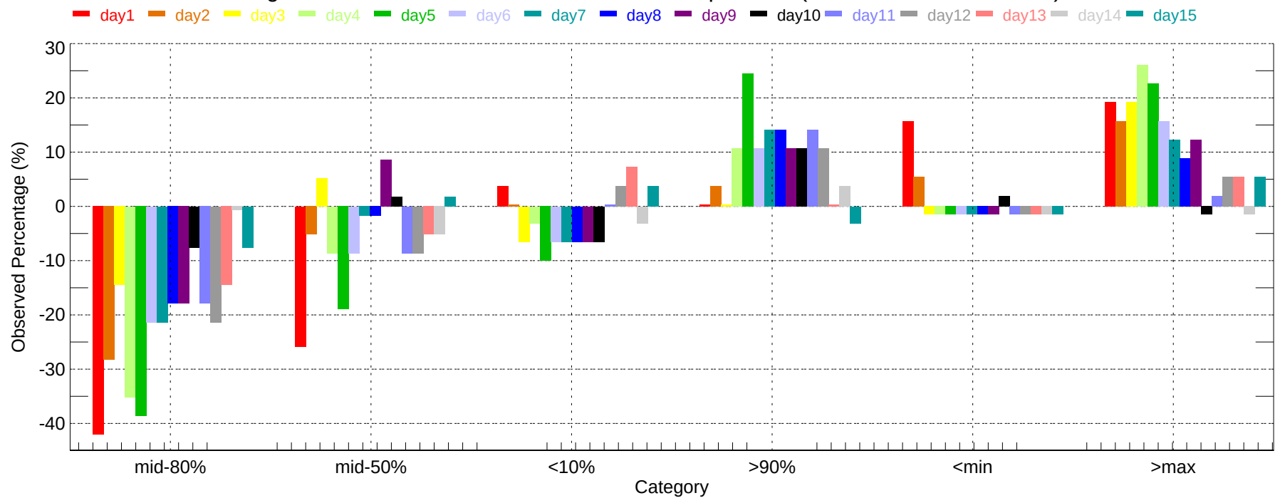
Observed Percentage Deviation of Ensembles - RDU: Min Temperature (2007-11-01~2007-11-30)
