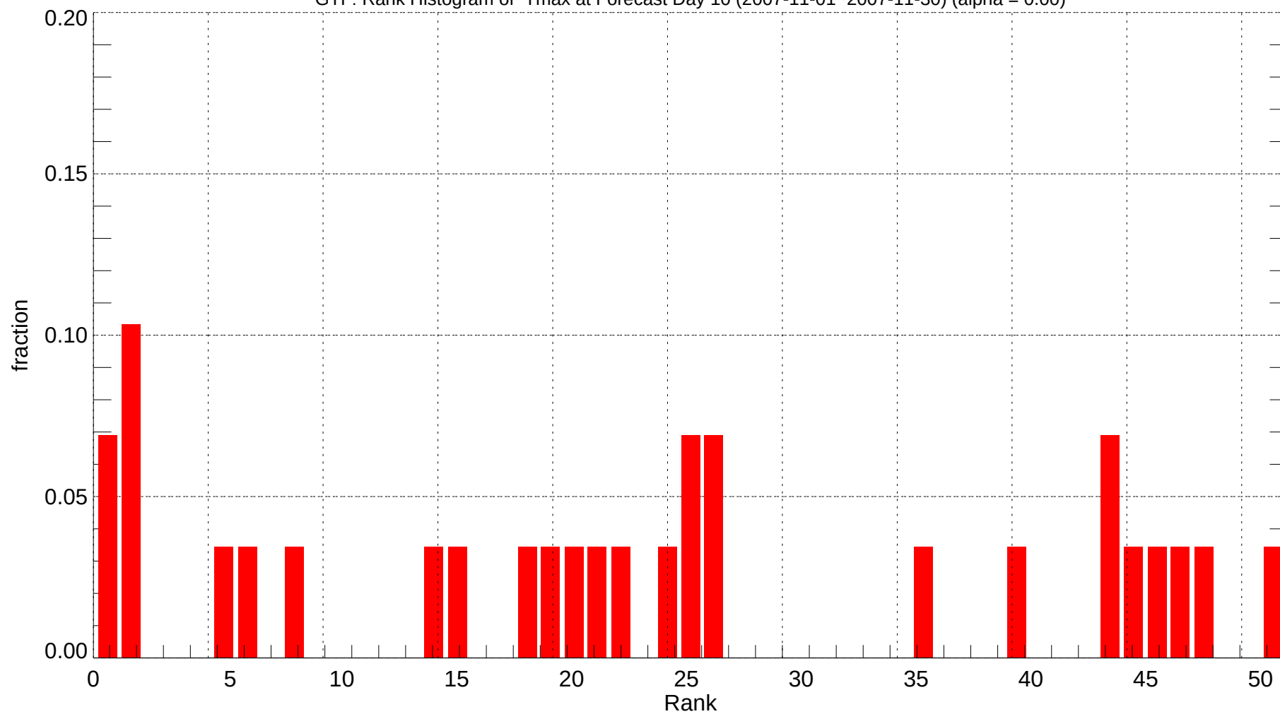
GTF: Rank Histogram of Tmax at Forecast Day 10 (2007-11-01~2007-11-30) (alpha = 0.00)
