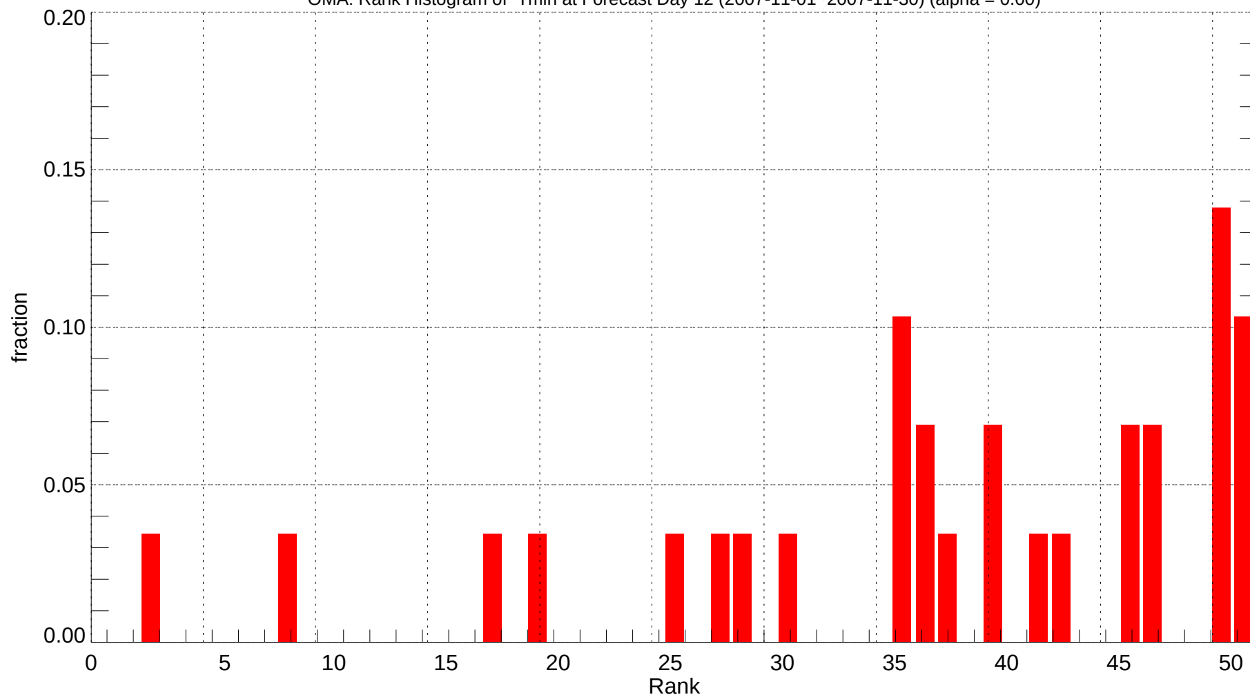
OMA: Rank Histogram of Tmin at Forecast Day 12 (2007-11-01~2007-11-30) (alpha = 0.00)
