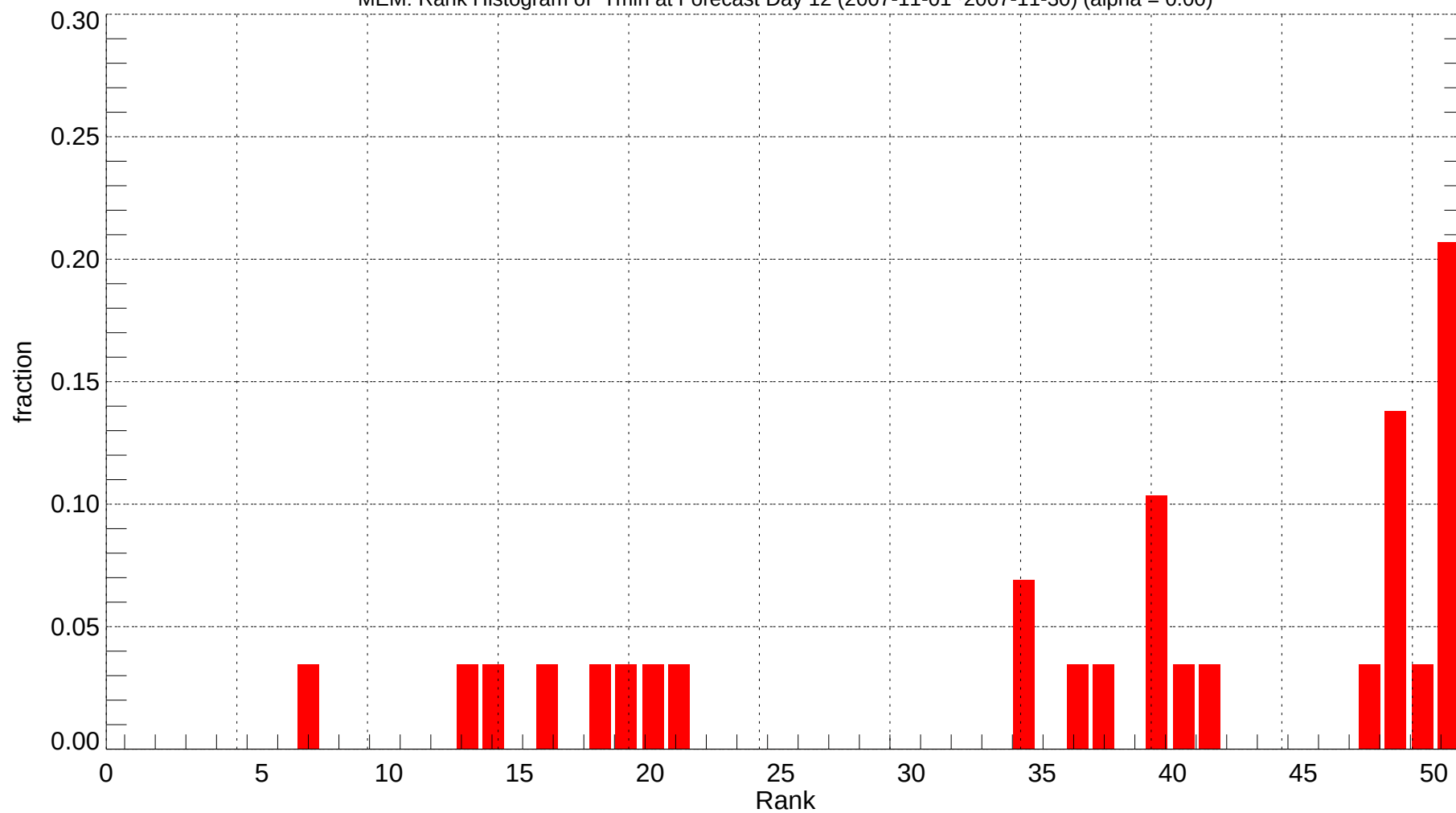
MEM: Rank Histogram of Tmin at Forecast Day 12 (2007-11-01~2007-11-30) (alpha = 0.00)
