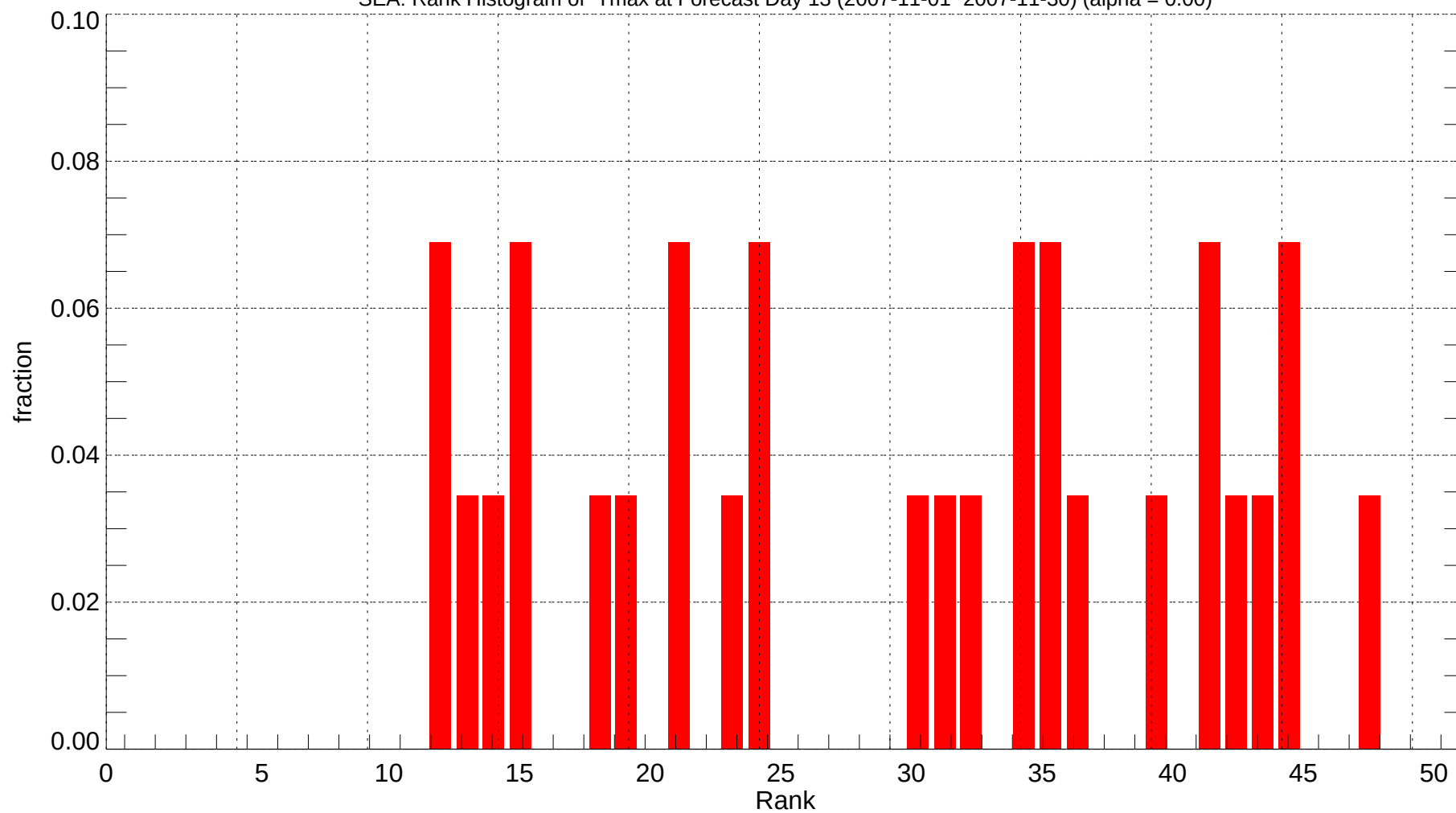
SEA: Rank Histogram of Tmax at Forecast Day 13 (2007-11-01~2007-11-30) (alpha = 0.00)
