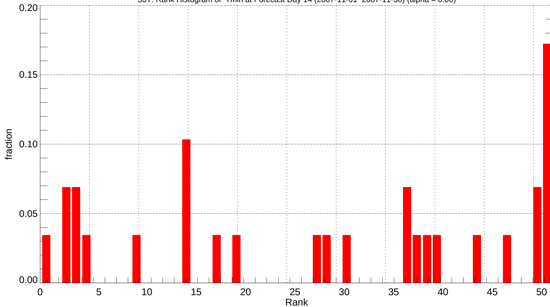
SJT: Rank Histogram of Tmin at Forecast Day 14 (2007-11-01~2007-11-30) (alpha = 0.00)
