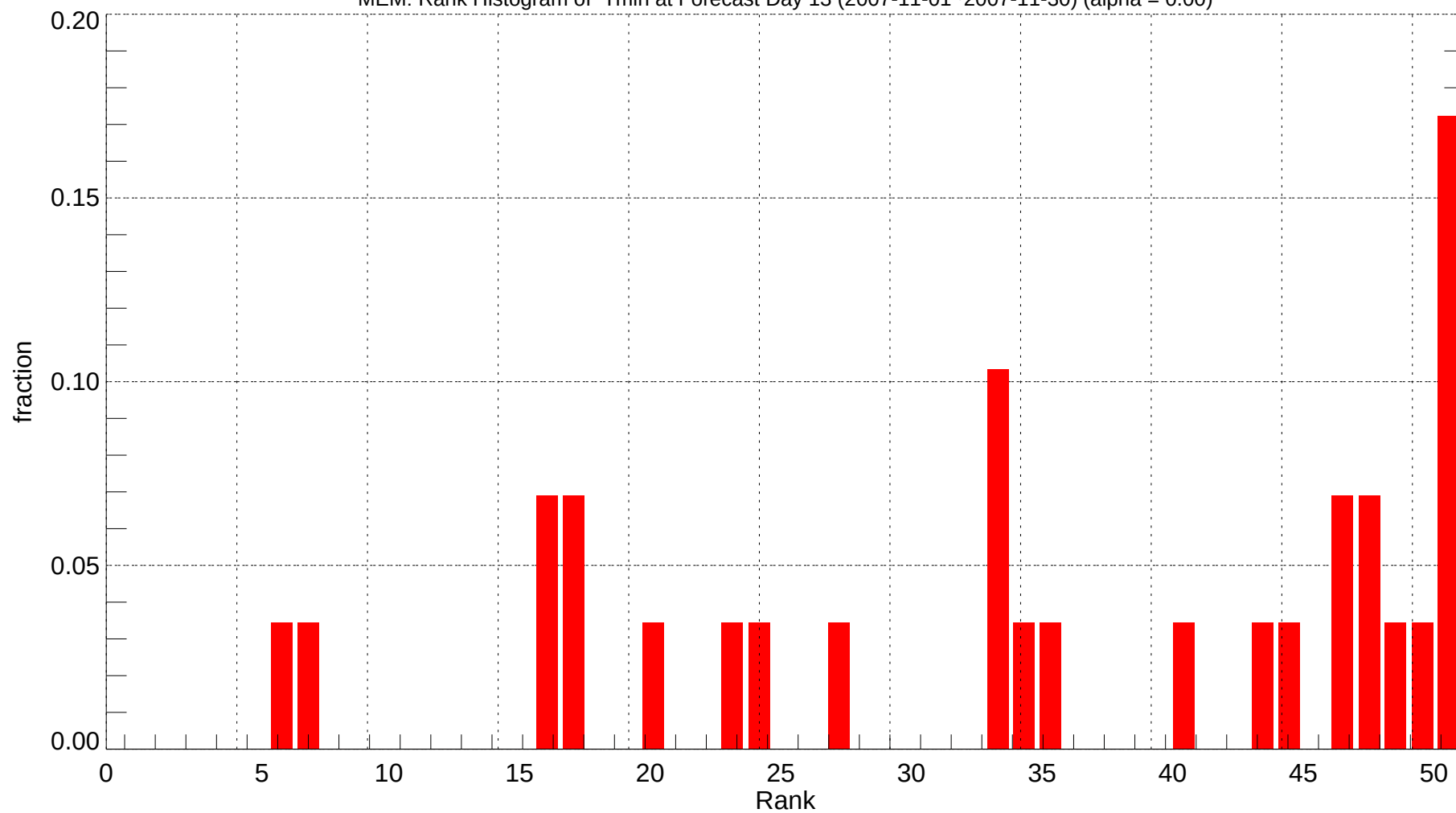
MEM: Rank Histogram of Tmin at Forecast Day 13 (2007-11-01~2007-11-30) (alpha = 0.00)
