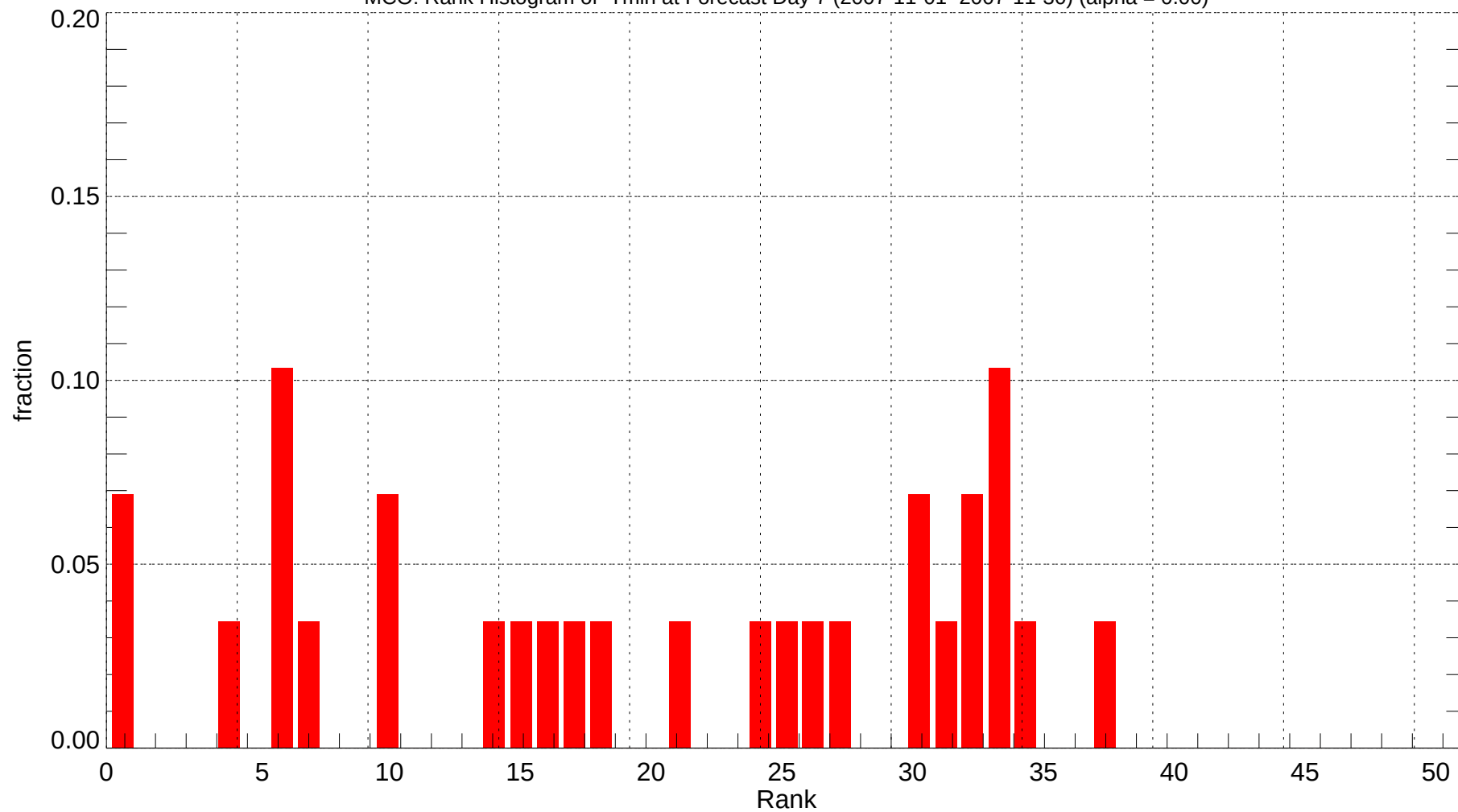
MCO: Rank Histogram of Tmin at Forecast Day 7 (2007-11-01~2007-11-30) (alpha = 0.00)
