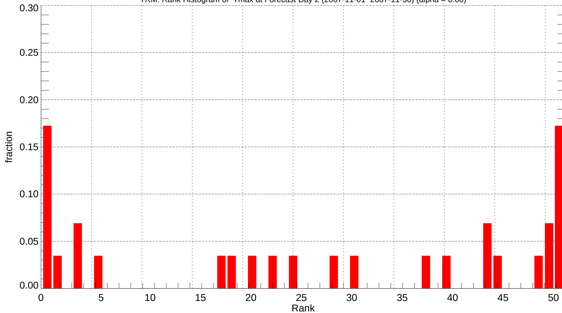
TRM: Rank Histogram of Tmax at Forecast Day 2 (2007-11-01~2007-11-30) (alpha = 0.00)
