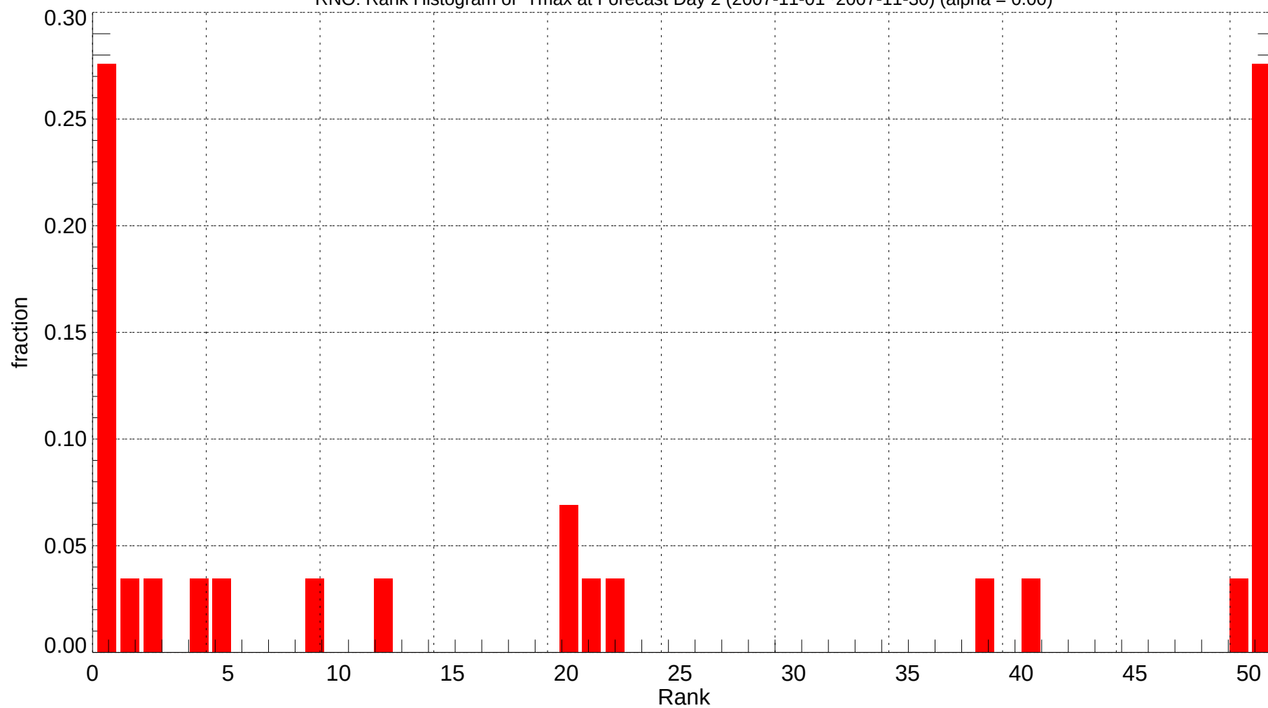
RNO: Rank Histogram of Tmax at Forecast Day 2 (2007-11-01~2007-11-30) (alpha = 0.00)
