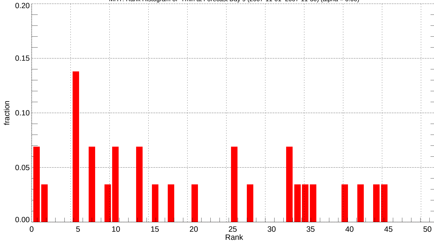
MHT: Rank Histogram of Tmin at Forecast Day 9 (2007-11-01~2007-11-30) (alpha = 0.00)
