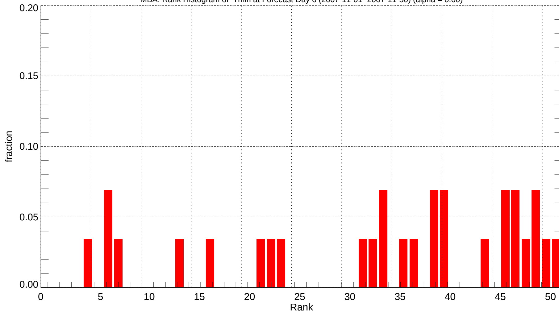
MBA: Rank Histogram of Tmin at Forecast Day 6 (2007-11-01~2007-11-30) (alpha = 0.00)
