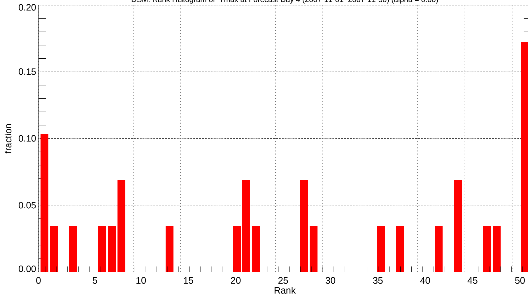
DSM: Rank Histogram of Tmax at Forecast Day 4 (2007-11-01~2007-11-30) (alpha = 0.00)
