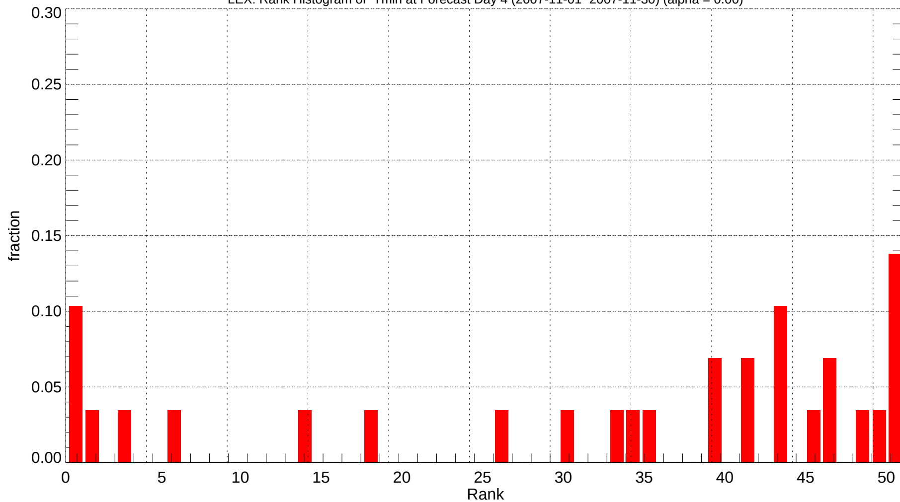
LEX: Rank Histogram of Tmin at Forecast Day 4 (2007-11-01~2007-11-30) (alpha = 0.00)
