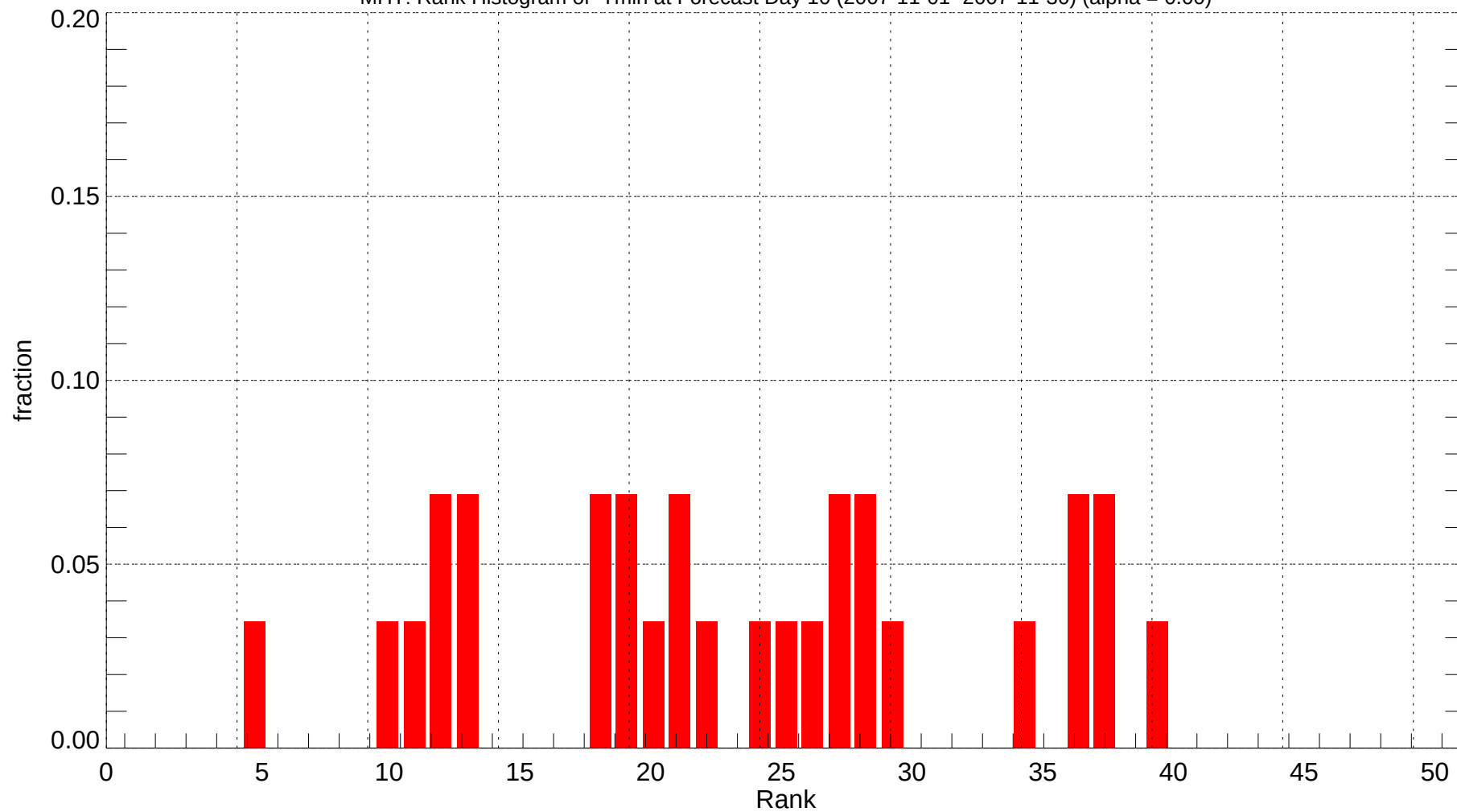
MHT: Rank Histogram of Tmin at Forecast Day 10 (2007-11-01~2007-11-30) (alpha = 0.00)
