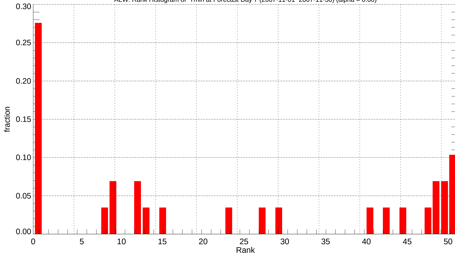
ALW: Rank Histogram of Tmin at Forecast Day 7 (2007-11-01~2007-11-30) (alpha = 0.00)
