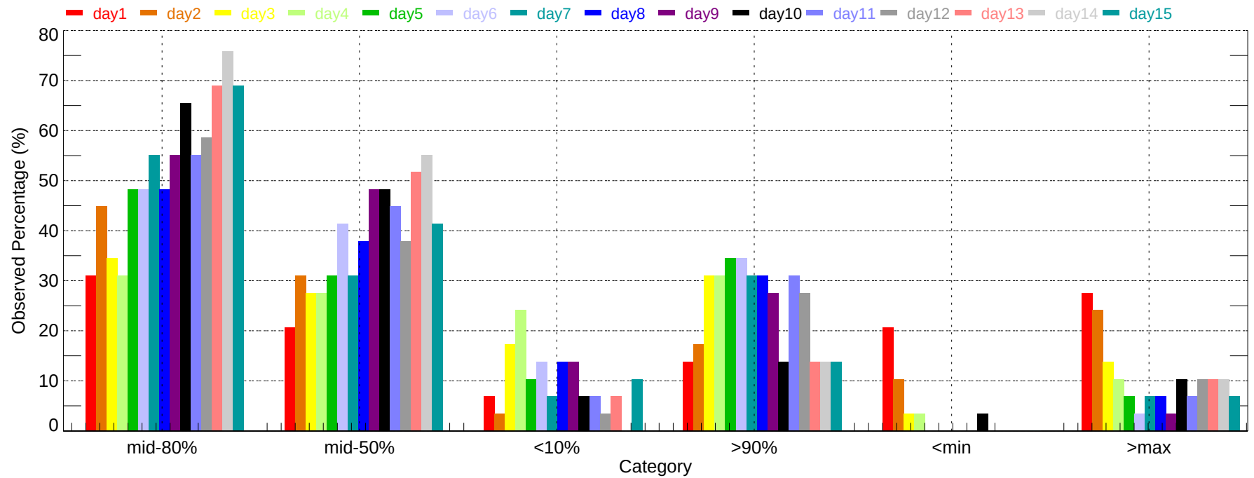
Observed Percentage of Ensembles - PIT: Max Temperature (2007-11-01~2007-11-30)
