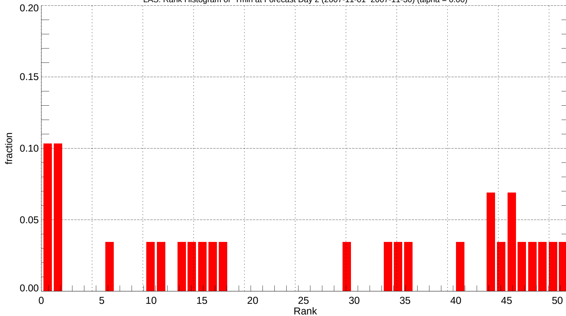
LAS: Rank Histogram of Tmin at Forecast Day 2 (2007-11-01~2007-11-30) (alpha = 0.00)
