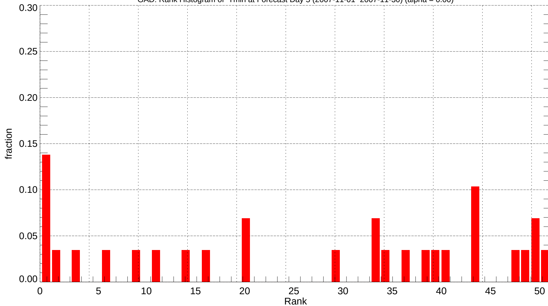
GAD: Rank Histogram of Tmin at Forecast Day 5 (2007-11-01~2007-11-30) (alpha = 0.00)
