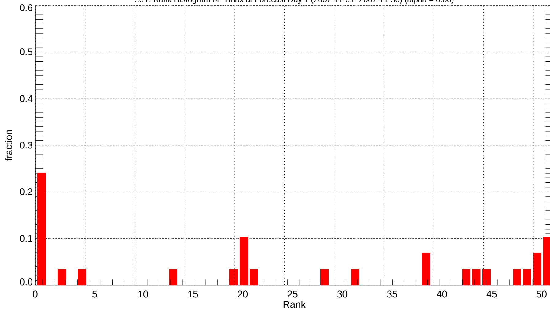
SJT: Rank Histogram of Tmax at Forecast Day 1 (2007-11-01~2007-11-30) (alpha = 0.00)
