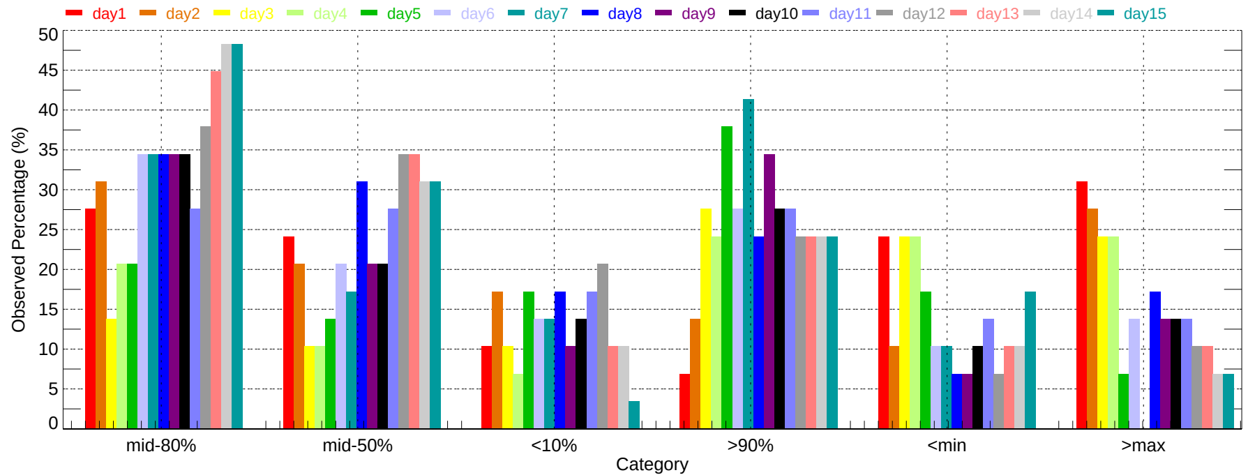
Observed Percentage of Ensembles - VCT: Max Temperature (2007-11-01~2007-11-30)
