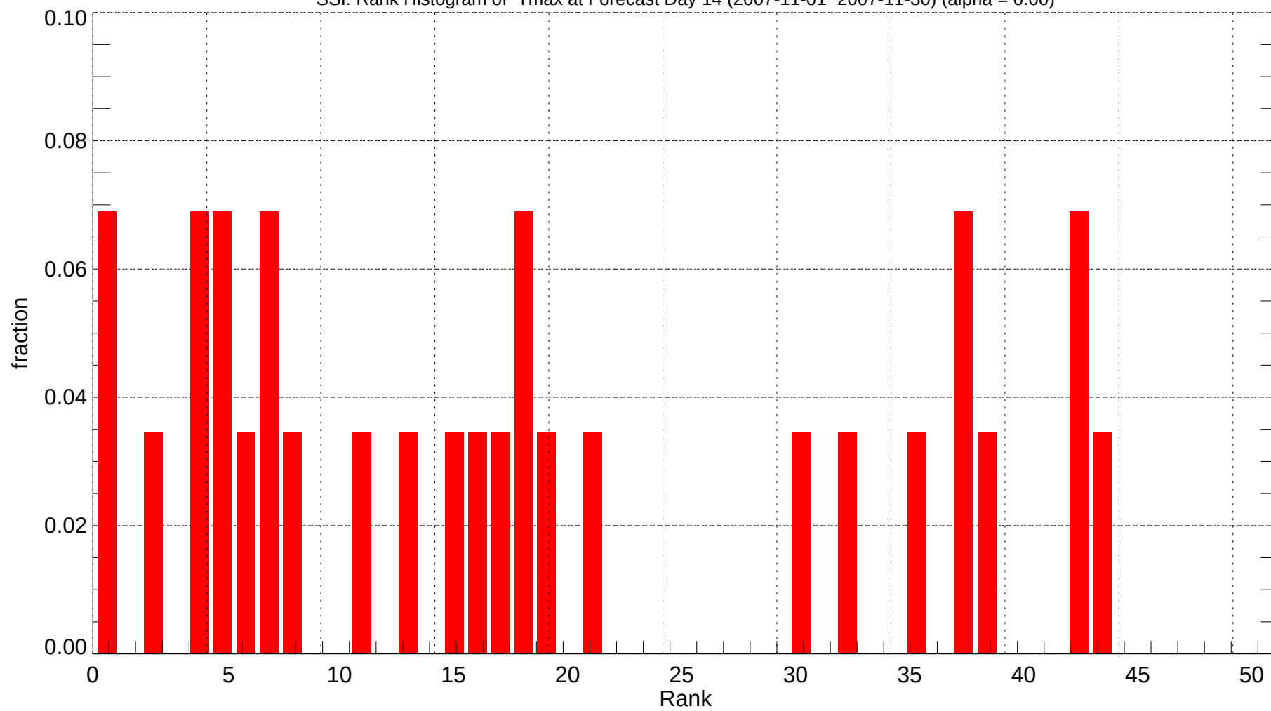
SSI: Rank Histogram of Tmax at Forecast Day 14 (2007-11-01~2007-11-30) (alpha = 0.00)
