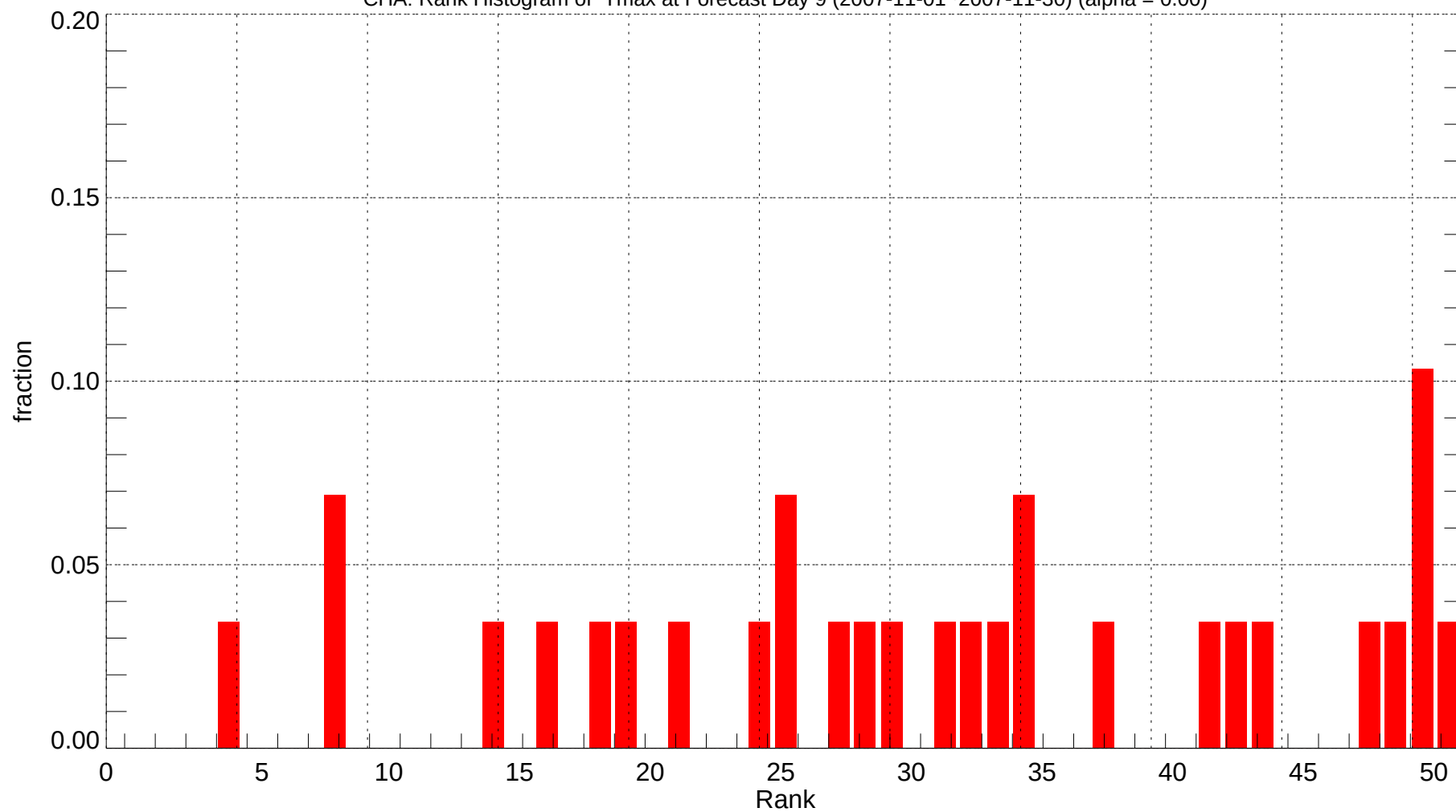
CHA: Rank Histogram of Tmax at Forecast Day 9 (2007-11-01~2007-11-30) (alpha = 0.00)
