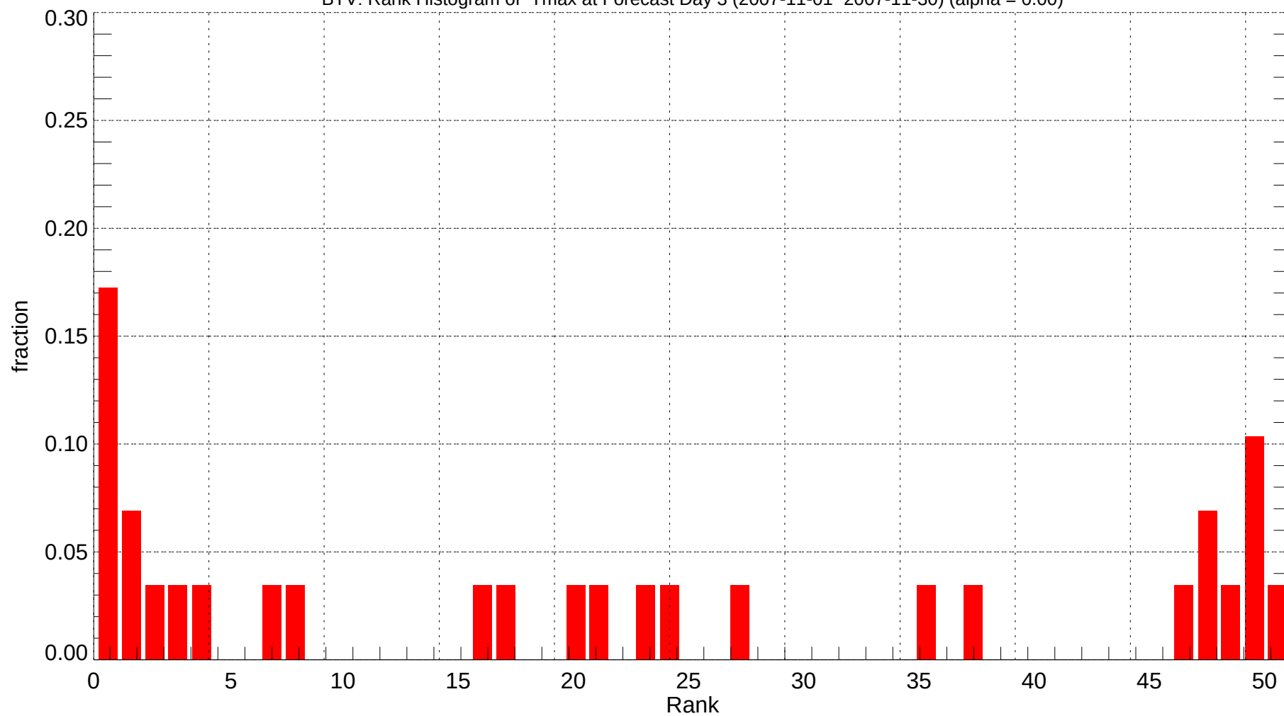
BTV: Rank Histogram of Tmax at Forecast Day 3 (2007-11-01~2007-11-30) (alpha = 0.00)
