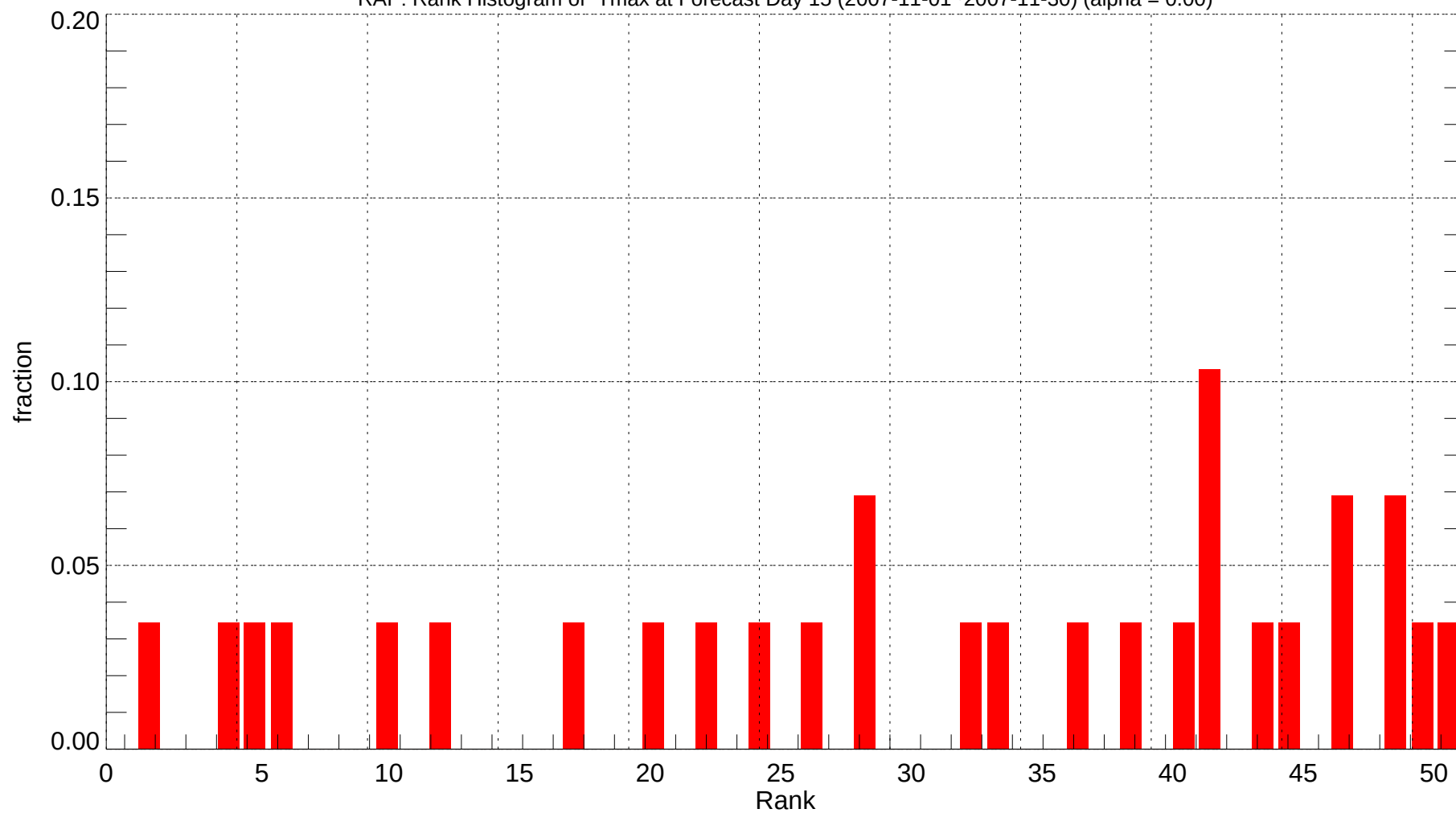
RAP: Rank Histogram of Tmax at Forecast Day 15 (2007-11-01~2007-11-30) (alpha = 0.00)
