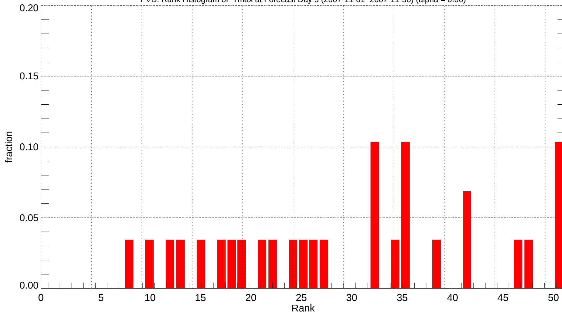
PVD: Rank Histogram of Tmax at Forecast Day 9 (2007-11-01~2007-11-30) (alpha = 0.00)
