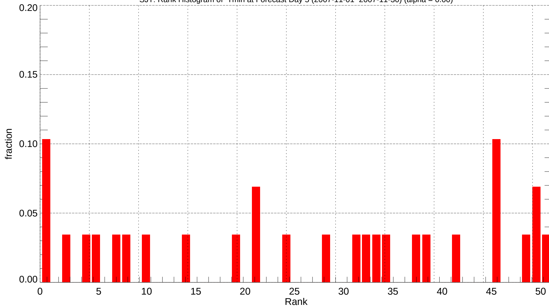
SJT: Rank Histogram of Tmin at Forecast Day 5 (2007-11-01~2007-11-30) (alpha = 0.00)
