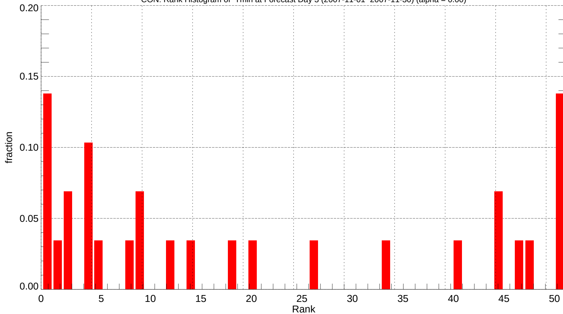
CON: Rank Histogram of Tmin at Forecast Day 3 (2007-11-01~2007-11-30) (alpha = 0.00)
