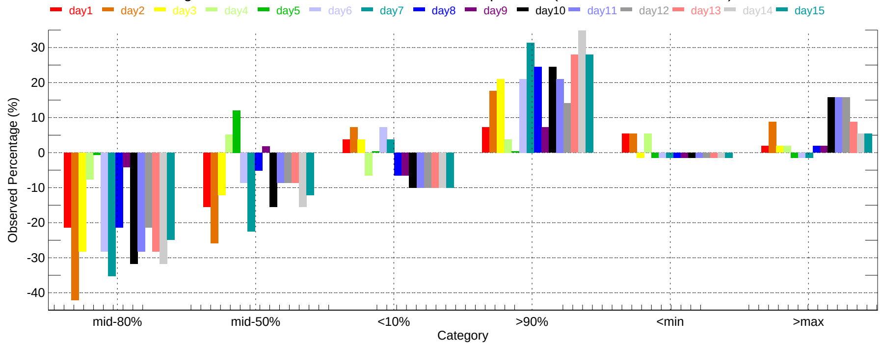
Observed Percentage Deviation of Ensembles - TUS: Max Temperature (2007-11-01~2007-11-30)
