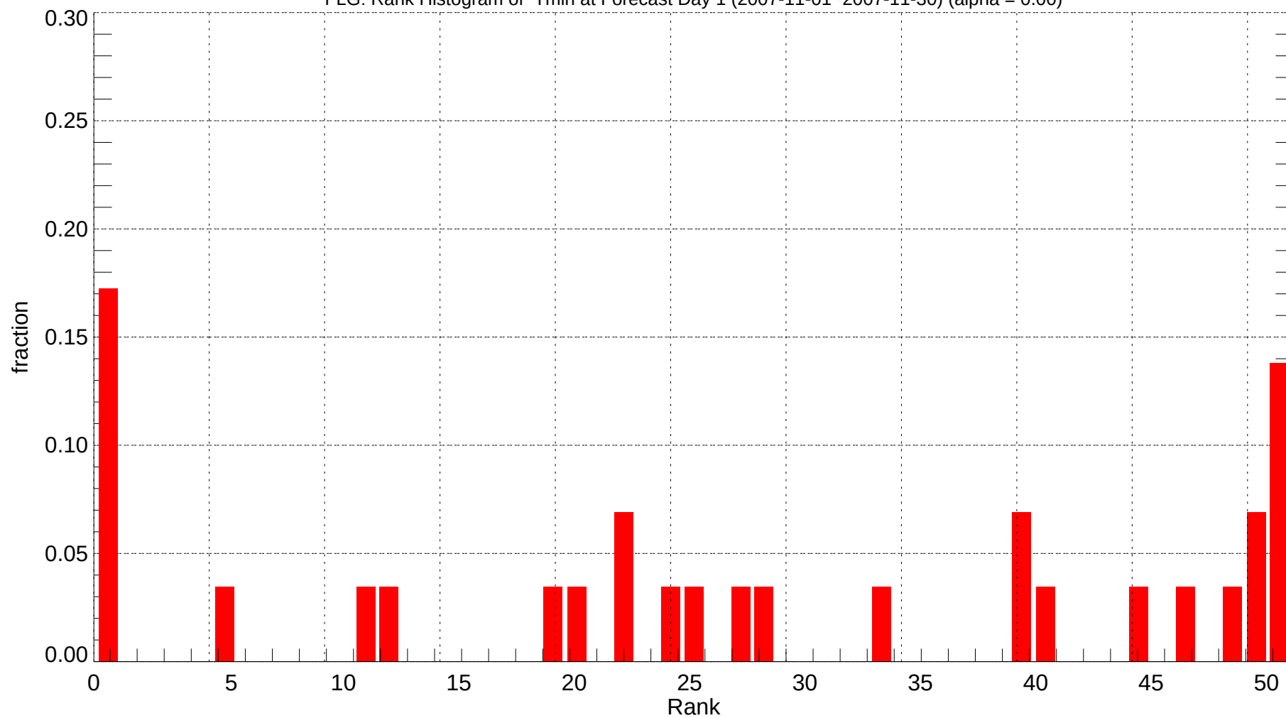
FLG: Rank Histogram of Tmin at Forecast Day 1 (2007-11-01~2007-11-30) (alpha = 0.00)
