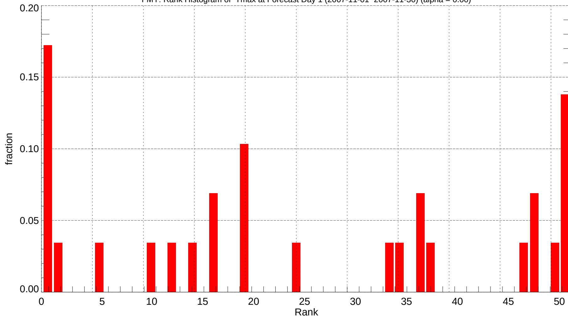
FMY: Rank Histogram of Tmax at Forecast Day 1 (2007-11-01~2007-11-30) (alpha = 0.00)
