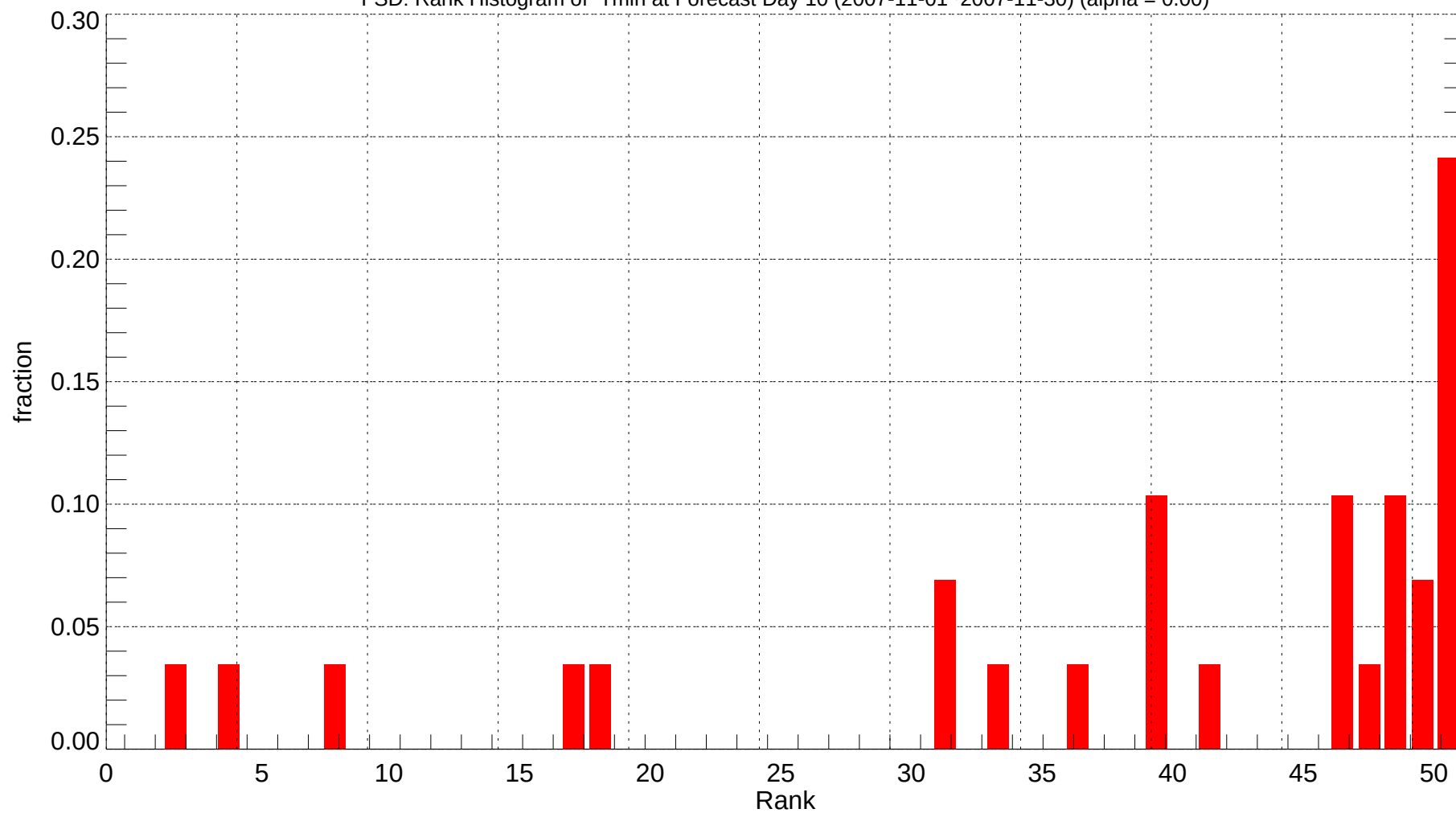
FSD: Rank Histogram of Tmin at Forecast Day 10 (2007-11-01~2007-11-30) (alpha = 0.00)
