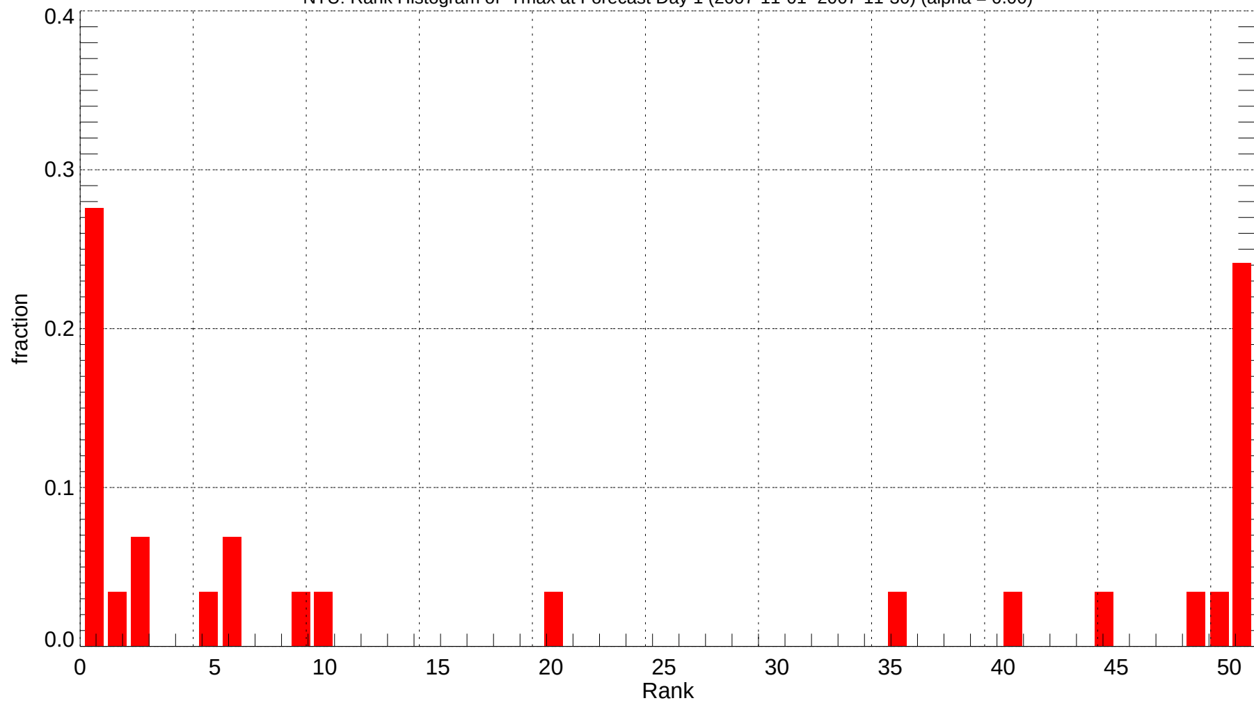
NTU: Rank Histogram of Tmax at Forecast Day 1 (2007-11-01~2007-11-30) (alpha = 0.00)
