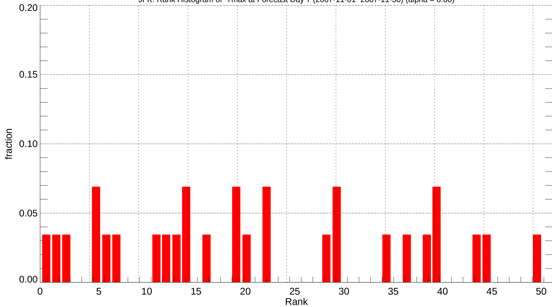
JFK: Rank Histogram of Tmax at Forecast Day 7 (2007-11-01~2007-11-30) (alpha = 0.00)
