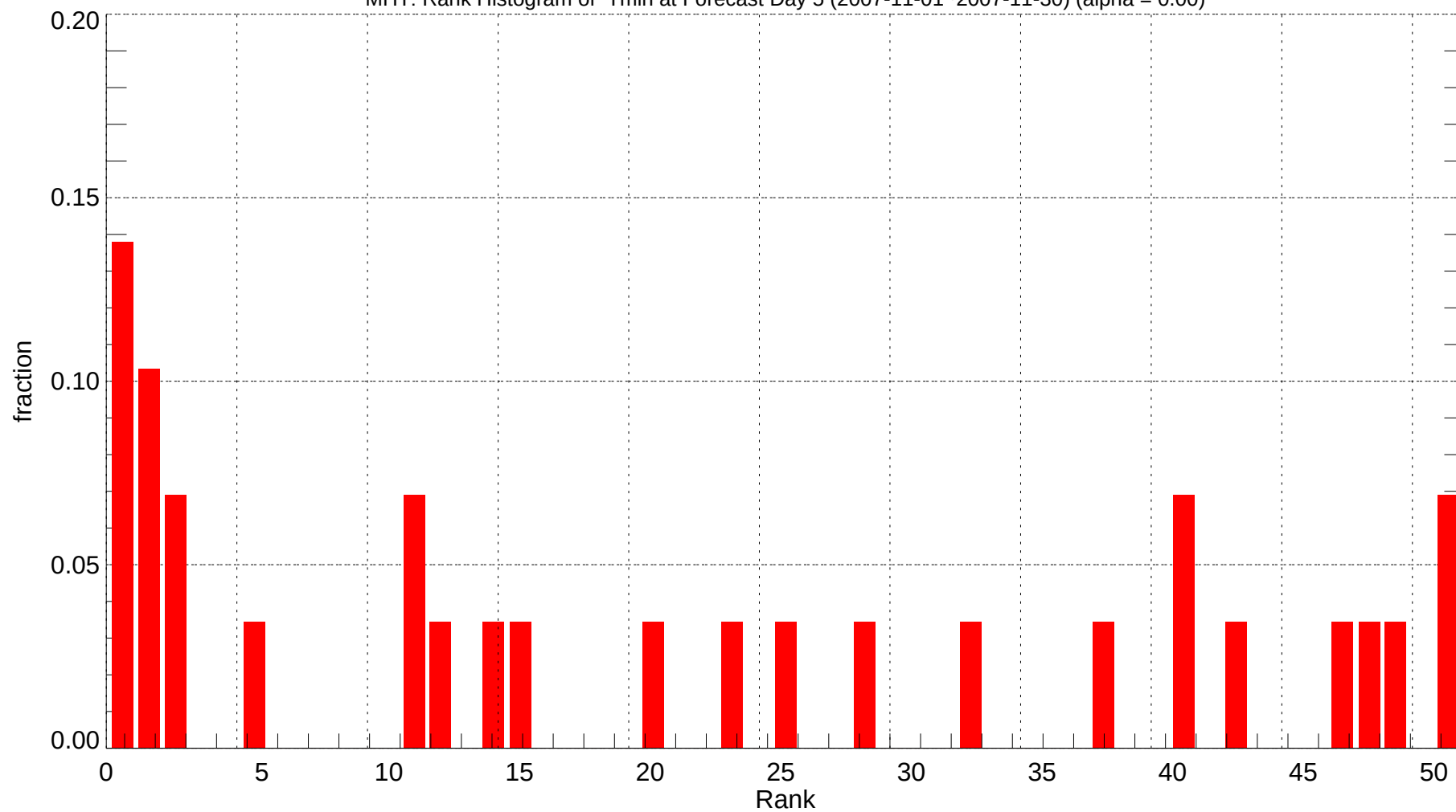
MHT: Rank Histogram of Tmin at Forecast Day 5 (2007-11-01~2007-11-30) (alpha = 0.00)
