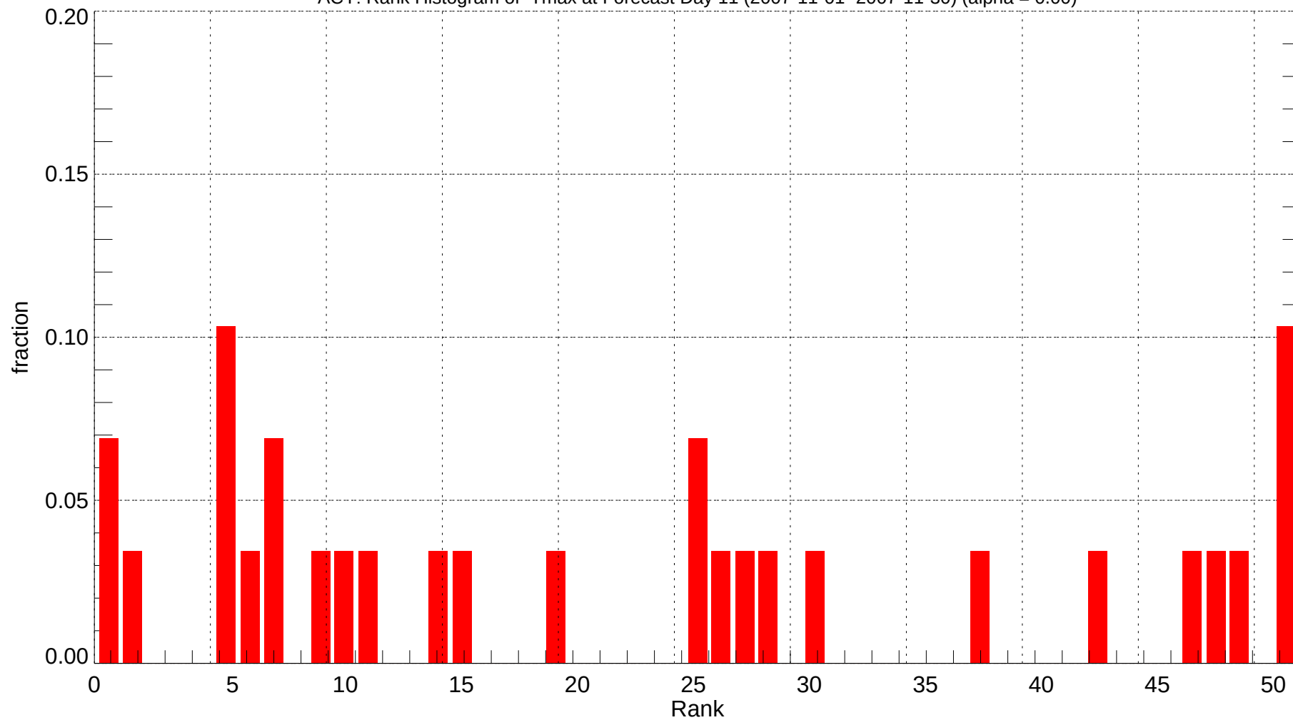
ACY: Rank Histogram of Tmax at Forecast Day 11 (2007-11-01~2007-11-30) (alpha = 0.00)
