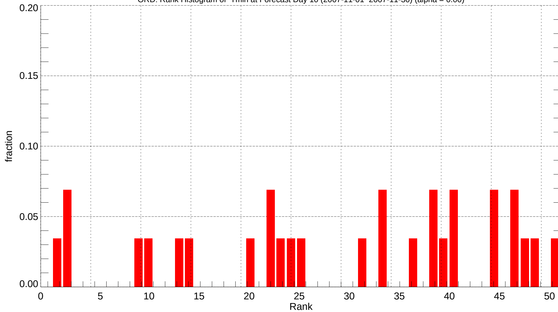
ORD: Rank Histogram of Tmin at Forecast Day 10 (2007-11-01~2007-11-30) (alpha = 0.00)
