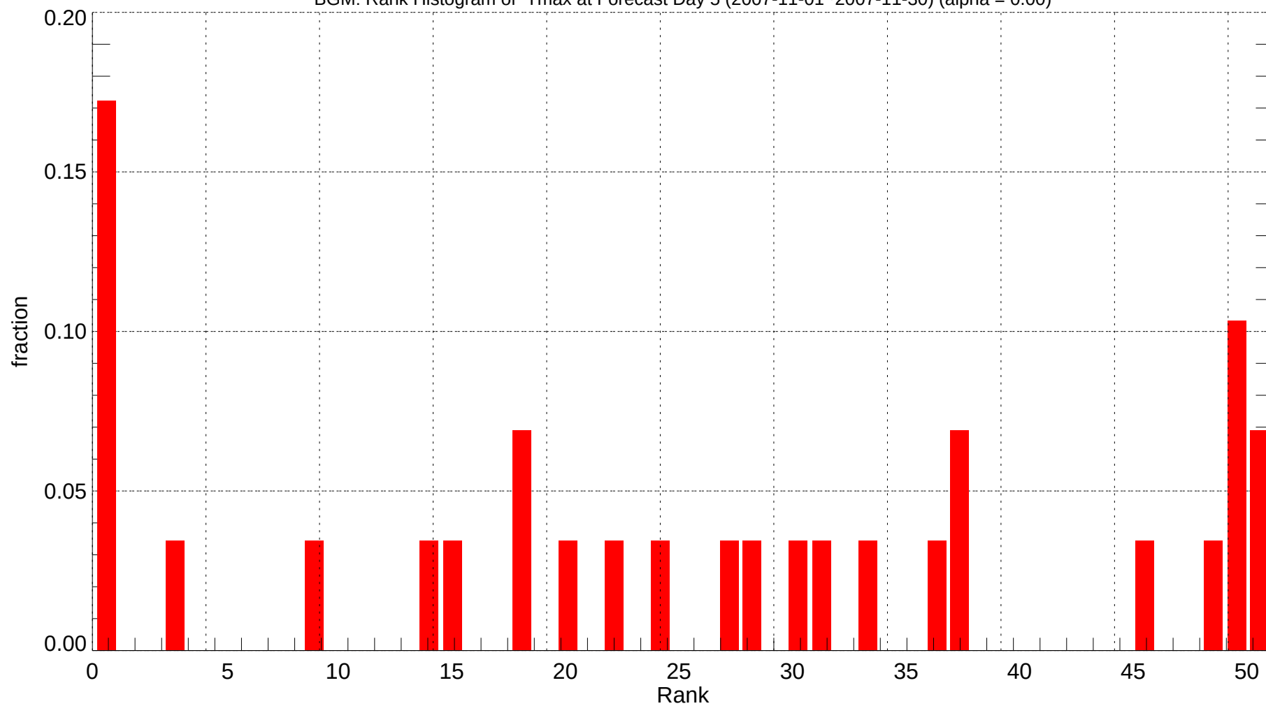
BGM: Rank Histogram of Tmax at Forecast Day 5 (2007-11-01~2007-11-30) (alpha = 0.00)
