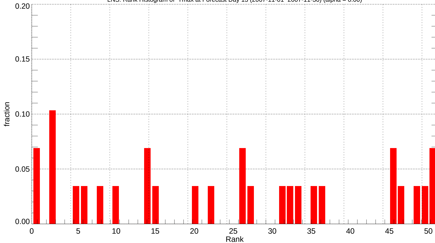
LNS: Rank Histogram of Tmax at Forecast Day 13 (2007-11-01~2007-11-30) (alpha = 0.00)
