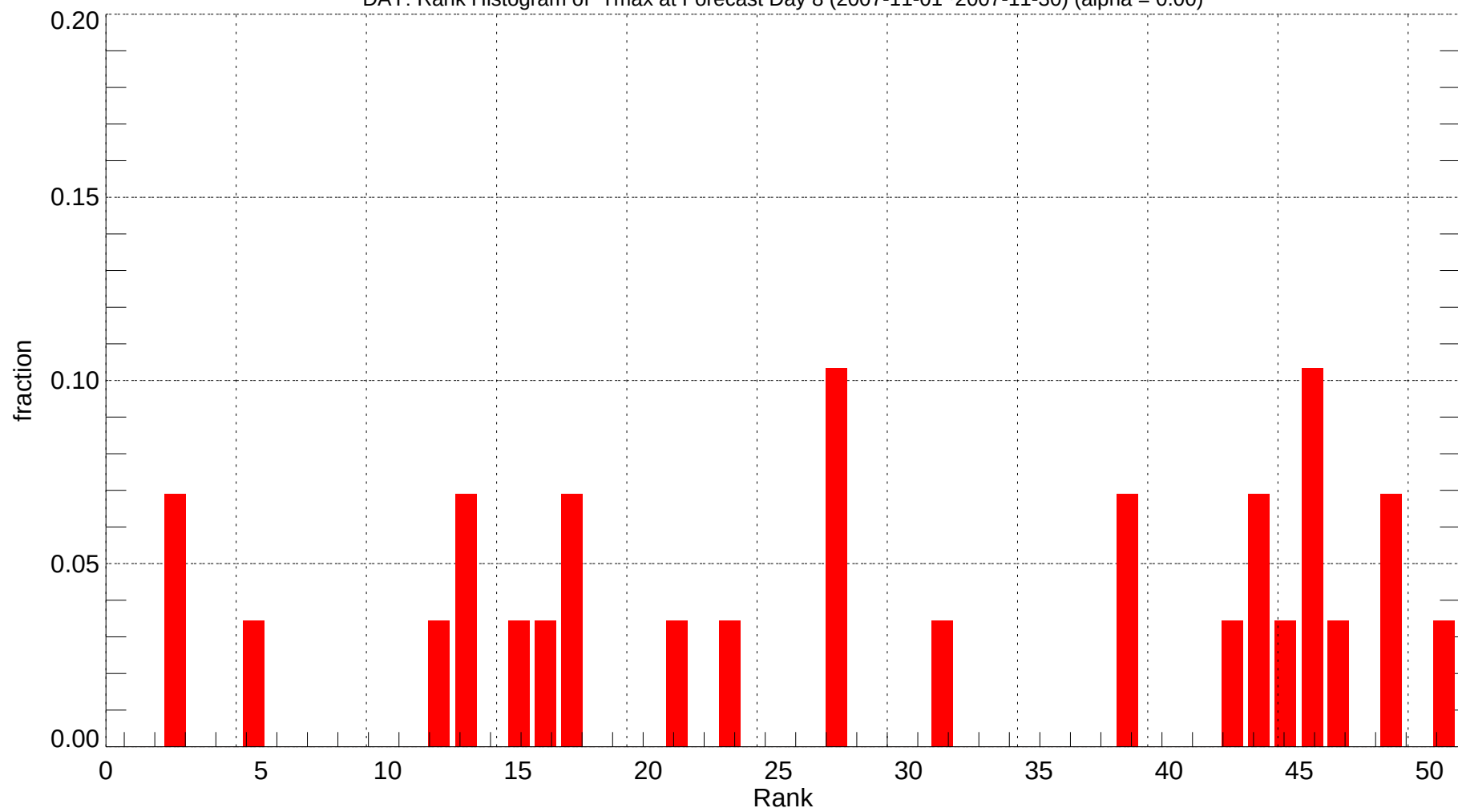
DAY: Rank Histogram of Tmax at Forecast Day 8 (2007-11-01~2007-11-30) (alpha = 0.00)
