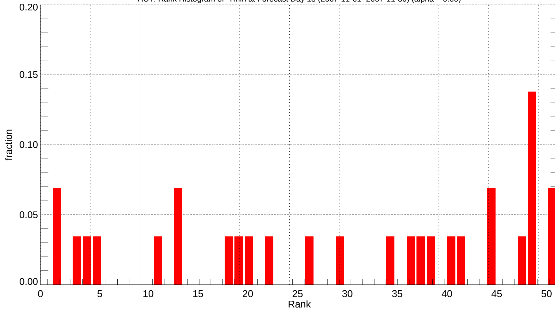
ACT: Rank Histogram of Tmin at Forecast Day 13 (2007-11-01~2007-11-30) (alpha = 0.00)
