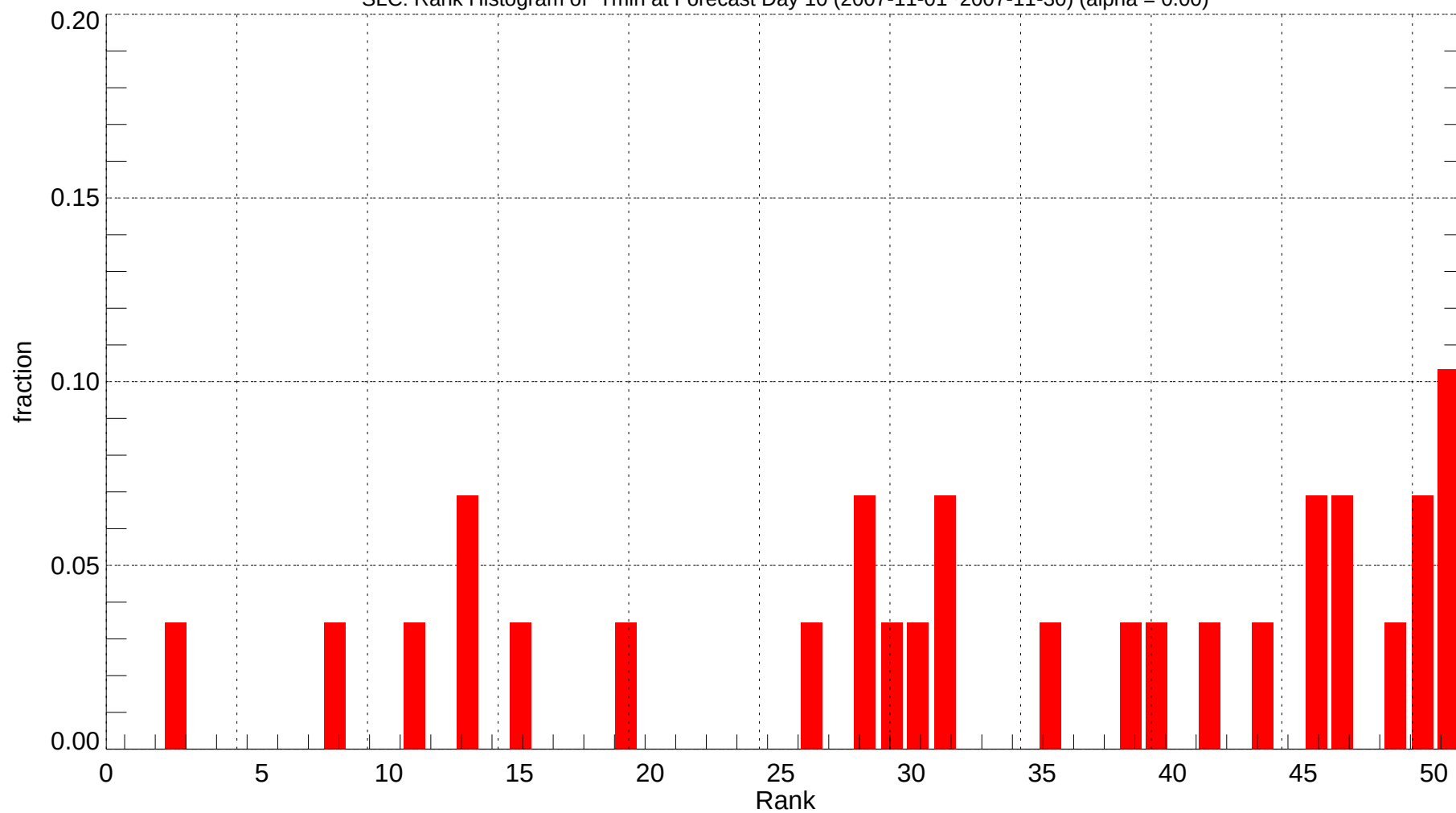
SLC: Rank Histogram of Tmin at Forecast Day 10 (2007-11-01~2007-11-30) (alpha = 0.00)
