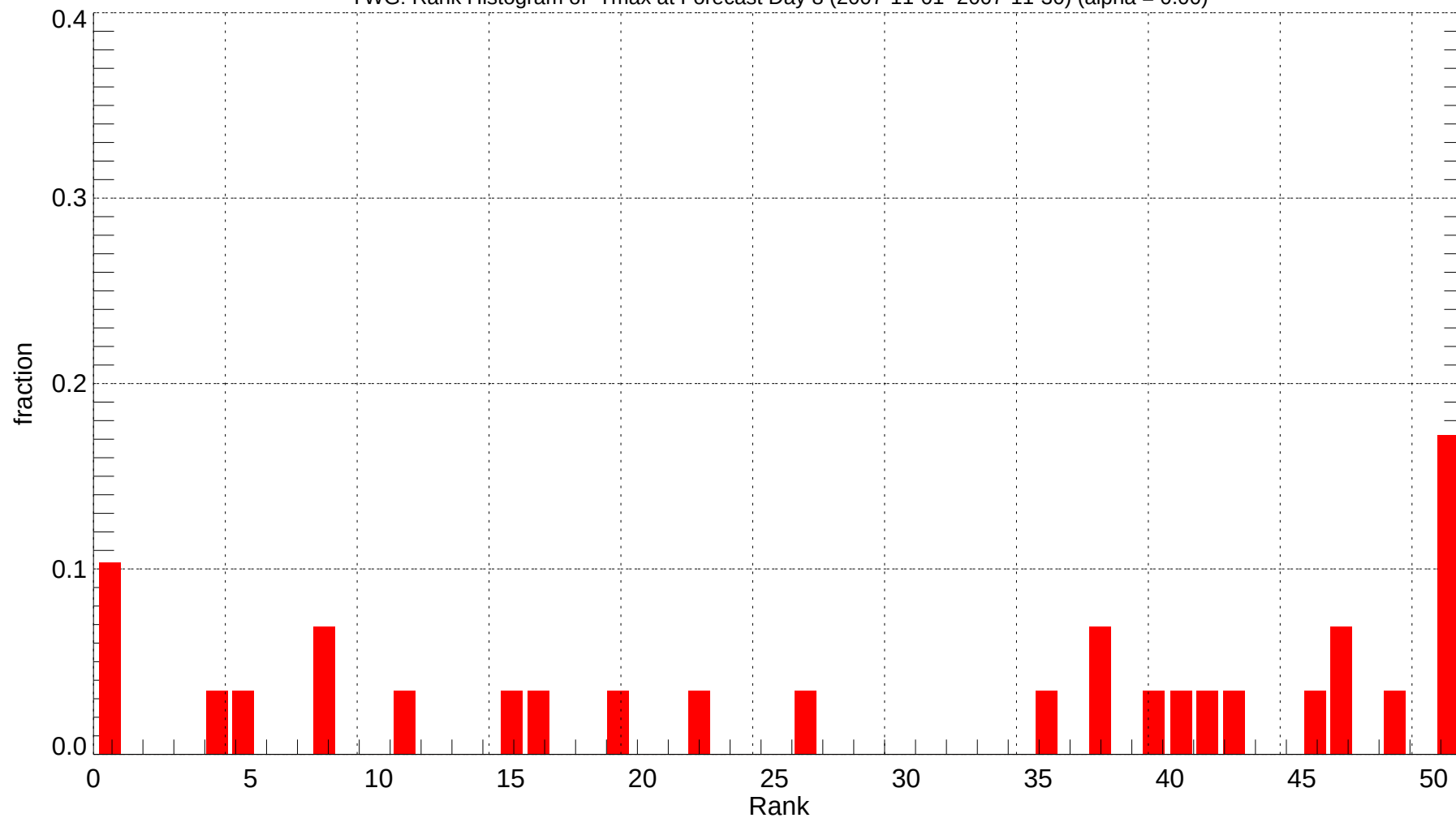
YWG: Rank Histogram of Tmax at Forecast Day 8 (2007-11-01~2007-11-30) (alpha = 0.00)
