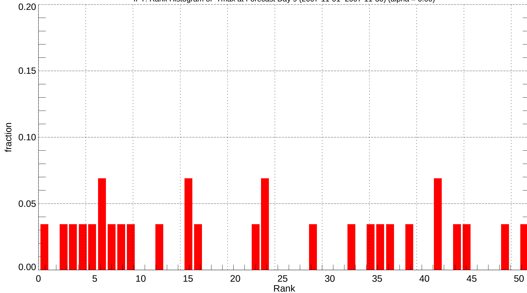
IPT: Rank Histogram of Tmax at Forecast Day 9 (2007-11-01~2007-11-30) (alpha = 0.00)
