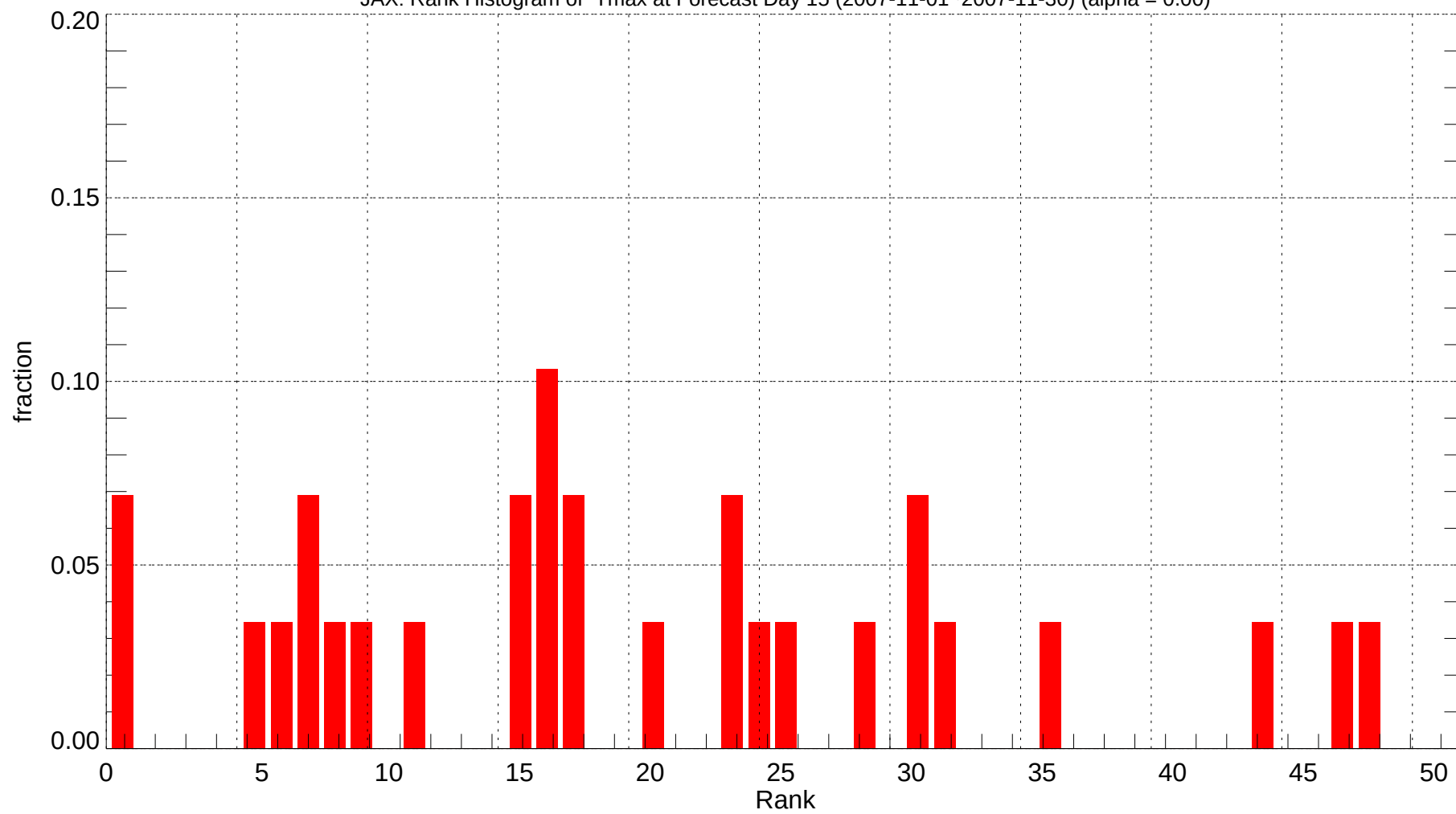
JAX: Rank Histogram of Tmax at Forecast Day 15 (2007-11-01~2007-11-30) (alpha = 0.00)
