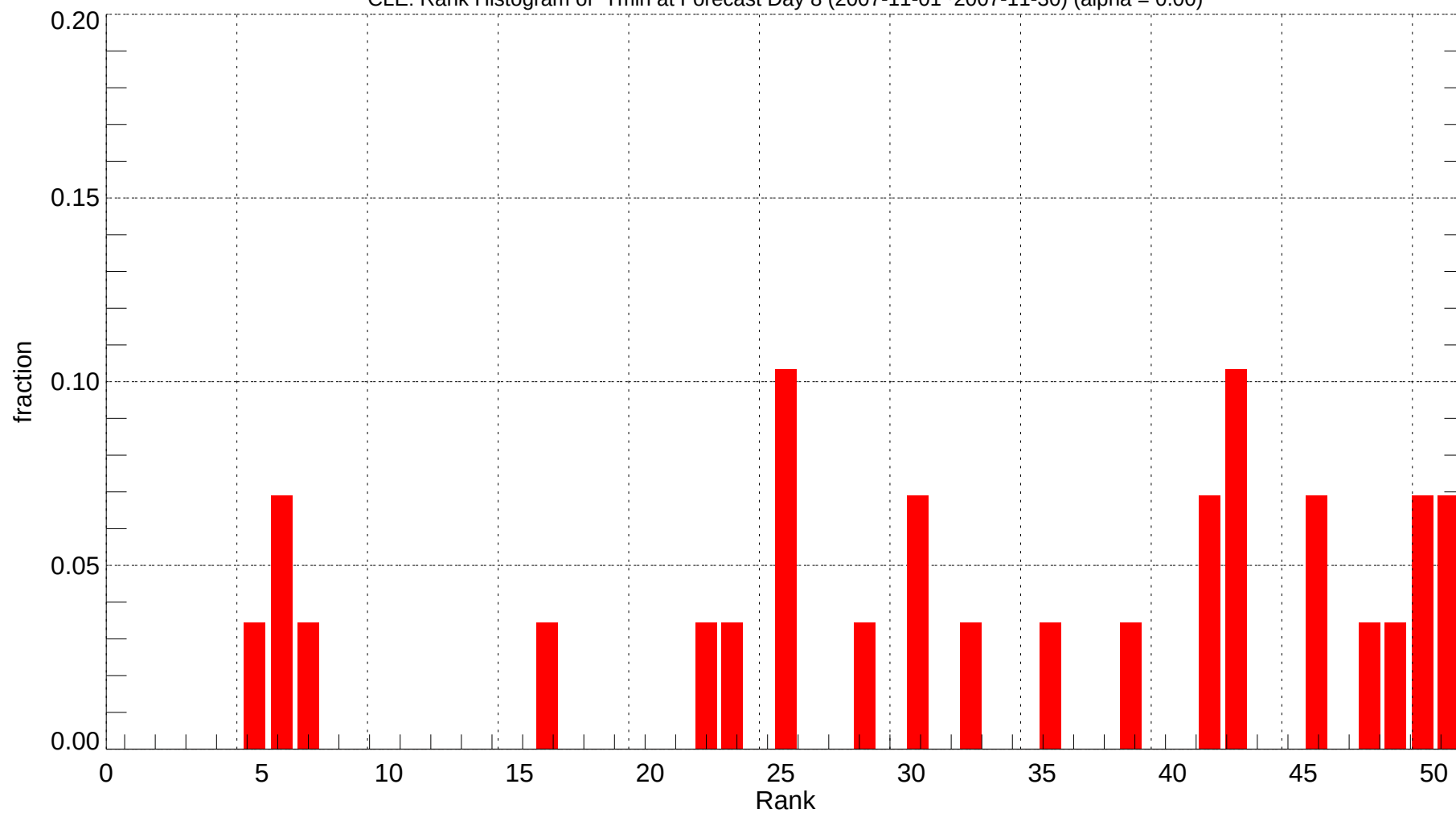
CLE: Rank Histogram of Tmin at Forecast Day 8 (2007-11-01~2007-11-30) (alpha = 0.00)
