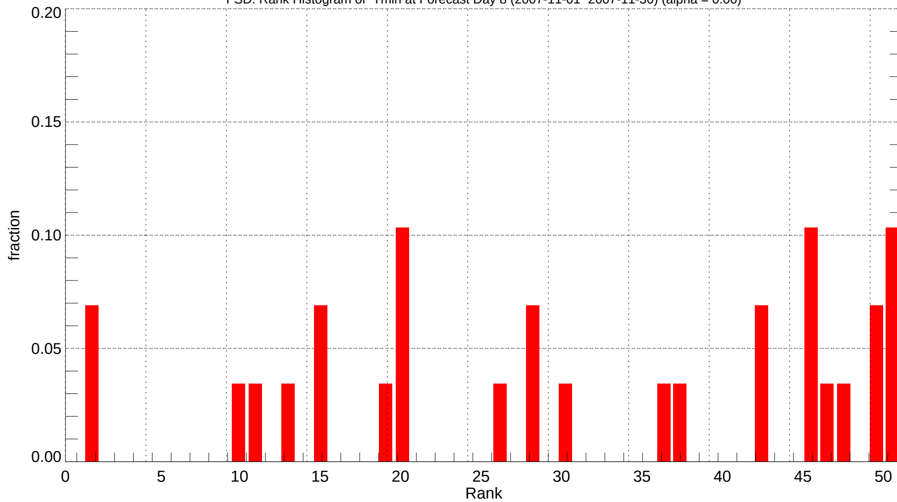
FSD: Rank Histogram of Tmin at Forecast Day 8 (2007-11-01~2007-11-30) (alpha = 0.00)
