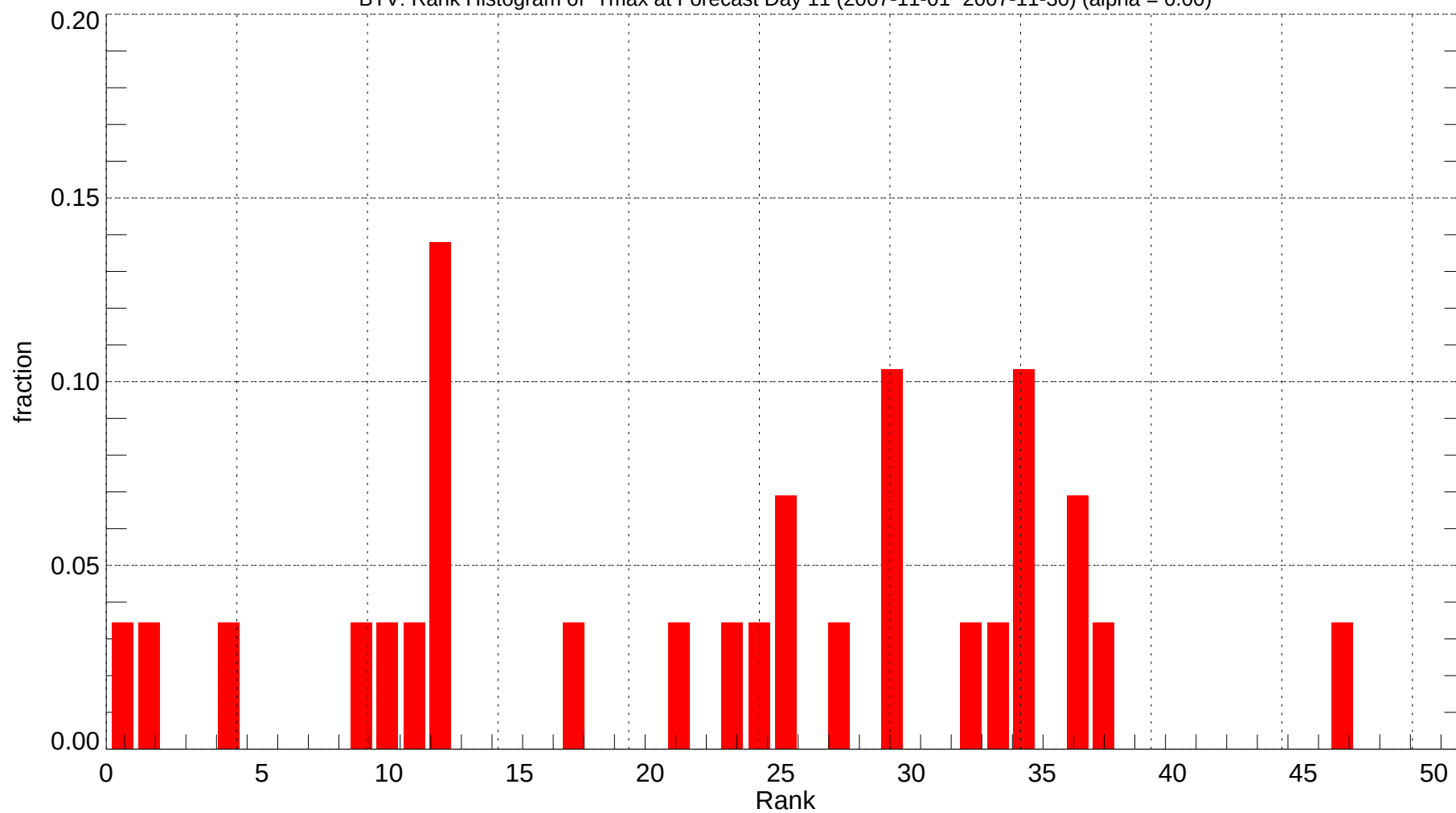
BTV: Rank Histogram of Tmax at Forecast Day 11 (2007-11-01~2007-11-30) (alpha = 0.00)
