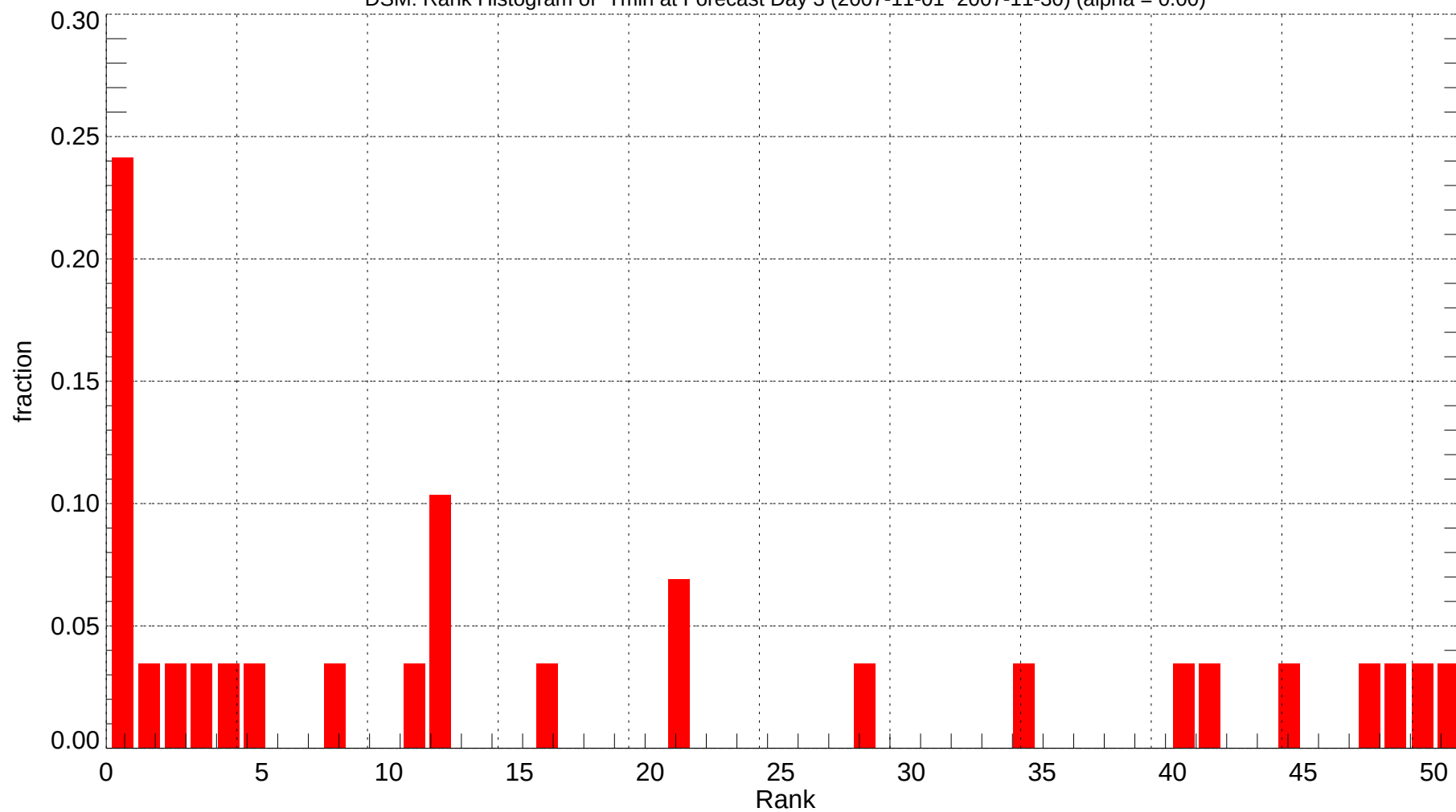
DSM: Rank Histogram of Tmin at Forecast Day 3 (2007-11-01~2007-11-30) (alpha = 0.00)
