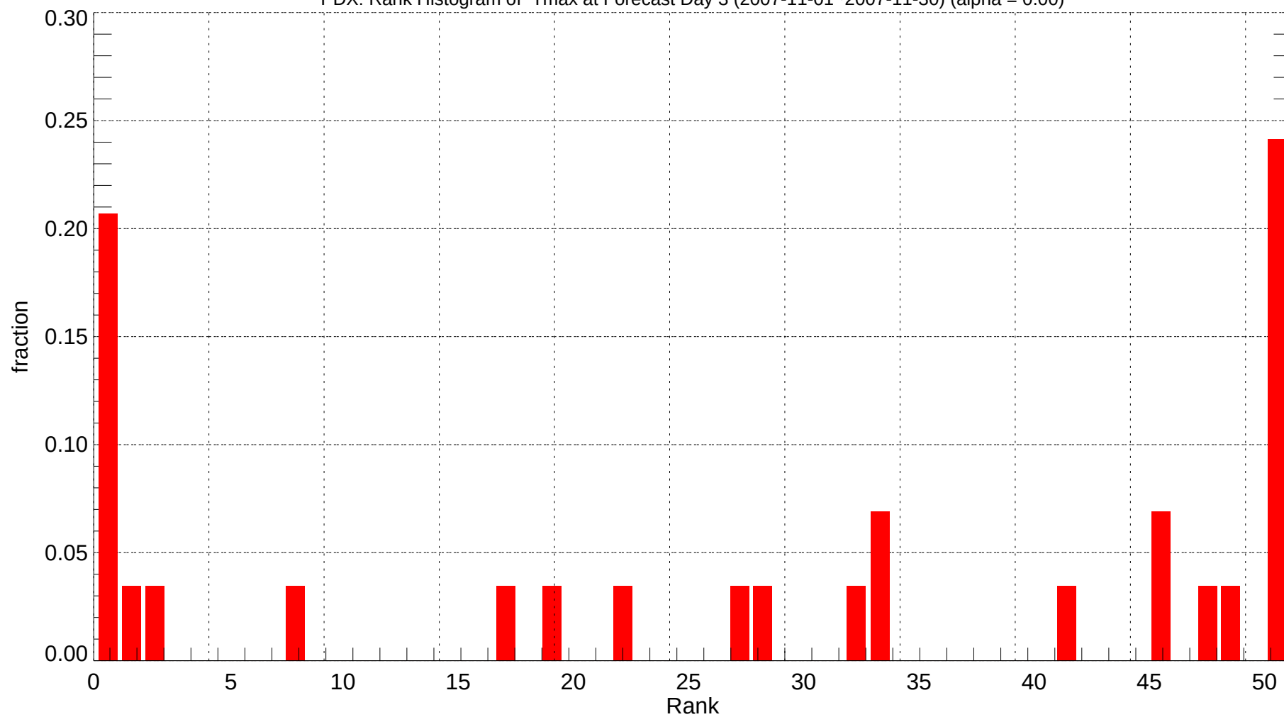
PDX: Rank Histogram of Tmax at Forecast Day 3 (2007-11-01~2007-11-30) (alpha = 0.00)
