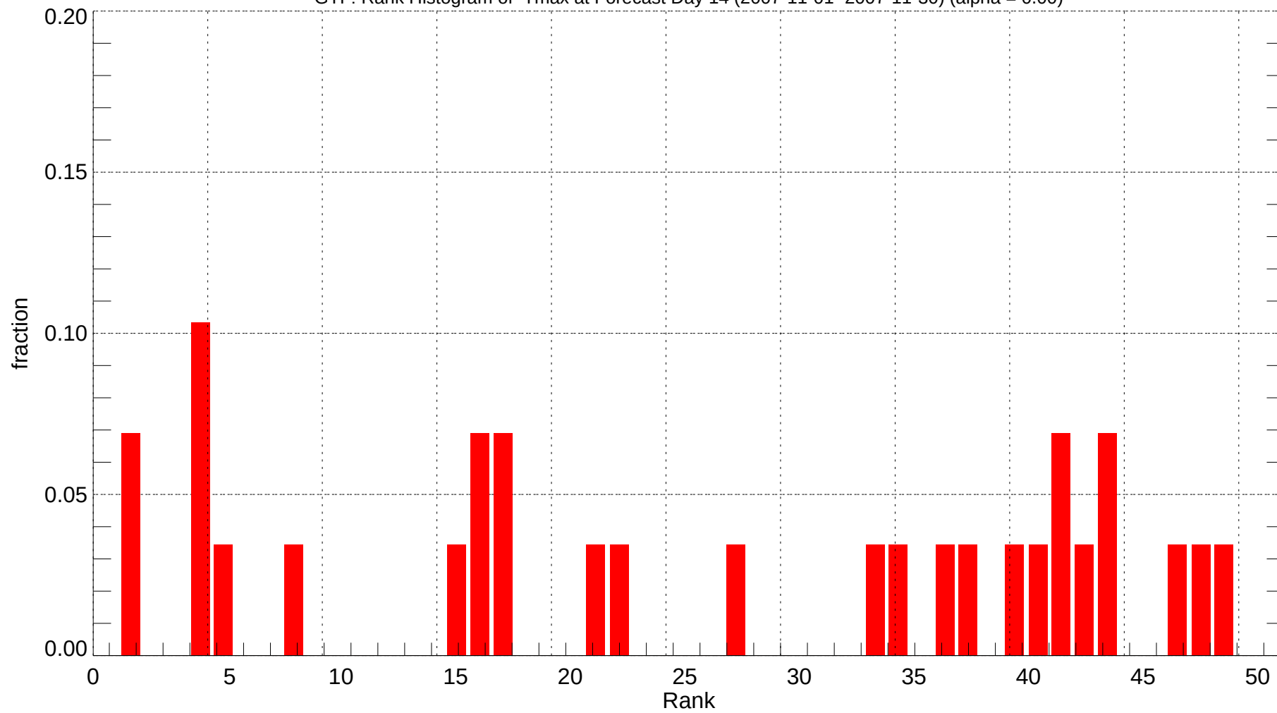
GTF: Rank Histogram of Tmax at Forecast Day 14 (2007-11-01~2007-11-30) (alpha = 0.00)
