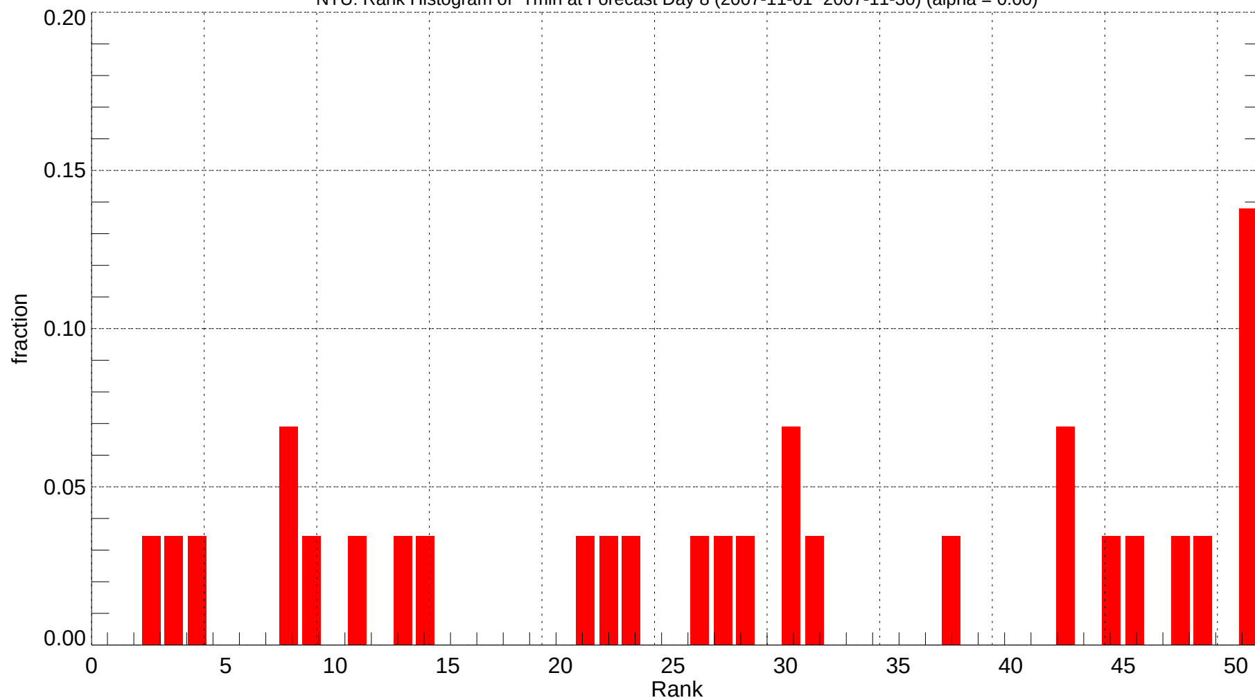
NTU: Rank Histogram of Tmin at Forecast Day 8 (2007-11-01~2007-11-30) (alpha = 0.00)
