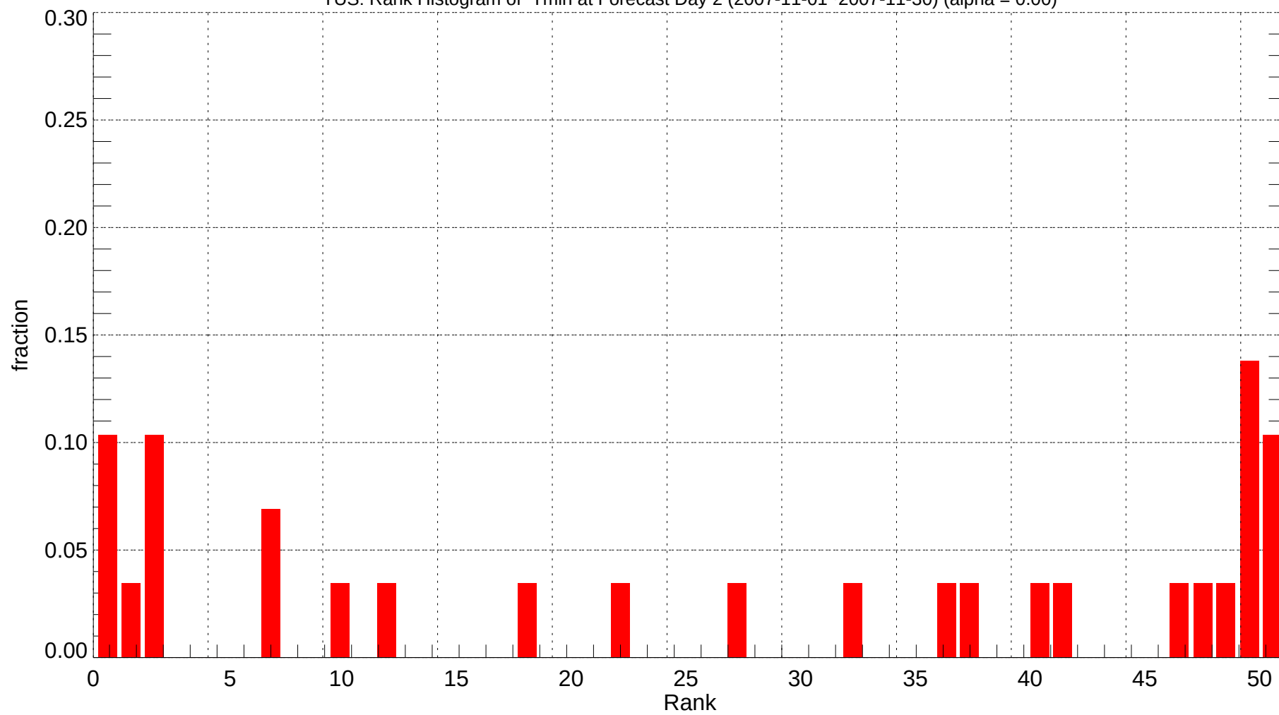
TUS: Rank Histogram of Tmin at Forecast Day 2 (2007-11-01~2007-11-30) (alpha = 0.00)
