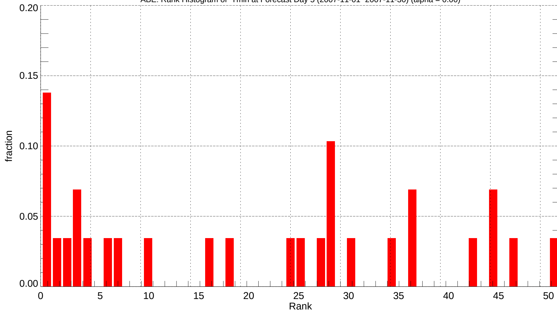
ABE: Rank Histogram of Tmin at Forecast Day 5 (2007-11-01~2007-11-30) (alpha = 0.00)
