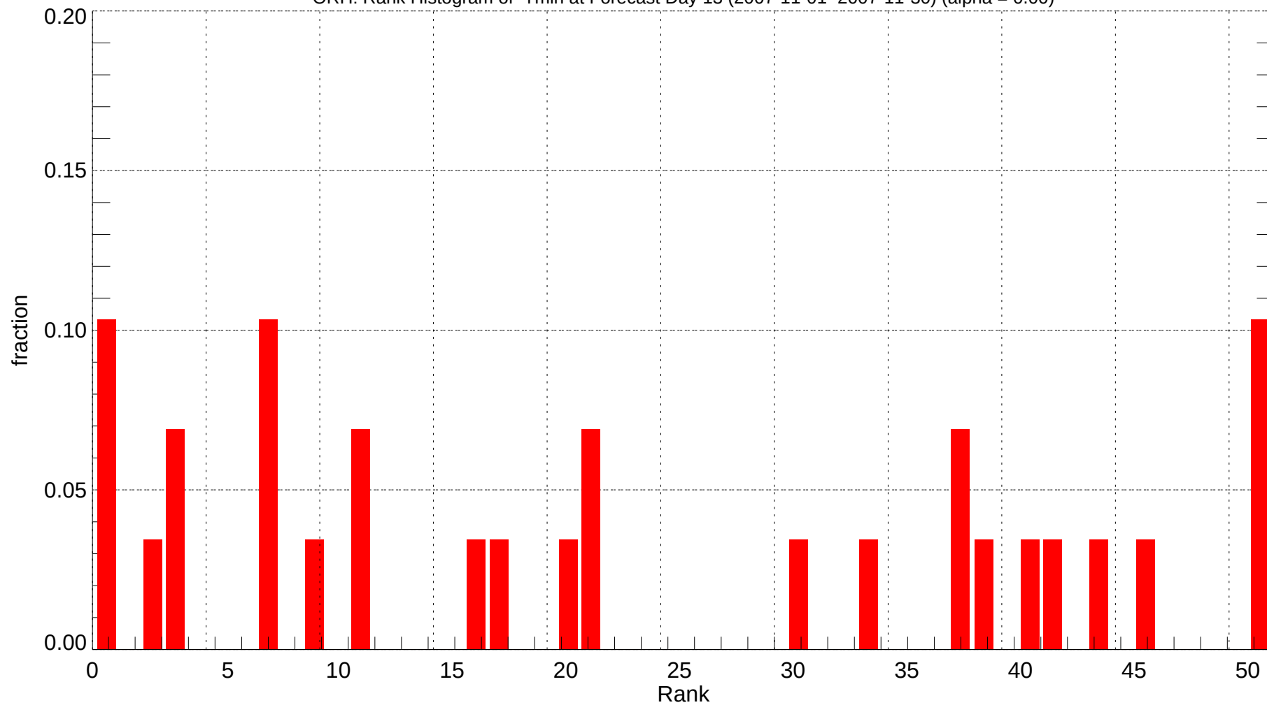
ORH: Rank Histogram of Tmin at Forecast Day 13 (2007-11-01~2007-11-30) (alpha = 0.00)
