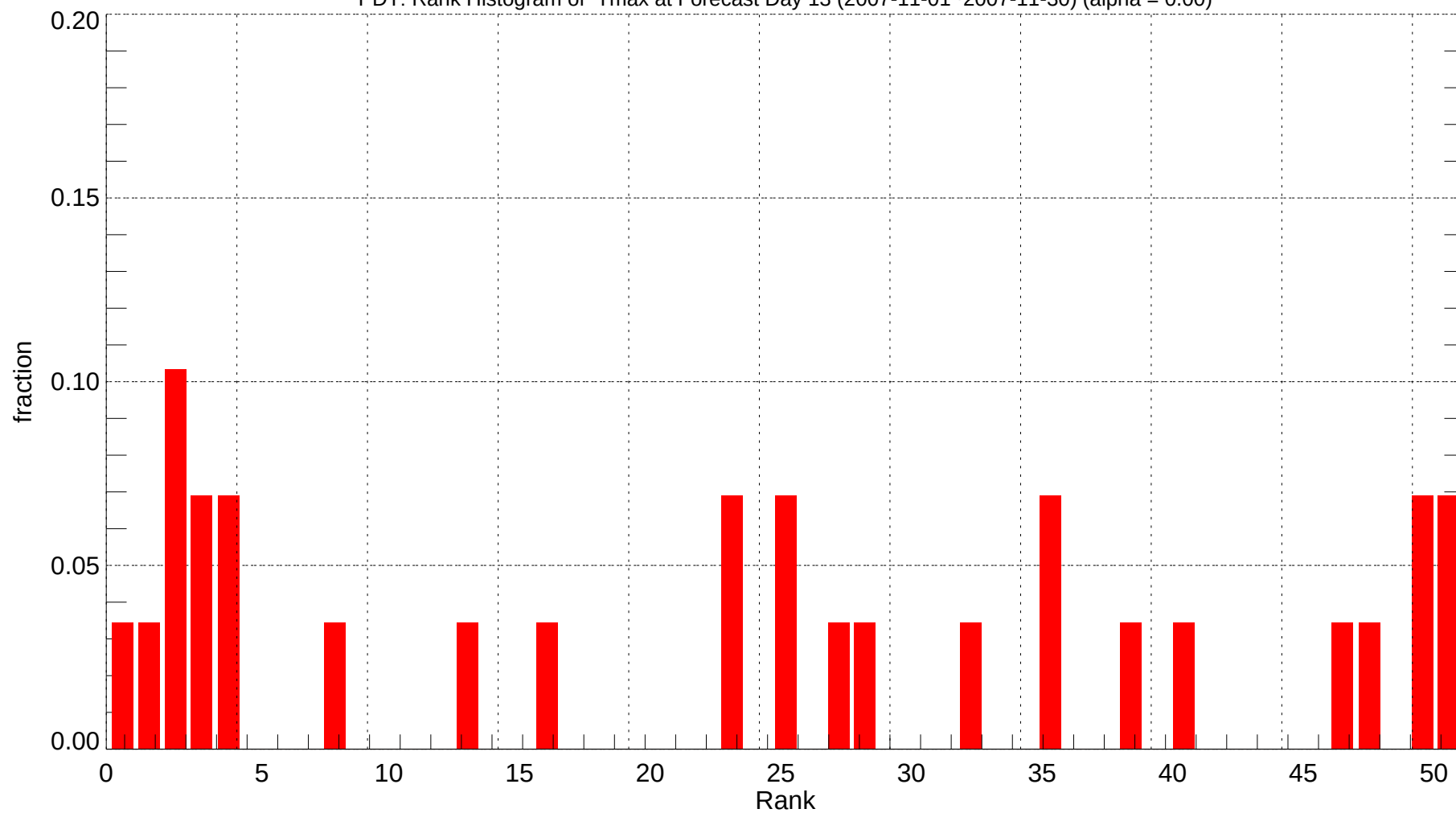
PDT: Rank Histogram of Tmax at Forecast Day 13 (2007-11-01~2007-11-30) (alpha = 0.00)
