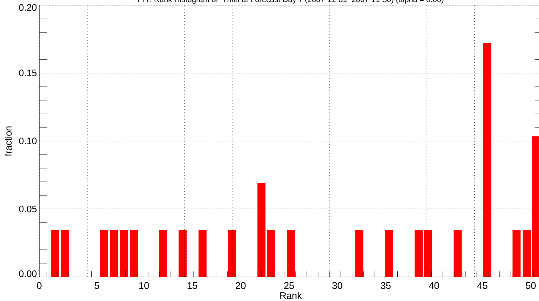
PIT: Rank Histogram of Tmin at Forecast Day 7 (2007-11-01~2007-11-30) (alpha = 0.00)
