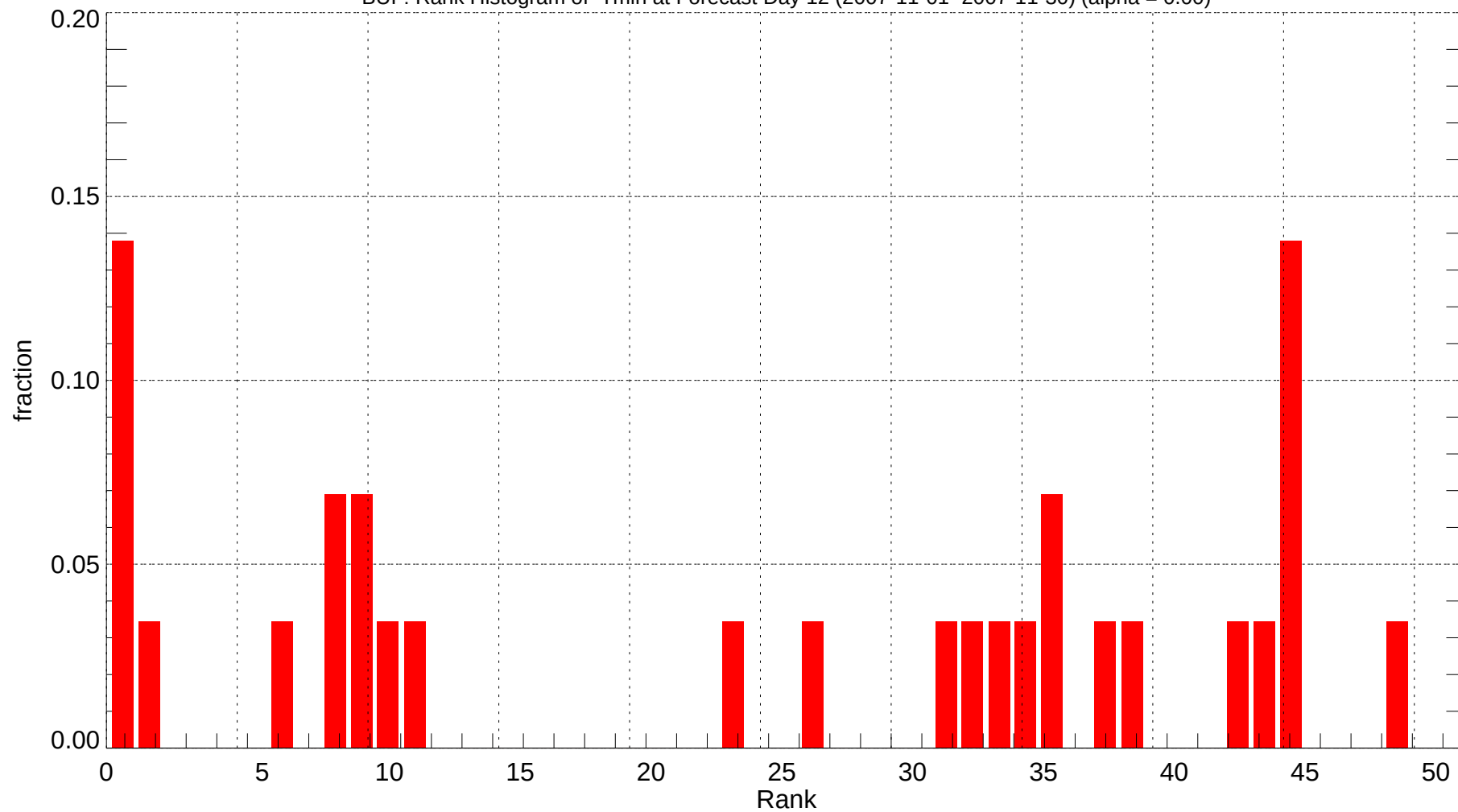
BUF: Rank Histogram of Tmin at Forecast Day 12 (2007-11-01~2007-11-30) (alpha = 0.00)
