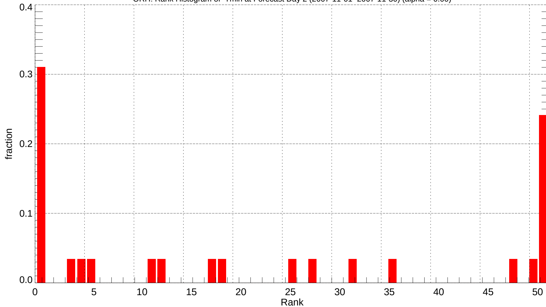
ORH: Rank Histogram of Tmin at Forecast Day 2 (2007-11-01~2007-11-30) (alpha = 0.00)
