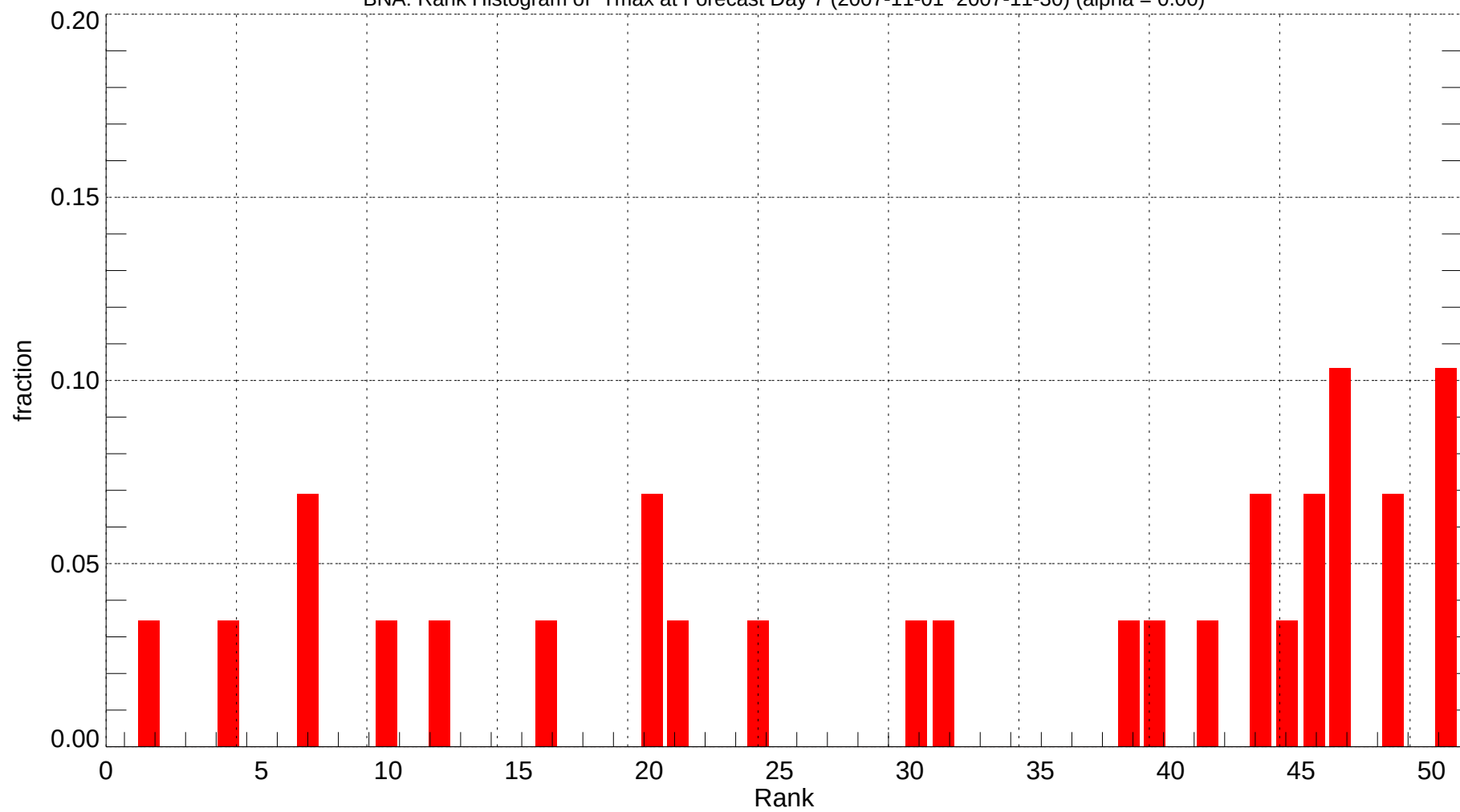
BNA: Rank Histogram of Tmax at Forecast Day 7 (2007-11-01~2007-11-30) (alpha = 0.00)
