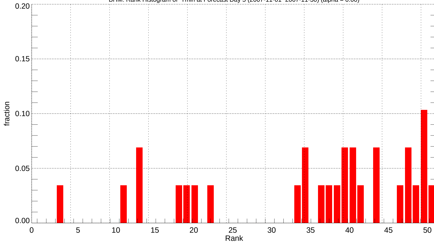
BHM: Rank Histogram of Tmin at Forecast Day 5 (2007-11-01~2007-11-30) (alpha = 0.00)
