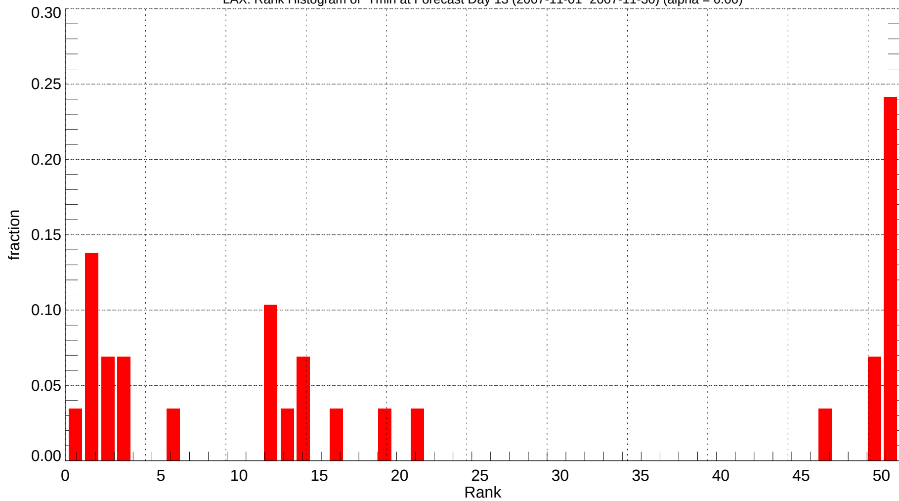
LAX: Rank Histogram of Tmin at Forecast Day 13 (2007-11-01~2007-11-30) (alpha = 0.00)
