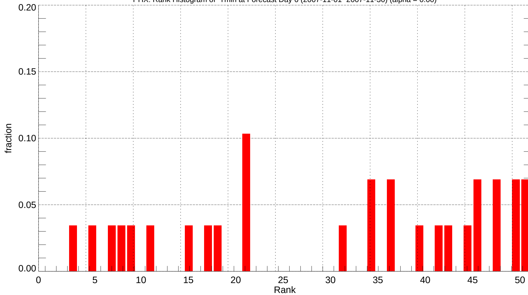
PHX: Rank Histogram of Tmin at Forecast Day 6 (2007-11-01~2007-11-30) (alpha = 0.00)
