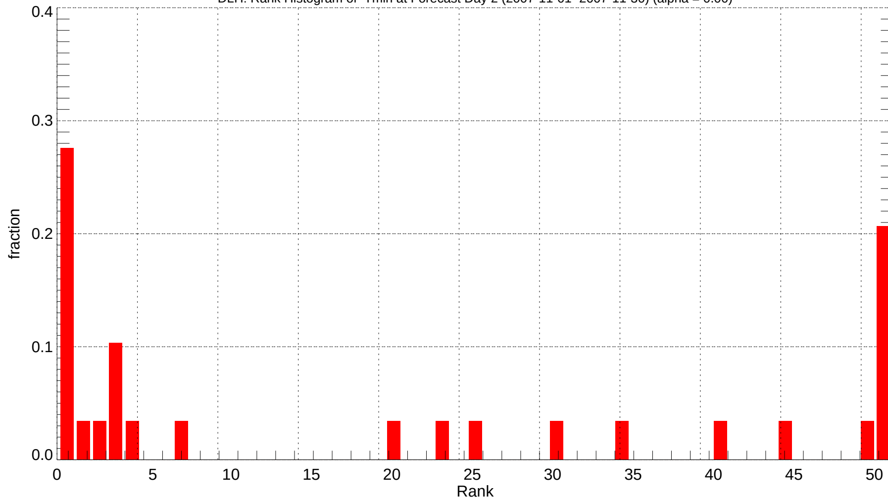
DLH: Rank Histogram of Tmin at Forecast Day 2 (2007-11-01~2007-11-30) (alpha = 0.00)
