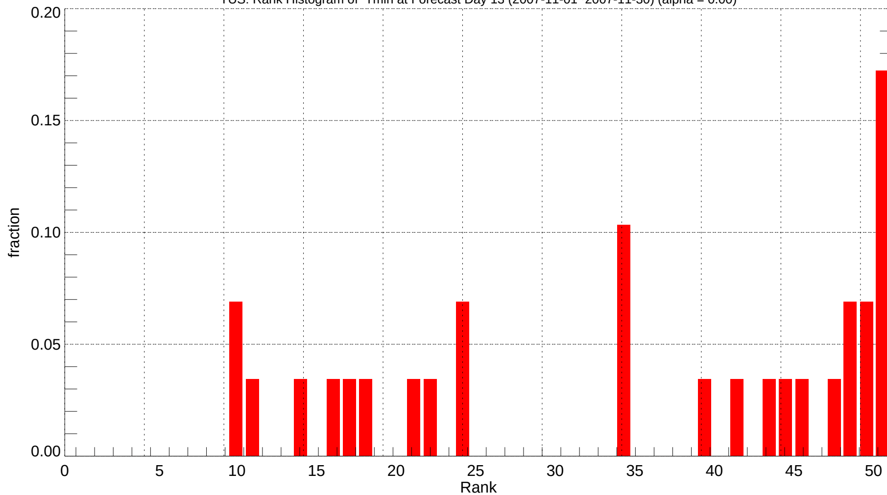
TUS: Rank Histogram of Tmin at Forecast Day 13 (2007-11-01~2007-11-30) (alpha = 0.00)
