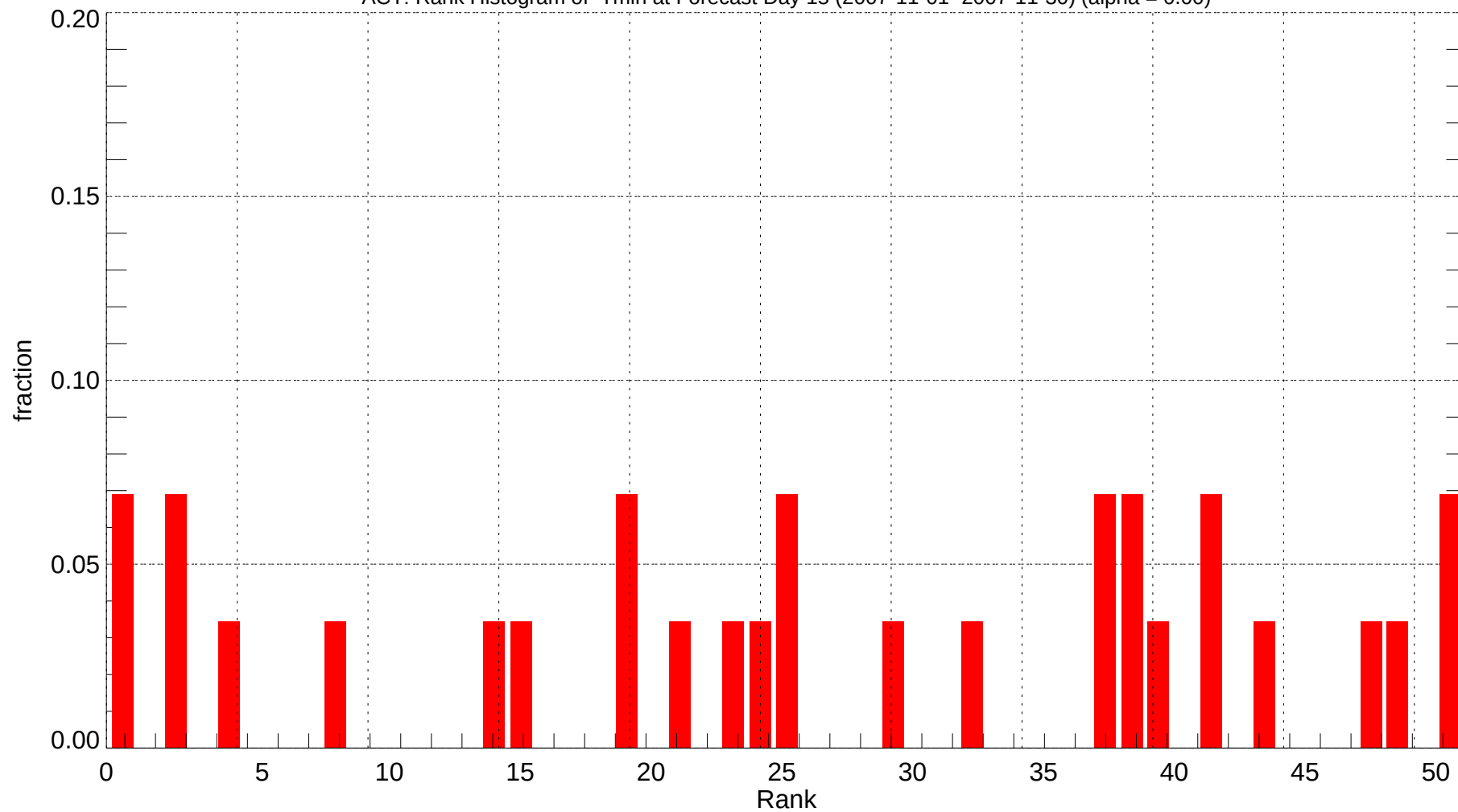
ACT: Rank Histogram of Tmin at Forecast Day 15 (2007-11-01~2007-11-30) (alpha = 0.00)
