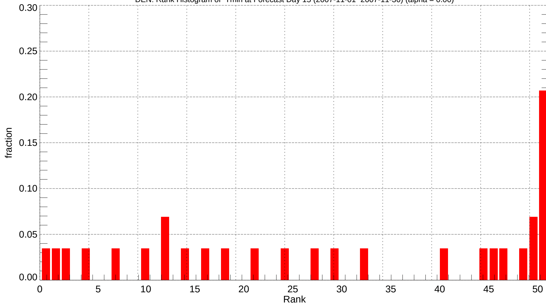
DEN: Rank Histogram of Tmin at Forecast Day 15 (2007-11-01~2007-11-30) (alpha = 0.00)
