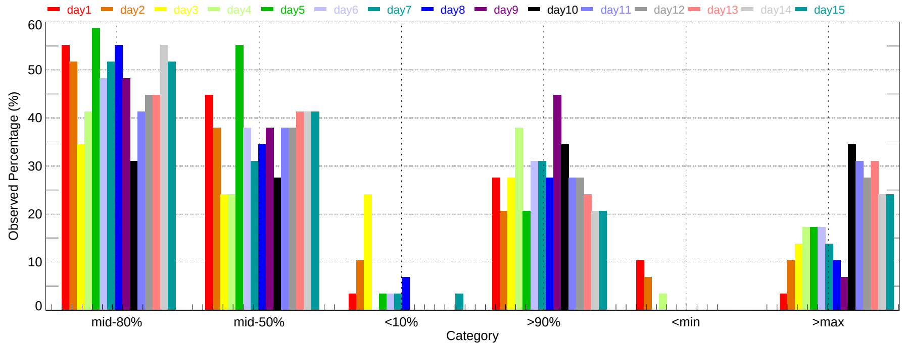
Observed Percentage of Ensembles - LIT: Max Temperature (2007-11-01~2007-11-30)
