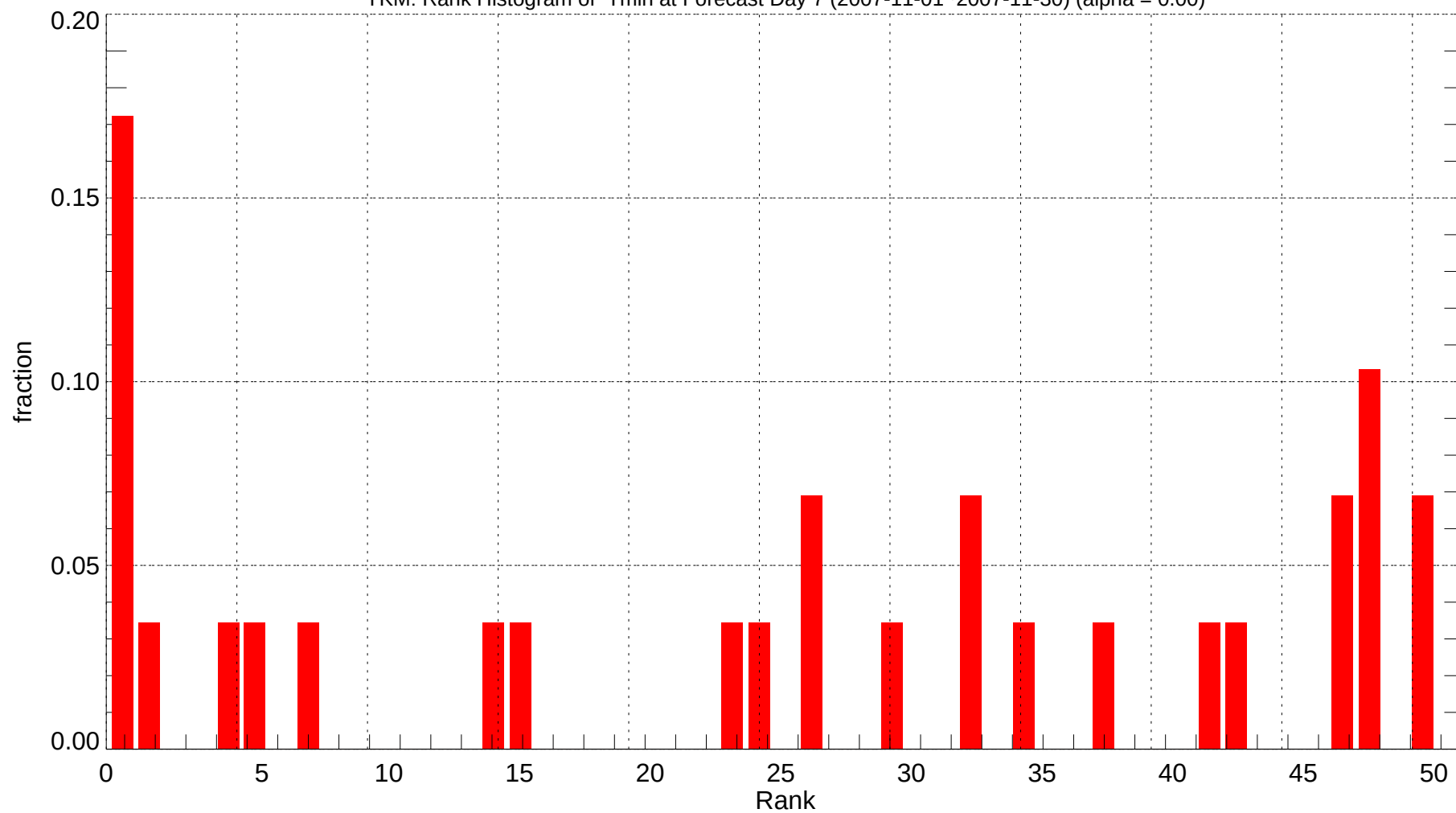
YKM: Rank Histogram of Tmin at Forecast Day 7 (2007-11-01~2007-11-30) (alpha = 0.00)
