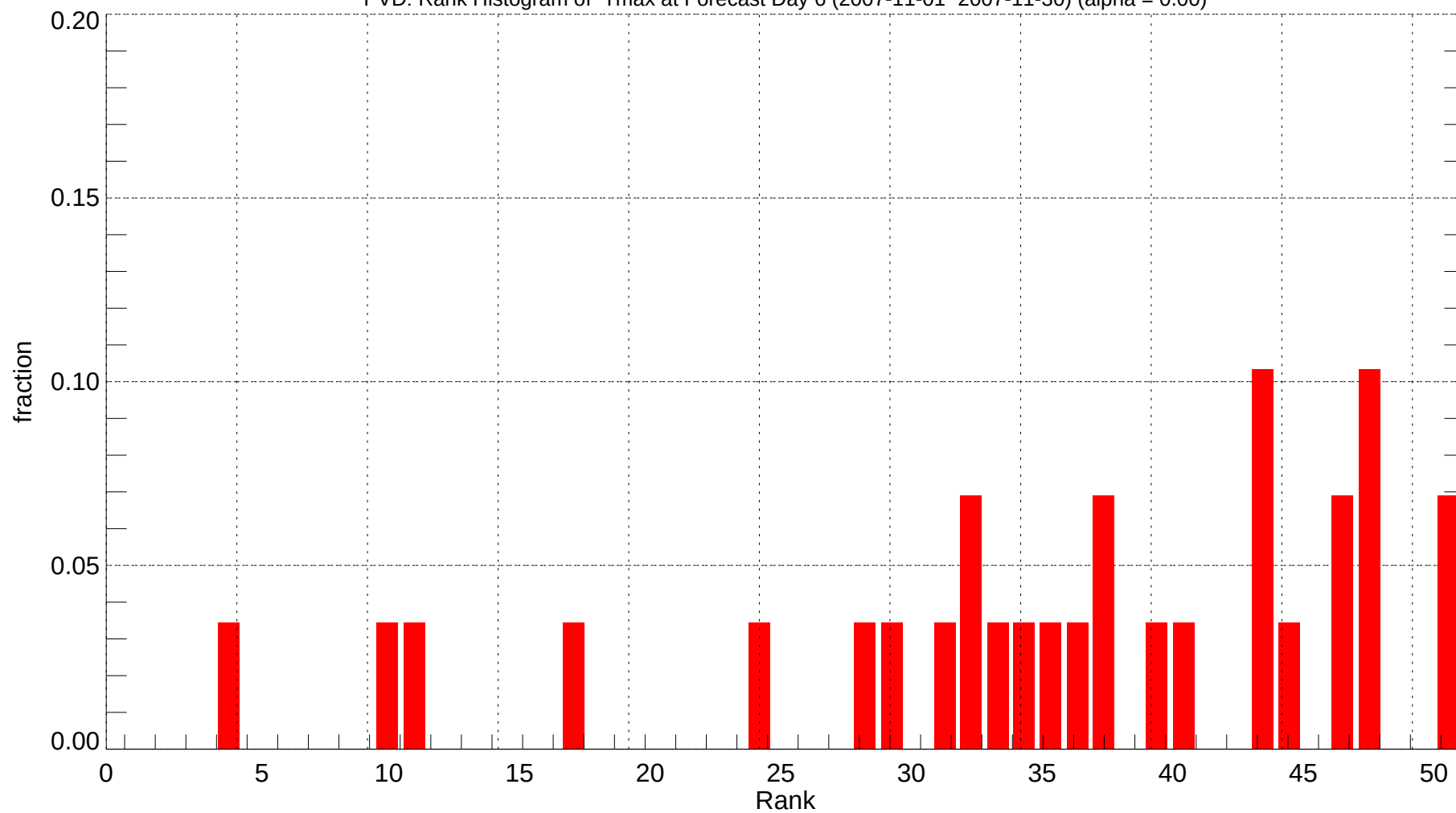
PVD: Rank Histogram of Tmax at Forecast Day 6 (2007-11-01~2007-11-30) (alpha = 0.00)
