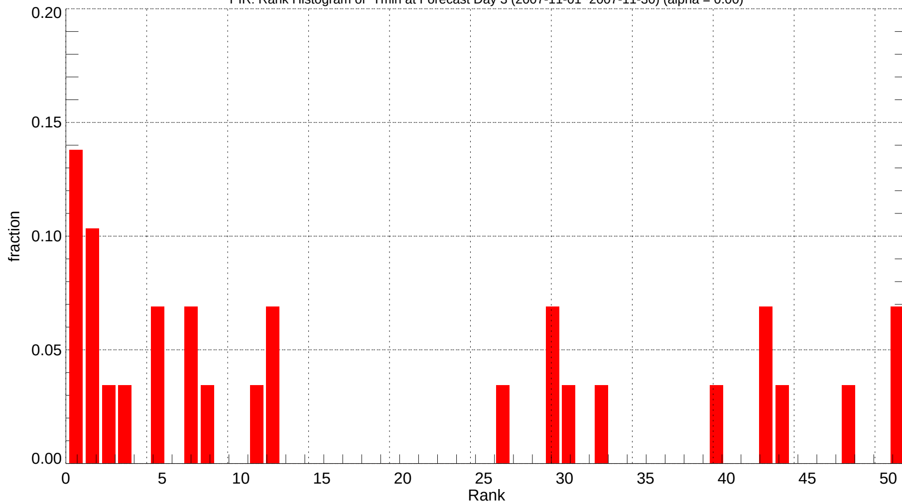
PIR: Rank Histogram of Tmin at Forecast Day 3 (2007-11-01~2007-11-30) (alpha = 0.00)
