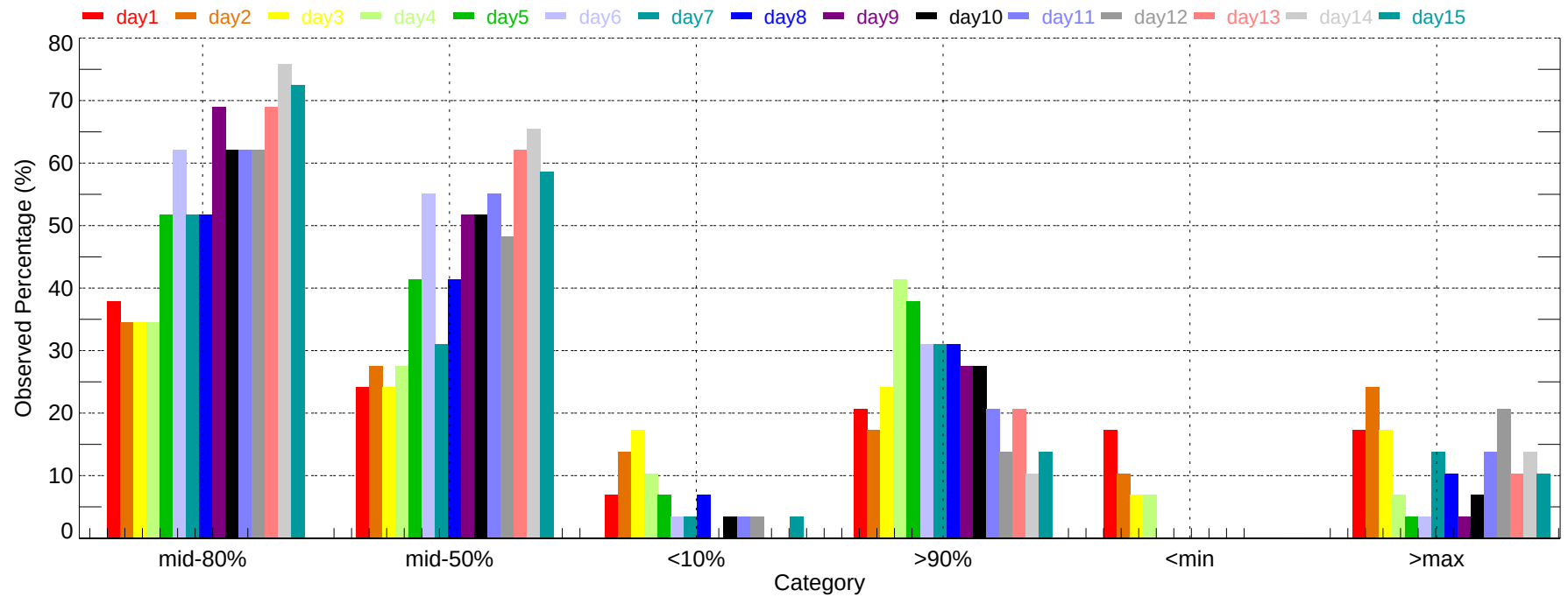
Observed Percentage of Ensembles - CMH: Min Temperature (2007-11-01~2007-11-30)
