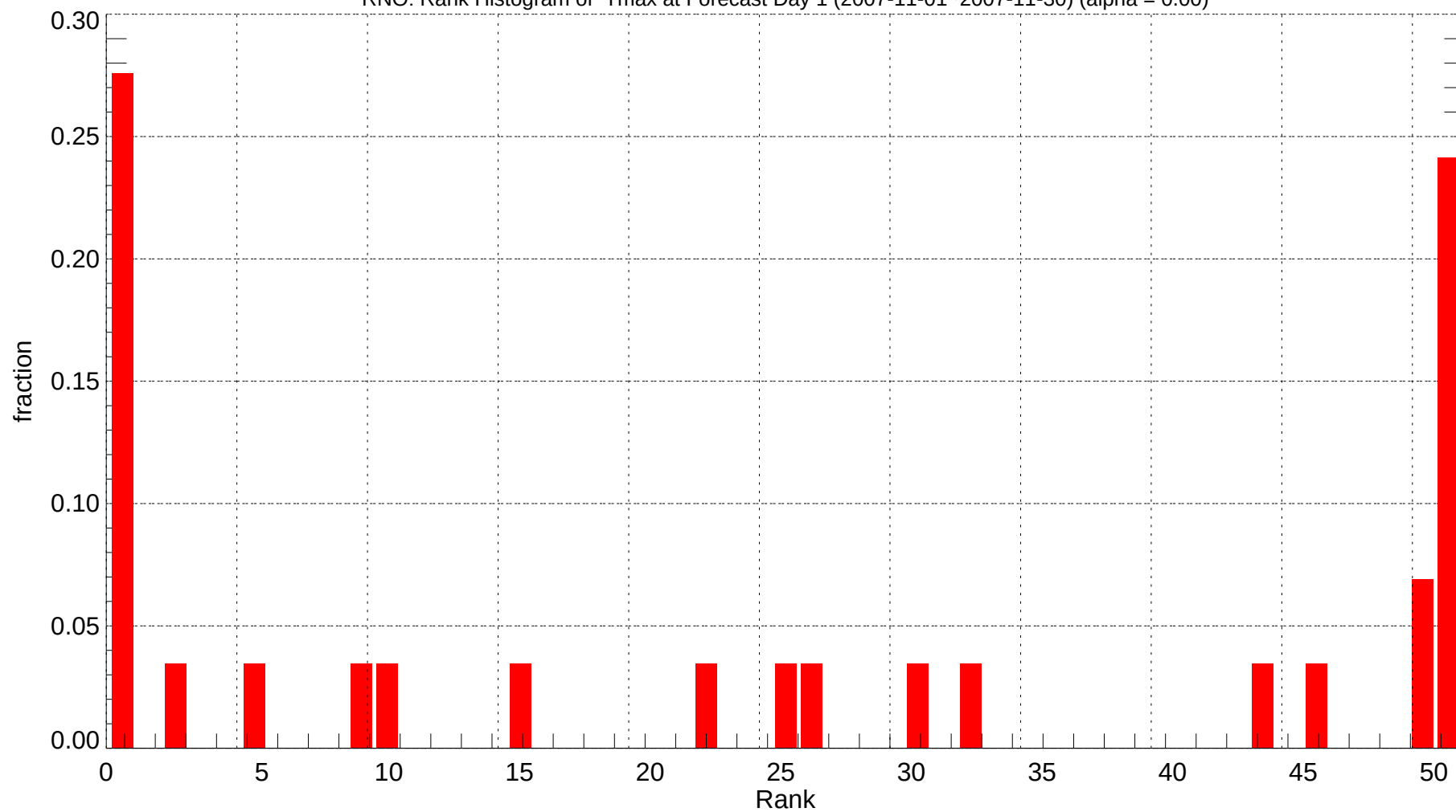
RNO: Rank Histogram of Tmax at Forecast Day 1 (2007-11-01~2007-11-30) (alpha = 0.00)
