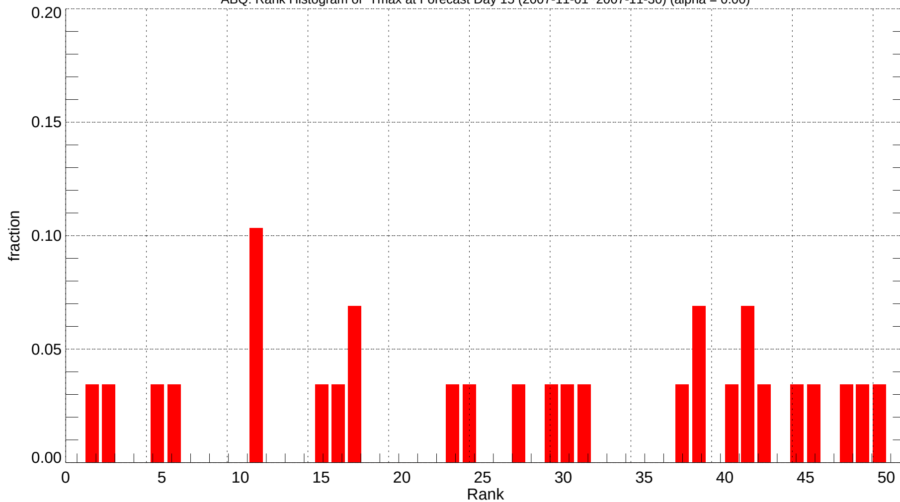
ABQ: Rank Histogram of Tmax at Forecast Day 15 (2007-11-01~2007-11-30) (alpha = 0.00)
