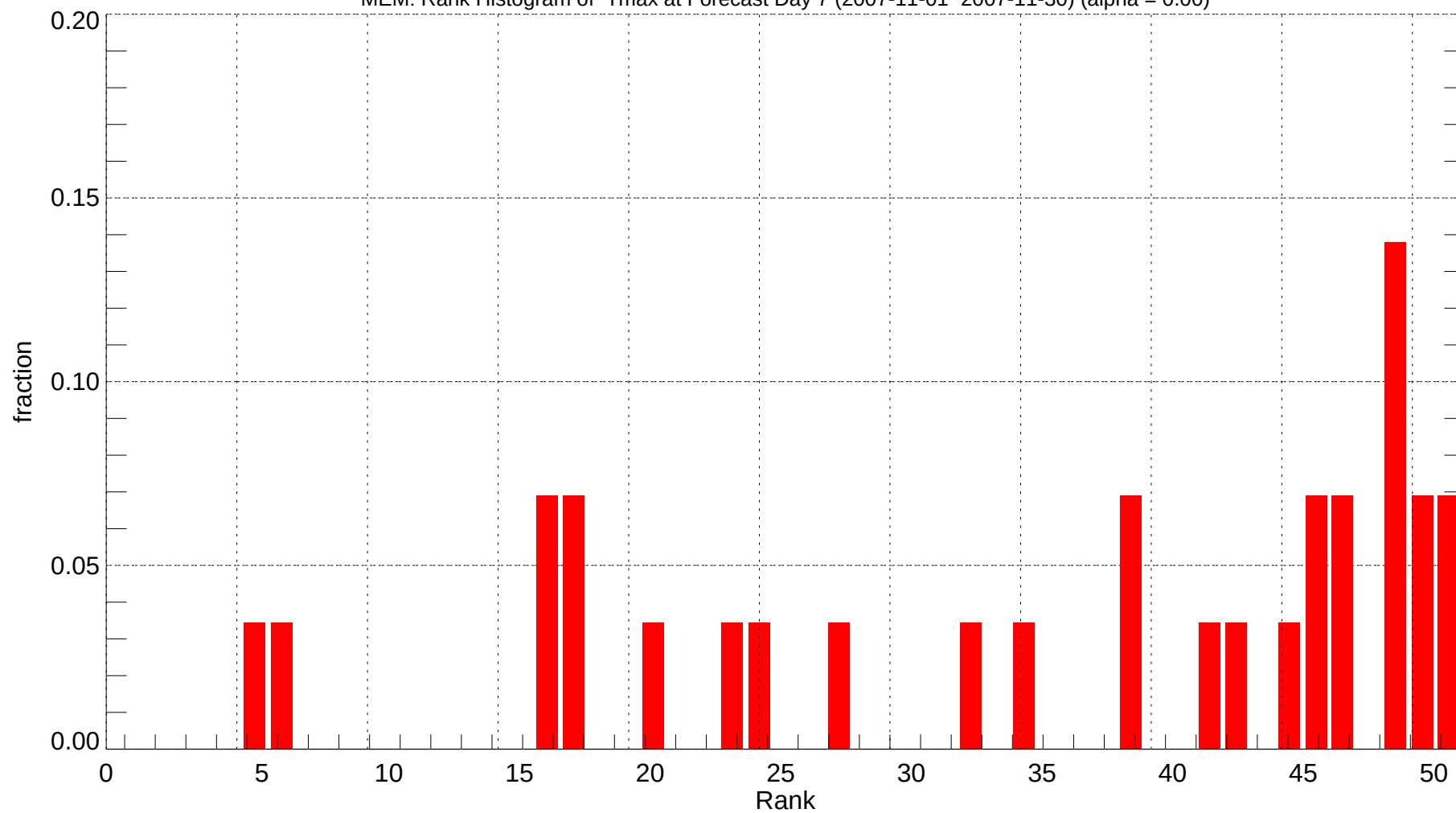
MEM: Rank Histogram of Tmax at Forecast Day 7 (2007-11-01~2007-11-30) (alpha = 0.00)
