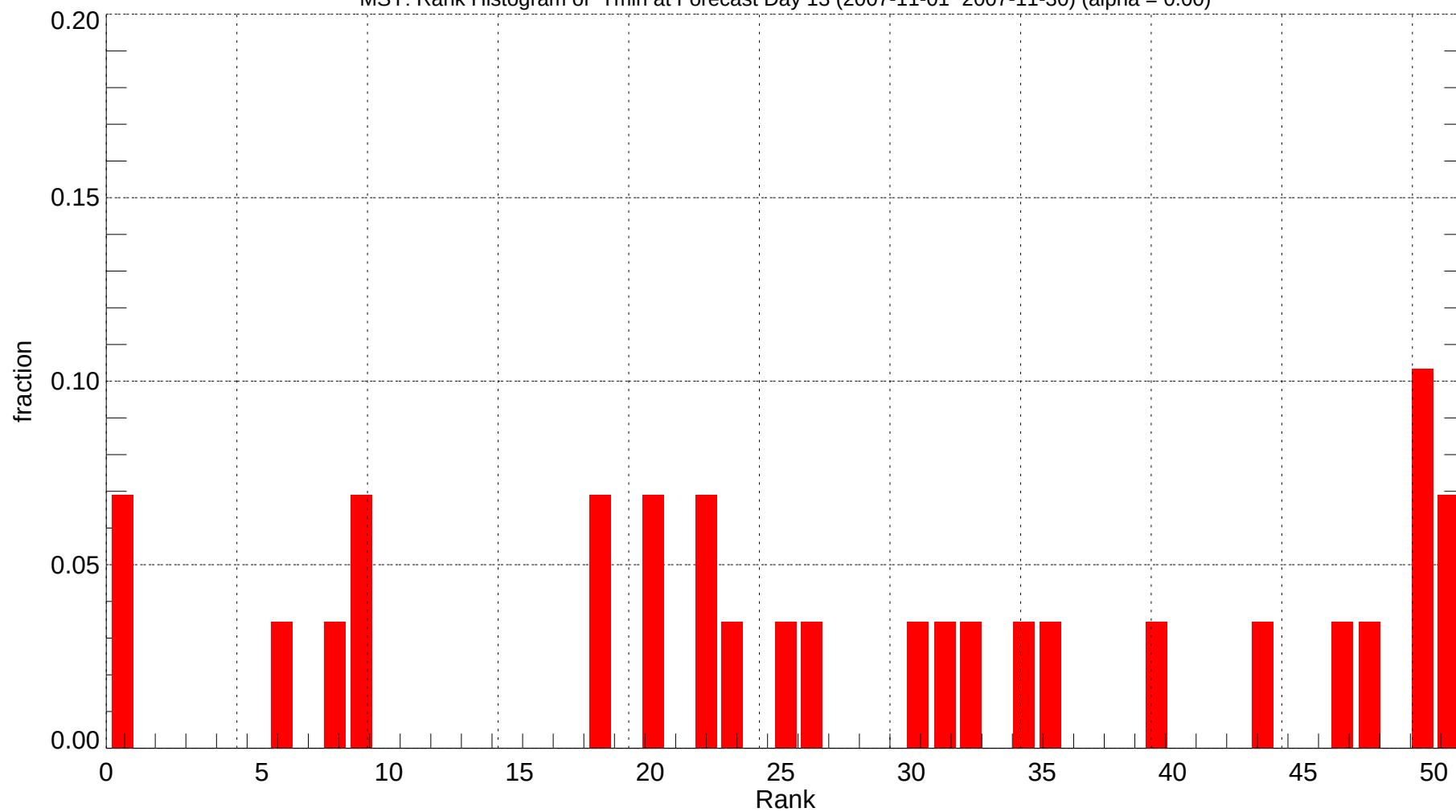
MSY: Rank Histogram of Tmin at Forecast Day 13 (2007-11-01~2007-11-30) (alpha = 0.00)
