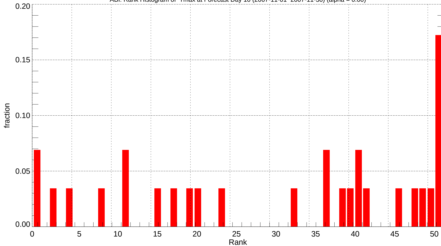
ABI: Rank Histogram of Tmax at Forecast Day 10 (2007-11-01~2007-11-30) (alpha = 0.00)
