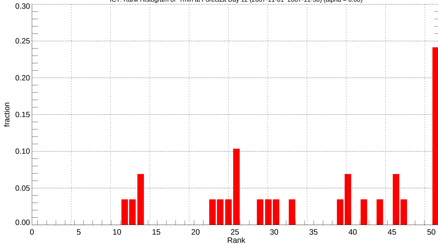
ICT: Rank Histogram of Tmin at Forecast Day 12 (2007-11-01~2007-11-30) (alpha = 0.00)
