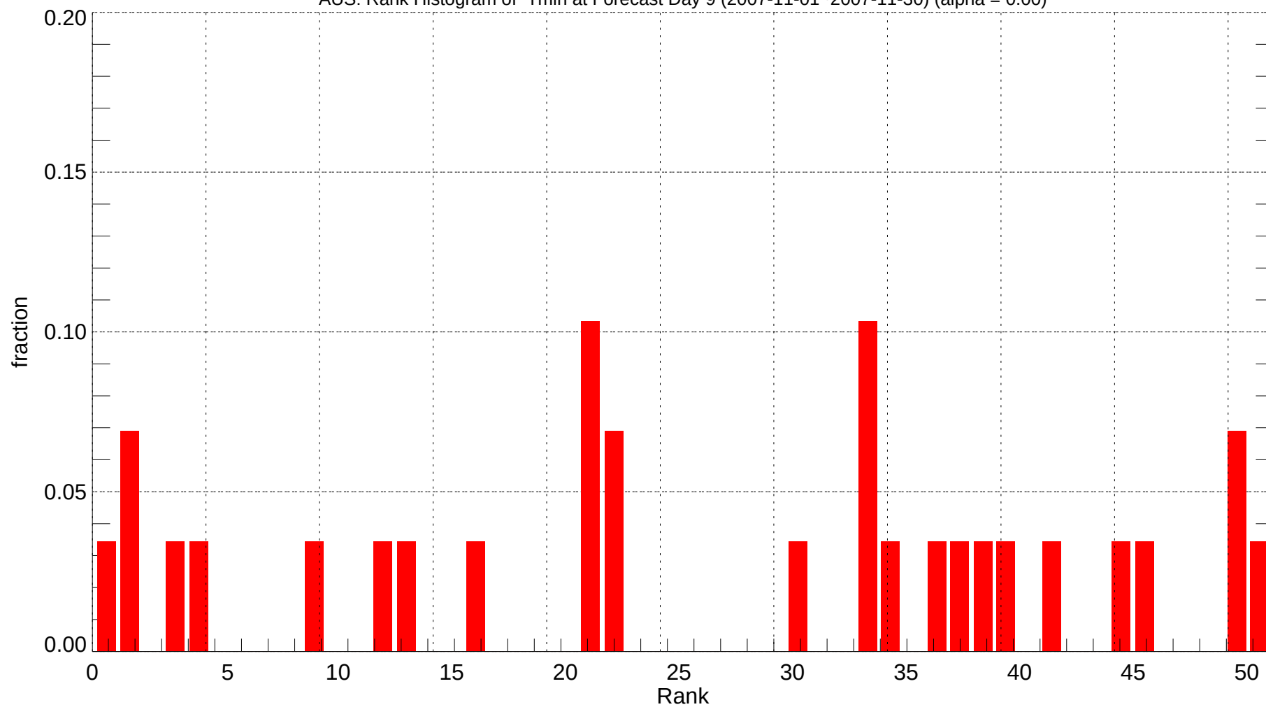
AUS: Rank Histogram of Tmin at Forecast Day 9 (2007-11-01~2007-11-30) (alpha = 0.00)
