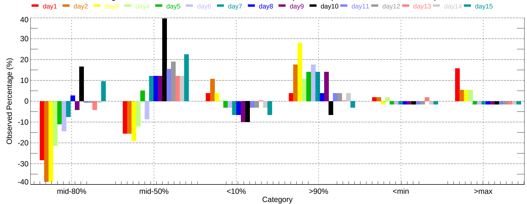
Observed Percentage Deviation of Ensembles - TLH: Max Temperature (2007-11-01~2007-11-30)
