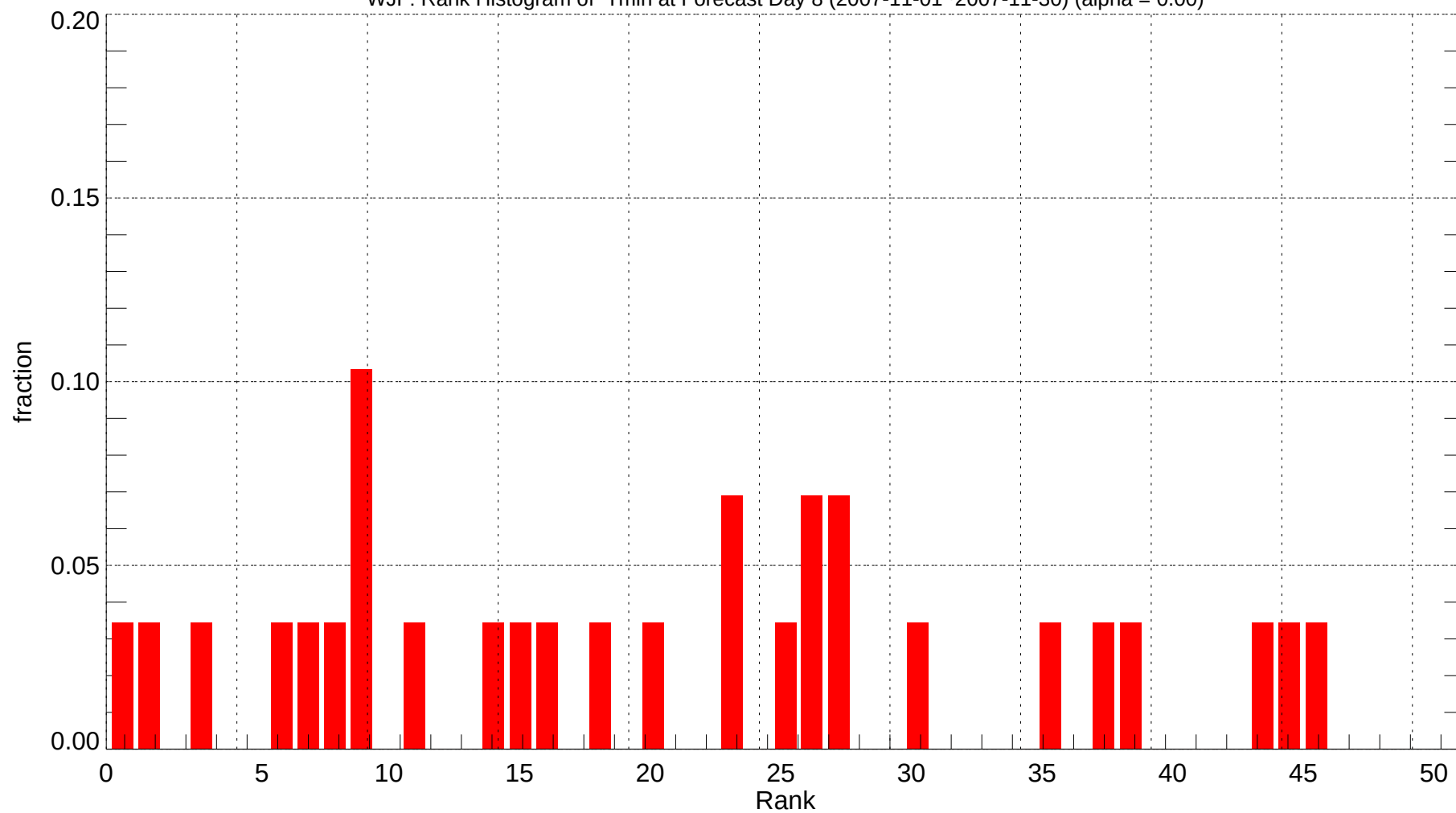
WJF: Rank Histogram of Tmin at Forecast Day 8 (2007-11-01~2007-11-30) (alpha = 0.00)
