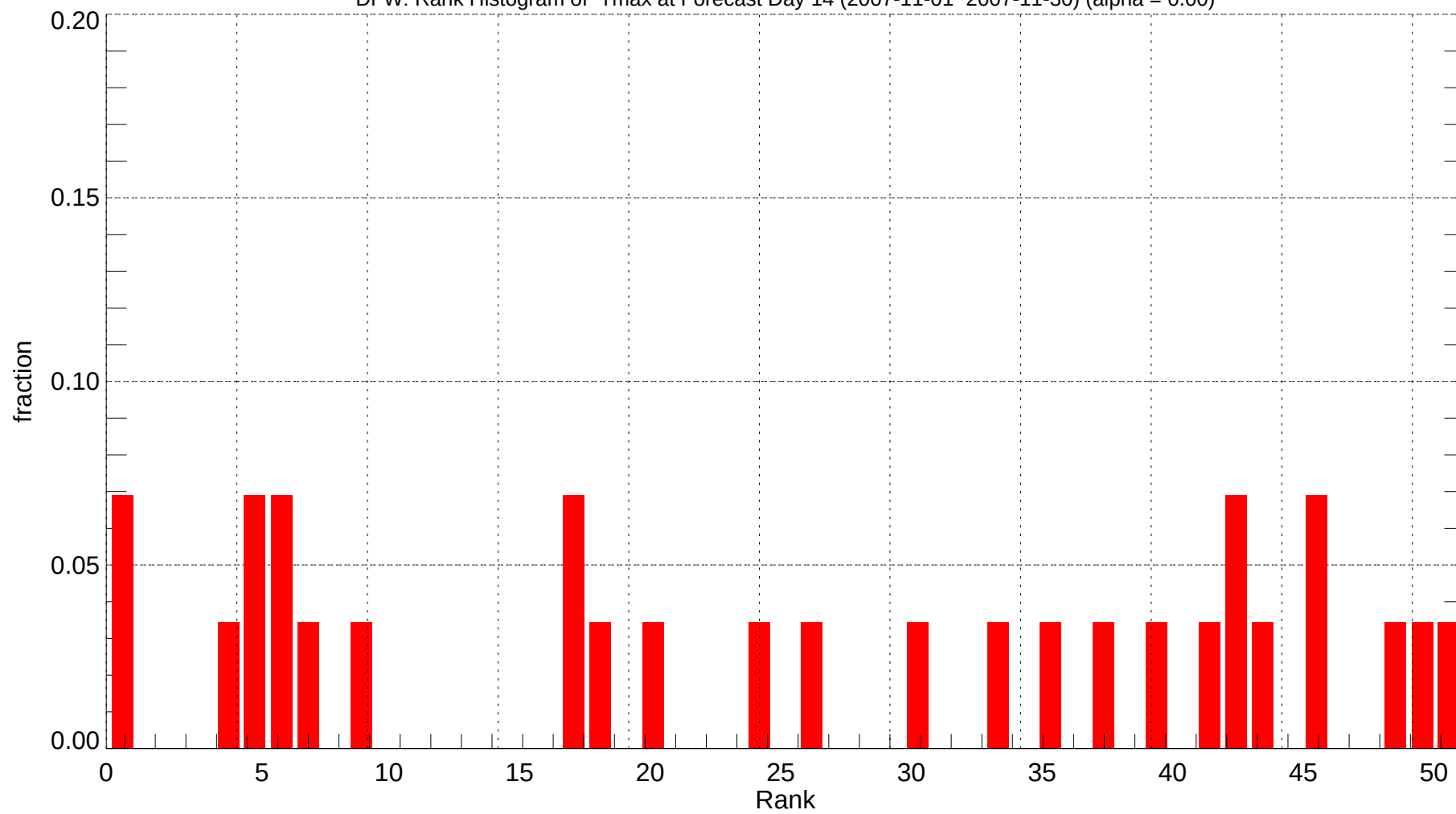
DFW: Rank Histogram of Tmax at Forecast Day 14 (2007-11-01~2007-11-30) (alpha = 0.00)
