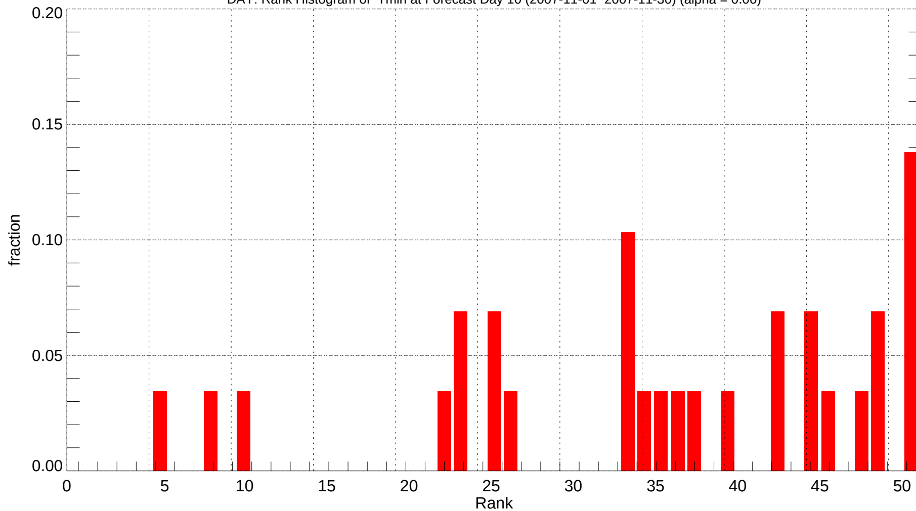
DAY: Rank Histogram of Tmin at Forecast Day 10 (2007-11-01~2007-11-30) (alpha = 0.00)
