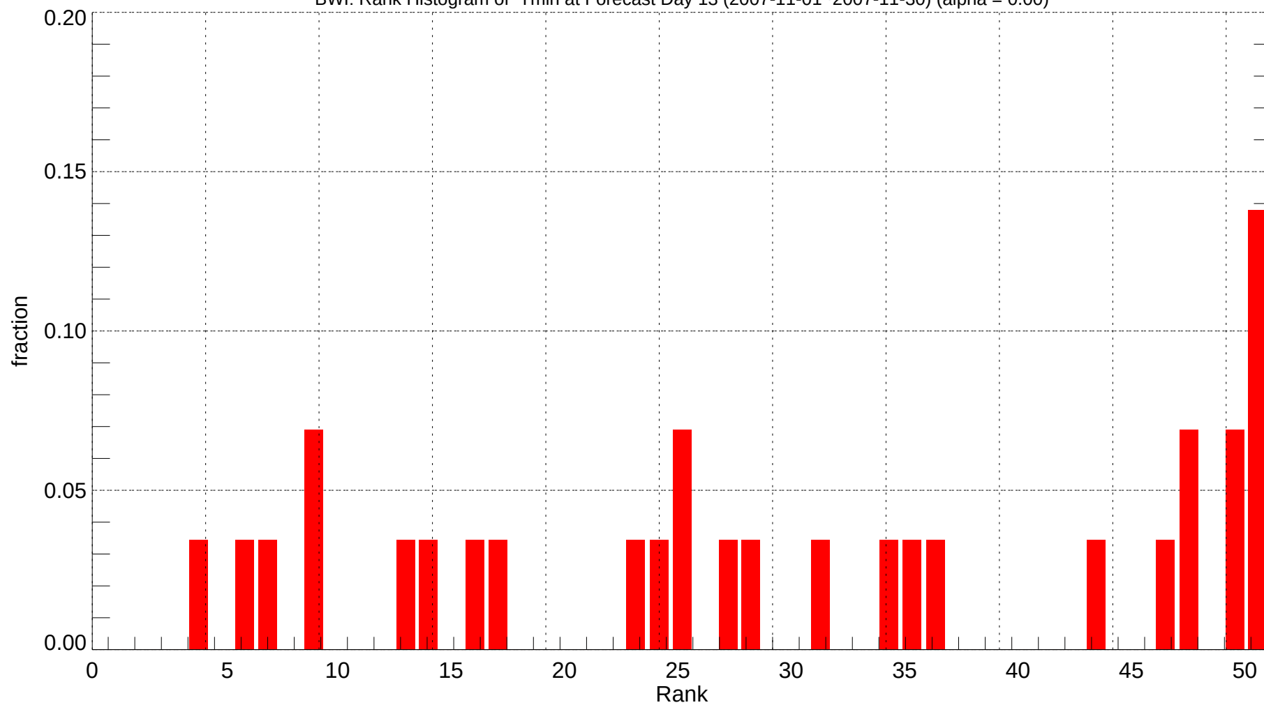
BWl: Rank Histogram of Tmin at Forecast Day 13 (2007-11-01~2007-11-30) (alpha = 0.00)
