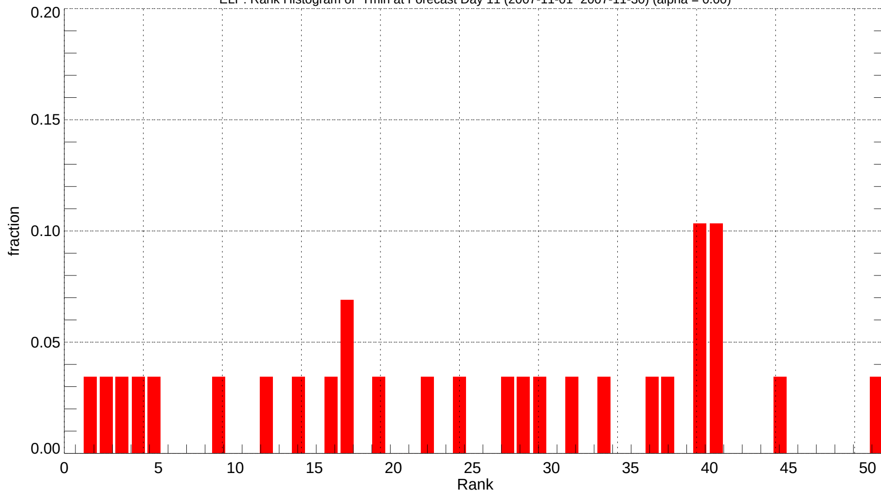
ELP: Rank Histogram of Tmin at Forecast Day 11 (2007-11-01~2007-11-30) (alpha = 0.00)
