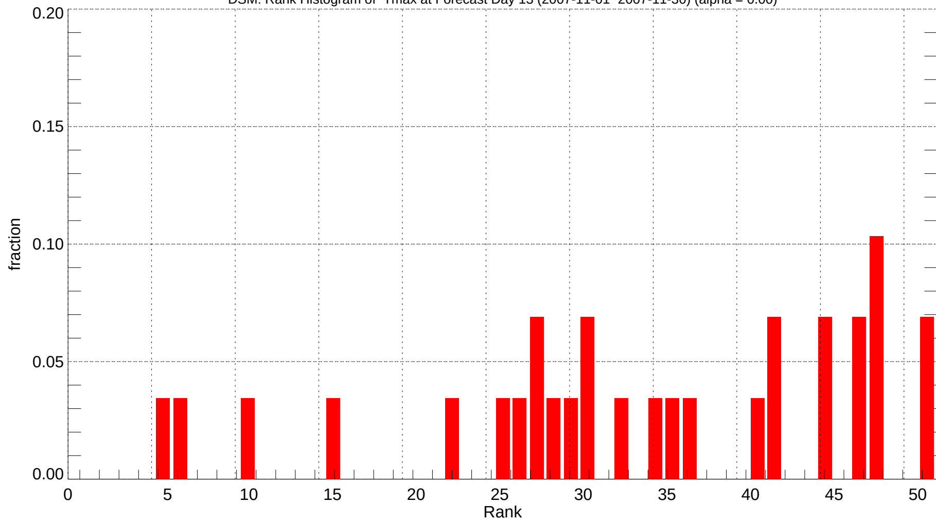
DSM: Rank Histogram of Tmax at Forecast Day 13 (2007-11-01~2007-11-30) (alpha = 0.00)
