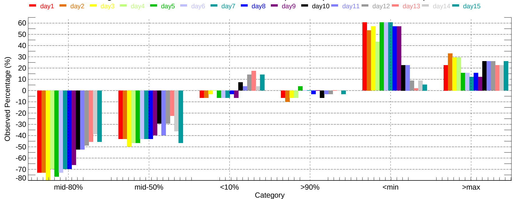
Observed Percentage Deviation of Ensembles - LAX: Max Temperature (2007-11-01~2007-11-30)
