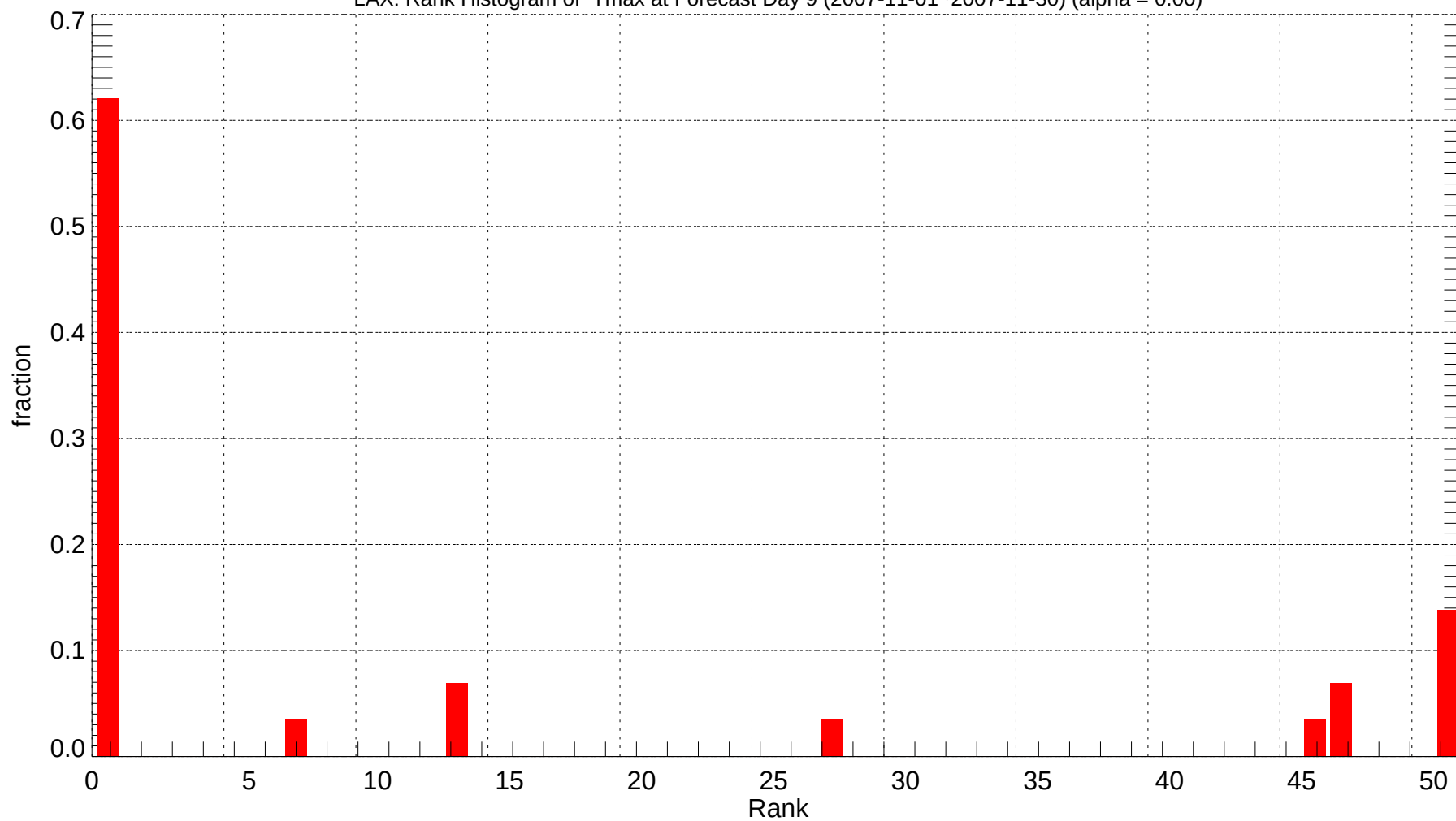
LAX: Rank Histogram of Tmax at Forecast Day 9 (2007-11-01~2007-11-30) (alpha = 0.00)
