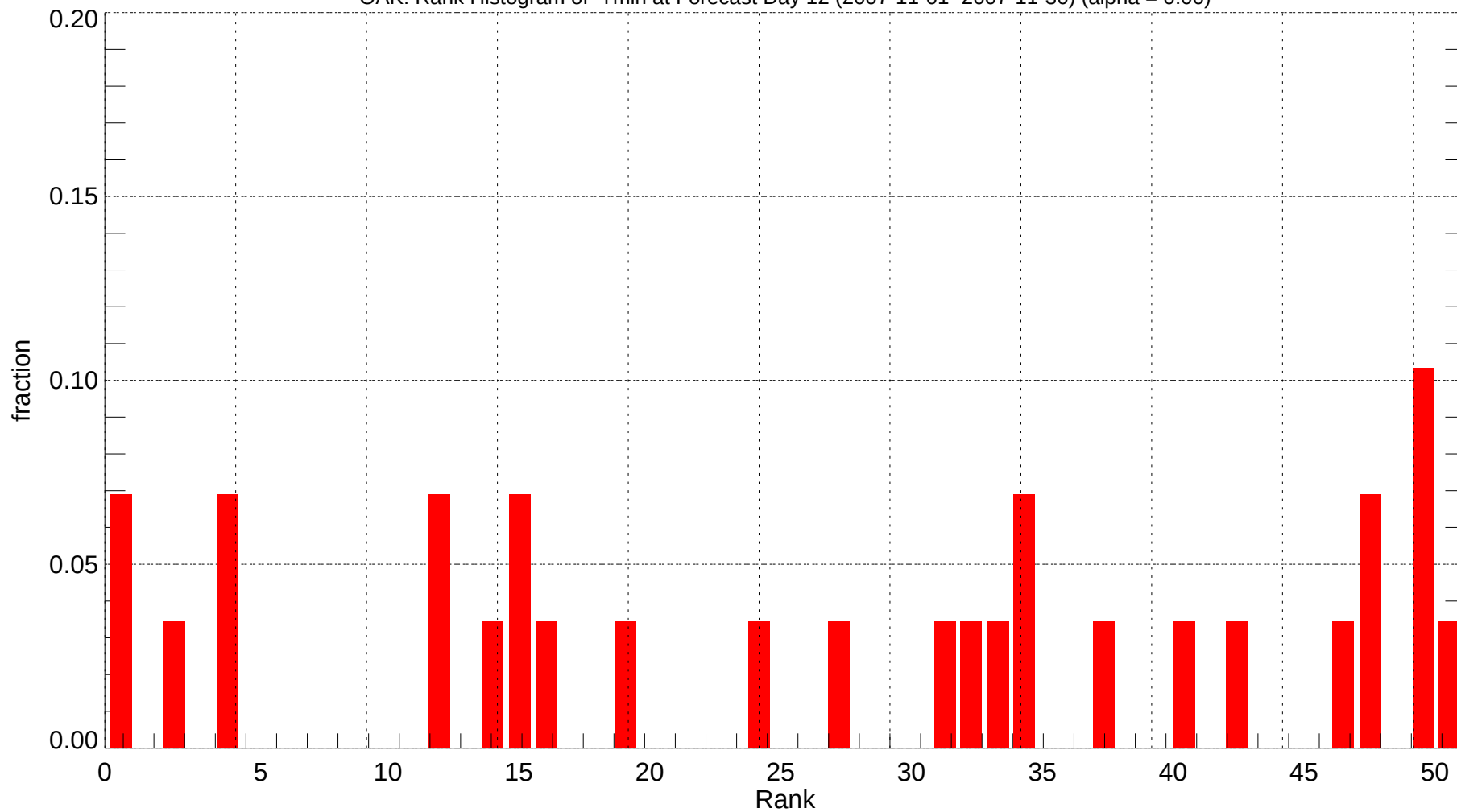
OAK: Rank Histogram of Tmin at Forecast Day 12 (2007-11-01~2007-11-30) (alpha = 0.00)
