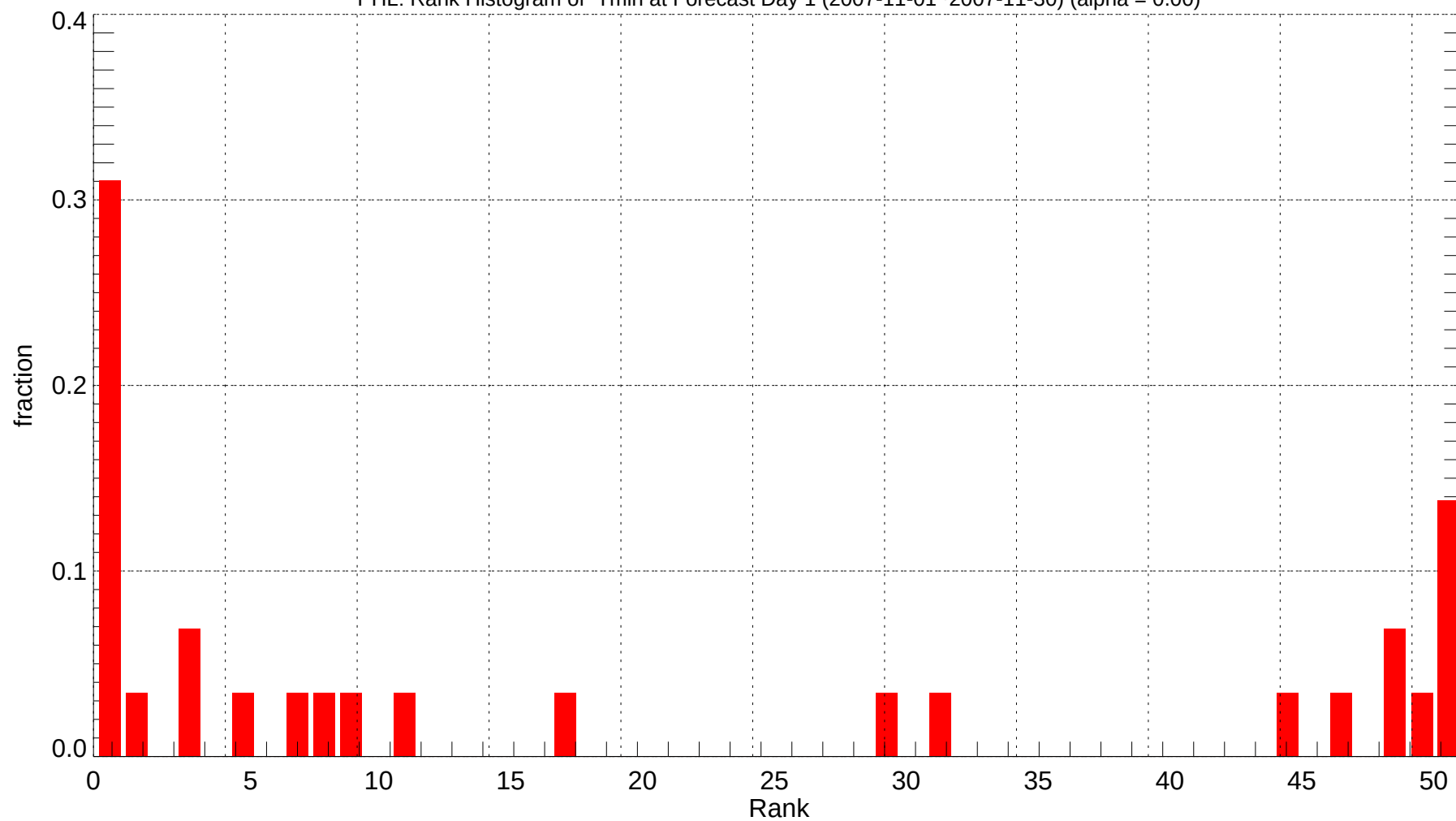
PHL: Rank Histogram of Tmin at Forecast Day 1 (2007-11-01~2007-11-30) (alpha = 0.00)
