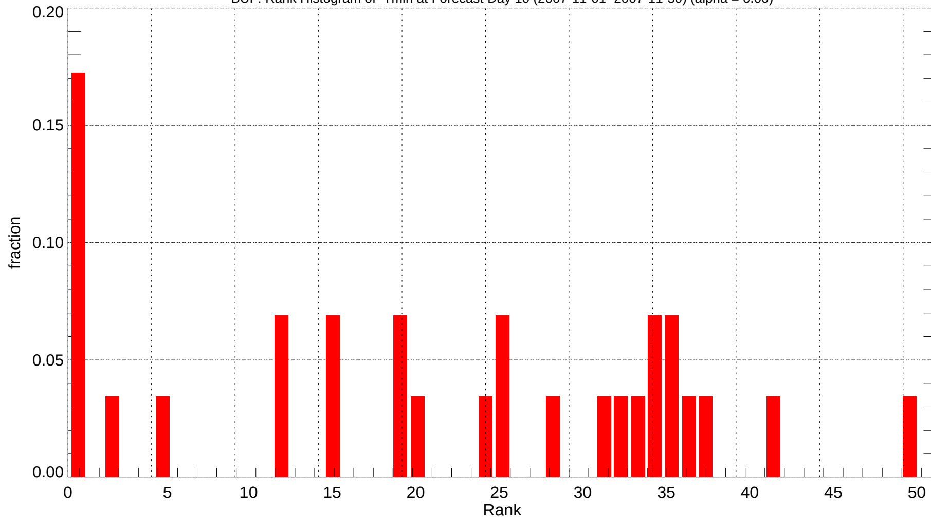
BUF: Rank Histogram of Tmin at Forecast Day 10 (2007-11-01~2007-11-30) (alpha = 0.00)
