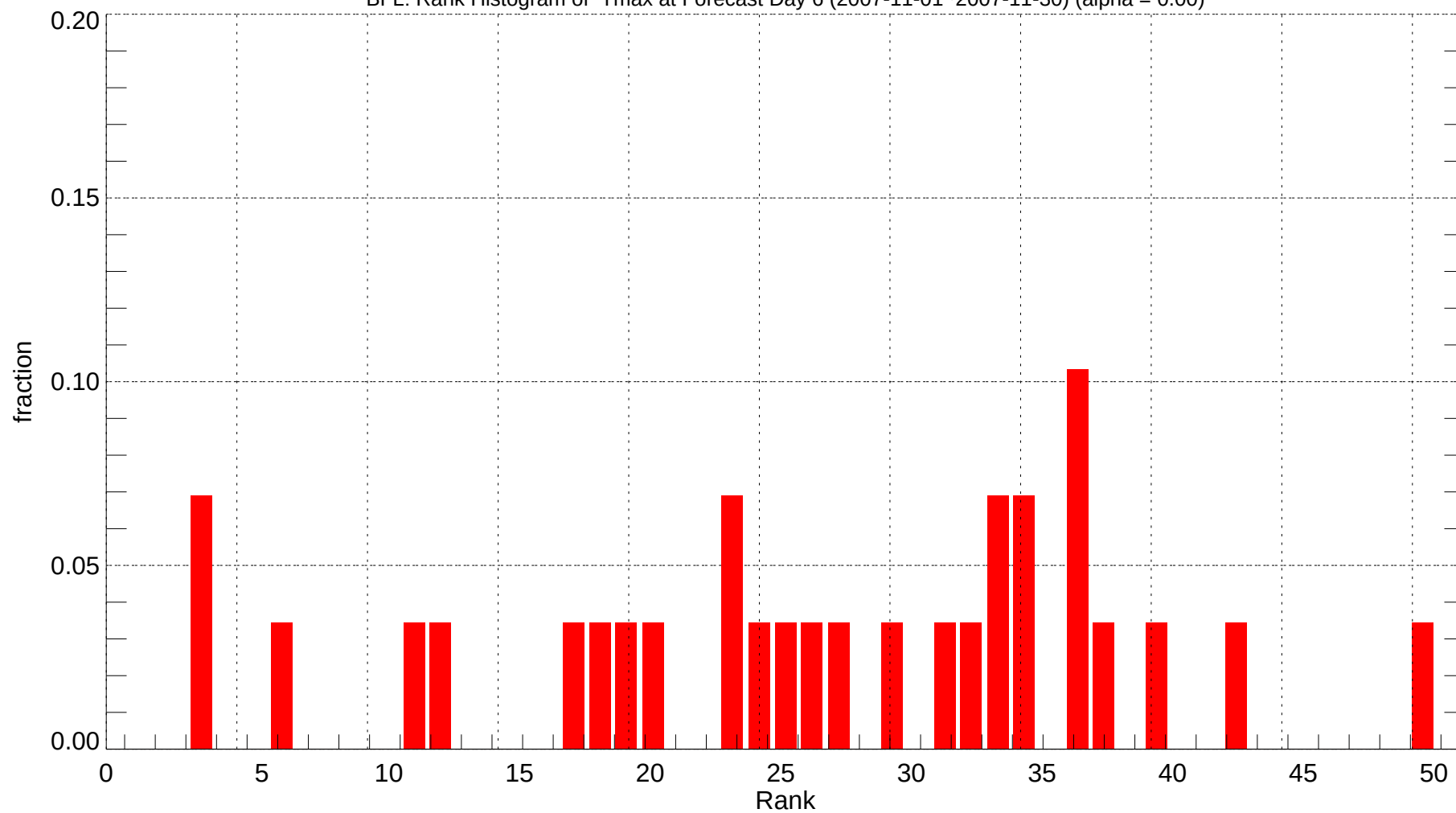
BFL: Rank Histogram of Tmax at Forecast Day 6 (2007-11-01~2007-11-30) (alpha = 0.00)
