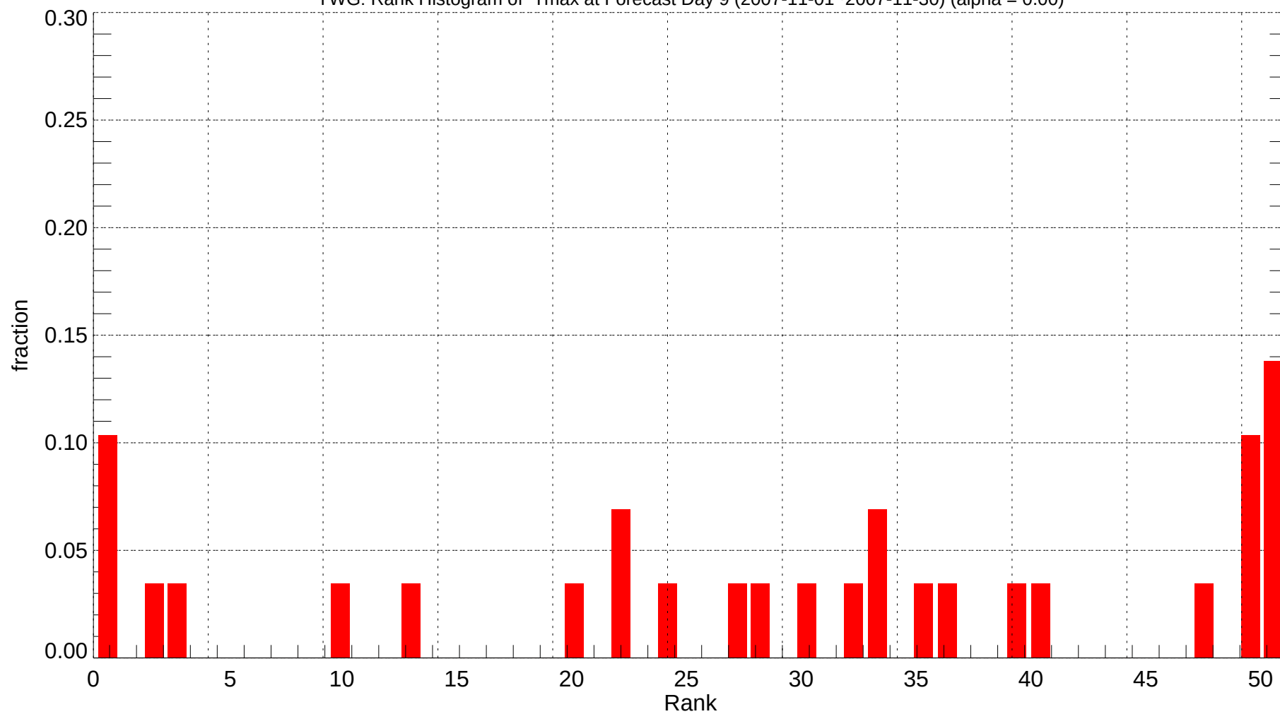
YWG: Rank Histogram of Tmax at Forecast Day 9 (2007-11-01~2007-11-30) (alpha = 0.00)
