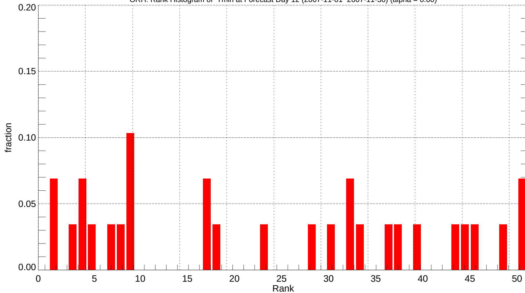
ORH: Rank Histogram of Tmin at Forecast Day 12 (2007-11-01~2007-11-30) (alpha = 0.00)
