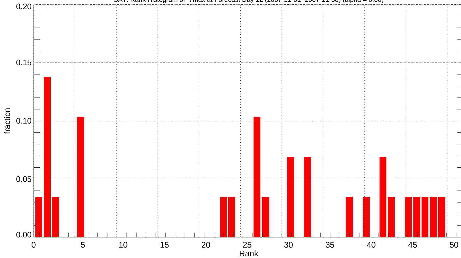
SAT: Rank Histogram of Tmax at Forecast Day 12 (2007-11-01~2007-11-30) (alpha = 0.00)
