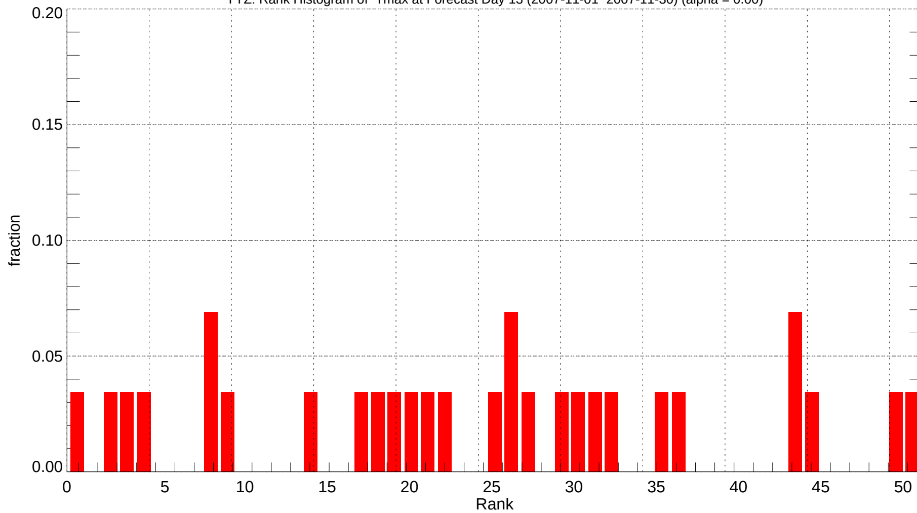
YYZ: Rank Histogram of Tmax at Forecast Day 13 (2007-11-01~2007-11-30) (alpha = 0.00)
