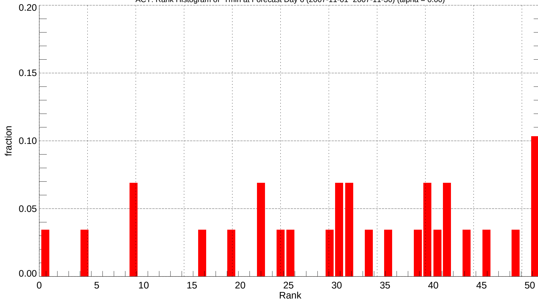
ACY: Rank Histogram of Tmin at Forecast Day 6 (2007-11-01~2007-11-30) (alpha = 0.00)
