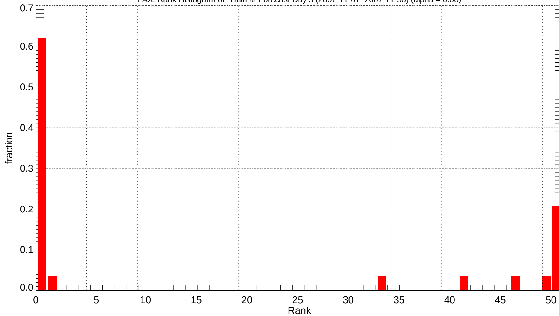
LAX: Rank Histogram of Tmin at Forecast Day 5 (2007-11-01~2007-11-30) (alpha = 0.00)
