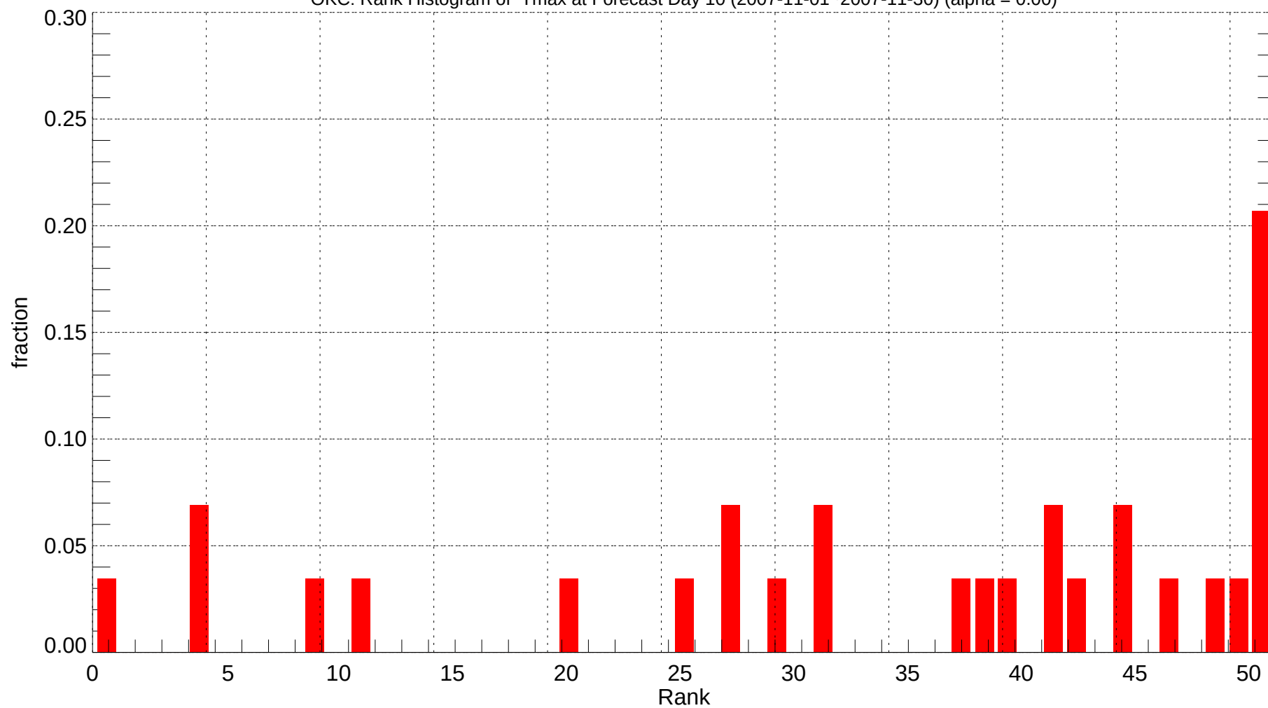
OKC: Rank Histogram of Tmax at Forecast Day 10 (2007-11-01~2007-11-30) (alpha = 0.00)
