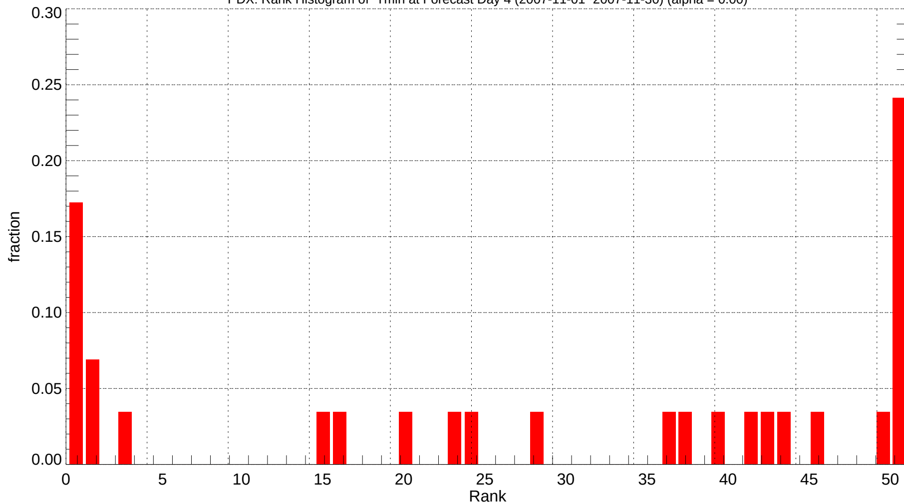
PDX: Rank Histogram of Tmin at Forecast Day 4 (2007-11-01~2007-11-30) (alpha = 0.00)
