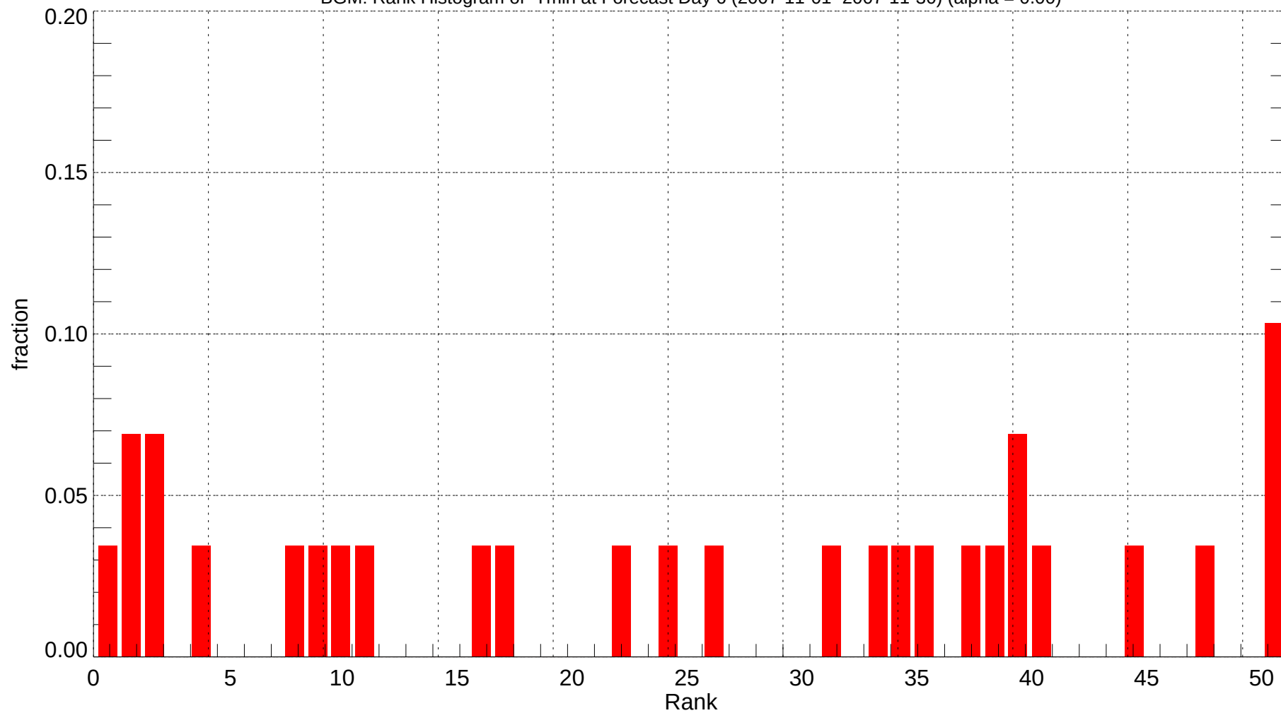
BGM: Rank Histogram of Tmin at Forecast Day 6 (2007-11-01~2007-11-30) (alpha = 0.00)
