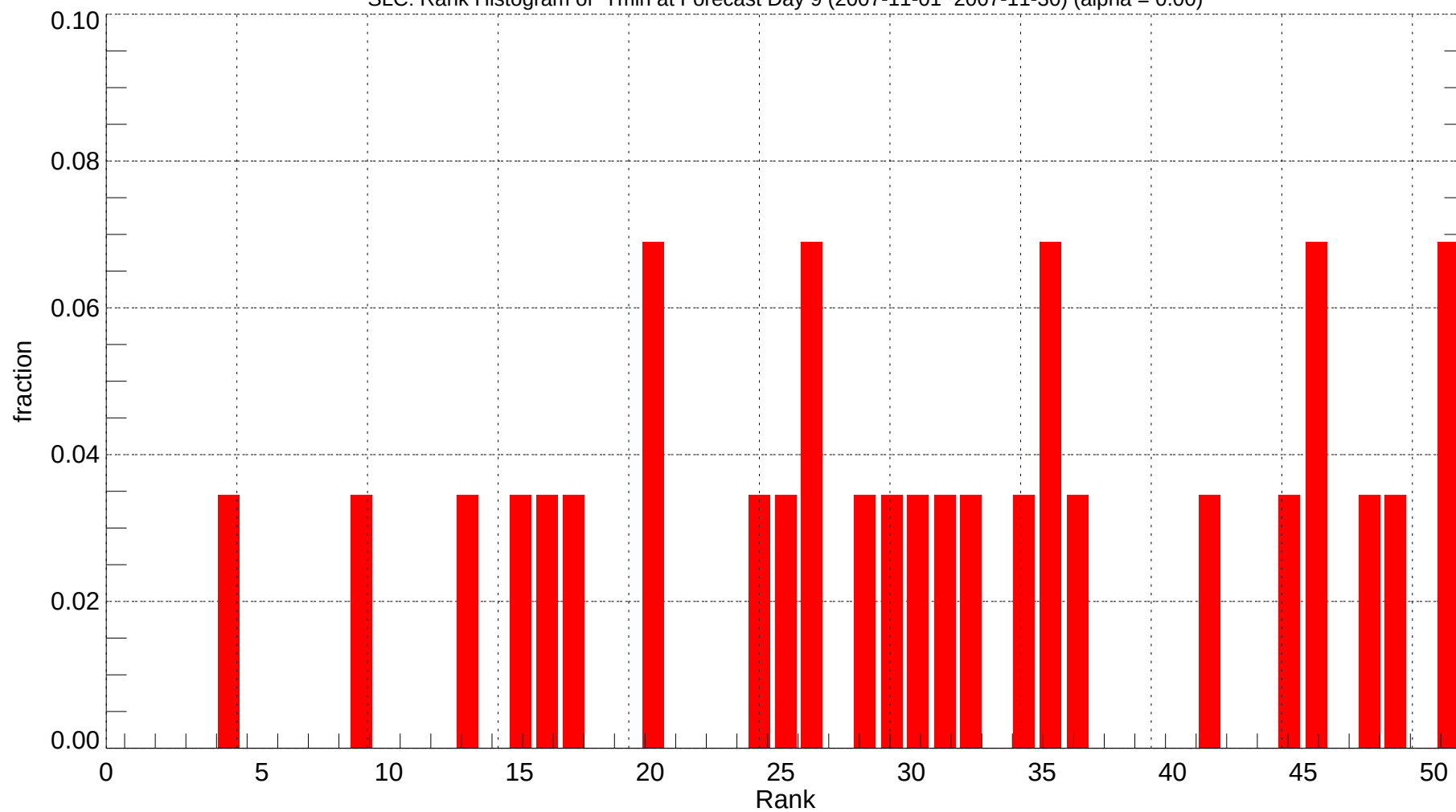
SLC: Rank Histogram of Tmin at Forecast Day 9 (2007-11-01~2007-11-30) (alpha = 0.00)
