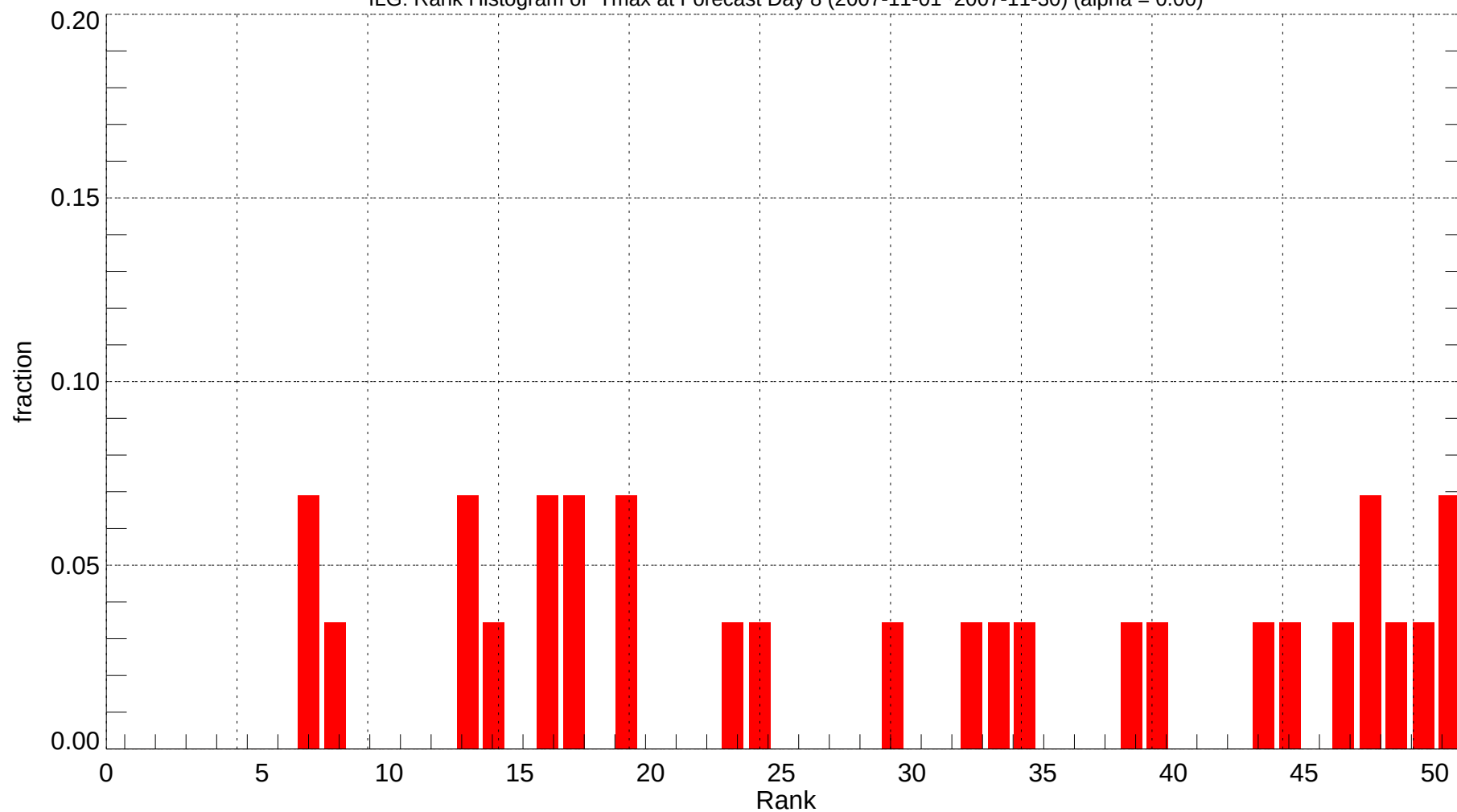
ILG: Rank Histogram of Tmax at Forecast Day 8 (2007-11-01~2007-11-30) (alpha = 0.00)
