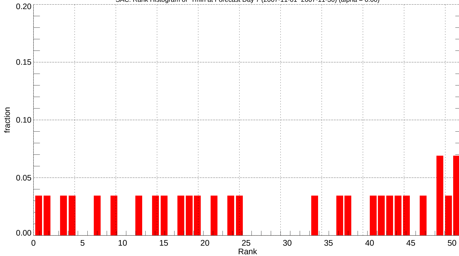
SAC: Rank Histogram of Tmin at Forecast Day 7 (2007-11-01~2007-11-30) (alpha = 0.00)
