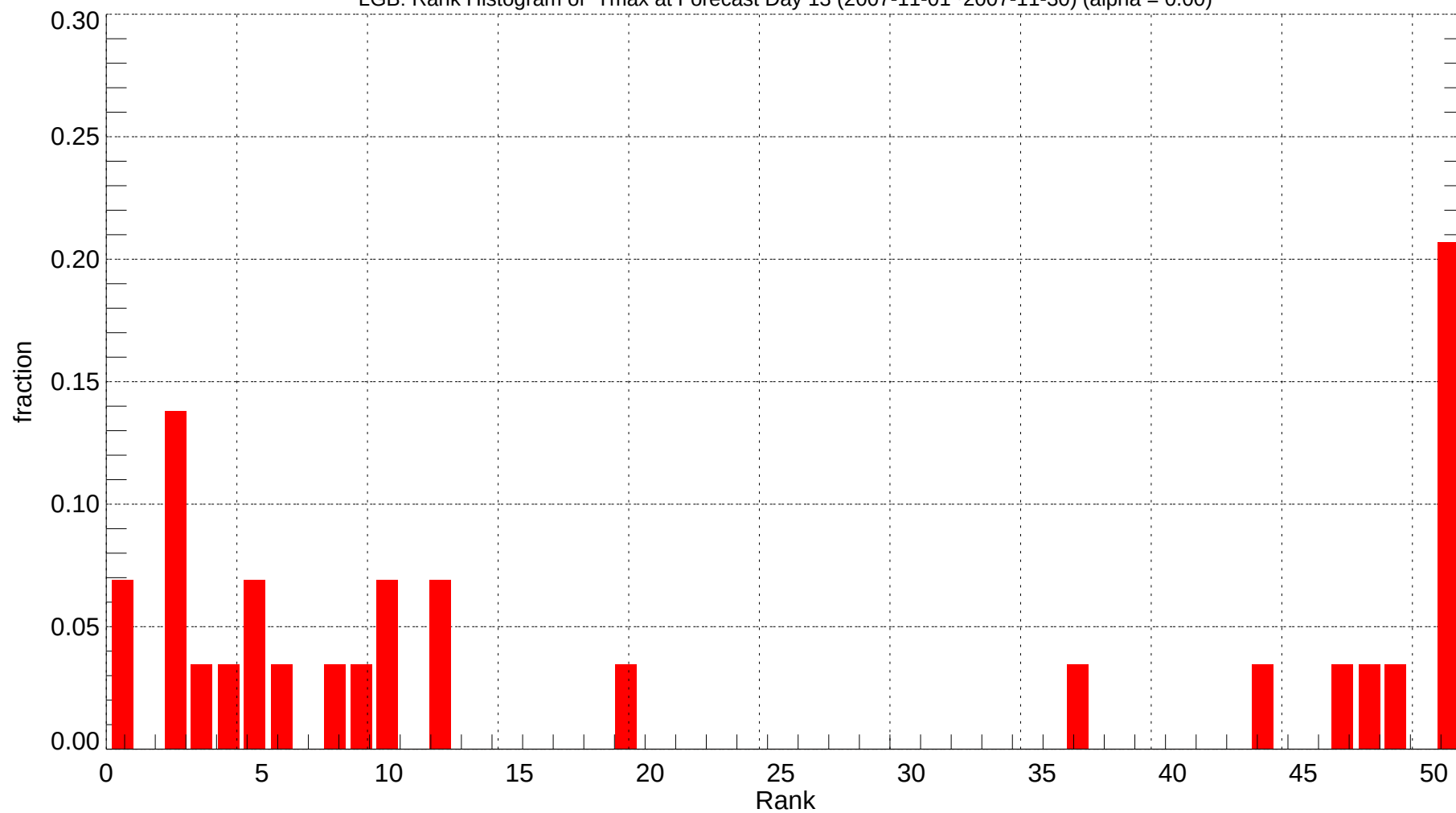
LGB: Rank Histogram of Tmax at Forecast Day 13 (2007-11-01~2007-11-30) (alpha = 0.00)
