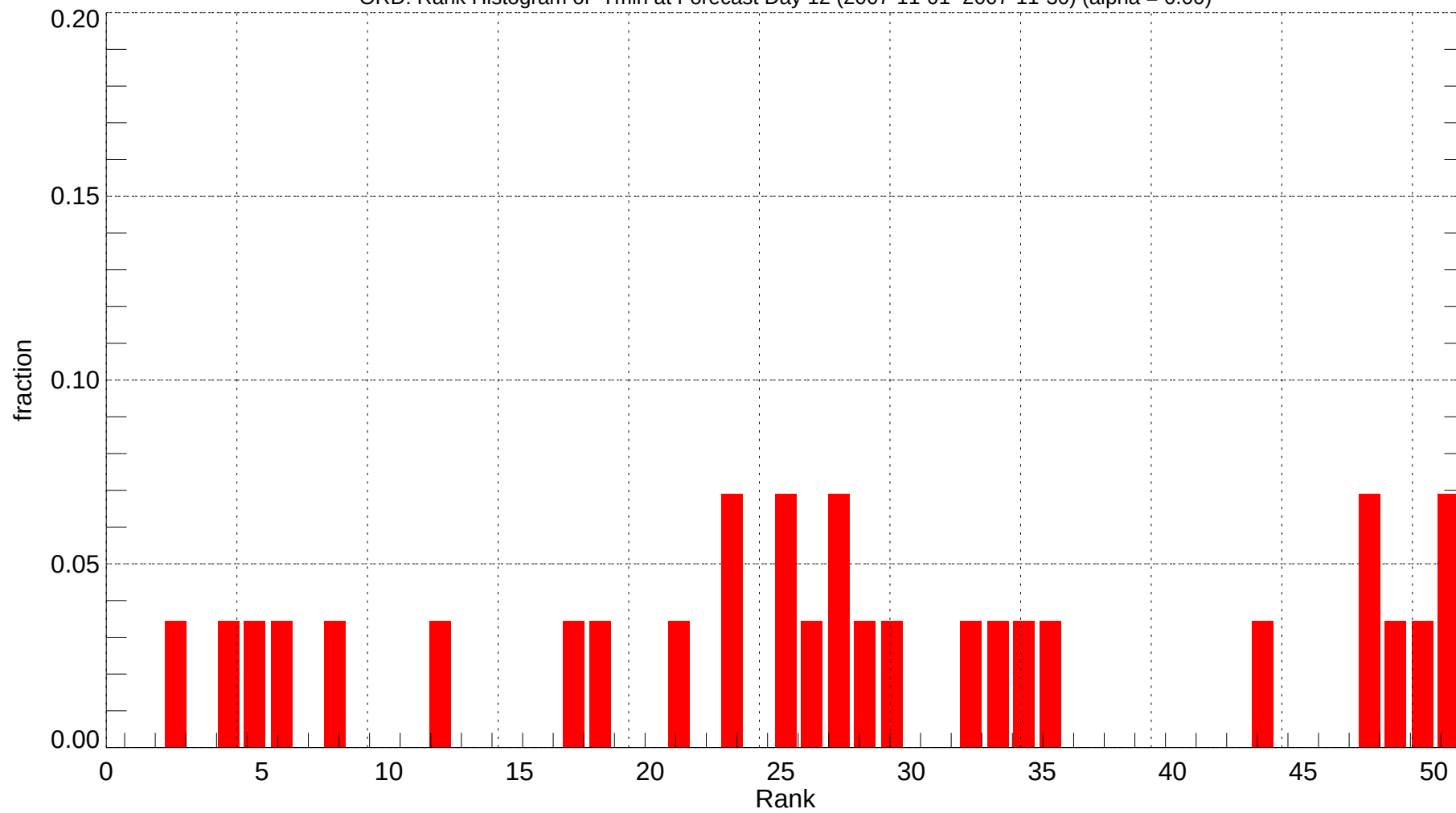
ORD: Rank Histogram of Tmin at Forecast Day 12 (2007-11-01~2007-11-30) (alpha = 0.00)
