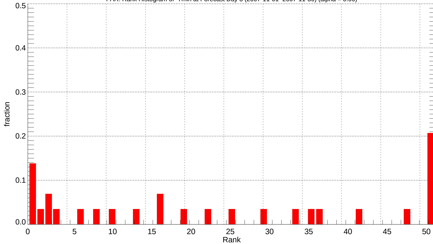
FAR: Rank Histogram of Tmin at Forecast Day 3 (2007-11-01~2007-11-30) (alpha = 0.00)
