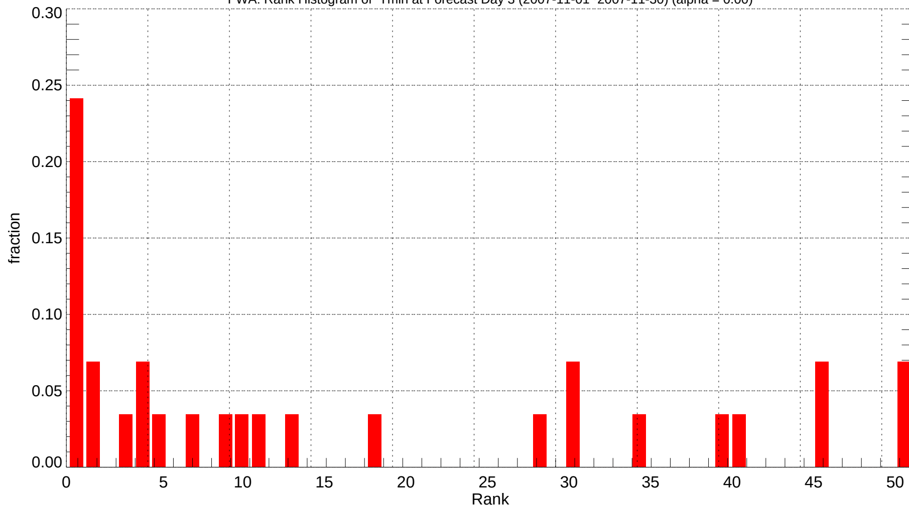
FWA: Rank Histogram of Tmin at Forecast Day 3 (2007-11-01~2007-11-30) (alpha = 0.00)
