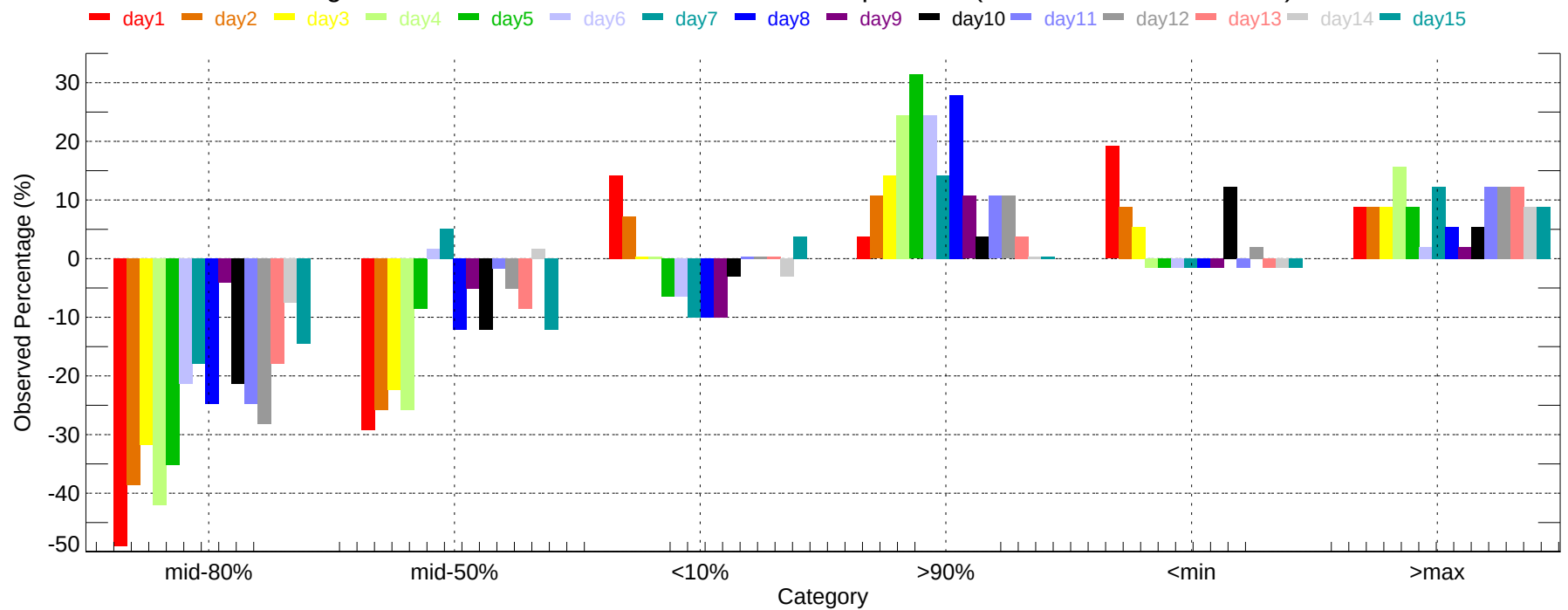
Observed Percentage Deviation of Ensembles - CLE: Min Temperature (2007-11-01~2007-11-30)
