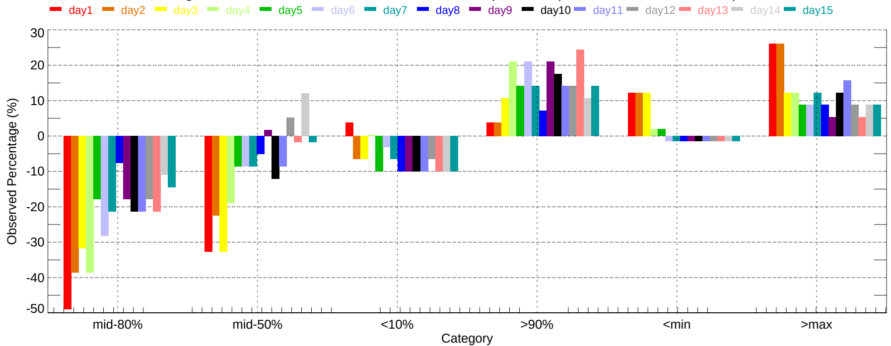
Observed Percentage Deviation of Ensembles - DEC: Min Temperature (2007-11-01~2007-11-30)
