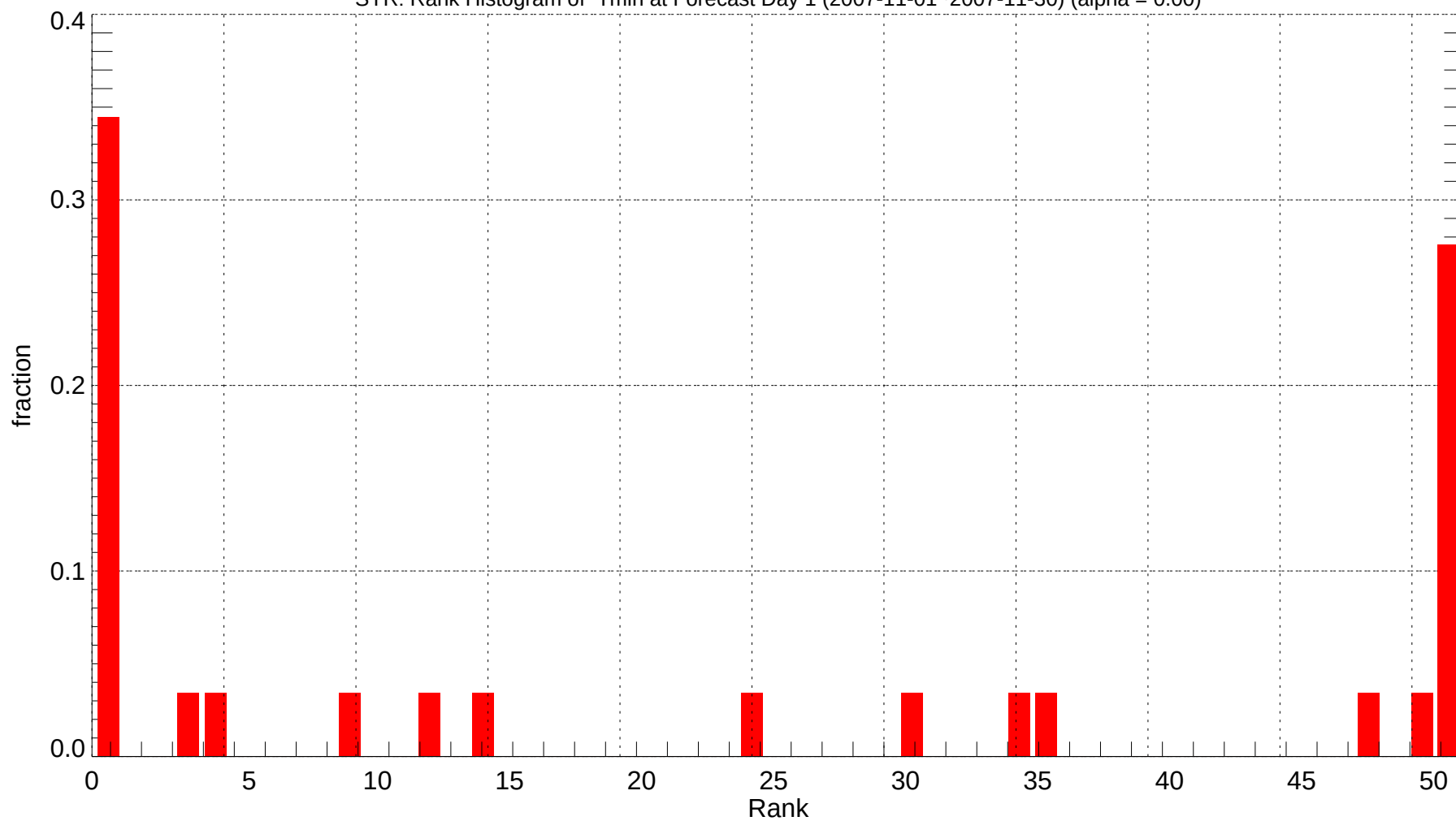
SYR: Rank Histogram of Tmin at Forecast Day 1 (2007-11-01~2007-11-30) (alpha = 0.00)
