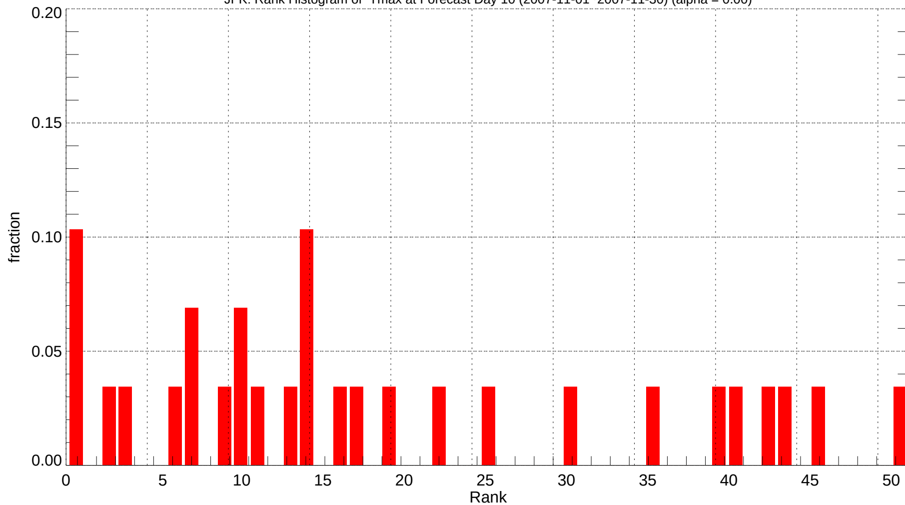
JFK: Rank Histogram of Tmax at Forecast Day 10 (2007-11-01~2007-11-30) (alpha = 0.00)
