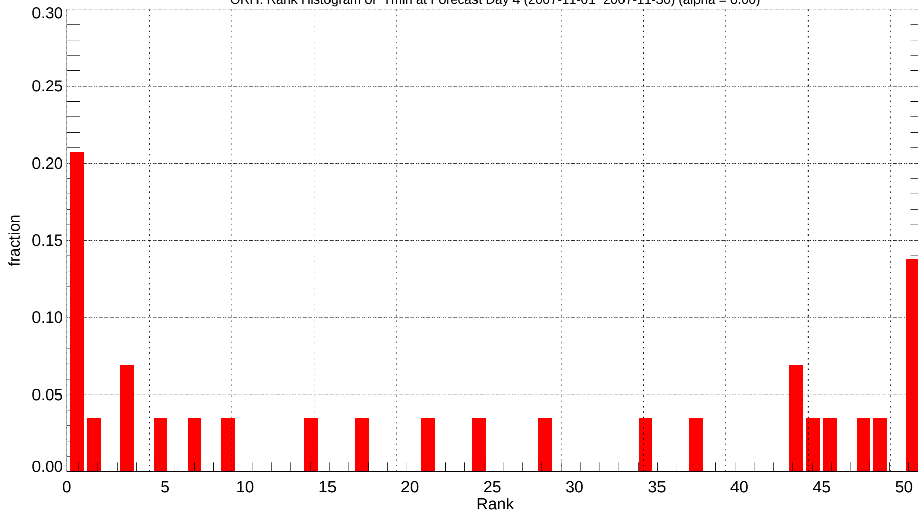
ORH: Rank Histogram of Tmin at Forecast Day 4 (2007-11-01~2007-11-30) (alpha = 0.00)
