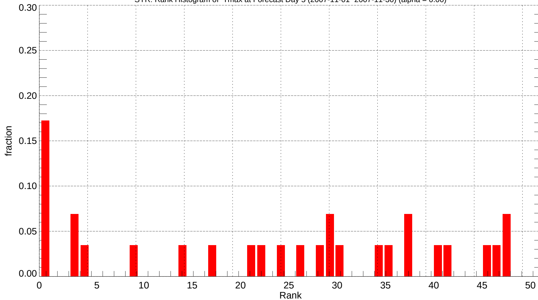
SYR: Rank Histogram of Tmax at Forecast Day 5 (2007-11-01~2007-11-30) (alpha = 0.00)
