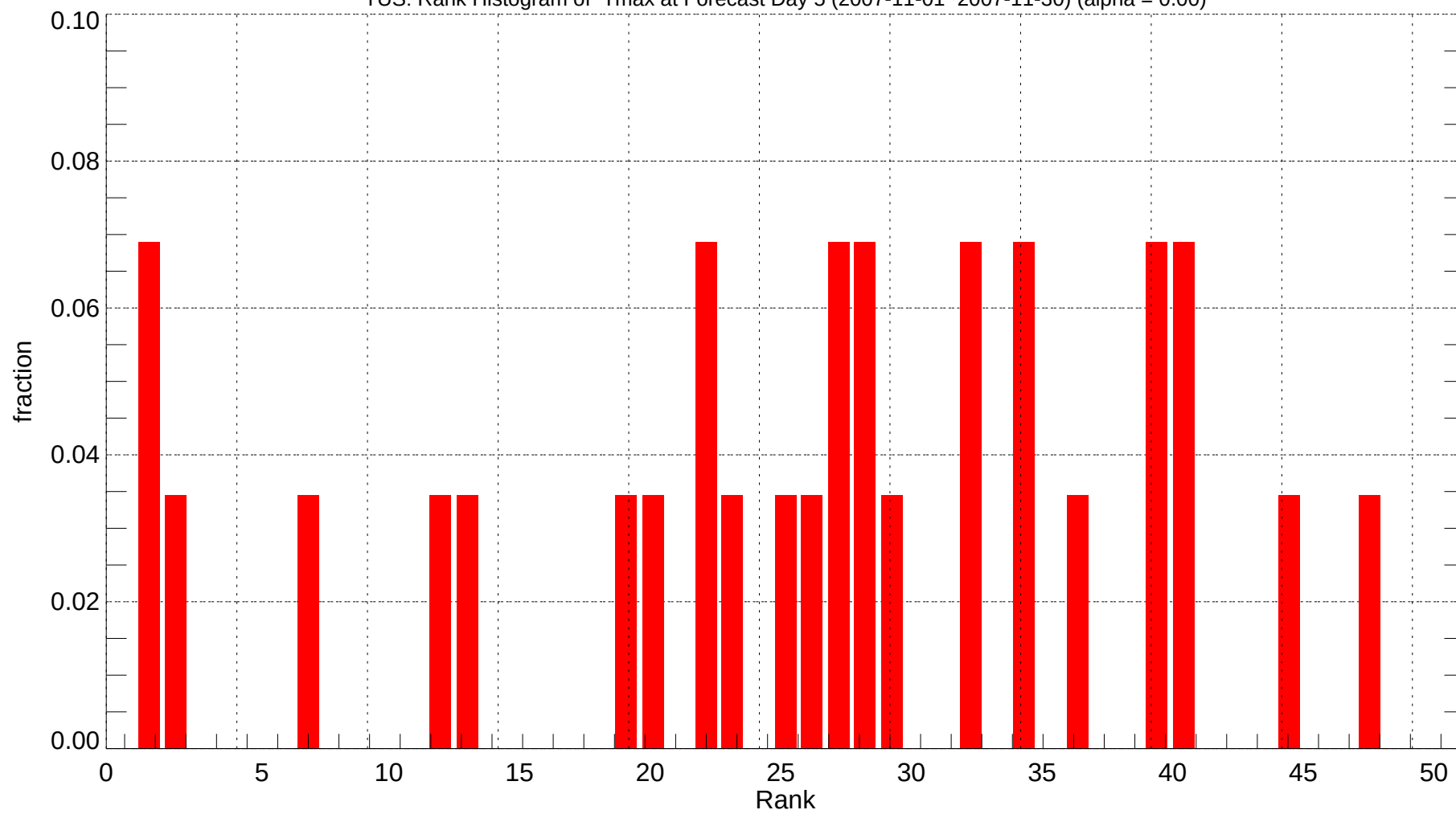
TUS: Rank Histogram of Tmax at Forecast Day 5 (2007-11-01~2007-11-30) (alpha = 0.00)
