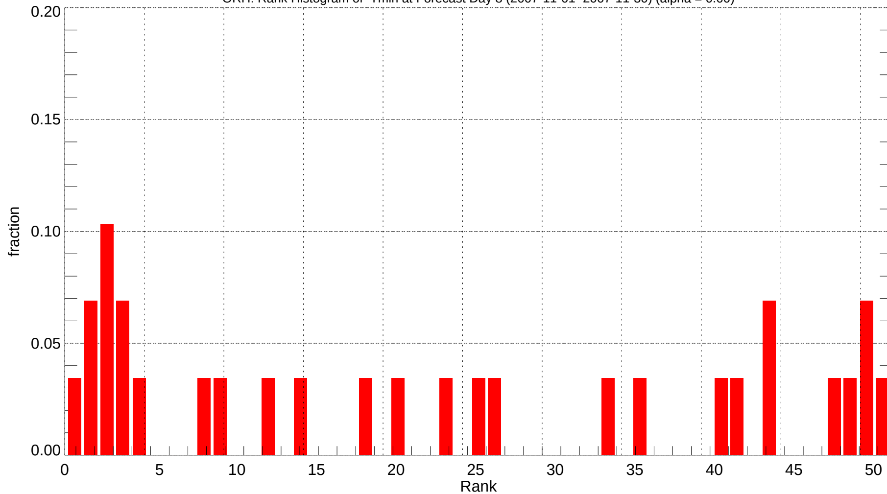
ORH: Rank Histogram of Tmin at Forecast Day 8 (2007-11-01~2007-11-30) (alpha = 0.00)
