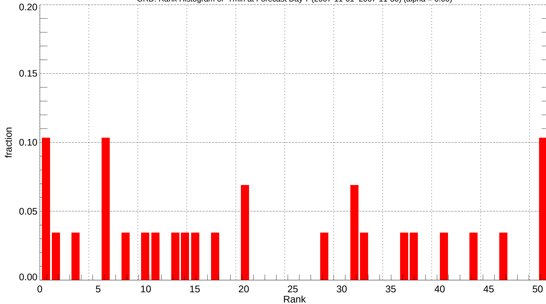
ORD: Rank Histogram of Tmin at Forecast Day 7 (2007-11-01~2007-11-30) (alpha = 0.00)
