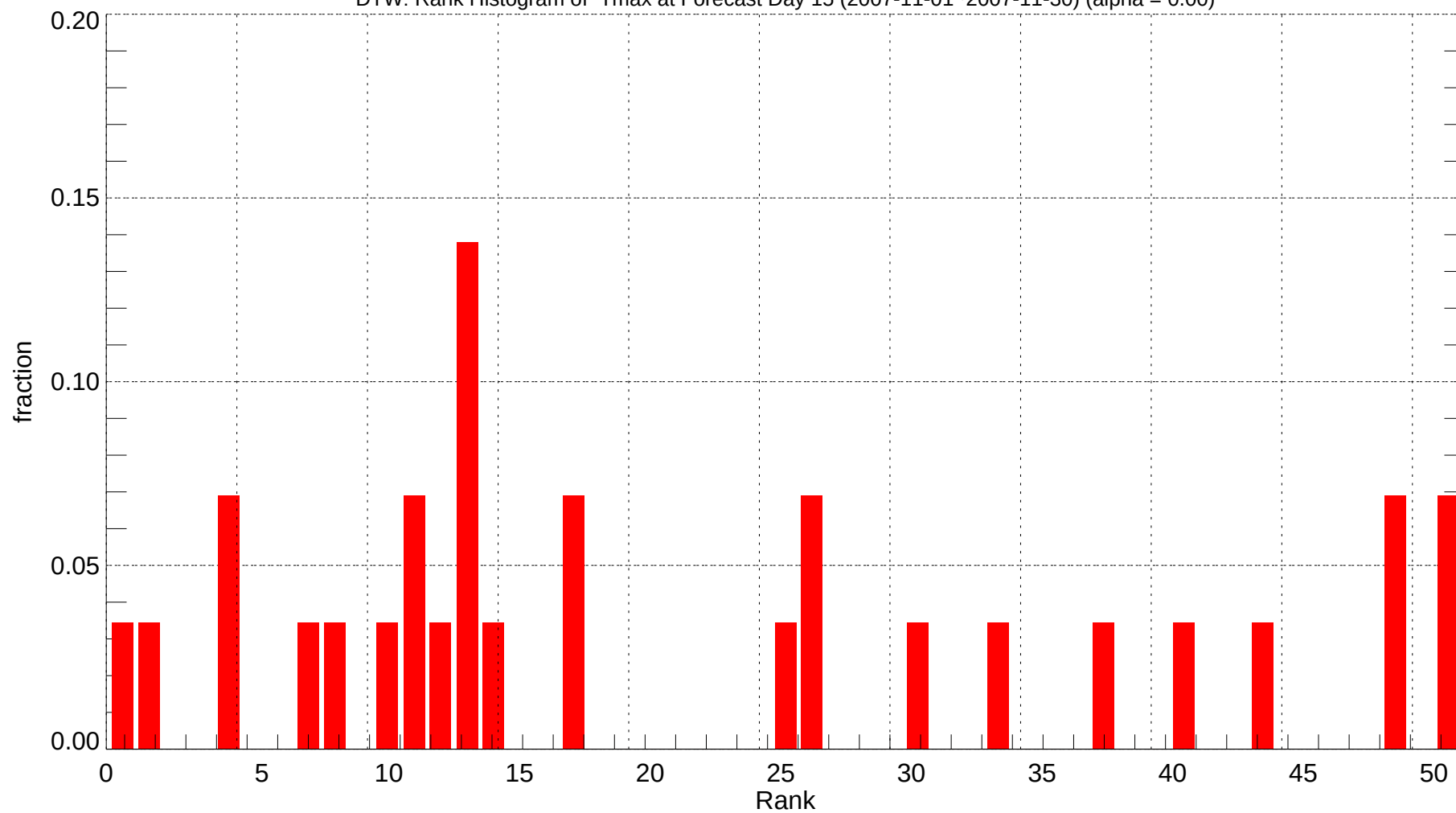
DTW: Rank Histogram of Tmax at Forecast Day 15 (2007-11-01~2007-11-30) (alpha = 0.00)
