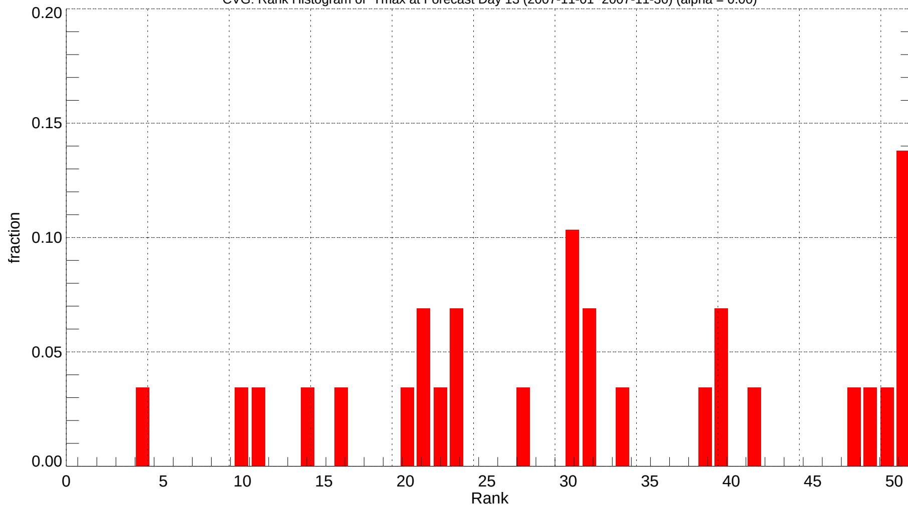
CVG: Rank Histogram of Tmax at Forecast Day 13 (2007-11-01~2007-11-30) (alpha = 0.00)
