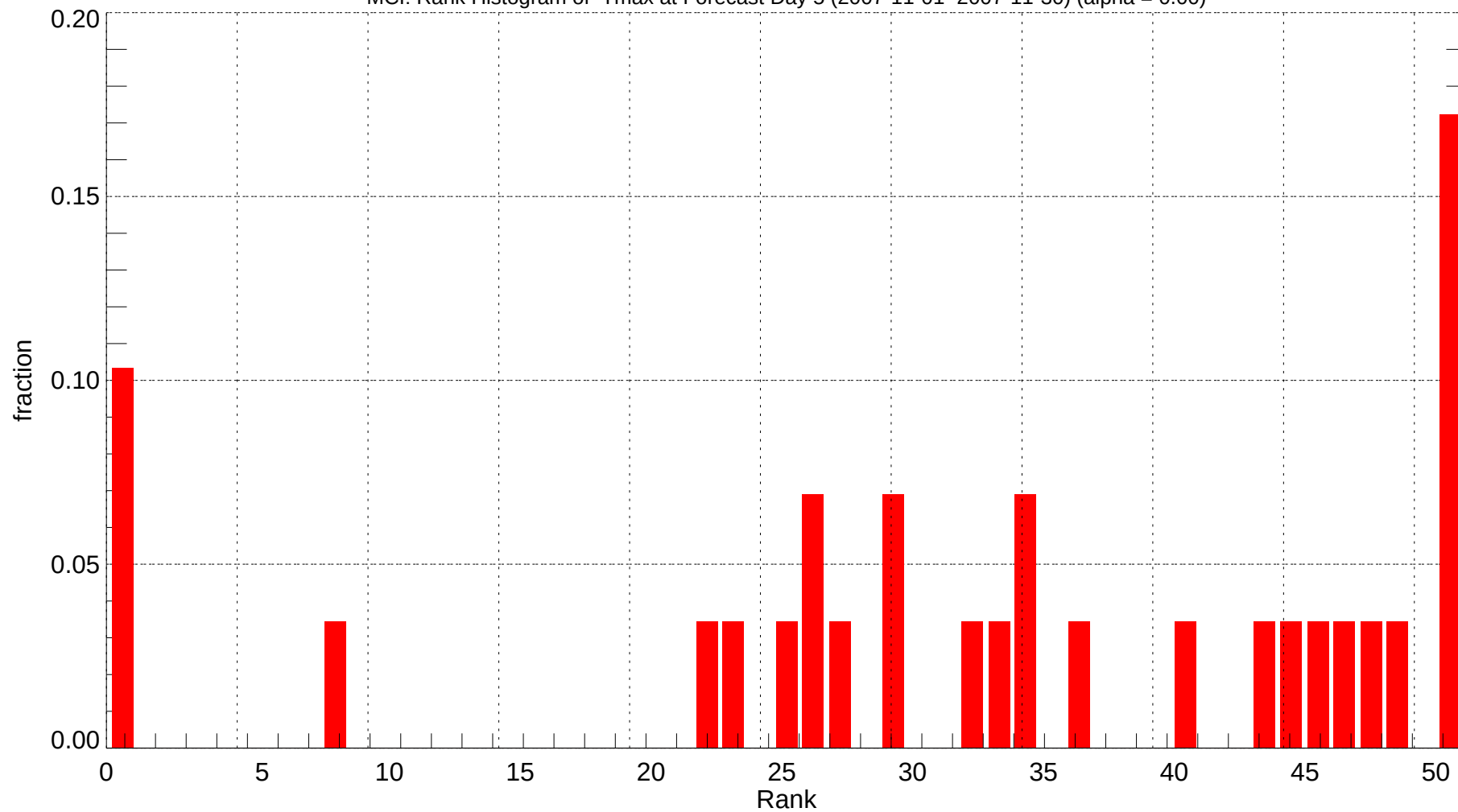
MCI: Rank Histogram of Tmax at Forecast Day 5 (2007-11-01~2007-11-30) (alpha = 0.00)
