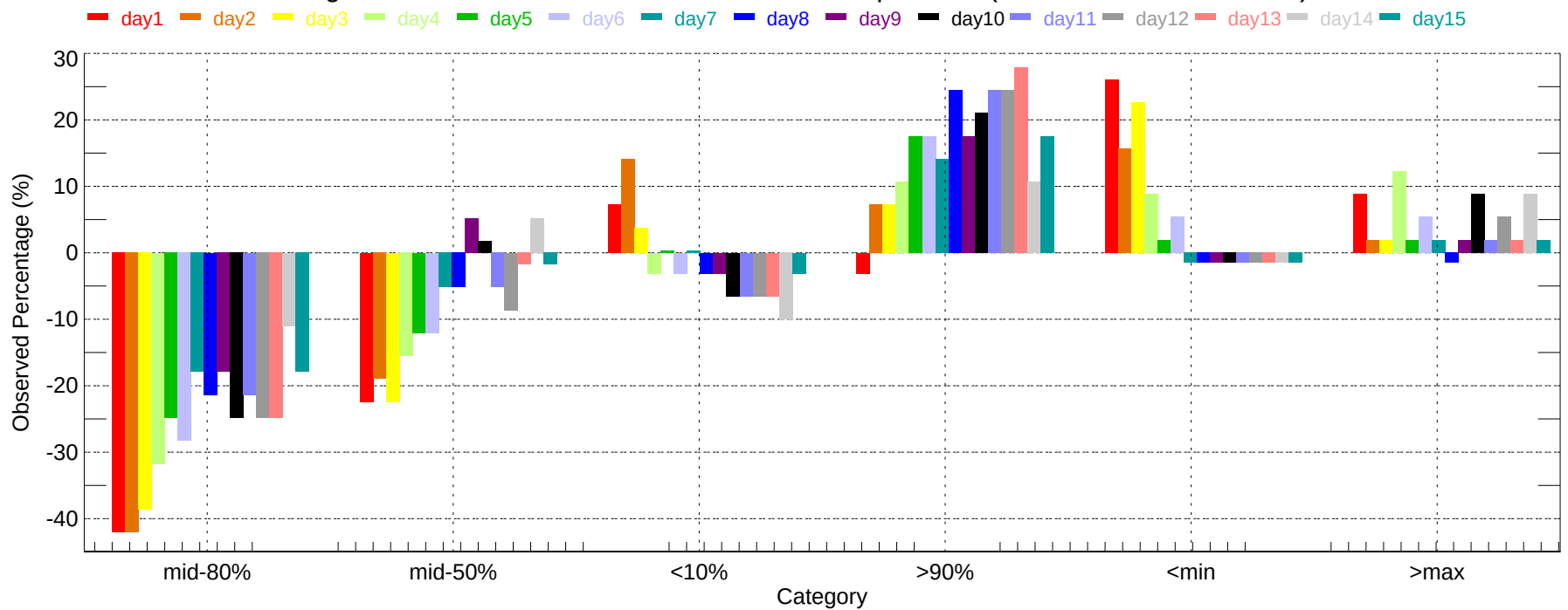
Observed Percentage Deviation of Ensembles - DSM: Max Temperature (2007-11-01~2007-11-30)
