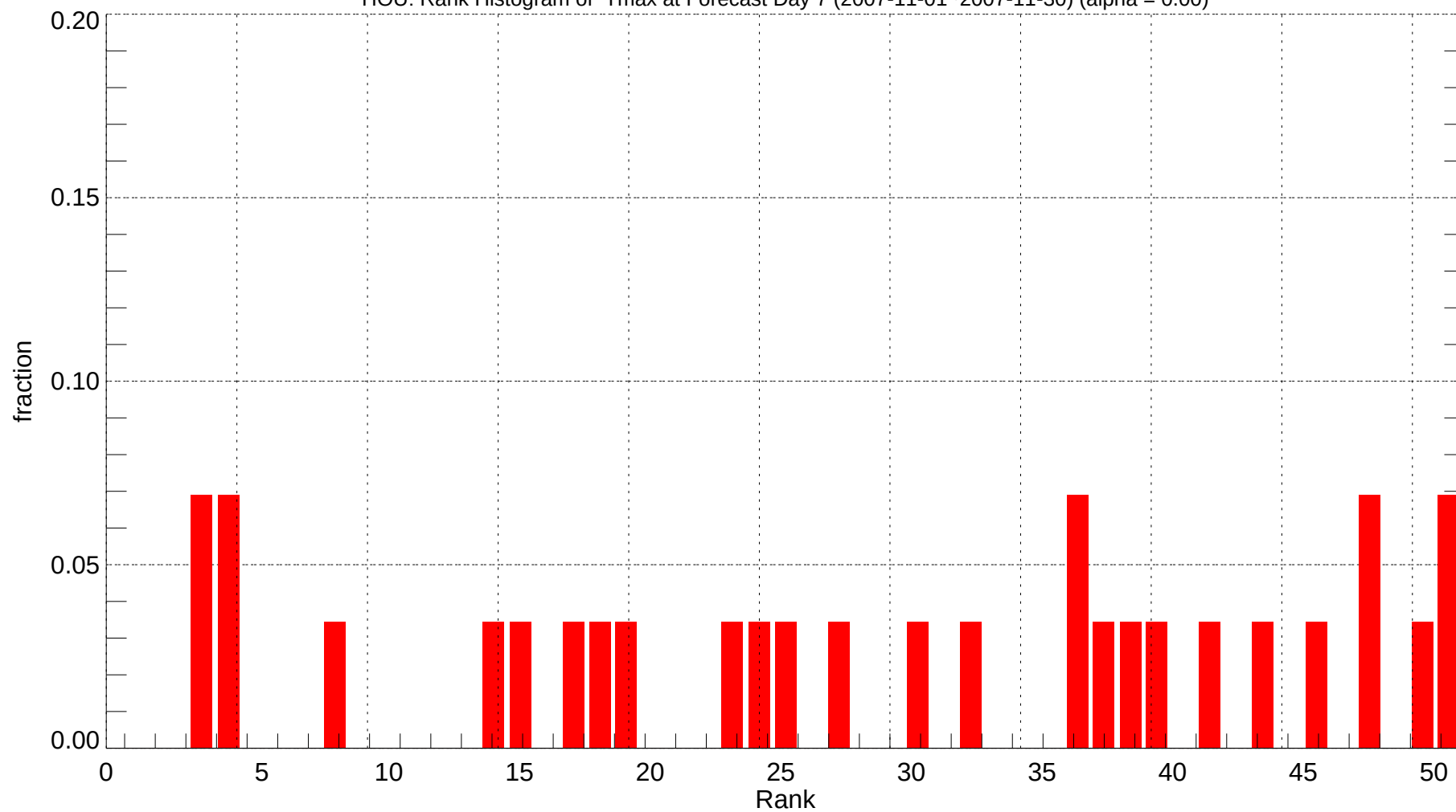
HOU: Rank Histogram of Tmax at Forecast Day 7 (2007-11-01~2007-11-30) (alpha = 0.00)
