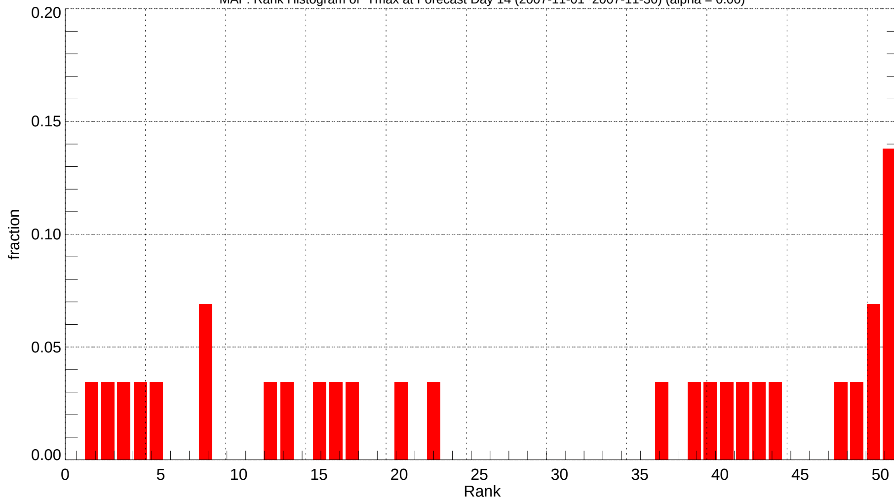
MAF: Rank Histogram of Tmax at Forecast Day 14 (2007-11-01~2007-11-30) (alpha = 0.00)
