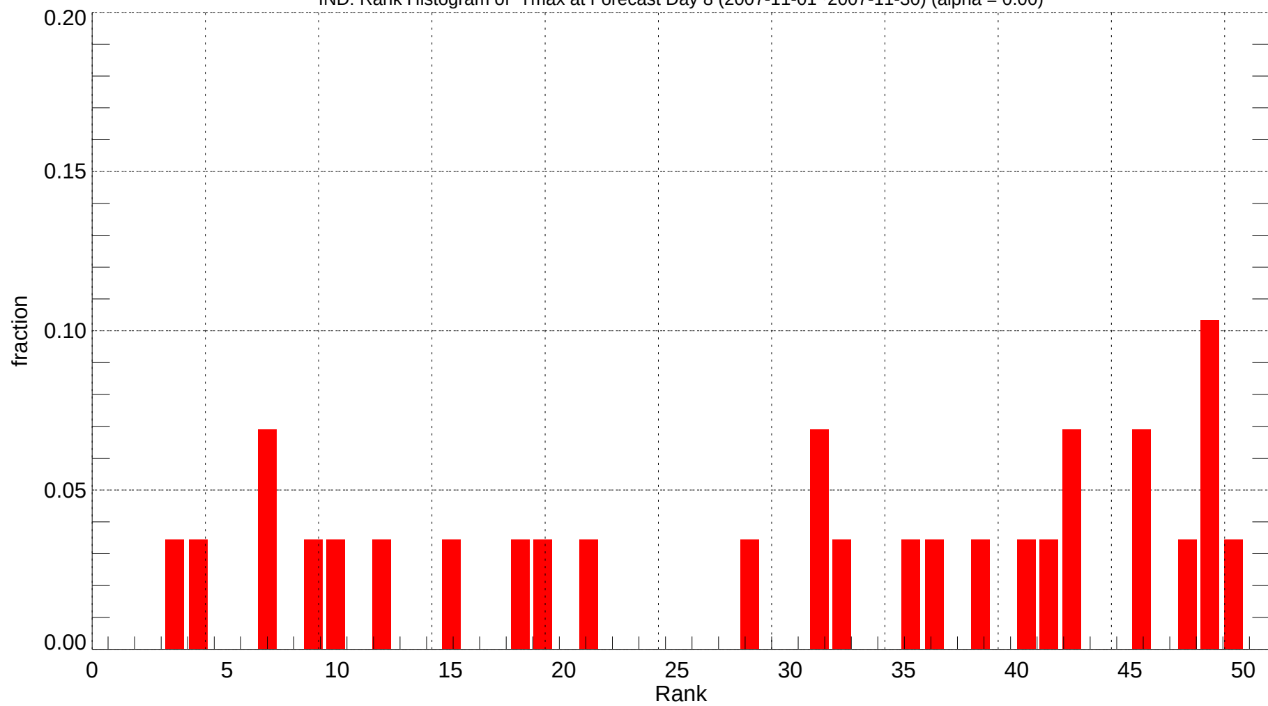
IND: Rank Histogram of Tmax at Forecast Day 8 (2007-11-01~2007-11-30) (alpha = 0.00)
