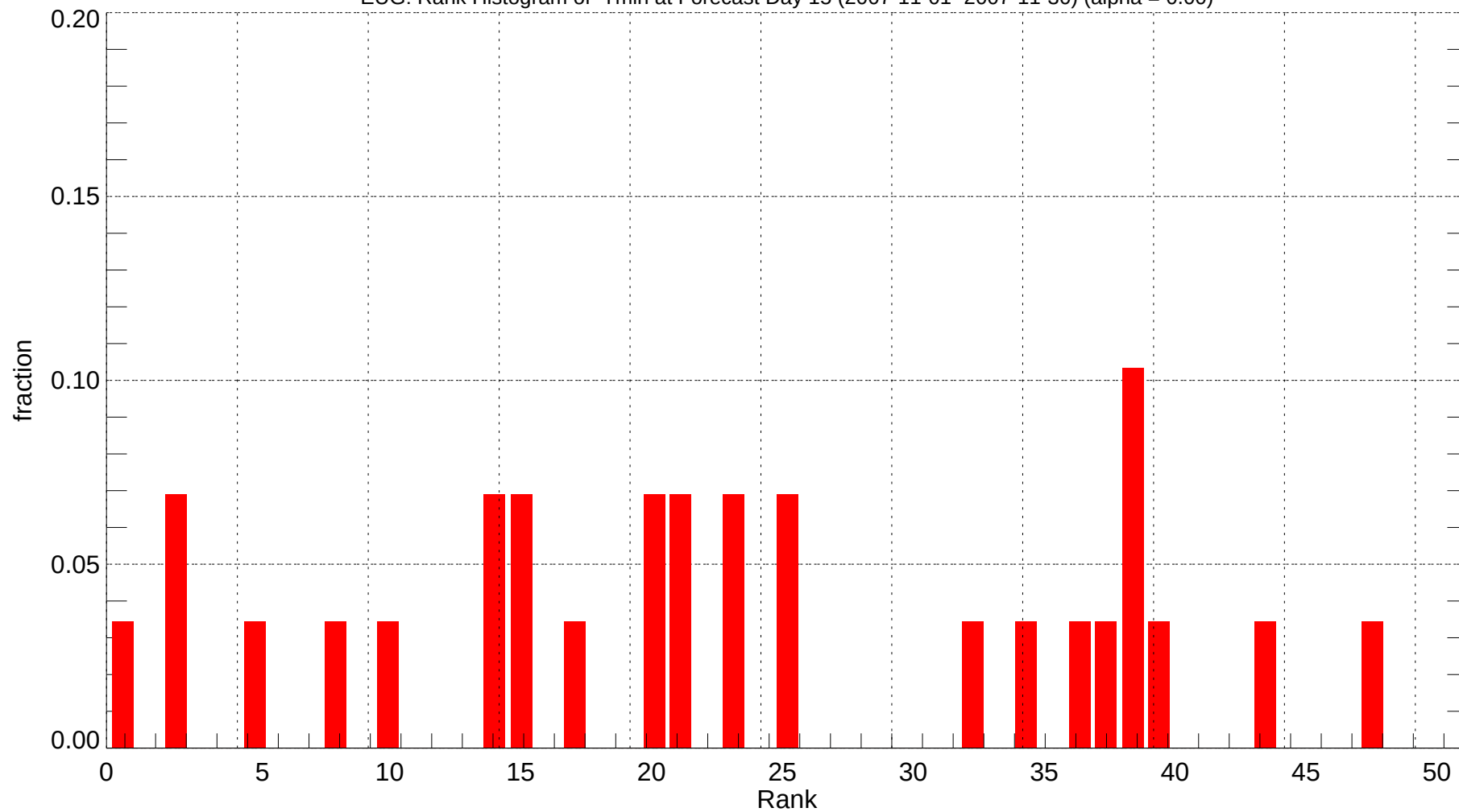
EUG: Rank Histogram of Tmin at Forecast Day 15 (2007-11-01~2007-11-30) (alpha = 0.00)
