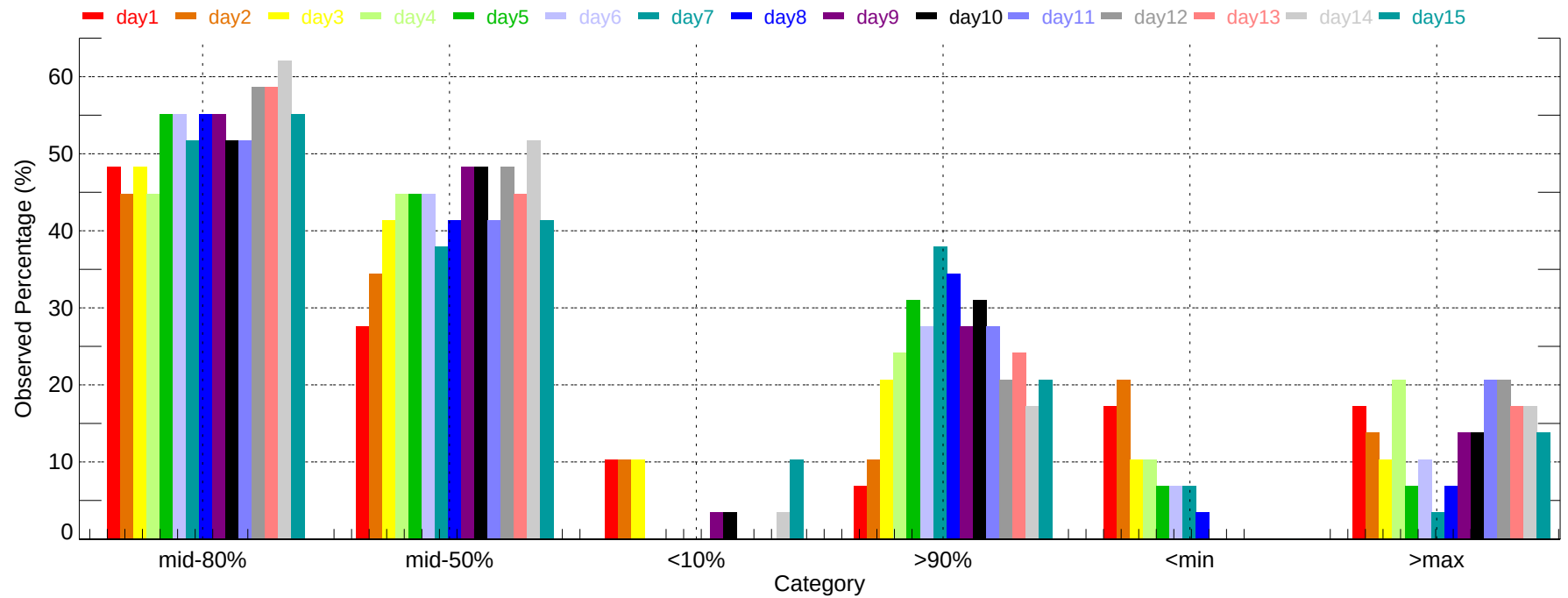
Observed Percentage of Ensembles - ICT: Max Temperature (2007-11-01~2007-11-30)
