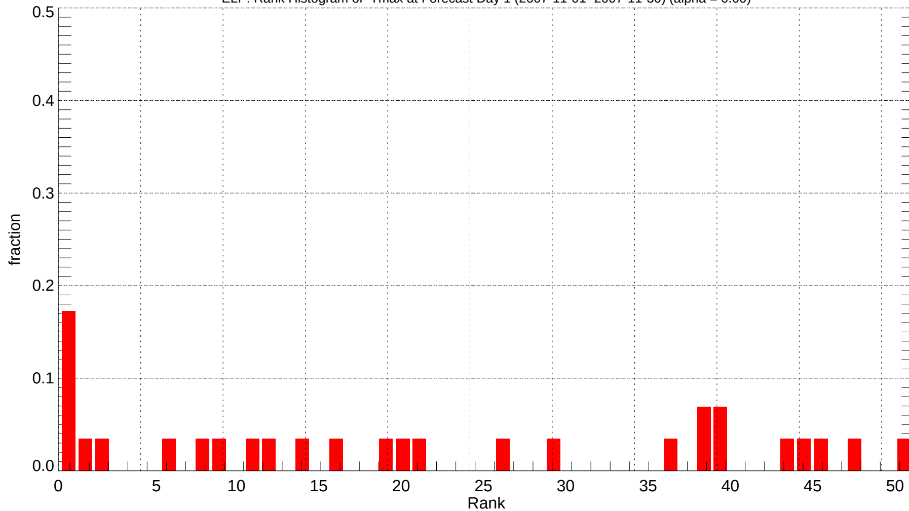
ELP: Rank Histogram of Tmax at Forecast Day 1 (2007-11-01~2007-11-30) (alpha = 0.00)
