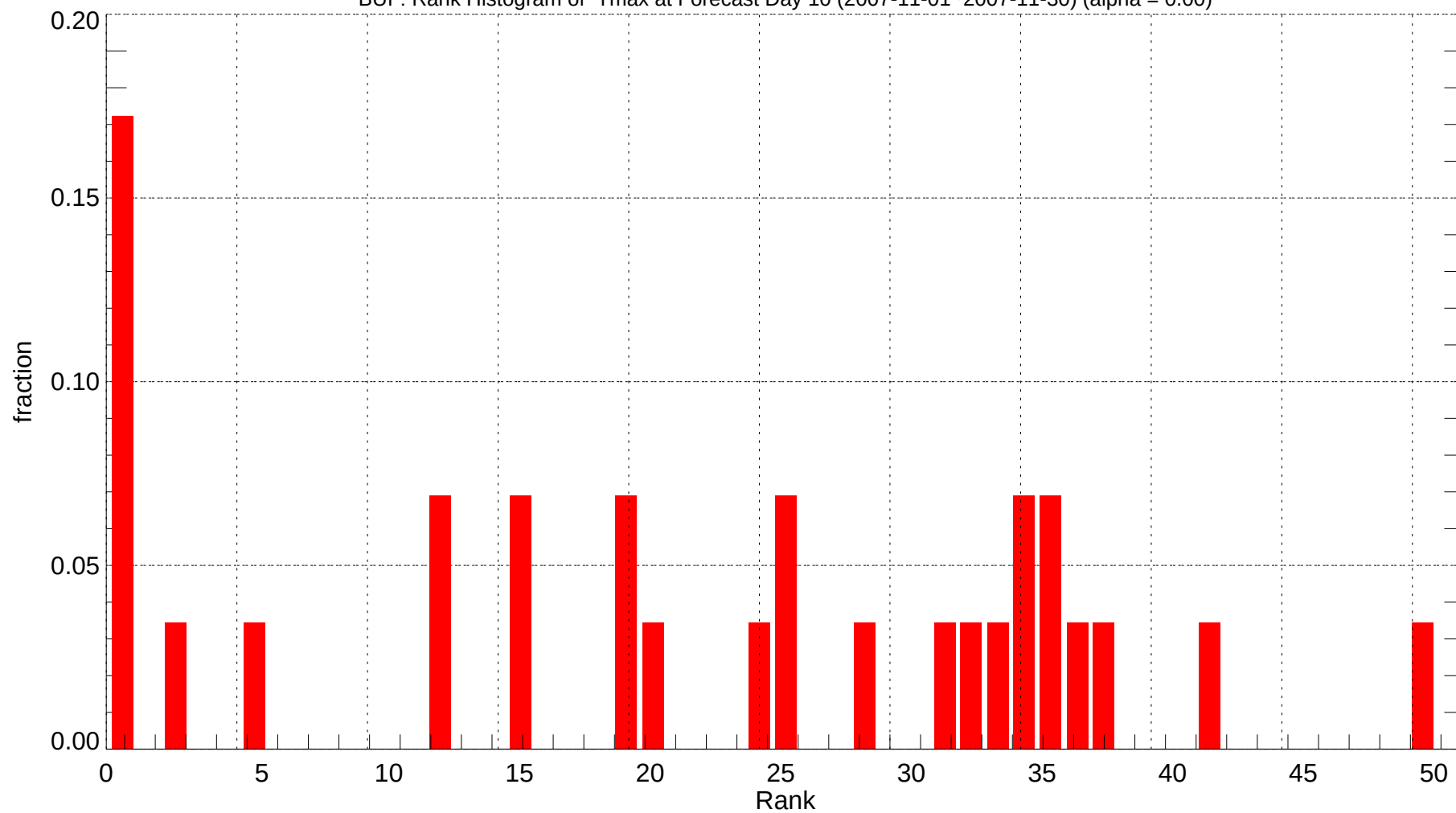
BUF: Rank Histogram of Tmax at Forecast Day 10 (2007-11-01~2007-11-30) (alpha = 0.00)
