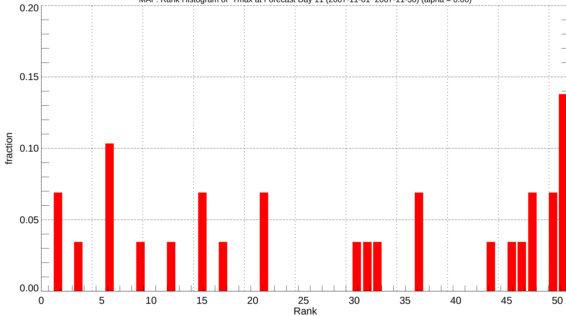
MAF: Rank Histogram of Tmax at Forecast Day 11 (2007-11-01~2007-11-30) (alpha = 0.00)
