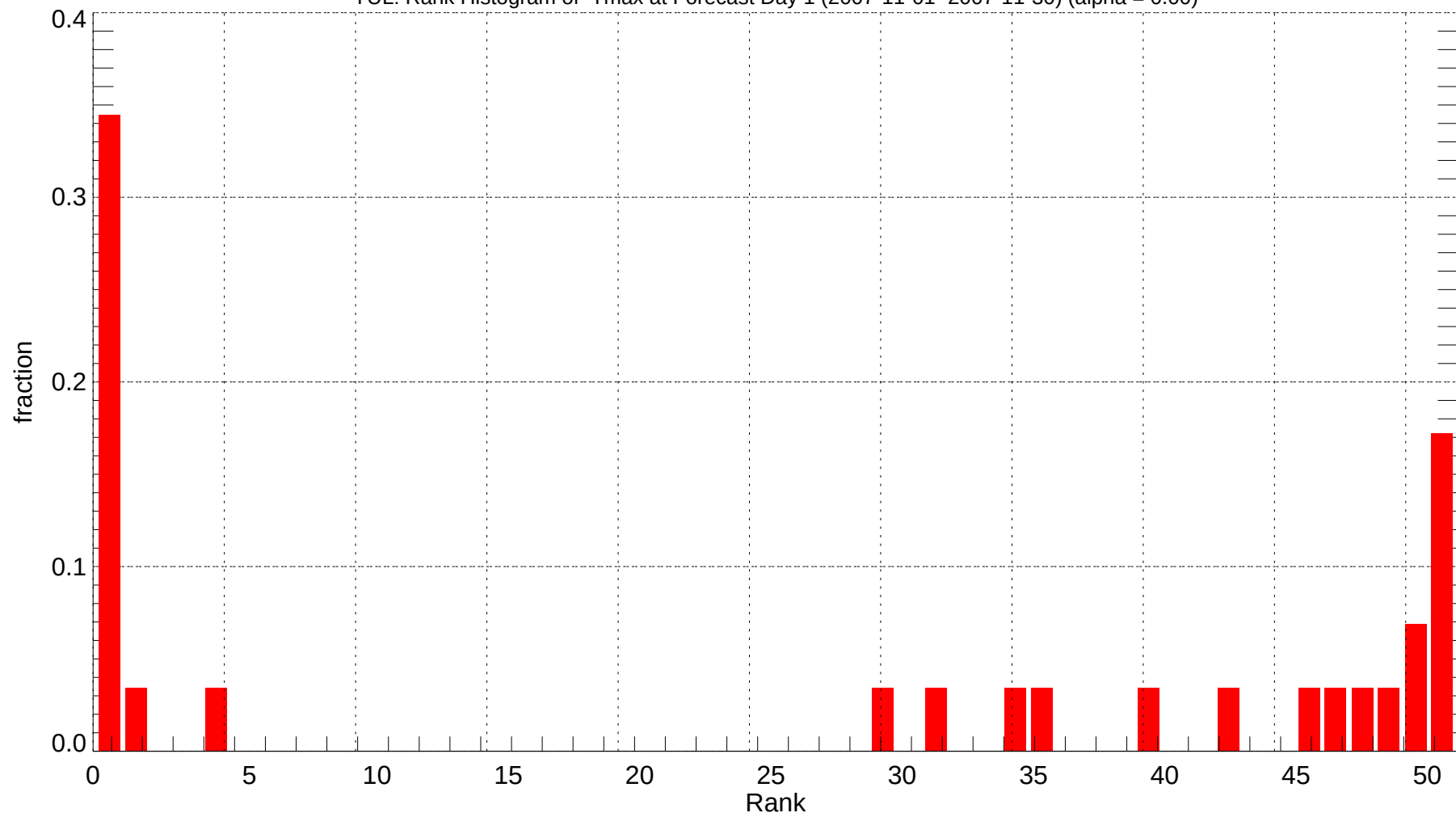
YUL: Rank Histogram of Tmax at Forecast Day 1 (2007-11-01~2007-11-30) (alpha = 0.00)
