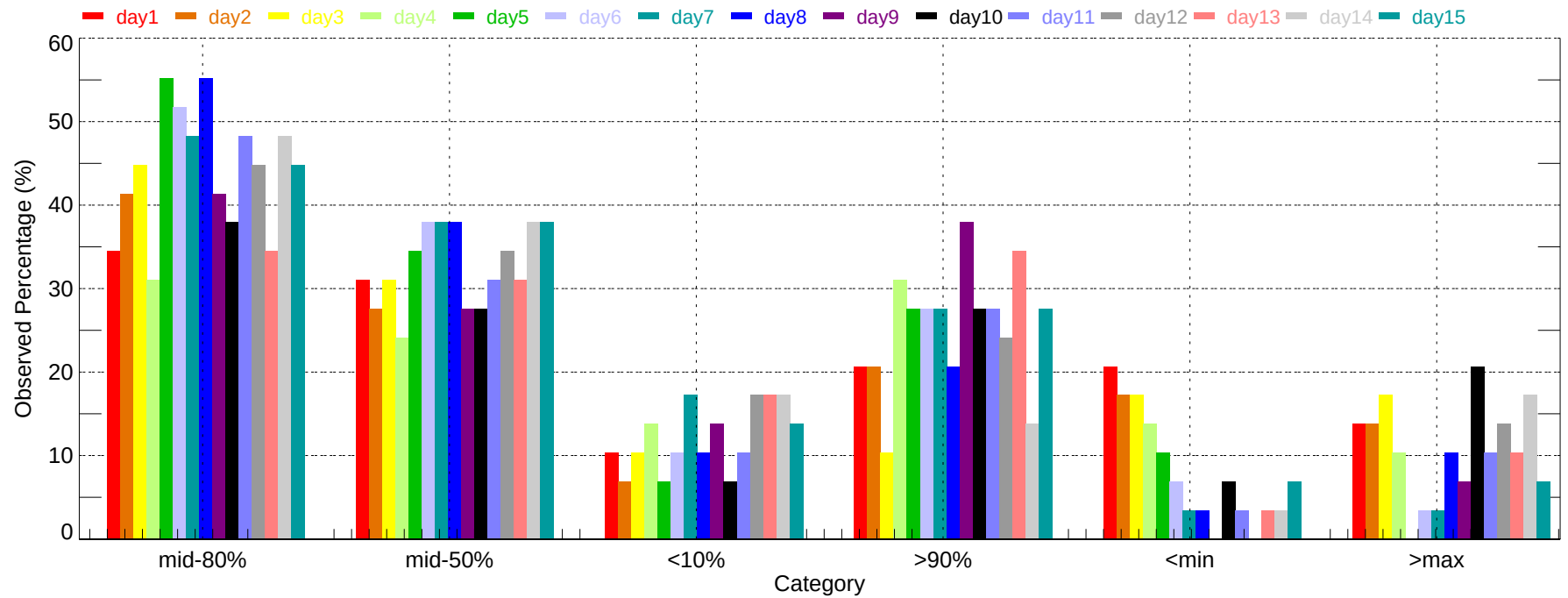
Observed Percentage of Ensembles - SJT: Min Temperature (2007-11-01~2007-11-30)
