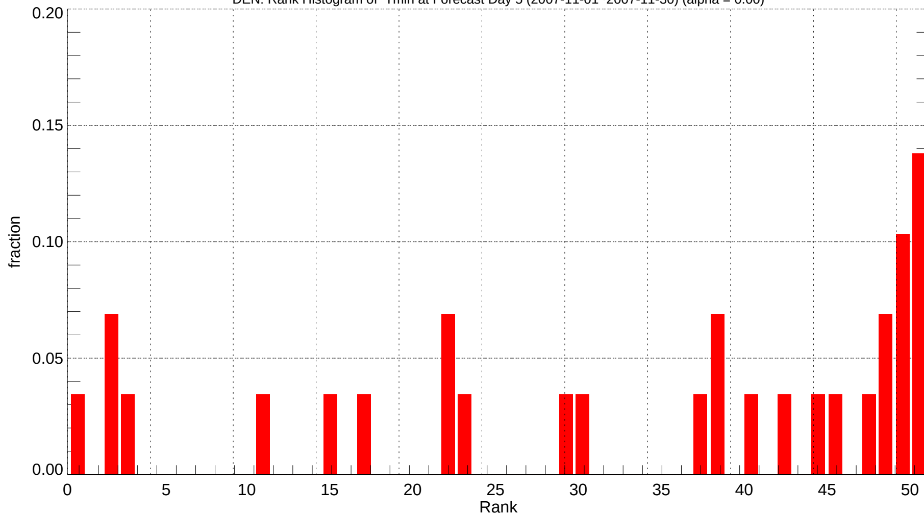
DEN: Rank Histogram of Tmin at Forecast Day 5 (2007-11-01~2007-11-30) (alpha = 0.00)
