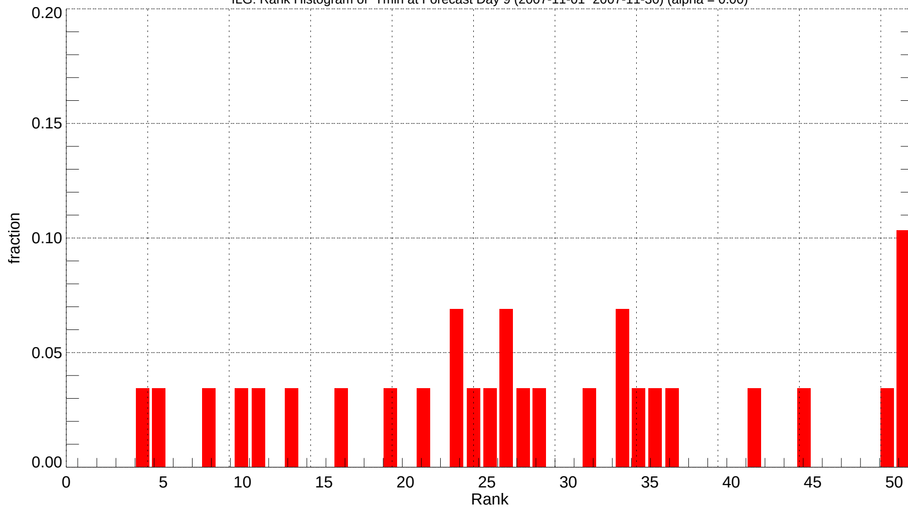
ILG: Rank Histogram of Tmin at Forecast Day 9 (2007-11-01~2007-11-30) (alpha = 0.00)
