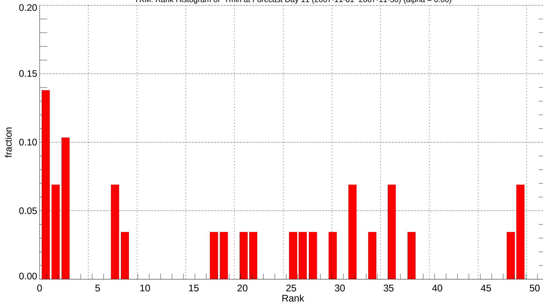
YKM: Rank Histogram of Tmin at Forecast Day 11 (2007-11-01~2007-11-30) (alpha = 0.00)
