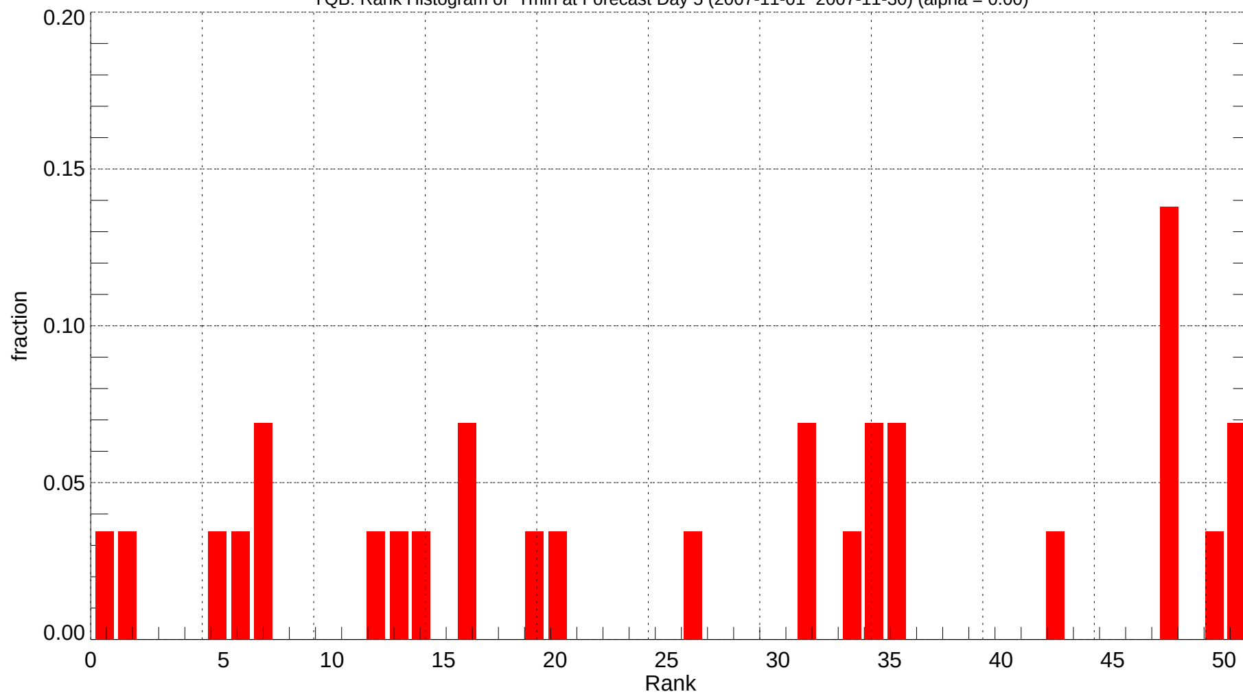
YQB: Rank Histogram of Tmin at Forecast Day 5 (2007-11-01~2007-11-30) (alpha = 0.00)
