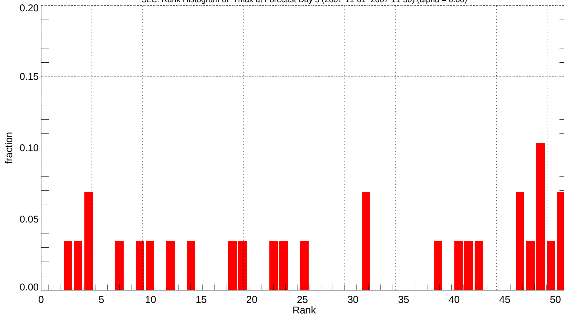
SLC: Rank Histogram of Tmax at Forecast Day 5 (2007-11-01~2007-11-30) (alpha = 0.00)
