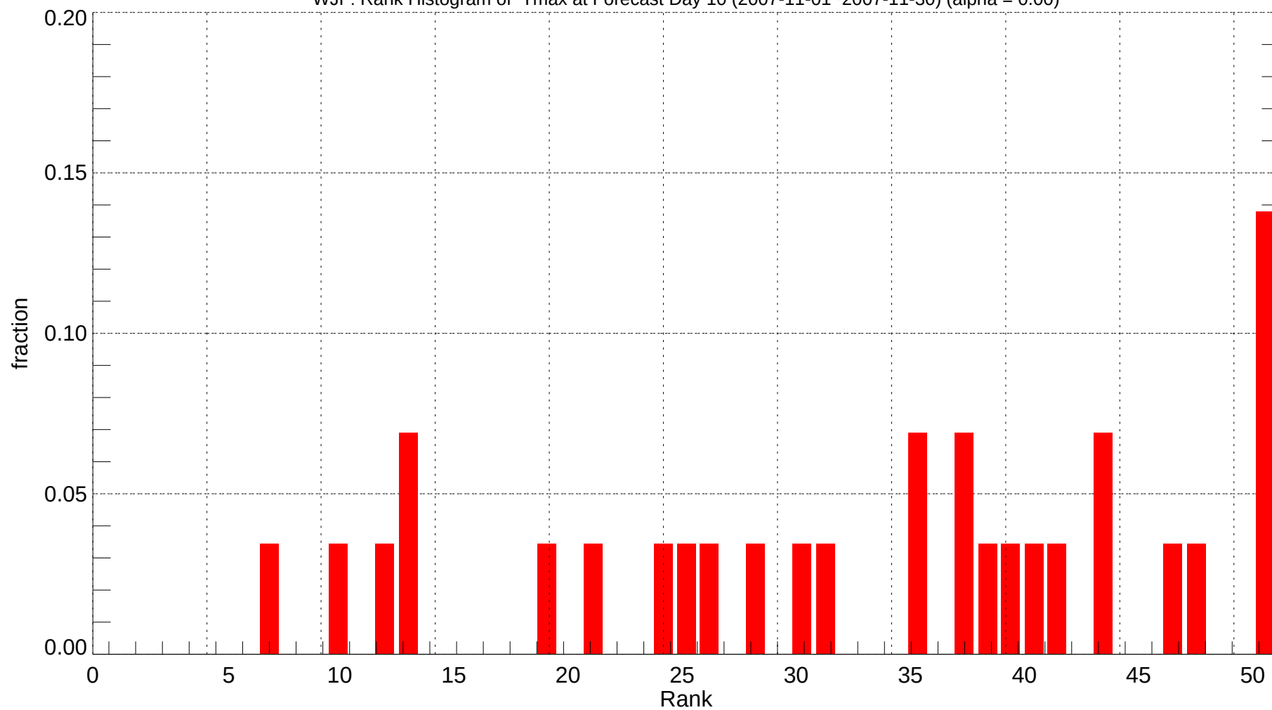
WJF: Rank Histogram of Tmax at Forecast Day 10 (2007-11-01~2007-11-30) (alpha = 0.00)
