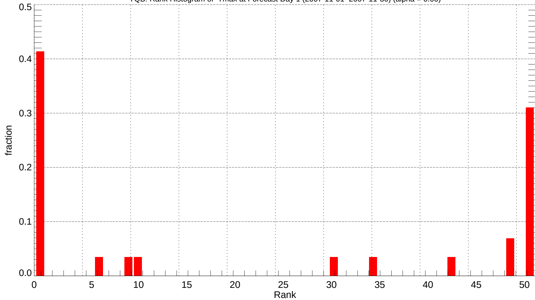
YQB: Rank Histogram of Tmax at Forecast Day 1 (2007-11-01~2007-11-30) (alpha = 0.00)
