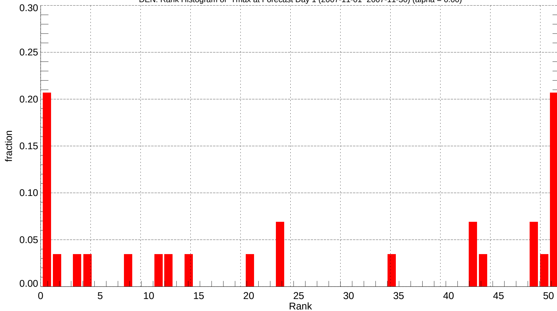
DEN: Rank Histogram of Tmax at Forecast Day 1 (2007-11-01~2007-11-30) (alpha = 0.00)
