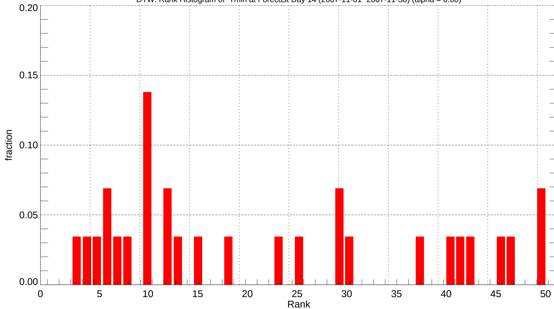
DTW: Rank Histogram of Tmin at Forecast Day 14 (2007-11-01~2007-11-30) (alpha = 0.00)
