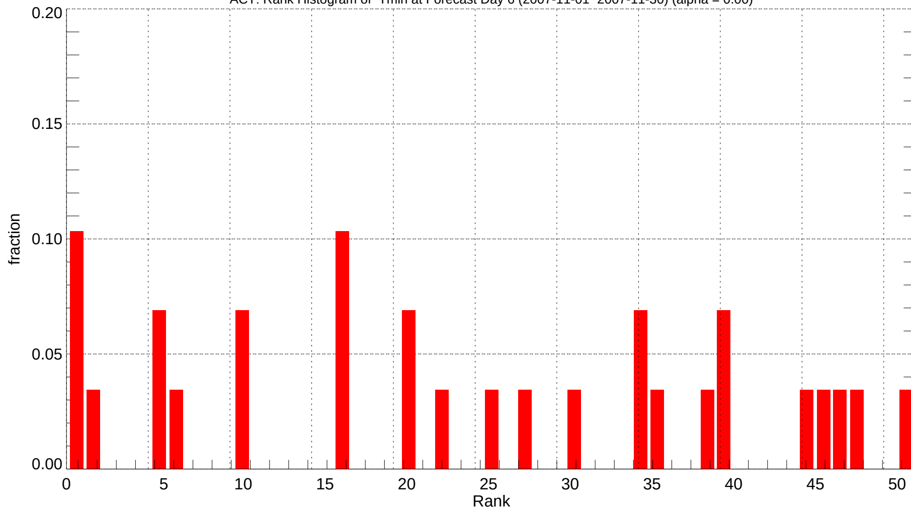
ACT: Rank Histogram of Tmin at Forecast Day 6 (2007-11-01~2007-11-30) (alpha = 0.00)
