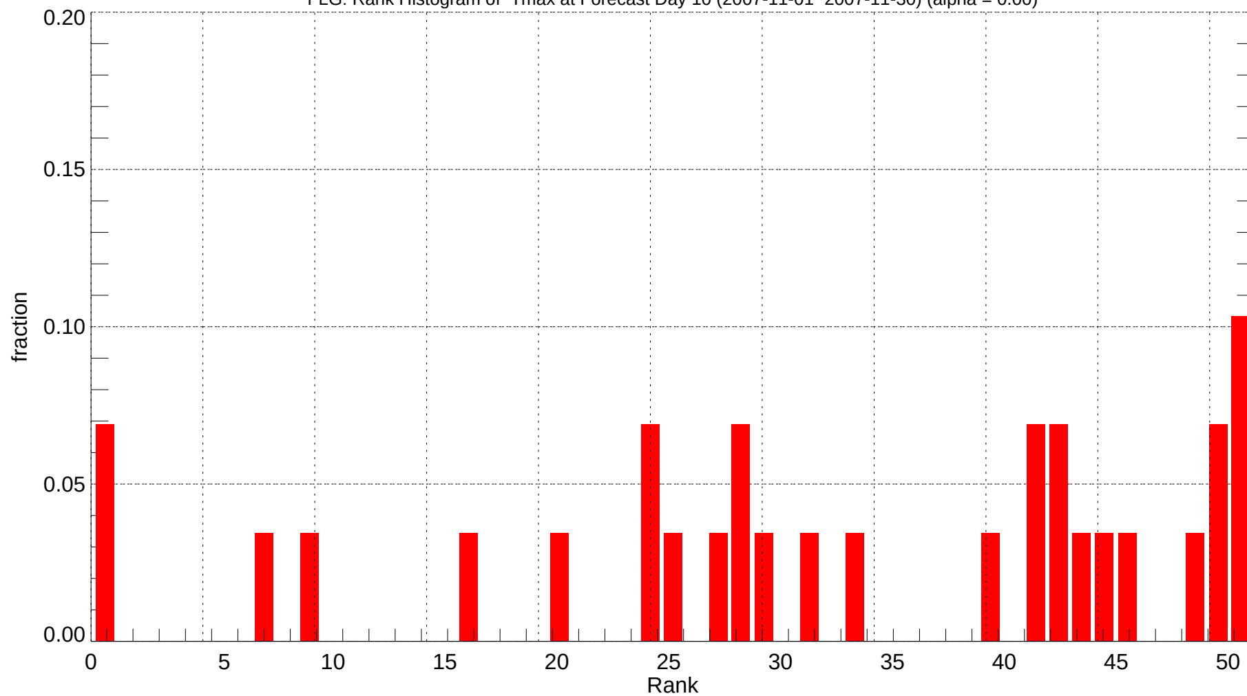
FLG: Rank Histogram of Tmax at Forecast Day 10 (2007-11-01~2007-11-30) (alpha = 0.00)
