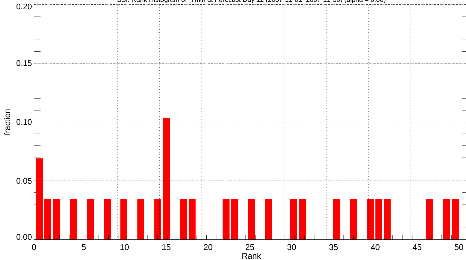
SSI: Rank Histogram of Tmin at Forecast Day 12 (2007-11-01~2007-11-30) (alpha = 0.00)
