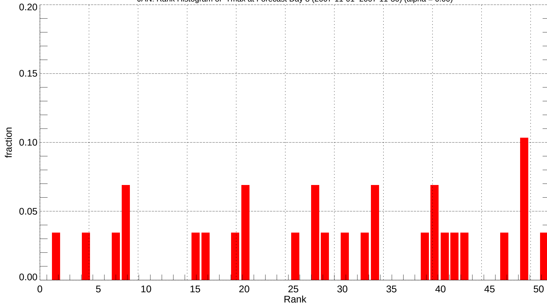
JAN: Rank Histogram of Tmax at Forecast Day 8 (2007-11-01~2007-11-30) (alpha = 0.00)
