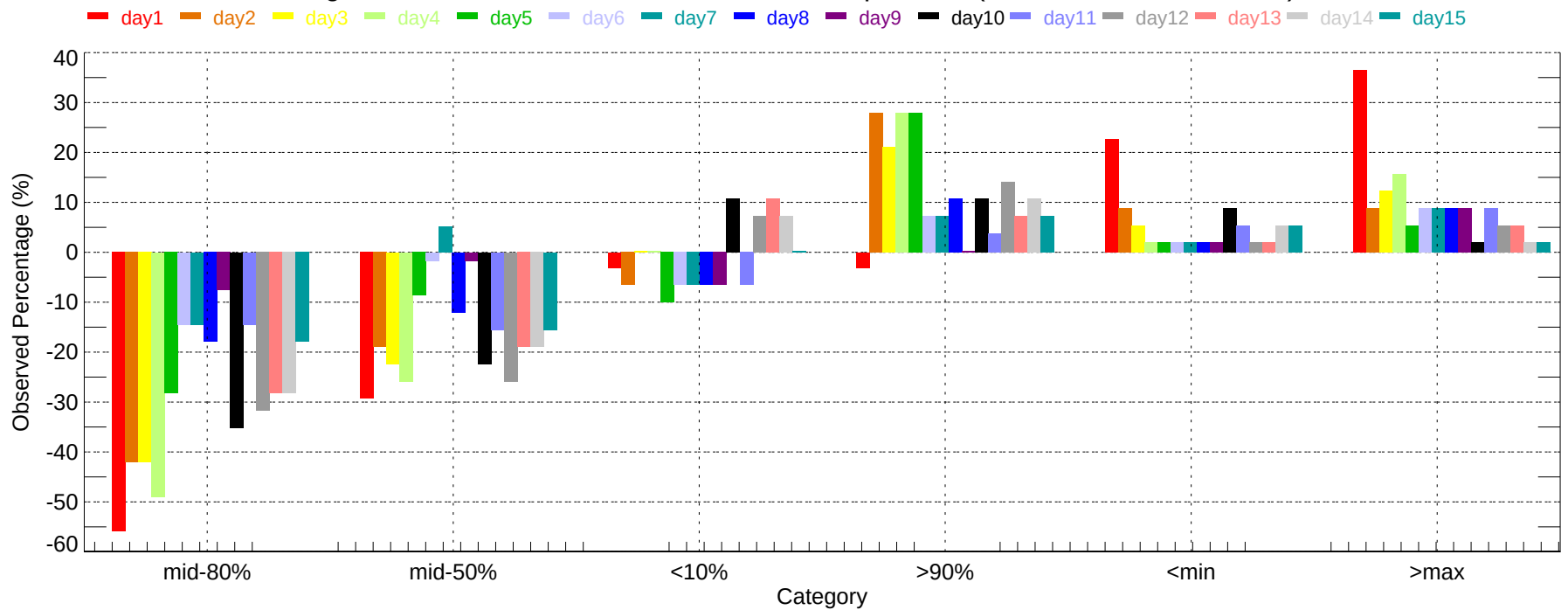
Observed Percentage Deviation of Ensembles - ACY: Min Temperature (2007-11-01~2007-11-30)
