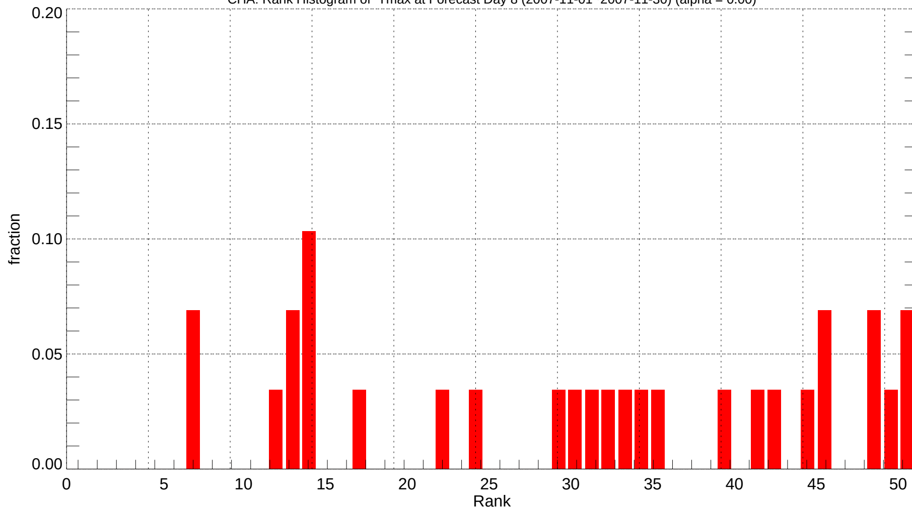
CHA: Rank Histogram of Tmax at Forecast Day 8 (2007-11-01~2007-11-30) (alpha = 0.00)
