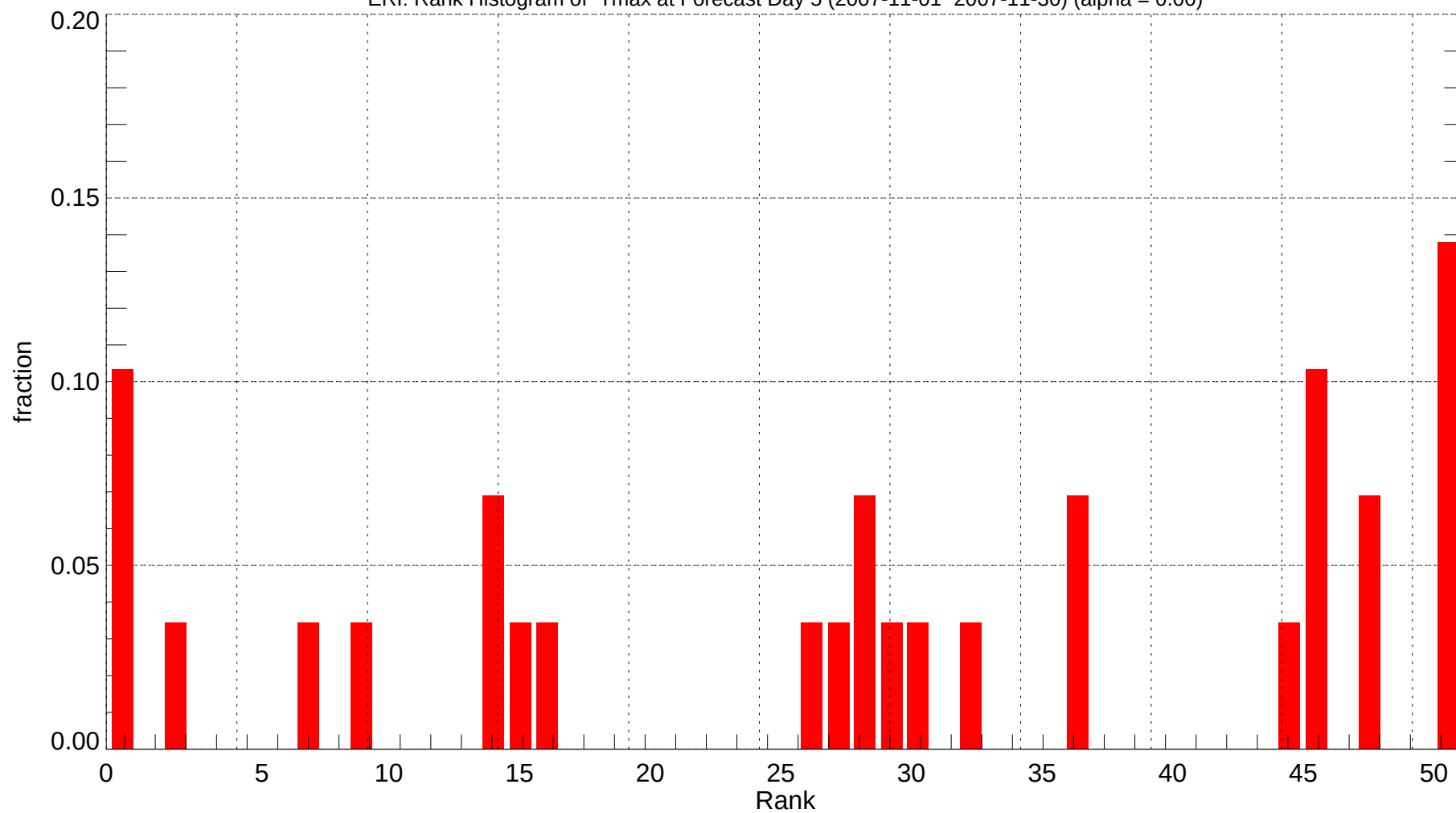
ERI: Rank Histogram of Tmax at Forecast Day 5 (2007-11-01~2007-11-30) (alpha = 0.00)
