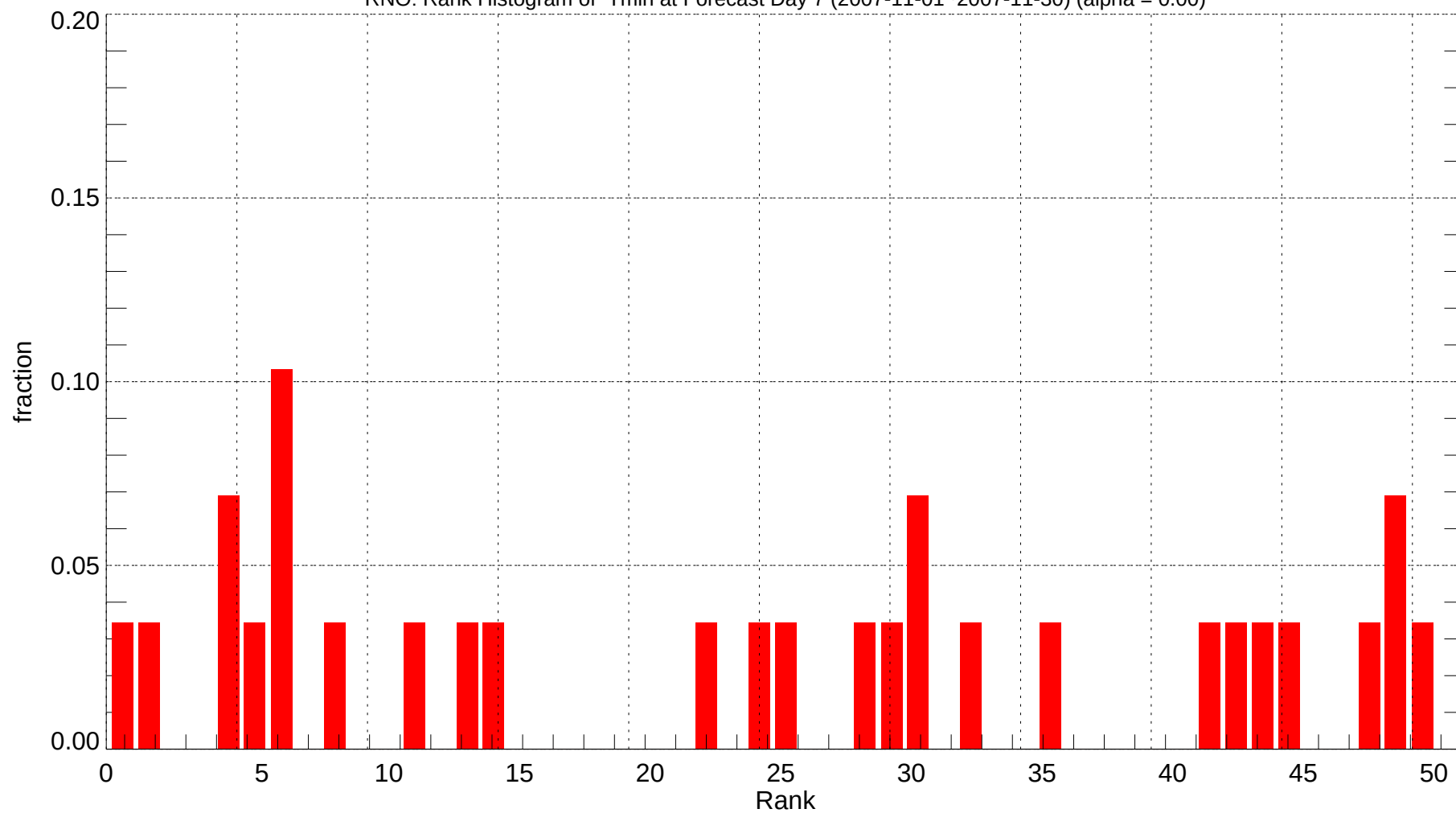
RNO: Rank Histogram of Tmin at Forecast Day 7 (2007-11-01~2007-11-30) (alpha = 0.00)
