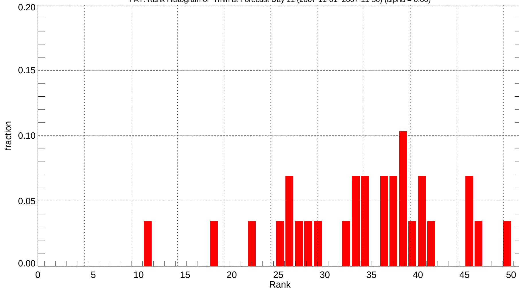
FAT: Rank Histogram of Tmin at Forecast Day 11 (2007-11-01~2007-11-30) (alpha = 0.00)
