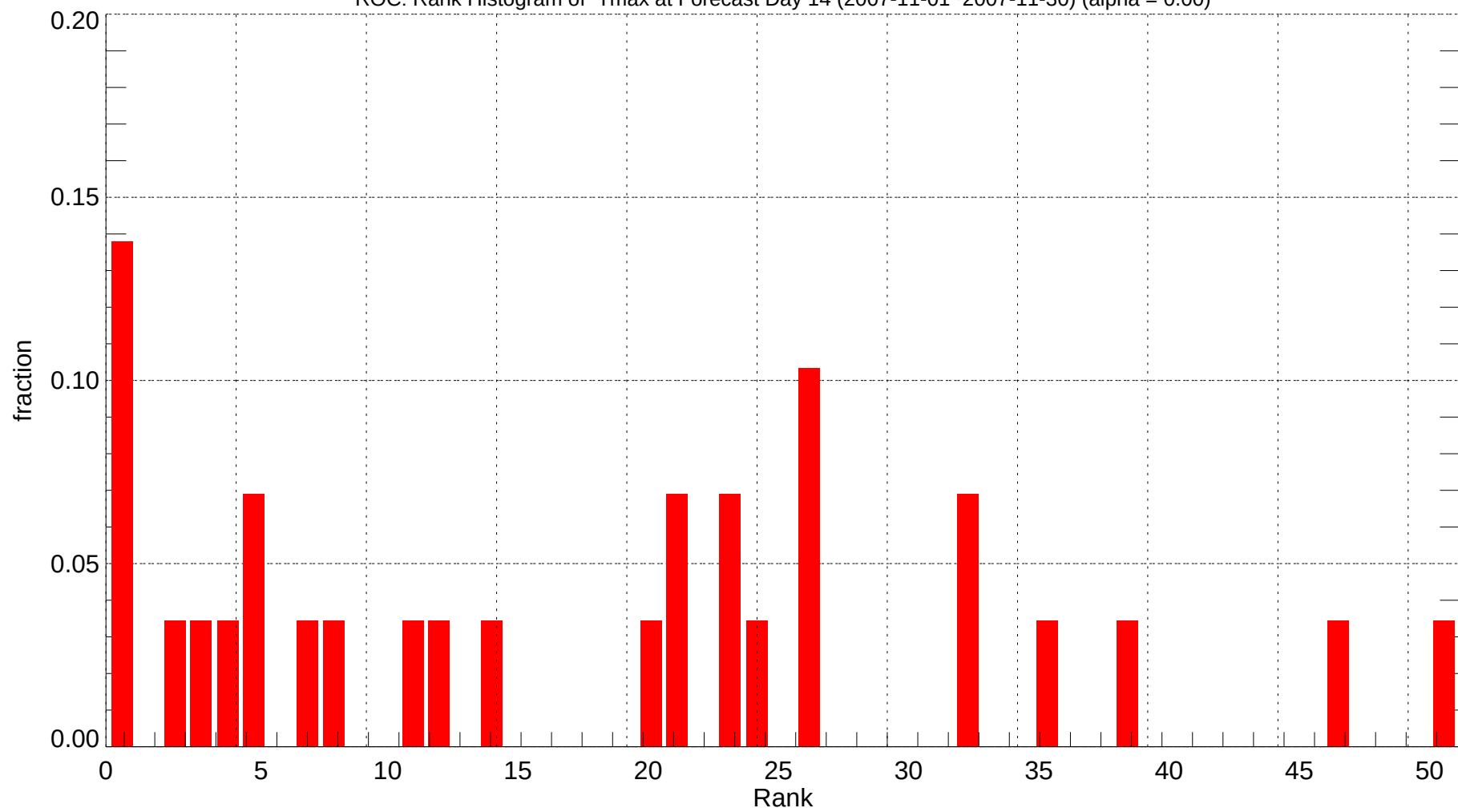
ROC: Rank Histogram of Tmax at Forecast Day 14 (2007-11-01~2007-11-30) (alpha = 0.00)
