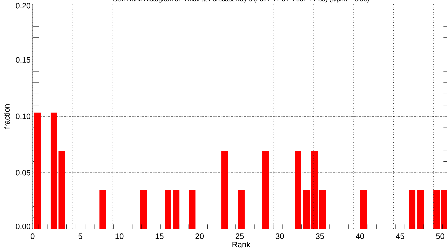
SSI: Rank Histogram of Tmax at Forecast Day 5 (2007-11-01~2007-11-30) (alpha = 0.00)
