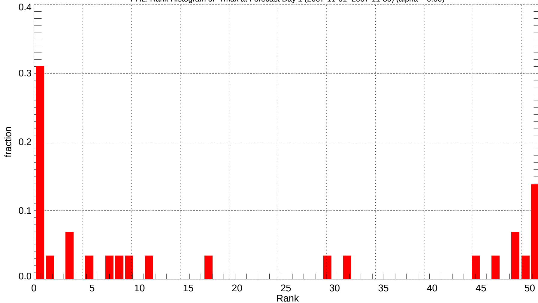
PHL: Rank Histogram of Tmax at Forecast Day 1 (2007-11-01~2007-11-30) (alpha = 0.00)
