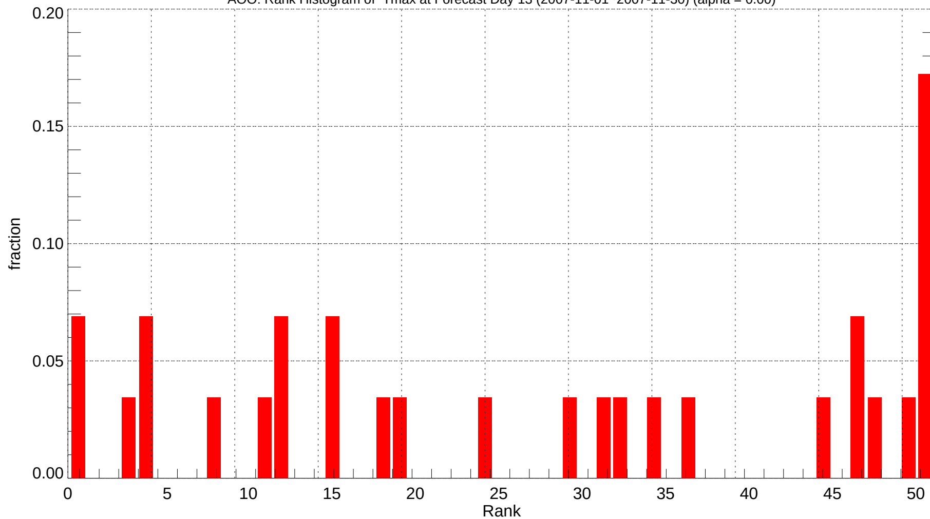
AOO: Rank Histogram of Tmax at Forecast Day 13 (2007-11-01~2007-11-30) (alpha = 0.00)
