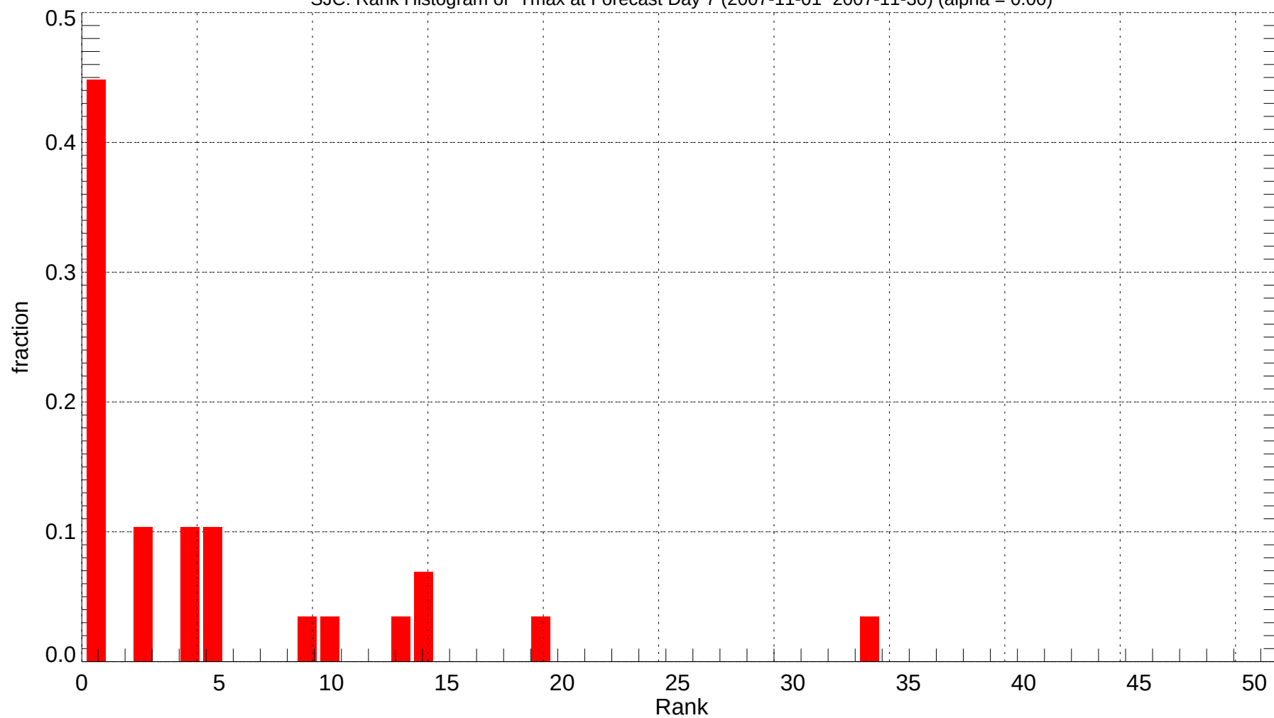
SJC: Rank Histogram of Tmax at Forecast Day 7 (2007-11-01~2007-11-30) (alpha = 0.00)
