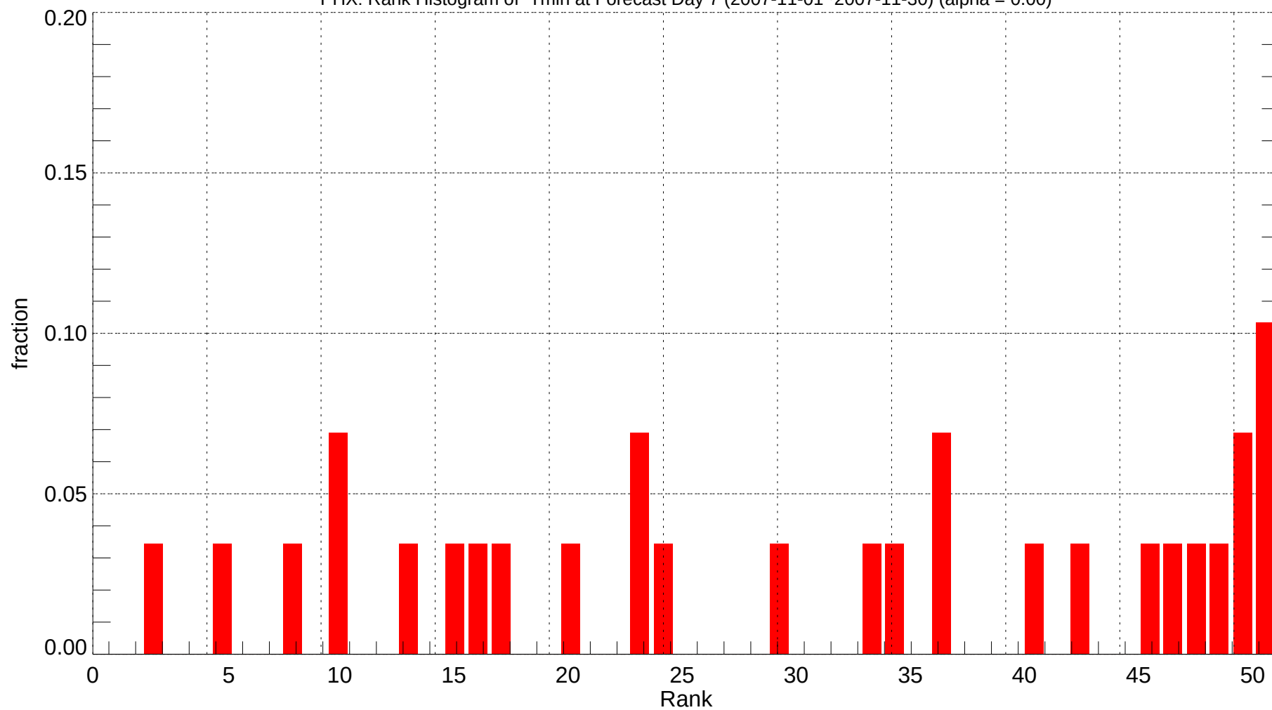
PHX: Rank Histogram of Tmin at Forecast Day 7 (2007-11-01~2007-11-30) (alpha = 0.00)
