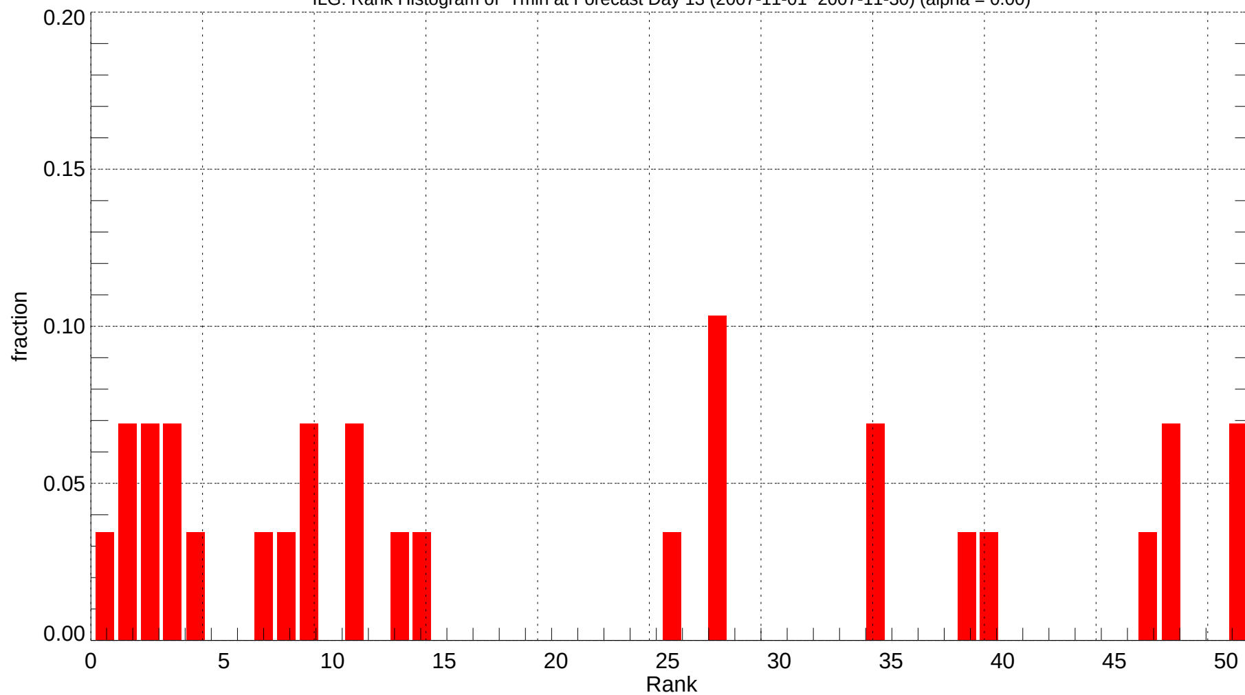
ILG: Rank Histogram of Tmin at Forecast Day 13 (2007-11-01~2007-11-30) (alpha = 0.00)
