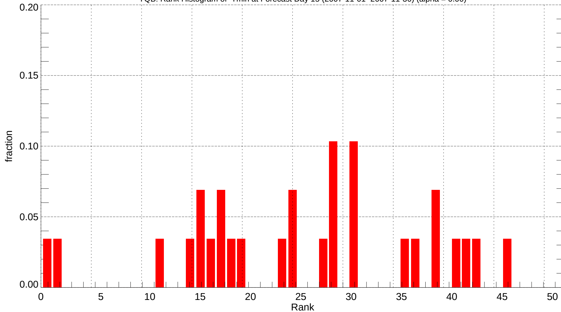
YQB: Rank Histogram of Tmin at Forecast Day 15 (2007-11-01~2007-11-30) (alpha = 0.00)
