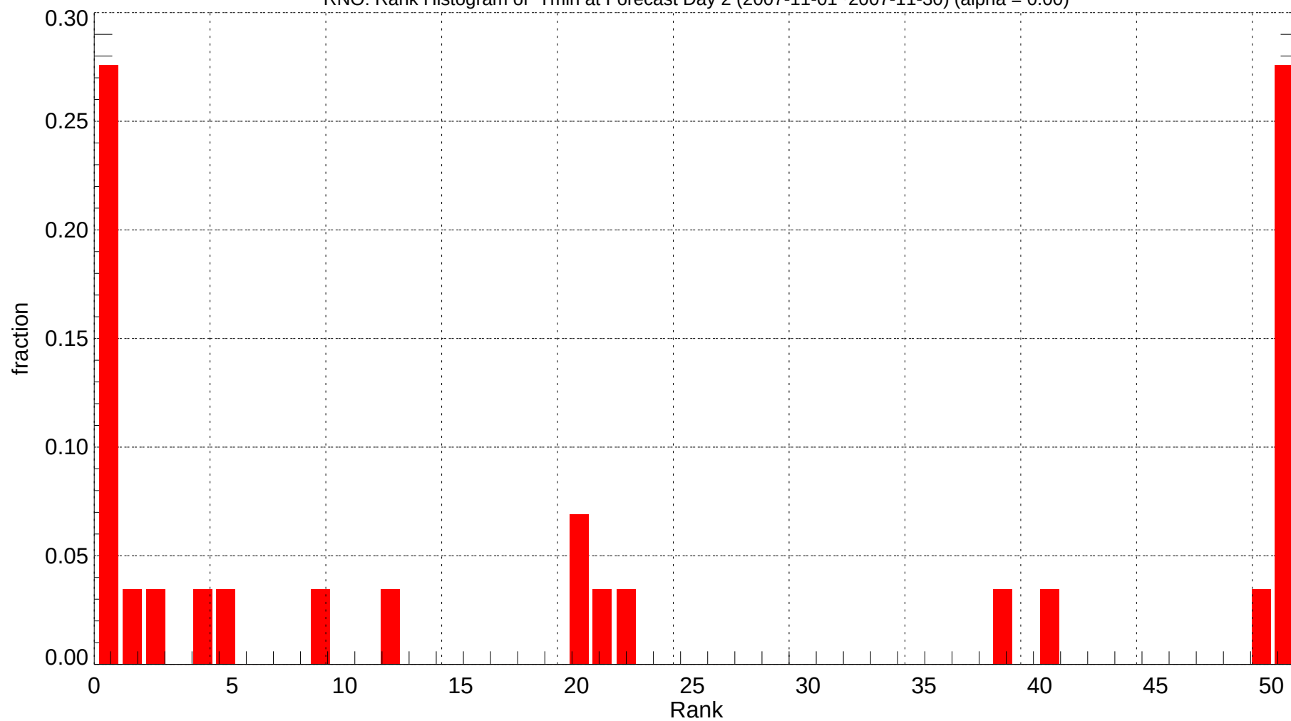
RNO: Rank Histogram of Tmin at Forecast Day 2 (2007-11-01~2007-11-30) (alpha = 0.00)
