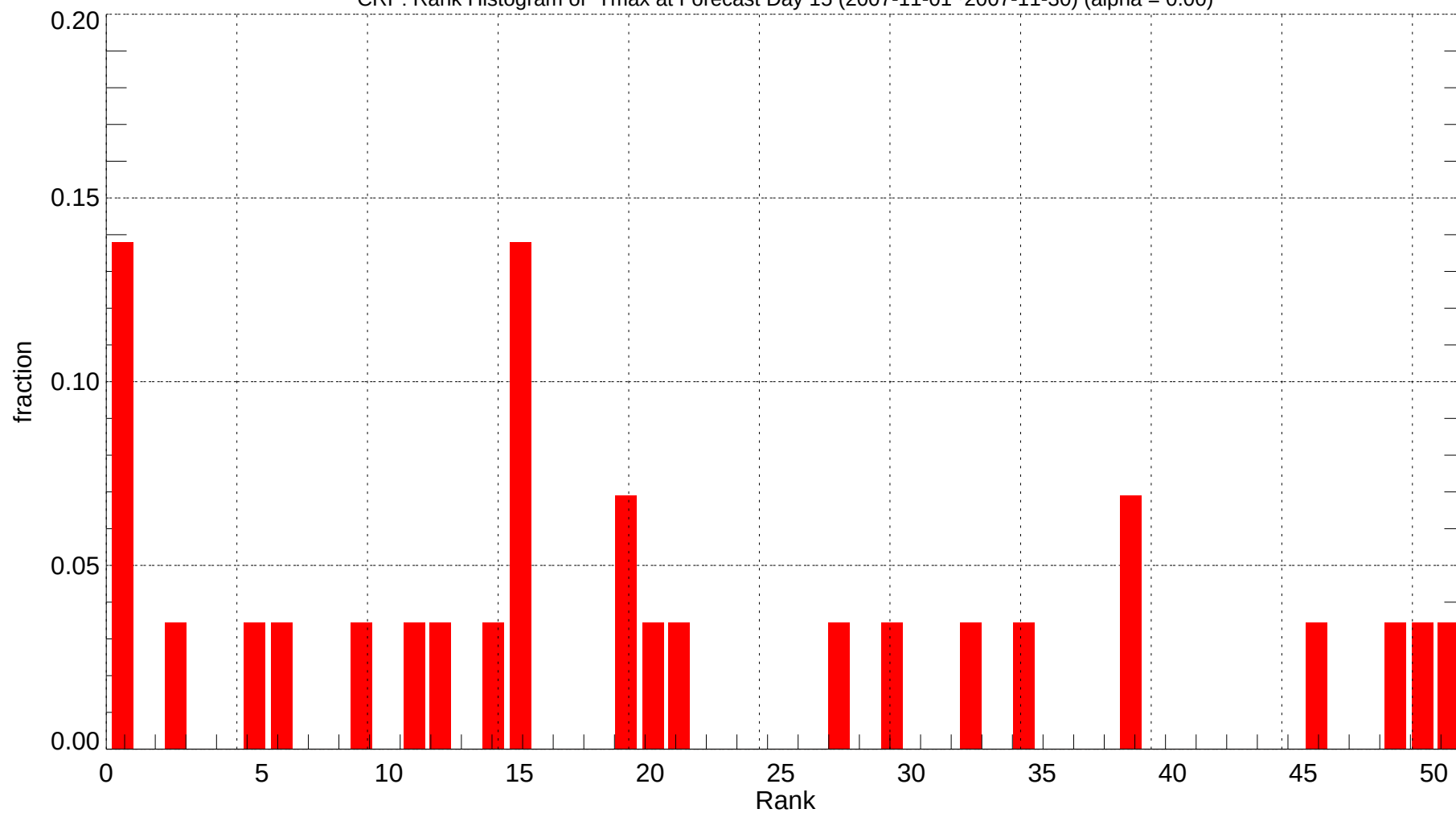
CRP: Rank Histogram of Tmax at Forecast Day 15 (2007-11-01~2007-11-30) (alpha = 0.00)
