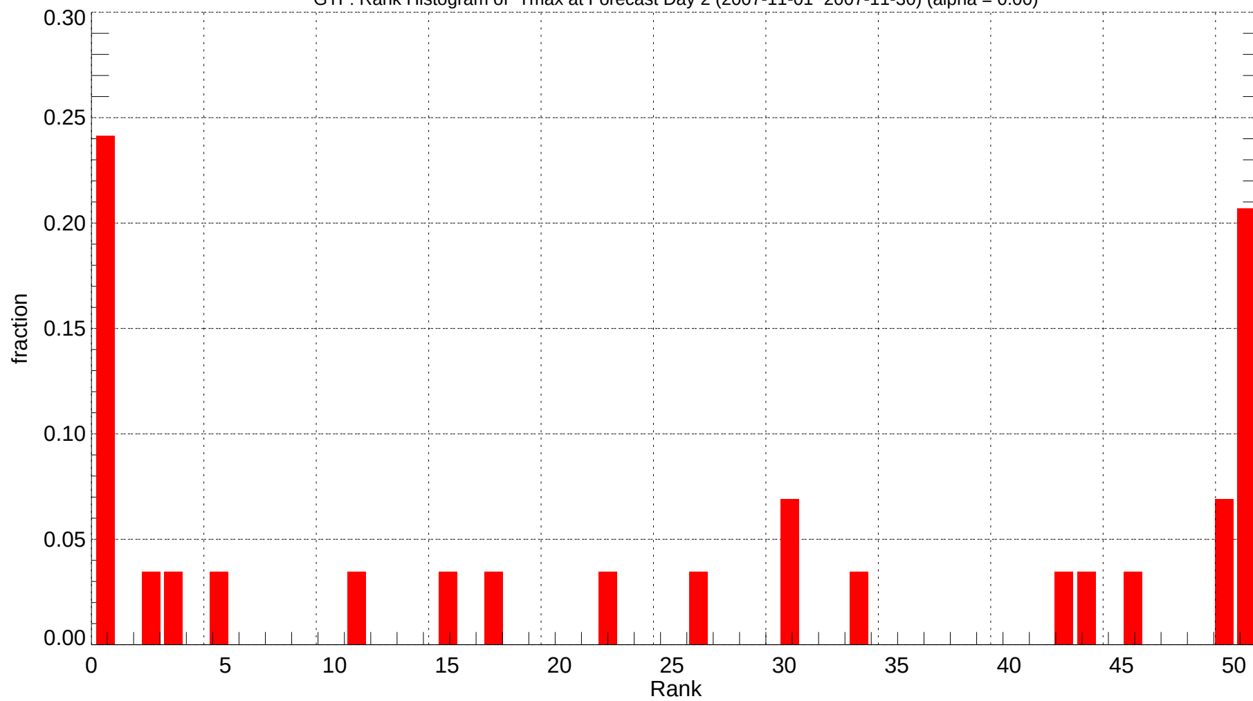
GTF: Rank Histogram of Tmax at Forecast Day 2 (2007-11-01~2007-11-30) (alpha = 0.00)
