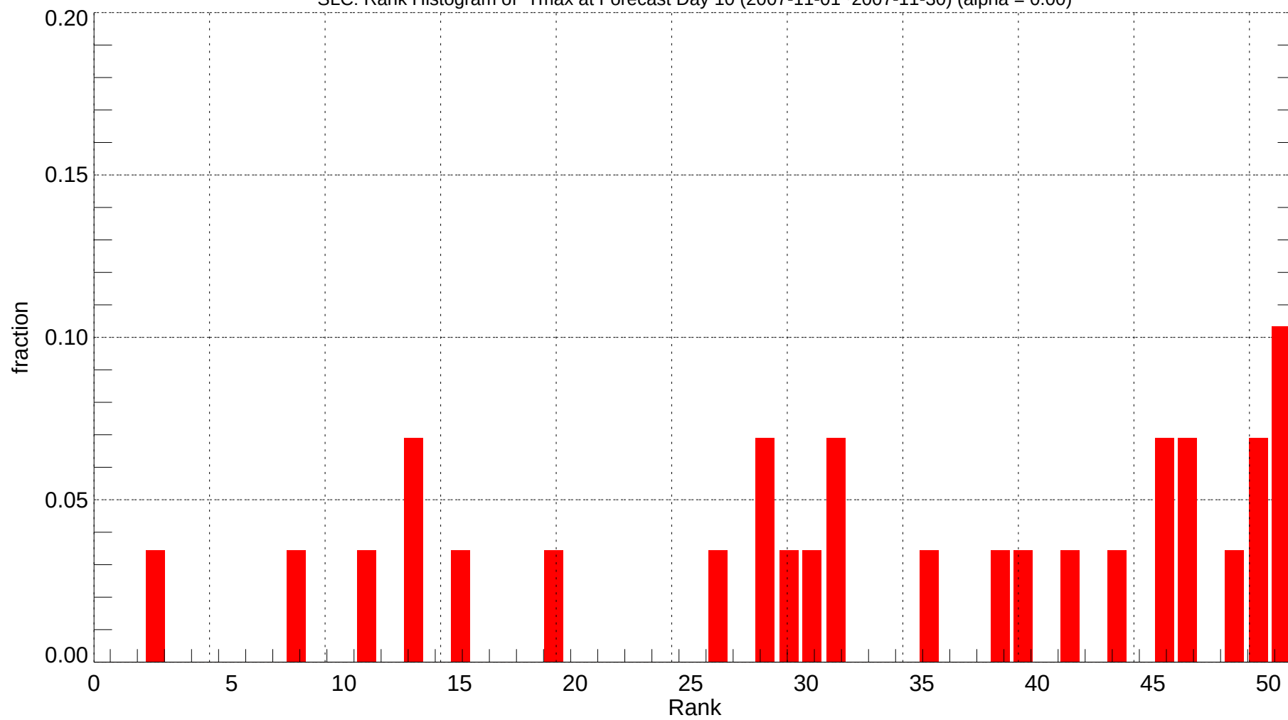
SLC: Rank Histogram of Tmax at Forecast Day 10 (2007-11-01~2007-11-30) (alpha = 0.00)
