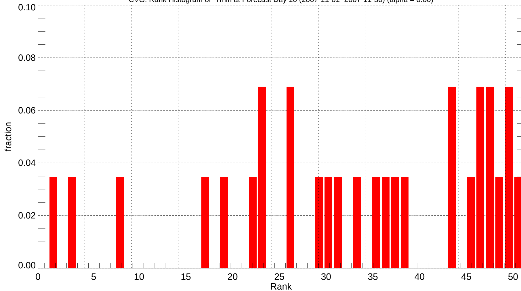
CVG: Rank Histogram of Tmin at Forecast Day 10 (2007-11-01~2007-11-30) (alpha = 0.00)
