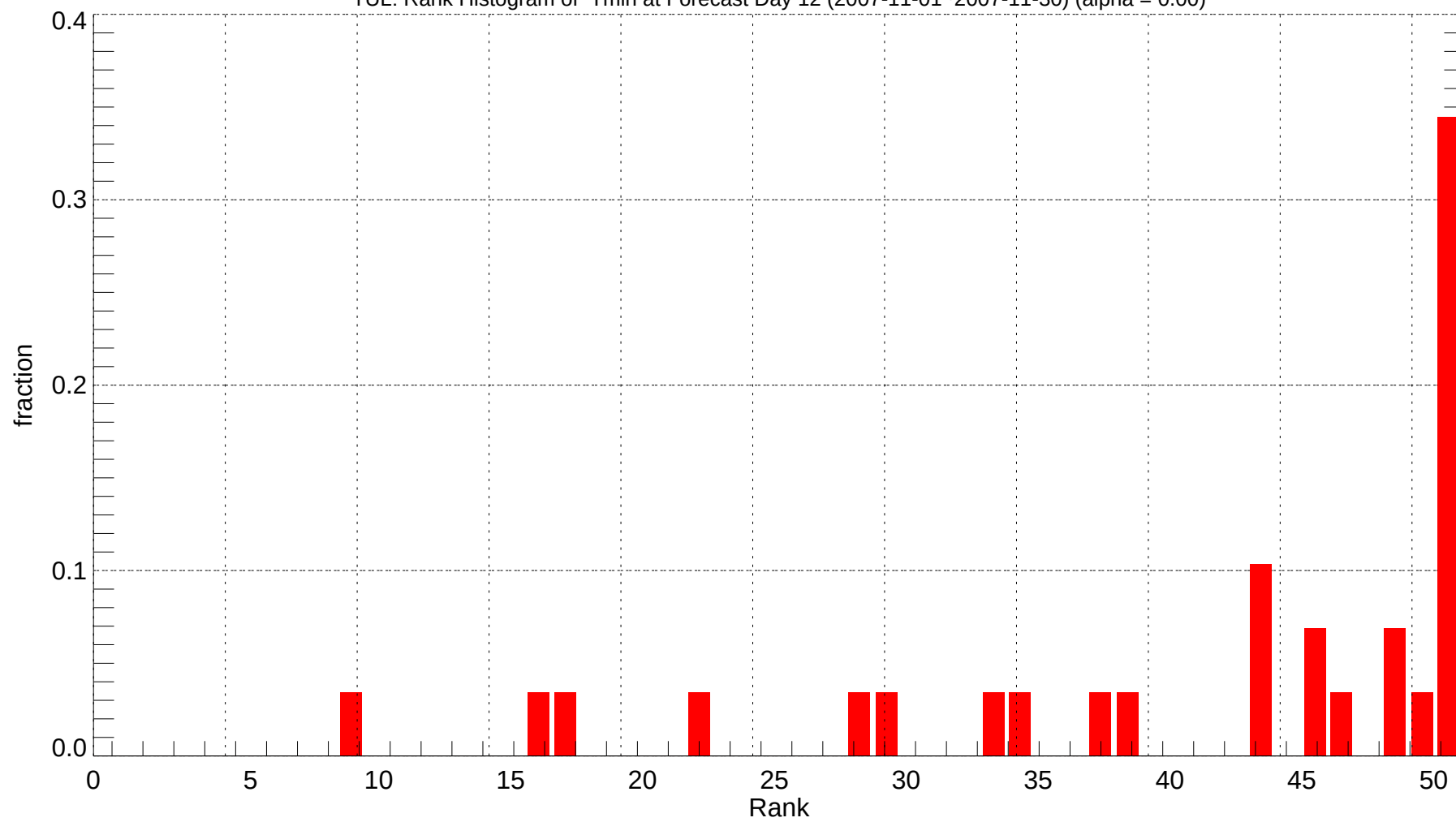
TUL: Rank Histogram of Tmin at Forecast Day 12 (2007-11-01~2007-11-30) (alpha = 0.00)
