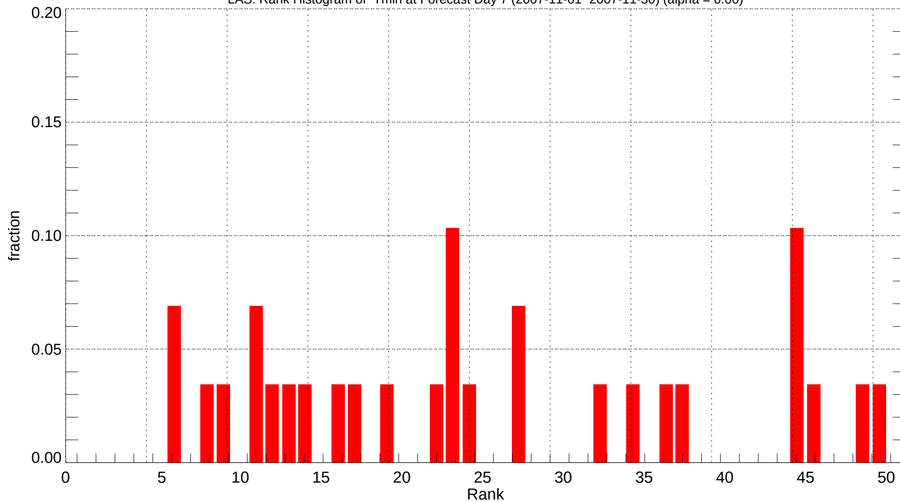
LAS: Rank Histogram of Tmin at Forecast Day 7 (2007-11-01~2007-11-30) (alpha = 0.00)
