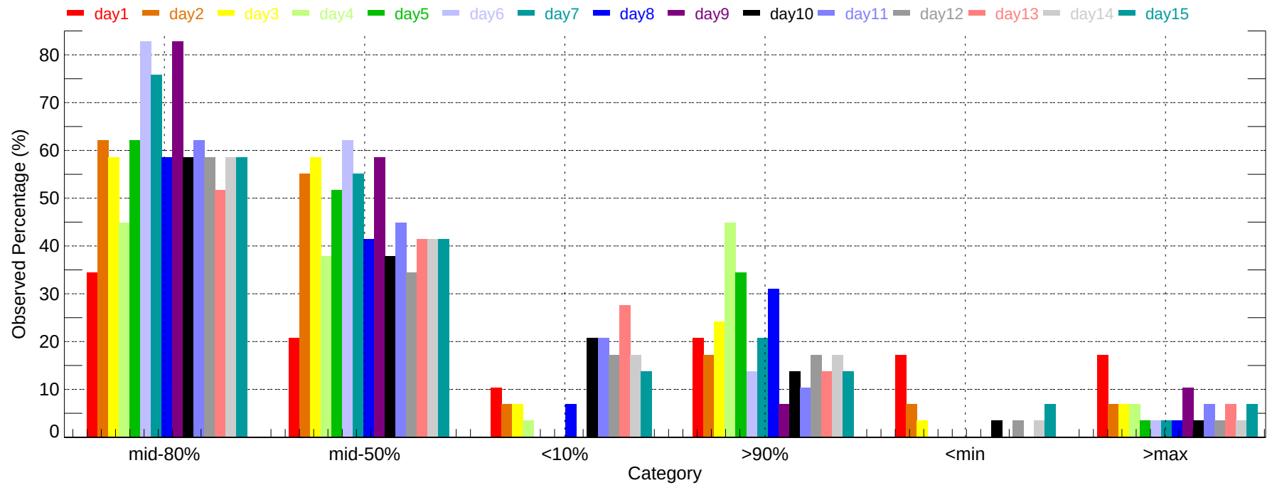
Observed Percentage of Ensembles - EWR: Min Temperature (2007-11-01~2007-11-30)
