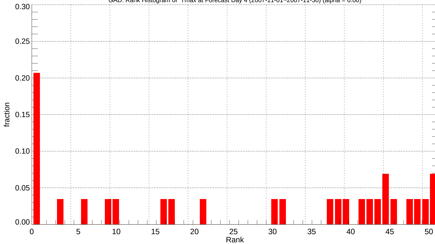
GAD: Rank Histogram of Tmax at Forecast Day 4 (2007-11-01~2007-11-30) (alpha = 0.00)
