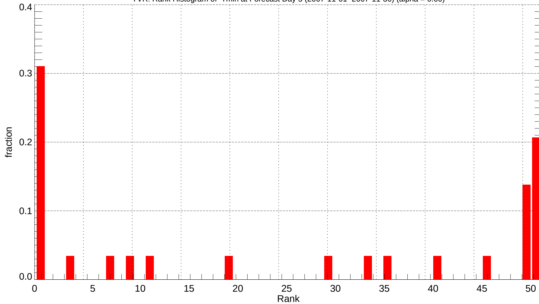
YVR: Rank Histogram of Tmin at Forecast Day 5 (2007-11-01~2007-11-30) (alpha = 0.00)
