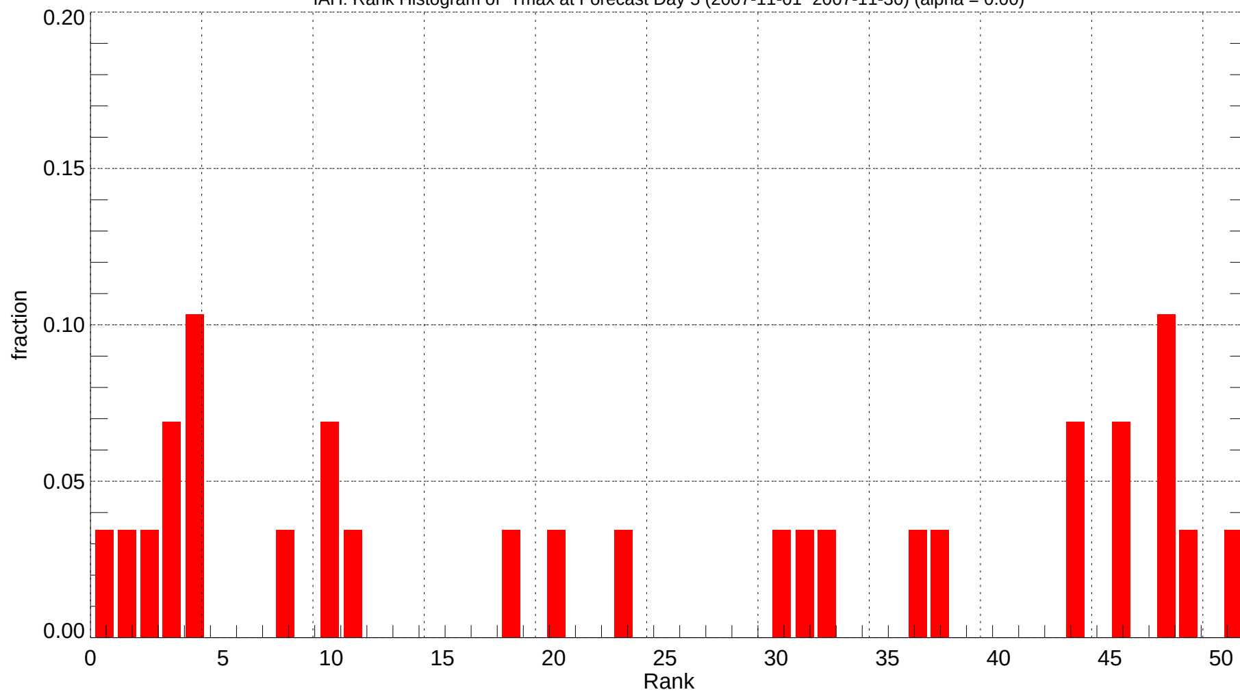
IAH: Rank Histogram of Tmax at Forecast Day 5 (2007-11-01~2007-11-30) (alpha = 0.00)
