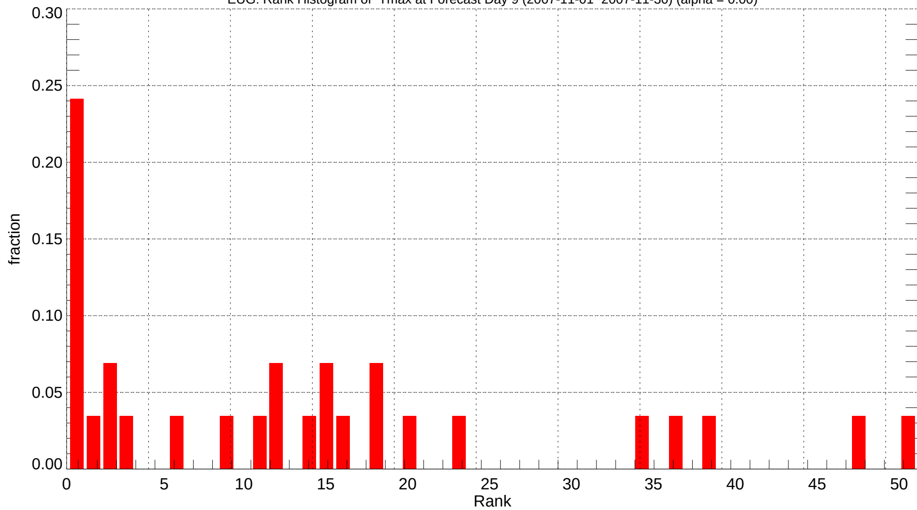
EUG: Rank Histogram of Tmax at Forecast Day 9 (2007-11-01~2007-11-30) (alpha = 0.00)
