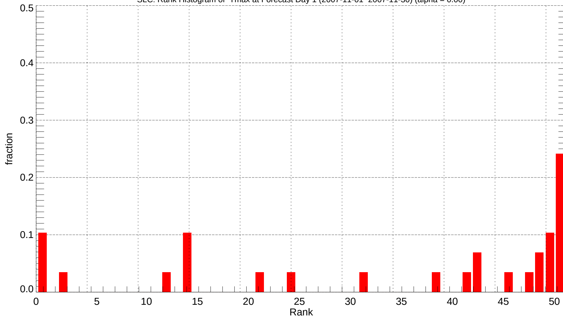
SLC: Rank Histogram of Tmax at Forecast Day 1 (2007-11-01~2007-11-30) (alpha = 0.00)
