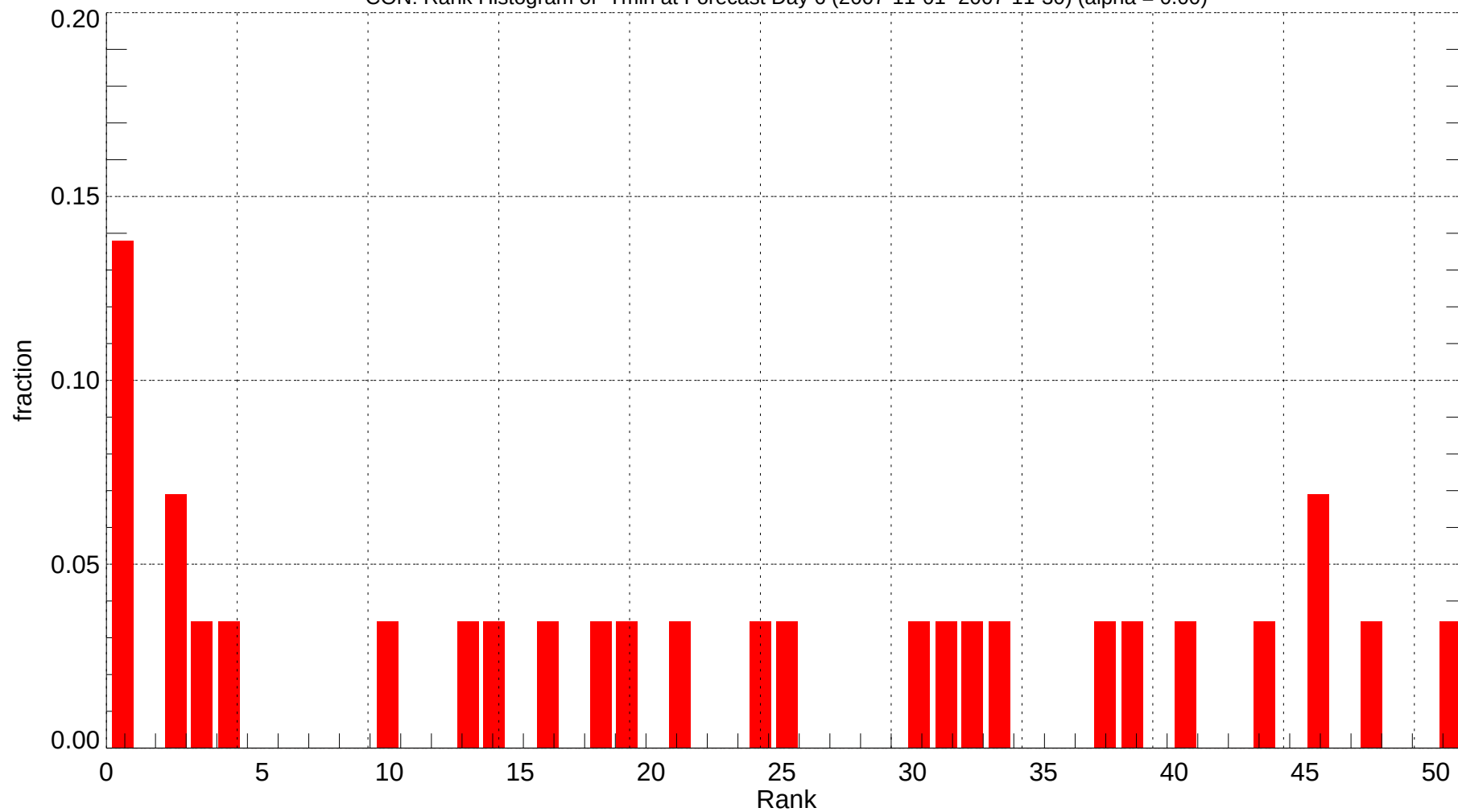
CON: Rank Histogram of Tmin at Forecast Day 6 (2007-11-01~2007-11-30) (alpha = 0.00)
