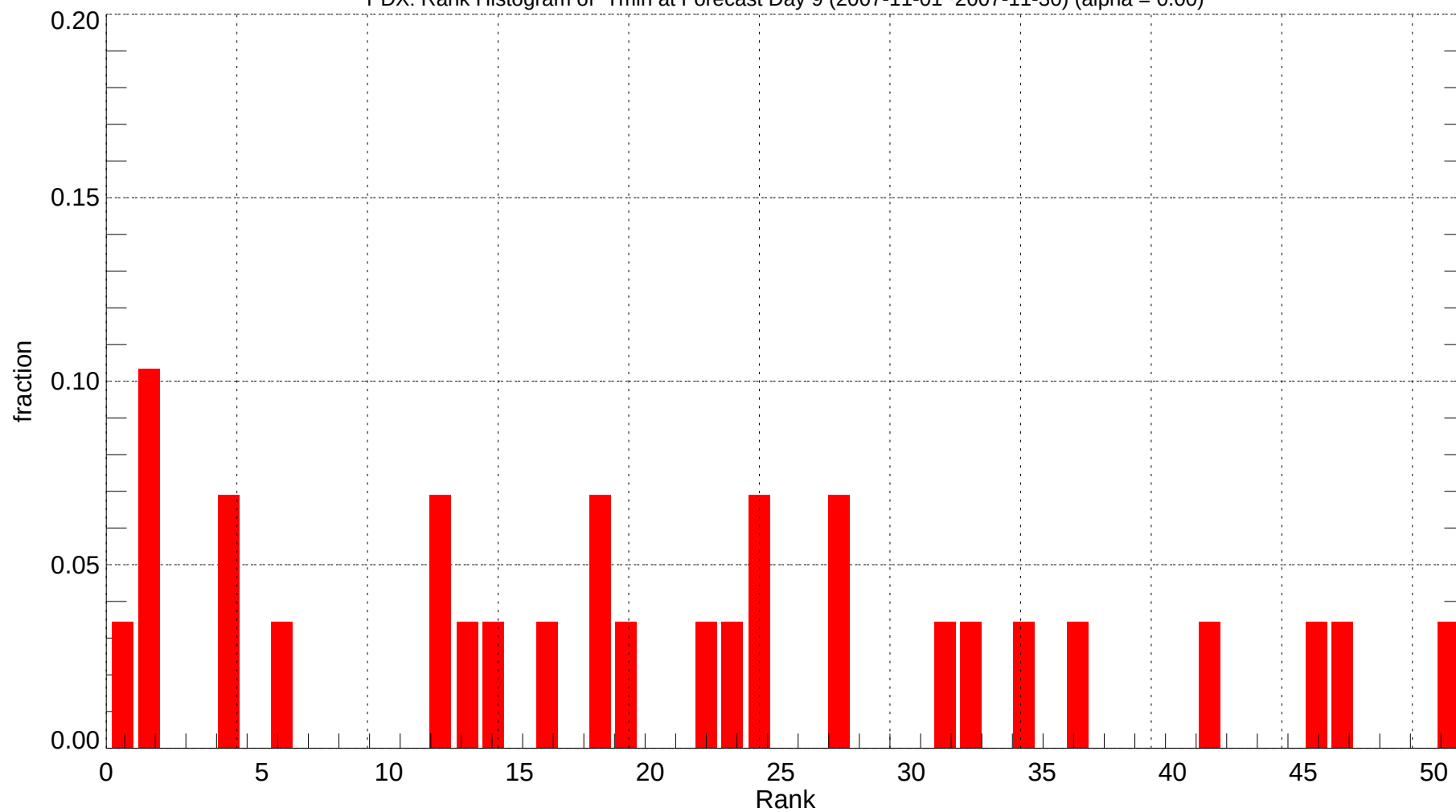
PDX: Rank Histogram of Tmin at Forecast Day 9 (2007-11-01~2007-11-30) (alpha = 0.00)
