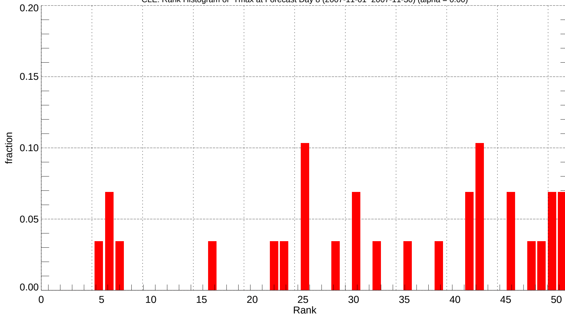
CLE: Rank Histogram of Tmax at Forecast Day 8 (2007-11-01~2007-11-30) (alpha = 0.00)
