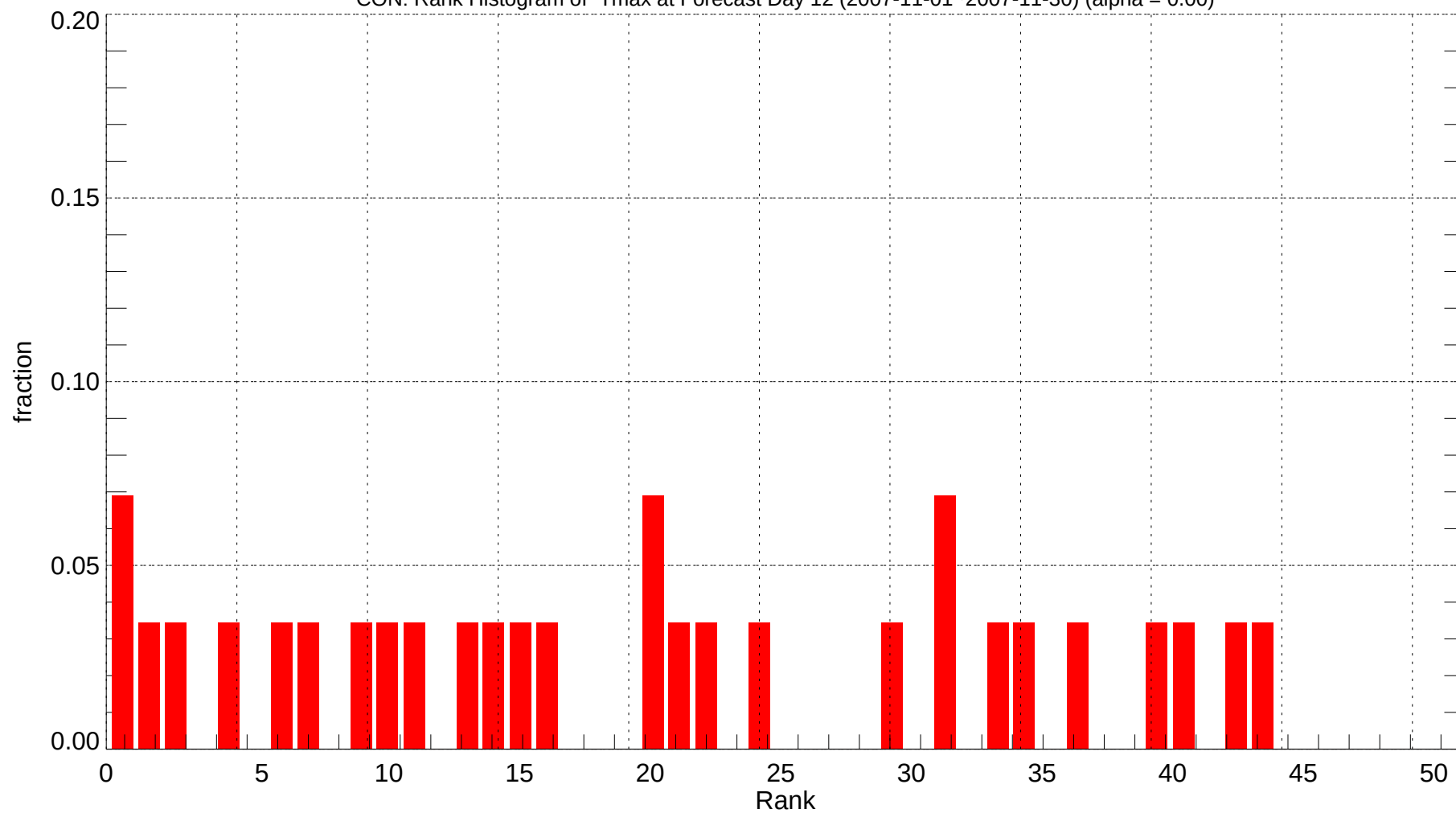
CON: Rank Histogram of Tmax at Forecast Day 12 (2007-11-01~2007-11-30) (alpha = 0.00)
