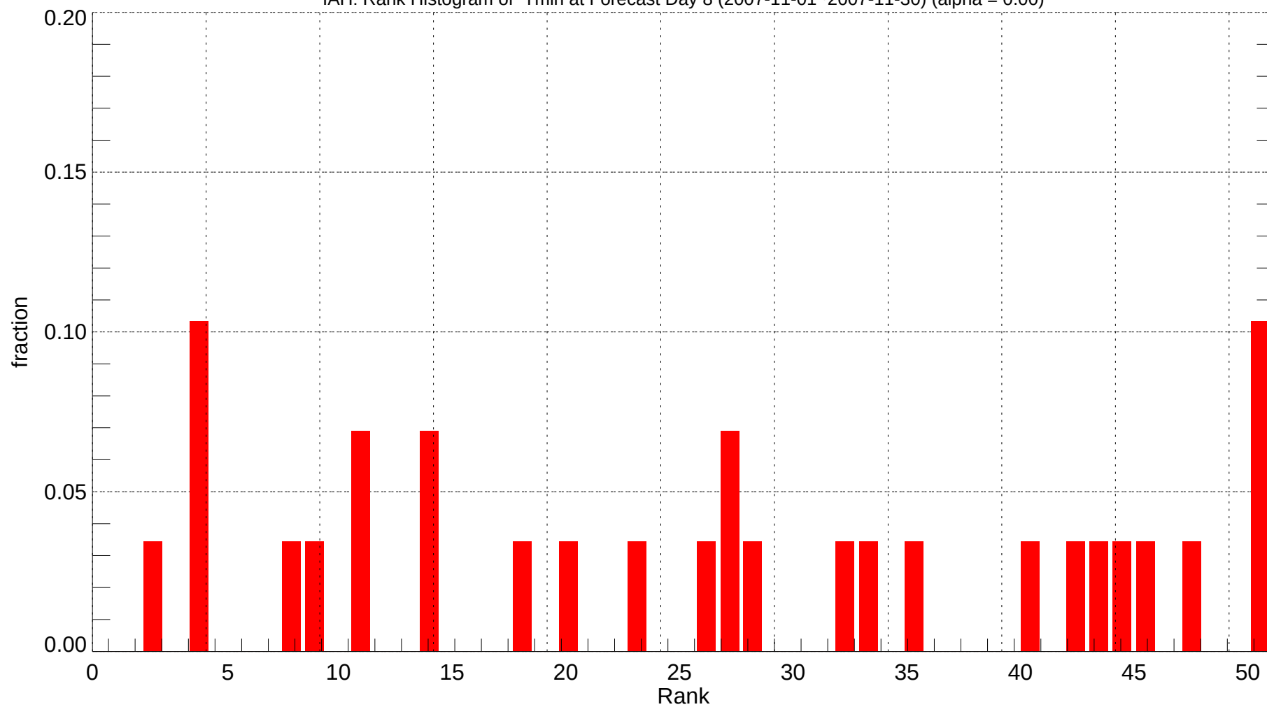
IAH: Rank Histogram of Tmin at Forecast Day 8 (2007-11-01~2007-11-30) (alpha = 0.00)
