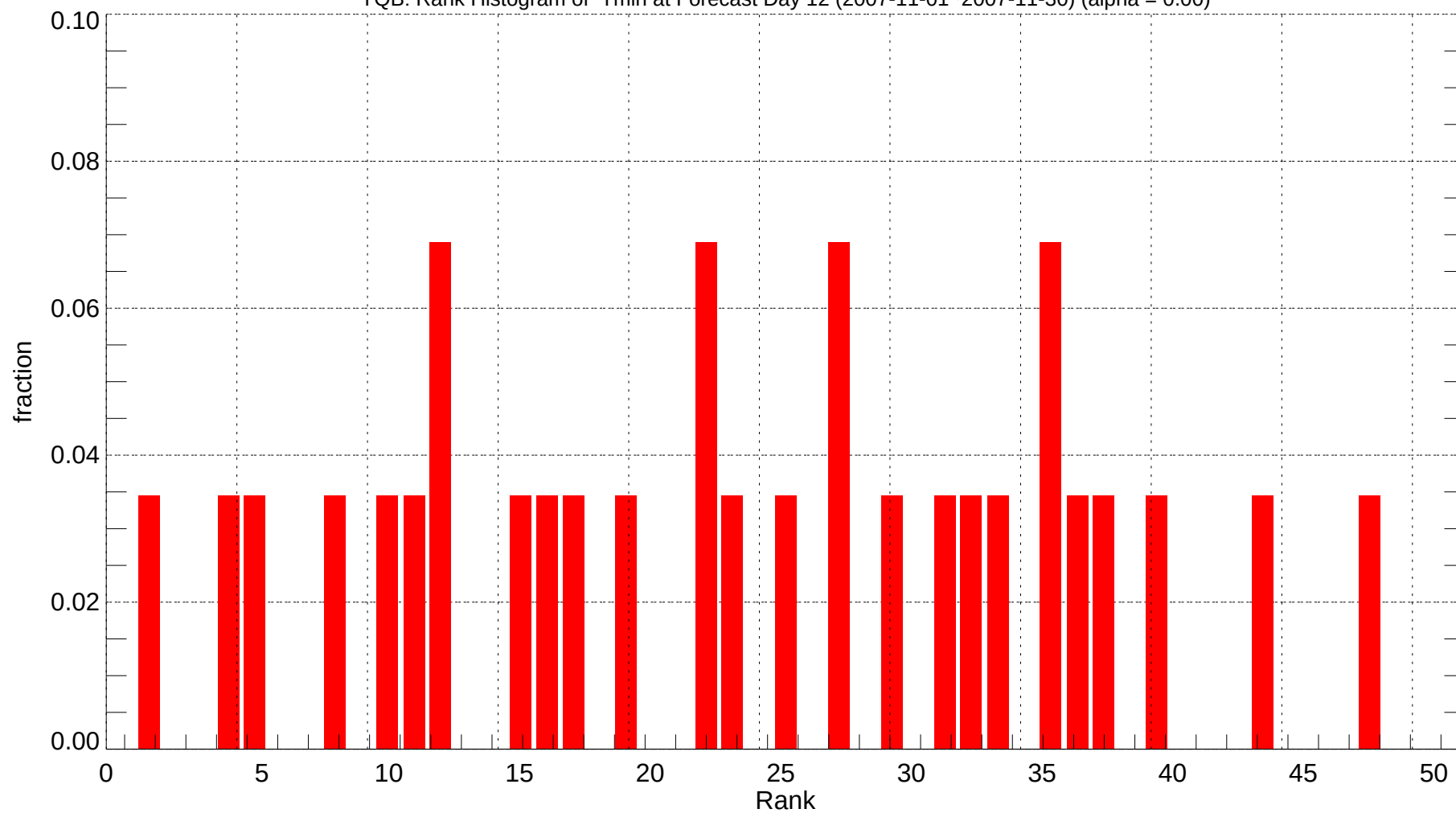
YQB: Rank Histogram of Tmin at Forecast Day 12 (2007-11-01~2007-11-30) (alpha = 0.00)
