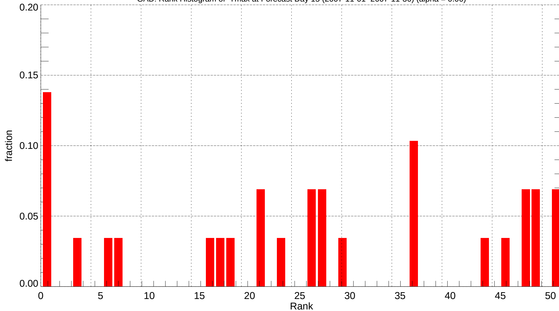
GAD: Rank Histogram of Tmax at Forecast Day 15 (2007-11-01~2007-11-30) (alpha = 0.00)
