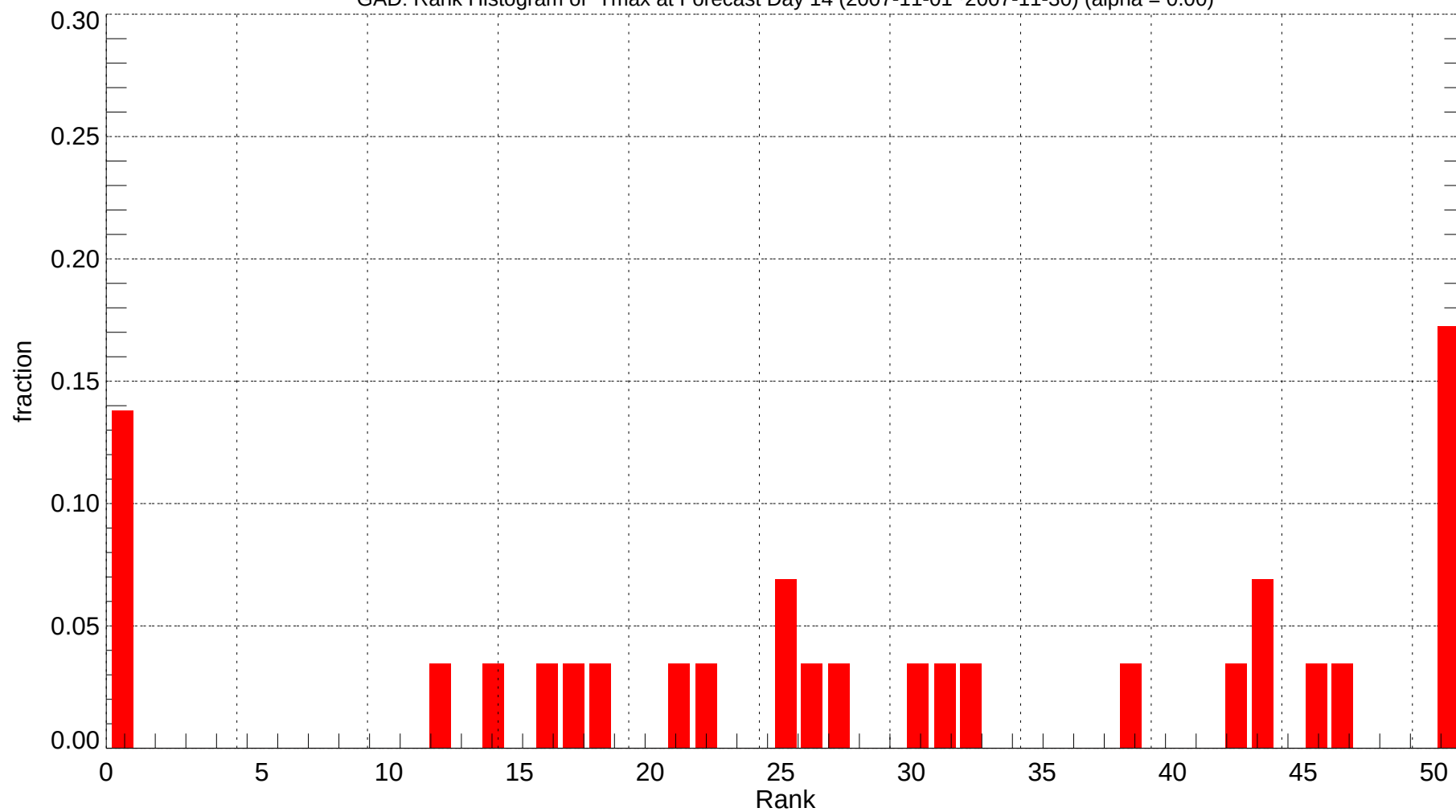
GAD: Rank Histogram of Tmax at Forecast Day 14 (2007-11-01~2007-11-30) (alpha = 0.00)
