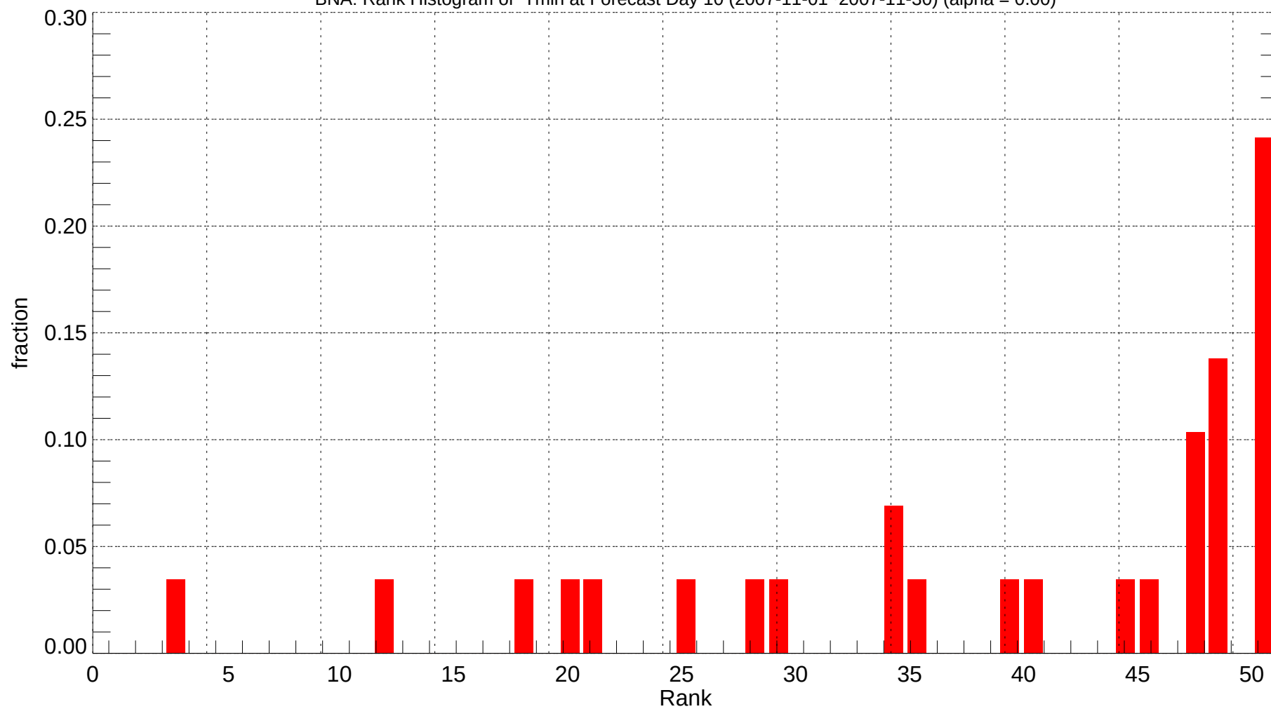
BNA: Rank Histogram of Tmin at Forecast Day 10 (2007-11-01~2007-11-30) (alpha = 0.00)
