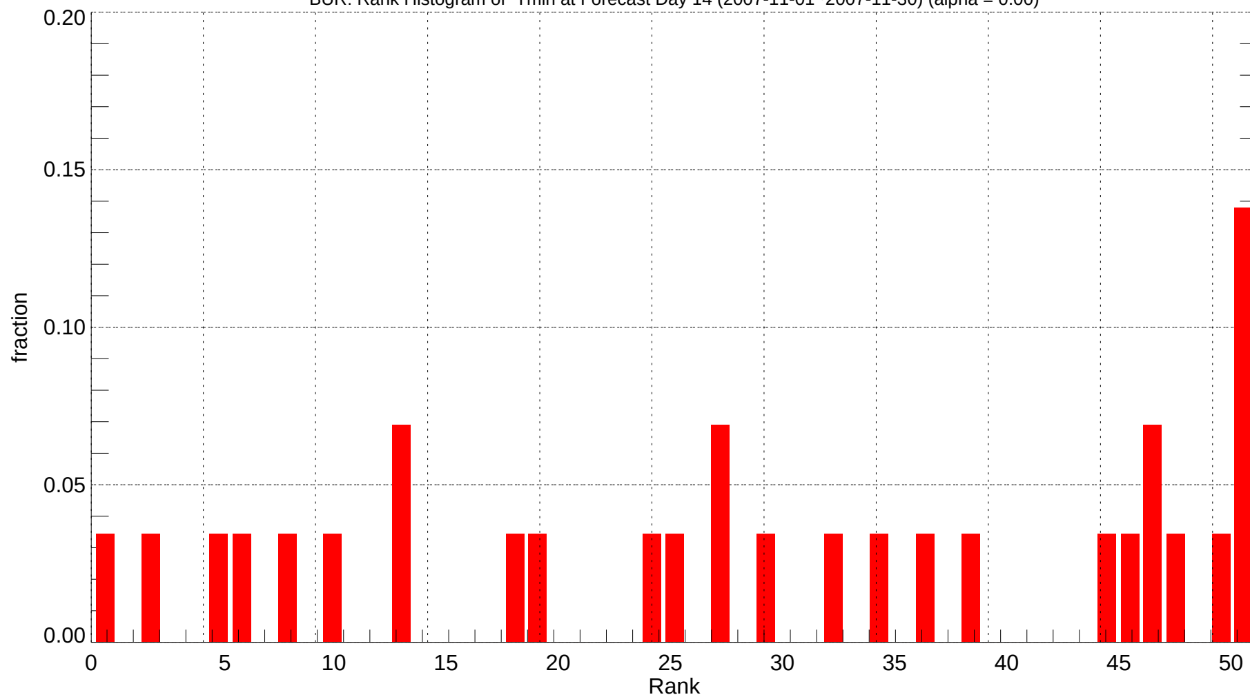
BUR: Rank Histogram of Tmin at Forecast Day 14 (2007-11-01~2007-11-30) (alpha = 0.00)
