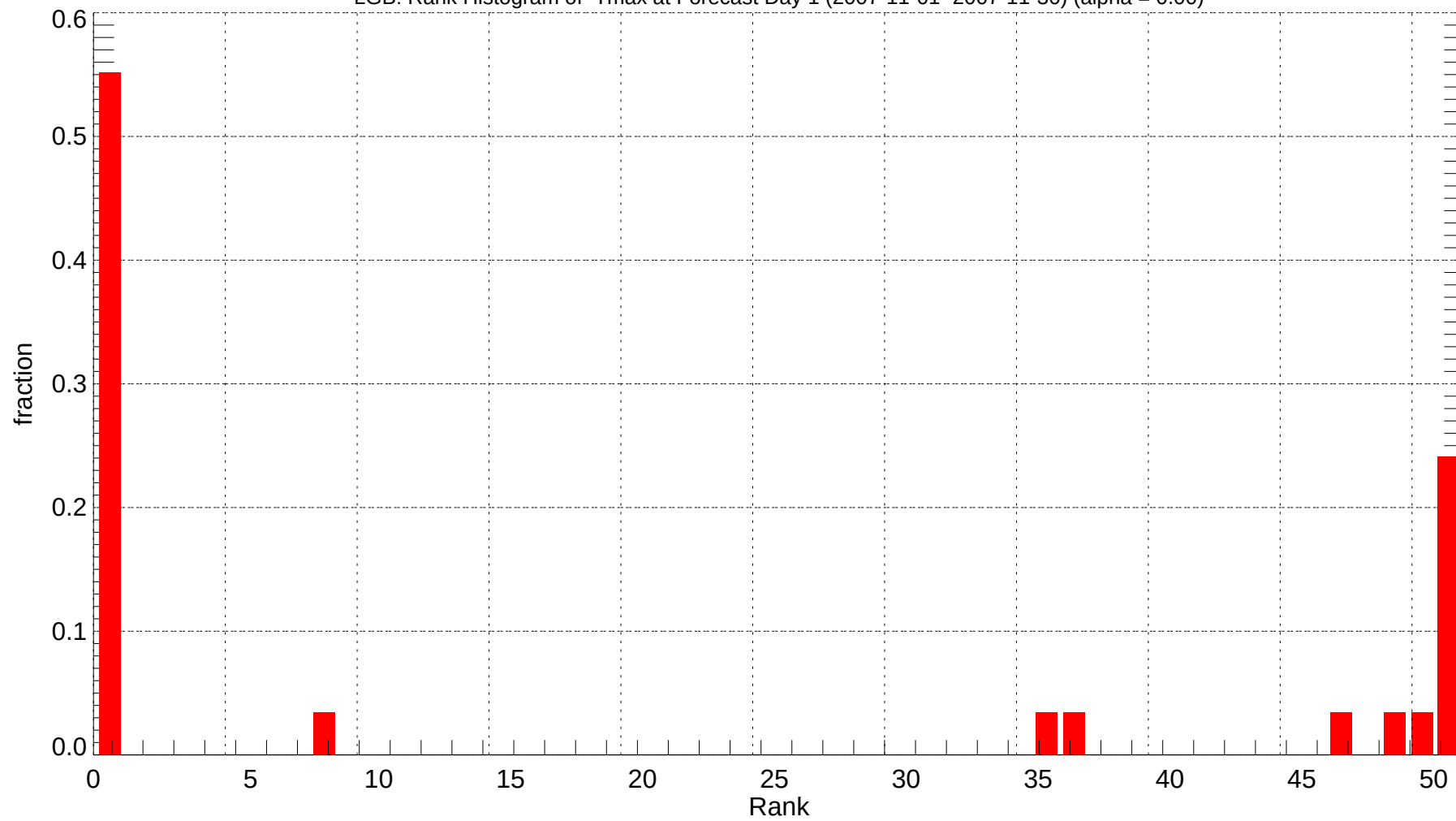
LGB: Rank Histogram of Tmax at Forecast Day 1 (2007-11-01~2007-11-30) (alpha = 0.00)
