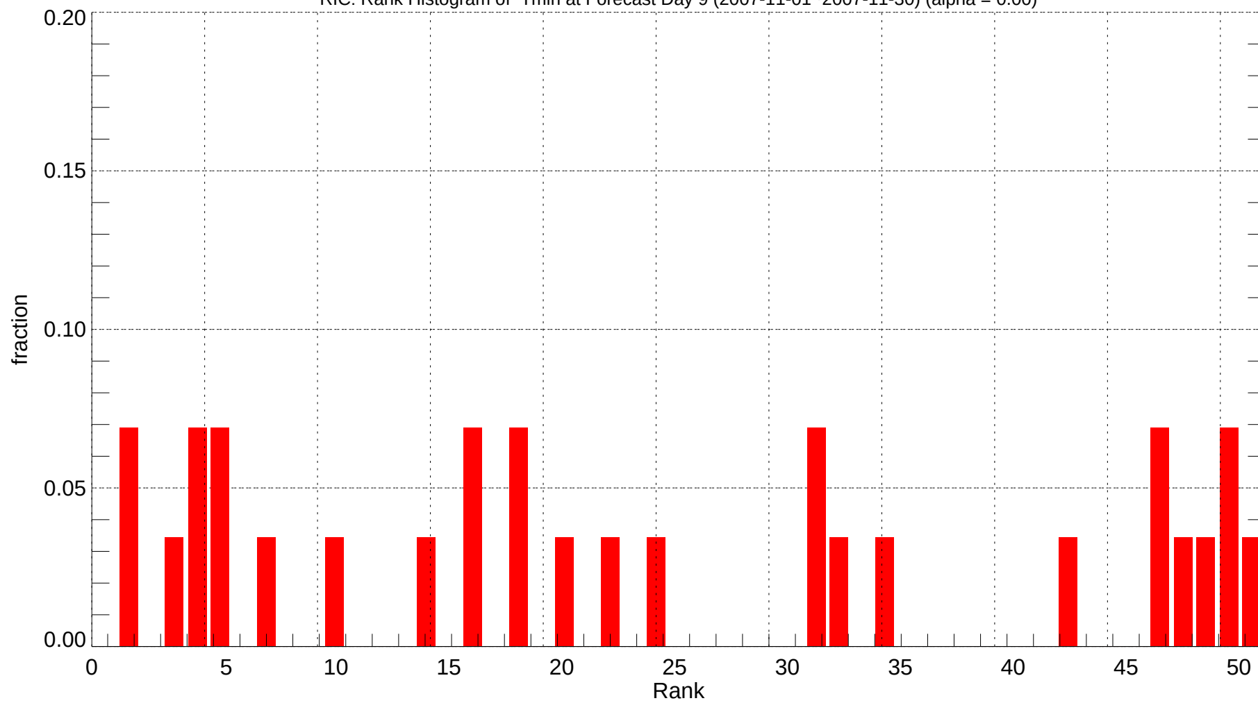
RIC: Rank Histogram of Tmin at Forecast Day 9 (2007-11-01~2007-11-30) (alpha = 0.00)
