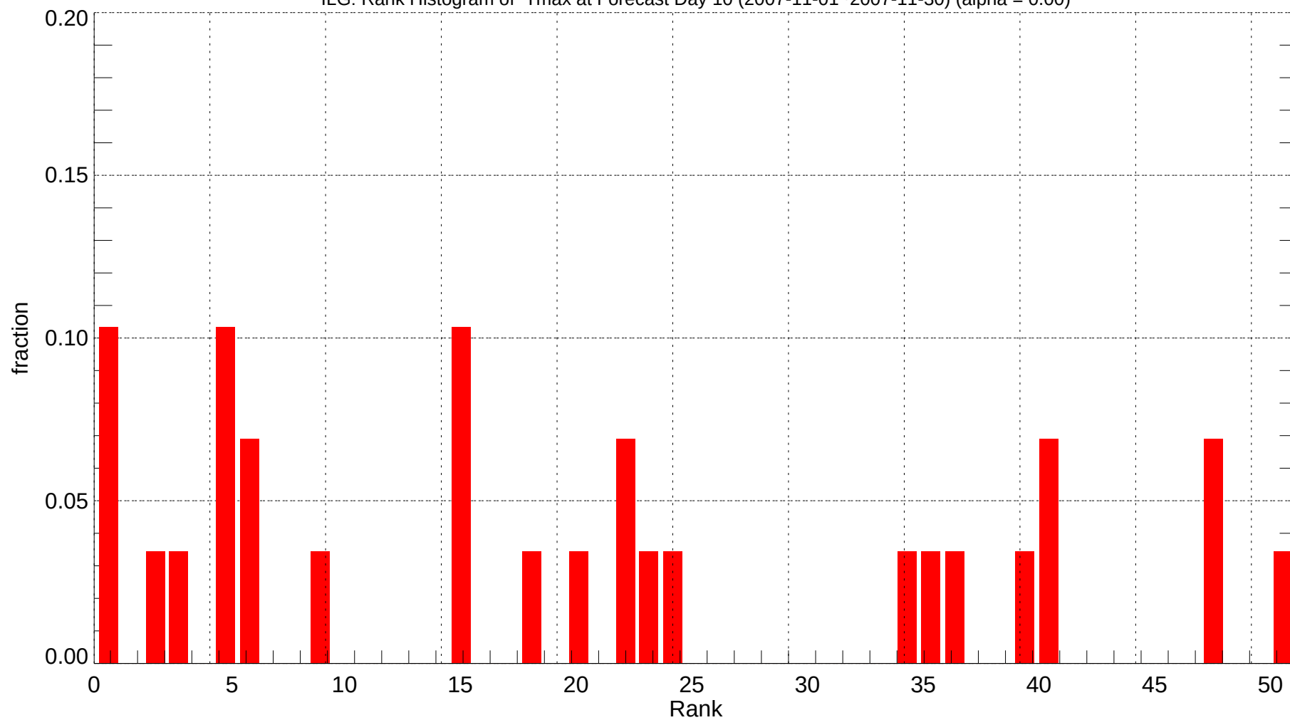
ILG: Rank Histogram of Tmax at Forecast Day 10 (2007-11-01~2007-11-30) (alpha = 0.00)
