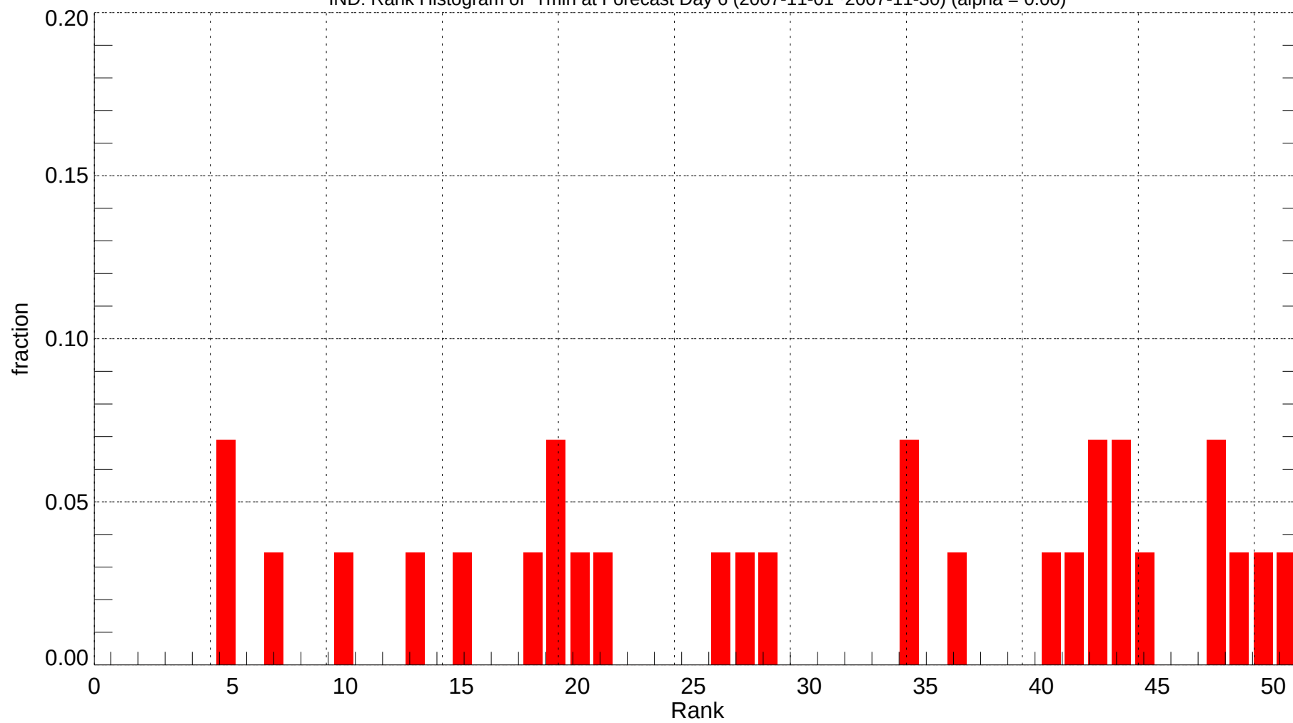
IND: Rank Histogram of Tmin at Forecast Day 6 (2007-11-01~2007-11-30) (alpha = 0.00)
