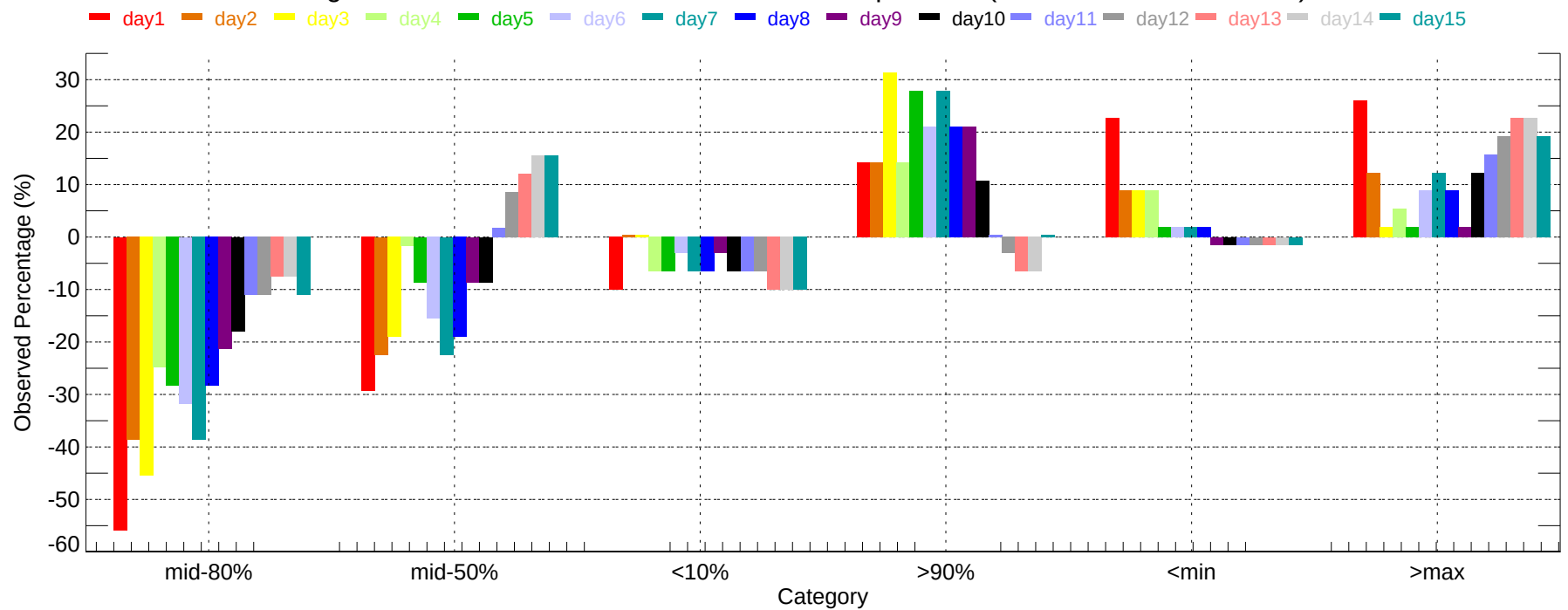
Observed Percentage Deviation of Ensembles - RDD: Max Temperature (2007-11-01~2007-11-30)
