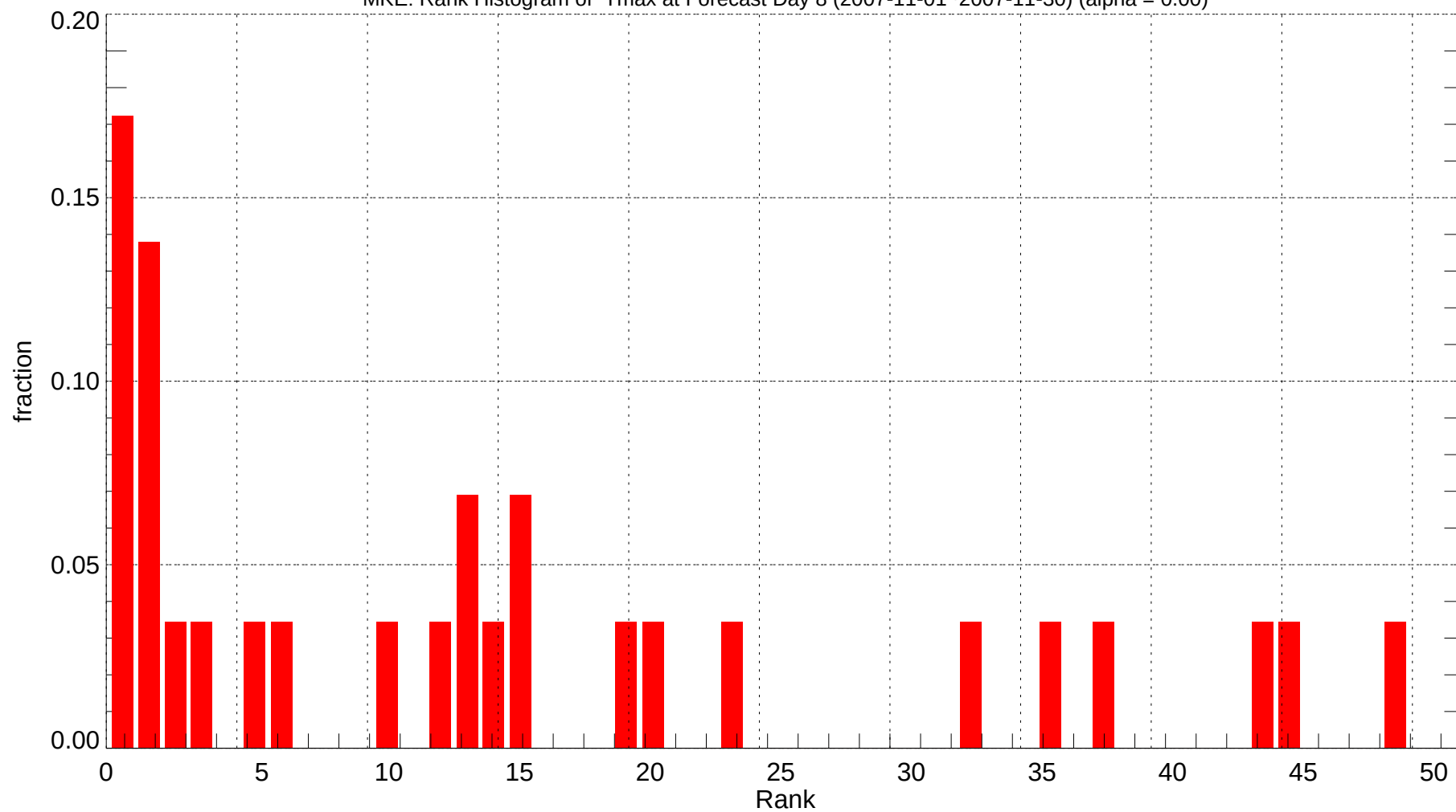
MKE: Rank Histogram of Tmax at Forecast Day 8 (2007-11-01~2007-11-30) (alpha = 0.00)
