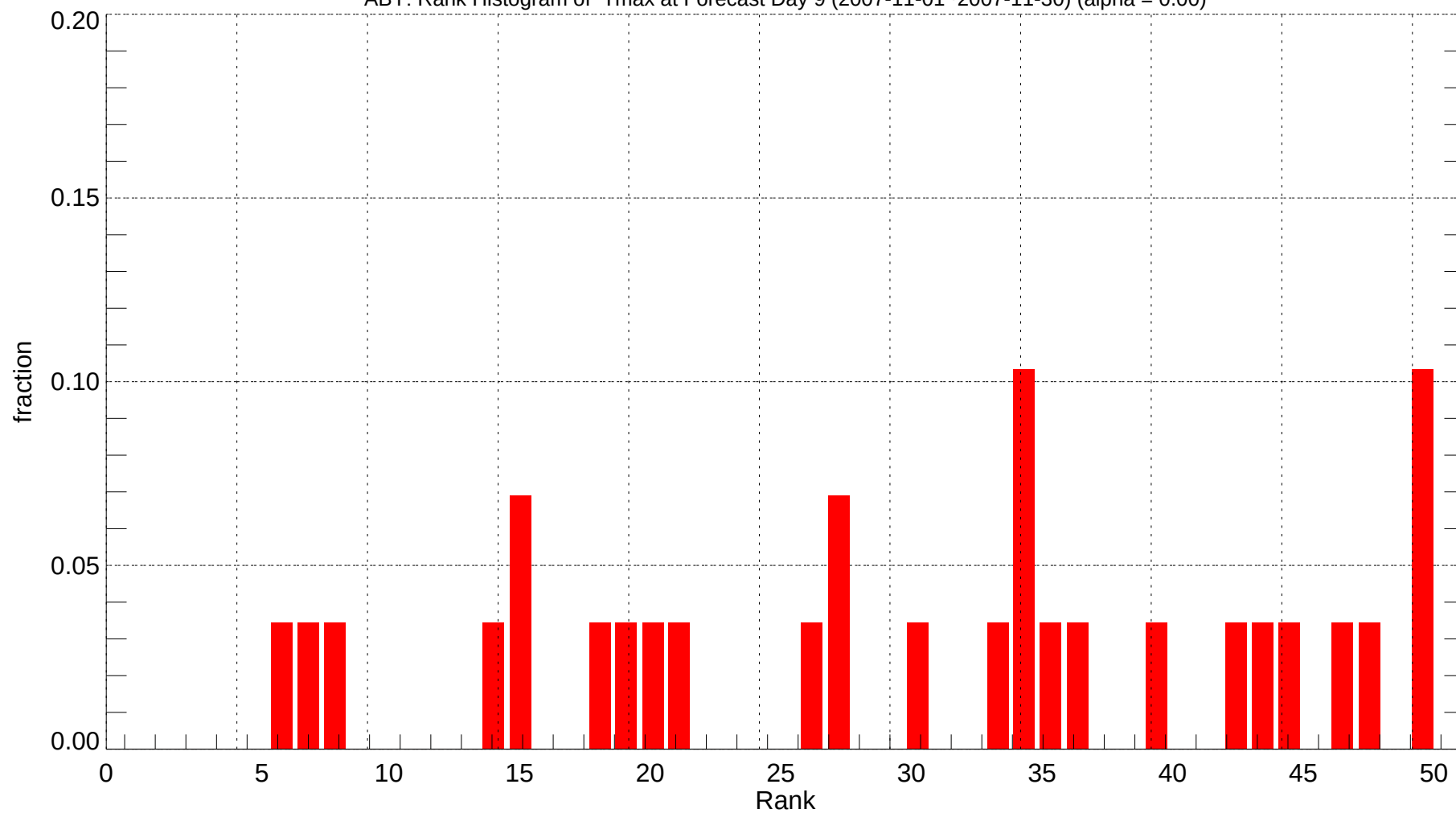
ABY: Rank Histogram of Tmax at Forecast Day 9 (2007-11-01~2007-11-30) (alpha = 0.00)
