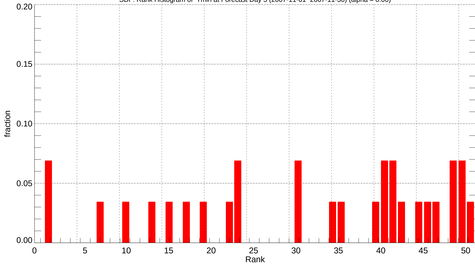
SDF: Rank Histogram of Tmin at Forecast Day 5 (2007-11-01~2007-11-30) (alpha = 0.00)
