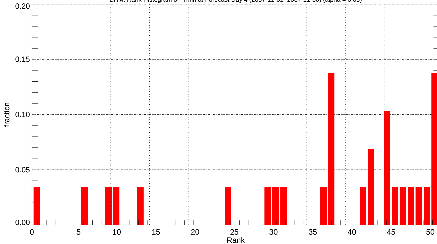
BHM: Rank Histogram of Tmin at Forecast Day 4 (2007-11-01~2007-11-30) (alpha = 0.00)
