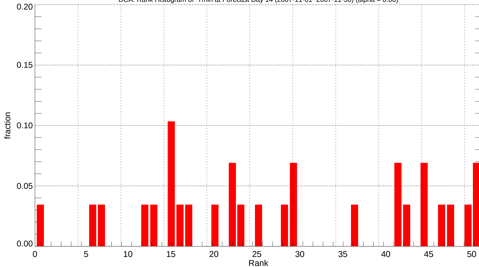
DCA: Rank Histogram of Tmin at Forecast Day 14 (2007-11-01~2007-11-30) (alpha = 0.00)
