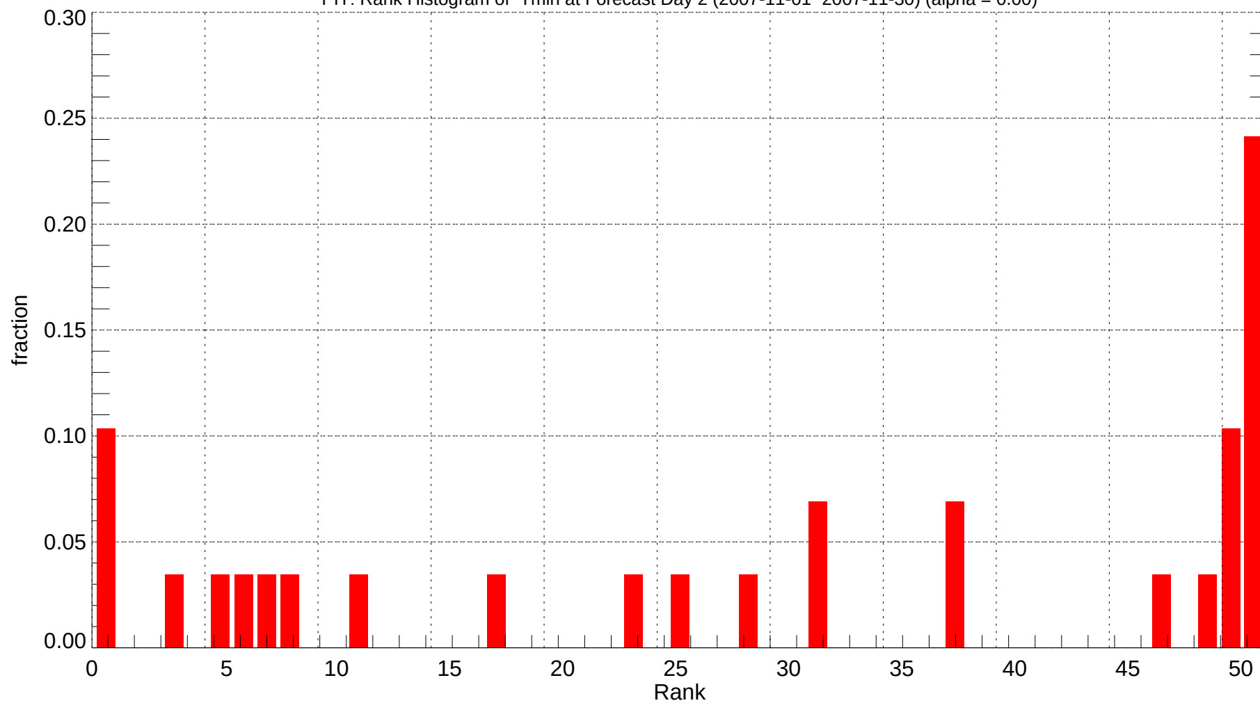
PIT: Rank Histogram of Tmin at Forecast Day 2 (2007-11-01~2007-11-30) (alpha = 0.00)
