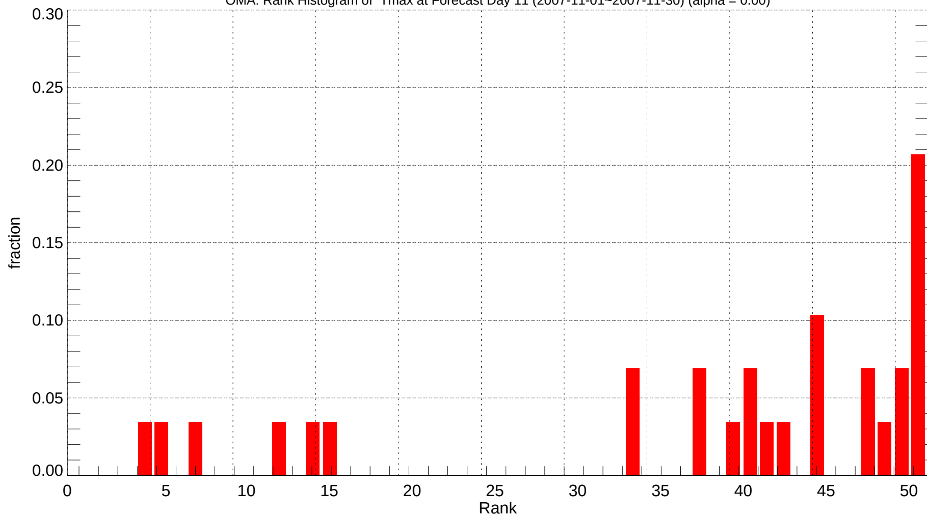
OMA: Rank Histogram of Tmax at Forecast Day 11 (2007-11-01~2007-11-30) (alpha = 0.00)
