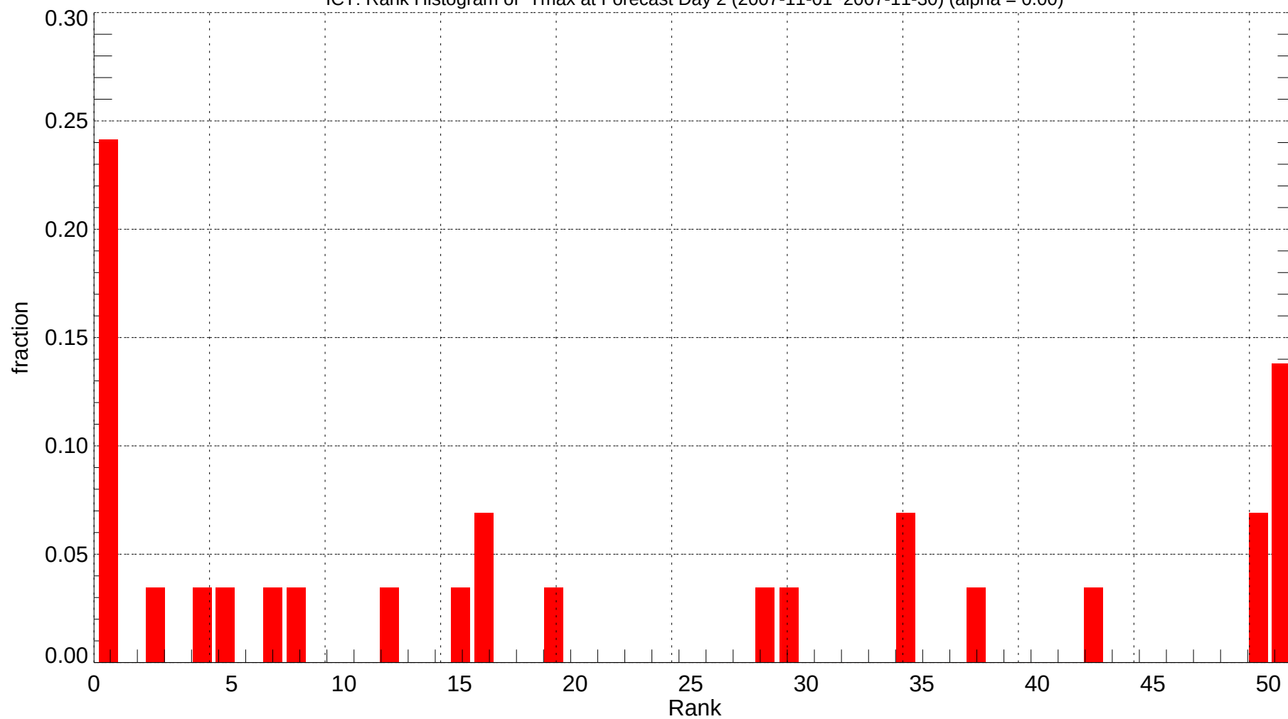
ICT: Rank Histogram of Tmax at Forecast Day 2 (2007-11-01~2007-11-30) (alpha = 0.00)
