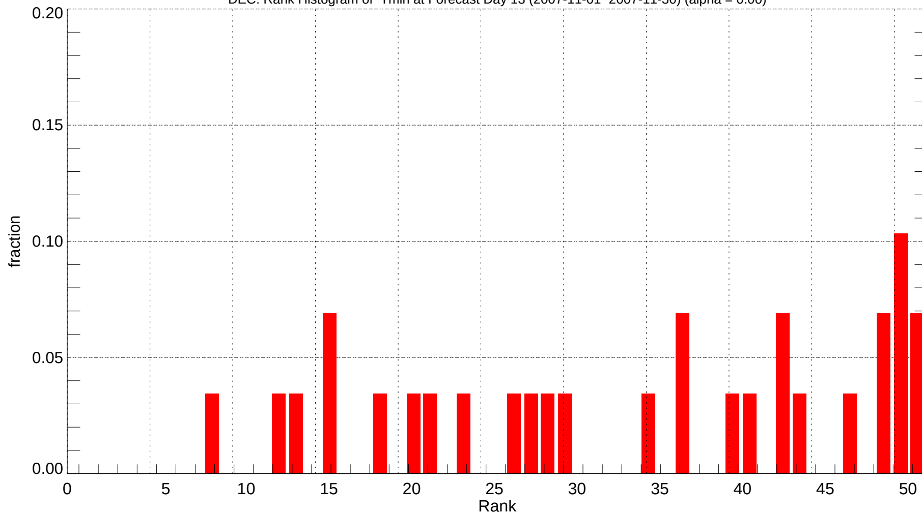
DEC: Rank Histogram of Tmin at Forecast Day 13 (2007-11-01~2007-11-30) (alpha = 0.00)
