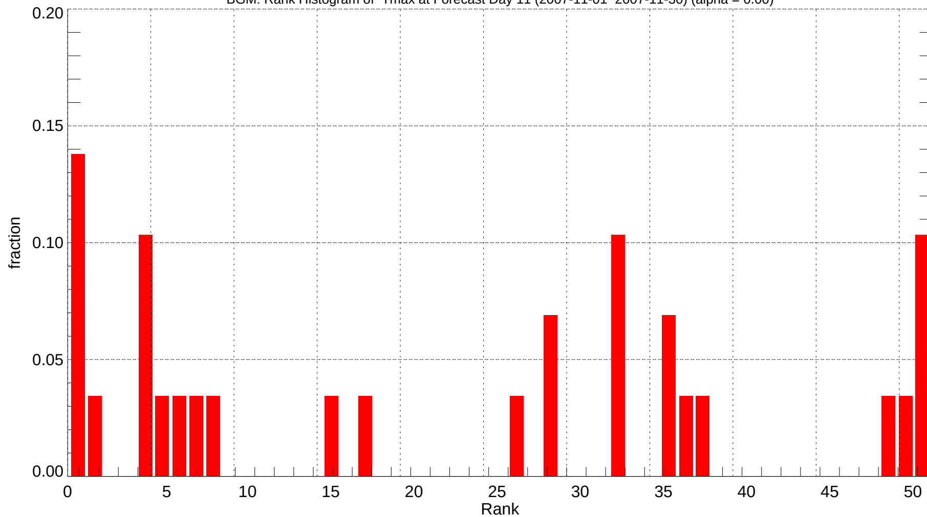
BGM: Rank Histogram of Tmax at Forecast Day 11 (2007-11-01~2007-11-30) (alpha = 0.00)
