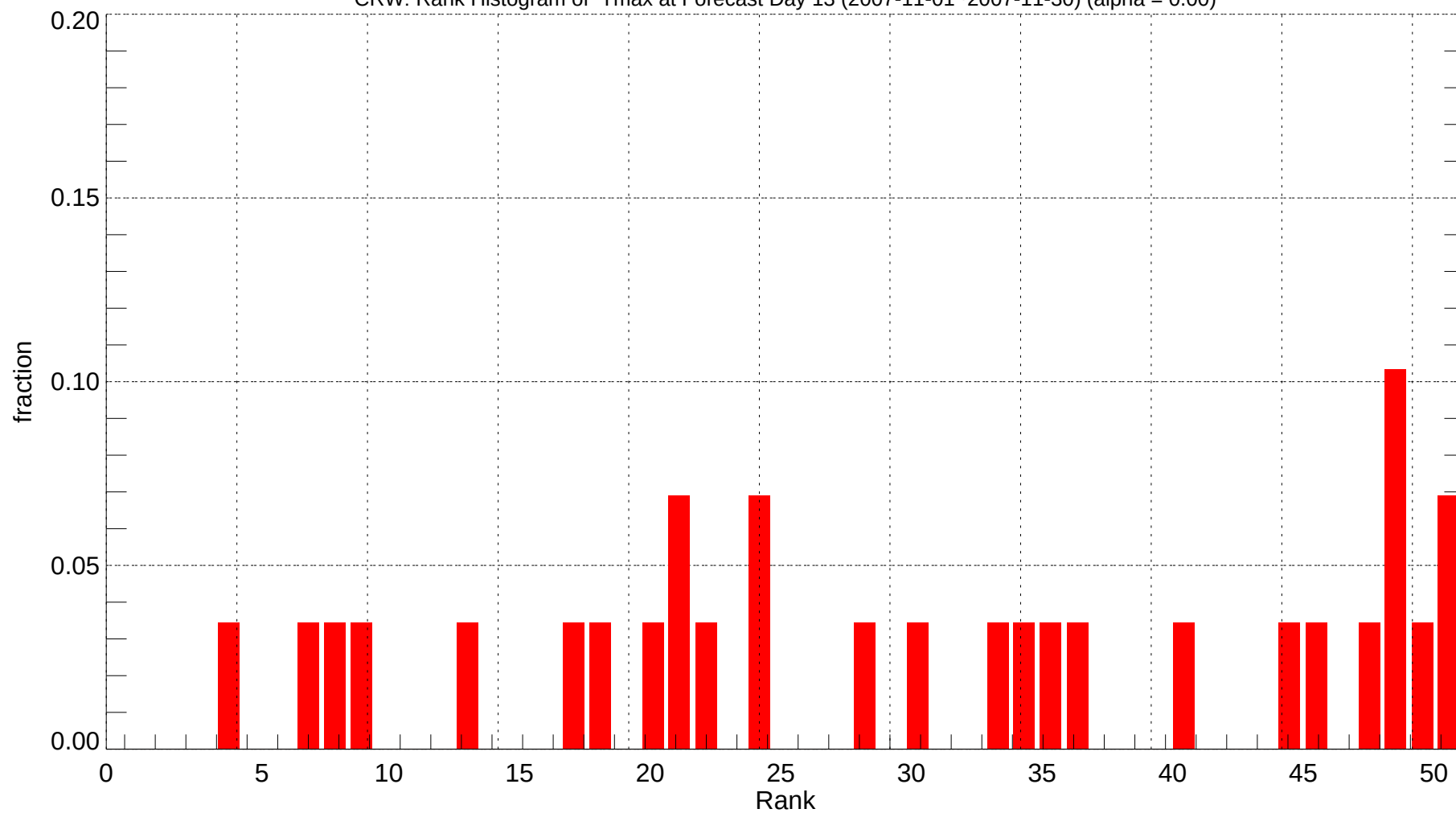
CRW: Rank Histogram of Tmax at Forecast Day 13 (2007-11-01~2007-11-30) (alpha = 0.00)
