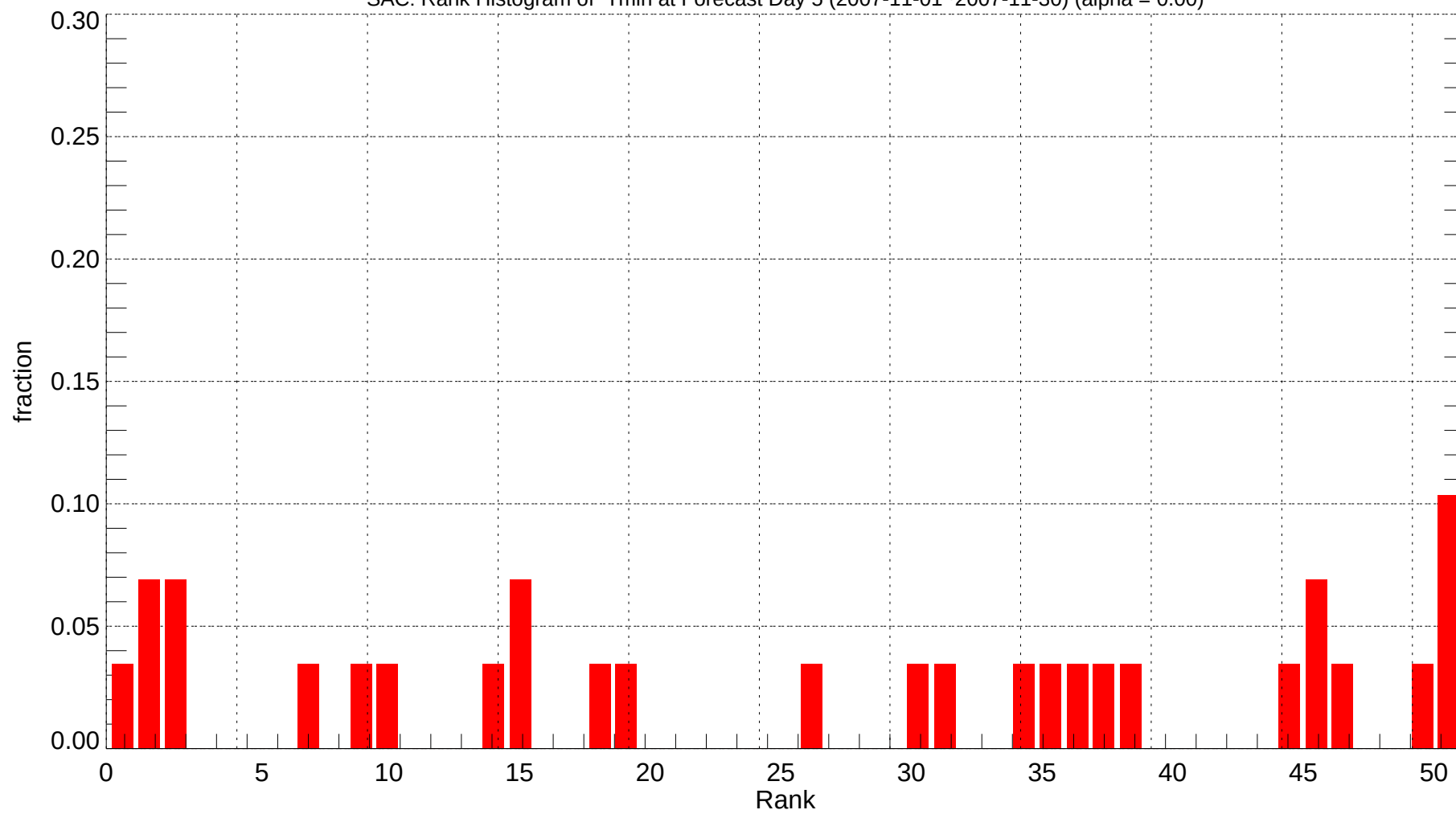
SAC: Rank Histogram of Tmin at Forecast Day 5 (2007-11-01~2007-11-30) (alpha = 0.00)
