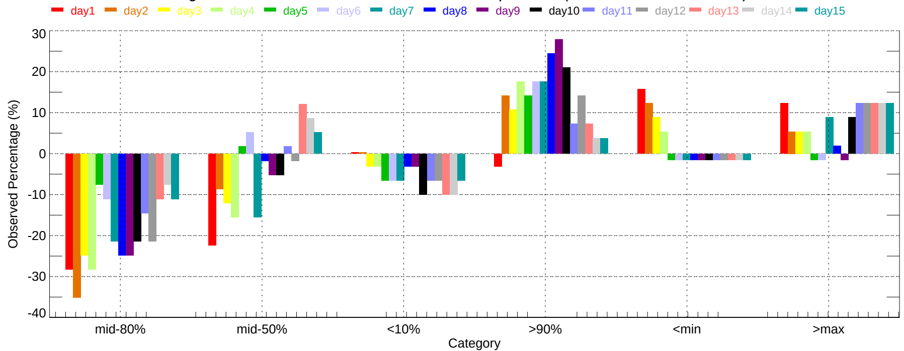
Observed Percentage Deviation of Ensembles - DAY: Min Temperature (2007-11-01~2007-11-30)
