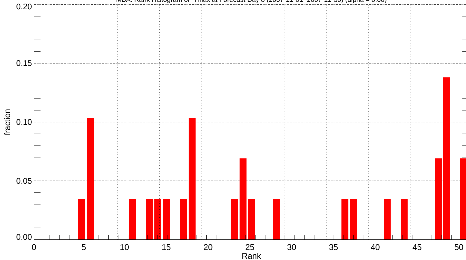
MBA: Rank Histogram of Tmax at Forecast Day 8 (2007-11-01~2007-11-30) (alpha = 0.00)
