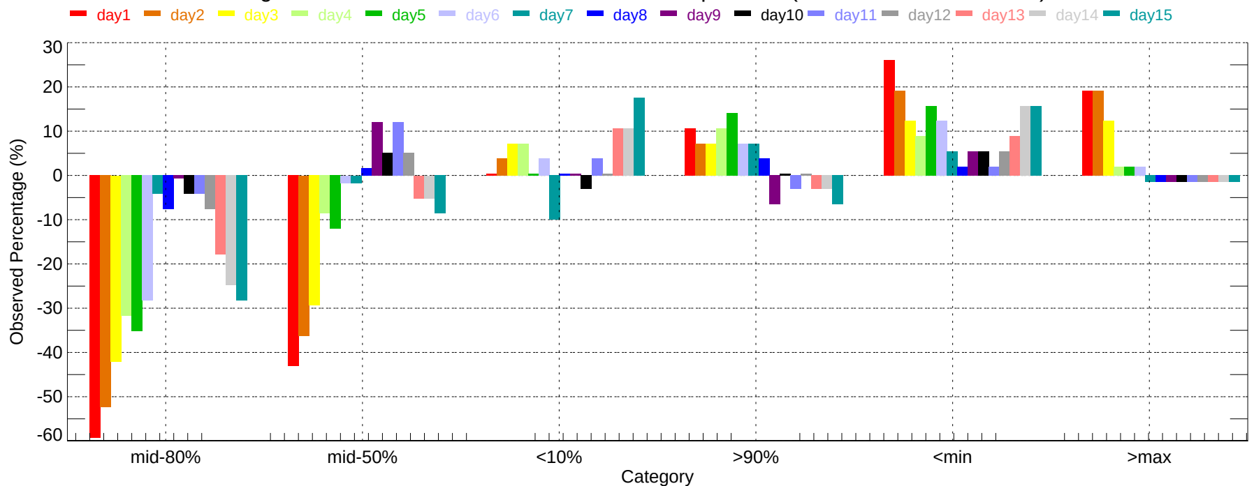
Observed Percentage Deviation of Ensembles - CON: Max Temperature (2007-11-01~2007-11-30)
