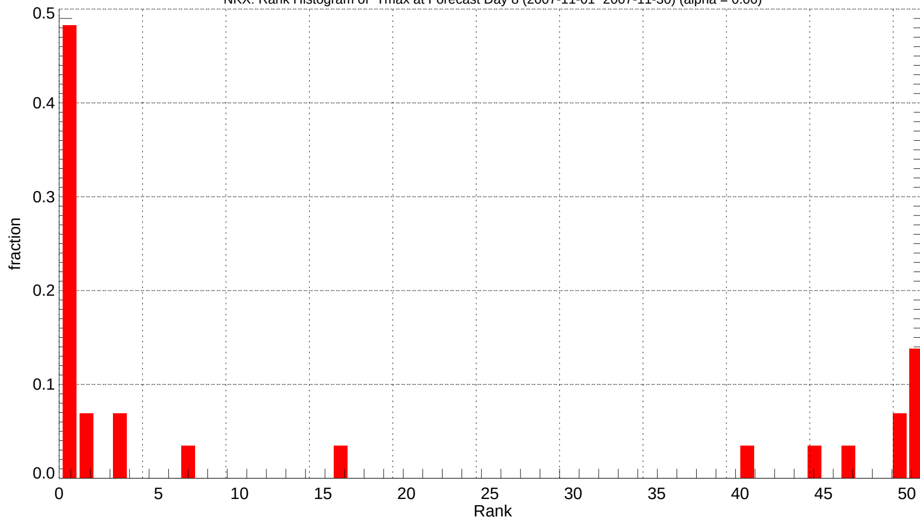
NKX: Rank Histogram of Tmax at Forecast Day 8 (2007-11-01~2007-11-30) (alpha = 0.00)
