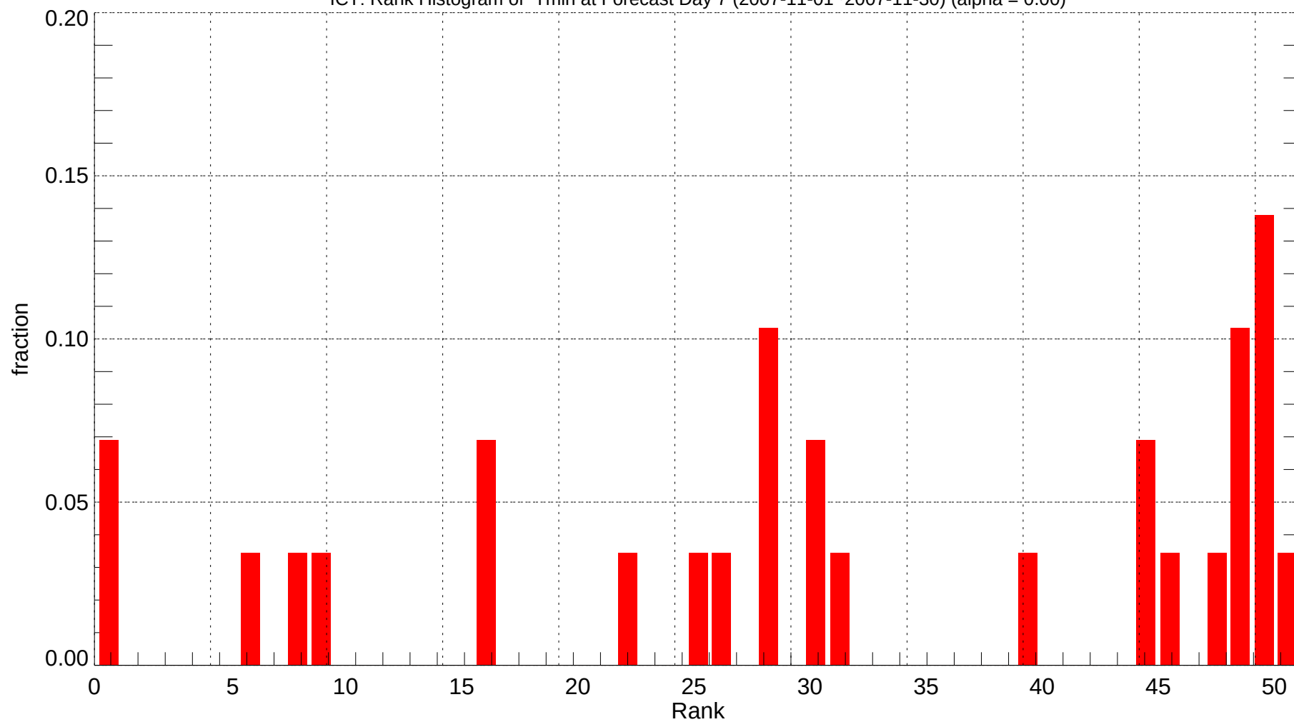
ICT: Rank Histogram of Tmin at Forecast Day 7 (2007-11-01~2007-11-30) (alpha = 0.00)
