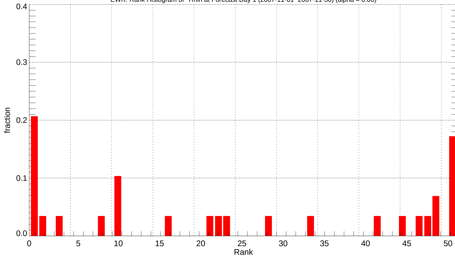
EWR: Rank Histogram of Tmin at Forecast Day 1 (2007-11-01~2007-11-30) (alpha = 0.00)
