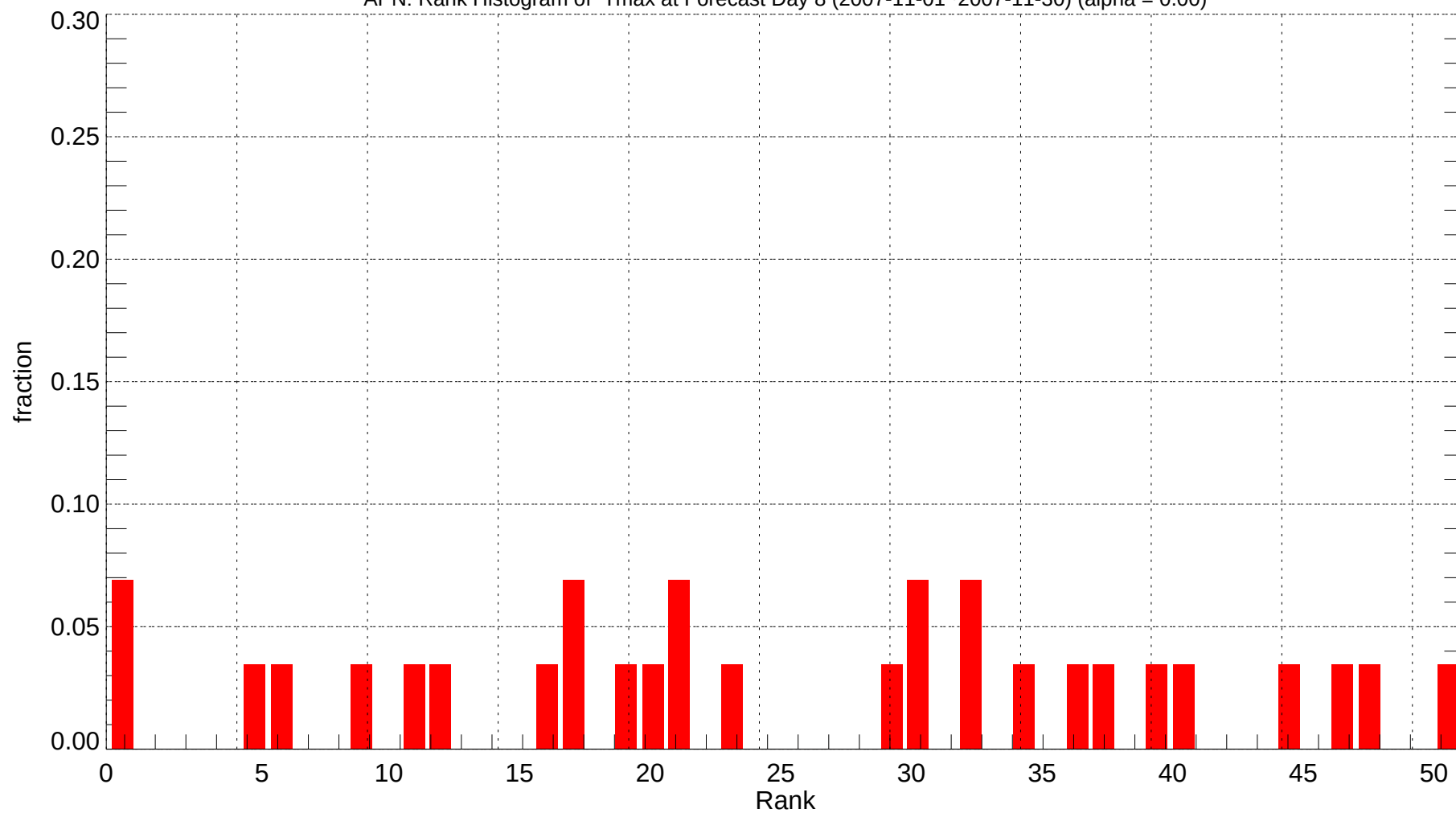
APN: Rank Histogram of Tmax at Forecast Day 8 (2007-11-01~2007-11-30) (alpha = 0.00)
