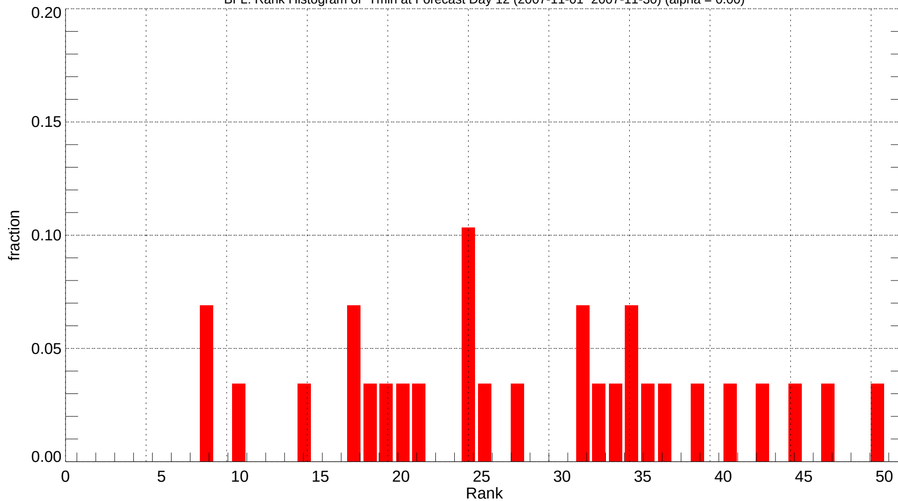
BFL: Rank Histogram of Tmin at Forecast Day 12 (2007-11-01~2007-11-30) (alpha = 0.00)
