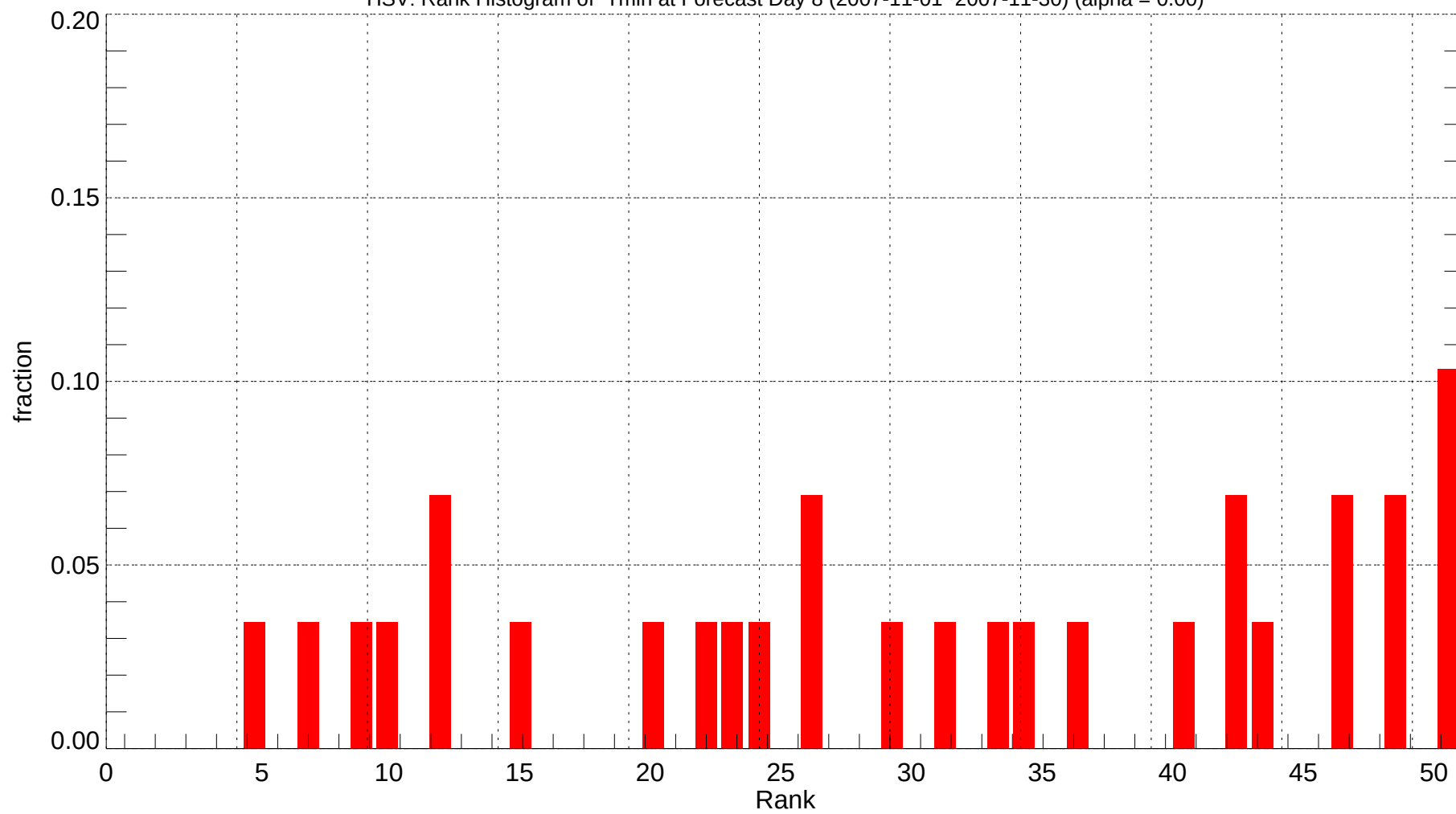
HSV: Rank Histogram of Tmin at Forecast Day 8 (2007-11-01~2007-11-30) (alpha = 0.00)
