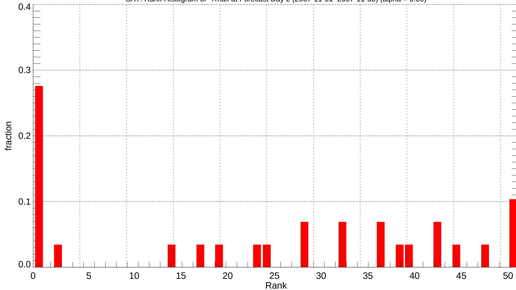
SAT: Rank Histogram of Tmax at Forecast Day 2 (2007-11-01~2007-11-30) (alpha = 0.00)
