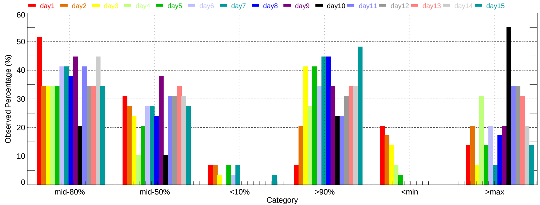
Observed Percentage of Ensembles - TUL: Max Temperature (2007-11-01~2007-11-30)
