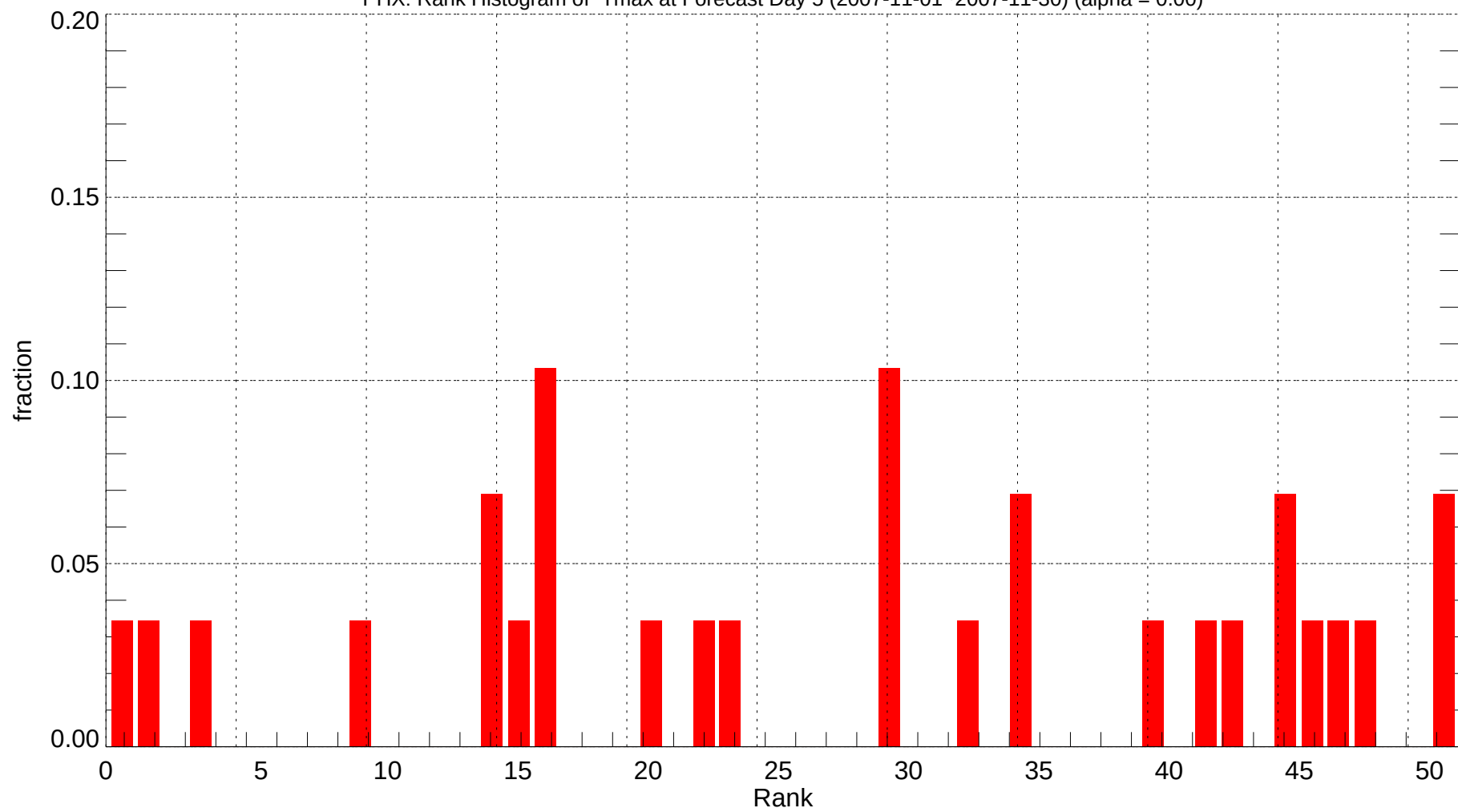
PHX: Rank Histogram of Tmax at Forecast Day 5 (2007-11-01~2007-11-30) (alpha = 0.00)
