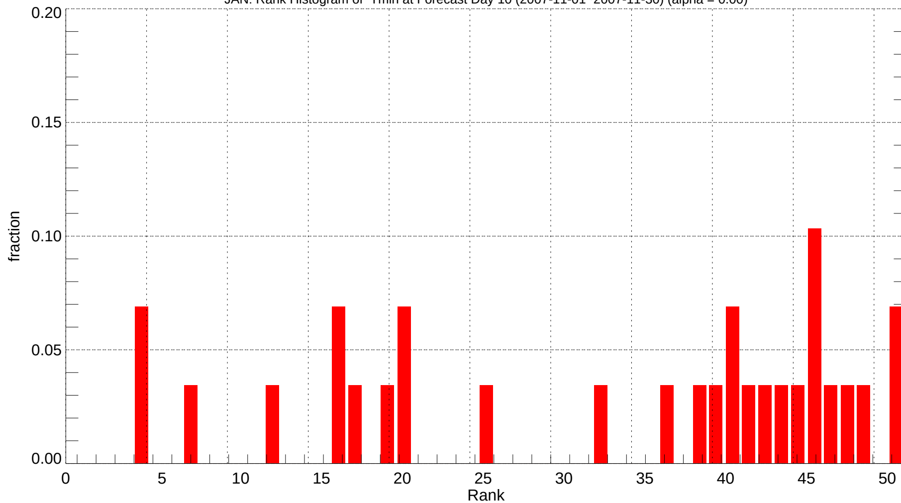
JAN: Rank Histogram of Tmin at Forecast Day 10 (2007-11-01~2007-11-30) (alpha = 0.00)
