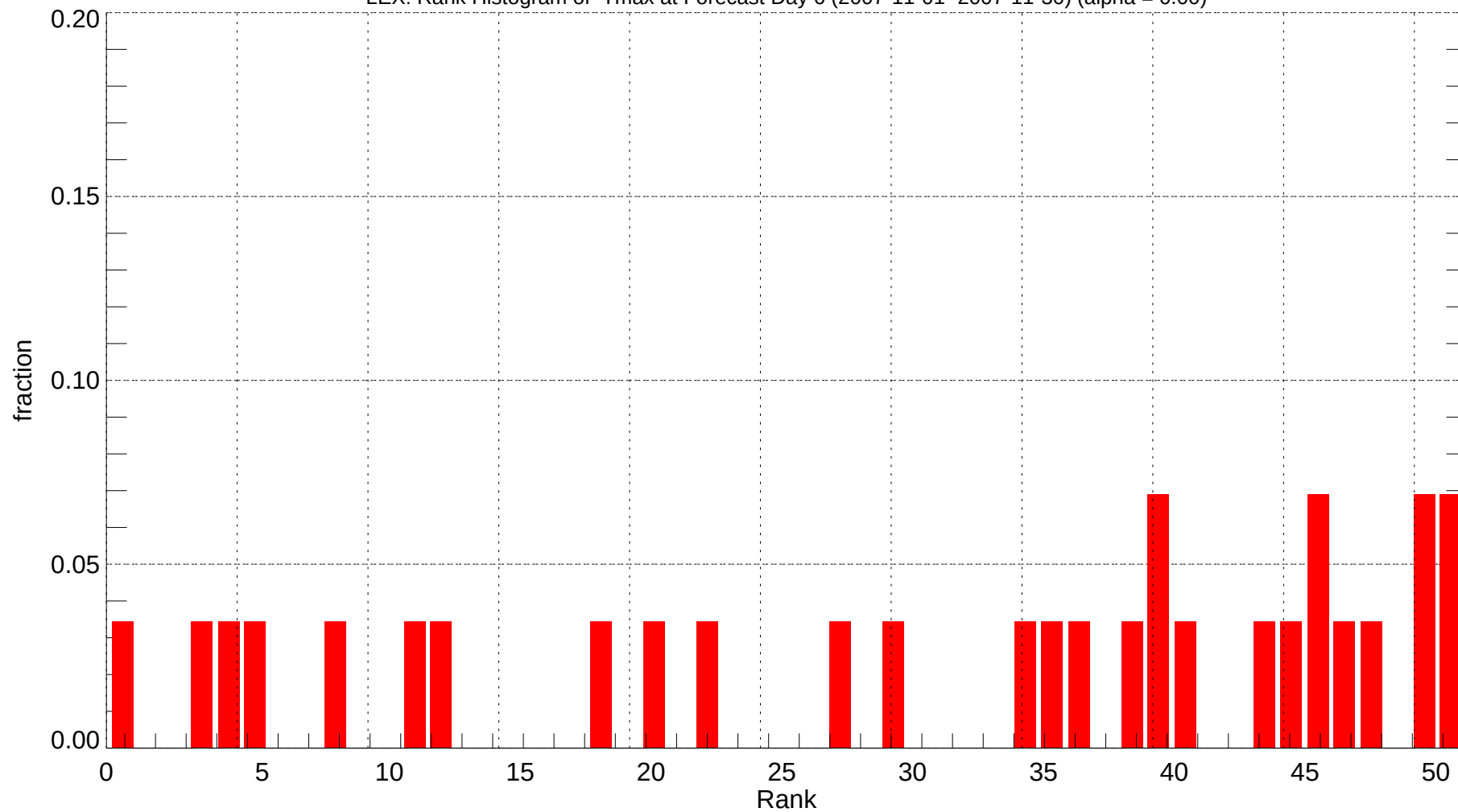
LEX: Rank Histogram of Tmax at Forecast Day 6 (2007-11-01~2007-11-30) (alpha = 0.00)
