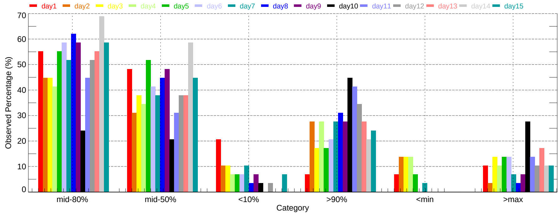
Observed Percentage of Ensembles - COU: Min Temperature (2007-11-01~2007-11-30)
