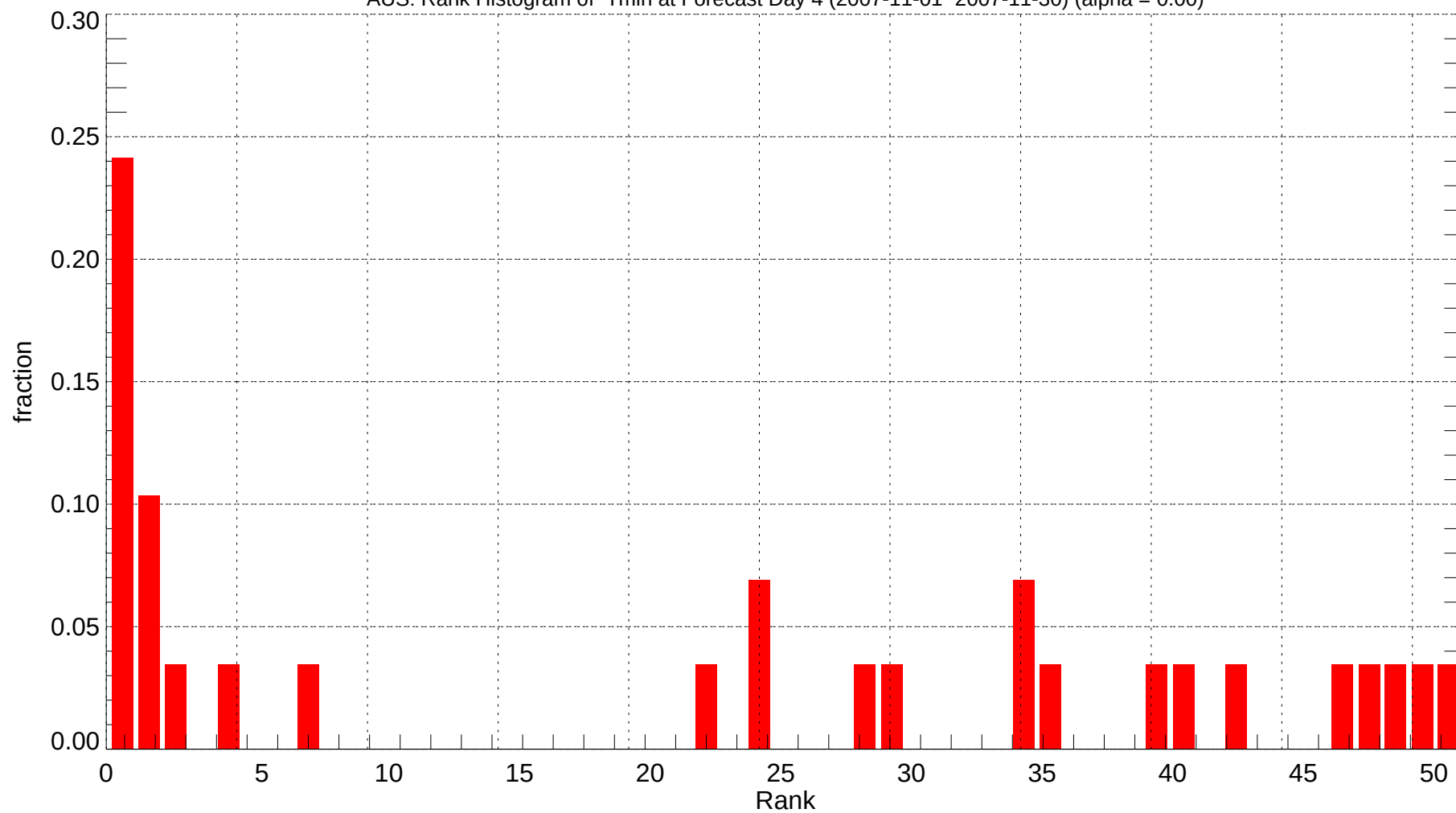
AUS: Rank Histogram of Tmin at Forecast Day 4 (2007-11-01~2007-11-30) (alpha = 0.00)
