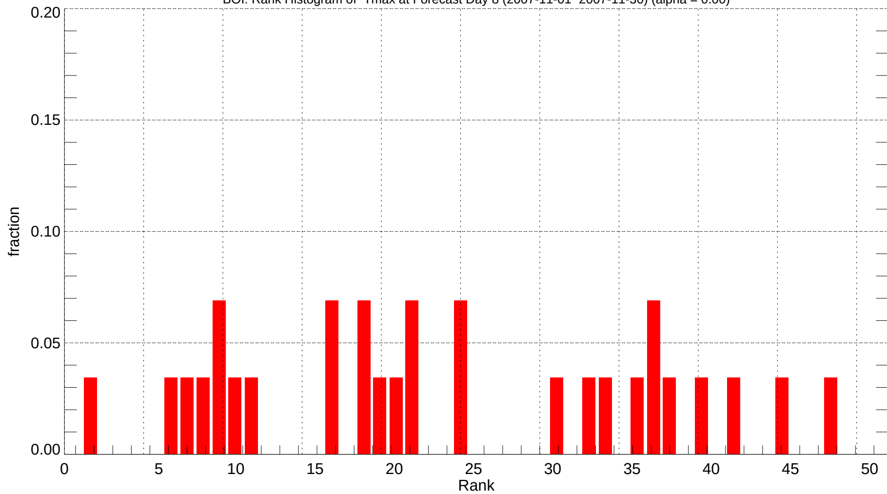
BOI: Rank Histogram of Tmax at Forecast Day 8 (2007-11-01~2007-11-30) (alpha = 0.00)
