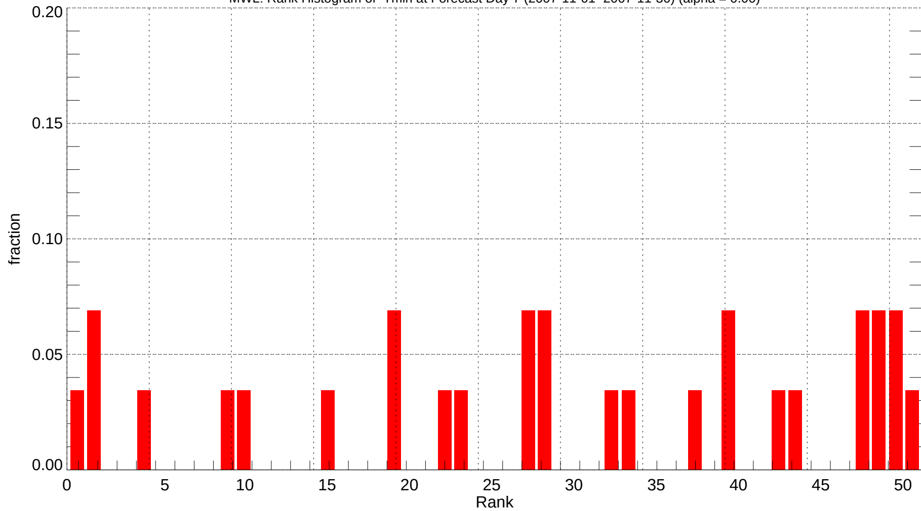
MWL: Rank Histogram of Tmin at Forecast Day 7 (2007-11-01~2007-11-30) (alpha = 0.00)
