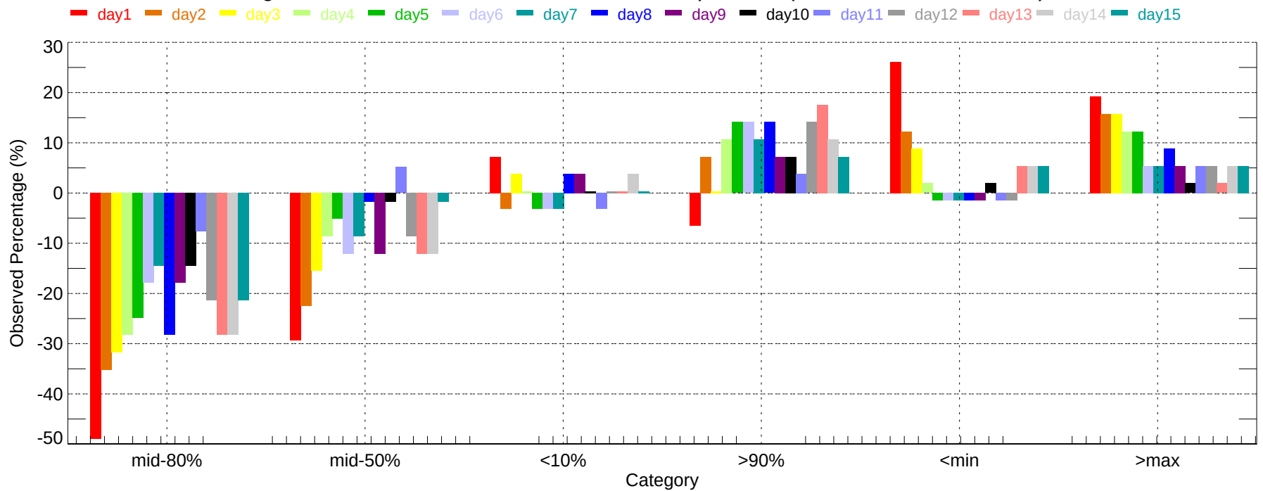
Observed Percentage Deviation of Ensembles - BOS: Min Temperature (2007-11-01~2007-11-30)
