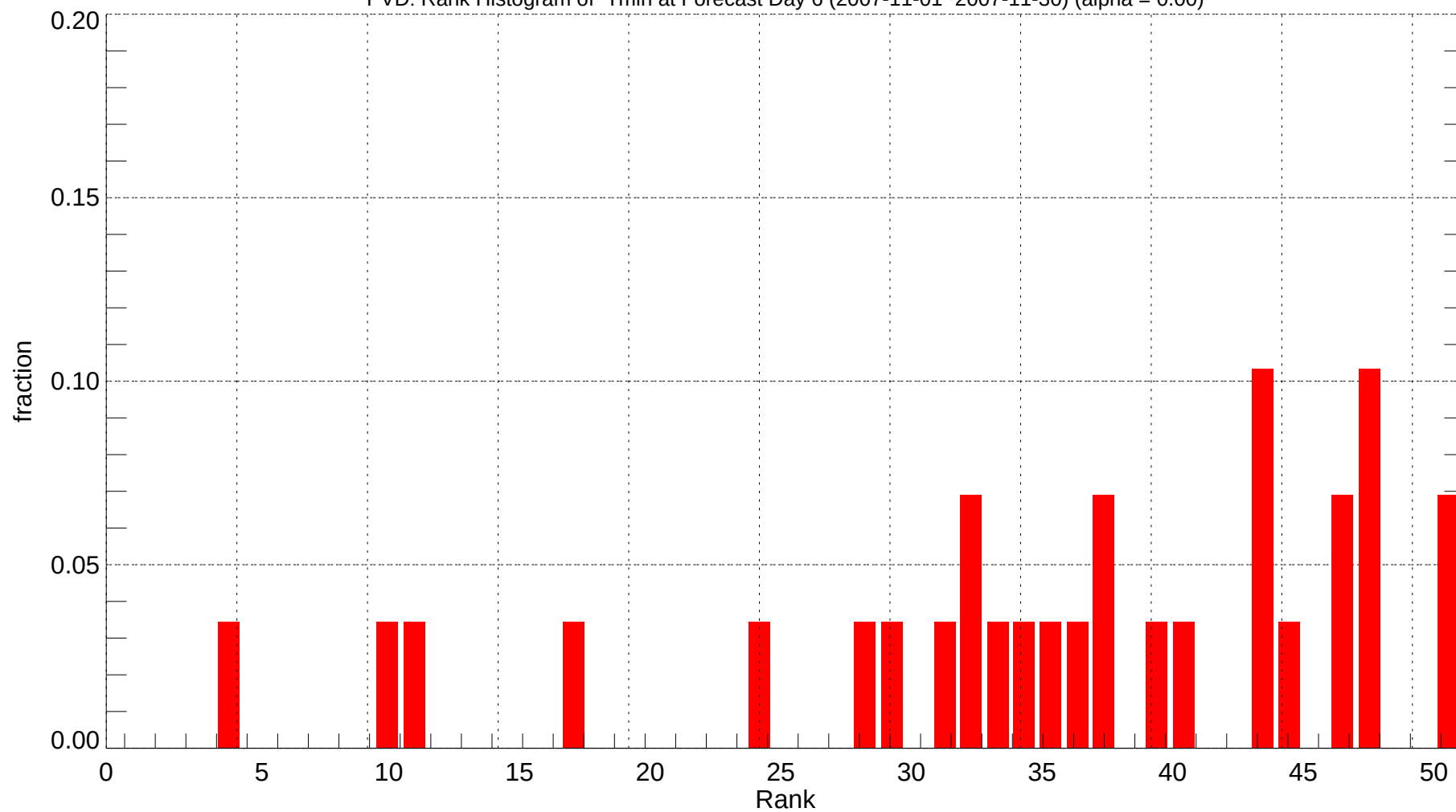
PVD: Rank Histogram of Tmin at Forecast Day 6 (2007-11-01~2007-11-30) (alpha = 0.00)
