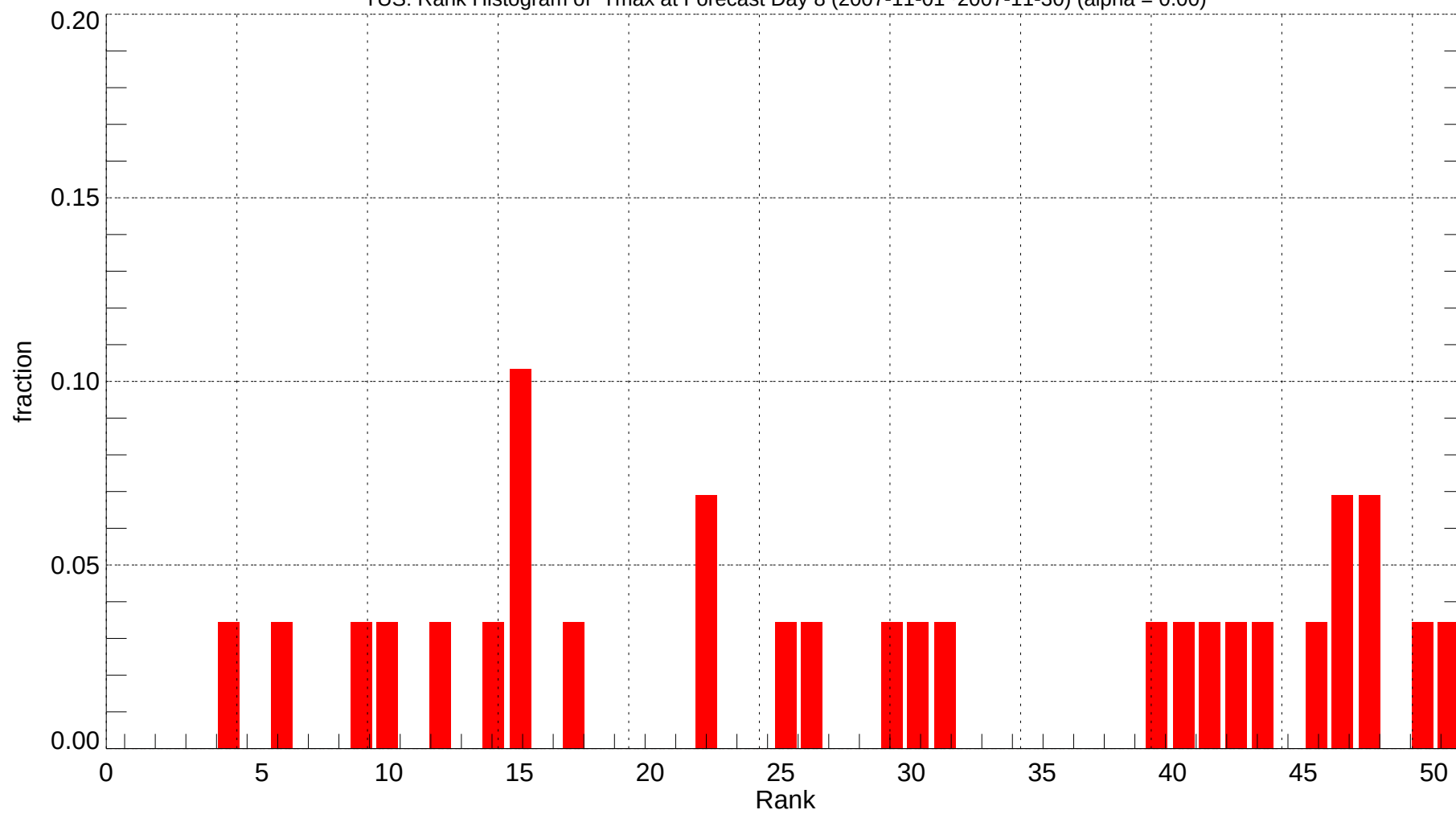
TUS: Rank Histogram of Tmax at Forecast Day 8 (2007-11-01~2007-11-30) (alpha = 0.00)
