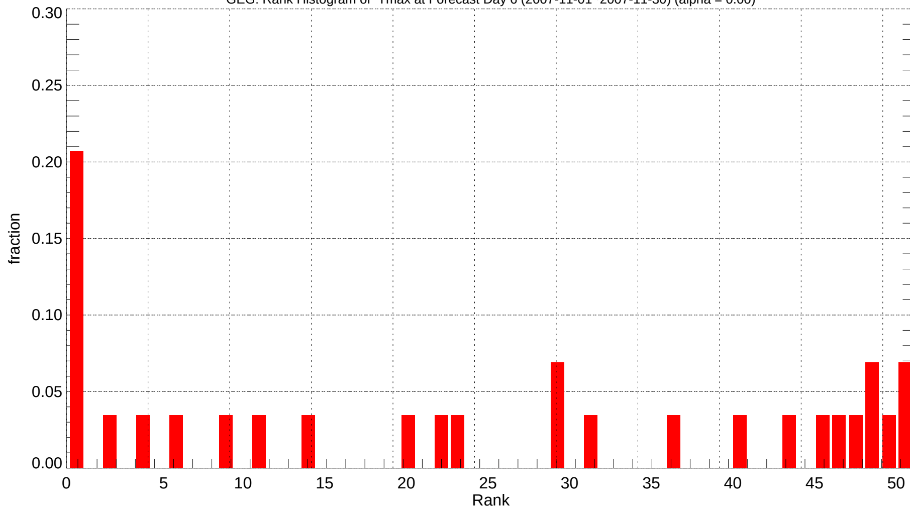
GEG: Rank Histogram of Tmax at Forecast Day 6 (2007-11-01~2007-11-30) (alpha = 0.00)
