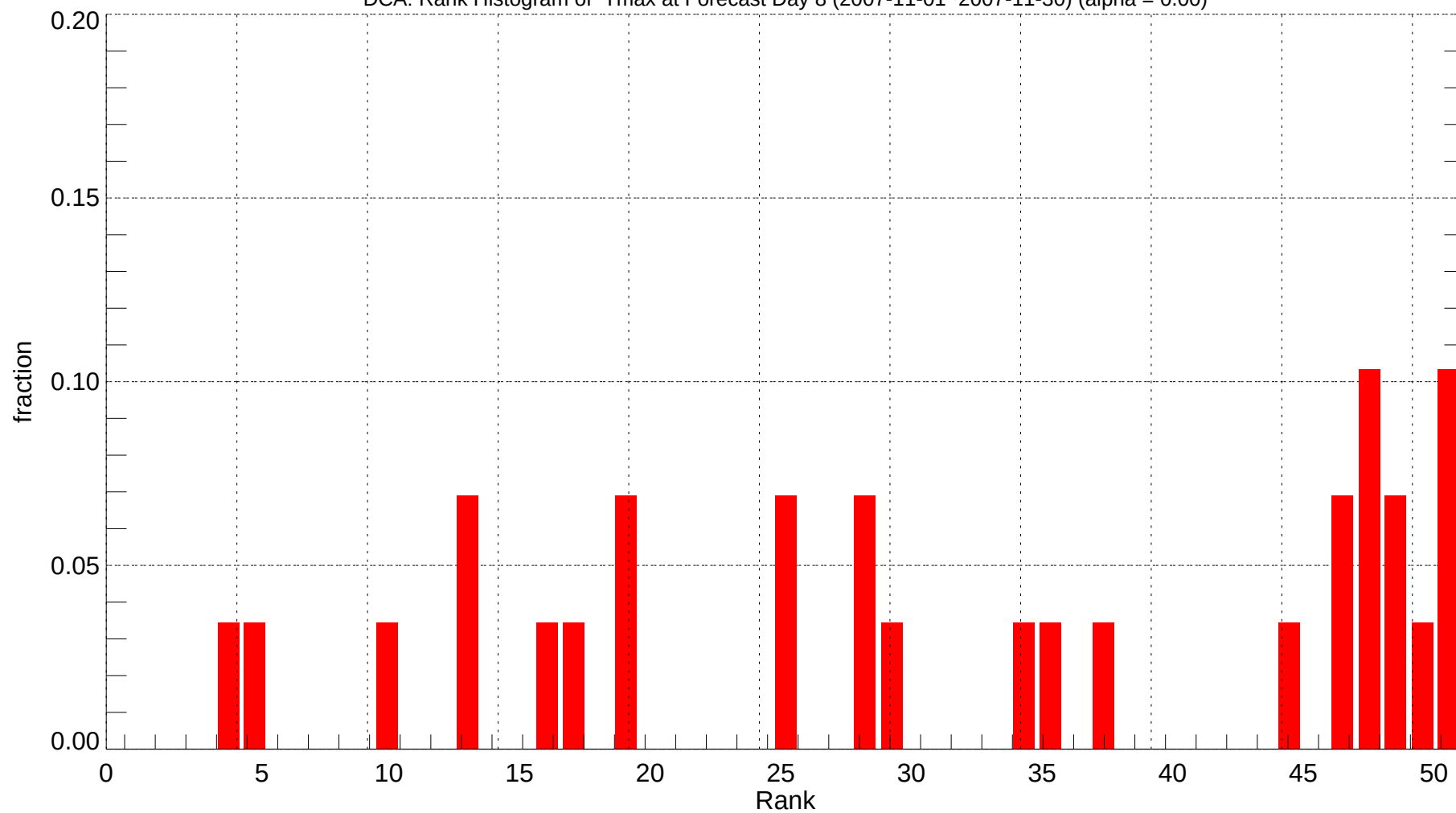
DCA: Rank Histogram of Tmax at Forecast Day 8 (2007-11-01~2007-11-30) (alpha = 0.00)
