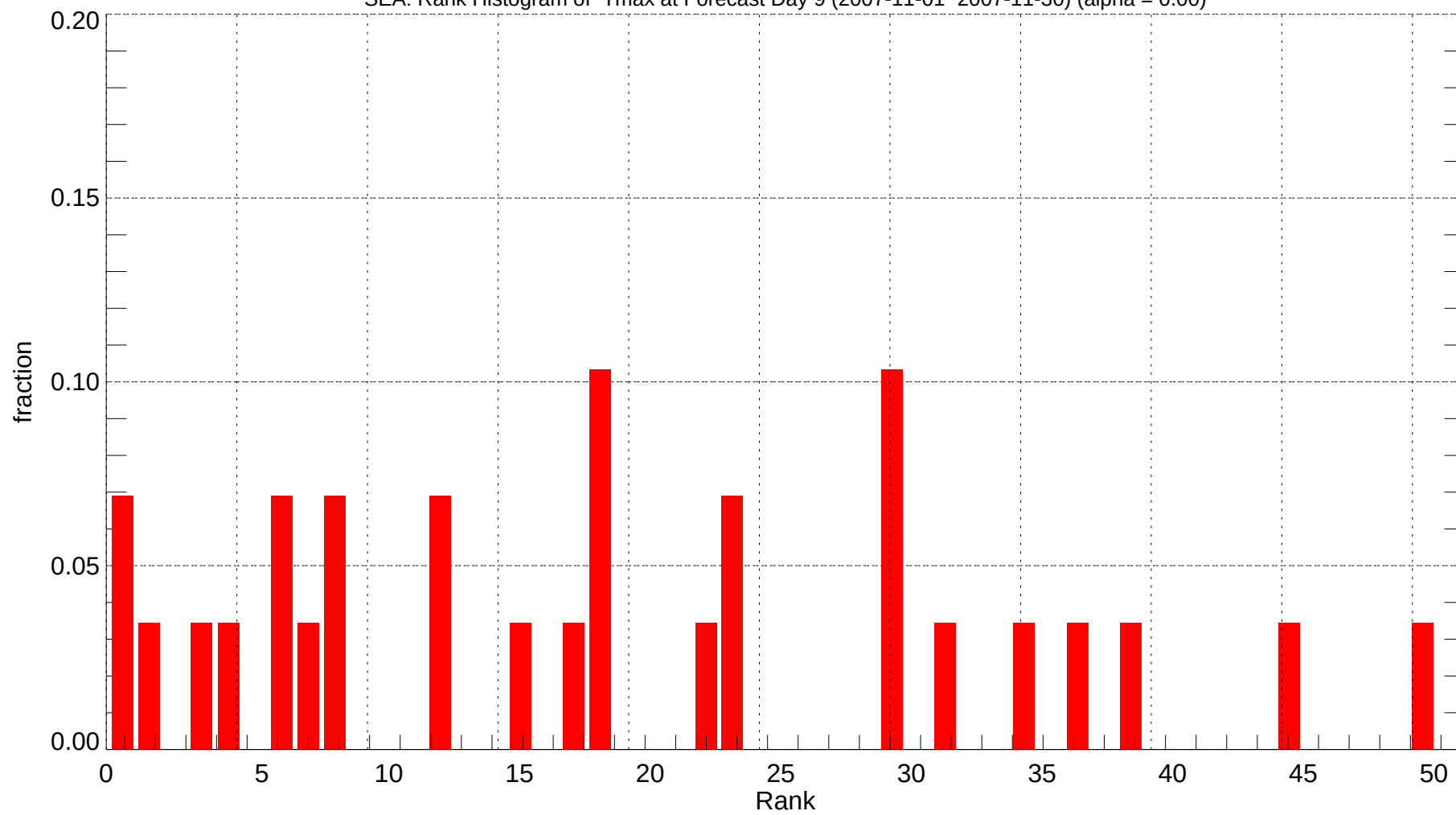
SEA: Rank Histogram of Tmax at Forecast Day 9 (2007-11-01~2007-11-30) (alpha = 0.00)
