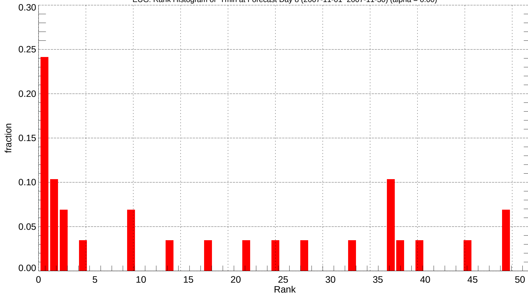
EUG: Rank Histogram of Tmin at Forecast Day 8 (2007-11-01~2007-11-30) (alpha = 0.00)
