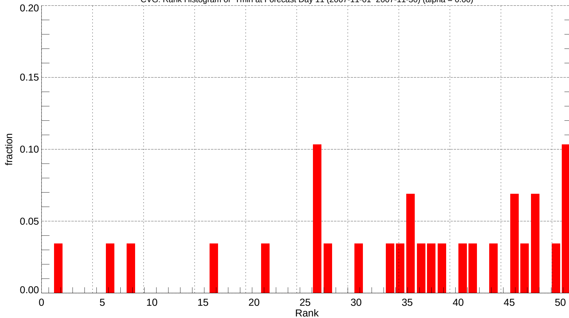
CVG: Rank Histogram of Tmin at Forecast Day 11 (2007-11-01~2007-11-30) (alpha = 0.00)
