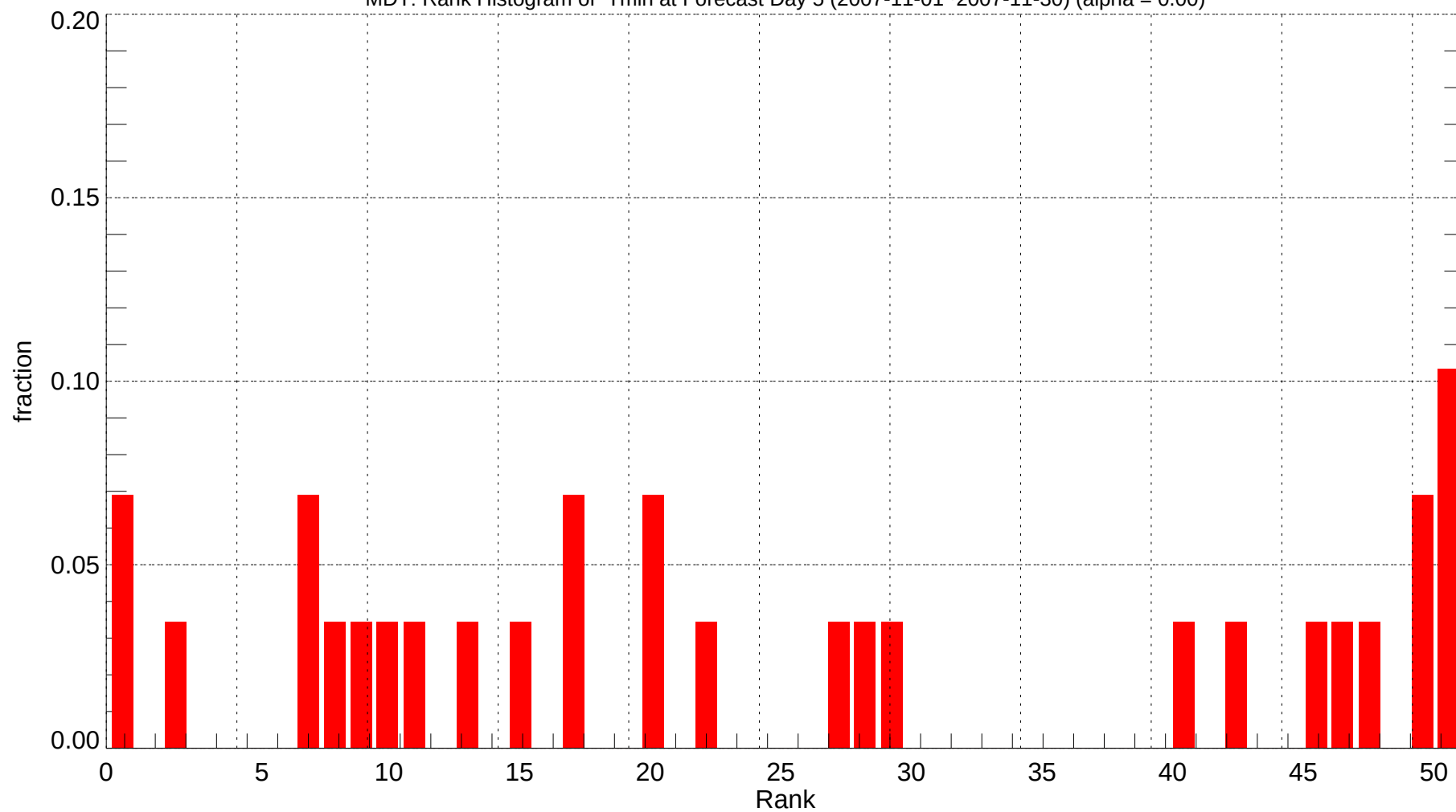
MDT: Rank Histogram of Tmin at Forecast Day 5 (2007-11-01~2007-11-30) (alpha = 0.00)
