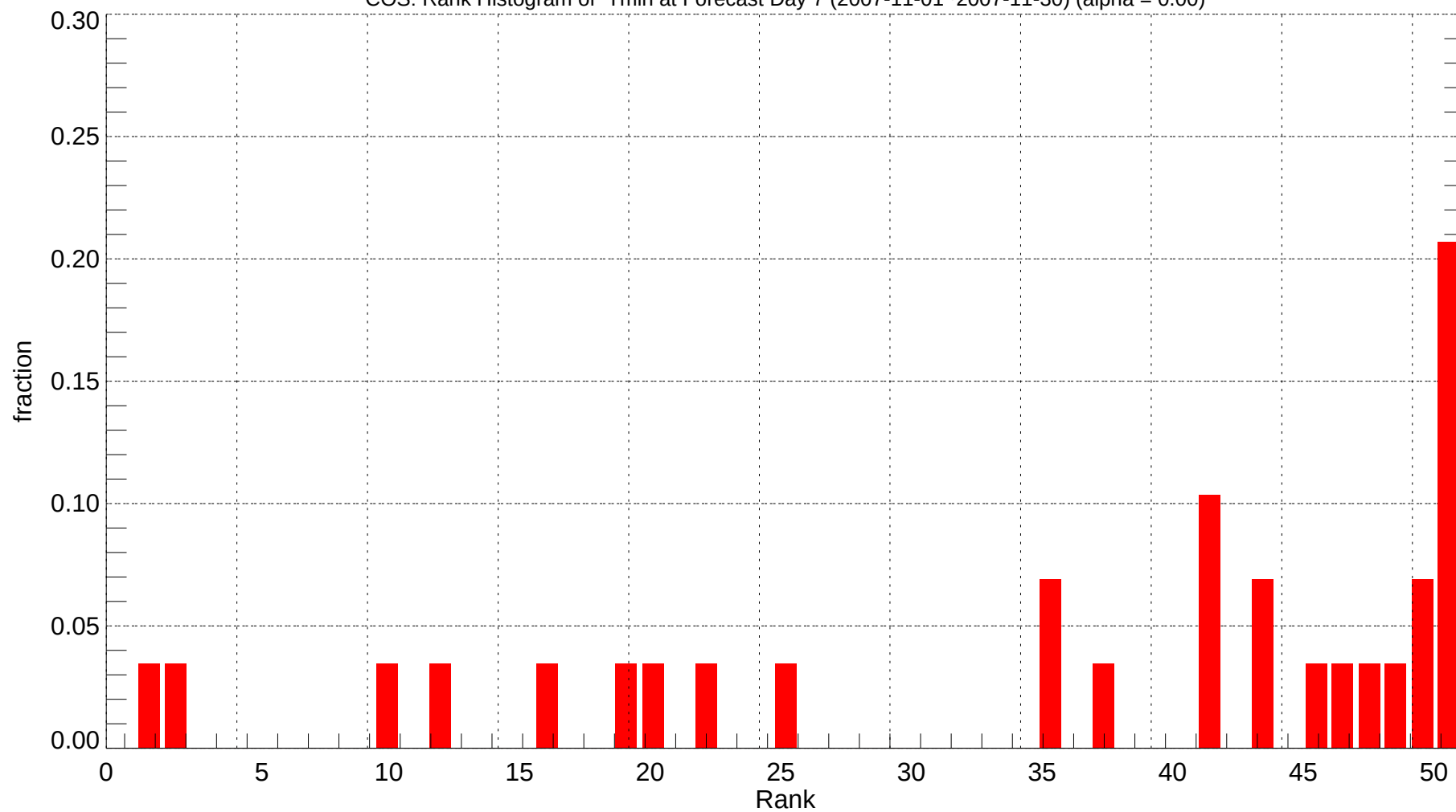
COS: Rank Histogram of Tmin at Forecast Day 7 (2007-11-01~2007-11-30) (alpha = 0.00)
