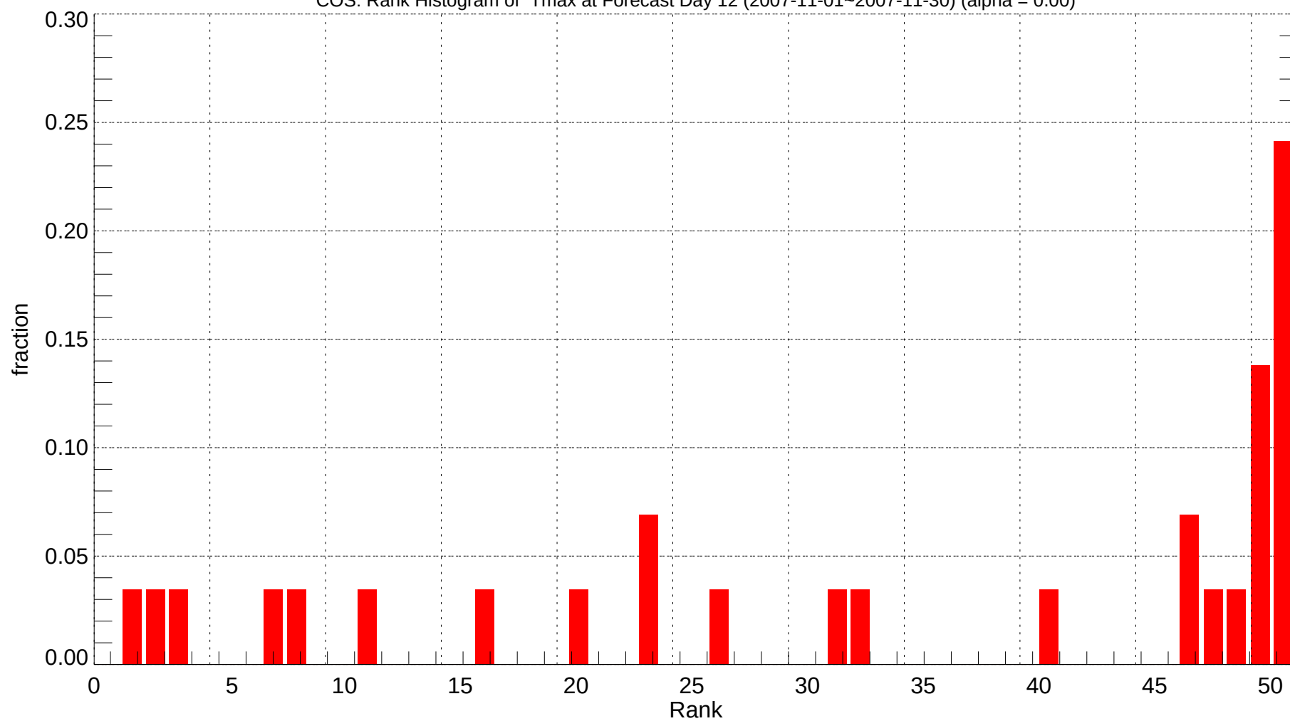
COS: Rank Histogram of Tmax at Forecast Day 12 (2007-11-01~2007-11-30) (alpha = 0.00)
