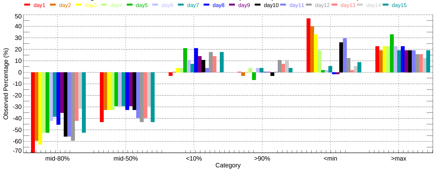
Observed Percentage Deviation of Ensembles - LGB: Min Temperature (2007-11-01~2007-11-30)
