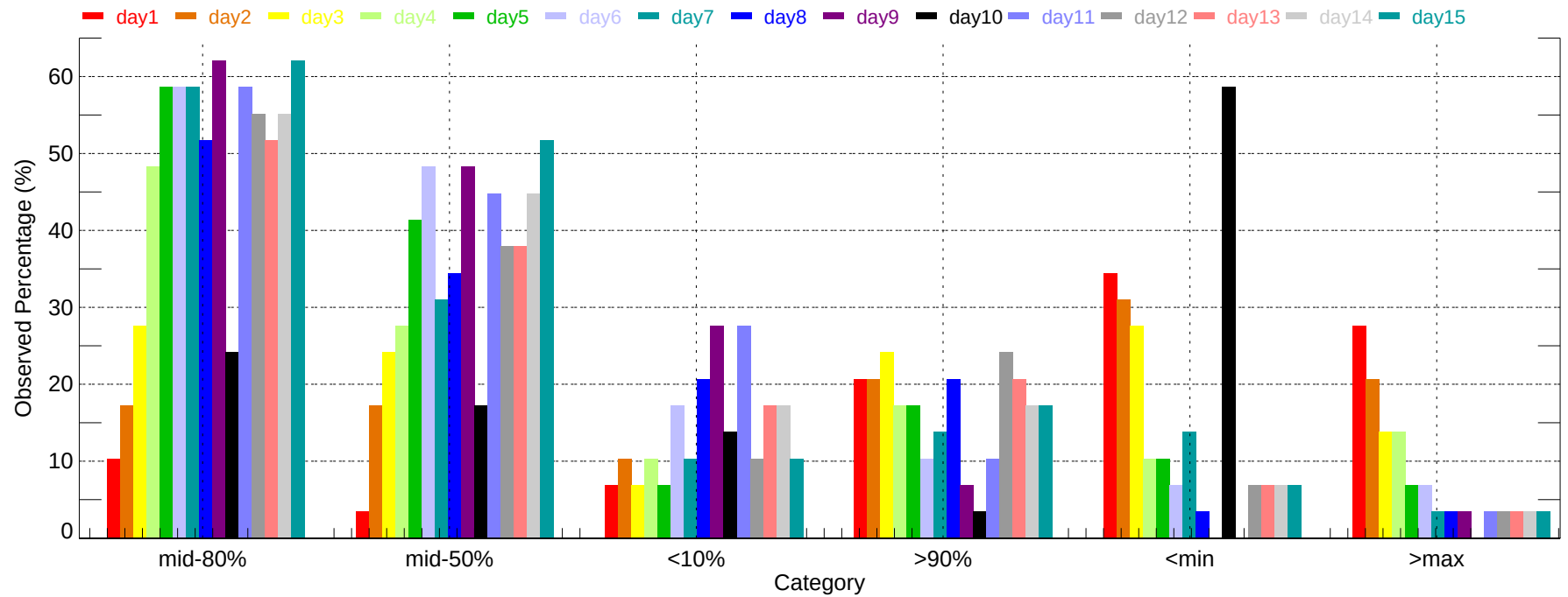
Observed Percentage of Ensembles - AVP: Max Temperature (2007-11-01~2007-11-30)
