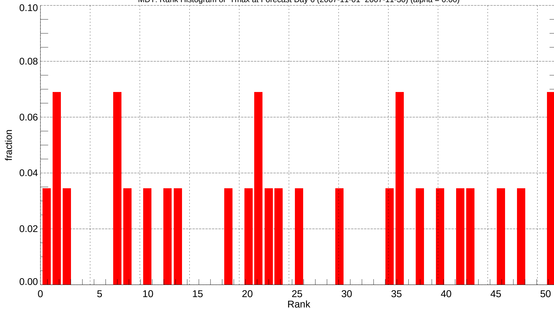
MDT: Rank Histogram of Tmax at Forecast Day 6 (2007-11-01~2007-11-30) (alpha = 0.00)
