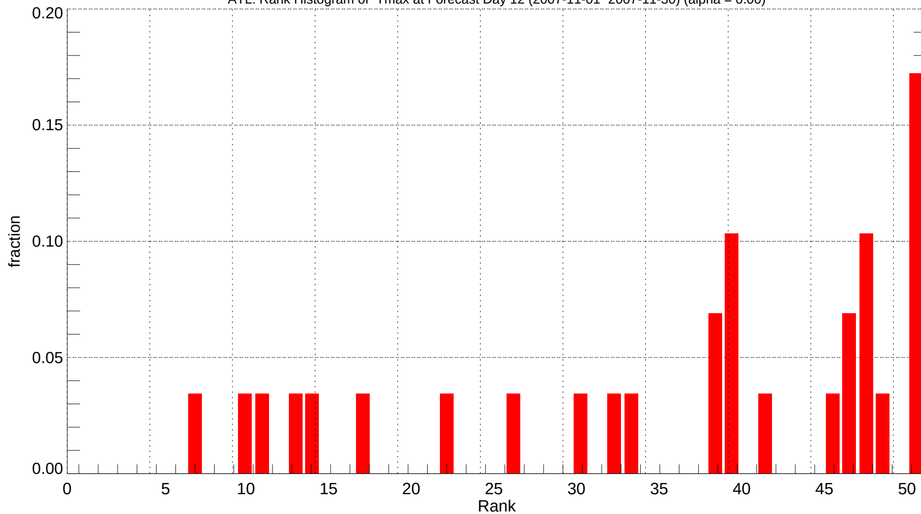
ATL: Rank Histogram of Tmax at Forecast Day 12 (2007-11-01~2007-11-30) (alpha = 0.00)
