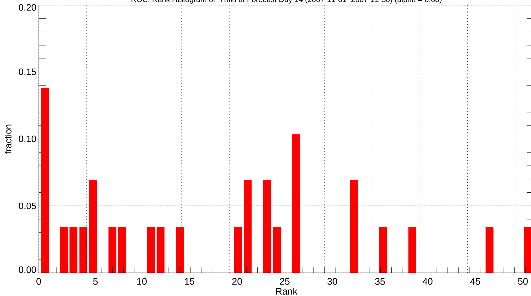
ROC: Rank Histogram of Tmin at Forecast Day 14 (2007-11-01~2007-11-30) (alpha = 0.00)
