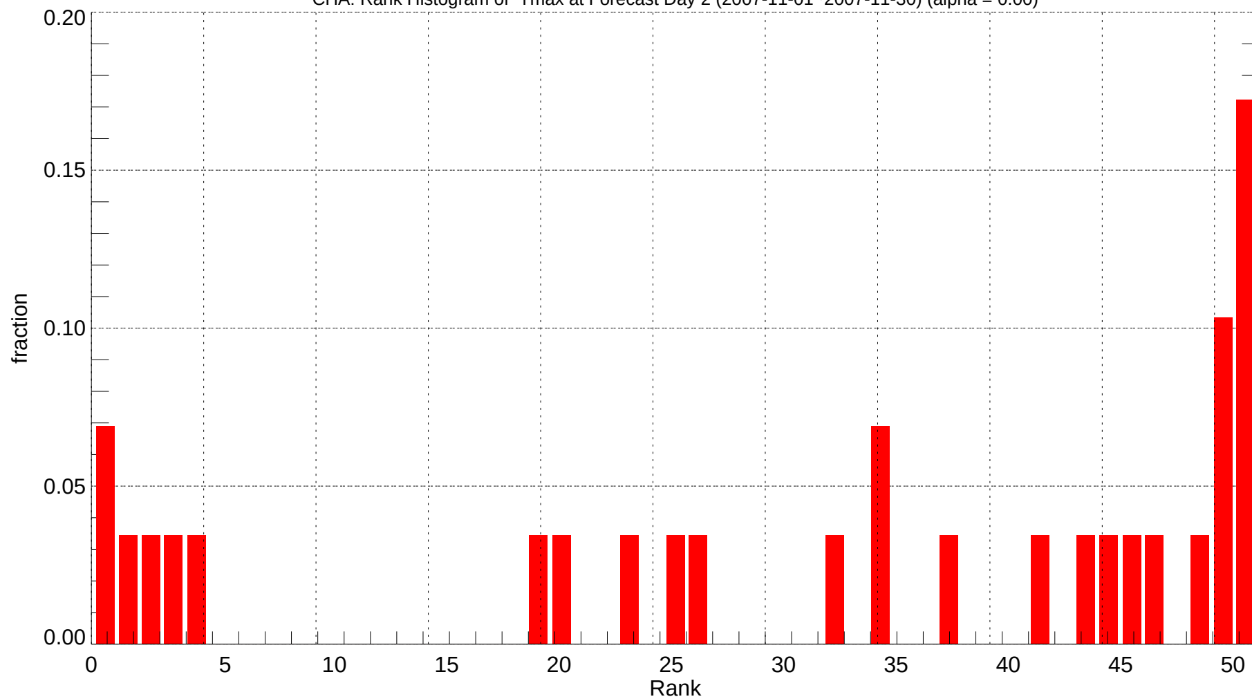
CHA: Rank Histogram of Tmax at Forecast Day 2 (2007-11-01~2007-11-30) (alpha = 0.00)
