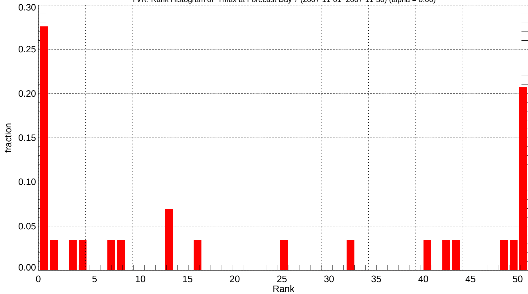
YVR: Rank Histogram of Tmax at Forecast Day 7 (2007-11-01~2007-11-30) (alpha = 0.00)
