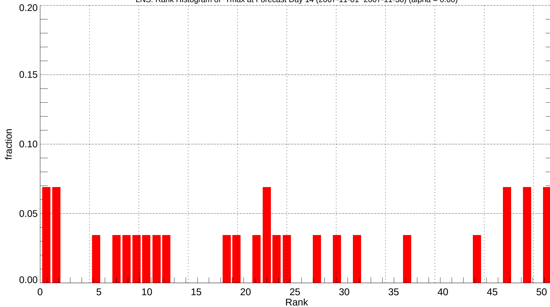
LNS: Rank Histogram of Tmax at Forecast Day 14 (2007-11-01~2007-11-30) (alpha = 0.00)
