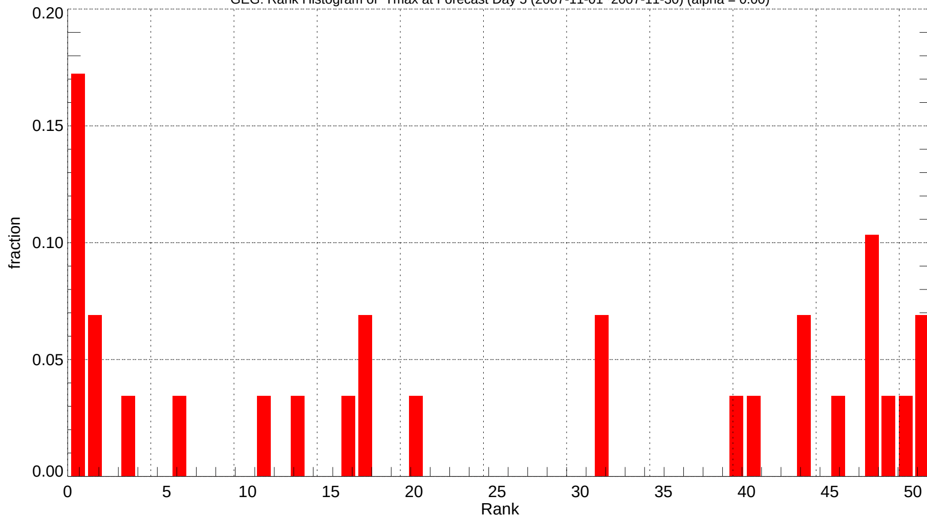
GEG: Rank Histogram of Tmax at Forecast Day 5 (2007-11-01~2007-11-30) (alpha = 0.00)
