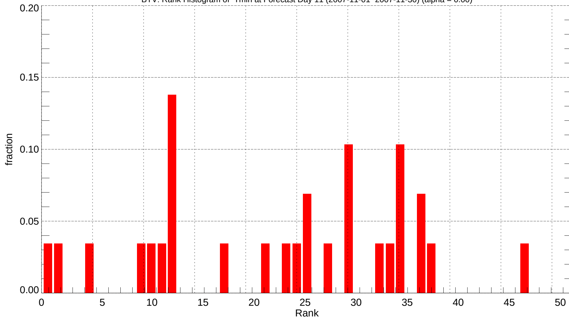
BTV: Rank Histogram of Tmin at Forecast Day 11 (2007-11-01~2007-11-30) (alpha = 0.00)
