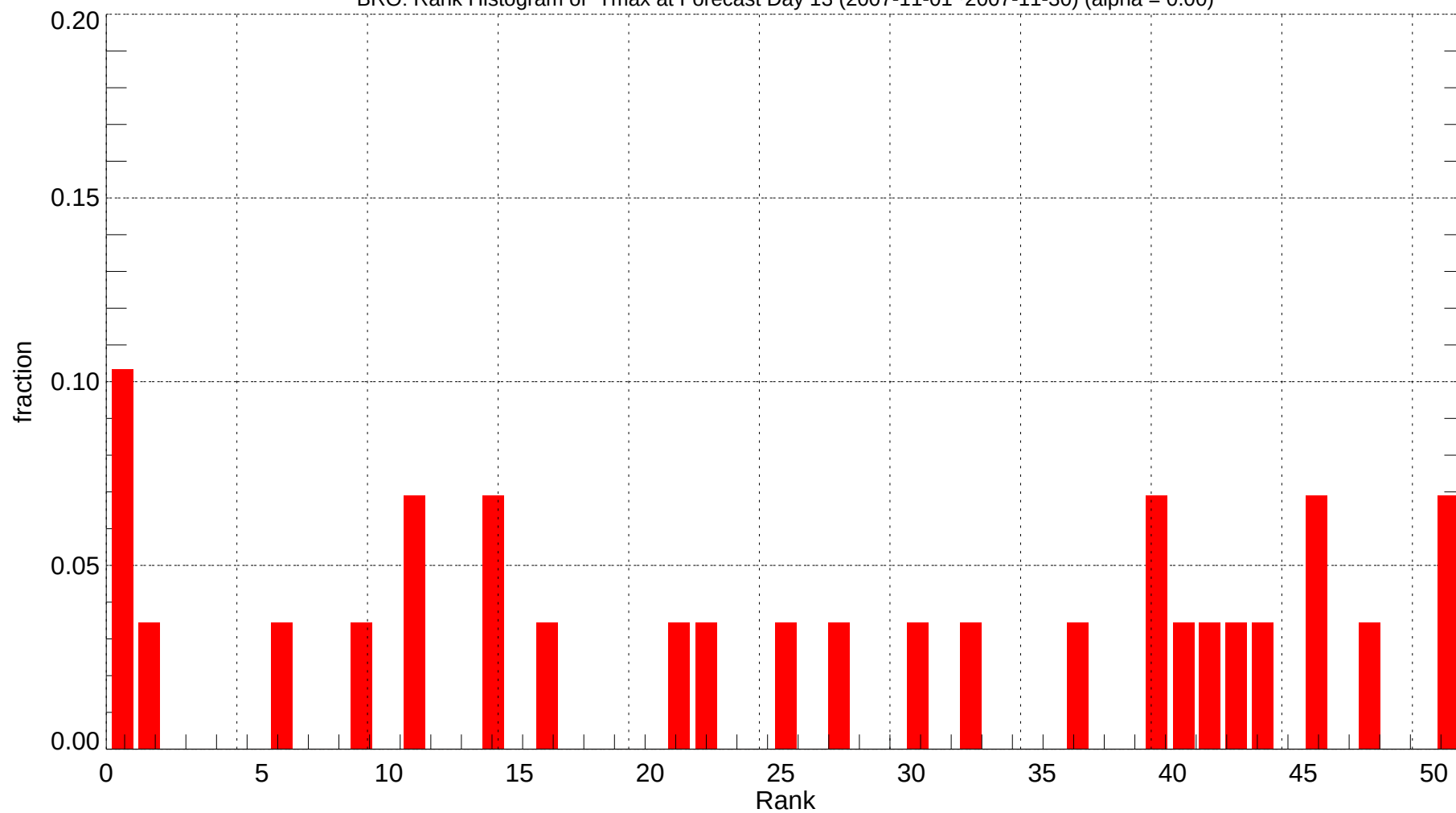
BRO: Rank Histogram of Tmax at Forecast Day 13 (2007-11-01~2007-11-30) (alpha = 0.00)
