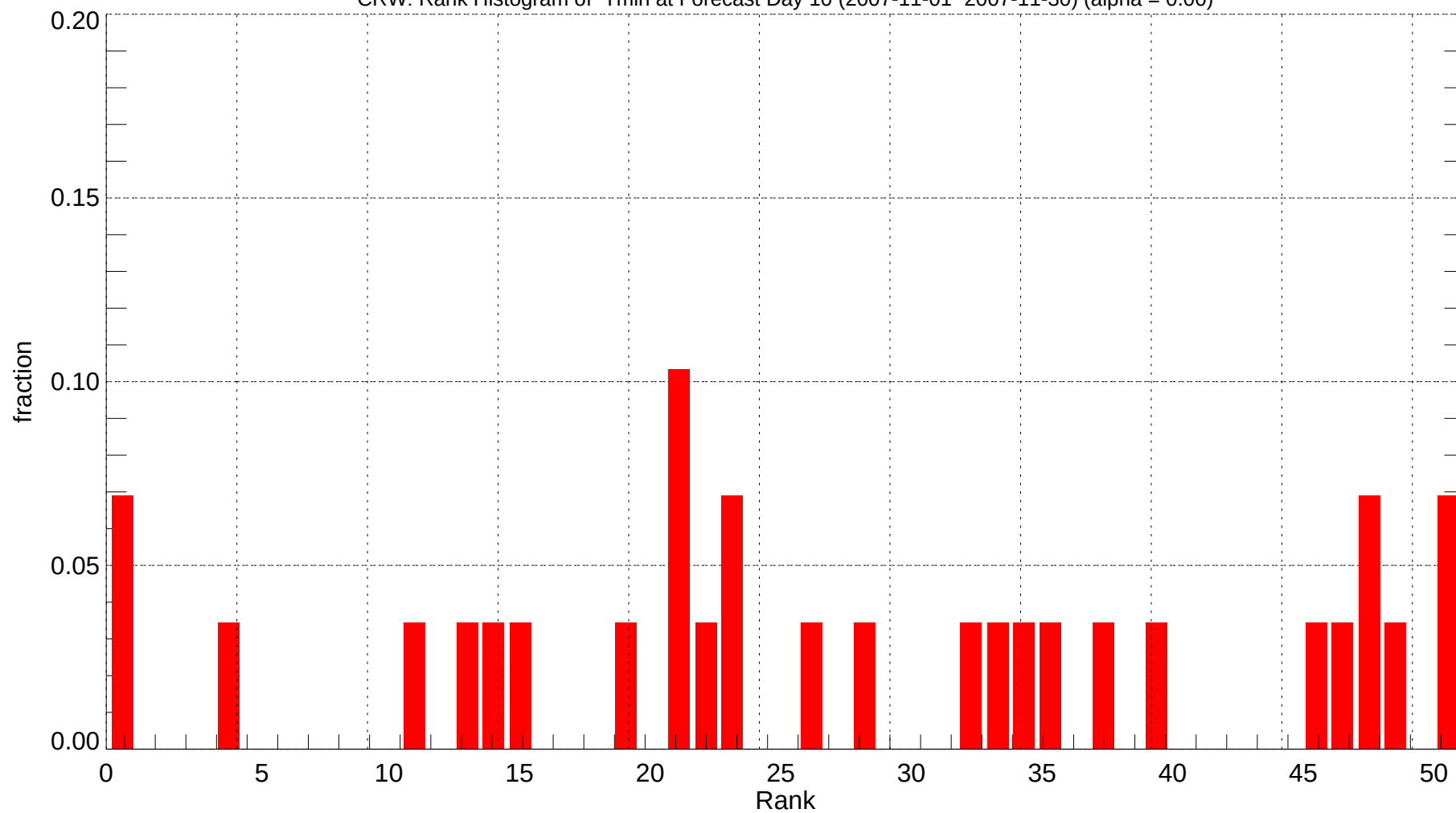
CRW: Rank Histogram of Tmin at Forecast Day 10 (2007-11-01~2007-11-30) (alpha = 0.00)
