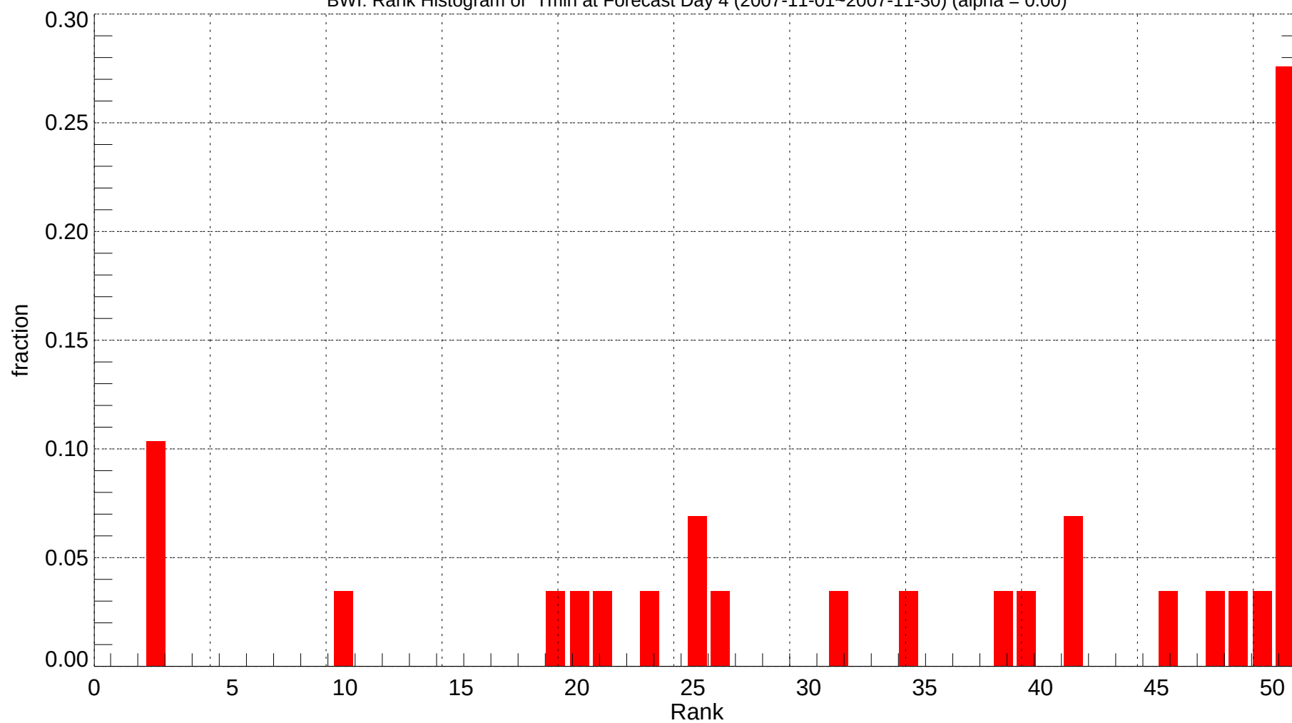
BWI: Rank Histogram of Tmin at Forecast Day 4 (2007-11-01~2007-11-30) (alpha = 0.00)
