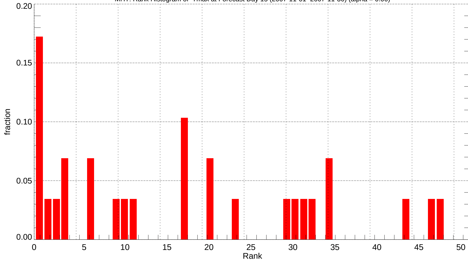
MHT: Rank Histogram of Tmax at Forecast Day 15 (2007-11-01~2007-11-30) (alpha = 0.00)
