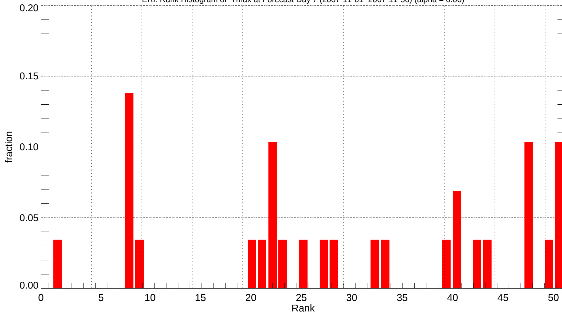
ERI: Rank Histogram of Tmax at Forecast Day 7 (2007-11-01~2007-11-30) (alpha = 0.00)
