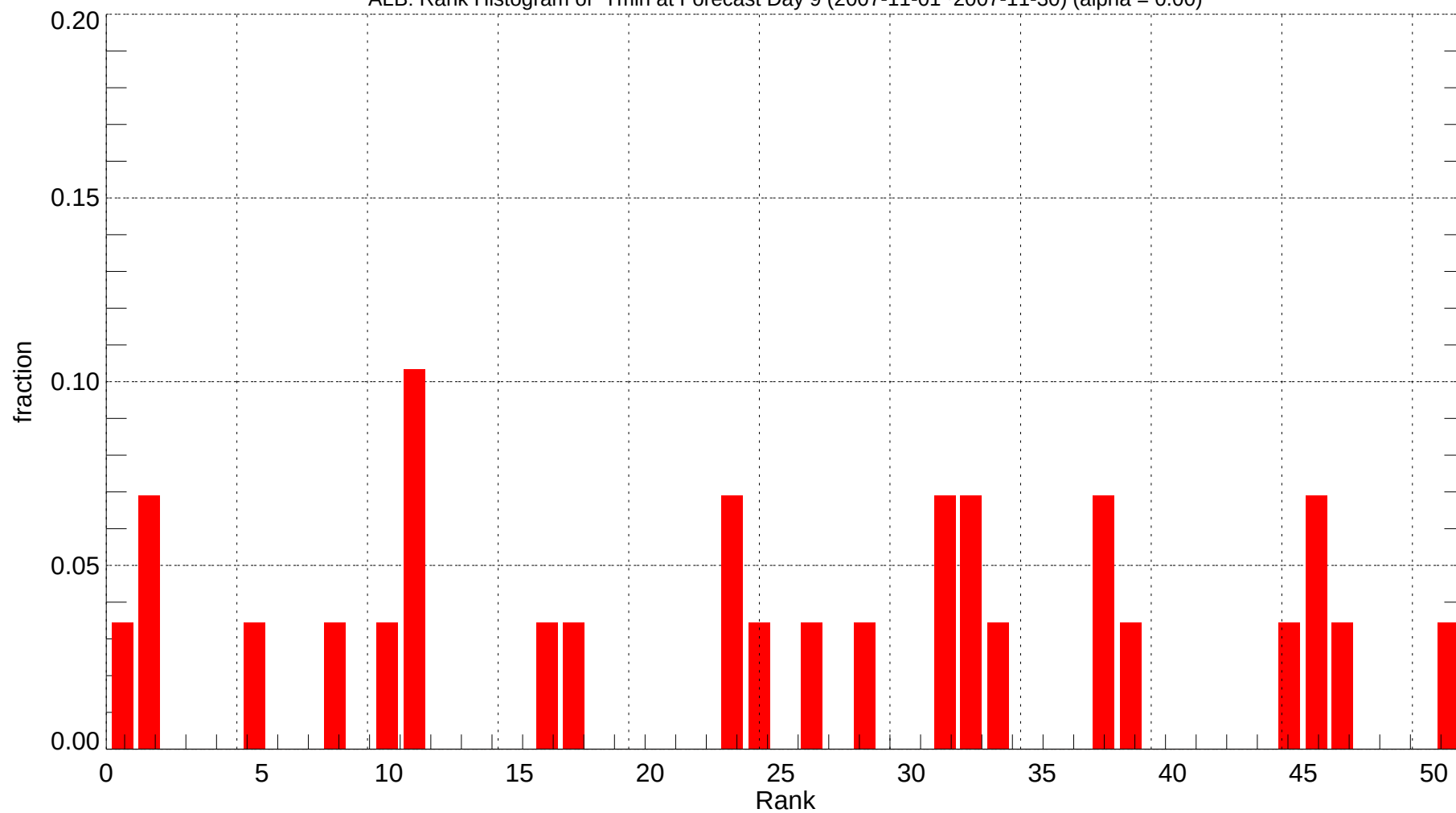
ALB: Rank Histogram of Tmin at Forecast Day 9 (2007-11-01~2007-11-30) (alpha = 0.00)
