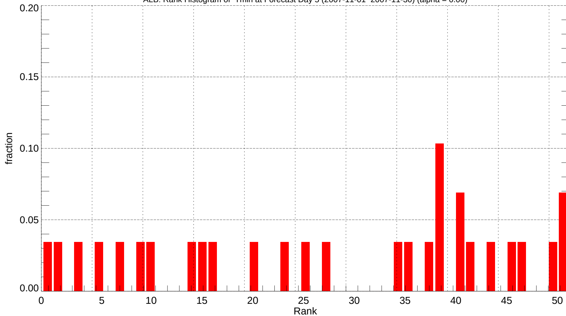
ALB: Rank Histogram of Tmin at Forecast Day 5 (2007-11-01~2007-11-30) (alpha = 0.00)
