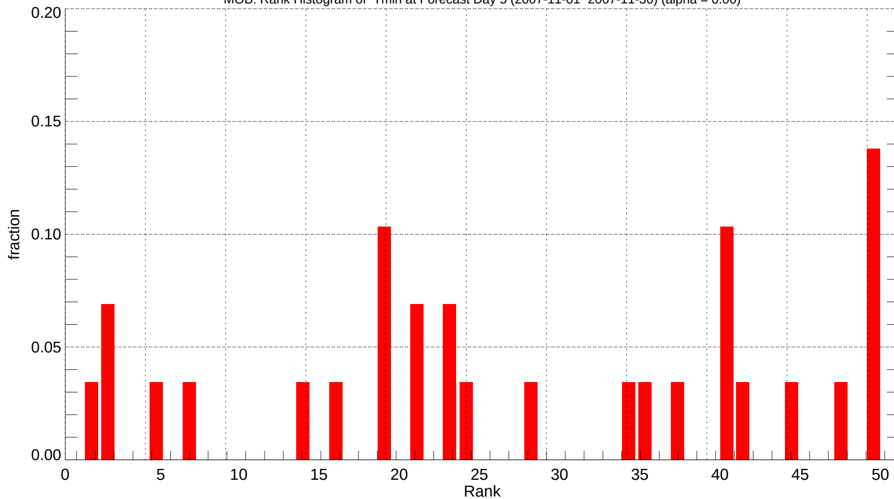
MOB: Rank Histogram of Tmin at Forecast Day 5 (2007-11-01~2007-11-30) (alpha = 0.00)
