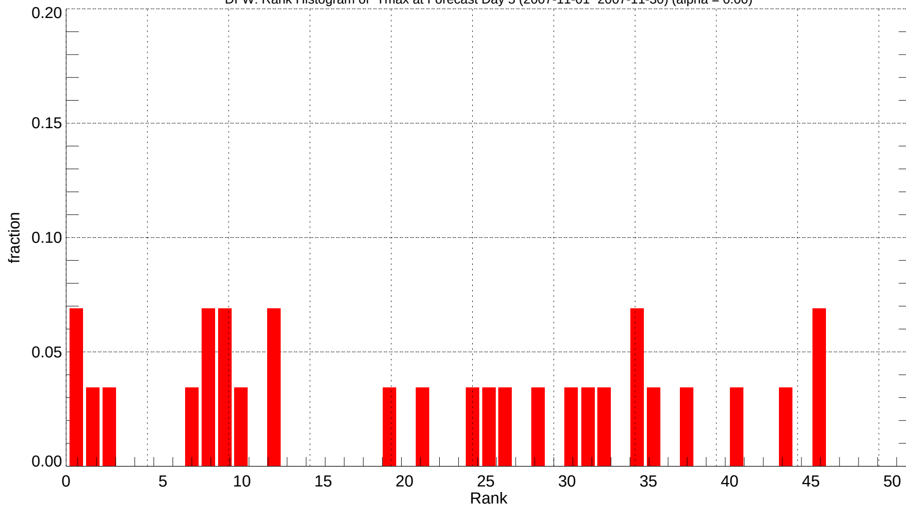
DFW: Rank Histogram of Tmax at Forecast Day 5 (2007-11-01~2007-11-30) (alpha = 0.00)
