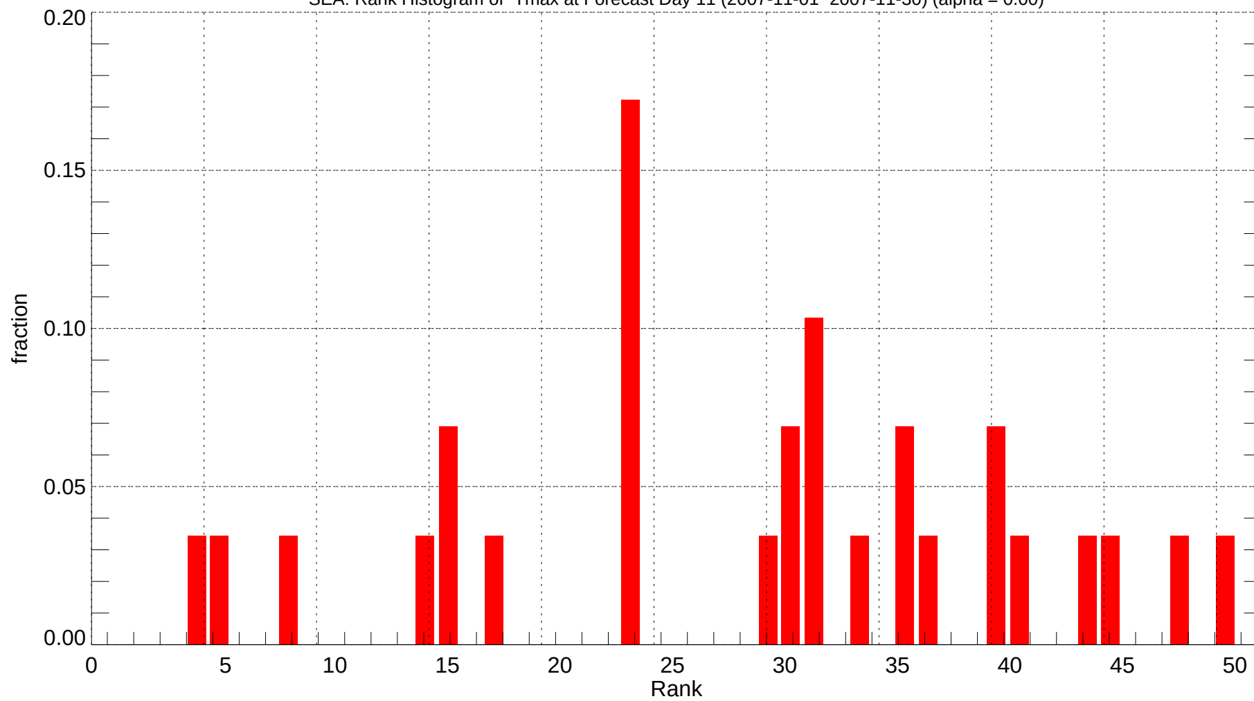
SEA: Rank Histogram of Tmax at Forecast Day 11 (2007-11-01~2007-11-30) (alpha = 0.00)
