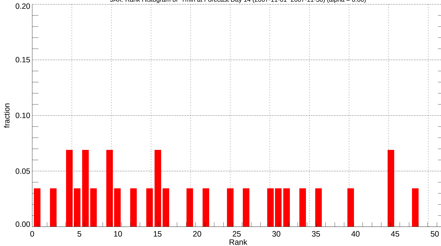
JAX: Rank Histogram of Tmin at Forecast Day 14 (2007-11-01~2007-11-30) (alpha = 0.00)
