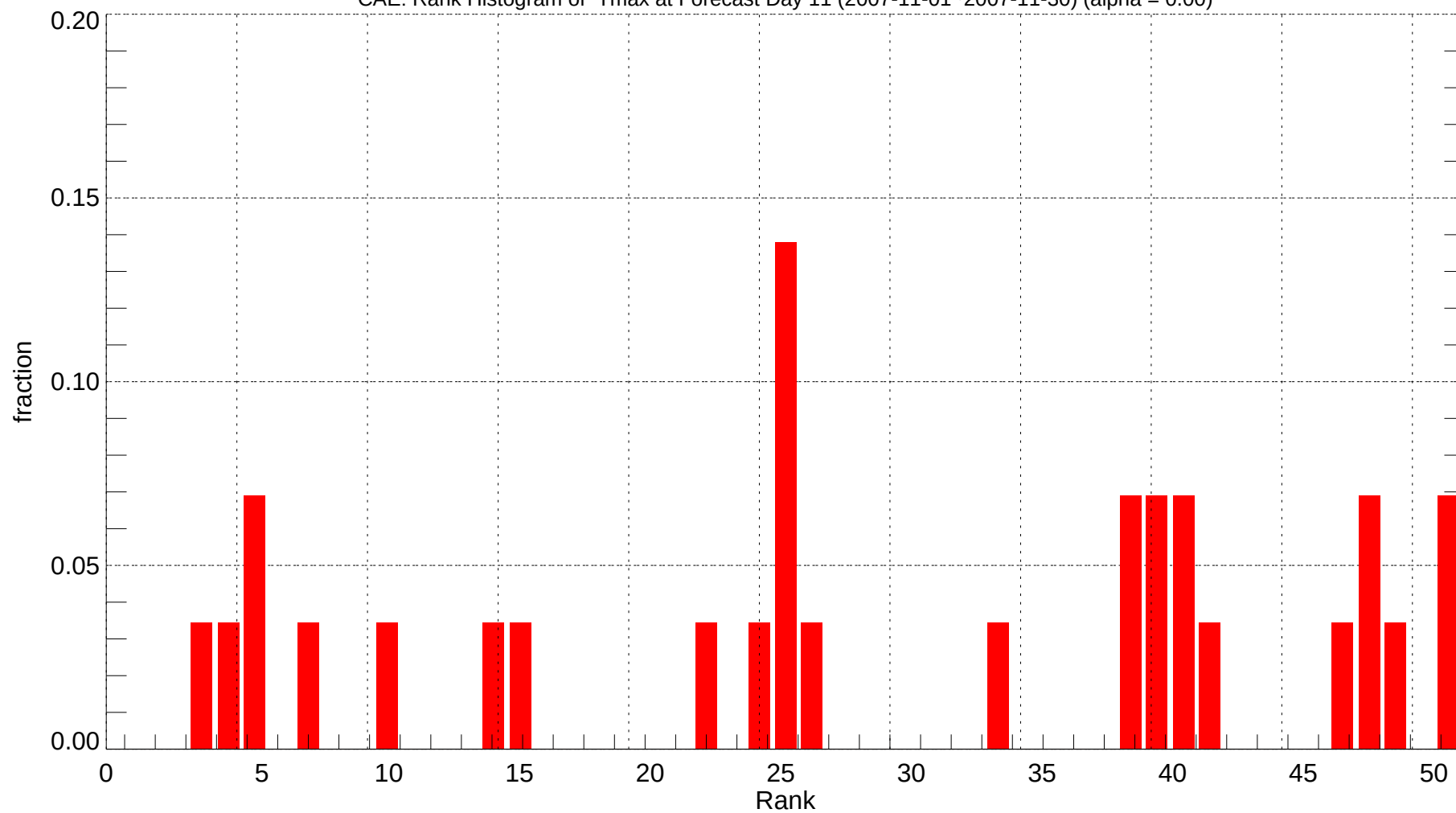
CAE: Rank Histogram of Tmax at Forecast Day 11 (2007-11-01~2007-11-30) (alpha = 0.00)
