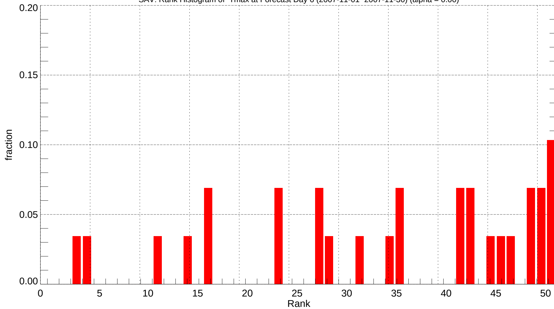
SAV: Rank Histogram of Tmax at Forecast Day 6 (2007-11-01~2007-11-30) (alpha = 0.00)
