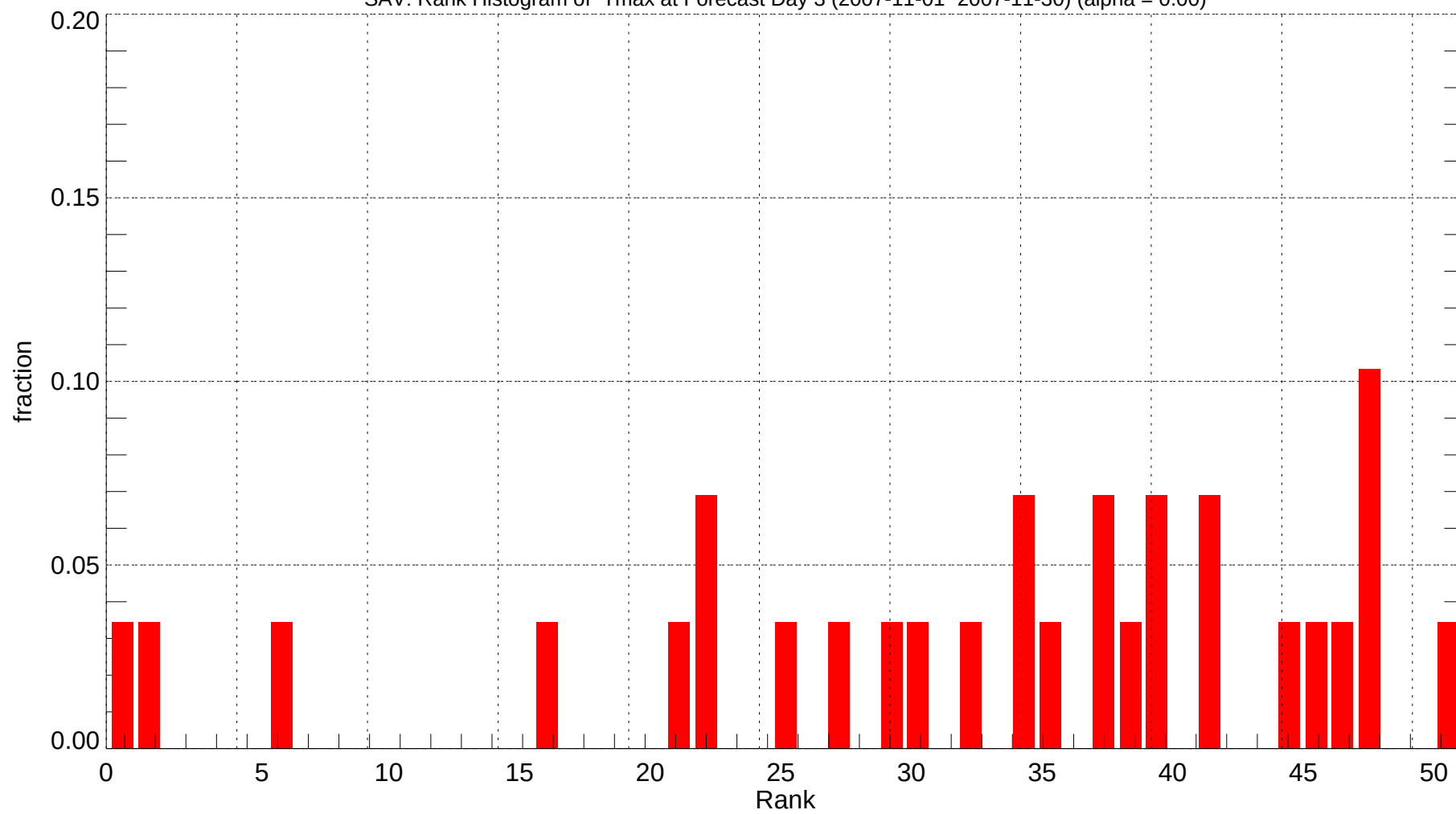
SAV: Rank Histogram of Tmax at Forecast Day 3 (2007-11-01~2007-11-30) (alpha = 0.00)
