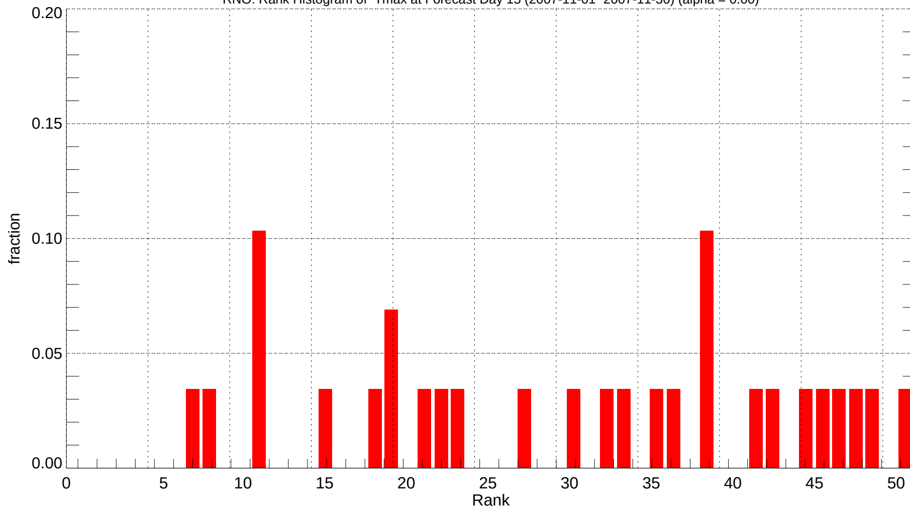
RNO: Rank Histogram of Tmax at Forecast Day 15 (2007-11-01~2007-11-30) (alpha = 0.00)
