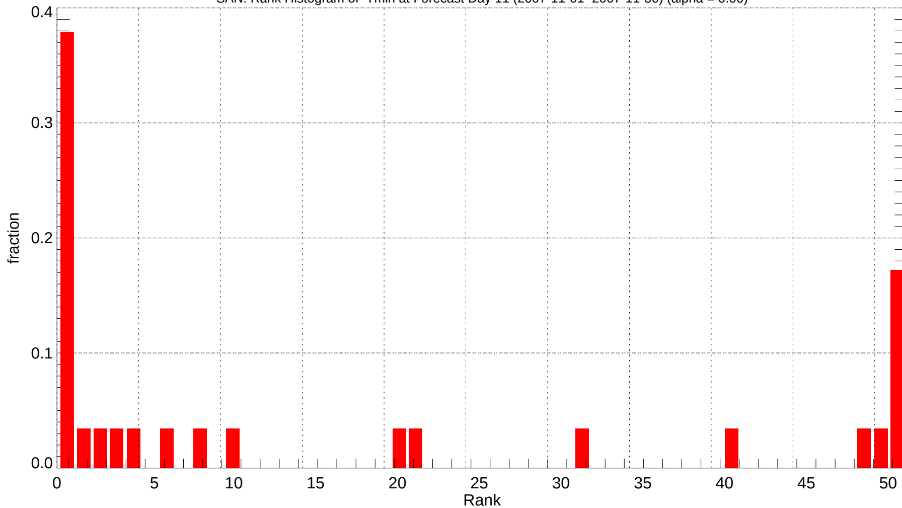
SAN: Rank Histogram of Tmin at Forecast Day 11 (2007-11-01~2007-11-30) (alpha = 0.00)
