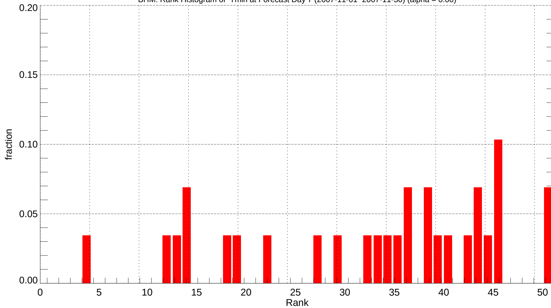
BHM: Rank Histogram of Tmin at Forecast Day 7 (2007-11-01~2007-11-30) (alpha = 0.00)
