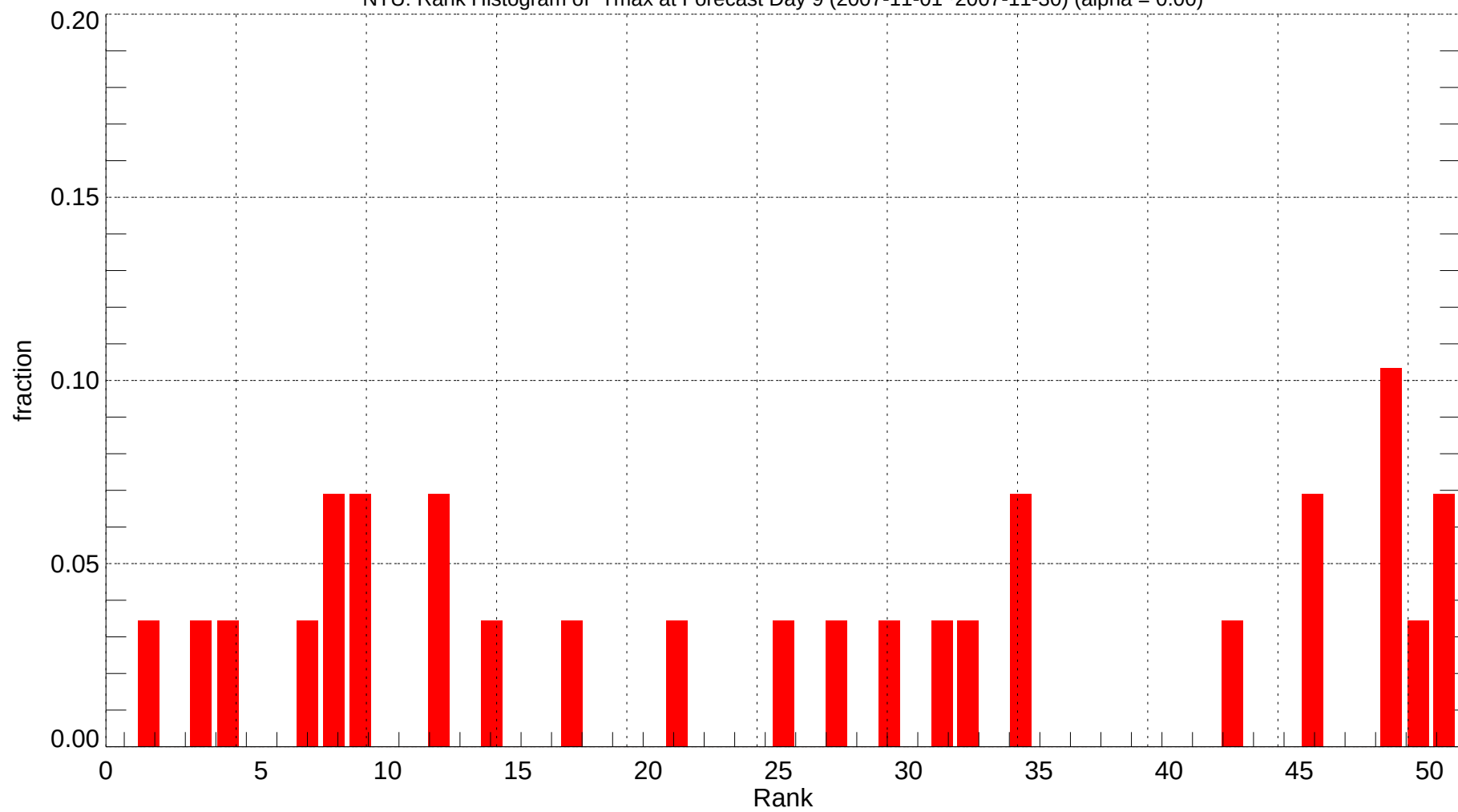
NTU: Rank Histogram of Tmax at Forecast Day 9 (2007-11-01~2007-11-30) (alpha = 0.00)
