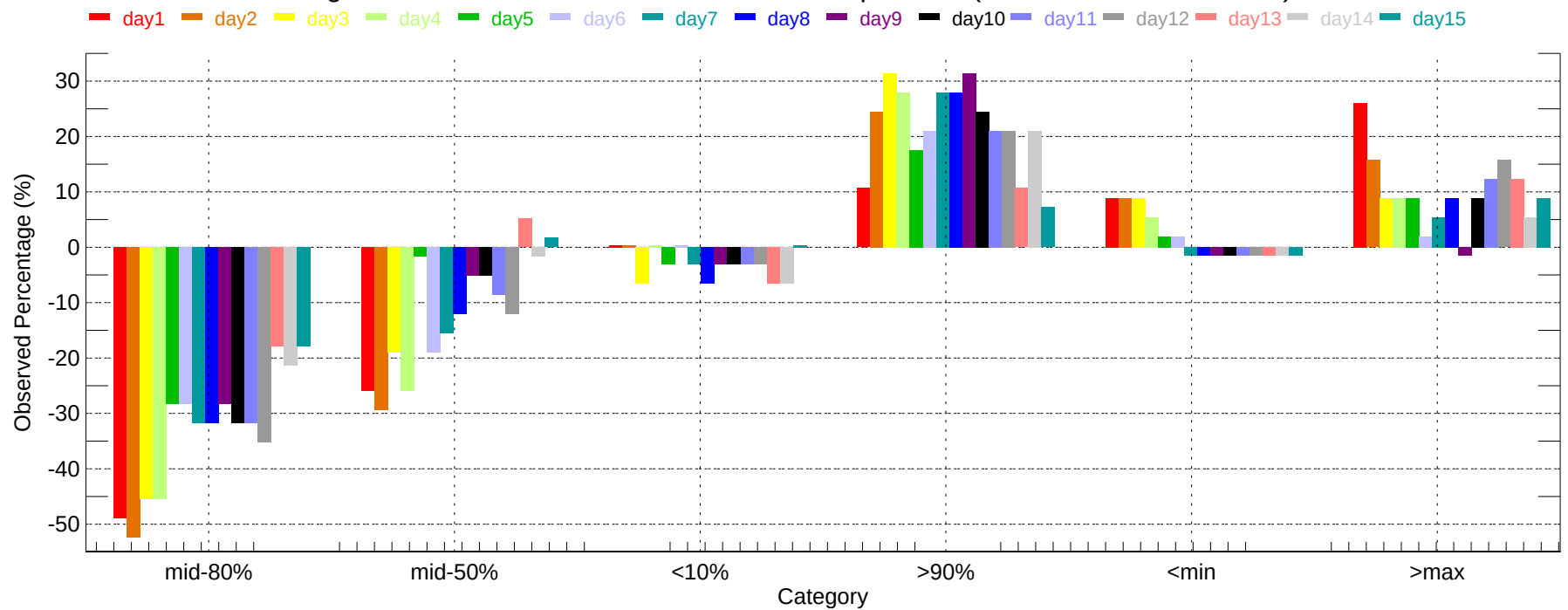
Observed Percentage Deviation of Ensembles - LEX: Min Temperature (2007-11-01~2007-11-30)
