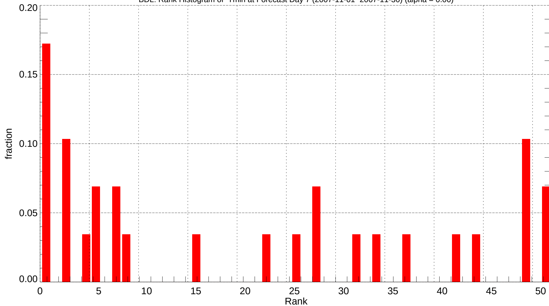
BDL: Rank Histogram of Tmin at Forecast Day 7 (2007-11-01~2007-11-30) (alpha = 0.00)
