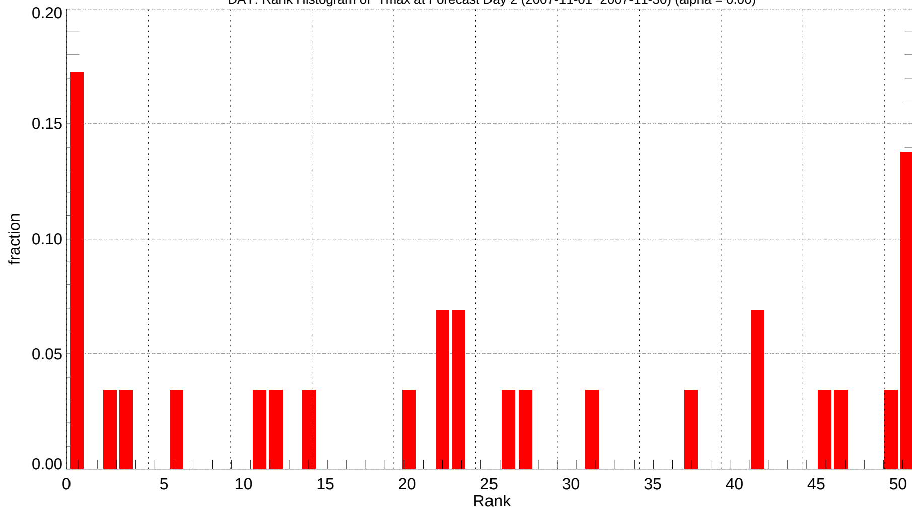
DAY: Rank Histogram of Tmax at Forecast Day 2 (2007-11-01~2007-11-30) (alpha = 0.00)
