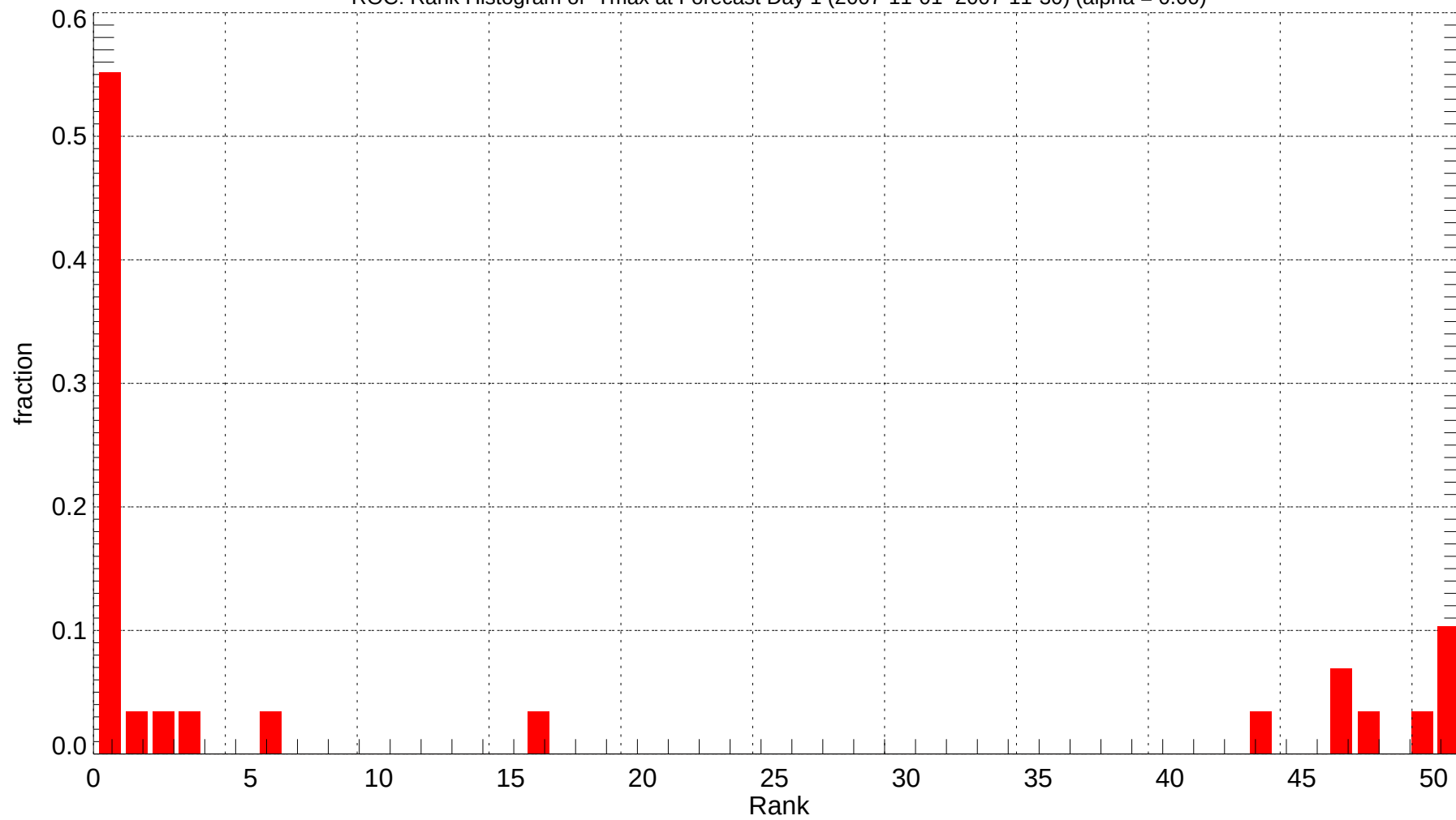
ROC: Rank Histogram of Tmax at Forecast Day 1 (2007-11-01~2007-11-30) (alpha = 0.00)
