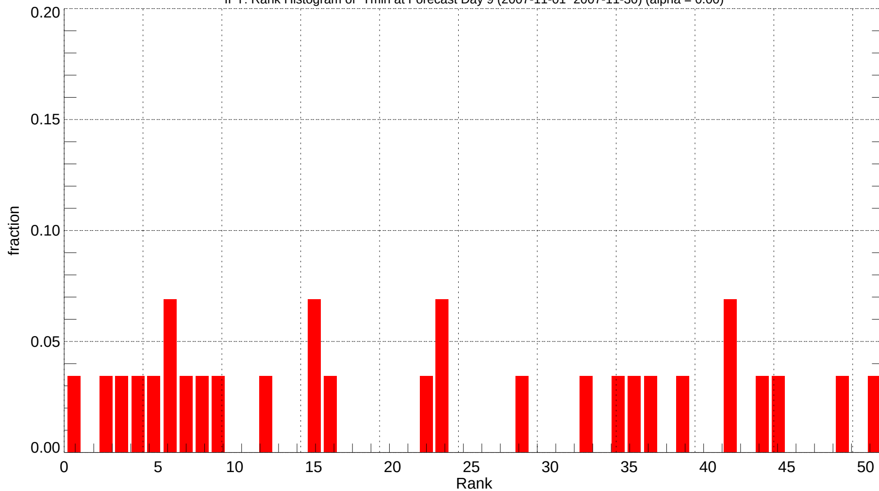
IPT: Rank Histogram of Tmin at Forecast Day 9 (2007-11-01~2007-11-30) (alpha = 0.00)
