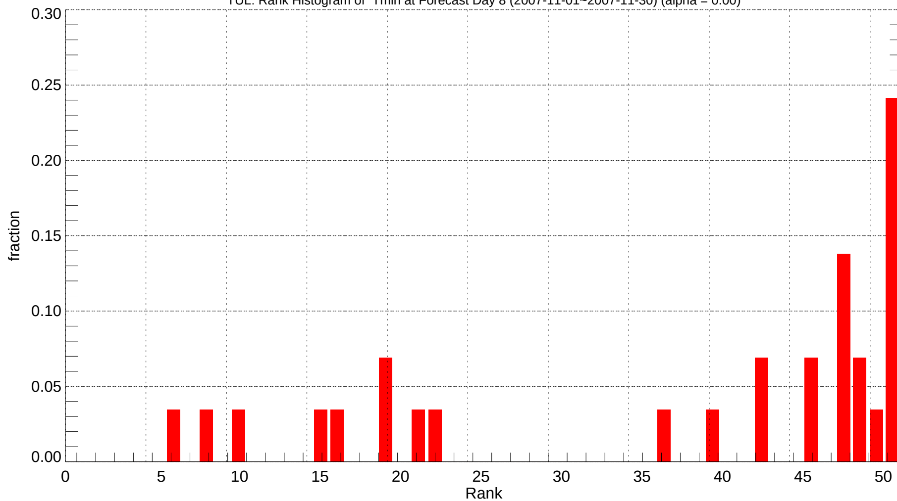
TUL: Rank Histogram of Tmin at Forecast Day 8 (2007-11-01~2007-11-30) (alpha = 0.00)
