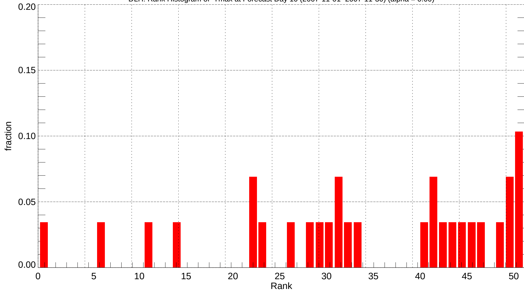
DLH: Rank Histogram of Tmax at Forecast Day 10 (2007-11-01~2007-11-30) (alpha = 0.00)
