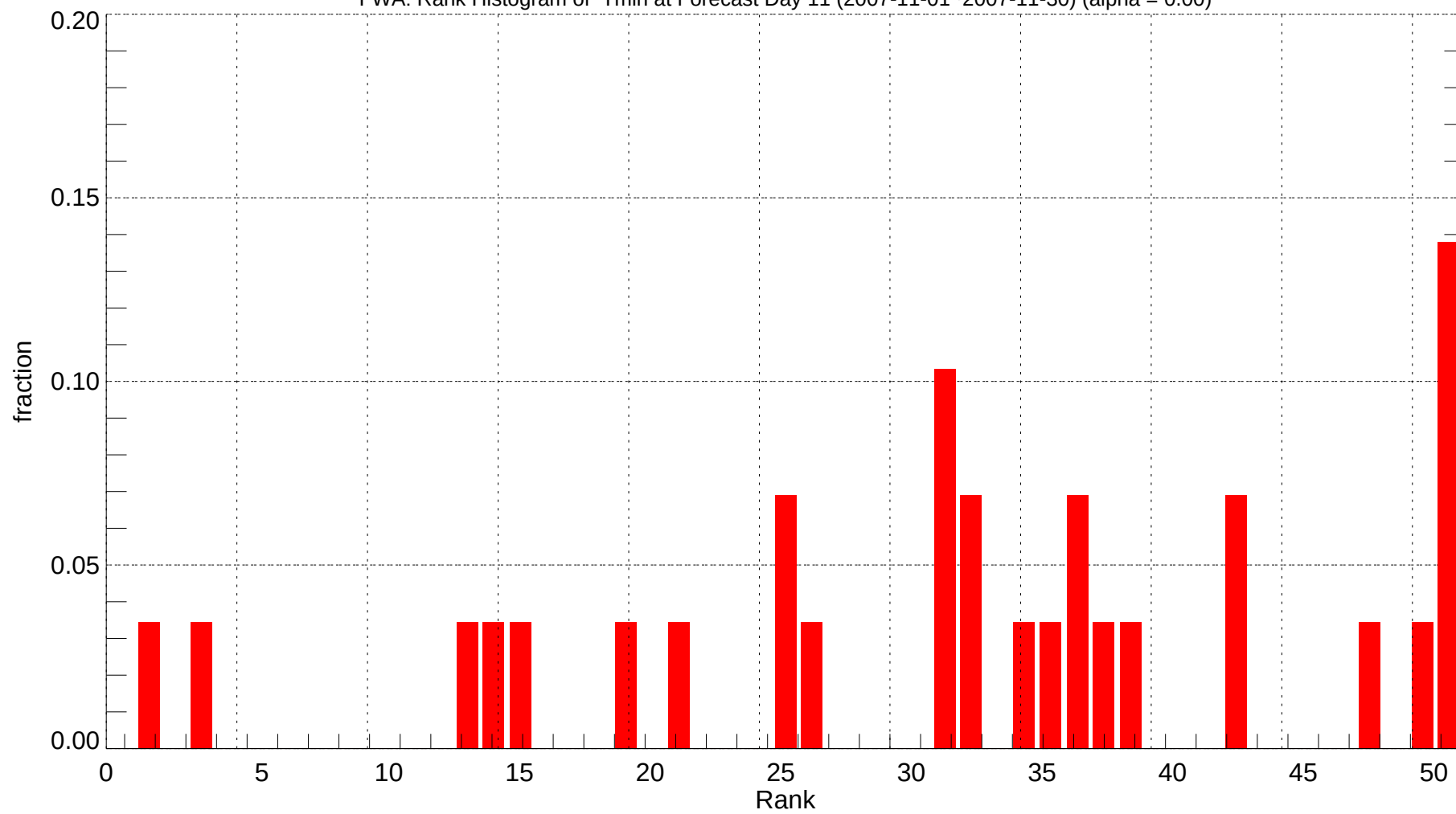
FWA: Rank Histogram of Tmin at Forecast Day 11 (2007-11-01~2007-11-30) (alpha = 0.00)
