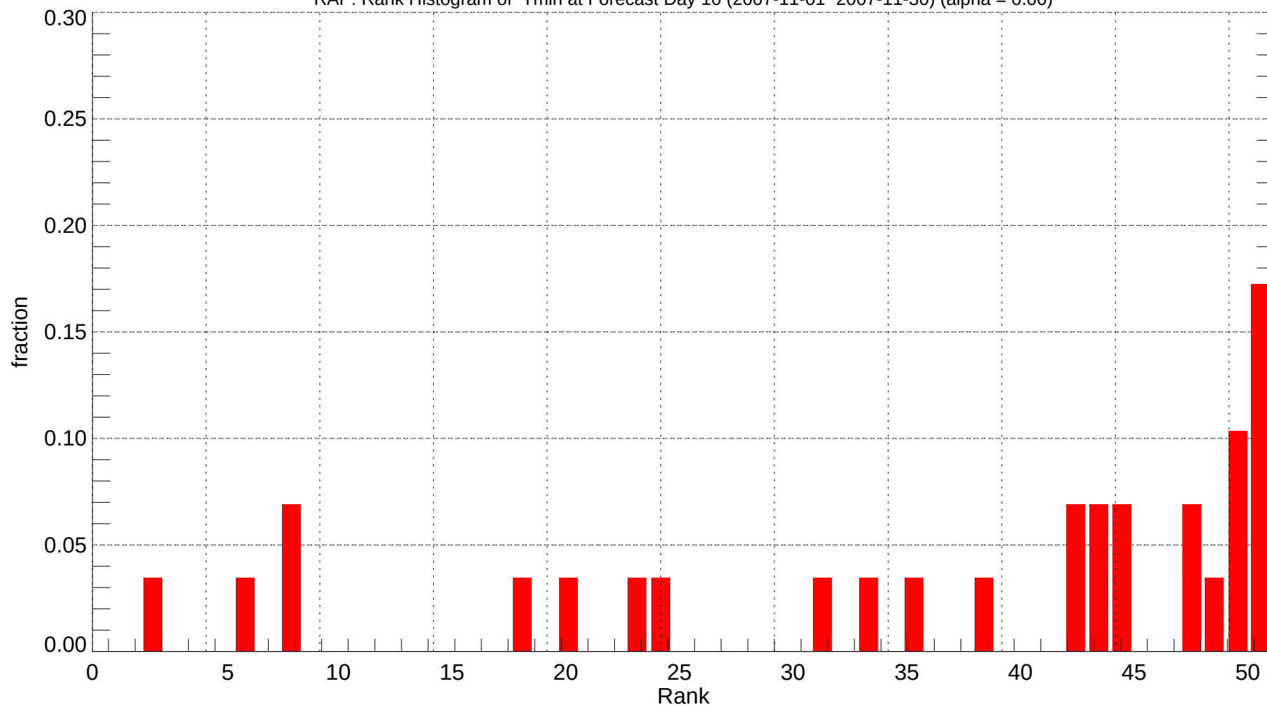
RAP: Rank Histogram of Tmin at Forecast Day 10 (2007-11-01~2007-11-30) (alpha = 0.00)
