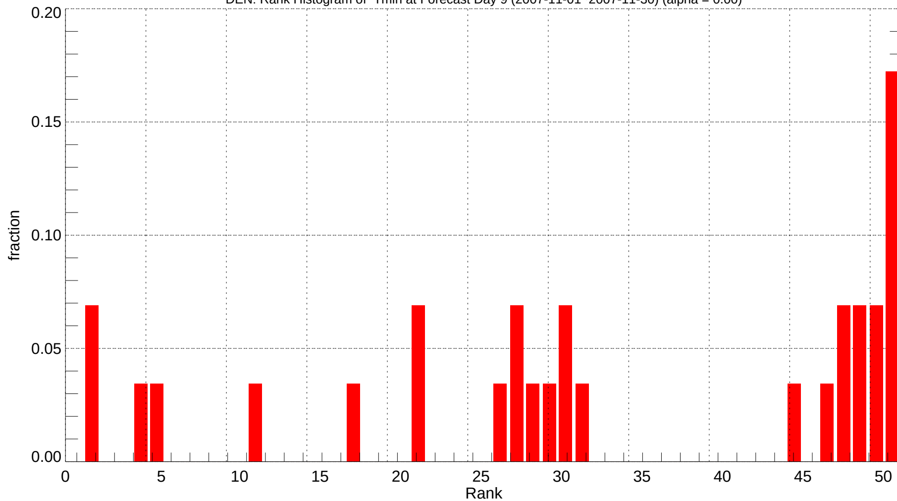
DEN: Rank Histogram of Tmin at Forecast Day 9 (2007-11-01~2007-11-30) (alpha = 0.00)
