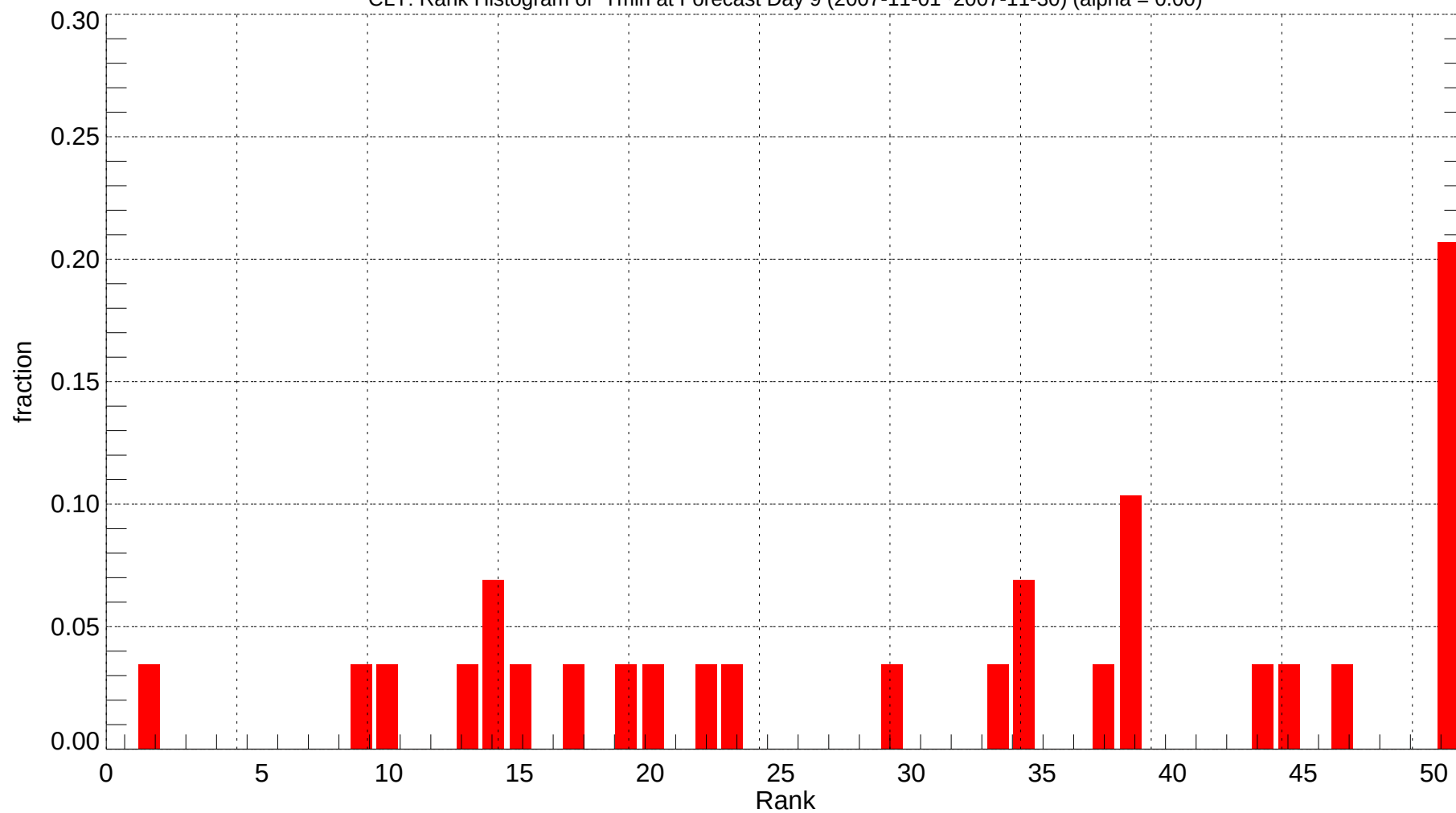
CLT: Rank Histogram of Tmin at Forecast Day 9 (2007-11-01~2007-11-30) (alpha = 0.00)
