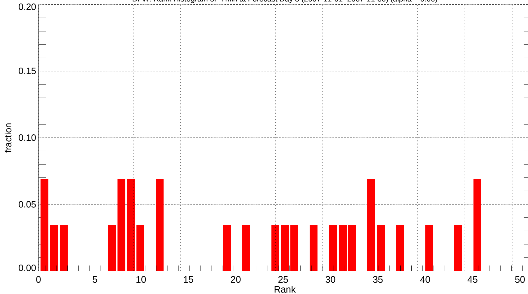
DFW: Rank Histogram of Tmin at Forecast Day 5 (2007-11-01~2007-11-30) (alpha = 0.00)
