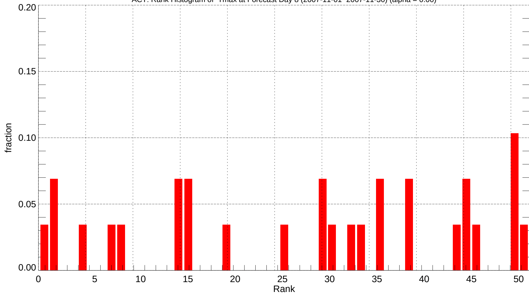
ACT: Rank Histogram of Tmax at Forecast Day 8 (2007-11-01~2007-11-30) (alpha = 0.00)
