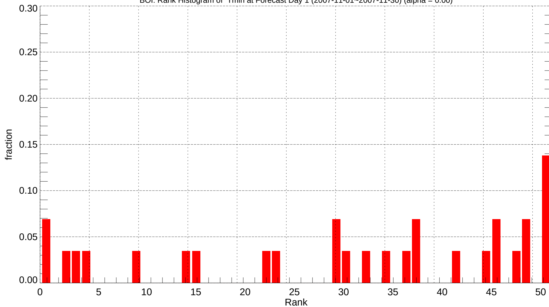
BOI: Rank Histogram of Tmin at Forecast Day 1 (2007-11-01~2007-11-30) (alpha = 0.00)
