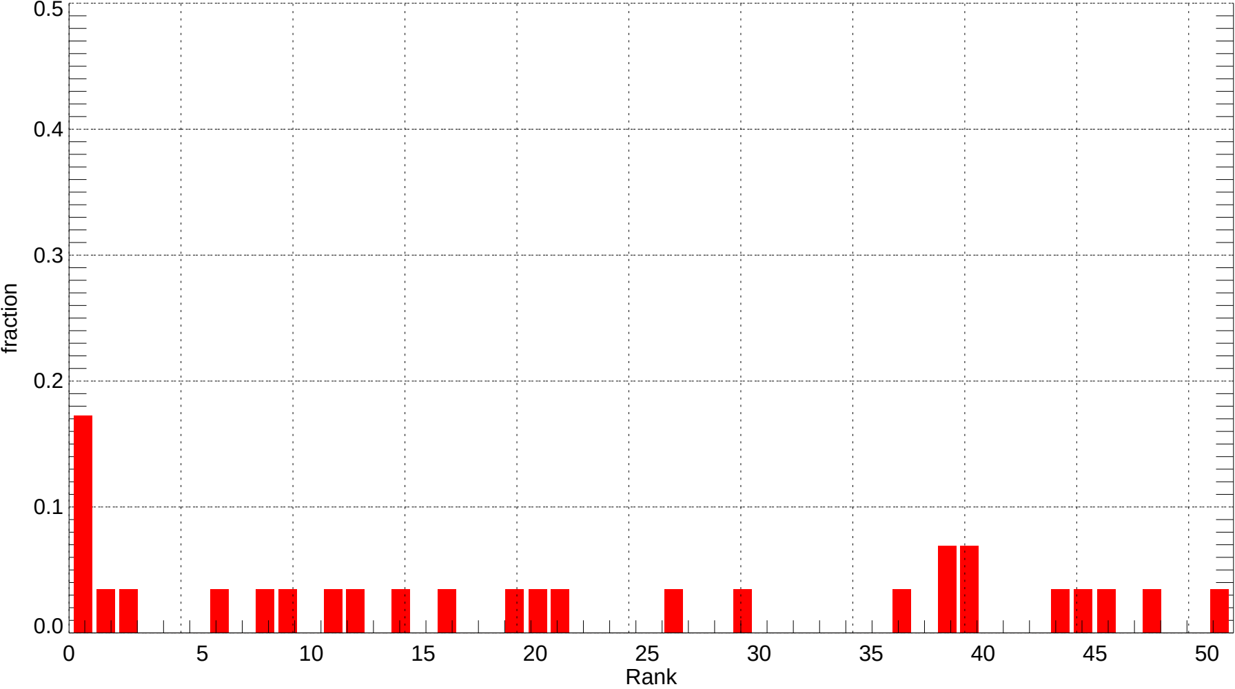
ELP: Rank Histogram of Tmin at Forecast Day 1 (2007-11-01~2007-11-30) (alpha = 0.00)
