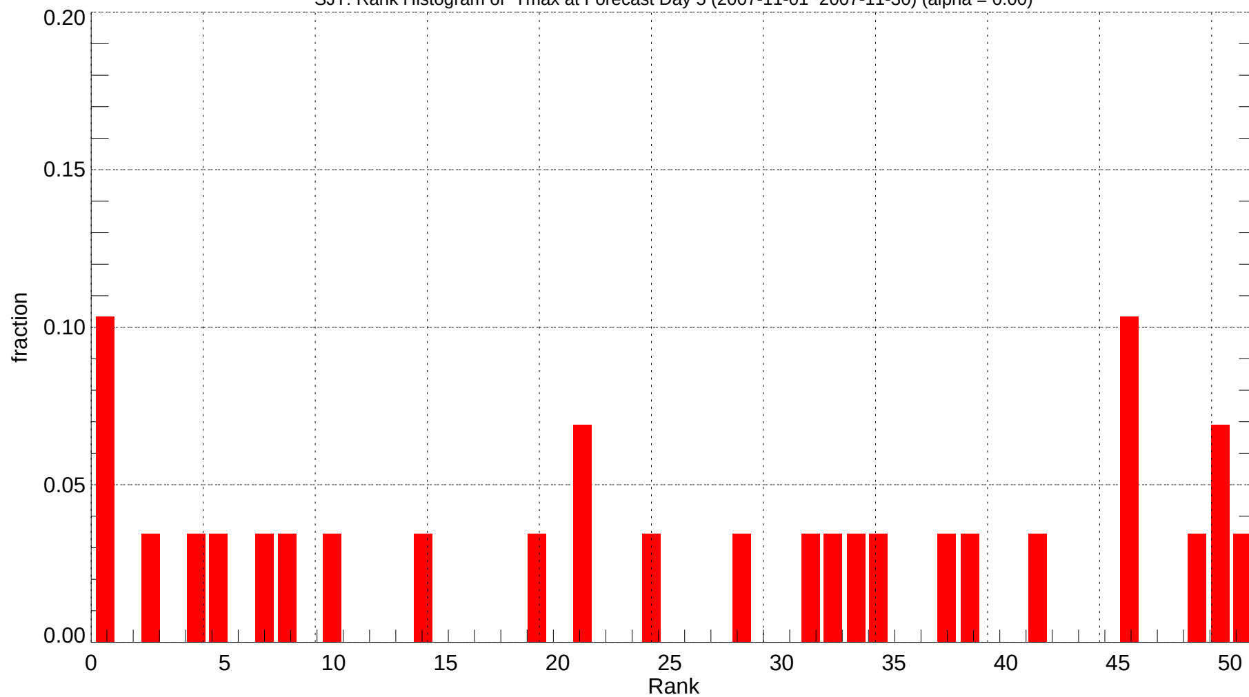
SJT: Rank Histogram of Tmax at Forecast Day 5 (2007-11-01~2007-11-30) (alpha = 0.00)
