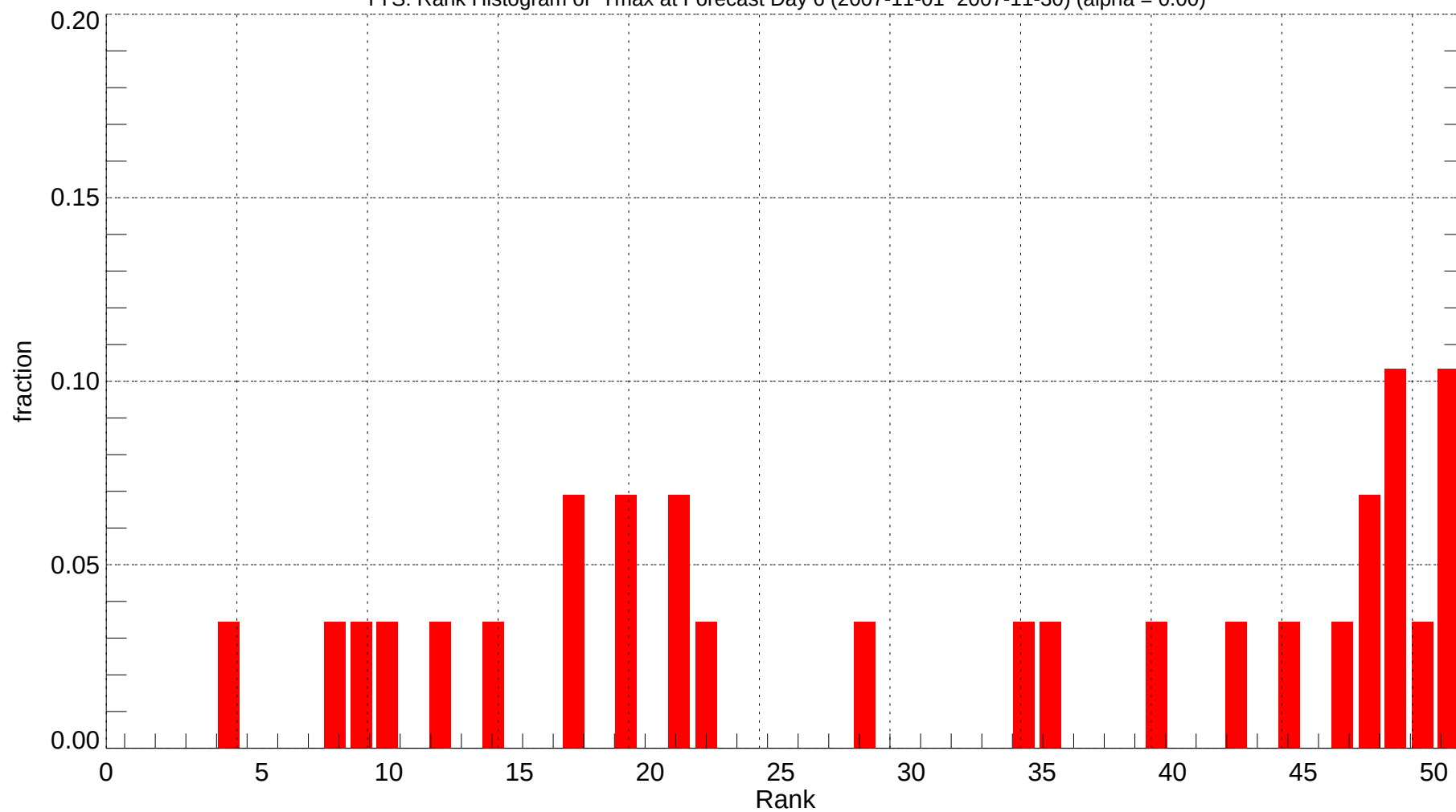
TYS: Rank Histogram of Tmax at Forecast Day 6 (2007-11-01~2007-11-30) (alpha = 0.00)
