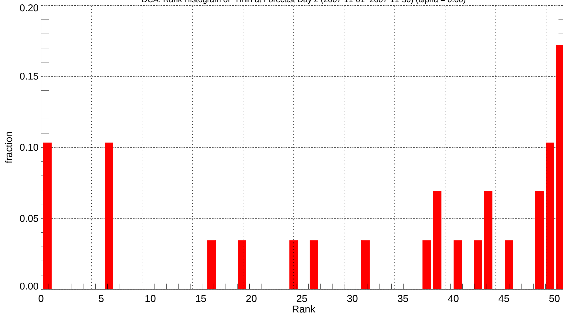
DCA: Rank Histogram of Tmin at Forecast Day 2 (2007-11-01~2007-11-30) (alpha = 0.00)
