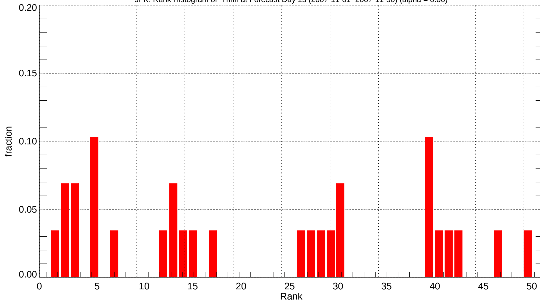
JFK: Rank Histogram of Tmin at Forecast Day 13 (2007-11-01~2007-11-30) (alpha = 0.00)
