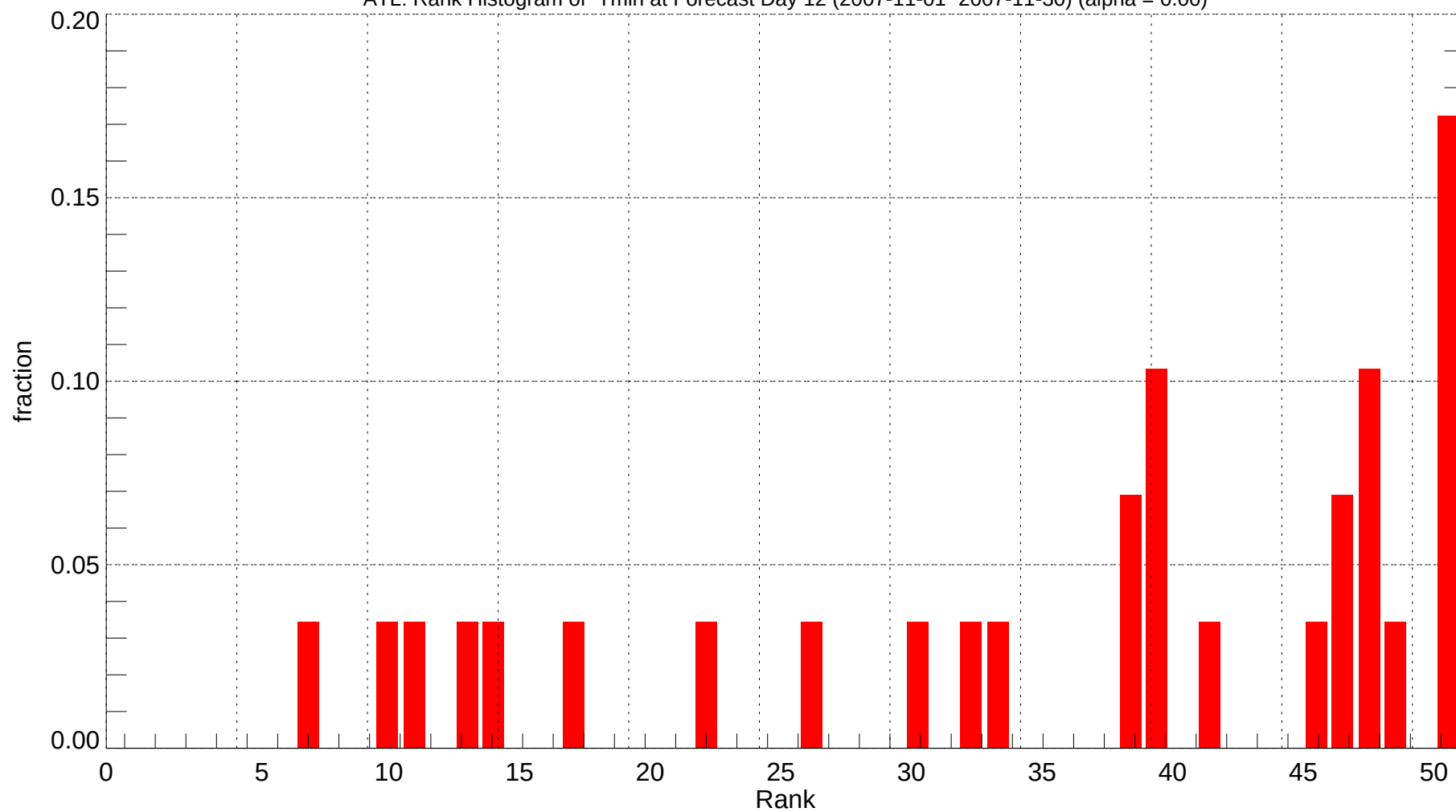
ATL: Rank Histogram of Tmin at Forecast Day 12 (2007-11-01~2007-11-30) (alpha = 0.00)
