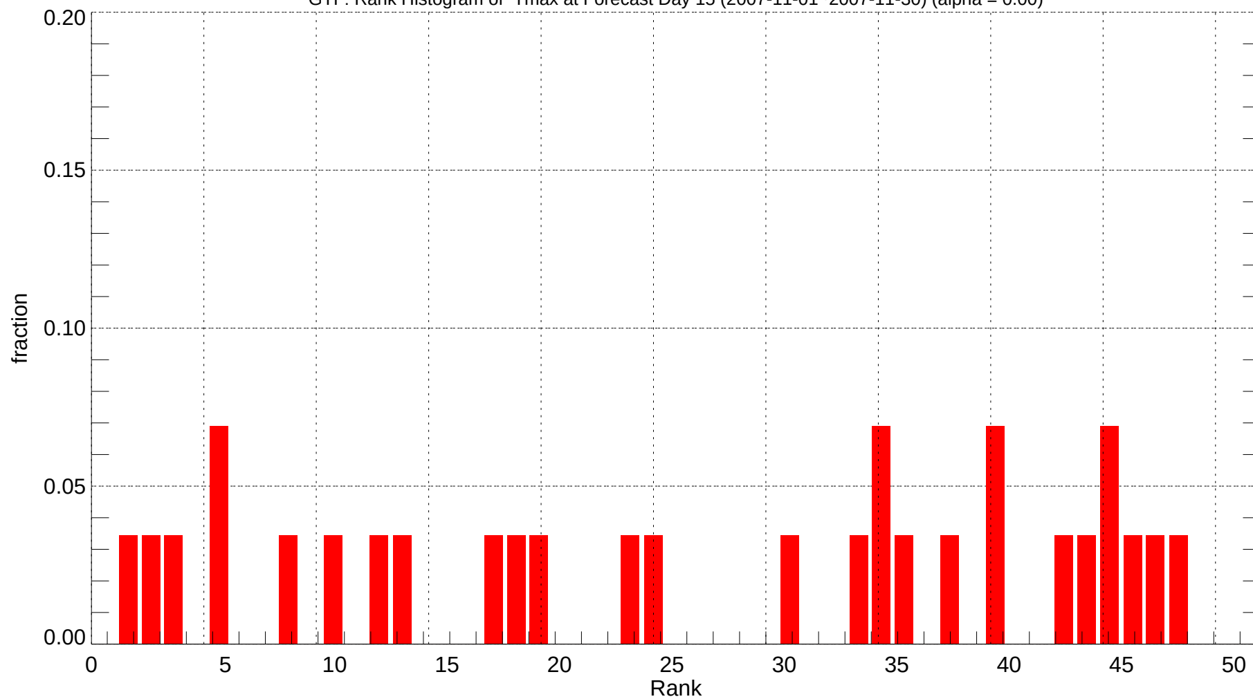
GTF: Rank Histogram of Tmax at Forecast Day 15 (2007-11-01~2007-11-30) (alpha = 0.00)
