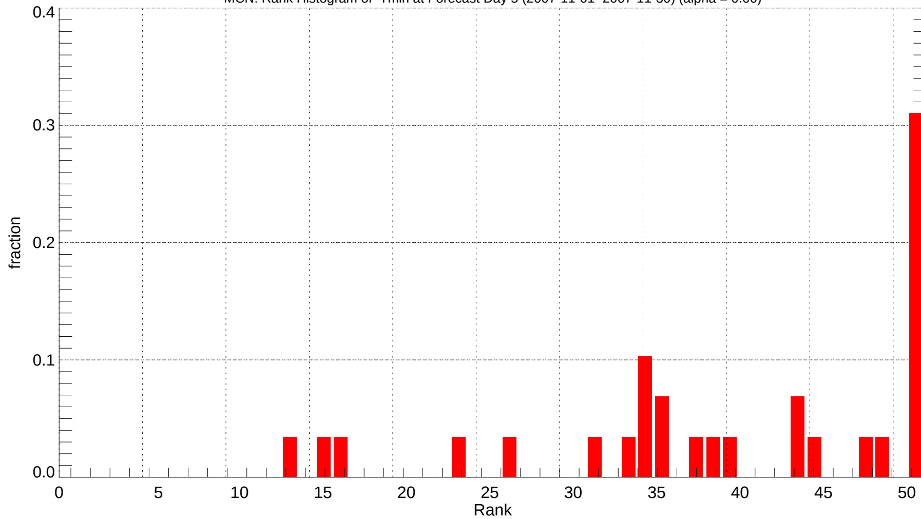
MCN: Rank Histogram of Tmin at Forecast Day 5 (2007-11-01~2007-11-30) (alpha = 0.00)
