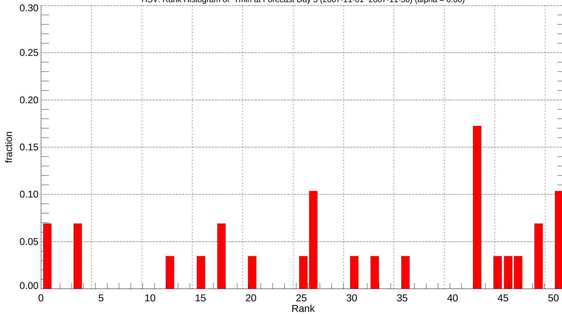
HSV: Rank Histogram of Tmin at Forecast Day 3 (2007-11-01~2007-11-30) (alpha = 0.00)
