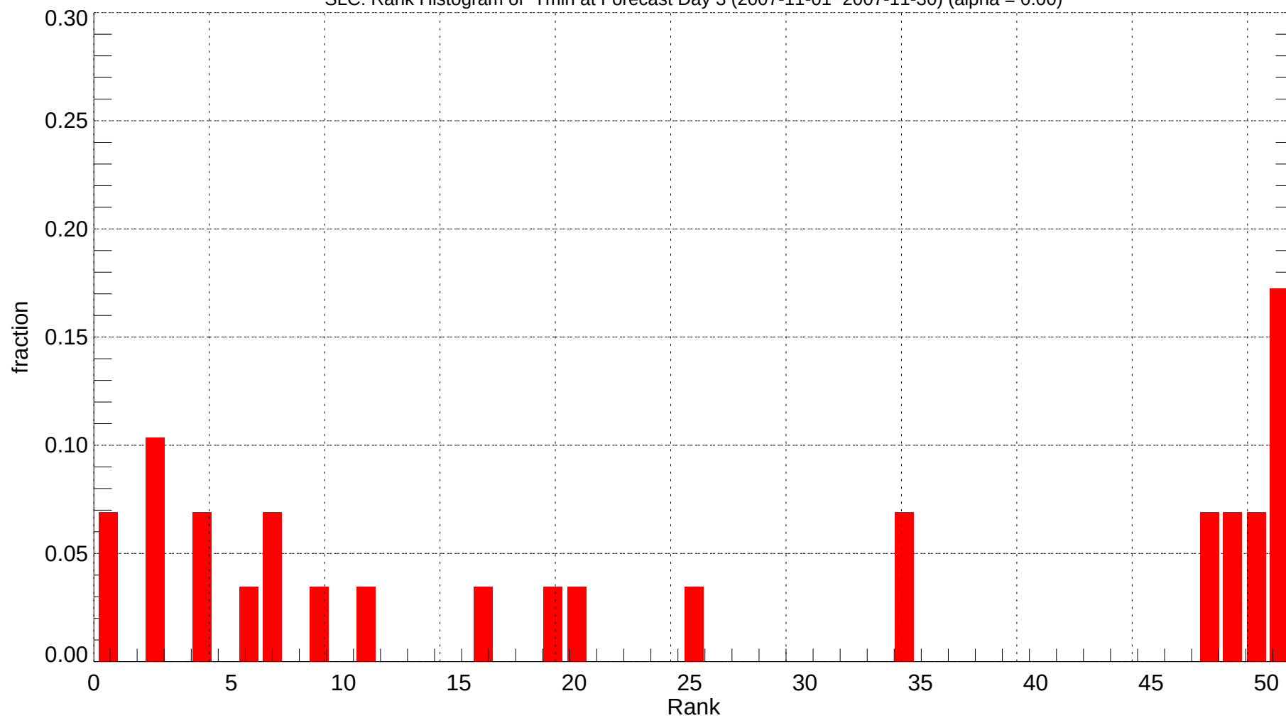
SLC: Rank Histogram of Tmin at Forecast Day 3 (2007-11-01~2007-11-30) (alpha = 0.00)
