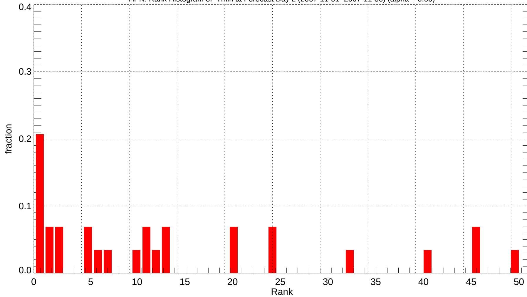
APN: Rank Histogram of Tmin at Forecast Day 2 (2007-11-01~2007-11-30) (alpha = 0.00)
