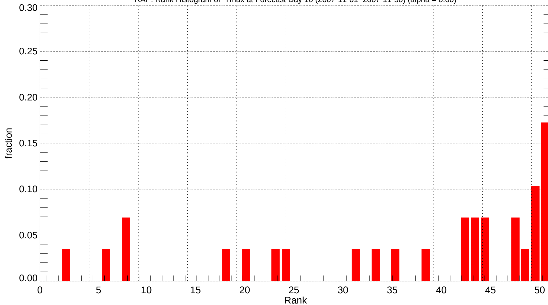
RAP: Rank Histogram of Tmax at Forecast Day 10 (2007-11-01~2007-11-30) (alpha = 0.00)
