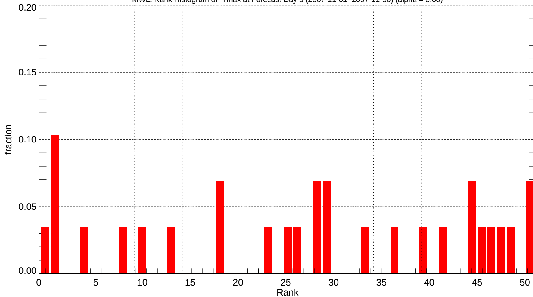
MWL: Rank Histogram of Tmax at Forecast Day 5 (2007-11-01~2007-11-30) (alpha = 0.00)
