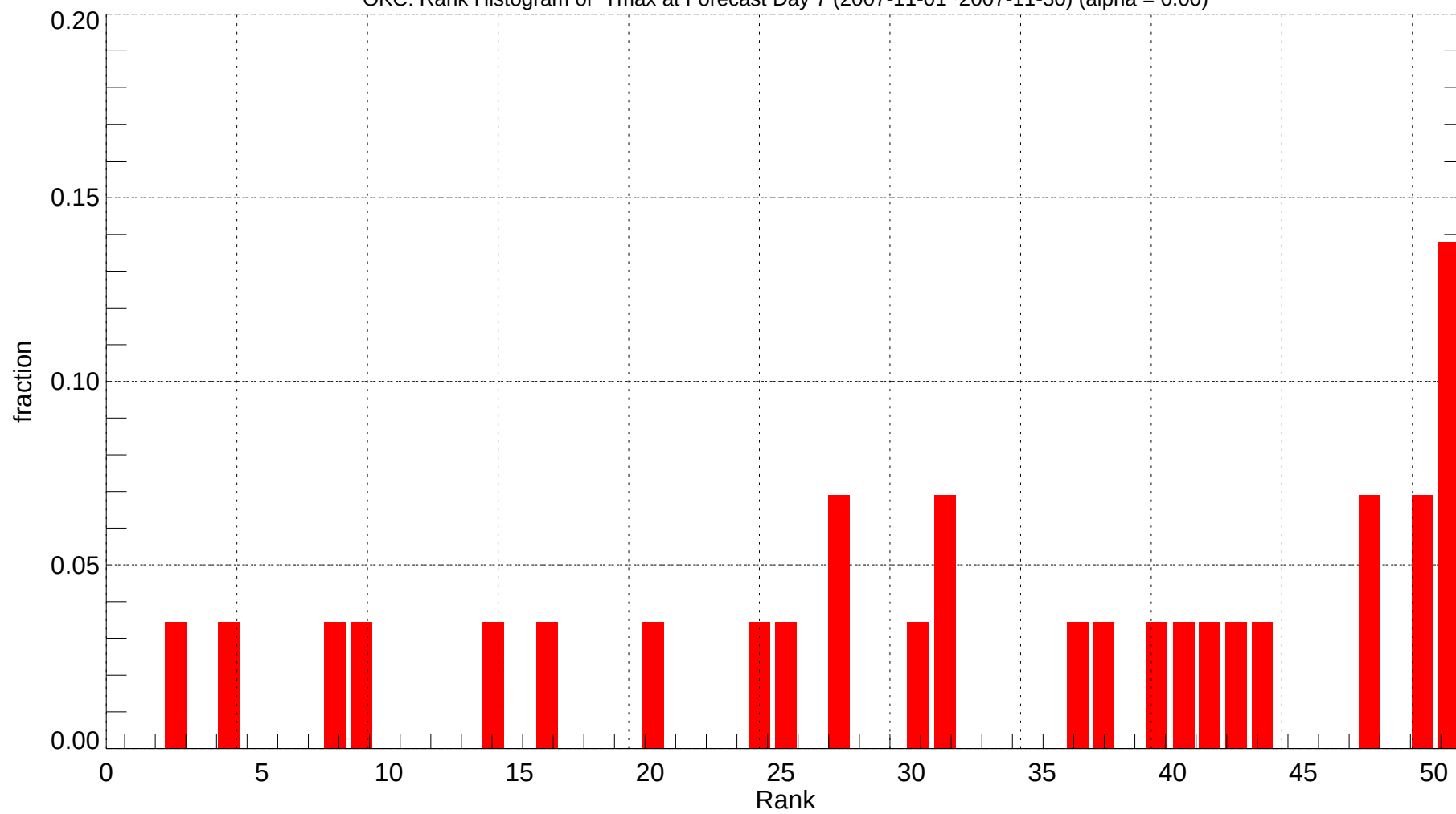
OKC: Rank Histogram of Tmax at Forecast Day 7 (2007-11-01~2007-11-30) (alpha = 0.00)
