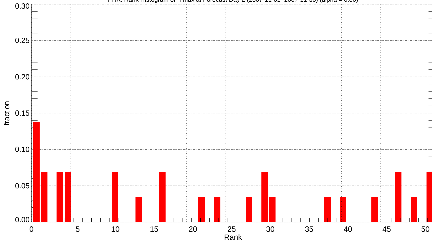
PHX: Rank Histogram of Tmax at Forecast Day 2 (2007-11-01~2007-11-30) (alpha = 0.00)
