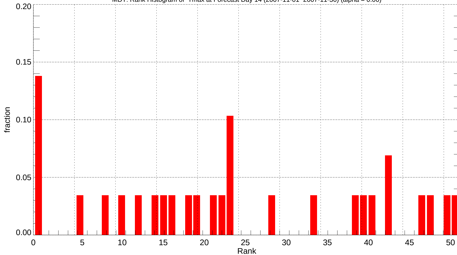
MDT: Rank Histogram of Tmax at Forecast Day 14 (2007-11-01~2007-11-30) (alpha = 0.00)
