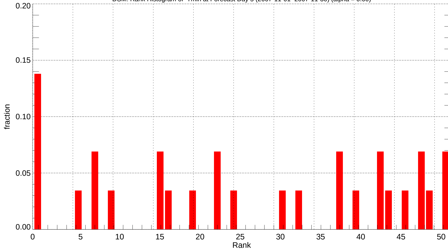
DSM: Rank Histogram of Tmin at Forecast Day 5 (2007-11-01~2007-11-30) (alpha = 0.00)
