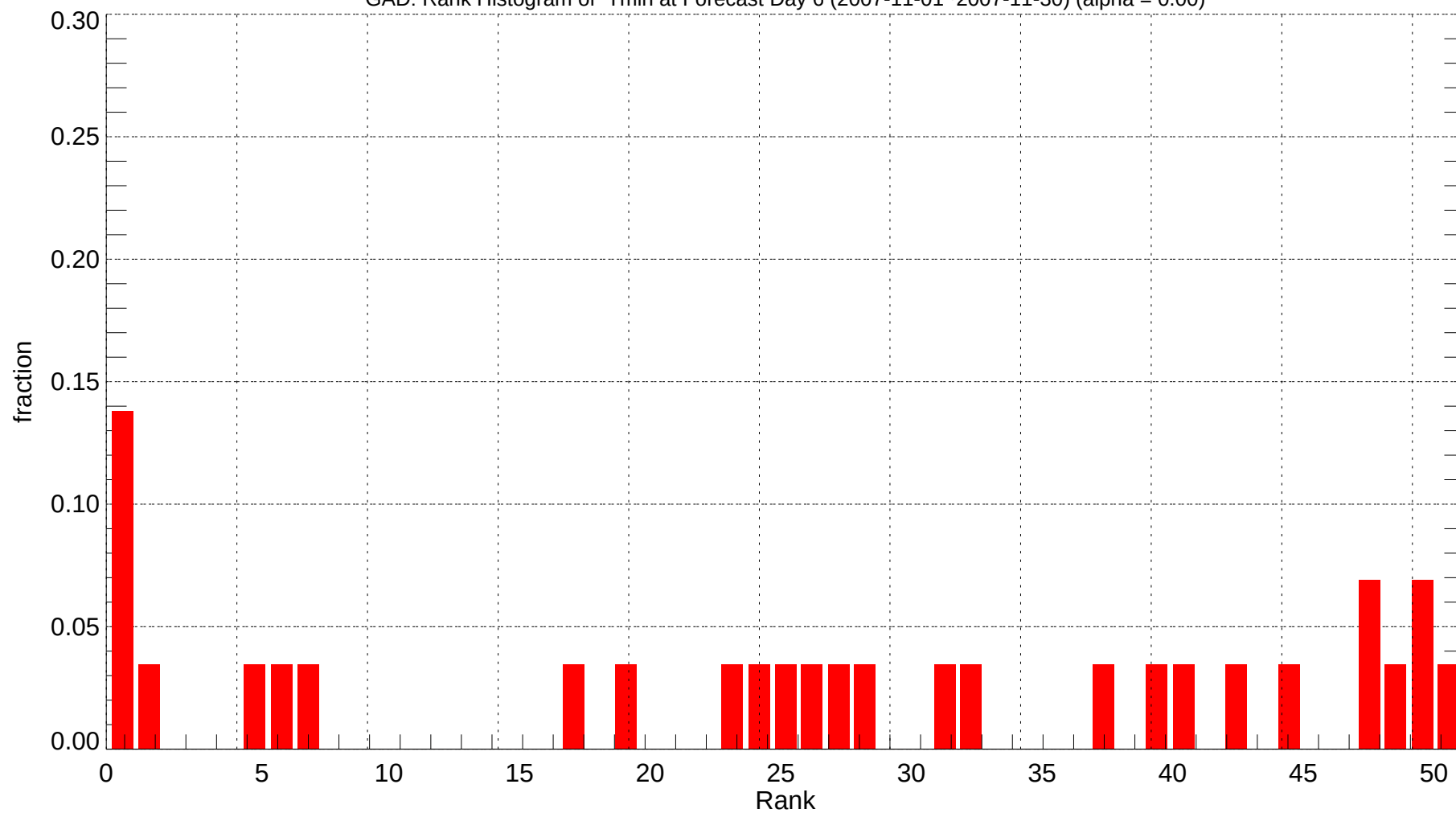
GAD: Rank Histogram of Tmin at Forecast Day 6 (2007-11-01~2007-11-30) (alpha = 0.00)
