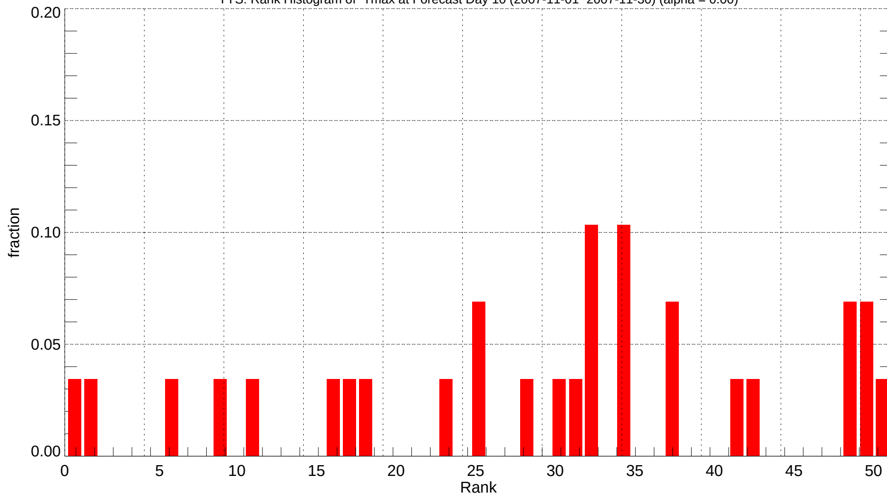
TYS: Rank Histogram of Tmax at Forecast Day 10 (2007-11-01~2007-11-30) (alpha = 0.00)
