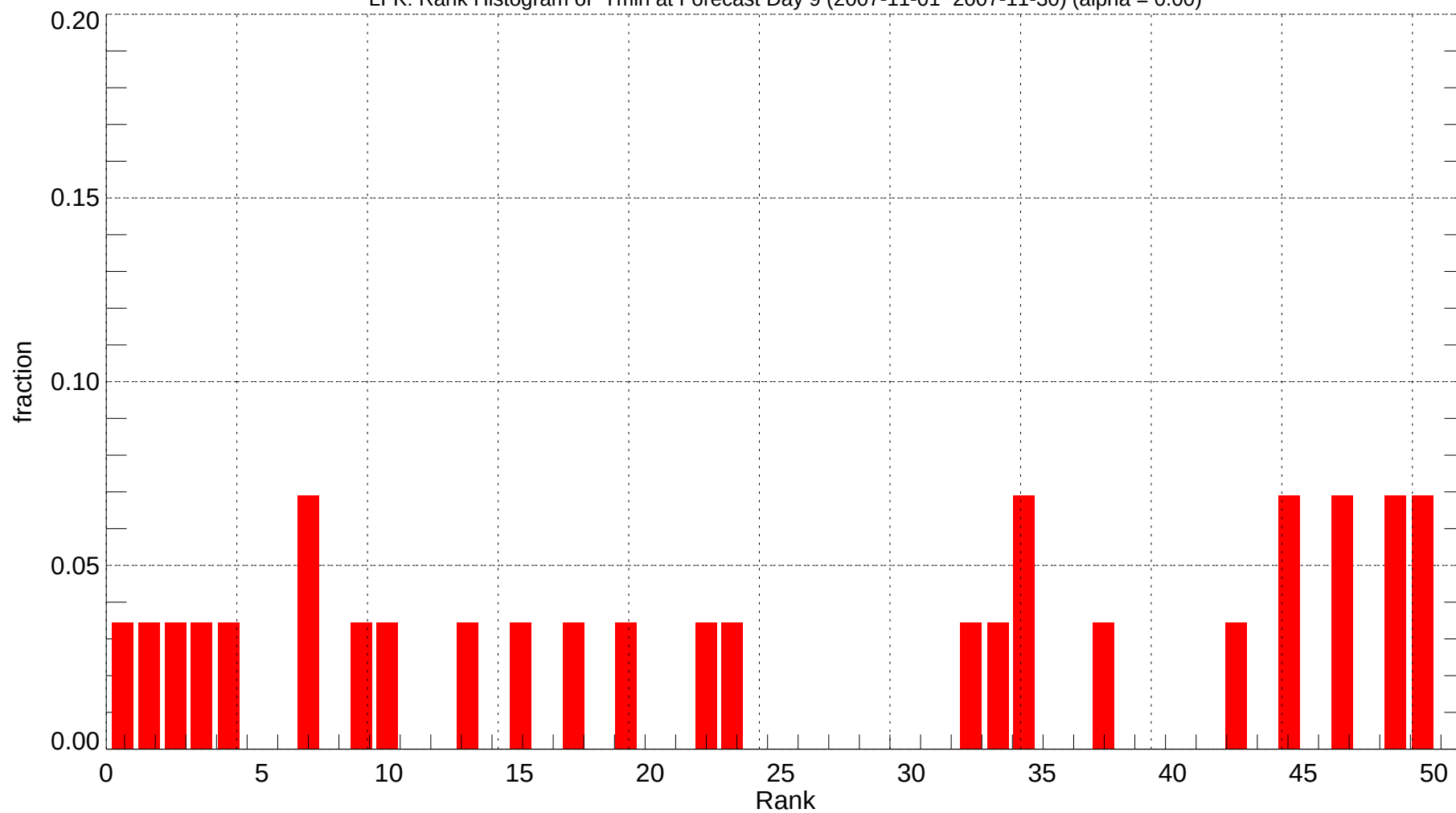
LFK: Rank Histogram of Tmin at Forecast Day 9 (2007-11-01~2007-11-30) (alpha = 0.00)
