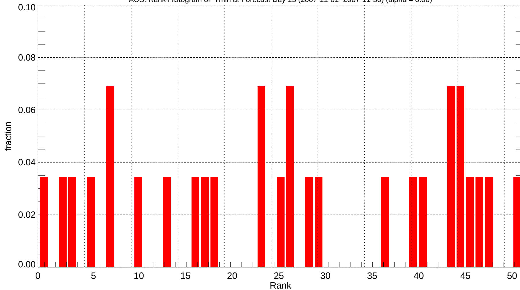
AUS: Rank Histogram of Tmin at Forecast Day 13 (2007-11-01~2007-11-30) (alpha = 0.00)
