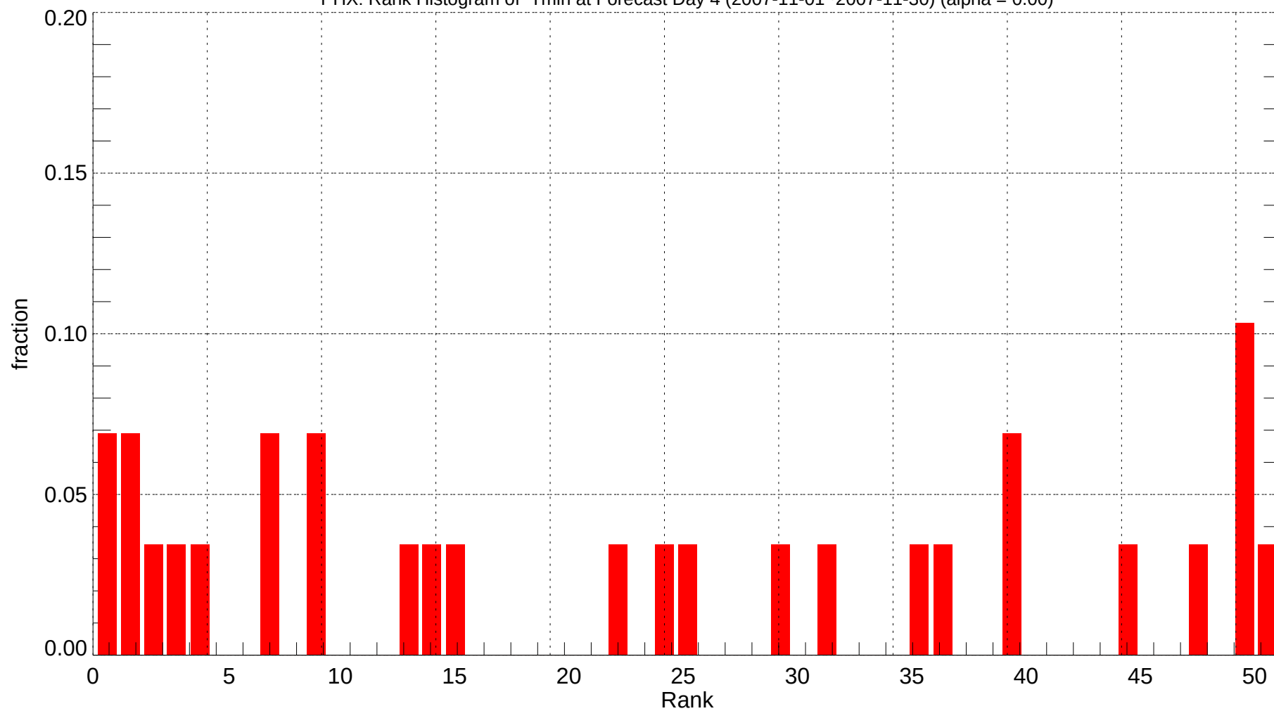
PHX: Rank Histogram of Tmin at Forecast Day 4 (2007-11-01~2007-11-30) (alpha = 0.00)
