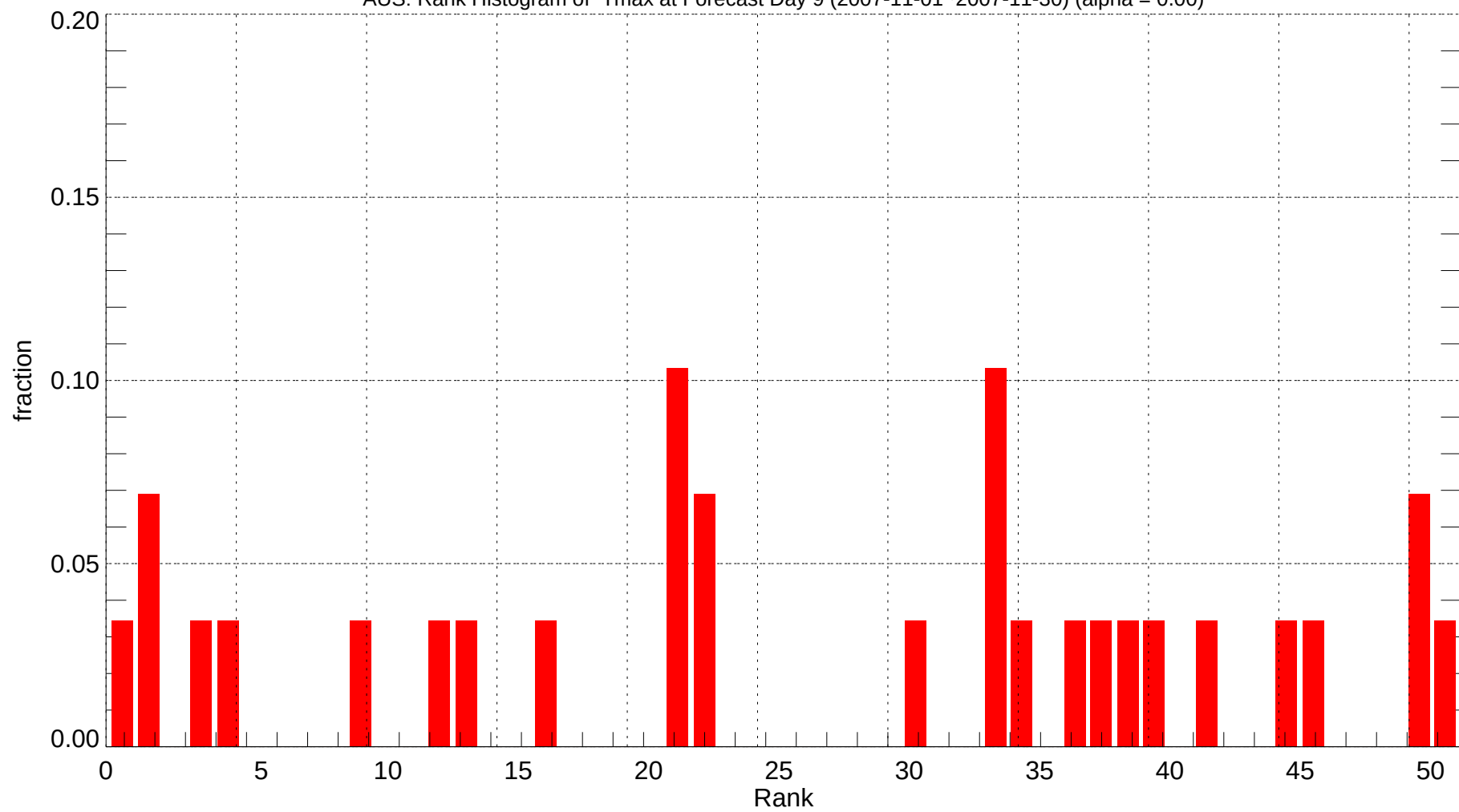
AUS: Rank Histogram of Tmax at Forecast Day 9 (2007-11-01~2007-11-30) (alpha = 0.00)
