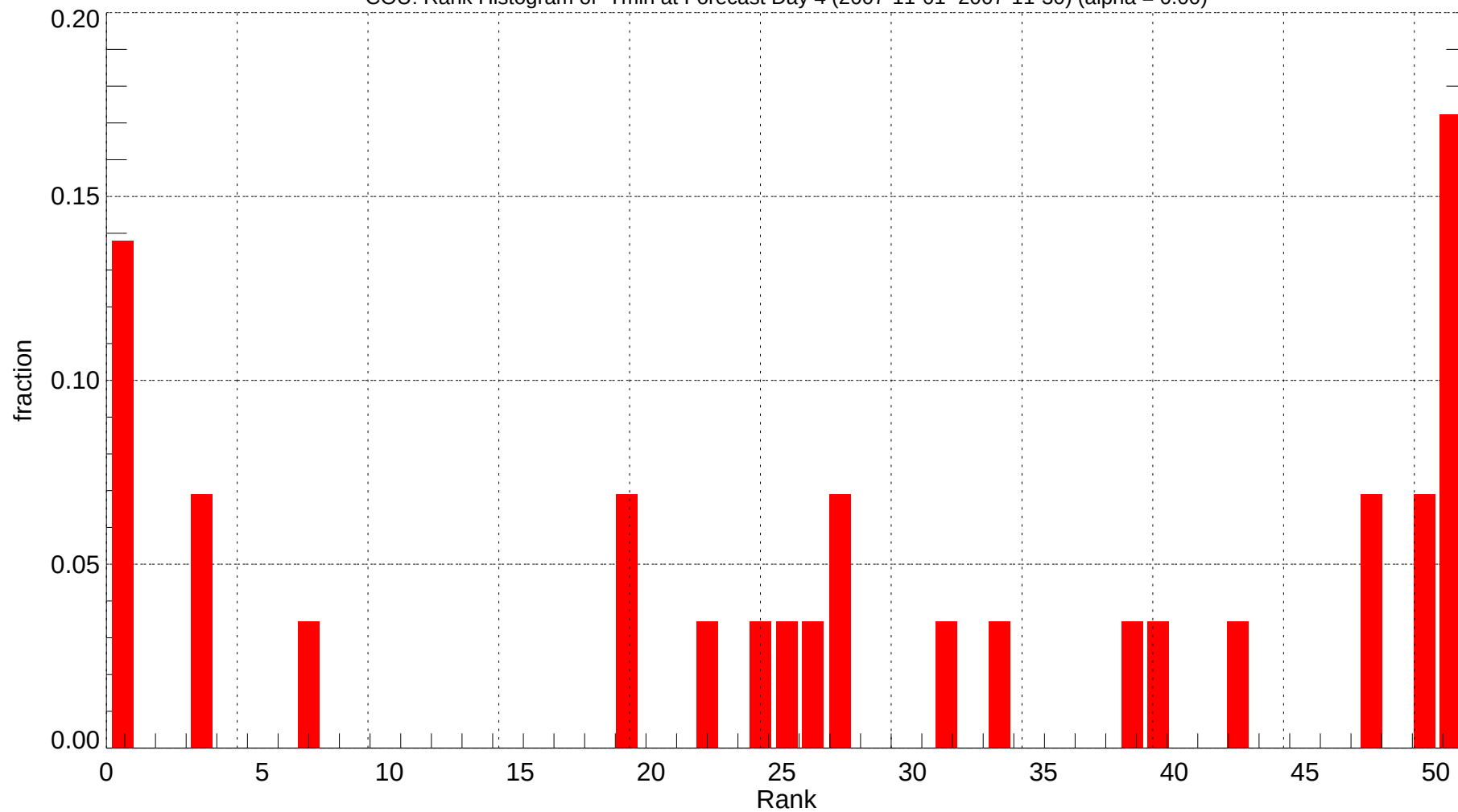
COU: Rank Histogram of Tmin at Forecast Day 4 (2007-11-01~2007-11-30) (alpha = 0.00)
