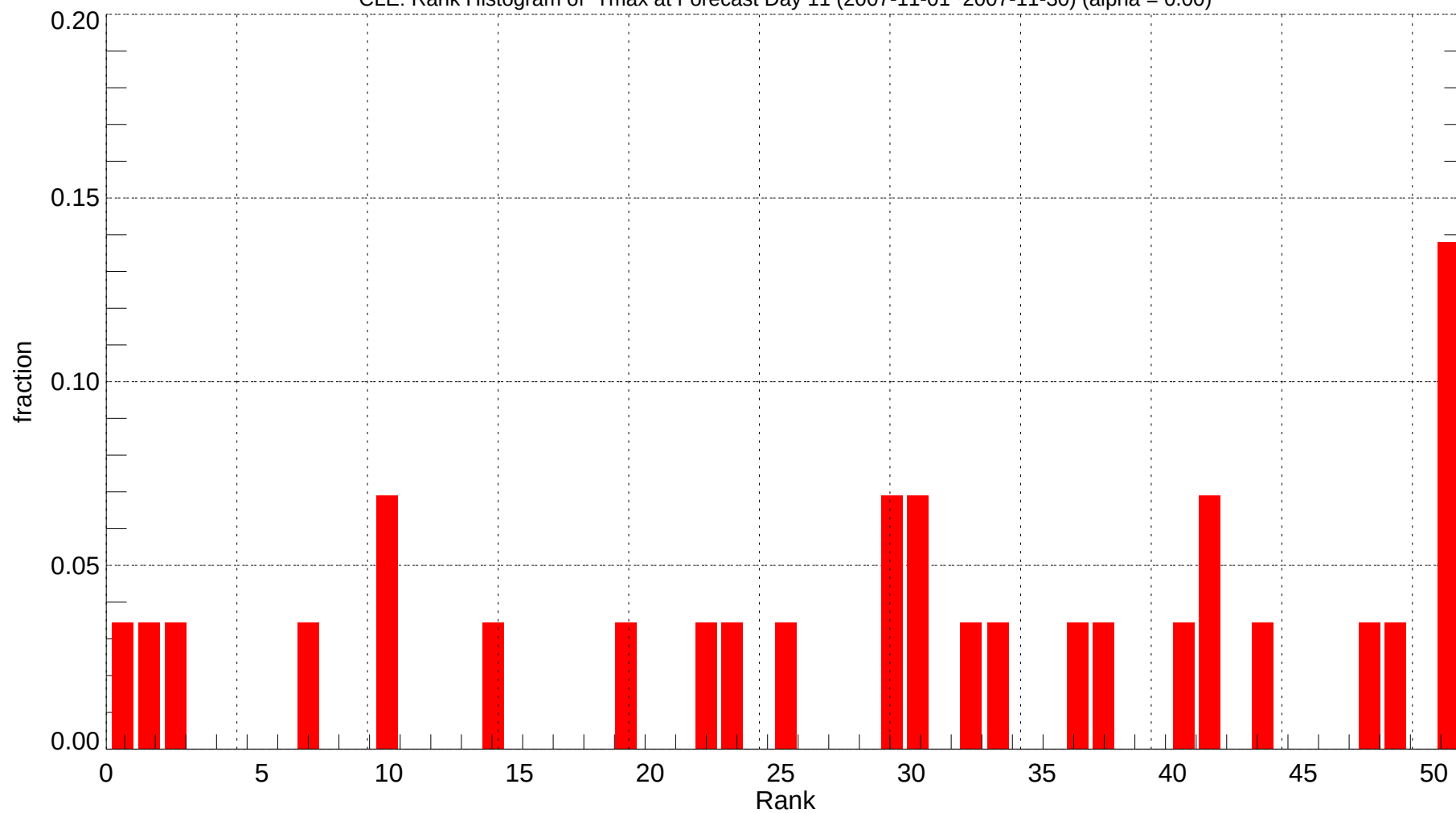
CLE: Rank Histogram of Tmax at Forecast Day 11 (2007-11-01~2007-11-30) (alpha = 0.00)
