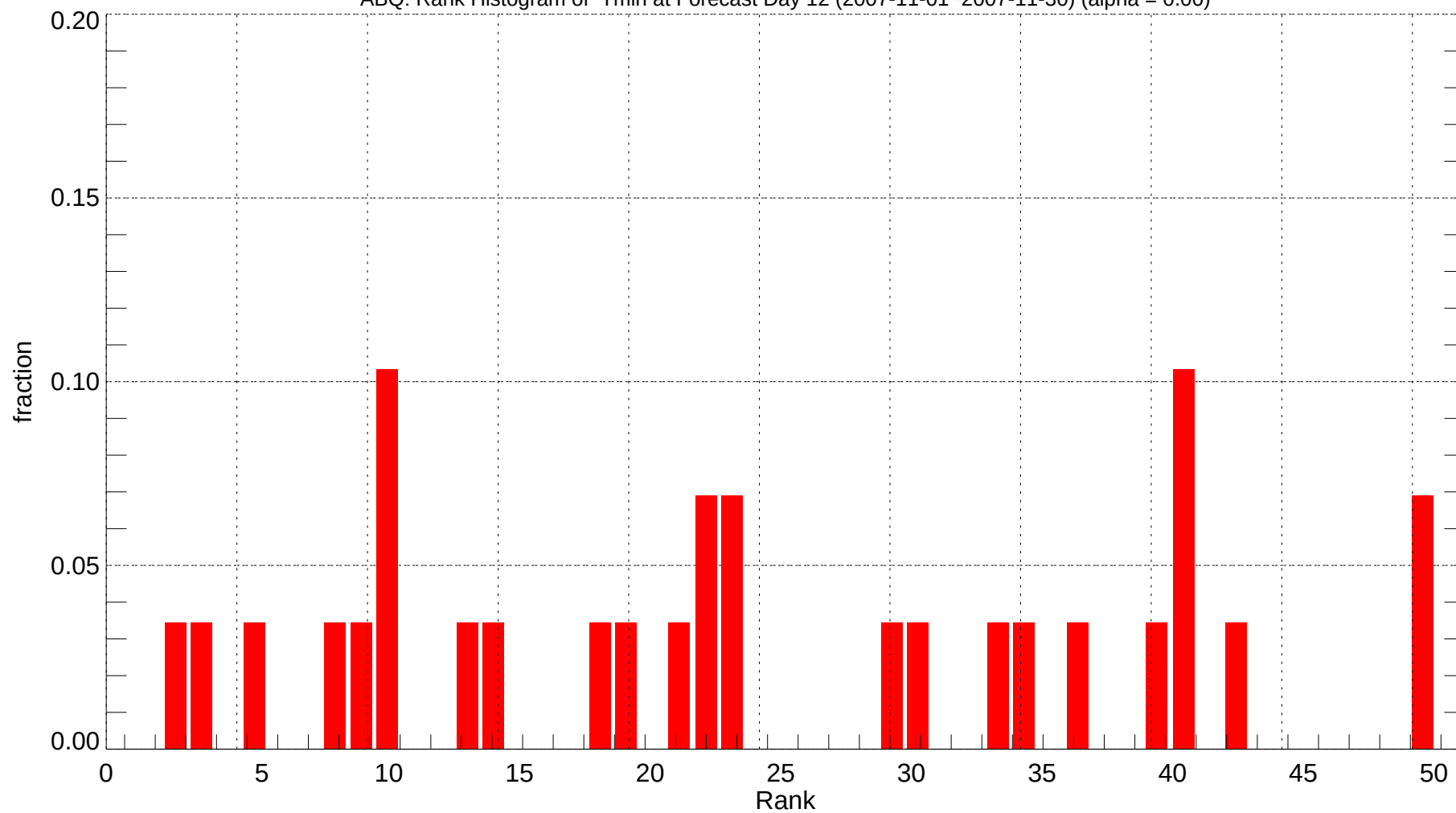
ABQ: Rank Histogram of Tmin at Forecast Day 12 (2007-11-01~2007-11-30) (alpha = 0.00)
