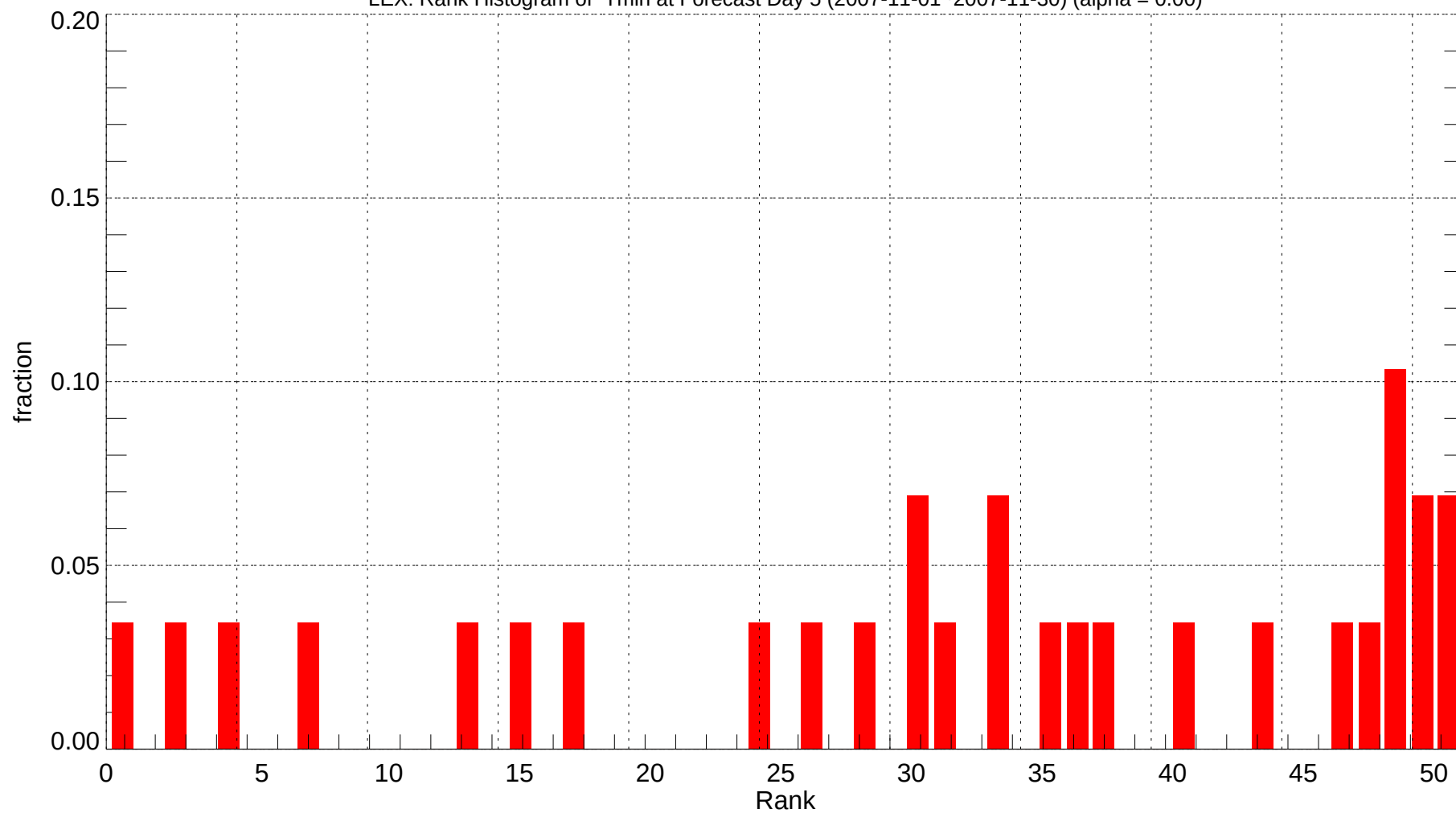
LEX: Rank Histogram of Tmin at Forecast Day 5 (2007-11-01~2007-11-30) (alpha = 0.00)
