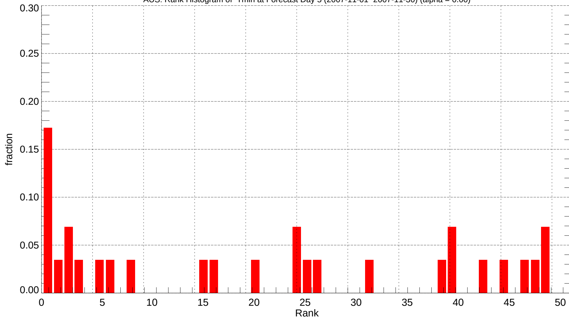
AUS: Rank Histogram of Tmin at Forecast Day 5 (2007-11-01~2007-11-30) (alpha = 0.00)
