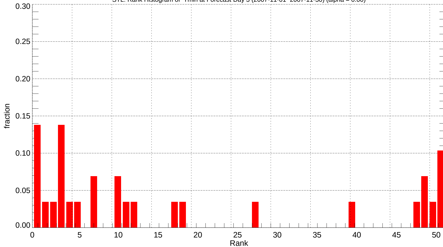
STL: Rank Histogram of Tmin at Forecast Day 3 (2007-11-01~2007-11-30) (alpha = 0.00)
