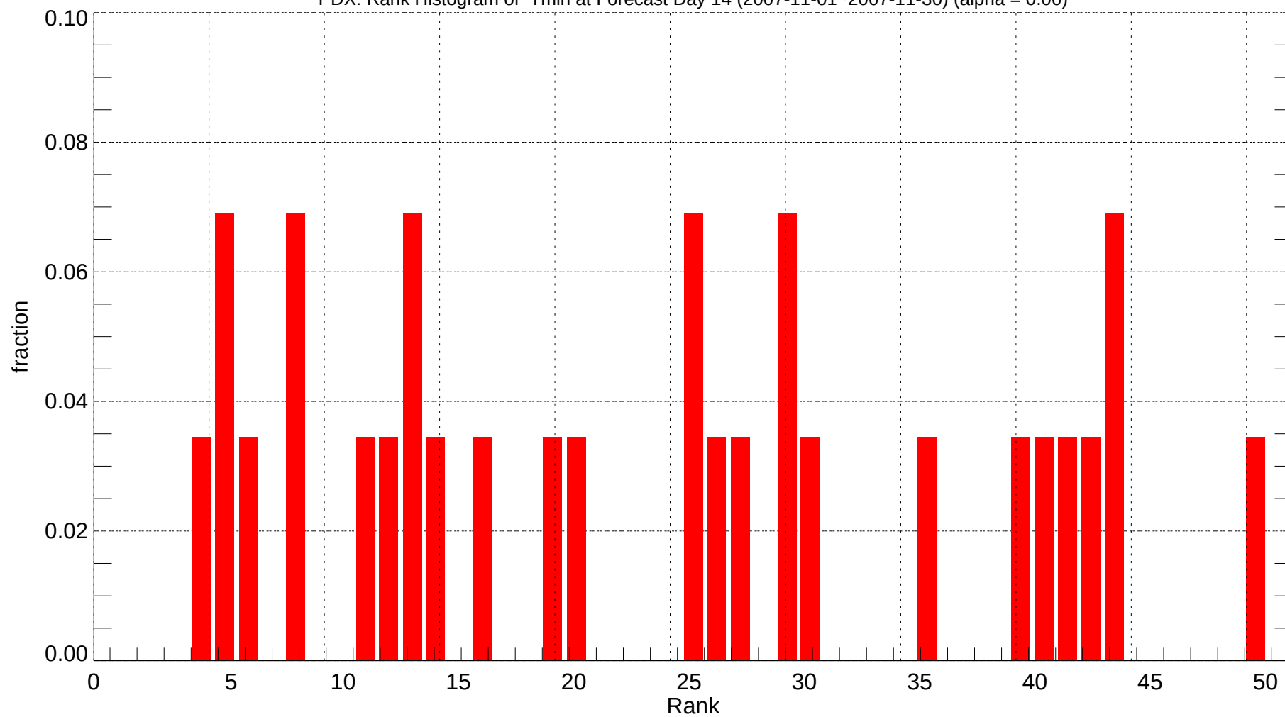
PDX: Rank Histogram of Tmin at Forecast Day 14 (2007-11-01~2007-11-30) (alpha = 0.00)
