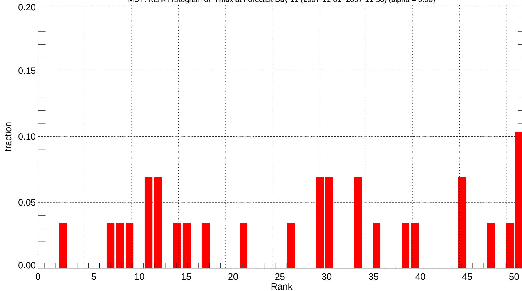
MDT: Rank Histogram of Tmax at Forecast Day 11 (2007-11-01~2007-11-30) (alpha = 0.00)
