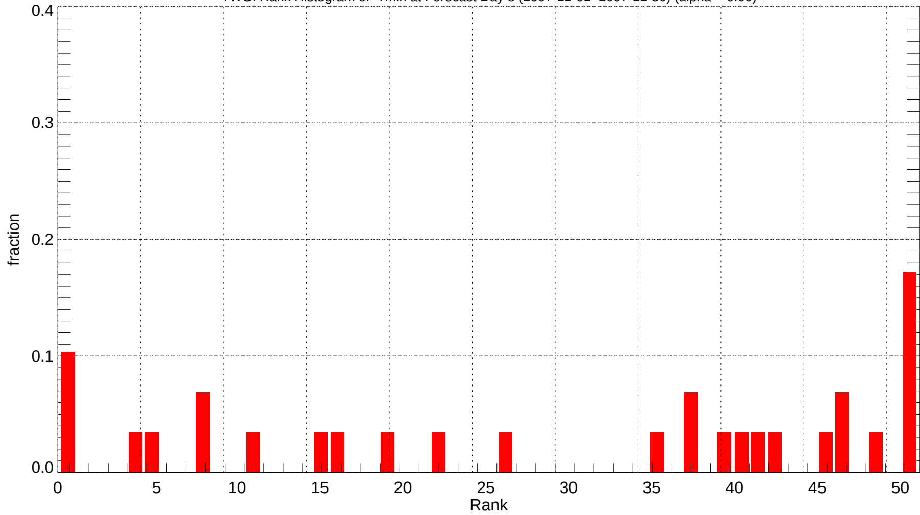
YWG: Rank Histogram of Tmin at Forecast Day 8 (2007-11-01~2007-11-30) (alpha = 0.00)
