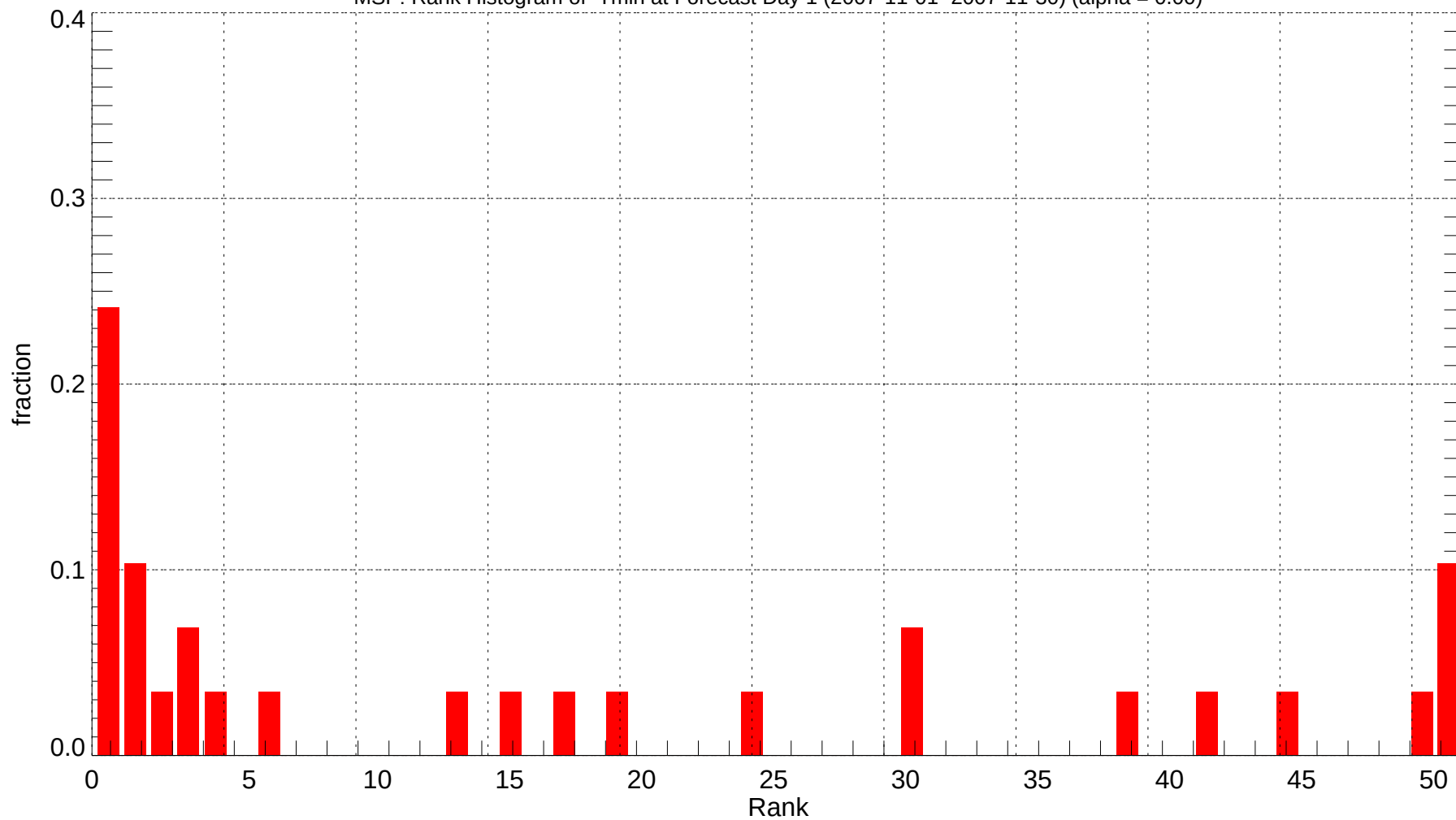
MSP: Rank Histogram of Tmin at Forecast Day 1 (2007-11-01~2007-11-30) (alpha = 0.00)
