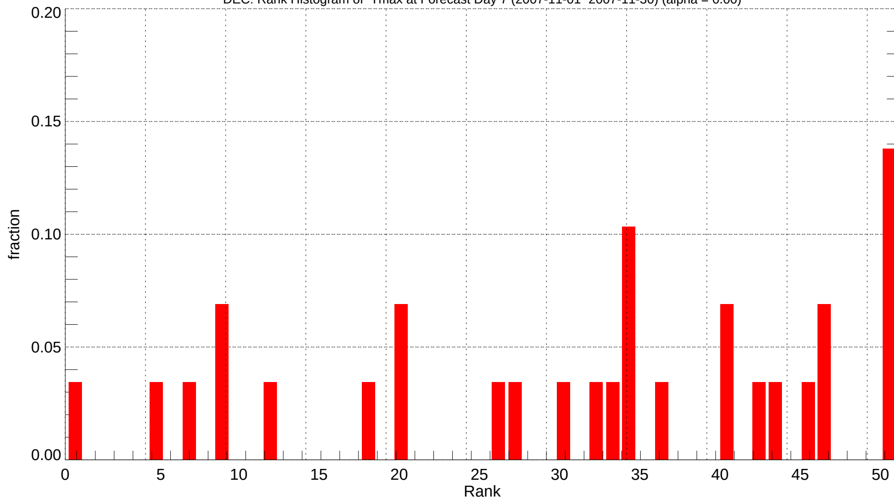
DEC: Rank Histogram of Tmax at Forecast Day 7 (2007-11-01~2007-11-30) (alpha = 0.00)
