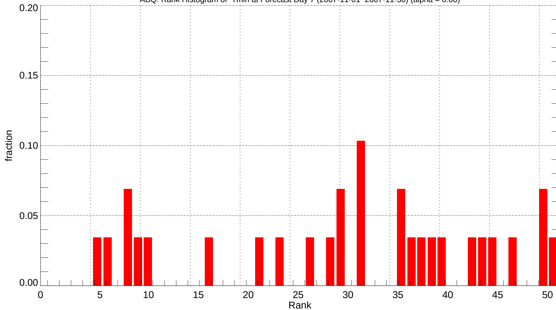
ABQ: Rank Histogram of Tmin at Forecast Day 7 (2007-11-01~2007-11-30) (alpha = 0.00)
