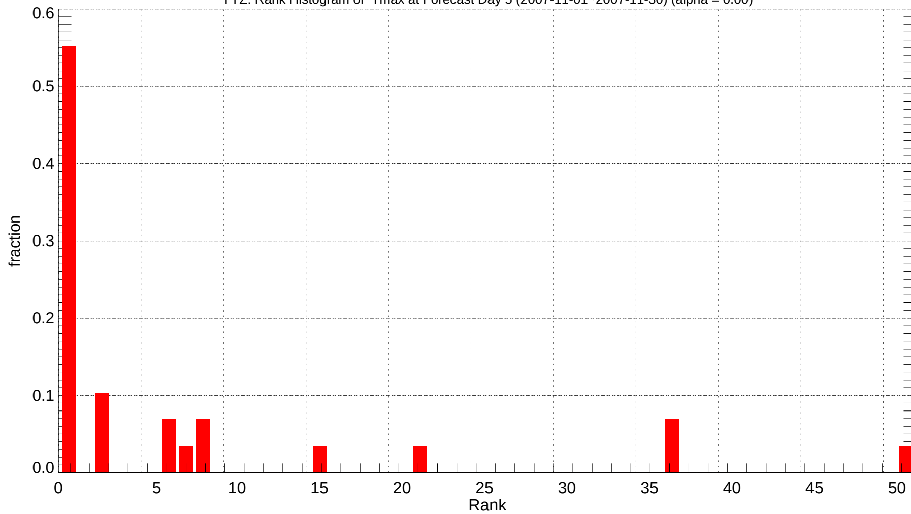
YYZ: Rank Histogram of Tmax at Forecast Day 5 (2007-11-01~2007-11-30) (alpha = 0.00)
