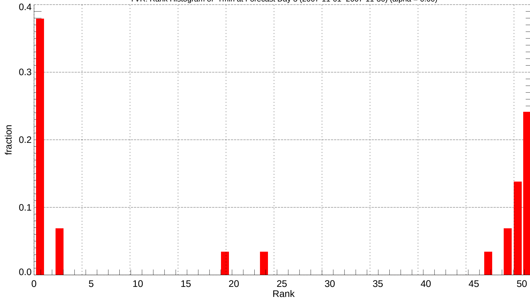
YVR: Rank Histogram of Tmin at Forecast Day 3 (2007-11-01~2007-11-30) (alpha = 0.00)
