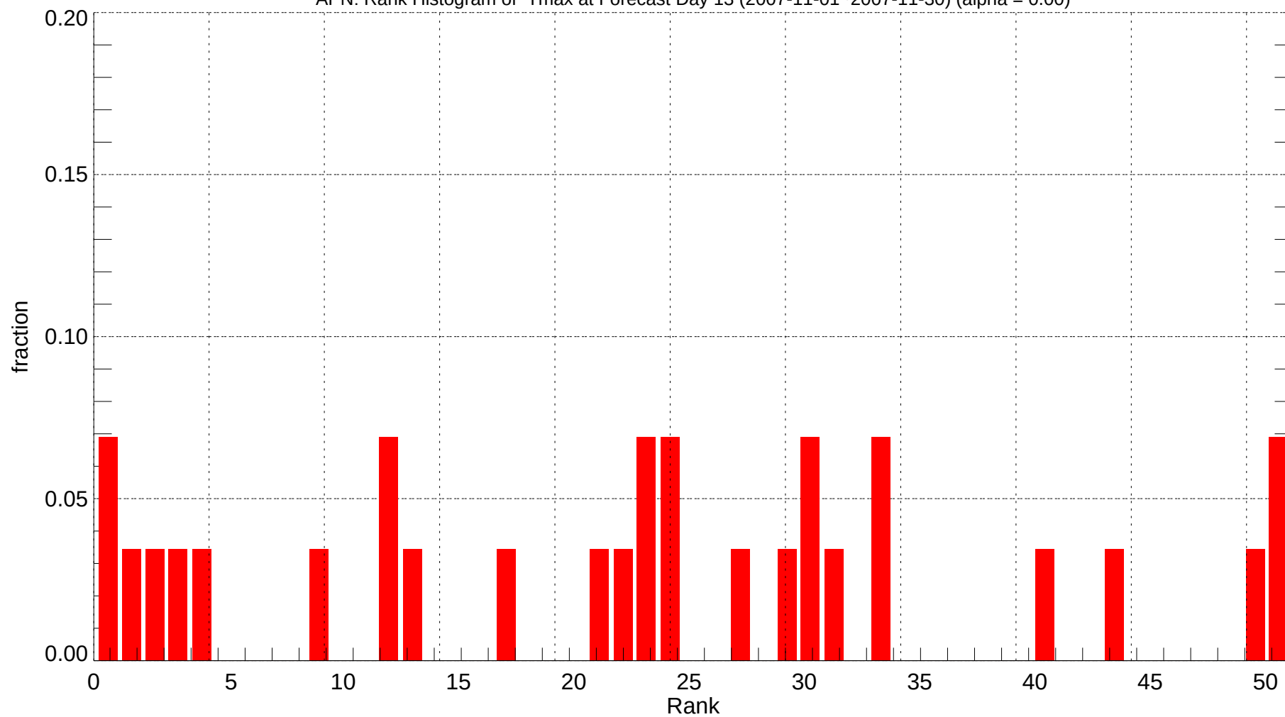
APN: Rank Histogram of Tmax at Forecast Day 13 (2007-11-01~2007-11-30) (alpha = 0.00)
