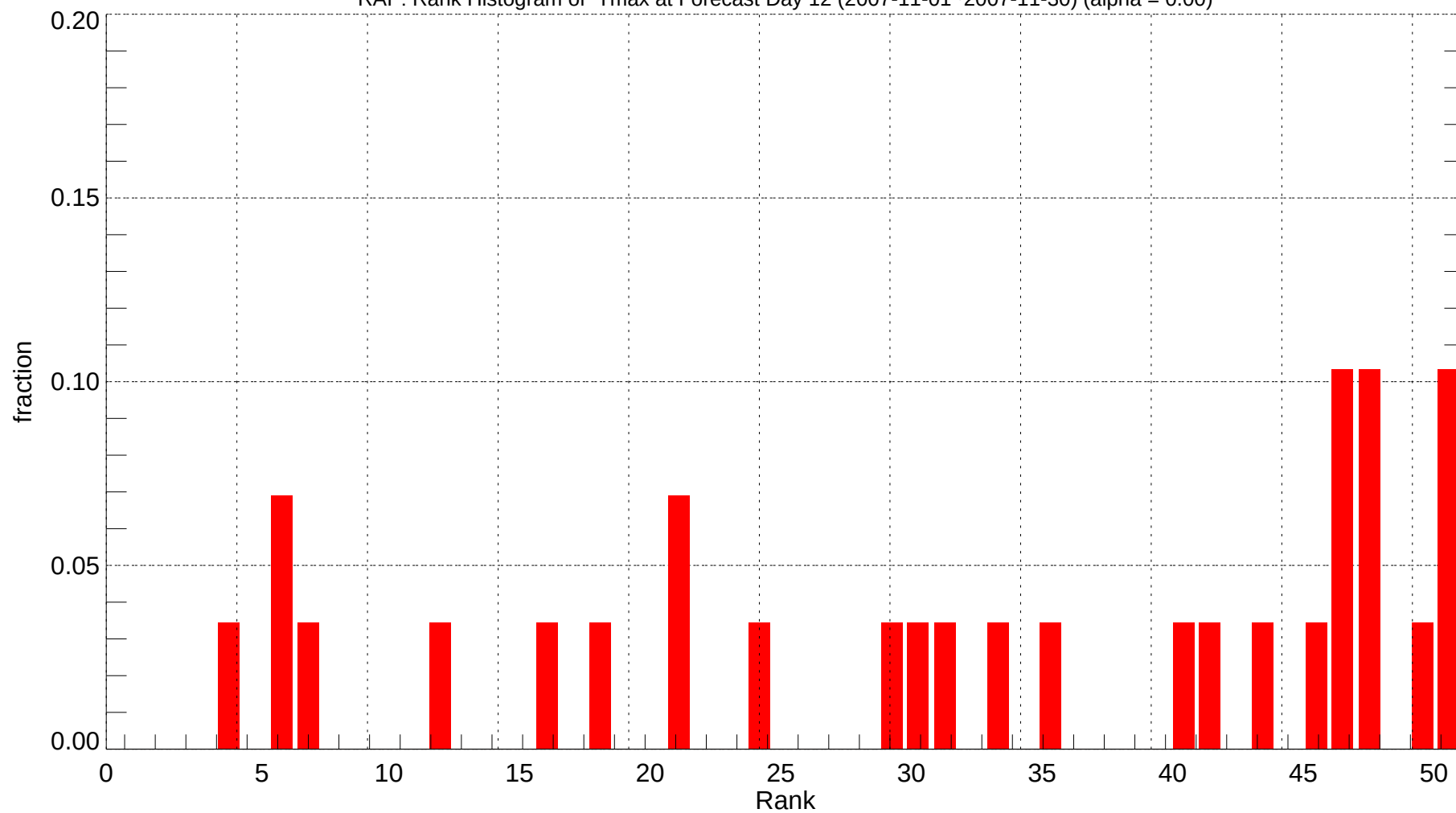
RAP: Rank Histogram of Tmax at Forecast Day 12 (2007-11-01~2007-11-30) (alpha = 0.00)
