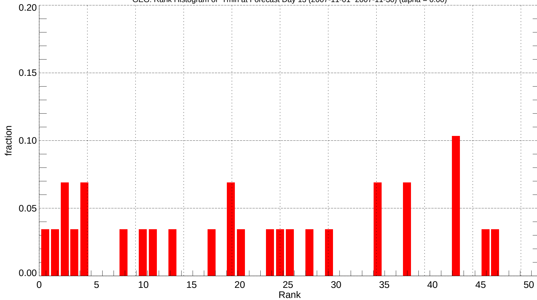
GEG: Rank Histogram of Tmin at Forecast Day 13 (2007-11-01~2007-11-30) (alpha = 0.00)
