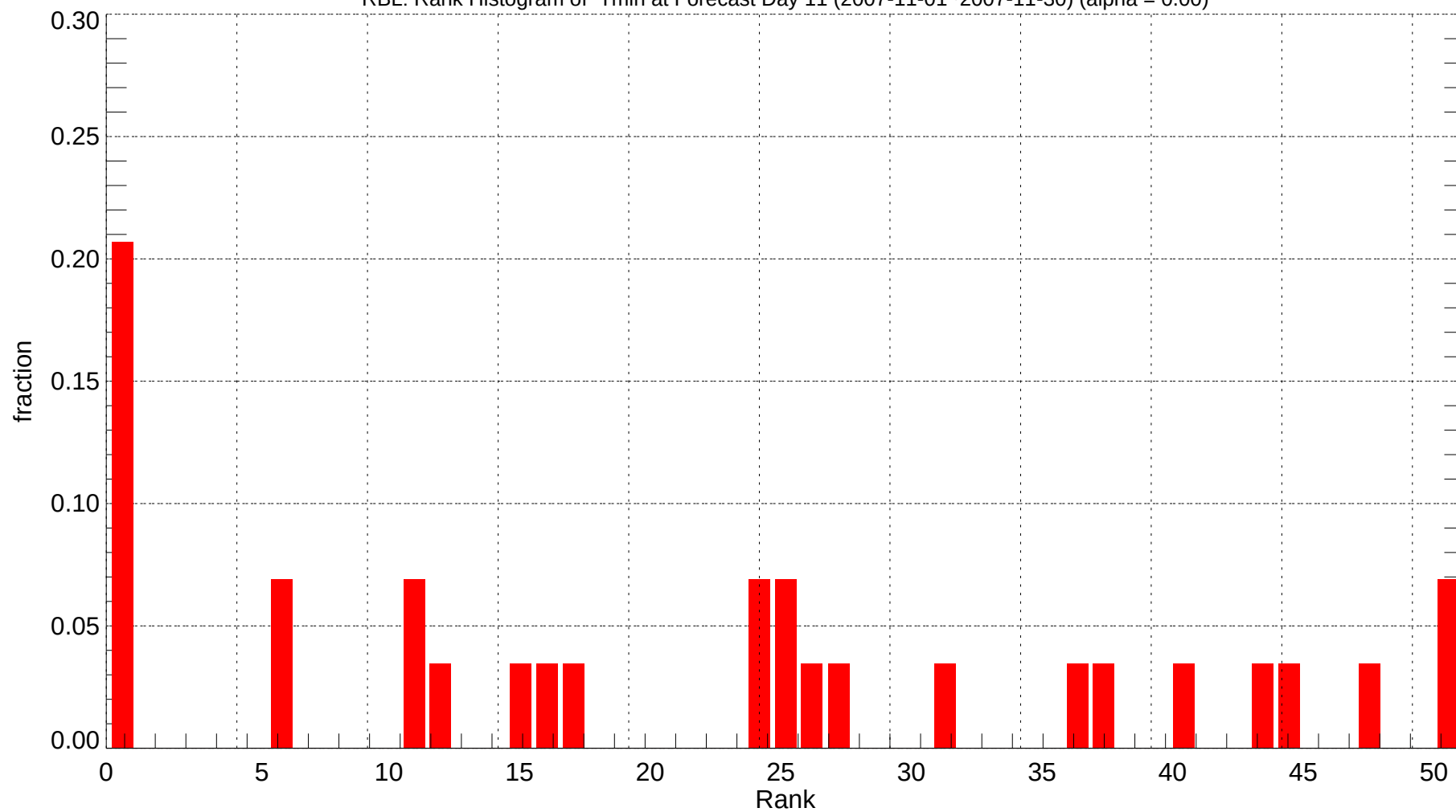
RBL: Rank Histogram of Tmin at Forecast Day 11 (2007-11-01~2007-11-30) (alpha = 0.00)
