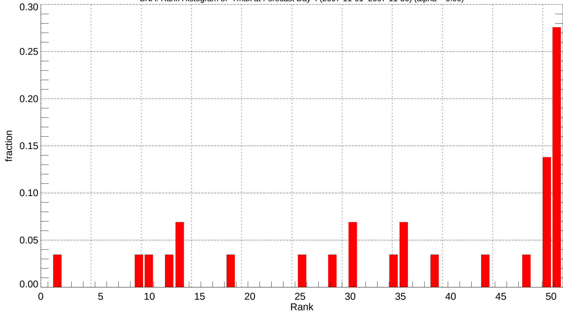
BNA: Rank Histogram of Tmax at Forecast Day 4 (2007-11-01~2007-11-30) (alpha = 0.00)
