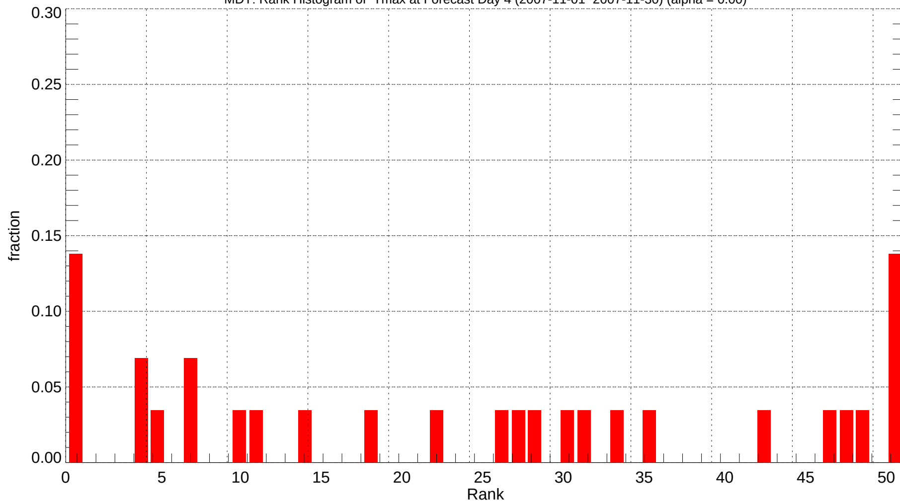
MDT: Rank Histogram of Tmax at Forecast Day 4 (2007-11-01~2007-11-30) (alpha = 0.00)
