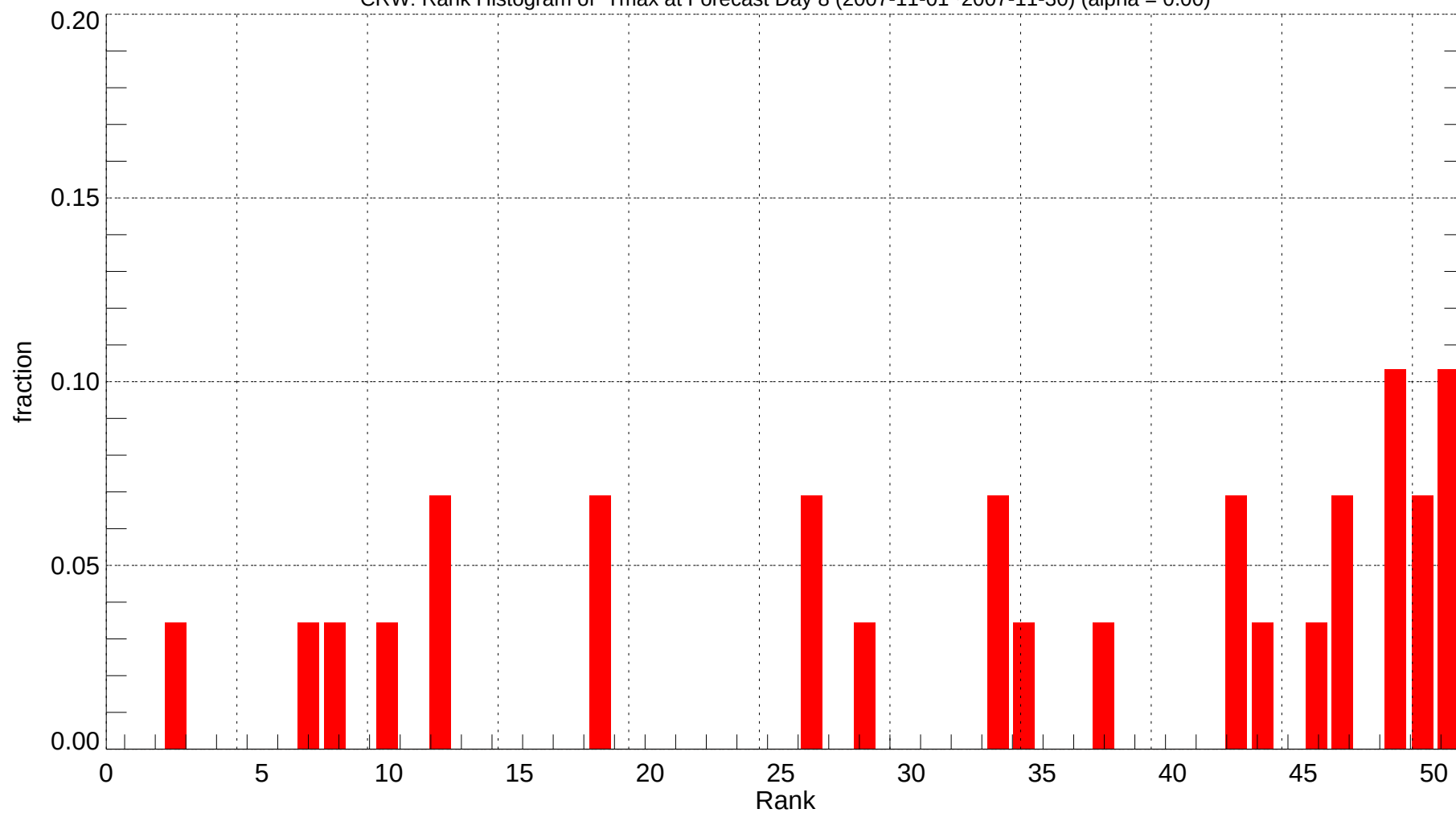
CRW: Rank Histogram of Tmax at Forecast Day 8 (2007-11-01~2007-11-30) (alpha = 0.00)
