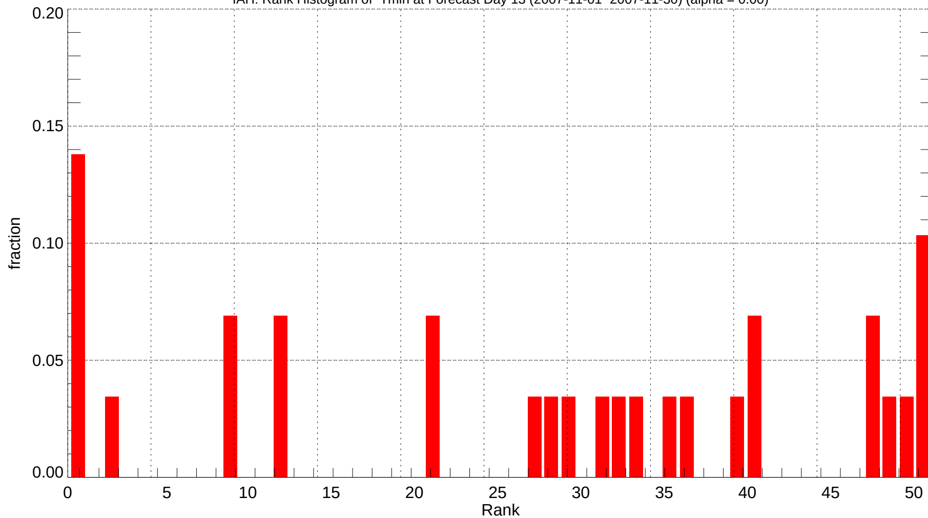
IAH: Rank Histogram of Tmin at Forecast Day 13 (2007-11-01~2007-11-30) (alpha = 0.00)
