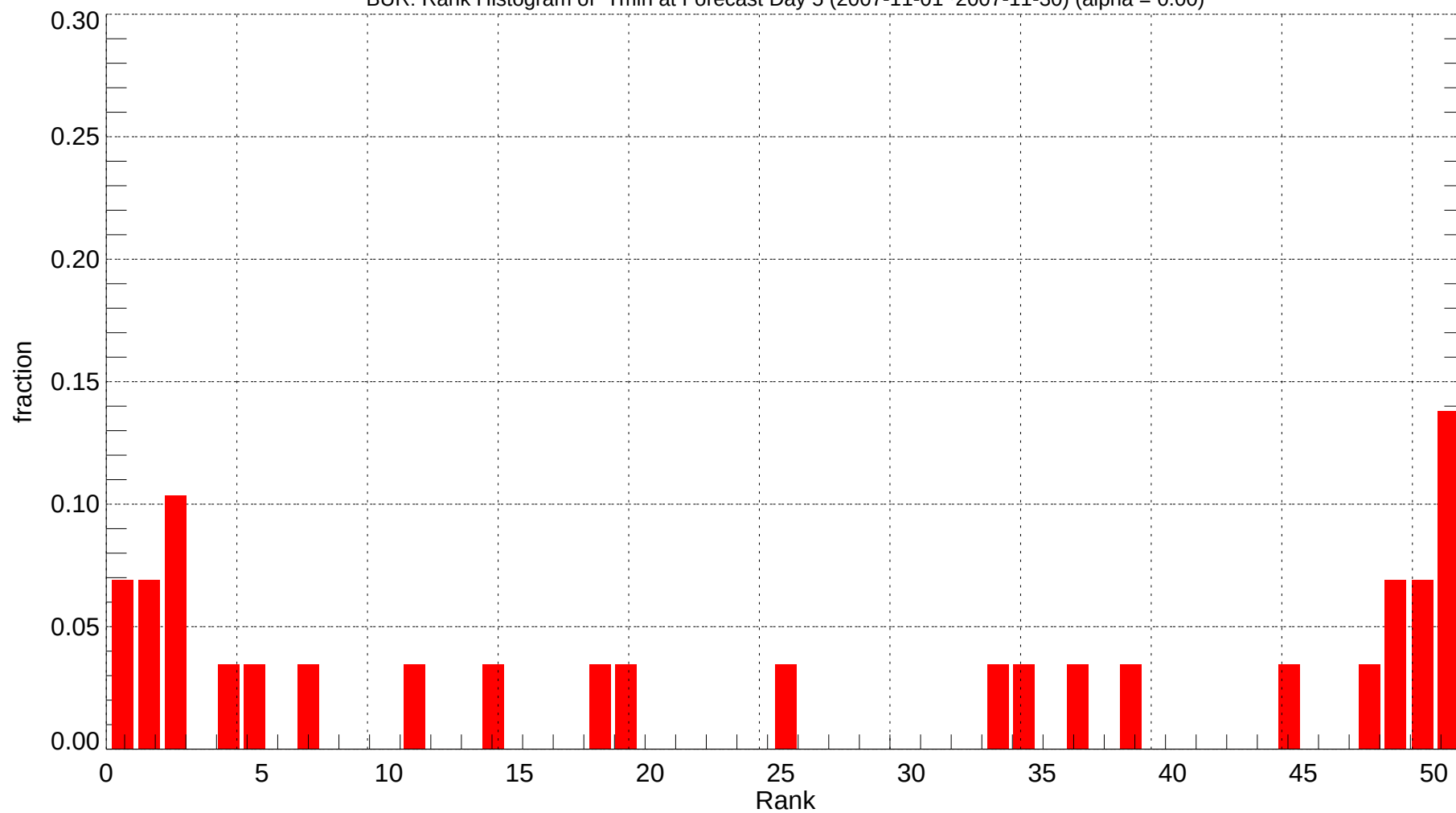
BUR: Rank Histogram of Tmin at Forecast Day 5 (2007-11-01~2007-11-30) (alpha = 0.00)
