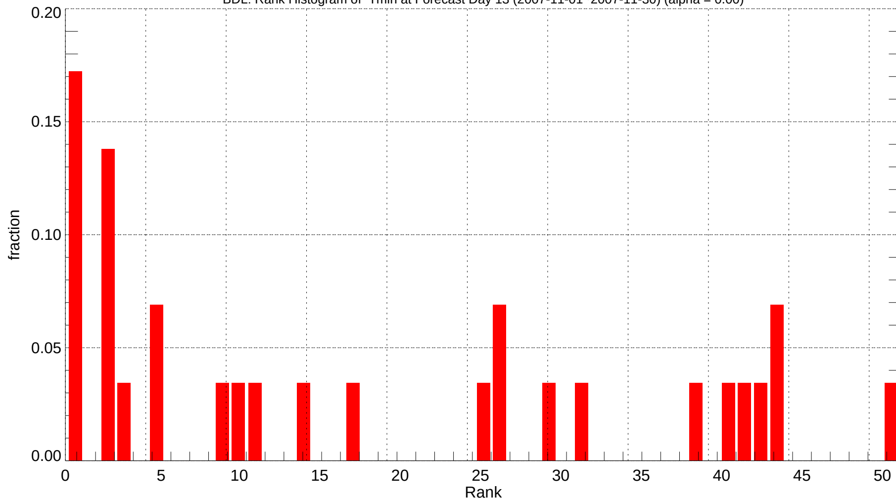
BDL: Rank Histogram of Tmin at Forecast Day 13 (2007-11-01~2007-11-30) (alpha = 0.00)
