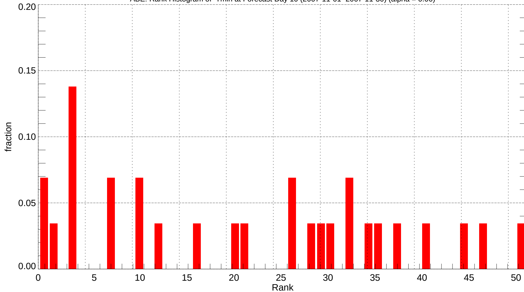
ABE: Rank Histogram of Tmin at Forecast Day 10 (2007-11-01~2007-11-30) (alpha = 0.00)
