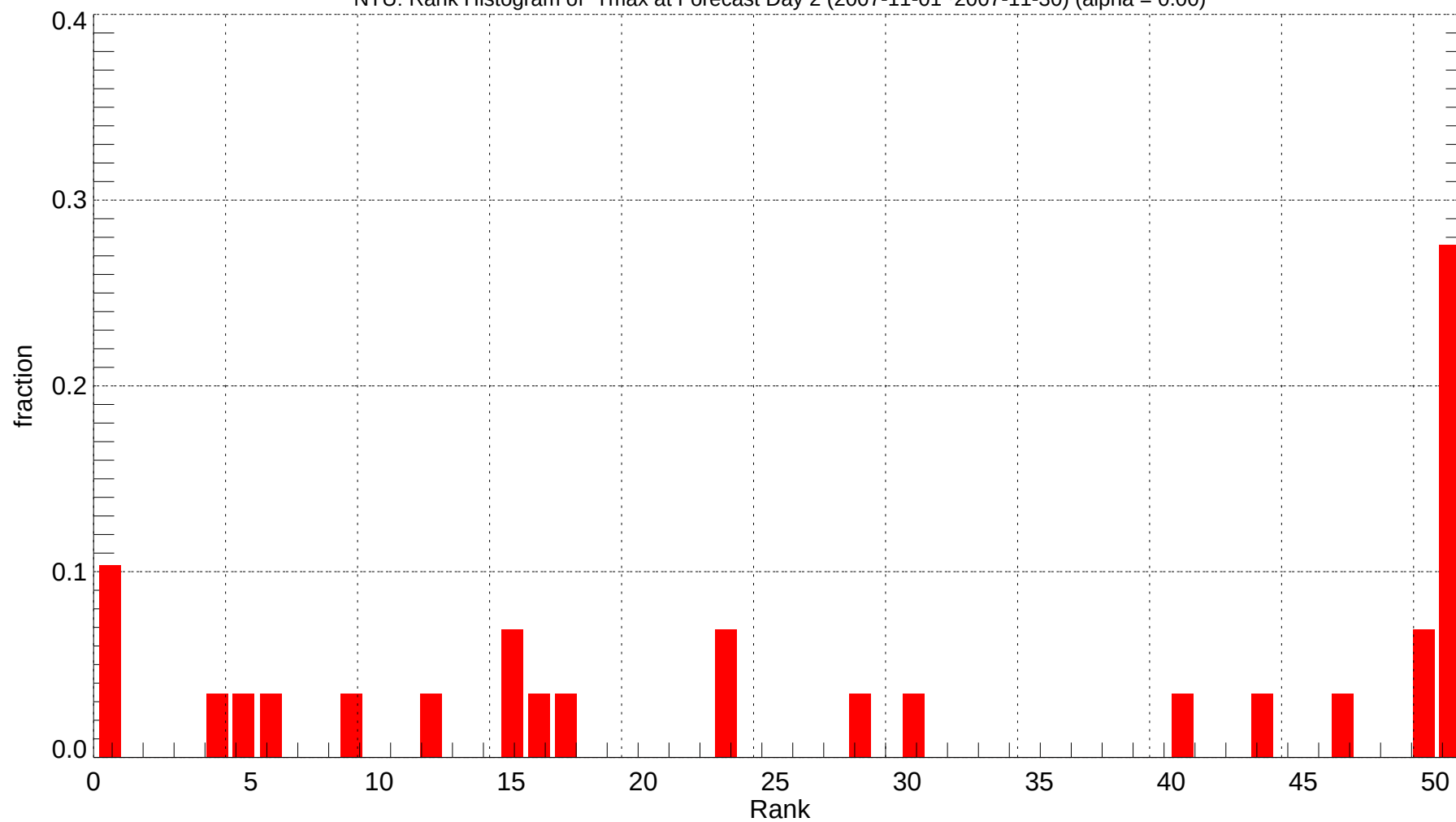
NTU: Rank Histogram of Tmax at Forecast Day 2 (2007-11-01~2007-11-30) (alpha = 0.00)
