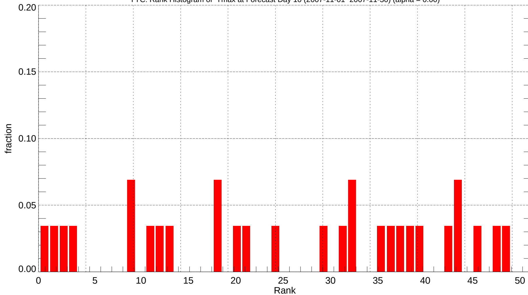
YYC: Rank Histogram of Tmax at Forecast Day 10 (2007-11-01~2007-11-30) (alpha = 0.00)
