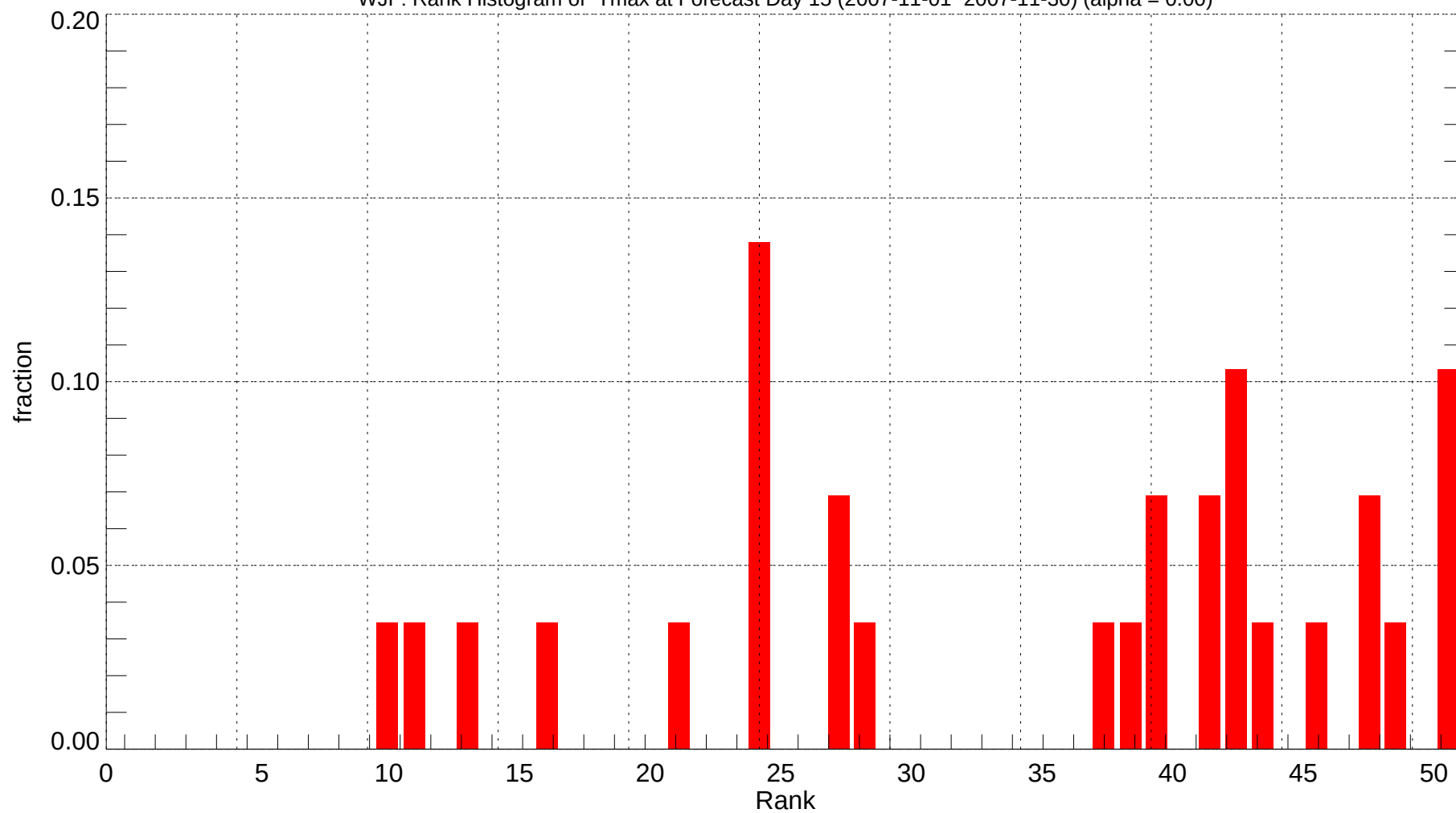
WJF: Rank Histogram of Tmax at Forecast Day 15 (2007-11-01~2007-11-30) (alpha = 0.00)
