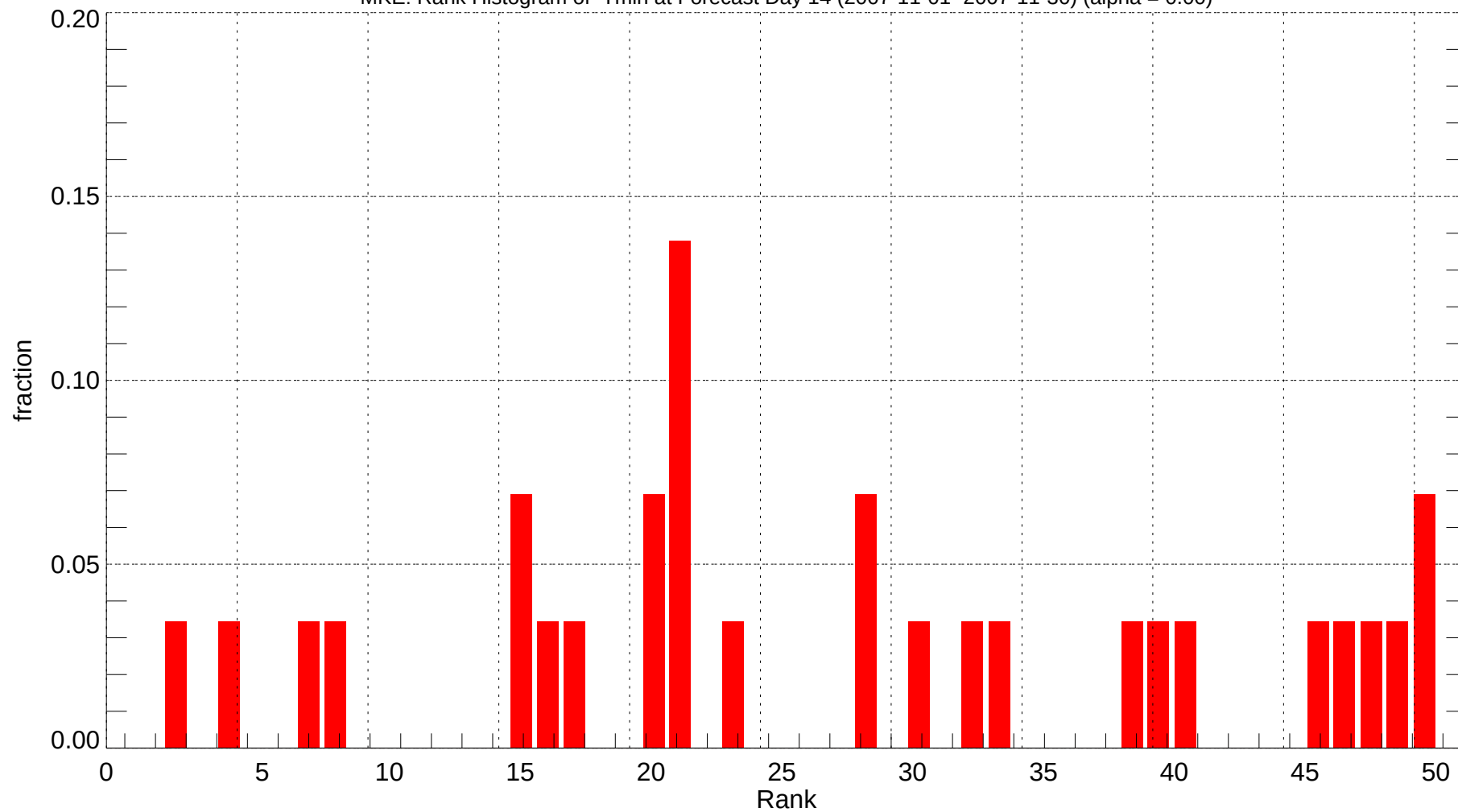
MKE: Rank Histogram of Tmin at Forecast Day 14 (2007-11-01~2007-11-30) (alpha = 0.00)
