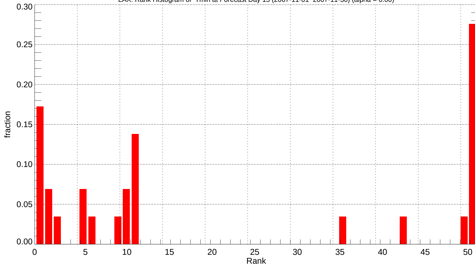
LAX: Rank Histogram of Tmin at Forecast Day 15 (2007-11-01~2007-11-30) (alpha = 0.00)
