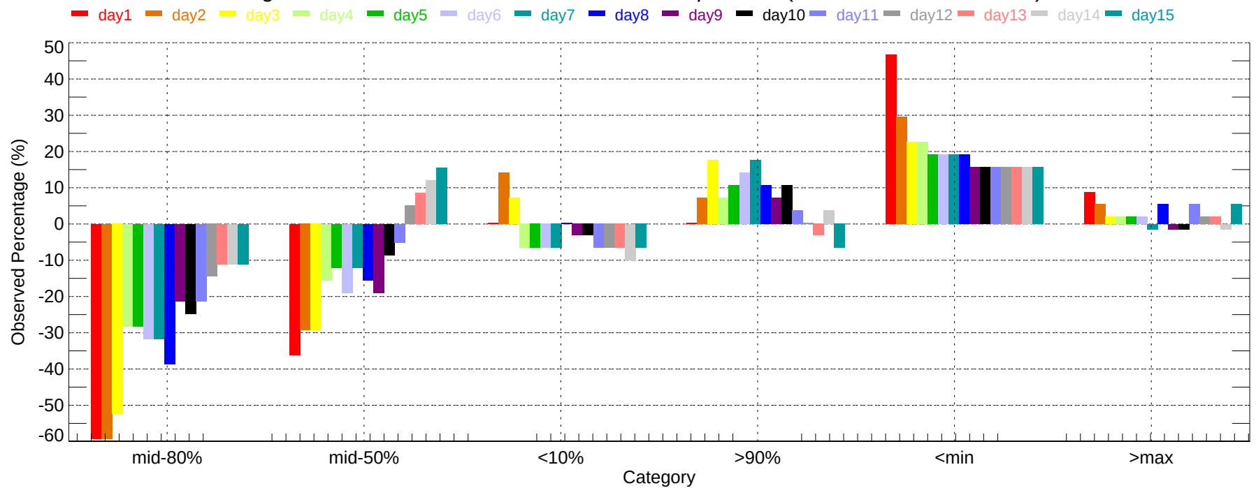
Observed Percentage Deviation of Ensembles - RBL: Max Temperature (2007-11-01~2007-11-30)
