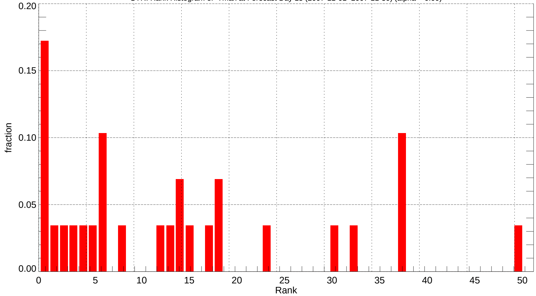
SYR: Rank Histogram of Tmax at Forecast Day 15 (2007-11-01~2007-11-30) (alpha = 0.00)
