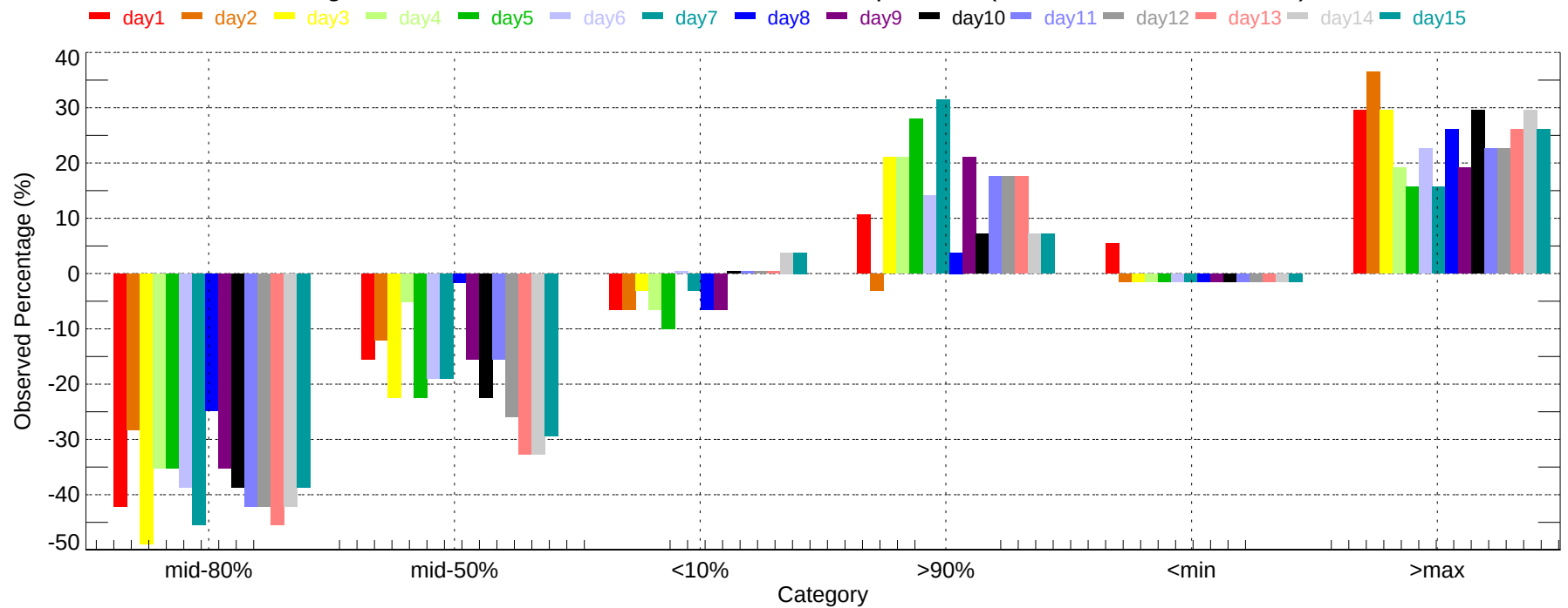
Observed Percentage Deviation of Ensembles - COS: Max Temperature (2007-11-01~2007-11-30)
