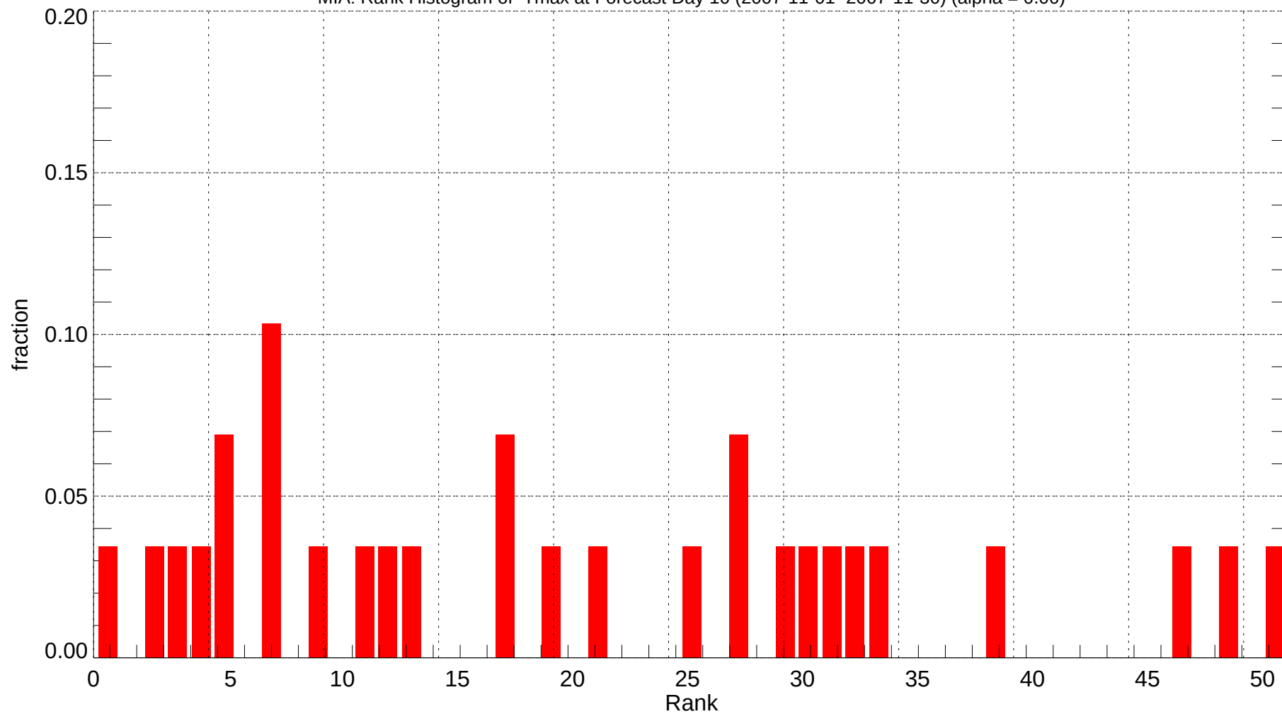
MIA: Rank Histogram of Tmax at Forecast Day 10 (2007-11-01~2007-11-30) (alpha = 0.00)
