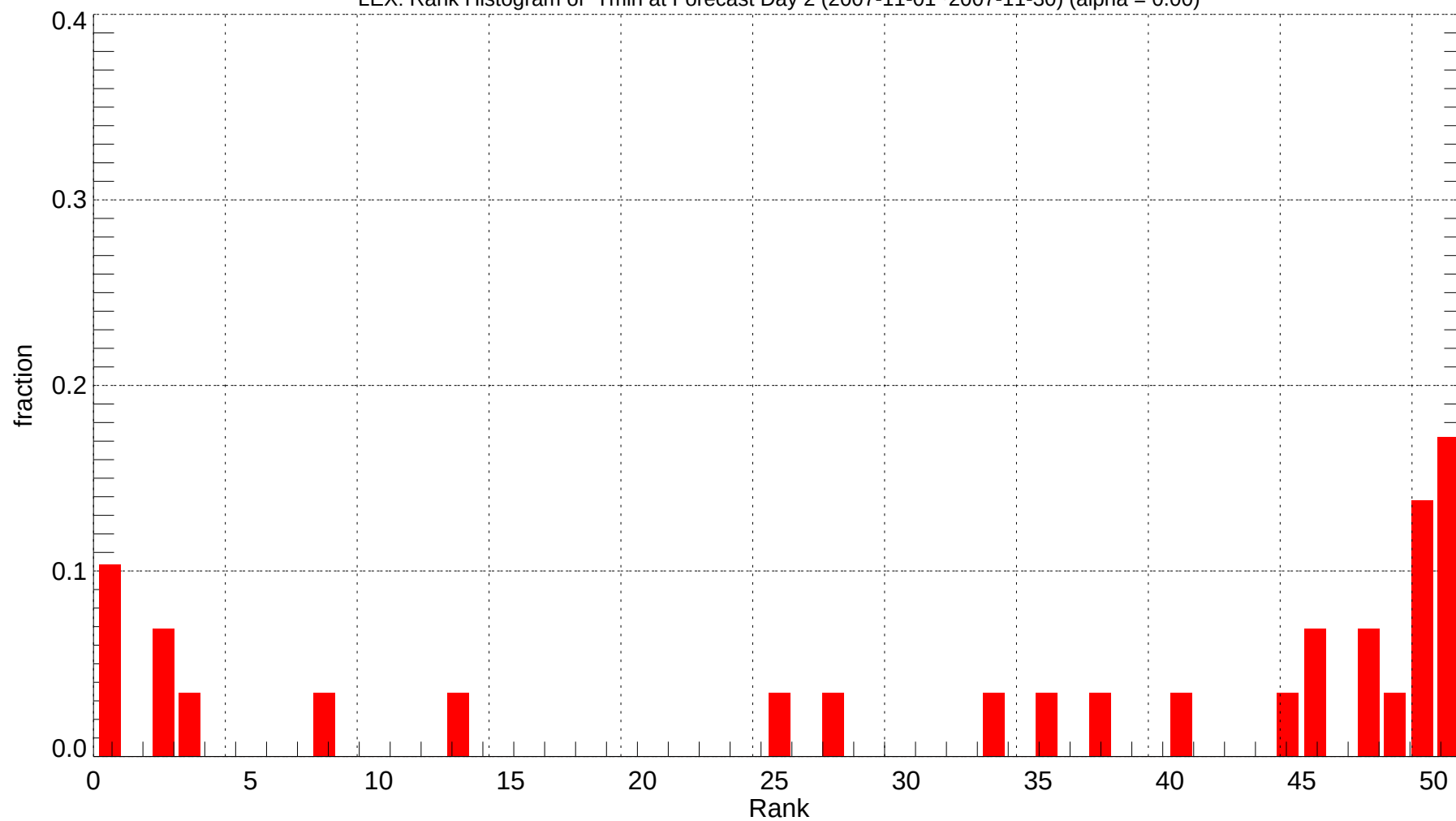
LEX: Rank Histogram of Tmin at Forecast Day 2 (2007-11-01~2007-11-30) (alpha = 0.00)
