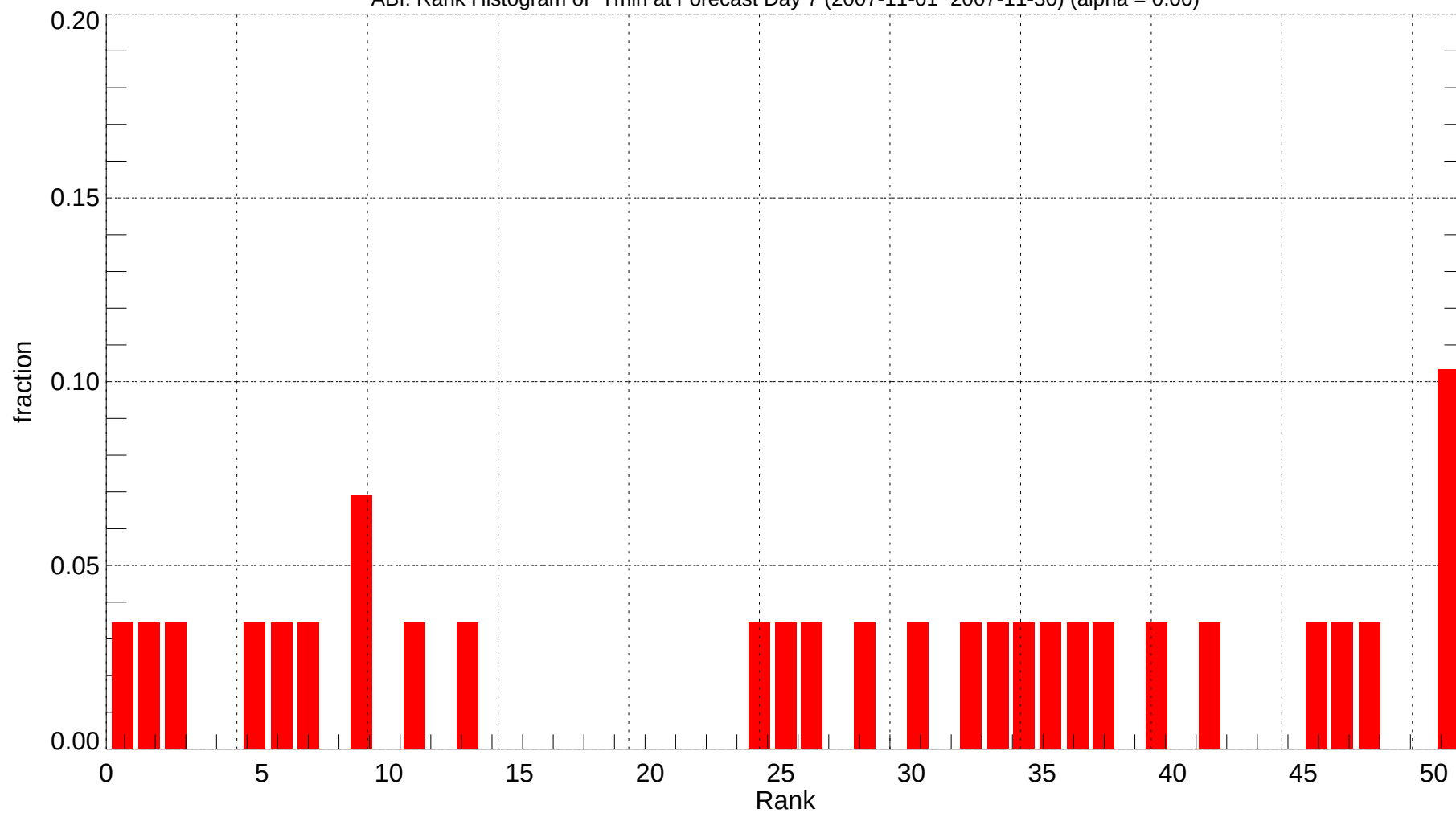
ABI: Rank Histogram of Tmin at Forecast Day 7 (2007-11-01~2007-11-30) (alpha = 0.00)
