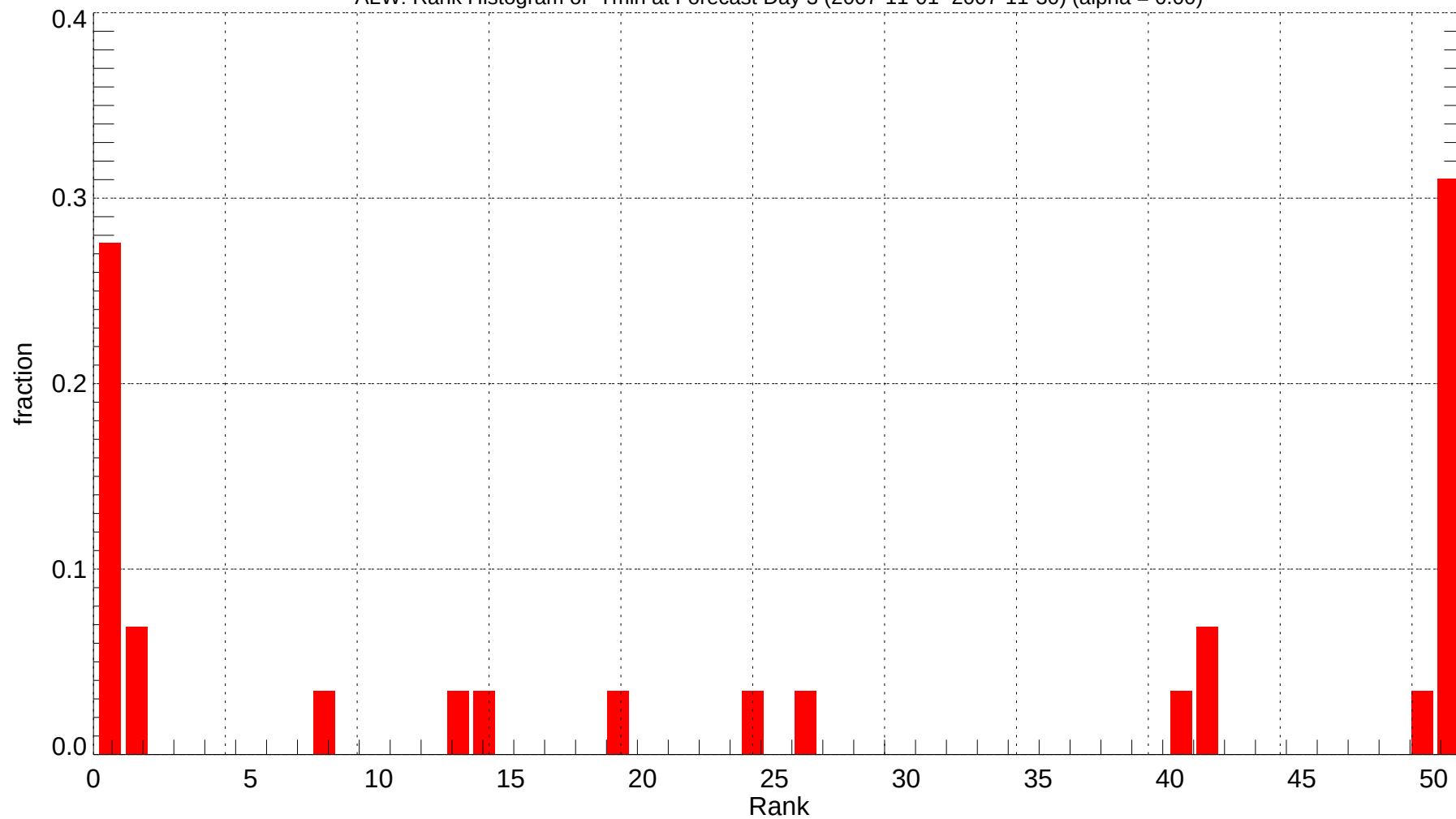
ALW: Rank Histogram of Tmin at Forecast Day 3 (2007-11-01~2007-11-30) (alpha = 0.00)
