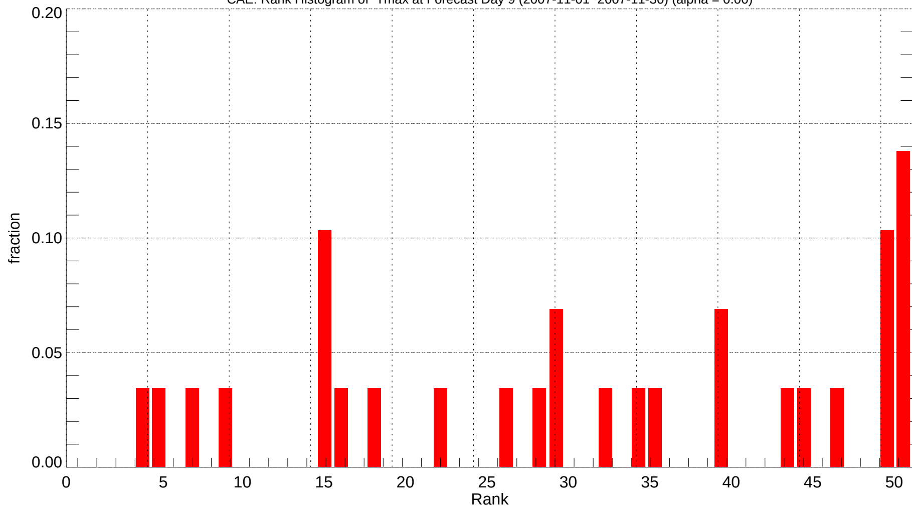
CAE: Rank Histogram of Tmax at Forecast Day 9 (2007-11-01~2007-11-30) (alpha = 0.00)
