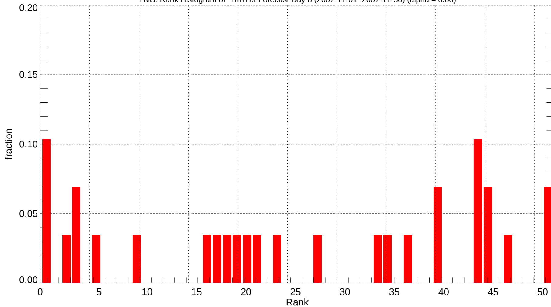
YNG: Rank Histogram of Tmin at Forecast Day 8 (2007-11-01~2007-11-30) (alpha = 0.00)
