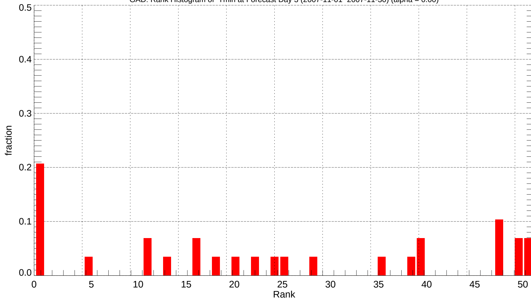
GAD: Rank Histogram of Tmin at Forecast Day 3 (2007-11-01~2007-11-30) (alpha = 0.00)
