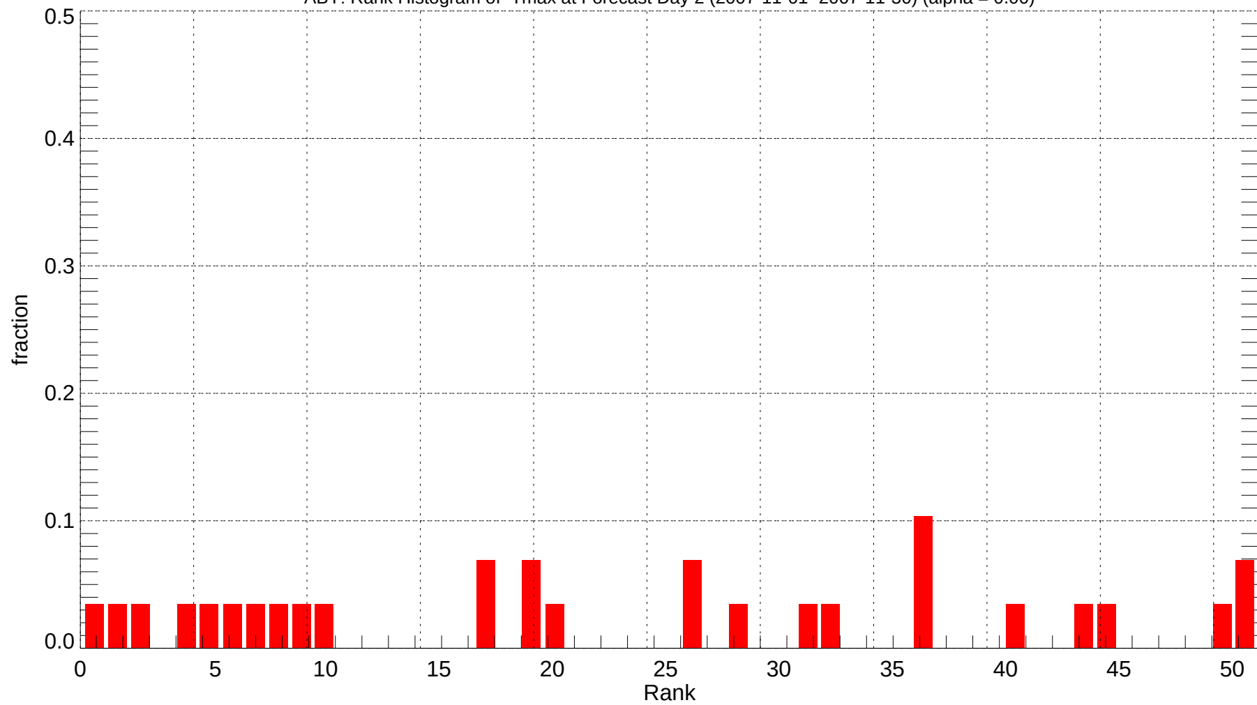
ABY: Rank Histogram of Tmax at Forecast Day 2 (2007-11-01~2007-11-30) (alpha = 0.00)
