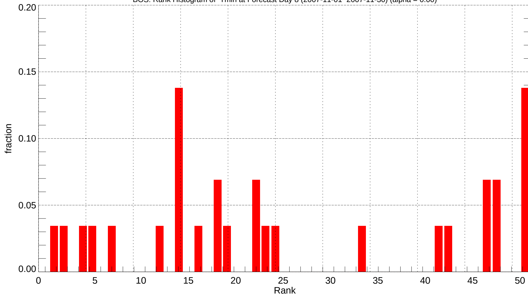
BOS: Rank Histogram of Tmin at Forecast Day 8 (2007-11-01~2007-11-30) (alpha = 0.00)
