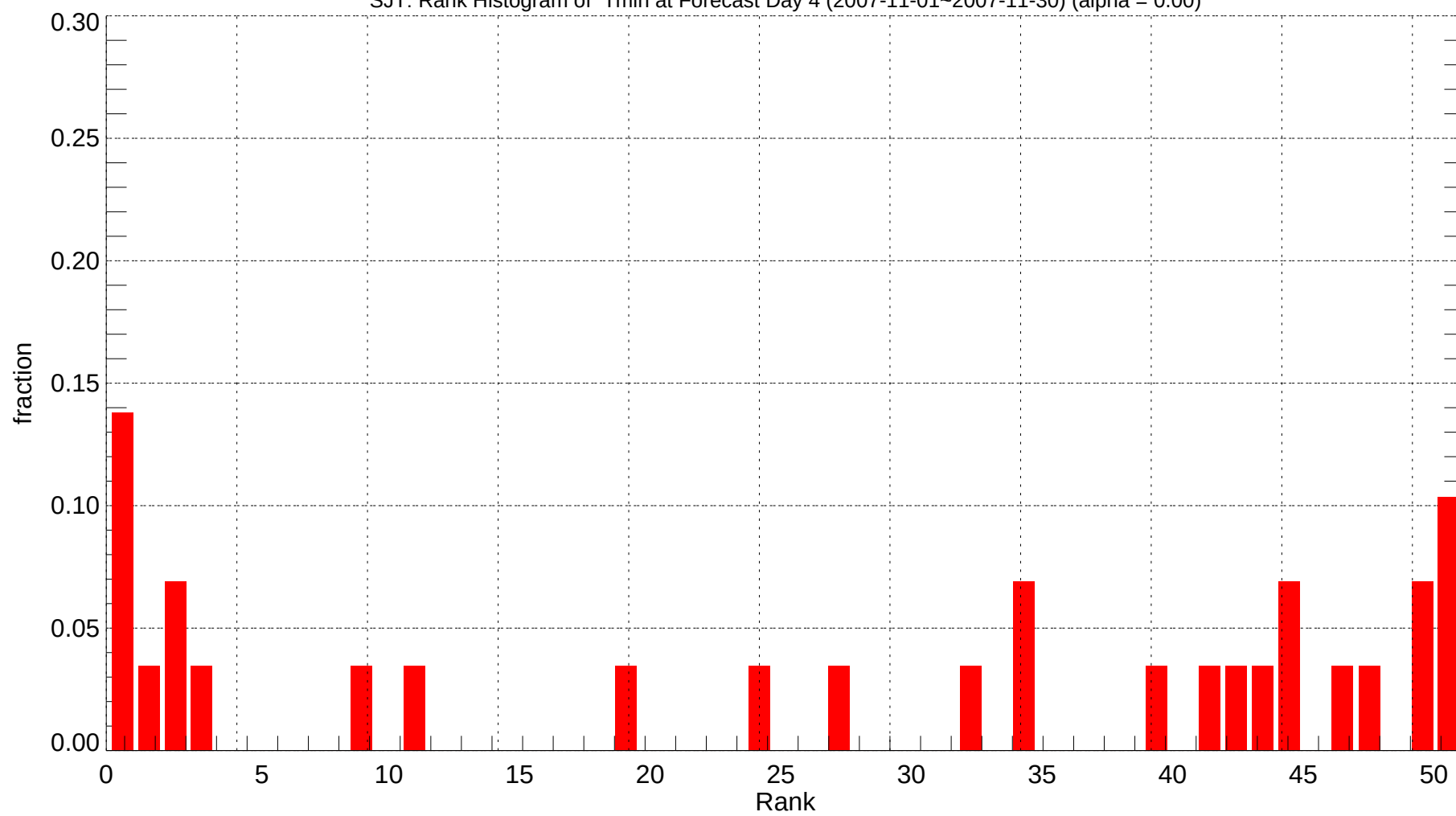
SJT: Rank Histogram of Tmin at Forecast Day 4 (2007-11-01~2007-11-30) (alpha = 0.00)
