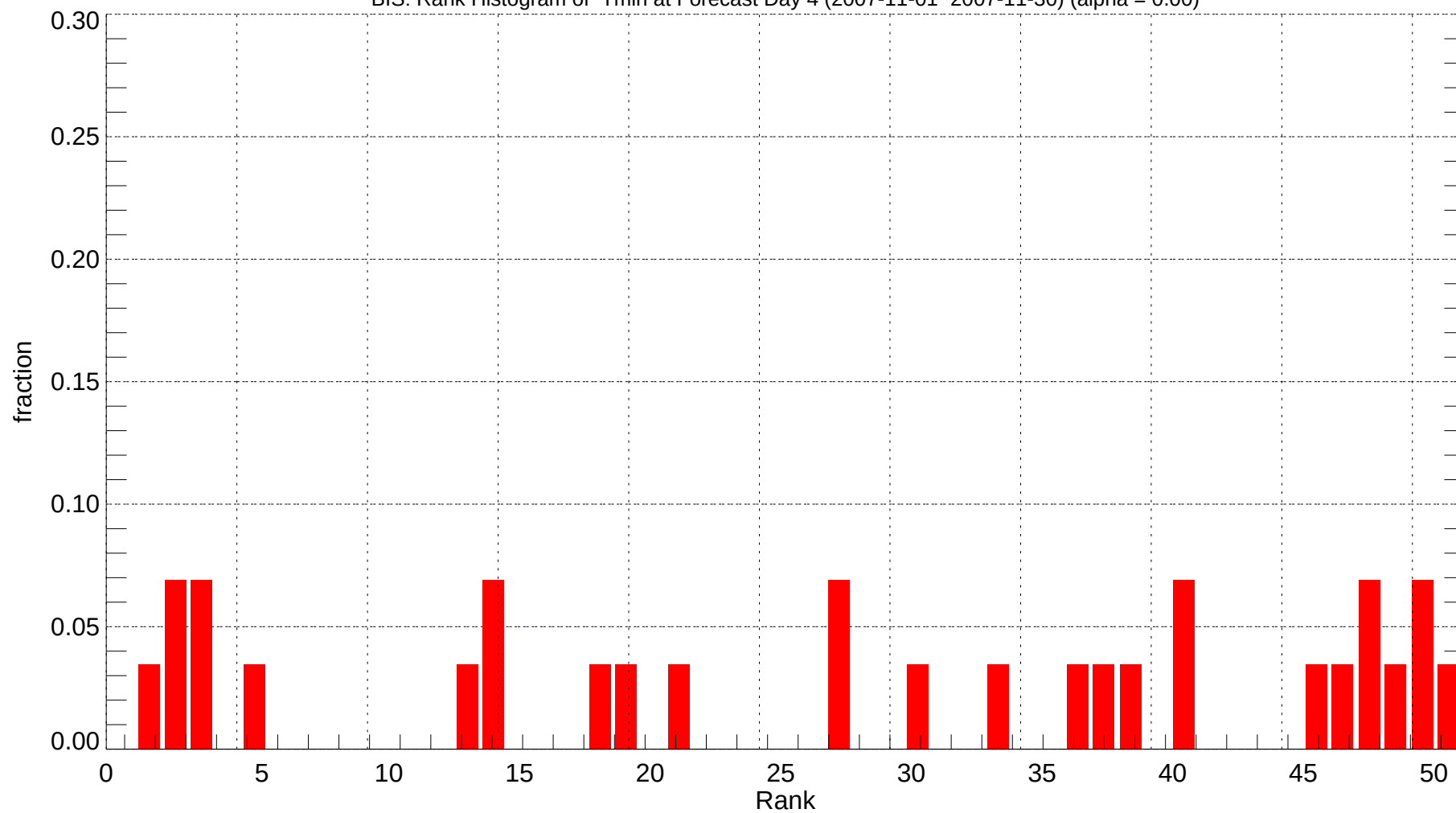
BIS: Rank Histogram of Tmin at Forecast Day 4 (2007-11-01~2007-11-30) (alpha = 0.00)
