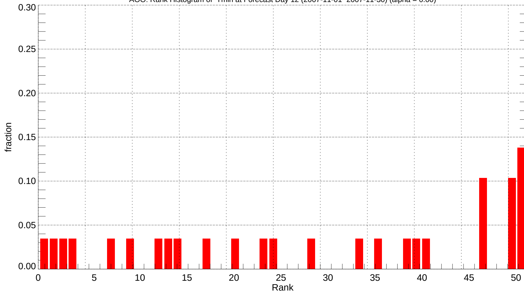
AOO: Rank Histogram of Tmin at Forecast Day 12 (2007-11-01~2007-11-30) (alpha = 0.00)
