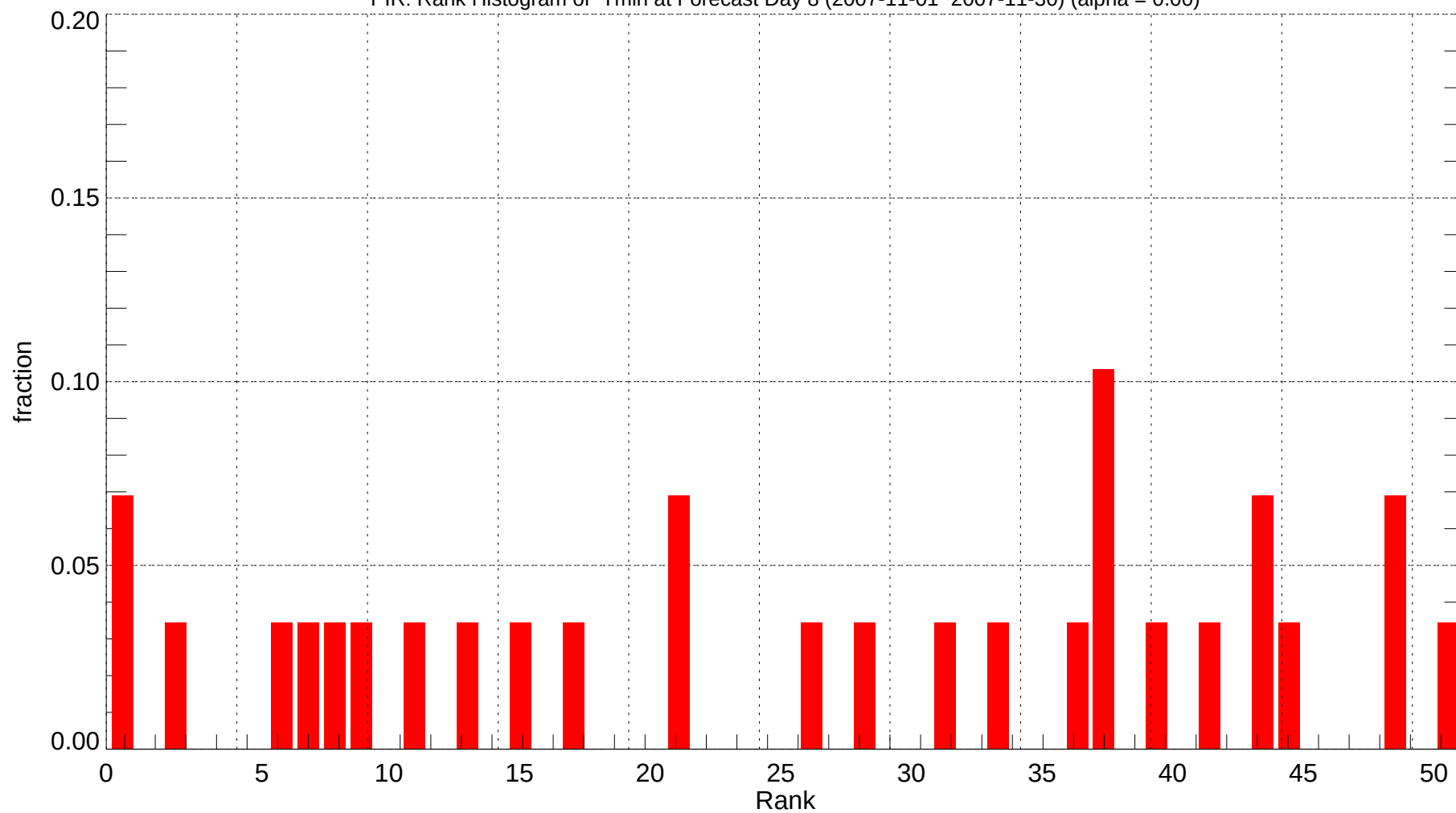
PIR: Rank Histogram of Tmin at Forecast Day 8 (2007-11-01~2007-11-30) (alpha = 0.00)
