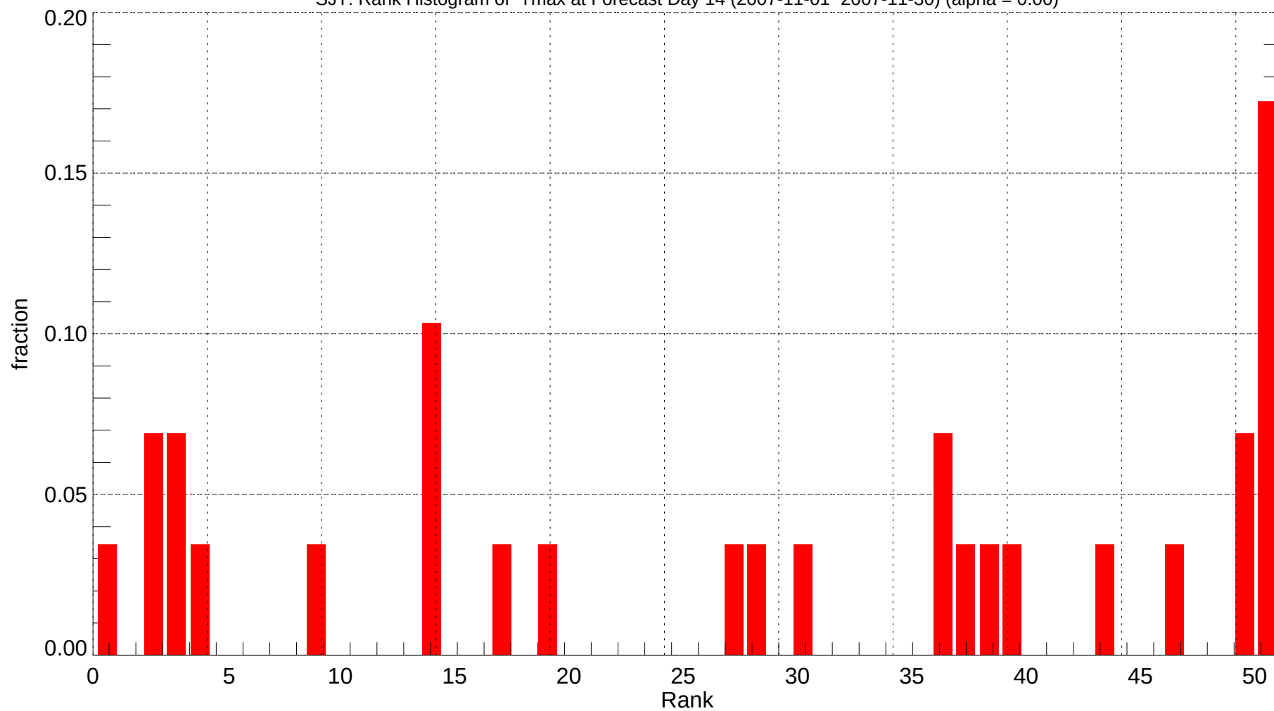
SJT: Rank Histogram of Tmax at Forecast Day 14 (2007-11-01~2007-11-30) (alpha = 0.00)
