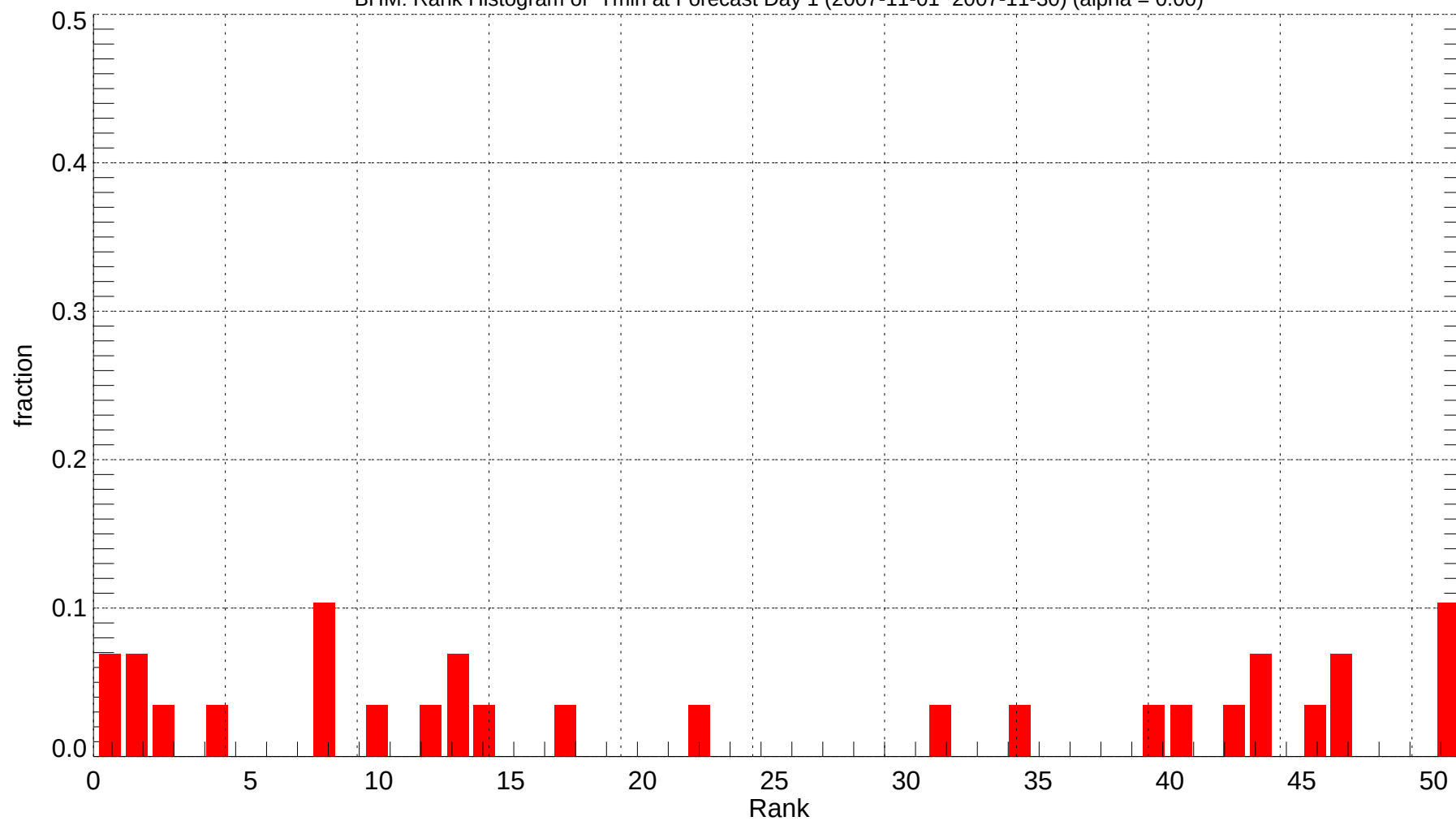
BHM: Rank Histogram of Tmin at Forecast Day 1 (2007-11-01~2007-11-30) (alpha = 0.00)
