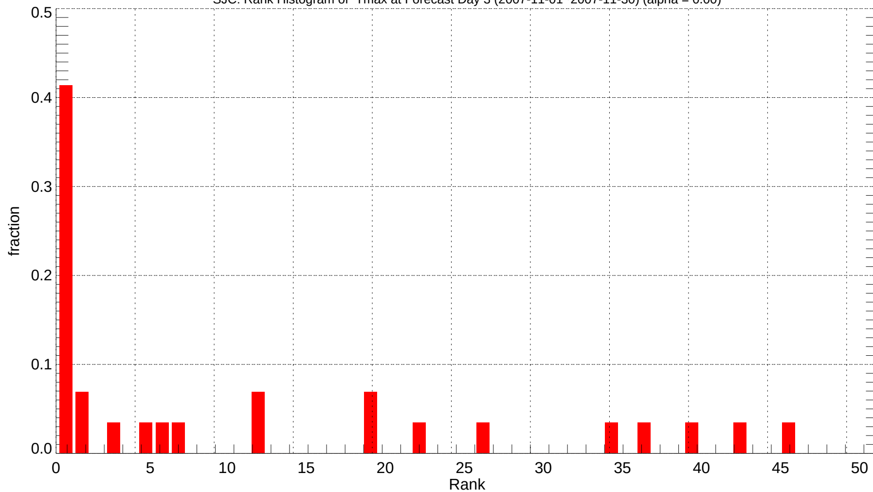
SJC: Rank Histogram of Tmax at Forecast Day 3 (2007-11-01~2007-11-30) (alpha = 0.00)
