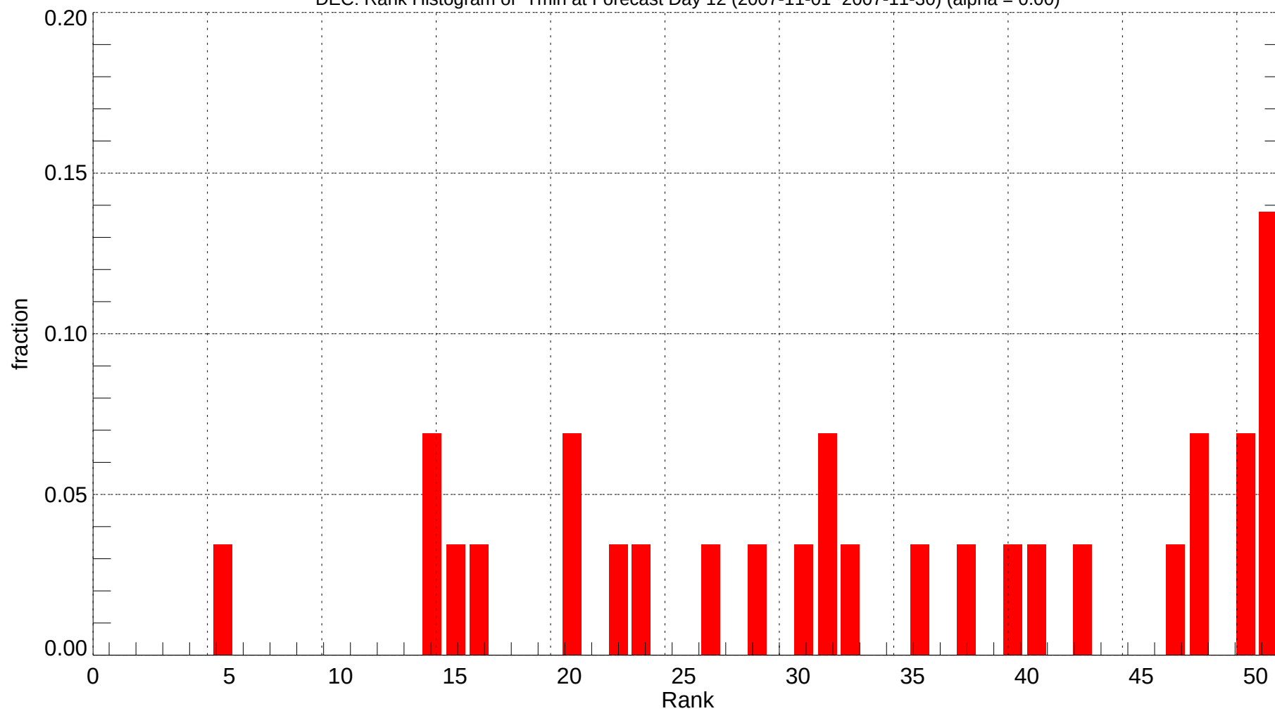
DEC: Rank Histogram of Tmin at Forecast Day 12 (2007-11-01~2007-11-30) (alpha = 0.00)
