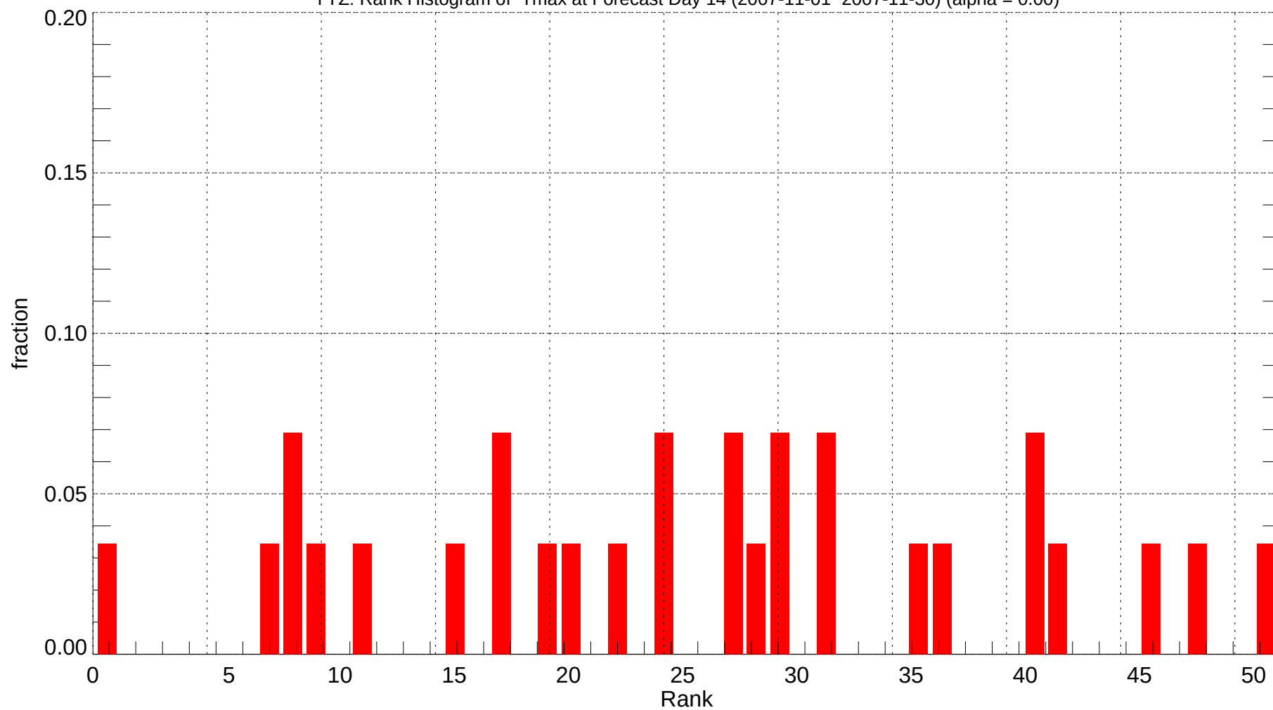
YYZ: Rank Histogram of Tmax at Forecast Day 14 (2007-11-01~2007-11-30) (alpha = 0.00)
