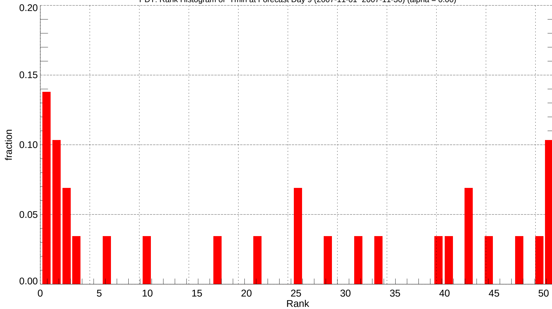
PDT: Rank Histogram of Tmin at Forecast Day 9 (2007-11-01~2007-11-30) (alpha = 0.00)
