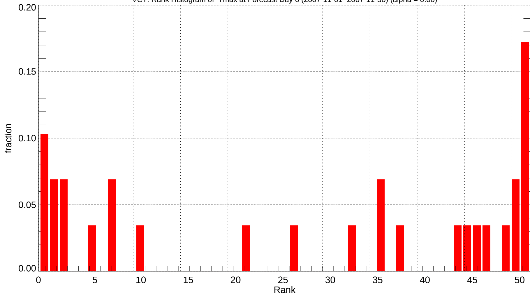
VCT: Rank Histogram of Tmax at Forecast Day 6 (2007-11-01~2007-11-30) (alpha = 0.00)
