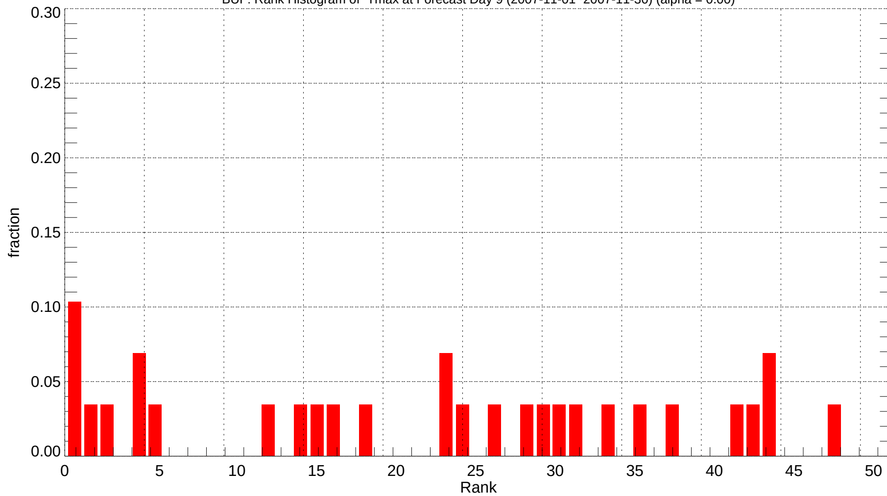
BUF: Rank Histogram of Tmax at Forecast Day 9 (2007-11-01~2007-11-30) (alpha = 0.00)
