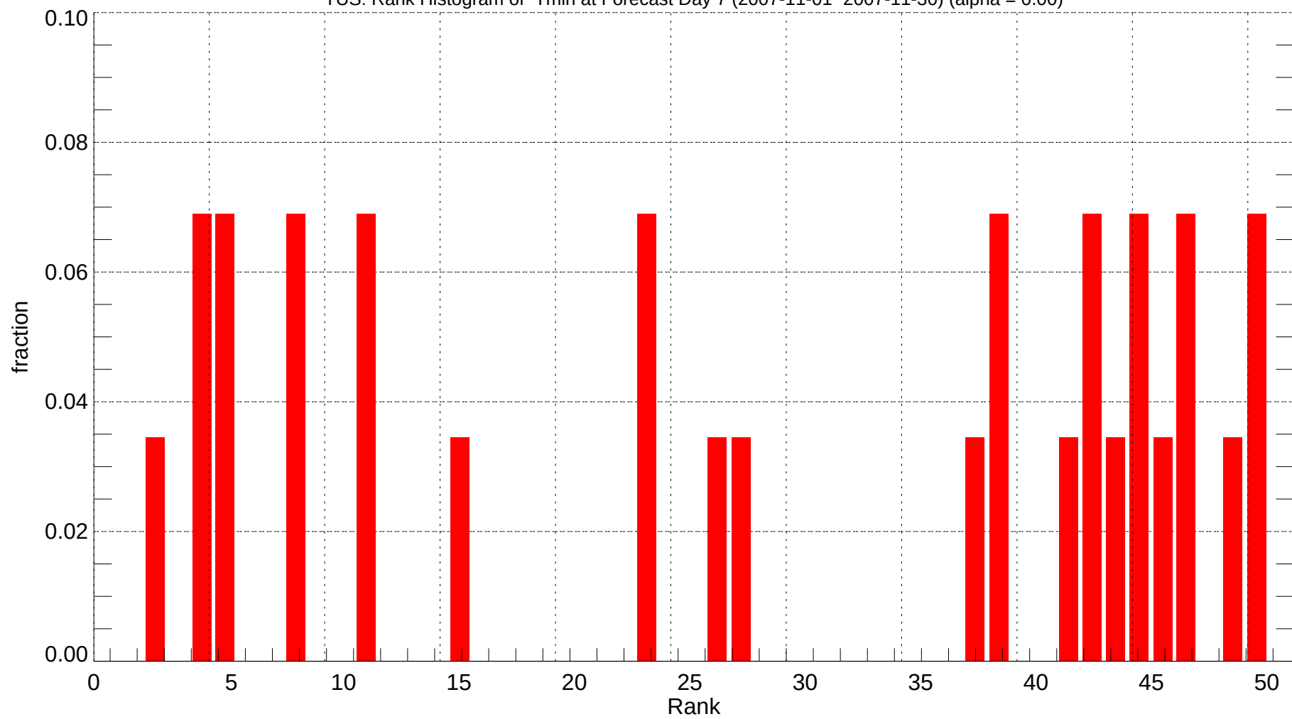
TUS: Rank Histogram of Tmin at Forecast Day 7 (2007-11-01~2007-11-30) (alpha = 0.00)
