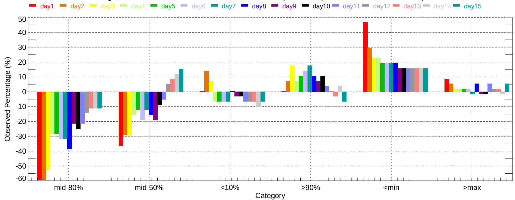
Observed Percentage Deviation of Ensembles - RBL: Min Temperature (2007-11-01~2007-11-30)
