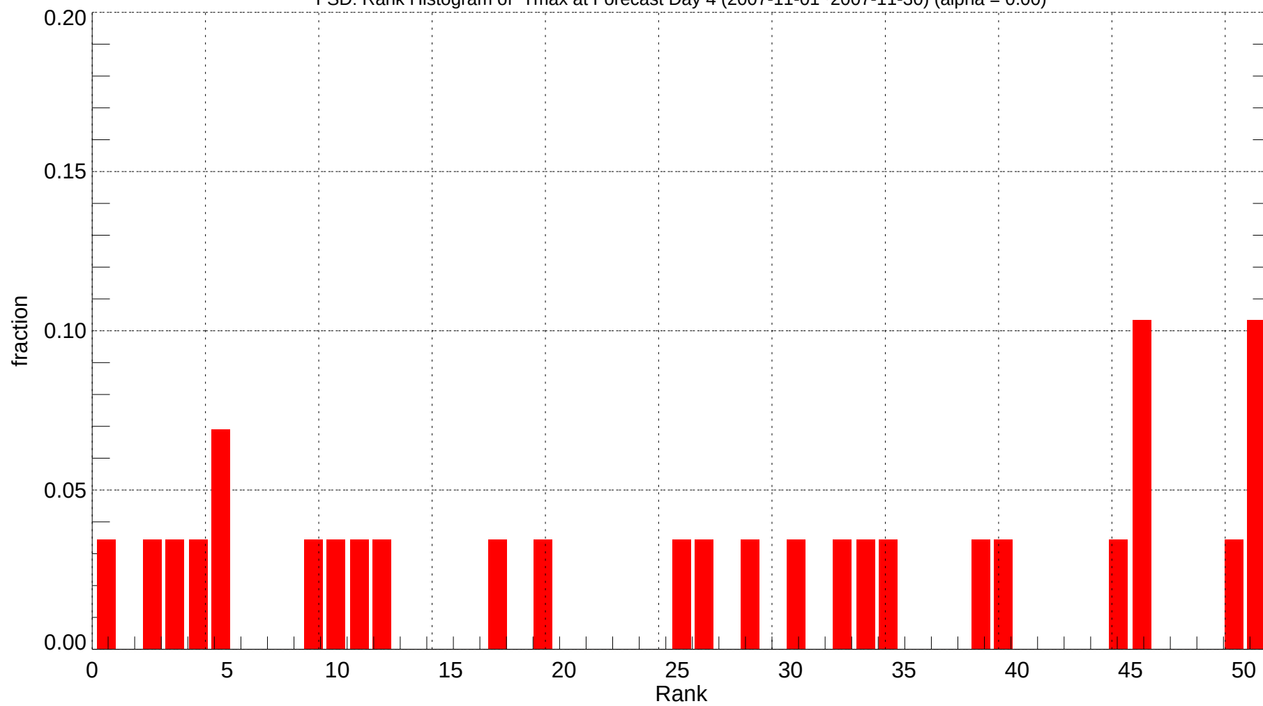
FSD: Rank Histogram of Tmax at Forecast Day 4 (2007-11-01~2007-11-30) (alpha = 0.00)
