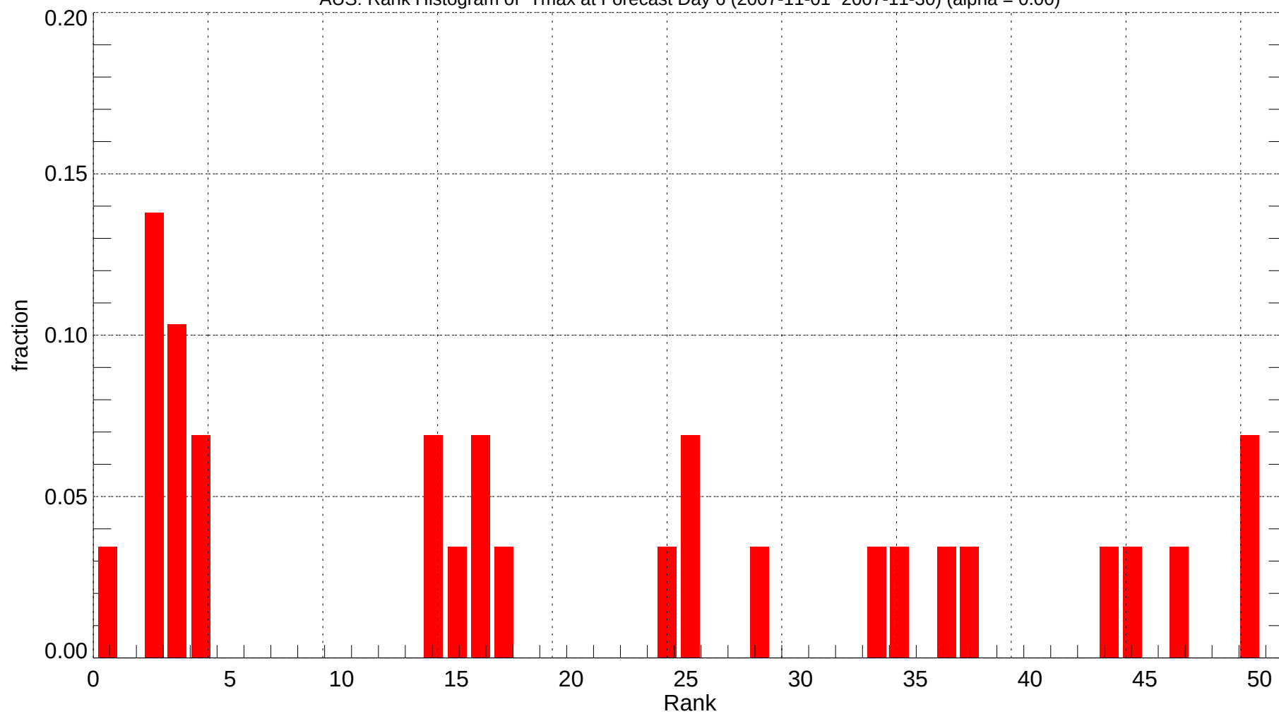
AUS: Rank Histogram of Tmax at Forecast Day 6 (2007-11-01~2007-11-30) (alpha = 0.00)
