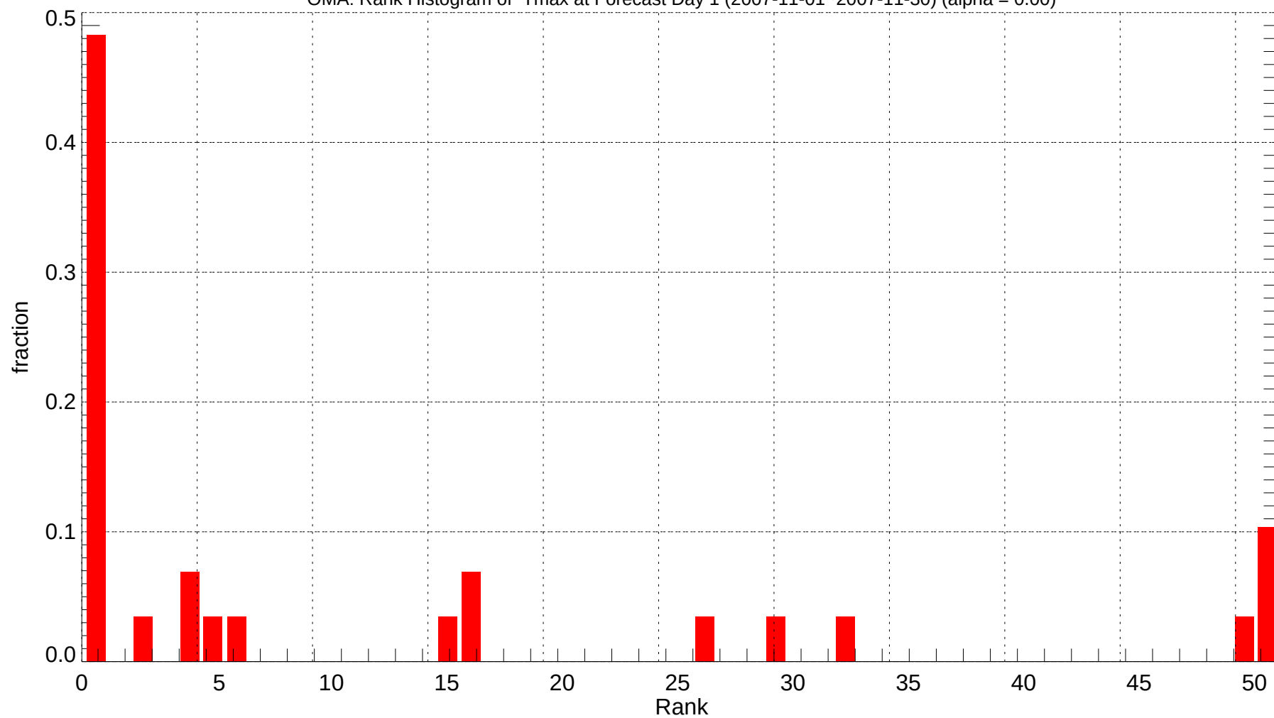
OMA: Rank Histogram of Tmax at Forecast Day 1 (2007-11-01~2007-11-30) (alpha = 0.00)
