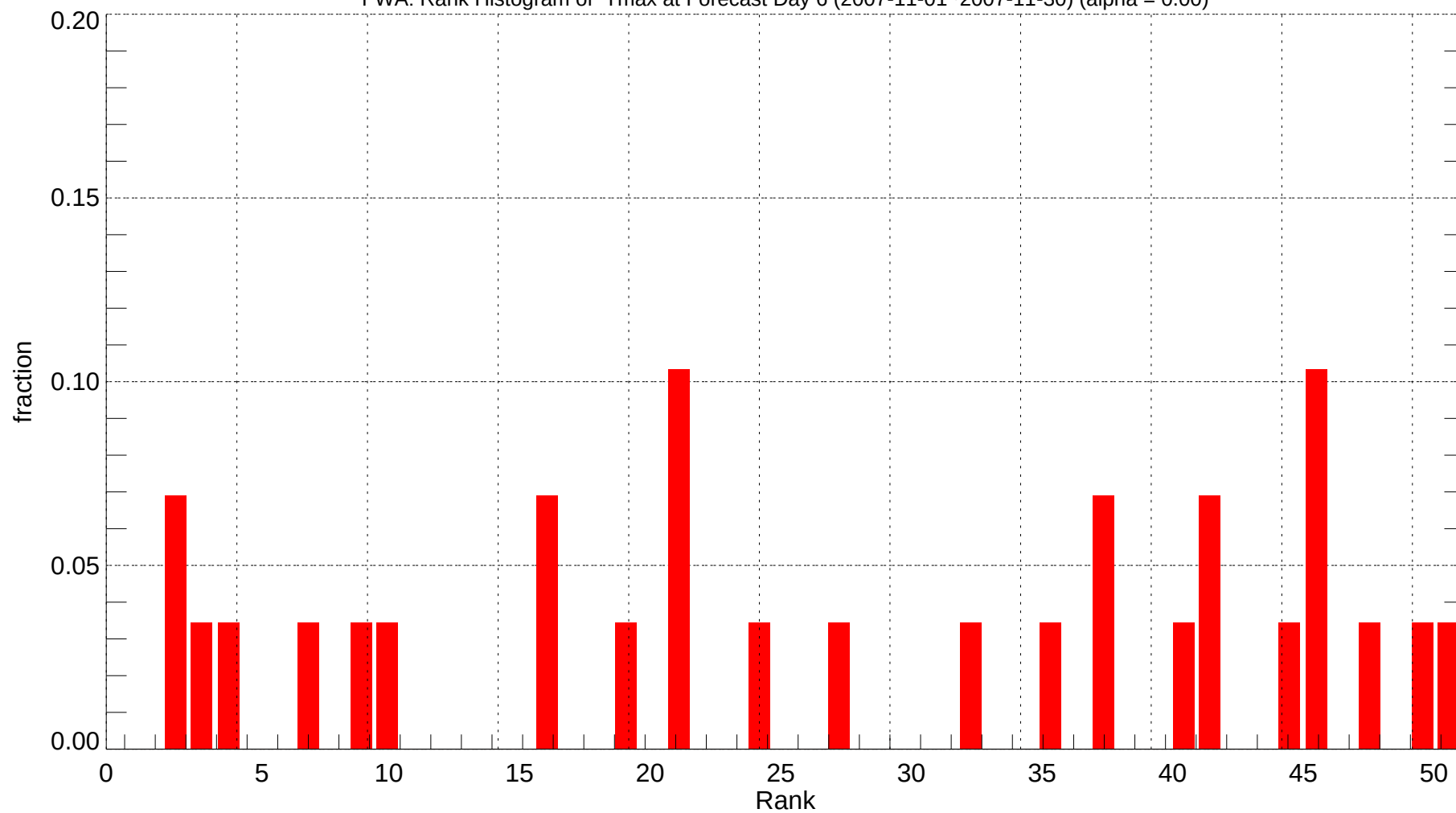
FWA: Rank Histogram of Tmax at Forecast Day 6 (2007-11-01~2007-11-30) (alpha = 0.00)
