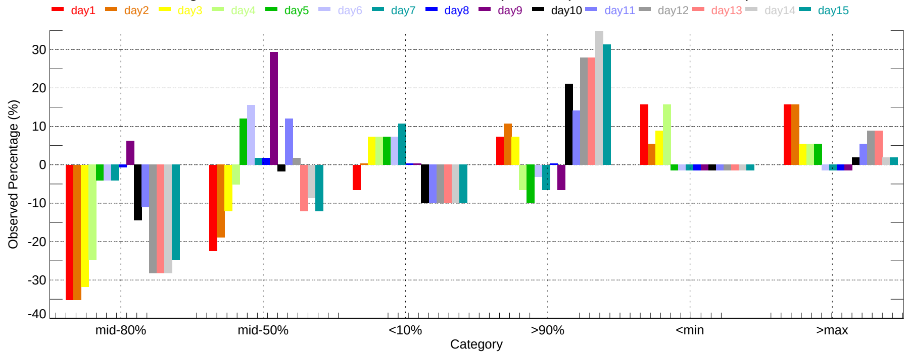
Observed Percentage Deviation of Ensembles - WJF: Min Temperature (2007-11-01~2007-11-30)
