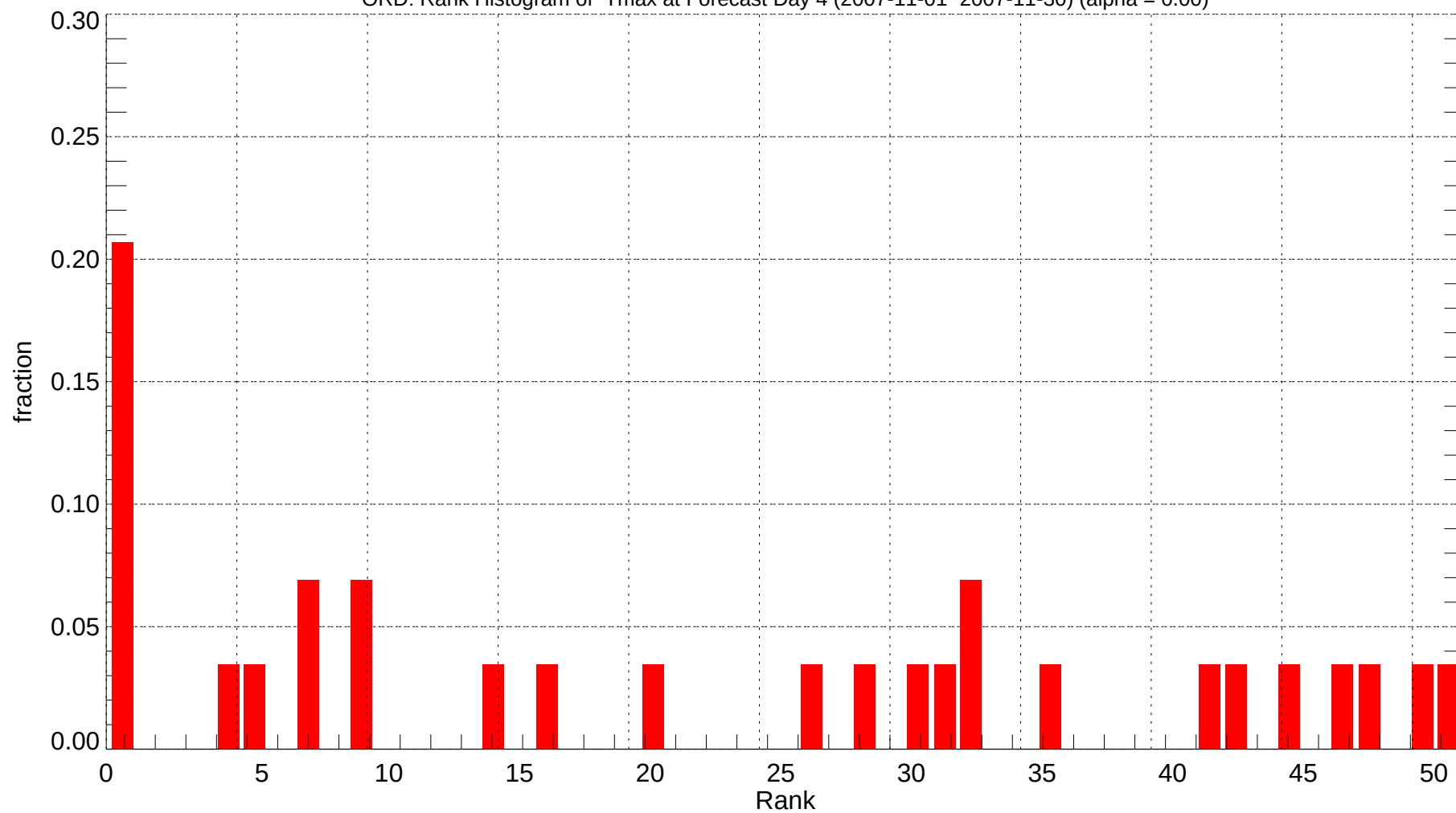
ORD: Rank Histogram of Tmax at Forecast Day 4 (2007-11-01~2007-11-30) (alpha = 0.00)
