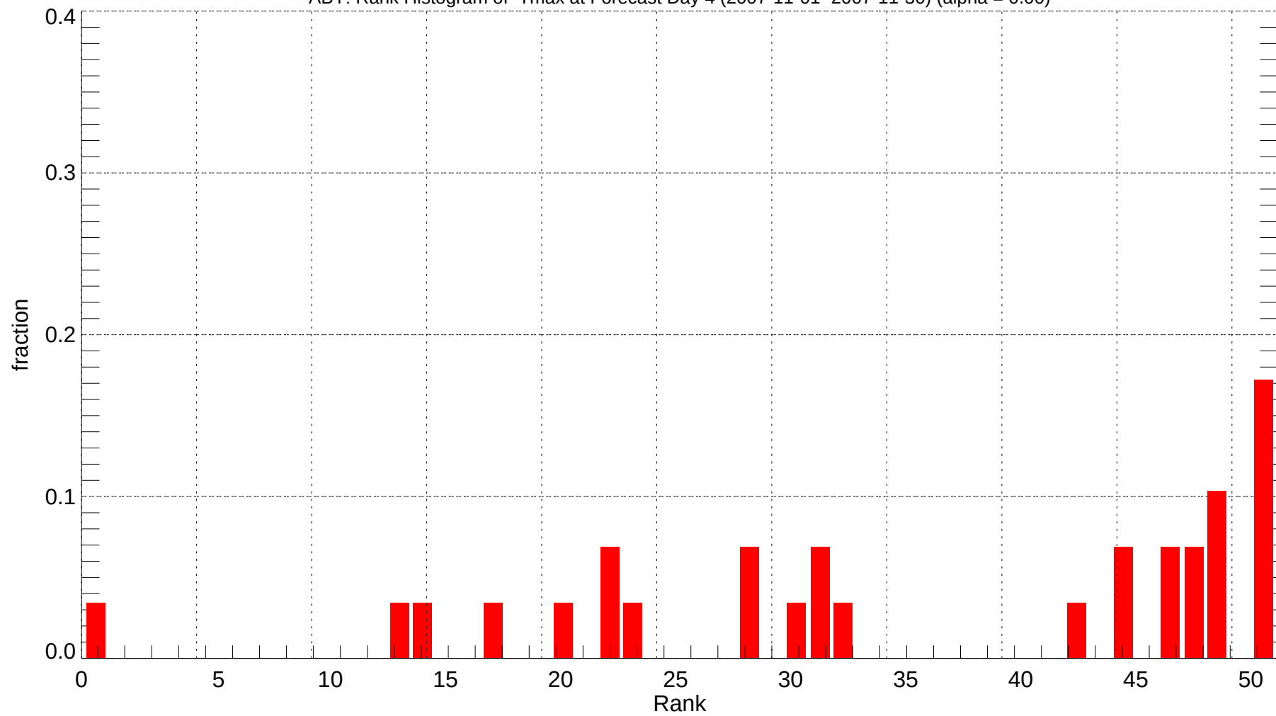
ABY: Rank Histogram of Tmax at Forecast Day 4 (2007-11-01~2007-11-30) (alpha = 0.00)
