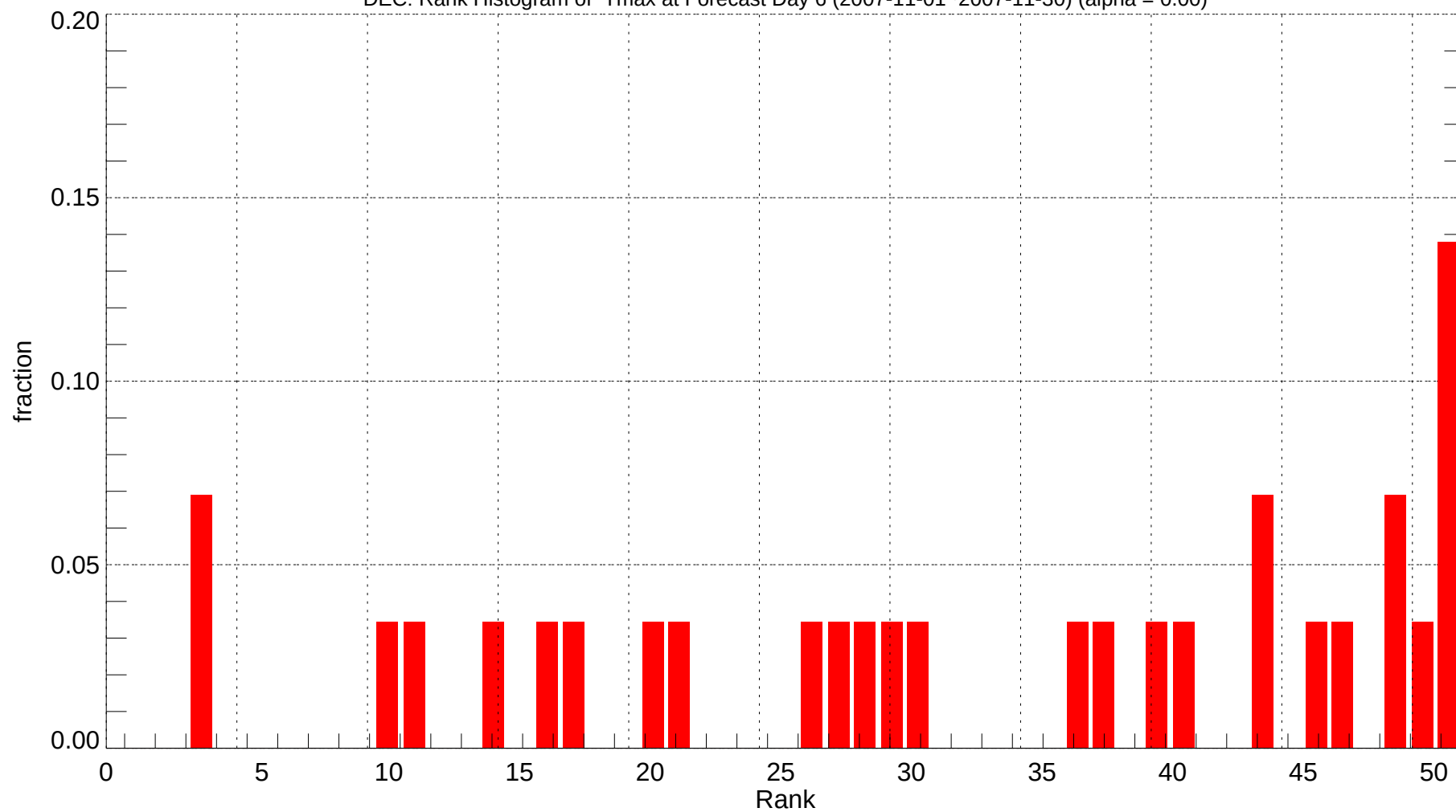
DEC: Rank Histogram of Tmax at Forecast Day 6 (2007-11-01~2007-11-30) (alpha = 0.00)
