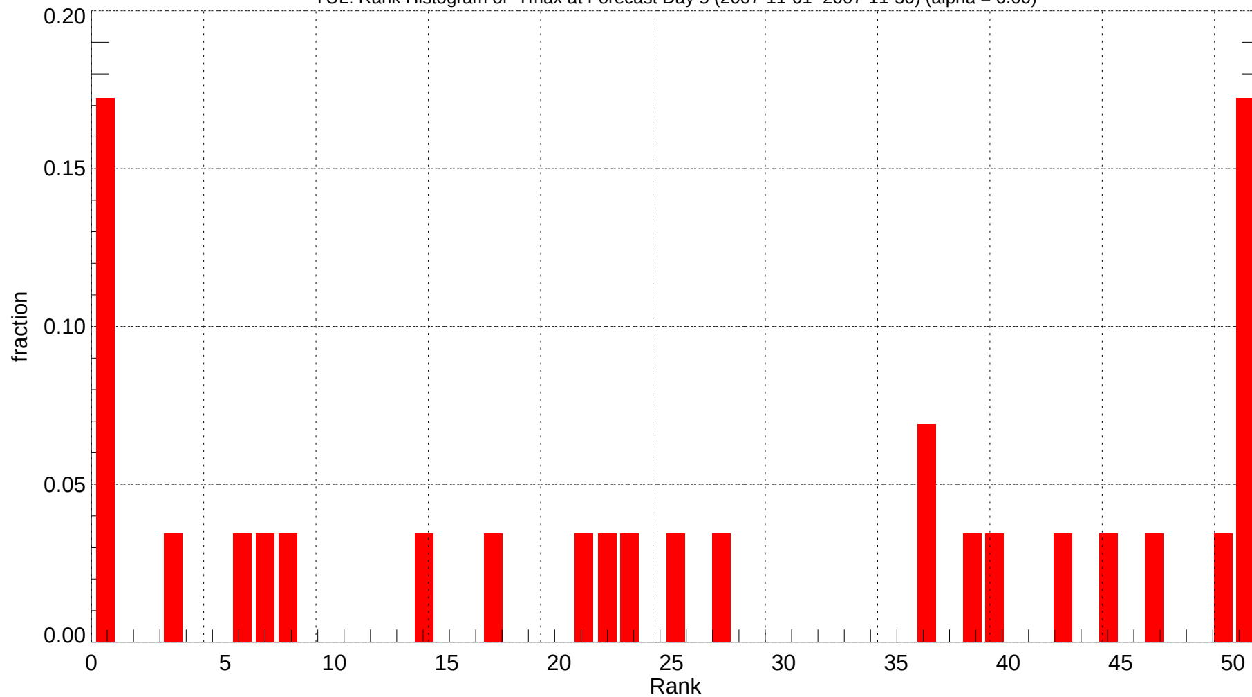
YUL: Rank Histogram of Tmax at Forecast Day 5 (2007-11-01~2007-11-30) (alpha = 0.00)
