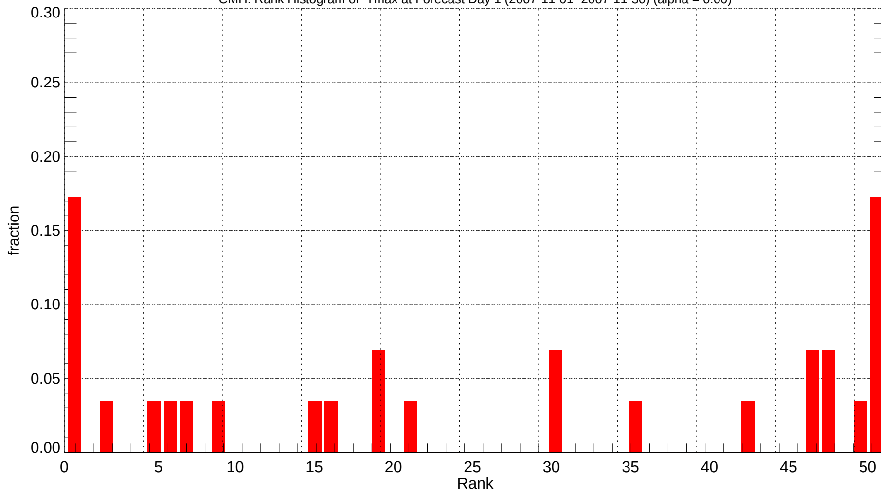
CMH: Rank Histogram of Tmax at Forecast Day 1 (2007-11-01~2007-11-30) (alpha = 0.00)
