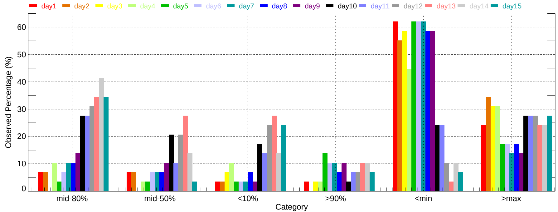
Observed Percentage of Ensembles - LAX: Min Temperature (2007-11-01~2007-11-30)
