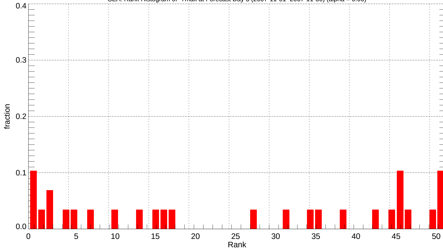
SEA: Rank Histogram of Tmax at Forecast Day 3 (2007-11-01~2007-11-30) (alpha = 0.00)
