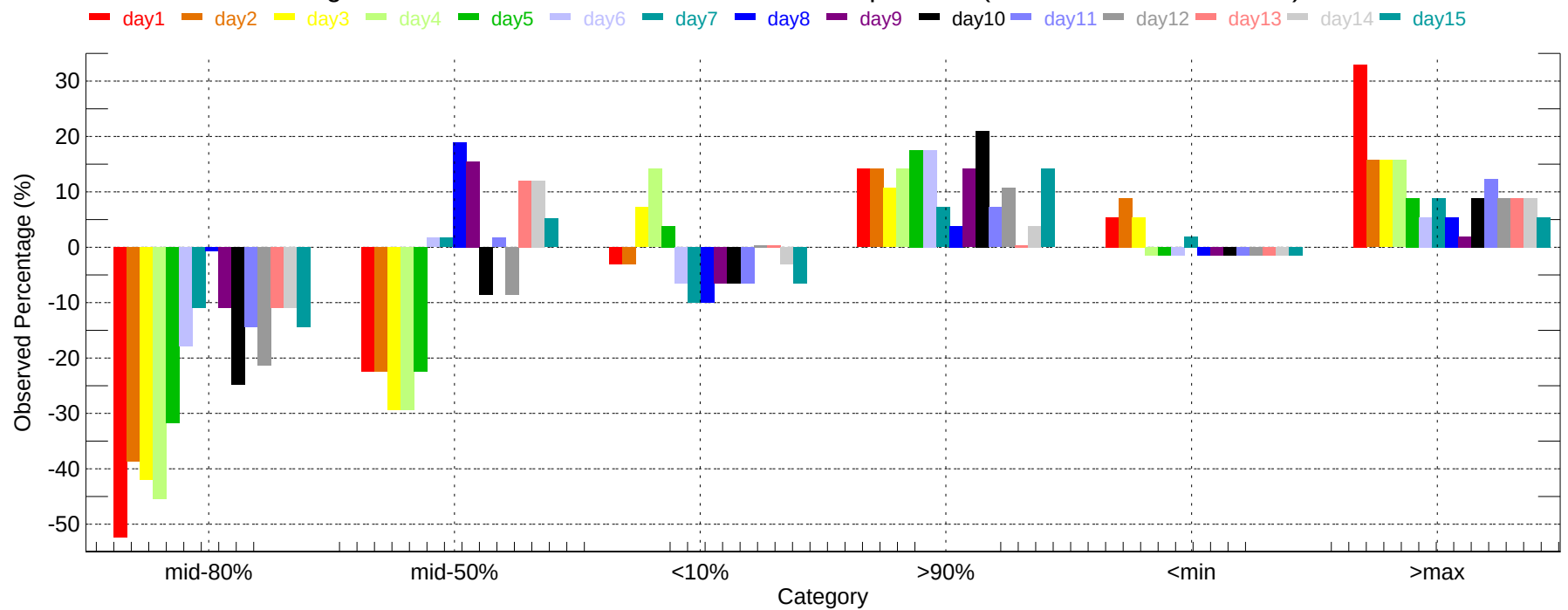
Observed Percentage Deviation of Ensembles - SLC: Max Temperature (2007-11-01~2007-11-30)
