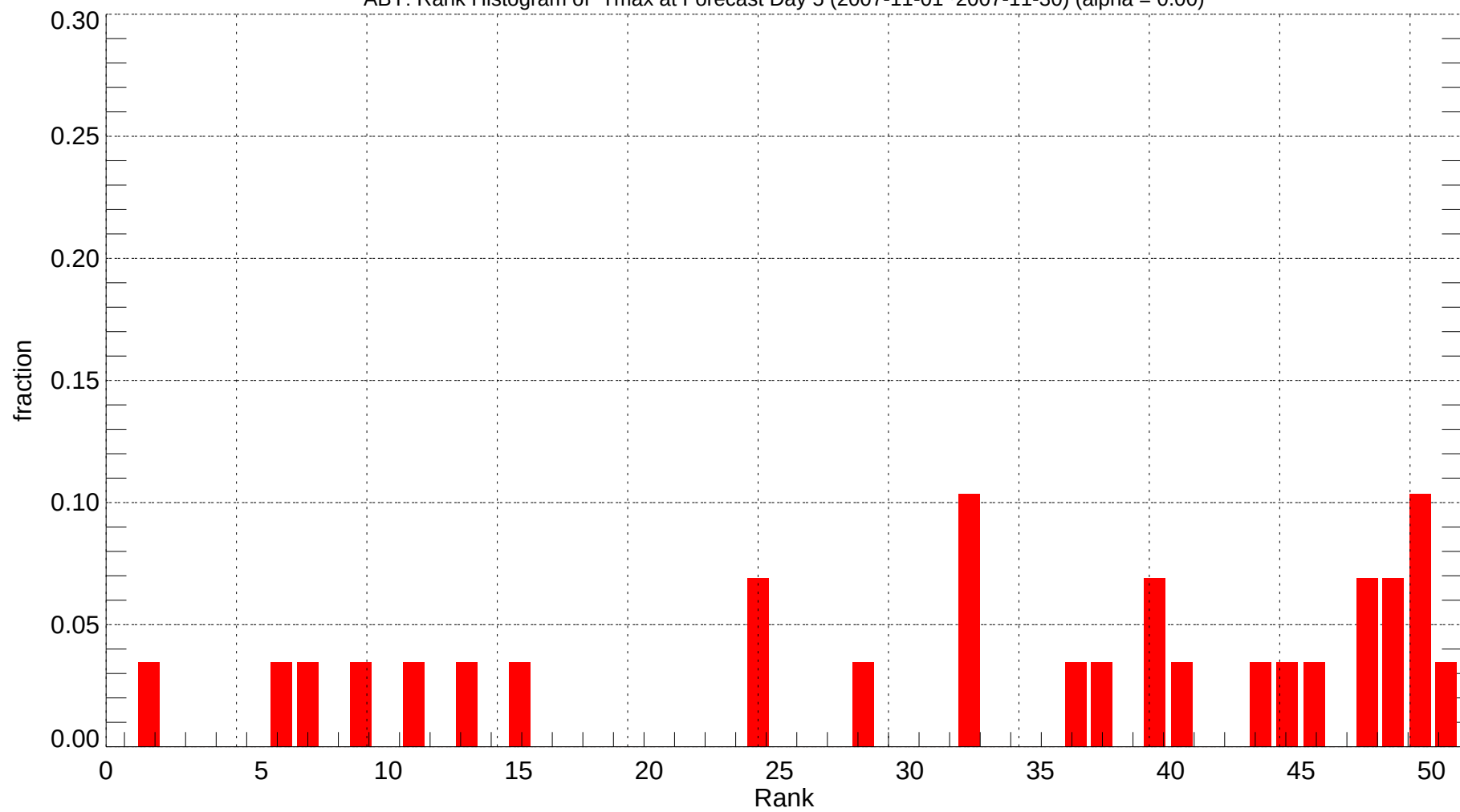
ABY: Rank Histogram of Tmax at Forecast Day 5 (2007-11-01~2007-11-30) (alpha = 0.00)
