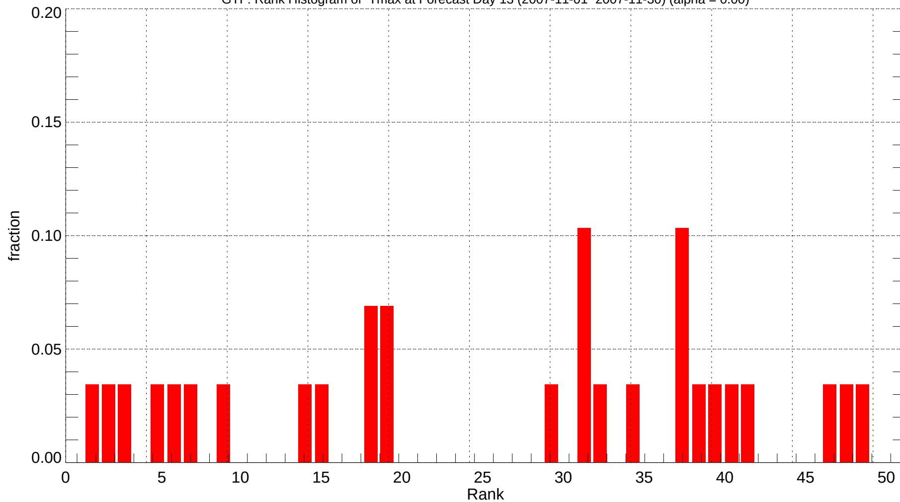
GTF: Rank Histogram of Tmax at Forecast Day 13 (2007-11-01~2007-11-30) (alpha = 0.00)
