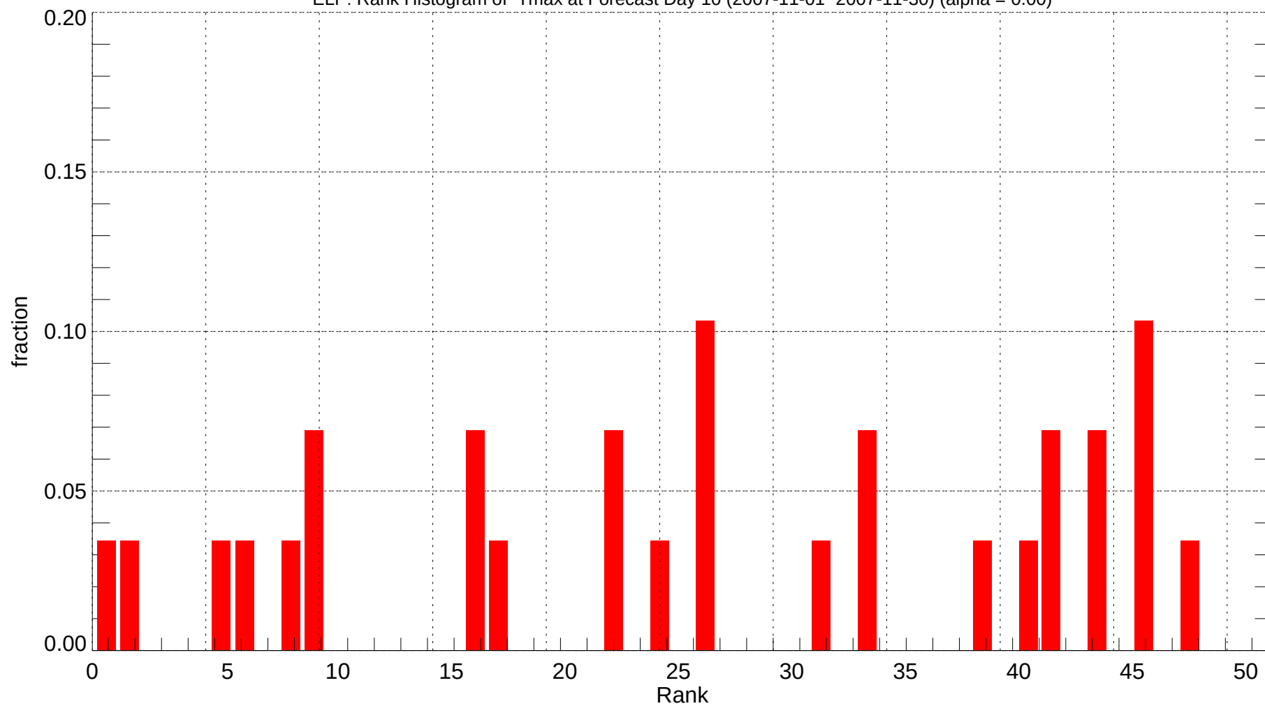
ELP: Rank Histogram of Tmax at Forecast Day 10 (2007-11-01~2007-11-30) (alpha = 0.00)
