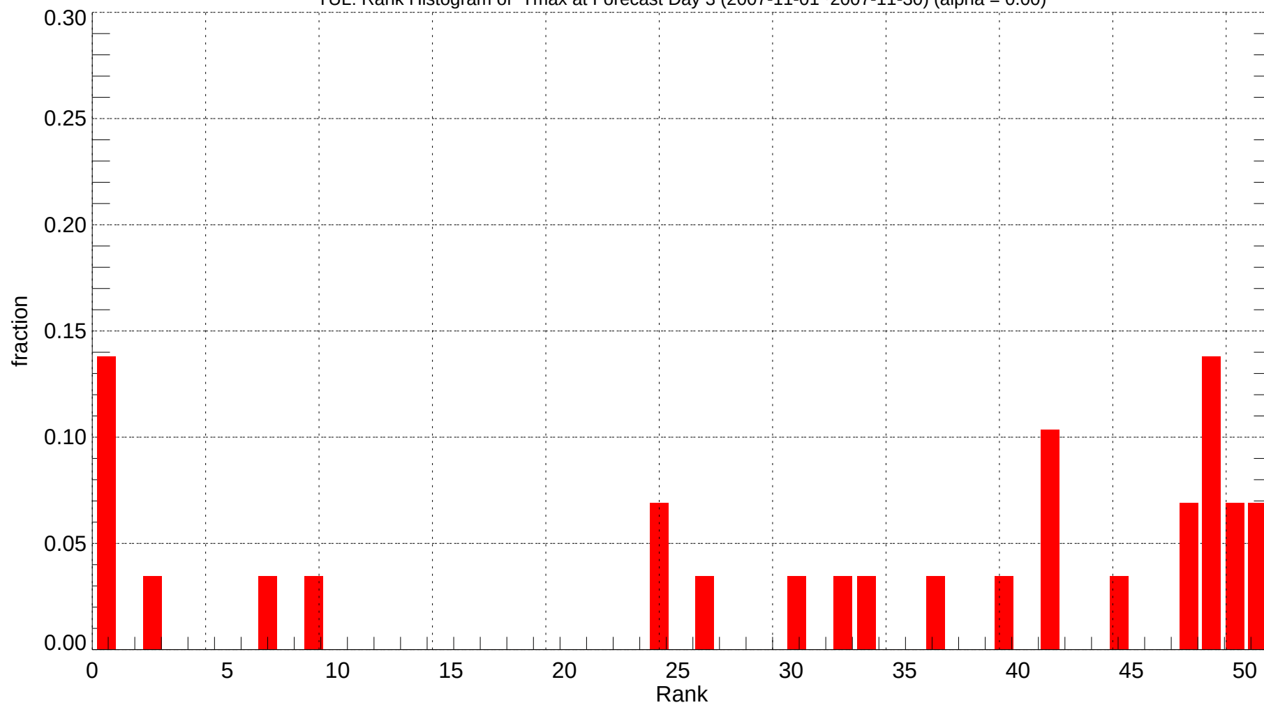
TUL: Rank Histogram of Tmax at Forecast Day 3 (2007-11-01~2007-11-30) (alpha = 0.00)
