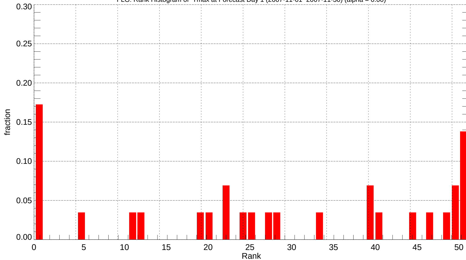
FLG: Rank Histogram of Tmax at Forecast Day 1 (2007-11-01~2007-11-30) (alpha = 0.00)
