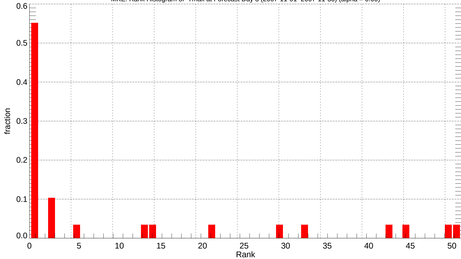
MKE: Rank Histogram of Tmax at Forecast Day 3 (2007-11-01~2007-11-30) (alpha = 0.00)
