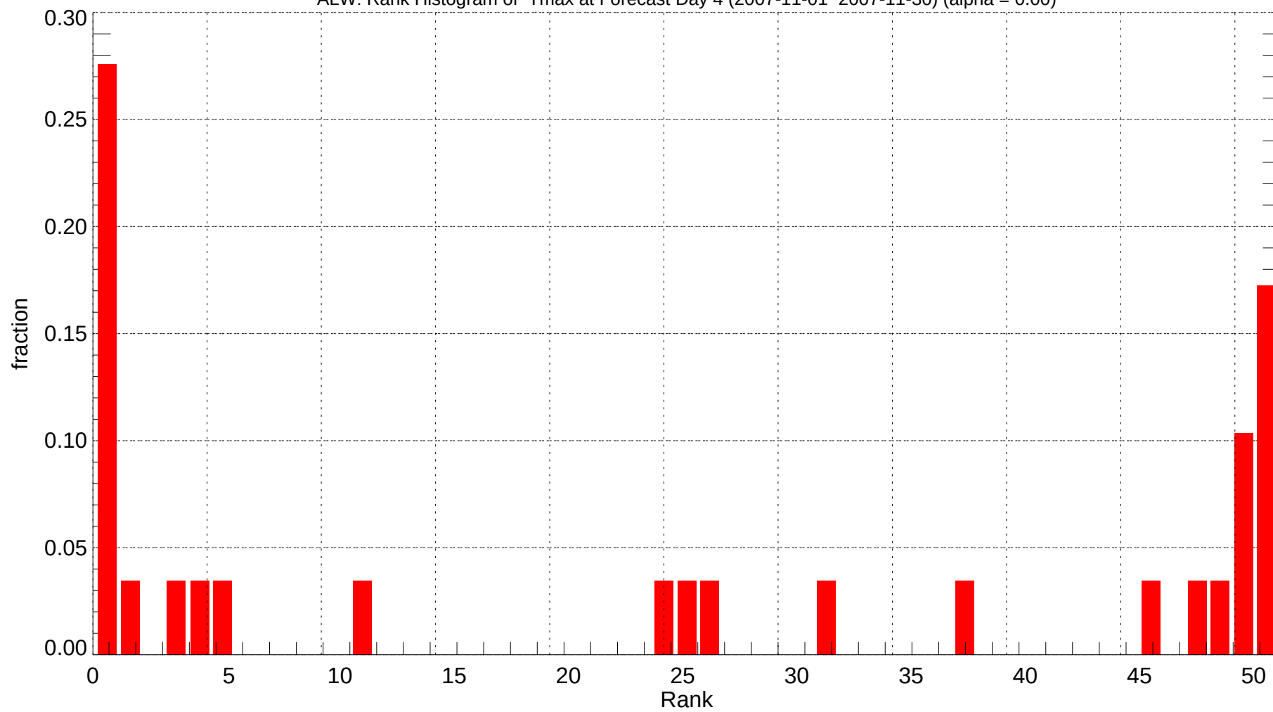
ALW: Rank Histogram of Tmax at Forecast Day 4 (2007-11-01~2007-11-30) (alpha = 0.00)
