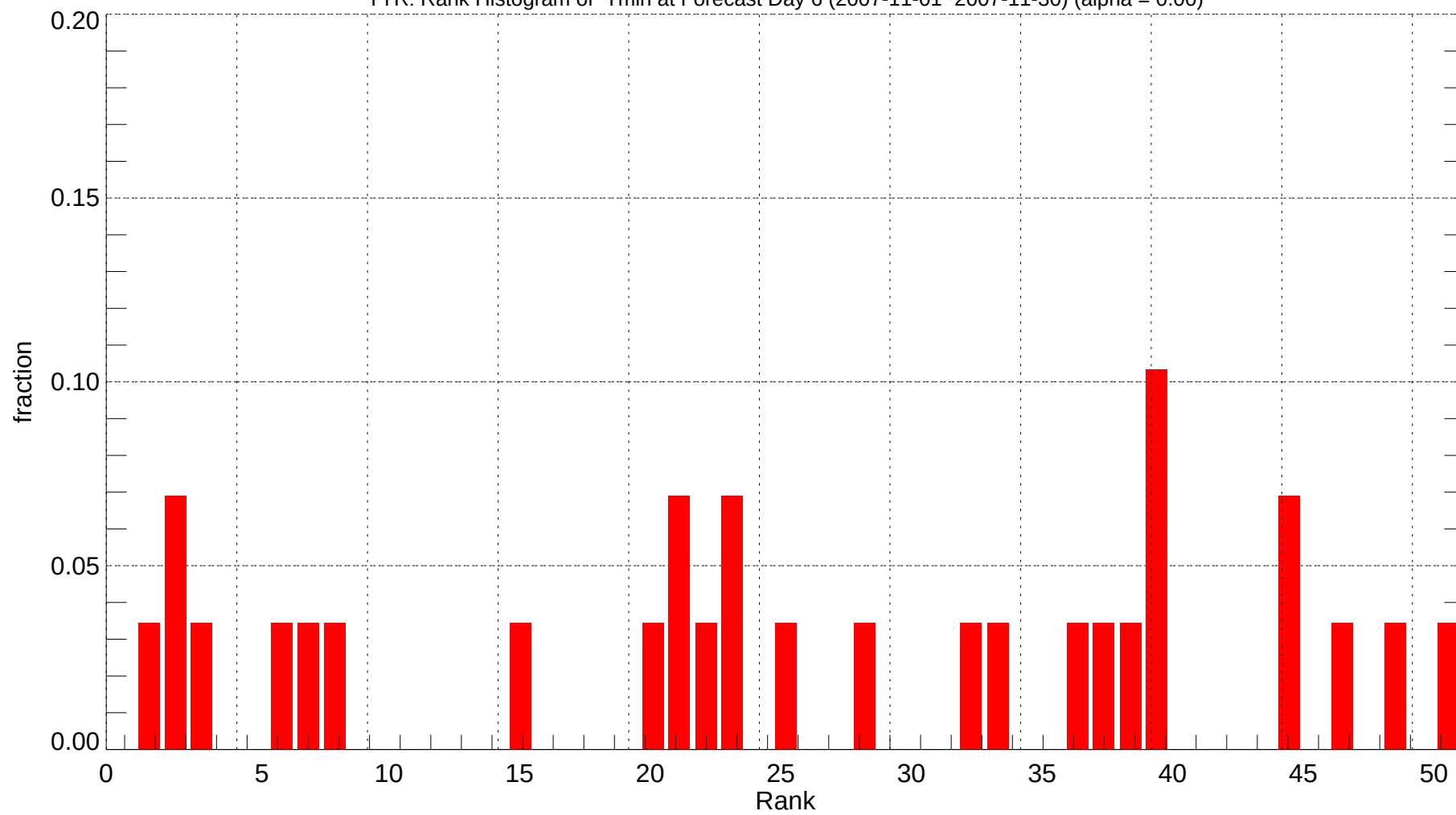
TYR: Rank Histogram of Tmin at Forecast Day 6 (2007-11-01~2007-11-30) (alpha = 0.00)
