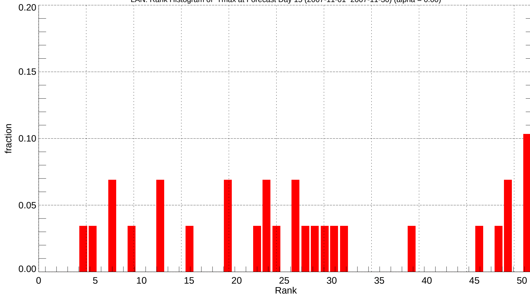
LAN: Rank Histogram of Tmax at Forecast Day 15 (2007-11-01~2007-11-30) (alpha = 0.00)
