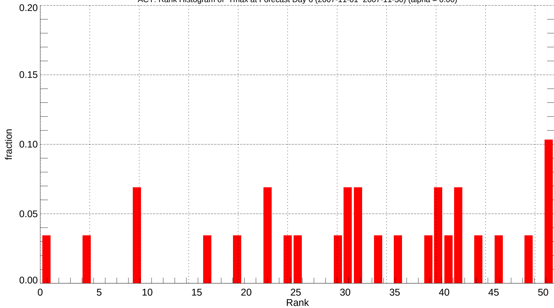
ACY: Rank Histogram of Tmax at Forecast Day 6 (2007-11-01~2007-11-30) (alpha = 0.00)
