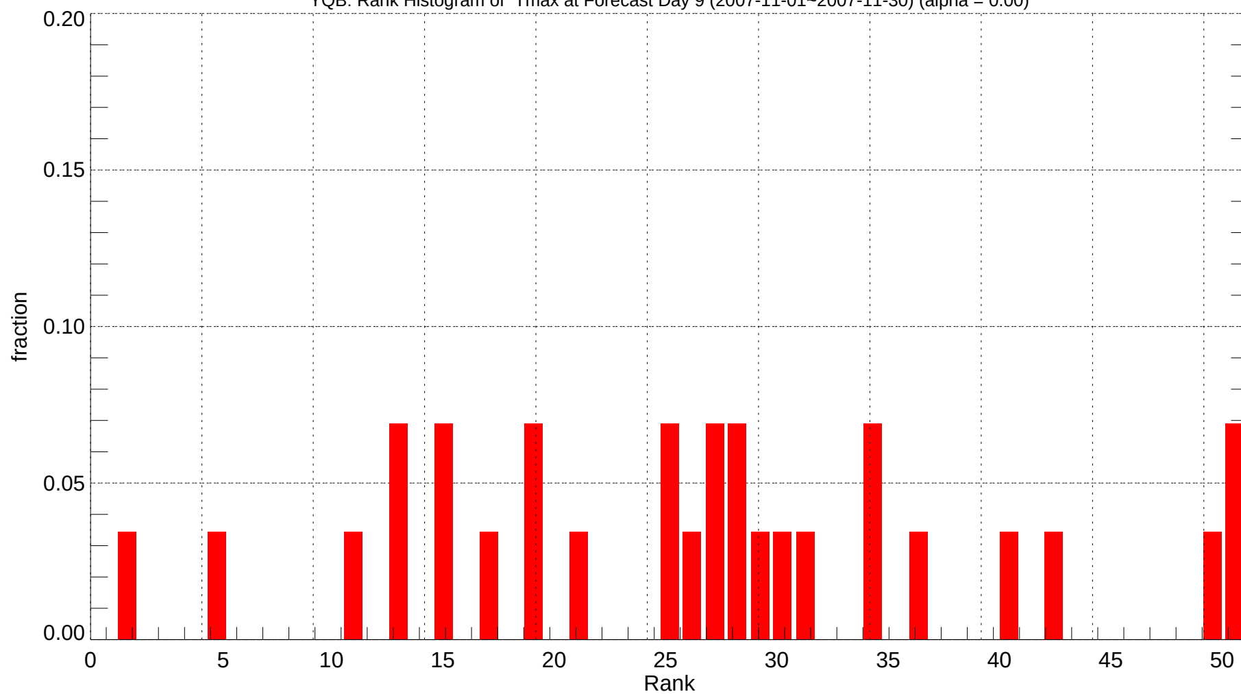
YQB: Rank Histogram of Tmax at Forecast Day 9 (2007-11-01~2007-11-30) (alpha = 0.00)
