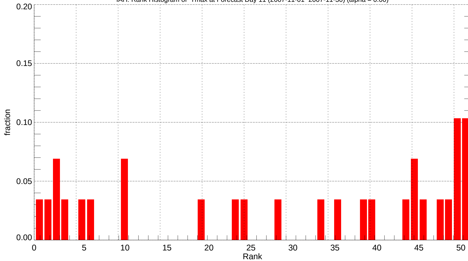
IAH: Rank Histogram of Tmax at Forecast Day 11 (2007-11-01~2007-11-30) (alpha = 0.00)
