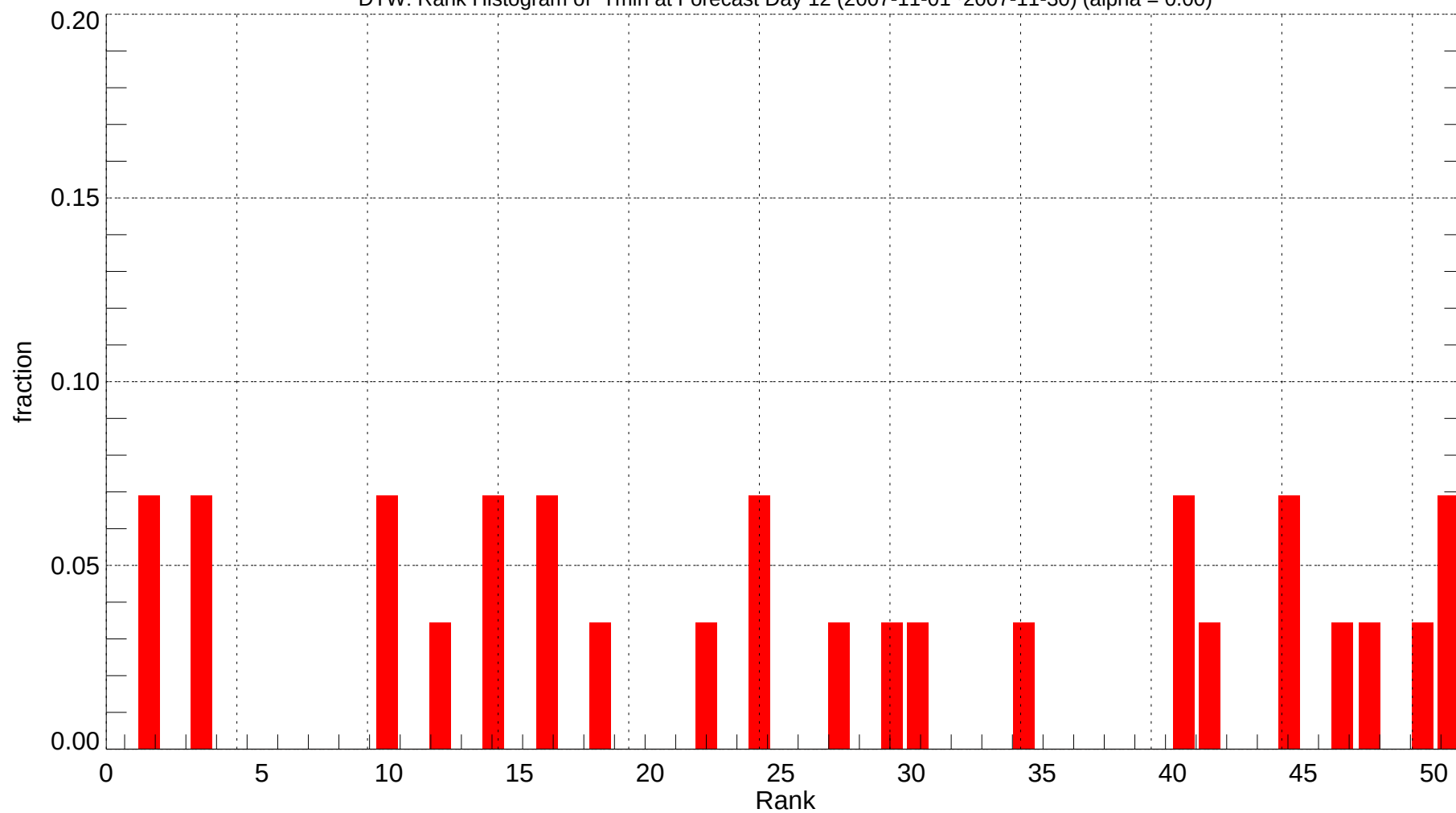
DTW: Rank Histogram of Tmin at Forecast Day 12 (2007-11-01~2007-11-30) (alpha = 0.00)
