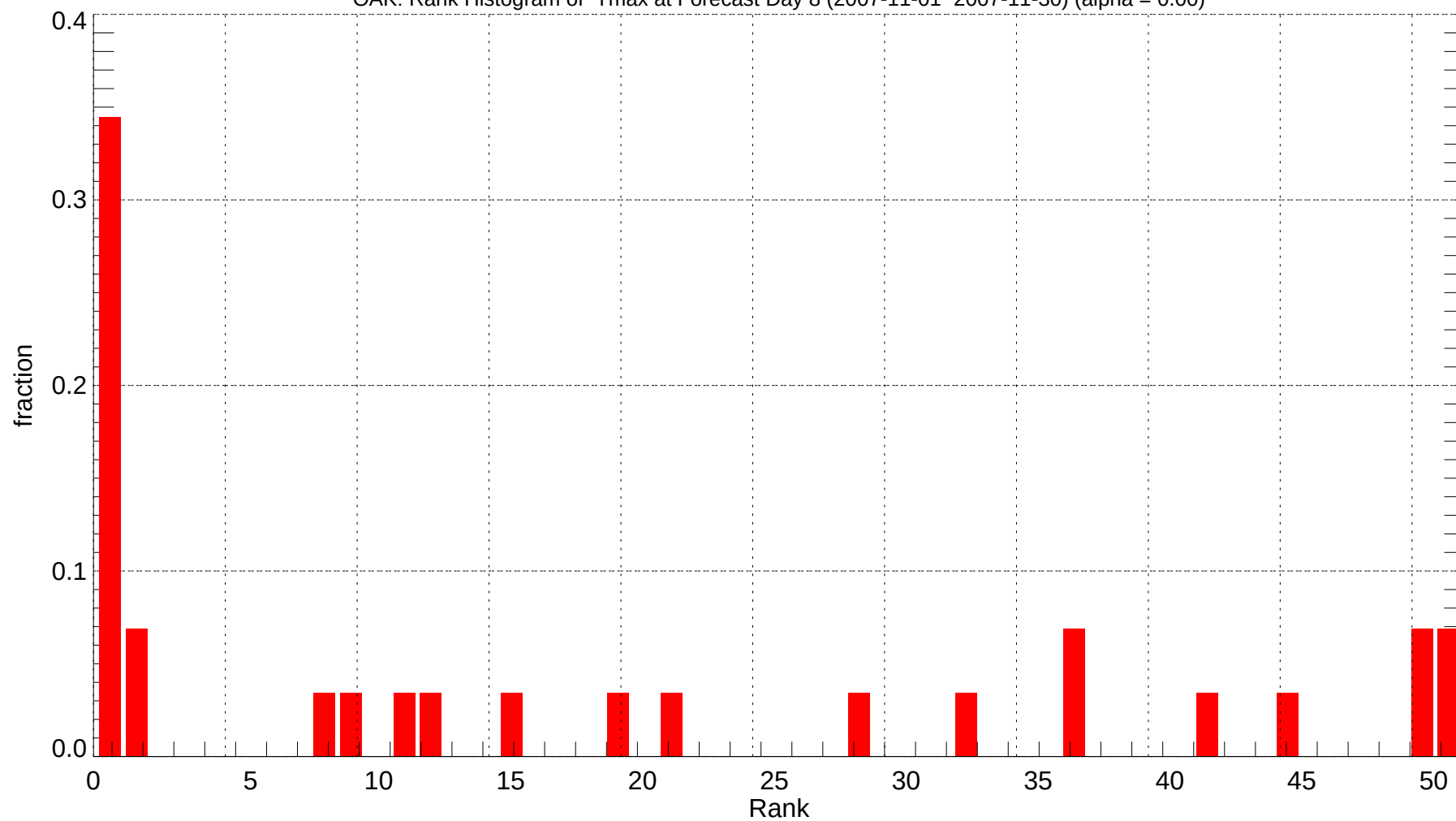
OAK: Rank Histogram of Tmax at Forecast Day 8 (2007-11-01~2007-11-30) (alpha = 0.00)
