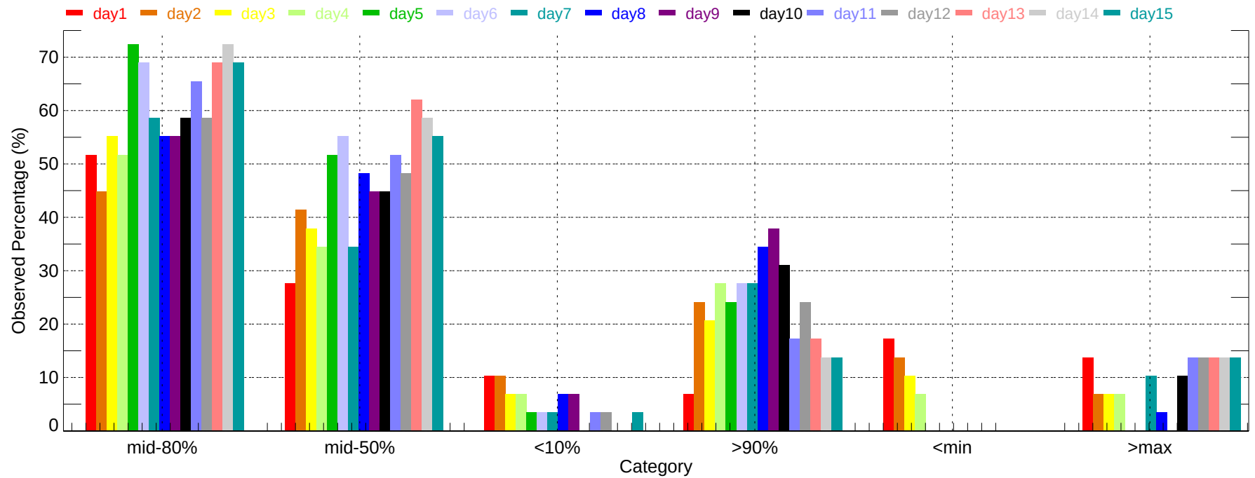
Observed Percentage of Ensembles - DAY: Min Temperature (2007-11-01~2007-11-30)
