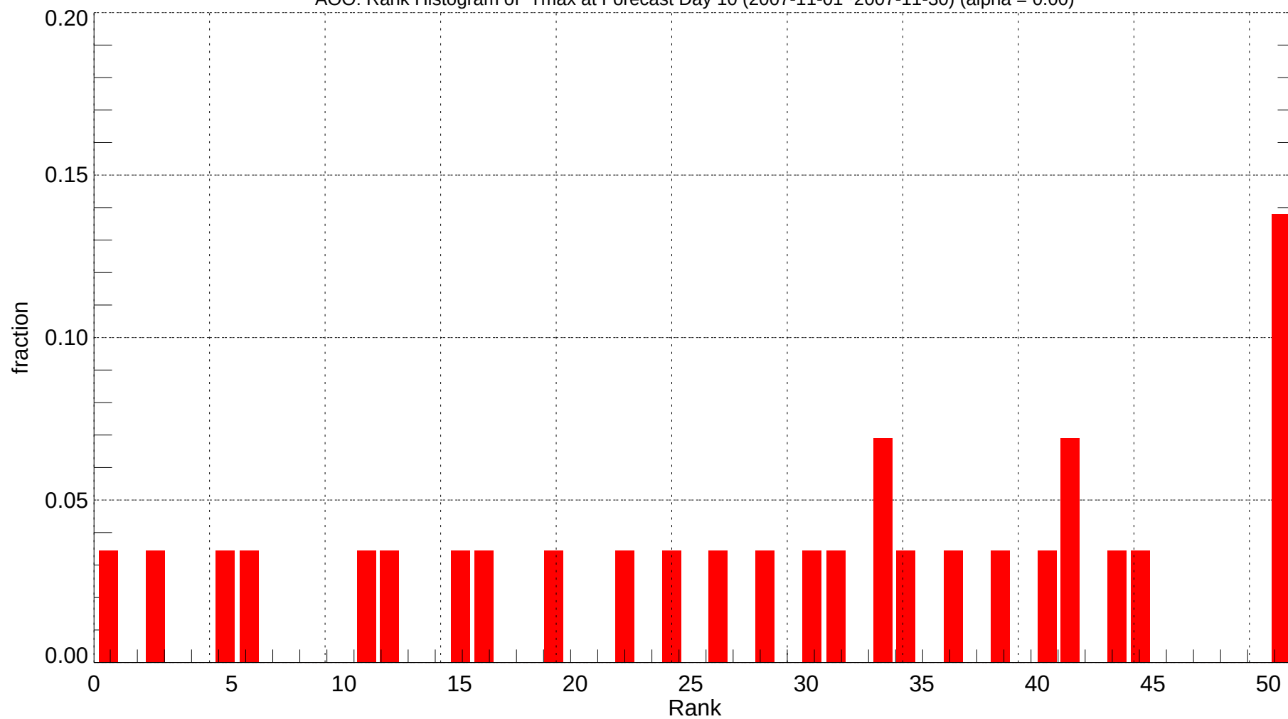
AOO: Rank Histogram of Tmax at Forecast Day 10 (2007-11-01~2007-11-30) (alpha = 0.00)
