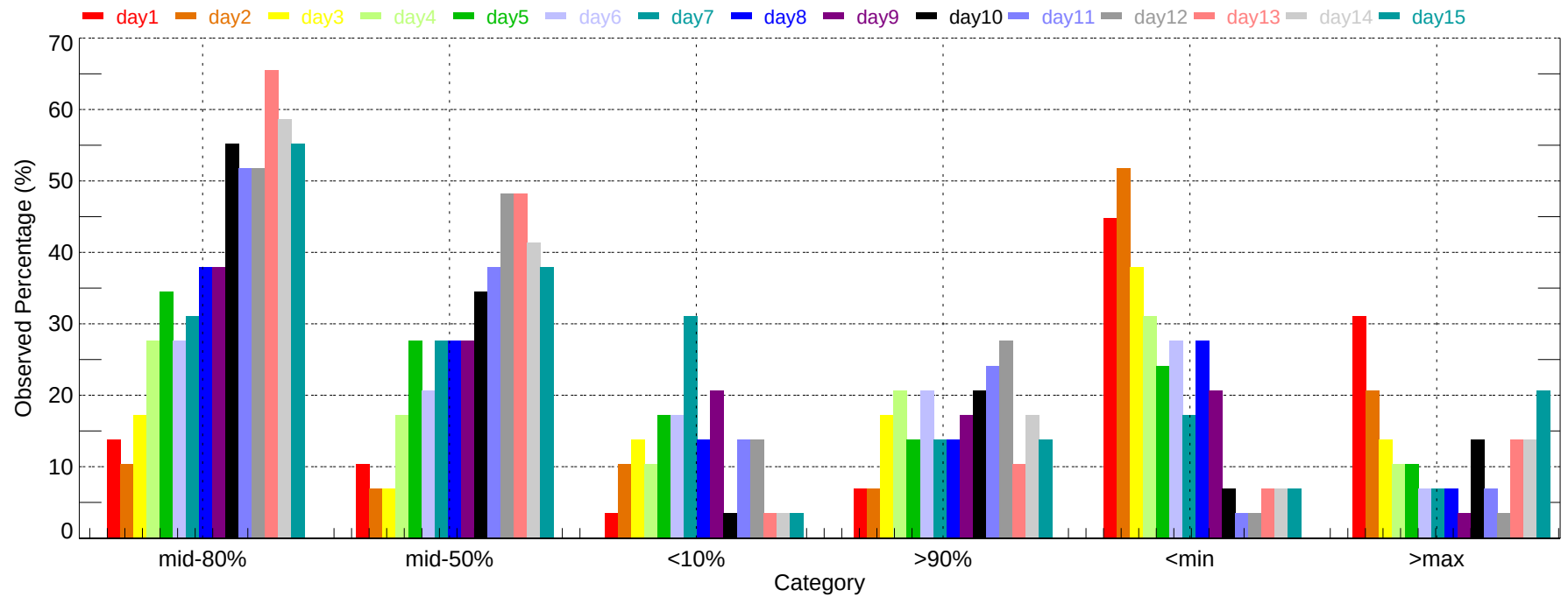
Observed Percentage of Ensembles - OAK: Max Temperature (2007-11-01~2007-11-30)
