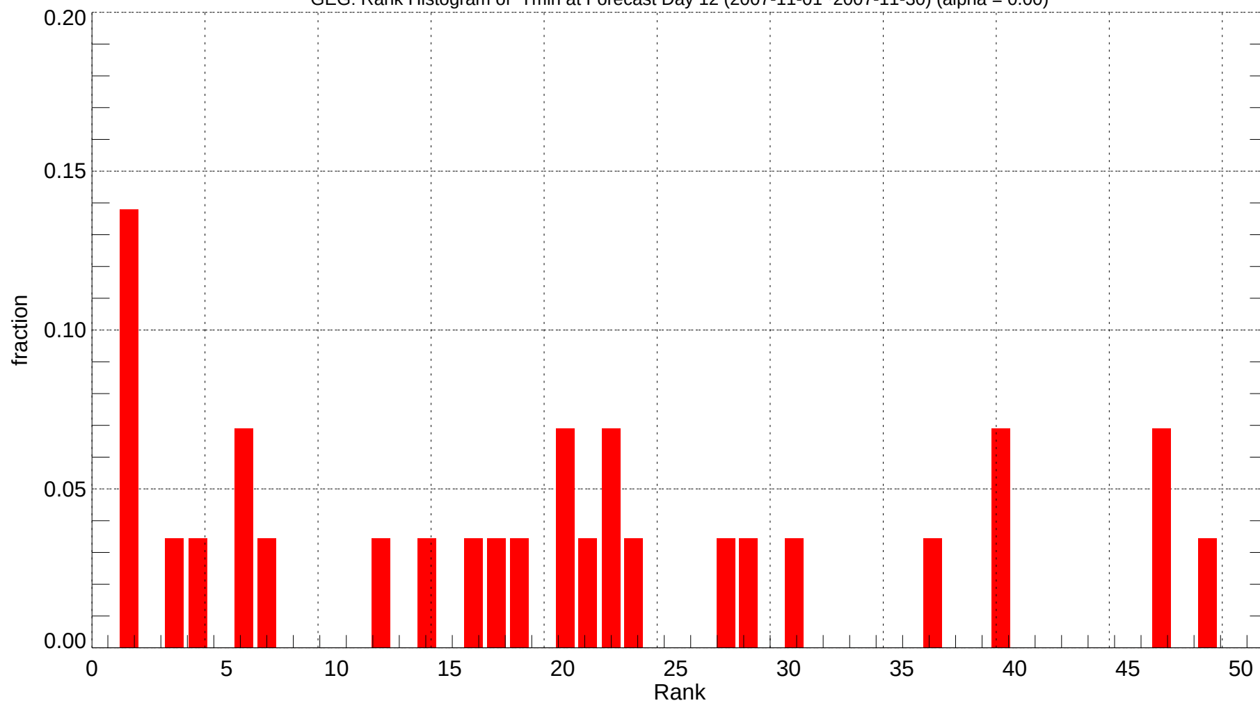
GEG: Rank Histogram of Tmin at Forecast Day 12 (2007-11-01~2007-11-30) (alpha = 0.00)
