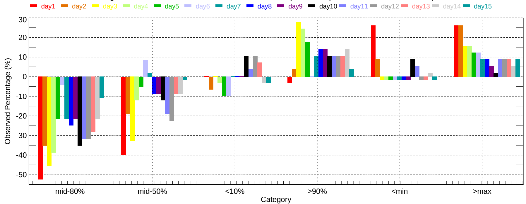
Observed Percentage Deviation of Ensembles - NTU: Min Temperature (2007-11-01~2007-11-30)
