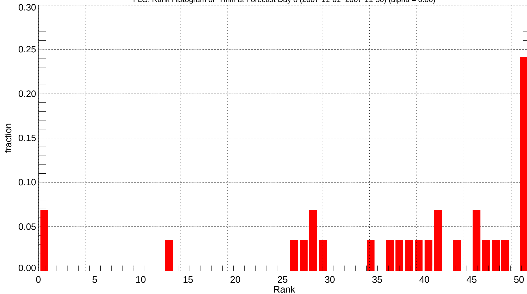
FLG: Rank Histogram of Tmin at Forecast Day 8 (2007-11-01~2007-11-30) (alpha = 0.00)
