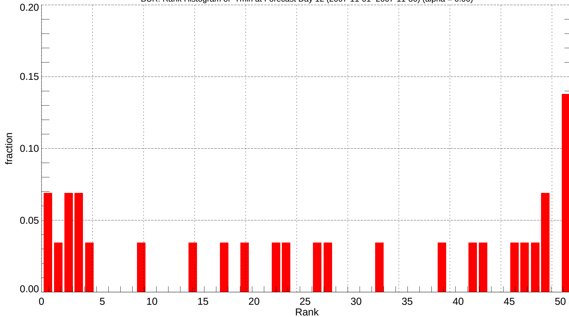
BUR: Rank Histogram of Tmin at Forecast Day 12 (2007-11-01~2007-11-30) (alpha = 0.00)
