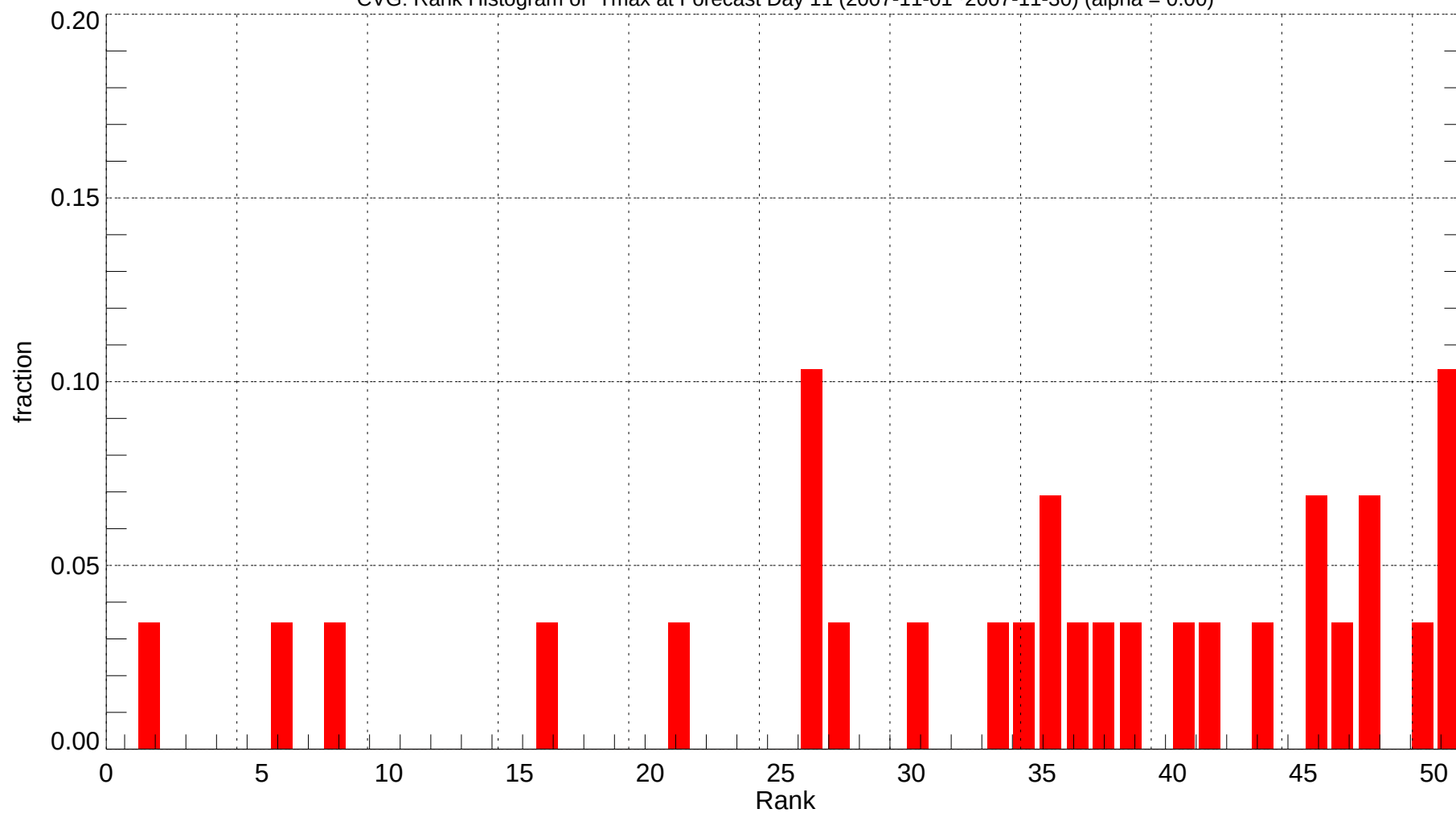
CVG: Rank Histogram of Tmax at Forecast Day 11 (2007-11-01~2007-11-30) (alpha = 0.00)
