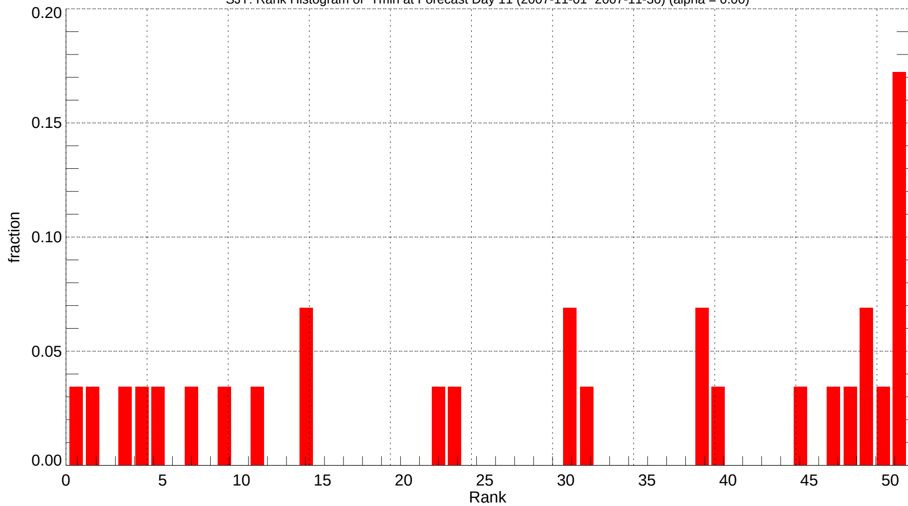
SJT: Rank Histogram of Tmin at Forecast Day 11 (2007-11-01~2007-11-30) (alpha = 0.00)
