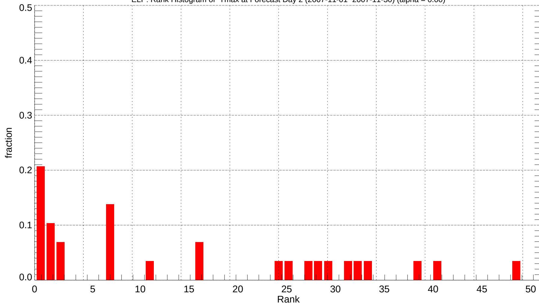
ELP: Rank Histogram of Tmax at Forecast Day 2 (2007-11-01~2007-11-30) (alpha = 0.00)
