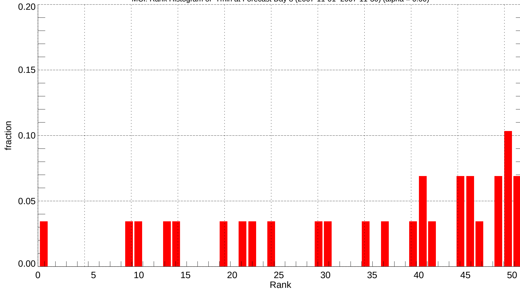
MCI: Rank Histogram of Tmin at Forecast Day 8 (2007-11-01~2007-11-30) (alpha = 0.00)
