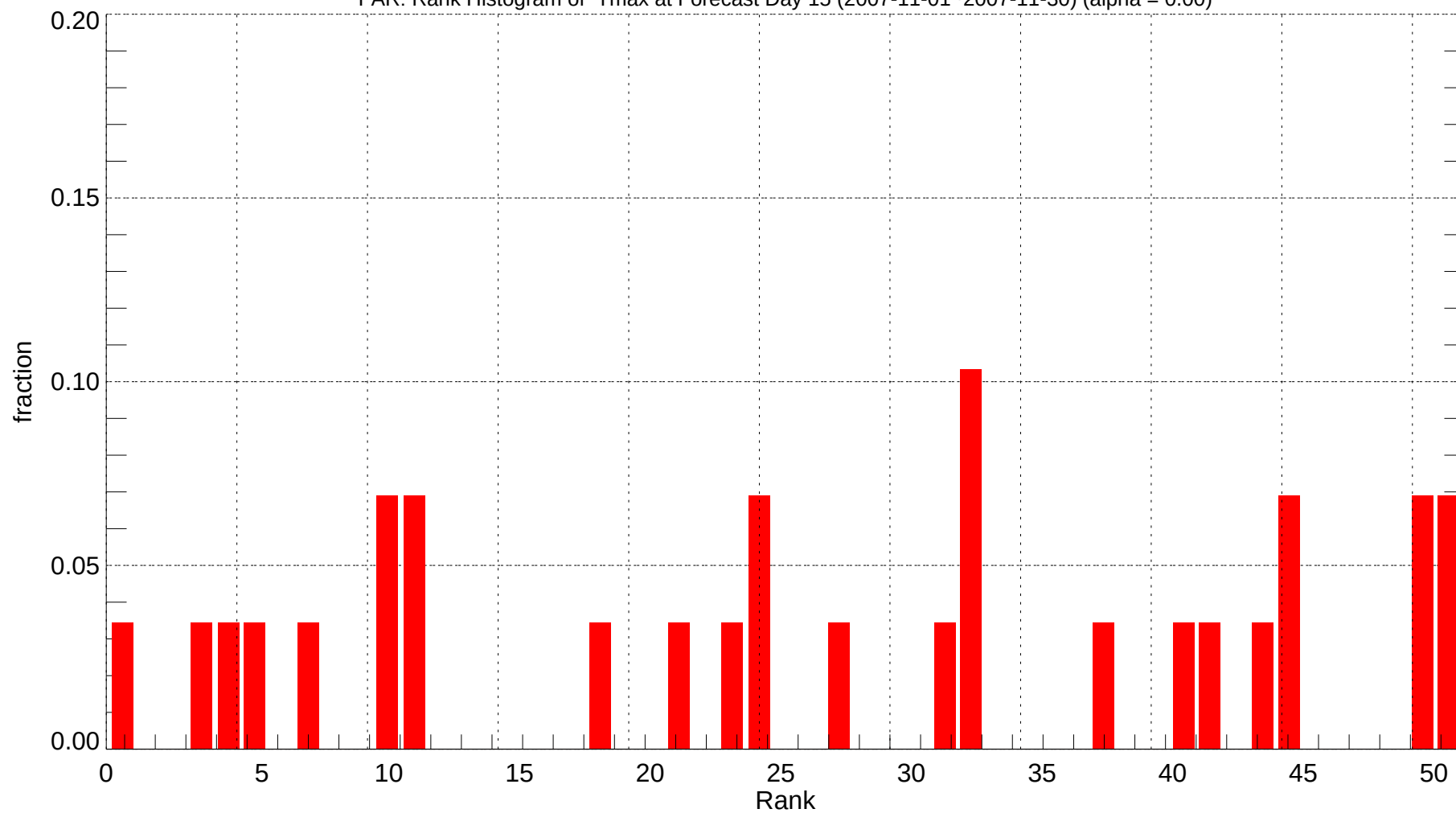
FAR: Rank Histogram of Tmax at Forecast Day 15 (2007-11-01~2007-11-30) (alpha = 0.00)
