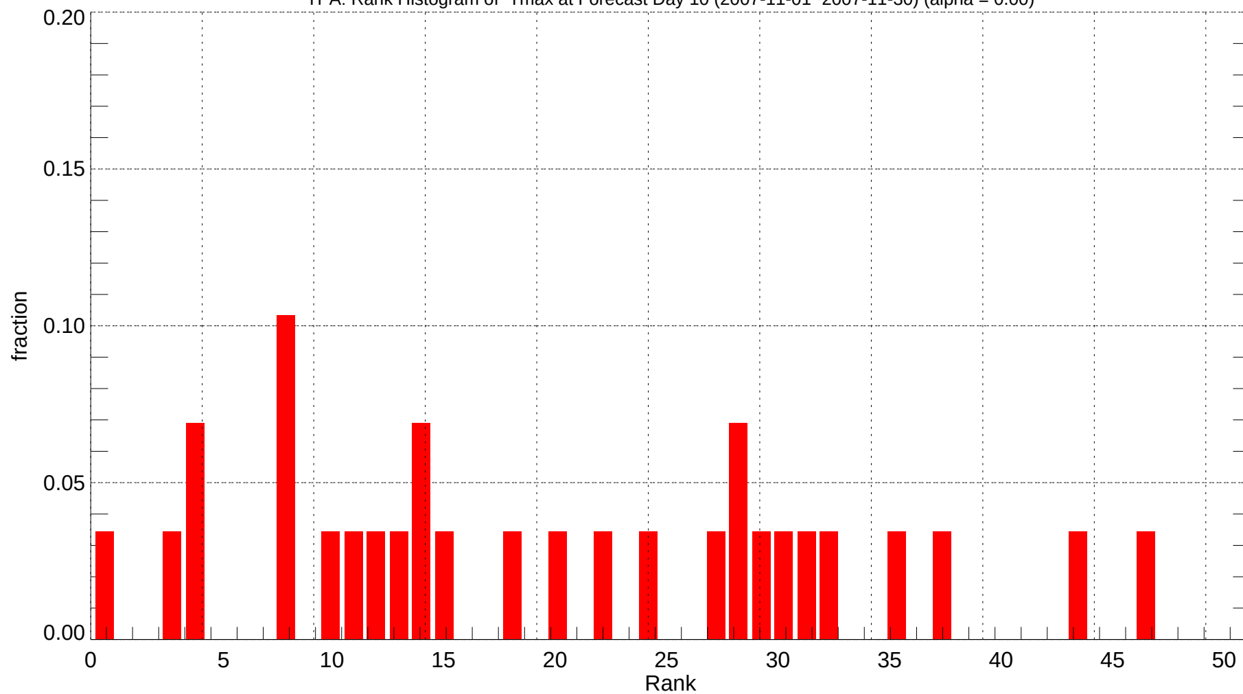
TPA: Rank Histogram of Tmax at Forecast Day 10 (2007-11-01~2007-11-30) (alpha = 0.00)
