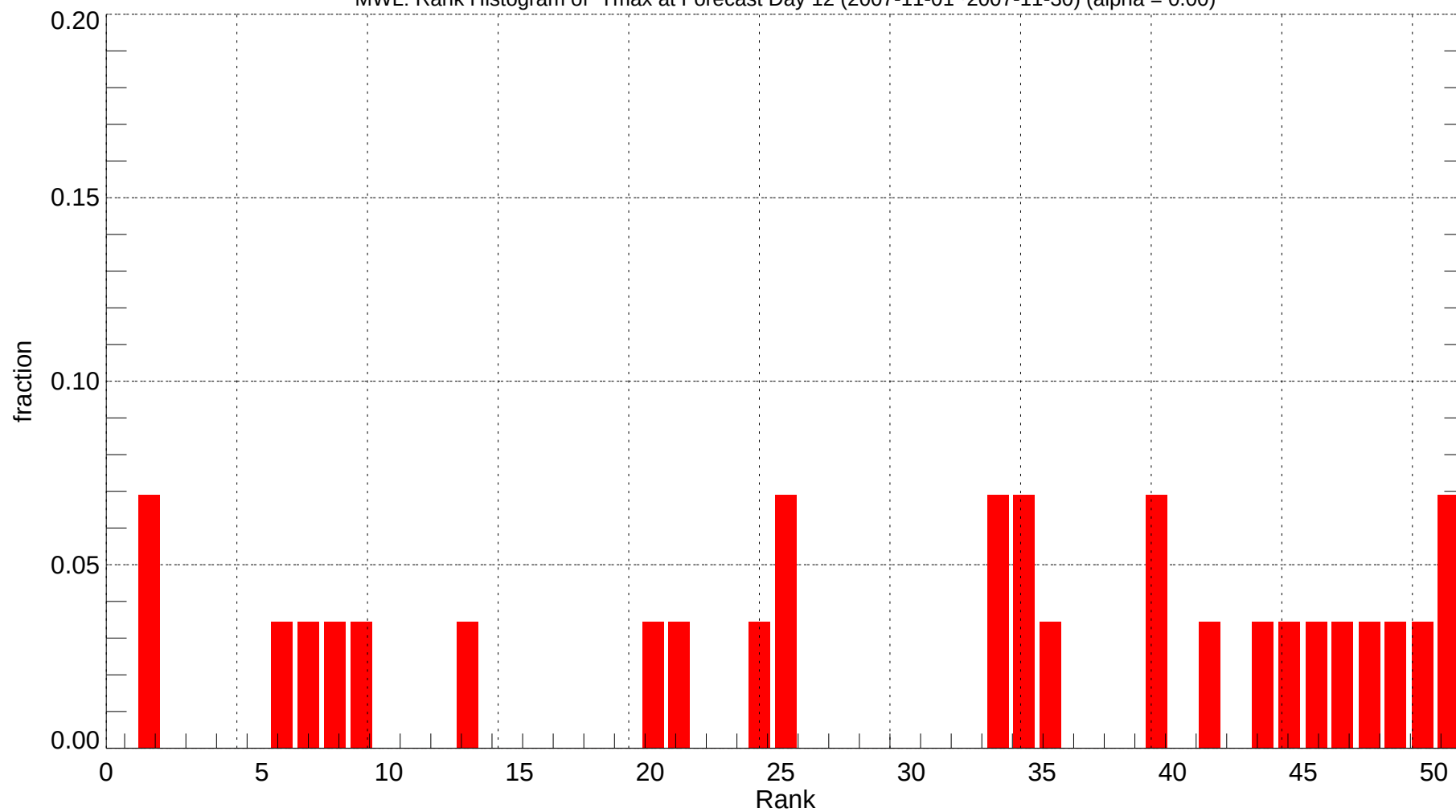
MWL: Rank Histogram of Tmax at Forecast Day 12 (2007-11-01~2007-11-30) (alpha = 0.00)
