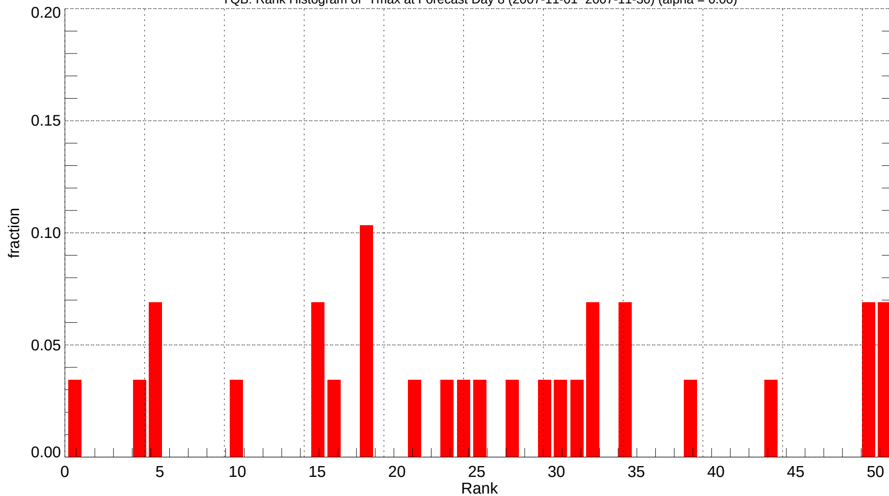
YQB: Rank Histogram of Tmax at Forecast Day 8 (2007-11-01~2007-11-30) (alpha = 0.00)
