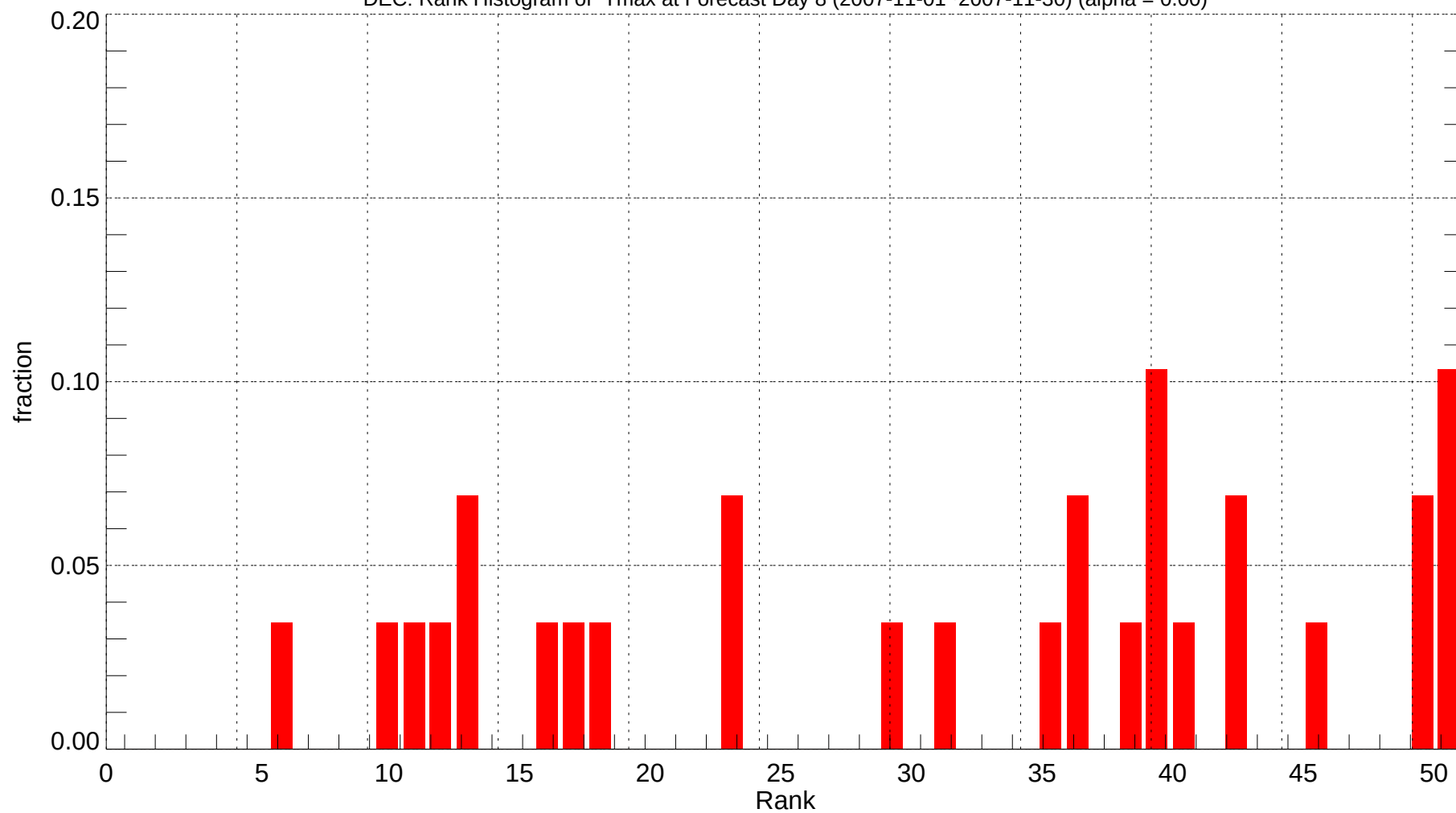
DEC: Rank Histogram of Tmax at Forecast Day 8 (2007-11-01~2007-11-30) (alpha = 0.00)
