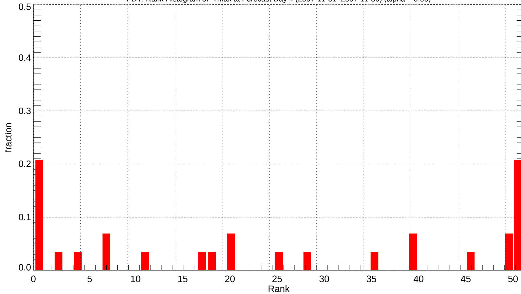
PDT: Rank Histogram of Tmax at Forecast Day 4 (2007-11-01~2007-11-30) (alpha = 0.00)
