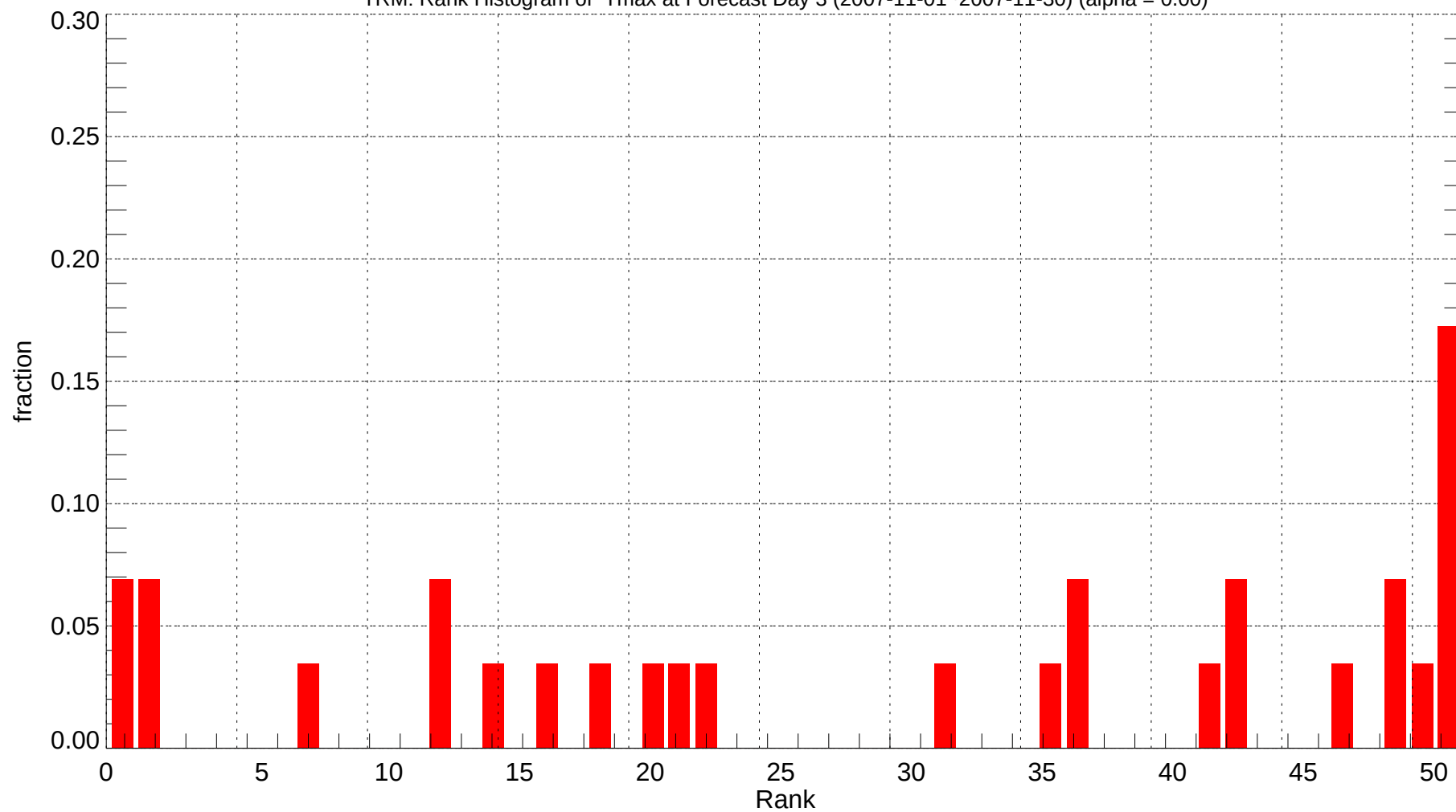
TRM: Rank Histogram of Tmax at Forecast Day 3 (2007-11-01~2007-11-30) (alpha = 0.00)
