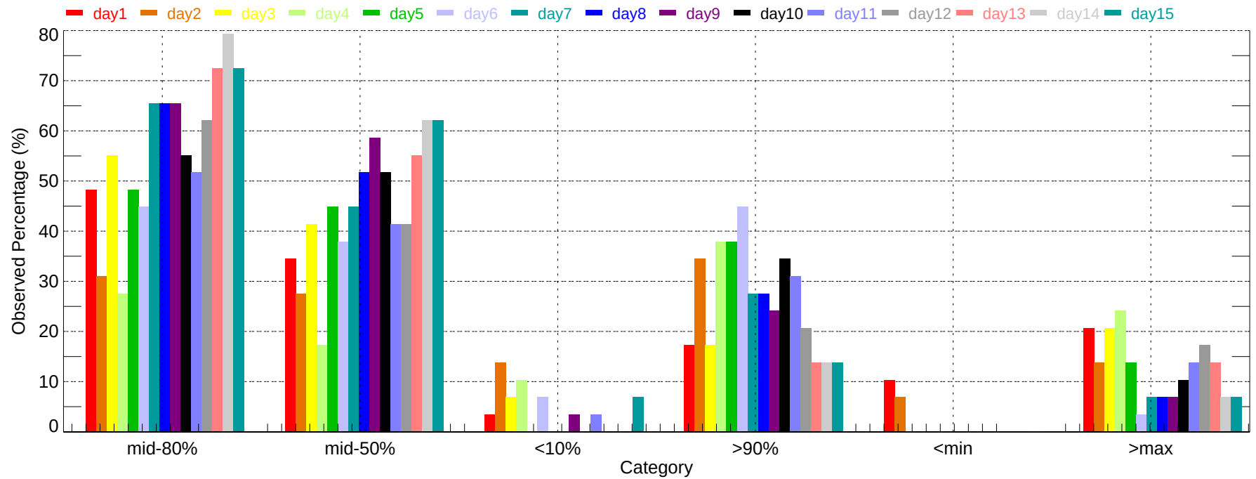
Observed Percentage of Ensembles - CHA: Max Temperature (2007-11-01~2007-11-30)
