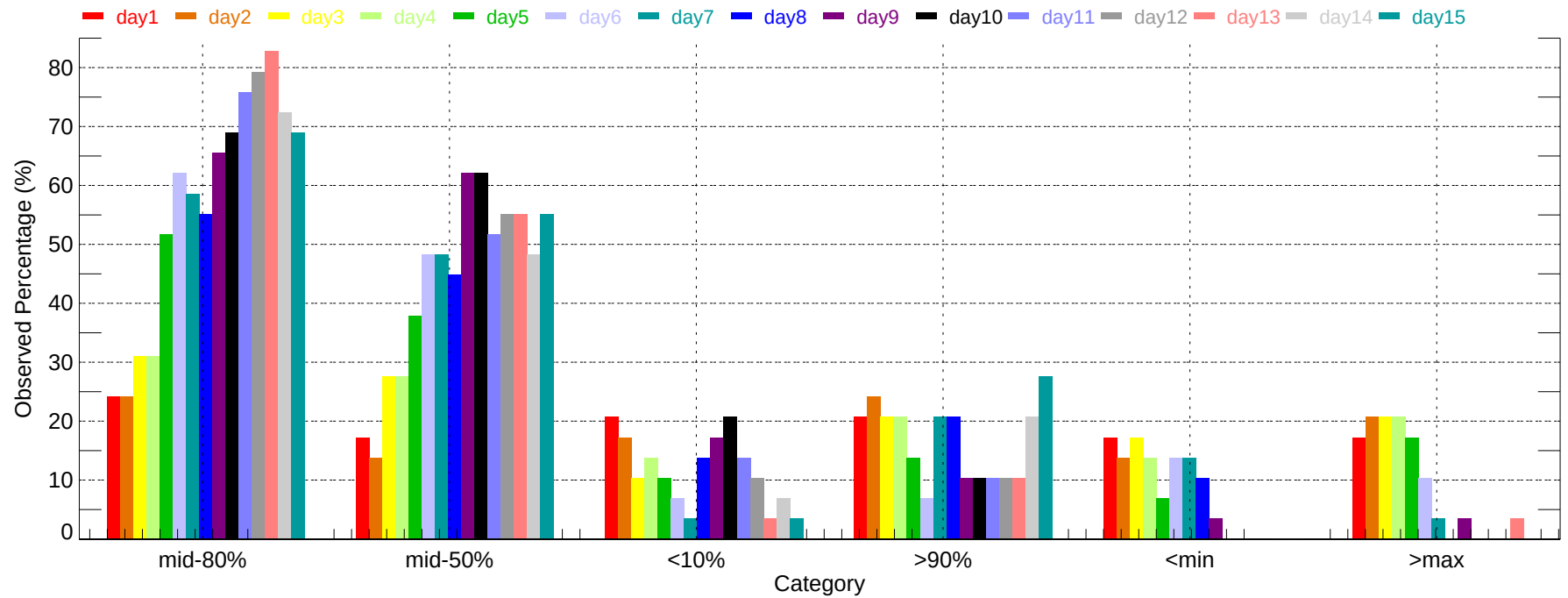
Observed Percentage of Ensembles - PDX: Max Temperature (2007-11-01~2007-11-30)
