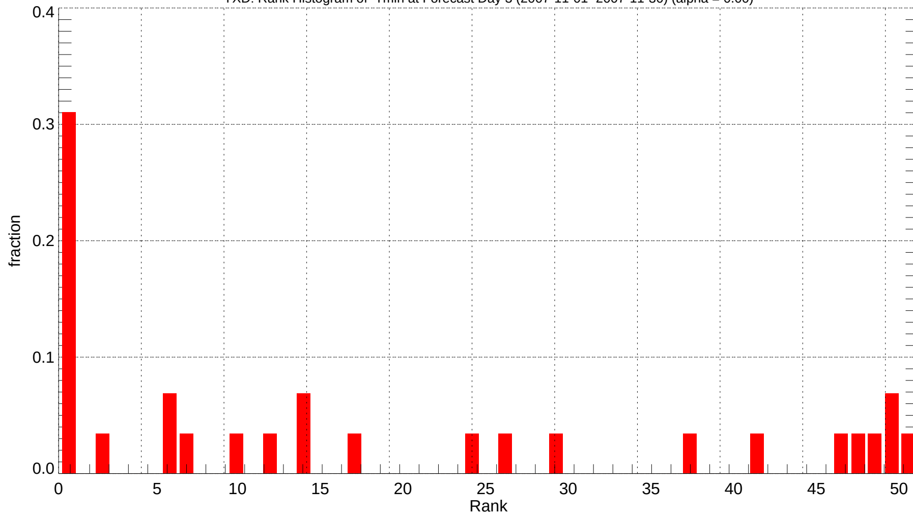
YXD: Rank Histogram of Tmin at Forecast Day 3 (2007-11-01~2007-11-30) (alpha = 0.00)
