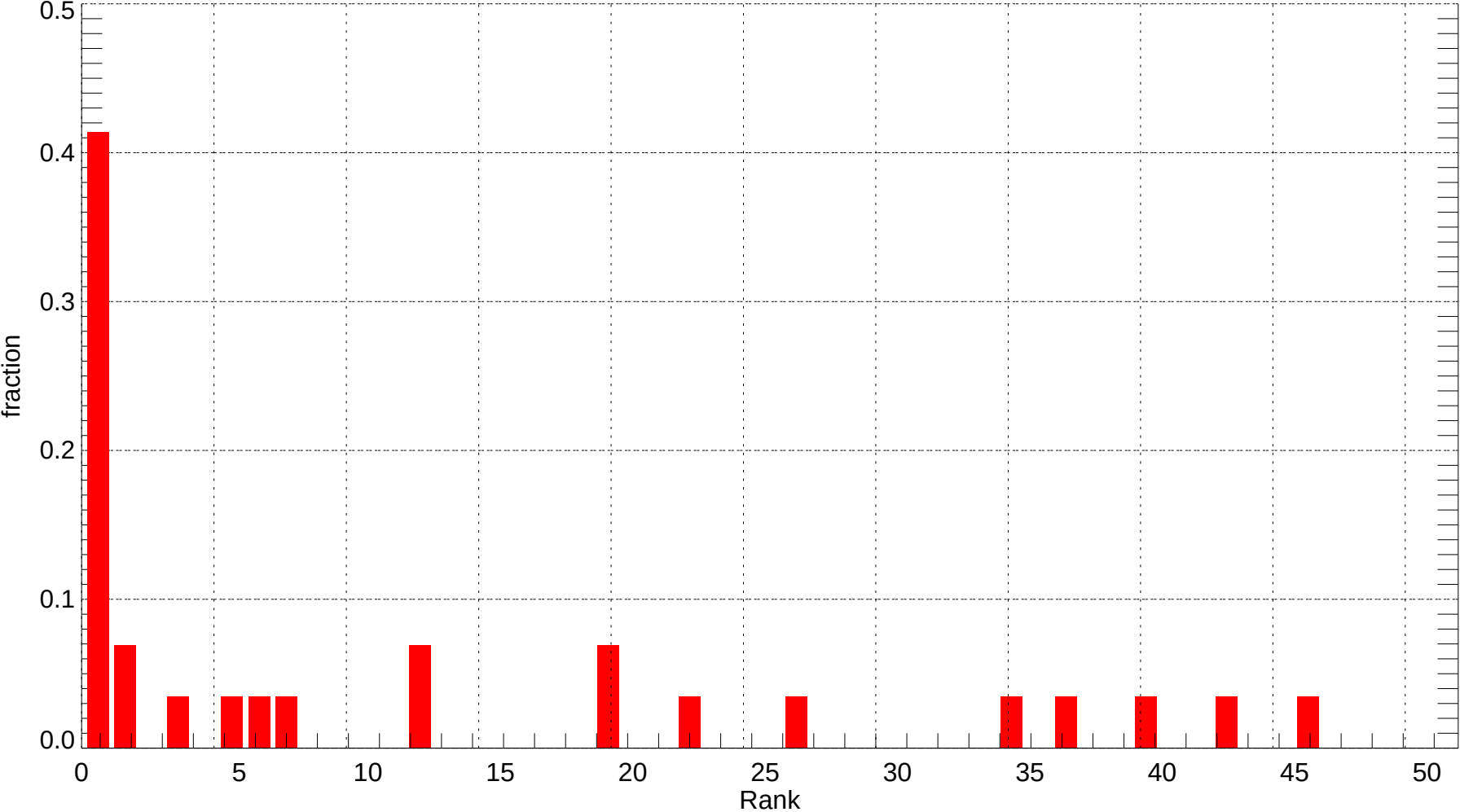
SJC: Rank Histogram of Tmin at Forecast Day 3 (2007-11-01~2007-11-30) (alpha = 0.00)
