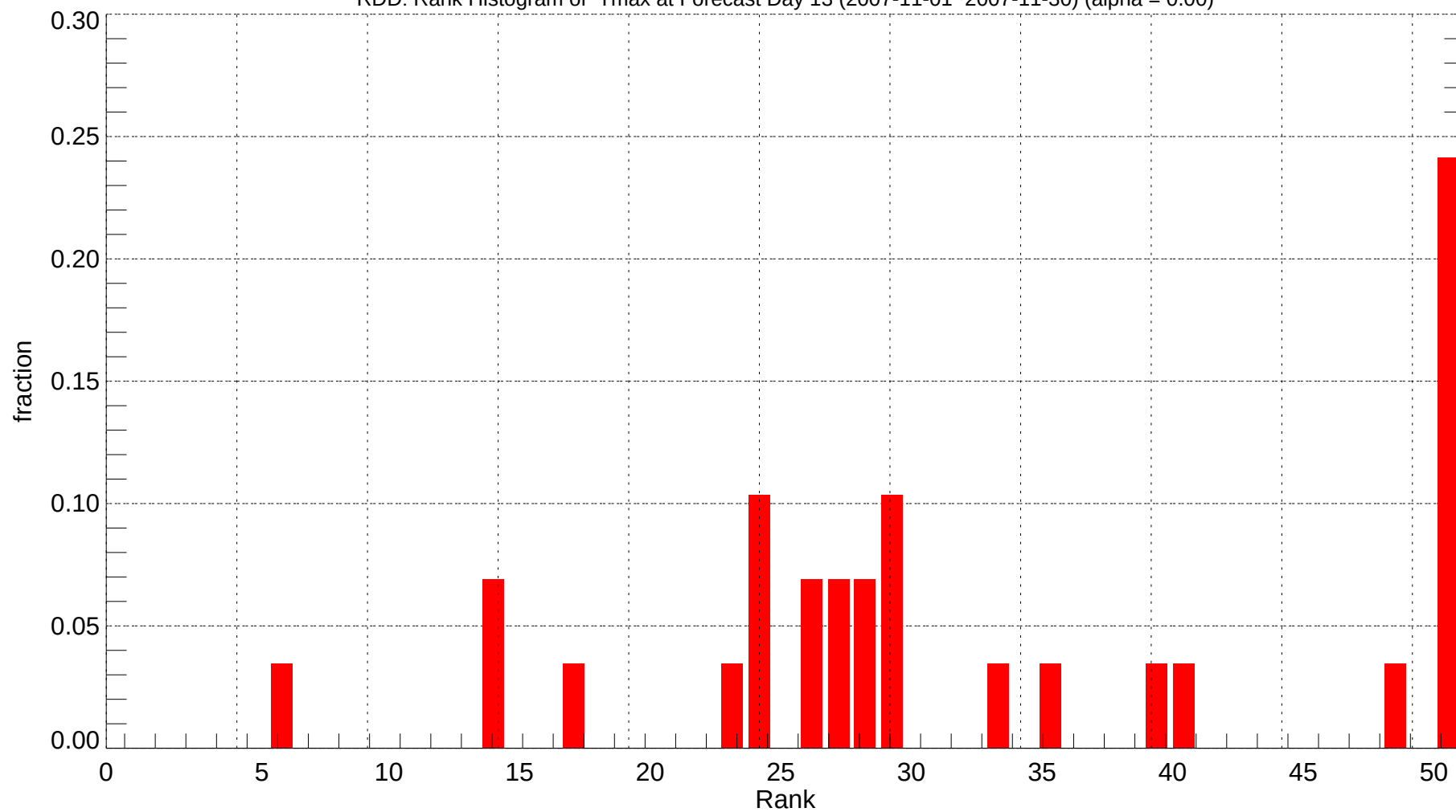
RDD: Rank Histogram of Tmax at Forecast Day 13 (2007-11-01~2007-11-30) (alpha = 0.00)
