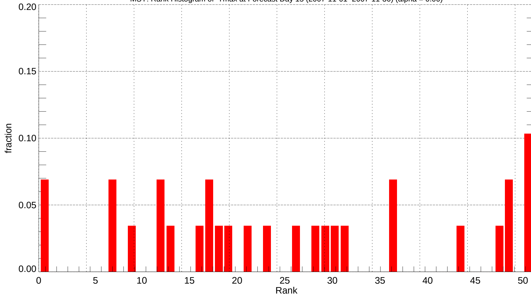
MSY: Rank Histogram of Tmax at Forecast Day 15 (2007-11-01~2007-11-30) (alpha = 0.00)
