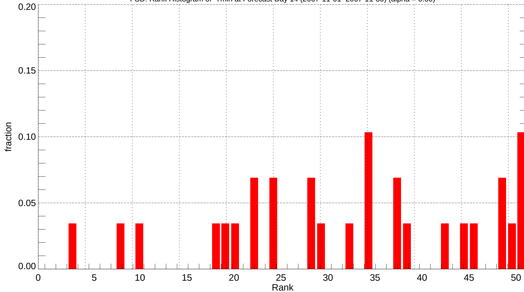
FSD: Rank Histogram of Tmin at Forecast Day 14 (2007-11-01~2007-11-30) (alpha = 0.00)
