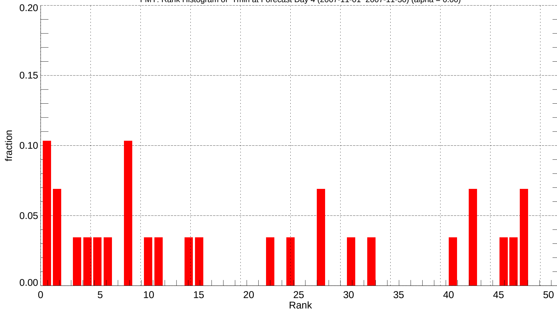
FMY: Rank Histogram of Tmin at Forecast Day 4 (2007-11-01~2007-11-30) (alpha = 0.00)
