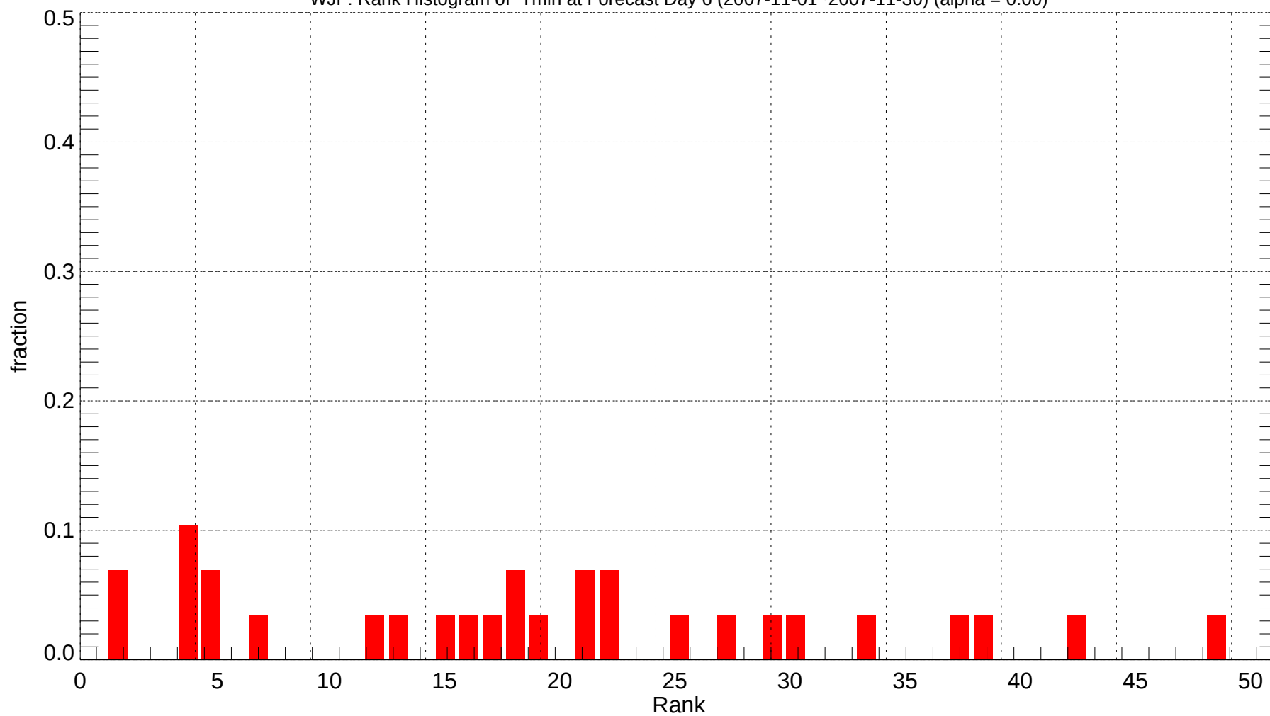
WJF: Rank Histogram of Tmin at Forecast Day 6 (2007-11-01~2007-11-30) (alpha = 0.00)
