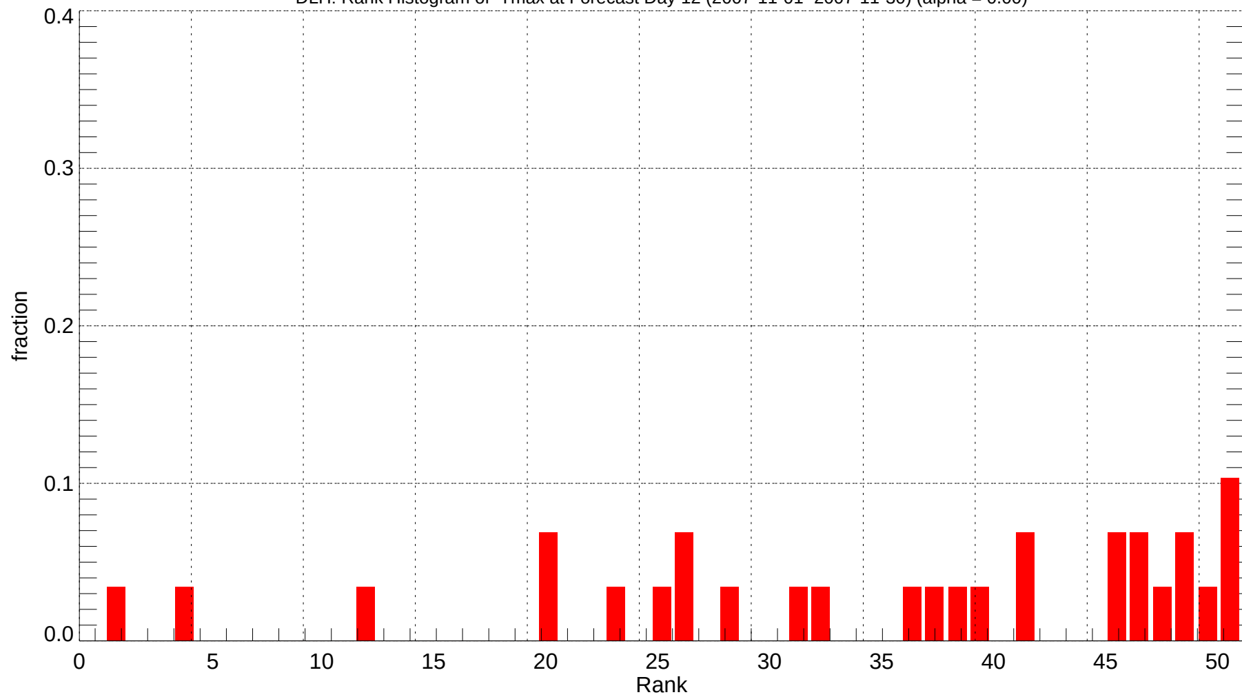
DLH: Rank Histogram of Tmax at Forecast Day 12 (2007-11-01~2007-11-30) (alpha = 0.00)
