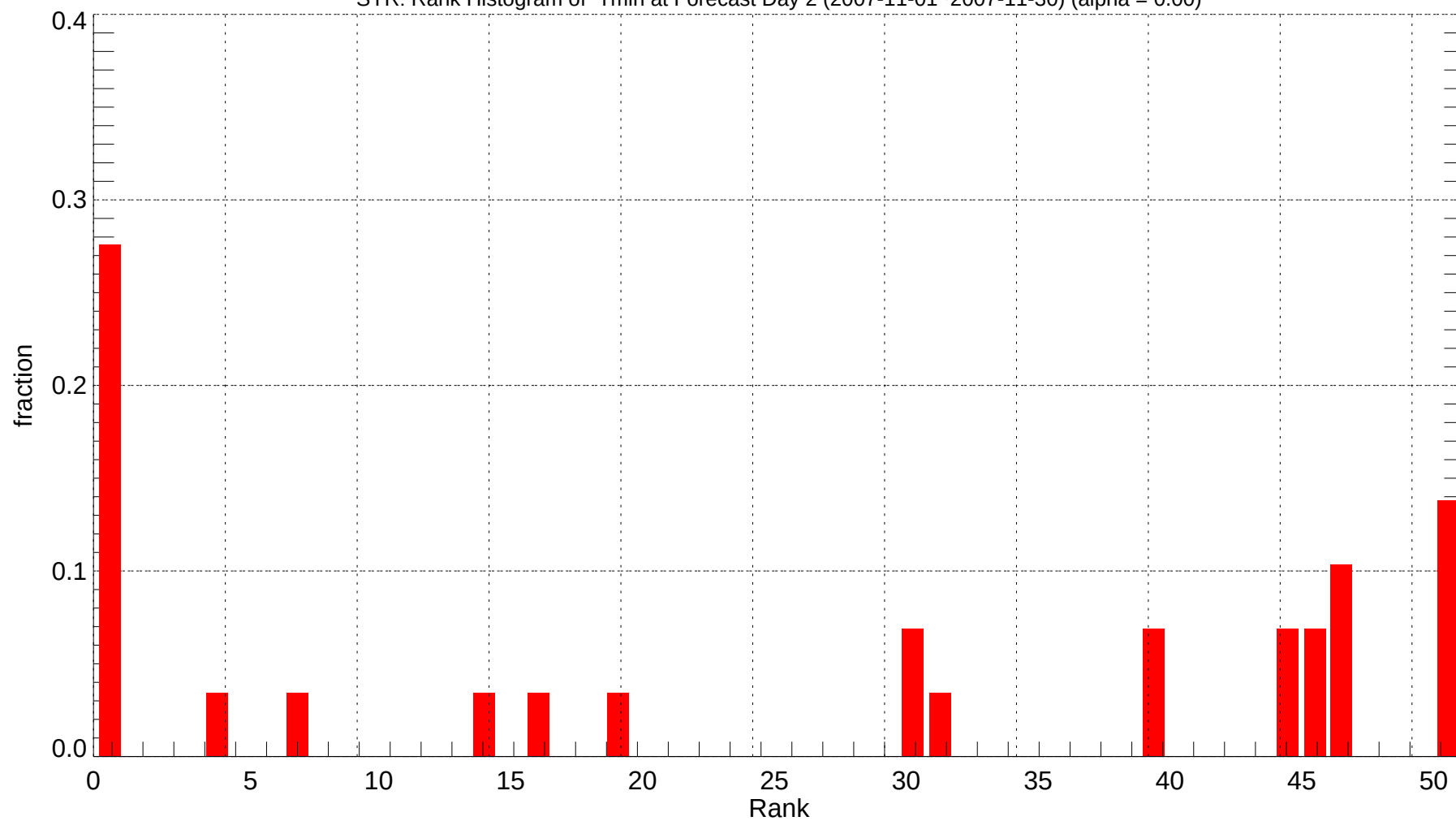
SYR: Rank Histogram of Tmin at Forecast Day 2 (2007-11-01~2007-11-30) (alpha = 0.00)
