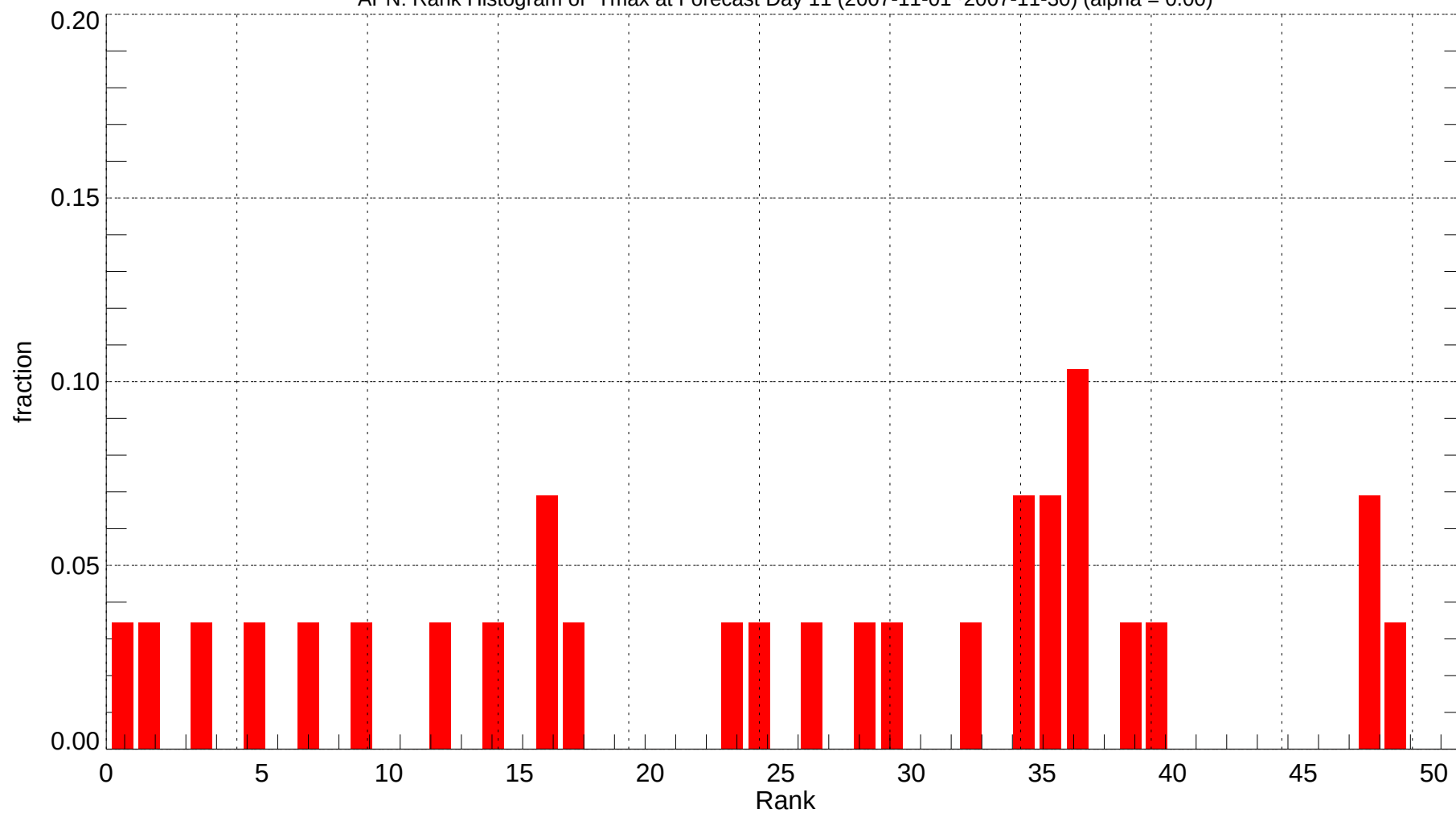
APN: Rank Histogram of Tmax at Forecast Day 11 (2007-11-01~2007-11-30) (alpha = 0.00)
