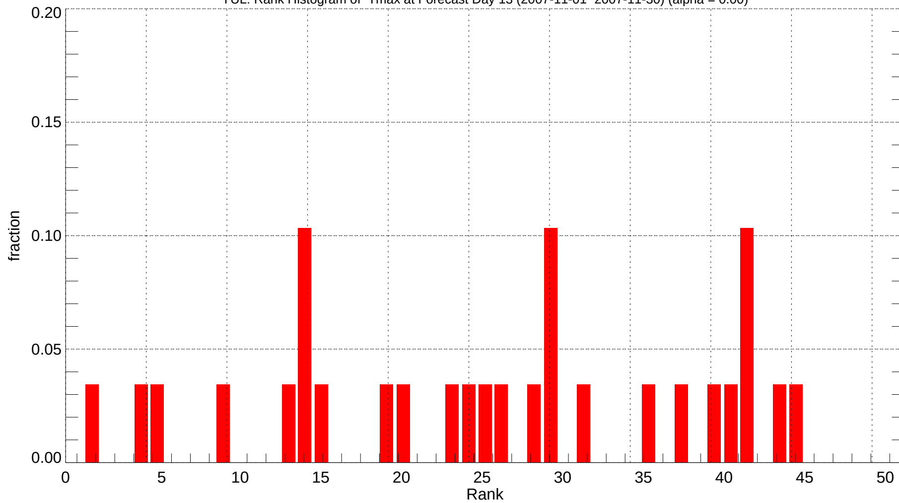
YUL: Rank Histogram of Tmax at Forecast Day 13 (2007-11-01~2007-11-30) (alpha = 0.00)
