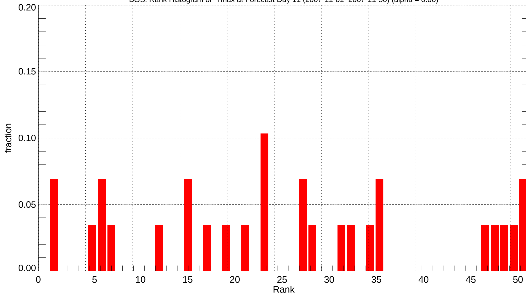
BOS: Rank Histogram of Tmax at Forecast Day 11 (2007-11-01~2007-11-30) (alpha = 0.00)
