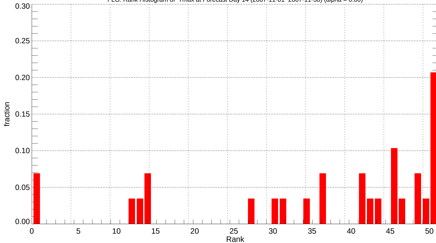
FLG: Rank Histogram of Tmax at Forecast Day 14 (2007-11-01~2007-11-30) (alpha = 0.00)
