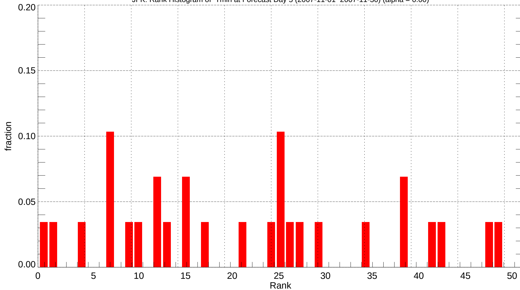
JFK: Rank Histogram of Tmin at Forecast Day 5 (2007-11-01~2007-11-30) (alpha = 0.00)
