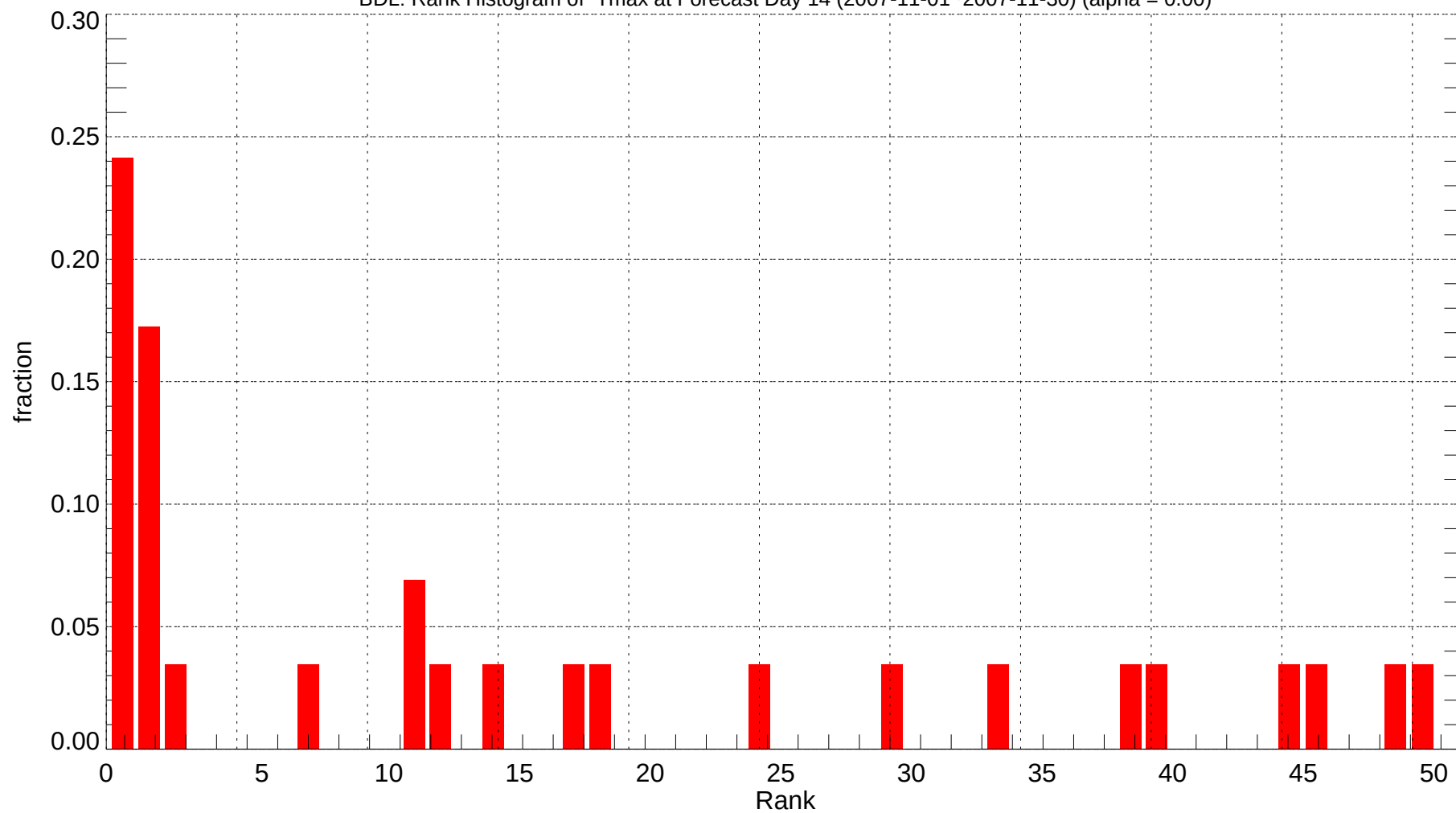
BDL: Rank Histogram of Tmax at Forecast Day 14 (2007-11-01~2007-11-30) (alpha = 0.00)
