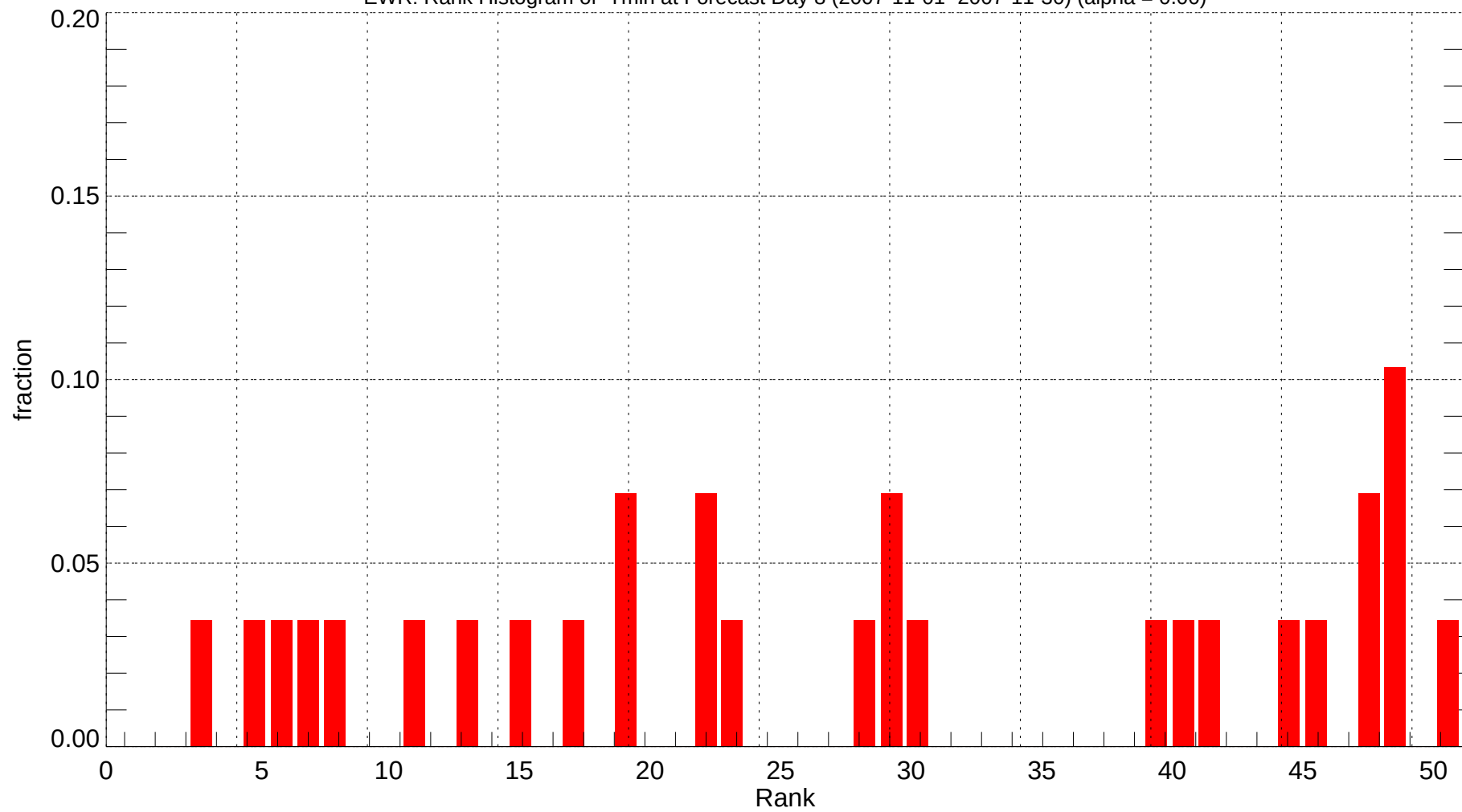
EWR: Rank Histogram of Tmin at Forecast Day 8 (2007-11-01~2007-11-30) (alpha = 0.00)
