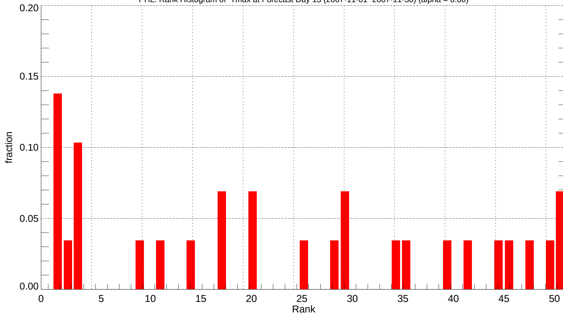
PHL: Rank Histogram of Tmax at Forecast Day 13 (2007-11-01~2007-11-30) (alpha = 0.00)
