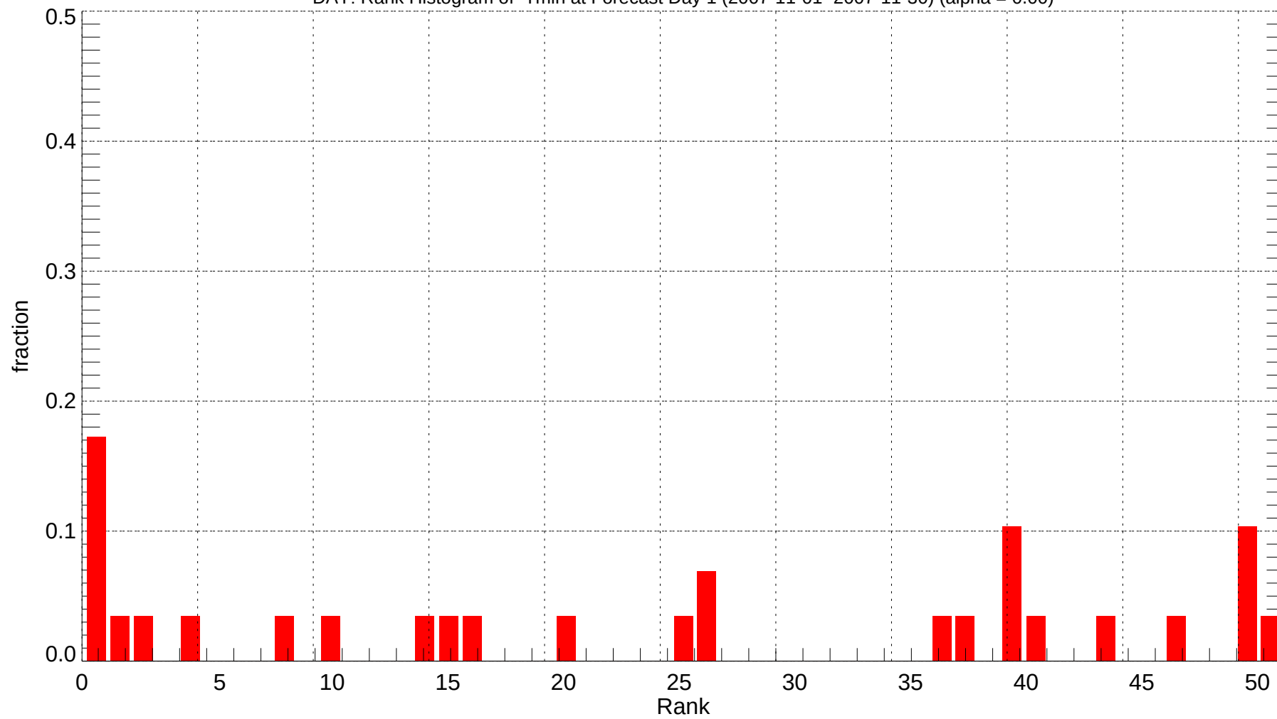
DAY: Rank Histogram of Tmin at Forecast Day 1 (2007-11-01~2007-11-30) (alpha = 0.00)
