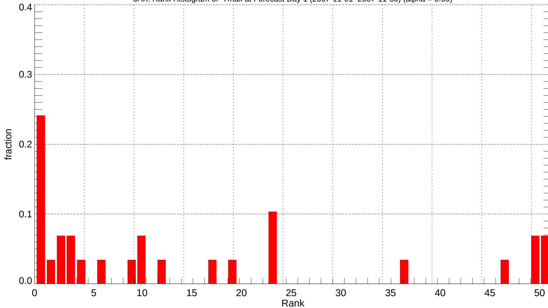
JAX: Rank Histogram of Tmax at Forecast Day 1 (2007-11-01~2007-11-30) (alpha = 0.00)
