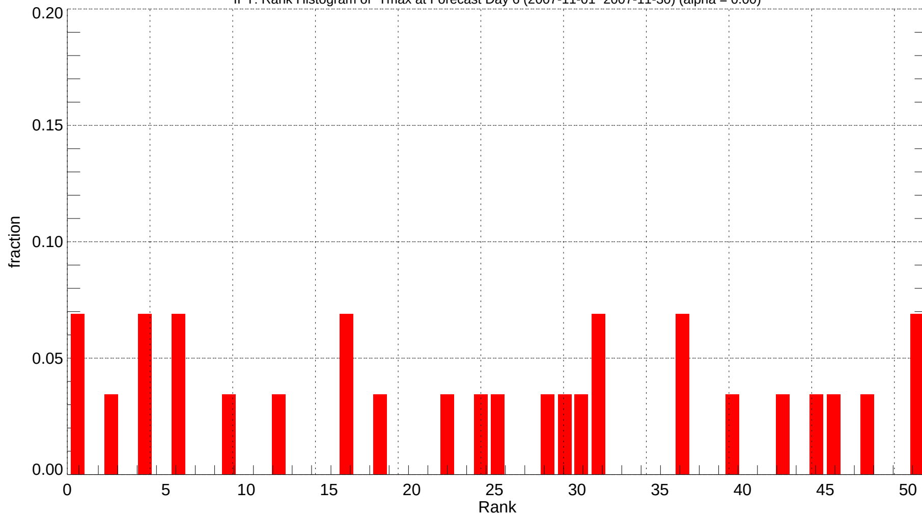
IPT: Rank Histogram of Tmax at Forecast Day 6 (2007-11-01~2007-11-30) (alpha = 0.00)
