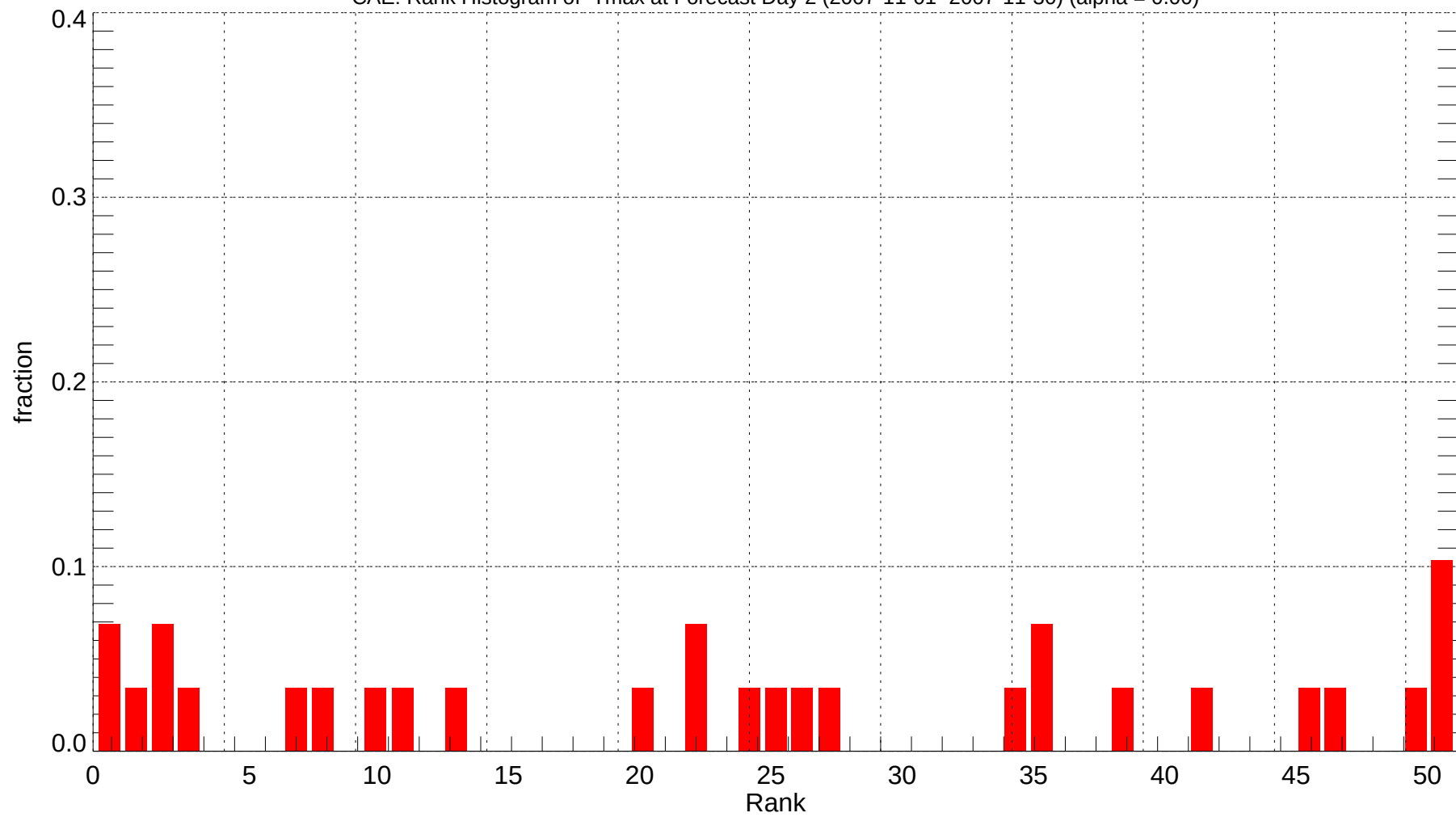
CAE: Rank Histogram of Tmax at Forecast Day 2 (2007-11-01~2007-11-30) (alpha = 0.00)
