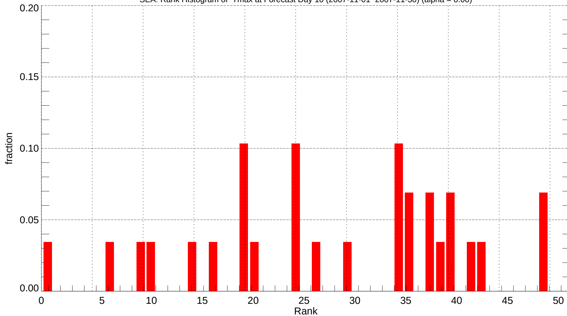
SEA: Rank Histogram of Tmax at Forecast Day 10 (2007-11-01~2007-11-30) (alpha = 0.00)
