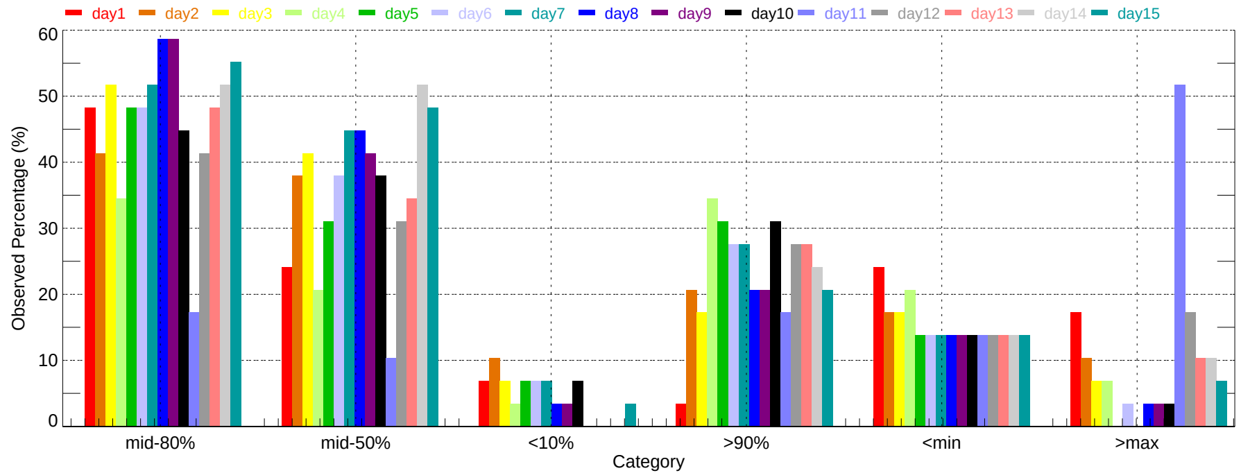
Observed Percentage of Ensembles - GAD: Max Temperature (2007-11-01~2007-11-30)
