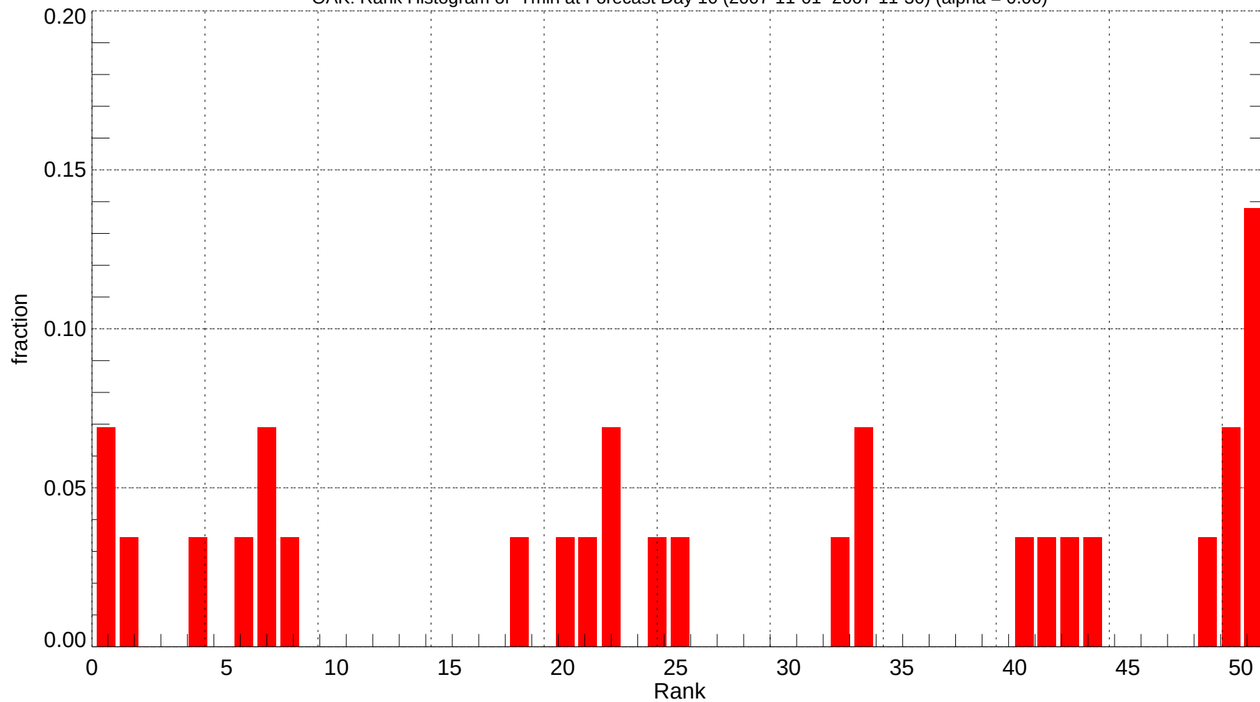
OAK: Rank Histogram of Tmin at Forecast Day 10 (2007-11-01~2007-11-30) (alpha = 0.00)
