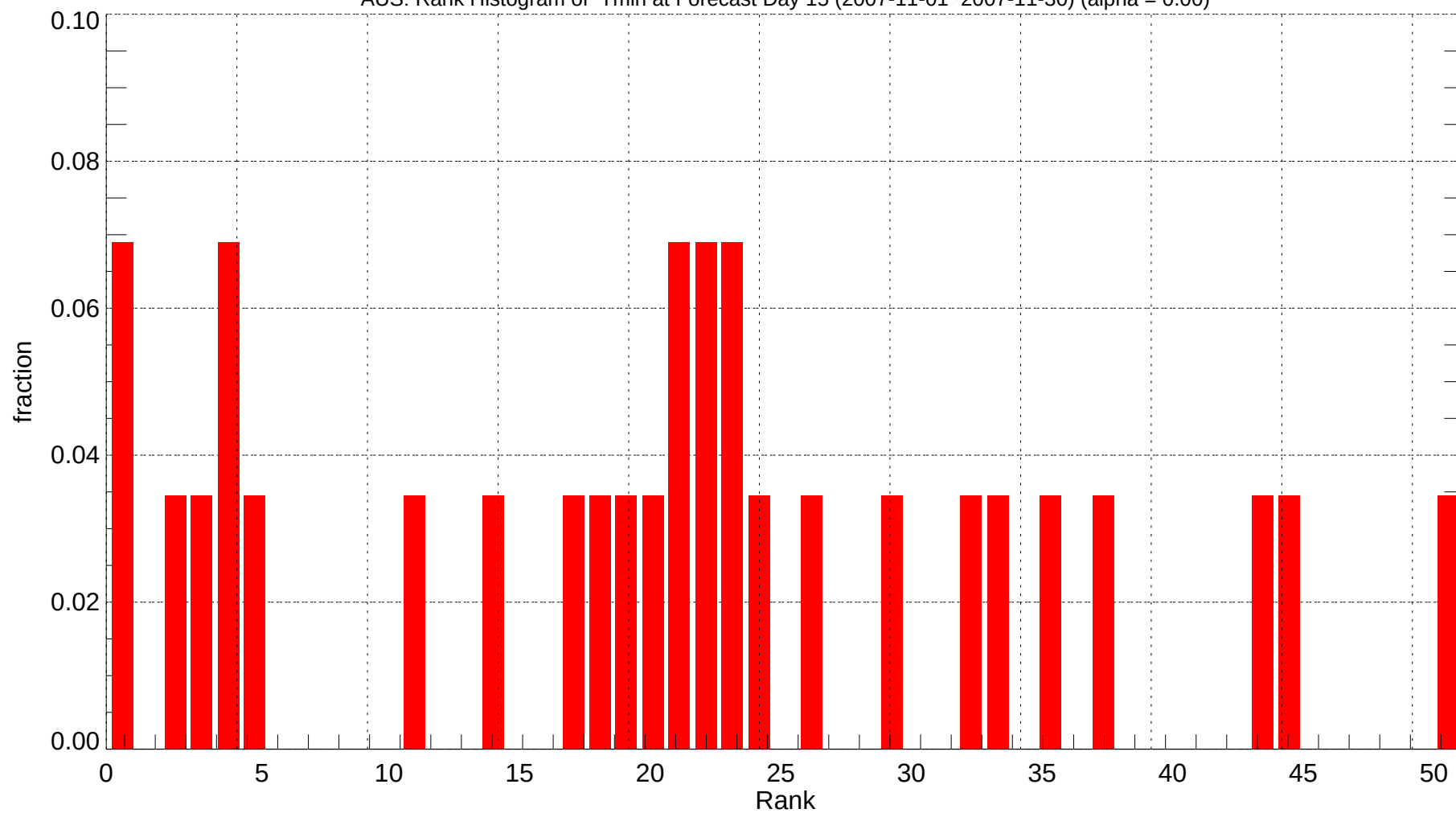
AUS: Rank Histogram of Tmin at Forecast Day 15 (2007-11-01~2007-11-30) (alpha = 0.00)
