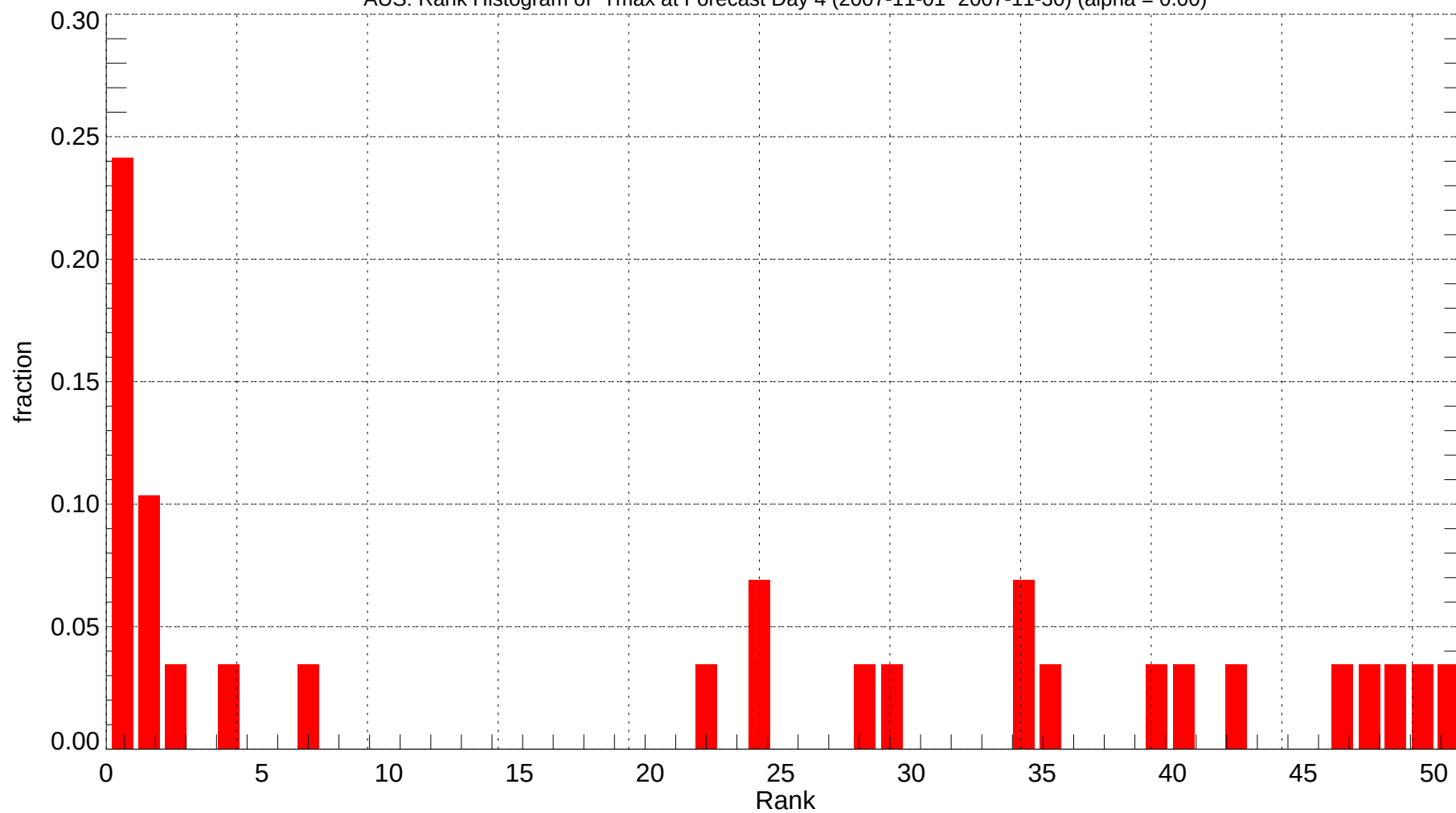
AUS: Rank Histogram of Tmax at Forecast Day 4 (2007-11-01~2007-11-30) (alpha = 0.00)
