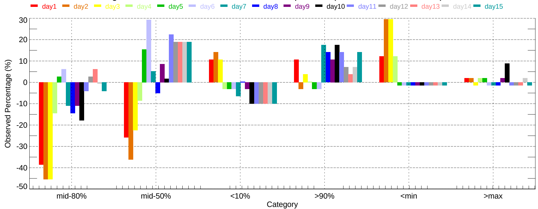
Observed Percentage Deviation of Ensembles - BFL: Min Temperature (2007-11-01~2007-11-30)
