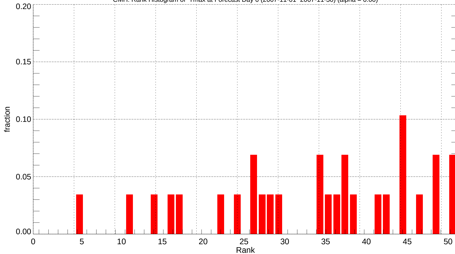
CMH: Rank Histogram of Tmax at Forecast Day 6 (2007-11-01~2007-11-30) (alpha = 0.00)
