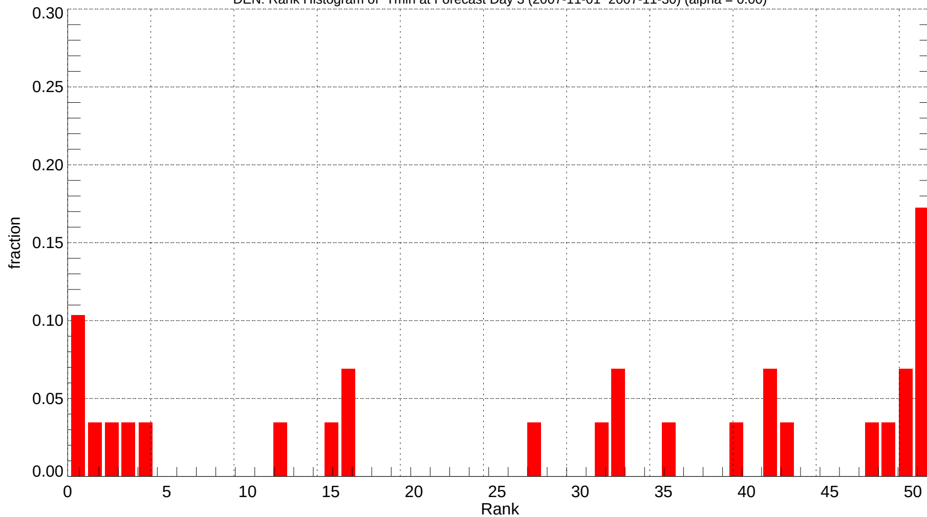
DEN: Rank Histogram of Tmin at Forecast Day 3 (2007-11-01~2007-11-30) (alpha = 0.00)
