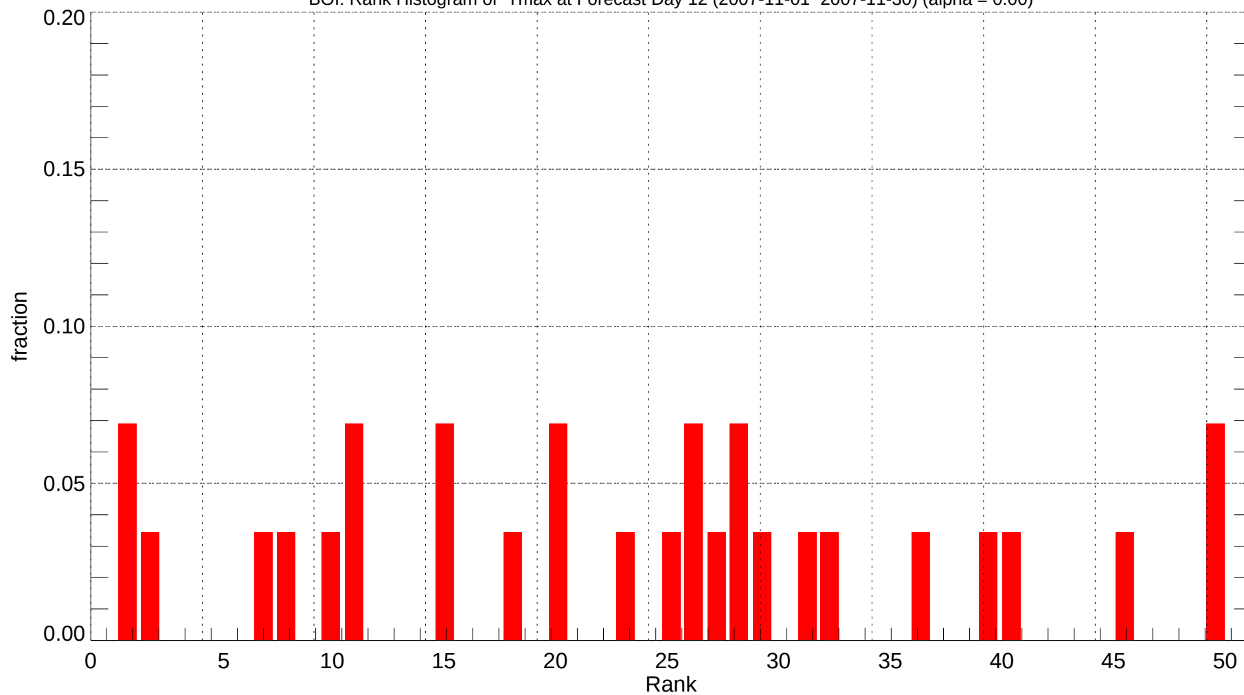
BOI: Rank Histogram of Tmax at Forecast Day 12 (2007-11-01~2007-11-30) (alpha = 0.00)
