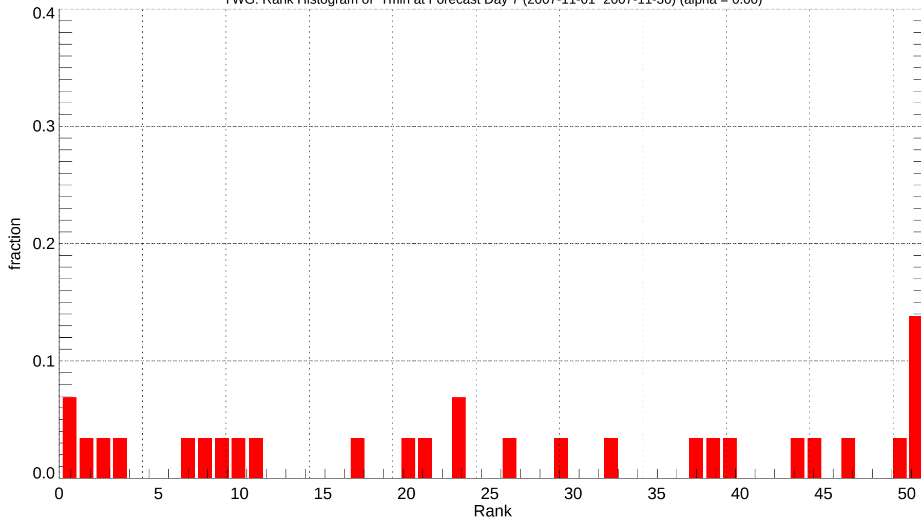
YWG: Rank Histogram of Tmin at Forecast Day 7 (2007-11-01~2007-11-30) (alpha = 0.00)
