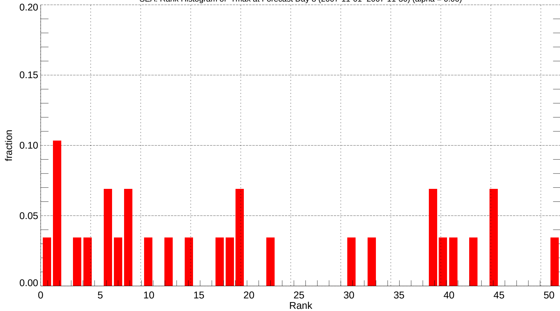
SEA: Rank Histogram of Tmax at Forecast Day 8 (2007-11-01~2007-11-30) (alpha = 0.00)
