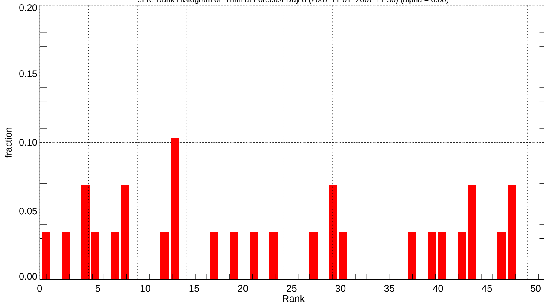
JFK: Rank Histogram of Tmin at Forecast Day 8 (2007-11-01~2007-11-30) (alpha = 0.00)
