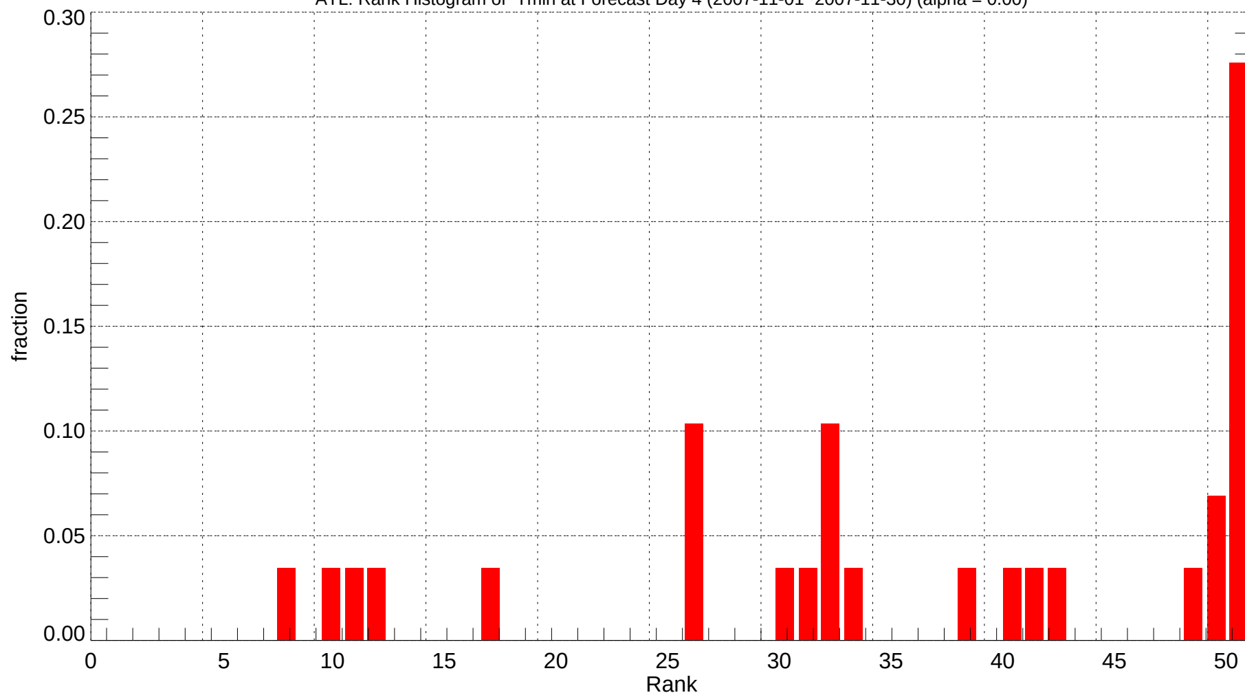
ATL: Rank Histogram of Tmin at Forecast Day 4 (2007-11-01~2007-11-30) (alpha = 0.00)
