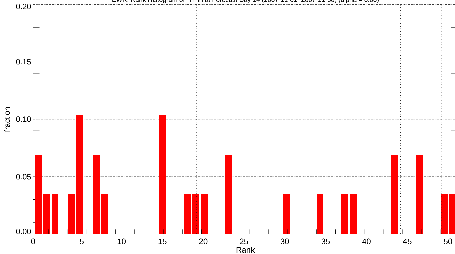
EWR: Rank Histogram of Tmin at Forecast Day 14 (2007-11-01~2007-11-30) (alpha = 0.00)
