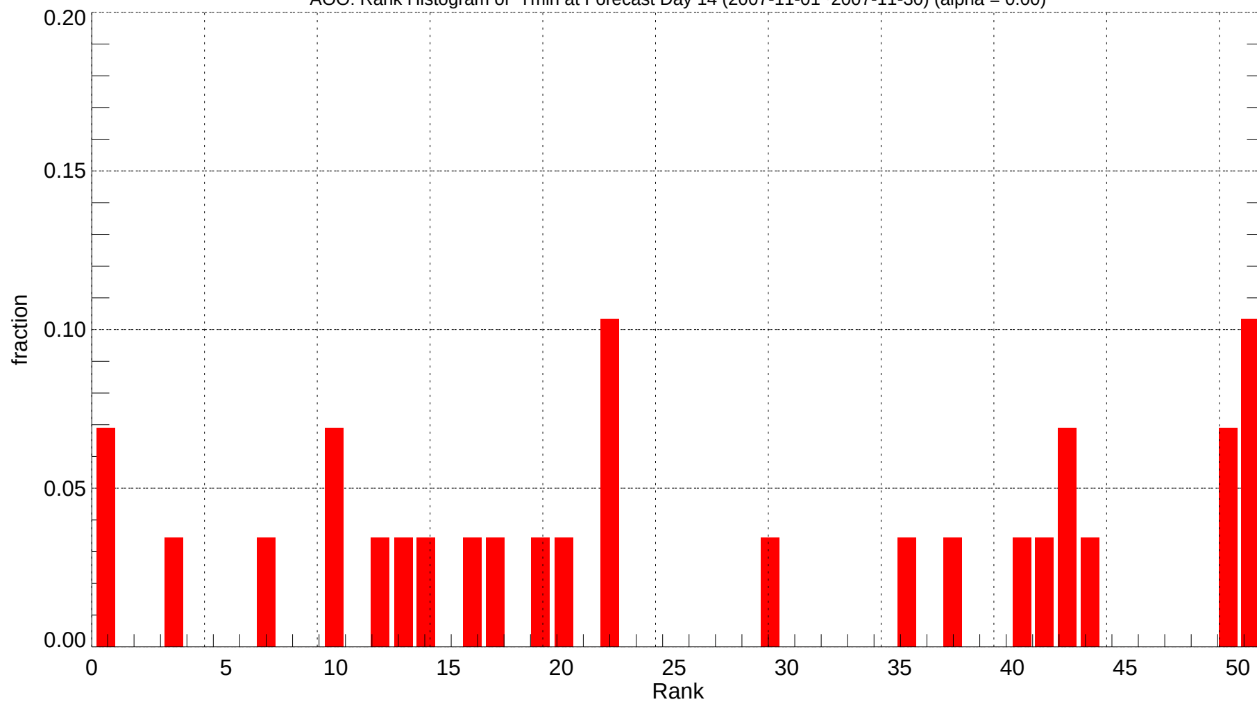
AOO: Rank Histogram of Tmin at Forecast Day 14 (2007-11-01~2007-11-30) (alpha = 0.00)
