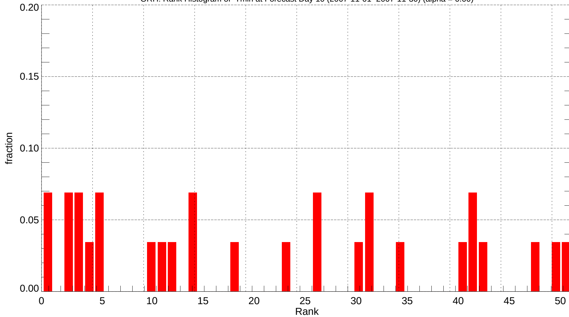
ORH: Rank Histogram of Tmin at Forecast Day 10 (2007-11-01~2007-11-30) (alpha = 0.00)
