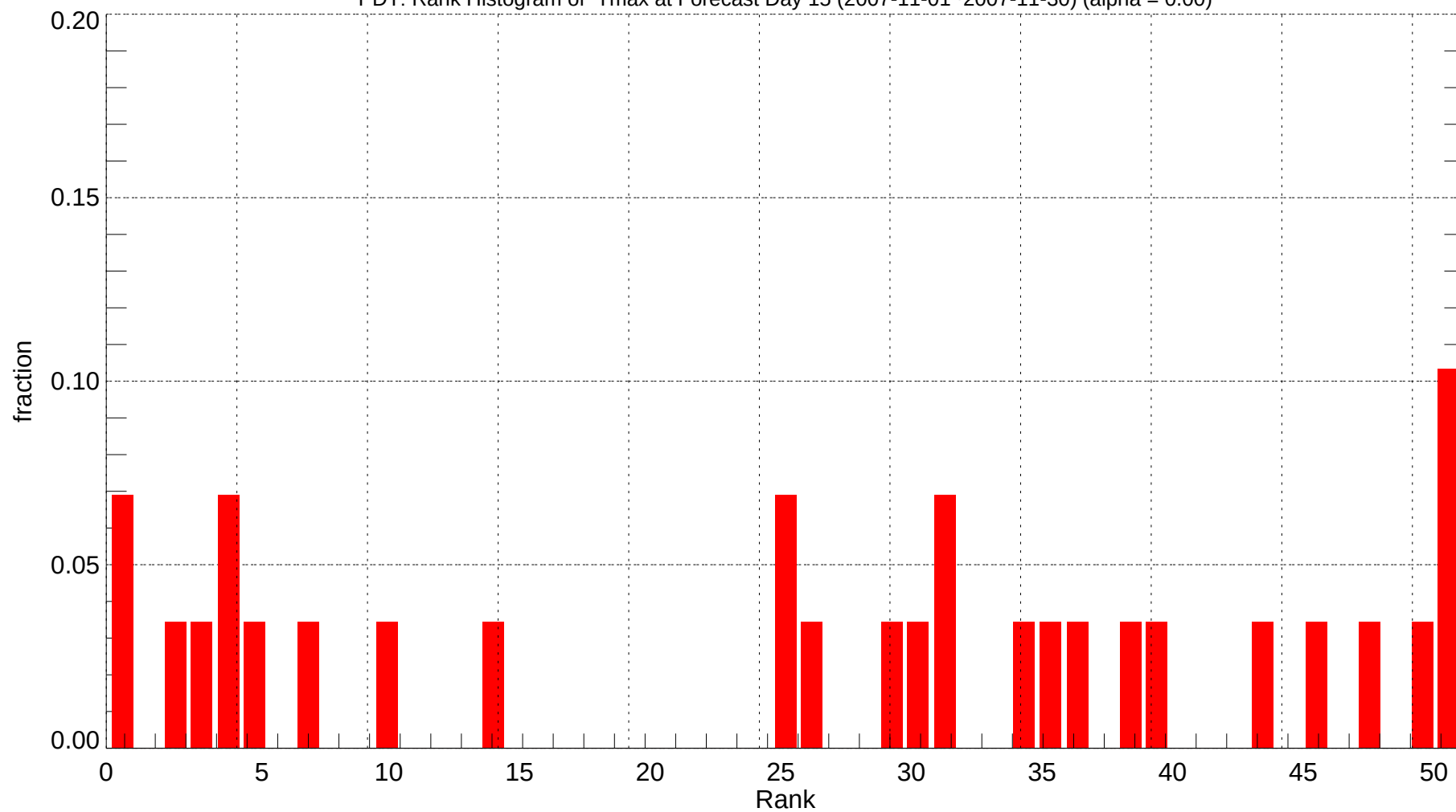
PDT: Rank Histogram of Tmax at Forecast Day 15 (2007-11-01~2007-11-30) (alpha = 0.00)
