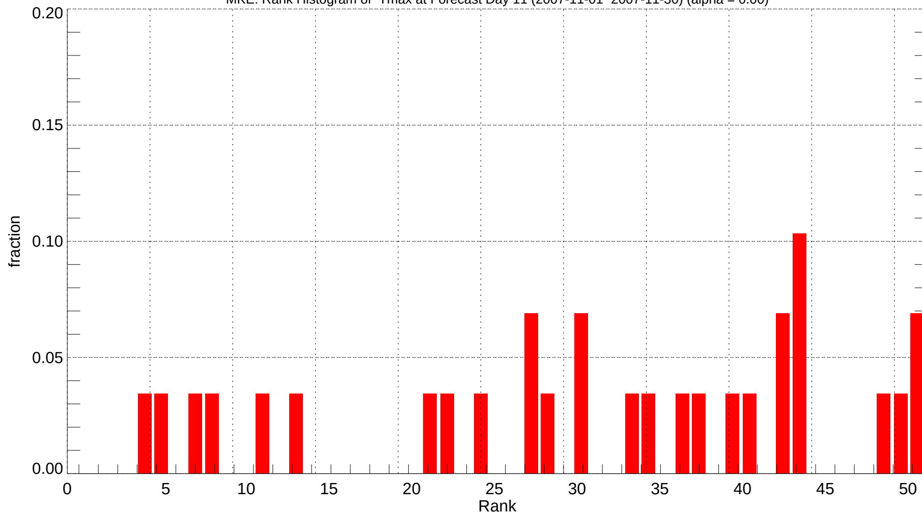
MKE: Rank Histogram of Tmax at Forecast Day 11 (2007-11-01~2007-11-30) (alpha = 0.00)
