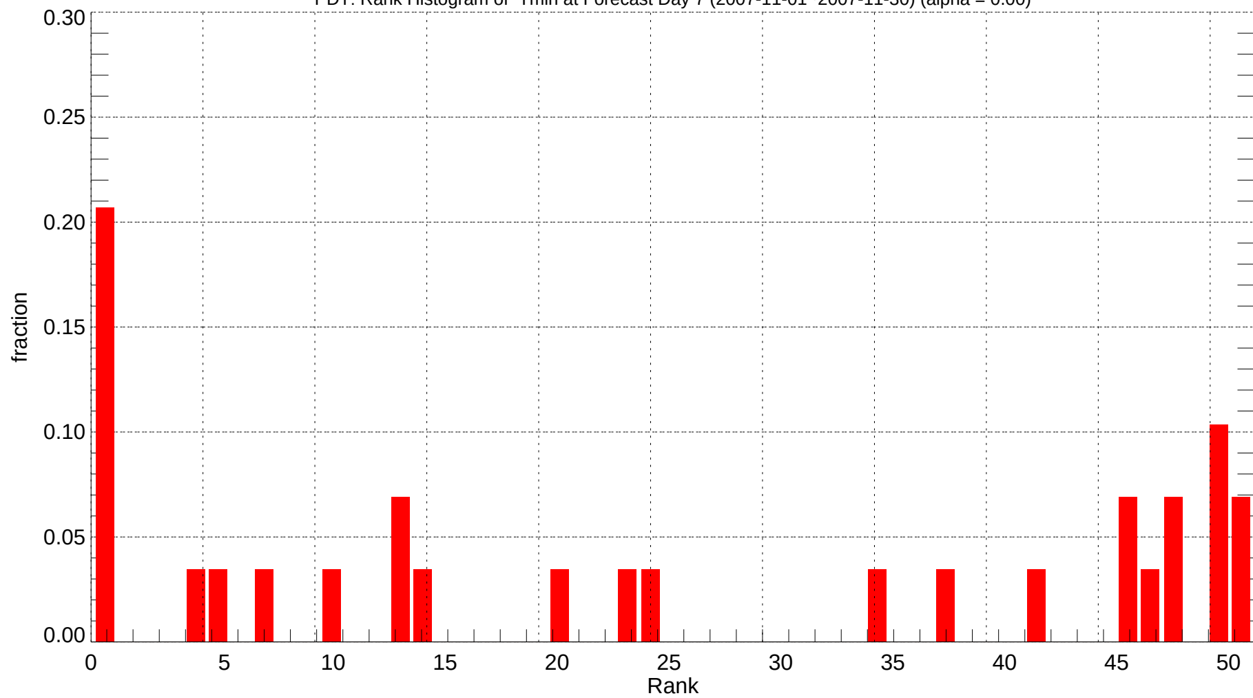
PDT: Rank Histogram of Tmin at Forecast Day 7 (2007-11-01~2007-11-30) (alpha = 0.00)
