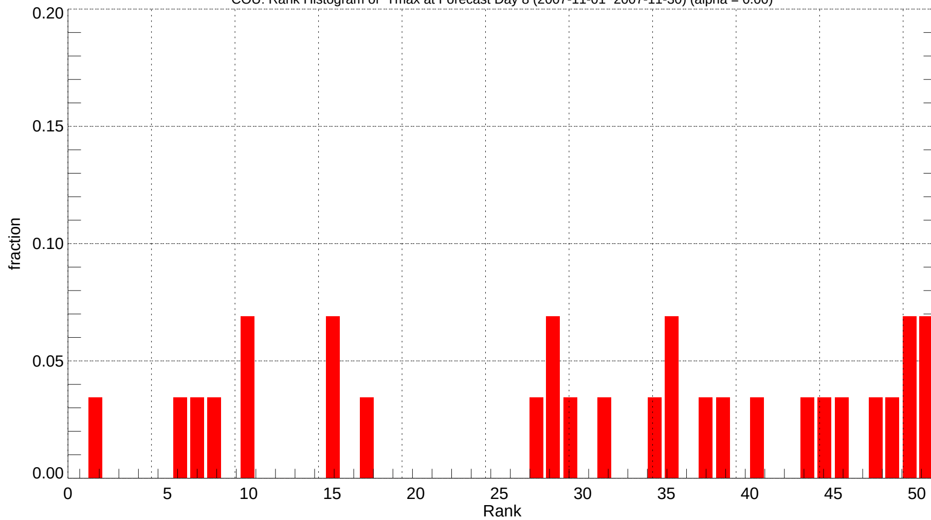
COU: Rank Histogram of Tmax at Forecast Day 8 (2007-11-01~2007-11-30) (alpha = 0.00)
