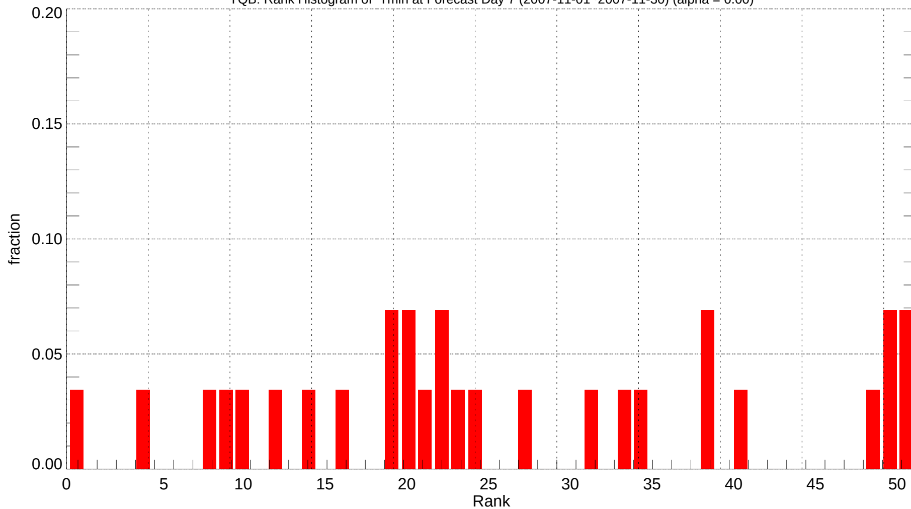
YQB: Rank Histogram of Tmin at Forecast Day 7 (2007-11-01~2007-11-30) (alpha = 0.00)
