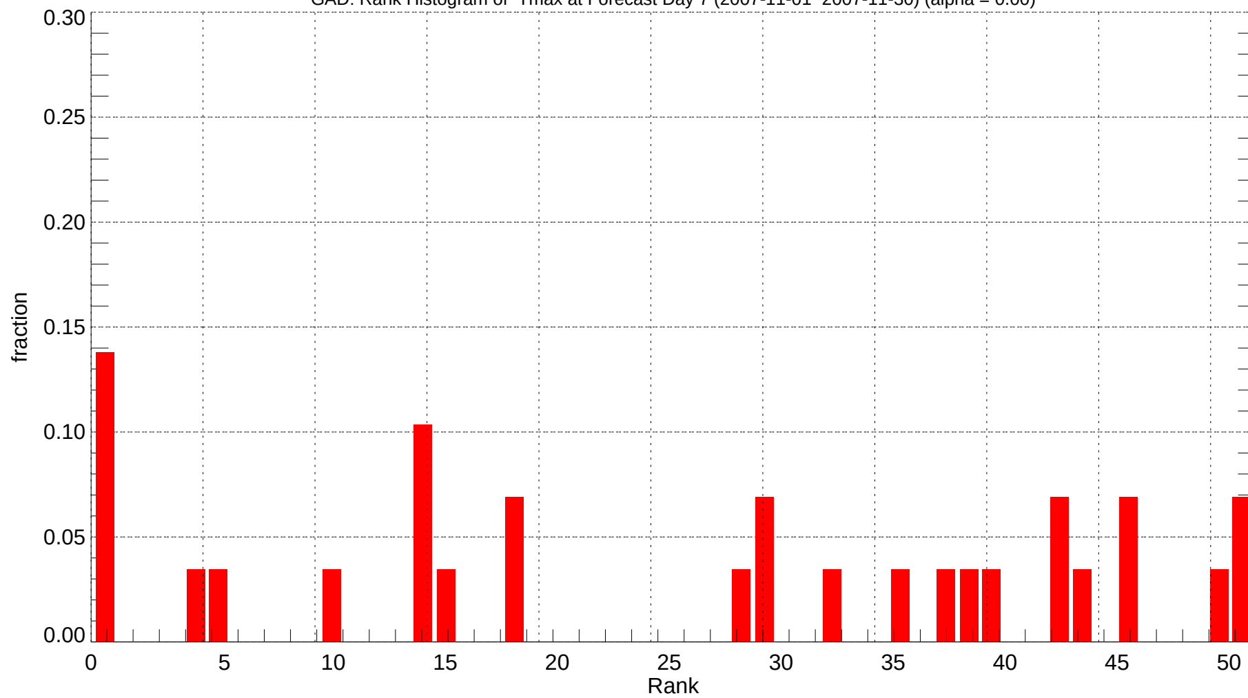
GAD: Rank Histogram of Tmax at Forecast Day 7 (2007-11-01~2007-11-30) (alpha = 0.00)
