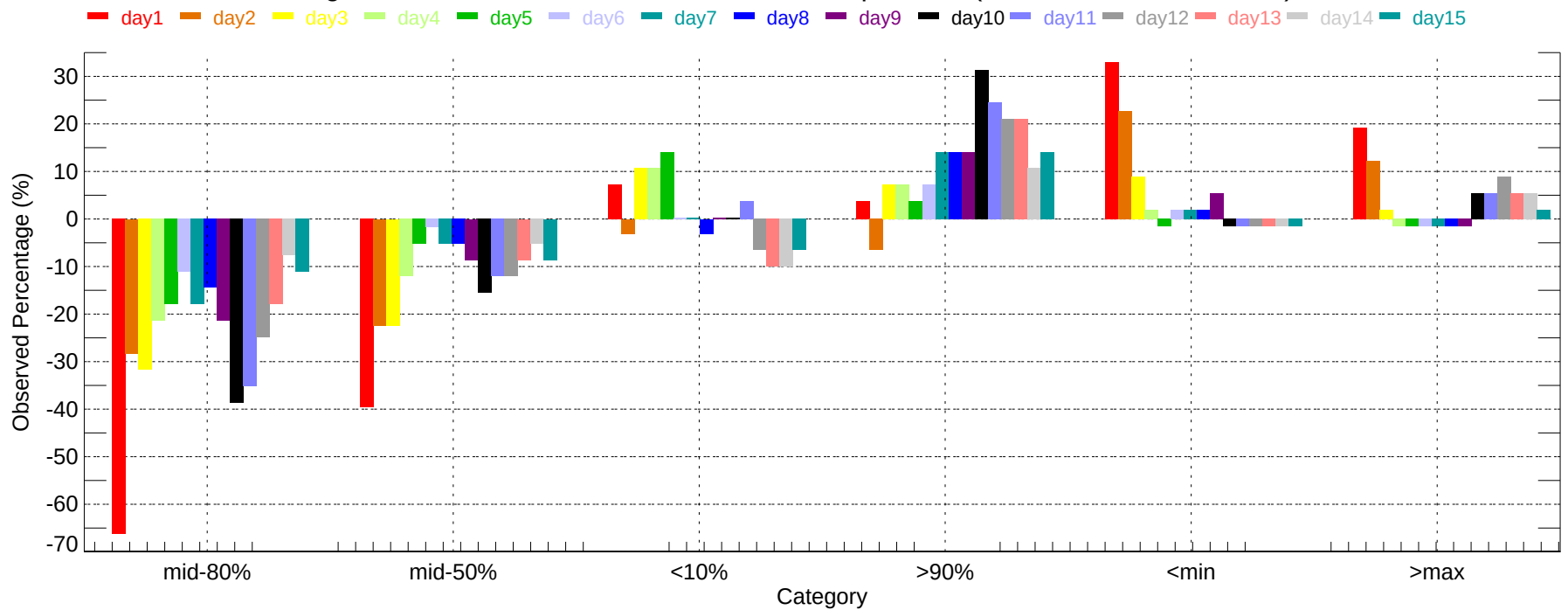
Observed Percentage Deviation of Ensembles - PIR: Max Temperature (2007-11-01~2007-11-30)
