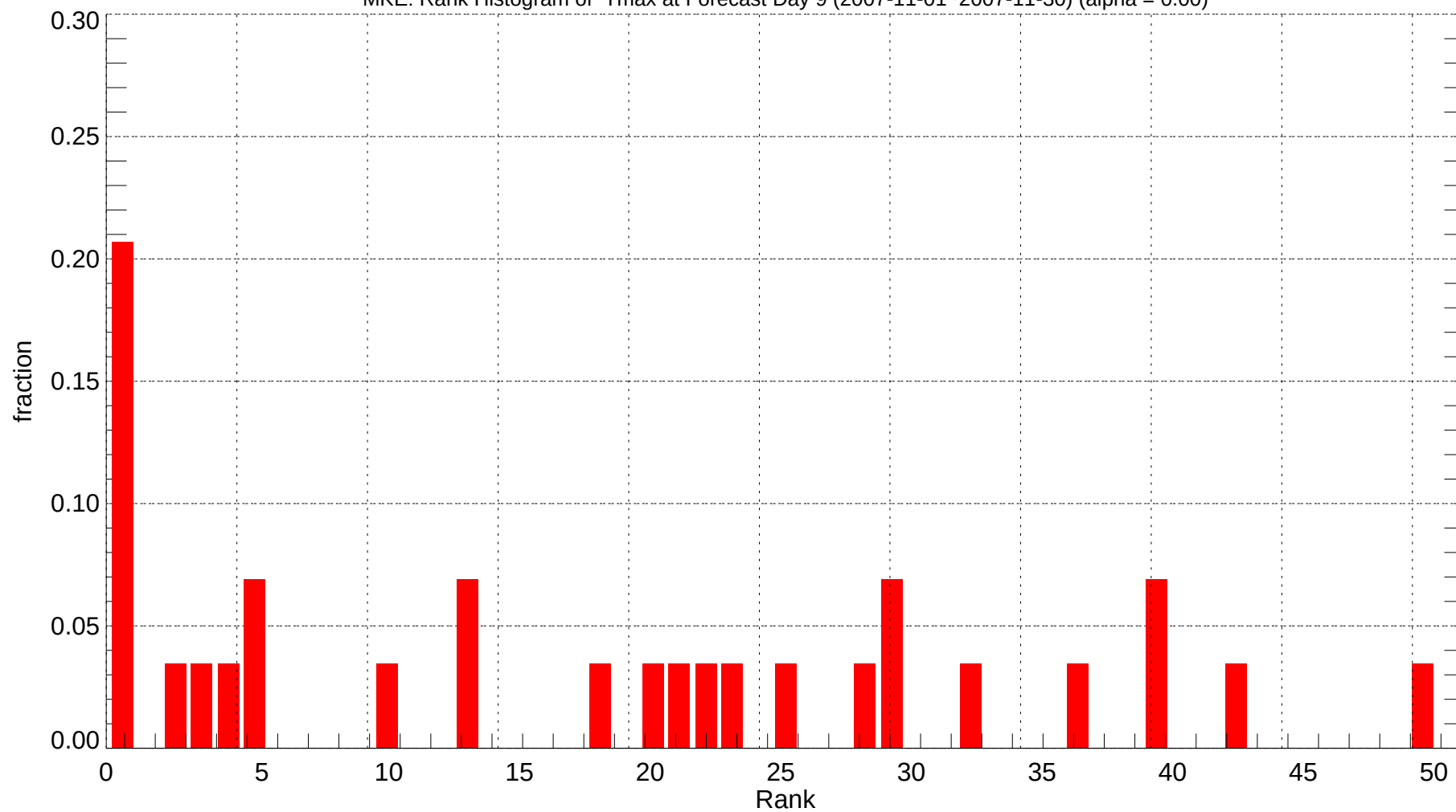
MKE: Rank Histogram of Tmax at Forecast Day 9 (2007-11-01~2007-11-30) (alpha = 0.00)
