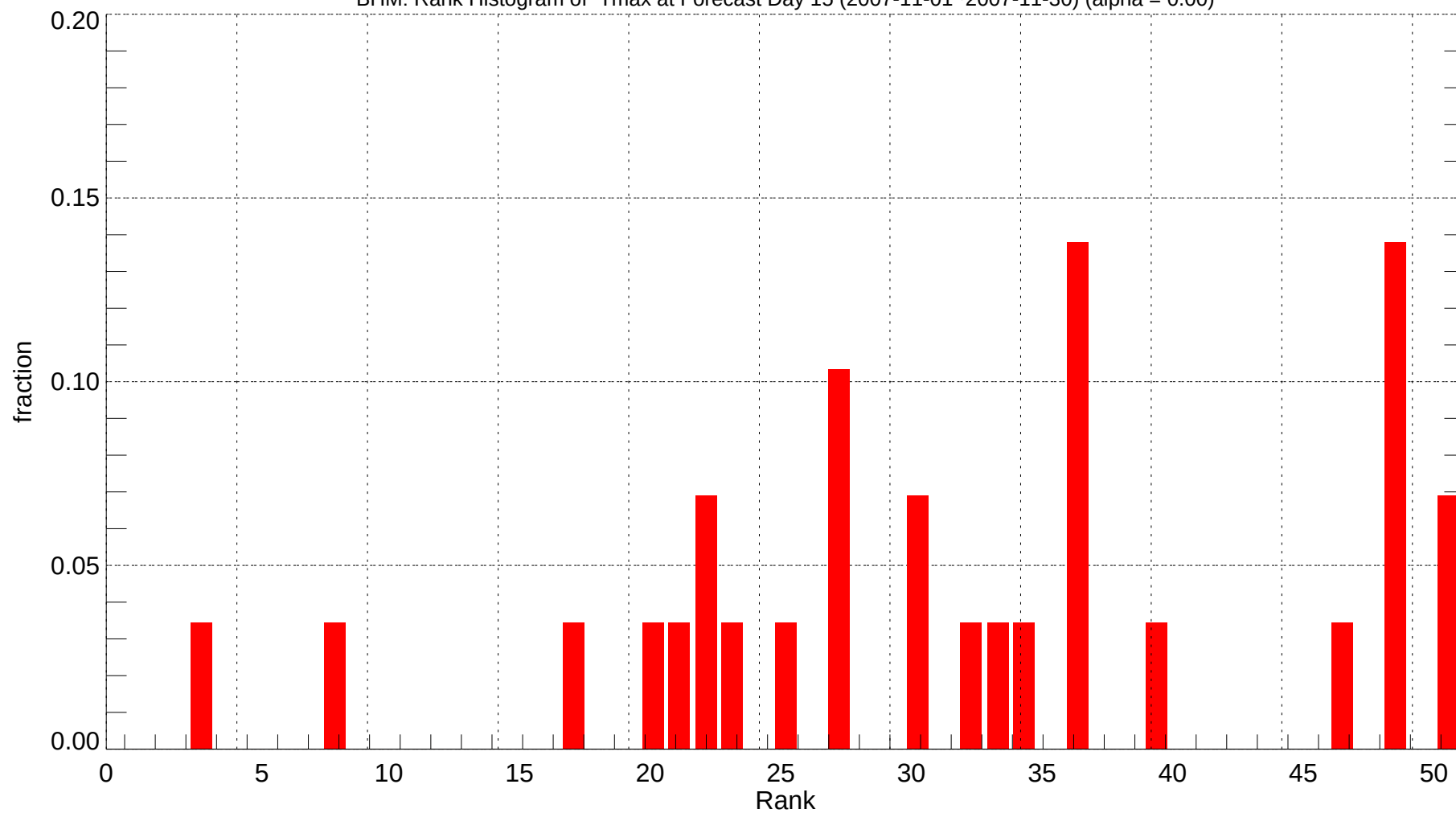
BHM: Rank Histogram of Tmax at Forecast Day 15 (2007-11-01~2007-11-30) (alpha = 0.00)
