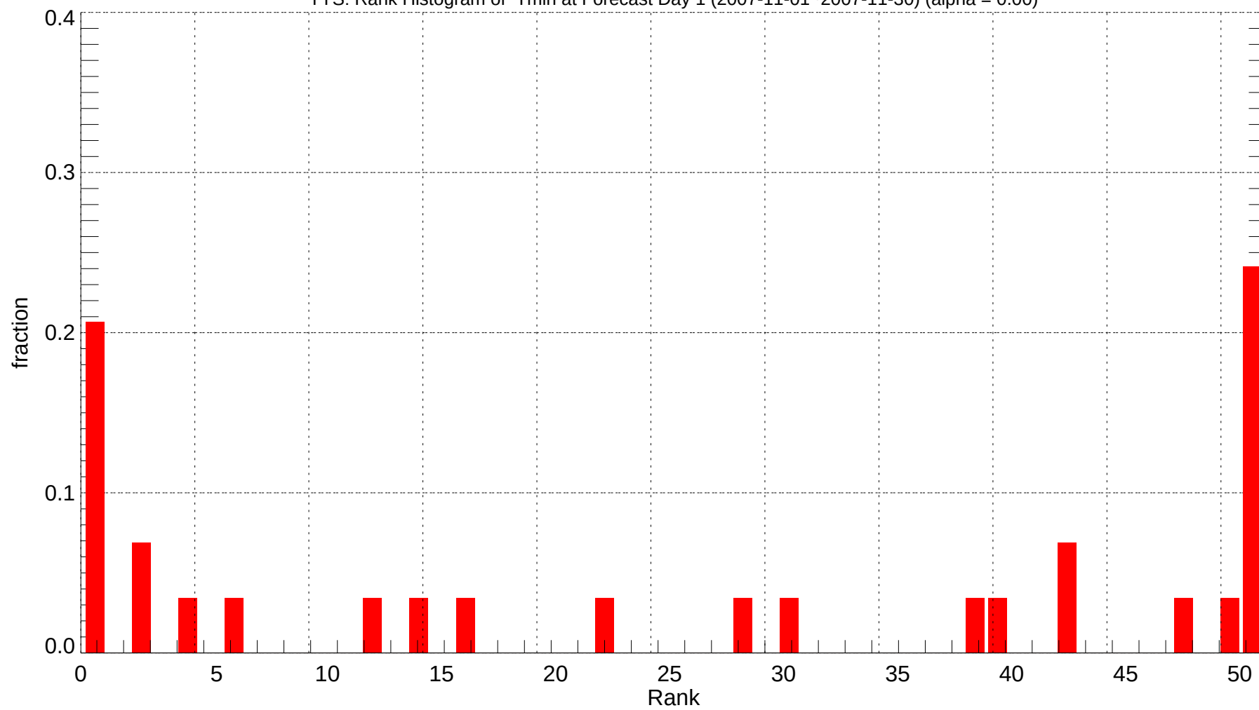
TYS: Rank Histogram of Tmin at Forecast Day 1 (2007-11-01~2007-11-30) (alpha = 0.00)
