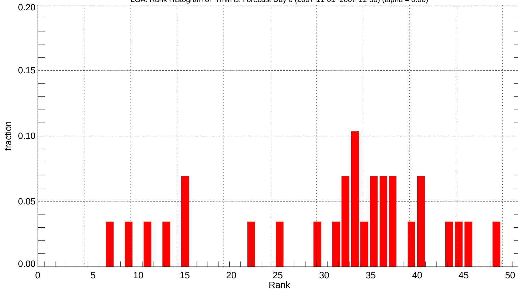
LGA: Rank Histogram of Tmin at Forecast Day 6 (2007-11-01~2007-11-30) (alpha = 0.00)
