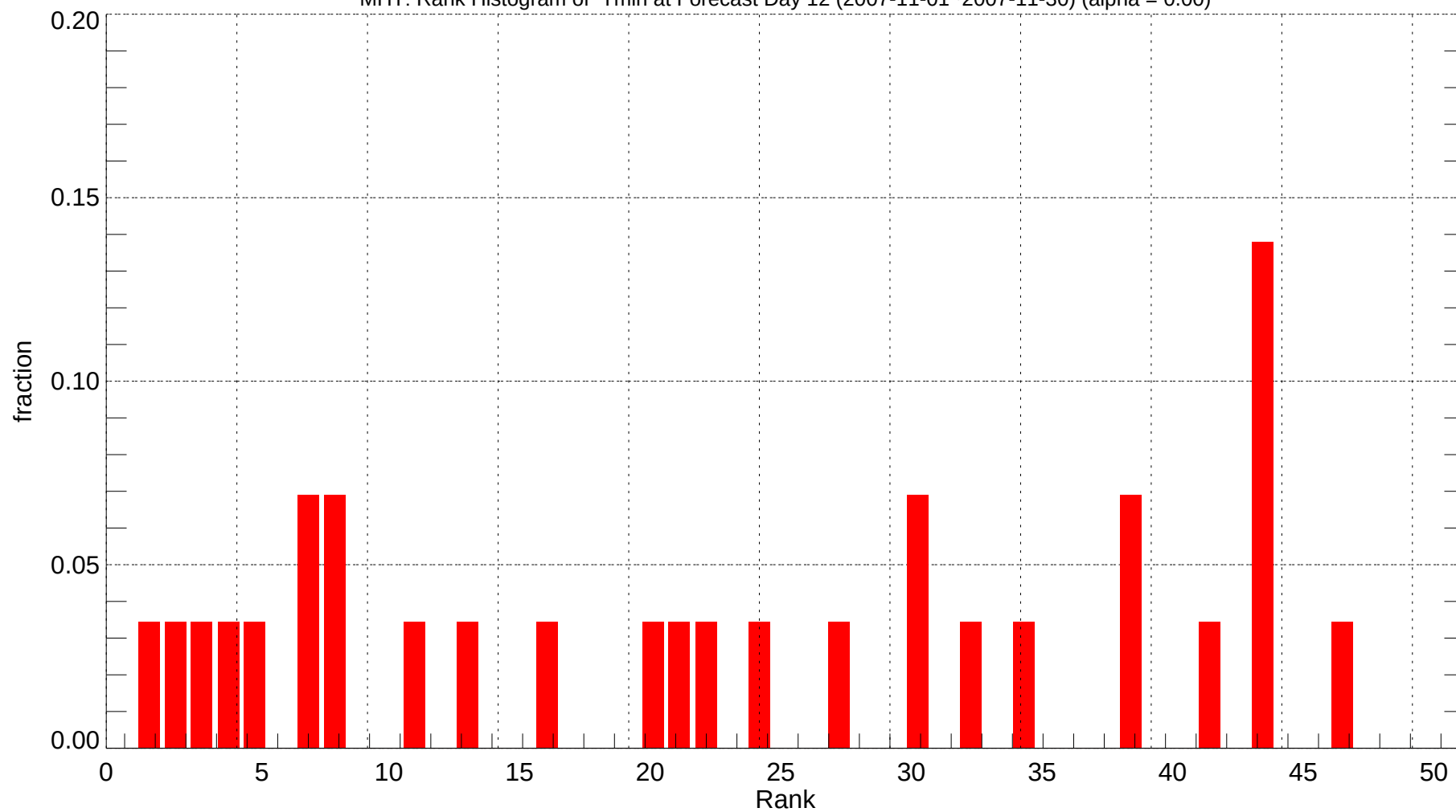
MHT: Rank Histogram of Tmin at Forecast Day 12 (2007-11-01~2007-11-30) (alpha = 0.00)
