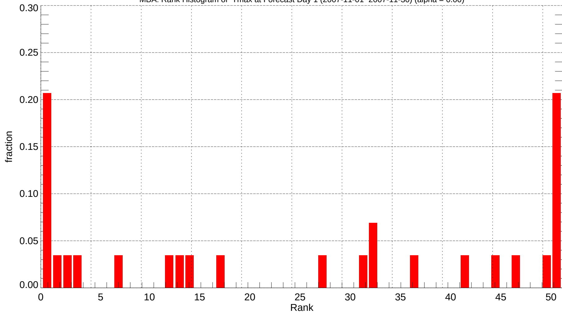
MBA: Rank Histogram of Tmax at Forecast Day 1 (2007-11-01~2007-11-30) (alpha = 0.00)
