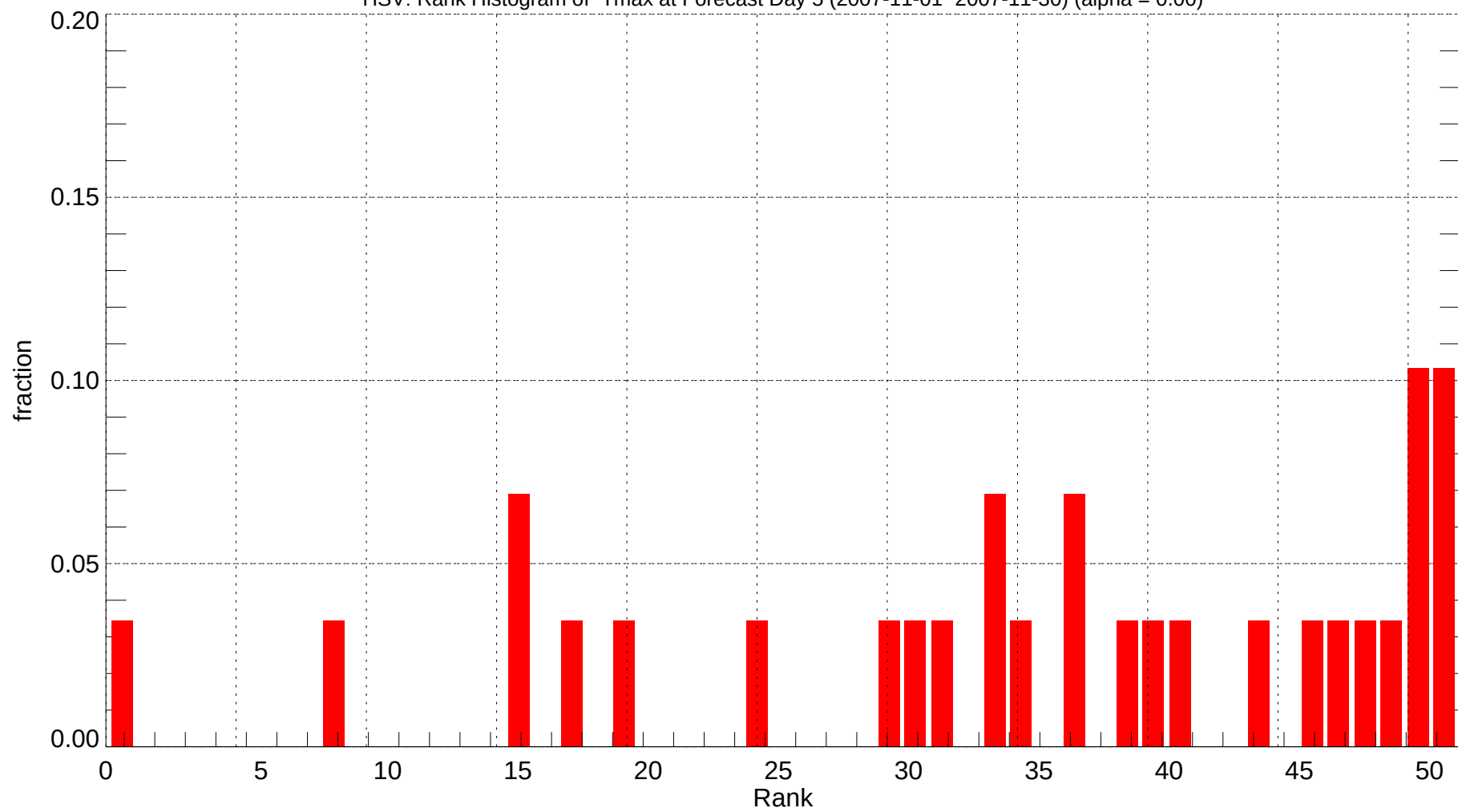
HSV: Rank Histogram of Tmax at Forecast Day 5 (2007-11-01~2007-11-30) (alpha = 0.00)
