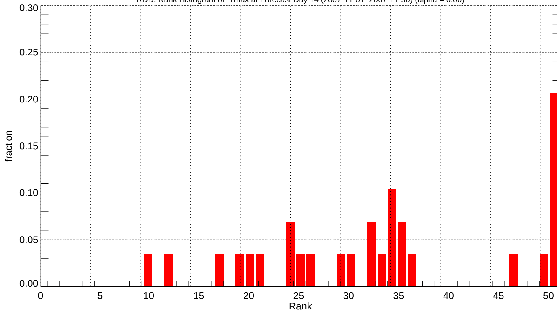
RDD: Rank Histogram of Tmax at Forecast Day 14 (2007-11-01~2007-11-30) (alpha = 0.00)
