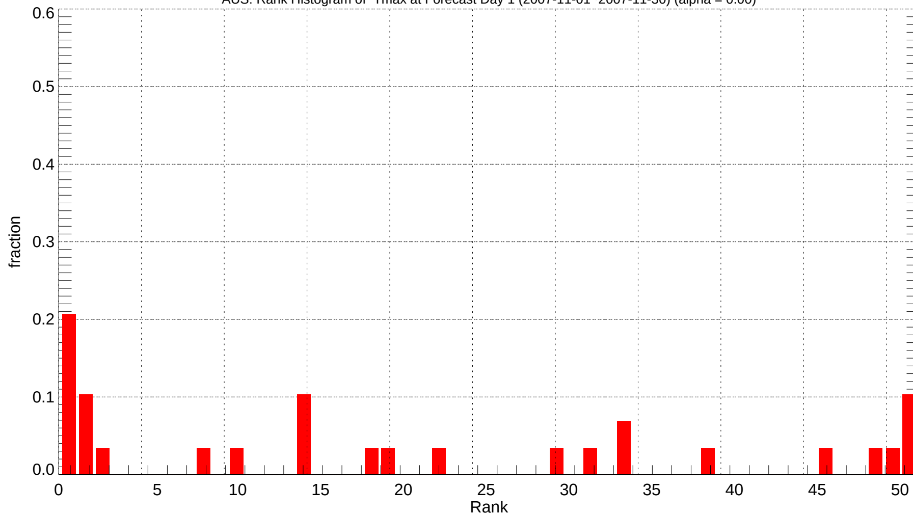
AUS: Rank Histogram of Tmax at Forecast Day 1 (2007-11-01~2007-11-30) (alpha = 0.00)
