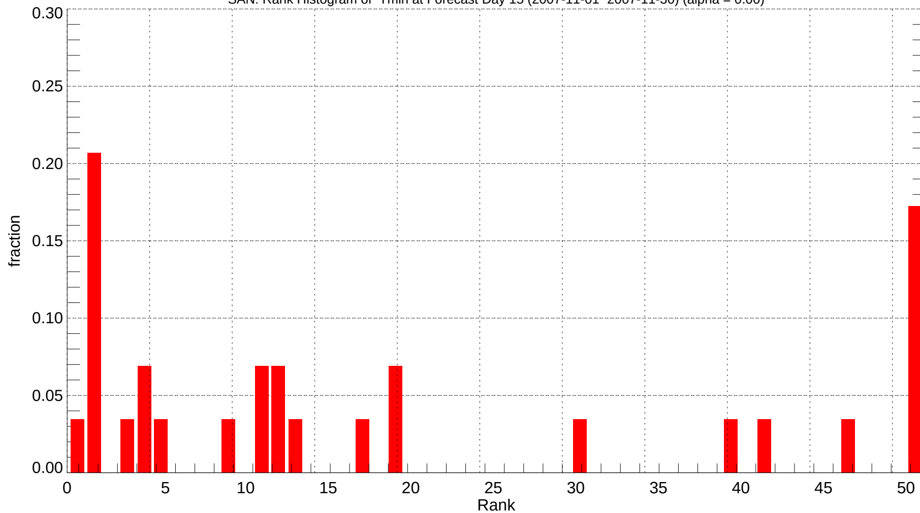
SAN: Rank Histogram of Tmin at Forecast Day 15 (2007-11-01~2007-11-30) (alpha = 0.00)
