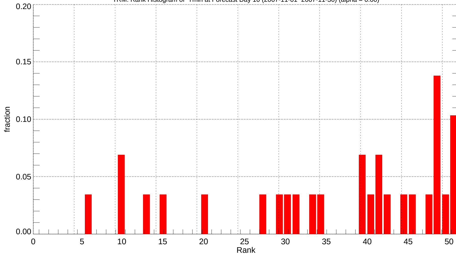
TRM: Rank Histogram of Tmin at Forecast Day 10 (2007-11-01~2007-11-30) (alpha = 0.00)
