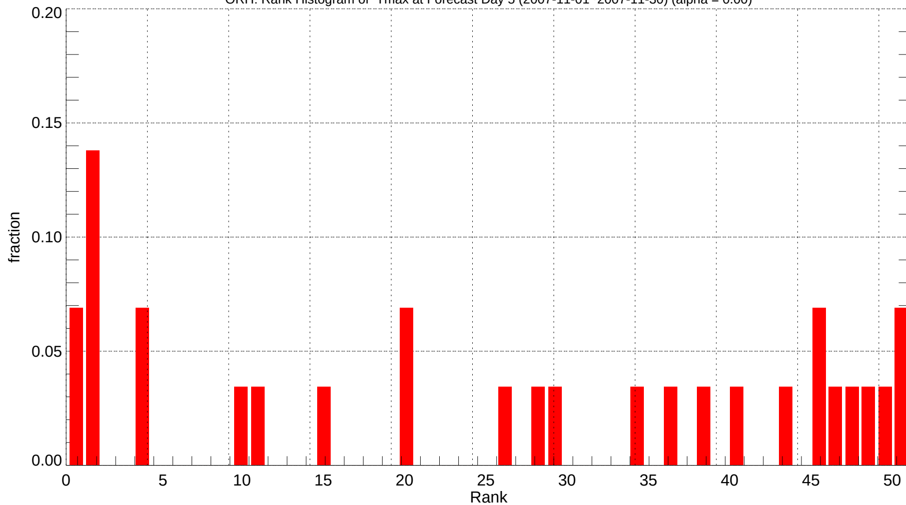
ORH: Rank Histogram of Tmax at Forecast Day 5 (2007-11-01~2007-11-30) (alpha = 0.00)
