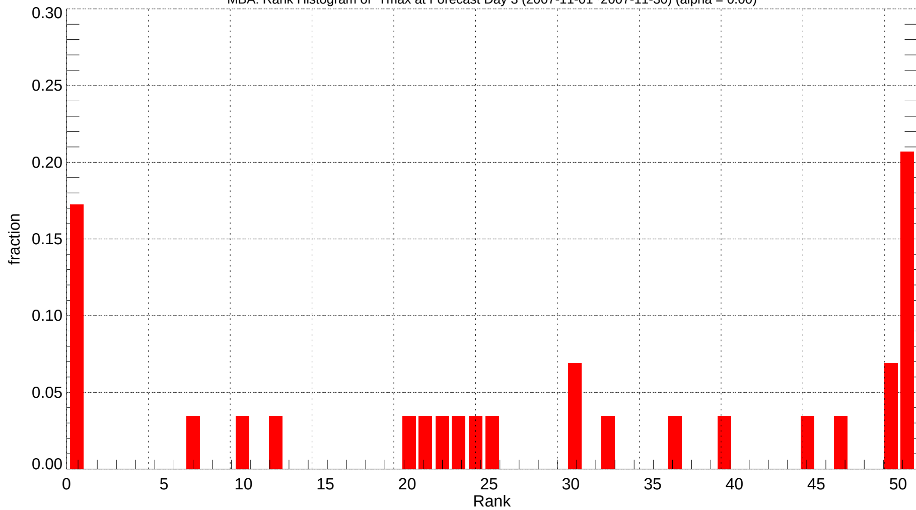
MBA: Rank Histogram of Tmax at Forecast Day 3 (2007-11-01~2007-11-30) (alpha = 0.00)
