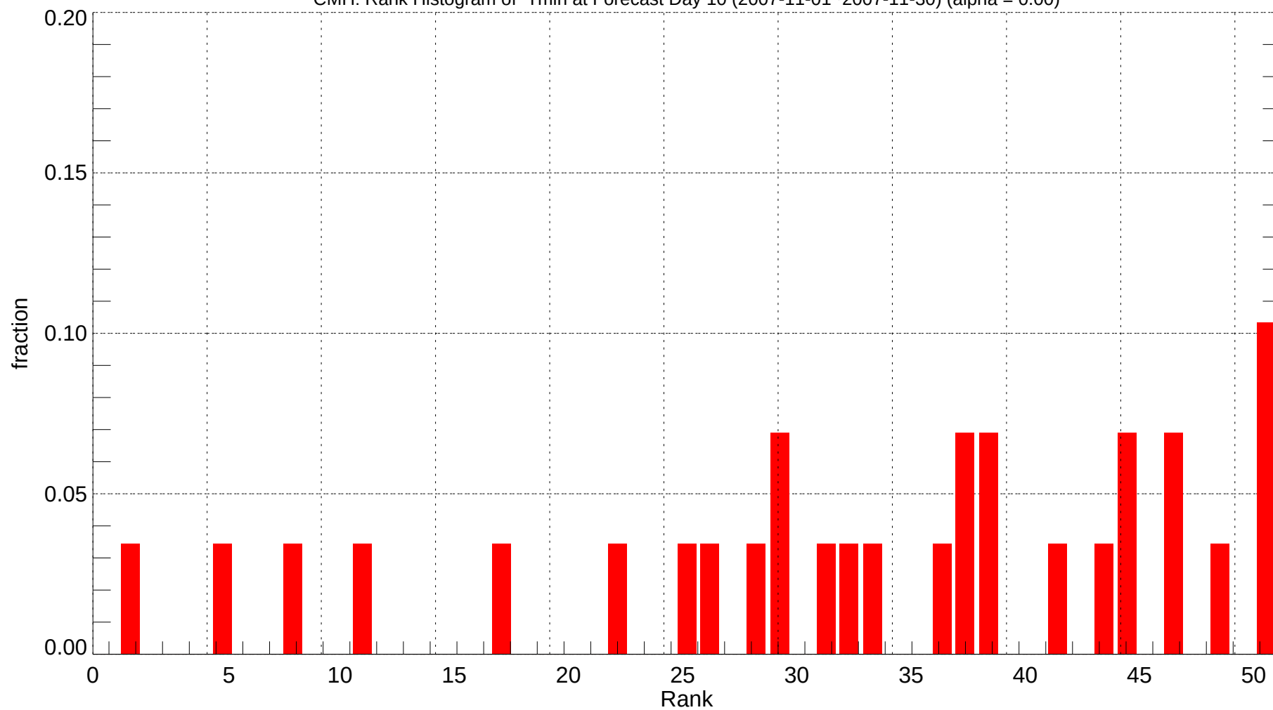
CMH: Rank Histogram of Tmin at Forecast Day 10 (2007-11-01~2007-11-30) (alpha = 0.00)
