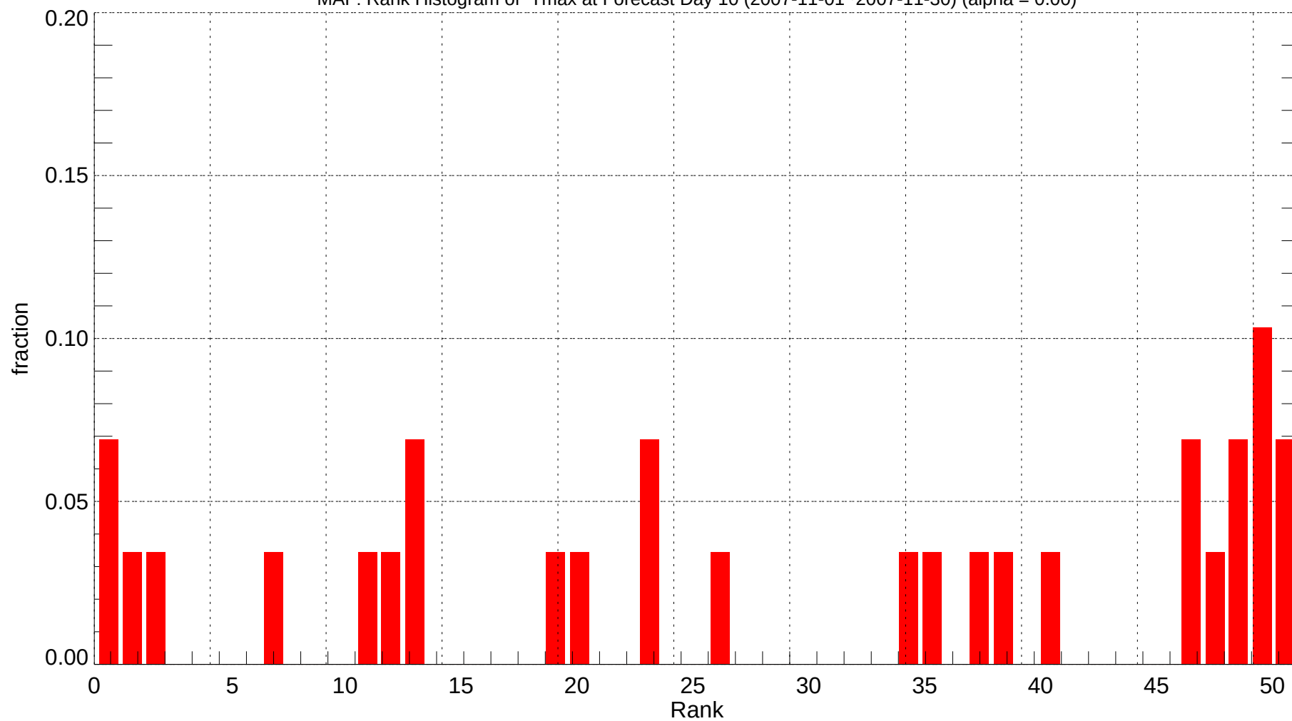
MAF: Rank Histogram of Tmax at Forecast Day 10 (2007-11-01~2007-11-30) (alpha = 0.00)
