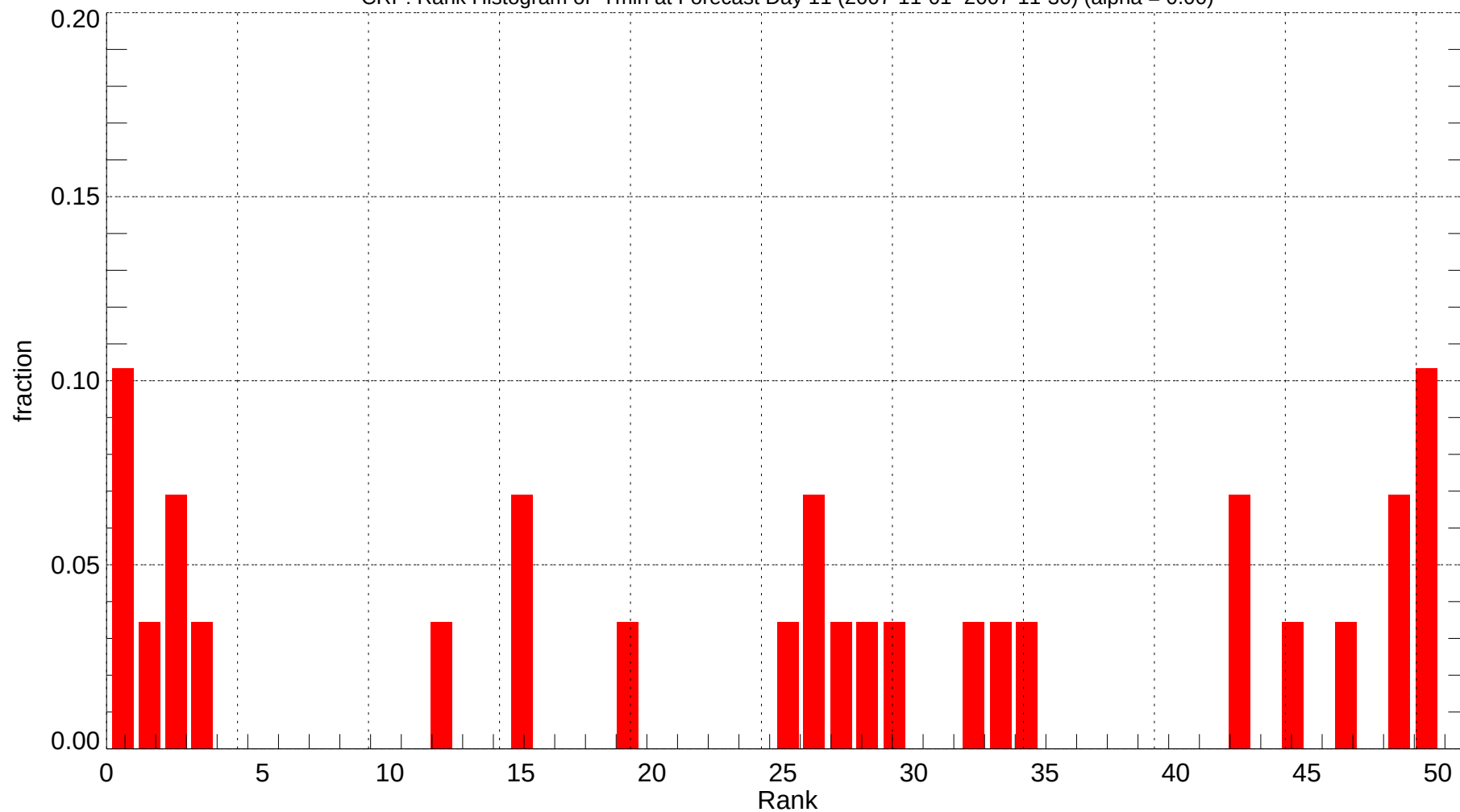
CRP: Rank Histogram of Tmin at Forecast Day 11 (2007-11-01~2007-11-30) (alpha = 0.00)
