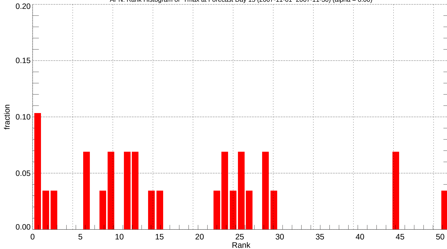
APN: Rank Histogram of Tmax at Forecast Day 15 (2007-11-01~2007-11-30) (alpha = 0.00)
