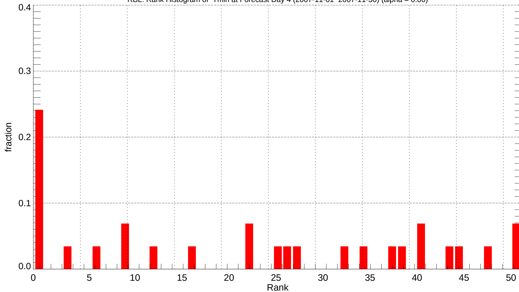
RBL: Rank Histogram of Tmin at Forecast Day 4 (2007-11-01~2007-11-30) (alpha = 0.00)
