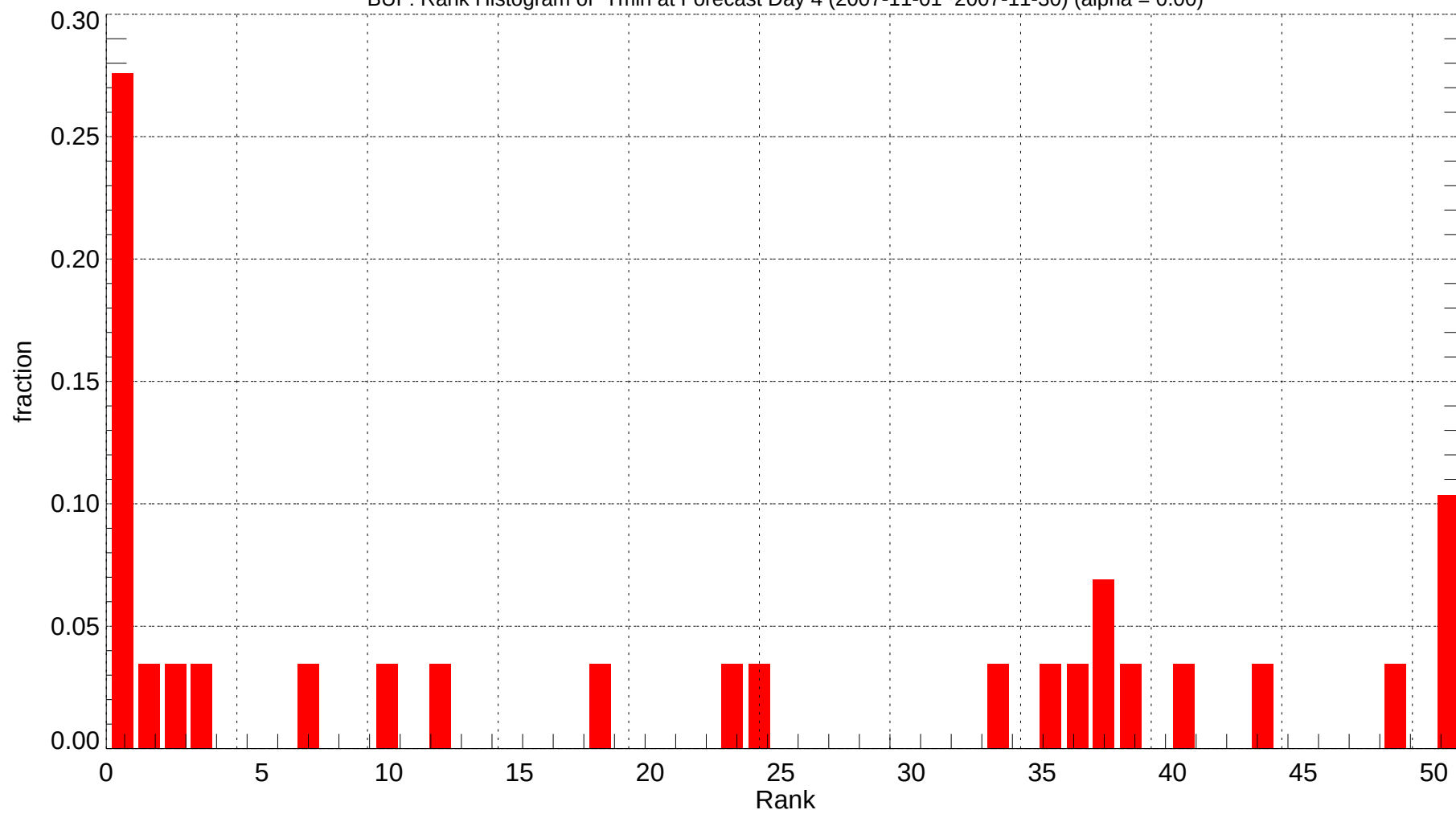
BUF: Rank Histogram of Tmin at Forecast Day 4 (2007-11-01~2007-11-30) (alpha = 0.00)
