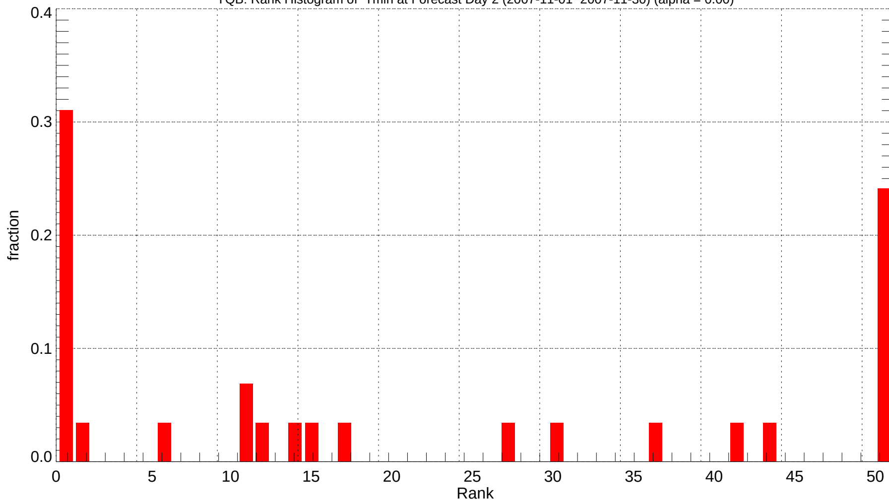
YQB: Rank Histogram of Tmin at Forecast Day 2 (2007-11-01~2007-11-30) (alpha = 0.00)
