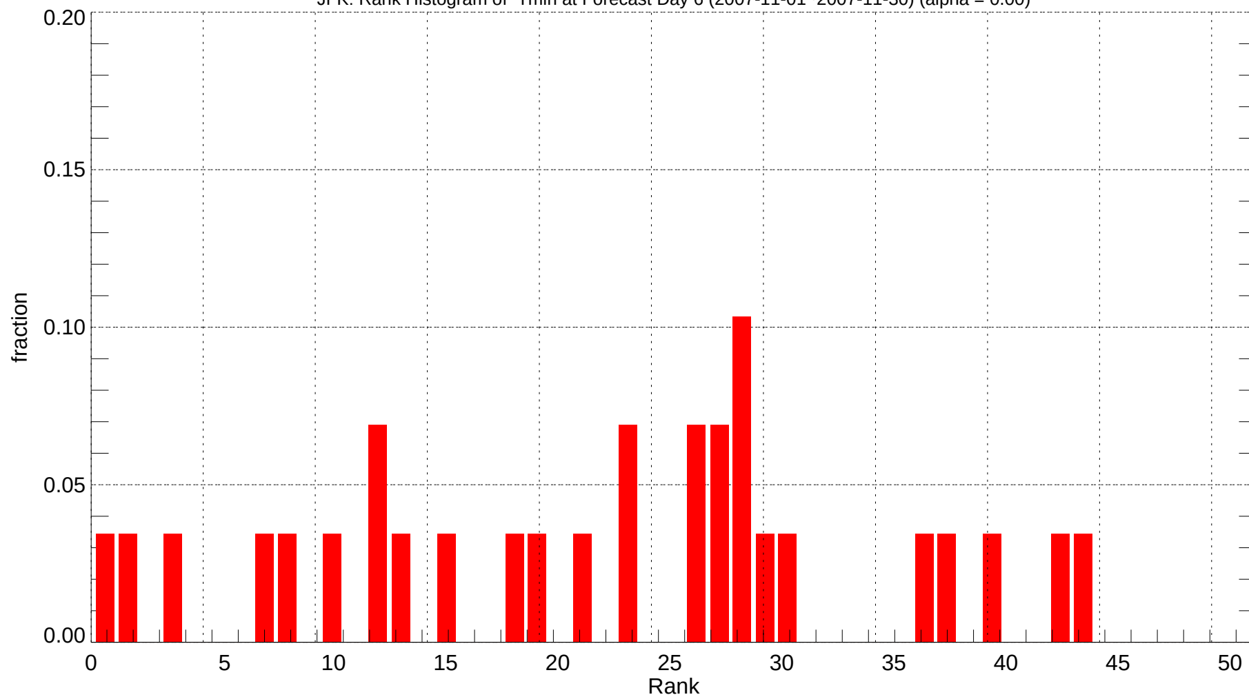
JFK: Rank Histogram of Tmin at Forecast Day 6 (2007-11-01~2007-11-30) (alpha = 0.00)
