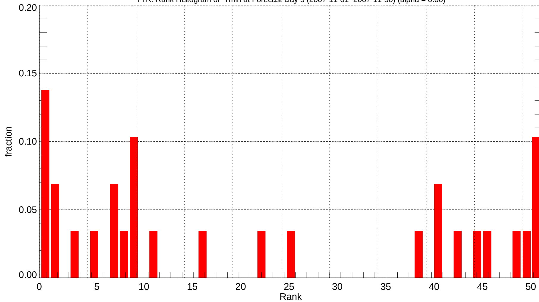
TYR: Rank Histogram of Tmin at Forecast Day 3 (2007-11-01~2007-11-30) (alpha = 0.00)
