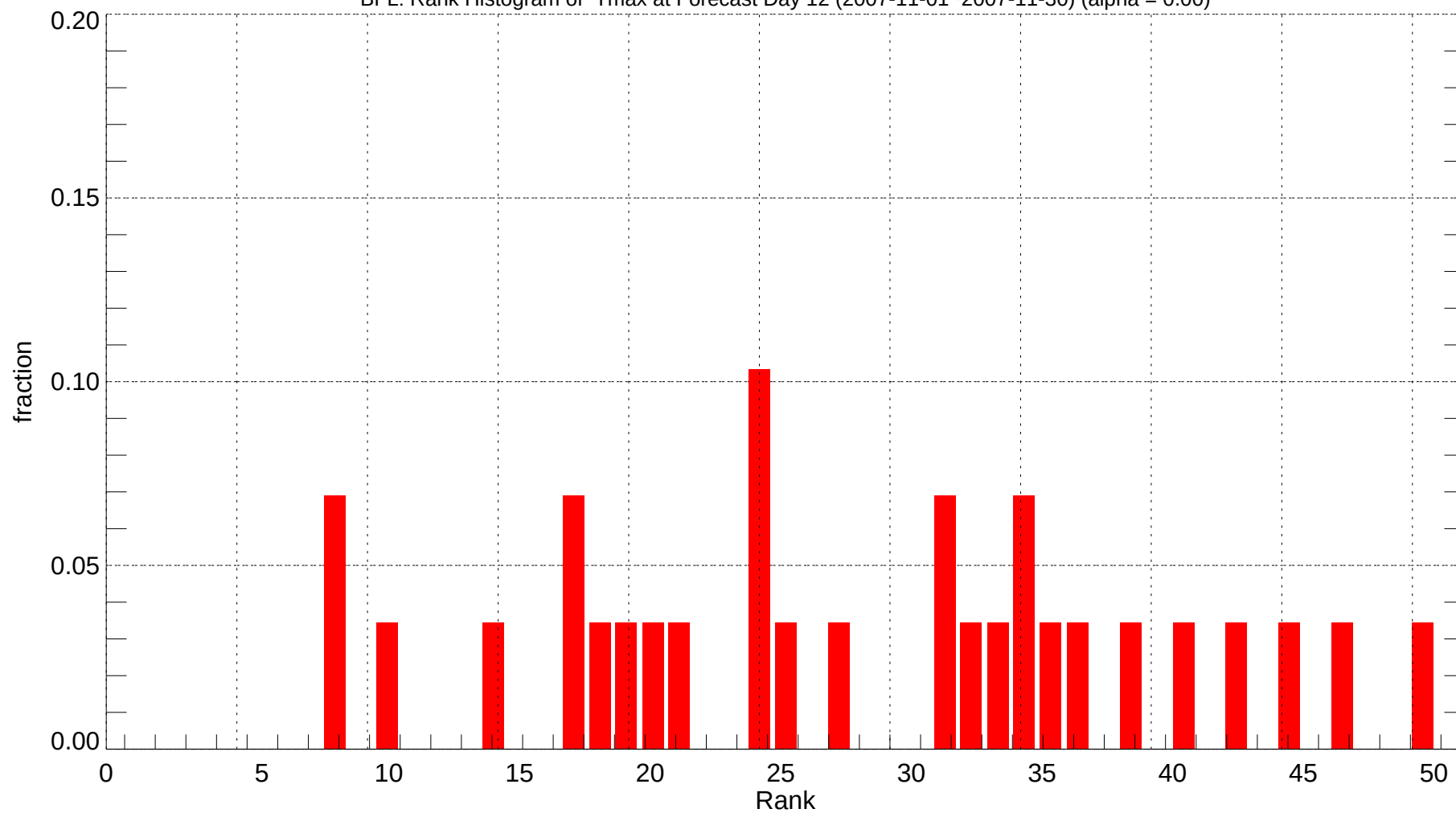
BFL: Rank Histogram of Tmax at Forecast Day 12 (2007-11-01~2007-11-30) (alpha = 0.00)
