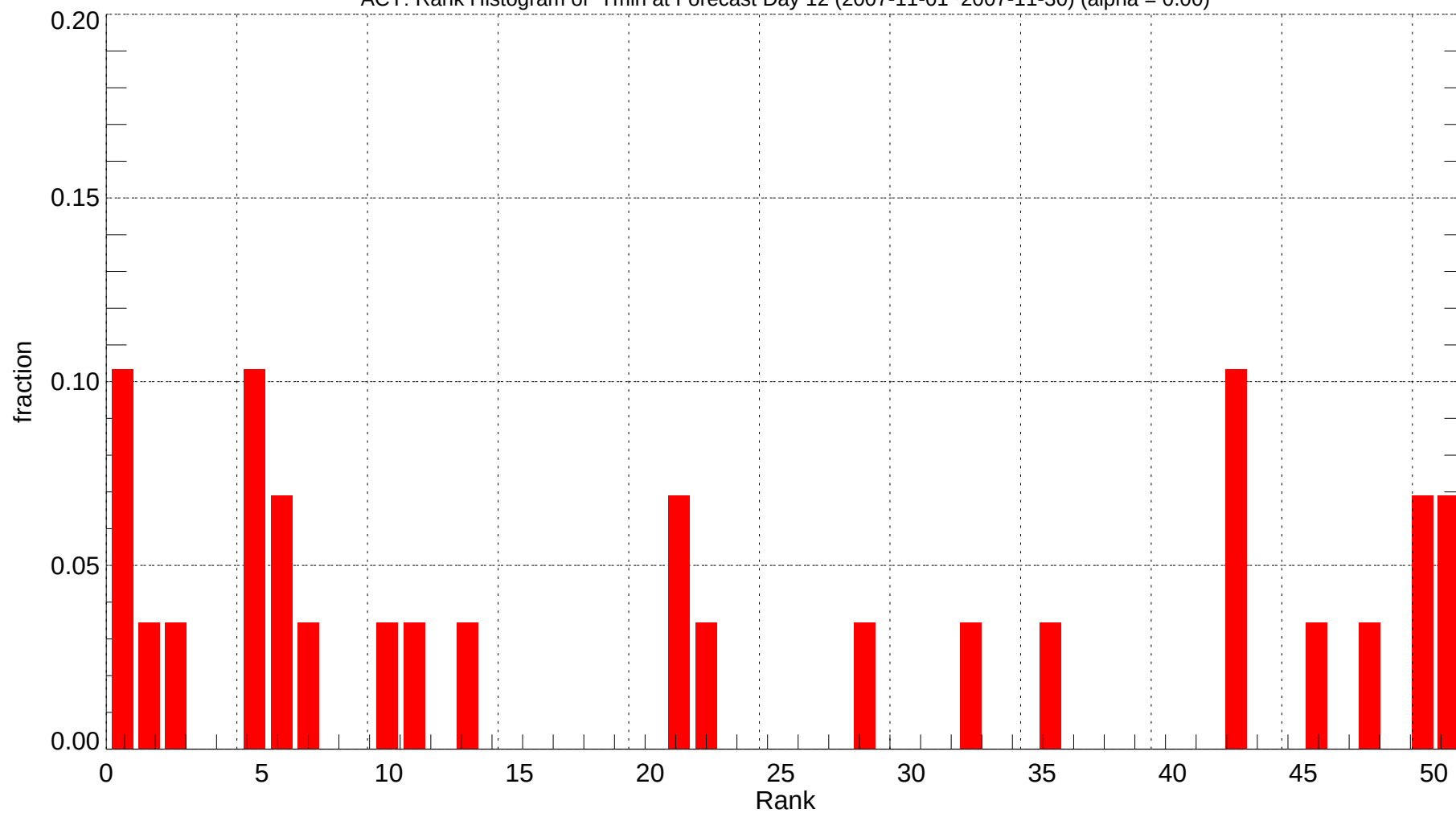
ACY: Rank Histogram of Tmin at Forecast Day 12 (2007-11-01~2007-11-30) (alpha = 0.00)
