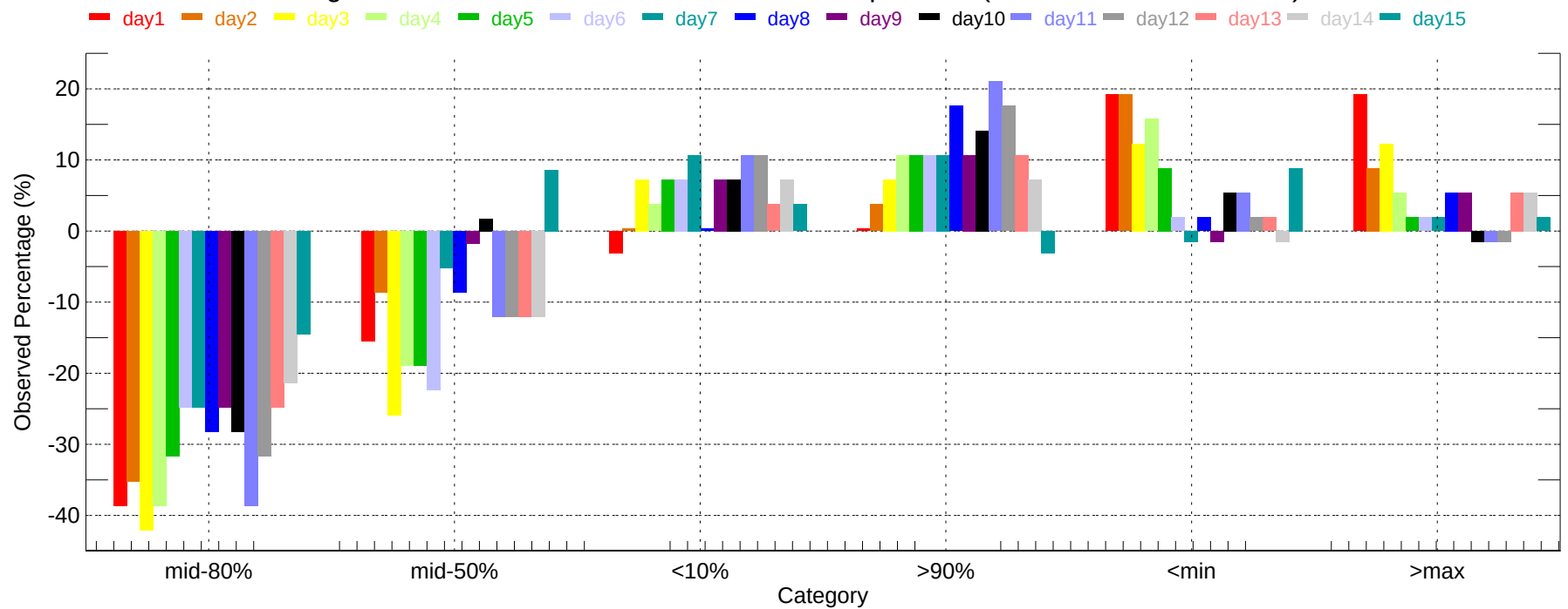
Observed Percentage Deviation of Ensembles - SAT: Max Temperature (2007-11-01~2007-11-30)
