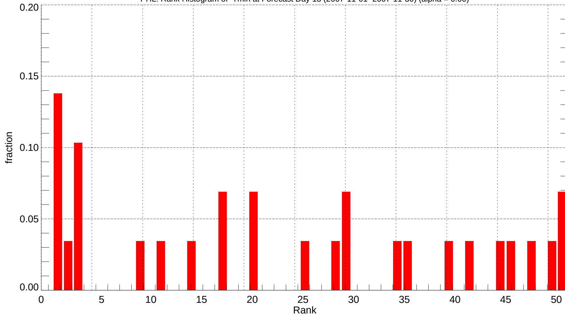
PHL: Rank Histogram of Tmin at Forecast Day 13 (2007-11-01~2007-11-30) (alpha = 0.00)
