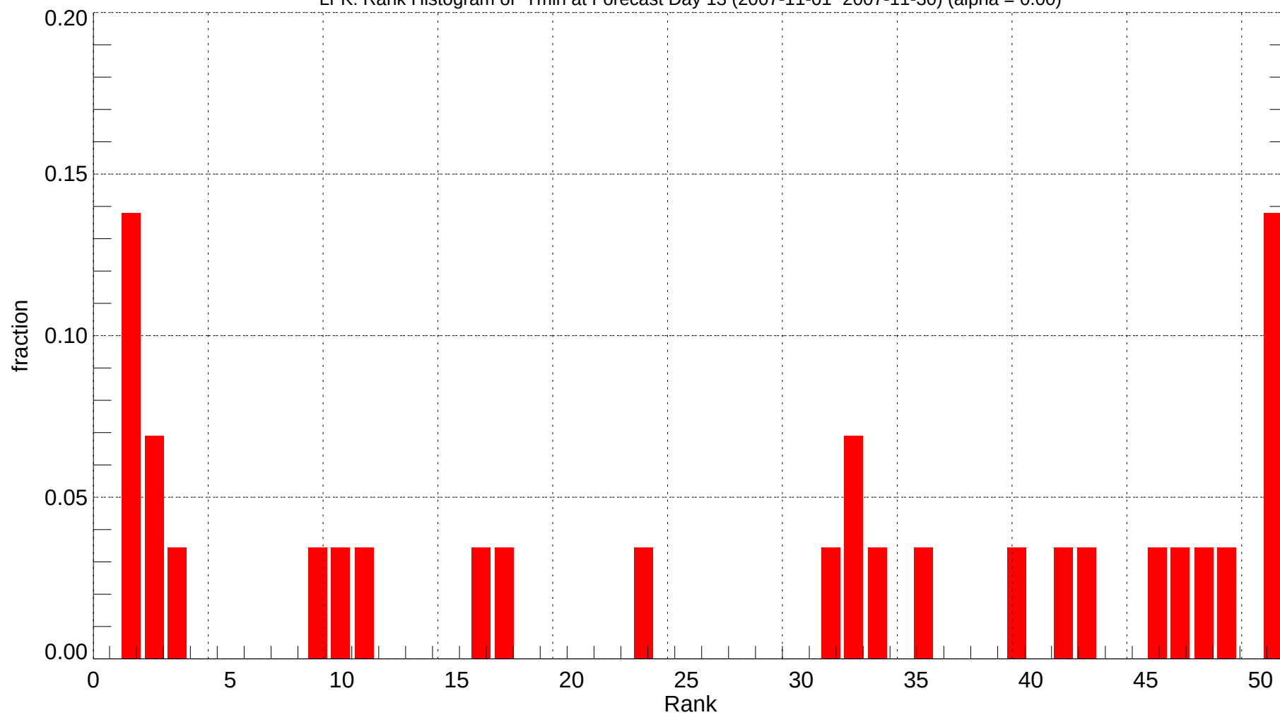
LFK: Rank Histogram of Tmin at Forecast Day 13 (2007-11-01~2007-11-30) (alpha = 0.00)
