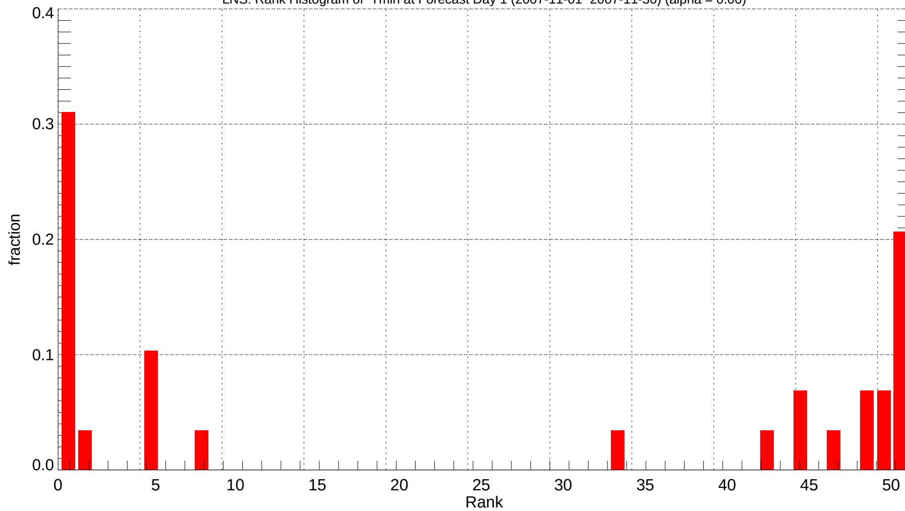
LNS: Rank Histogram of Tmin at Forecast Day 1 (2007-11-01~2007-11-30) (alpha = 0.00)
