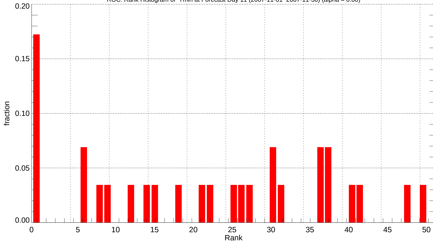
ROC: Rank Histogram of Tmin at Forecast Day 11 (2007-11-01~2007-11-30) (alpha = 0.00)
