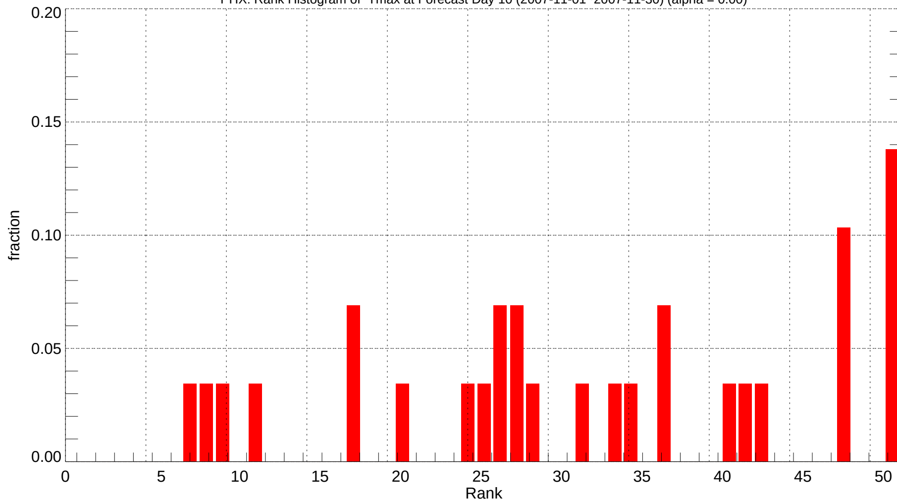
PHX: Rank Histogram of Tmax at Forecast Day 10 (2007-11-01~2007-11-30) (alpha = 0.00)
