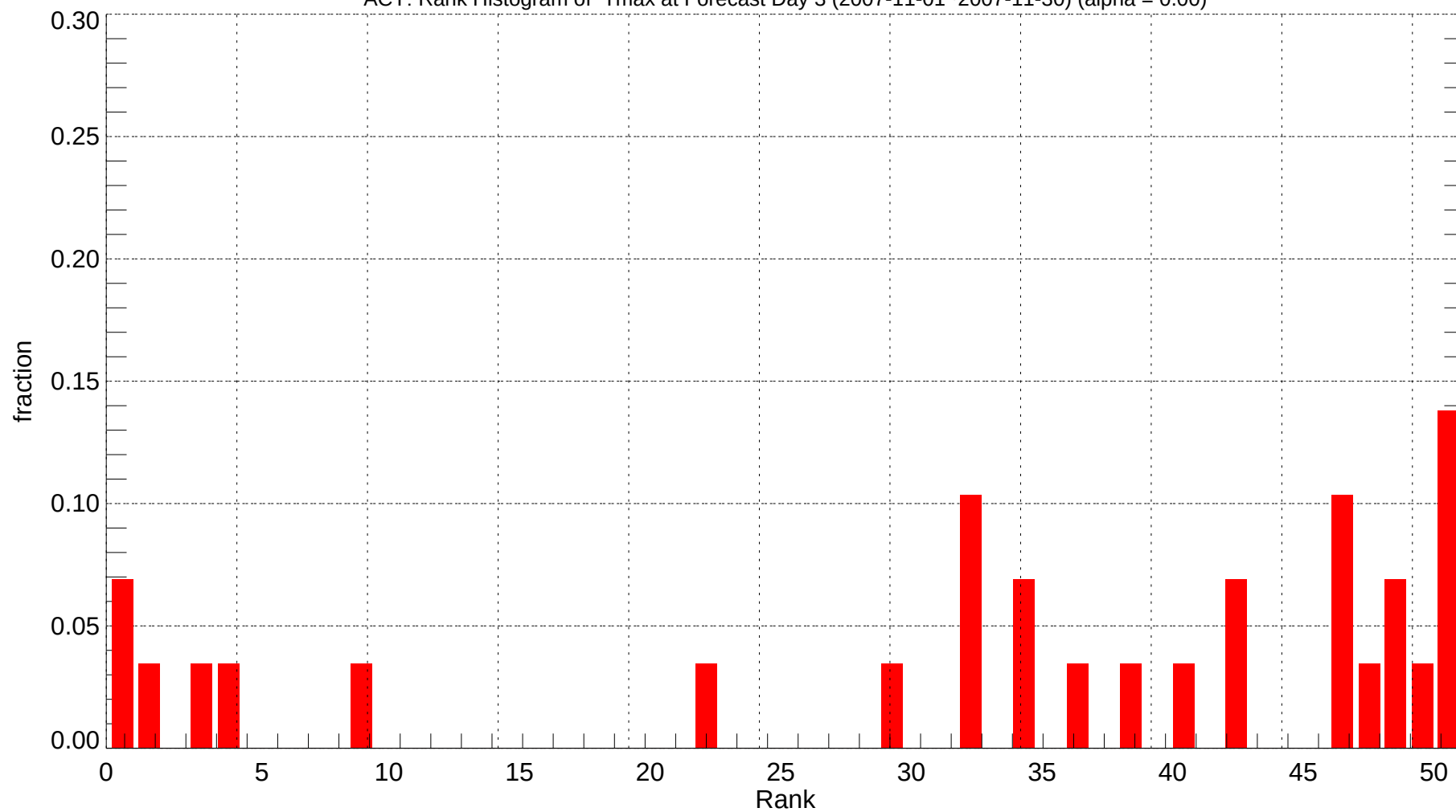
ACY: Rank Histogram of Tmax at Forecast Day 3 (2007-11-01~2007-11-30) (alpha = 0.00)
