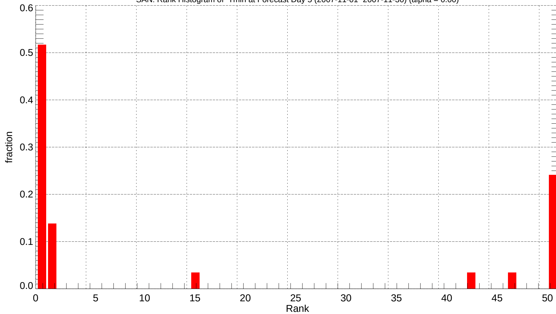
SAN: Rank Histogram of Tmin at Forecast Day 5 (2007-11-01~2007-11-30) (alpha = 0.00)
