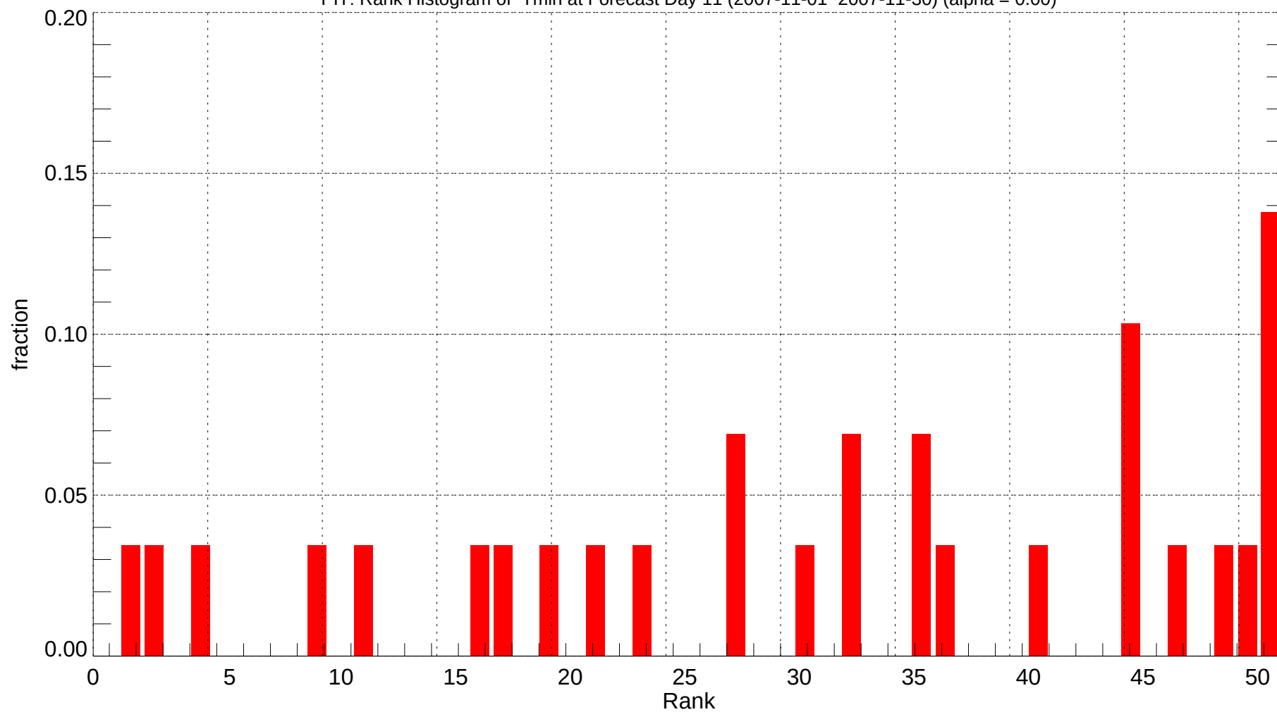
PIT: Rank Histogram of Tmin at Forecast Day 11 (2007-11-01~2007-11-30) (alpha = 0.00)
