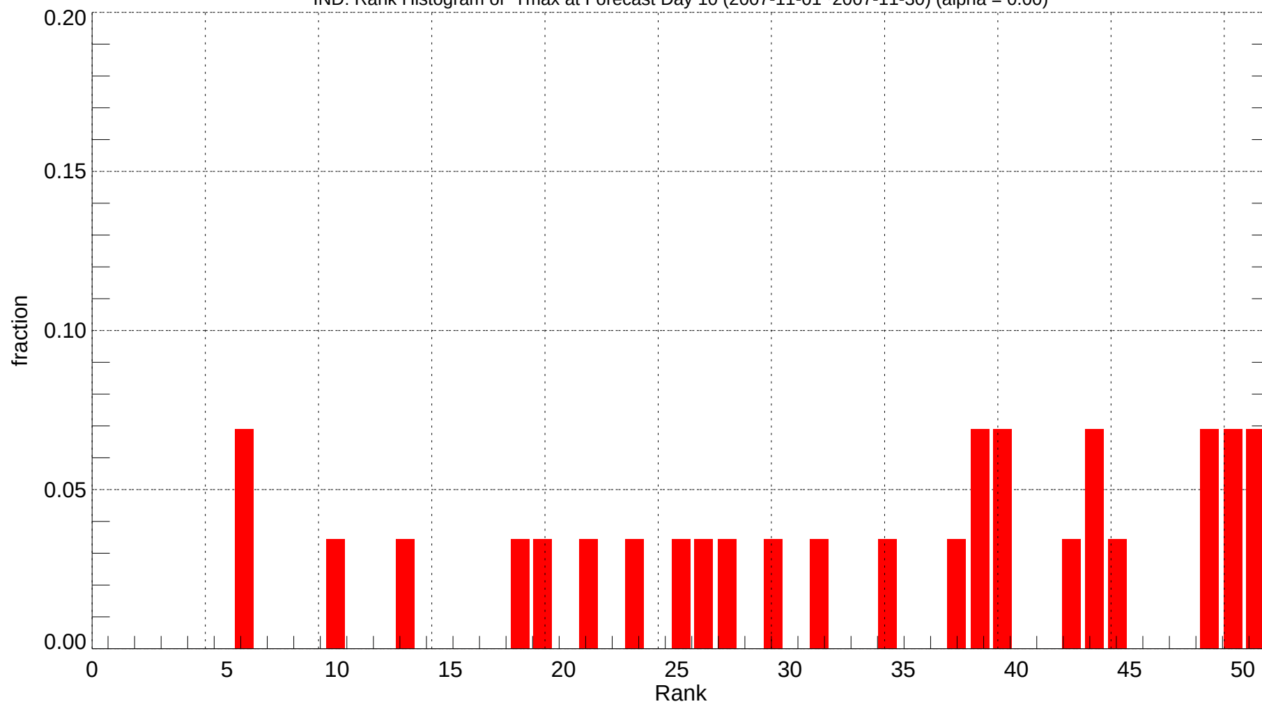
IND: Rank Histogram of Tmax at Forecast Day 10 (2007-11-01~2007-11-30) (alpha = 0.00)
