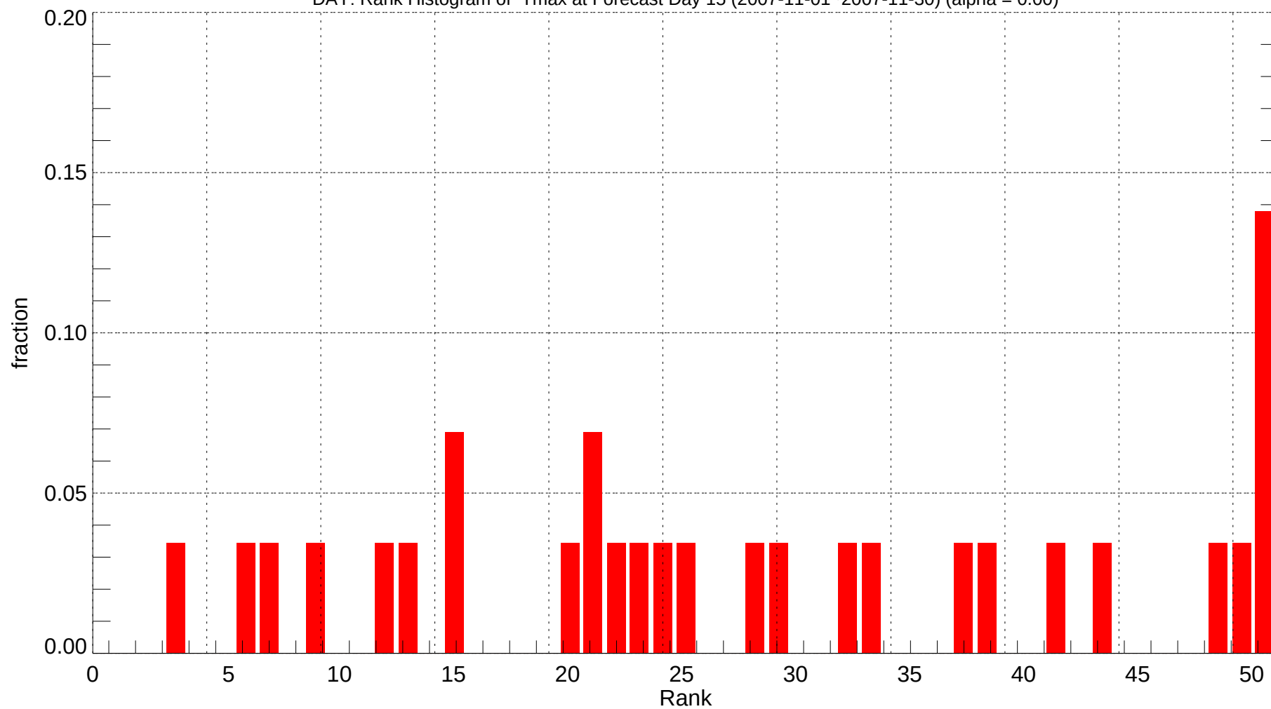
DAY: Rank Histogram of Tmax at Forecast Day 15 (2007-11-01~2007-11-30) (alpha = 0.00)
