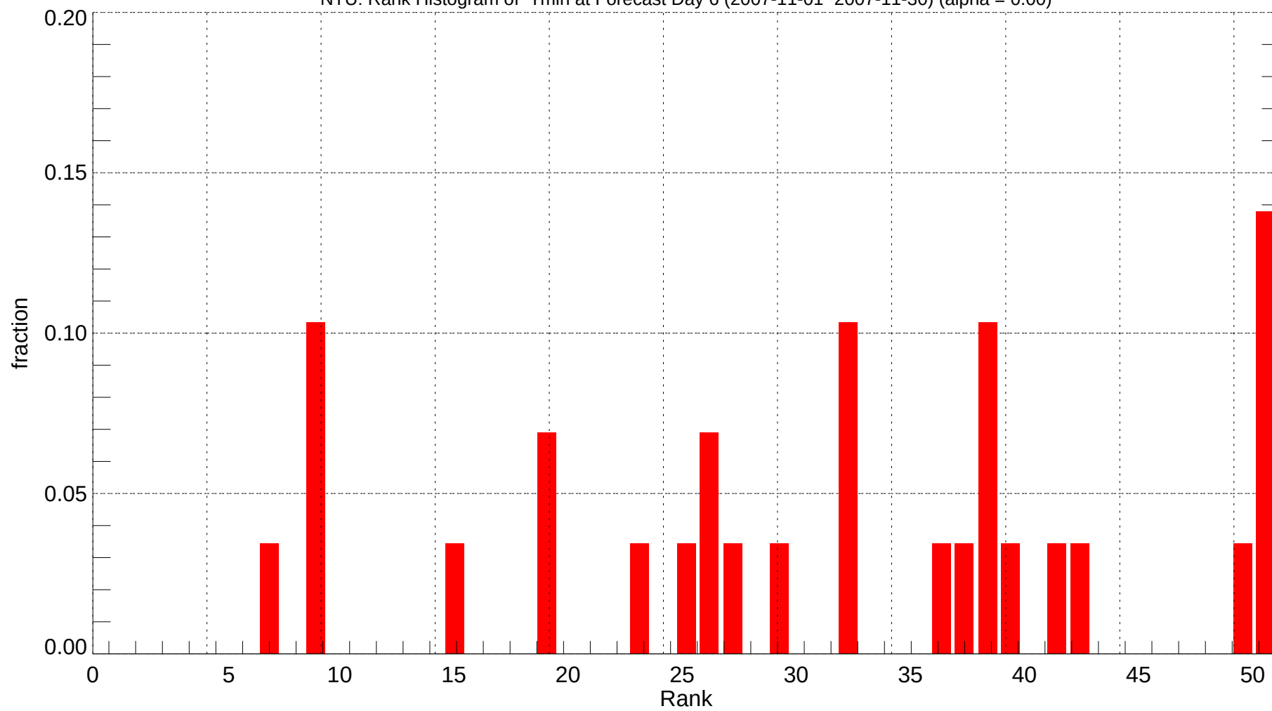
NTU: Rank Histogram of Tmin at Forecast Day 6 (2007-11-01~2007-11-30) (alpha = 0.00)
