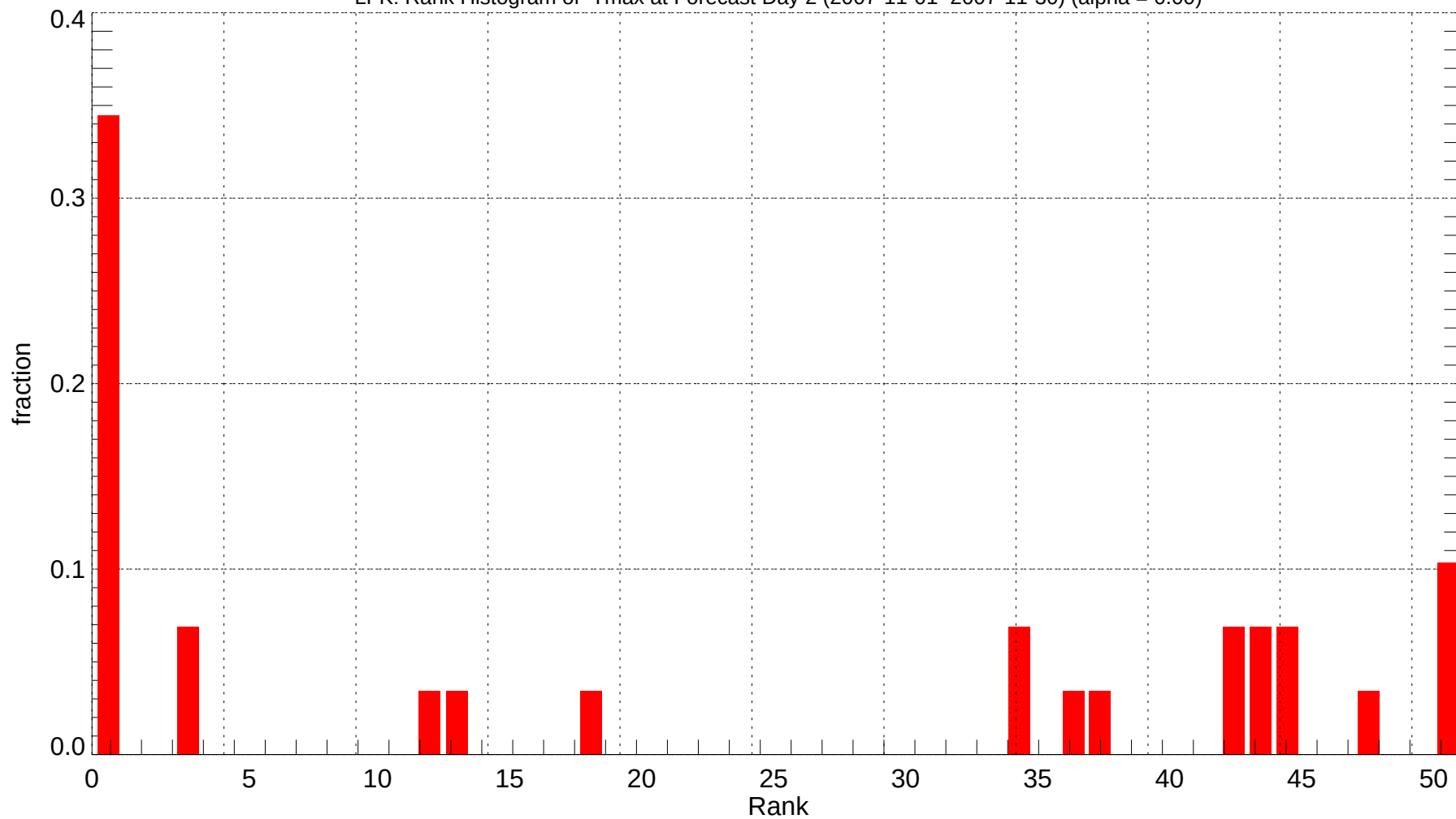
LFK: Rank Histogram of Tmax at Forecast Day 2 (2007-11-01~2007-11-30) (alpha = 0.00)
