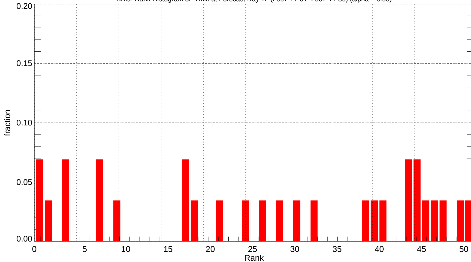
BRO: Rank Histogram of Tmin at Forecast Day 12 (2007-11-01~2007-11-30) (alpha = 0.00)
