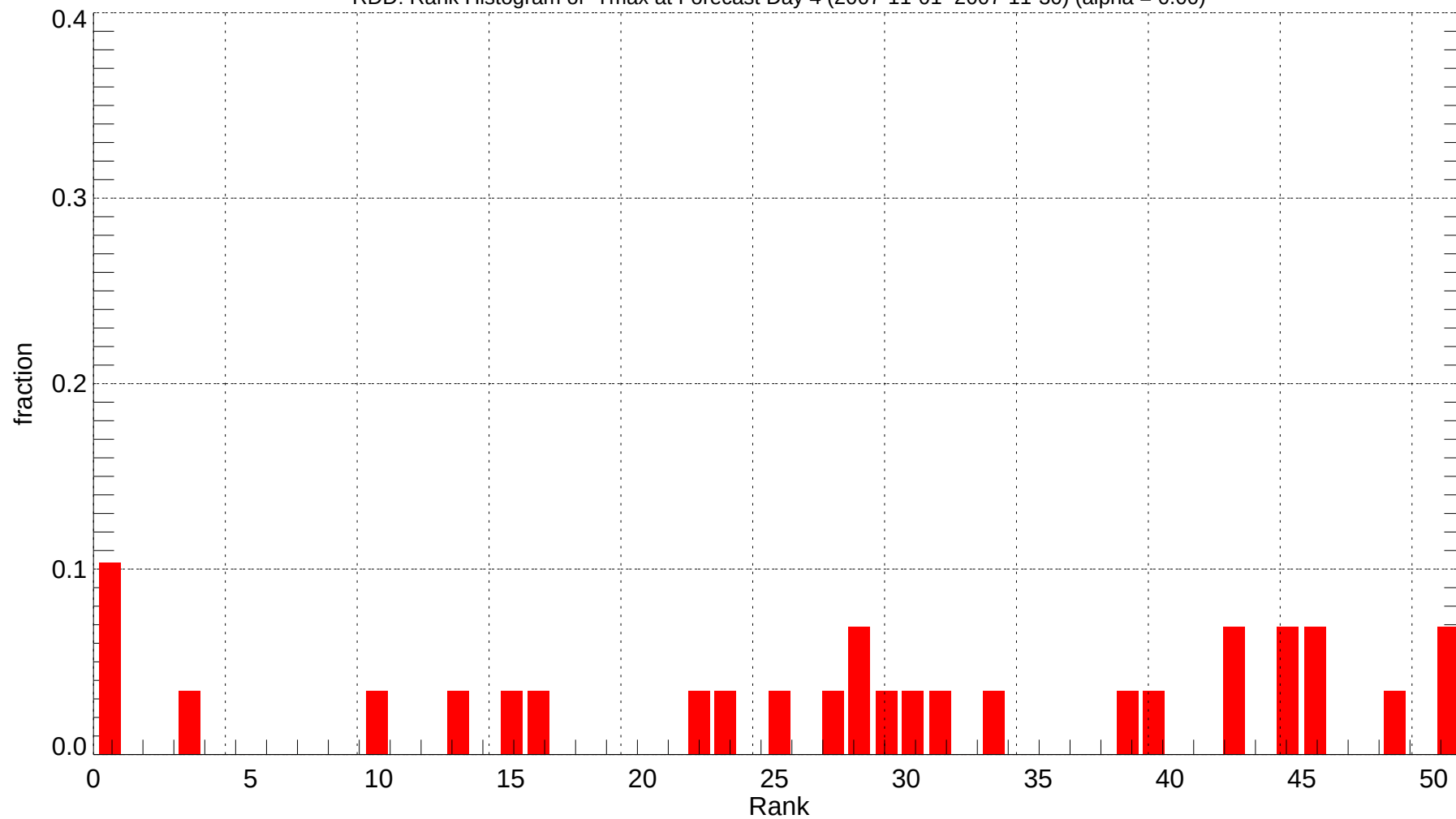
RDD: Rank Histogram of Tmax at Forecast Day 4 (2007-11-01~2007-11-30) (alpha = 0.00)
