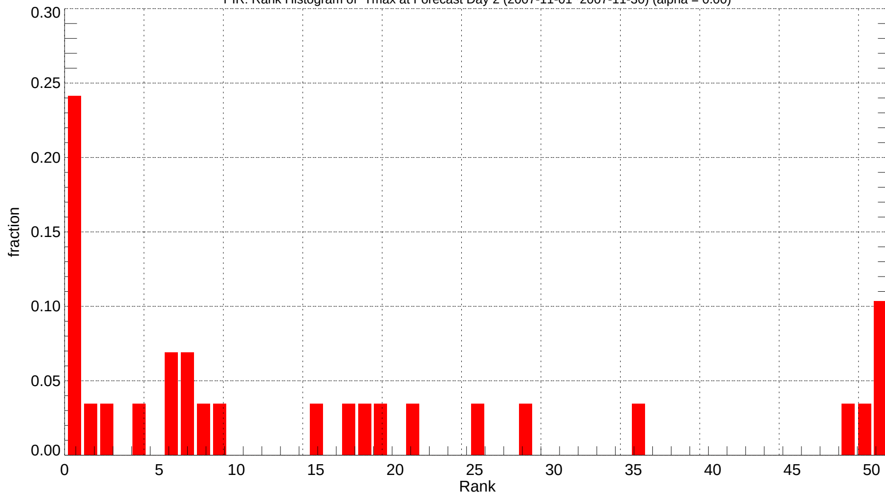
PIR: Rank Histogram of Tmax at Forecast Day 2 (2007-11-01~2007-11-30) (alpha = 0.00)
