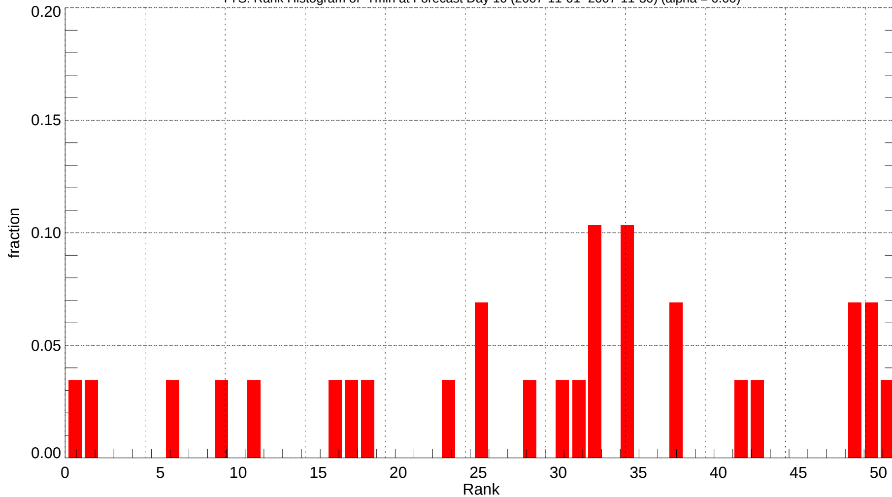
TYS: Rank Histogram of Tmin at Forecast Day 10 (2007-11-01~2007-11-30) (alpha = 0.00)
