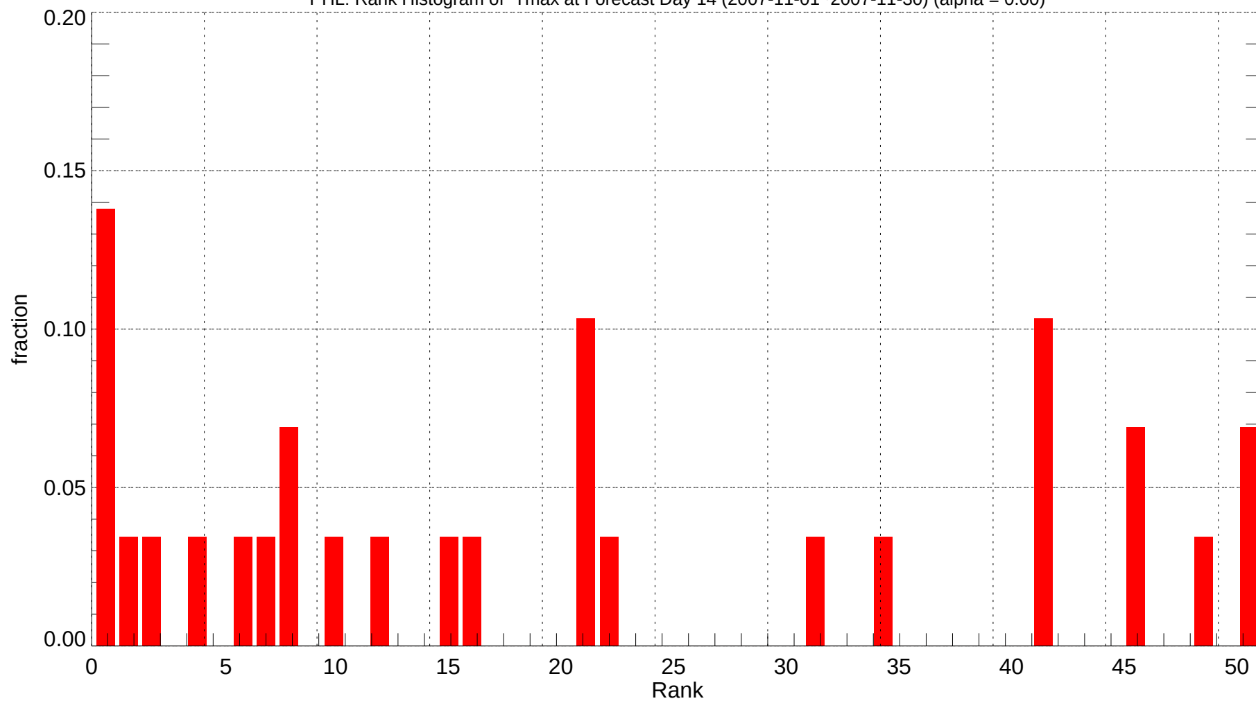
PHL: Rank Histogram of Tmax at Forecast Day 14 (2007-11-01~2007-11-30) (alpha = 0.00)
