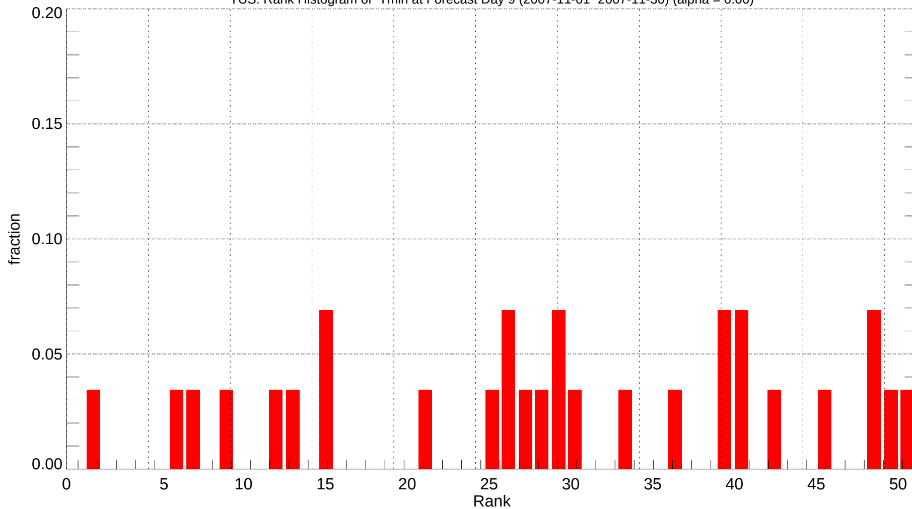
TUS: Rank Histogram of Tmin at Forecast Day 9 (2007-11-01~2007-11-30) (alpha = 0.00)
