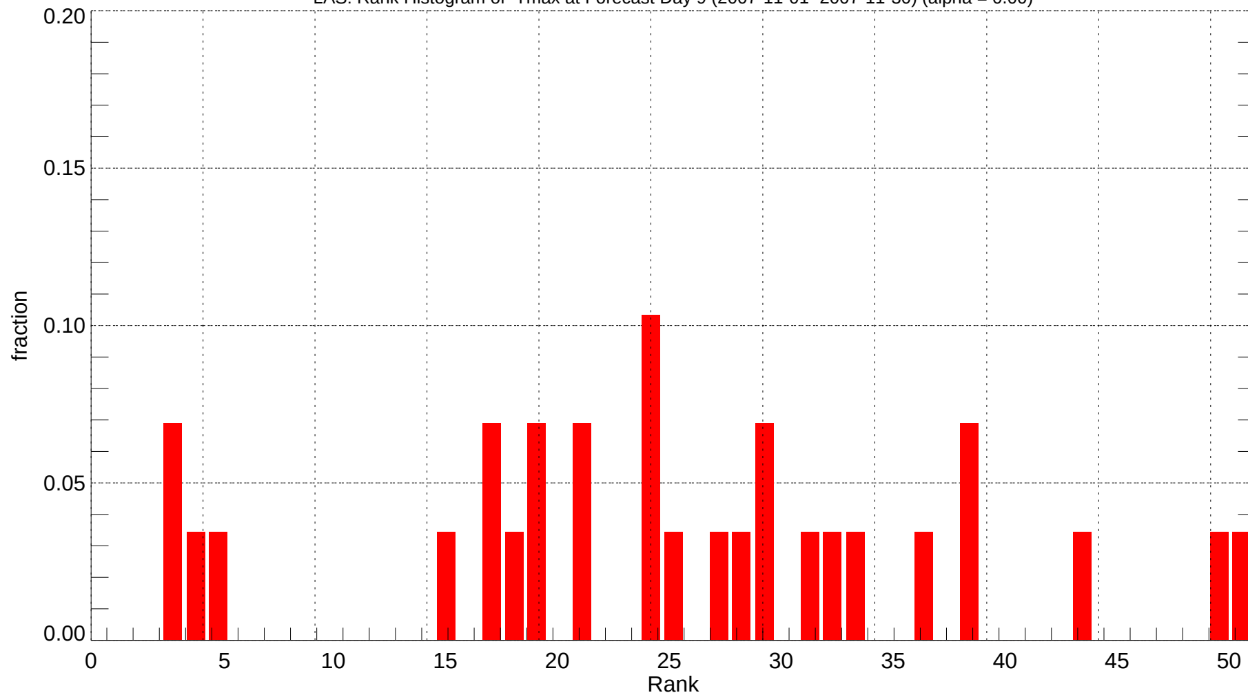
LAS: Rank Histogram of Tmax at Forecast Day 9 (2007-11-01~2007-11-30) (alpha = 0.00)
