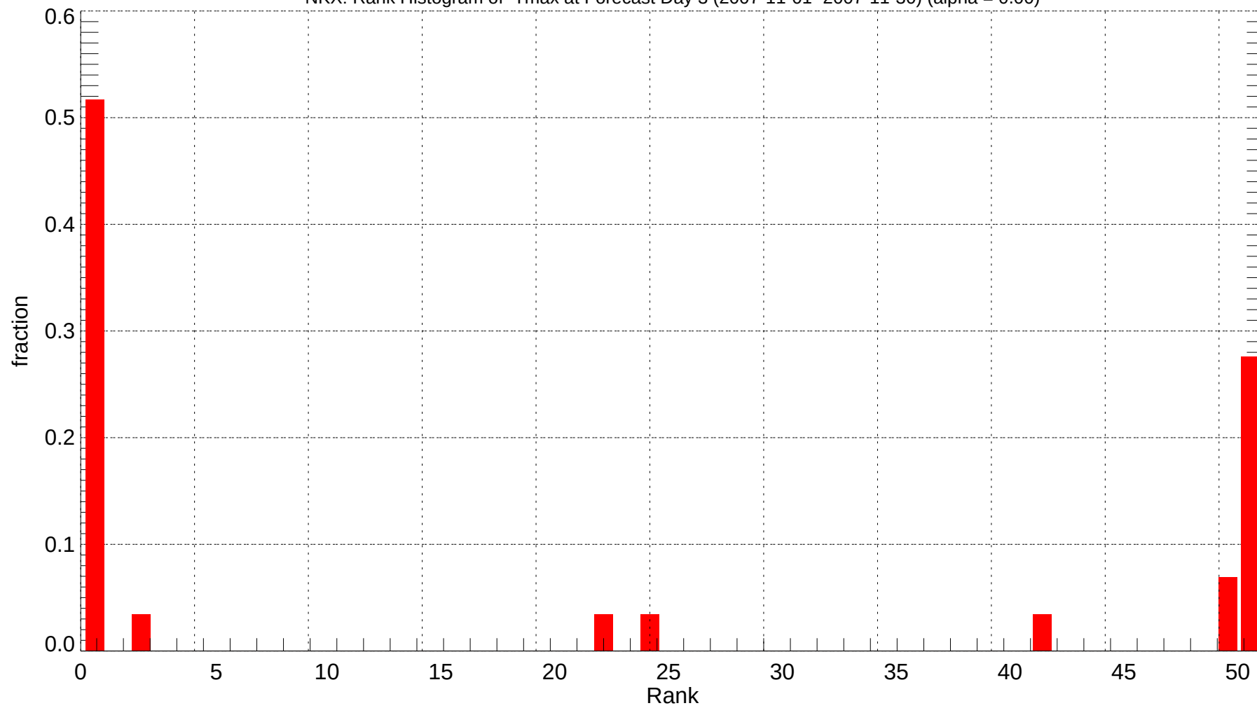
NKX: Rank Histogram of Tmax at Forecast Day 3 (2007-11-01~2007-11-30) (alpha = 0.00)
