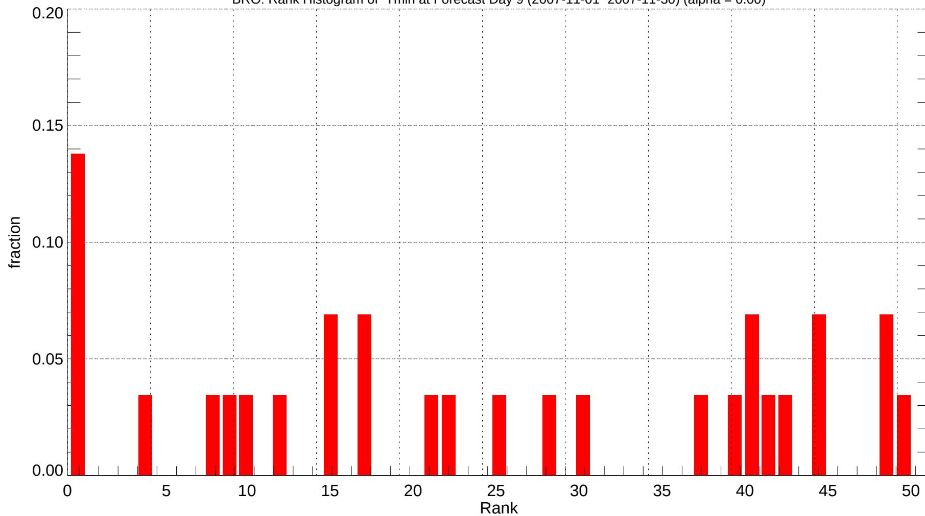
BRO: Rank Histogram of Tmin at Forecast Day 9 (2007-11-01~2007-11-30) (alpha = 0.00)
