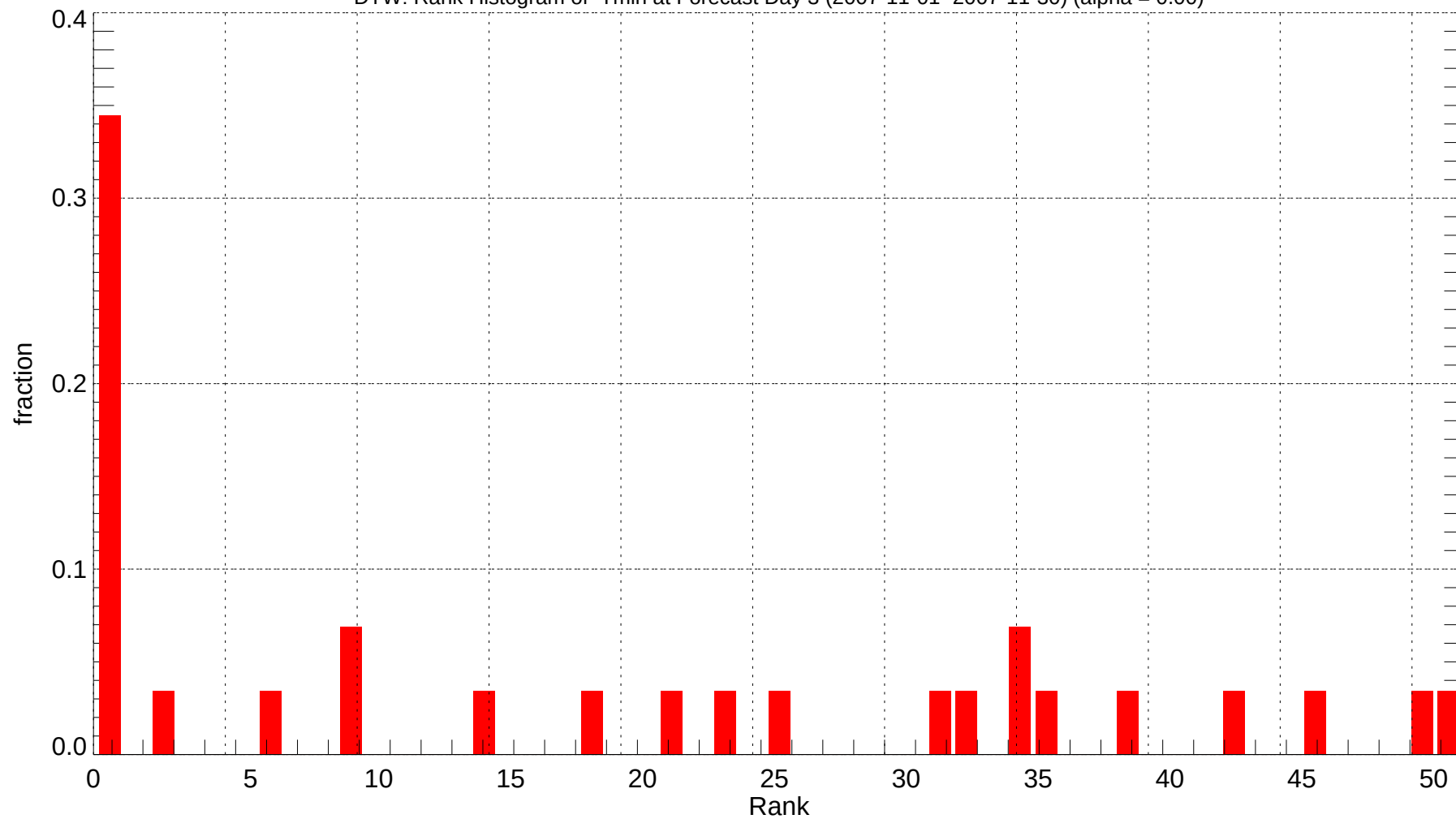
DTW: Rank Histogram of Tmin at Forecast Day 3 (2007-11-01~2007-11-30) (alpha = 0.00)
