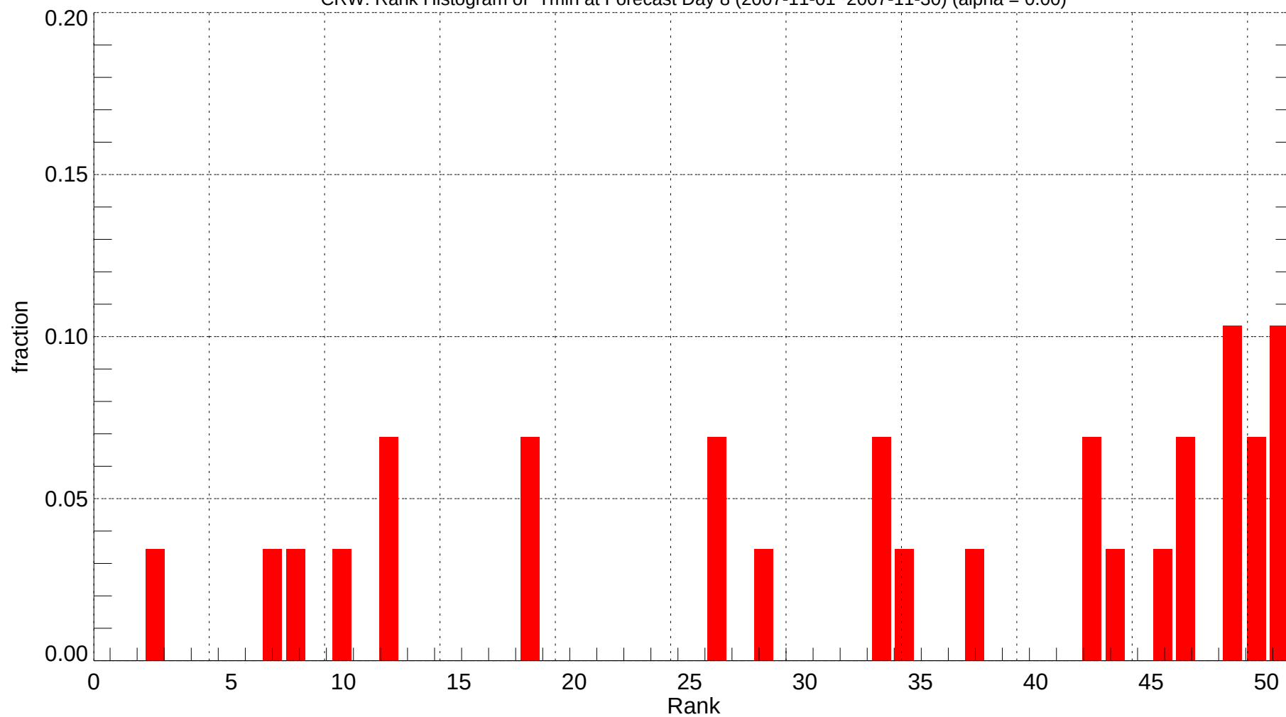
CRW: Rank Histogram of Tmin at Forecast Day 8 (2007-11-01~2007-11-30) (alpha = 0.00)
