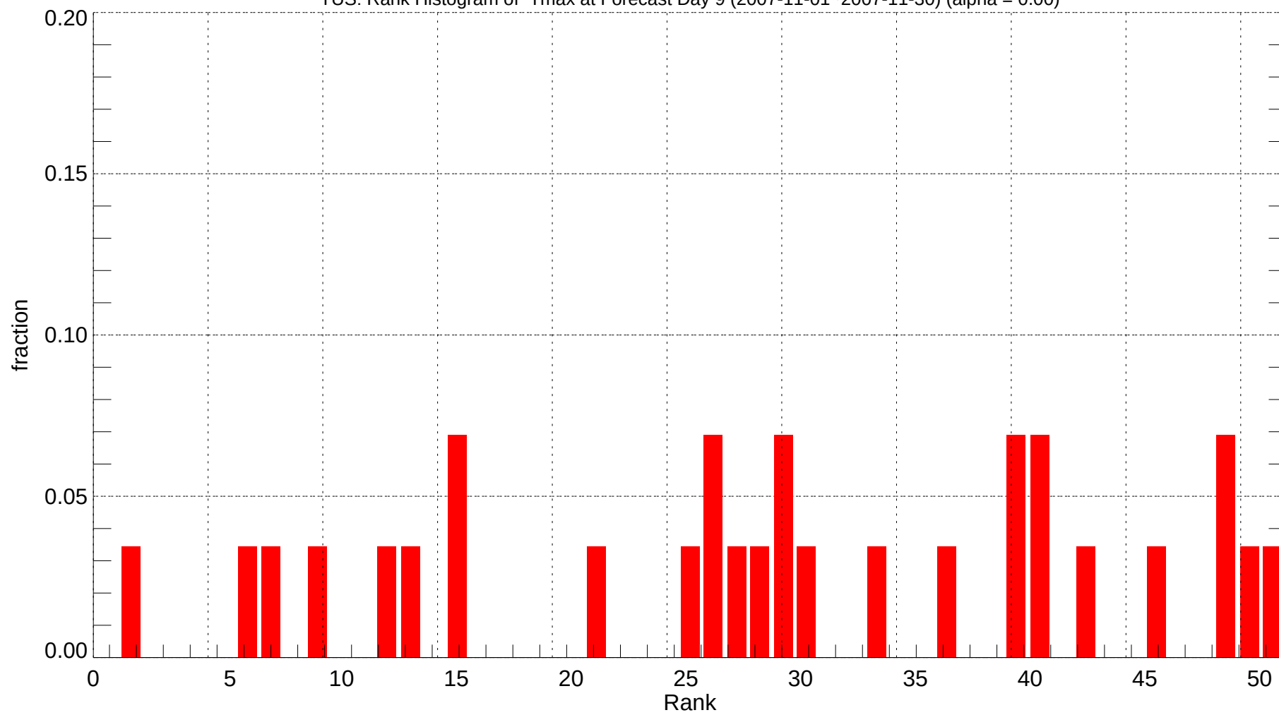
TUS: Rank Histogram of Tmax at Forecast Day 9 (2007-11-01~2007-11-30) (alpha = 0.00)
