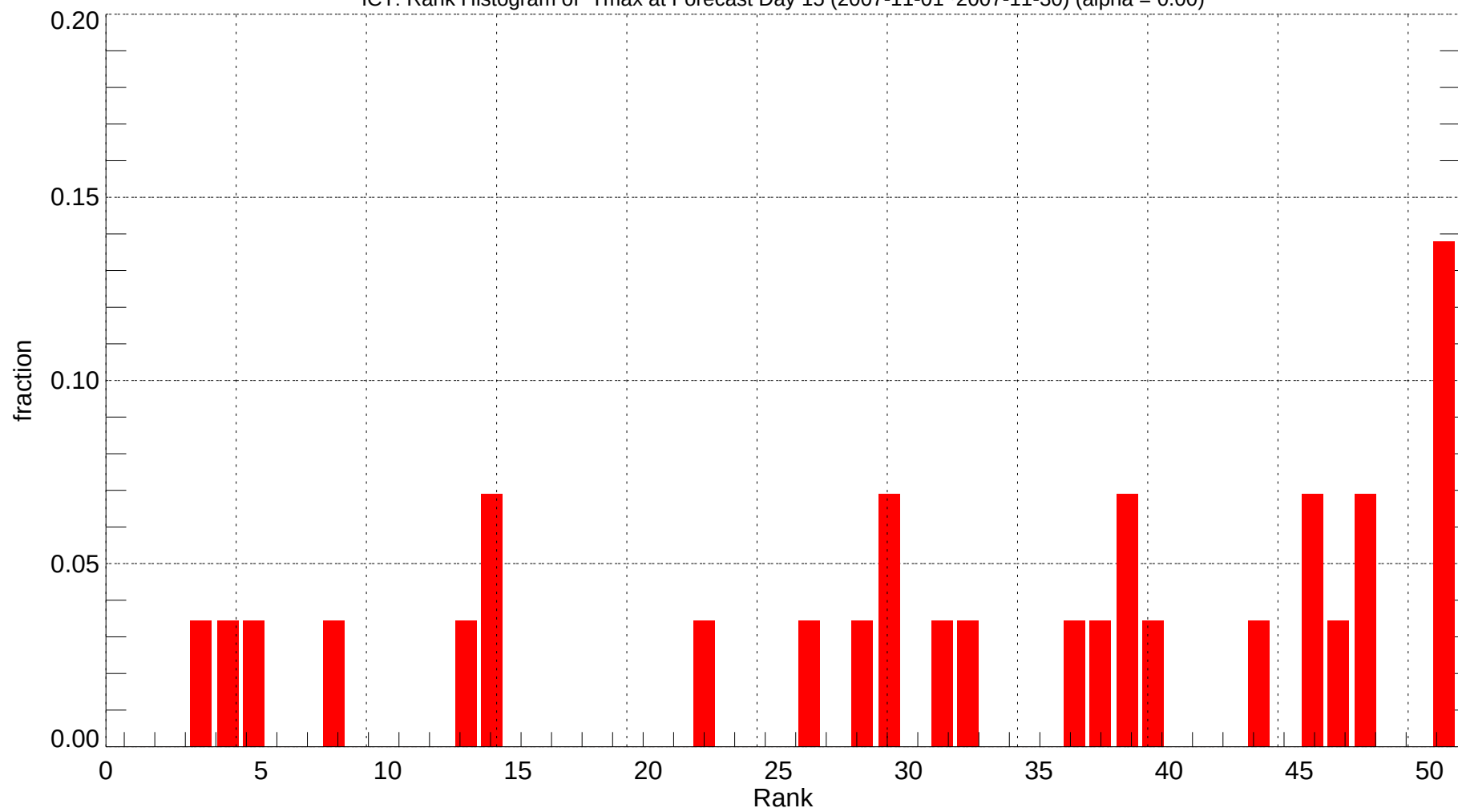
ICT: Rank Histogram of Tmax at Forecast Day 15 (2007-11-01~2007-11-30) (alpha = 0.00)
