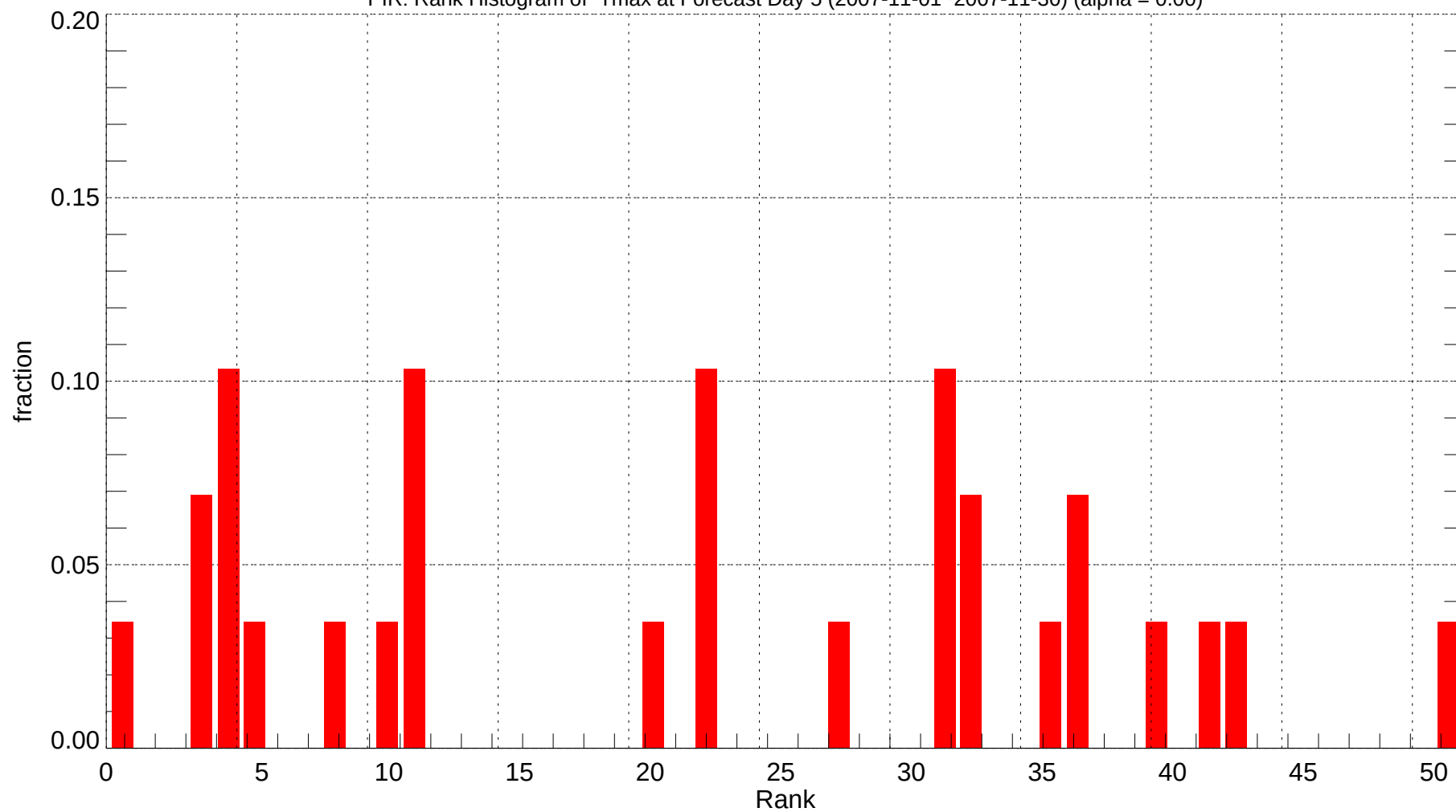
PIR: Rank Histogram of Tmax at Forecast Day 5 (2007-11-01~2007-11-30) (alpha = 0.00)
