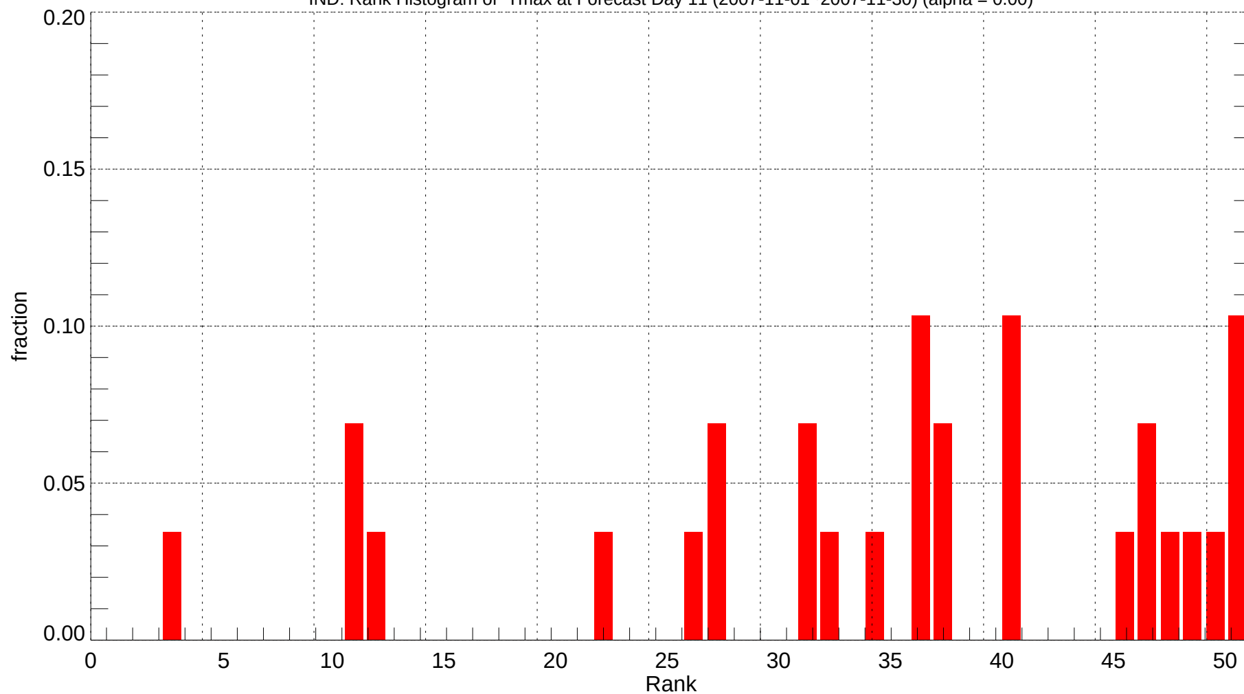
IND: Rank Histogram of Tmax at Forecast Day 11 (2007-11-01~2007-11-30) (alpha = 0.00)
