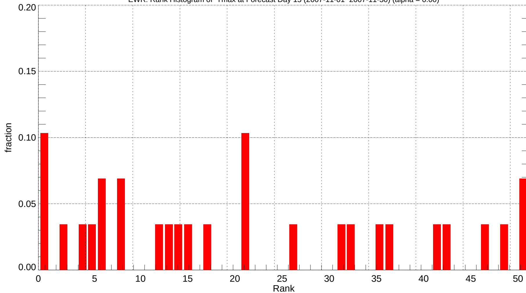
EWR: Rank Histogram of Tmax at Forecast Day 15 (2007-11-01~2007-11-30) (alpha = 0.00)
