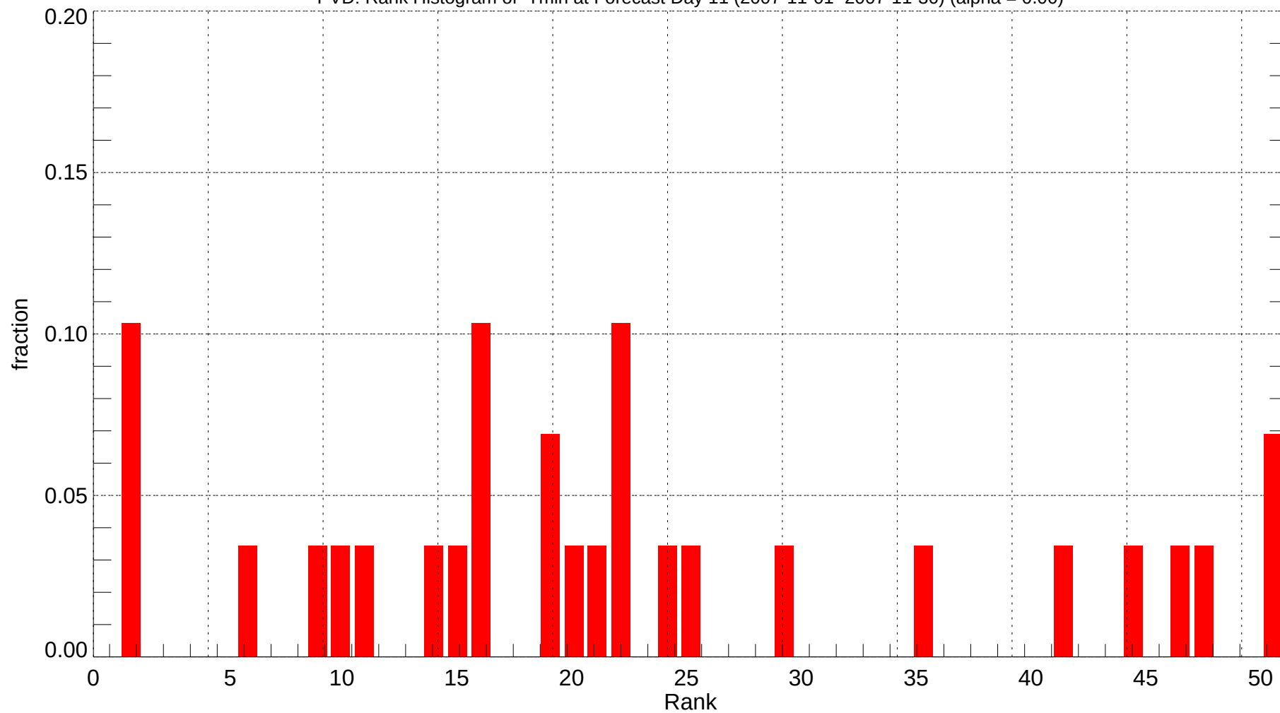
PVD: Rank Histogram of Tmin at Forecast Day 11 (2007-11-01~2007-11-30) (alpha = 0.00)
