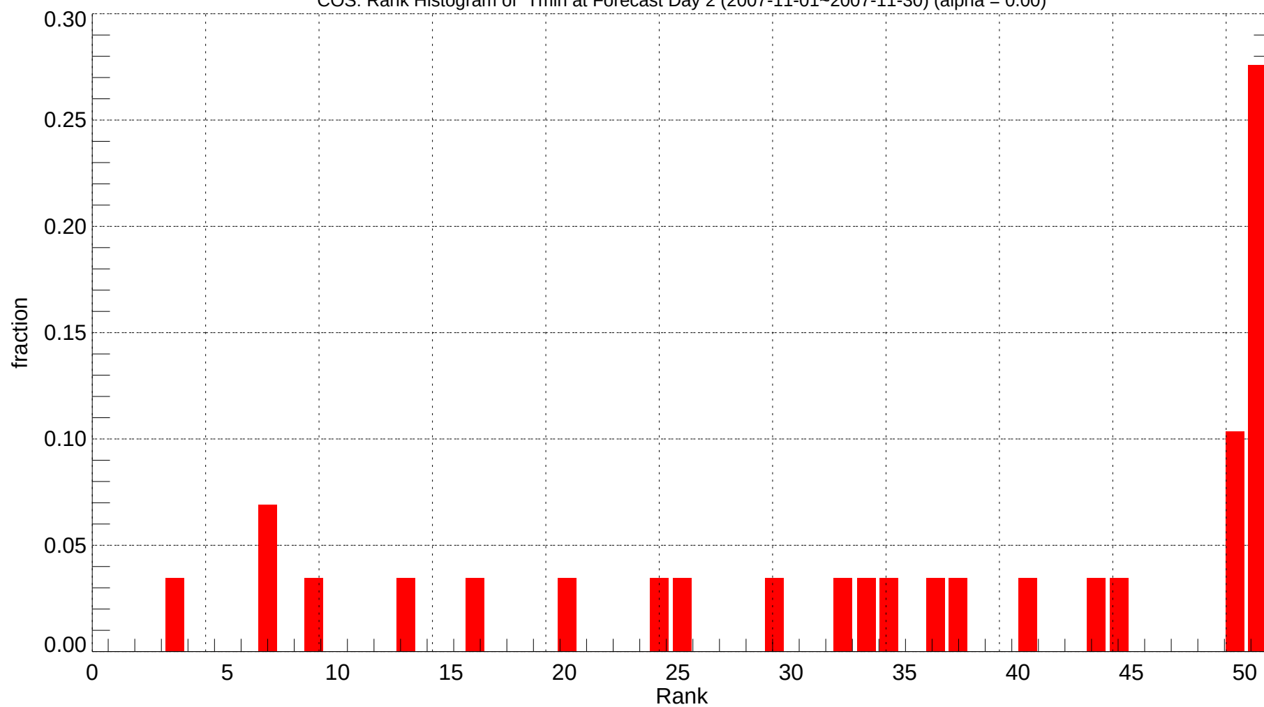
COS: Rank Histogram of Tmin at Forecast Day 2 (2007-11-01~2007-11-30) (alpha = 0.00)
