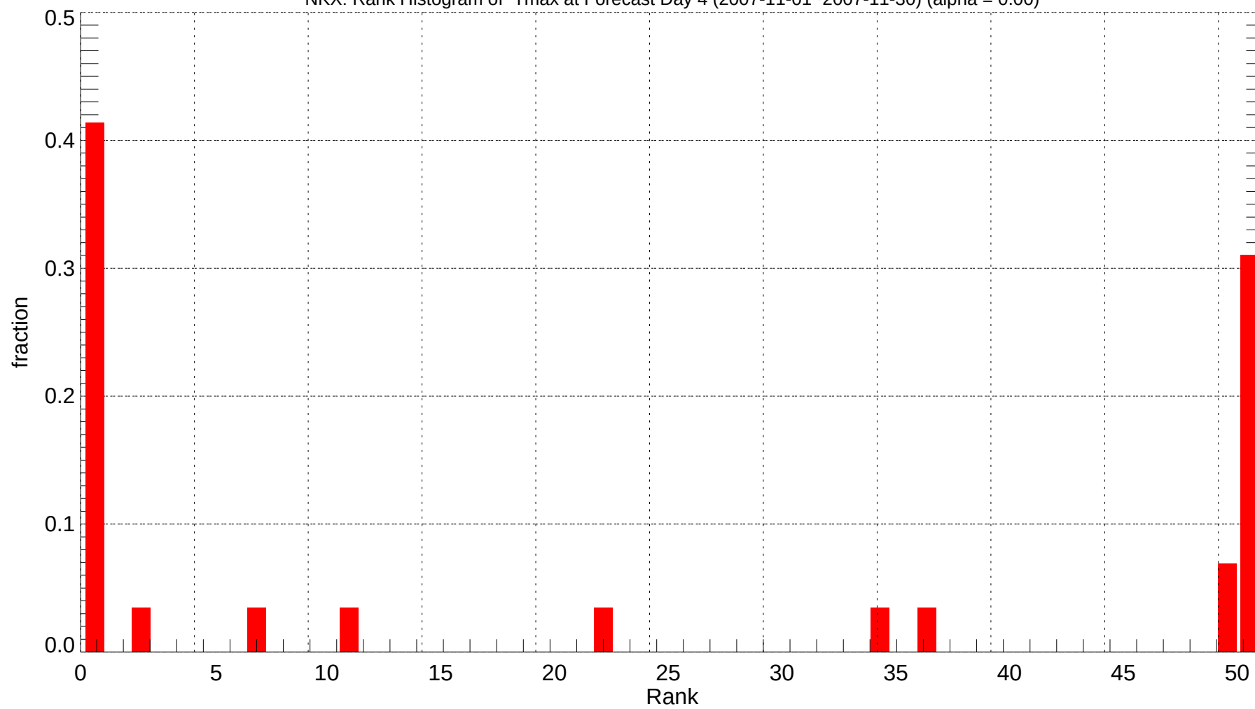
NKX: Rank Histogram of Tmax at Forecast Day 4 (2007-11-01~2007-11-30) (alpha = 0.00)
