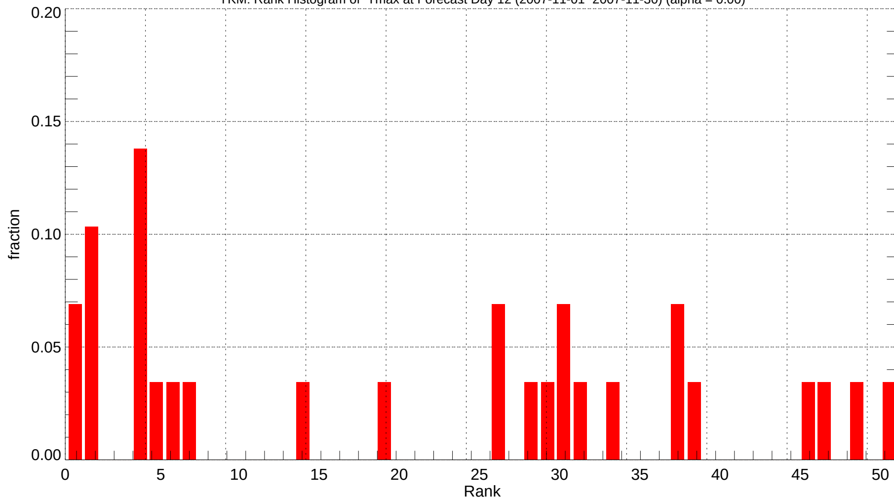
YKM: Rank Histogram of Tmax at Forecast Day 12 (2007-11-01~2007-11-30) (alpha = 0.00)
