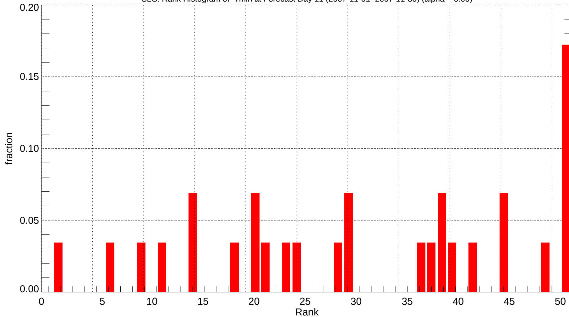
SLC: Rank Histogram of Tmin at Forecast Day 11 (2007-11-01~2007-11-30) (alpha = 0.00)
