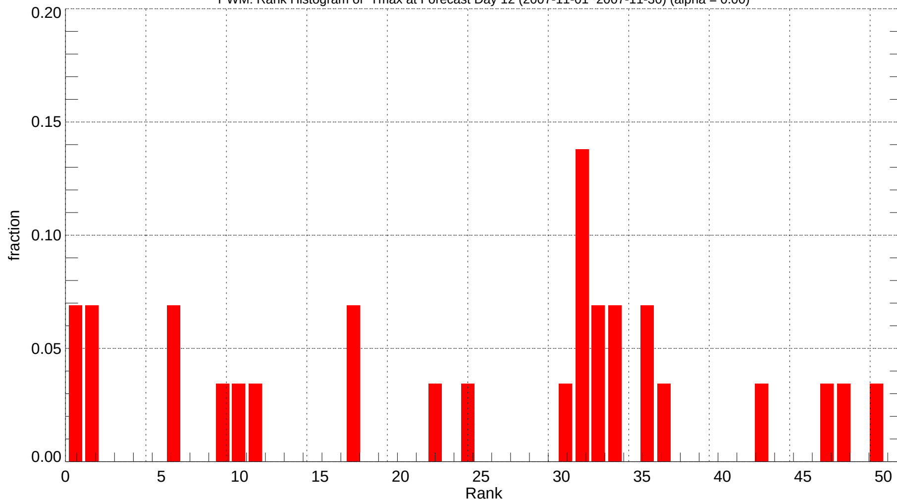
PWM: Rank Histogram of Tmax at Forecast Day 12 (2007-11-01~2007-11-30) (alpha = 0.00)
