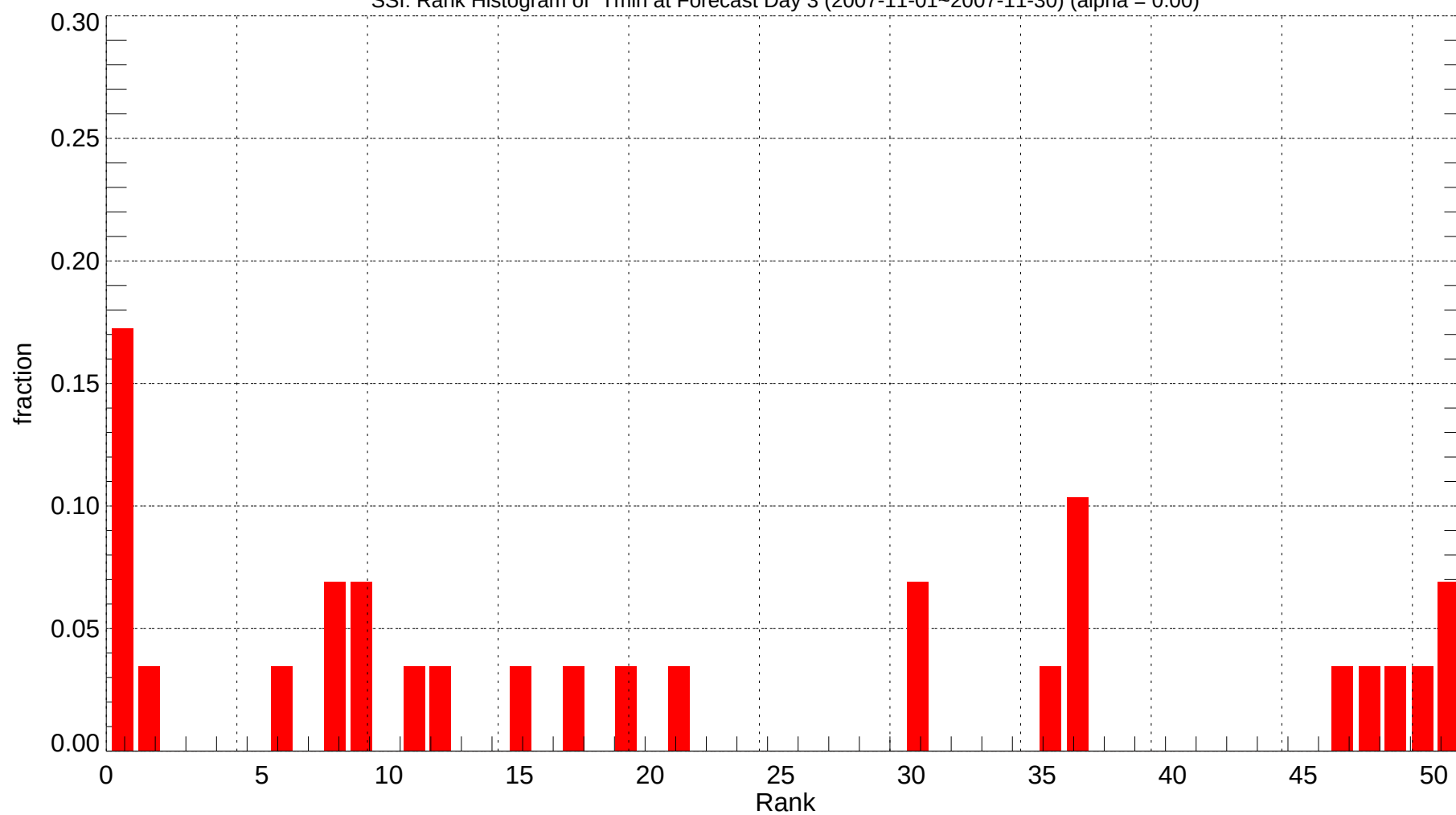
SSI: Rank Histogram of Tmin at Forecast Day 3 (2007-11-01~2007-11-30) (alpha = 0.00)
