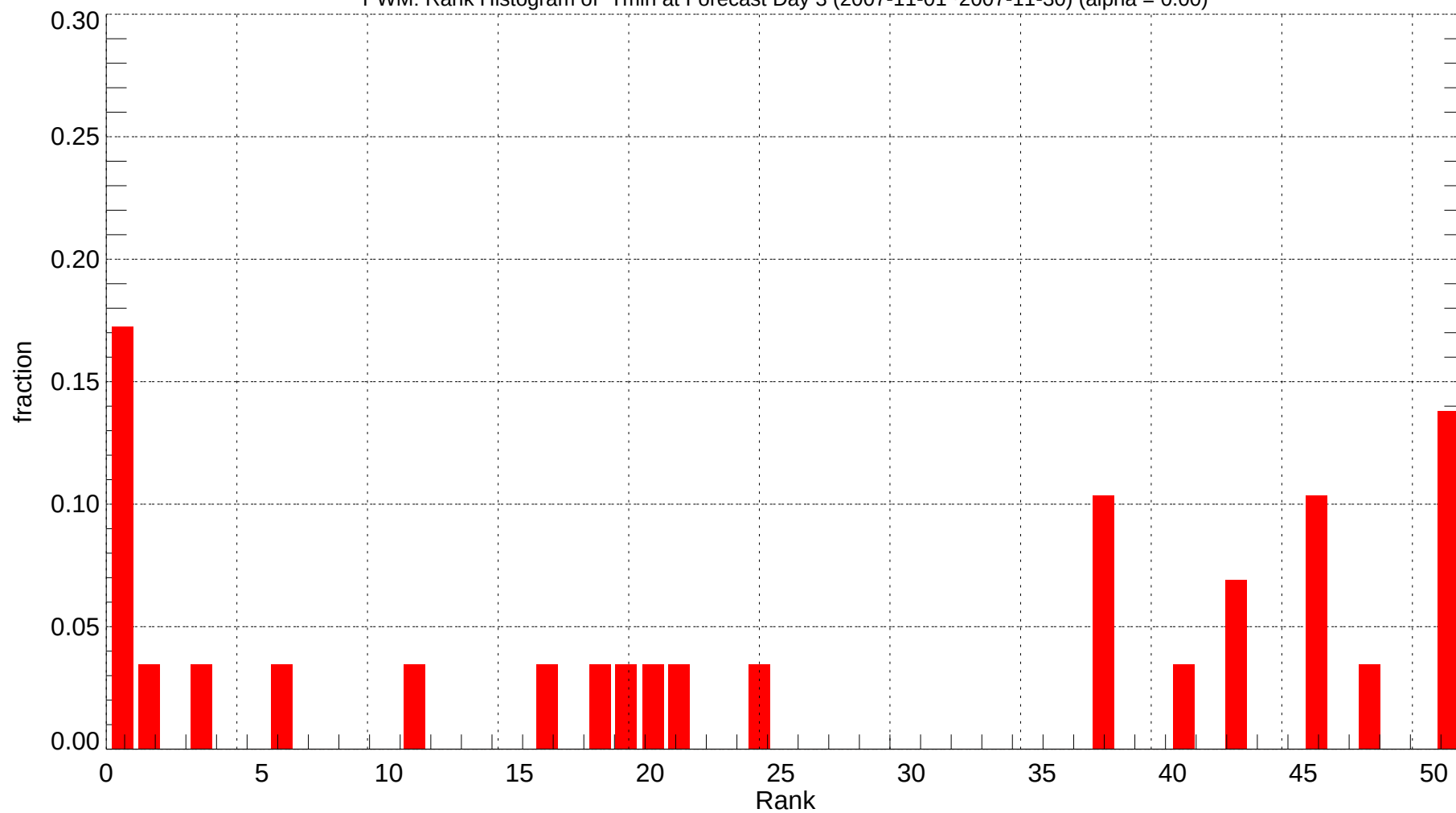
PWM: Rank Histogram of Tmin at Forecast Day 3 (2007-11-01~2007-11-30) (alpha = 0.00)
