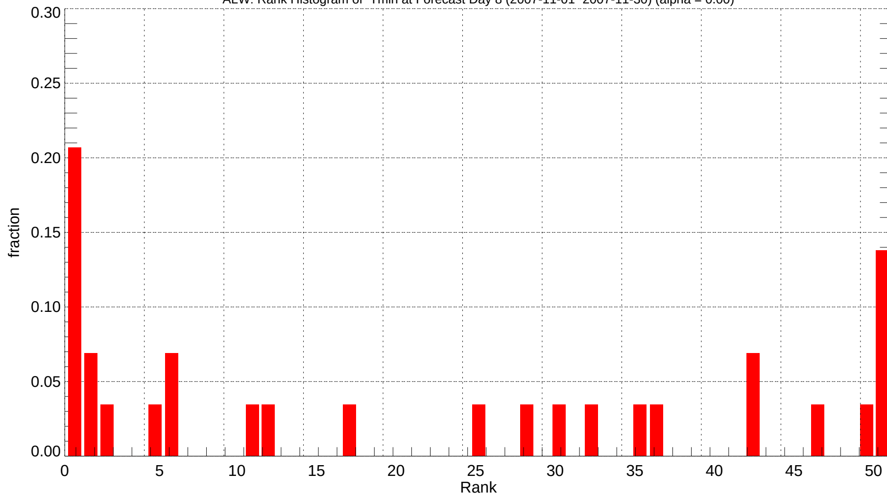
ALW: Rank Histogram of Tmin at Forecast Day 8 (2007-11-01~2007-11-30) (alpha = 0.00)
