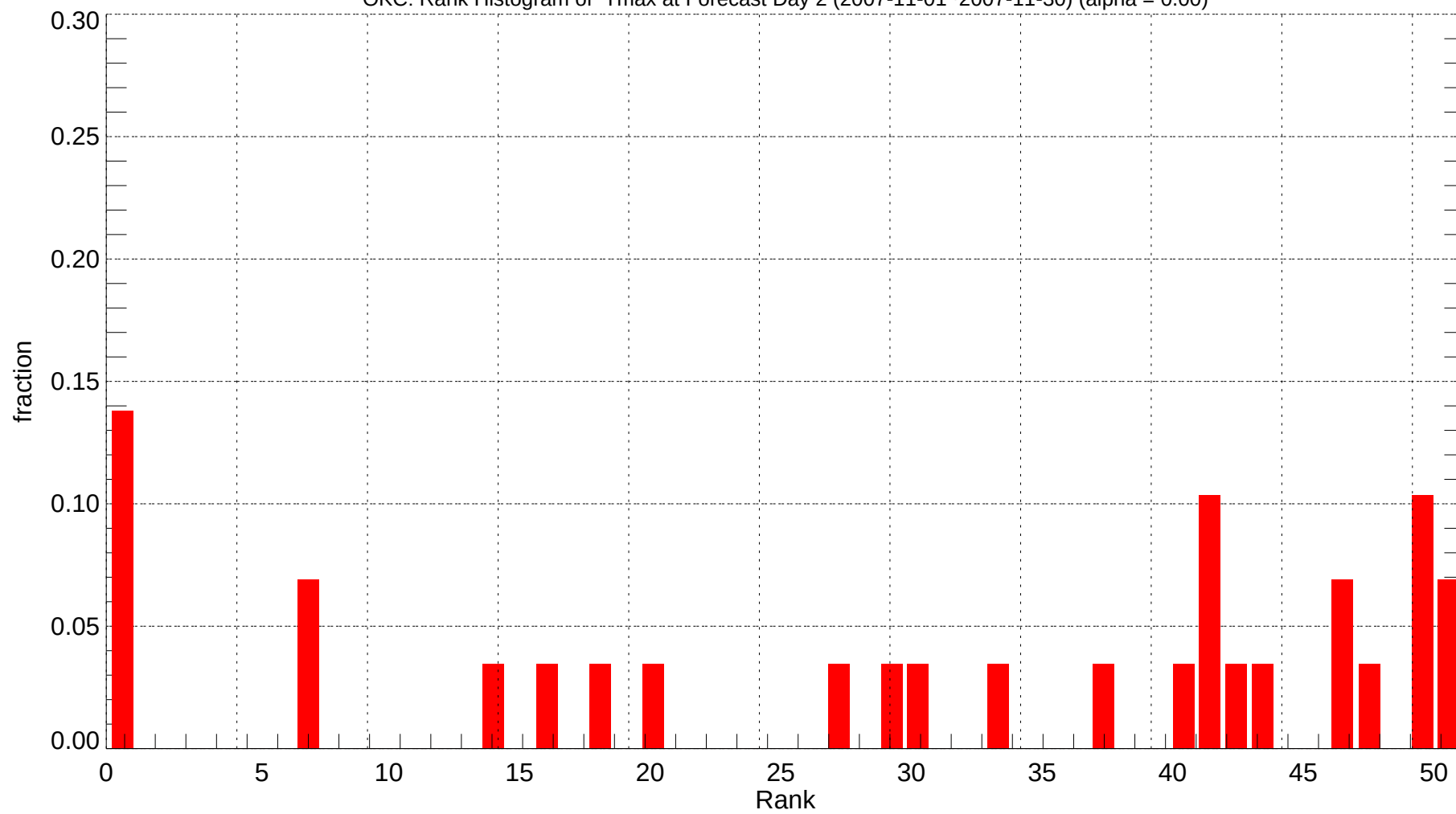
OKC: Rank Histogram of Tmax at Forecast Day 2 (2007-11-01~2007-11-30) (alpha = 0.00)
