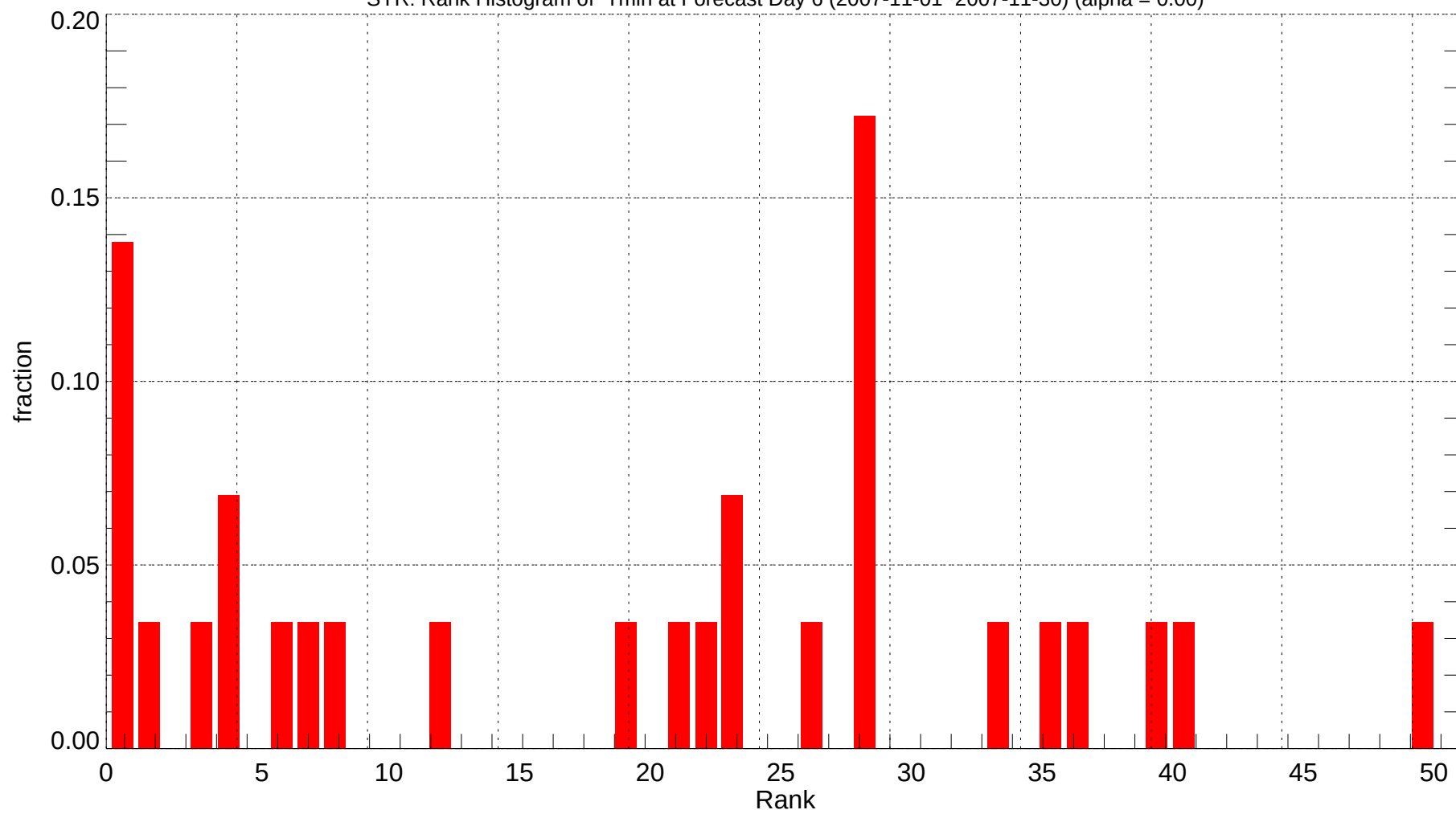
SYR: Rank Histogram of Tmin at Forecast Day 6 (2007-11-01~2007-11-30) (alpha = 0.00)
