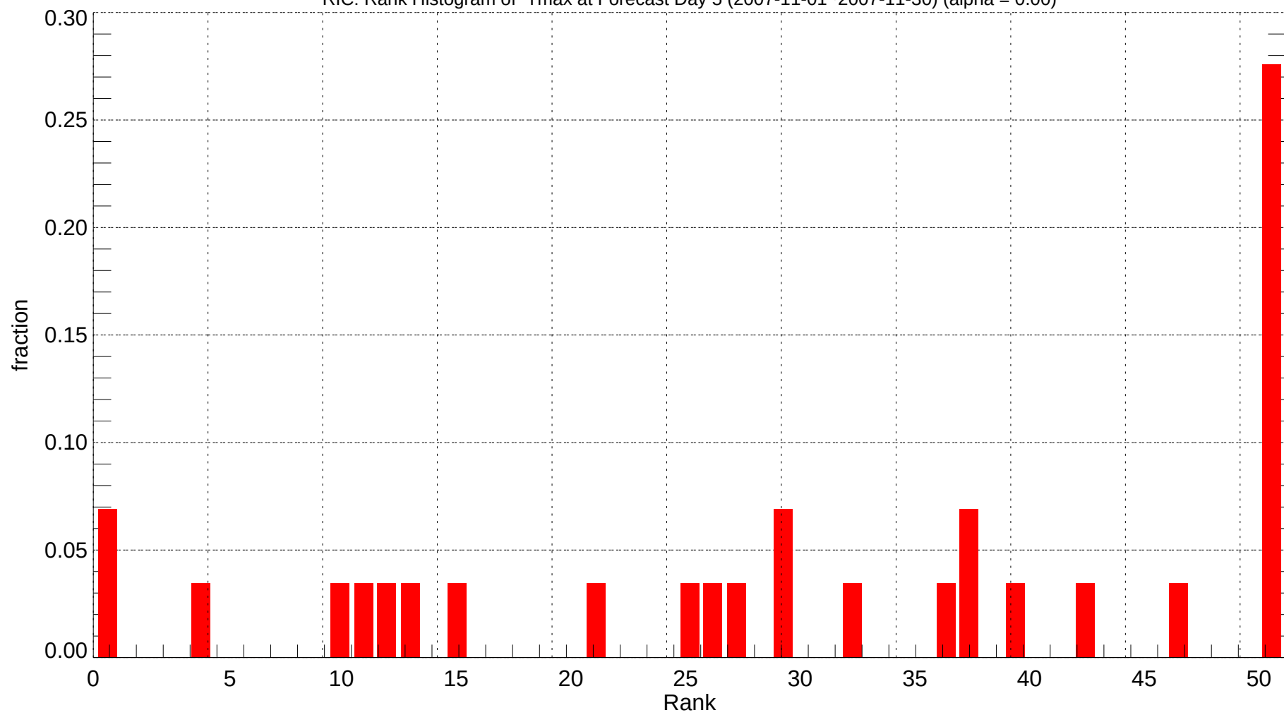
RIC: Rank Histogram of Tmax at Forecast Day 5 (2007-11-01~2007-11-30) (alpha = 0.00)
