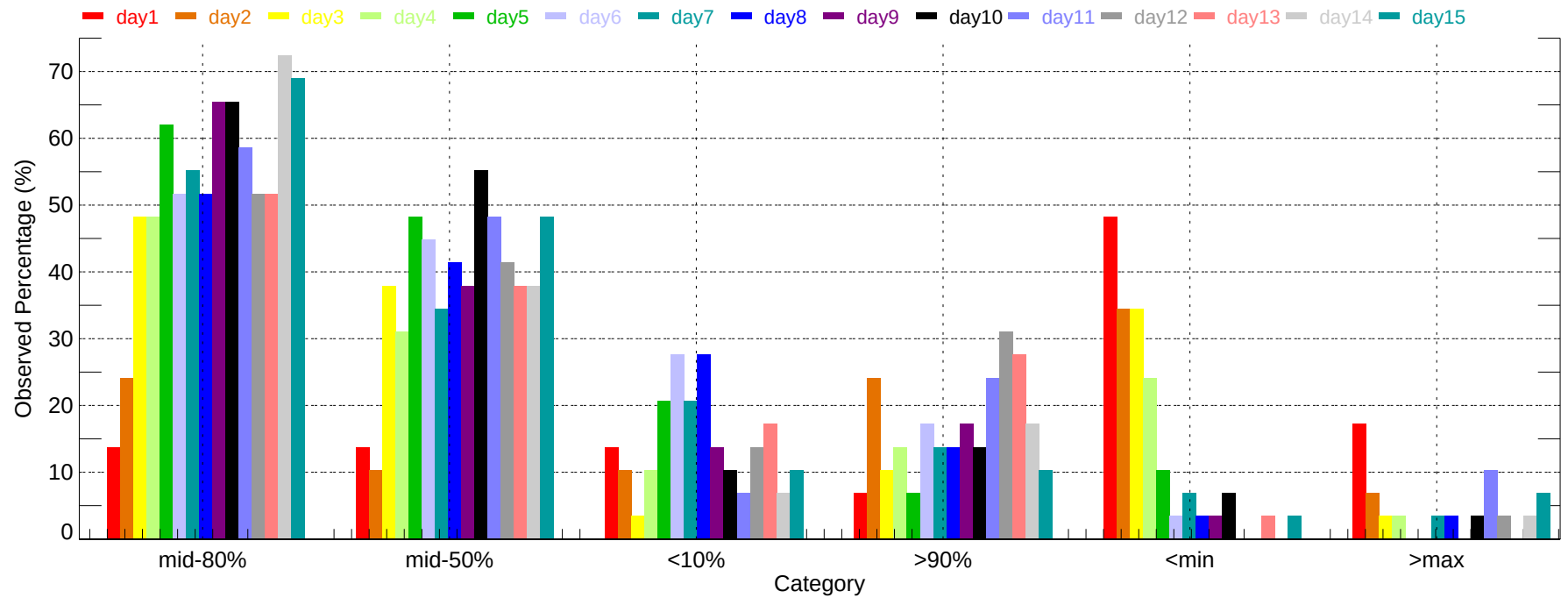
Observed Percentage of Ensembles - DTW: Max Temperature (2007-11-01~2007-11-30)
