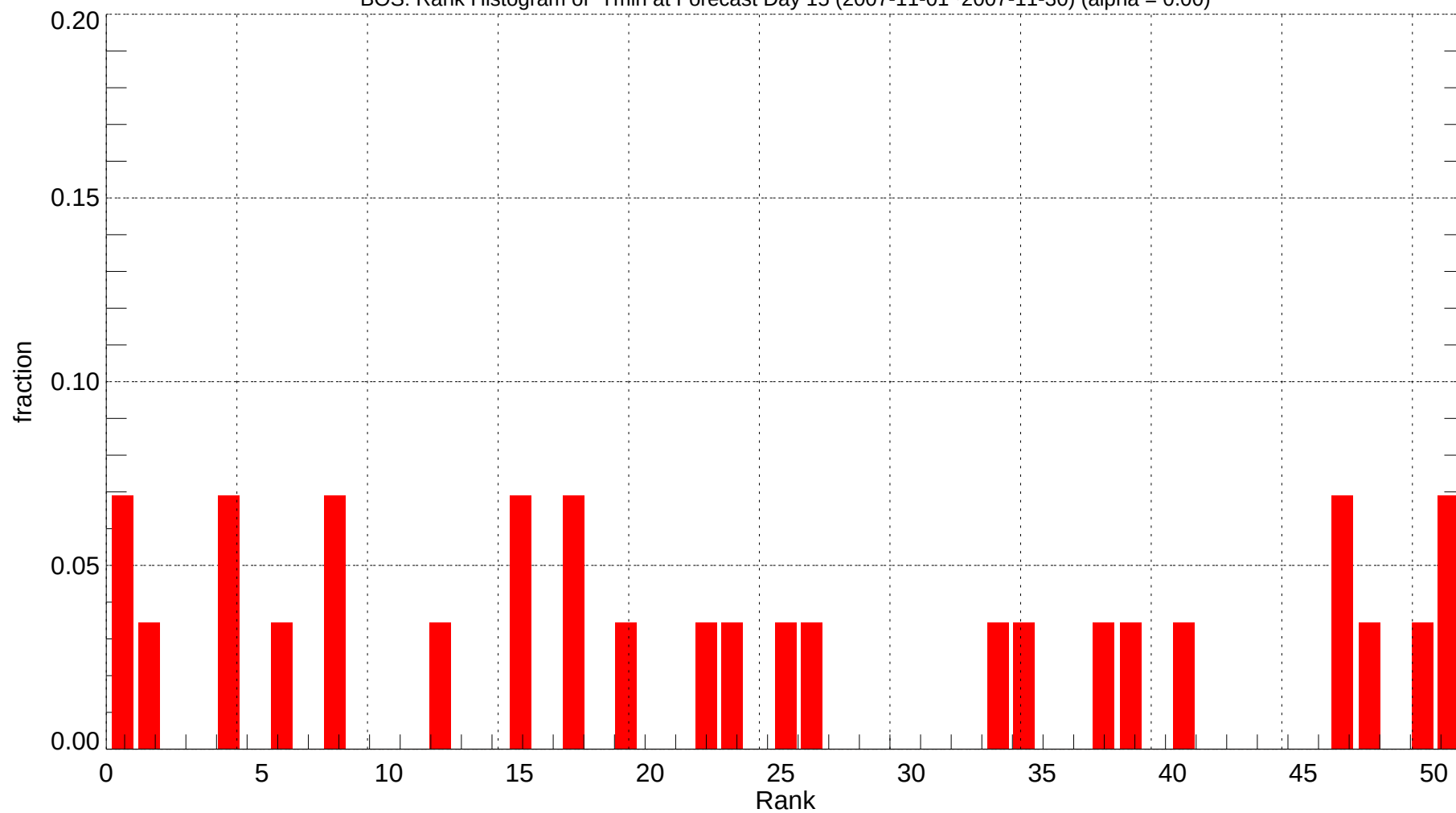
BOS: Rank Histogram of Tmin at Forecast Day 15 (2007-11-01~2007-11-30) (alpha = 0.00)
