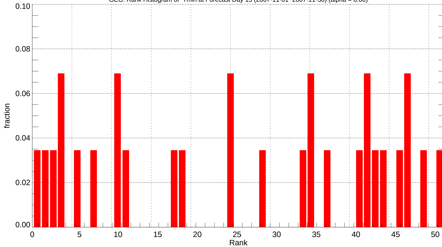
GEG: Rank Histogram of Tmin at Forecast Day 15 (2007-11-01~2007-11-30) (alpha = 0.00)
