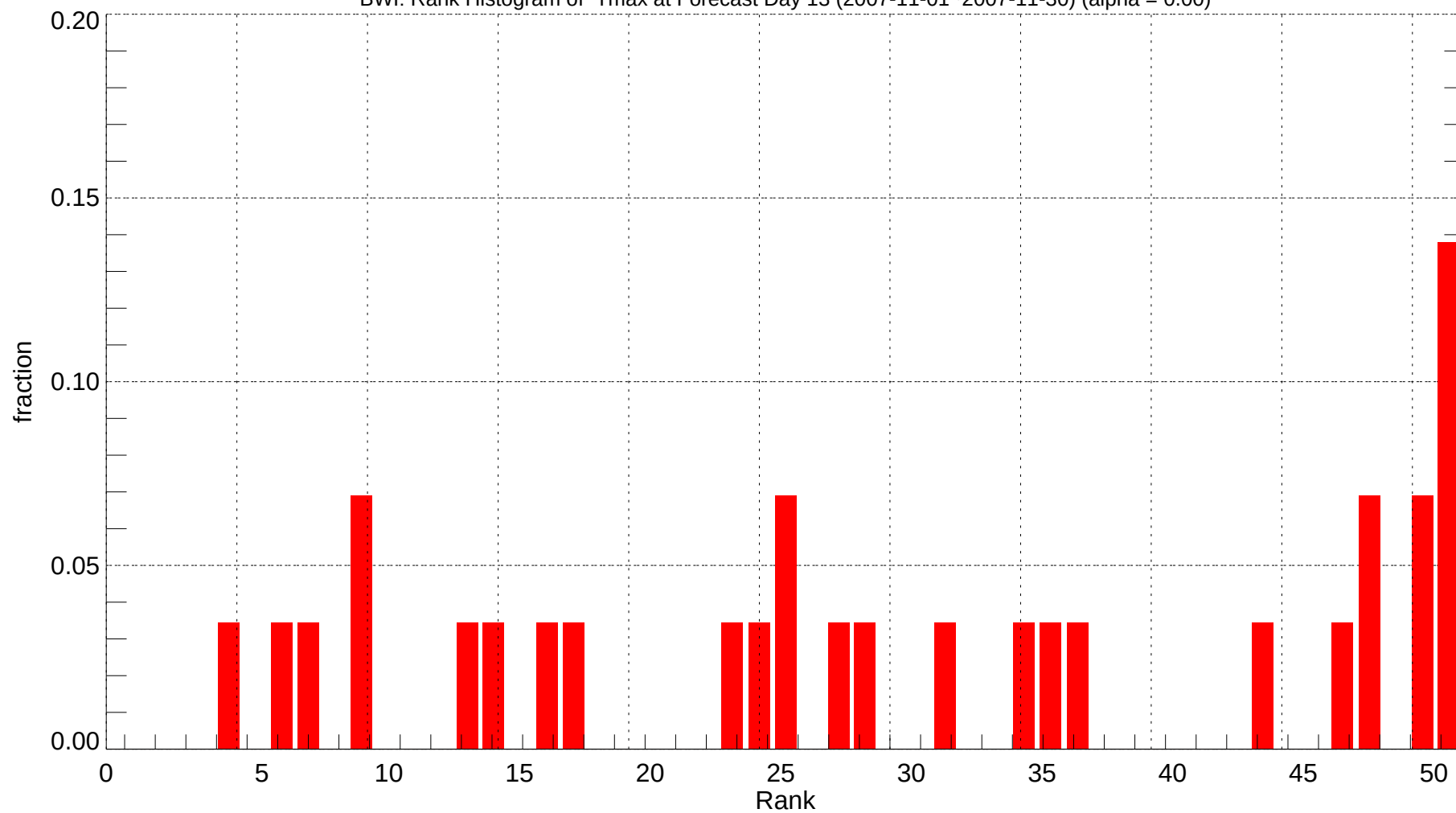
BWI: Rank Histogram of Tmax at Forecast Day 13 (2007-11-01~2007-11-30) (alpha = 0.00)
