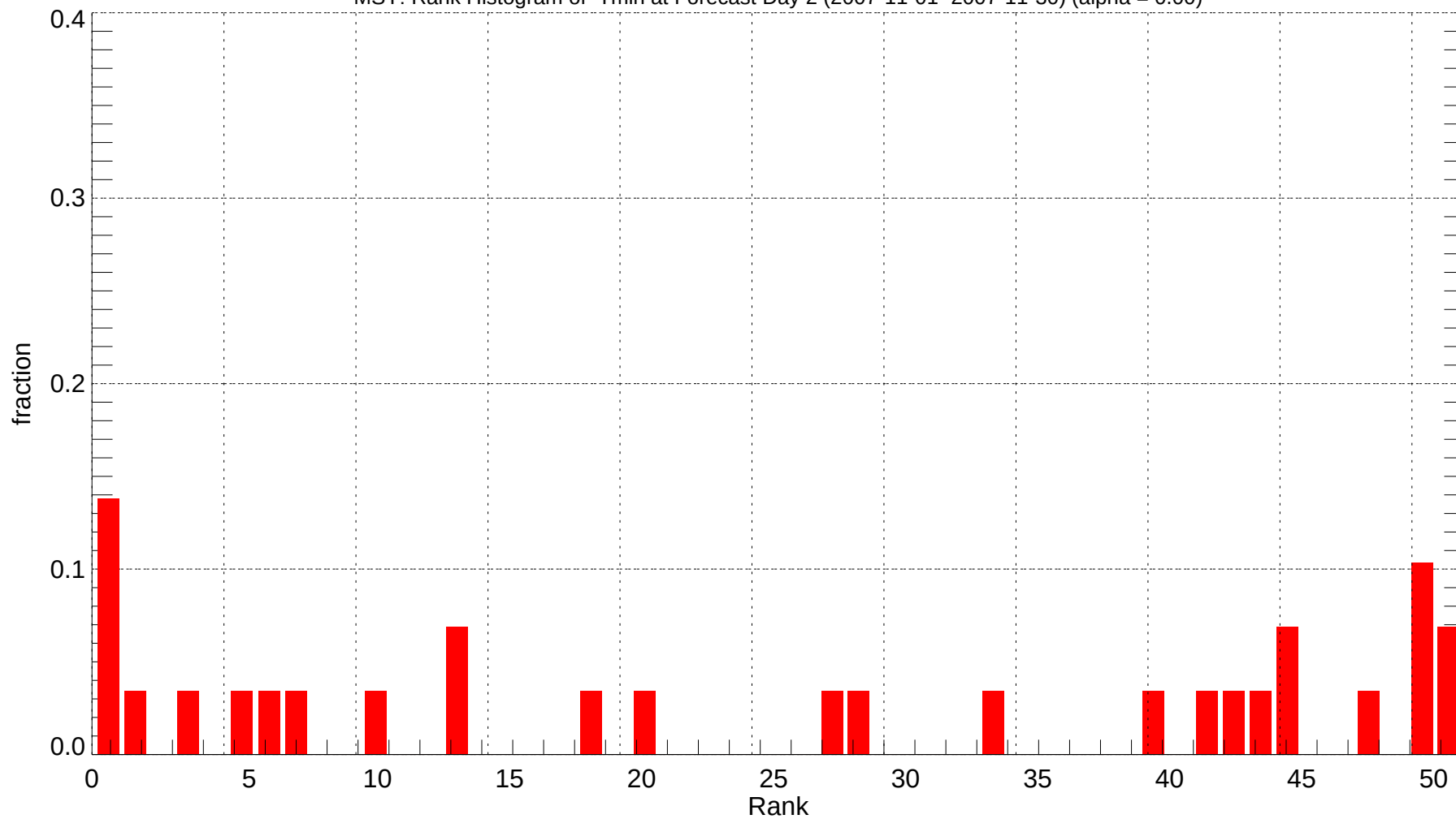
MSY: Rank Histogram of Tmin at Forecast Day 2 (2007-11-01~2007-11-30) (alpha = 0.00)
