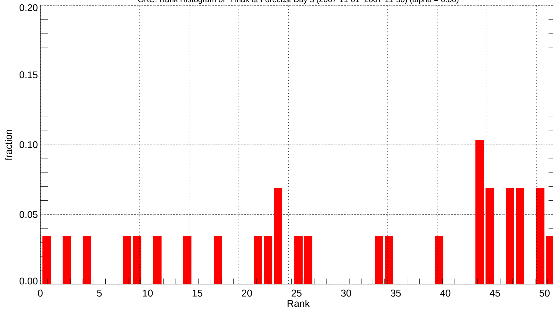
OKC: Rank Histogram of Tmax at Forecast Day 3 (2007-11-01~2007-11-30) (alpha = 0.00)
