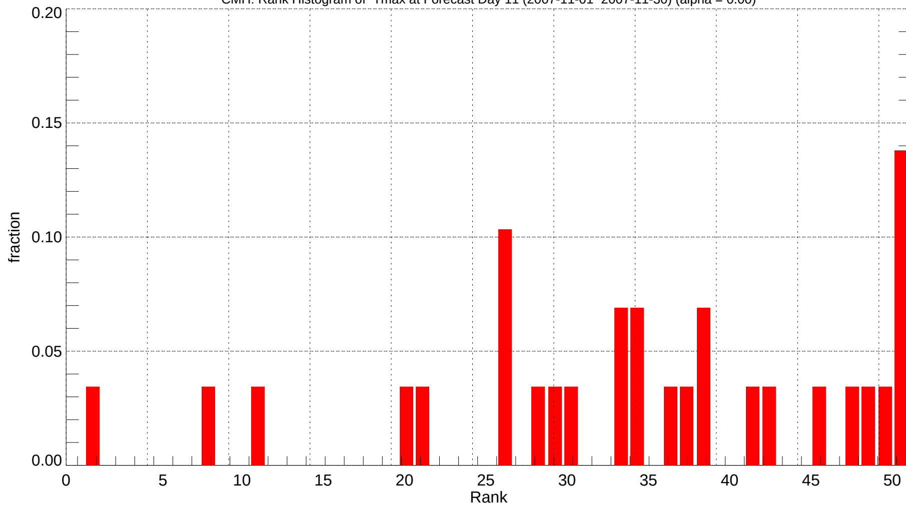
CMH: Rank Histogram of Tmax at Forecast Day 11 (2007-11-01~2007-11-30) (alpha = 0.00)
