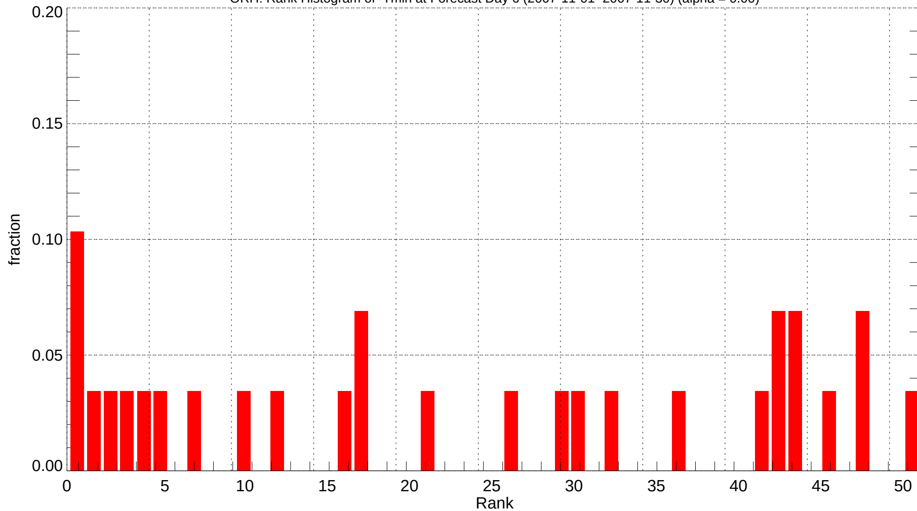
ORH: Rank Histogram of Tmin at Forecast Day 6 (2007-11-01~2007-11-30) (alpha = 0.00)
