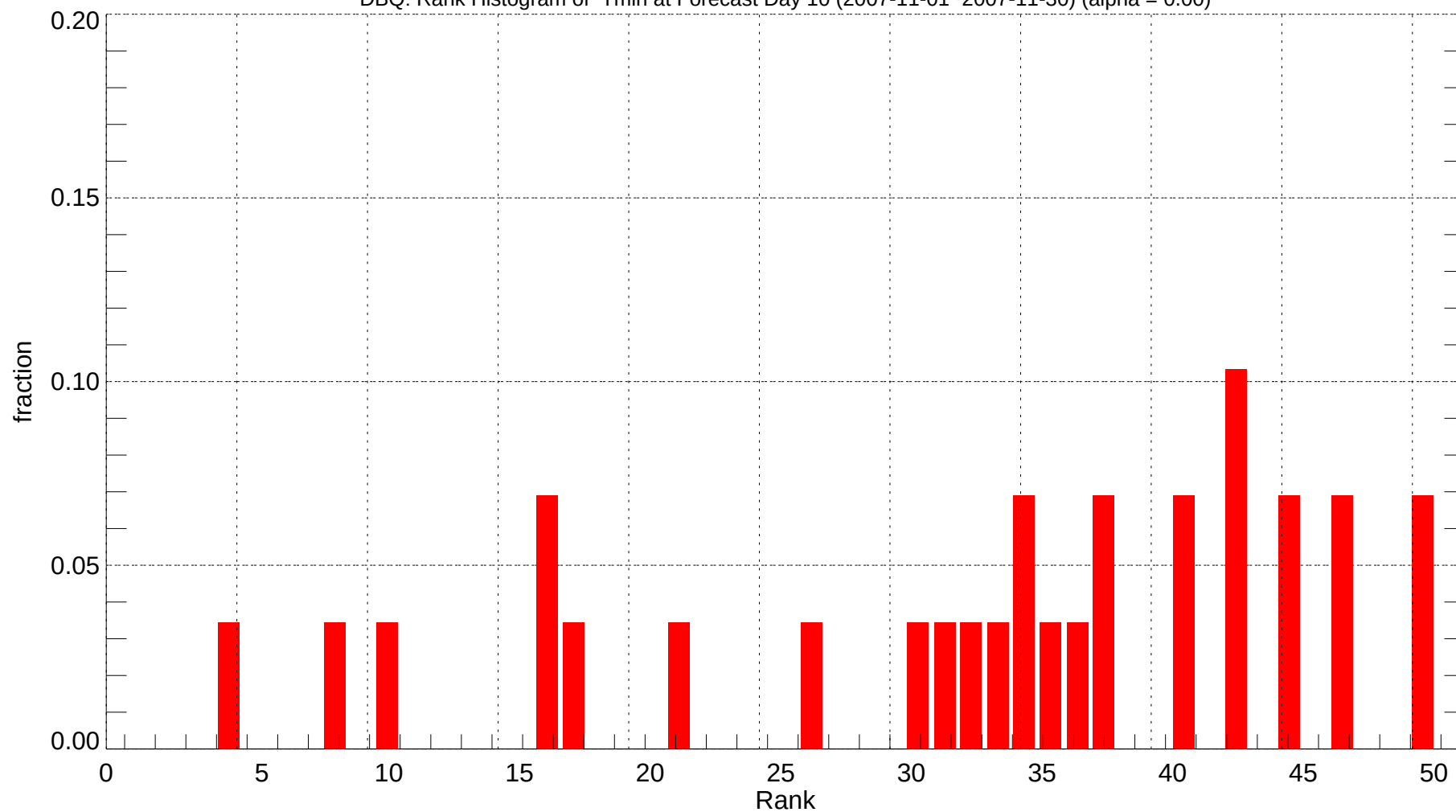
DBQ: Rank Histogram of Tmin at Forecast Day 10 (2007-11-01~2007-11-30) (alpha = 0.00)
