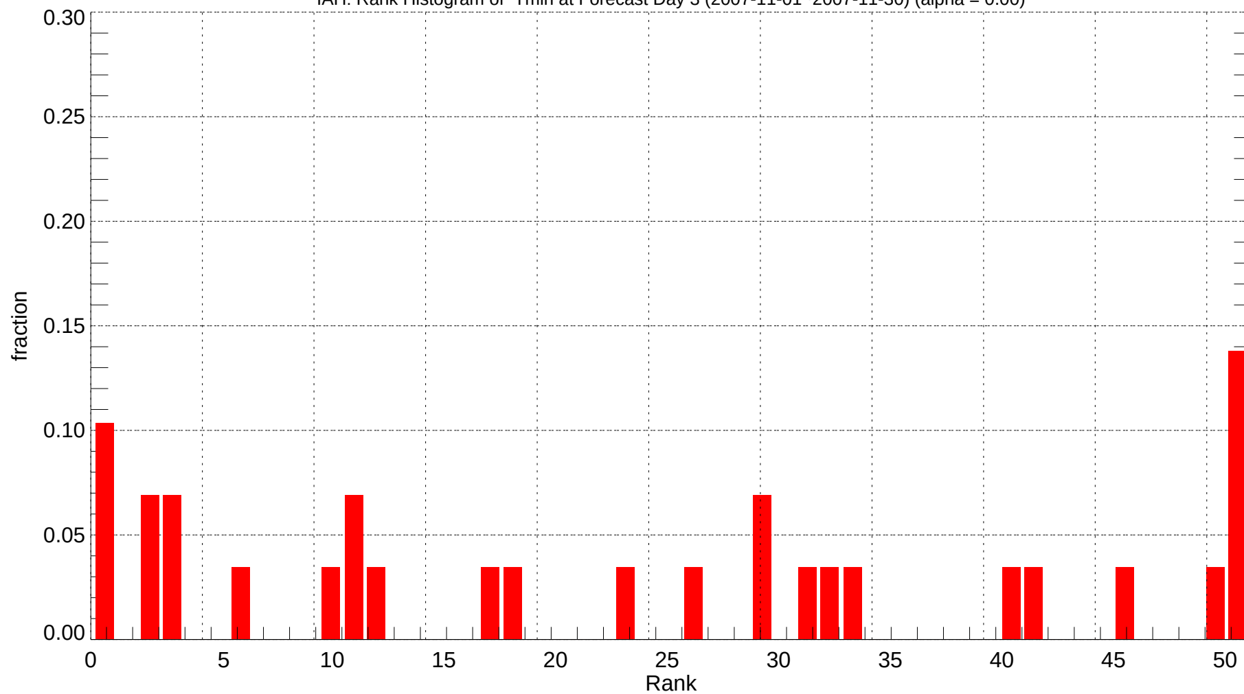
IAH: Rank Histogram of Tmin at Forecast Day 3 (2007-11-01~2007-11-30) (alpha = 0.00)
