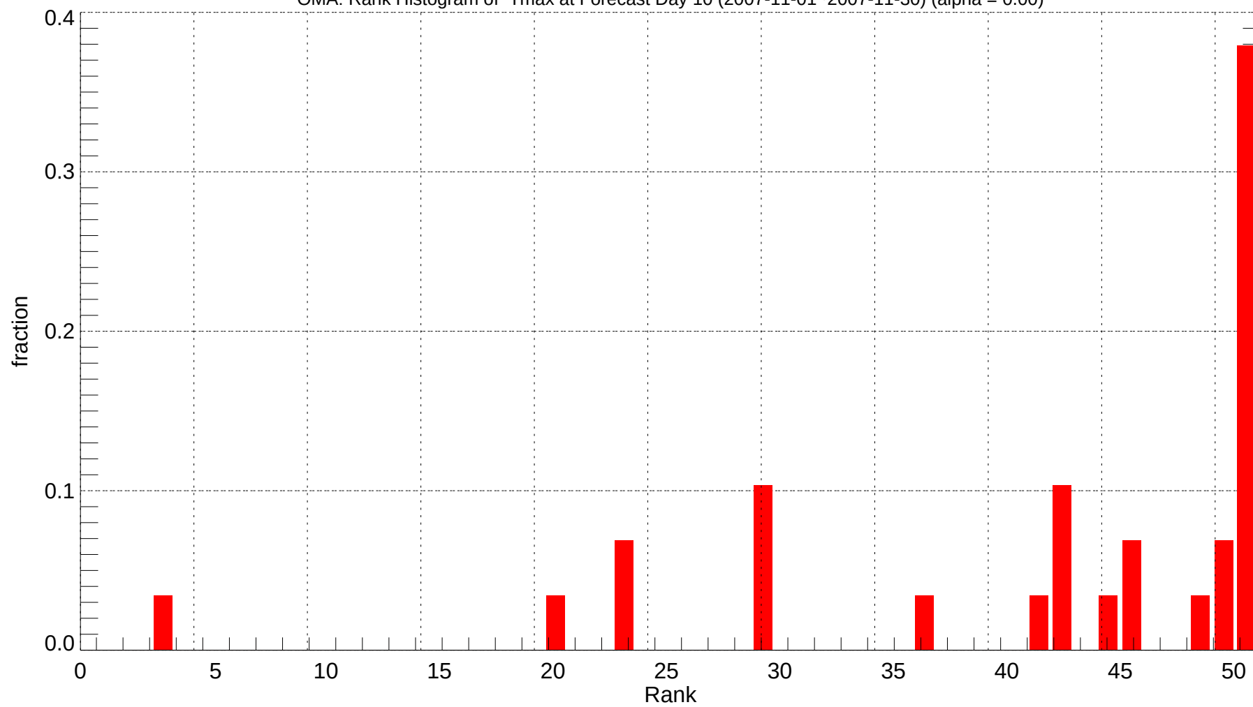
OMA: Rank Histogram of Tmax at Forecast Day 10 (2007-11-01~2007-11-30) (alpha = 0.00)
