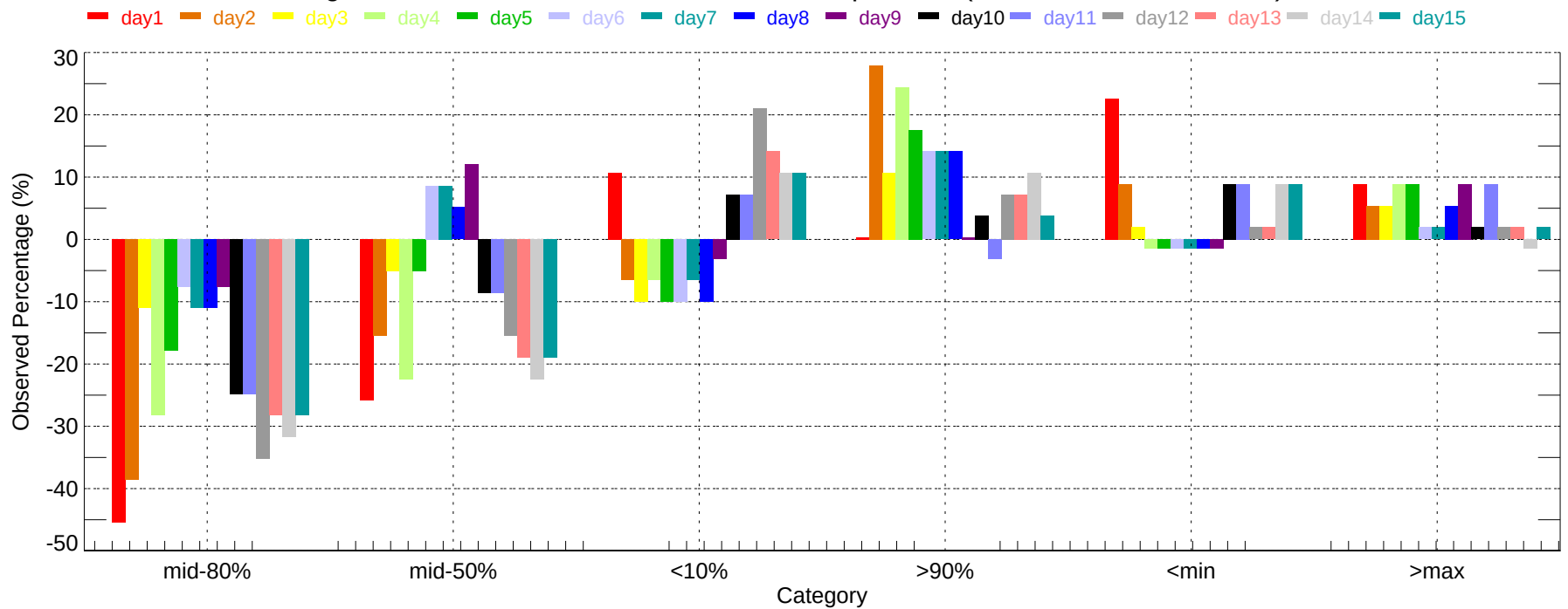
Observed Percentage Deviation of Ensembles - ILG: Min Temperature (2007-11-01~2007-11-30)
