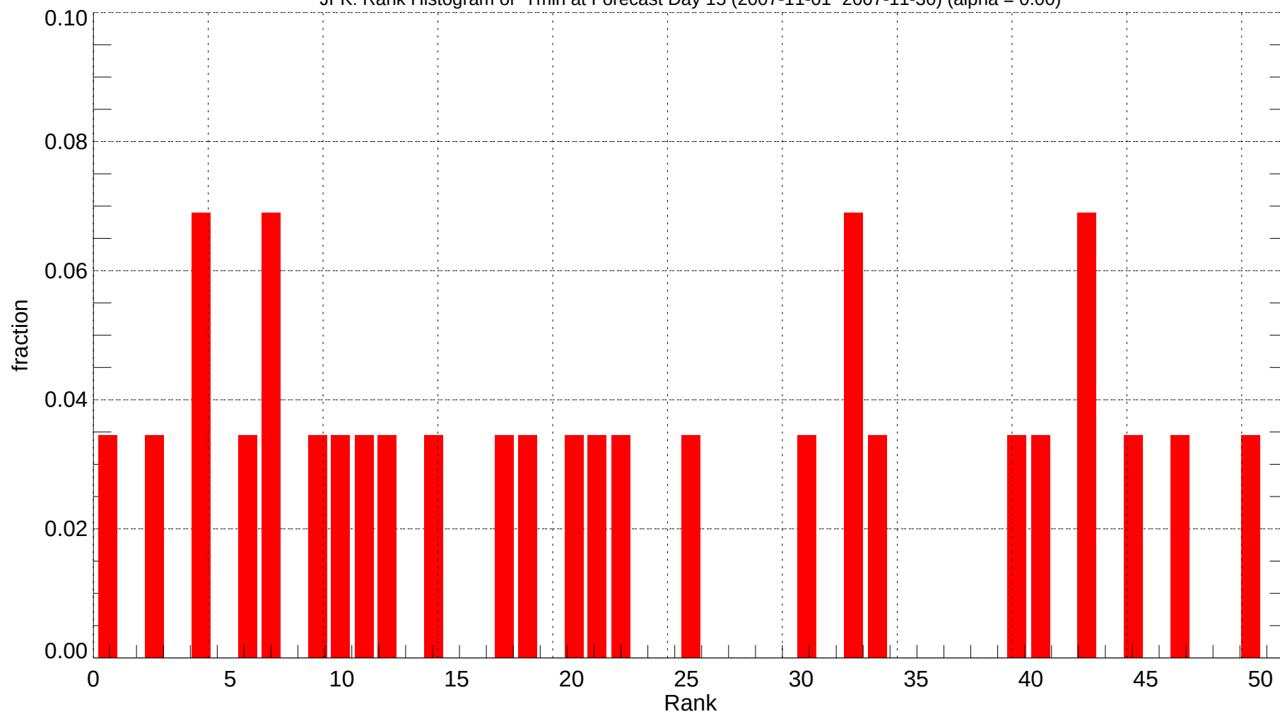
JFK: Rank Histogram of Tmin at Forecast Day 15 (2007-11-01~2007-11-30) (alpha = 0.00)
