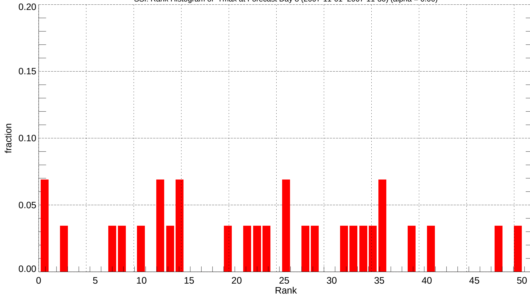
SSI: Rank Histogram of Tmax at Forecast Day 8 (2007-11-01~2007-11-30) (alpha = 0.00)
