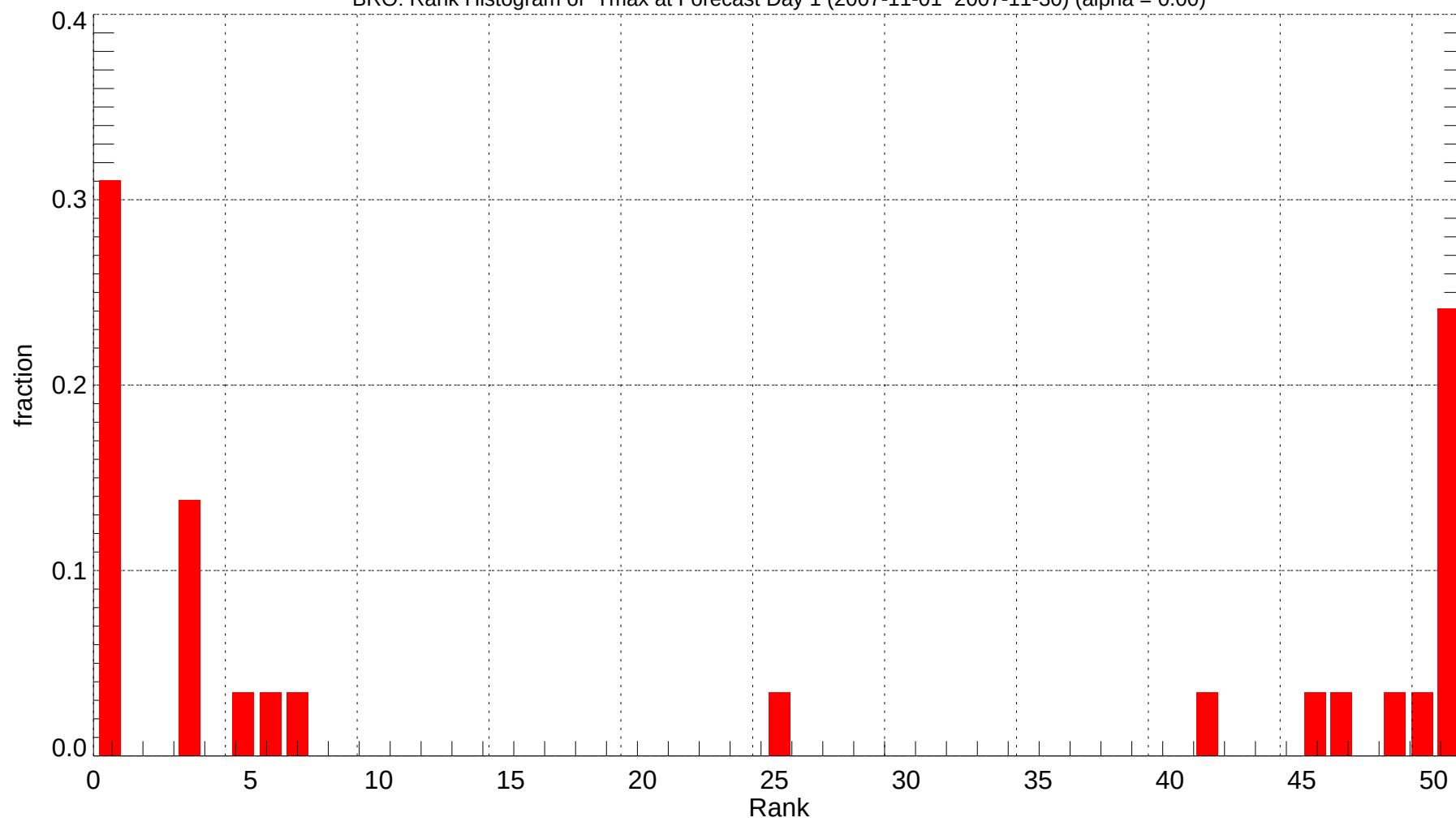
BRO: Rank Histogram of Tmax at Forecast Day 1 (2007-11-01~2007-11-30) (alpha = 0.00)
