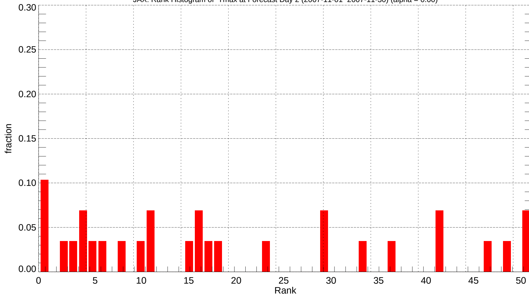
JAX: Rank Histogram of Tmax at Forecast Day 2 (2007-11-01~2007-11-30) (alpha = 0.00)
