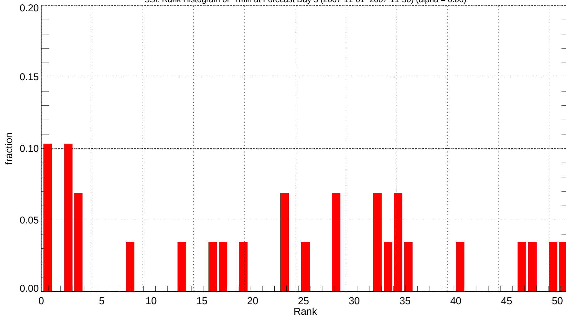
SSI: Rank Histogram of Tmin at Forecast Day 5 (2007-11-01~2007-11-30) (alpha = 0.00)
