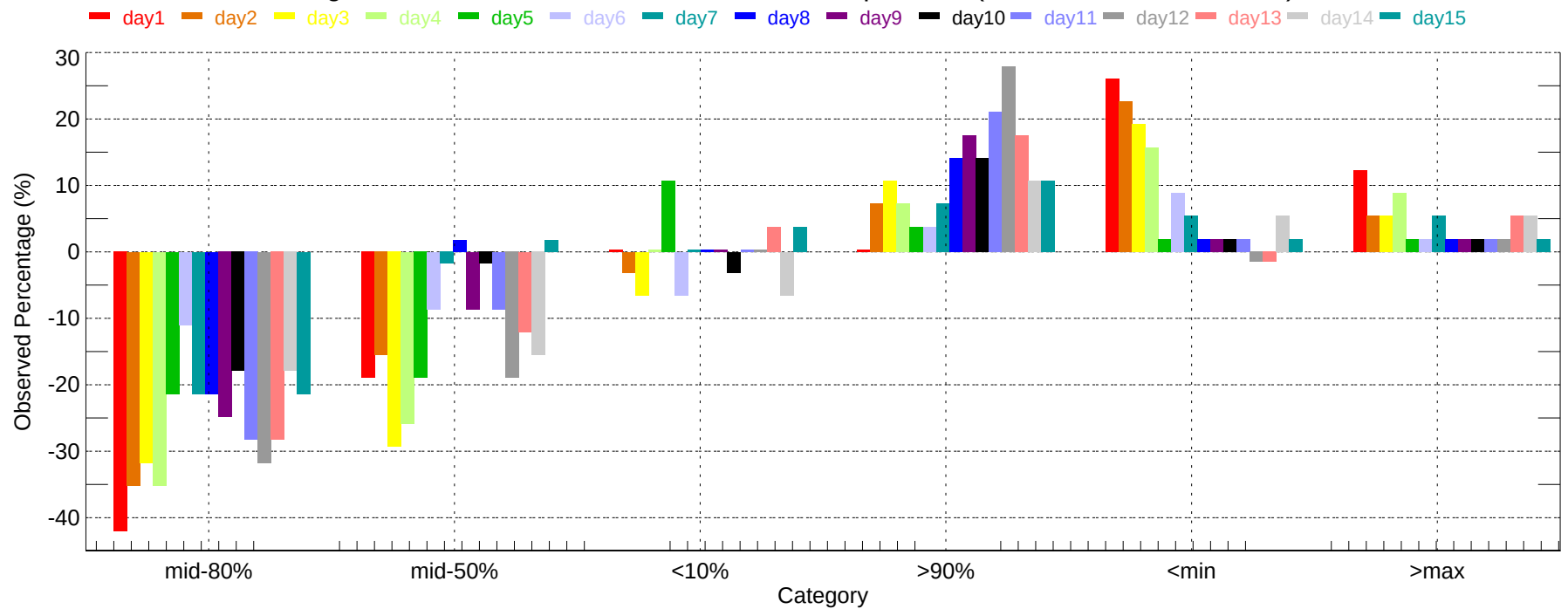
Observed Percentage Deviation of Ensembles - ACT: Min Temperature (2007-11-01~2007-11-30)
