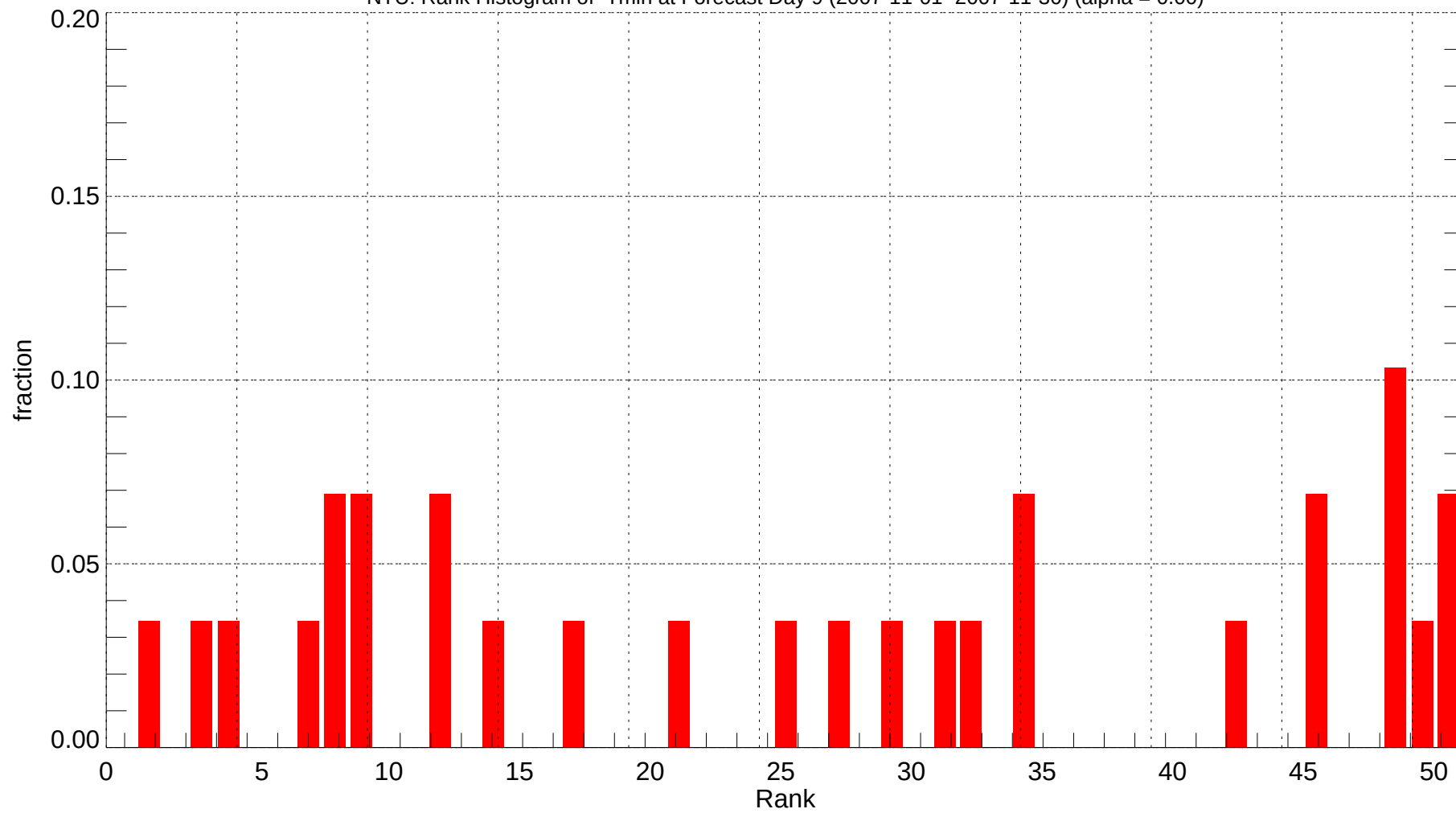
NTU: Rank Histogram of Tmin at Forecast Day 9 (2007-11-01~2007-11-30) (alpha = 0.00)
