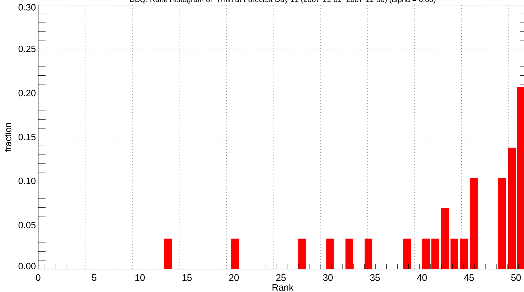
DBQ: Rank Histogram of Tmin at Forecast Day 11 (2007-11-01~2007-11-30) (alpha = 0.00)
