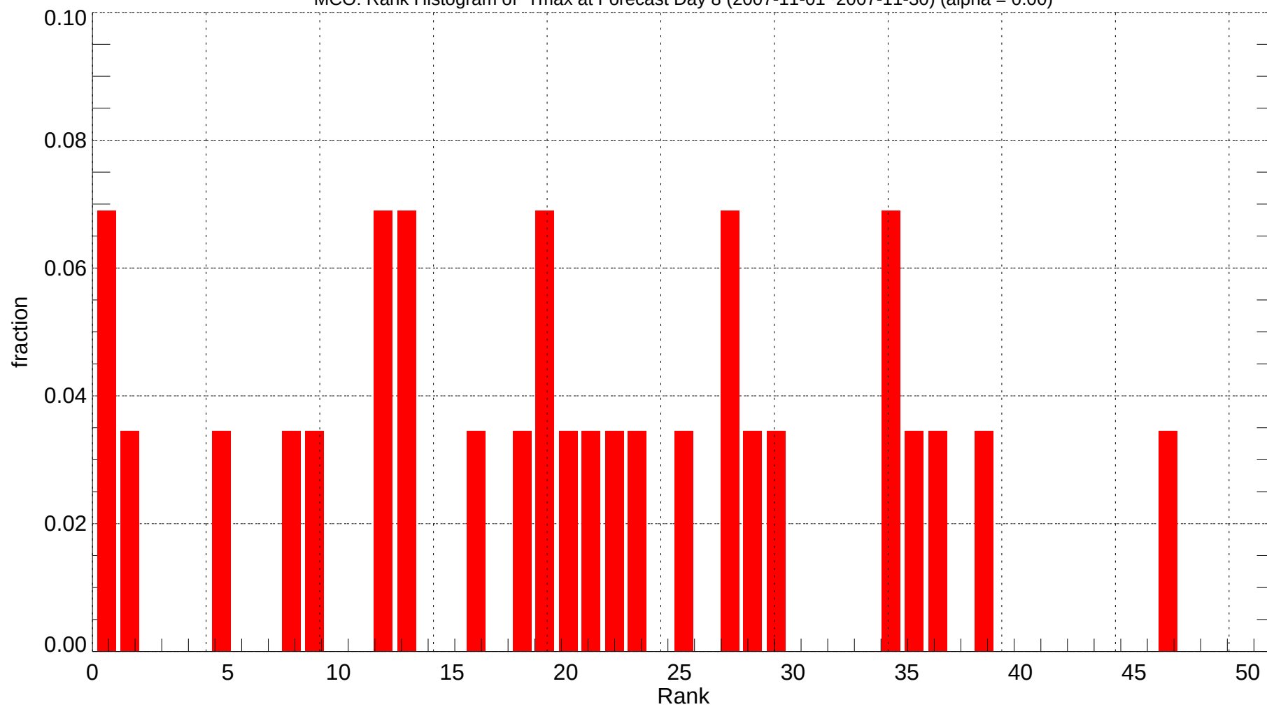
MCO: Rank Histogram of Tmax at Forecast Day 8 (2007-11-01~2007-11-30) (alpha = 0.00)
