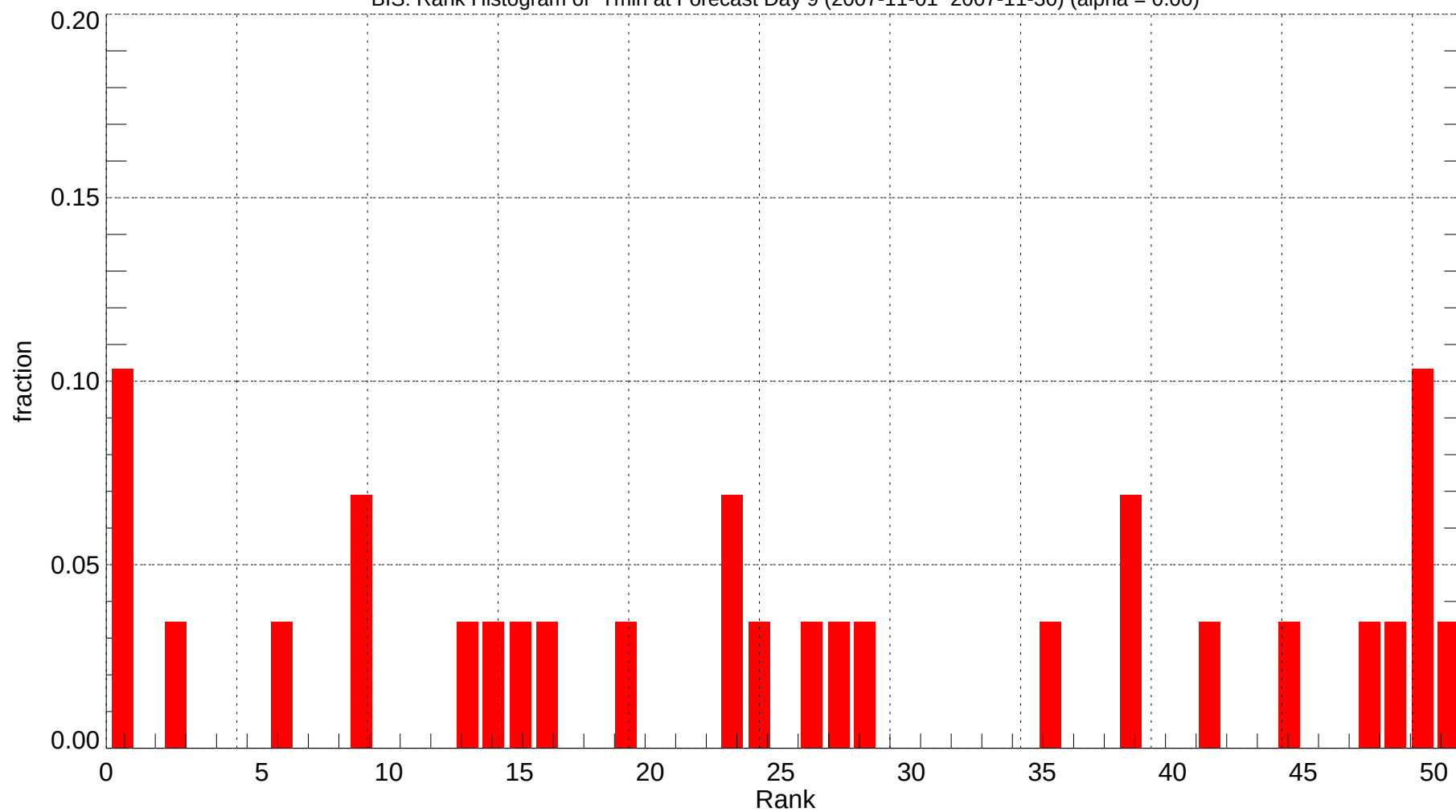
BIS: Rank Histogram of Tmin at Forecast Day 9 (2007-11-01~2007-11-30) (alpha = 0.00)
