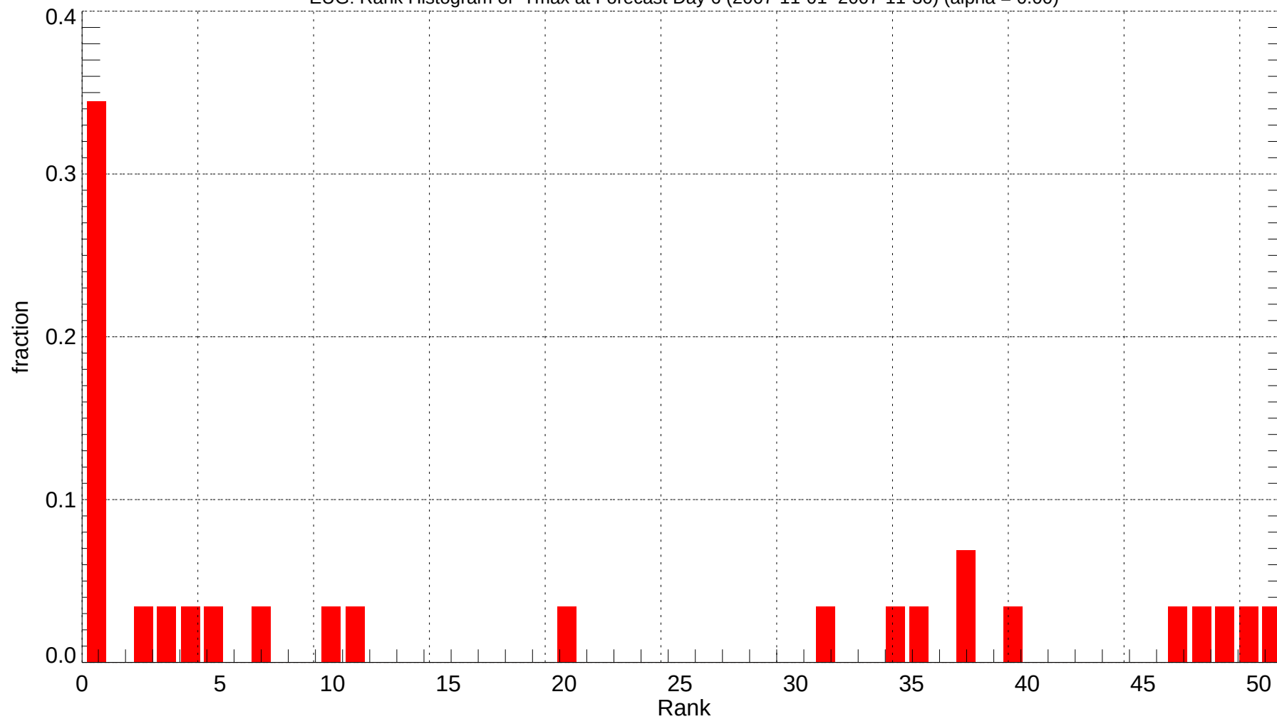
EUG: Rank Histogram of Tmax at Forecast Day 6 (2007-11-01~2007-11-30) (alpha = 0.00)
