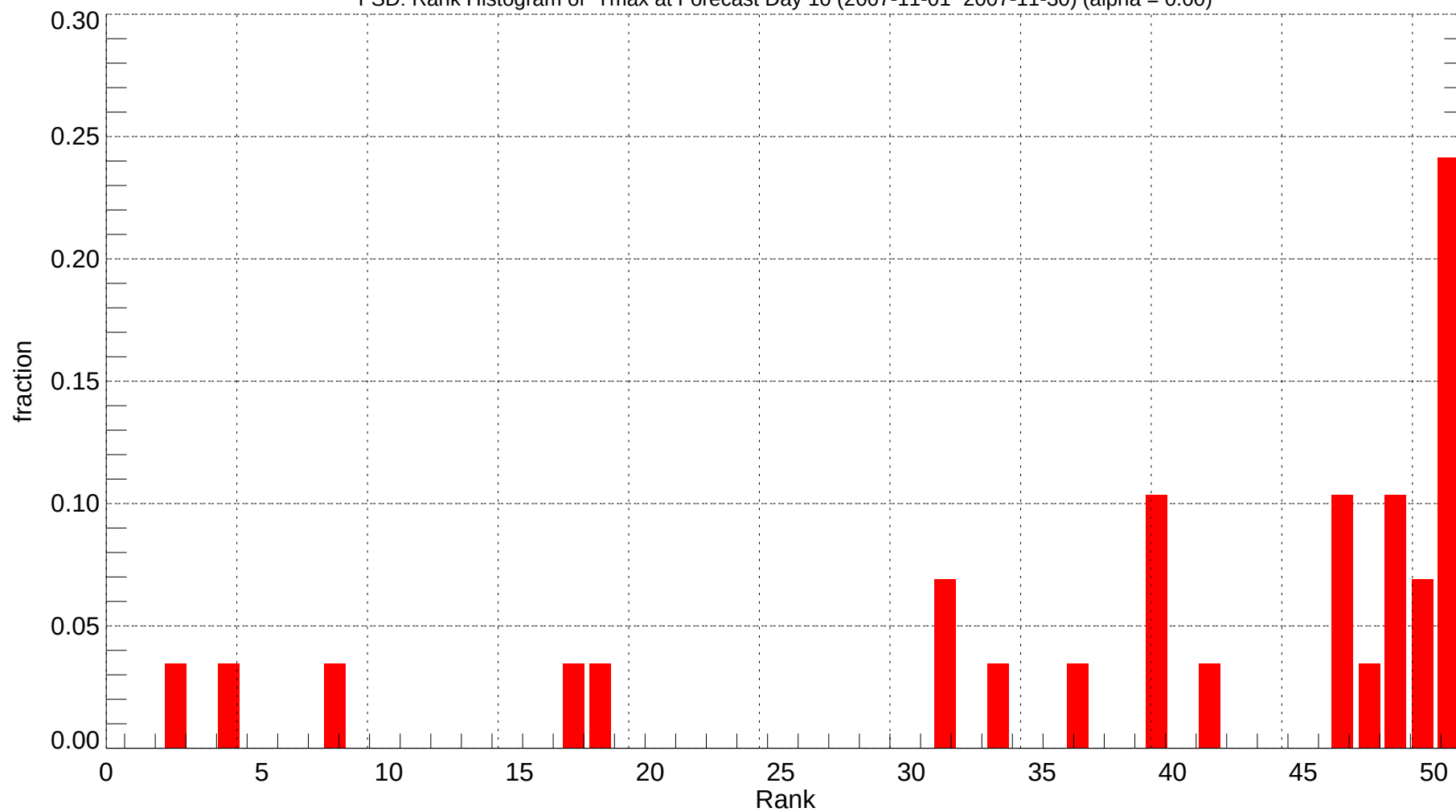
FSD: Rank Histogram of Tmax at Forecast Day 10 (2007-11-01~2007-11-30) (alpha = 0.00)
