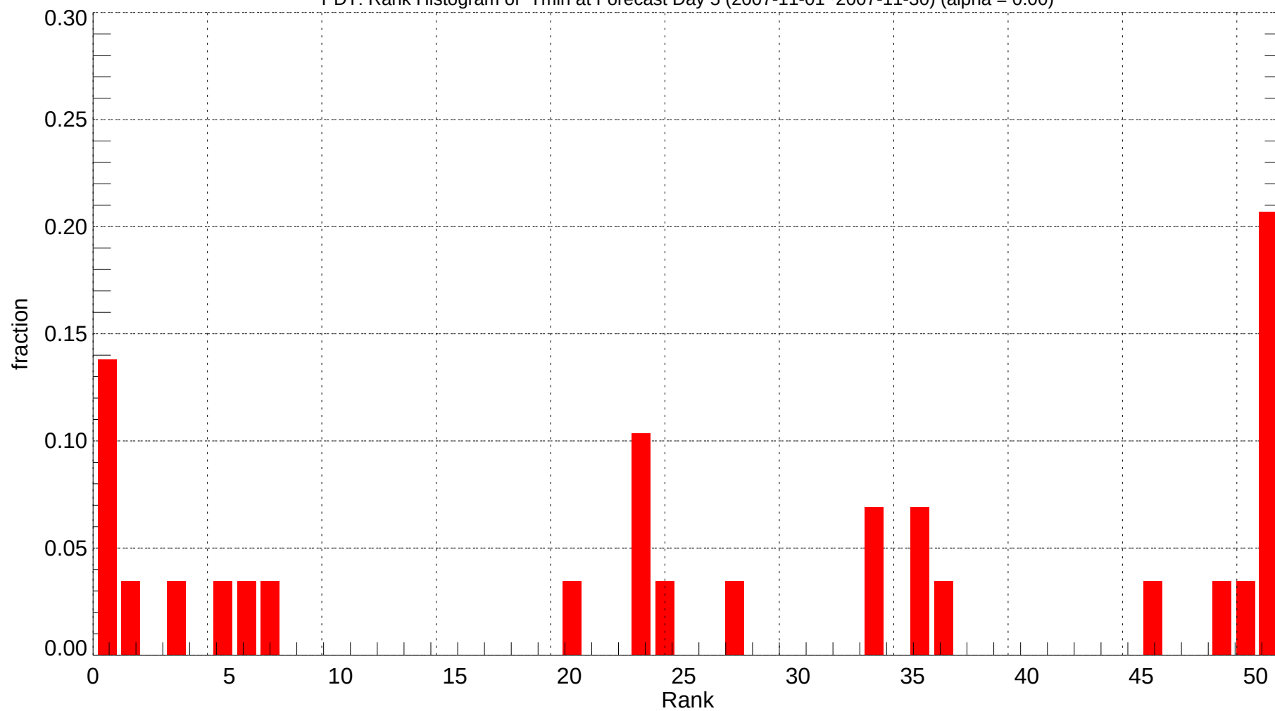
PDT: Rank Histogram of Tmin at Forecast Day 5 (2007-11-01~2007-11-30) (alpha = 0.00)
