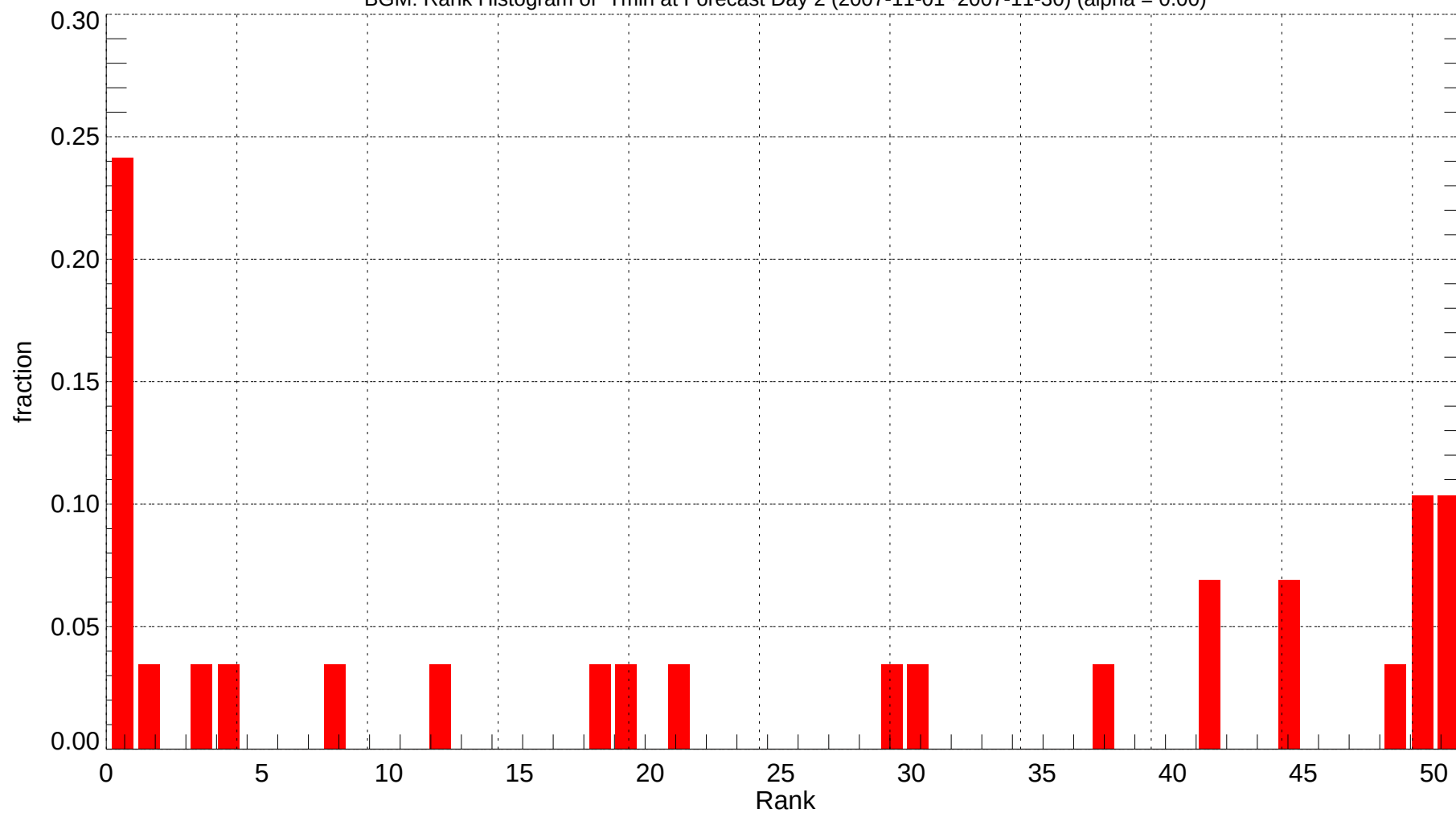
BGM: Rank Histogram of Tmin at Forecast Day 2 (2007-11-01~2007-11-30) (alpha = 0.00)
