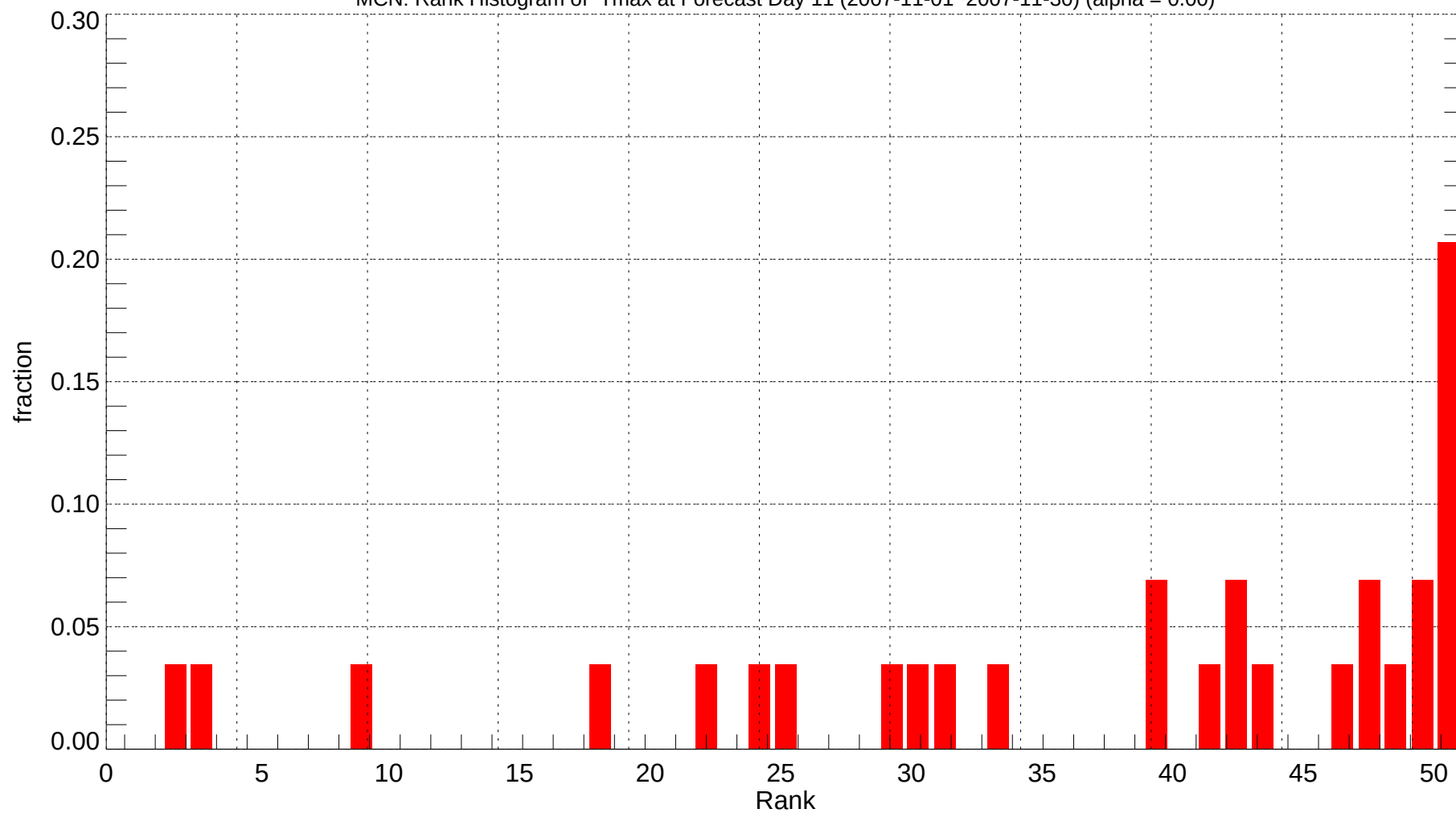
MCN: Rank Histogram of Tmax at Forecast Day 11 (2007-11-01~2007-11-30) (alpha = 0.00)
