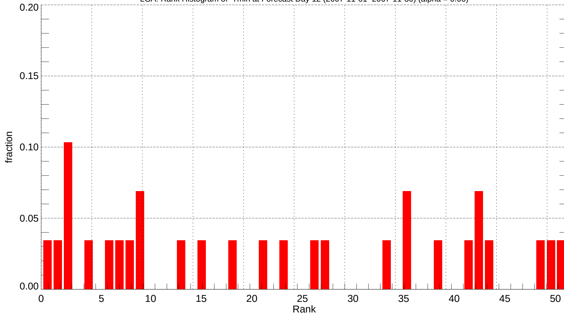
LGA: Rank Histogram of Tmin at Forecast Day 12 (2007-11-01~2007-11-30) (alpha = 0.00)
