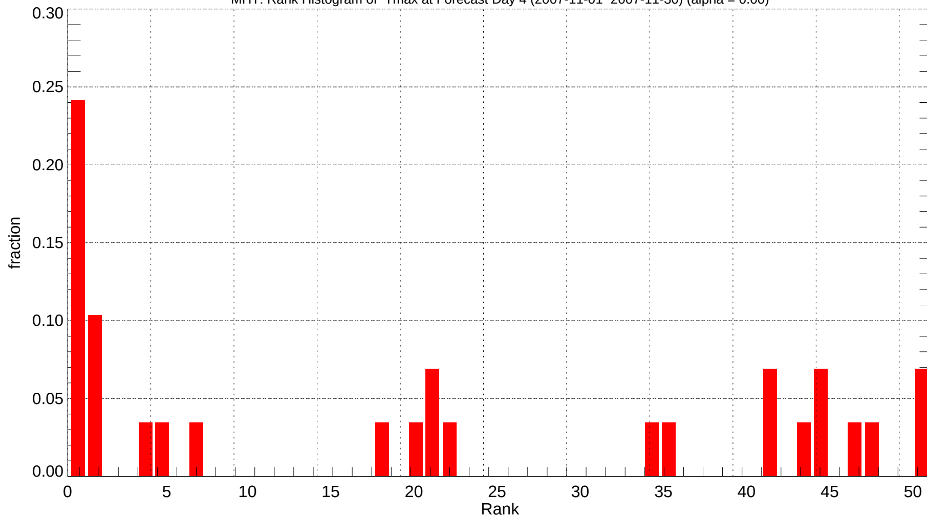
MHT: Rank Histogram of Tmax at Forecast Day 4 (2007-11-01~2007-11-30) (alpha = 0.00)
