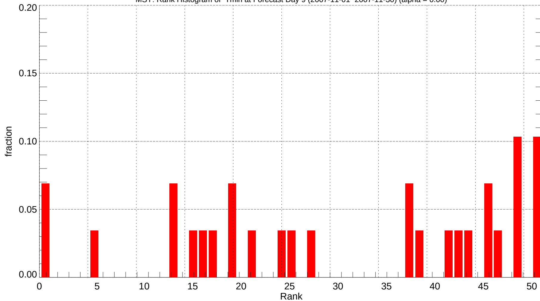
MSY: Rank Histogram of Tmin at Forecast Day 9 (2007-11-01~2007-11-30) (alpha = 0.00)
