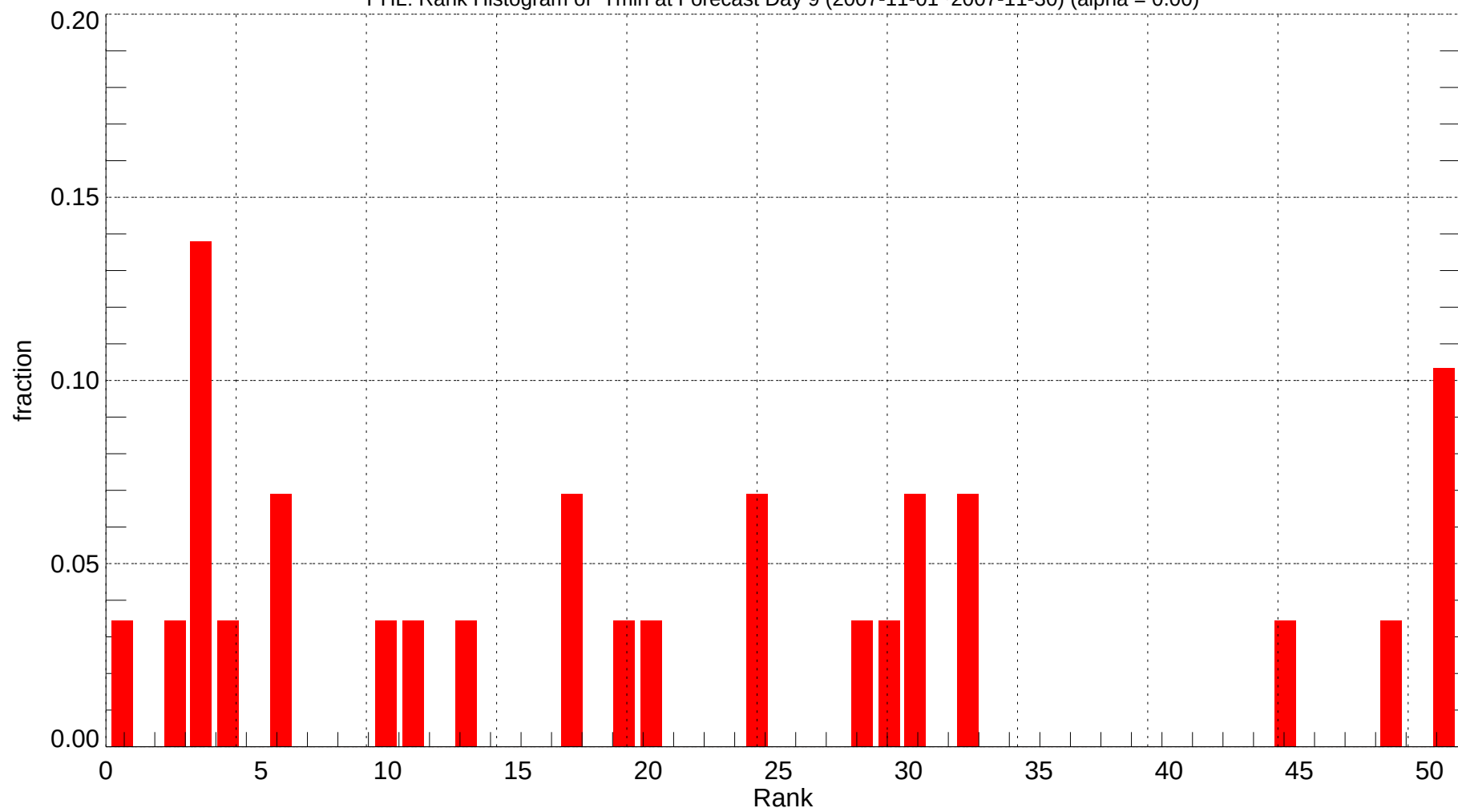
PHL: Rank Histogram of Tmin at Forecast Day 9 (2007-11-01~2007-11-30) (alpha = 0.00)
