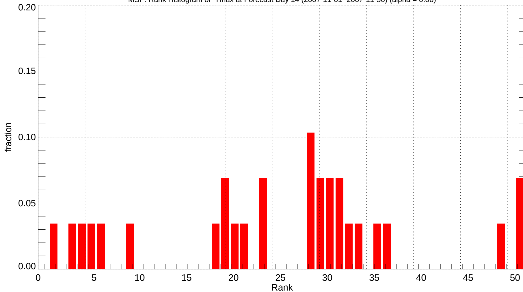
MSP: Rank Histogram of Tmax at Forecast Day 14 (2007-11-01~2007-11-30) (alpha = 0.00)
