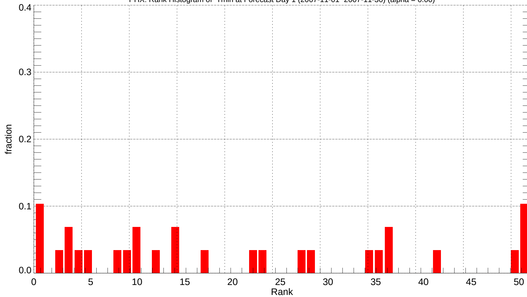
PHX: Rank Histogram of Tmin at Forecast Day 1 (2007-11-01~2007-11-30) (alpha = 0.00)
