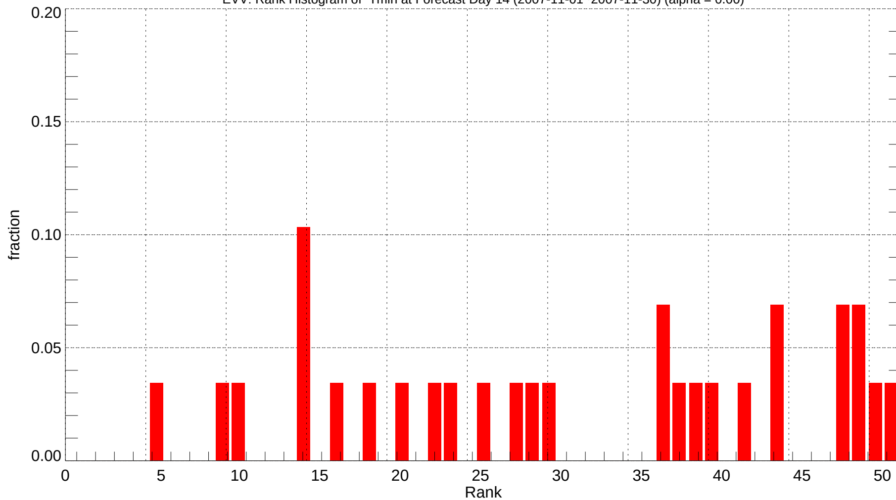
EVV: Rank Histogram of Tmin at Forecast Day 14 (2007-11-01~2007-11-30) (alpha = 0.00)
