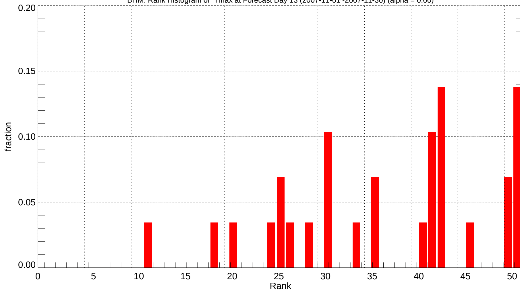
BHM: Rank Histogram of Tmax at Forecast Day 13 (2007-11-01~2007-11-30) (alpha = 0.00)
