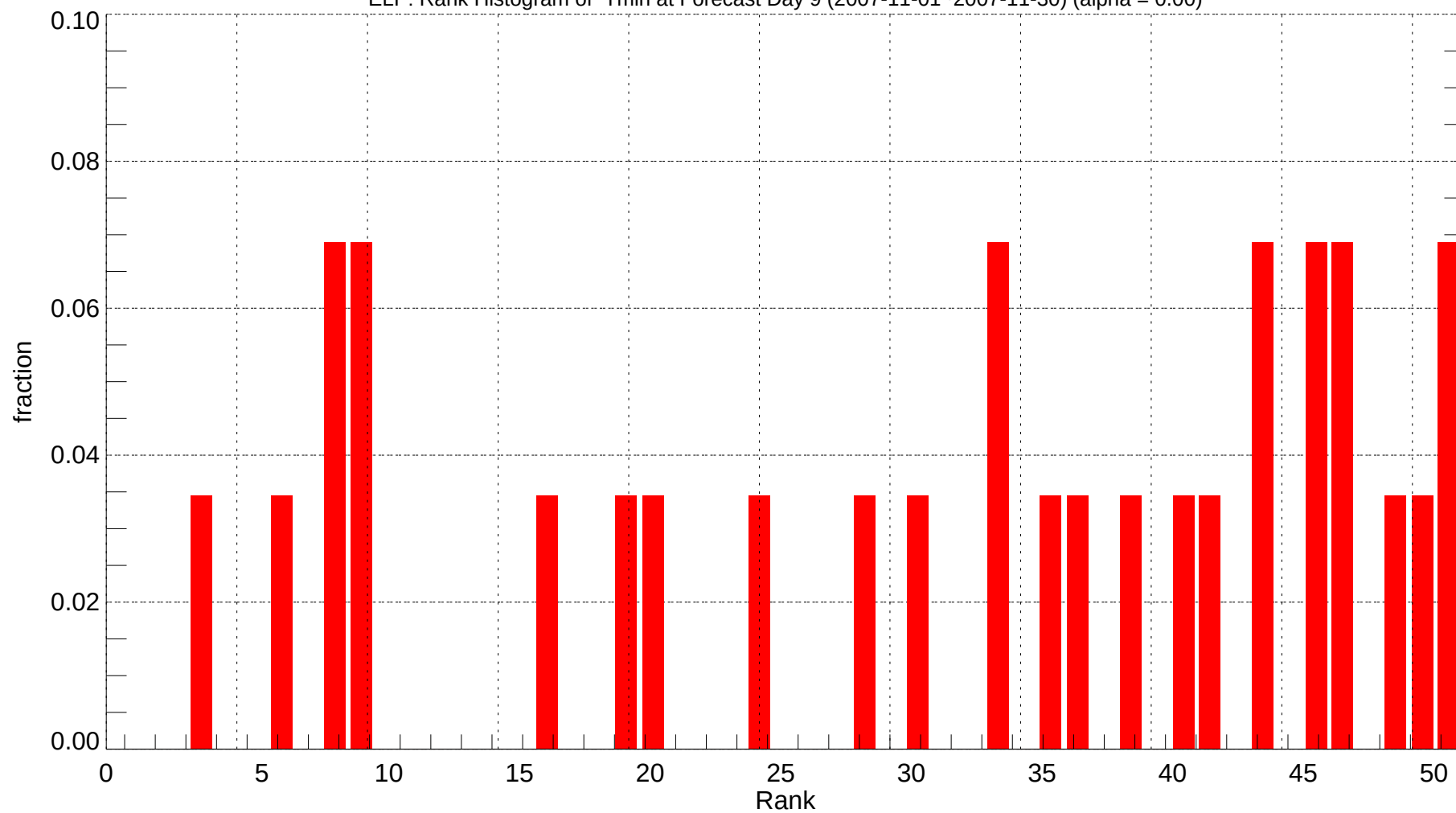
ELP: Rank Histogram of Tmin at Forecast Day 9 (2007-11-01~2007-11-30) (alpha = 0.00)
