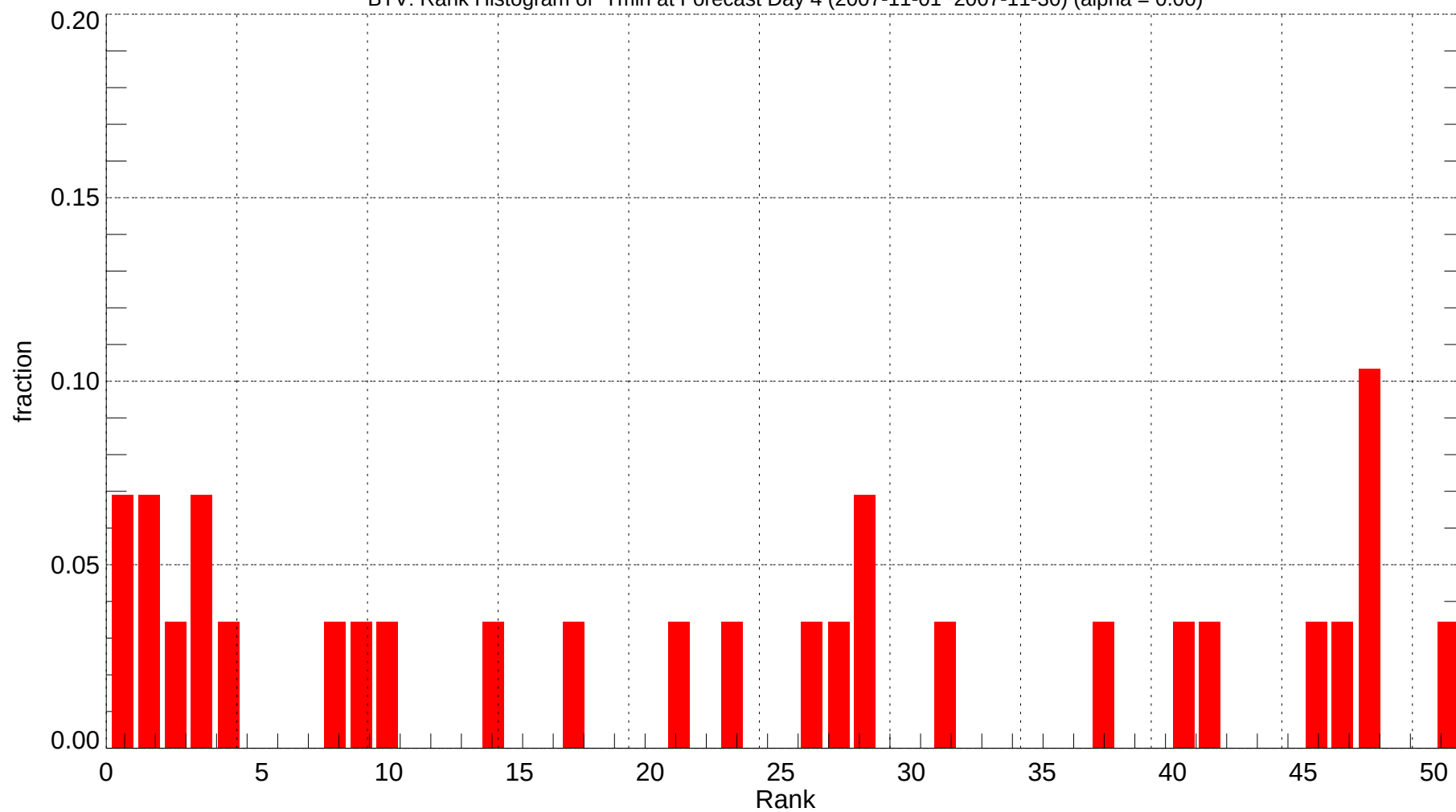
BTV: Rank Histogram of Tmin at Forecast Day 4 (2007-11-01~2007-11-30) (alpha = 0.00)
