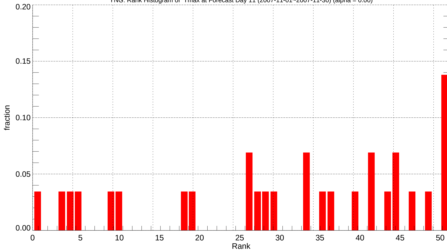
YNG: Rank Histogram of Tmax at Forecast Day 11 (2007-11-01~2007-11-30) (alpha = 0.00)
