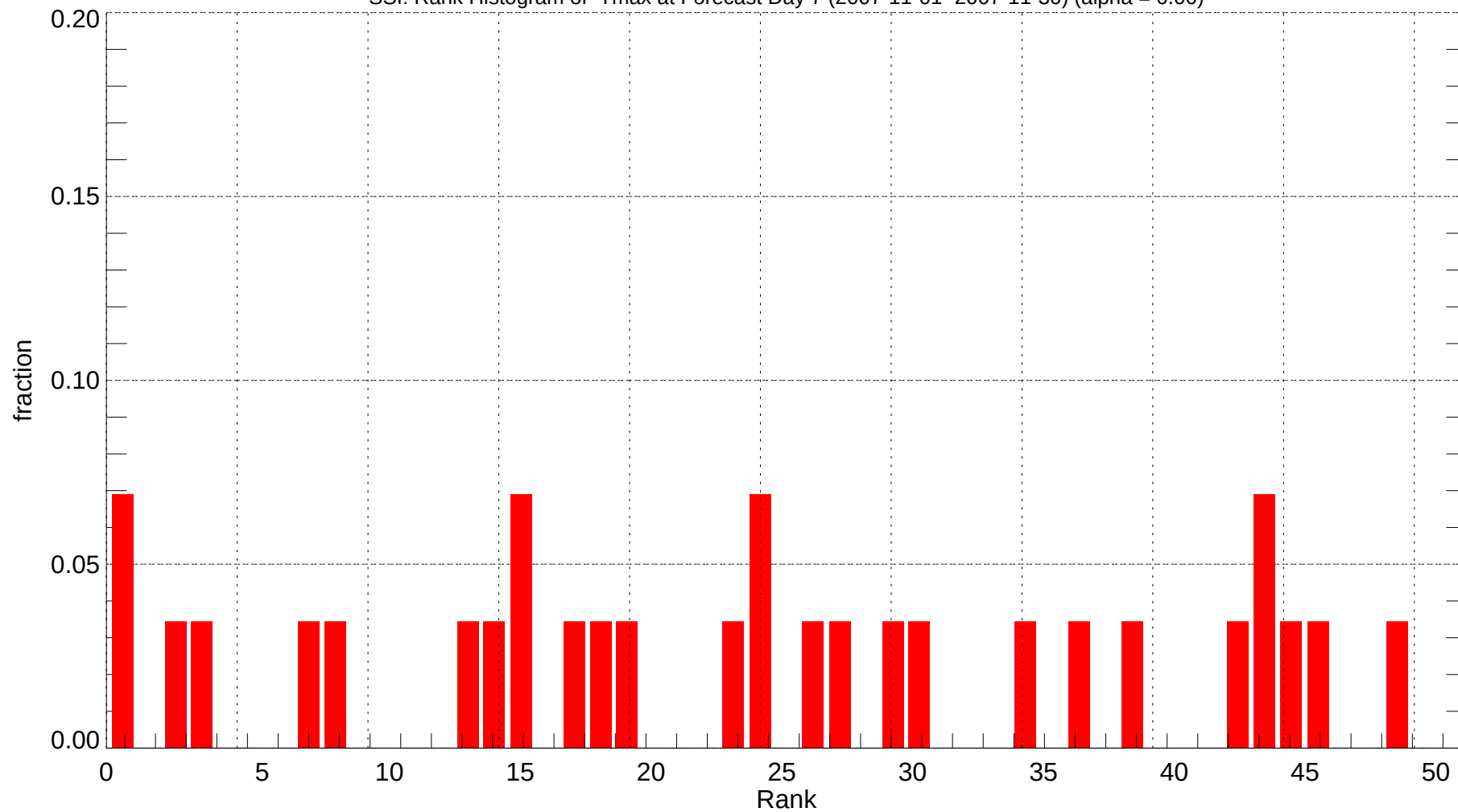
SSI: Rank Histogram of Tmax at Forecast Day 7 (2007-11-01~2007-11-30) (alpha = 0.00)
