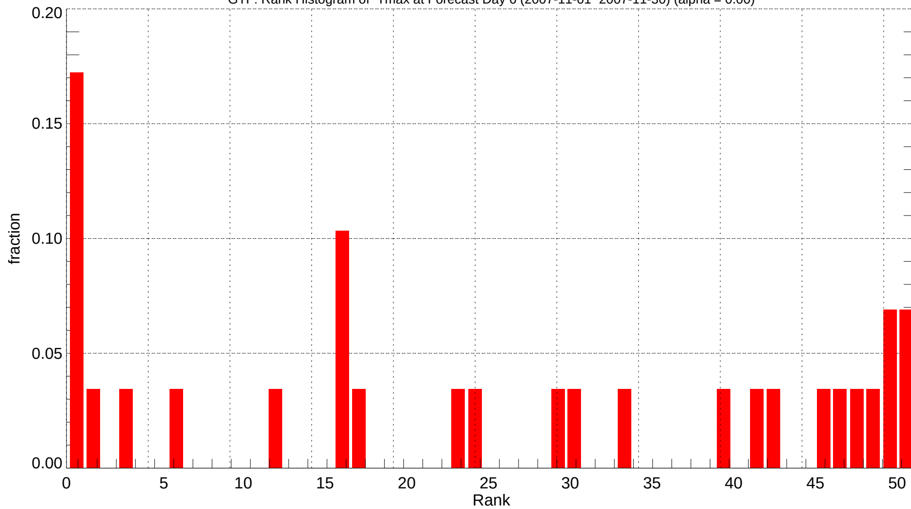
GTF: Rank Histogram of Tmax at Forecast Day 6 (2007-11-01~2007-11-30) (alpha = 0.00)
