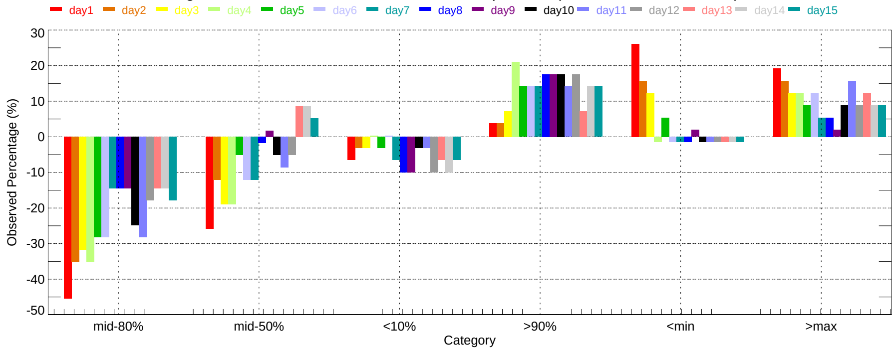
Observed Percentage Deviation of Ensembles - ERI: Max Temperature (2007-11-01~2007-11-30)
