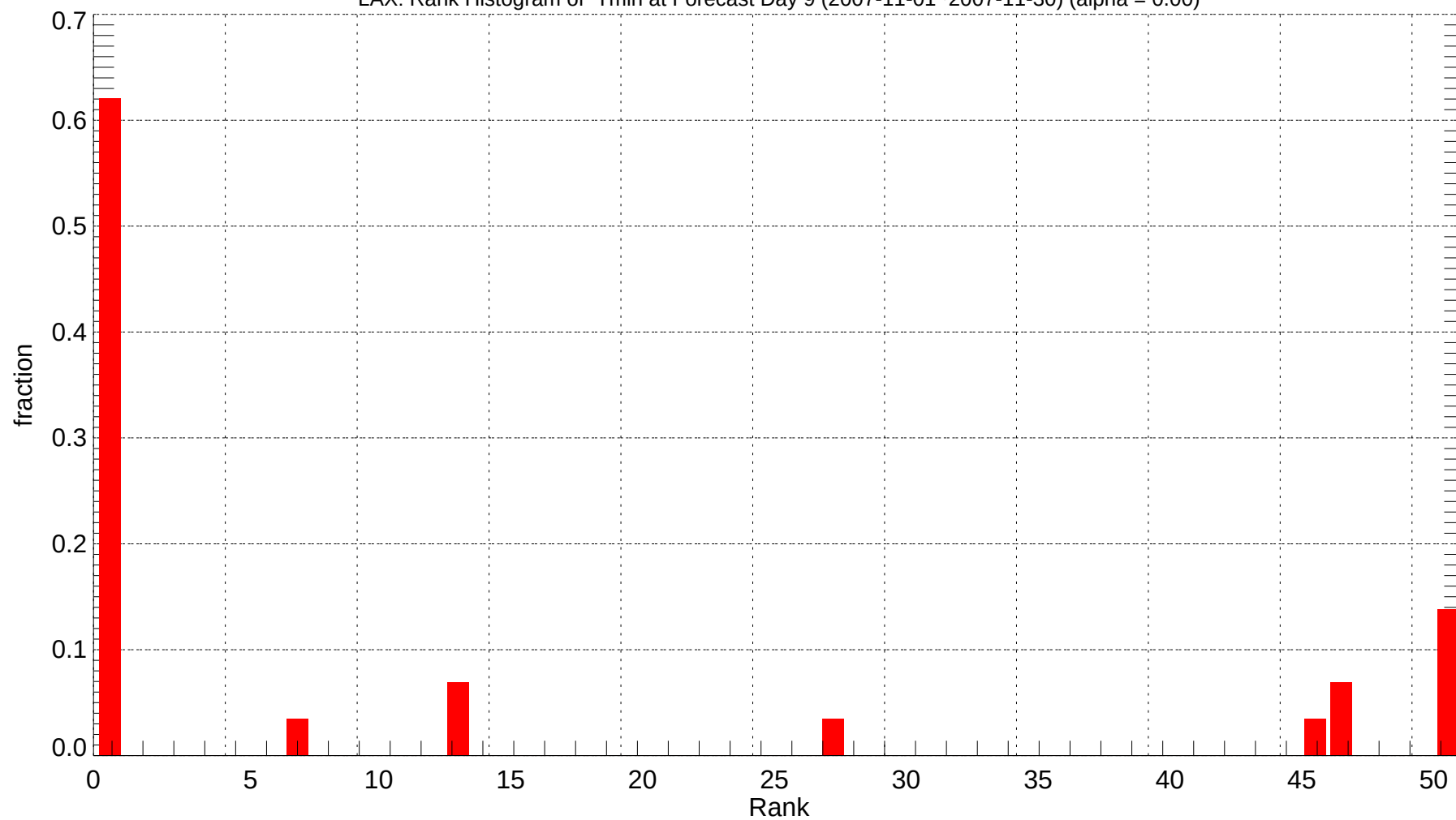
LAX: Rank Histogram of Tmin at Forecast Day 9 (2007-11-01~2007-11-30) (alpha = 0.00)
