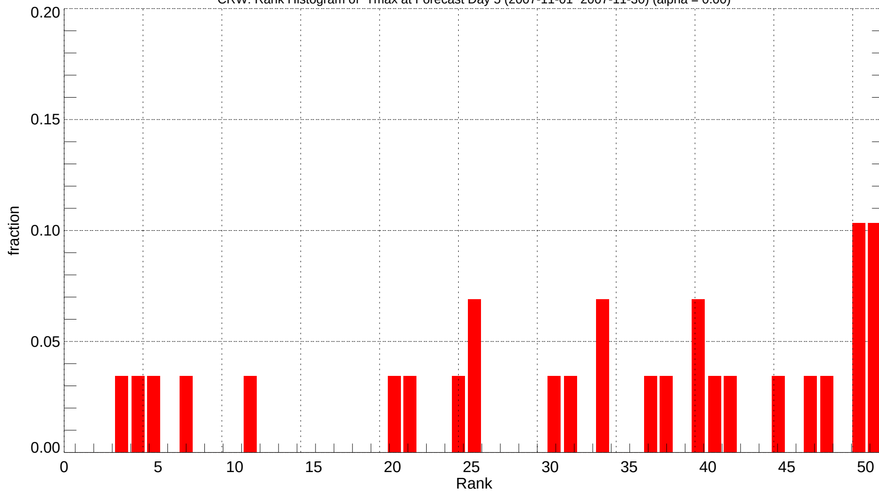
CRW: Rank Histogram of Tmax at Forecast Day 5 (2007-11-01~2007-11-30) (alpha = 0.00)
