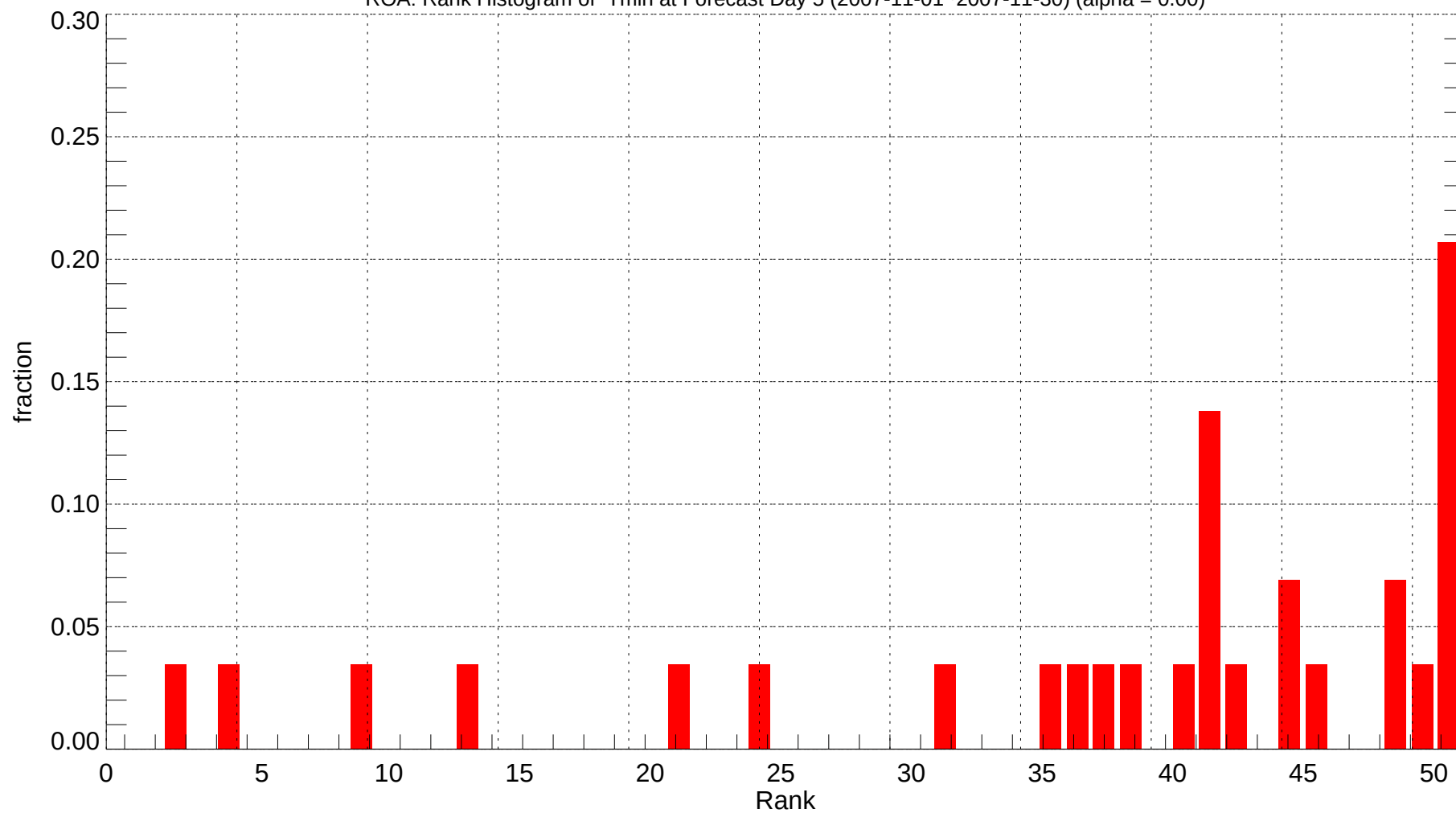
ROA: Rank Histogram of Tmin at Forecast Day 5 (2007-11-01~2007-11-30) (alpha = 0.00)
