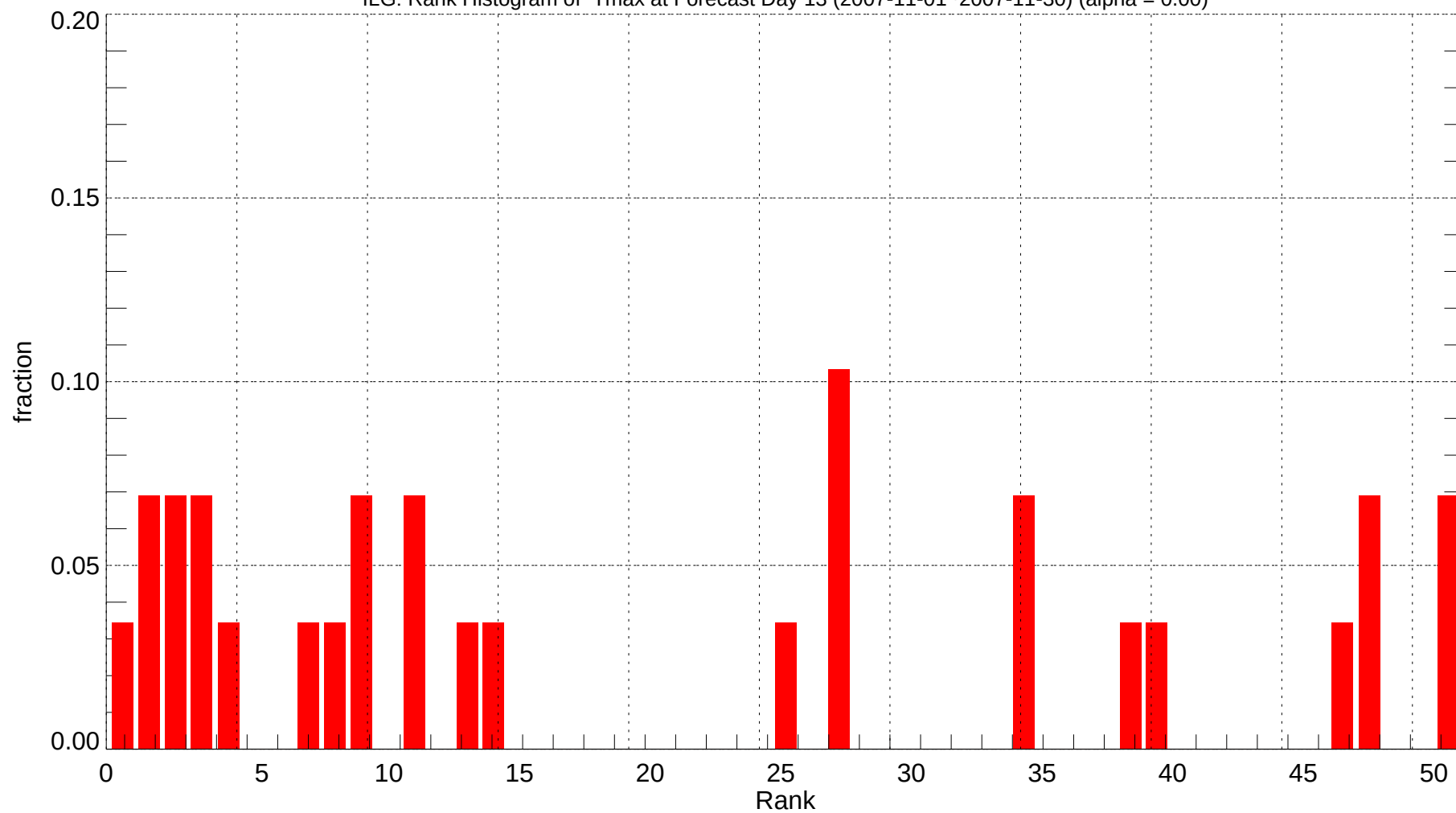
ILG: Rank Histogram of Tmax at Forecast Day 13 (2007-11-01~2007-11-30) (alpha = 0.00)
