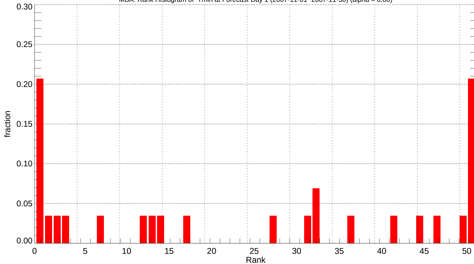
MBA: Rank Histogram of Tmin at Forecast Day 1 (2007-11-01~2007-11-30) (alpha = 0.00)
