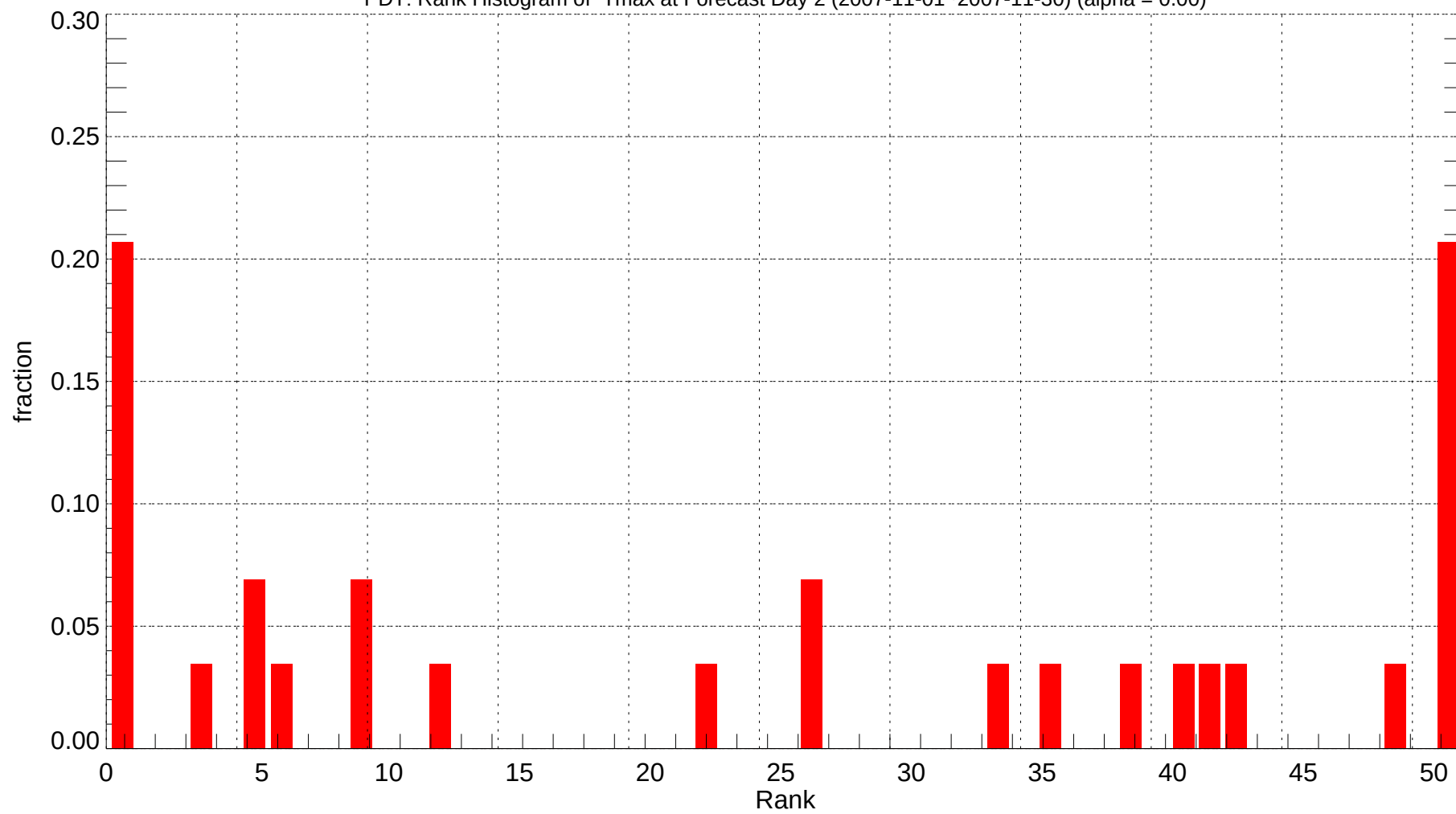
PDT: Rank Histogram of Tmax at Forecast Day 2 (2007-11-01~2007-11-30) (alpha = 0.00)
