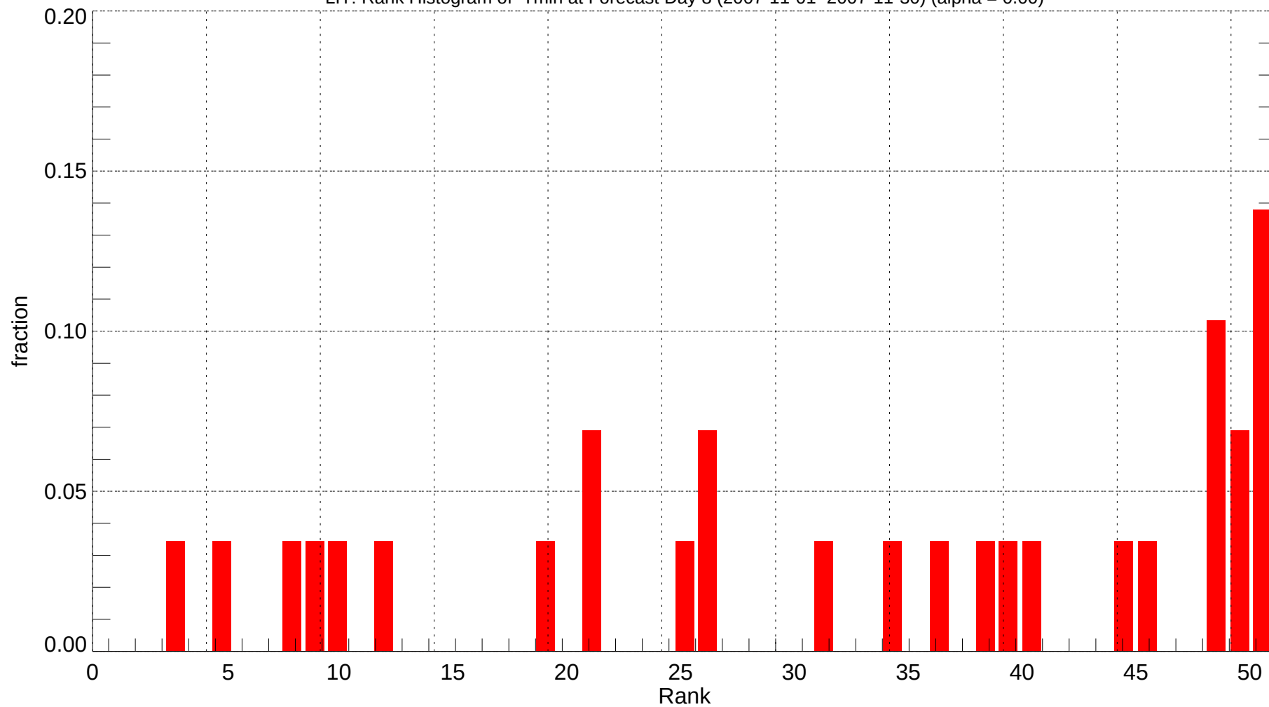
LIT: Rank Histogram of Tmin at Forecast Day 8 (2007-11-01~2007-11-30) (alpha = 0.00)
