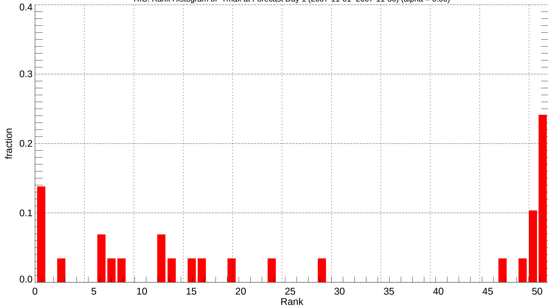
RIC: Rank Histogram of Tmax at Forecast Day 1 (2007-11-01~2007-11-30) (alpha = 0.00)
