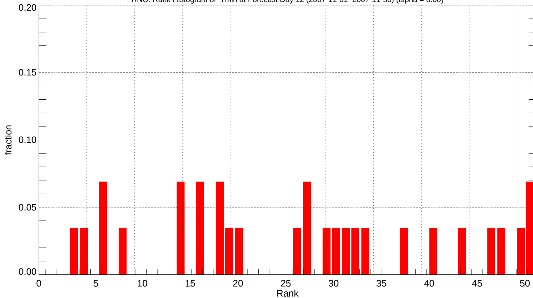
RNO: Rank Histogram of Tmin at Forecast Day 12 (2007-11-01~2007-11-30) (alpha = 0.00)
