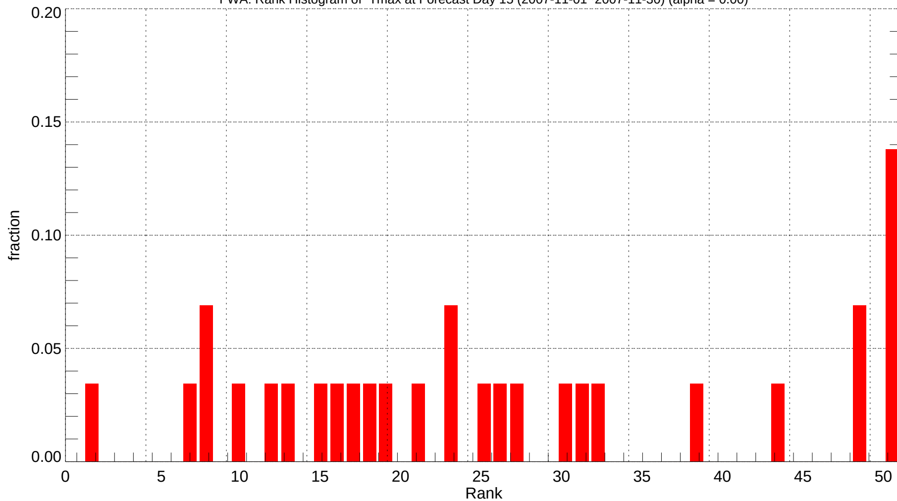
FWA: Rank Histogram of Tmax at Forecast Day 15 (2007-11-01~2007-11-30) (alpha = 0.00)
