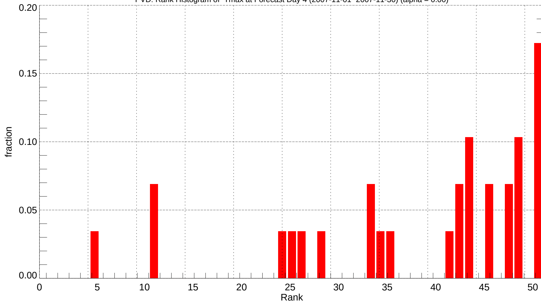
PVD: Rank Histogram of Tmax at Forecast Day 4 (2007-11-01~2007-11-30) (alpha = 0.00)
