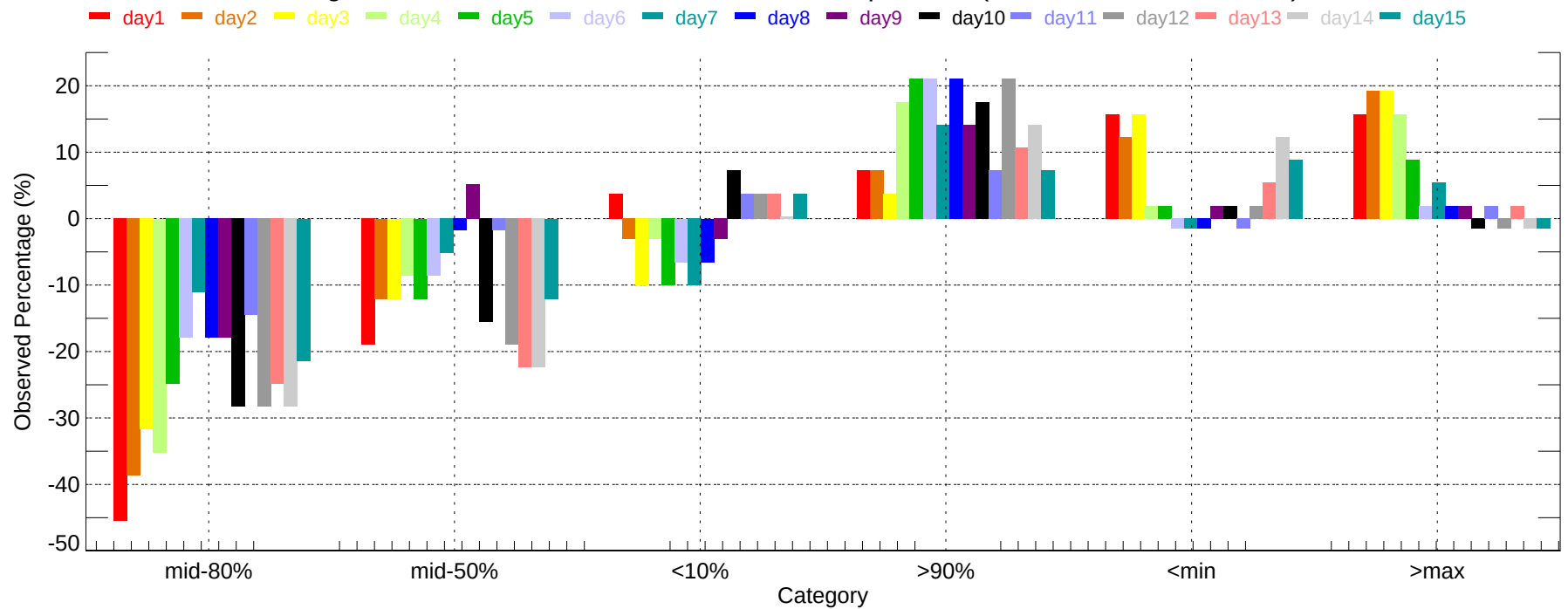
Observed Percentage Deviation of Ensembles - MBA: Min Temperature (2007-11-01~2007-11-30)
