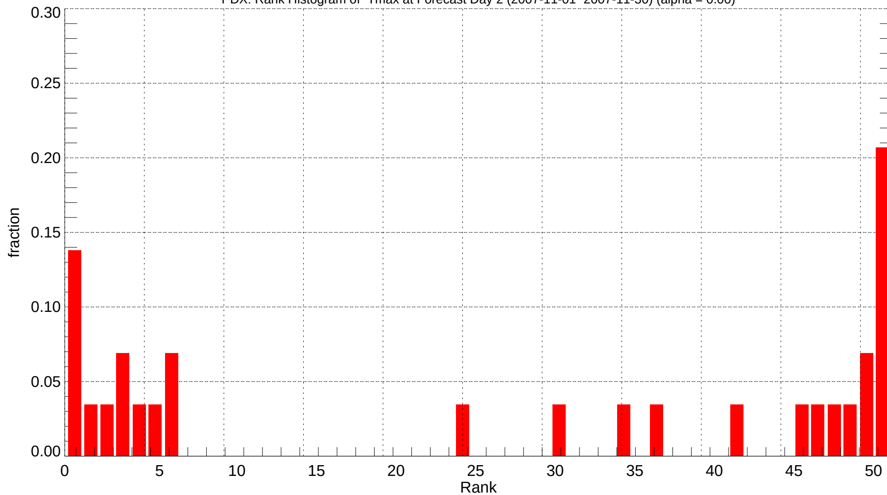
PDX: Rank Histogram of Tmax at Forecast Day 2 (2007-11-01~2007-11-30) (alpha = 0.00)
