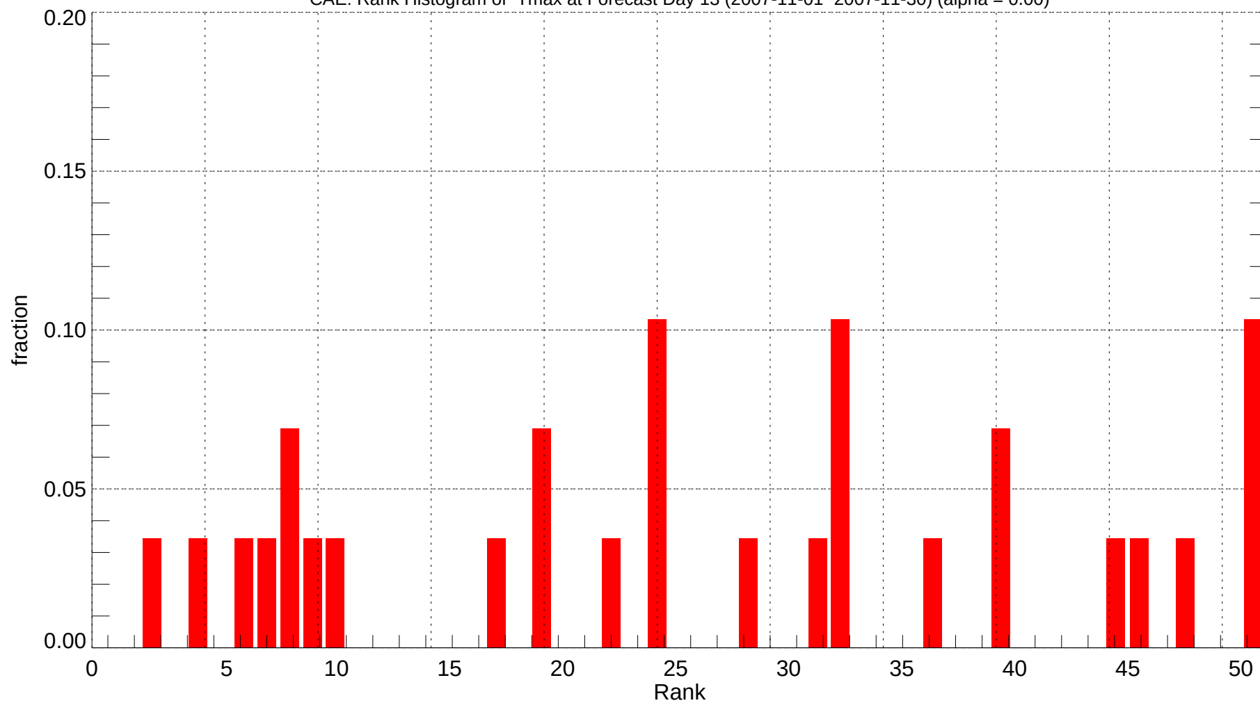
CAE: Rank Histogram of Tmax at Forecast Day 13 (2007-11-01~2007-11-30) (alpha = 0.00)
