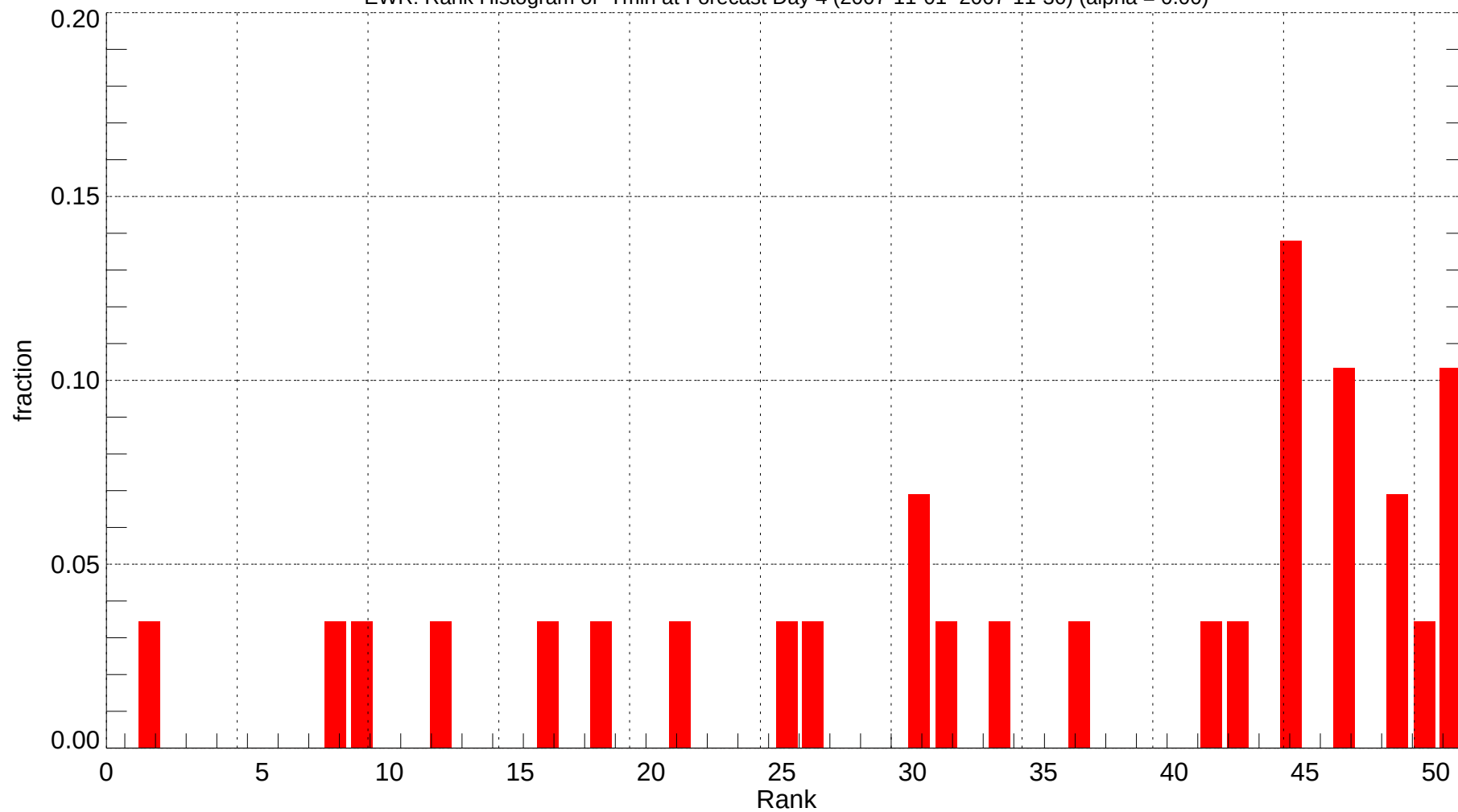
EWR: Rank Histogram of Tmin at Forecast Day 4 (2007-11-01~2007-11-30) (alpha = 0.00)
