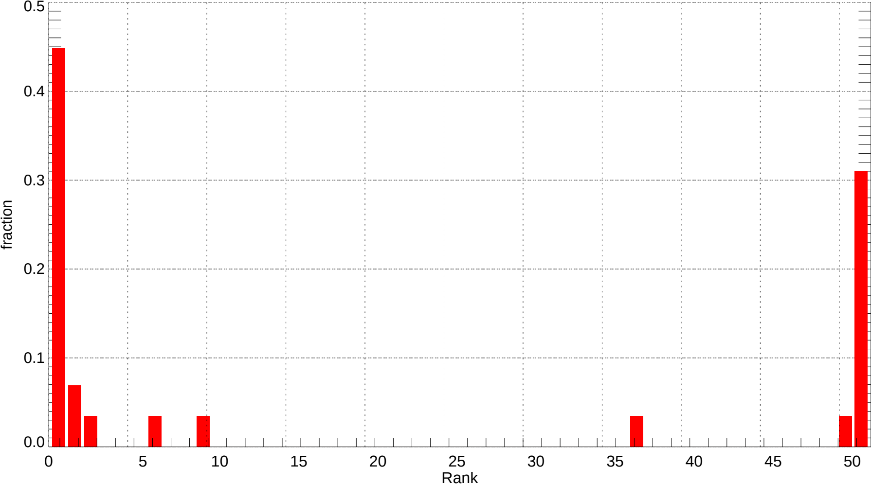
LAX: Rank Histogram of Tmin at Forecast Day 4 (2007-11-01~2007-11-30) (alpha = 0.00)
