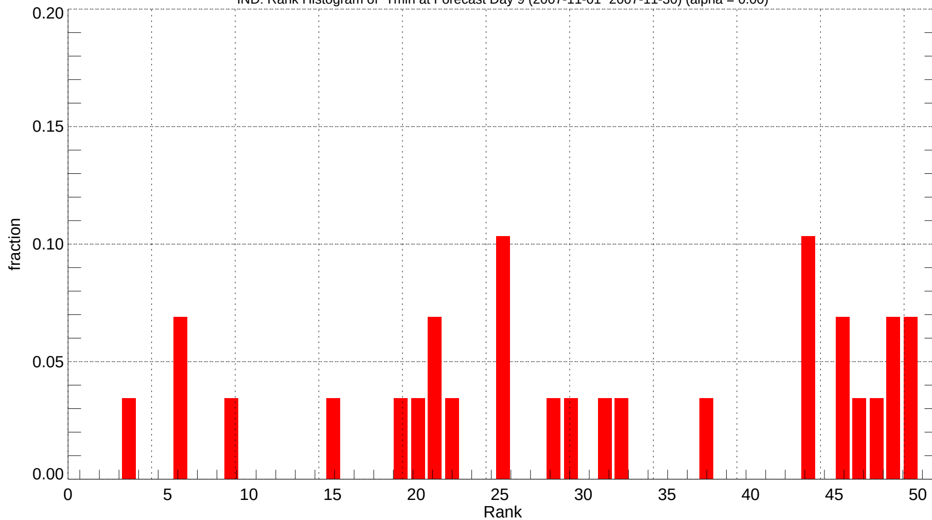
IND: Rank Histogram of Tmin at Forecast Day 9 (2007-11-01~2007-11-30) (alpha = 0.00)
