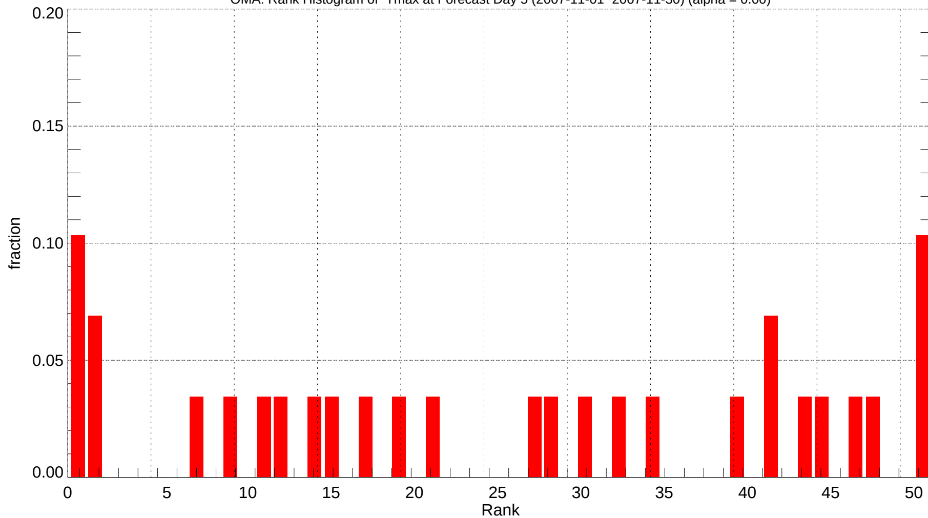
OMA: Rank Histogram of Tmax at Forecast Day 5 (2007-11-01~2007-11-30) (alpha = 0.00)
