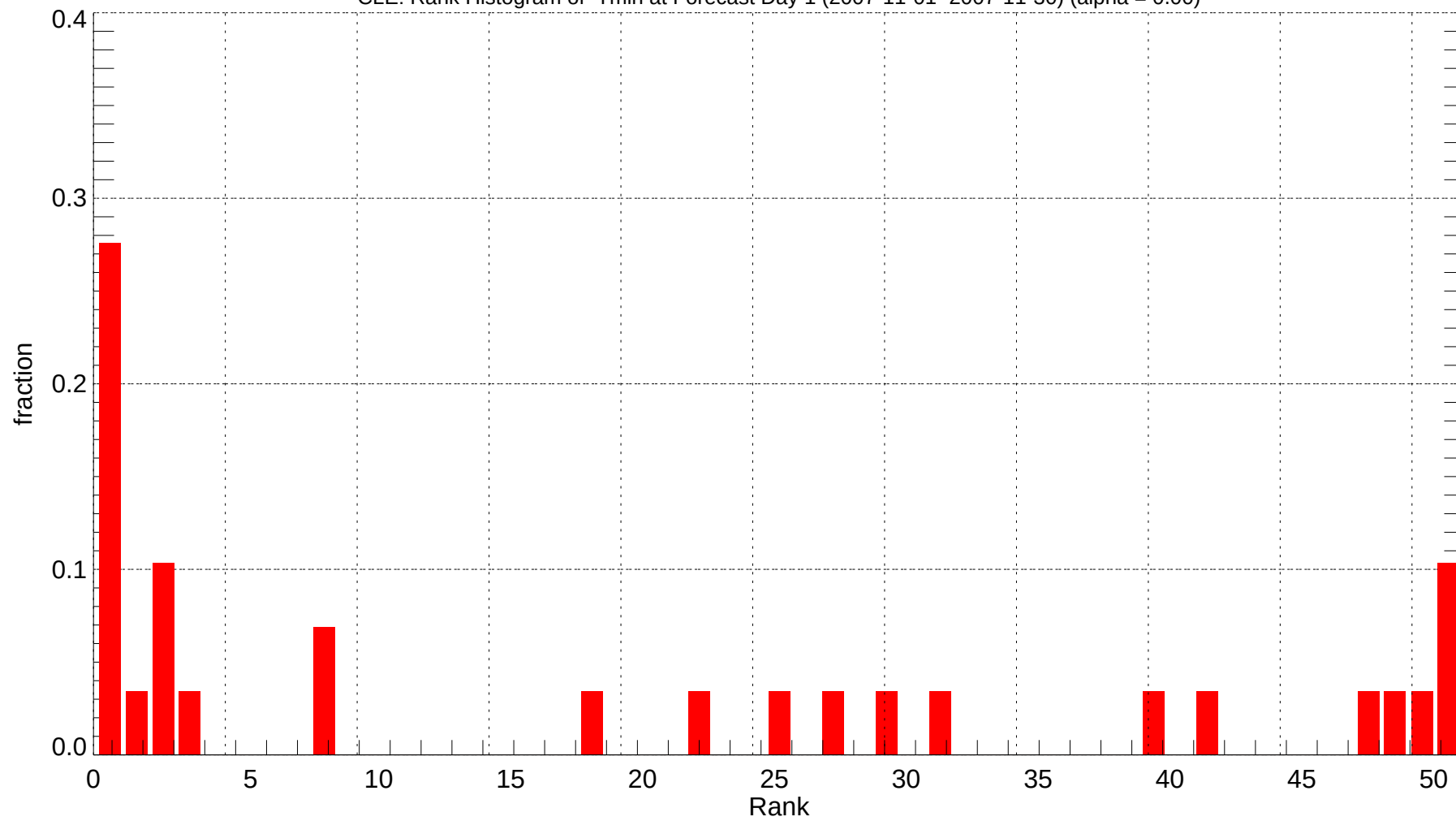
CLE: Rank Histogram of Tmin at Forecast Day 1 (2007-11-01~2007-11-30) (alpha = 0.00)
