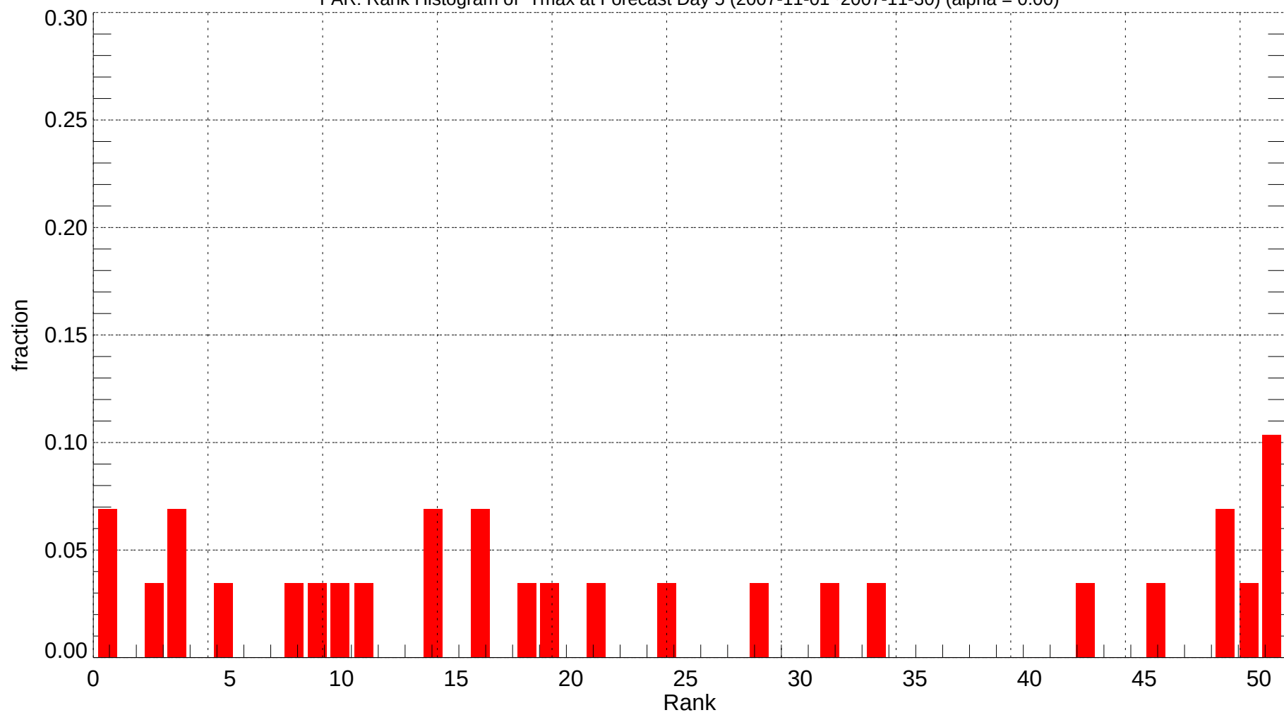
FAR: Rank Histogram of Tmax at Forecast Day 5 (2007-11-01~2007-11-30) (alpha = 0.00)
