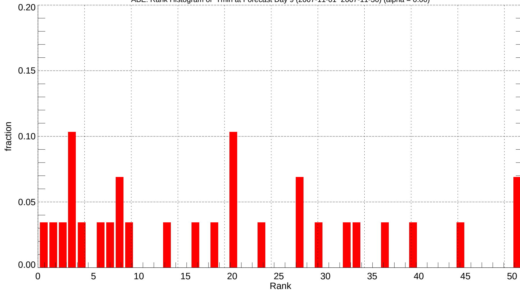
ABE: Rank Histogram of Tmin at Forecast Day 9 (2007-11-01~2007-11-30) (alpha = 0.00)
