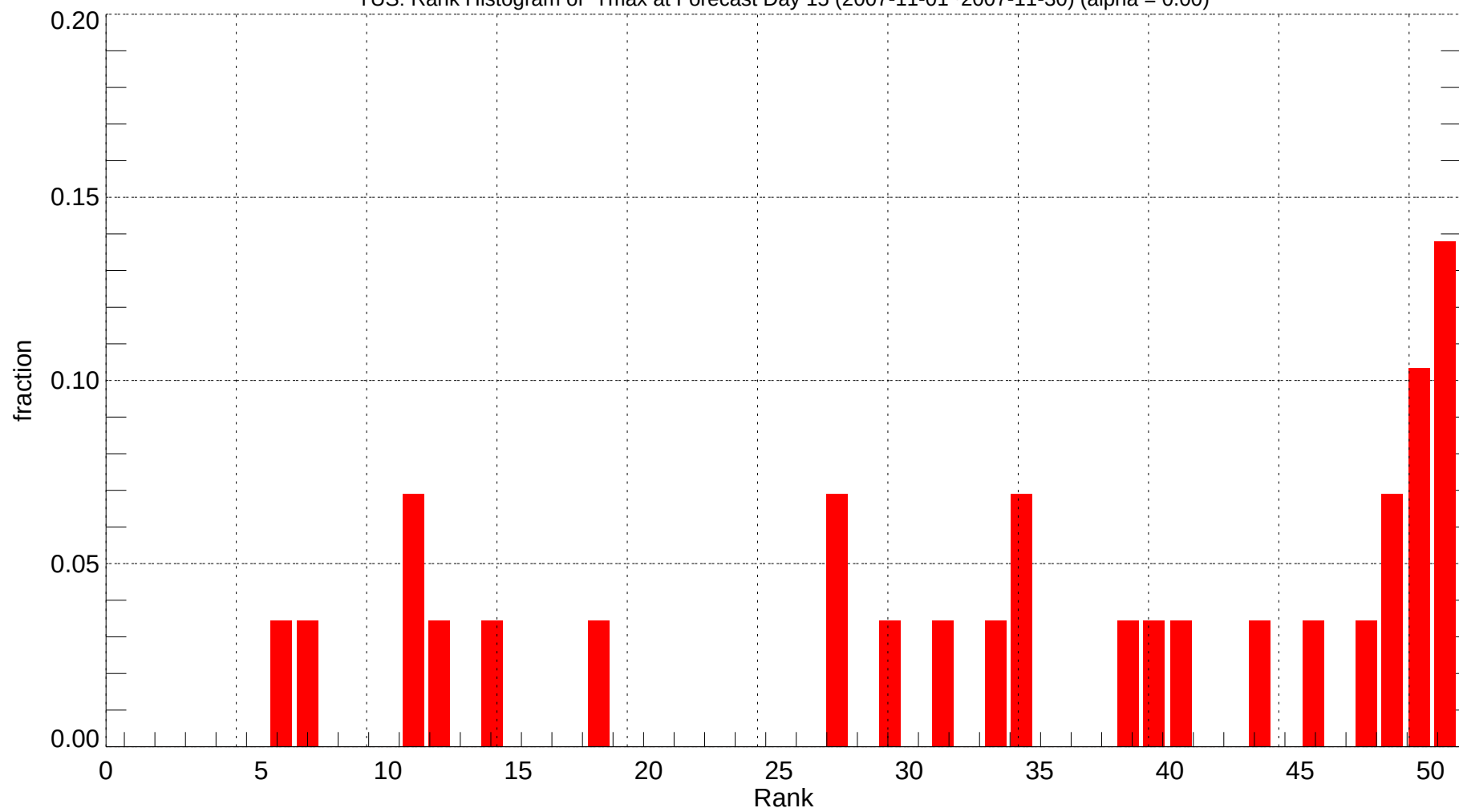
TUS: Rank Histogram of Tmax at Forecast Day 15 (2007-11-01~2007-11-30) (alpha = 0.00)
