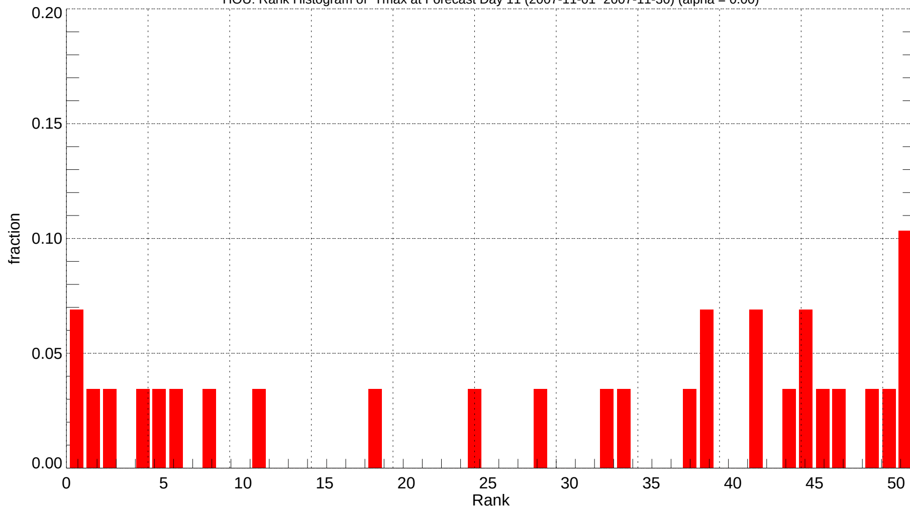
HOU: Rank Histogram of Tmax at Forecast Day 11 (2007-11-01~2007-11-30) (alpha = 0.00)
