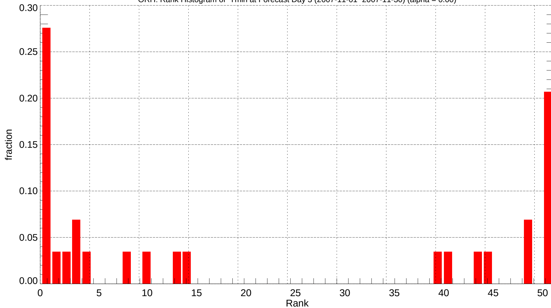
ORH: Rank Histogram of Tmin at Forecast Day 3 (2007-11-01~2007-11-30) (alpha = 0.00)
