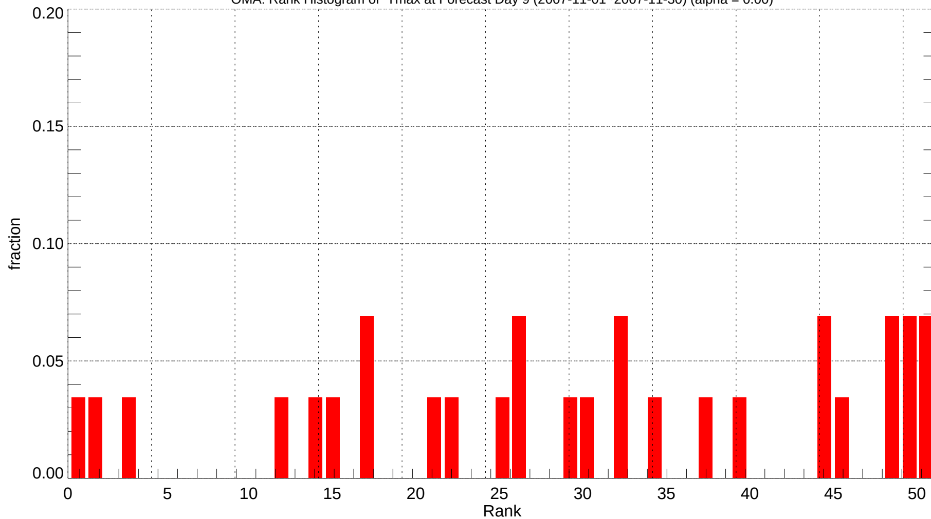
OMA: Rank Histogram of Tmax at Forecast Day 9 (2007-11-01~2007-11-30) (alpha = 0.00)
