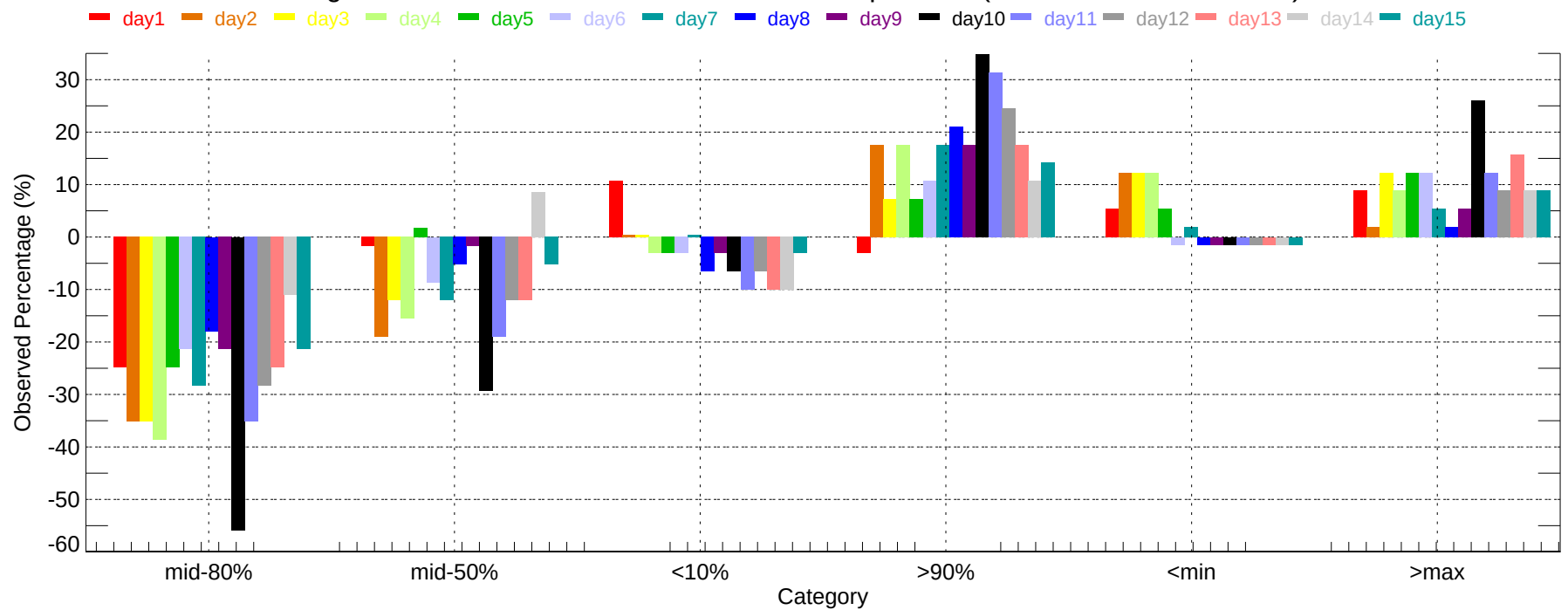
Observed Percentage Deviation of Ensembles - COU: Min Temperature (2007-11-01~2007-11-30)
