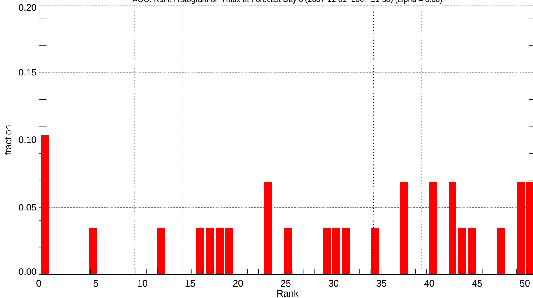
AOO: Rank Histogram of Tmax at Forecast Day 6 (2007-11-01~2007-11-30) (alpha = 0.00)
