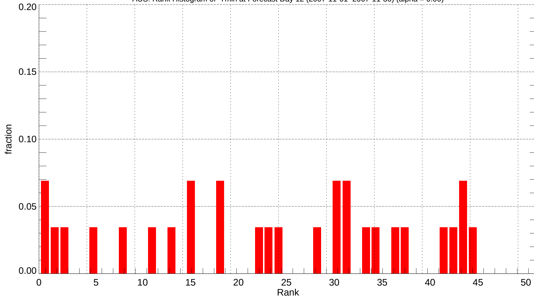
AUS: Rank Histogram of Tmin at Forecast Day 12 (2007-11-01~2007-11-30) (alpha = 0.00)
