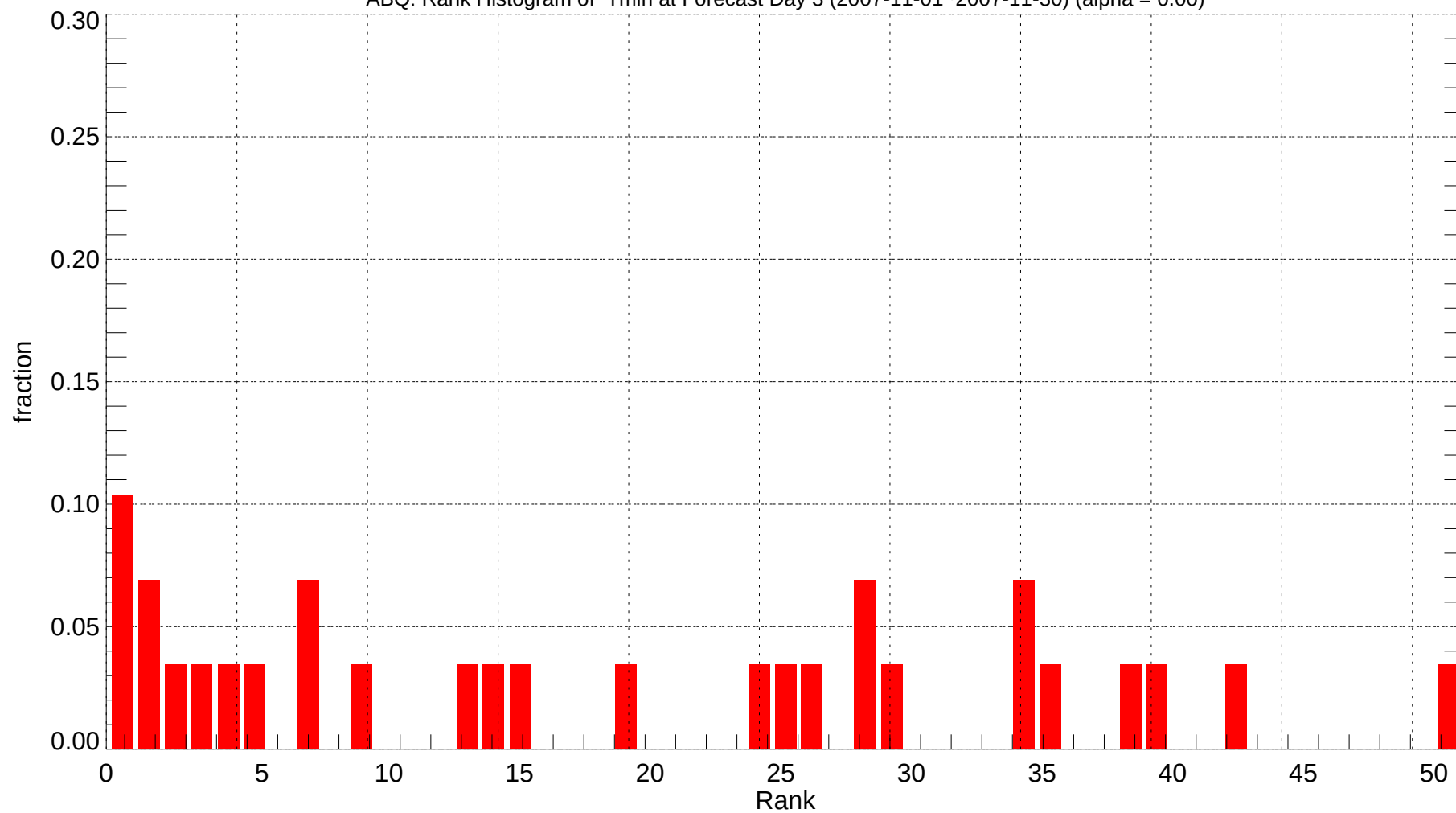
ABQ: Rank Histogram of Tmin at Forecast Day 3 (2007-11-01~2007-11-30) (alpha = 0.00)
