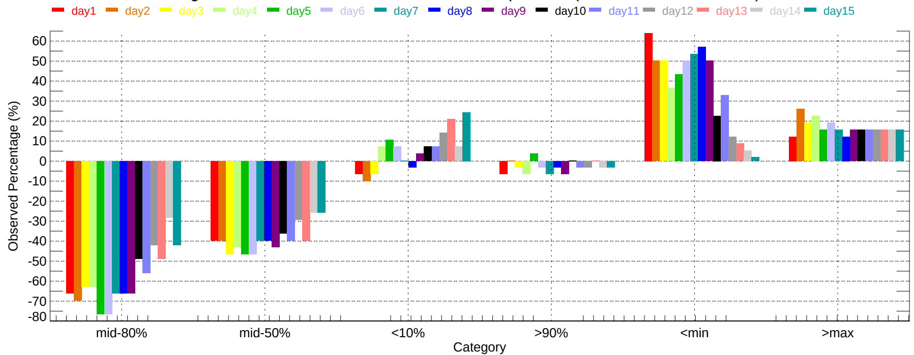
Observed Percentage Deviation of Ensembles - SAN: Max Temperature (2007-11-01~2007-11-30)
