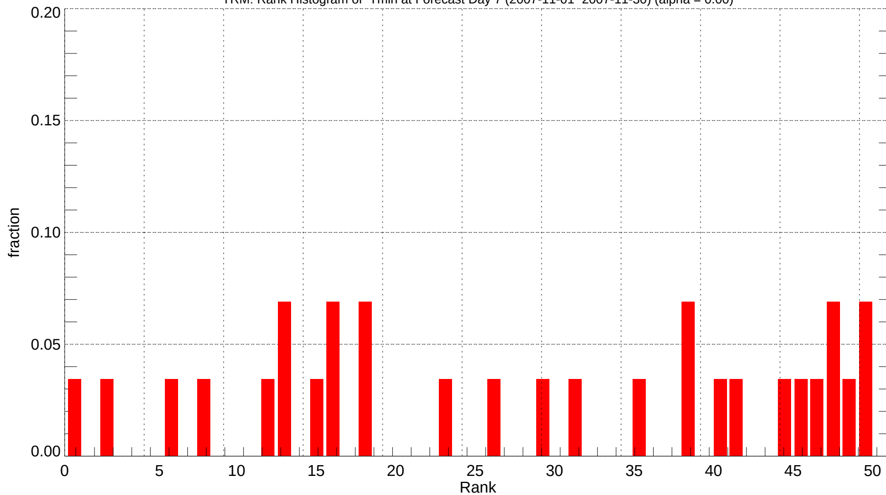
TRM: Rank Histogram of Tmin at Forecast Day 7 (2007-11-01~2007-11-30) (alpha = 0.00)
