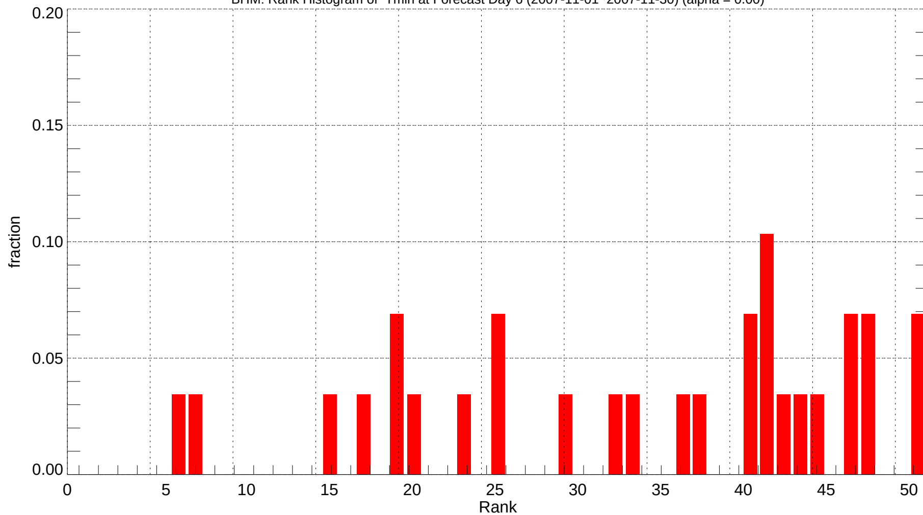
BHM: Rank Histogram of Tmin at Forecast Day 6 (2007-11-01~2007-11-30) (alpha = 0.00)
