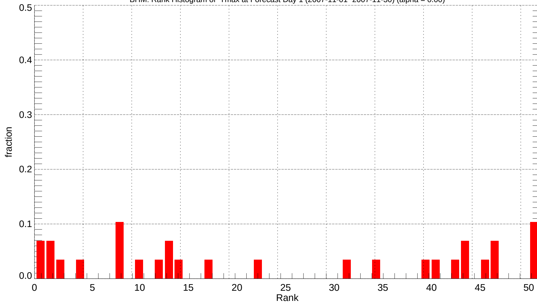
BHM: Rank Histogram of Tmax at Forecast Day 1 (2007-11-01~2007-11-30) (alpha = 0.00)
