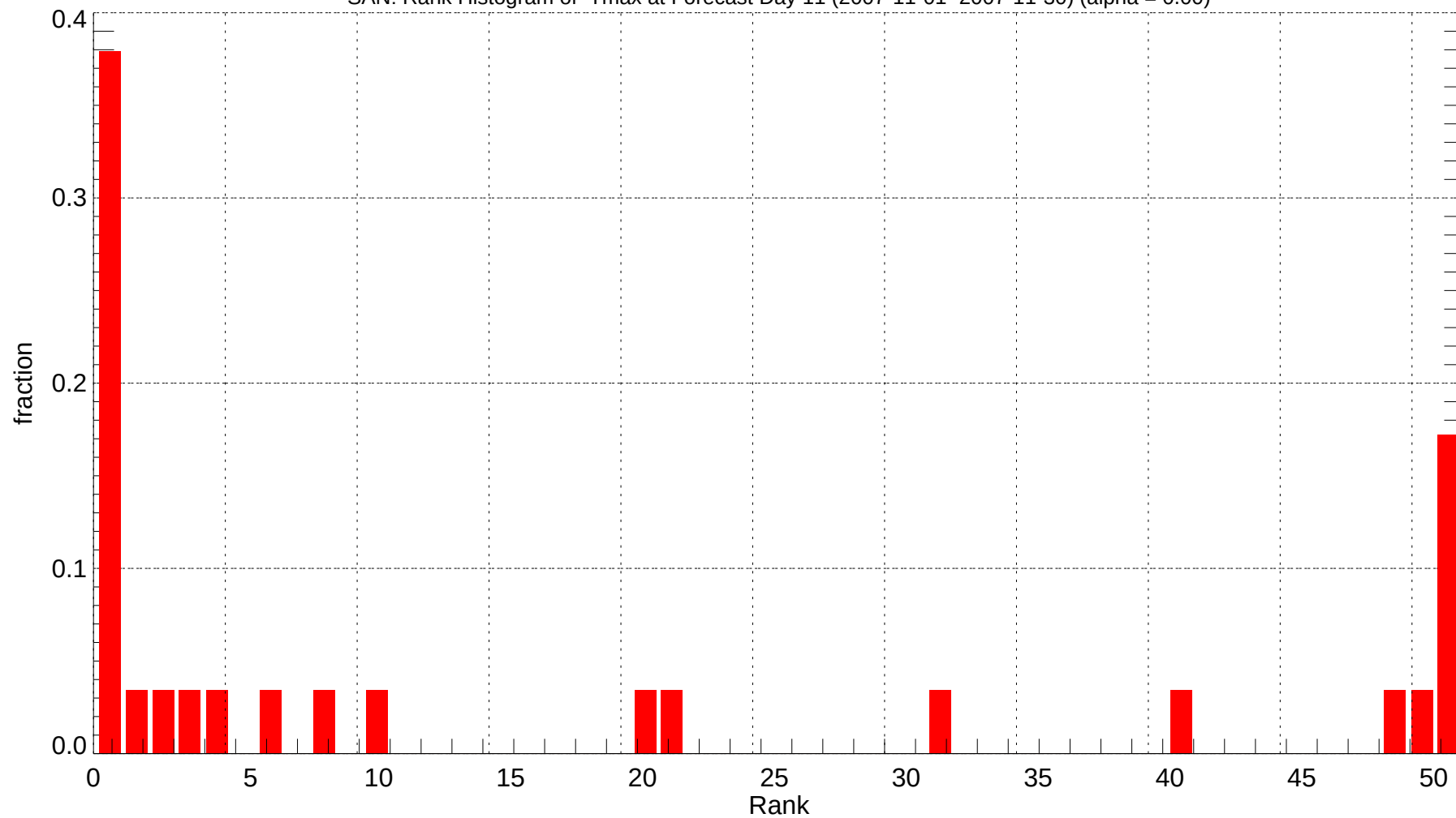
SAN: Rank Histogram of Tmax at Forecast Day 11 (2007-11-01~2007-11-30) (alpha = 0.00)
