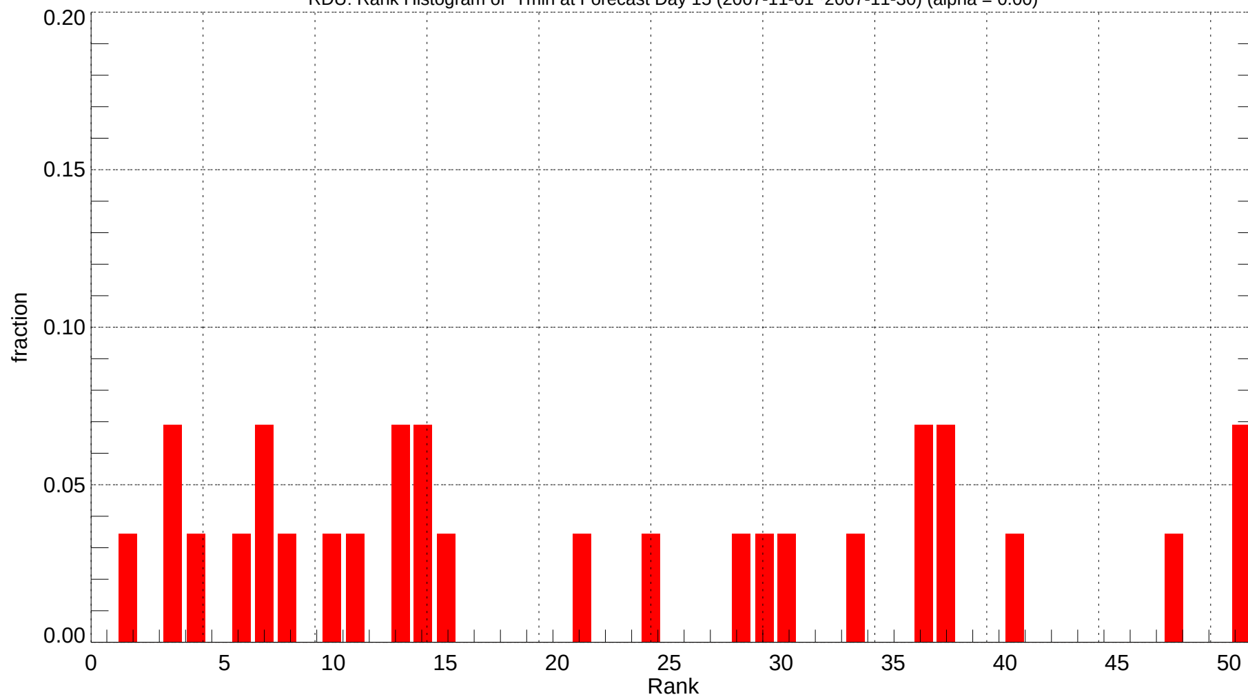
RDU: Rank Histogram of Tmin at Forecast Day 15 (2007-11-01~2007-11-30) (alpha = 0.00)
