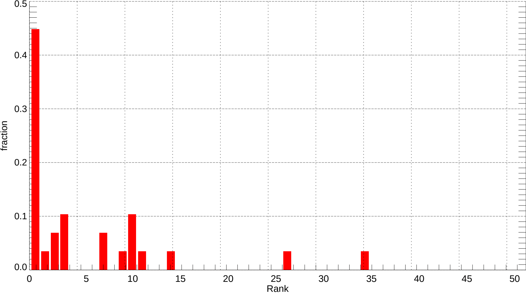
SJC: Rank Histogram of Tmin at Forecast Day 5 (2007-11-01~2007-11-30) (alpha = 0.00)
