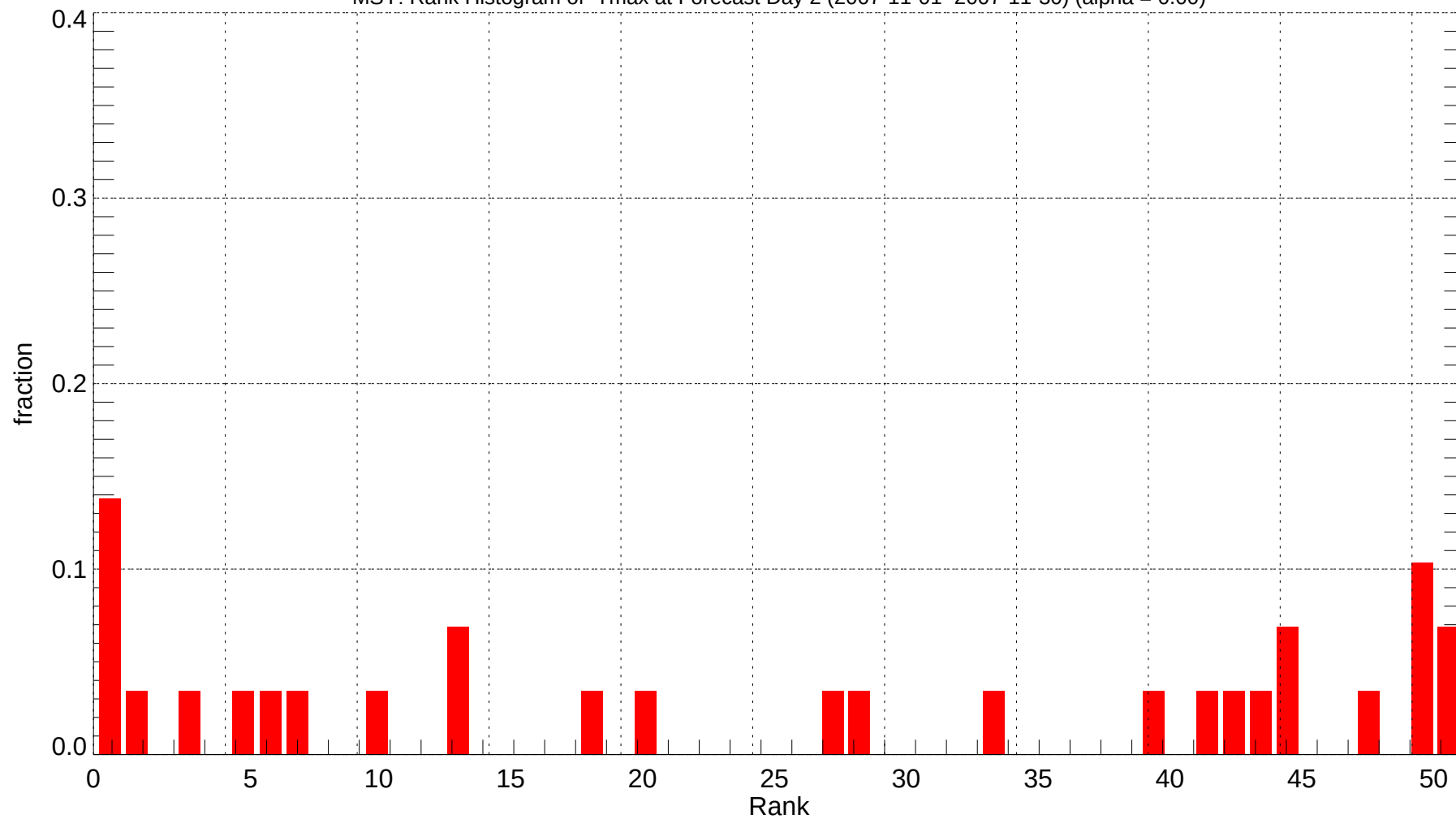
MSY: Rank Histogram of Tmax at Forecast Day 2 (2007-11-01~2007-11-30) (alpha = 0.00)
