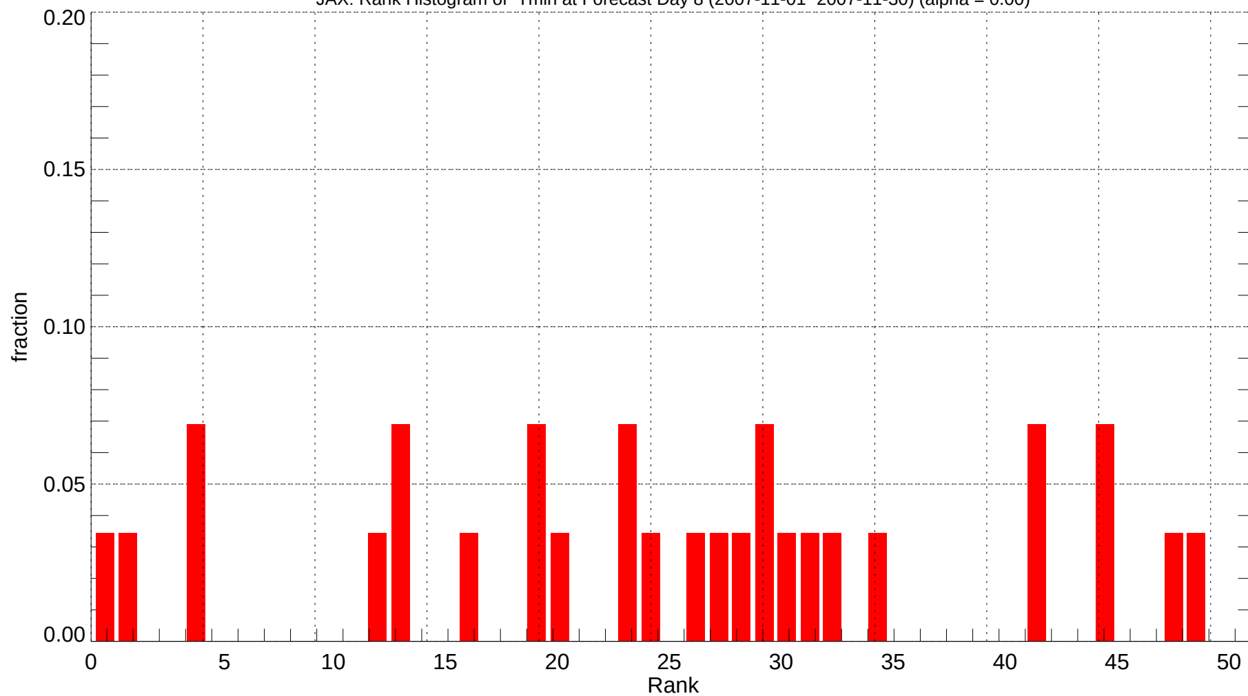
JAX: Rank Histogram of Tmin at Forecast Day 8 (2007-11-01~2007-11-30) (alpha = 0.00)
