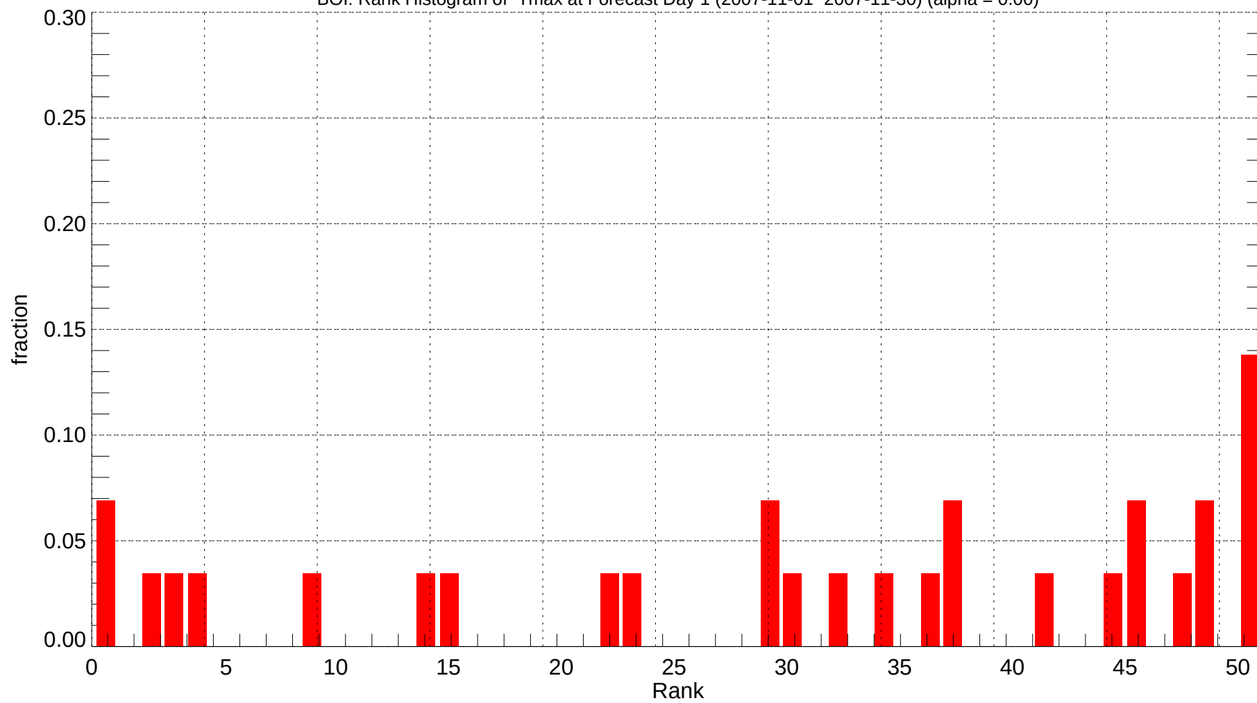
BOI: Rank Histogram of Tmax at Forecast Day 1 (2007-11-01~2007-11-30) (alpha = 0.00)
