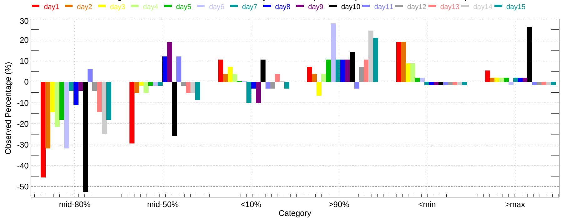
Observed Percentage Deviation of Ensembles - ABQ: Max Temperature (2007-11-01~2007-11-30)
