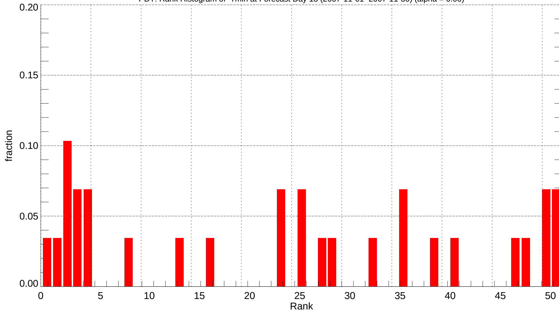
PDT: Rank Histogram of Tmin at Forecast Day 13 (2007-11-01~2007-11-30) (alpha = 0.00)
