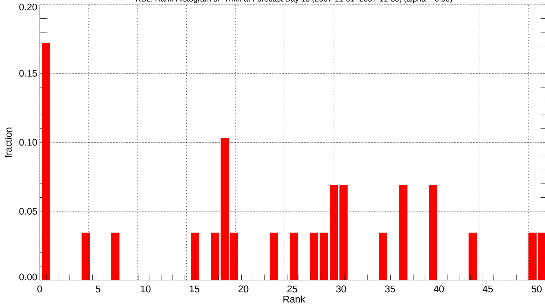
RBL: Rank Histogram of Tmin at Forecast Day 13 (2007-11-01~2007-11-30) (alpha = 0.00)
