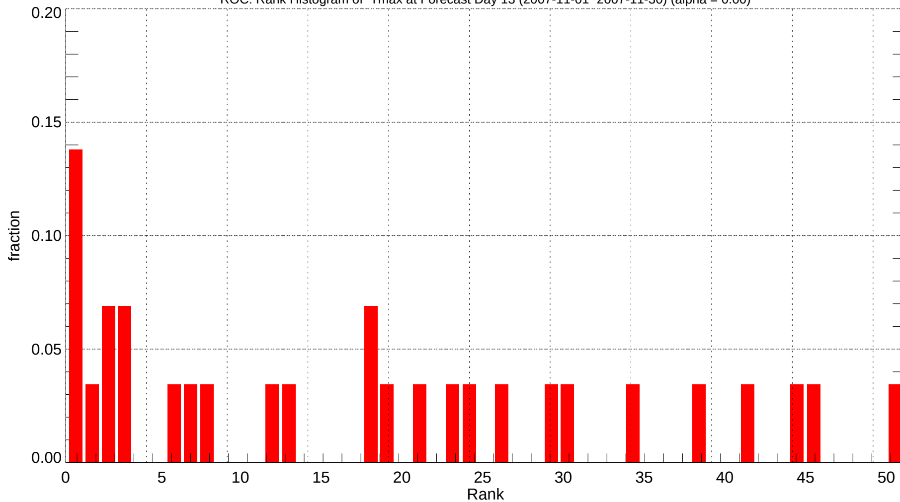
ROC: Rank Histogram of Tmax at Forecast Day 13 (2007-11-01~2007-11-30) (alpha = 0.00)
