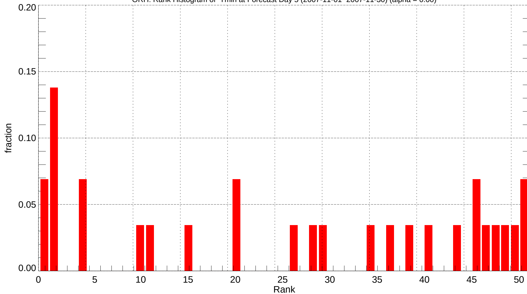
ORH: Rank Histogram of Tmin at Forecast Day 5 (2007-11-01~2007-11-30) (alpha = 0.00)
