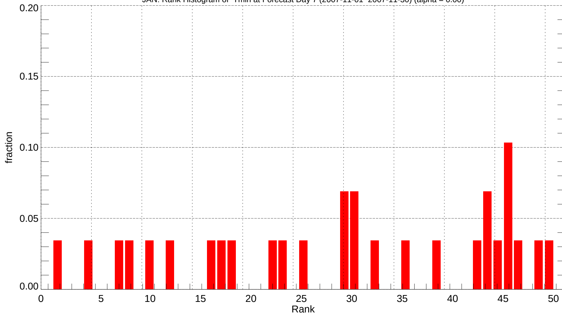
JAN: Rank Histogram of Tmin at Forecast Day 7 (2007-11-01~2007-11-30) (alpha = 0.00)
