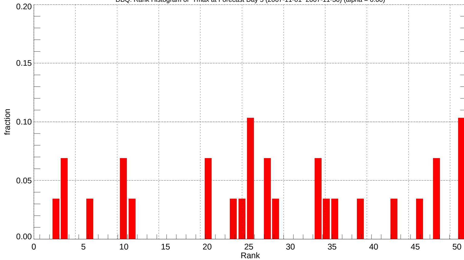
DBQ: Rank Histogram of Tmax at Forecast Day 5 (2007-11-01~2007-11-30) (alpha = 0.00)
