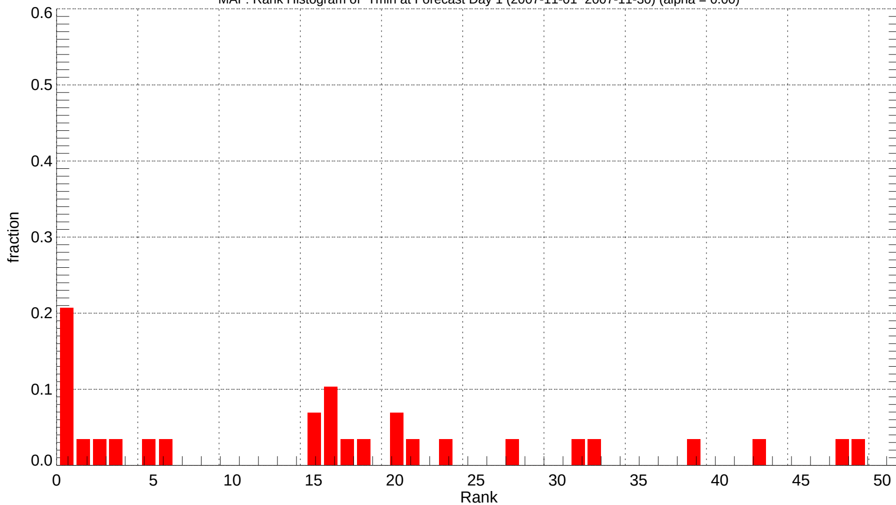
MAF: Rank Histogram of Tmin at Forecast Day 1 (2007-11-01~2007-11-30) (alpha = 0.00)
