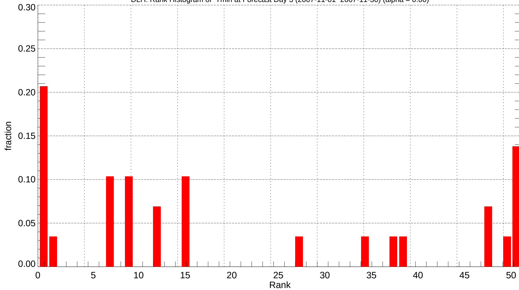
DLH: Rank Histogram of Tmin at Forecast Day 3 (2007-11-01~2007-11-30) (alpha = 0.00)
