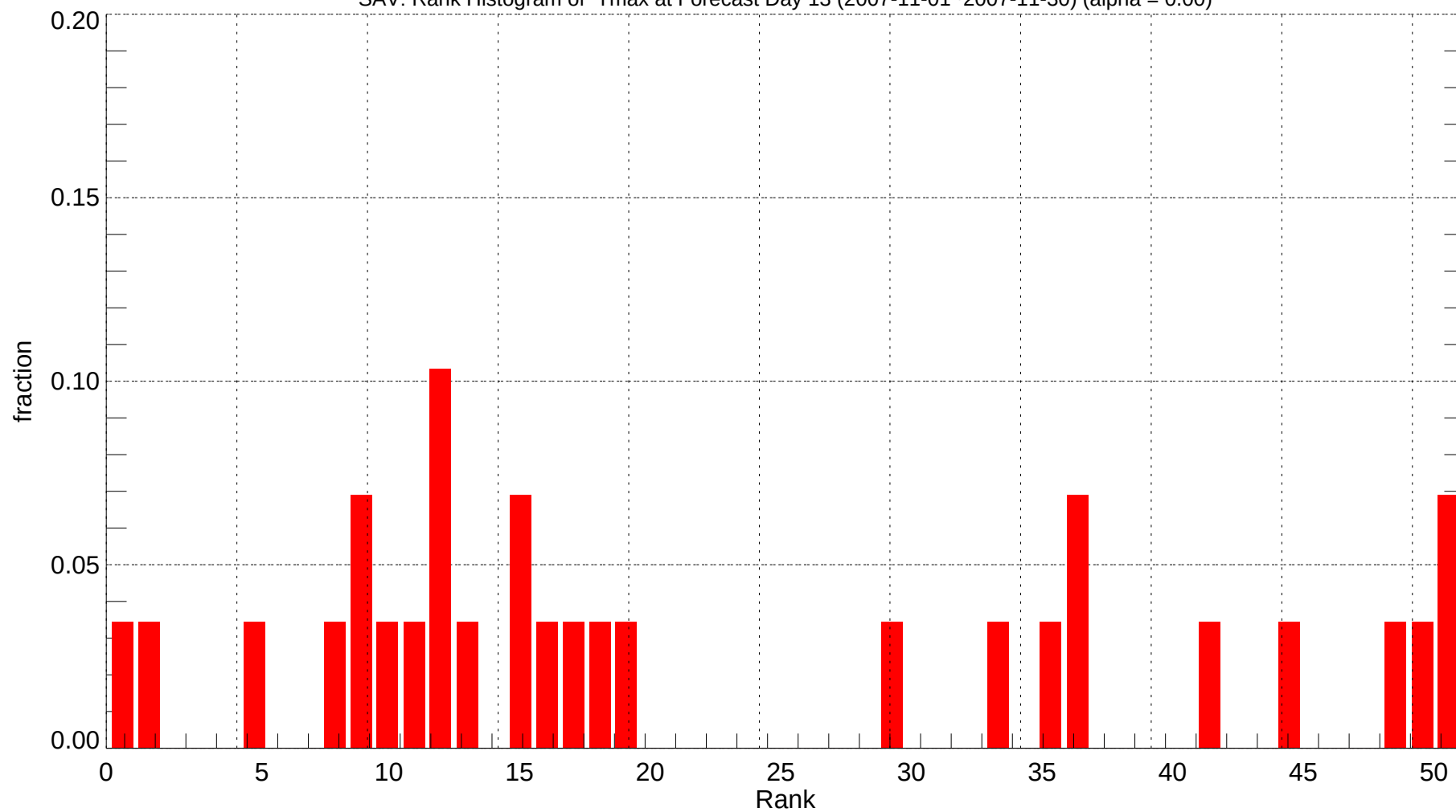
SAV: Rank Histogram of Tmax at Forecast Day 13 (2007-11-01~2007-11-30) (alpha = 0.00)
