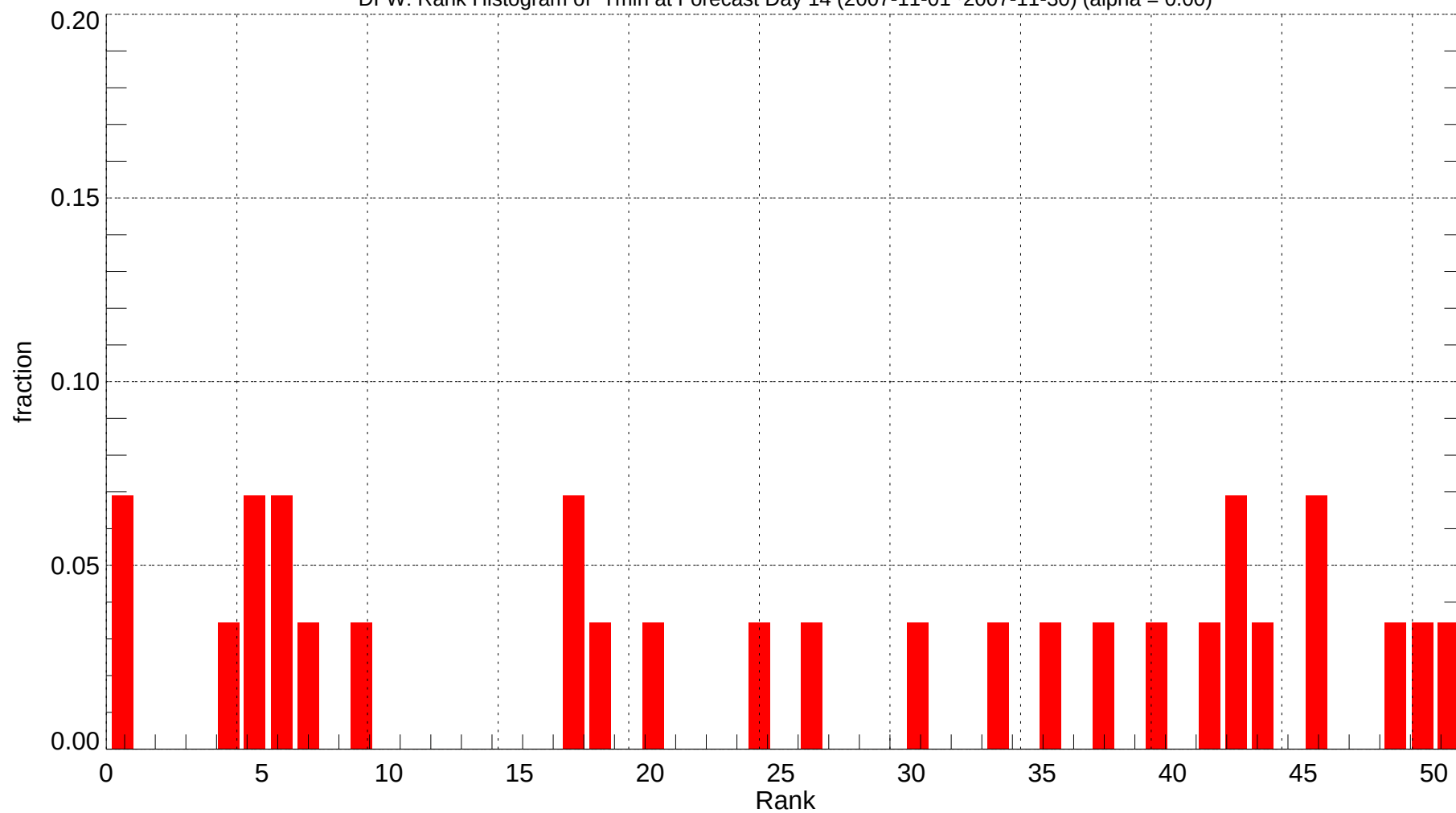
DFW: Rank Histogram of Tmin at Forecast Day 14 (2007-11-01~2007-11-30) (alpha = 0.00)
