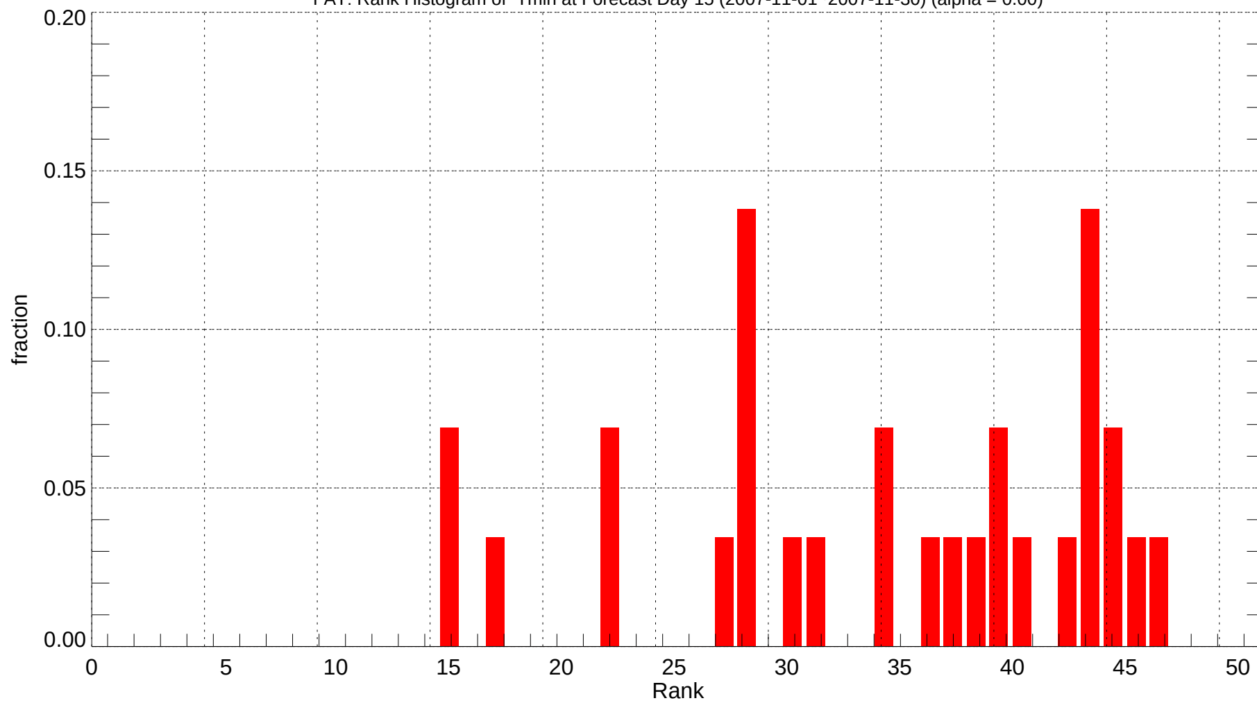
FAT: Rank Histogram of Tmin at Forecast Day 15 (2007-11-01~2007-11-30) (alpha = 0.00)
