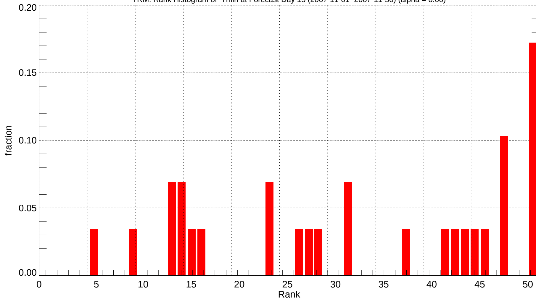
TRM: Rank Histogram of Tmin at Forecast Day 13 (2007-11-01~2007-11-30) (alpha = 0.00)
