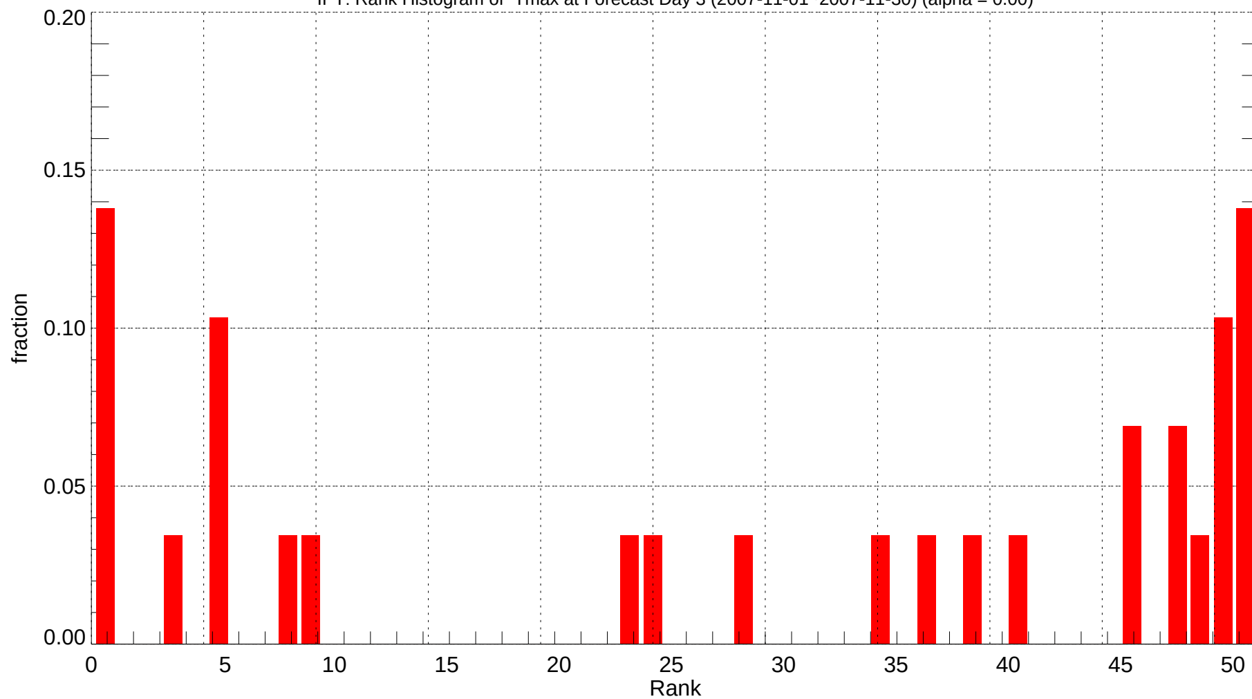
IPT: Rank Histogram of Tmax at Forecast Day 3 (2007-11-01~2007-11-30) (alpha = 0.00)
