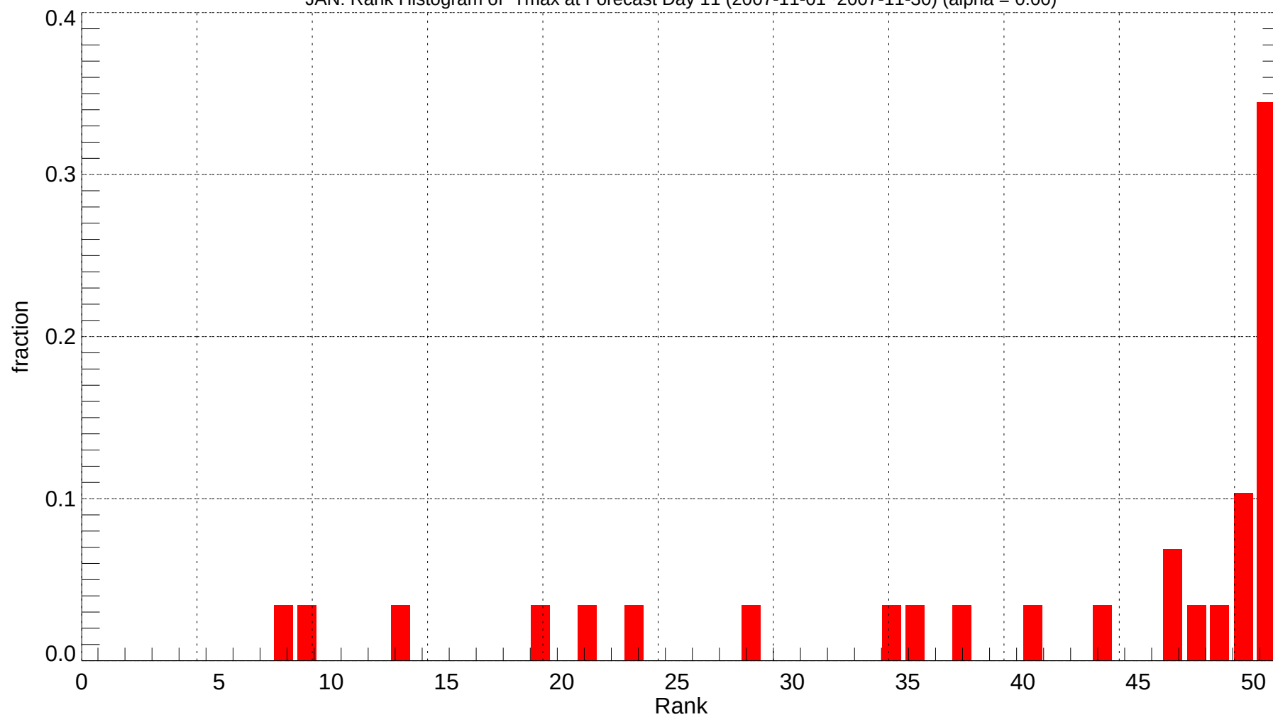
JAN: Rank Histogram of Tmax at Forecast Day 11 (2007-11-01~2007-11-30) (alpha = 0.00)
