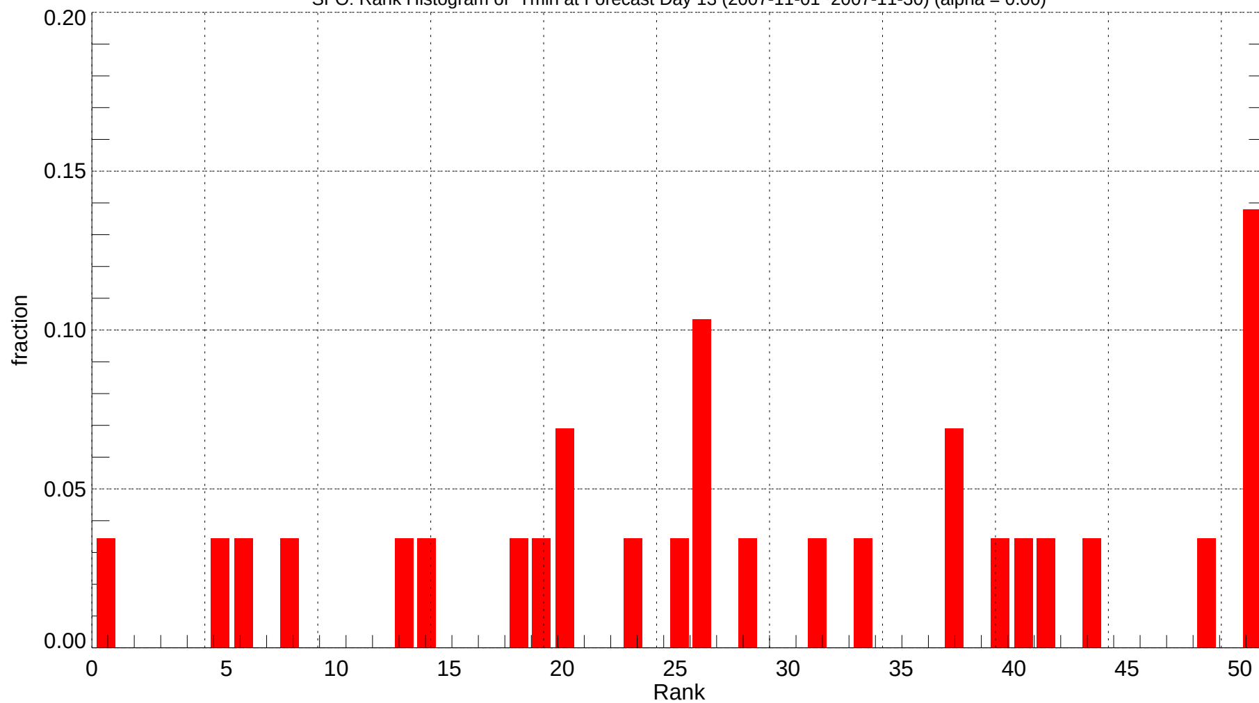
SFO: Rank Histogram of Tmin at Forecast Day 13 (2007-11-01~2007-11-30) (alpha = 0.00)
