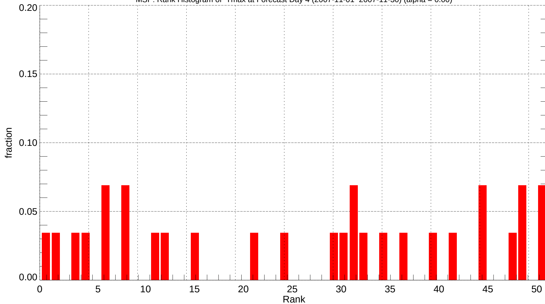
MSP: Rank Histogram of Tmax at Forecast Day 4 (2007-11-01~2007-11-30) (alpha = 0.00)
