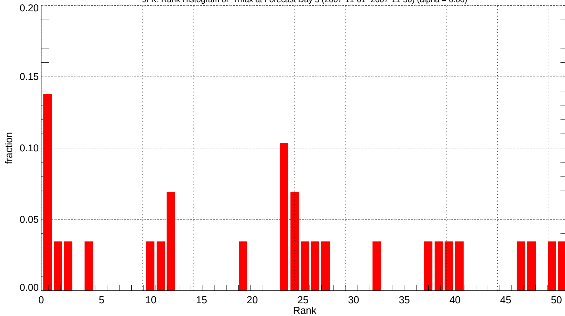
JFK: Rank Histogram of Tmax at Forecast Day 3 (2007-11-01~2007-11-30) (alpha = 0.00)
