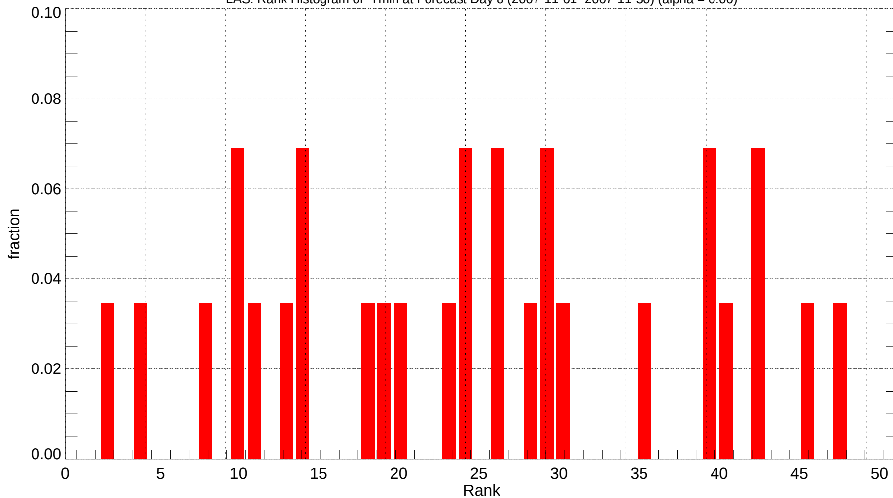
LAS: Rank Histogram of Tmin at Forecast Day 8 (2007-11-01~2007-11-30) (alpha = 0.00)
