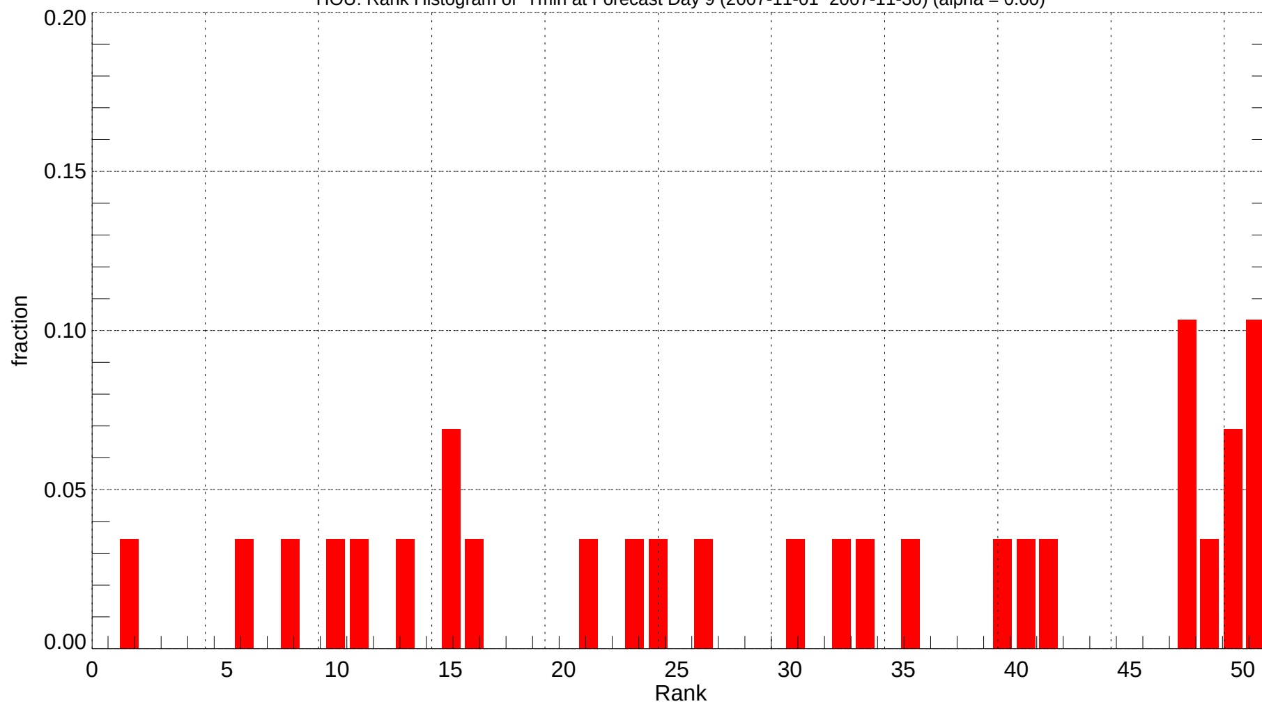
HOU: Rank Histogram of Tmin at Forecast Day 9 (2007-11-01~2007-11-30) (alpha = 0.00)
