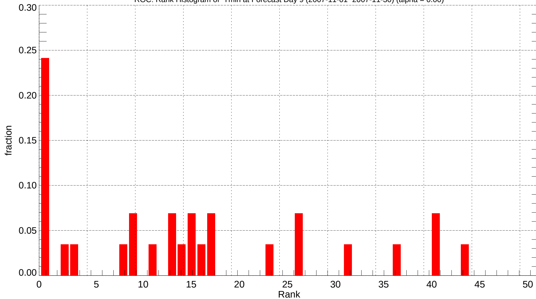
ROC: Rank Histogram of Tmin at Forecast Day 9 (2007-11-01~2007-11-30) (alpha = 0.00)
