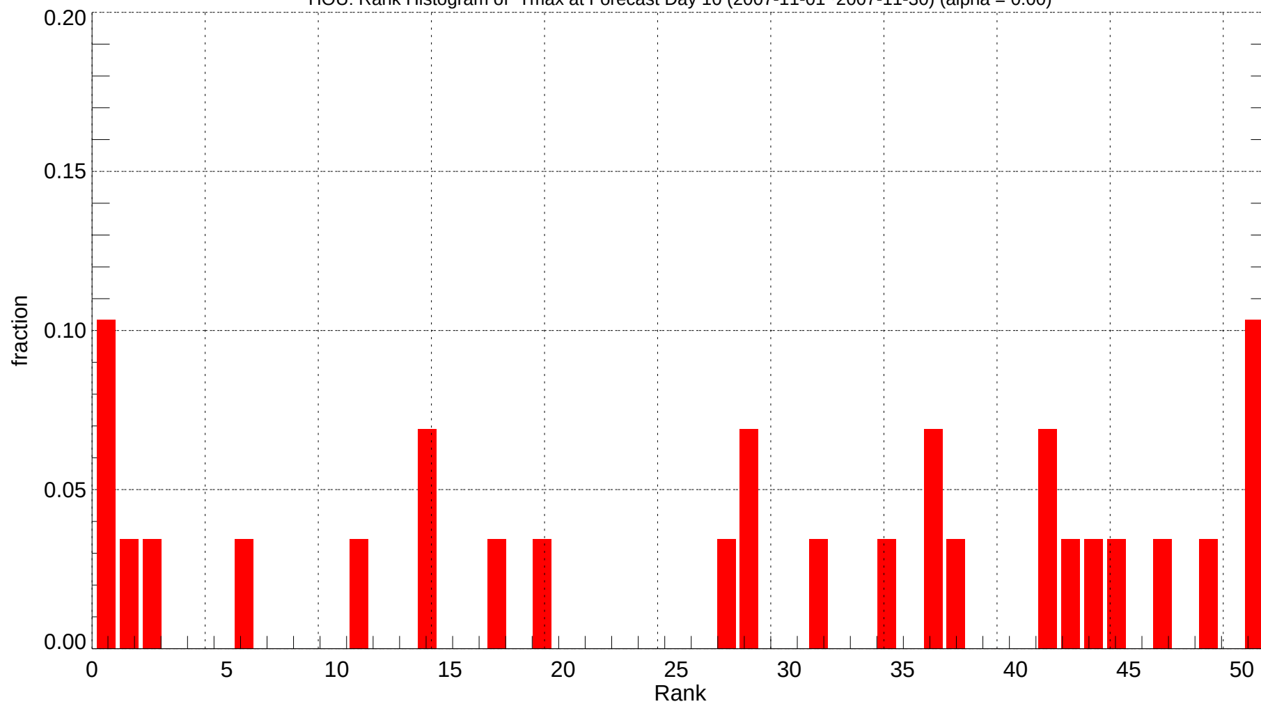
HOU: Rank Histogram of Tmax at Forecast Day 10 (2007-11-01~2007-11-30) (alpha = 0.00)
