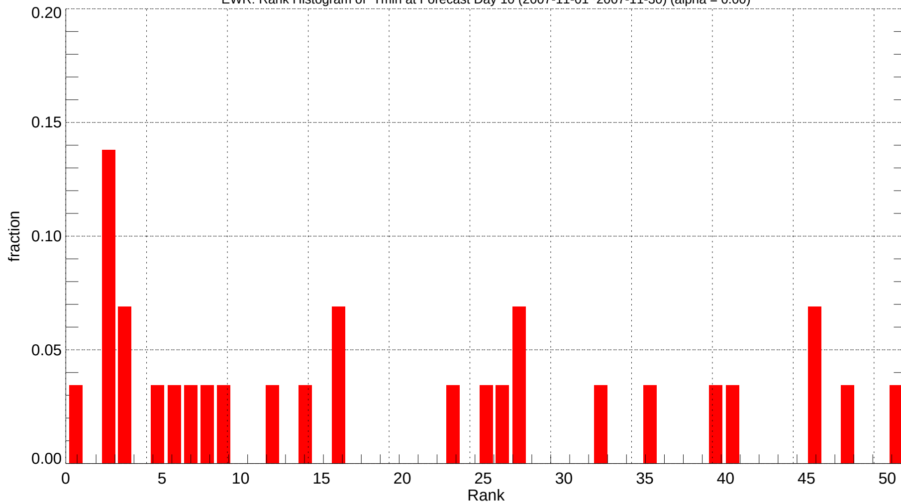
EWR: Rank Histogram of Tmin at Forecast Day 10 (2007-11-01~2007-11-30) (alpha = 0.00)
