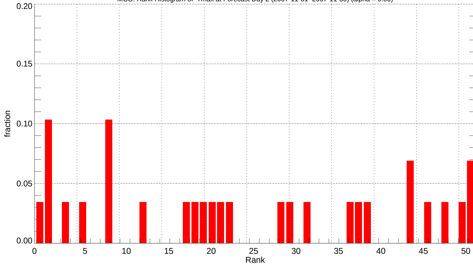
MCO: Rank Histogram of Tmax at Forecast Day 2 (2007-11-01~2007-11-30) (alpha = 0.00)
