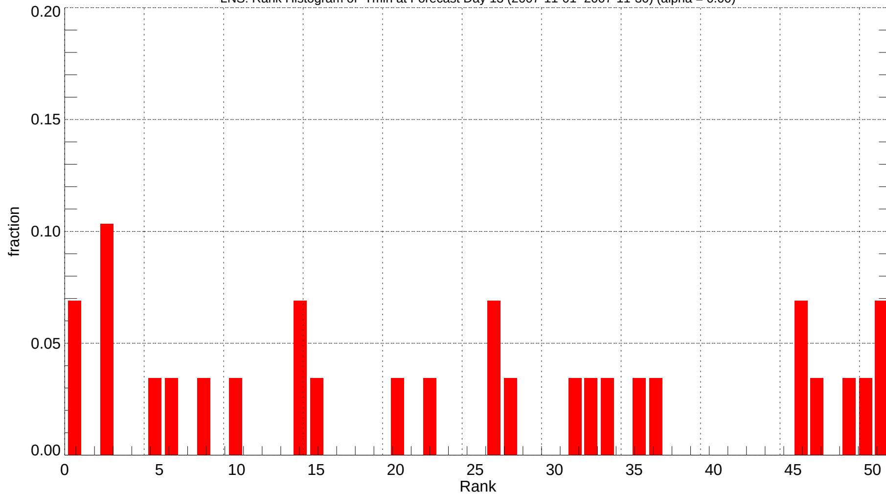
LNS: Rank Histogram of Tmin at Forecast Day 13 (2007-11-01~2007-11-30) (alpha = 0.00)
