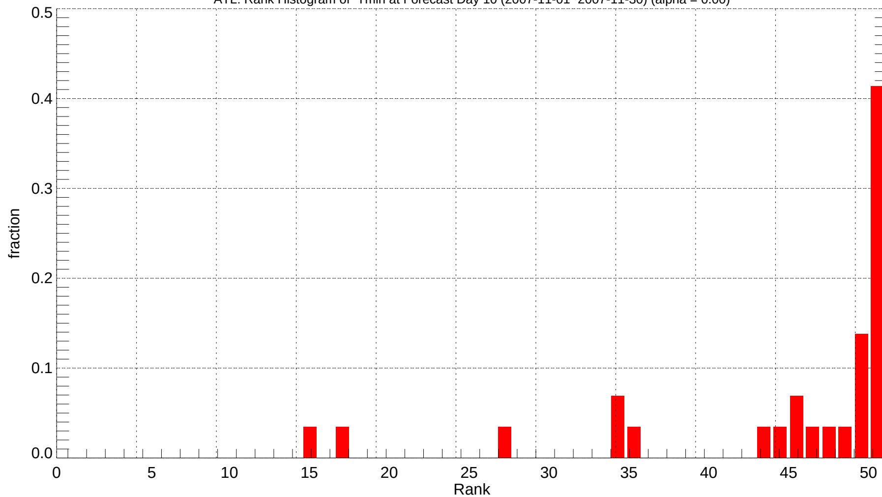
ATL: Rank Histogram of Tmin at Forecast Day 10 (2007-11-01~2007-11-30) (alpha = 0.00)
