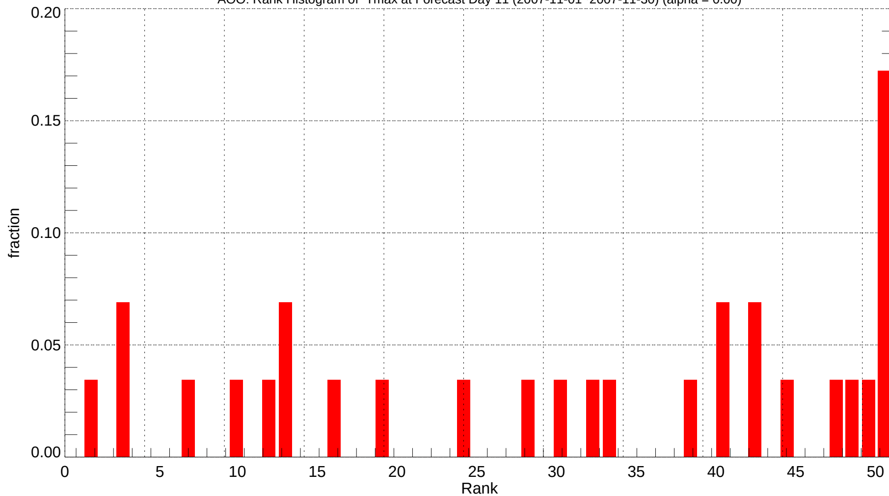
AOO: Rank Histogram of Tmax at Forecast Day 11 (2007-11-01~2007-11-30) (alpha = 0.00)
