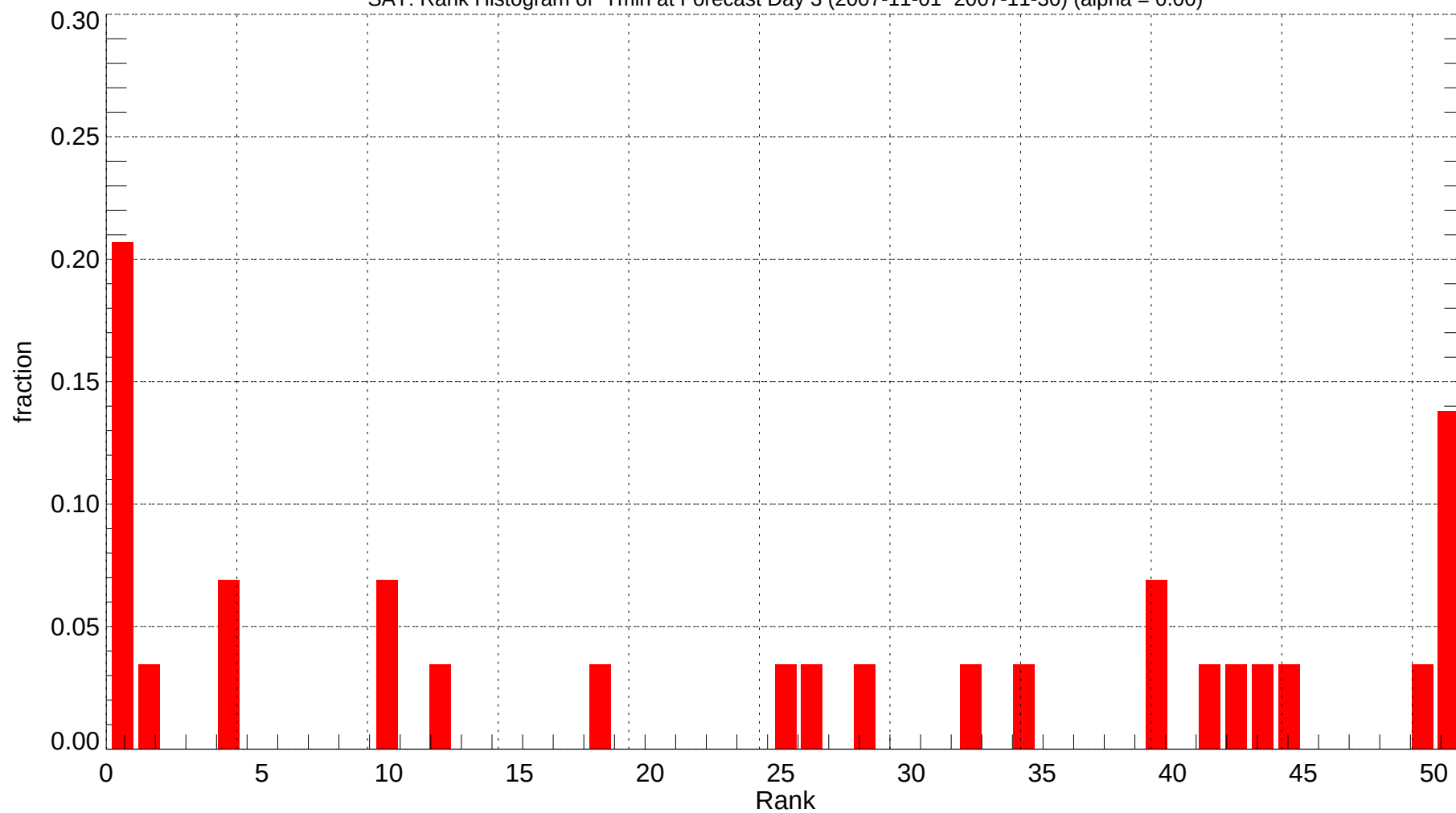
SAT: Rank Histogram of Tmin at Forecast Day 3 (2007-11-01~2007-11-30) (alpha = 0.00)
