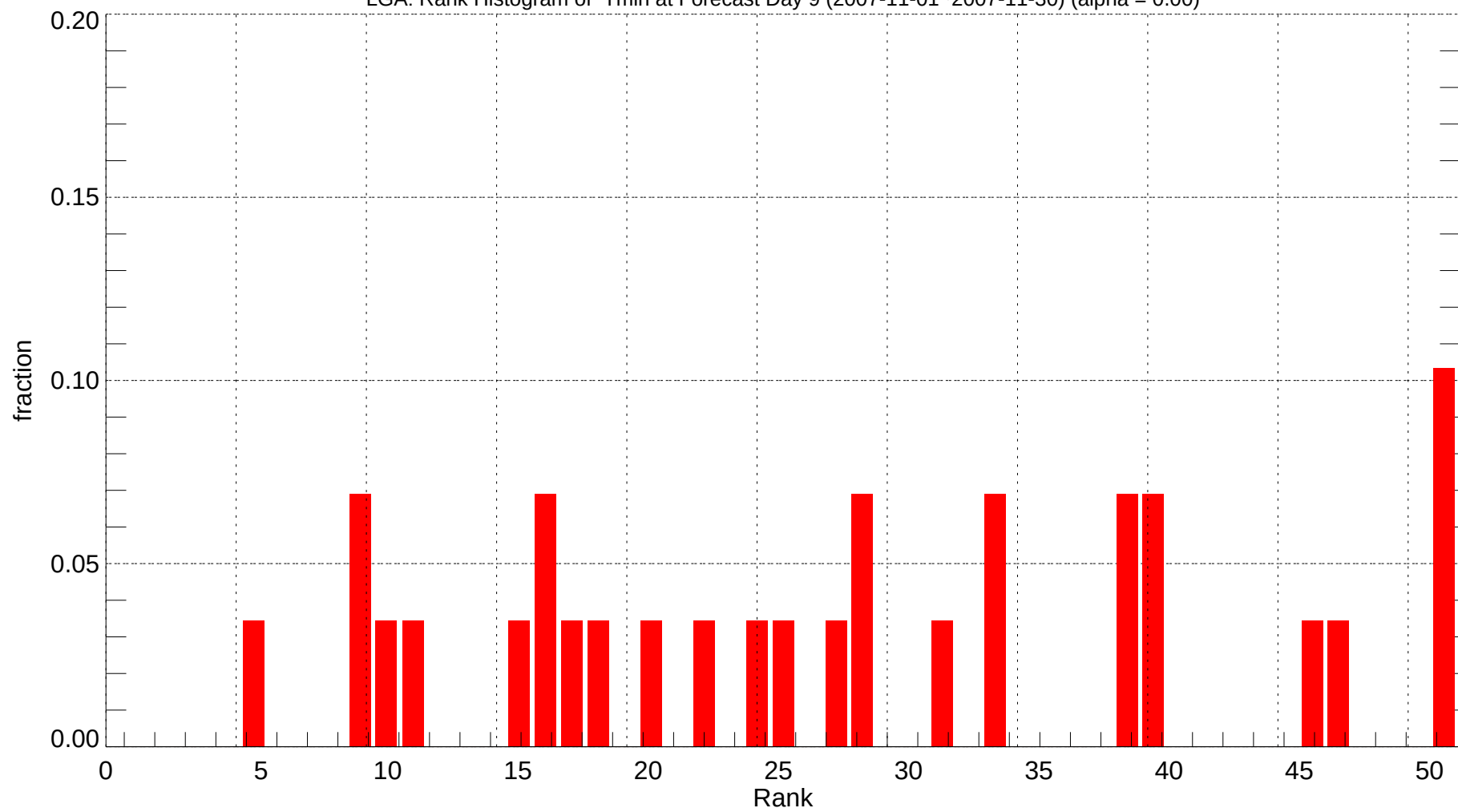
LGA: Rank Histogram of Tmin at Forecast Day 9 (2007-11-01~2007-11-30) (alpha = 0.00)
