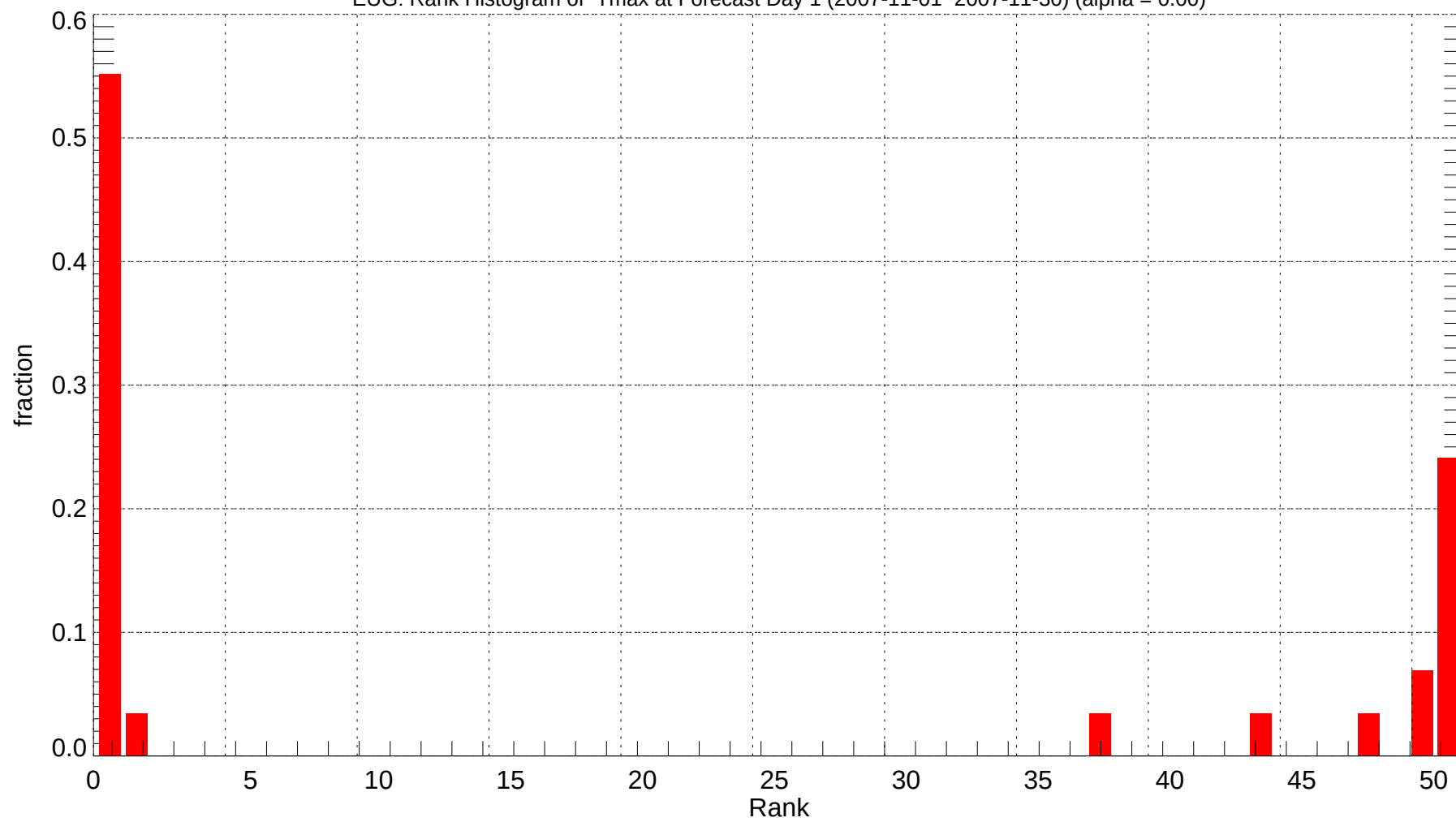
EUG: Rank Histogram of Tmax at Forecast Day 1 (2007-11-01~2007-11-30) (alpha = 0.00)
