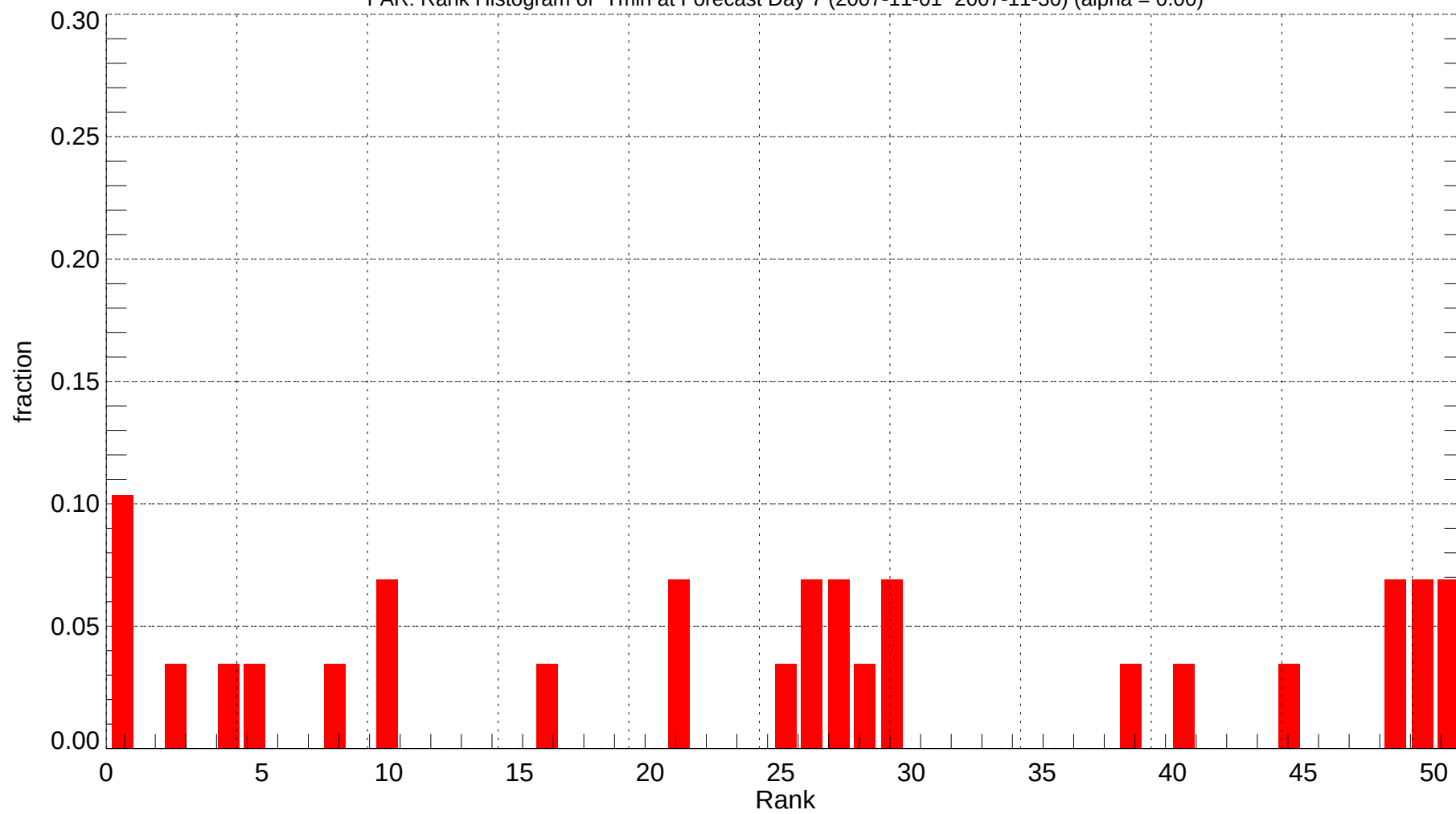
FAR: Rank Histogram of Tmin at Forecast Day 7 (2007-11-01~2007-11-30) (alpha = 0.00)
