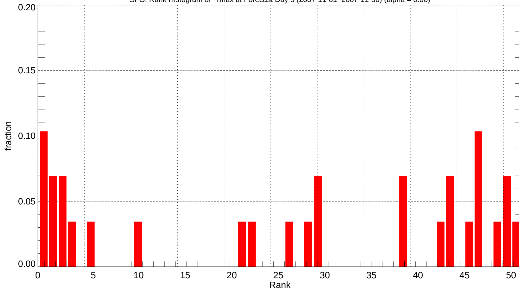
SFO: Rank Histogram of Tmax at Forecast Day 5 (2007-11-01~2007-11-30) (alpha = 0.00)
