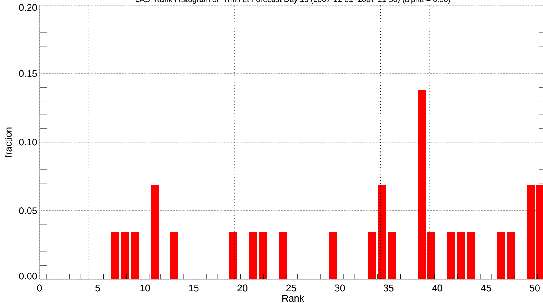
LAS: Rank Histogram of Tmin at Forecast Day 13 (2007-11-01~2007-11-30) (alpha = 0.00)
