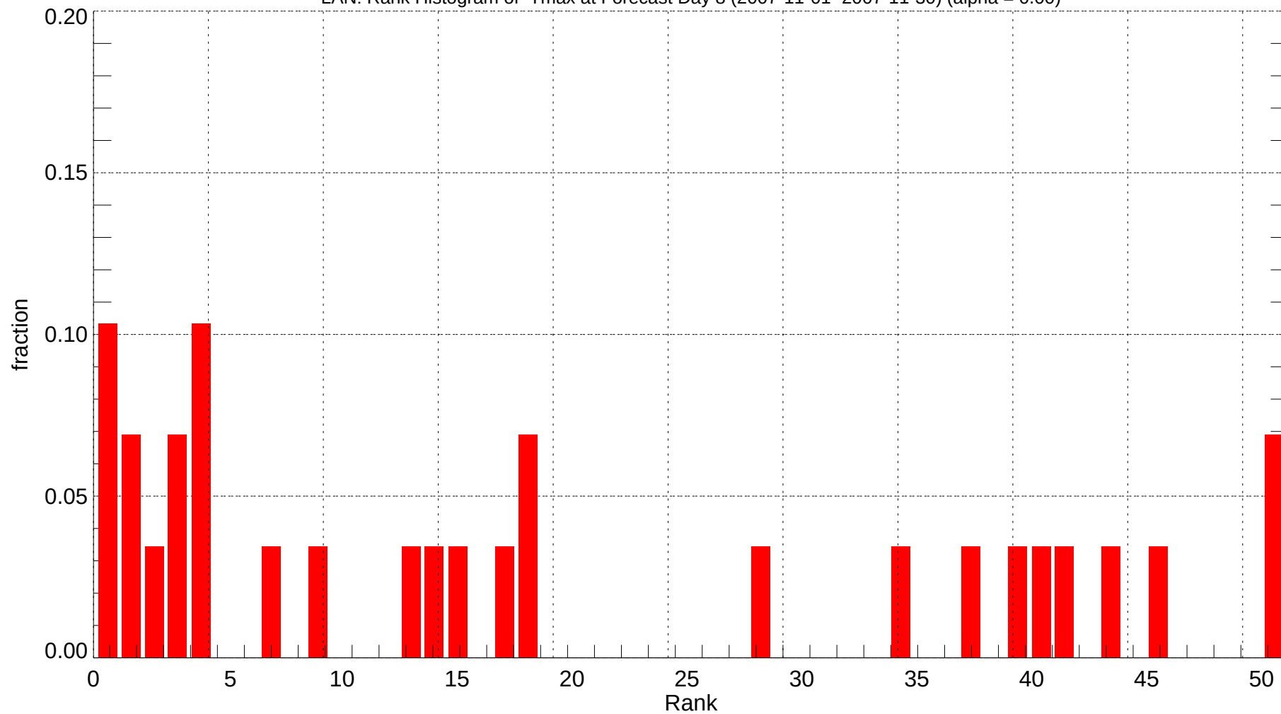
LAN: Rank Histogram of Tmax at Forecast Day 8 (2007-11-01~2007-11-30) (alpha = 0.00)
