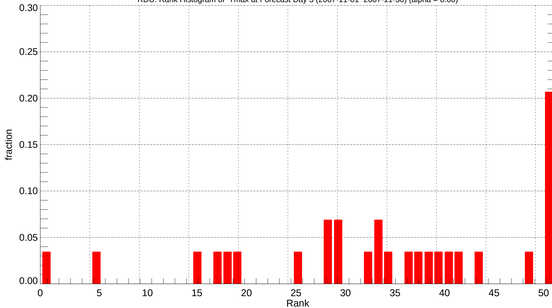
RDU: Rank Histogram of Tmax at Forecast Day 3 (2007-11-01~2007-11-30) (alpha = 0.00)
