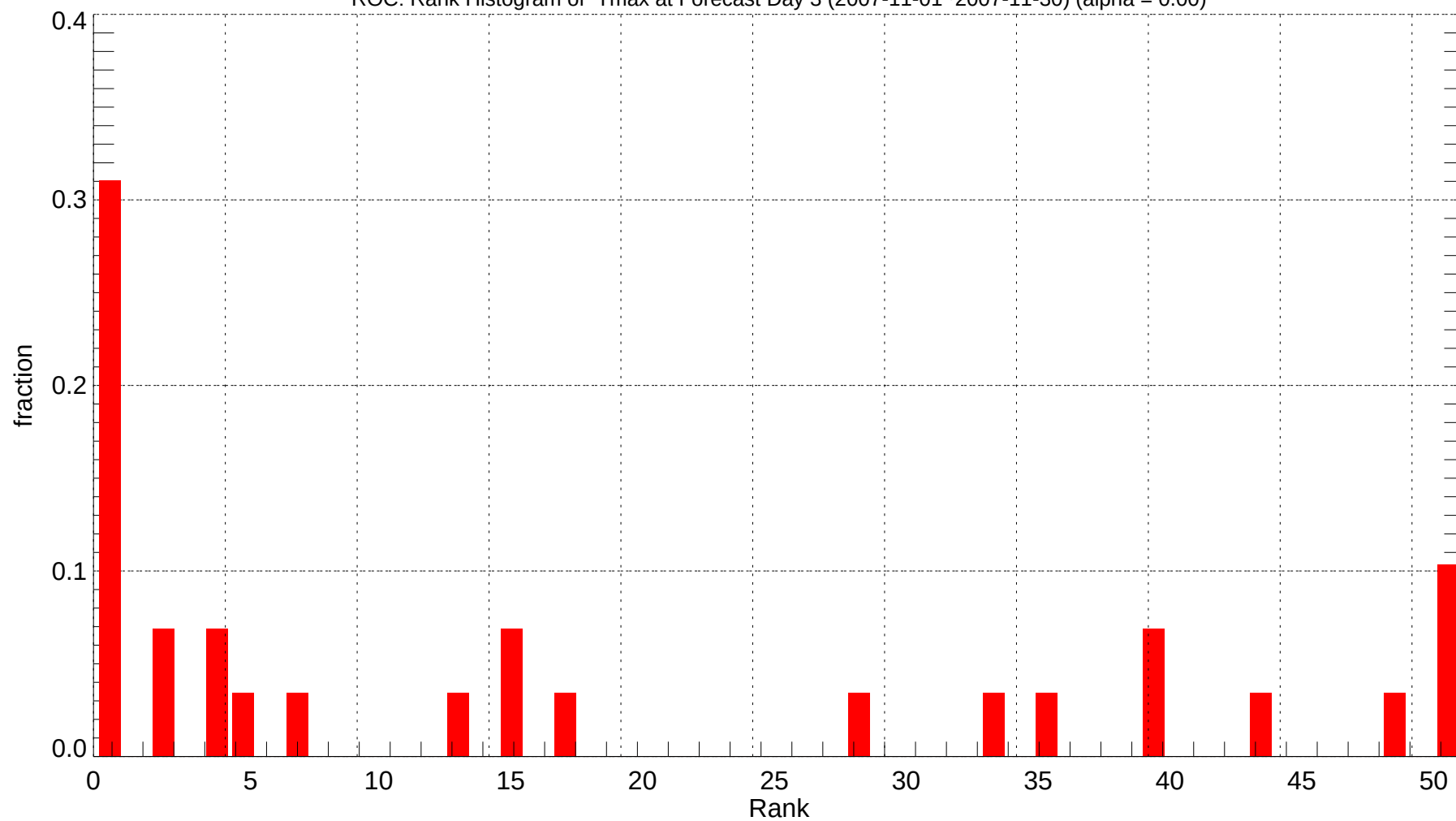
ROC: Rank Histogram of Tmax at Forecast Day 3 (2007-11-01~2007-11-30) (alpha = 0.00)
