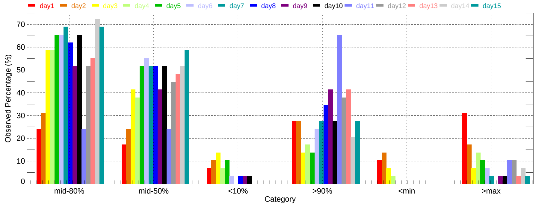
Observed Percentage of Ensembles - DBQ: Min Temperature (2007-11-01~2007-11-30)
