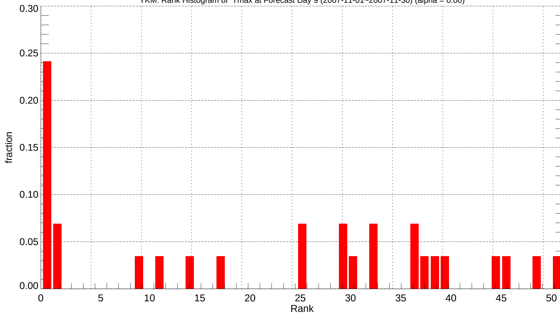
YKM: Rank Histogram of Tmax at Forecast Day 9 (2007-11-01~2007-11-30) (alpha = 0.00)
