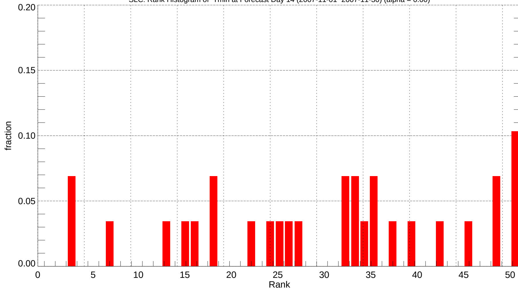
SLC: Rank Histogram of Tmin at Forecast Day 14 (2007-11-01~2007-11-30) (alpha = 0.00)
