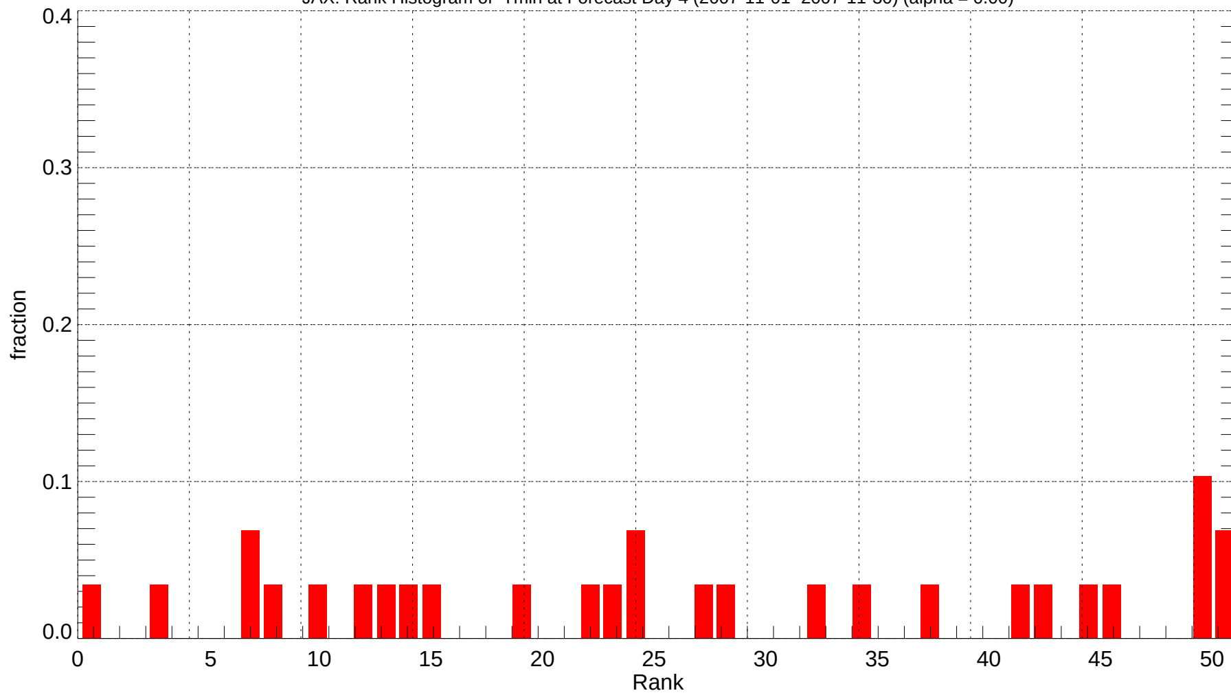
JAX: Rank Histogram of Tmin at Forecast Day 4 (2007-11-01~2007-11-30) (alpha = 0.00)
