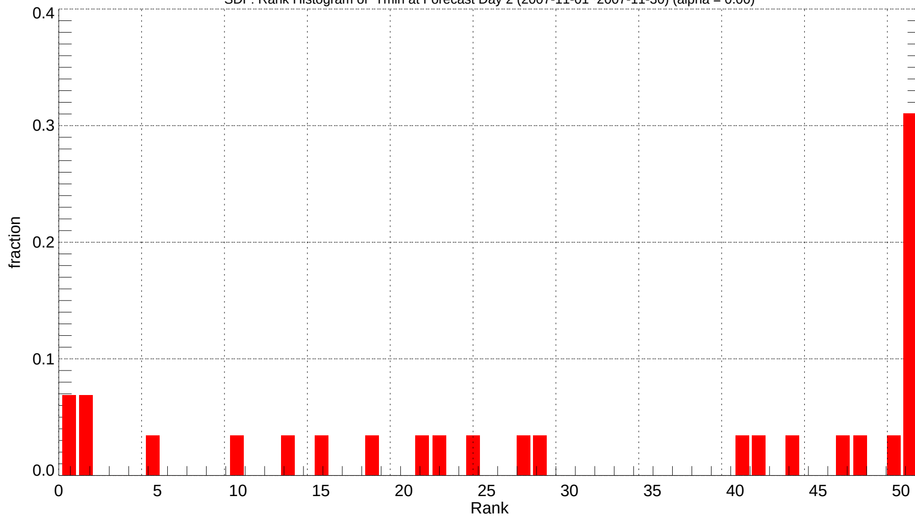
SDF: Rank Histogram of Tmin at Forecast Day 2 (2007-11-01~2007-11-30) (alpha = 0.00)
