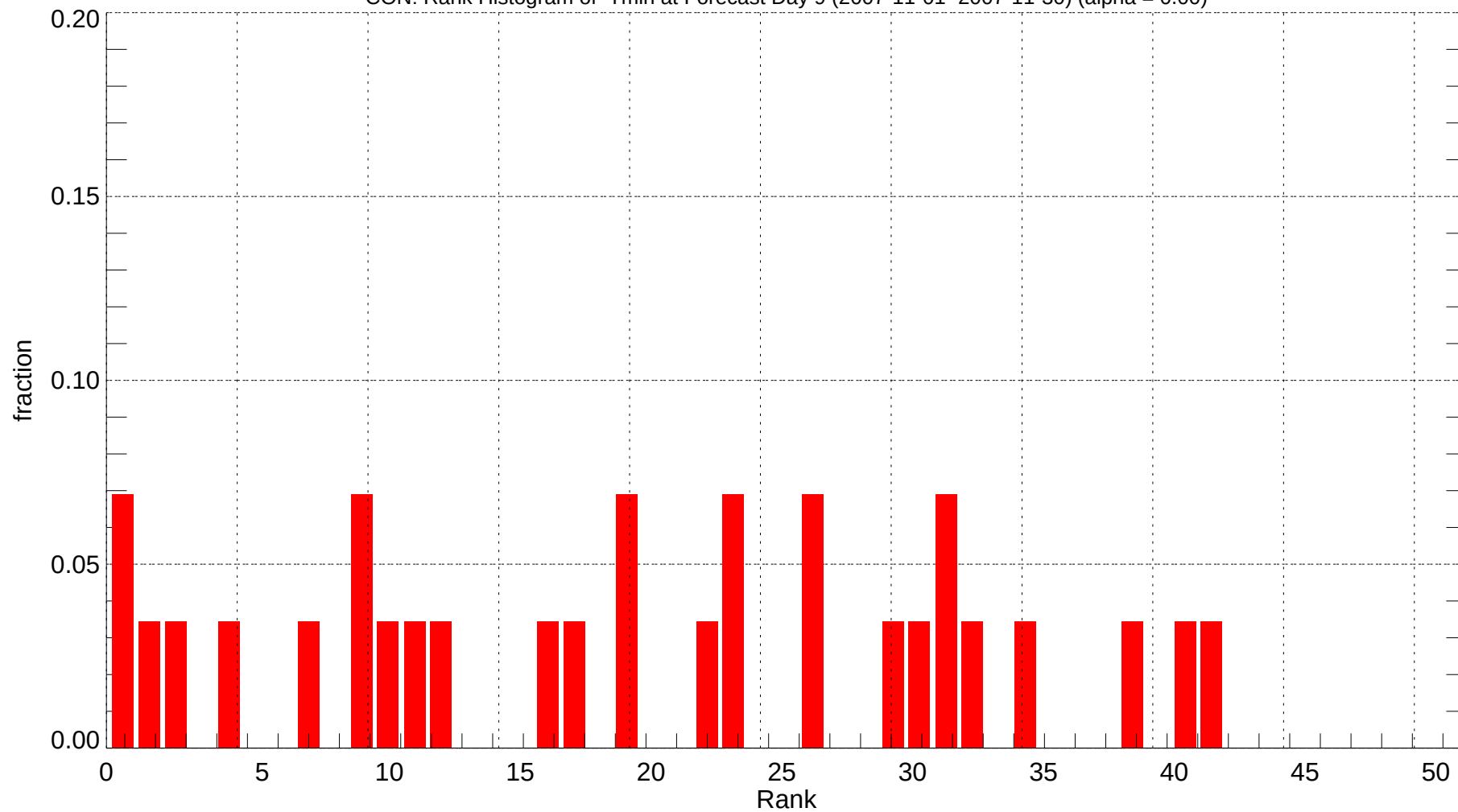
CON: Rank Histogram of Tmin at Forecast Day 9 (2007-11-01~2007-11-30) (alpha = 0.00)
