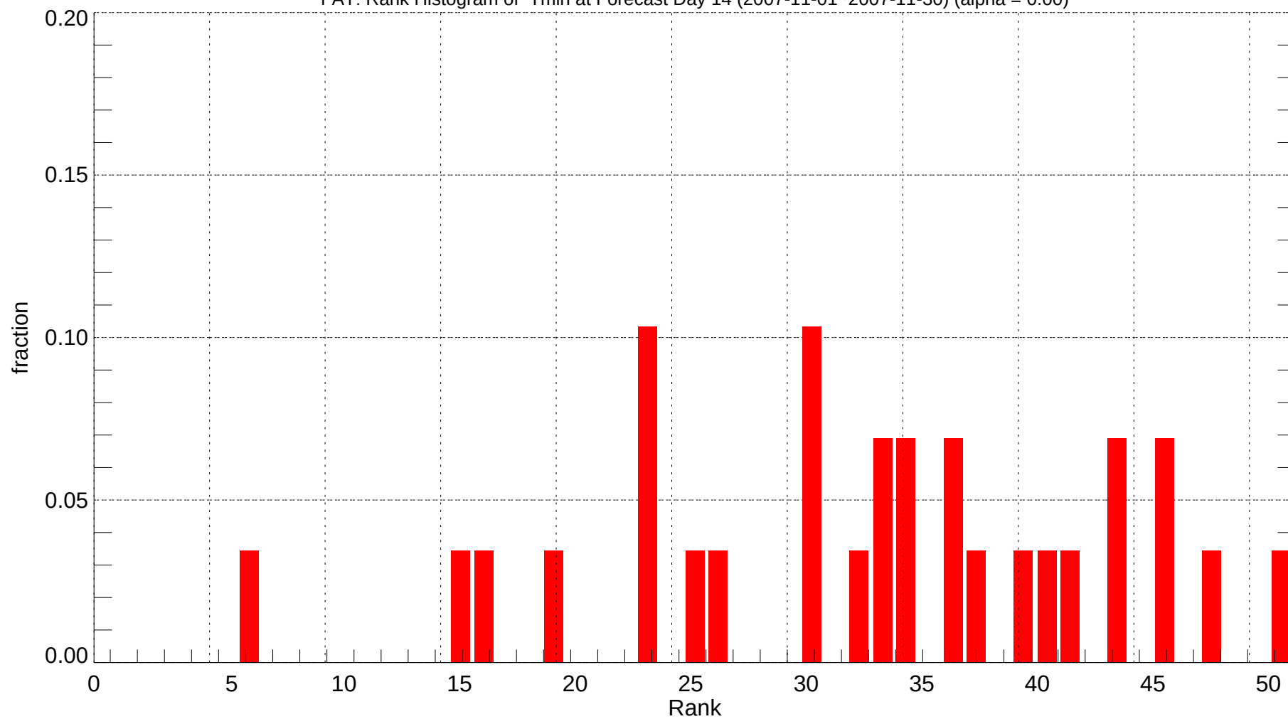
FAT: Rank Histogram of Tmin at Forecast Day 14 (2007-11-01~2007-11-30) (alpha = 0.00)
