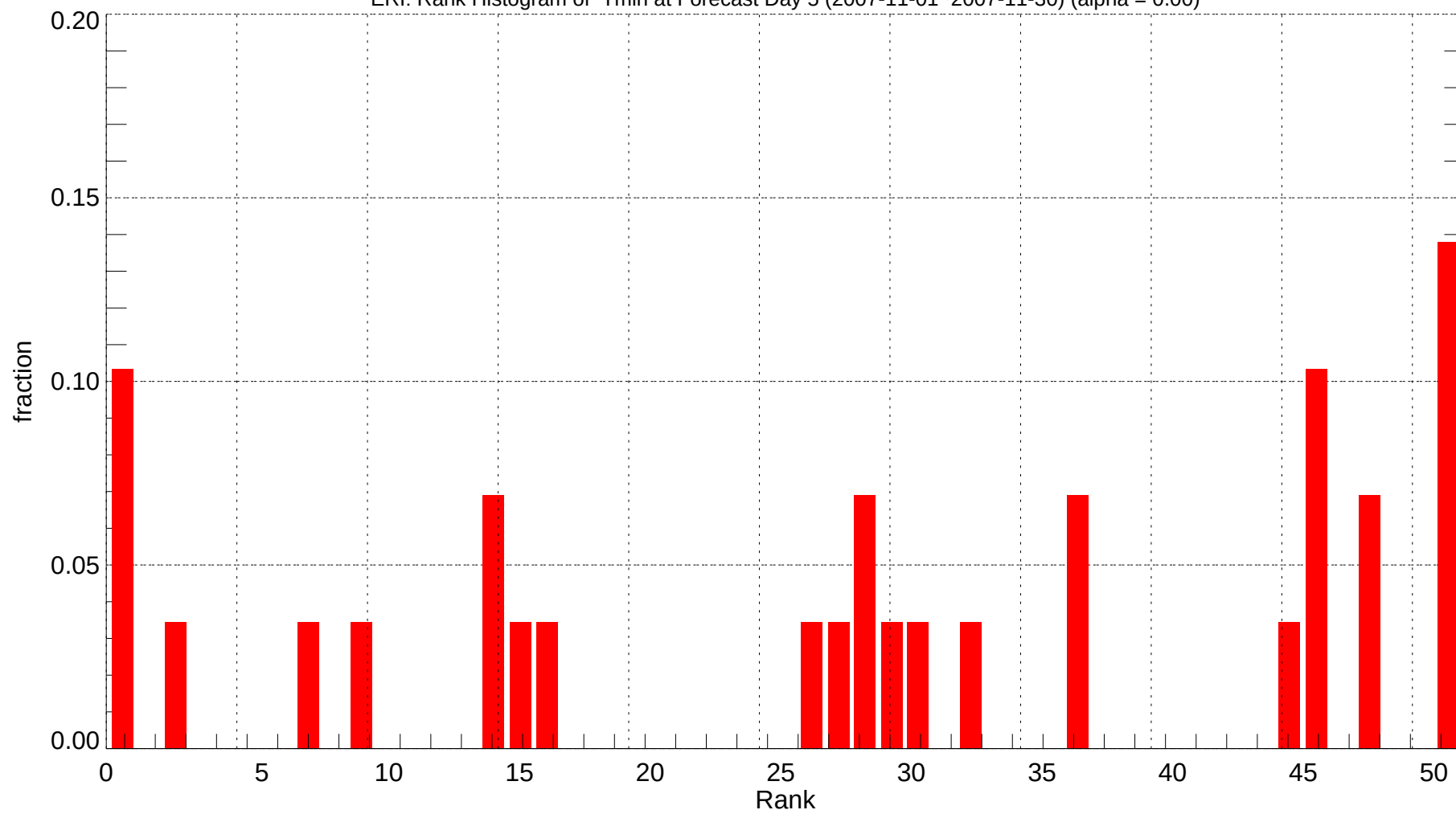
ERI: Rank Histogram of Tmin at Forecast Day 5 (2007-11-01~2007-11-30) (alpha = 0.00)
