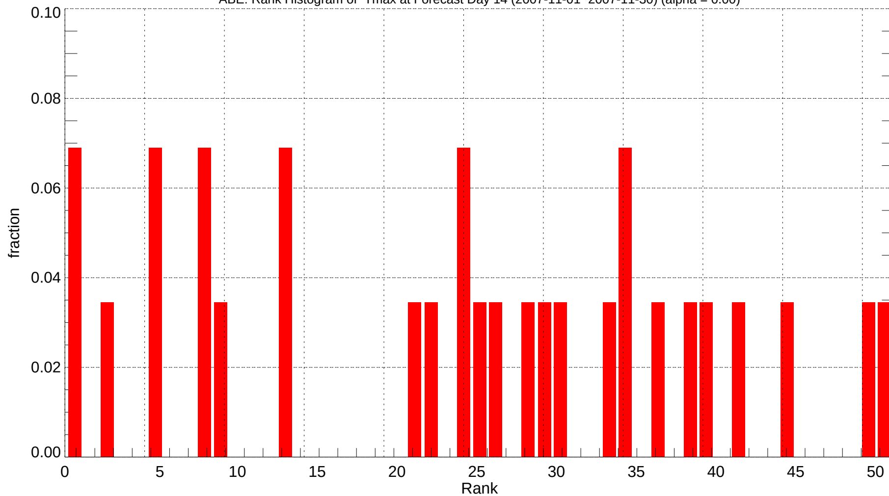
ABE: Rank Histogram of Tmax at Forecast Day 14 (2007-11-01~2007-11-30) (alpha = 0.00)
