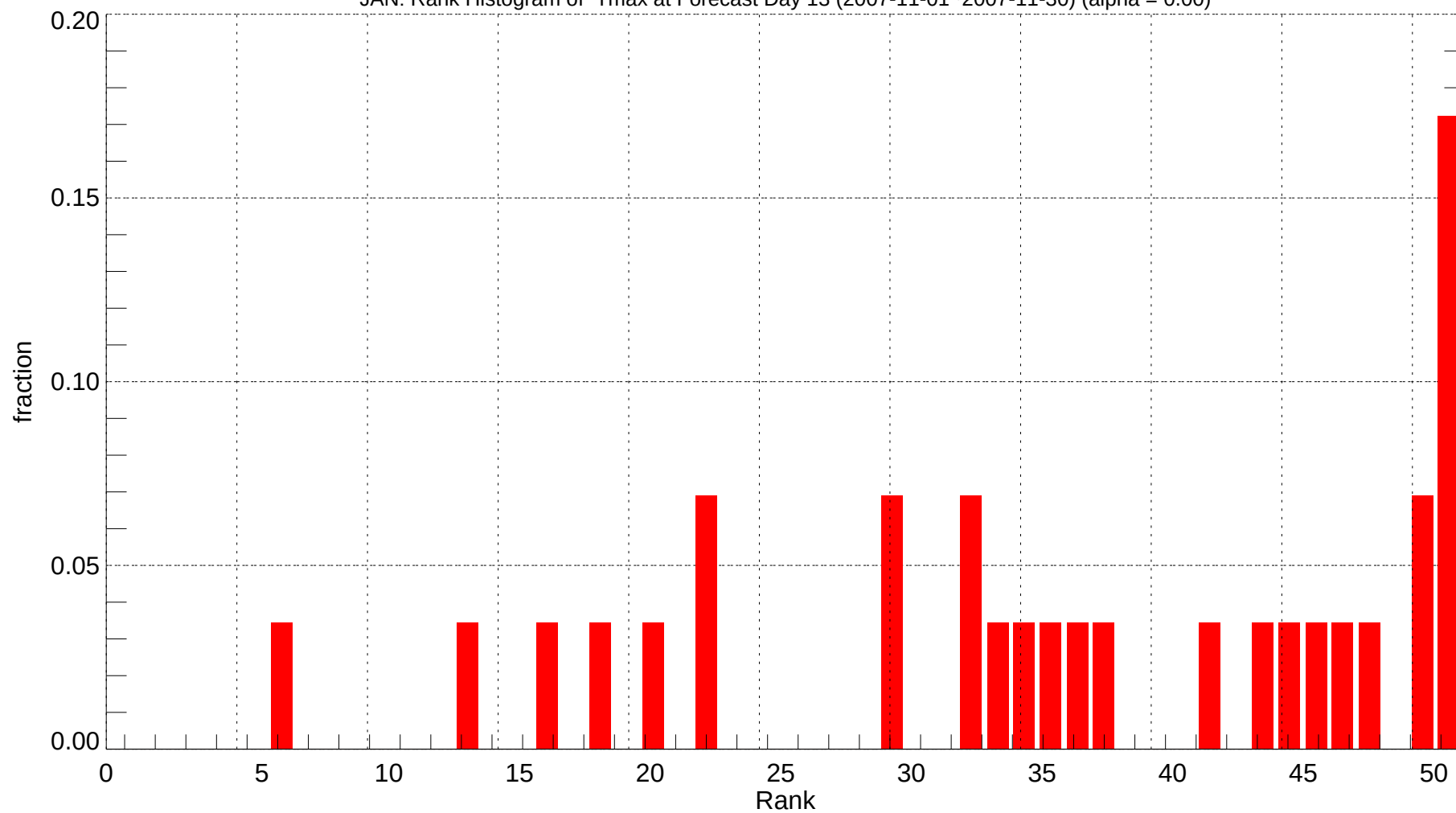
JAN: Rank Histogram of Tmax at Forecast Day 13 (2007-11-01~2007-11-30) (alpha = 0.00)
