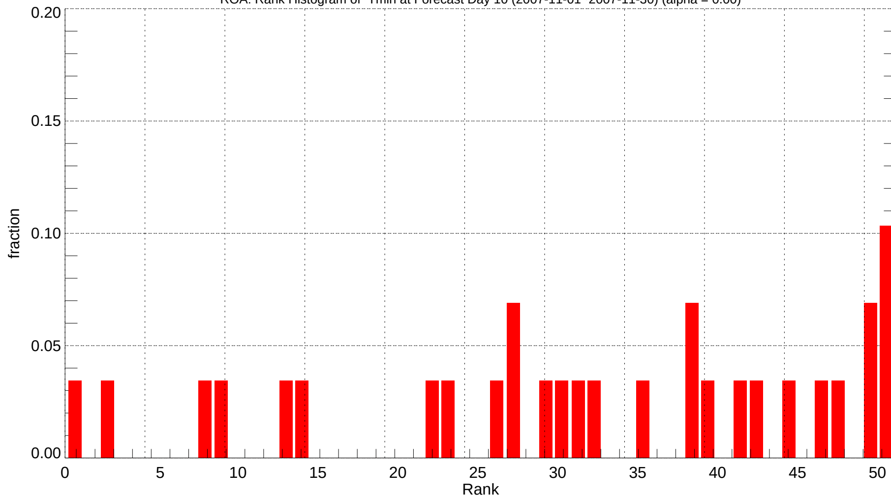
ROA: Rank Histogram of Tmin at Forecast Day 10 (2007-11-01~2007-11-30) (alpha = 0.00)
