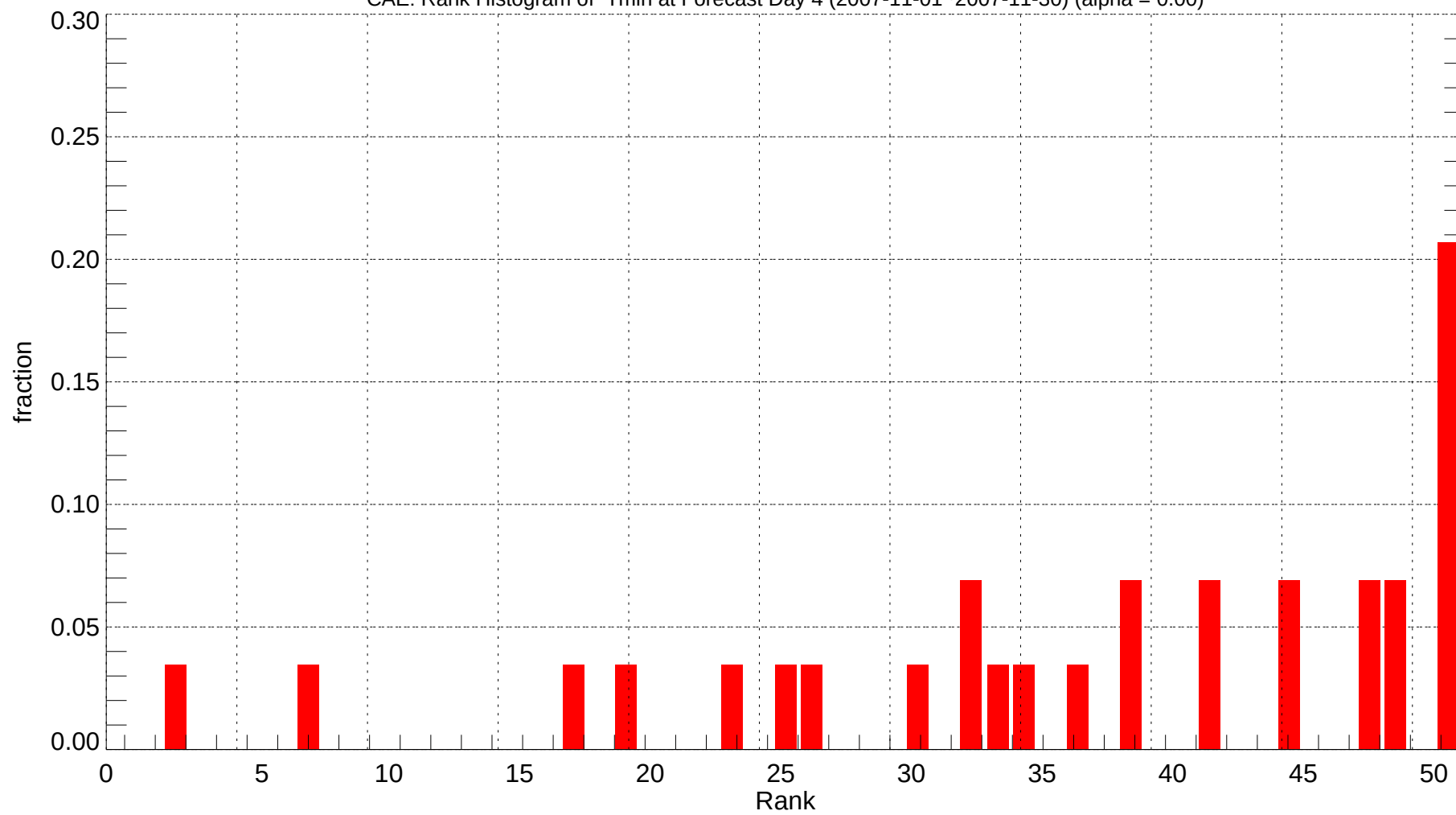
CAE: Rank Histogram of Tmin at Forecast Day 4 (2007-11-01~2007-11-30) (alpha = 0.00)
