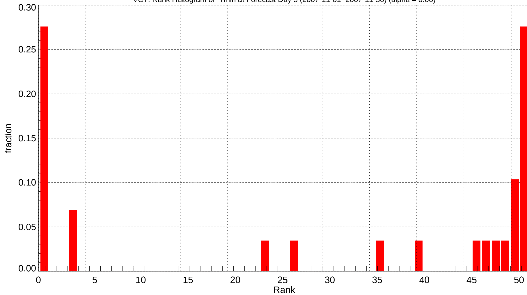
VCT: Rank Histogram of Tmin at Forecast Day 3 (2007-11-01~2007-11-30) (alpha = 0.00)
