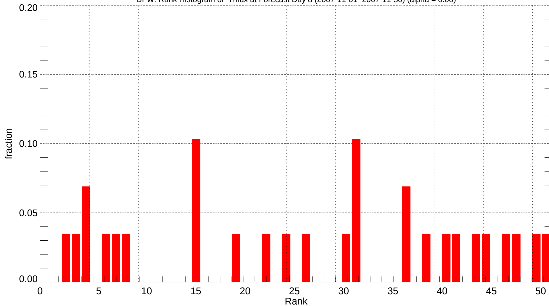
DFW: Rank Histogram of Tmax at Forecast Day 8 (2007-11-01~2007-11-30) (alpha = 0.00)
