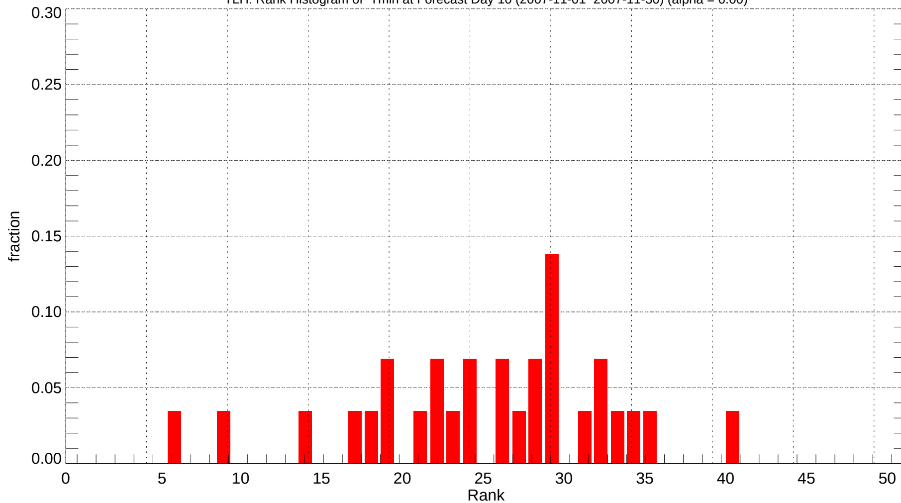
TLH: Rank Histogram of Tmin at Forecast Day 10 (2007-11-01~2007-11-30) (alpha = 0.00)
