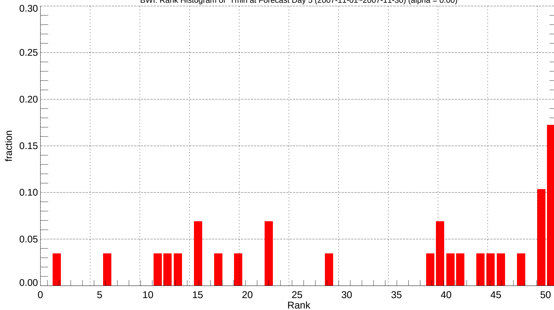
BWI: Rank Histogram of Tmin at Forecast Day 5 (2007-11-01~2007-11-30) (alpha = 0.00)
