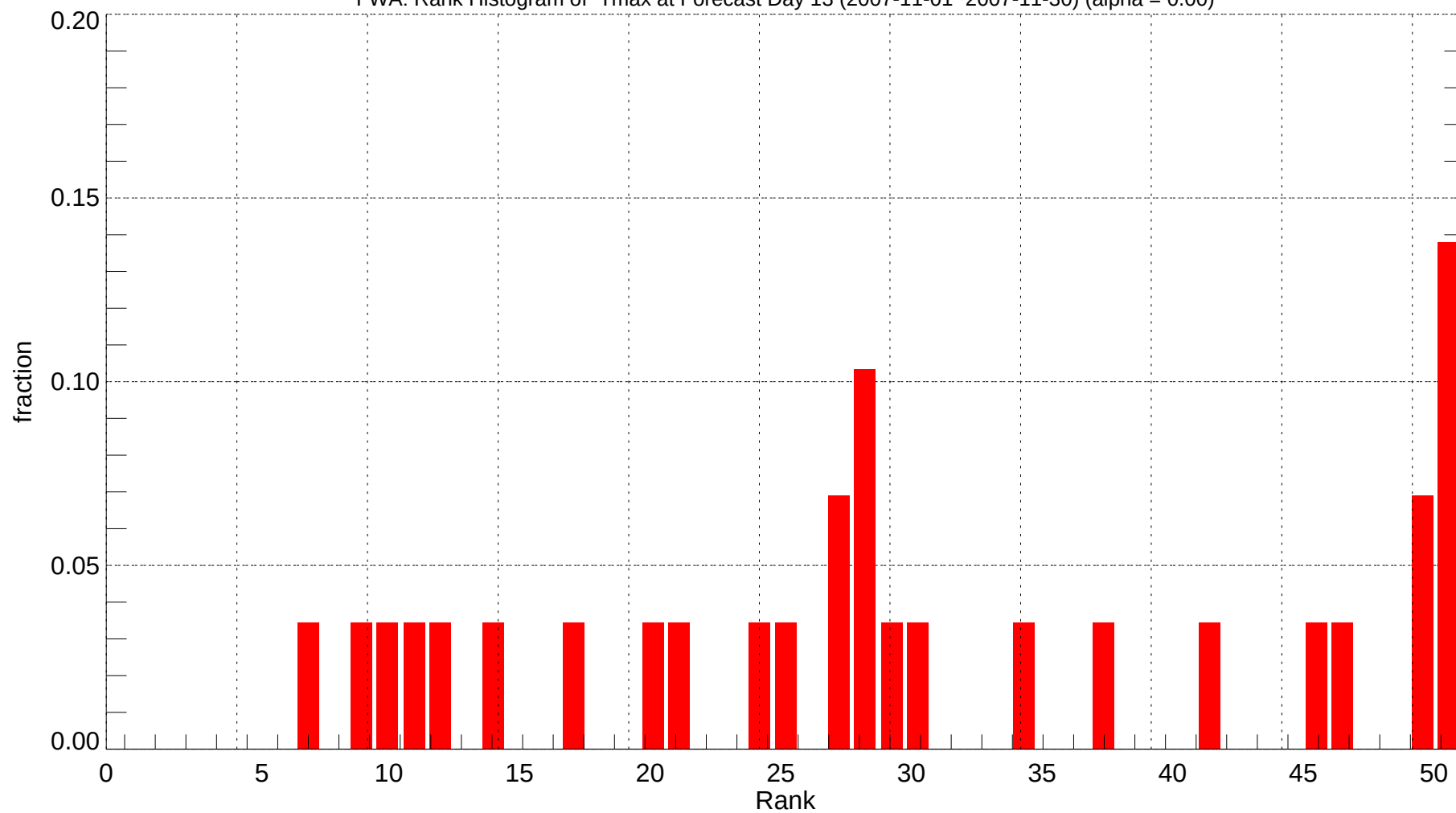
FWA: Rank Histogram of Tmax at Forecast Day 13 (2007-11-01~2007-11-30) (alpha = 0.00)
