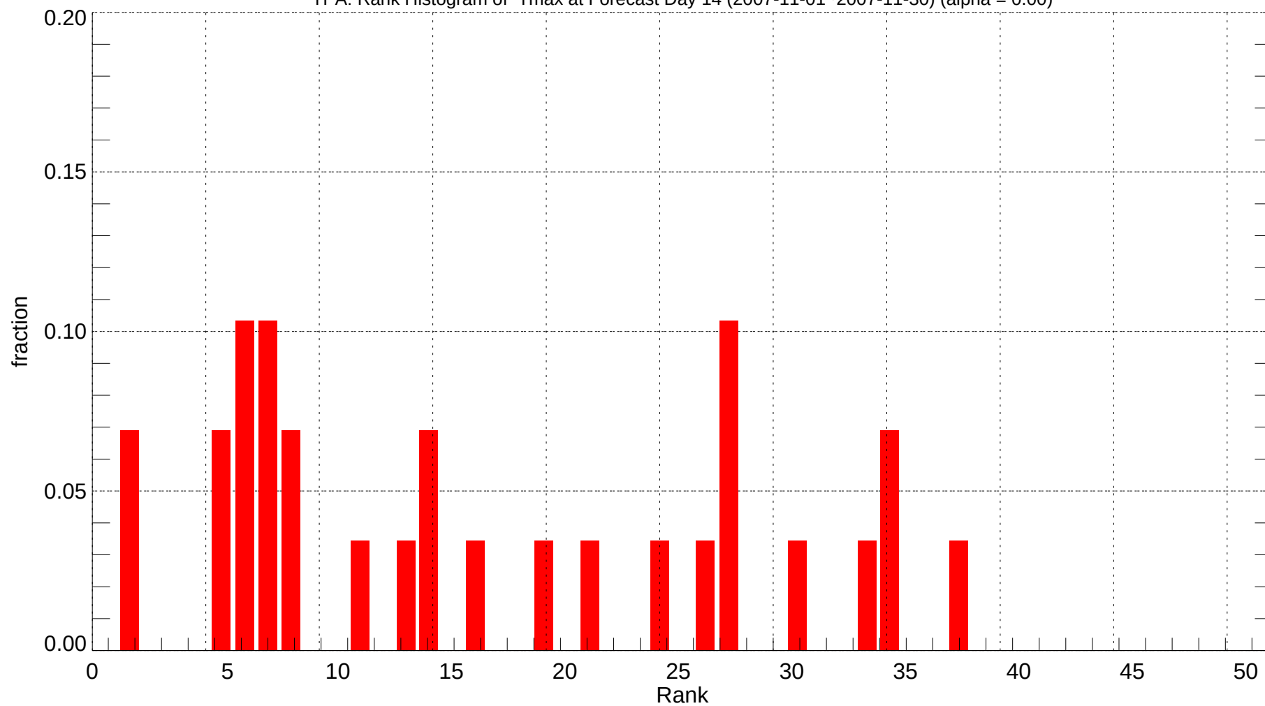
TPA: Rank Histogram of Tmax at Forecast Day 14 (2007-11-01~2007-11-30) (alpha = 0.00)
