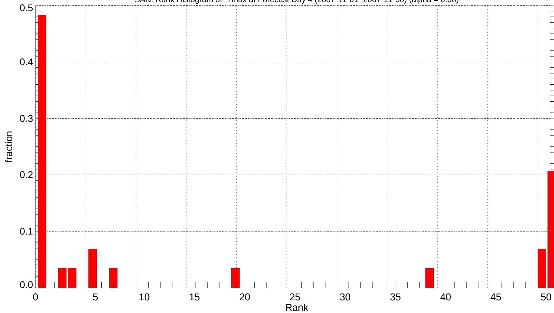
SAN: Rank Histogram of Tmax at Forecast Day 4 (2007-11-01~2007-11-30) (alpha = 0.00)
