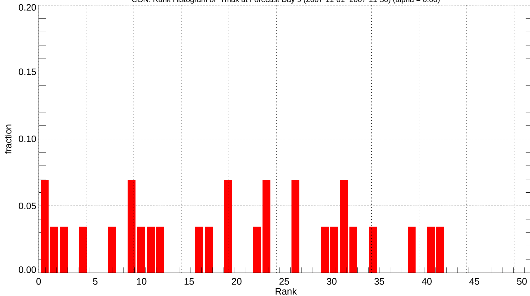
CON: Rank Histogram of Tmax at Forecast Day 9 (2007-11-01~2007-11-30) (alpha = 0.00)
