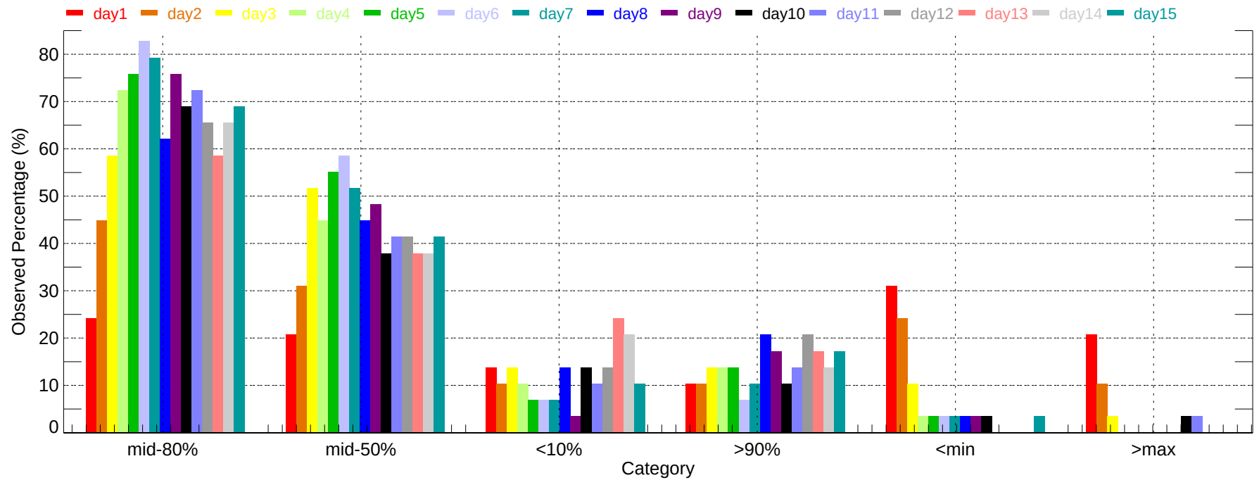
Observed Percentage of Ensembles - JFK: Max Temperature (2007-11-01~2007-11-30)
