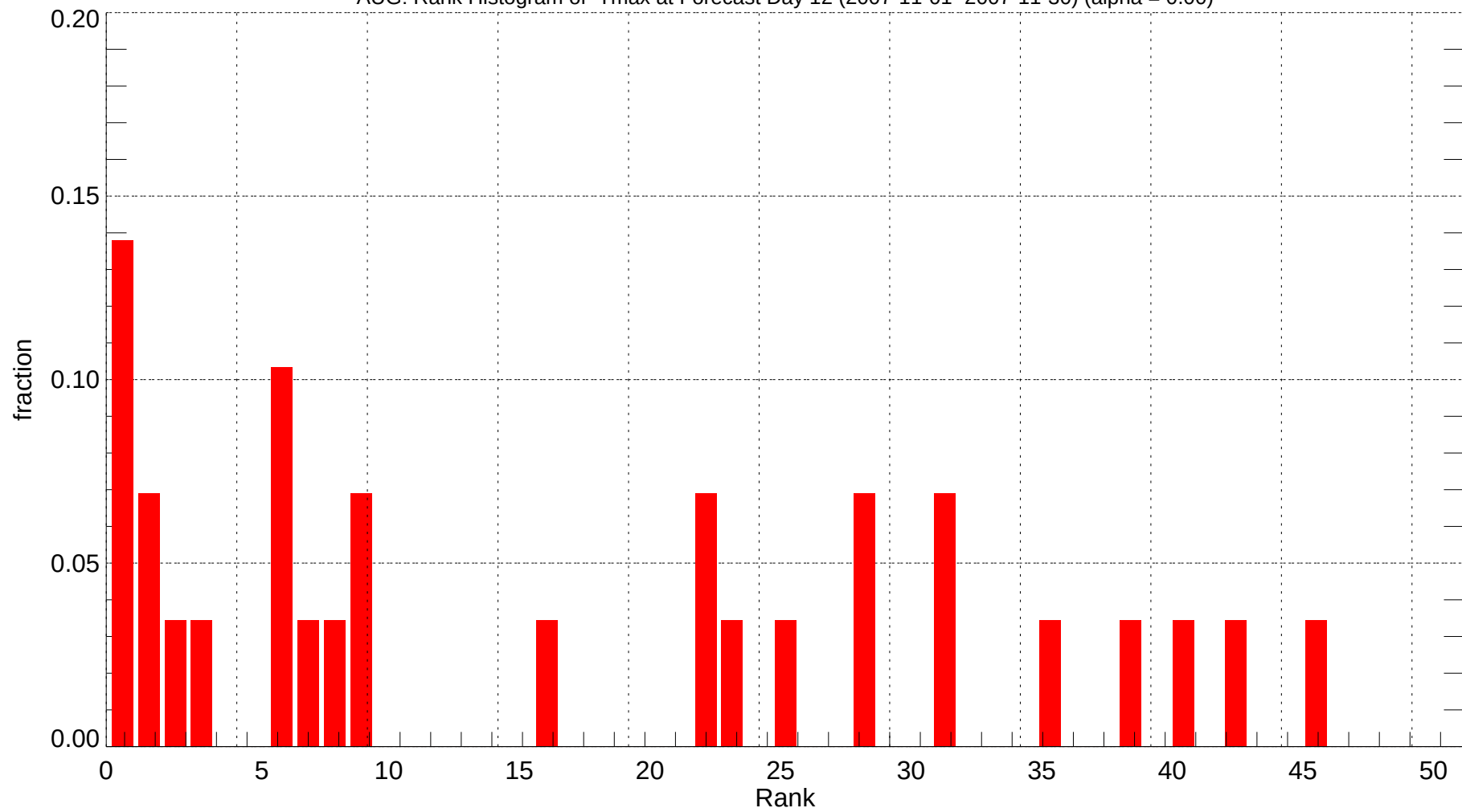
AUG: Rank Histogram of Tmax at Forecast Day 12 (2007-11-01~2007-11-30) (alpha = 0.00)
