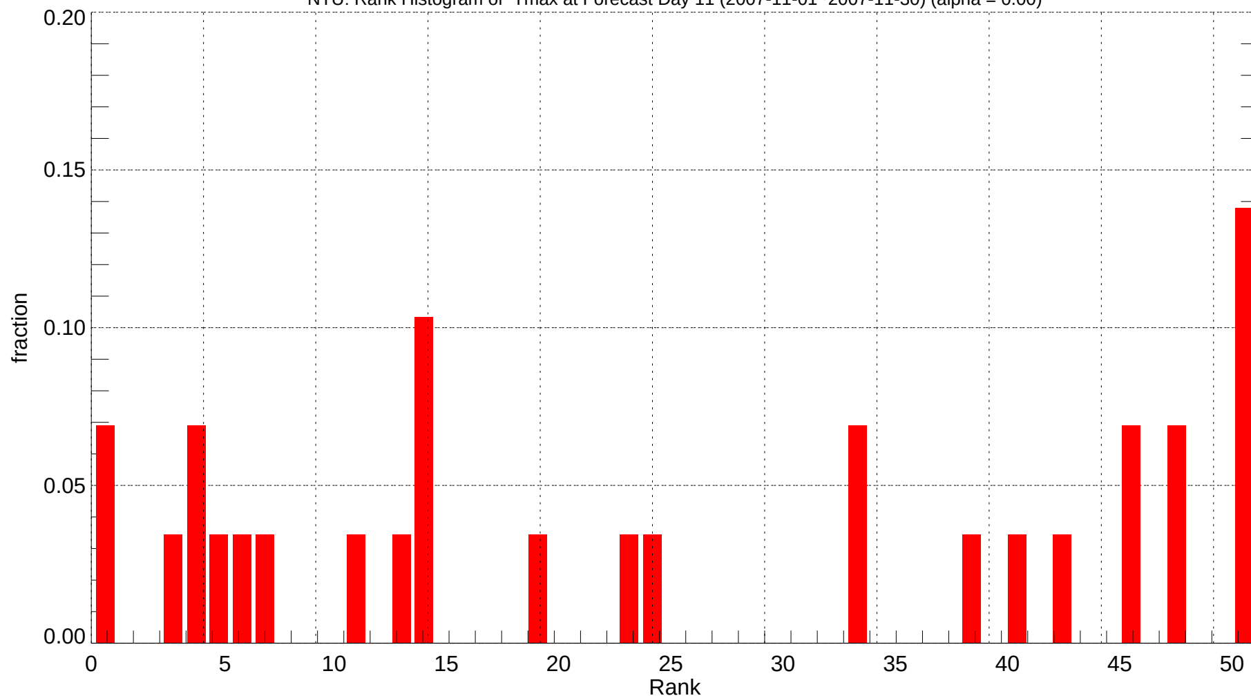
NTU: Rank Histogram of Tmax at Forecast Day 11 (2007-11-01~2007-11-30) (alpha = 0.00)
