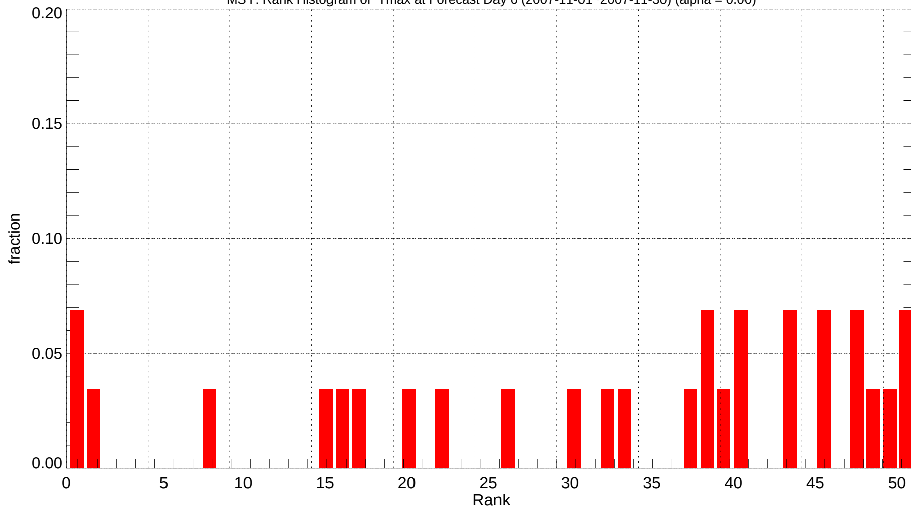
MSY: Rank Histogram of Tmax at Forecast Day 6 (2007-11-01~2007-11-30) (alpha = 0.00)
