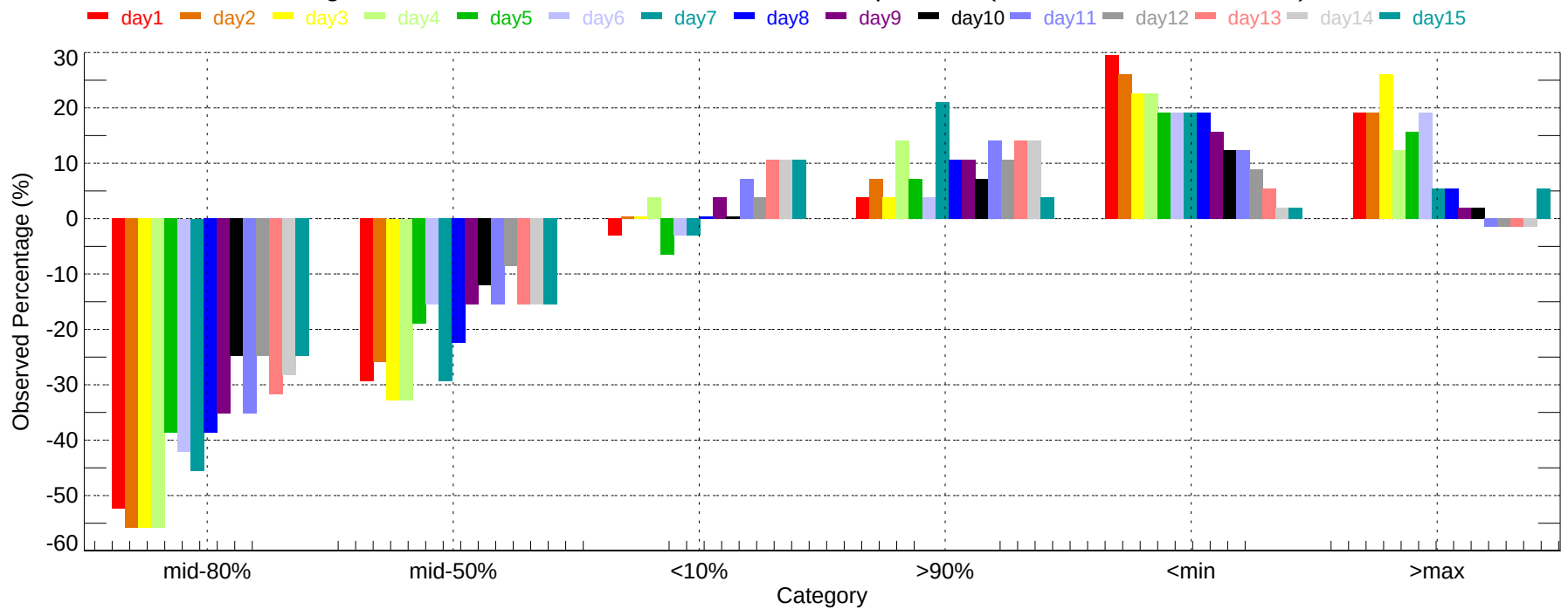
Observed Percentage Deviation of Ensembles - ALW: Max Temperature (2007-11-01~2007-11-30)
