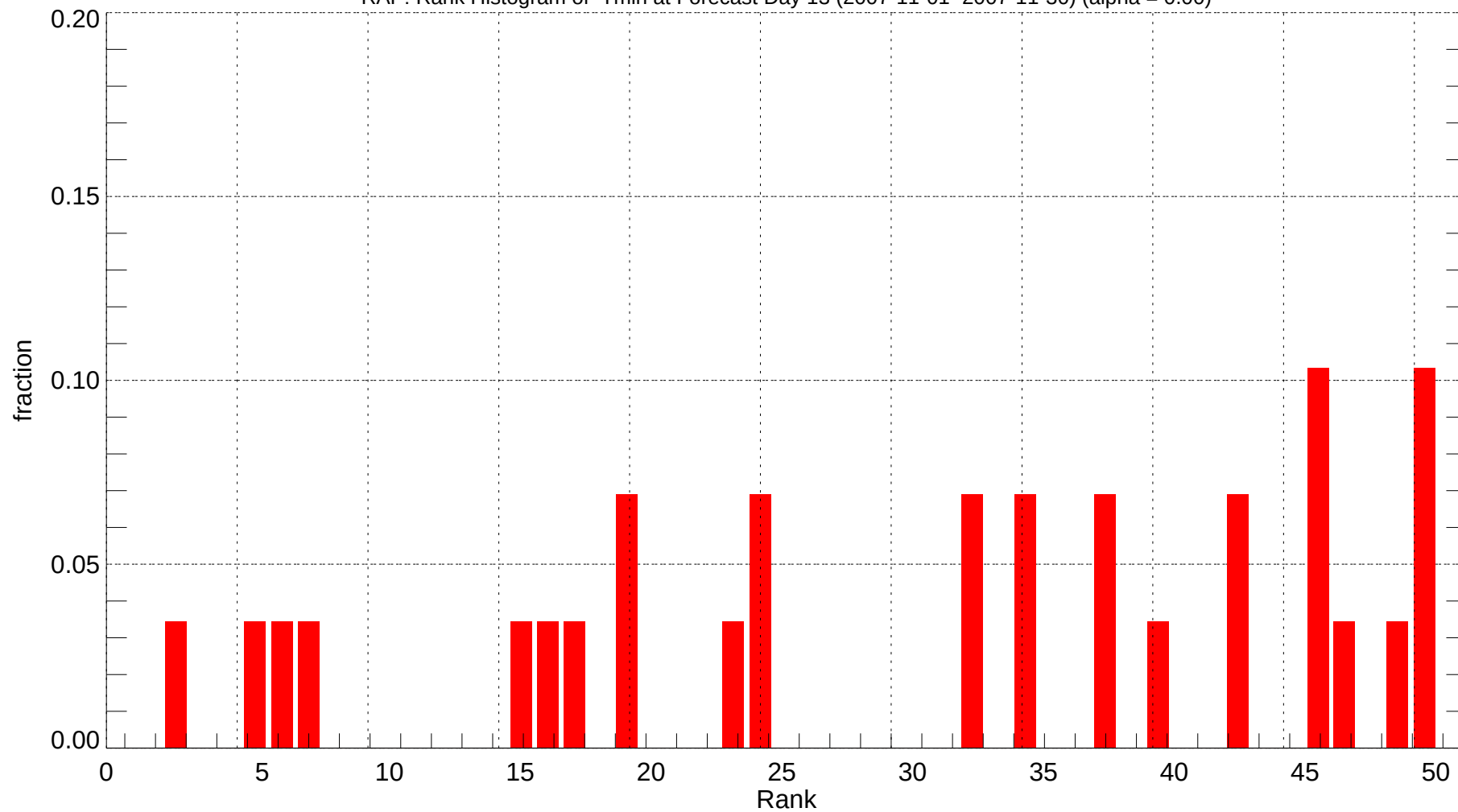
RAP: Rank Histogram of Tmin at Forecast Day 13 (2007-11-01~2007-11-30) (alpha = 0.00)
