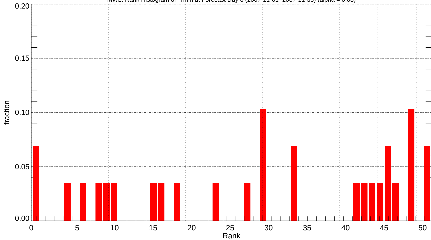
MWL: Rank Histogram of Tmin at Forecast Day 6 (2007-11-01~2007-11-30) (alpha = 0.00)
