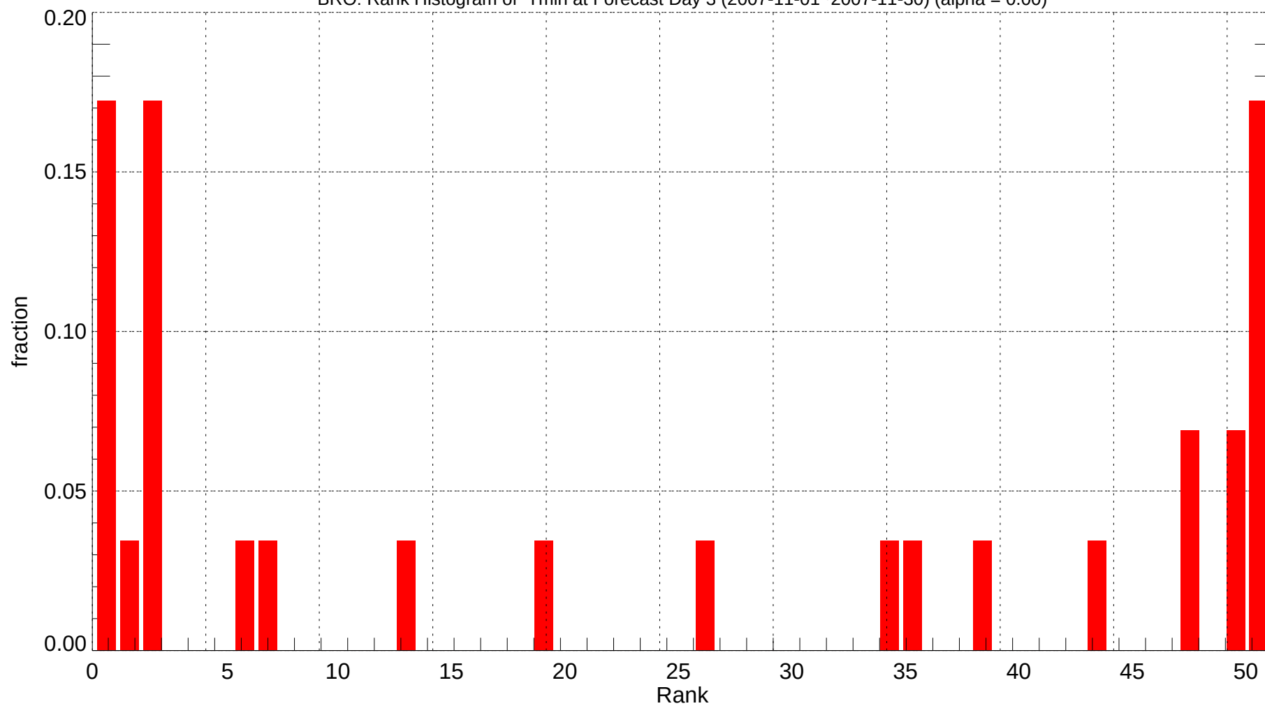
BRO: Rank Histogram of Tmin at Forecast Day 3 (2007-11-01~2007-11-30) (alpha = 0.00)
