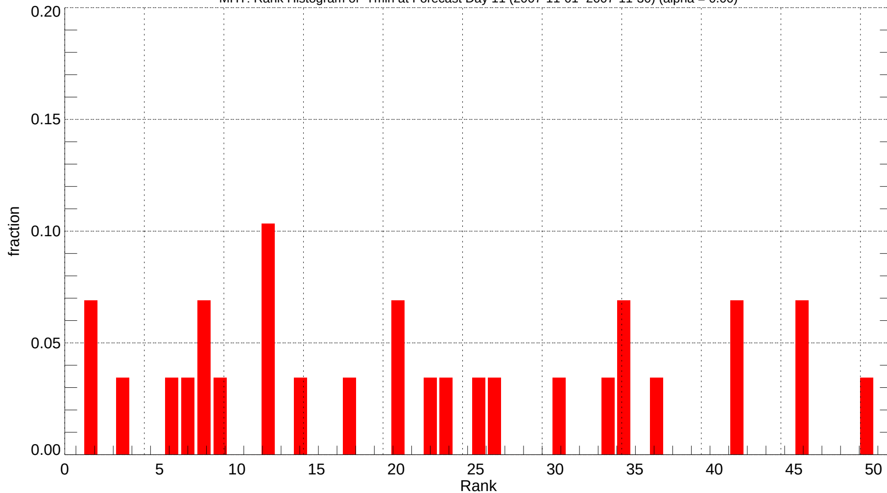
MHT: Rank Histogram of Tmin at Forecast Day 11 (2007-11-01~2007-11-30) (alpha = 0.00)
