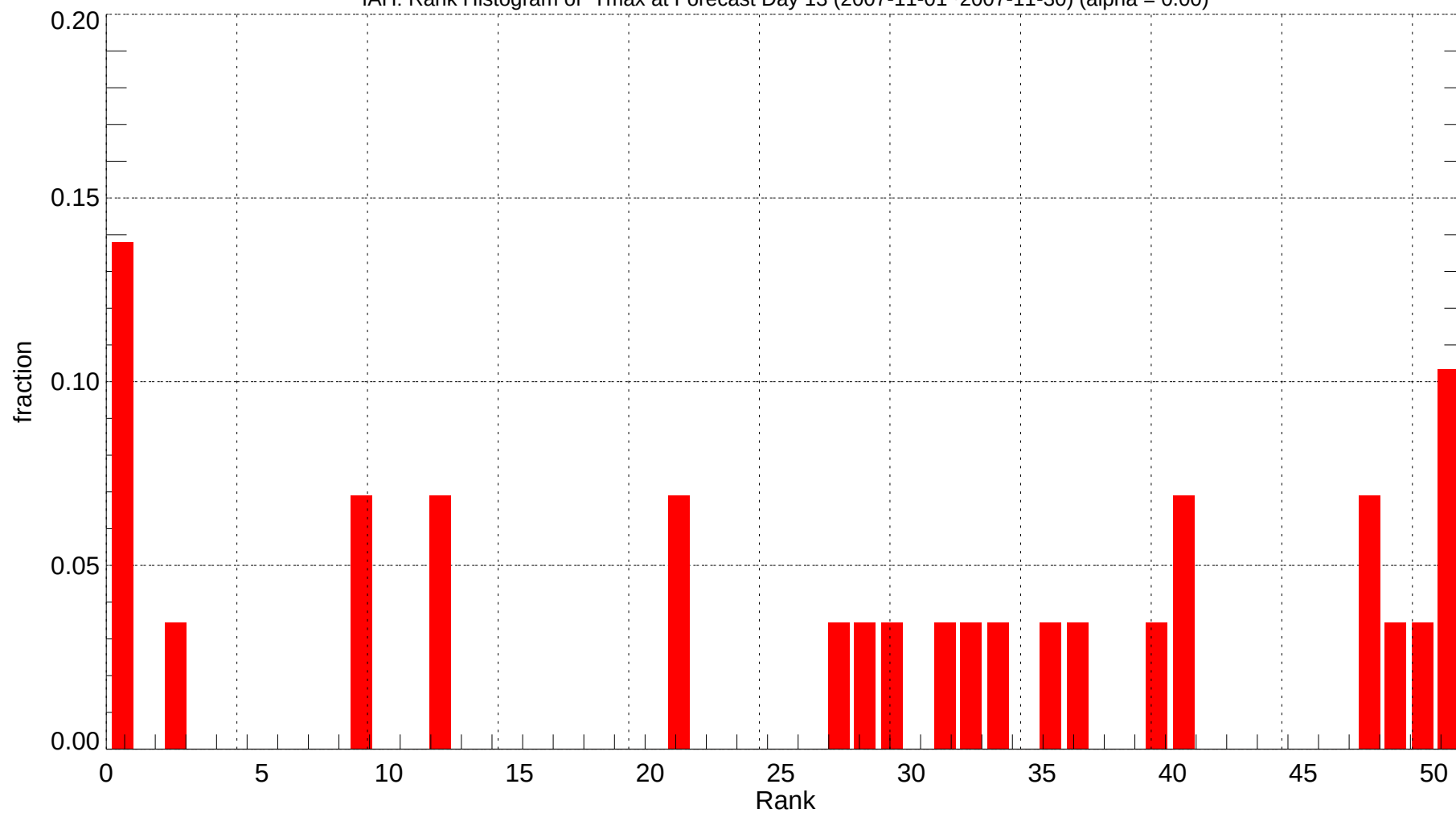
IAH: Rank Histogram of Tmax at Forecast Day 13 (2007-11-01~2007-11-30) (alpha = 0.00)
