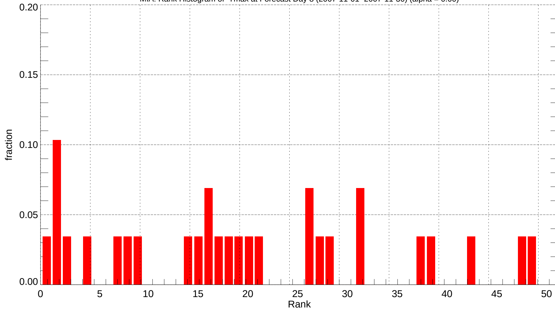
MIA: Rank Histogram of Tmax at Forecast Day 8 (2007-11-01~2007-11-30) (alpha = 0.00)
