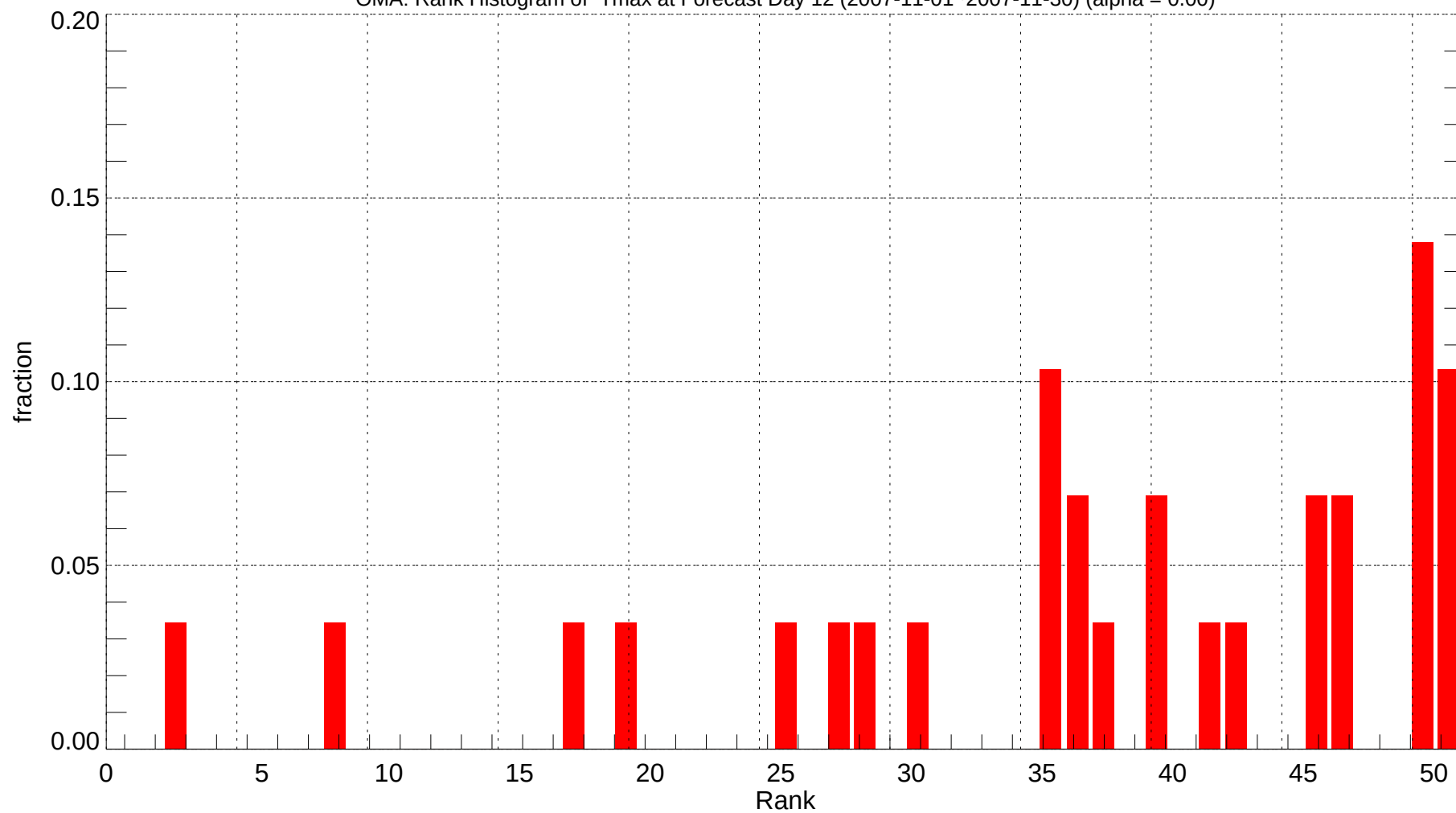
OMA: Rank Histogram of Tmax at Forecast Day 12 (2007-11-01~2007-11-30) (alpha = 0.00)
