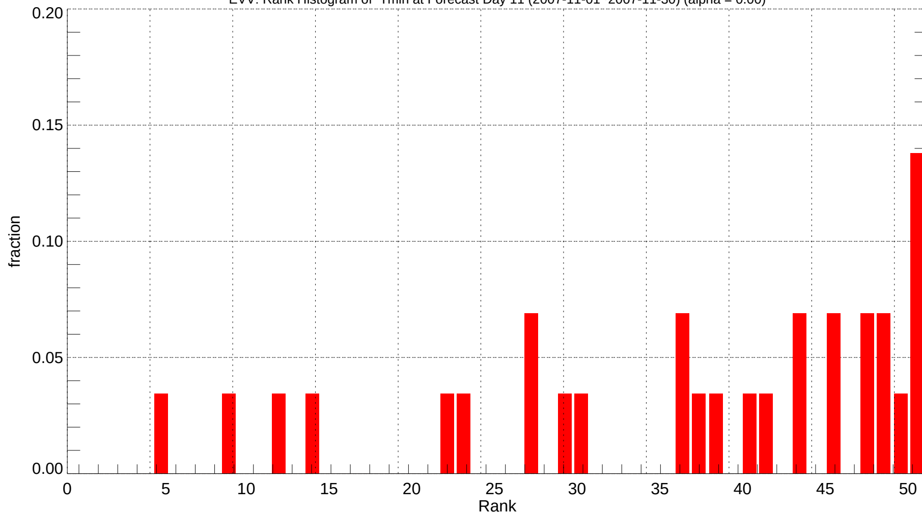
EVV: Rank Histogram of Tmin at Forecast Day 11 (2007-11-01~2007-11-30) (alpha = 0.00)
