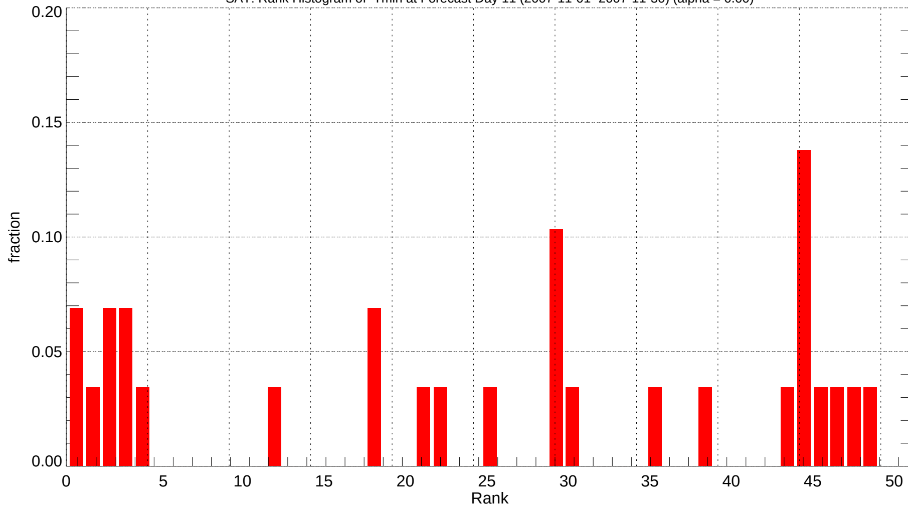
SAT: Rank Histogram of Tmin at Forecast Day 11 (2007-11-01~2007-11-30) (alpha = 0.00)
