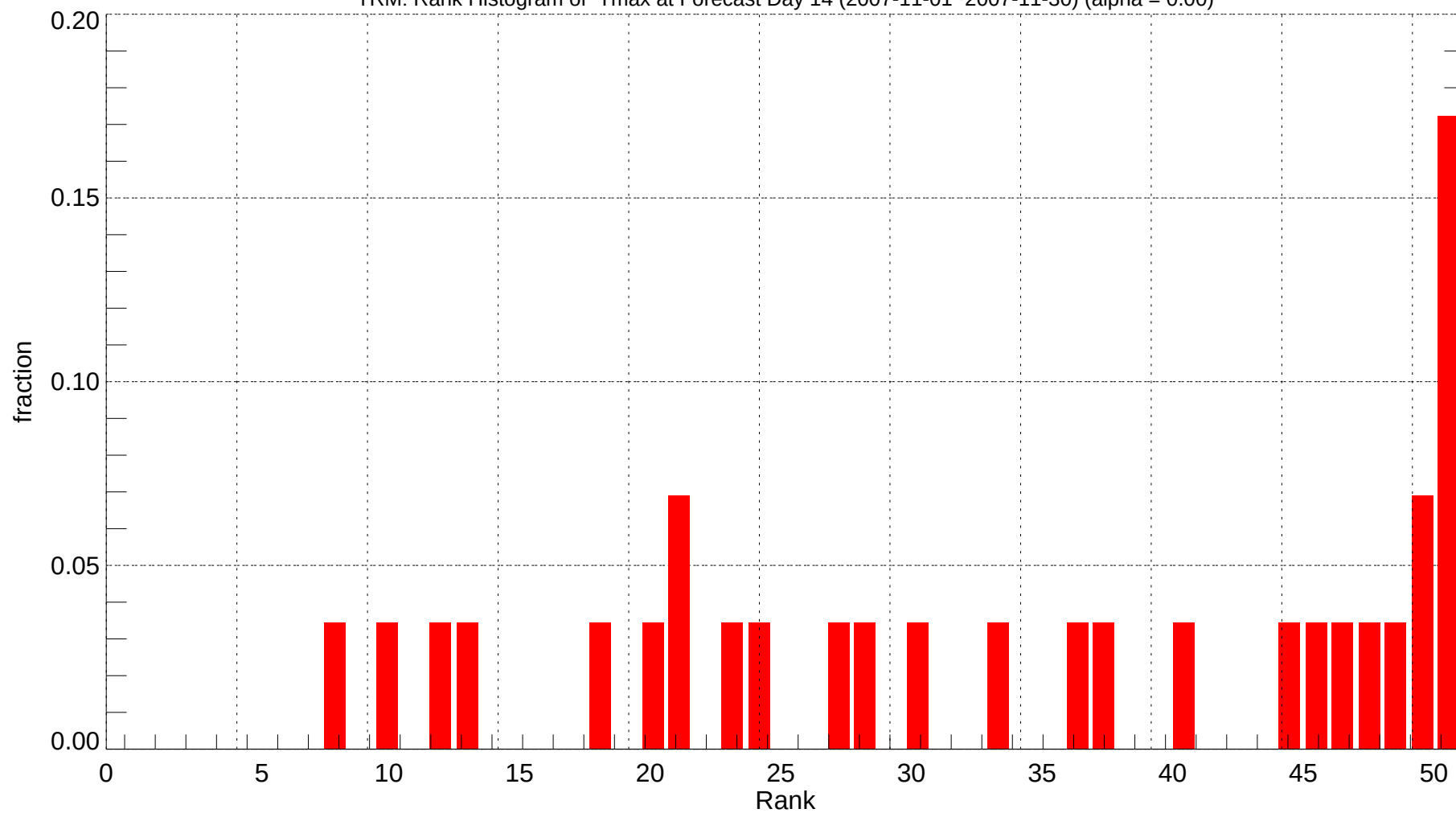
TRM: Rank Histogram of Tmax at Forecast Day 14 (2007-11-01~2007-11-30) (alpha = 0.00)
