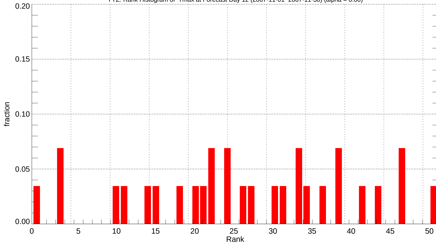
YYZ: Rank Histogram of Tmax at Forecast Day 12 (2007-11-01~2007-11-30) (alpha = 0.00)
