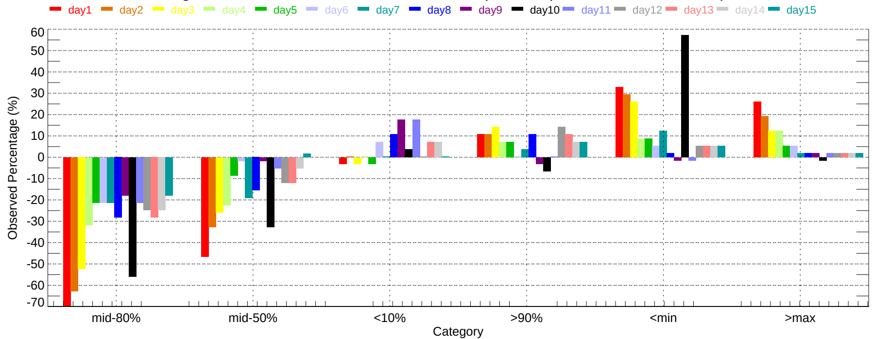
Observed Percentage Deviation of Ensembles - AVP: Max Temperature (2007-11-01~2007-11-30)
