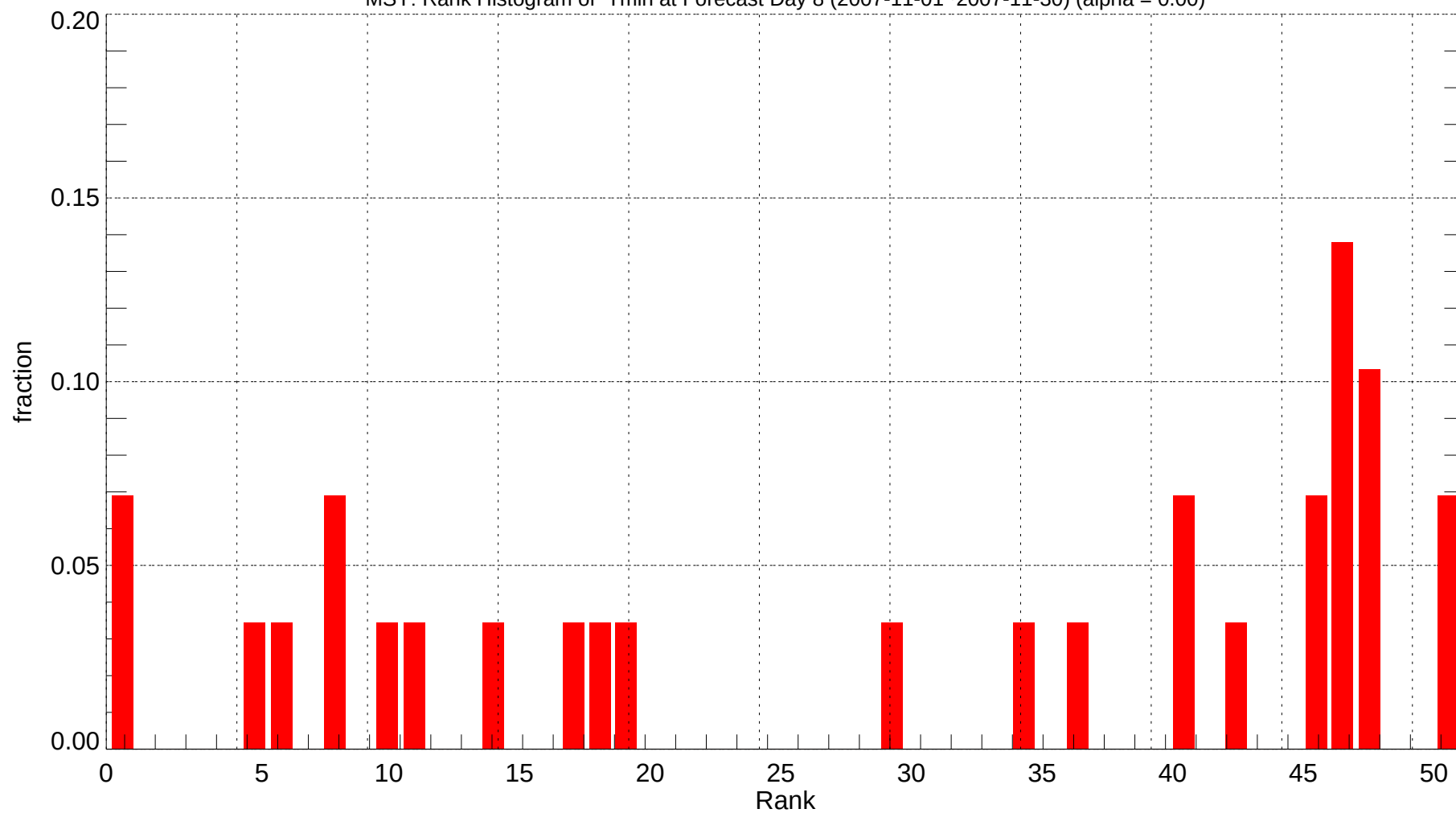
MSY: Rank Histogram of Tmin at Forecast Day 8 (2007-11-01~2007-11-30) (alpha = 0.00)
