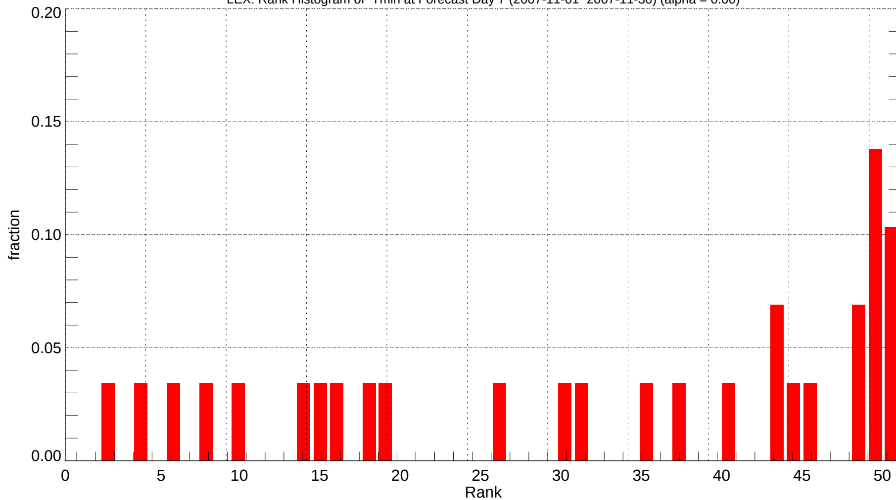
LEX: Rank Histogram of Tmin at Forecast Day 7 (2007-11-01~2007-11-30) (alpha = 0.00)
