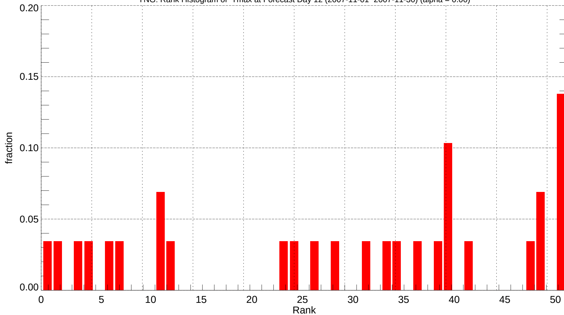
YNG: Rank Histogram of Tmax at Forecast Day 12 (2007-11-01~2007-11-30) (alpha = 0.00)
