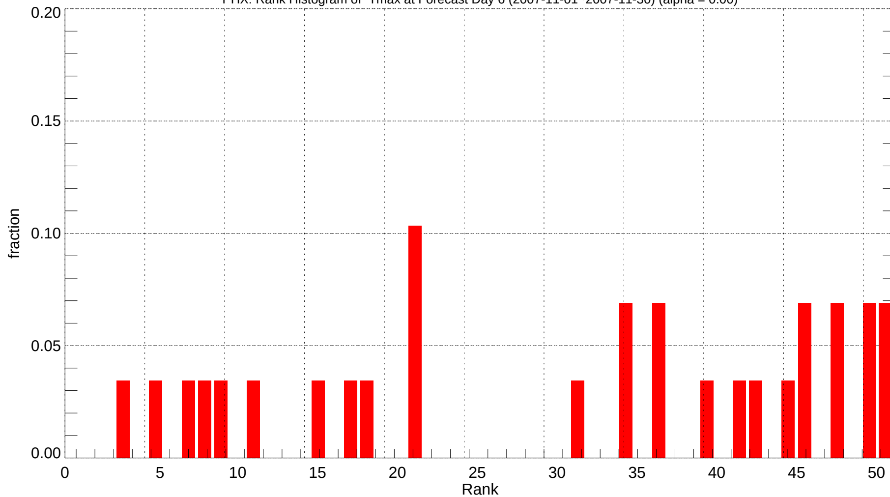
PHX: Rank Histogram of Tmax at Forecast Day 6 (2007-11-01~2007-11-30) (alpha = 0.00)
