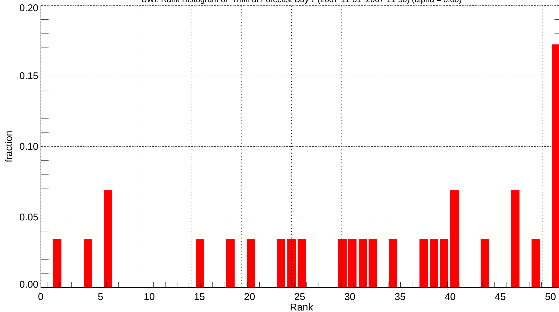
BWI: Rank Histogram of Tmin at Forecast Day 7 (2007-11-01~2007-11-30) (alpha = 0.00)
