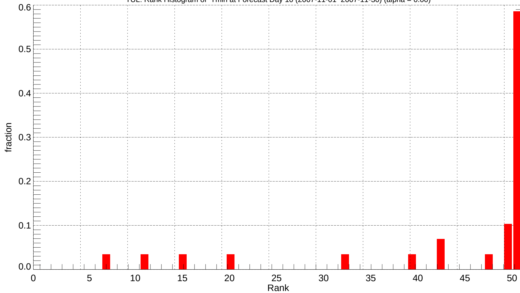
TUL: Rank Histogram of Tmin at Forecast Day 10 (2007-11-01~2007-11-30) (alpha = 0.00)
