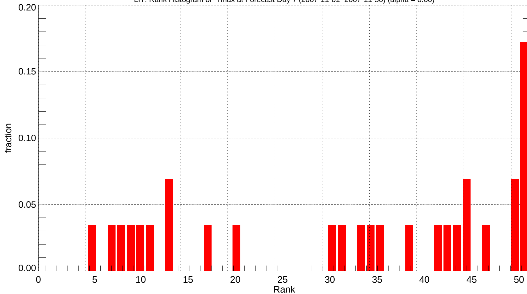
LIT: Rank Histogram of Tmax at Forecast Day 7 (2007-11-01~2007-11-30) (alpha = 0.00)
