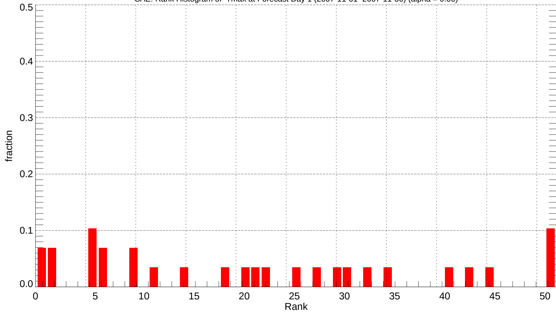
CAE: Rank Histogram of Tmax at Forecast Day 1 (2007-11-01~2007-11-30) (alpha = 0.00)
