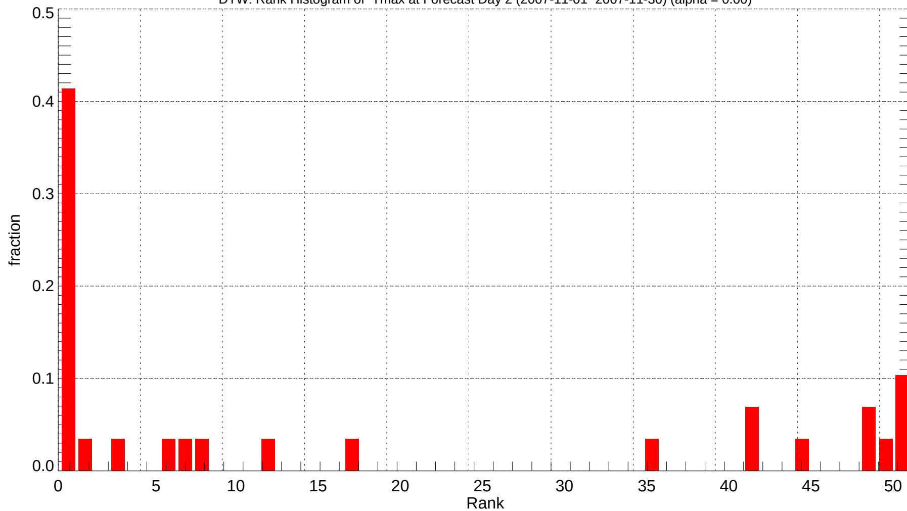
DTW: Rank Histogram of Tmax at Forecast Day 2 (2007-11-01~2007-11-30) (alpha = 0.00)
