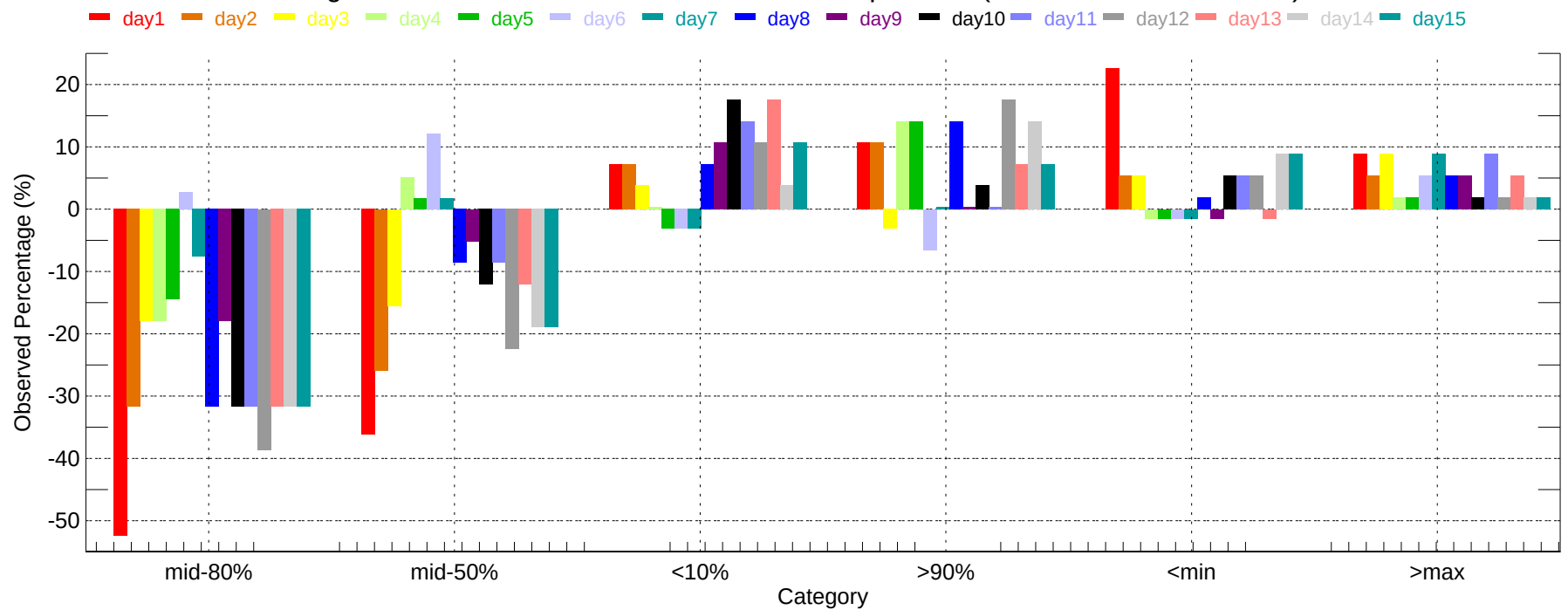
Observed Percentage Deviation of Ensembles - PHL: Max Temperature (2007-11-01~2007-11-30)
