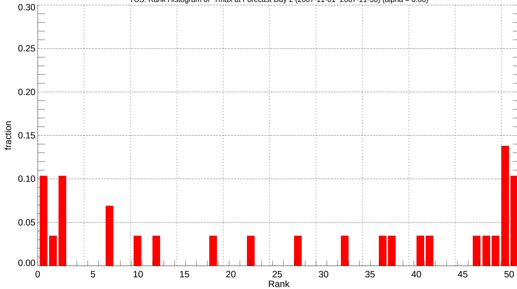
TUS: Rank Histogram of Tmax at Forecast Day 2 (2007-11-01~2007-11-30) (alpha = 0.00)
