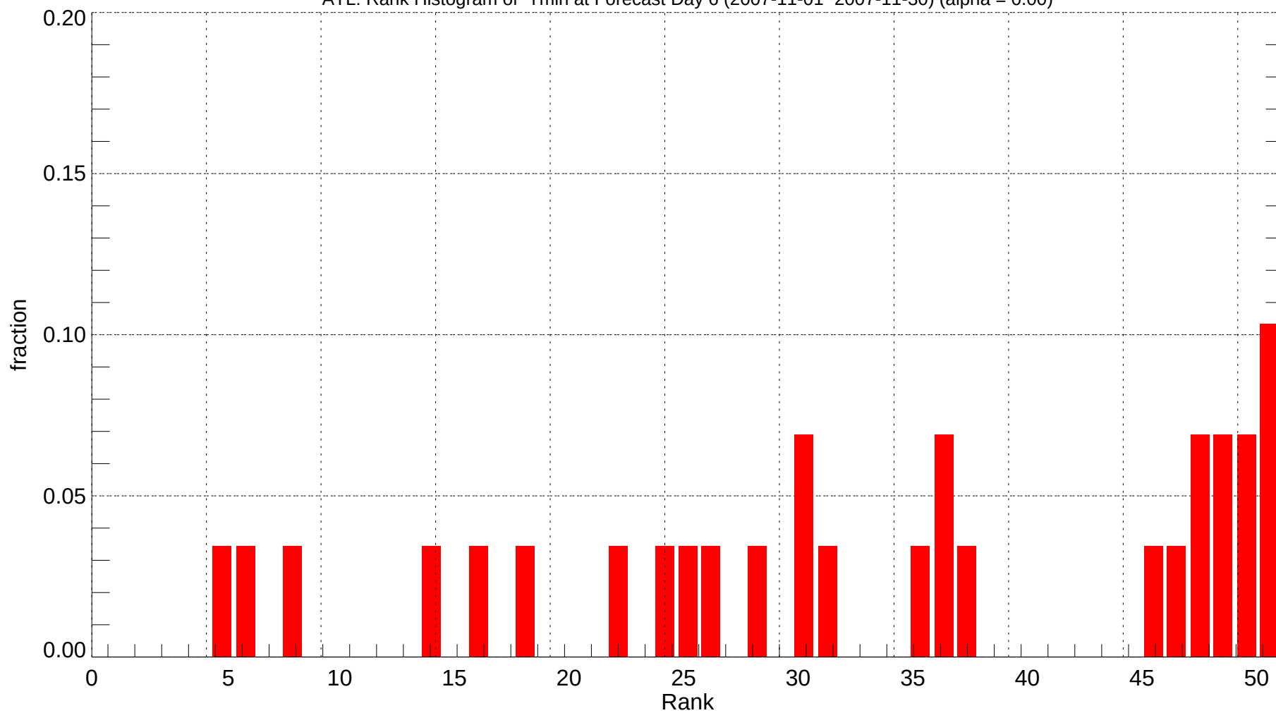
ATL: Rank Histogram of Tmin at Forecast Day 6 (2007-11-01~2007-11-30) (alpha = 0.00)
