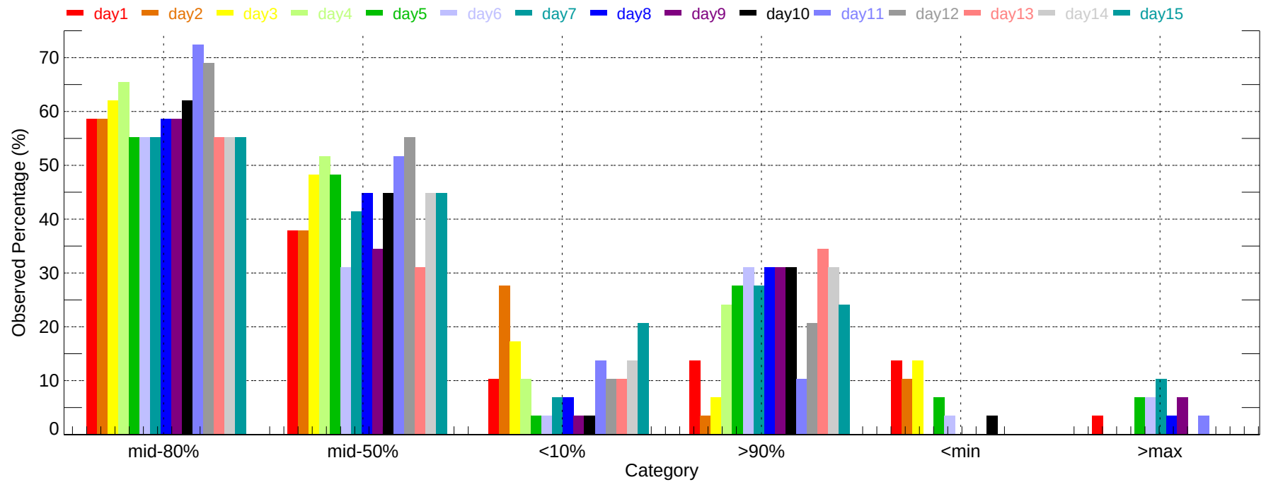
Observed Percentage of Ensembles - ELP: Min Temperature (2007-11-01~2007-11-30)
