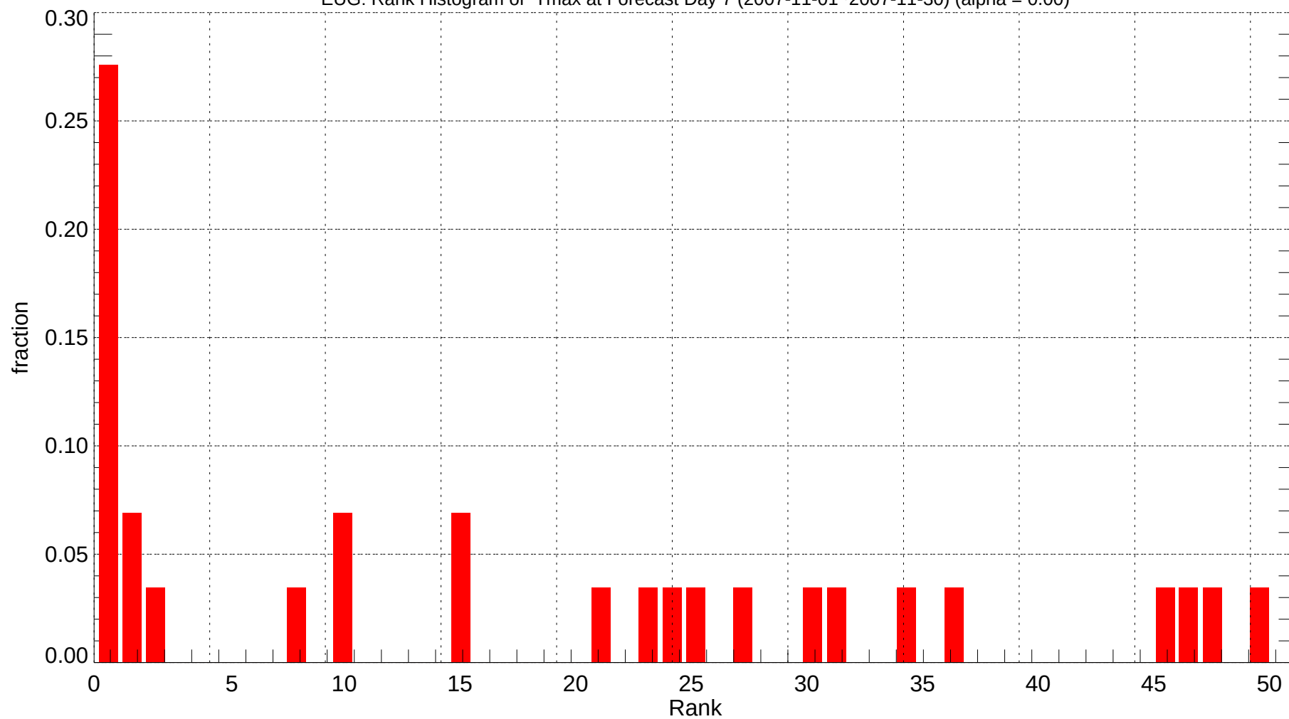
EUG: Rank Histogram of Tmax at Forecast Day 7 (2007-11-01~2007-11-30) (alpha = 0.00)
