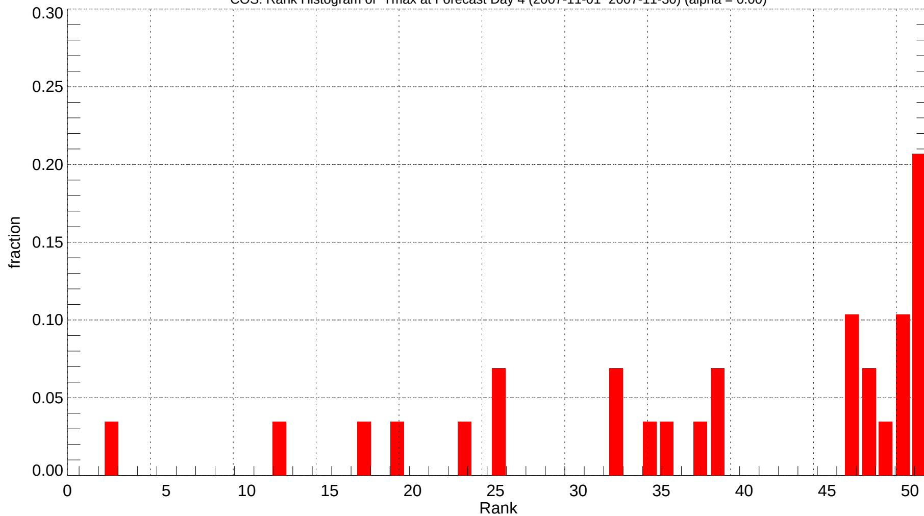
COS: Rank Histogram of Tmax at Forecast Day 4 (2007-11-01~2007-11-30) (alpha = 0.00)
