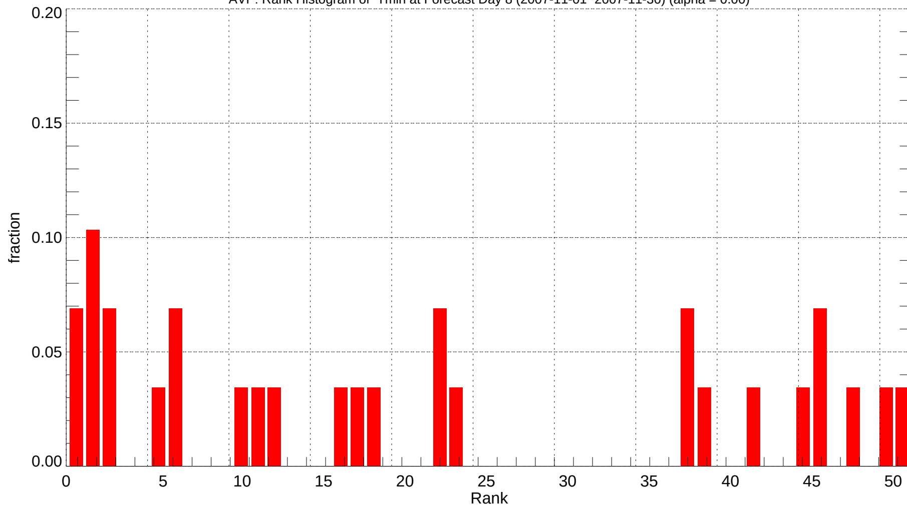
AVP: Rank Histogram of Tmin at Forecast Day 8 (2007-11-01~2007-11-30) (alpha = 0.00)
