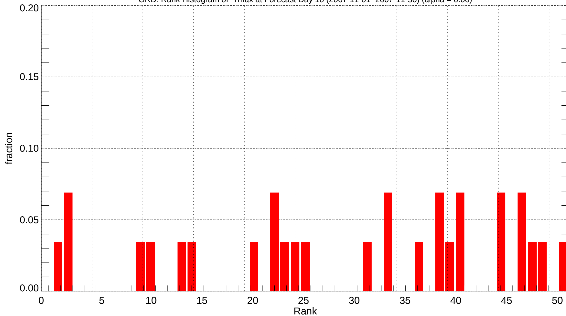
ORD: Rank Histogram of Tmax at Forecast Day 10 (2007-11-01~2007-11-30) (alpha = 0.00)
