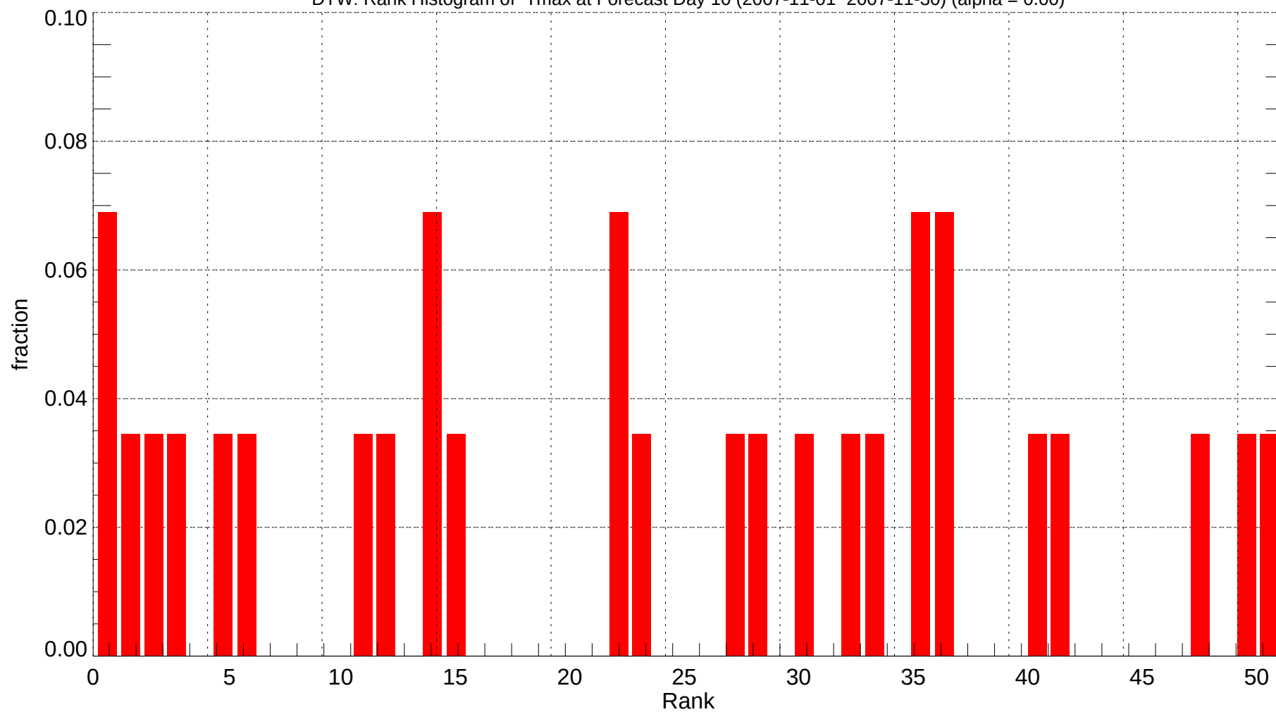
DTW: Rank Histogram of Tmax at Forecast Day 10 (2007-11-01~2007-11-30) (alpha = 0.00)
