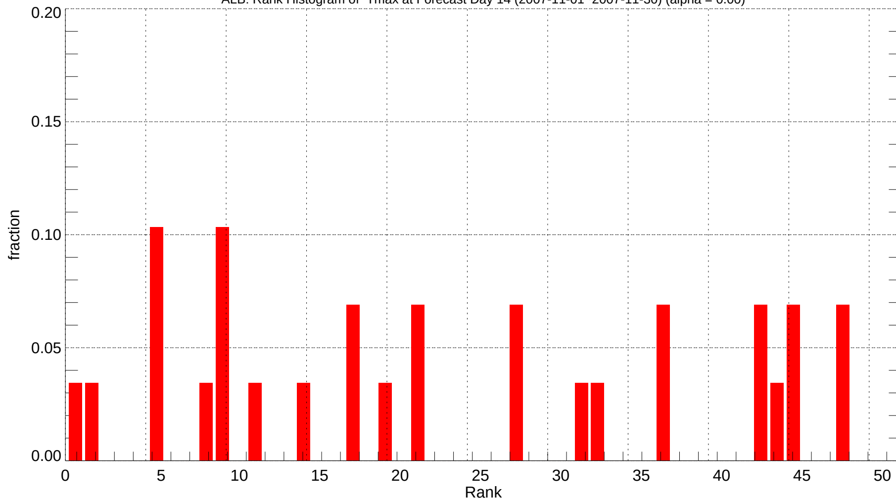
ALB: Rank Histogram of Tmax at Forecast Day 14 (2007-11-01~2007-11-30) (alpha = 0.00)
