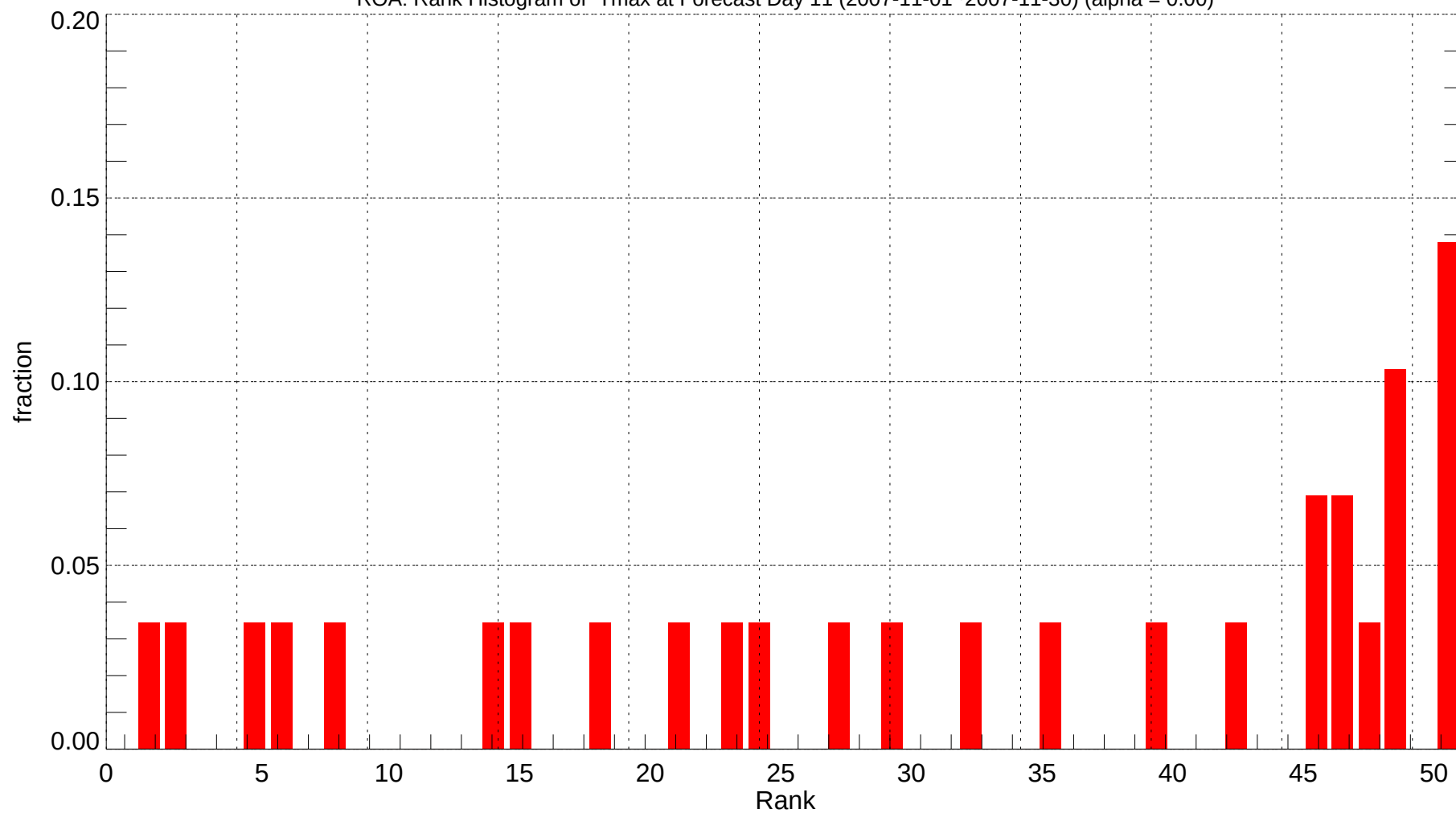
ROA: Rank Histogram of Tmax at Forecast Day 11 (2007-11-01~2007-11-30) (alpha = 0.00)
