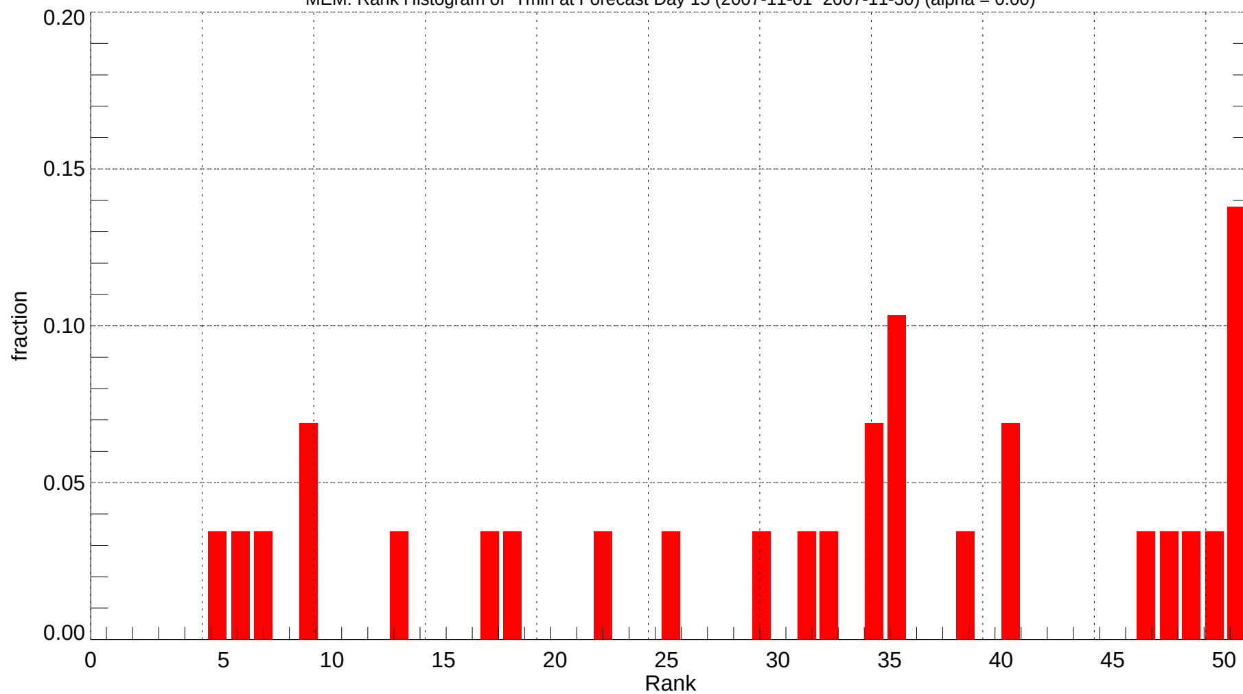
MEM: Rank Histogram of Tmin at Forecast Day 15 (2007-11-01~2007-11-30) (alpha = 0.00)
