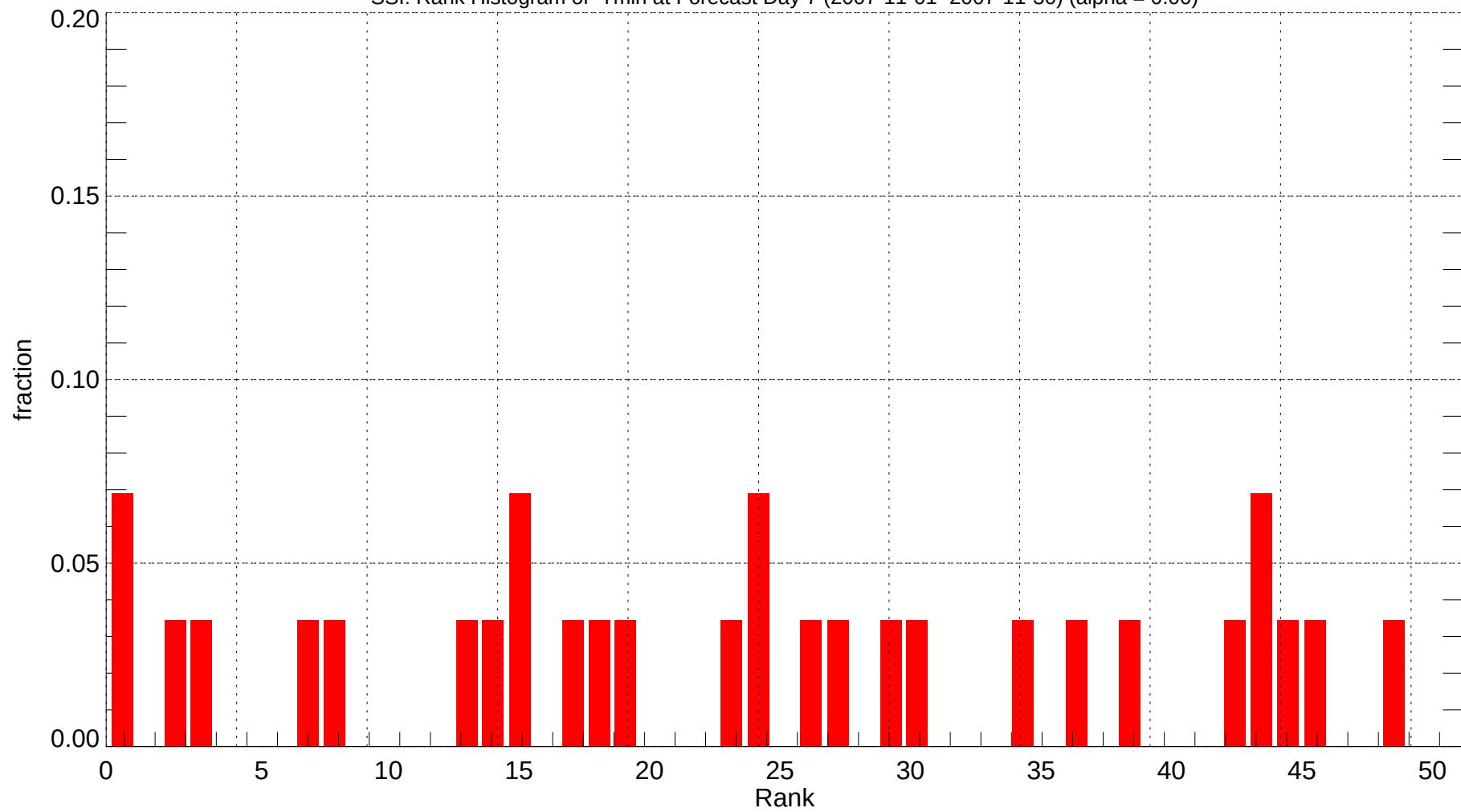
SSI: Rank Histogram of Tmin at Forecast Day 7 (2007-11-01~2007-11-30) (alpha = 0.00)
