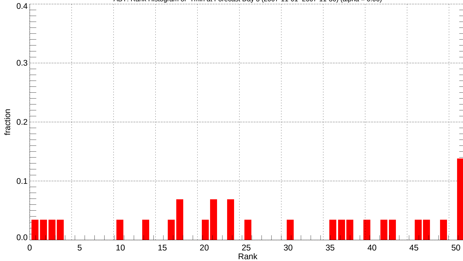
ABY: Rank Histogram of Tmin at Forecast Day 3 (2007-11-01~2007-11-30) (alpha = 0.00)
