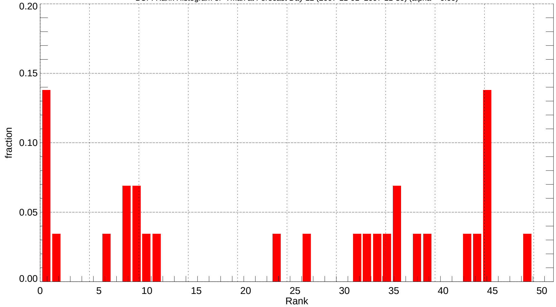
BUF: Rank Histogram of Tmax at Forecast Day 12 (2007-11-01~2007-11-30) (alpha = 0.00)
