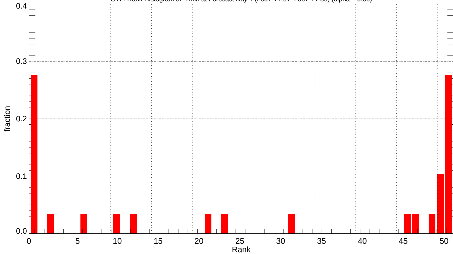
GTF: Rank Histogram of Tmin at Forecast Day 1 (2007-11-01~2007-11-30) (alpha = 0.00)
