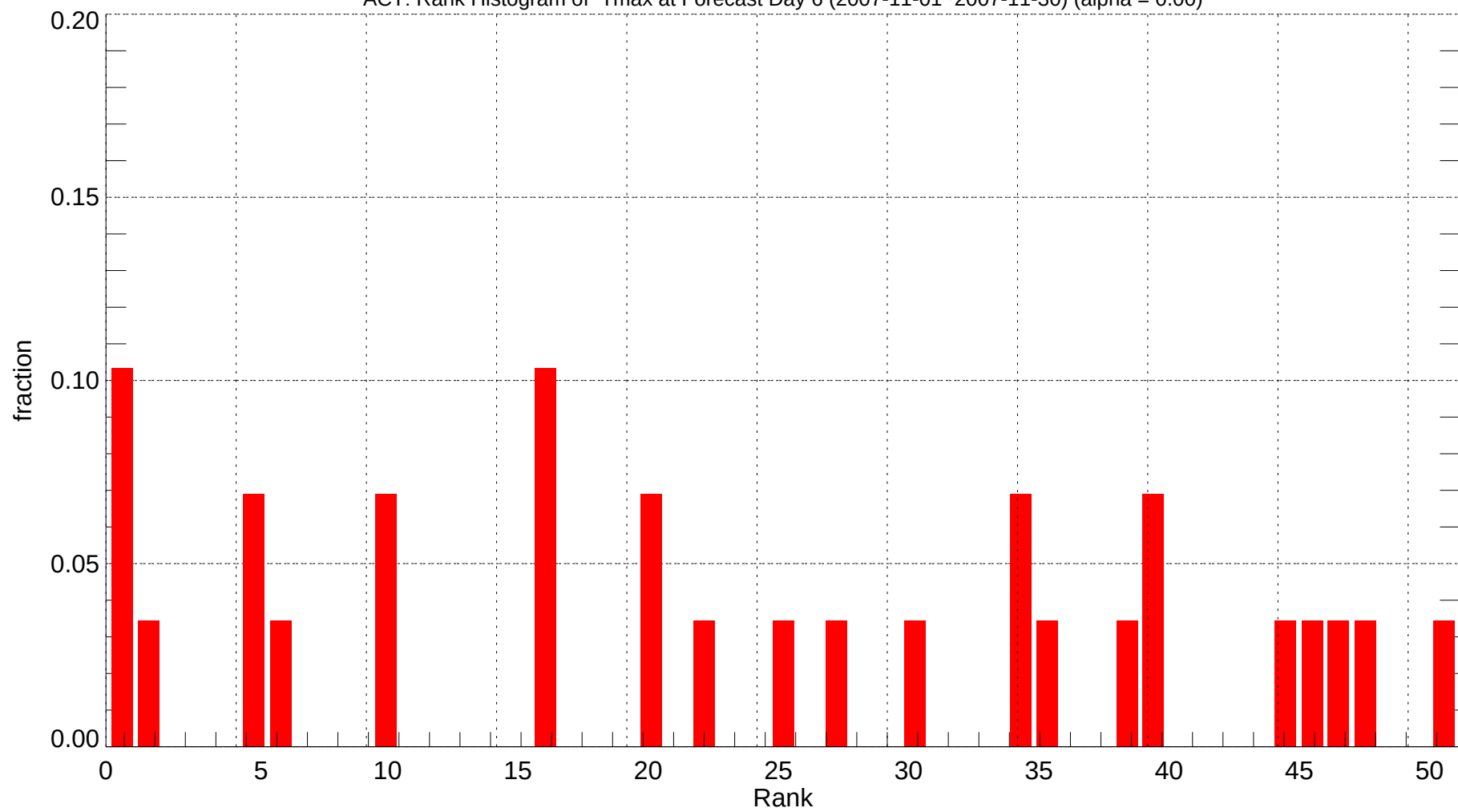
ACT: Rank Histogram of Tmax at Forecast Day 6 (2007-11-01~2007-11-30) (alpha = 0.00)
