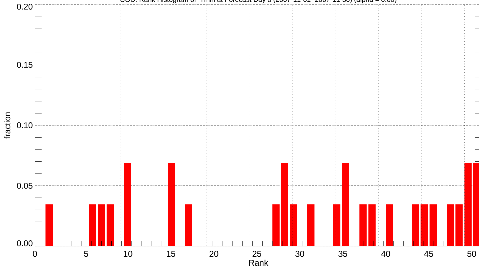
COU: Rank Histogram of Tmin at Forecast Day 8 (2007-11-01~2007-11-30) (alpha = 0.00)
