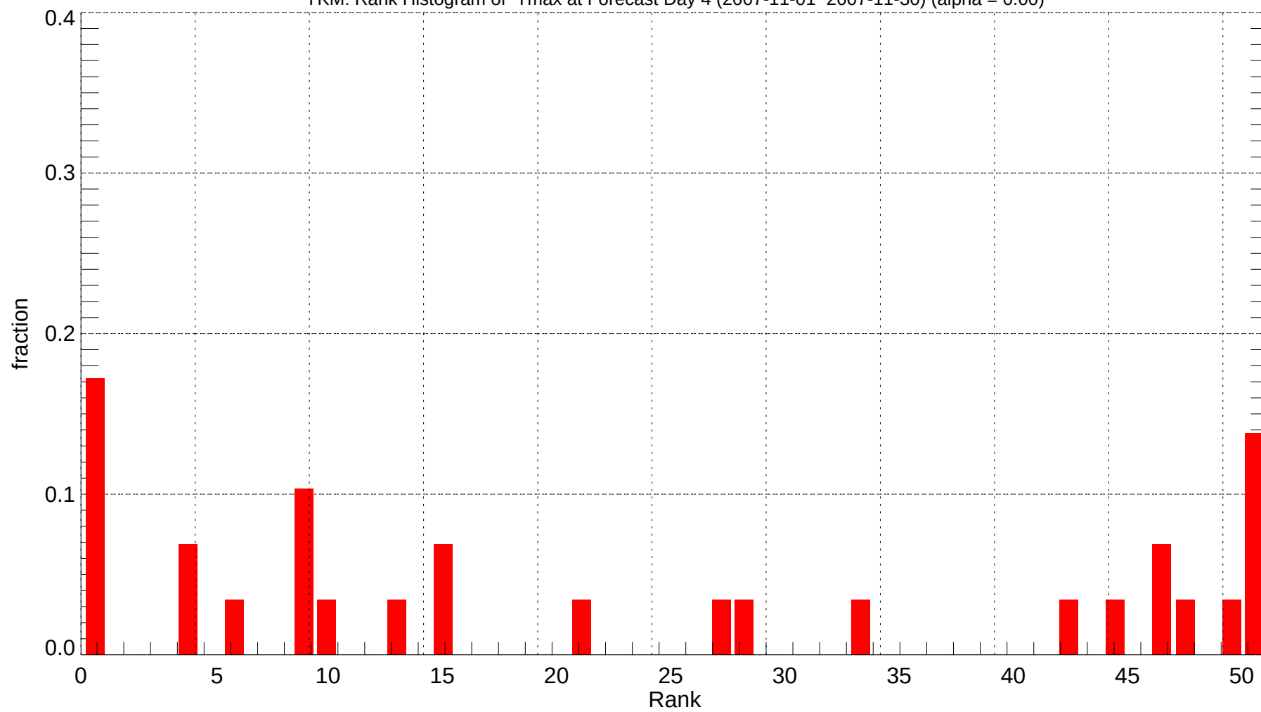
YKM: Rank Histogram of Tmax at Forecast Day 4 (2007-11-01~2007-11-30) (alpha = 0.00)
