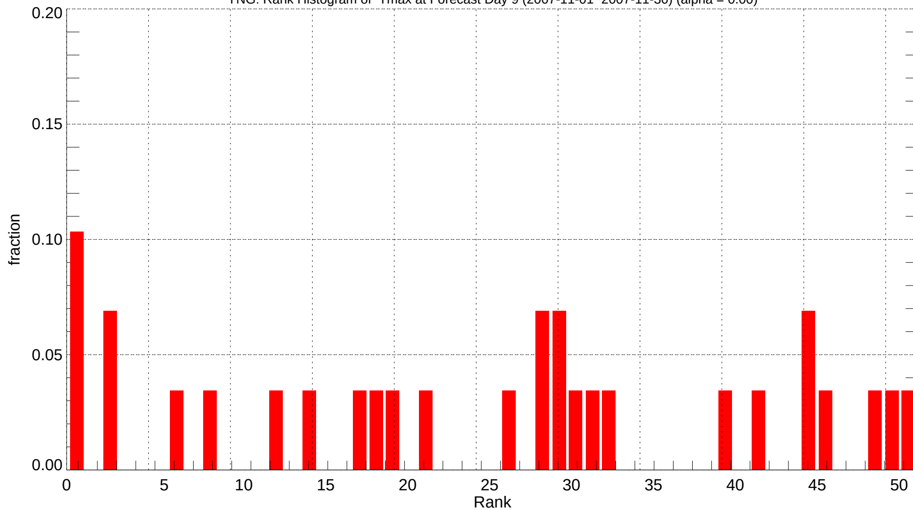
YNG: Rank Histogram of Tmax at Forecast Day 9 (2007-11-01~2007-11-30) (alpha = 0.00)
