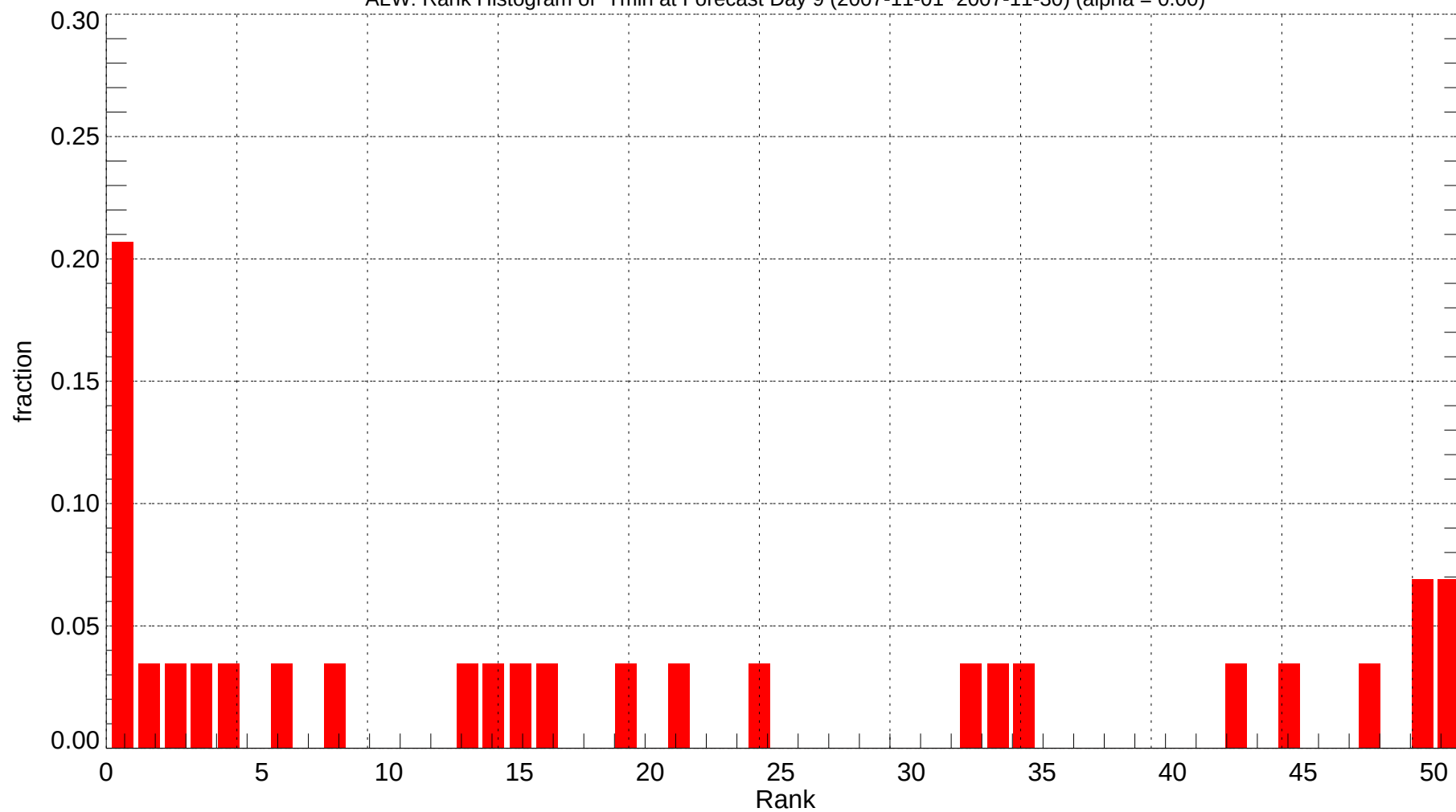
ALW: Rank Histogram of Tmin at Forecast Day 9 (2007-11-01~2007-11-30) (alpha = 0.00)
