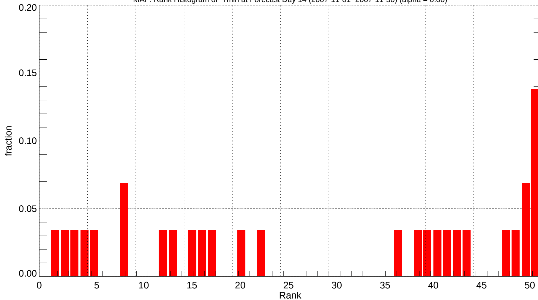
MAF: Rank Histogram of Tmin at Forecast Day 14 (2007-11-01~2007-11-30) (alpha = 0.00)
