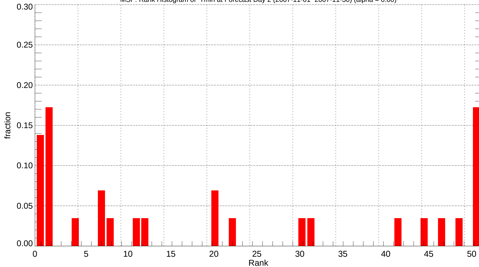
MSP: Rank Histogram of Tmin at Forecast Day 2 (2007-11-01~2007-11-30) (alpha = 0.00)
