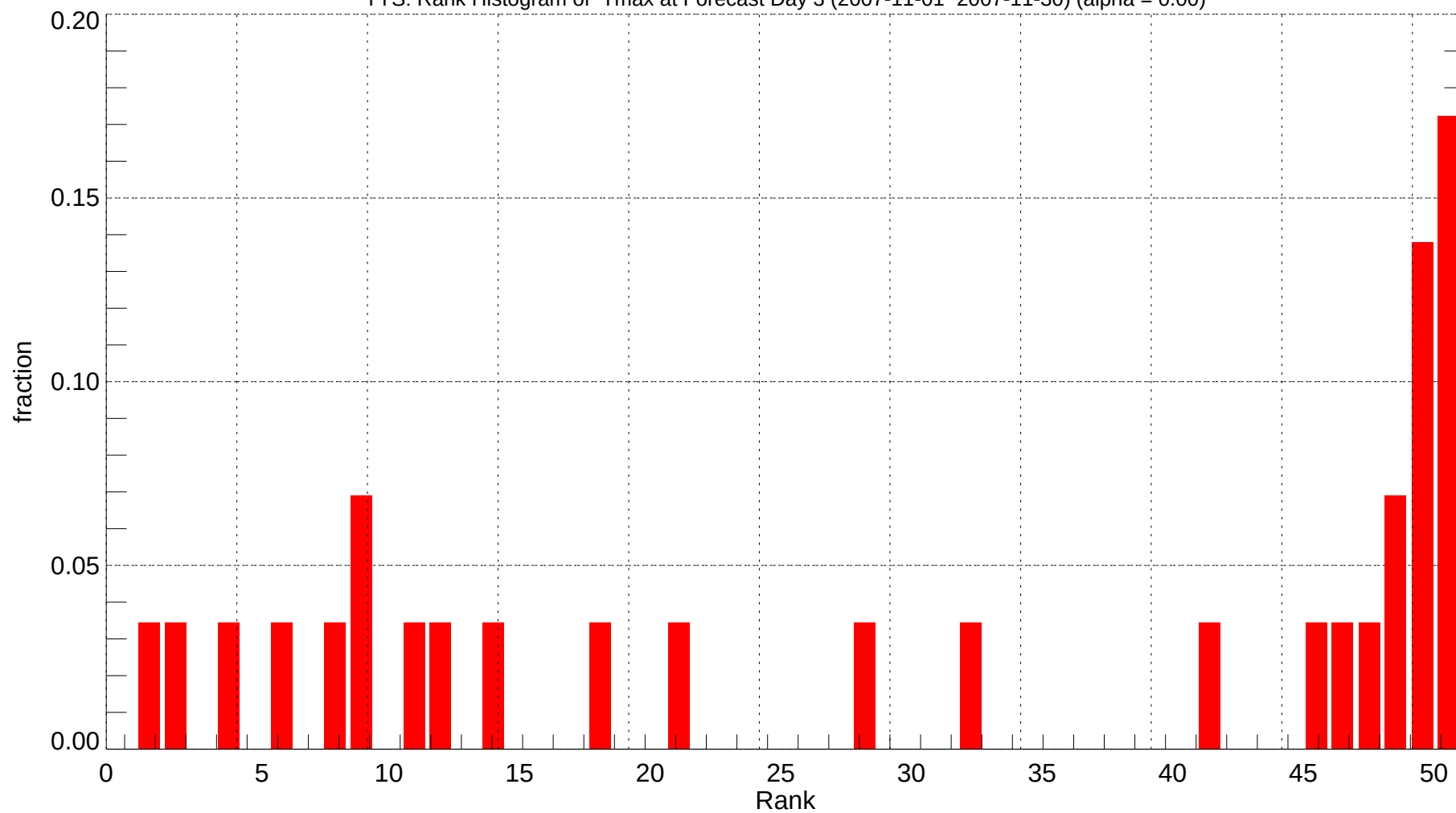
TYS: Rank Histogram of Tmax at Forecast Day 3 (2007-11-01~2007-11-30) (alpha = 0.00)
