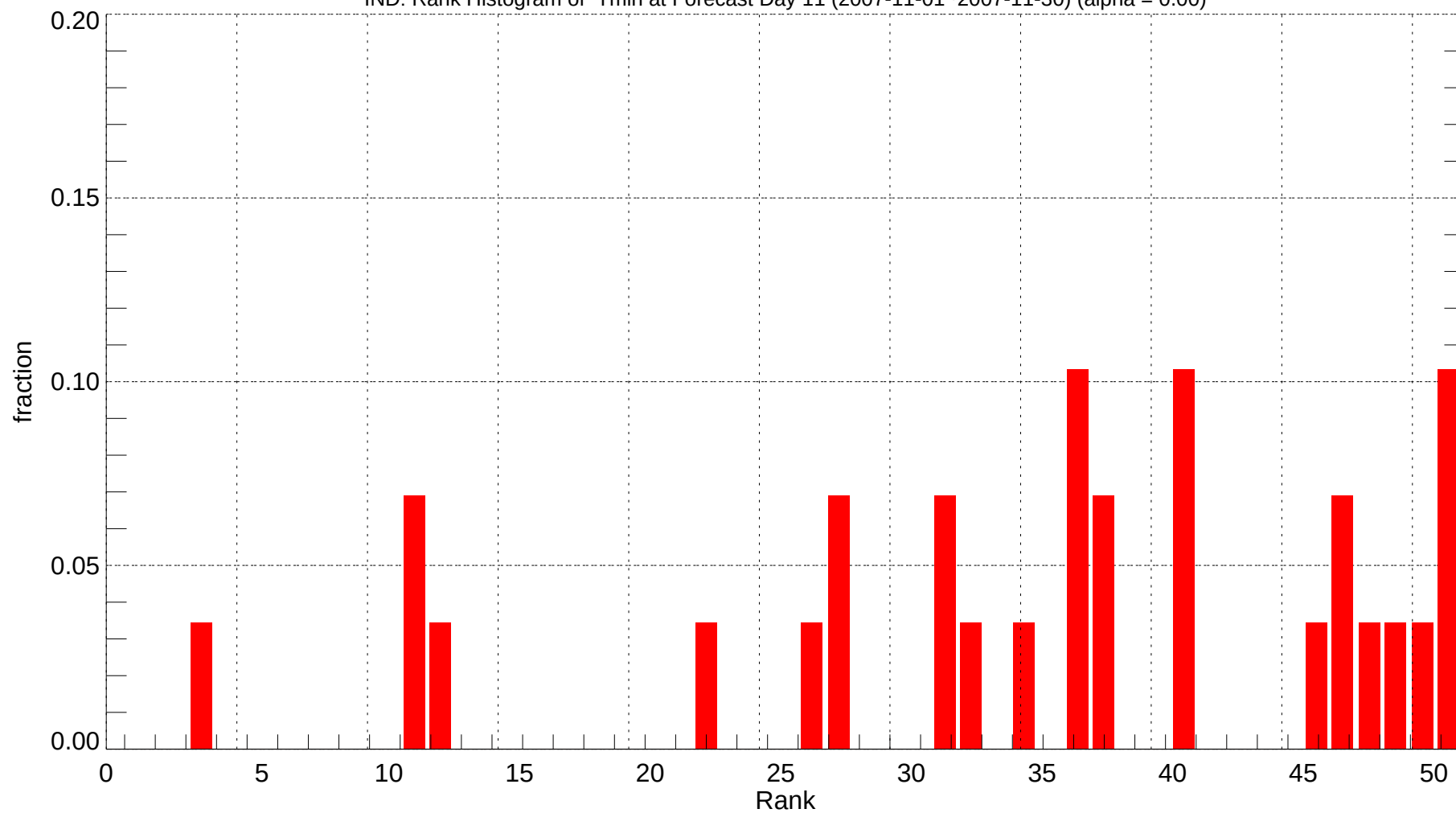
IND: Rank Histogram of Tmin at Forecast Day 11 (2007-11-01~2007-11-30) (alpha = 0.00)
