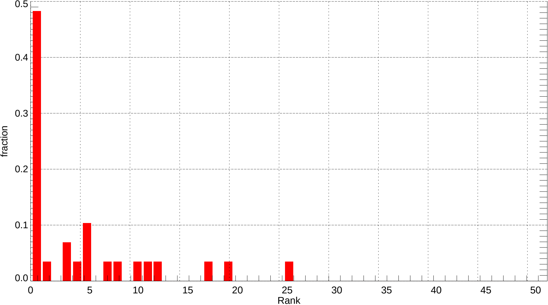
SJC: Rank Histogram of Tmin at Forecast Day 6 (2007-11-01~2007-11-30) (alpha = 0.00)
