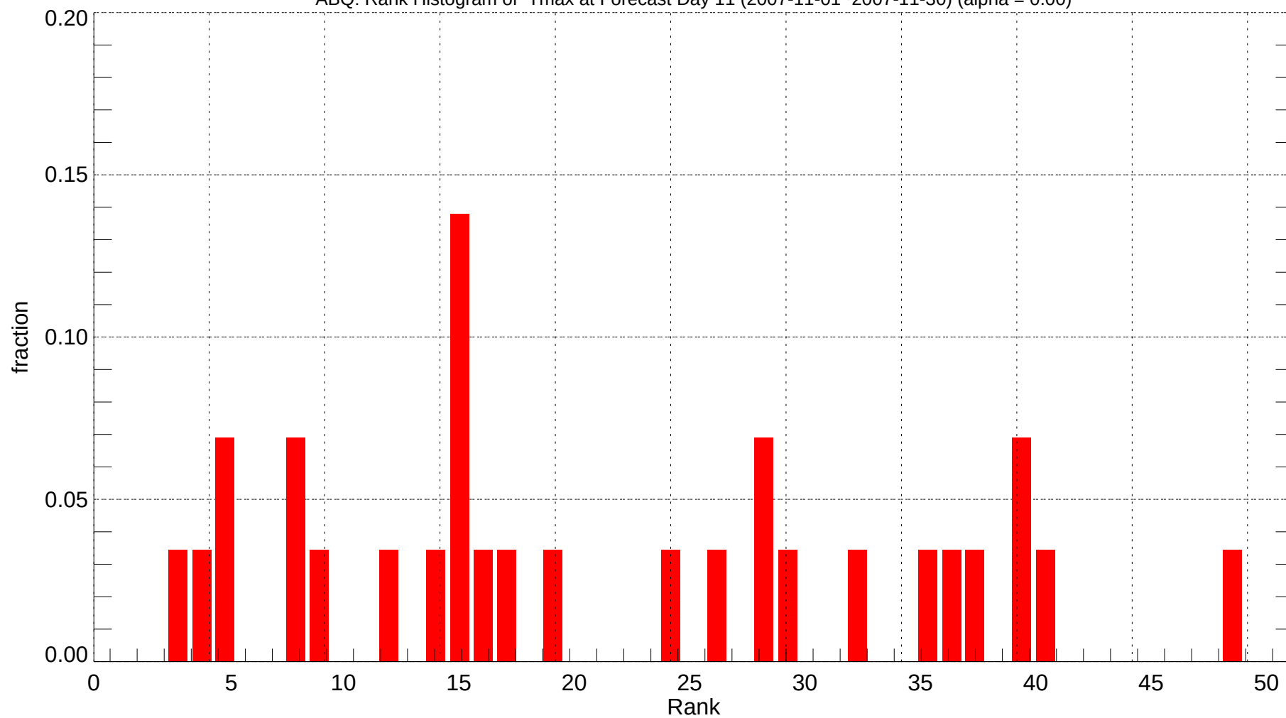
ABQ: Rank Histogram of Tmax at Forecast Day 11 (2007-11-01~2007-11-30) (alpha = 0.00)
