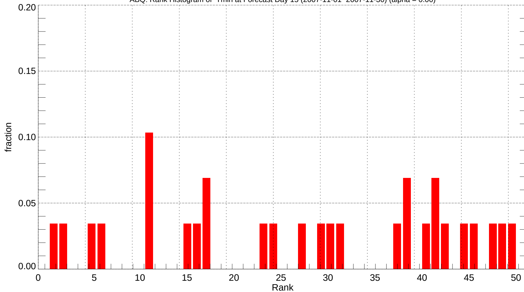
ABQ: Rank Histogram of Tmin at Forecast Day 15 (2007-11-01~2007-11-30) (alpha = 0.00)
