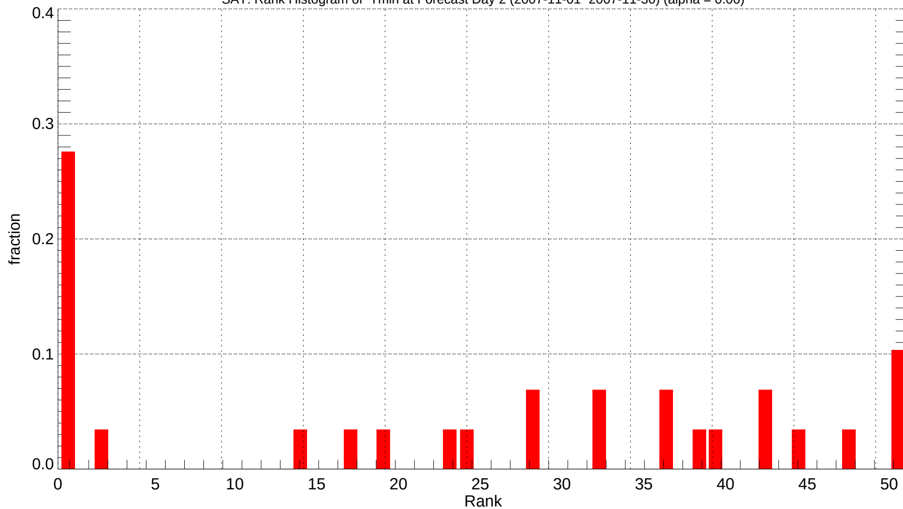
SAT: Rank Histogram of Tmin at Forecast Day 2 (2007-11-01~2007-11-30) (alpha = 0.00)
