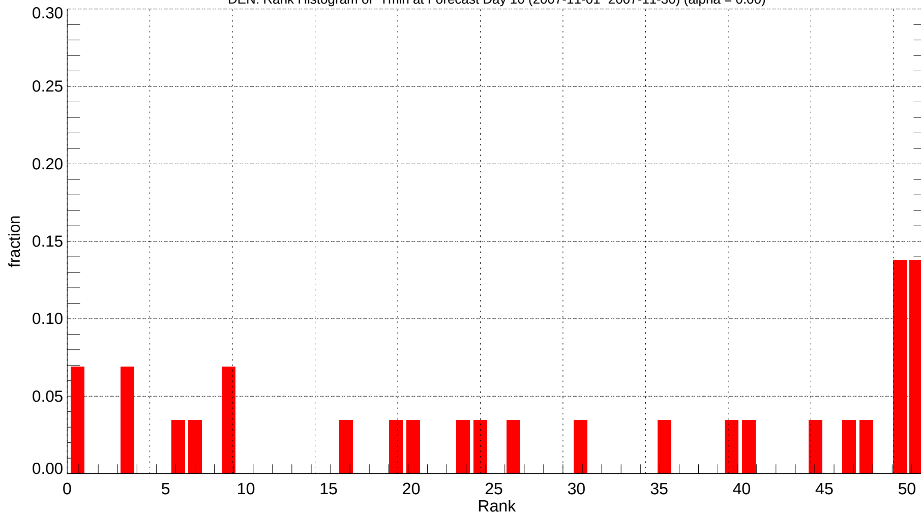
DEN: Rank Histogram of Tmin at Forecast Day 10 (2007-11-01~2007-11-30) (alpha = 0.00)
