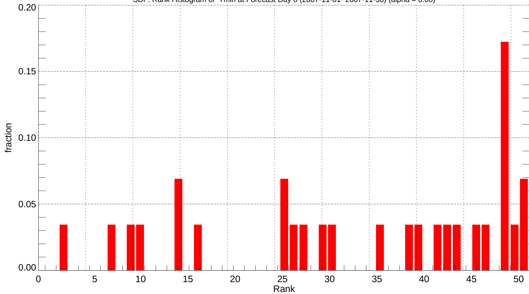
SDF: Rank Histogram of Tmin at Forecast Day 8 (2007-11-01~2007-11-30) (alpha = 0.00)
