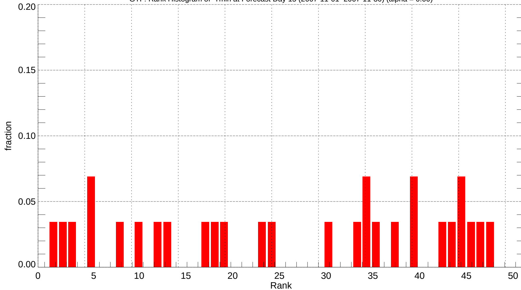
GTF: Rank Histogram of Tmin at Forecast Day 15 (2007-11-01~2007-11-30) (alpha = 0.00)
