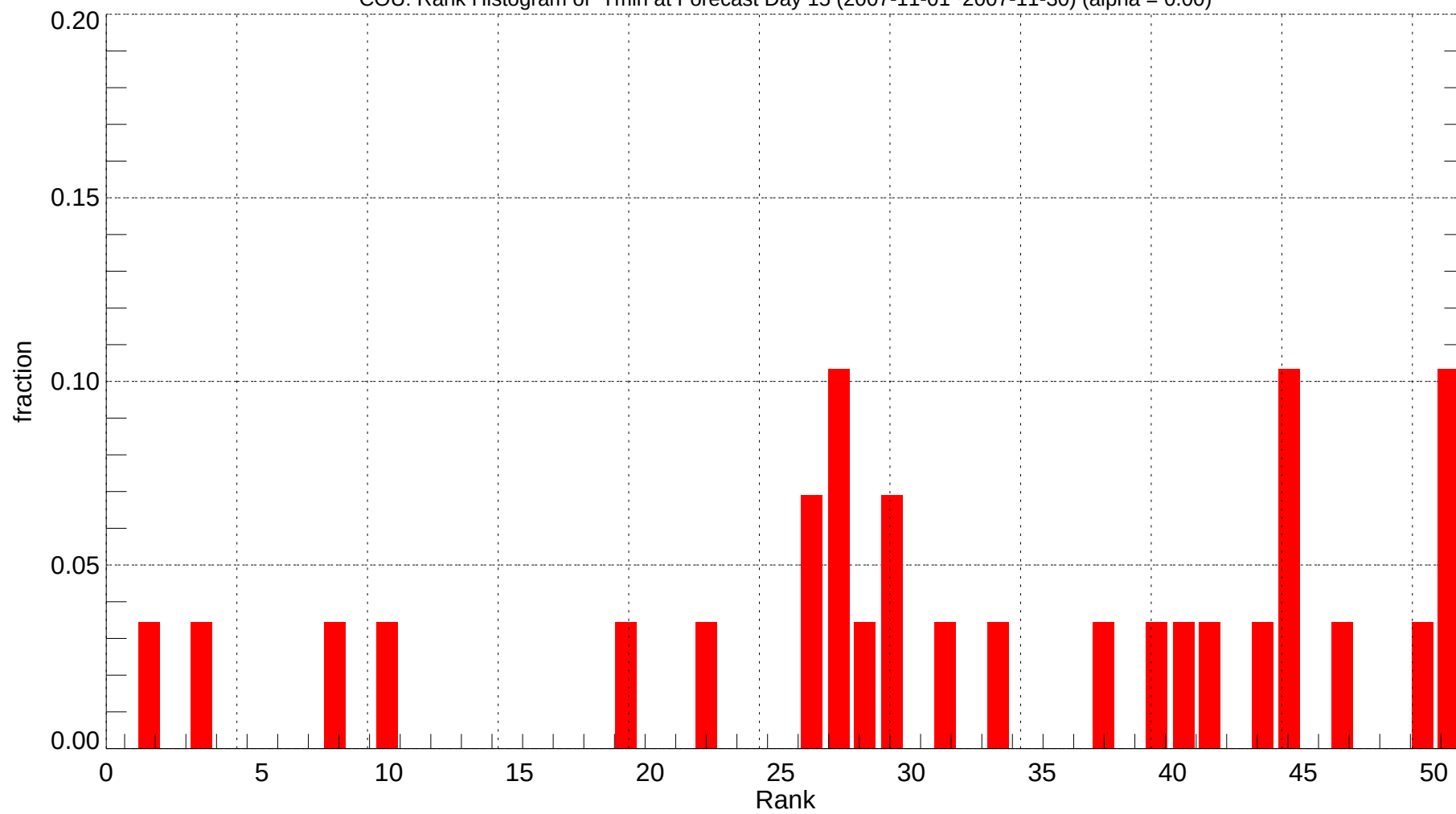
COU: Rank Histogram of Tmin at Forecast Day 15 (2007-11-01~2007-11-30) (alpha = 0.00)
