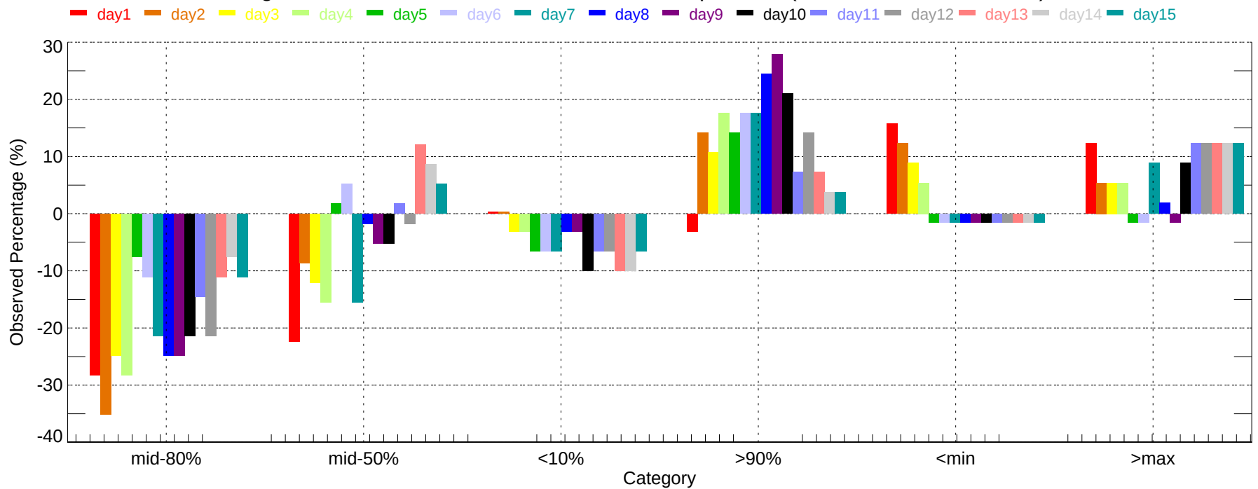
Observed Percentage Deviation of Ensembles - DAY: Max Temperature (2007-11-01~2007-11-30)
