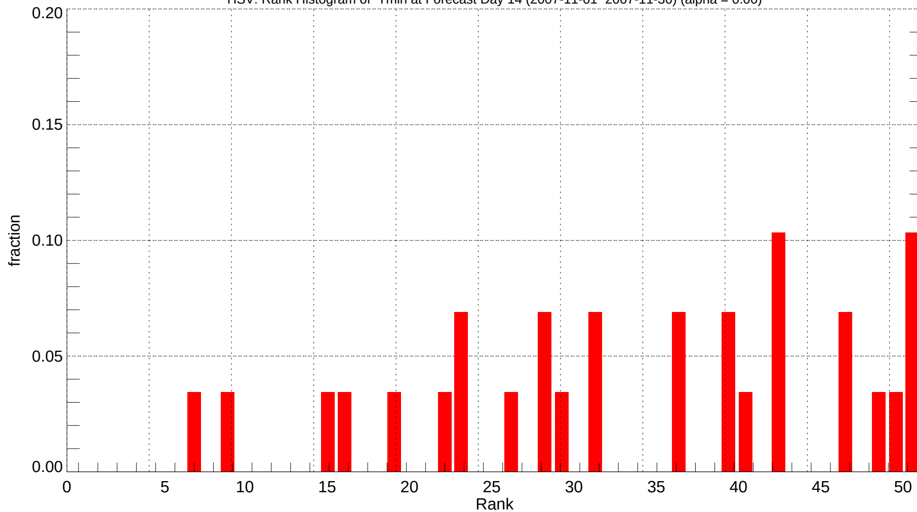
HSV: Rank Histogram of Tmin at Forecast Day 14 (2007-11-01~2007-11-30) (alpha = 0.00)
