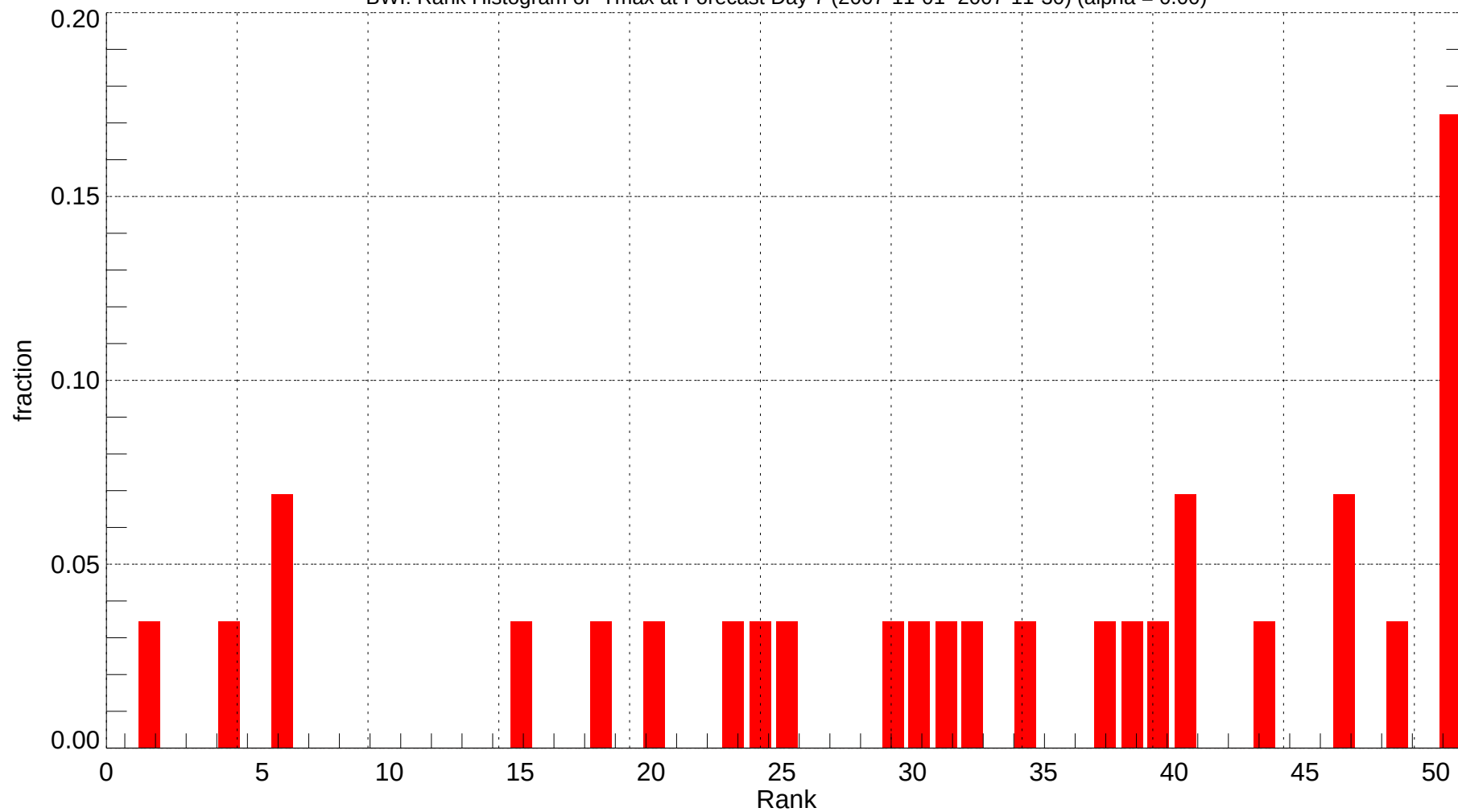
BWI: Rank Histogram of Tmax at Forecast Day 7 (2007-11-01~2007-11-30) (alpha = 0.00)
