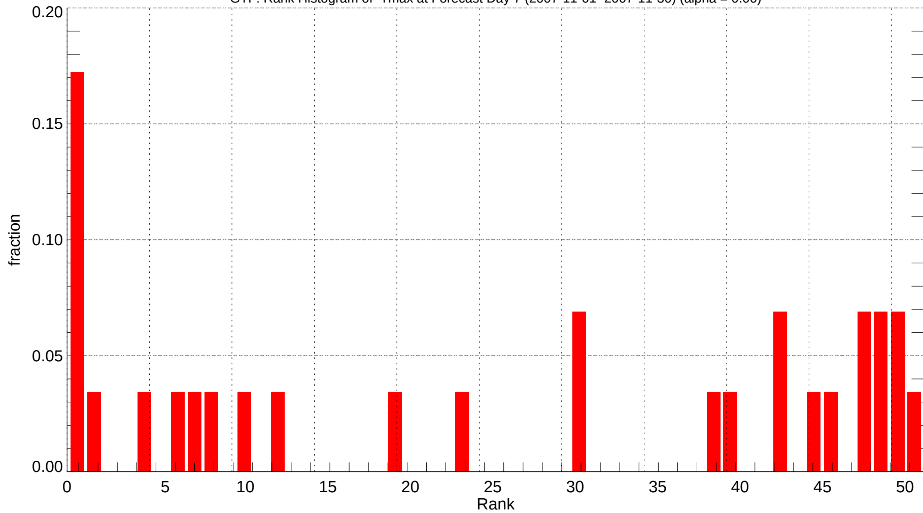
GTF: Rank Histogram of Tmax at Forecast Day 7 (2007-11-01~2007-11-30) (alpha = 0.00)
