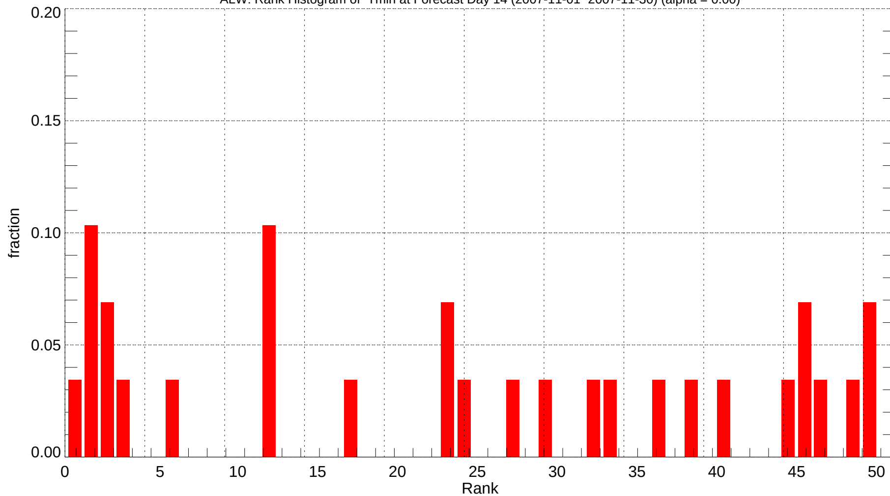
ALW: Rank Histogram of Tmin at Forecast Day 14 (2007-11-01~2007-11-30) (alpha = 0.00)
