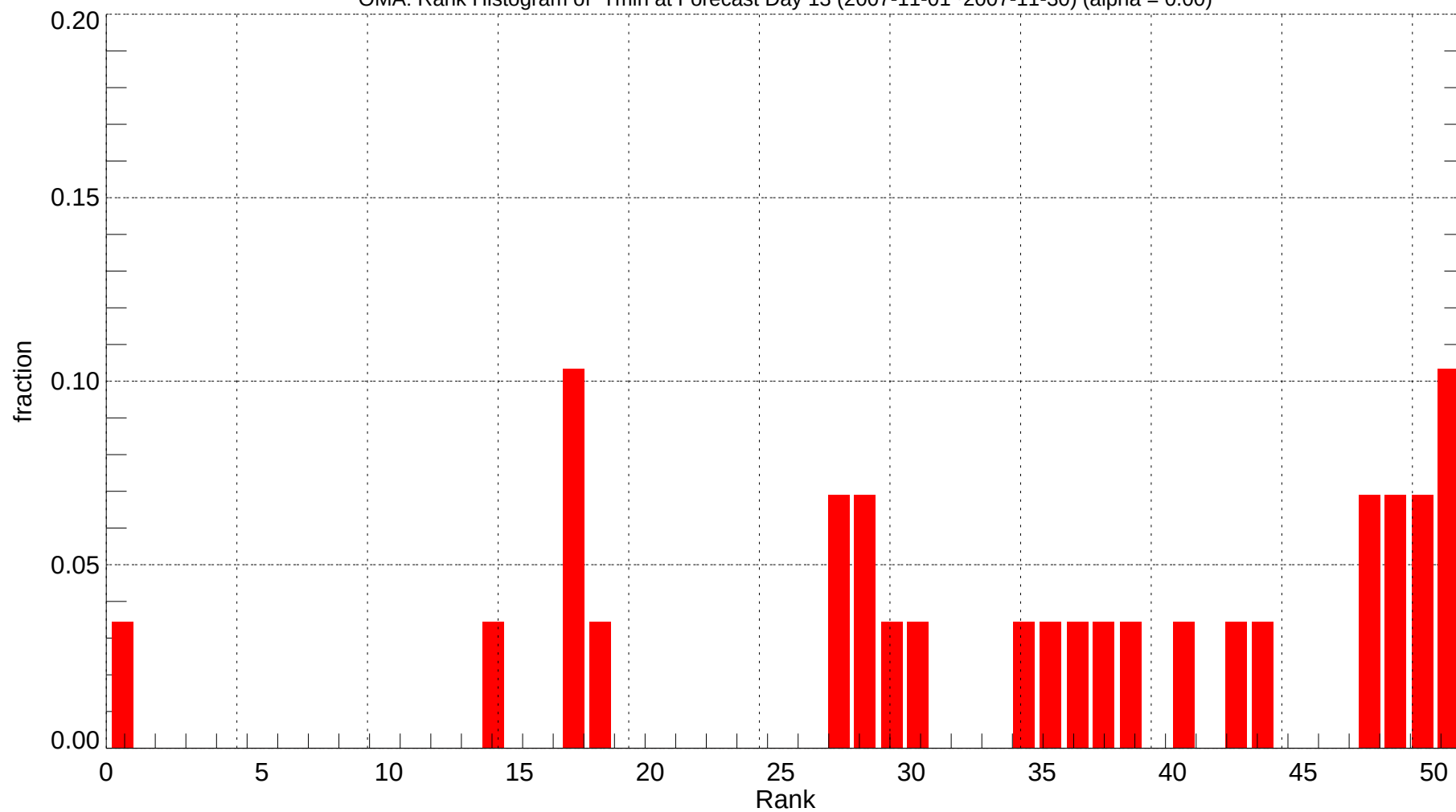
OMA: Rank Histogram of Tmin at Forecast Day 13 (2007-11-01~2007-11-30) (alpha = 0.00)
