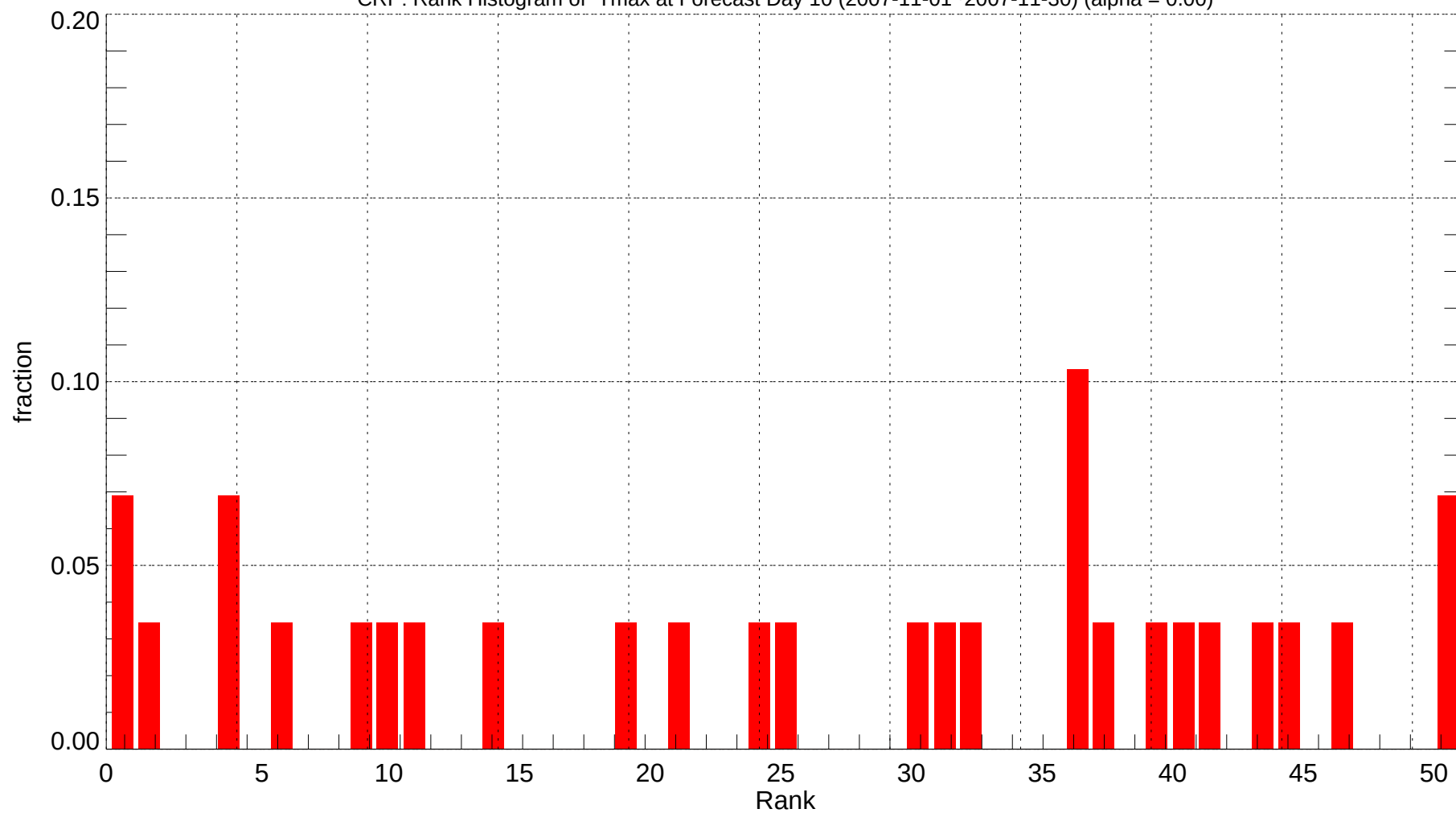
CRP: Rank Histogram of Tmax at Forecast Day 10 (2007-11-01~2007-11-30) (alpha = 0.00)
