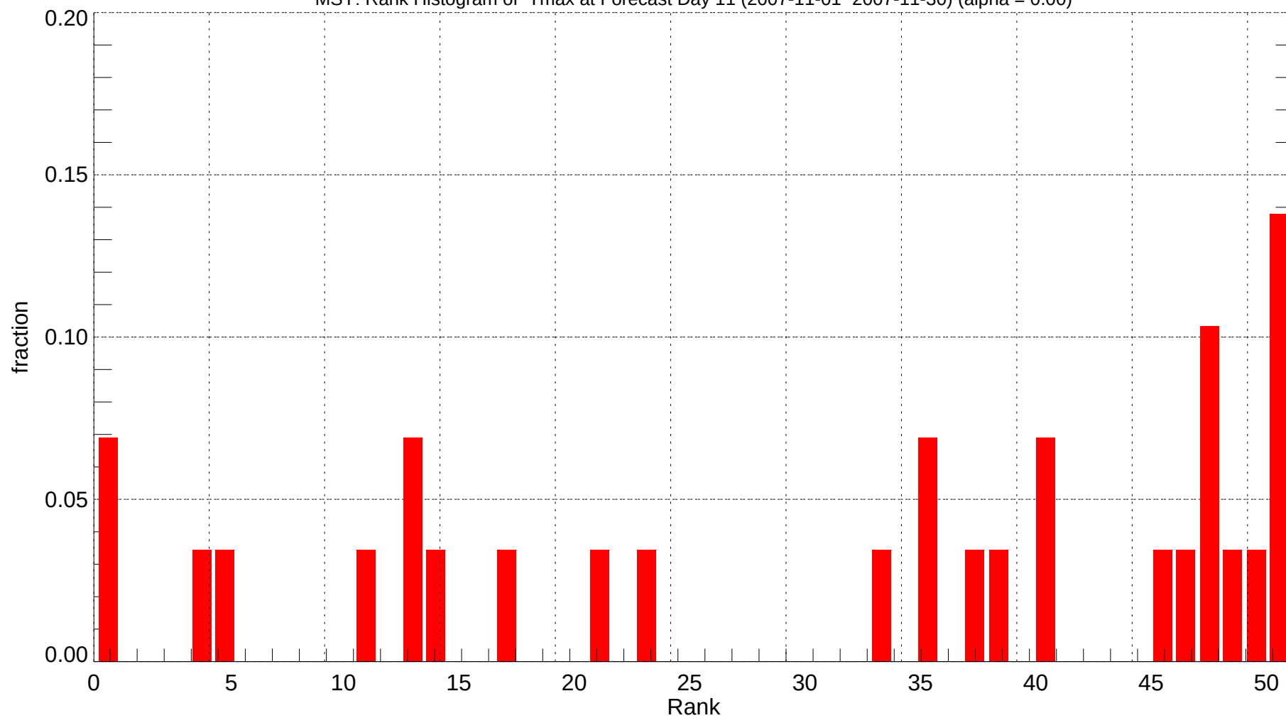
MSY: Rank Histogram of Tmax at Forecast Day 11 (2007-11-01~2007-11-30) (alpha = 0.00)
