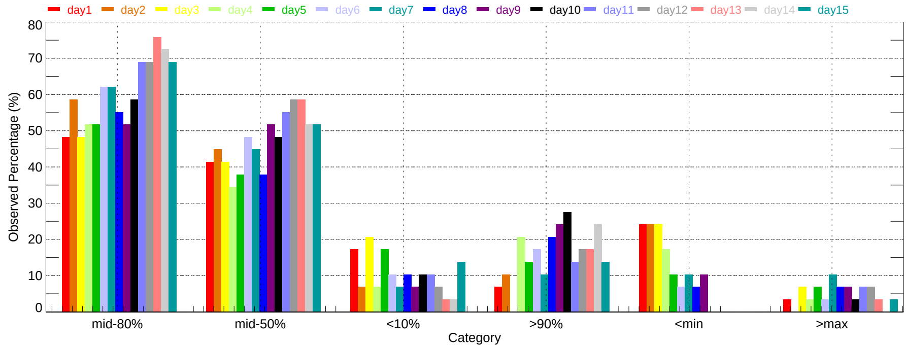
Observed Percentage of Ensembles - ORD: Max Temperature (2007-11-01~2007-11-30)
