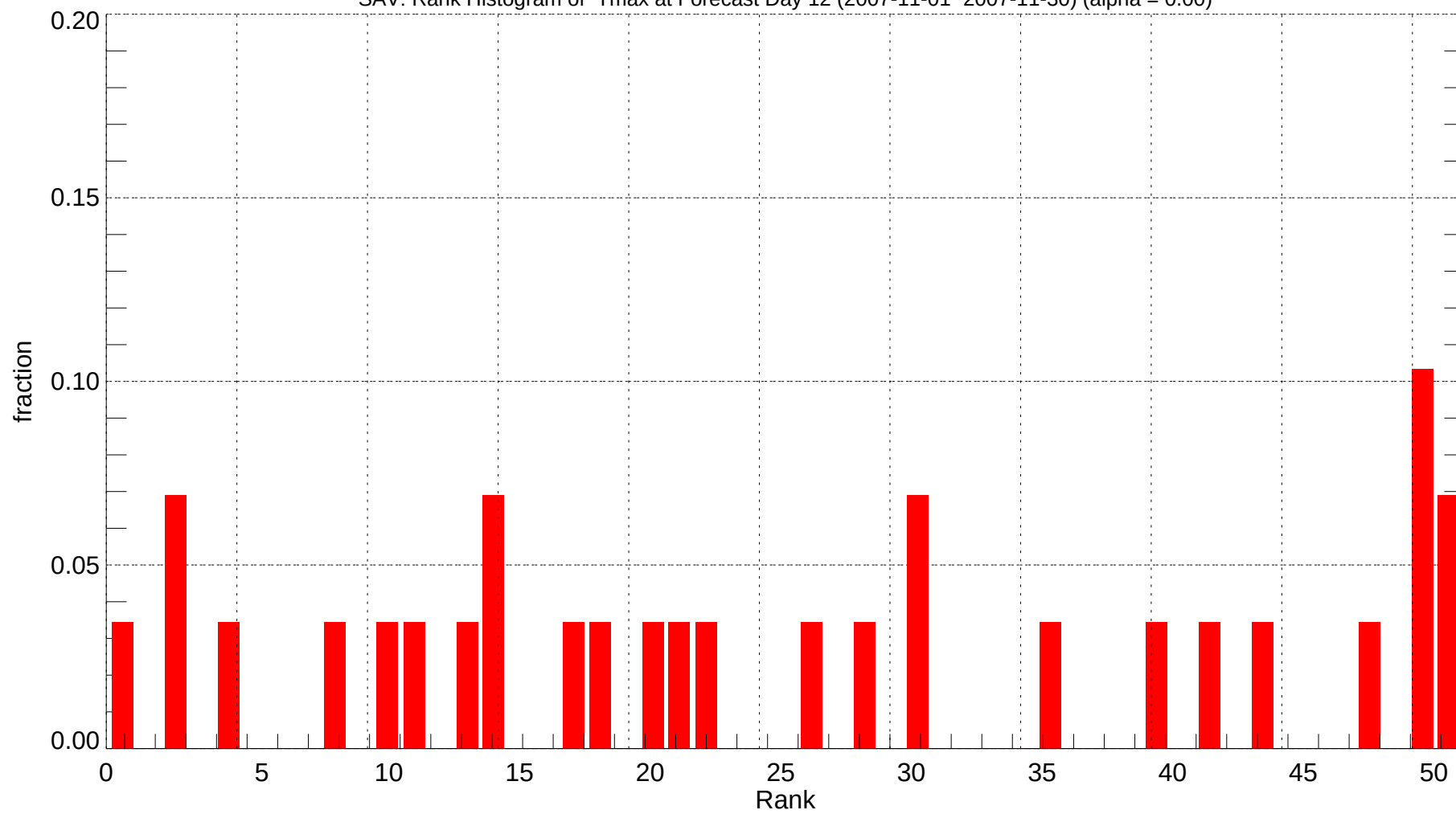
SAV: Rank Histogram of Tmax at Forecast Day 12 (2007-11-01~2007-11-30) (alpha = 0.00)
