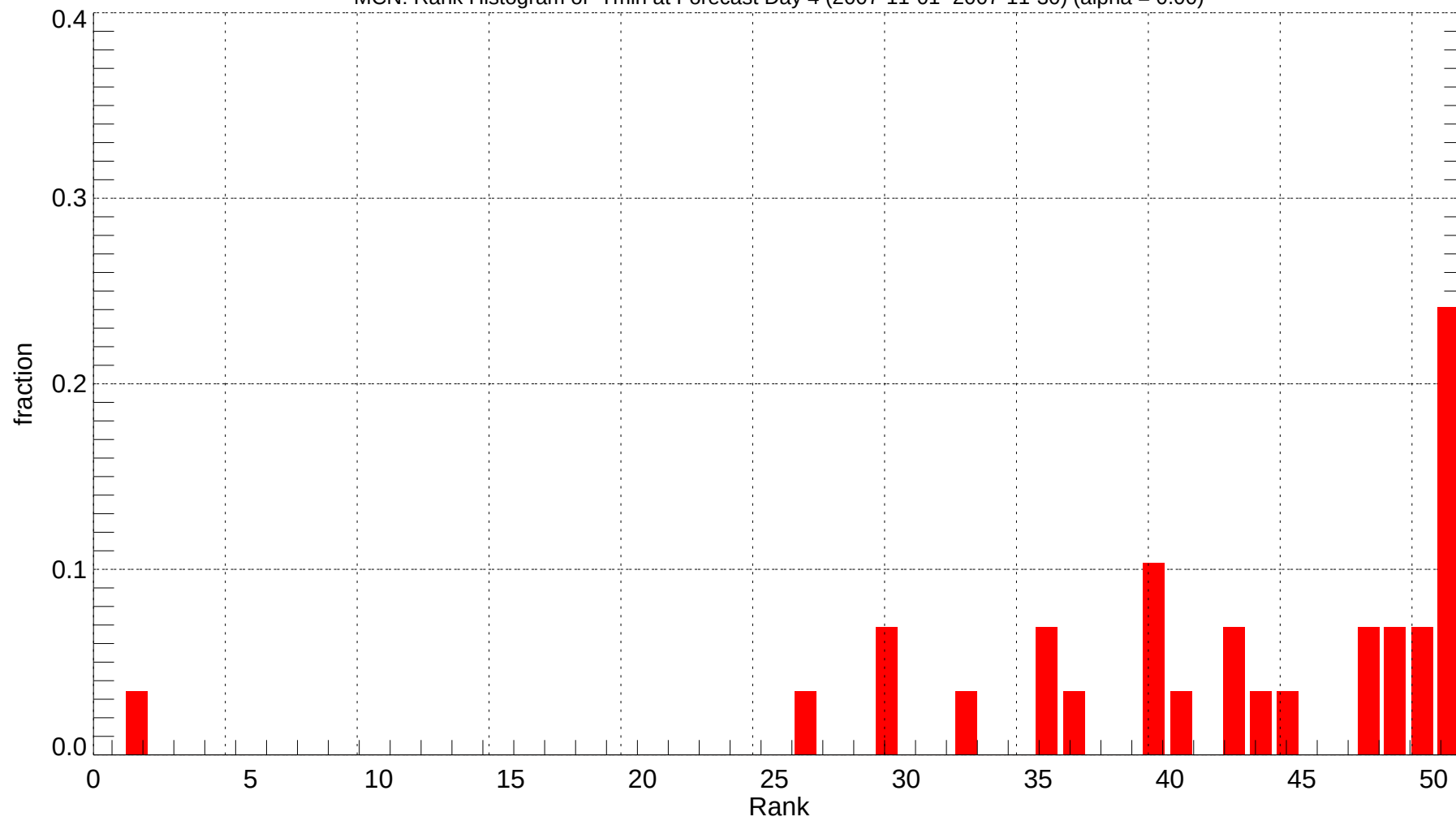
MCN: Rank Histogram of Tmin at Forecast Day 4 (2007-11-01~2007-11-30) (alpha = 0.00)
