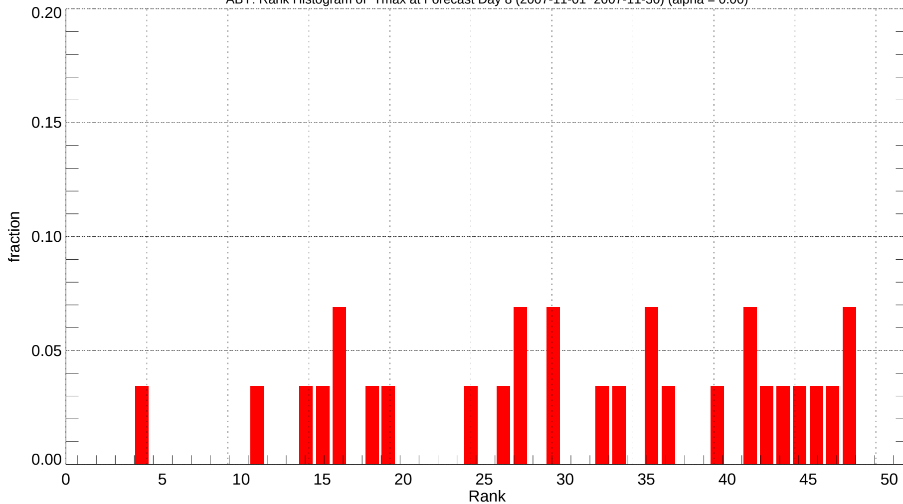
ABY: Rank Histogram of Tmax at Forecast Day 8 (2007-11-01~2007-11-30) (alpha = 0.00)
