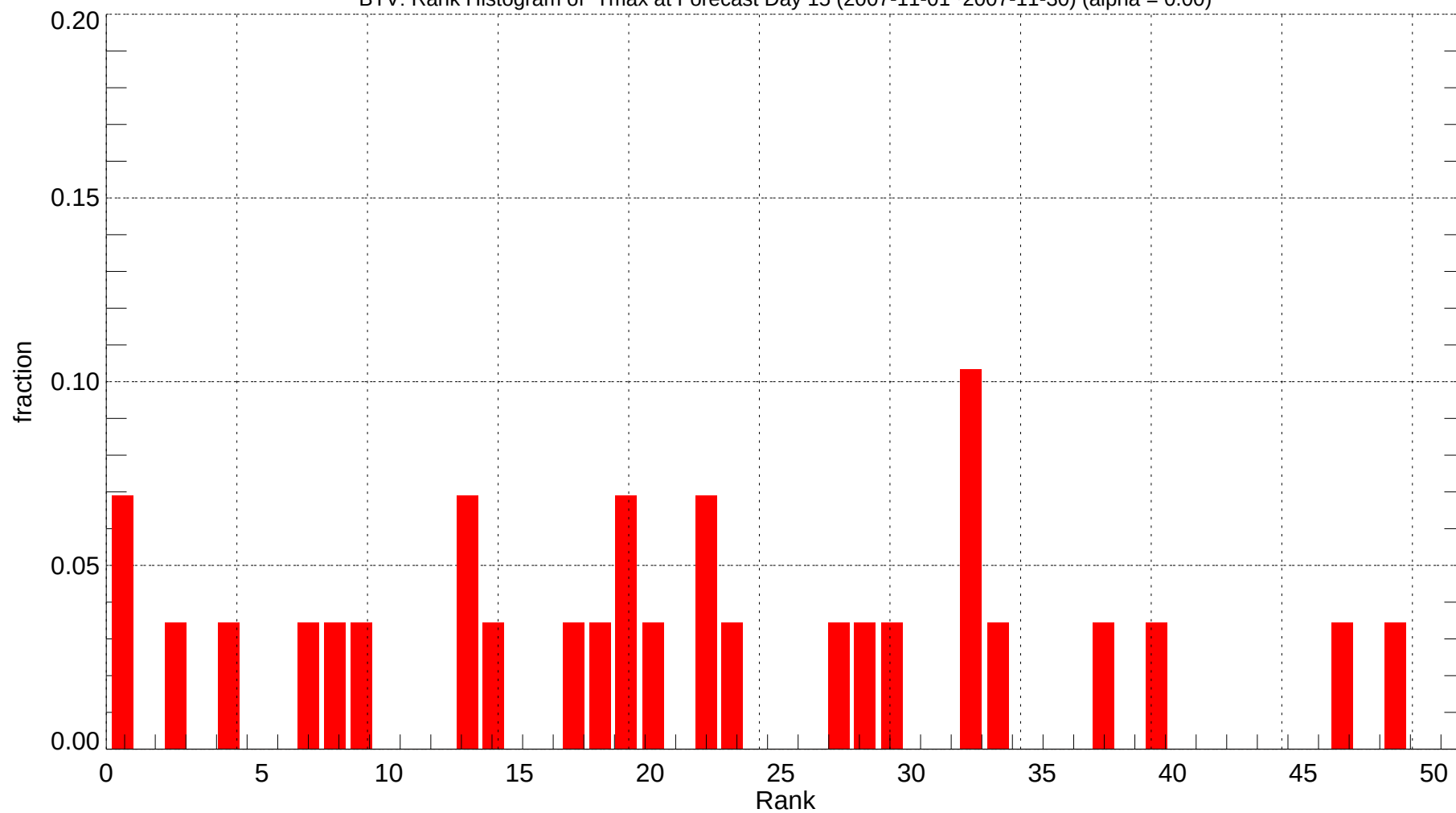
BTV: Rank Histogram of Tmax at Forecast Day 15 (2007-11-01~2007-11-30) (alpha = 0.00)
