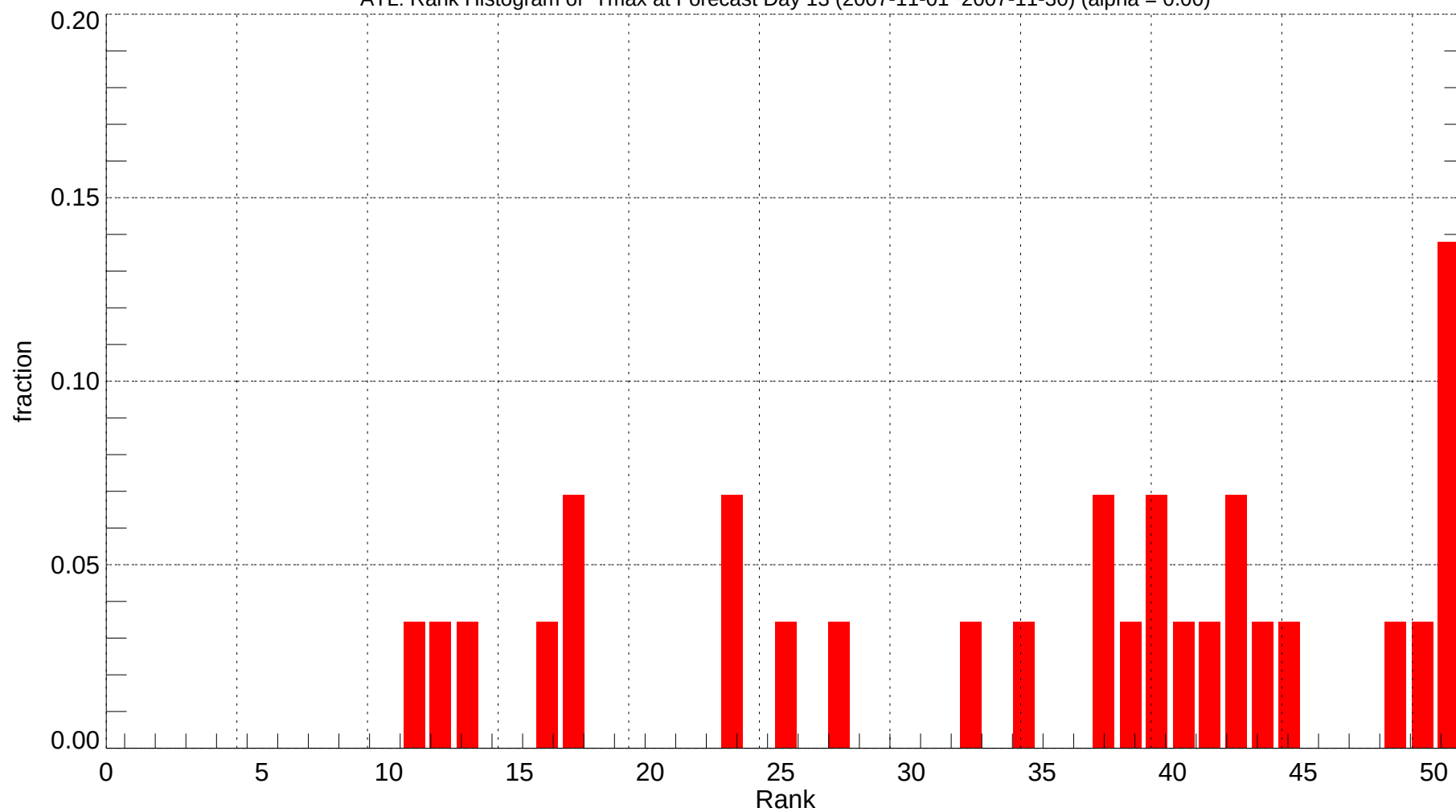
ATL: Rank Histogram of Tmax at Forecast Day 13 (2007-11-01~2007-11-30) (alpha = 0.00)
