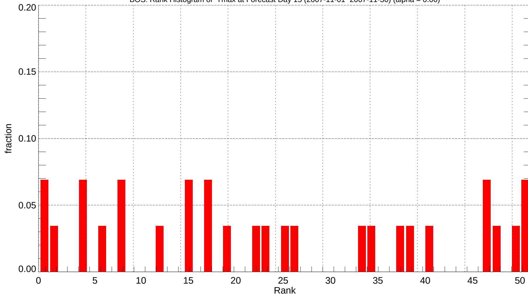
BOS: Rank Histogram of Tmax at Forecast Day 15 (2007-11-01~2007-11-30) (alpha = 0.00)
