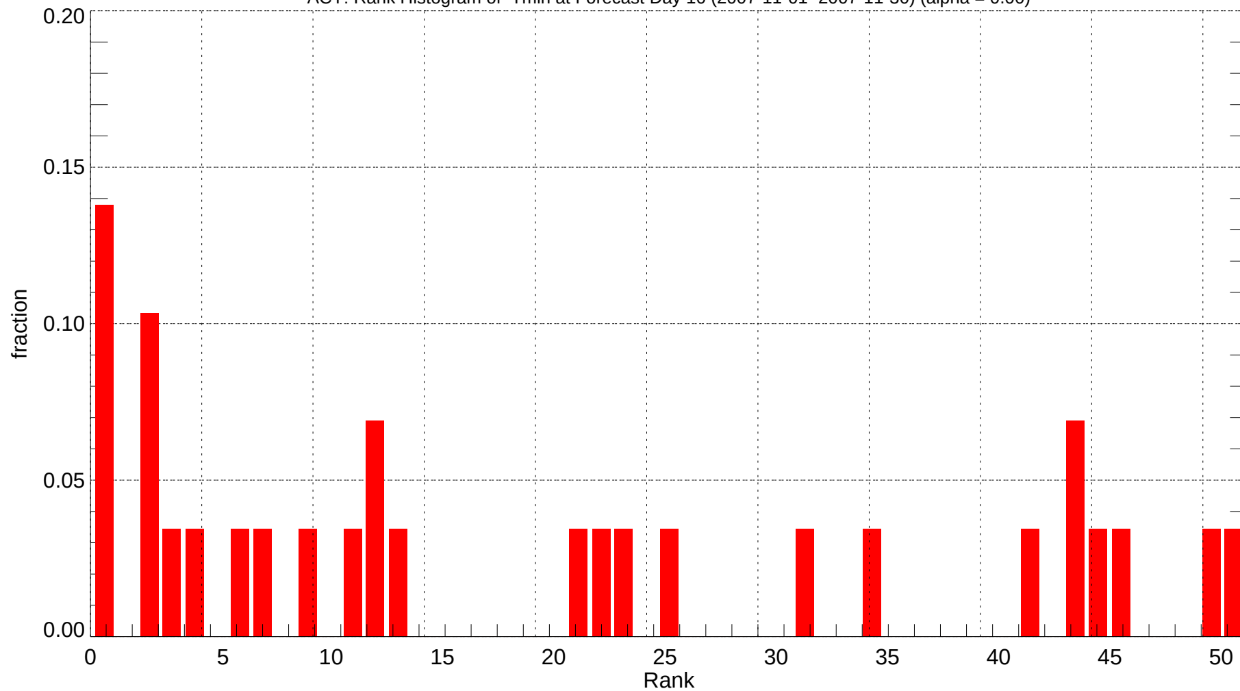
ACY: Rank Histogram of Tmin at Forecast Day 10 (2007-11-01~2007-11-30) (alpha = 0.00)
