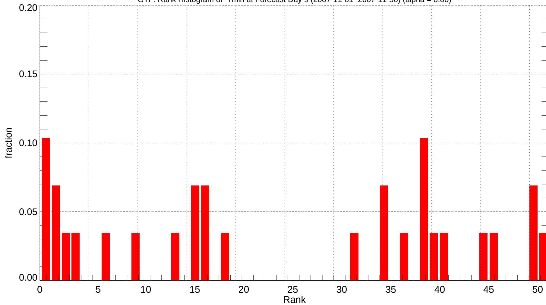
GTF: Rank Histogram of Tmin at Forecast Day 9 (2007-11-01~2007-11-30) (alpha = 0.00)
