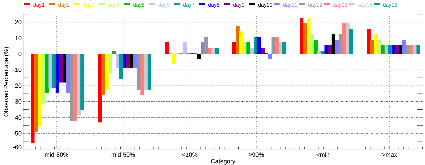
Observed Percentage Deviation of Ensembles - BGM: Min Temperature (2007-11-01~2007-11-30)
