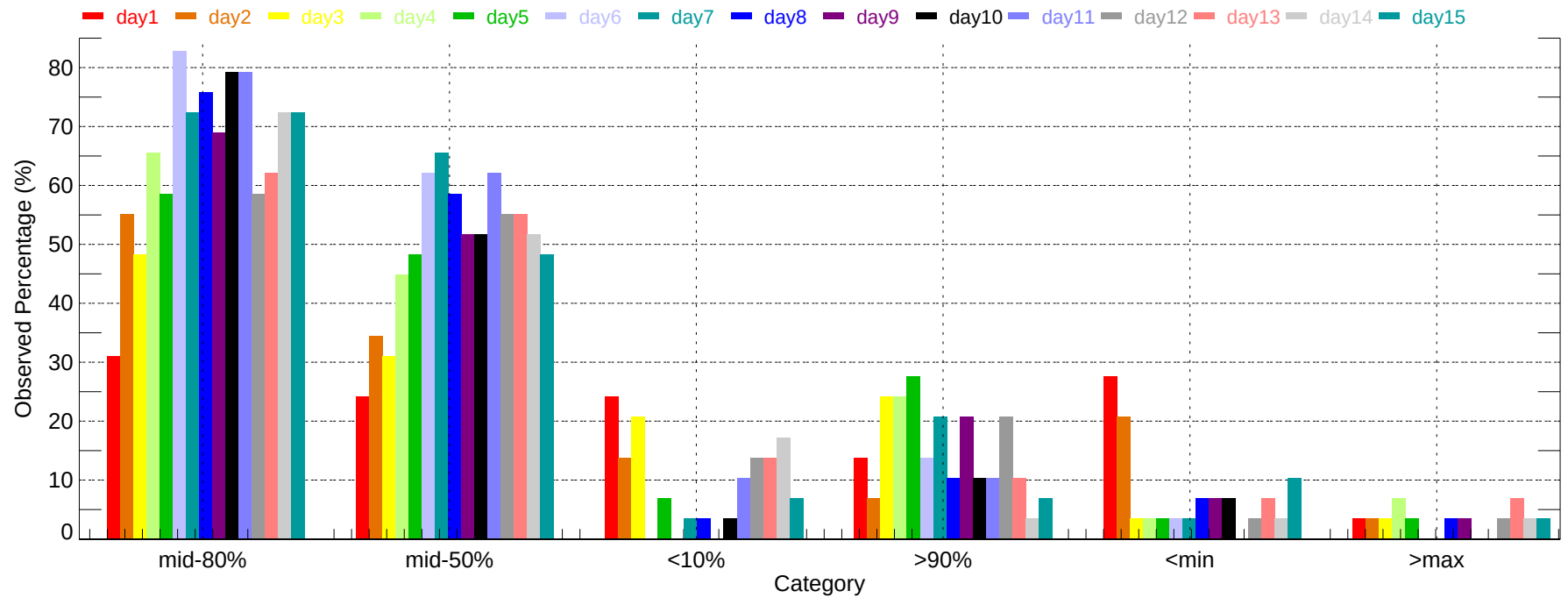
Observed Percentage of Ensembles - APN: Max Temperature (2007-11-01~2007-11-30)
