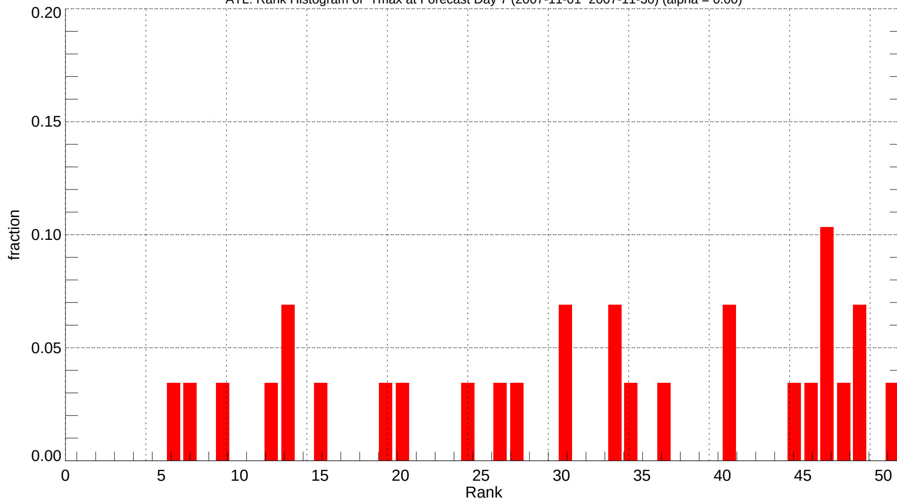
ATL: Rank Histogram of Tmax at Forecast Day 7 (2007-11-01~2007-11-30) (alpha = 0.00)
