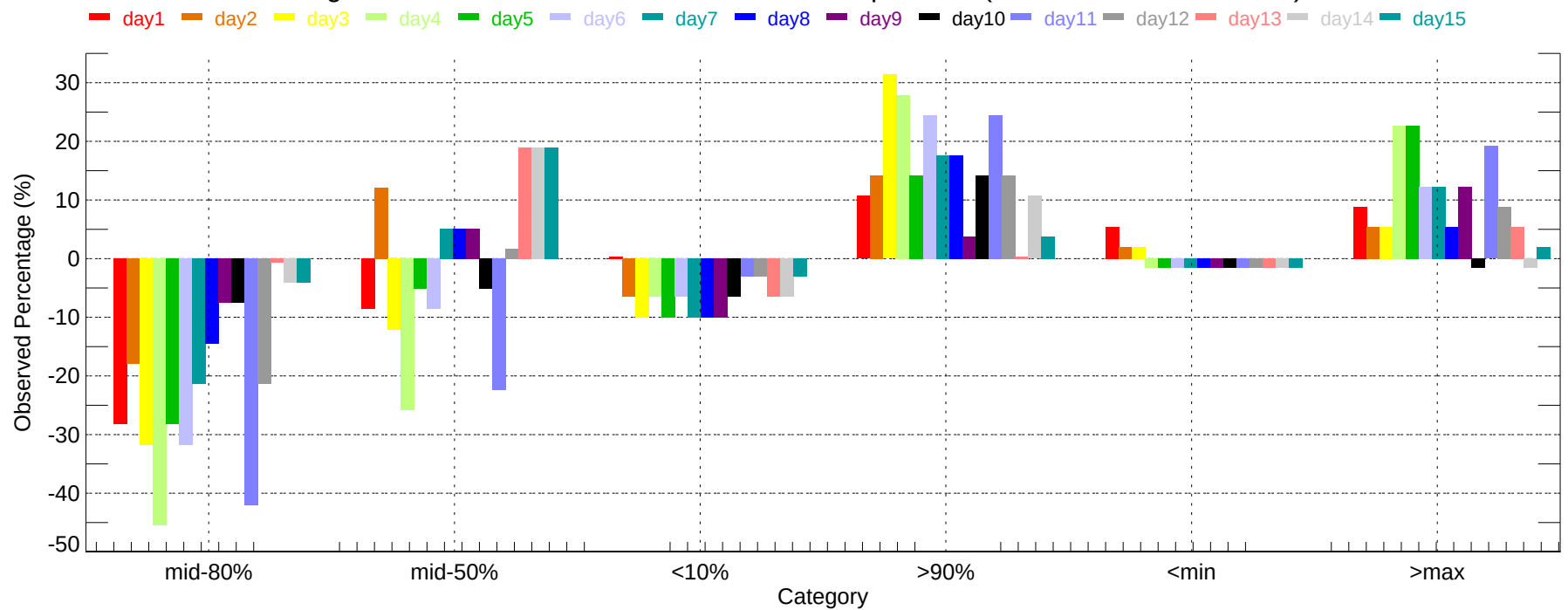
Observed Percentage Deviation of Ensembles - MCN: Min Temperature (2007-11-01~2007-11-30)
