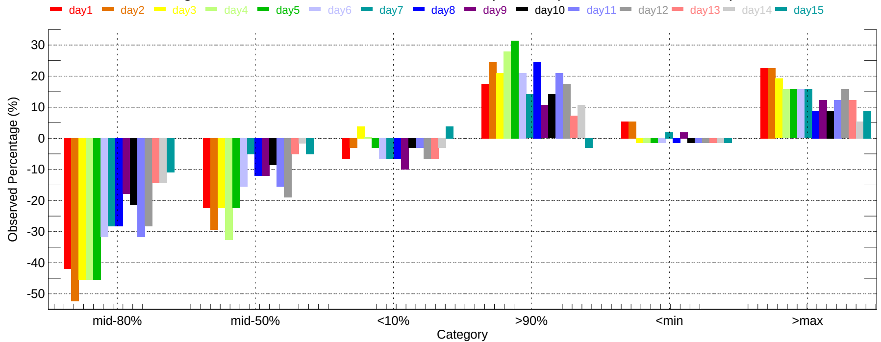
Observed Percentage Deviation of Ensembles - ROA: Max Temperature (2007-11-01~2007-11-30)
