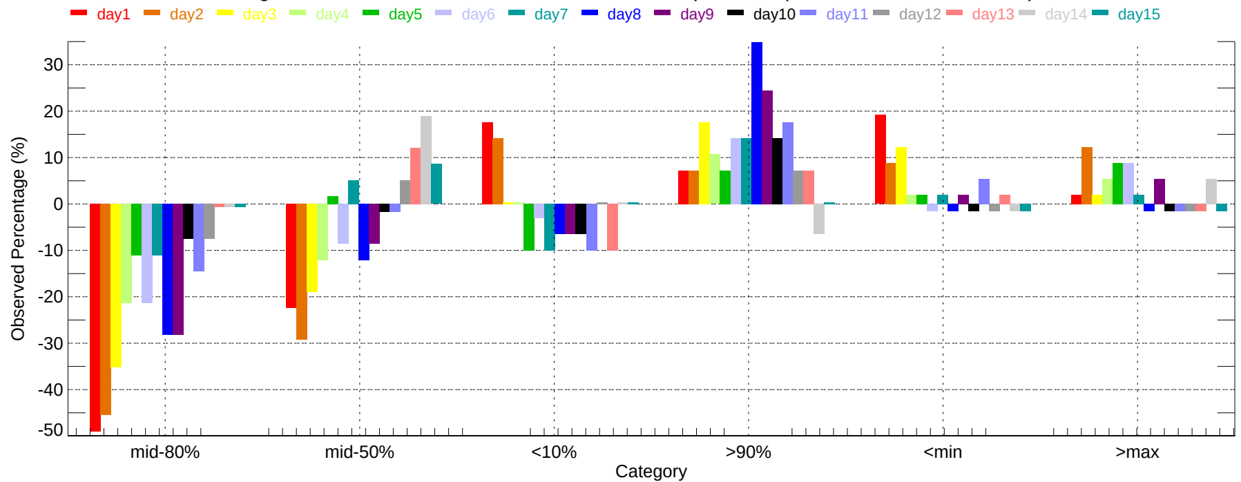
Observed Percentage Deviation of Ensembles - MSP: Max Temperature (2007-11-01~2007-11-30)
