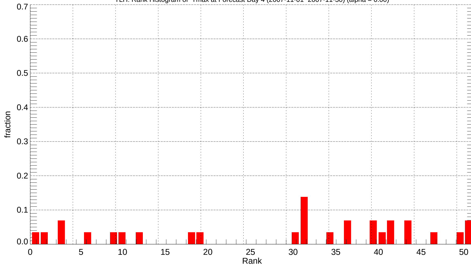
TLH: Rank Histogram of Tmax at Forecast Day 4 (2007-11-01~2007-11-30) (alpha = 0.00)
