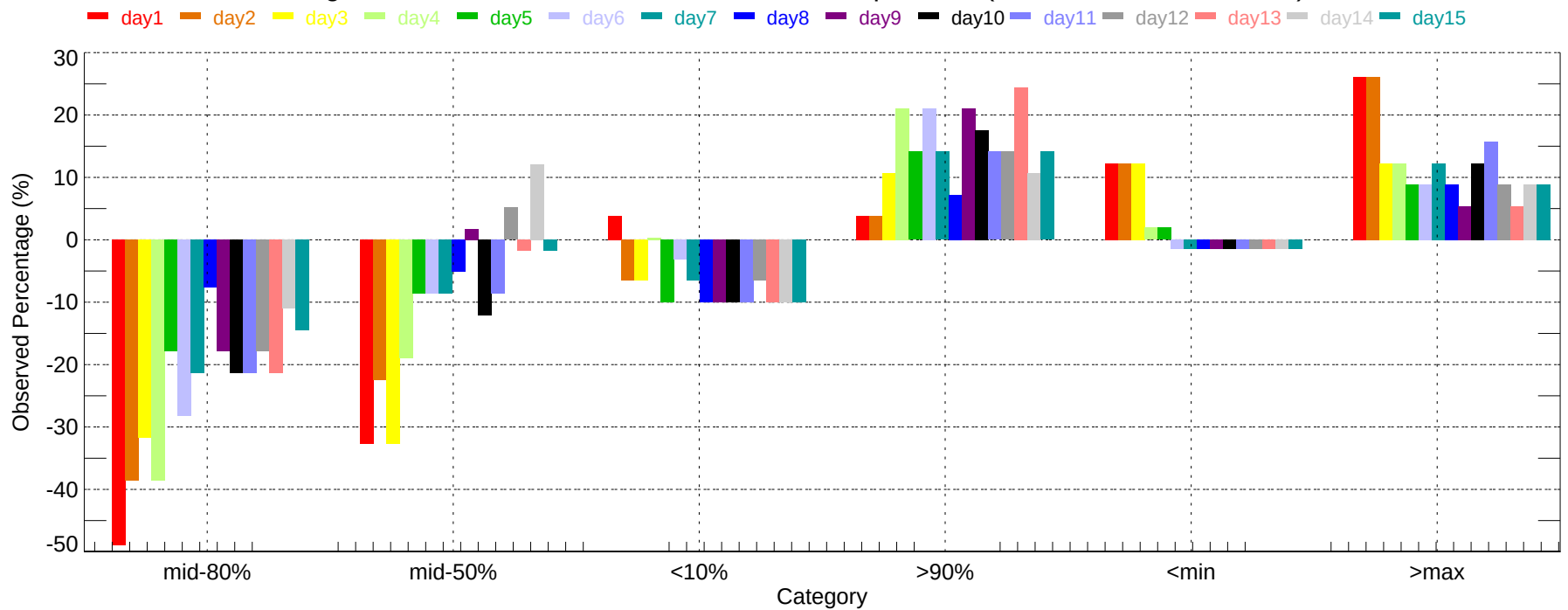
Observed Percentage Deviation of Ensembles - DEC: Max Temperature (2007-11-01~2007-11-30)
