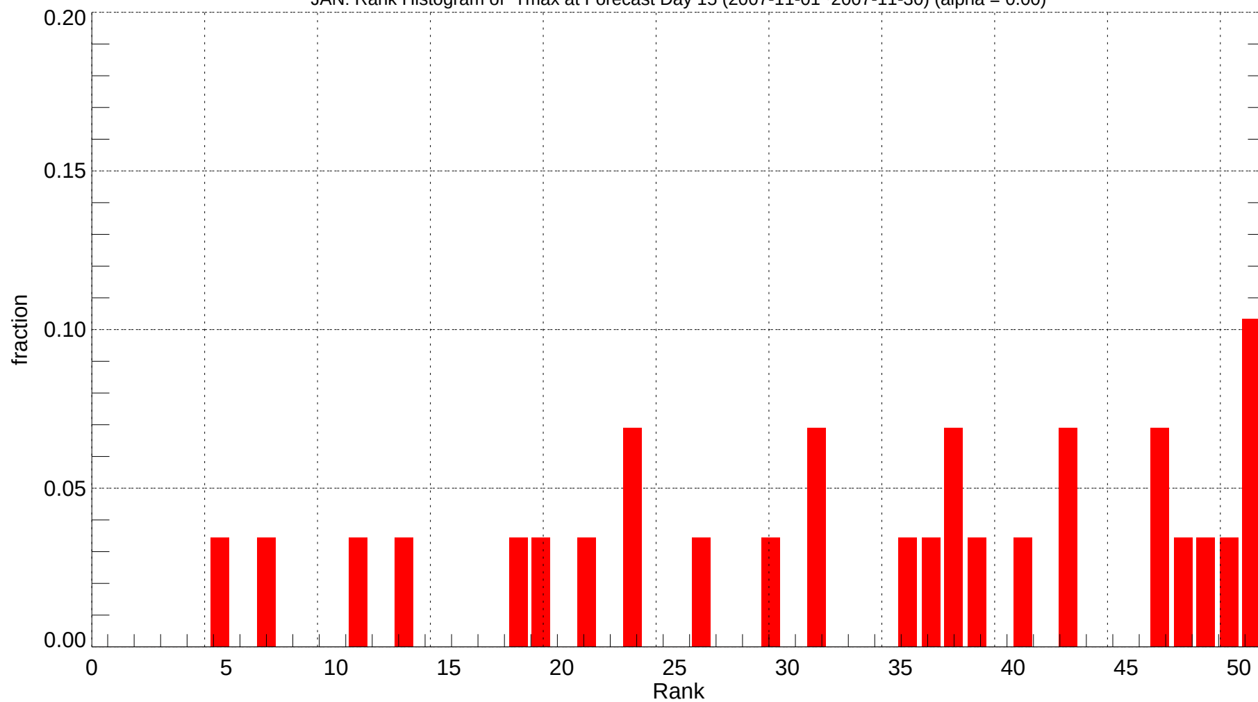
JAN: Rank Histogram of Tmax at Forecast Day 15 (2007-11-01~2007-11-30) (alpha = 0.00)
