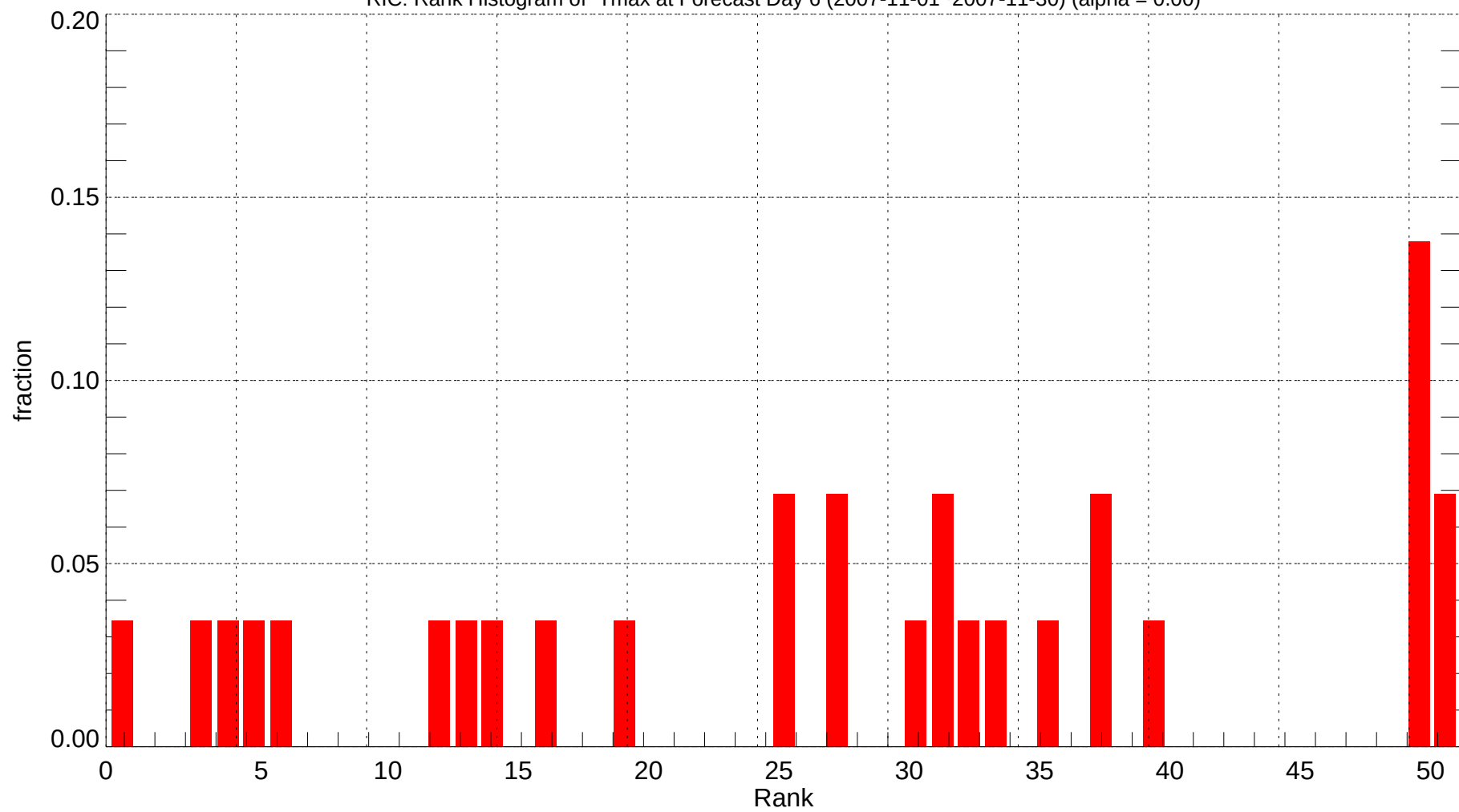
RIC: Rank Histogram of Tmax at Forecast Day 6 (2007-11-01~2007-11-30) (alpha = 0.00)
