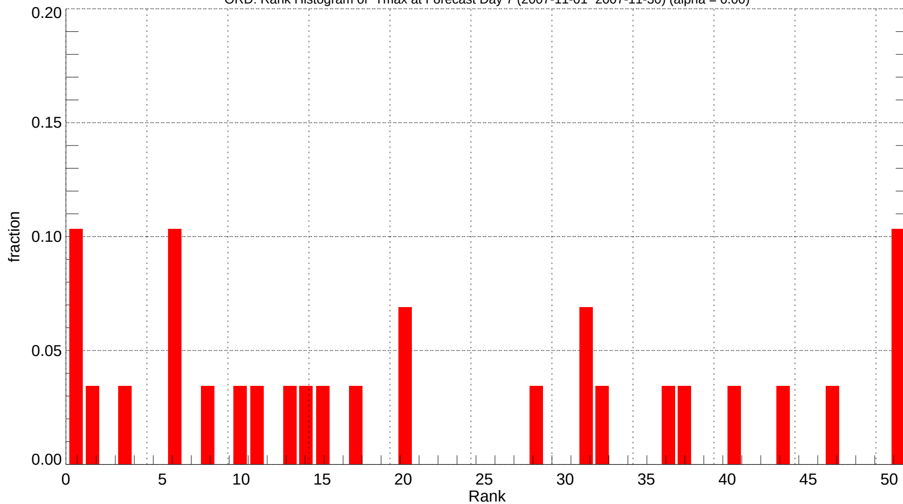
ORD: Rank Histogram of Tmax at Forecast Day 7 (2007-11-01~2007-11-30) (alpha = 0.00)
