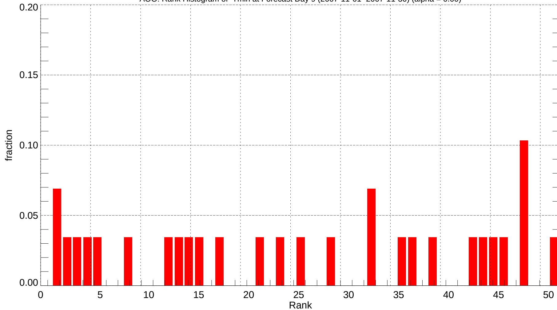
AOO: Rank Histogram of Tmin at Forecast Day 9 (2007-11-01~2007-11-30) (alpha = 0.00)
