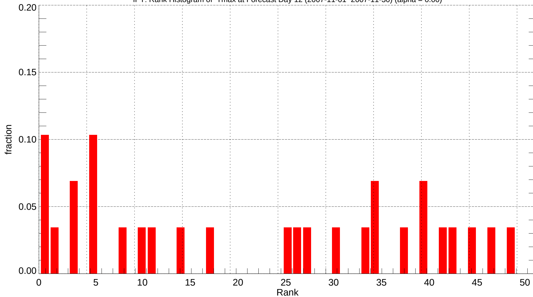
IPT: Rank Histogram of Tmax at Forecast Day 12 (2007-11-01~2007-11-30) (alpha = 0.00)
