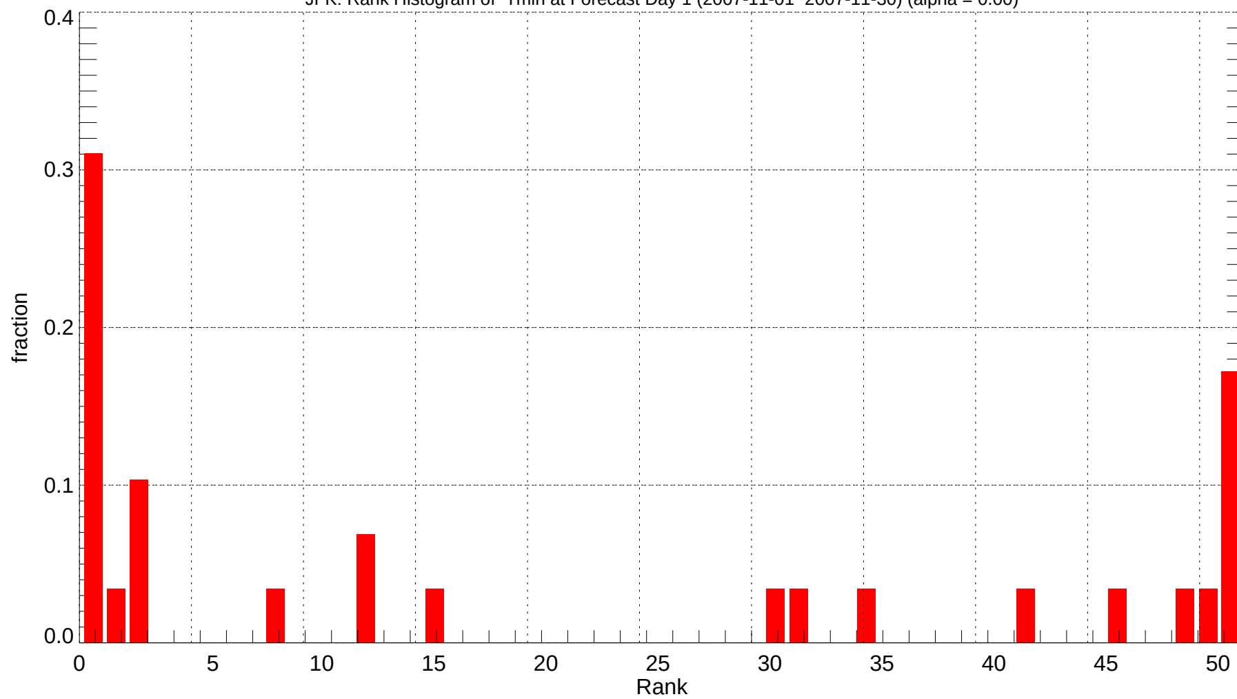
JFK: Rank Histogram of Tmin at Forecast Day 1 (2007-11-01~2007-11-30) (alpha = 0.00)
