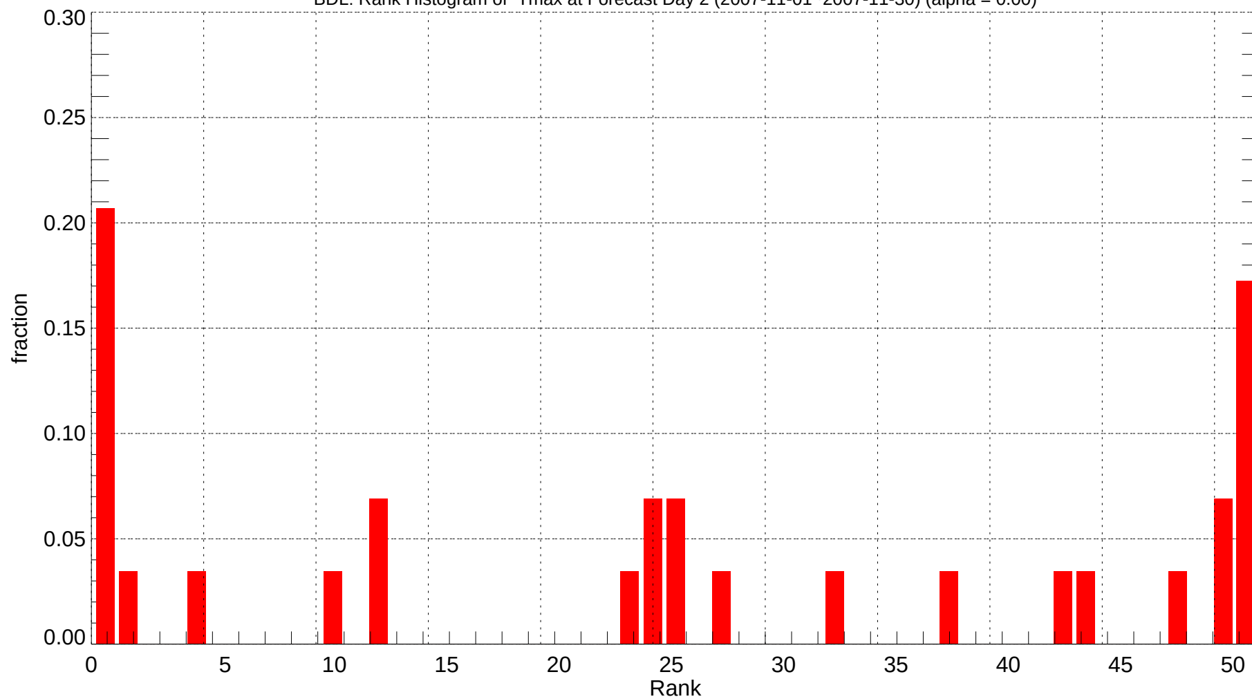
BDL: Rank Histogram of Tmax at Forecast Day 2 (2007-11-01~2007-11-30) (alpha = 0.00)
