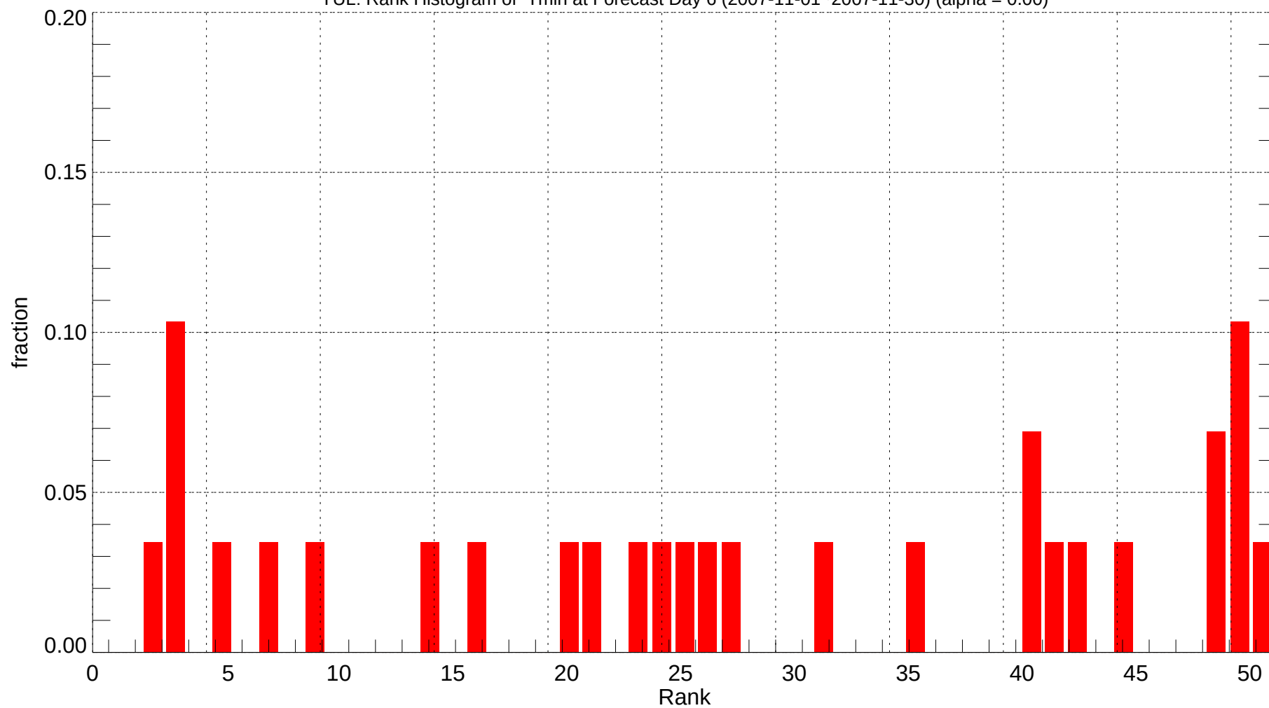
YUL: Rank Histogram of Tmin at Forecast Day 6 (2007-11-01~2007-11-30) (alpha = 0.00)
