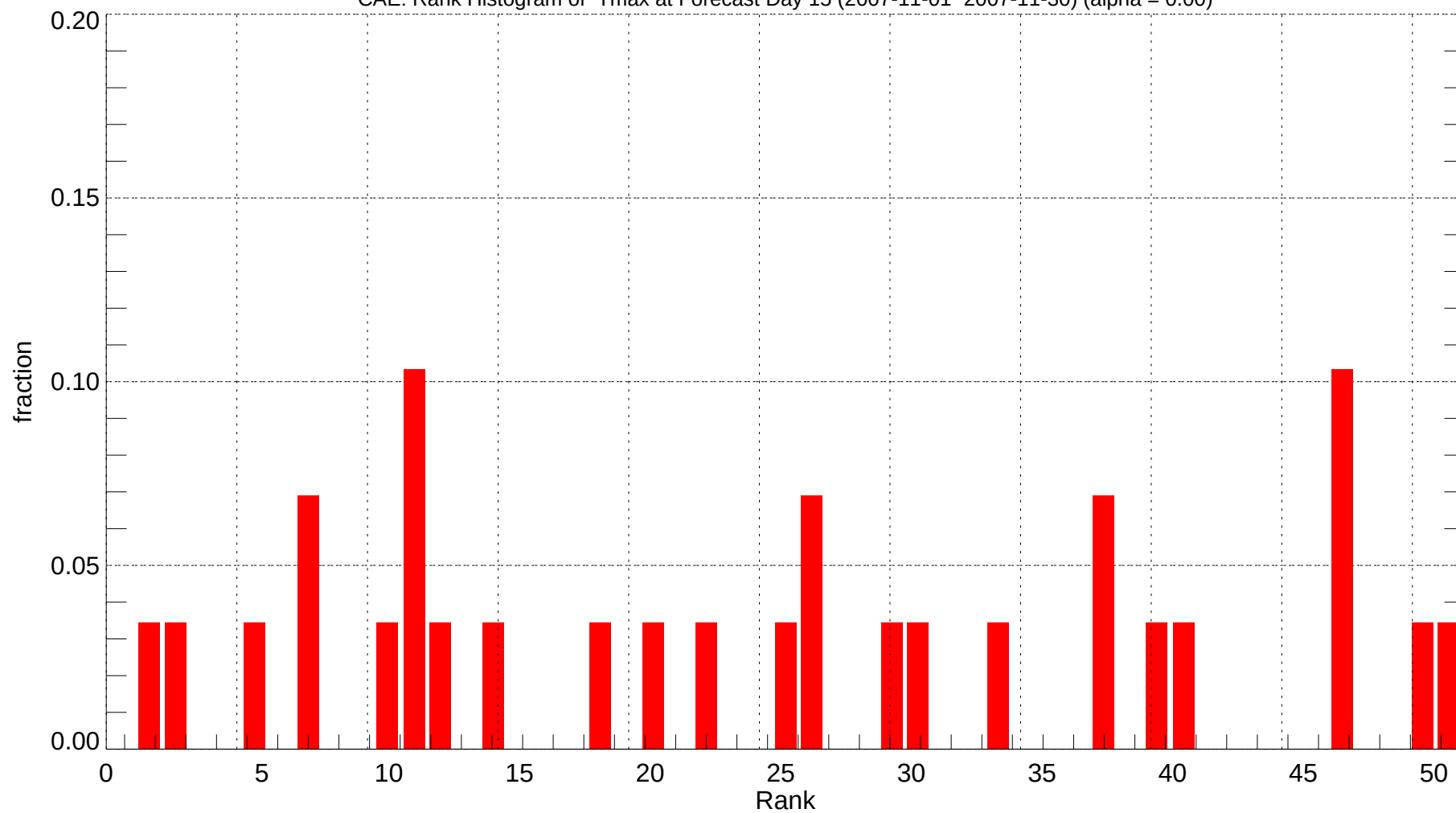
CAE: Rank Histogram of Tmax at Forecast Day 15 (2007-11-01~2007-11-30) (alpha = 0.00)
