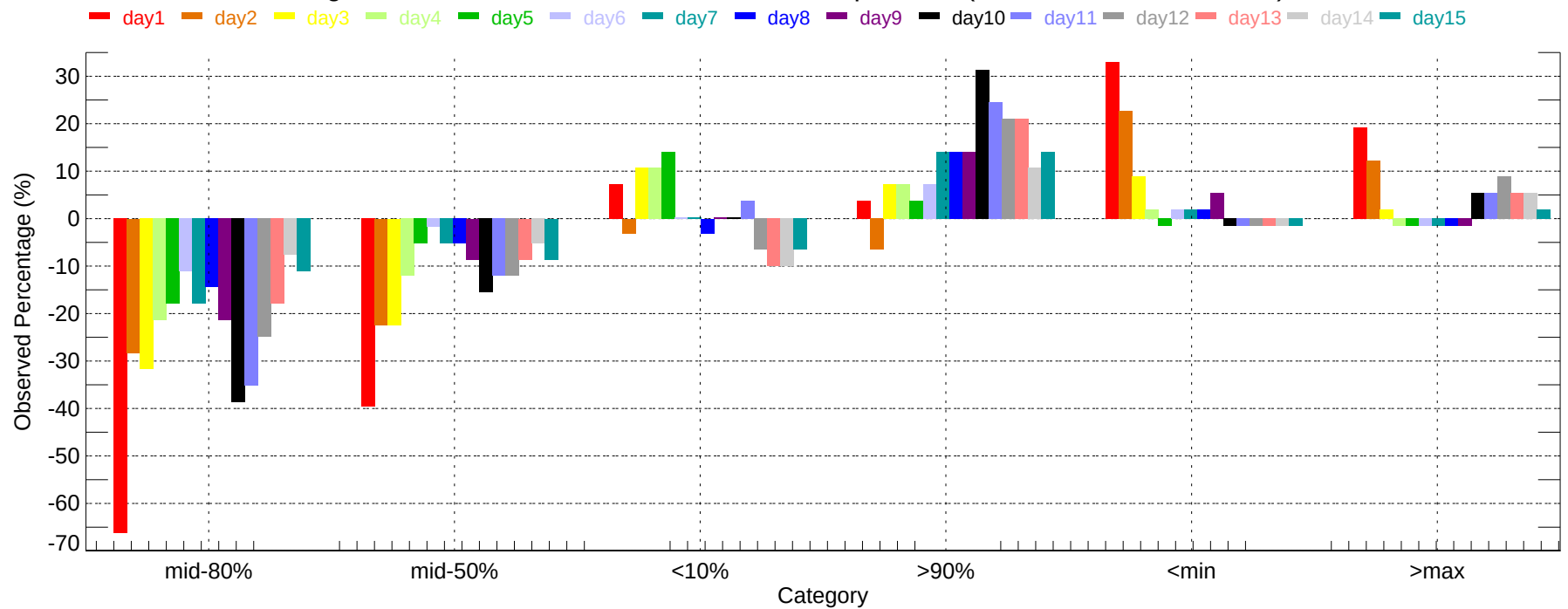
Observed Percentage Deviation of Ensembles - PIR: Min Temperature (2007-11-01~2007-11-30)
