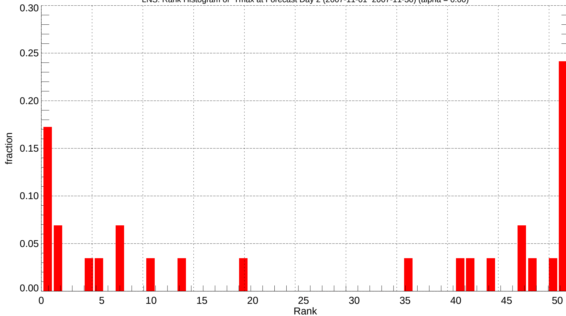
LNS: Rank Histogram of Tmax at Forecast Day 2 (2007-11-01~2007-11-30) (alpha = 0.00)
