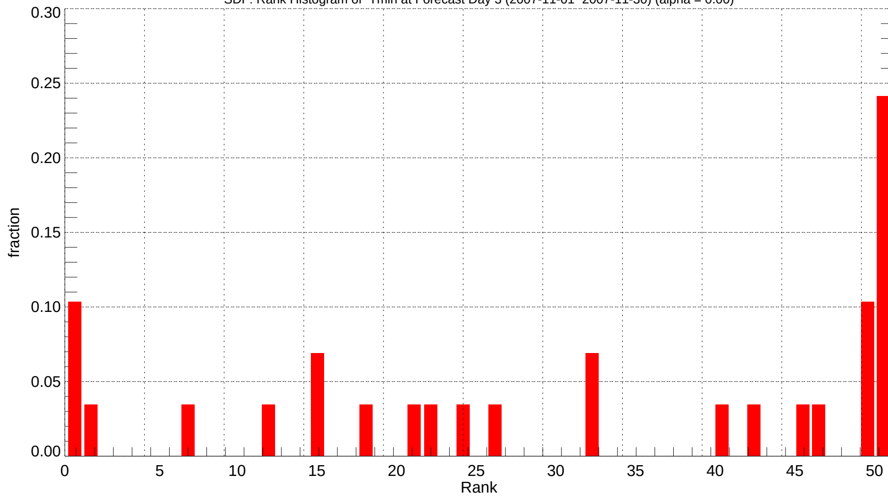
SDF: Rank Histogram of Tmin at Forecast Day 3 (2007-11-01~2007-11-30) (alpha = 0.00)
