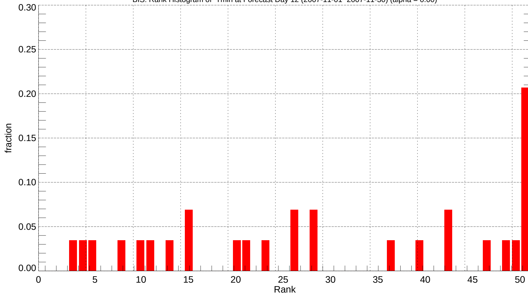
BIS: Rank Histogram of Tmin at Forecast Day 12 (2007-11-01~2007-11-30) (alpha = 0.00)
