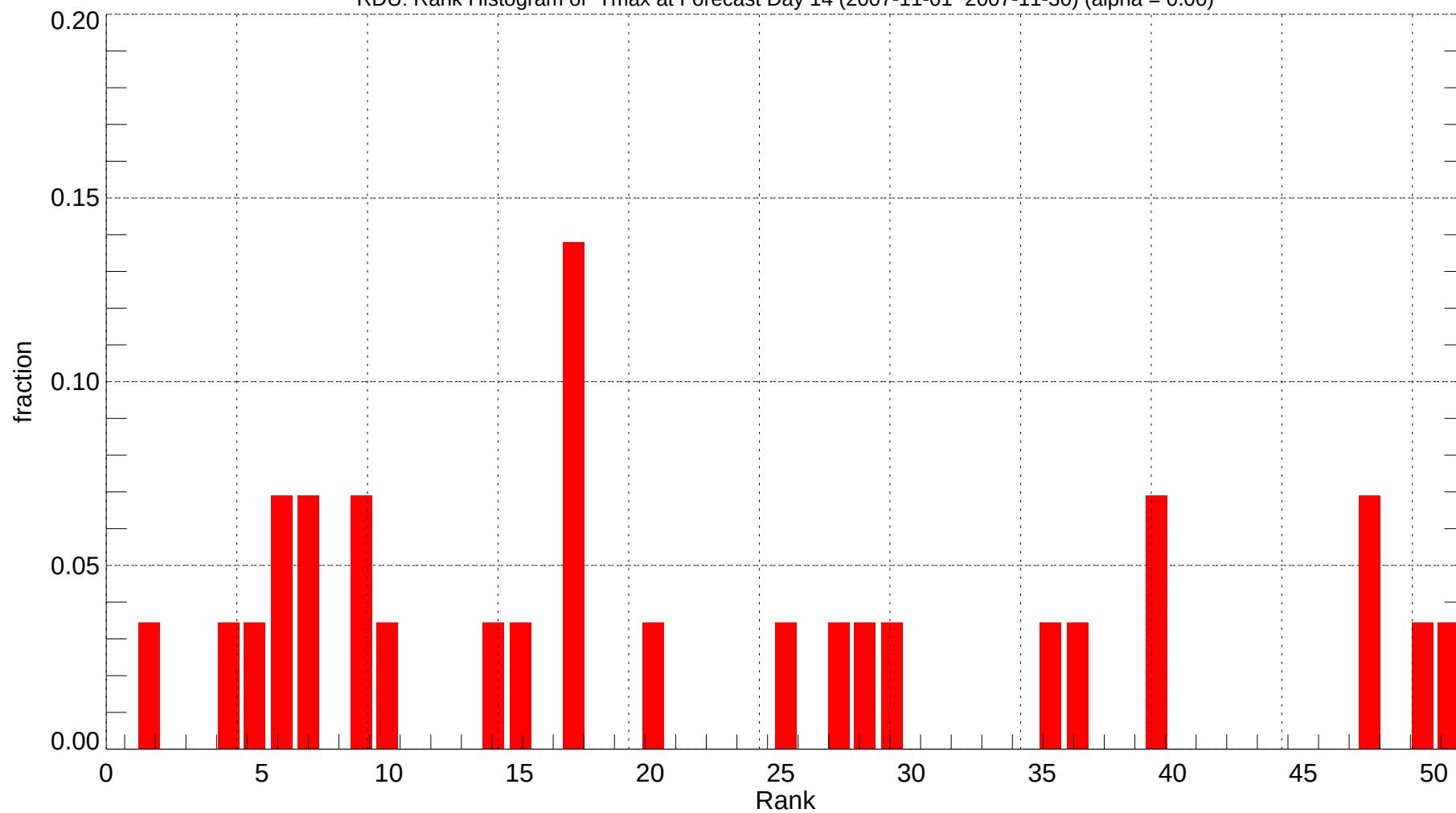
RDU: Rank Histogram of Tmax at Forecast Day 14 (2007-11-01~2007-11-30) (alpha = 0.00)
