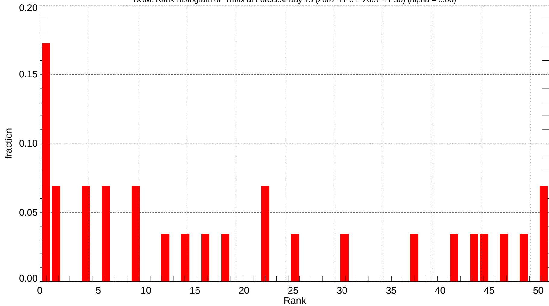
BGM: Rank Histogram of Tmax at Forecast Day 15 (2007-11-01~2007-11-30) (alpha = 0.00)
