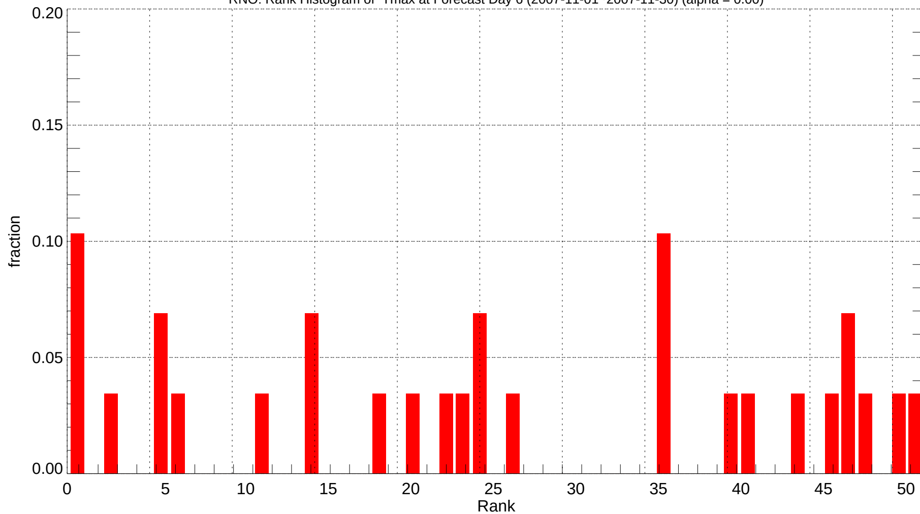
RNO: Rank Histogram of Tmax at Forecast Day 6 (2007-11-01~2007-11-30) (alpha = 0.00)
