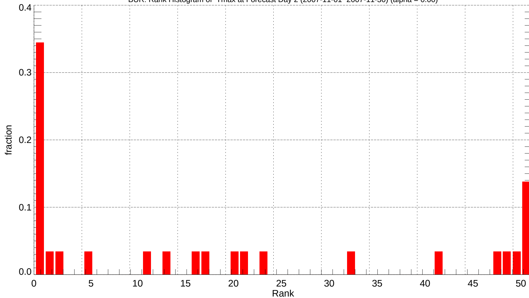
BUR: Rank Histogram of Tmax at Forecast Day 2 (2007-11-01~2007-11-30) (alpha = 0.00)
