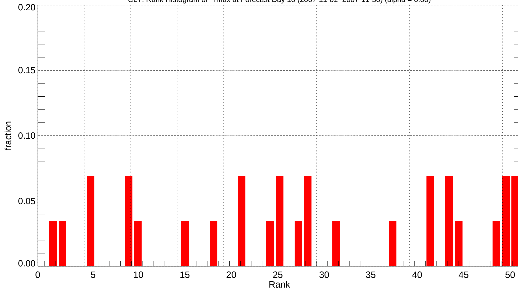
CLT: Rank Histogram of Tmax at Forecast Day 10 (2007-11-01~2007-11-30) (alpha = 0.00)
