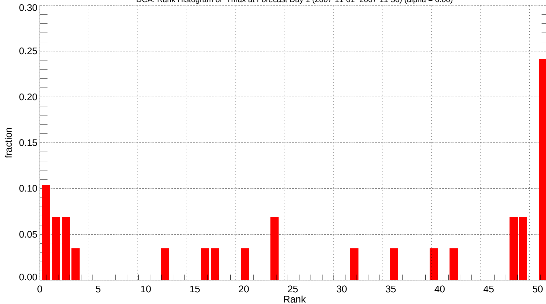
DCA: Rank Histogram of Tmax at Forecast Day 1 (2007-11-01~2007-11-30) (alpha = 0.00)
