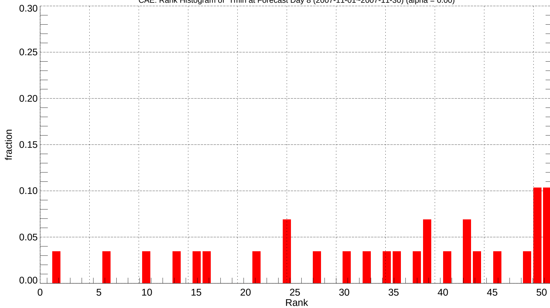
CAE: Rank Histogram of Tmin at Forecast Day 8 (2007-11-01~2007-11-30) (alpha = 0.00)
