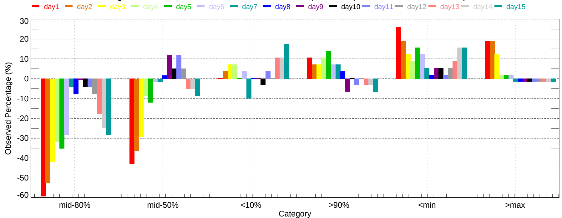
Observed Percentage Deviation of Ensembles - CON: Min Temperature (2007-11-01~2007-11-30)
