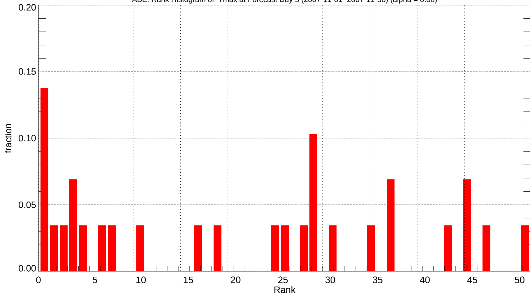
ABE: Rank Histogram of Tmax at Forecast Day 5 (2007-11-01~2007-11-30) (alpha = 0.00)
