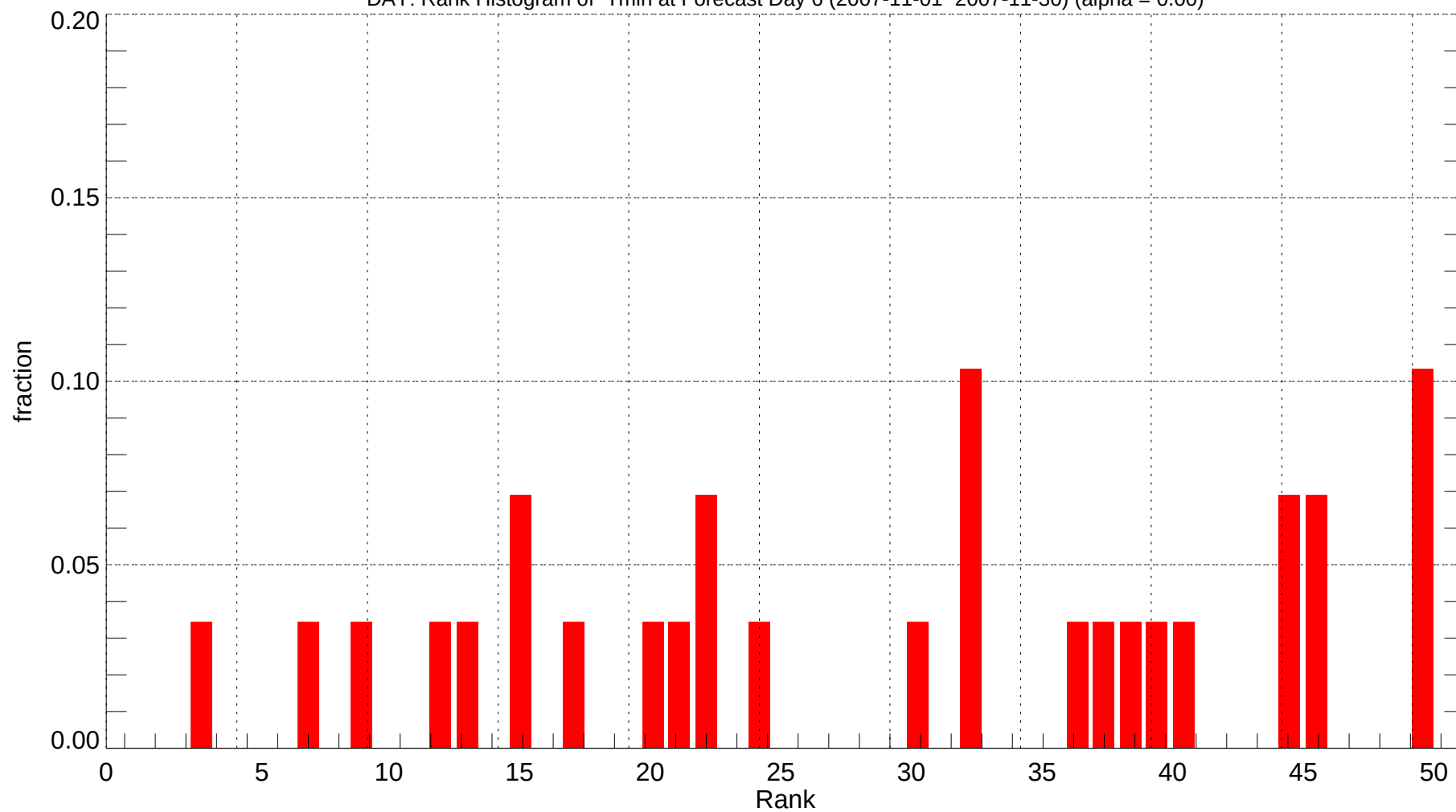
DAY: Rank Histogram of Tmin at Forecast Day 6 (2007-11-01~2007-11-30) (alpha = 0.00)
