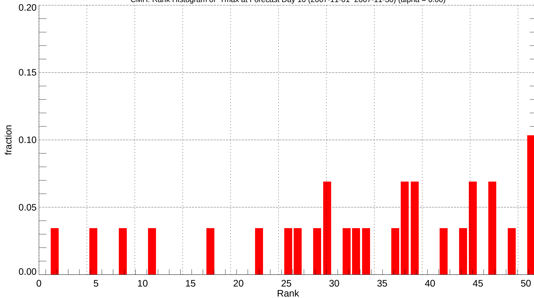
CMH: Rank Histogram of Tmax at Forecast Day 10 (2007-11-01~2007-11-30) (alpha = 0.00)
