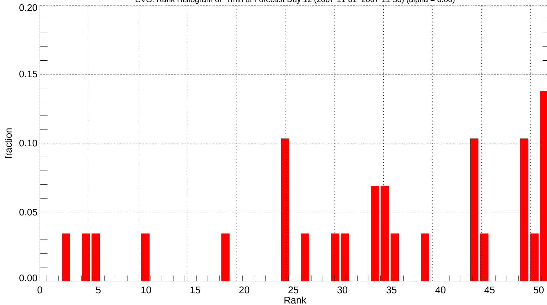
CVG: Rank Histogram of Tmin at Forecast Day 12 (2007-11-01~2007-11-30) (alpha = 0.00)
