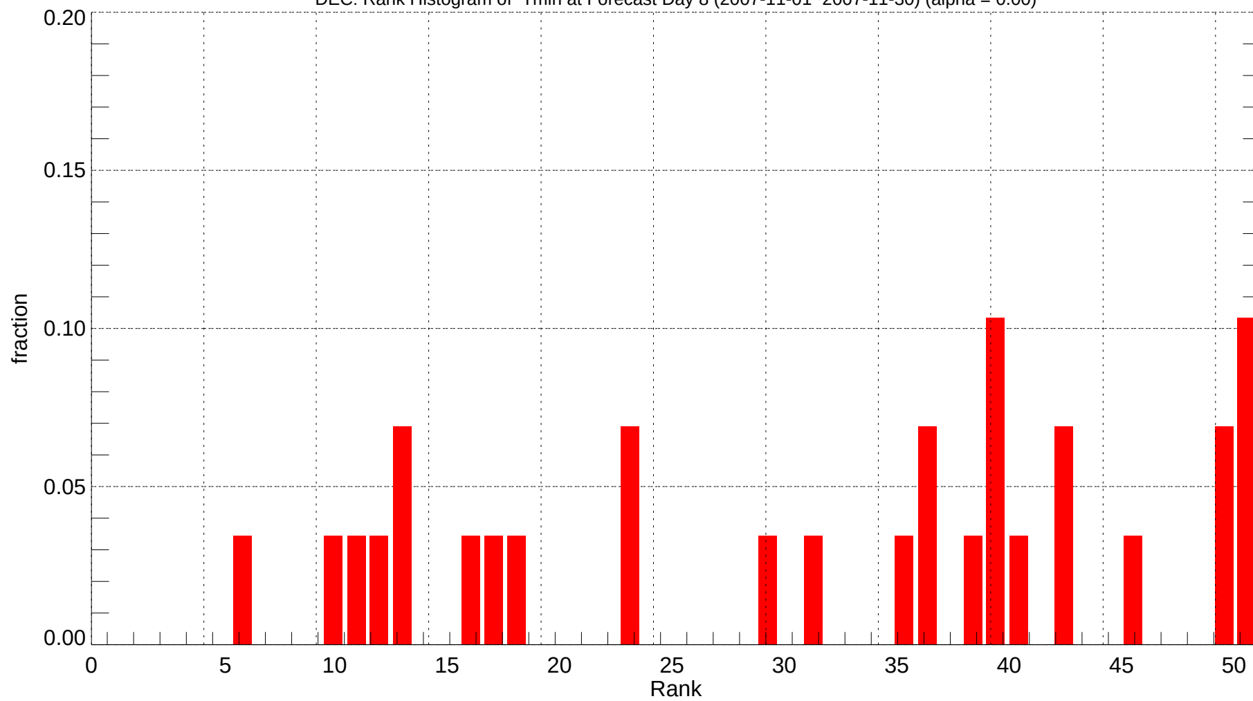
DEC: Rank Histogram of Tmin at Forecast Day 8 (2007-11-01~2007-11-30) (alpha = 0.00)
