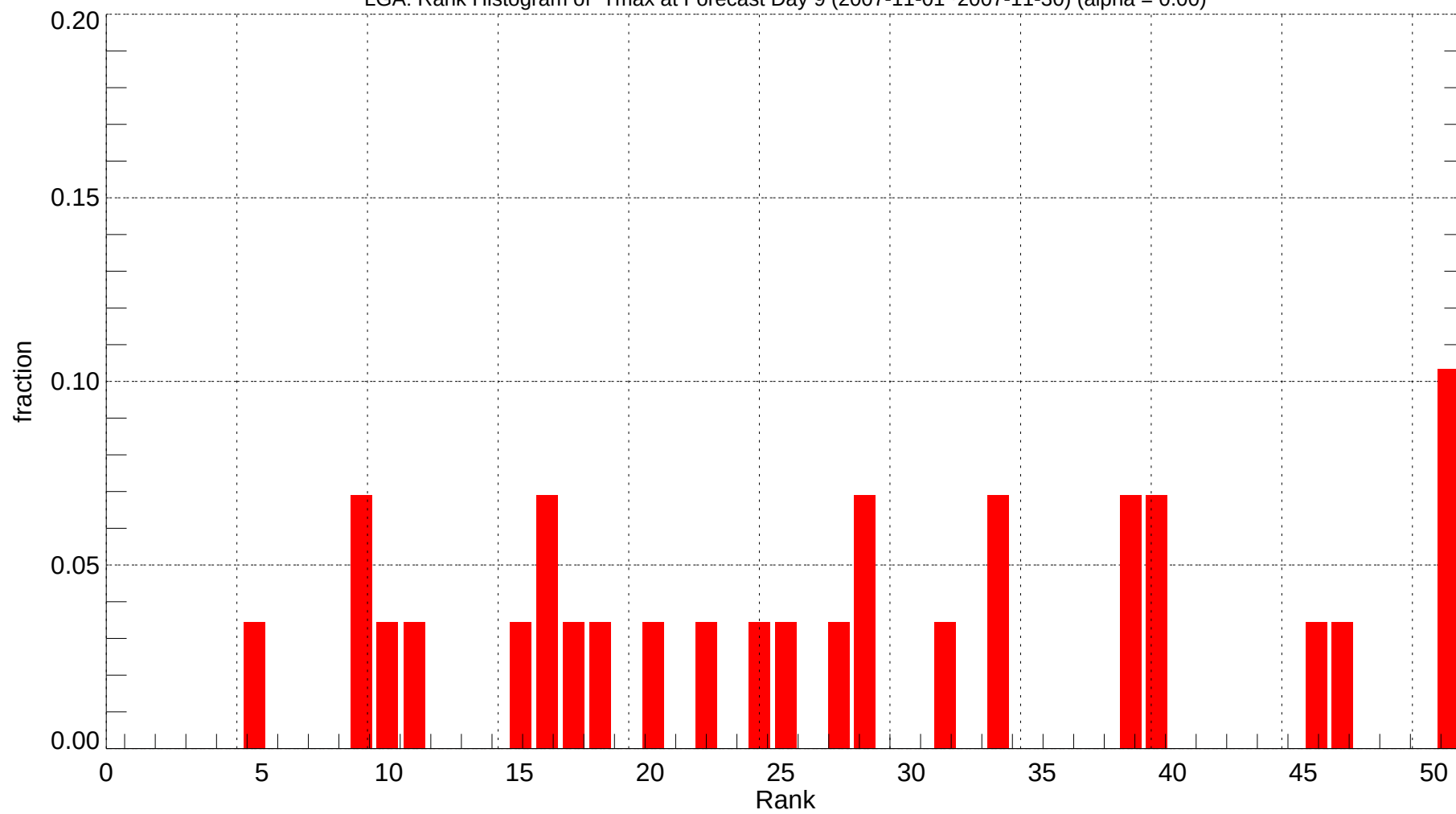
LGA: Rank Histogram of Tmax at Forecast Day 9 (2007-11-01~2007-11-30) (alpha = 0.00)
