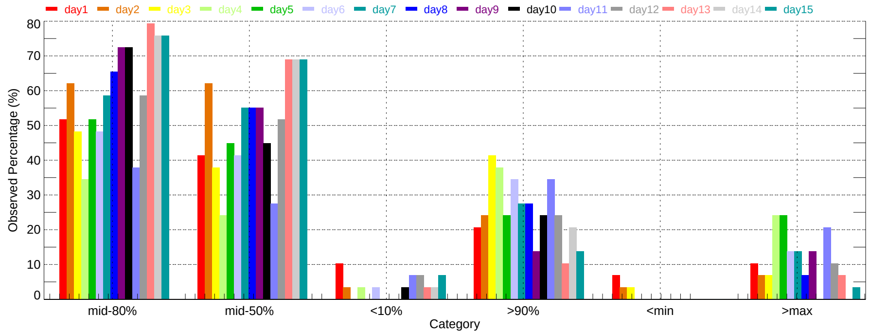
Observed Percentage of Ensembles - MCN: Max Temperature (2007-11-01~2007-11-30)
