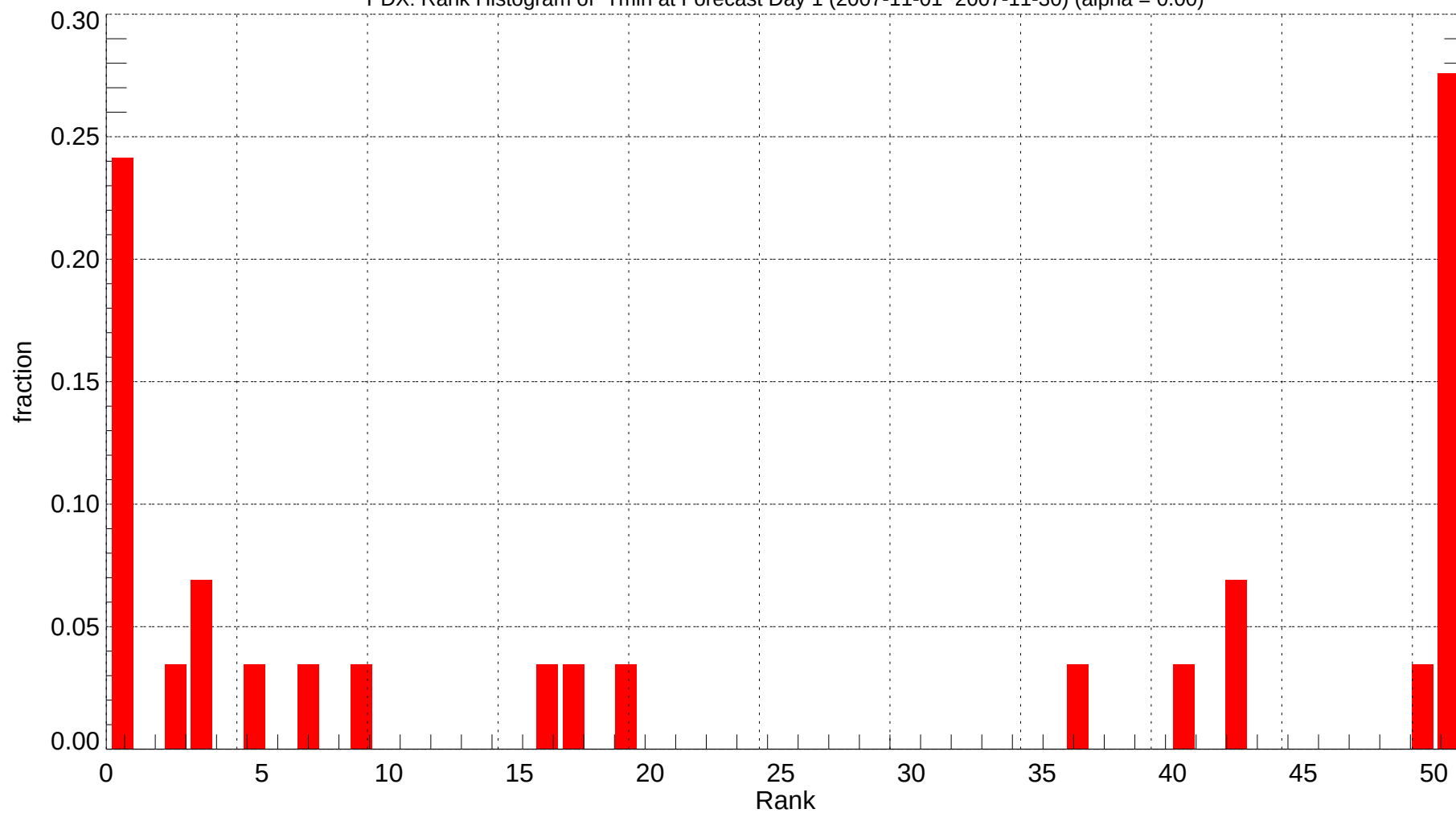
PDX: Rank Histogram of Tmin at Forecast Day 1 (2007-11-01~2007-11-30) (alpha = 0.00)
