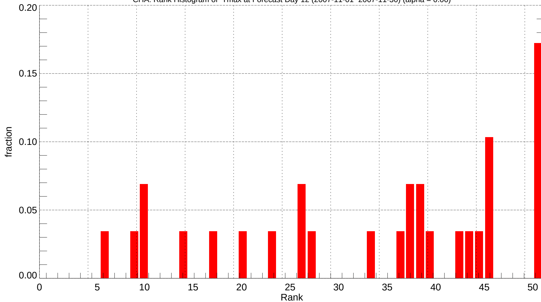
CHA: Rank Histogram of Tmax at Forecast Day 12 (2007-11-01~2007-11-30) (alpha = 0.00)
