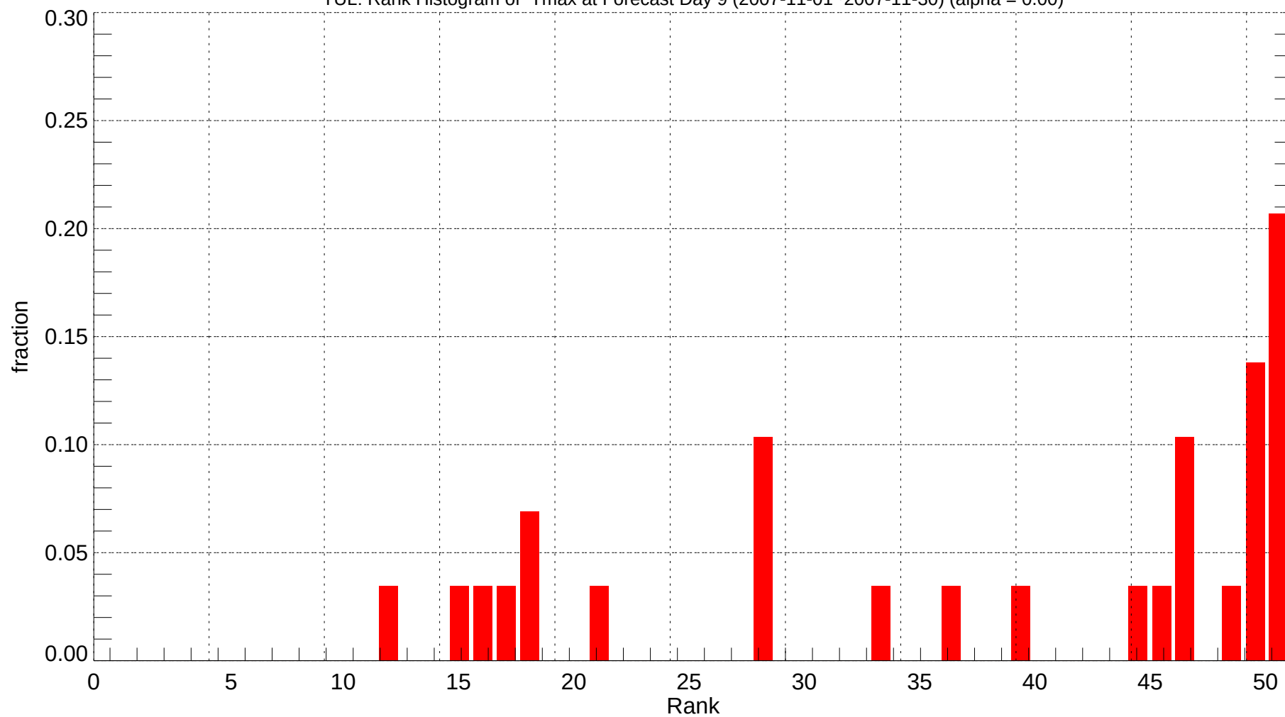
TUL: Rank Histogram of Tmax at Forecast Day 9 (2007-11-01~2007-11-30) (alpha = 0.00)
