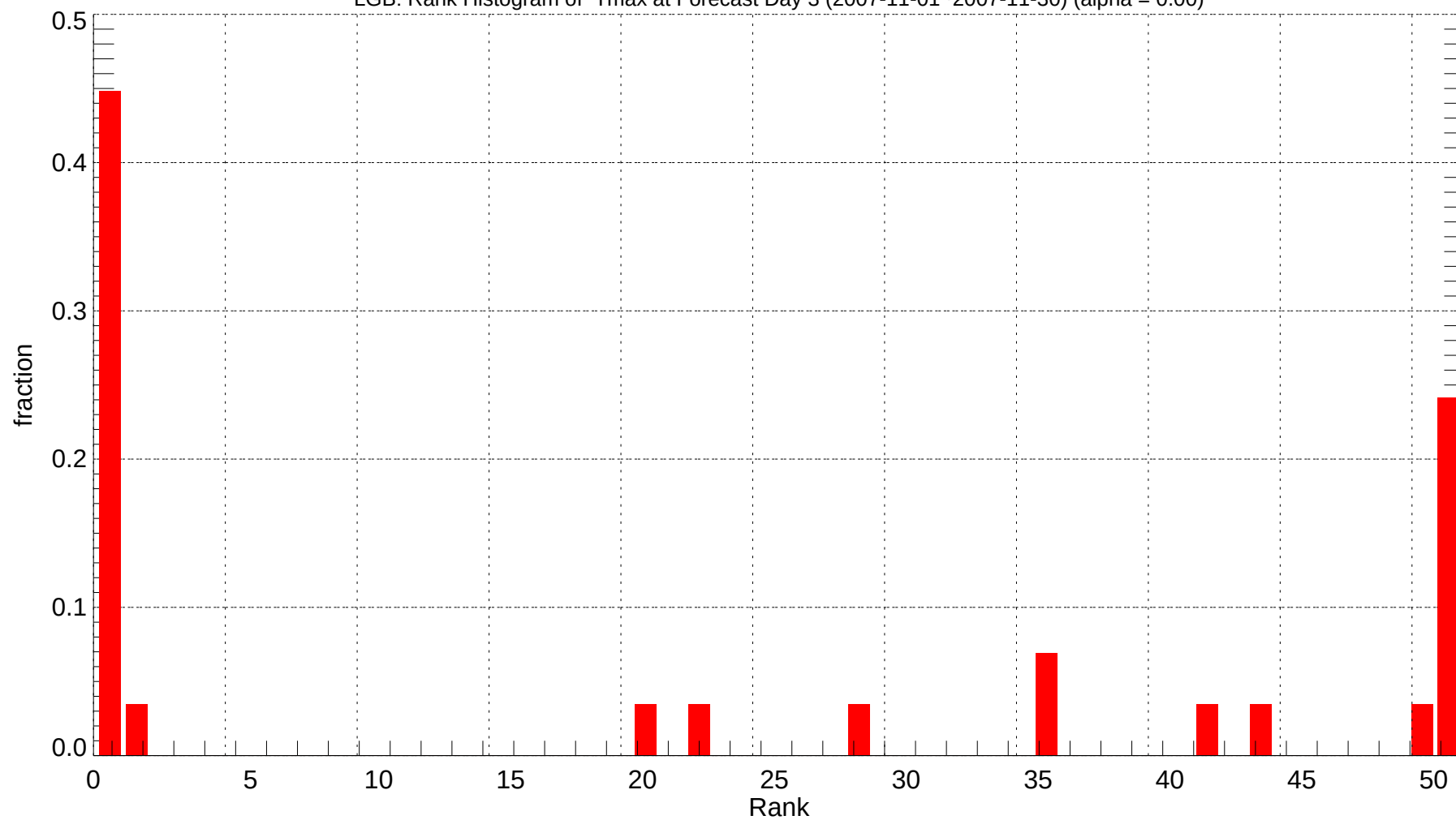
LGB: Rank Histogram of Tmax at Forecast Day 3 (2007-11-01~2007-11-30) (alpha = 0.00)
