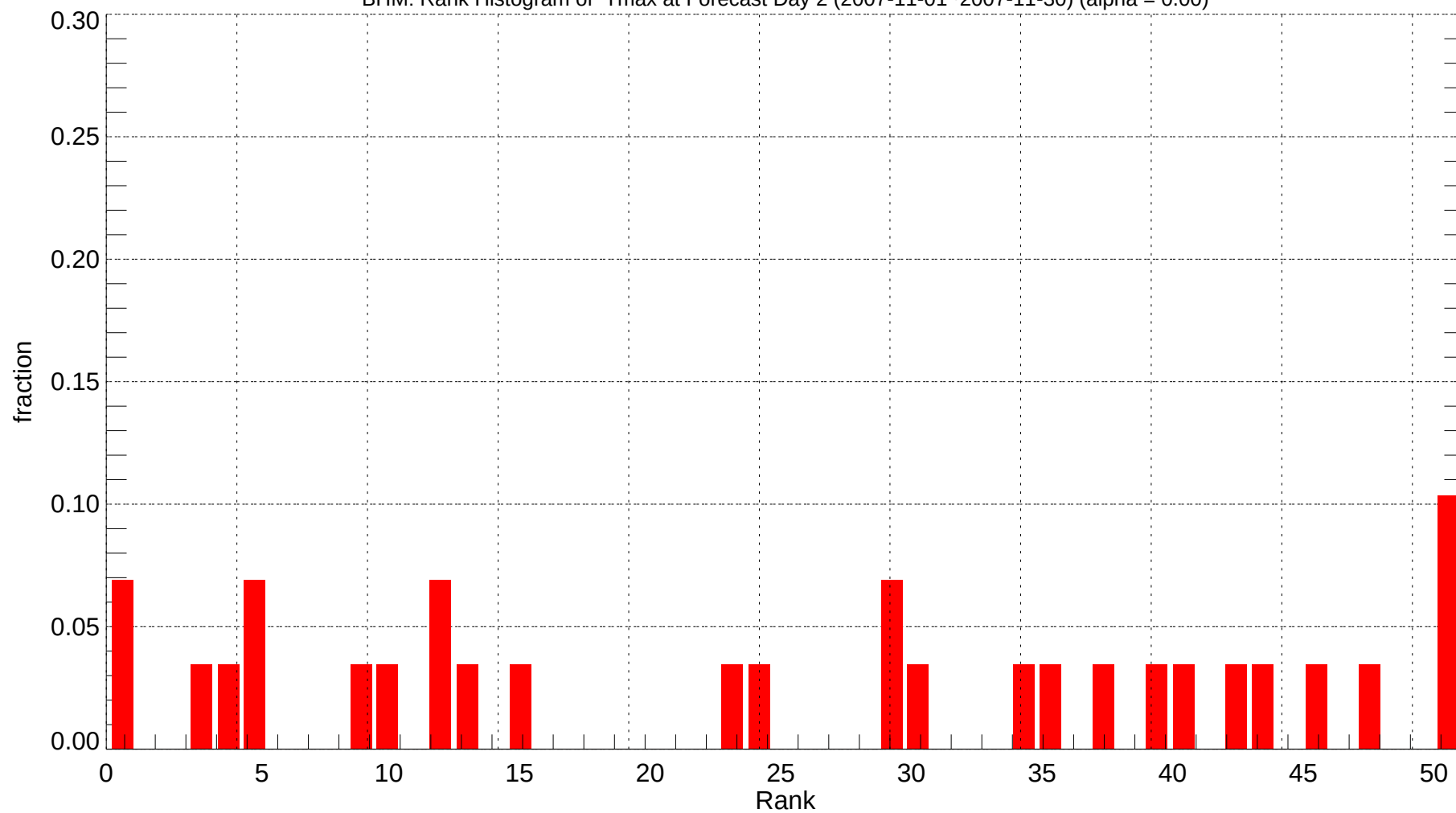
BHM: Rank Histogram of Tmax at Forecast Day 2 (2007-11-01~2007-11-30) (alpha = 0.00)
