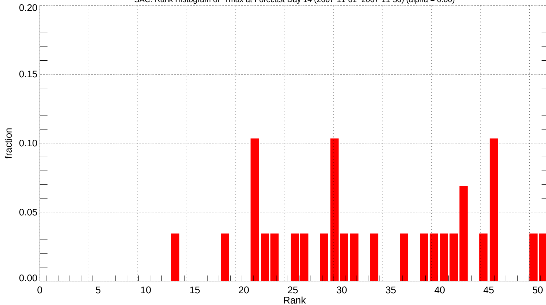
SAC: Rank Histogram of Tmax at Forecast Day 14 (2007-11-01~2007-11-30) (alpha = 0.00)
