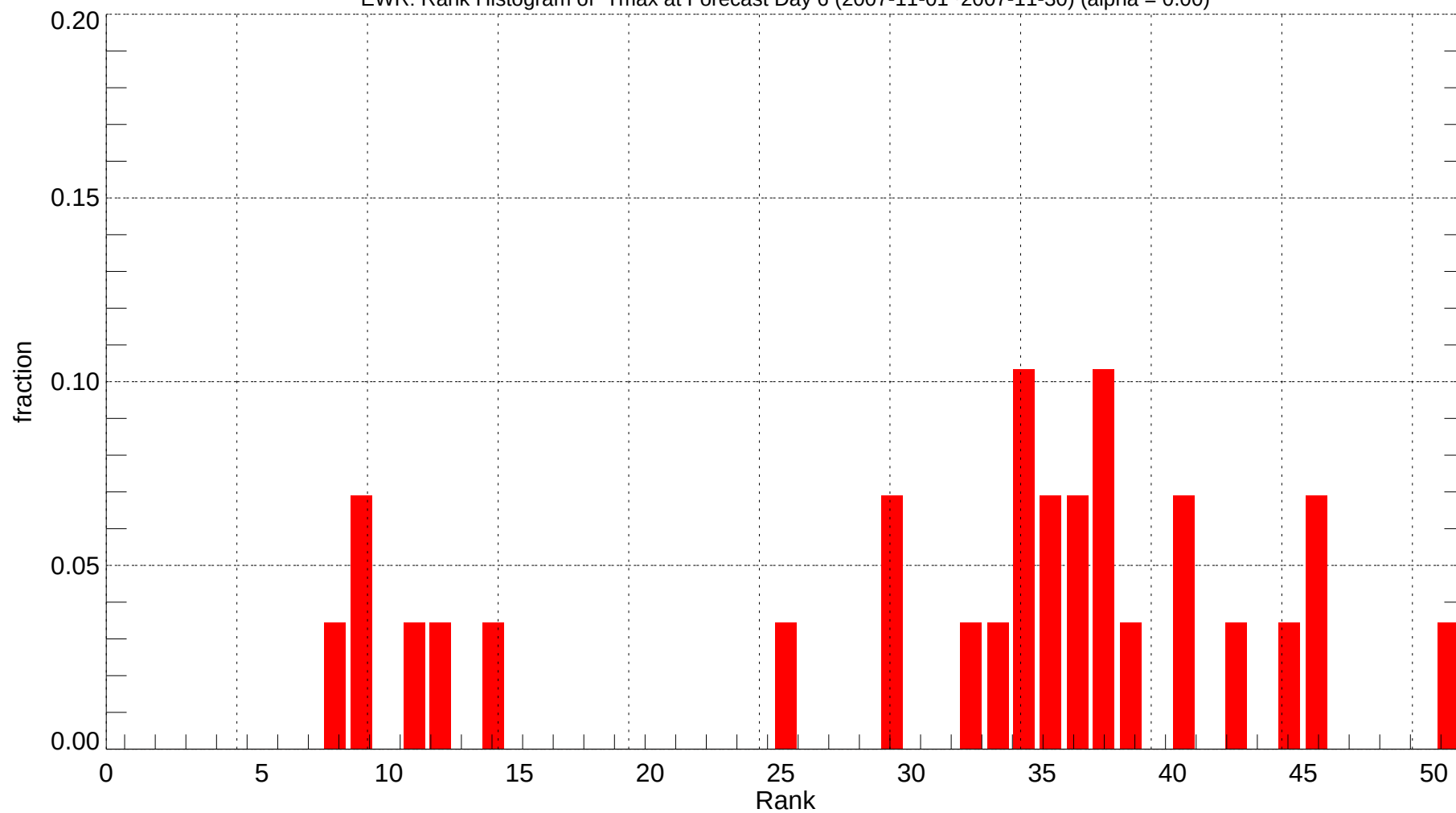
EW: Rank Histogram of Tmax at Forecast Day 6 (2007-11-01~2007-11-30) (alpha = 0.00)
