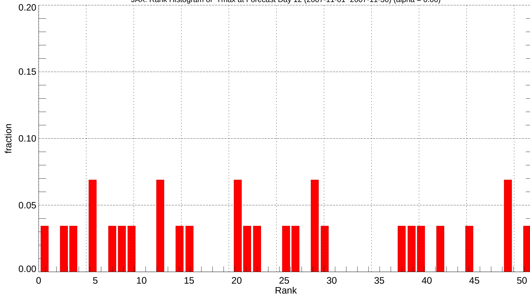
JAX: Rank Histogram of Tmax at Forecast Day 12 (2007-11-01~2007-11-30) (alpha = 0.00)
