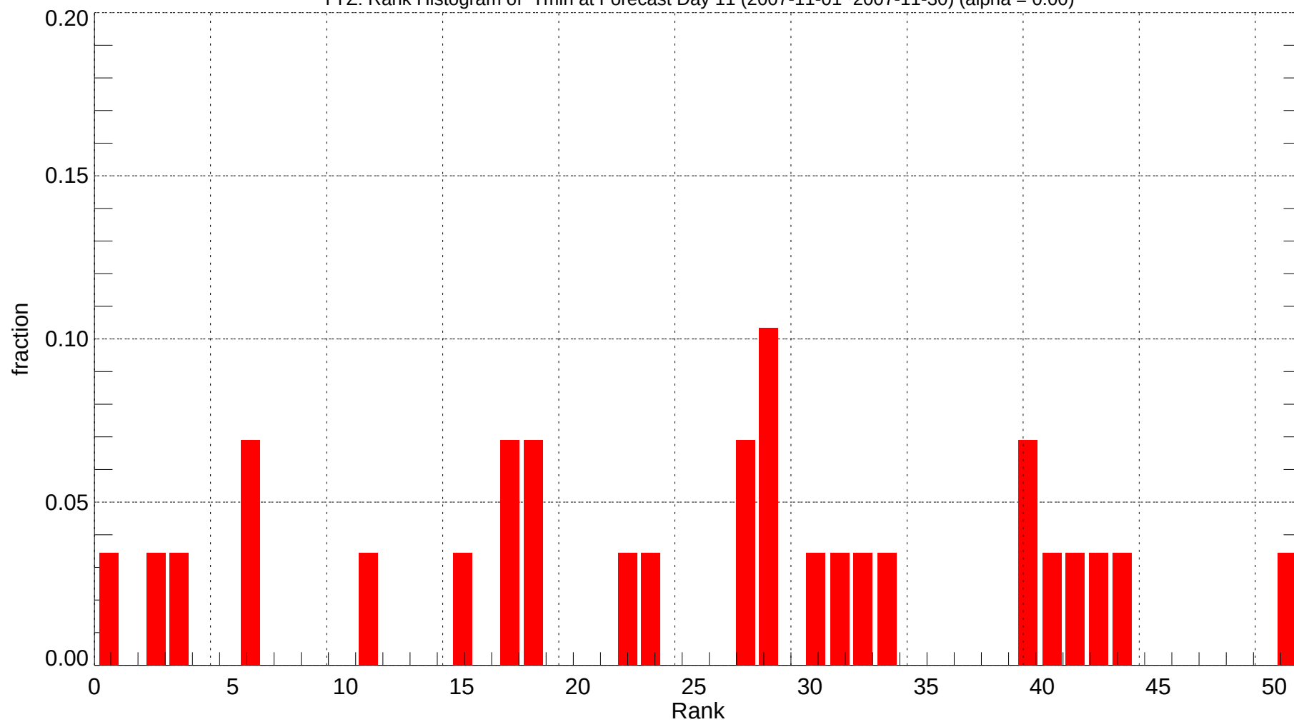
YYZ: Rank Histogram of Tmin at Forecast Day 11 (2007-11-01~2007-11-30) (alpha = 0.00)
