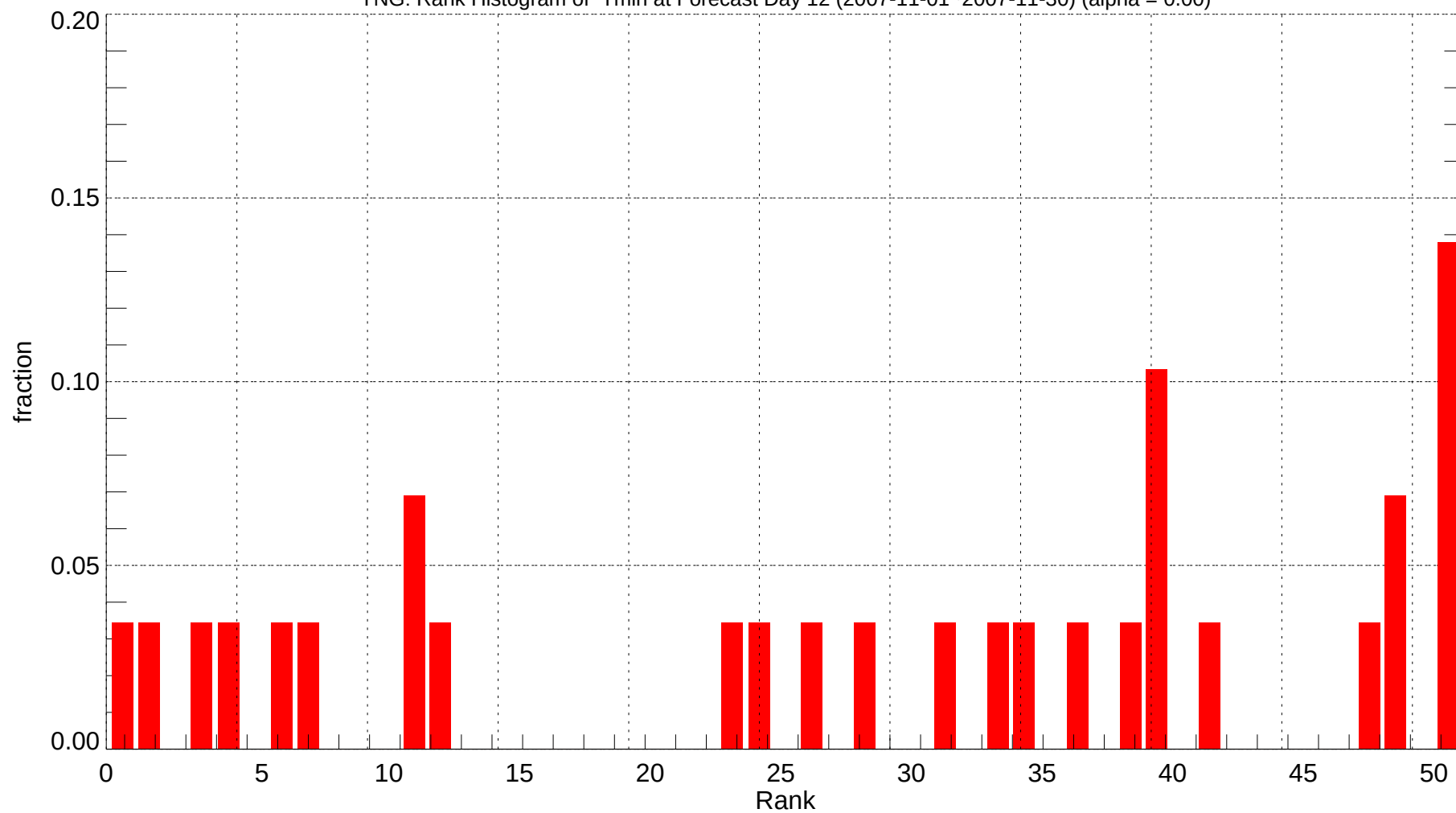
YNG: Rank Histogram of Tmin at Forecast Day 12 (2007-11-01~2007-11-30) (alpha = 0.00)
