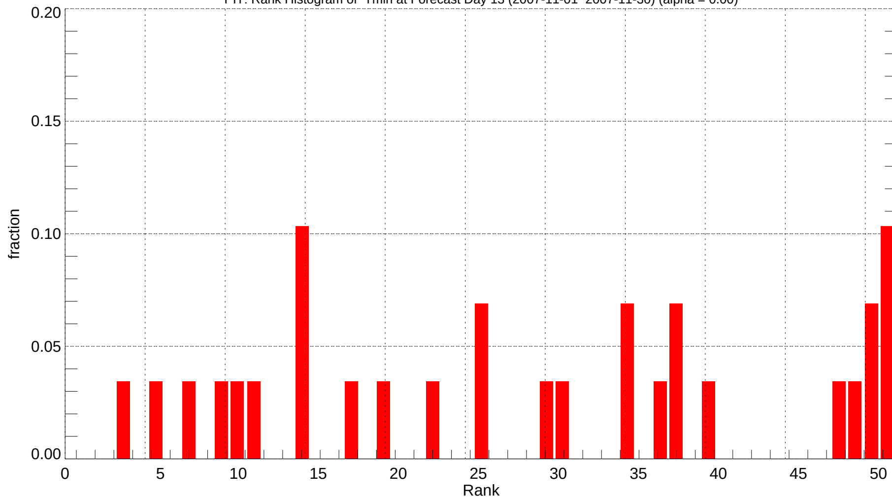
PIT: Rank Histogram of Tmin at Forecast Day 13 (2007-11-01~2007-11-30) (alpha = 0.00)
