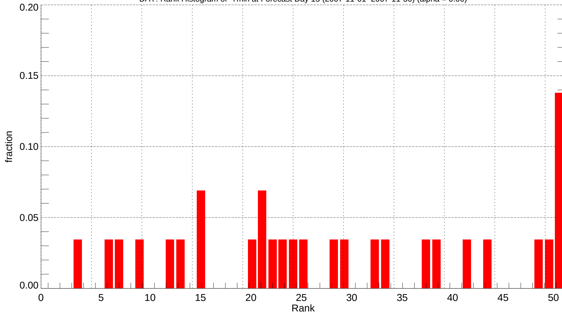
DAY: Rank Histogram of Tmin at Forecast Day 15 (2007-11-01~2007-11-30) (alpha = 0.00)
