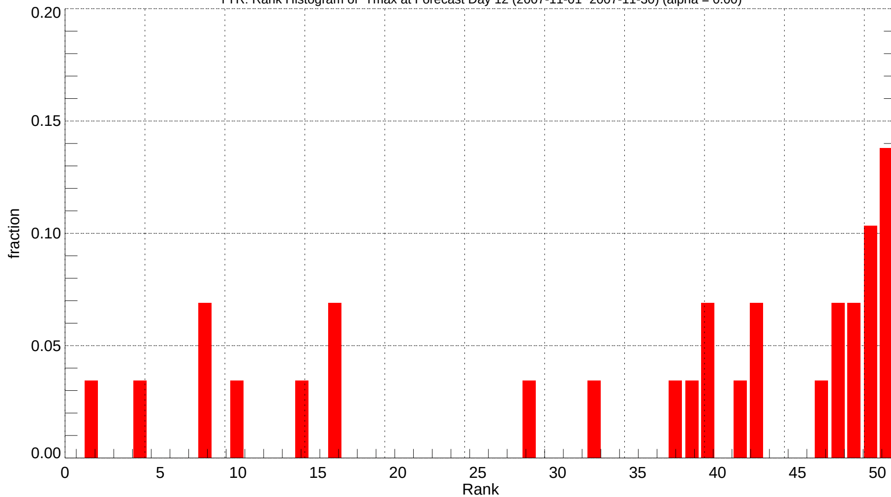
TYR: Rank Histogram of Tmax at Forecast Day 12 (2007-11-01~2007-11-30) (alpha = 0.00)
