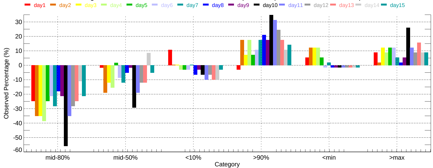
Observed Percentage Deviation of Ensembles - COU: Max Temperature (2007-11-01~2007-11-30)
