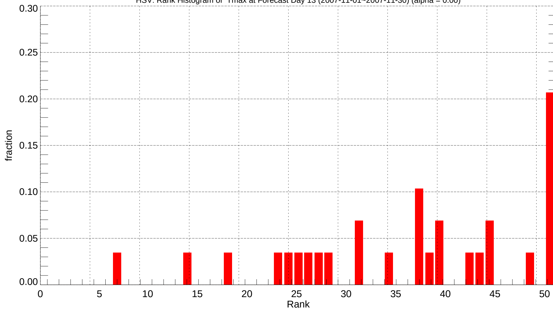
HSV: Rank Histogram of Tmax at Forecast Day 13 (2007-11-01~2007-11-30) (alpha = 0.00)
