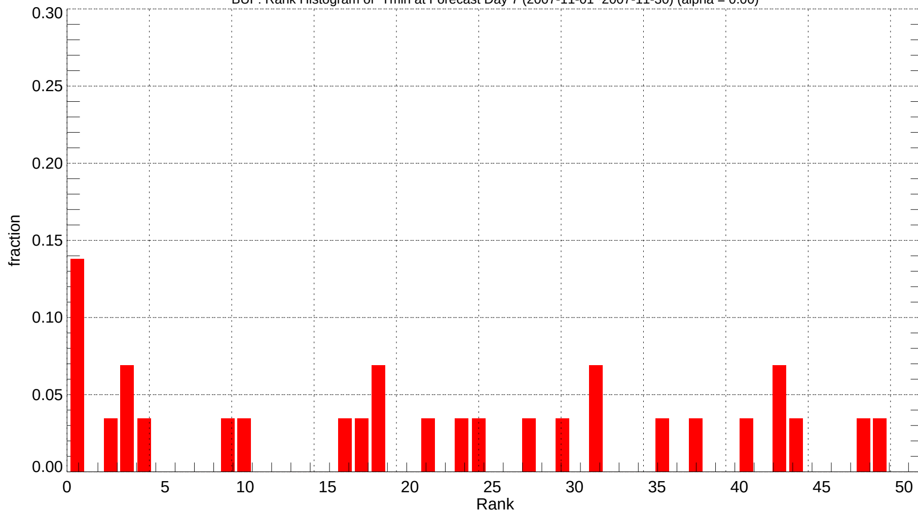
BUF: Rank Histogram of Tmin at Forecast Day 7 (2007-11-01~2007-11-30) (alpha = 0.00)
