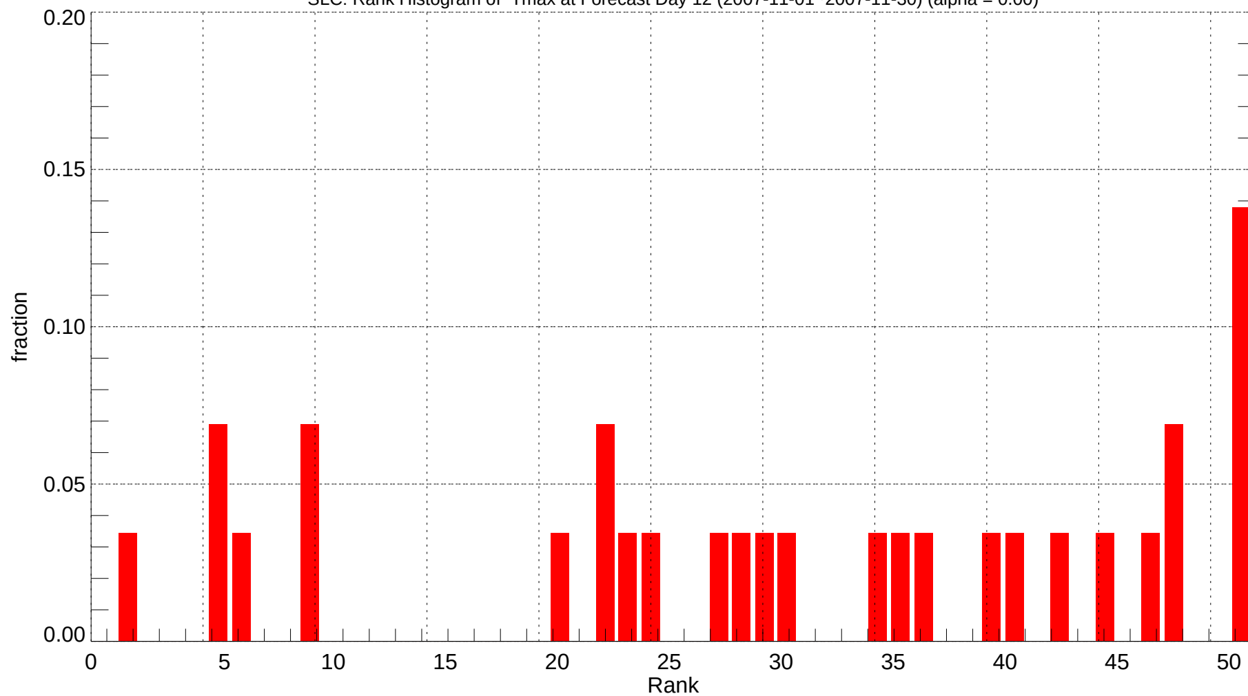
SLC: Rank Histogram of Tmax at Forecast Day 12 (2007-11-01~2007-11-30) (alpha = 0.00)
