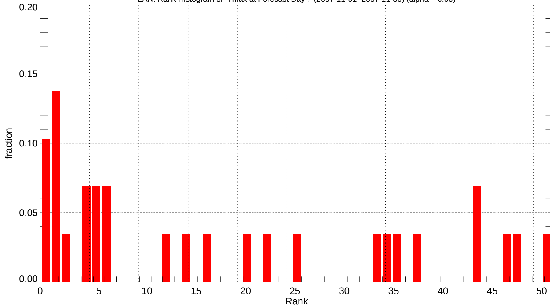
LAN: Rank Histogram of Tmax at Forecast Day 7 (2007-11-01~2007-11-30) (alpha = 0.00)
