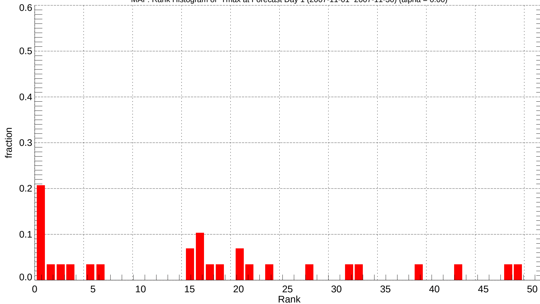
MAF: Rank Histogram of Tmax at Forecast Day 1 (2007-11-01~2007-11-30) (alpha = 0.00)
