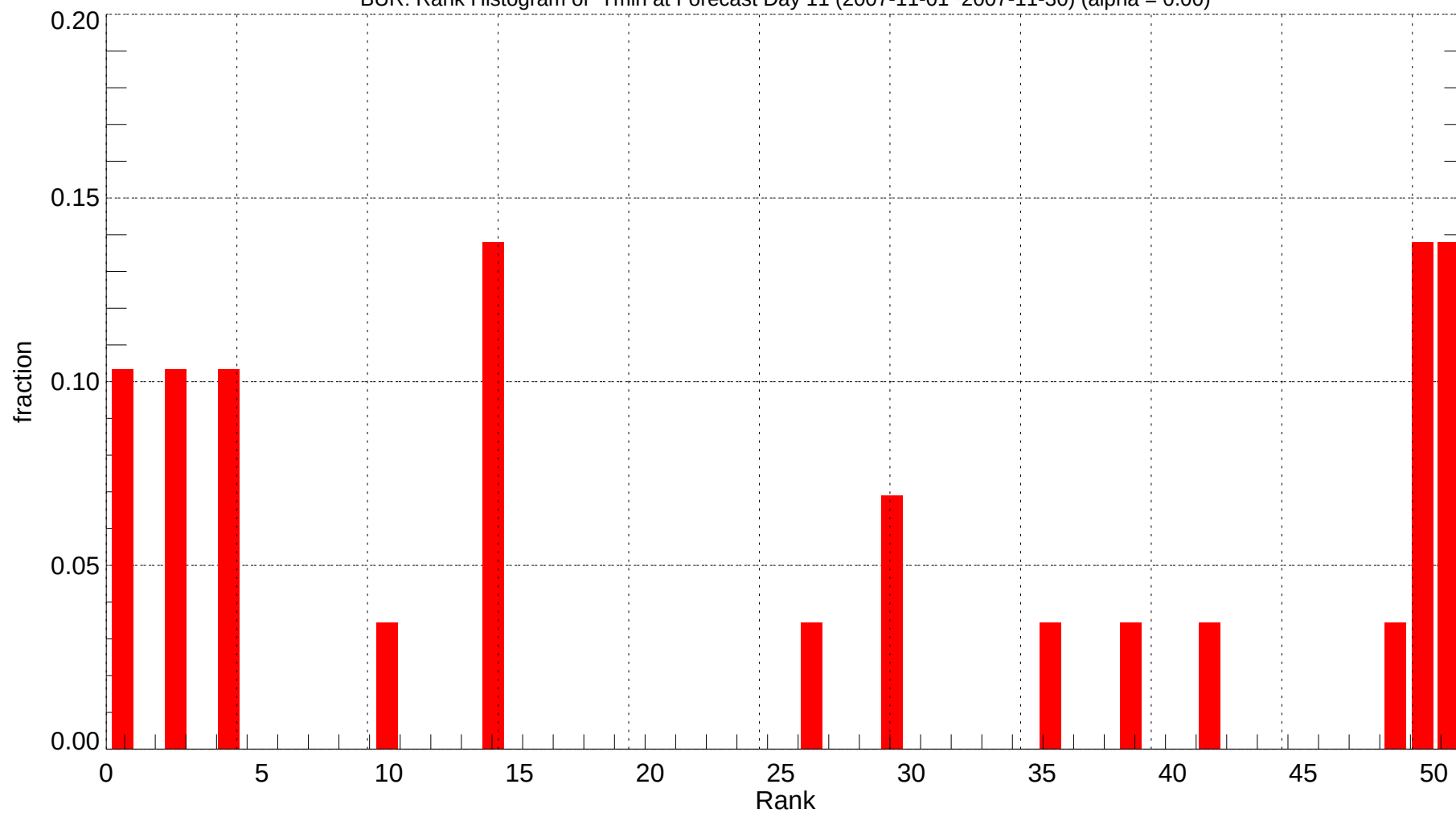
BUR: Rank Histogram of Tmin at Forecast Day 11 (2007-11-01~2007-11-30) (alpha = 0.00)
