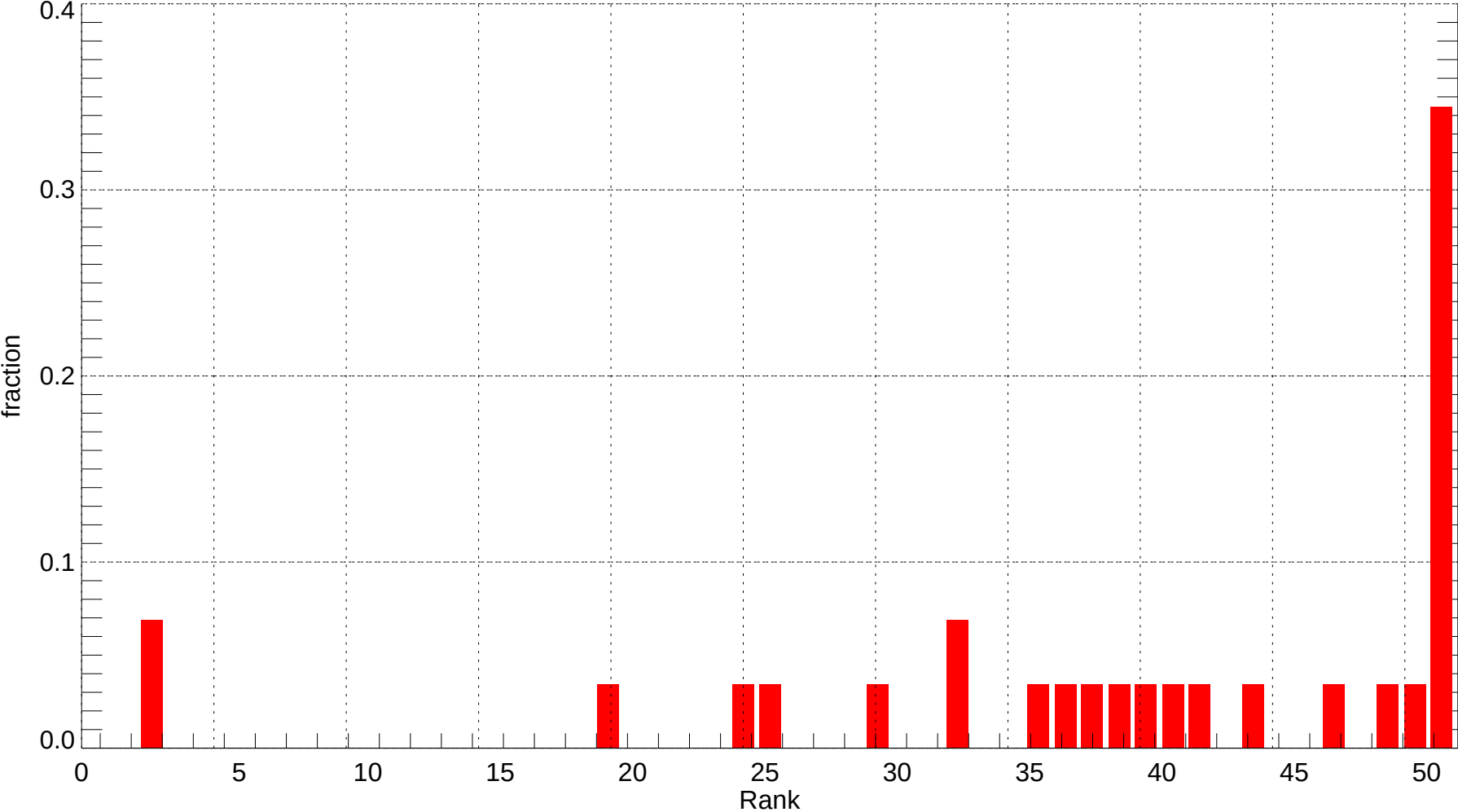
CLT: Rank Histogram of Tmin at Forecast Day 4 (2007-11-01~2007-11-30) (alpha = 0.00)
