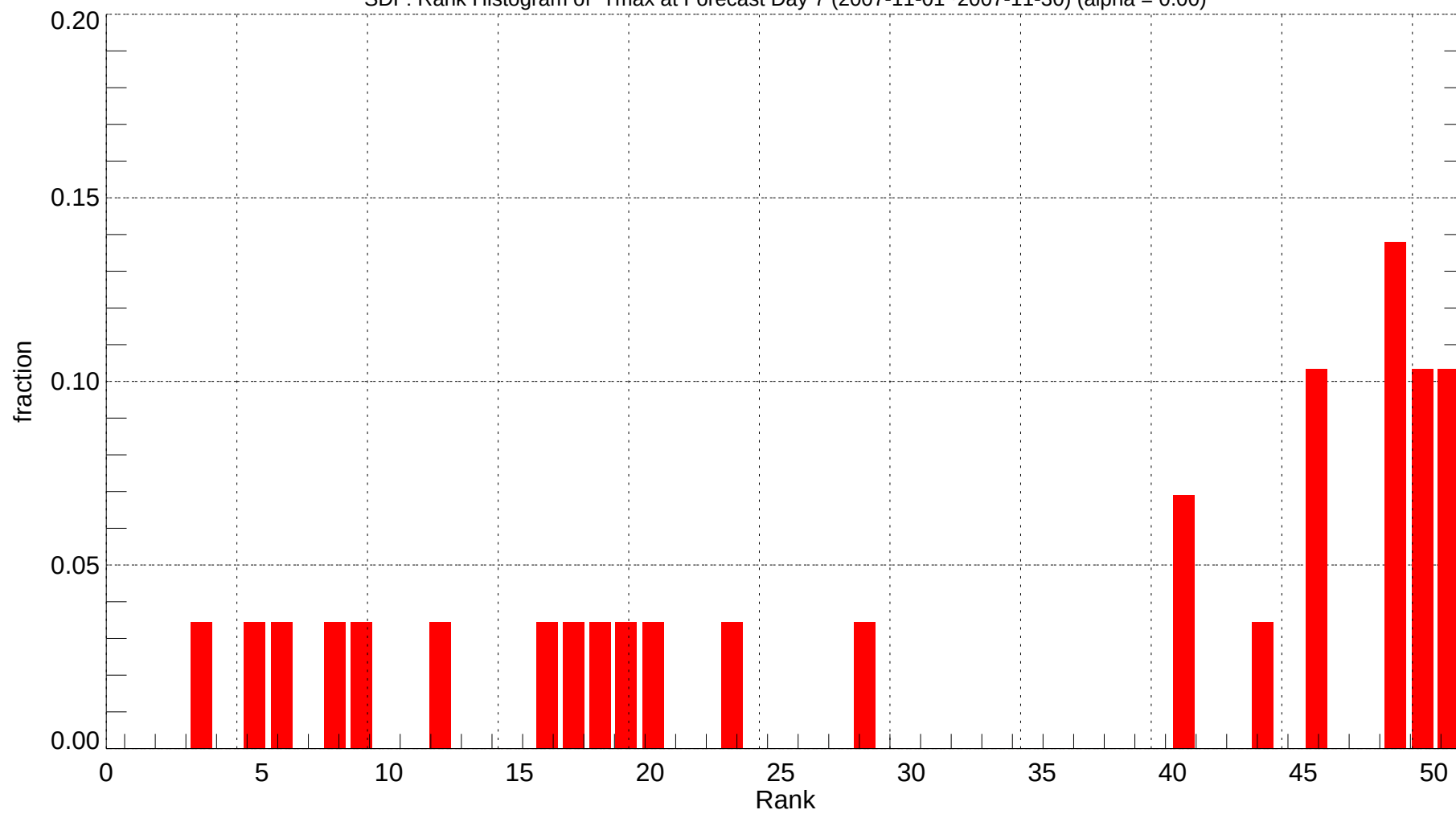
SDF: Rank Histogram of Tmax at Forecast Day 7 (2007-11-01~2007-11-30) (alpha = 0.00)
