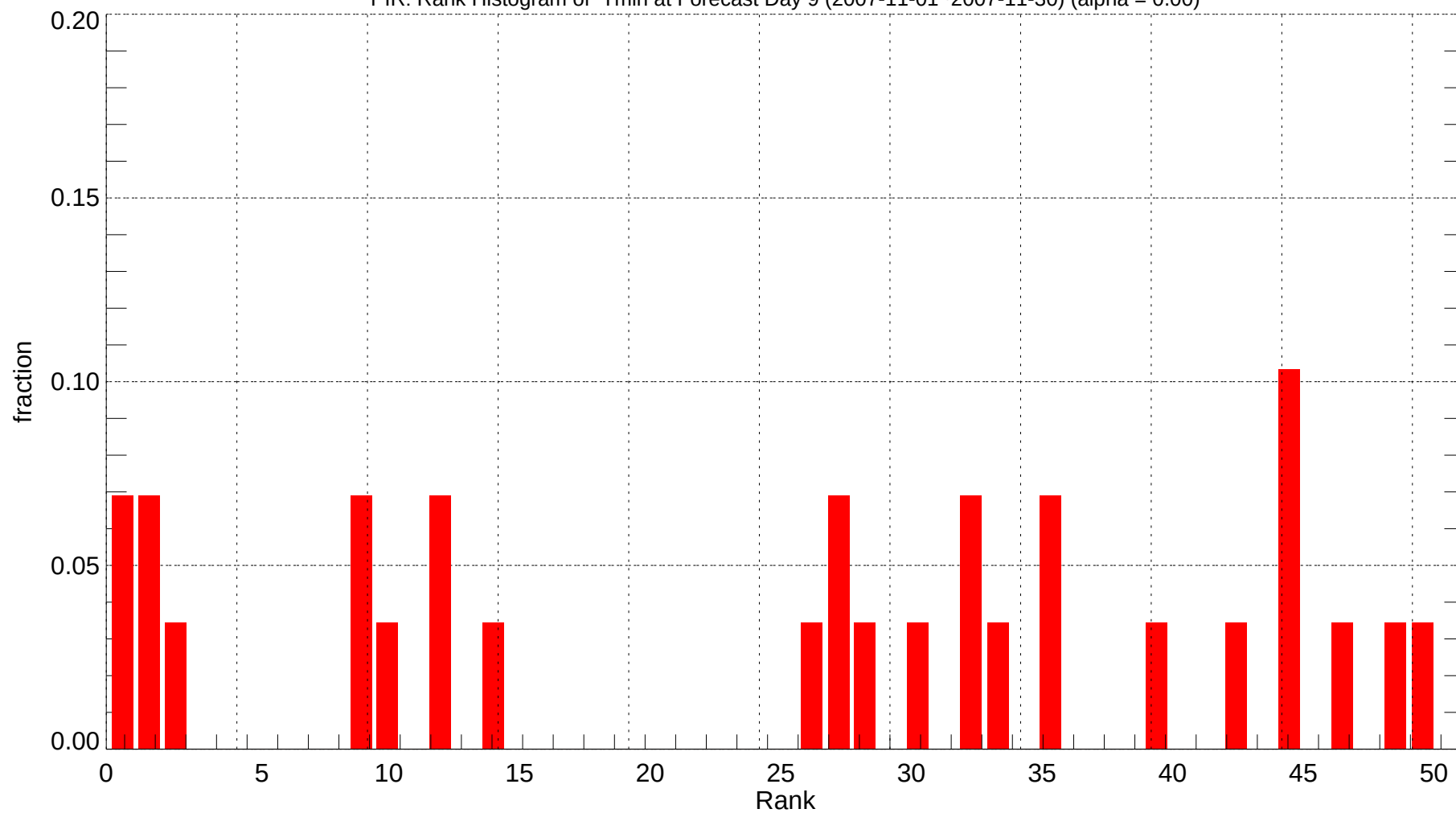
PIR: Rank Histogram of Tmin at Forecast Day 9 (2007-11-01~2007-11-30) (alpha = 0.00)
