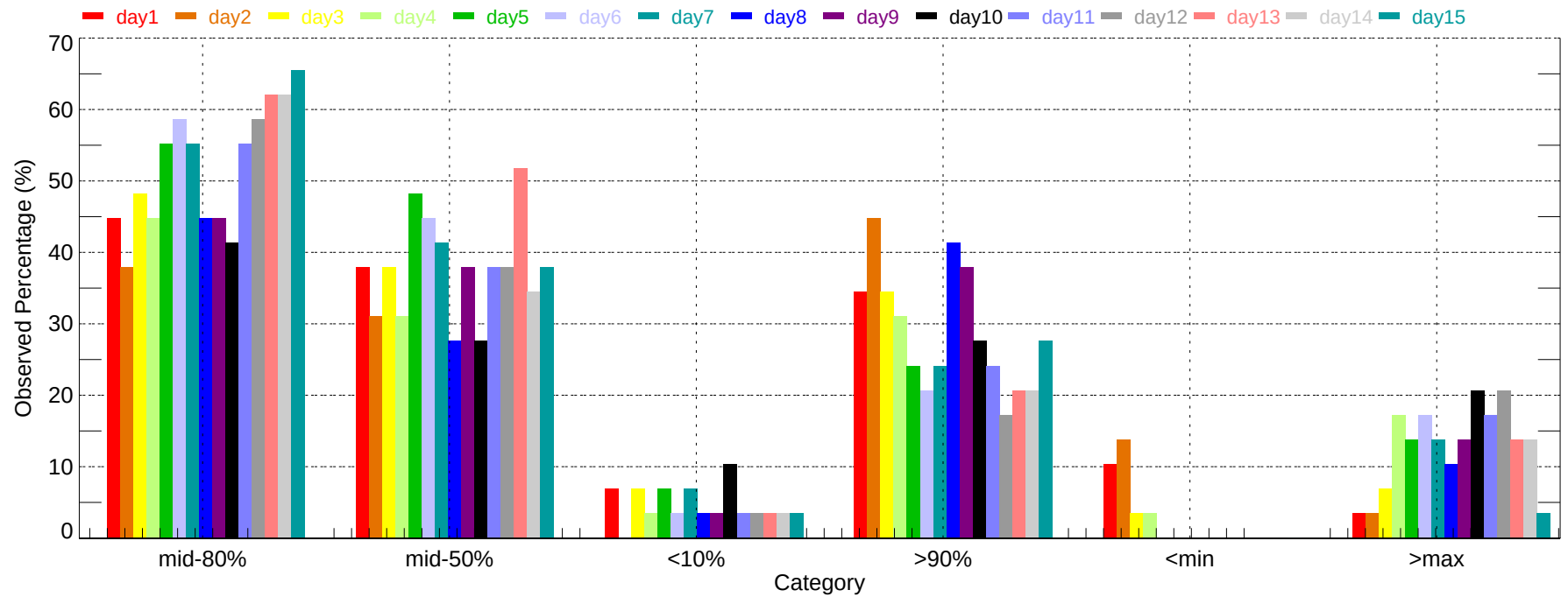
Observed Percentage of Ensembles - OKC: Max Temperature (2007-11-01~2007-11-30)
