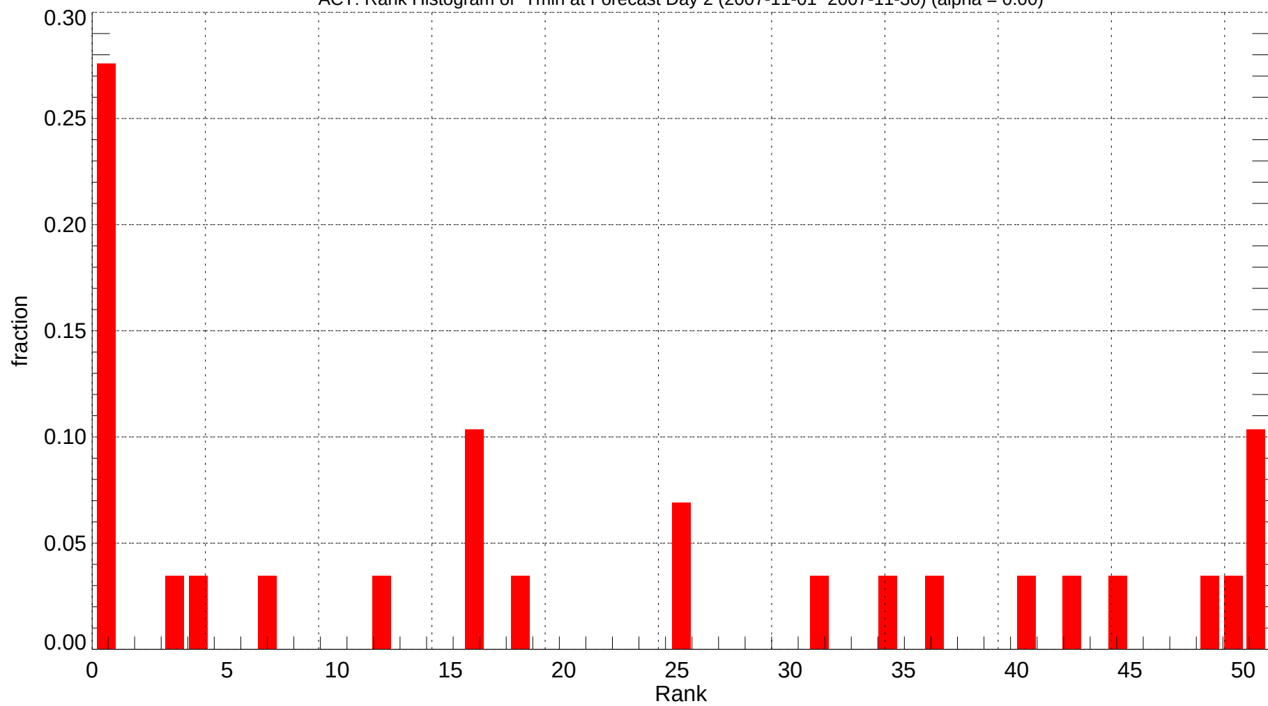
ACT: Rank Histogram of Tmin at Forecast Day 2 (2007-11-01~2007-11-30) (alpha = 0.00)
