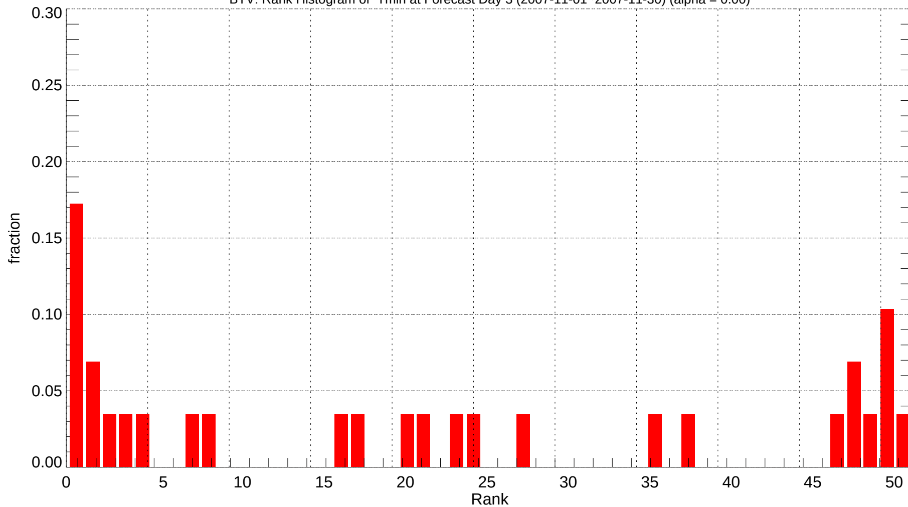
BTV: Rank Histogram of Tmin at Forecast Day 3 (2007-11-01~2007-11-30) (alpha = 0.00)
