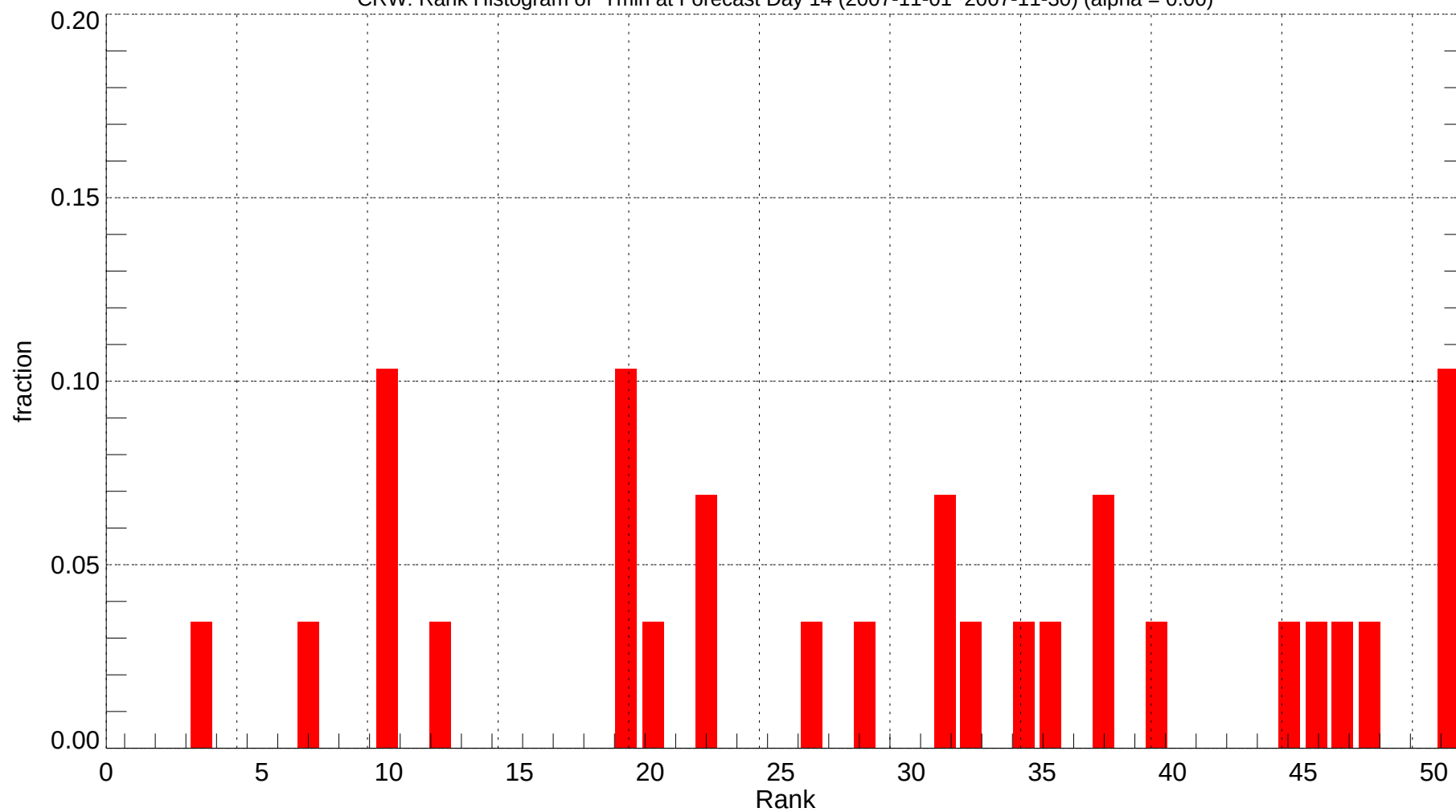
CRW: Rank Histogram of Tmin at Forecast Day 14 (2007-11-01~2007-11-30) (alpha = 0.00)
