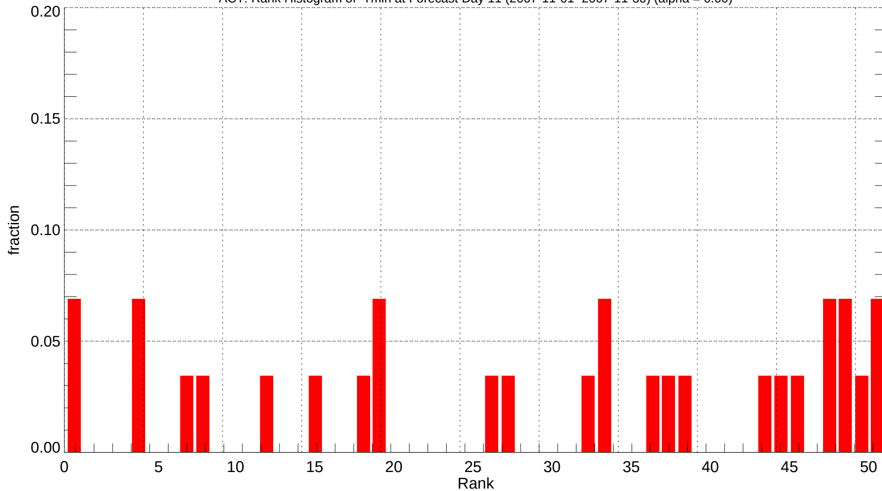
ACT: Rank Histogram of Tmin at Forecast Day 11 (2007-11-01~2007-11-30) (alpha = 0.00)
