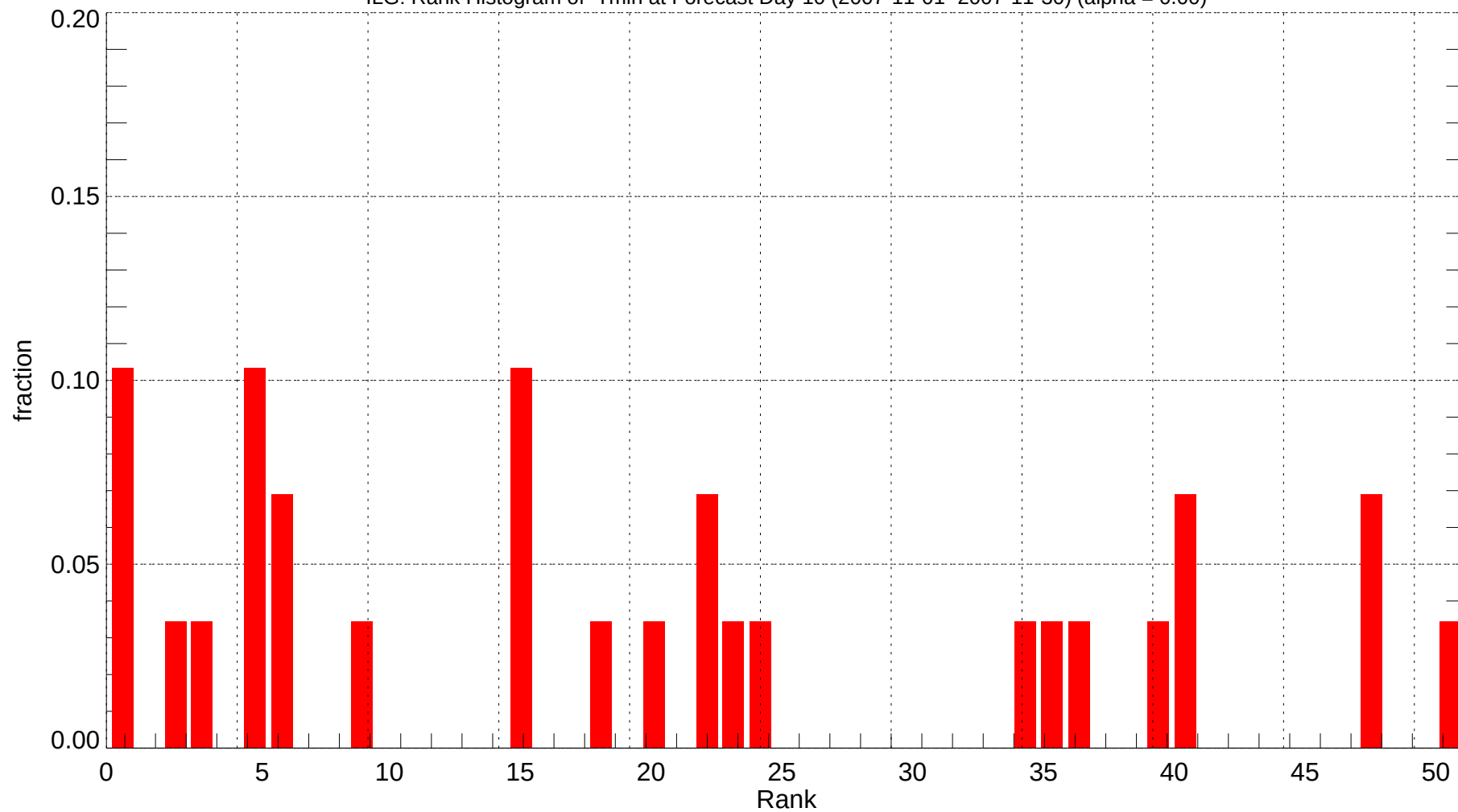
ILG: Rank Histogram of Tmin at Forecast Day 10 (2007-11-01~2007-11-30) (alpha = 0.00)
