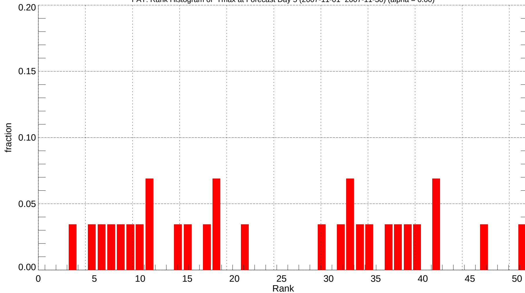
FAT: Rank Histogram of Tmax at Forecast Day 5 (2007-11-01~2007-11-30) (alpha = 0.00)
