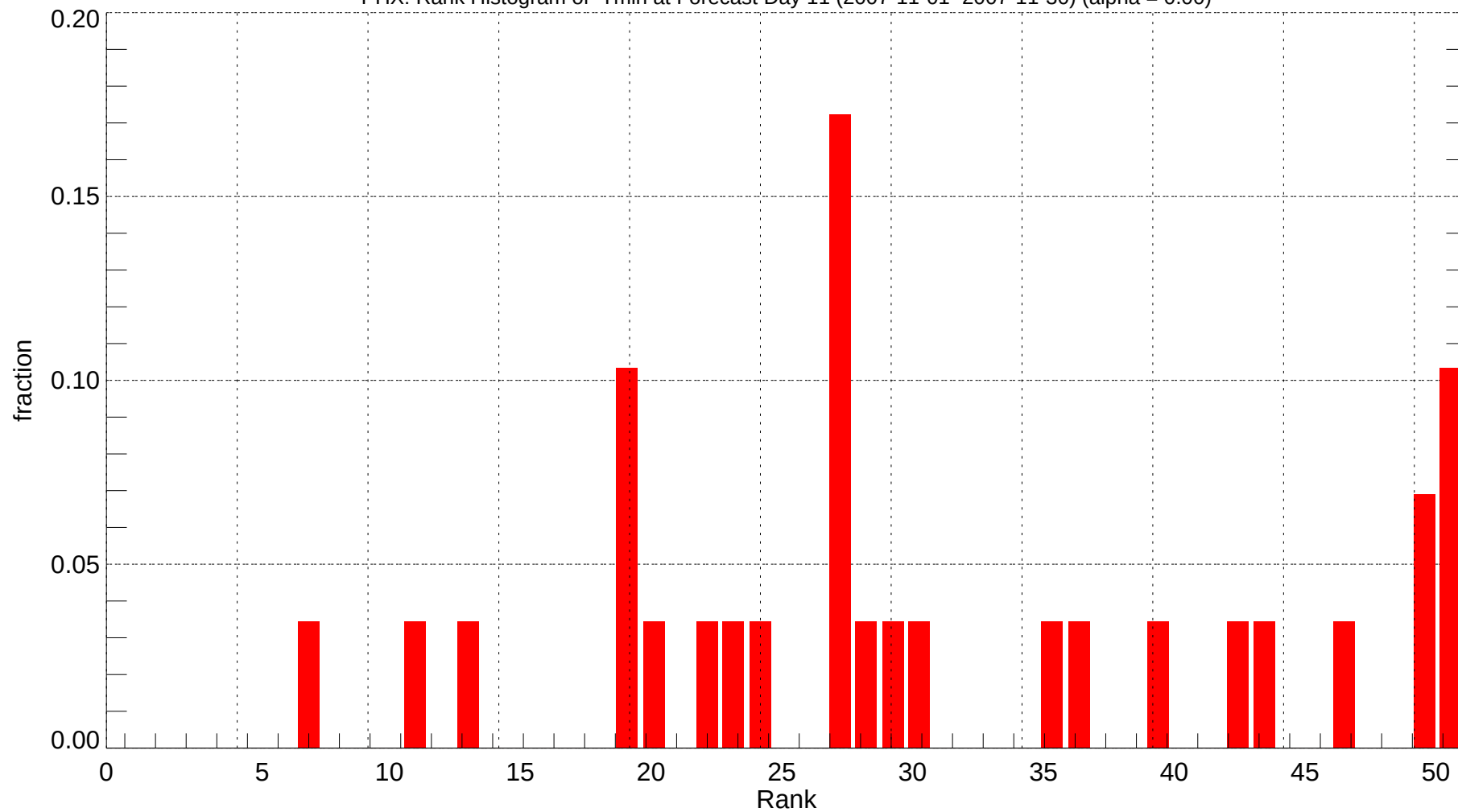
PHX: Rank Histogram of Tmin at Forecast Day 11 (2007-11-01~2007-11-30) (alpha = 0.00)
