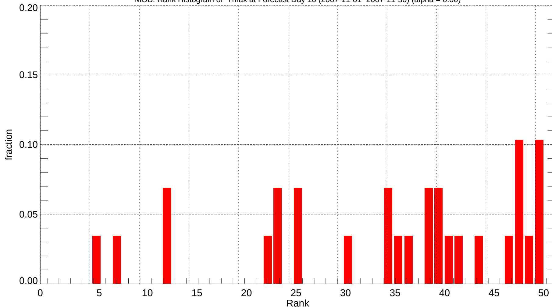
MOB: Rank Histogram of Tmax at Forecast Day 10 (2007-11-01~2007-11-30) (alpha = 0.00)
