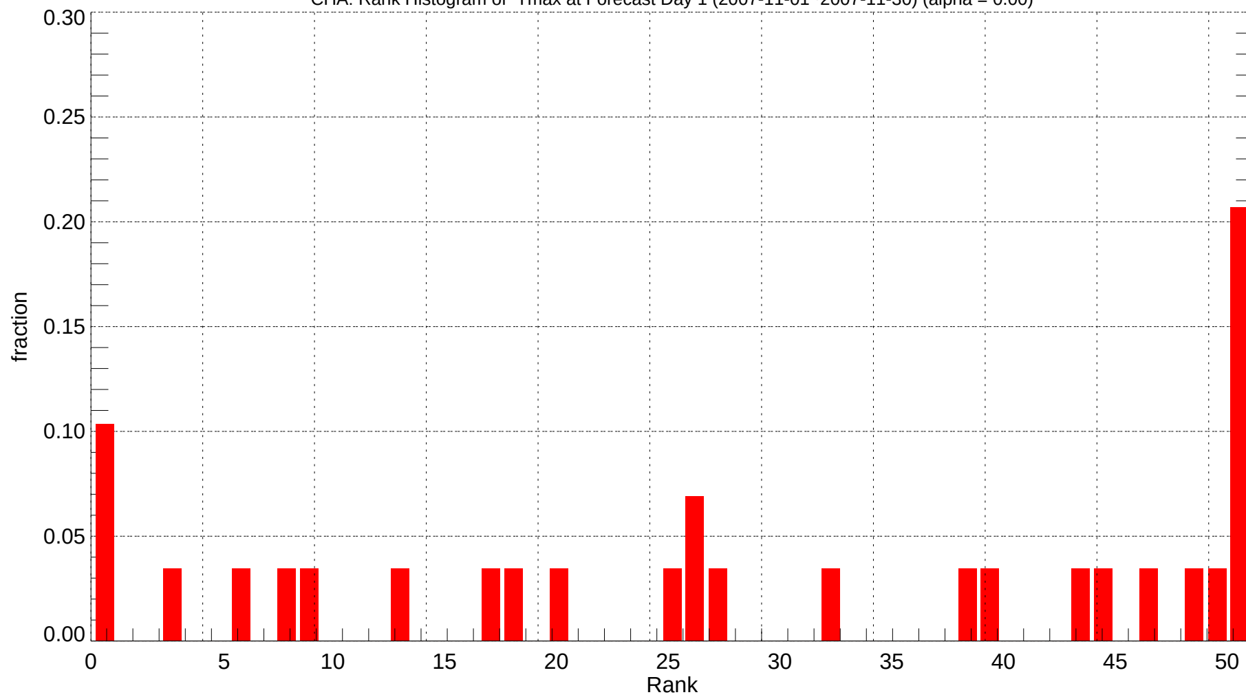
CHA: Rank Histogram of Tmax at Forecast Day 1 (2007-11-01~2007-11-30) (alpha = 0.00)
