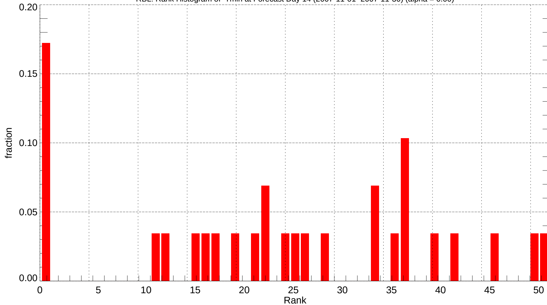
RBL: Rank Histogram of Tmin at Forecast Day 14 (2007-11-01~2007-11-30) (alpha = 0.00)
