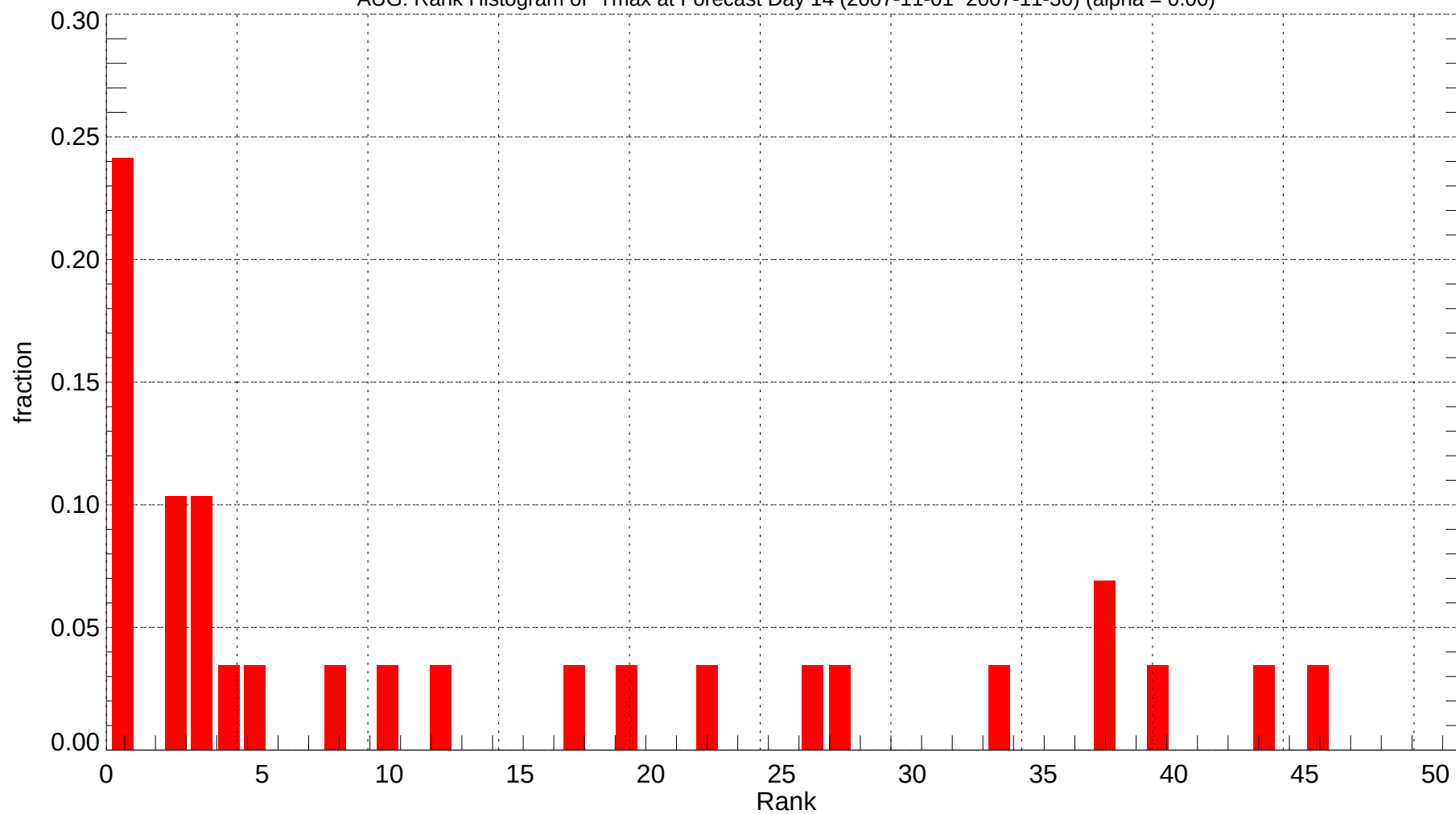
AUG: Rank Histogram of Tmax at Forecast Day 14 (2007-11-01~2007-11-30) (alpha = 0.00)
