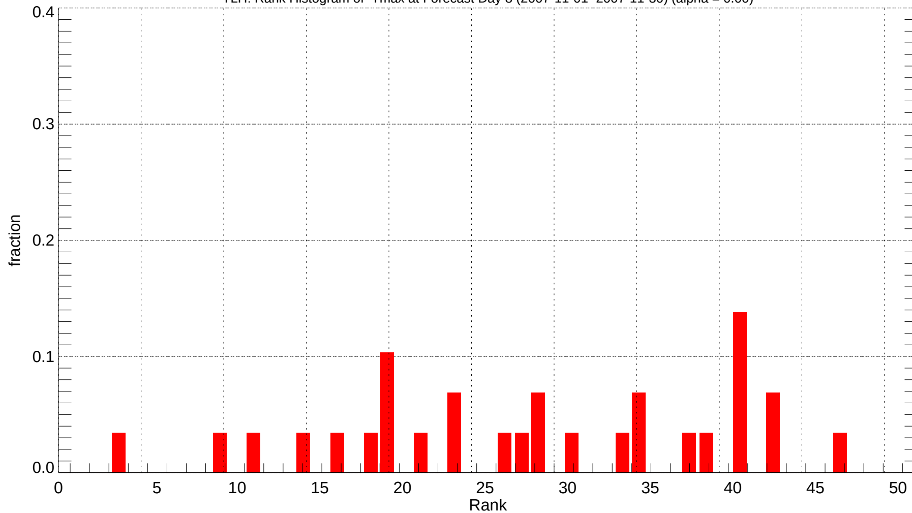
TLH: Rank Histogram of Tmax at Forecast Day 8 (2007-11-01~2007-11-30) (alpha = 0.00)
