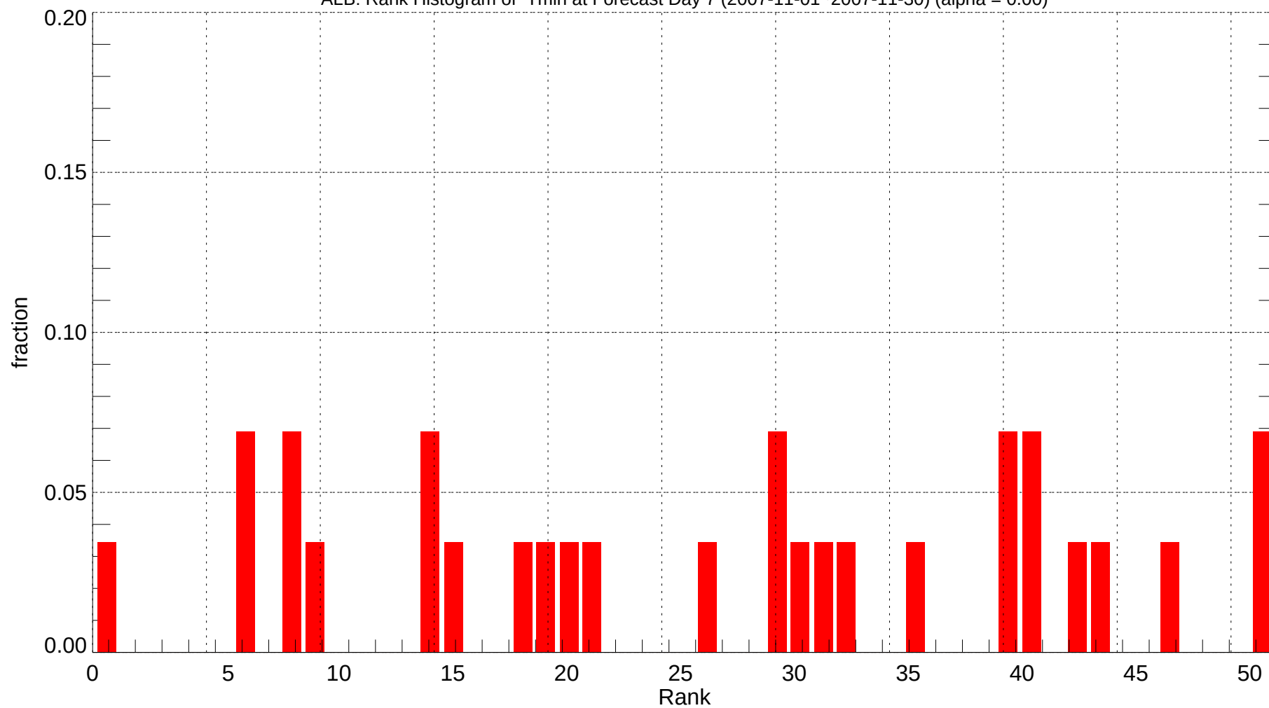
ALB: Rank Histogram of Tmin at Forecast Day 7 (2007-11-01~2007-11-30) (alpha = 0.00)
