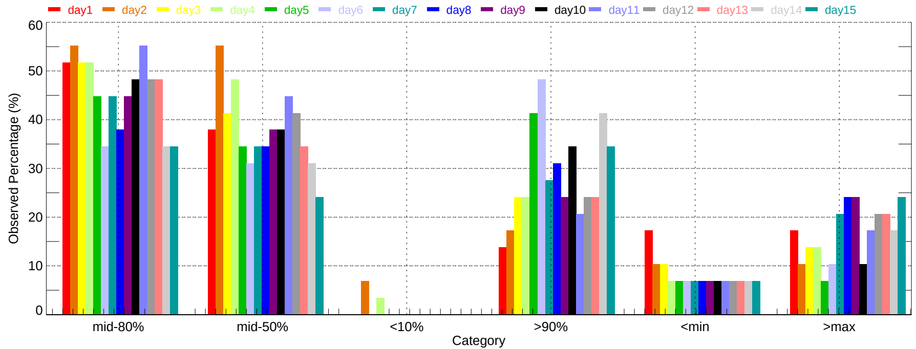
Observed Percentage of Ensembles - FLG: Min Temperature (2007-11-01~2007-11-30)
