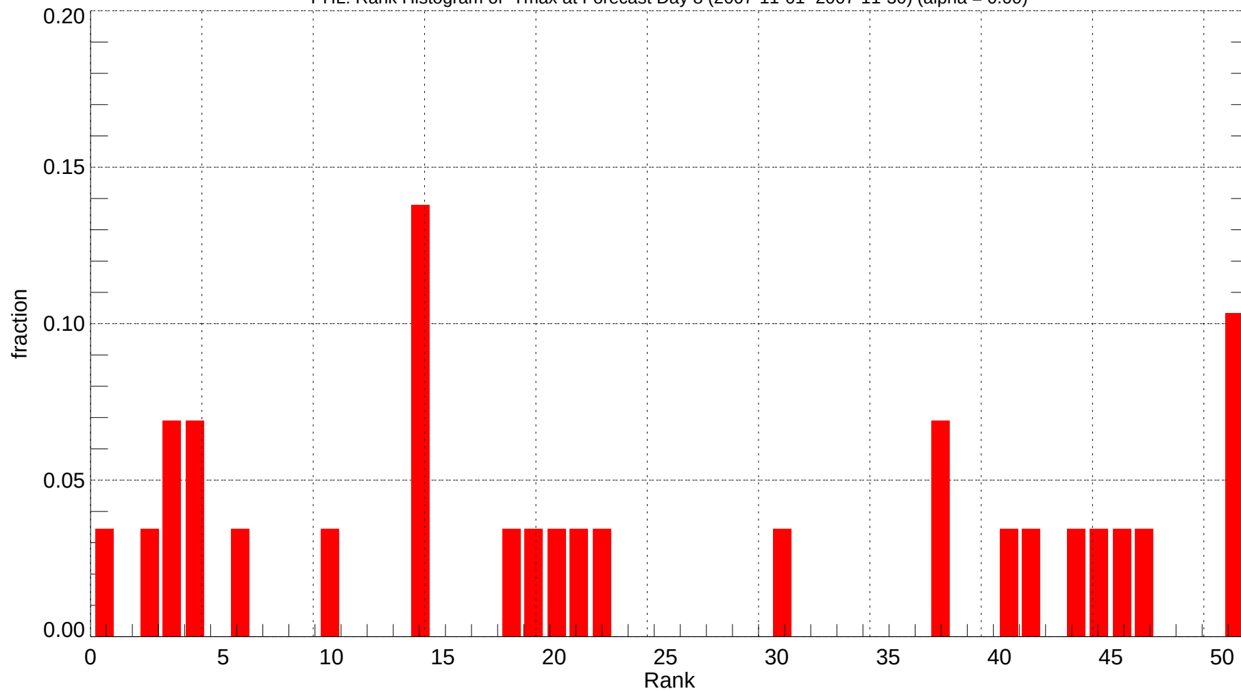
PHL: Rank Histogram of Tmax at Forecast Day 8 (2007-11-01~2007-11-30) (alpha = 0.00)
