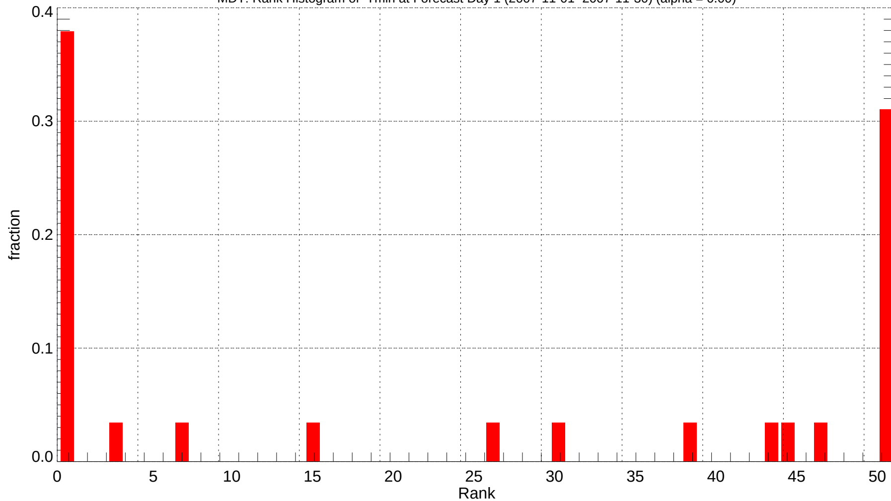
MDT: Rank Histogram of Tmin at Forecast Day 1 (2007-11-01~2007-11-30) (alpha = 0.00)
