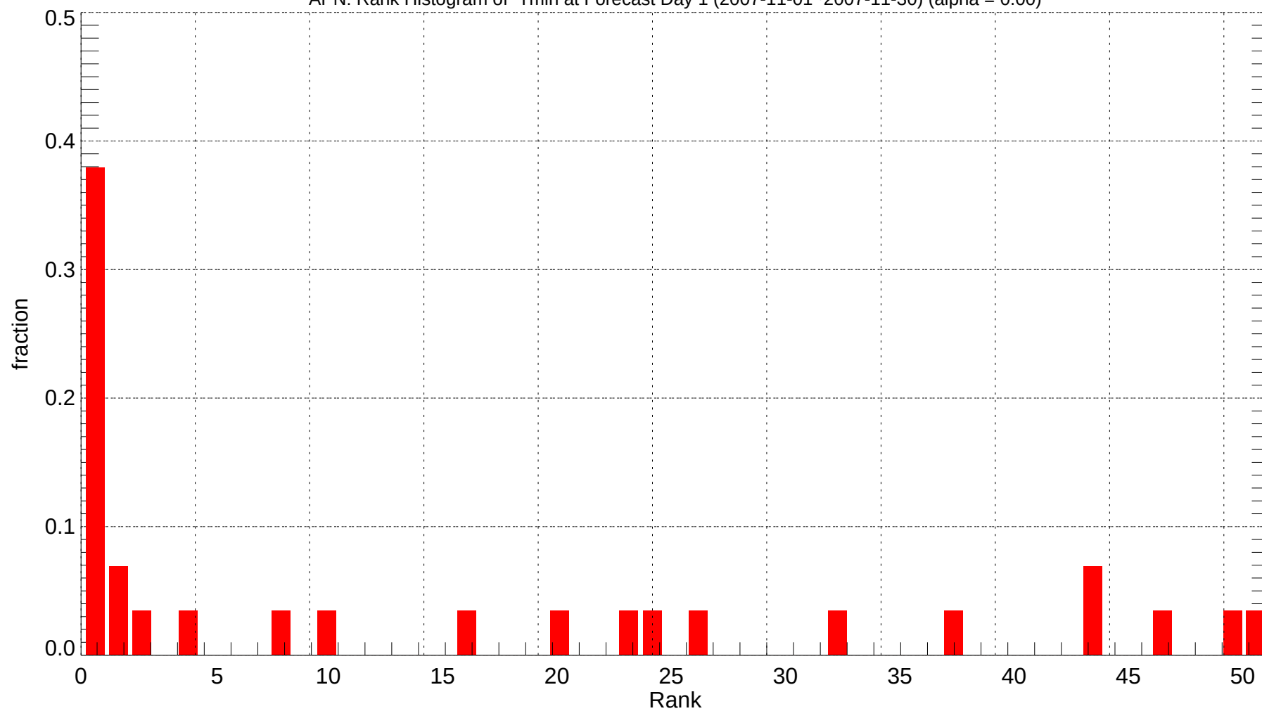
APN: Rank Histogram of Tmin at Forecast Day 1 (2007-11-01~2007-11-30) (alpha = 0.00)
