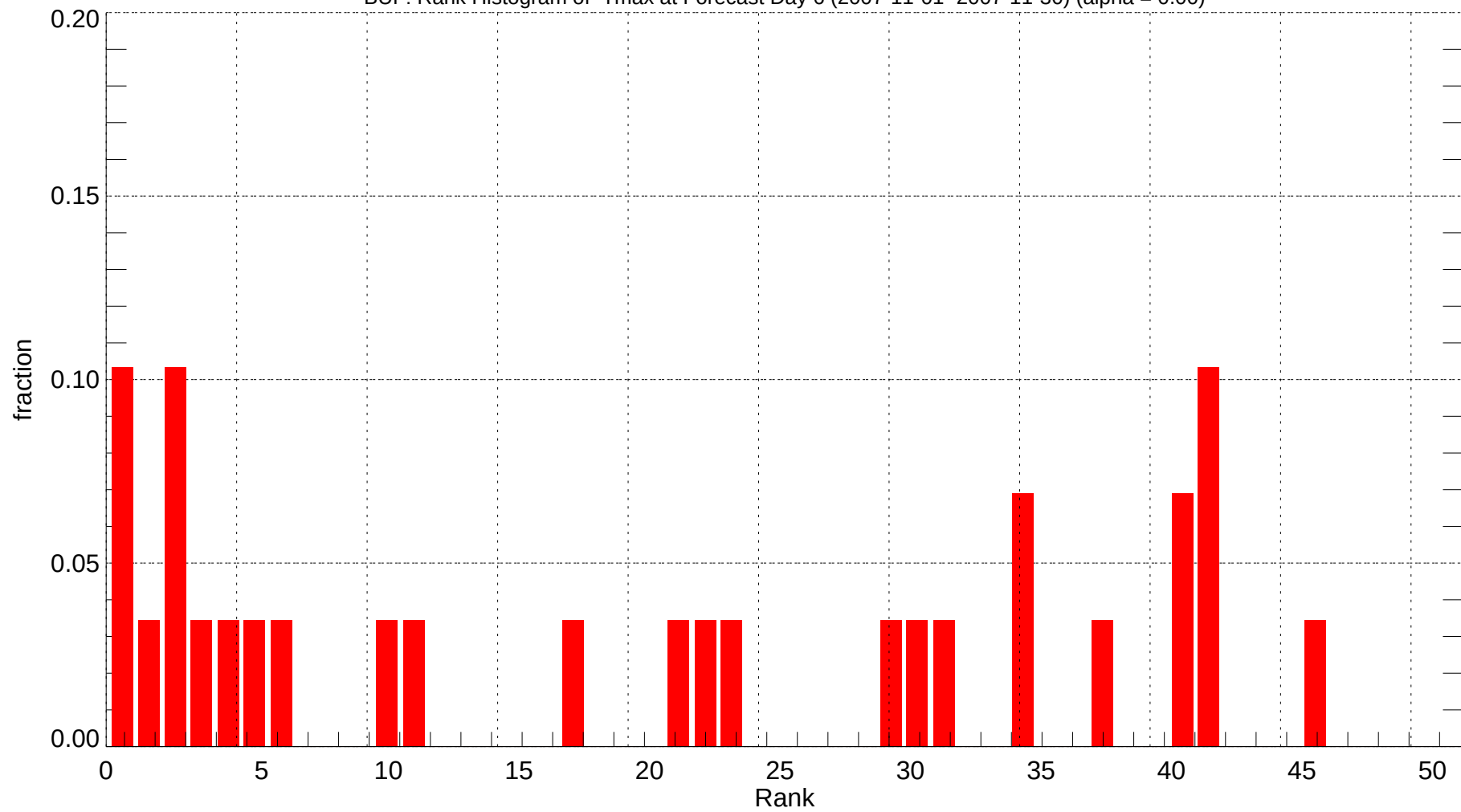
BUF: Rank Histogram of Tmax at Forecast Day 6 (2007-11-01~2007-11-30) (alpha = 0.00)
