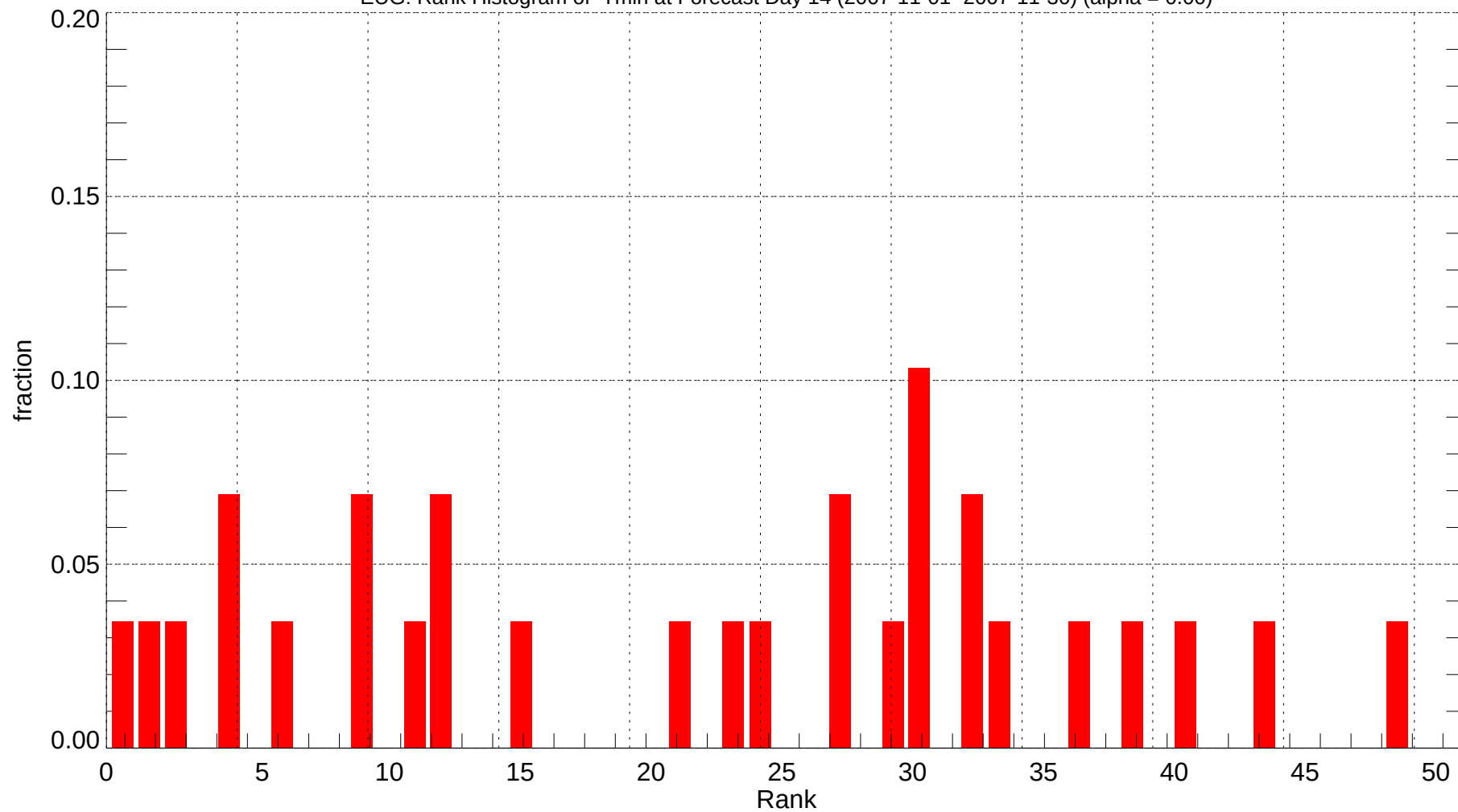
EUG: Rank Histogram of Tmin at Forecast Day 14 (2007-11-01~2007-11-30) (alpha = 0.00)
