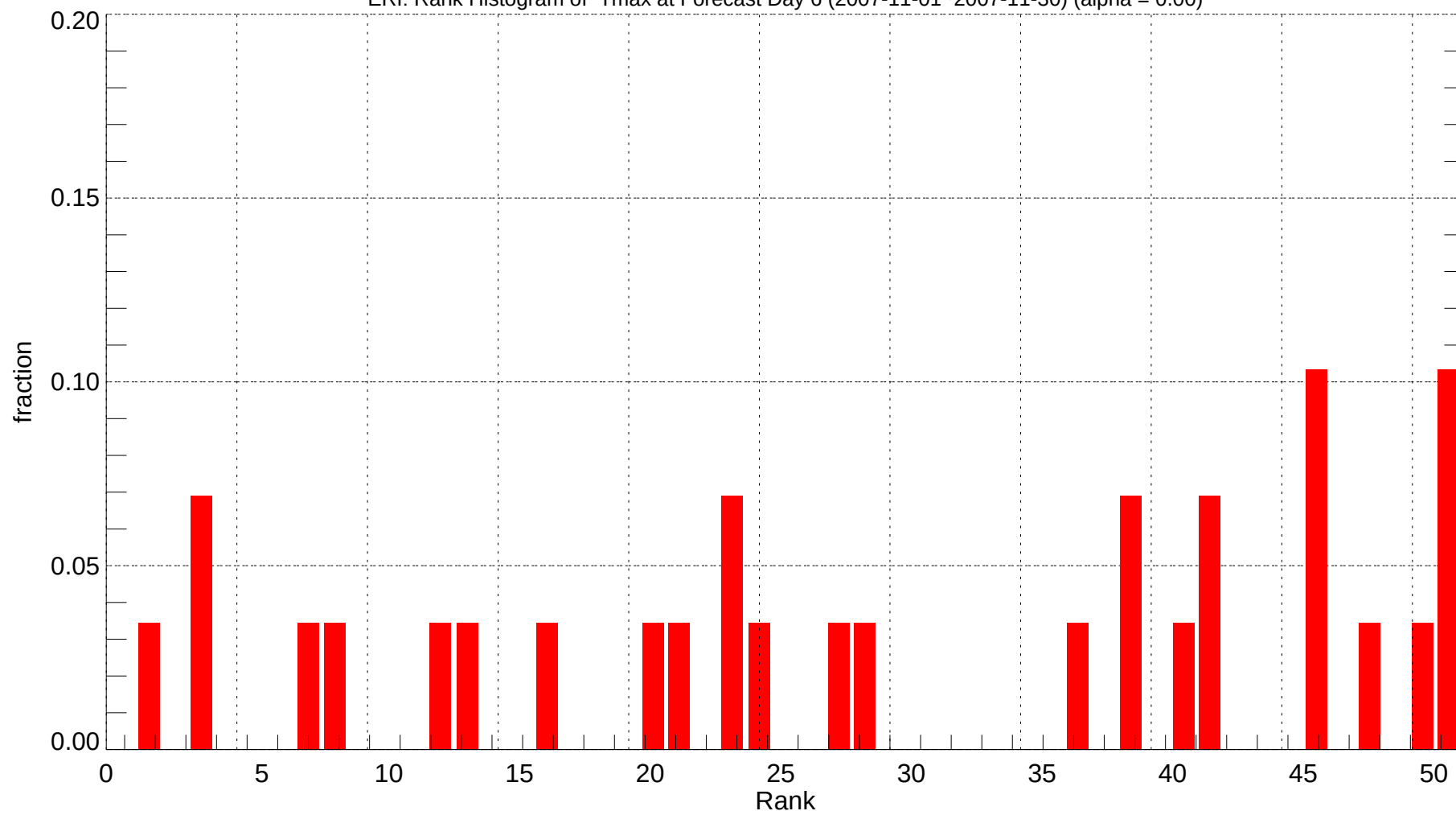
ERI: Rank Histogram of Tmax at Forecast Day 6 (2007-11-01~2007-11-30) (alpha = 0.00)
