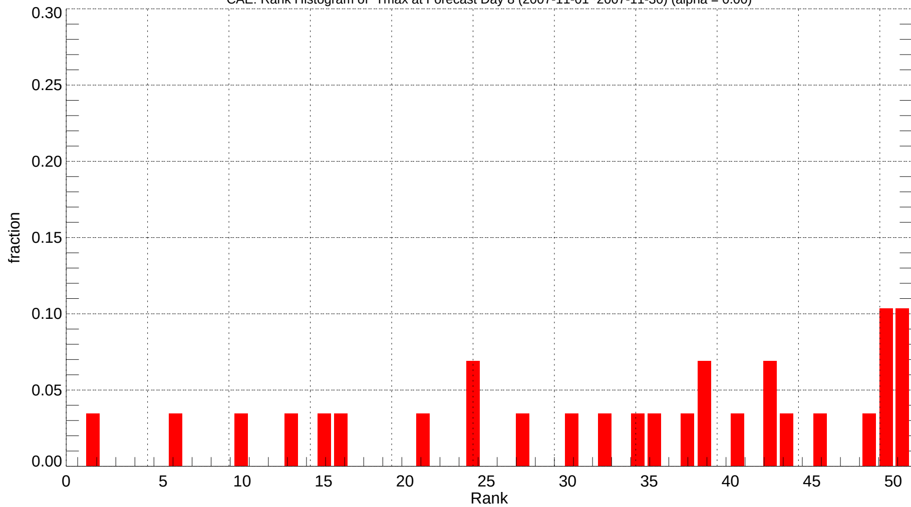
CAE: Rank Histogram of Tmax at Forecast Day 8 (2007-11-01~2007-11-30) (alpha = 0.00)
