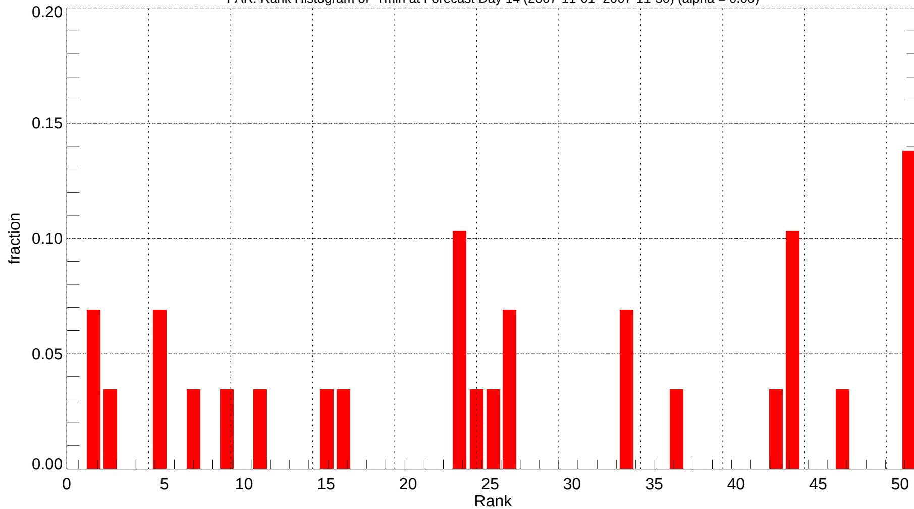
FAR: Rank Histogram of Tmin at Forecast Day 14 (2007-11-01~2007-11-30) (alpha = 0.00)
