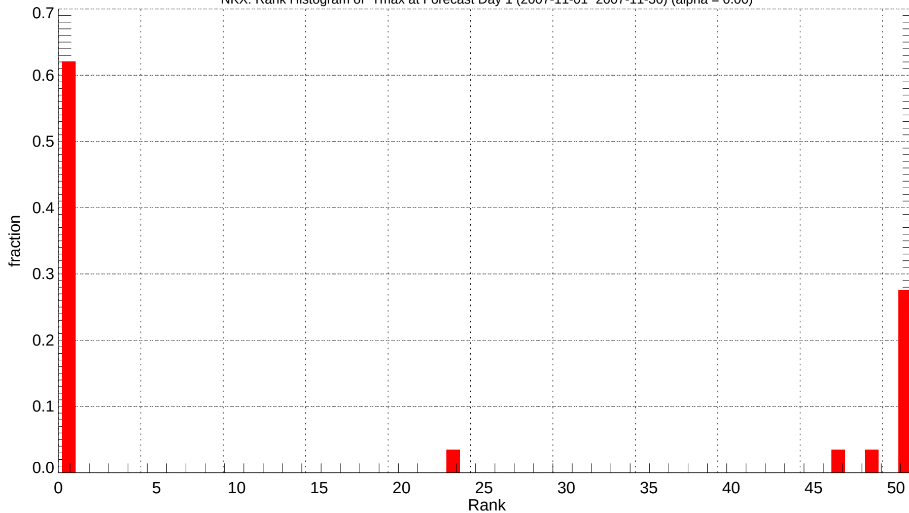
NKX: Rank Histogram of Tmax at Forecast Day 1 (2007-11-01~2007-11-30) (alpha = 0.00)
