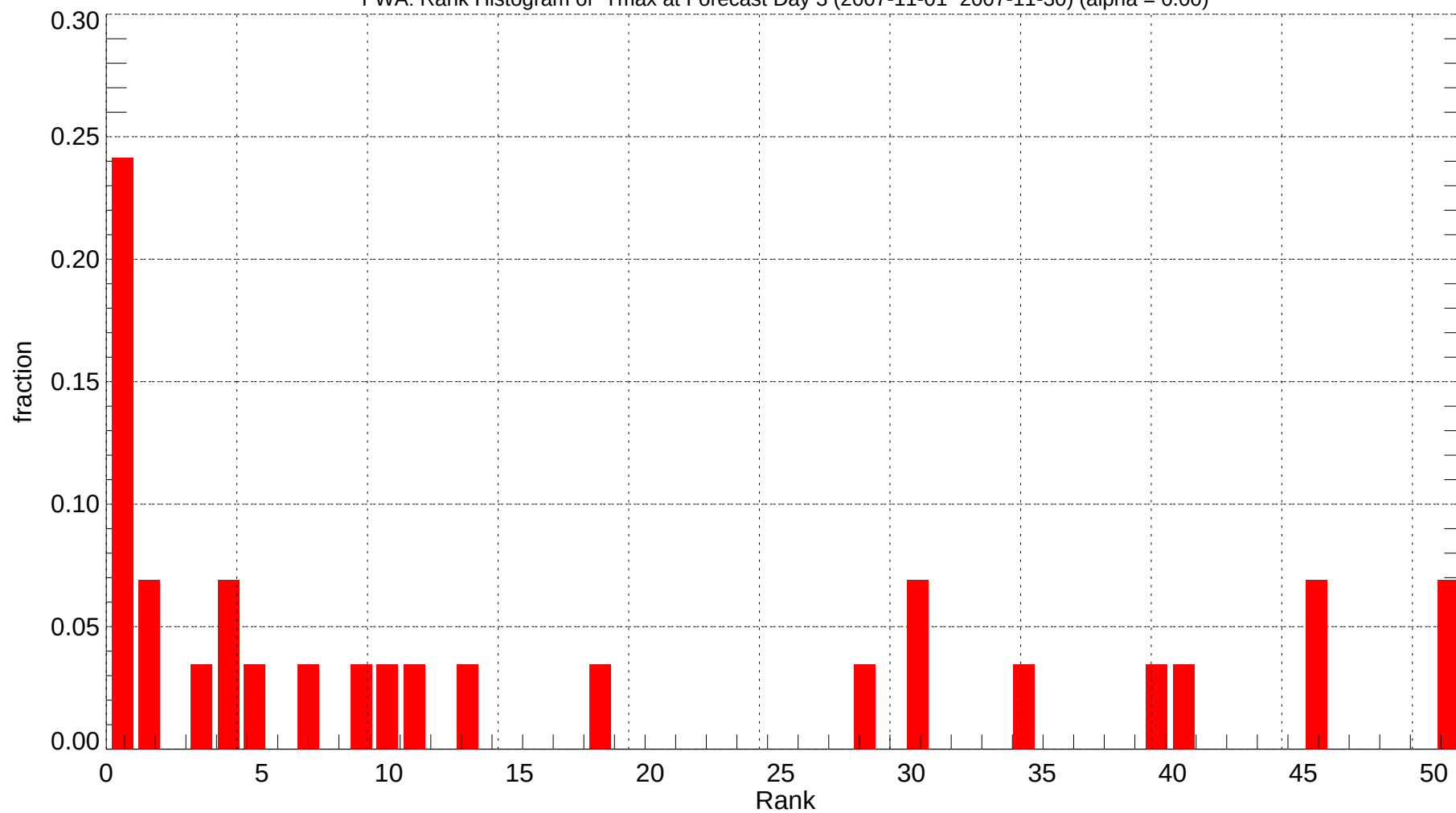
FWA: Rank Histogram of Tmax at Forecast Day 3 (2007-11-01~2007-11-30) (alpha = 0.00)
