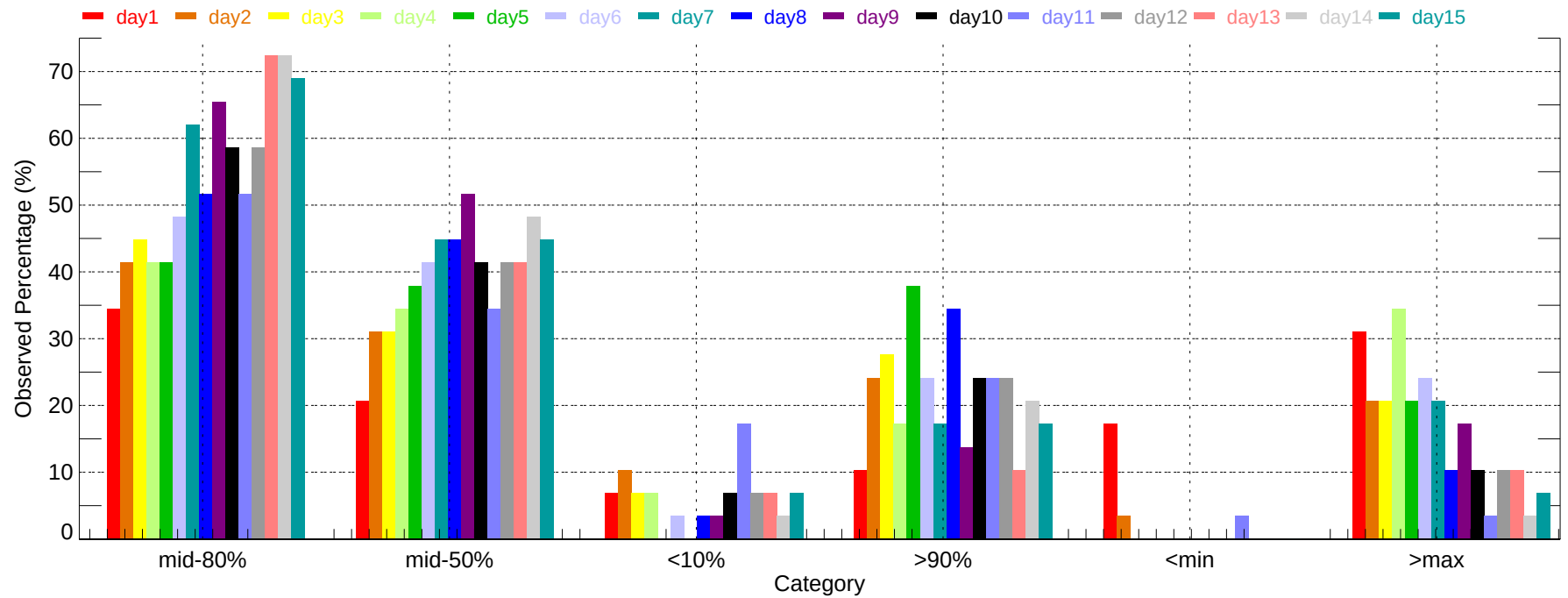
Observed Percentage of Ensembles - CLT: Max Temperature (2007-11-01~2007-11-30)
