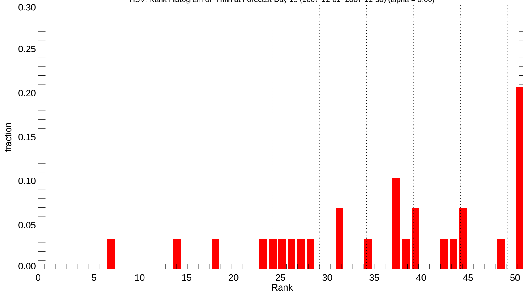
HSV: Rank Histogram of Tmin at Forecast Day 13 (2007-11-01~2007-11-30) (alpha = 0.00)
