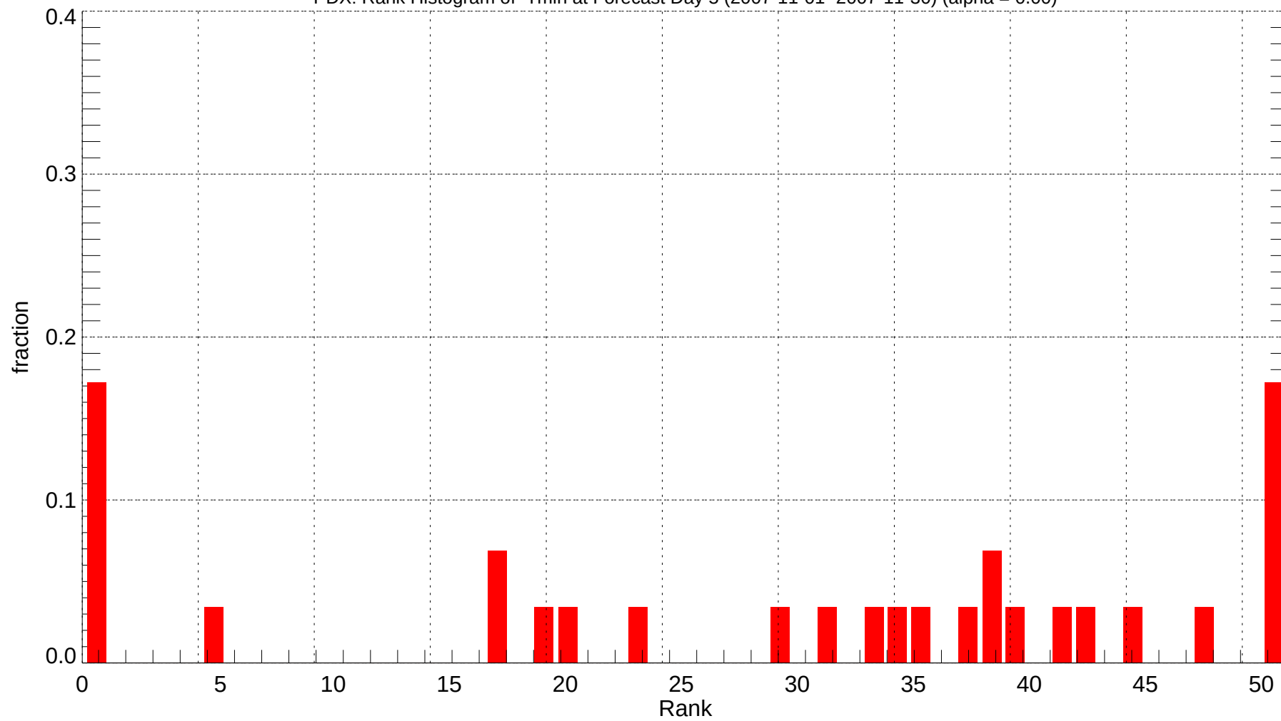
PDX: Rank Histogram of Tmin at Forecast Day 5 (2007-11-01~2007-11-30) (alpha = 0.00)
