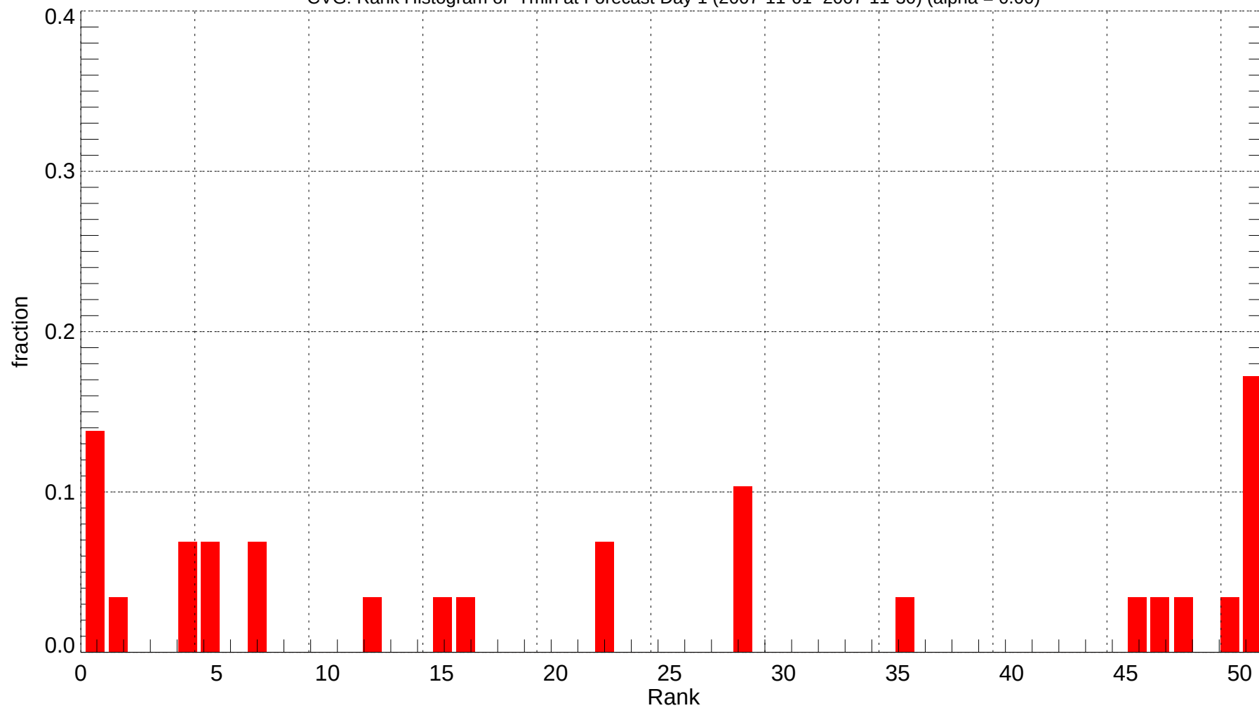
CVG: Rank Histogram of Tmin at Forecast Day 1 (2007-11-01~2007-11-30) (alpha = 0.00)
