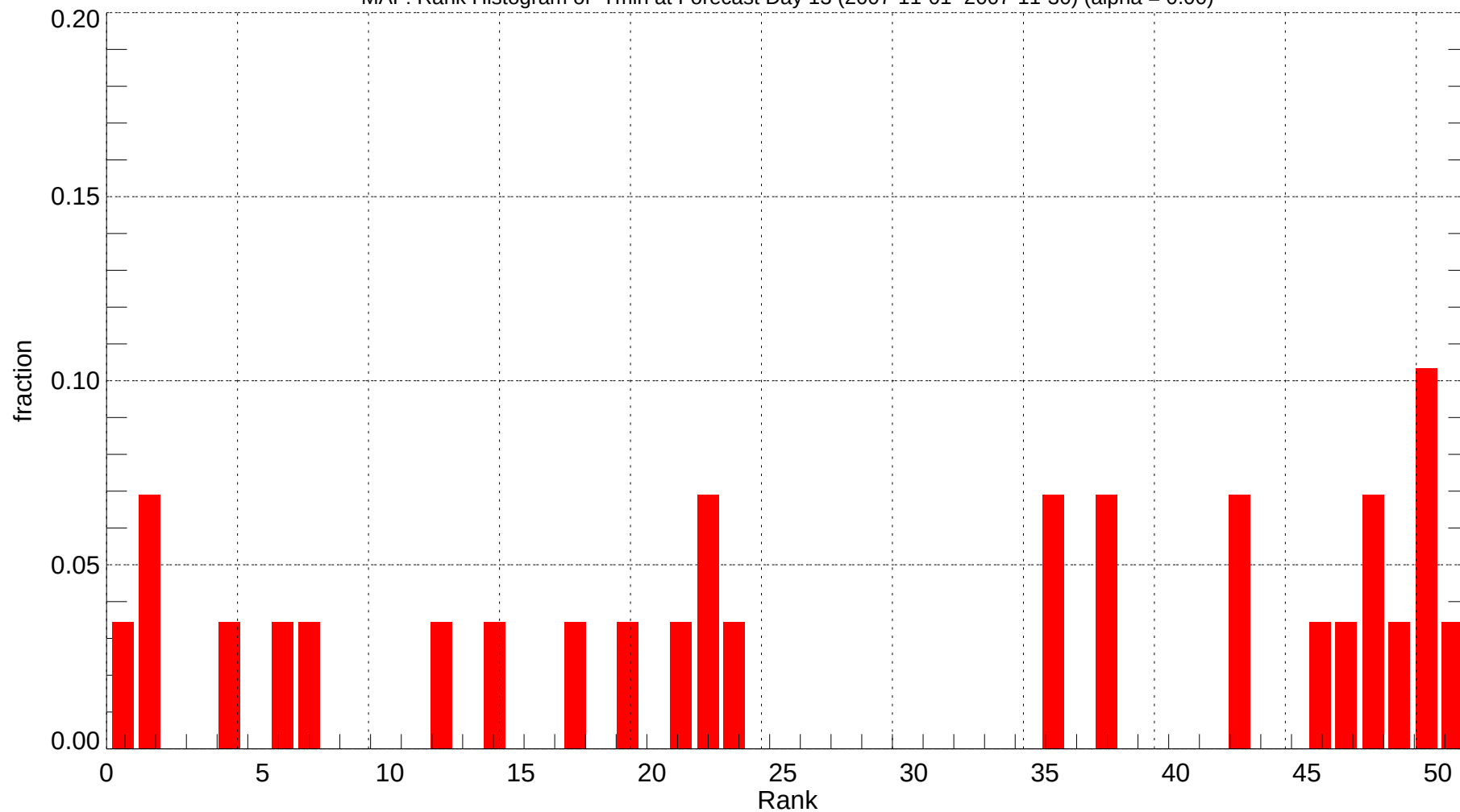
MAF: Rank Histogram of Tmin at Forecast Day 13 (2007-11-01~2007-11-30) (alpha = 0.00)
