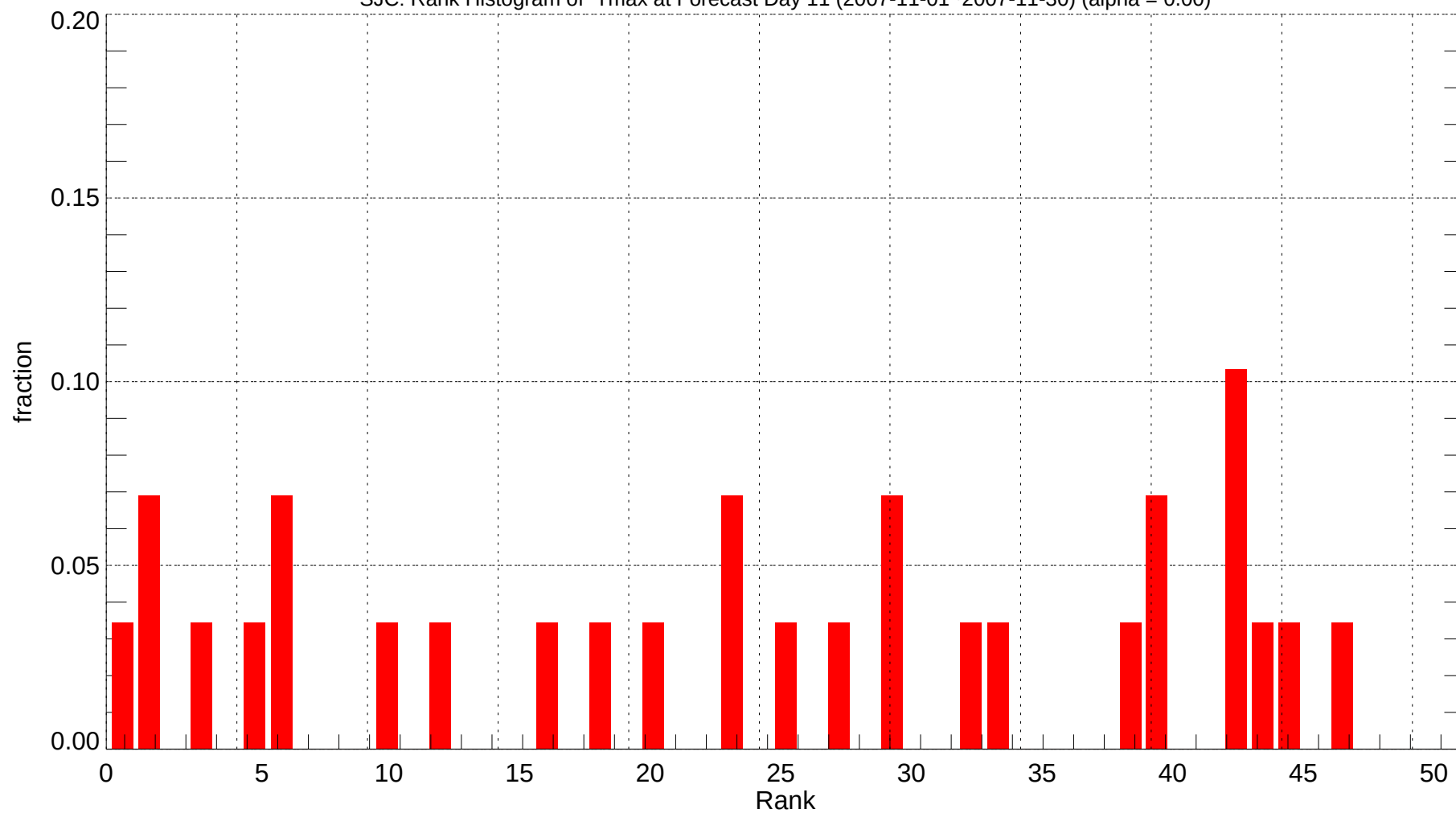
SJC: Rank Histogram of Tmax at Forecast Day 11 (2007-11-01~2007-11-30) (alpha = 0.00)
