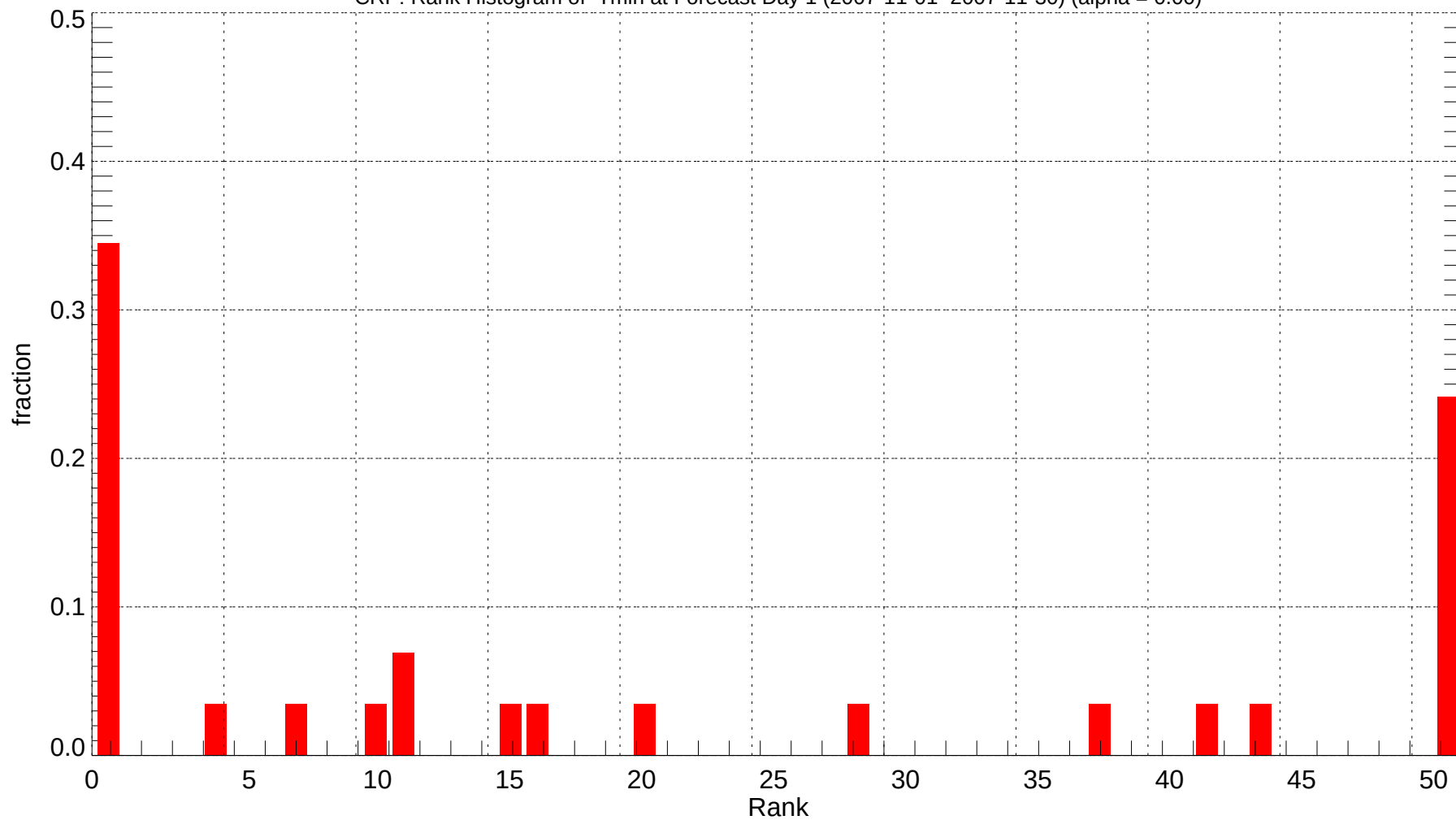
CRP: Rank Histogram of Tmin at Forecast Day 1 (2007-11-01~2007-11-30) (alpha = 0.00)
