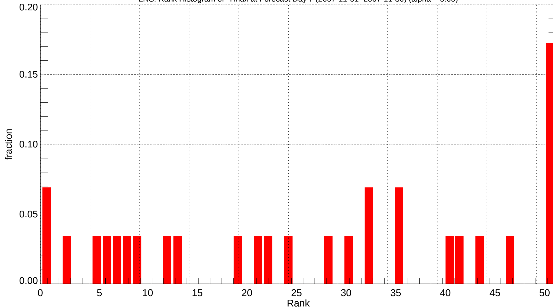
LNS: Rank Histogram of Tmax at Forecast Day 7 (2007-11-01~2007-11-30) (alpha = 0.00)
