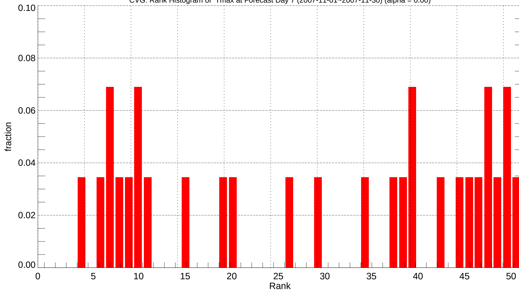
CVG: Rank Histogram of Tmax at Forecast Day 7 (2007-11-01~2007-11-30) (alpha = 0.00)
