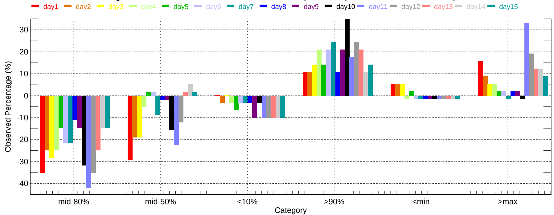
Observed Percentage Deviation of Ensembles - JAN: Min Temperature (2007-11-01~2007-11-30)
