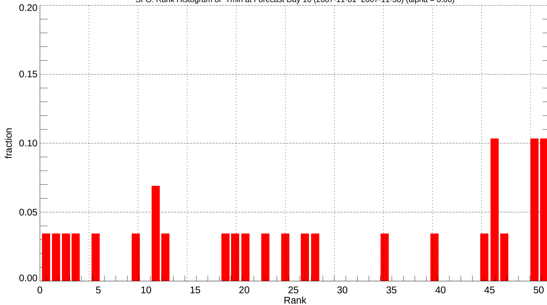
SFO: Rank Histogram of Tmin at Forecast Day 10 (2007-11-01~2007-11-30) (alpha = 0.00)
