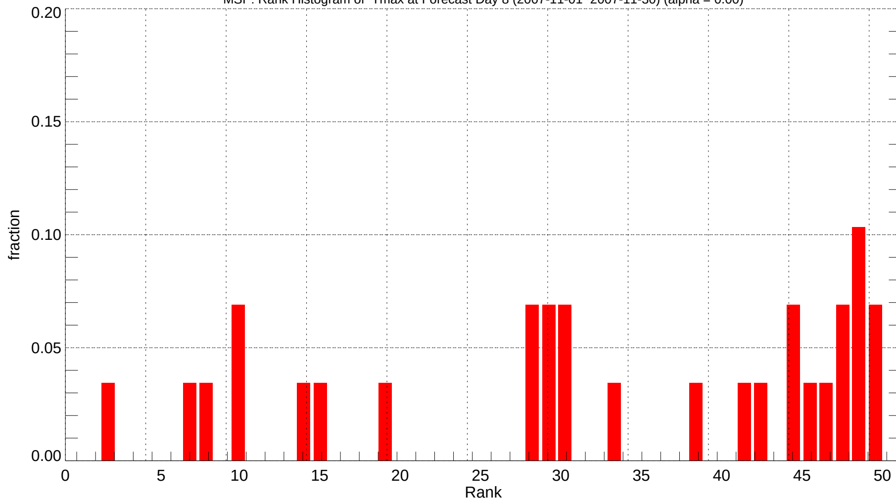
MSP: Rank Histogram of Tmax at Forecast Day 8 (2007-11-01~2007-11-30) (alpha = 0.00)
