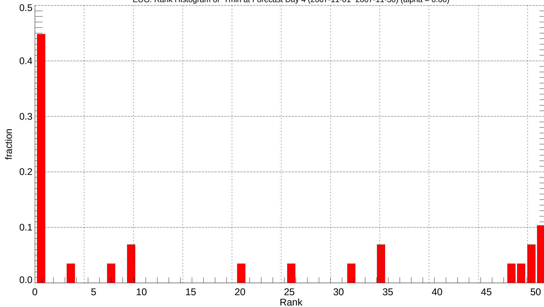
EUG: Rank Histogram of Tmin at Forecast Day 4 (2007-11-01~2007-11-30) (alpha = 0.00)
