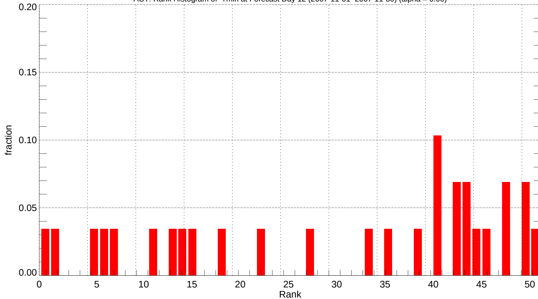
ACT: Rank Histogram of Tmin at Forecast Day 12 (2007-11-01~2007-11-30) (alpha = 0.00)
