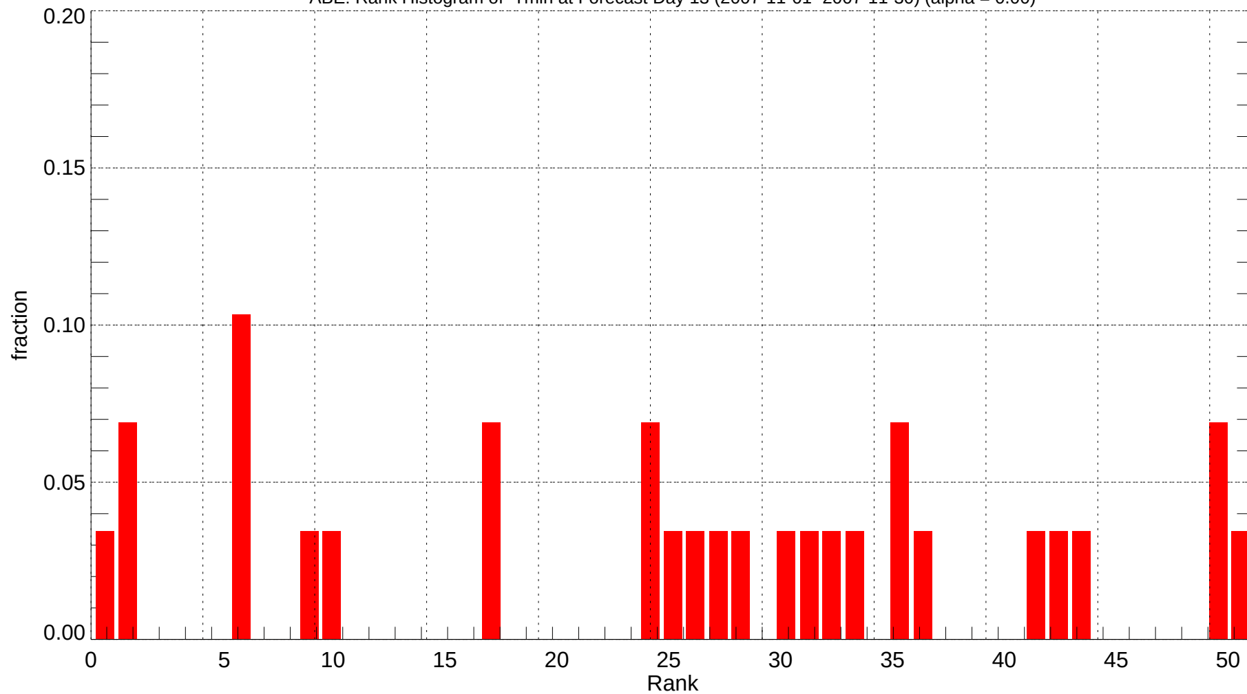
ABE: Rank Histogram of Tmin at Forecast Day 13 (2007-11-01~2007-11-30) (alpha = 0.00)
