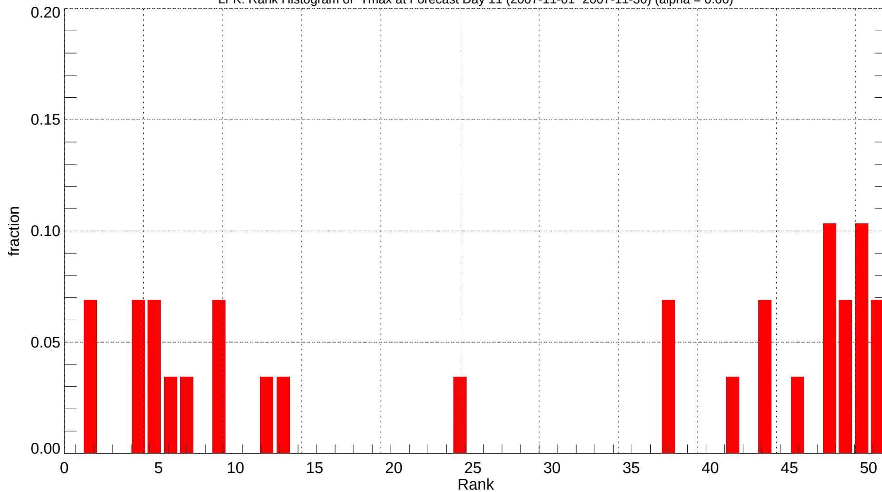
LFK: Rank Histogram of Tmax at Forecast Day 11 (2007-11-01~2007-11-30) (alpha = 0.00)
