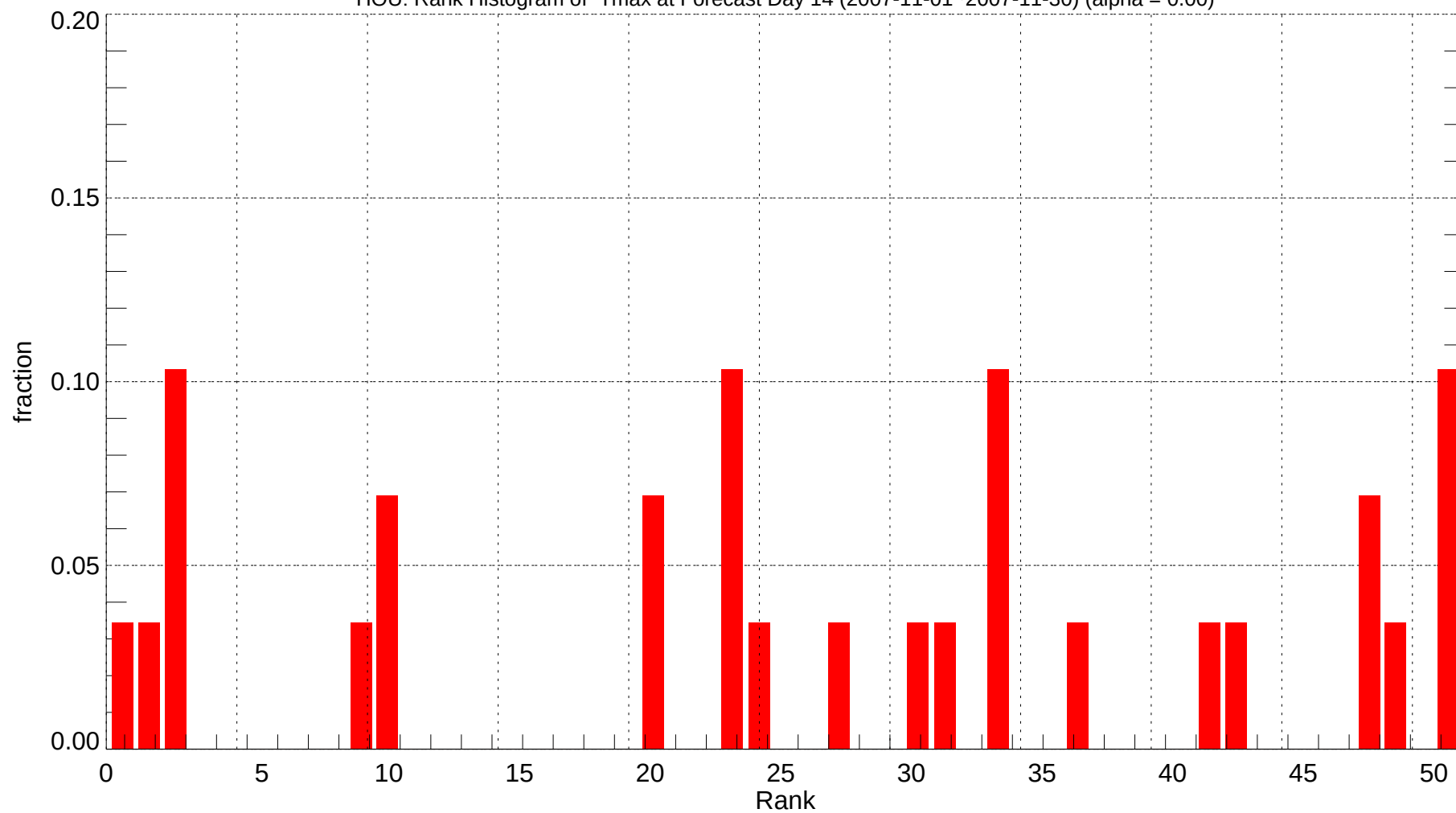
HOU: Rank Histogram of Tmax at Forecast Day 14 (2007-11-01~2007-11-30) (alpha = 0.00)
