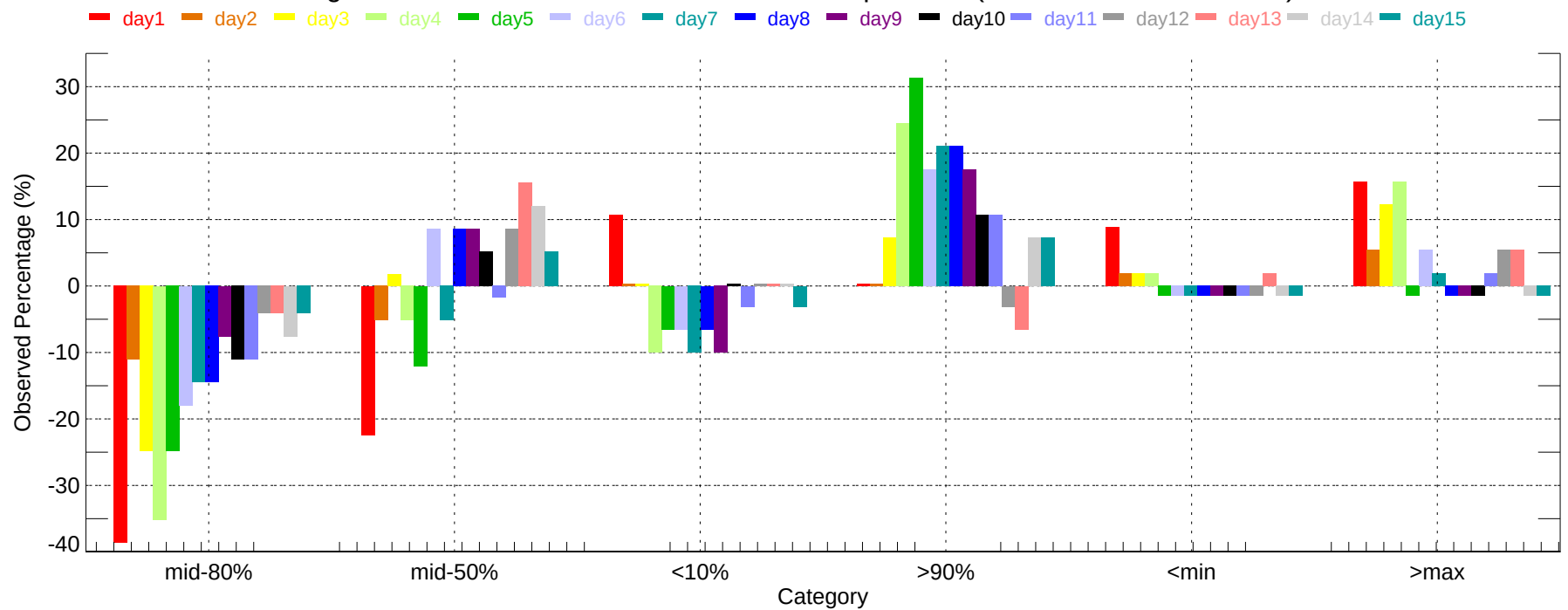
Observed Percentage Deviation of Ensembles - ABY: Min Temperature (2007-11-01~2007-11-30)
