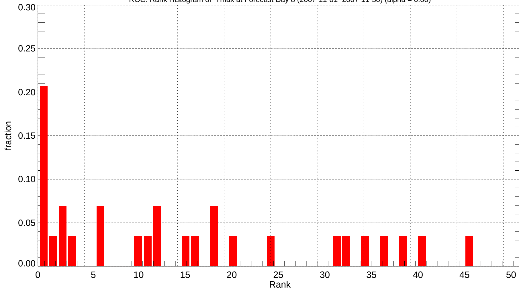
ROC: Rank Histogram of Tmax at Forecast Day 8 (2007-11-01~2007-11-30) (alpha = 0.00)
