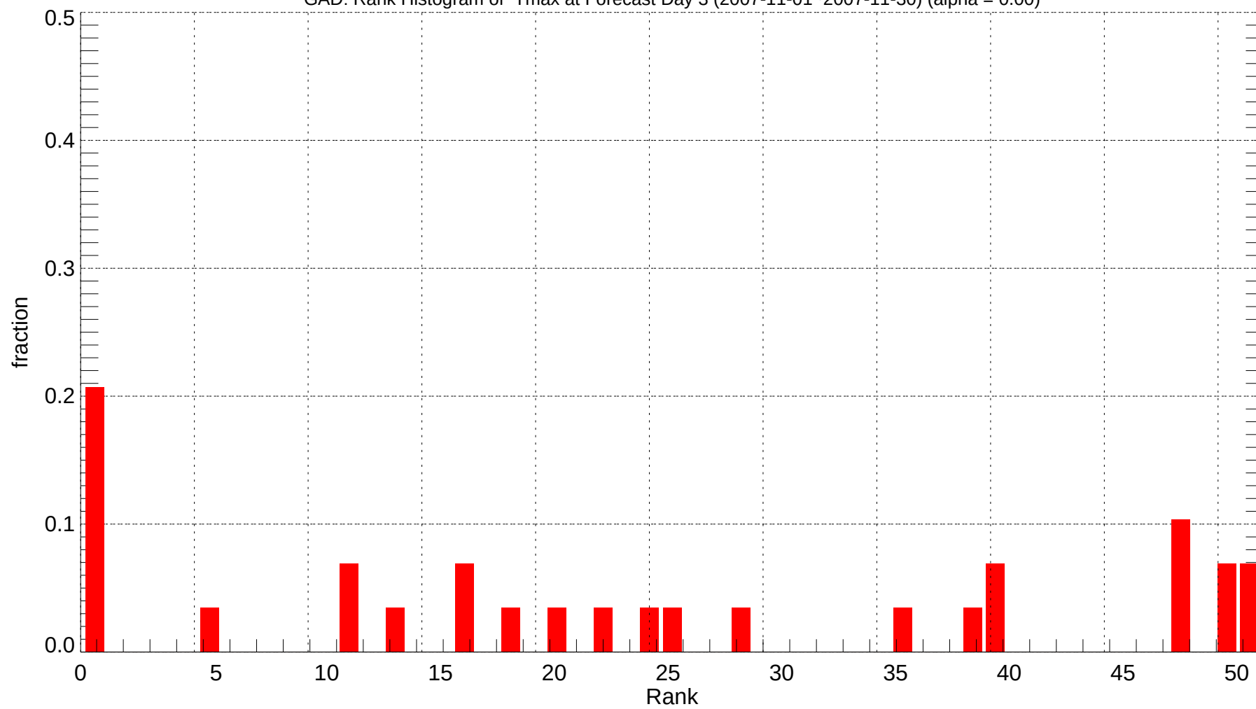
GAD: Rank Histogram of Tmax at Forecast Day 3 (2007-11-01~2007-11-30) (alpha = 0.00)
