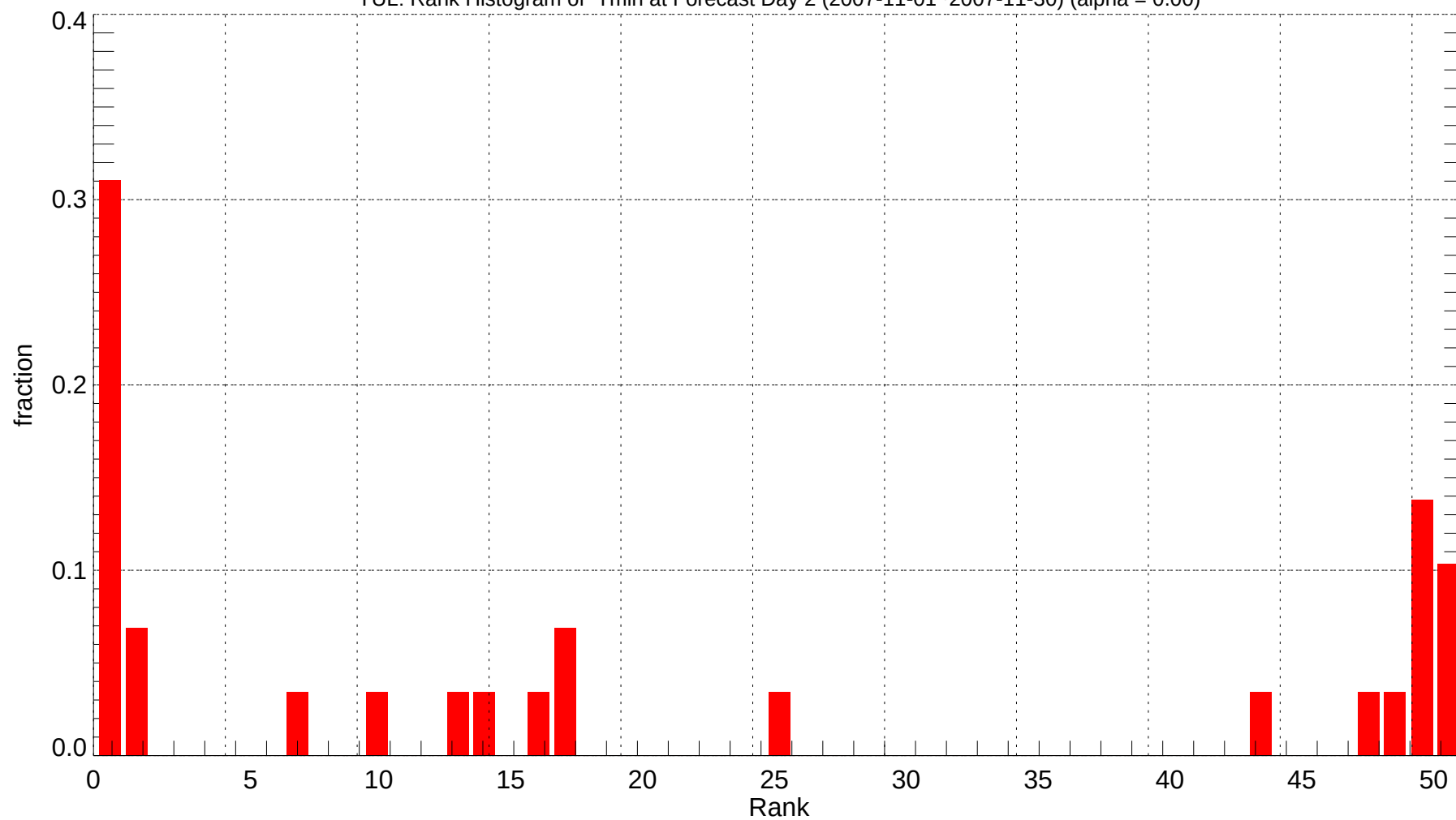
YUL: Rank Histogram of Tmin at Forecast Day 2 (2007-11-01~2007-11-30) (alpha = 0.00)
