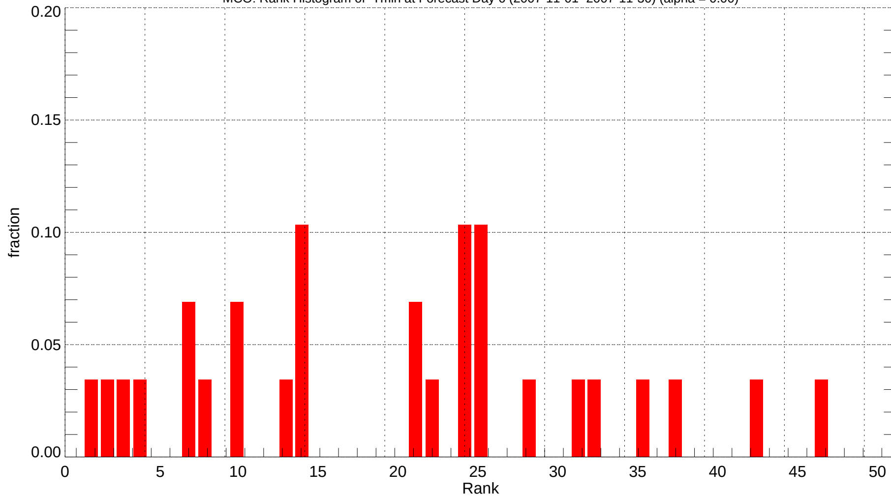
MCO: Rank Histogram of Tmin at Forecast Day 6 (2007-11-01~2007-11-30) (alpha = 0.00)
