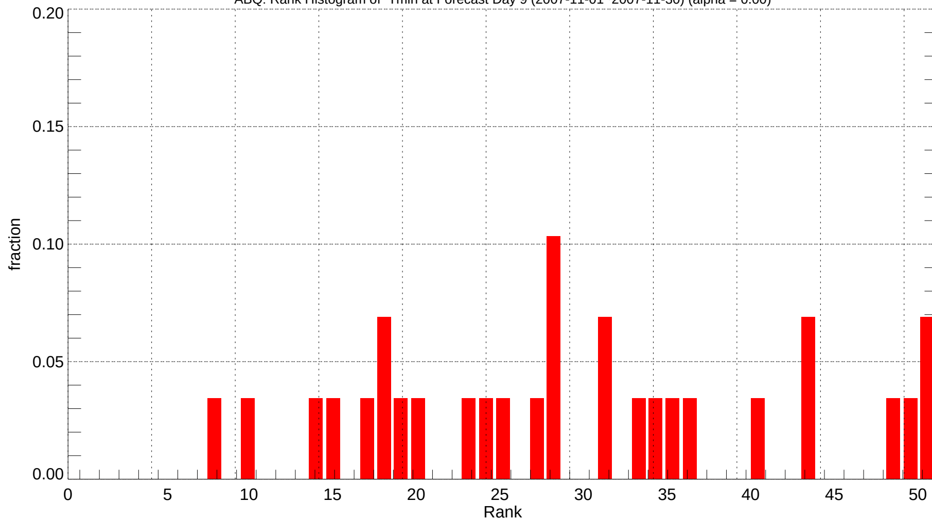
ABQ: Rank Histogram of Tmin at Forecast Day 9 (2007-11-01~2007-11-30) (alpha = 0.00)
