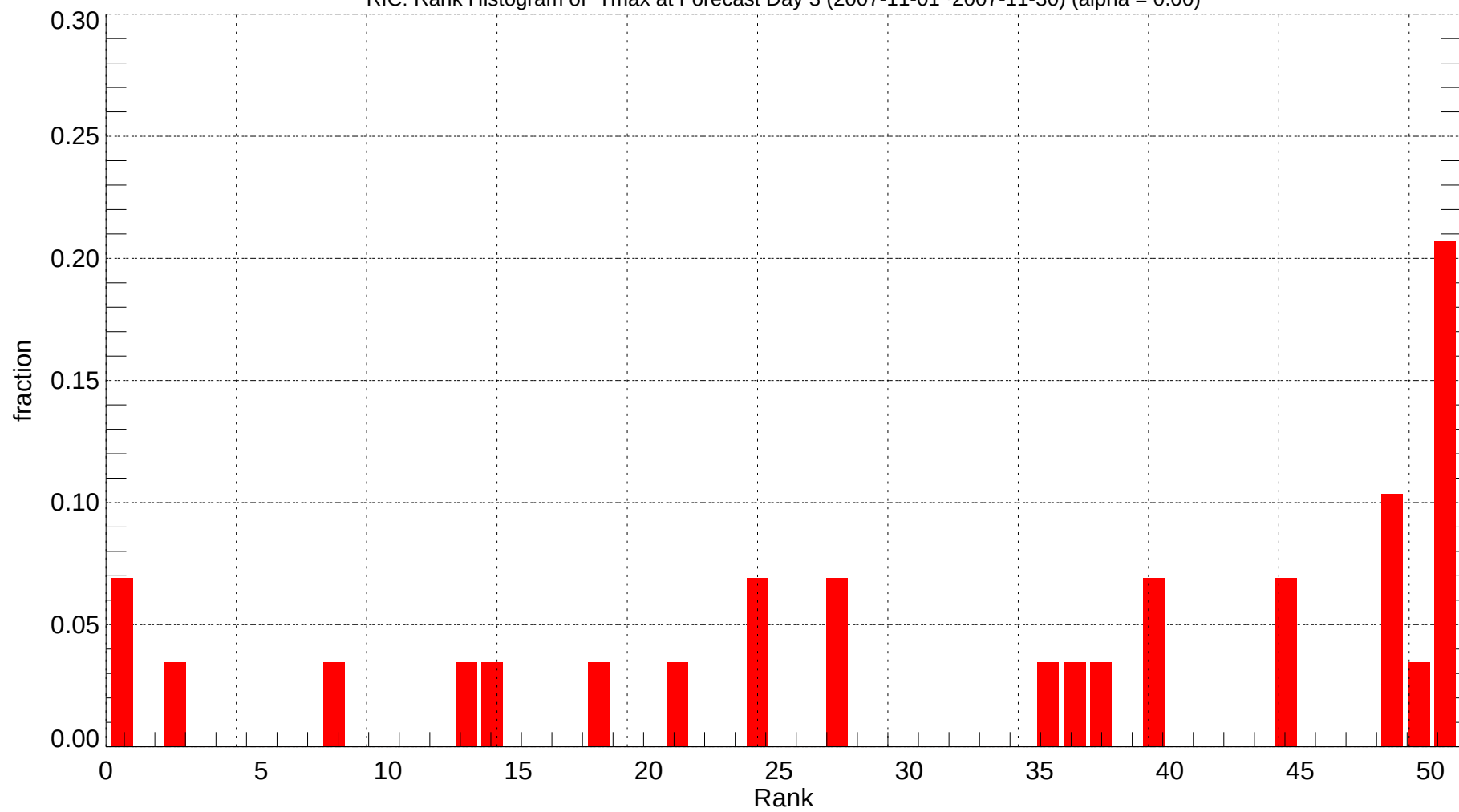
RIC: Rank Histogram of Tmax at Forecast Day 3 (2007-11-01~2007-11-30) (alpha = 0.00)
