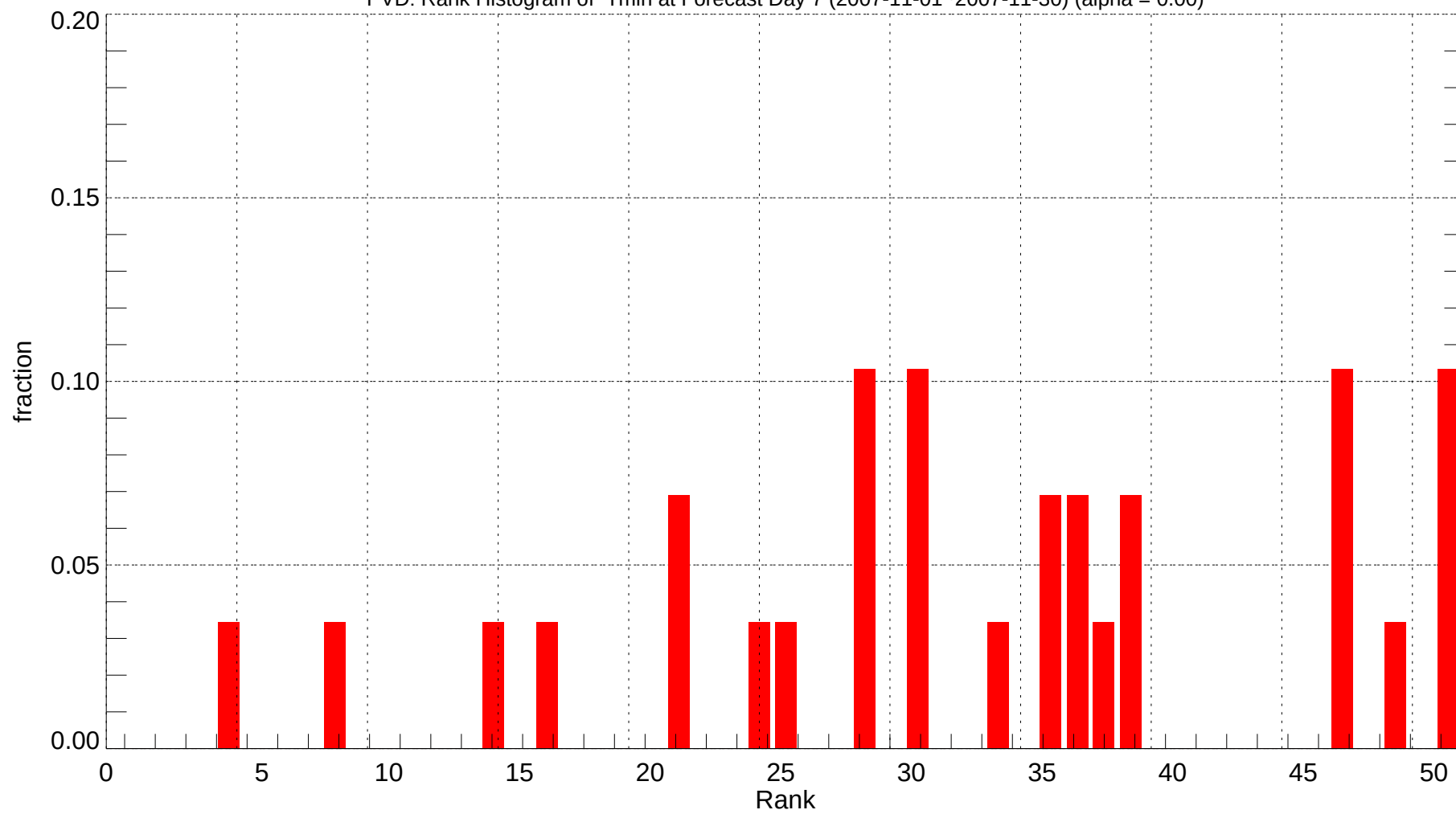
PVD: Rank Histogram of Tmin at Forecast Day 7 (2007-11-01~2007-11-30) (alpha = 0.00)
