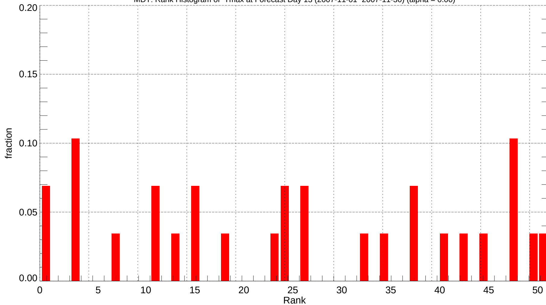
MDT: Rank Histogram of Tmax at Forecast Day 13 (2007-11-01~2007-11-30) (alpha = 0.00)
