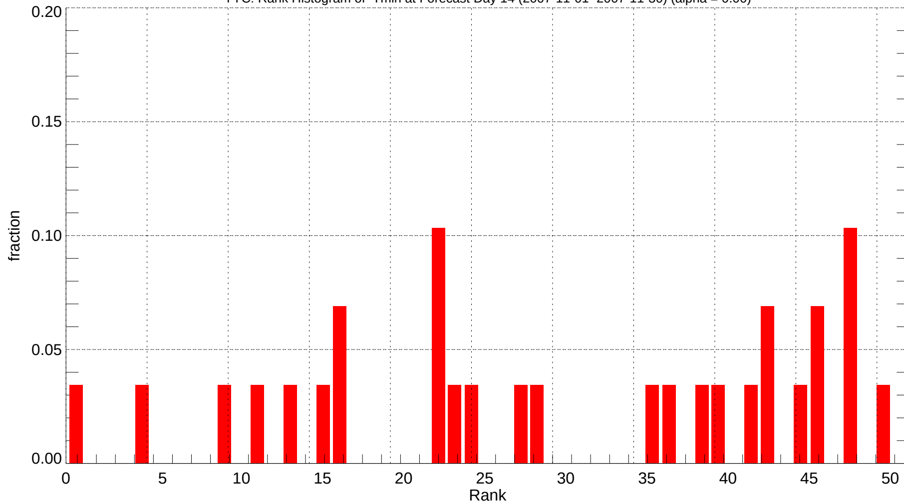
YYC: Rank Histogram of Tmin at Forecast Day 14 (2007-11-01~2007-11-30) (alpha = 0.00)
