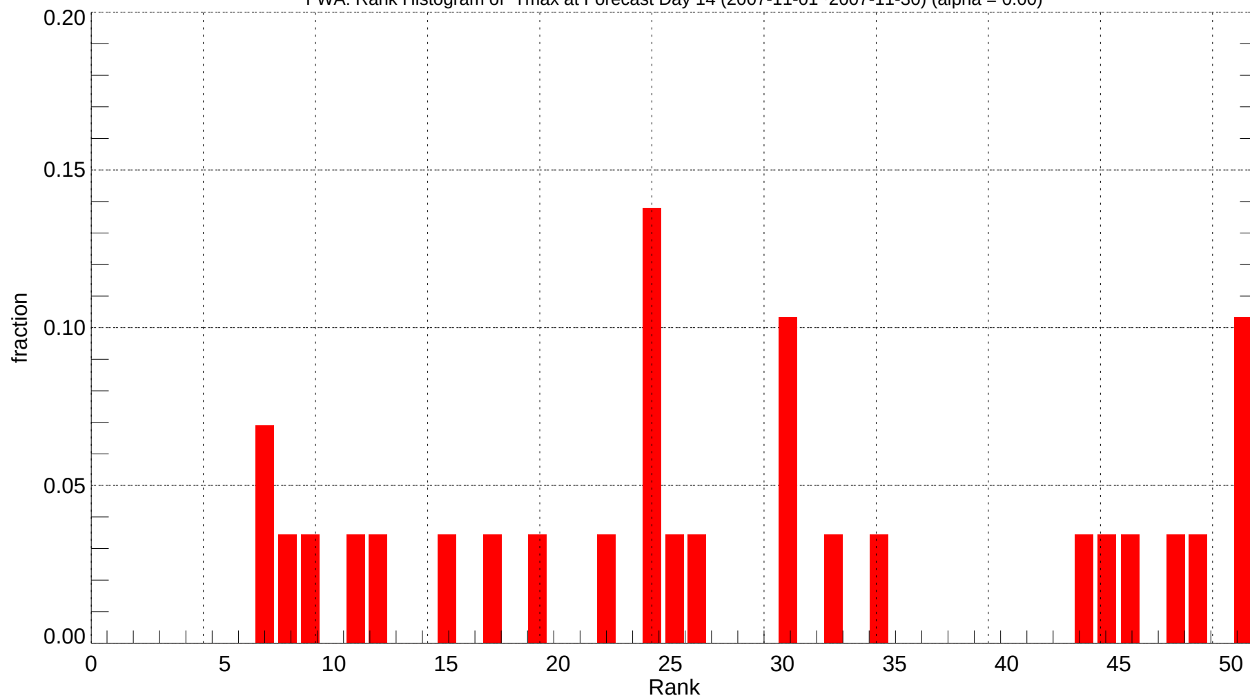
FWA: Rank Histogram of Tmax at Forecast Day 14 (2007-11-01~2007-11-30) (alpha = 0.00)
