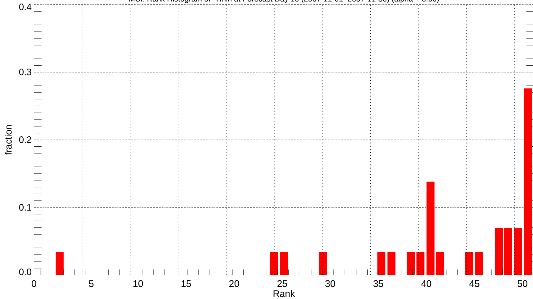
MCI: Rank Histogram of Tmin at Forecast Day 10 (2007-11-01~2007-11-30) (alpha = 0.00)
