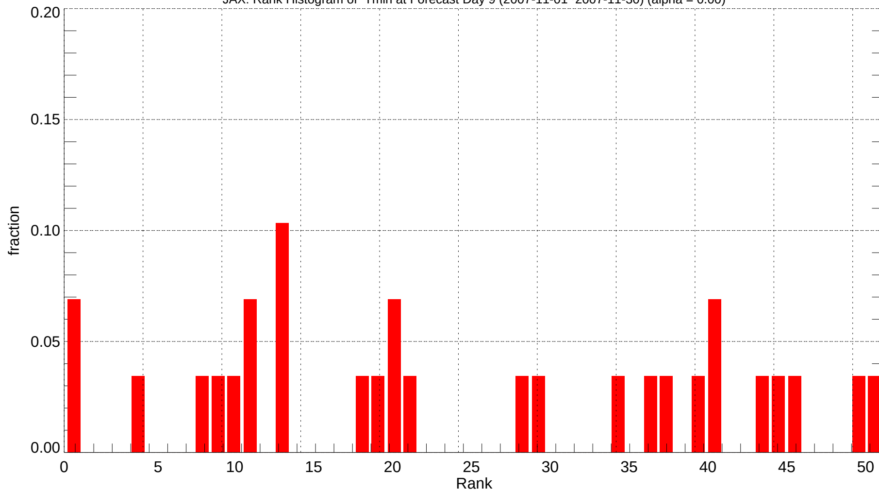
JAX: Rank Histogram of Tmin at Forecast Day 9 (2007-11-01~2007-11-30) (alpha = 0.00)
