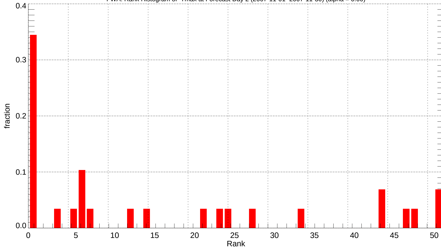
FWA: Rank Histogram of Tmax at Forecast Day 2 (2007-11-01~2007-11-30) (alpha = 0.00)
