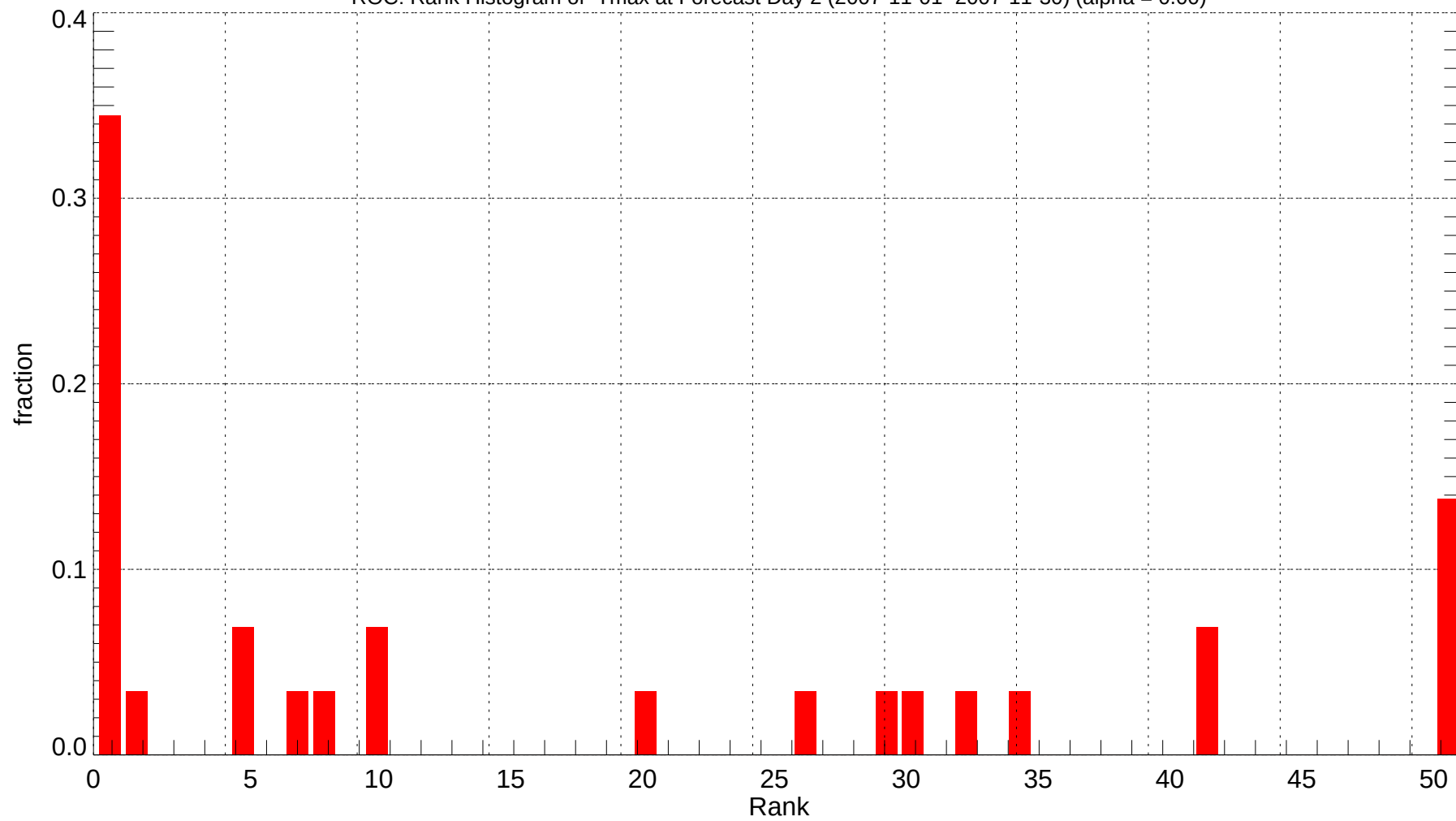
ROC: Rank Histogram of Tmax at Forecast Day 2 (2007-11-01~2007-11-30) (alpha = 0.00)
