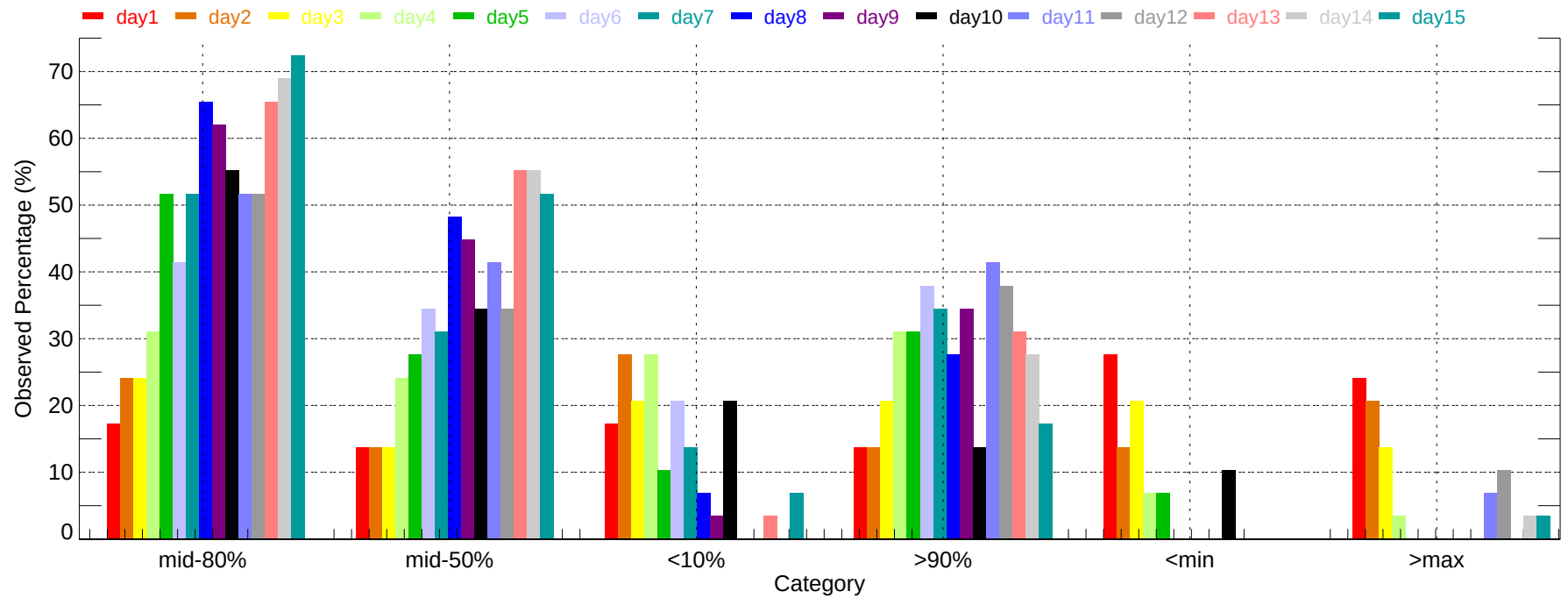
Observed Percentage of Ensembles - EVV: Min Temperature (2007-11-01~2007-11-30)
