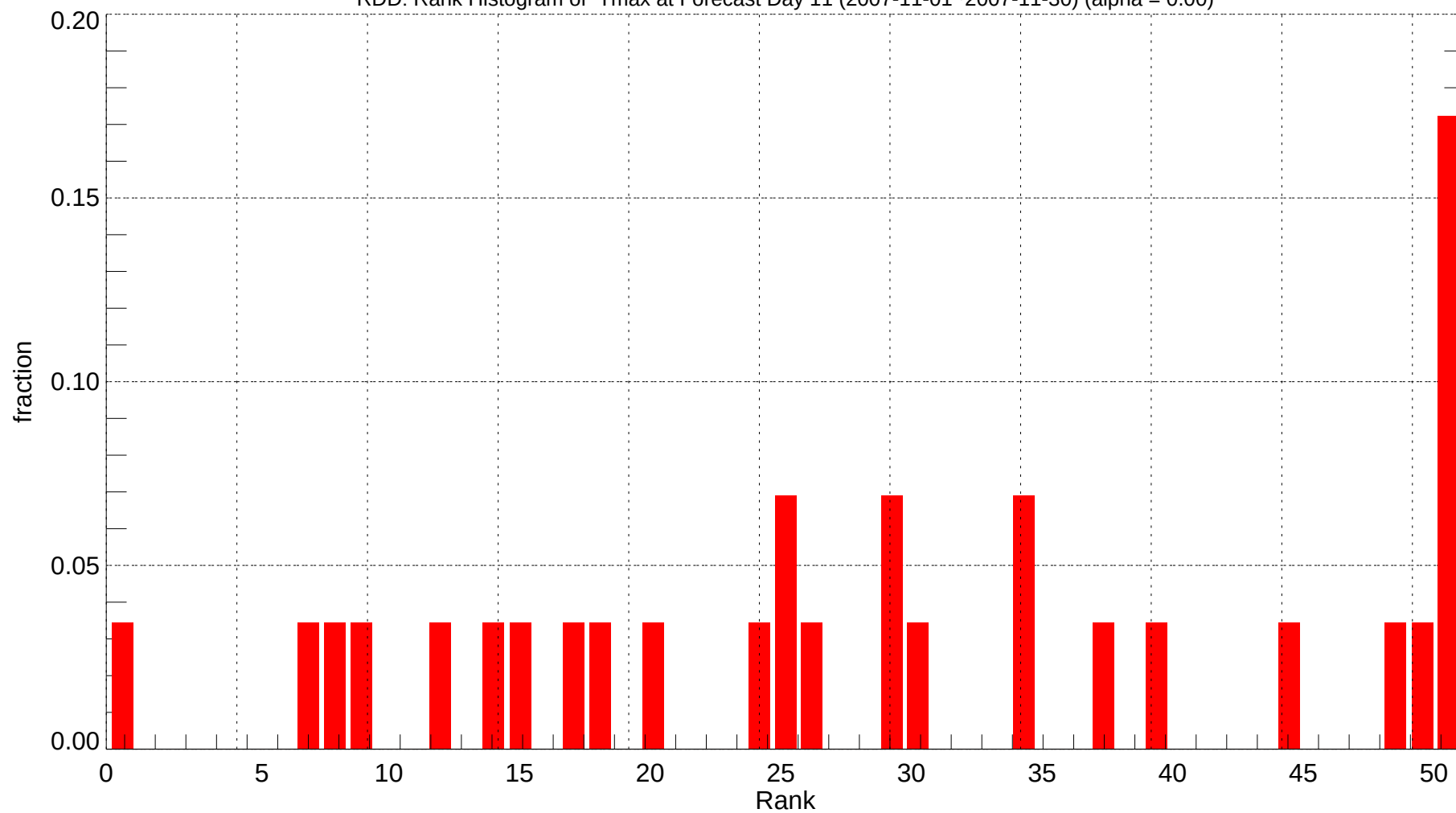
RDD: Rank Histogram of Tmax at Forecast Day 11 (2007-11-01~2007-11-30) (alpha = 0.00)
