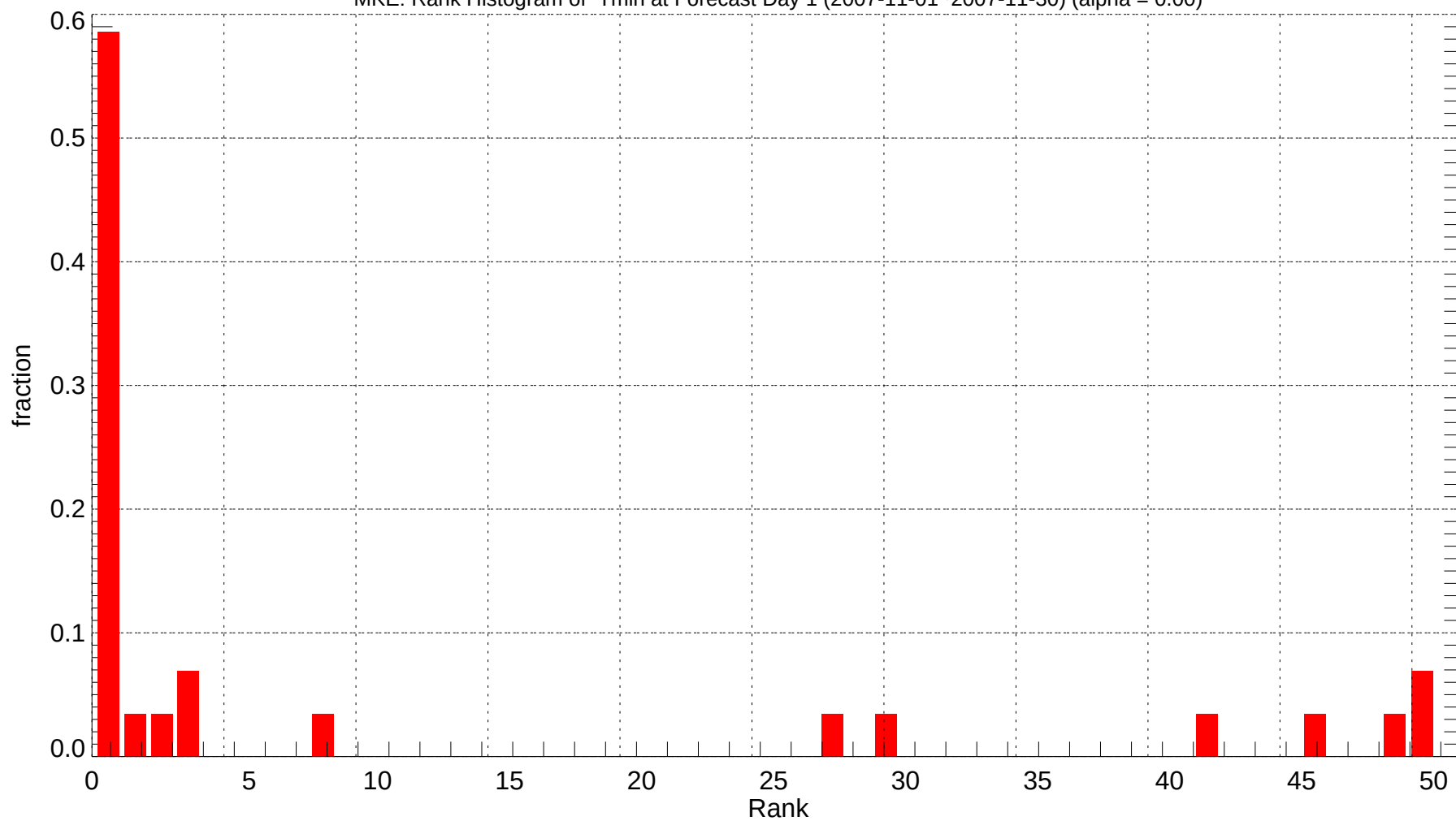
MKE: Rank Histogram of Tmin at Forecast Day 1 (2007-11-01~2007-11-30) (alpha = 0.00)
