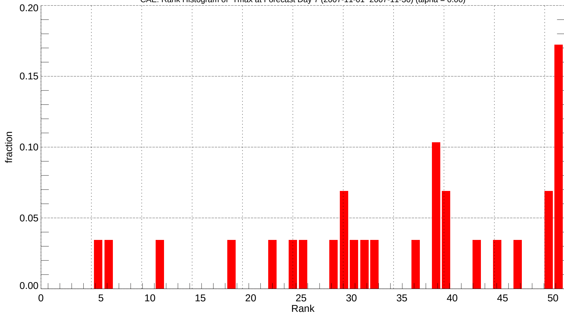
CAE: Rank Histogram of Tmax at Forecast Day 7 (2007-11-01~2007-11-30) (alpha = 0.00)
