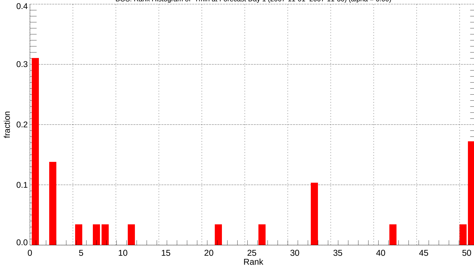
BOS: Rank Histogram of Tmin at Forecast Day 1 (2007-11-01~2007-11-30) (alpha = 0.00)
