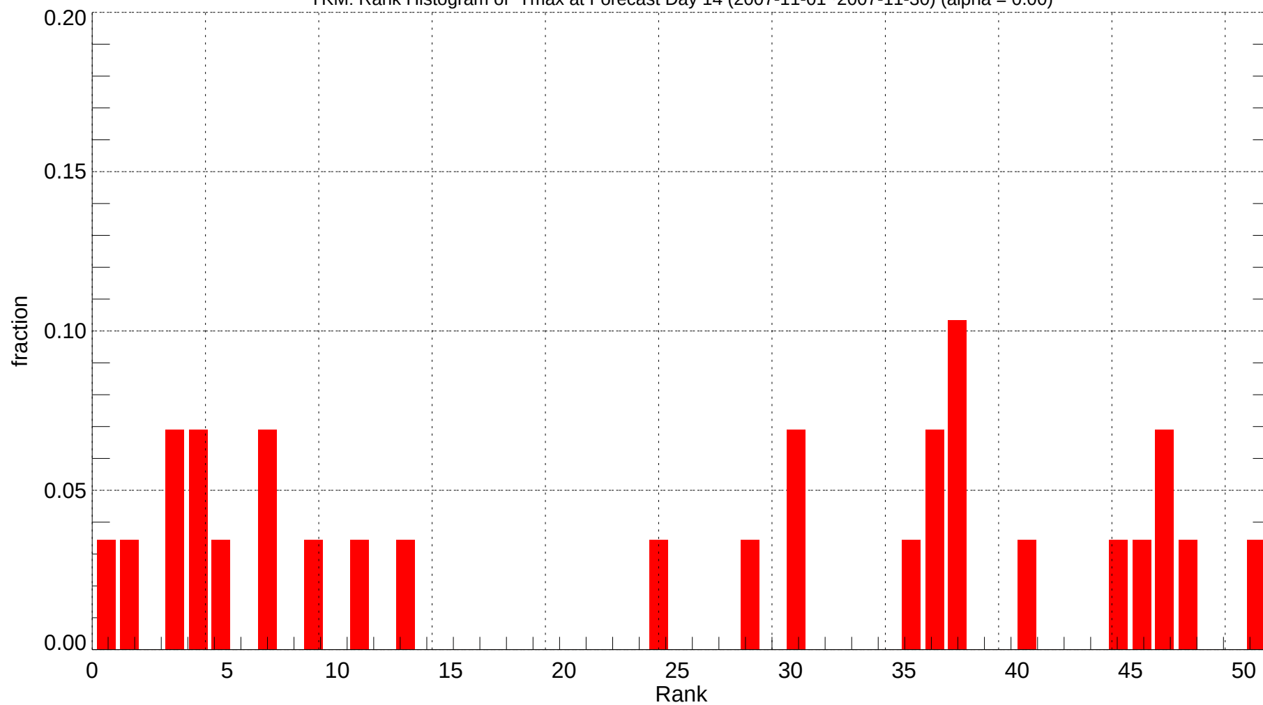
YKM: Rank Histogram of Tmax at Forecast Day 14 (2007-11-01~2007-11-30) (alpha = 0.00)
