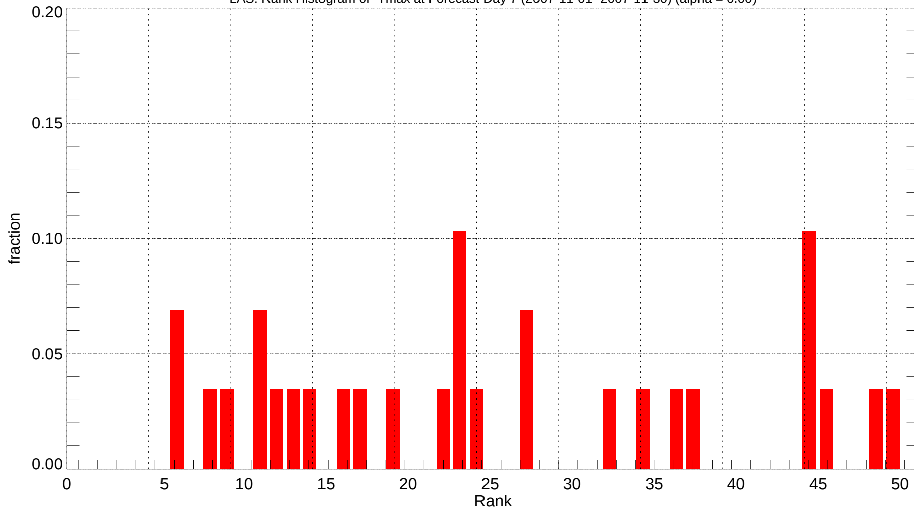
LAS: Rank Histogram of Tmax at Forecast Day 7 (2007-11-01~2007-11-30) (alpha = 0.00)
