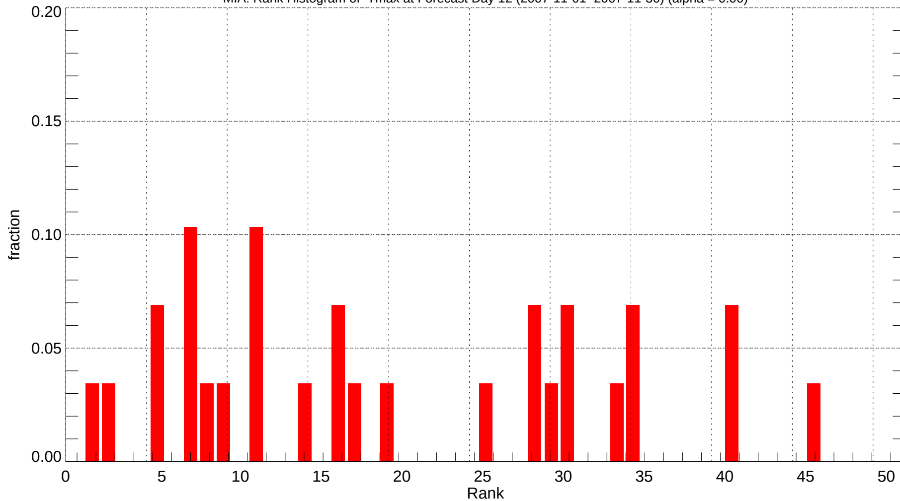
MIA: Rank Histogram of Tmax at Forecast Day 12 (2007-11-01~2007-11-30) (alpha = 0.00)
