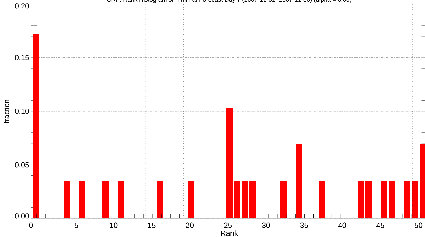
CRP: Rank Histogram of Tmin at Forecast Day 7 (2007-11-01~2007-11-30) (alpha = 0.00)
