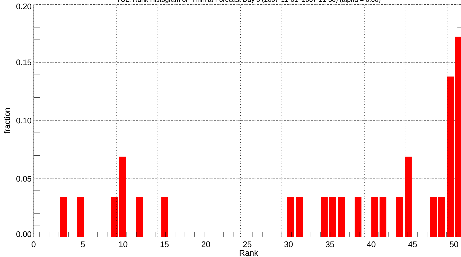
TUL: Rank Histogram of Tmin at Forecast Day 6 (2007-11-01~2007-11-30) (alpha = 0.00)
