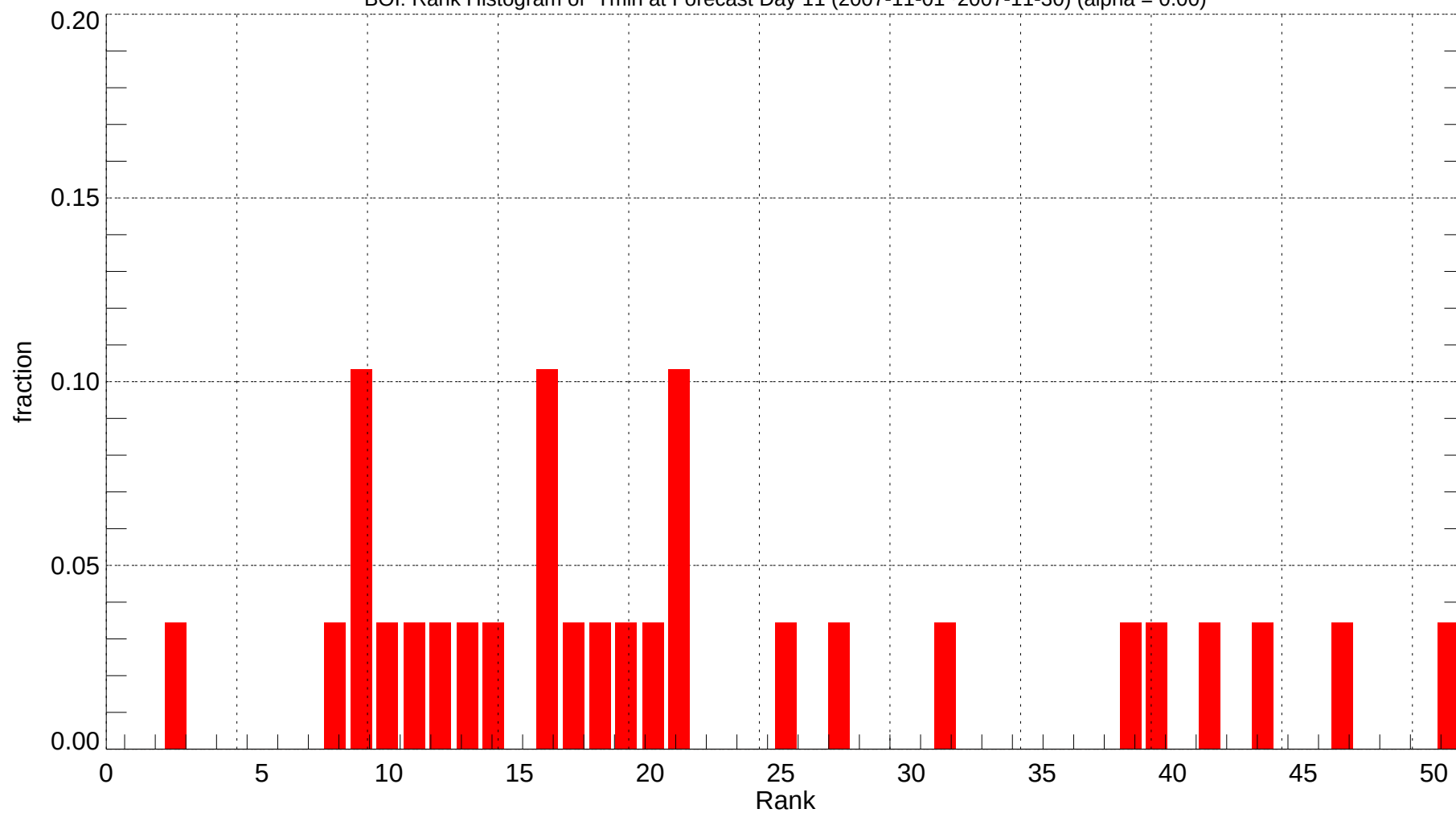
BOI: Rank Histogram of Tmin at Forecast Day 11 (2007-11-01~2007-11-30) (alpha = 0.00)
