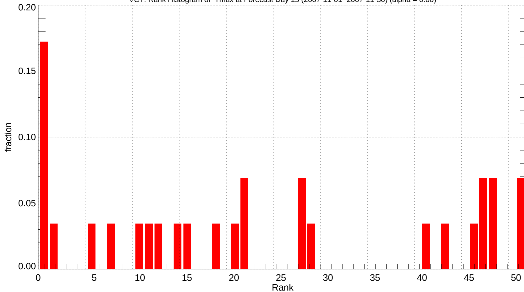
VCT: Rank Histogram of Tmax at Forecast Day 15 (2007-11-01~2007-11-30) (alpha = 0.00)
