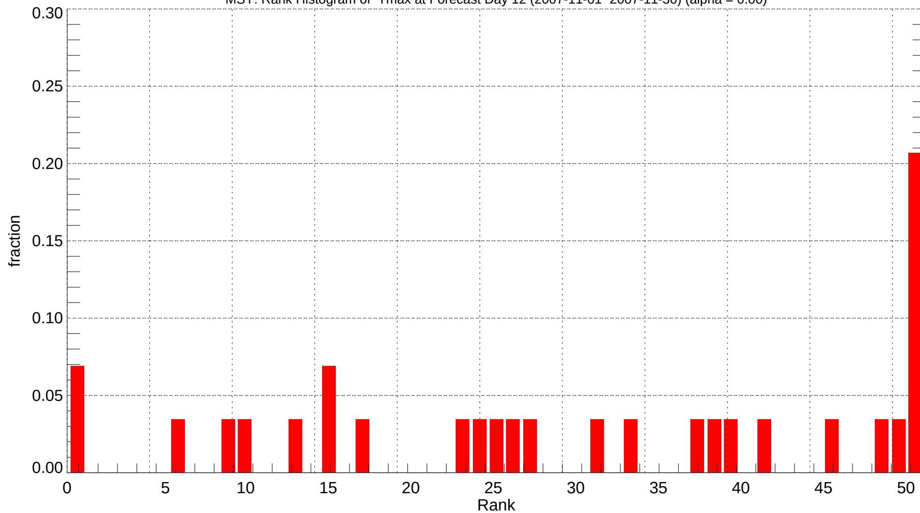
MSY: Rank Histogram of Tmax at Forecast Day 12 (2007-11-01~2007-11-30) (alpha = 0.00)
