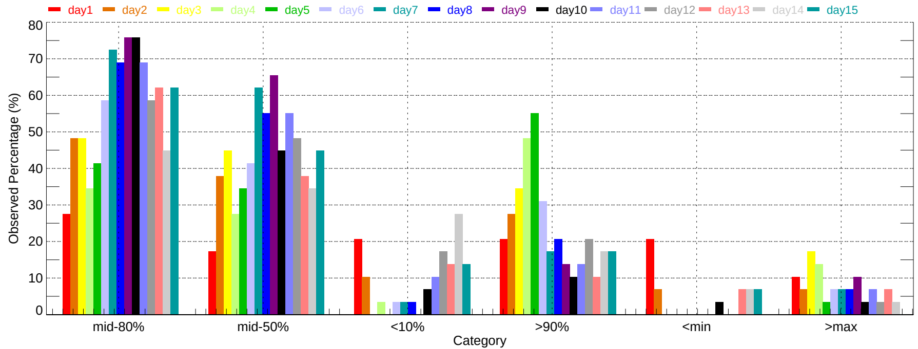
Observed Percentage of Ensembles - PVD: Max Temperature (2007-11-01~2007-11-30)
