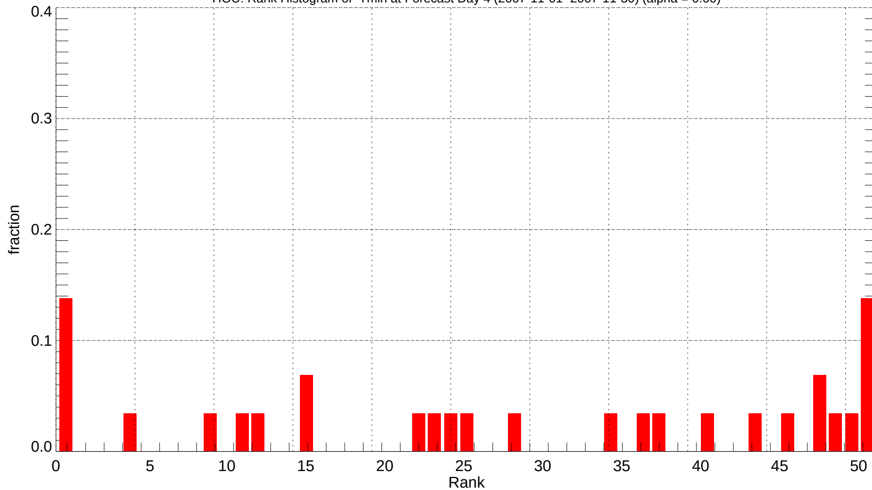
HOU: Rank Histogram of Tmin at Forecast Day 4 (2007-11-01~2007-11-30) (alpha = 0.00)
