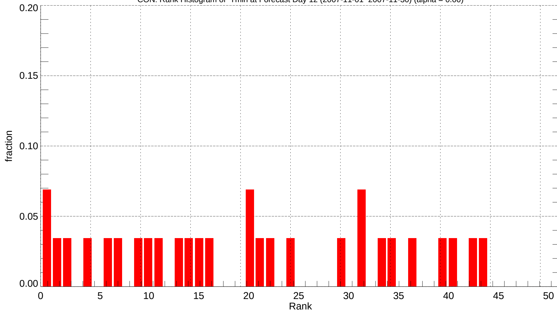
CON: Rank Histogram of Tmin at Forecast Day 12 (2007-11-01~2007-11-30) (alpha = 0.00)
