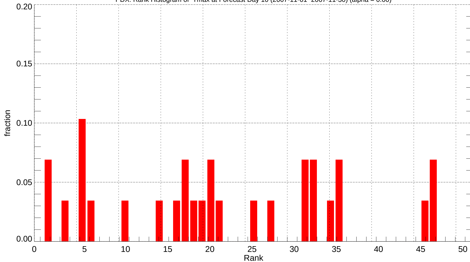
PDX: Rank Histogram of Tmax at Forecast Day 10 (2007-11-01~2007-11-30) (alpha = 0.00)
