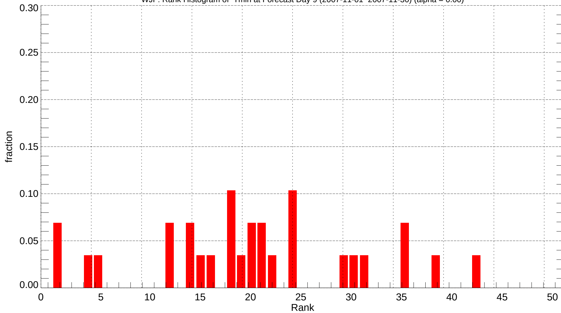
WJF: Rank Histogram of Tmin at Forecast Day 9 (2007-11-01~2007-11-30) (alpha = 0.00)
