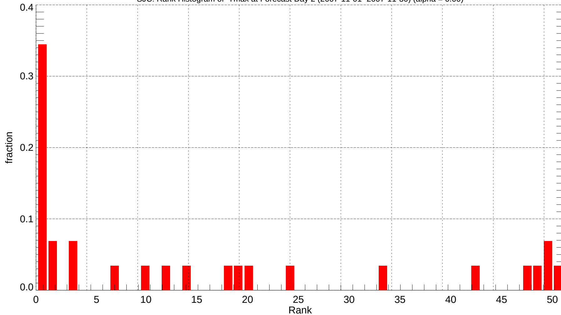
SJC: Rank Histogram of Tmax at Forecast Day 2 (2007-11-01~2007-11-30) (alpha = 0.00)
