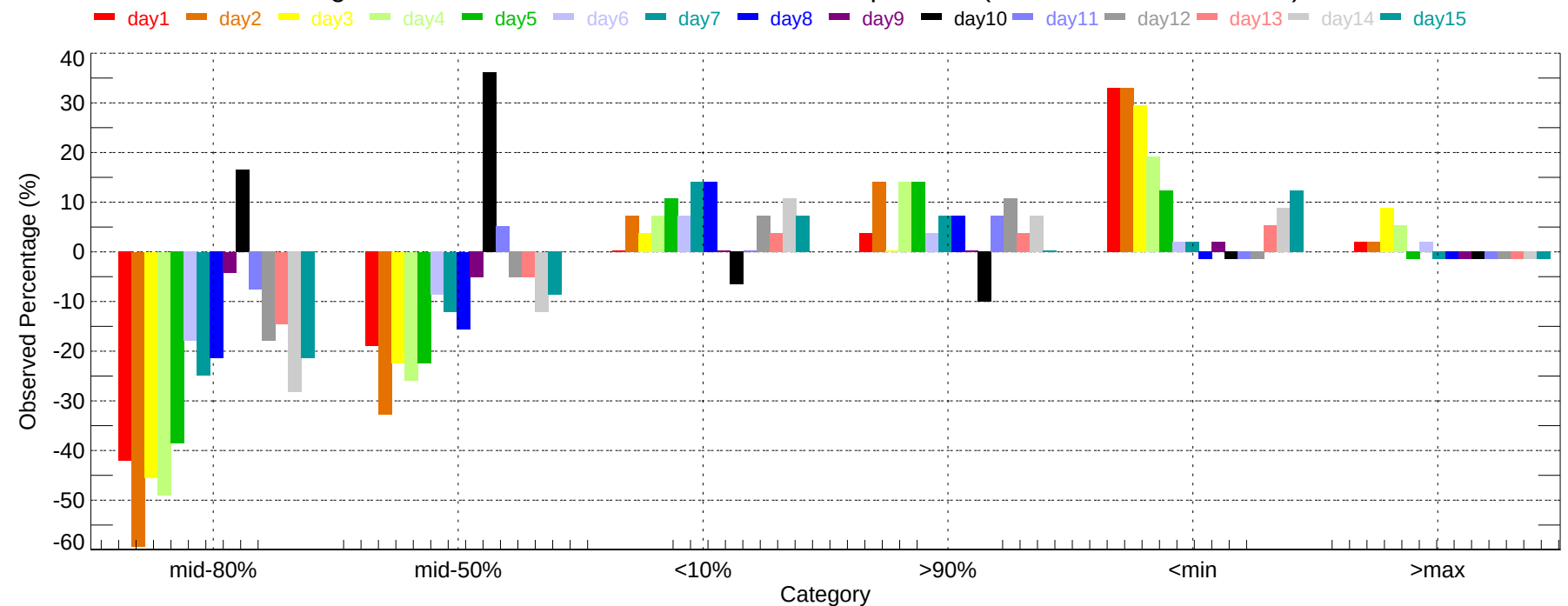
Observed Percentage Deviation of Ensembles - MHT: Min Temperature (2007-11-01~2007-11-30)
