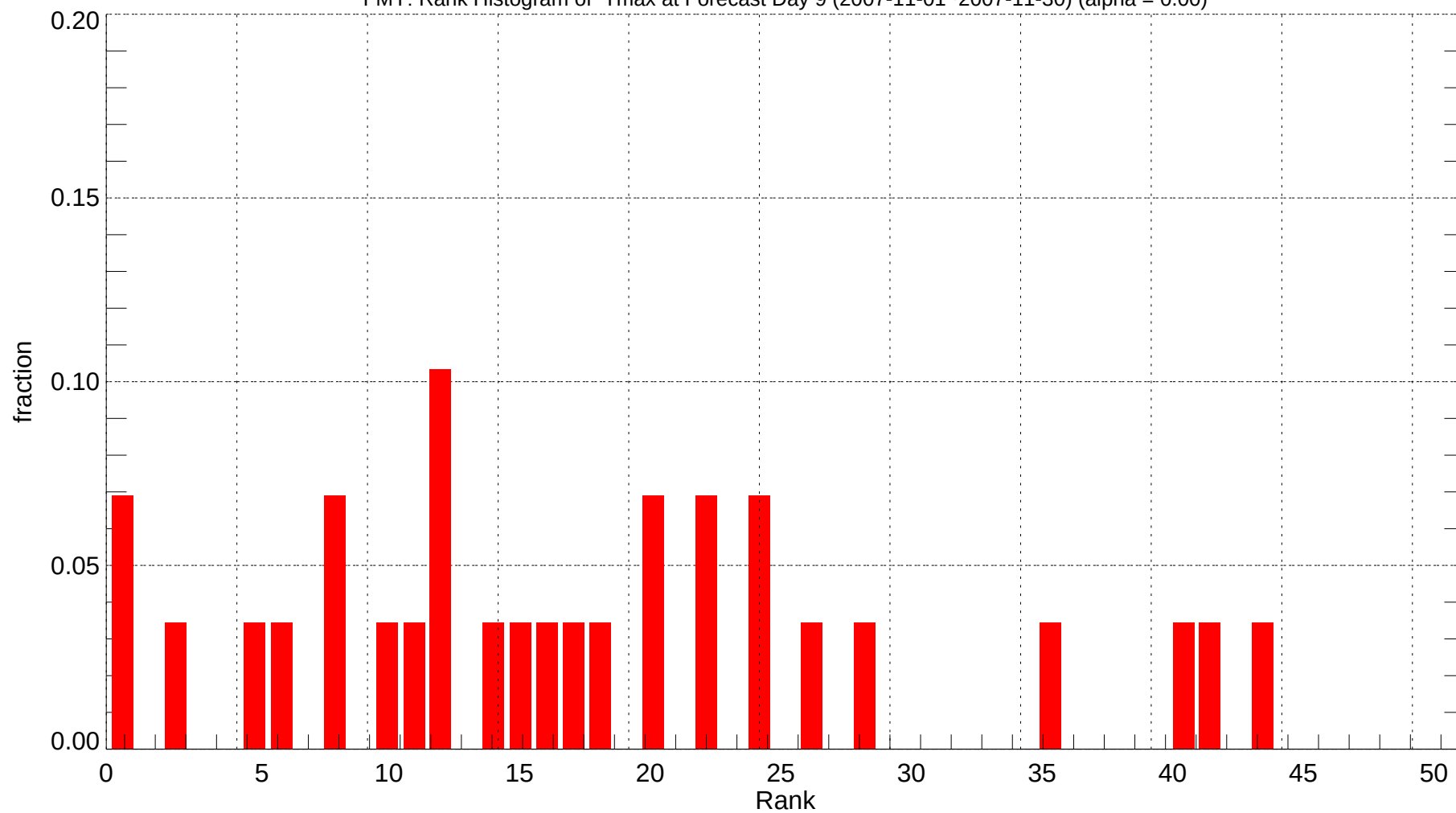
FMY: Rank Histogram of Tmax at Forecast Day 9 (2007-11-01~2007-11-30) (alpha = 0.00)
