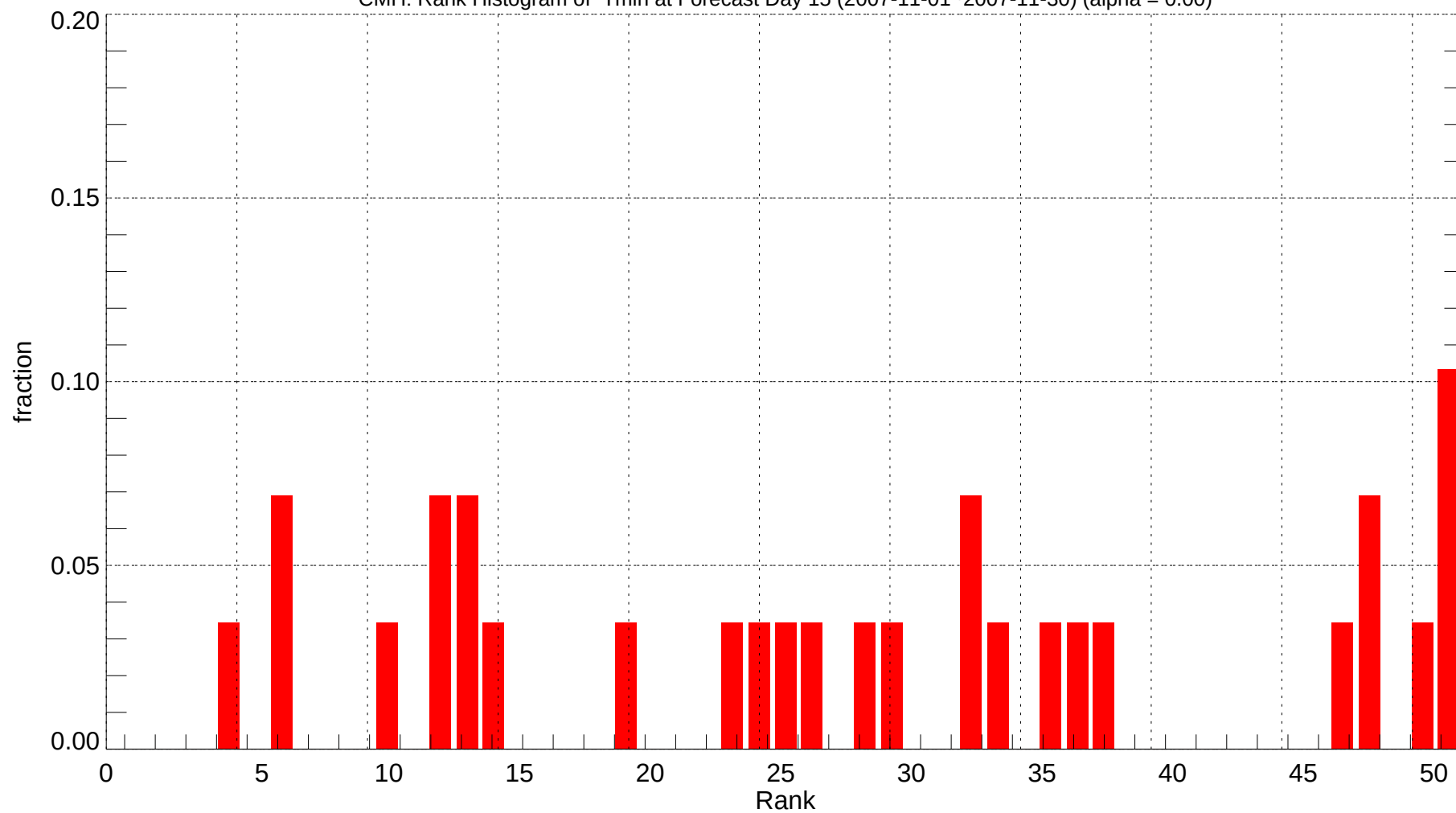
CMH: Rank Histogram of Tmin at Forecast Day 15 (2007-11-01~2007-11-30) (alpha = 0.00)
