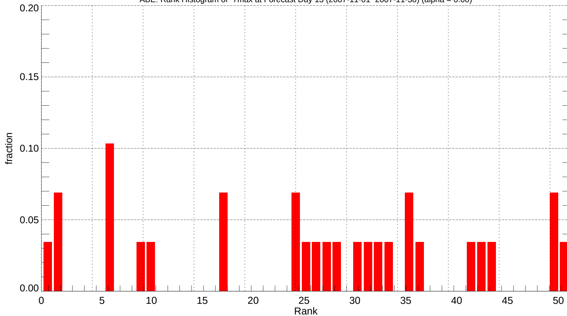
ABE: Rank Histogram of Tmax at Forecast Day 13 (2007-11-01~2007-11-30) (alpha = 0.00)
