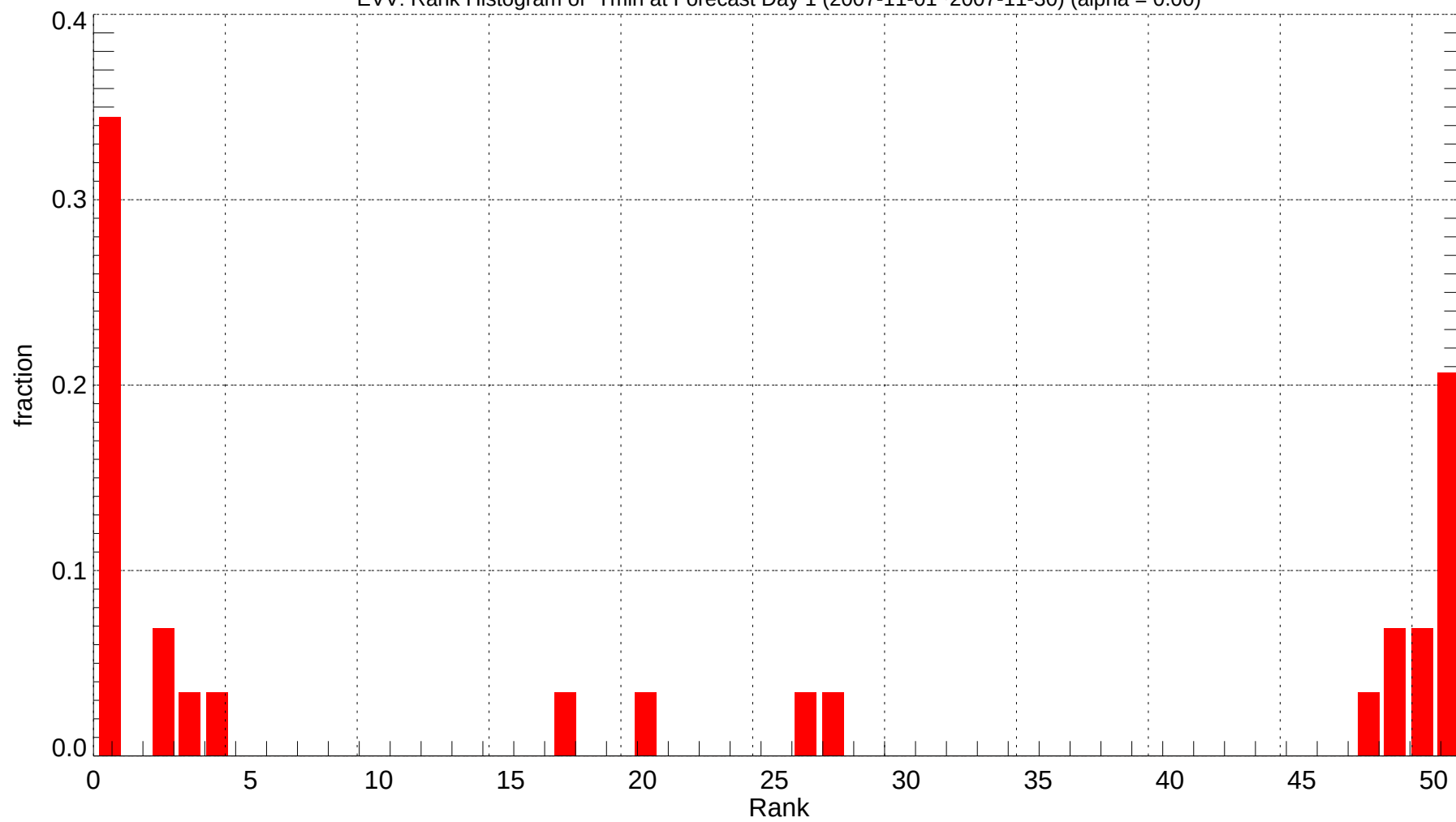
EVV: Rank Histogram of Tmin at Forecast Day 1 (2007-11-01~2007-11-30) (alpha = 0.00)
