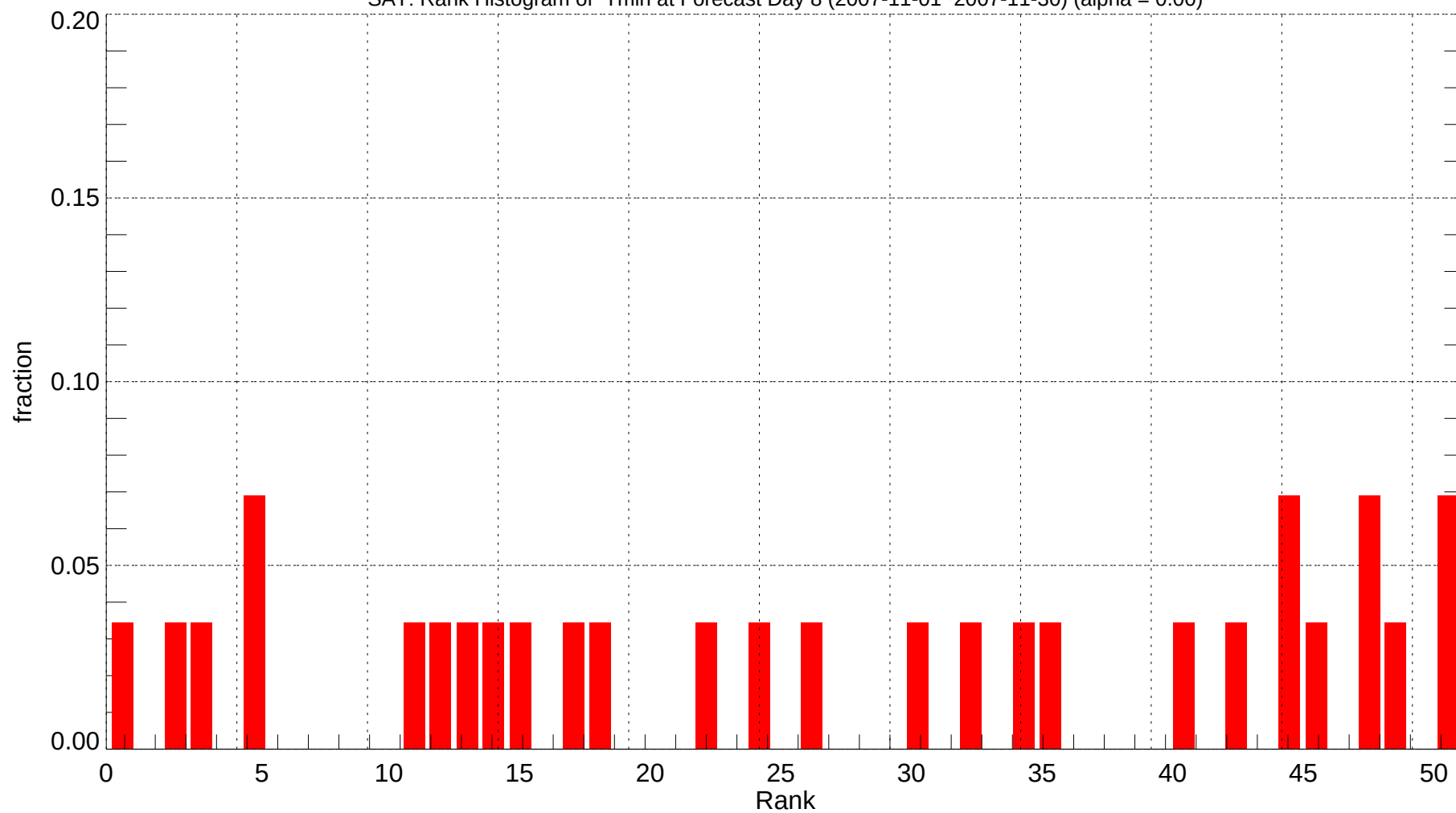
SAT: Rank Histogram of Tmin at Forecast Day 8 (2007-11-01~2007-11-30) (alpha = 0.00)
