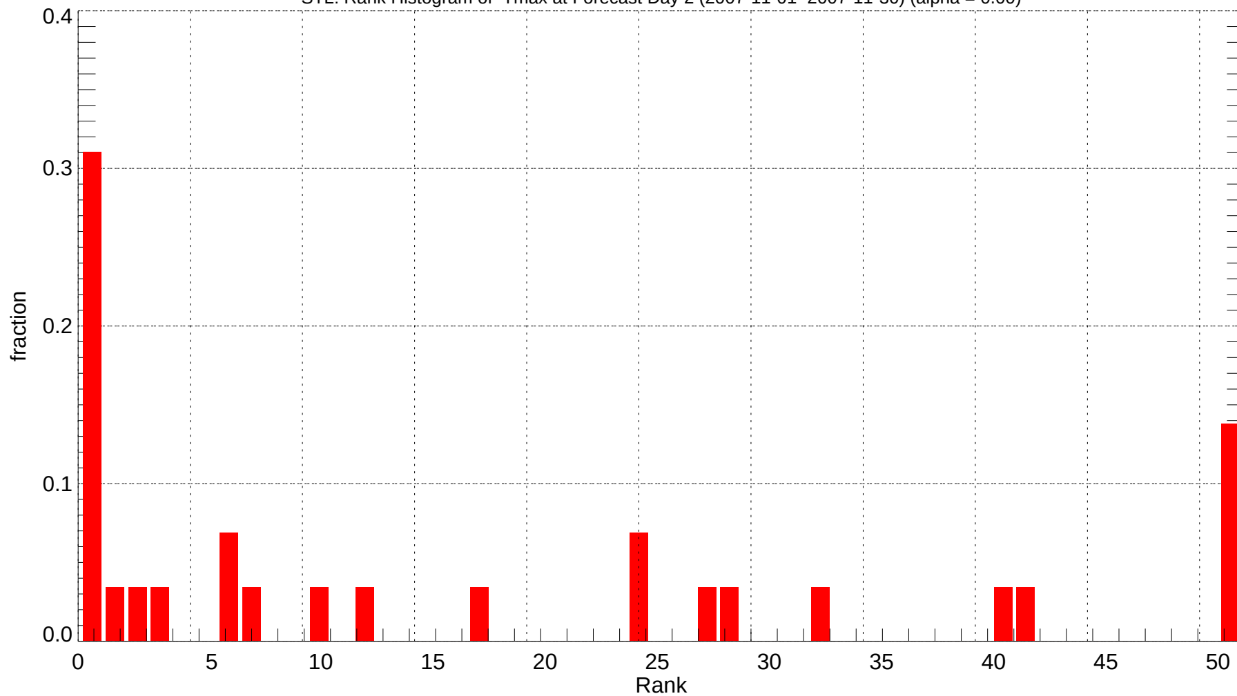
STL: Rank Histogram of Tmax at Forecast Day 2 (2007-11-01~2007-11-30) (alpha = 0.00)
