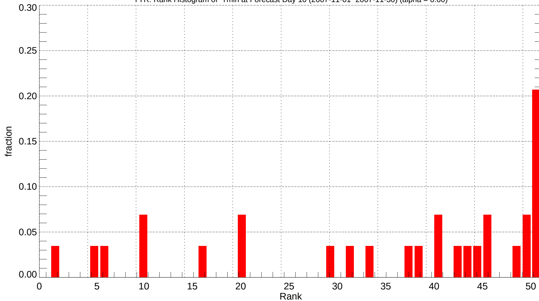
TYR: Rank Histogram of Tmin at Forecast Day 10 (2007-11-01~2007-11-30) (alpha = 0.00)
