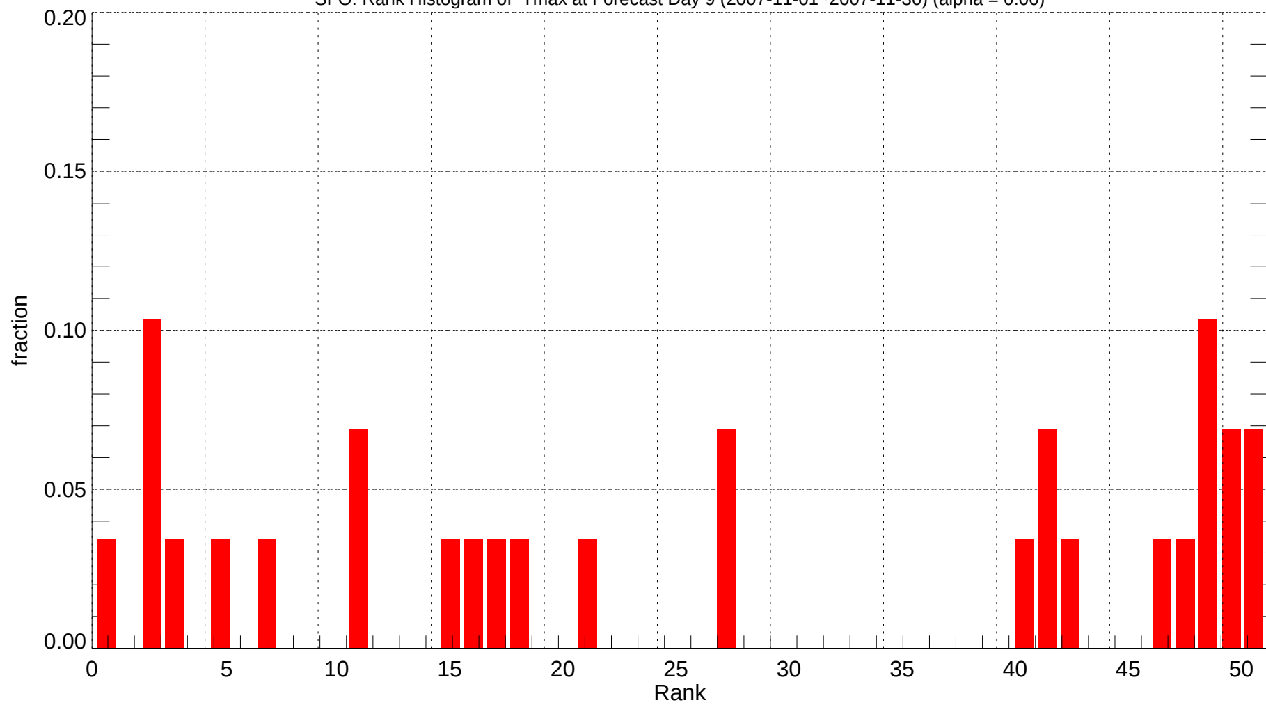
SFO: Rank Histogram of Tmax at Forecast Day 9 (2007-11-01~2007-11-30) (alpha = 0.00)
