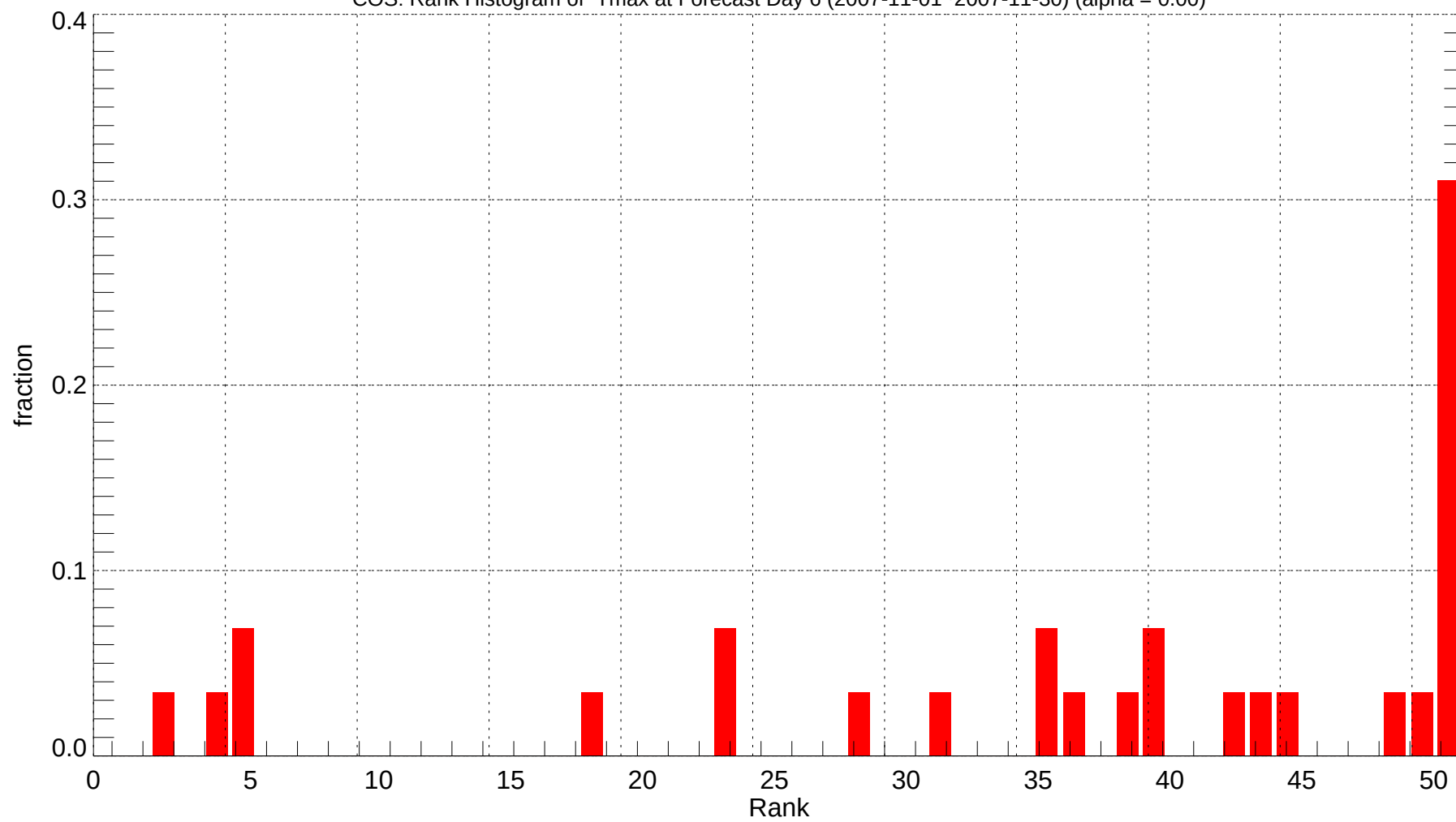
COS: Rank Histogram of Tmax at Forecast Day 6 (2007-11-01~2007-11-30) (alpha = 0.00)
