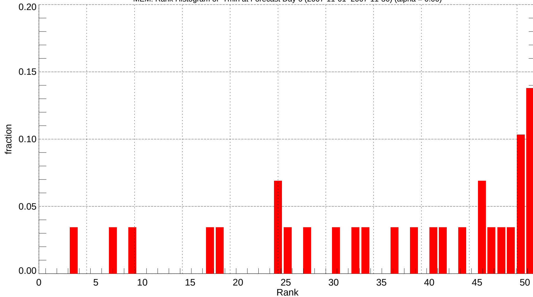
MEM: Rank Histogram of Tmin at Forecast Day 6 (2007-11-01~2007-11-30) (alpha = 0.00)
