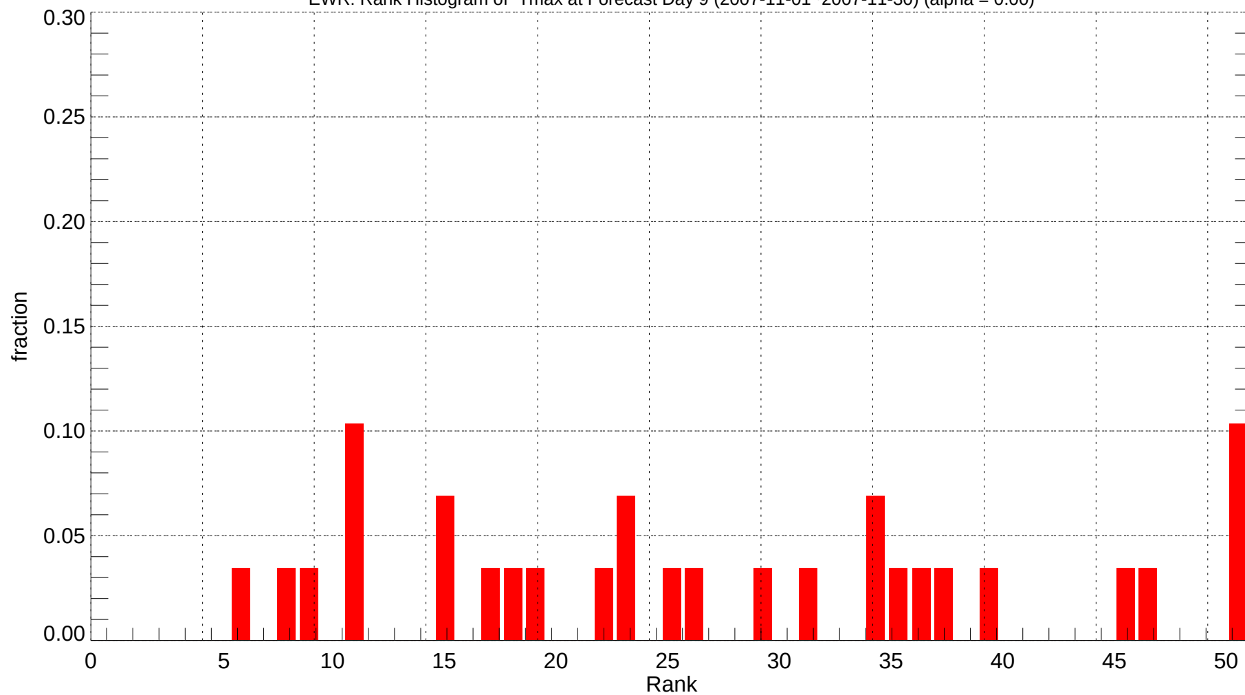
EWR: Rank Histogram of Tmax at Forecast Day 9 (2007-11-01~2007-11-30) (alpha = 0.00)
