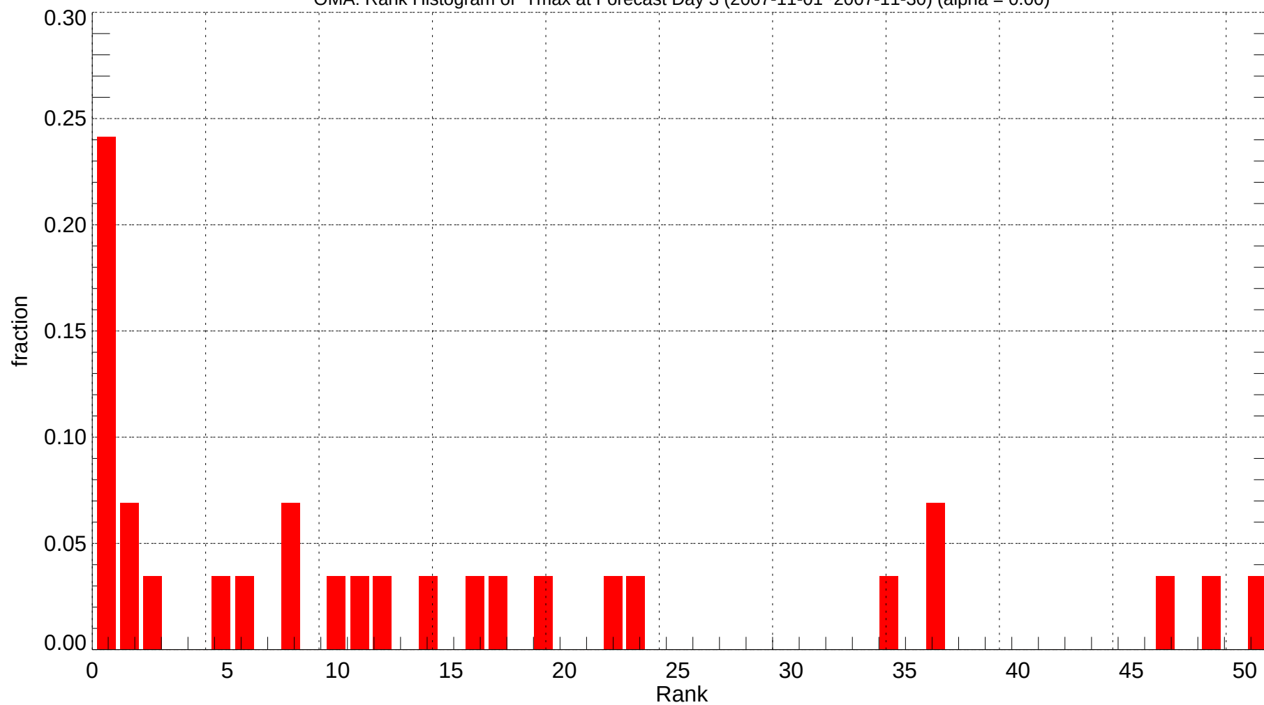
OMA: Rank Histogram of Tmax at Forecast Day 3 (2007-11-01~2007-11-30) (alpha = 0.00)
