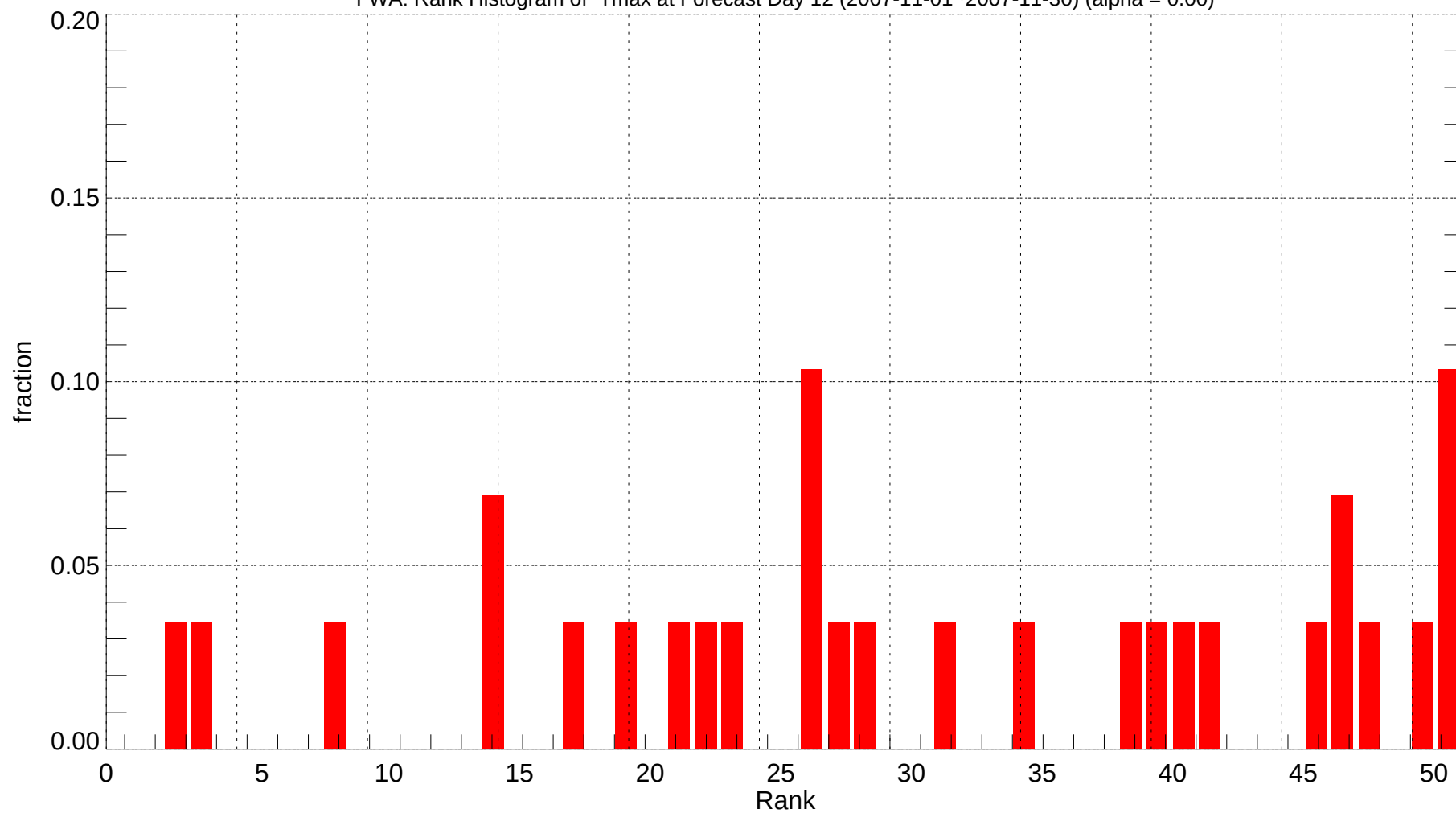
FWA: Rank Histogram of Tmax at Forecast Day 12 (2007-11-01~2007-11-30) (alpha = 0.00)
