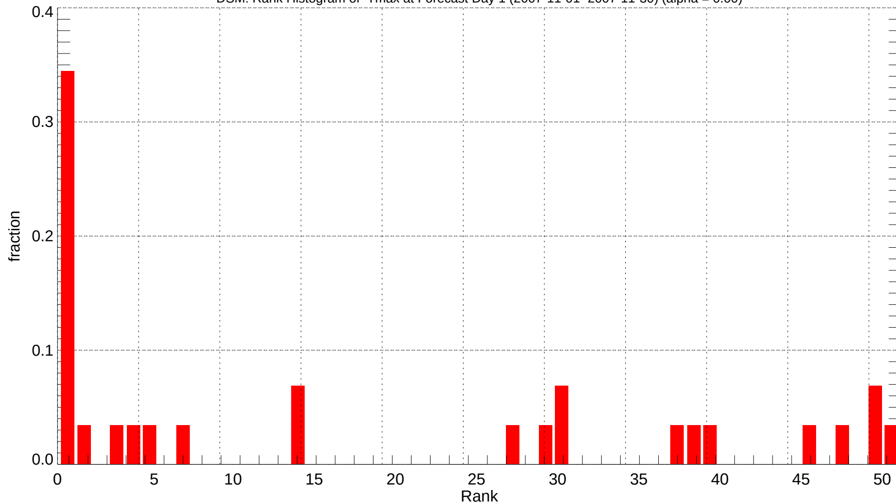
DSM: Rank Histogram of Tmax at Forecast Day 1 (2007-11-01~2007-11-30) (alpha = 0.00)
