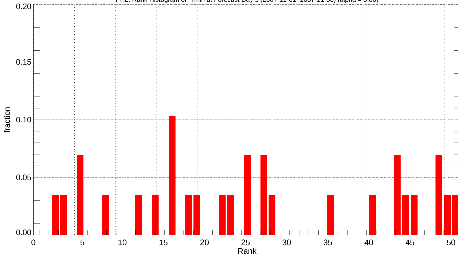
PHL: Rank Histogram of Tmin at Forecast Day 5 (2007-11-01~2007-11-30) (alpha = 0.00)
