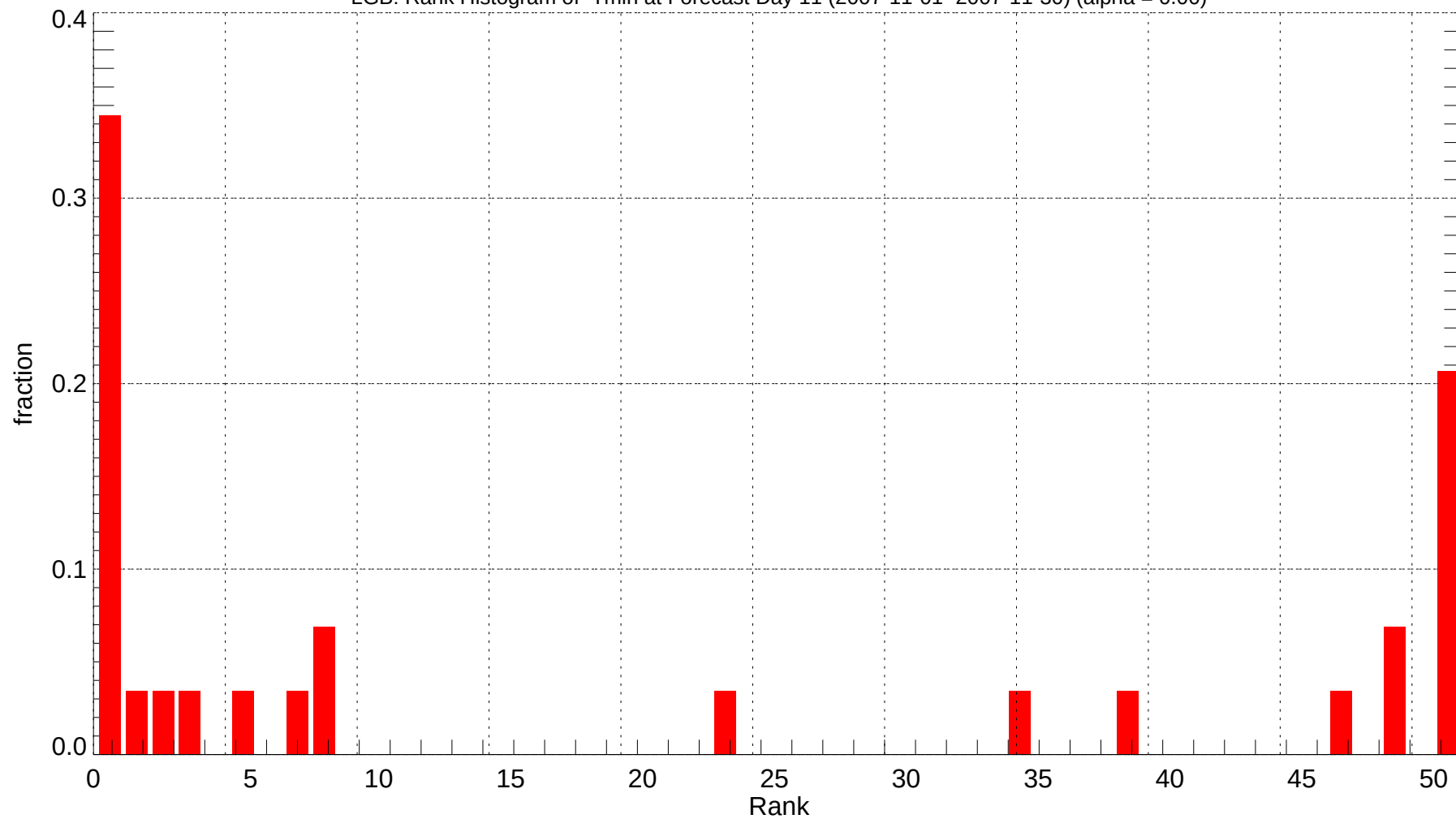
LGB: Rank Histogram of Tmin at Forecast Day 11 (2007-11-01~2007-11-30) (alpha = 0.00)
