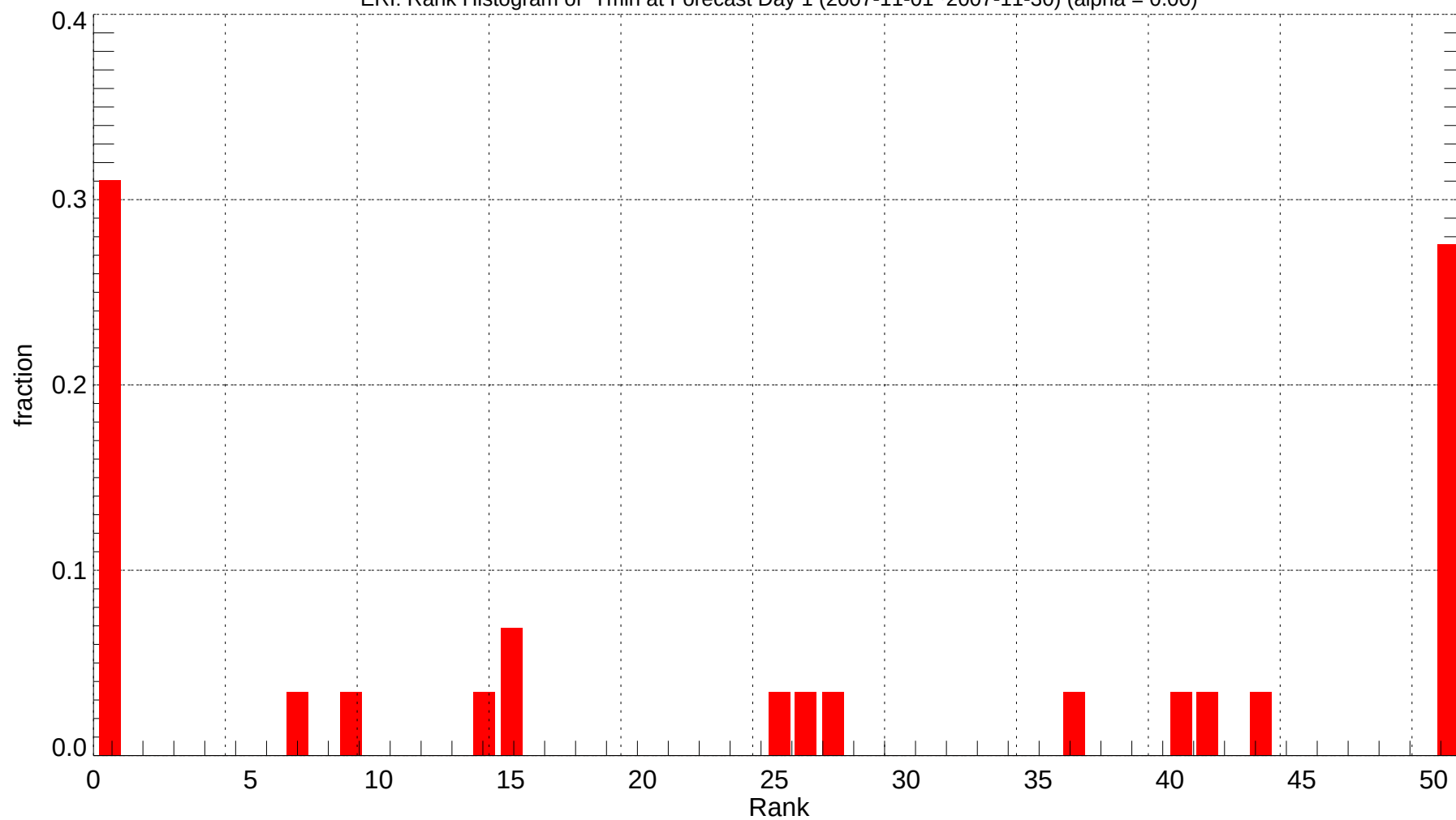
ERI: Rank Histogram of Tmin at Forecast Day 1 (2007-11-01~2007-11-30) (alpha = 0.00)
