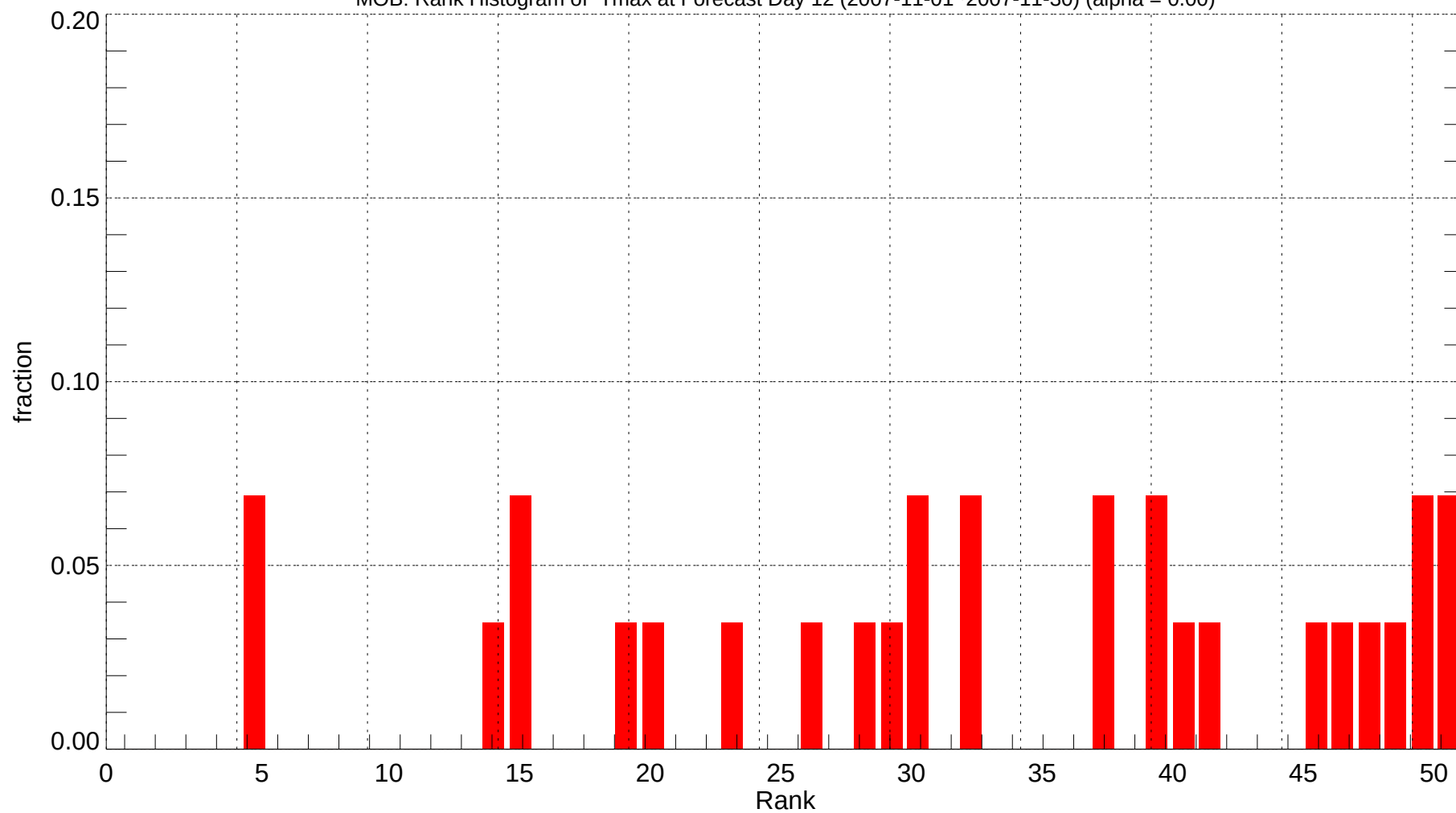
MOB: Rank Histogram of Tmax at Forecast Day 12 (2007-11-01~2007-11-30) (alpha = 0.00)
