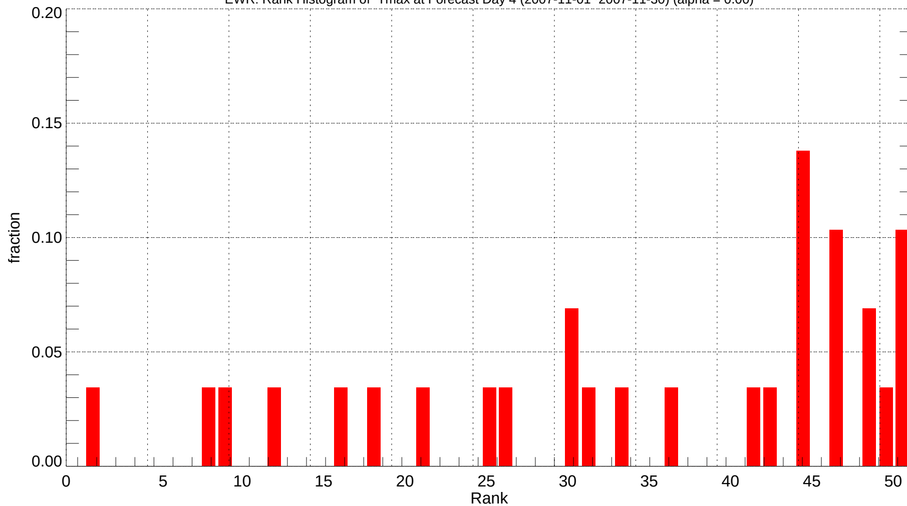
EWR: Rank Histogram of Tmax at Forecast Day 4 (2007-11-01~2007-11-30) (alpha = 0.00)
