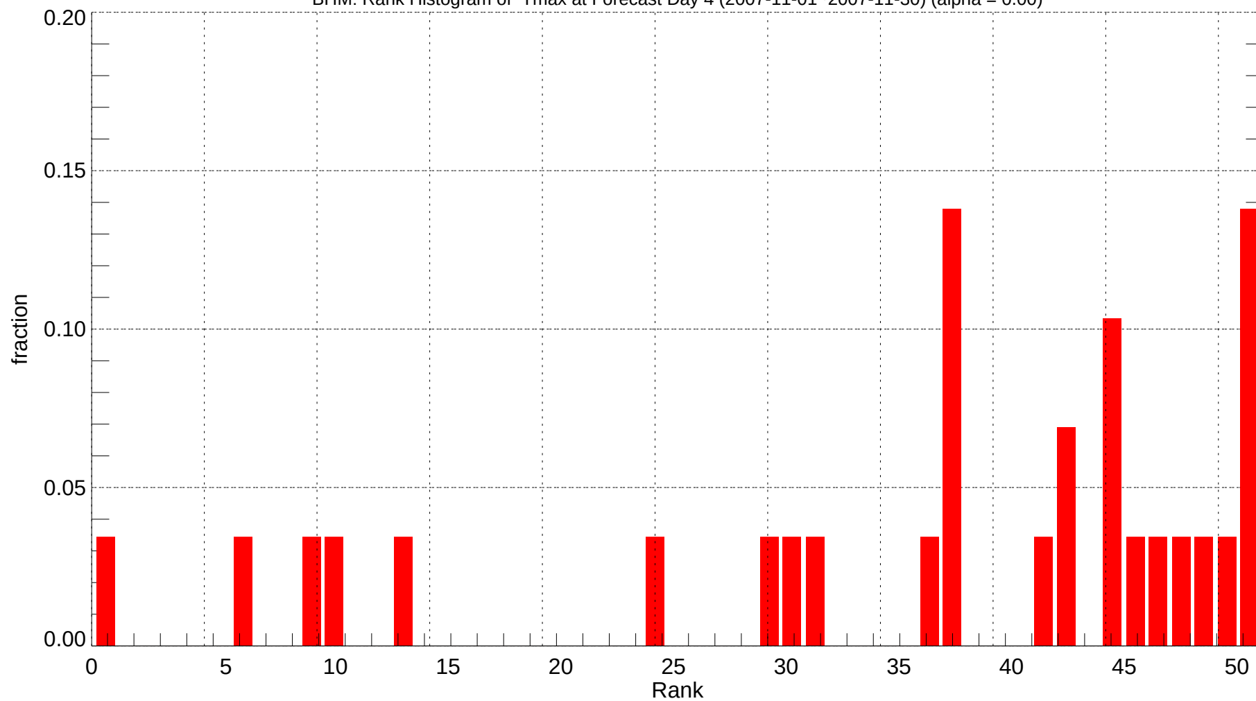
BHM: Rank Histogram of Tmax at Forecast Day 4 (2007-11-01~2007-11-30) (alpha = 0.00)
