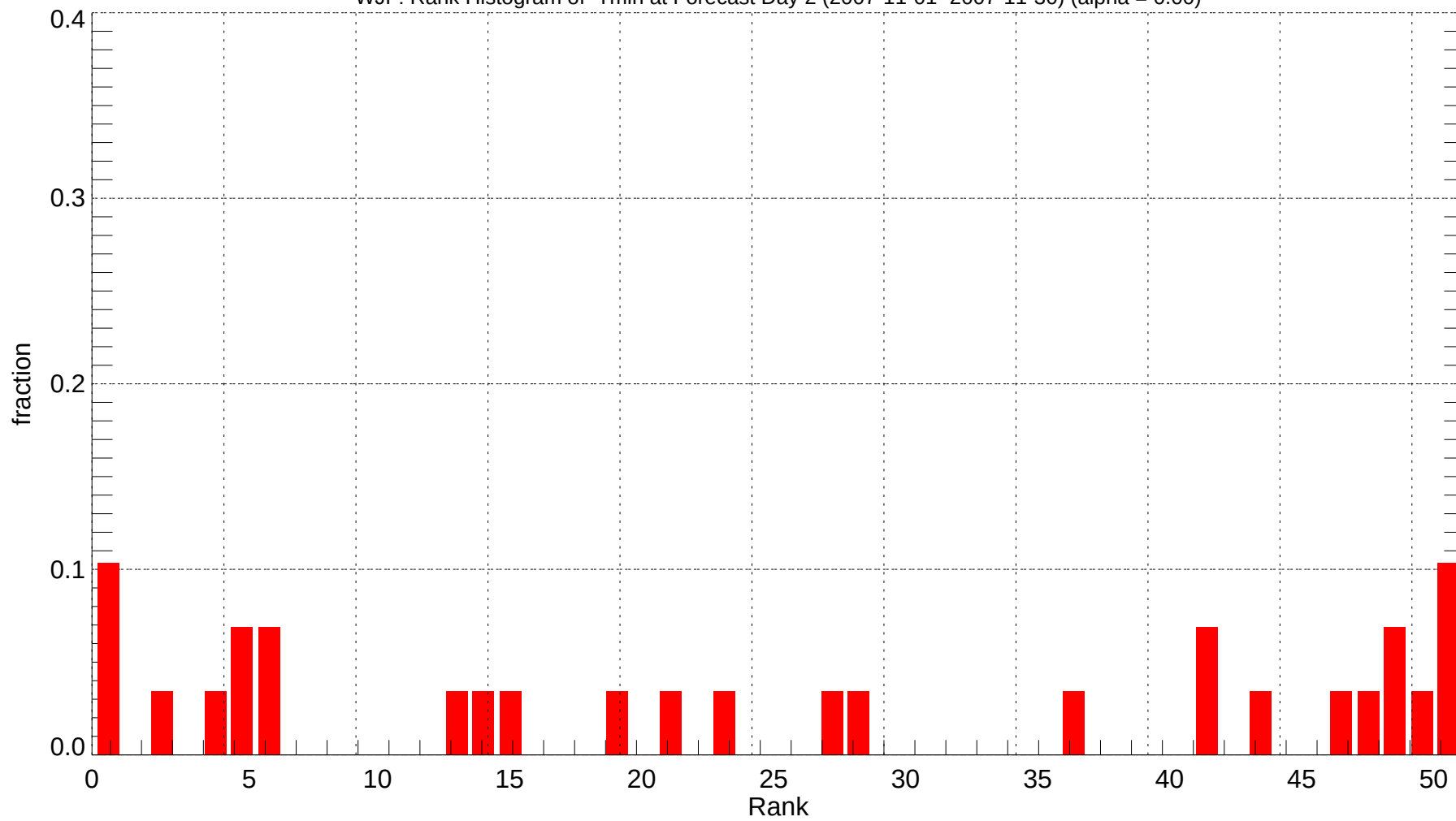
WJF: Rank Histogram of Tmin at Forecast Day 2 (2007-11-01~2007-11-30) (alpha = 0.00)
