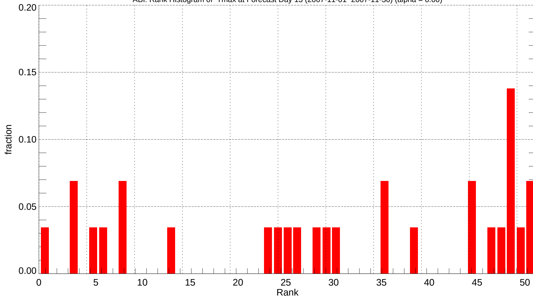
ABI: Rank Histogram of Tmax at Forecast Day 13 (2007-11-01~2007-11-30) (alpha = 0.00)
