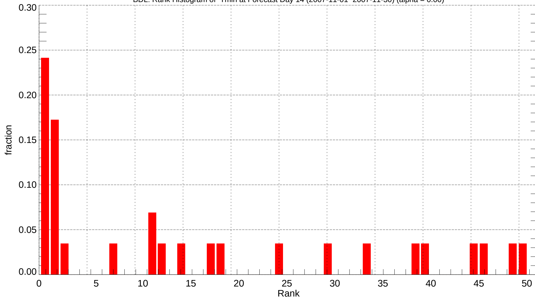
BDL: Rank Histogram of Tmin at Forecast Day 14 (2007-11-01~2007-11-30) (alpha = 0.00)
