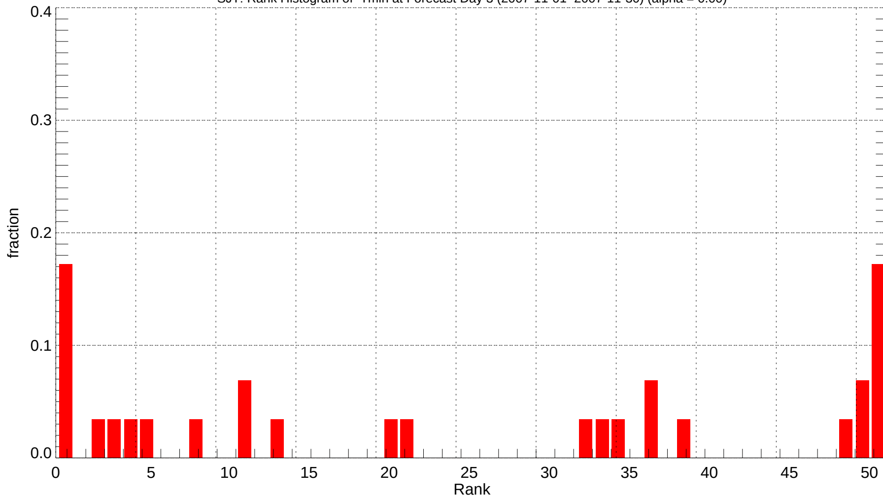
SJT: Rank Histogram of Tmin at Forecast Day 3 (2007-11-01~2007-11-30) (alpha = 0.00)
