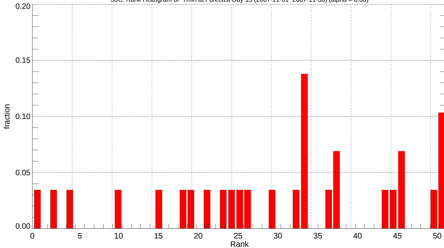
SJC: Rank Histogram of Tmin at Forecast Day 15 (2007-11-01~2007-11-30) (alpha = 0.00)
