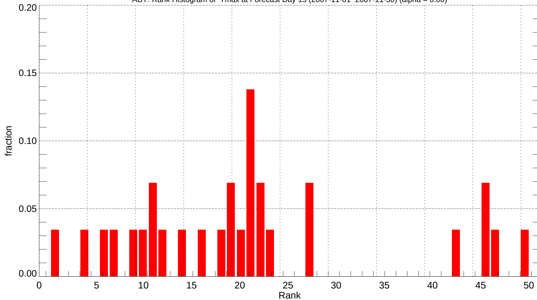
ABY: Rank Histogram of Tmax at Forecast Day 15 (2007-11-01~2007-11-30) (alpha = 0.00)
