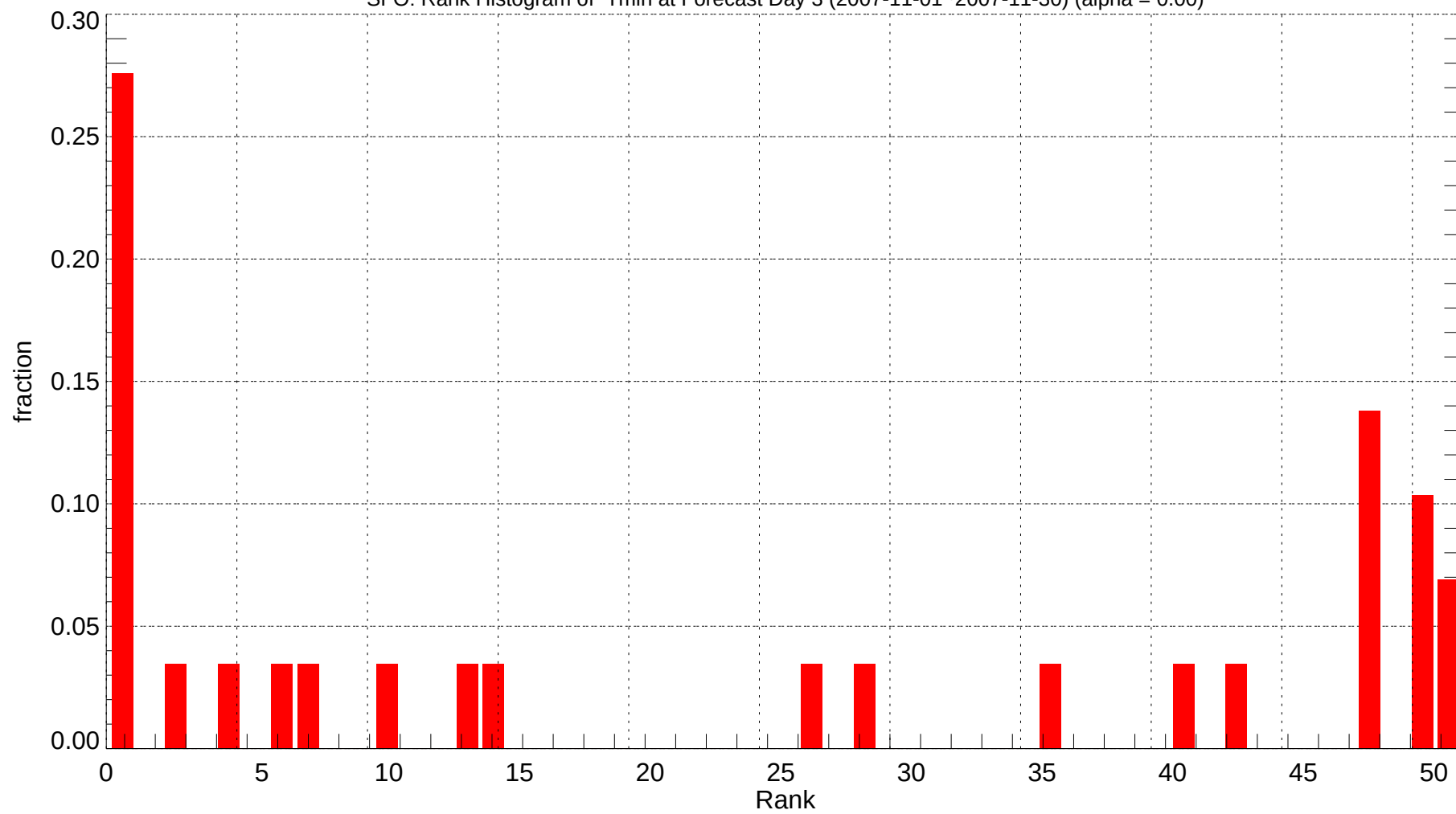
SFO: Rank Histogram of Tmin at Forecast Day 3 (2007-11-01~2007-11-30) (alpha = 0.00)
