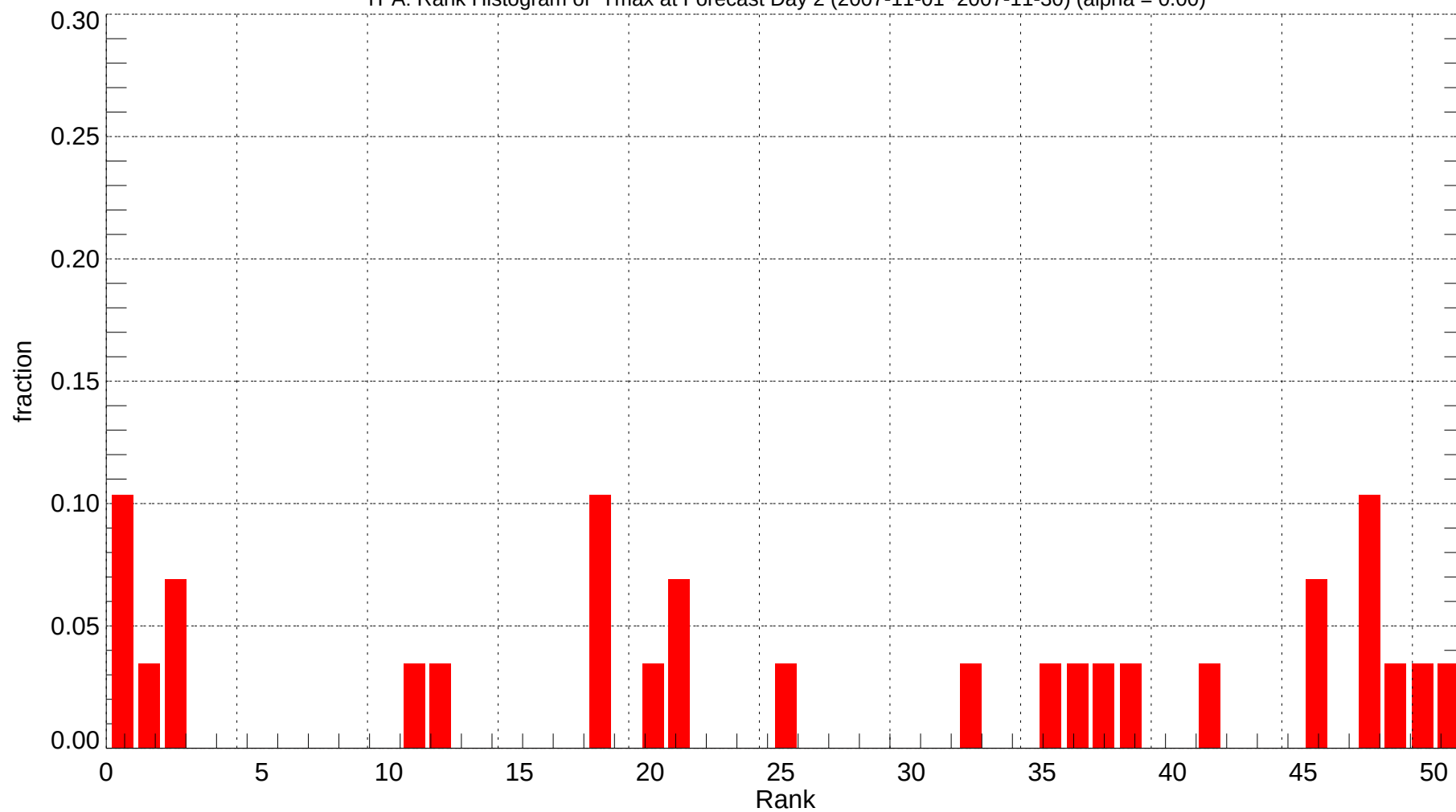
TPA: Rank Histogram of Tmax at Forecast Day 2 (2007-11-01~2007-11-30) (alpha = 0.00)
