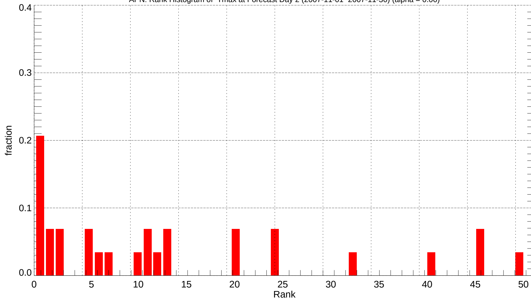
APN: Rank Histogram of Tmax at Forecast Day 2 (2007-11-01~2007-11-30) (alpha = 0.00)
