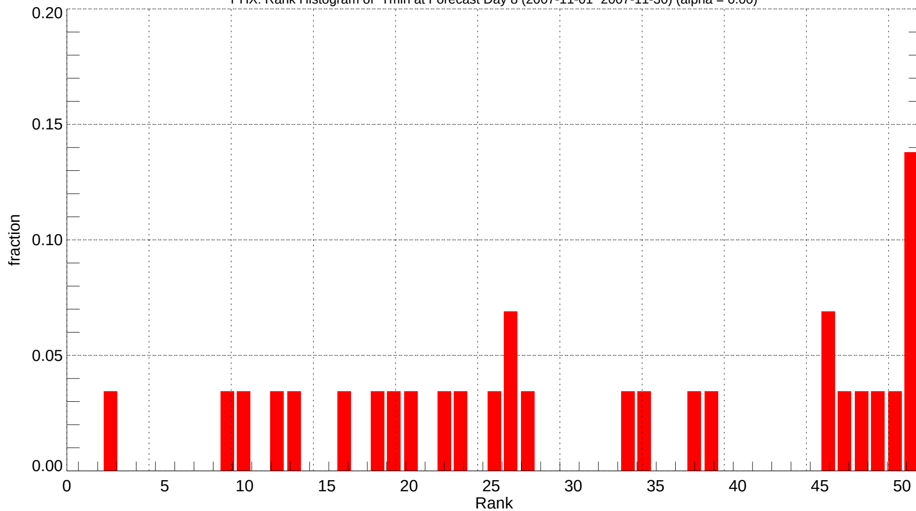
PHX: Rank Histogram of Tmin at Forecast Day 8 (2007-11-01~2007-11-30) (alpha = 0.00)
