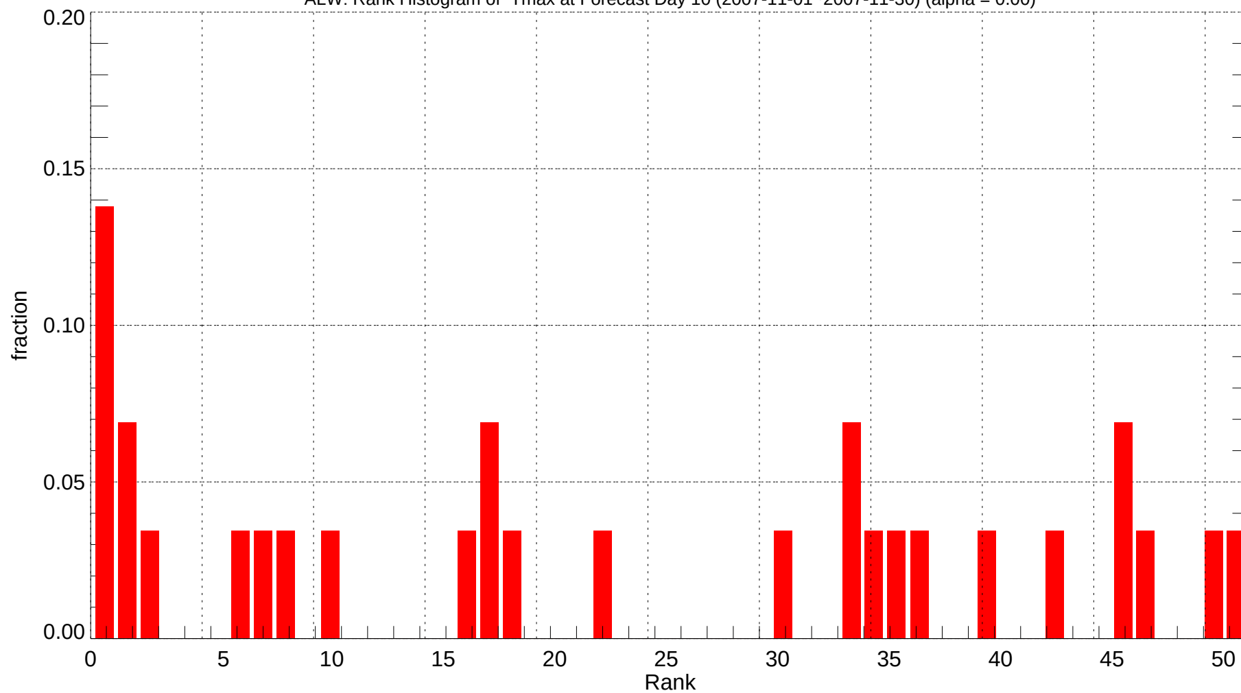
ALW: Rank Histogram of Tmax at Forecast Day 10 (2007-11-01~2007-11-30) (alpha = 0.00)
