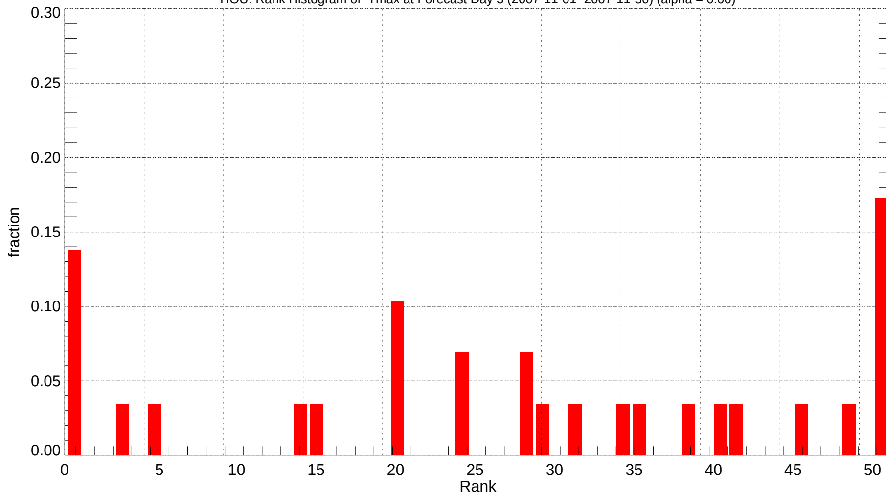
HOU: Rank Histogram of Tmax at Forecast Day 3 (2007-11-01~2007-11-30) (alpha = 0.00)
