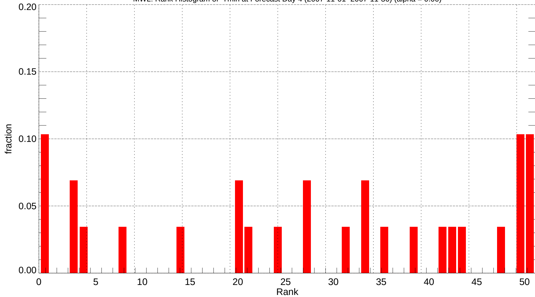
MWL: Rank Histogram of Tmin at Forecast Day 4 (2007-11-01~2007-11-30) (alpha = 0.00)
