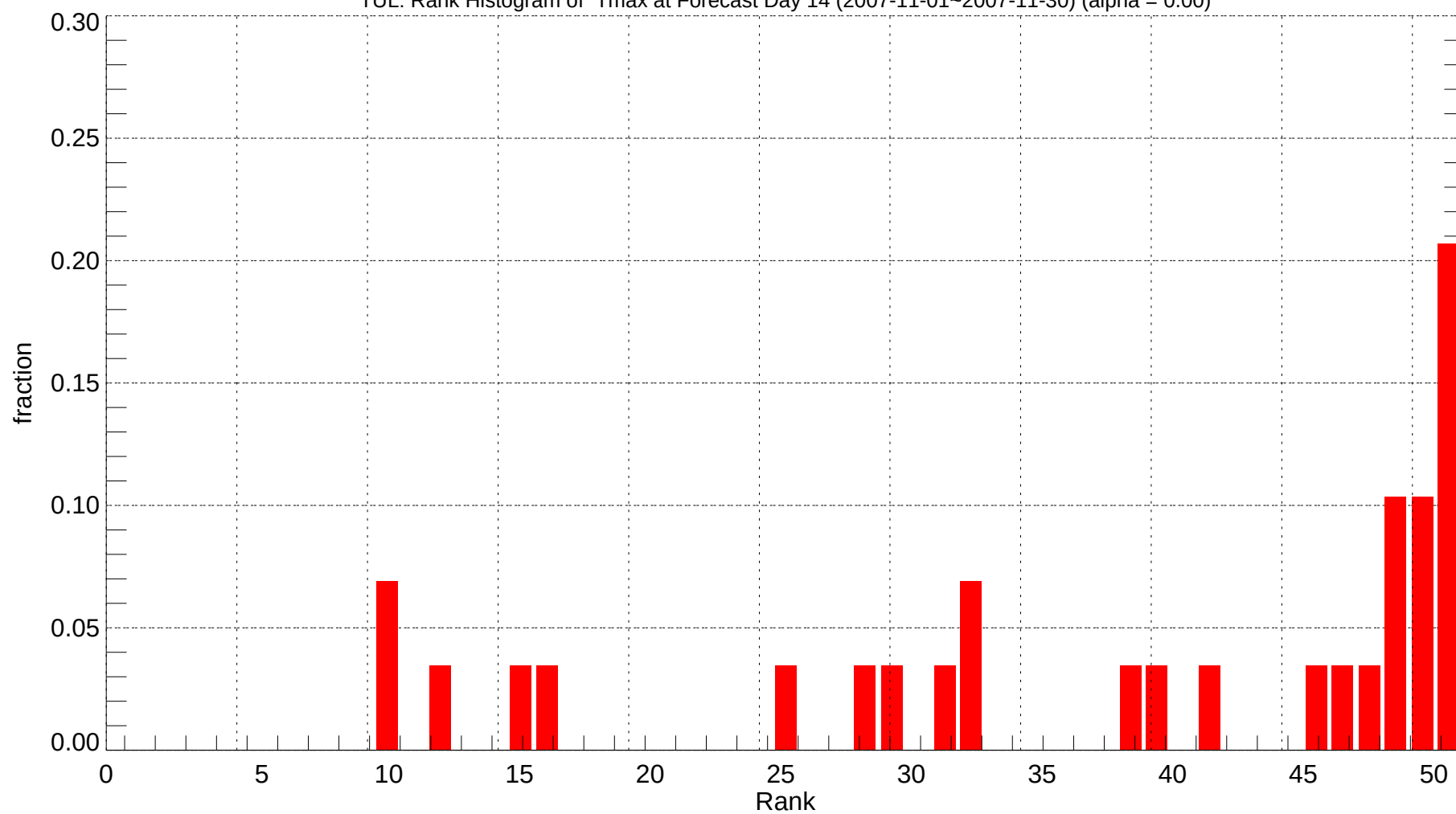
TUL: Rank Histogram of Tmax at Forecast Day 14 (2007-11-01~2007-11-30) (alpha = 0.00)
