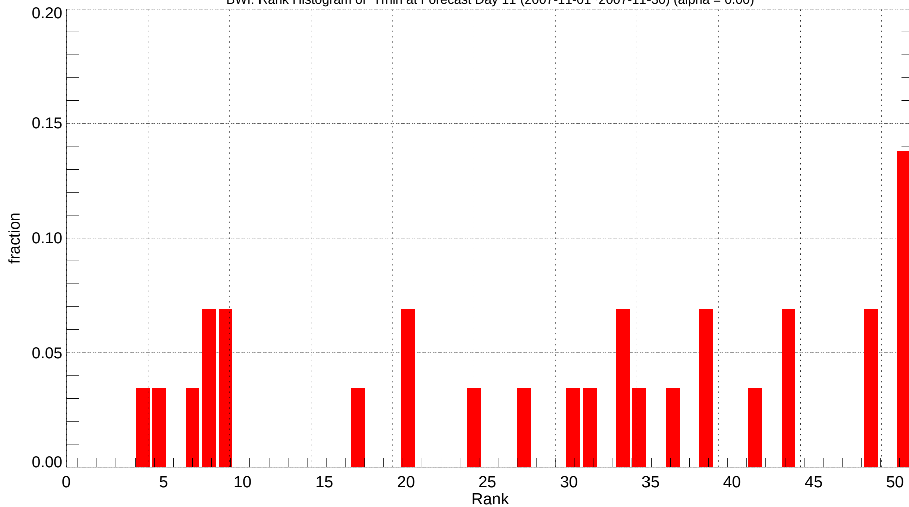
BWl: Rank Histogram of Tmin at Forecast Day 11 (2007-11-01~2007-11-30) (alpha = 0.00)
