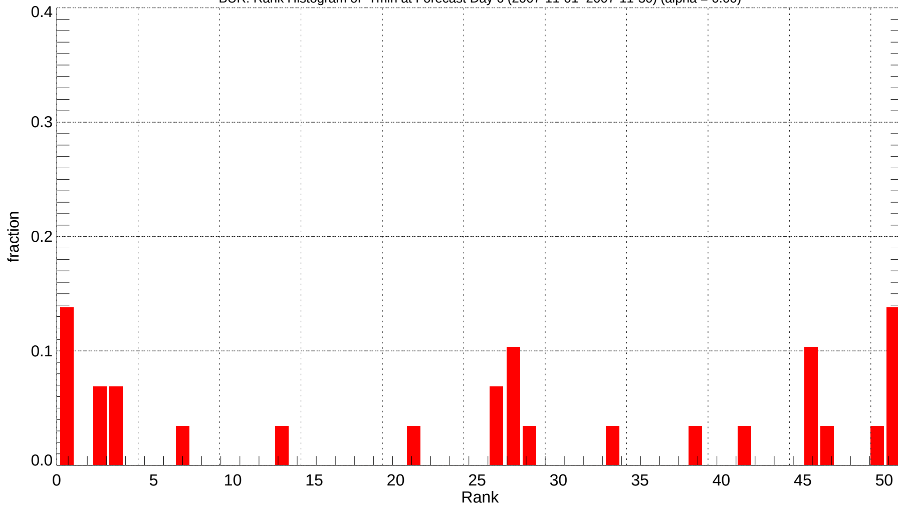
BUR: Rank Histogram of Tmin at Forecast Day 6 (2007-11-01~2007-11-30) (alpha = 0.00)
