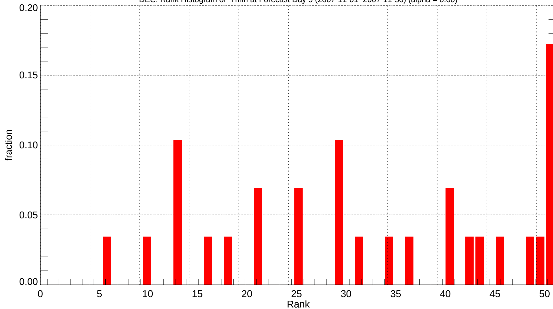
DEC: Rank Histogram of Tmin at Forecast Day 9 (2007-11-01~2007-11-30) (alpha = 0.00)
