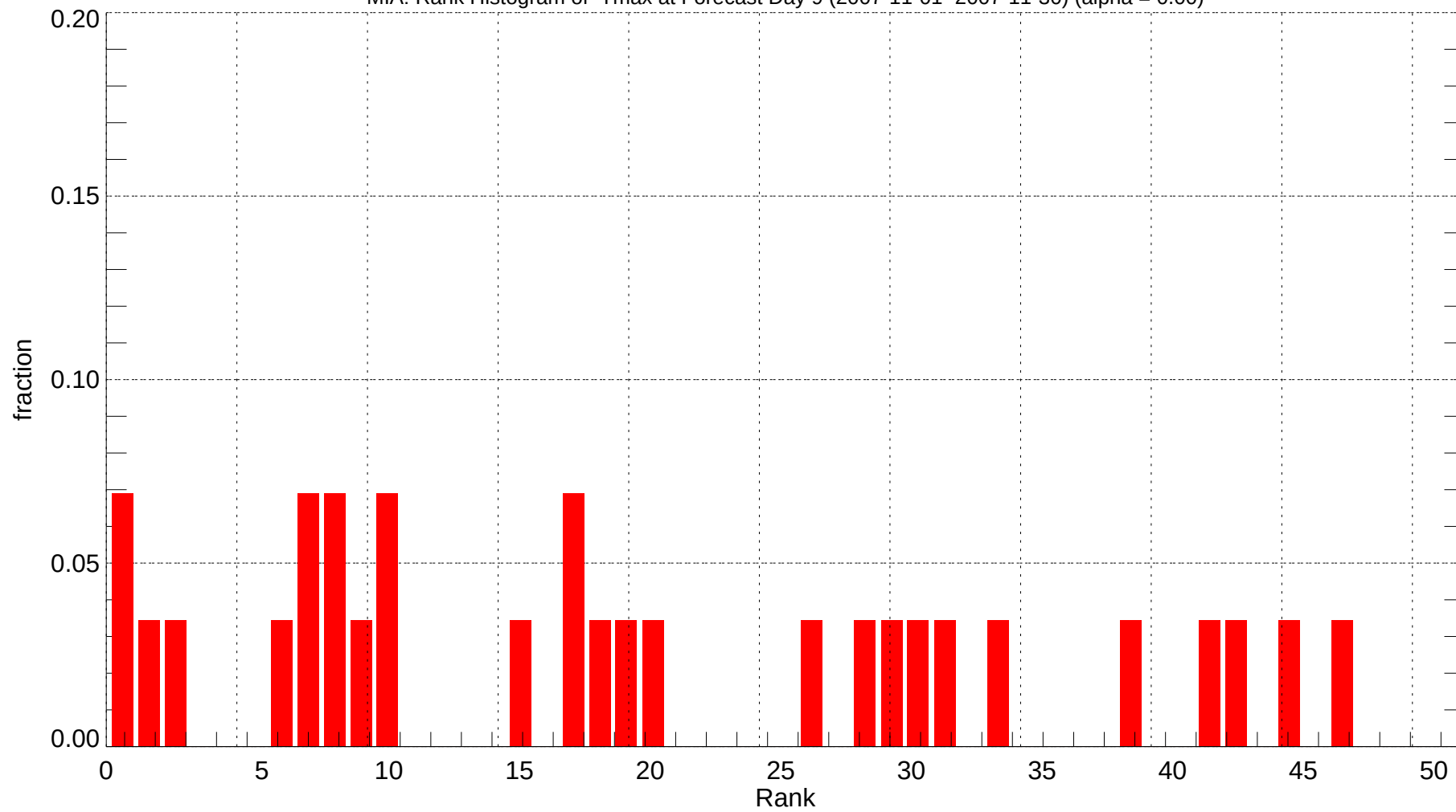
MIA: Rank Histogram of Tmax at Forecast Day 9 (2007-11-01~2007-11-30) (alpha = 0.00)
