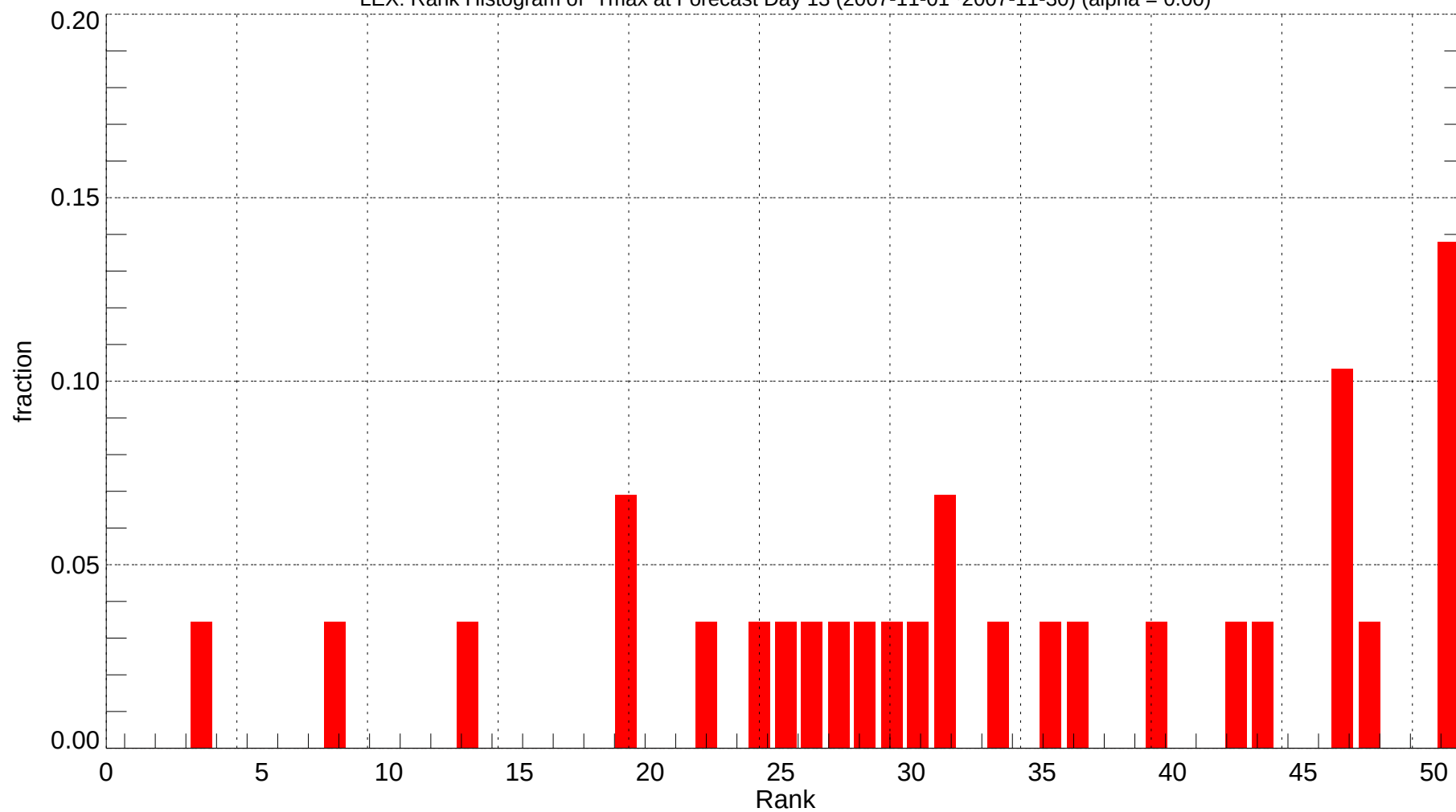
LEX: Rank Histogram of Tmax at Forecast Day 13 (2007-11-01~2007-11-30) (alpha = 0.00)
