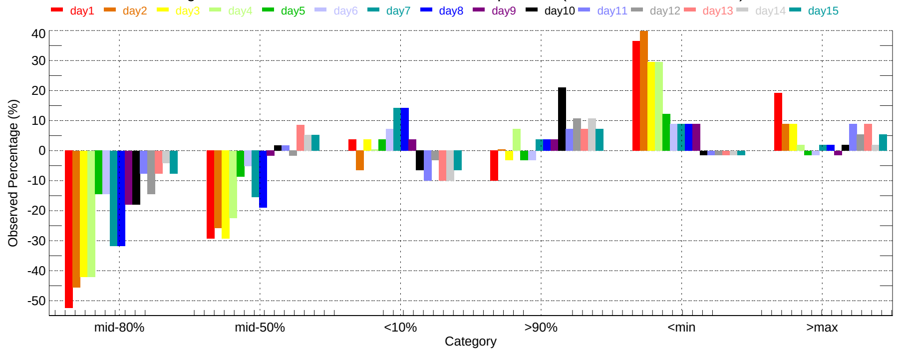
Observed Percentage Deviation of Ensembles - LAN: Max Temperature (2007-11-01~2007-11-30)
