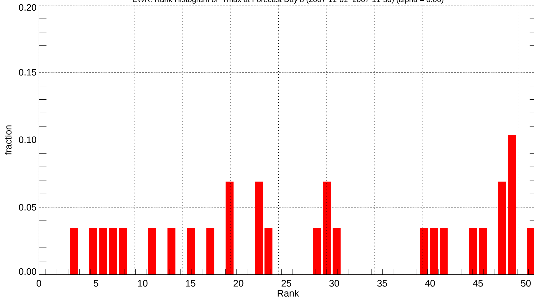
EWR: Rank Histogram of Tmax at Forecast Day 8 (2007-11-01~2007-11-30) (alpha = 0.00)
