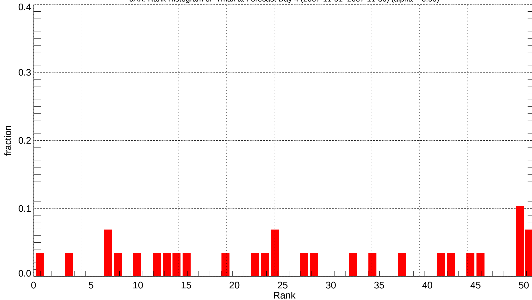
JAX: Rank Histogram of Tmax at Forecast Day 4 (2007-11-01~2007-11-30) (alpha = 0.00)
