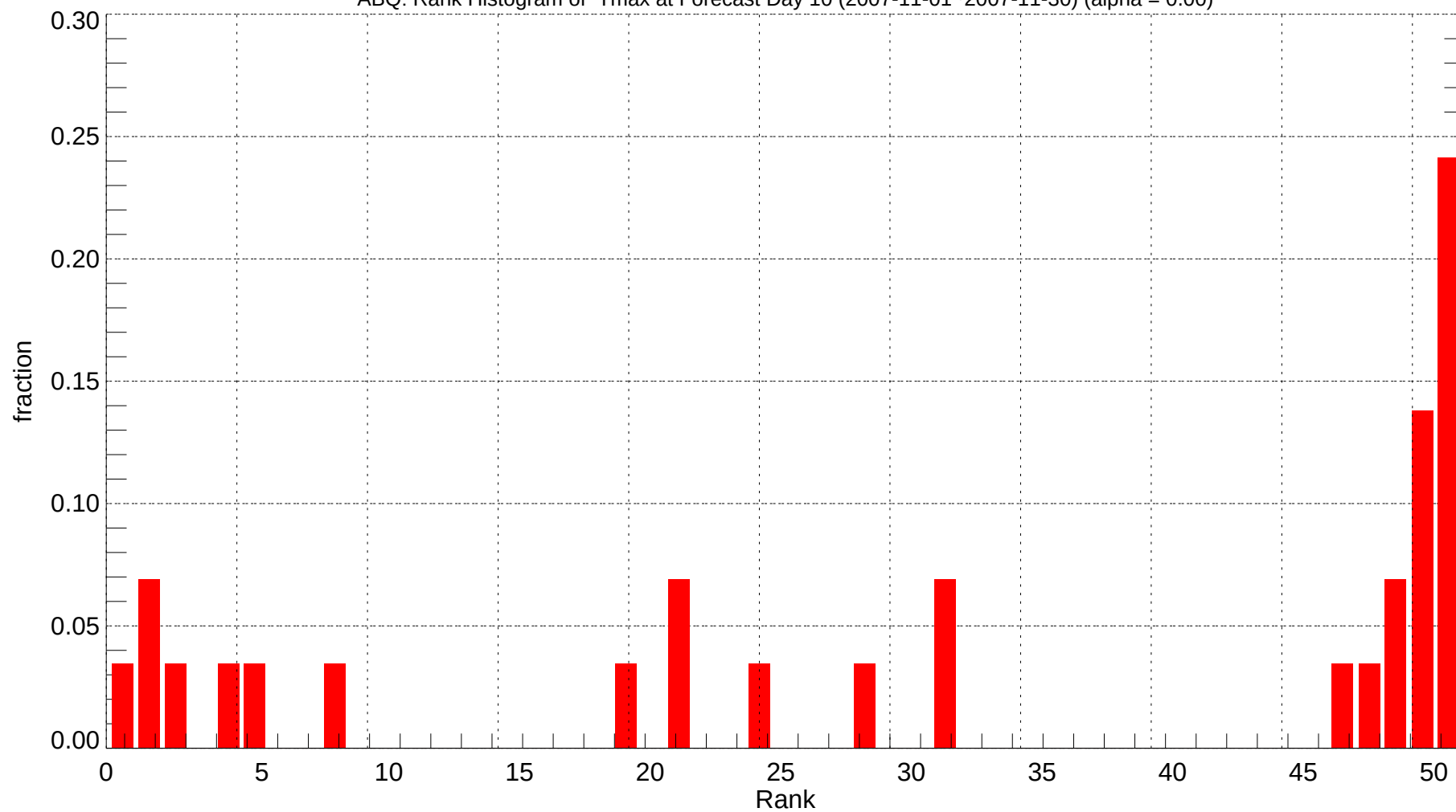
ABQ: Rank Histogram of Tmax at Forecast Day 10 (2007-11-01~2007-11-30) (alpha = 0.00)
