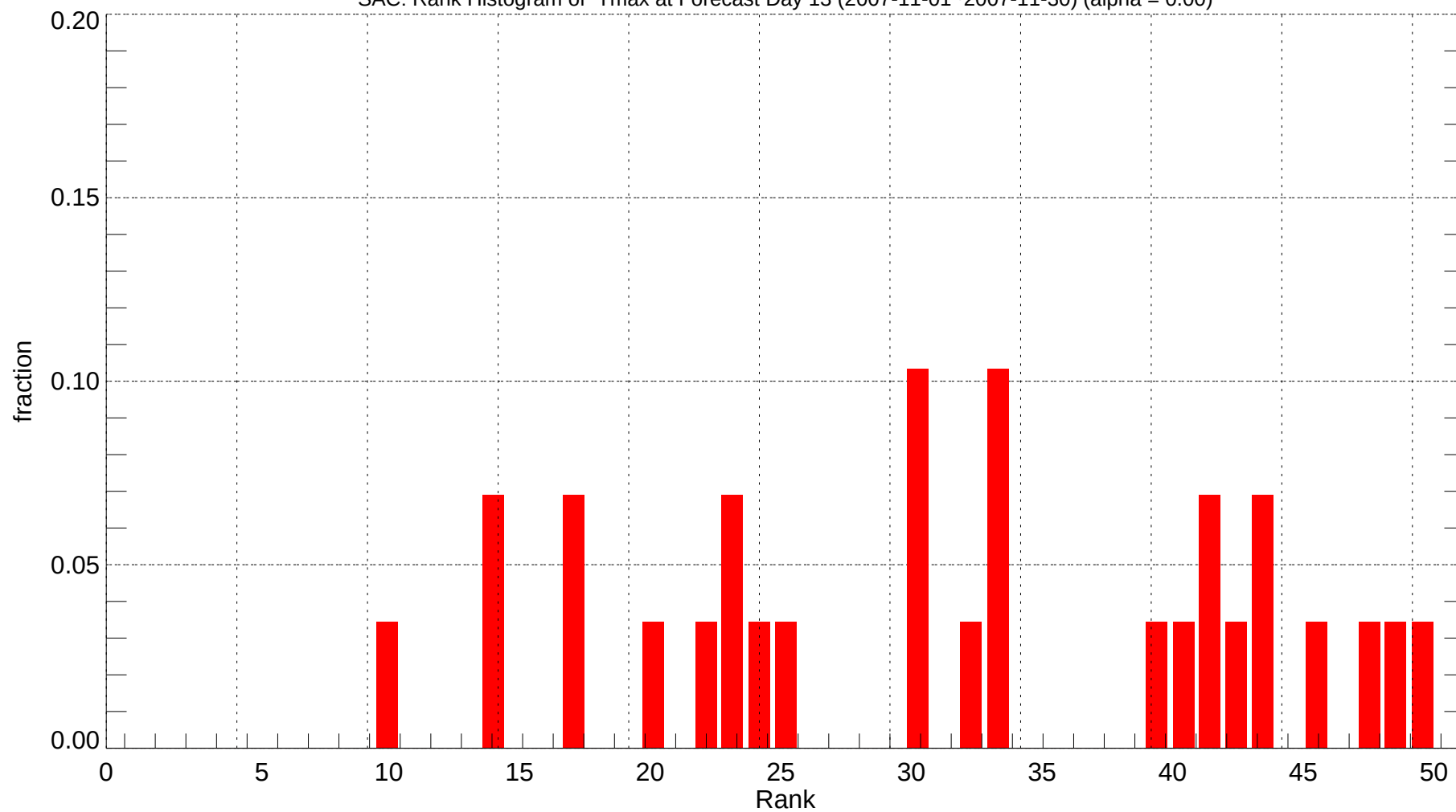
SAC: Rank Histogram of Tmax at Forecast Day 13 (2007-11-01~2007-11-30) (alpha = 0.00)
