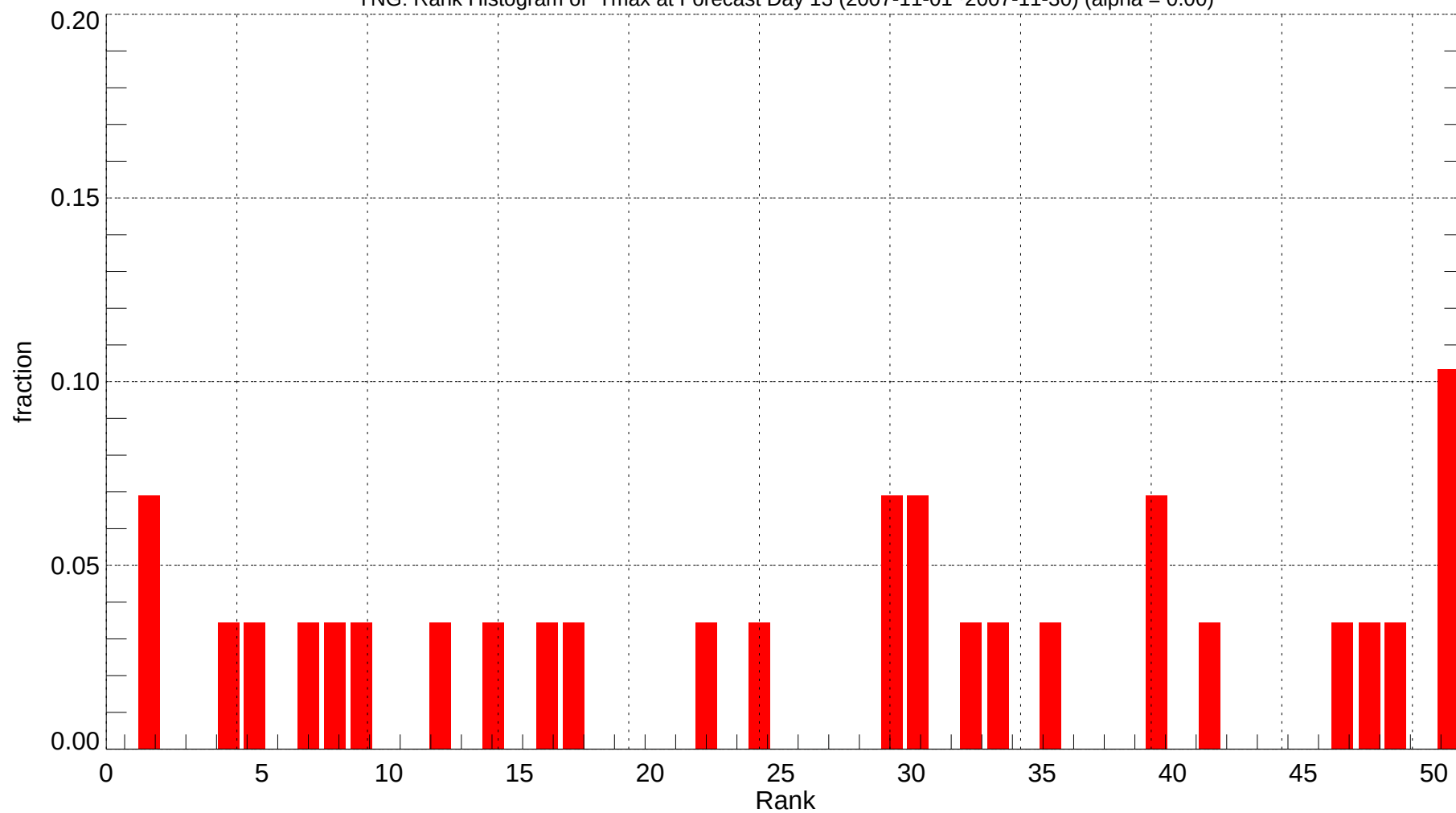
YNG: Rank Histogram of Tmax at Forecast Day 13 (2007-11-01~2007-11-30) (alpha = 0.00)
