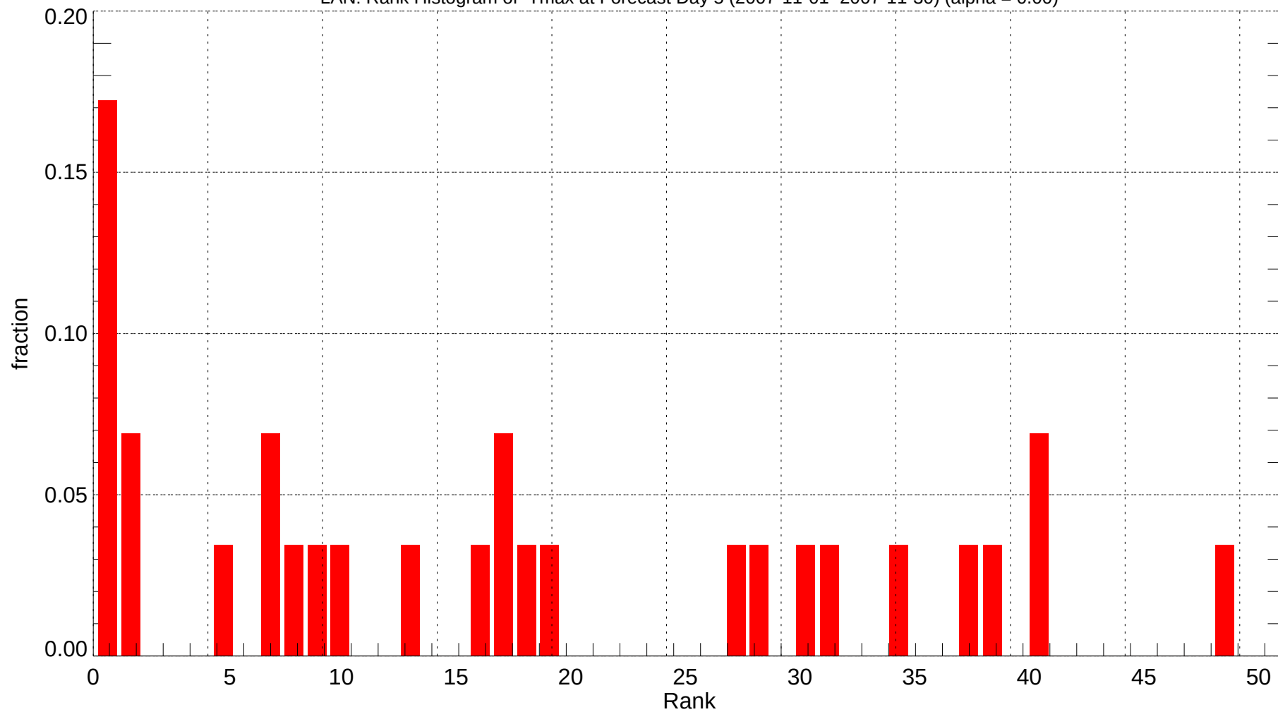
LAN: Rank Histogram of Tmax at Forecast Day 5 (2007-11-01~2007-11-30) (alpha = 0.00)
