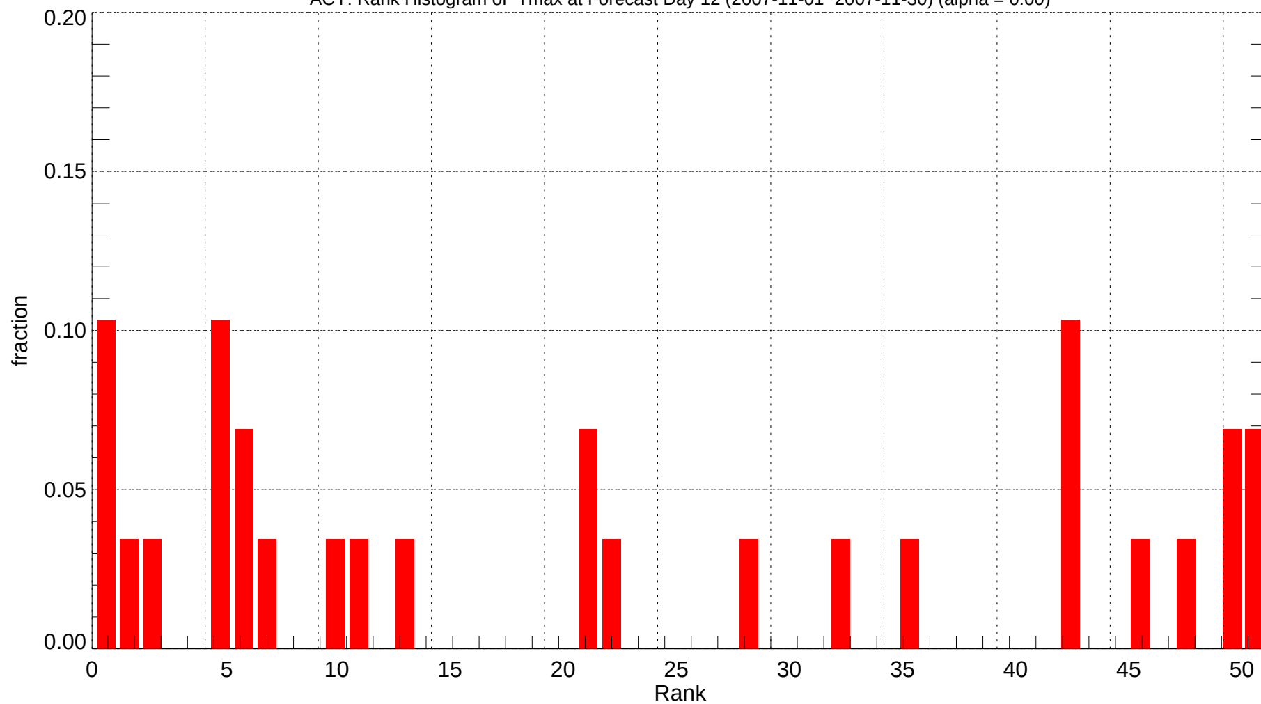
ACY: Rank Histogram of Tmax at Forecast Day 12 (2007-11-01~2007-11-30) (alpha = 0.00)
