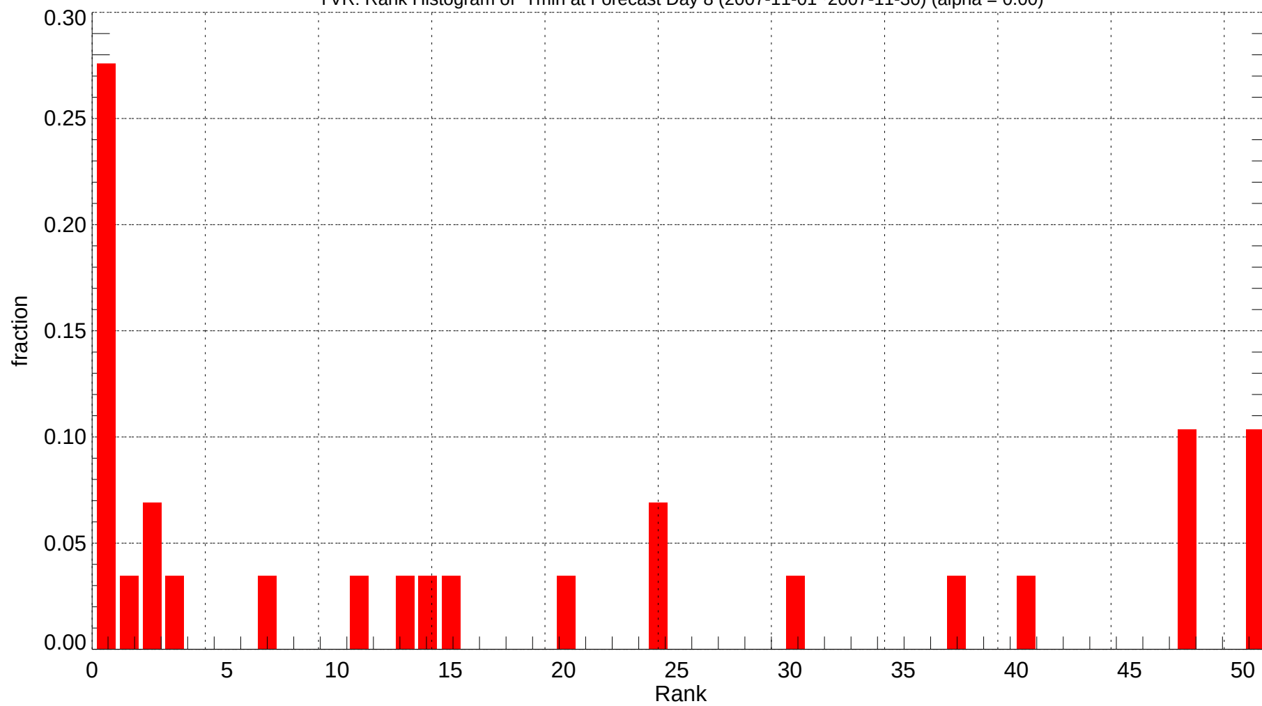
YVR: Rank Histogram of Tmin at Forecast Day 8 (2007-11-01~2007-11-30) (alpha = 0.00)
