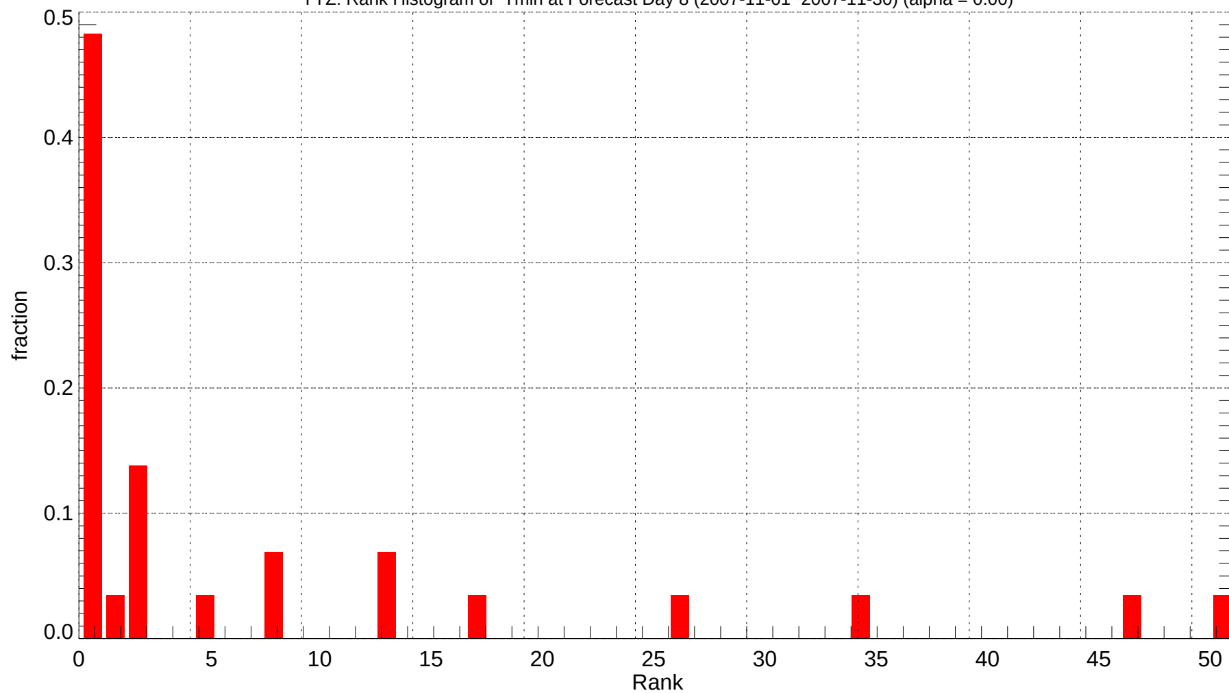
YYZ: Rank Histogram of Tmin at Forecast Day 8 (2007-11-01~2007-11-30) (alpha = 0.00)
