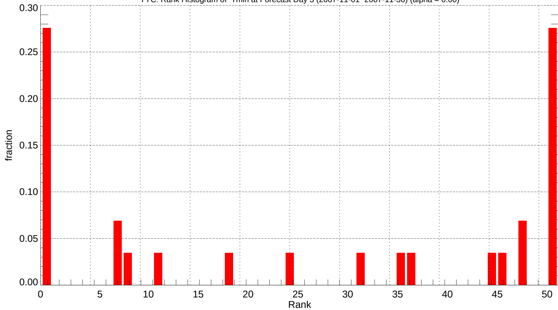
YYC: Rank Histogram of Tmin at Forecast Day 3 (2007-11-01~2007-11-30) (alpha = 0.00)
