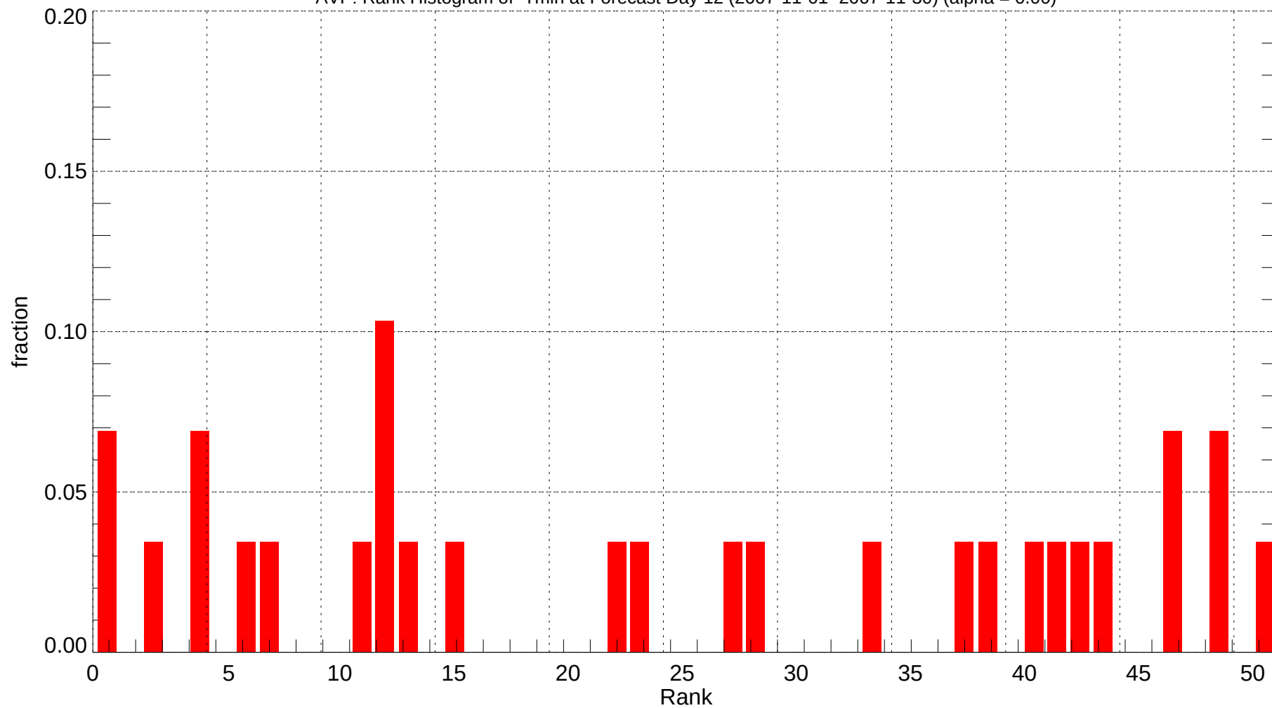
AVP: Rank Histogram of Tmin at Forecast Day 12 (2007-11-01~2007-11-30) (alpha = 0.00)
