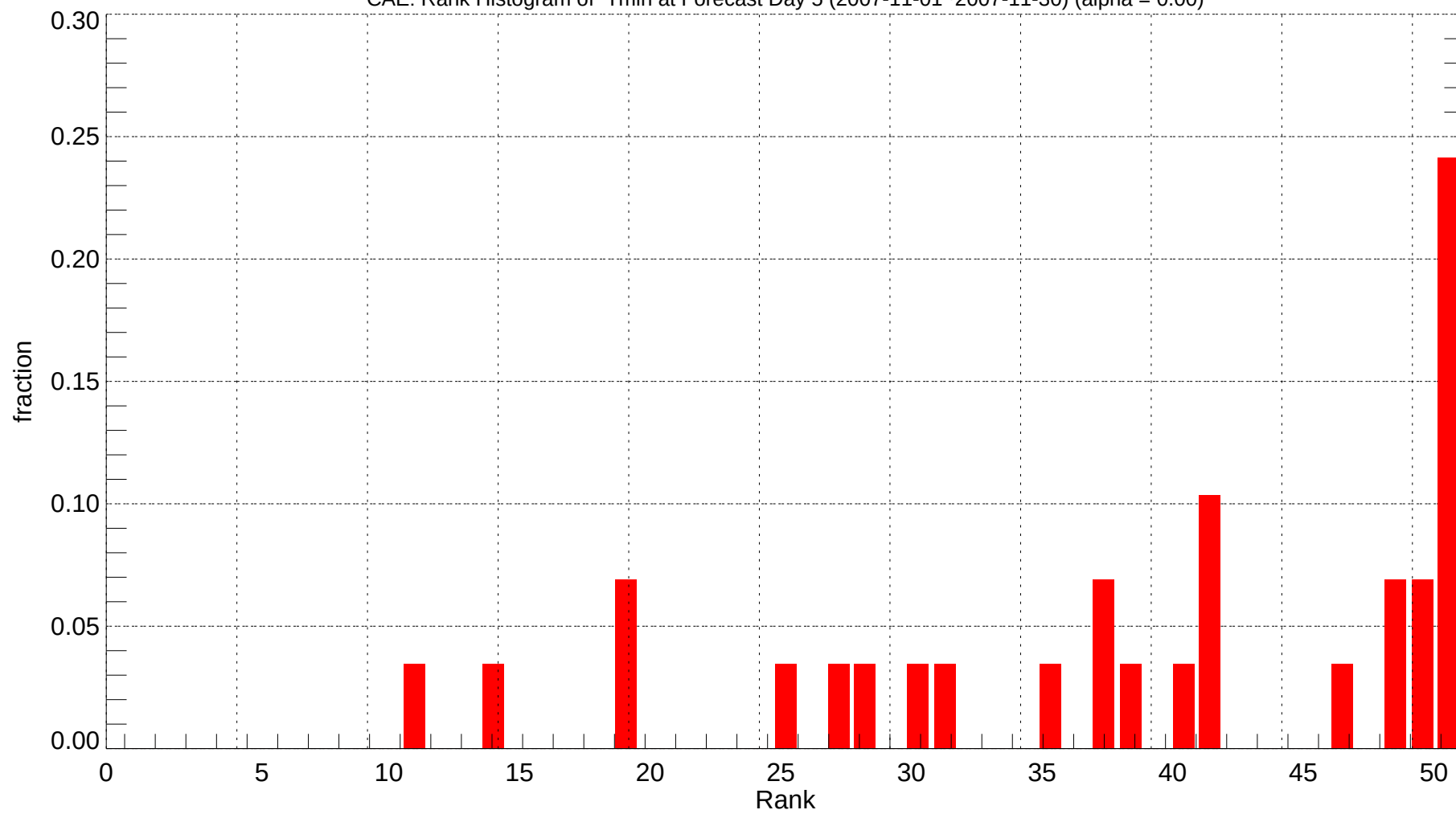
CAE: Rank Histogram of Tmin at Forecast Day 5 (2007-11-01~2007-11-30) (alpha = 0.00)
