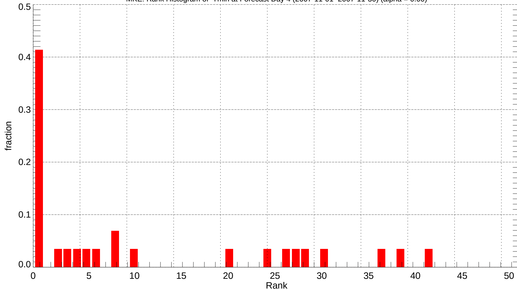
MKE: Rank Histogram of Tmin at Forecast Day 4 (2007-11-01~2007-11-30) (alpha = 0.00)
