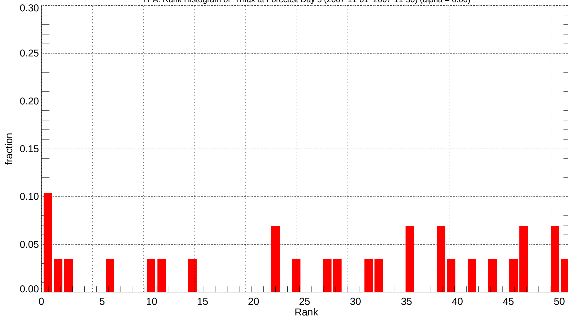
TPA: Rank Histogram of Tmax at Forecast Day 3 (2007-11-01~2007-11-30) (alpha = 0.00)
