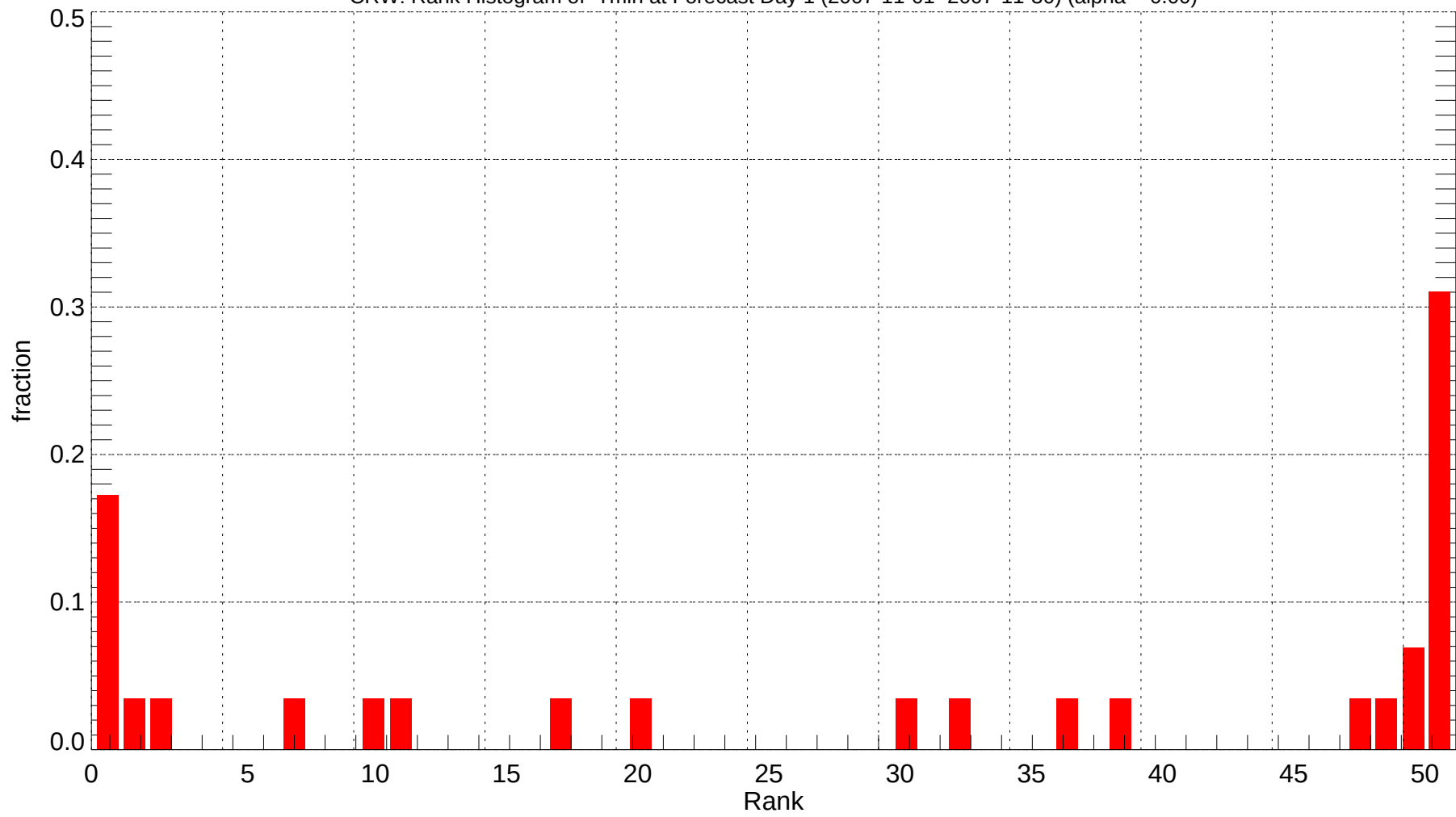
CRW: Rank Histogram of Tmin at Forecast Day 1 (2007-11-01~2007-11-30) (alpha = 0.00)
