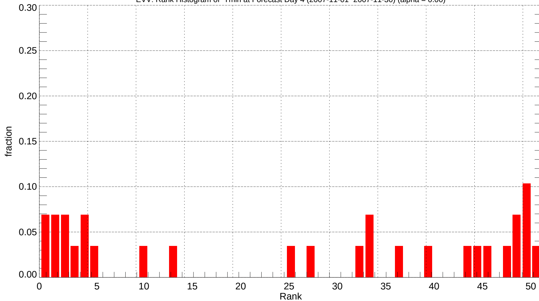
EVV: Rank Histogram of Tmin at Forecast Day 4 (2007-11-01~2007-11-30) (alpha = 0.00)
