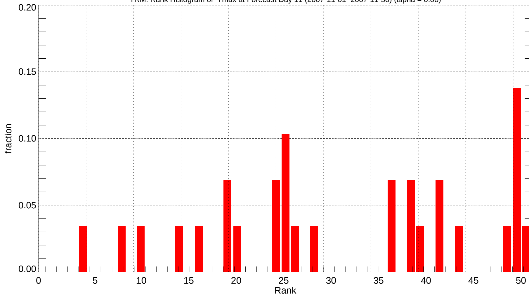
TRM: Rank Histogram of Tmax at Forecast Day 11 (2007-11-01~2007-11-30) (alpha = 0.00)
