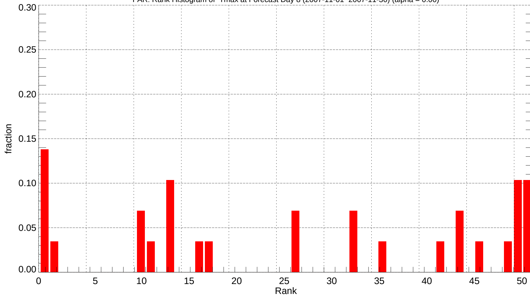
FAR: Rank Histogram of Tmax at Forecast Day 8 (2007-11-01~2007-11-30) (alpha = 0.00)
