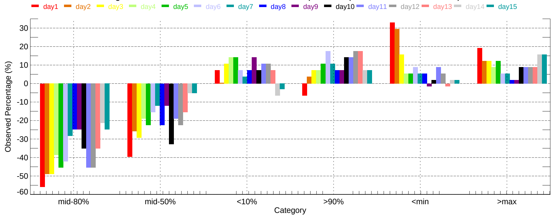
Observed Percentage Deviation of Ensembles - BUR: Max Temperature (2007-11-01~2007-11-30)
