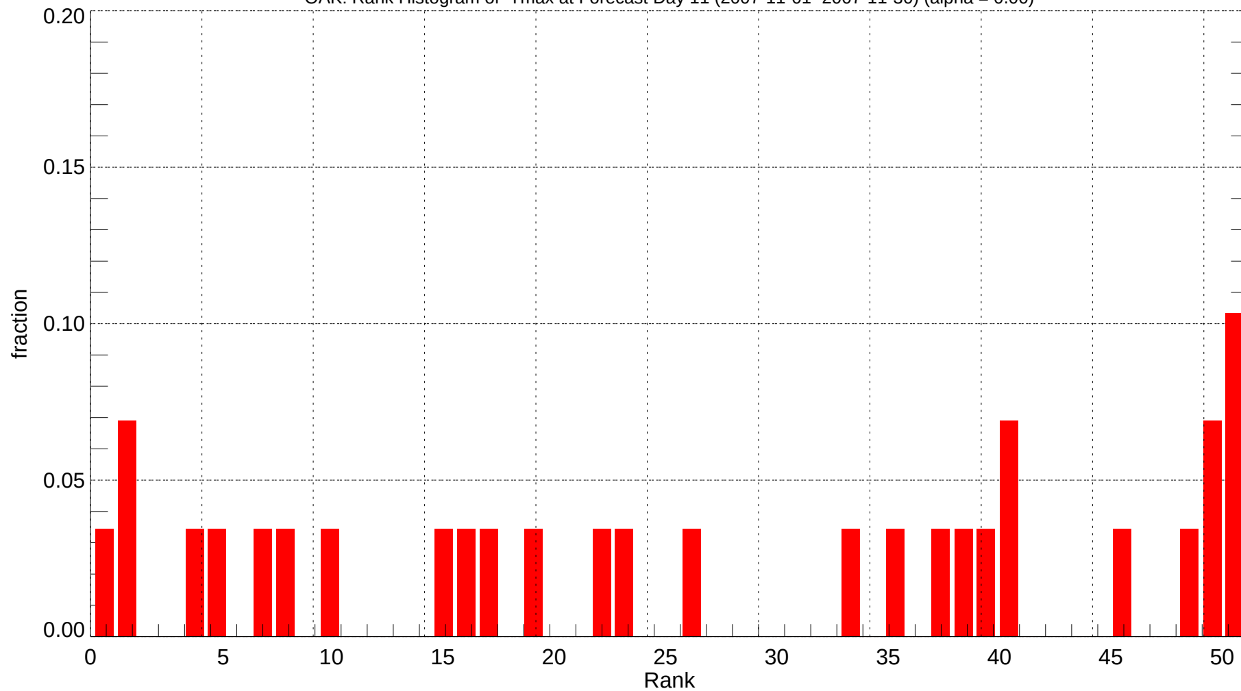
OAK: Rank Histogram of Tmax at Forecast Day 11 (2007-11-01~2007-11-30) (alpha = 0.00)
