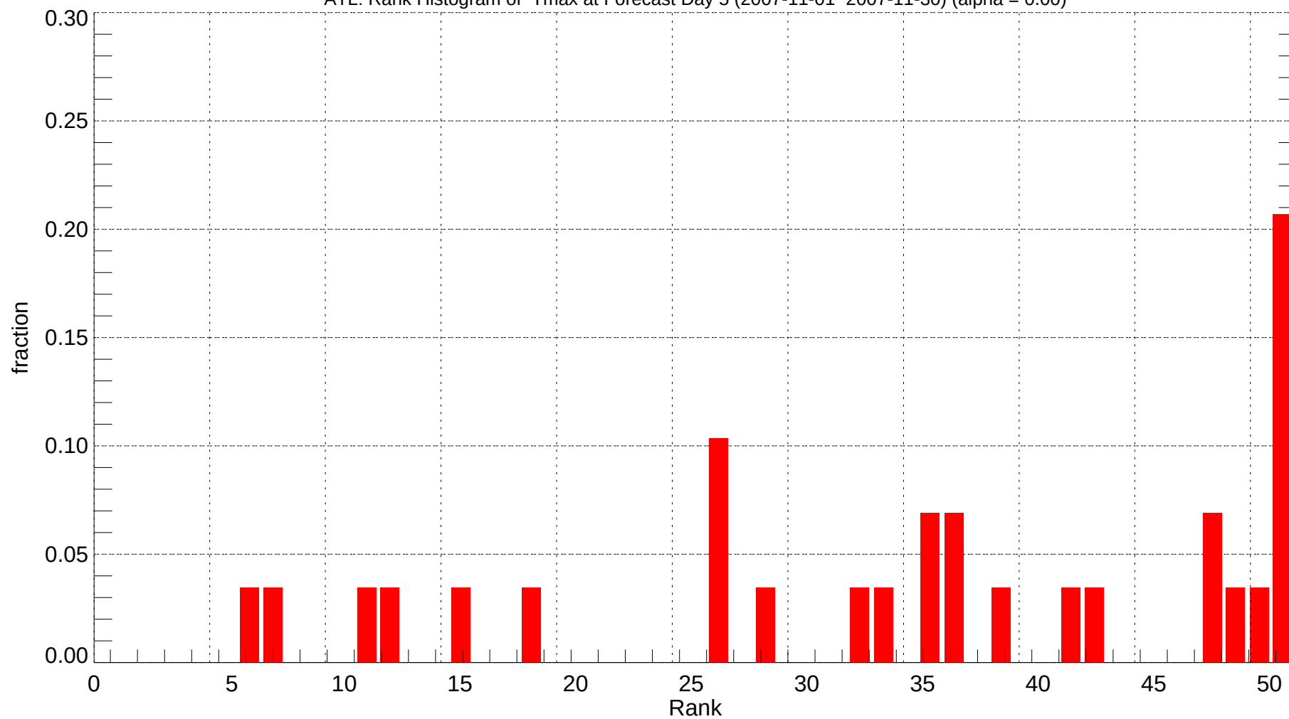
ATL: Rank Histogram of Tmax at Forecast Day 5 (2007-11-01~2007-11-30) (alpha = 0.00)
