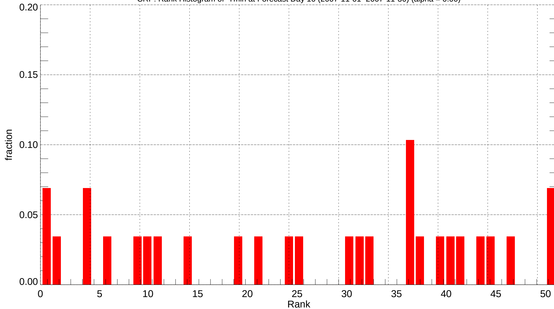
CRP: Rank Histogram of Tmin at Forecast Day 10 (2007-11-01~2007-11-30) (alpha = 0.00)
