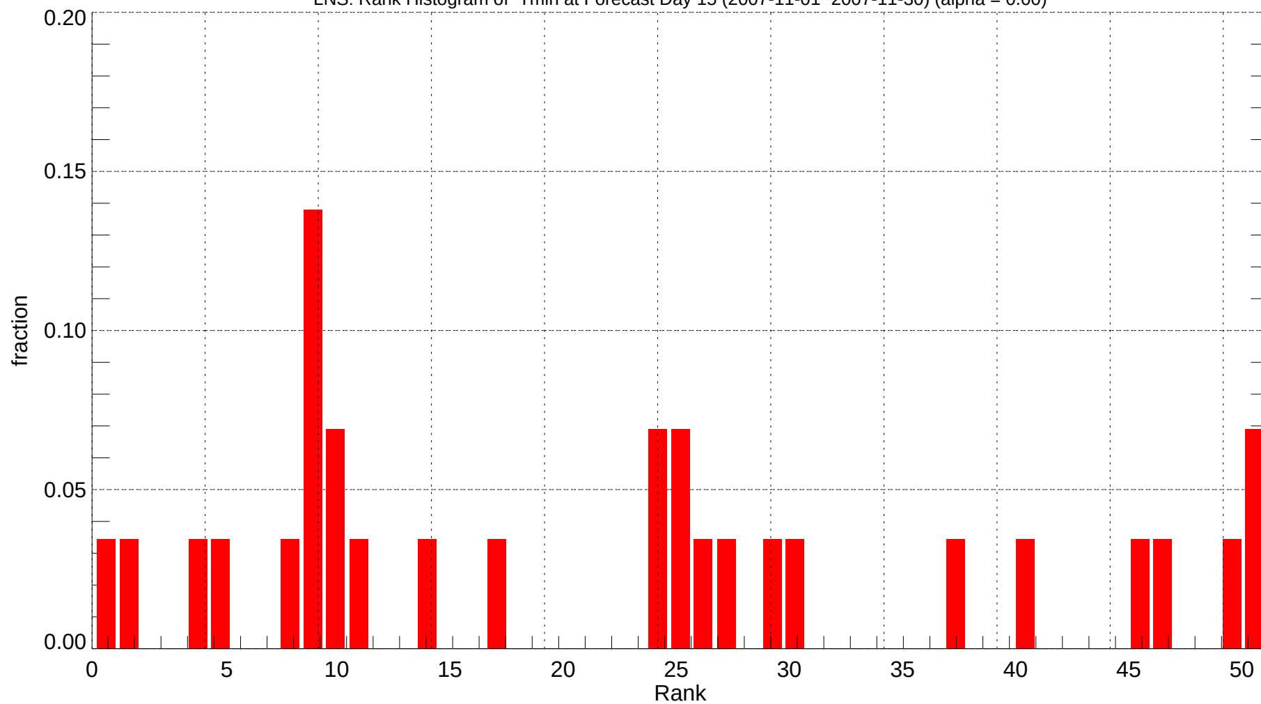
LNS: Rank Histogram of Tmin at Forecast Day 15 (2007-11-01~2007-11-30) (alpha = 0.00)
