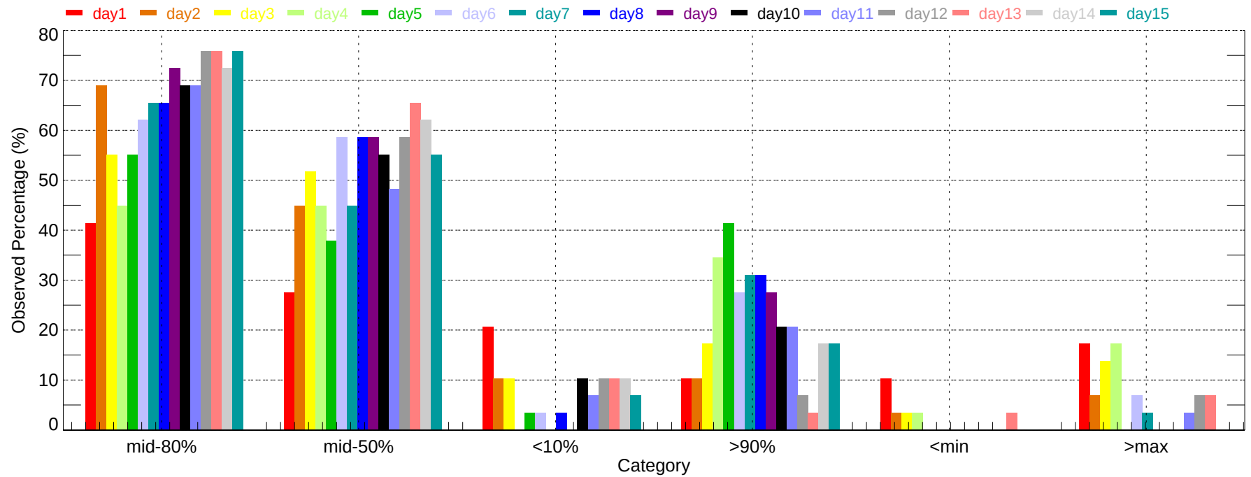
Observed Percentage of Ensembles - ABY: Min Temperature (2007-11-01~2007-11-30)
