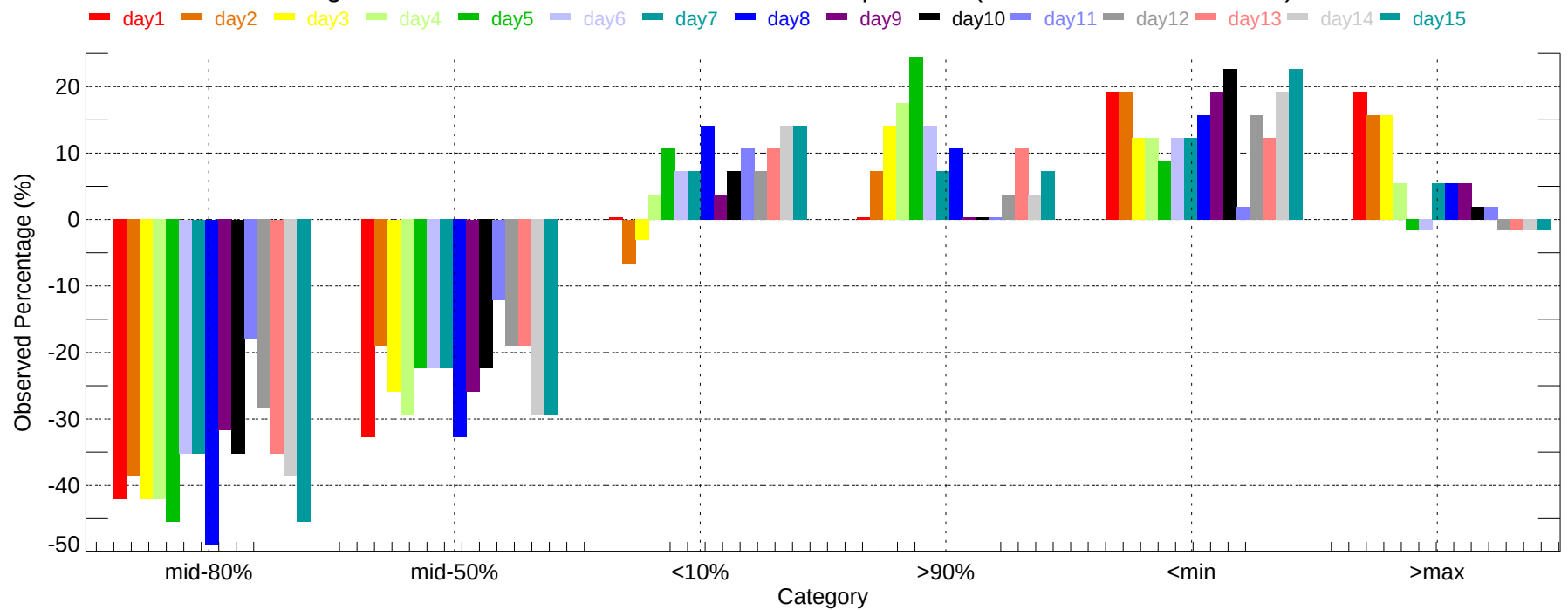
Observed Percentage Deviation of Ensembles - BDL: Min Temperature (2007-11-01~2007-11-30)
