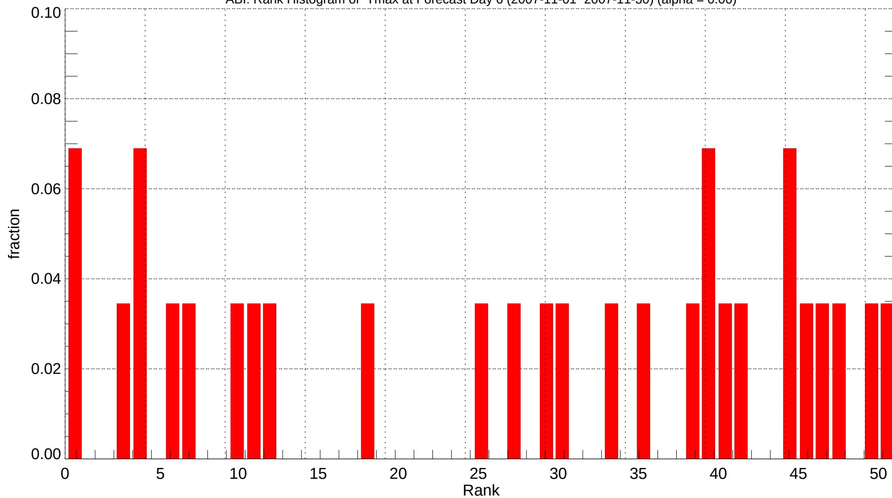
ABI: Rank Histogram of Tmax at Forecast Day 6 (2007-11-01~2007-11-30) (alpha = 0.00)
