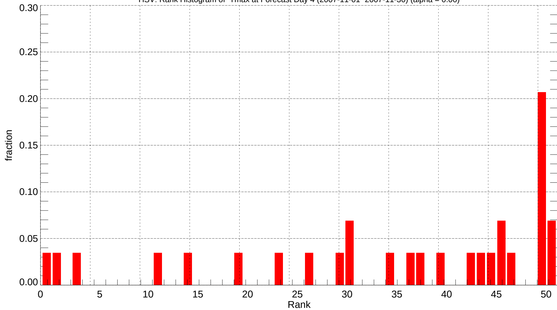
HSV: Rank Histogram of Tmax at Forecast Day 4 (2007-11-01~2007-11-30) (alpha = 0.00)
