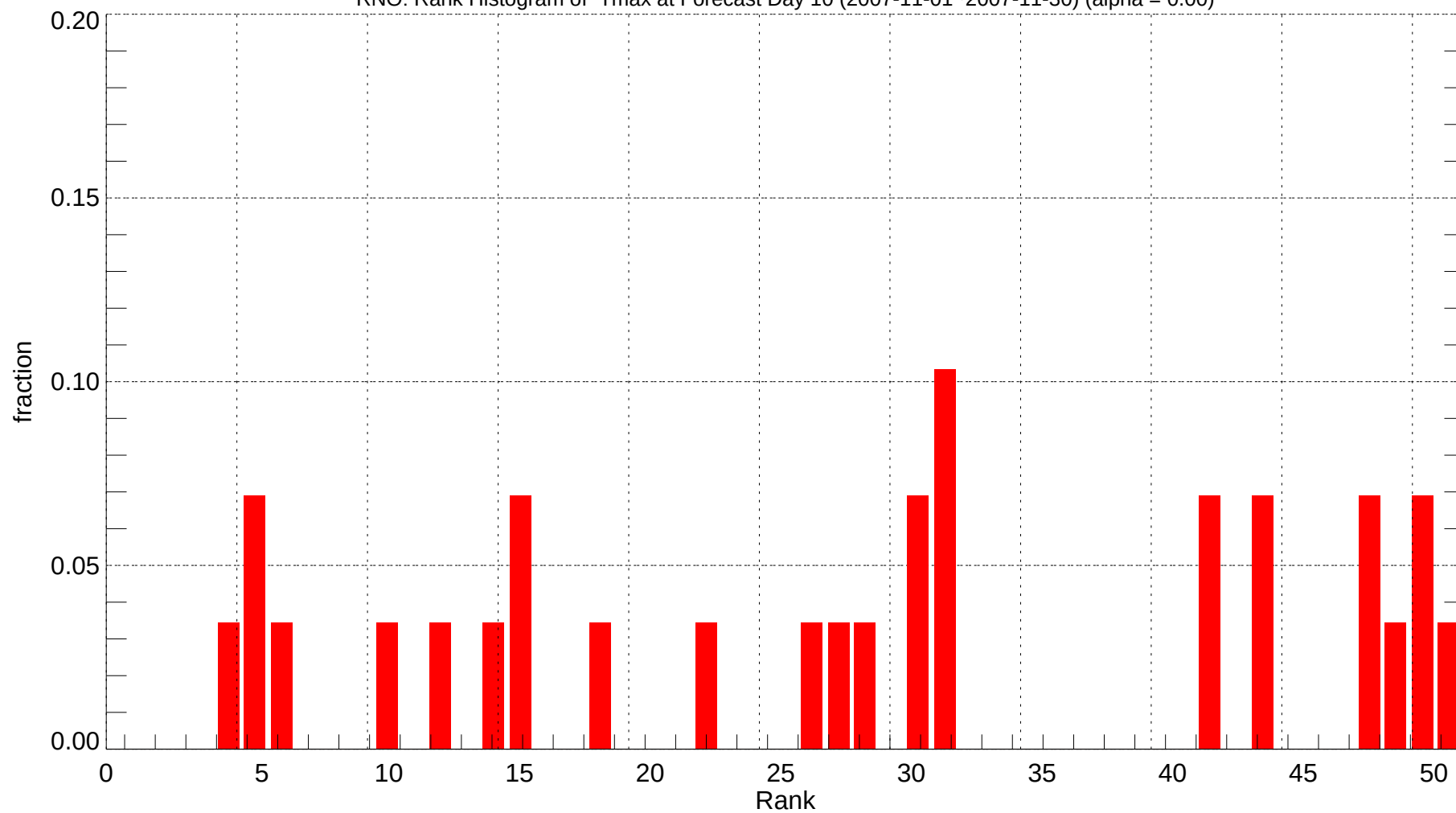
RNO: Rank Histogram of Tmax at Forecast Day 10 (2007-11-01~2007-11-30) (alpha = 0.00)
