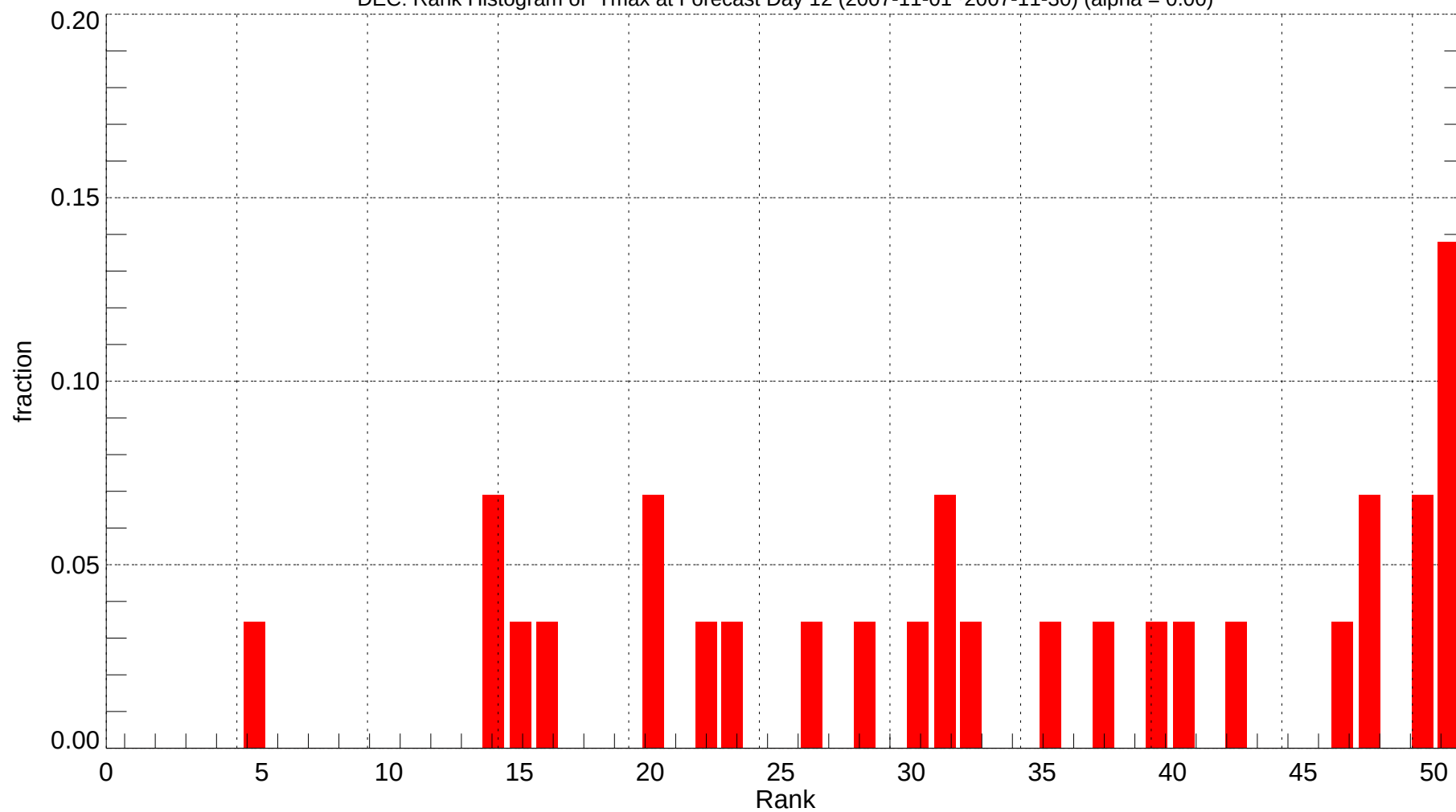
DEC: Rank Histogram of Tmax at Forecast Day 12 (2007-11-01~2007-11-30) (alpha = 0.00)
