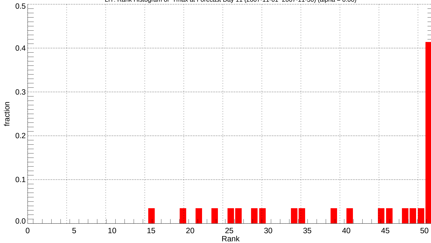
LIT: Rank Histogram of Tmax at Forecast Day 11 (2007-11-01~2007-11-30) (alpha = 0.00)
