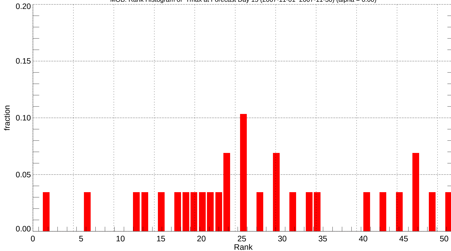
MOB: Rank Histogram of Tmax at Forecast Day 15 (2007-11-01~2007-11-30) (alpha = 0.00)
