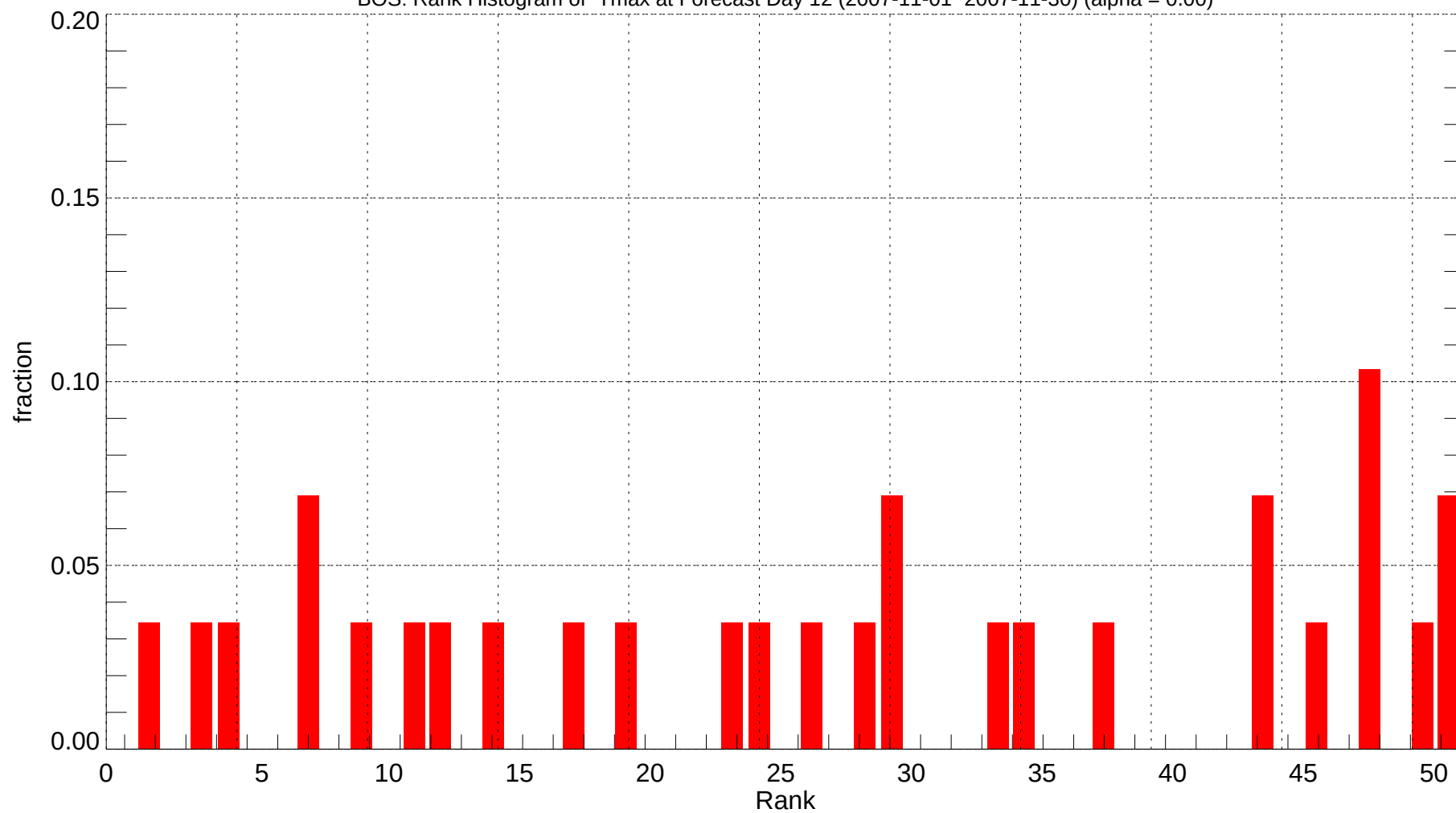
BOS: Rank Histogram of Tmax at Forecast Day 12 (2007-11-01~2007-11-30) (alpha = 0.00)
