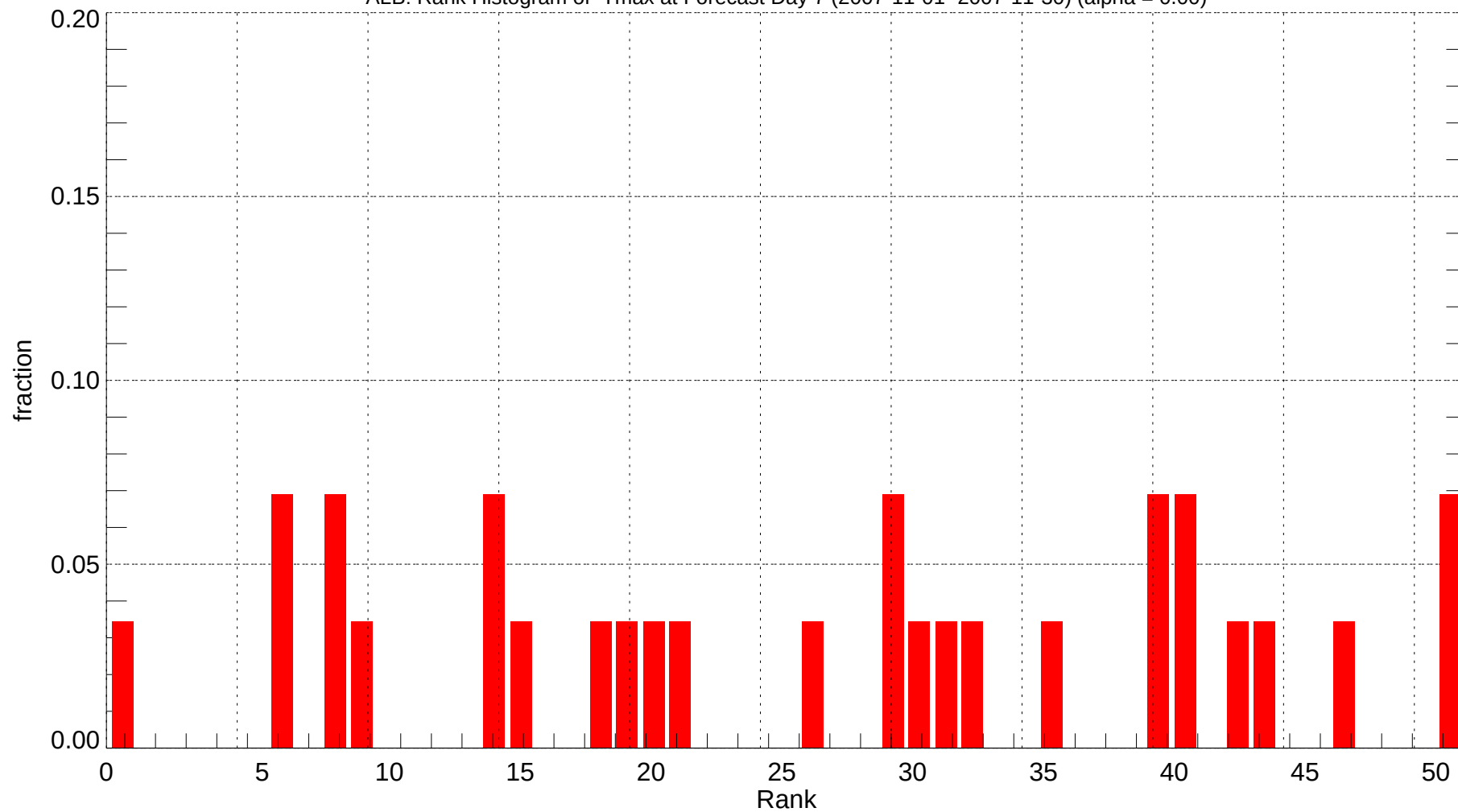
ALB: Rank Histogram of Tmax at Forecast Day 7 (2007-11-01~2007-11-30) (alpha = 0.00)
