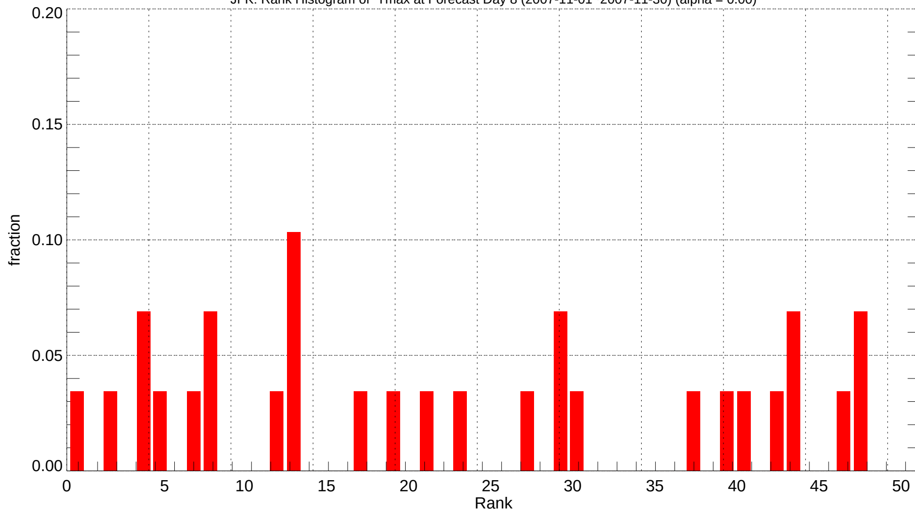
JFK: Rank Histogram of Tmax at Forecast Day 8 (2007-11-01~2007-11-30) (alpha = 0.00)
