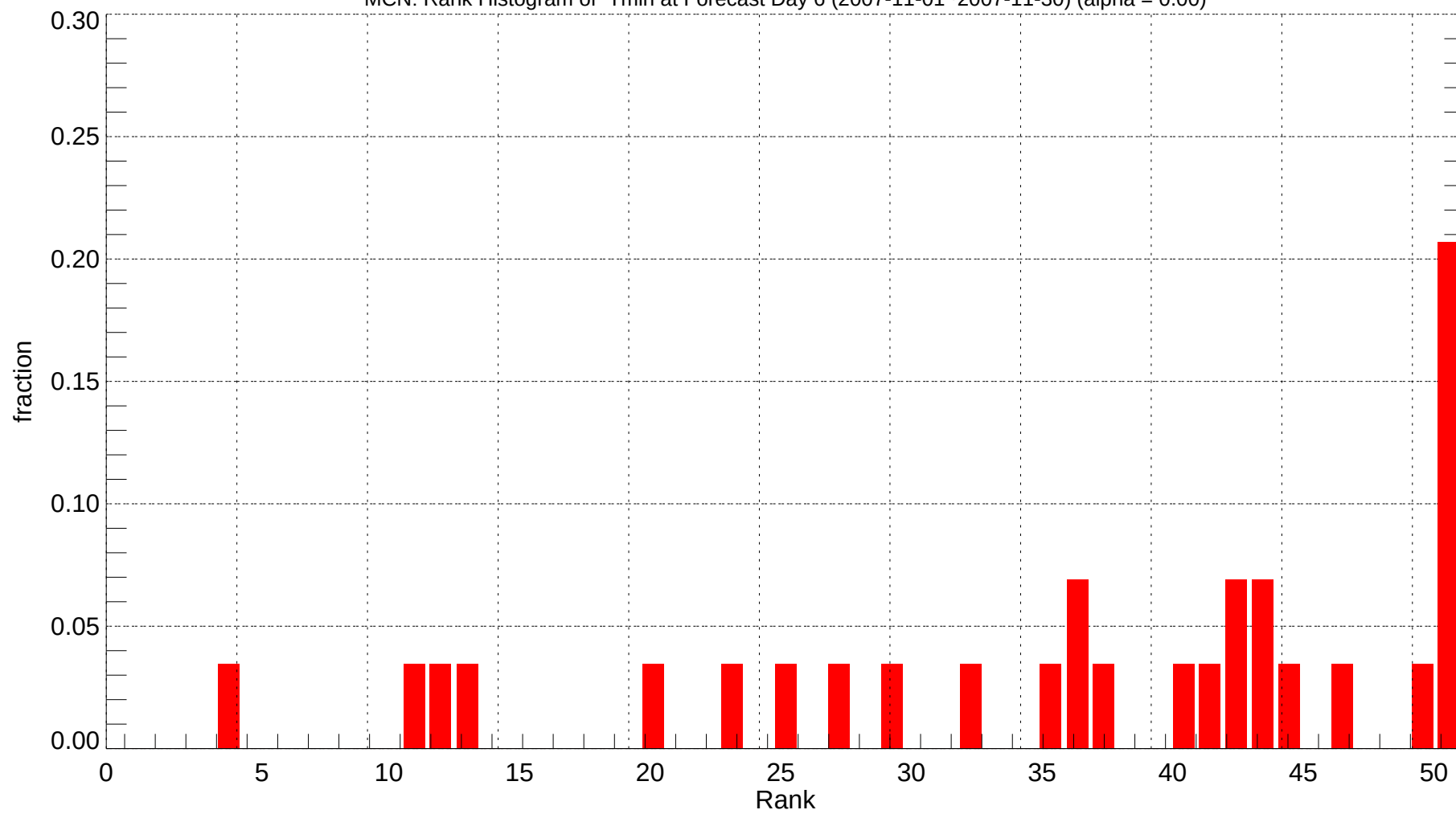
MCN: Rank Histogram of Tmin at Forecast Day 6 (2007-11-01~2007-11-30) (alpha = 0.00)
