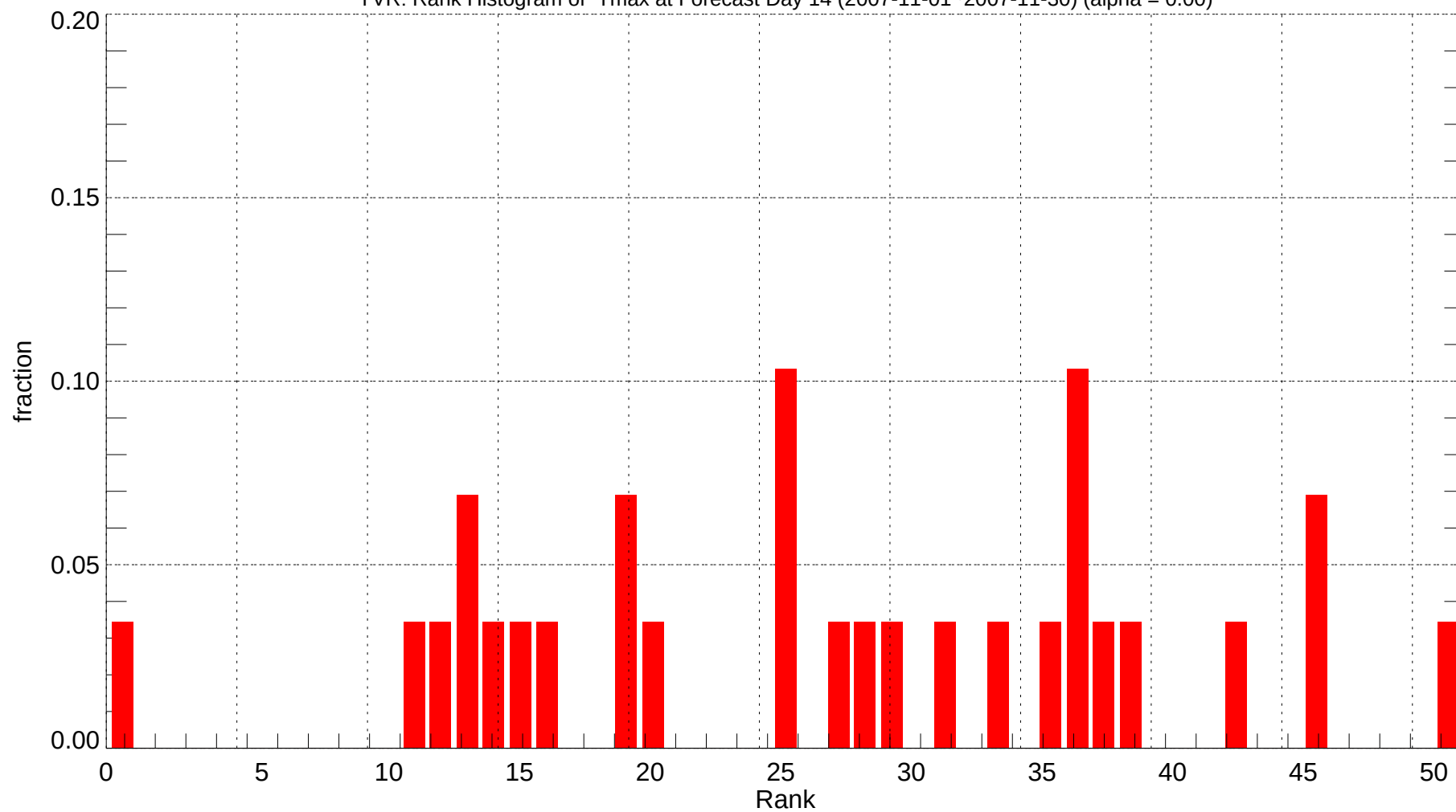
YVR: Rank Histogram of Tmax at Forecast Day 14 (2007-11-01~2007-11-30) (alpha = 0.00)
