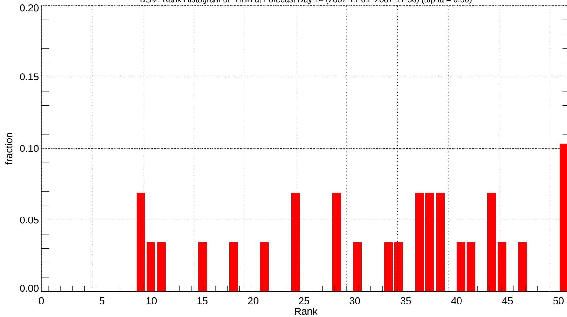
DSM: Rank Histogram of Tmin at Forecast Day 14 (2007-11-01~2007-11-30) (alpha = 0.00)
