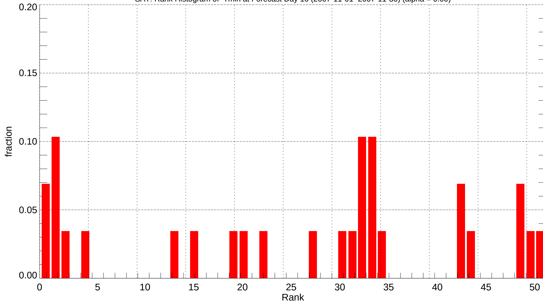
SAT: Rank Histogram of Tmin at Forecast Day 10 (2007-11-01~2007-11-30) (alpha = 0.00)
