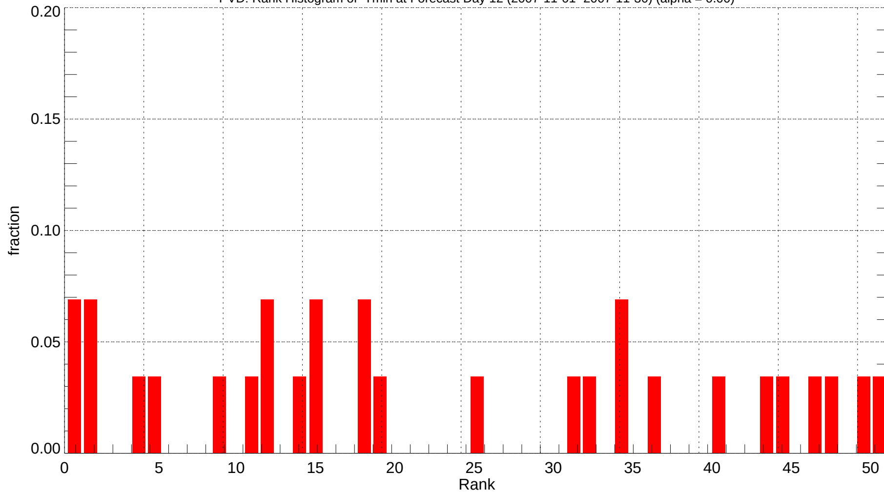
PVD: Rank Histogram of Tmin at Forecast Day 12 (2007-11-01~2007-11-30) (alpha = 0.00)
