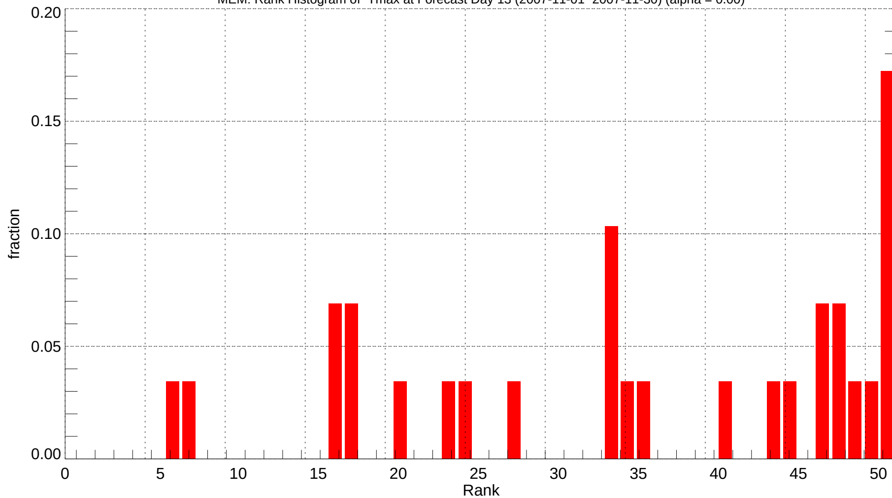
MEM: Rank Histogram of Tmax at Forecast Day 13 (2007-11-01~2007-11-30) (alpha = 0.00)
