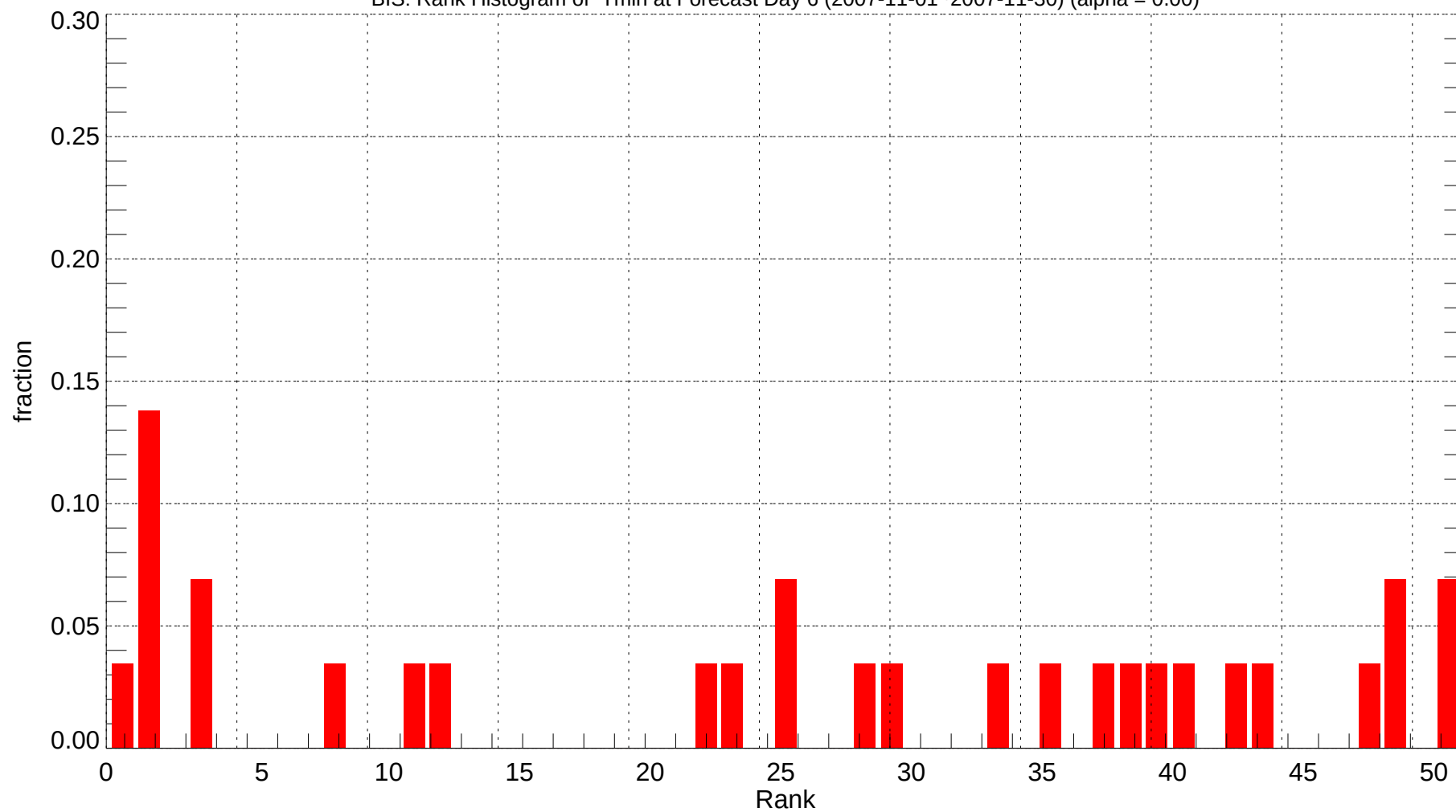
BIS: Rank Histogram of Tmin at Forecast Day 6 (2007-11-01~2007-11-30) (alpha = 0.00)
