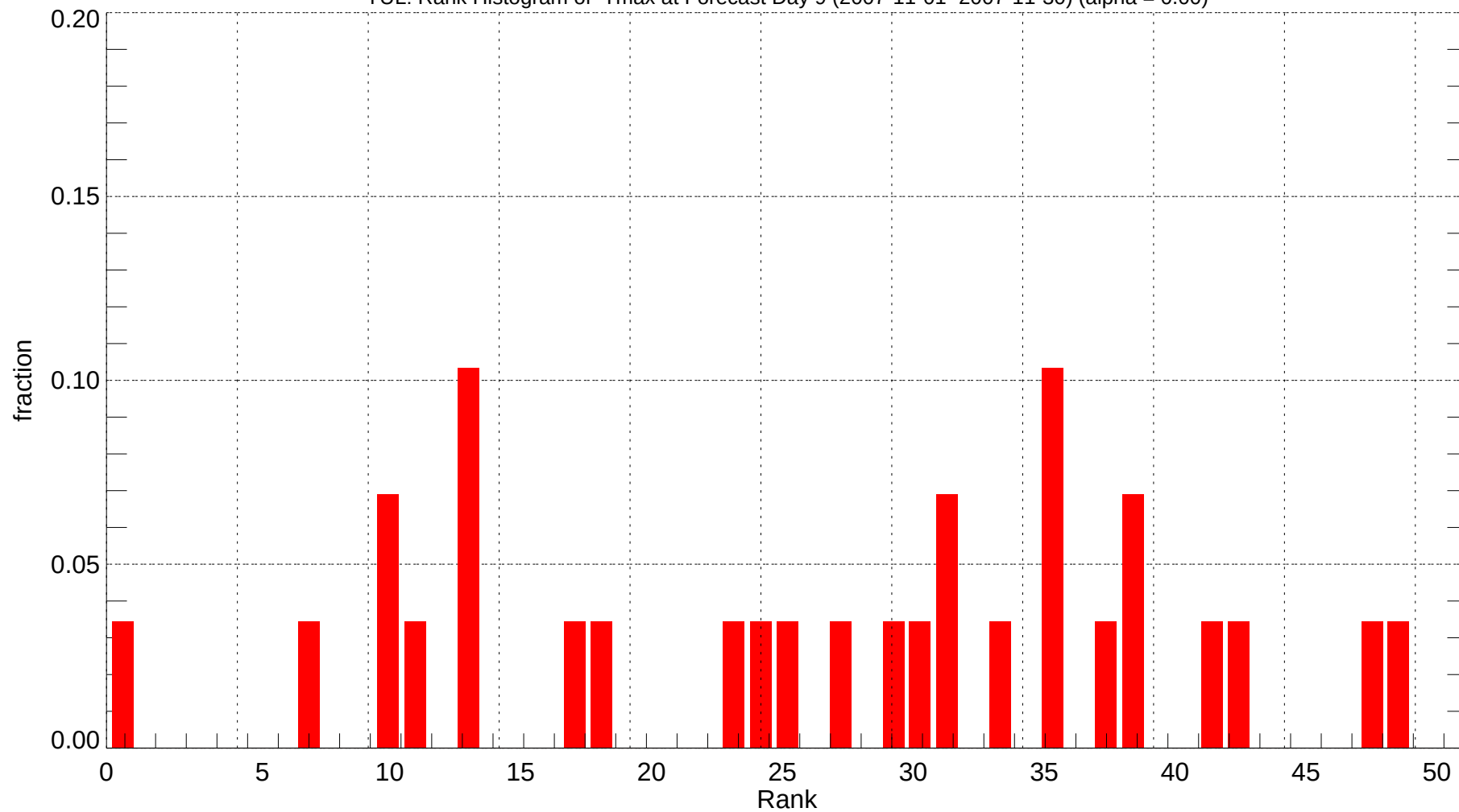
YUL: Rank Histogram of Tmax at Forecast Day 9 (2007-11-01~2007-11-30) (alpha = 0.00)
