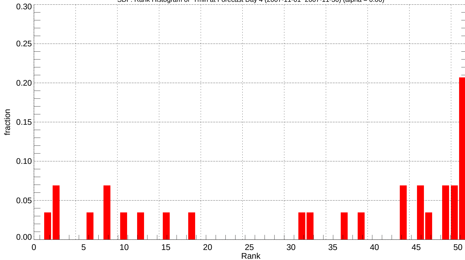
SDF: Rank Histogram of Tmin at Forecast Day 4 (2007-11-01~2007-11-30) (alpha = 0.00)
