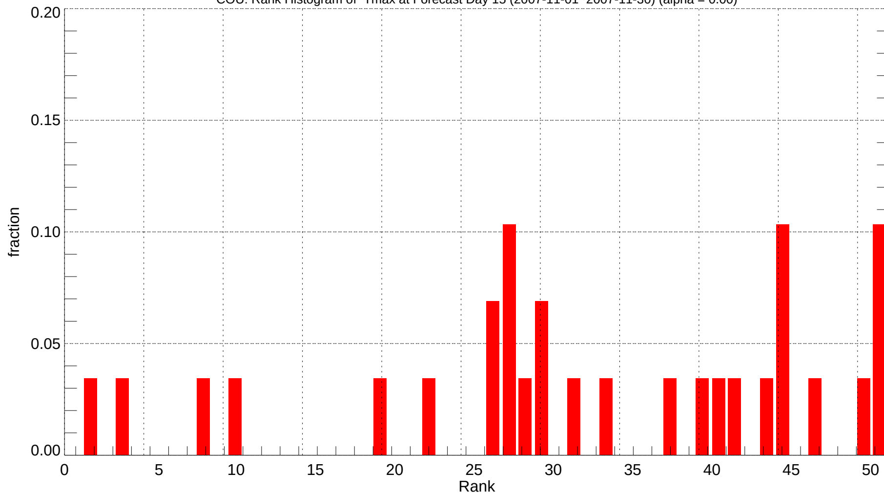
COU: Rank Histogram of Tmax at Forecast Day 15 (2007-11-01~2007-11-30) (alpha = 0.00)
