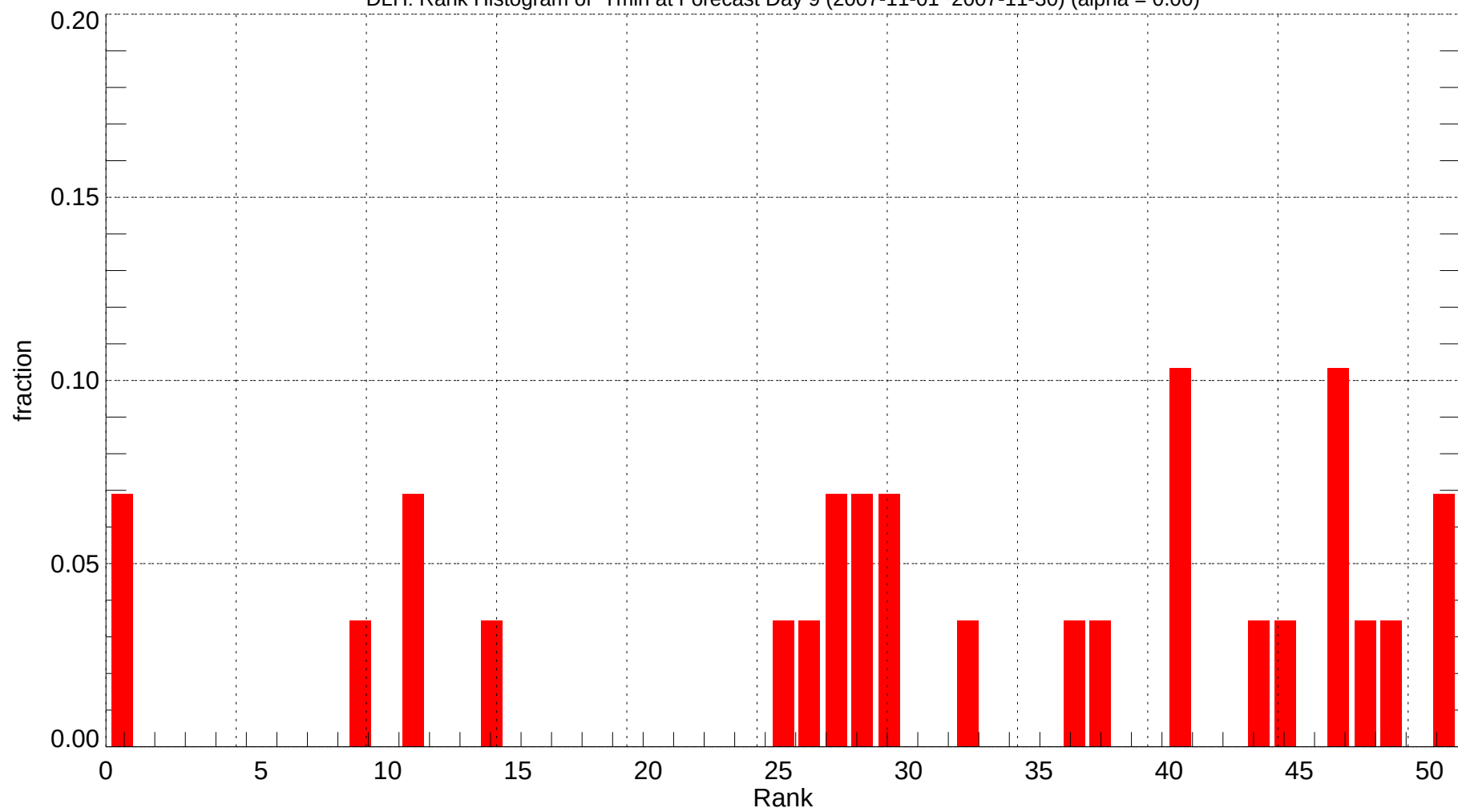
DLH: Rank Histogram of Tmin at Forecast Day 9 (2007-11-01~2007-11-30) (alpha = 0.00)
