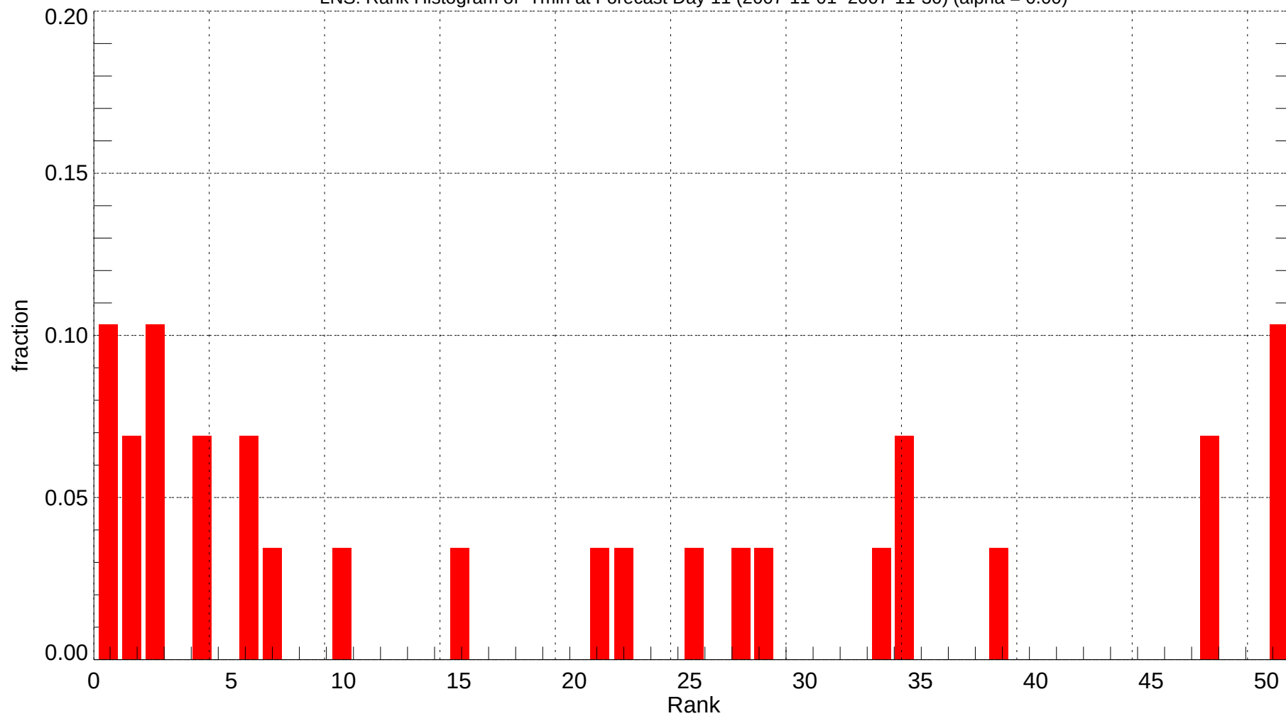
LNS: Rank Histogram of Tmin at Forecast Day 11 (2007-11-01~2007-11-30) (alpha = 0.00)
