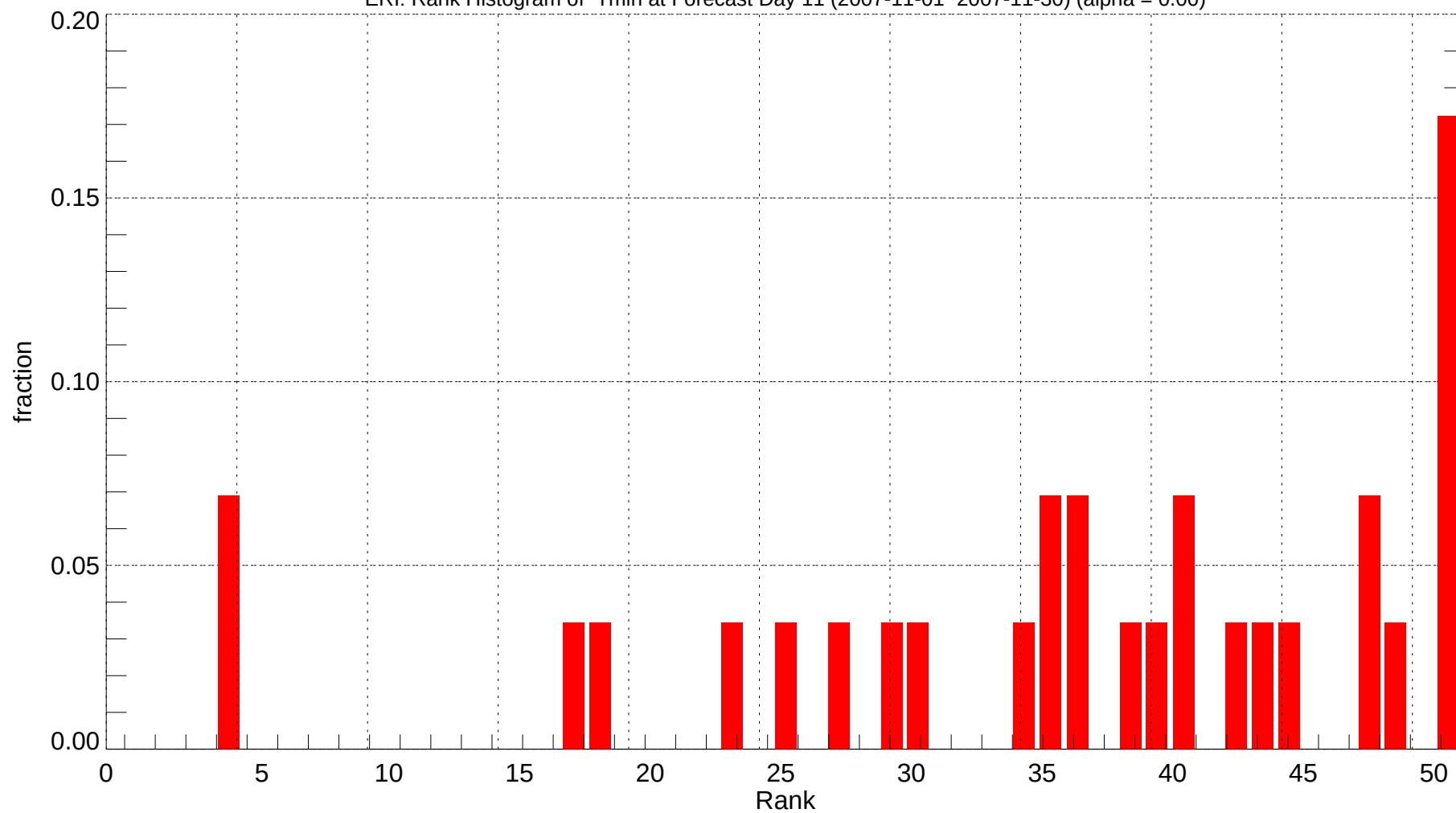
ERI: Rank Histogram of Tmin at Forecast Day 11 (2007-11-01~2007-11-30) (alpha = 0.00)
