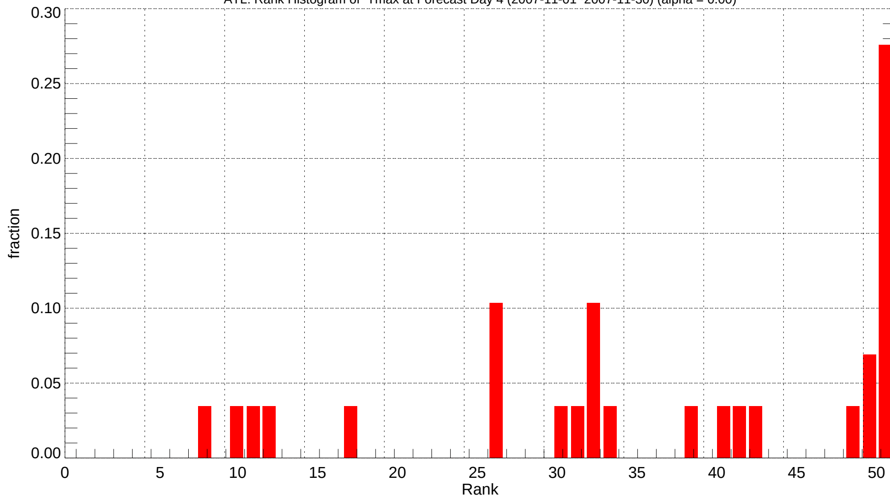
ATL: Rank Histogram of Tmax at Forecast Day 4 (2007-11-01~2007-11-30) (alpha = 0.00)
