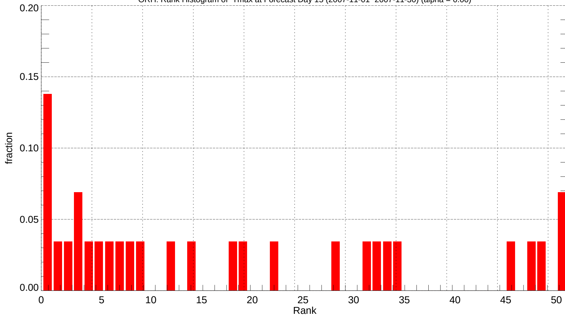
ORH: Rank Histogram of Tmax at Forecast Day 15 (2007-11-01~2007-11-30) (alpha = 0.00)
