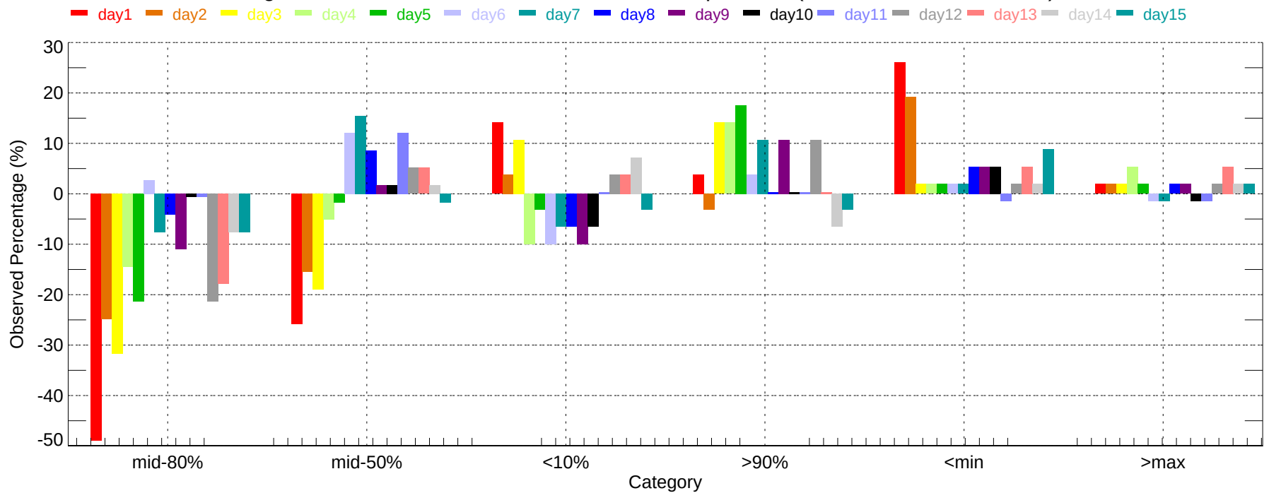
Observed Percentage Deviation of Ensembles - APN: Max Temperature (2007-11-01~2007-11-30)
