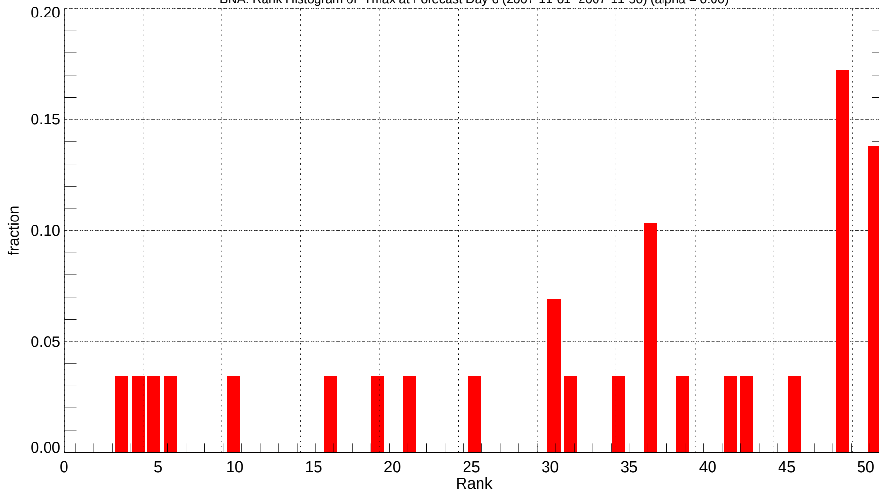
BNA: Rank Histogram of Tmax at Forecast Day 6 (2007-11-01~2007-11-30) (alpha = 0.00)
