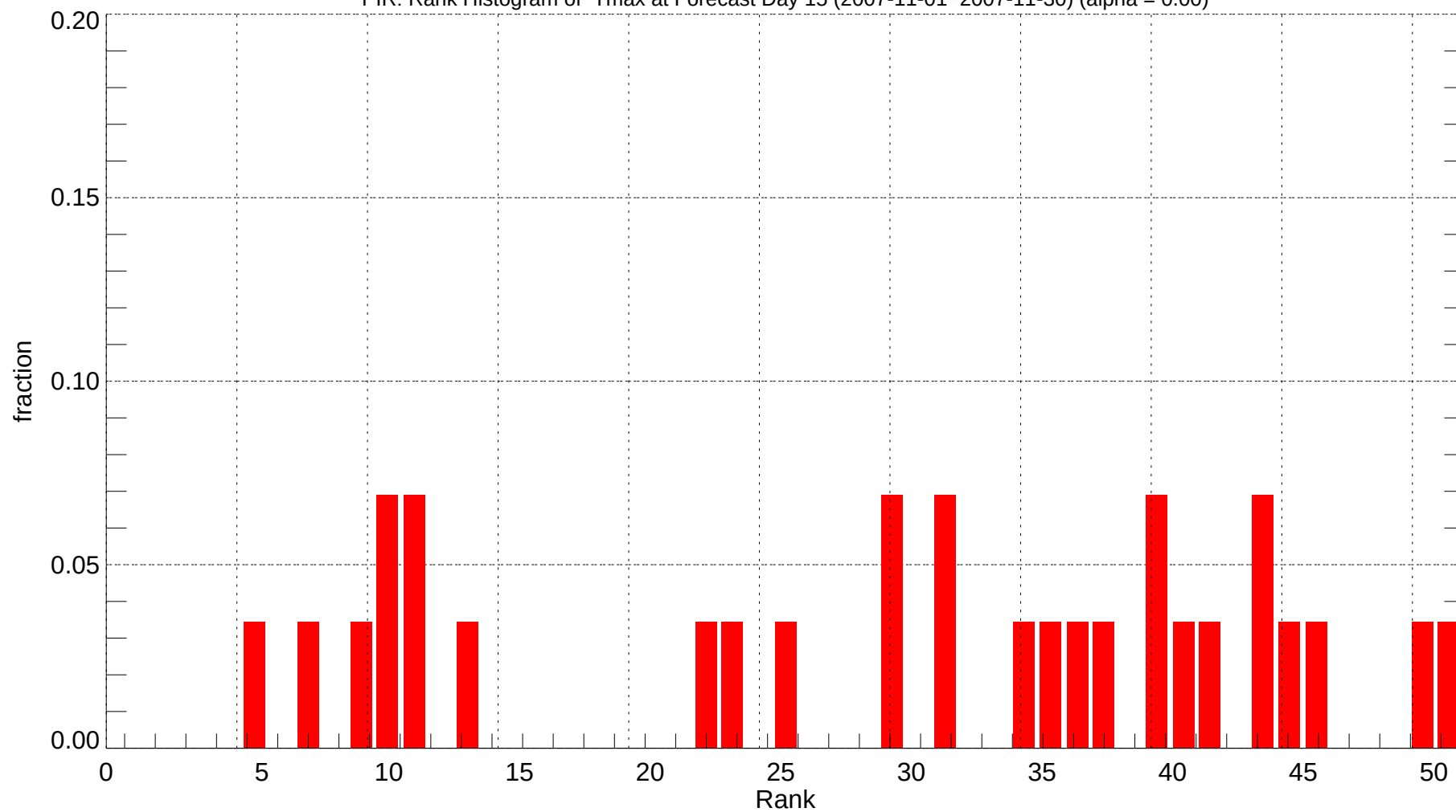
PIR: Rank Histogram of Tmax at Forecast Day 15 (2007-11-01~2007-11-30) (alpha = 0.00)
