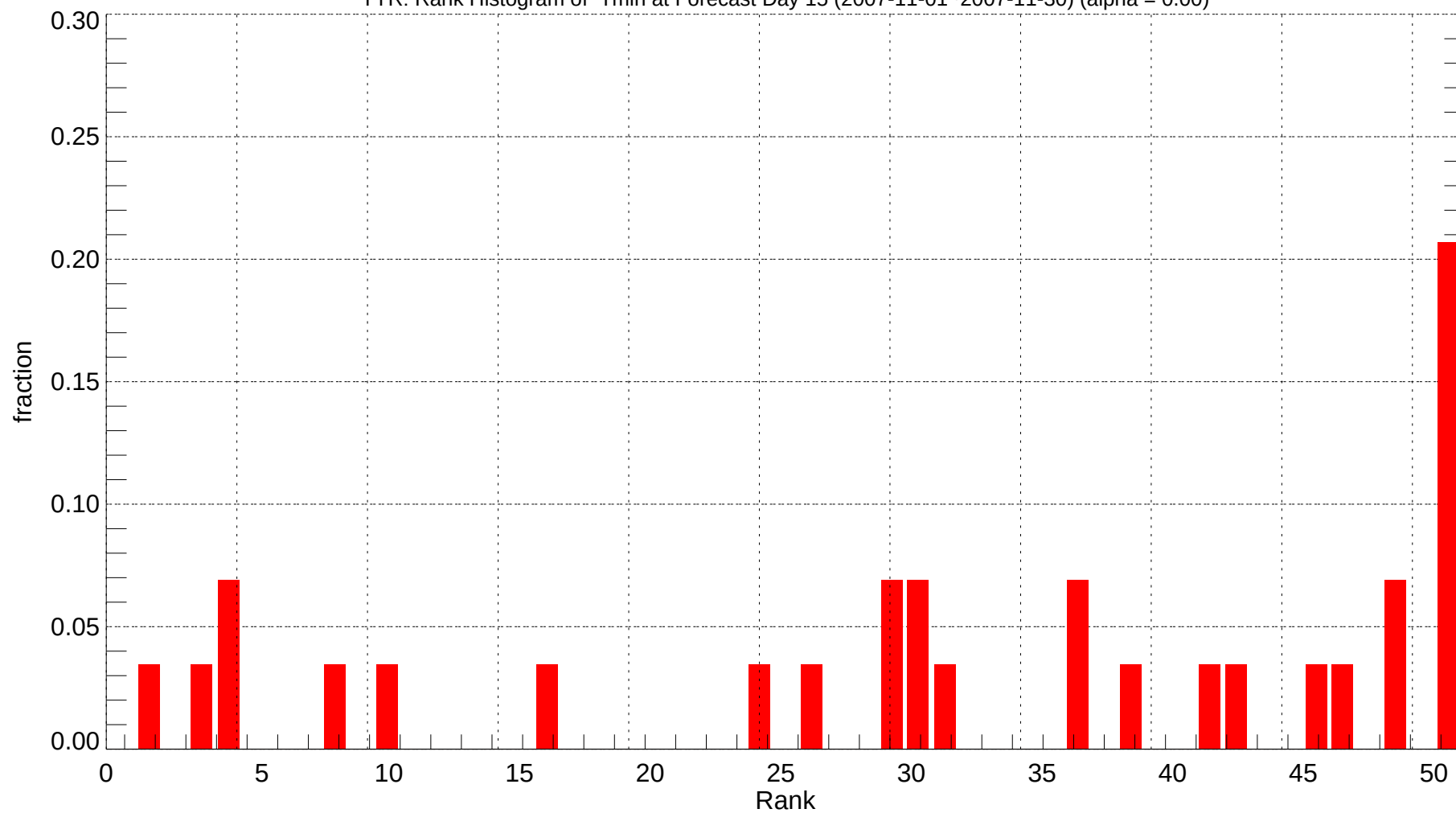
TYR: Rank Histogram of Tmin at Forecast Day 15 (2007-11-01~2007-11-30) (alpha = 0.00)
