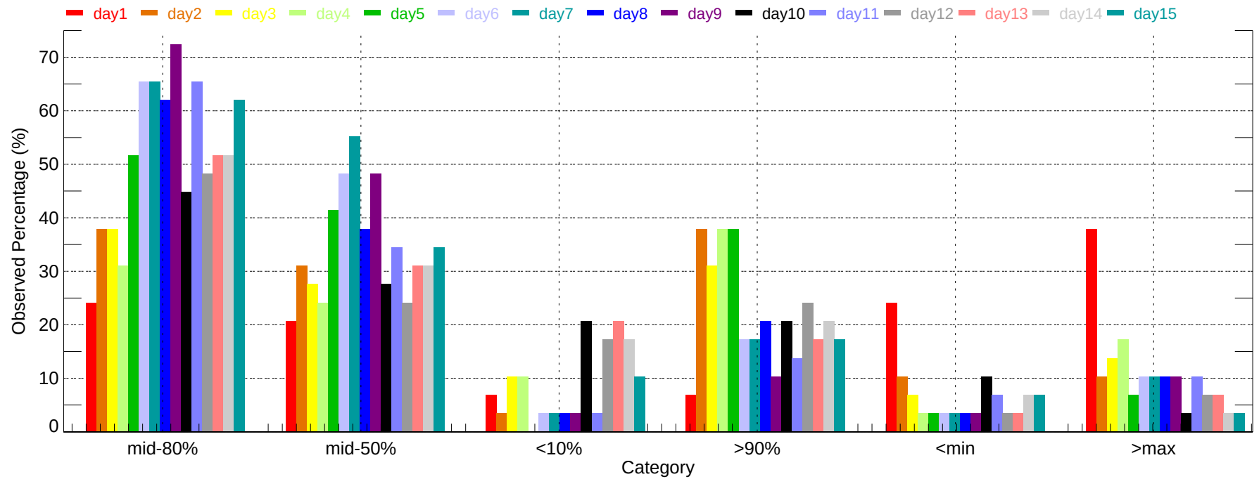
Observed Percentage of Ensembles - ACY: Max Temperature (2007-11-01~2007-11-30)
