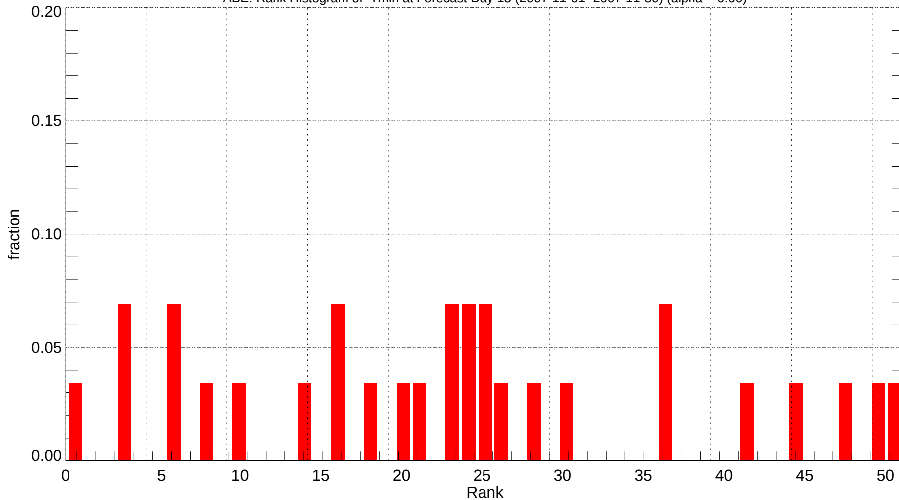
ABE: Rank Histogram of Tmin at Forecast Day 15 (2007-11-01~2007-11-30) (alpha = 0.00)
