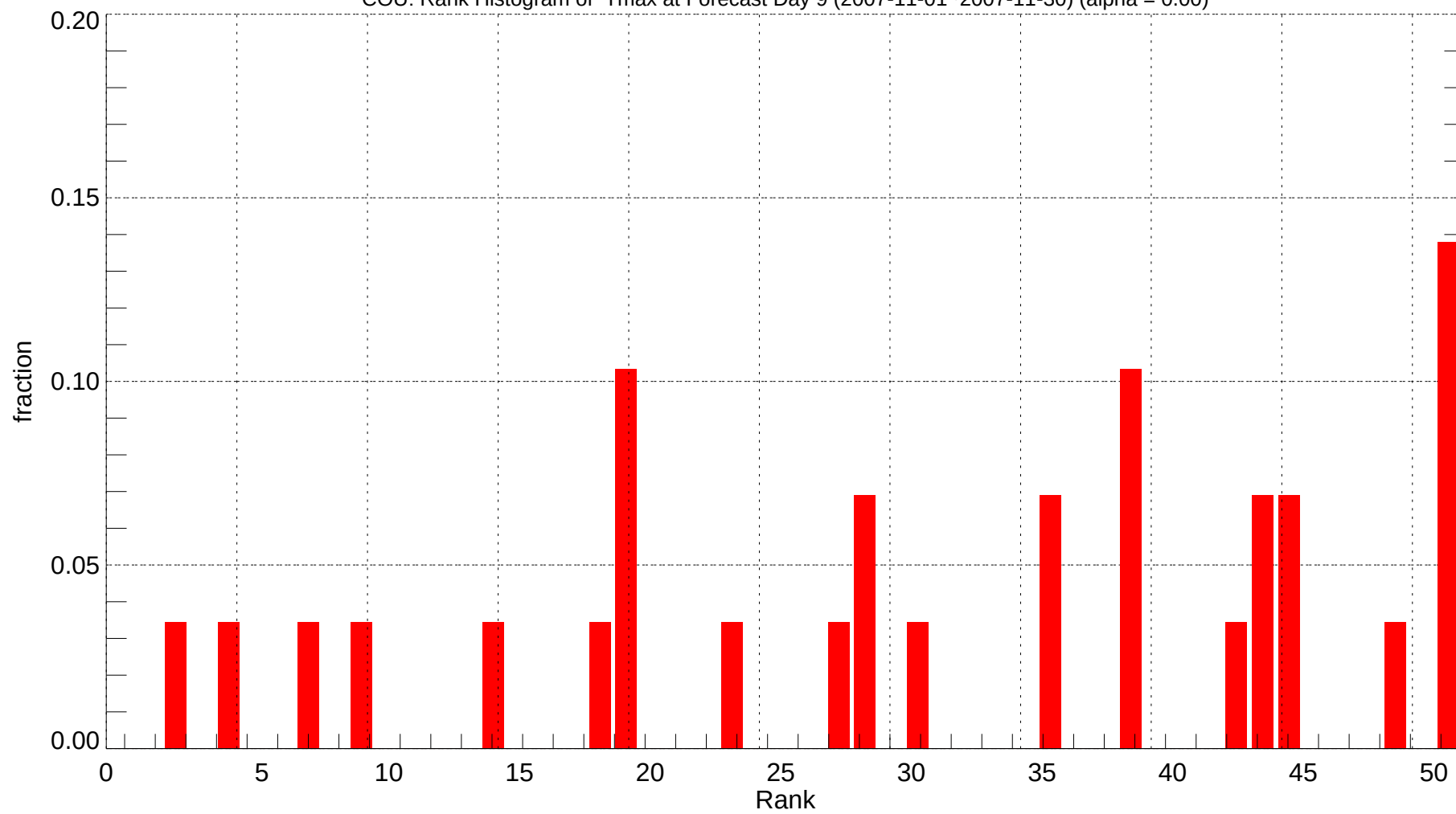
COU: Rank Histogram of Tmax at Forecast Day 9 (2007-11-01~2007-11-30) (alpha = 0.00)
