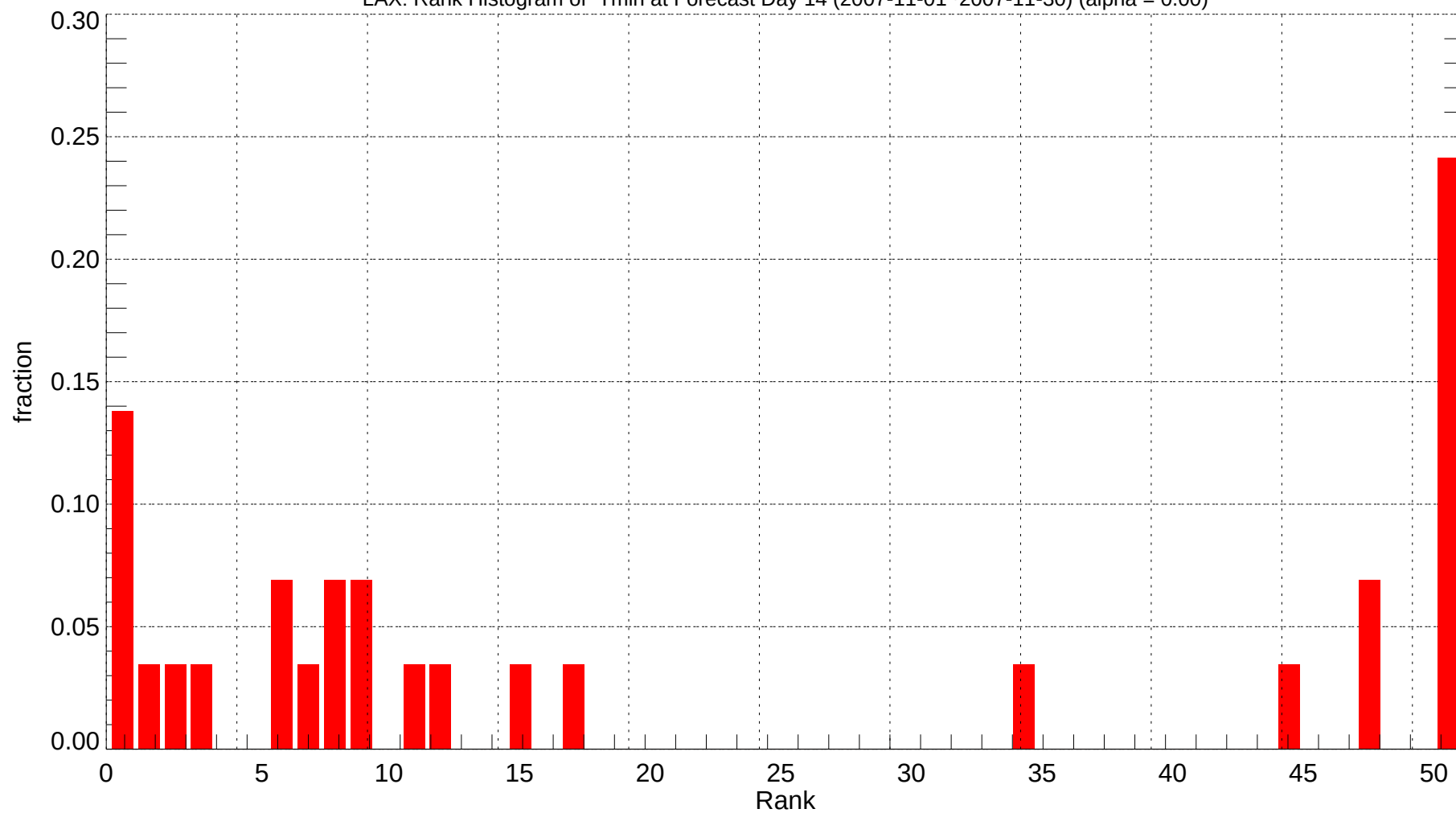
LAX: Rank Histogram of Tmin at Forecast Day 14 (2007-11-01~2007-11-30) (alpha = 0.00)
