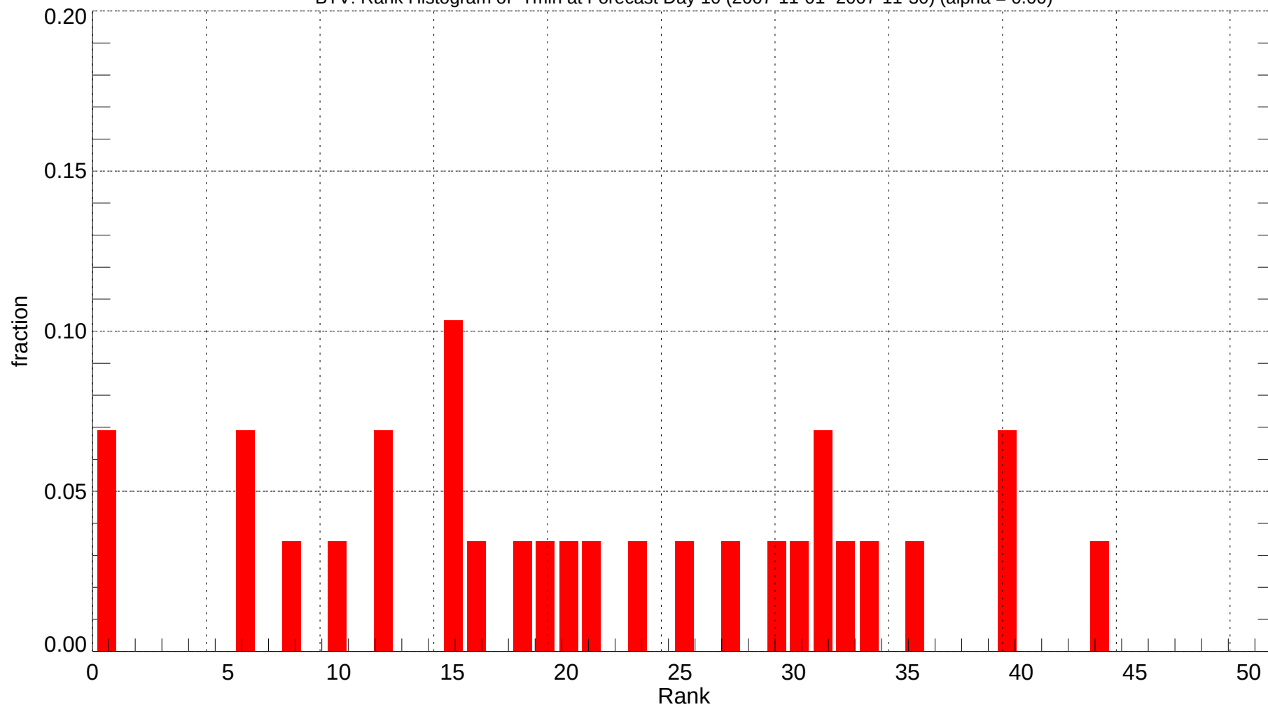
BTV: Rank Histogram of Tmin at Forecast Day 10 (2007-11-01~2007-11-30) (alpha = 0.00)
