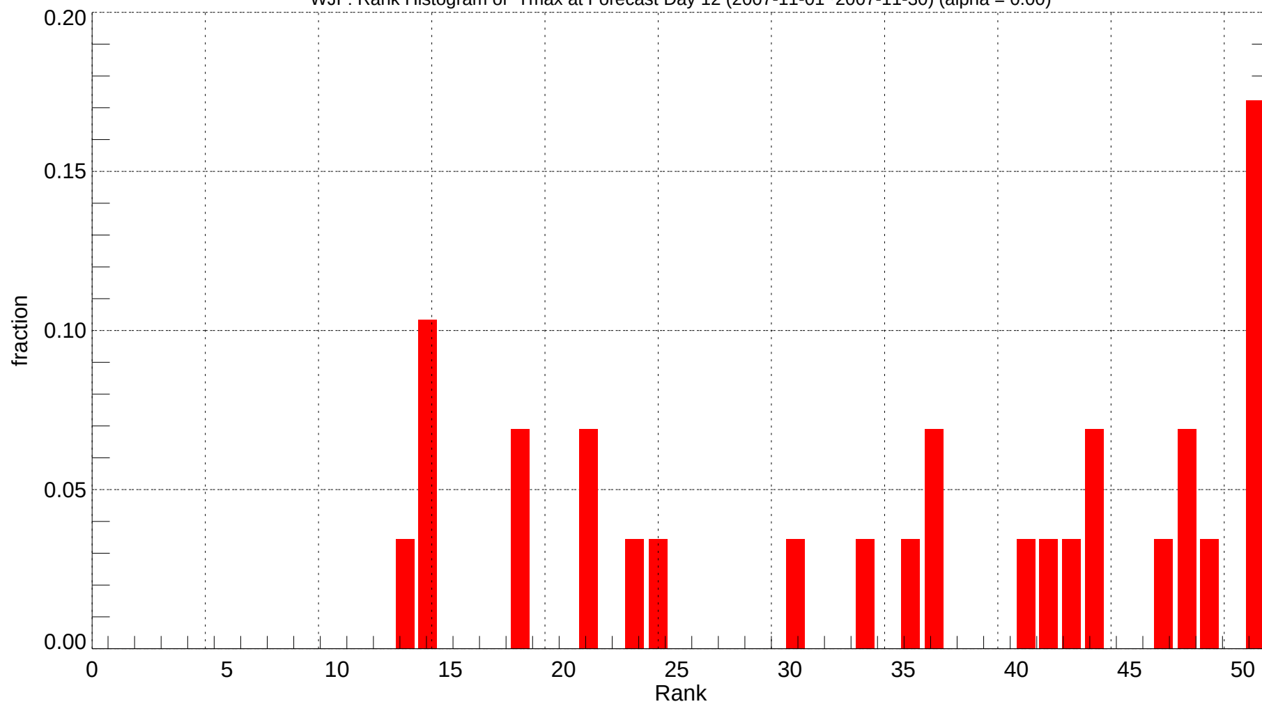
WJF: Rank Histogram of Tmax at Forecast Day 12 (2007-11-01~2007-11-30) (alpha = 0.00)
