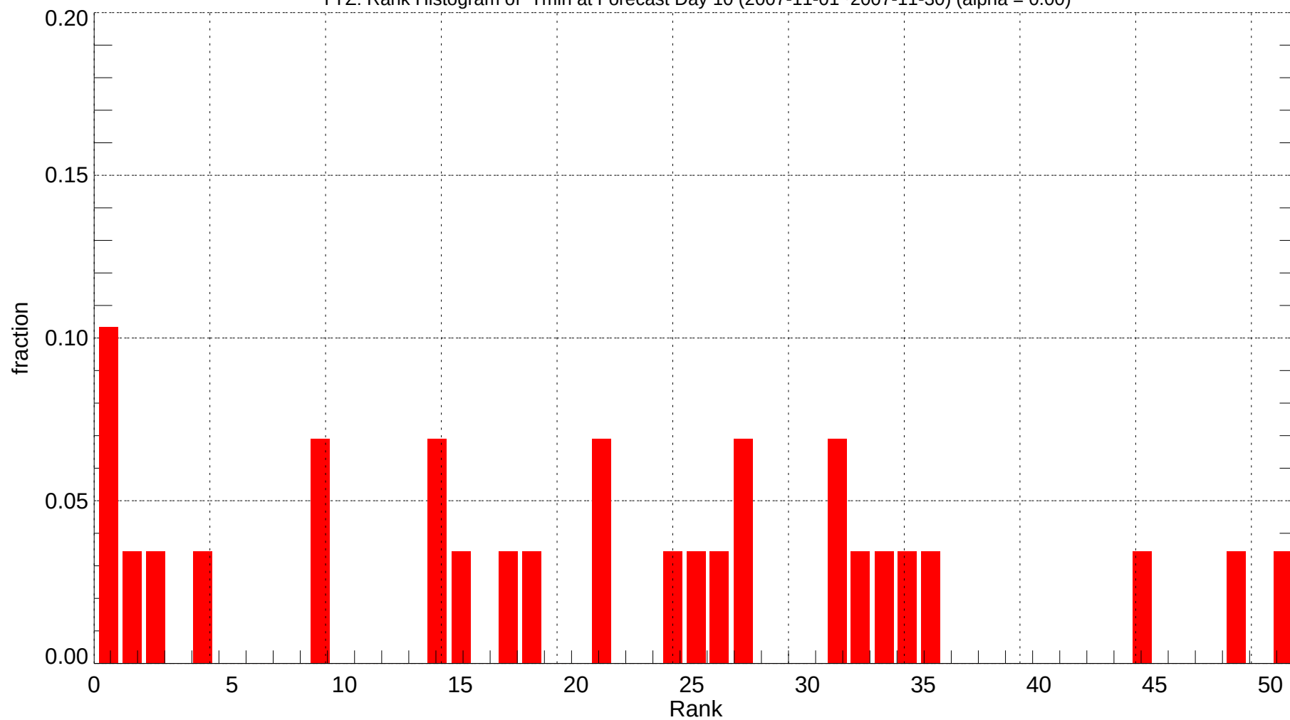
YYZ: Rank Histogram of Tmin at Forecast Day 10 (2007-11-01~2007-11-30) (alpha = 0.00)
