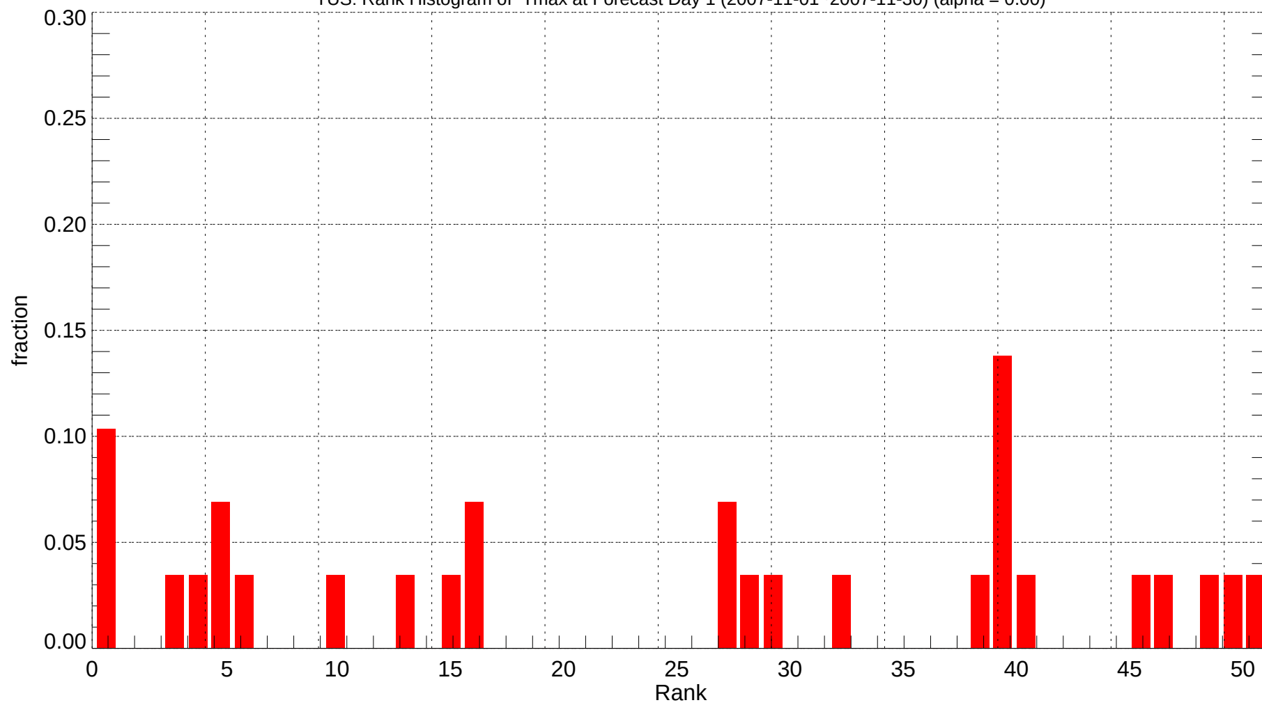
TUS: Rank Histogram of Tmax at Forecast Day 1 (2007-11-01~2007-11-30) (alpha = 0.00)
