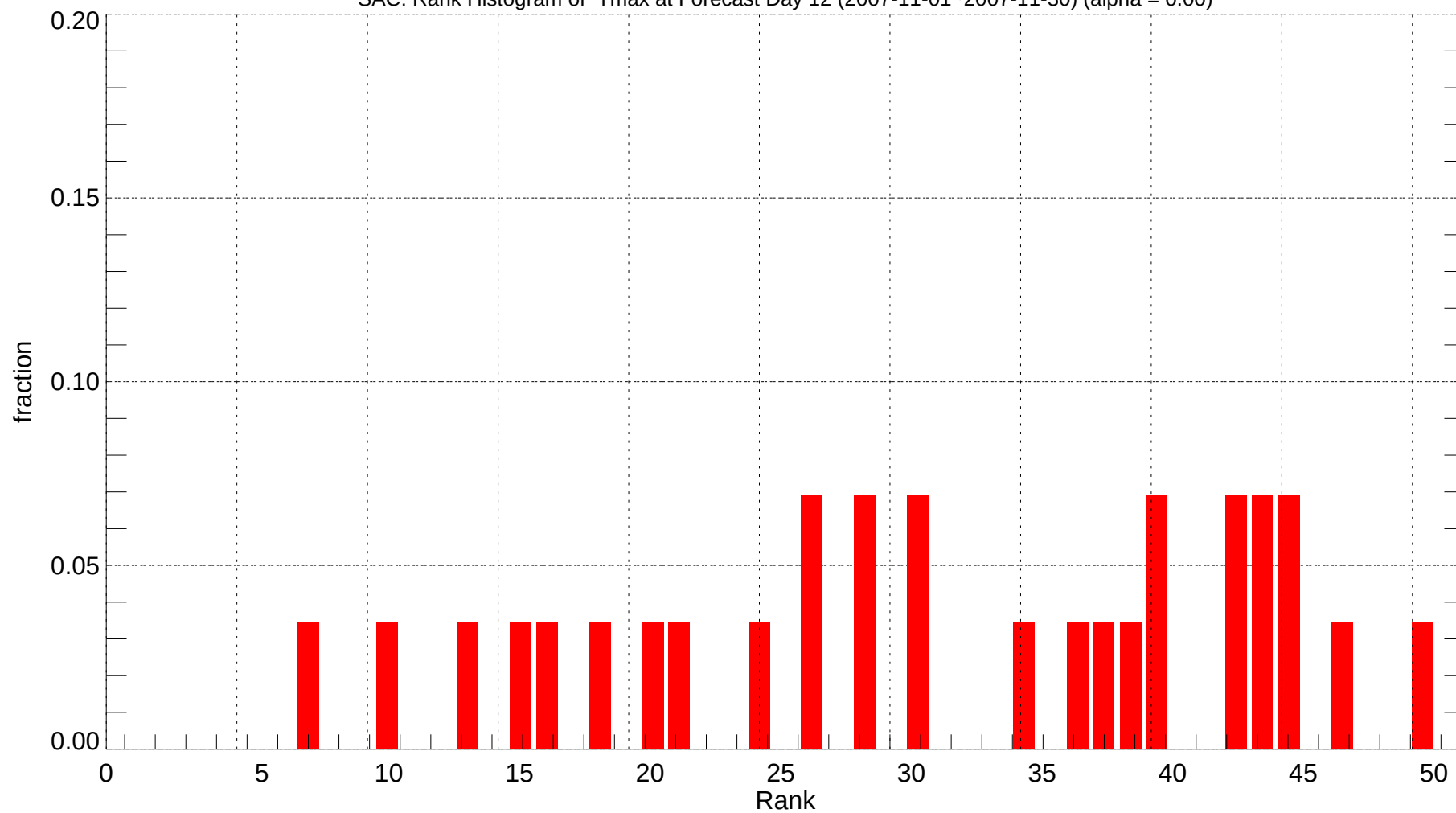
SAC: Rank Histogram of Tmax at Forecast Day 12 (2007-11-01~2007-11-30) (alpha = 0.00)
