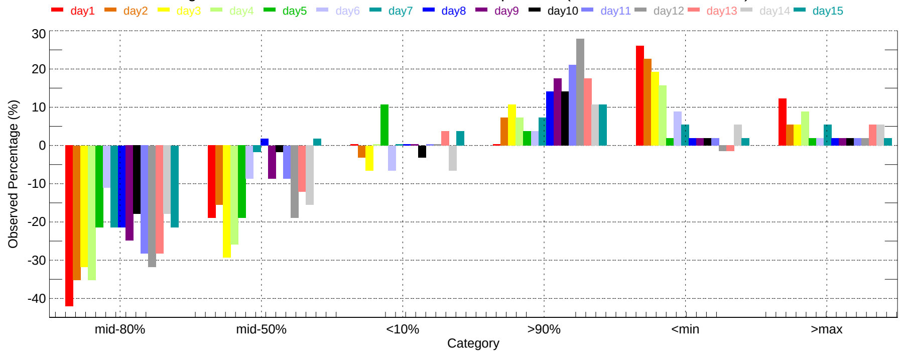
Observed Percentage Deviation of Ensembles - ACT: Max Temperature (2007-11-01~2007-11-30)
