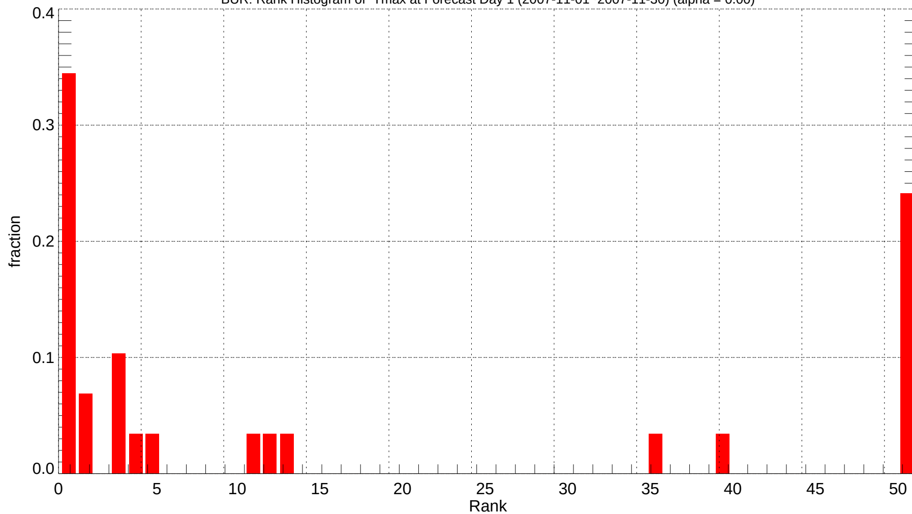
BUR: Rank Histogram of Tmax at Forecast Day 1 (2007-11-01~2007-11-30) (alpha = 0.00)
