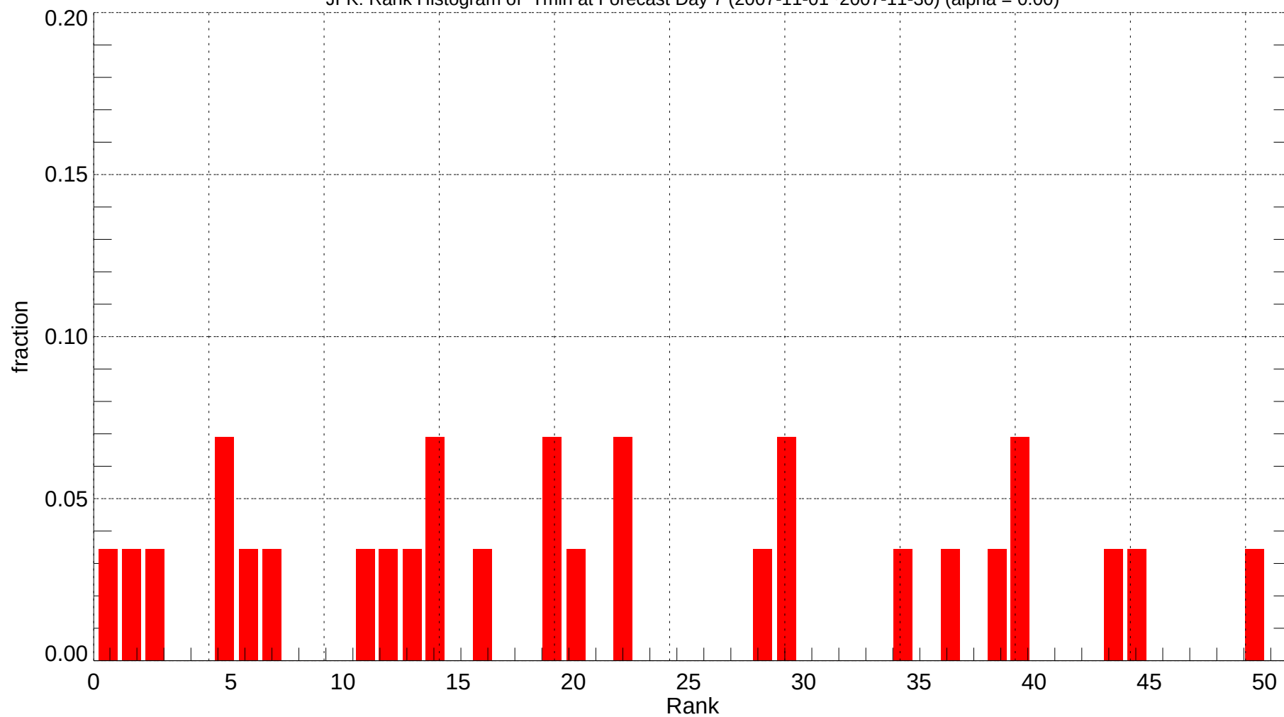
JFK: Rank Histogram of Tmin at Forecast Day 7 (2007-11-01~2007-11-30) (alpha = 0.00)
