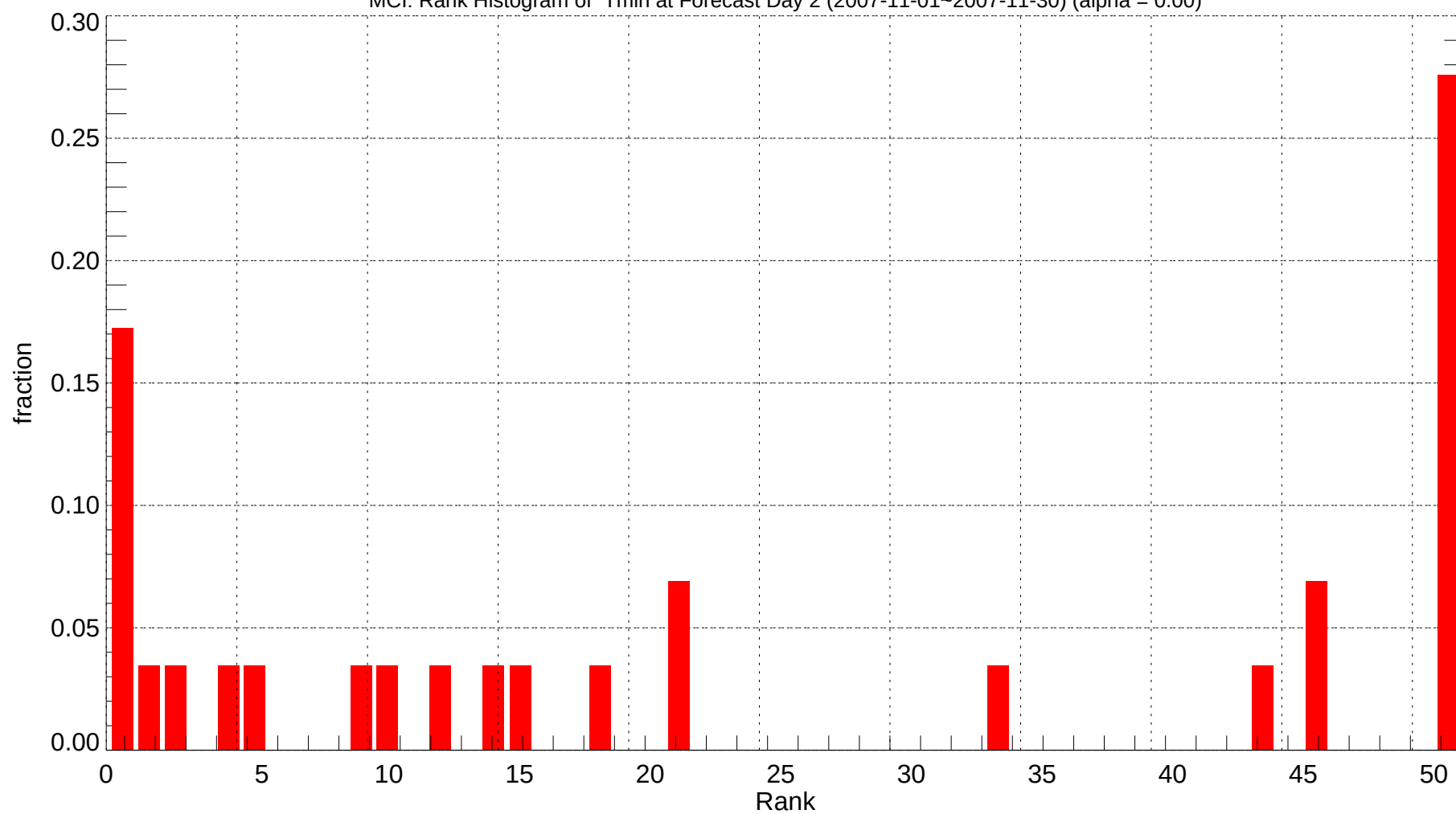
MCI: Rank Histogram of Tmin at Forecast Day 2 (2007-11-01~2007-11-30) (alpha = 0.00)
