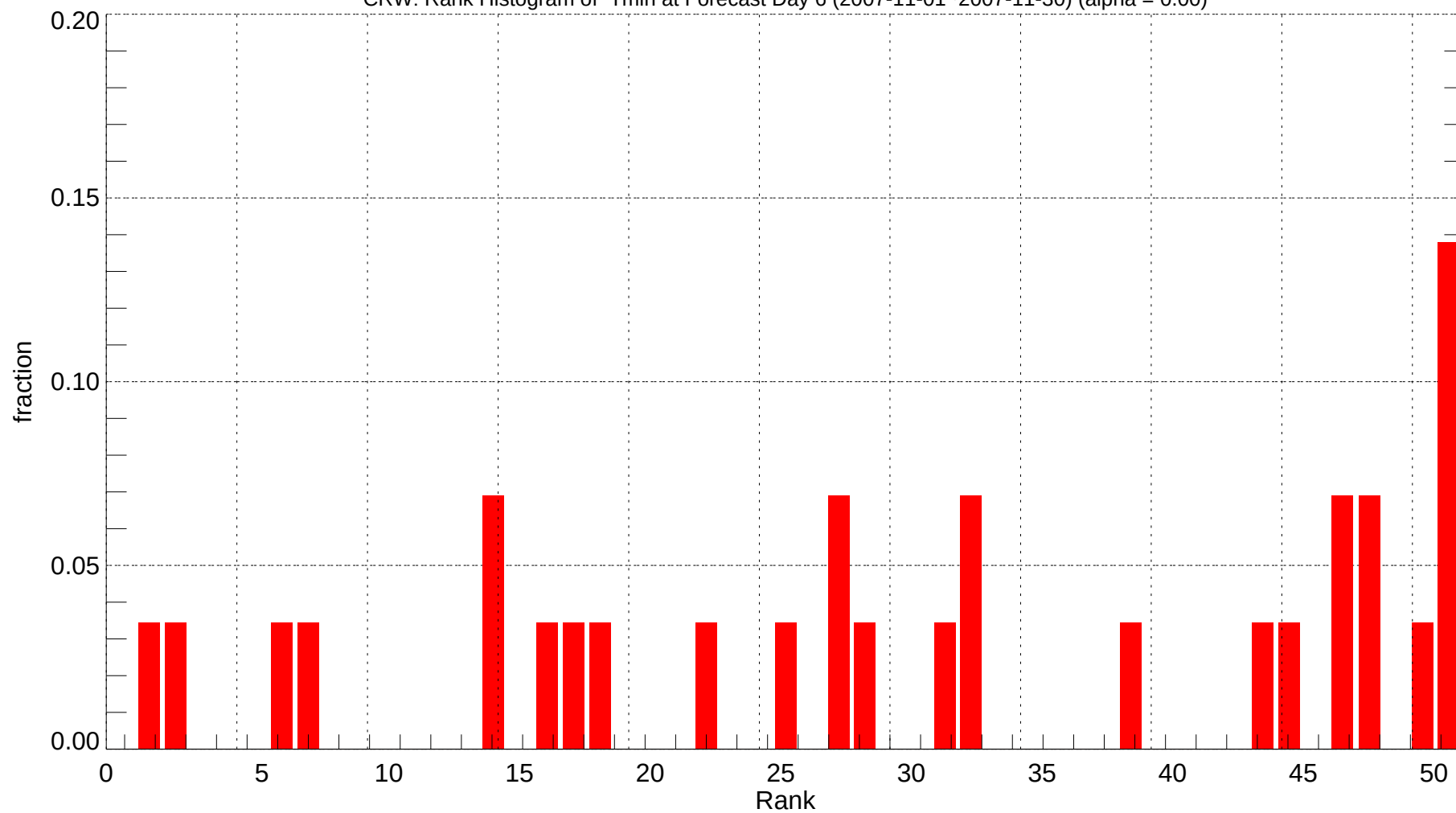
CRW: Rank Histogram of Tmin at Forecast Day 6 (2007-11-01~2007-11-30) (alpha = 0.00)
