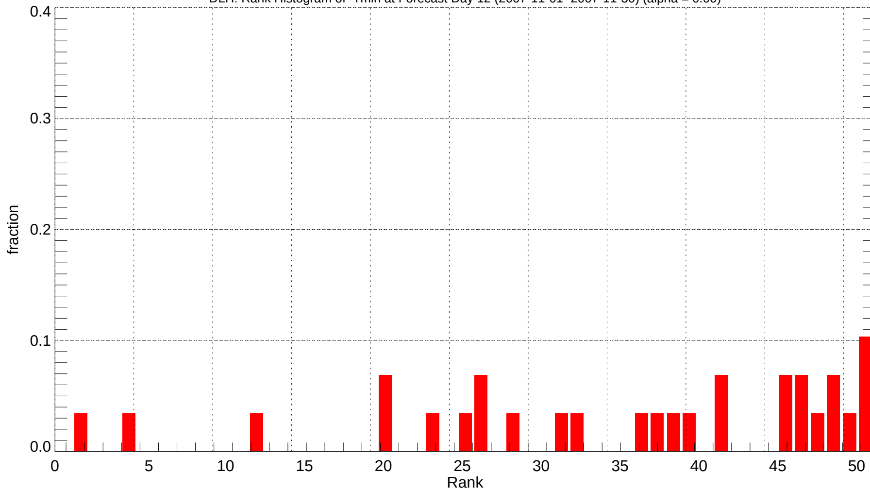
DLH: Rank Histogram of Tmin at Forecast Day 12 (2007-11-01~2007-11-30) (alpha = 0.00)
