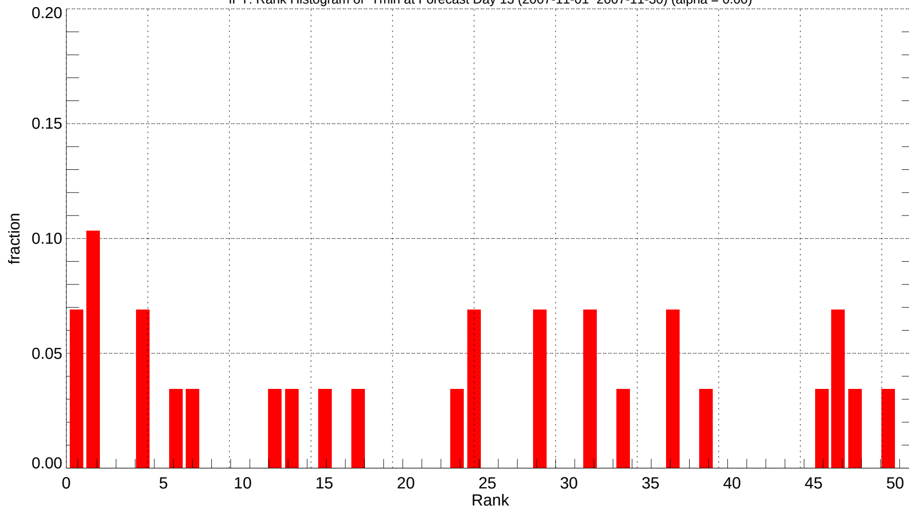
IPT: Rank Histogram of Tmin at Forecast Day 13 (2007-11-01~2007-11-30) (alpha = 0.00)
