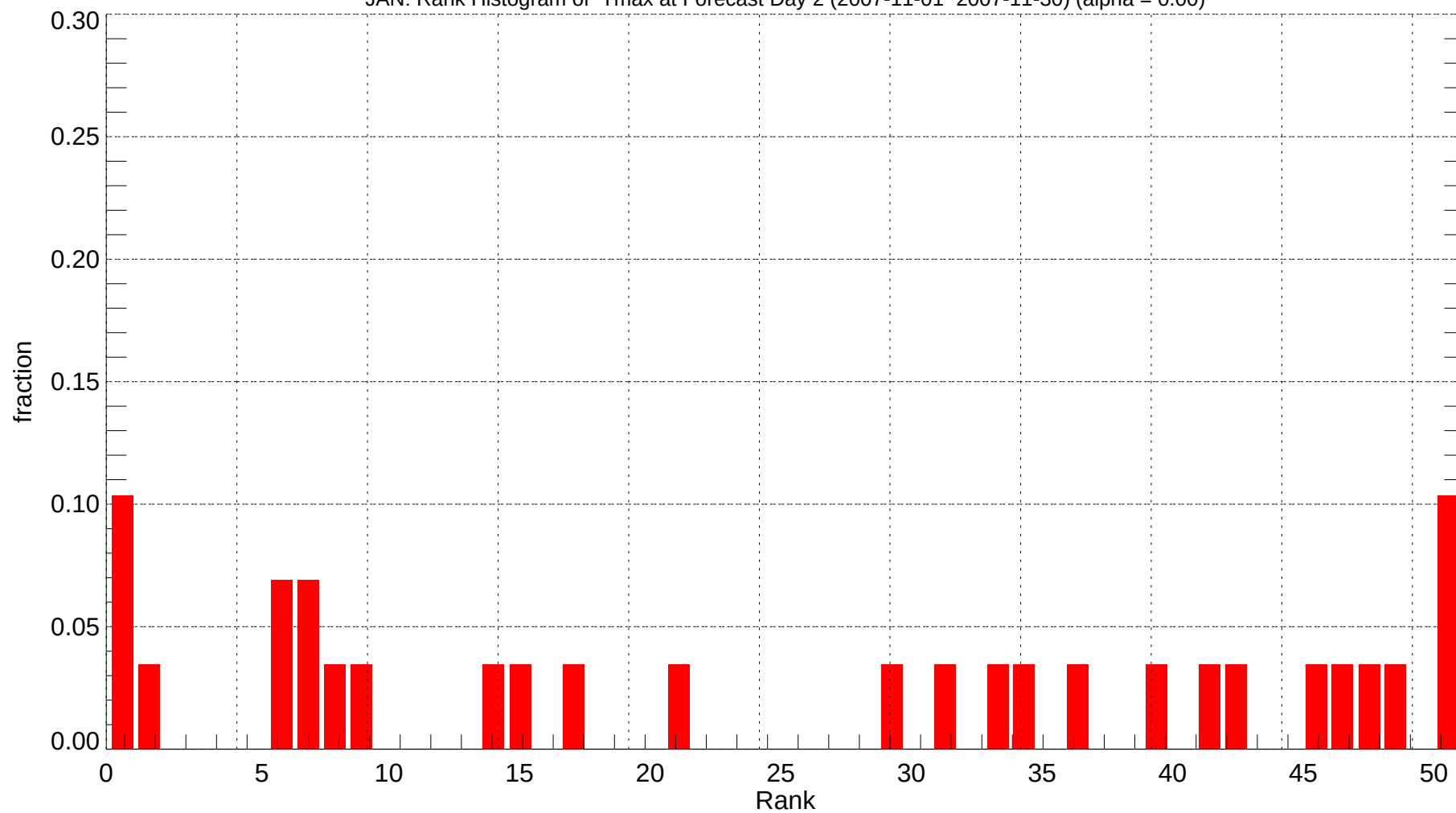
JAN: Rank Histogram of Tmax at Forecast Day 2 (2007-11-01~2007-11-30) (alpha = 0.00)
