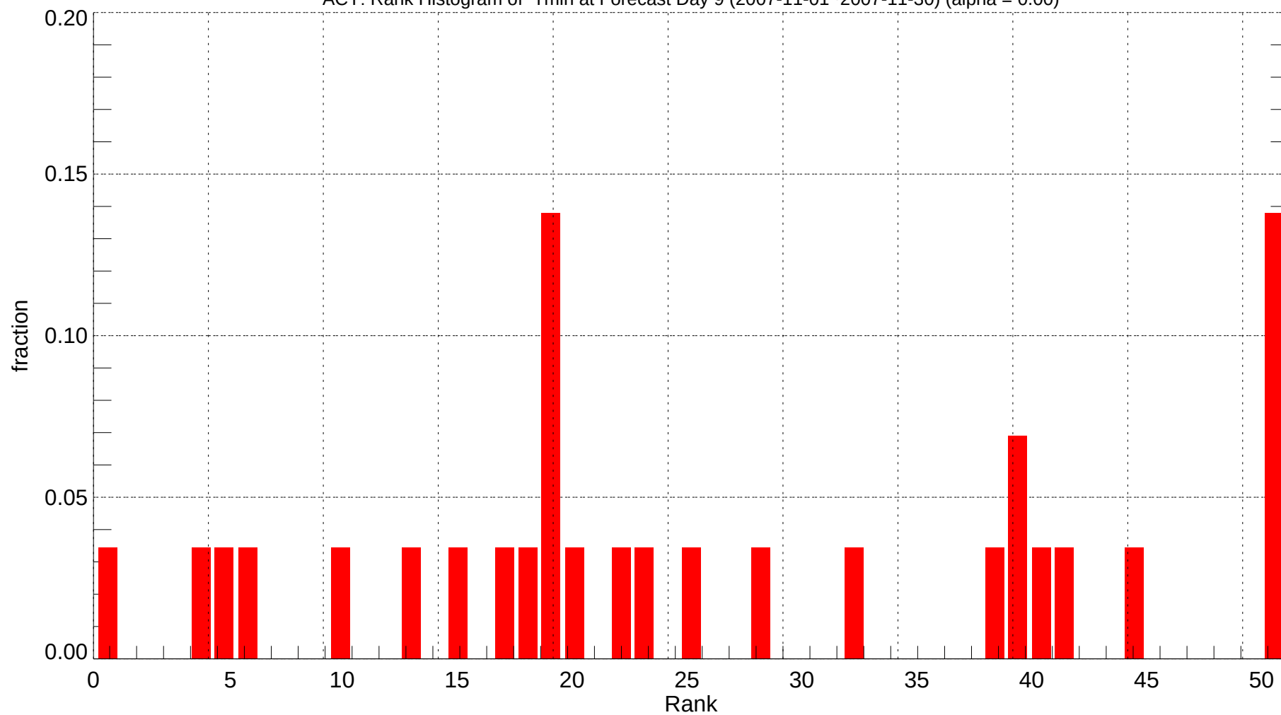
ACY: Rank Histogram of Tmin at Forecast Day 9 (2007-11-01~2007-11-30) (alpha = 0.00)
