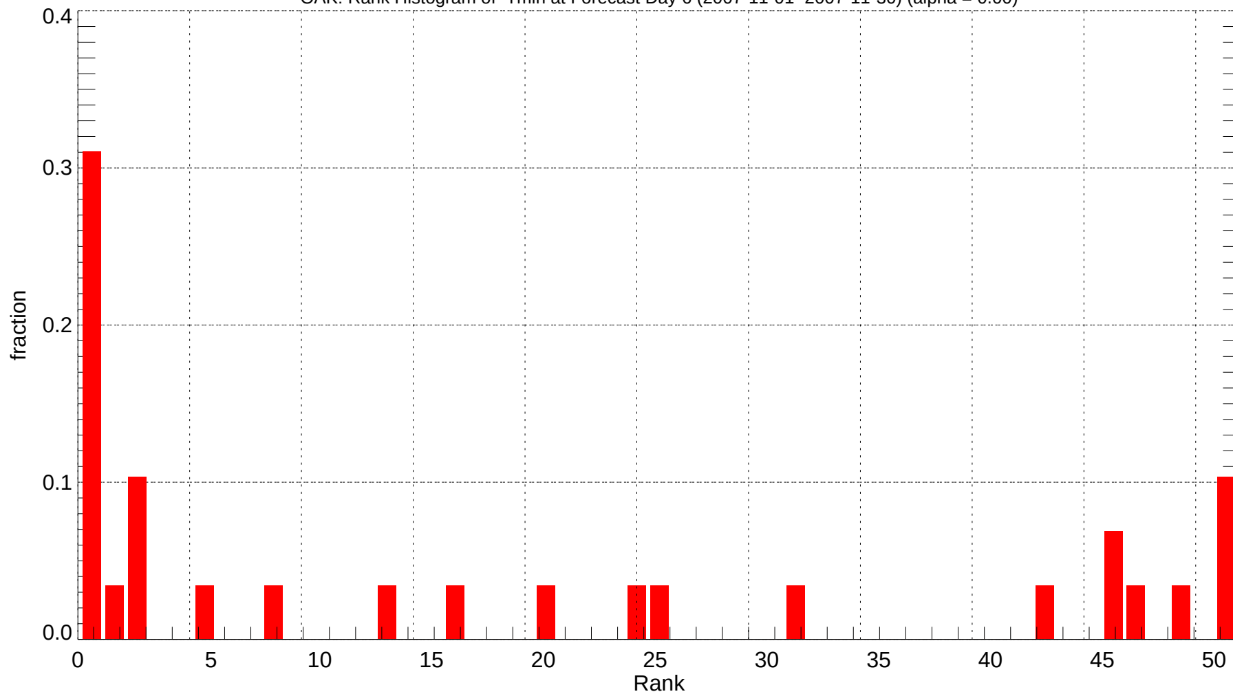
OAK: Rank Histogram of Tmin at Forecast Day 6 (2007-11-01~2007-11-30) (alpha = 0.00)
