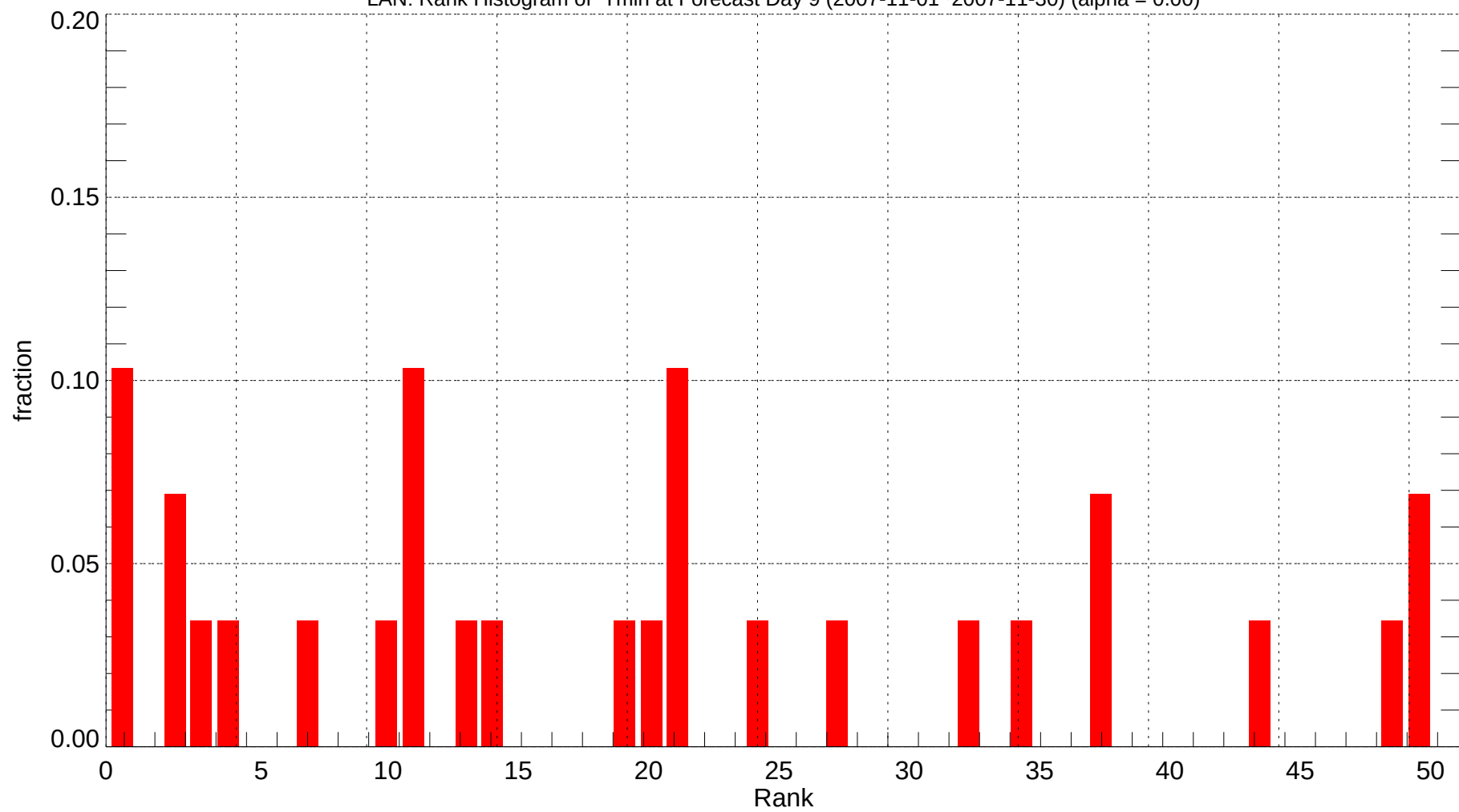
LAN: Rank Histogram of Tmin at Forecast Day 9 (2007-11-01~2007-11-30) (alpha = 0.00)
