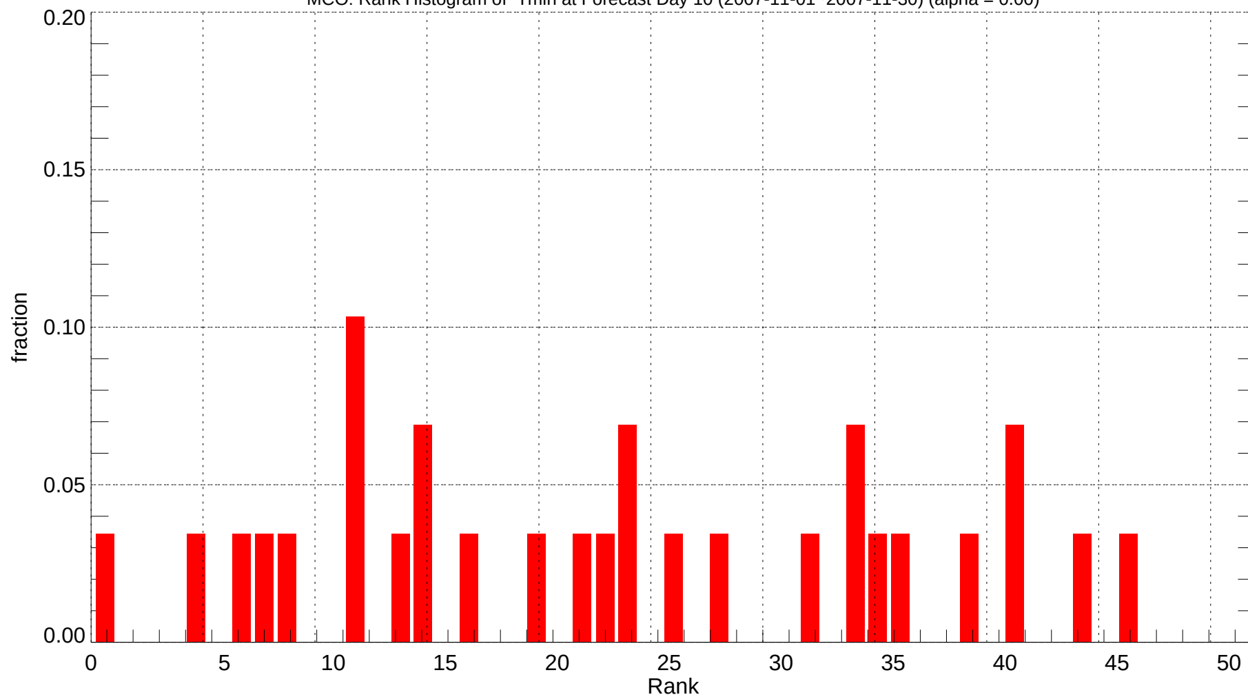
MCO: Rank Histogram of Tmin at Forecast Day 10 (2007-11-01~2007-11-30) (alpha = 0.00)
