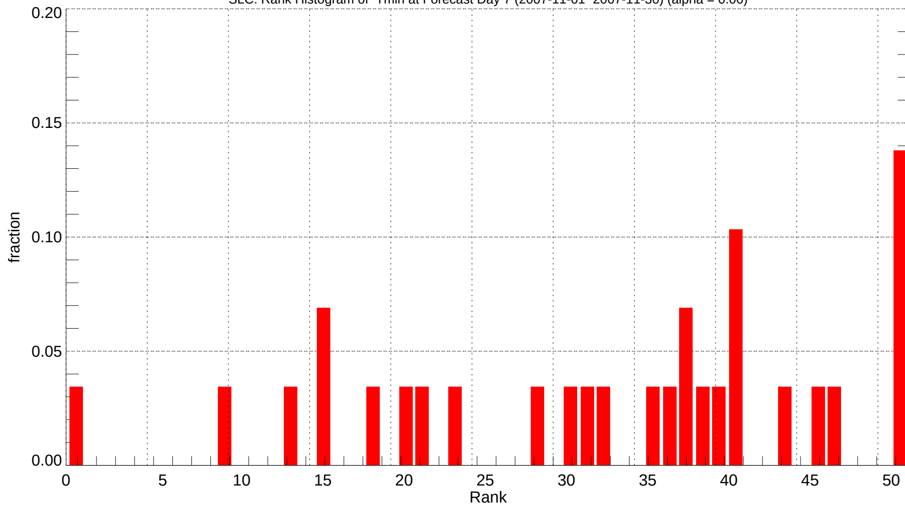
SLC: Rank Histogram of Tmin at Forecast Day 7 (2007-11-01~2007-11-30) (alpha = 0.00)
