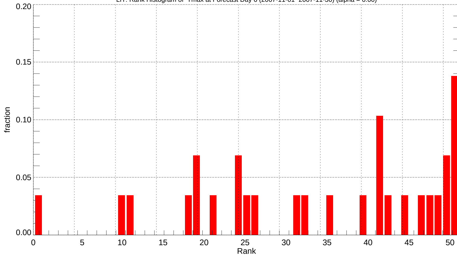
LIT: Rank Histogram of Tmax at Forecast Day 6 (2007-11-01~2007-11-30) (alpha = 0.00)
