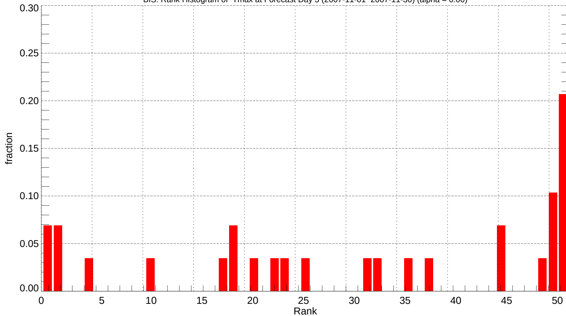
BIS: Rank Histogram of Tmax at Forecast Day 3 (2007-11-01~2007-11-30) (alpha = 0.00)
