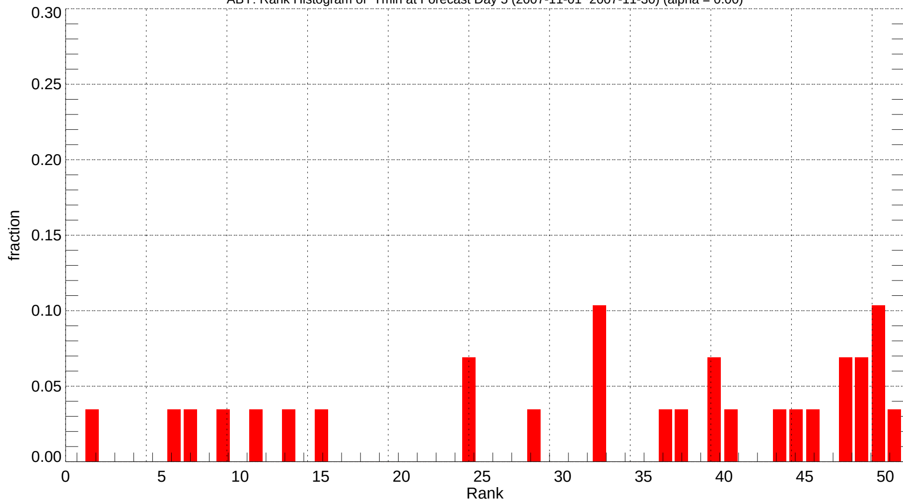
ABY: Rank Histogram of Tmin at Forecast Day 5 (2007-11-01~2007-11-30) (alpha = 0.00)
