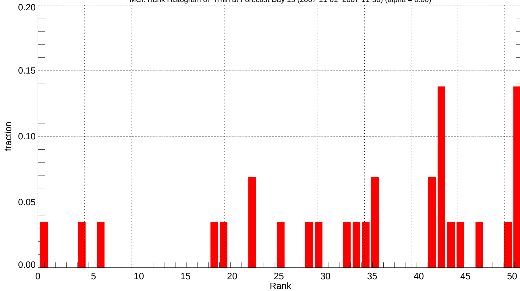
MCI: Rank Histogram of Tmin at Forecast Day 15 (2007-11-01~2007-11-30) (alpha = 0.00)
