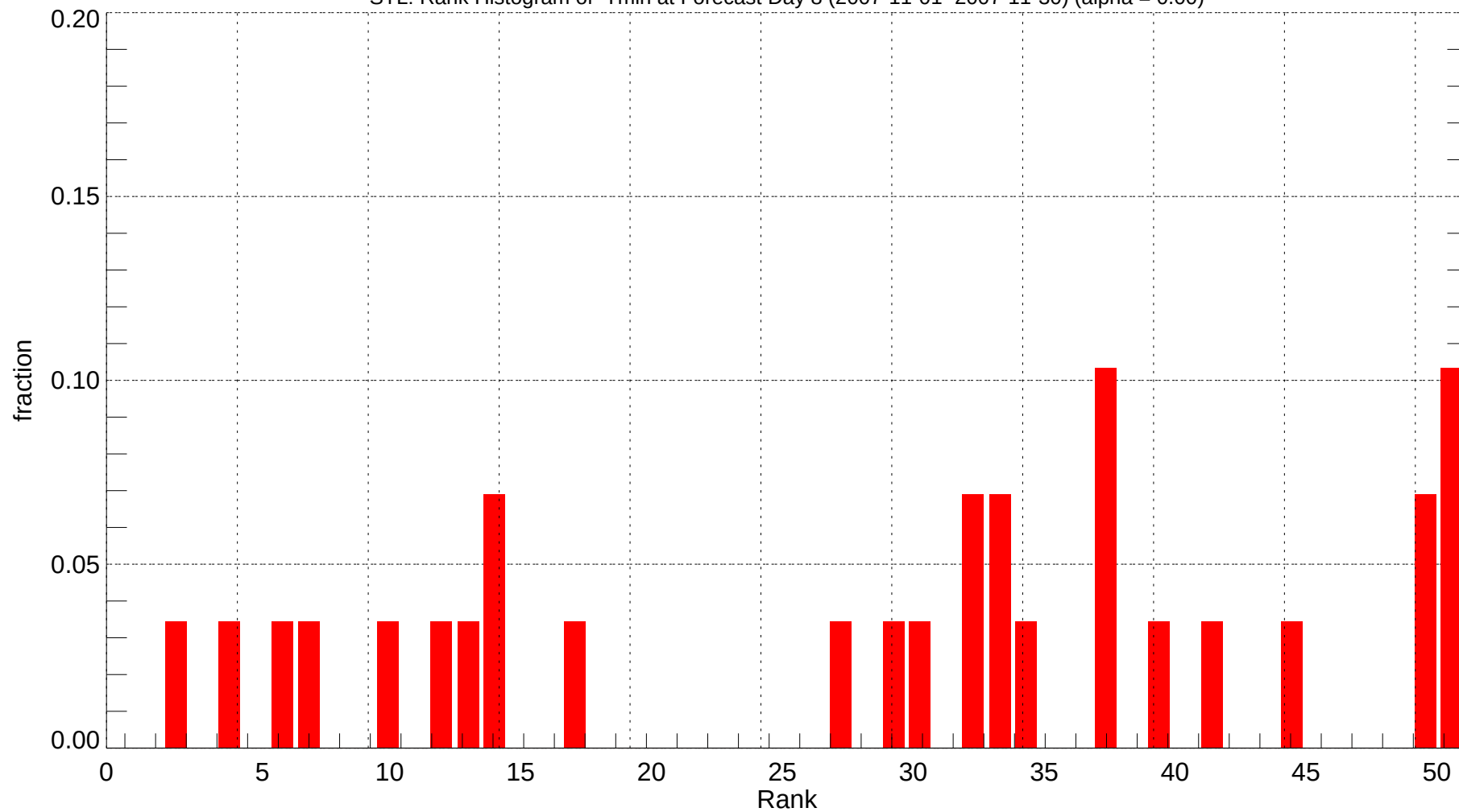
STL: Rank Histogram of Tmin at Forecast Day 8 (2007-11-01~2007-11-30) (alpha = 0.00)
