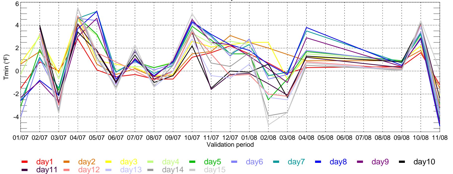
HOU: ECMWF BIAS of Tmin for Monthly Period from 2007-01-01 ~ 2008-11-30
