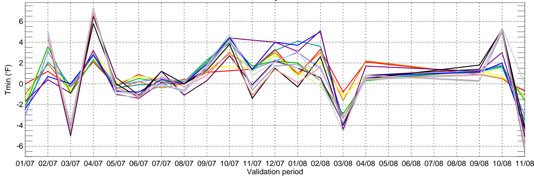
AUS: ECMWF BIAS of Tmin for Monthly Period from 2007-01-01 ~ 2008-11-30
