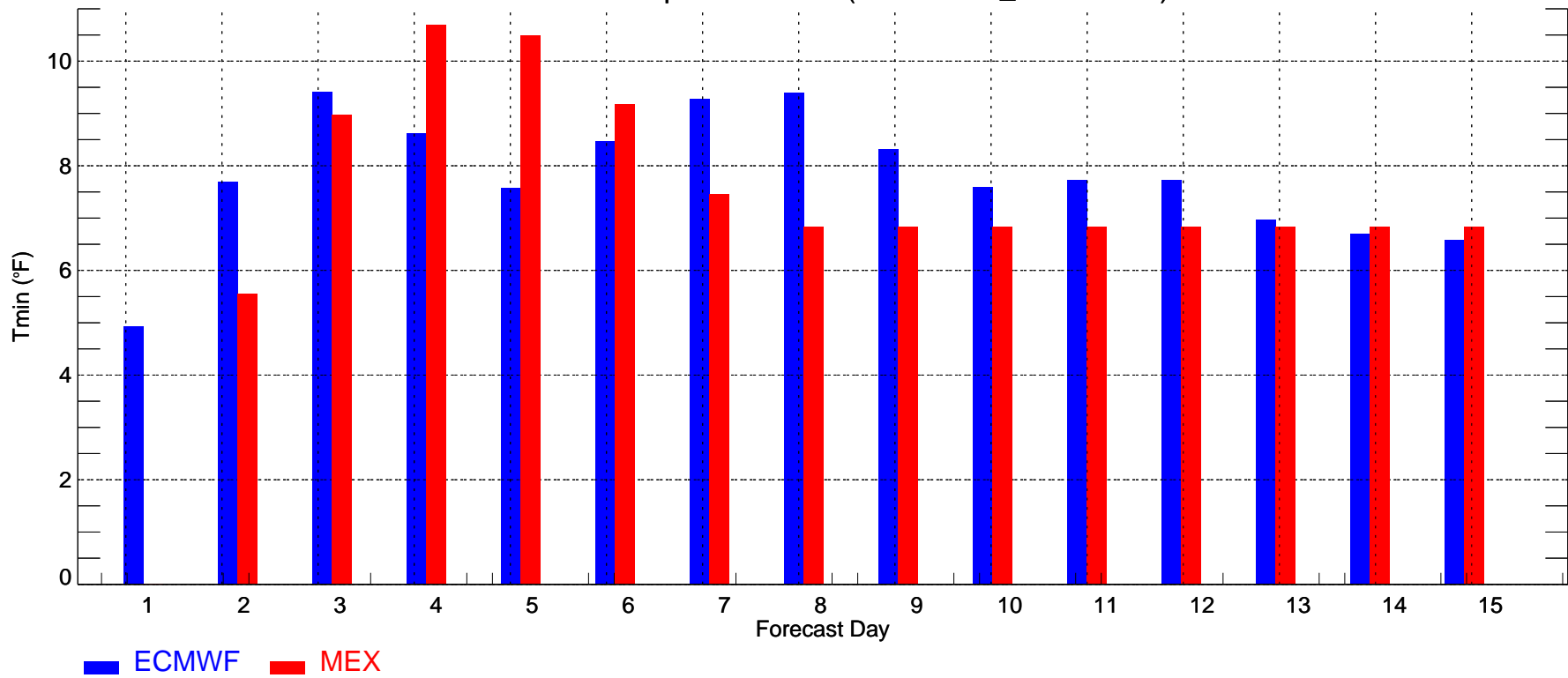
HOU: Min Temperature MAE (2008-11-01_2008-11-30)
