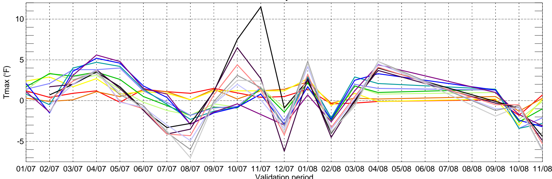
AUS: ECMWF BIAS of Tmax for Monthly Period from 2007-01-01 ~ 2008-11-30
