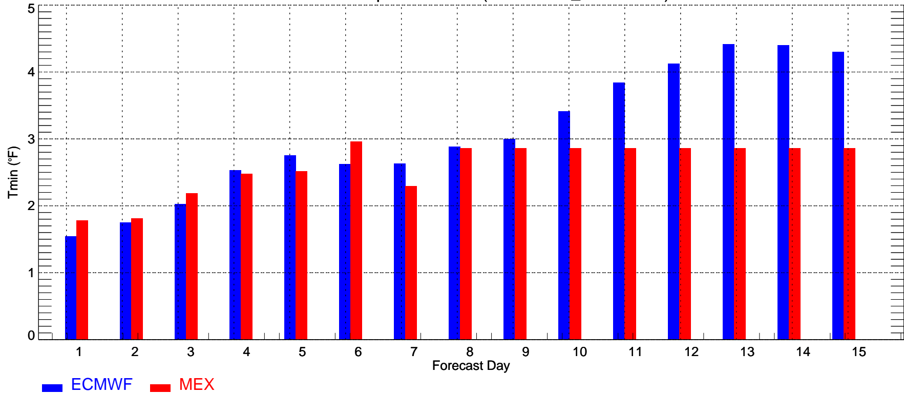
LAX: Min Temperature MAE (2008-06-01_2008-06-30)
