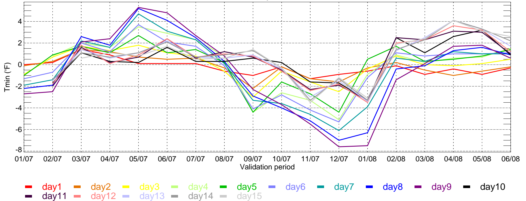
LAX: ECMWF BIAS of Tmin for Monthly Period from 2007-01-01 ~ 2008-06-30
