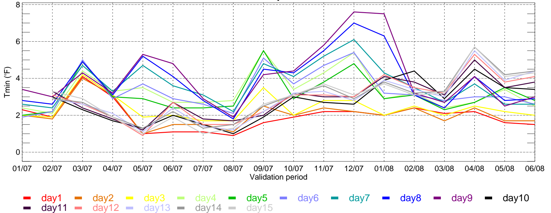
LAX: ECMWF MAE of Tmin for Monthly Period from 2007-01-01 ~ 2008-06-30
