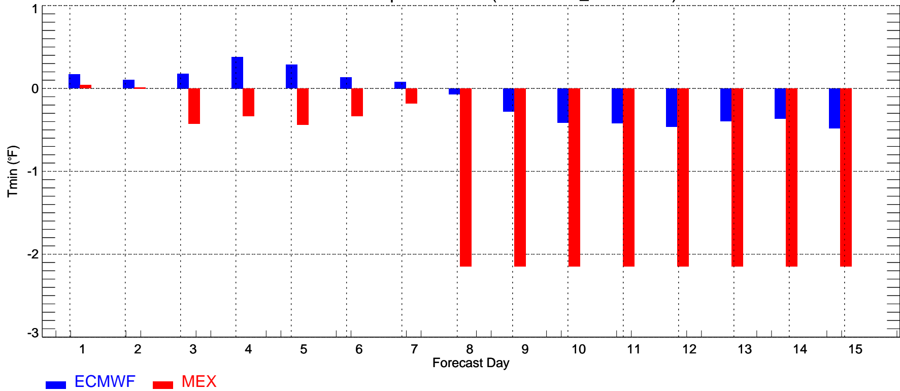
CUST2: Min Temperature Bias (2008-06-01_2008-06-30)
