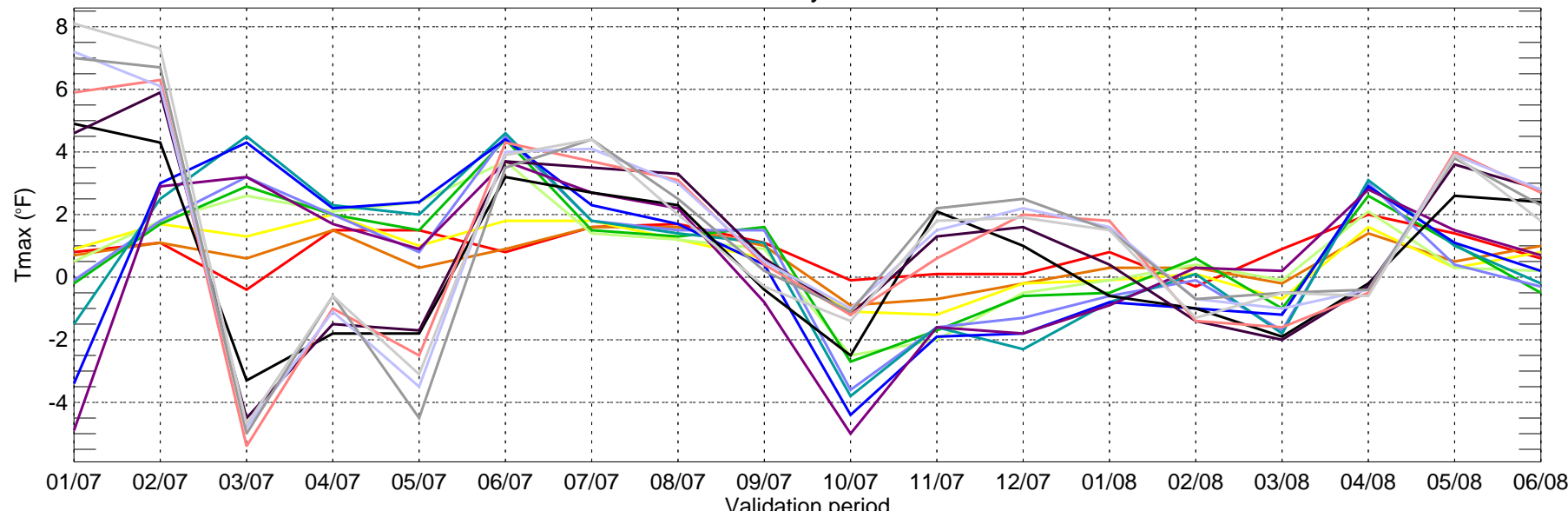
LGA: ECMWF BIAS of Tmax for Monthly Period from 2007-01-01 ~ 2008-06-30
