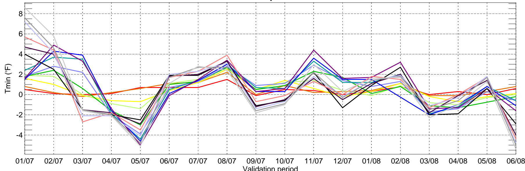
LGA: ECMWF BIAS of Tmin for Monthly Period from 2007-01-01 ~ 2008-06-30
