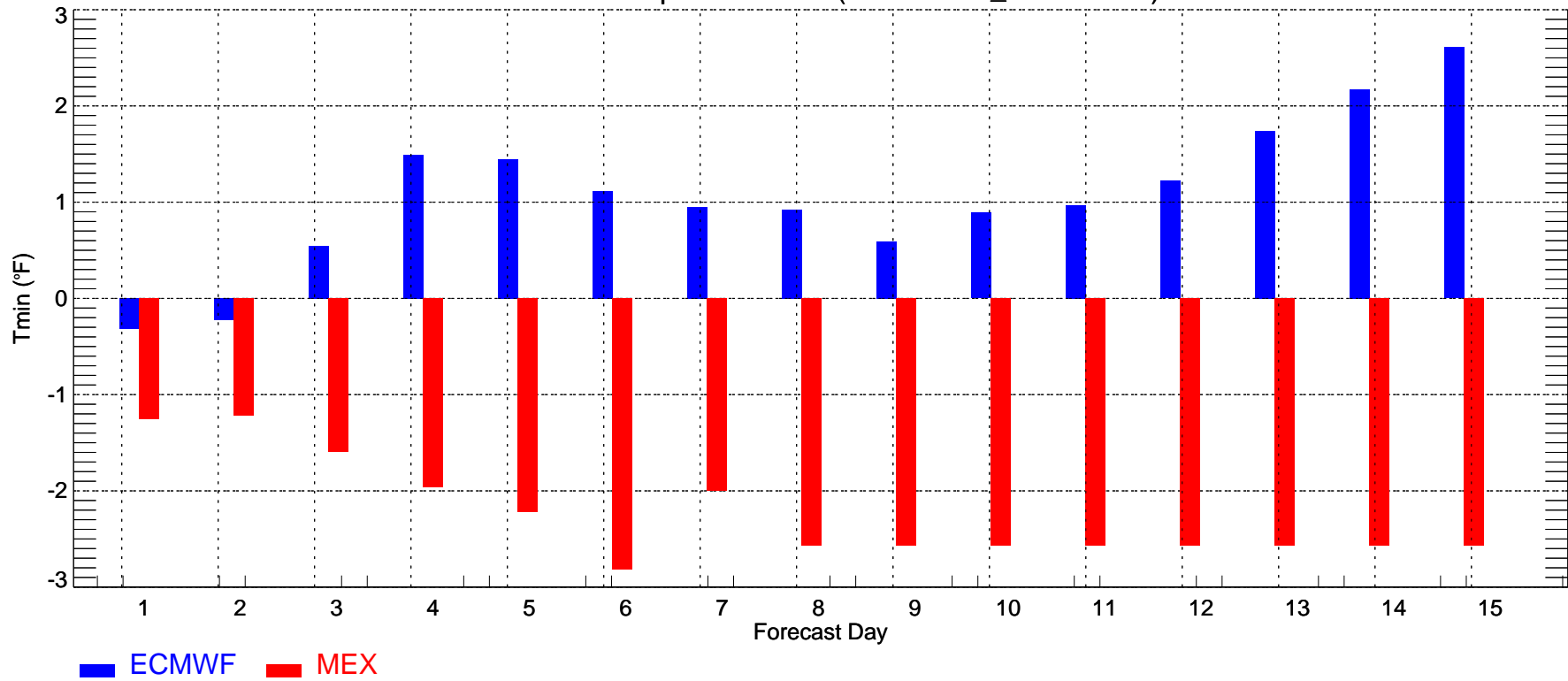
LAX: Min Temperature Bias (2008-06-01_2008-06-30)
