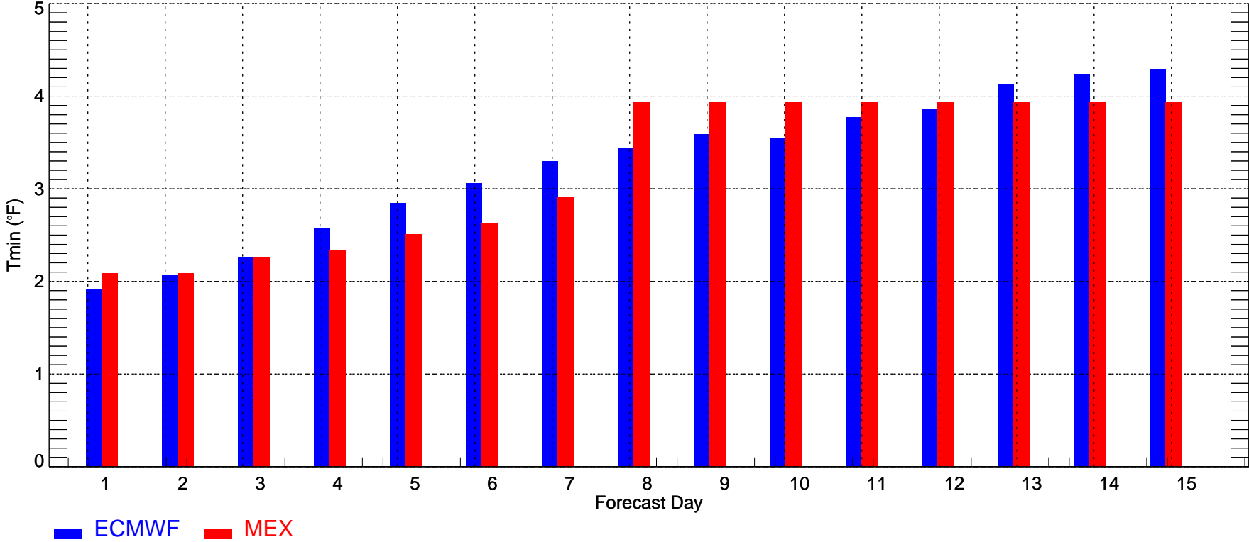
CUST2: Min Temperature MAE (2008-06-01_2008-06-30)
