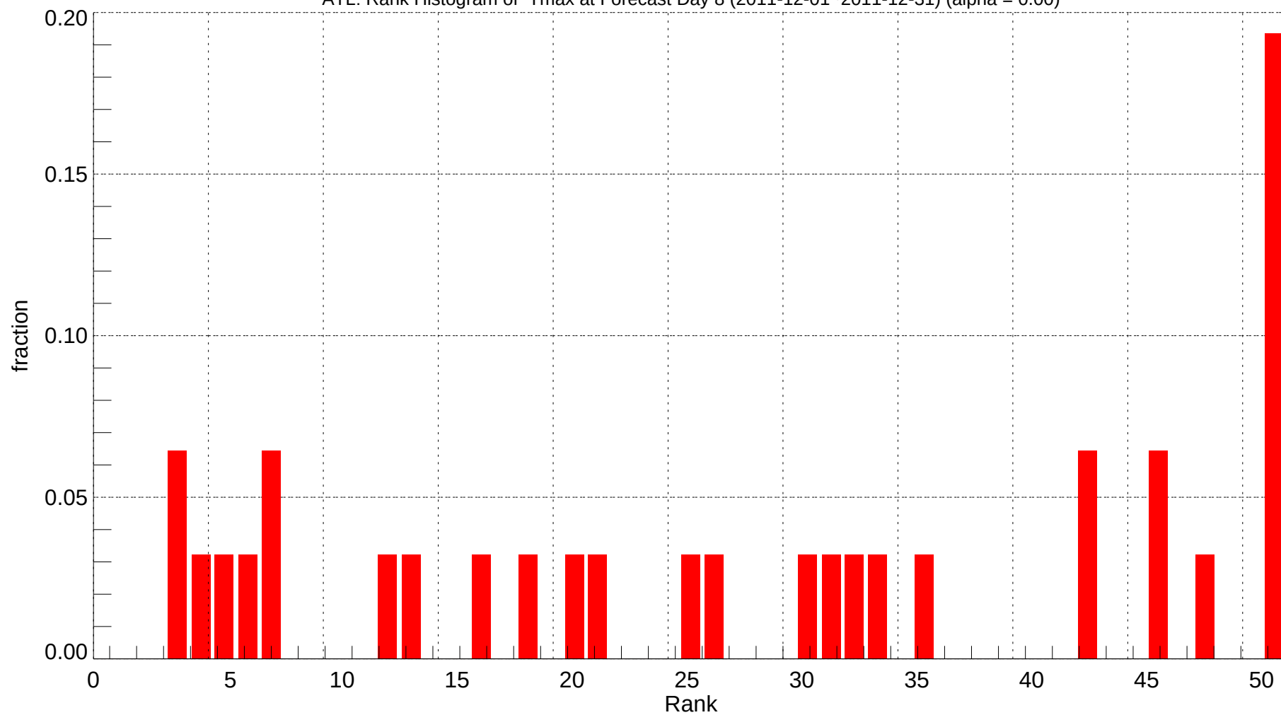
ATL: Rank Histogram of Tmax at Forecast Day 8 (2011-12-01~2011-12-31) (alpha = 0.00)
