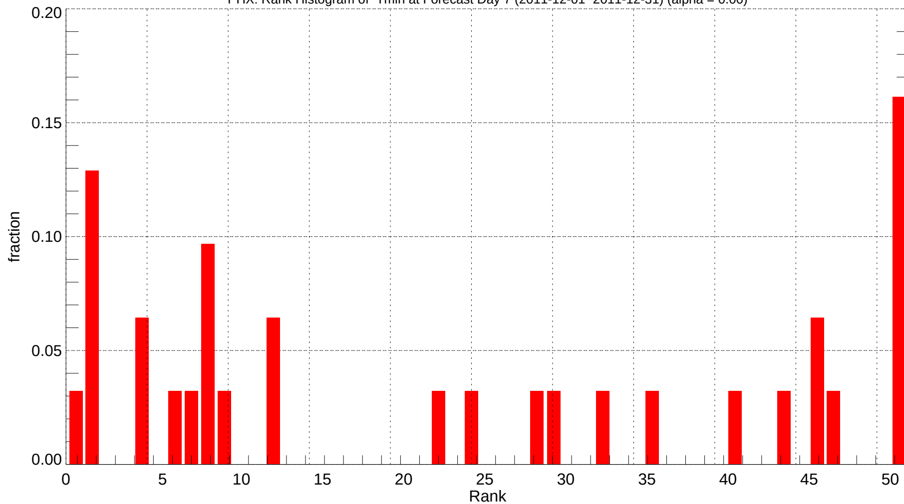
PHX: Rank Histogram of Tmin at Forecast Day 7 (2011-12-01~2011-12-31) (alpha = 0.00)
