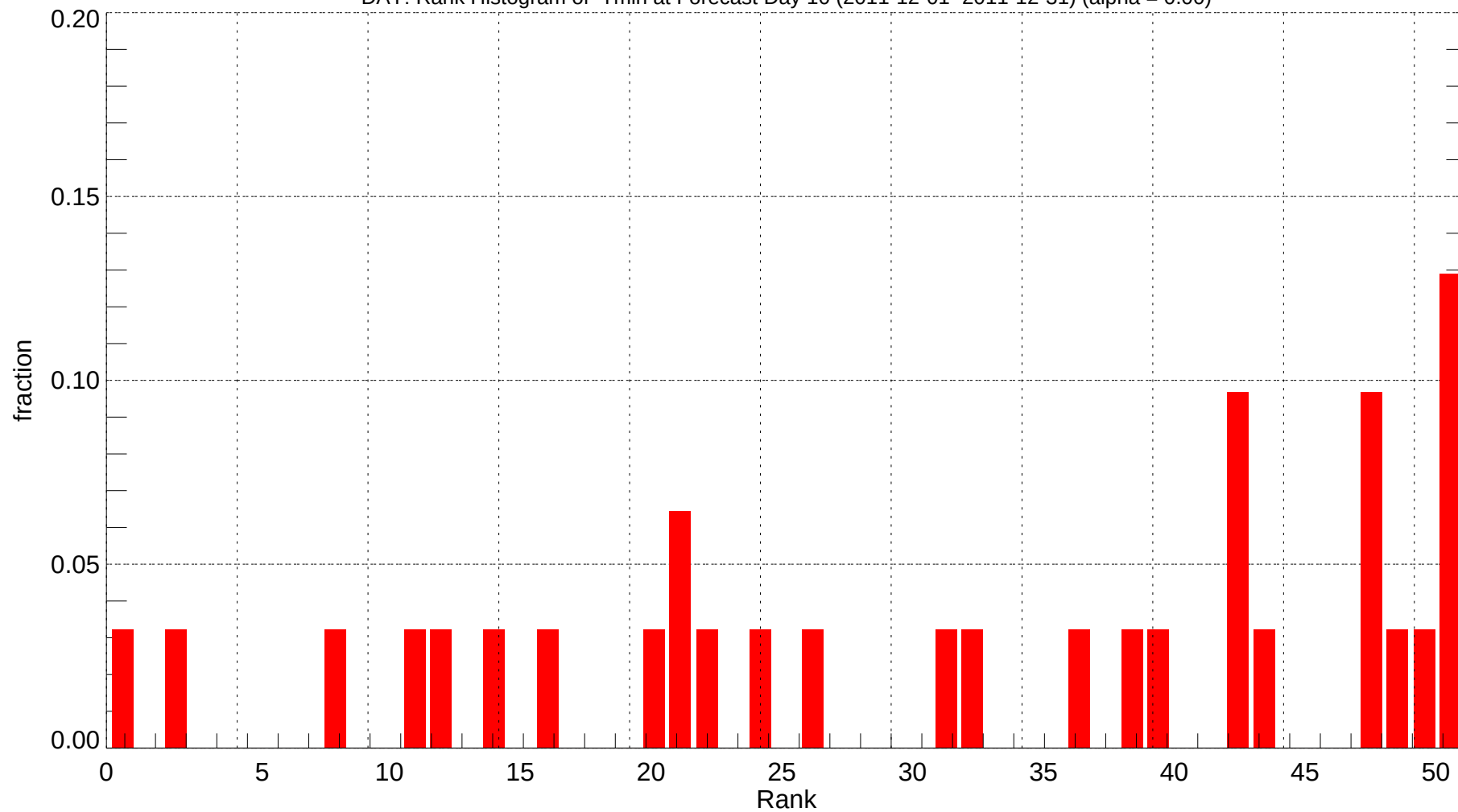
DAY: Rank Histogram of Tmin at Forecast Day 10 (2011-12-01~2011-12-31) (alpha = 0.00)
