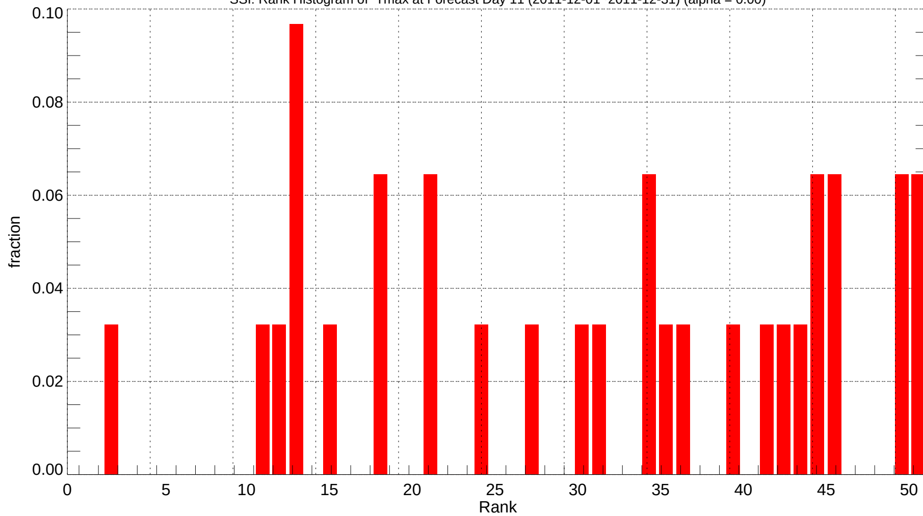
SSI: Rank Histogram of Tmax at Forecast Day 11 (2011-12-01~2011-12-31) (alpha = 0.00)
