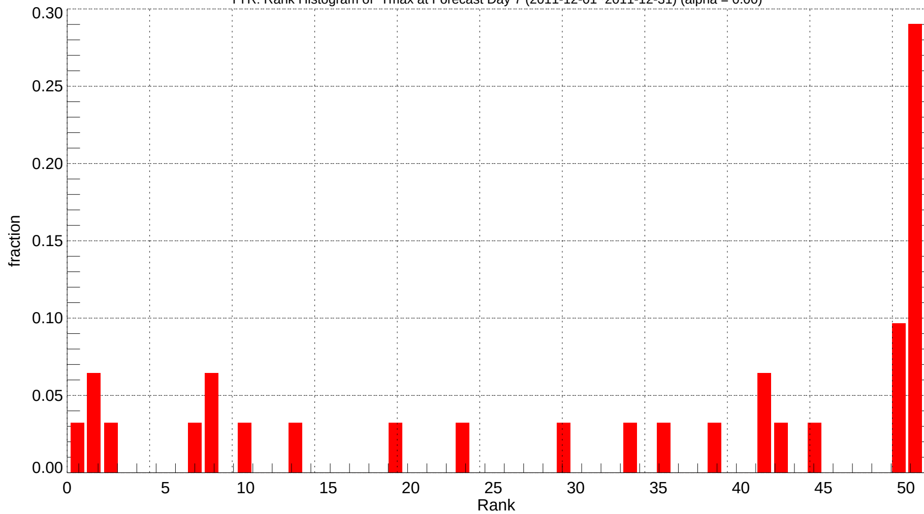
TYR: Rank Histogram of Tmax at Forecast Day 7 (2011-12-01~2011-12-31) (alpha = 0.00)
