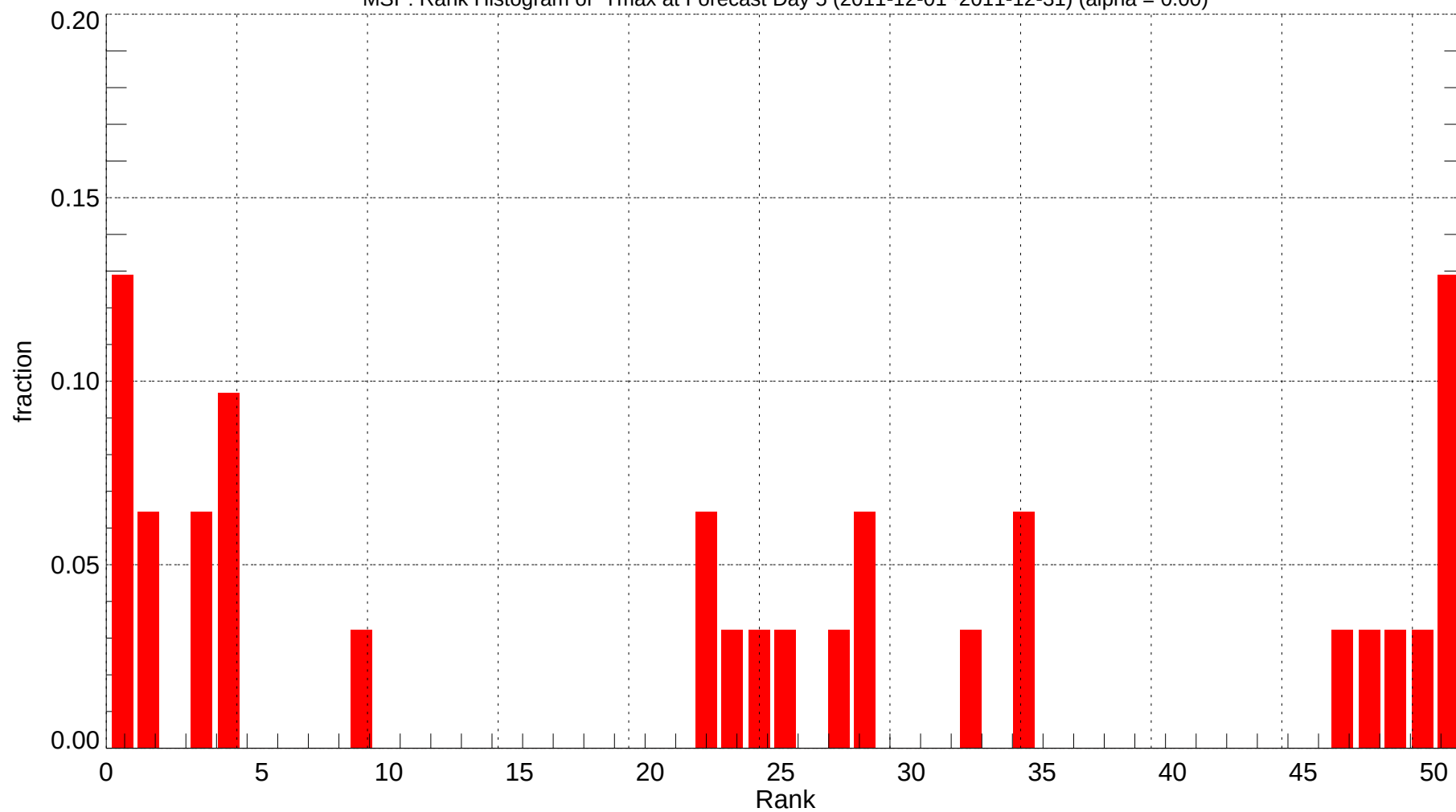
MSP: Rank Histogram of Tmax at Forecast Day 5 (2011-12-01~2011-12-31) (alpha = 0.00)
