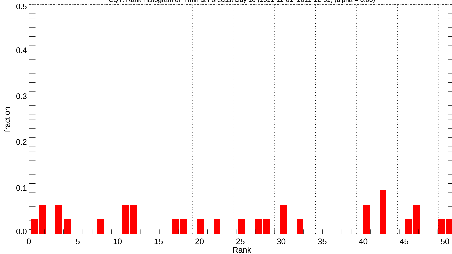
CQT: Rank Histogram of Tmin at Forecast Day 10 (2011-12-01~2011-12-31) (alpha = 0.00)
