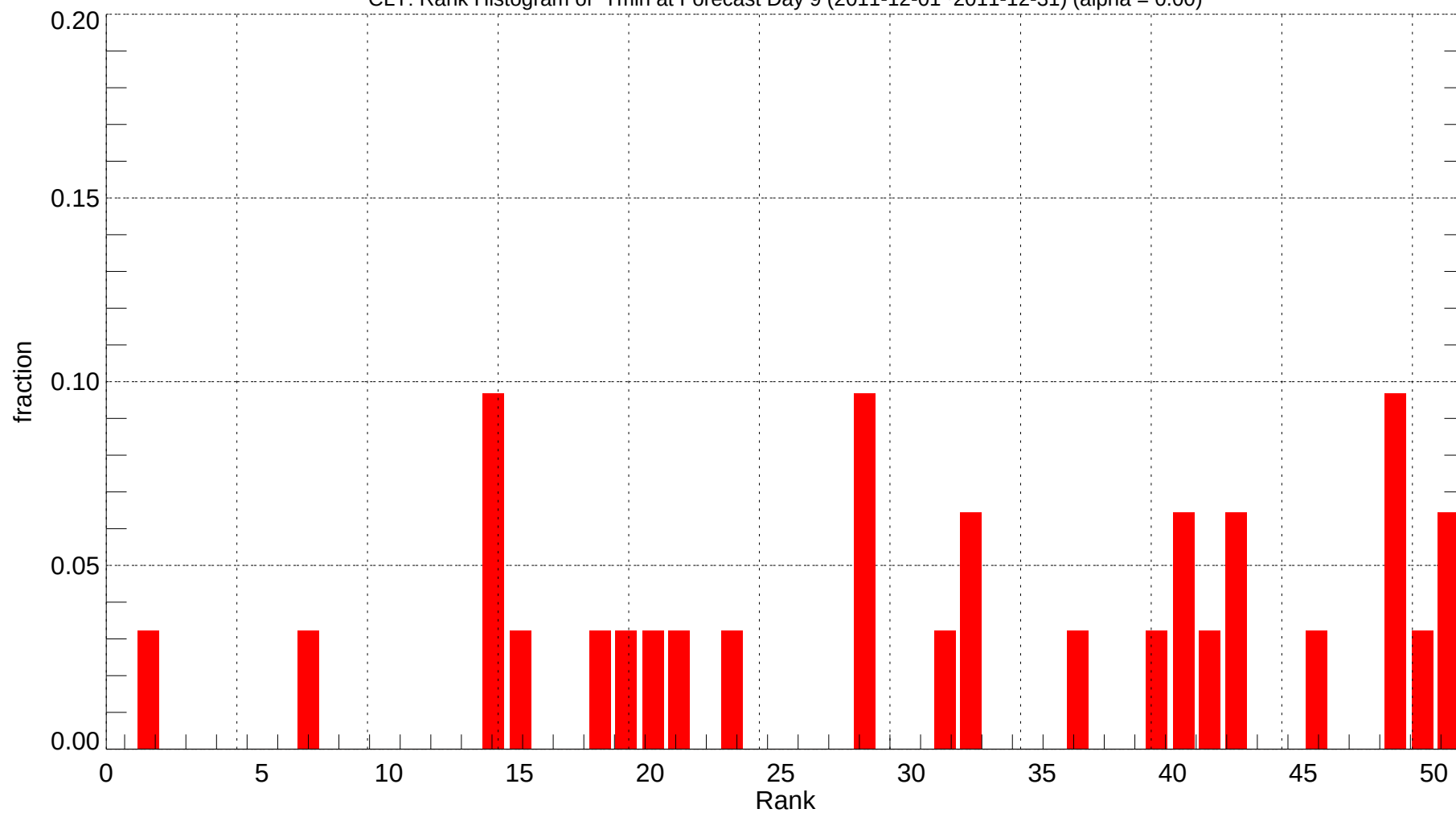
CLT: Rank Histogram of Tmin at Forecast Day 9 (2011-12-01~2011-12-31) (alpha = 0.00)
