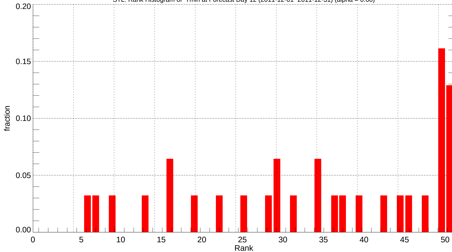
STL: Rank Histogram of Tmin at Forecast Day 12 (2011-12-01~2011-12-31) (alpha = 0.00)
