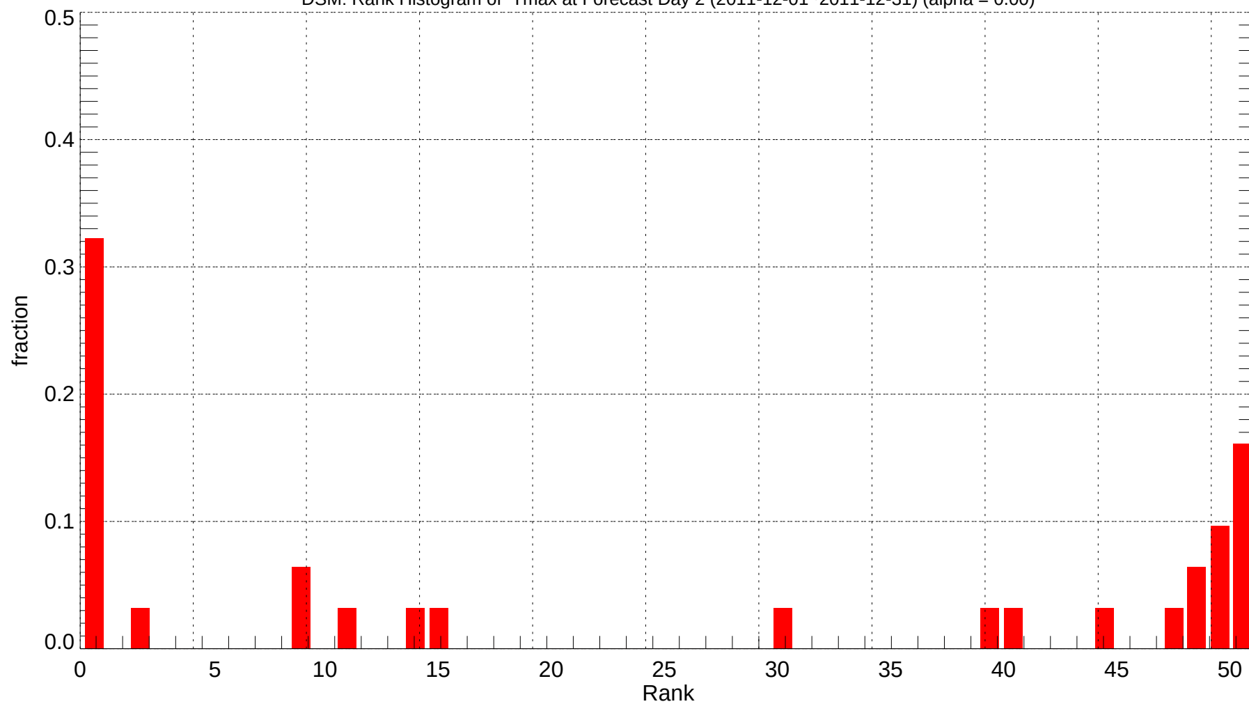
DSM: Rank Histogram of Tmax at Forecast Day 2 (2011-12-01~2011-12-31) (alpha = 0.00)
