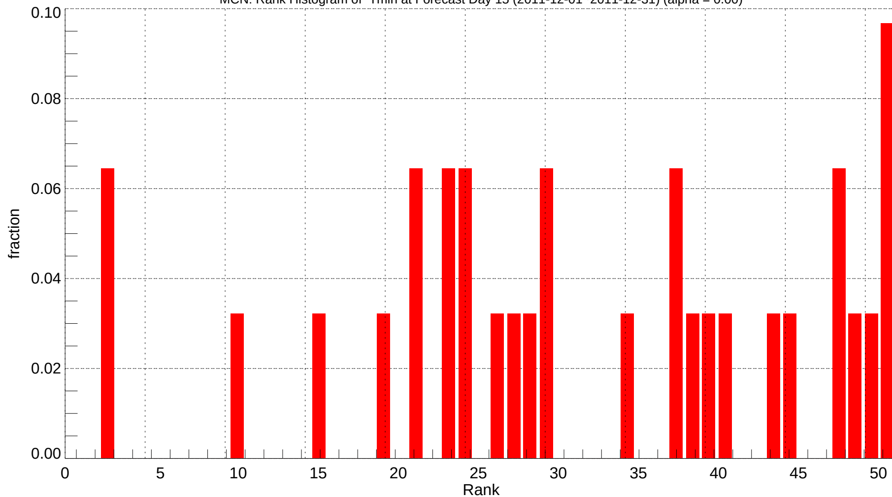
MCN: Rank Histogram of Tmin at Forecast Day 15 (2011-12-01~2011-12-31) (alpha = 0.00)
