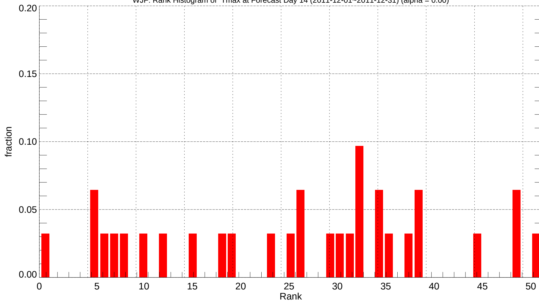
WJF: Rank Histogram of Tmax at Forecast Day 14 (2011-12-01~2011-12-31) (alpha = 0.00)
