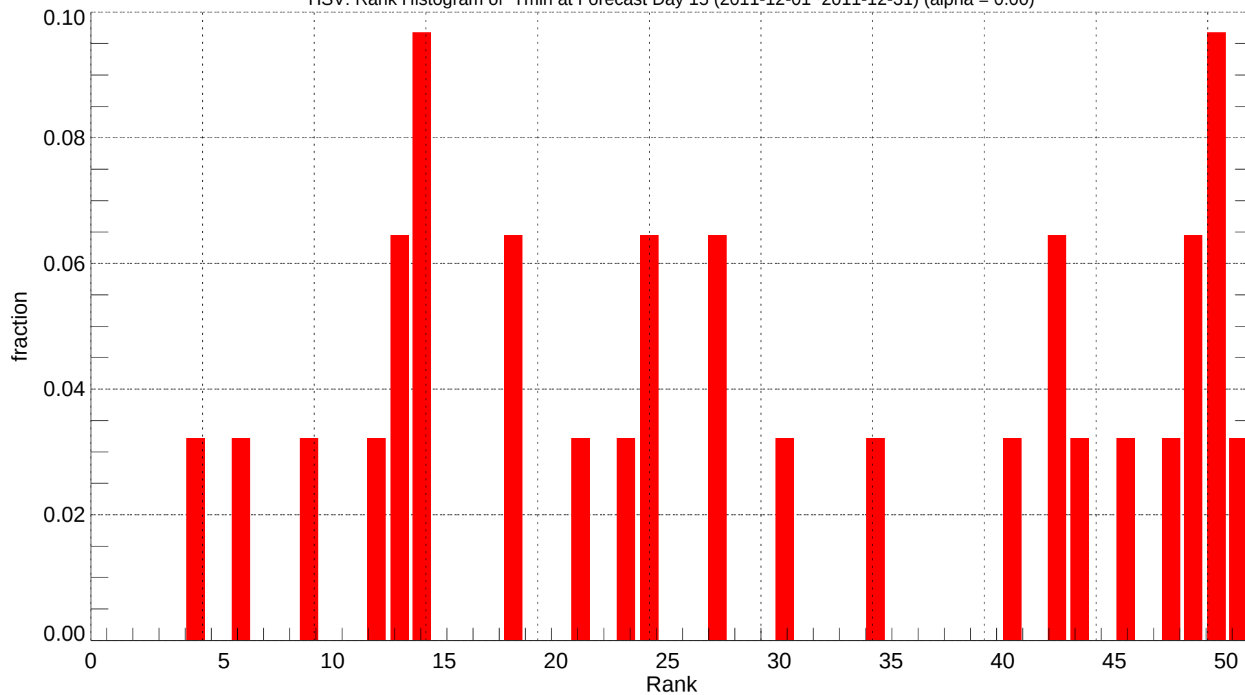
HSV: Rank Histogram of Tmin at Forecast Day 15 (2011-12-01~2011-12-31) (alpha = 0.00)
