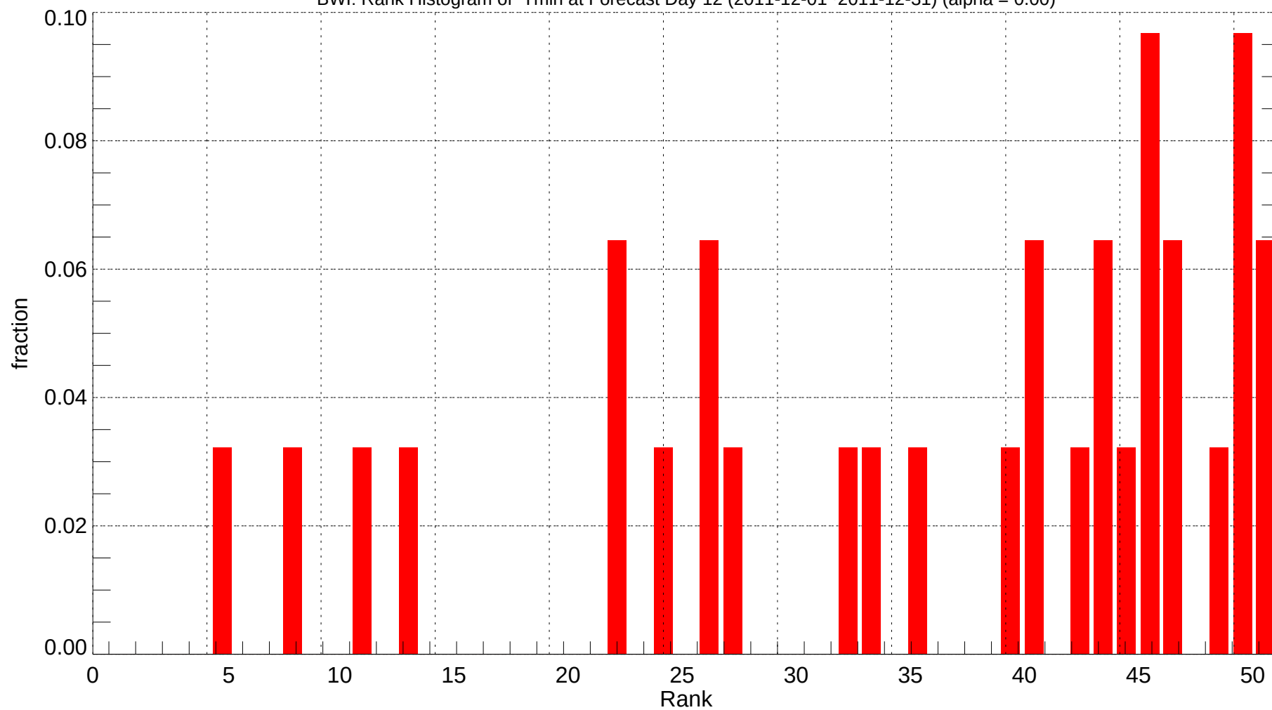
BWI: Rank Histogram of Tmin at Forecast Day 12 (2011-12-01~2011-12-31) (alpha = 0.00)
