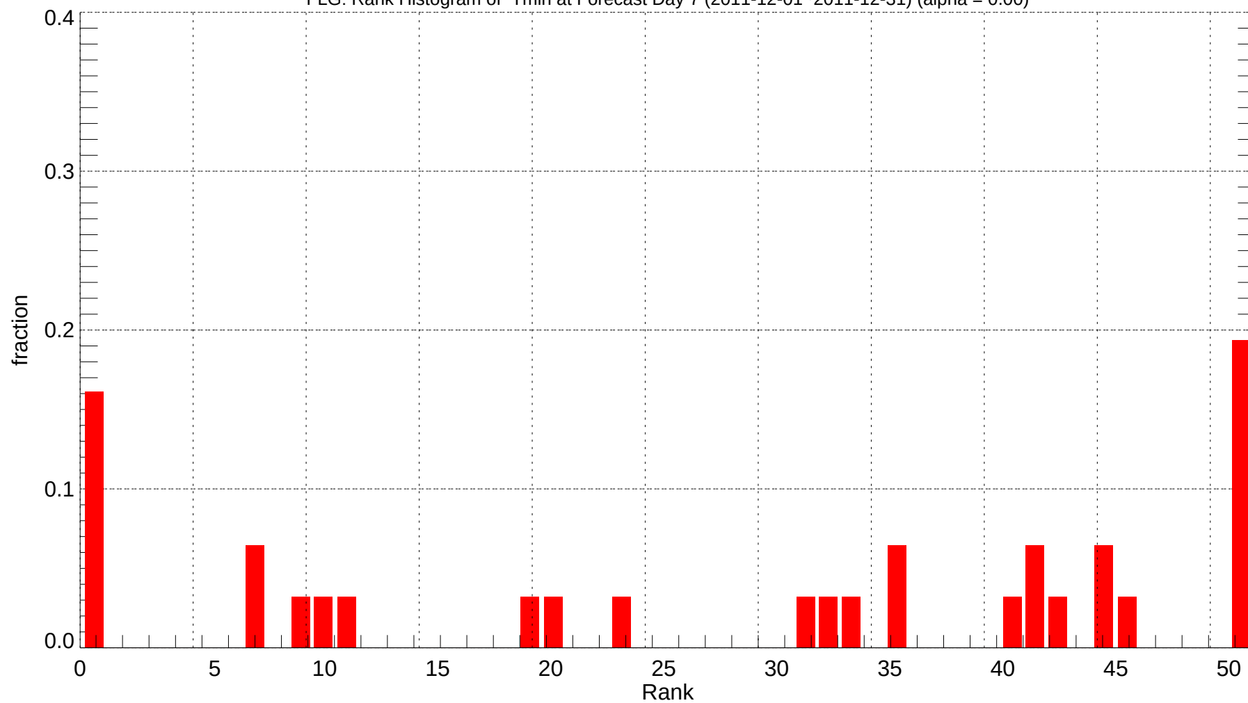
FLG: Rank Histogram of Tmin at Forecast Day 7 (2011-12-01~2011-12-31) (alpha = 0.00)
