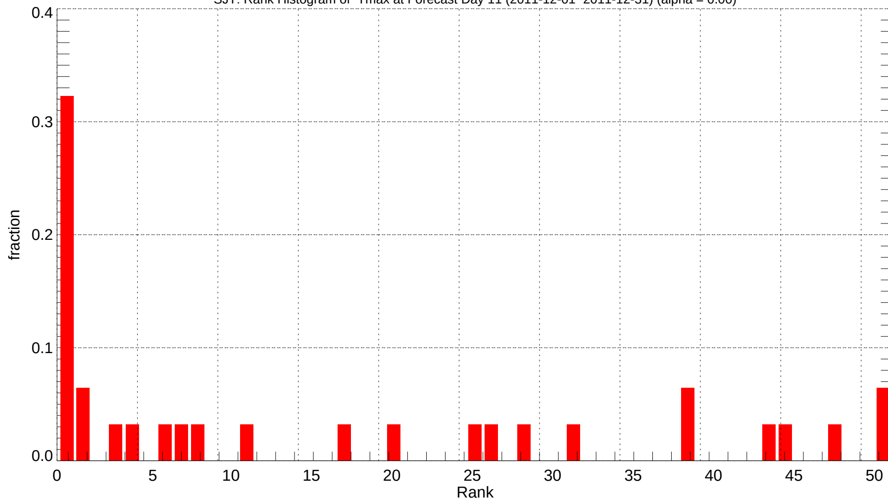
SJT: Rank Histogram of Tmax at Forecast Day 11 (2011-12-01~2011-12-31) (alpha = 0.00)
