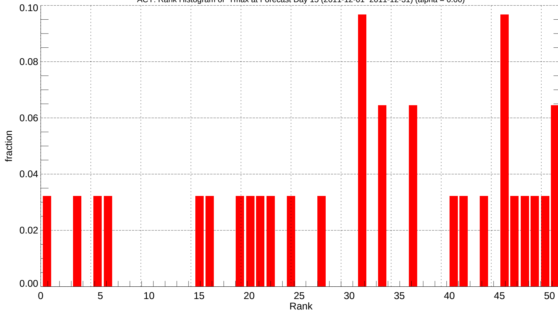
ACY: Rank Histogram of Tmax at Forecast Day 15 (2011-12-01~2011-12-31) (alpha = 0.00)
