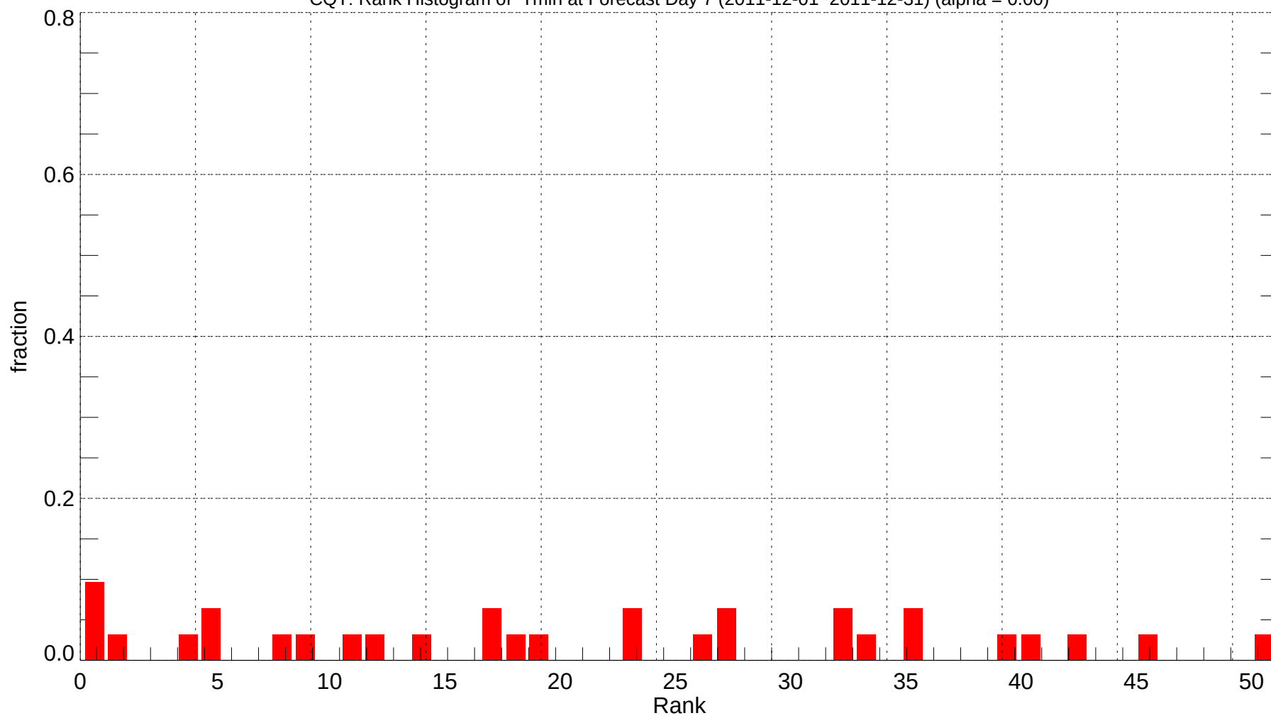
CQT: Rank Histogram of Tmin at Forecast Day 7 (2011-12-01~2011-12-31) (alpha = 0.00)
