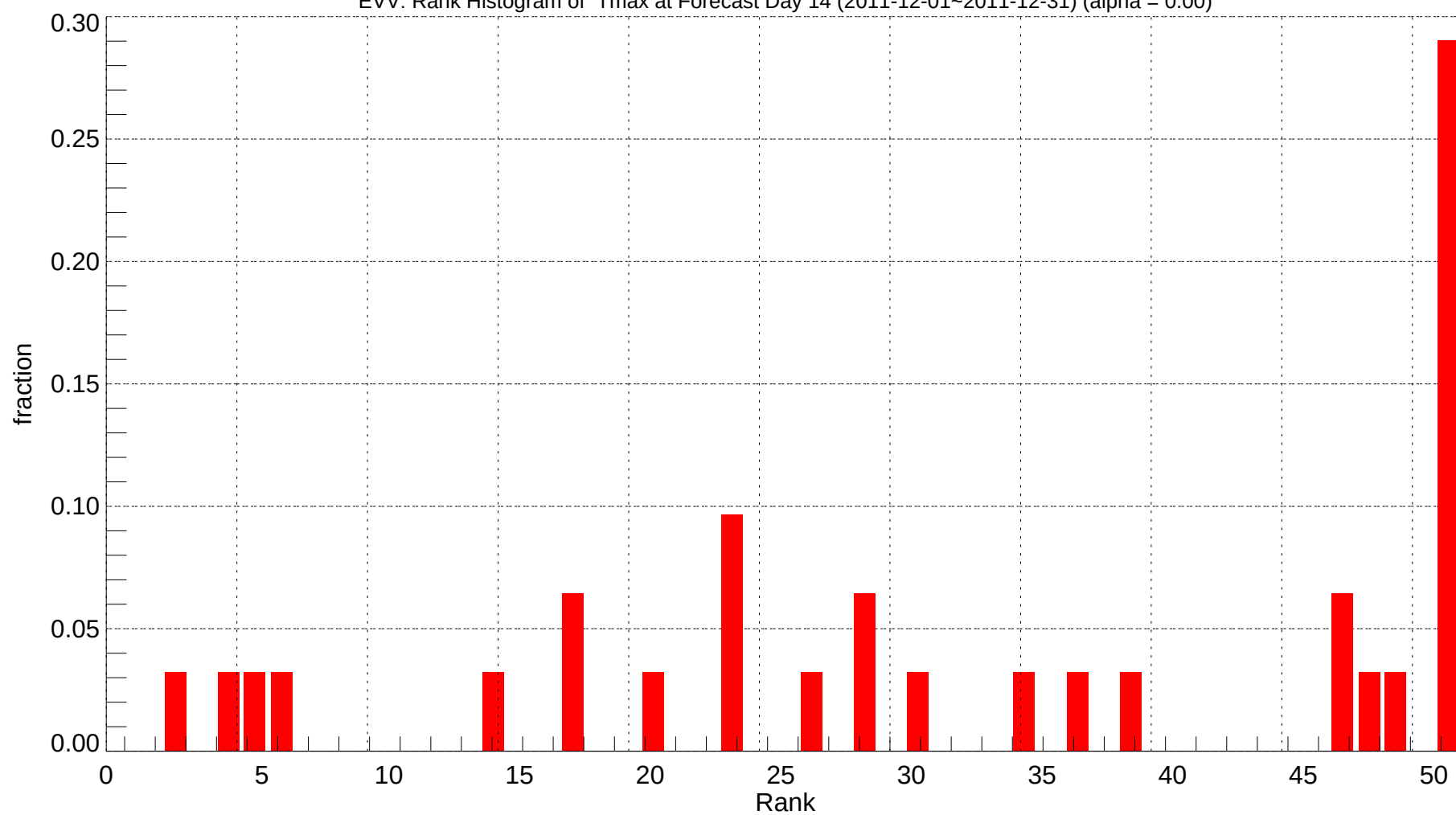
EVV: Rank Histogram of Tmax at Forecast Day 14 (2011-12-01~2011-12-31) (alpha = 0.00)
