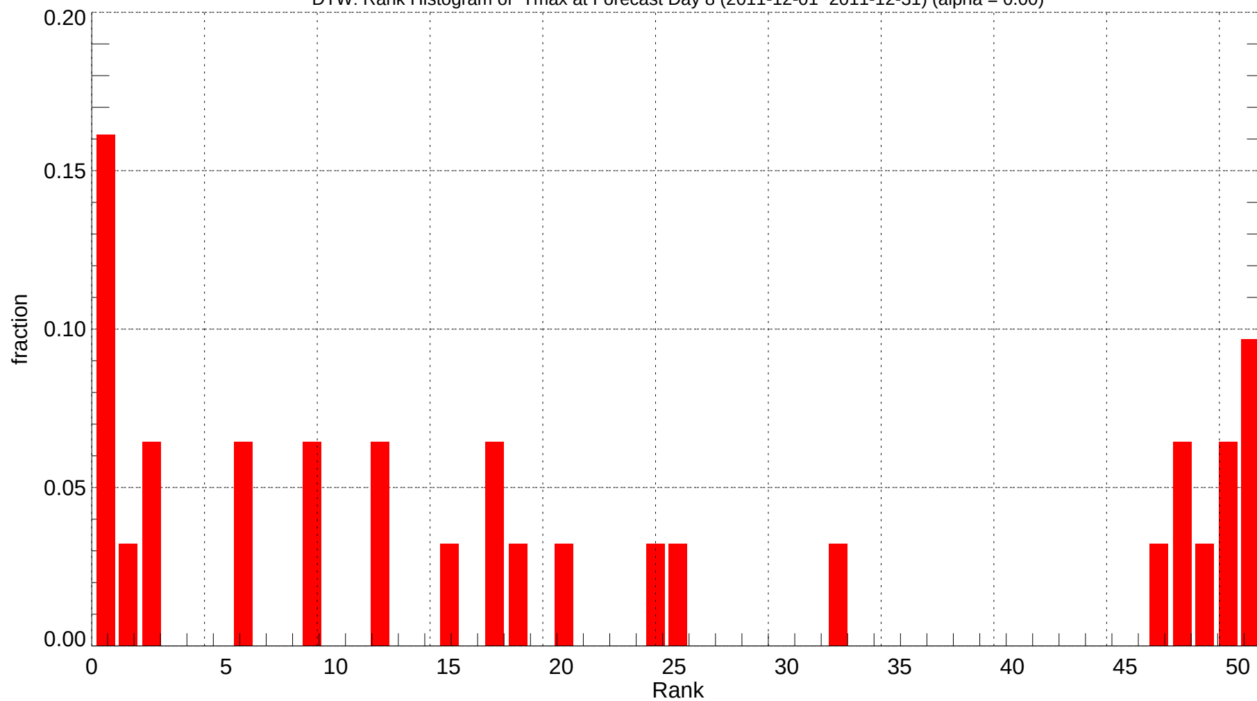
DTW: Rank Histogram of Tmax at Forecast Day 8 (2011-12-01~2011-12-31) (alpha = 0.00)
