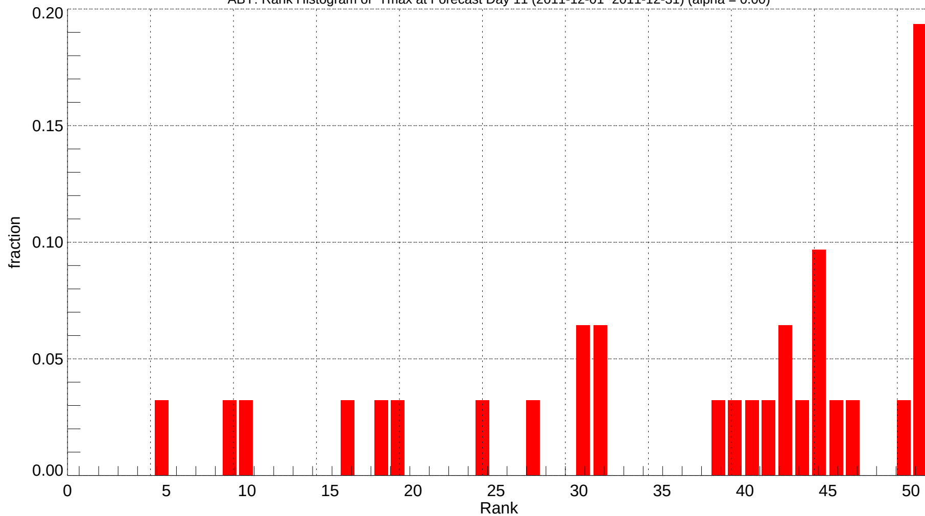
ABY: Rank Histogram of Tmax at Forecast Day 11 (2011-12-01~2011-12-31) (alpha = 0.00)
