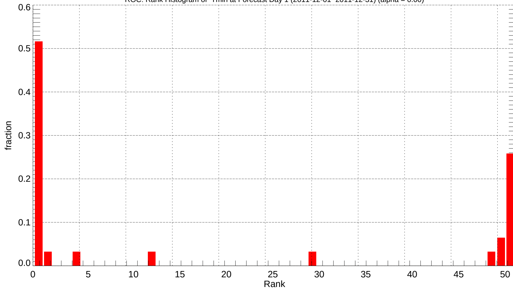
ROC: Rank Histogram of Tmin at Forecast Day 1 (2011-12-01~2011-12-31) (alpha = 0.00)
