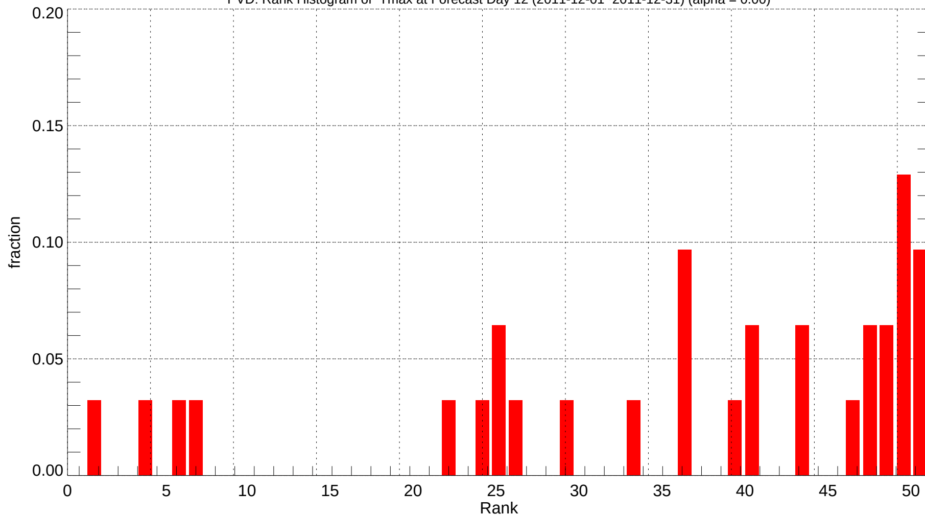
PVD: Rank Histogram of Tmax at Forecast Day 12 (2011-12-01~2011-12-31) (alpha = 0.00)
