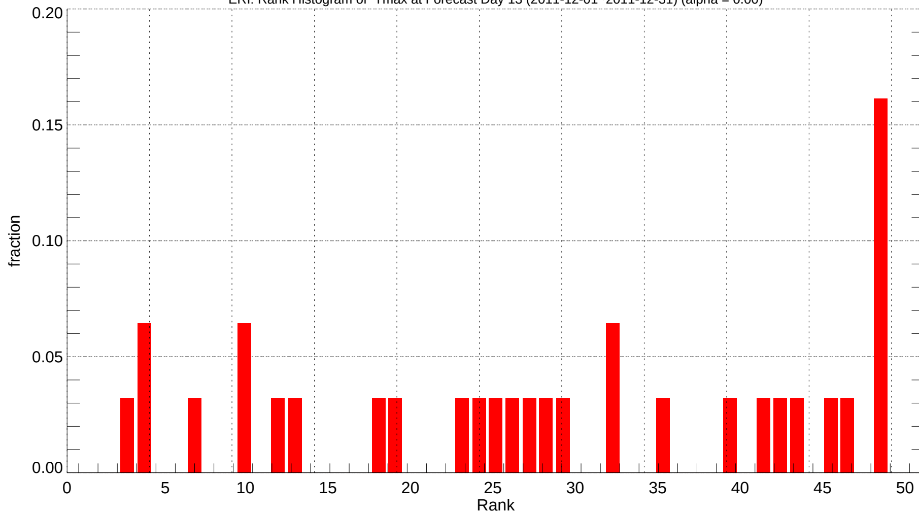
ERI: Rank Histogram of Tmax at Forecast Day 13 (2011-12-01~2011-12-31) (alpha = 0.00)
