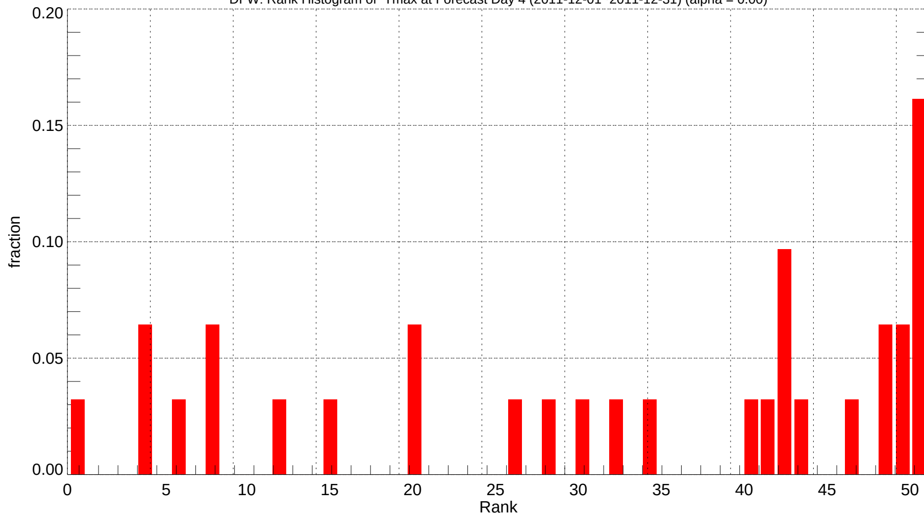
DFW: Rank Histogram of Tmax at Forecast Day 4 (2011-12-01~2011-12-31) (alpha = 0.00)
