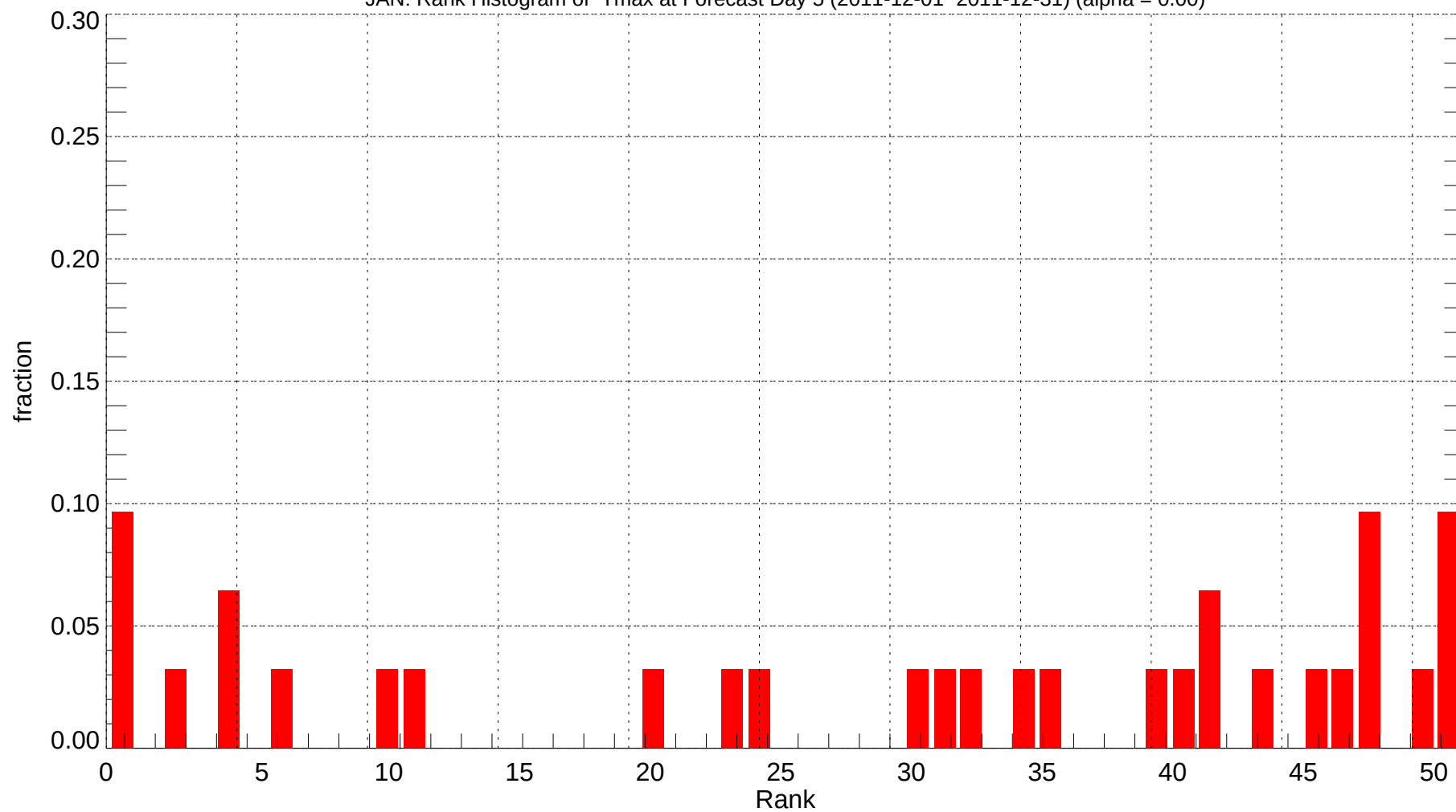
JAN: Rank Histogram of Tmax at Forecast Day 5 (2011-12-01~2011-12-31) (alpha = 0.00)
