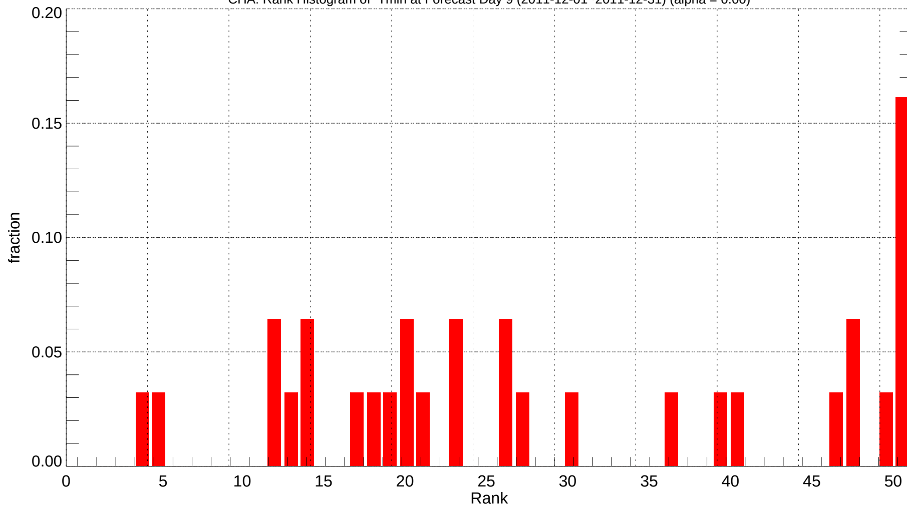
CHA: Rank Histogram of Tmin at Forecast Day 9 (2011-12-01~2011-12-31) (alpha = 0.00)
