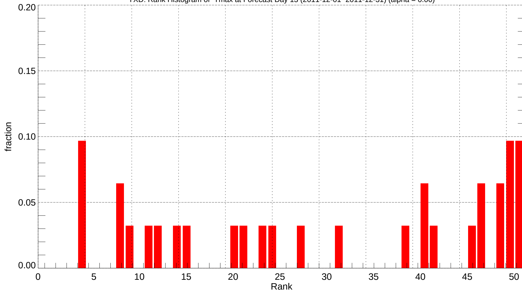
YXD: Rank Histogram of Tmax at Forecast Day 13 (2011-12-01~2011-12-31) (alpha = 0.00)
