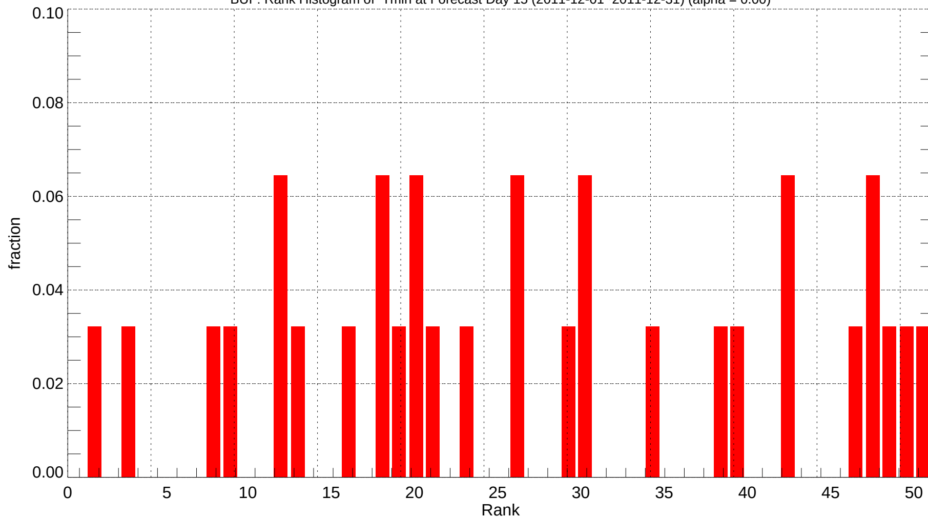
BUF: Rank Histogram of Tmin at Forecast Day 15 (2011-12-01~2011-12-31) (alpha = 0.00)
