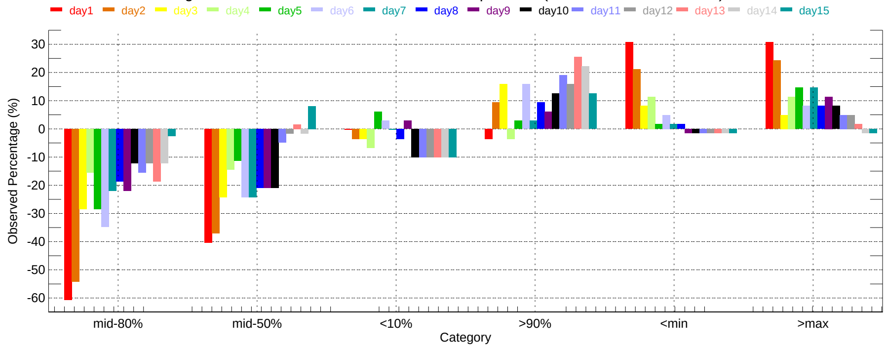
Observed Percentage Deviation of Ensembles - LIT: Min Temperature (2011-12-01~2011-12-31)
