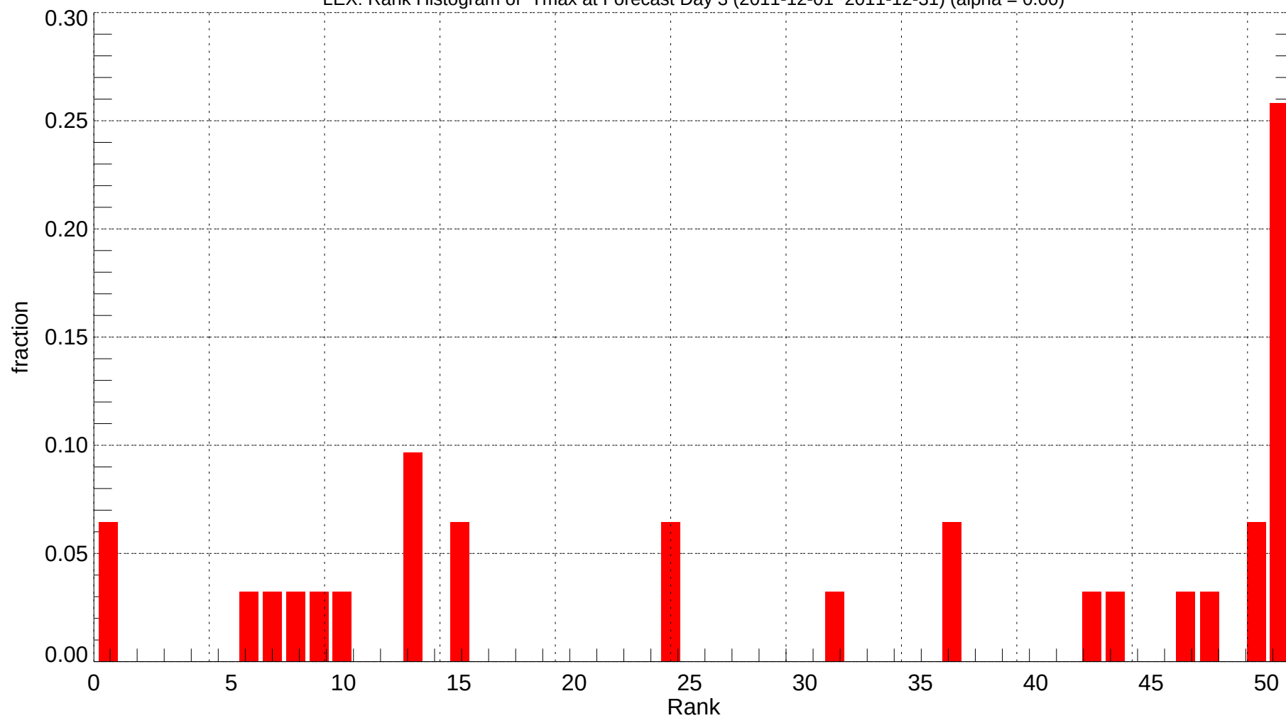
LEX: Rank Histogram of Tmax at Forecast Day 3 (2011-12-01~2011-12-31) (alpha = 0.00)
