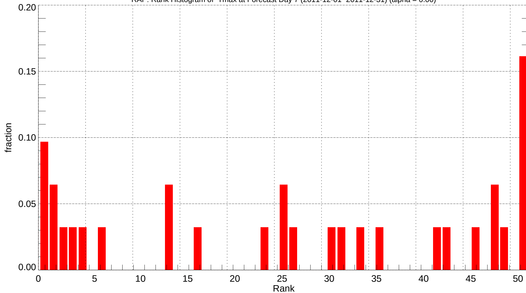
RAP: Rank Histogram of Tmax at Forecast Day 7 (2011-12-01~2011-12-31) (alpha = 0.00)
