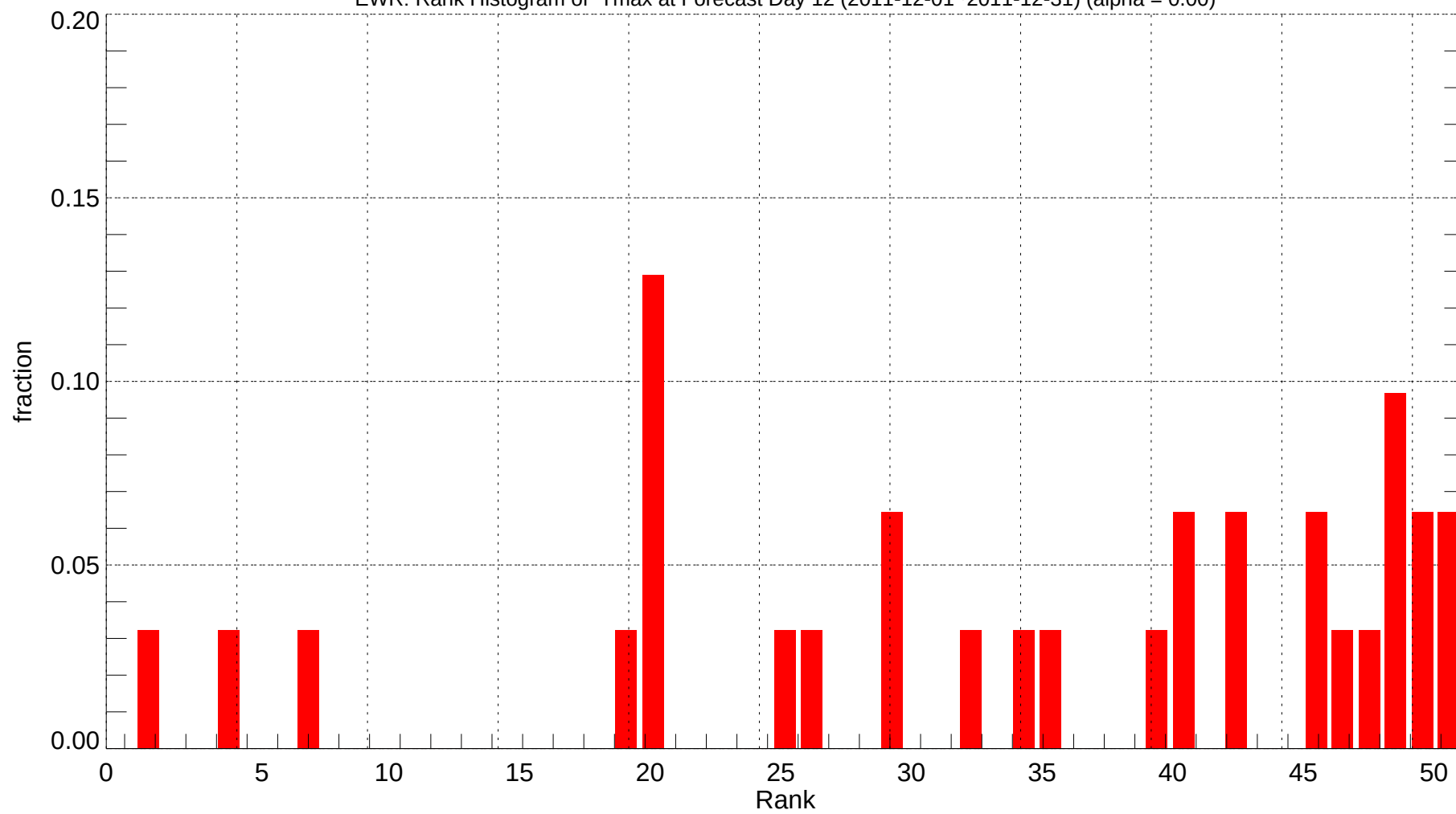
EWR: Rank Histogram of Tmax at Forecast Day 12 (2011-12-01~2011-12-31) (alpha = 0.00)
