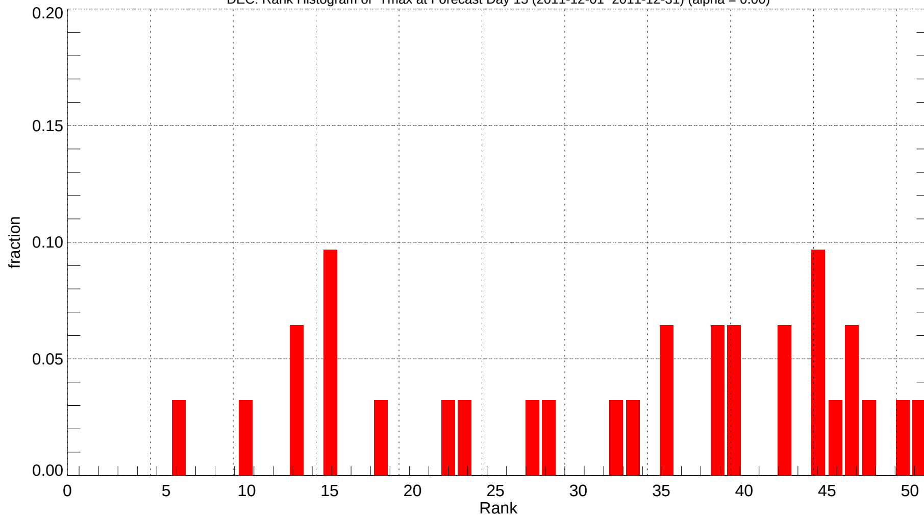
DEC: Rank Histogram of Tmax at Forecast Day 15 (2011-12-01~2011-12-31) (alpha = 0.00)
