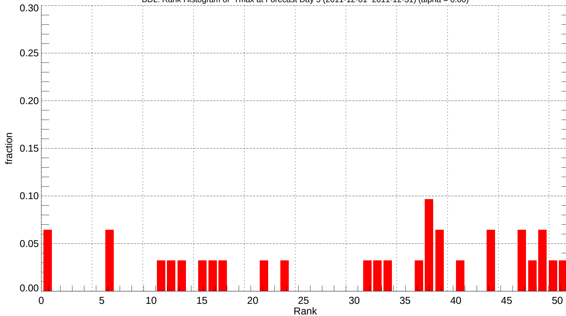
BDL: Rank Histogram of Tmax at Forecast Day 5 (2011-12-01~2011-12-31) (alpha = 0.00)
