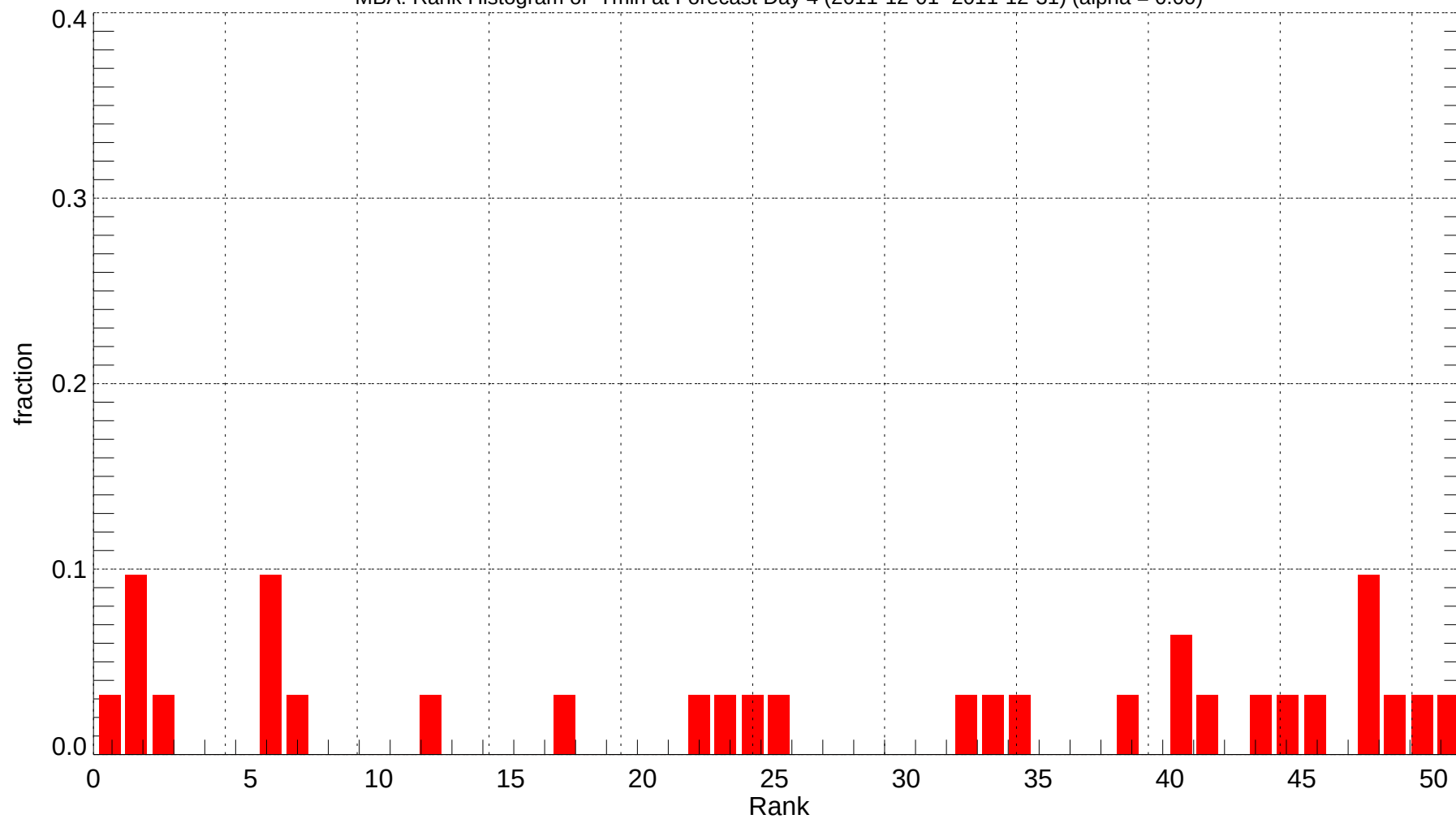
MBA: Rank Histogram of Tmin at Forecast Day 4 (2011-12-01~2011-12-31) (alpha = 0.00)
