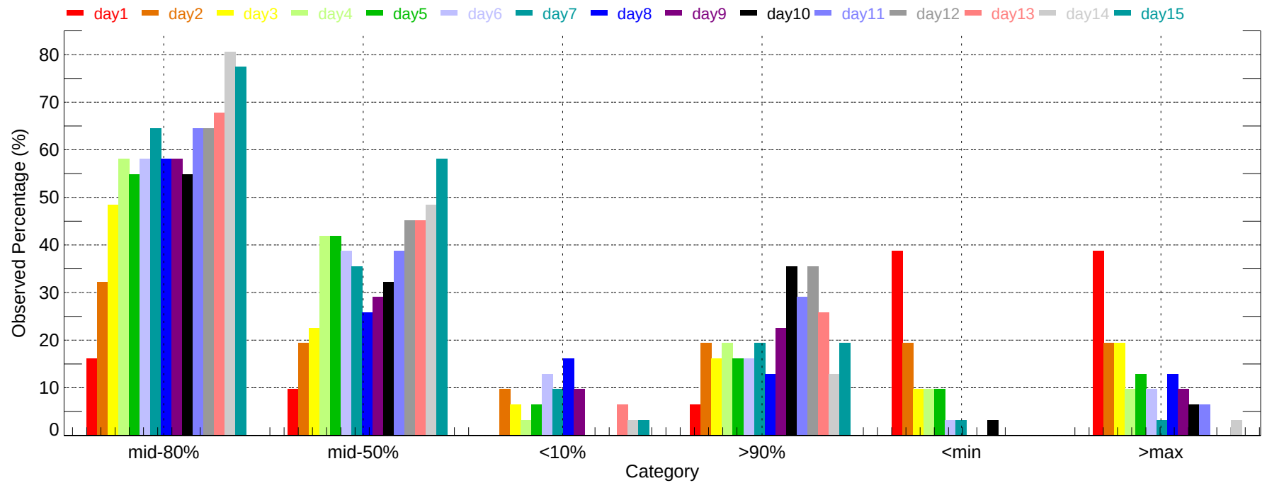
Observed Percentage of Ensembles - BNA: Min Temperature (2011-12-01~2011-12-31)
