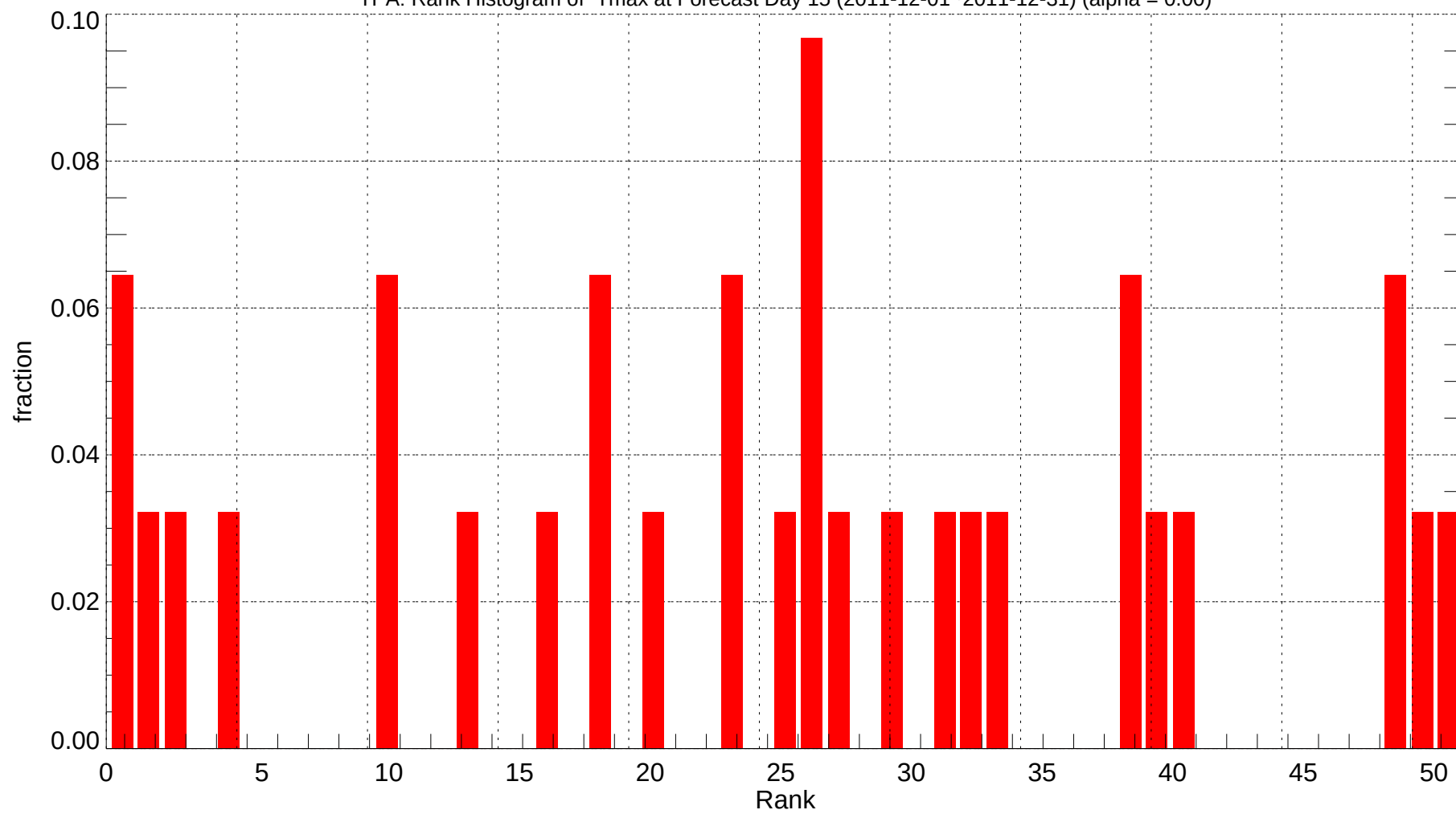
TPA: Rank Histogram of Tmax at Forecast Day 15 (2011-12-01~2011-12-31) (alpha = 0.00)
