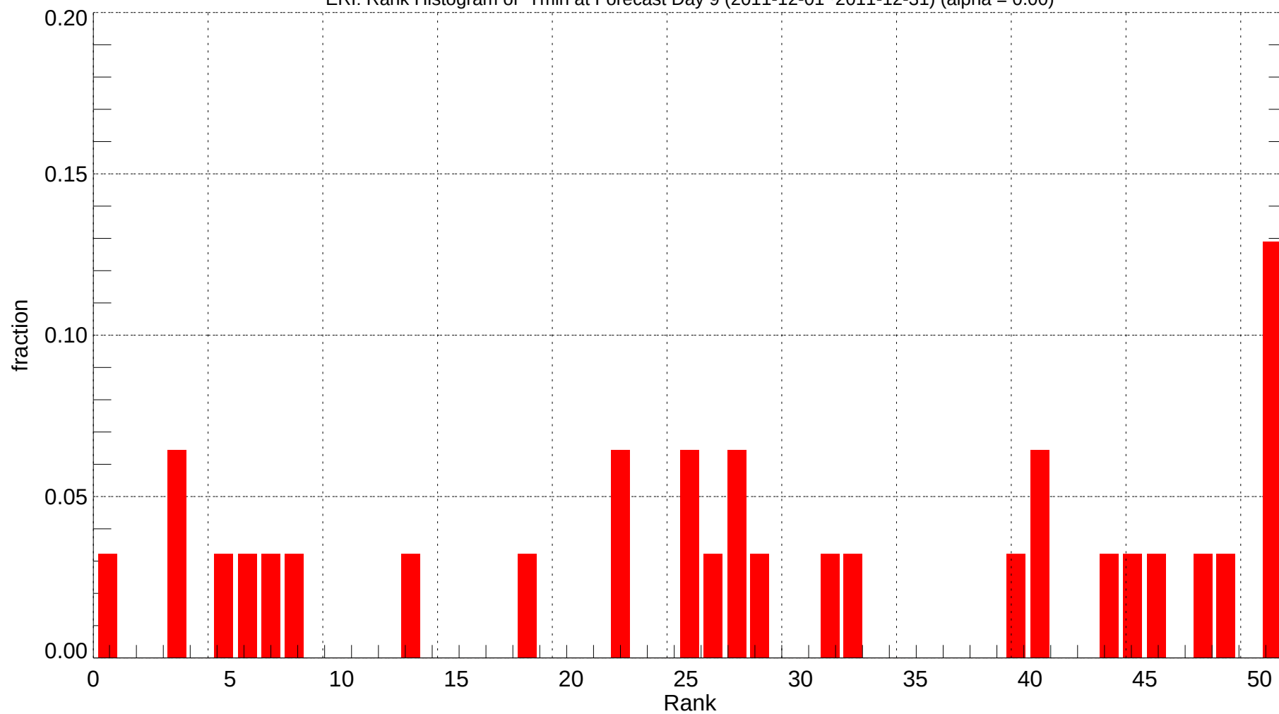
ERI: Rank Histogram of Tmin at Forecast Day 9 (2011-12-01~2011-12-31) (alpha = 0.00)
