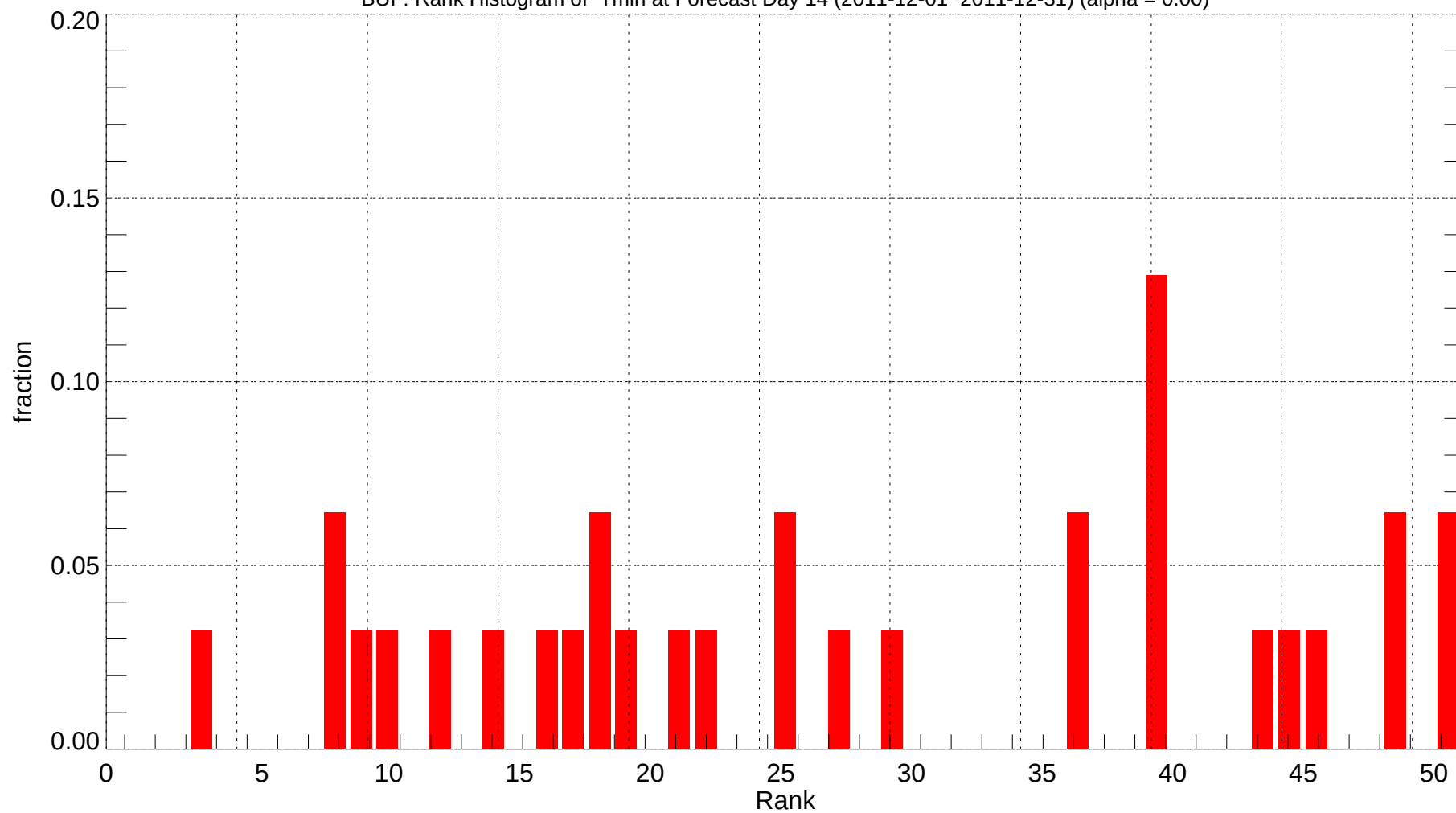
BUF: Rank Histogram of Tmin at Forecast Day 14 (2011-12-01~2011-12-31) (alpha = 0.00)
