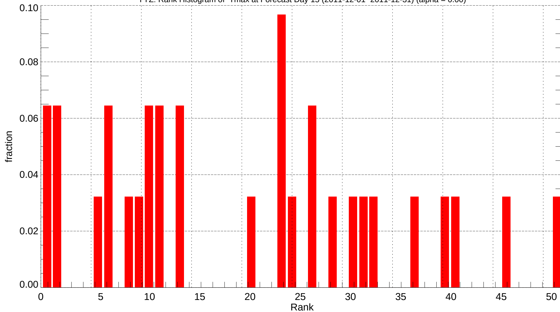
YYZ: Rank Histogram of Tmax at Forecast Day 15 (2011-12-01~2011-12-31) (alpha = 0.00)
