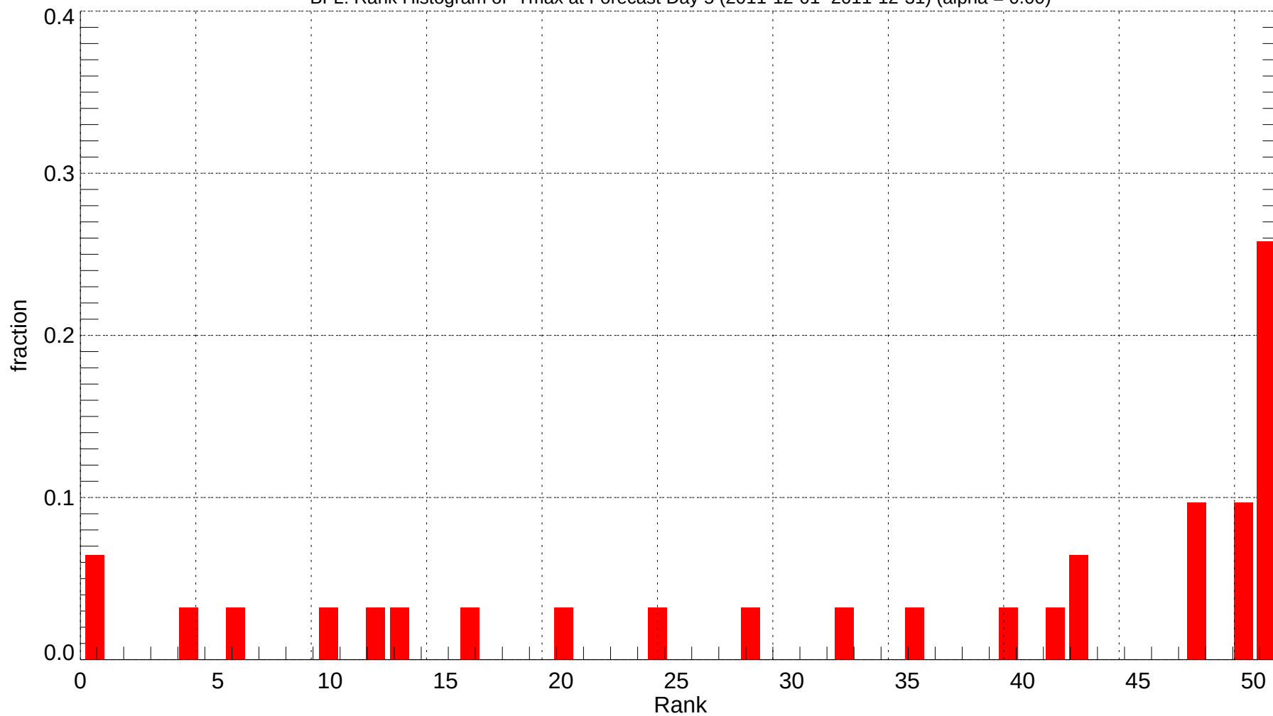
BFL: Rank Histogram of Tmax at Forecast Day 5 (2011-12-01~2011-12-31) (alpha = 0.00)
