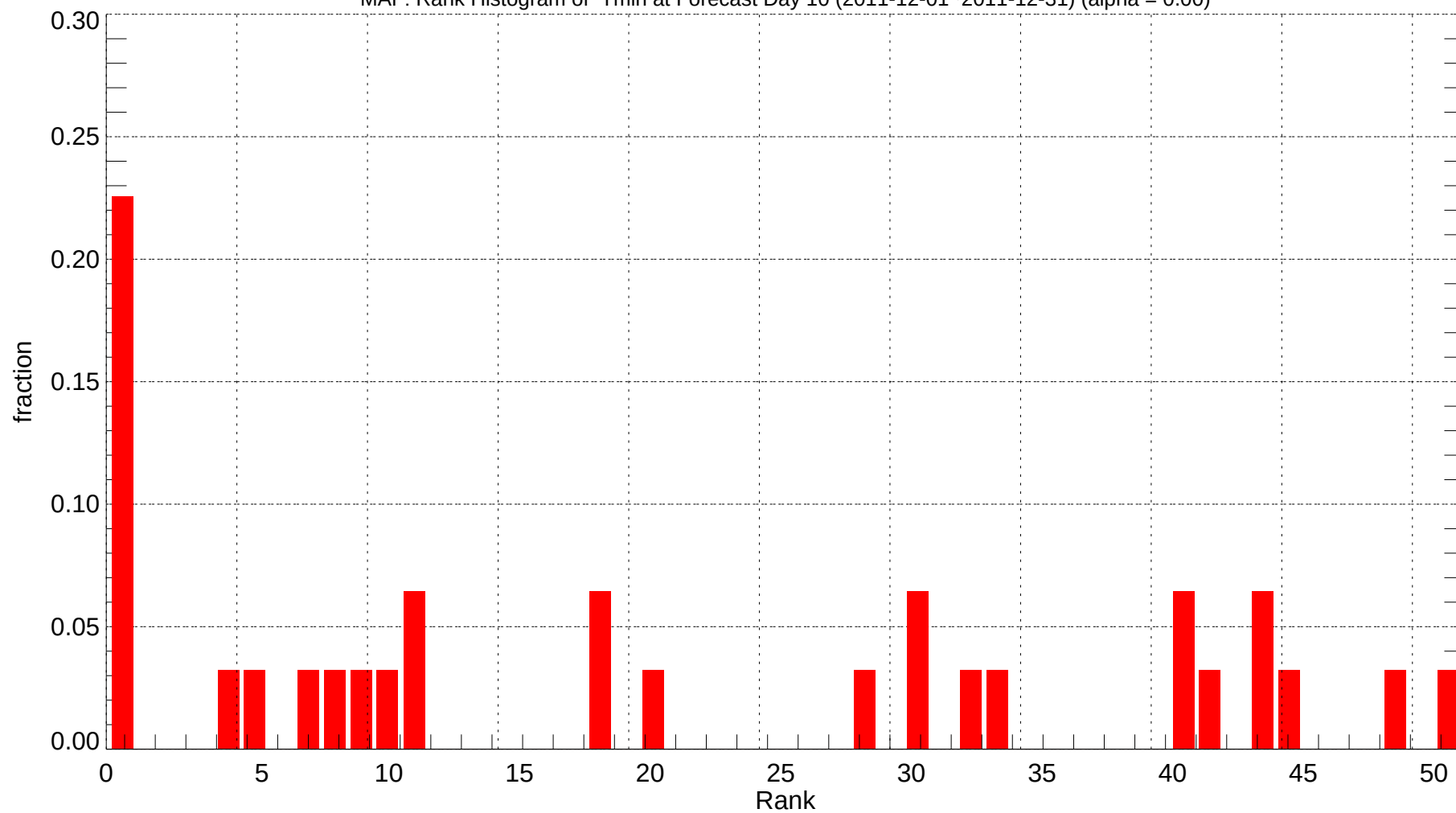
MAF: Rank Histogram of Tmin at Forecast Day 10 (2011-12-01~2011-12-31) (alpha = 0.00)
