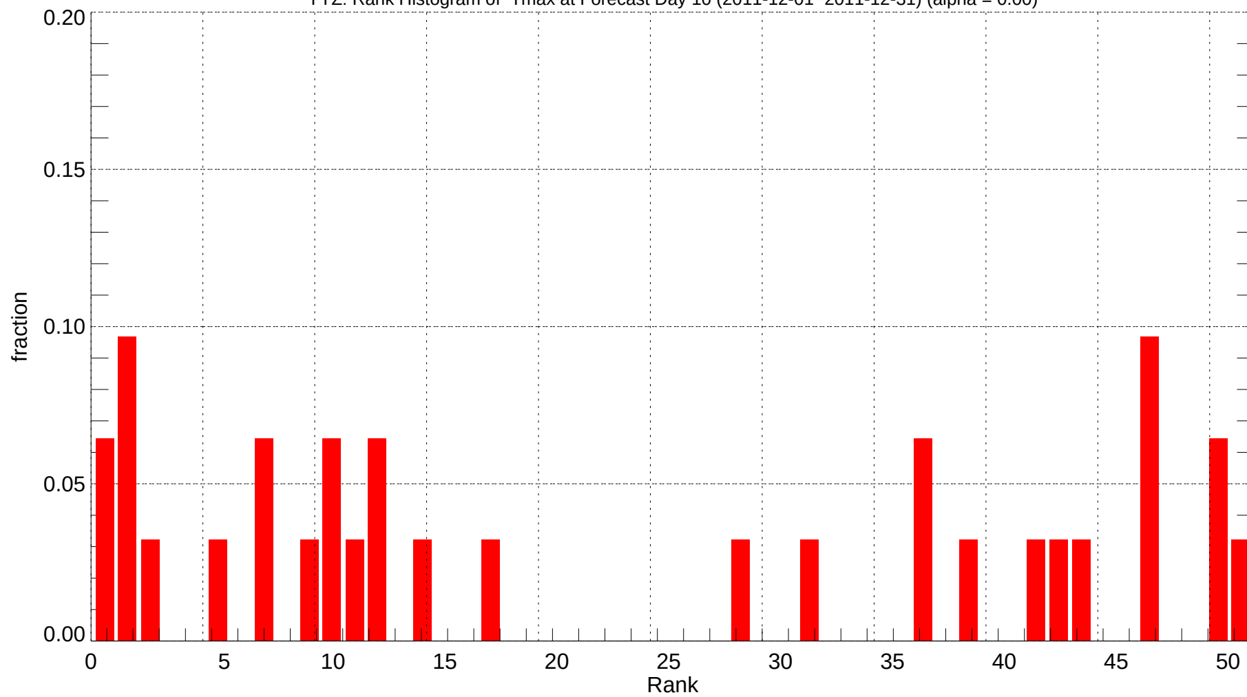
YYZ: Rank Histogram of Tmax at Forecast Day 10 (2011-12-01~2011-12-31) (alpha = 0.00)
