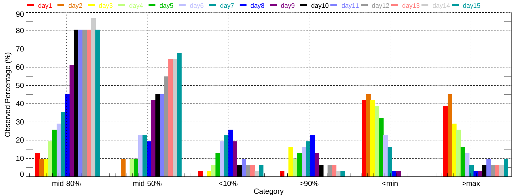
Observed Percentage of Ensembles - PDT: Min Temperature (2011-12-01~2011-12-31)
