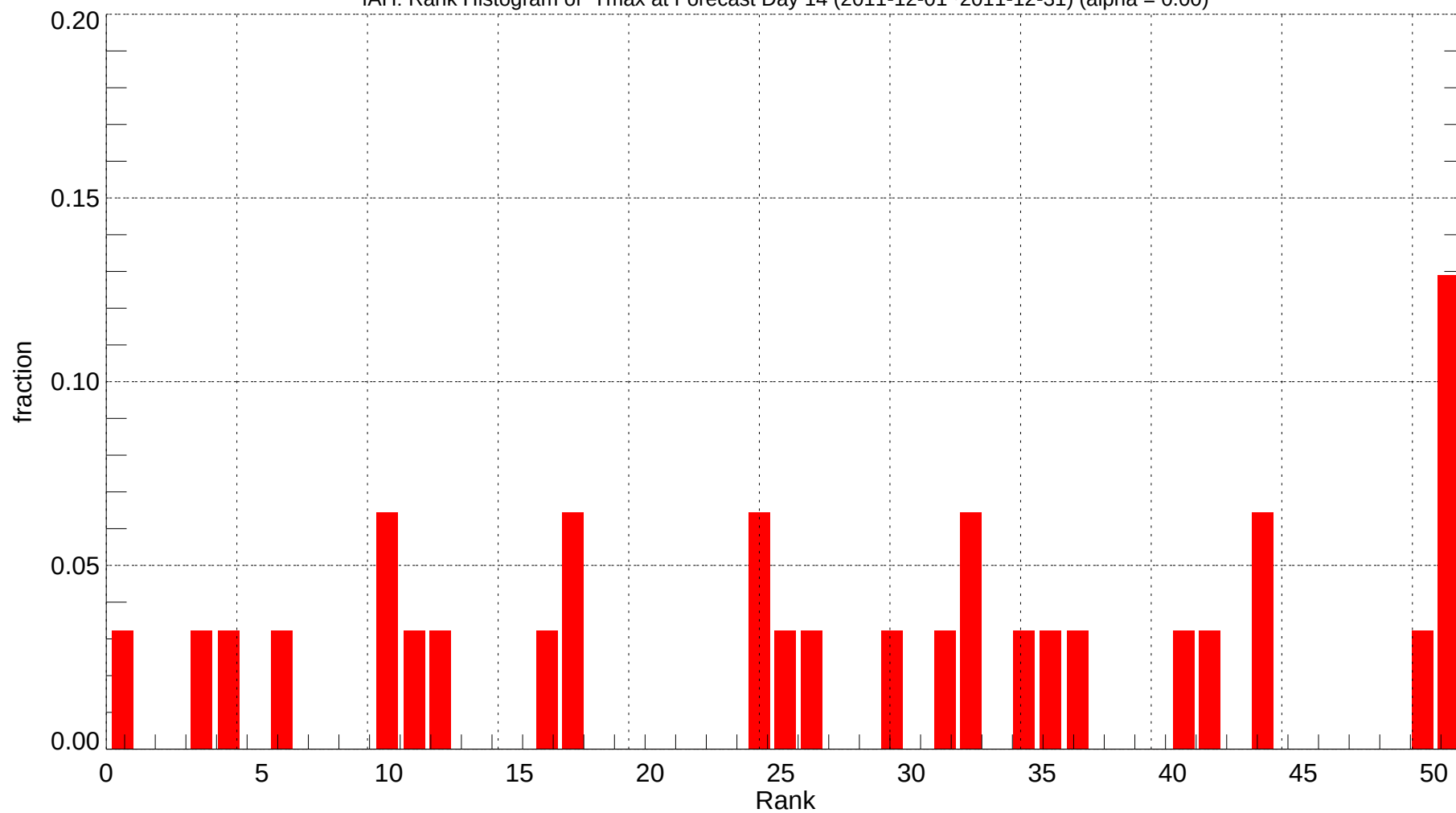
IAH: Rank Histogram of Tmax at Forecast Day 14 (2011-12-01~2011-12-31) (alpha = 0.00)
