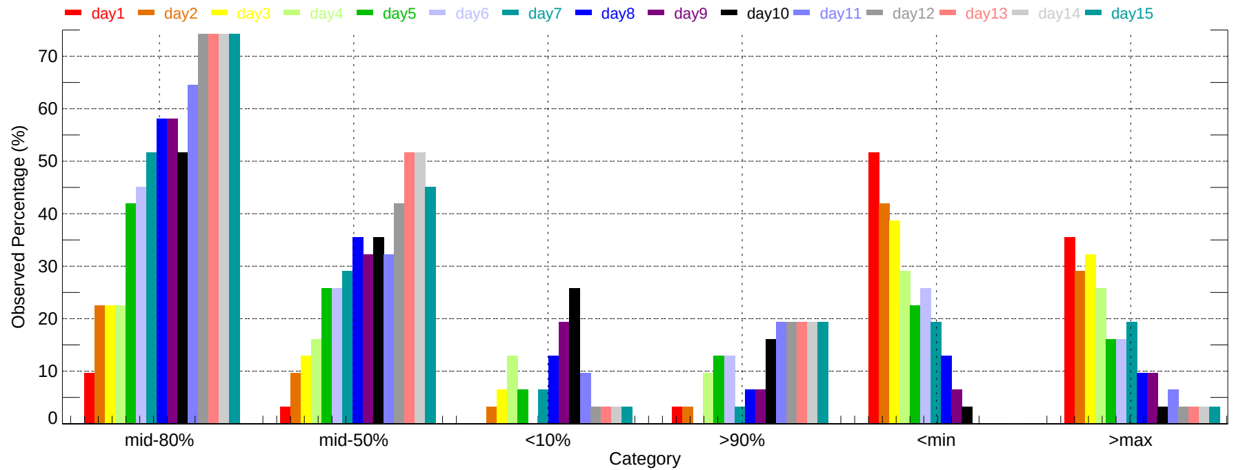
Observed Percentage of Ensembles - BUR: Min Temperature (2011-12-01~2011-12-31)
