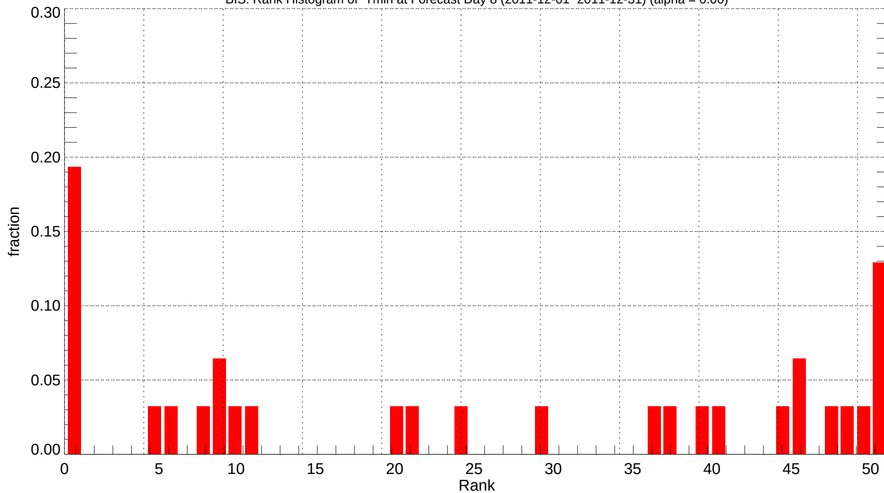
BIS: Rank Histogram of Tmin at Forecast Day 8 (2011-12-01~2011-12-31) (alpha = 0.00)
