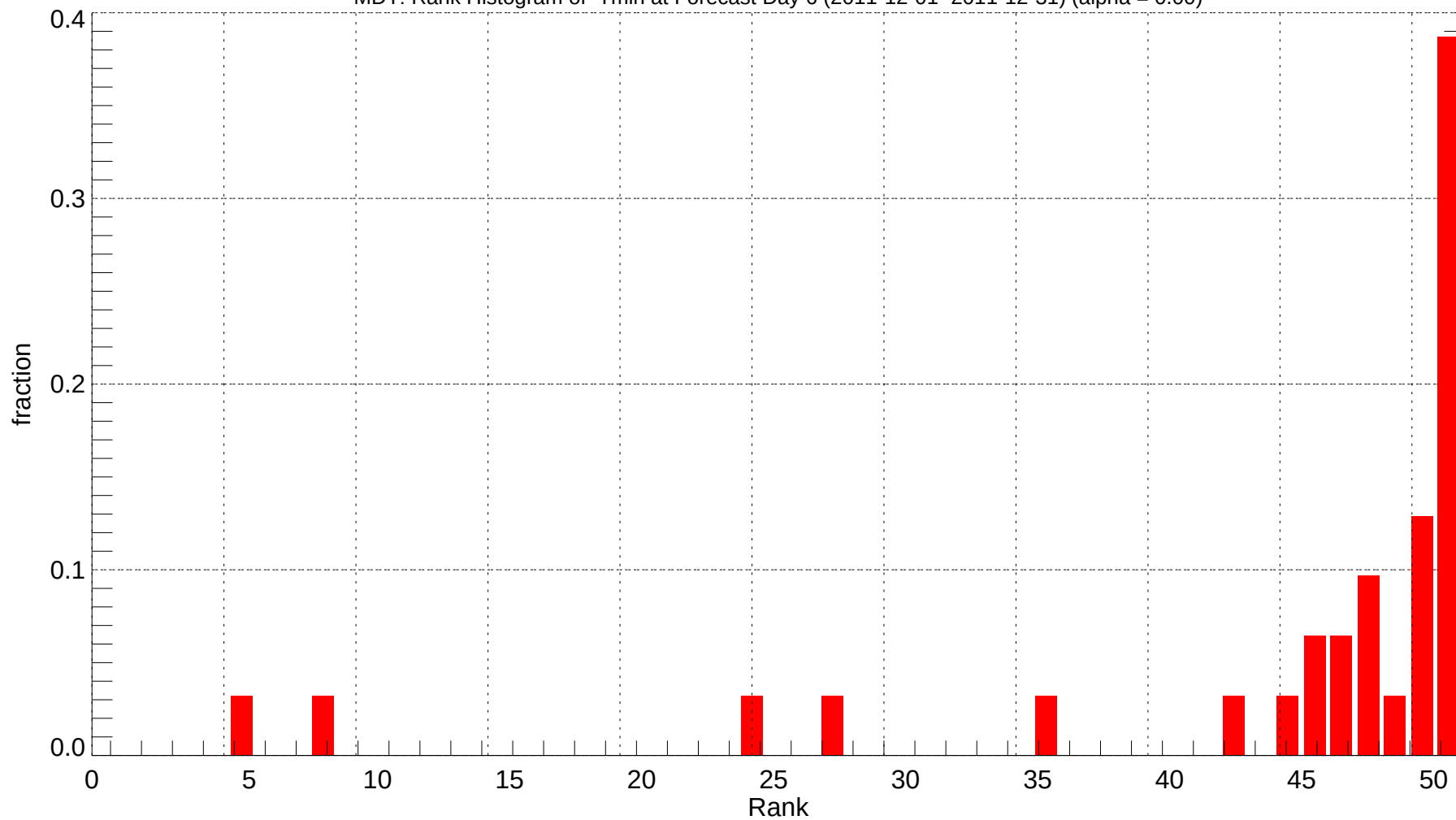
MDT: Rank Histogram of Tmin at Forecast Day 6 (2011-12-01~2011-12-31) (alpha = 0.00)
