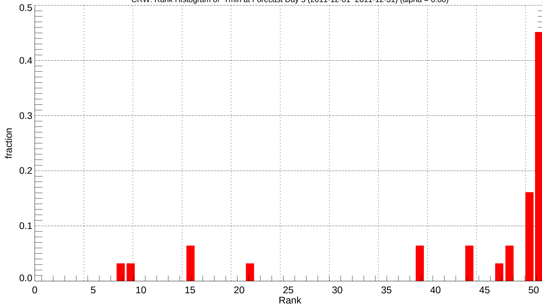
CRW: Rank Histogram of Tmin at Forecast Day 5 (2011-12-01~2011-12-31) (alpha = 0.00)
