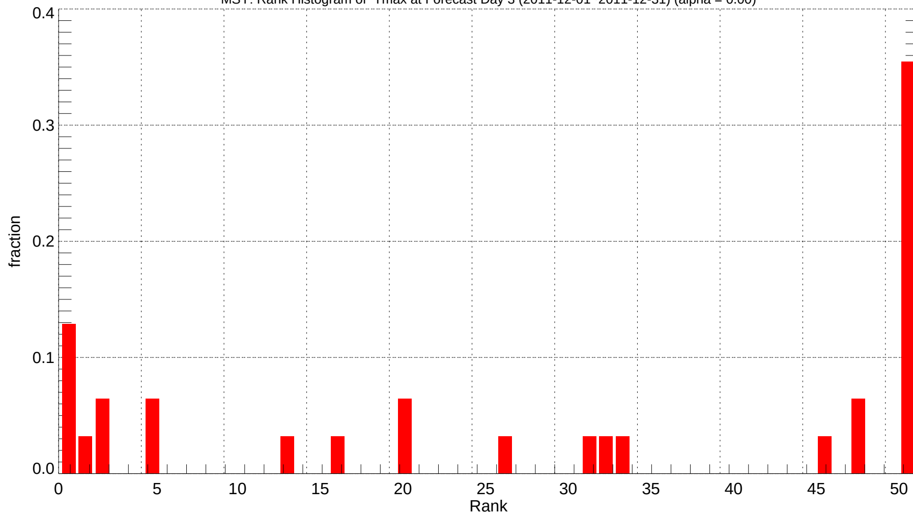
MSY: Rank Histogram of Tmax at Forecast Day 3 (2011-12-01~2011-12-31) (alpha = 0.00)
