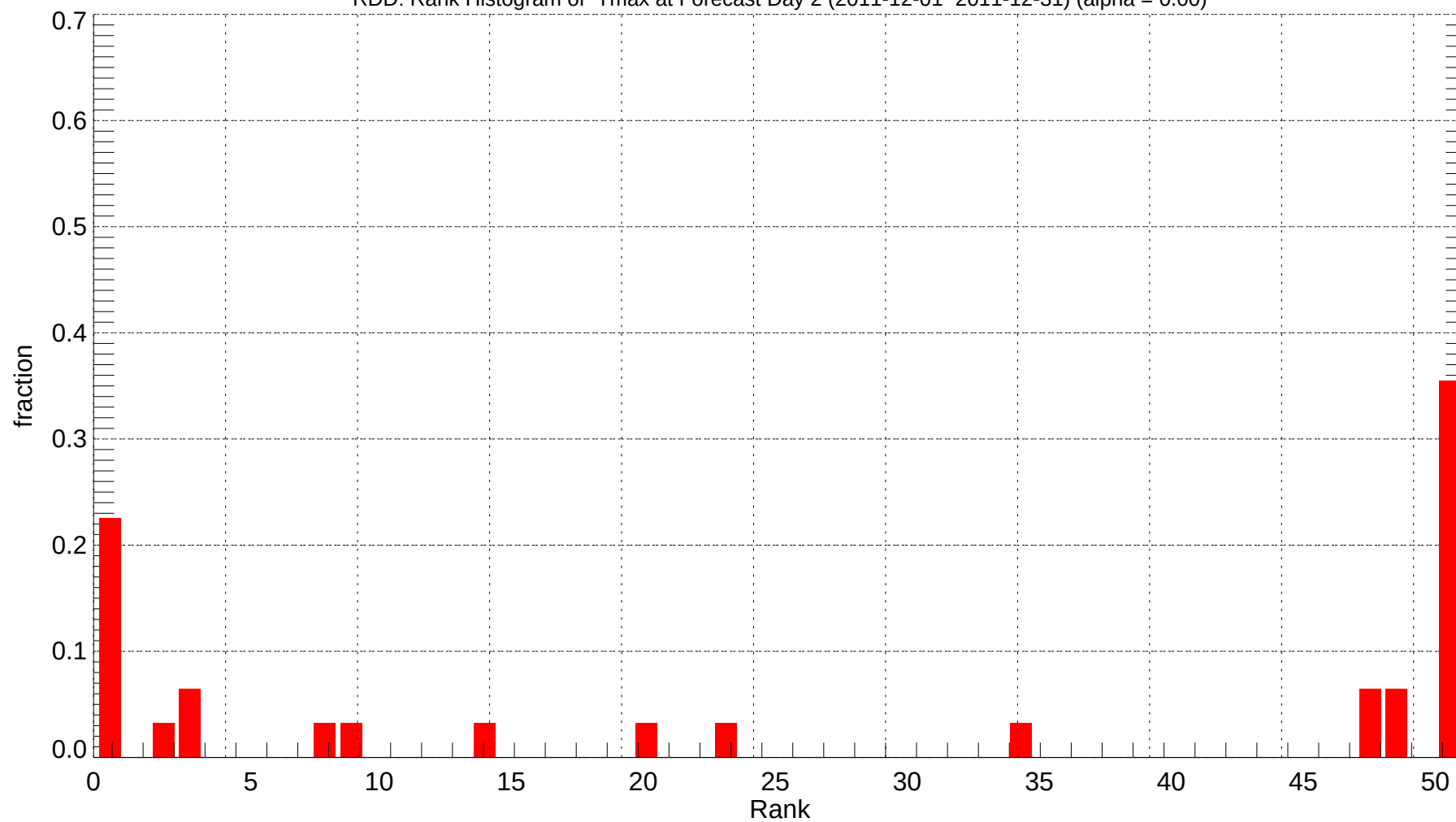
RDD: Rank Histogram of Tmax at Forecast Day 2 (2011-12-01~2011-12-31) (alpha = 0.00)
