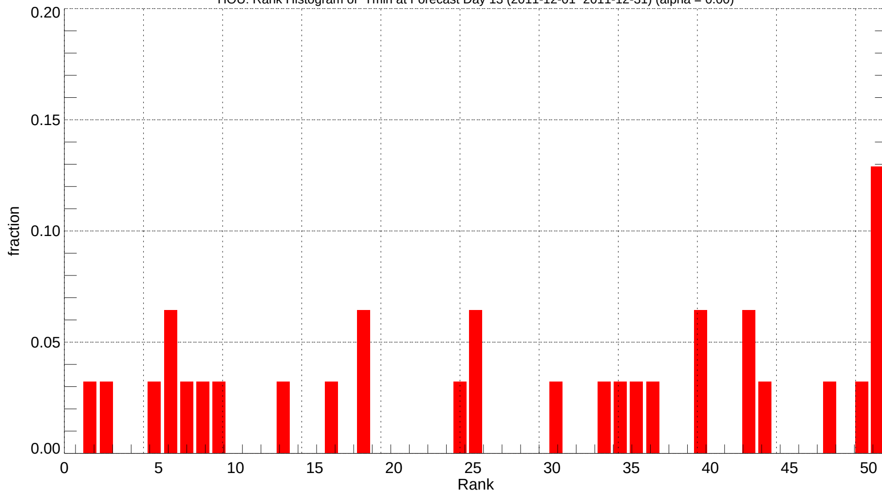
HOU: Rank Histogram of Tmin at Forecast Day 13 (2011-12-01~2011-12-31) (alpha = 0.00)
