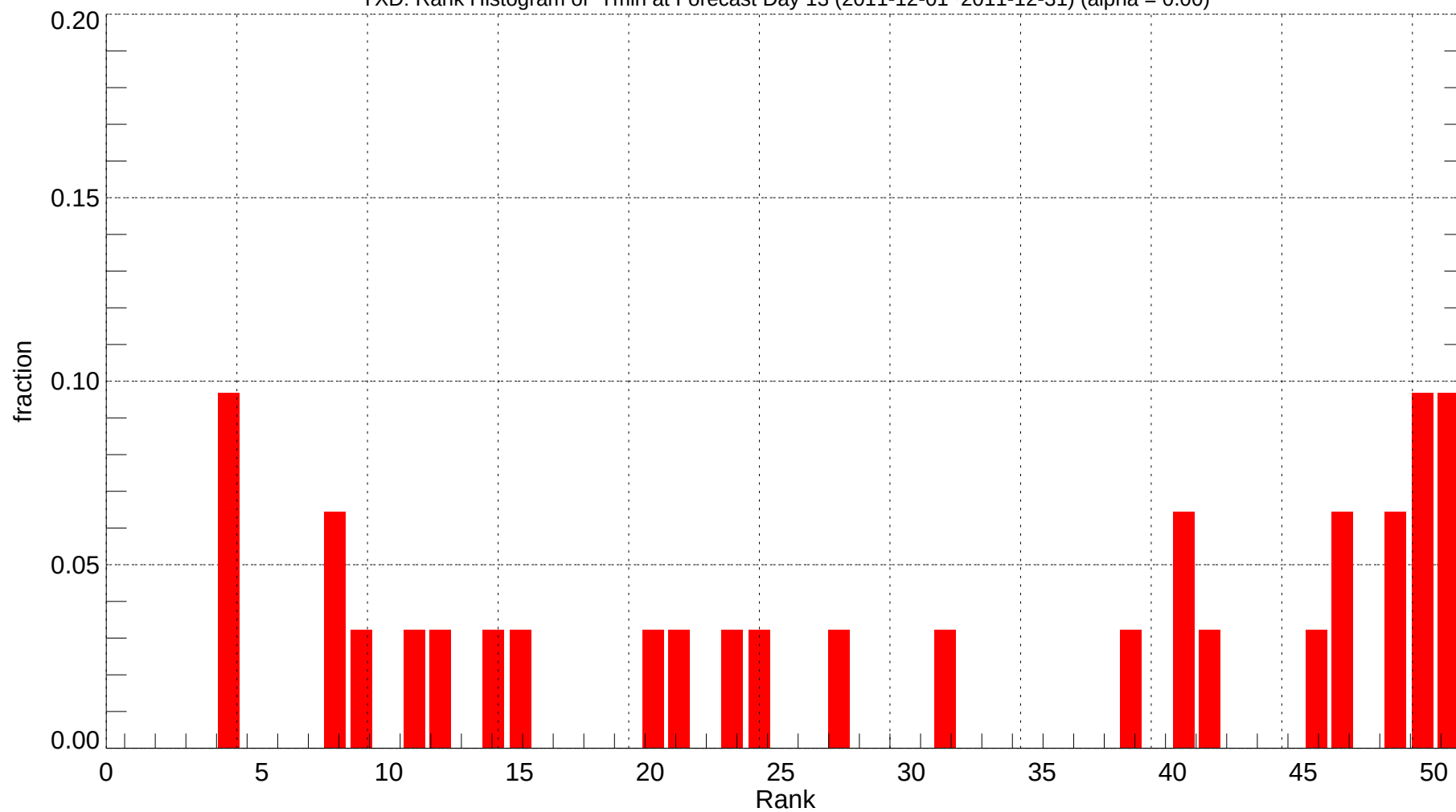
YXD: Rank Histogram of Tmin at Forecast Day 13 (2011-12-01~2011-12-31) (alpha = 0.00)
