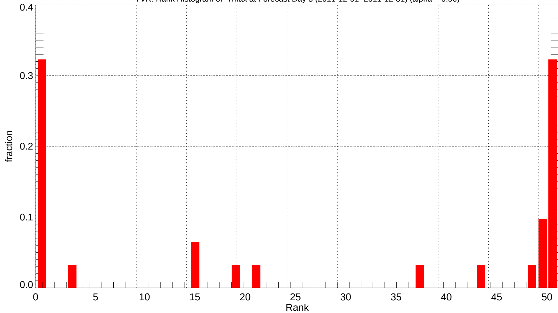
YVR: Rank Histogram of Tmax at Forecast Day 5 (2011-12-01~2011-12-31) (alpha = 0.00)
