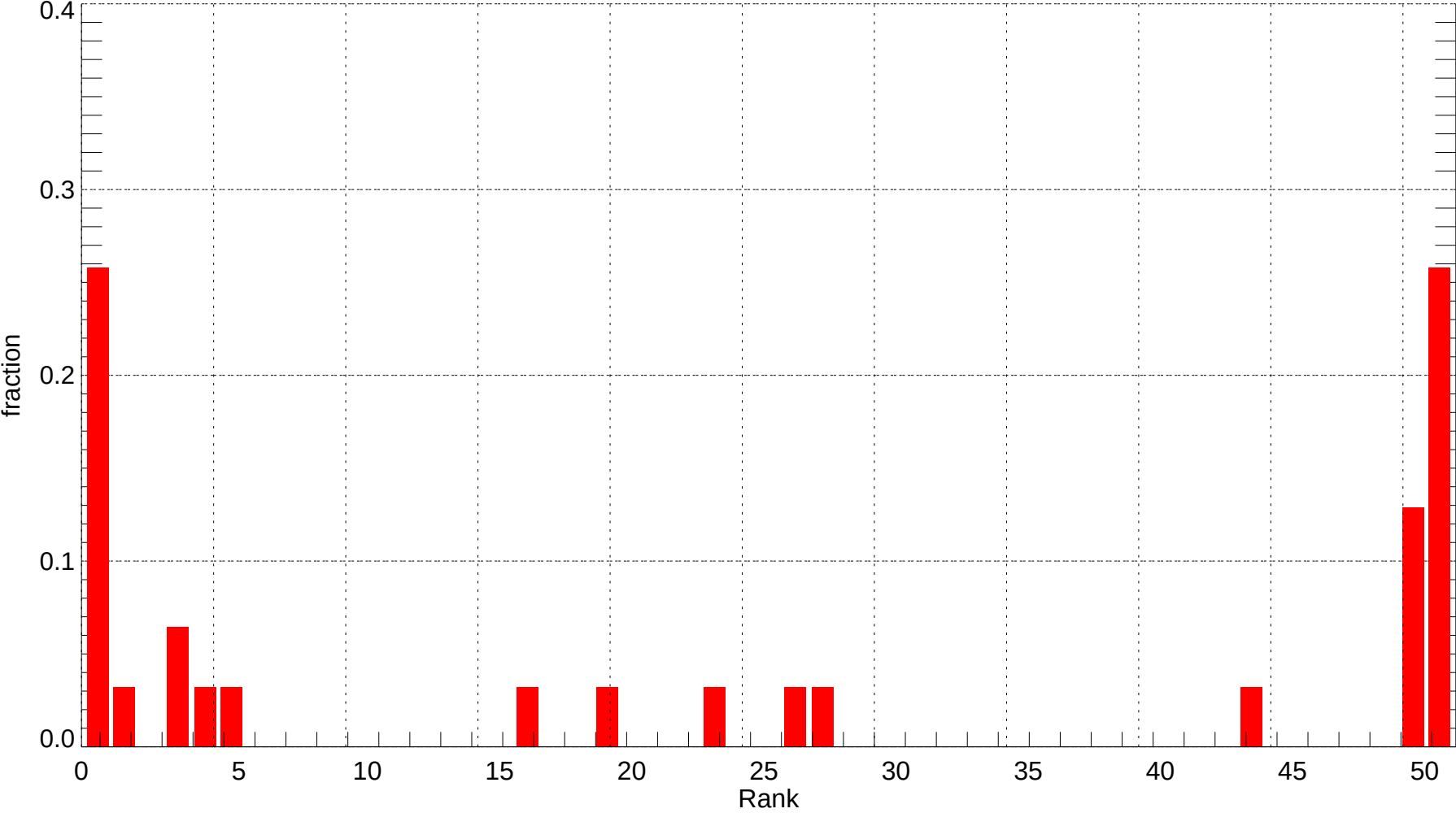
MCI: Rank Histogram of Tmin at Forecast Day 1 (2011-12-01~2011-12-31) (alpha = 0.00)
