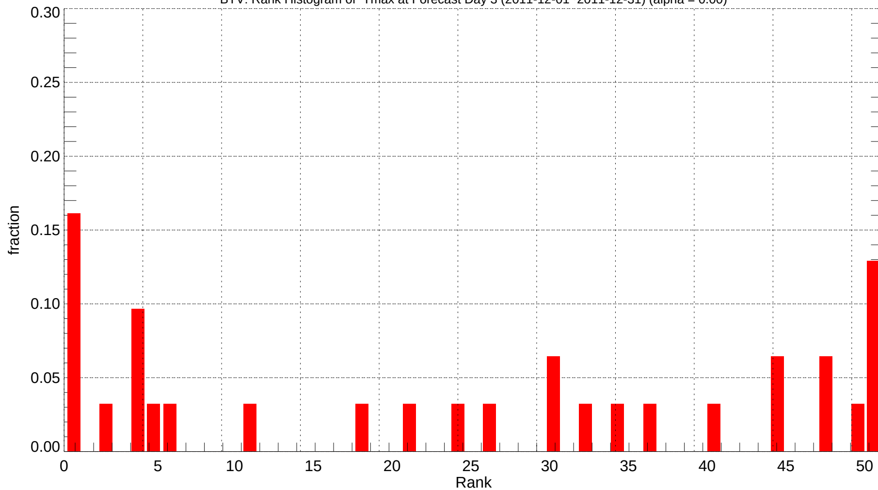
BTV: Rank Histogram of Tmax at Forecast Day 3 (2011-12-01~2011-12-31) (alpha = 0.00)
