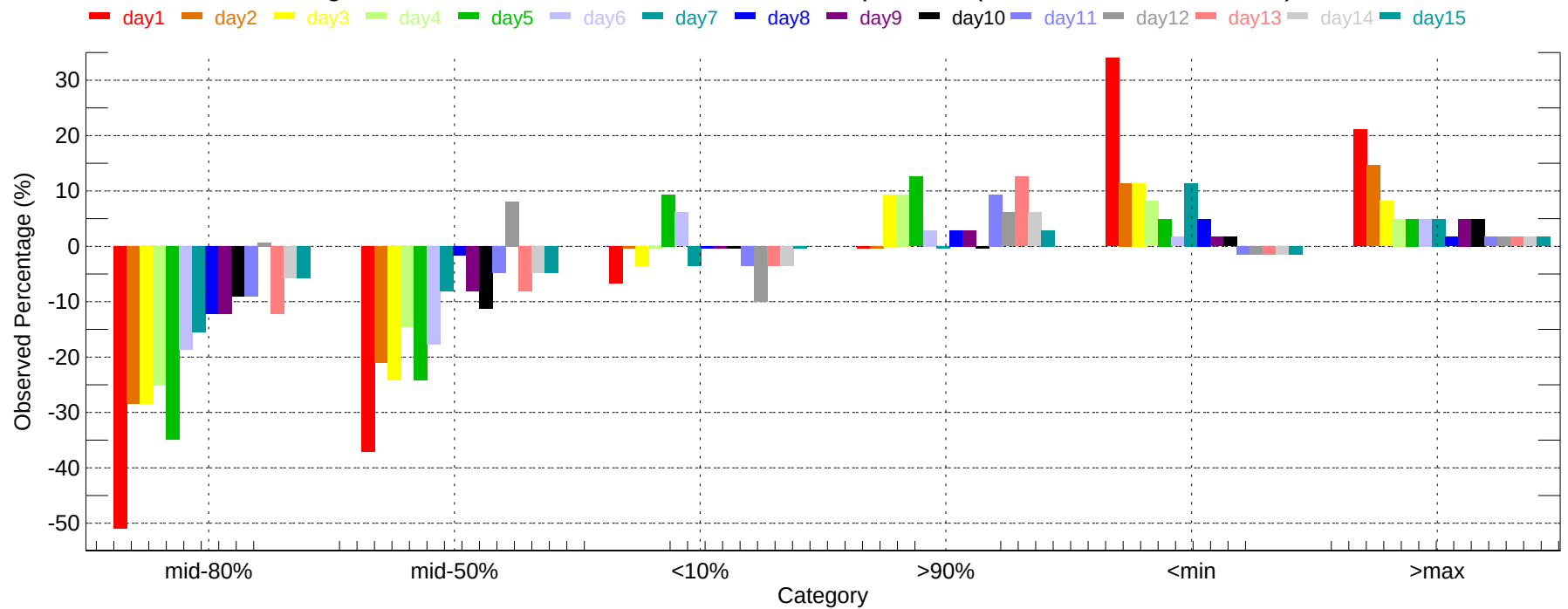
Observed Percentage Deviation of Ensembles - LNS: Min Temperature (2011-12-01~2011-12-31)
