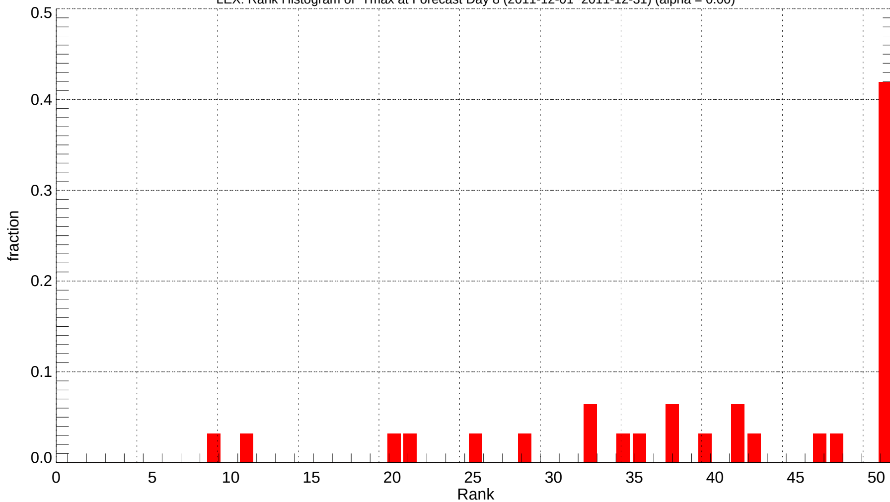
LEX: Rank Histogram of Tmax at Forecast Day 8 (2011-12-01~2011-12-31) (alpha = 0.00)
