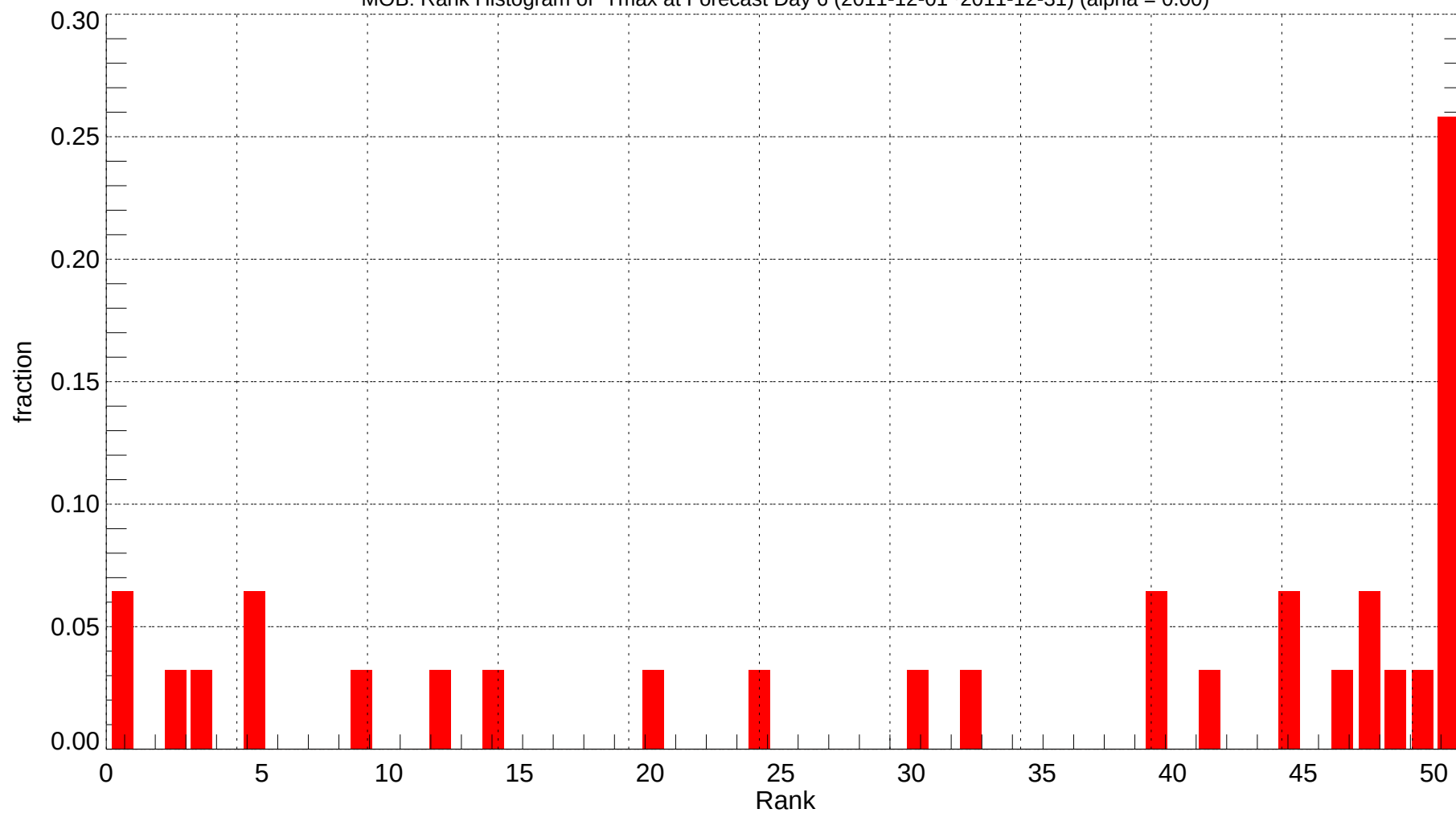
MOB: Rank Histogram of Tmax at Forecast Day 6 (2011-12-01~2011-12-31) (alpha = 0.00)
