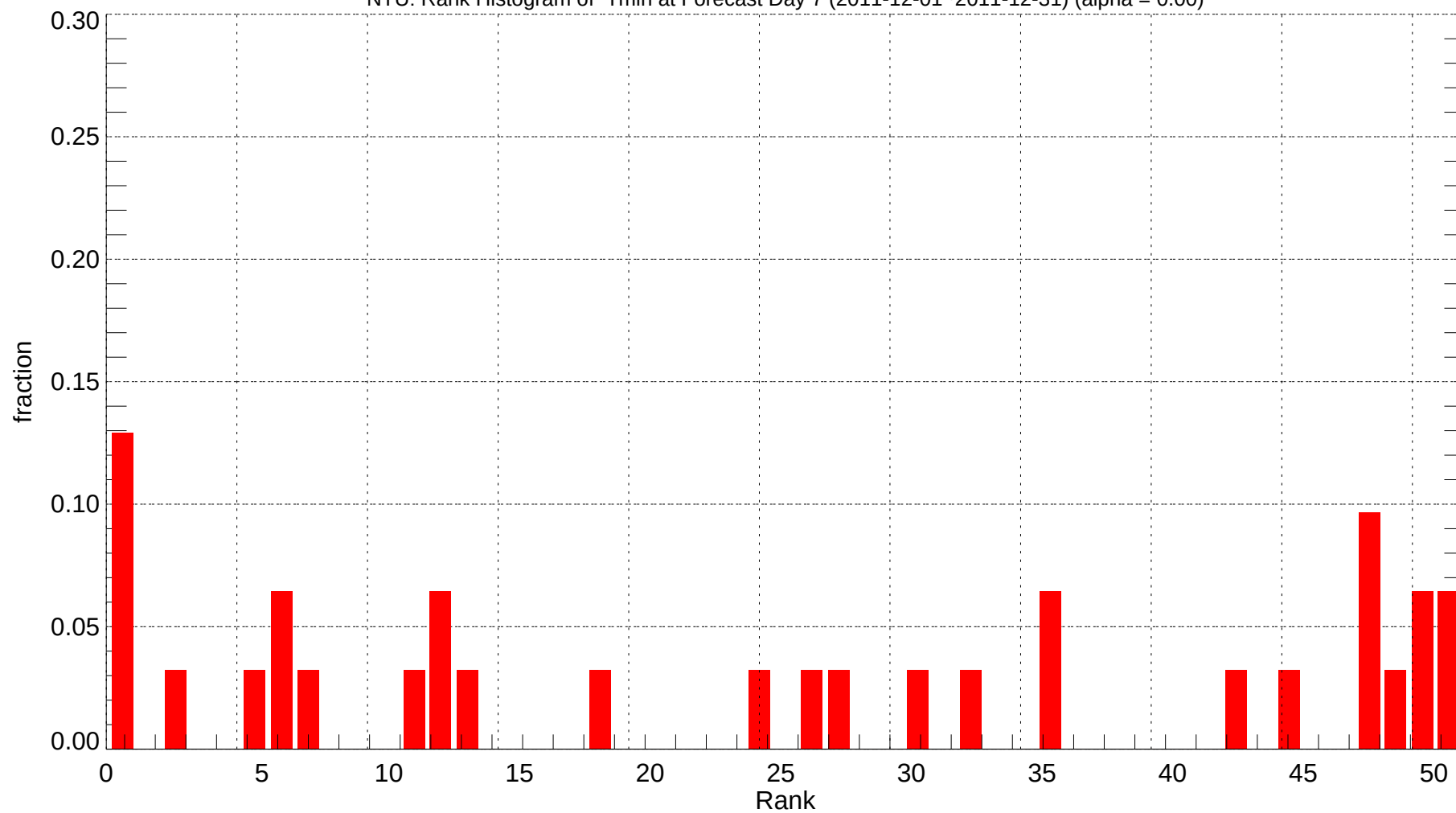
NTU: Rank Histogram of Tmin at Forecast Day 7 (2011-12-01~2011-12-31) (alpha = 0.00)
