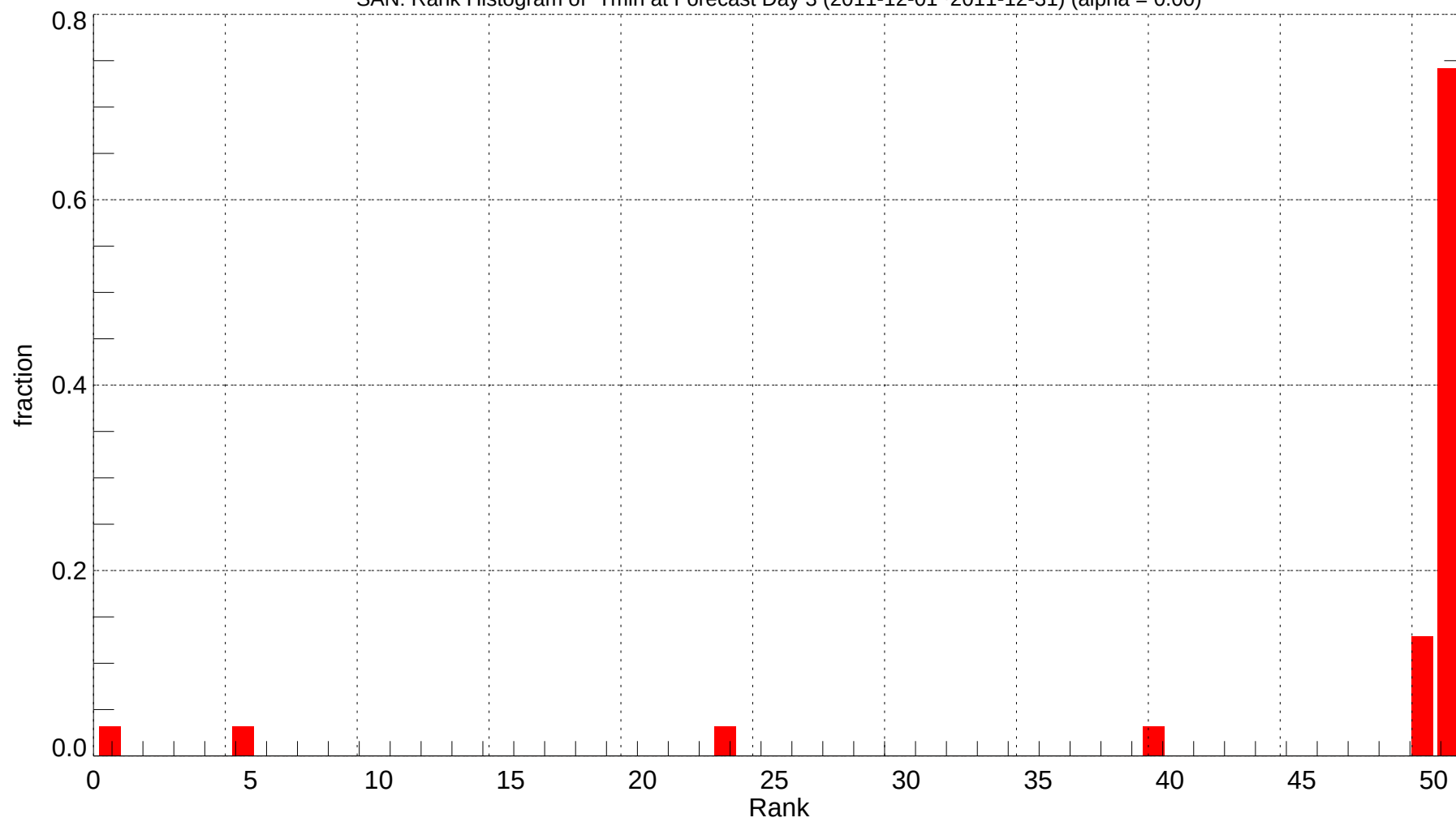
SAN: Rank Histogram of Tmin at Forecast Day 3 (2011-12-01~2011-12-31) (alpha = 0.00)
