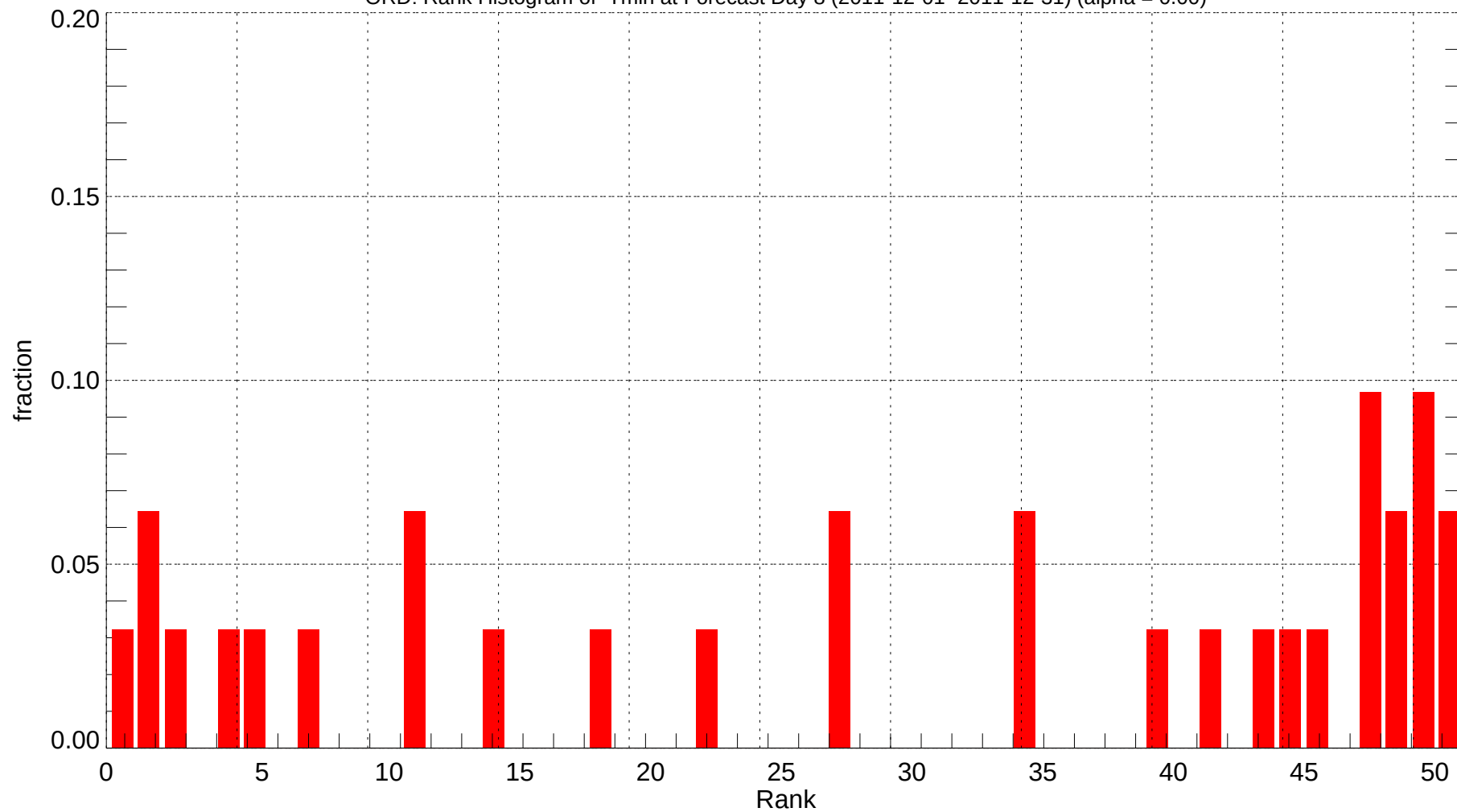
ORD: Rank Histogram of Tmin at Forecast Day 8 (2011-12-01~2011-12-31) (alpha = 0.00)
