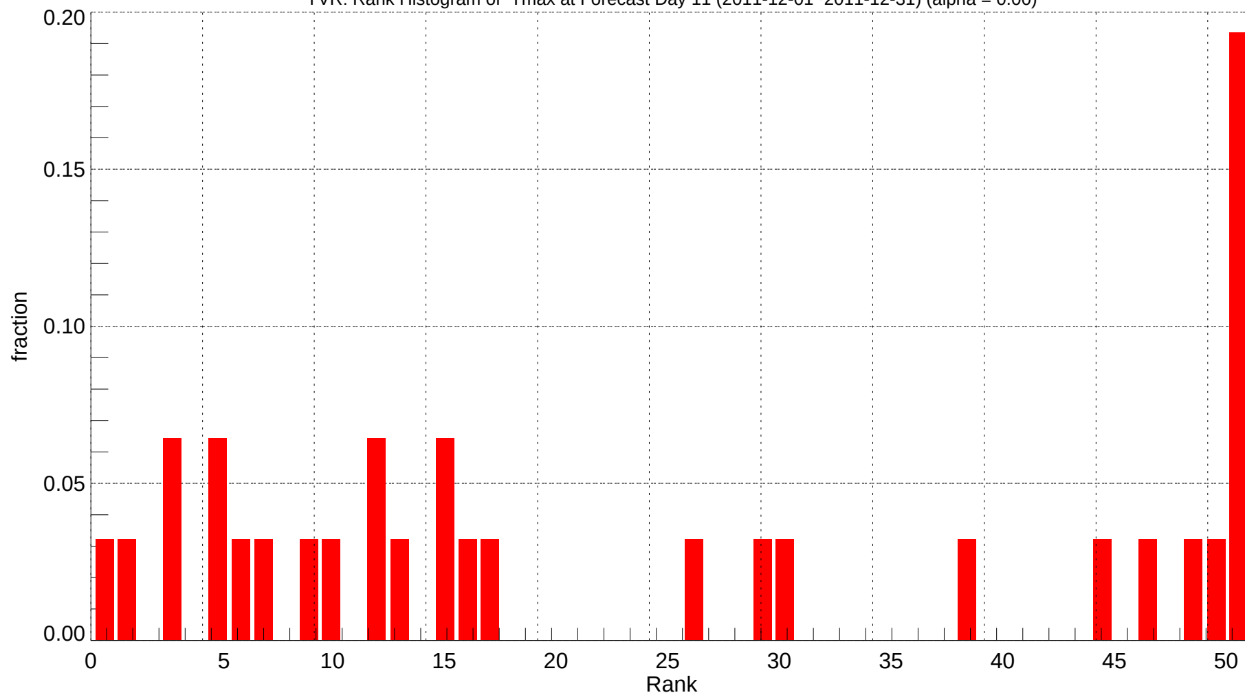
YVR: Rank Histogram of Tmax at Forecast Day 11 (2011-12-01~2011-12-31) (alpha = 0.00)
