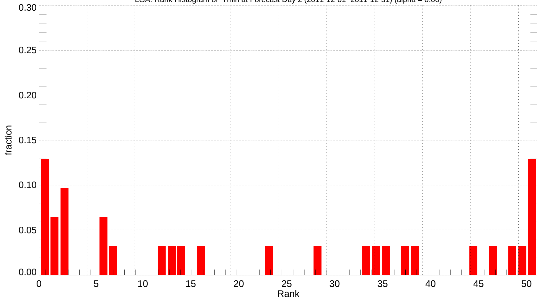
LGA: Rank Histogram of Tmin at Forecast Day 2 (2011-12-01~2011-12-31) (alpha = 0.00)
