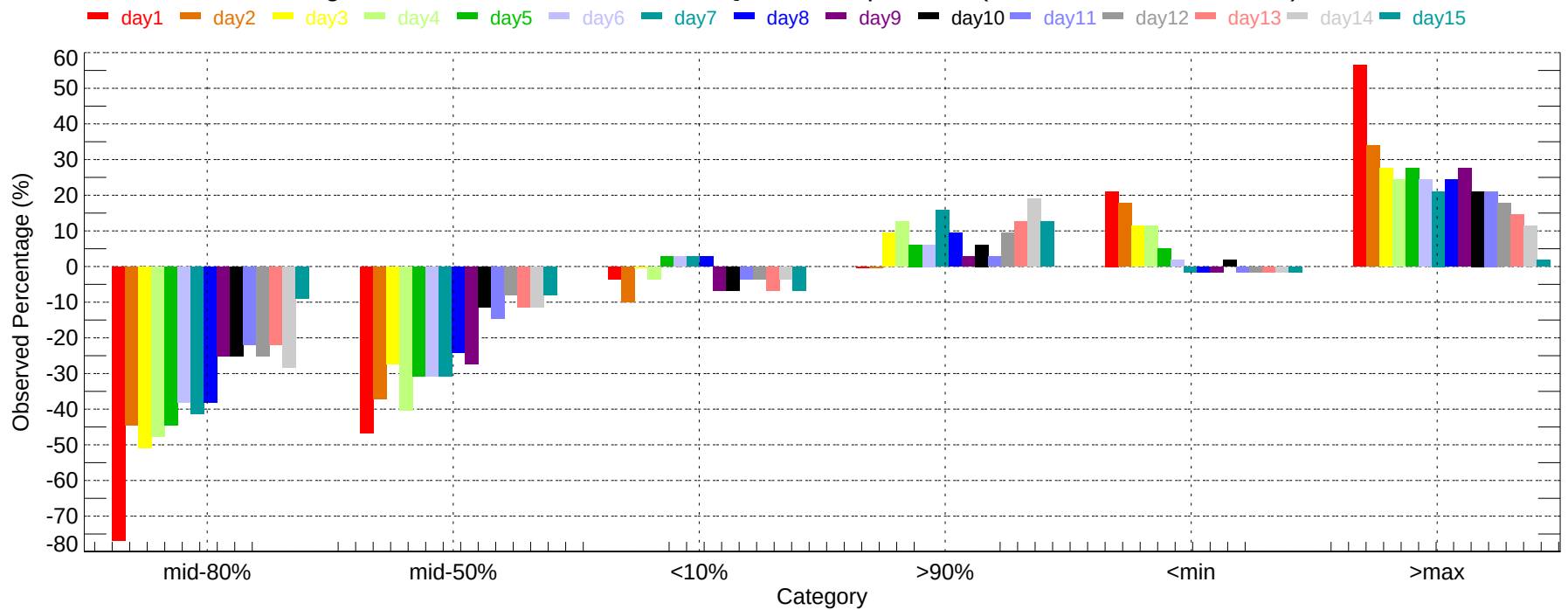
Observed Percentage Deviation of Ensembles - DBQ: Min Temperature (2011-12-01~2011-12-31)
