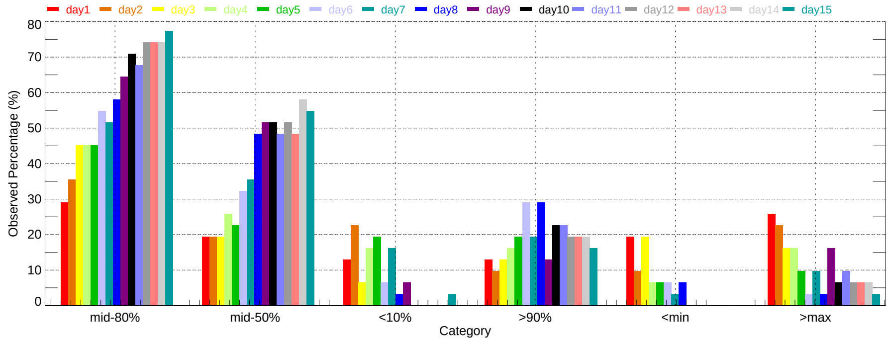
Observed Percentage of Ensembles - CAE: Max Temperature (2011-12-01~2011-12-31)
