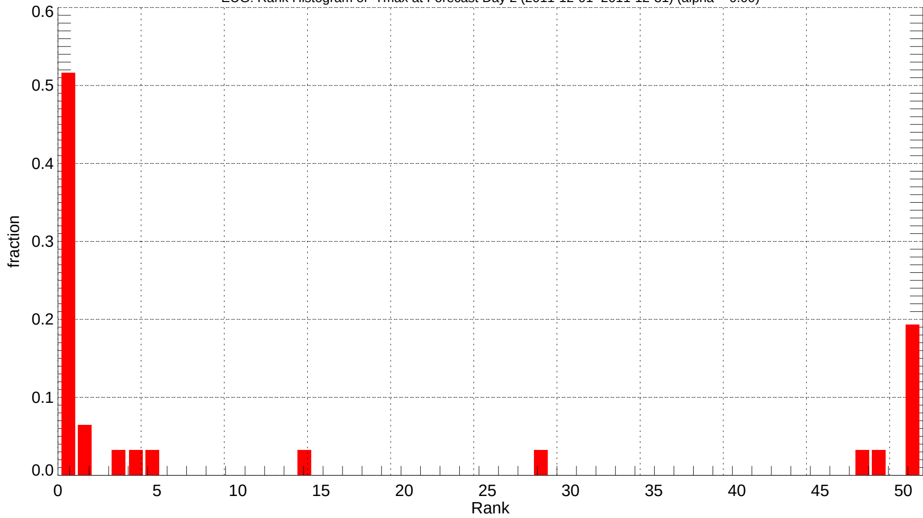
EUG: Rank Histogram of Tmax at Forecast Day 2 (2011-12-01~2011-12-31) (alpha = 0.00)
