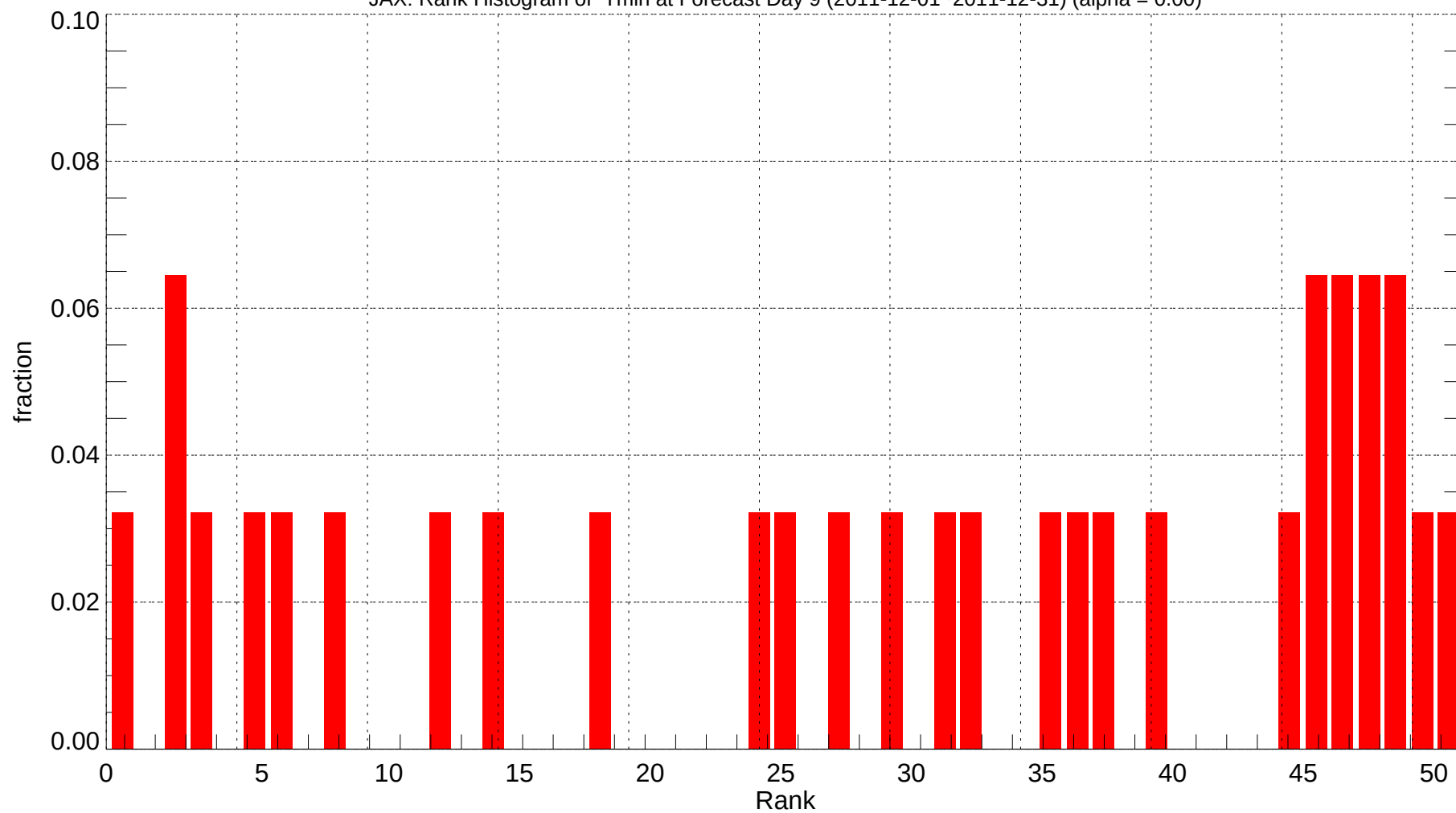
JAX: Rank Histogram of Tmin at Forecast Day 9 (2011-12-01~2011-12-31) (alpha = 0.00)
