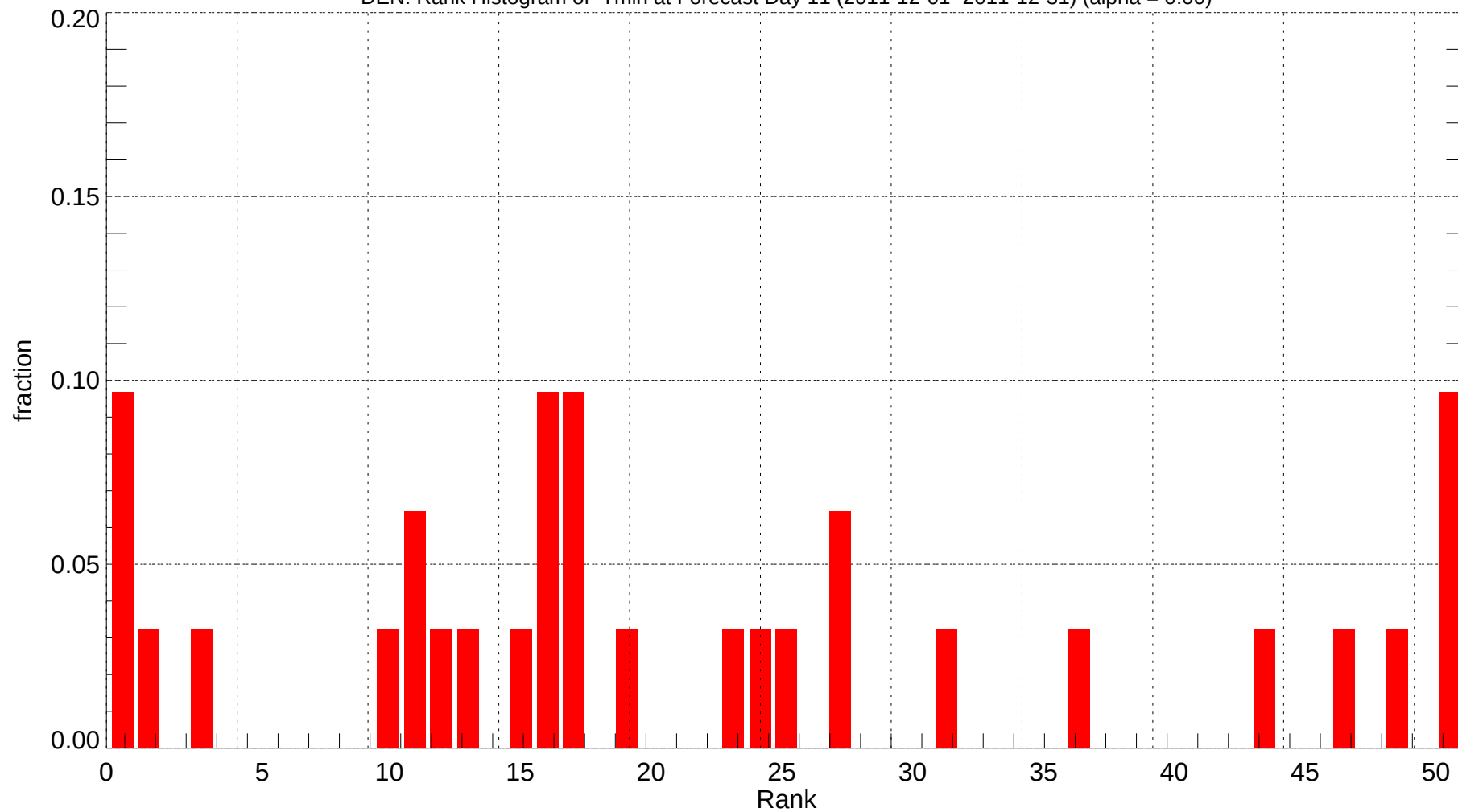
DEN: Rank Histogram of Tmin at Forecast Day 11 (2011-12-01~2011-12-31) (alpha = 0.00)
