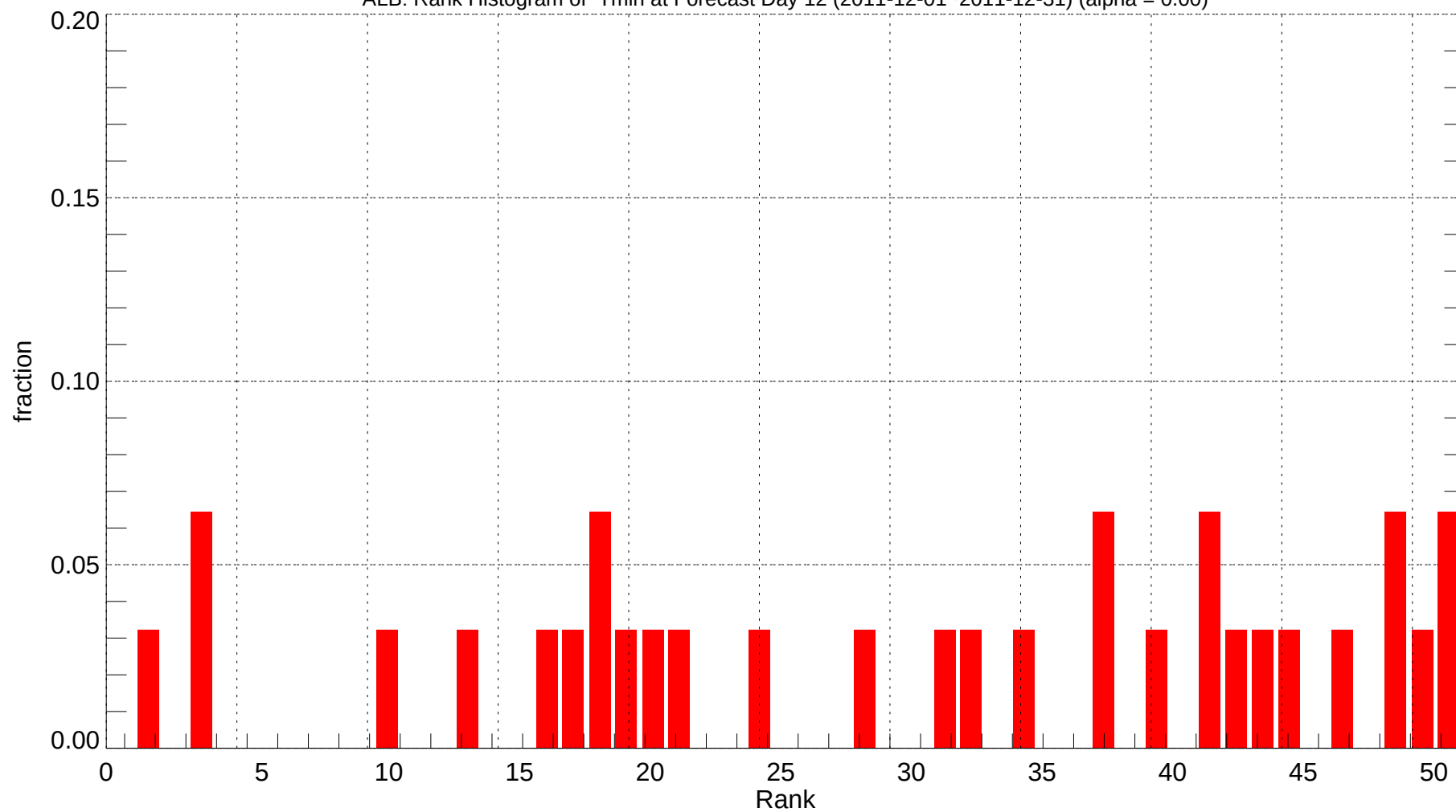
ALB: Rank Histogram of Tmin at Forecast Day 12 (2011-12-01~2011-12-31) (alpha = 0.00)
