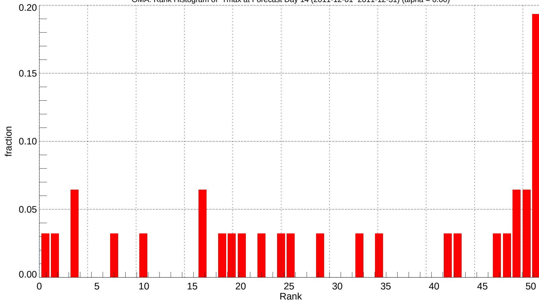
OMA: Rank Histogram of Tmax at Forecast Day 14 (2011-12-01~2011-12-31) (alpha = 0.00)
