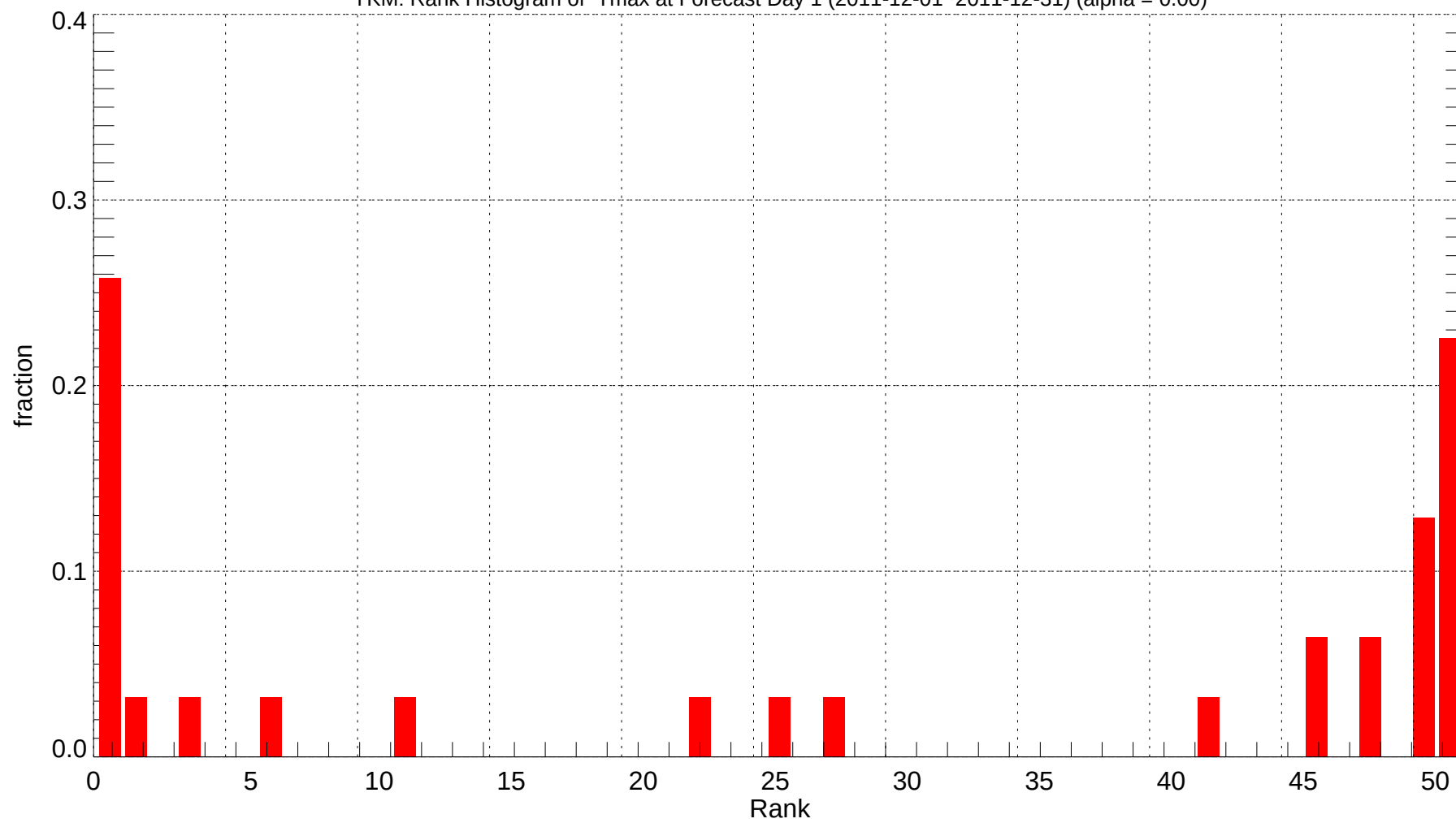
YKM: Rank Histogram of Tmax at Forecast Day 1 (2011-12-01~2011-12-31) (alpha = 0.00)
