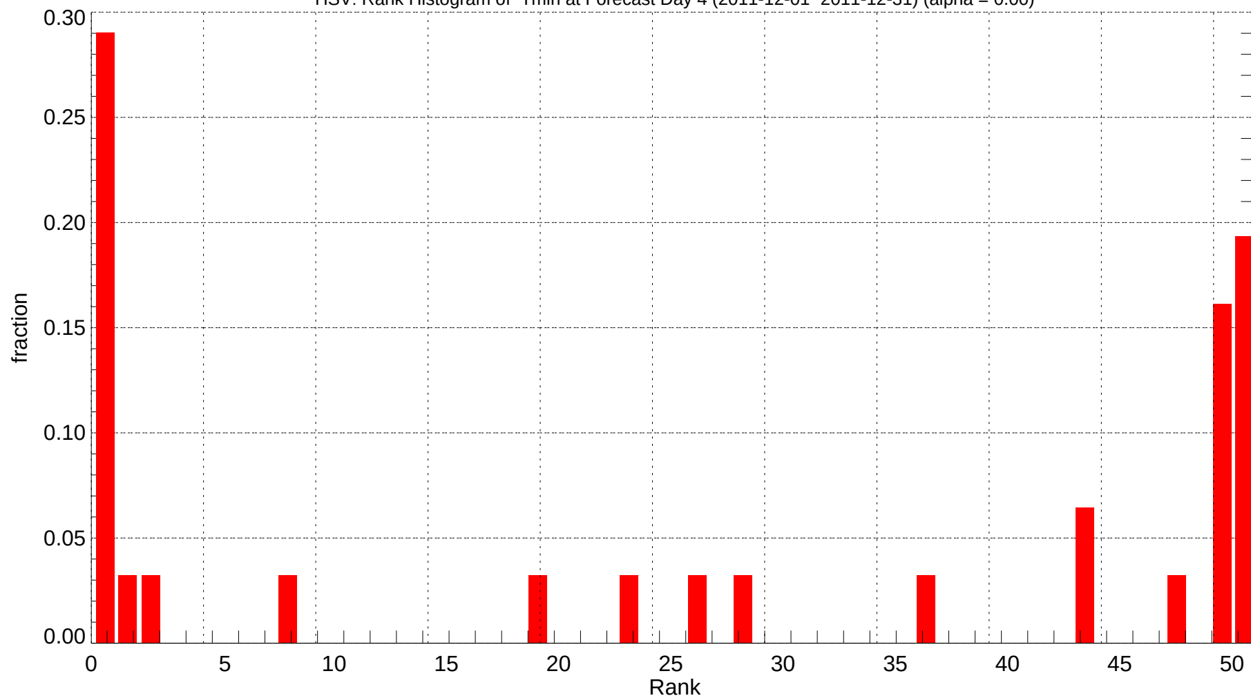
HSV: Rank Histogram of Tmin at Forecast Day 4 (2011-12-01~2011-12-31) (alpha = 0.00)
