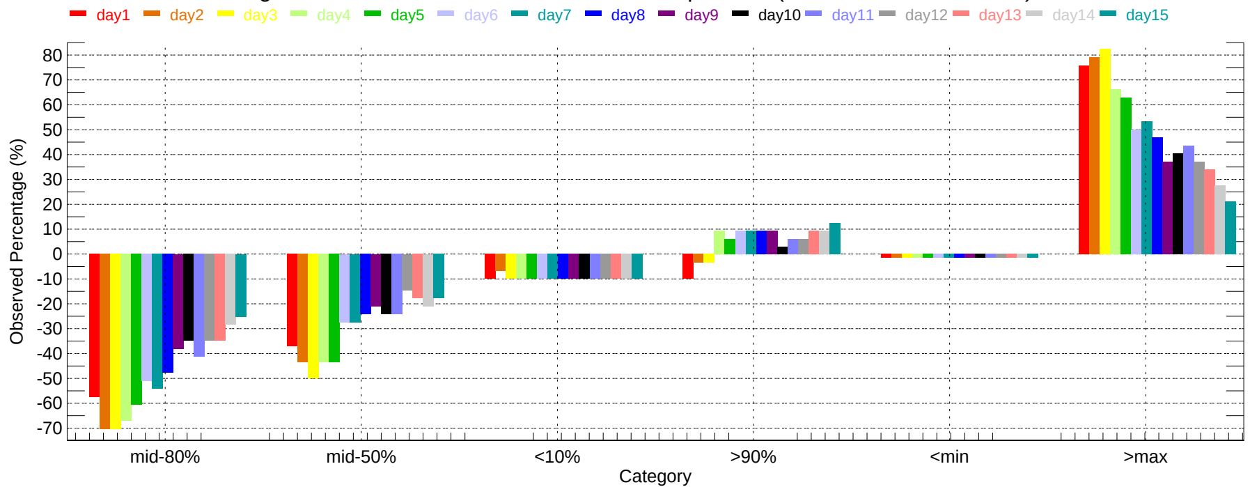
Observed Percentage Deviation of Ensembles - GTF: Min Temperature (2011-12-01~2011-12-31)
