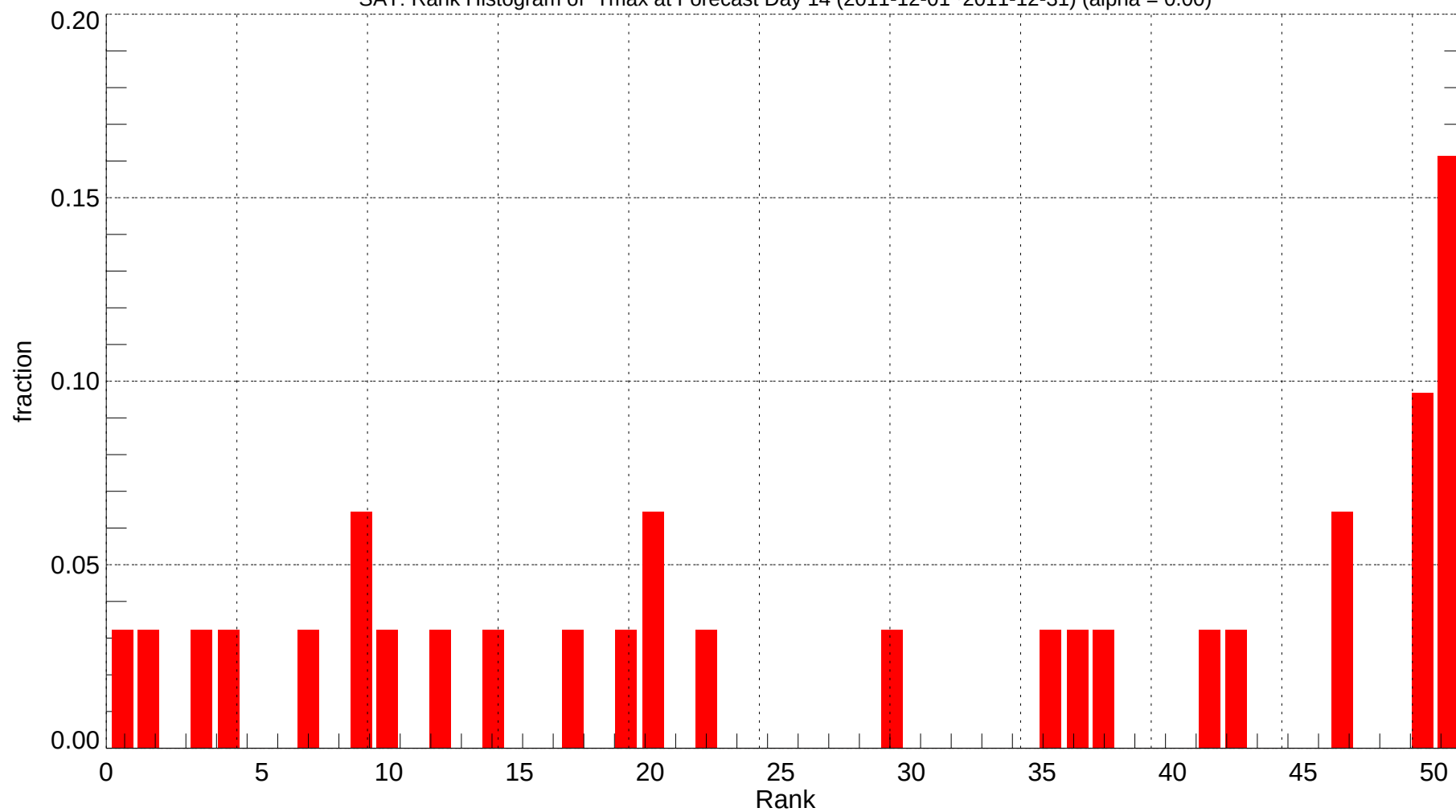
SAT: Rank Histogram of Tmax at Forecast Day 14 (2011-12-01~2011-12-31) (alpha = 0.00)
