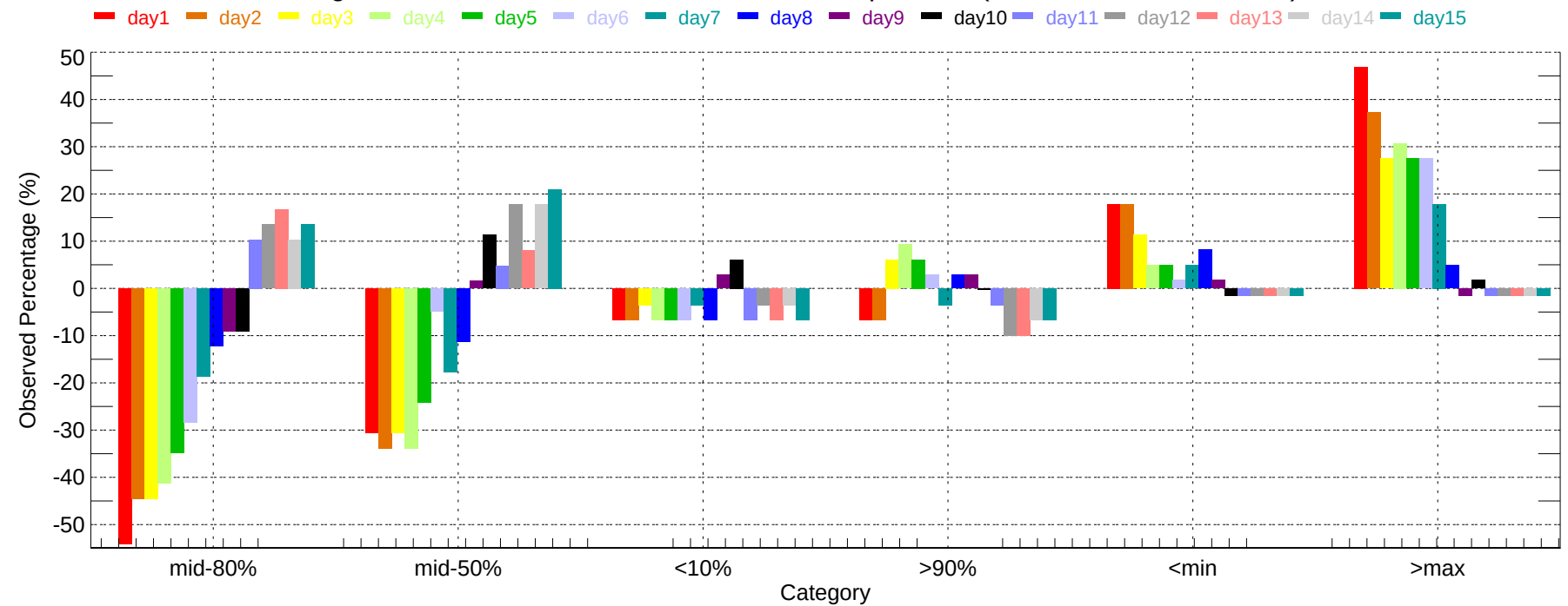
Observed Percentage Deviation of Ensembles - BFL: Max Temperature (2011-12-01~2011-12-31)
