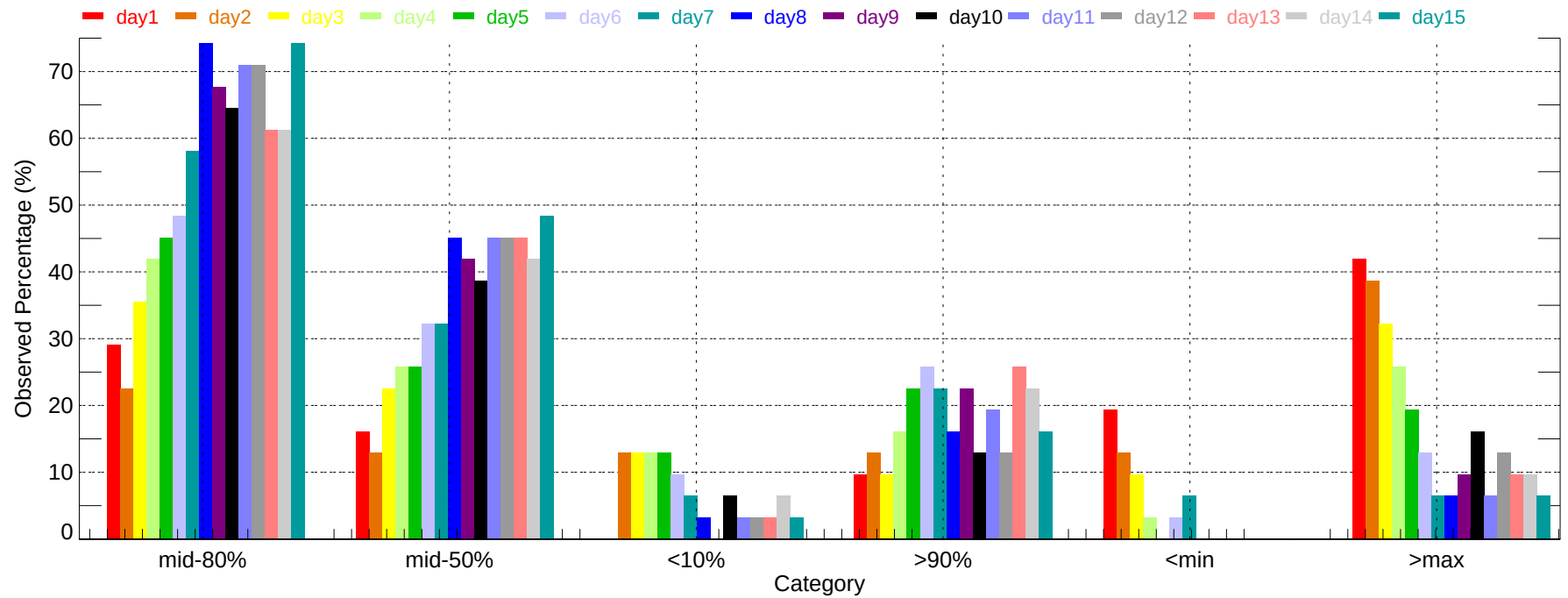
Observed Percentage of Ensembles - LIT: Max Temperature (2011-12-01~2011-12-31)
