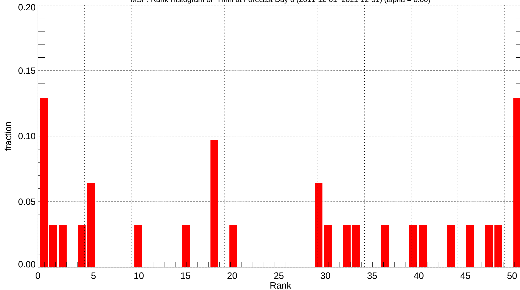
MSP: Rank Histogram of Tmin at Forecast Day 6 (2011-12-01~2011-12-31) (alpha = 0.00)
