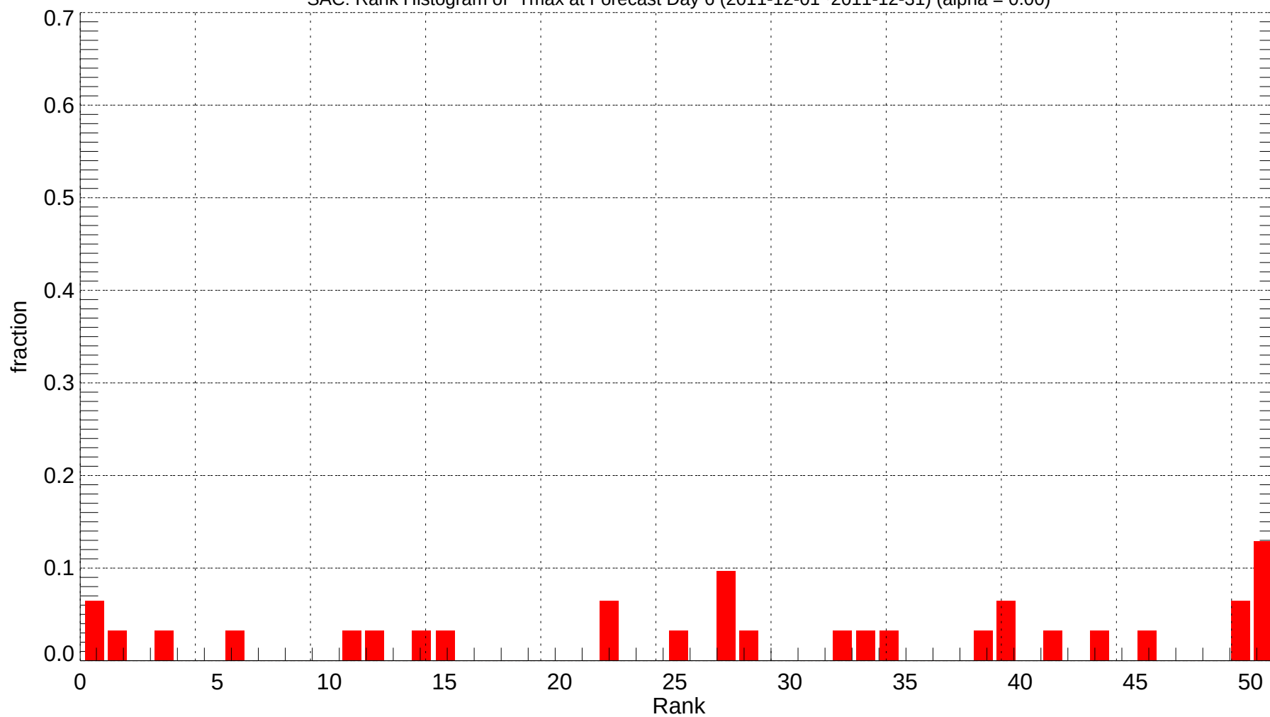
SAC: Rank Histogram of Tmax at Forecast Day 6 (2011-12-01~2011-12-31) (alpha = 0.00)
