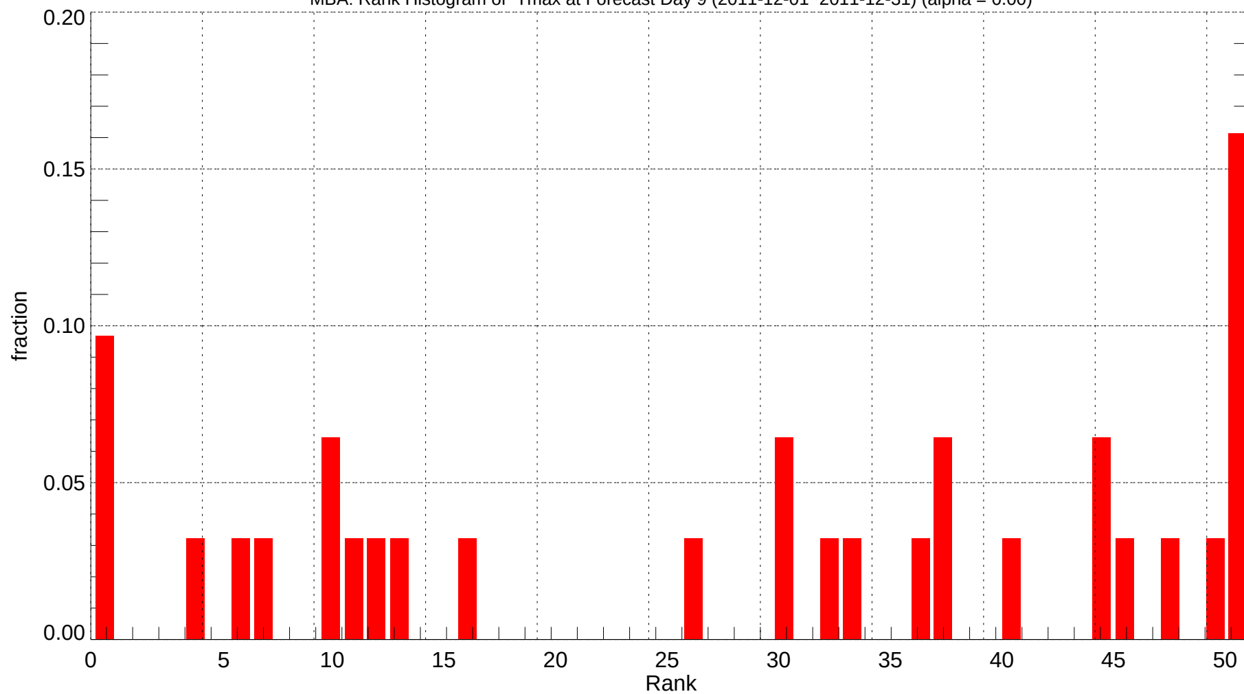
MBA: Rank Histogram of Tmax at Forecast Day 9 (2011-12-01~2011-12-31) (alpha = 0.00)
