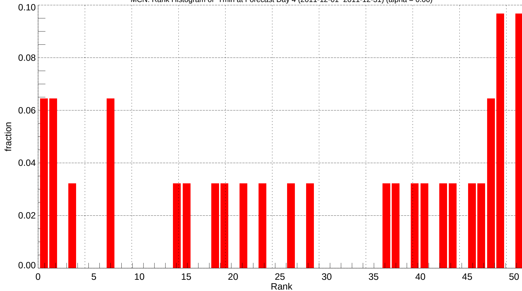
MCN: Rank Histogram of Tmin at Forecast Day 4 (2011-12-01~2011-12-31) (alpha = 0.00)
