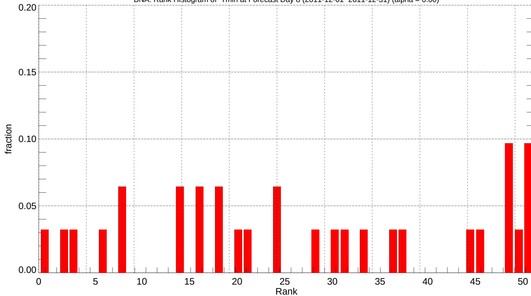
BNA: Rank Histogram of Tmin at Forecast Day 8 (2011-12-01~2011-12-31) (alpha = 0.00)
