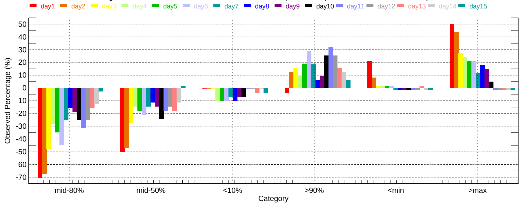
Observed Percentage Deviation of Ensembles - LEX: Min Temperature (2011-12-01~2011-12-31)
