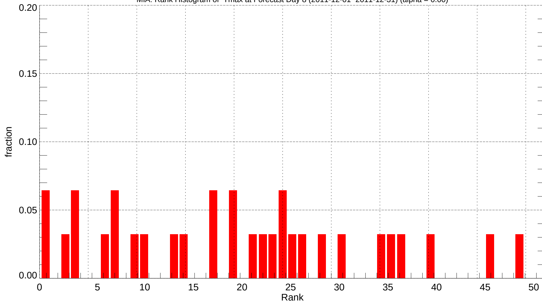
MIA: Rank Histogram of Tmax at Forecast Day 8 (2011-12-01~2011-12-31) (alpha = 0.00)
