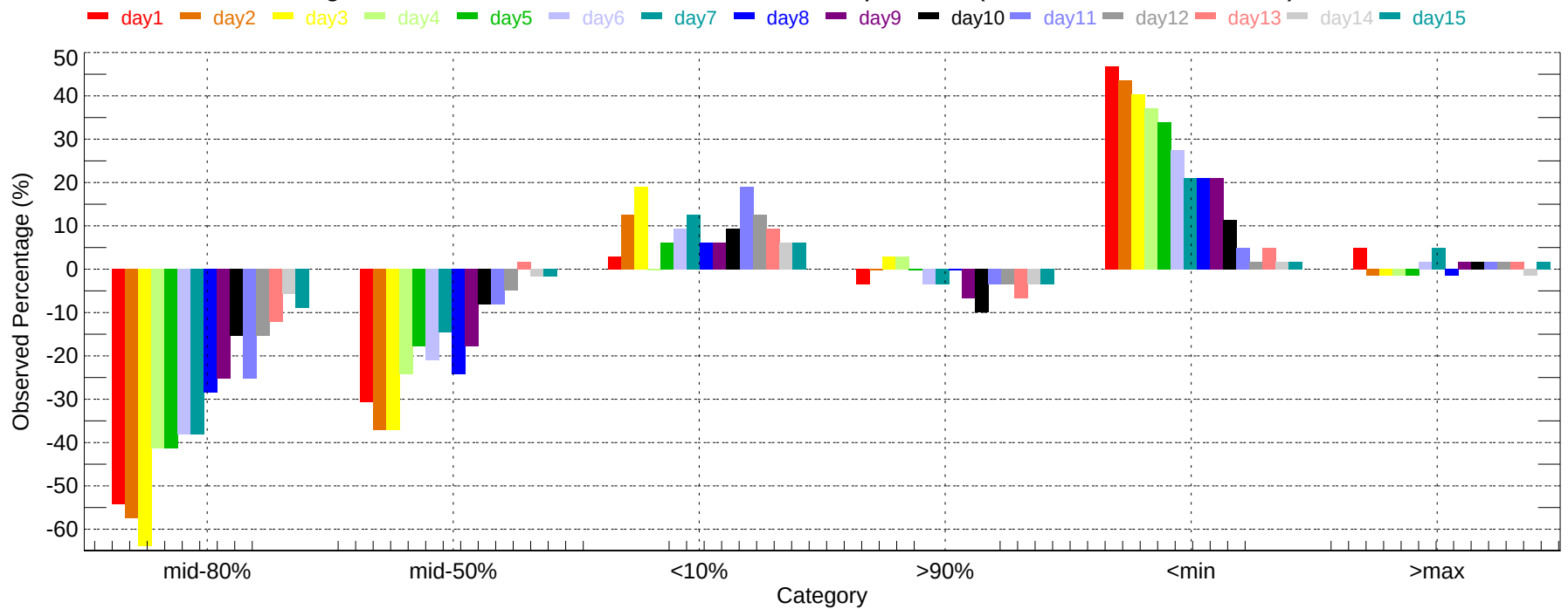
Observed Percentage Deviation of Ensembles - PDX: Min Temperature (2011-12-01~2011-12-31)
