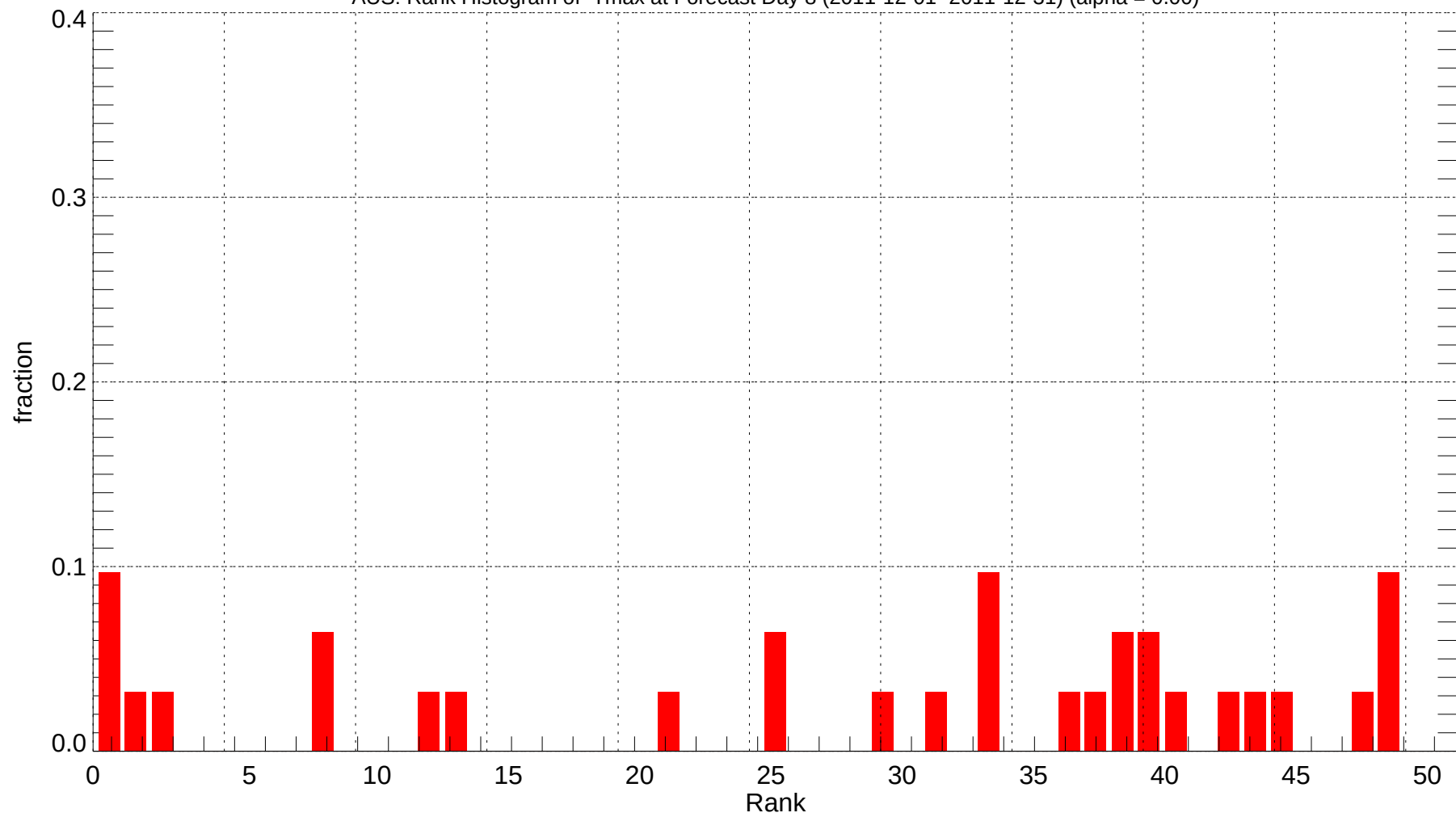
AUS: Rank Histogram of Tmax at Forecast Day 8 (2011-12-01~2011-12-31) (alpha = 0.00)
