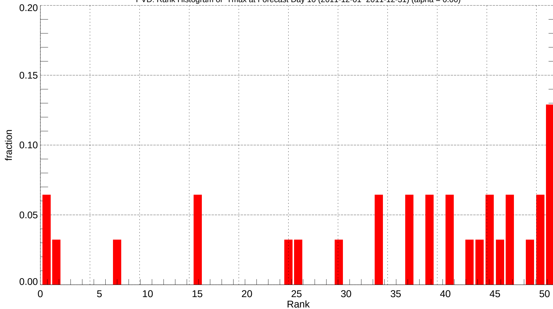
PVD: Rank Histogram of Tmax at Forecast Day 10 (2011-12-01~2011-12-31) (alpha = 0.00)
