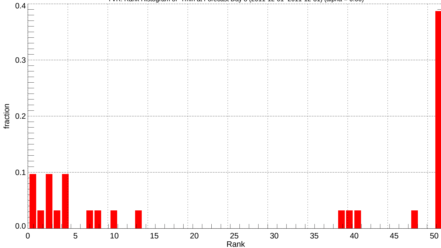
YVR: Rank Histogram of Tmin at Forecast Day 8 (2011-12-01~2011-12-31) (alpha = 0.00)
