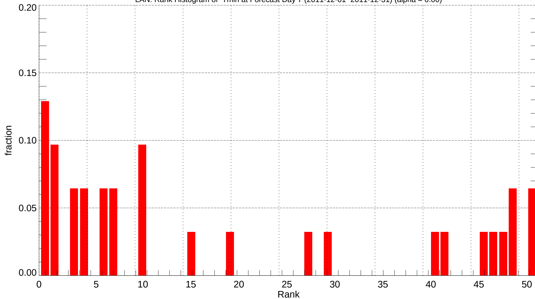
LAN: Rank Histogram of Tmin at Forecast Day 7 (2011-12-01~2011-12-31) (alpha = 0.00)
