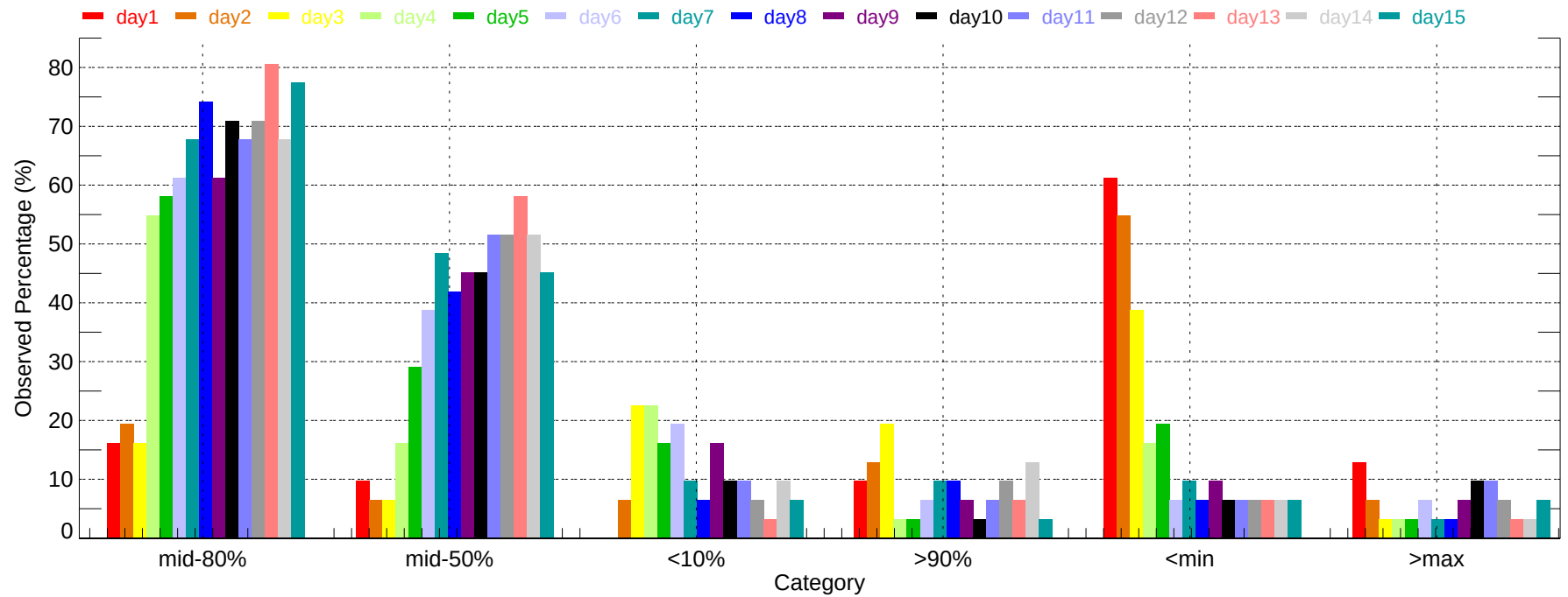
Observed Percentage of Ensembles - DEN: Max Temperature (2011-12-01~2011-12-31)
