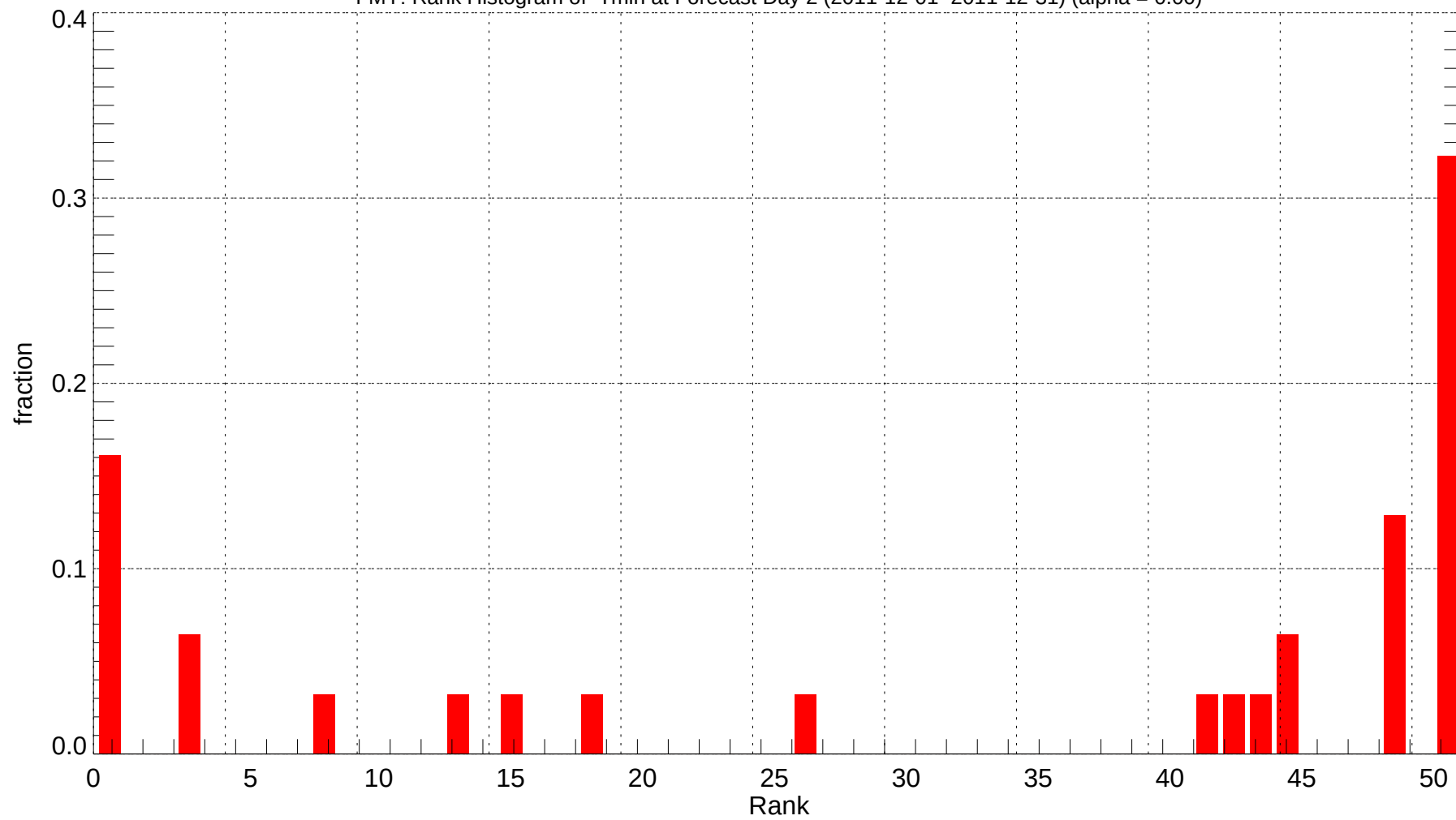
FMY: Rank Histogram of Tmin at Forecast Day 2 (2011-12-01~2011-12-31) (alpha = 0.00)
