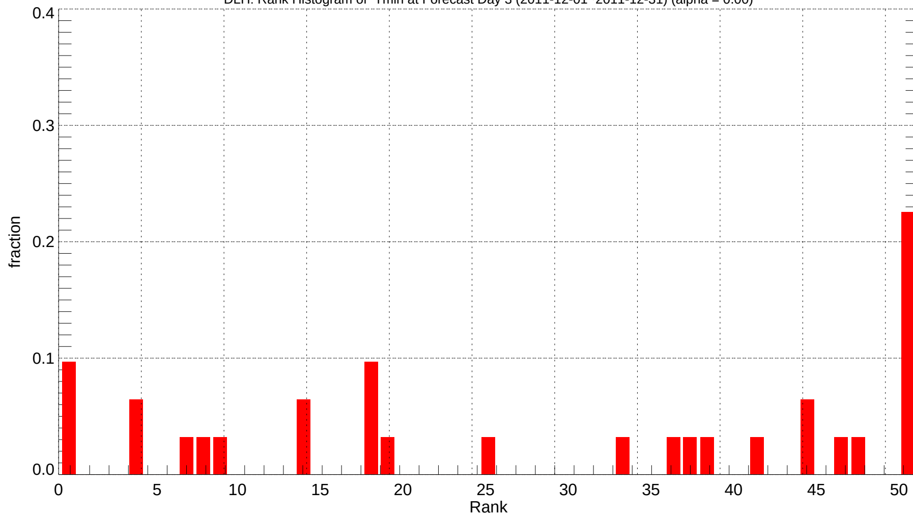
DLH: Rank Histogram of Tmin at Forecast Day 3 (2011-12-01~2011-12-31) (alpha = 0.00)
