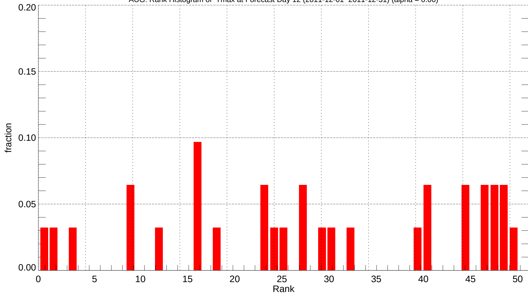
AUG: Rank Histogram of Tmax at Forecast Day 12 (2011-12-01~2011-12-31) (alpha = 0.00)
