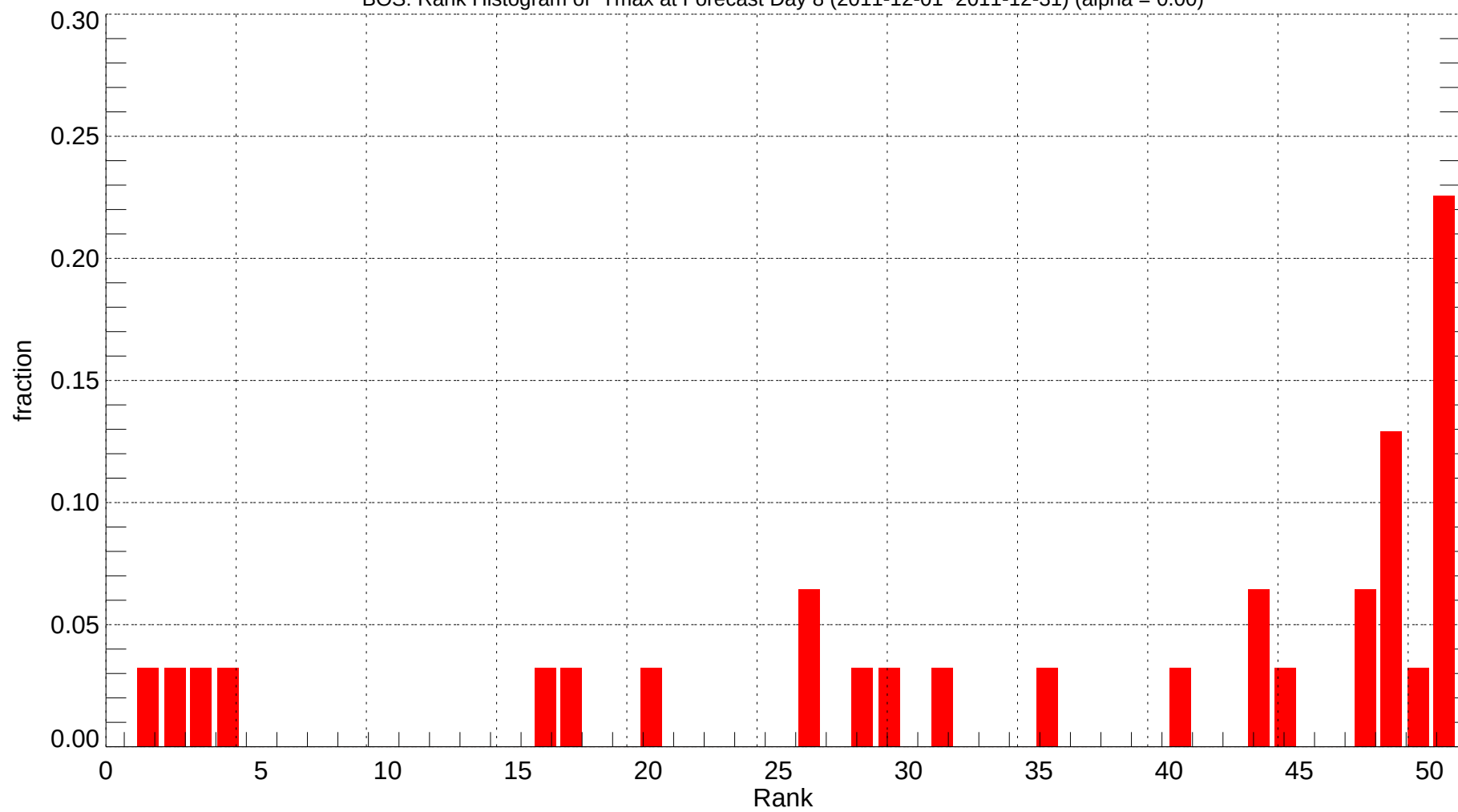
BOS: Rank Histogram of Tmax at Forecast Day 8 (2011-12-01~2011-12-31) (alpha = 0.00)
