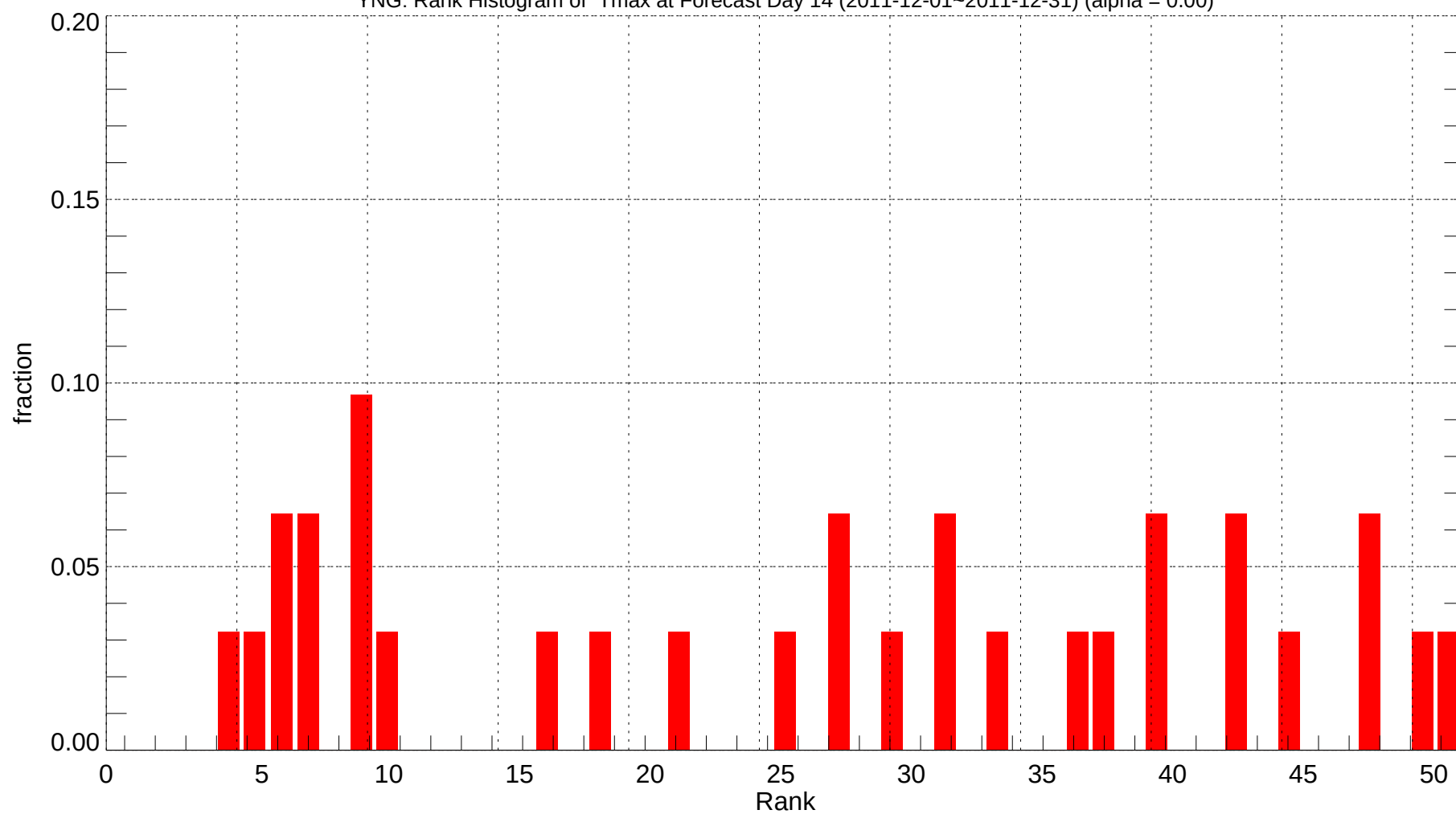
YNG: Rank Histogram of Tmax at Forecast Day 14 (2011-12-01~2011-12-31) (alpha = 0.00)
