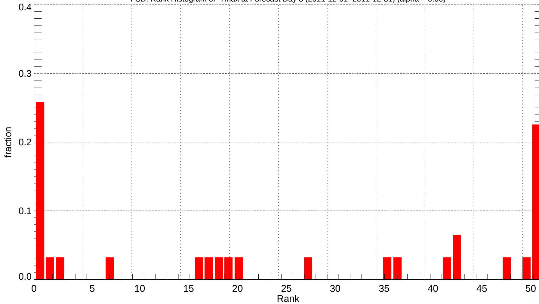
FSD: Rank Histogram of Tmax at Forecast Day 3 (2011-12-01~2011-12-31) (alpha = 0.00)
