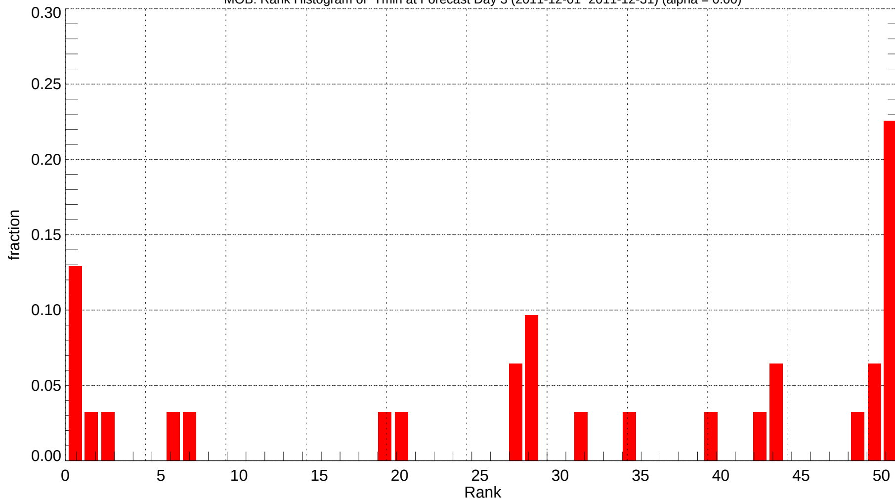
MOB: Rank Histogram of Tmin at Forecast Day 3 (2011-12-01~2011-12-31) (alpha = 0.00)
