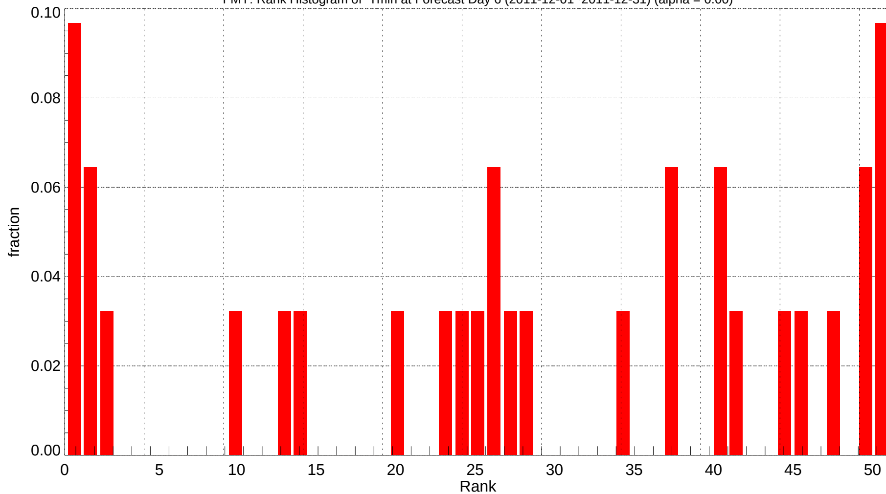
FMY: Rank Histogram of Tmin at Forecast Day 6 (2011-12-01~2011-12-31) (alpha = 0.00)
