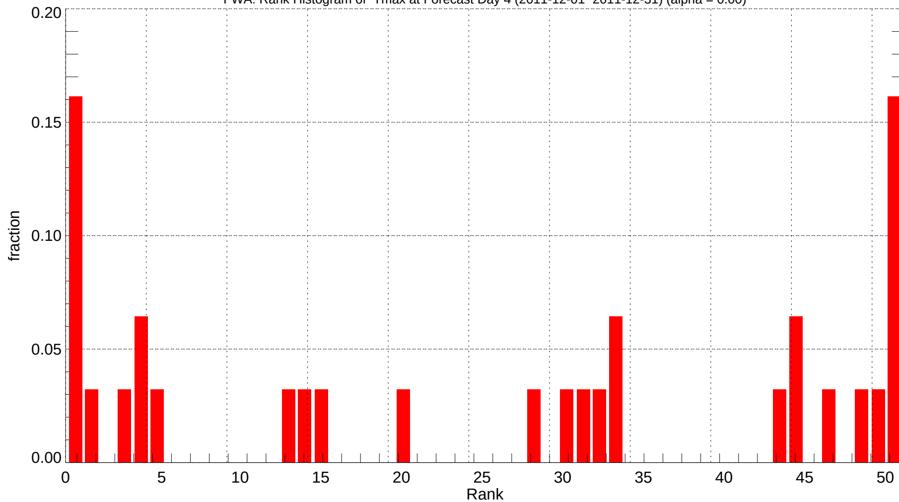
FWA: Rank Histogram of Tmax at Forecast Day 4 (2011-12-01~2011-12-31) (alpha = 0.00)
