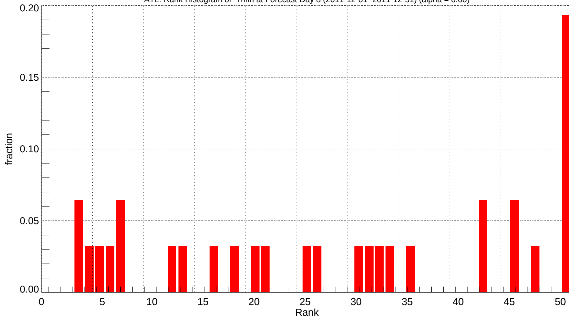
ATL: Rank Histogram of Tmin at Forecast Day 8 (2011-12-01~2011-12-31) (alpha = 0.00)
