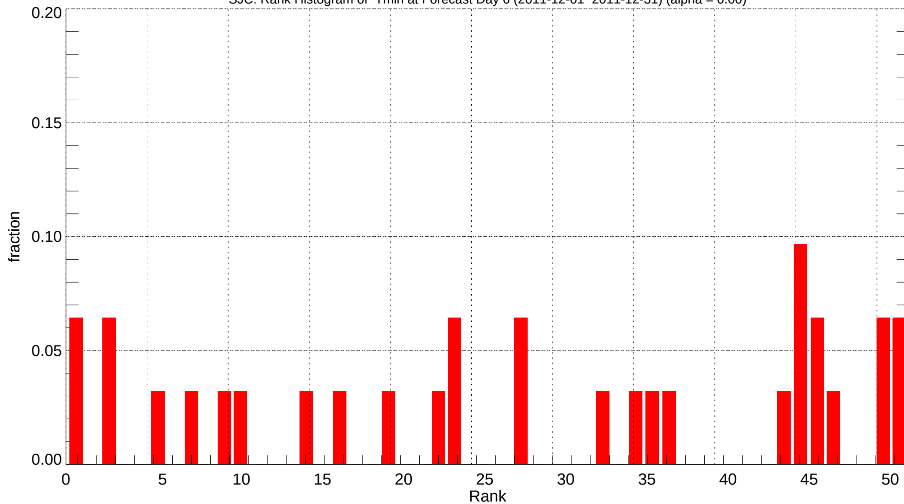
SJC: Rank Histogram of Tmin at Forecast Day 6 (2011-12-01~2011-12-31) (alpha = 0.00)
