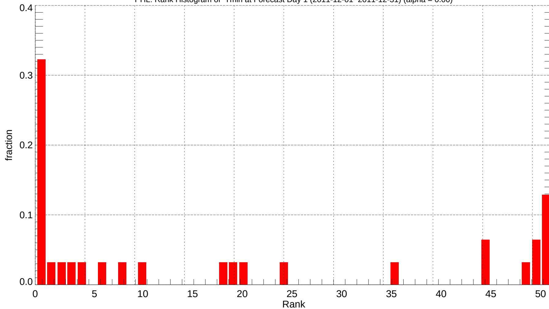
PHL: Rank Histogram of Tmin at Forecast Day 1 (2011-12-01~2011-12-31) (alpha = 0.00)
