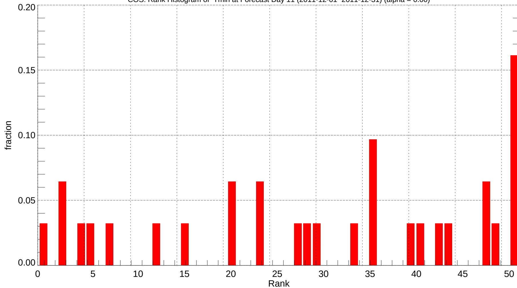
COS: Rank Histogram of Tmin at Forecast Day 11 (2011-12-01~2011-12-31) (alpha = 0.00)
