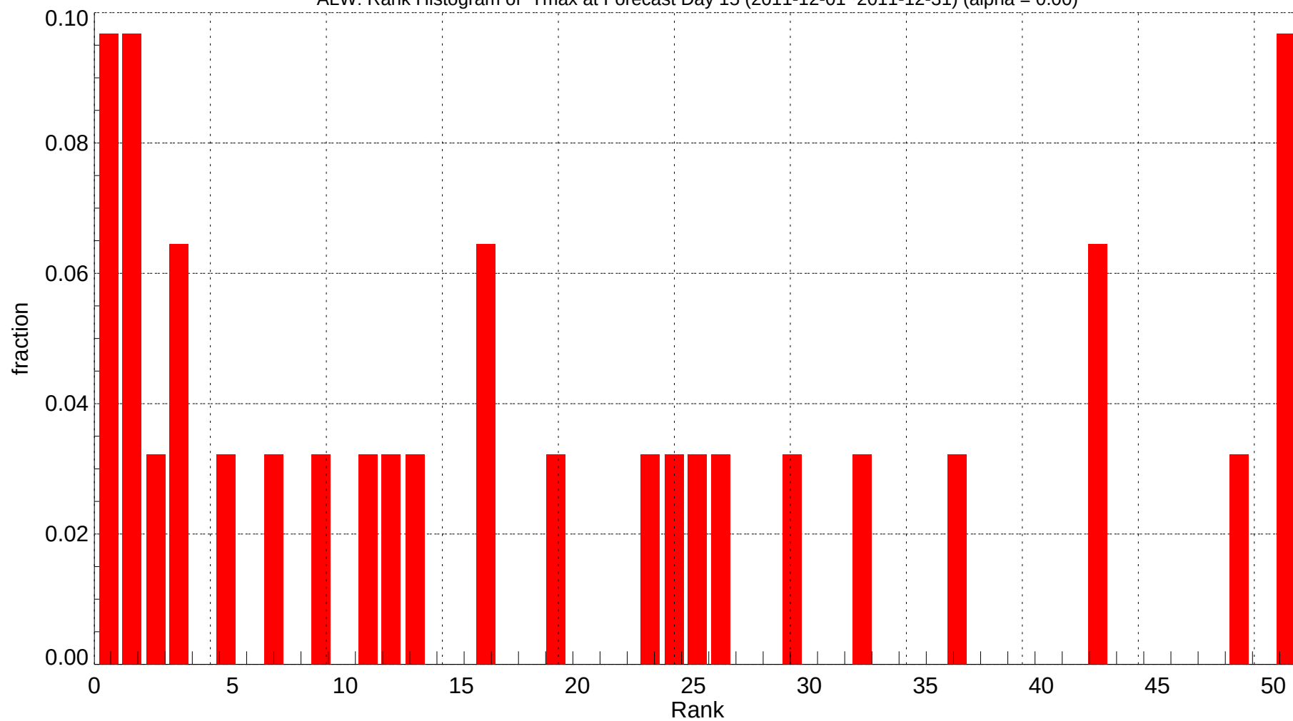
ALW: Rank Histogram of Tmax at Forecast Day 15 (2011-12-01~2011-12-31) (alpha = 0.00)
