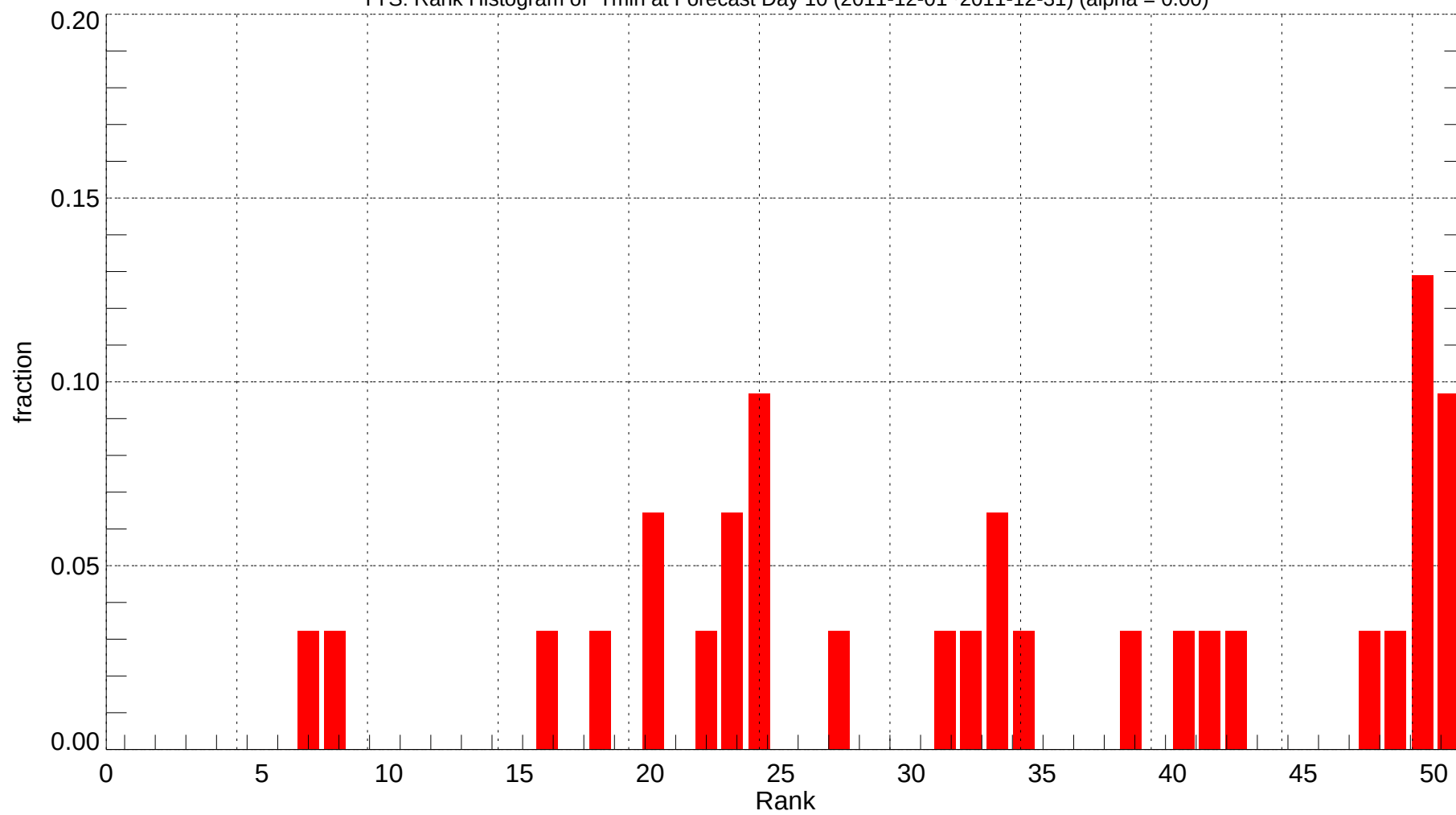
TYS: Rank Histogram of Tmin at Forecast Day 10 (2011-12-01~2011-12-31) (alpha = 0.00)
