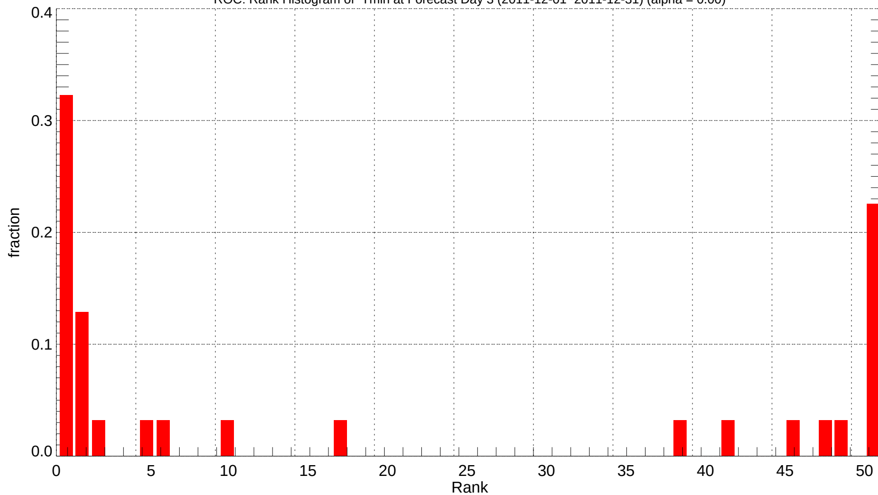
ROC: Rank Histogram of Tmin at Forecast Day 3 (2011-12-01~2011-12-31) (alpha = 0.00)
