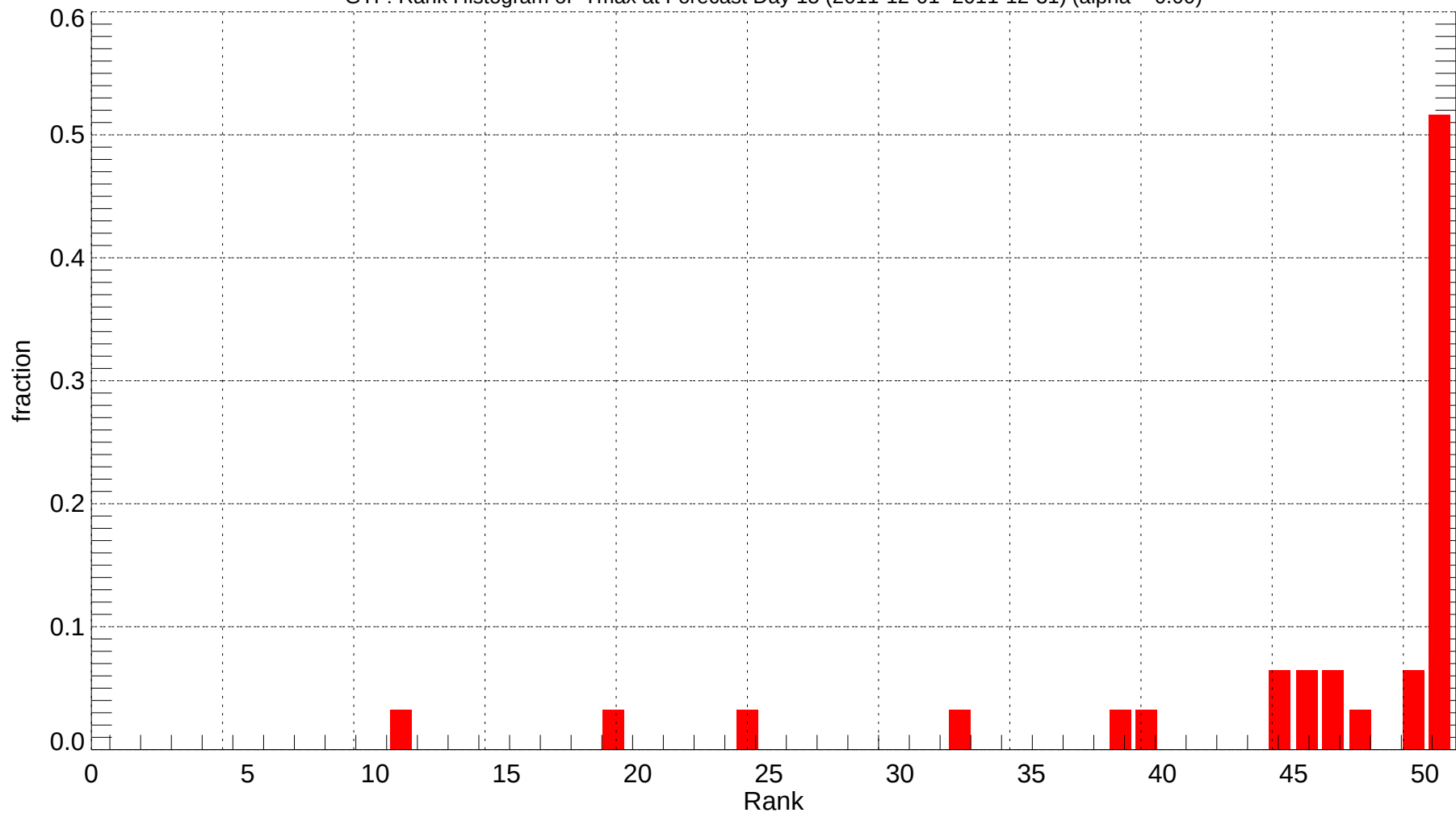
GTF: Rank Histogram of Tmax at Forecast Day 15 (2011-12-01~2011-12-31) (alpha = 0.00)
