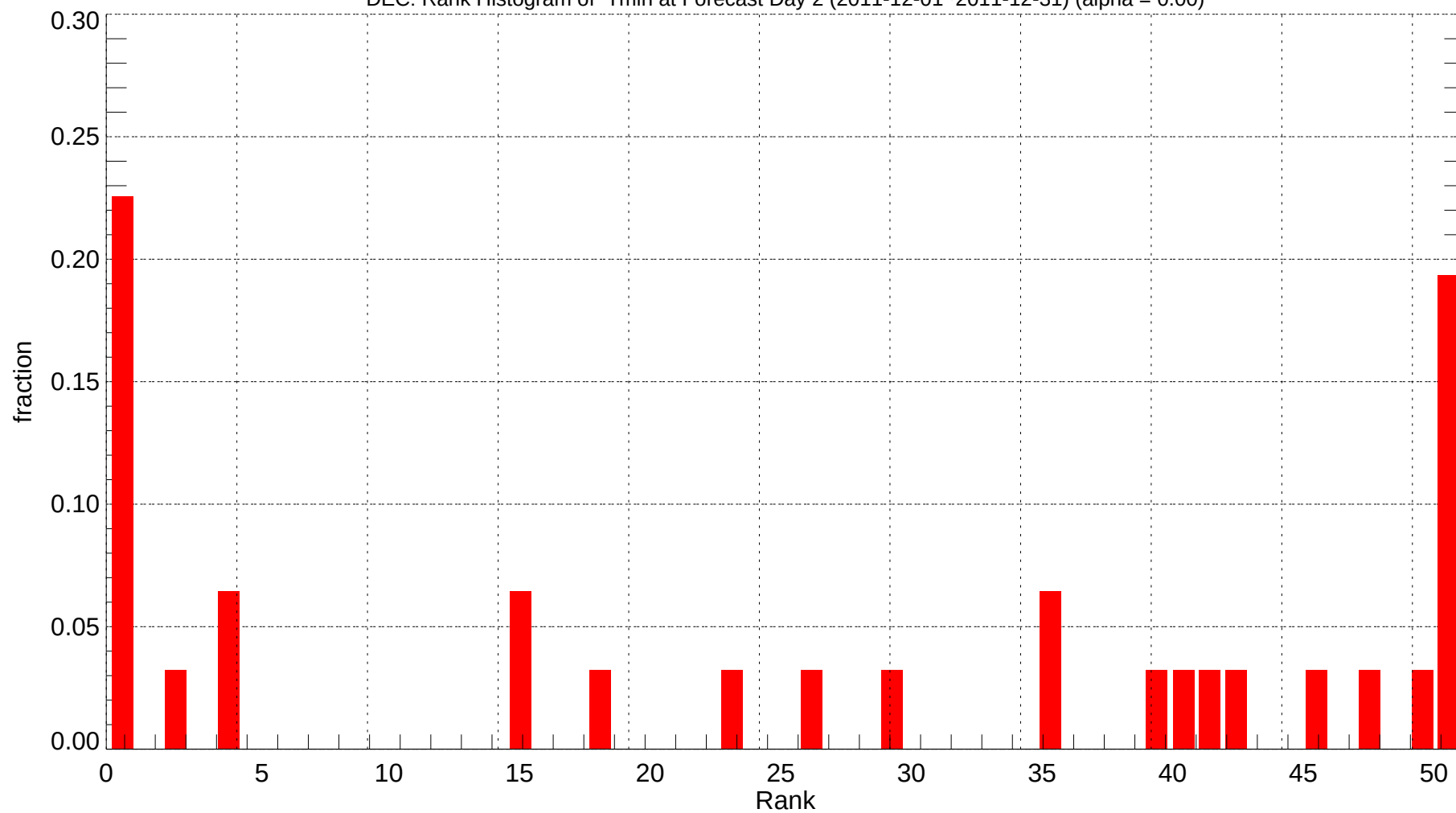
DEC: Rank Histogram of Tmin at Forecast Day 2 (2011-12-01~2011-12-31) (alpha = 0.00)
