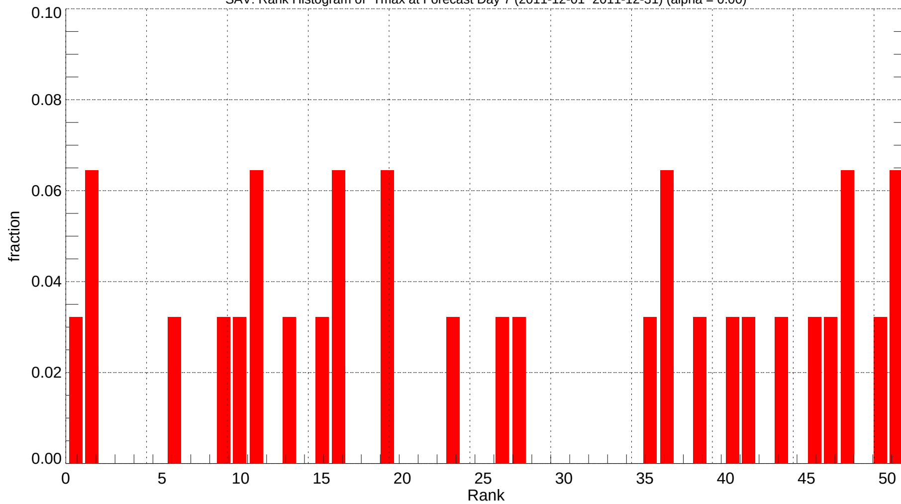
SAV: Rank Histogram of Tmax at Forecast Day 7 (2011-12-01~2011-12-31) (alpha = 0.00)
