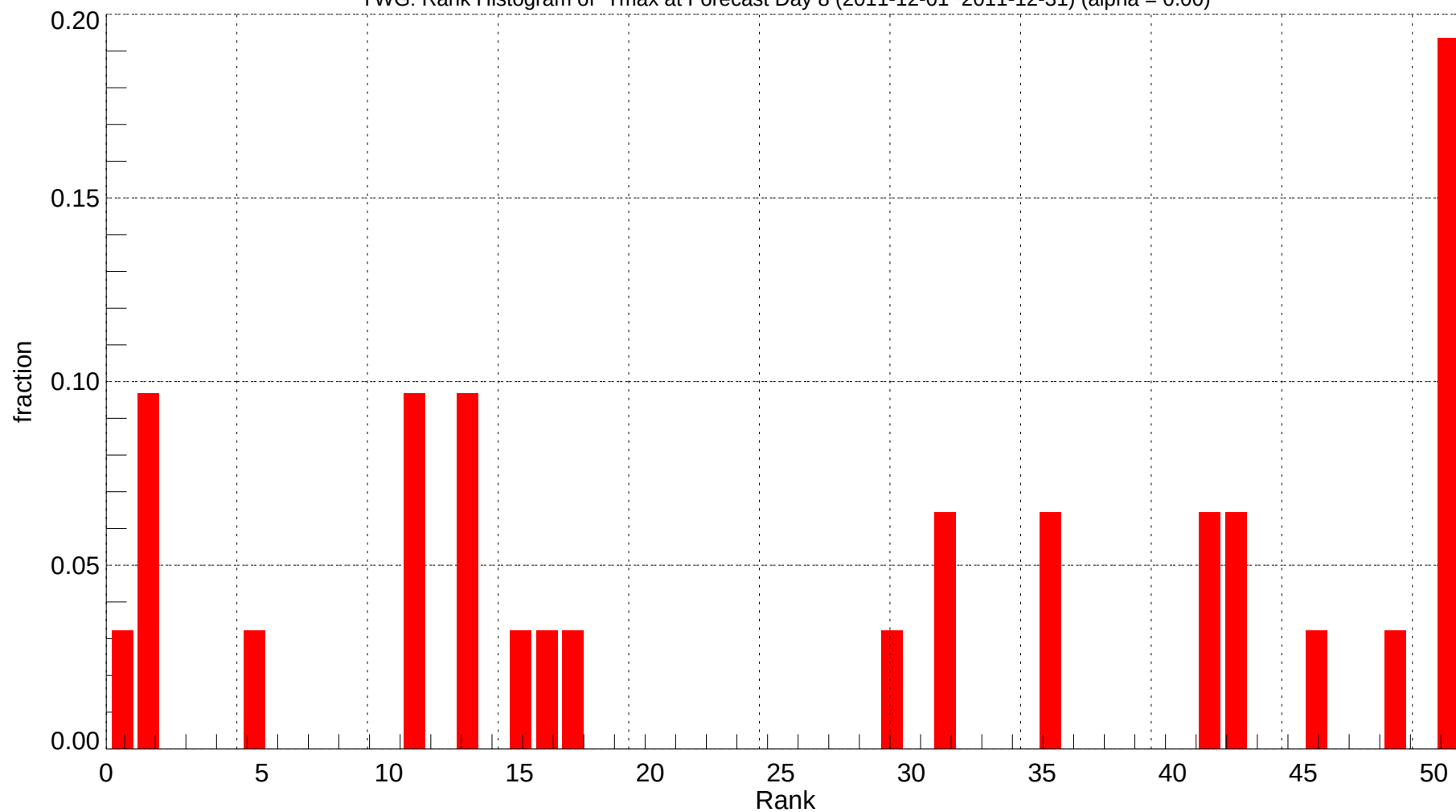
YWG: Rank Histogram of Tmax at Forecast Day 8 (2011-12-01~2011-12-31) (alpha = 0.00)
