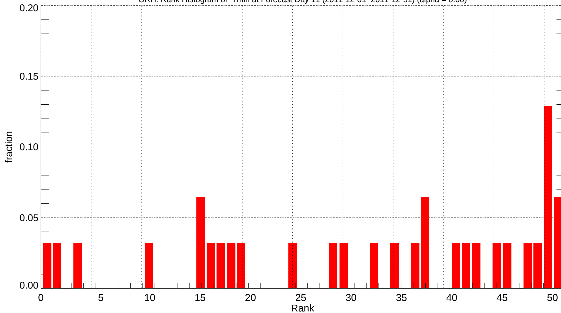
ORH: Rank Histogram of Tmin at Forecast Day 11 (2011-12-01~2011-12-31) (alpha = 0.00)
