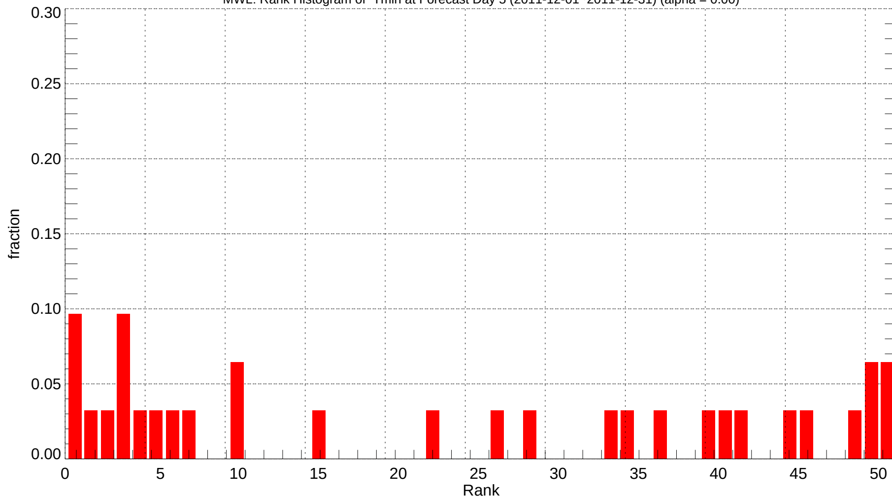
MWL: Rank Histogram of Tmin at Forecast Day 5 (2011-12-01~2011-12-31) (alpha = 0.00)
