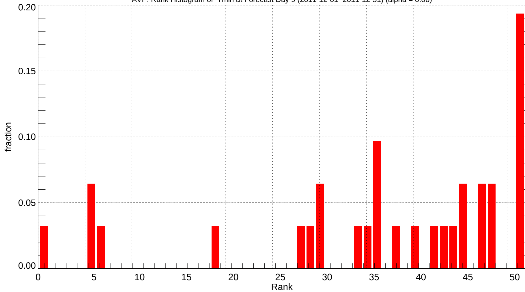
AVP: Rank Histogram of Tmin at Forecast Day 9 (2011-12-01~2011-12-31) (alpha = 0.00)
