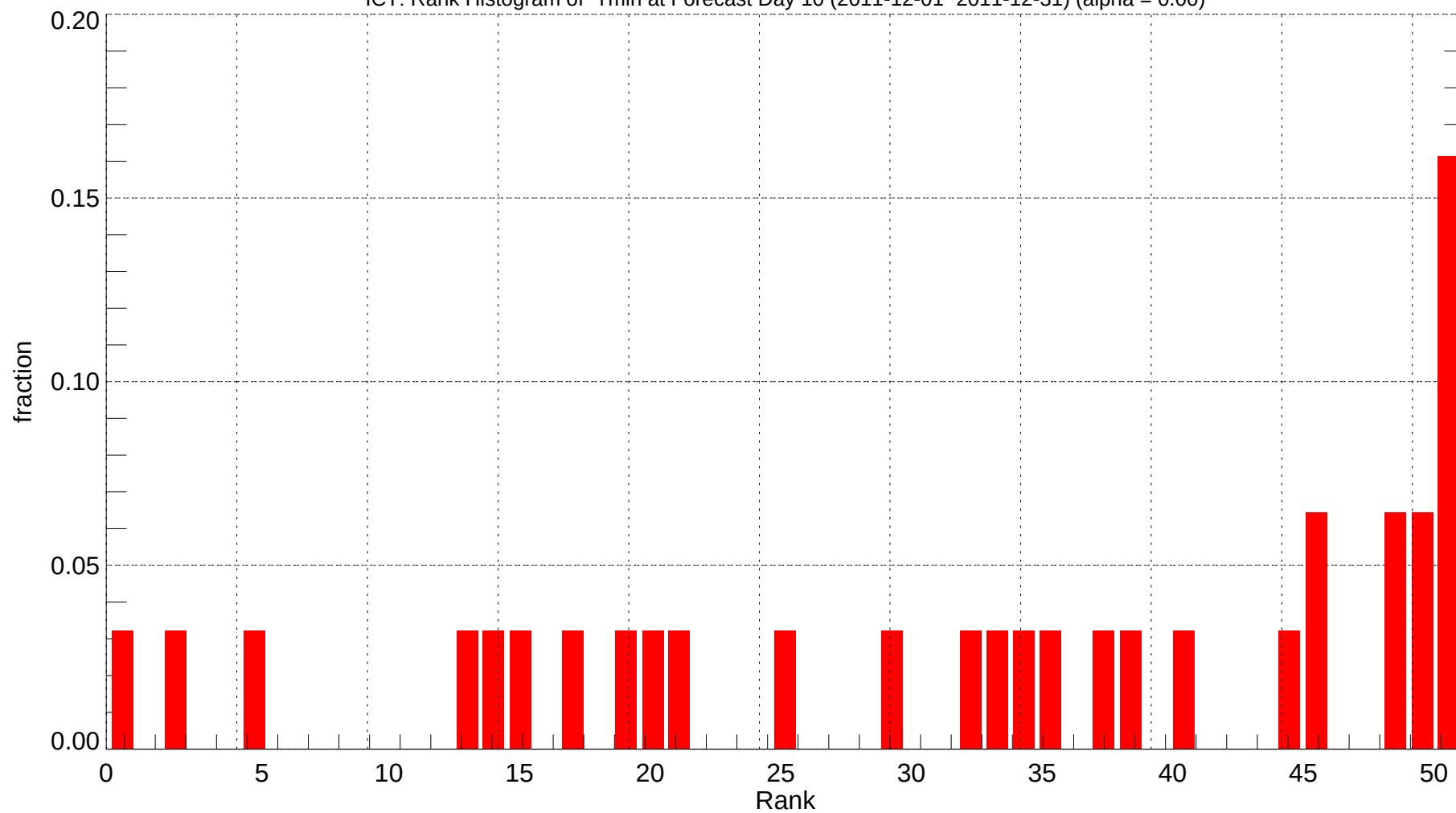
ICT: Rank Histogram of Tmin at Forecast Day 10 (2011-12-01~2011-12-31) (alpha = 0.00)
