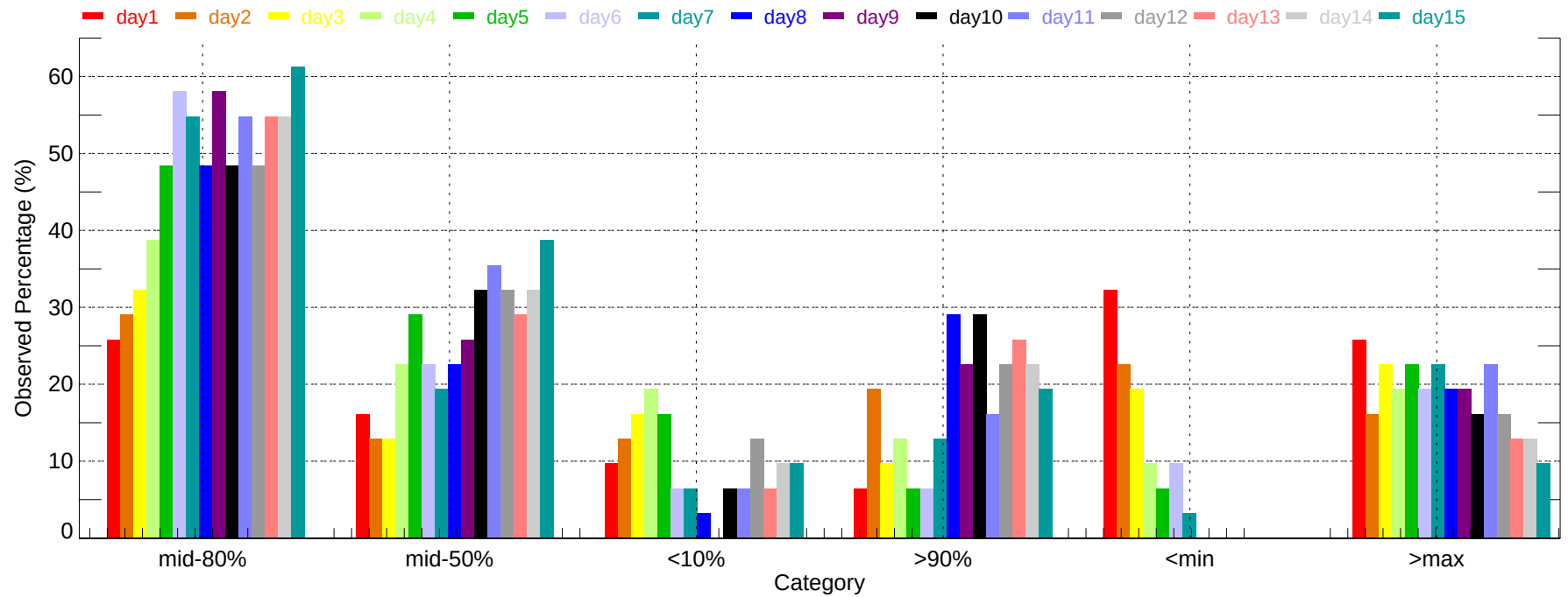
Observed Percentage of Ensembles - DSM: Max Temperature (2011-12-01~2011-12-31)
