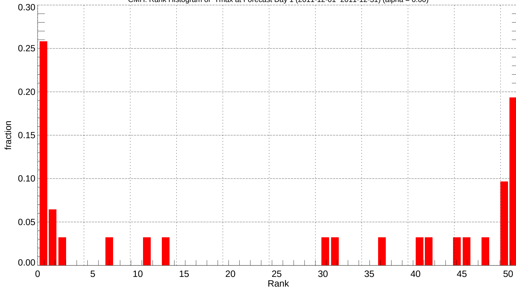
CMH: Rank Histogram of Tmax at Forecast Day 1 (2011-12-01~2011-12-31) (alpha = 0.00)
