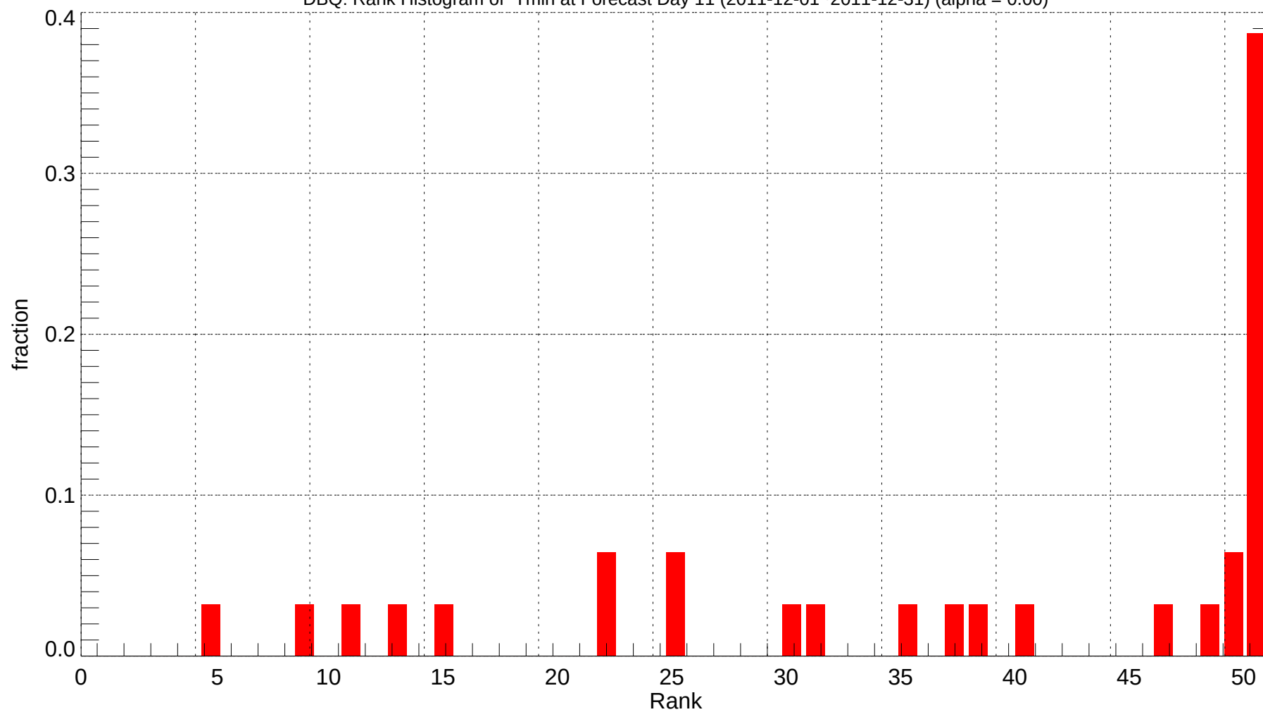
DBQ: Rank Histogram of Tmin at Forecast Day 11 (2011-12-01~2011-12-31) (alpha = 0.00)
