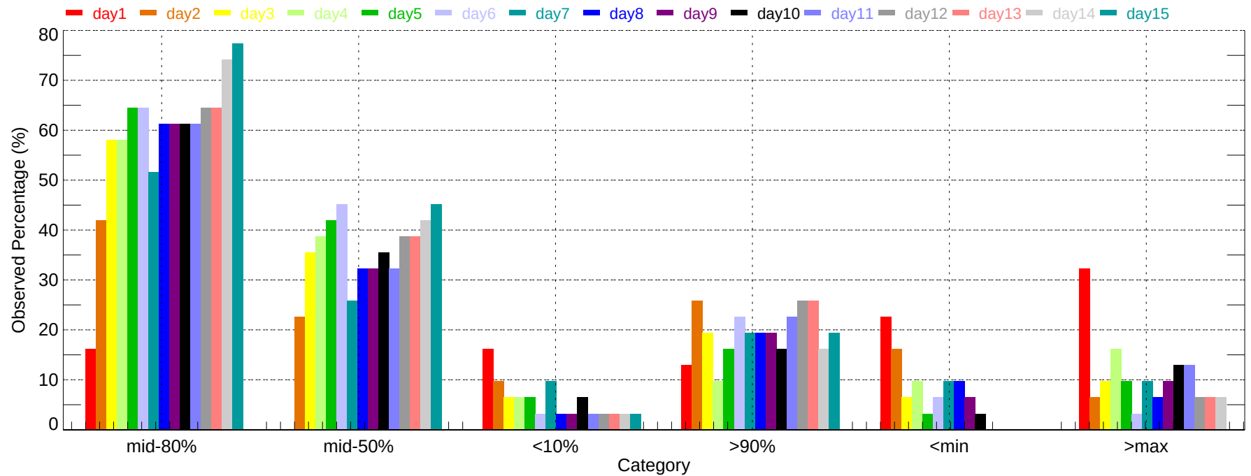
Observed Percentage of Ensembles - LNS: Max Temperature (2011-12-01~2011-12-31)
