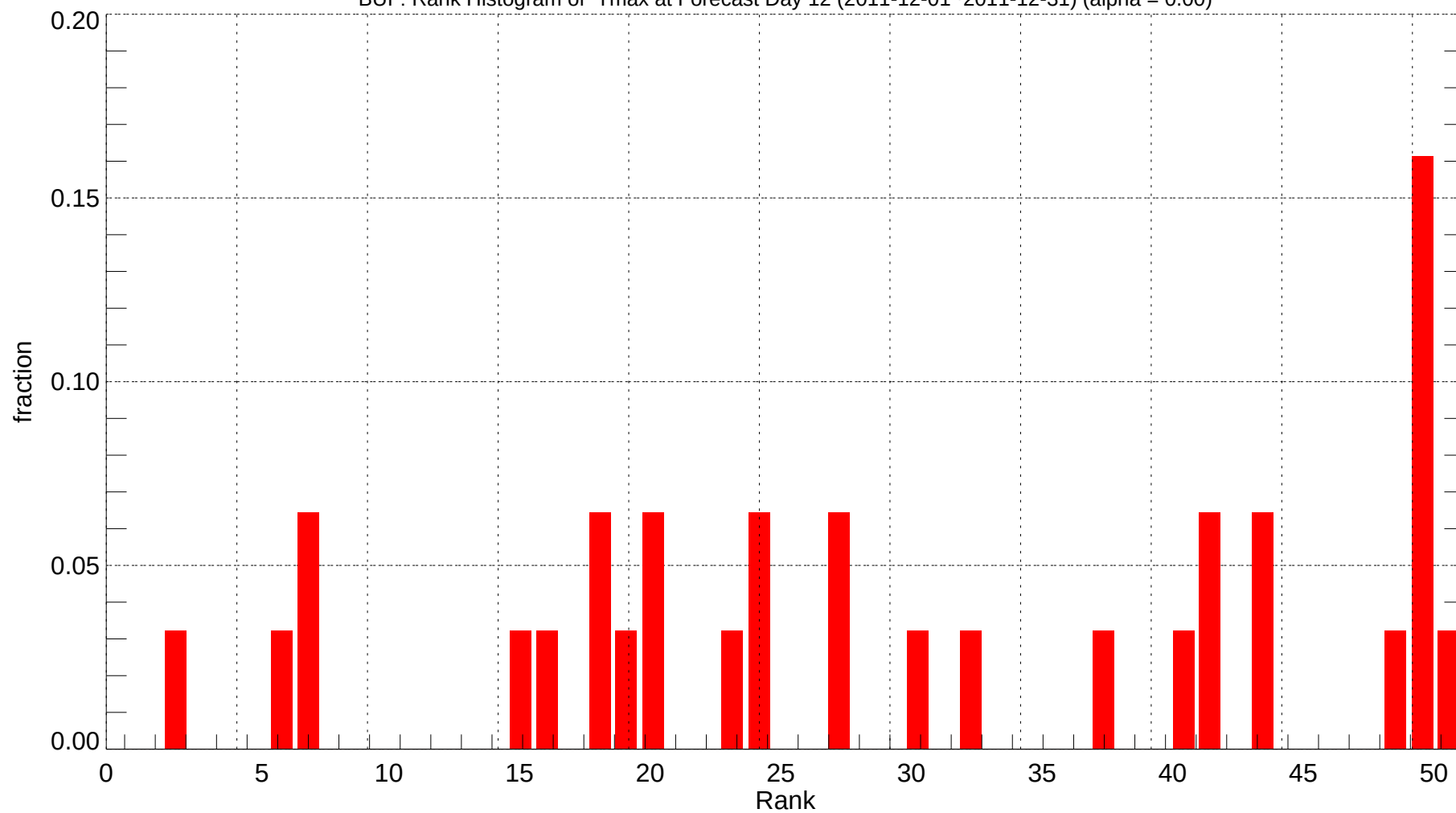
BUF: Rank Histogram of Tmax at Forecast Day 12 (2011-12-01~2011-12-31) (alpha = 0.00)
