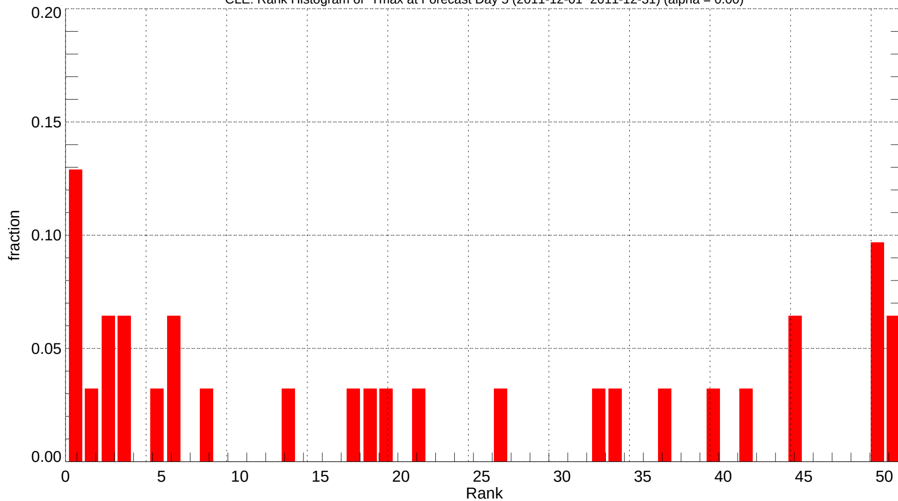
CLE: Rank Histogram of Tmax at Forecast Day 5 (2011-12-01~2011-12-31) (alpha = 0.00)
