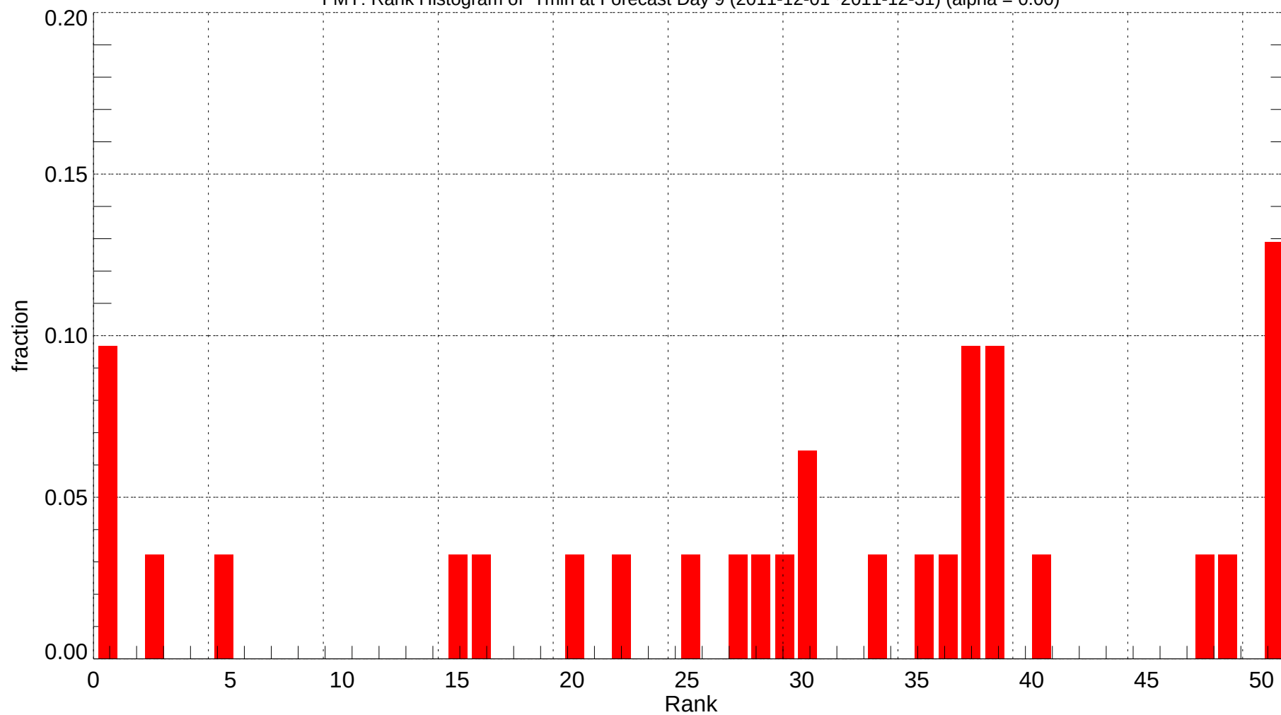
FMY: Rank Histogram of Tmin at Forecast Day 9 (2011-12-01~2011-12-31) (alpha = 0.00)
