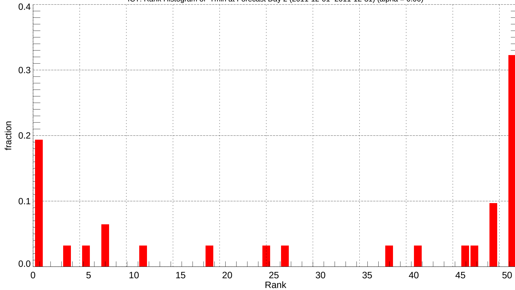
ICT: Rank Histogram of Tmin at Forecast Day 2 (2011-12-01~2011-12-31) (alpha = 0.00)
