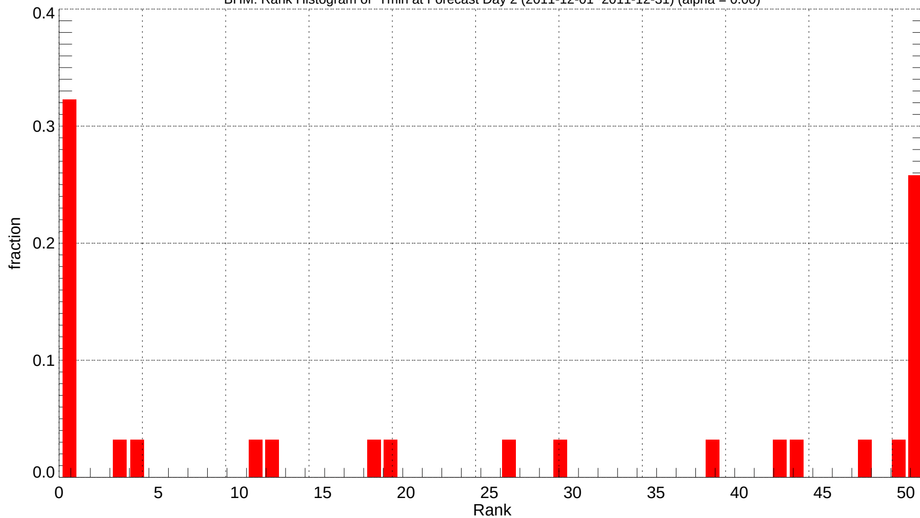
BHM: Rank Histogram of Tmin at Forecast Day 2 (2011-12-01~2011-12-31) (alpha = 0.00)
