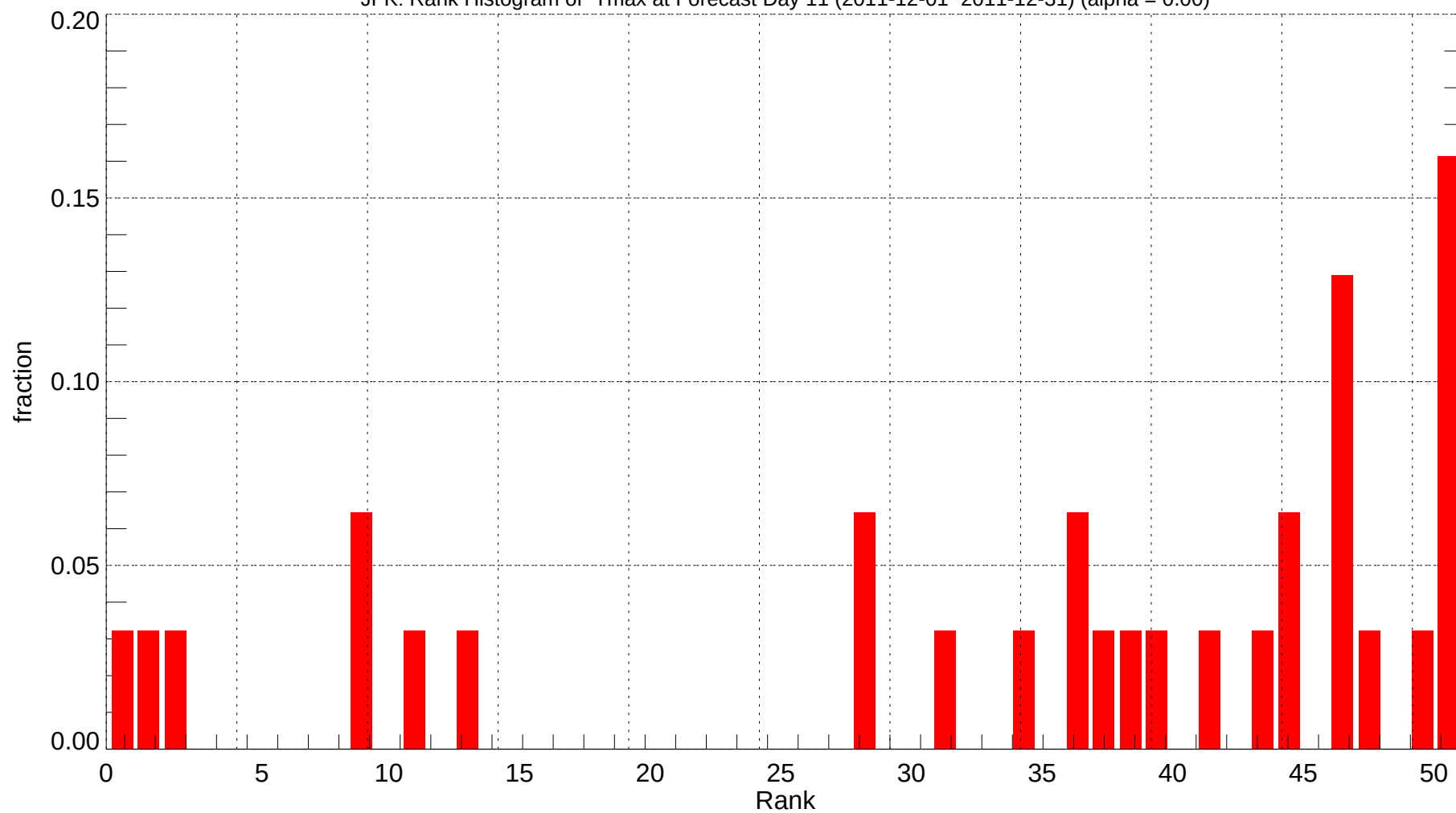
JFK: Rank Histogram of Tmax at Forecast Day 11 (2011-12-01~2011-12-31) (alpha = 0.00)
