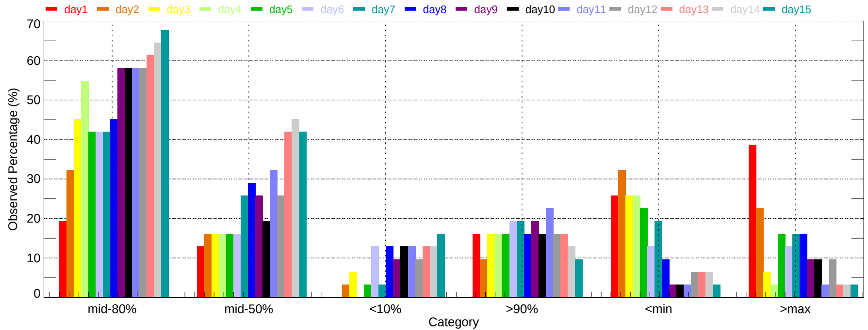
Observed Percentage of Ensembles - MOB: Min Temperature (2011-12-01~2011-12-31)
