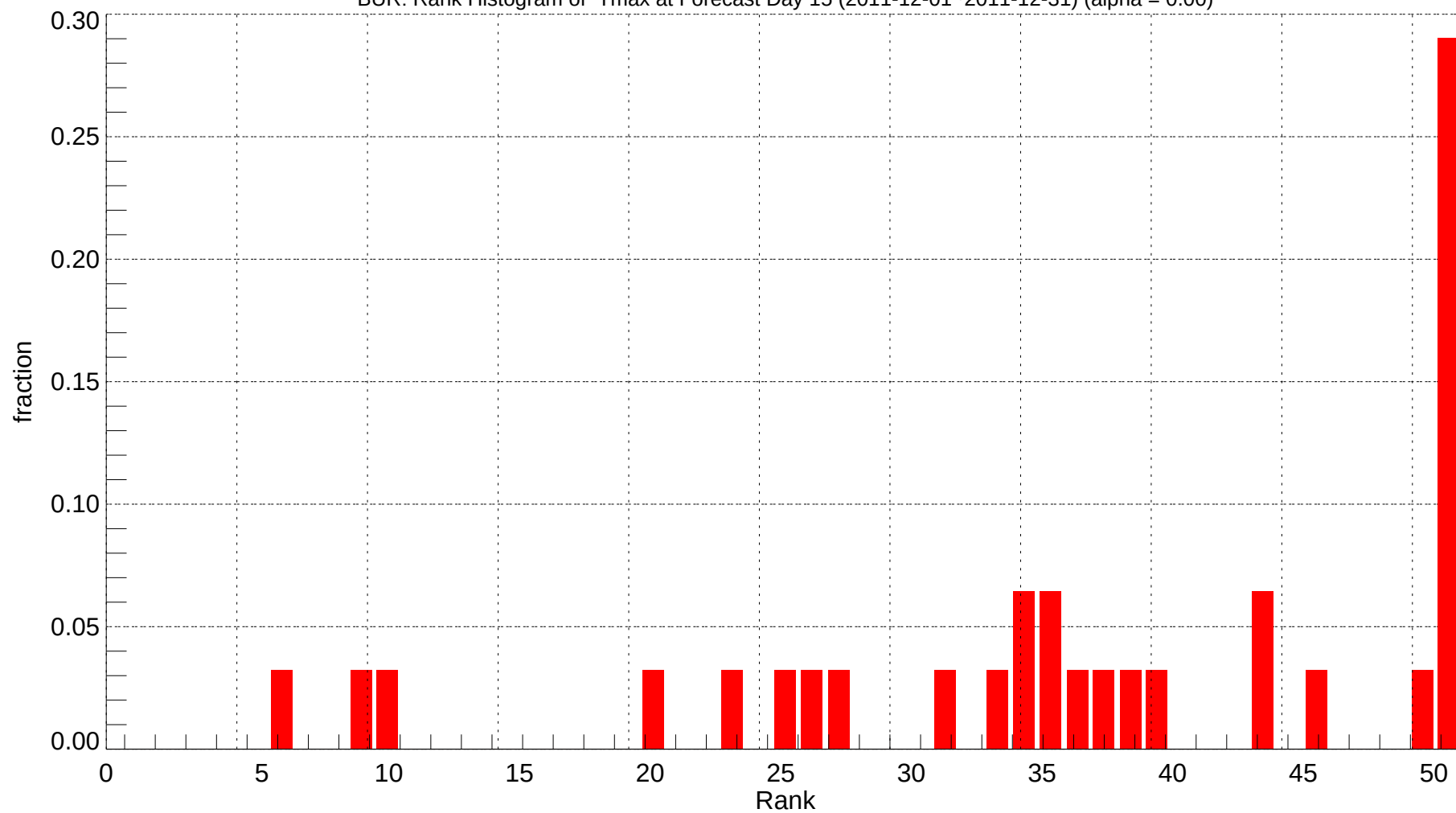
BUR: Rank Histogram of Tmax at Forecast Day 15 (2011-12-01~2011-12-31) (alpha = 0.00)
