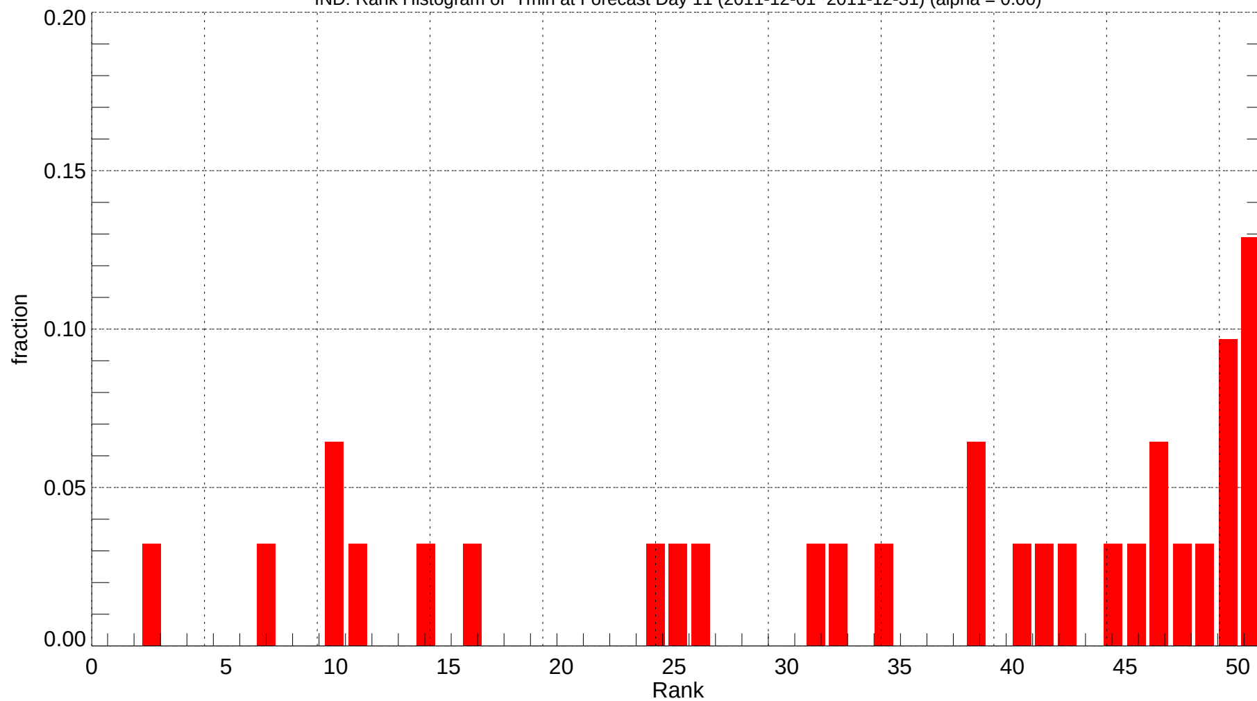
IND: Rank Histogram of Tmin at Forecast Day 11 (2011-12-01~2011-12-31) (alpha = 0.00)
