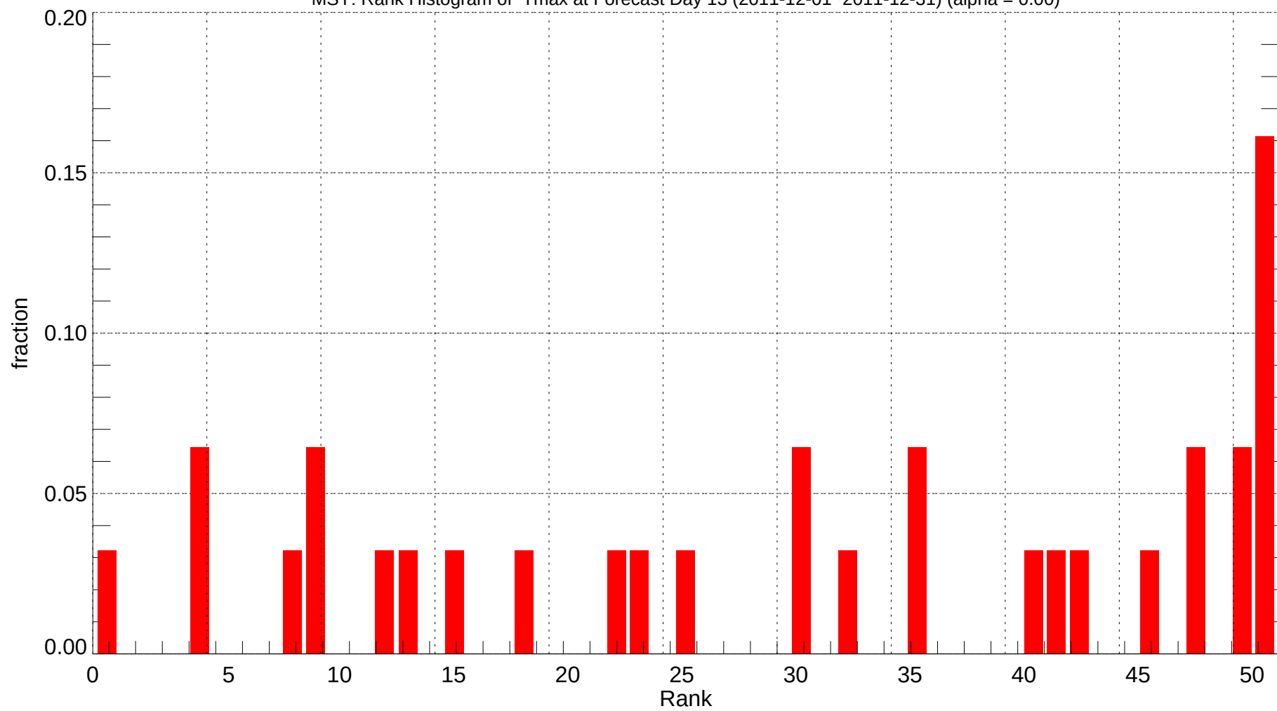
MSY: Rank Histogram of Tmax at Forecast Day 13 (2011-12-01~2011-12-31) (alpha = 0.00)
