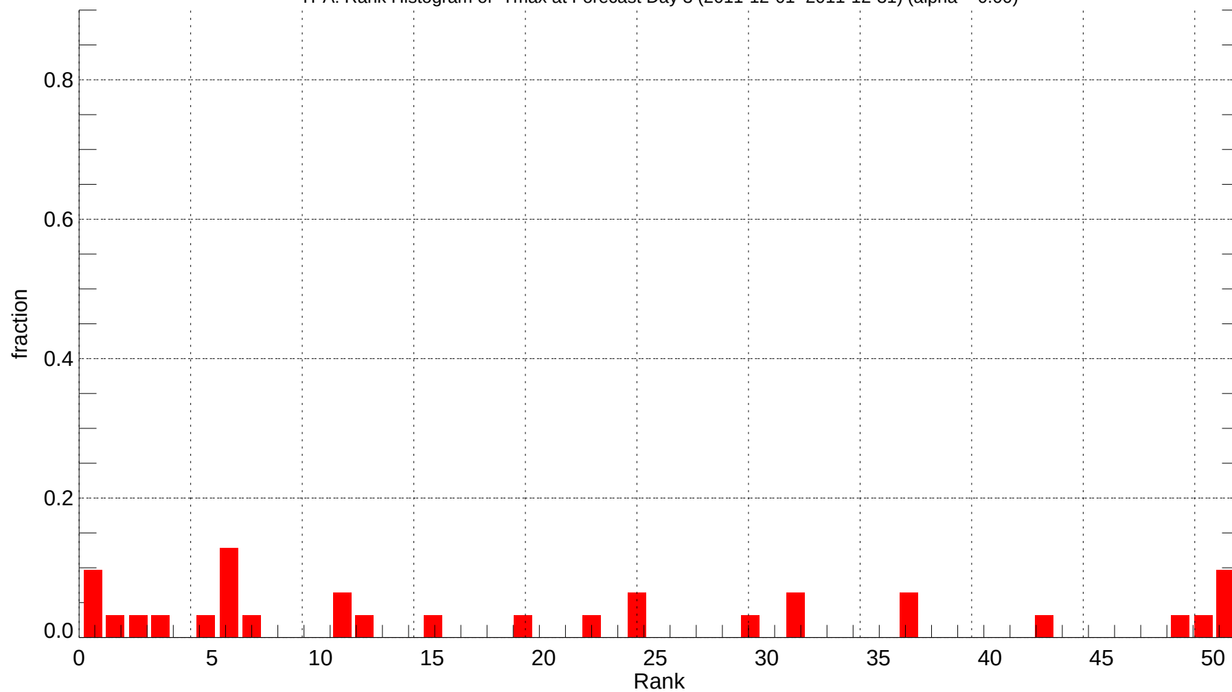
TPA: Rank Histogram of Tmax at Forecast Day 3 (2011-12-01~2011-12-31) (alpha = 0.00)
