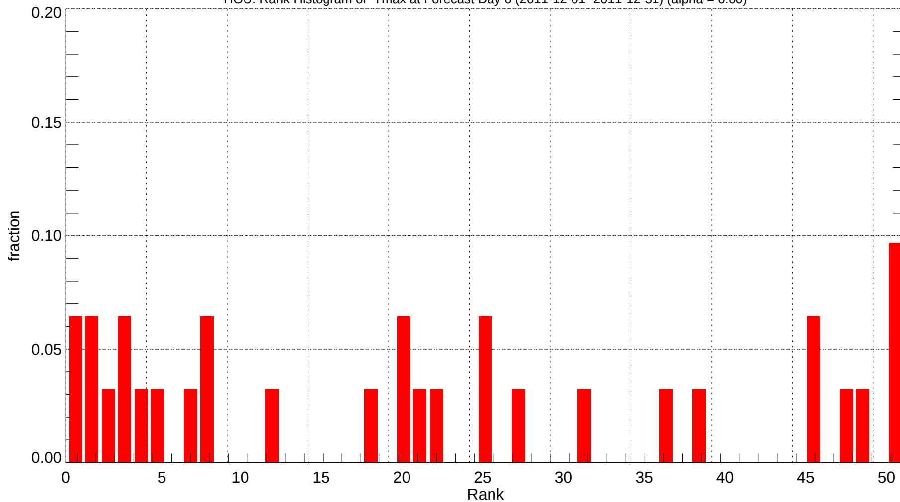
HOU: Rank Histogram of Tmax at Forecast Day 6 (2011-12-01~2011-12-31) (alpha = 0.00)
