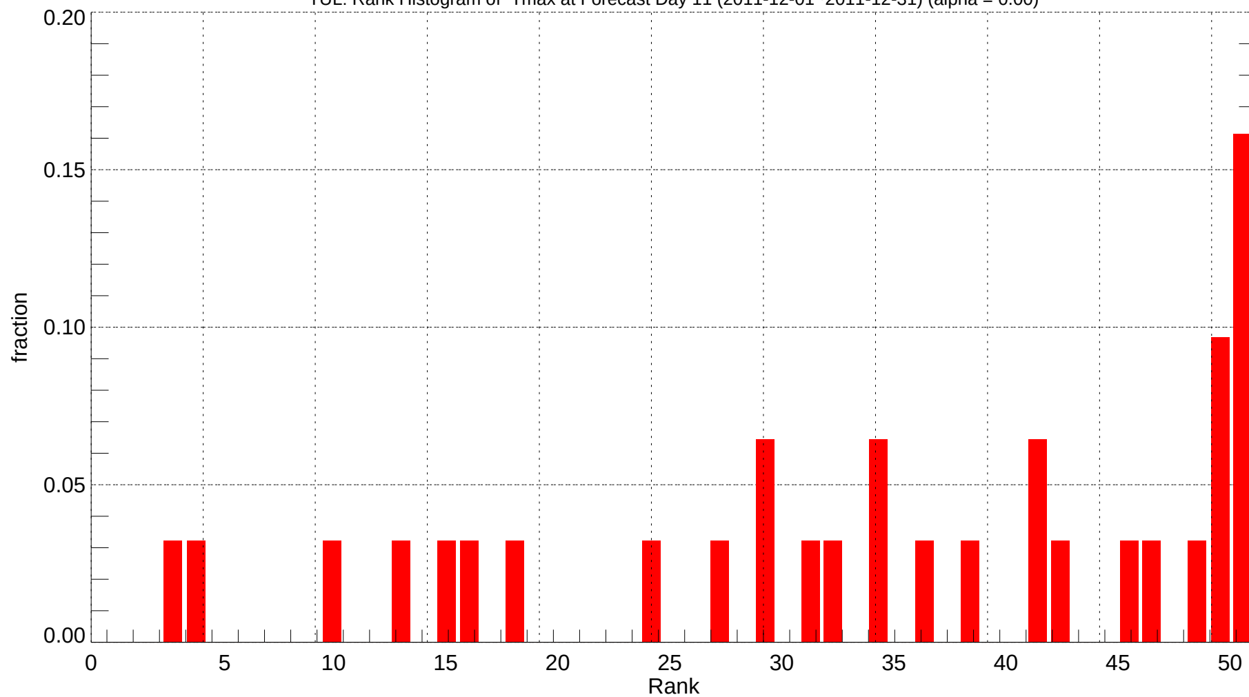
TUL: Rank Histogram of Tmax at Forecast Day 11 (2011-12-01~2011-12-31) (alpha = 0.00)
