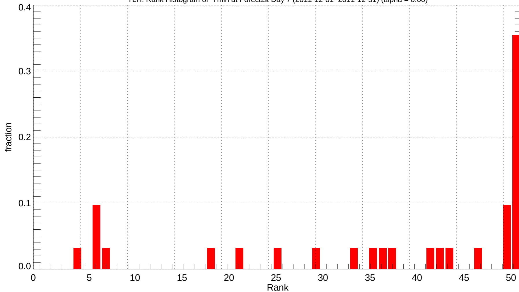
TLH: Rank Histogram of Tmin at Forecast Day 7 (2011-12-01~2011-12-31) (alpha = 0.00)
