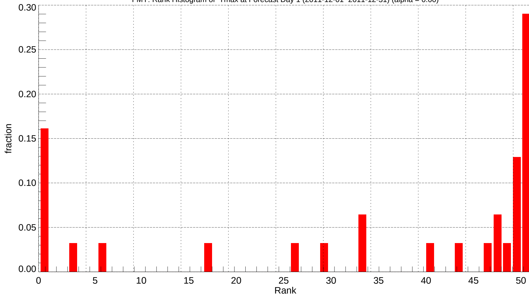
FMY: Rank Histogram of Tmax at Forecast Day 1 (2011-12-01~2011-12-31) (alpha = 0.00)
