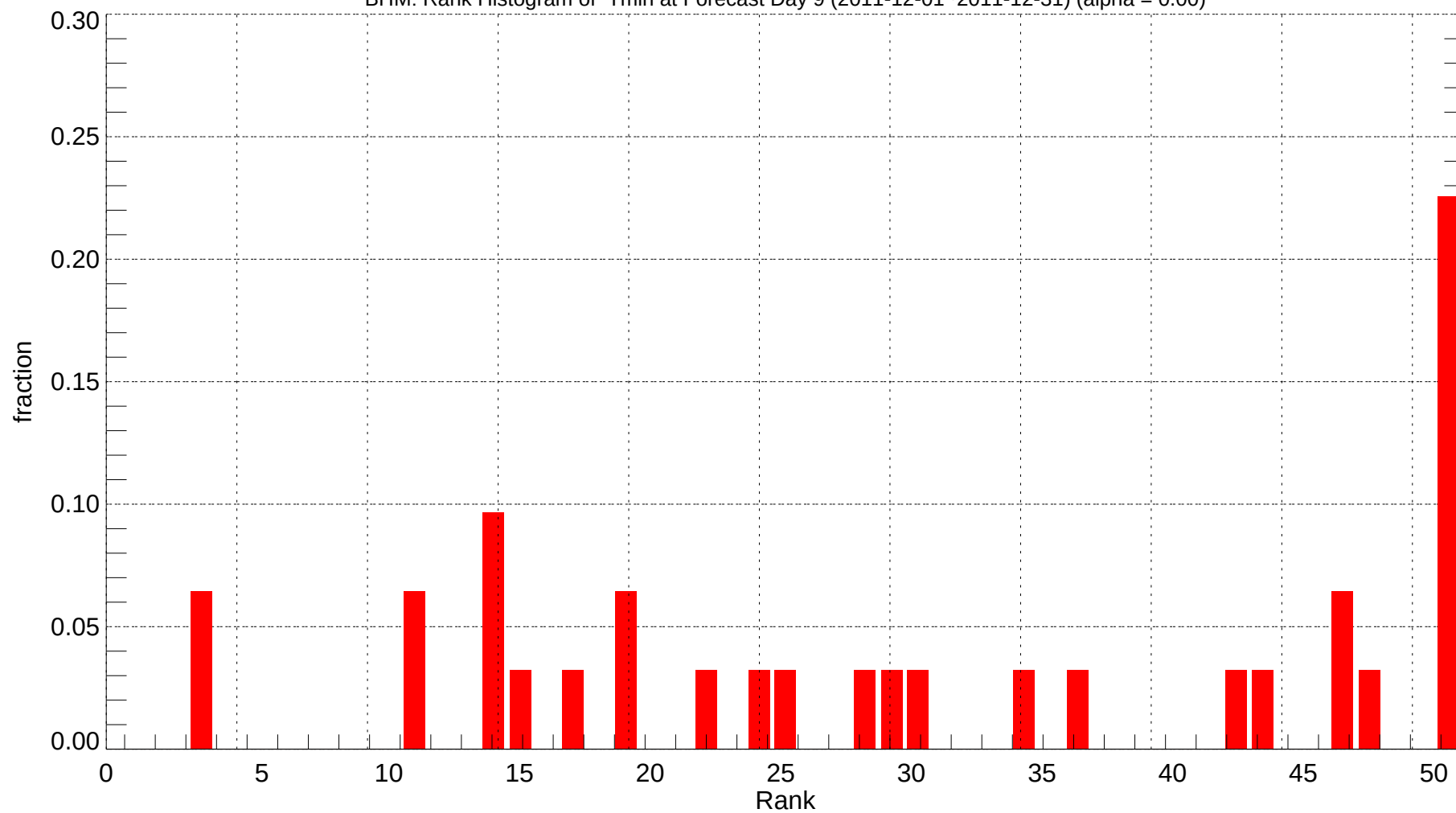
BHM: Rank Histogram of Tmin at Forecast Day 9 (2011-12-01~2011-12-31) (alpha = 0.00)
