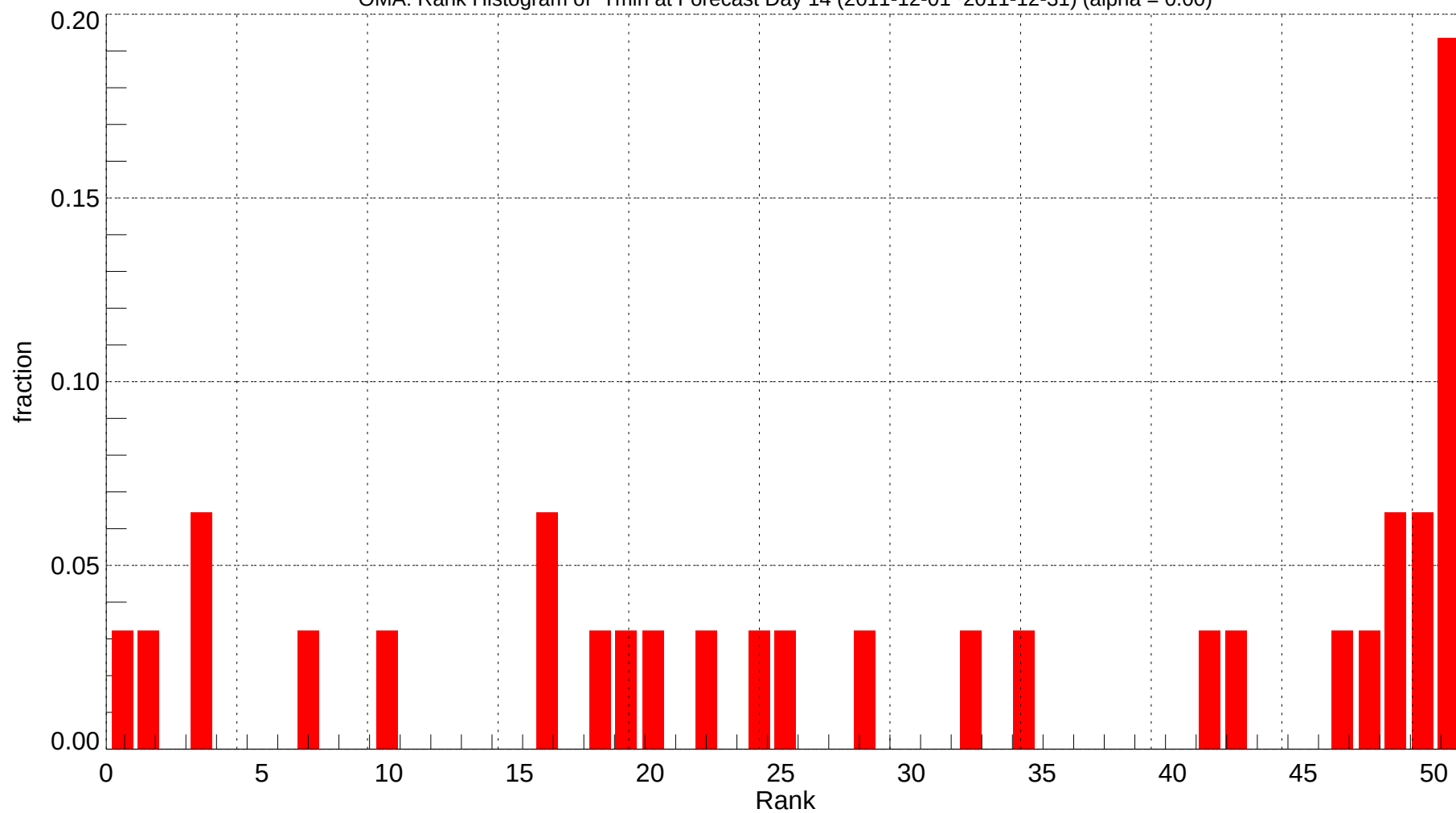
OMA: Rank Histogram of Tmin at Forecast Day 14 (2011-12-01~2011-12-31) (alpha = 0.00)
