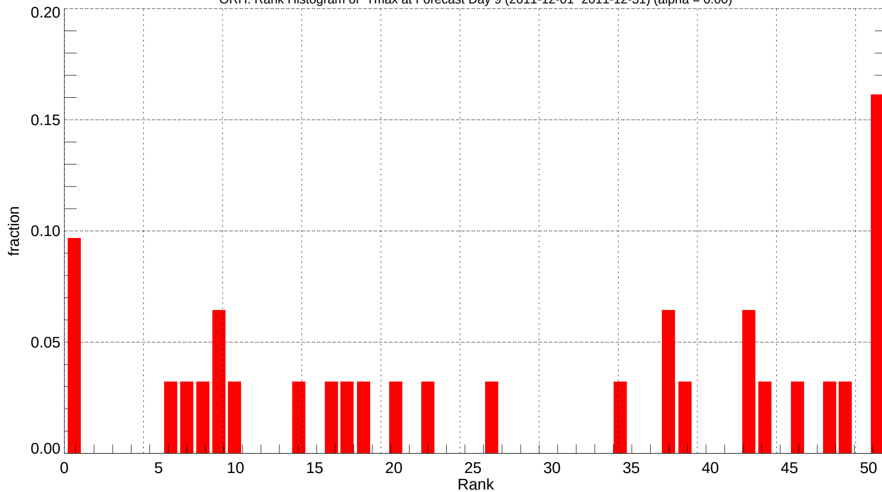
ORH: Rank Histogram of Tmax at Forecast Day 9 (2011-12-01~2011-12-31) (alpha = 0.00)
