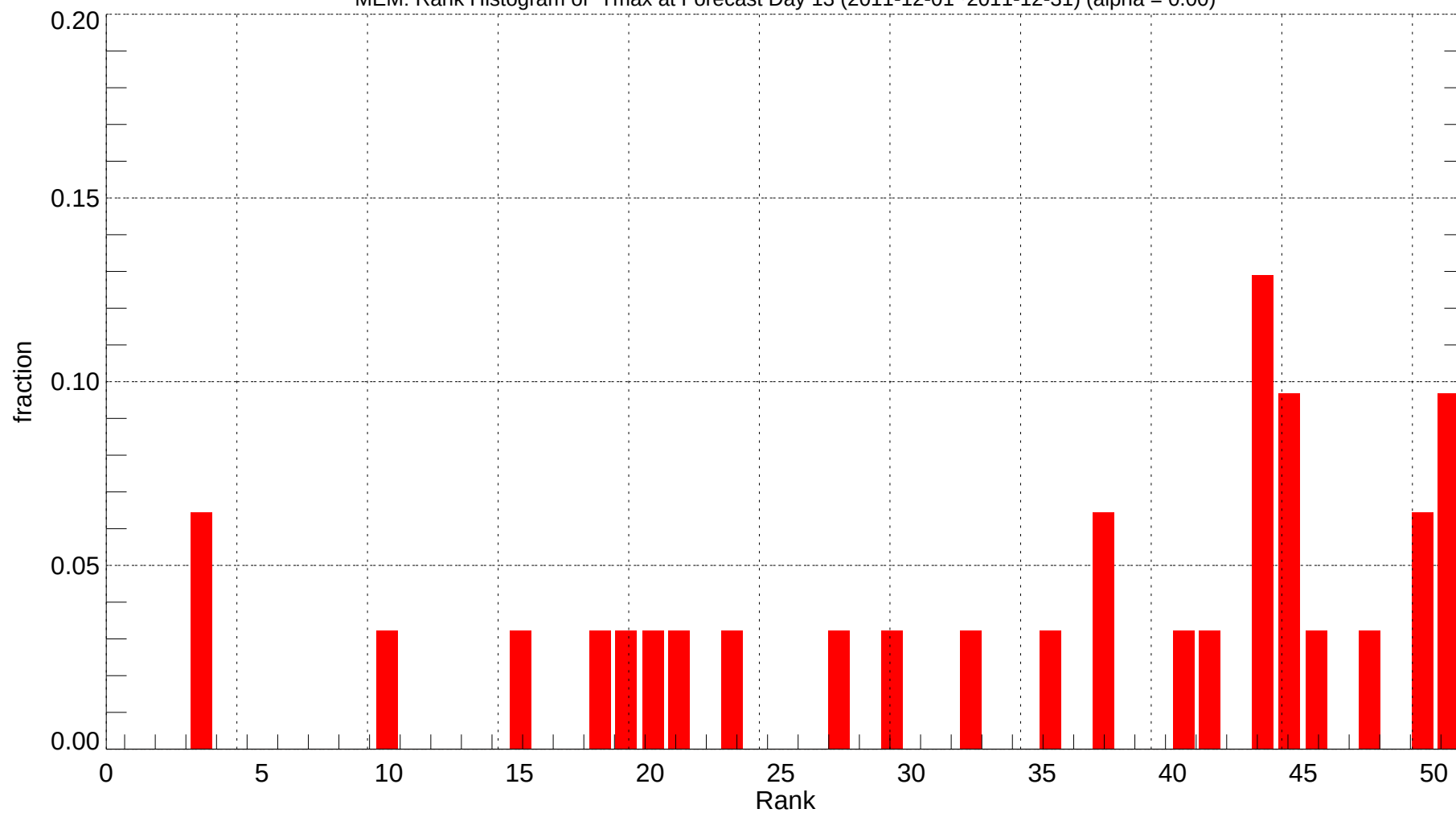
MEM: Rank Histogram of Tmax at Forecast Day 13 (2011-12-01~2011-12-31) (alpha = 0.00)
