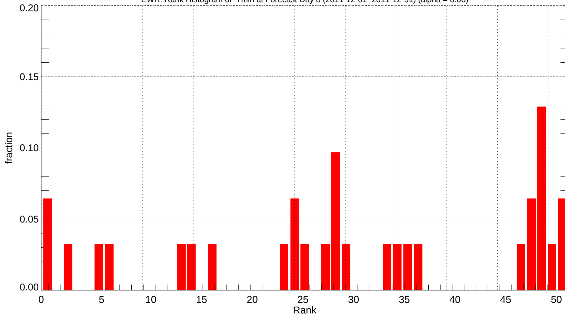
EWR: Rank Histogram of Tmin at Forecast Day 8 (2011-12-01~2011-12-31) (alpha = 0.00)
