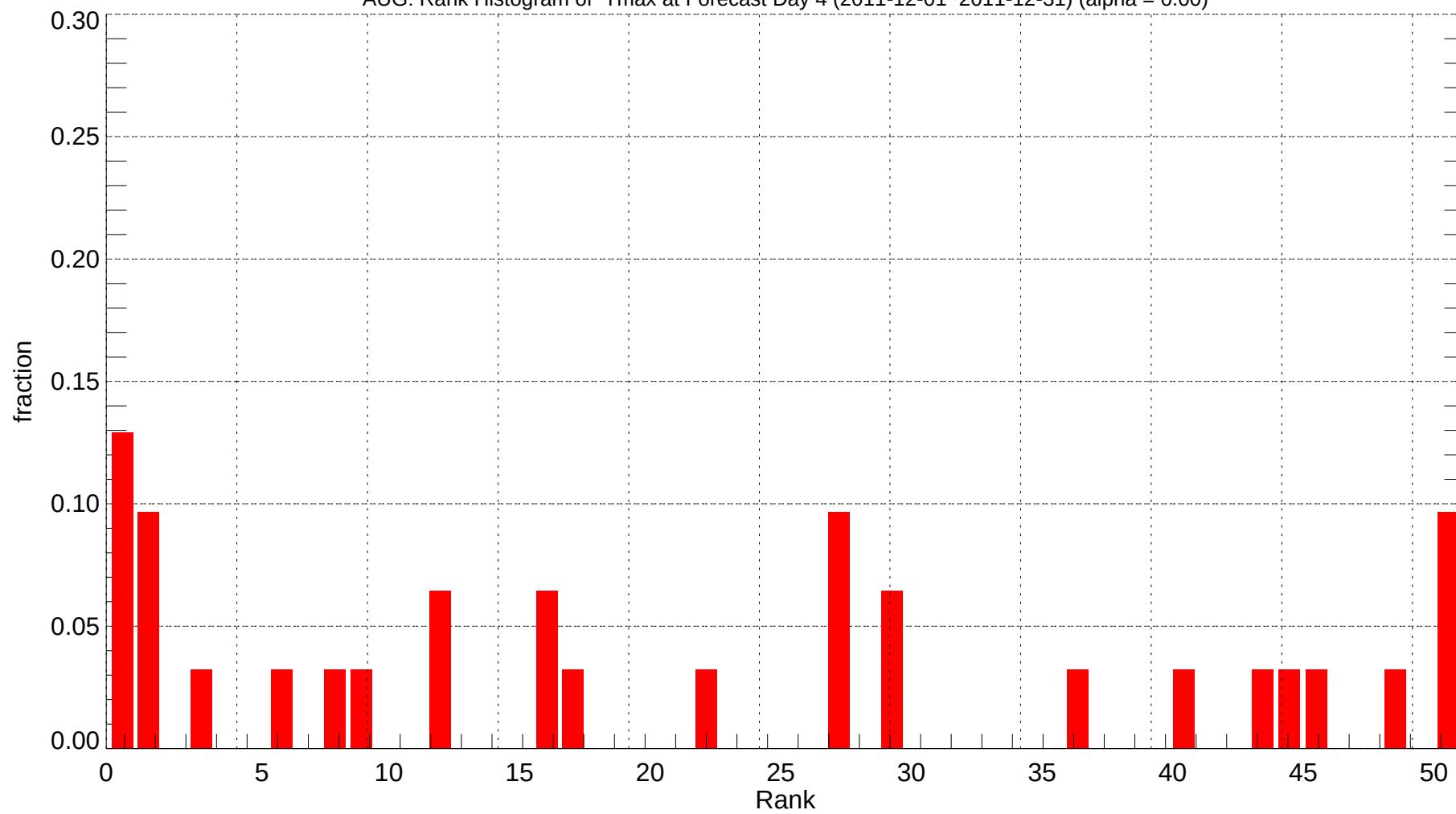
AUG: Rank Histogram of Tmax at Forecast Day 4 (2011-12-01~2011-12-31) (alpha = 0.00)
