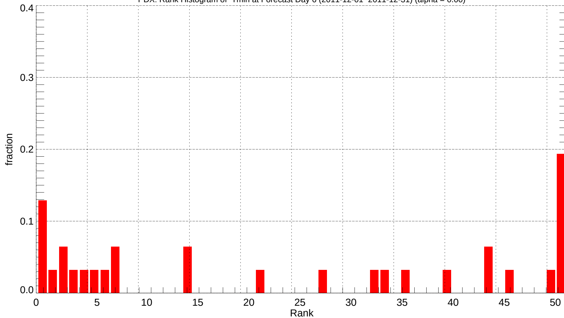
PDX: Rank Histogram of Tmin at Forecast Day 6 (2011-12-01~2011-12-31) (alpha = 0.00)
