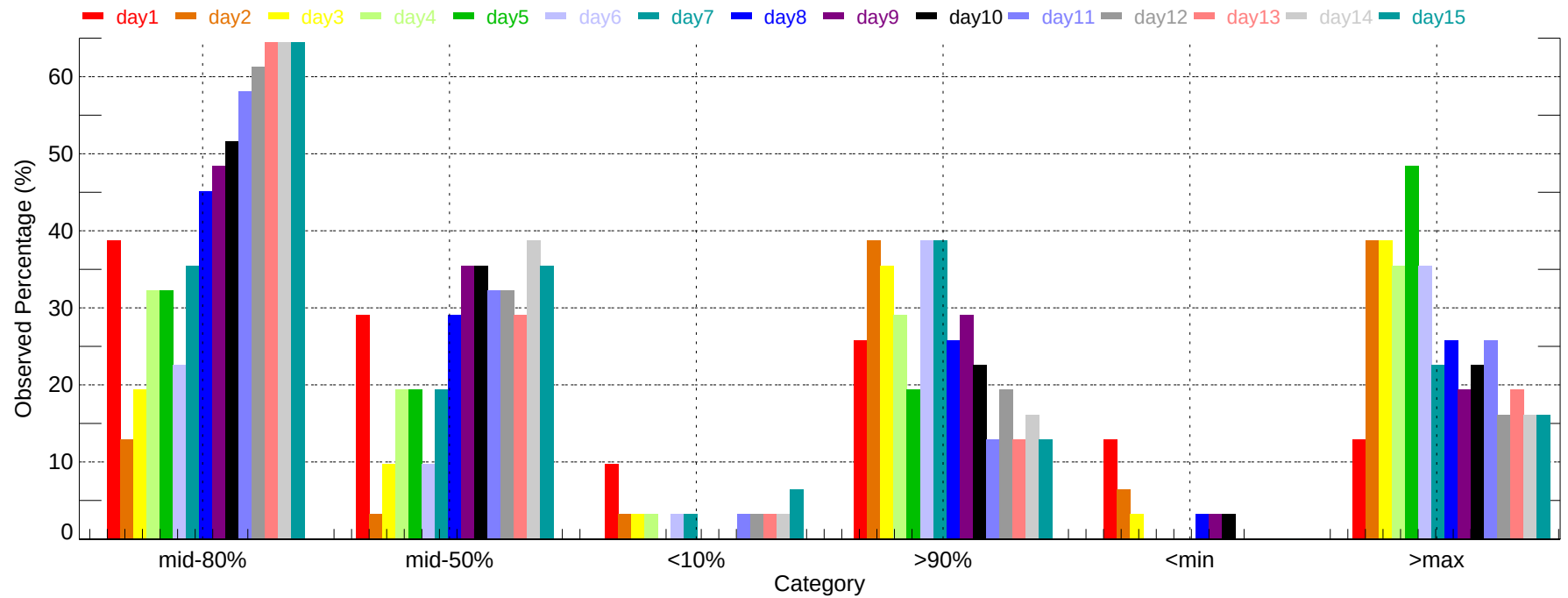
Observed Percentage of Ensembles - MDT: Max Temperature (2011-12-01~2011-12-31)
