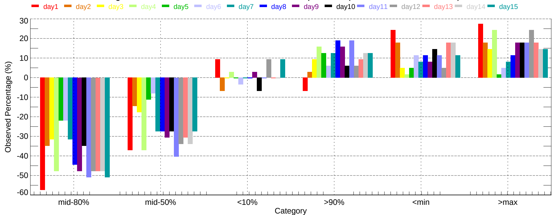
Observed Percentage Deviation of Ensembles - VCT: Max Temperature (2011-12-01~2011-12-31)
