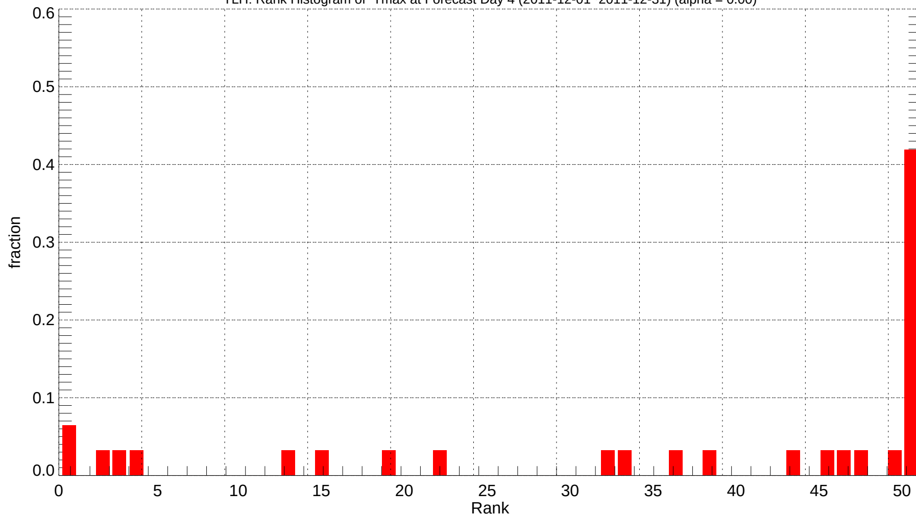
TLH: Rank Histogram of Tmax at Forecast Day 4 (2011-12-01~2011-12-31) (alpha = 0.00)
