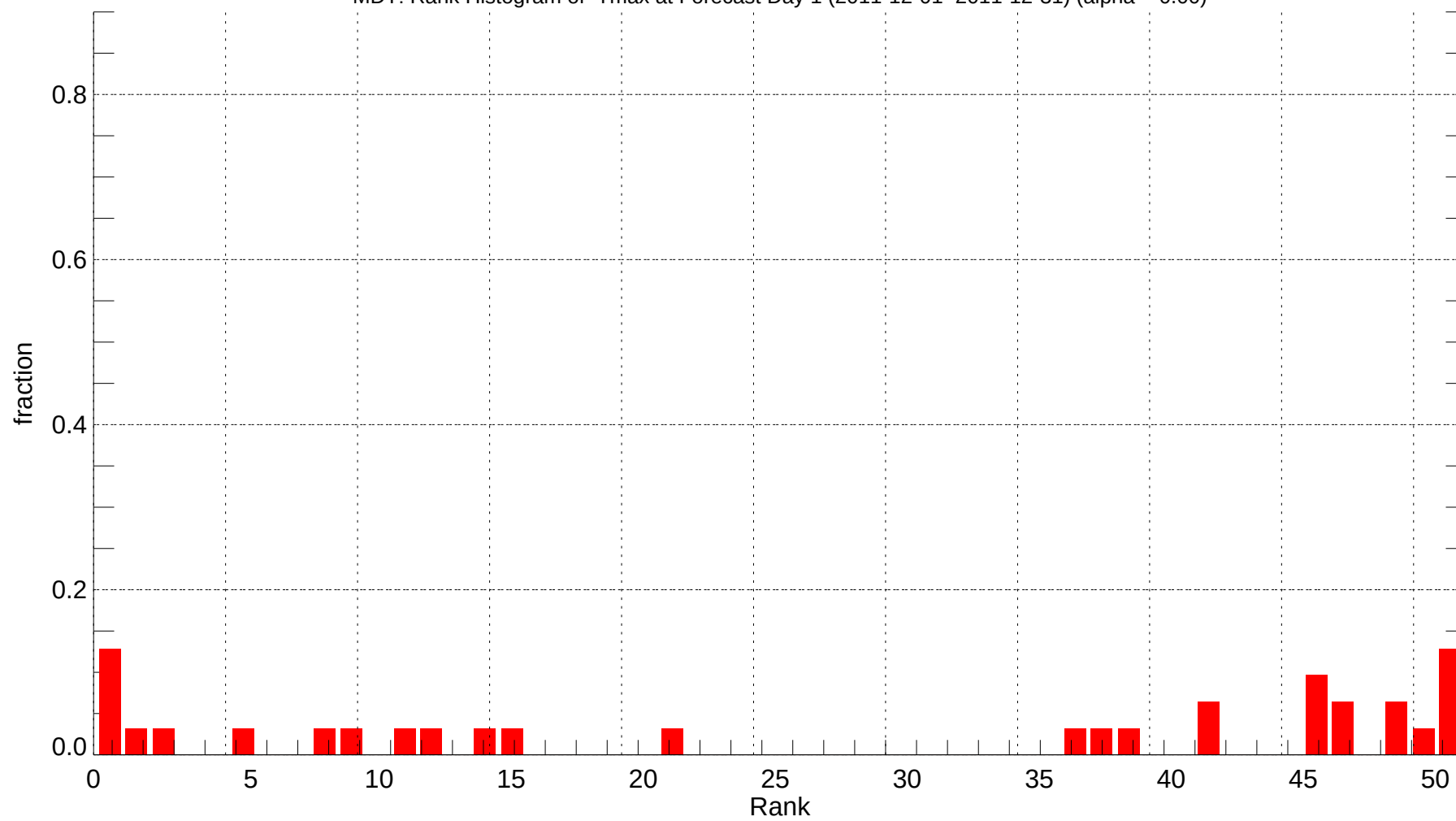
MDT: Rank Histogram of Tmax at Forecast Day 1 (2011-12-01~2011-12-31) (alpha = 0.00)
