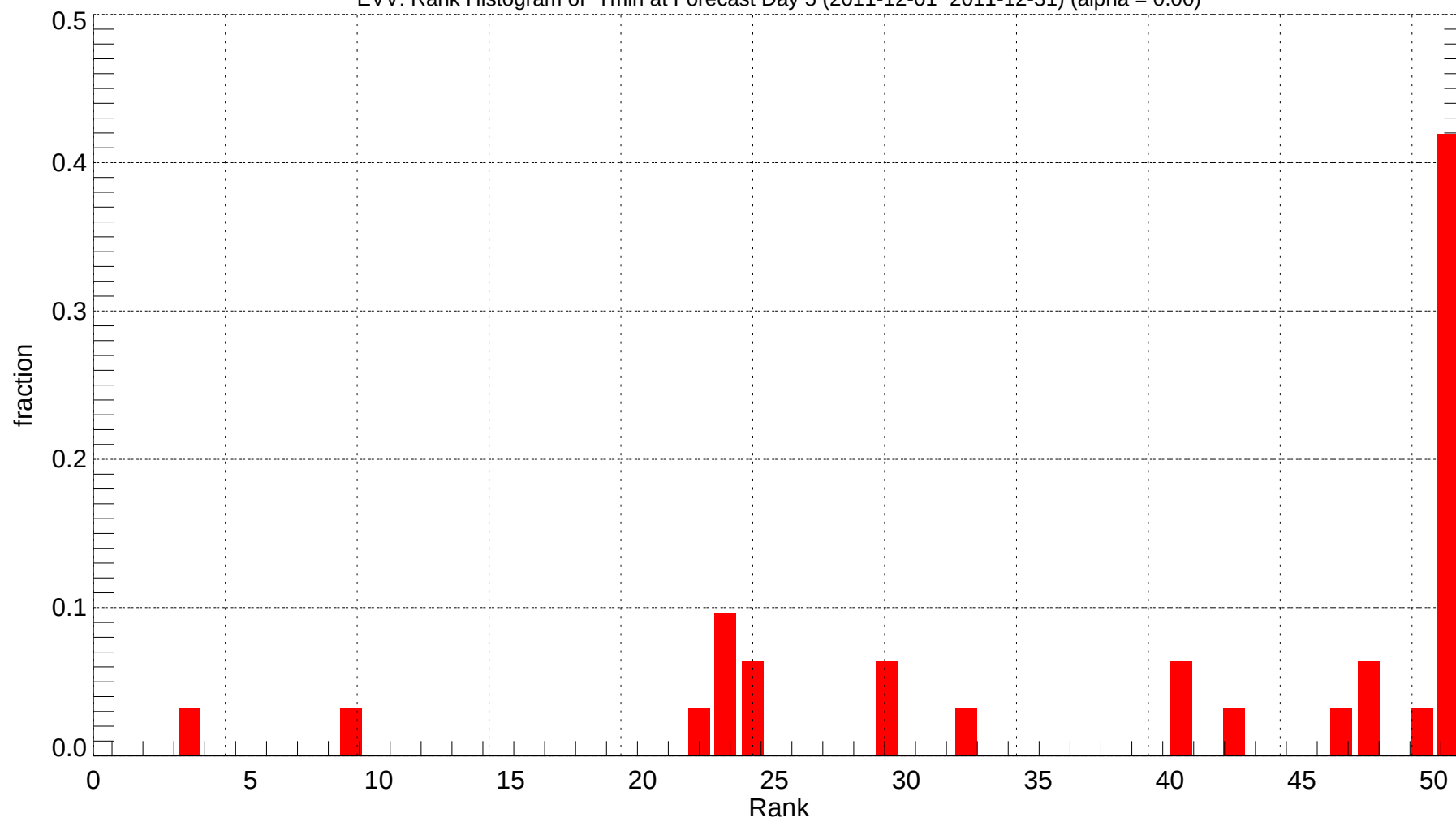
EVV: Rank Histogram of Tmin at Forecast Day 5 (2011-12-01~2011-12-31) (alpha = 0.00)
