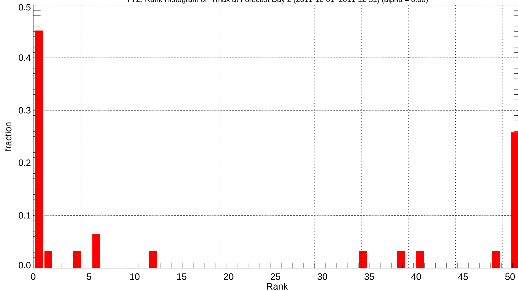
YYZ: Rank Histogram of Tmax at Forecast Day 2 (2011-12-01~2011-12-31) (alpha = 0.00)
