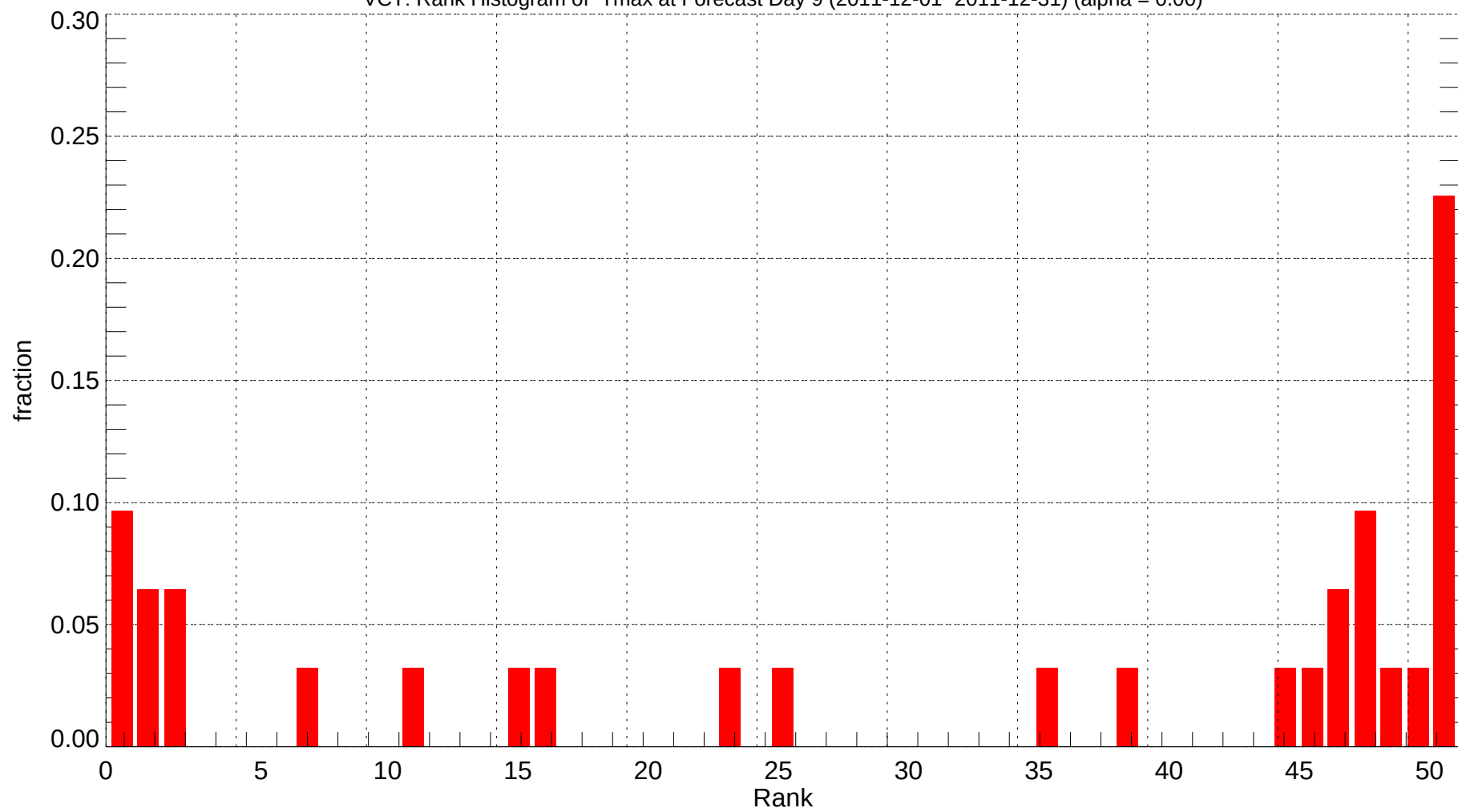
VCT: Rank Histogram of Tmax at Forecast Day 9 (2011-12-01~2011-12-31) (alpha = 0.00)
