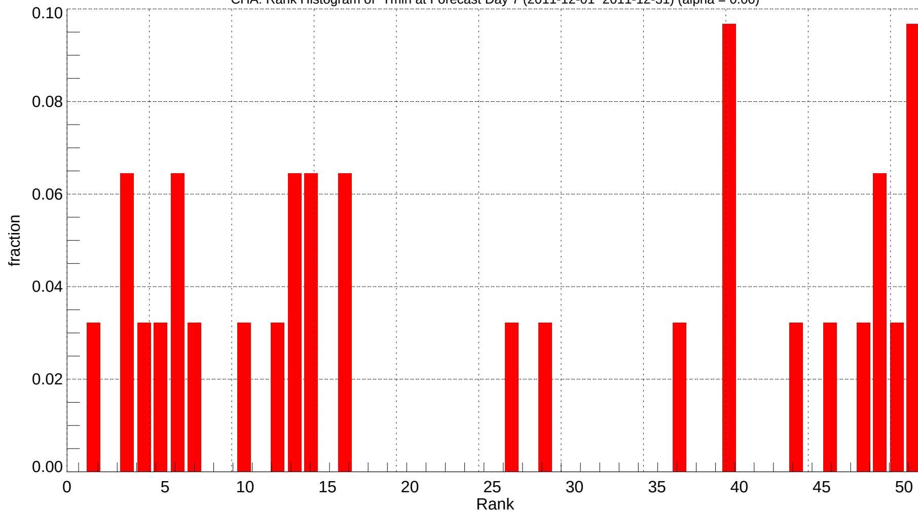
CHA: Rank Histogram of Tmin at Forecast Day 7 (2011-12-01~2011-12-31) (alpha = 0.00)
