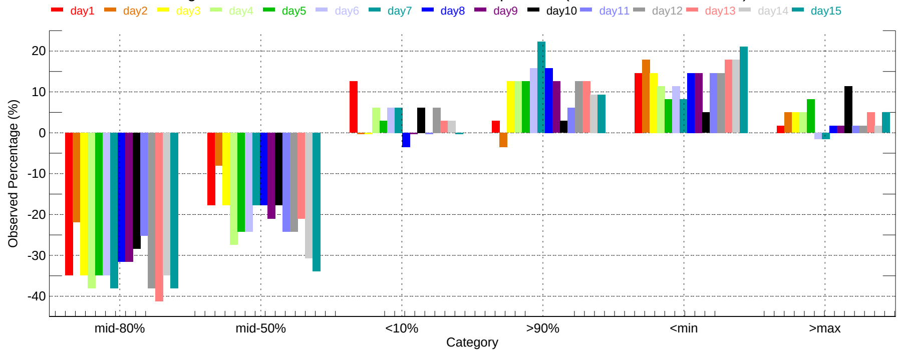
Observed Percentage Deviation of Ensembles - ACT: Max Temperature (2011-12-01~2011-12-31)
