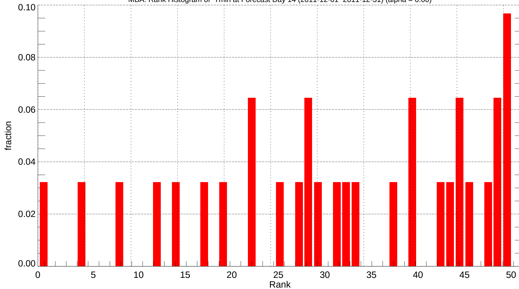
MBA: Rank Histogram of Tmin at Forecast Day 14 (2011-12-01~2011-12-31) (alpha = 0.00)
