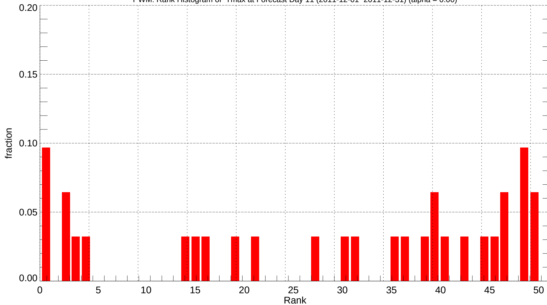
PWM: Rank Histogram of Tmax at Forecast Day 11 (2011-12-01~2011-12-31) (alpha = 0.00)
