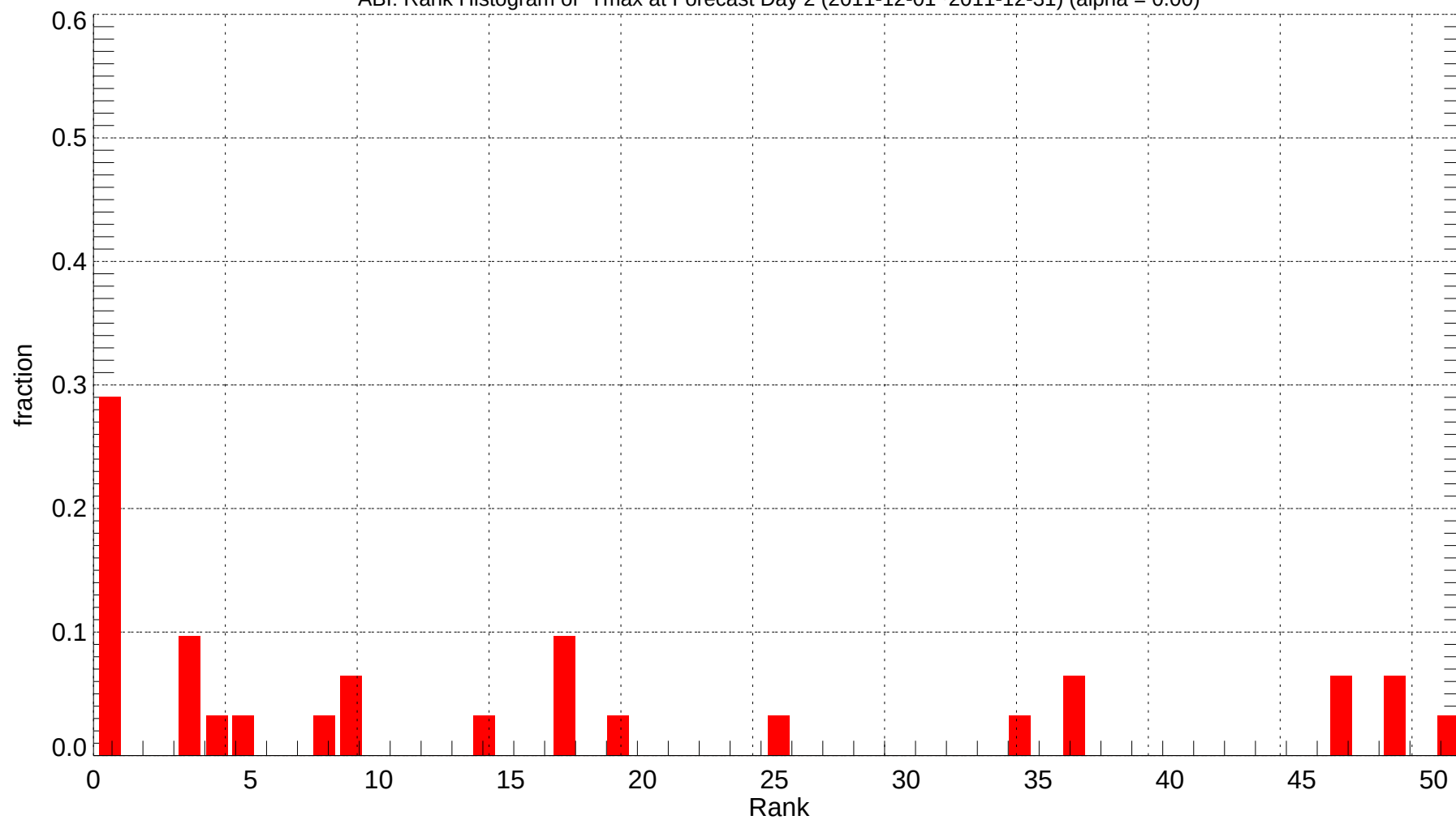
ABI: Rank Histogram of Tmax at Forecast Day 2 (2011-12-01~2011-12-31) (alpha = 0.00)
