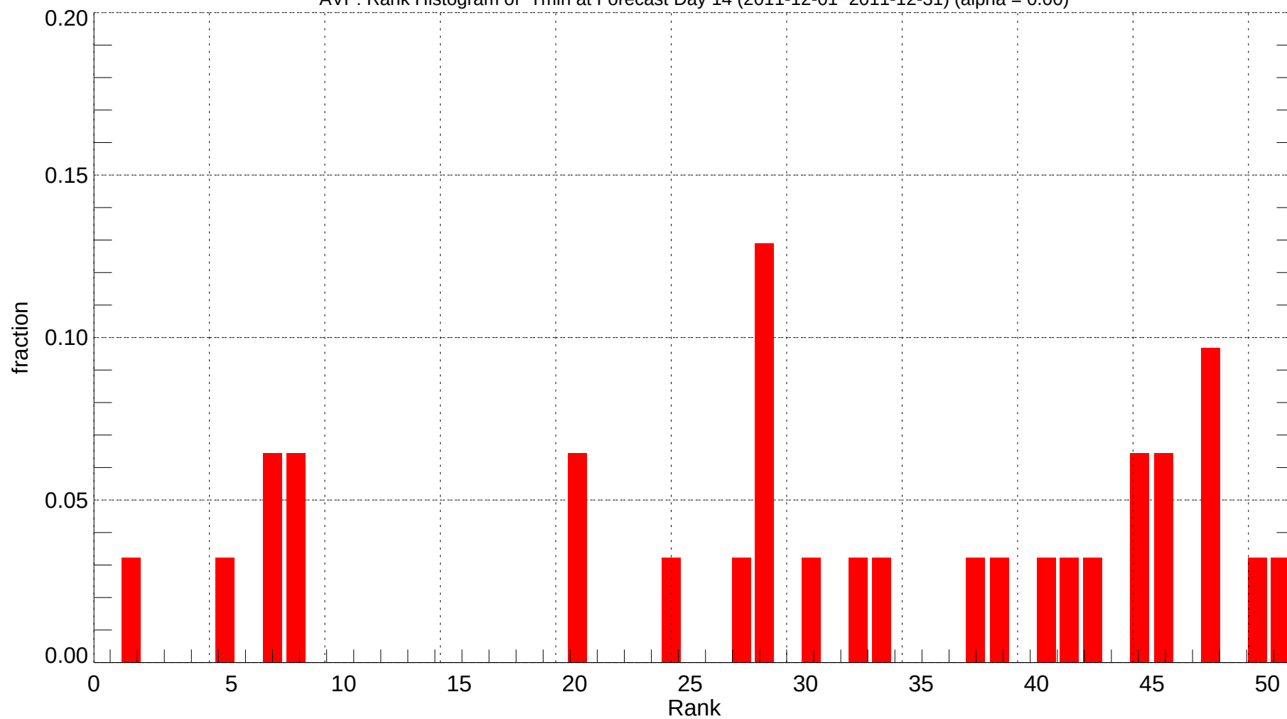
AVP: Rank Histogram of Tmin at Forecast Day 14 (2011-12-01~2011-12-31) (alpha = 0.00)
