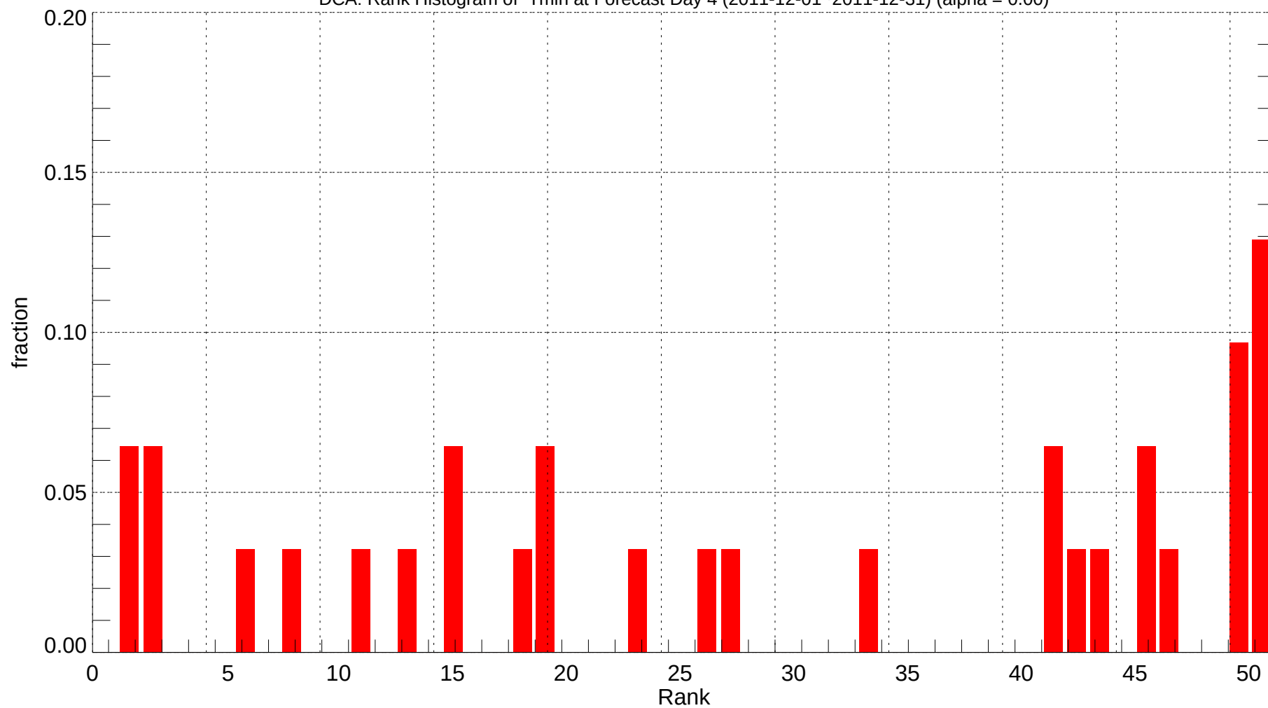
DCA: Rank Histogram of Tmin at Forecast Day 4 (2011-12-01~2011-12-31) (alpha = 0.00)
