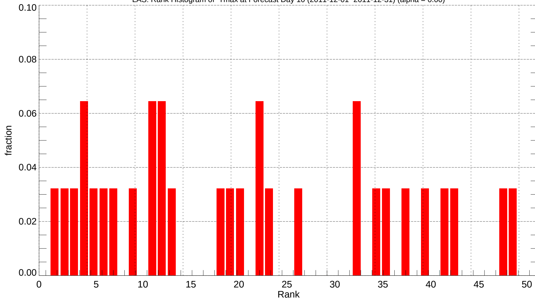
LAS: Rank Histogram of Tmax at Forecast Day 10 (2011-12-01~2011-12-31) (alpha = 0.00)
