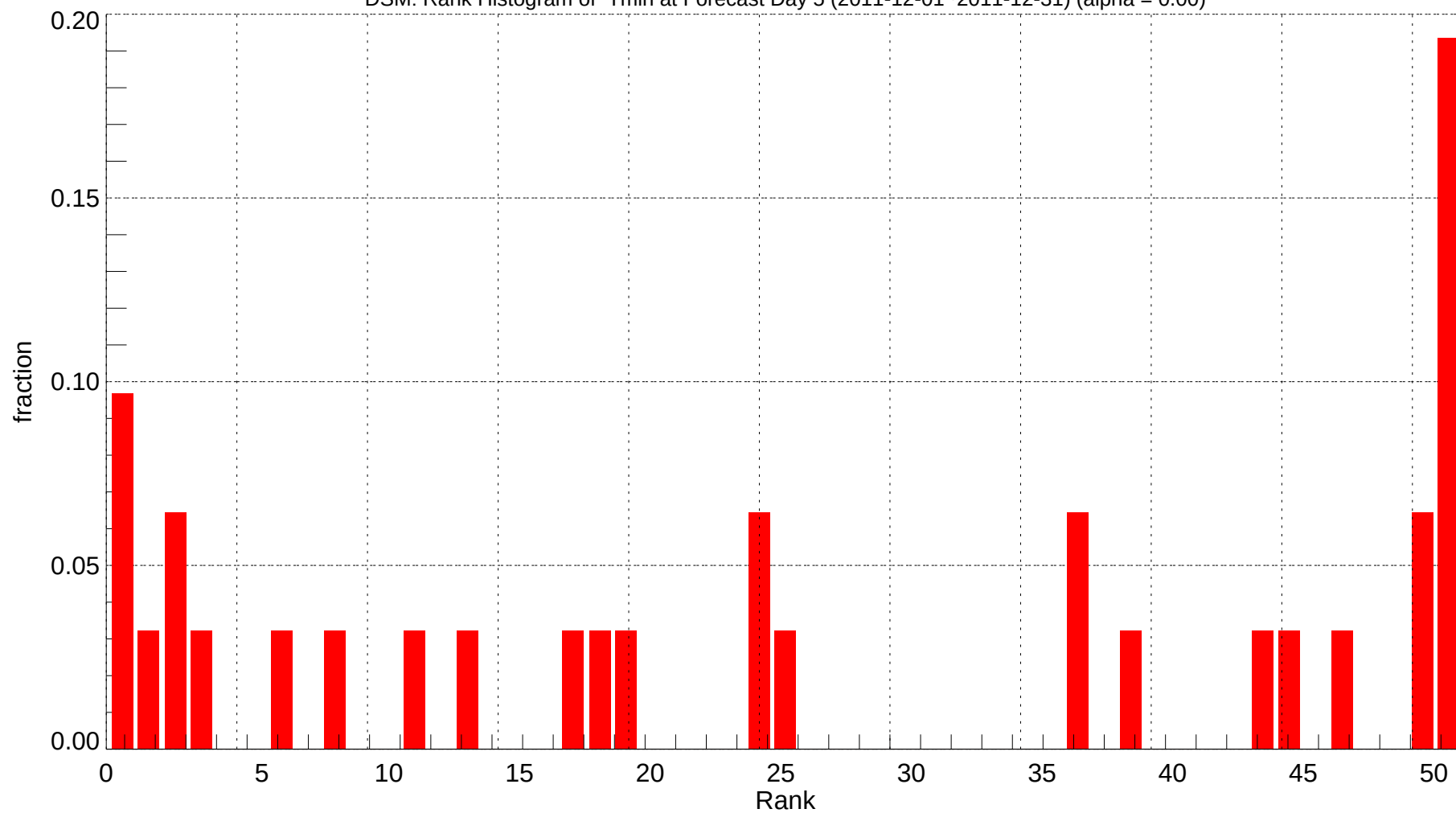
DSM: Rank Histogram of Tmin at Forecast Day 5 (2011-12-01~2011-12-31) (alpha = 0.00)
