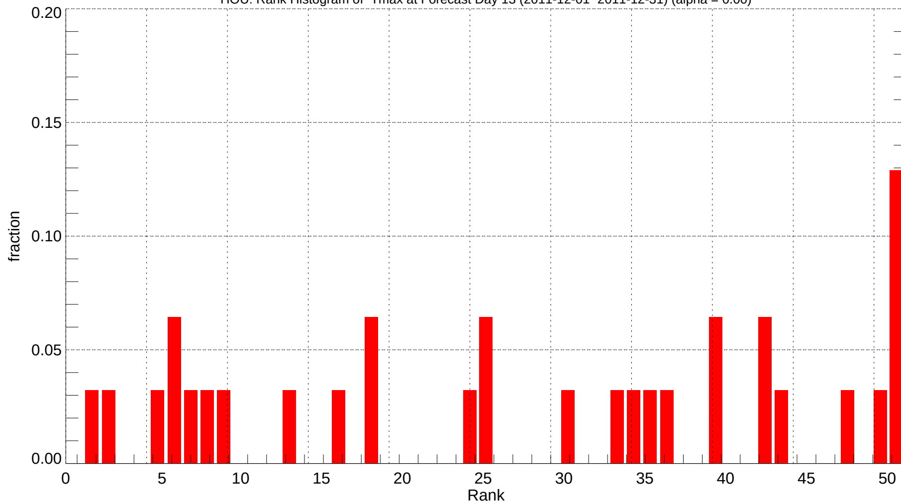
HOU: Rank Histogram of Tmax at Forecast Day 13 (2011-12-01~2011-12-31) (alpha = 0.00)
