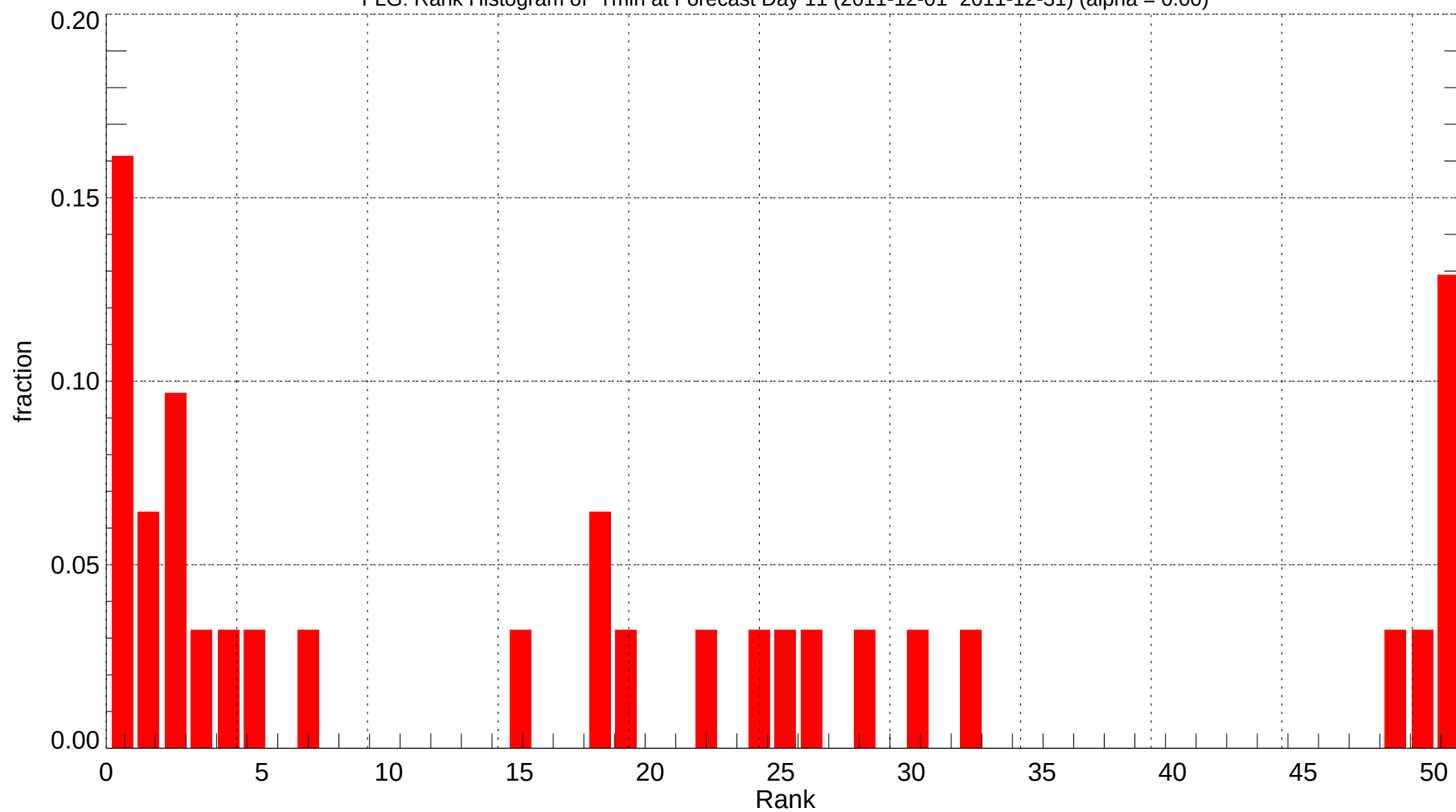
FLG: Rank Histogram of Tmin at Forecast Day 11 (2011-12-01~2011-12-31) (alpha = 0.00)
