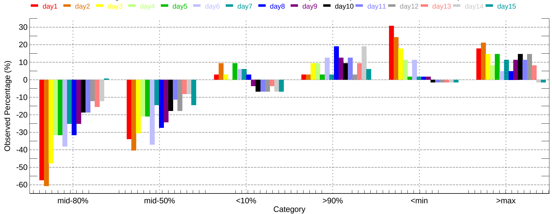
Observed Percentage Deviation of Ensembles - ORD: Max Temperature (2011-12-01~2011-12-31)
