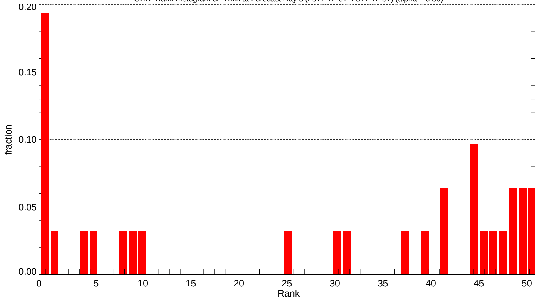
ORD: Rank Histogram of Tmin at Forecast Day 6 (2011-12-01~2011-12-31) (alpha = 0.00)
