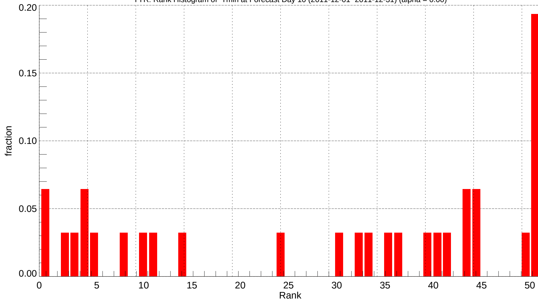
TYR: Rank Histogram of Tmin at Forecast Day 10 (2011-12-01~2011-12-31) (alpha = 0.00)
