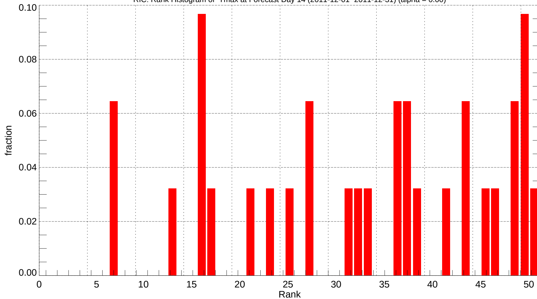
RIC: Rank Histogram of Tmax at Forecast Day 14 (2011-12-01~2011-12-31) (alpha = 0.00)
