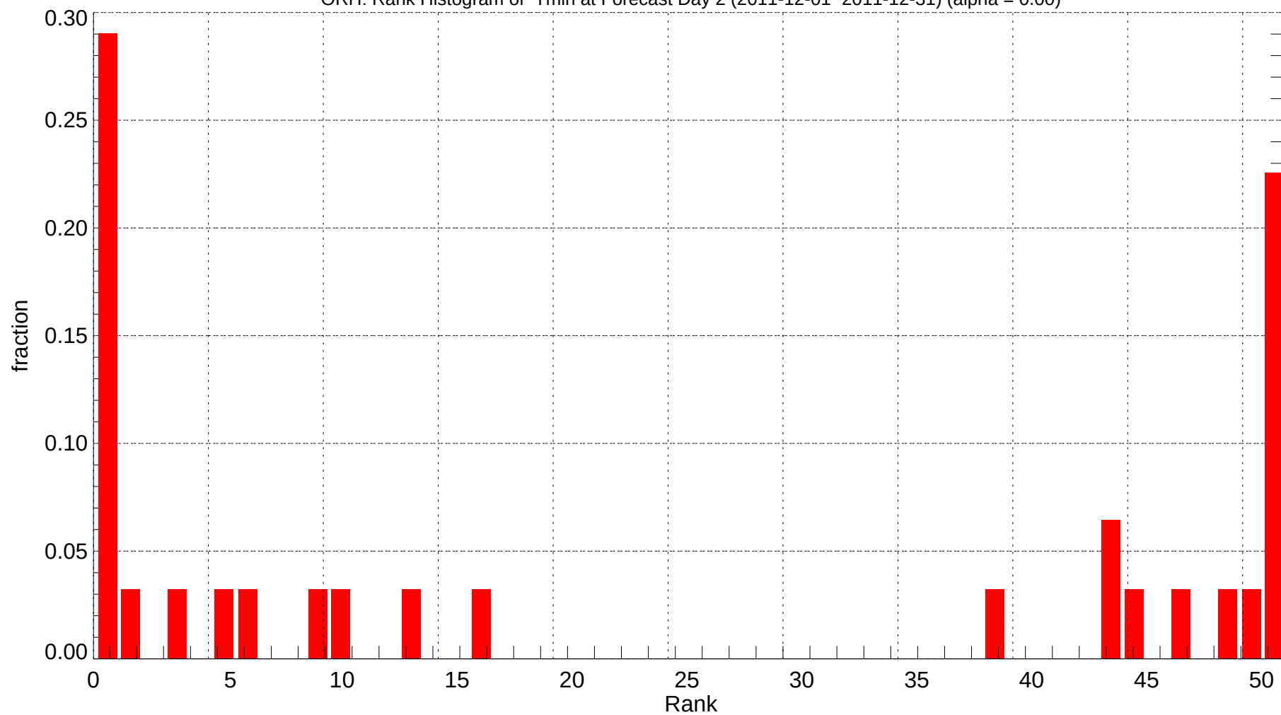
ORH: Rank Histogram of Tmin at Forecast Day 2 (2011-12-01~2011-12-31) (alpha = 0.00)
