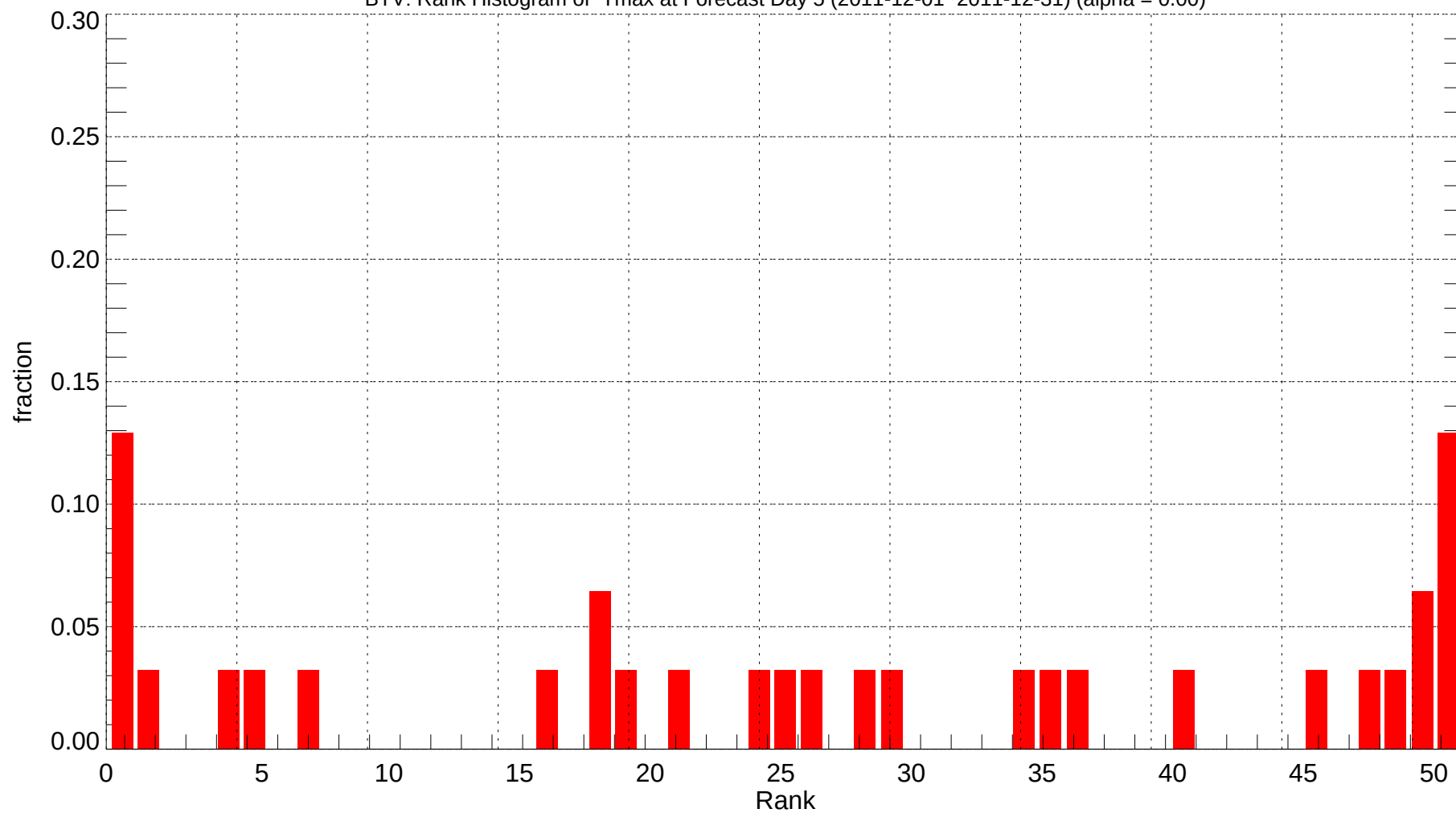
BTV: Rank Histogram of Tmax at Forecast Day 5 (2011-12-01~2011-12-31) (alpha = 0.00)
