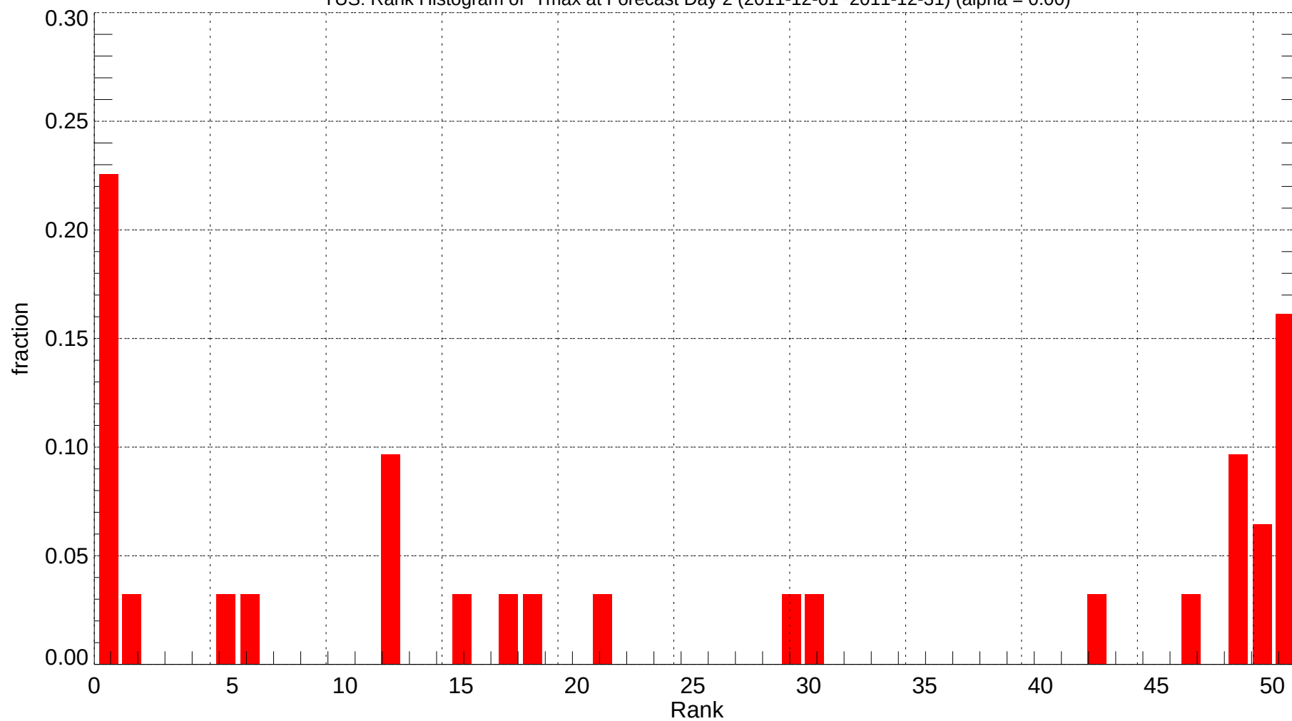
TUS: Rank Histogram of Tmax at Forecast Day 2 (2011-12-01~2011-12-31) (alpha = 0.00)
