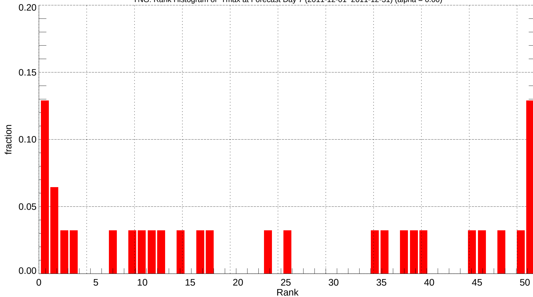
YNG: Rank Histogram of Tmax at Forecast Day 7 (2011-12-01~2011-12-31) (alpha = 0.00)
