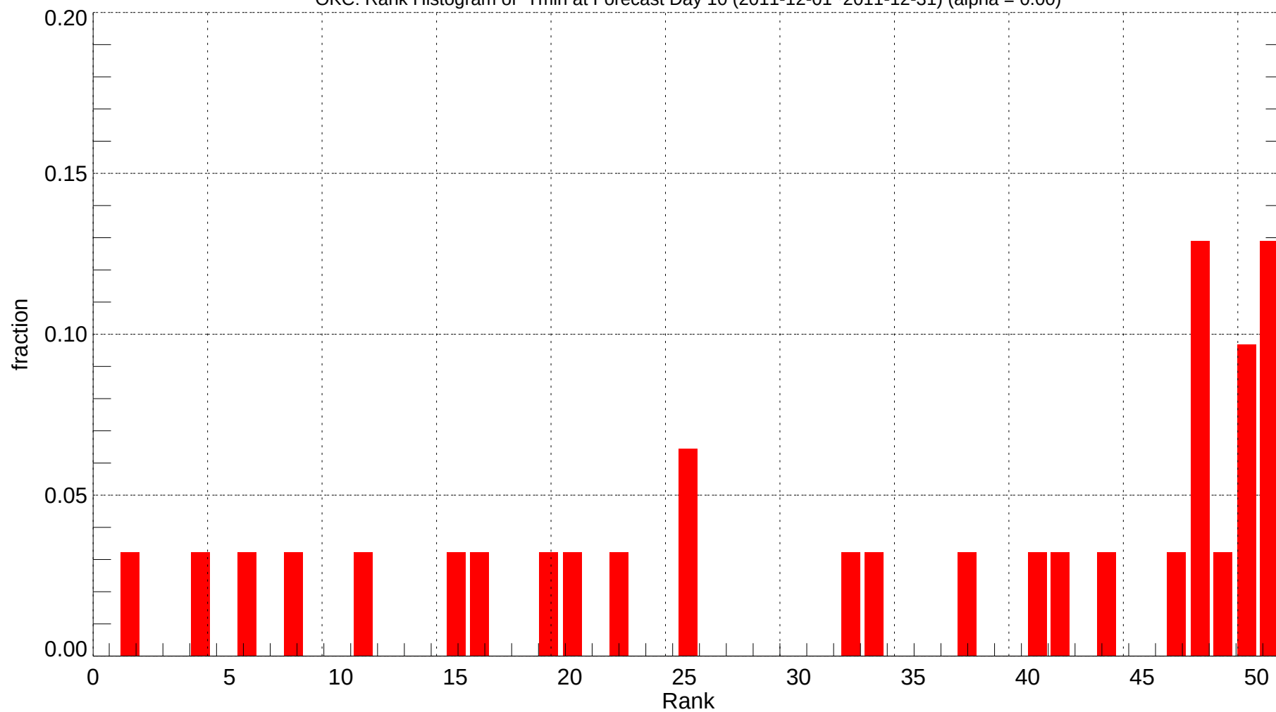
OKC: Rank Histogram of Tmin at Forecast Day 10 (2011-12-01~2011-12-31) (alpha = 0.00)
