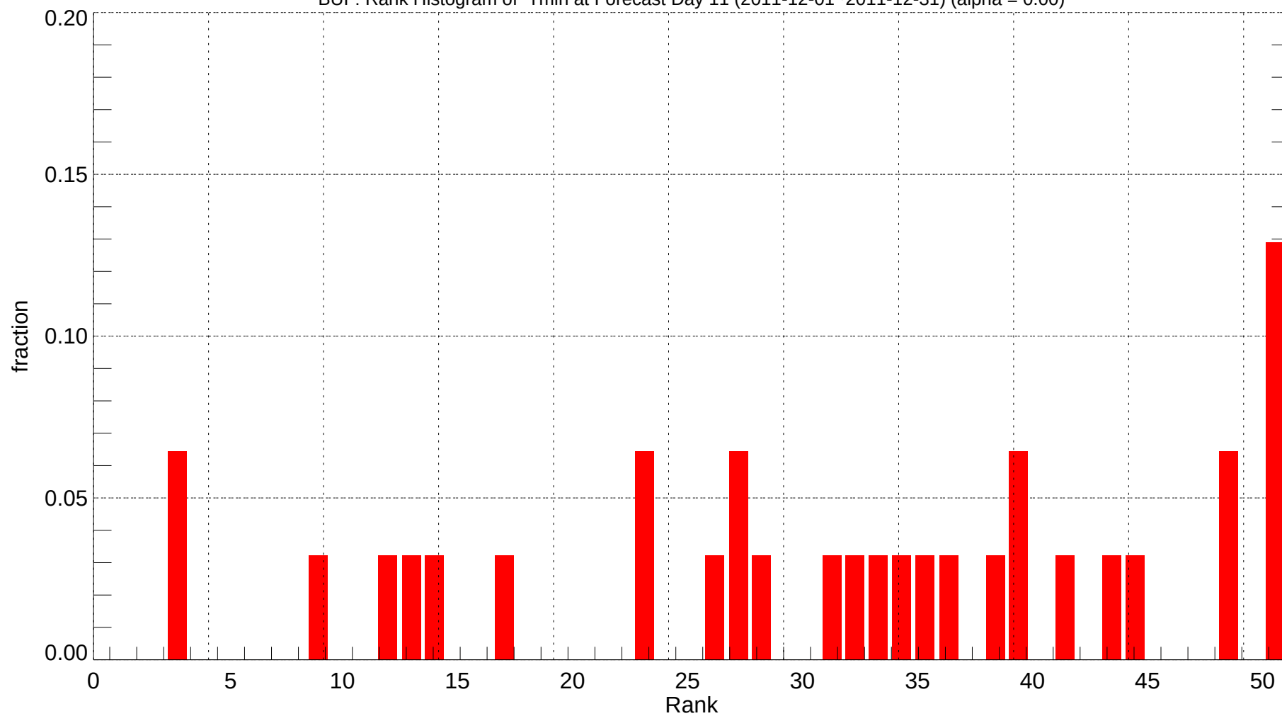
BUF: Rank Histogram of Tmin at Forecast Day 11 (2011-12-01~2011-12-31) (alpha = 0.00)
