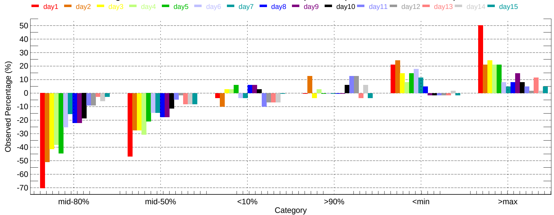
Observed Percentage Deviation of Ensembles - ALB: Min Temperature (2011-12-01~2011-12-31)
