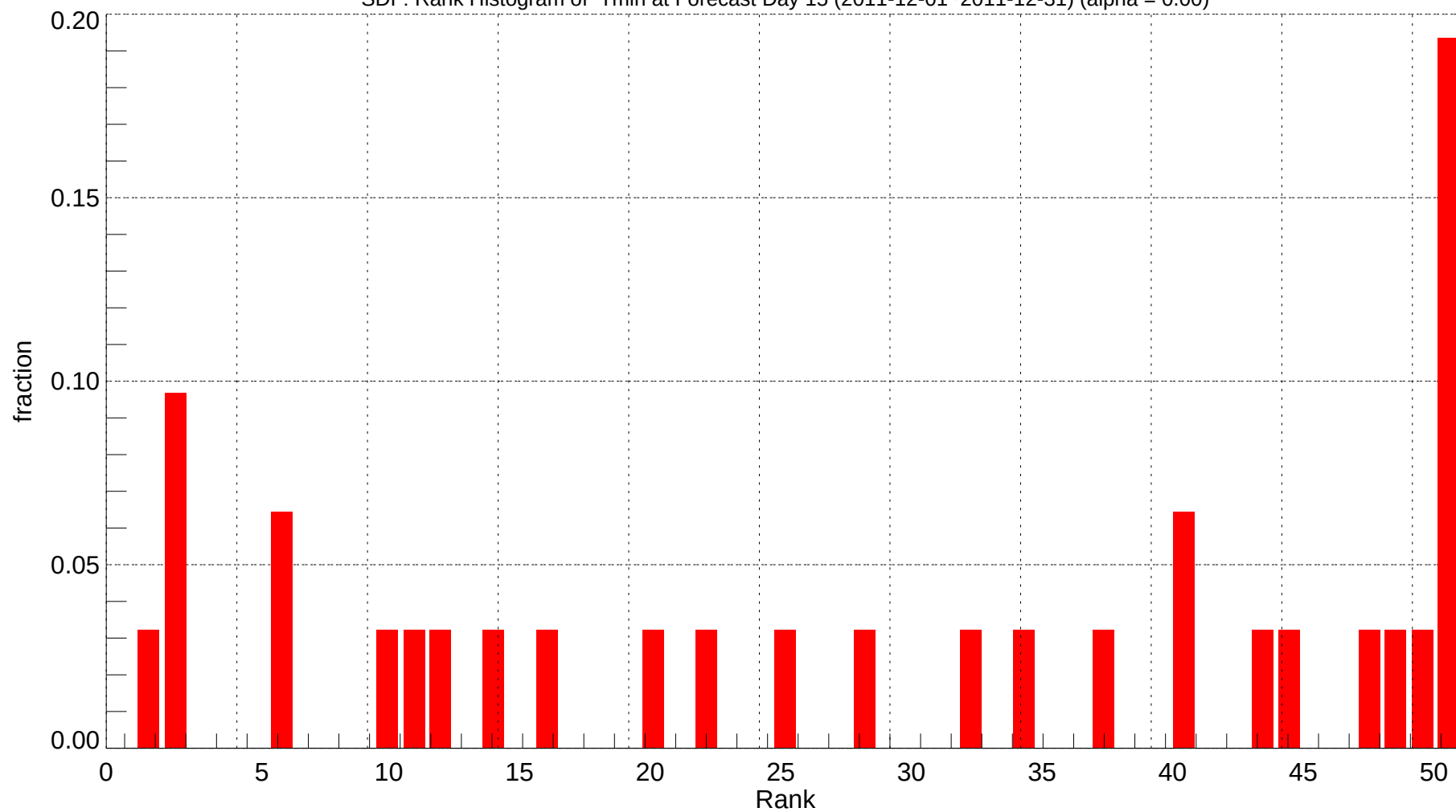
SDF: Rank Histogram of Tmin at Forecast Day 15 (2011-12-01~2011-12-31) (alpha = 0.00)
