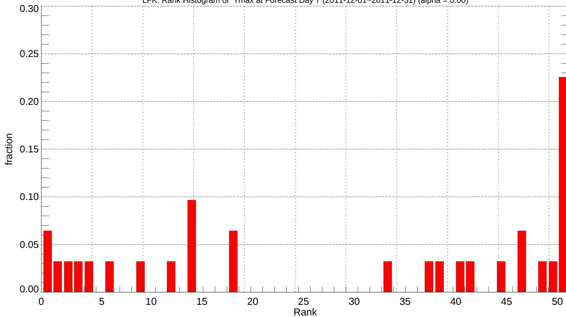
LFK: Rank Histogram of Tmax at Forecast Day 7 (2011-12-01~2011-12-31) (alpha = 0.00)
