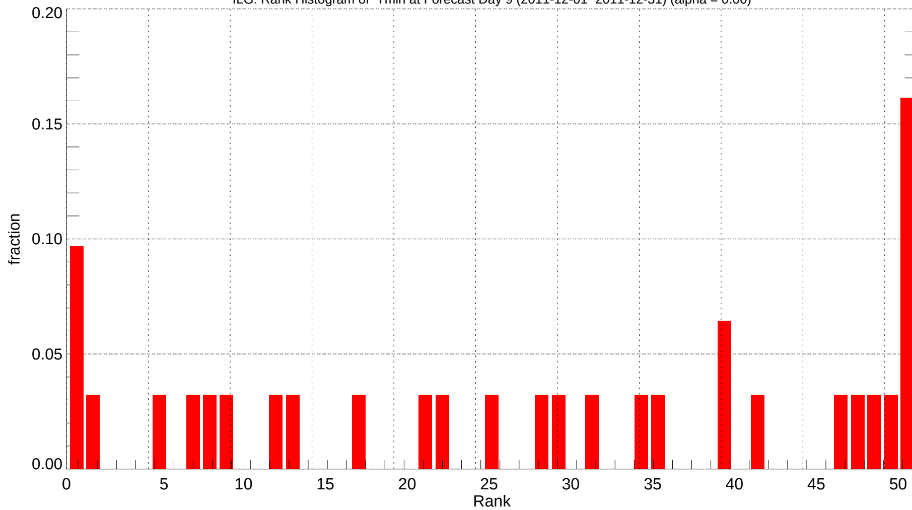
ILG: Rank Histogram of Tmin at Forecast Day 9 (2011-12-01~2011-12-31) (alpha = 0.00)
