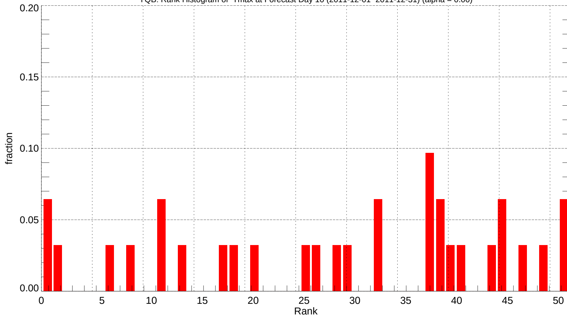
YQB: Rank Histogram of Tmax at Forecast Day 10 (2011-12-01~2011-12-31) (alpha = 0.00)
