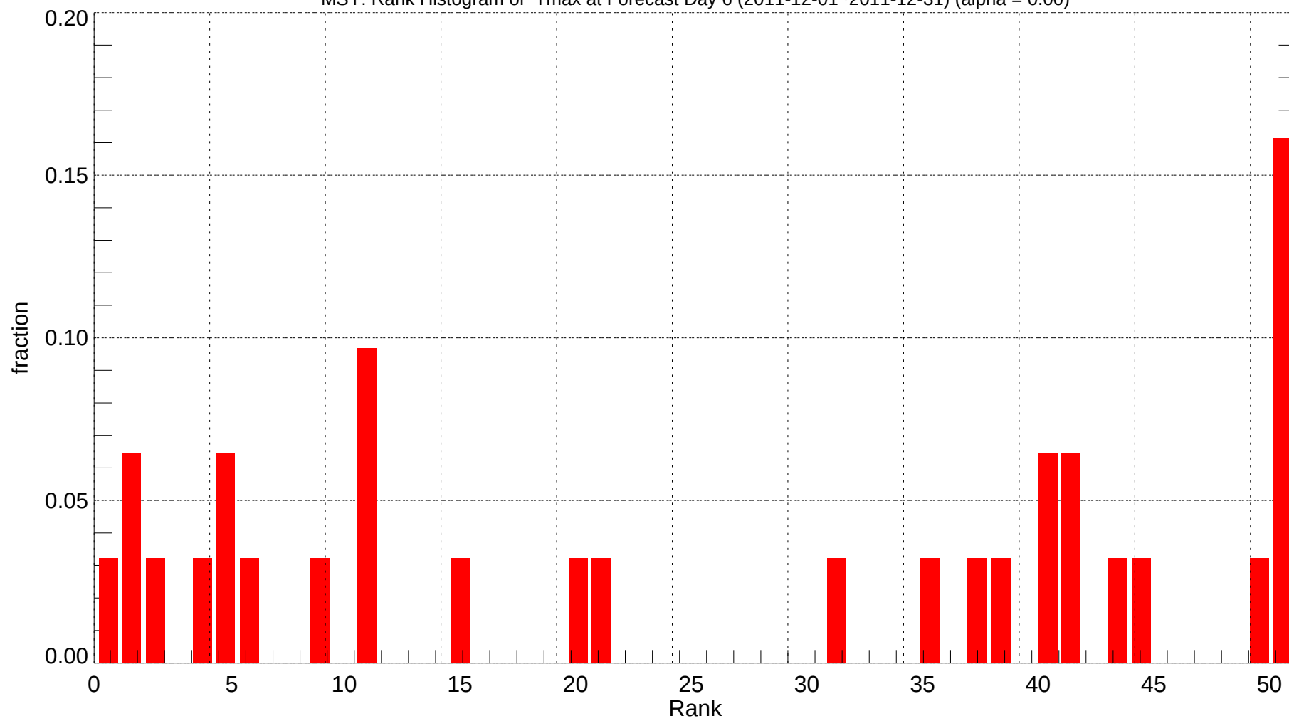
MSY: Rank Histogram of Tmax at Forecast Day 6 (2011-12-01~2011-12-31) (alpha = 0.00)
