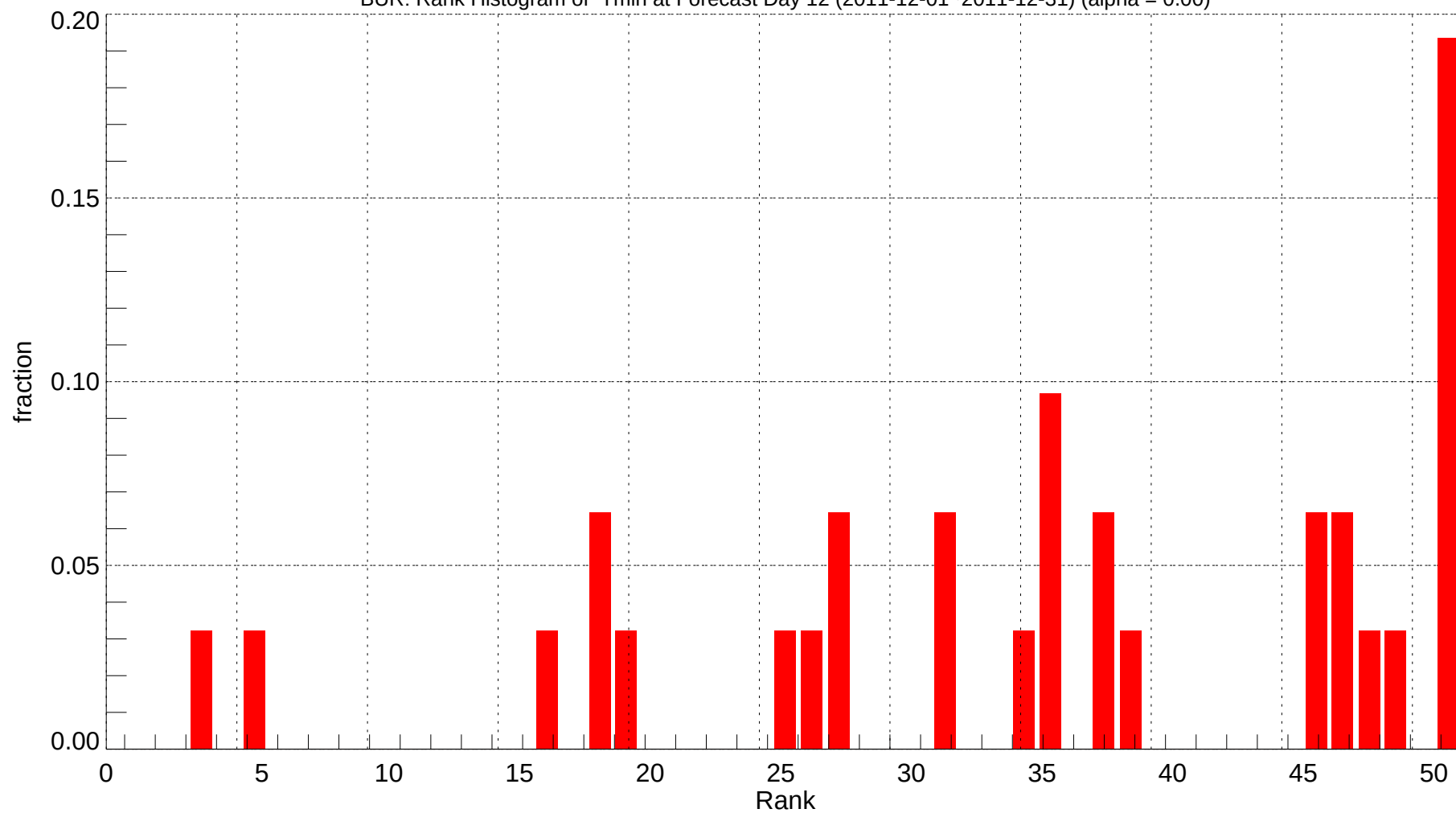
BUR: Rank Histogram of Tmin at Forecast Day 12 (2011-12-01~2011-12-31) (alpha = 0.00)
