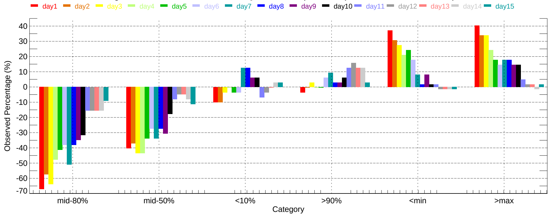
Observed Percentage Deviation of Ensembles - YQB: Min Temperature (2011-12-01~2011-12-31)
