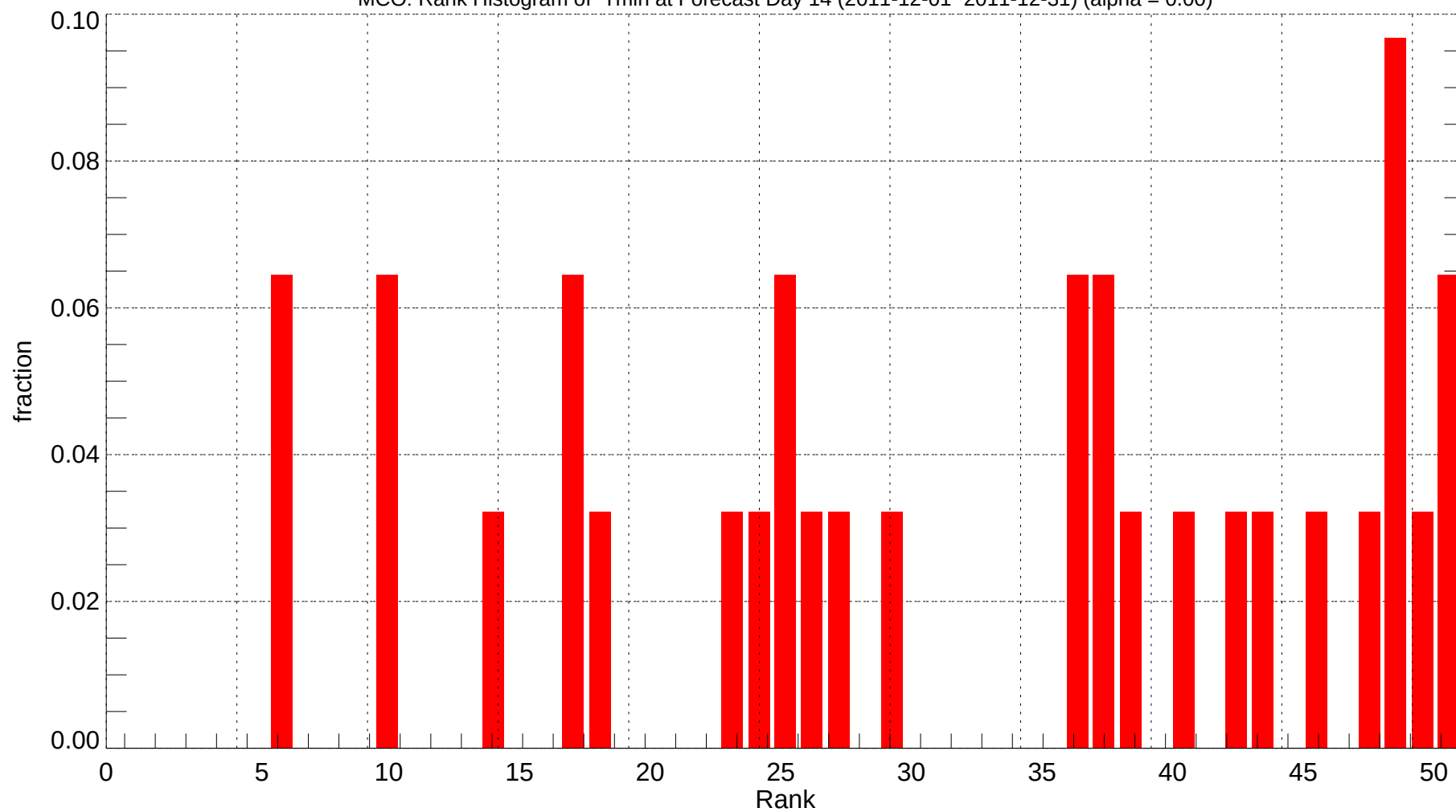
MCO: Rank Histogram of Tmin at Forecast Day 14 (2011-12-01~2011-12-31) (alpha = 0.00)
