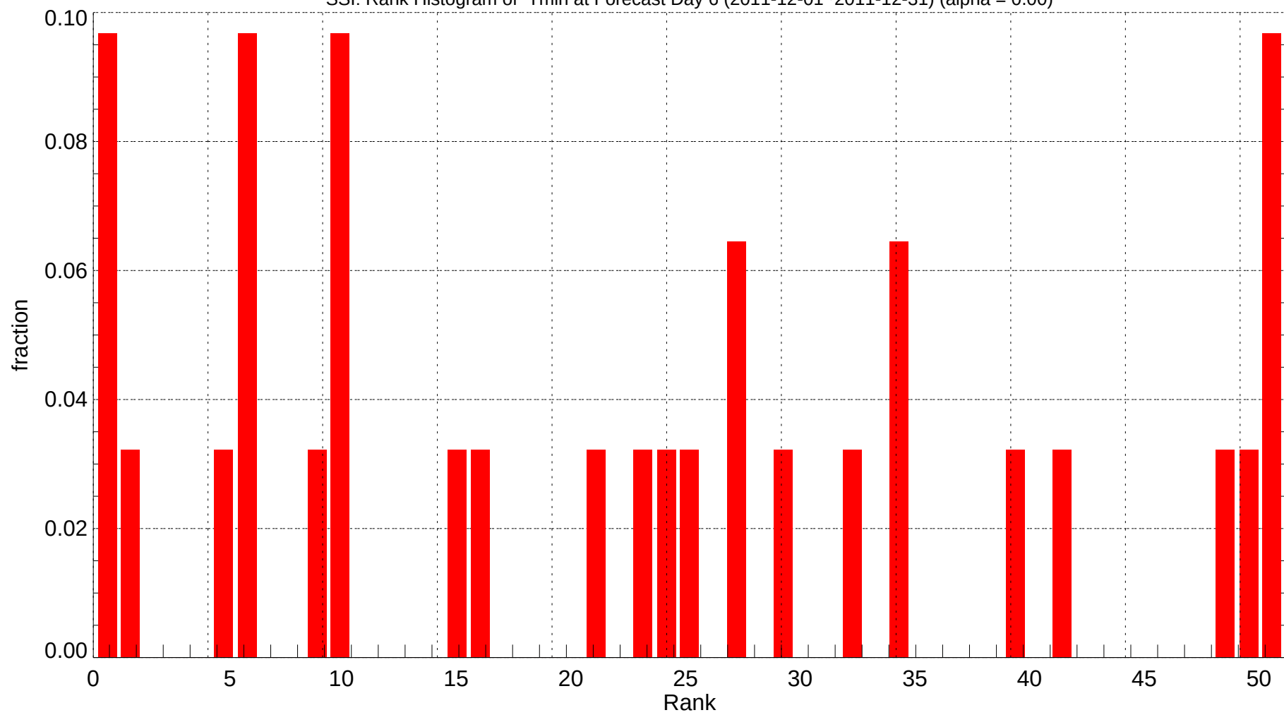
SSI: Rank Histogram of Tmin at Forecast Day 6 (2011-12-01~2011-12-31) (alpha = 0.00)
