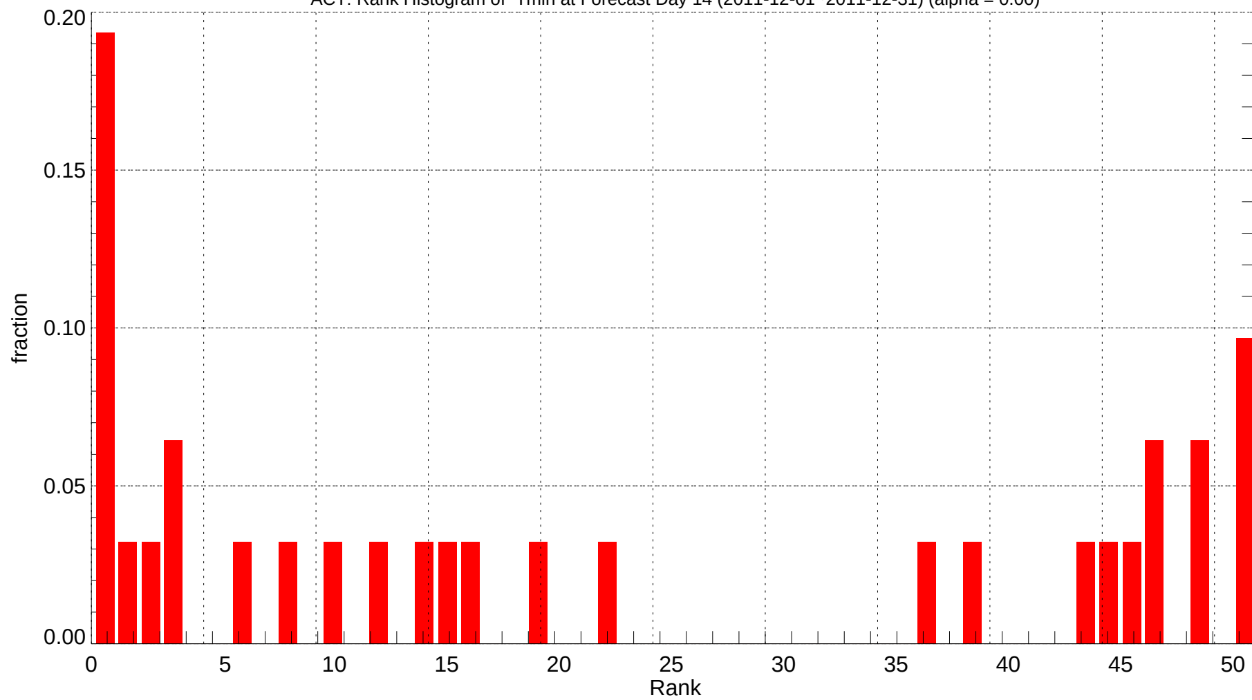
ACT: Rank Histogram of Tmin at Forecast Day 14 (2011-12-01~2011-12-31) (alpha = 0.00)
