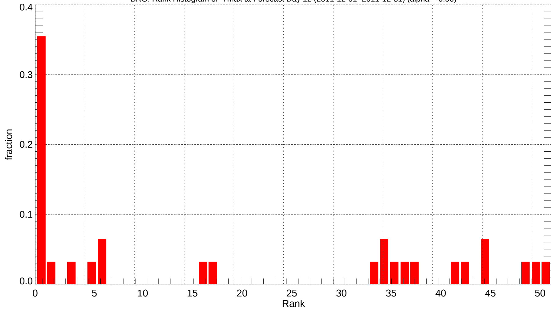
BRO: Rank Histogram of Tmax at Forecast Day 12 (2011-12-01~2011-12-31) (alpha = 0.00)
