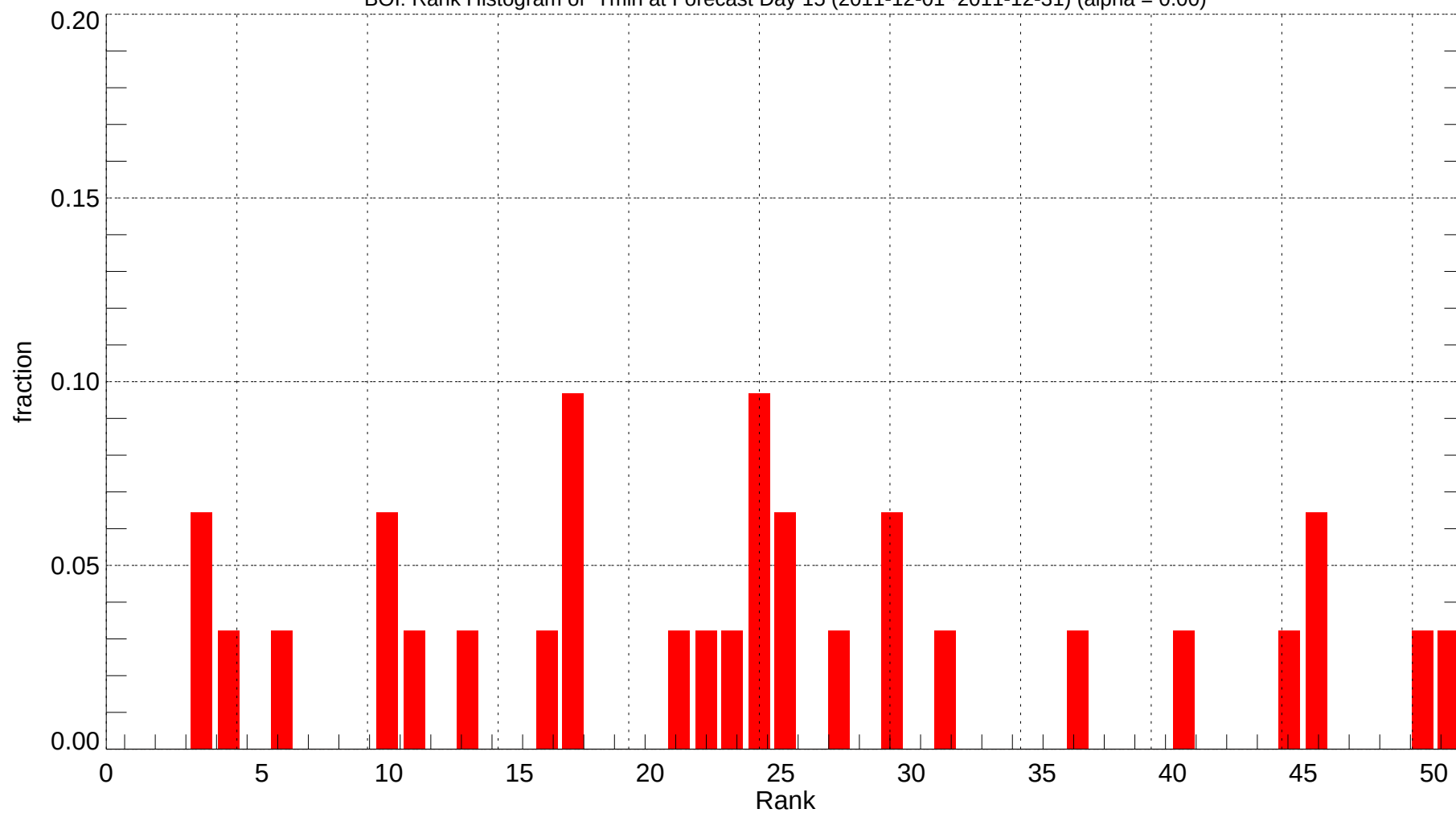
BOI: Rank Histogram of Tmin at Forecast Day 15 (2011-12-01~2011-12-31) (alpha = 0.00)
