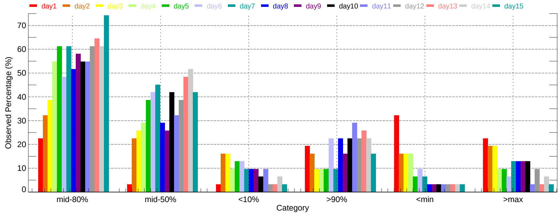
Observed Percentage of Ensembles - RAP: Min Temperature (2011-12-01~2011-12-31)
