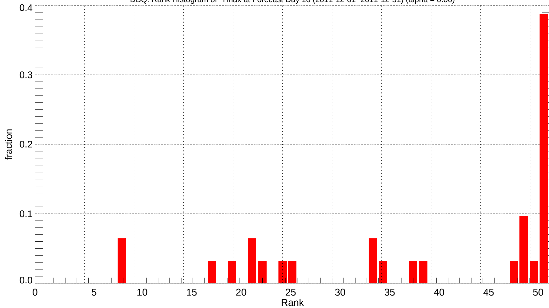
DBQ: Rank Histogram of Tmax at Forecast Day 10 (2011-12-01~2011-12-31) (alpha = 0.00)
