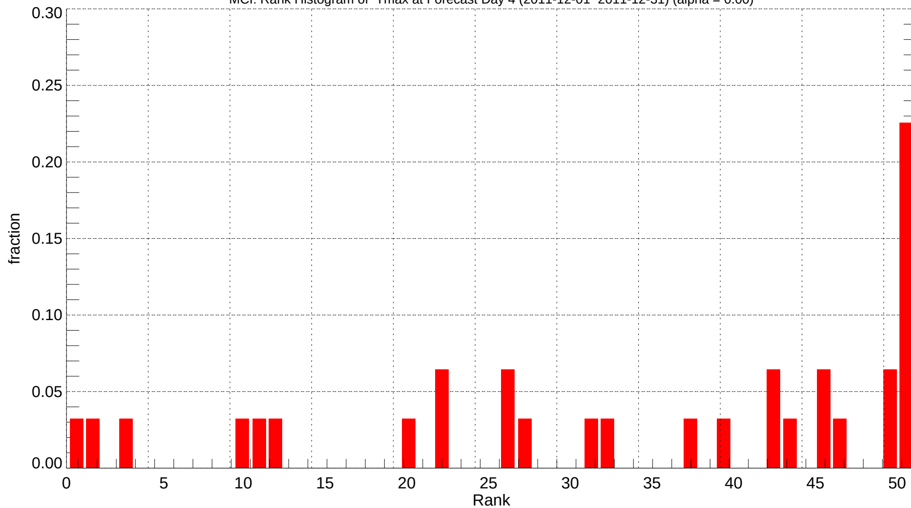
MCI: Rank Histogram of Tmax at Forecast Day 4 (2011-12-01~2011-12-31) (alpha = 0.00)
