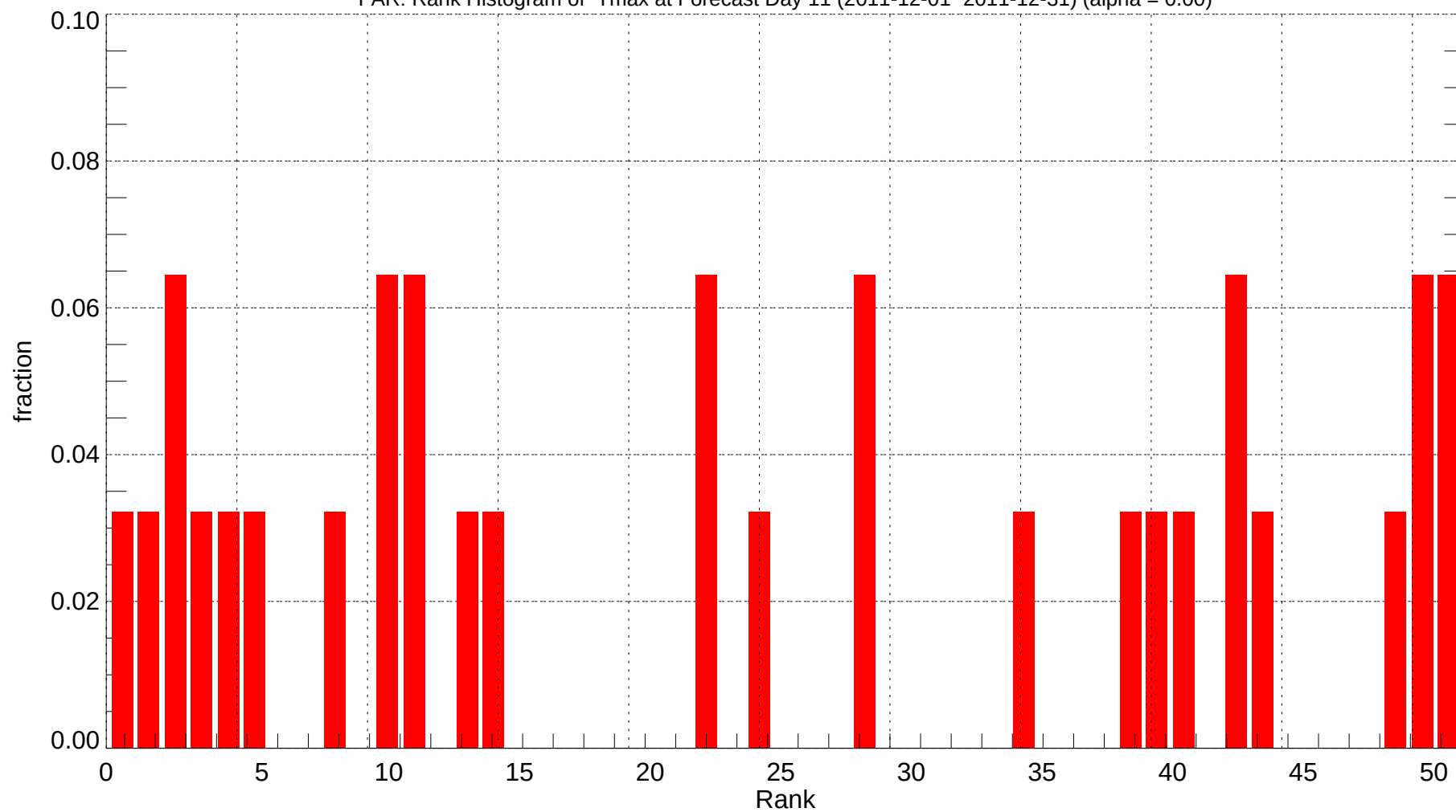
FAR: Rank Histogram of Tmax at Forecast Day 11 (2011-12-01~2011-12-31) (alpha = 0.00)
