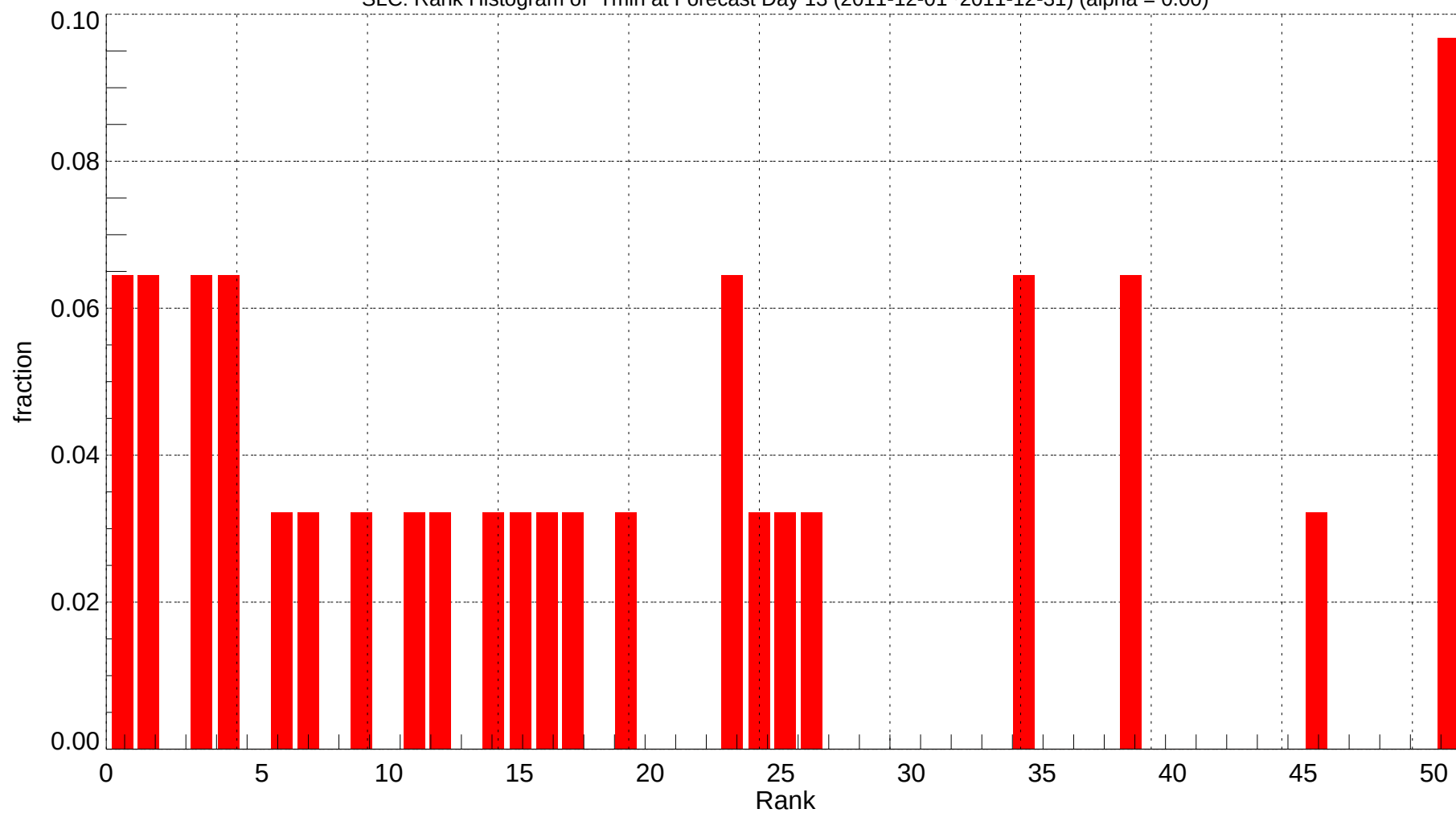
SLC: Rank Histogram of Tmin at Forecast Day 13 (2011-12-01~2011-12-31) (alpha = 0.00)
