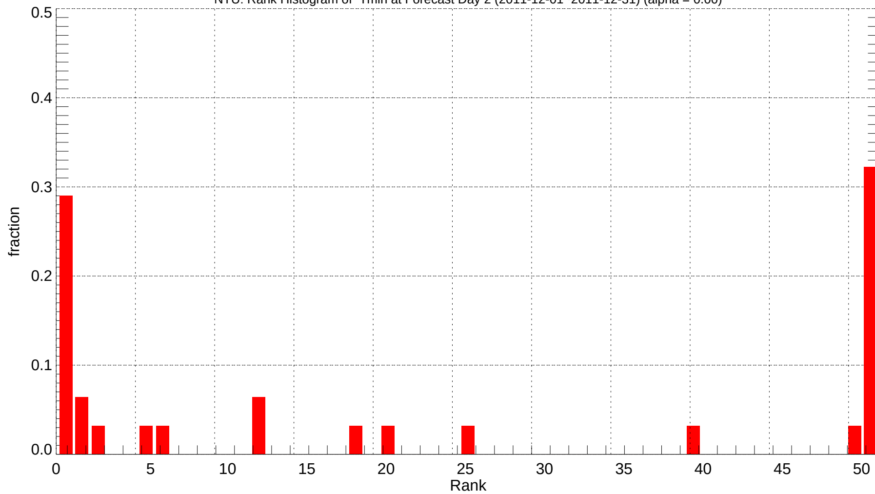
NTU: Rank Histogram of Tmin at Forecast Day 2 (2011-12-01~2011-12-31) (alpha = 0.00)
