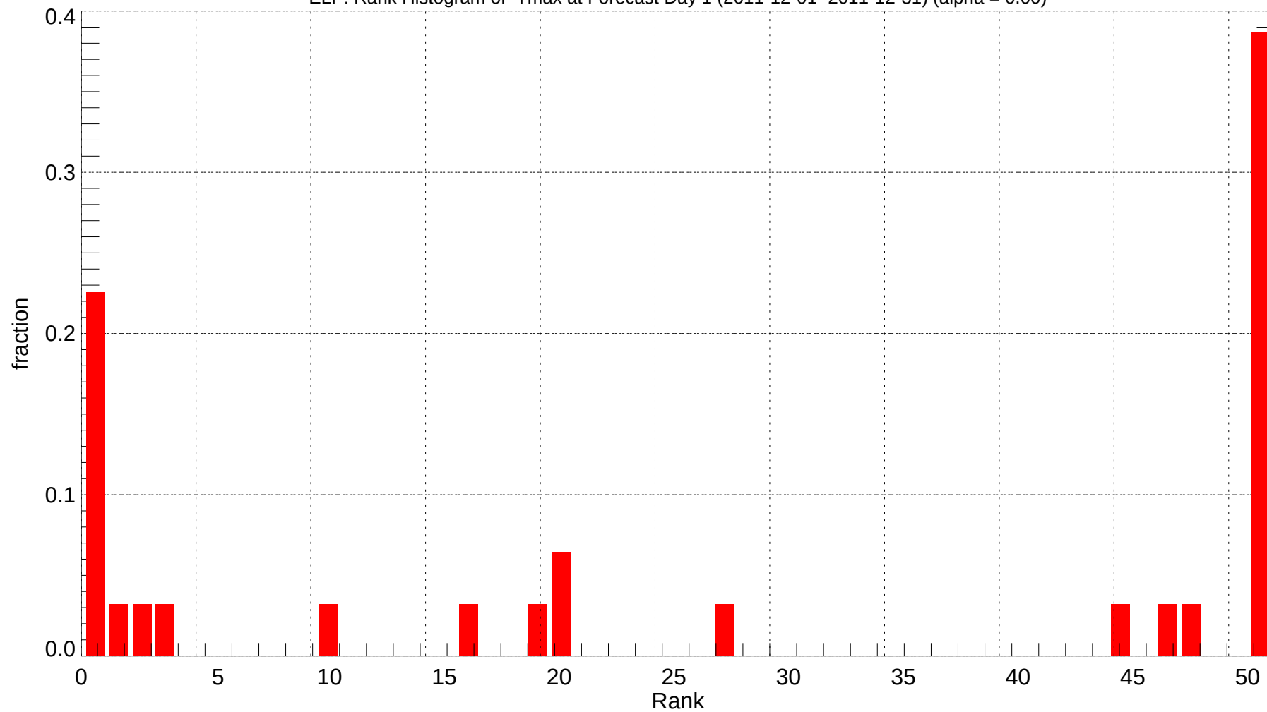
ELP: Rank Histogram of Tmax at Forecast Day 1 (2011-12-01~2011-12-31) (alpha = 0.00)
