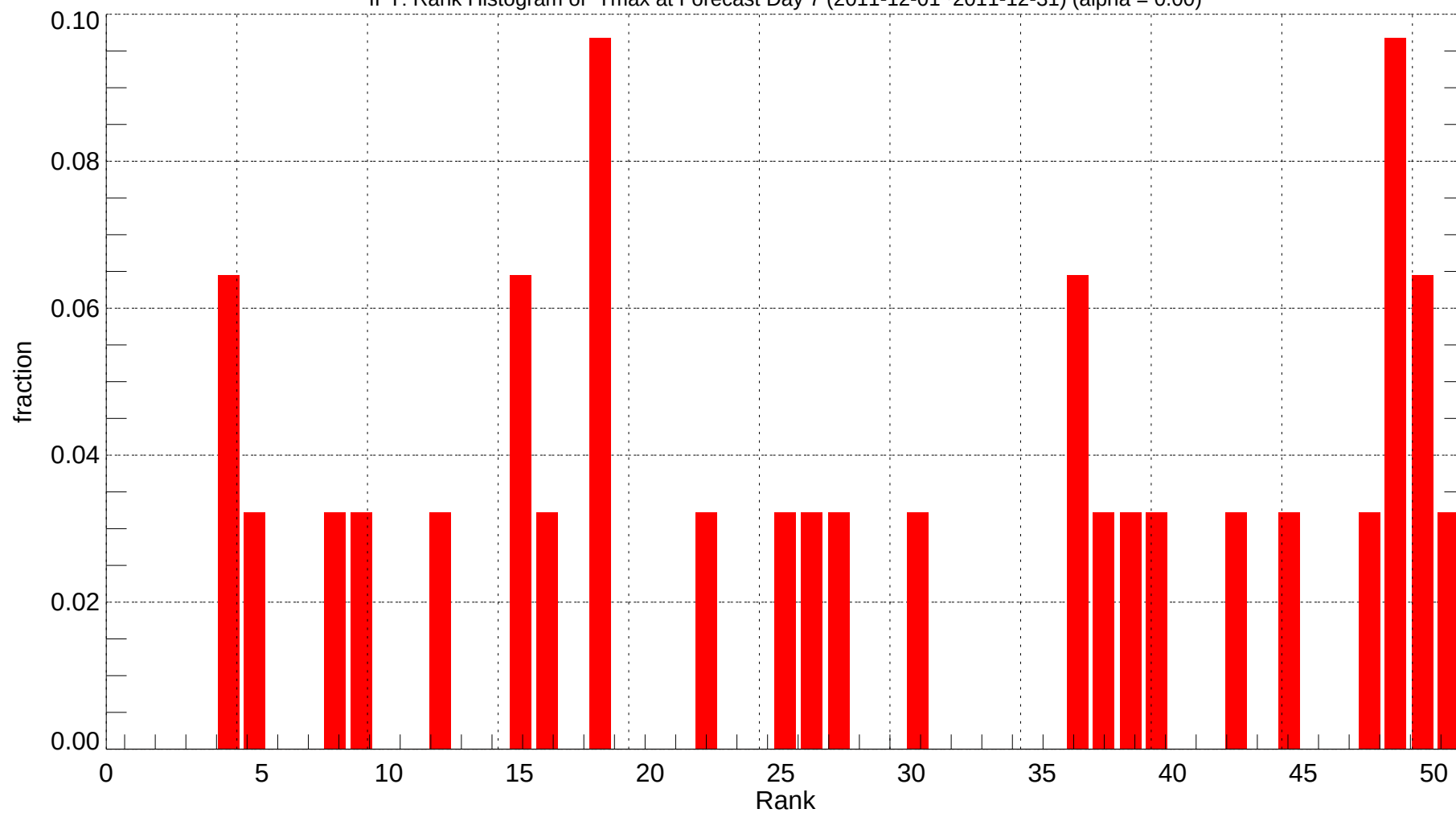
IPT: Rank Histogram of Tmax at Forecast Day 7 (2011-12-01~2011-12-31) (alpha = 0.00)
