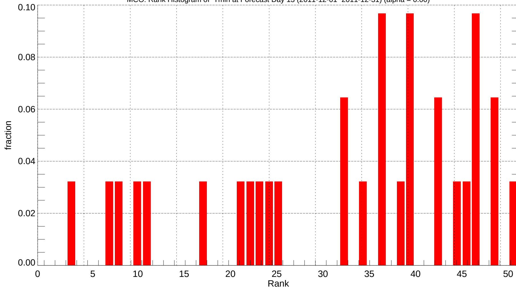
MCO: Rank Histogram of Tmin at Forecast Day 13 (2011-12-01~2011-12-31) (alpha = 0.00)
