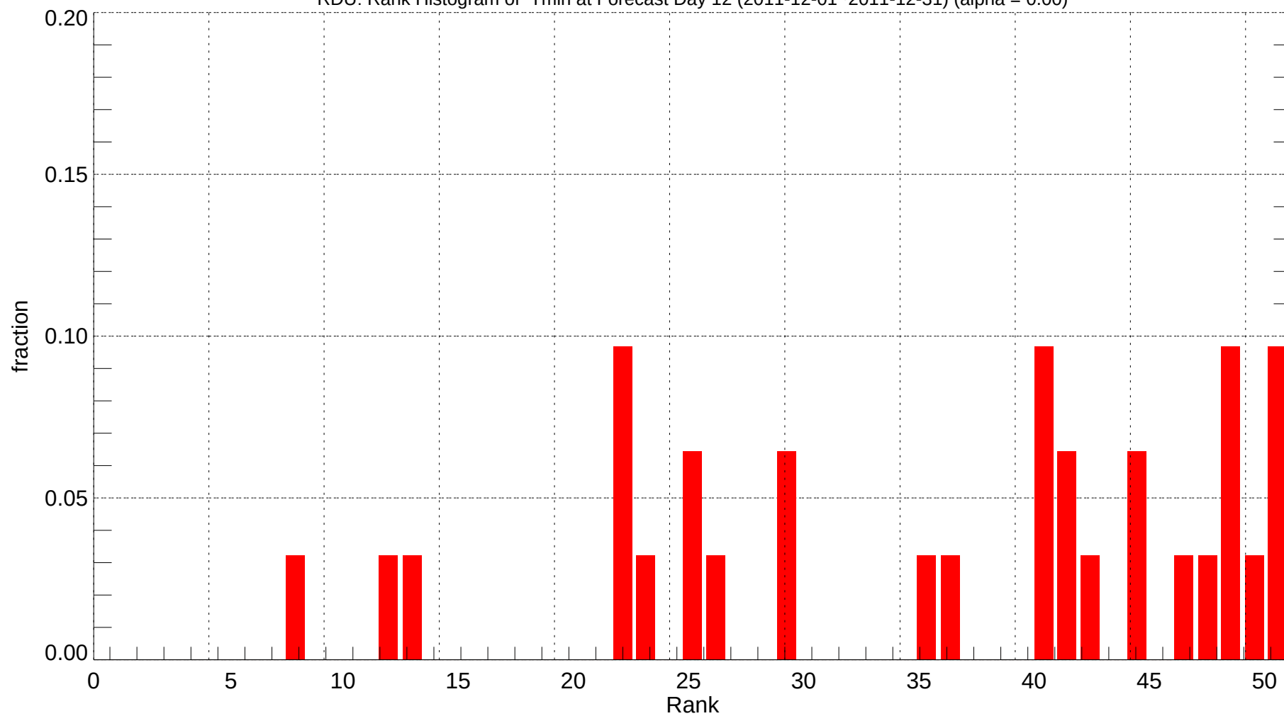
RDU: Rank Histogram of Tmin at Forecast Day 12 (2011-12-01~2011-12-31) (alpha = 0.00)
