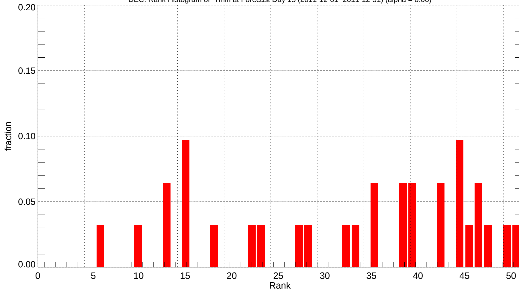
DEC: Rank Histogram of Tmin at Forecast Day 15 (2011-12-01~2011-12-31) (alpha = 0.00)
