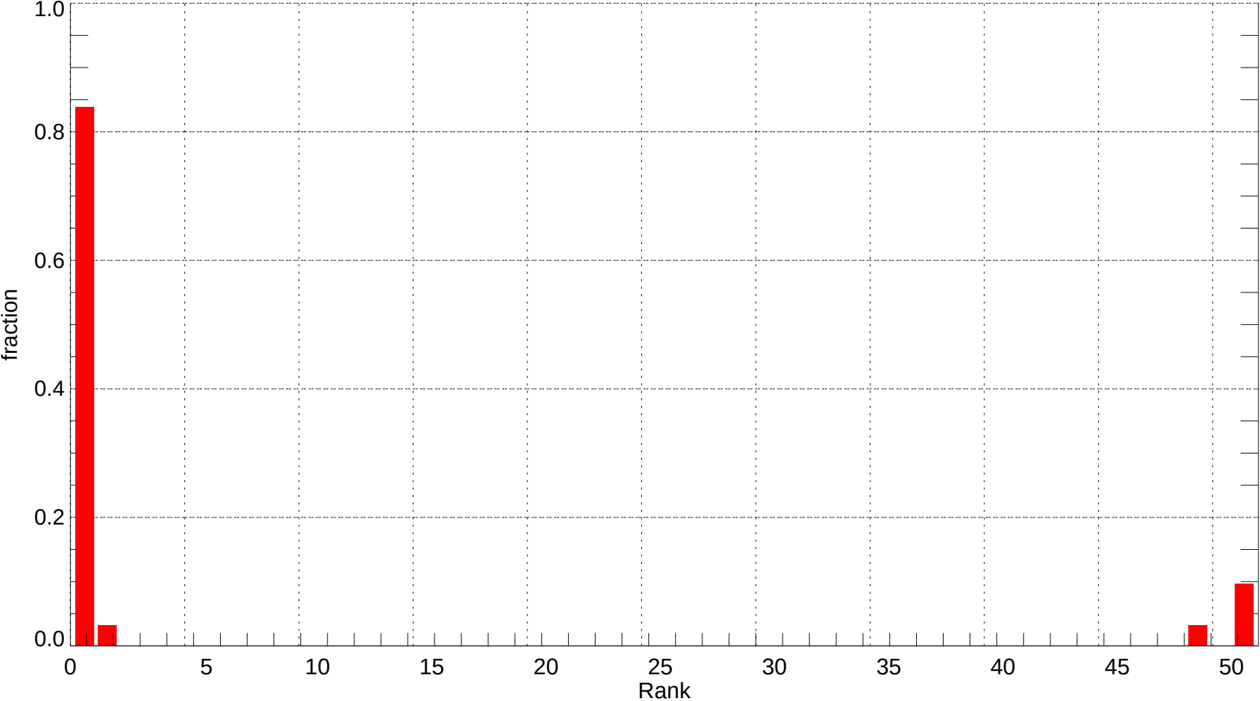
RBL: Rank Histogram of Tmin at Forecast Day 1 (2011-12-01~2011-12-31) (alpha = 0.00)
