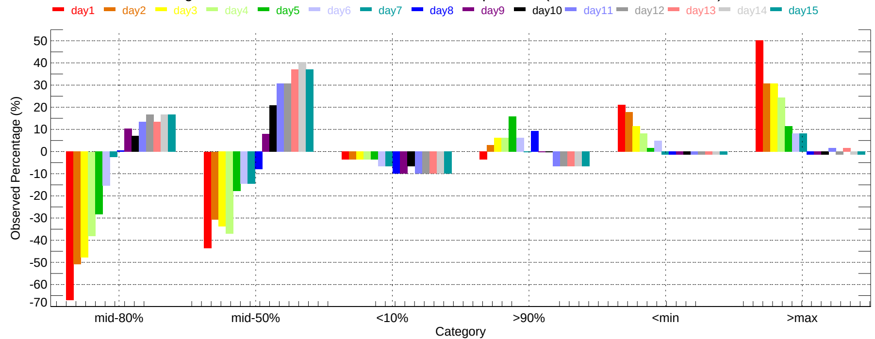
Observed Percentage Deviation of Ensembles - SLC: Min Temperature (2011-12-01~2011-12-31)
