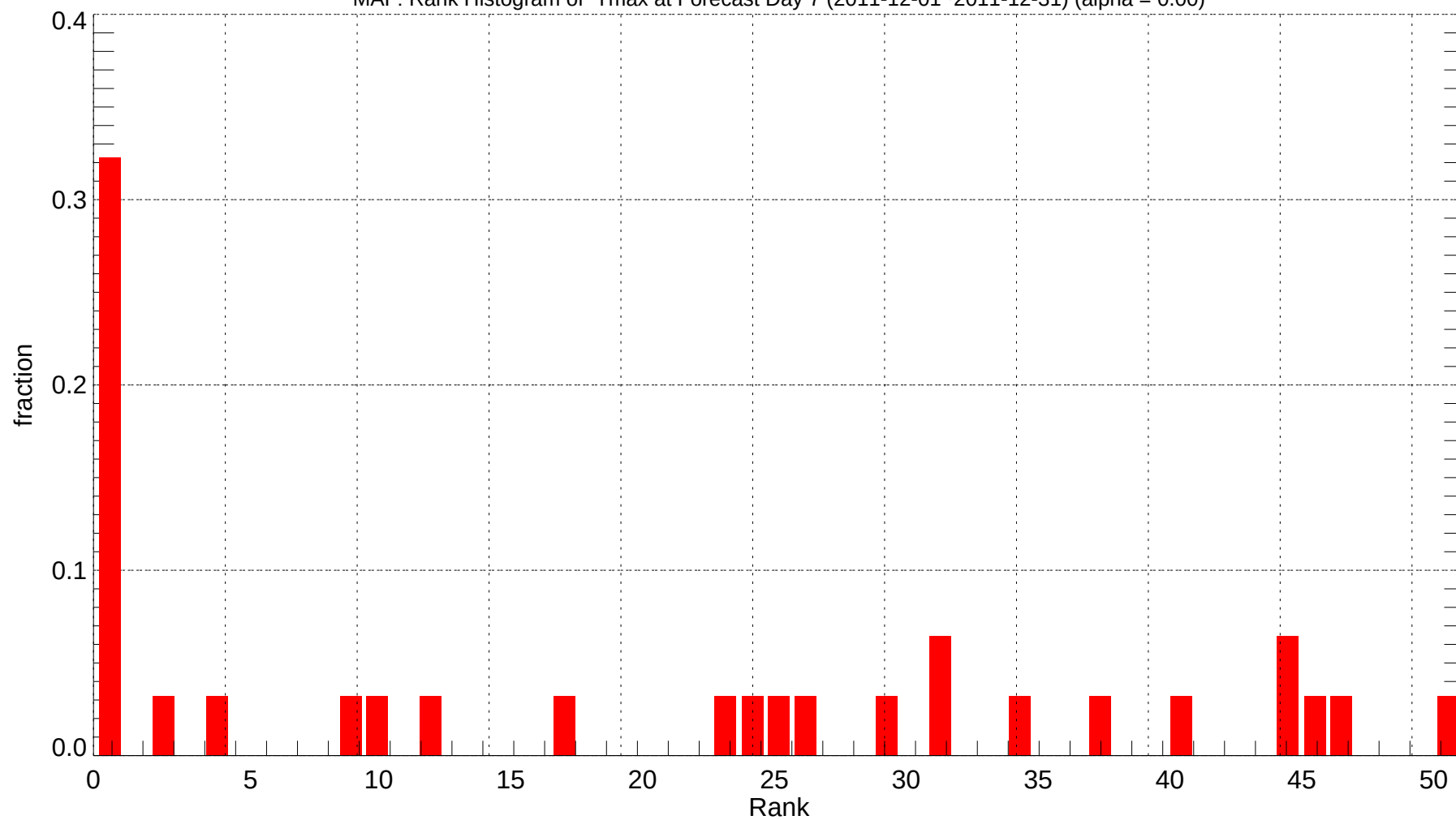
MAF: Rank Histogram of Tmax at Forecast Day 7 (2011-12-01~2011-12-31) (alpha = 0.00)
