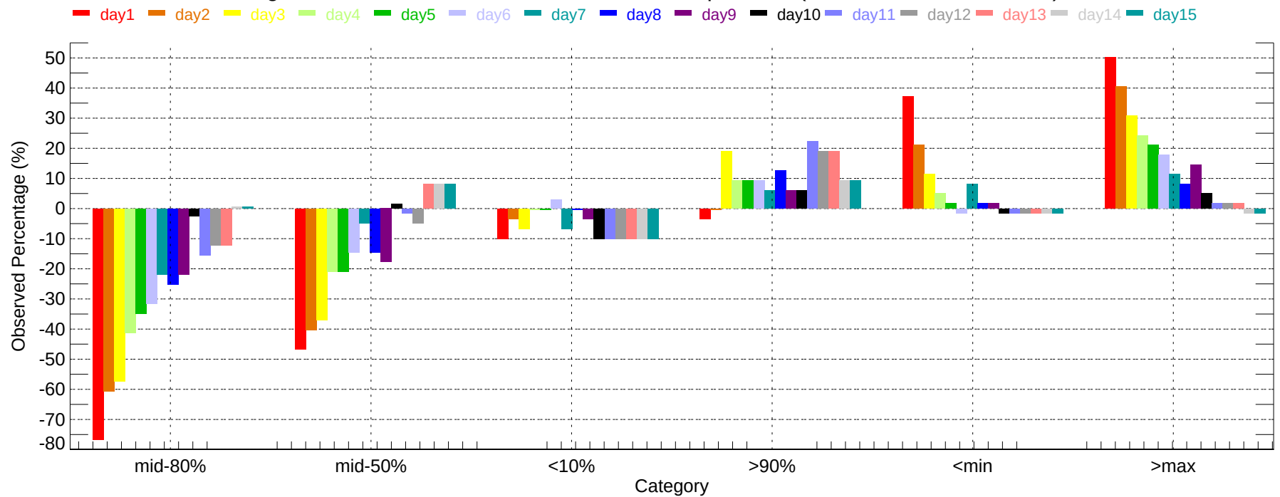
Observed Percentage Deviation of Ensembles - DCA: Min Temperature (2011-12-01~2011-12-31)
