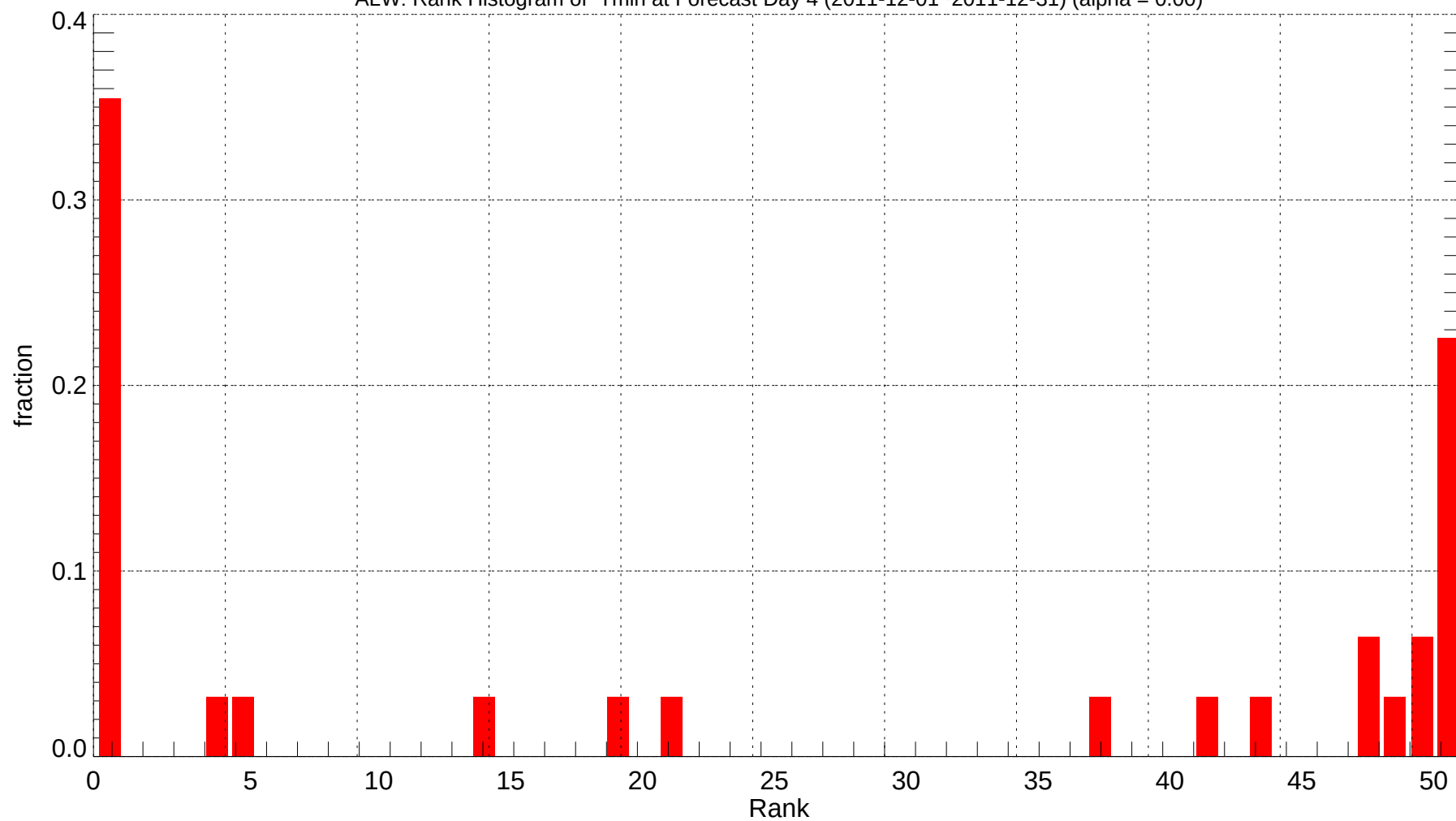
ALW: Rank Histogram of Tmin at Forecast Day 4 (2011-12-01~2011-12-31) (alpha = 0.00)
