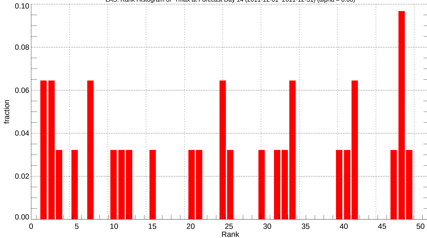
LAS: Rank Histogram of Tmax at Forecast Day 14 (2011-12-01~2011-12-31) (alpha = 0.00)
