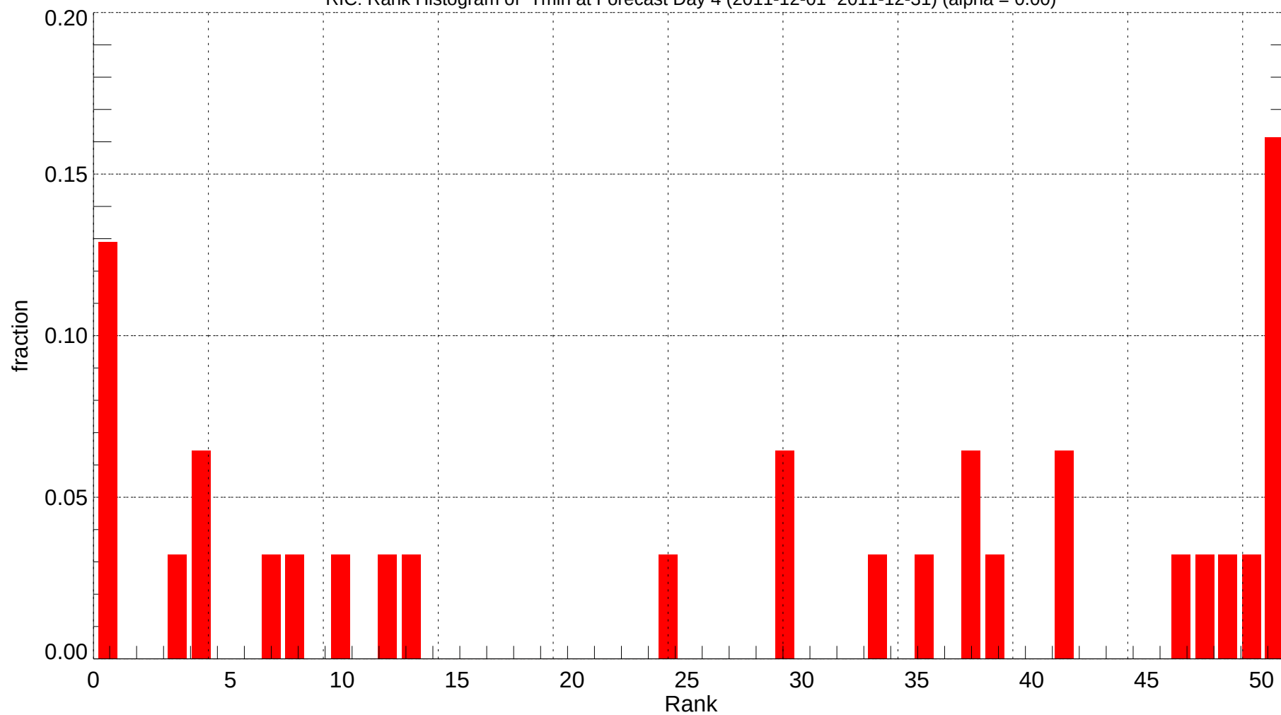
RIC: Rank Histogram of Tmin at Forecast Day 4 (2011-12-01~2011-12-31) (alpha = 0.00)
