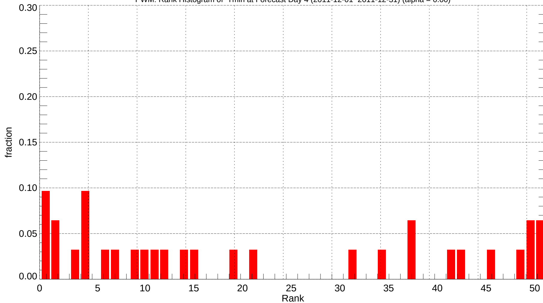
PWM: Rank Histogram of Tmin at Forecast Day 4 (2011-12-01~2011-12-31) (alpha = 0.00)
