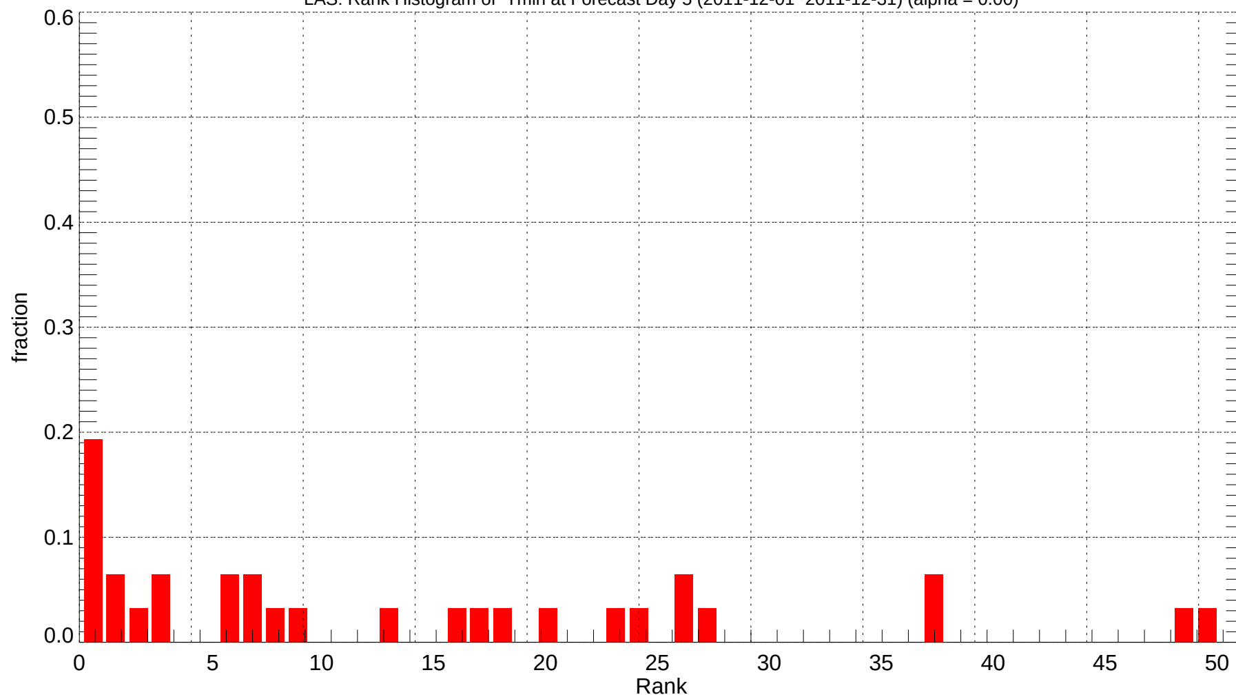
LAS: Rank Histogram of Tmin at Forecast Day 5 (2011-12-01~2011-12-31) (alpha = 0.00)
