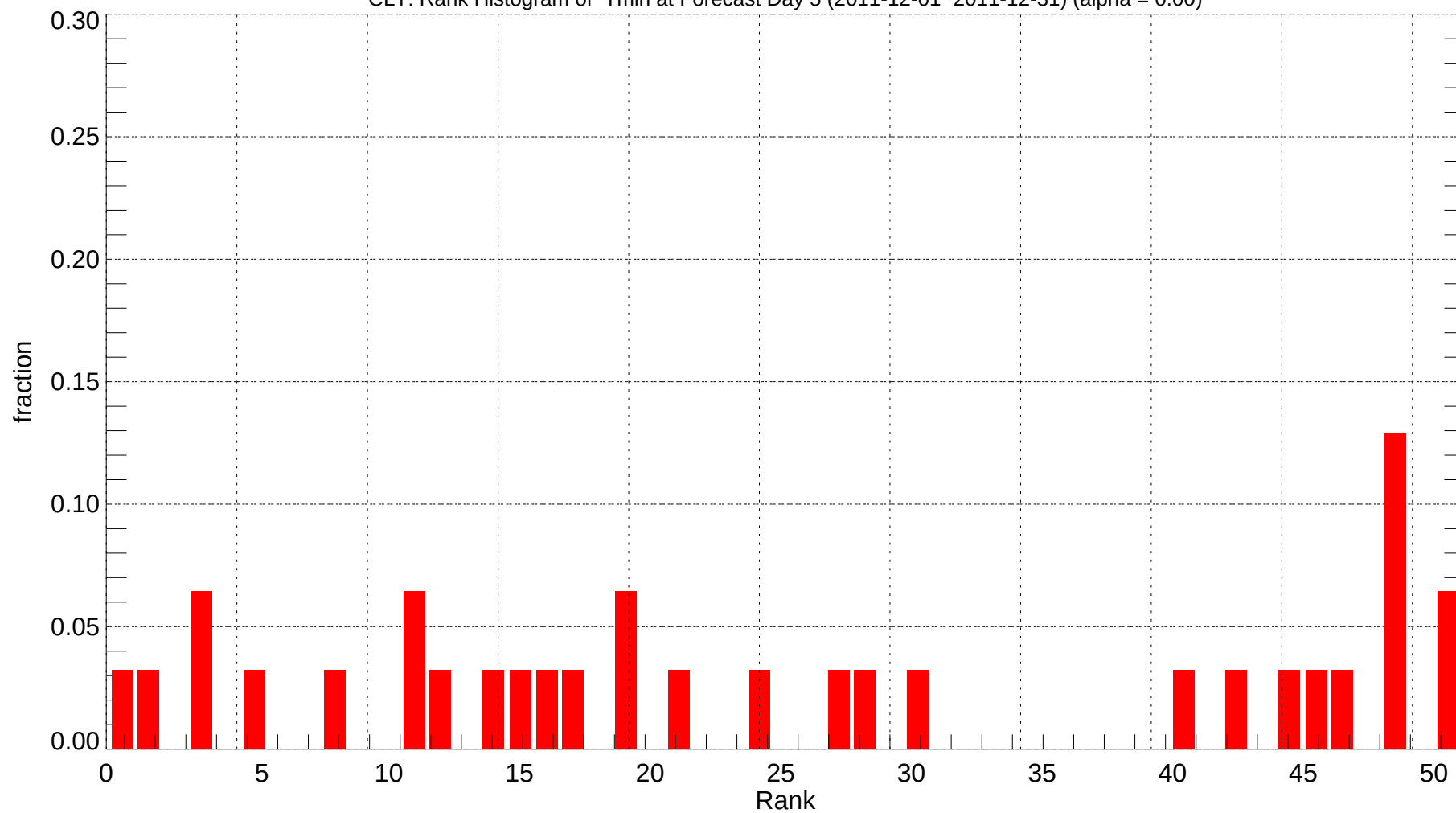
CLT: Rank Histogram of Tmin at Forecast Day 5 (2011-12-01~2011-12-31) (alpha = 0.00)
