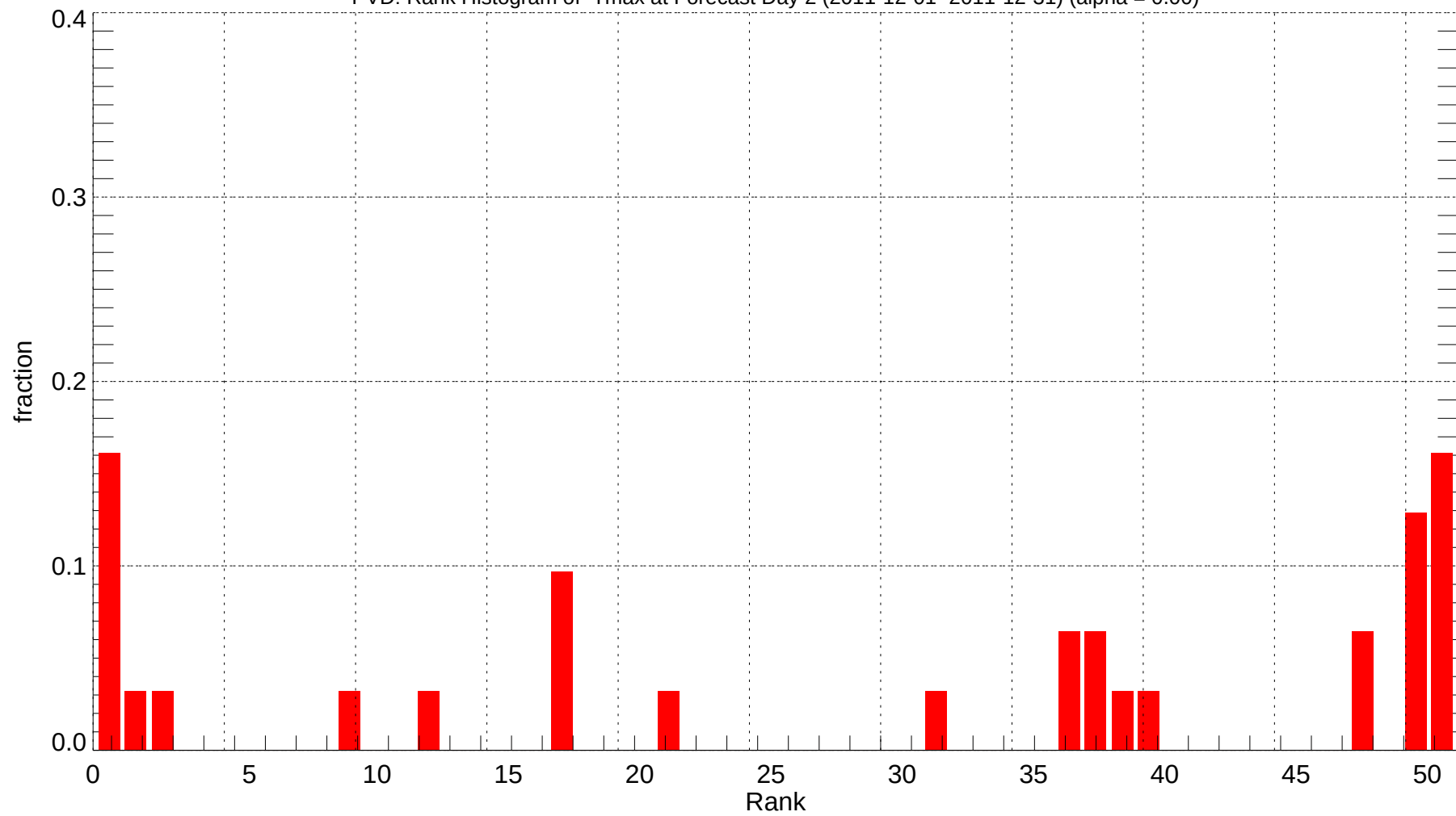
PVD: Rank Histogram of Tmax at Forecast Day 2 (2011-12-01~2011-12-31) (alpha = 0.00)
