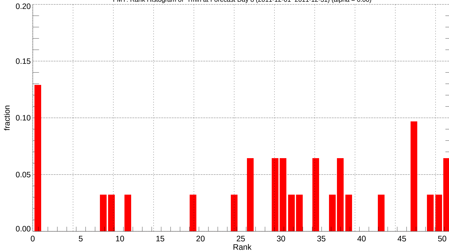
FMY: Rank Histogram of Tmin at Forecast Day 8 (2011-12-01~2011-12-31) (alpha = 0.00)
