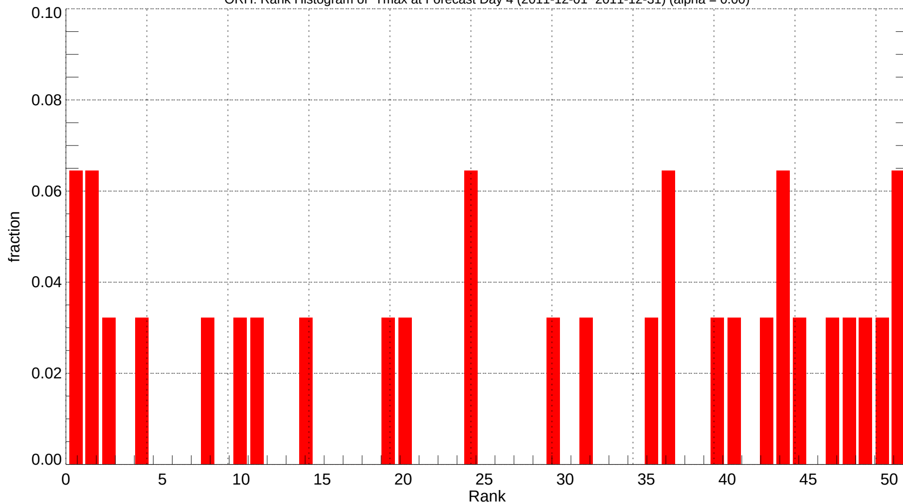
ORH: Rank Histogram of Tmax at Forecast Day 4 (2011-12-01~2011-12-31) (alpha = 0.00)
