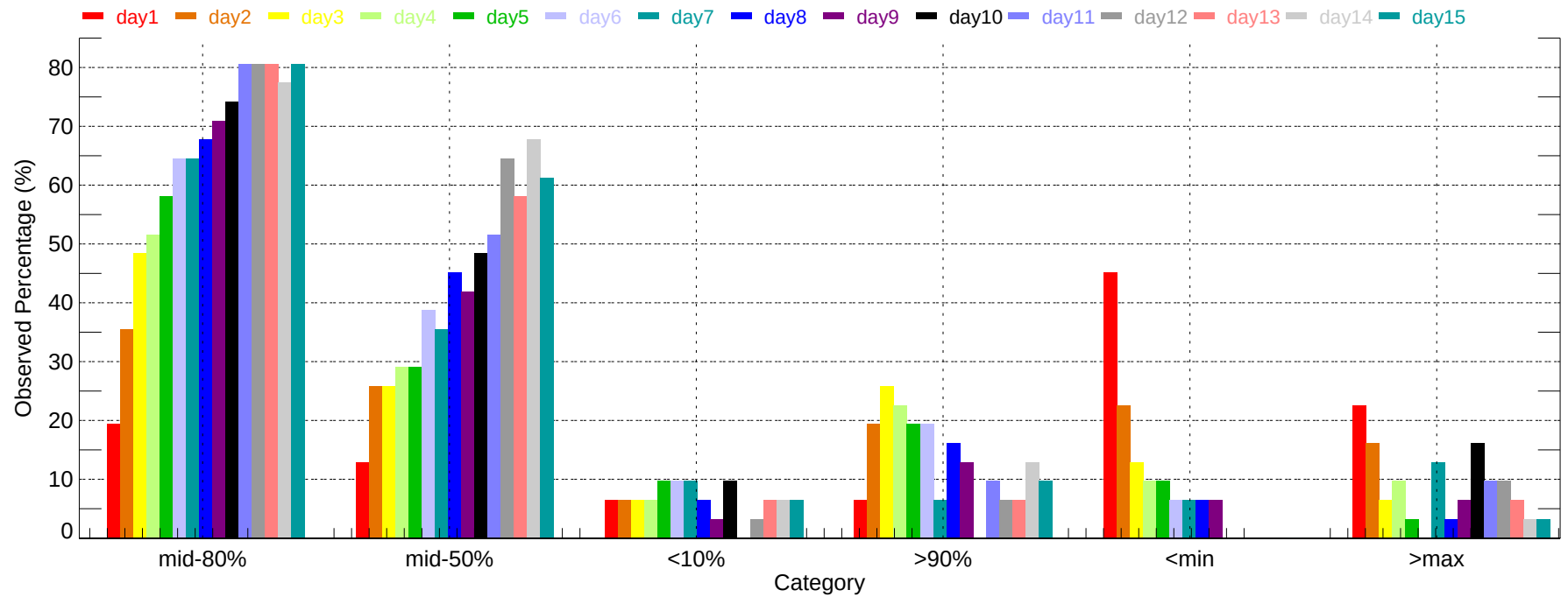
Observed Percentage of Ensembles - ORH: Min Temperature (2011-12-01~2011-12-31)
