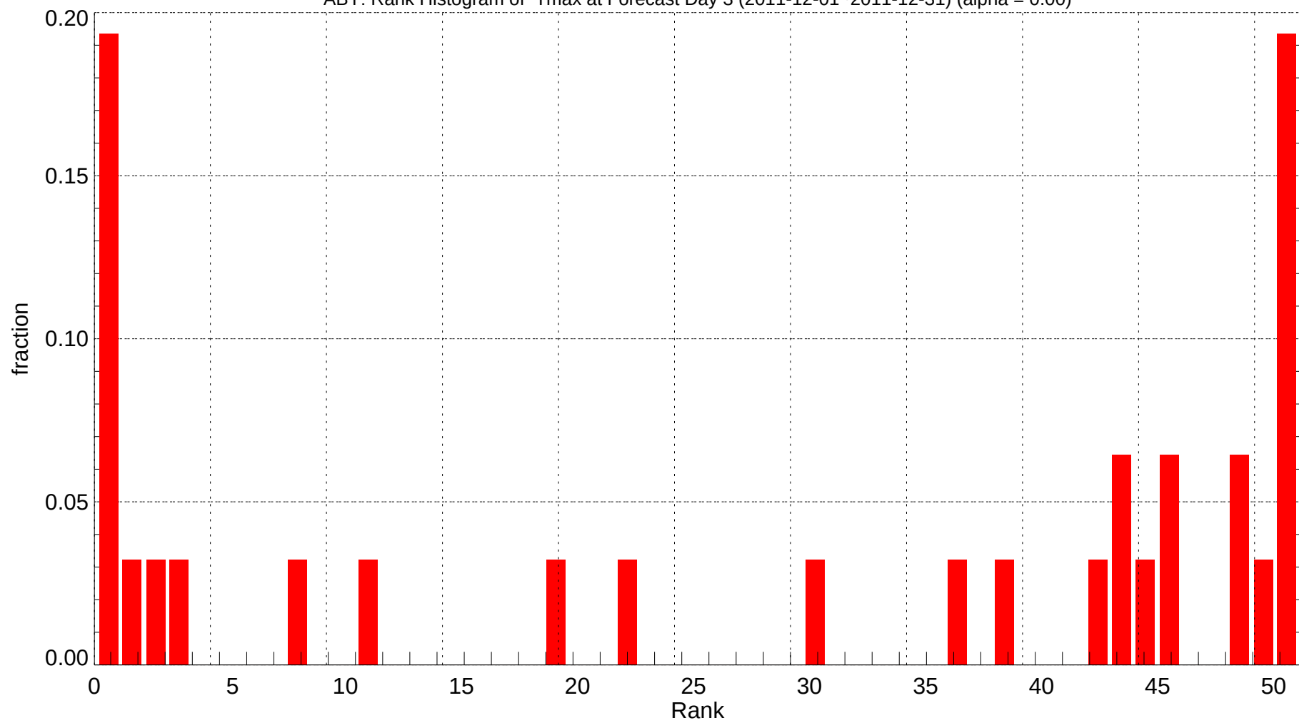
ABY: Rank Histogram of Tmax at Forecast Day 3 (2011-12-01~2011-12-31) (alpha = 0.00)
