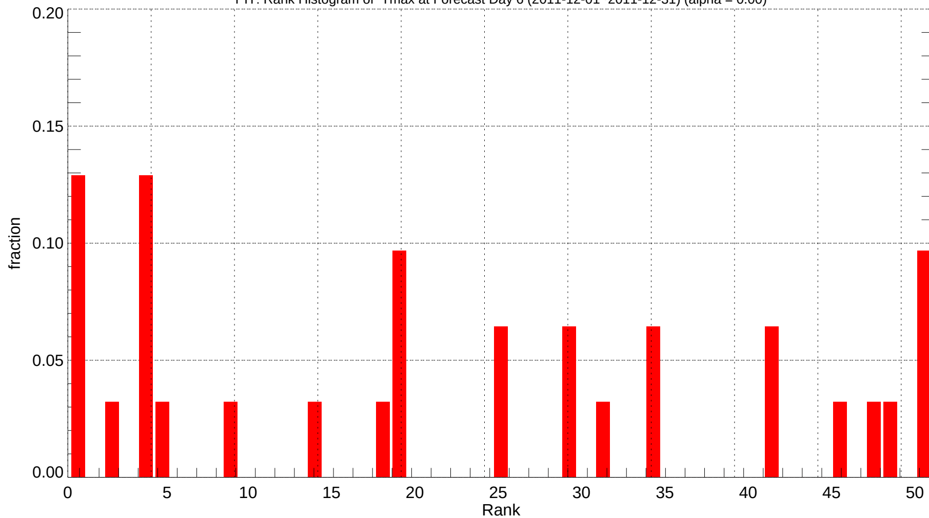
PIT: Rank Histogram of Tmax at Forecast Day 6 (2011-12-01~2011-12-31) (alpha = 0.00)
