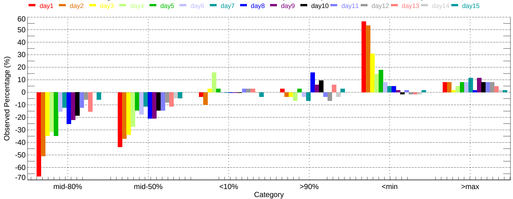
Observed Percentage Deviation of Ensembles - SYR: Min Temperature (2011-12-01~2011-12-31)
