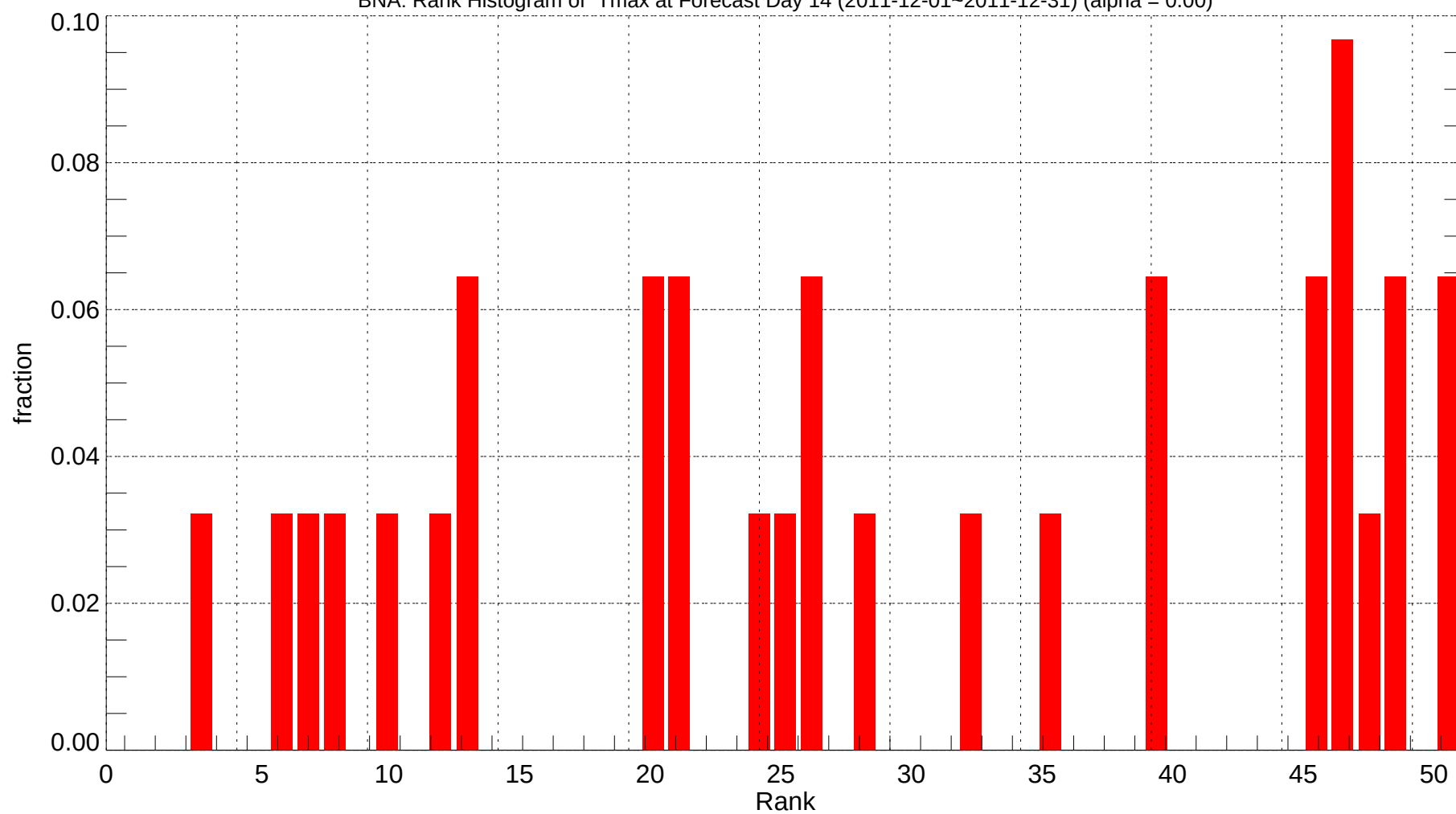
BNA: Rank Histogram of Tmax at Forecast Day 14 (2011-12-01~2011-12-31) (alpha = 0.00)
