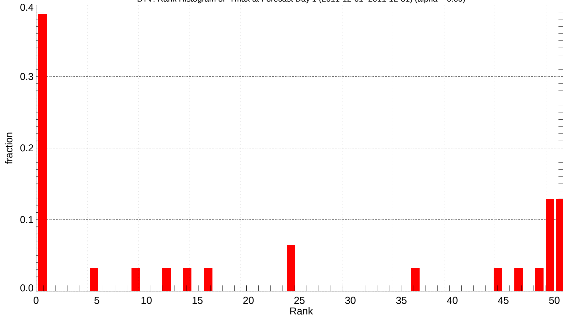
BTV: Rank Histogram of Tmax at Forecast Day 1 (2011-12-01~2011-12-31) (alpha = 0.00)
