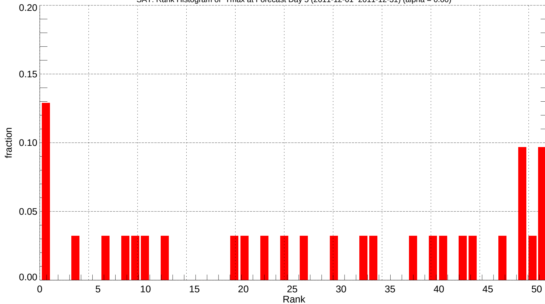
SAT: Rank Histogram of Tmax at Forecast Day 5 (2011-12-01~2011-12-31) (alpha = 0.00)
