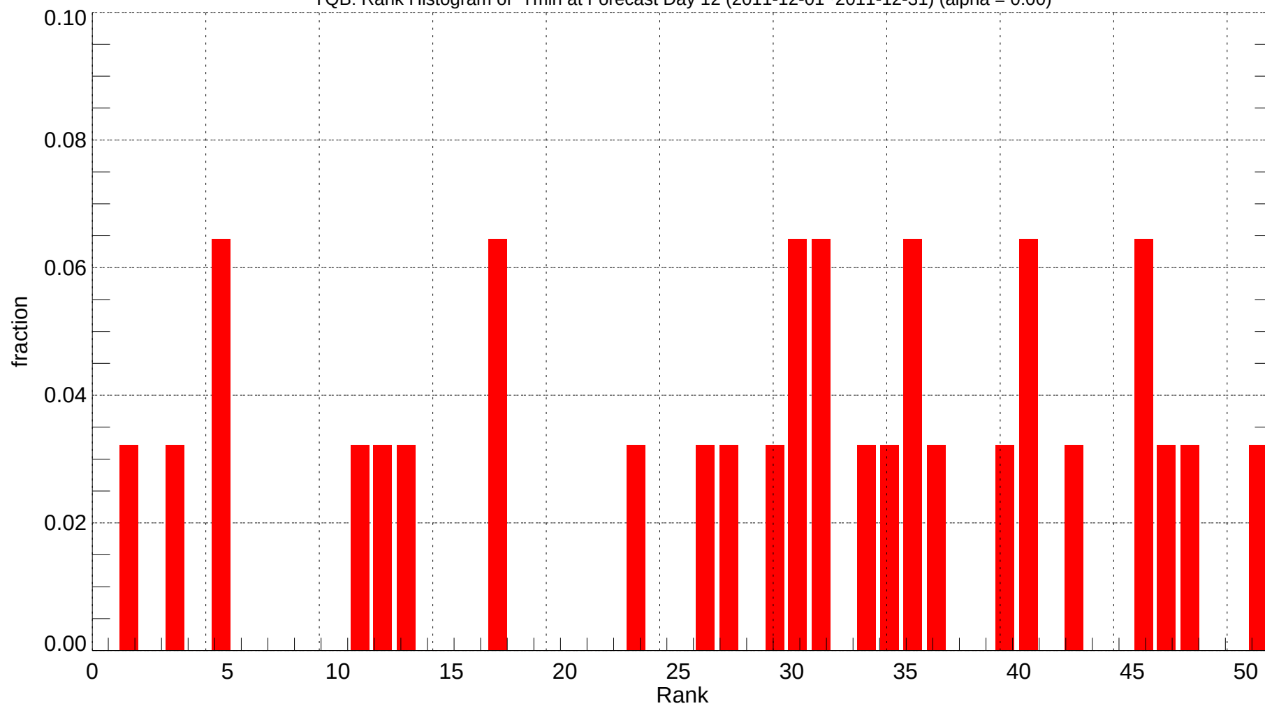
YQB: Rank Histogram of Tmin at Forecast Day 12 (2011-12-01~2011-12-31) (alpha = 0.00)
