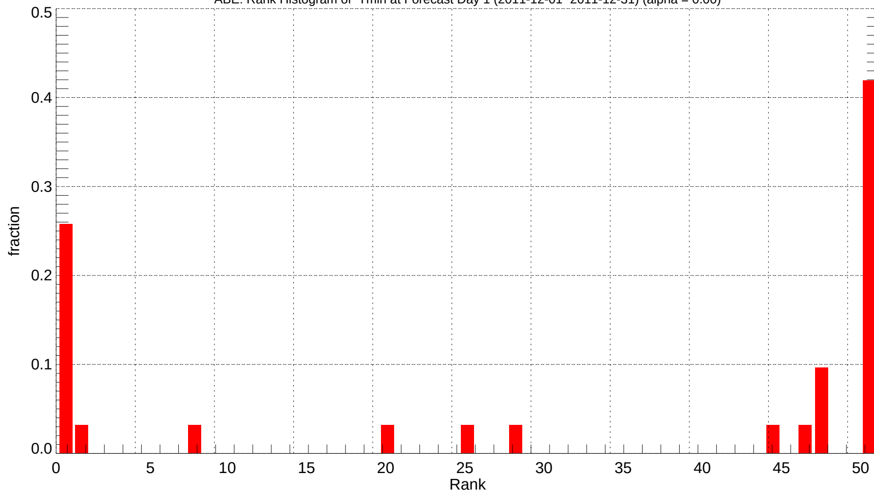
ABE: Rank Histogram of Tmin at Forecast Day 1 (2011-12-01~2011-12-31) (alpha = 0.00)
