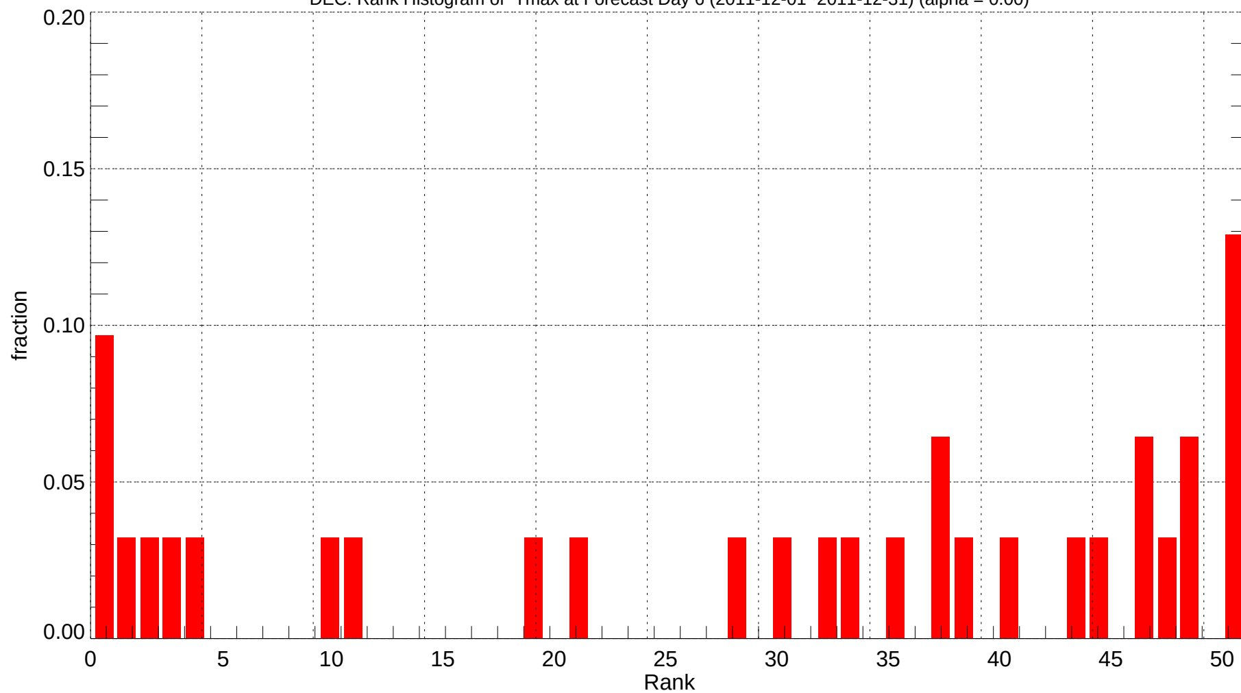
DEC: Rank Histogram of Tmax at Forecast Day 6 (2011-12-01~2011-12-31) (alpha = 0.00)
