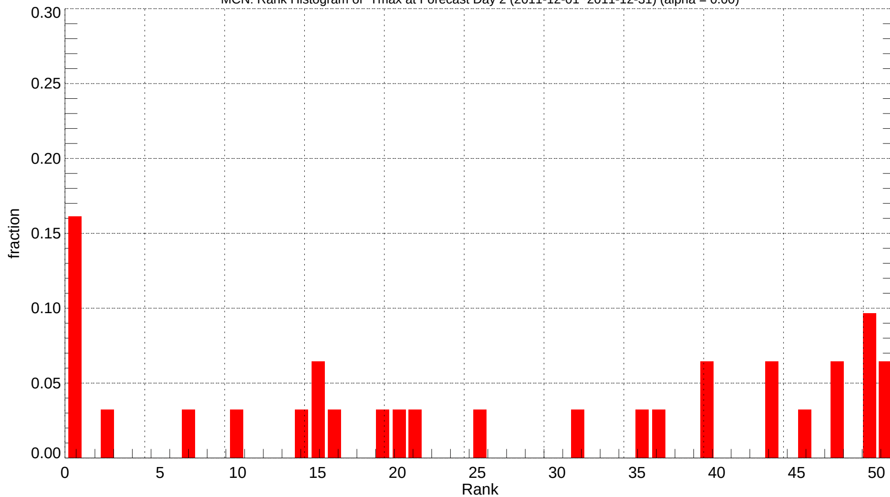
MCN: Rank Histogram of Tmax at Forecast Day 2 (2011-12-01~2011-12-31) (alpha = 0.00)
