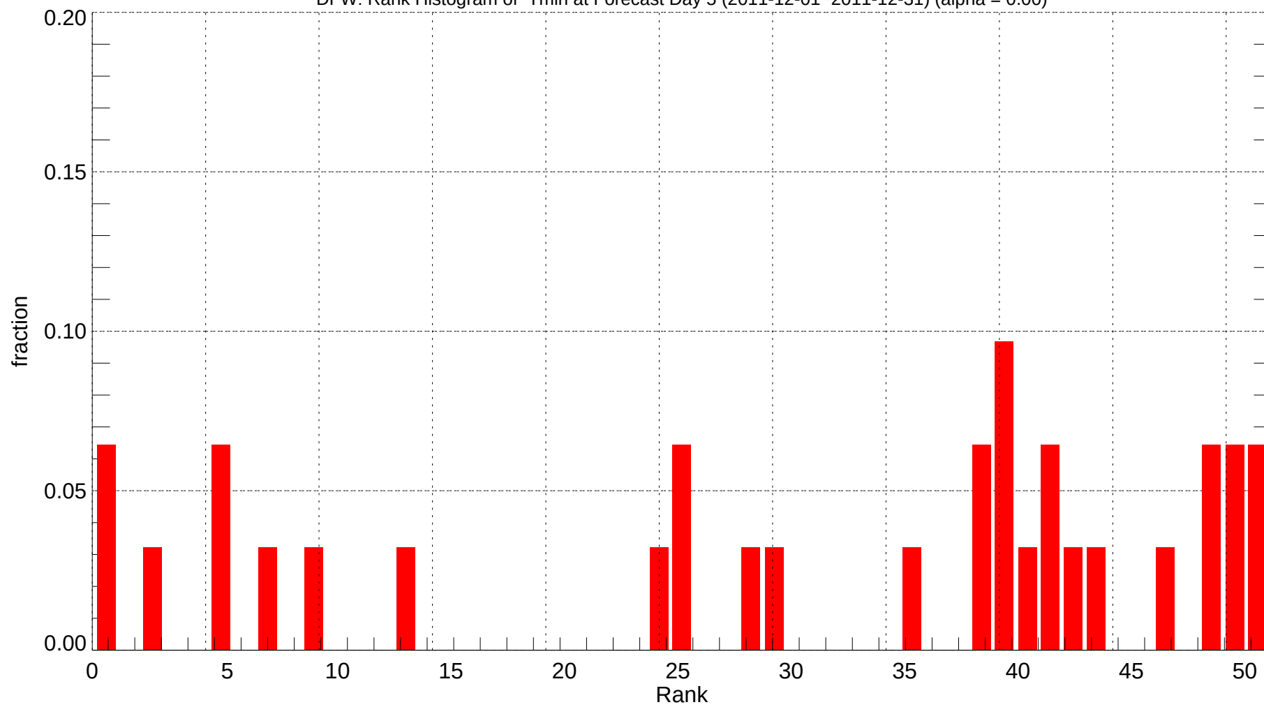
DFW: Rank Histogram of Tmin at Forecast Day 5 (2011-12-01~2011-12-31) (alpha = 0.00)
