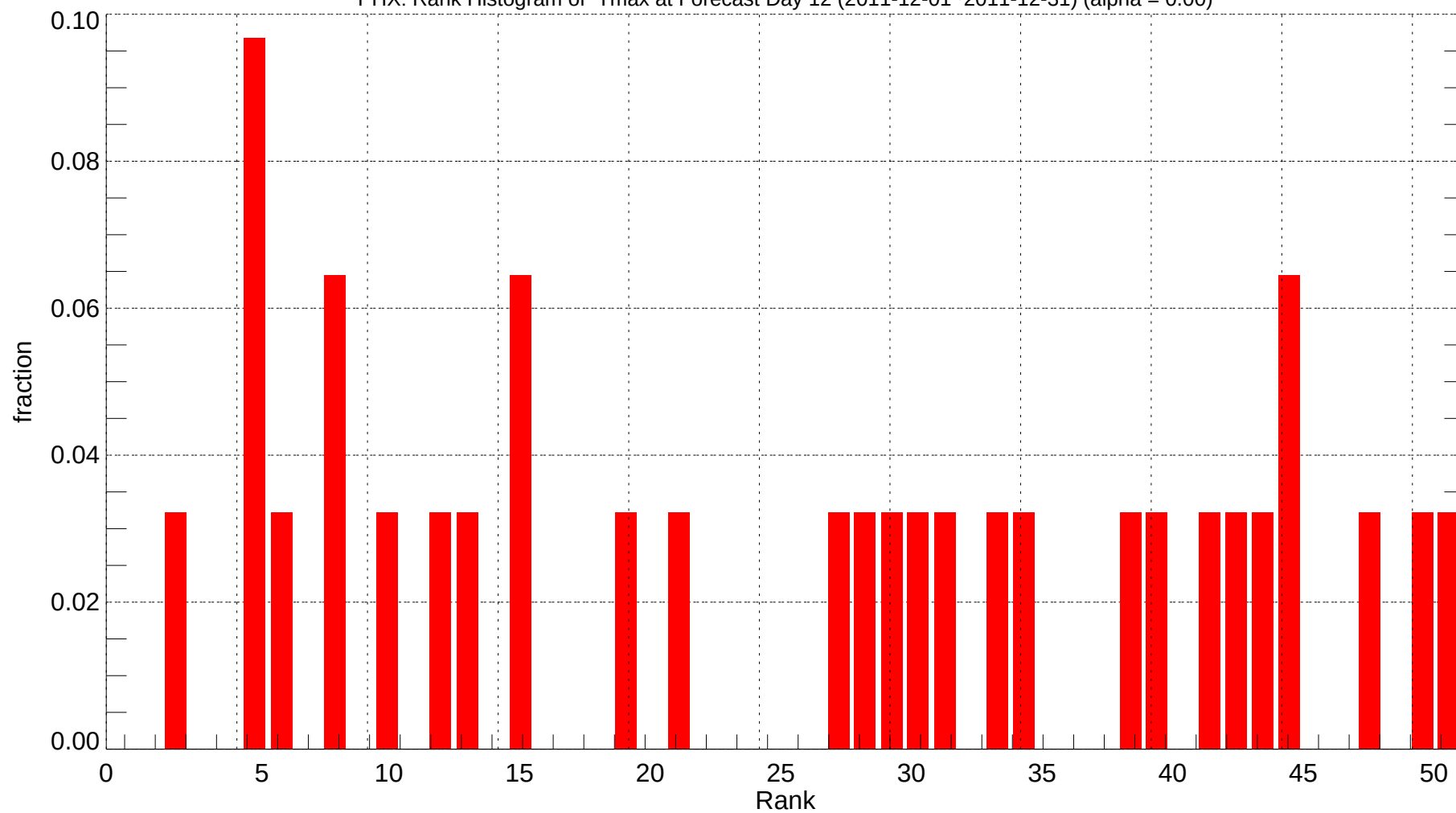
PHX: Rank Histogram of Tmax at Forecast Day 12 (2011-12-01~2011-12-31) (alpha = 0.00)
