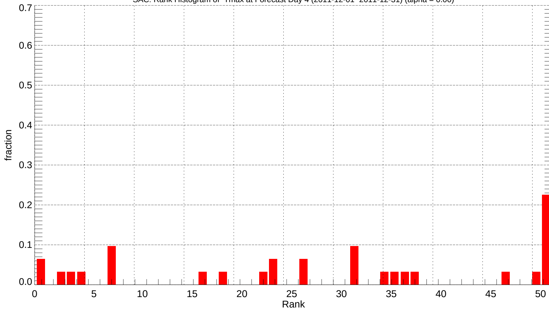
SAC: Rank Histogram of Tmax at Forecast Day 4 (2011-12-01~2011-12-31) (alpha = 0.00)
