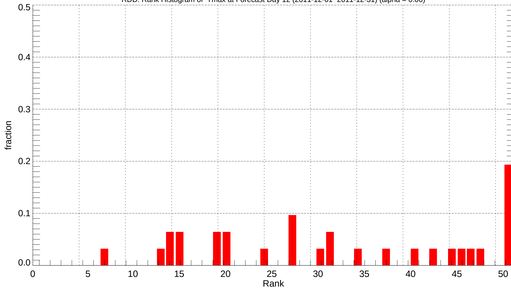
RDD: Rank Histogram of Tmax at Forecast Day 12 (2011-12-01~2011-12-31) (alpha = 0.00)
