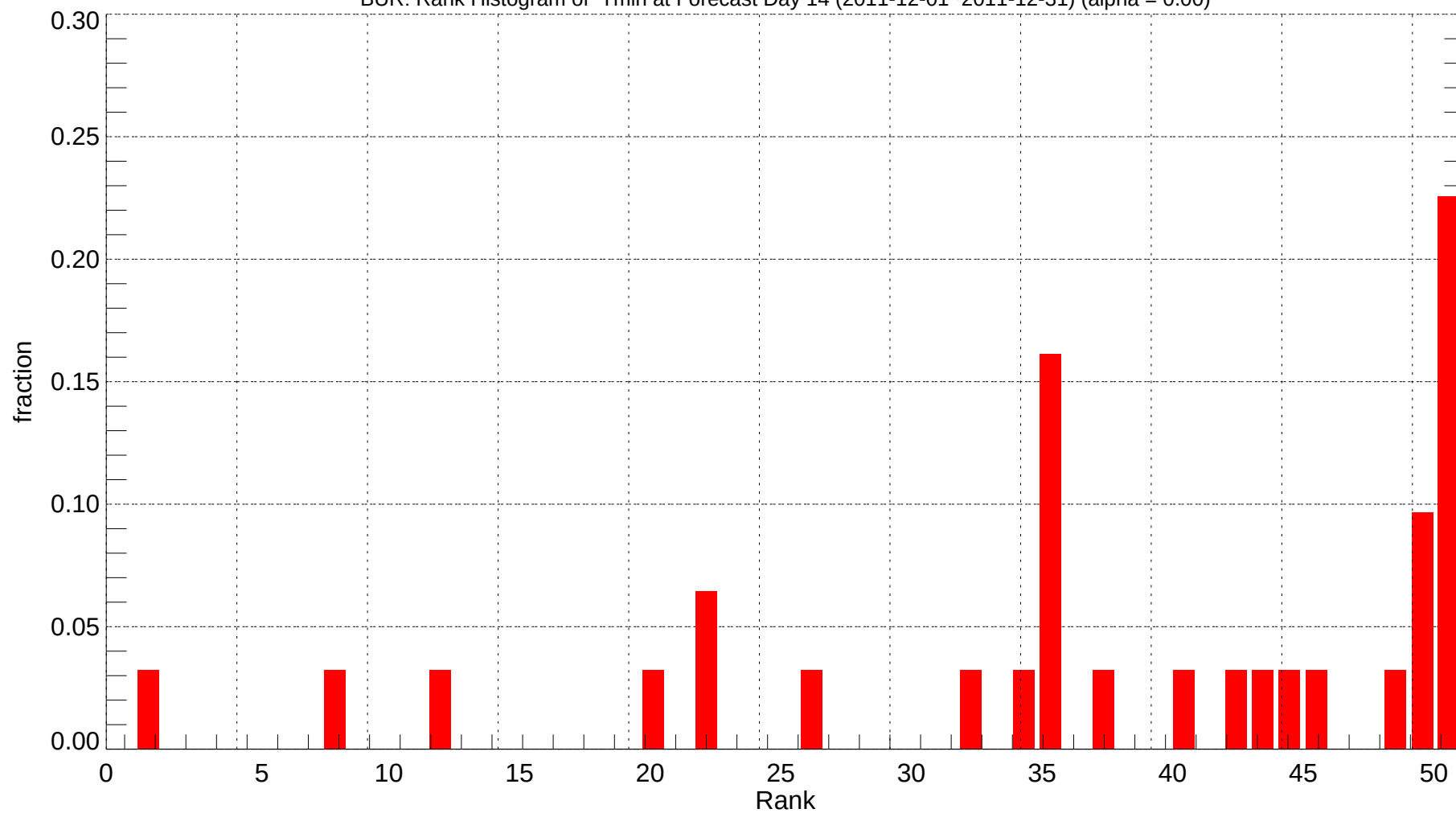
BUR: Rank Histogram of Tmin at Forecast Day 14 (2011-12-01~2011-12-31) (alpha = 0.00)
