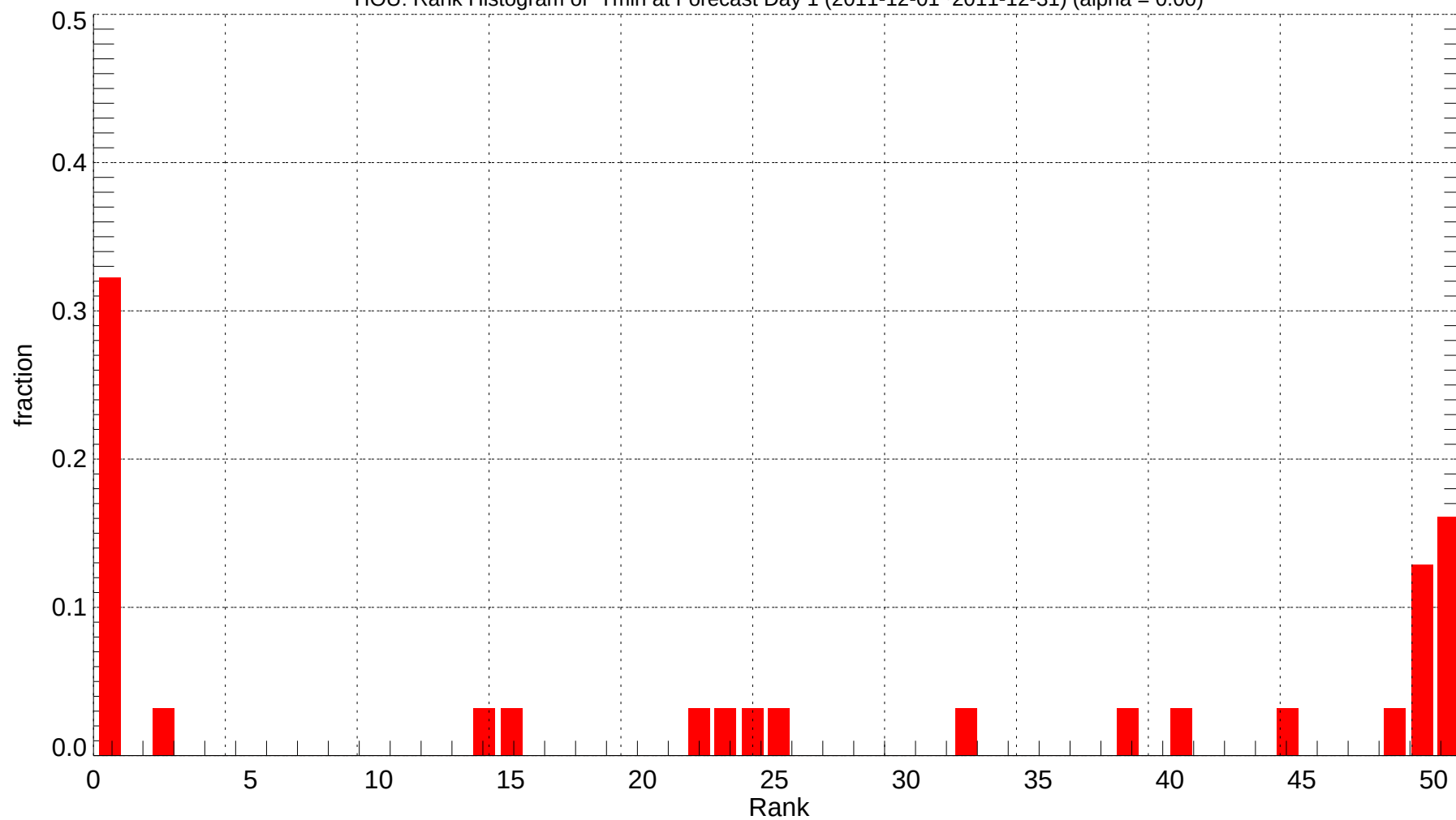
HOU: Rank Histogram of Tmin at Forecast Day 1 (2011-12-01~2011-12-31) (alpha = 0.00)
