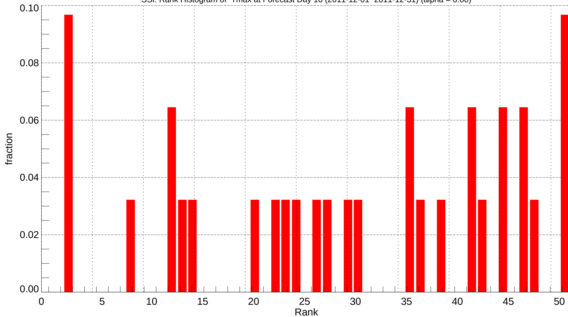
SSI: Rank Histogram of Tmax at Forecast Day 10 (2011-12-01~2011-12-31) (alpha = 0.00)
