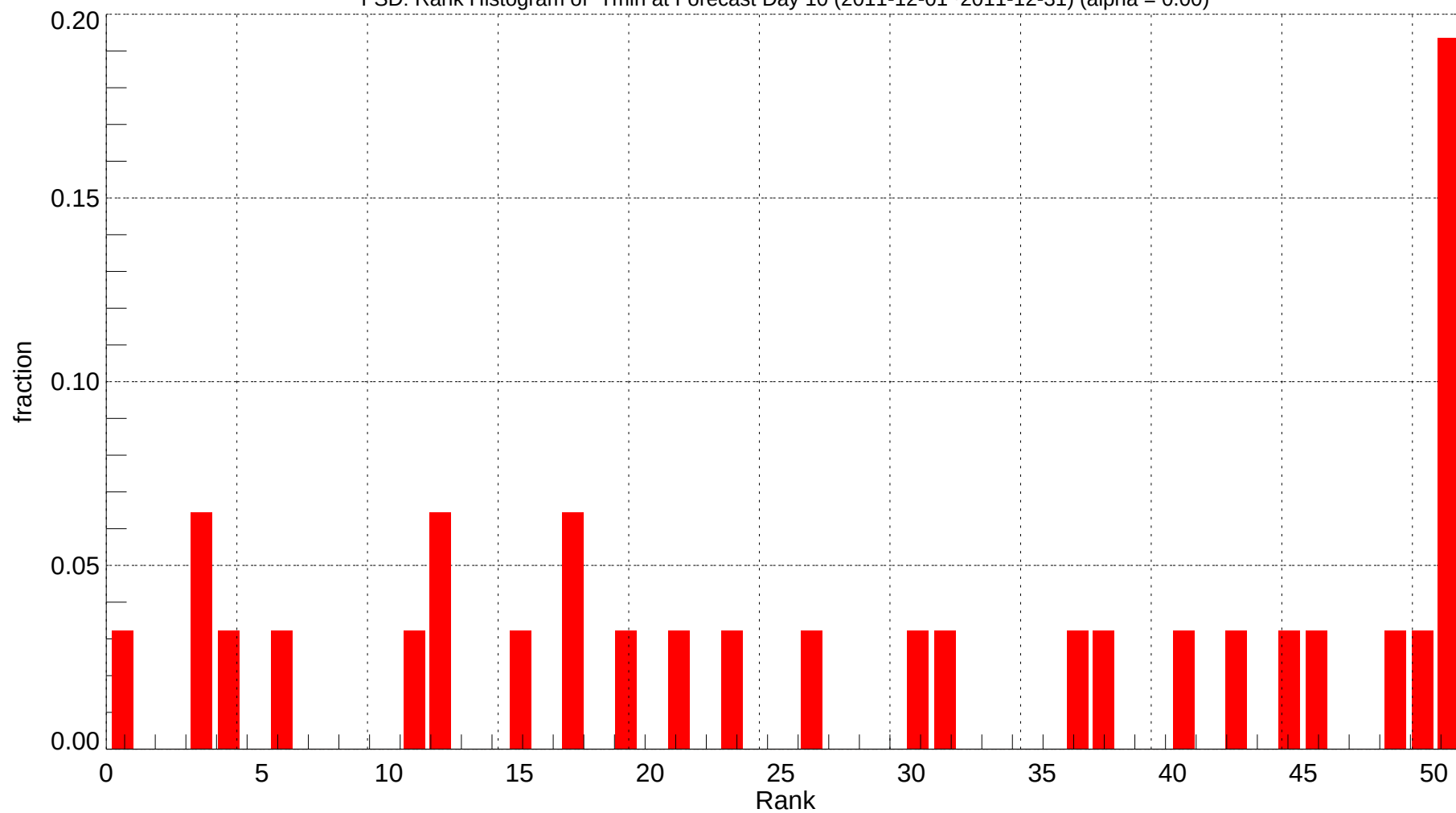
FSD: Rank Histogram of Tmin at Forecast Day 10 (2011-12-01~2011-12-31) (alpha = 0.00)
