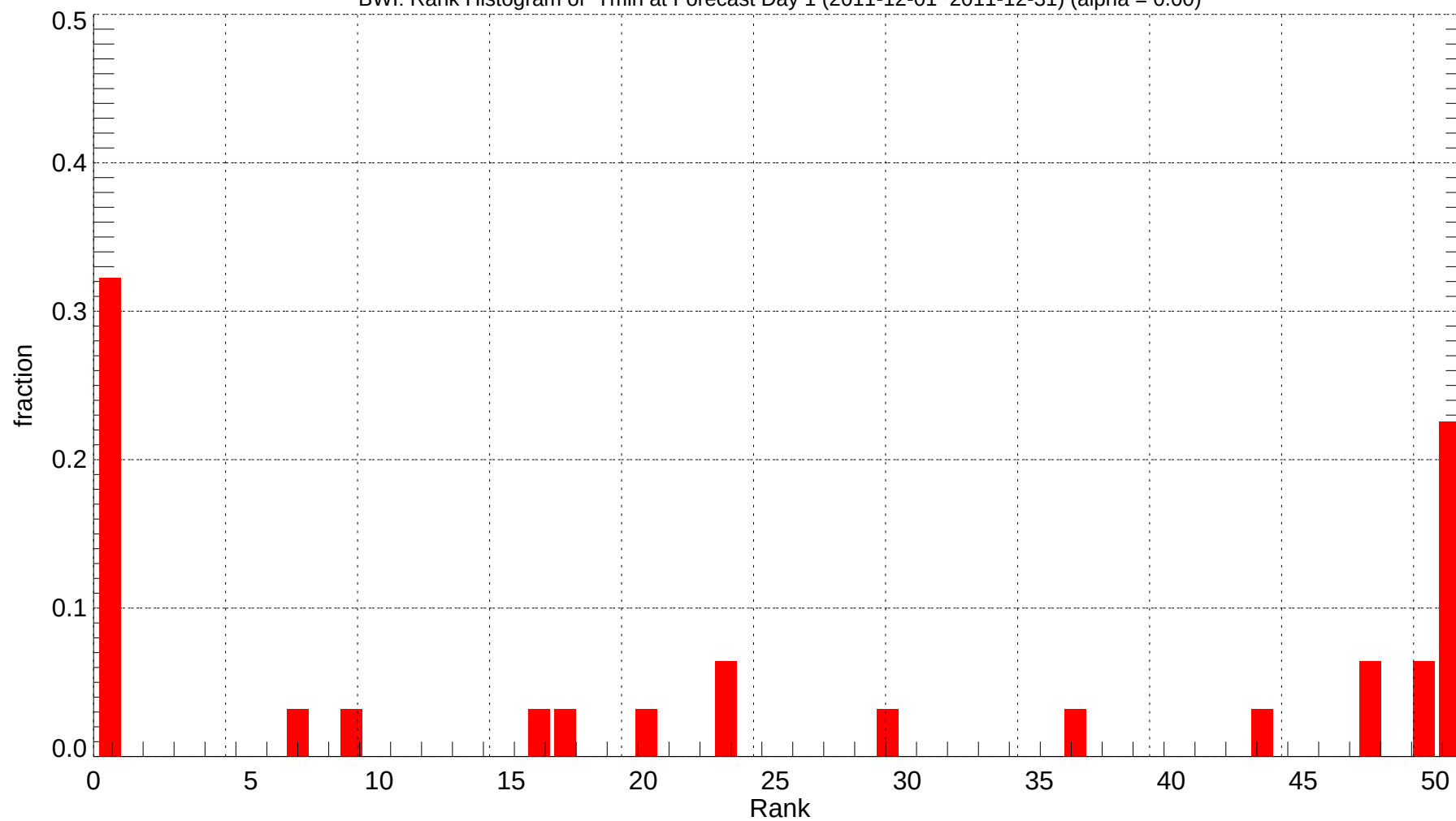
BWI: Rank Histogram of Tmin at Forecast Day 1 (2011-12-01~2011-12-31) (alpha = 0.00)
