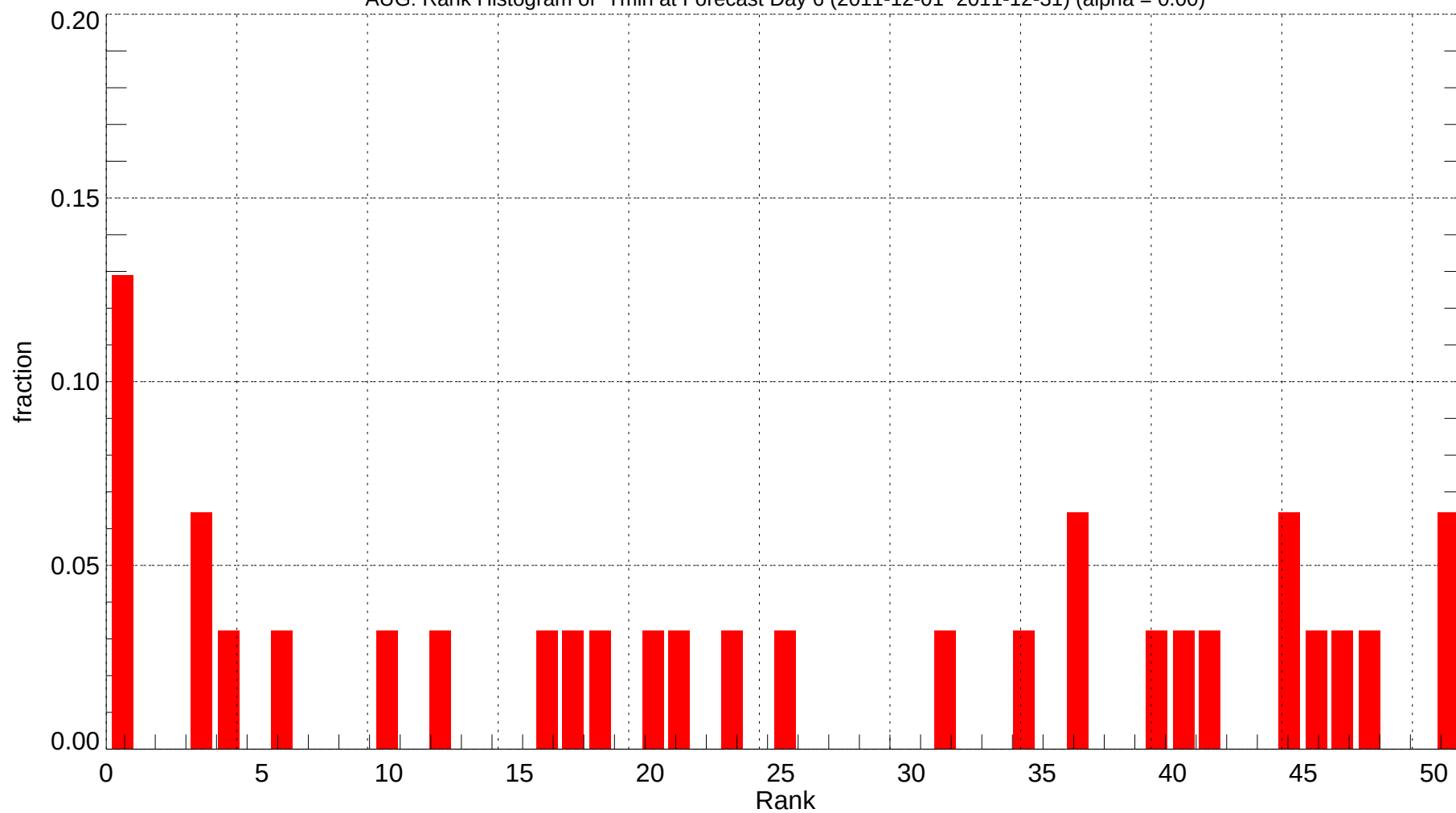
AUG: Rank Histogram of Tmin at Forecast Day 6 (2011-12-01~2011-12-31) (alpha = 0.00)
