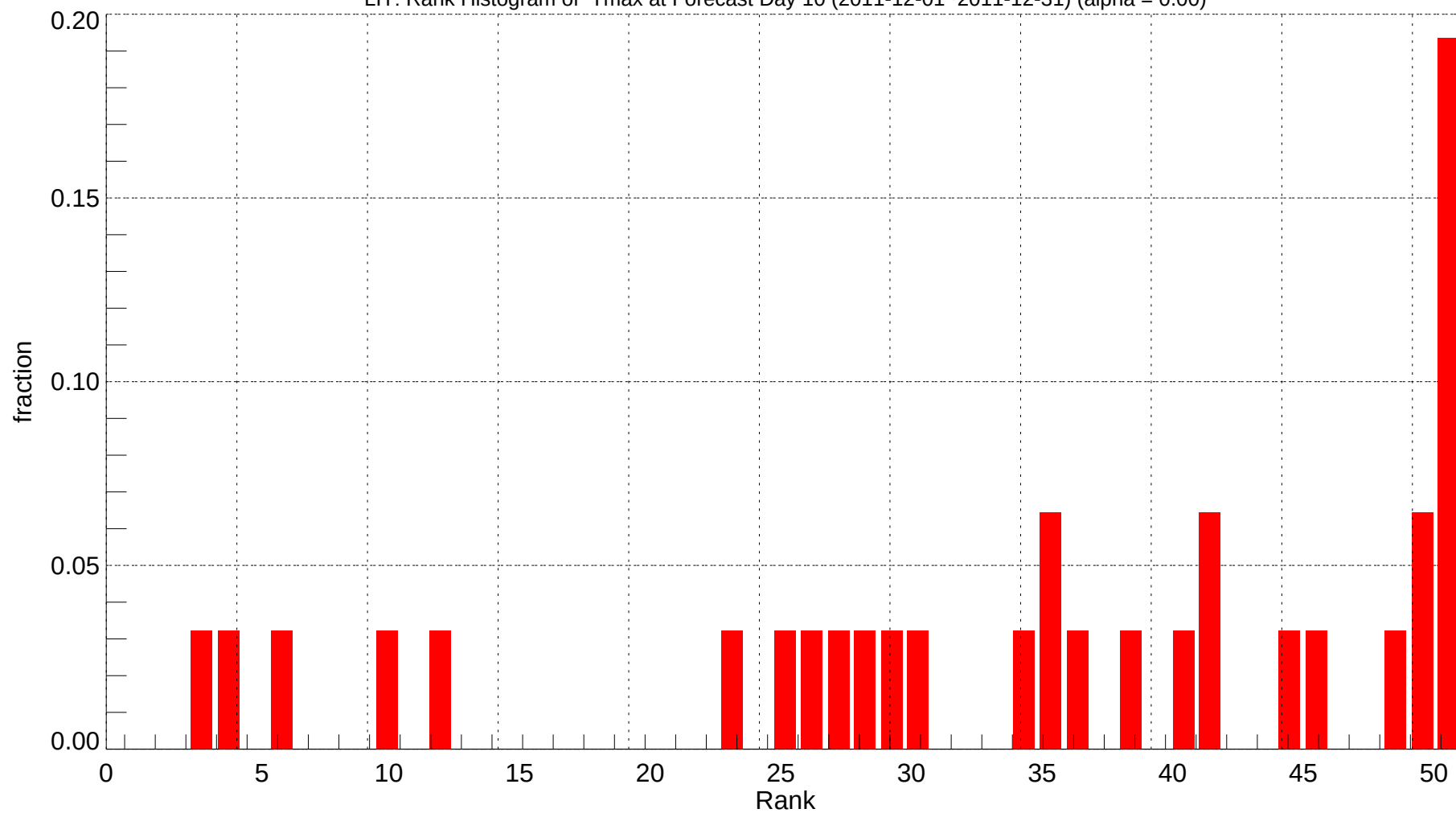
LIT: Rank Histogram of Tmax at Forecast Day 10 (2011-12-01~2011-12-31) (alpha = 0.00)
