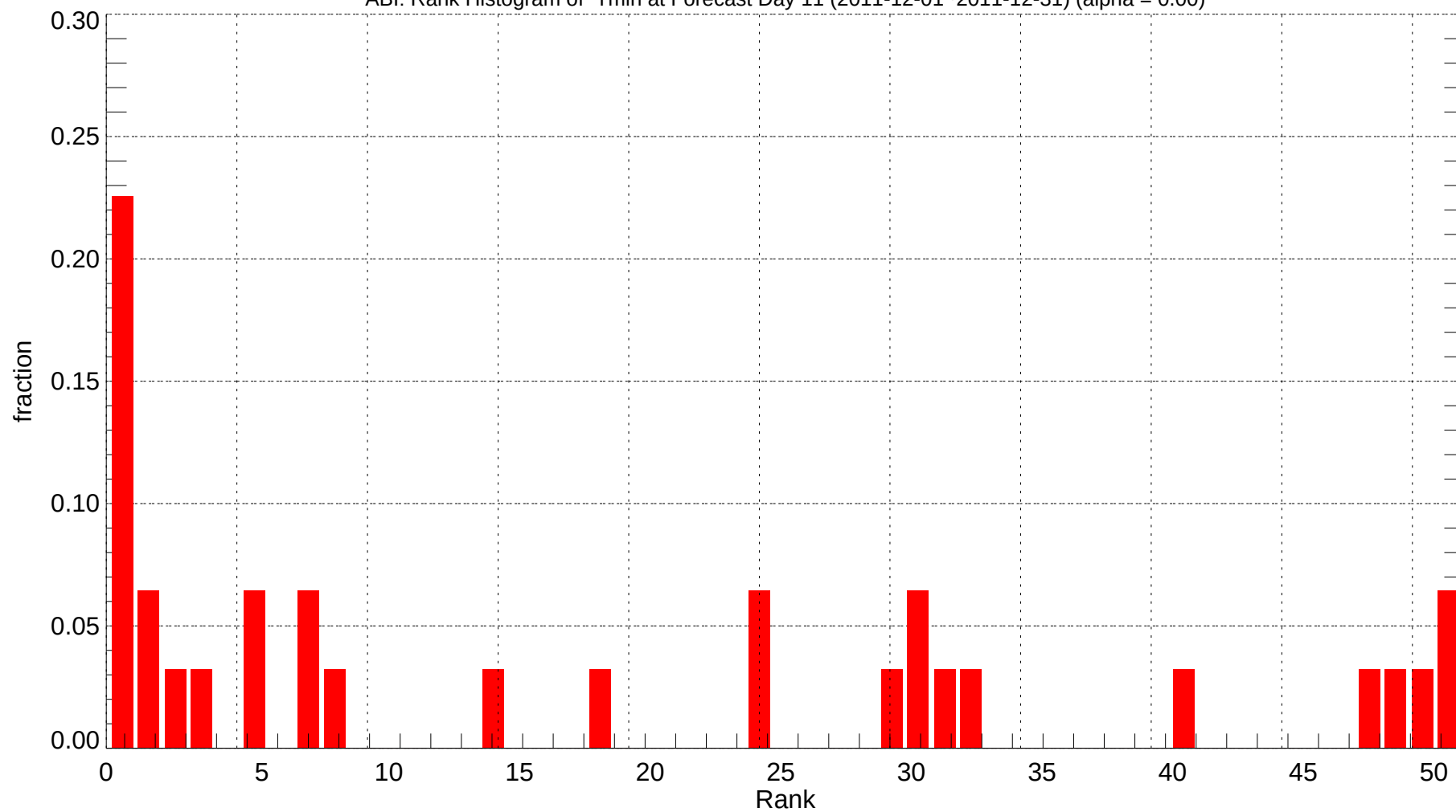
ABI: Rank Histogram of Tmin at Forecast Day 11 (2011-12-01~2011-12-31) (alpha = 0.00)
