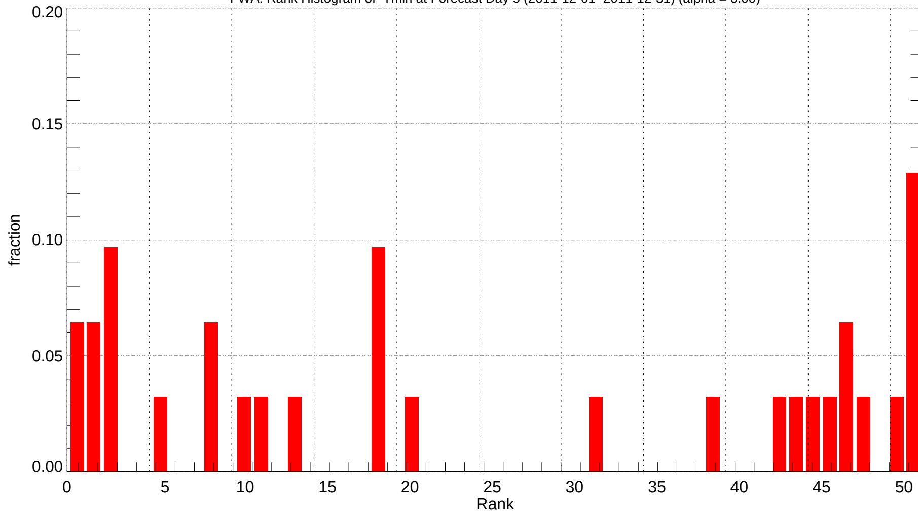
FWA: Rank Histogram of Tmin at Forecast Day 5 (2011-12-01~2011-12-31) (alpha = 0.00)
