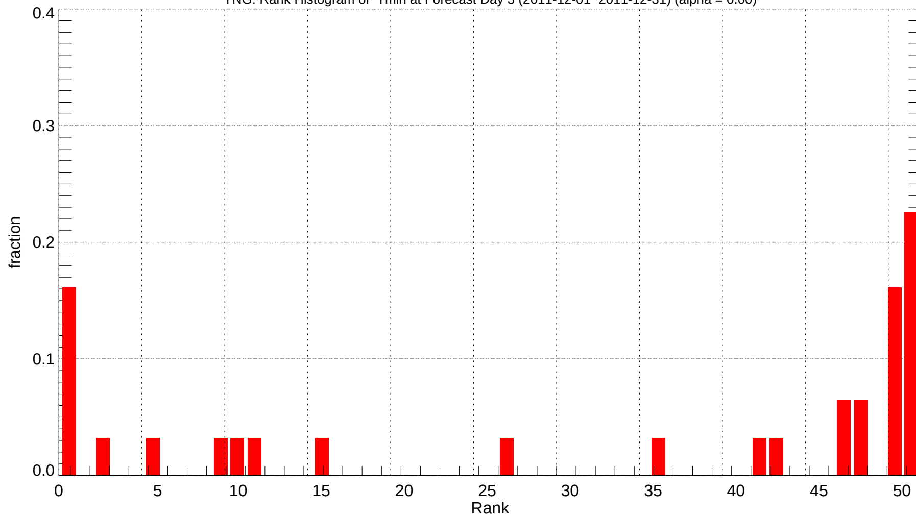
YNG: Rank Histogram of Tmin at Forecast Day 3 (2011-12-01~2011-12-31) (alpha = 0.00)
