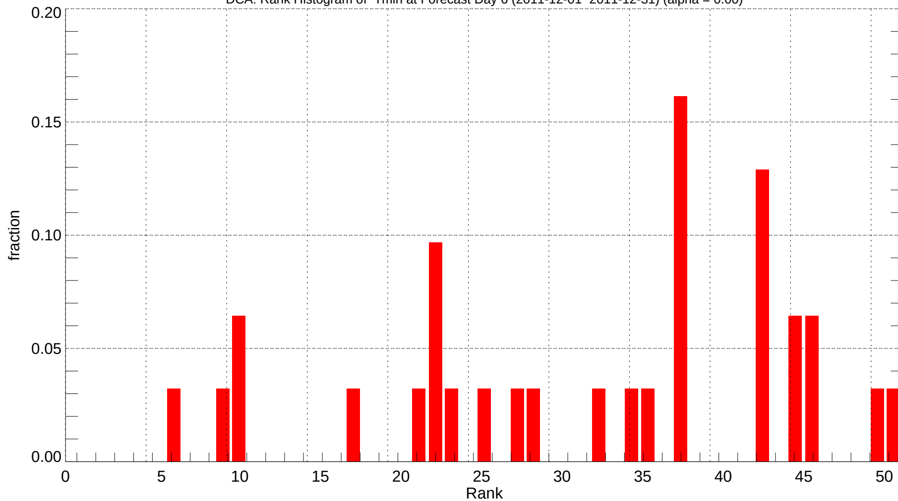
DCA: Rank Histogram of Tmin at Forecast Day 6 (2011-12-01~2011-12-31) (alpha = 0.00)
