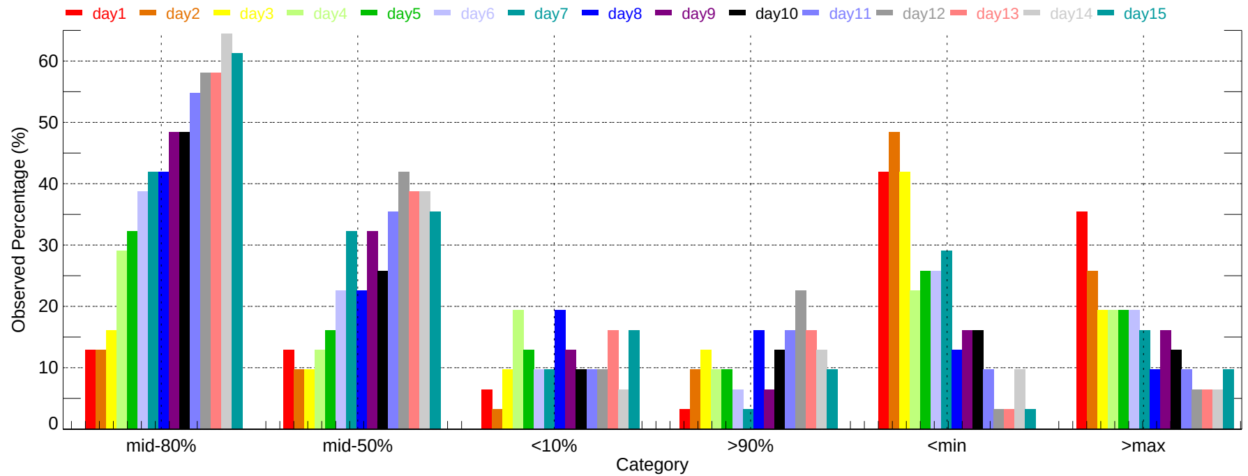
Observed Percentage of Ensembles - ACY: Min Temperature (2011-12-01~2011-12-31)
