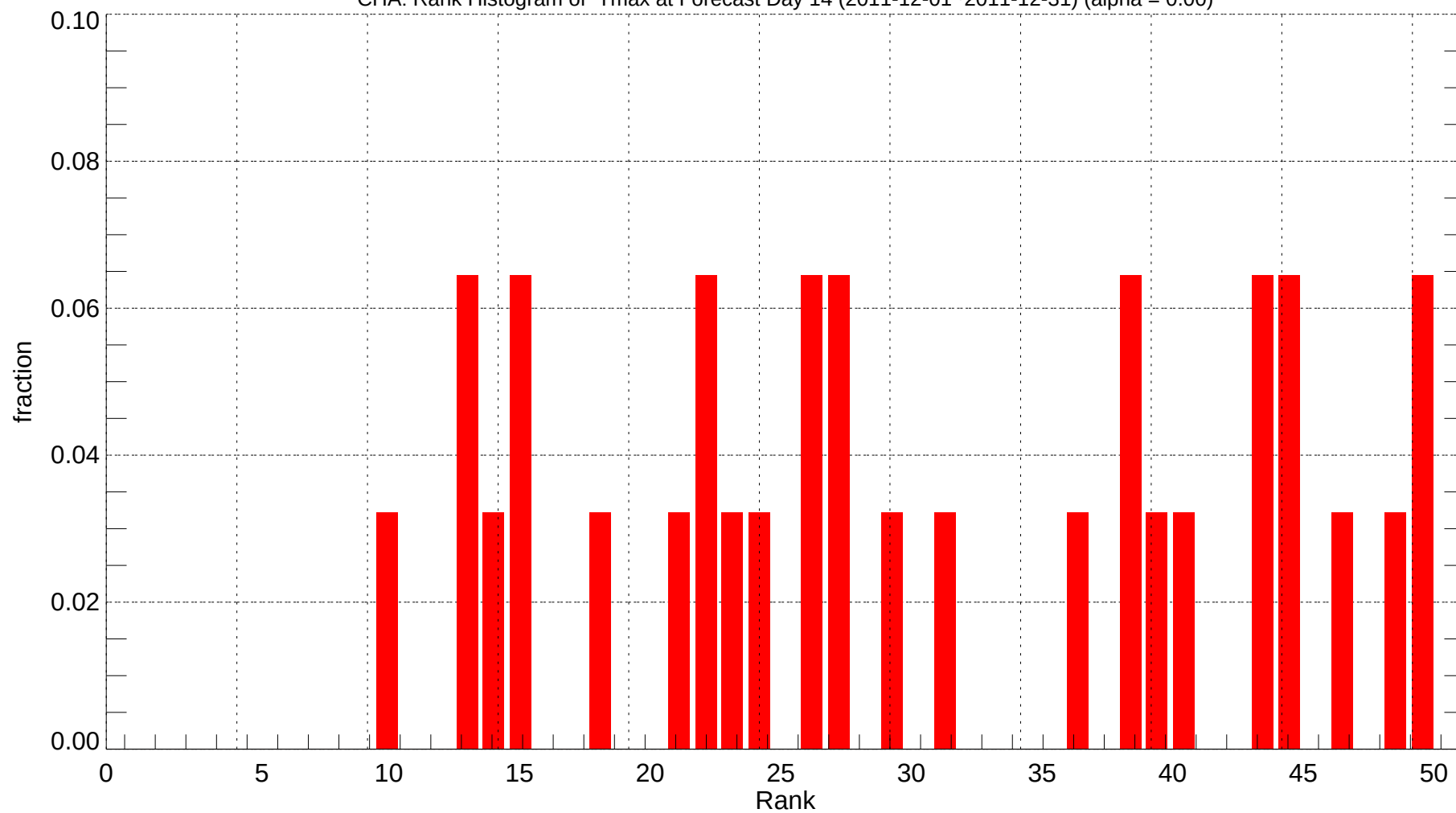
CHA: Rank Histogram of Tmax at Forecast Day 14 (2011-12-01~2011-12-31) (alpha = 0.00)
