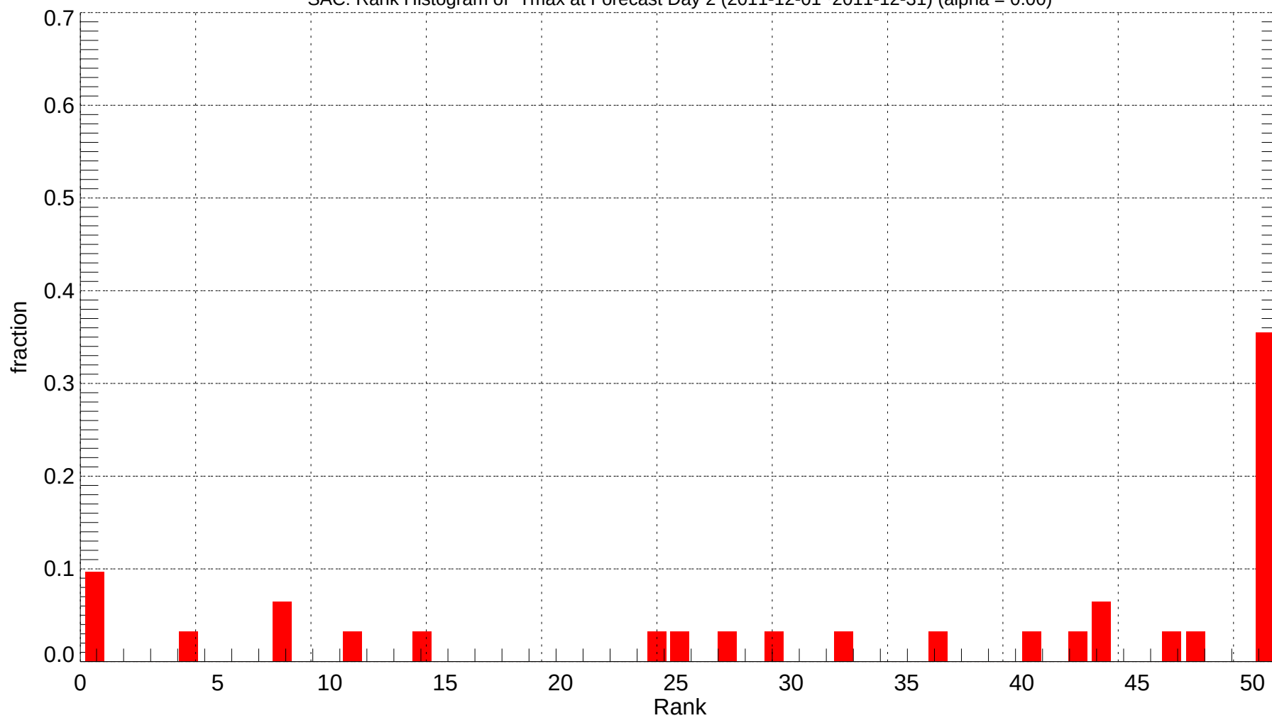
SAC: Rank Histogram of Tmax at Forecast Day 2 (2011-12-01~2011-12-31) (alpha = 0.00)
