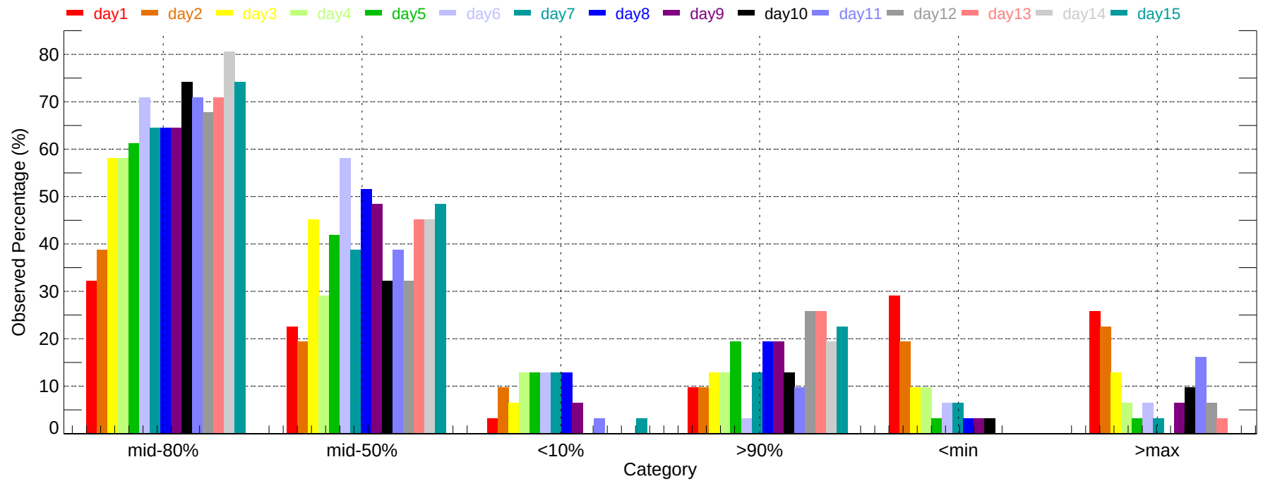
Observed Percentage of Ensembles - BWI: Max Temperature (2011-12-01~2011-12-31)
