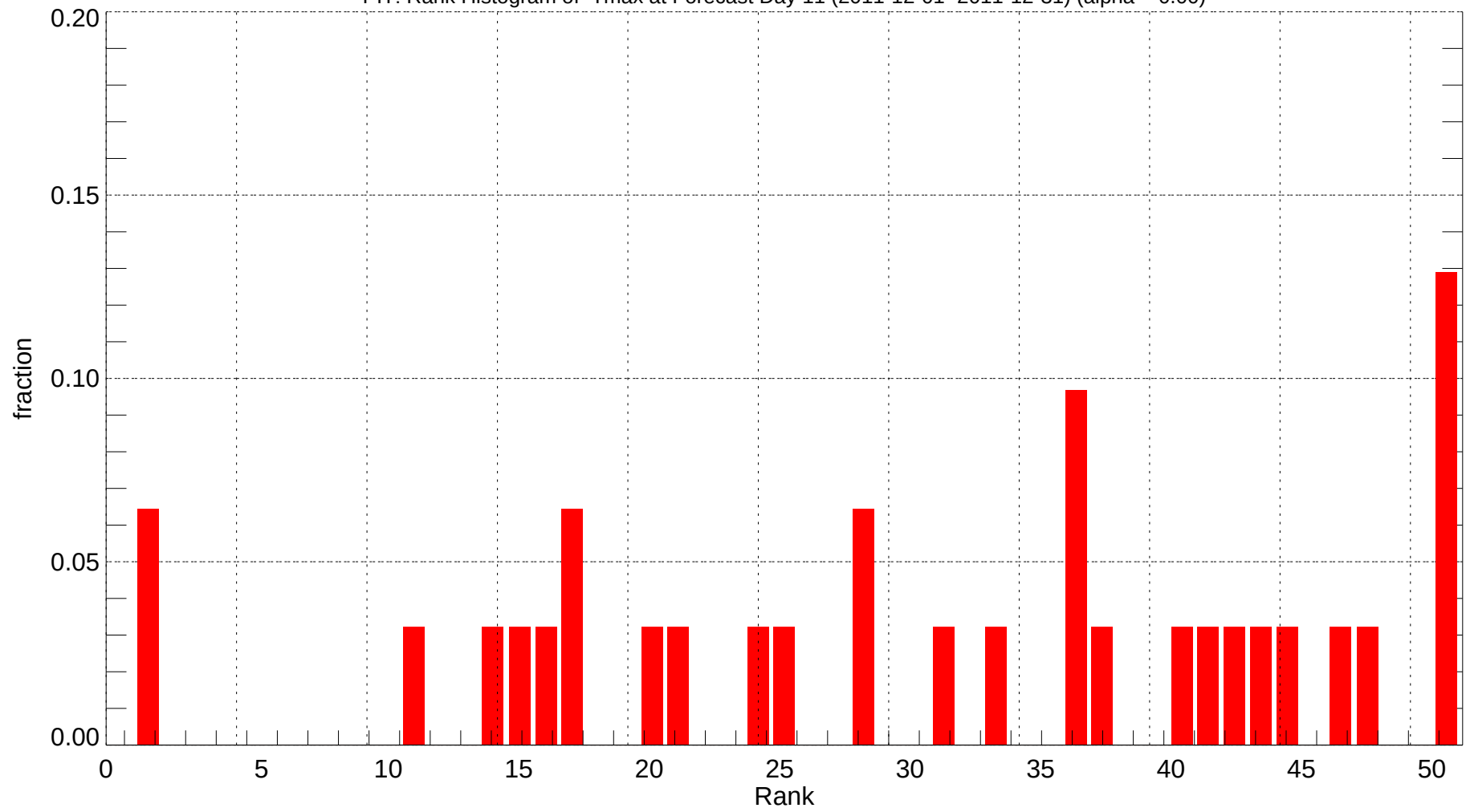
PIT: Rank Histogram of Tmax at Forecast Day 11 (2011-12-01~2011-12-31) (alpha = 0.00)
