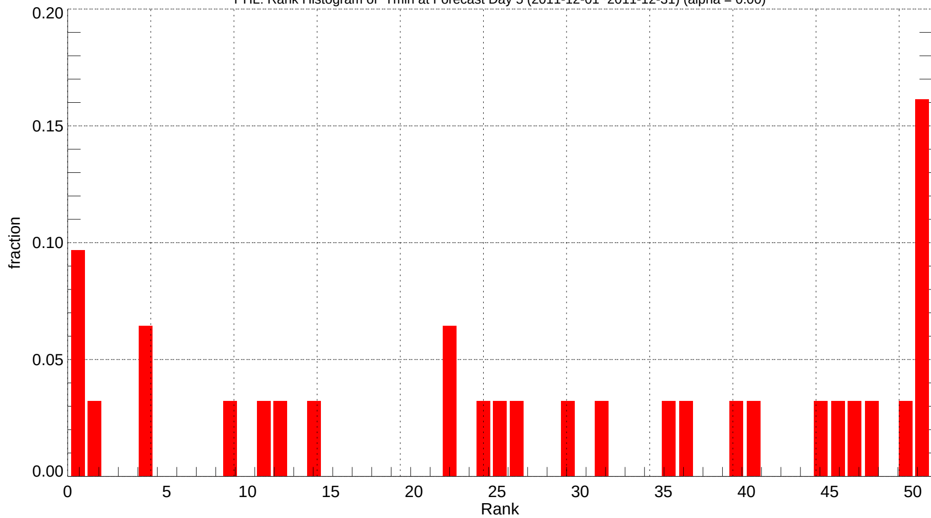
PHL: Rank Histogram of Tmin at Forecast Day 5 (2011-12-01~2011-12-31) (alpha = 0.00)
