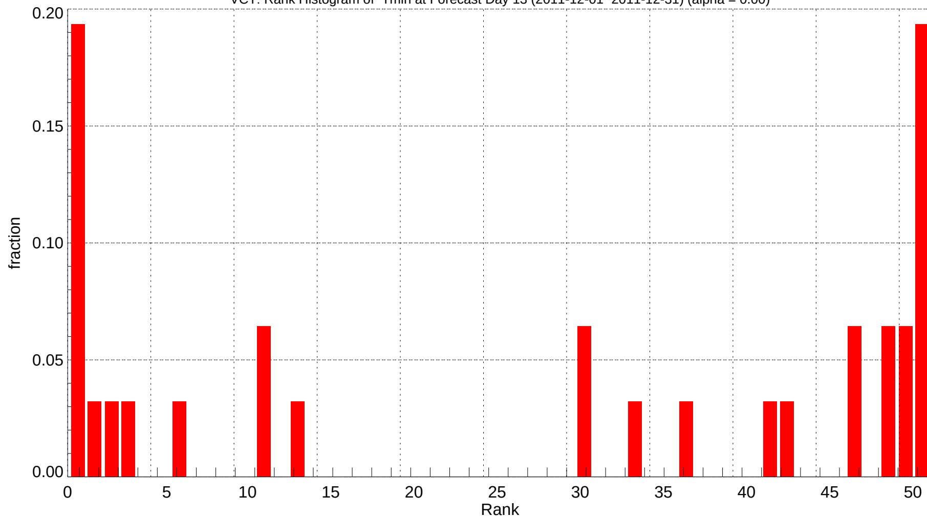
VCT: Rank Histogram of Tmin at Forecast Day 13 (2011-12-01~2011-12-31) (alpha = 0.00)
