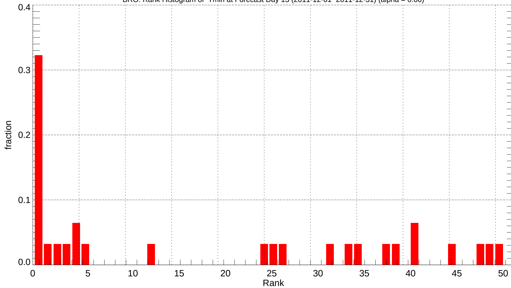
BRO: Rank Histogram of Tmin at Forecast Day 13 (2011-12-01~2011-12-31) (alpha = 0.00)
