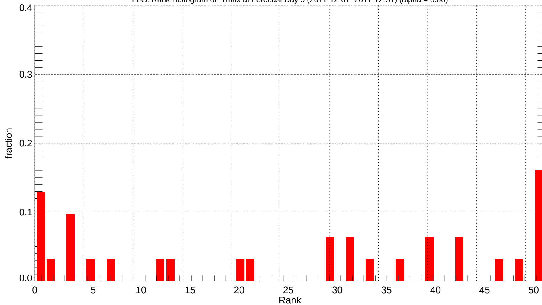
FLG: Rank Histogram of Tmax at Forecast Day 9 (2011-12-01~2011-12-31) (alpha = 0.00)
