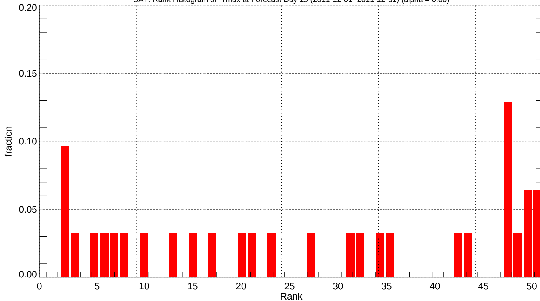
SAT: Rank Histogram of Tmax at Forecast Day 15 (2011-12-01~2011-12-31) (alpha = 0.00)
