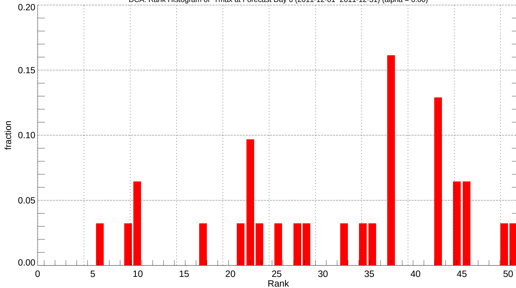
DCA: Rank Histogram of Tmax at Forecast Day 6 (2011-12-01~2011-12-31) (alpha = 0.00)
