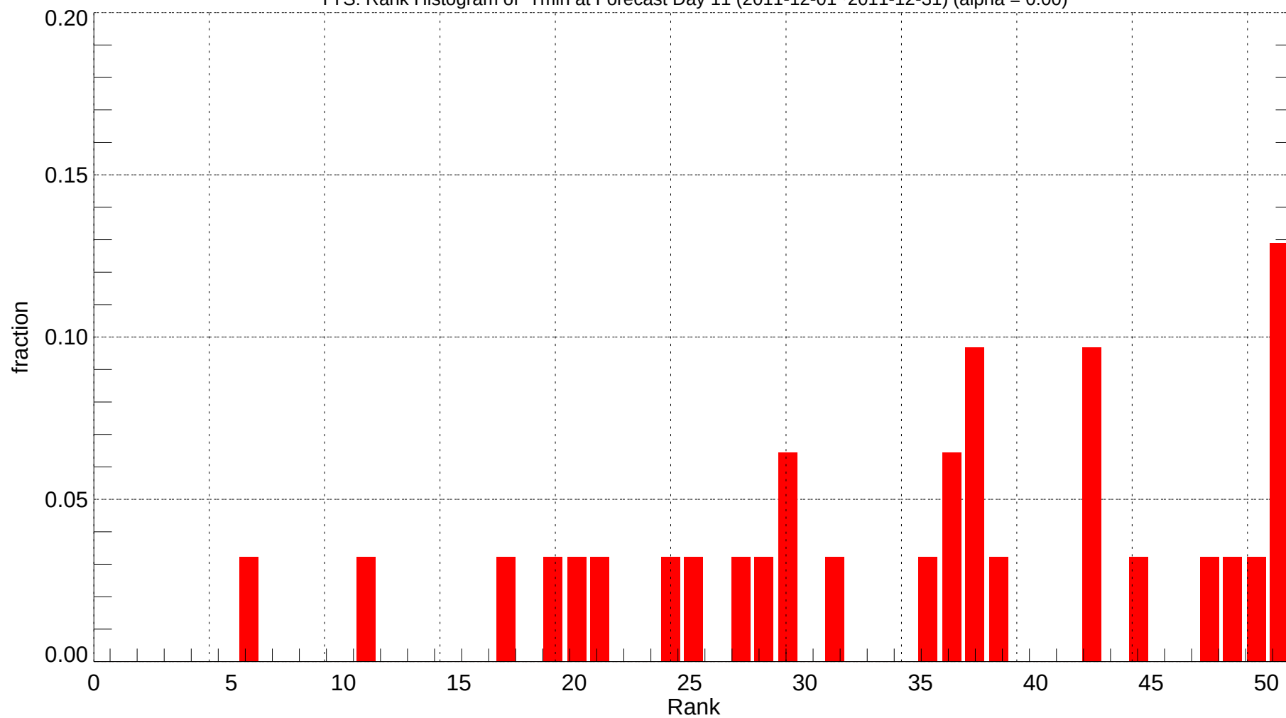
TYS: Rank Histogram of Tmin at Forecast Day 11 (2011-12-01~2011-12-31) (alpha = 0.00)
