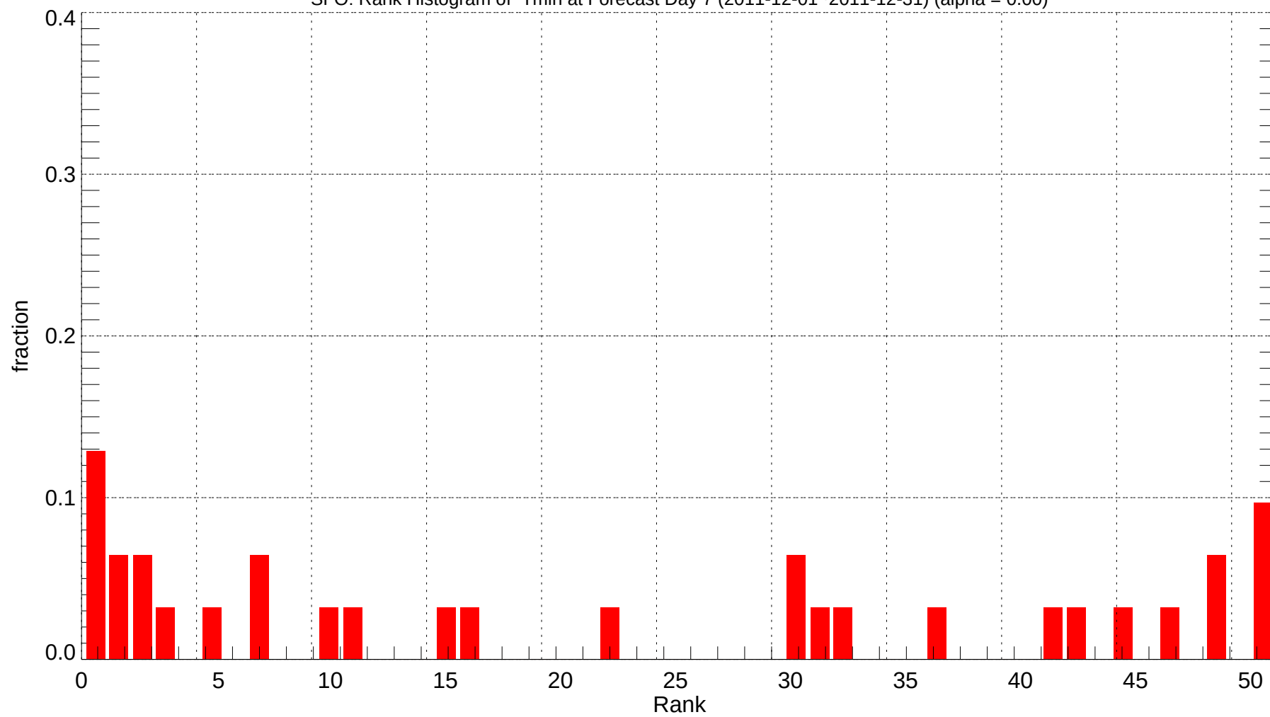
SFO: Rank Histogram of Tmin at Forecast Day 7 (2011-12-01~2011-12-31) (alpha = 0.00)
