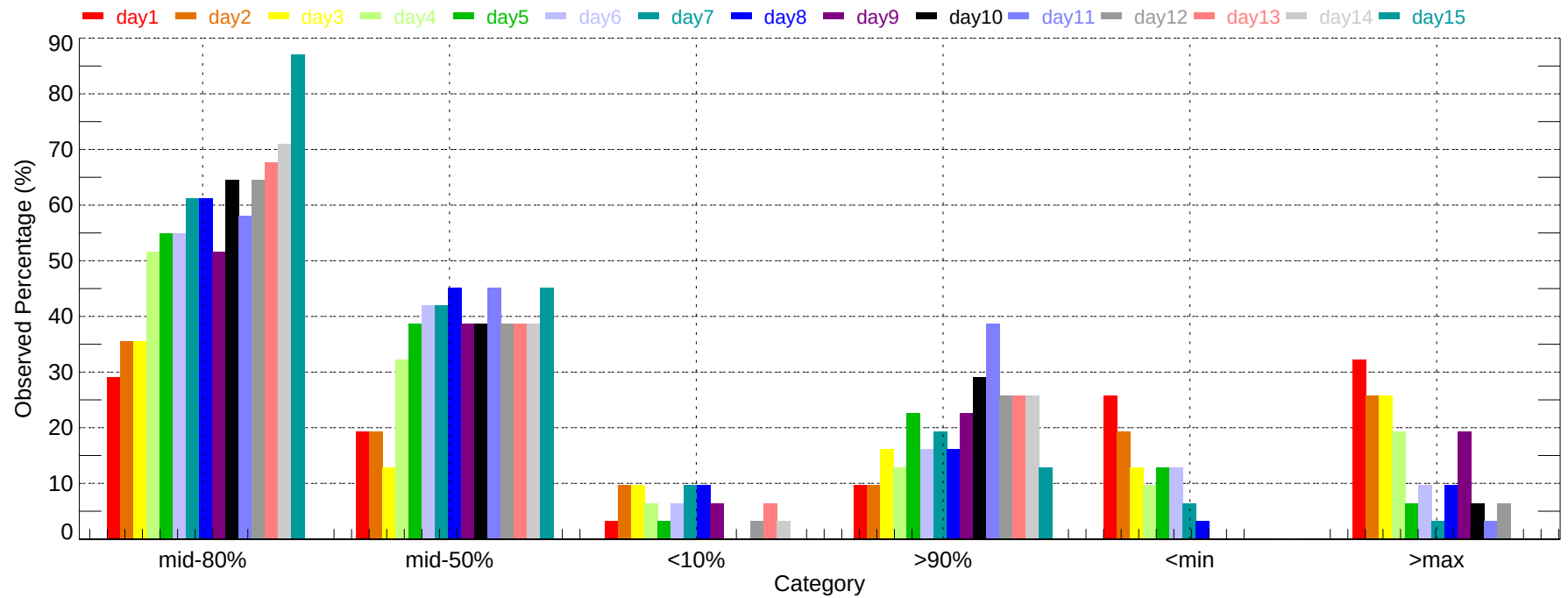
Observed Percentage of Ensembles - CLE: Min Temperature (2011-12-01~2011-12-31)
