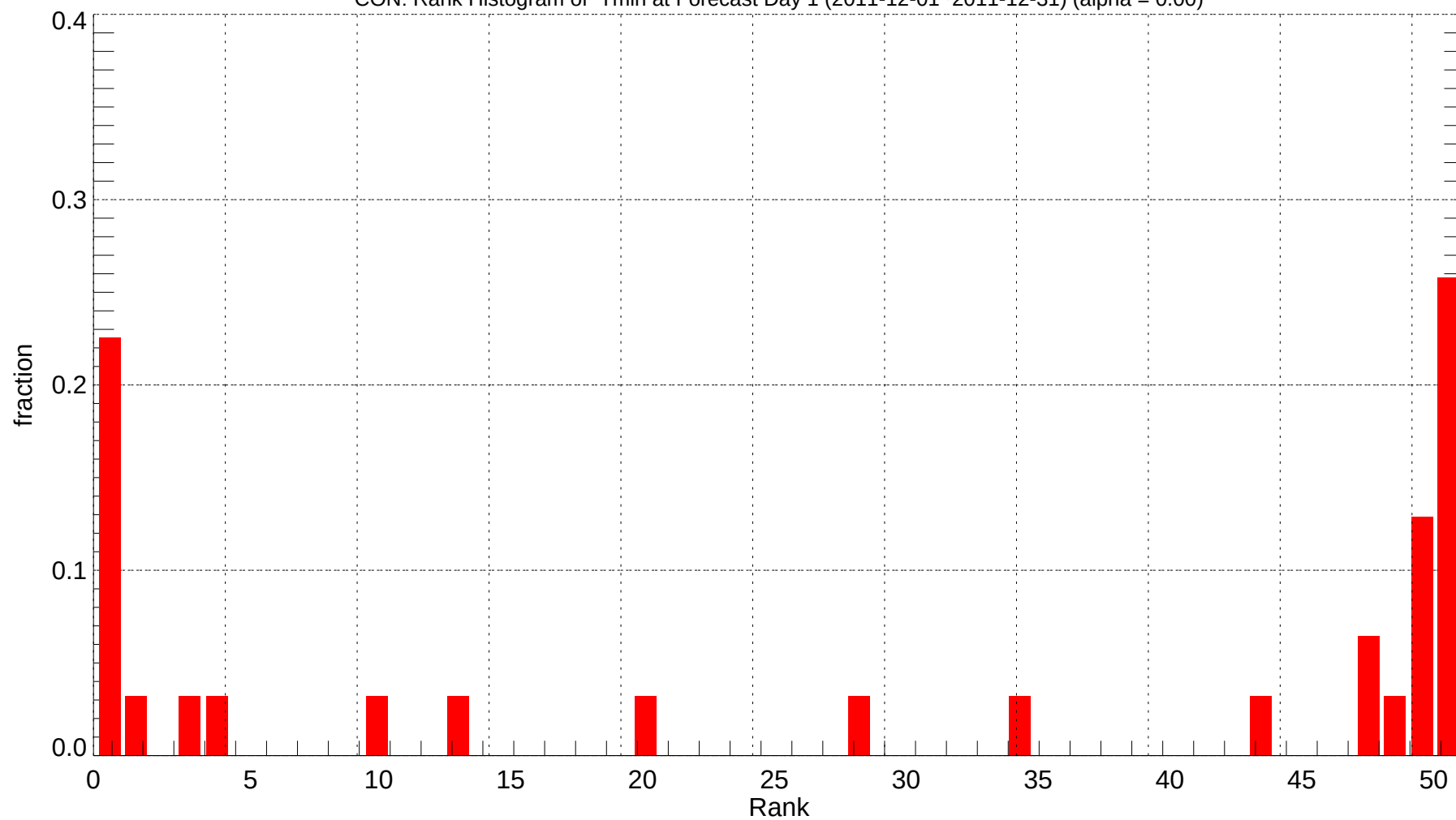
CON: Rank Histogram of Tmin at Forecast Day 1 (2011-12-01~2011-12-31) (alpha = 0.00)
