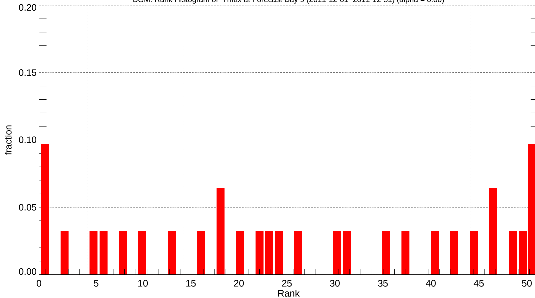
BGM: Rank Histogram of Tmax at Forecast Day 9 (2011-12-01~2011-12-31) (alpha = 0.00)
