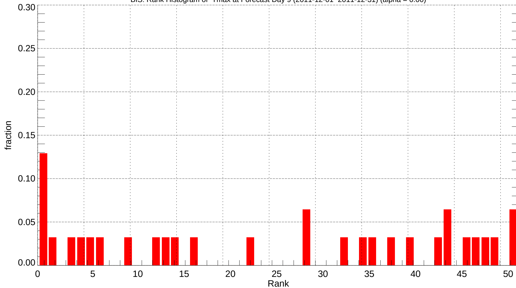
BIS: Rank Histogram of Tmax at Forecast Day 9 (2011-12-01~2011-12-31) (alpha = 0.00)
