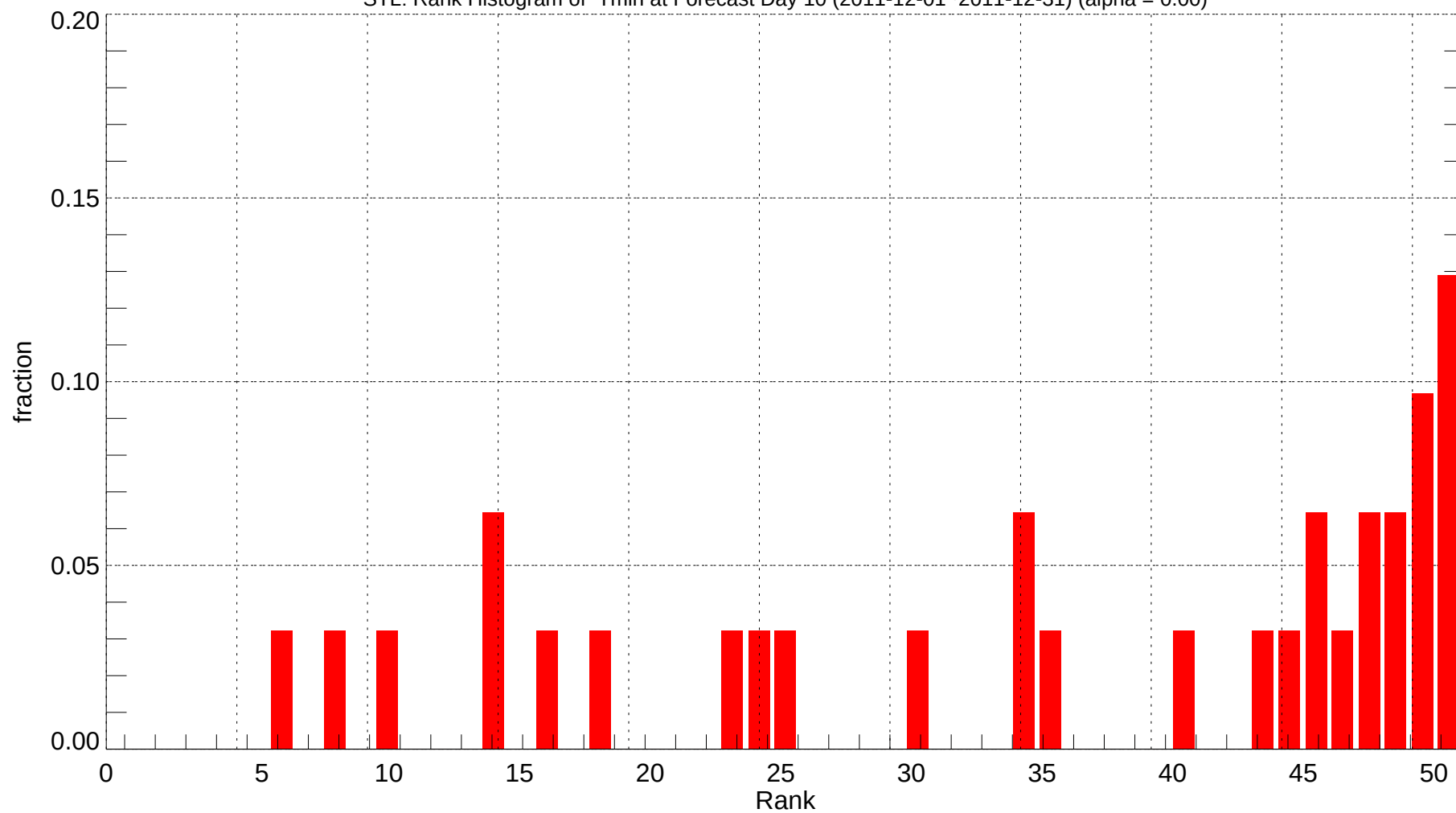
STL: Rank Histogram of Tmin at Forecast Day 10 (2011-12-01~2011-12-31) (alpha = 0.00)
