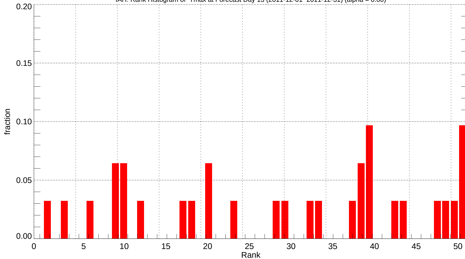
IAH: Rank Histogram of Tmax at Forecast Day 13 (2011-12-01~2011-12-31) (alpha = 0.00)
