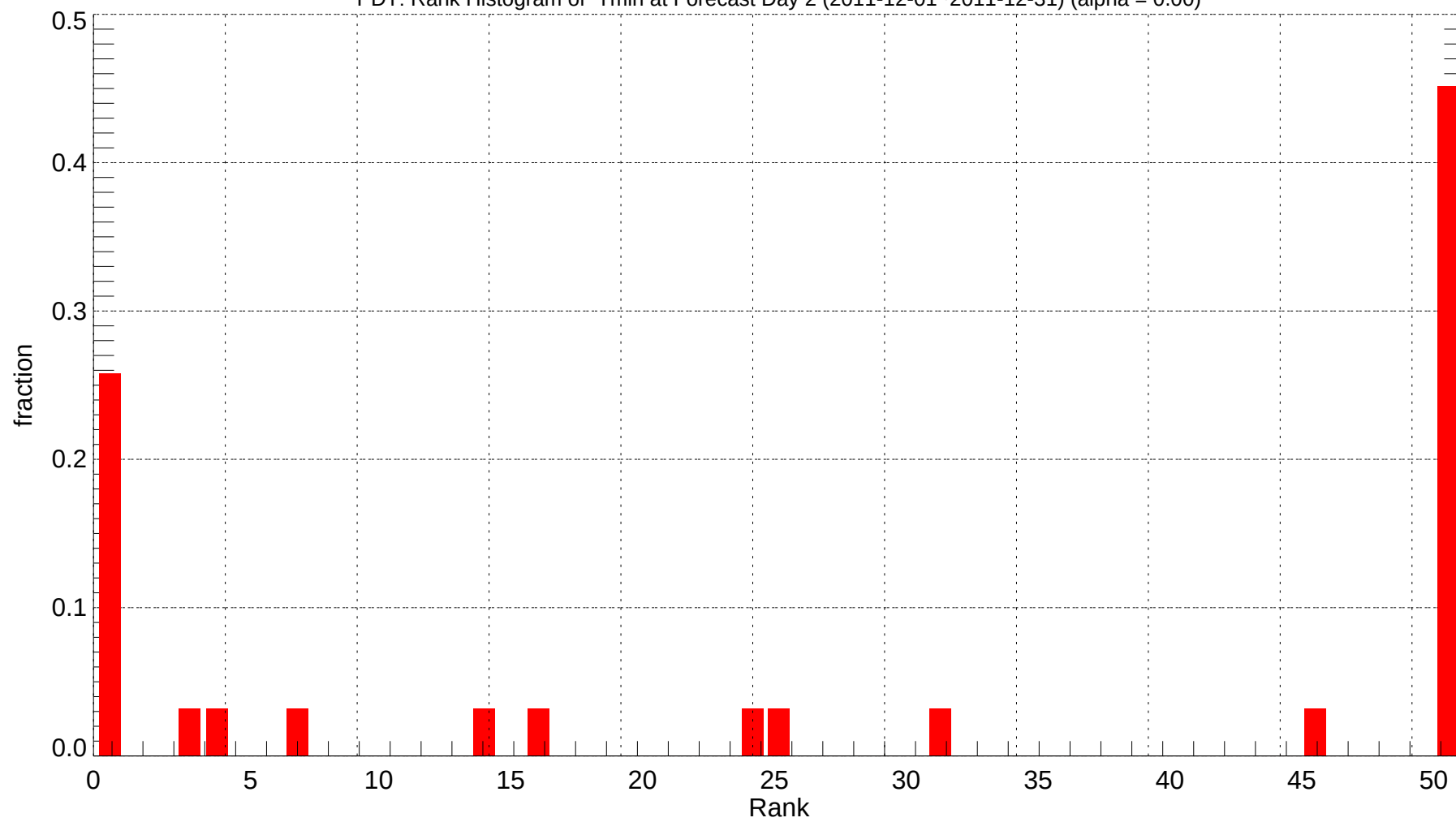
PDT: Rank Histogram of Tmin at Forecast Day 2 (2011-12-01~2011-12-31) (alpha = 0.00)
