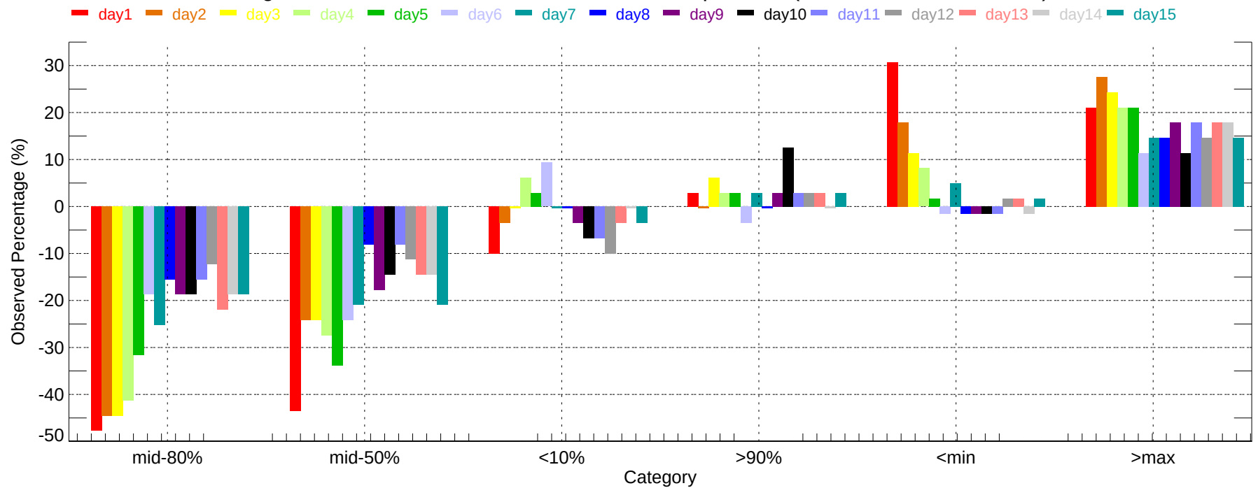
Observed Percentage Deviation of Ensembles - MSY: Max Temperature (2011-12-01~2011-12-31)
