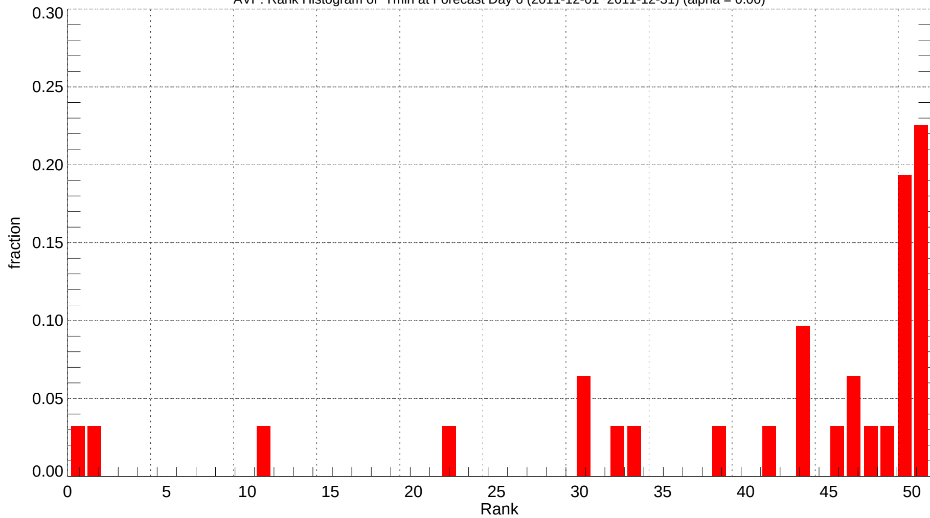
AVP: Rank Histogram of Tmin at Forecast Day 6 (2011-12-01~2011-12-31) (alpha = 0.00)
