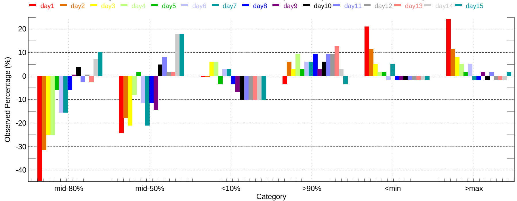
Observed Percentage Deviation of Ensembles - JAX: Min Temperature (2011-12-01~2011-12-31)
