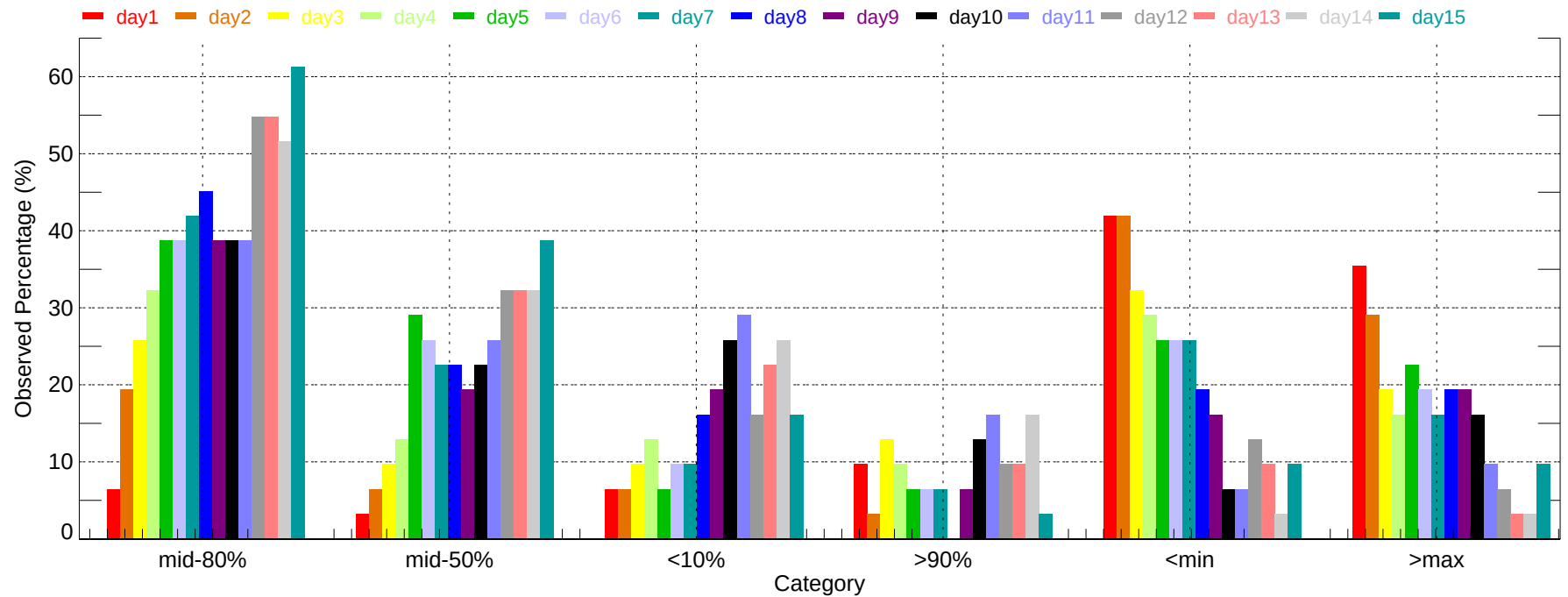
Observed Percentage of Ensembles - TRM: Min Temperature (2011-12-01~2011-12-31)
