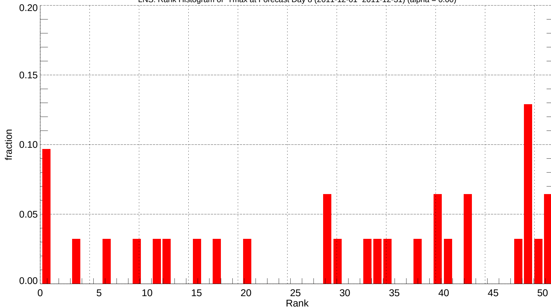
LNS: Rank Histogram of Tmax at Forecast Day 8 (2011-12-01~2011-12-31) (alpha = 0.00)
