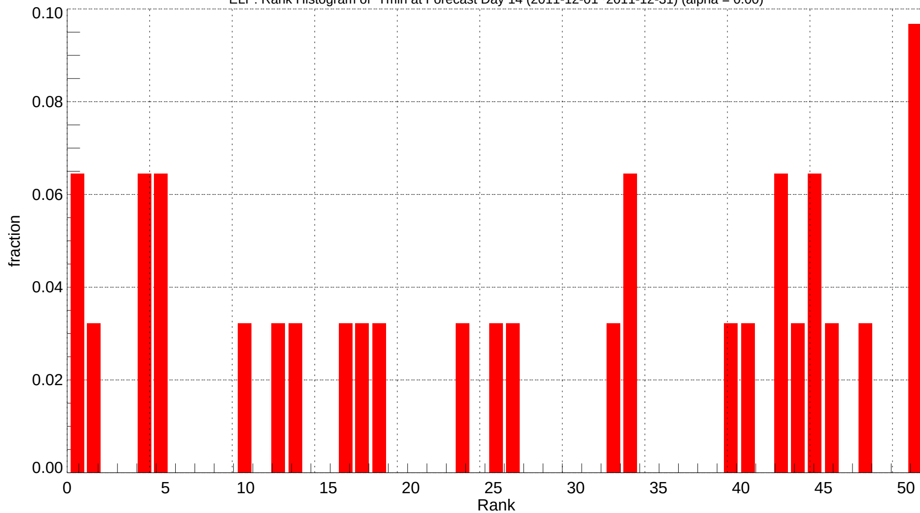
ELP: Rank Histogram of Tmin at Forecast Day 14 (2011-12-01~2011-12-31) (alpha = 0.00)
