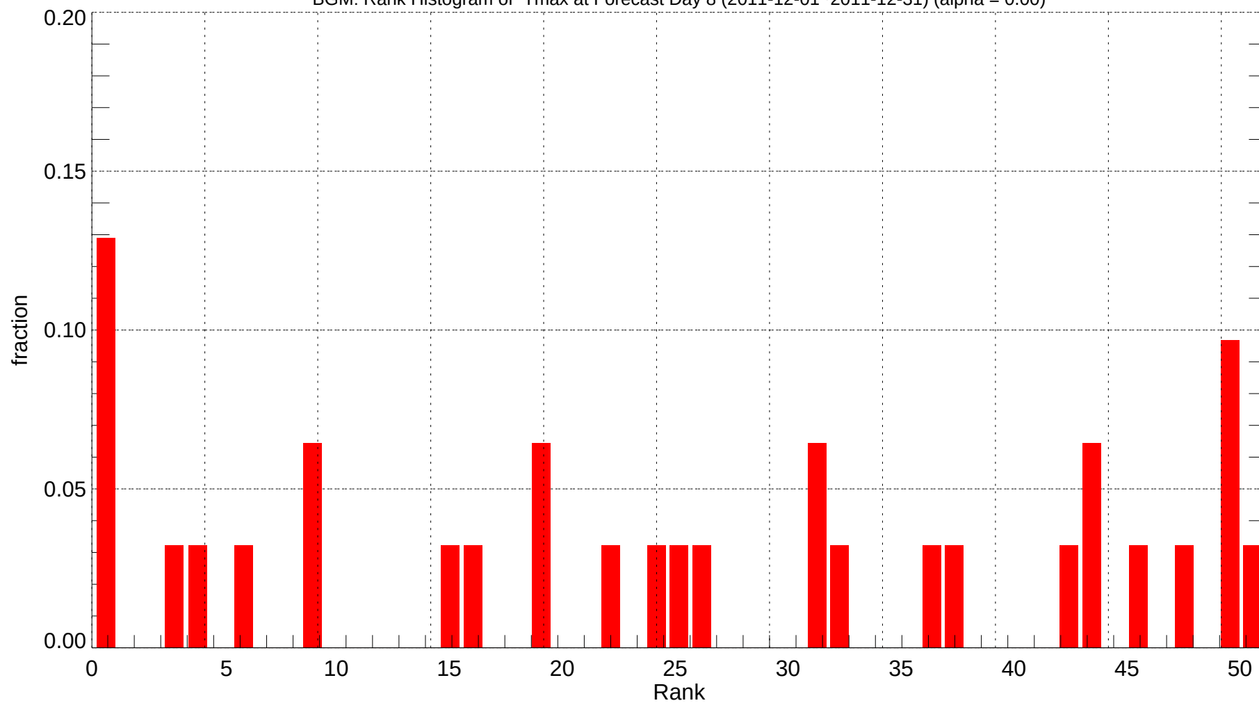
BGM: Rank Histogram of Tmax at Forecast Day 8 (2011-12-01~2011-12-31) (alpha = 0.00)
