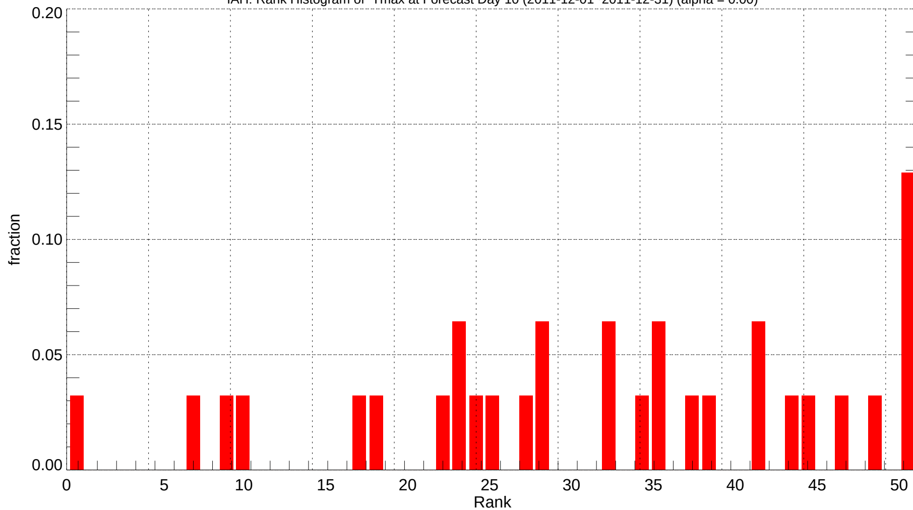
IAH: Rank Histogram of Tmax at Forecast Day 10 (2011-12-01~2011-12-31) (alpha = 0.00)
