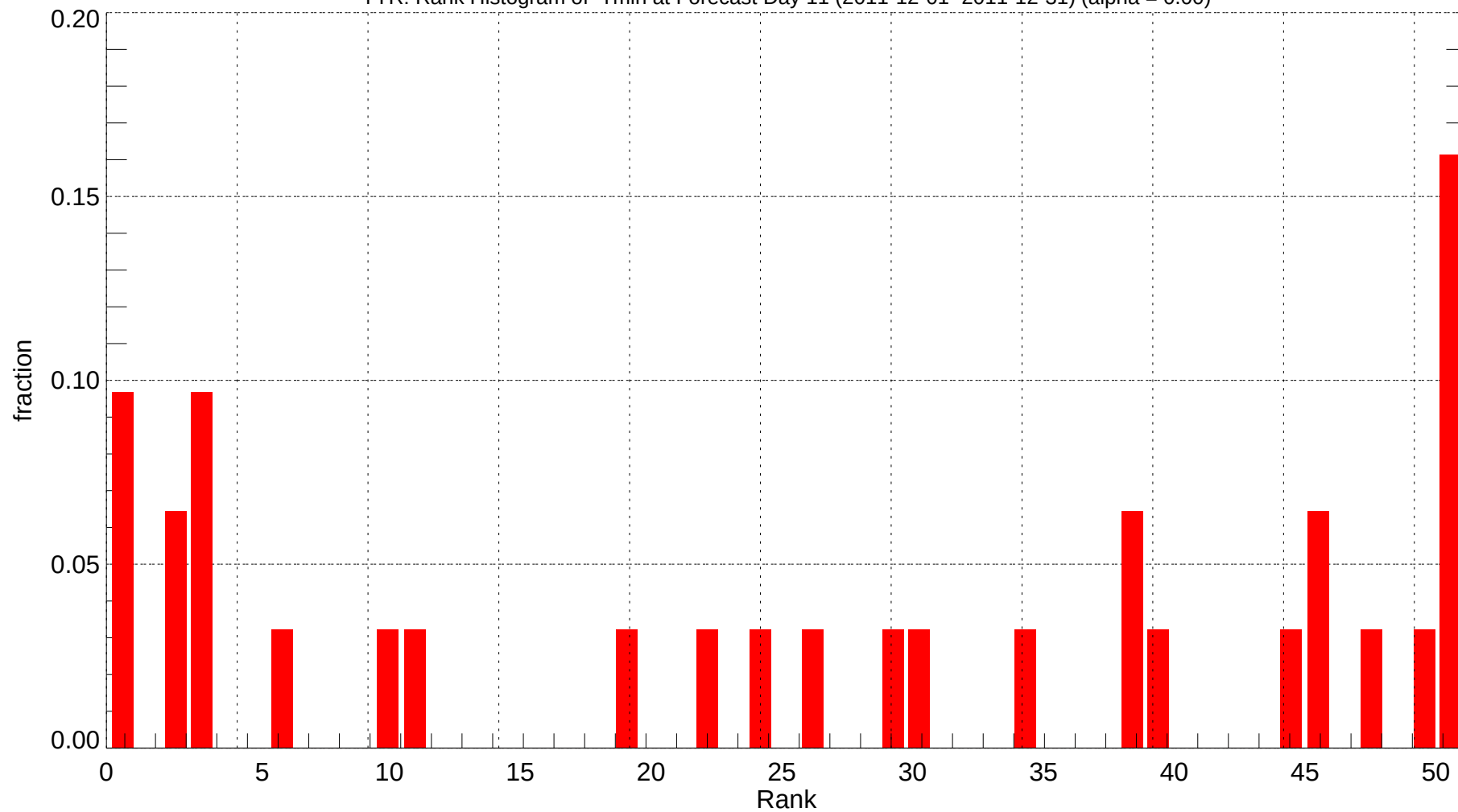
TYR: Rank Histogram of Tmin at Forecast Day 11 (2011-12-01~2011-12-31) (alpha = 0.00)
