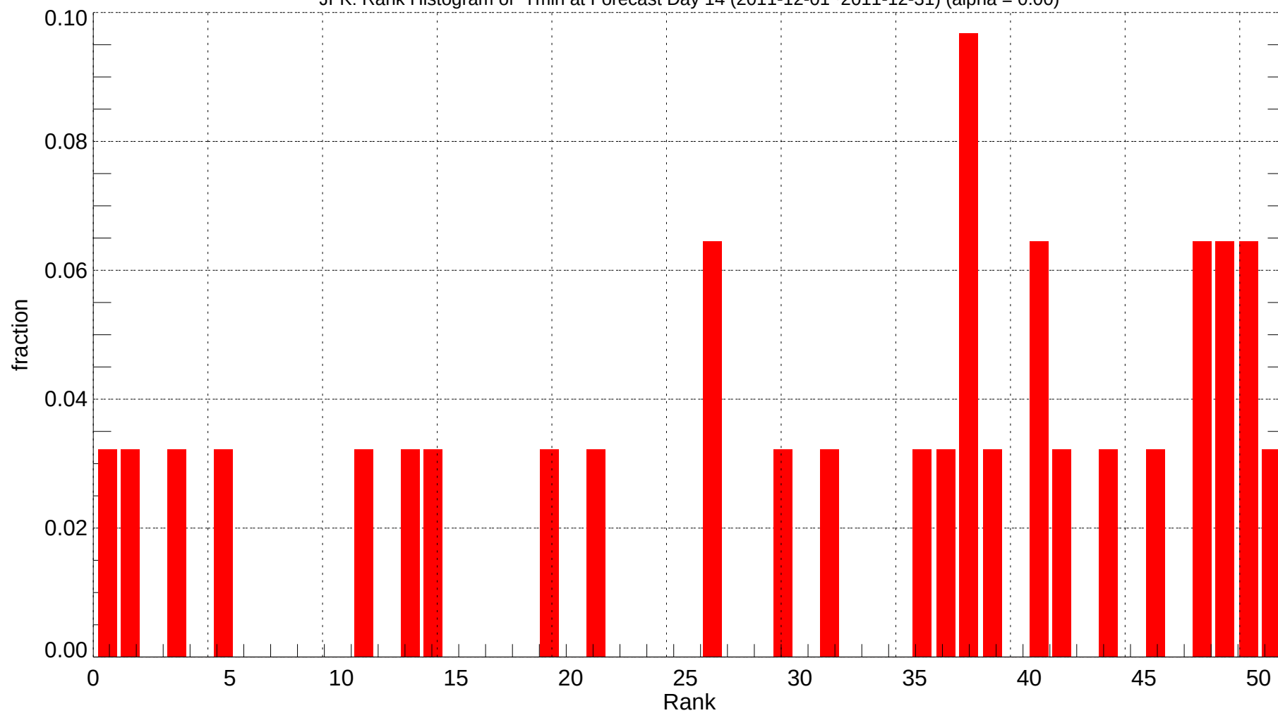
JFK: Rank Histogram of Tmin at Forecast Day 14 (2011-12-01~2011-12-31) (alpha = 0.00)
