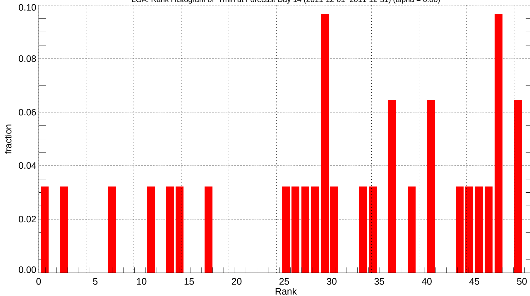
LGA: Rank Histogram of Tmin at Forecast Day 14 (2011-12-01~2011-12-31) (alpha = 0.00)
