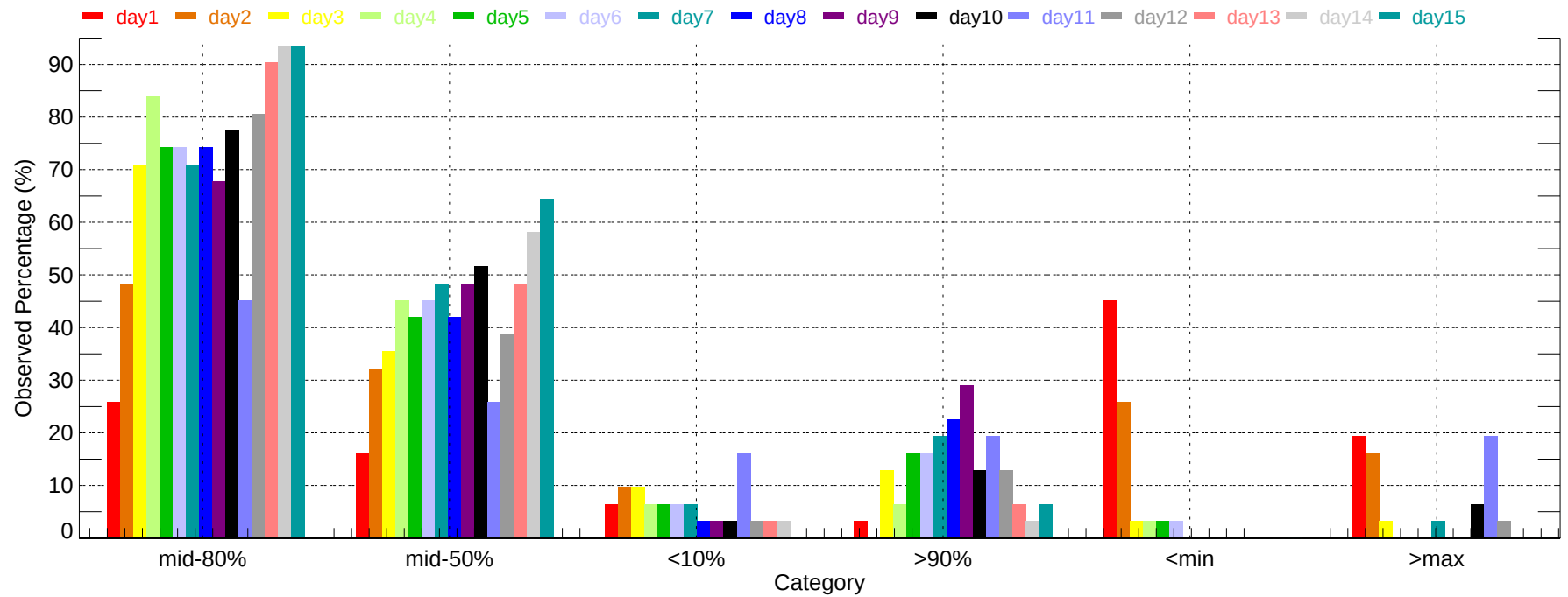
Observed Percentage of Ensembles - IPT: Max Temperature (2011-12-01~2011-12-31)
