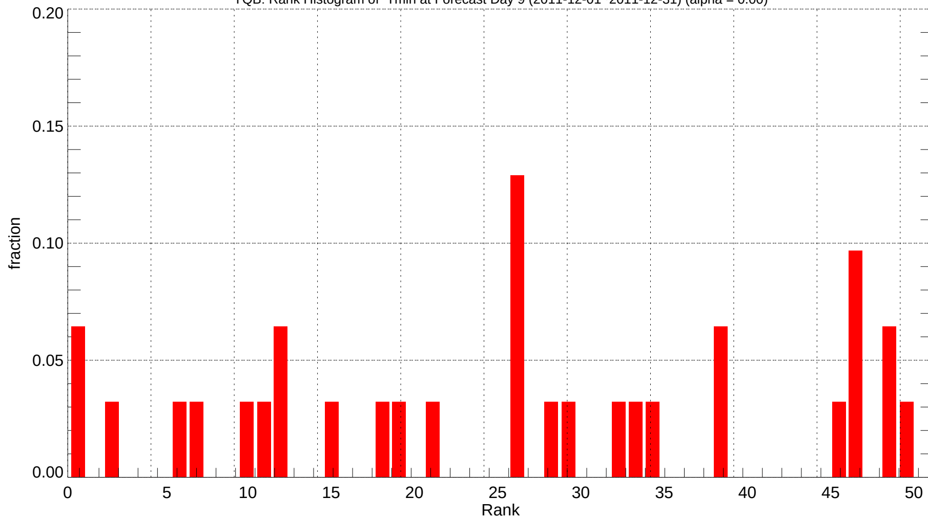
YQB: Rank Histogram of Tmin at Forecast Day 9 (2011-12-01~2011-12-31) (alpha = 0.00)
