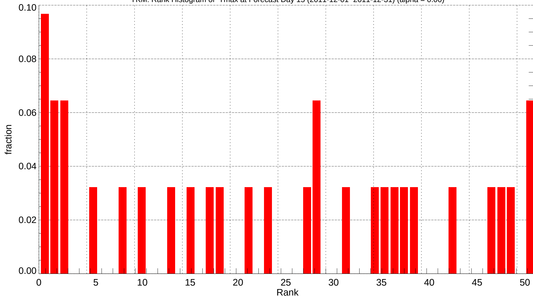
YKM: Rank Histogram of Tmax at Forecast Day 15 (2011-12-01~2011-12-31) (alpha = 0.00)
