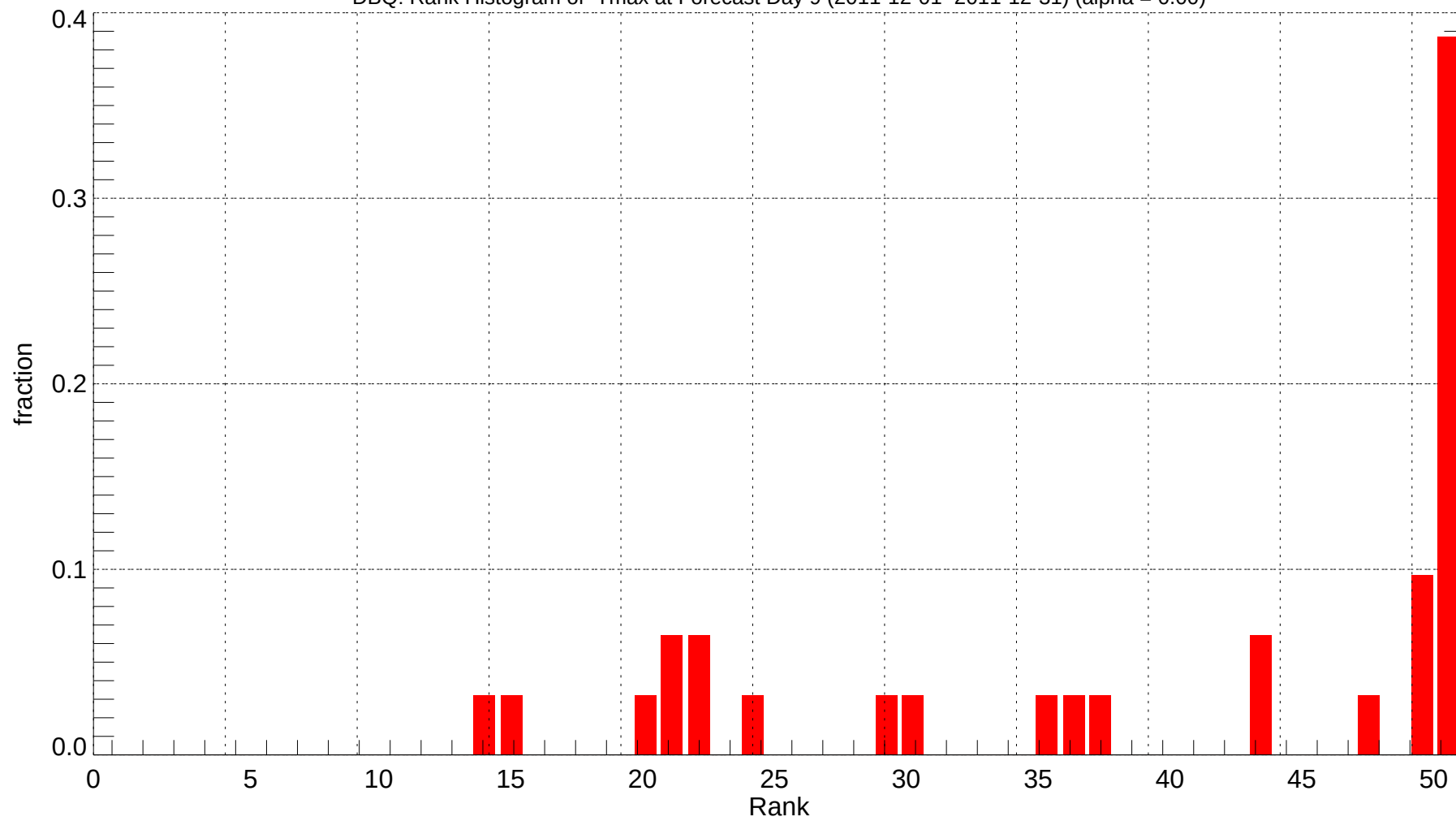
DBQ: Rank Histogram of Tmax at Forecast Day 9 (2011-12-01~2011-12-31) (alpha = 0.00)
