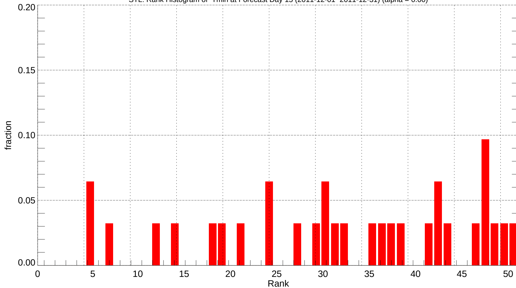
STL: Rank Histogram of Tmin at Forecast Day 15 (2011-12-01~2011-12-31) (alpha = 0.00)
