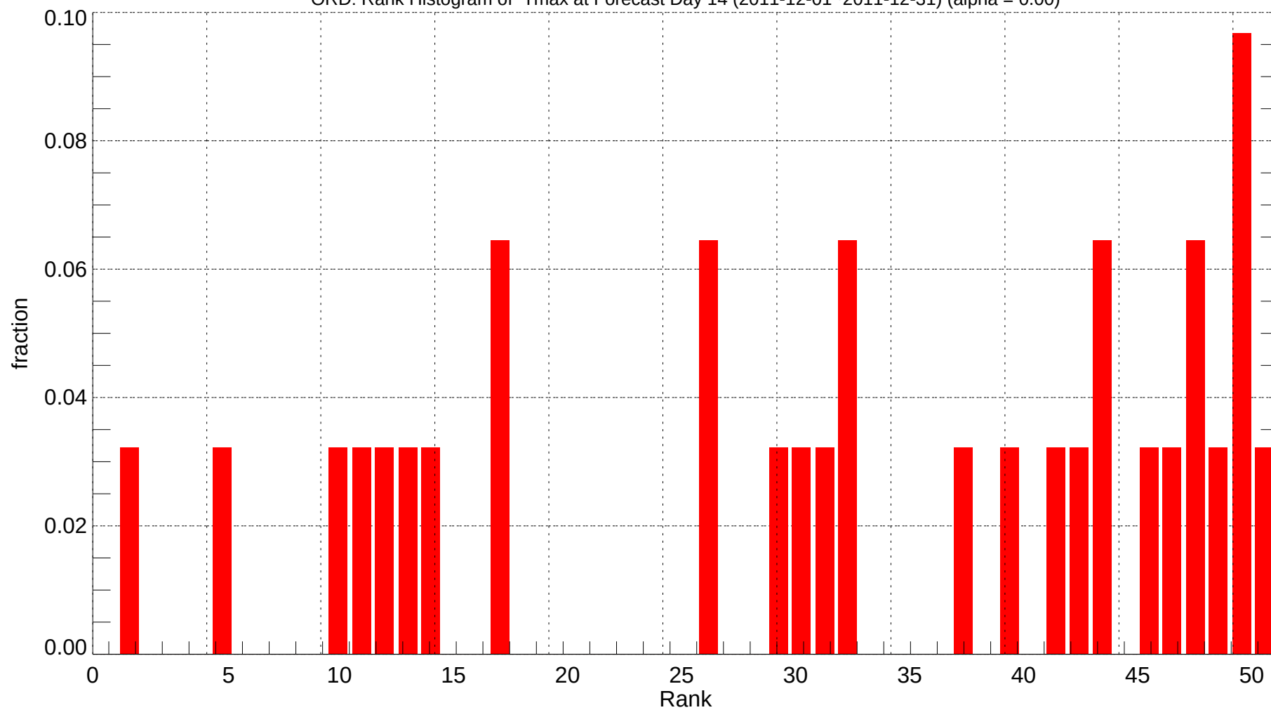
ORD: Rank Histogram of Tmax at Forecast Day 14 (2011-12-01~2011-12-31) (alpha = 0.00)
