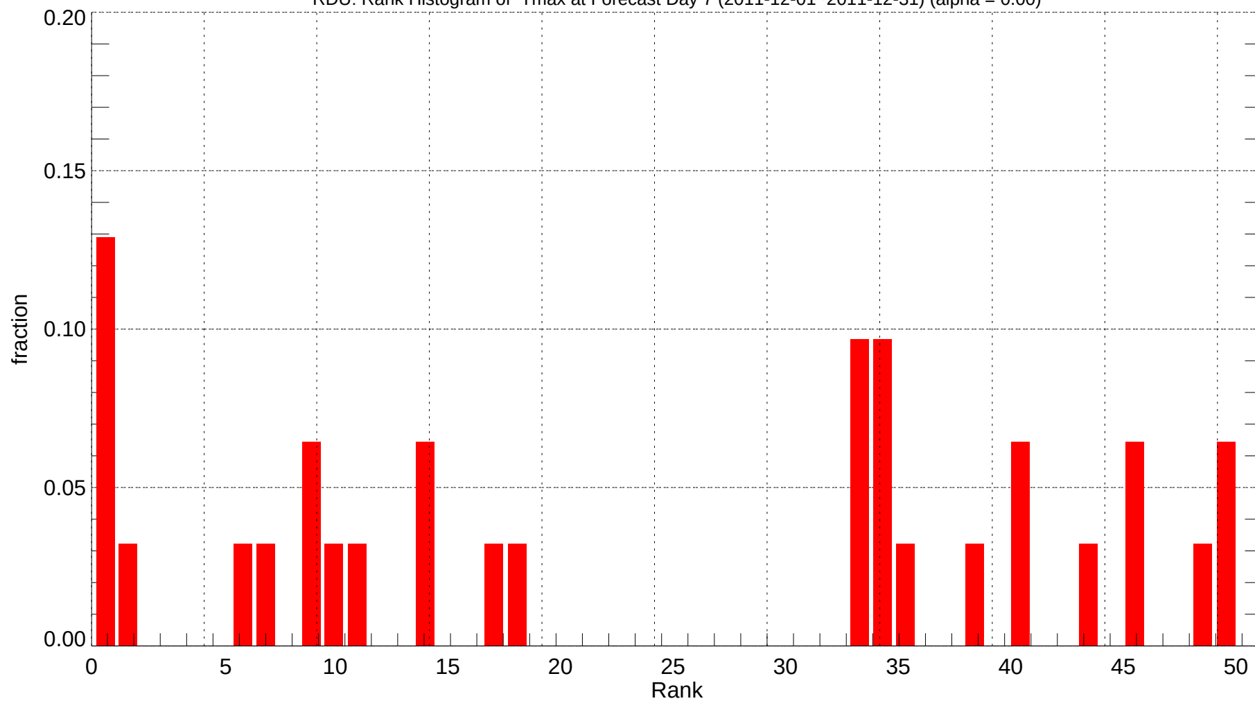
RDU: Rank Histogram of Tmax at Forecast Day 7 (2011-12-01~2011-12-31) (alpha = 0.00)
