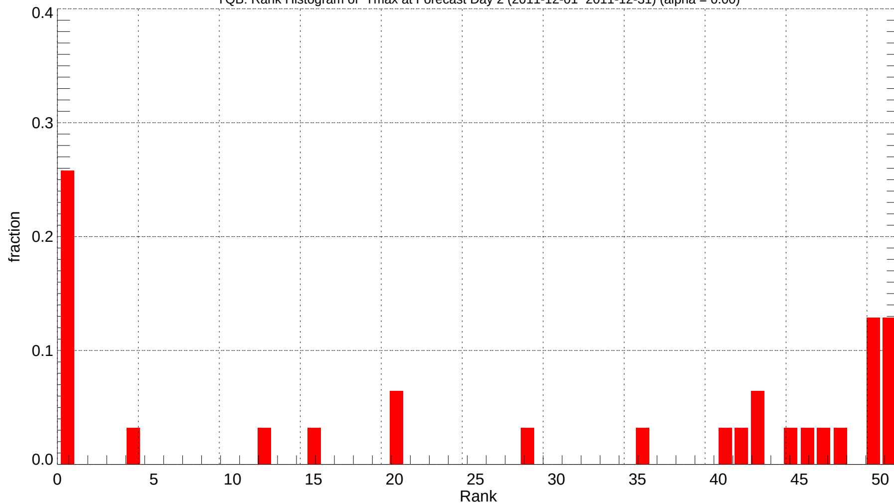
YQB: Rank Histogram of Tmax at Forecast Day 2 (2011-12-01~2011-12-31) (alpha = 0.00)
