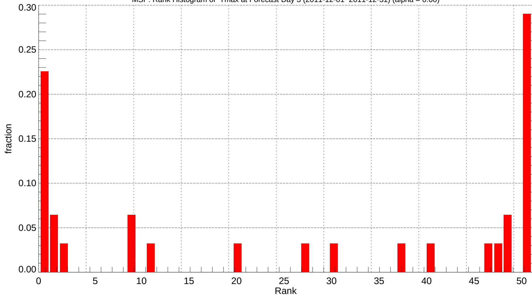
MSP: Rank Histogram of Tmax at Forecast Day 3 (2011-12-01~2011-12-31) (alpha = 0.00)
