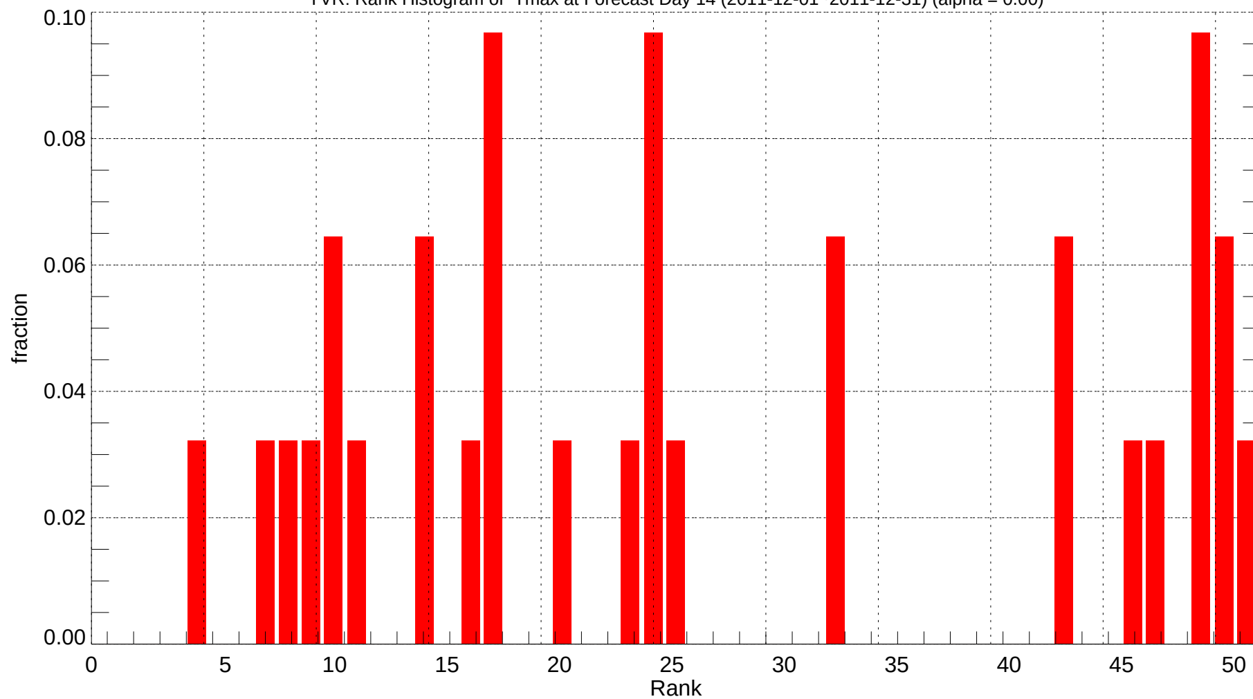
YVR: Rank Histogram of Tmax at Forecast Day 14 (2011-12-01~2011-12-31) (alpha = 0.00)
