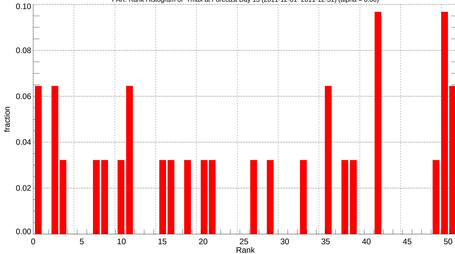
FAR: Rank Histogram of Tmax at Forecast Day 13 (2011-12-01~2011-12-31) (alpha = 0.00)
