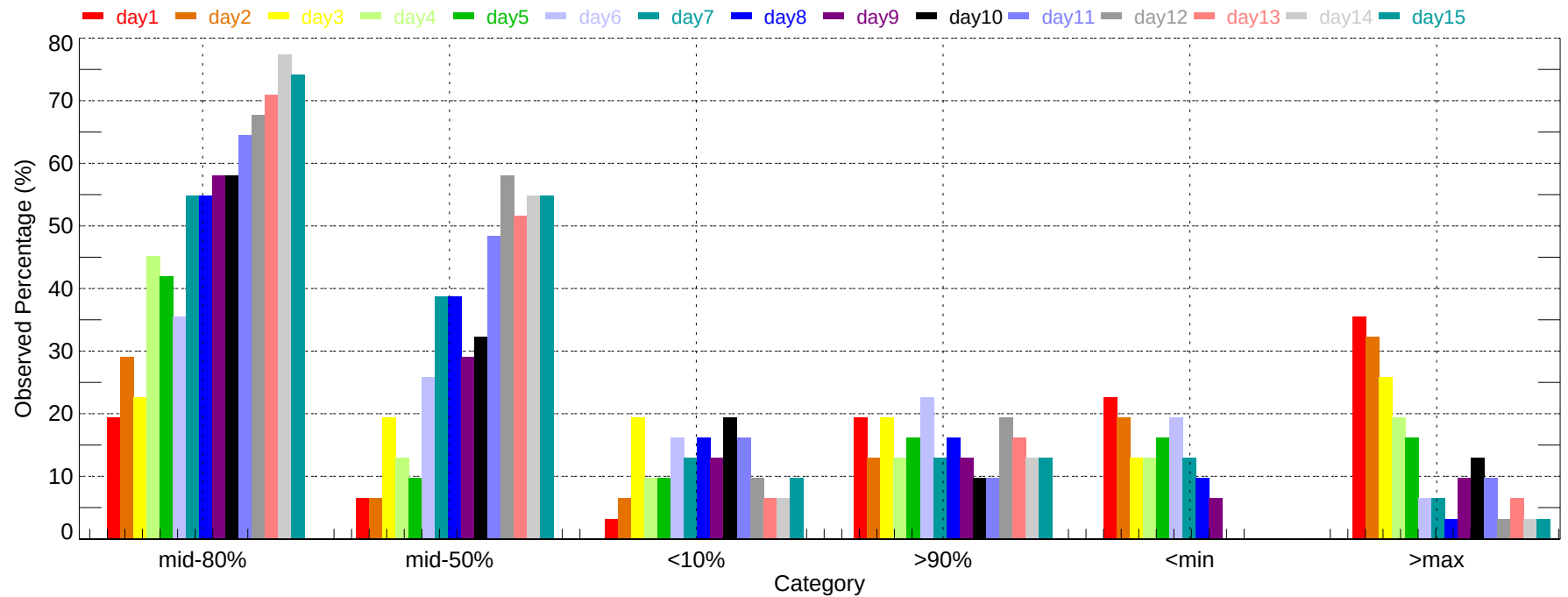
Observed Percentage of Ensembles - MHT: Min Temperature (2011-12-01~2011-12-31)
