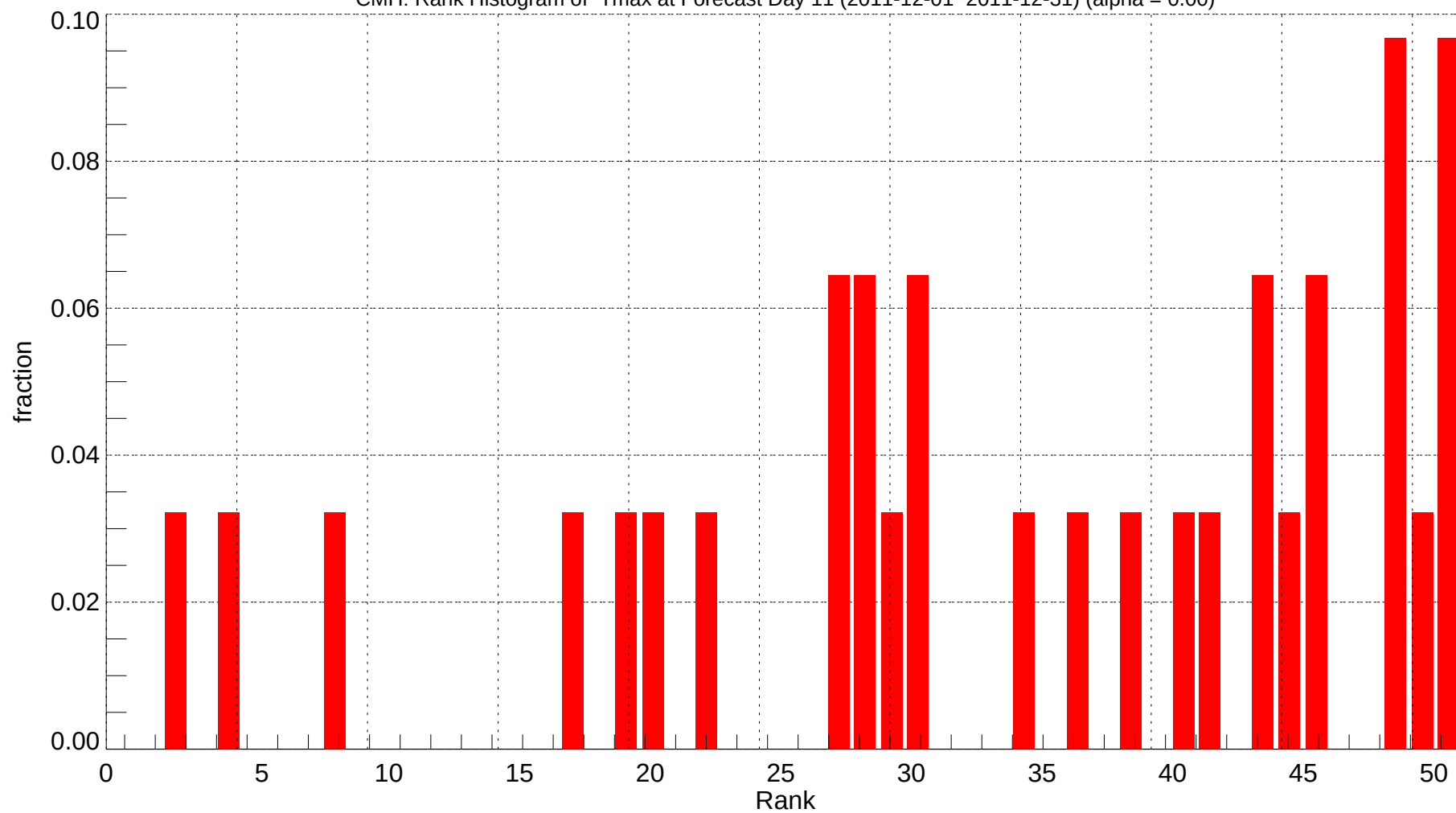
CMH: Rank Histogram of Tmax at Forecast Day 11 (2011-12-01~2011-12-31) (alpha = 0.00)
