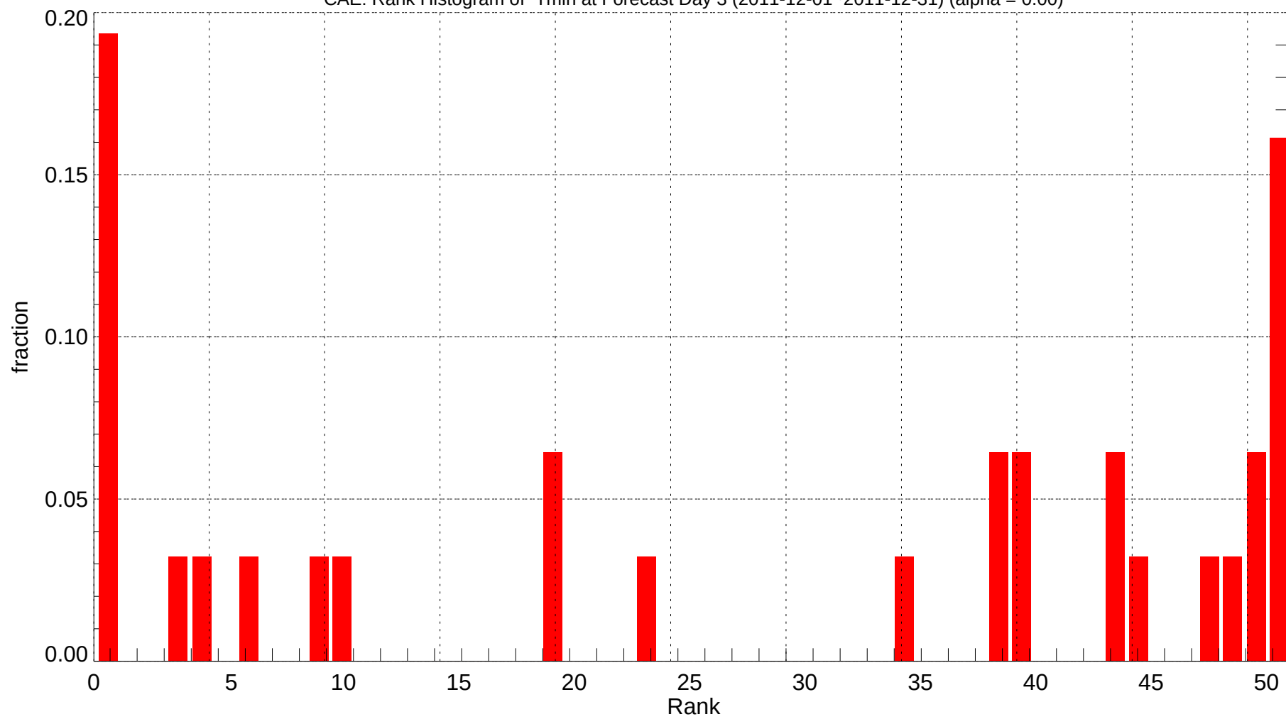
CAE: Rank Histogram of Tmin at Forecast Day 3 (2011-12-01~2011-12-31) (alpha = 0.00)
