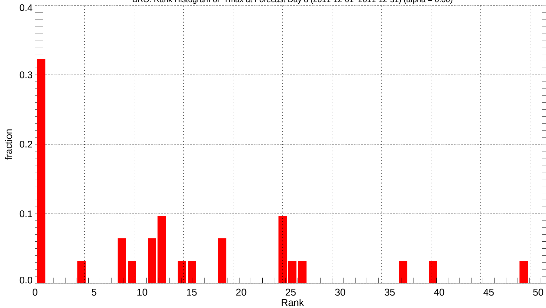
BRO: Rank Histogram of Tmax at Forecast Day 8 (2011-12-01~2011-12-31) (alpha = 0.00)
