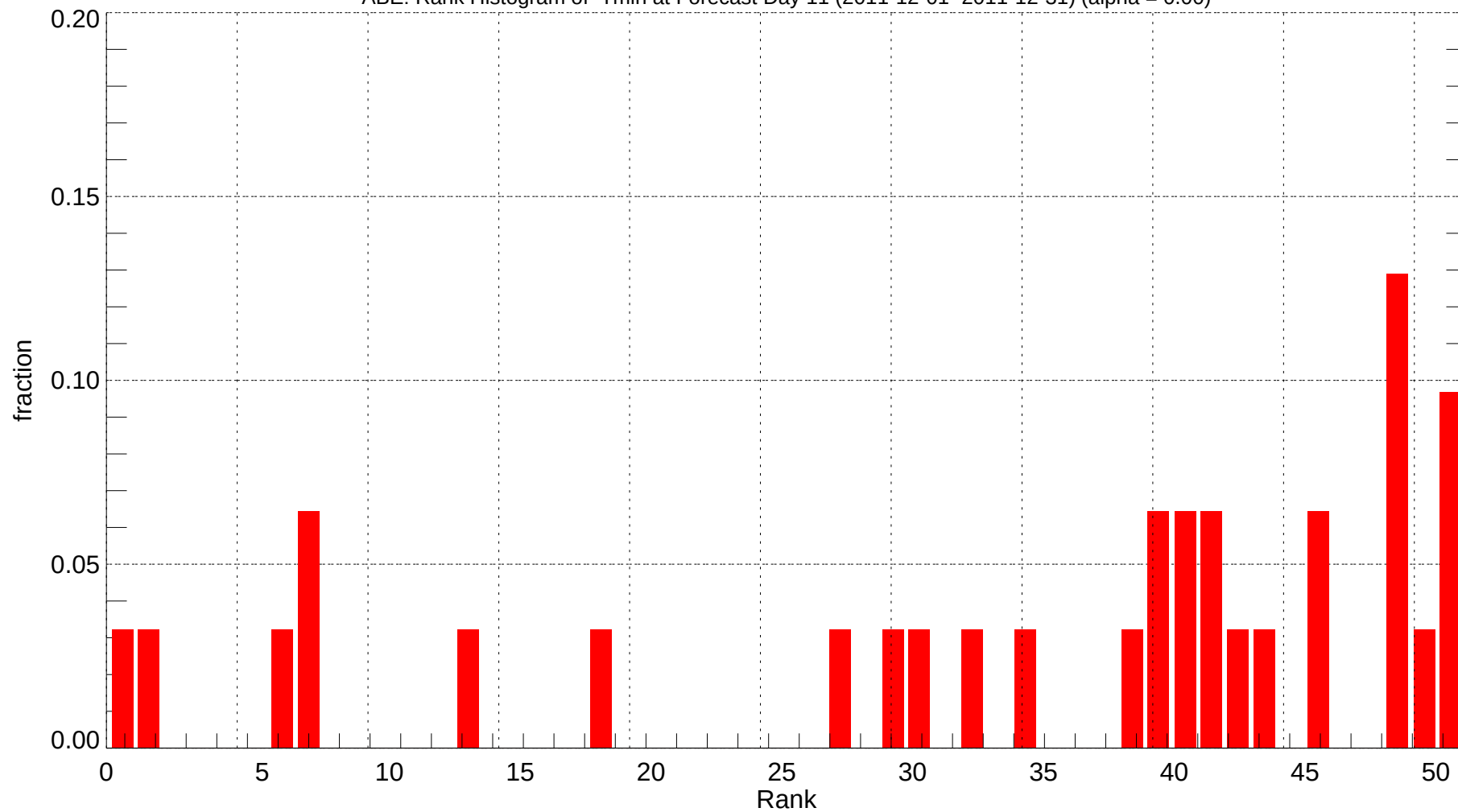
ABE: Rank Histogram of Tmin at Forecast Day 11 (2011-12-01~2011-12-31) (alpha = 0.00)
