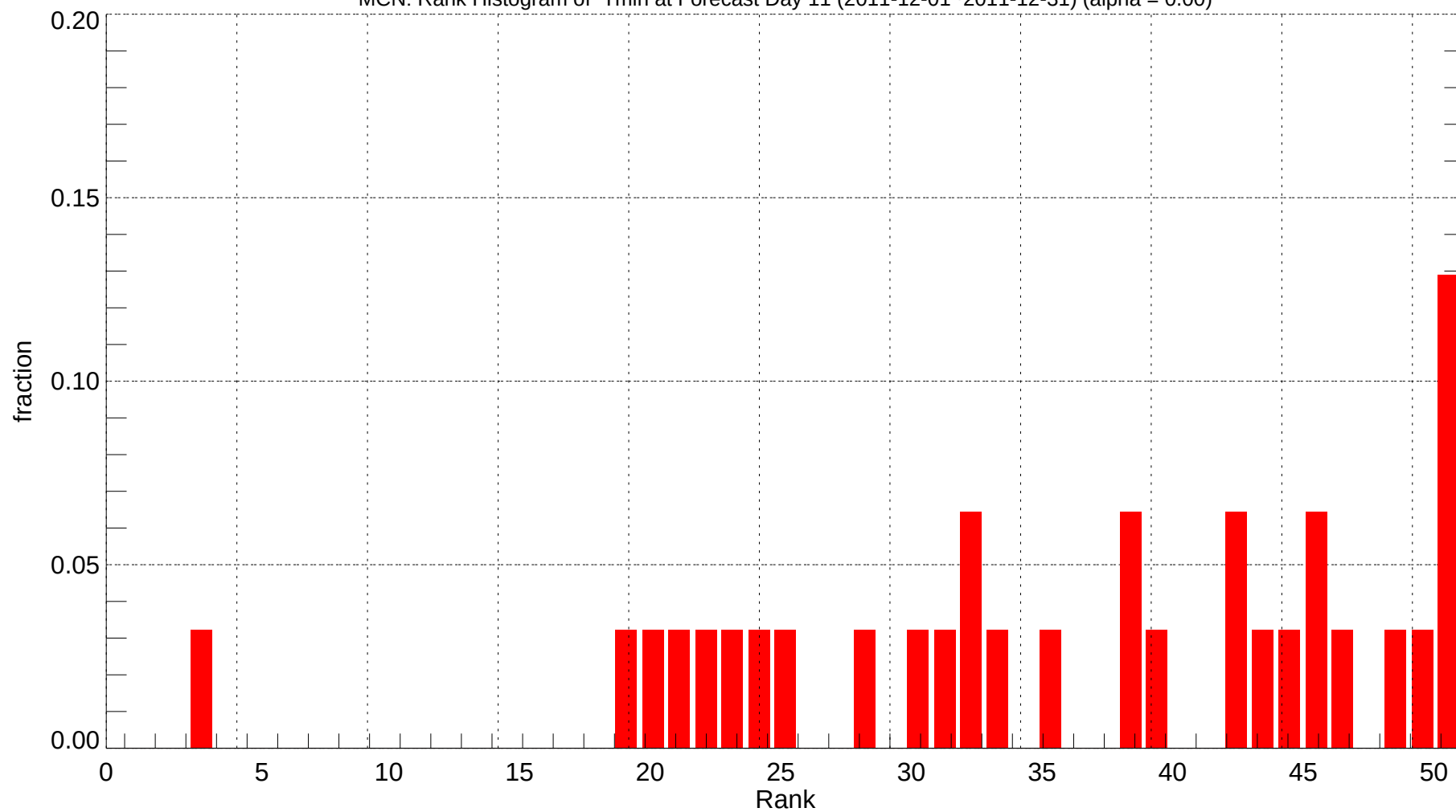
MCN: Rank Histogram of Tmin at Forecast Day 11 (2011-12-01~2011-12-31) (alpha = 0.00)
