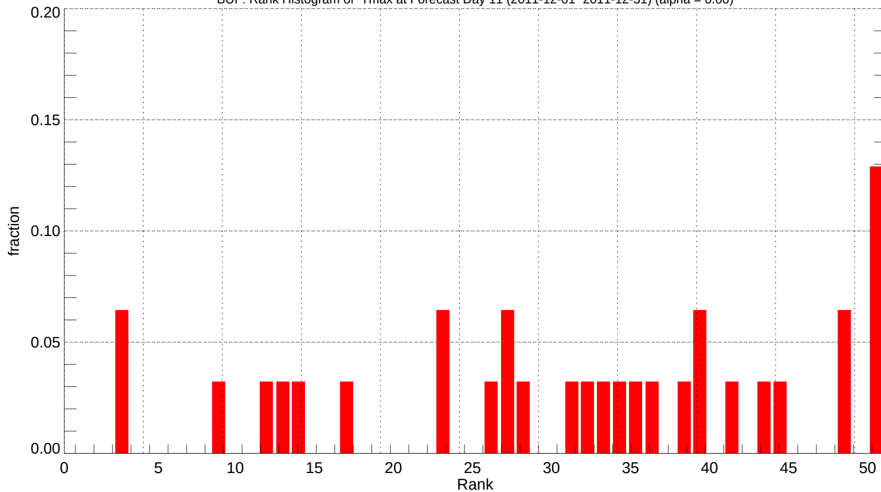
BUF: Rank Histogram of Tmax at Forecast Day 11 (2011-12-01~2011-12-31) (alpha = 0.00)
