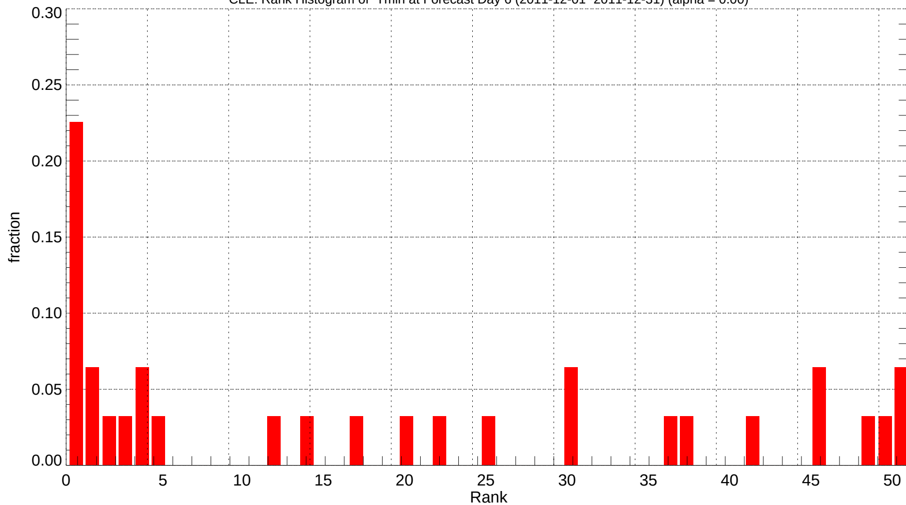
CLE: Rank Histogram of Tmin at Forecast Day 6 (2011-12-01~2011-12-31) (alpha = 0.00)
