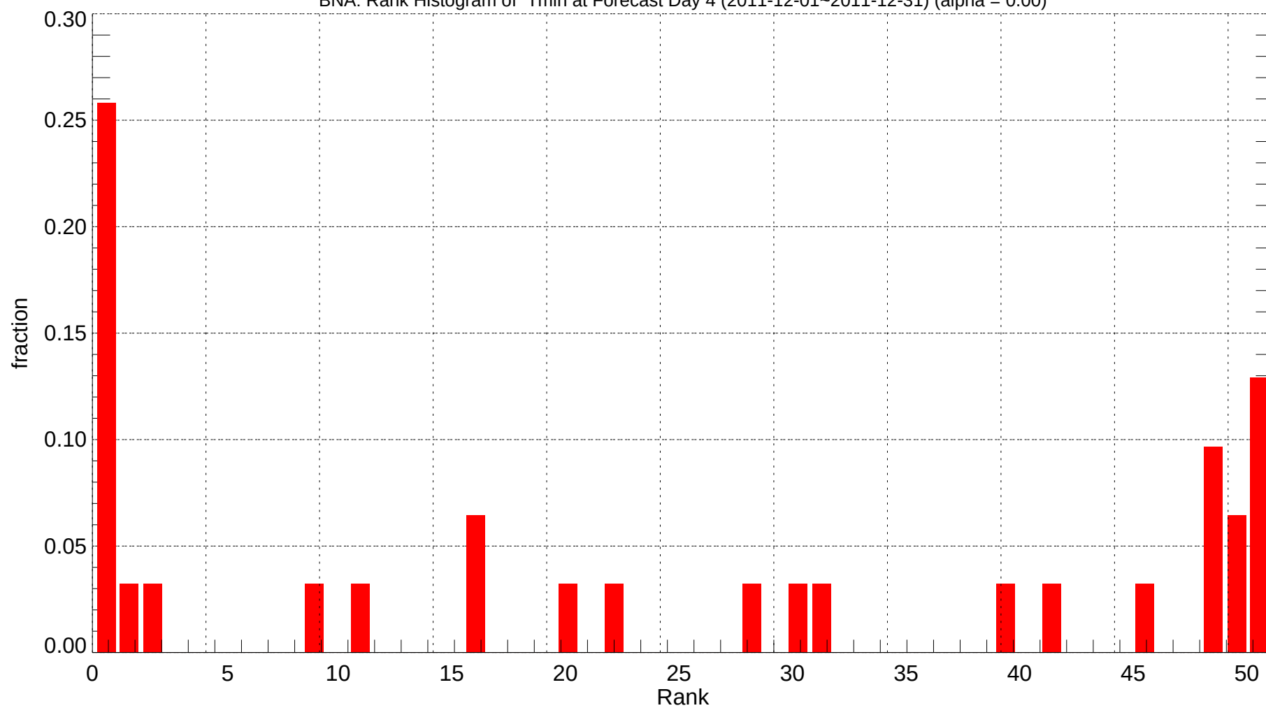
BNA: Rank Histogram of Tmin at Forecast Day 4 (2011-12-01~2011-12-31) (alpha = 0.00)
