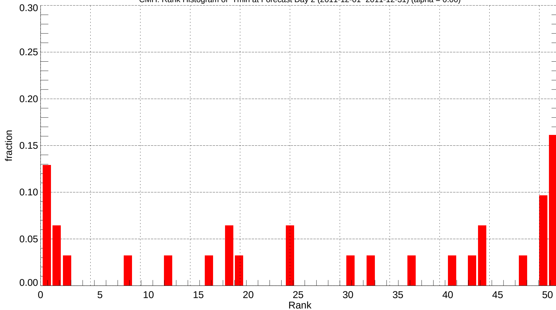
CMH: Rank Histogram of Tmin at Forecast Day 2 (2011-12-01~2011-12-31) (alpha = 0.00)
