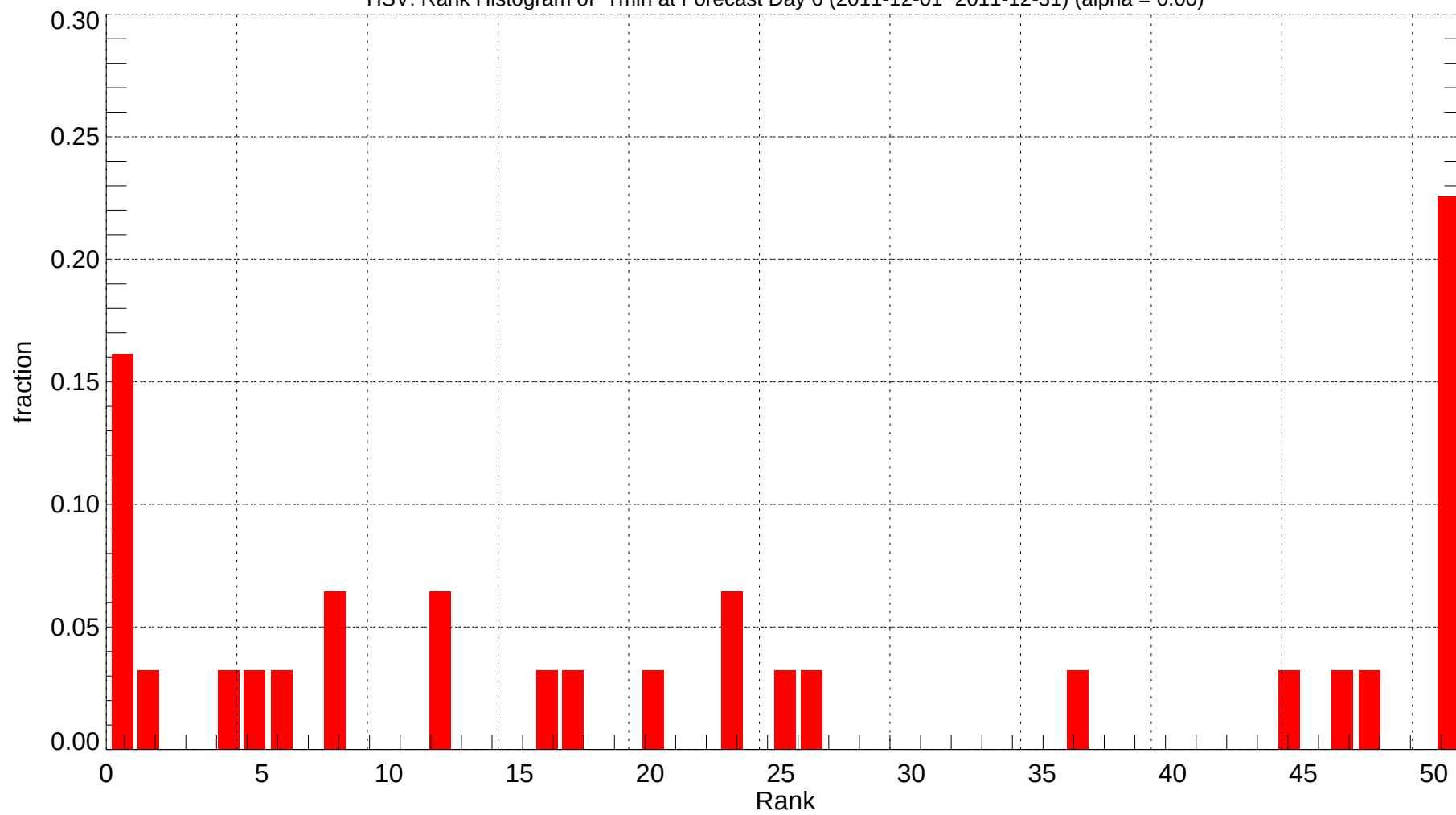
HSV: Rank Histogram of Tmin at Forecast Day 6 (2011-12-01~2011-12-31) (alpha = 0.00)
