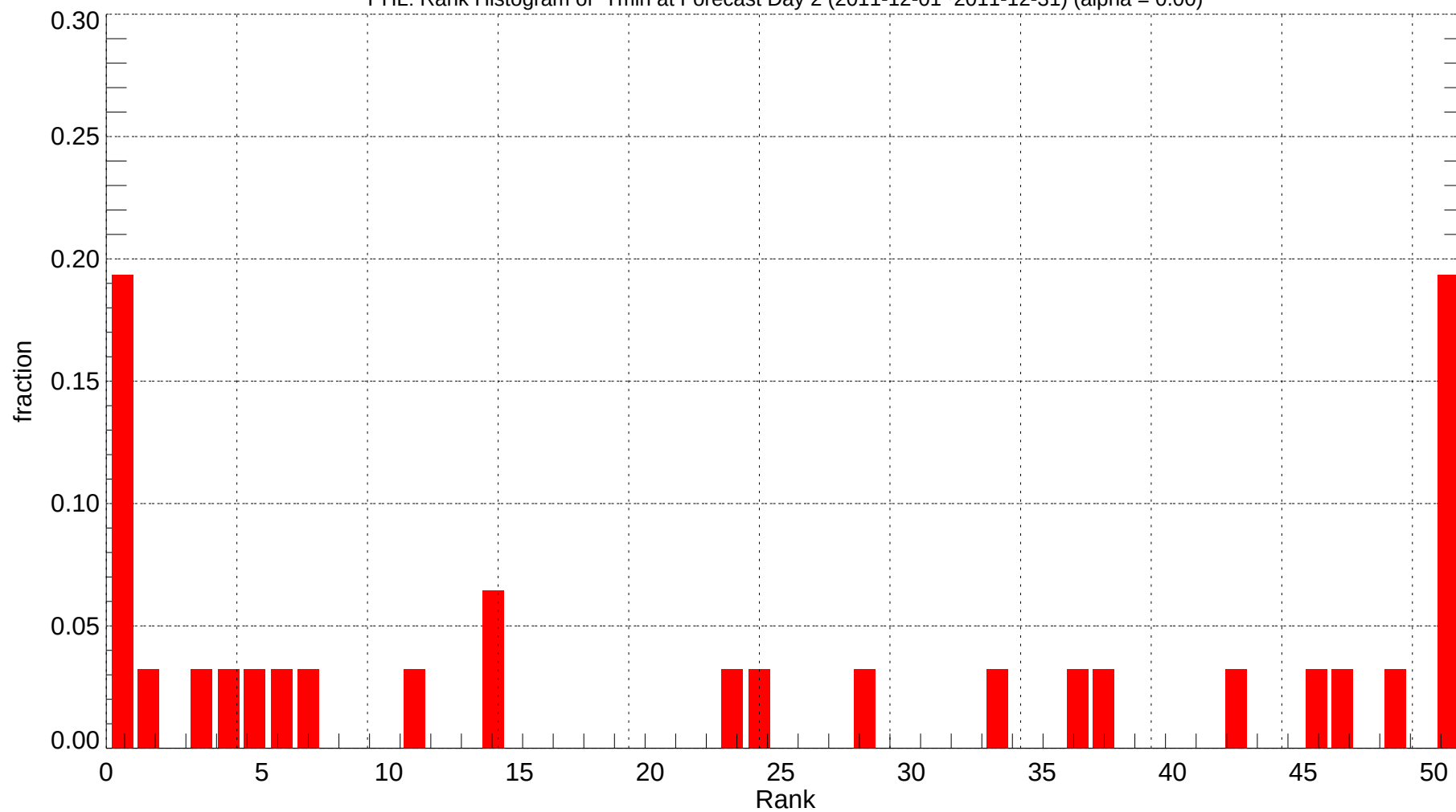
PHL: Rank Histogram of Tmin at Forecast Day 2 (2011-12-01~2011-12-31) (alpha = 0.00)
