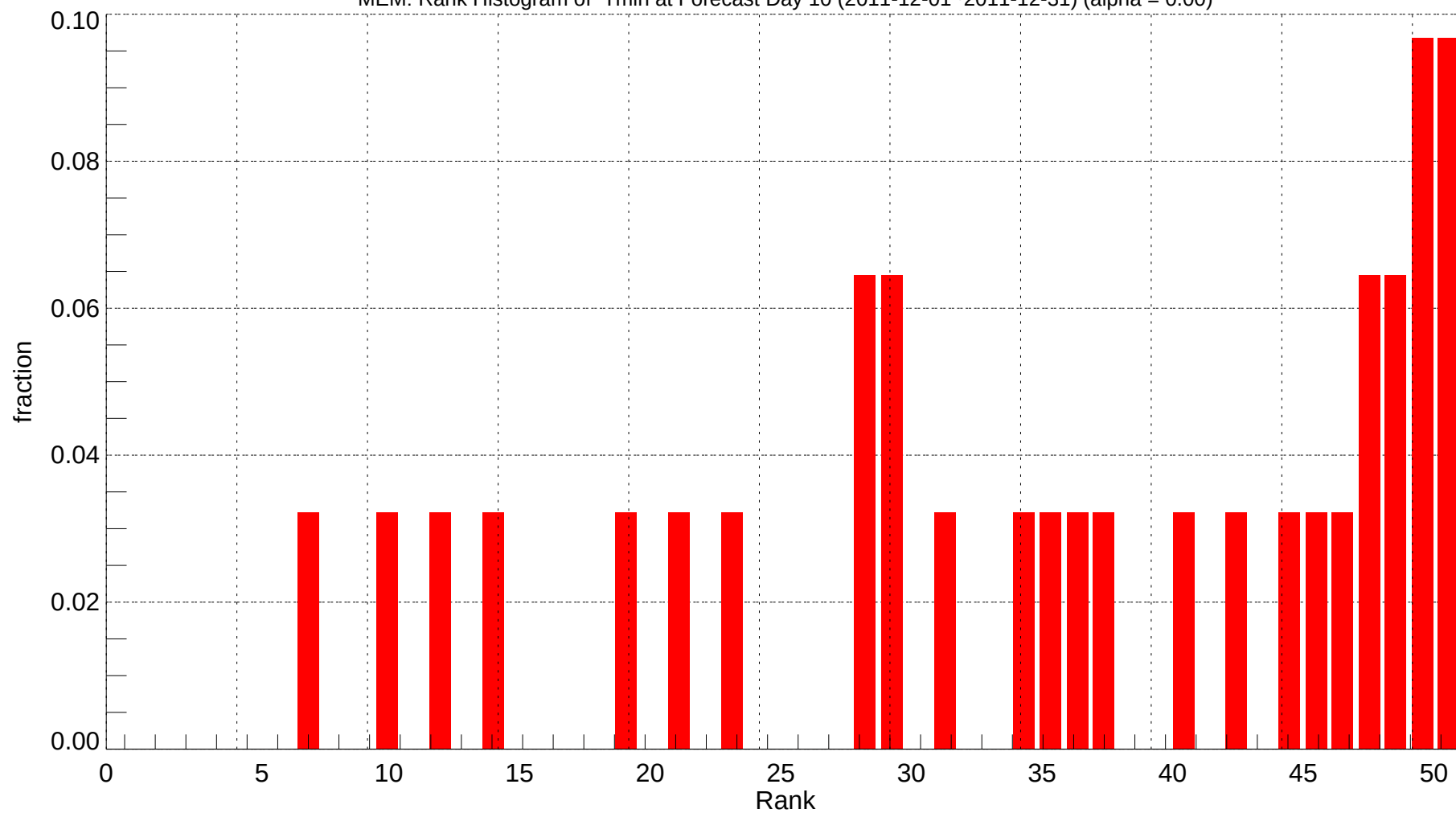
MEM: Rank Histogram of Tmin at Forecast Day 10 (2011-12-01~2011-12-31) (alpha = 0.00)
