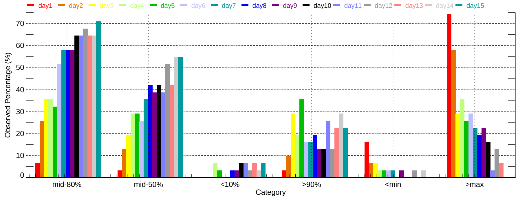
Observed Percentage of Ensembles - COU: Min Temperature (2011-12-01~2011-12-31)
