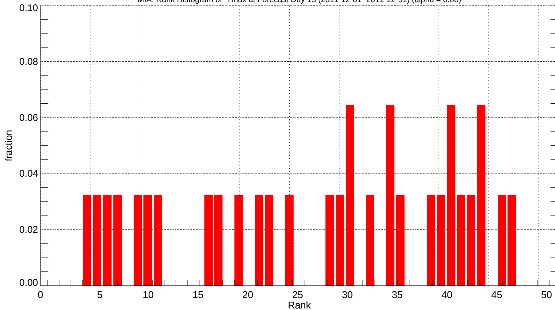
MIA: Rank Histogram of Tmax at Forecast Day 13 (2011-12-01~2011-12-31) (alpha = 0.00)
