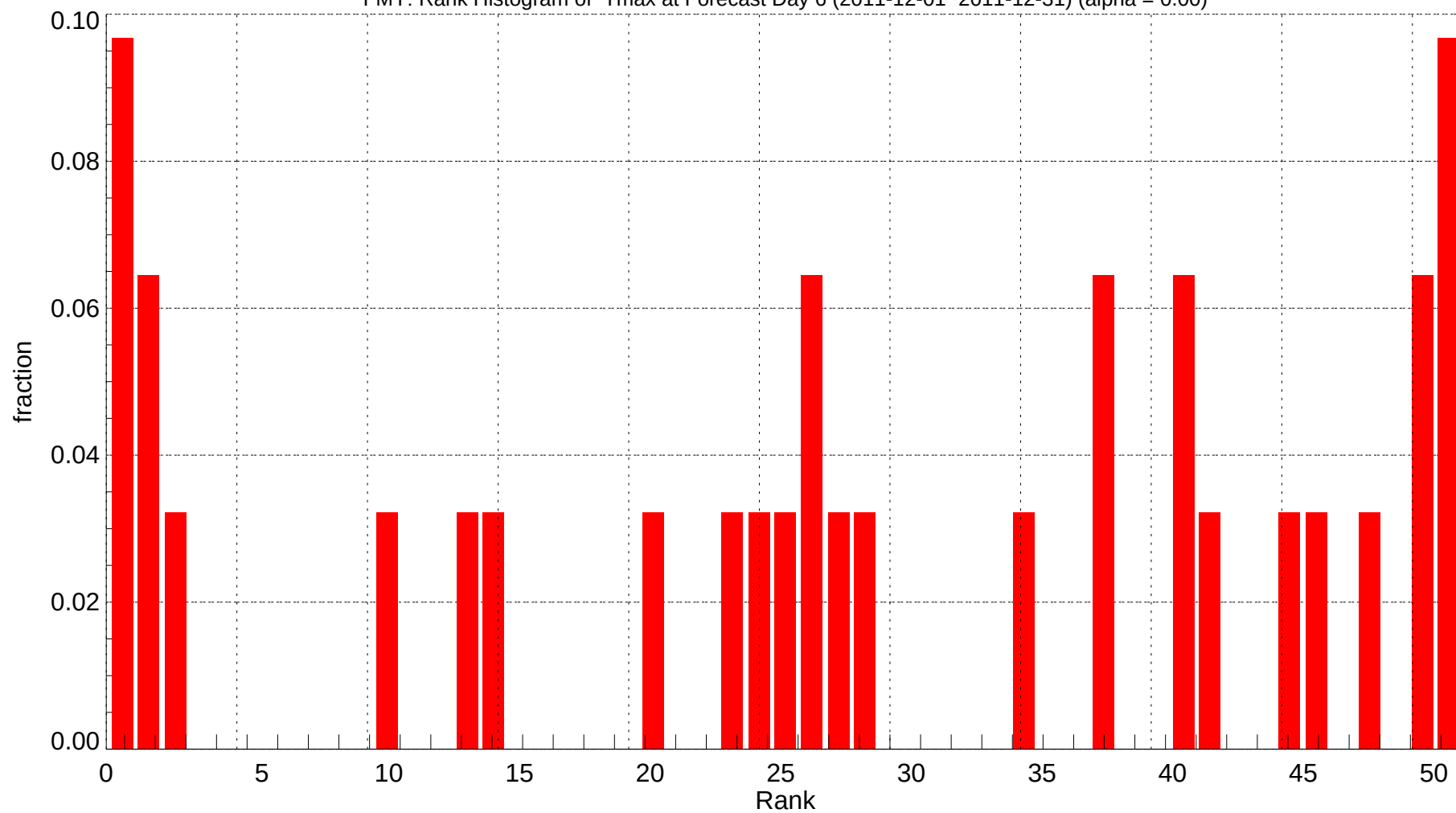
FMY: Rank Histogram of Tmax at Forecast Day 6 (2011-12-01~2011-12-31) (alpha = 0.00)
