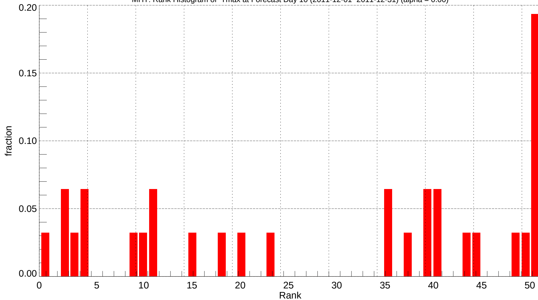
MHT: Rank Histogram of Tmax at Forecast Day 10 (2011-12-01~2011-12-31) (alpha = 0.00)
