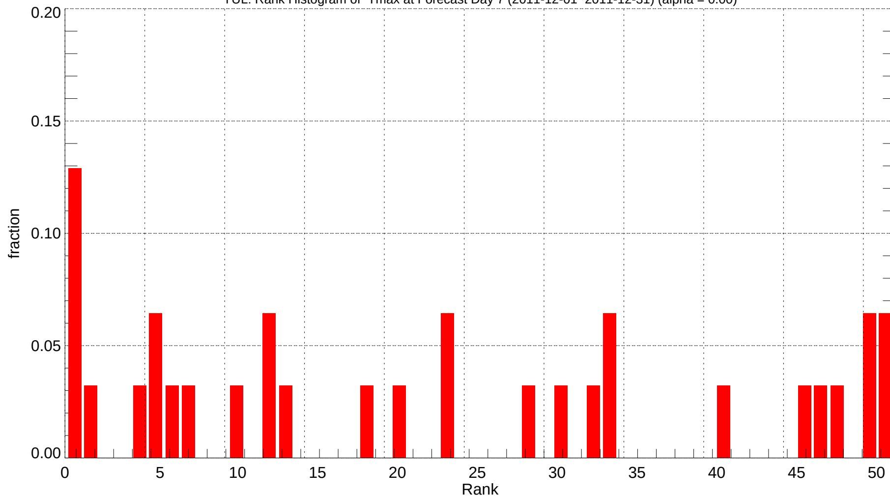
YUL: Rank Histogram of Tmax at Forecast Day 7 (2011-12-01~2011-12-31) (alpha = 0.00)
