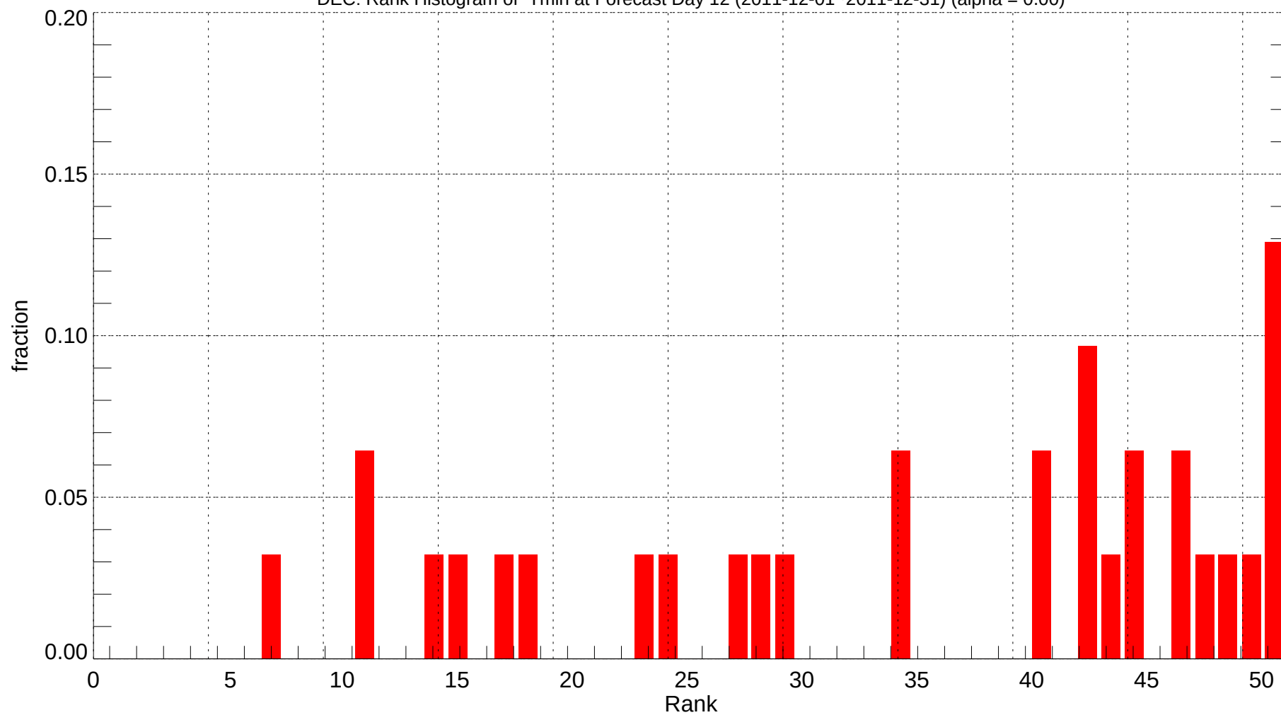
DEC: Rank Histogram of Tmin at Forecast Day 12 (2011-12-01~2011-12-31) (alpha = 0.00)
