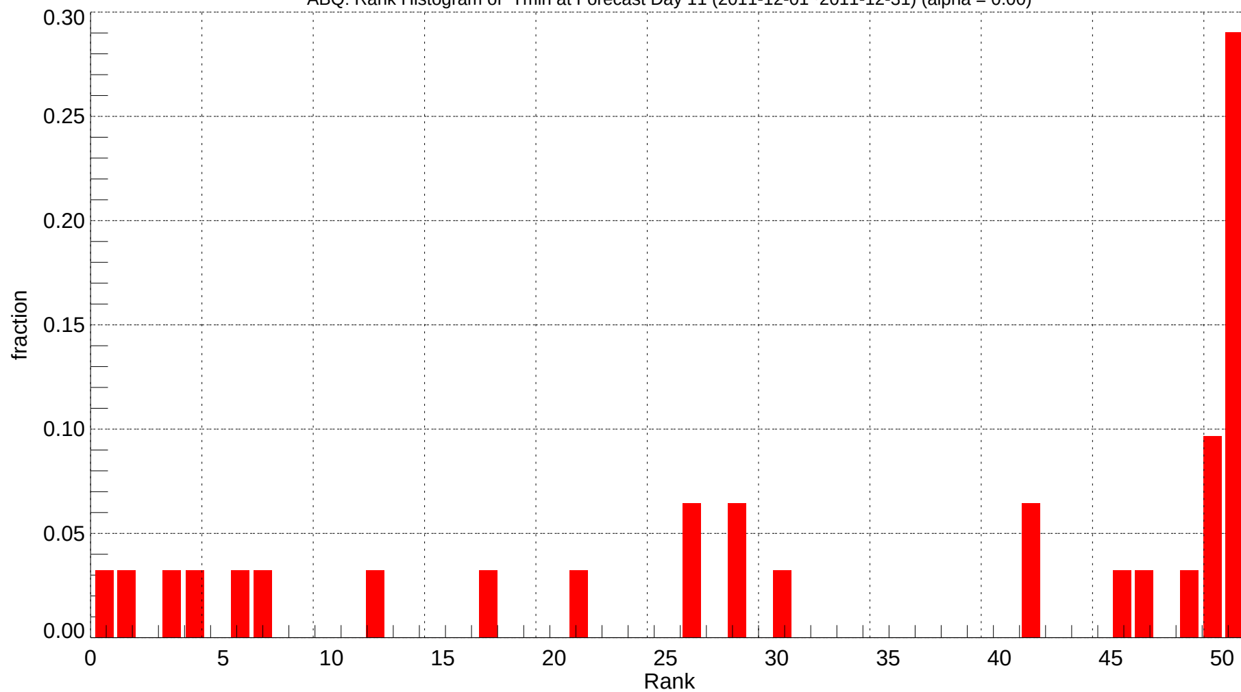
ABQ: Rank Histogram of Tmin at Forecast Day 11 (2011-12-01~2011-12-31) (alpha = 0.00)
