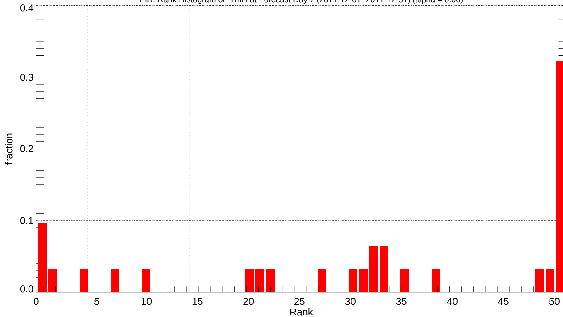
PIR: Rank Histogram of Tmin at Forecast Day 7 (2011-12-01~2011-12-31) (alpha = 0.00)
