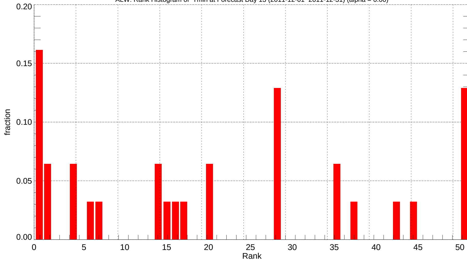
ALW: Rank Histogram of Tmin at Forecast Day 13 (2011-12-01~2011-12-31) (alpha = 0.00)
