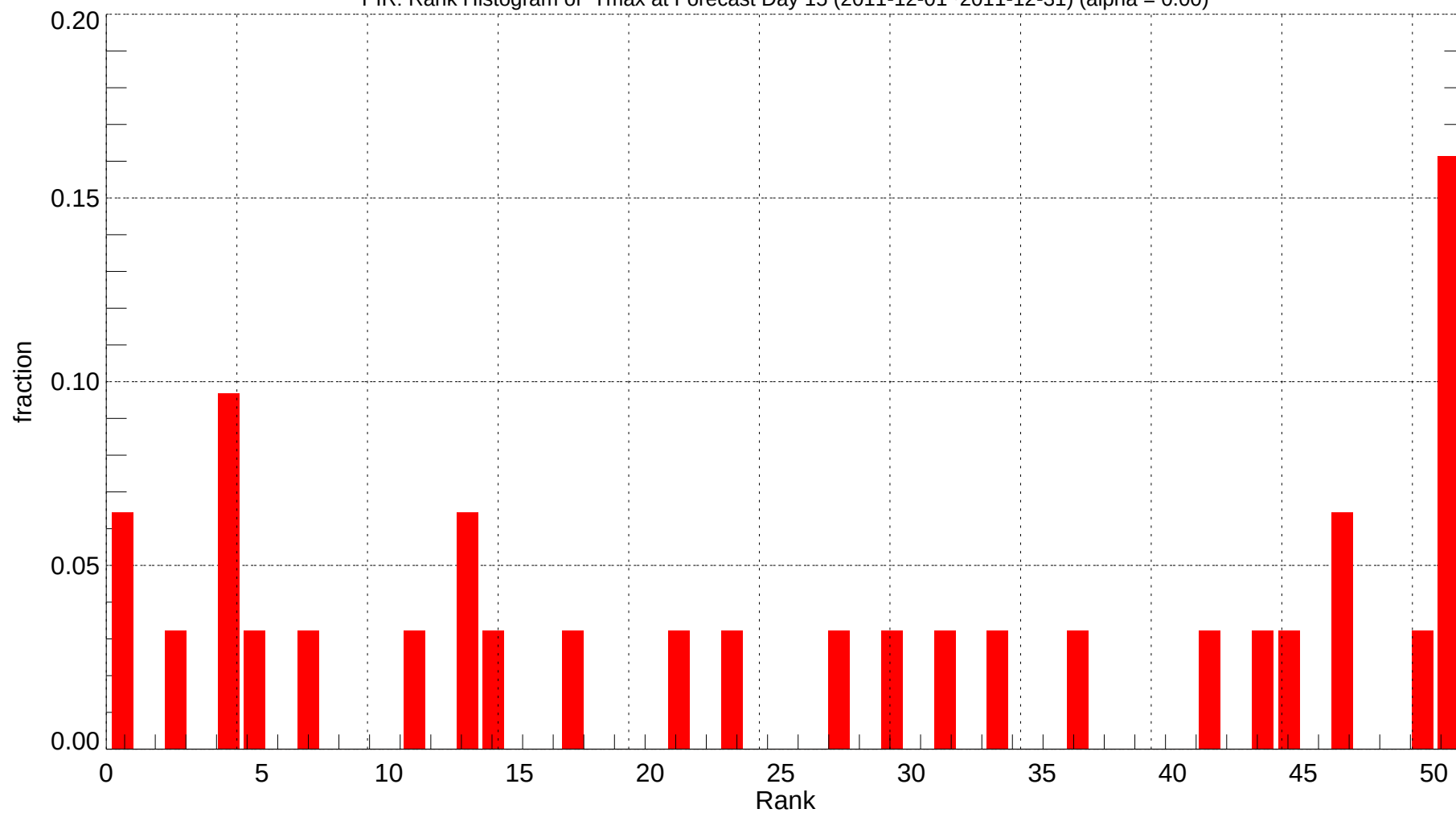
PIR: Rank Histogram of Tmax at Forecast Day 15 (2011-12-01~2011-12-31) (alpha = 0.00)
