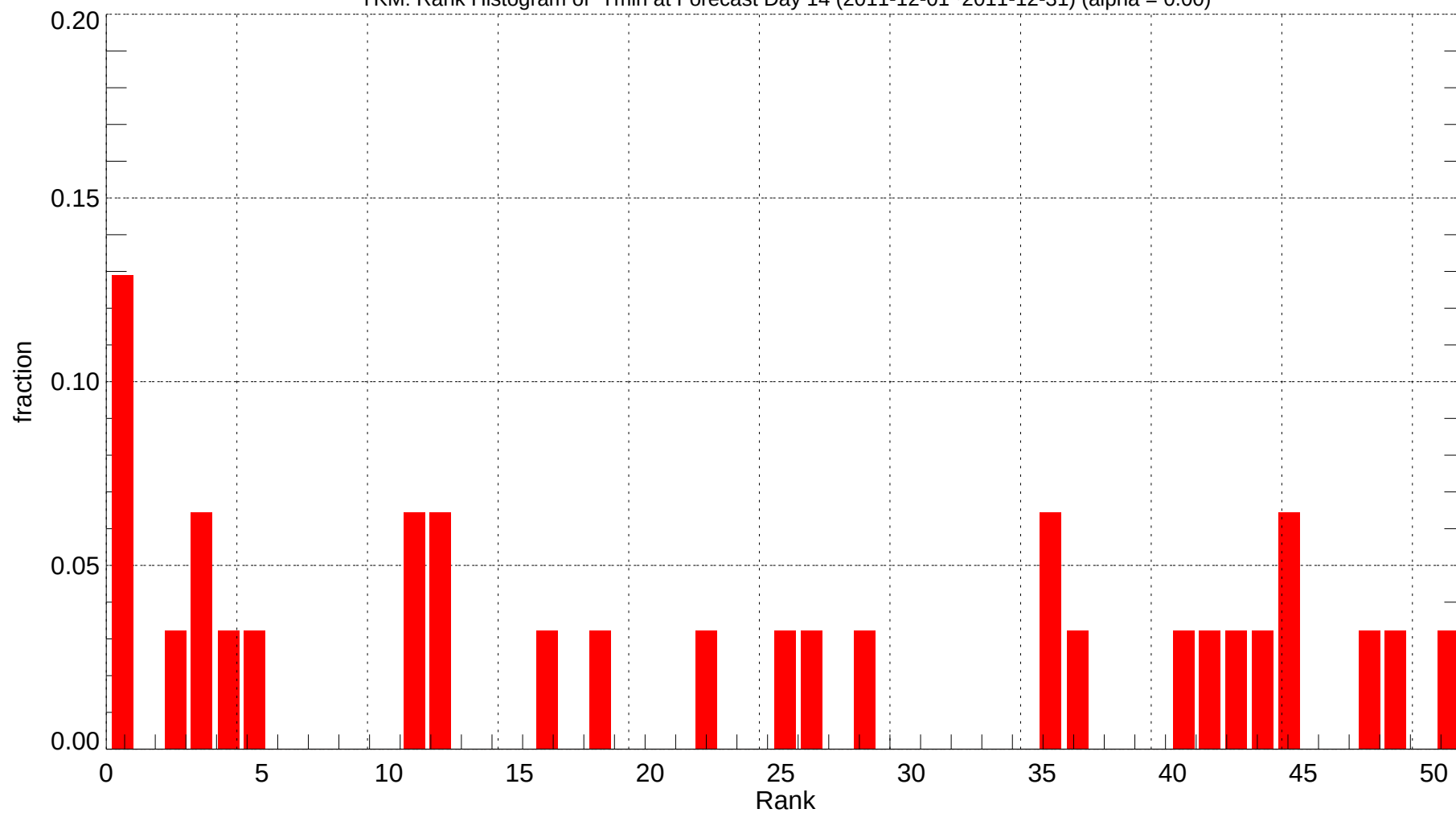
YKM: Rank Histogram of Tmin at Forecast Day 14 (2011-12-01~2011-12-31) (alpha = 0.00)
