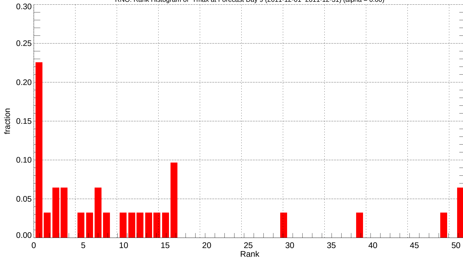
RNO: Rank Histogram of Tmax at Forecast Day 9 (2011-12-01~2011-12-31) (alpha = 0.00)
