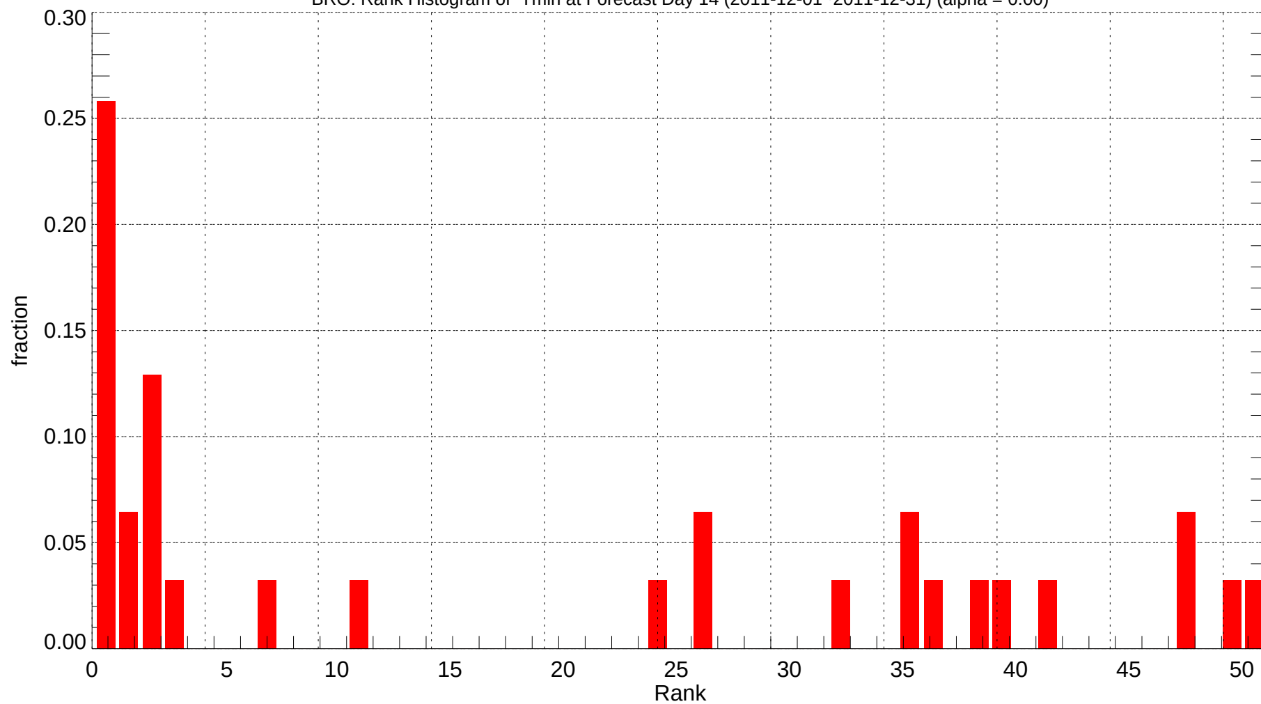
BRO: Rank Histogram of Tmin at Forecast Day 14 (2011-12-01~2011-12-31) (alpha = 0.00)
