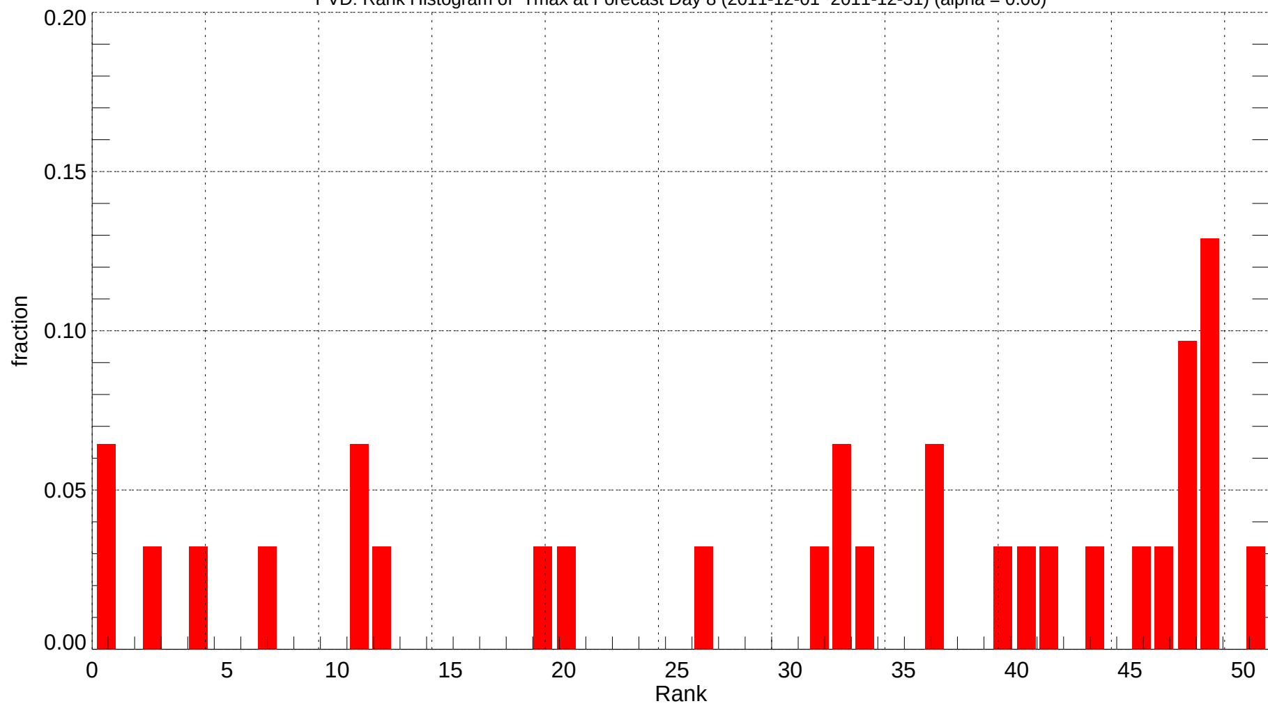
PVD: Rank Histogram of Tmax at Forecast Day 8 (2011-12-01~2011-12-31) (alpha = 0.00)
