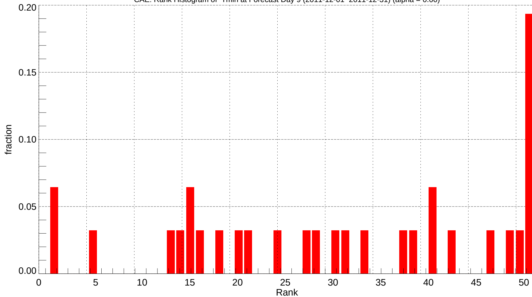
CAE: Rank Histogram of Tmin at Forecast Day 9 (2011-12-01~2011-12-31) (alpha = 0.00)
