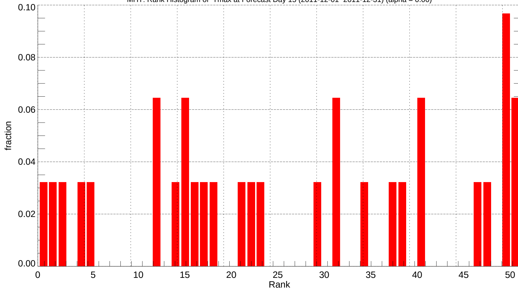
MHT: Rank Histogram of Tmax at Forecast Day 15 (2011-12-01~2011-12-31) (alpha = 0.00)
