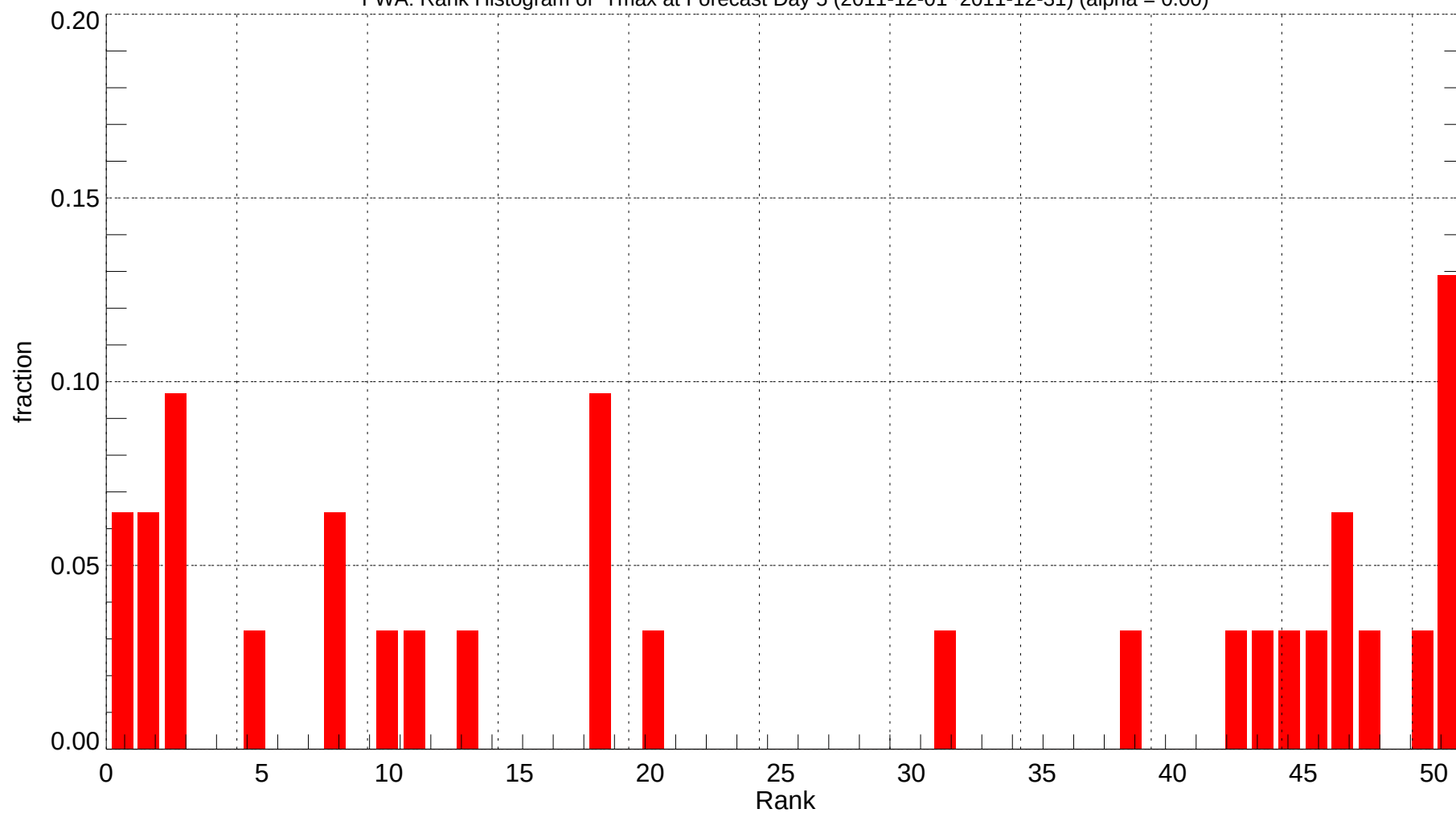
FWA: Rank Histogram of Tmax at Forecast Day 5 (2011-12-01~2011-12-31) (alpha = 0.00)
