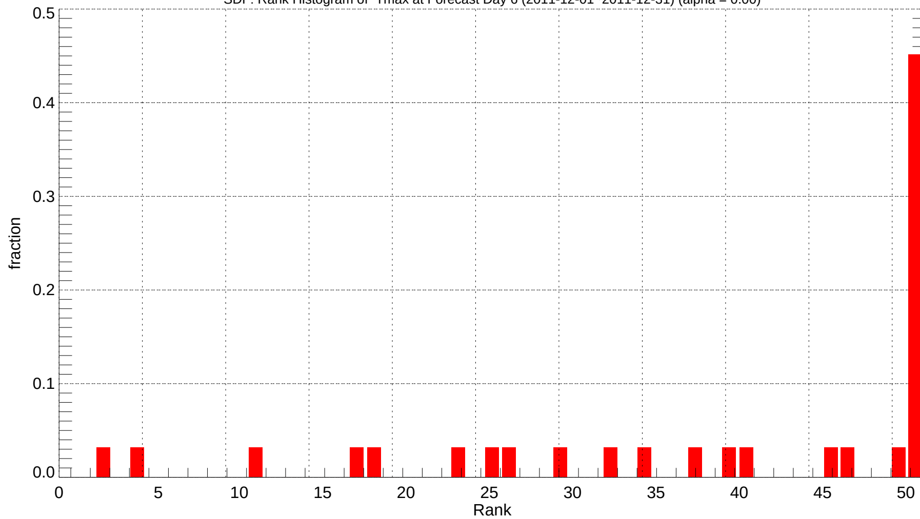
SDF: Rank Histogram of Tmax at Forecast Day 6 (2011-12-01~2011-12-31) (alpha = 0.00)
