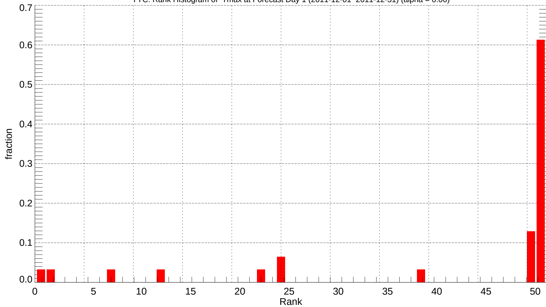
YYC: Rank Histogram of Tmax at Forecast Day 1 (2011-12-01~2011-12-31) (alpha = 0.00)
