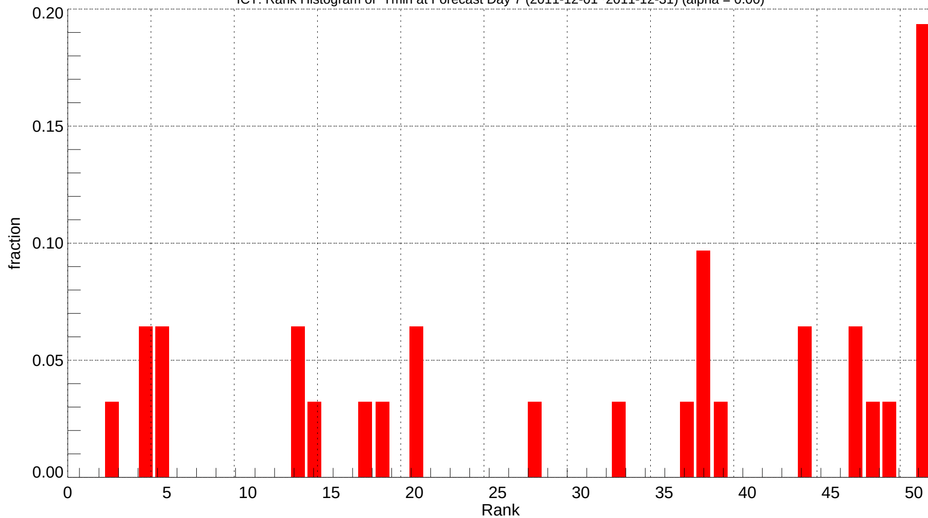
ICT: Rank Histogram of Tmin at Forecast Day 7 (2011-12-01~2011-12-31) (alpha = 0.00)
