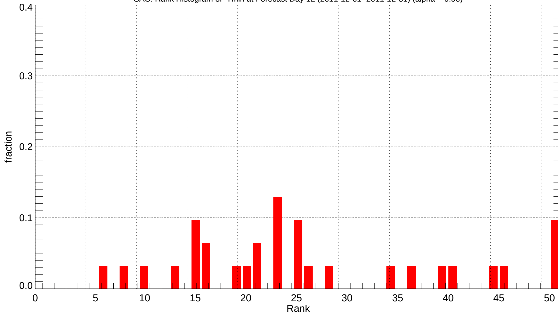
SAC: Rank Histogram of Tmin at Forecast Day 12 (2011-12-01~2011-12-31) (alpha = 0.00)
