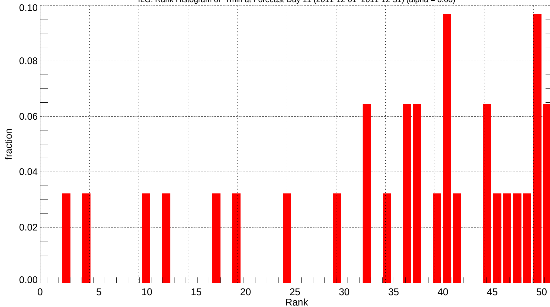
ILG: Rank Histogram of Tmin at Forecast Day 11 (2011-12-01~2011-12-31) (alpha = 0.00)
