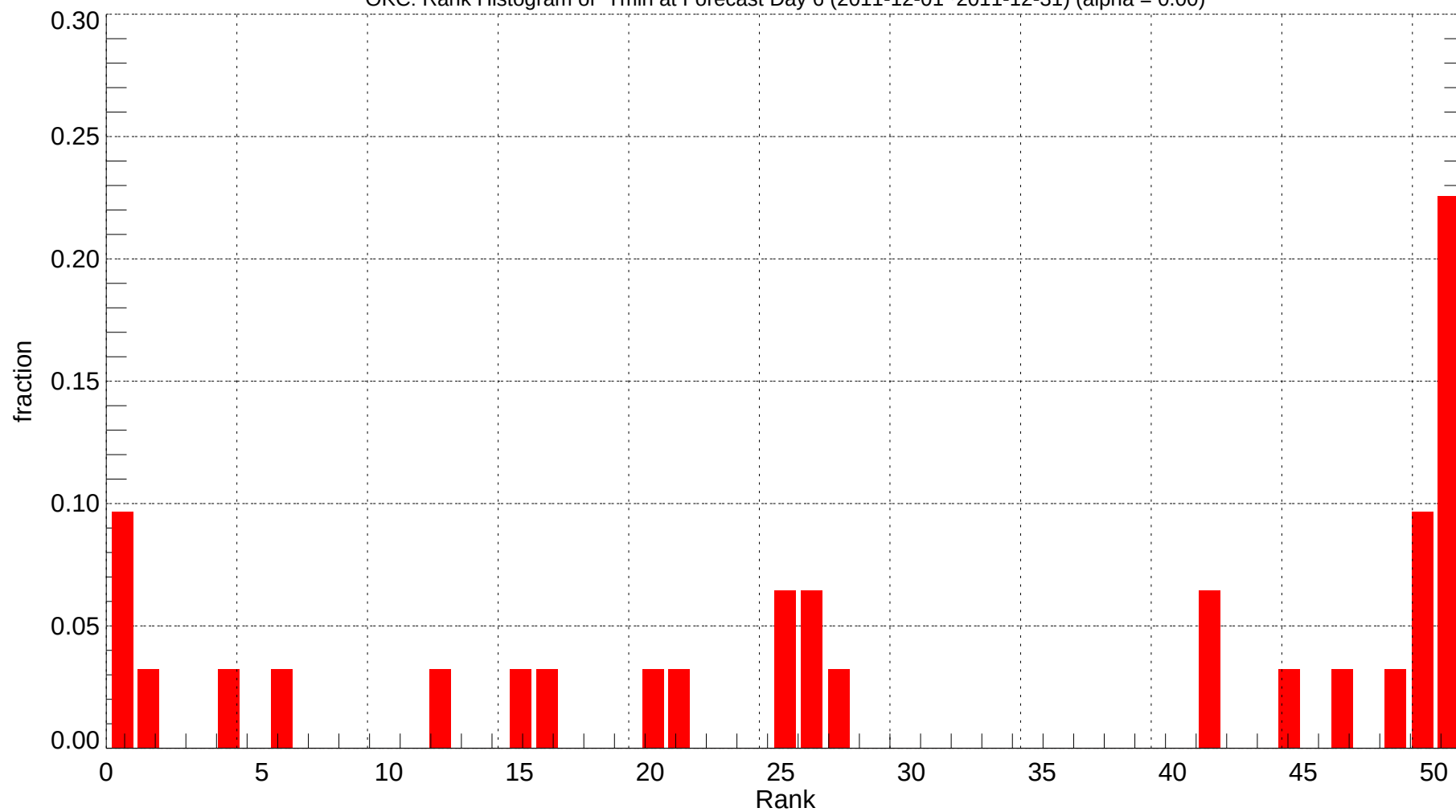
OKC: Rank Histogram of Tmin at Forecast Day 6 (2011-12-01~2011-12-31) (alpha = 0.00)
