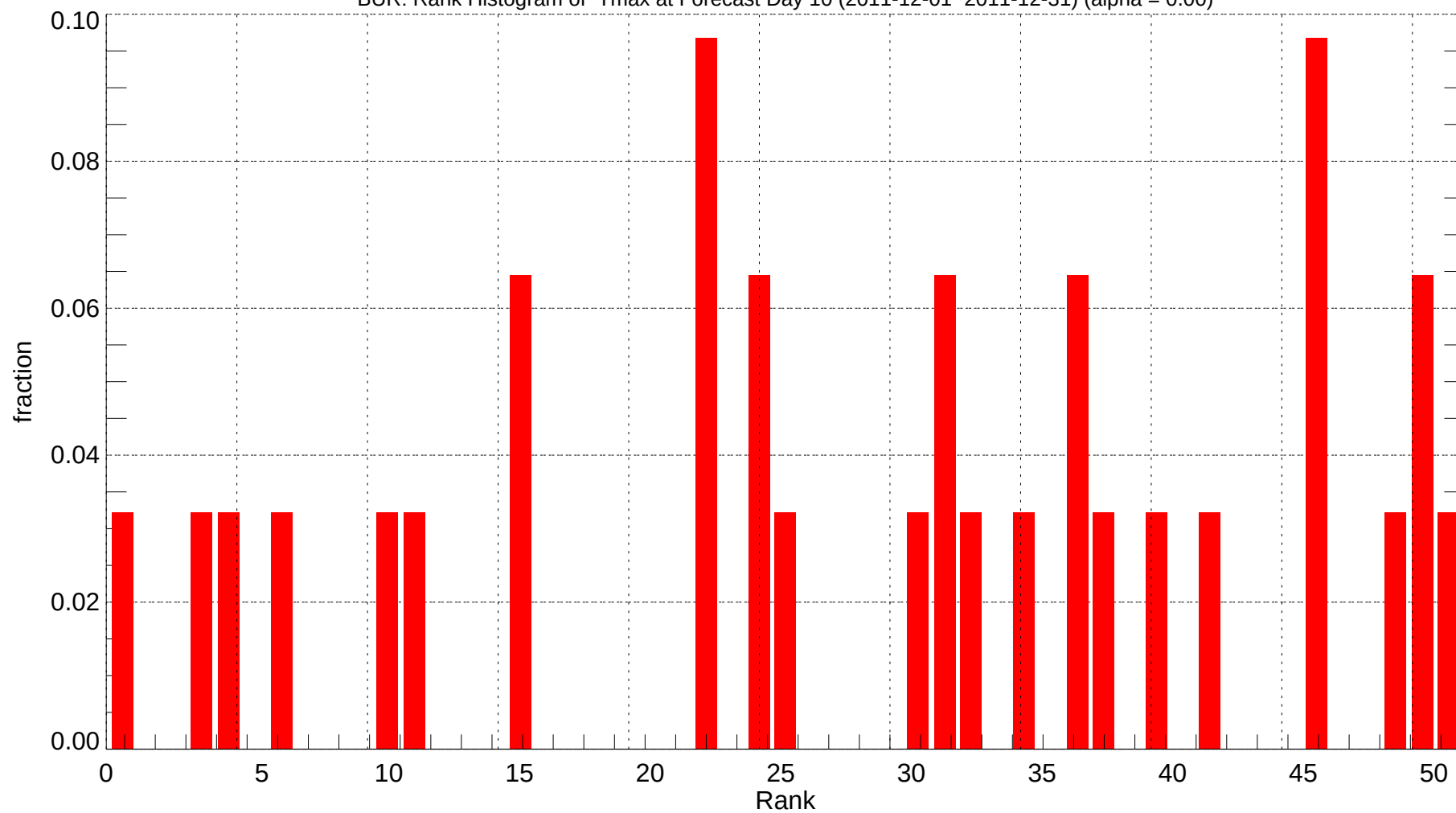
BUR: Rank Histogram of Tmax at Forecast Day 10 (2011-12-01~2011-12-31) (alpha = 0.00)
