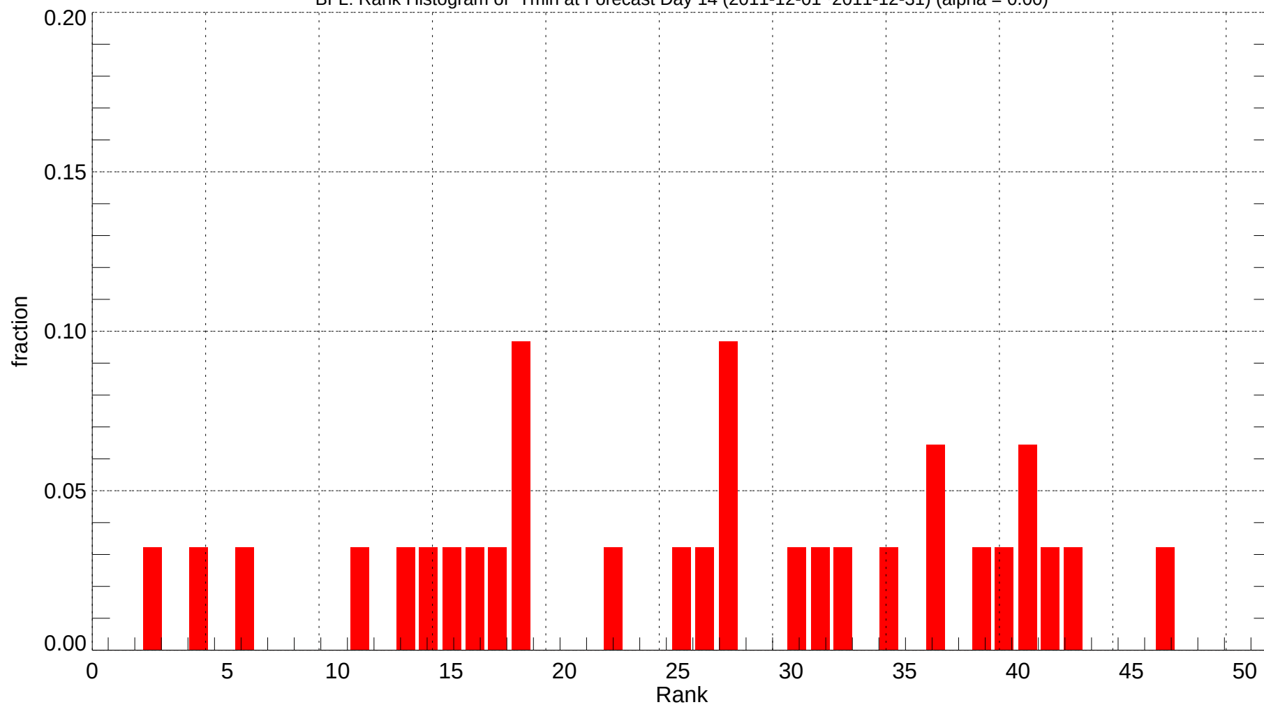
BFL: Rank Histogram of Tmin at Forecast Day 14 (2011-12-01~2011-12-31) (alpha = 0.00)
