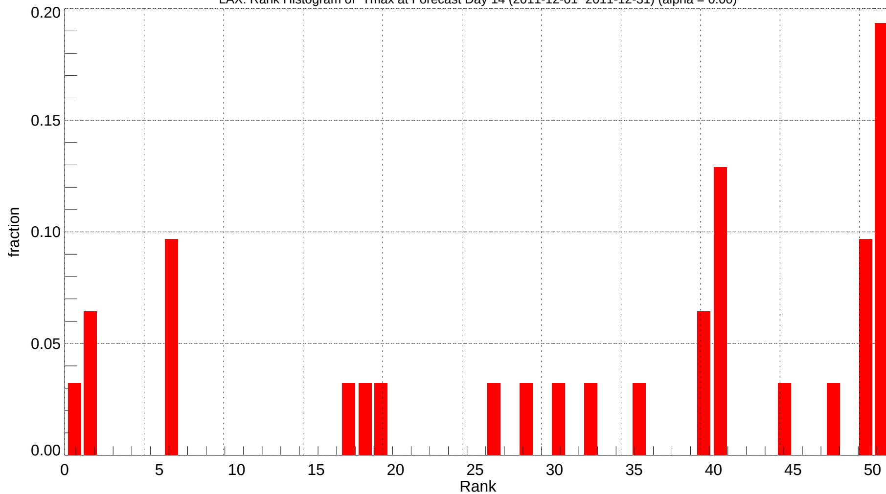
LAX: Rank Histogram of Tmax at Forecast Day 14 (2011-12-01~2011-12-31) (alpha = 0.00)
