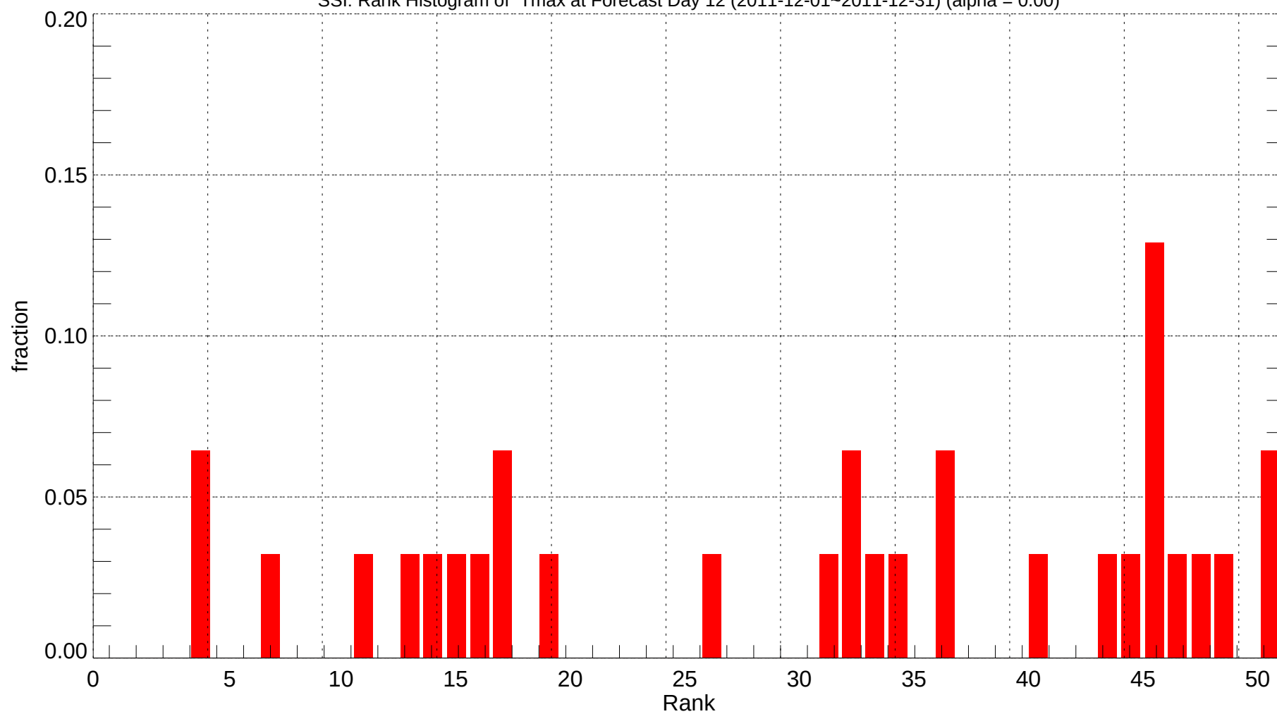
SSI: Rank Histogram of Tmax at Forecast Day 12 (2011-12-01~2011-12-31) (alpha = 0.00)
