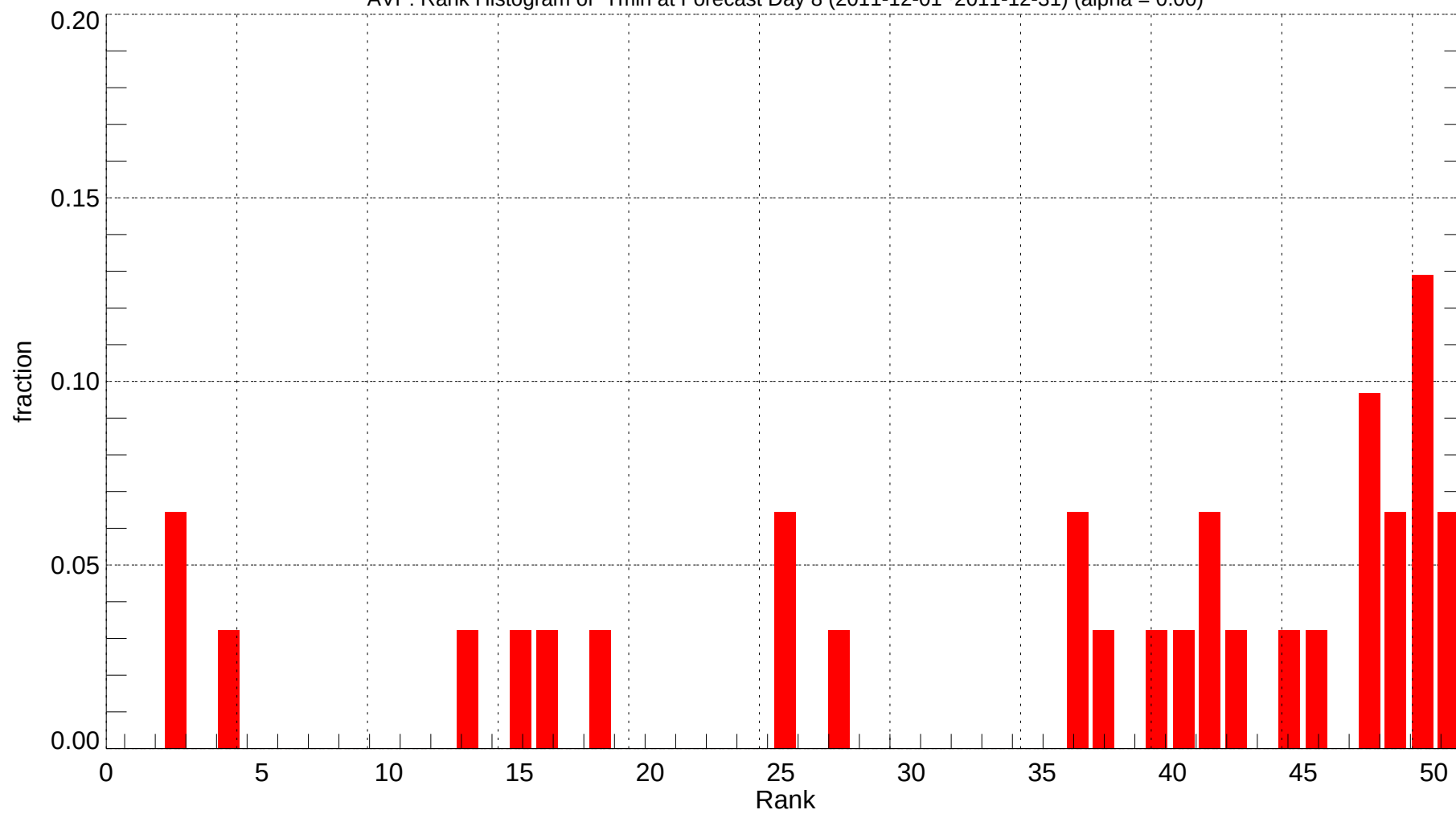
AVP: Rank Histogram of Tmin at Forecast Day 8 (2011-12-01~2011-12-31) (alpha = 0.00)
