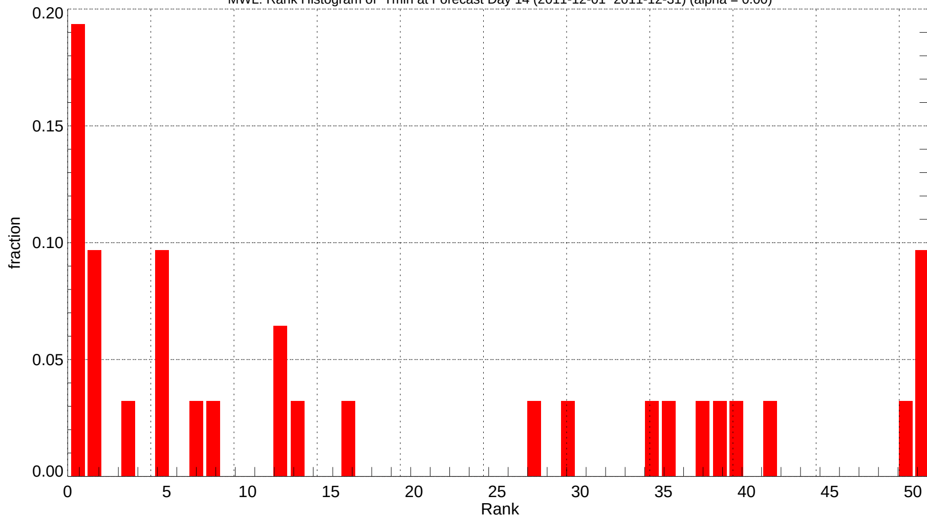
MWL: Rank Histogram of Tmin at Forecast Day 14 (2011-12-01~2011-12-31) (alpha = 0.00)
