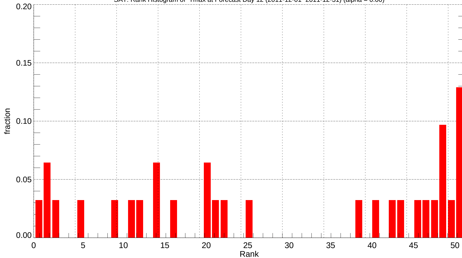
SAT: Rank Histogram of Tmax at Forecast Day 12 (2011-12-01~2011-12-31) (alpha = 0.00)
