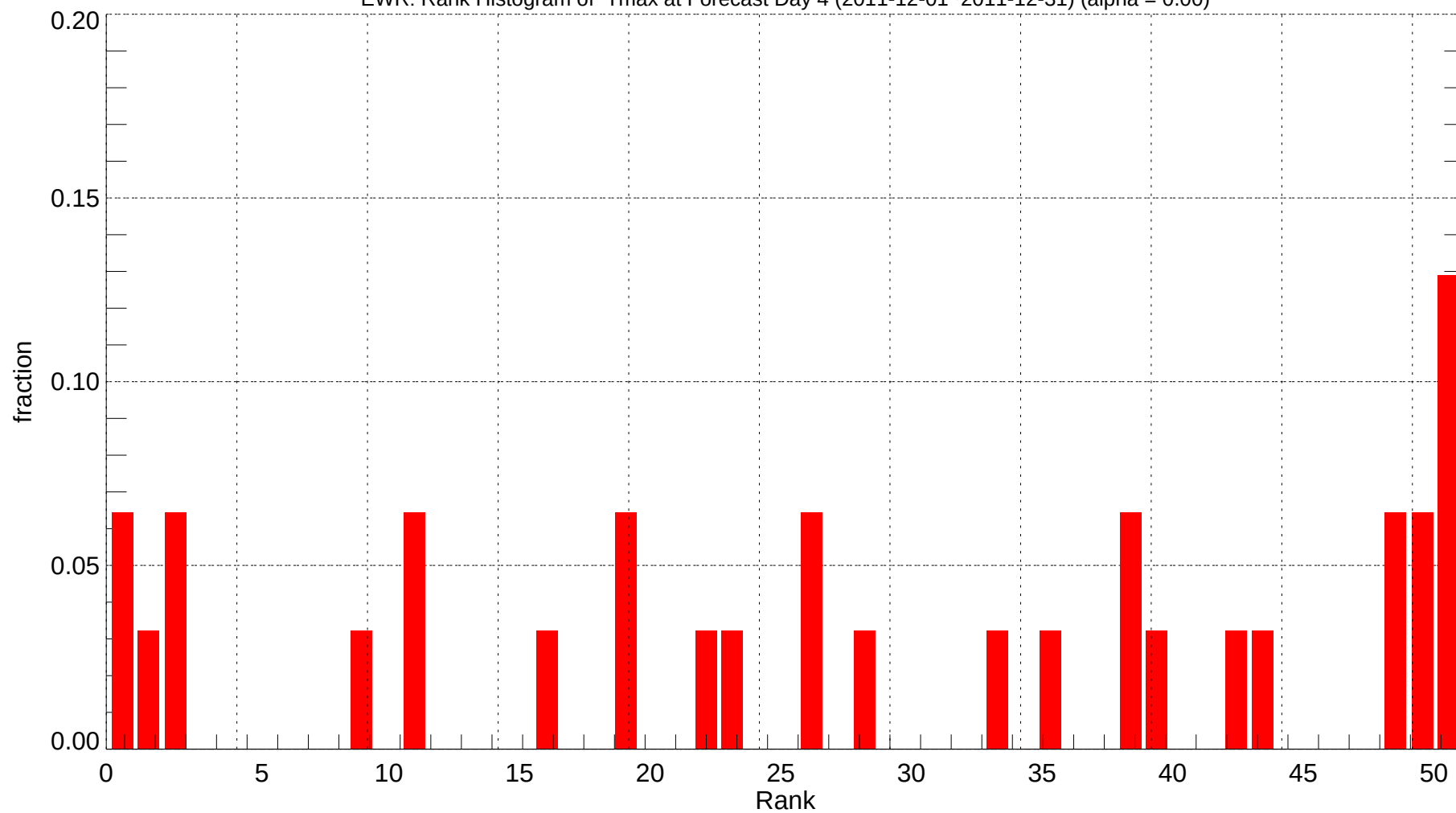
EWR: Rank Histogram of Tmax at Forecast Day 4 (2011-12-01~2011-12-31) (alpha = 0.00)
