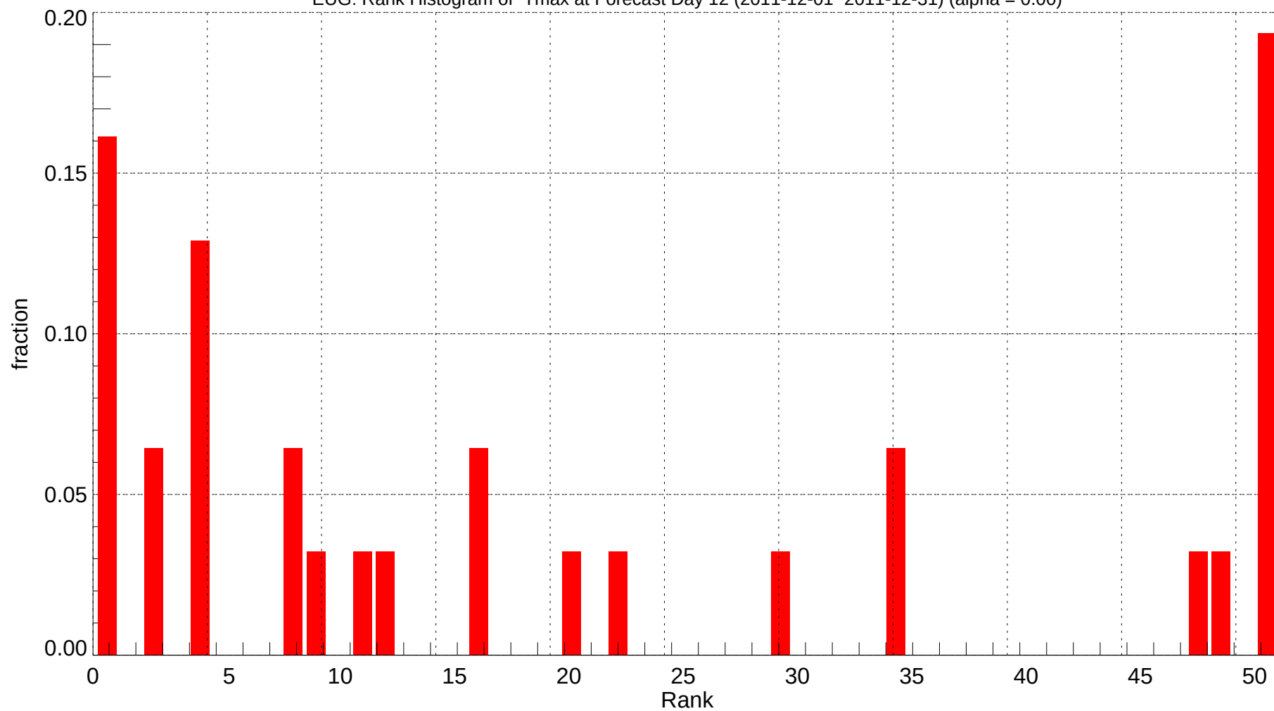
EUG: Rank Histogram of Tmax at Forecast Day 12 (2011-12-01~2011-12-31) (alpha = 0.00)
