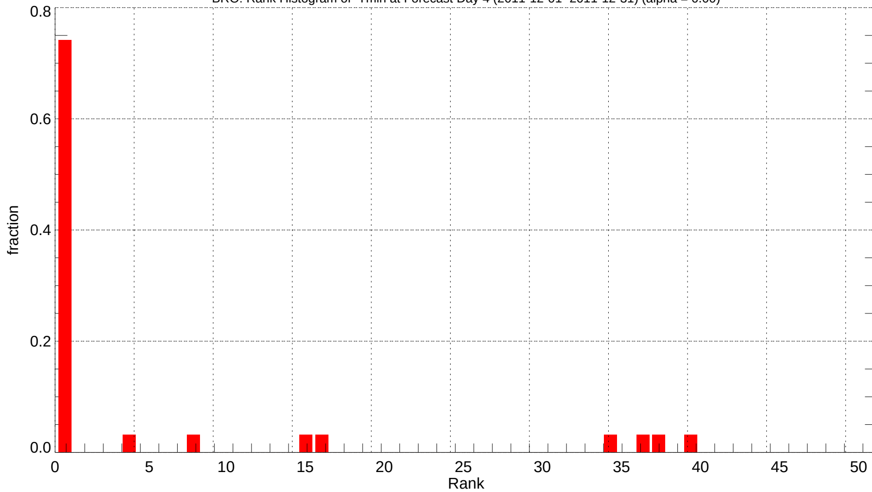
BRO: Rank Histogram of Tmin at Forecast Day 4 (2011-12-01~2011-12-31) (alpha = 0.00)
