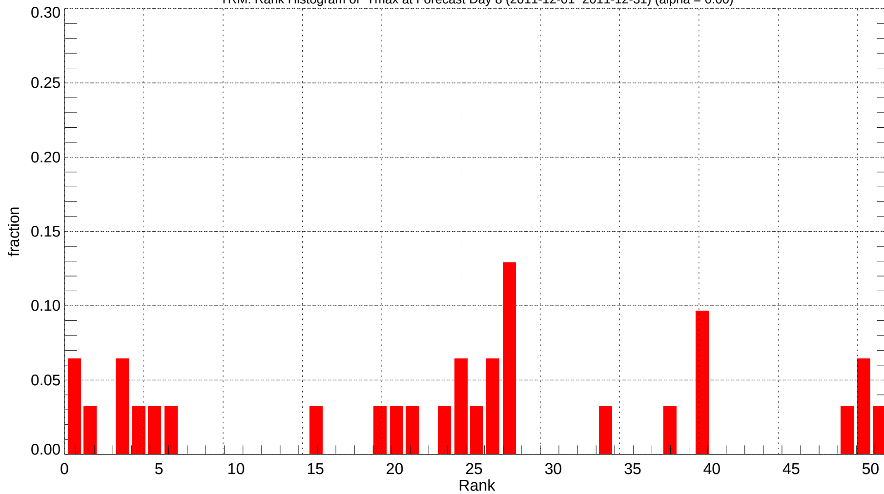
TRM: Rank Histogram of Tmax at Forecast Day 8 (2011-12-01~2011-12-31) (alpha = 0.00)
