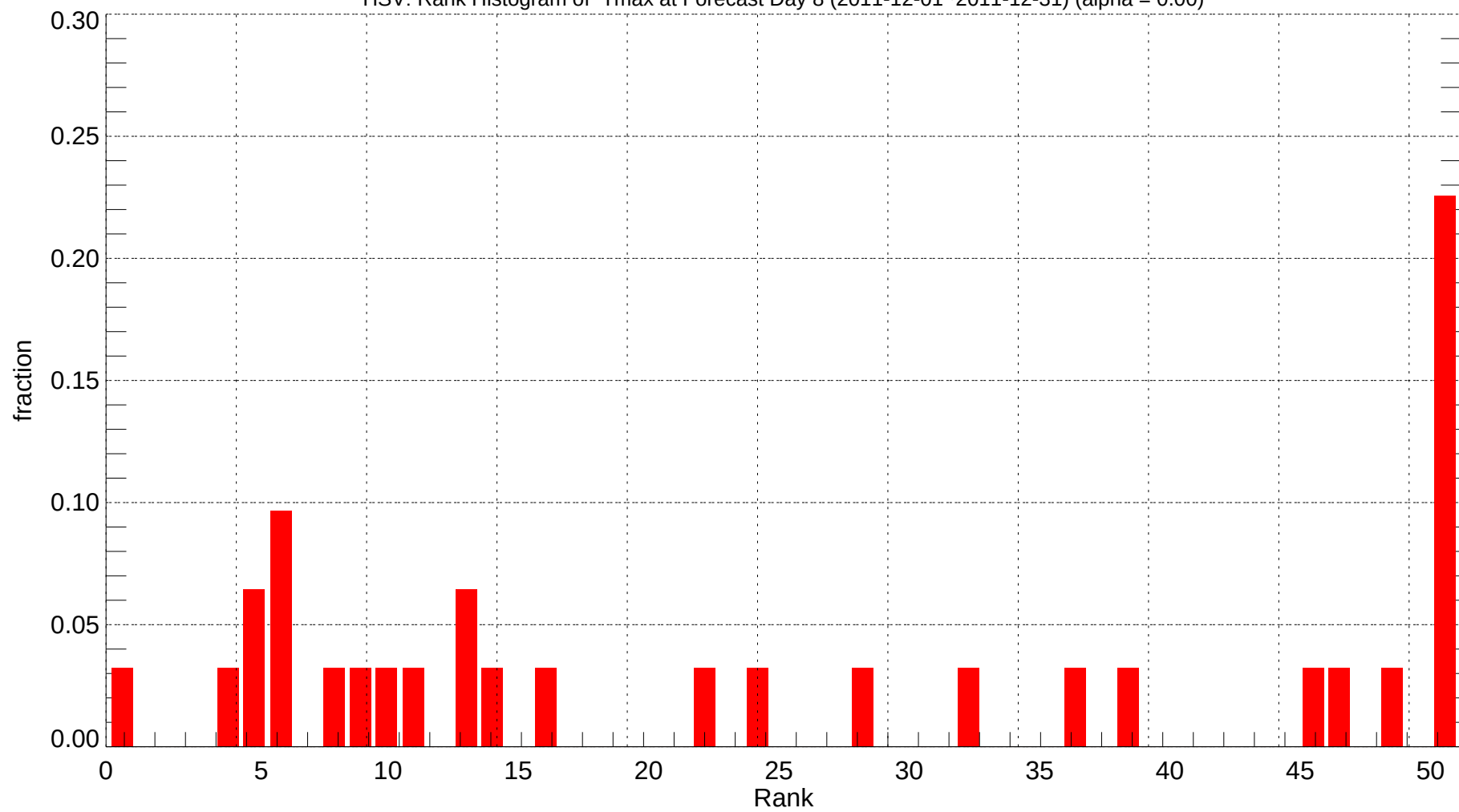
HSV: Rank Histogram of Tmax at Forecast Day 8 (2011-12-01~2011-12-31) (alpha = 0.00)
