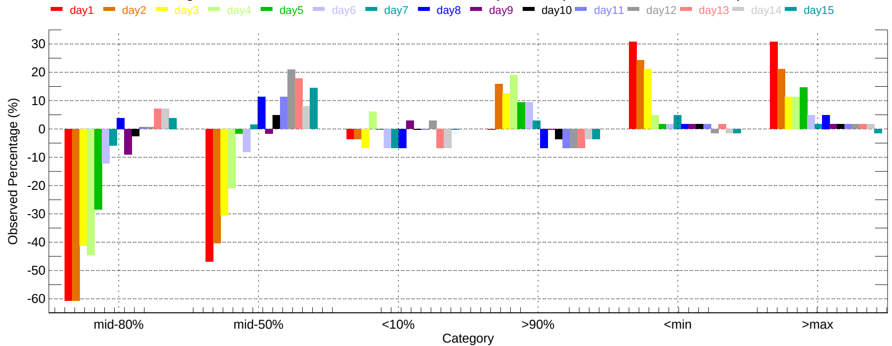
Observed Percentage Deviation of Ensembles - WJF: Max Temperature (2011-12-01~2011-12-31)
