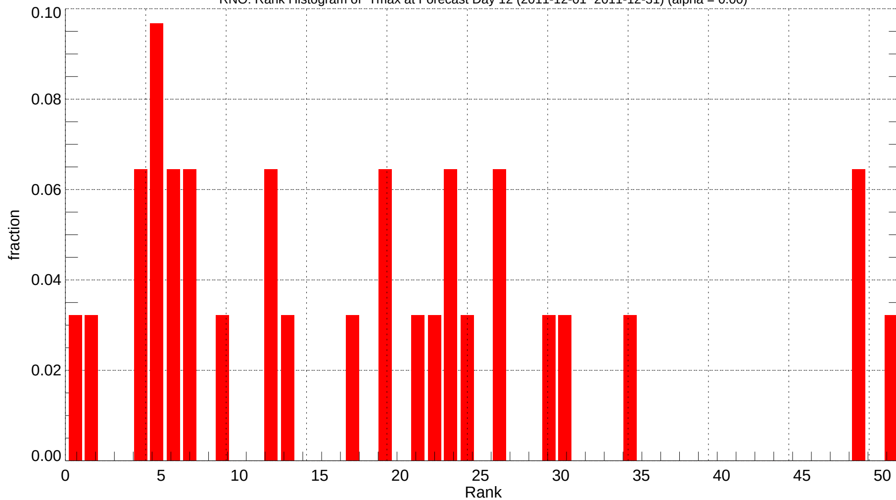
RNO: Rank Histogram of Tmax at Forecast Day 12 (2011-12-01~2011-12-31) (alpha = 0.00)
