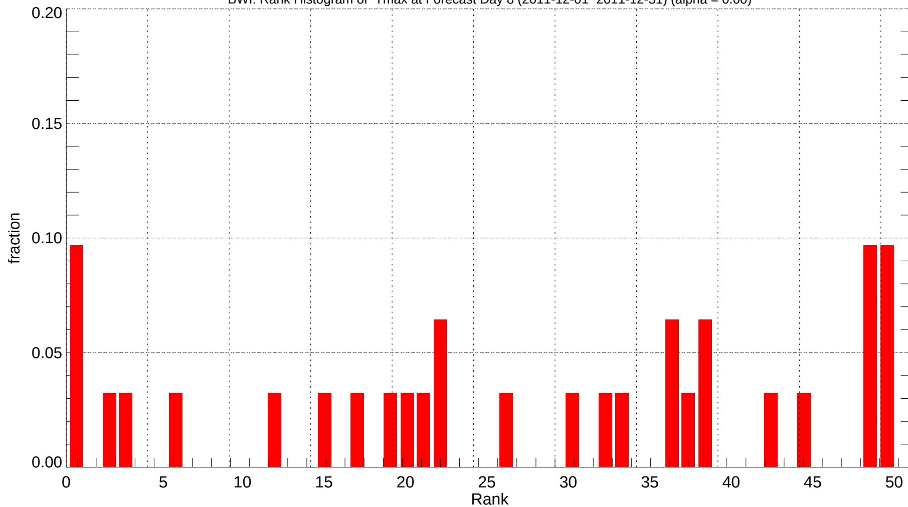
BWI: Rank Histogram of Tmax at Forecast Day 8 (2011-12-01~2011-12-31) (alpha = 0.00)
