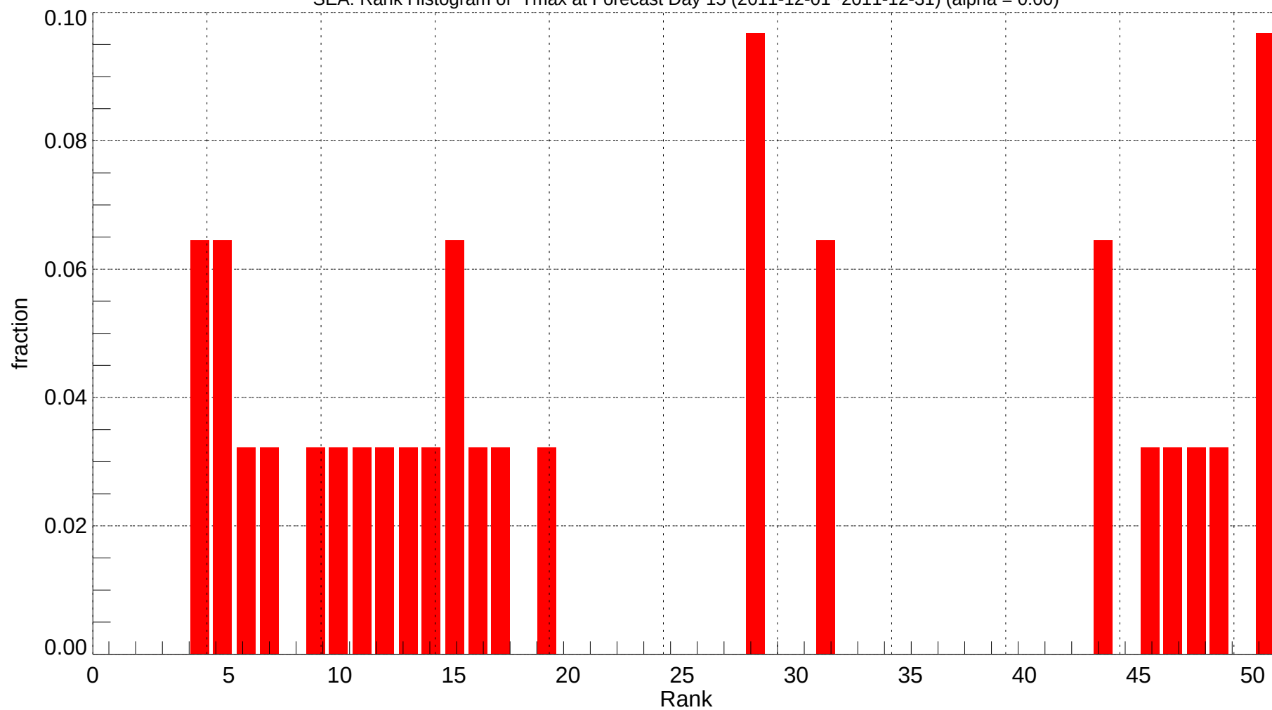
SEA: Rank Histogram of Tmax at Forecast Day 15 (2011-12-01~2011-12-31) (alpha = 0.00)
