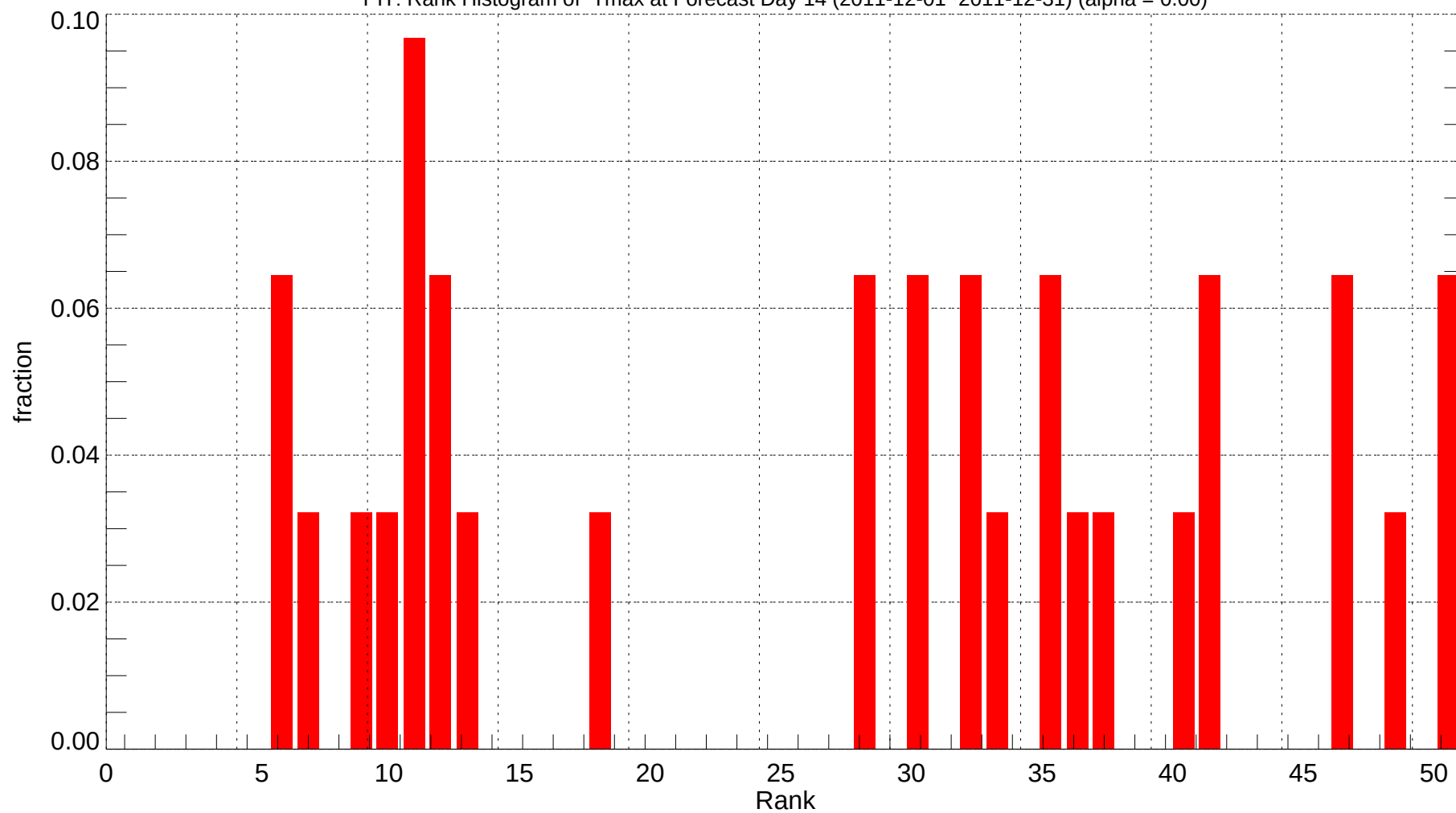
PIT: Rank Histogram of Tmax at Forecast Day 14 (2011-12-01~2011-12-31) (alpha = 0.00)
