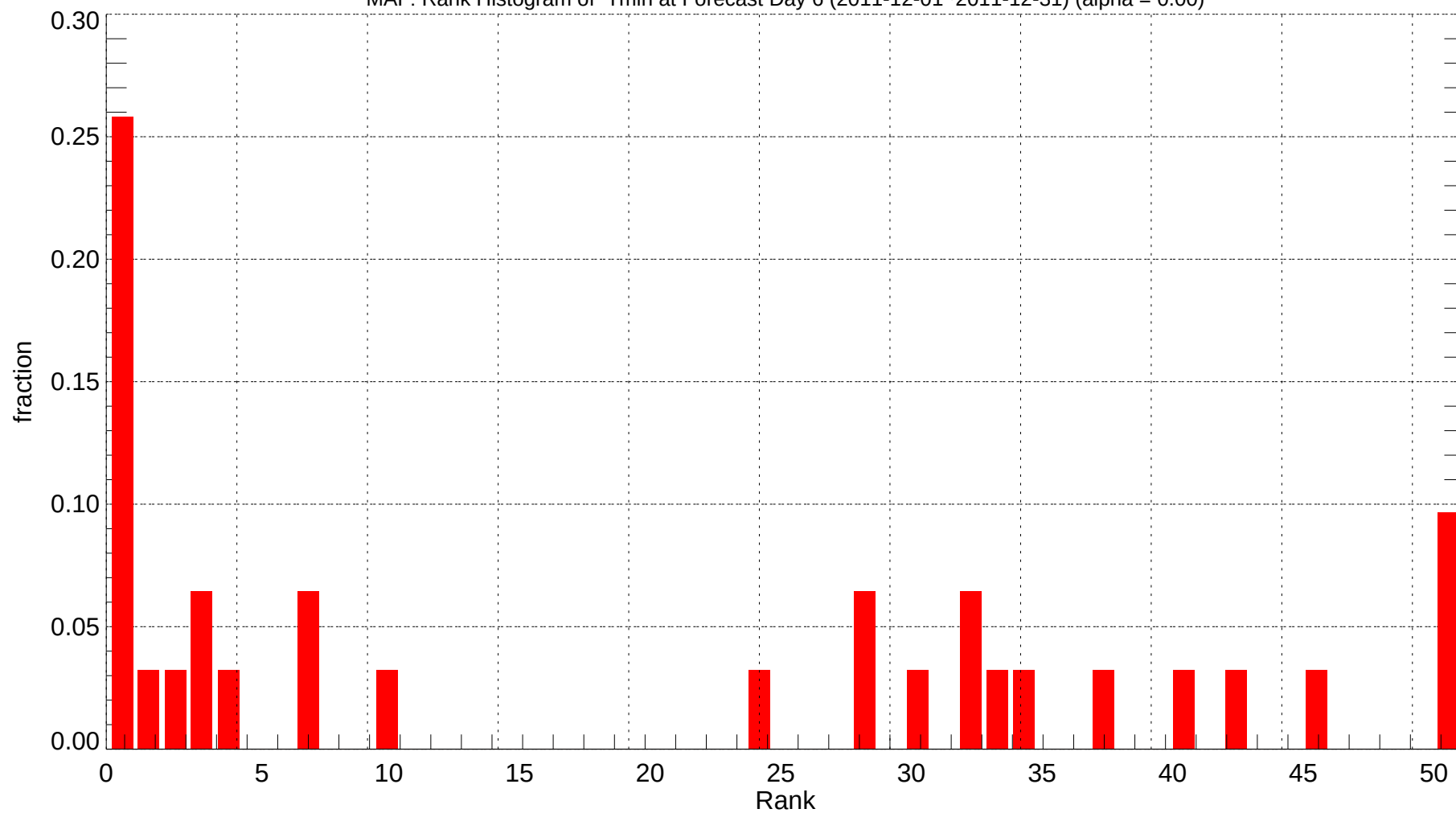
MAF: Rank Histogram of Tmin at Forecast Day 6 (2011-12-01~2011-12-31) (alpha = 0.00)
