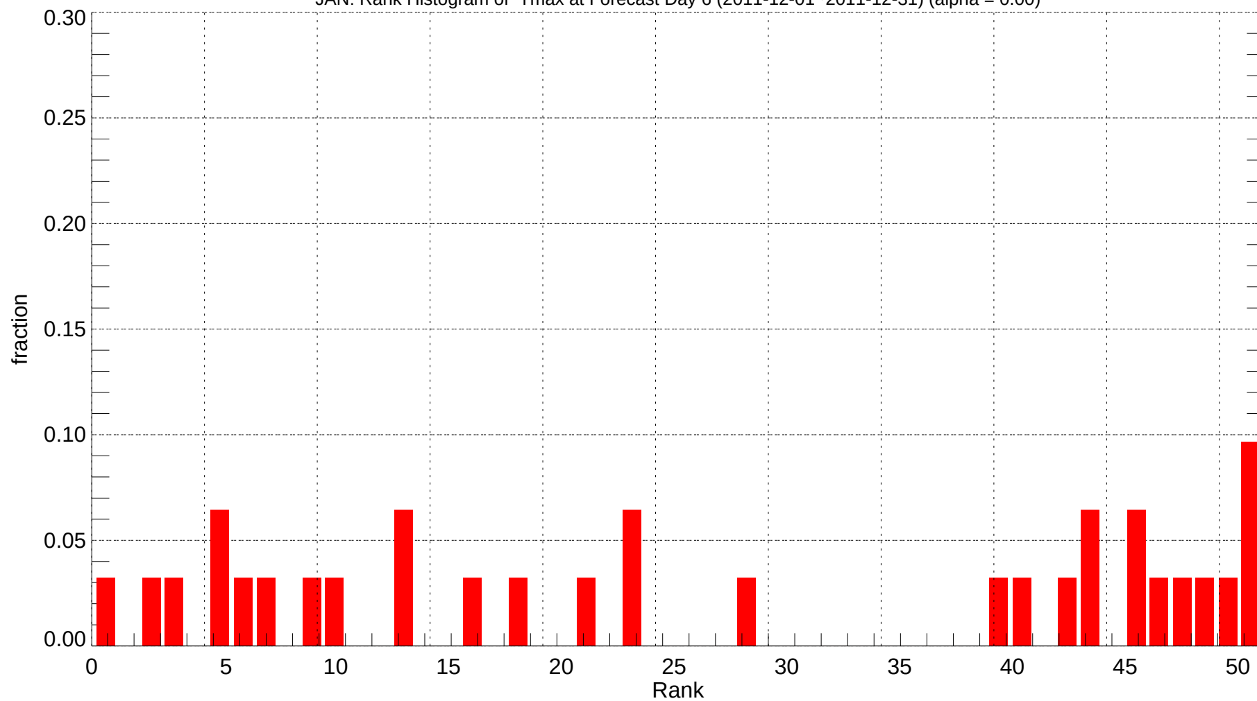
JAN: Rank Histogram of Tmax at Forecast Day 6 (2011-12-01~2011-12-31) (alpha = 0.00)
