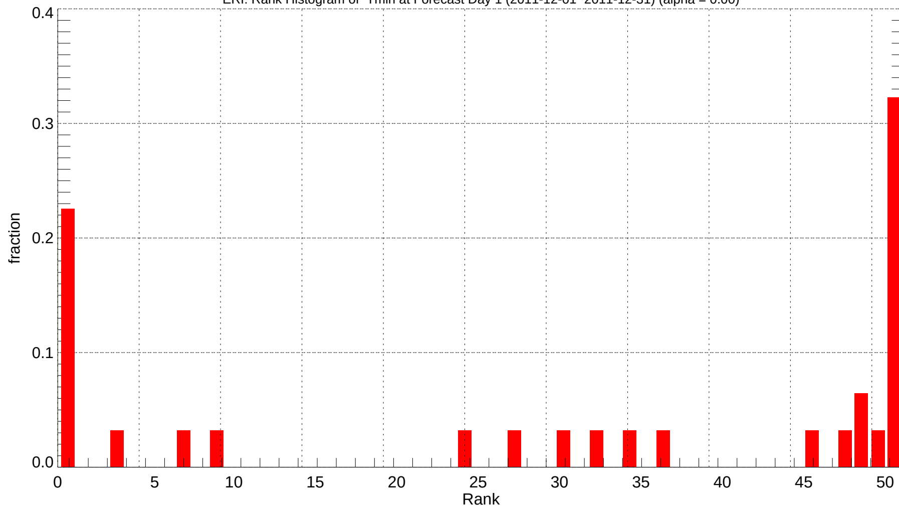
ERI: Rank Histogram of Tmin at Forecast Day 1 (2011-12-01~2011-12-31) (alpha = 0.00)
