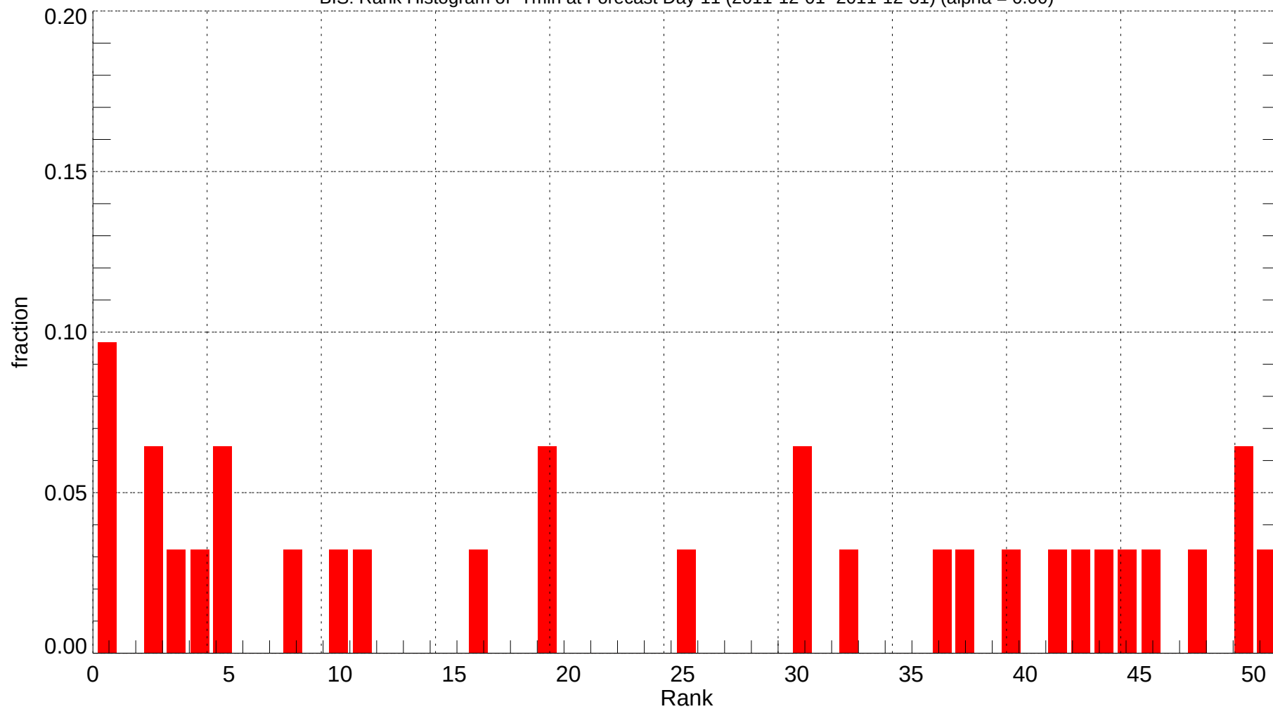
BIS: Rank Histogram of Tmin at Forecast Day 11 (2011-12-01~2011-12-31) (alpha = 0.00)
