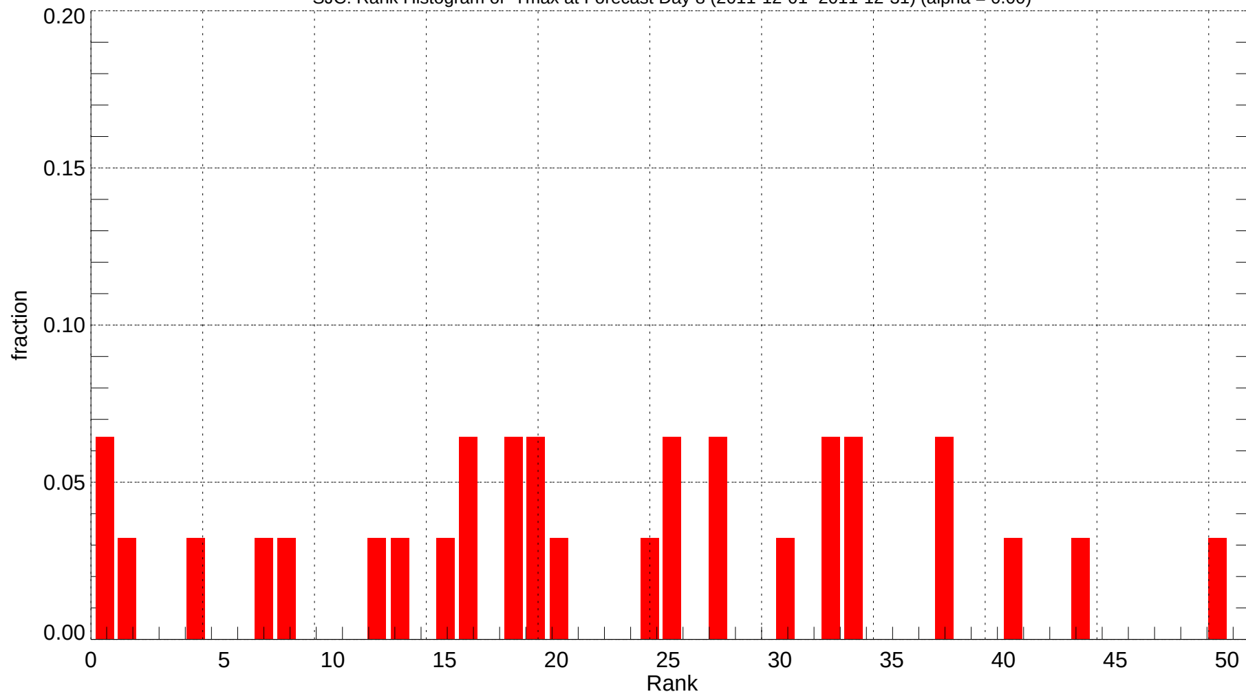
SJC: Rank Histogram of Tmax at Forecast Day 8 (2011-12-01~2011-12-31) (alpha = 0.00)
