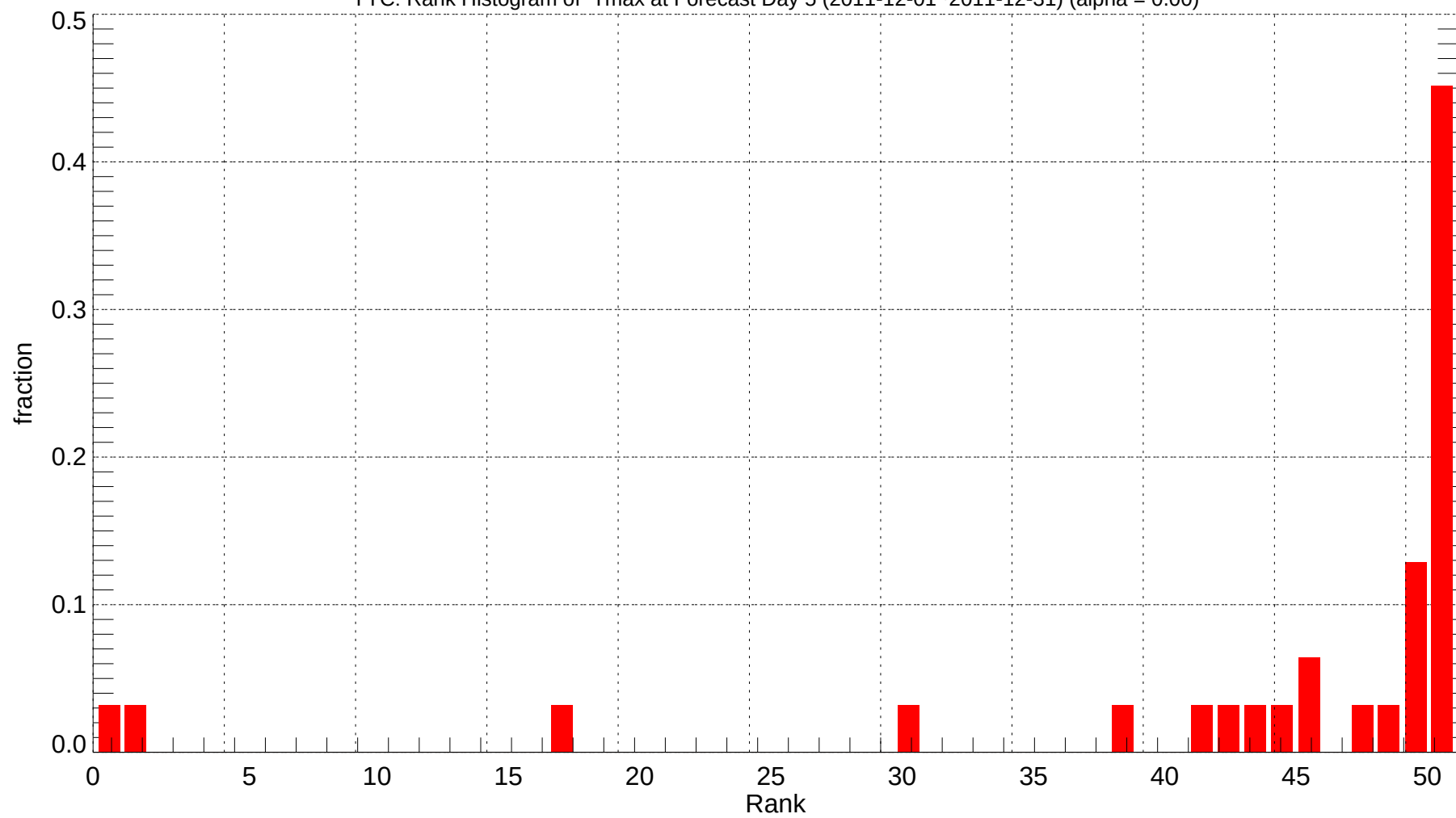
YYC: Rank Histogram of Tmax at Forecast Day 5 (2011-12-01~2011-12-31) (alpha = 0.00)
