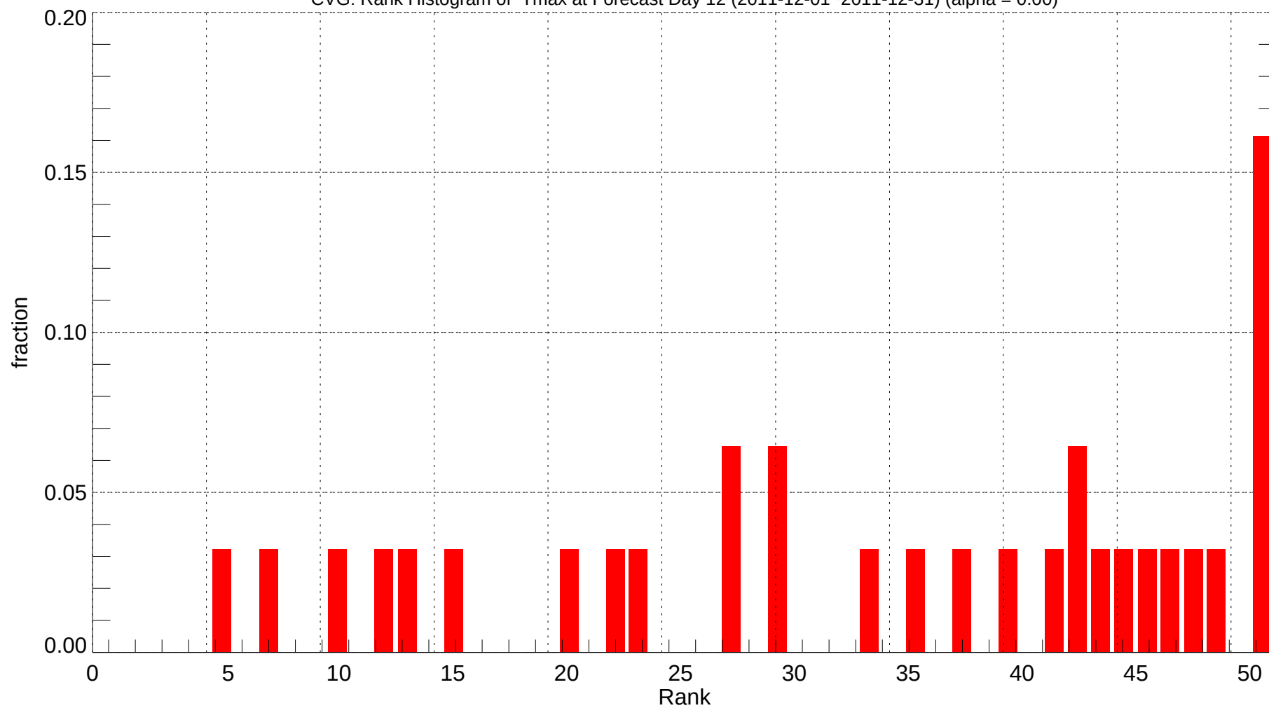
CVG: Rank Histogram of Tmax at Forecast Day 12 (2011-12-01~2011-12-31) (alpha = 0.00)
