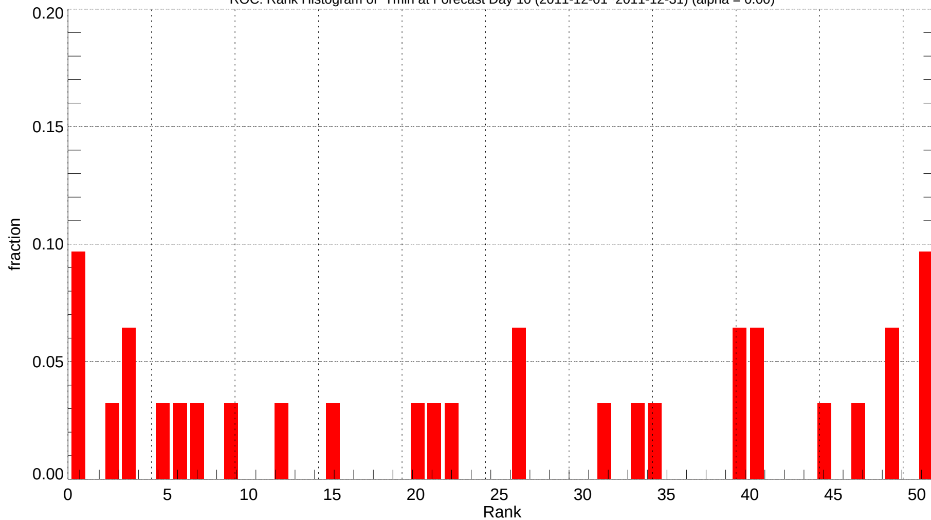
ROC: Rank Histogram of Tmin at Forecast Day 10 (2011-12-01~2011-12-31) (alpha = 0.00)
