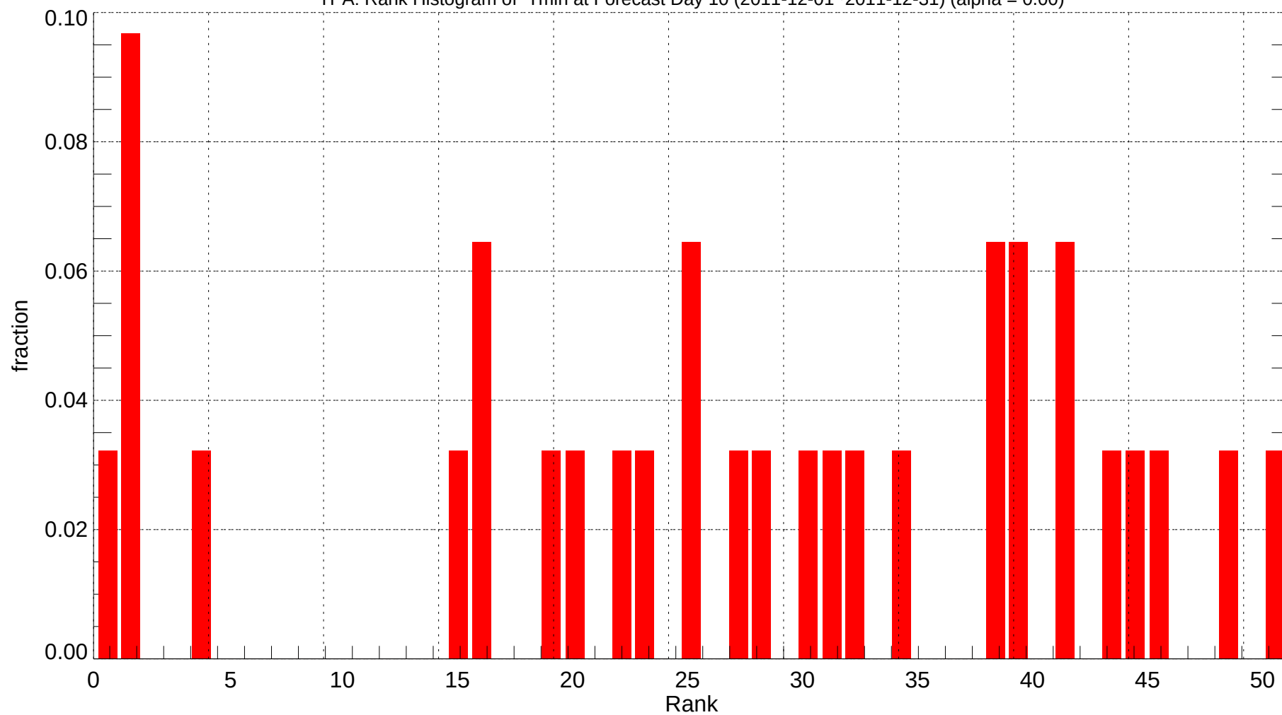
TPA: Rank Histogram of Tmin at Forecast Day 10 (2011-12-01~2011-12-31) (alpha = 0.00)
