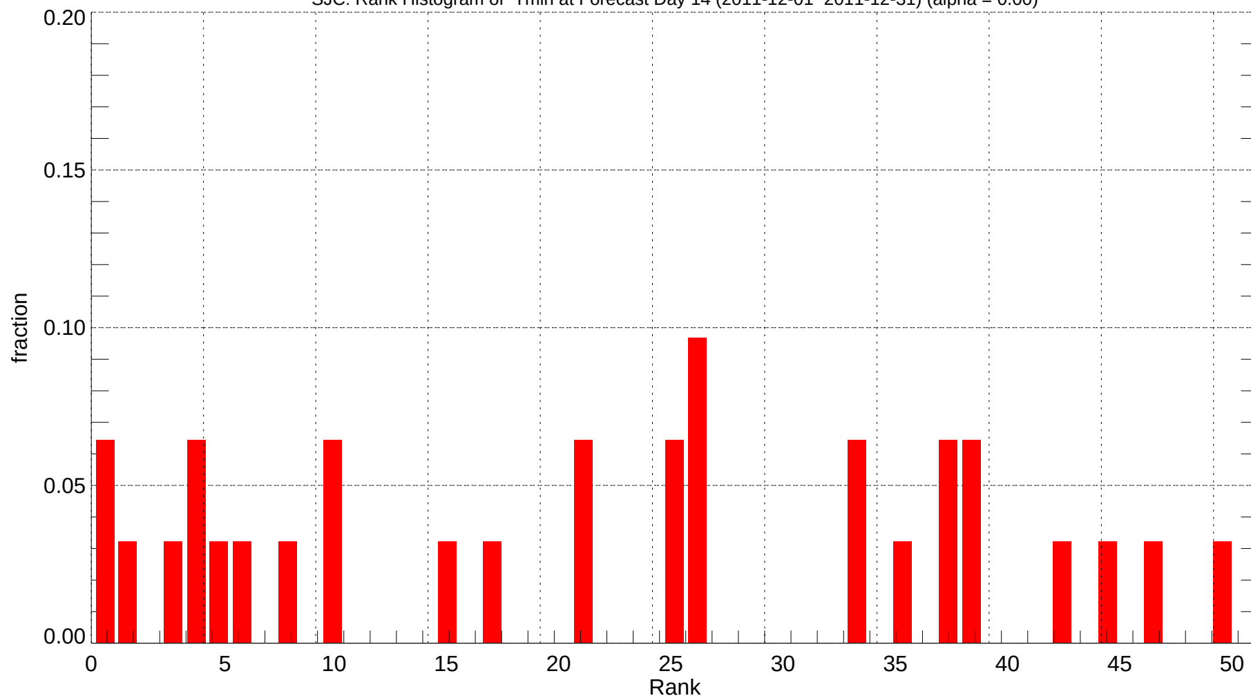
SJC: Rank Histogram of Tmin at Forecast Day 14 (2011-12-01~2011-12-31) (alpha = 0.00)
