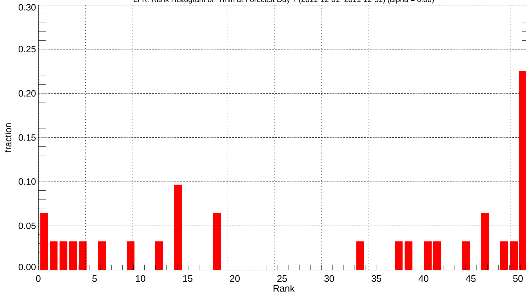
LFK: Rank Histogram of Tmin at Forecast Day 7 (2011-12-01~2011-12-31) (alpha = 0.00)
