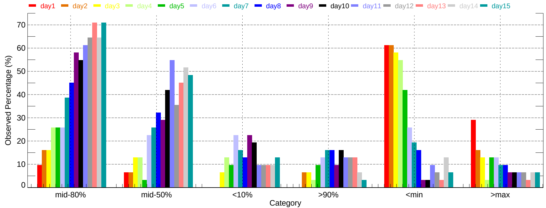
Observed Percentage of Ensembles - TLH: Min Temperature (2011-12-01~2011-12-31)
