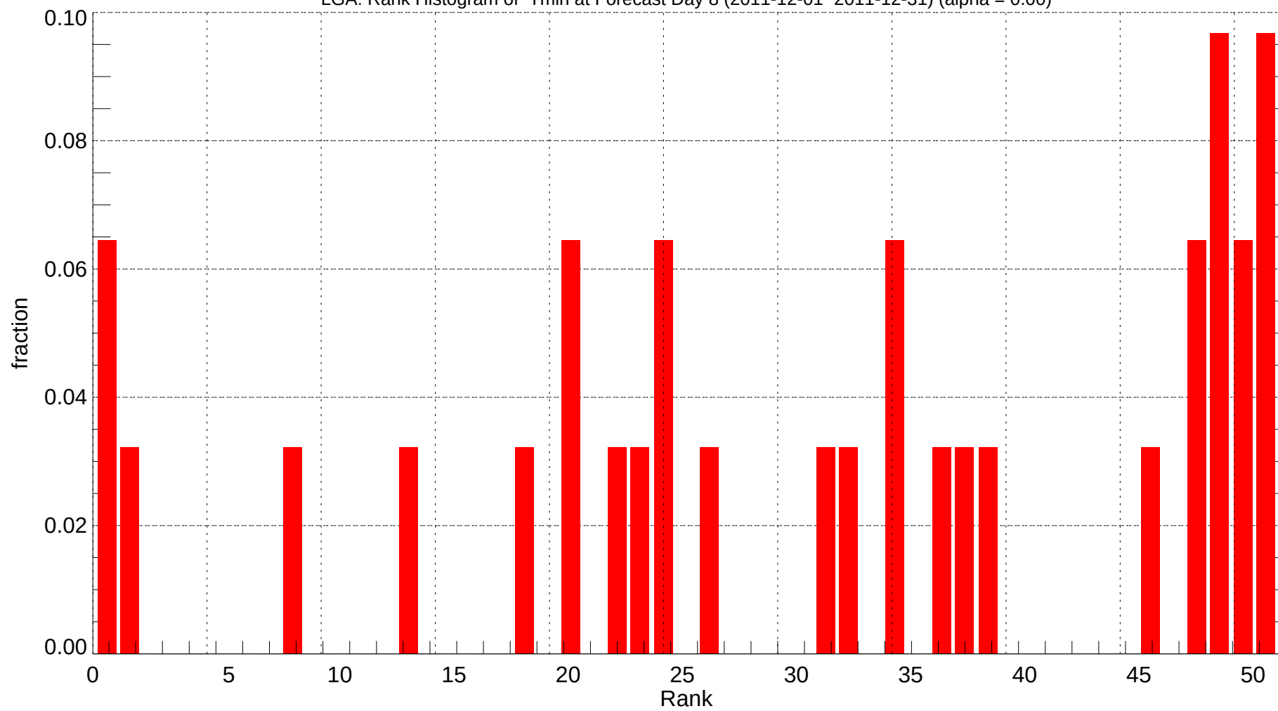
LGA: Rank Histogram of Tmin at Forecast Day 8 (2011-12-01~2011-12-31) (alpha = 0.00)
