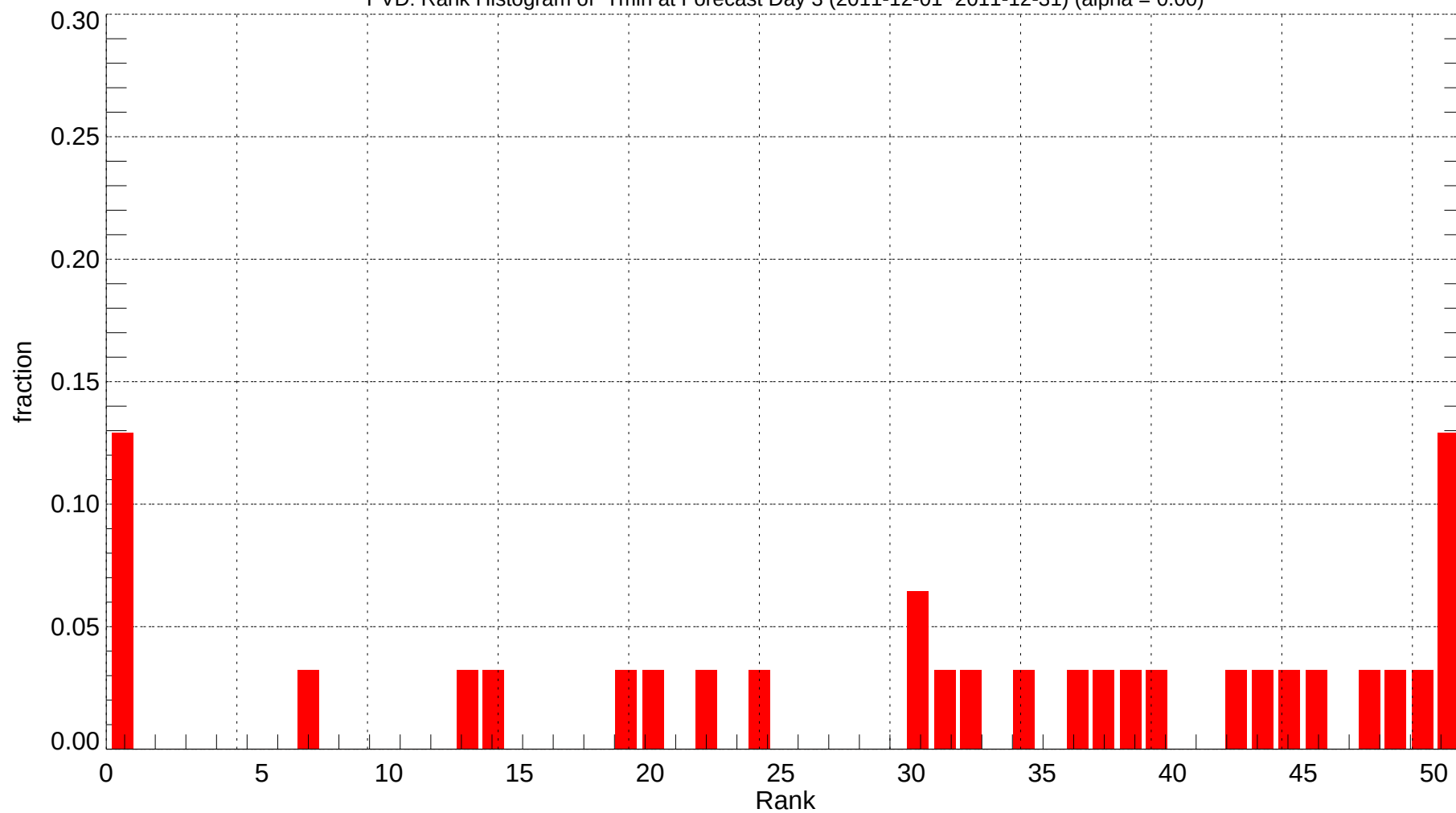
PVD: Rank Histogram of Tmin at Forecast Day 3 (2011-12-01~2011-12-31) (alpha = 0.00)
