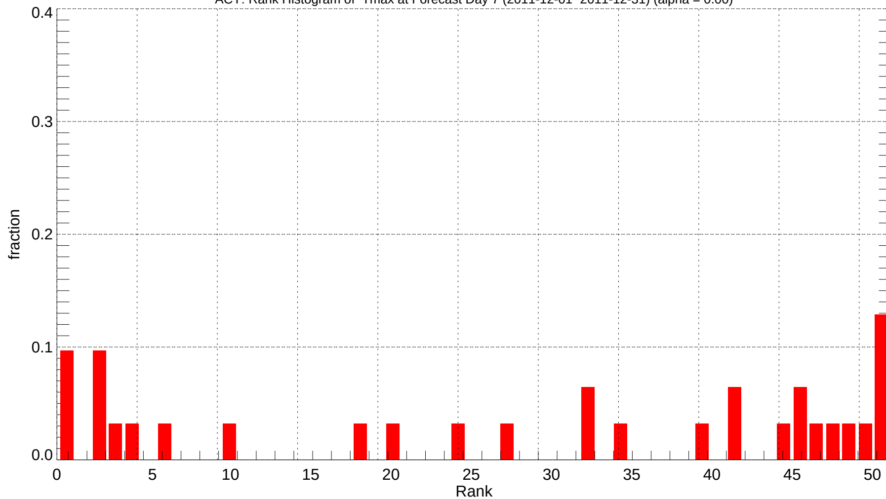
ACY: Rank Histogram of Tmax at Forecast Day 7 (2011-12-01~2011-12-31) (alpha = 0.00)
