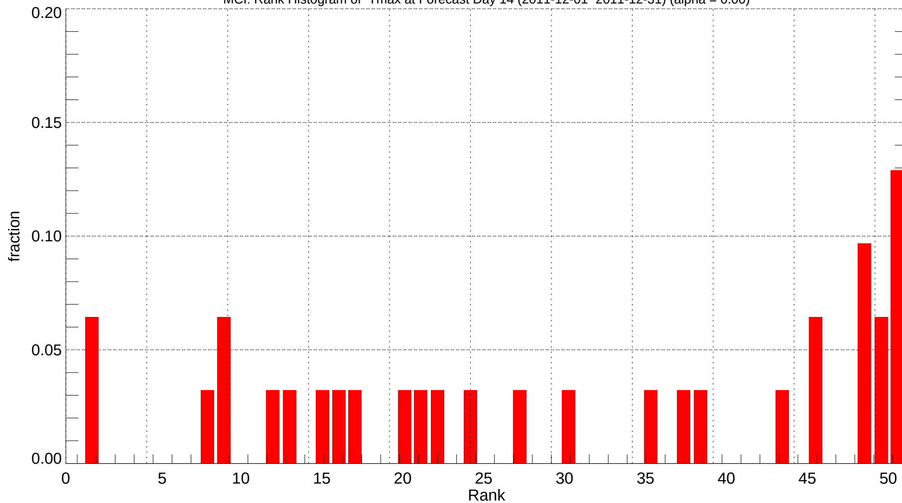
MCI: Rank Histogram of Tmax at Forecast Day 14 (2011-12-01~2011-12-31) (alpha = 0.00)
