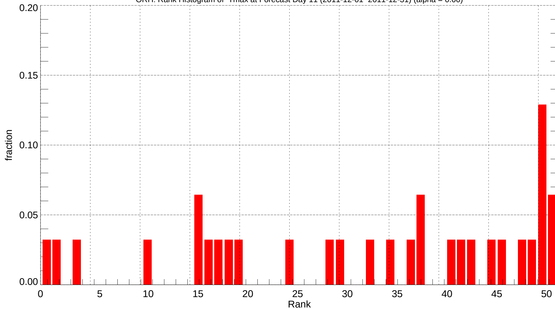
ORH: Rank Histogram of Tmax at Forecast Day 11 (2011-12-01~2011-12-31) (alpha = 0.00)
