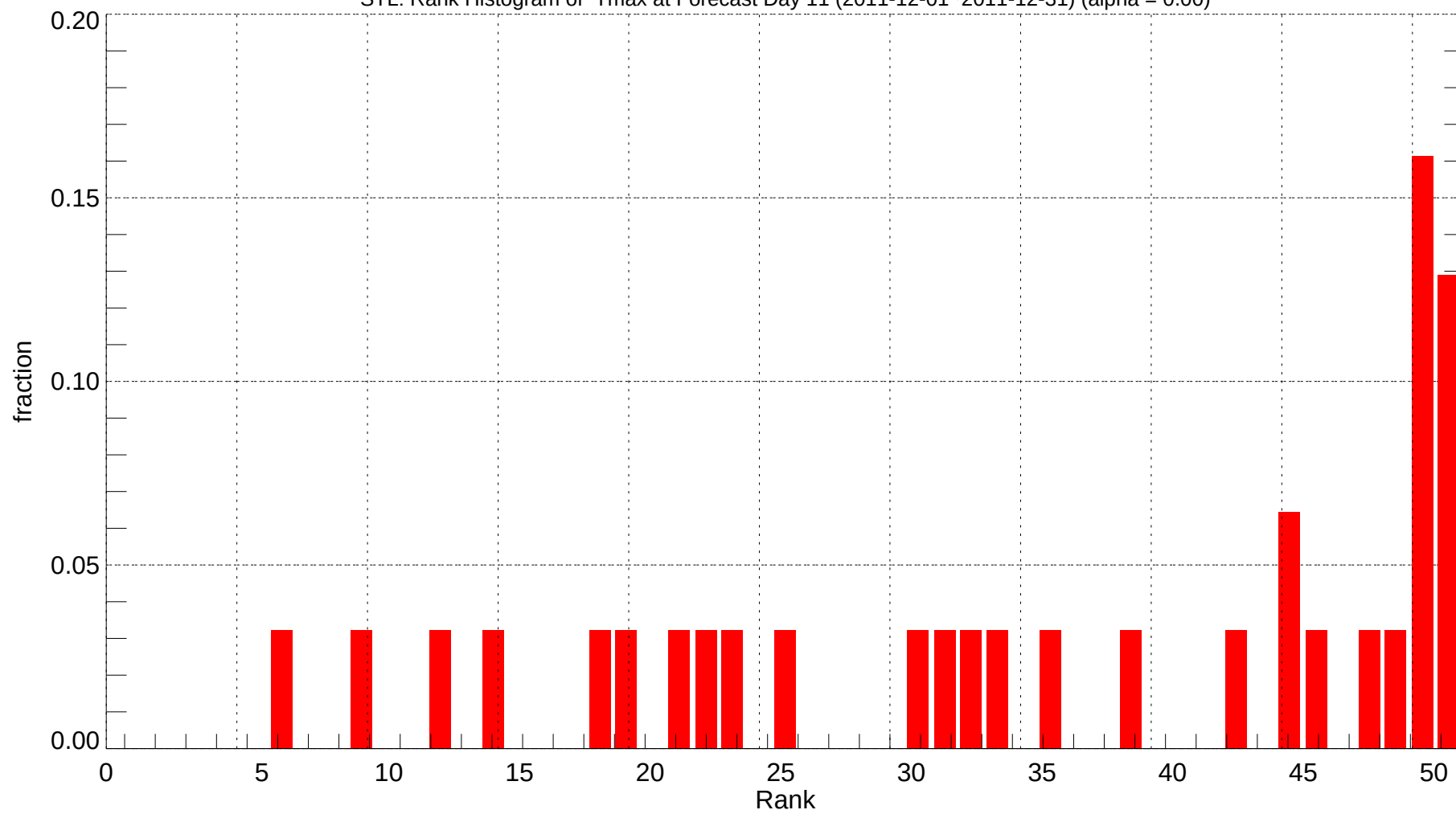
STL: Rank Histogram of Tmax at Forecast Day 11 (2011-12-01~2011-12-31) (alpha = 0.00)
