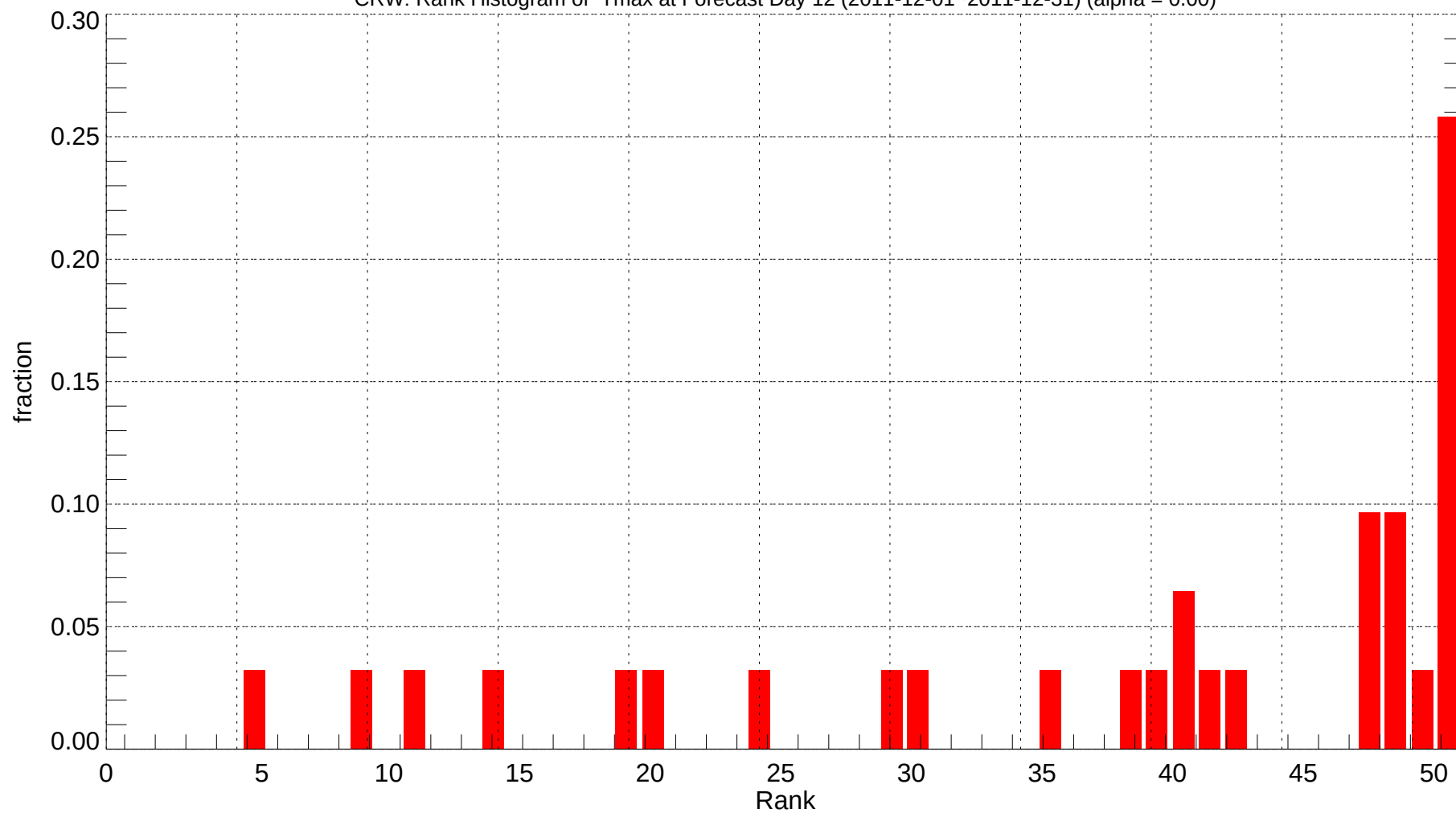
CRW: Rank Histogram of Tmax at Forecast Day 12 (2011-12-01~2011-12-31) (alpha = 0.00)
