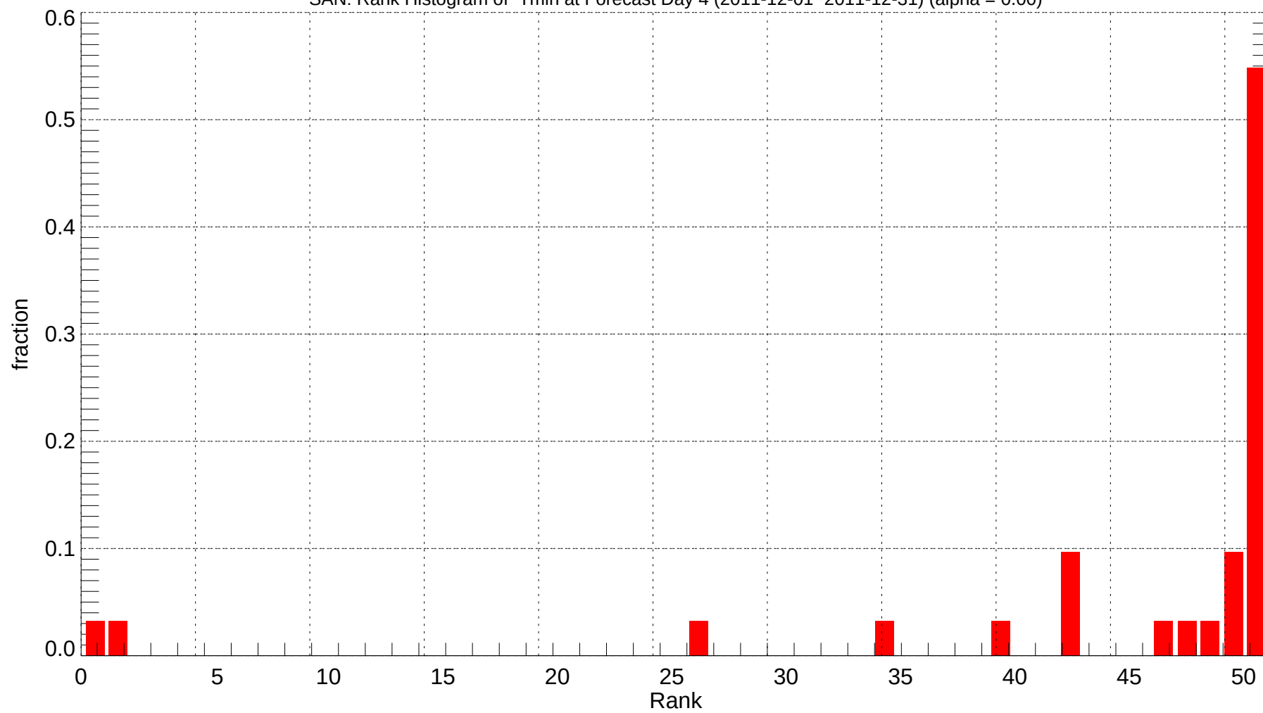
SAN: Rank Histogram of Tmin at Forecast Day 4 (2011-12-01~2011-12-31) (alpha = 0.00)
