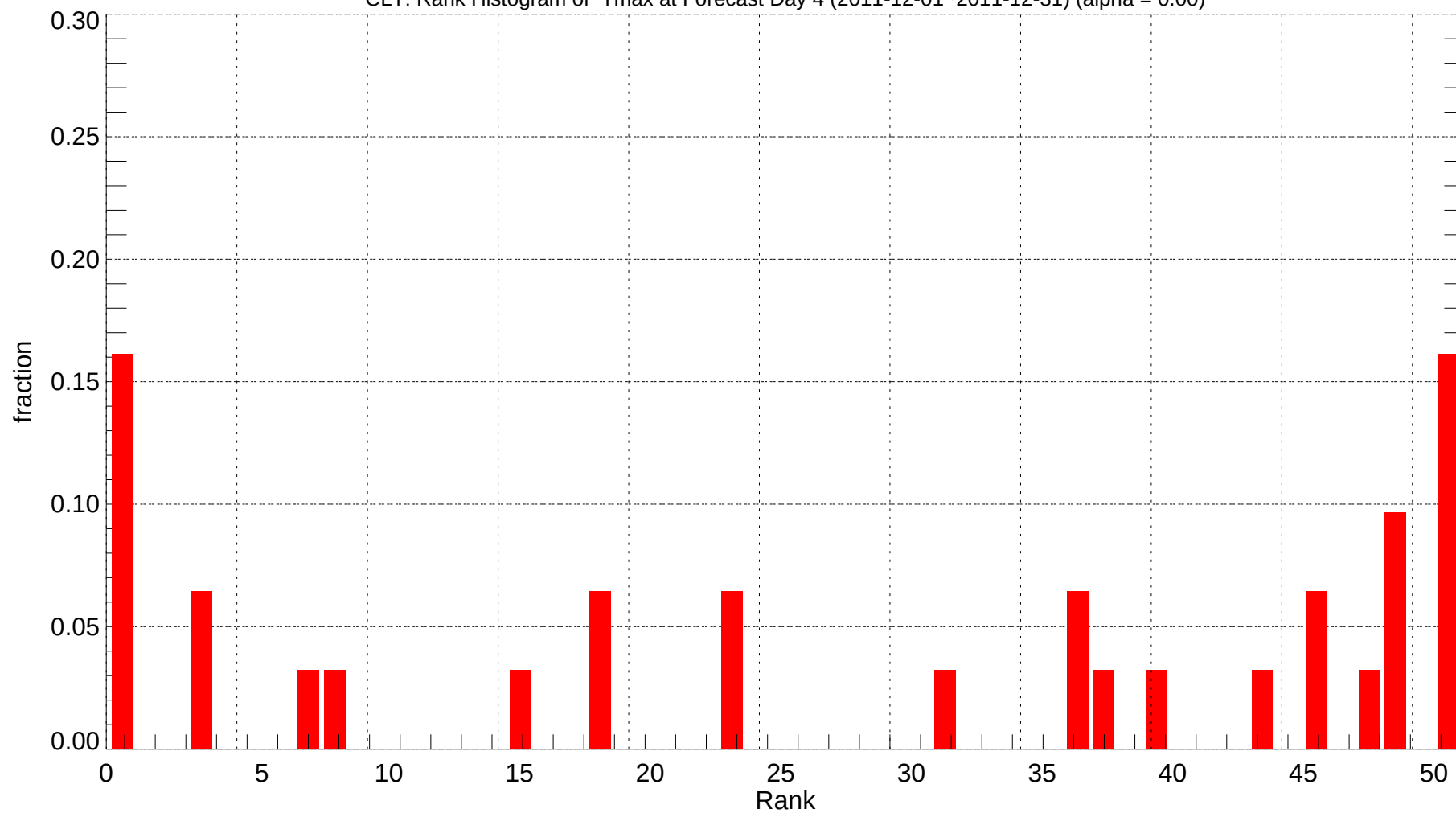
CLT: Rank Histogram of Tmax at Forecast Day 4 (2011-12-01~2011-12-31) (alpha = 0.00)
