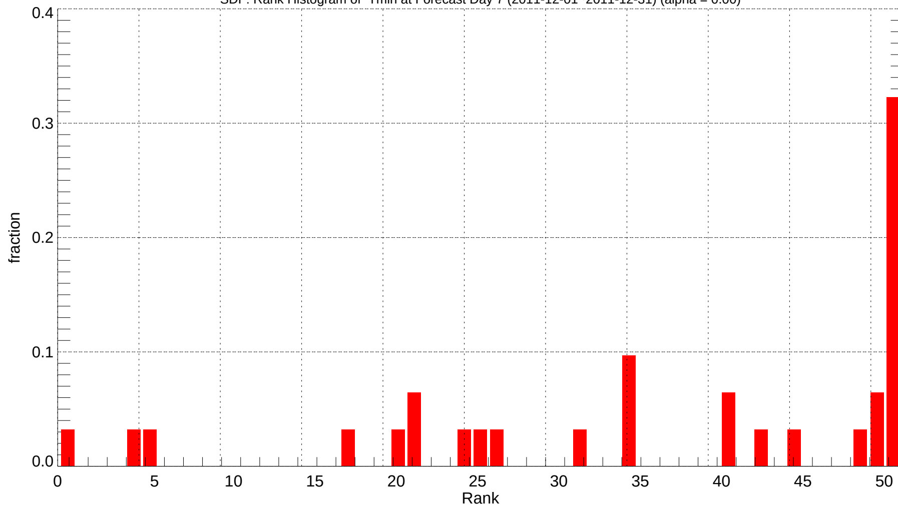
SDF: Rank Histogram of Tmin at Forecast Day 7 (2011-12-01~2011-12-31) (alpha = 0.00)
