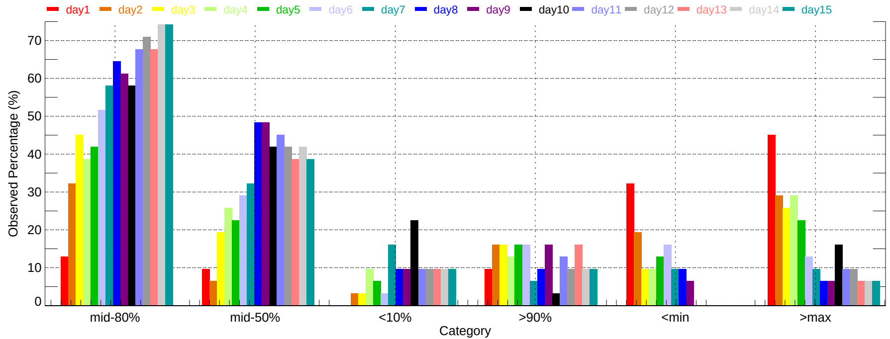
Observed Percentage of Ensembles - BDL: Min Temperature (2011-12-01~2011-12-31)
