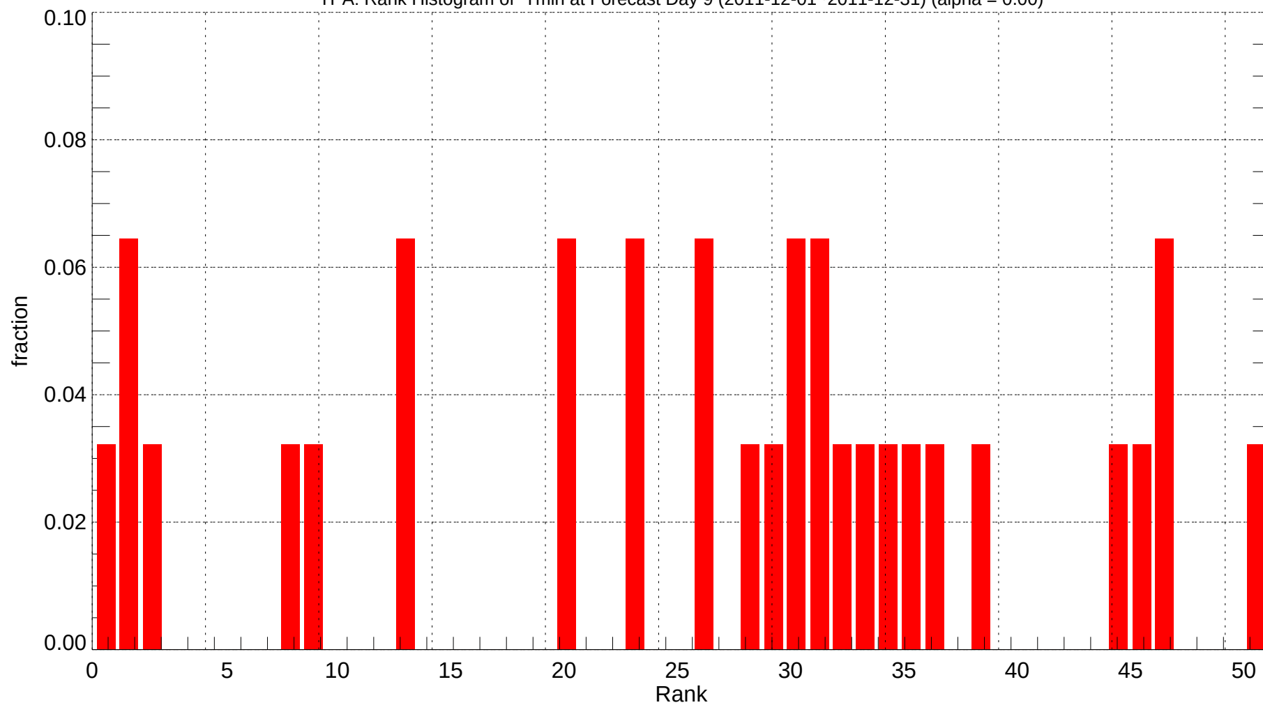
TPA: Rank Histogram of Tmin at Forecast Day 9 (2011-12-01~2011-12-31) (alpha = 0.00)
