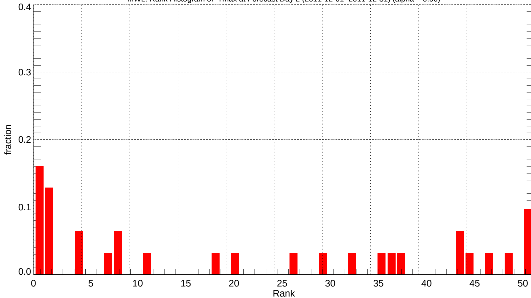
MWL: Rank Histogram of Tmax at Forecast Day 2 (2011-12-01~2011-12-31) (alpha = 0.00)
