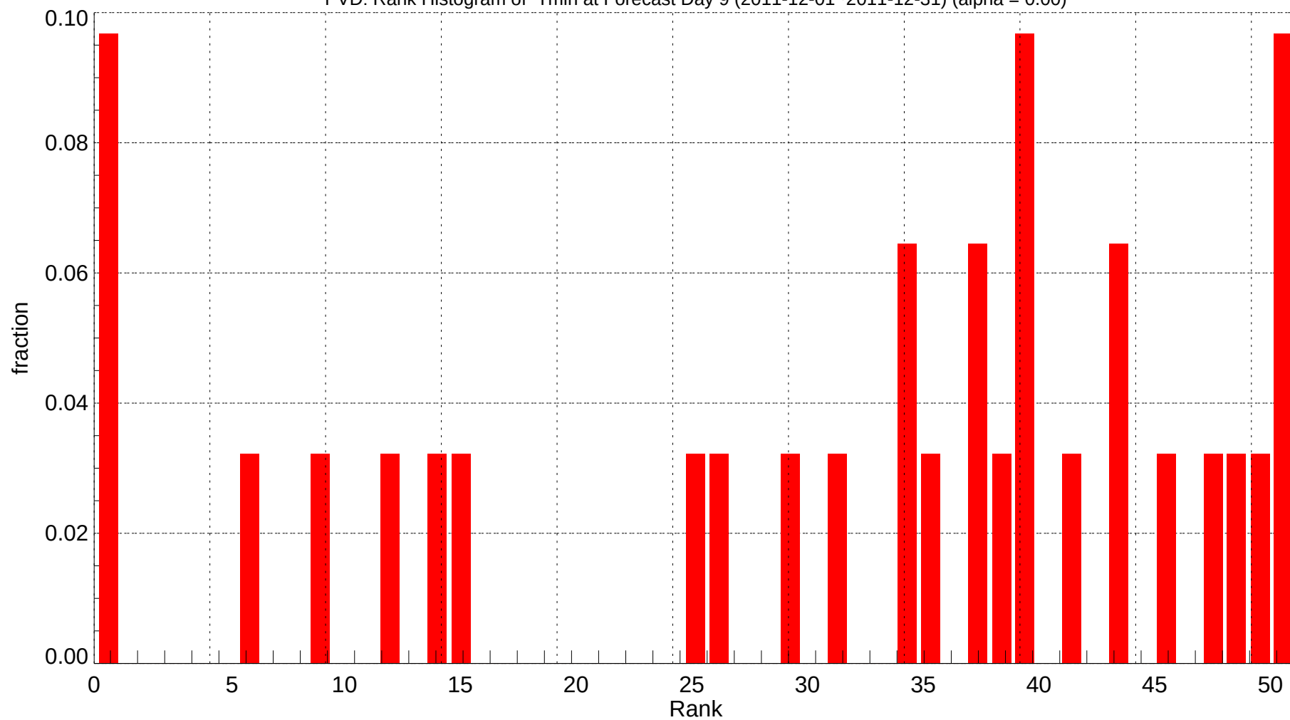
PVD: Rank Histogram of Tmin at Forecast Day 9 (2011-12-01~2011-12-31) (alpha = 0.00)
