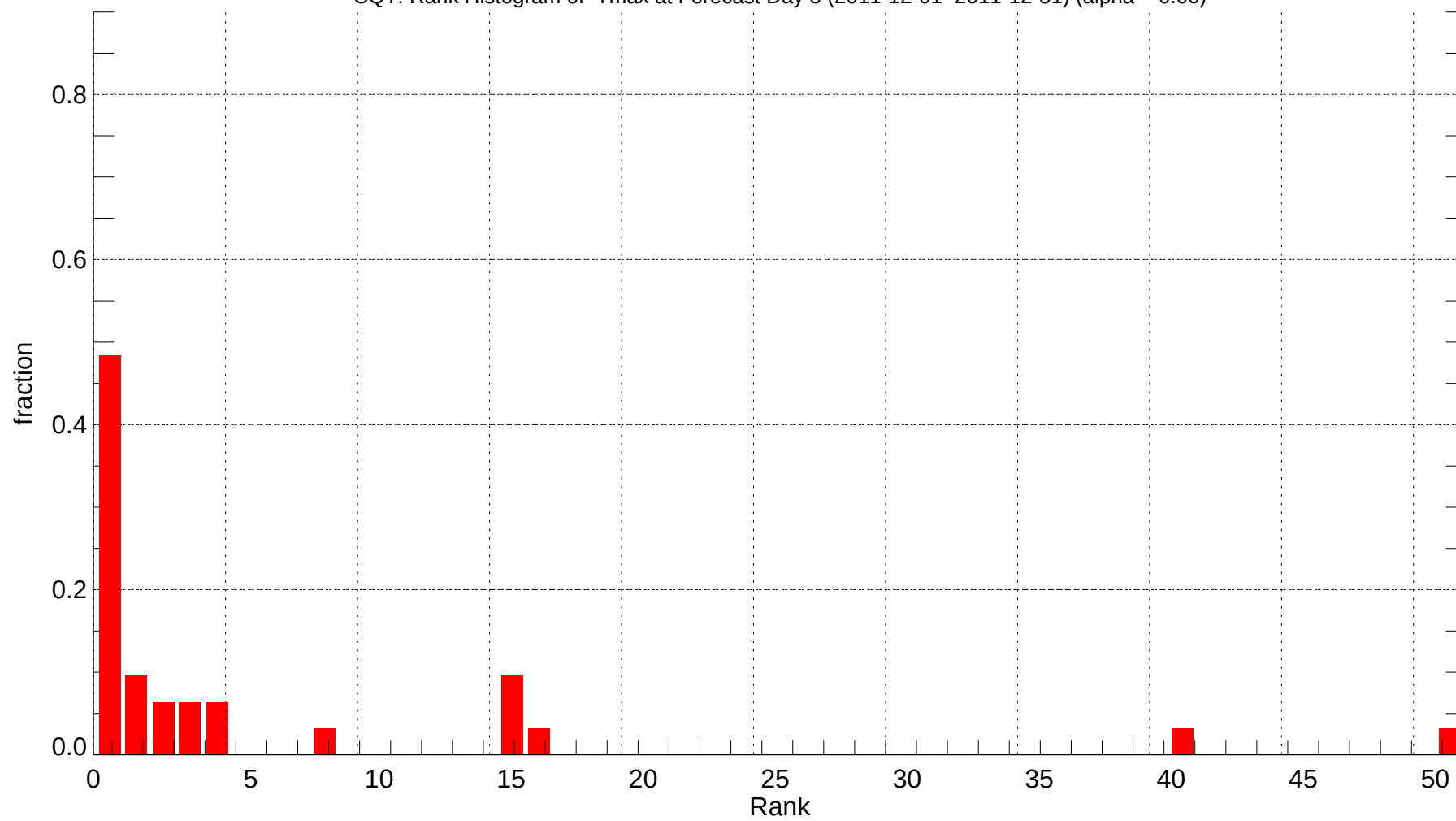
CQT: Rank Histogram of Tmax at Forecast Day 5 (2011-12-01~2011-12-31) (alpha = 0.00)
