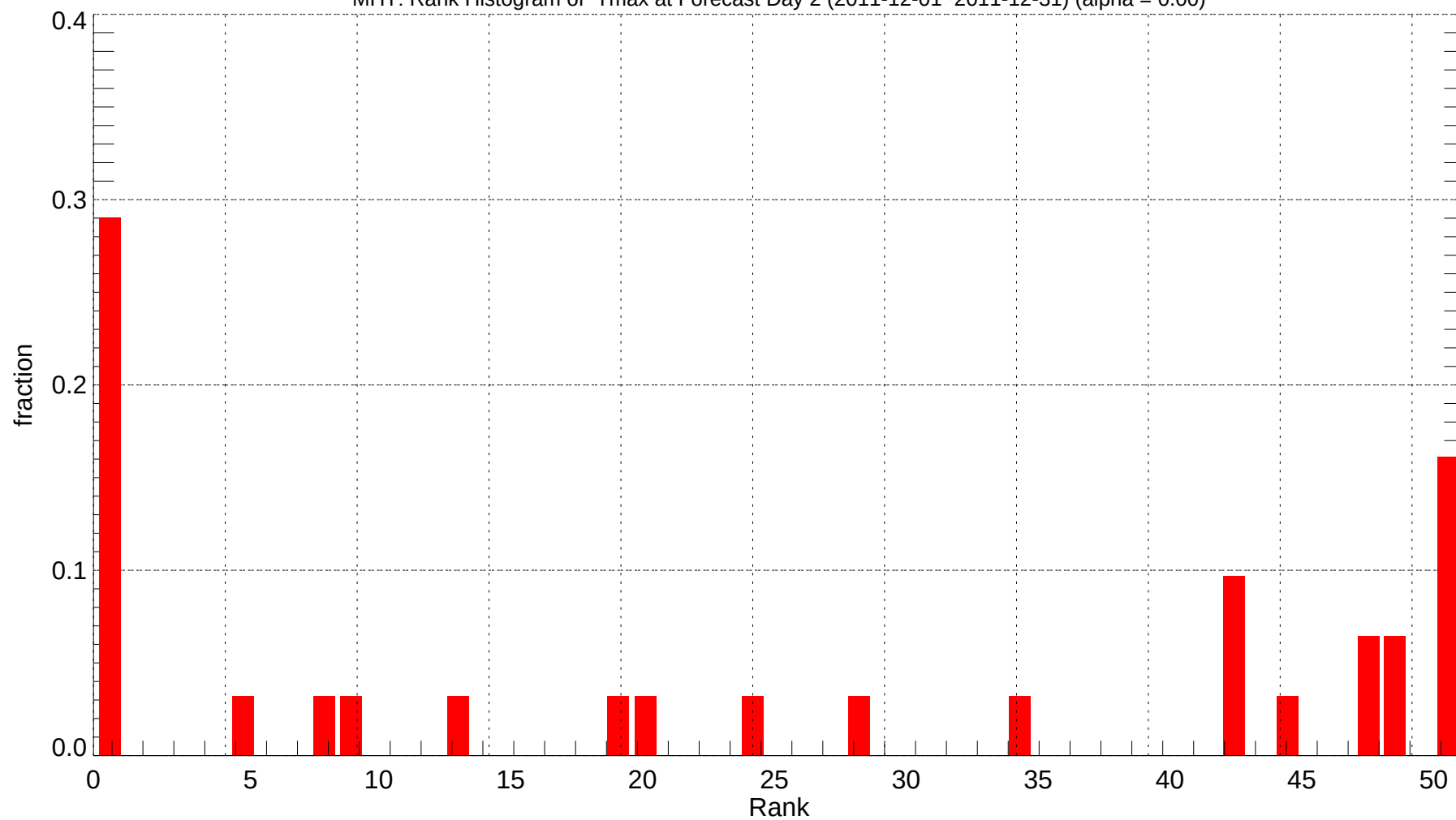
MHT: Rank Histogram of Tmax at Forecast Day 2 (2011-12-01~2011-12-31) (alpha = 0.00)
