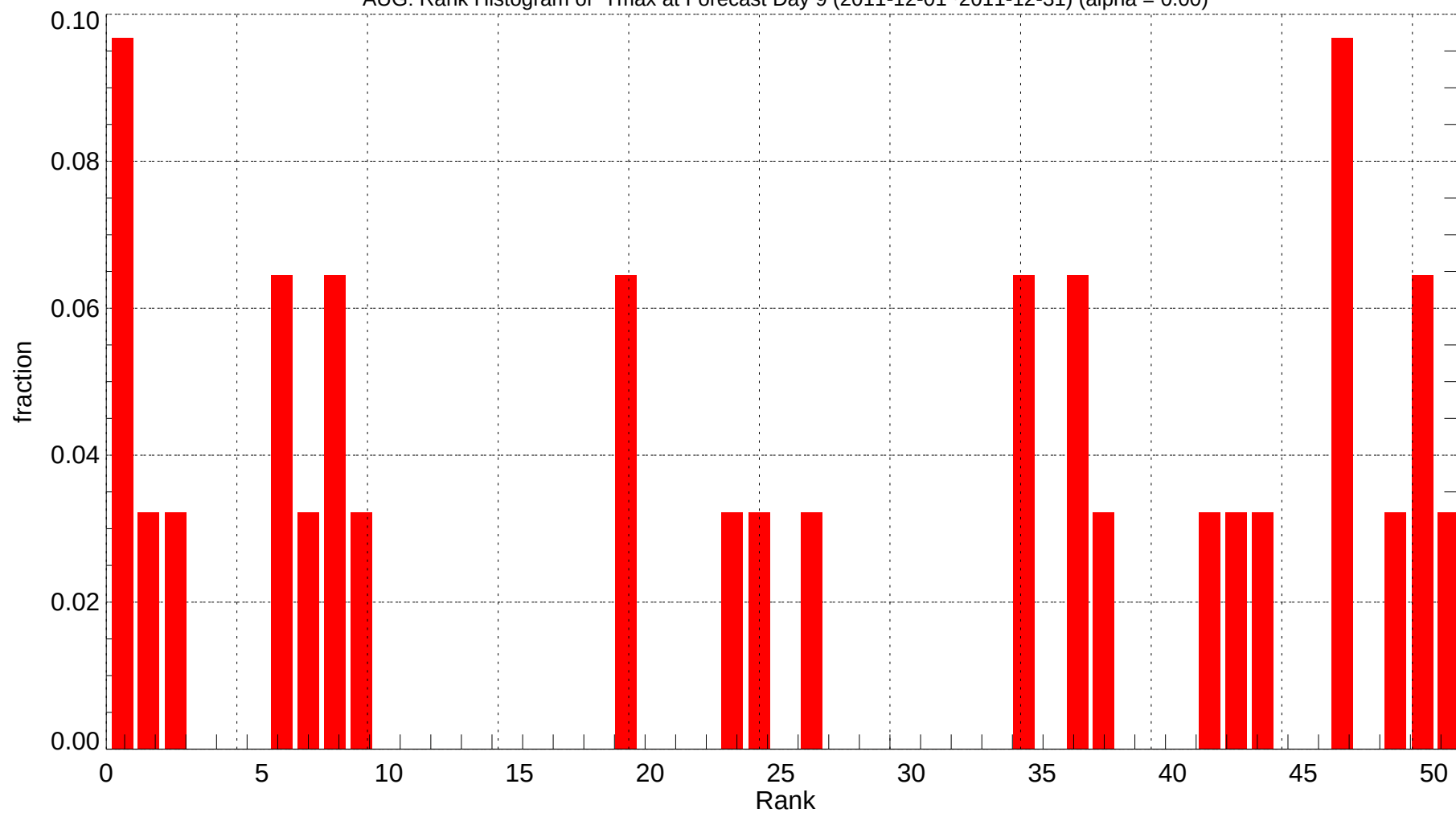
AUG: Rank Histogram of Tmax at Forecast Day 9 (2011-12-01~2011-12-31) (alpha = 0.00)
