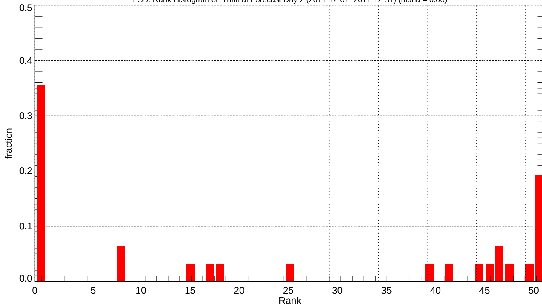
FSD: Rank Histogram of Tmin at Forecast Day 2 (2011-12-01~2011-12-31) (alpha = 0.00)
