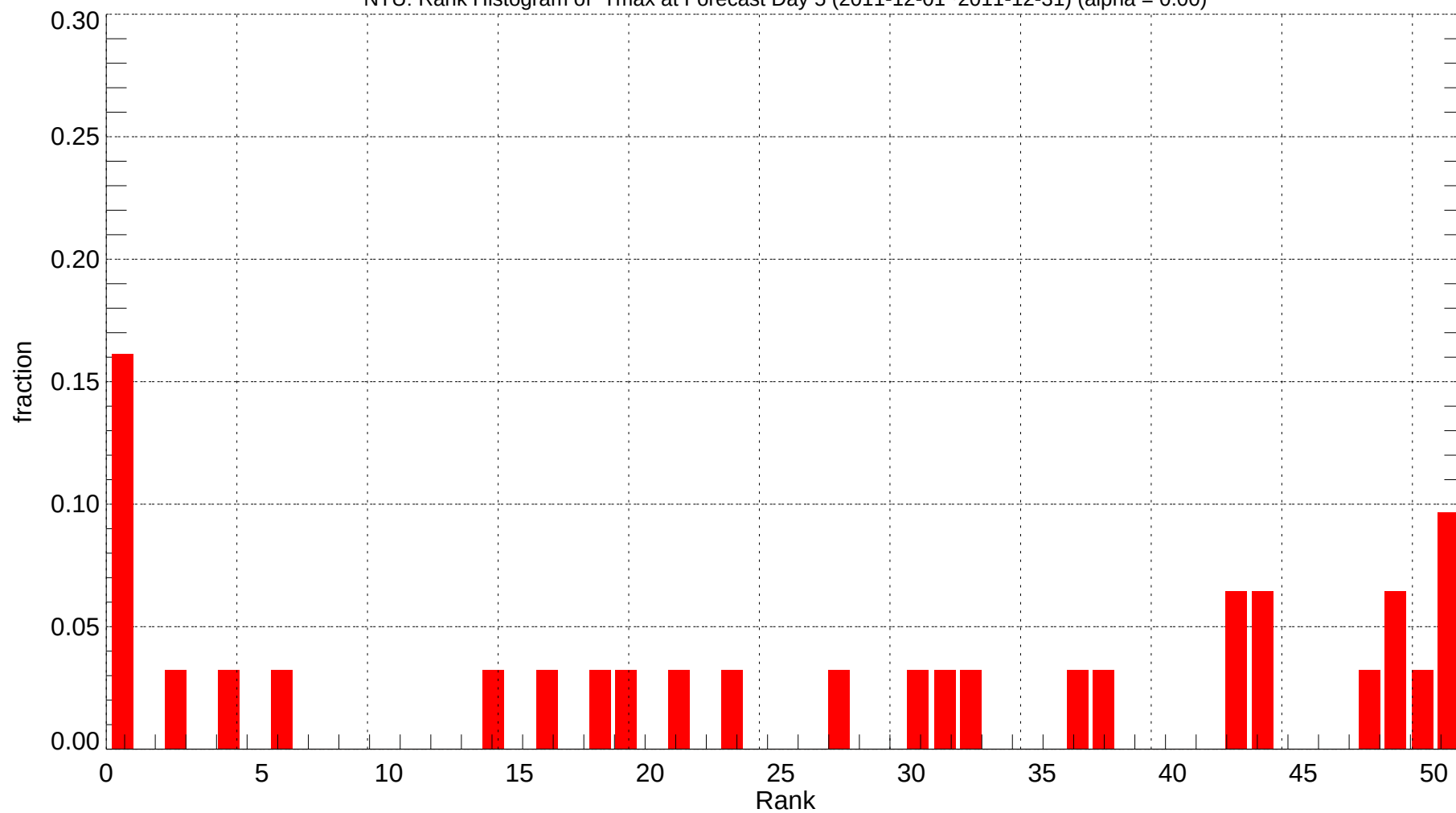
NTU: Rank Histogram of Tmax at Forecast Day 5 (2011-12-01~2011-12-31) (alpha = 0.00)
