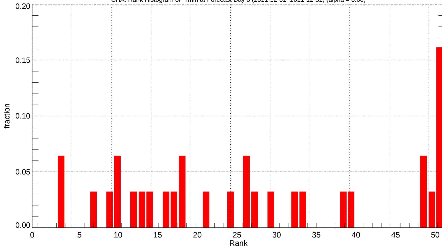
CHA: Rank Histogram of Tmin at Forecast Day 8 (2011-12-01~2011-12-31) (alpha = 0.00)
