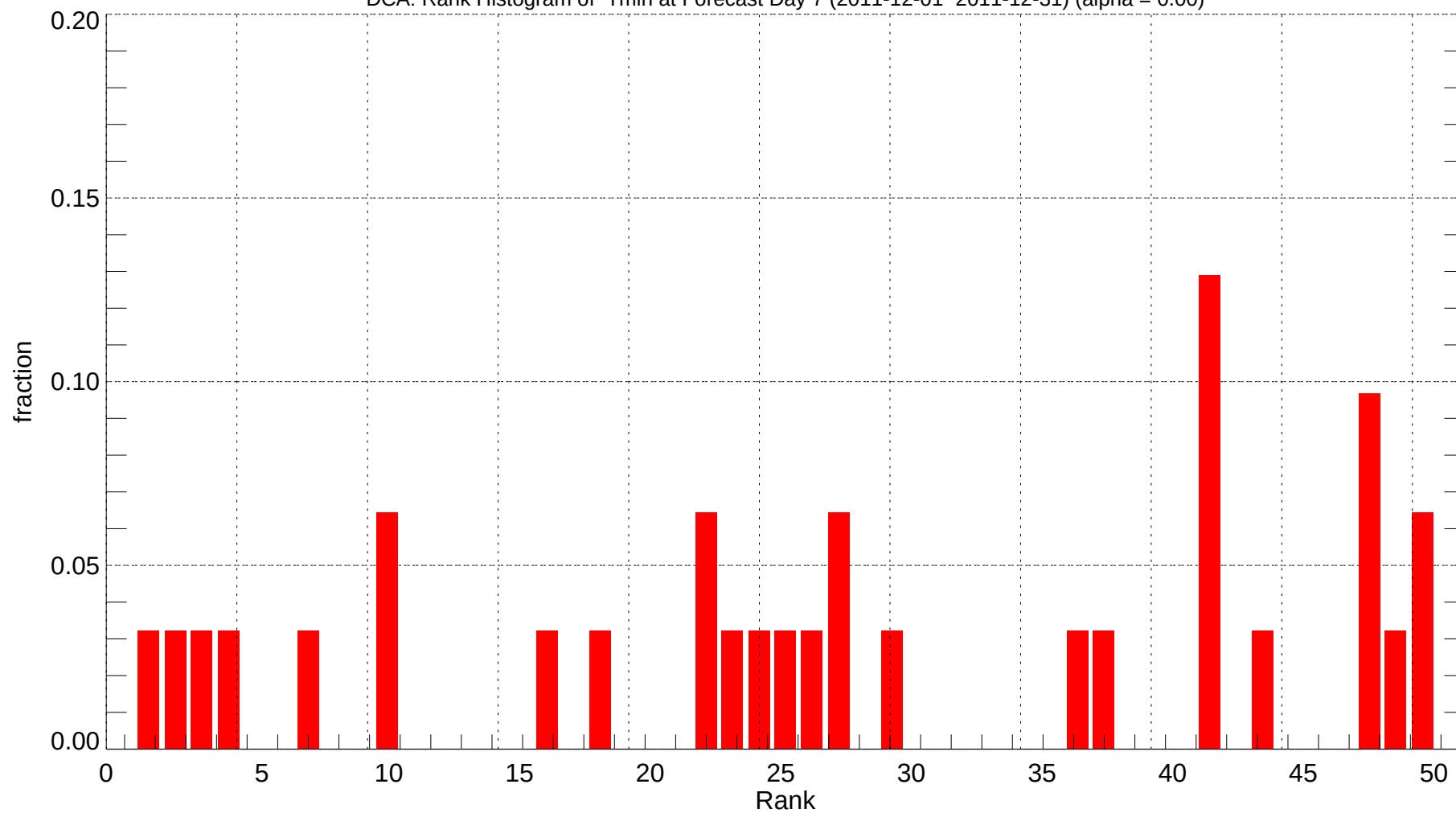
DCA: Rank Histogram of Tmin at Forecast Day 7 (2011-12-01~2011-12-31) (alpha = 0.00)
