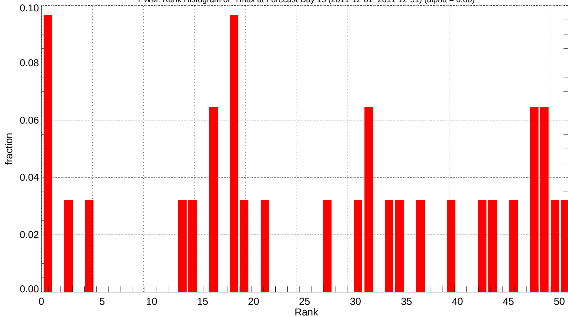
PWM: Rank Histogram of Tmax at Forecast Day 15 (2011-12-01~2011-12-31) (alpha = 0.00)
