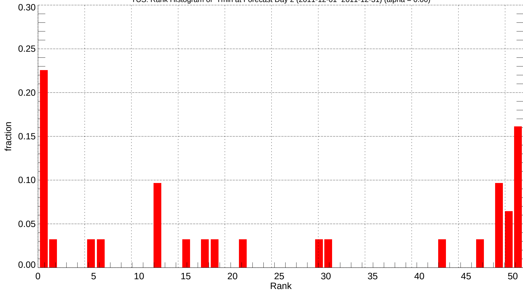
TUS: Rank Histogram of Tmin at Forecast Day 2 (2011-12-01~2011-12-31) (alpha = 0.00)
