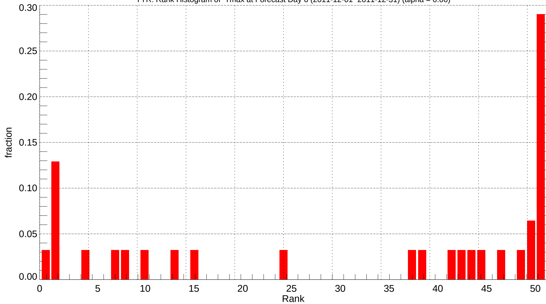
TYR: Rank Histogram of Tmax at Forecast Day 6 (2011-12-01~2011-12-31) (alpha = 0.00)
