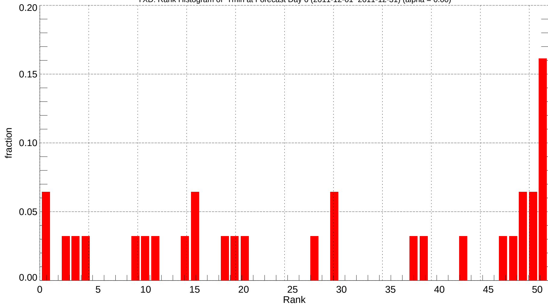
YXD: Rank Histogram of Tmin at Forecast Day 6 (2011-12-01~2011-12-31) (alpha = 0.00)
