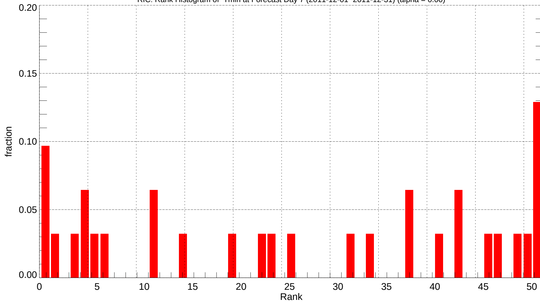
RIC: Rank Histogram of Tmin at Forecast Day 7 (2011-12-01~2011-12-31) (alpha = 0.00)
