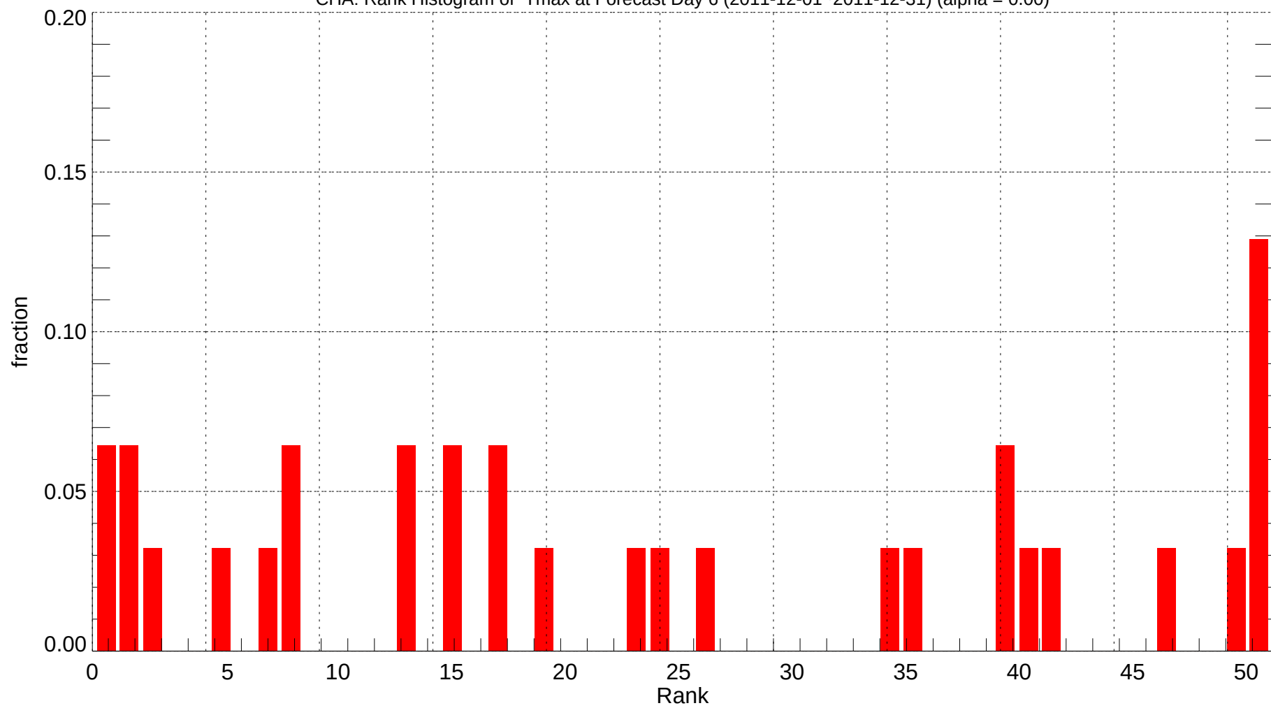
CHA: Rank Histogram of Tmax at Forecast Day 6 (2011-12-01~2011-12-31) (alpha = 0.00)
