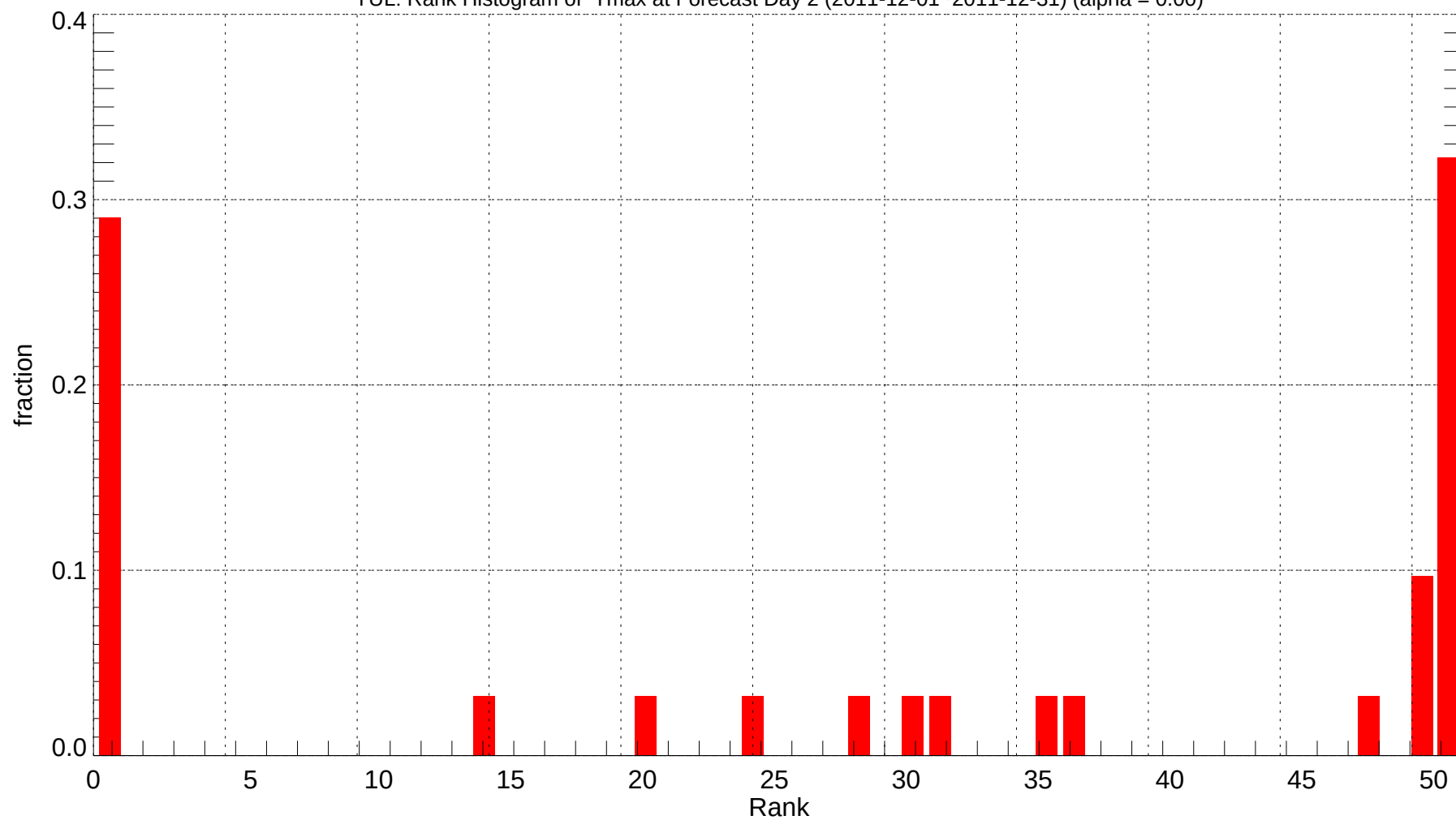
YUL: Rank Histogram of Tmax at Forecast Day 2 (2011-12-01~2011-12-31) (alpha = 0.00)
