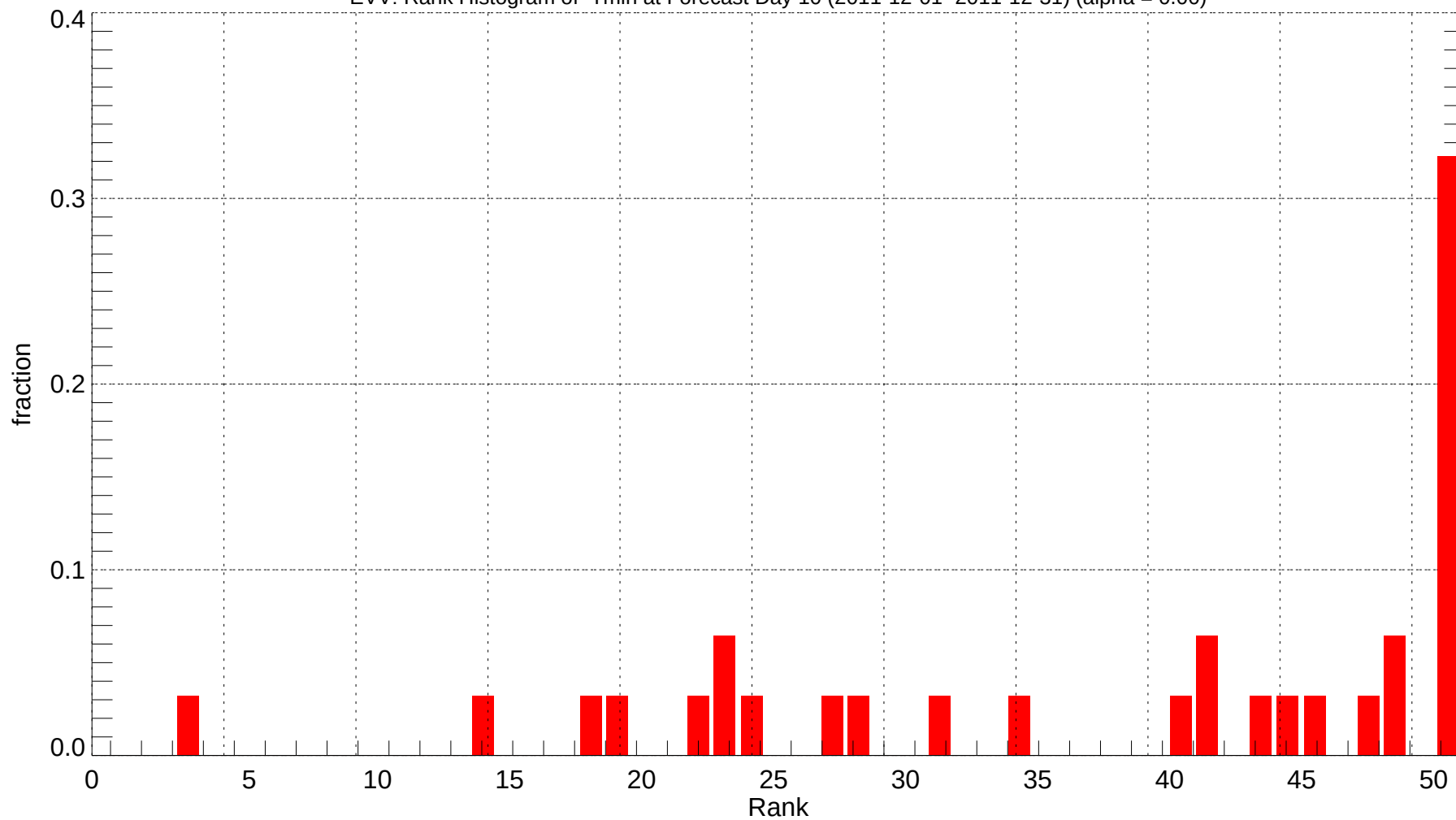
EVV: Rank Histogram of Tmin at Forecast Day 10 (2011-12-01~2011-12-31) (alpha = 0.00)
