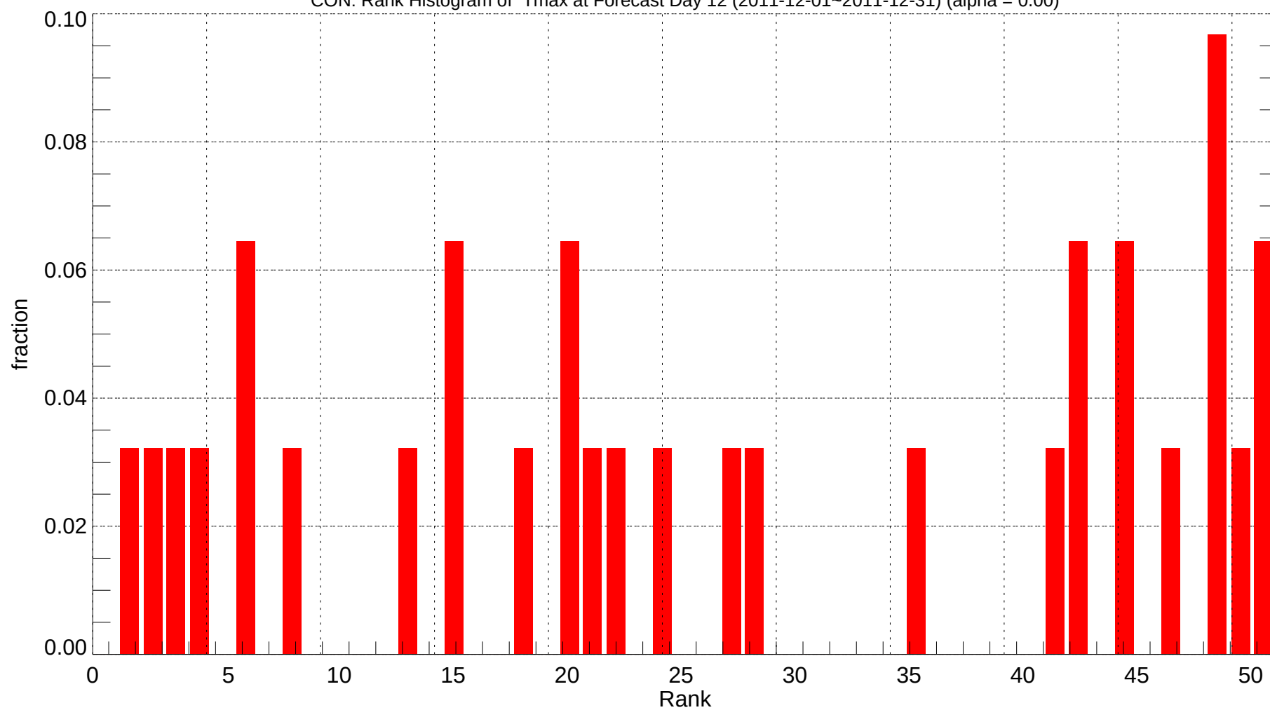
CON: Rank Histogram of Tmax at Forecast Day 12 (2011-12-01~2011-12-31) (alpha = 0.00)
