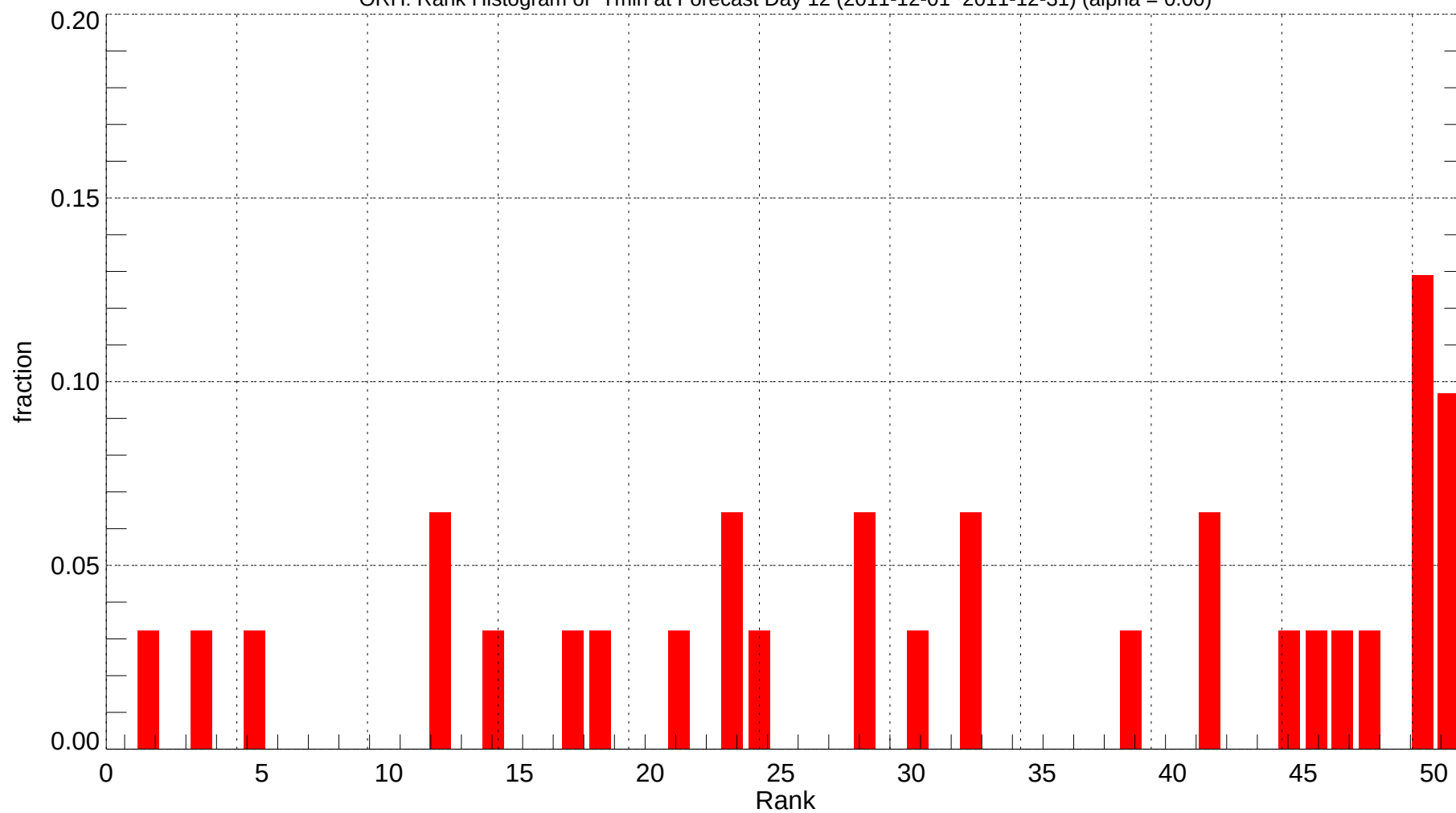
ORH: Rank Histogram of Tmin at Forecast Day 12 (2011-12-01~2011-12-31) (alpha = 0.00)
