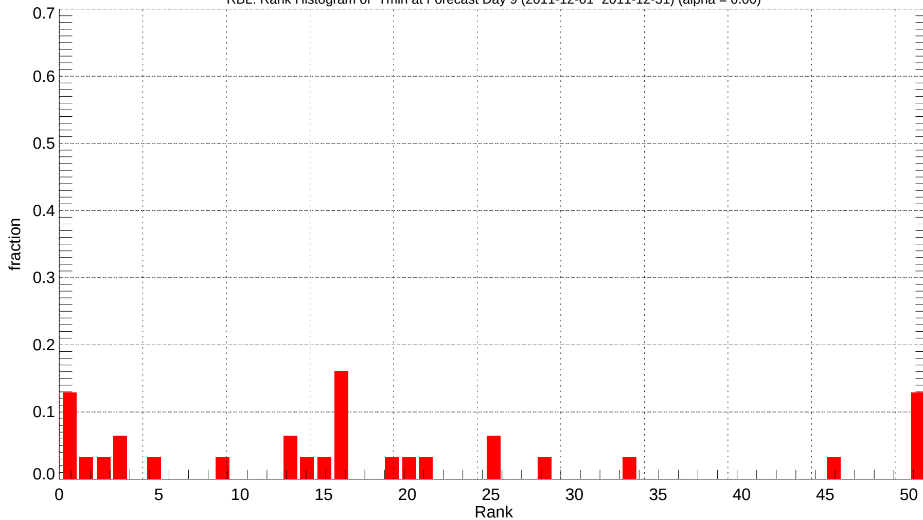
RBL: Rank Histogram of Tmin at Forecast Day 9 (2011-12-01~2011-12-31) (alpha = 0.00)
