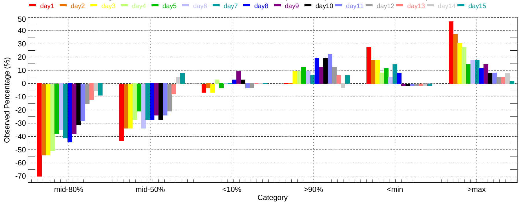
Observed Percentage Deviation of Ensembles - SAT: Min Temperature (2011-12-01~2011-12-31)
