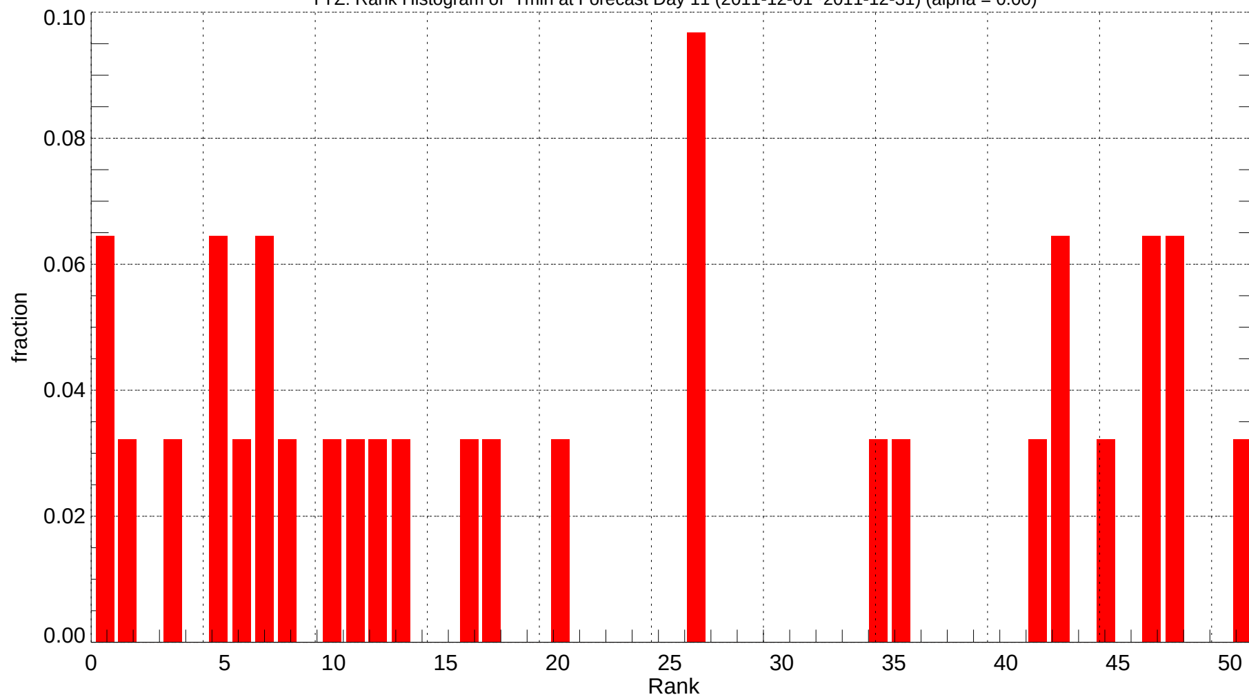
YYZ: Rank Histogram of Tmin at Forecast Day 11 (2011-12-01~2011-12-31) (alpha = 0.00)
