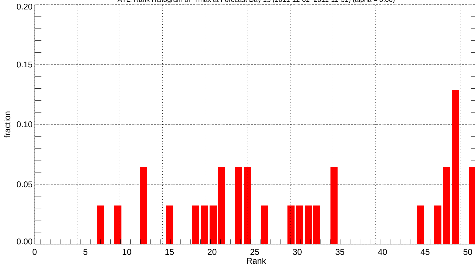
ATL: Rank Histogram of Tmax at Forecast Day 15 (2011-12-01~2011-12-31) (alpha = 0.00)
