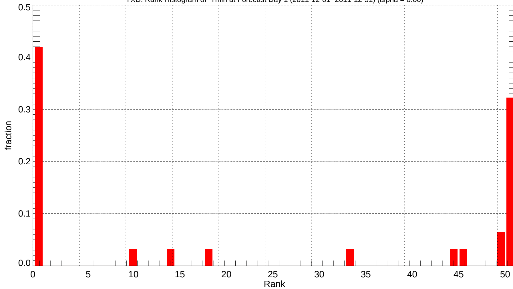
YXD: Rank Histogram of Tmin at Forecast Day 1 (2011-12-01~2011-12-31) (alpha = 0.00)
