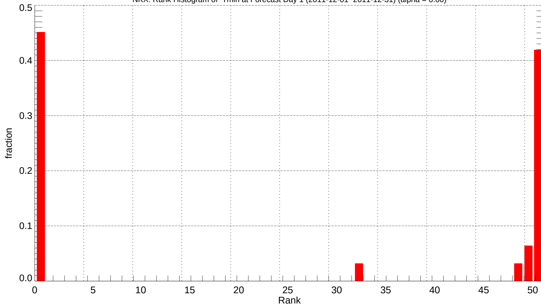
NKX: Rank Histogram of Tmin at Forecast Day 1 (2011-12-01~2011-12-31) (alpha = 0.00)
