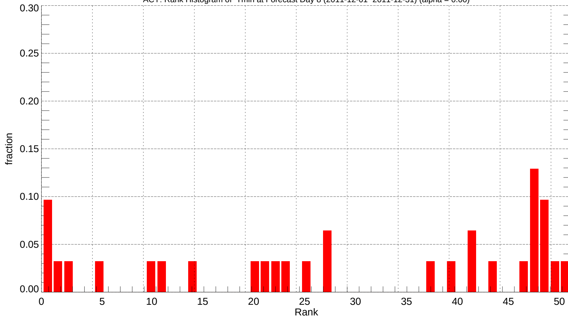
ACY: Rank Histogram of Tmin at Forecast Day 8 (2011-12-01~2011-12-31) (alpha = 0.00)
