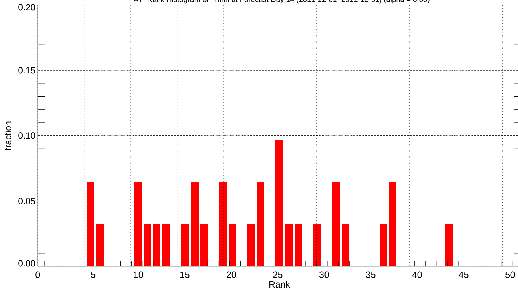
FAT: Rank Histogram of Tmin at Forecast Day 14 (2011-12-01~2011-12-31) (alpha = 0.00)
