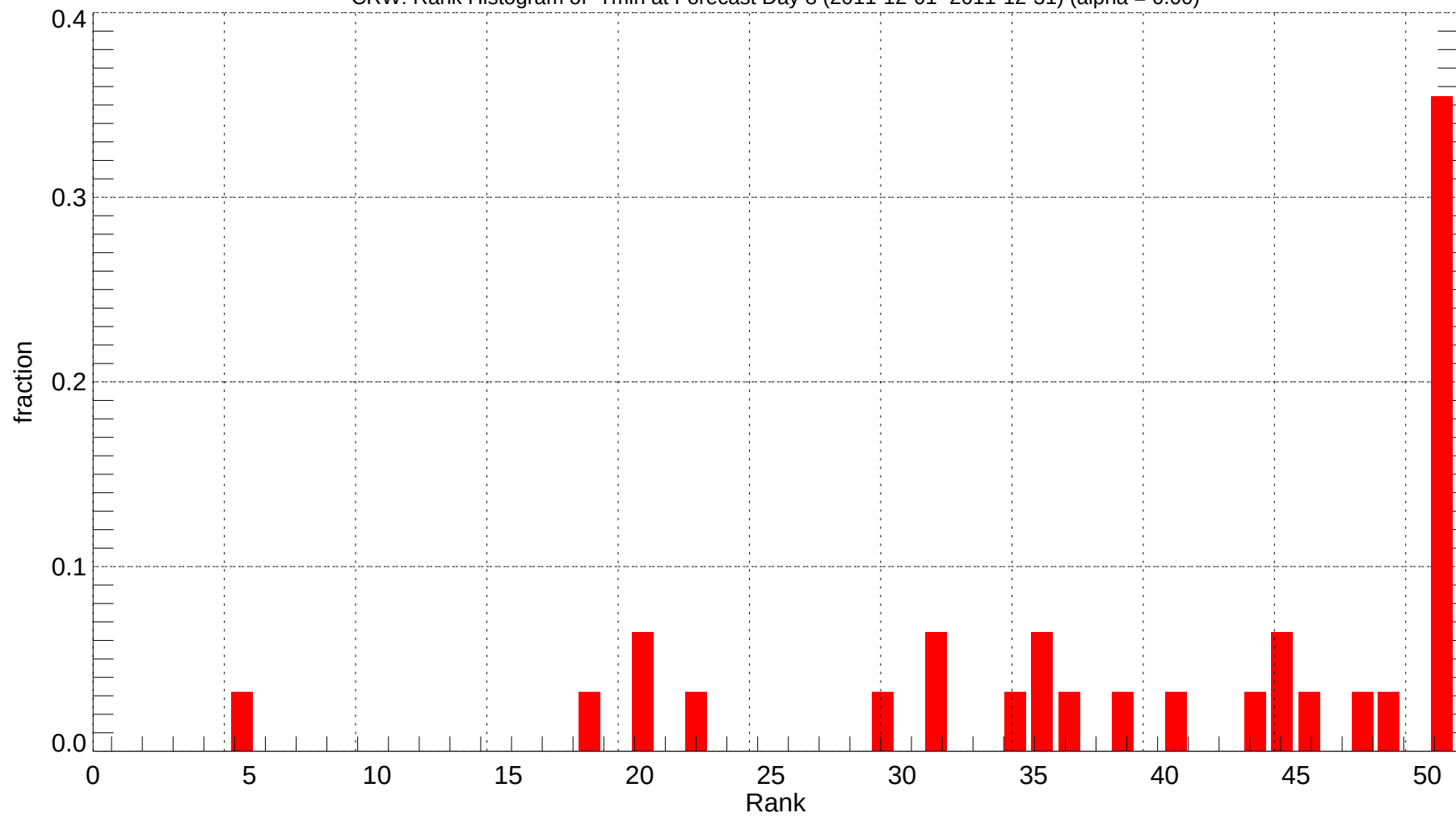
CRW: Rank Histogram of Tmin at Forecast Day 8 (2011-12-01~2011-12-31) (alpha = 0.00)
