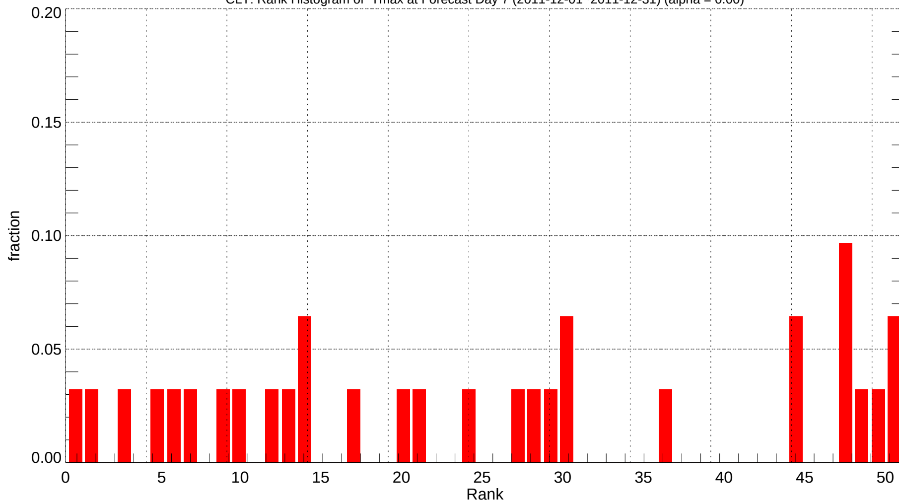
CLT: Rank Histogram of Tmax at Forecast Day 7 (2011-12-01~2011-12-31) (alpha = 0.00)
