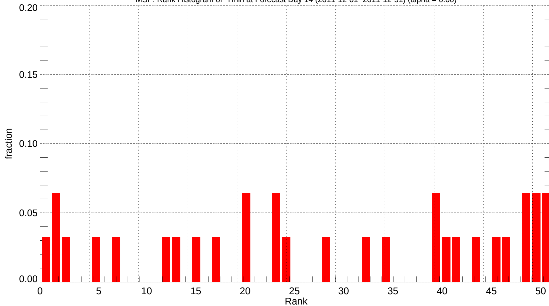
MSP: Rank Histogram of Tmin at Forecast Day 14 (2011-12-01~2011-12-31) (alpha = 0.00)
