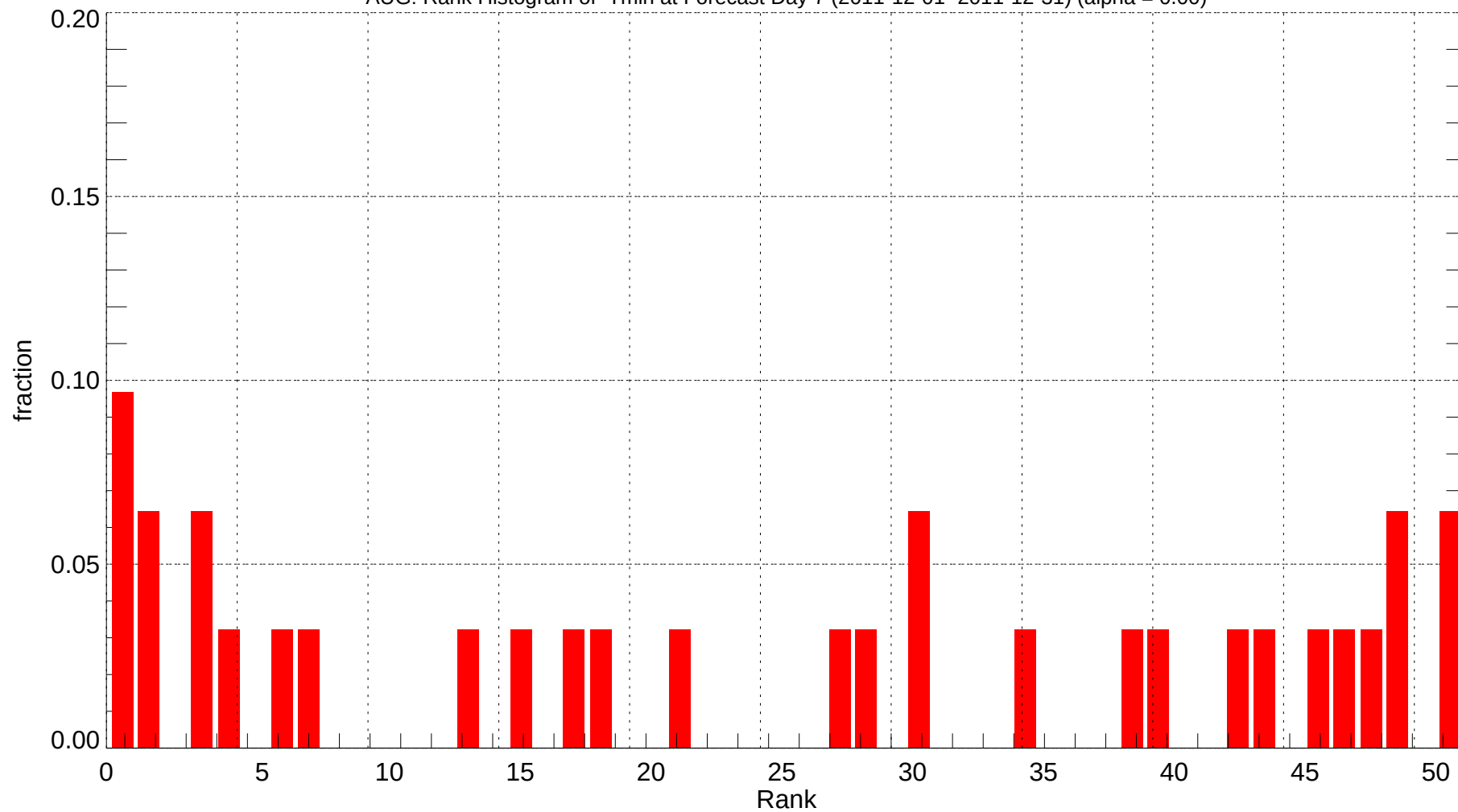
AUG: Rank Histogram of Tmin at Forecast Day 7 (2011-12-01~2011-12-31) (alpha = 0.00)
