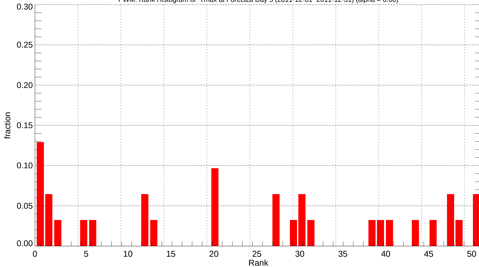
PWM: Rank Histogram of Tmax at Forecast Day 5 (2011-12-01~2011-12-31) (alpha = 0.00)
