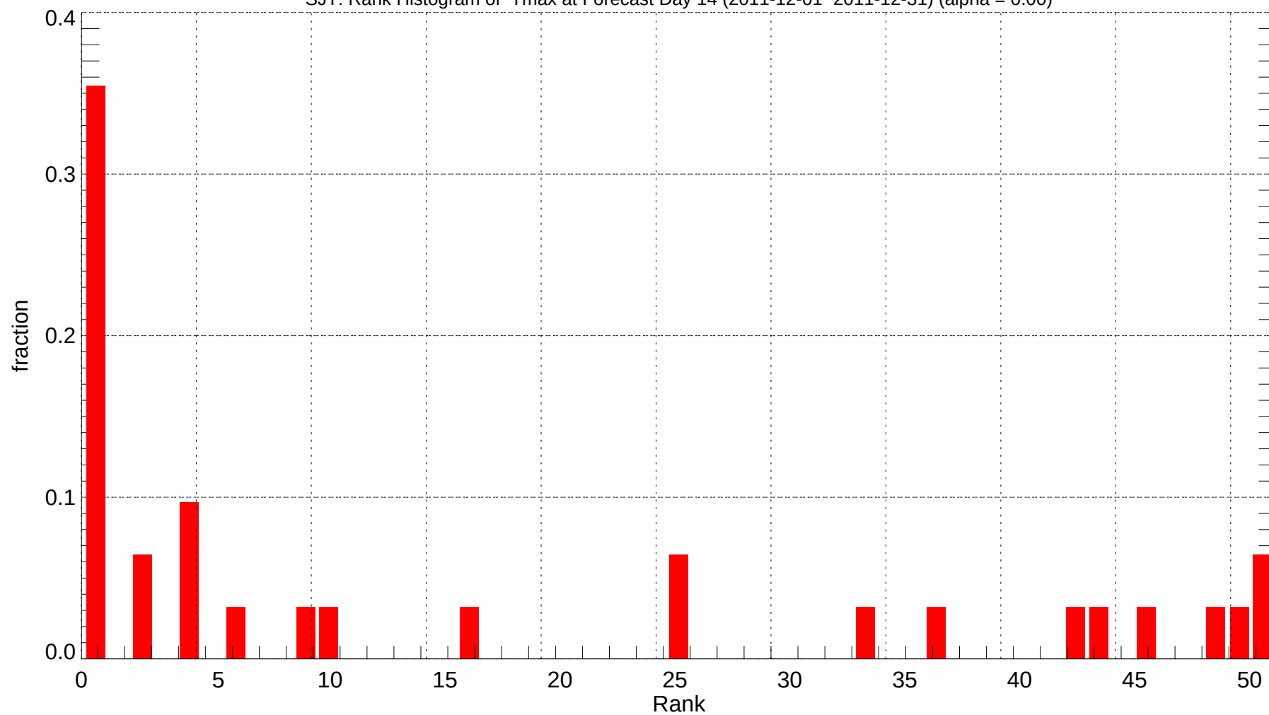
SJT: Rank Histogram of Tmax at Forecast Day 14 (2011-12-01~2011-12-31) (alpha = 0.00)
