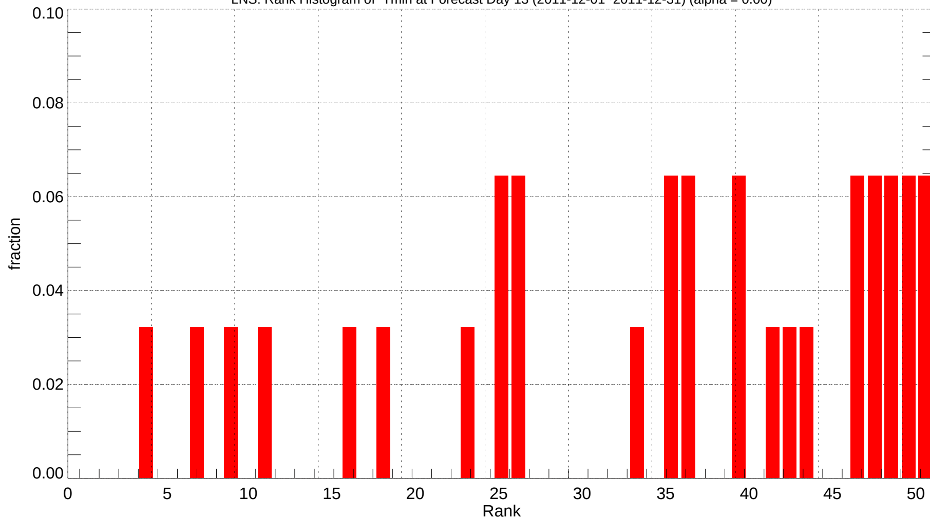
LNS: Rank Histogram of Tmin at Forecast Day 13 (2011-12-01~2011-12-31) (alpha = 0.00)
