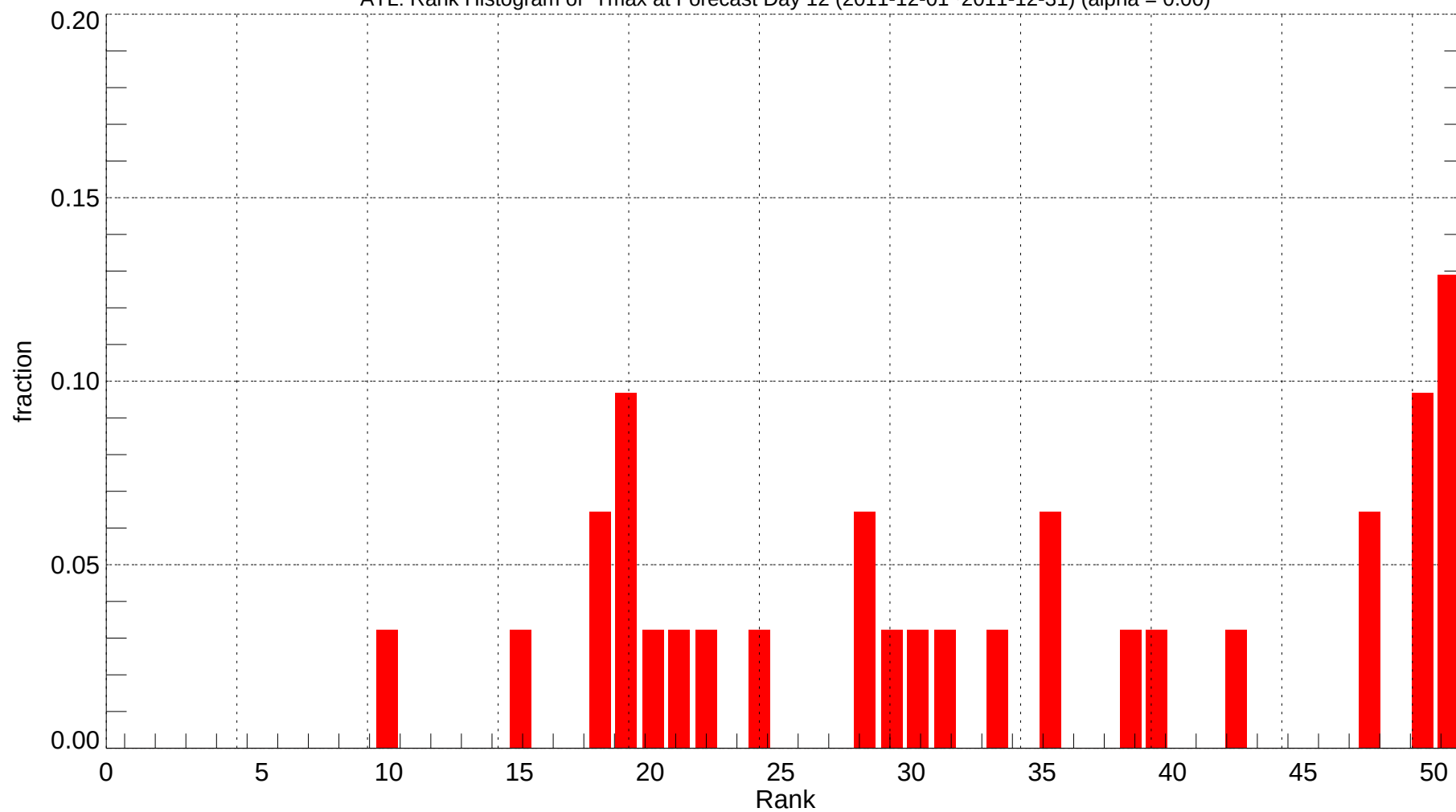
ATL: Rank Histogram of Tmax at Forecast Day 12 (2011-12-01~2011-12-31) (alpha = 0.00)
