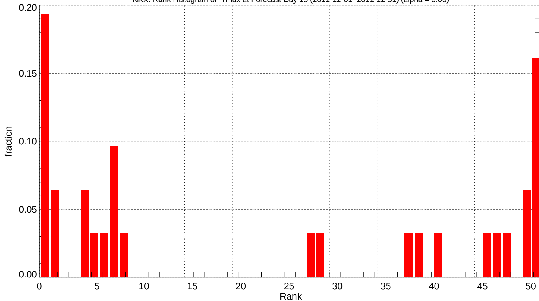
NKX: Rank Histogram of Tmax at Forecast Day 15 (2011-12-01~2011-12-31) (alpha = 0.00)
