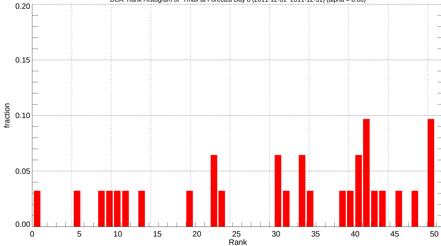
DCA: Rank Histogram of Tmax at Forecast Day 8 (2011-12-01~2011-12-31) (alpha = 0.00)
