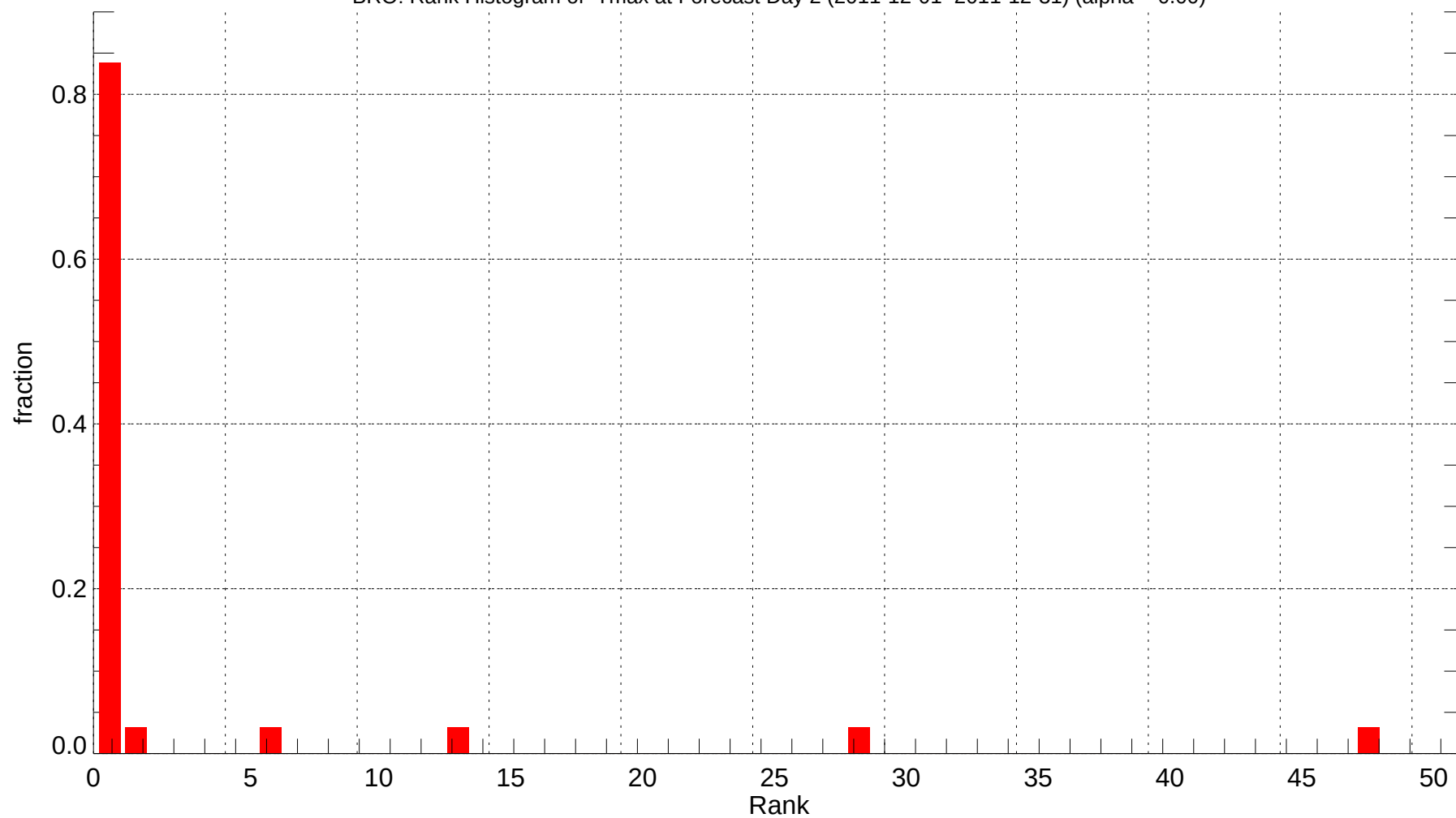
BRO: Rank Histogram of Tmax at Forecast Day 2 (2011-12-01~2011-12-31) (alpha = 0.00)
