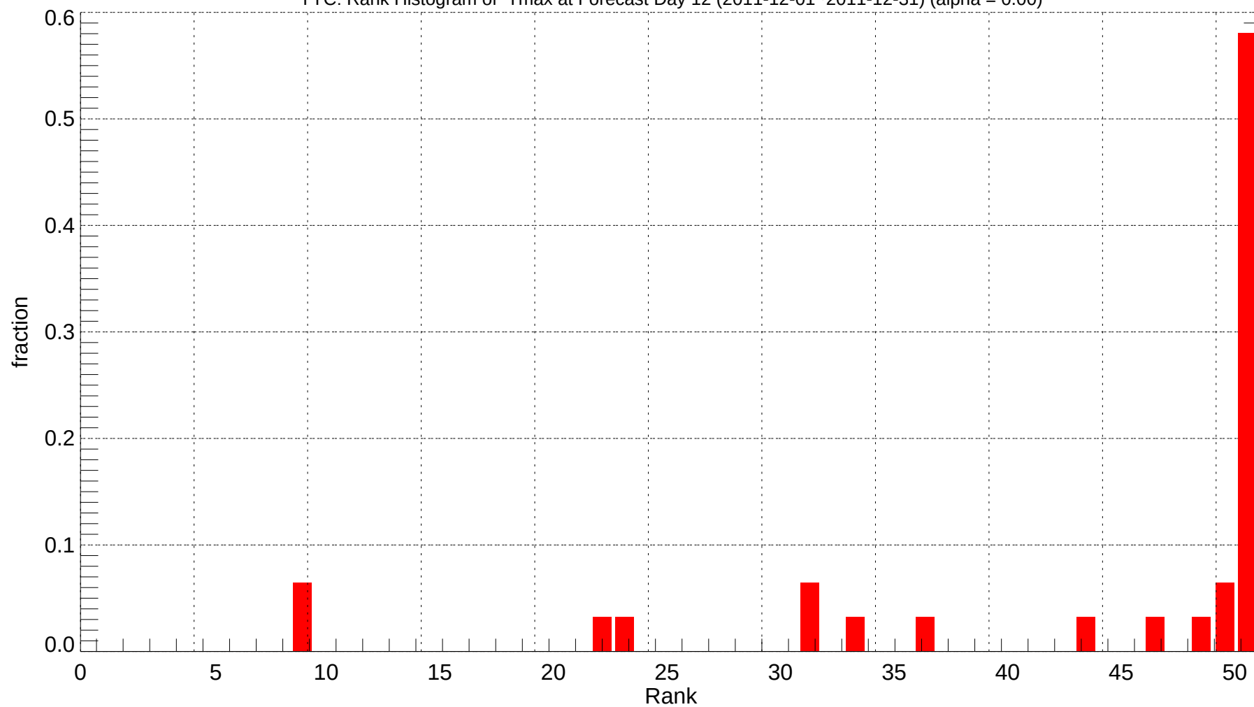
YYC: Rank Histogram of Tmax at Forecast Day 12 (2011-12-01~2011-12-31) (alpha = 0.00)
