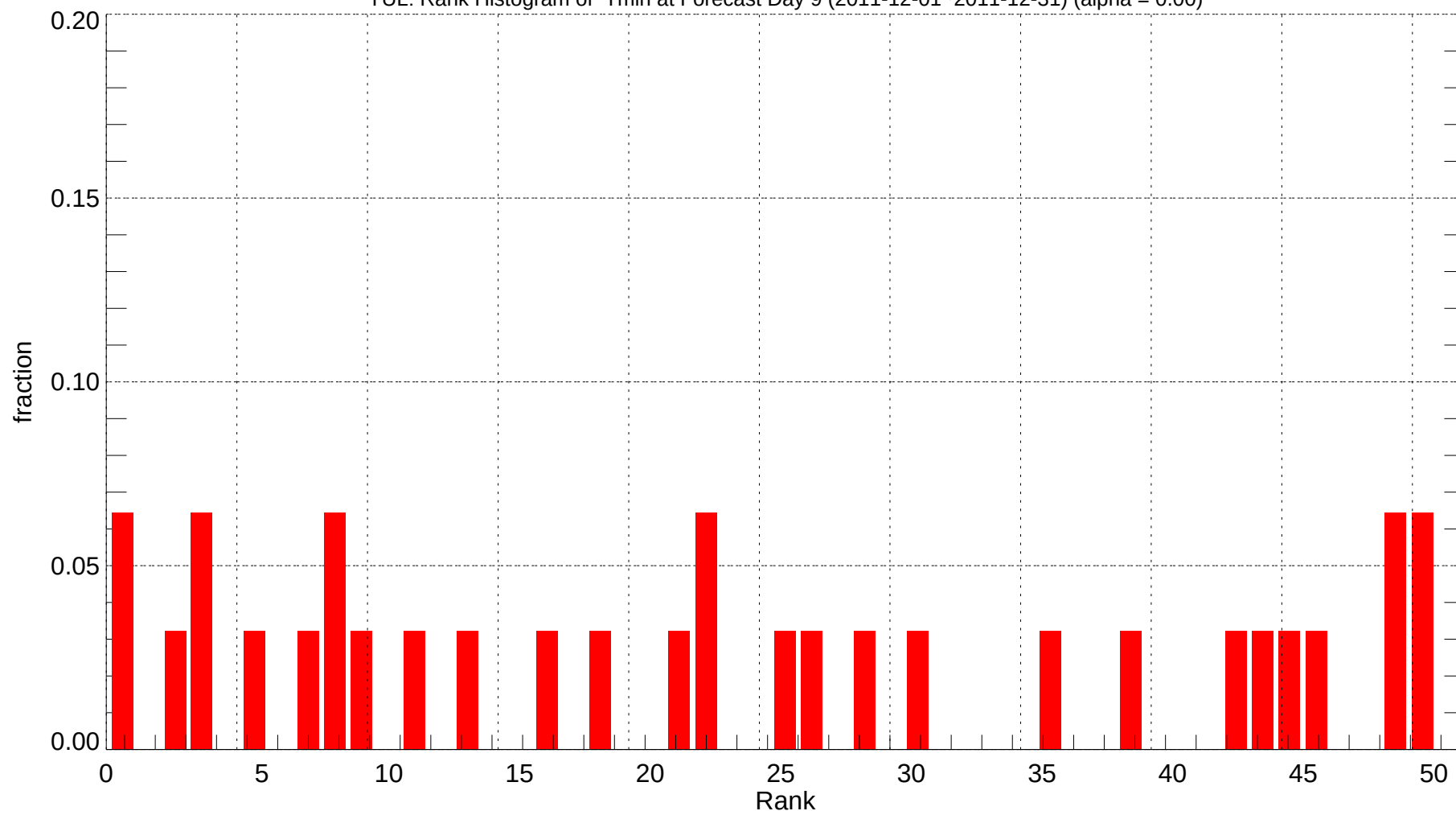
YUL: Rank Histogram of Tmin at Forecast Day 9 (2011-12-01~2011-12-31) (alpha = 0.00)
