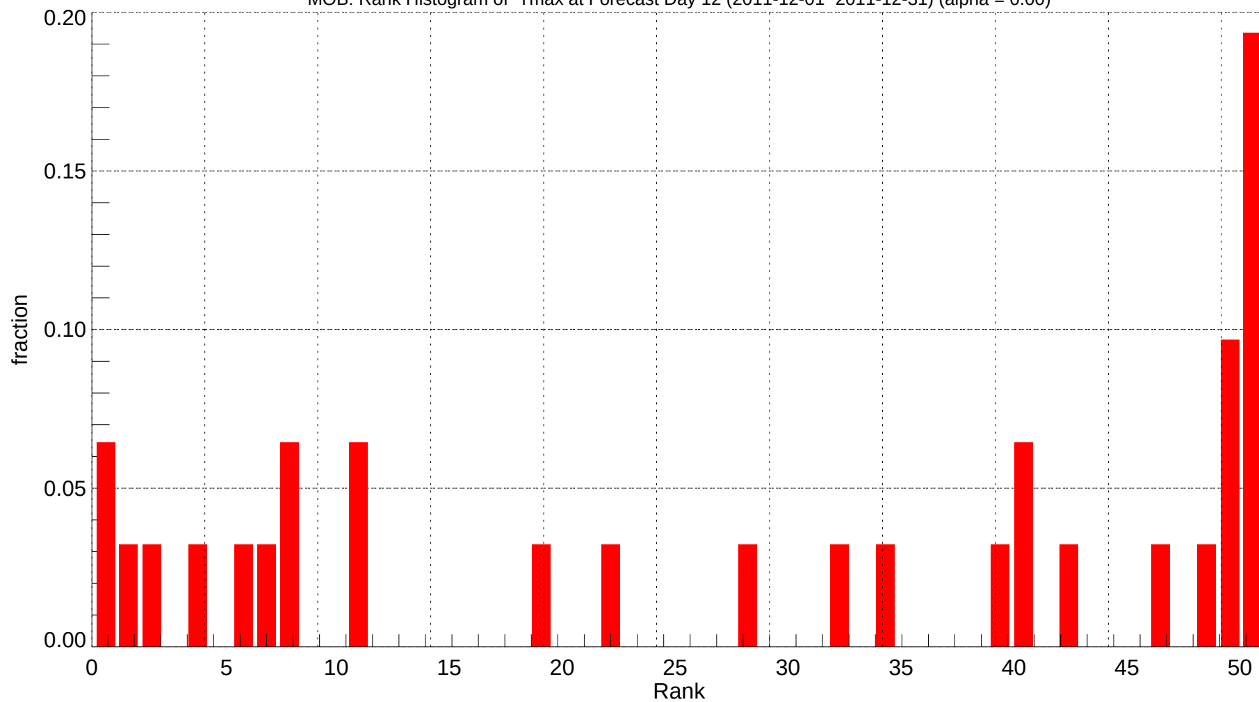
MOB: Rank Histogram of Tmax at Forecast Day 12 (2011-12-01~2011-12-31) (alpha = 0.00)
