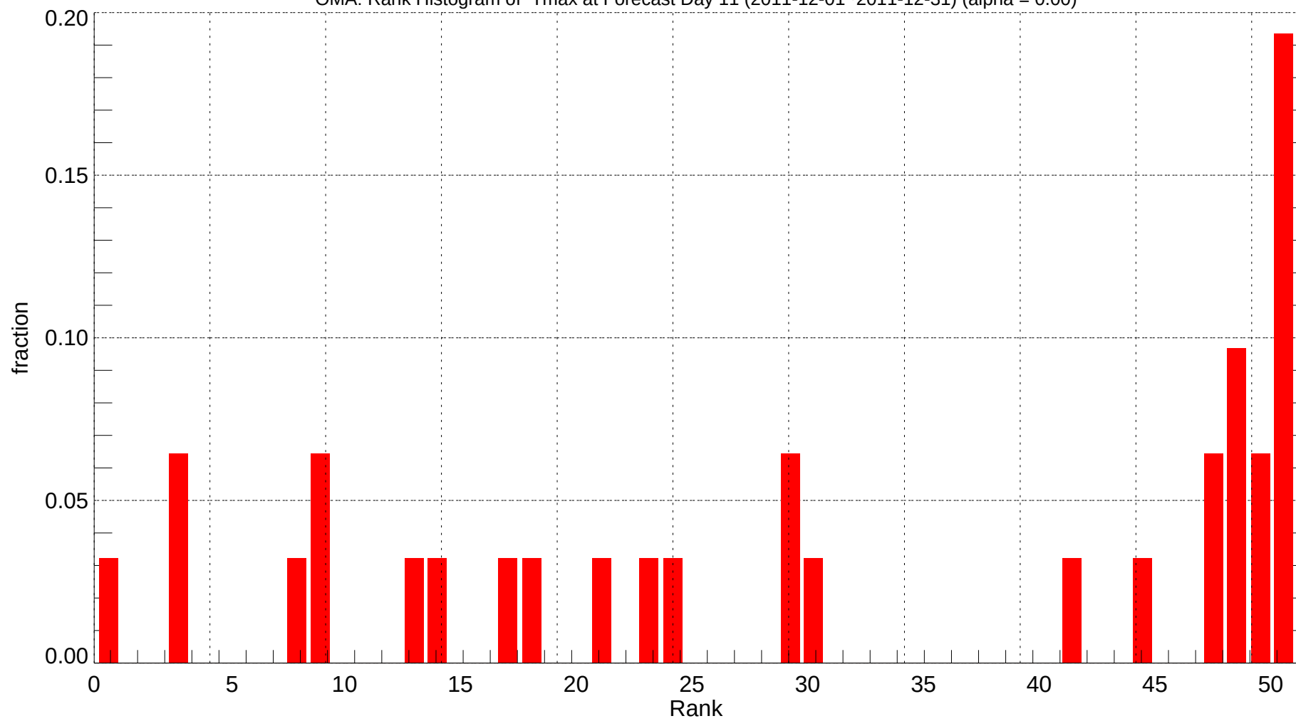
OMA: Rank Histogram of Tmax at Forecast Day 11 (2011-12-01~2011-12-31) (alpha = 0.00)
