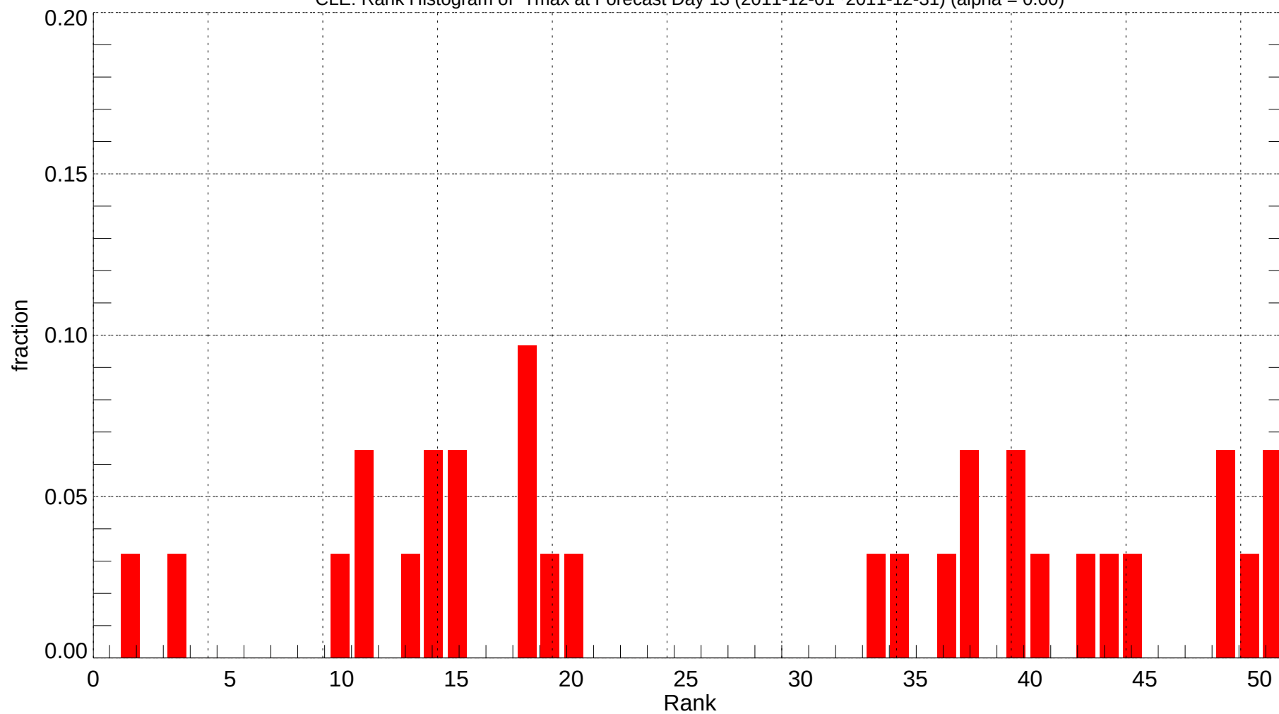
CLE: Rank Histogram of Tmax at Forecast Day 13 (2011-12-01~2011-12-31) (alpha = 0.00)
