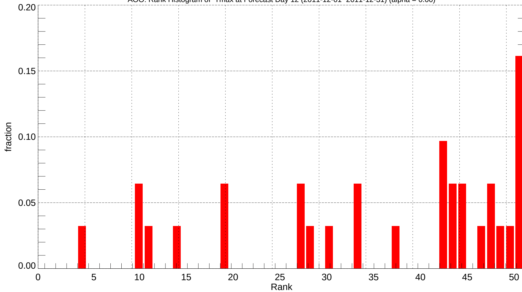
AOO: Rank Histogram of Tmax at Forecast Day 12 (2011-12-01~2011-12-31) (alpha = 0.00)
