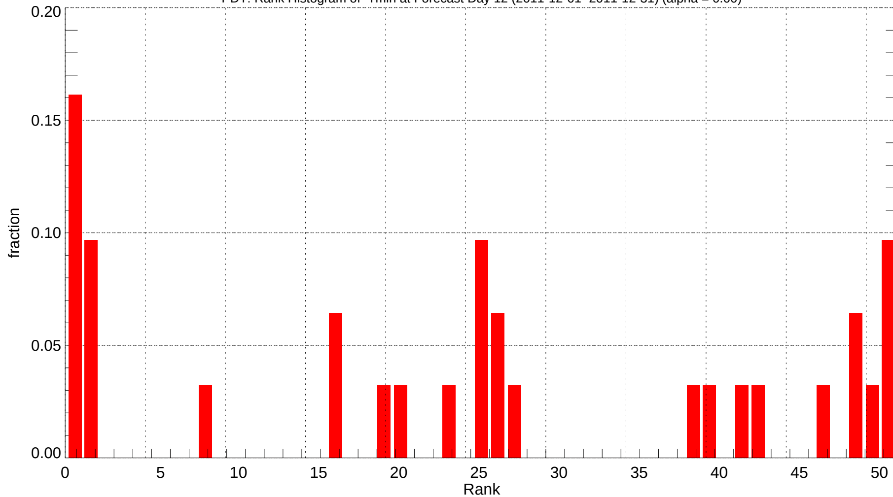
PDT: Rank Histogram of Tmin at Forecast Day 12 (2011-12-01~2011-12-31) (alpha = 0.00)
