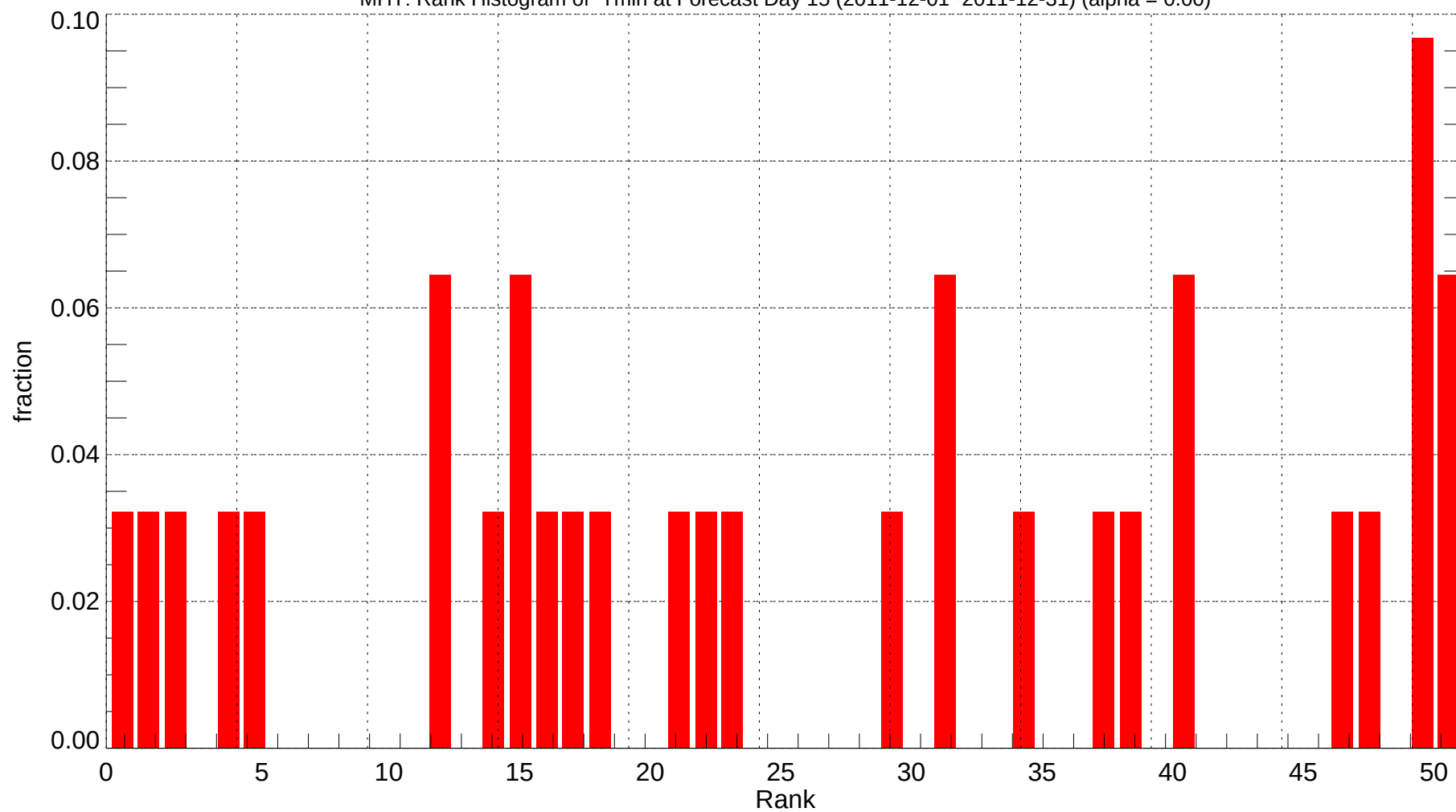
MHT: Rank Histogram of Tmin at Forecast Day 15 (2011-12-01~2011-12-31) (alpha = 0.00)
