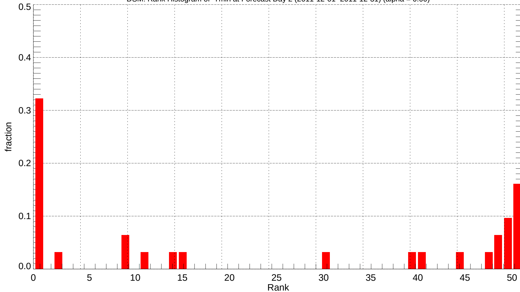
DSM: Rank Histogram of Tmin at Forecast Day 2 (2011-12-01~2011-12-31) (alpha = 0.00)
