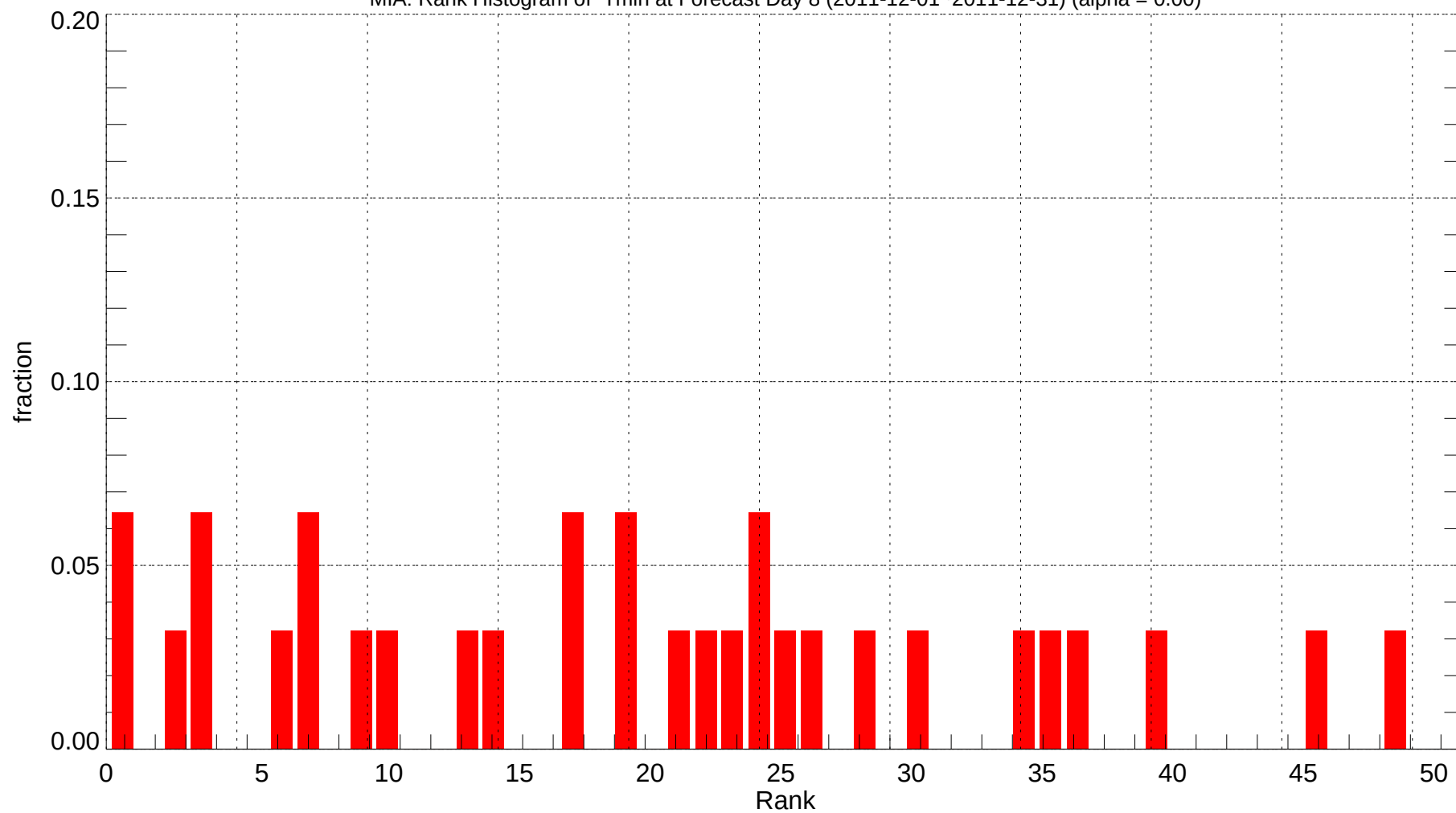
MIA: Rank Histogram of Tmin at Forecast Day 8 (2011-12-01~2011-12-31) (alpha = 0.00)
