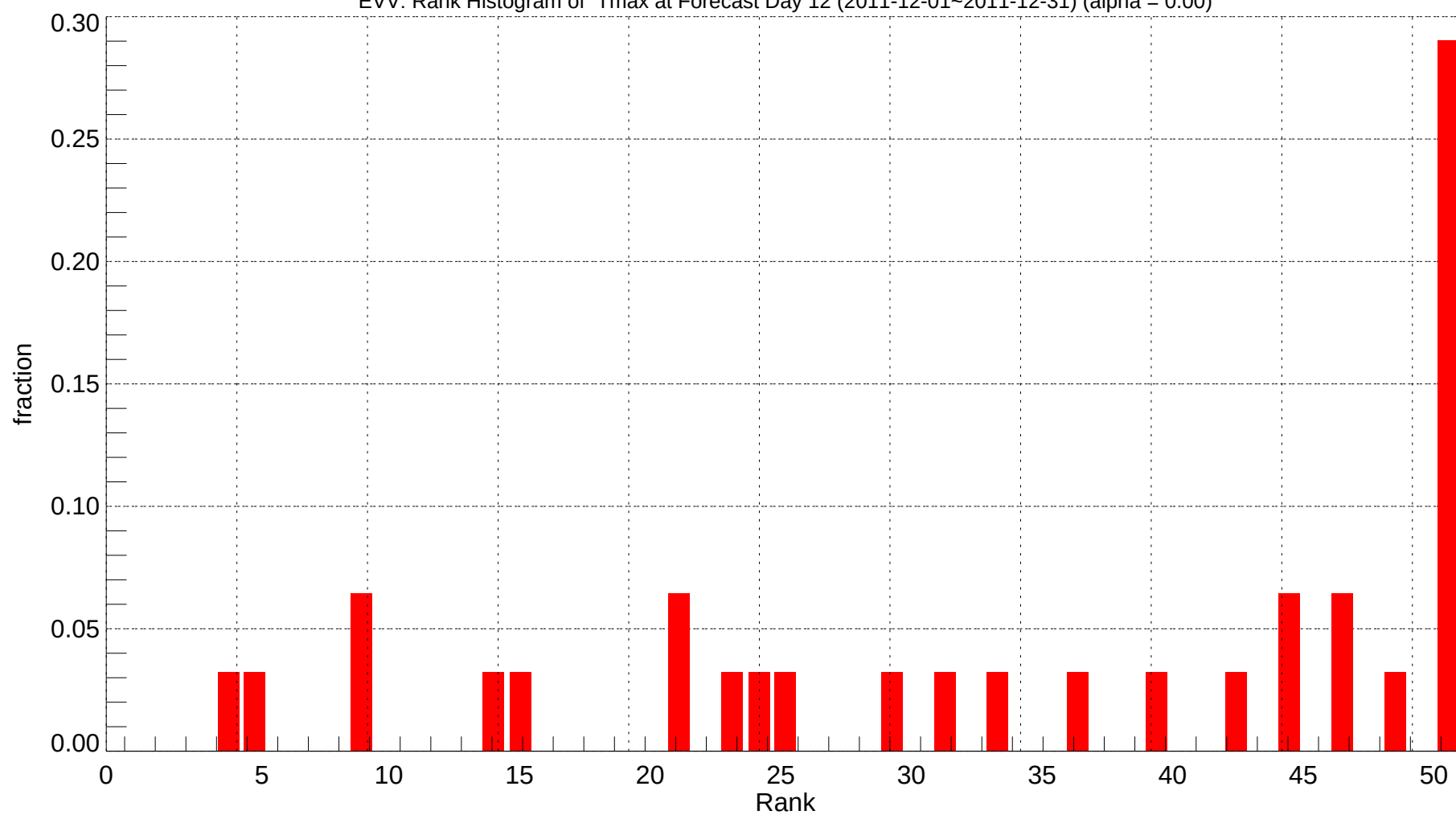
EVV: Rank Histogram of Tmax at Forecast Day 12 (2011-12-01~2011-12-31) (alpha = 0.00)
