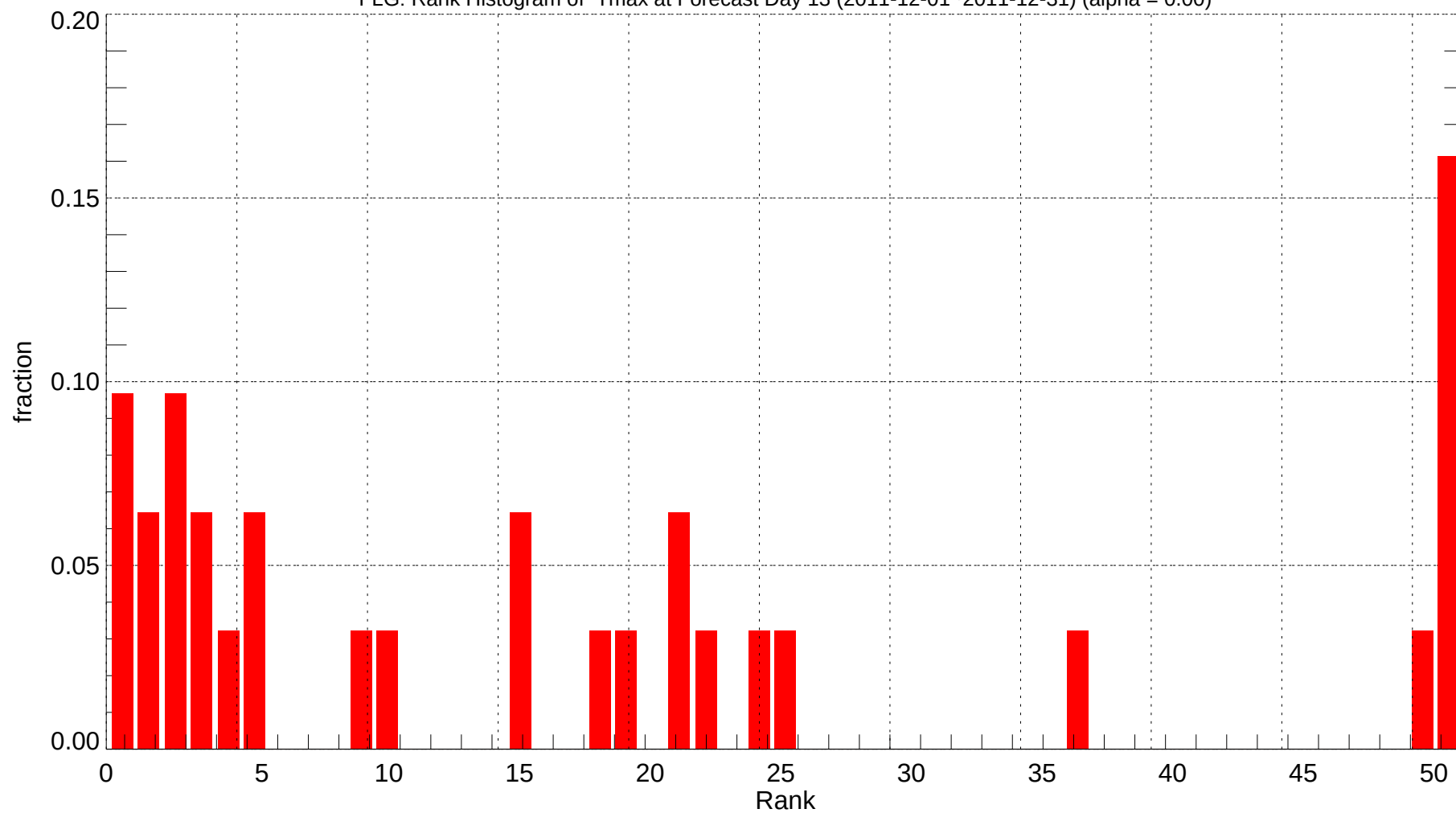
FLG: Rank Histogram of Tmax at Forecast Day 13 (2011-12-01~2011-12-31) (alpha = 0.00)
