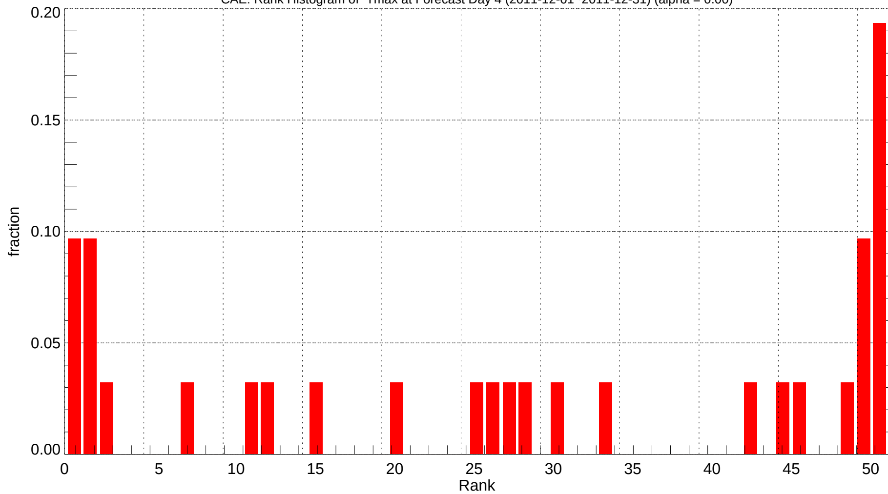
CAE: Rank Histogram of Tmax at Forecast Day 4 (2011-12-01~2011-12-31) (alpha = 0.00)
