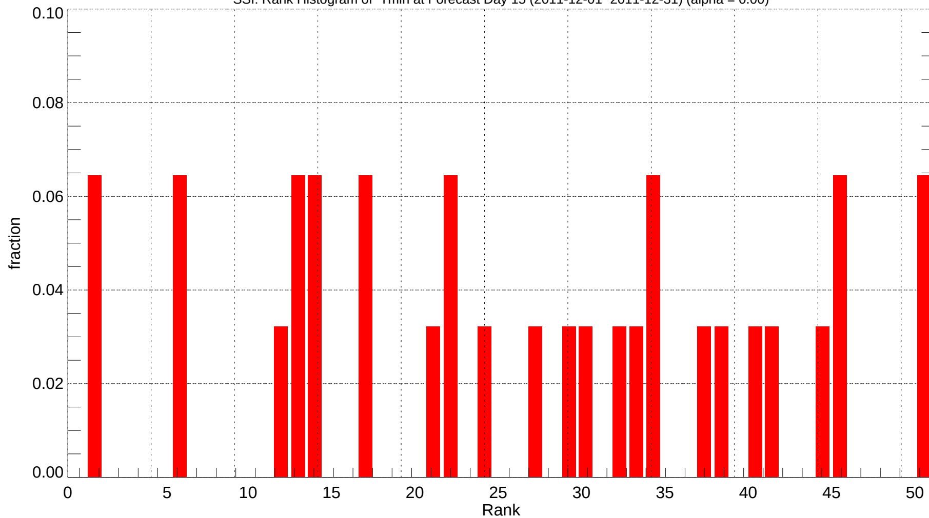
SSI: Rank Histogram of Tmin at Forecast Day 15 (2011-12-01~2011-12-31) (alpha = 0.00)
