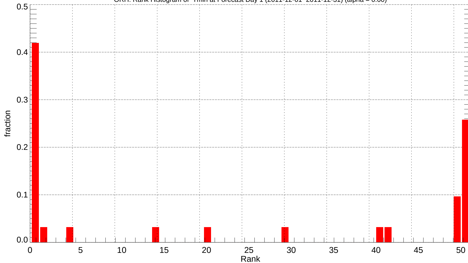
ORH: Rank Histogram of Tmin at Forecast Day 1 (2011-12-01~2011-12-31) (alpha = 0.00)
