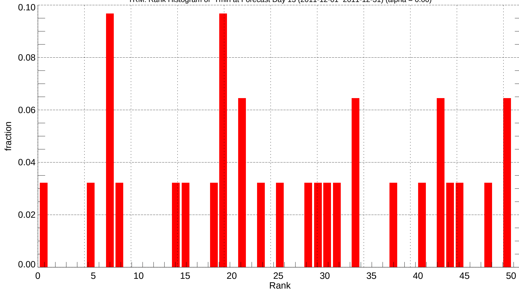
TRM: Rank Histogram of Tmin at Forecast Day 13 (2011-12-01~2011-12-31) (alpha = 0.00)
