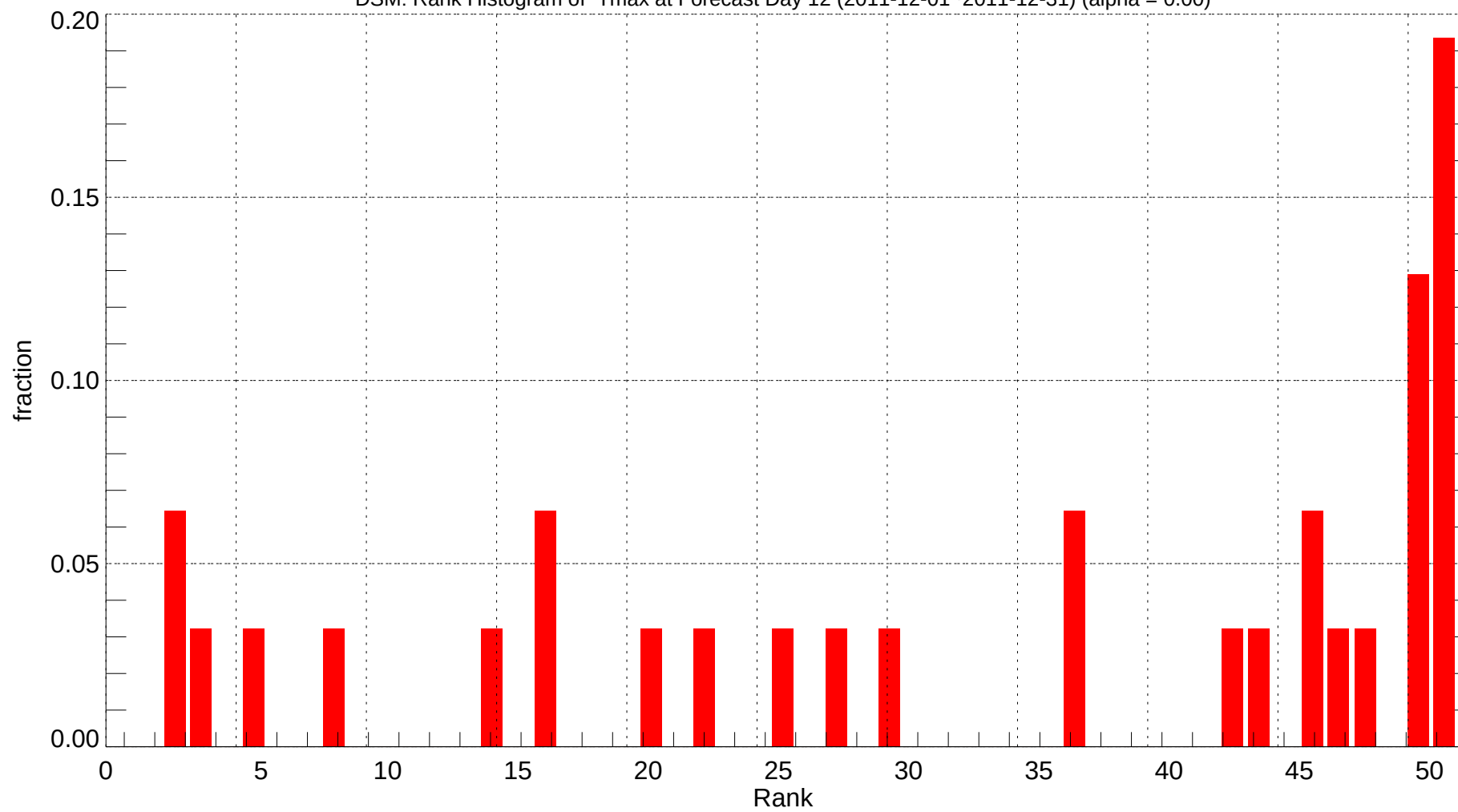
DSM: Rank Histogram of Tmax at Forecast Day 12 (2011-12-01~2011-12-31) (alpha = 0.00)
