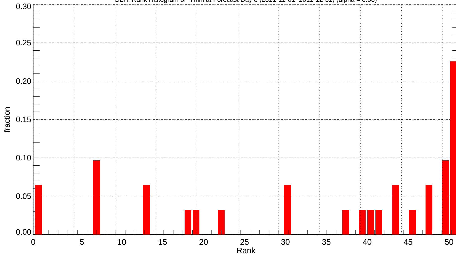
DLH: Rank Histogram of Tmin at Forecast Day 8 (2011-12-01~2011-12-31) (alpha = 0.00)
