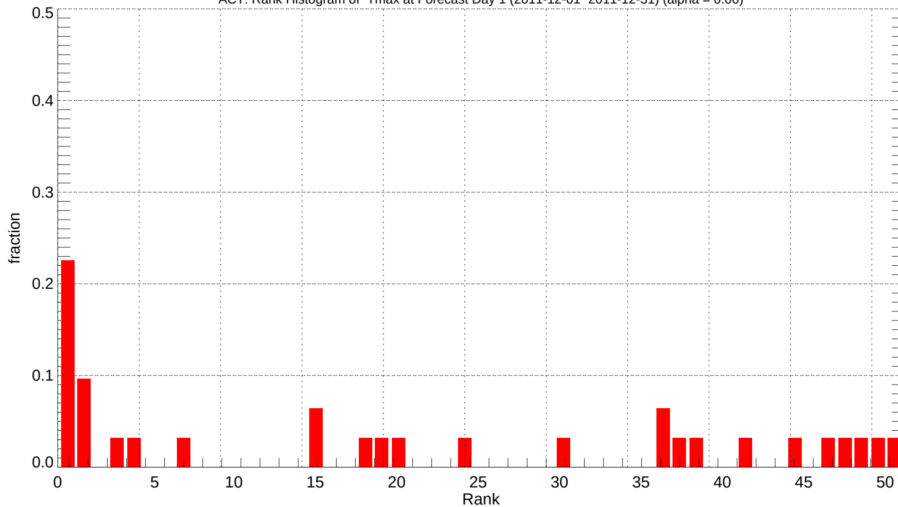
ACT: Rank Histogram of Tmax at Forecast Day 1 (2011-12-01~2011-12-31) (alpha = 0.00)
