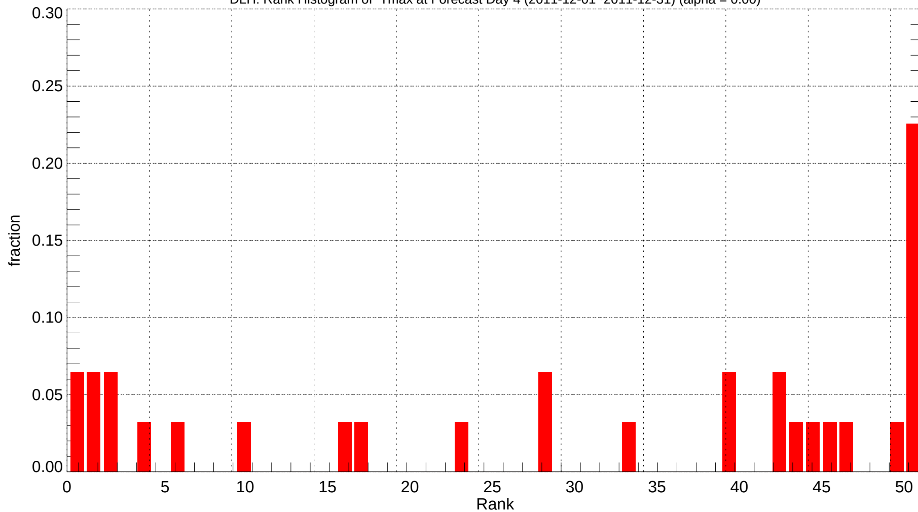
DLH: Rank Histogram of Tmax at Forecast Day 4 (2011-12-01~2011-12-31) (alpha = 0.00)
