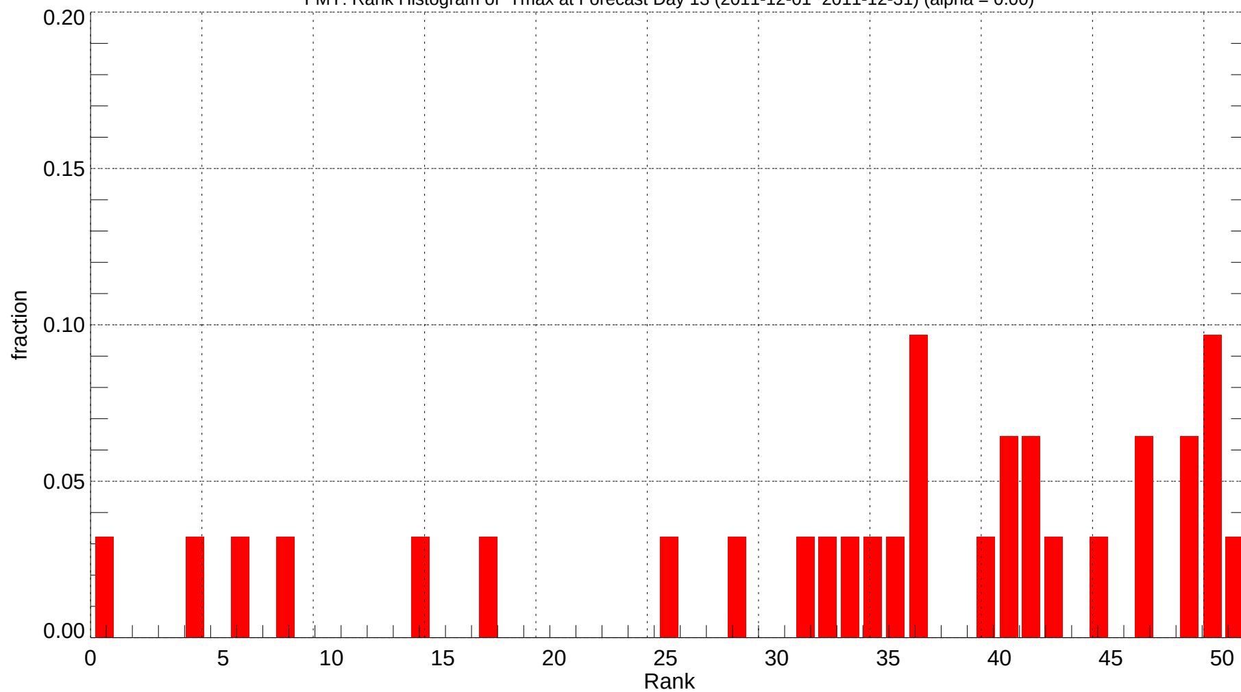
FMY: Rank Histogram of Tmax at Forecast Day 13 (2011-12-01~2011-12-31) (alpha = 0.00)
