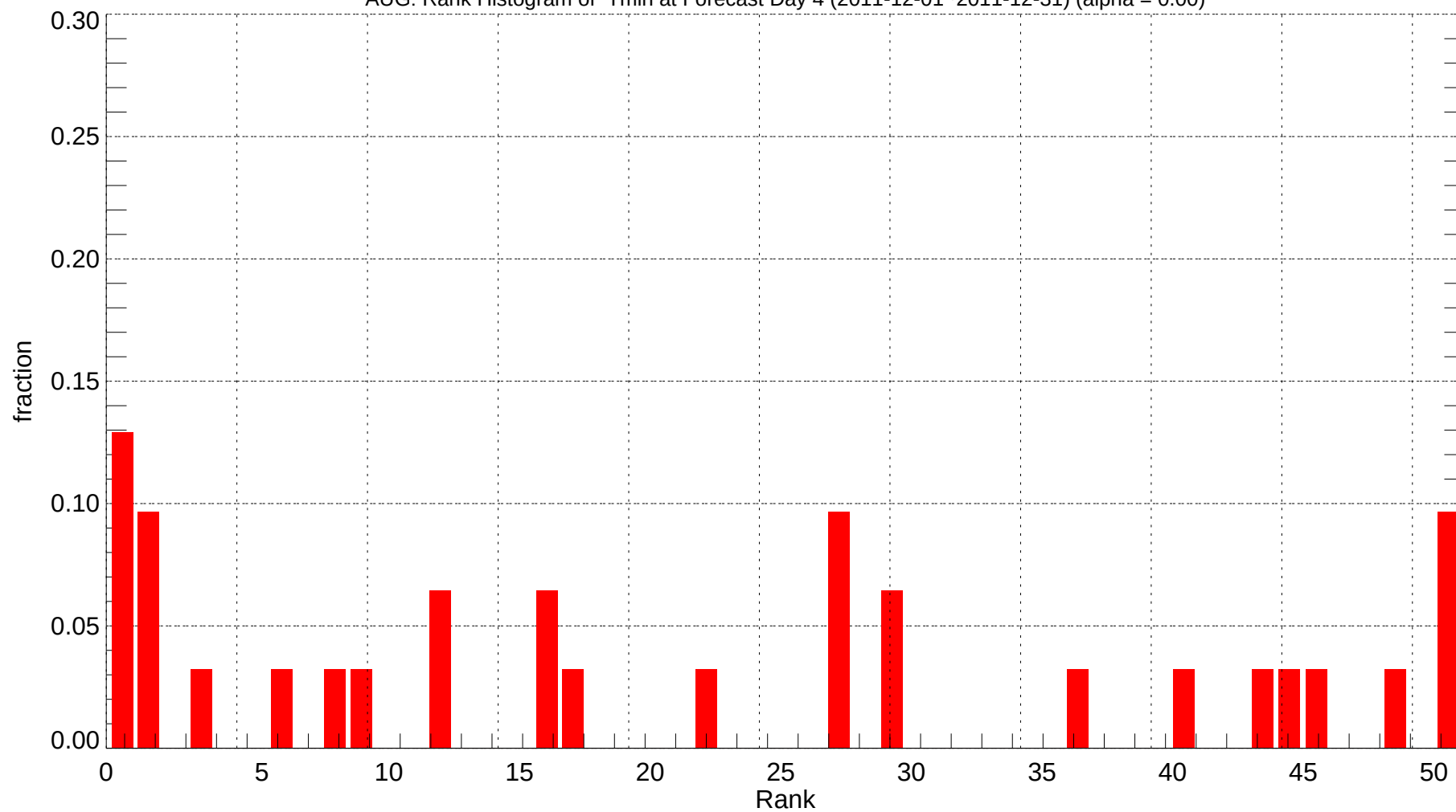
AUG: Rank Histogram of Tmin at Forecast Day 4 (2011-12-01~2011-12-31) (alpha = 0.00)
