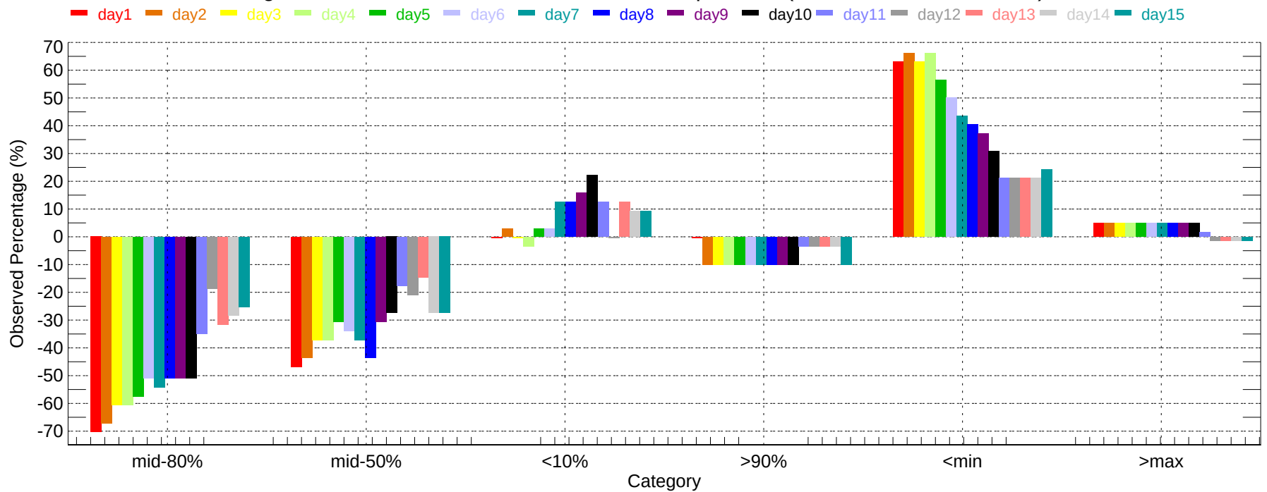
Observed Percentage Deviation of Ensembles - RAL: Min Temperature (2011-12-01~2011-12-31)
