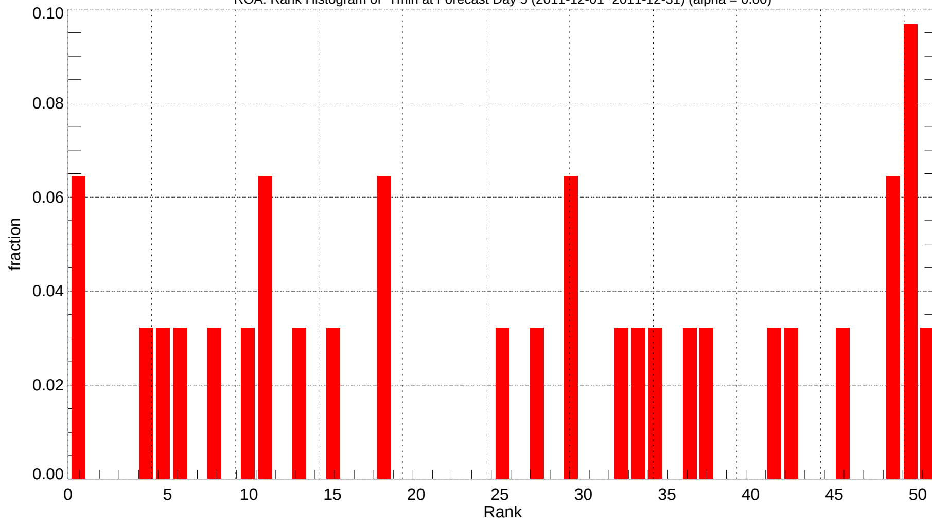
ROA: Rank Histogram of Tmin at Forecast Day 5 (2011-12-01~2011-12-31) (alpha = 0.00)
