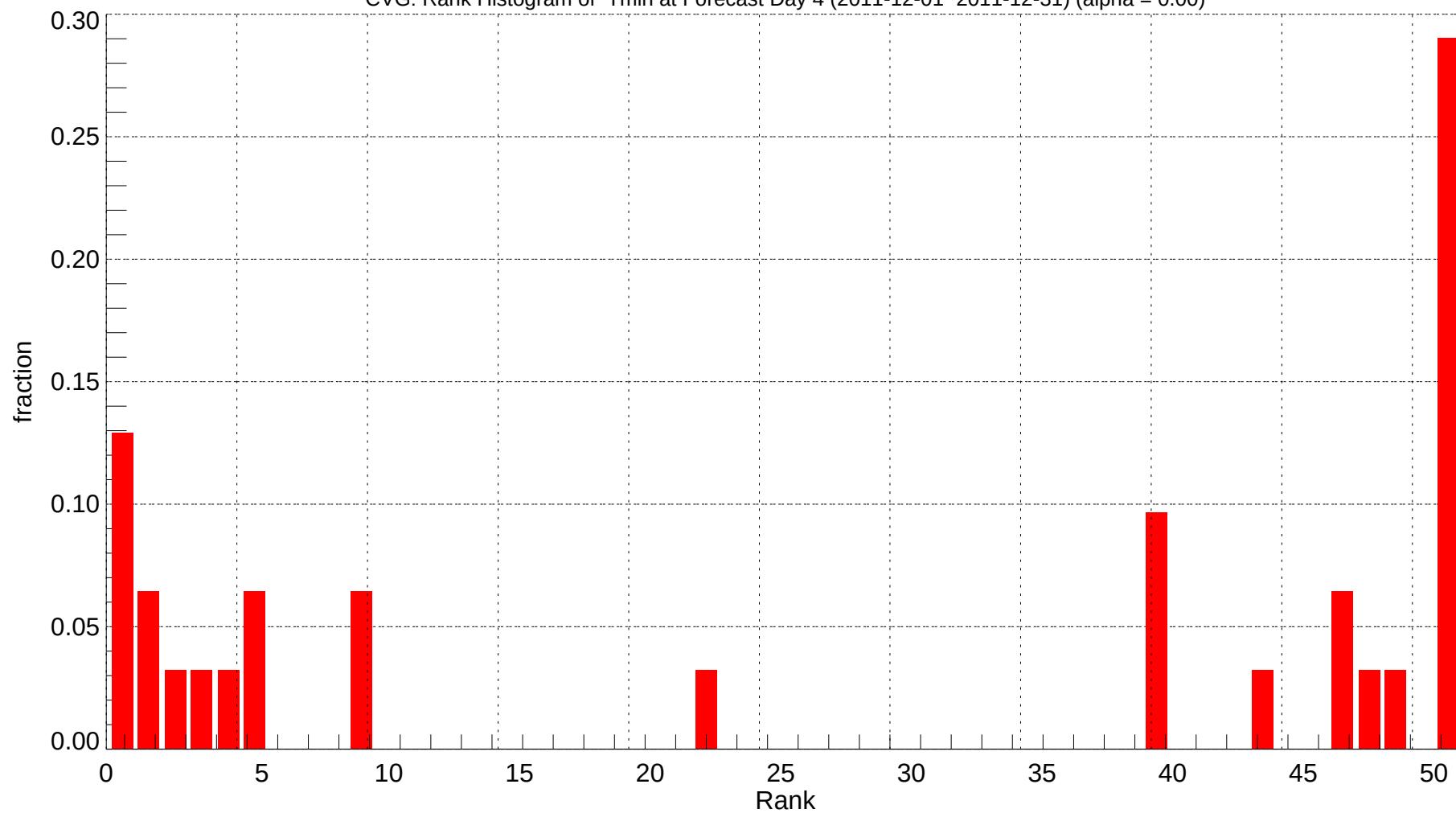
CVG: Rank Histogram of Tmin at Forecast Day 4 (2011-12-01~2011-12-31) (alpha = 0.00)
