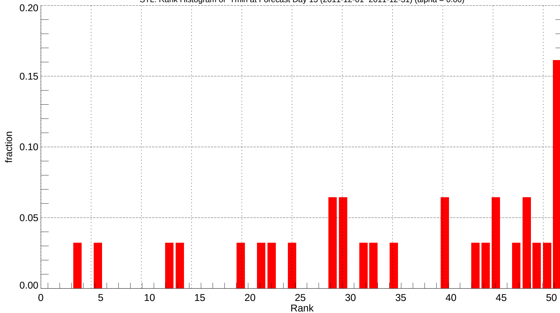
STL: Rank Histogram of Tmin at Forecast Day 13 (2011-12-01~2011-12-31) (alpha = 0.00)
