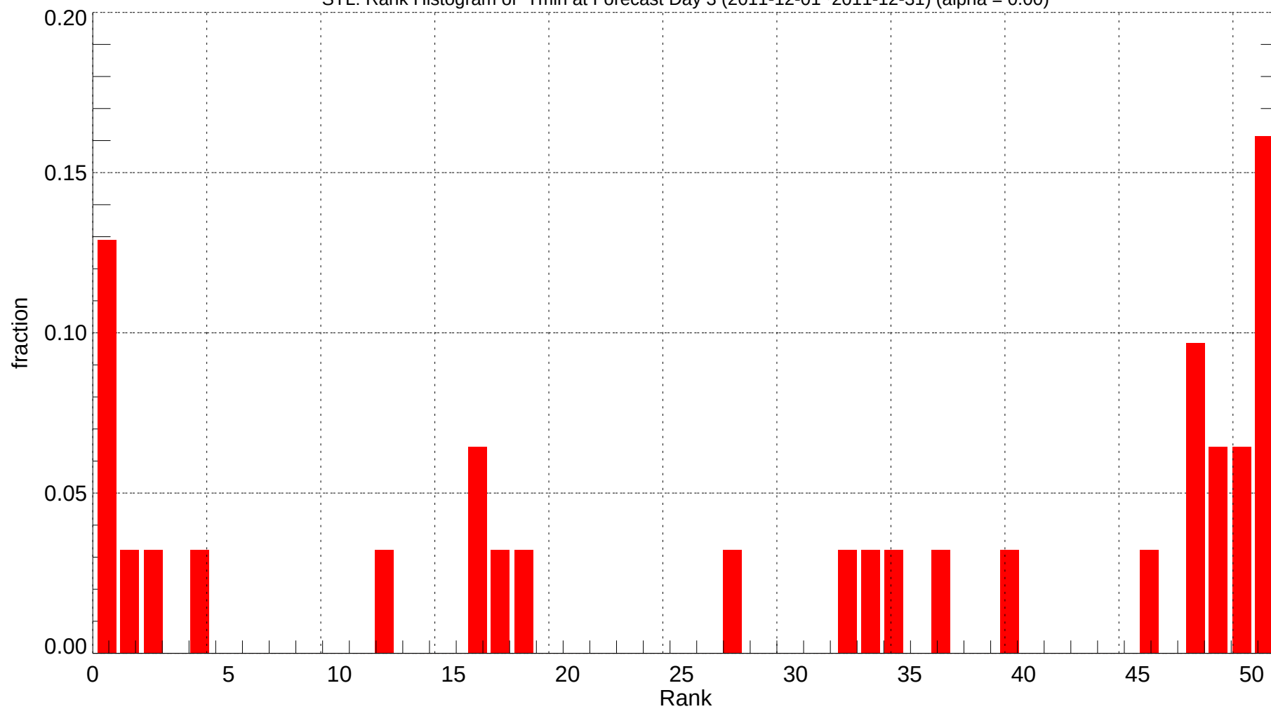
STL: Rank Histogram of Tmin at Forecast Day 3 (2011-12-01~2011-12-31) (alpha = 0.00)
