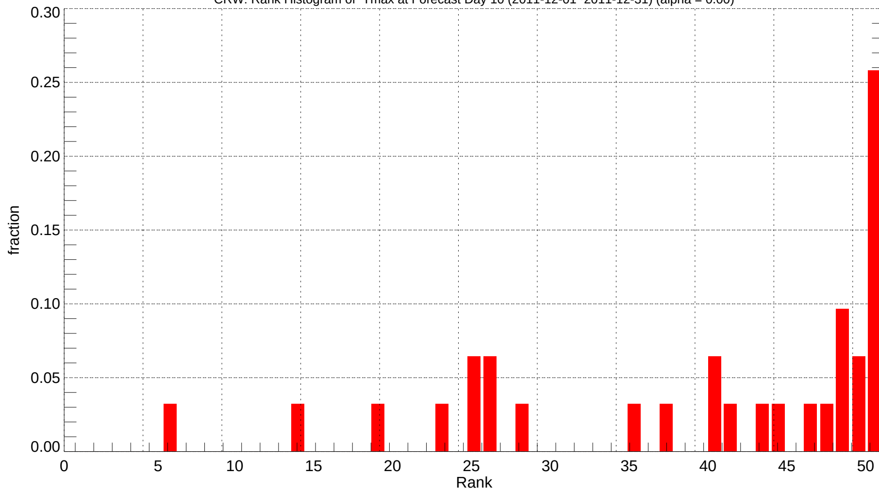
CRW: Rank Histogram of Tmax at Forecast Day 10 (2011-12-01~2011-12-31) (alpha = 0.00)
