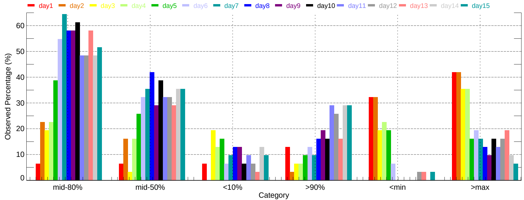
Observed Percentage of Ensembles - OMA: Max Temperature (2011-12-01~2011-12-31)
