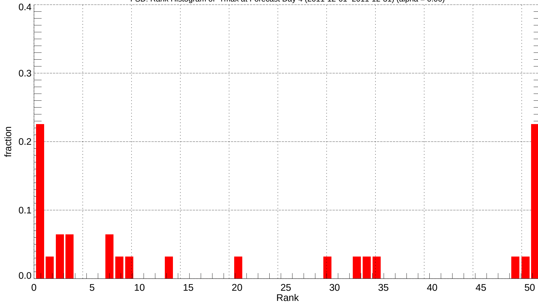
FSD: Rank Histogram of Tmax at Forecast Day 4 (2011-12-01~2011-12-31) (alpha = 0.00)
