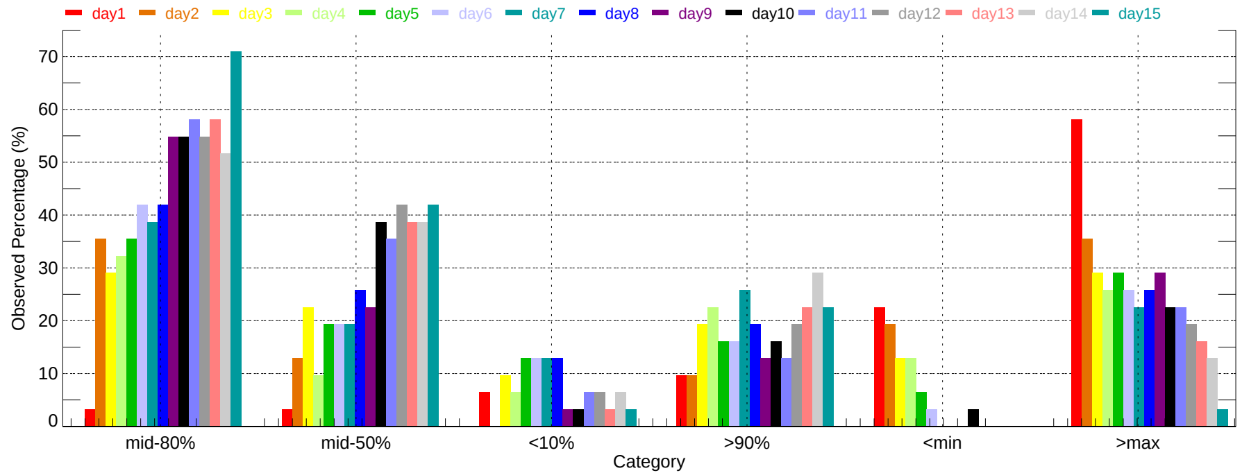
Observed Percentage of Ensembles - DBQ: Min Temperature (2011-12-01~2011-12-31)
