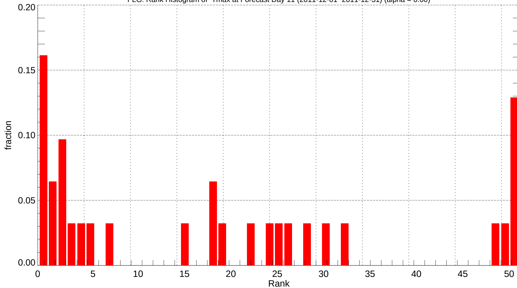
FLG: Rank Histogram of Tmax at Forecast Day 11 (2011-12-01~2011-12-31) (alpha = 0.00)
