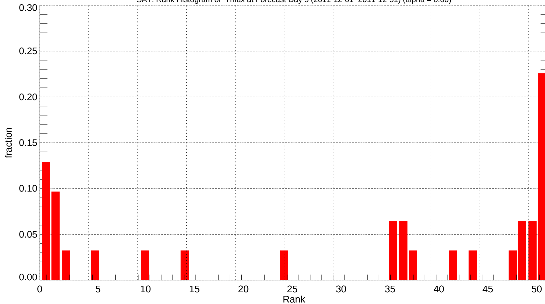
SAT: Rank Histogram of Tmax at Forecast Day 3 (2011-12-01~2011-12-31) (alpha = 0.00)
