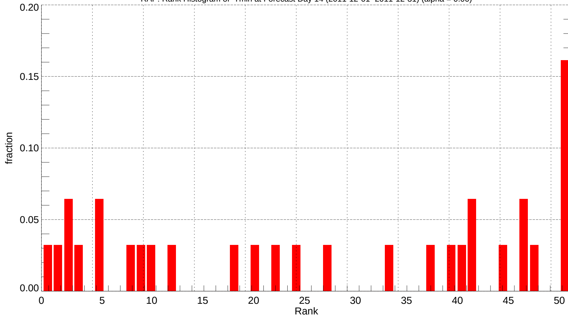
RAP: Rank Histogram of Tmin at Forecast Day 14 (2011-12-01~2011-12-31) (alpha = 0.00)
