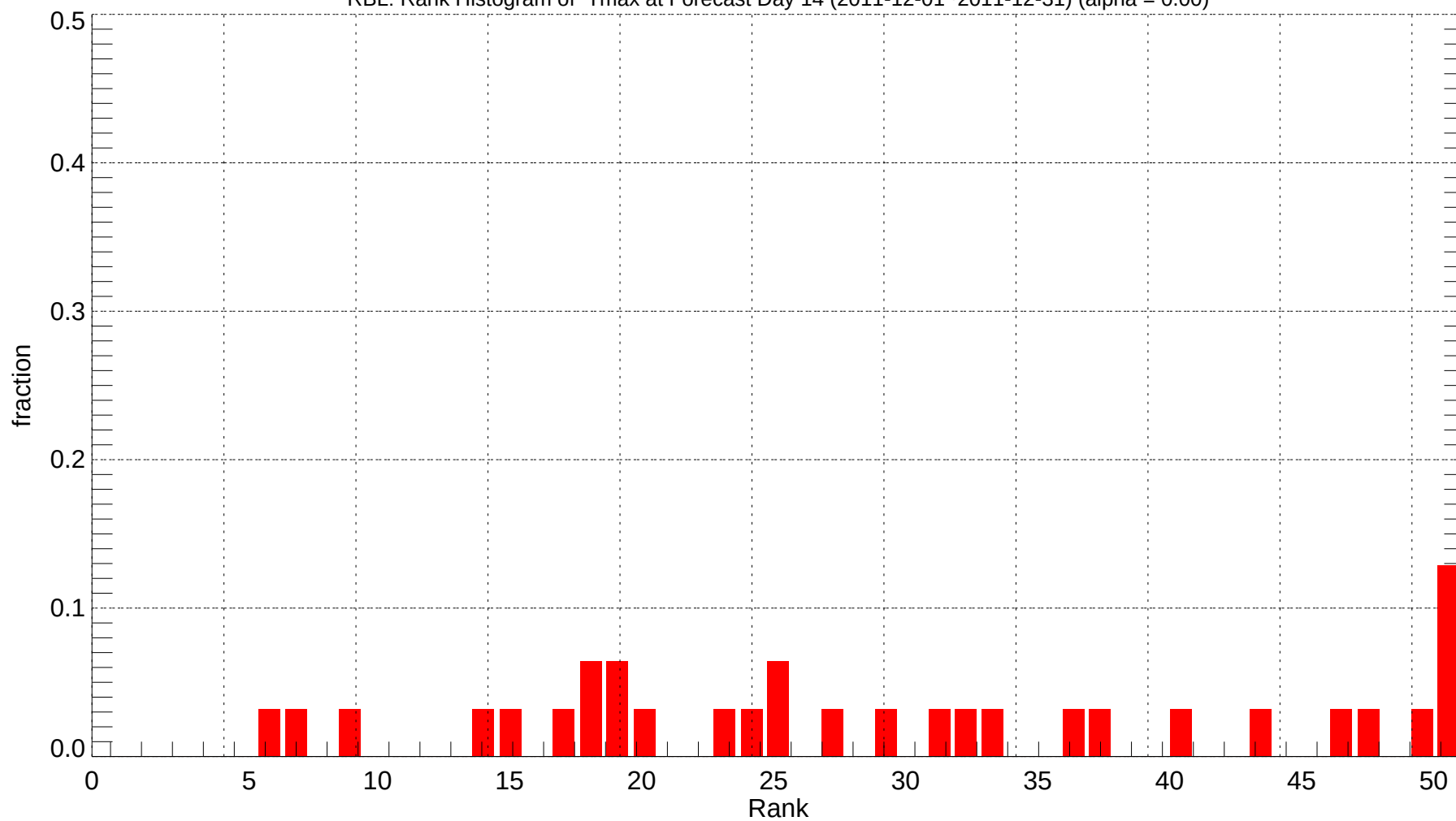
RBL: Rank Histogram of Tmax at Forecast Day 14 (2011-12-01~2011-12-31) (alpha = 0.00)
