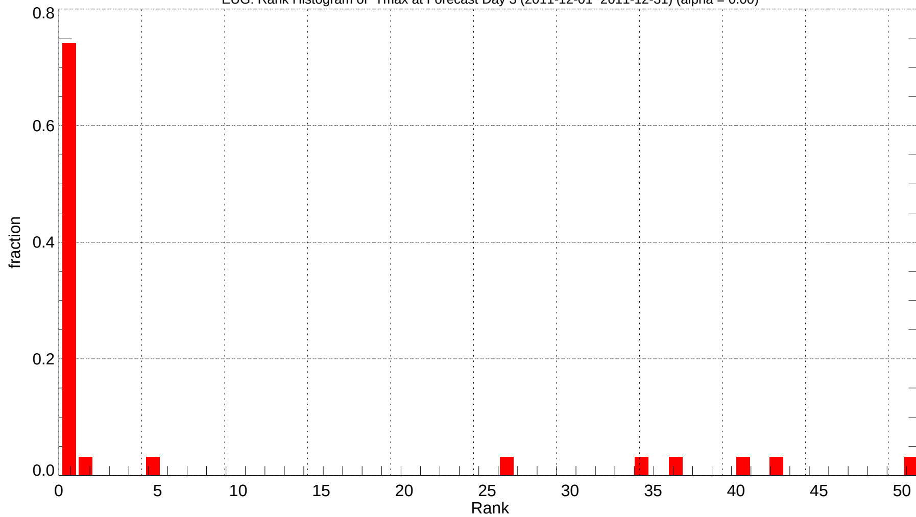
EUG: Rank Histogram of Tmax at Forecast Day 3 (2011-12-01~2011-12-31) (alpha = 0.00)
