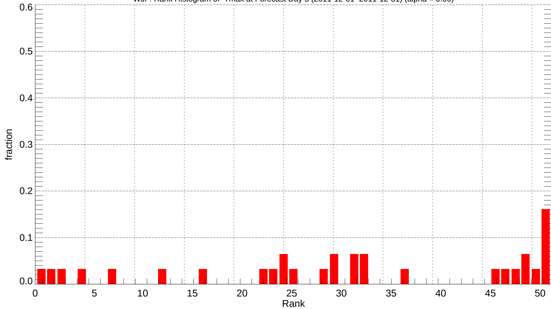
WJF: Rank Histogram of Tmax at Forecast Day 5 (2011-12-01~2011-12-31) (alpha = 0.00)
