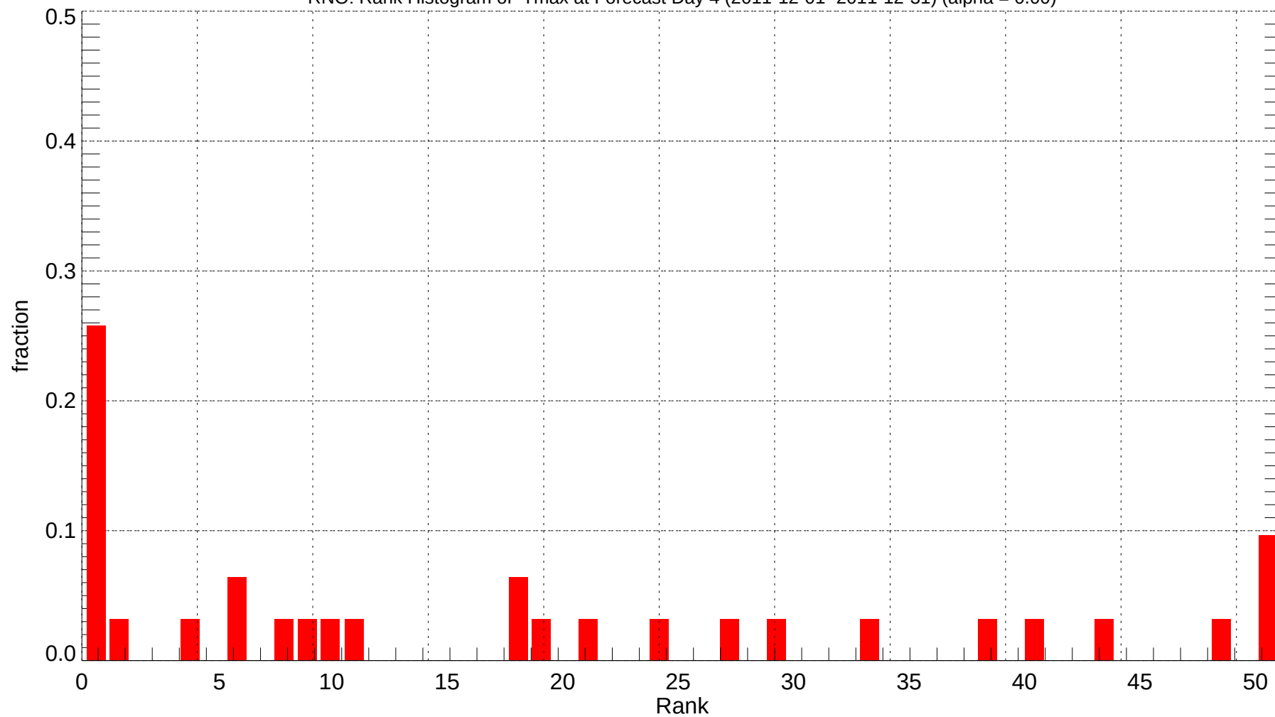
RNO: Rank Histogram of Tmax at Forecast Day 4 (2011-12-01~2011-12-31) (alpha = 0.00)
