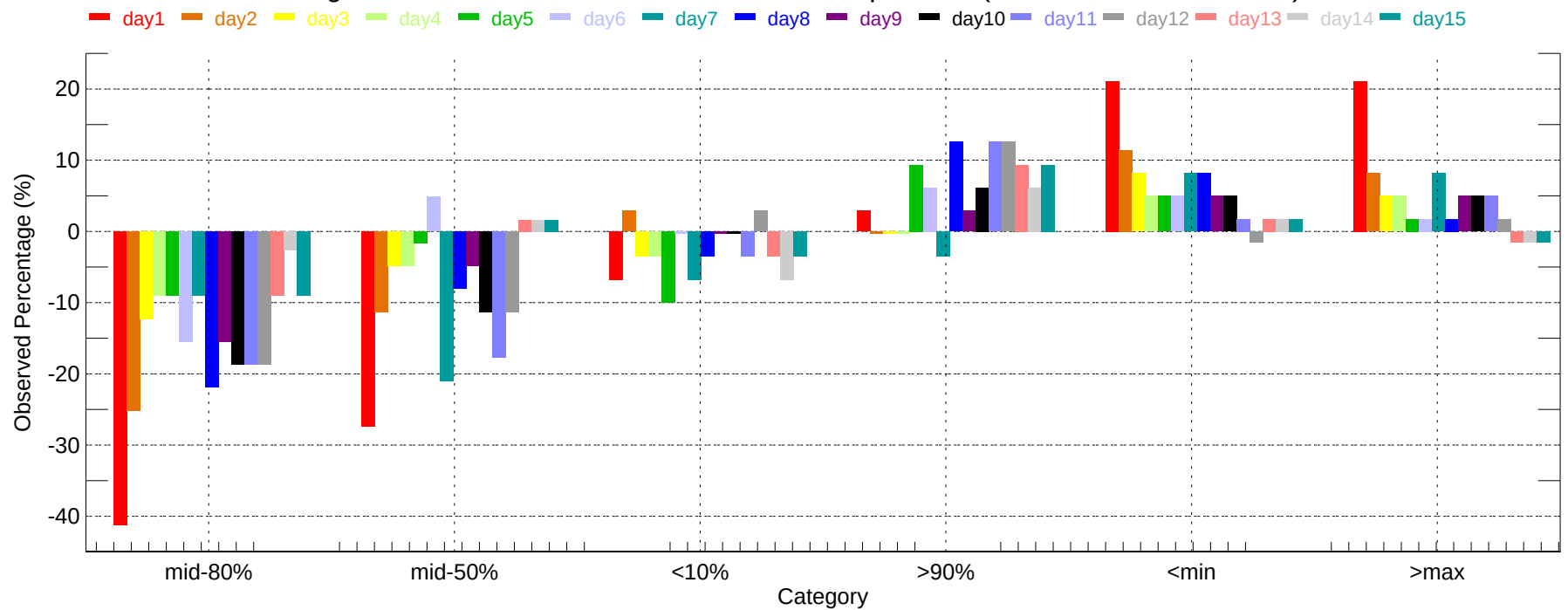
Observed Percentage Deviation of Ensembles - BDL: Max Temperature (2011-12-01~2011-12-31)
