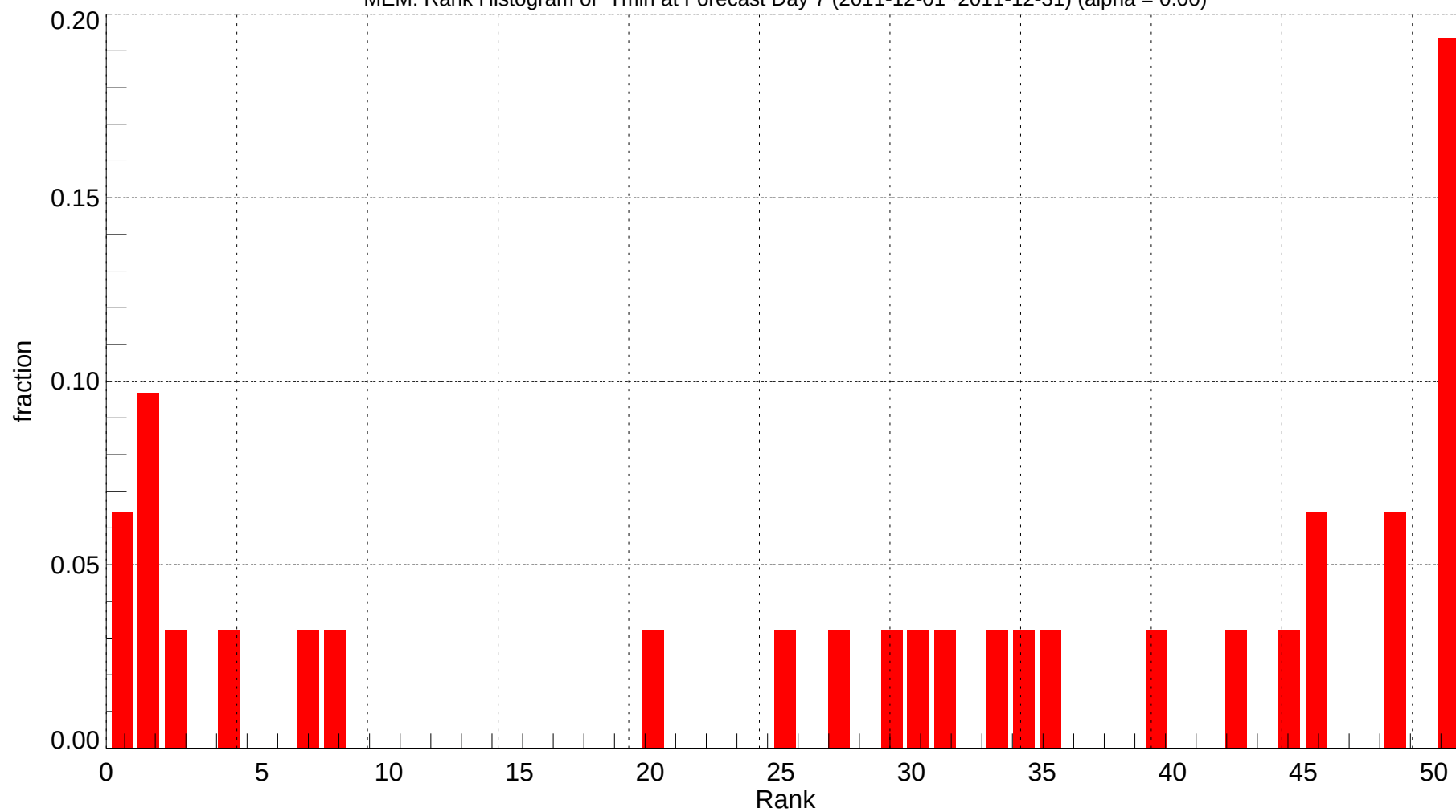
MEM: Rank Histogram of Tmin at Forecast Day 7 (2011-12-01~2011-12-31) (alpha = 0.00)
