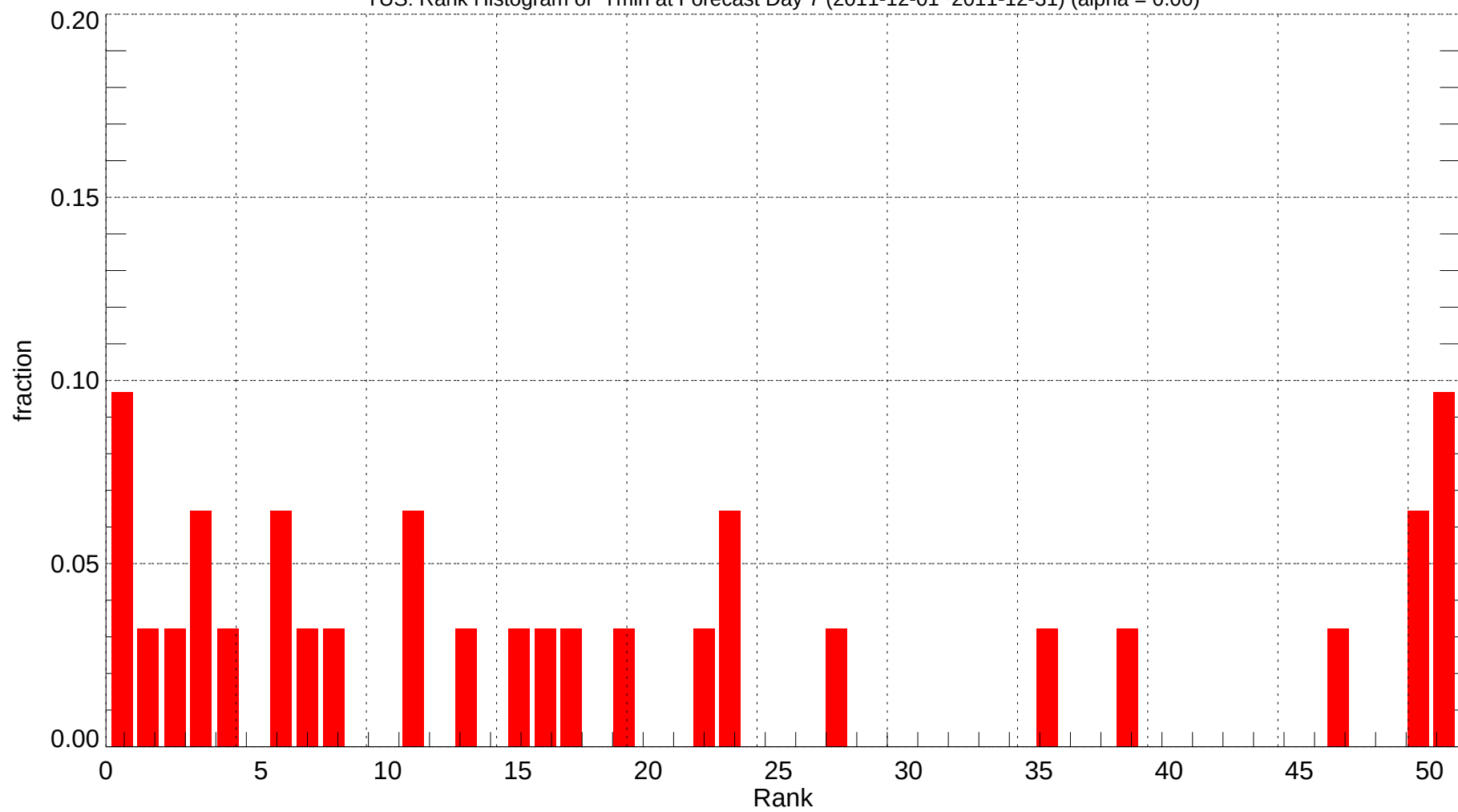
TUS: Rank Histogram of Tmin at Forecast Day 7 (2011-12-01~2011-12-31) (alpha = 0.00)
