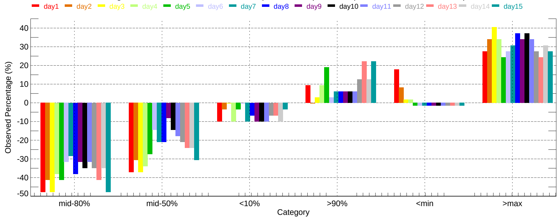
Observed Percentage Deviation of Ensembles - DBQ: Max Temperature (2011-12-01~2011-12-31)
