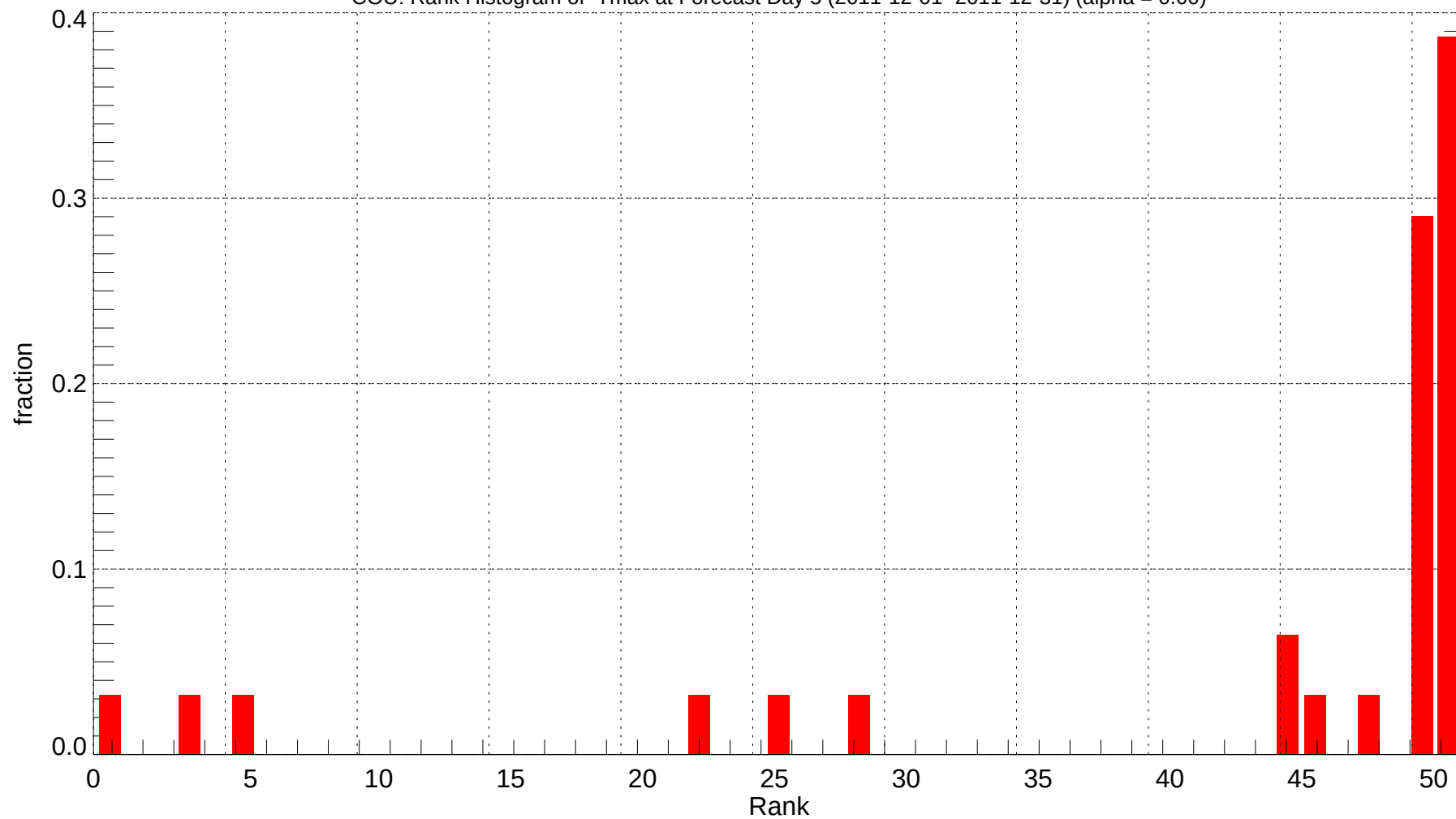
COU: Rank Histogram of Tmax at Forecast Day 5 (2011-12-01~2011-12-31) (alpha = 0.00)
