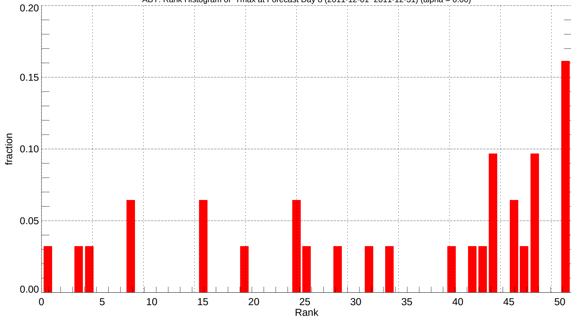
ABY: Rank Histogram of Tmax at Forecast Day 8 (2011-12-01~2011-12-31) (alpha = 0.00)
