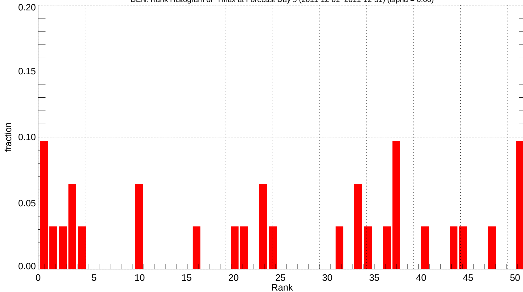
DEN: Rank Histogram of Tmax at Forecast Day 9 (2011-12-01~2011-12-31) (alpha = 0.00)
