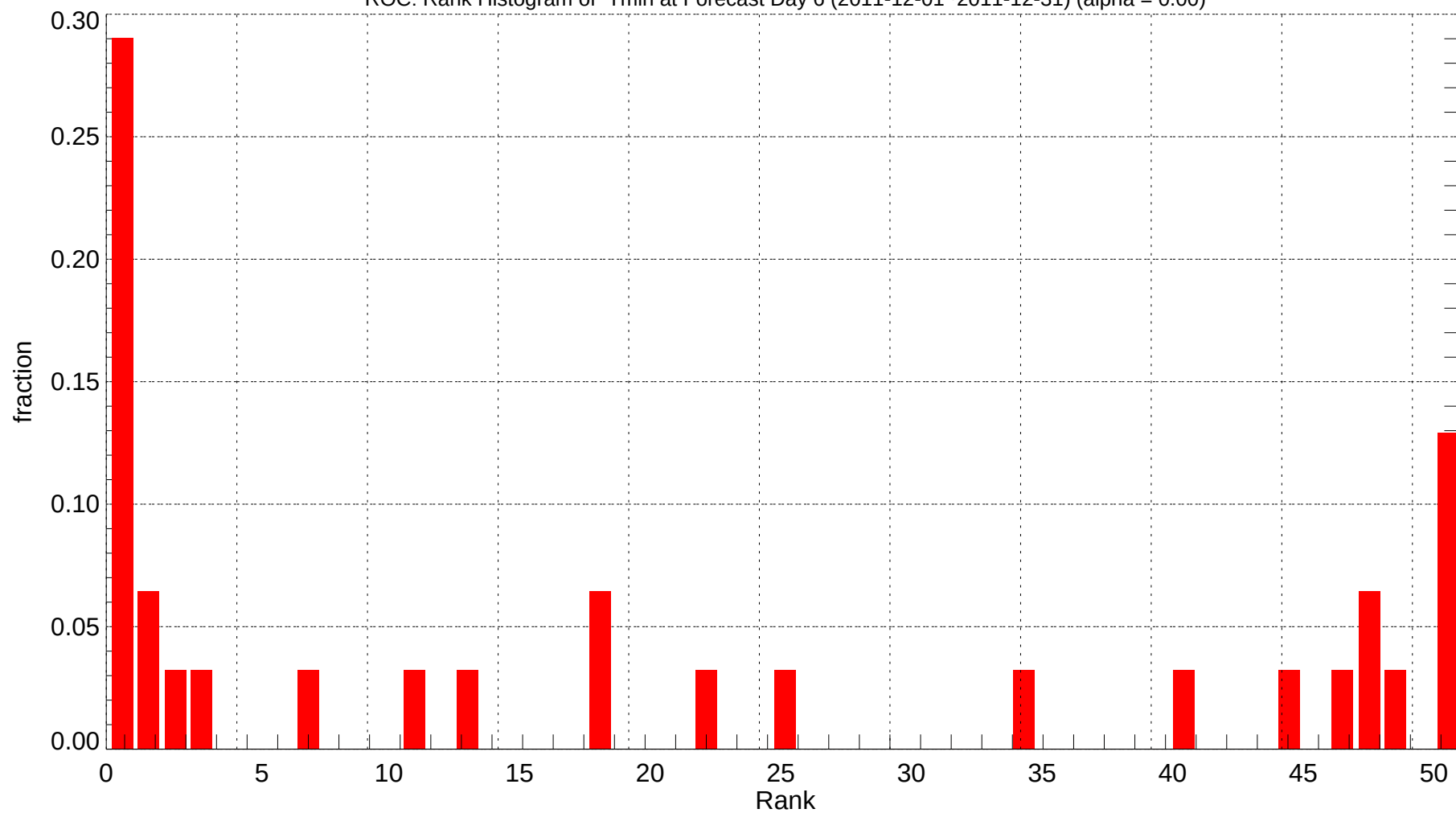
ROC: Rank Histogram of Tmin at Forecast Day 6 (2011-12-01~2011-12-31) (alpha = 0.00)
