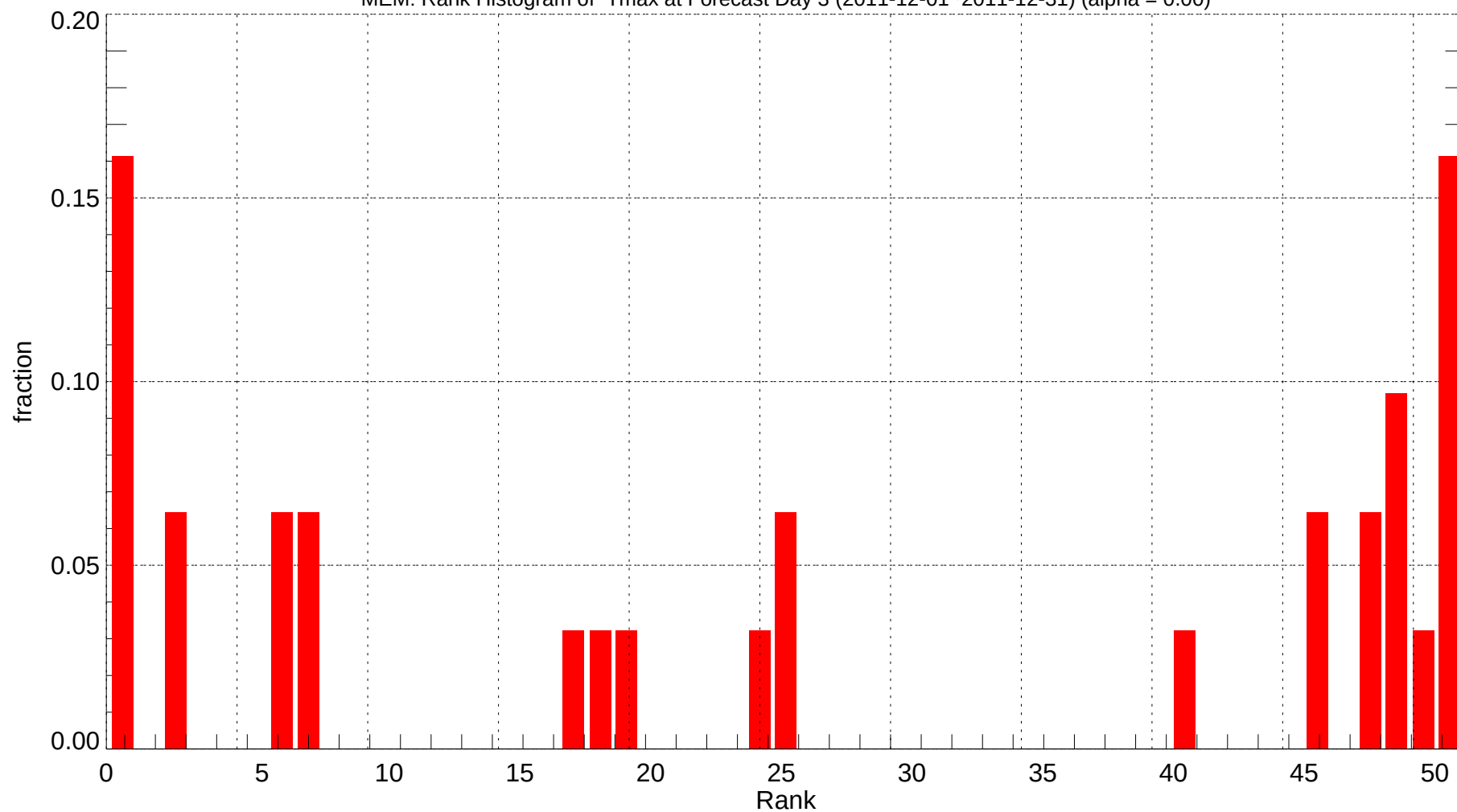
MEM: Rank Histogram of Tmax at Forecast Day 3 (2011-12-01~2011-12-31) (alpha = 0.00)
