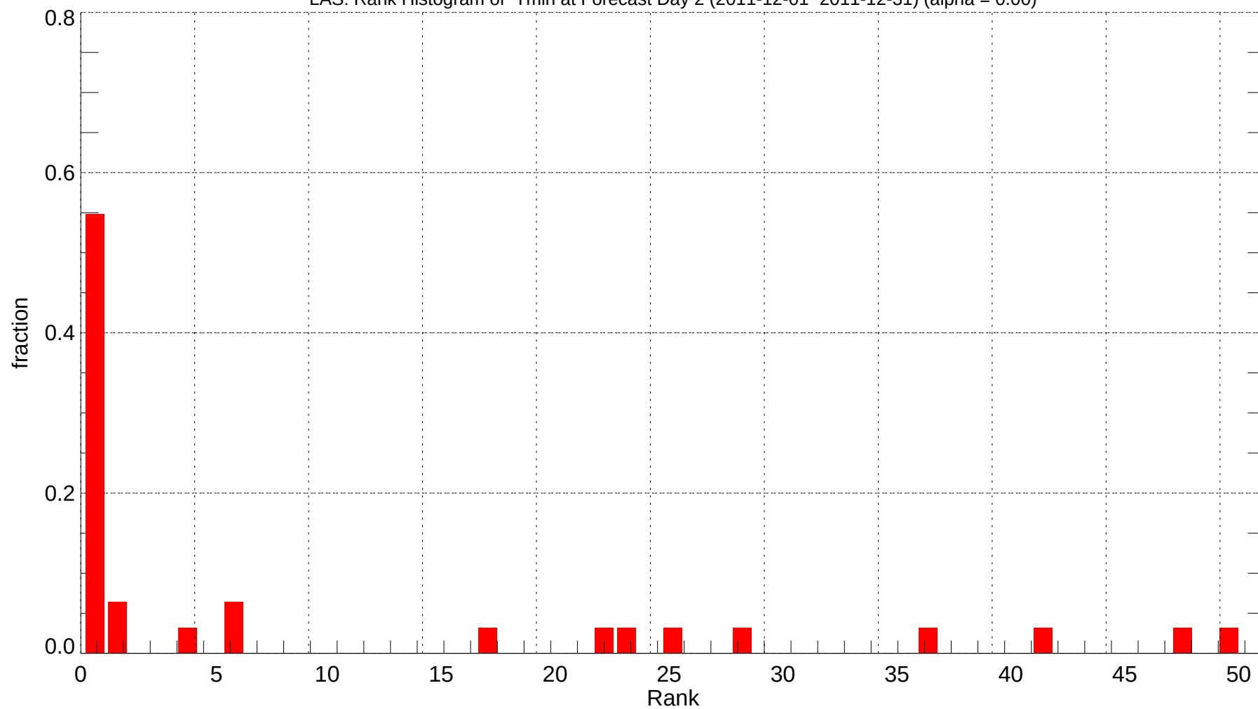
LAS: Rank Histogram of Tmin at Forecast Day 2 (2011-12-01~2011-12-31) (alpha = 0.00)
