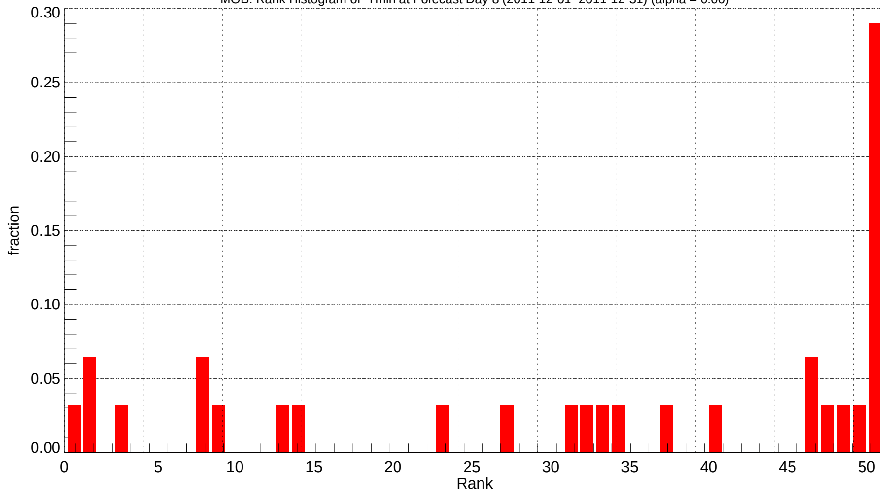
MOB: Rank Histogram of Tmin at Forecast Day 8 (2011-12-01~2011-12-31) (alpha = 0.00)
