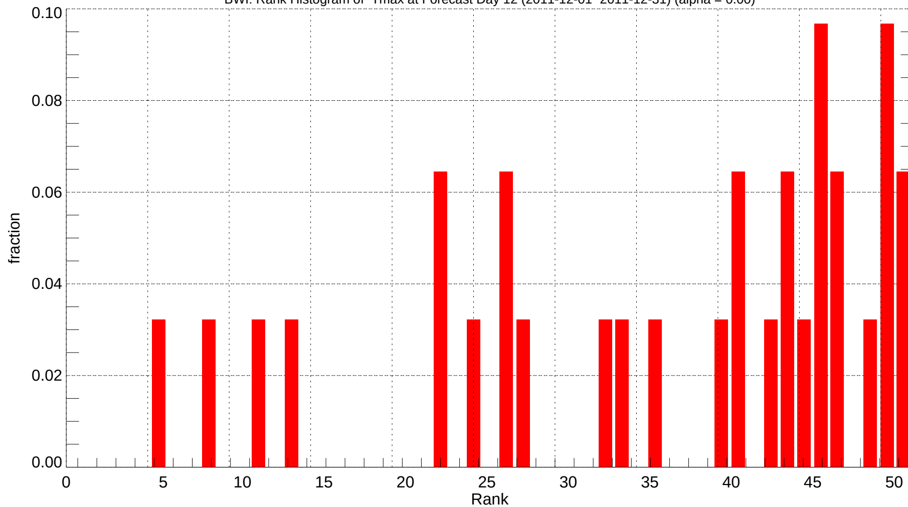
BWI: Rank Histogram of Tmax at Forecast Day 12 (2011-12-01~2011-12-31) (alpha = 0.00)
