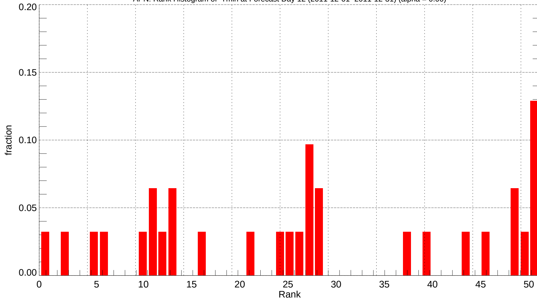
APN: Rank Histogram of Tmin at Forecast Day 12 (2011-12-01~2011-12-31) (alpha = 0.00)
