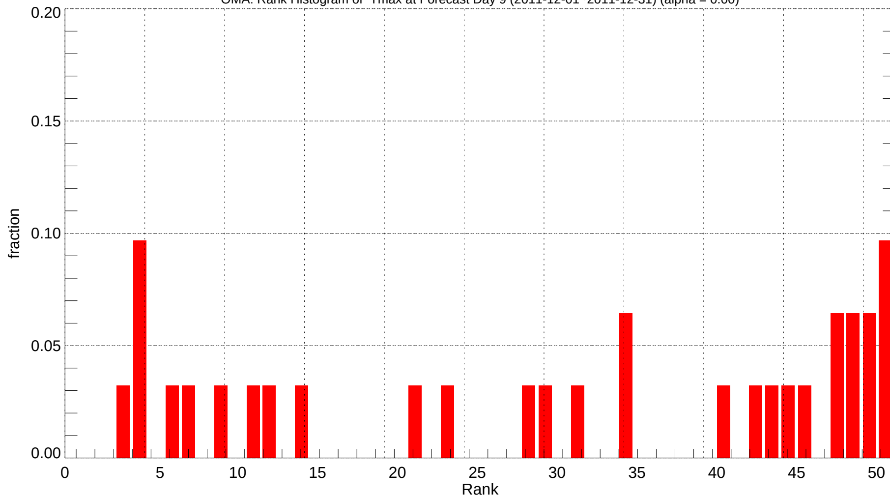
OMA: Rank Histogram of Tmax at Forecast Day 9 (2011-12-01~2011-12-31) (alpha = 0.00)
