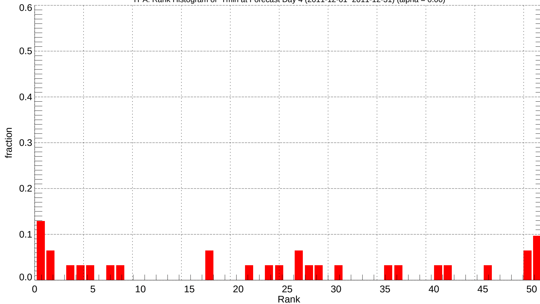
TPA: Rank Histogram of Tmin at Forecast Day 4 (2011-12-01~2011-12-31) (alpha = 0.00)
