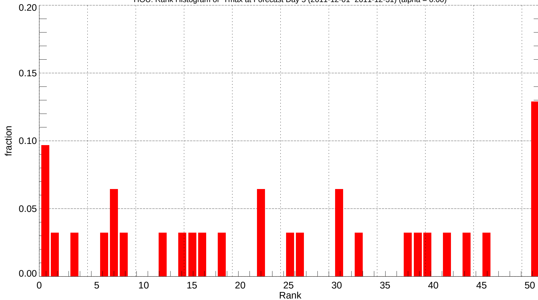
HOU: Rank Histogram of Tmax at Forecast Day 5 (2011-12-01~2011-12-31) (alpha = 0.00)
