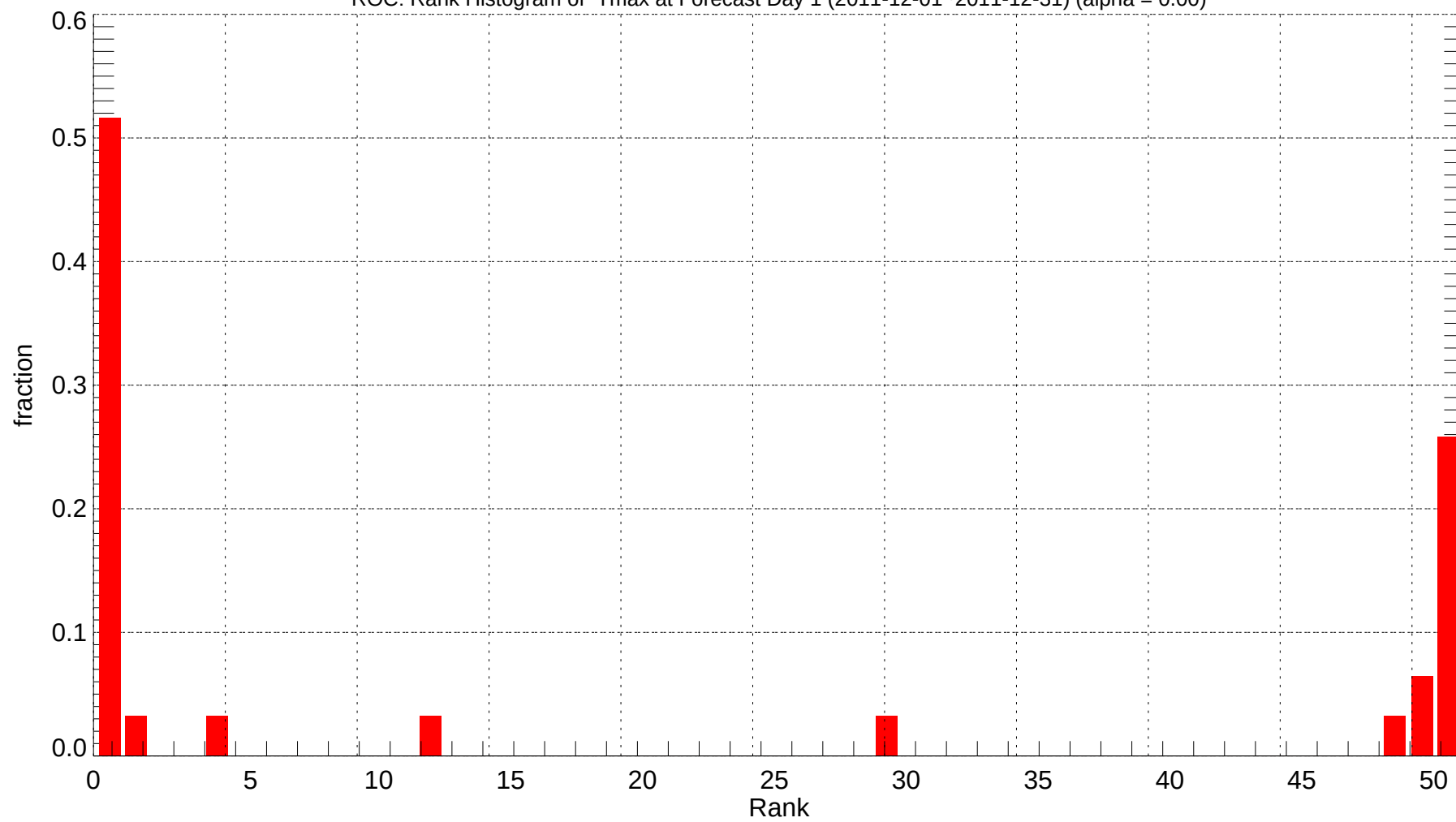
ROC: Rank Histogram of Tmax at Forecast Day 1 (2011-12-01~2011-12-31) (alpha = 0.00)
