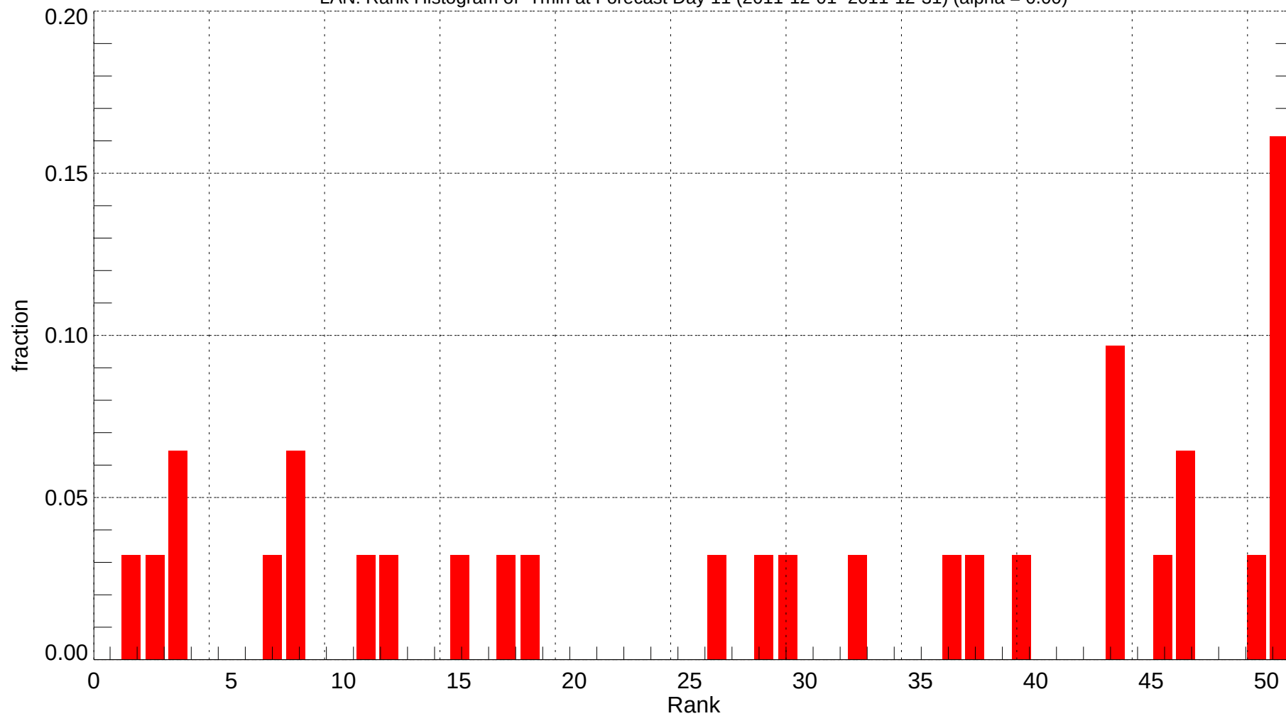
LAN: Rank Histogram of Tmin at Forecast Day 11 (2011-12-01~2011-12-31) (alpha = 0.00)
