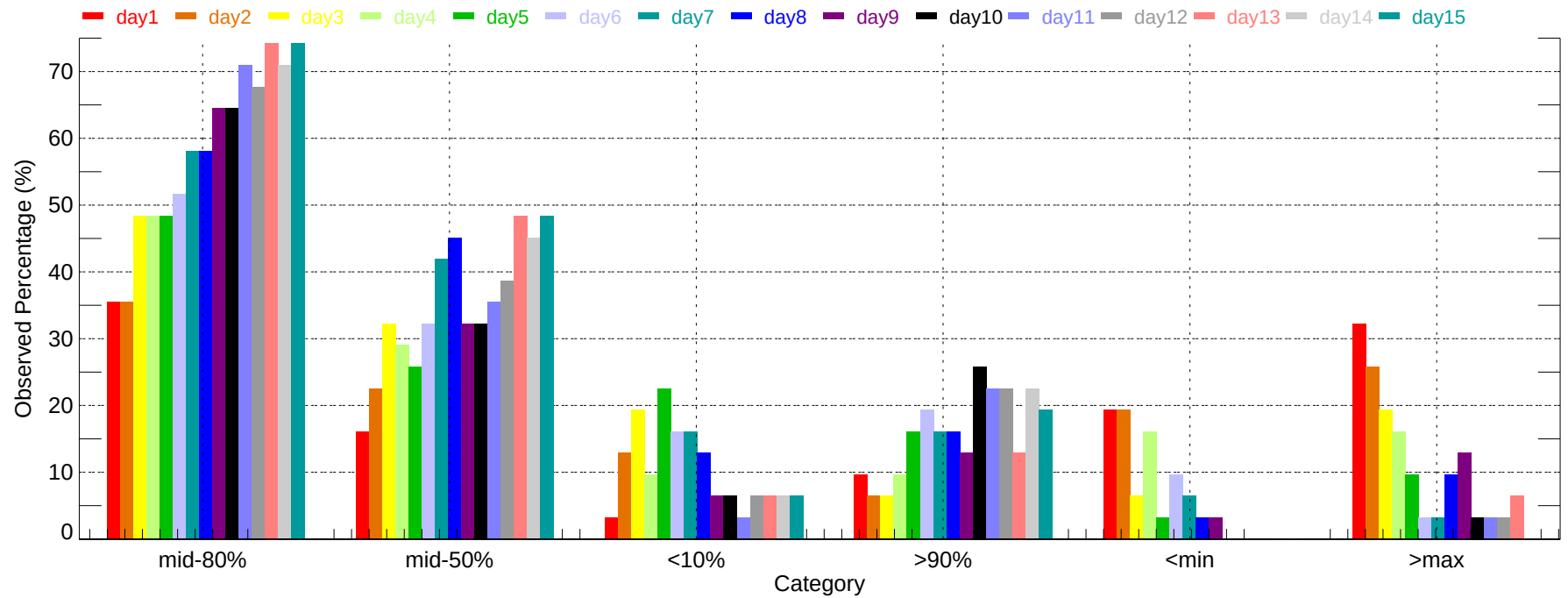
Observed Percentage of Ensembles - FWA: Max Temperature (2011-12-01~2011-12-31)
