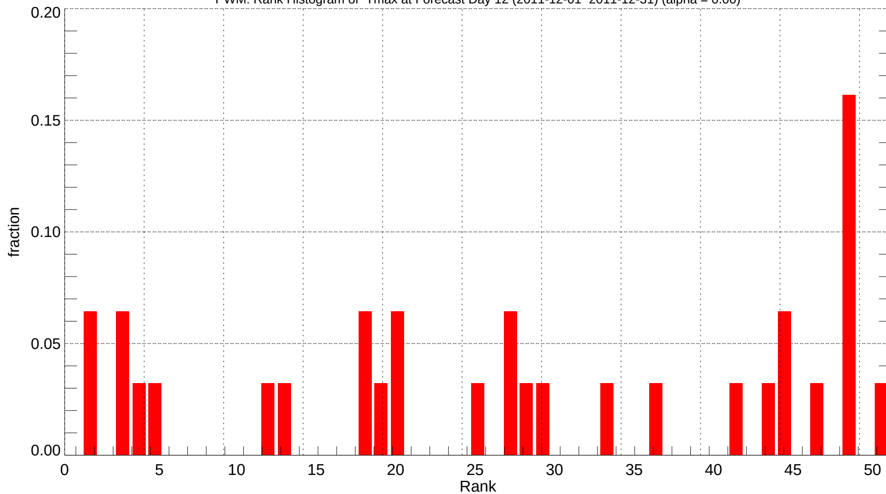
PWM: Rank Histogram of Tmax at Forecast Day 12 (2011-12-01~2011-12-31) (alpha = 0.00)
