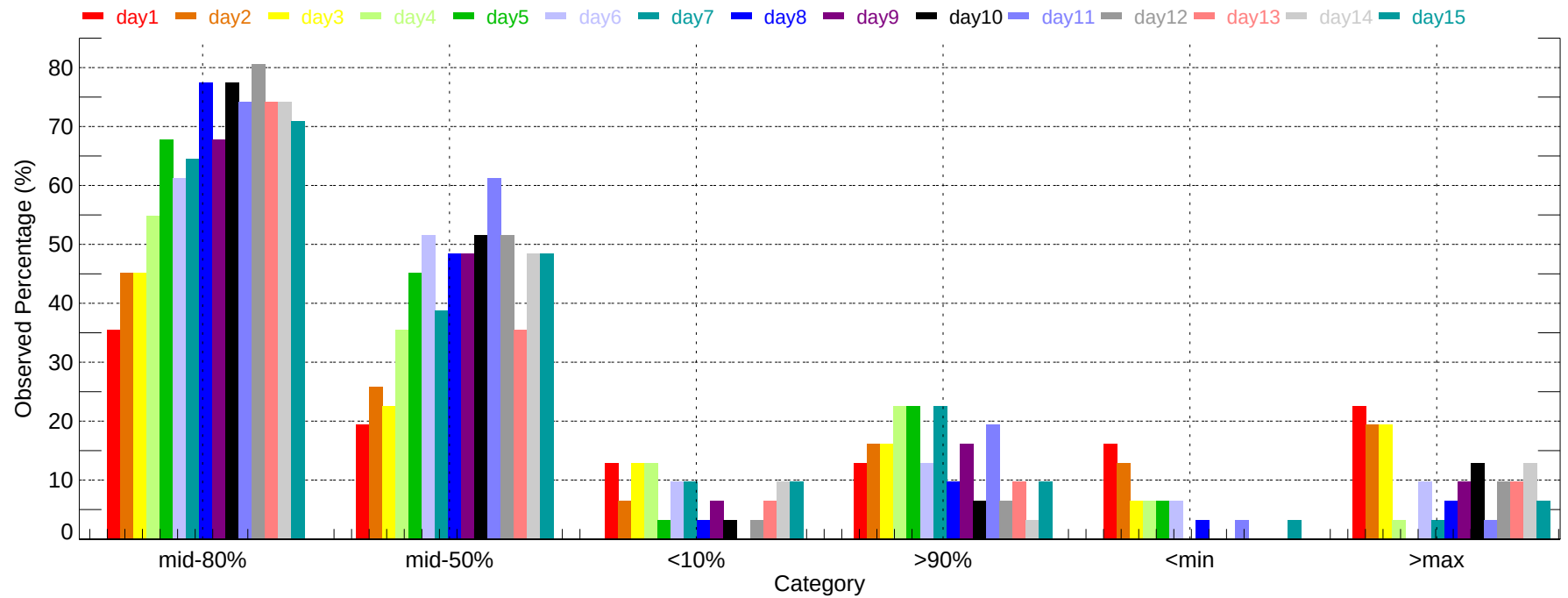
Observed Percentage of Ensembles - IAH: Max Temperature (2011-12-01~2011-12-31)
