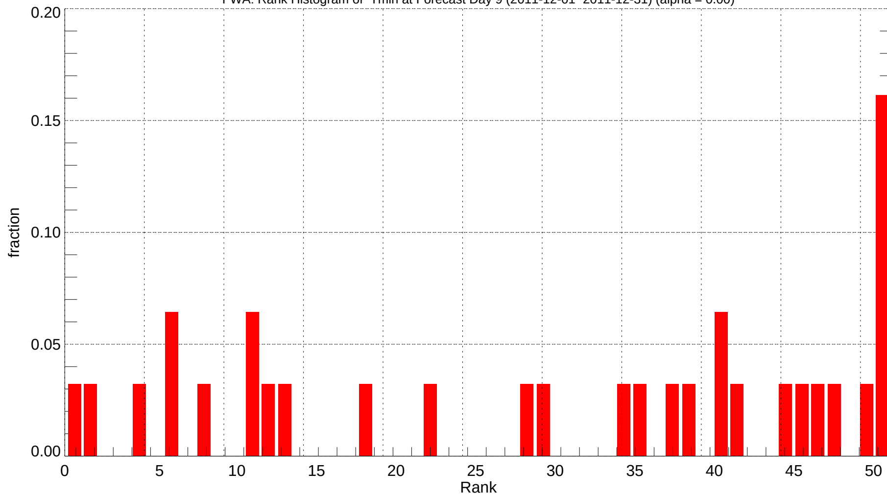
FWA: Rank Histogram of Tmin at Forecast Day 9 (2011-12-01~2011-12-31) (alpha = 0.00)
