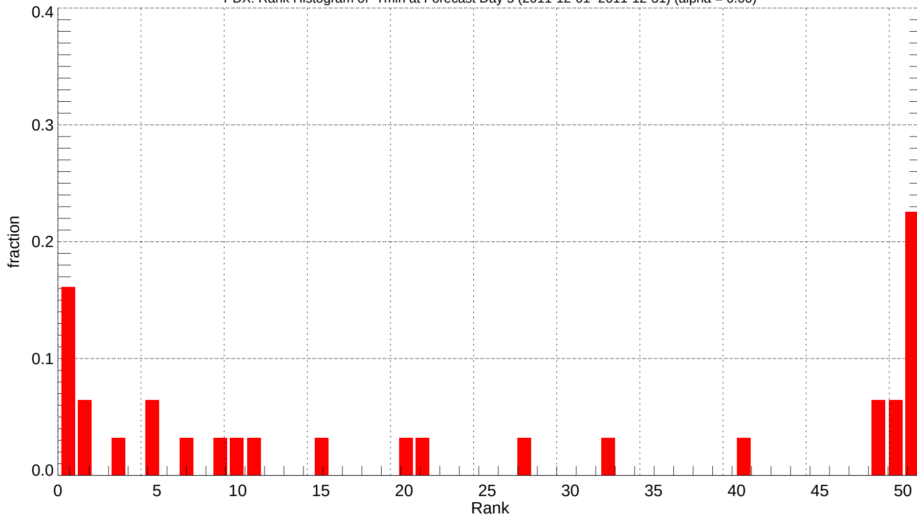
PDX: Rank Histogram of Tmin at Forecast Day 5 (2011-12-01~2011-12-31) (alpha = 0.00)
