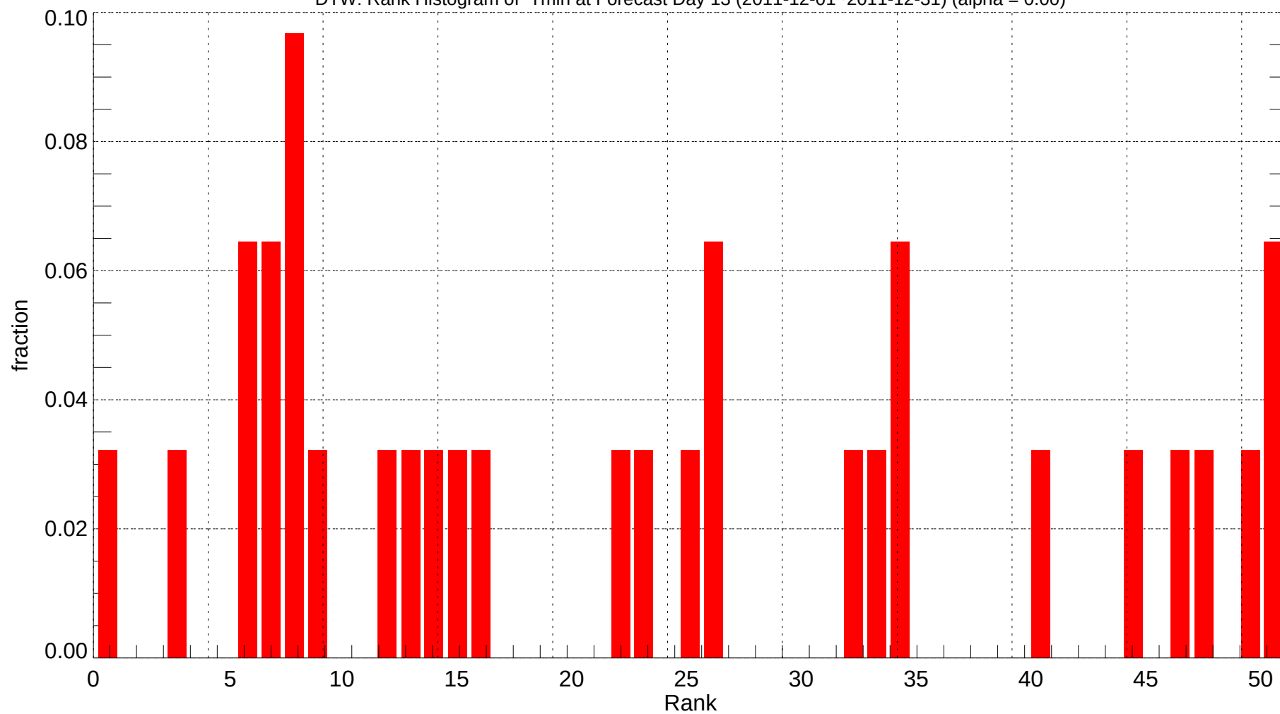
DTW: Rank Histogram of Tmin at Forecast Day 13 (2011-12-01~2011-12-31) (alpha = 0.00)
