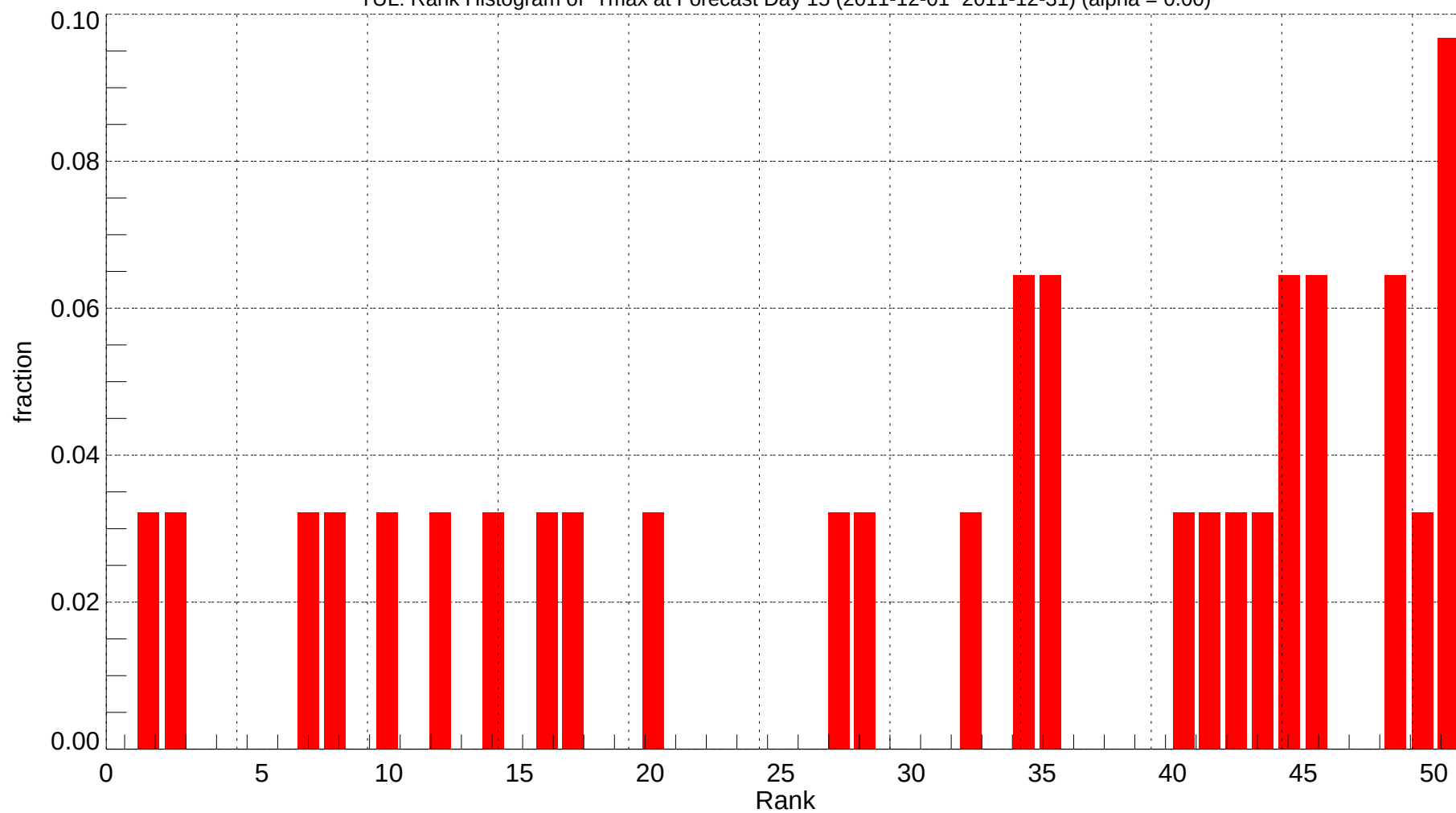
TUL: Rank Histogram of Tmax at Forecast Day 15 (2011-12-01~2011-12-31) (alpha = 0.00)
