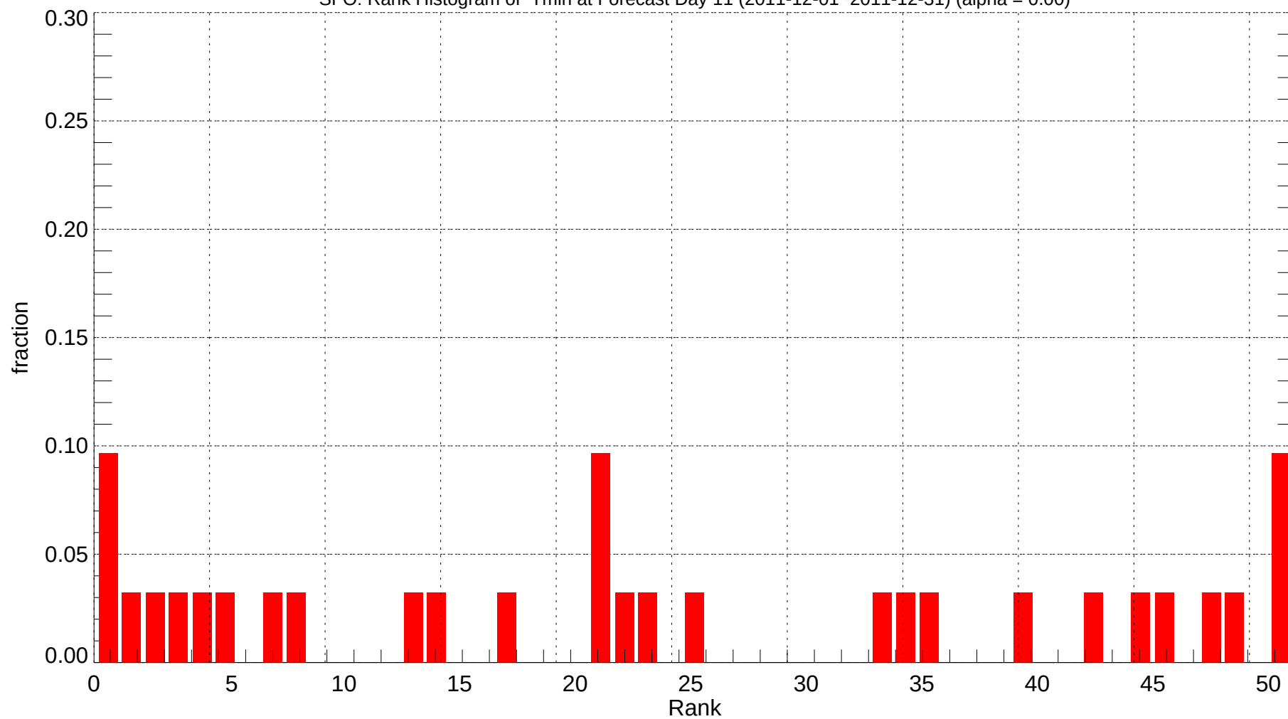
SFO: Rank Histogram of Tmin at Forecast Day 11 (2011-12-01~2011-12-31) (alpha = 0.00)
