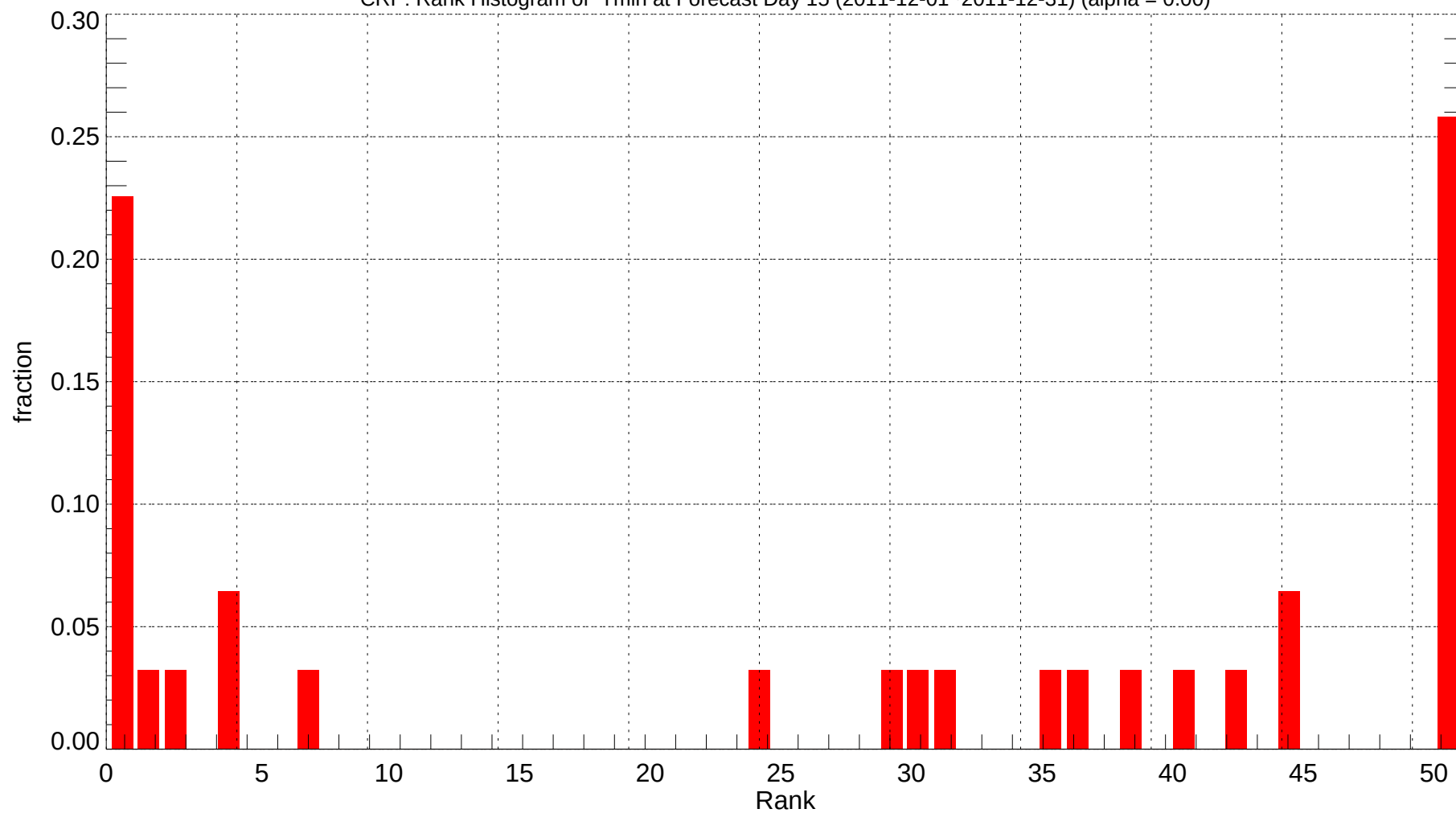
CRP: Rank Histogram of Tmin at Forecast Day 15 (2011-12-01~2011-12-31) (alpha = 0.00)
