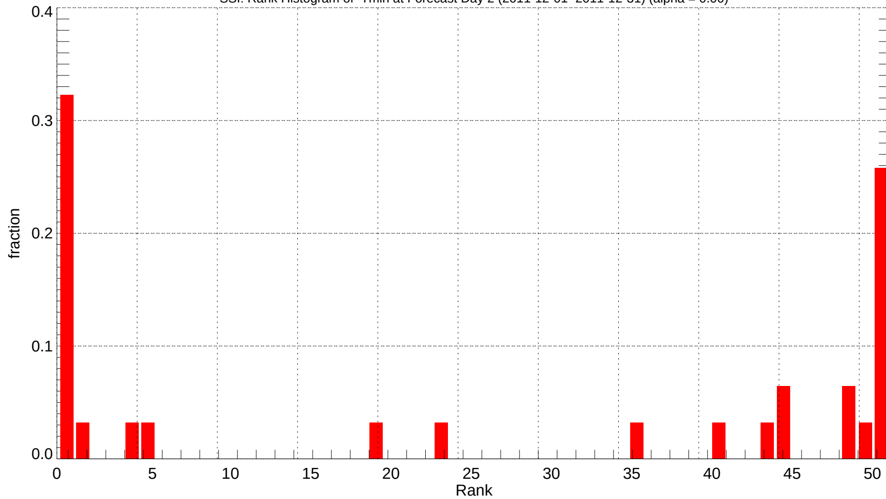
SSI: Rank Histogram of Tmin at Forecast Day 2 (2011-12-01~2011-12-31) (alpha = 0.00)
