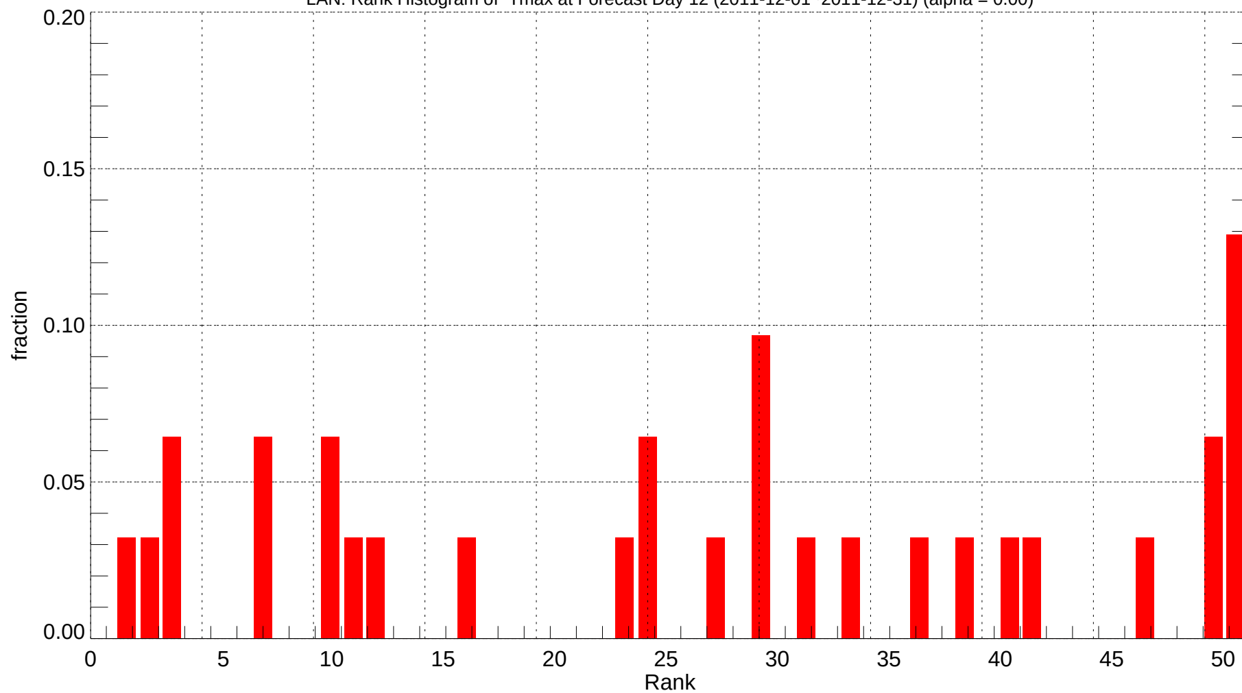
LAN: Rank Histogram of Tmax at Forecast Day 12 (2011-12-01~2011-12-31) (alpha = 0.00)
