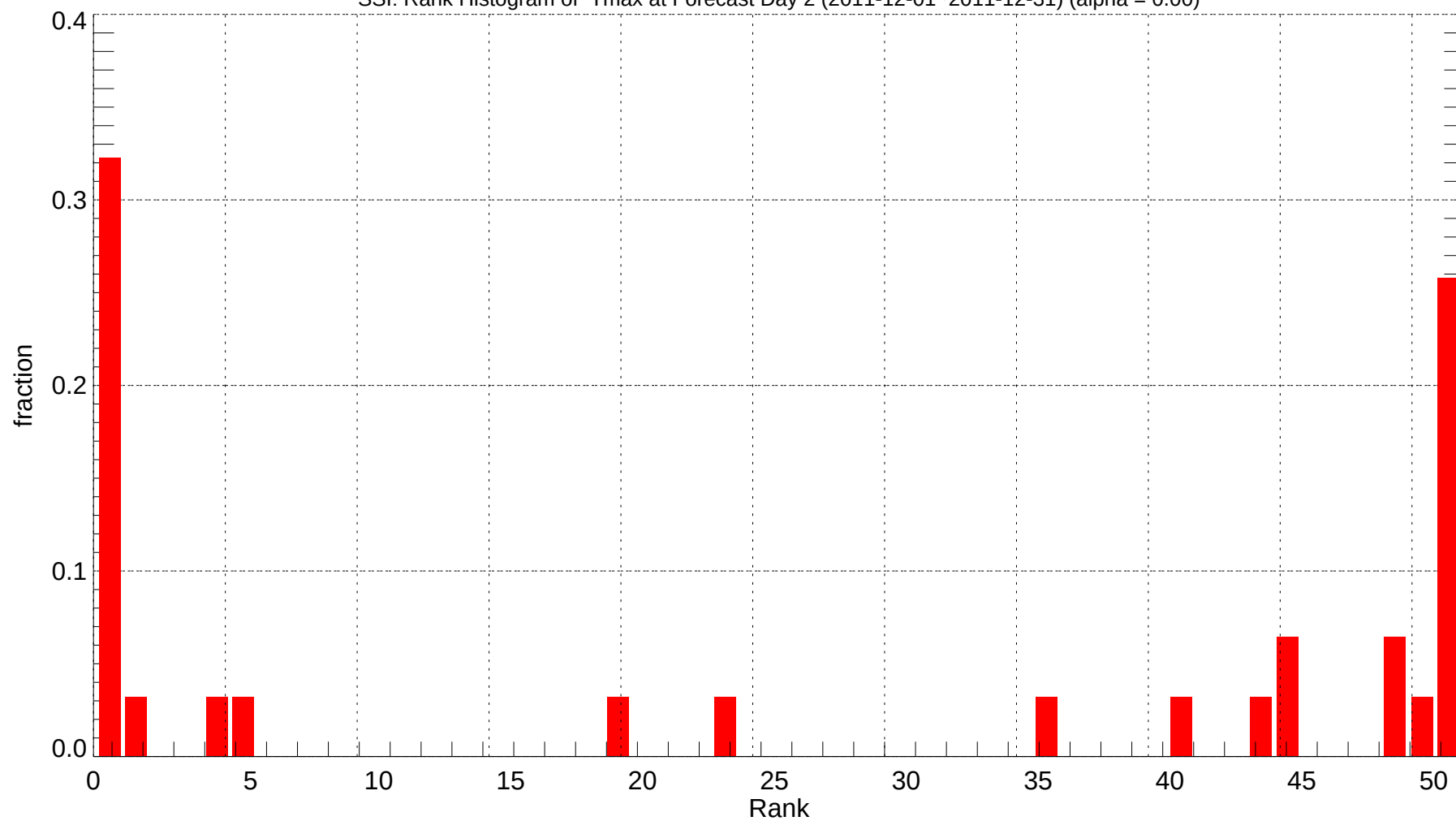
SSI: Rank Histogram of Tmax at Forecast Day 2 (2011-12-01~2011-12-31) (alpha = 0.00)
