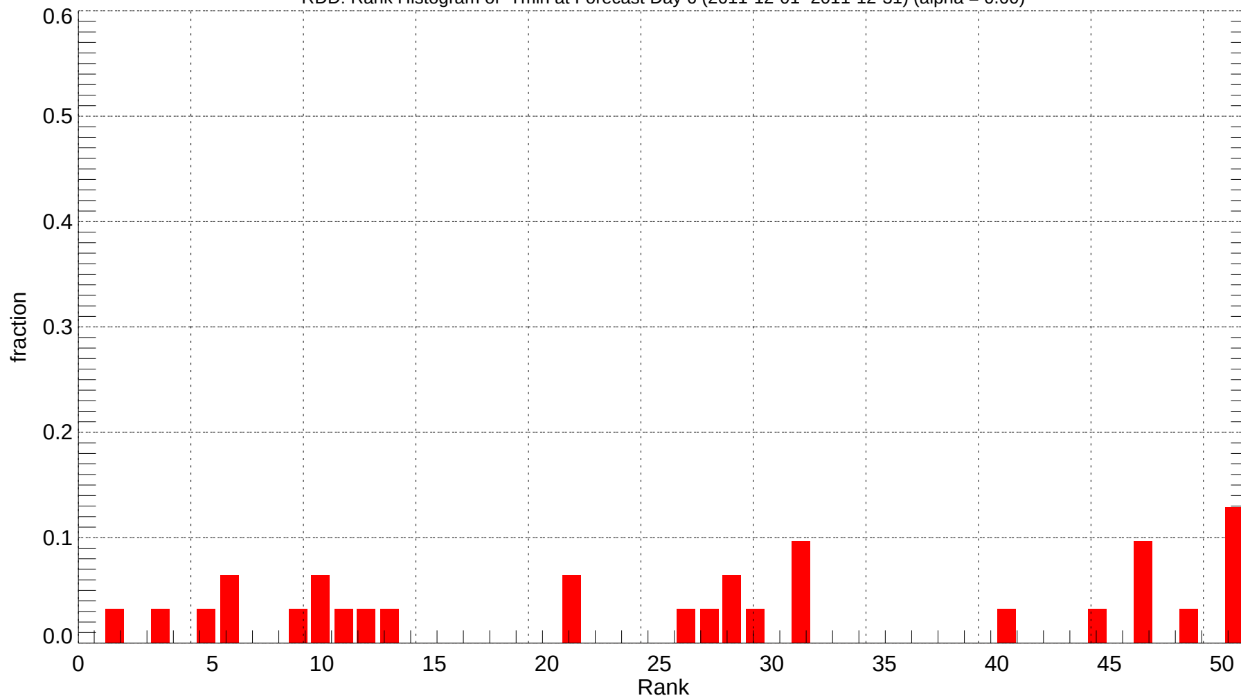
RDD: Rank Histogram of Tmin at Forecast Day 6 (2011-12-01~2011-12-31) (alpha = 0.00)
