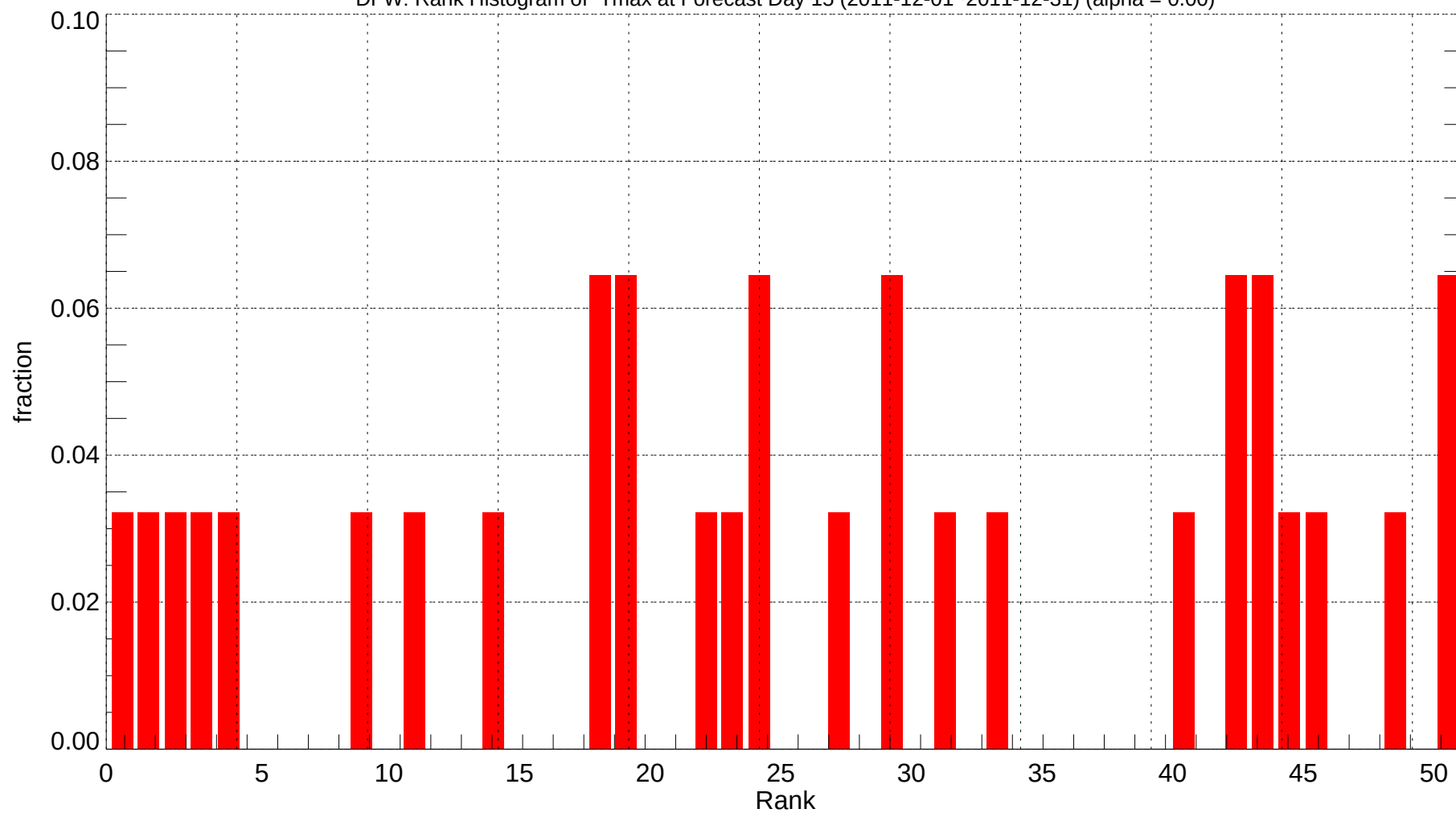
DFW: Rank Histogram of Tmax at Forecast Day 15 (2011-12-01~2011-12-31) (alpha = 0.00)
