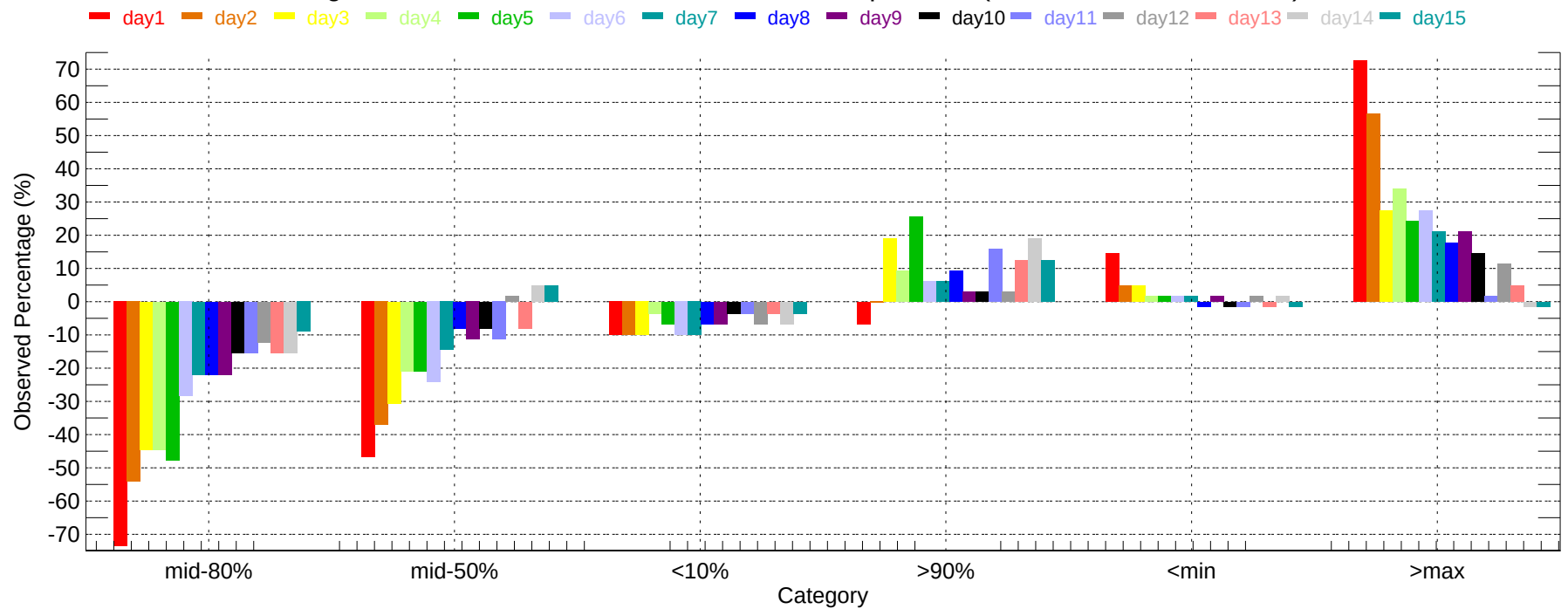
Observed Percentage Deviation of Ensembles - COU: Min Temperature (2011-12-01~2011-12-31)
