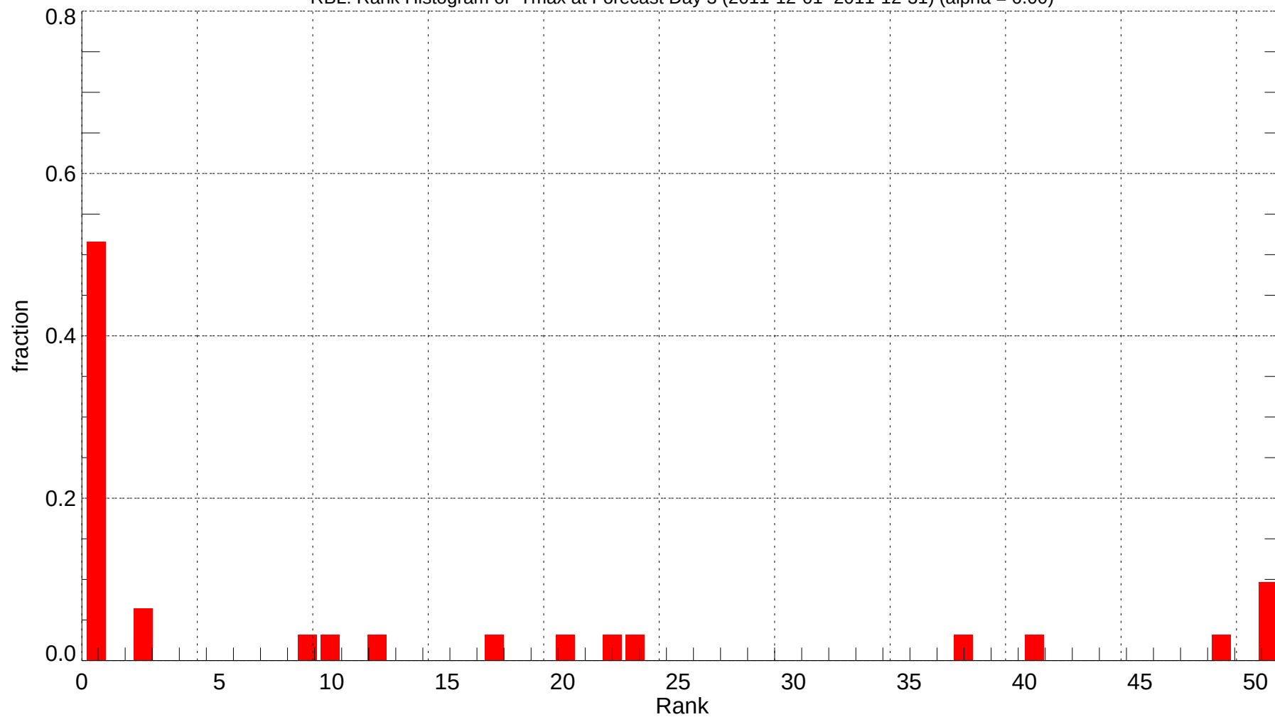
RBL: Rank Histogram of Tmax at Forecast Day 3 (2011-12-01~2011-12-31) (alpha = 0.00)
