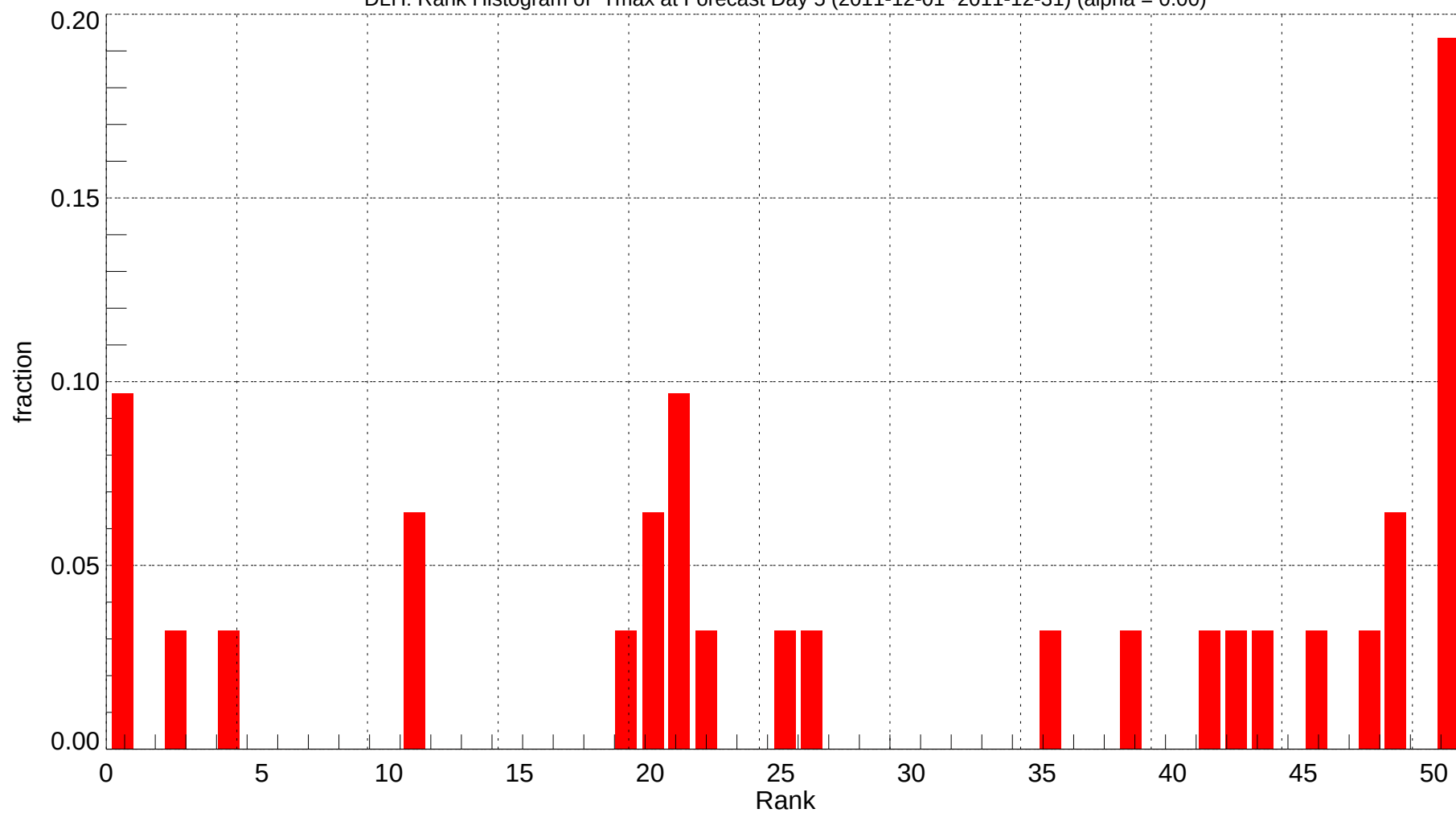
DLH: Rank Histogram of Tmax at Forecast Day 5 (2011-12-01~2011-12-31) (alpha = 0.00)
