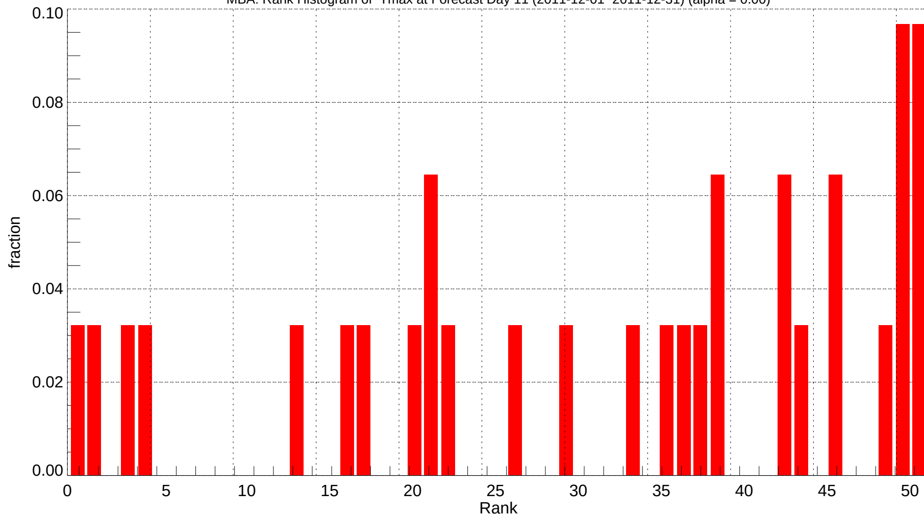
MBA: Rank Histogram of Tmax at Forecast Day 11 (2011-12-01~2011-12-31) (alpha = 0.00)
