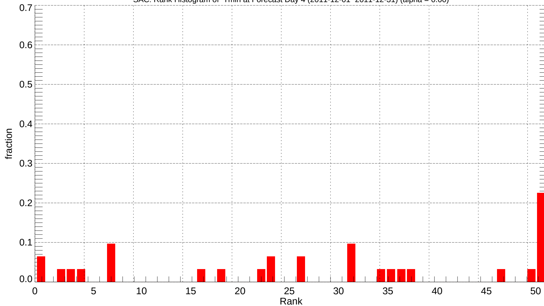
SAC: Rank Histogram of Tmin at Forecast Day 4 (2011-12-01~2011-12-31) (alpha = 0.00)
