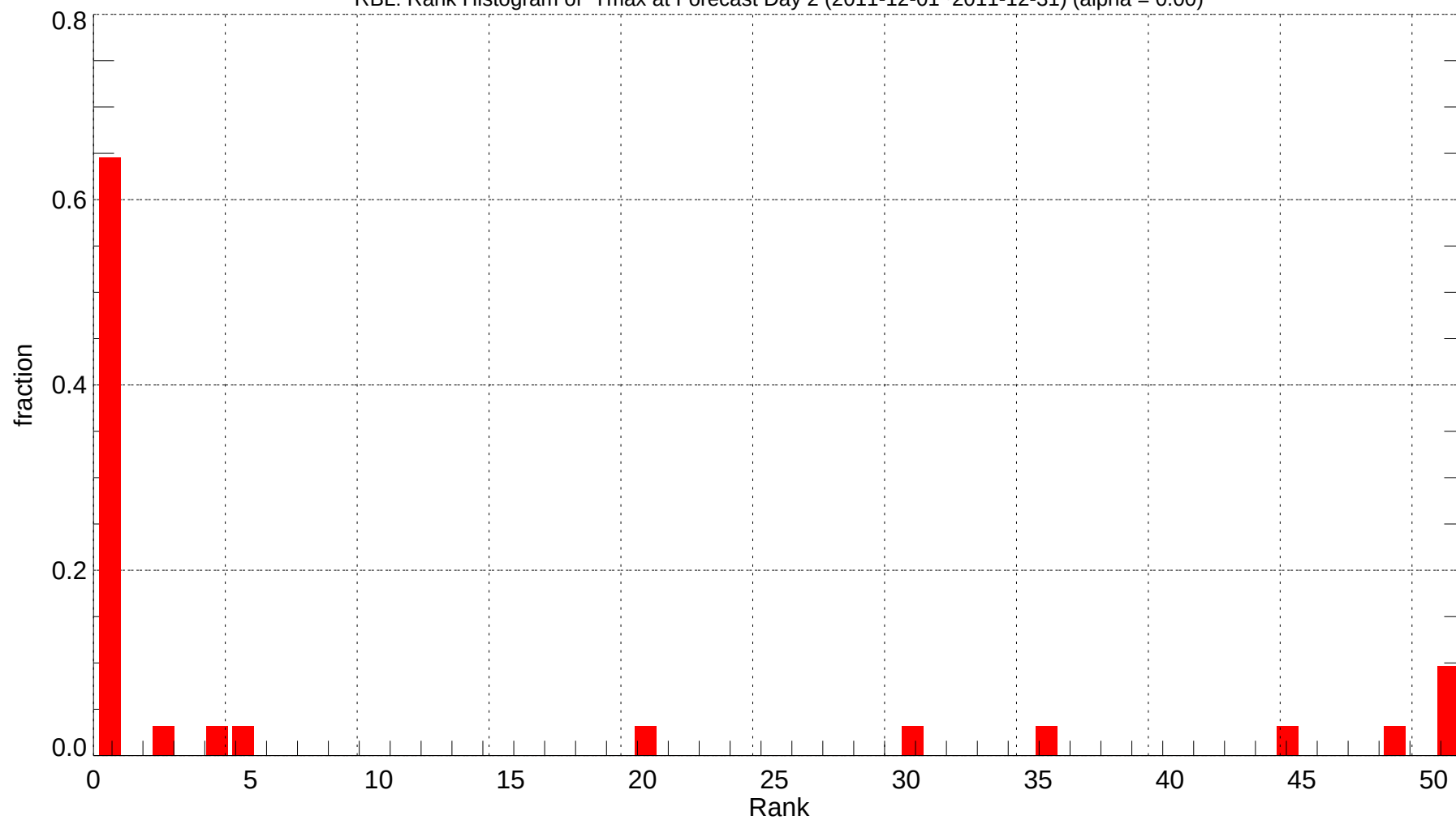
RBL: Rank Histogram of Tmax at Forecast Day 2 (2011-12-01~2011-12-31) (alpha = 0.00)
