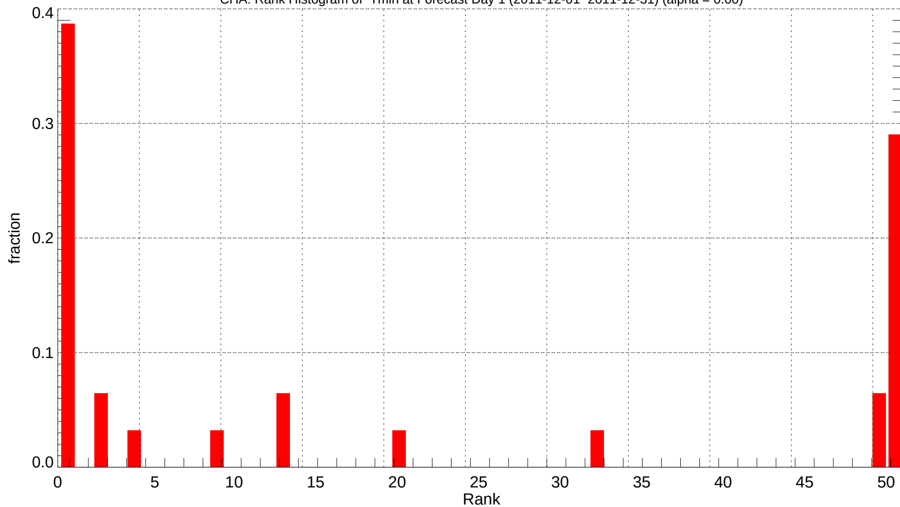
CHA: Rank Histogram of Tmin at Forecast Day 1 (2011-12-01~2011-12-31) (alpha = 0.00)
