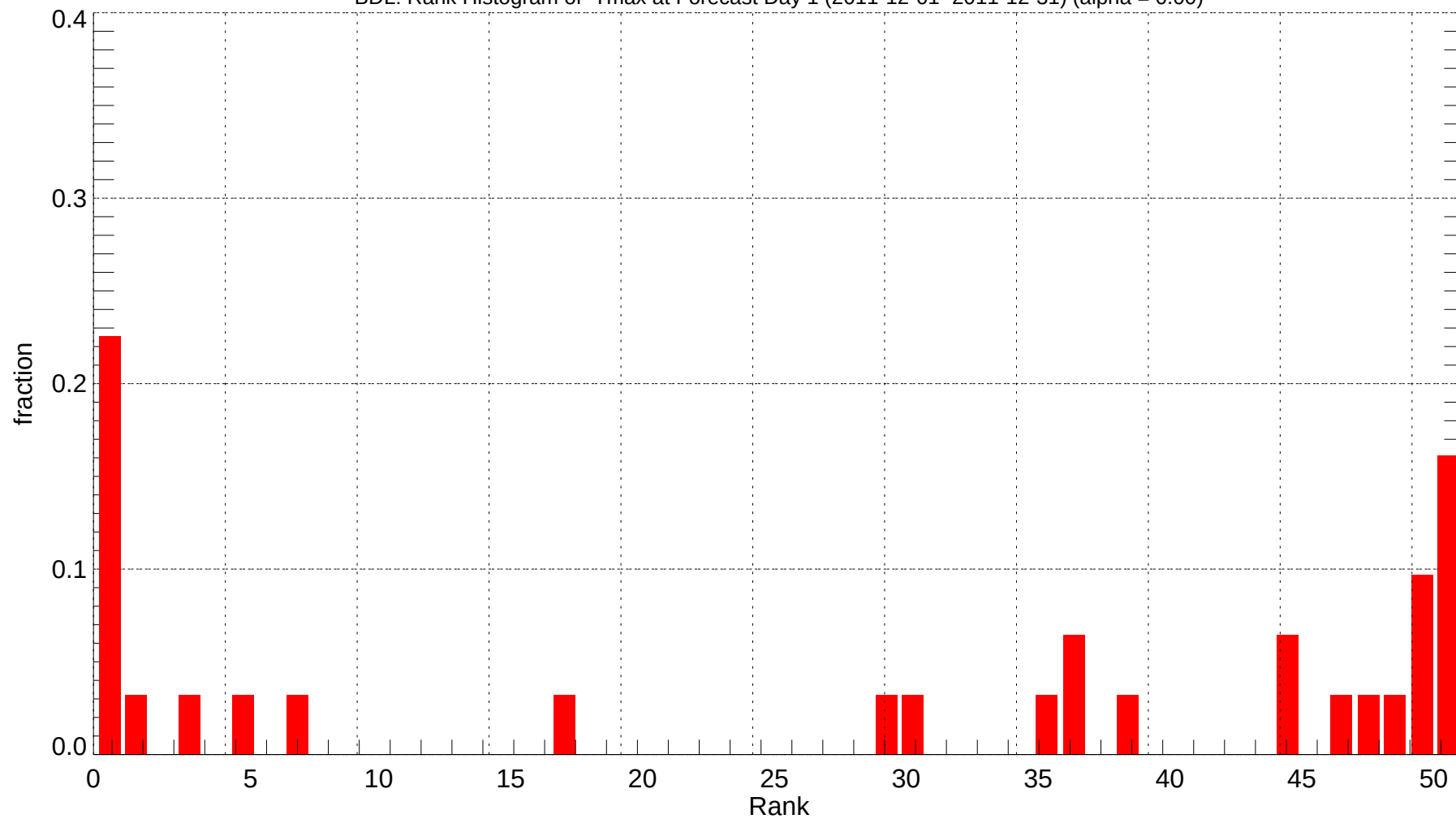
BDL: Rank Histogram of Tmax at Forecast Day 1 (2011-12-01~2011-12-31) (alpha = 0.00)
