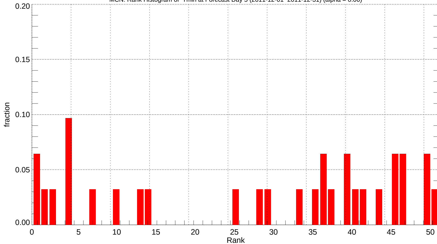
MCN: Rank Histogram of Tmin at Forecast Day 5 (2011-12-01~2011-12-31) (alpha = 0.00)
