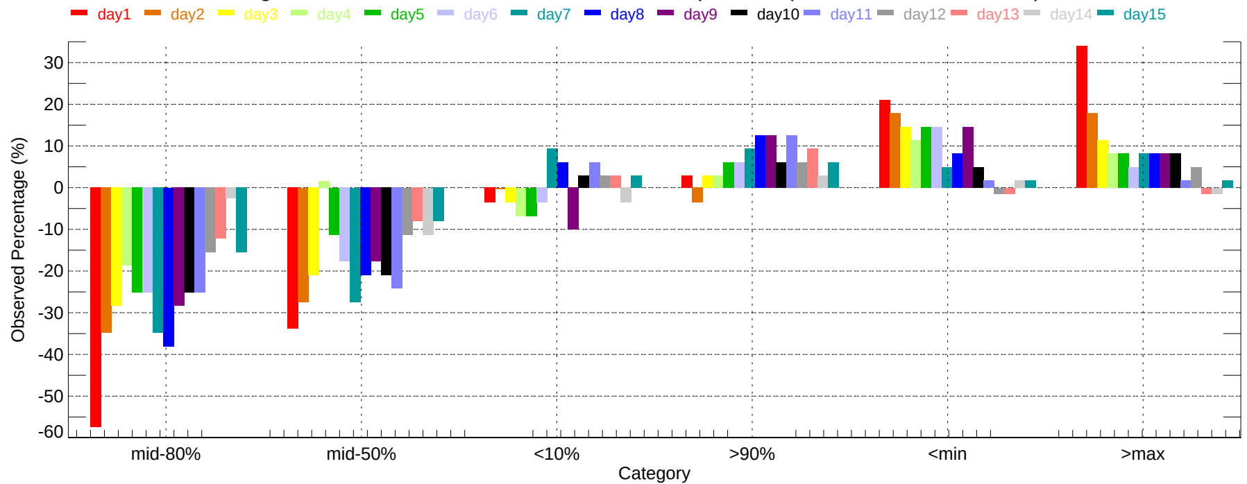
Observed Percentage Deviation of Ensembles - CON: Max Temperature (2011-12-01~2011-12-31)
