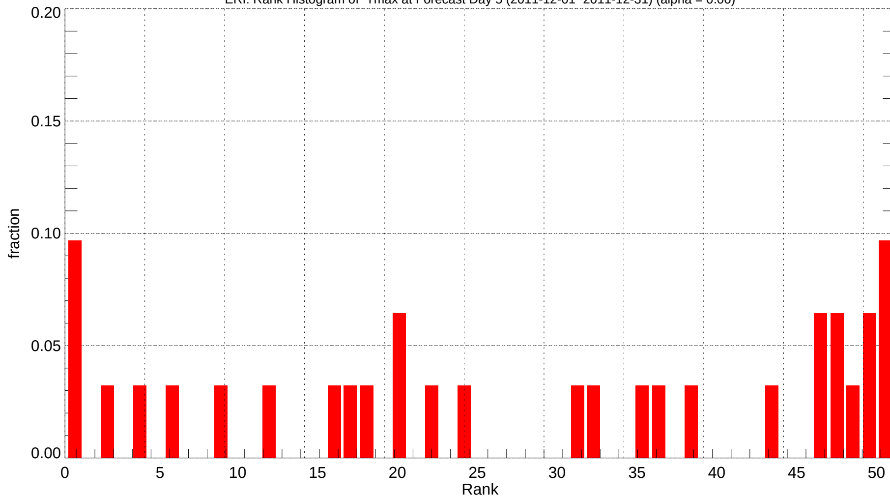
ERI: Rank Histogram of Tmax at Forecast Day 5 (2011-12-01~2011-12-31) (alpha = 0.00)
