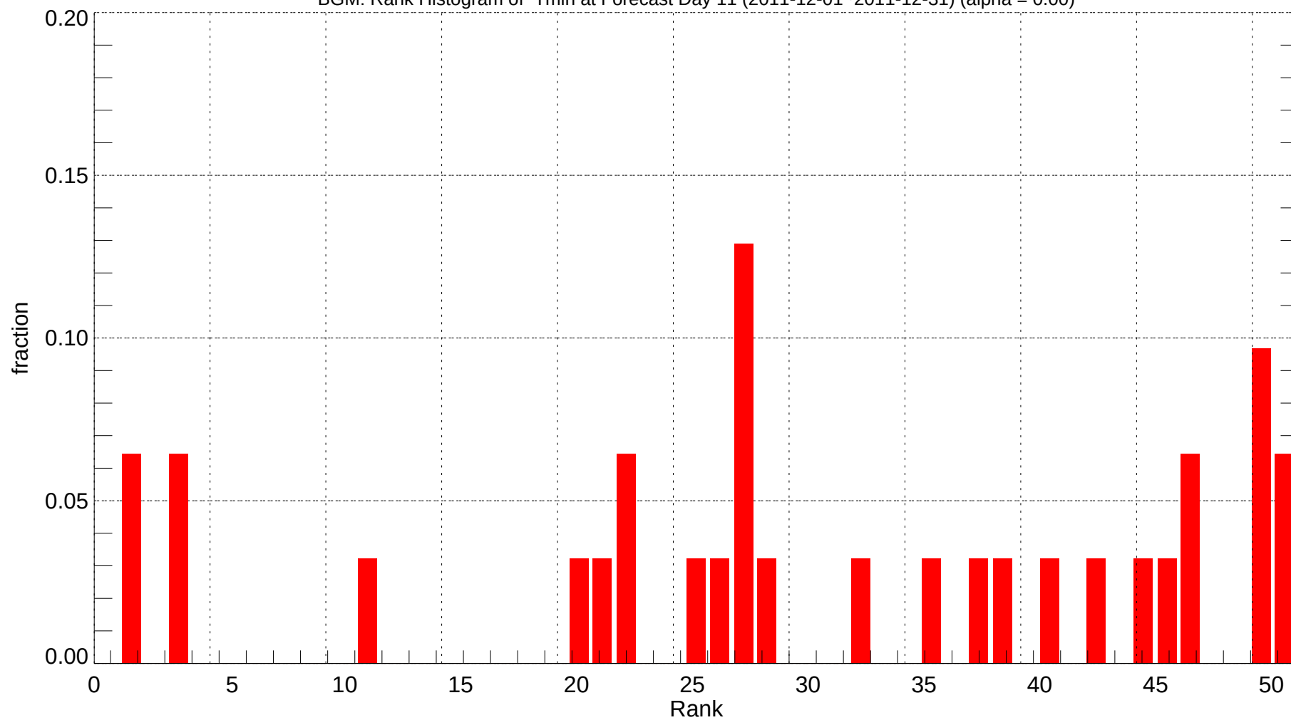
BGM: Rank Histogram of Tmin at Forecast Day 11 (2011-12-01~2011-12-31) (alpha = 0.00)
