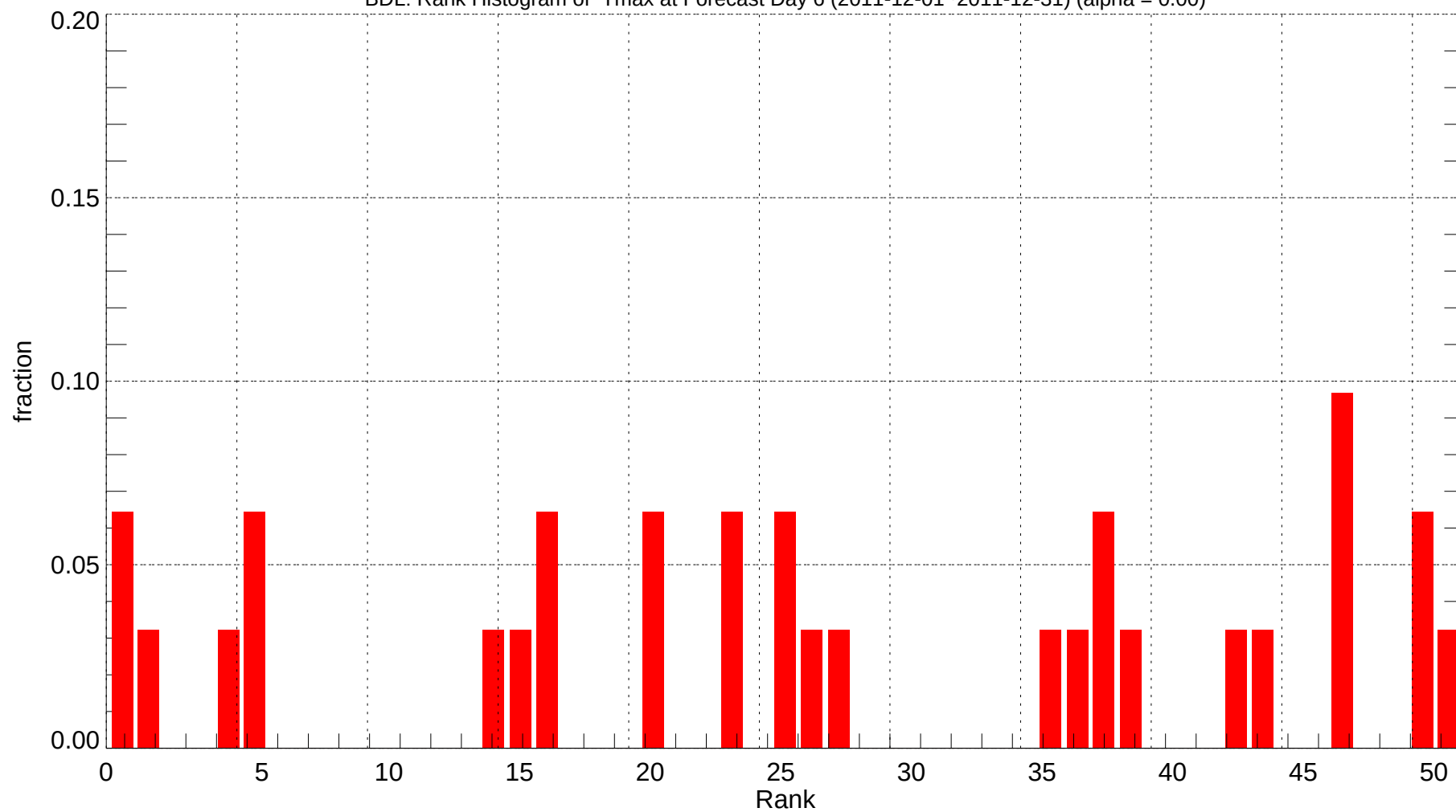
BDL: Rank Histogram of Tmax at Forecast Day 6 (2011-12-01~2011-12-31) (alpha = 0.00)
