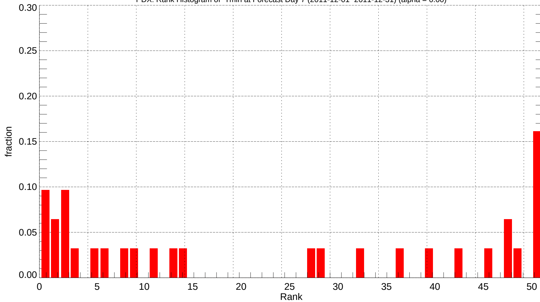
PDX: Rank Histogram of Tmin at Forecast Day 7 (2011-12-01~2011-12-31) (alpha = 0.00)
