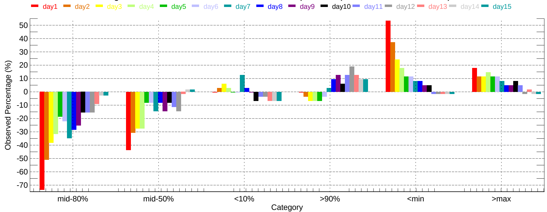
Observed Percentage Deviation of Ensembles - ILG: Max Temperature (2011-12-01~2011-12-31)
