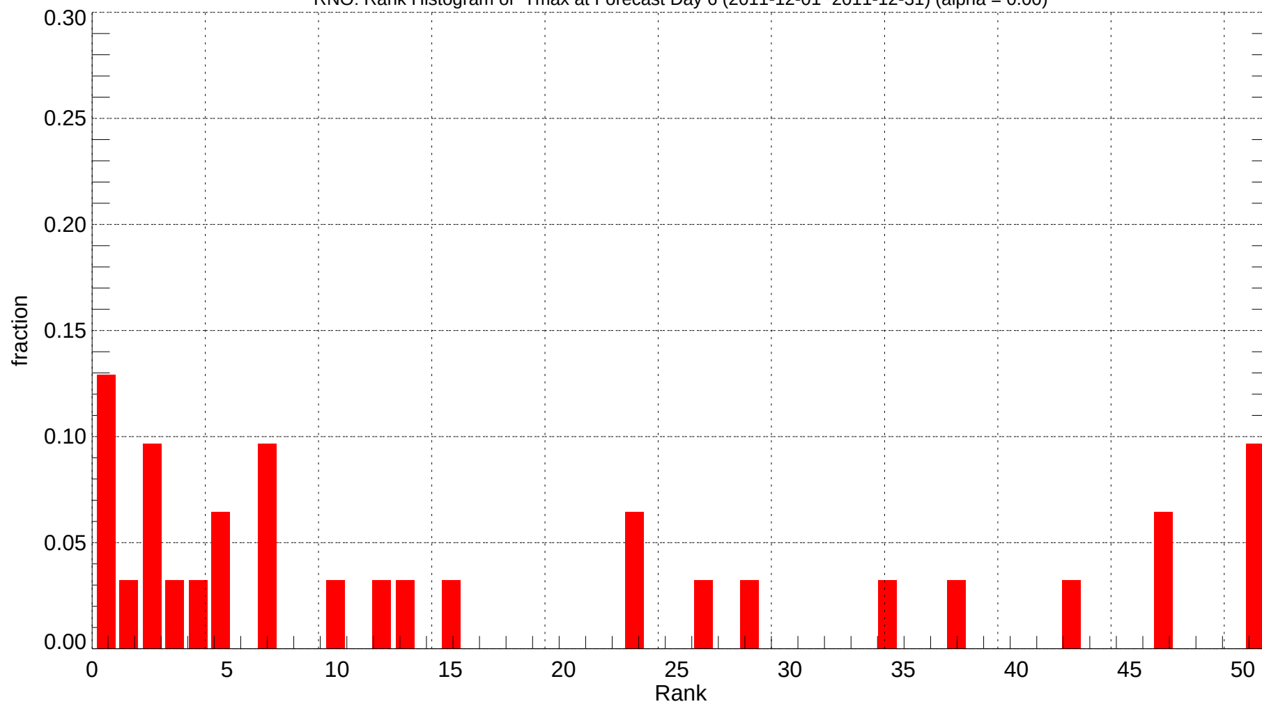
RNO: Rank Histogram of Tmax at Forecast Day 6 (2011-12-01~2011-12-31) (alpha = 0.00)
