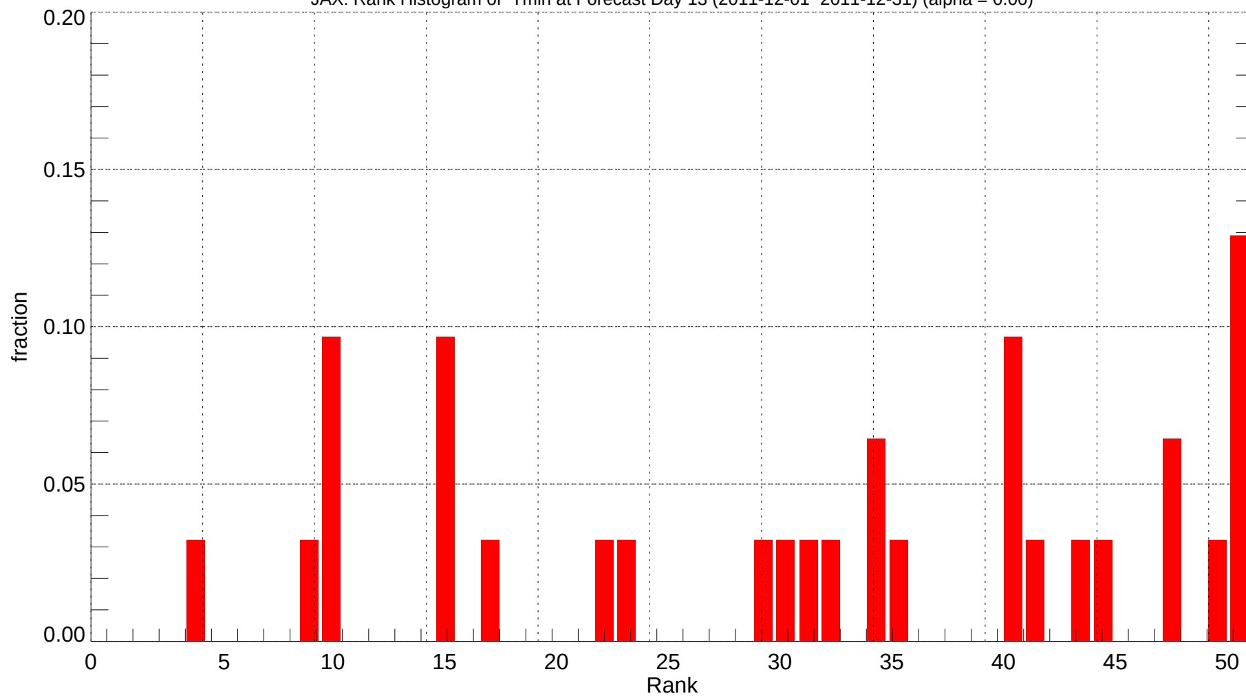
JAX: Rank Histogram of Tmin at Forecast Day 13 (2011-12-01~2011-12-31) (alpha = 0.00)
