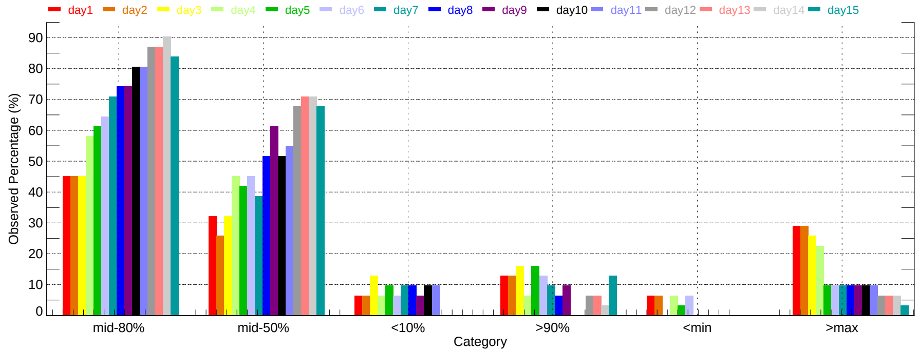
Observed Percentage of Ensembles - SAC: Max Temperature (2011-12-01~2011-12-31)
