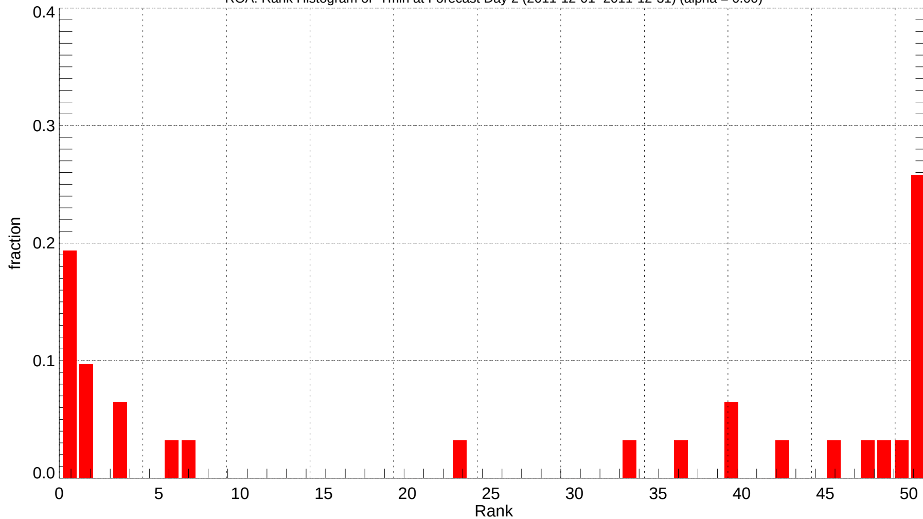
ROA: Rank Histogram of Tmin at Forecast Day 2 (2011-12-01~2011-12-31) (alpha = 0.00)
