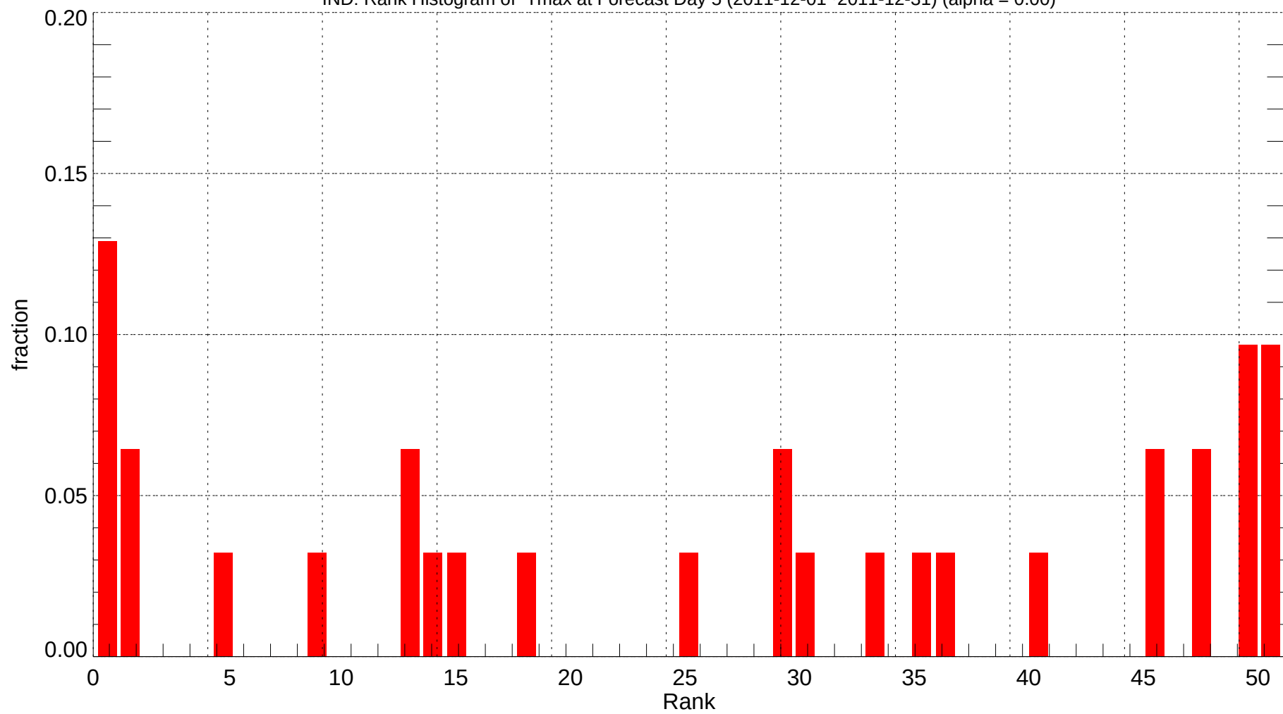
IND: Rank Histogram of Tmax at Forecast Day 5 (2011-12-01~2011-12-31) (alpha = 0.00)
