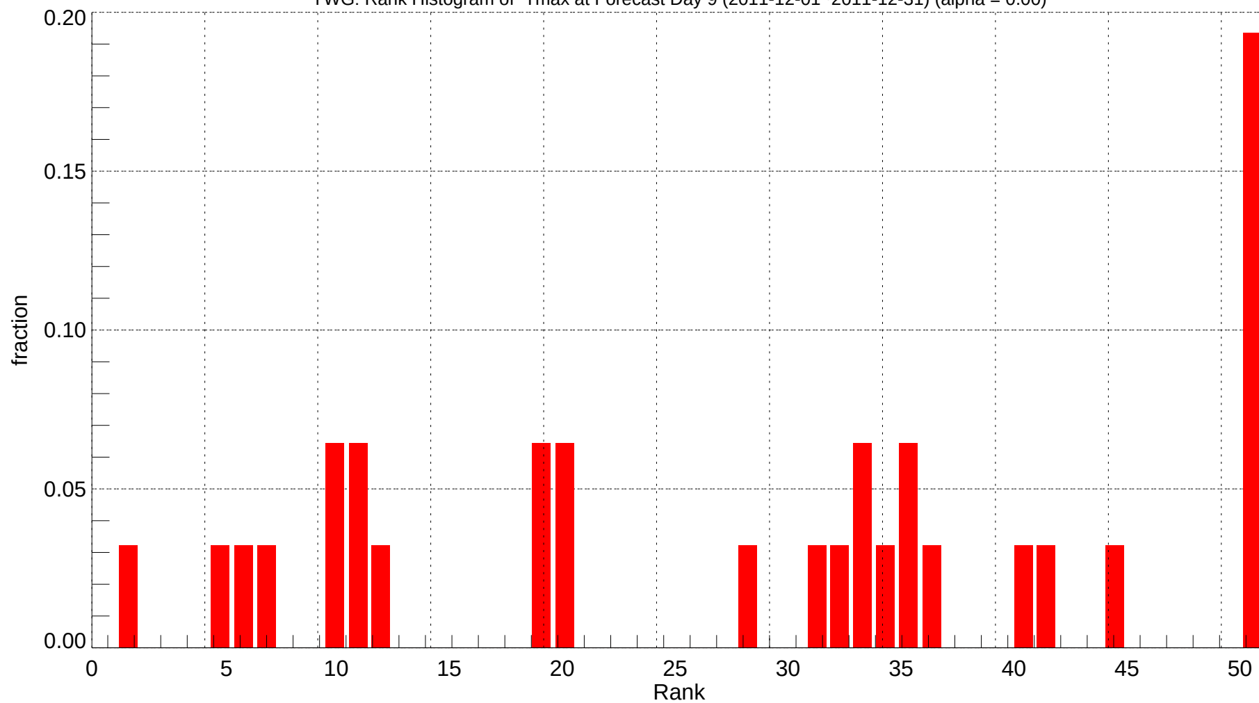
YWG: Rank Histogram of Tmax at Forecast Day 9 (2011-12-01~2011-12-31) (alpha = 0.00)
