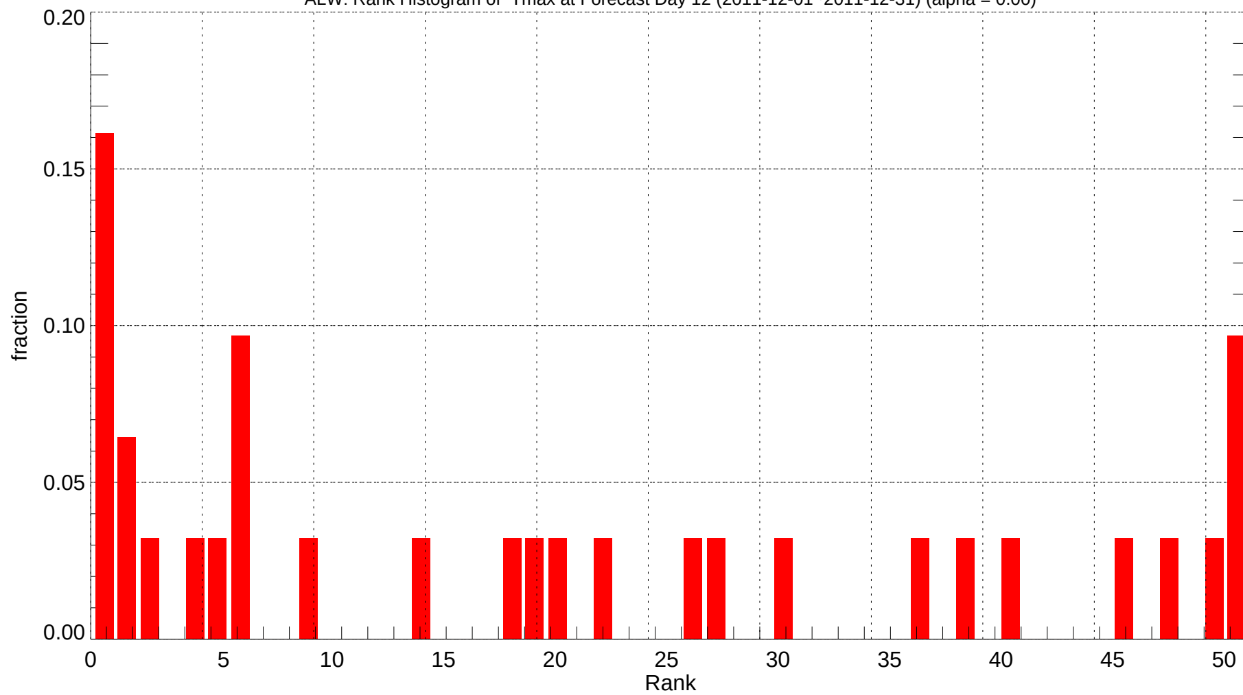
ALW: Rank Histogram of Tmax at Forecast Day 12 (2011-12-01~2011-12-31) (alpha = 0.00)
