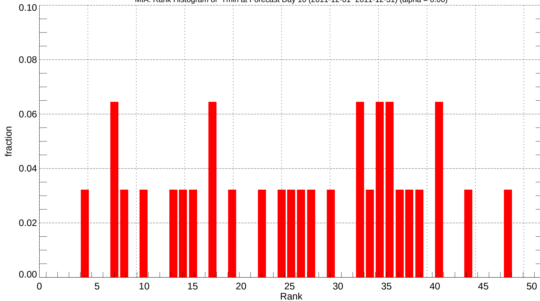
MIA: Rank Histogram of Tmin at Forecast Day 10 (2011-12-01~2011-12-31) (alpha = 0.00)
