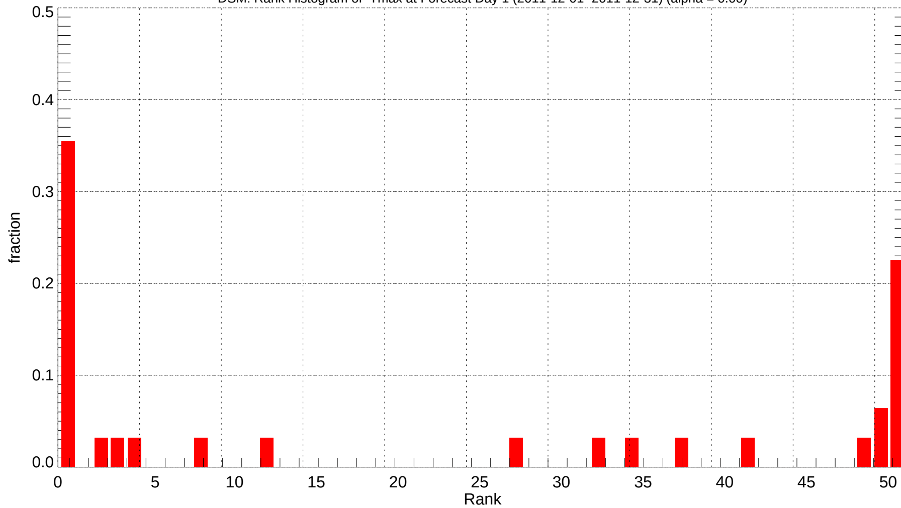
DSM: Rank Histogram of Tmax at Forecast Day 1 (2011-12-01~2011-12-31) (alpha = 0.00)
