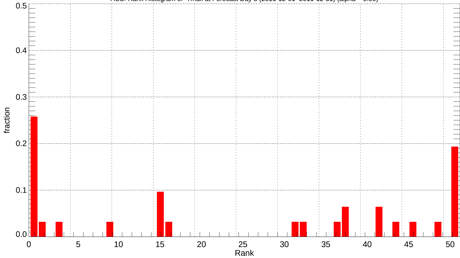
AUS: Rank Histogram of Tmax at Forecast Day 3 (2011-12-01~2011-12-31) (alpha = 0.00)
