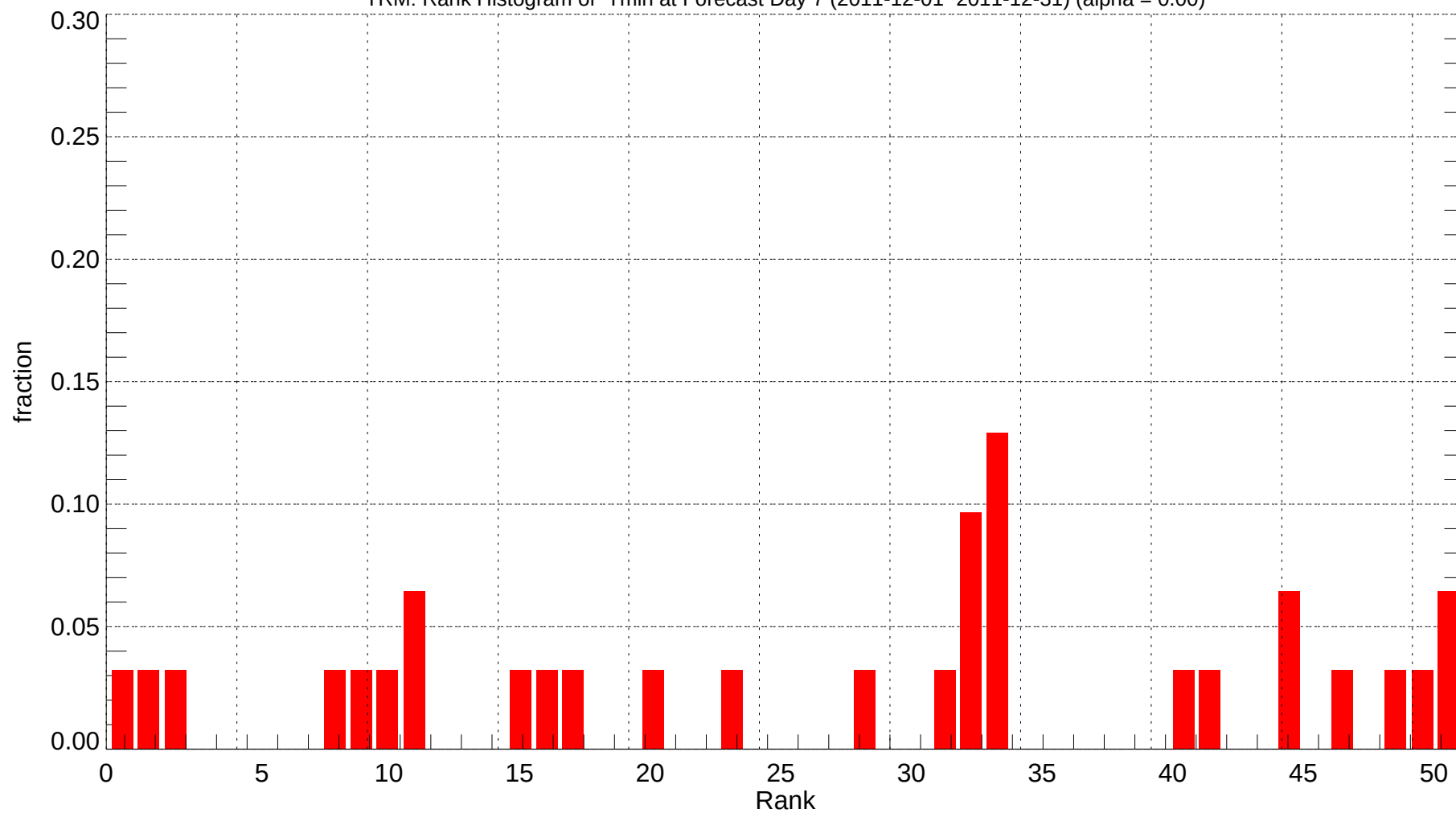
TRM: Rank Histogram of Tmin at Forecast Day 7 (2011-12-01~2011-12-31) (alpha = 0.00)
