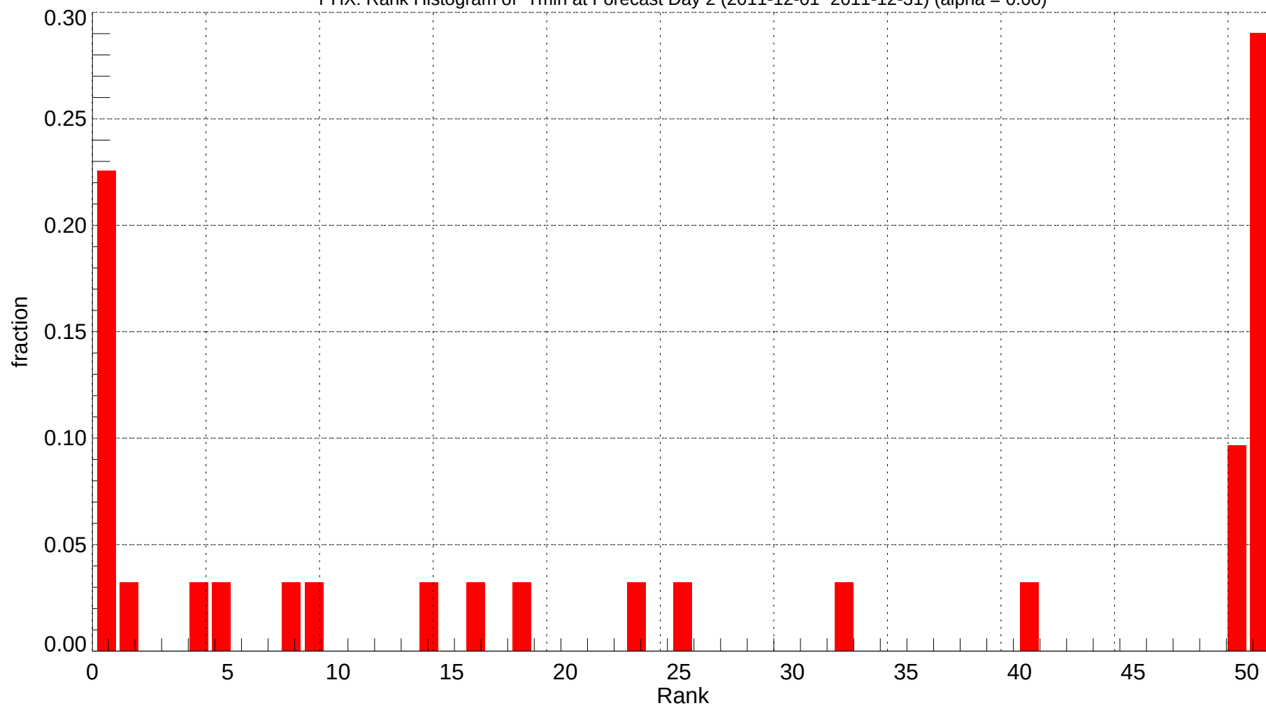
PHX: Rank Histogram of Tmin at Forecast Day 2 (2011-12-01~2011-12-31) (alpha = 0.00)
