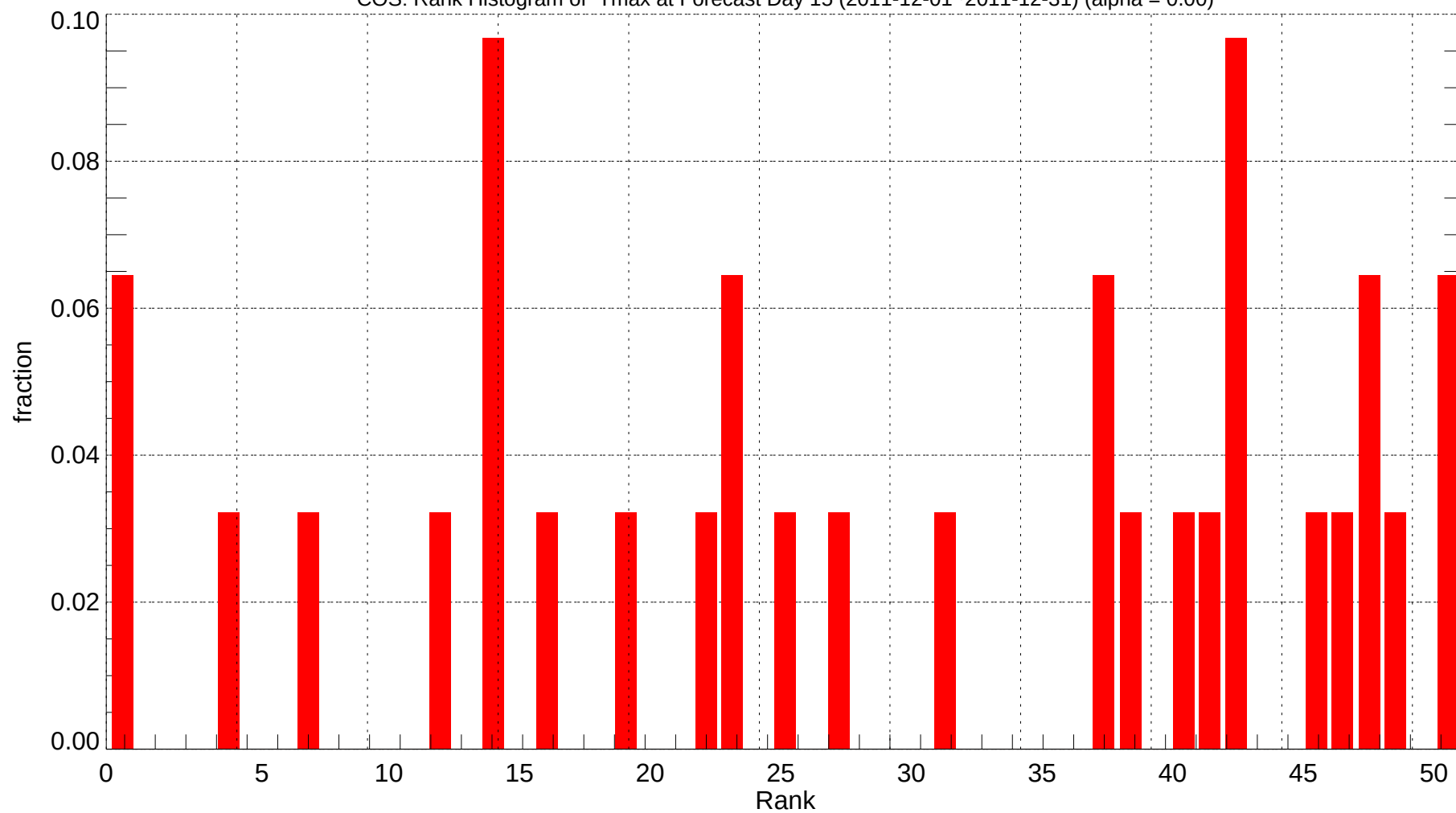
COS: Rank Histogram of Tmax at Forecast Day 15 (2011-12-01~2011-12-31) (alpha = 0.00)
