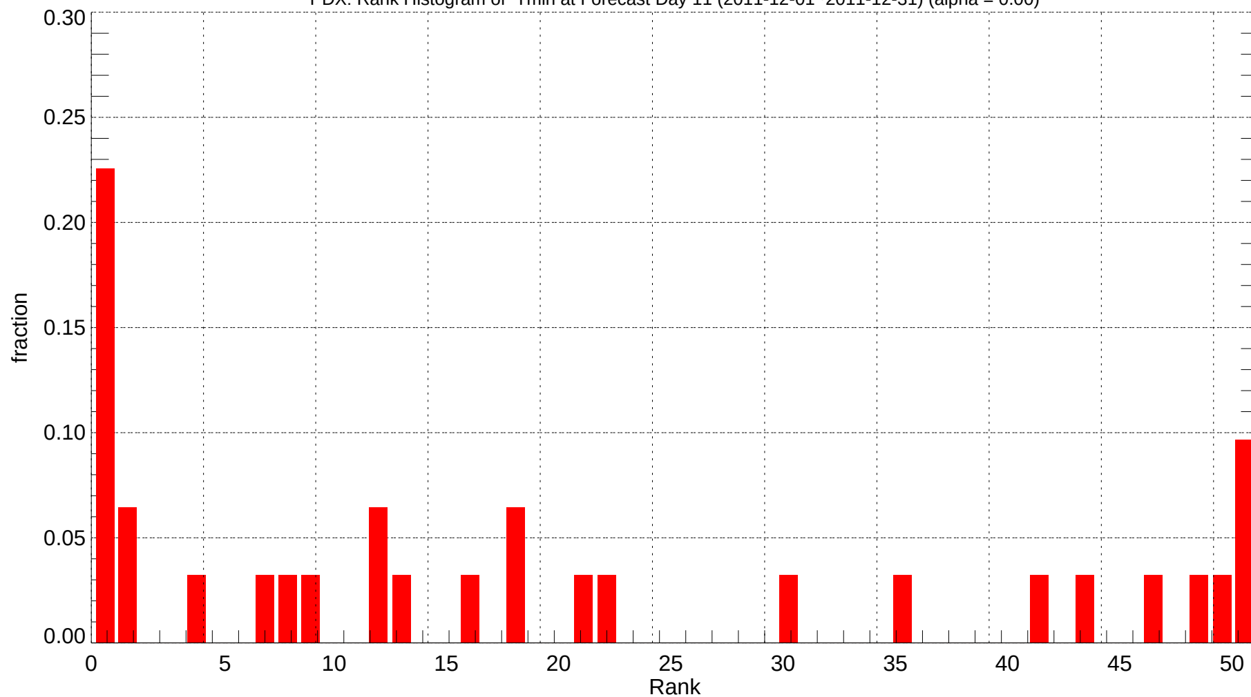
PDX: Rank Histogram of Tmin at Forecast Day 11 (2011-12-01~2011-12-31) (alpha = 0.00)
