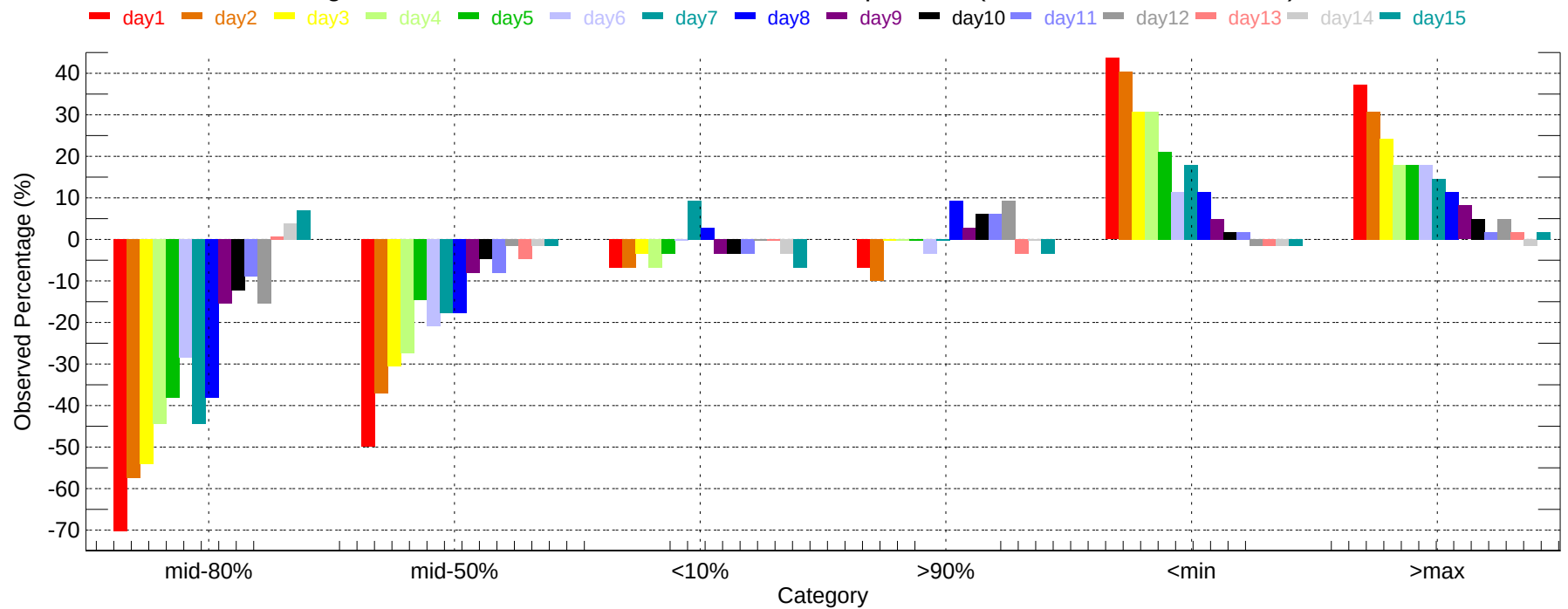
Observed Percentage Deviation of Ensembles - NTU: Min Temperature (2011-12-01~2011-12-31)
