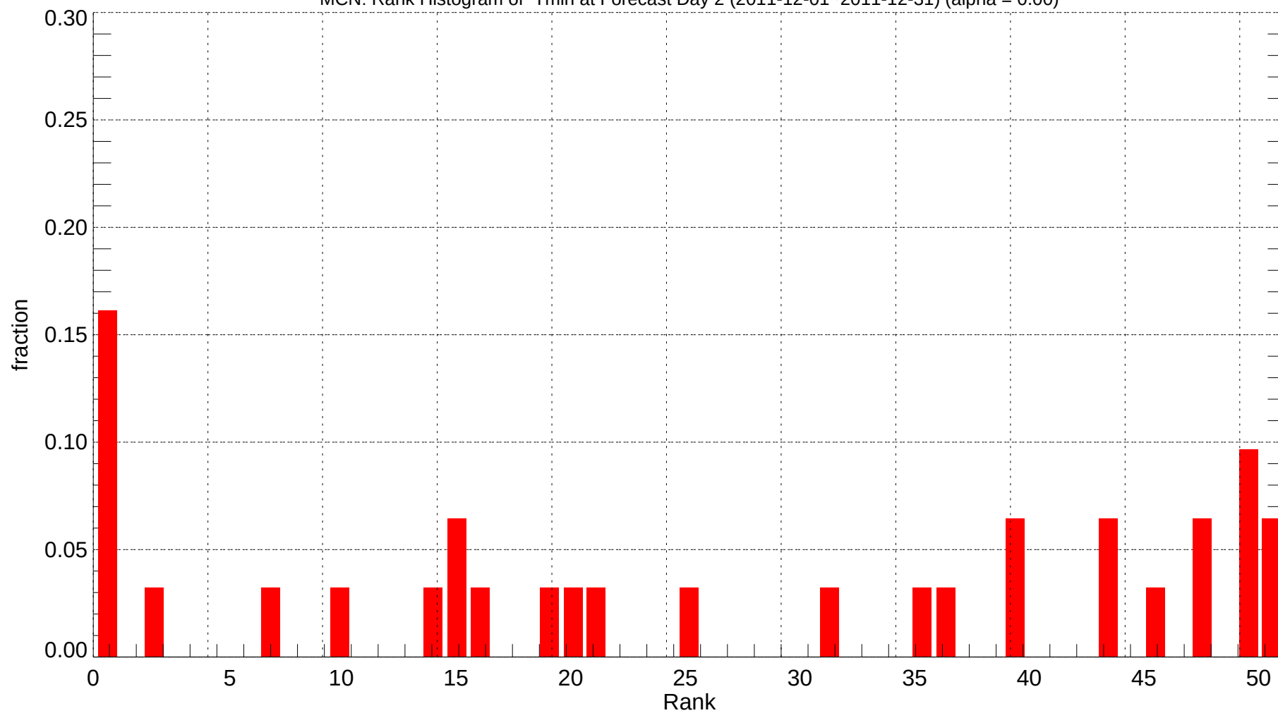
MCN: Rank Histogram of Tmin at Forecast Day 2 (2011-12-01~2011-12-31) (alpha = 0.00)
