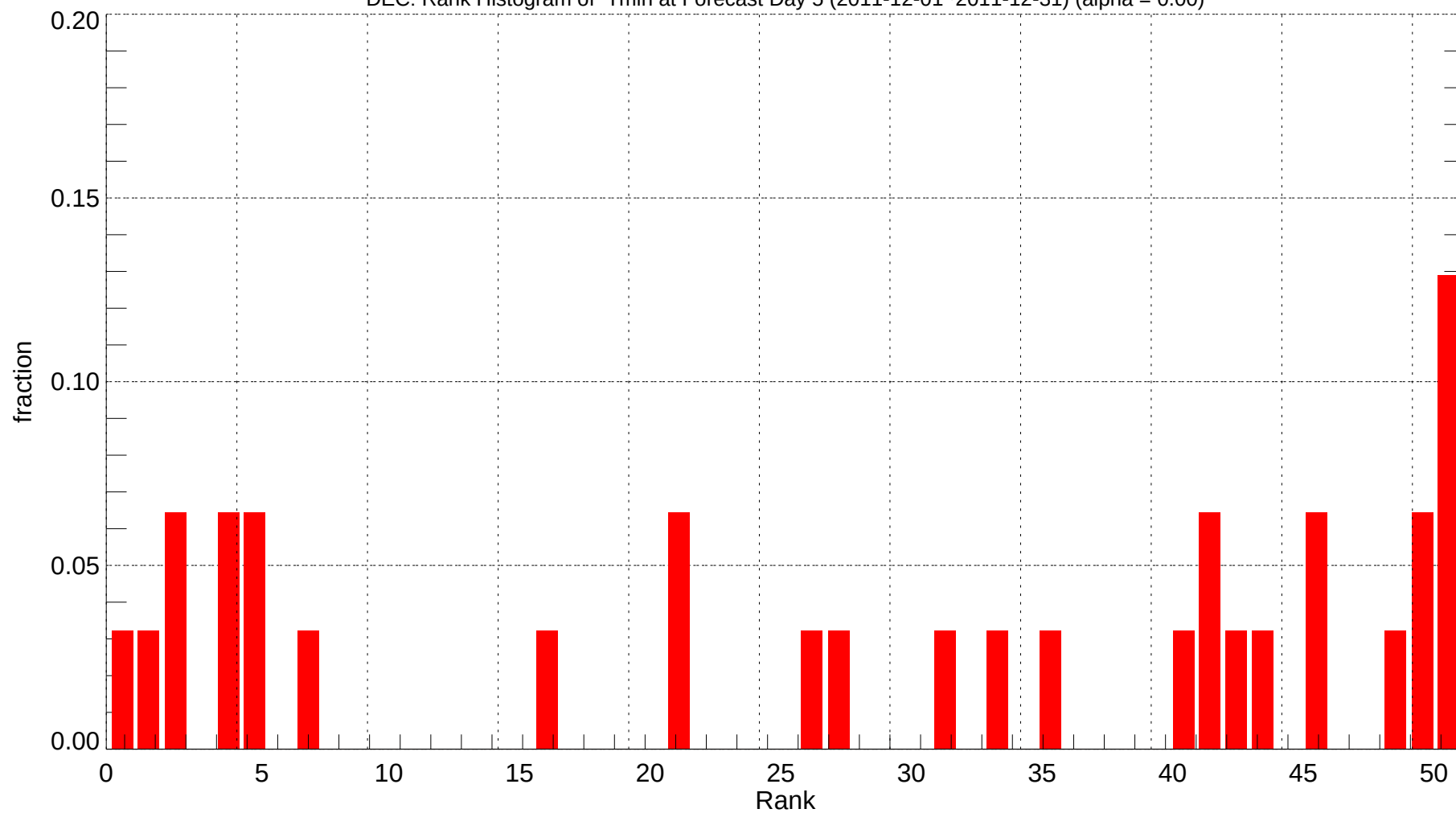
DEC: Rank Histogram of Tmin at Forecast Day 5 (2011-12-01~2011-12-31) (alpha = 0.00)
