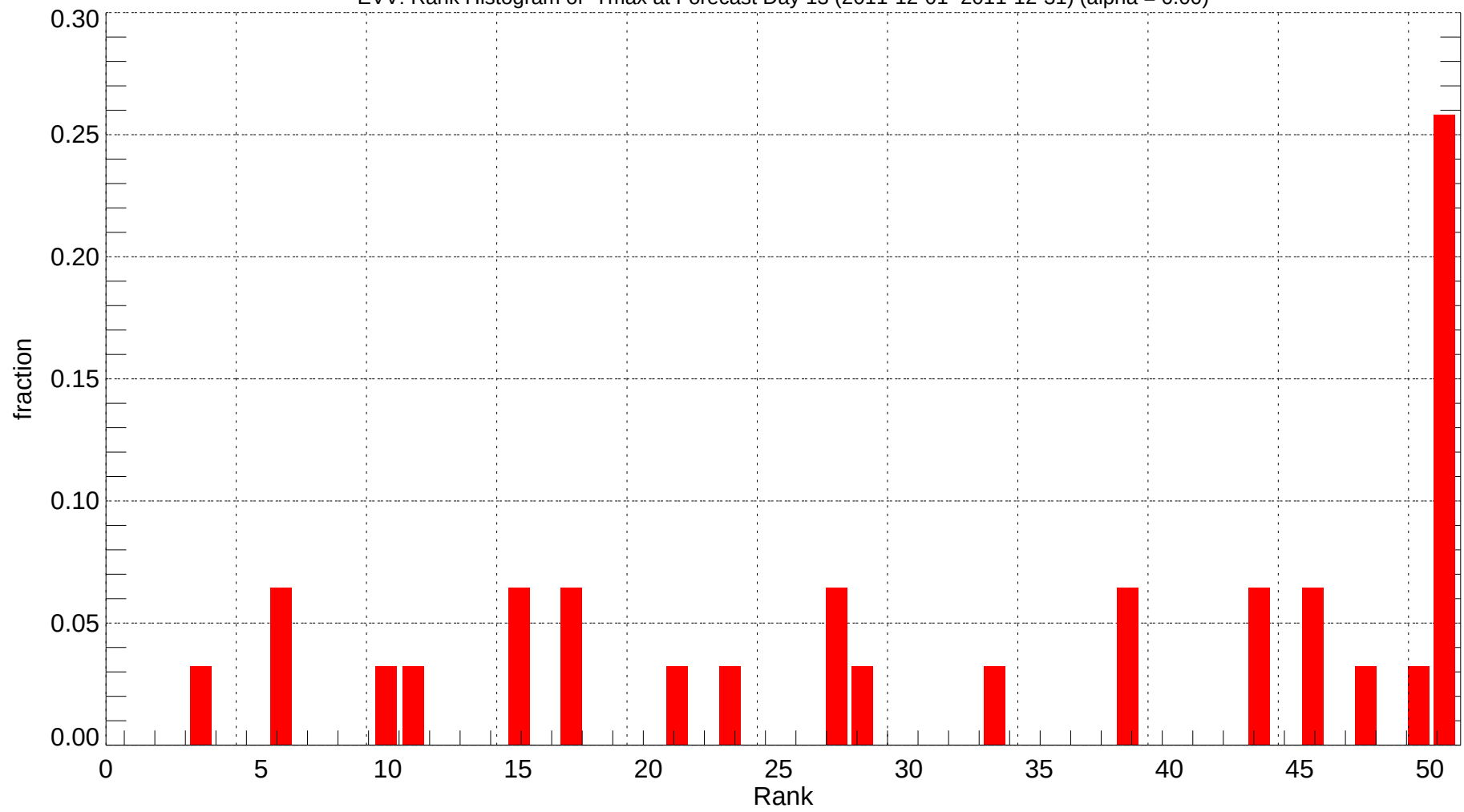
EVV: Rank Histogram of Tmax at Forecast Day 13 (2011-12-01~2011-12-31) (alpha = 0.00)
