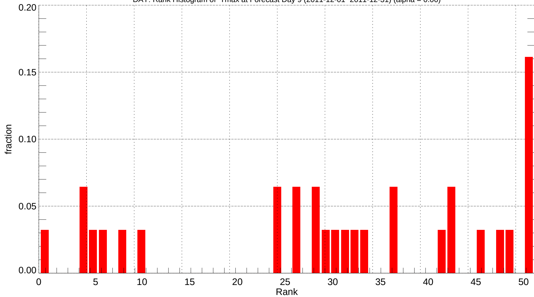
DAY: Rank Histogram of Tmax at Forecast Day 9 (2011-12-01~2011-12-31) (alpha = 0.00)
