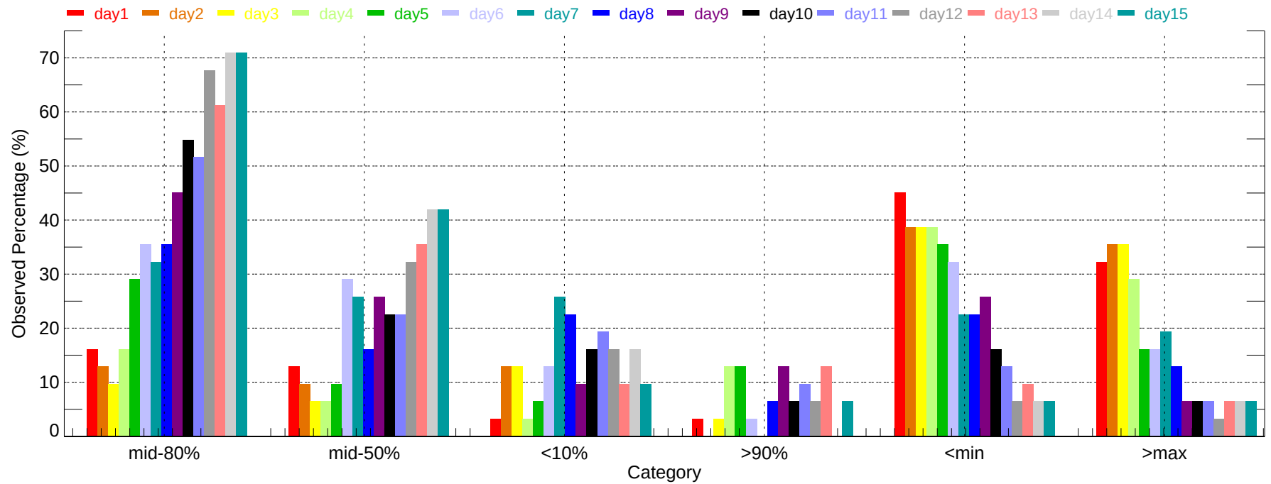
Observed Percentage of Ensembles - GEG: Max Temperature (2011-12-01~2011-12-31)
