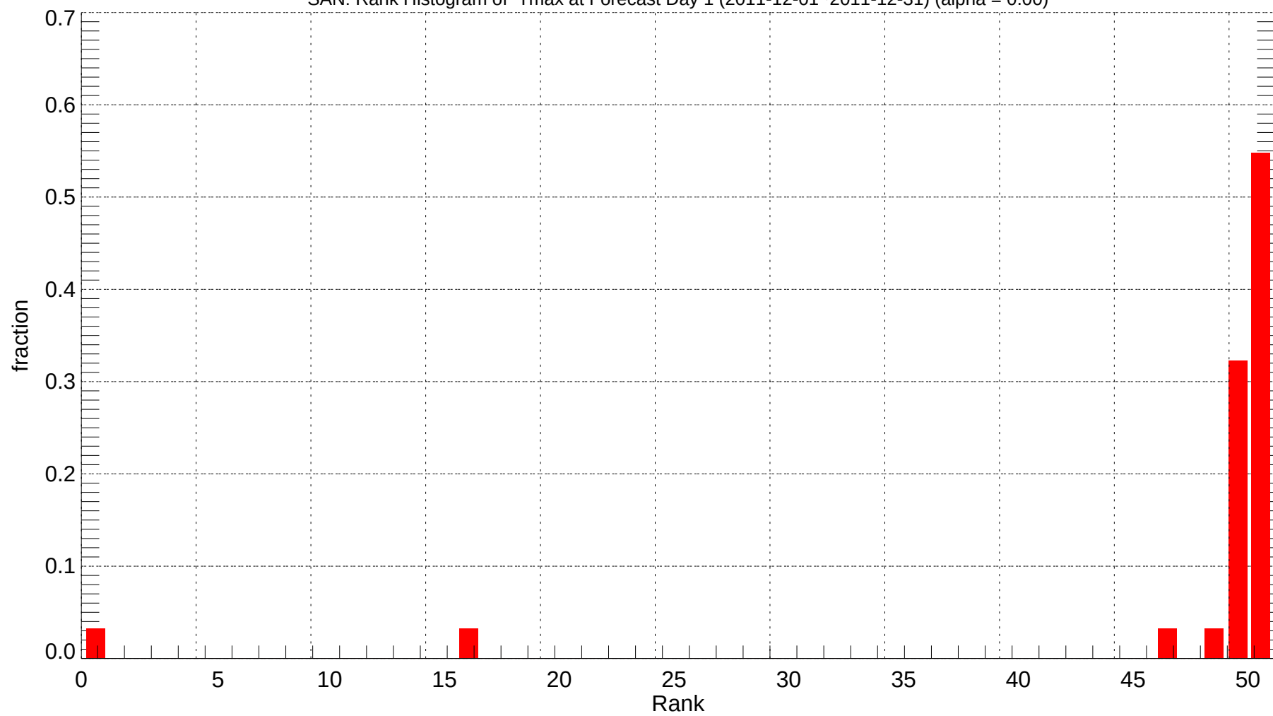
SAN: Rank Histogram of Tmax at Forecast Day 1 (2011-12-01~2011-12-31) (alpha = 0.00)
