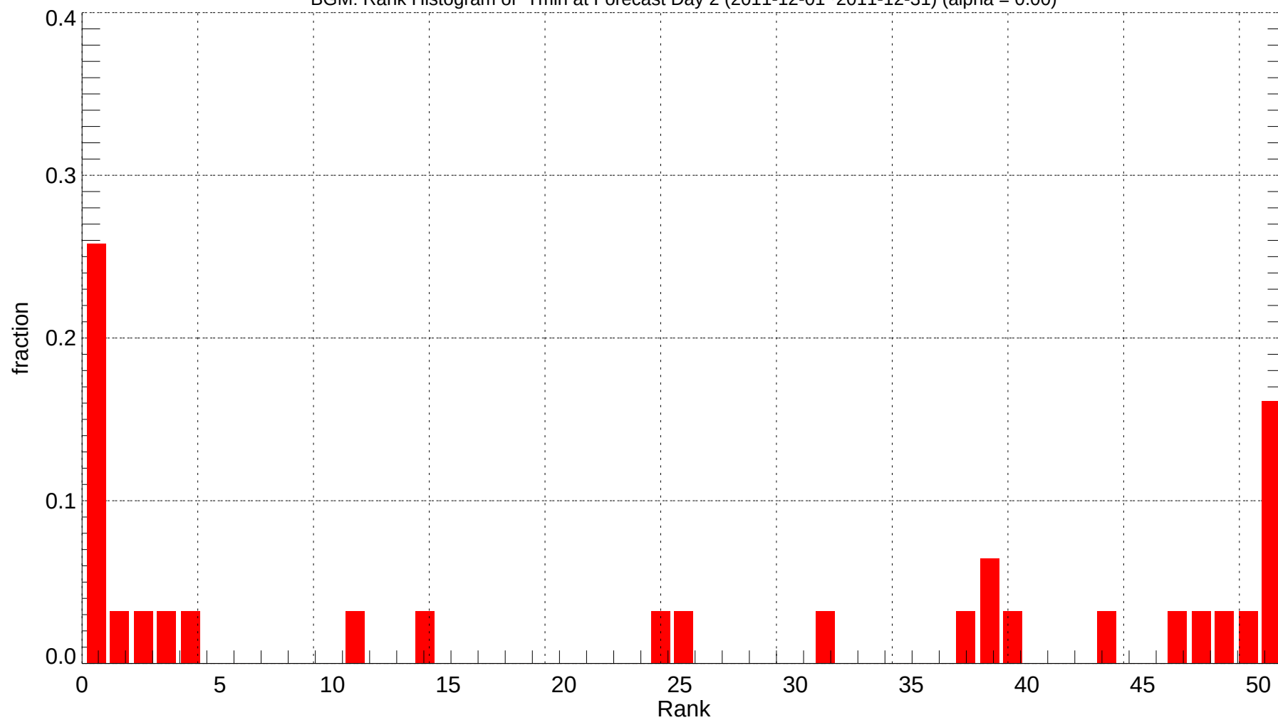
BGM: Rank Histogram of Tmin at Forecast Day 2 (2011-12-01~2011-12-31) (alpha = 0.00)
