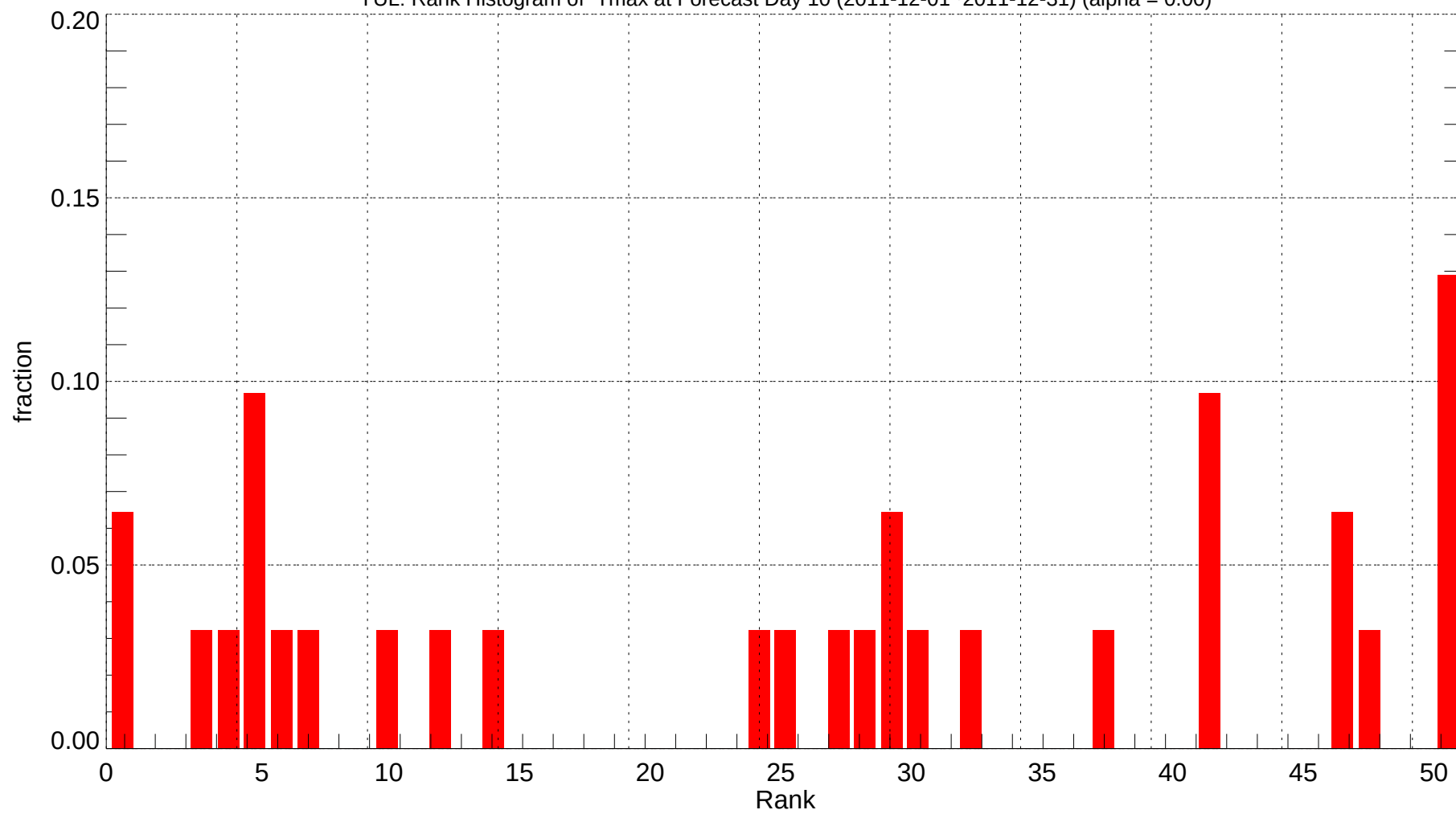
YUL: Rank Histogram of Tmax at Forecast Day 10 (2011-12-01~2011-12-31) (alpha = 0.00)
