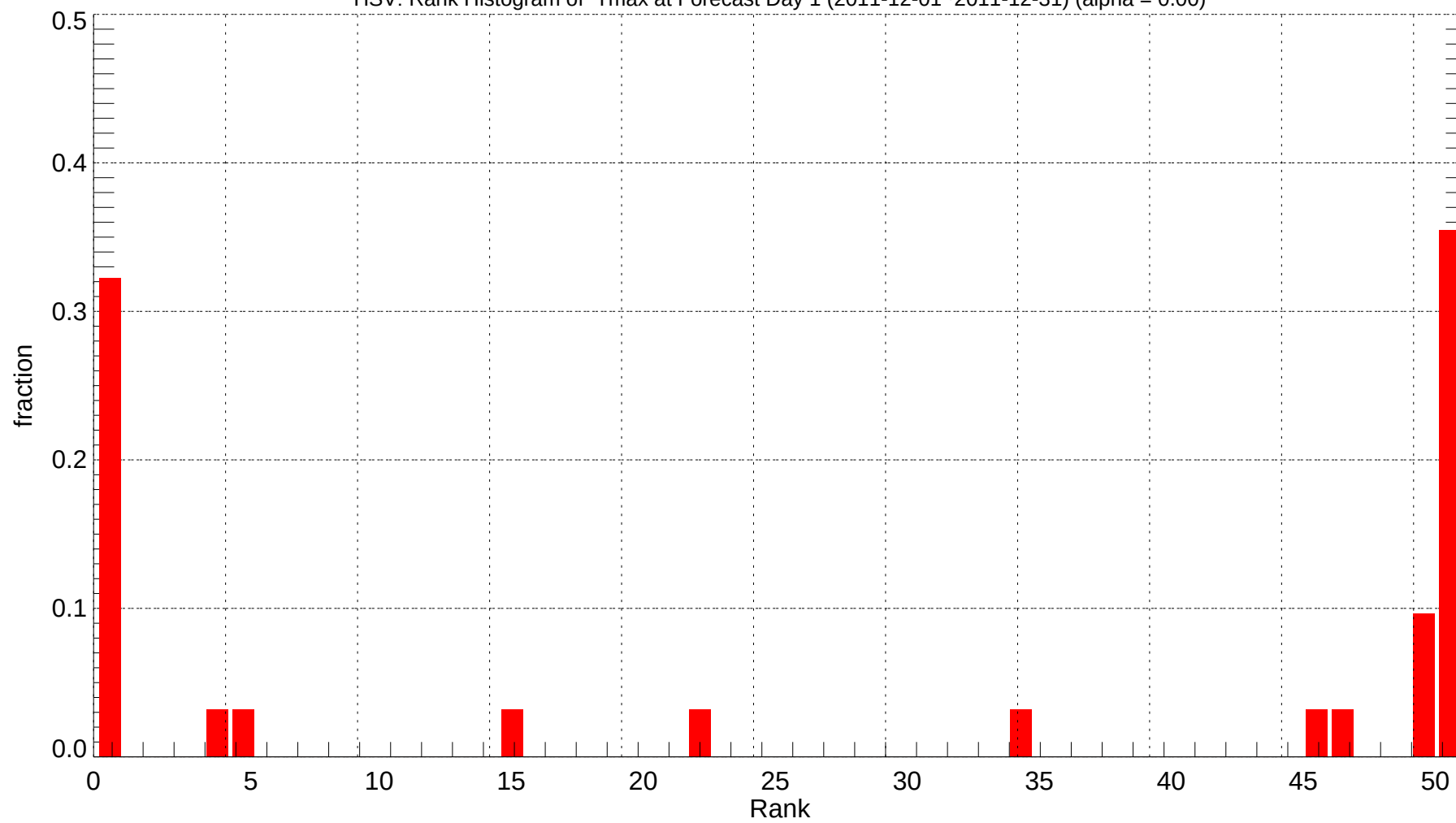
HSV: Rank Histogram of Tmax at Forecast Day 1 (2011-12-01~2011-12-31) (alpha = 0.00)
