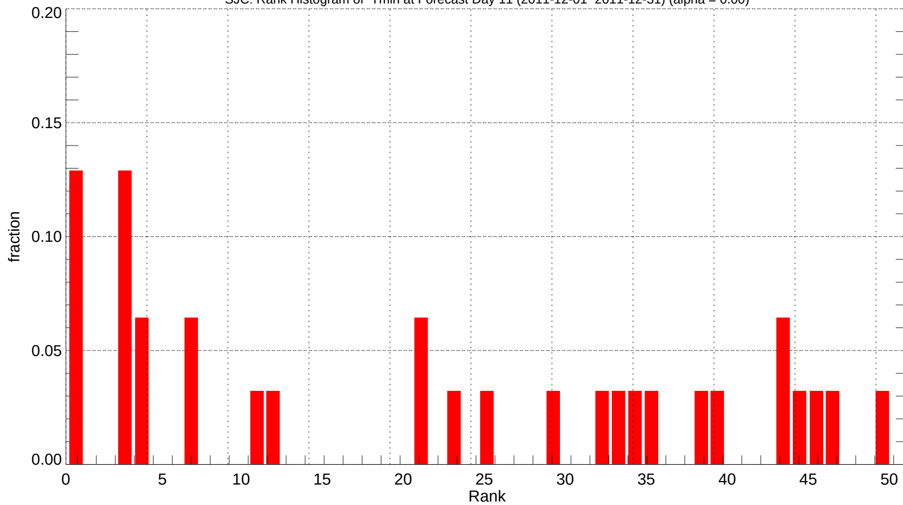
SJC: Rank Histogram of Tmin at Forecast Day 11 (2011-12-01~2011-12-31) (alpha = 0.00)
