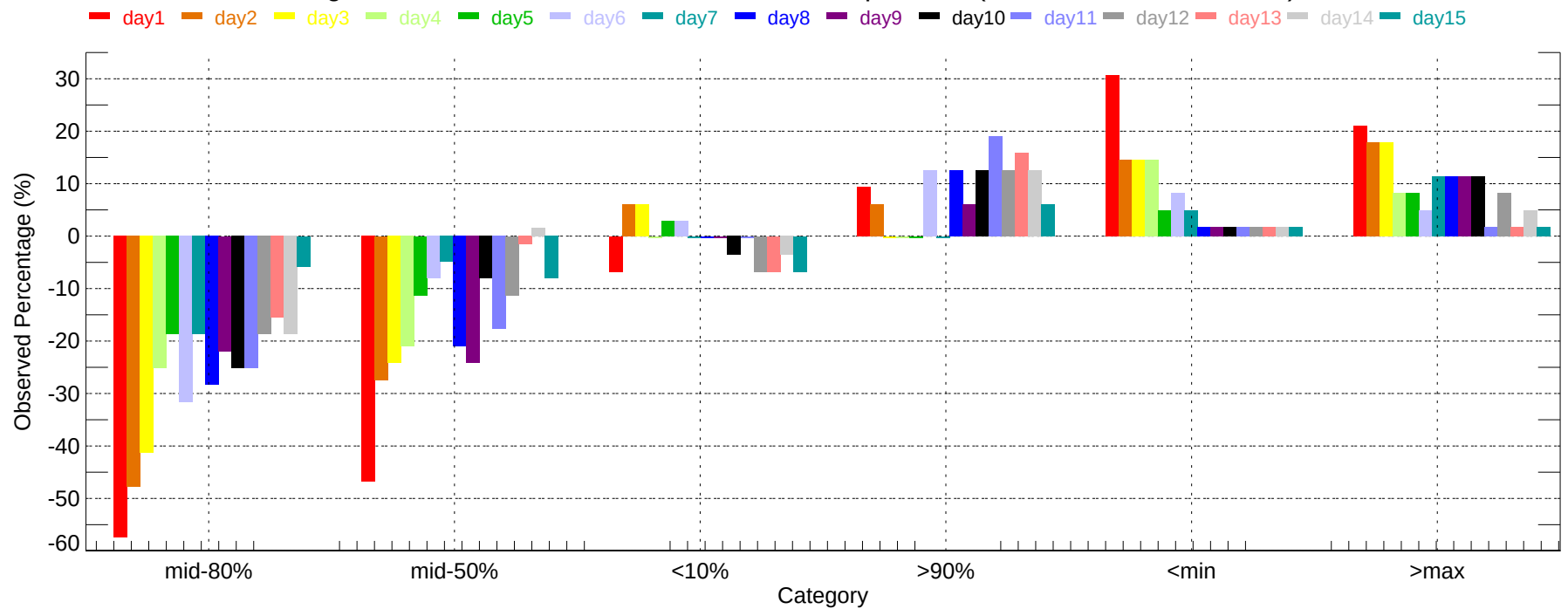
Observed Percentage Deviation of Ensembles - RAP: Min Temperature (2011-12-01~2011-12-31)
