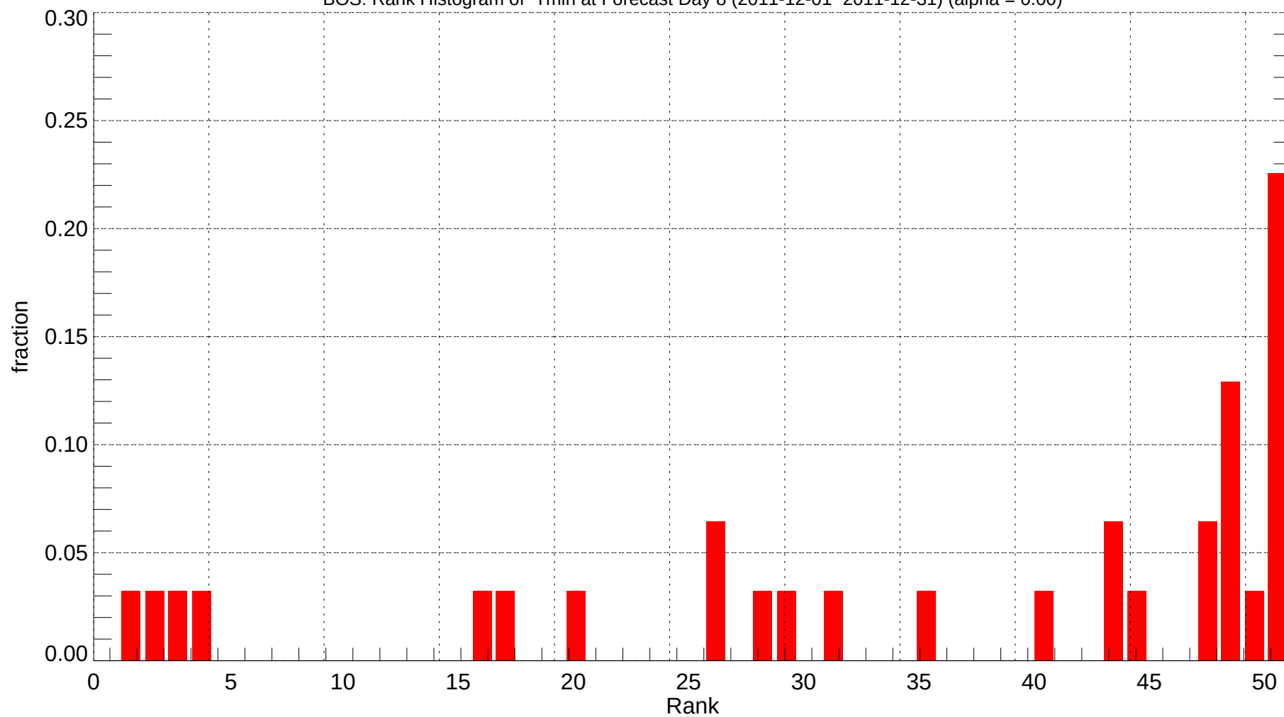
BOS: Rank Histogram of Tmin at Forecast Day 8 (2011-12-01~2011-12-31) (alpha = 0.00)
