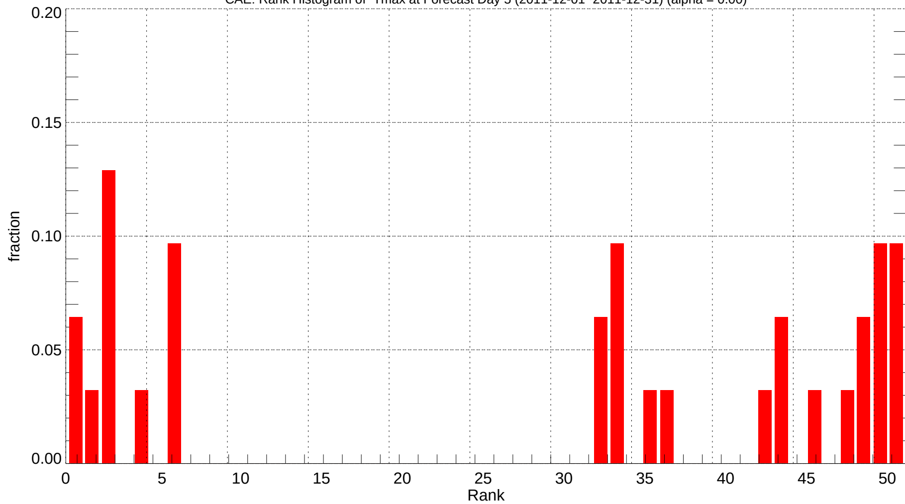
CAE: Rank Histogram of Tmax at Forecast Day 5 (2011-12-01~2011-12-31) (alpha = 0.00)
