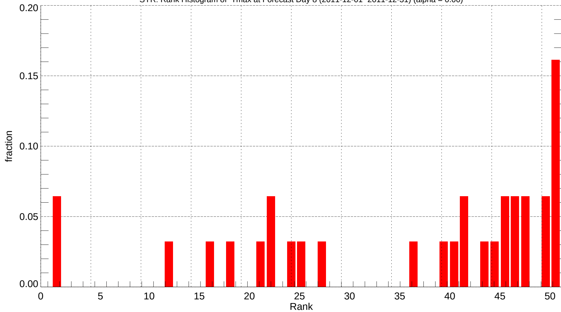
SYR: Rank Histogram of Tmax at Forecast Day 8 (2011-12-01~2011-12-31) (alpha = 0.00)
