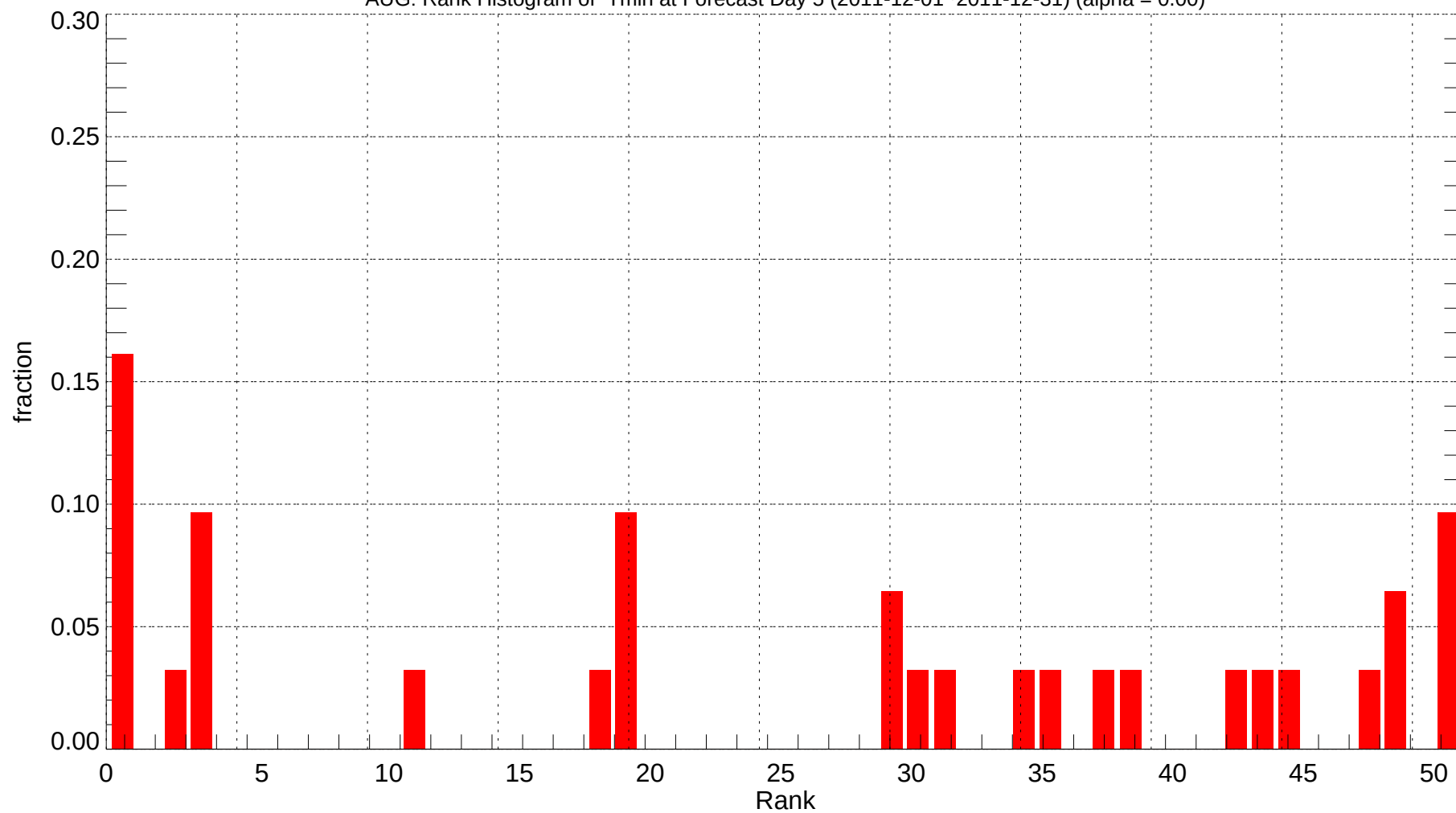
AUG: Rank Histogram of Tmin at Forecast Day 5 (2011-12-01~2011-12-31) (alpha = 0.00)
