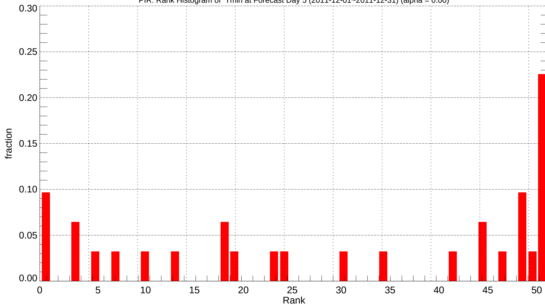
PIR: Rank Histogram of Tmin at Forecast Day 5 (2011-12-01~2011-12-31) (alpha = 0.00)
