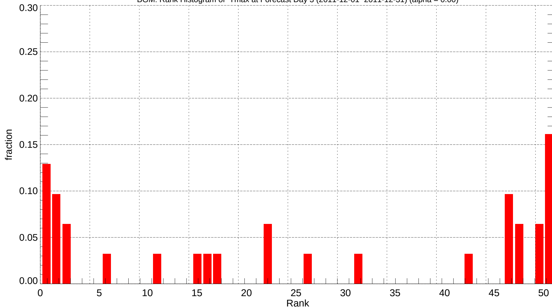
BGM: Rank Histogram of Tmax at Forecast Day 3 (2011-12-01~2011-12-31) (alpha = 0.00)
