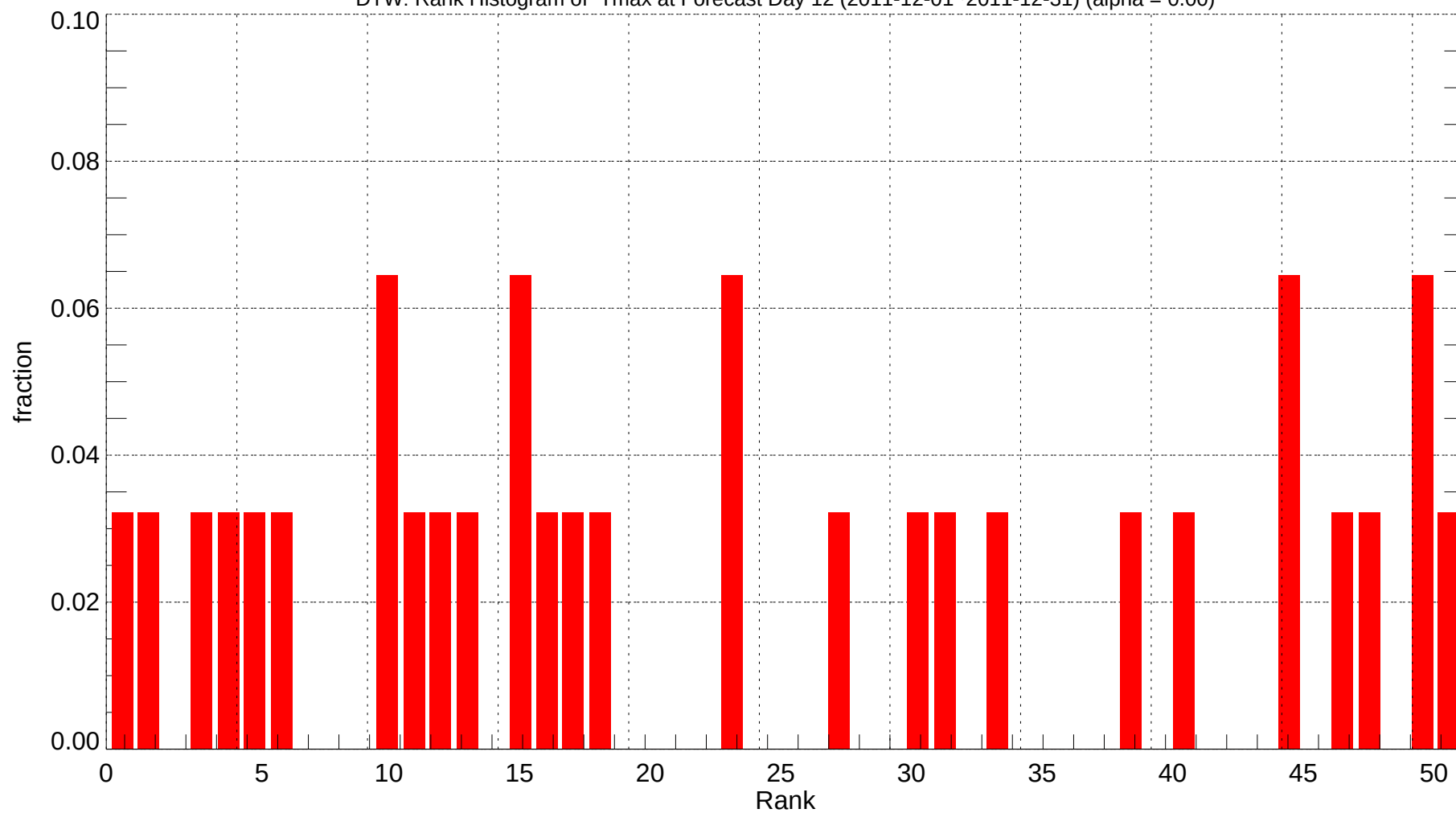
DTW: Rank Histogram of Tmax at Forecast Day 12 (2011-12-01~2011-12-31) (alpha = 0.00)
