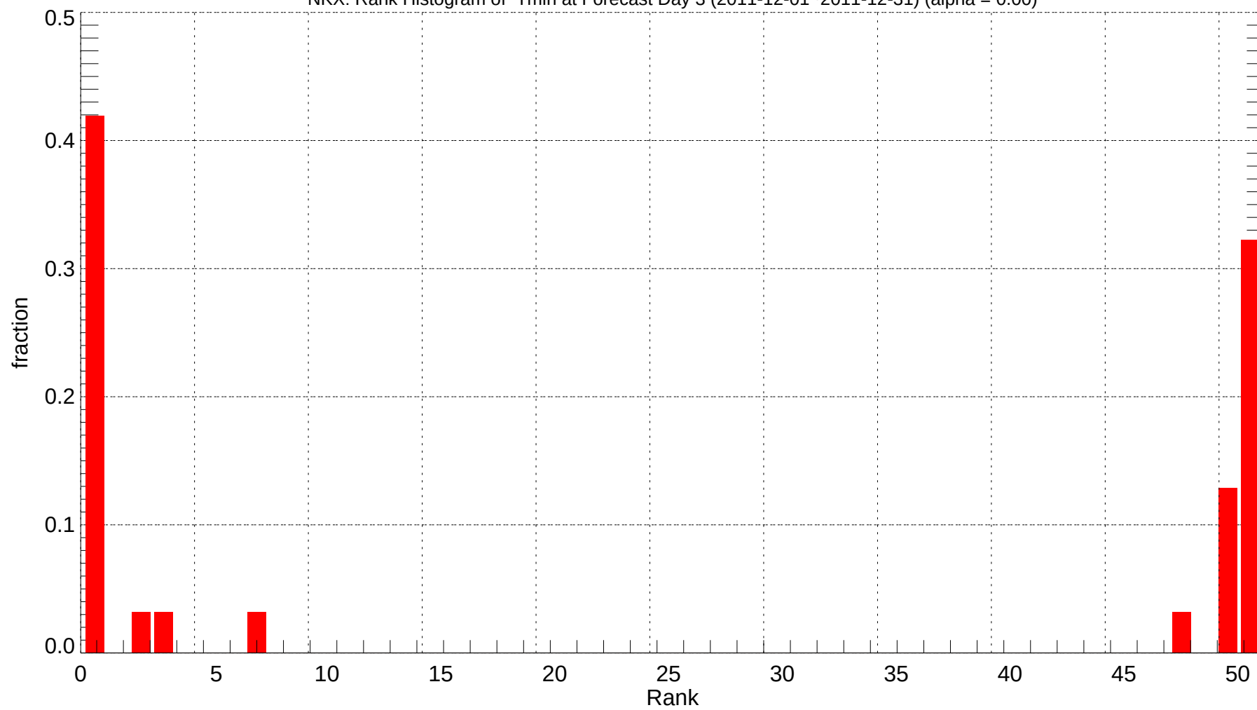
NKX: Rank Histogram of Tmin at Forecast Day 3 (2011-12-01~2011-12-31) (alpha = 0.00)
