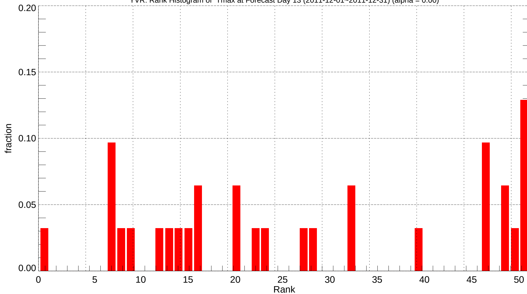
YVR: Rank Histogram of Tmax at Forecast Day 13 (2011-12-01~2011-12-31) (alpha = 0.00)
