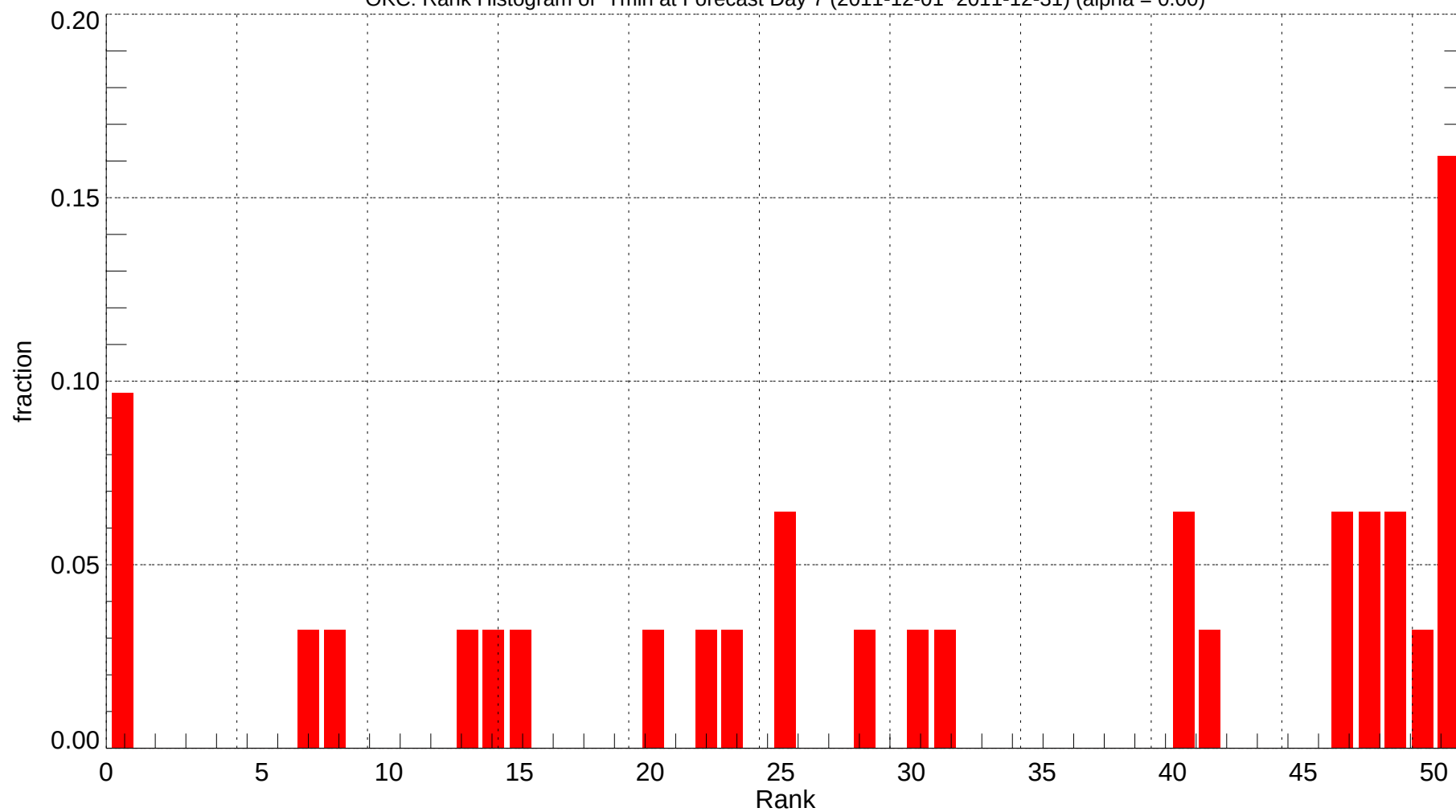
OKC: Rank Histogram of Tmin at Forecast Day 7 (2011-12-01~2011-12-31) (alpha = 0.00)
