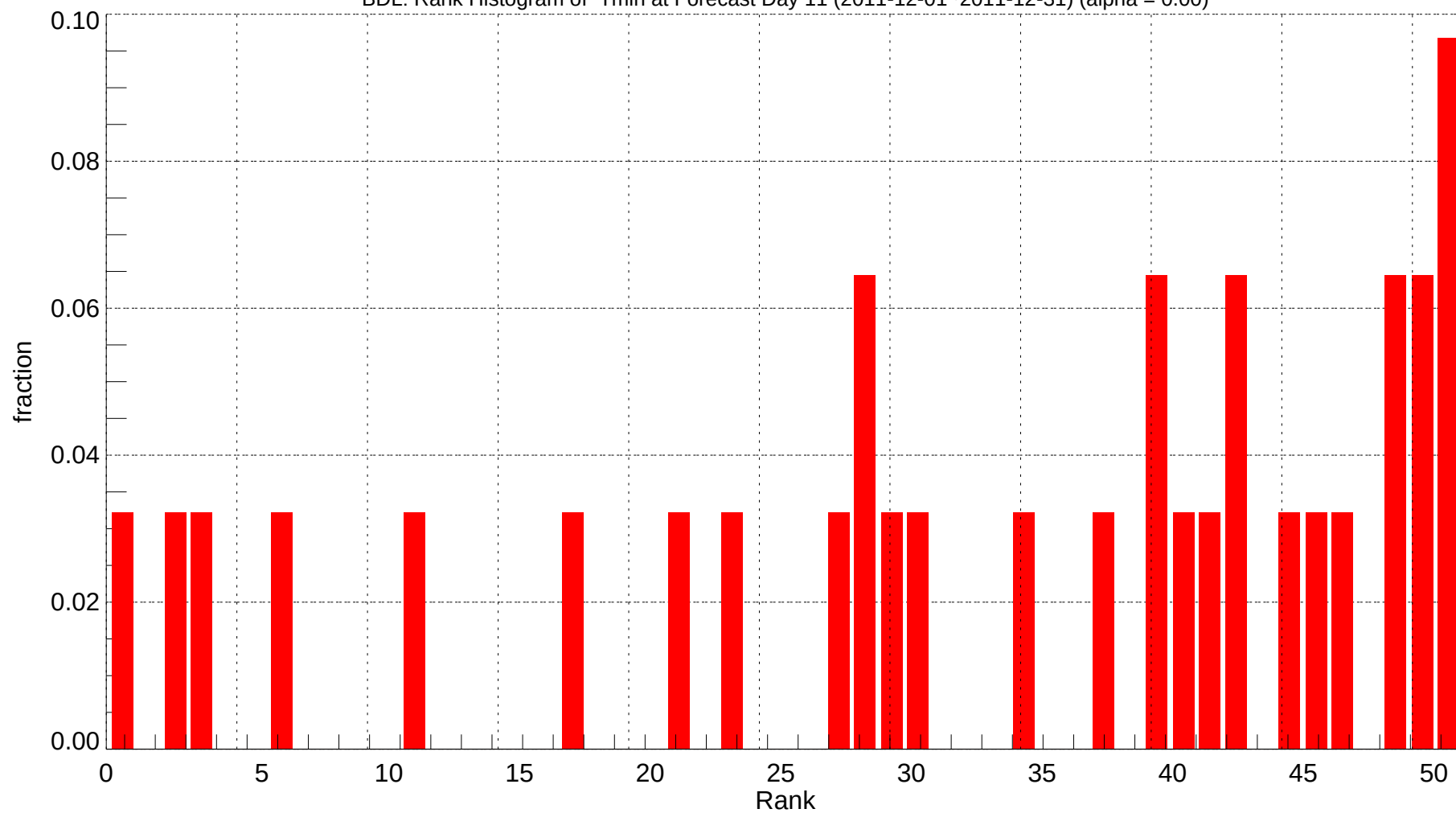
BDL: Rank Histogram of Tmin at Forecast Day 11 (2011-12-01~2011-12-31) (alpha = 0.00)
