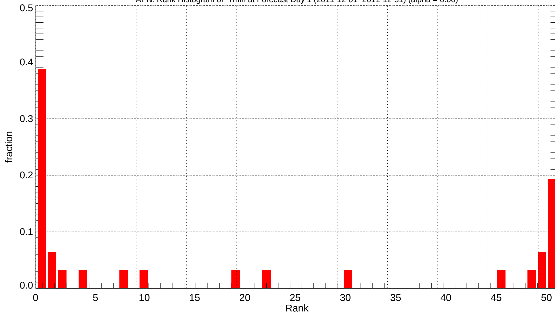
APN: Rank Histogram of Tmin at Forecast Day 1 (2011-12-01~2011-12-31) (alpha = 0.00)
