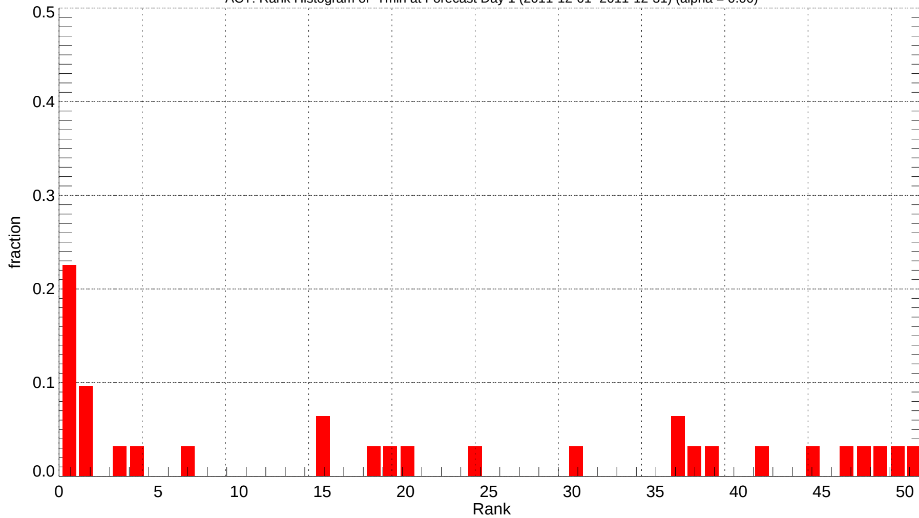
ACT: Rank Histogram of Tmin at Forecast Day 1 (2011-12-01~2011-12-31) (alpha = 0.00)
