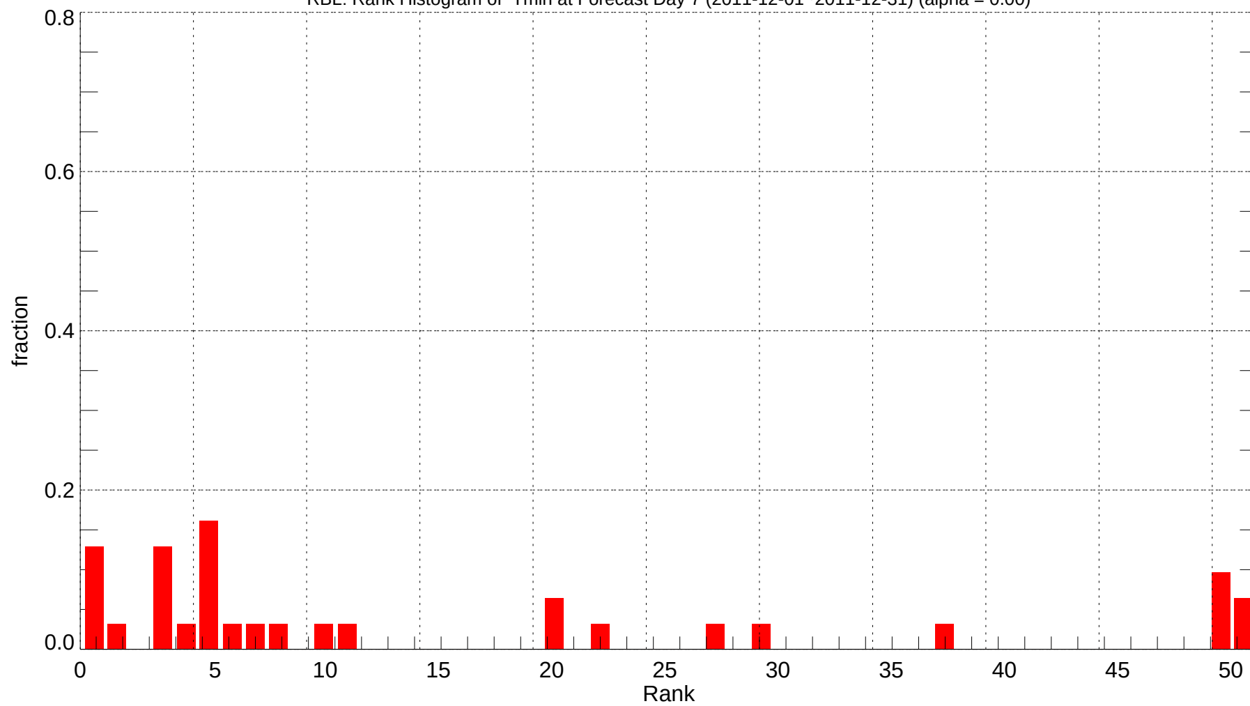
RBL: Rank Histogram of Tmin at Forecast Day 7 (2011-12-01~2011-12-31) (alpha = 0.00)
