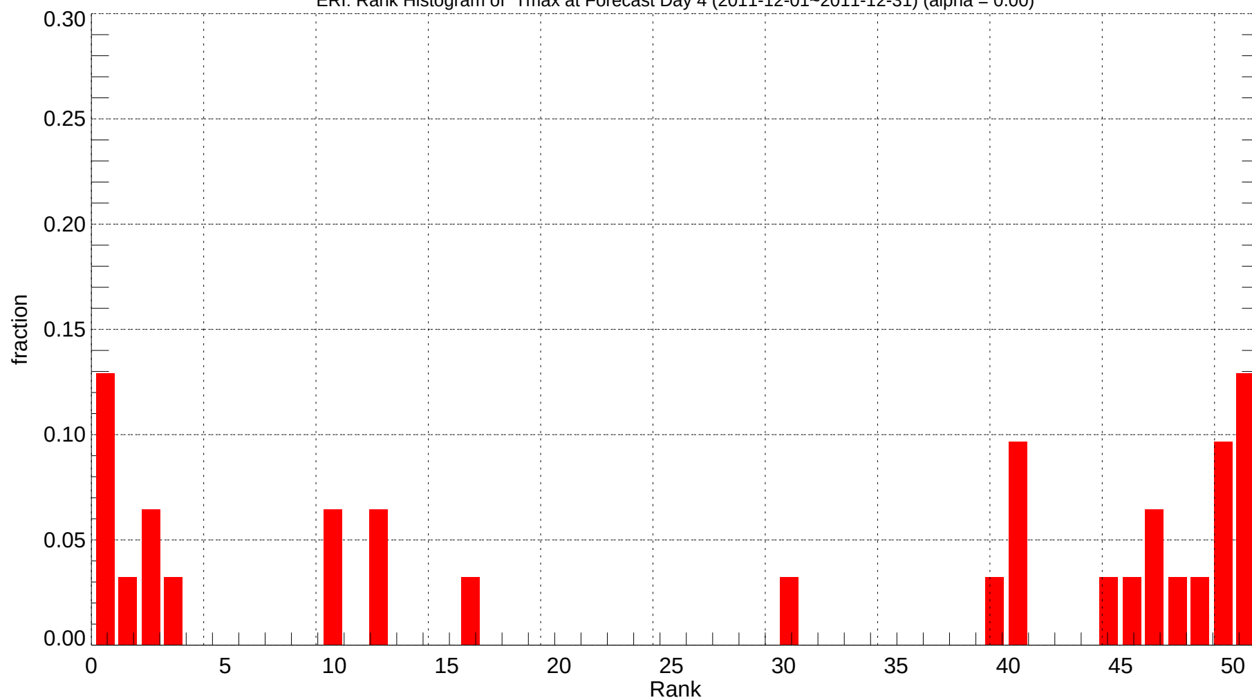
ERI: Rank Histogram of Tmax at Forecast Day 4 (2011-12-01~2011-12-31) (alpha = 0.00)
