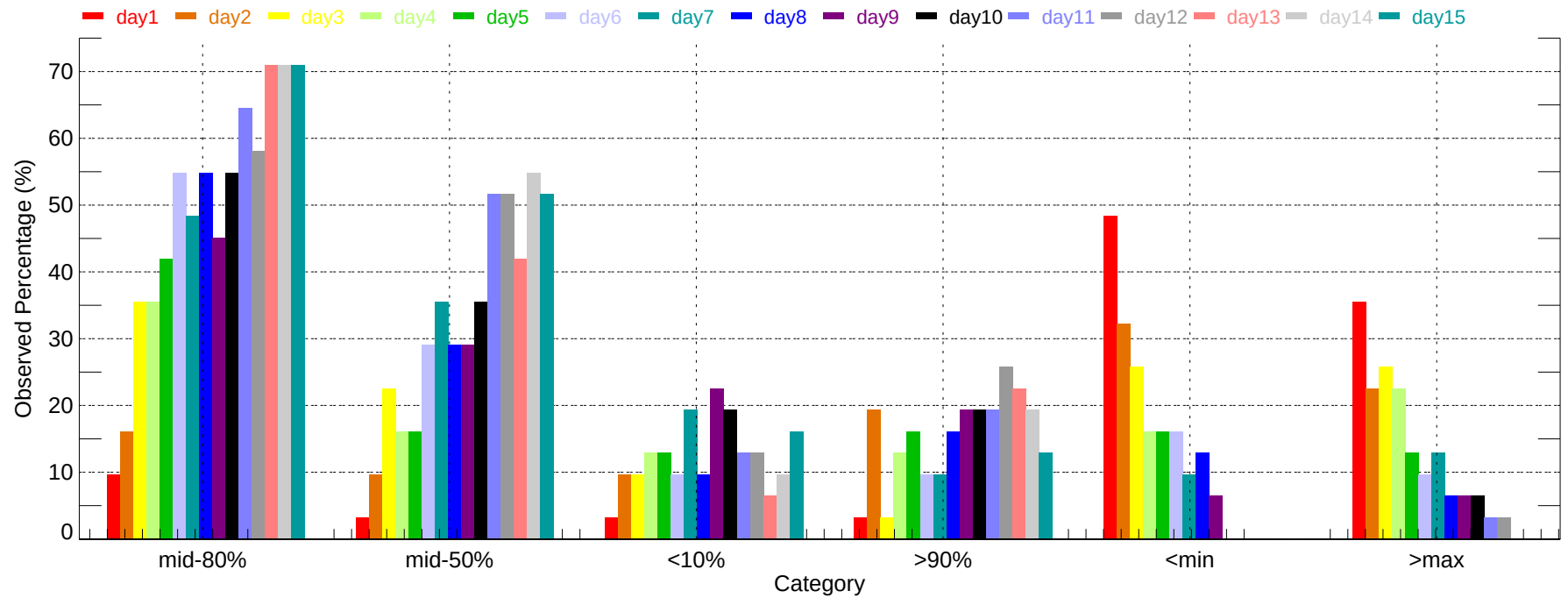
Observed Percentage of Ensembles - AUG: Min Temperature (2011-12-01~2011-12-31)
