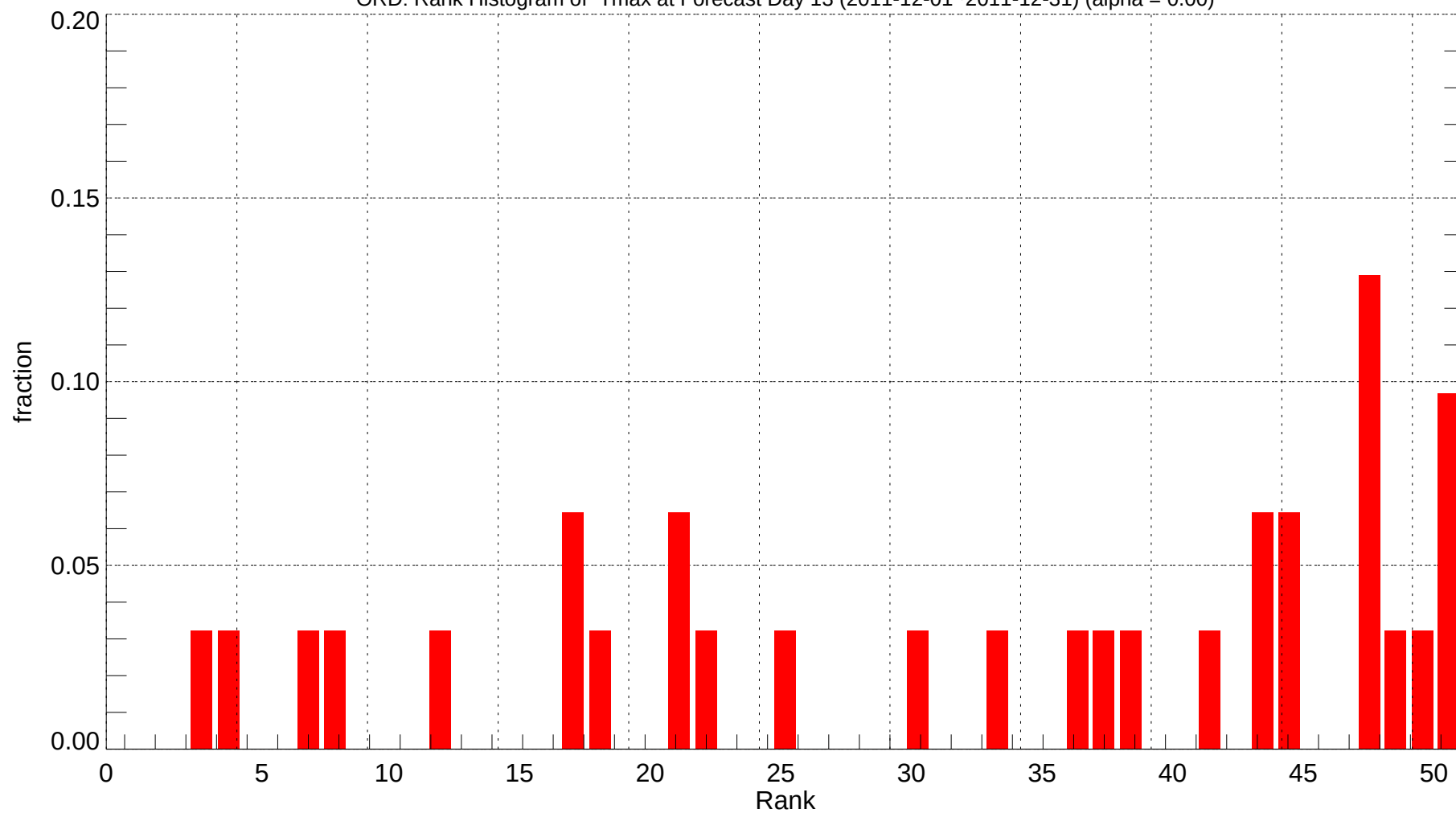
ORD: Rank Histogram of Tmax at Forecast Day 13 (2011-12-01~2011-12-31) (alpha = 0.00)
