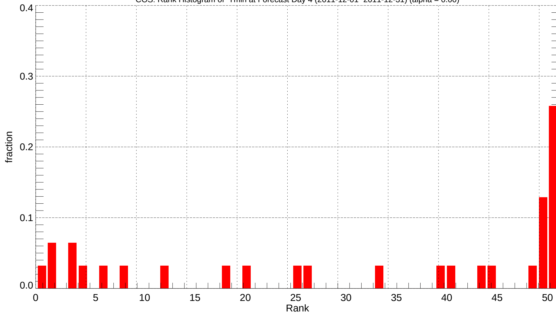
COS: Rank Histogram of Tmin at Forecast Day 4 (2011-12-01~2011-12-31) (alpha = 0.00)
