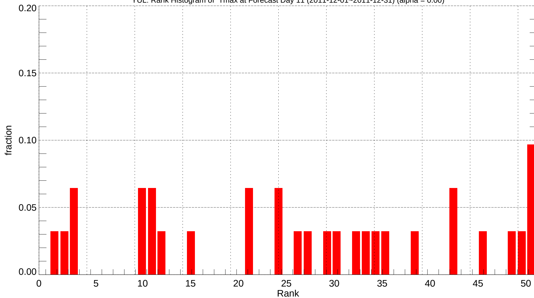
YUL: Rank Histogram of Tmax at Forecast Day 11 (2011-12-01~2011-12-31) (alpha = 0.00)
