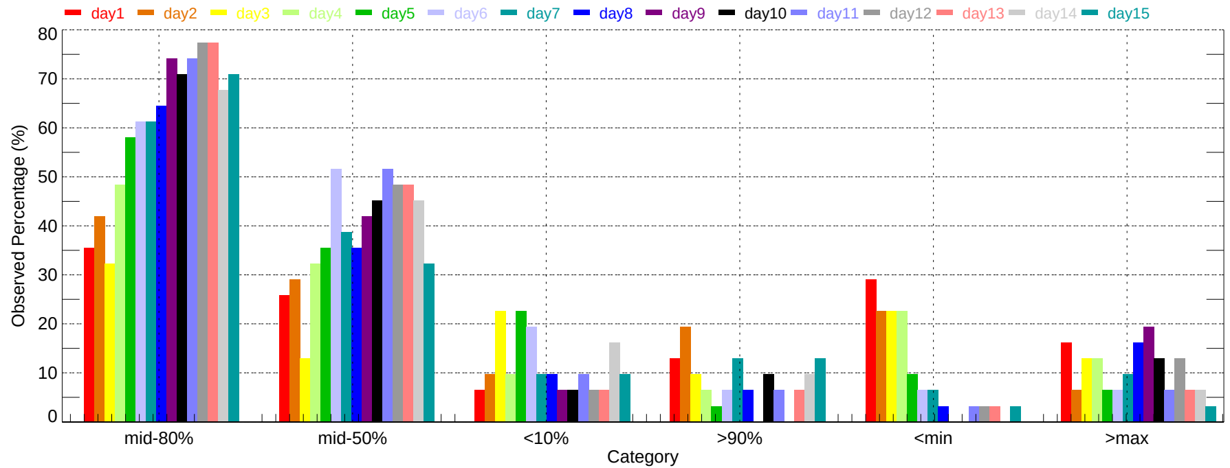
Observed Percentage of Ensembles - YWG: Max Temperature (2011-12-01~2011-12-31)
