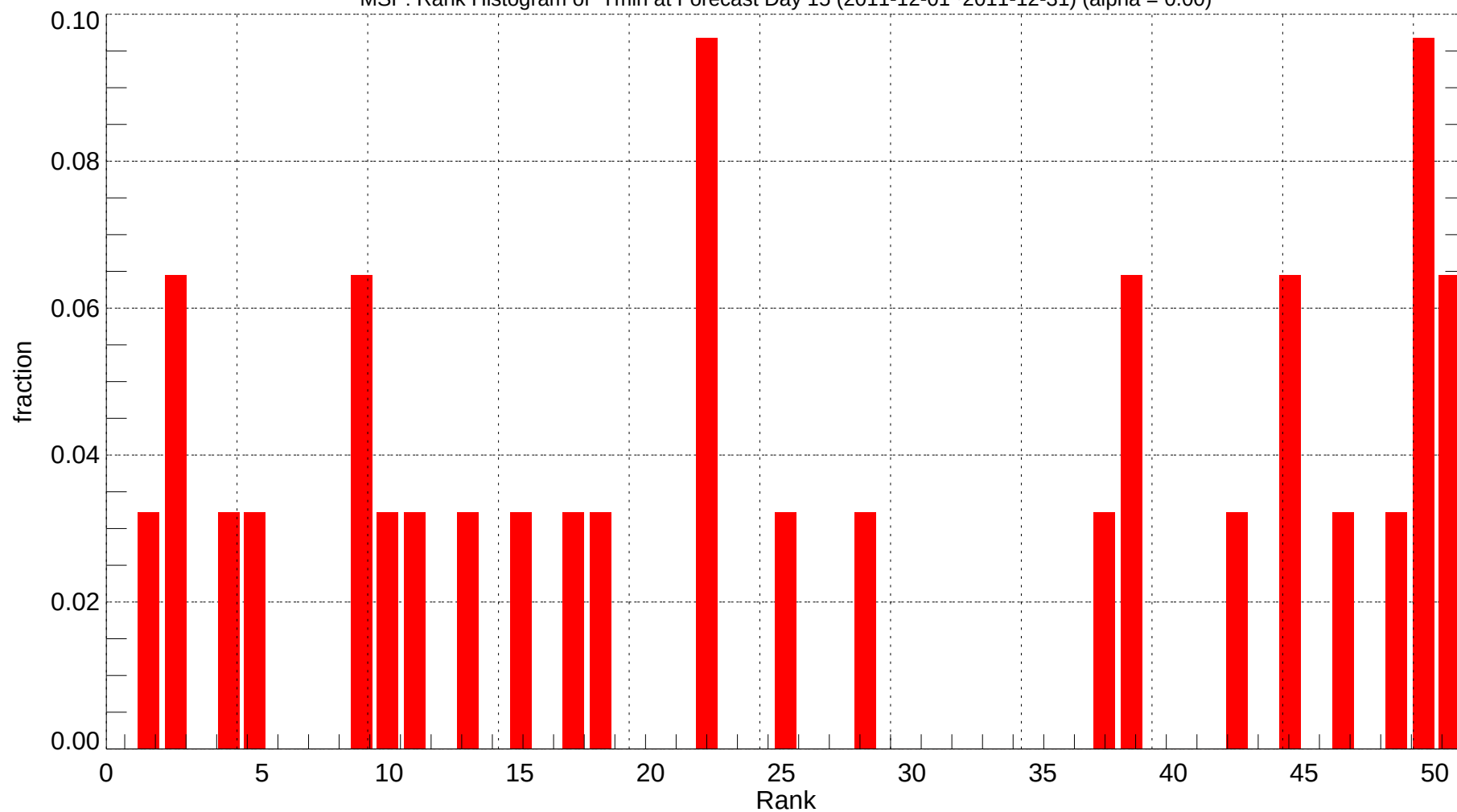
MSP: Rank Histogram of Tmin at Forecast Day 15 (2011-12-01~2011-12-31) (alpha = 0.00)
