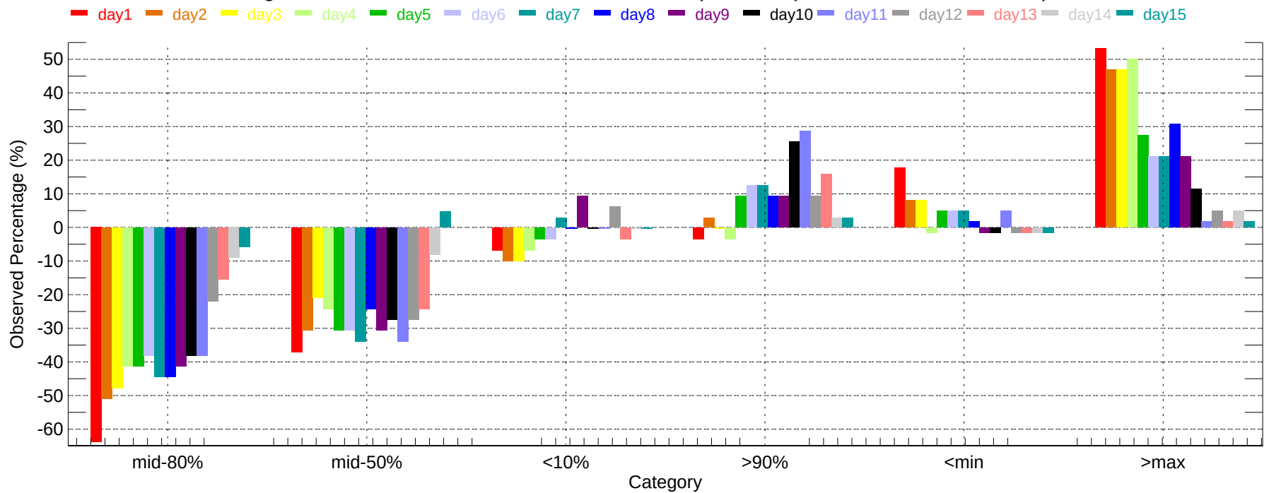
Observed Percentage Deviation of Ensembles - AUS: Min Temperature (2011-12-01~2011-12-31)
