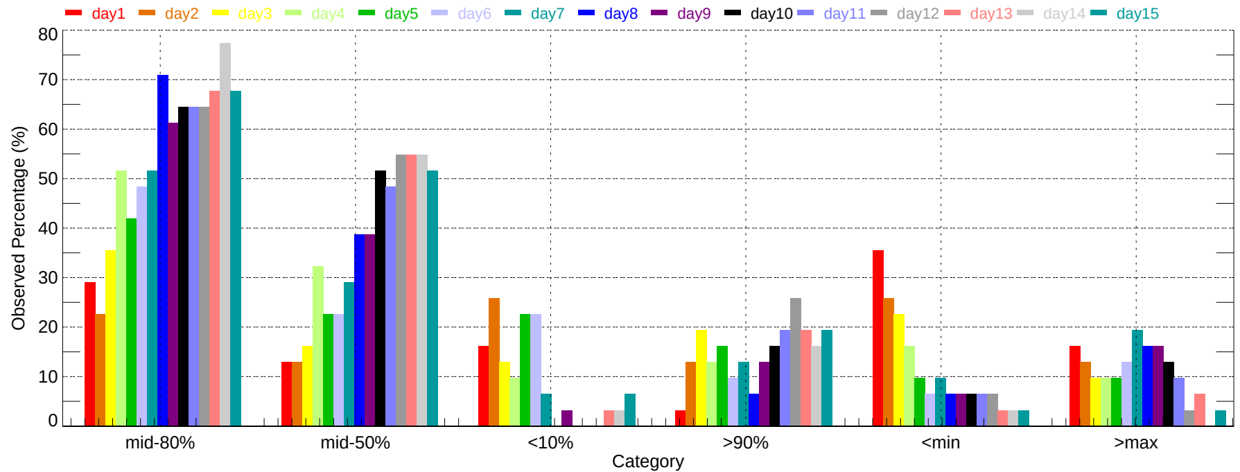
Observed Percentage of Ensembles - GAD: Max Temperature (2011-12-01~2011-12-31)
