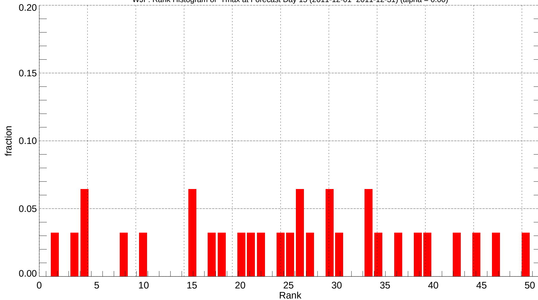
WJF: Rank Histogram of Tmax at Forecast Day 15 (2011-12-01~2011-12-31) (alpha = 0.00)
