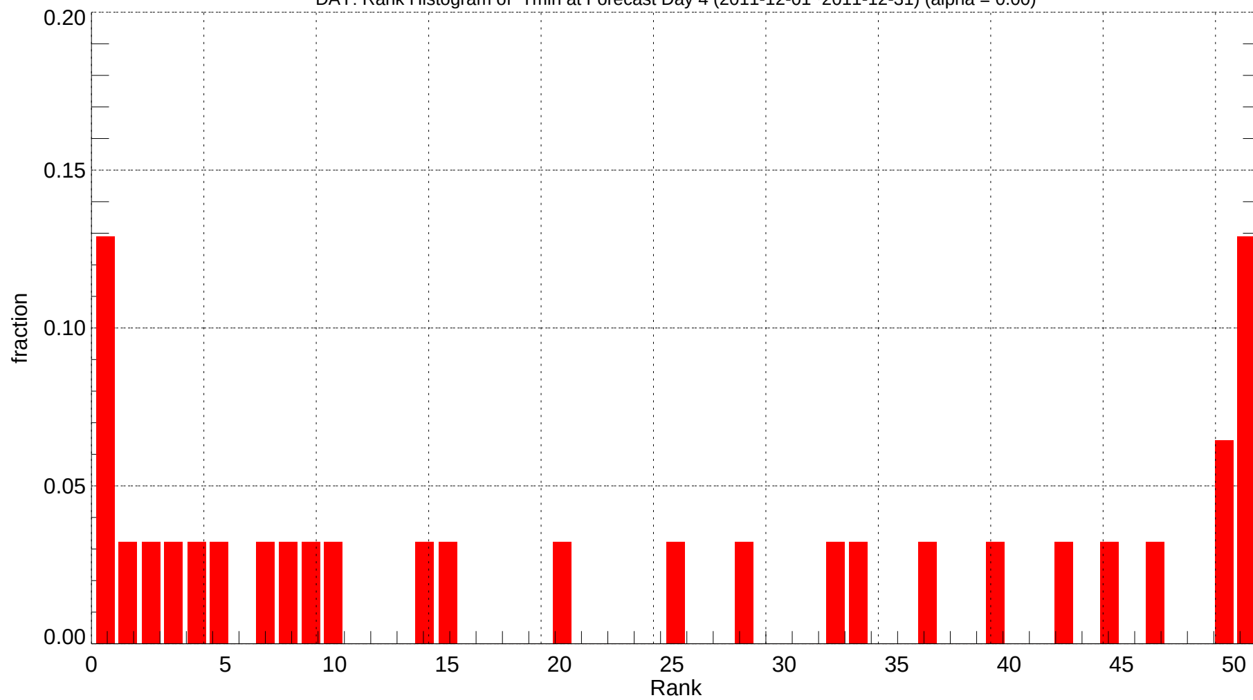
DAY: Rank Histogram of Tmin at Forecast Day 4 (2011-12-01~2011-12-31) (alpha = 0.00)
