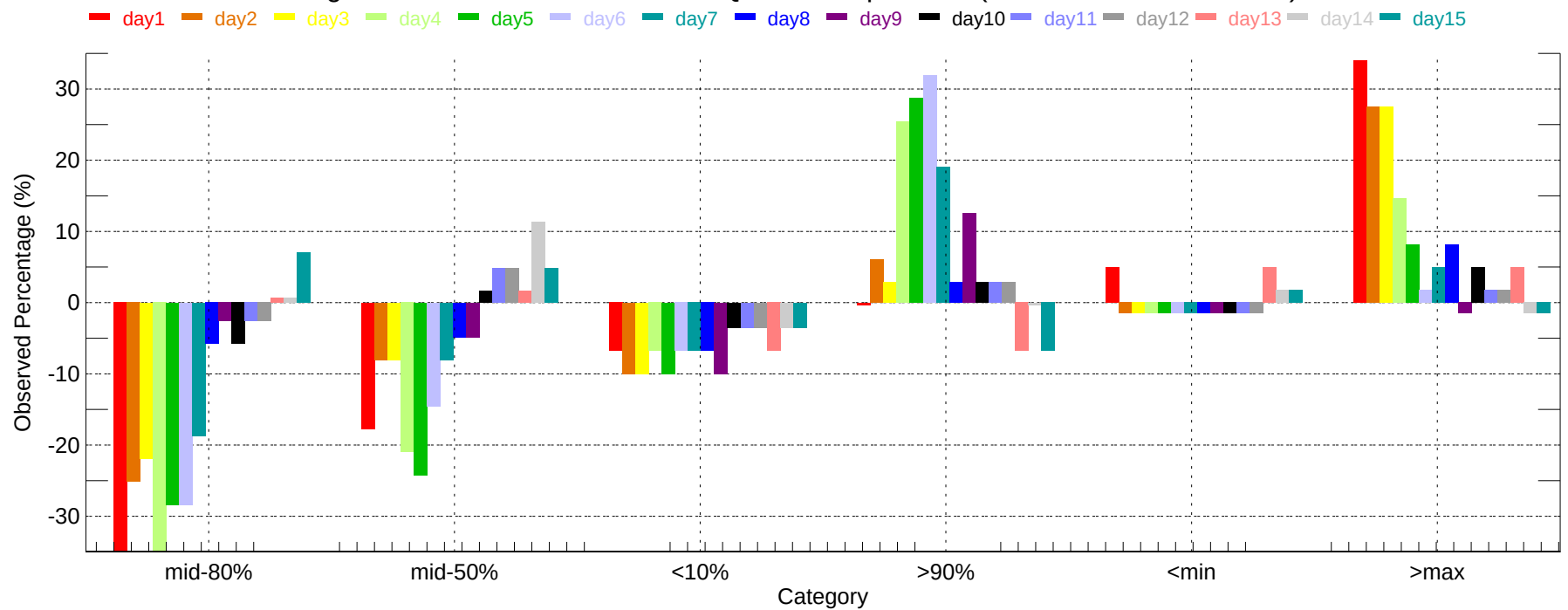
Observed Percentage Deviation of Ensembles - ABQ: Min Temperature (2011-12-01~2011-12-31)
