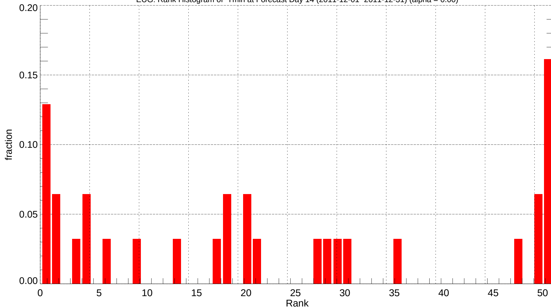
EUG: Rank Histogram of Tmin at Forecast Day 14 (2011-12-01~2011-12-31) (alpha = 0.00)
