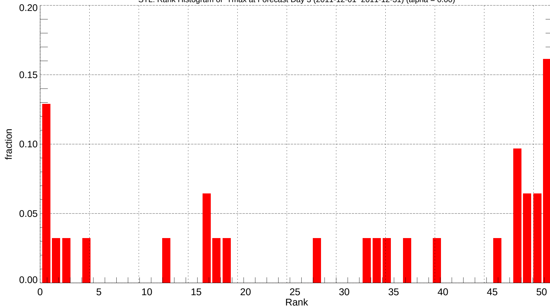
STL: Rank Histogram of Tmax at Forecast Day 3 (2011-12-01~2011-12-31) (alpha = 0.00)
