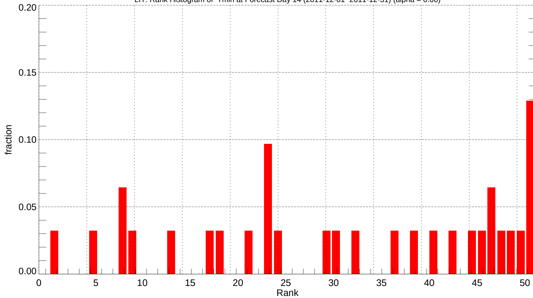
LIT: Rank Histogram of Tmin at Forecast Day 14 (2011-12-01~2011-12-31) (alpha = 0.00)
