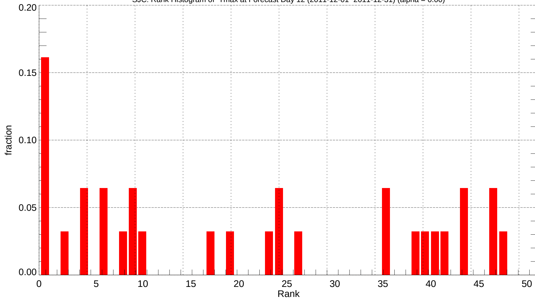
SJC: Rank Histogram of Tmax at Forecast Day 12 (2011-12-01~2011-12-31) (alpha = 0.00)
