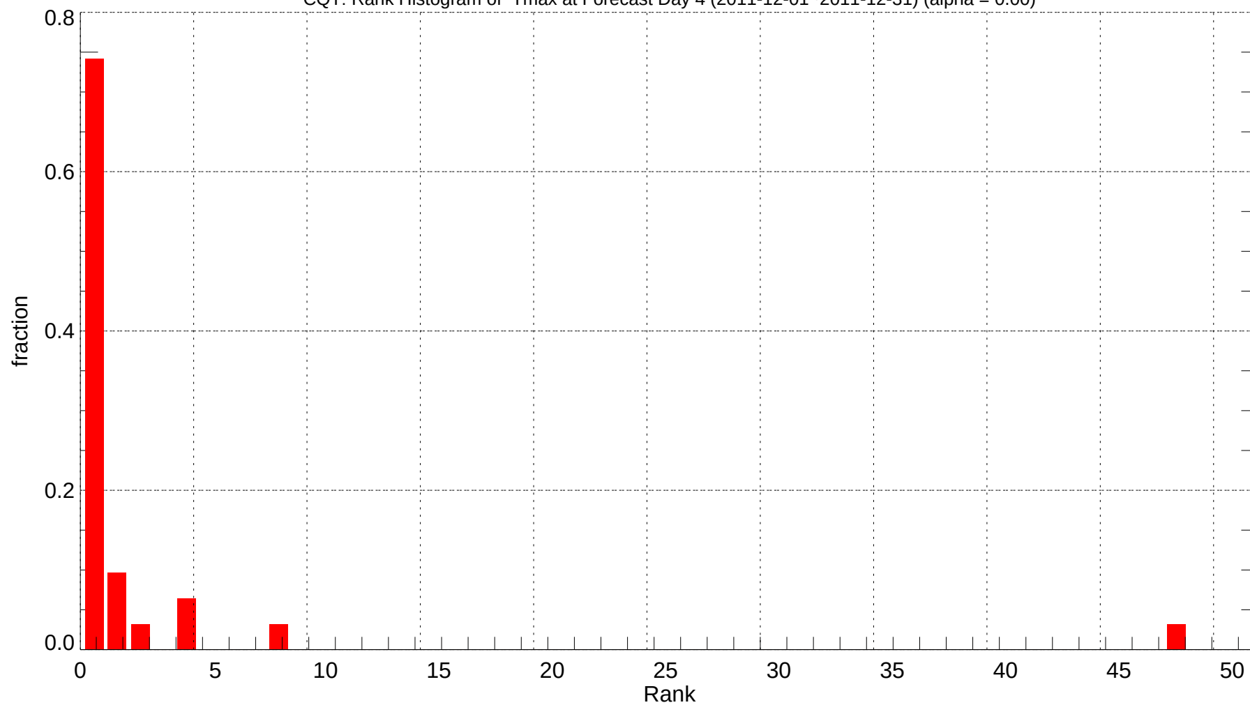
CQT: Rank Histogram of Tmax at Forecast Day 4 (2011-12-01~2011-12-31) (alpha = 0.00)
