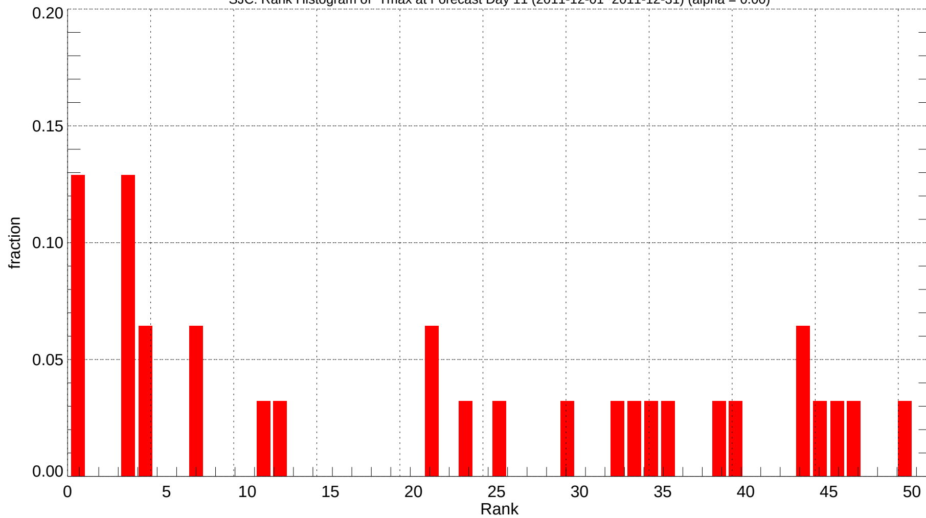
SJC: Rank Histogram of Tmax at Forecast Day 11 (2011-12-01~2011-12-31) (alpha = 0.00)
