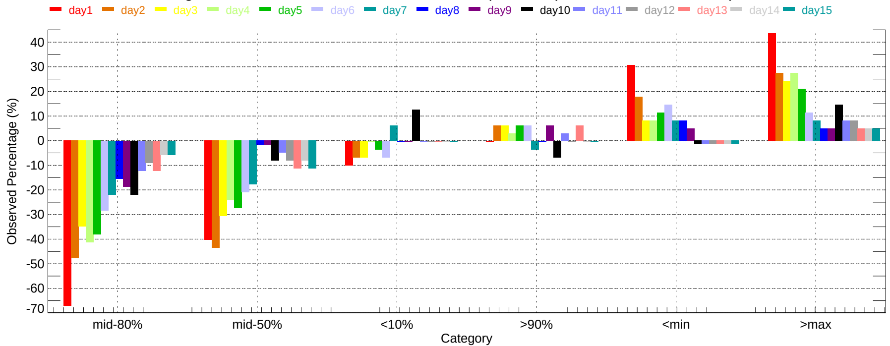
Observed Percentage Deviation of Ensembles - BDL: Min Temperature (2011-12-01~2011-12-31)
