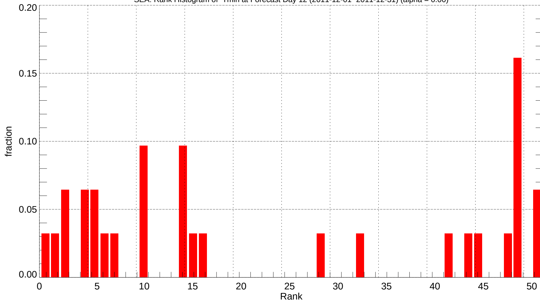
SEA: Rank Histogram of Tmin at Forecast Day 12 (2011-12-01~2011-12-31) (alpha = 0.00)
