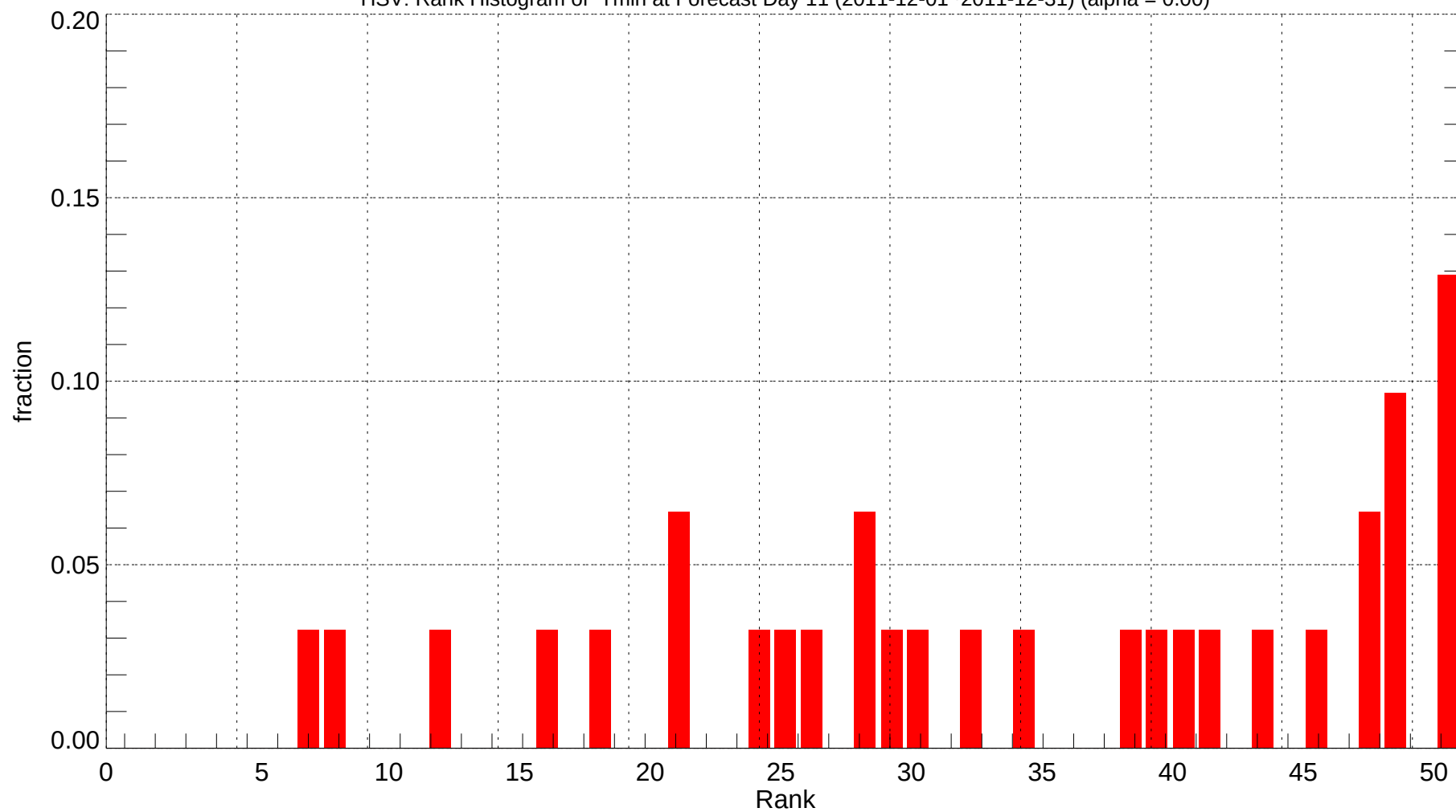
HSV: Rank Histogram of Tmin at Forecast Day 11 (2011-12-01~2011-12-31) (alpha = 0.00)
