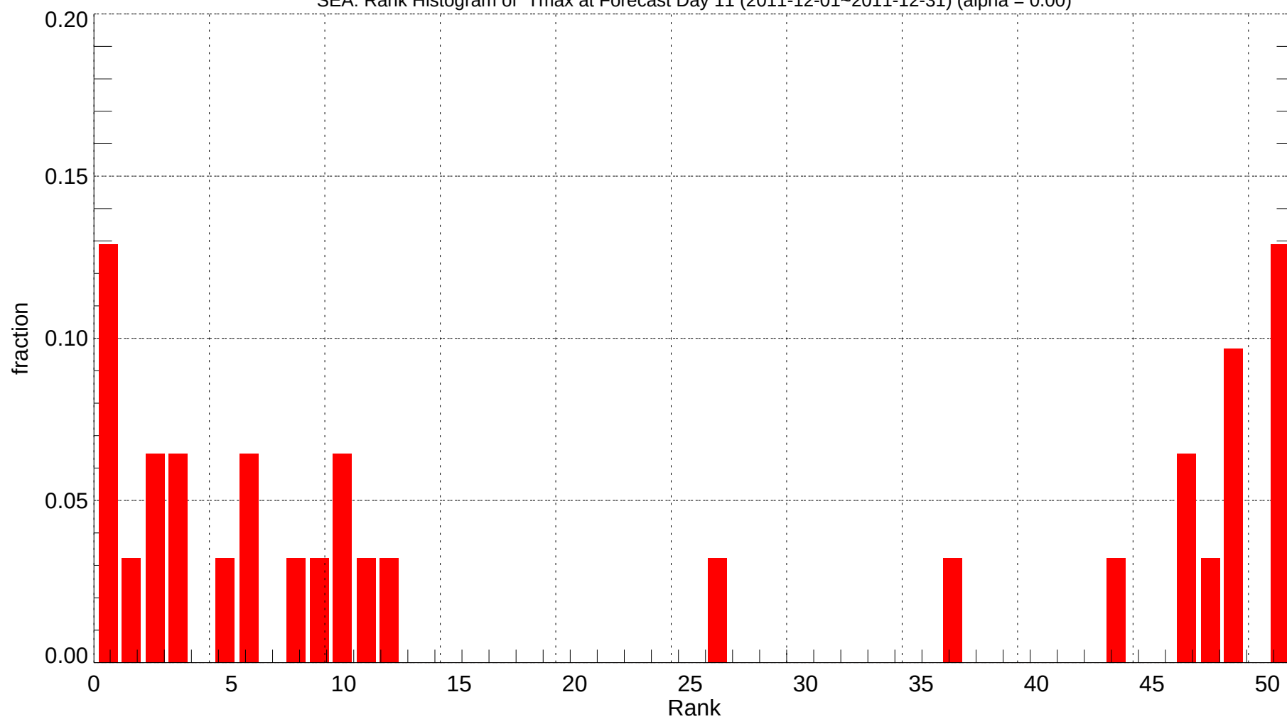
SEA: Rank Histogram of Tmax at Forecast Day 11 (2011-12-01~2011-12-31) (alpha = 0.00)
