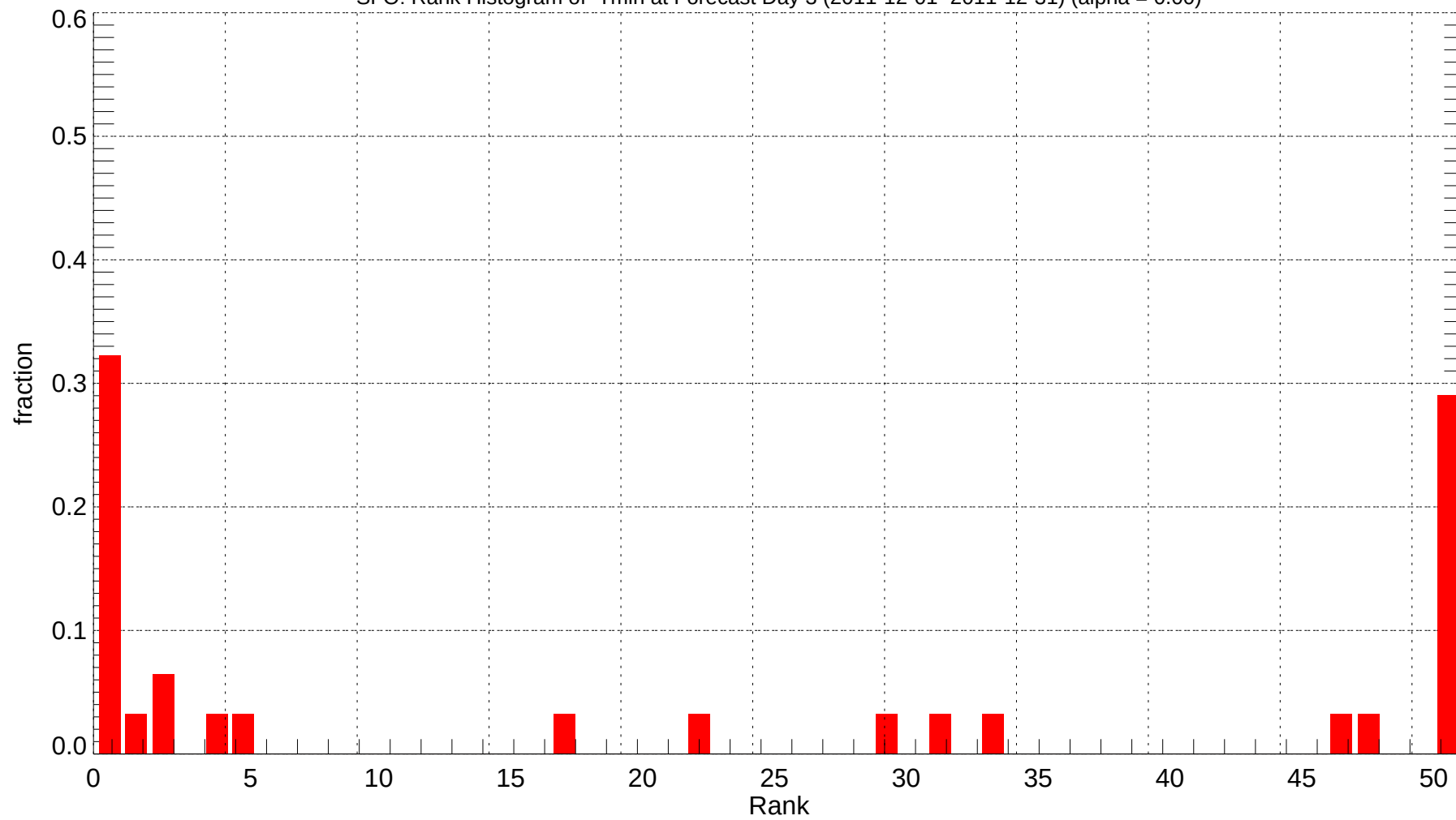
SFO: Rank Histogram of Tmin at Forecast Day 3 (2011-12-01~2011-12-31) (alpha = 0.00)
