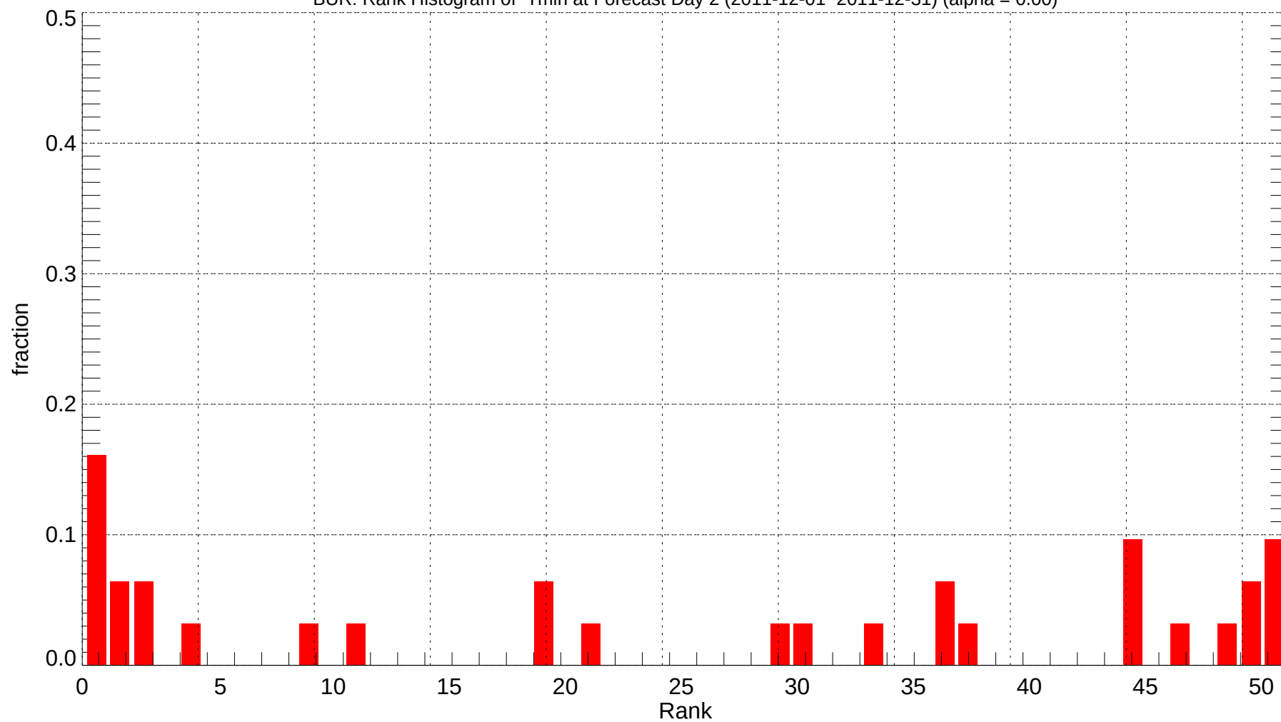
BUR: Rank Histogram of Tmin at Forecast Day 2 (2011-12-01~2011-12-31) (alpha = 0.00)
