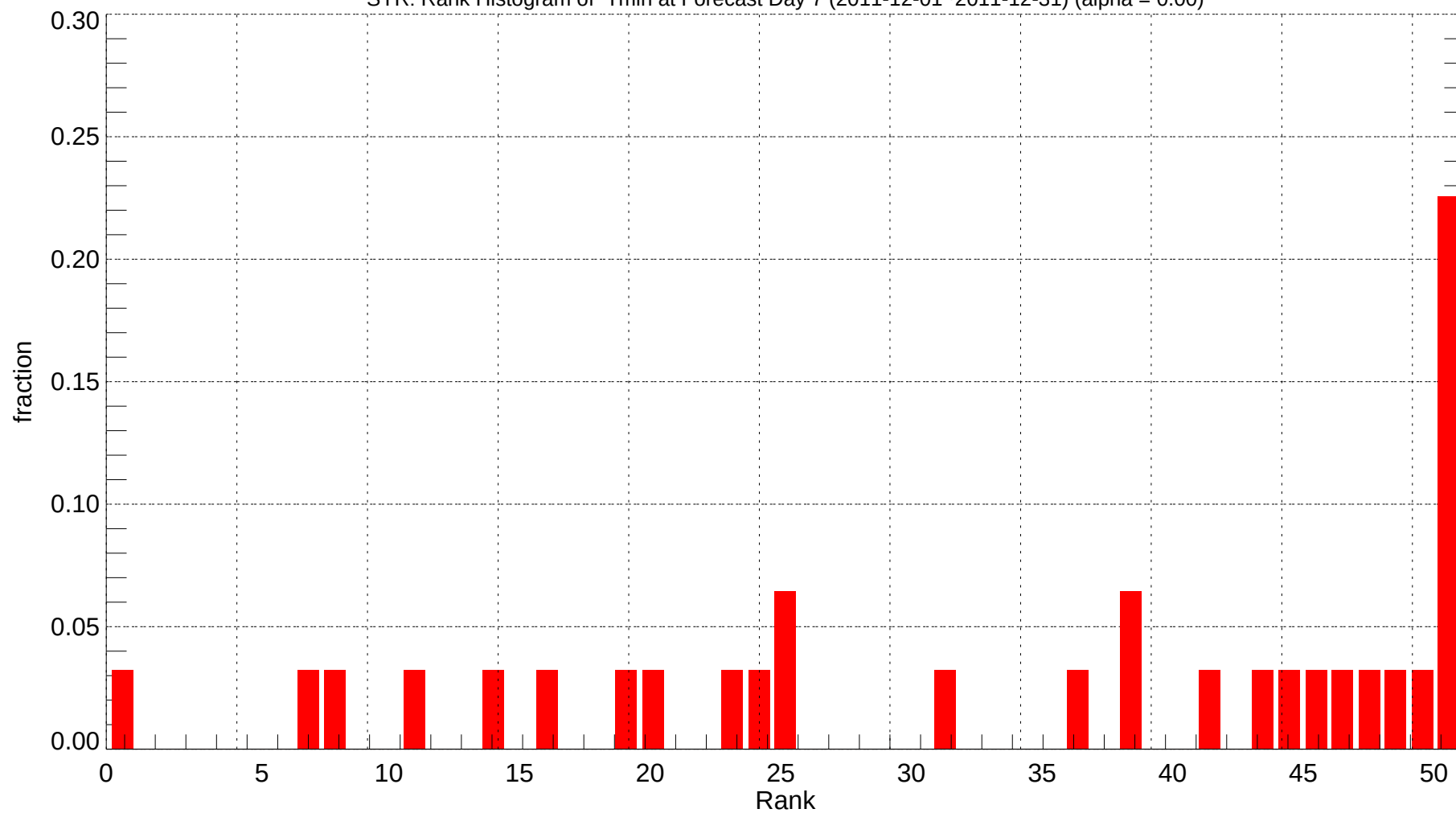
SYR: Rank Histogram of Tmin at Forecast Day 7 (2011-12-01~2011-12-31) (alpha = 0.00)
