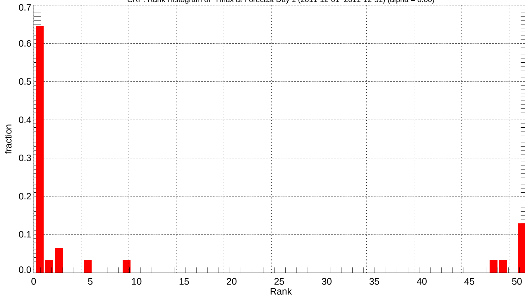
CRP: Rank Histogram of Tmax at Forecast Day 1 (2011-12-01~2011-12-31) (alpha = 0.00)
