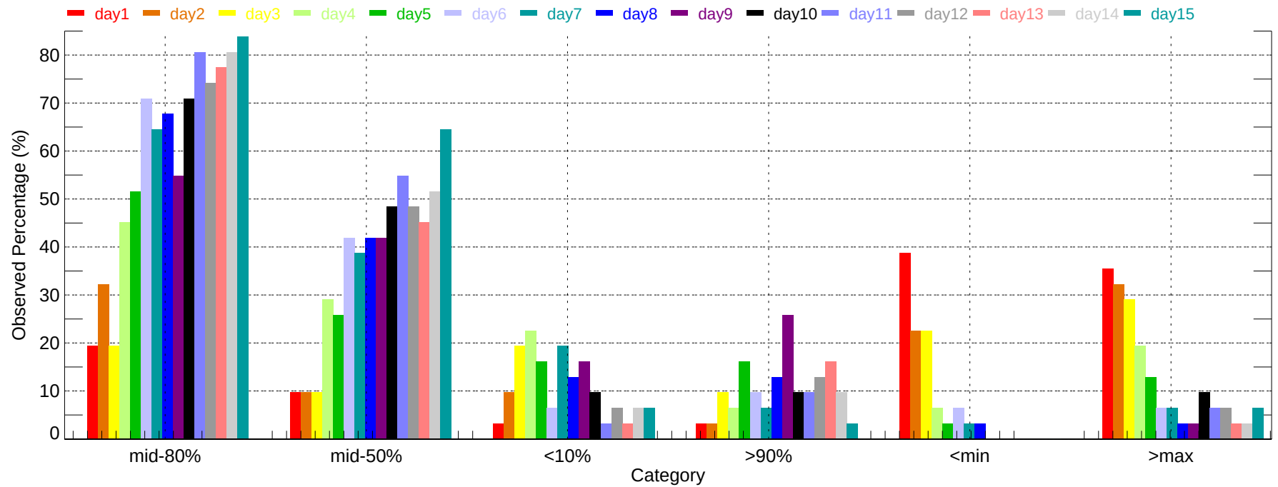
Observed Percentage of Ensembles - SSI: Max Temperature (2011-12-01~2011-12-31)
