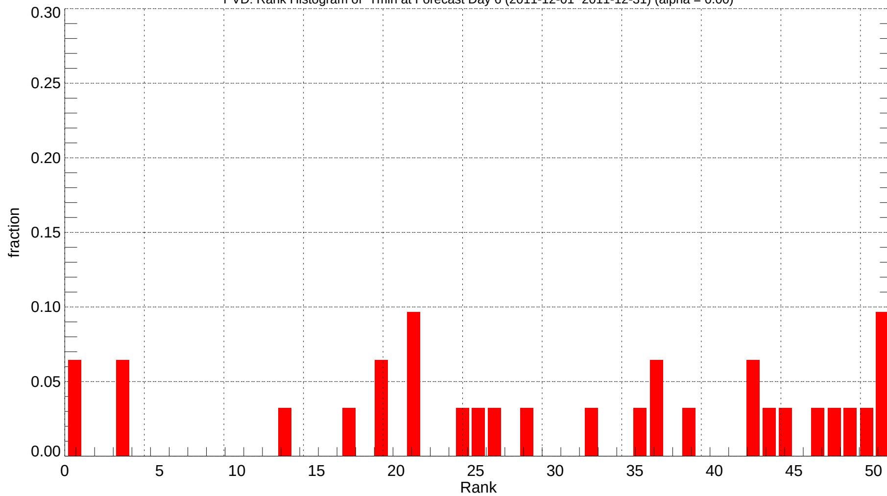
PVD: Rank Histogram of Tmin at Forecast Day 6 (2011-12-01~2011-12-31) (alpha = 0.00)
