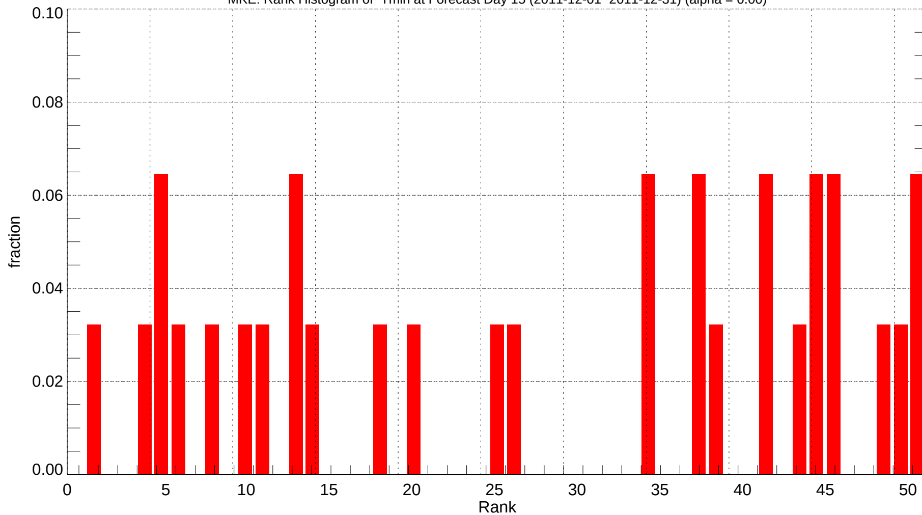
MKE: Rank Histogram of Tmin at Forecast Day 15 (2011-12-01~2011-12-31) (alpha = 0.00)
