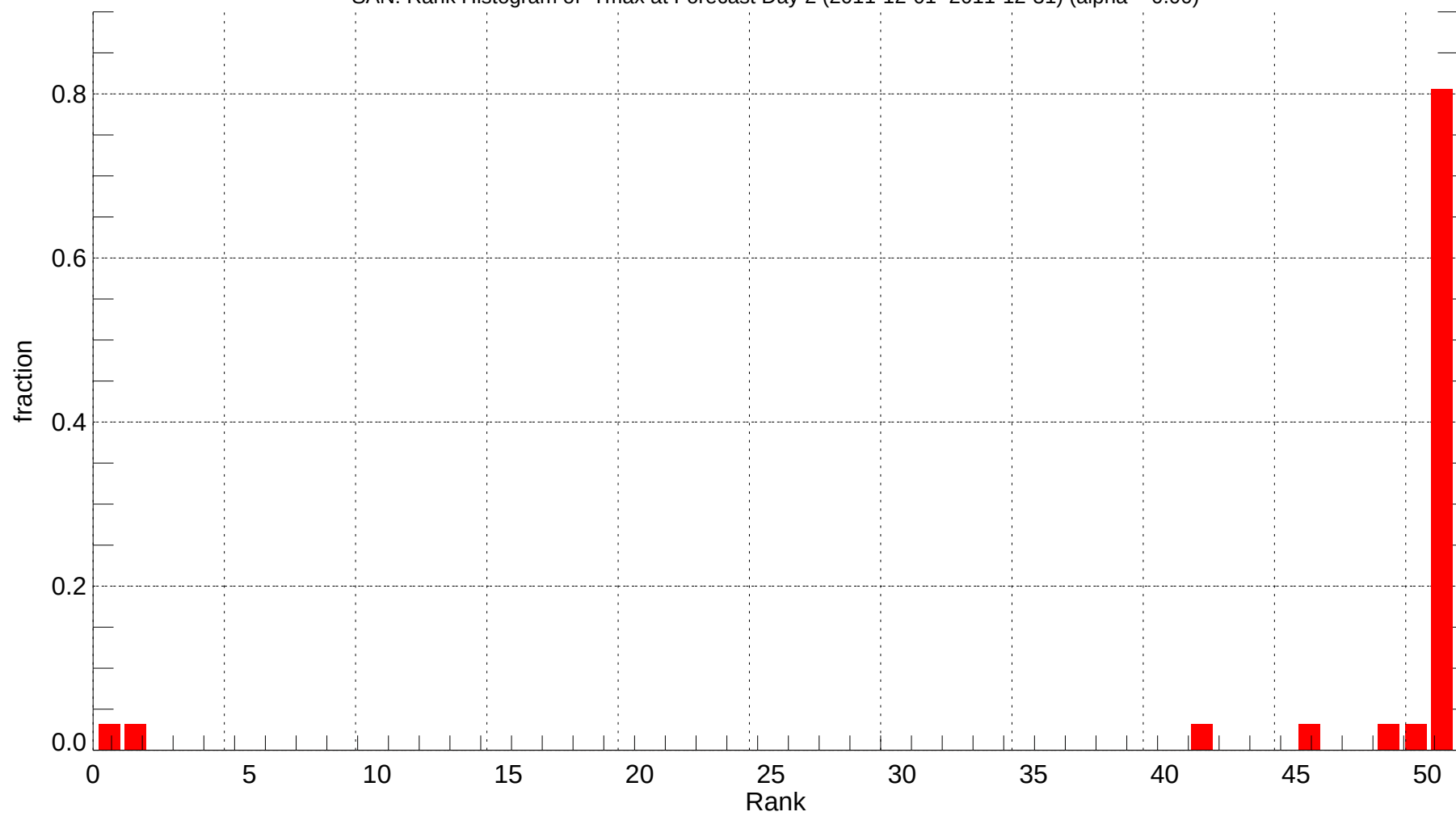
SAN: Rank Histogram of Tmax at Forecast Day 2 (2011-12-01~2011-12-31) (alpha = 0.00)
