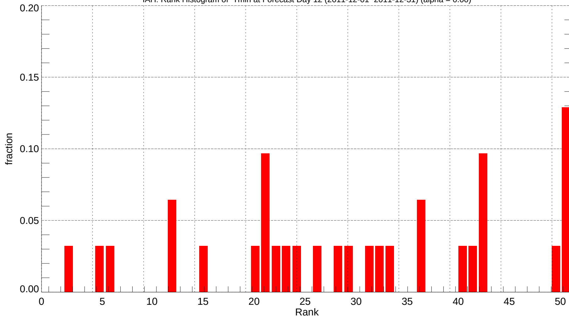
IAH: Rank Histogram of Tmin at Forecast Day 12 (2011-12-01~2011-12-31) (alpha = 0.00)
