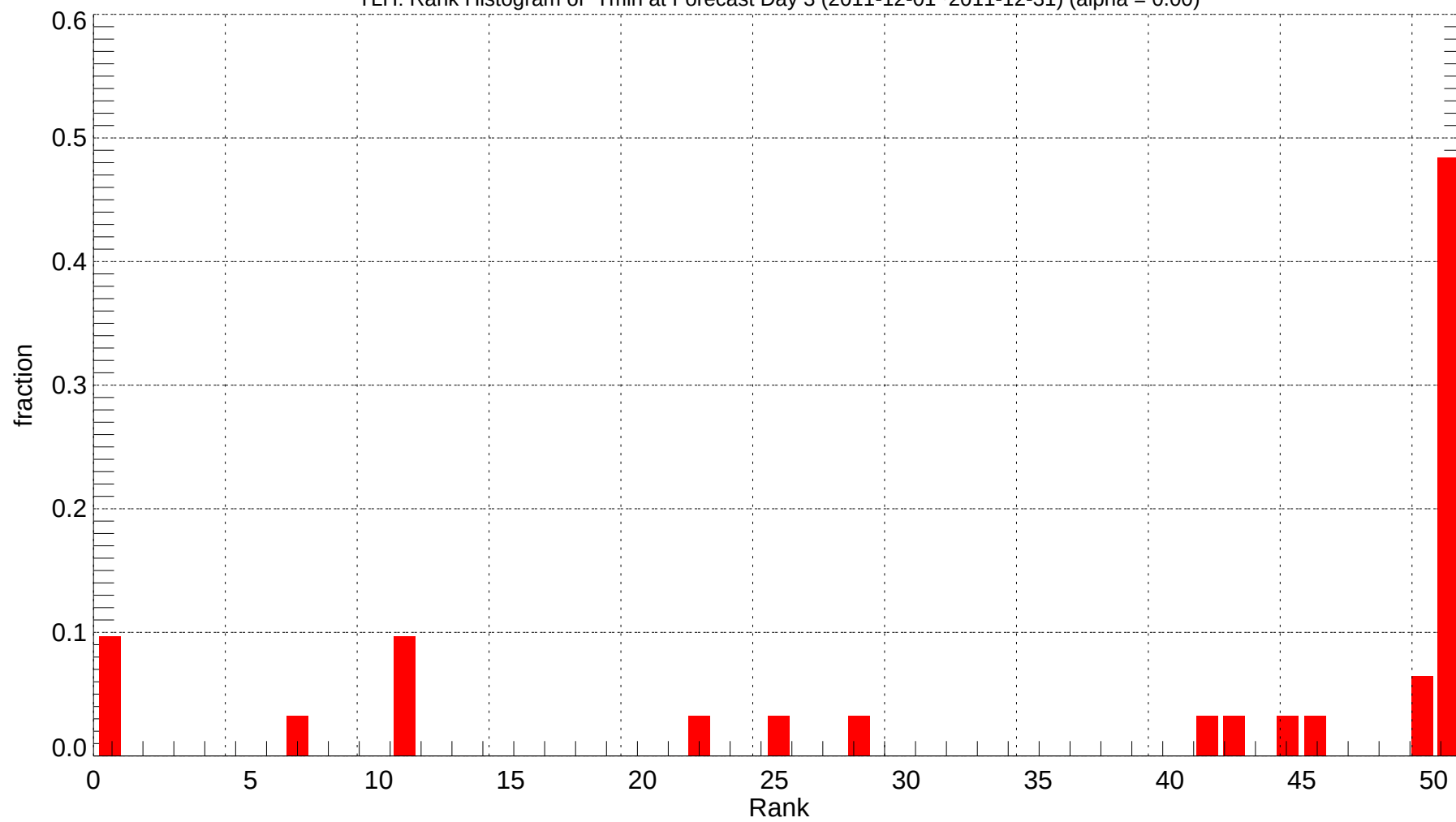
TLH: Rank Histogram of Tmin at Forecast Day 3 (2011-12-01~2011-12-31) (alpha = 0.00)
