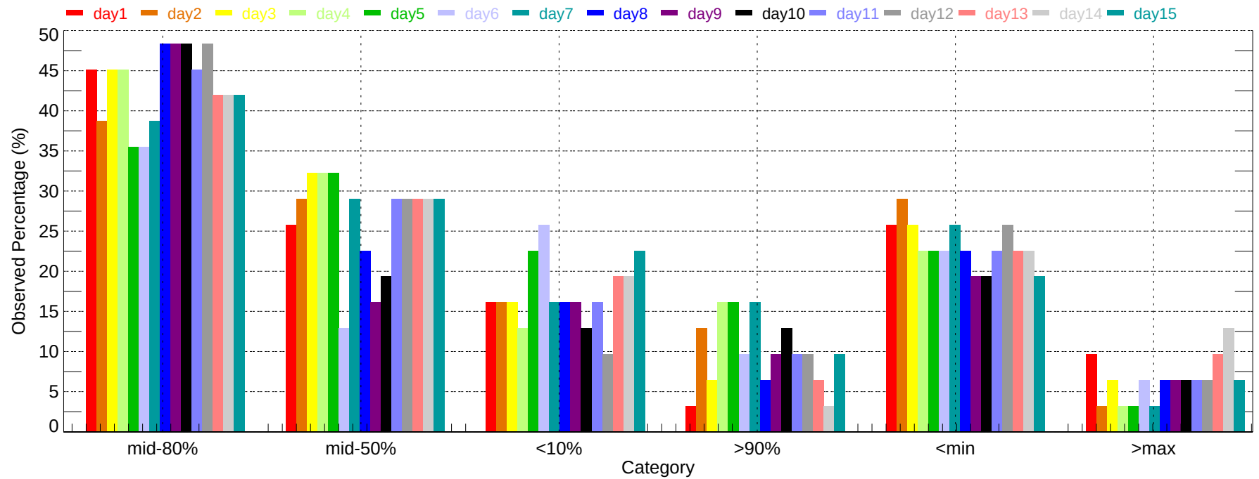
Observed Percentage of Ensembles - ABI: Max Temperature (2011-12-01~2011-12-31)
