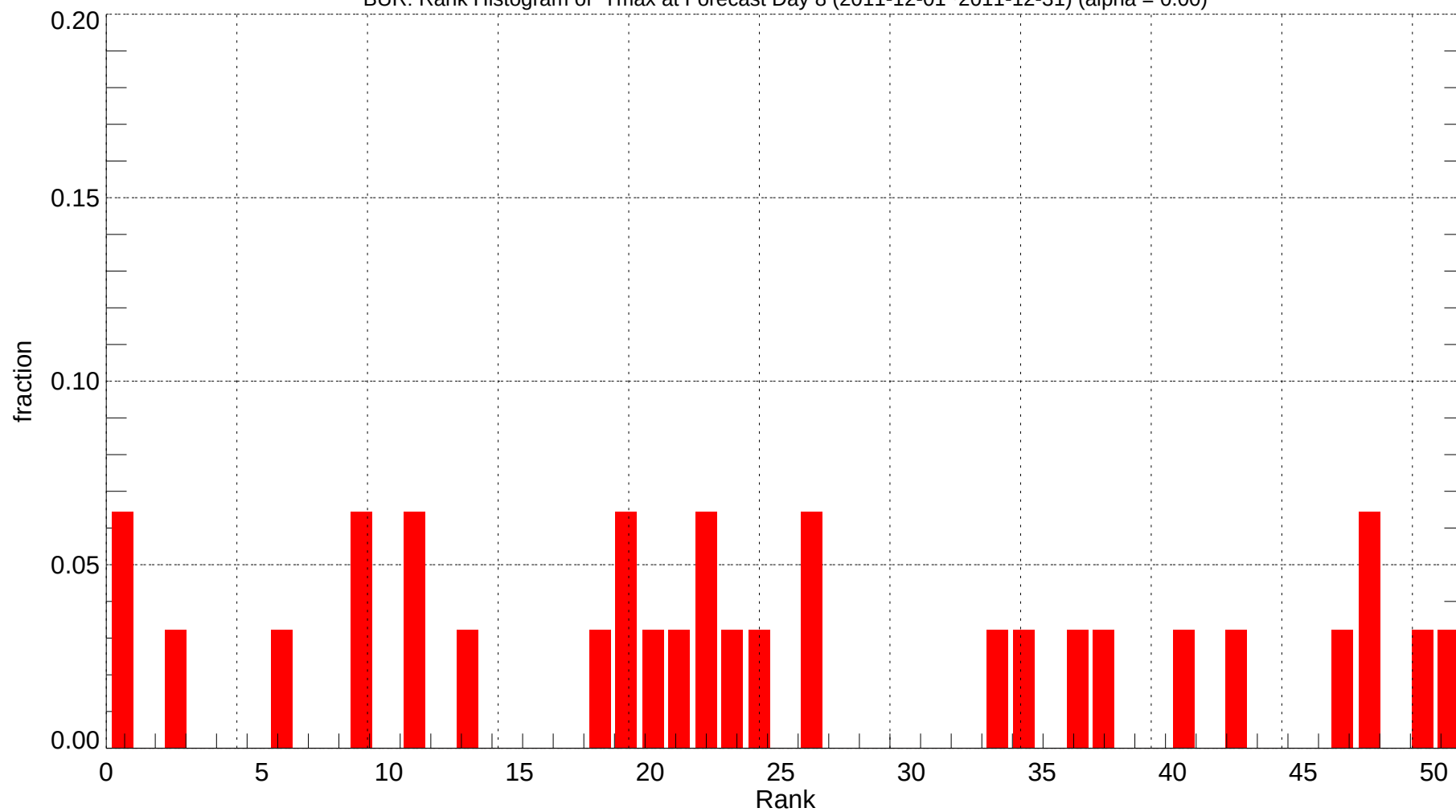
BUR: Rank Histogram of Tmax at Forecast Day 8 (2011-12-01~2011-12-31) (alpha = 0.00)
