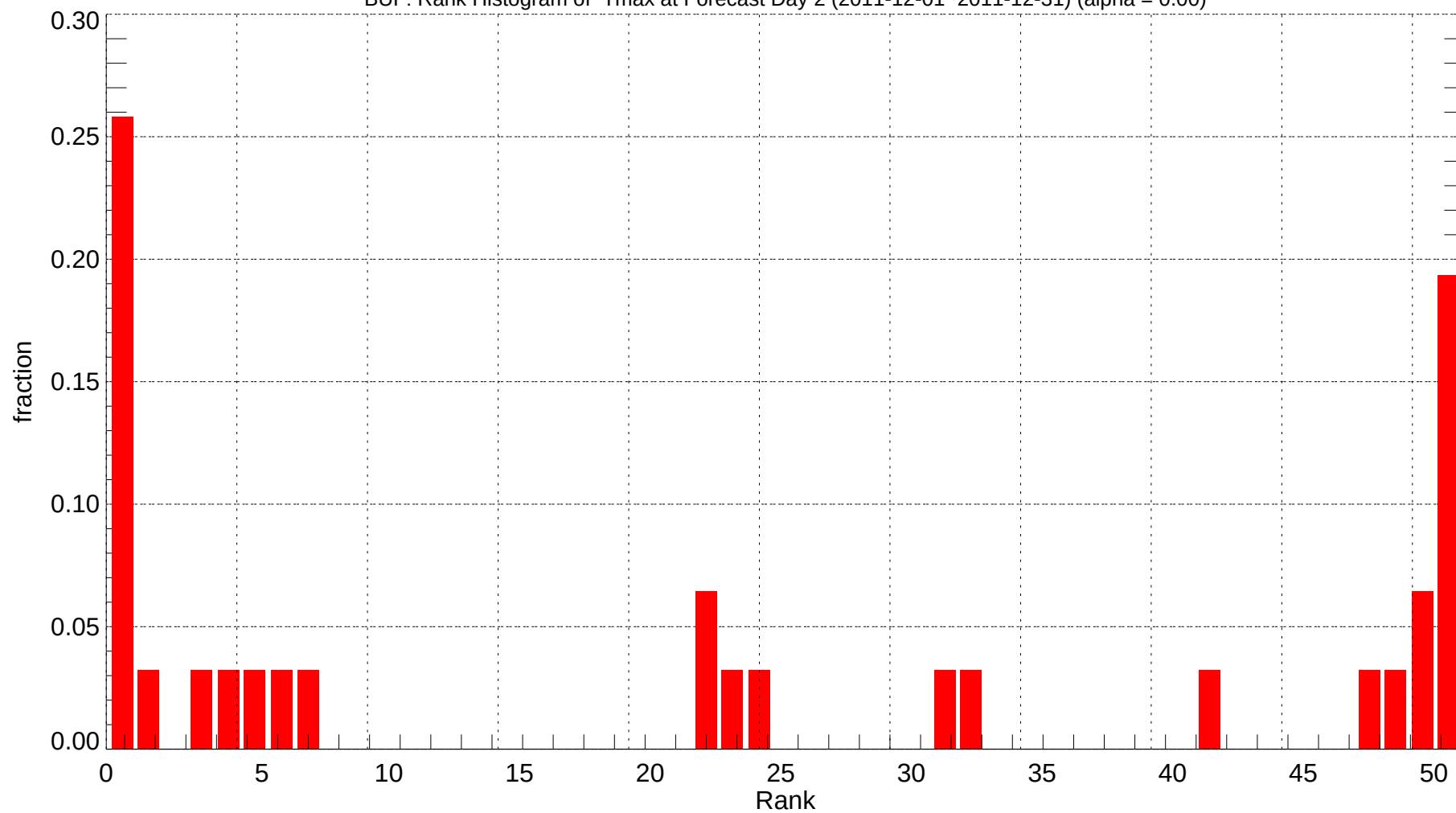
BUF: Rank Histogram of Tmax at Forecast Day 2 (2011-12-01~2011-12-31) (alpha = 0.00)
