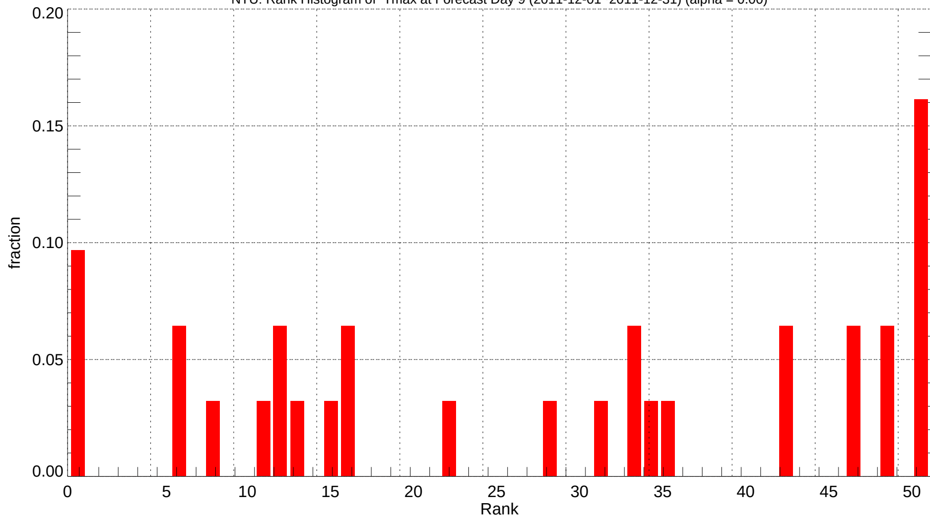
NTU: Rank Histogram of Tmax at Forecast Day 9 (2011-12-01~2011-12-31) (alpha = 0.00)
