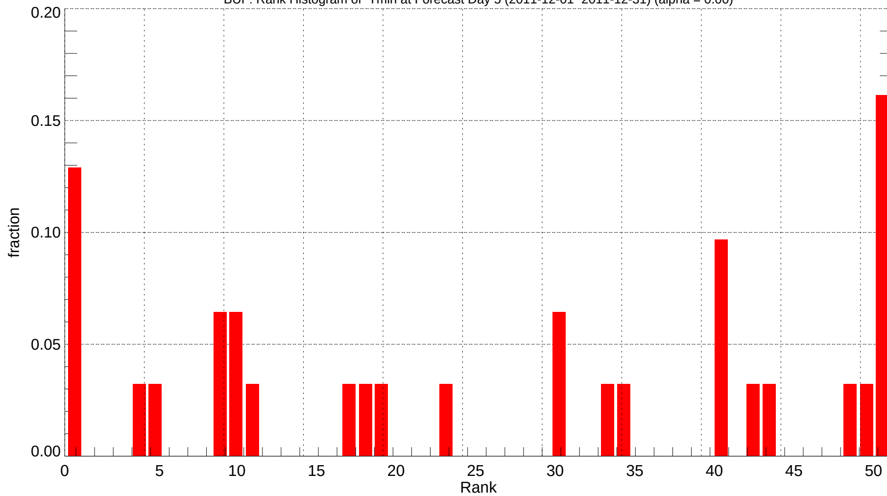
BUF: Rank Histogram of Tmin at Forecast Day 5 (2011-12-01~2011-12-31) (alpha = 0.00)
