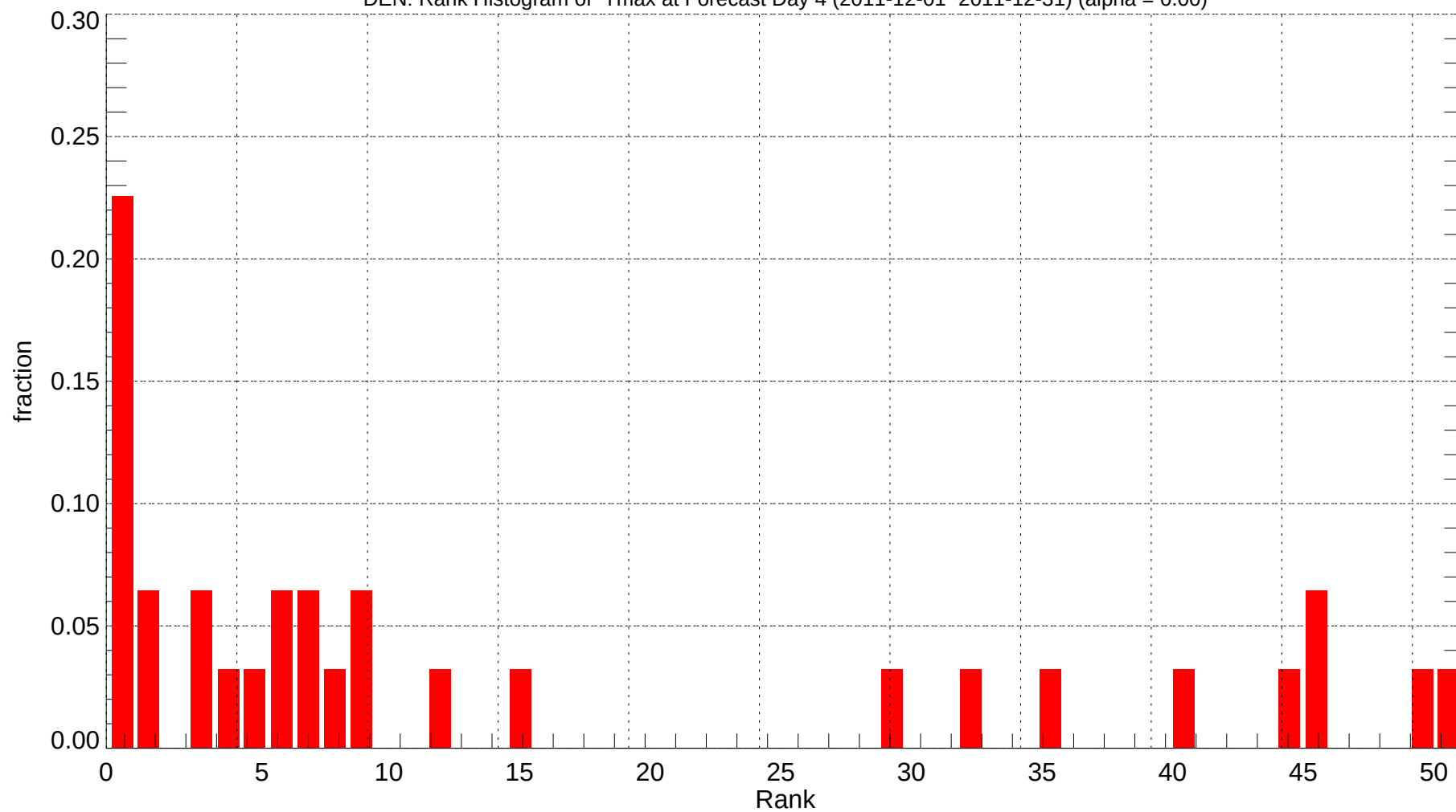
DEN: Rank Histogram of Tmax at Forecast Day 4 (2011-12-01~2011-12-31) (alpha = 0.00)
