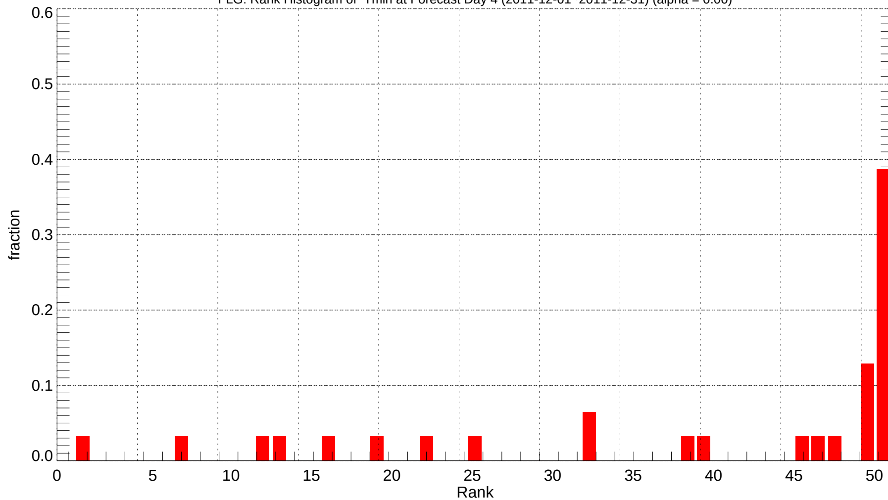
FLG: Rank Histogram of Tmin at Forecast Day 4 (2011-12-01~2011-12-31) (alpha = 0.00)
