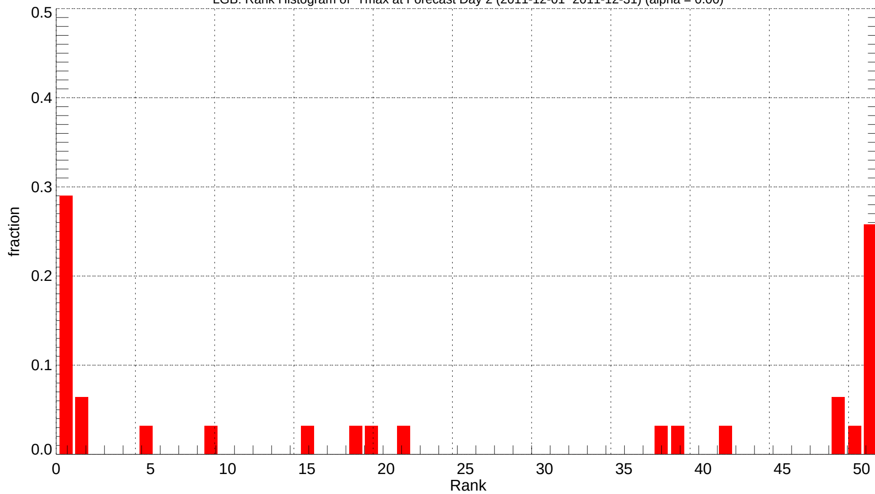
LGB: Rank Histogram of Tmax at Forecast Day 2 (2011-12-01~2011-12-31) (alpha = 0.00)
