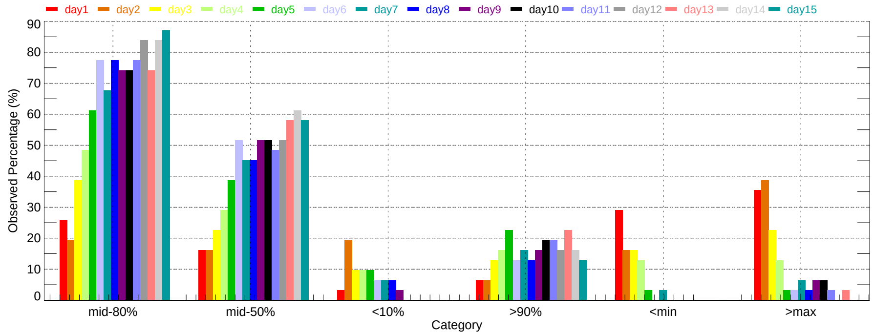
Observed Percentage of Ensembles - CLT: Max Temperature (2011-12-01~2011-12-31)
