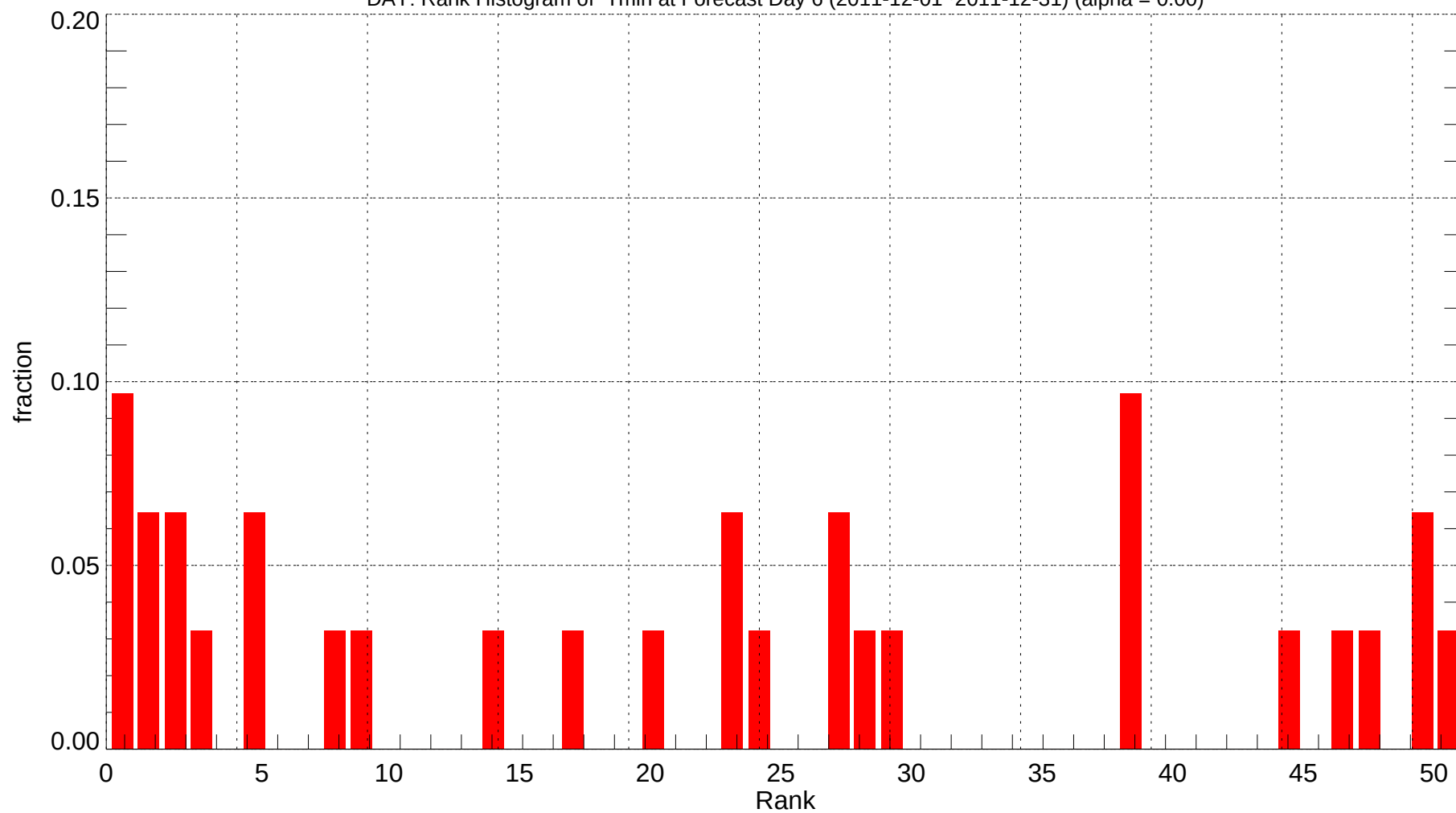
DAY: Rank Histogram of Tmin at Forecast Day 6 (2011-12-01~2011-12-31) (alpha = 0.00)
