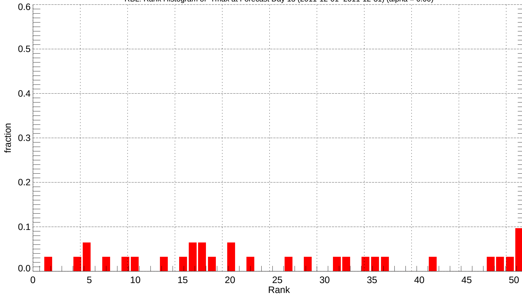
RBL: Rank Histogram of Tmax at Forecast Day 13 (2011-12-01~2011-12-31) (alpha = 0.00)
