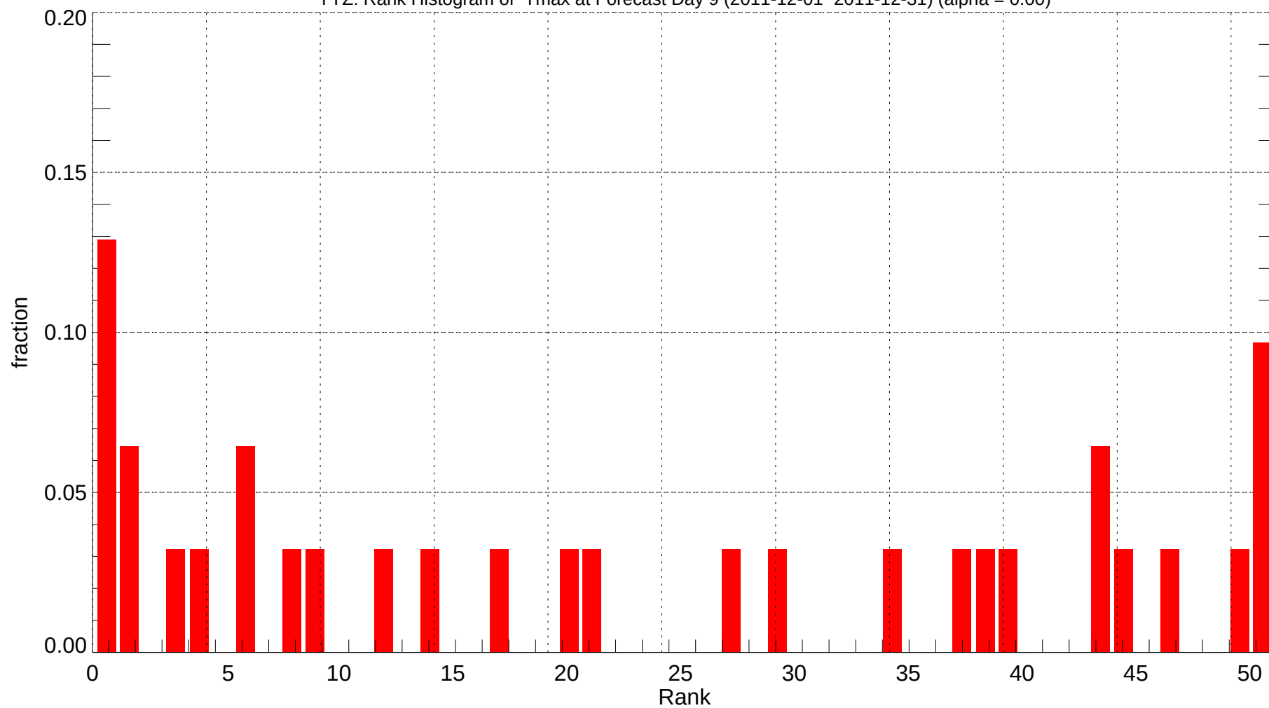
YYZ: Rank Histogram of Tmax at Forecast Day 9 (2011-12-01~2011-12-31) (alpha = 0.00)
