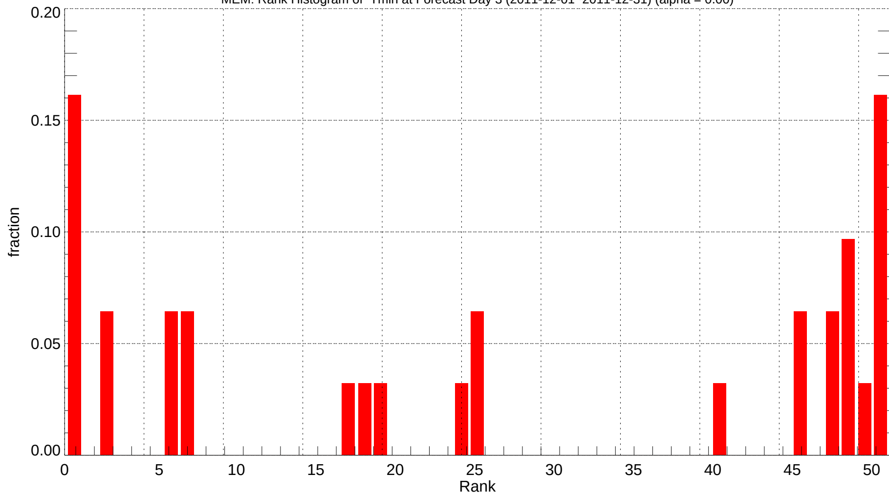
MEM: Rank Histogram of Tmin at Forecast Day 3 (2011-12-01~2011-12-31) (alpha = 0.00)
