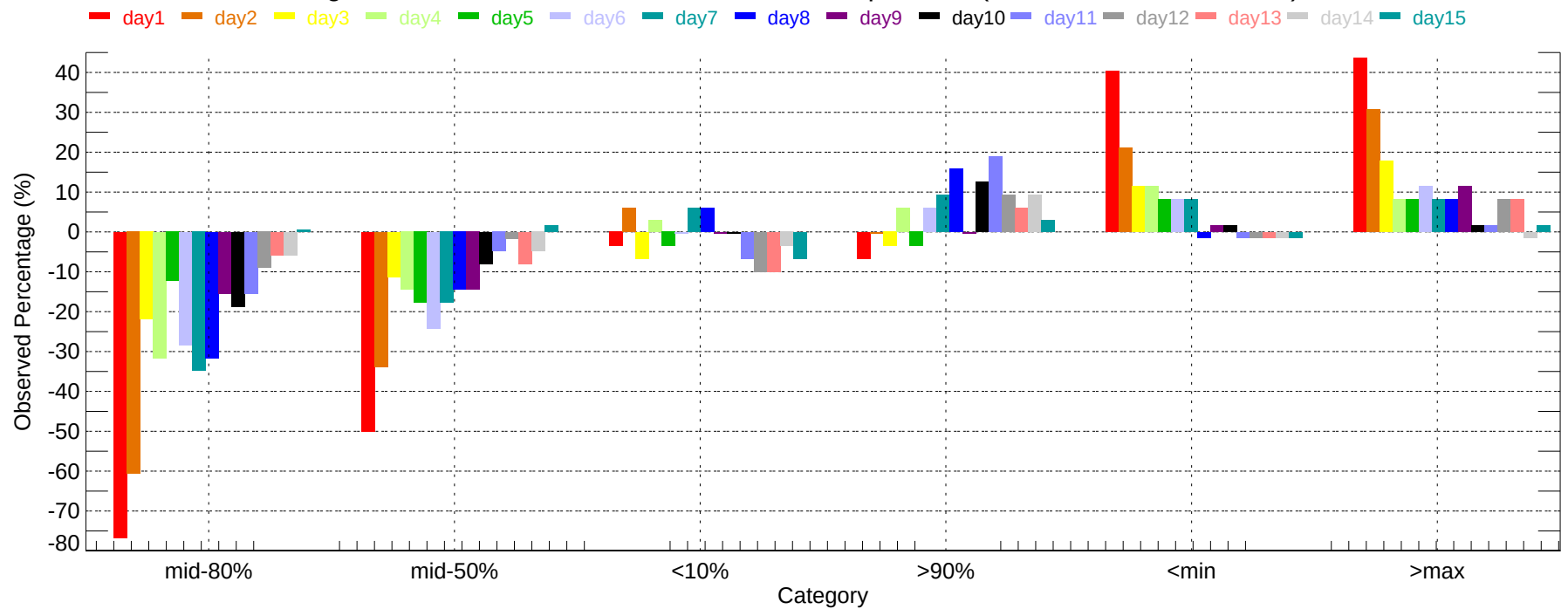
Observed Percentage Deviation of Ensembles - ROA: Min Temperature (2011-12-01~2011-12-31)
