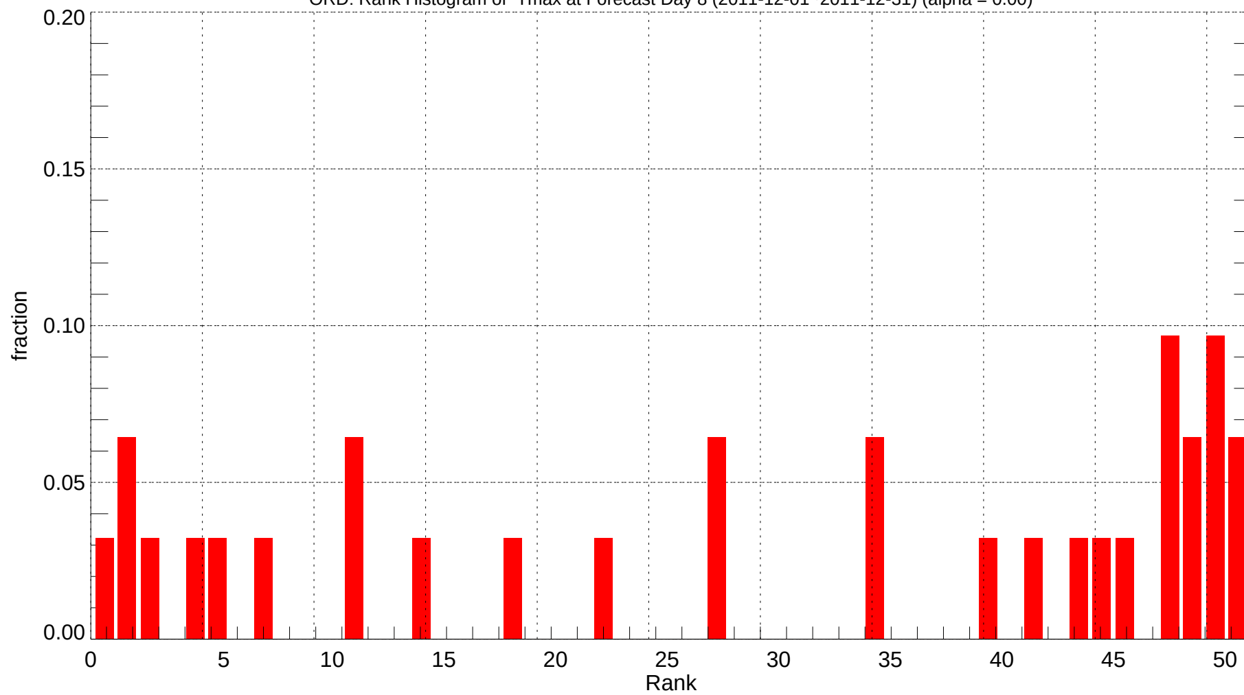
ORD: Rank Histogram of Tmax at Forecast Day 8 (2011-12-01~2011-12-31) (alpha = 0.00)
