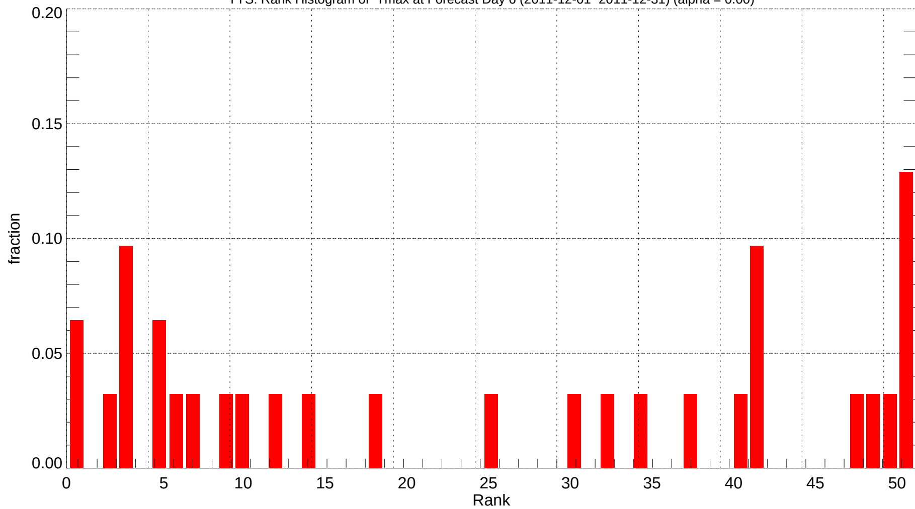
TYS: Rank Histogram of Tmax at Forecast Day 6 (2011-12-01~2011-12-31) (alpha = 0.00)
