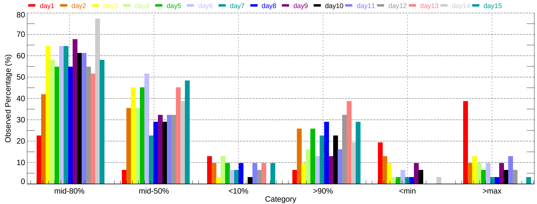
Observed Percentage of Ensembles - PVD: Max Temperature (2011-12-01~2011-12-31)
