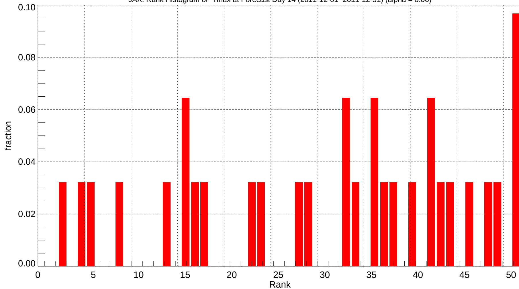
JAX: Rank Histogram of Tmax at Forecast Day 14 (2011-12-01~2011-12-31) (alpha = 0.00)
