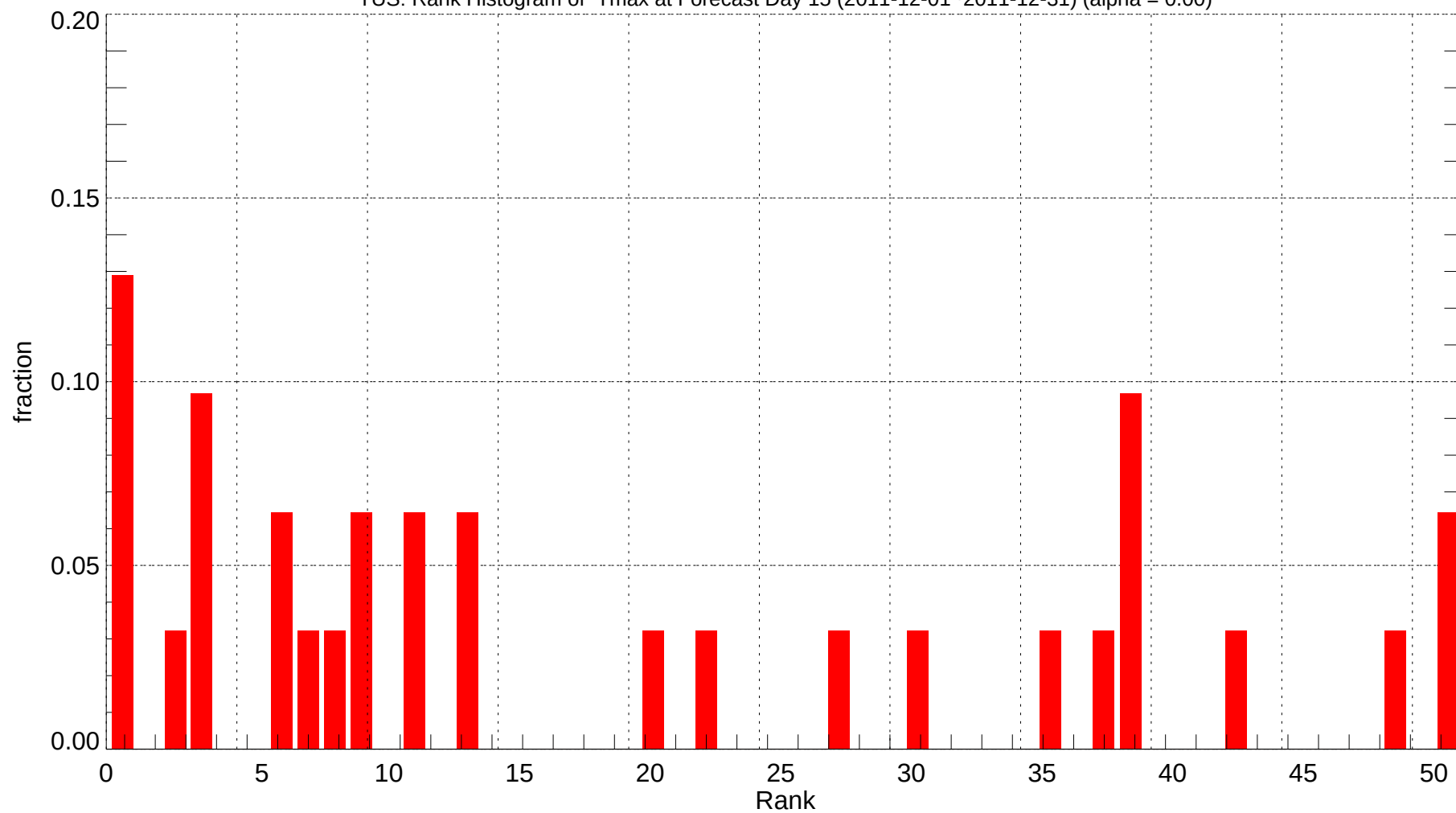
TUS: Rank Histogram of Tmax at Forecast Day 15 (2011-12-01~2011-12-31) (alpha = 0.00)
