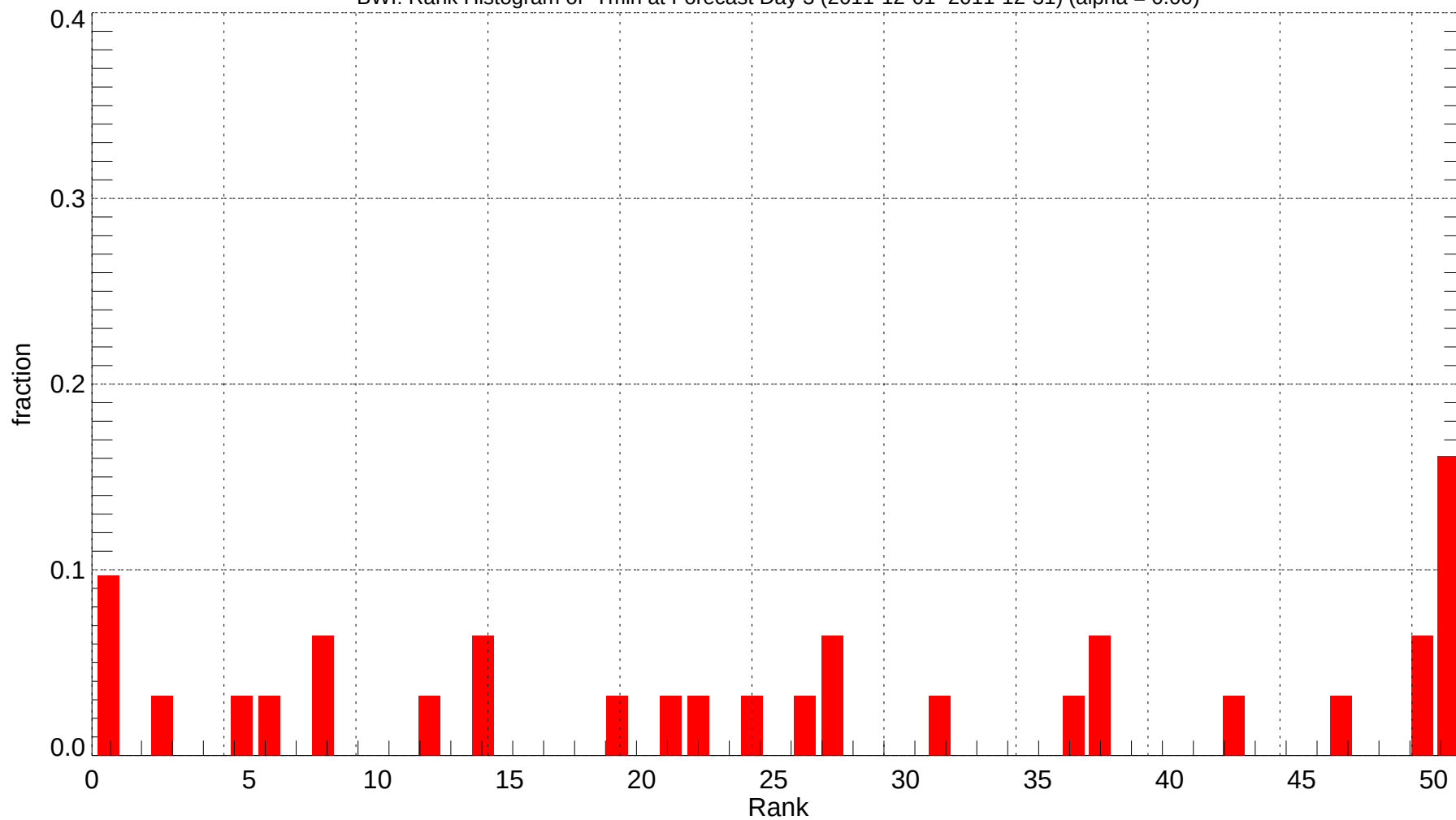
BWI: Rank Histogram of Tmin at Forecast Day 3 (2011-12-01~2011-12-31) (alpha = 0.00)
