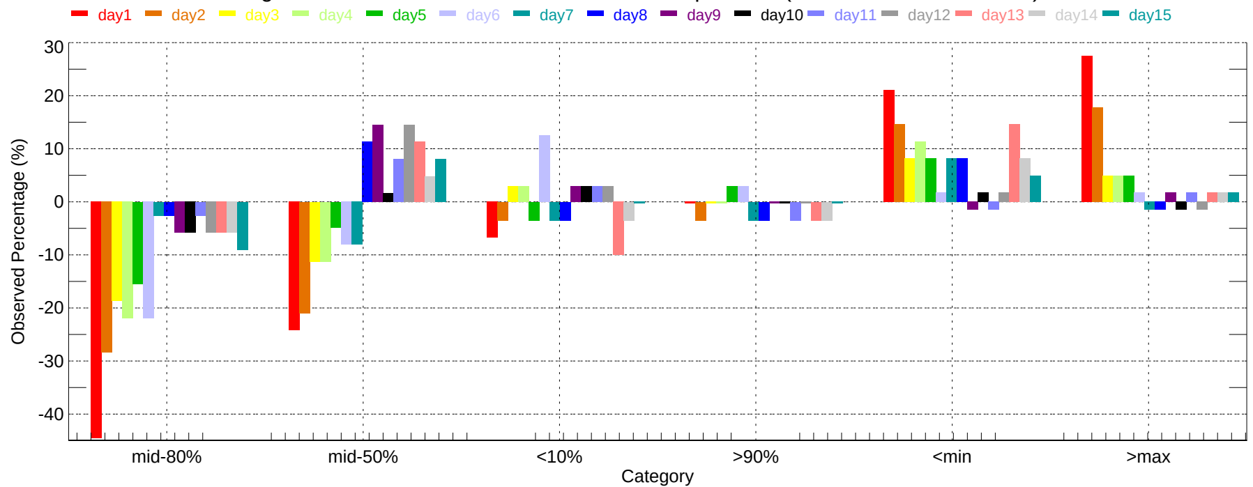
Observed Percentage Deviation of Ensembles - TPA: Max Temperature (2011-12-01~2011-12-31)
