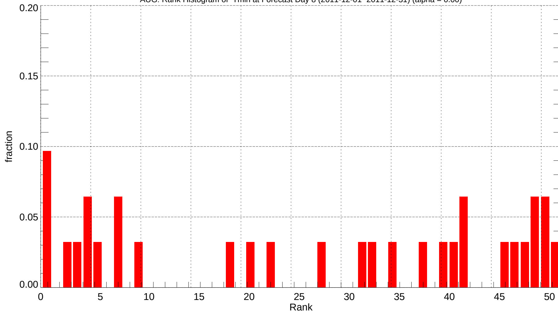
AUG: Rank Histogram of Tmin at Forecast Day 8 (2011-12-01~2011-12-31) (alpha = 0.00)
