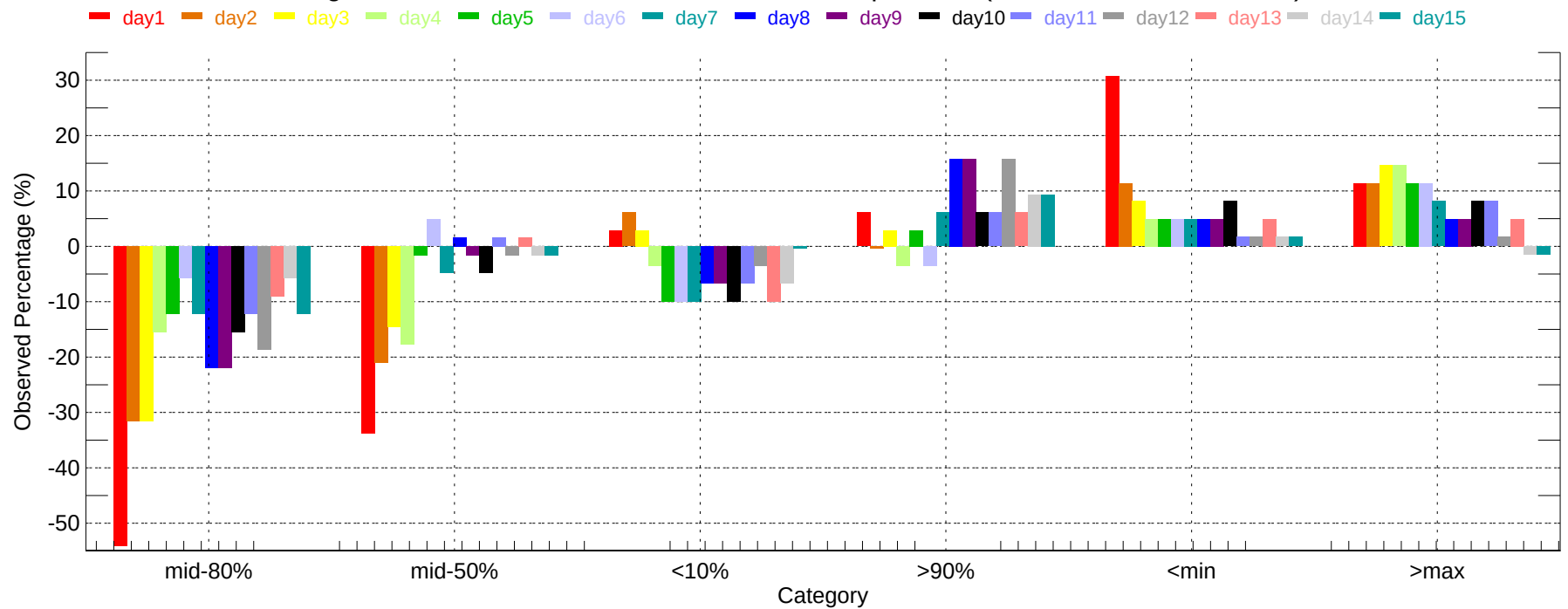
Observed Percentage Deviation of Ensembles - LGA: Max Temperature (2011-12-01~2011-12-31)
