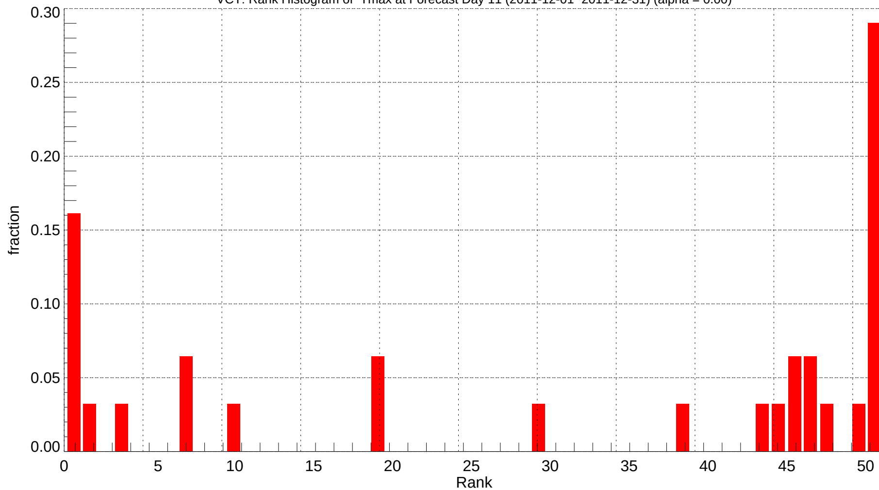
VCT: Rank Histogram of Tmax at Forecast Day 11 (2011-12-01~2011-12-31) (alpha = 0.00)
