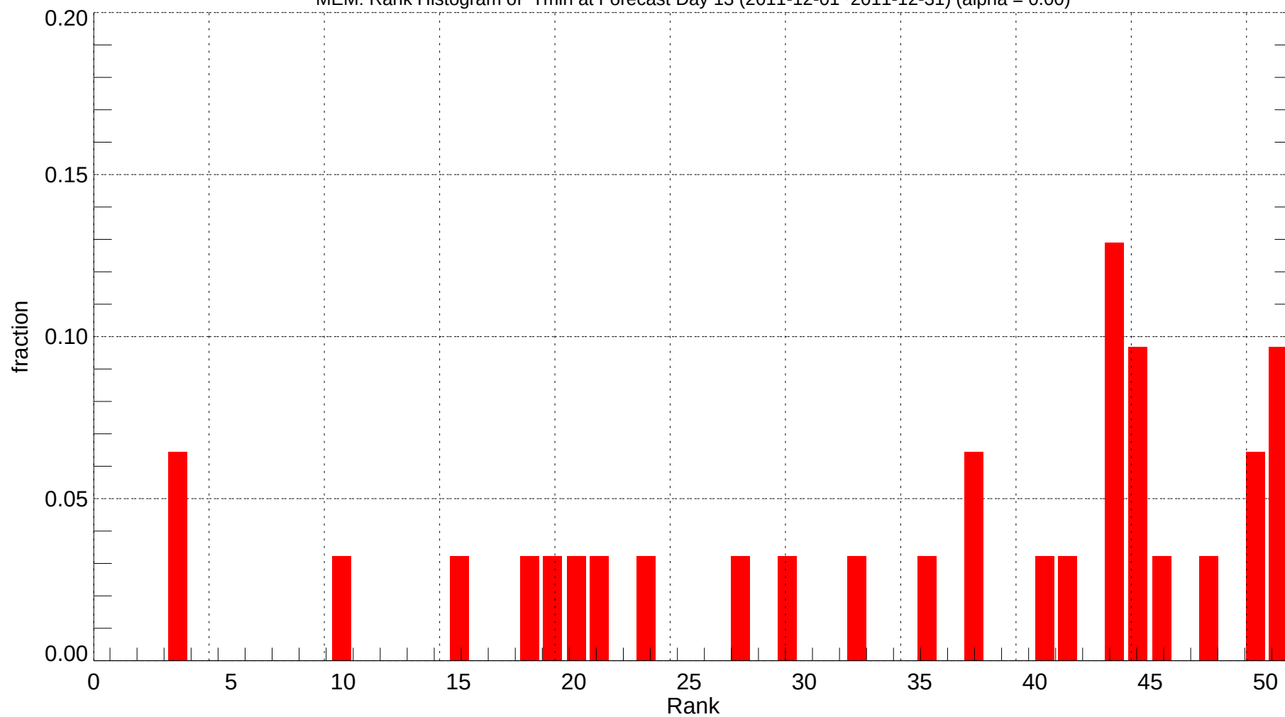
MEM: Rank Histogram of Tmin at Forecast Day 13 (2011-12-01~2011-12-31) (alpha = 0.00)
