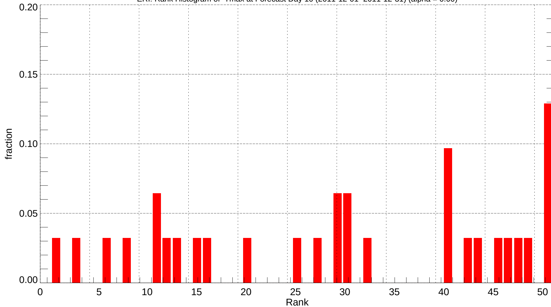
ERI: Rank Histogram of Tmax at Forecast Day 10 (2011-12-01~2011-12-31) (alpha = 0.00)
