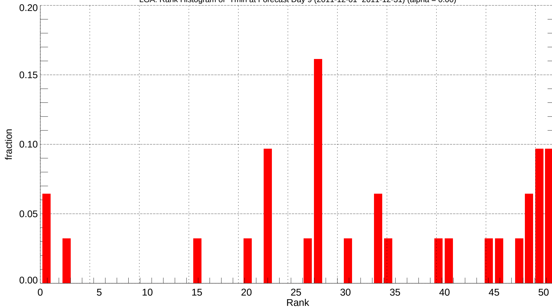
LGA: Rank Histogram of Tmin at Forecast Day 9 (2011-12-01~2011-12-31) (alpha = 0.00)
