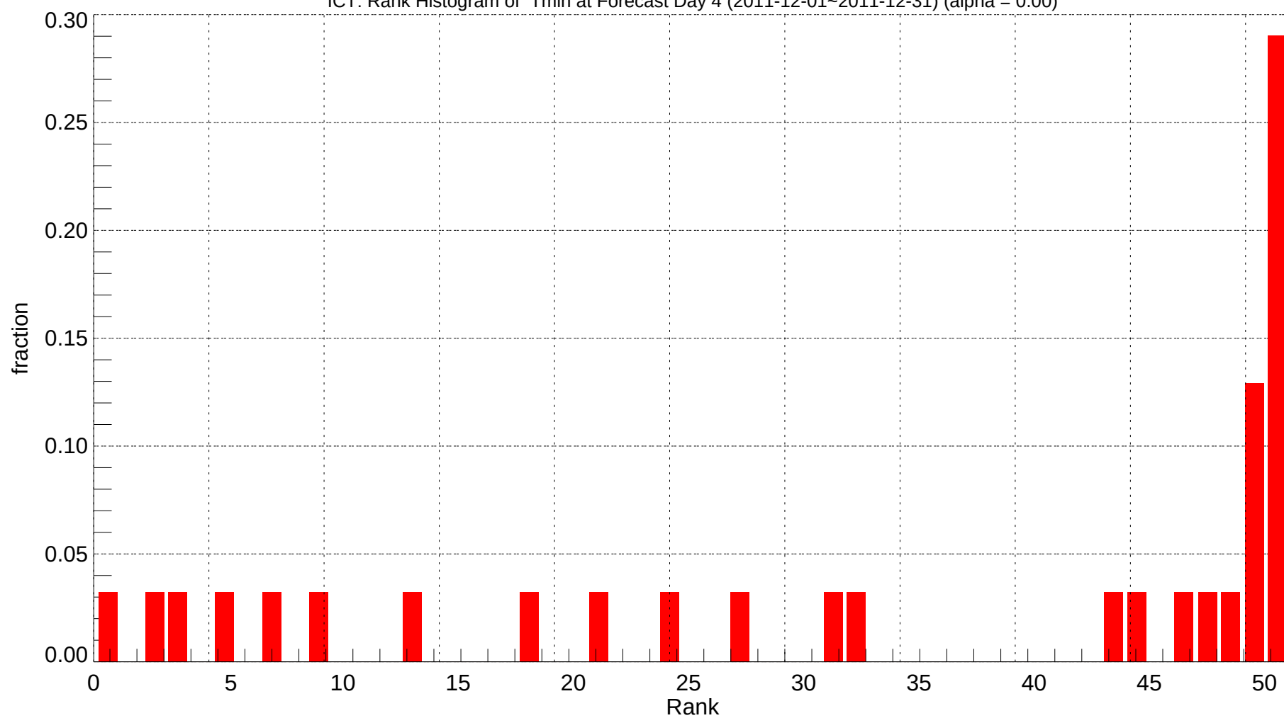
ICT: Rank Histogram of Tmin at Forecast Day 4 (2011-12-01~2011-12-31) (alpha = 0.00)
