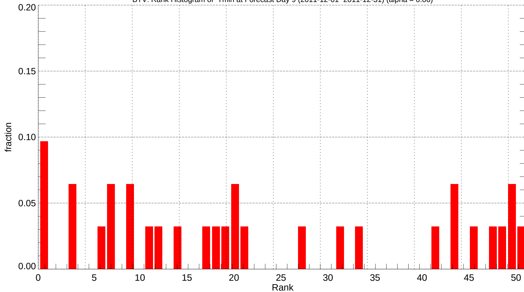
BTV: Rank Histogram of Tmin at Forecast Day 9 (2011-12-01~2011-12-31) (alpha = 0.00)
