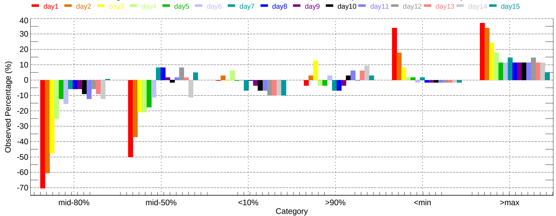
Observed Percentage Deviation of Ensembles - RDD: Max Temperature (2011-12-01~2011-12-31)
