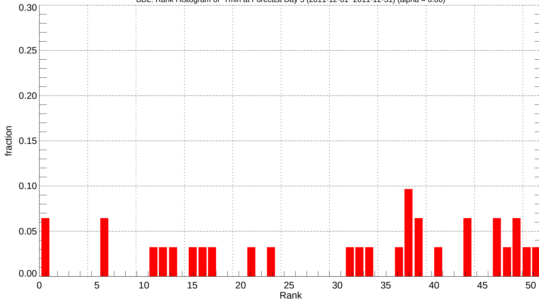
BDL: Rank Histogram of Tmin at Forecast Day 5 (2011-12-01~2011-12-31) (alpha = 0.00)
