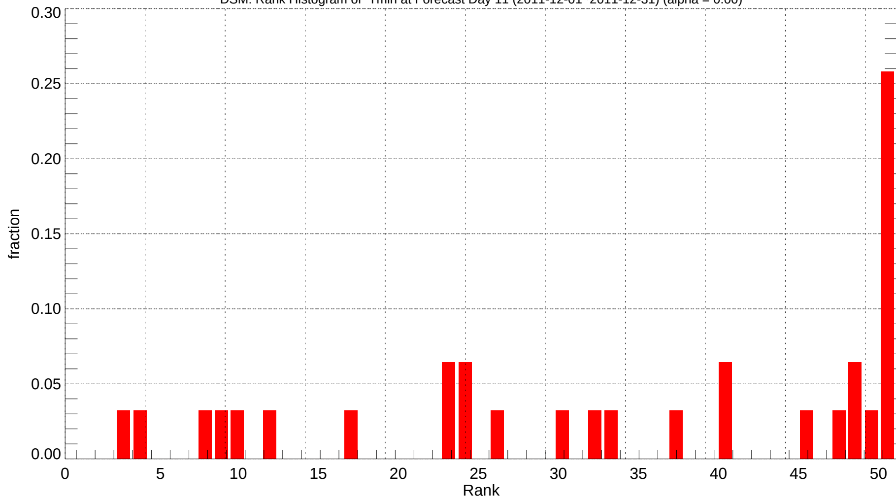
DSM: Rank Histogram of Tmin at Forecast Day 11 (2011-12-01~2011-12-31) (alpha = 0.00)
