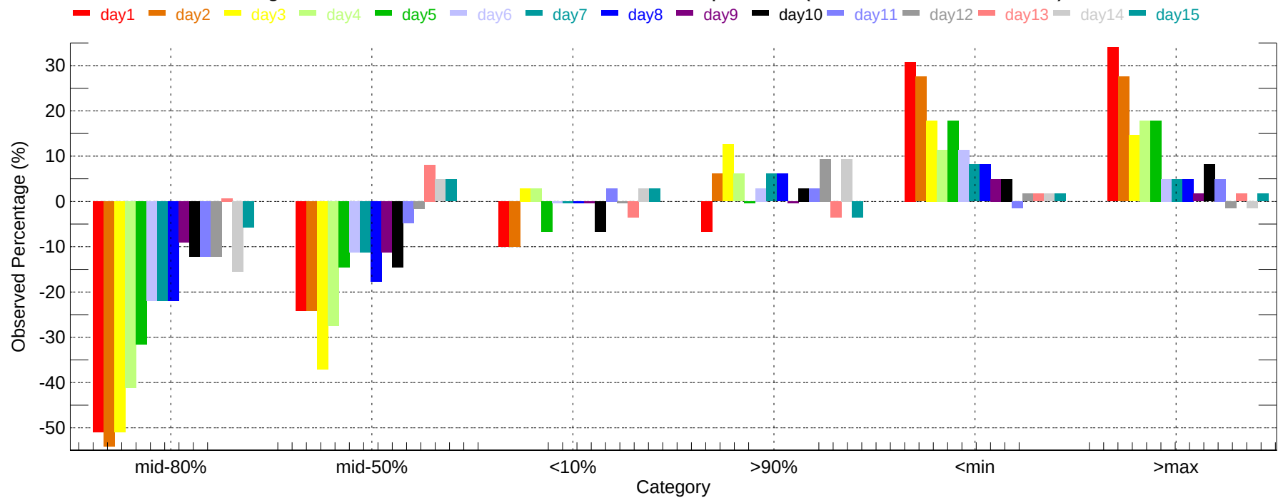
Observed Percentage Deviation of Ensembles - YUL: Max Temperature (2011-12-01~2011-12-31)
