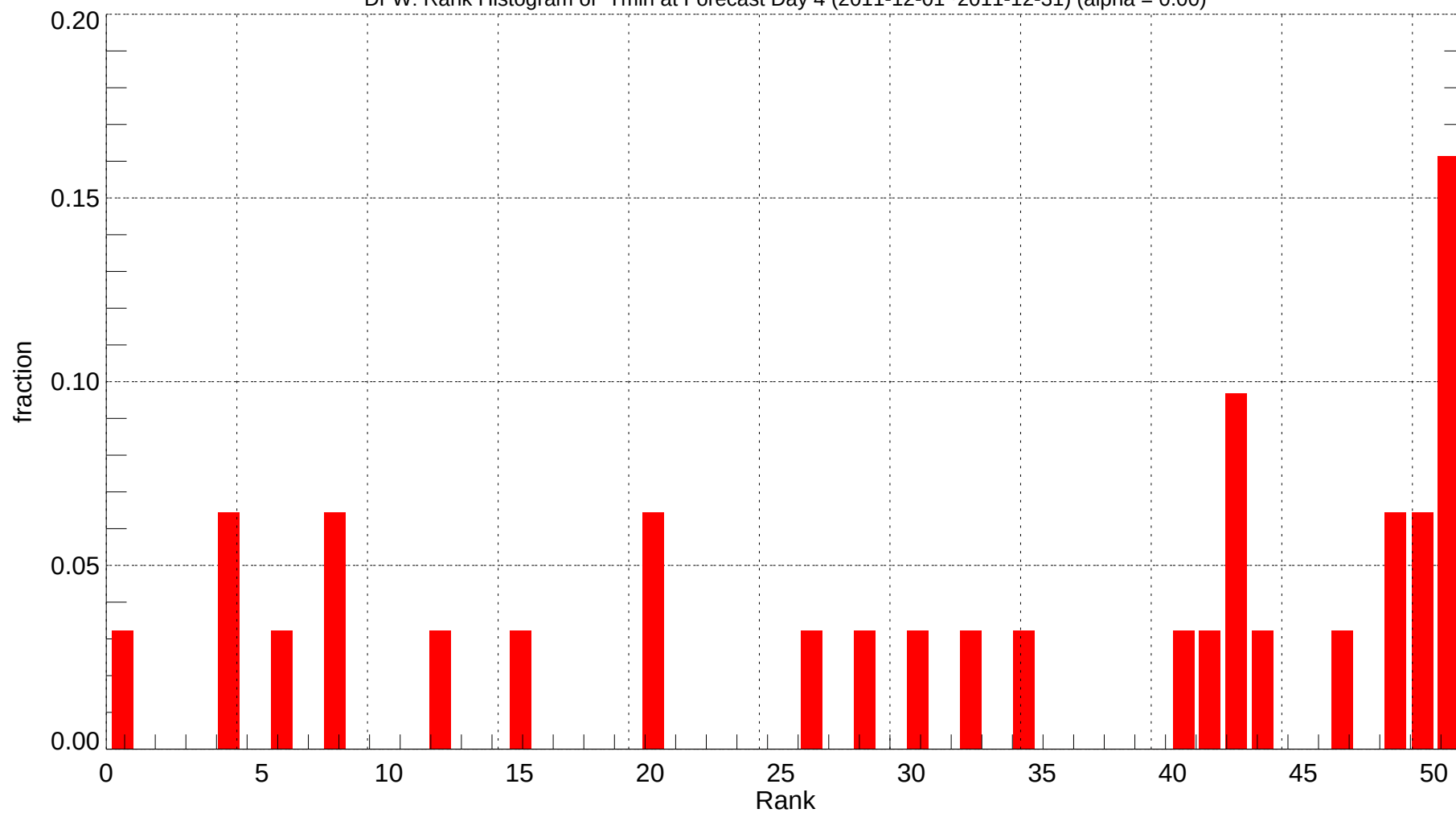
DFW: Rank Histogram of Tmin at Forecast Day 4 (2011-12-01~2011-12-31) (alpha = 0.00)
