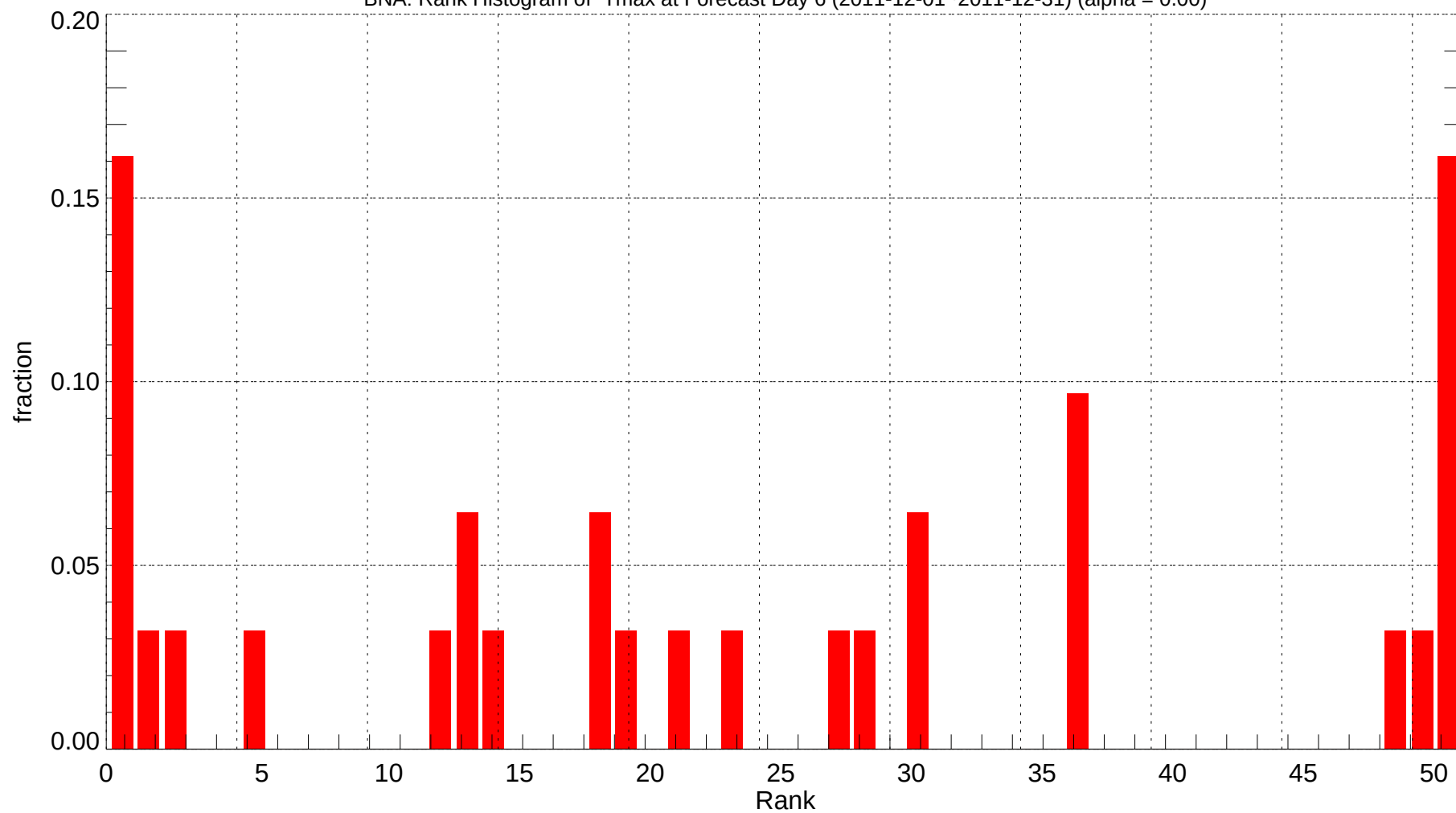
BNA: Rank Histogram of Tmax at Forecast Day 6 (2011-12-01~2011-12-31) (alpha = 0.00)
