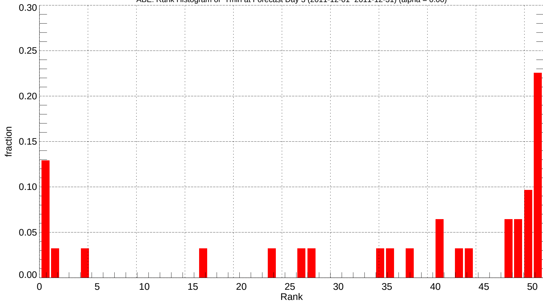
ABE: Rank Histogram of Tmin at Forecast Day 3 (2011-12-01~2011-12-31) (alpha = 0.00)
