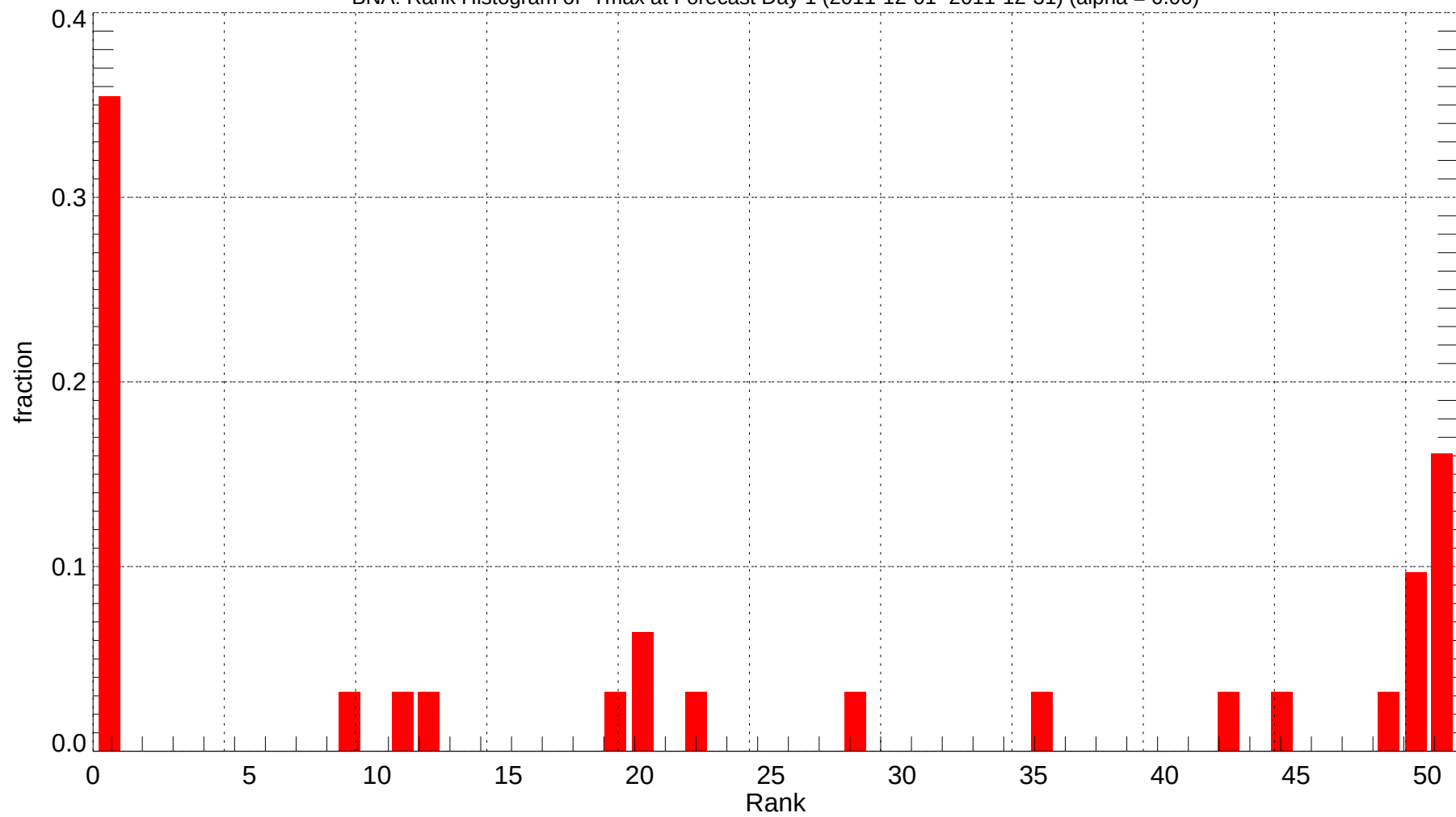
BNA: Rank Histogram of Tmax at Forecast Day 1 (2011-12-01~2011-12-31) (alpha = 0.00)
