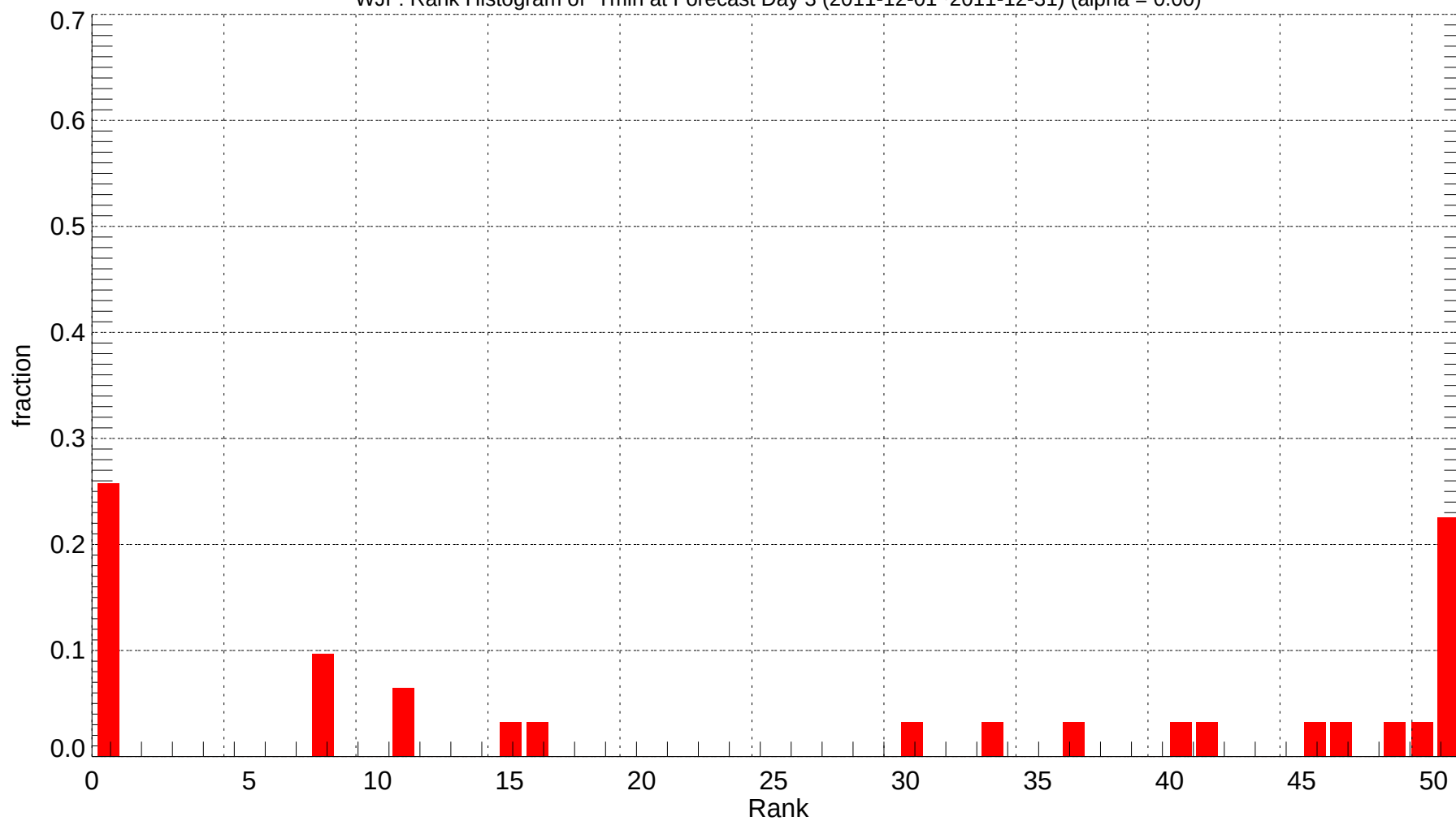
WJF: Rank Histogram of Tmin at Forecast Day 3 (2011-12-01~2011-12-31) (alpha = 0.00)
