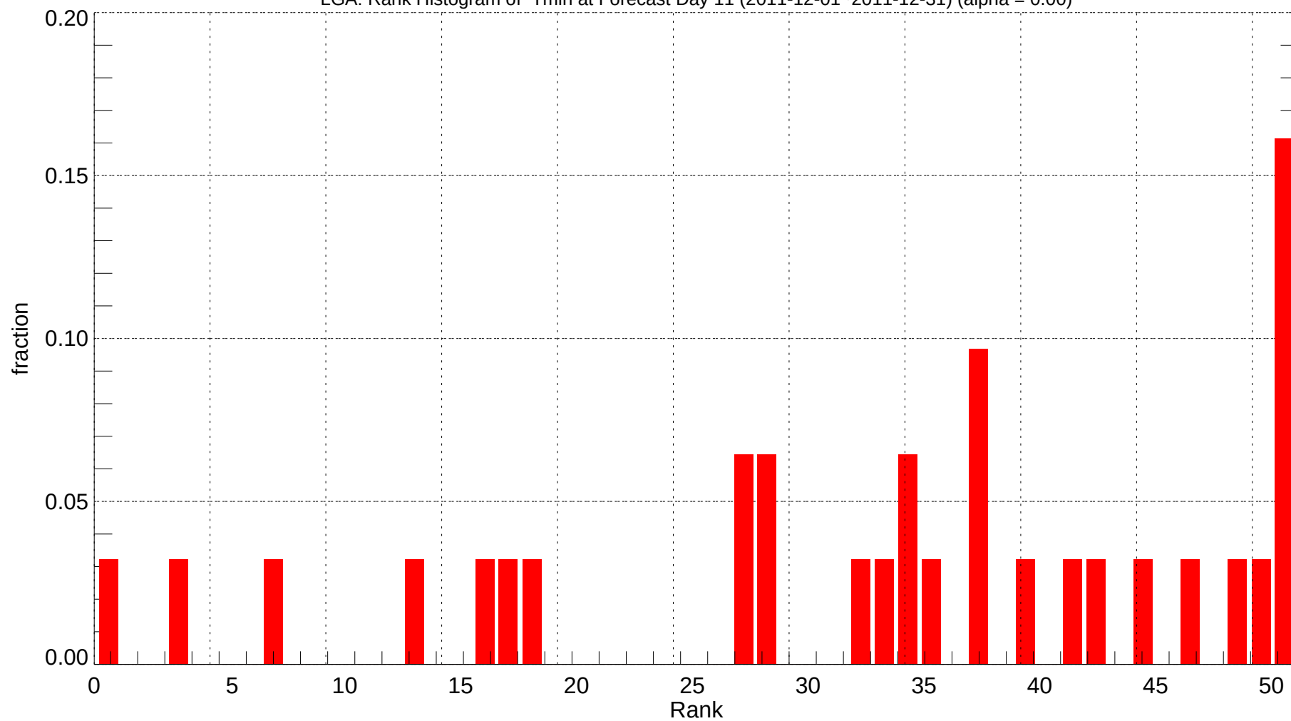
LGA: Rank Histogram of Tmin at Forecast Day 11 (2011-12-01~2011-12-31) (alpha = 0.00)
