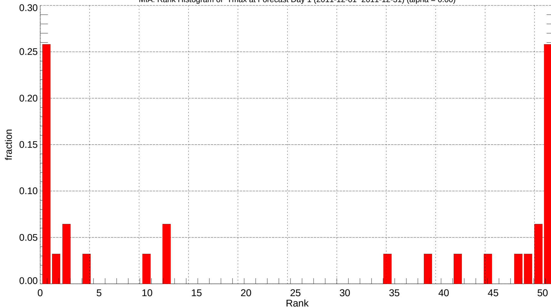
MIA: Rank Histogram of Tmax at Forecast Day 1 (2011-12-01~2011-12-31) (alpha = 0.00)
