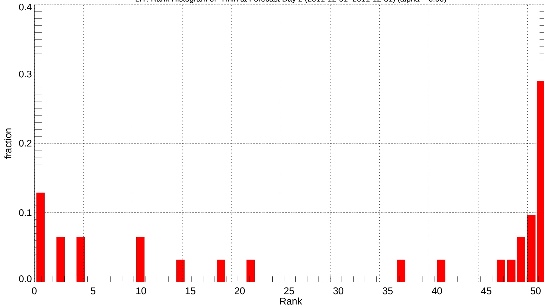
LIT: Rank Histogram of Tmin at Forecast Day 2 (2011-12-01~2011-12-31) (alpha = 0.00)
