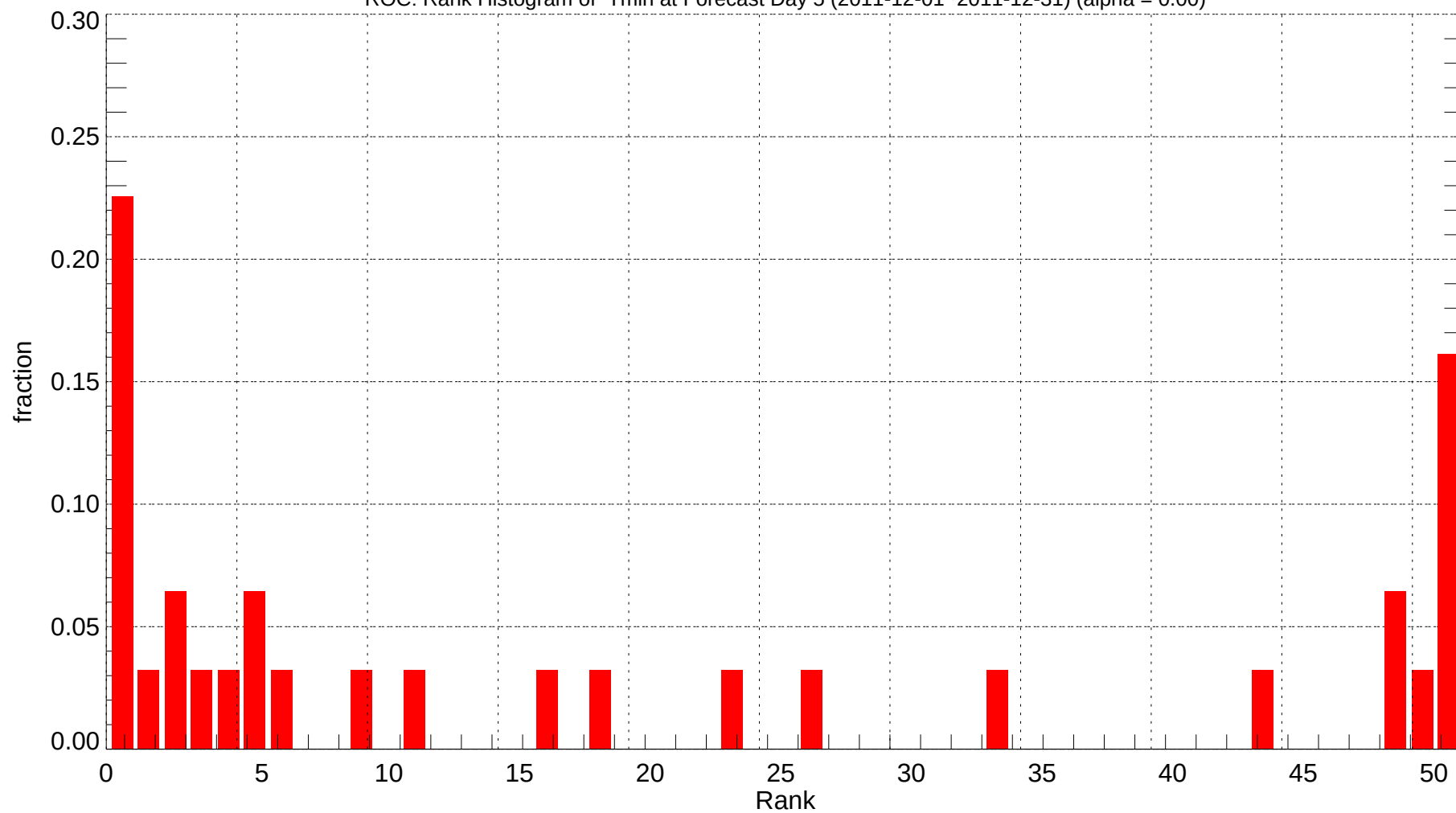
ROC: Rank Histogram of Tmin at Forecast Day 5 (2011-12-01~2011-12-31) (alpha = 0.00)
