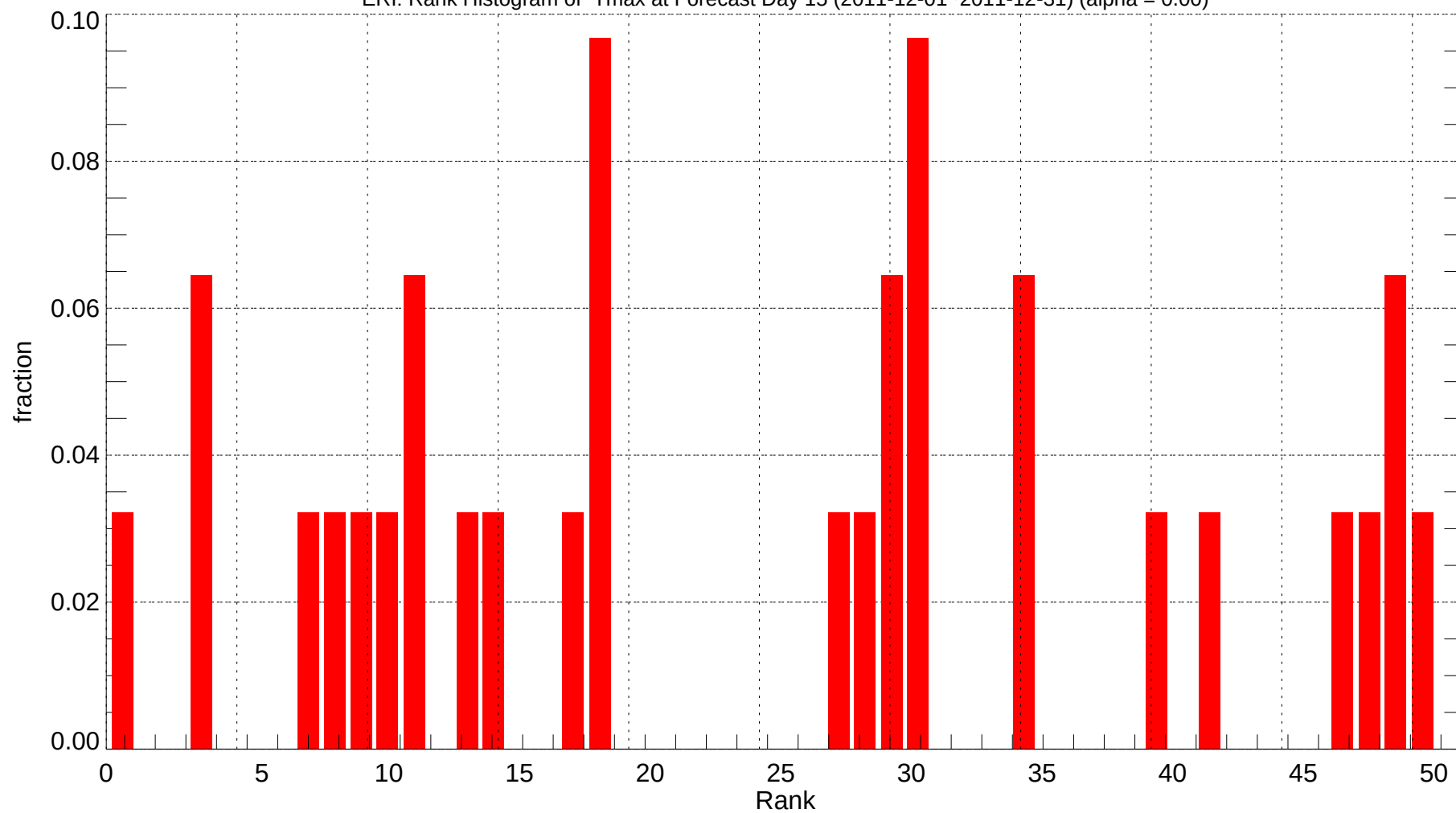
ERI: Rank Histogram of Tmax at Forecast Day 15 (2011-12-01~2011-12-31) (alpha = 0.00)
