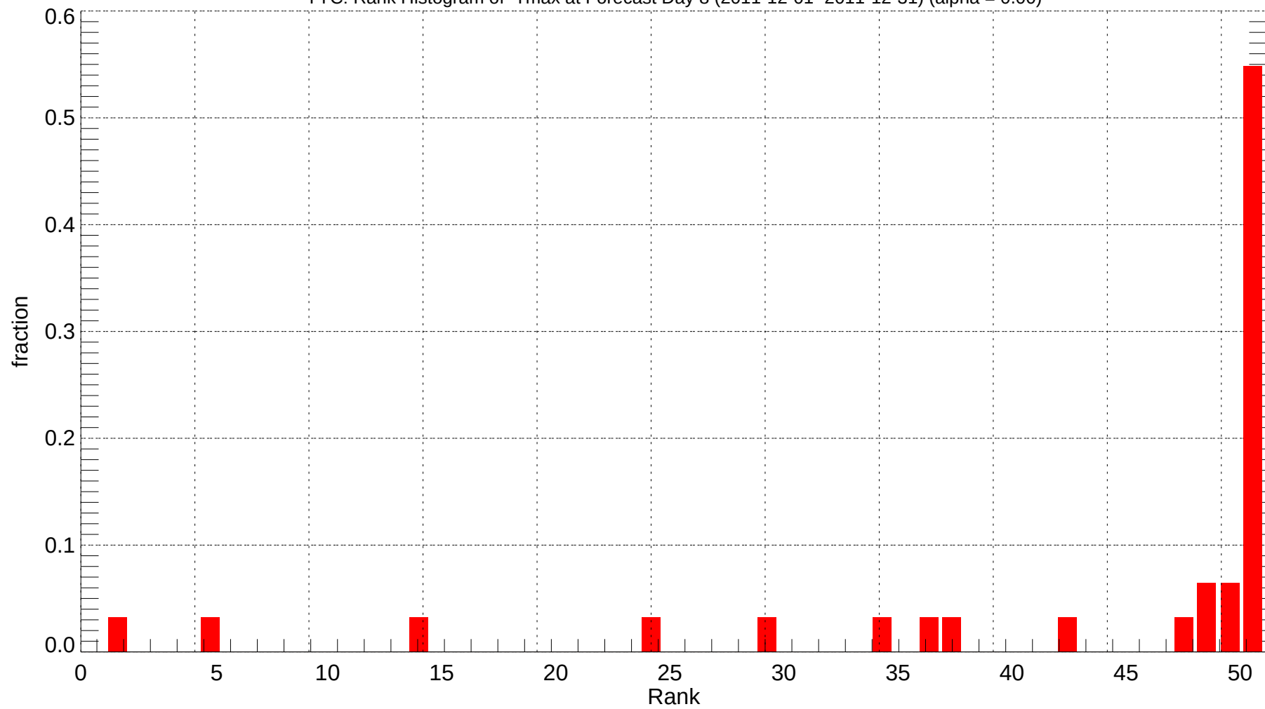
YYC: Rank Histogram of Tmax at Forecast Day 8 (2011-12-01~2011-12-31) (alpha = 0.00)
