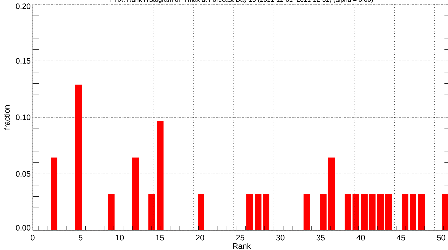
PHX: Rank Histogram of Tmax at Forecast Day 13 (2011-12-01~2011-12-31) (alpha = 0.00)
