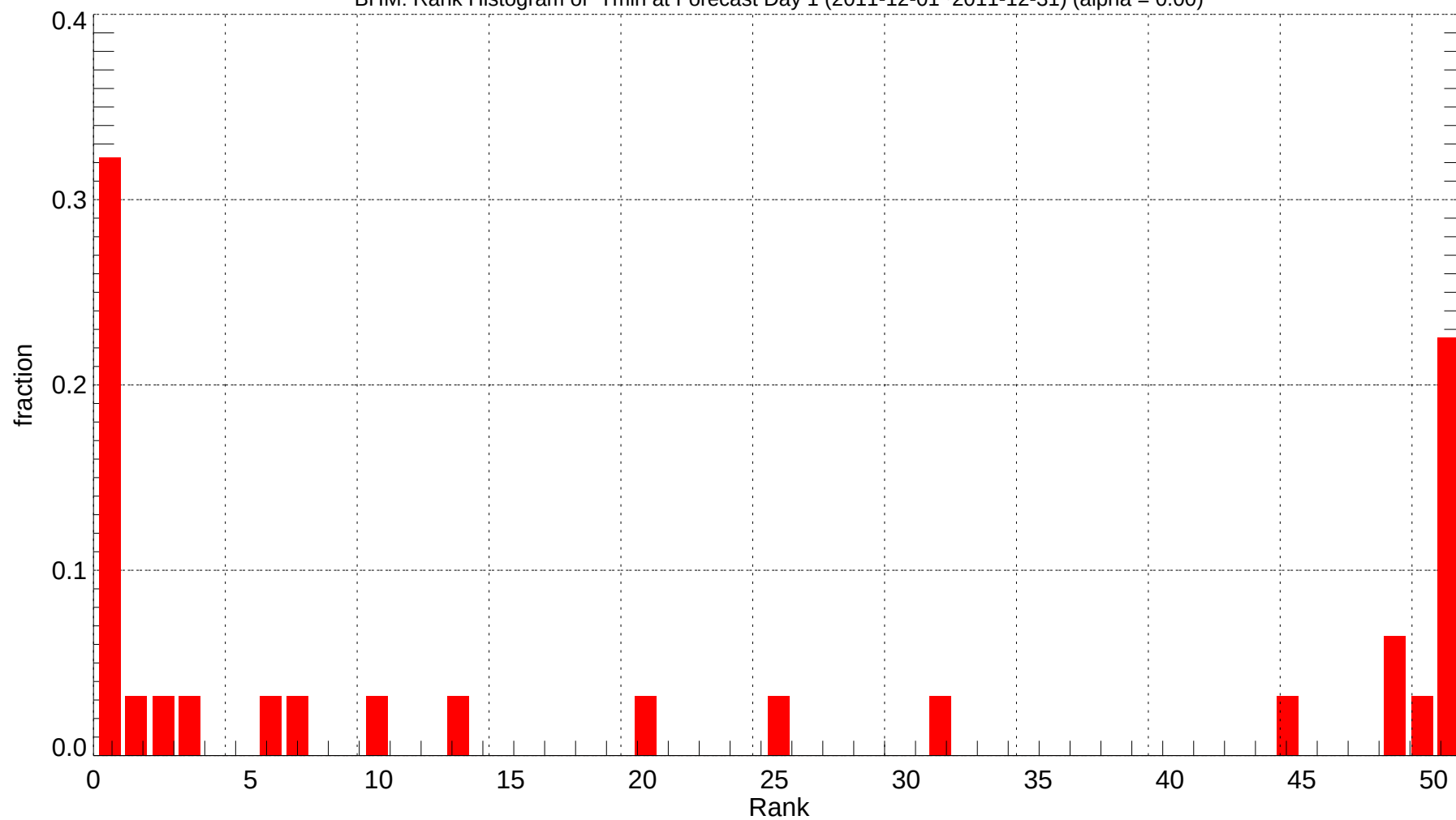
BHM: Rank Histogram of Tmin at Forecast Day 1 (2011-12-01~2011-12-31) (alpha = 0.00)
