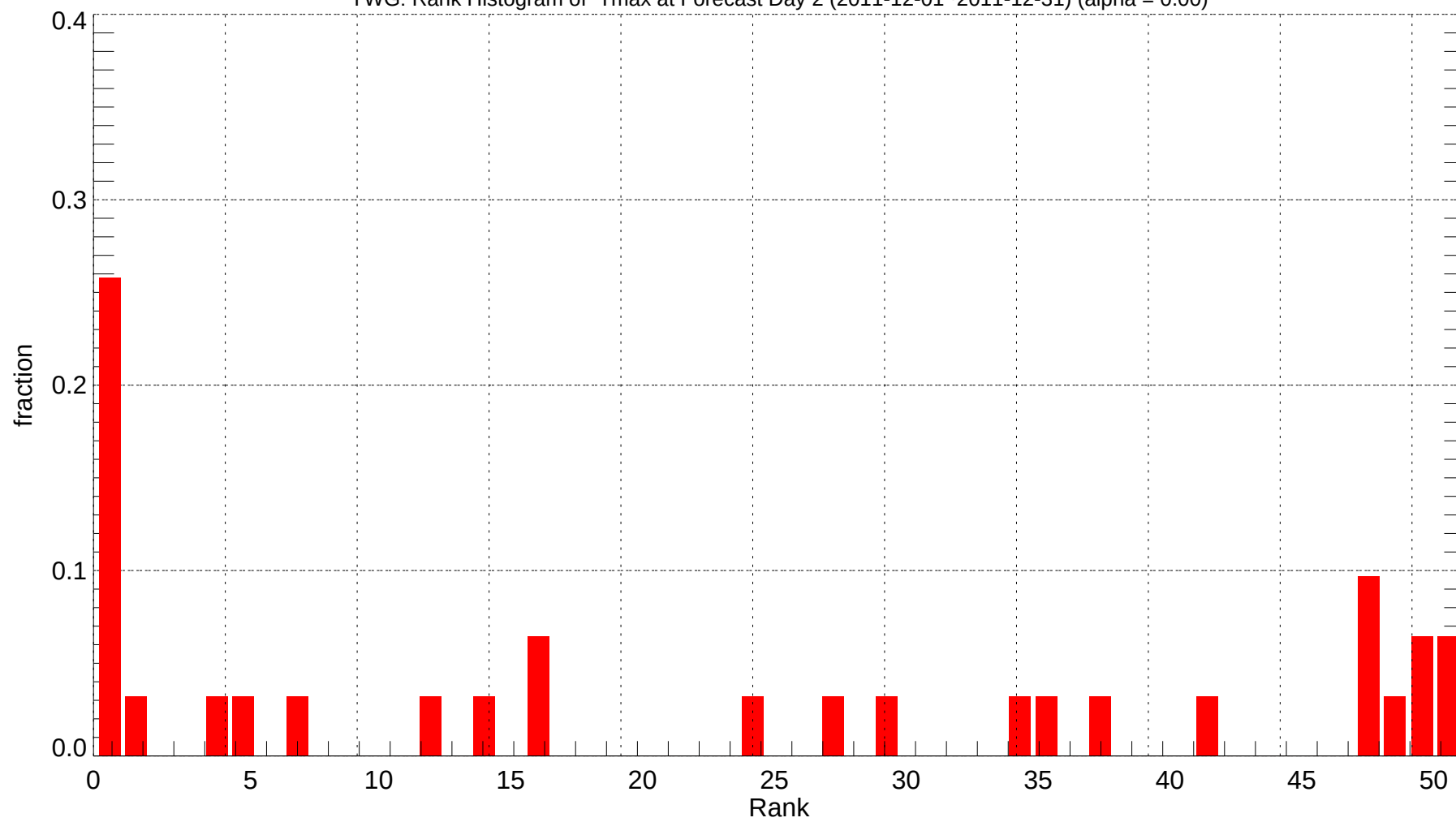
YWG: Rank Histogram of Tmax at Forecast Day 2 (2011-12-01~2011-12-31) (alpha = 0.00)
