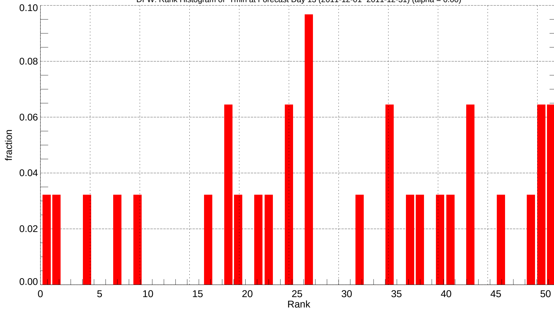
DFW: Rank Histogram of Tmin at Forecast Day 13 (2011-12-01~2011-12-31) (alpha = 0.00)
