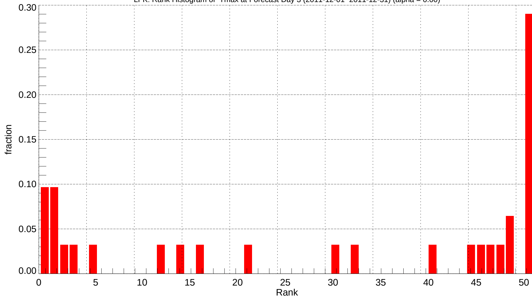
LFK: Rank Histogram of Tmax at Forecast Day 3 (2011-12-01~2011-12-31) (alpha = 0.00)
