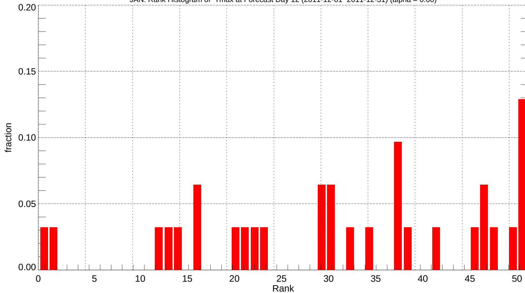
JAN: Rank Histogram of Tmax at Forecast Day 12 (2011-12-01~2011-12-31) (alpha = 0.00)
