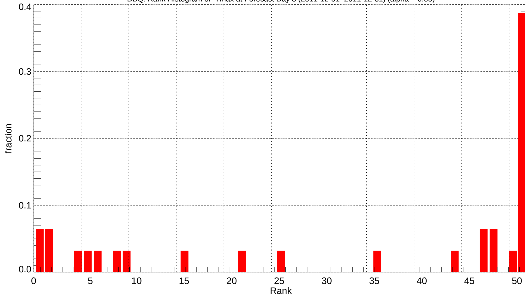
DBQ: Rank Histogram of Tmax at Forecast Day 3 (2011-12-01~2011-12-31) (alpha = 0.00)
