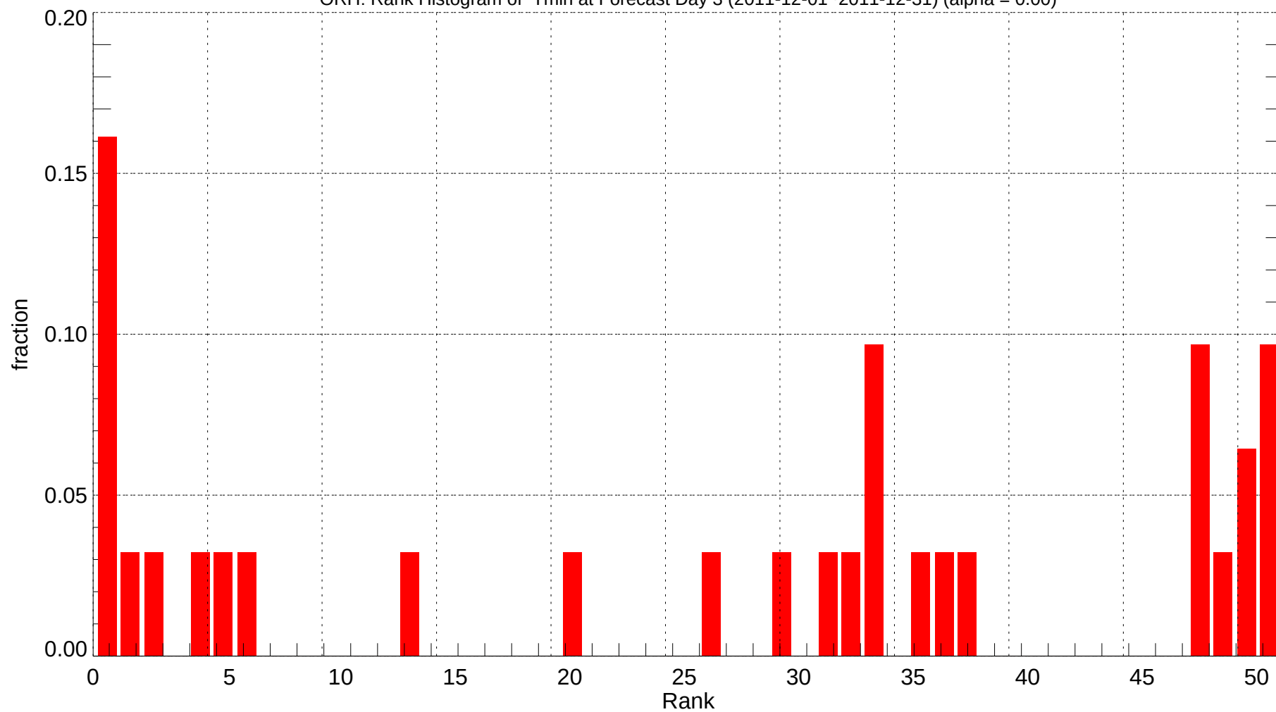
ORH: Rank Histogram of Tmin at Forecast Day 3 (2011-12-01~2011-12-31) (alpha = 0.00)
