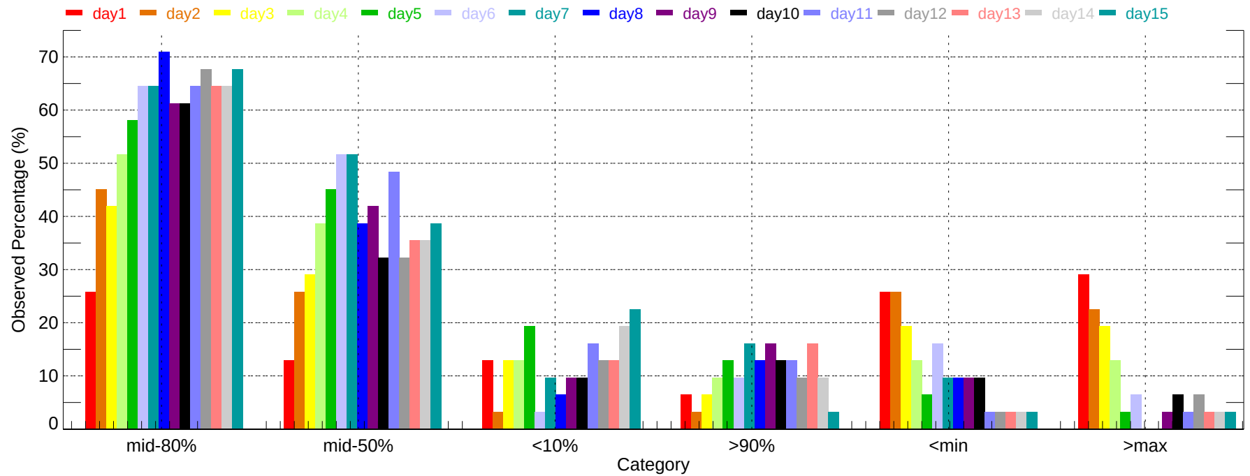
Observed Percentage of Ensembles - AUS: Max Temperature (2011-12-01~2011-12-31)
