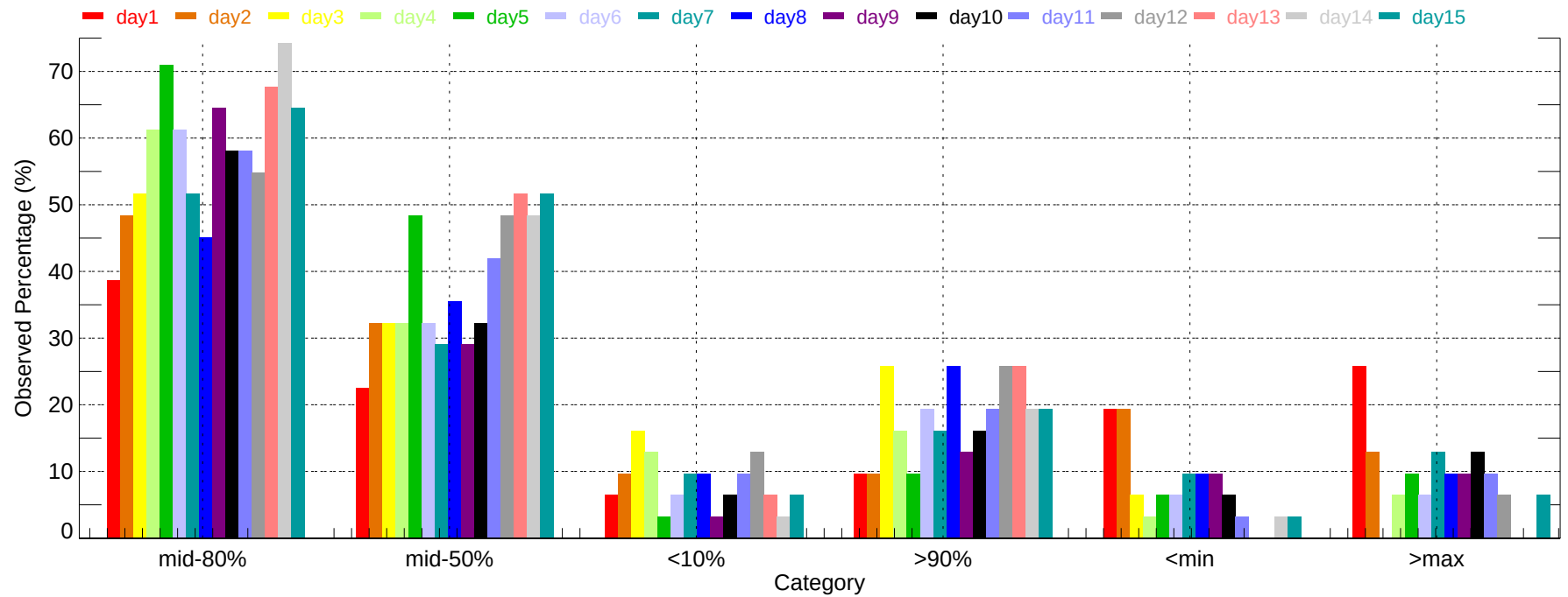
Observed Percentage of Ensembles - MBA: Max Temperature (2011-12-01~2011-12-31)
