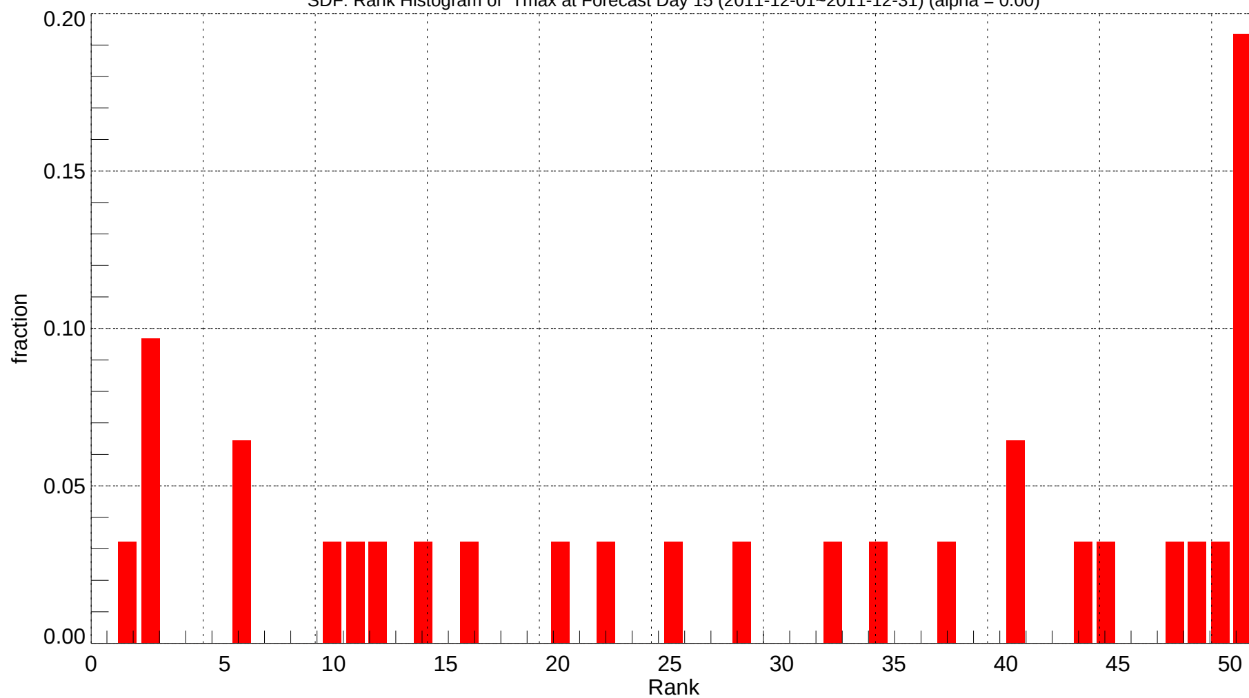
SDF: Rank Histogram of Tmax at Forecast Day 15 (2011-12-01~2011-12-31) (alpha = 0.00)
