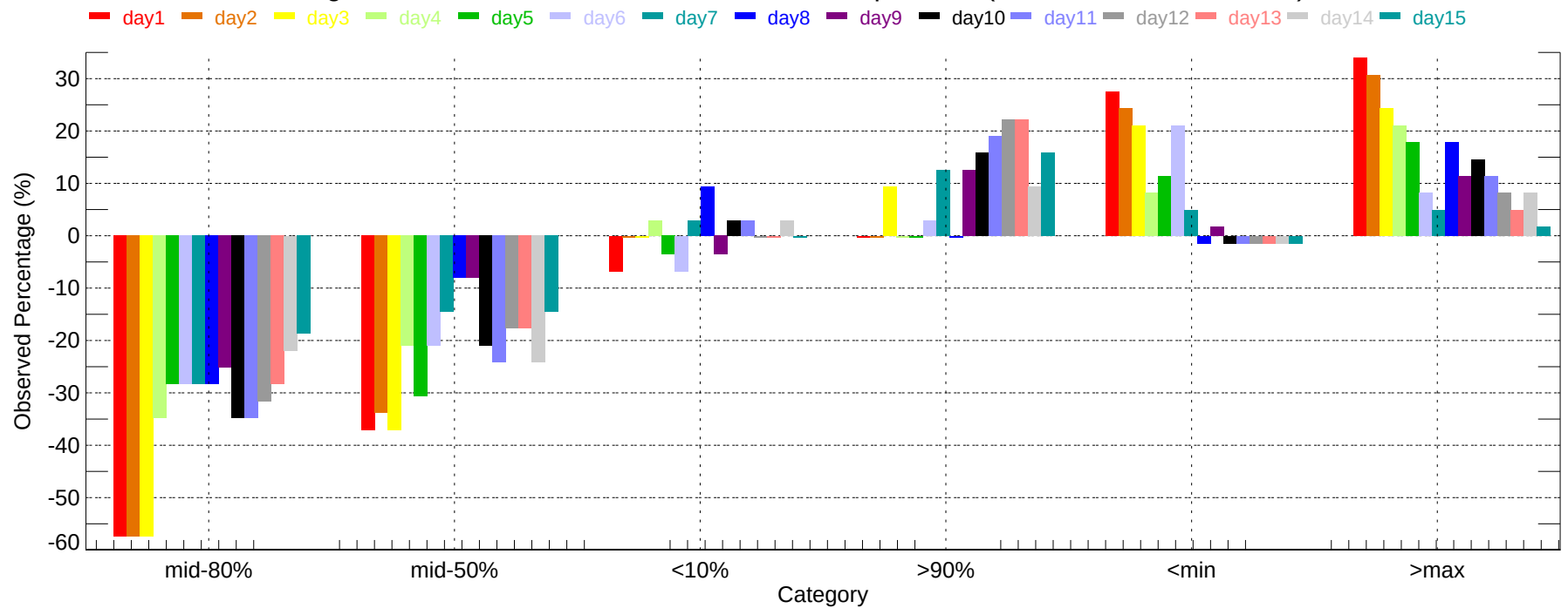
Observed Percentage Deviation of Ensembles - YWG: Min Temperature (2011-12-01~2011-12-31)
