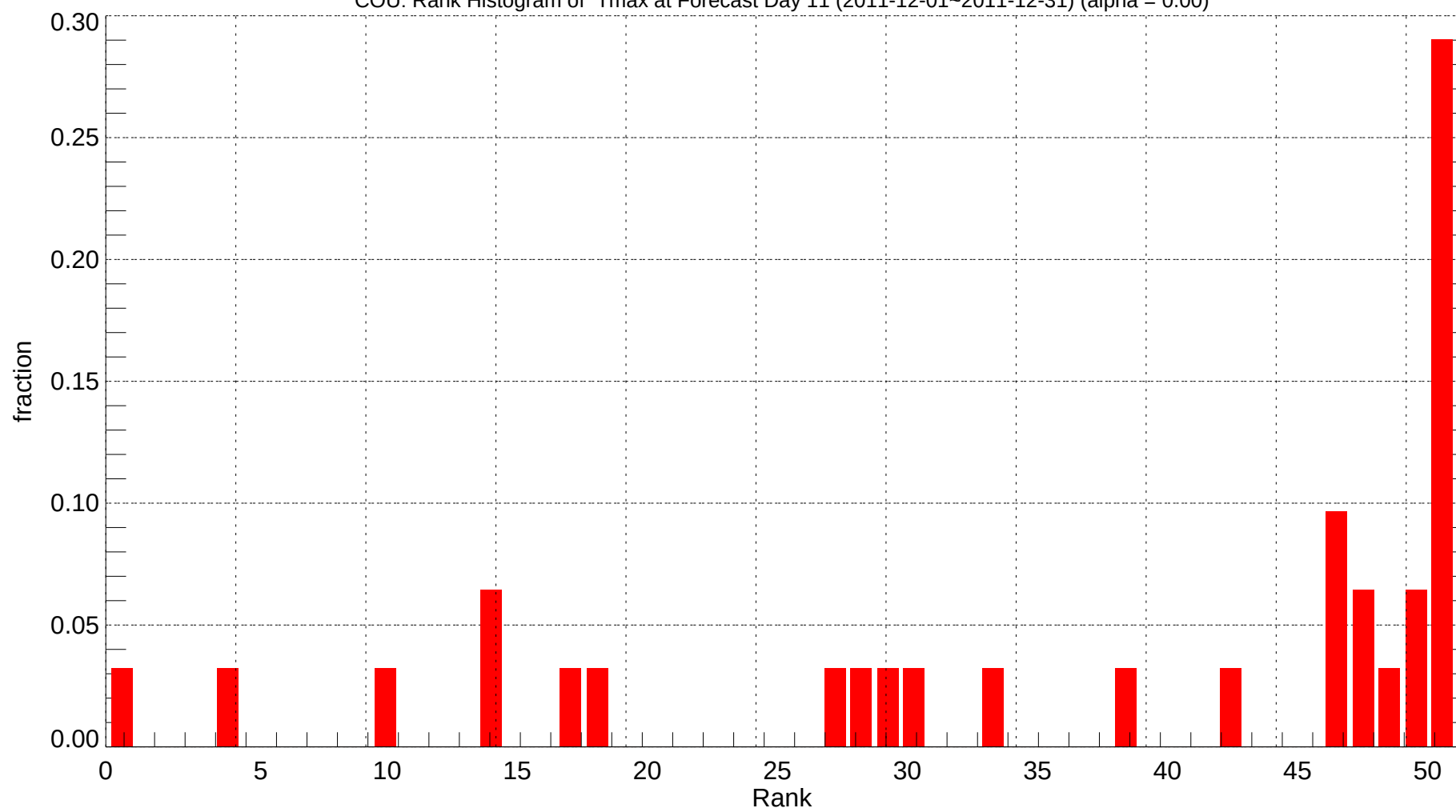
COU: Rank Histogram of Tmax at Forecast Day 11 (2011-12-01~2011-12-31) (alpha = 0.00)
