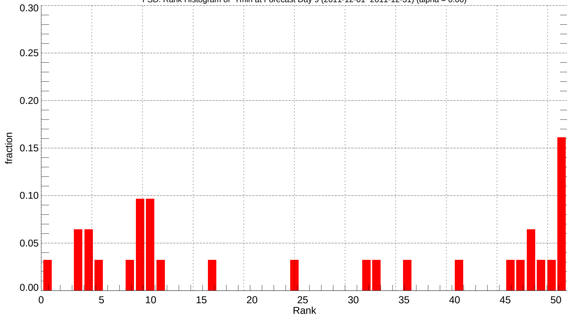
FSD: Rank Histogram of Tmin at Forecast Day 9 (2011-12-01~2011-12-31) (alpha = 0.00)
