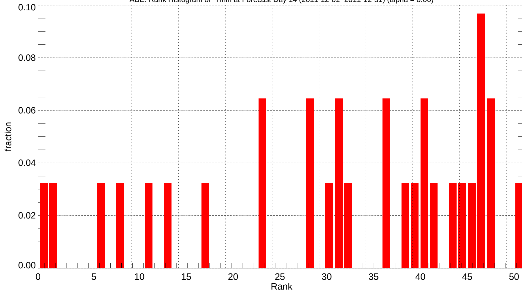
ABE: Rank Histogram of Tmin at Forecast Day 14 (2011-12-01~2011-12-31) (alpha = 0.00)
