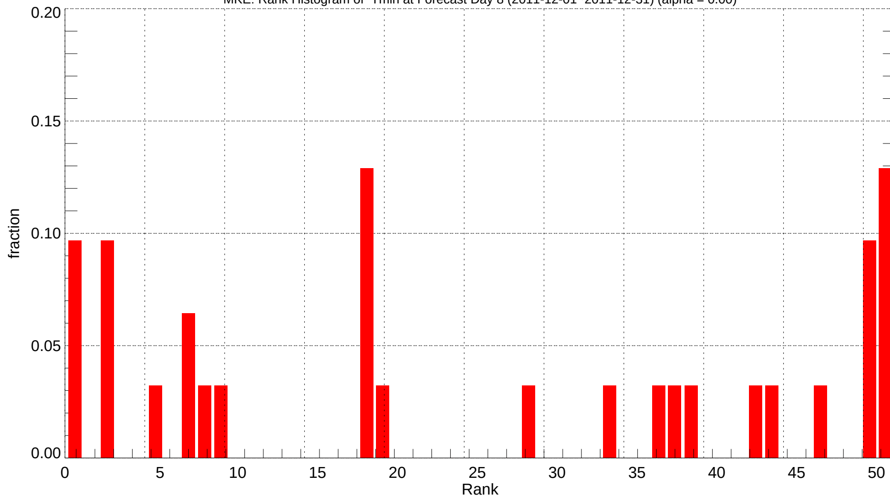
MKE: Rank Histogram of Tmin at Forecast Day 8 (2011-12-01~2011-12-31) (alpha = 0.00)
