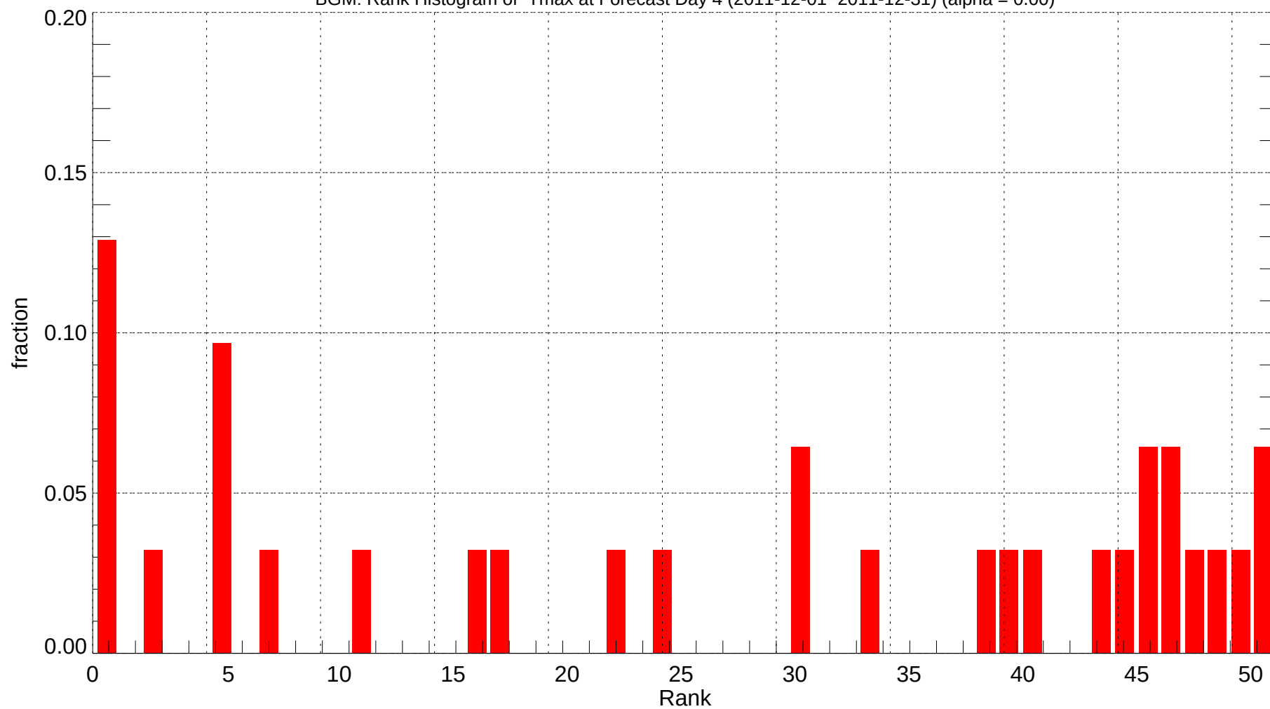
BGM: Rank Histogram of Tmax at Forecast Day 4 (2011-12-01~2011-12-31) (alpha = 0.00)
