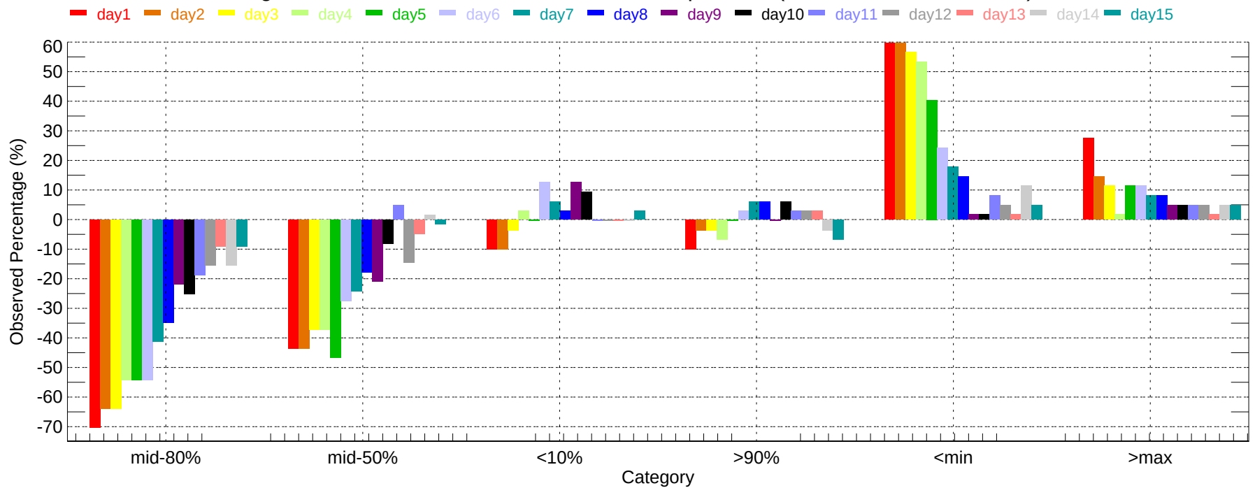
Observed Percentage Deviation of Ensembles - TLH: Min Temperature (2011-12-01~2011-12-31)
