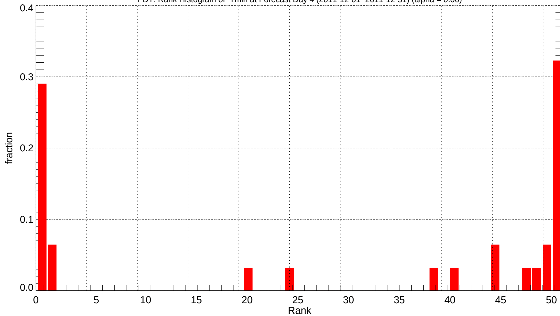
PDT: Rank Histogram of Tmin at Forecast Day 4 (2011-12-01~2011-12-31) (alpha = 0.00)
