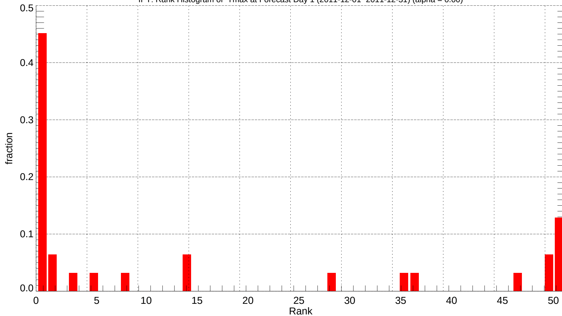
IPT: Rank Histogram of Tmax at Forecast Day 1 (2011-12-01~2011-12-31) (alpha = 0.00)
