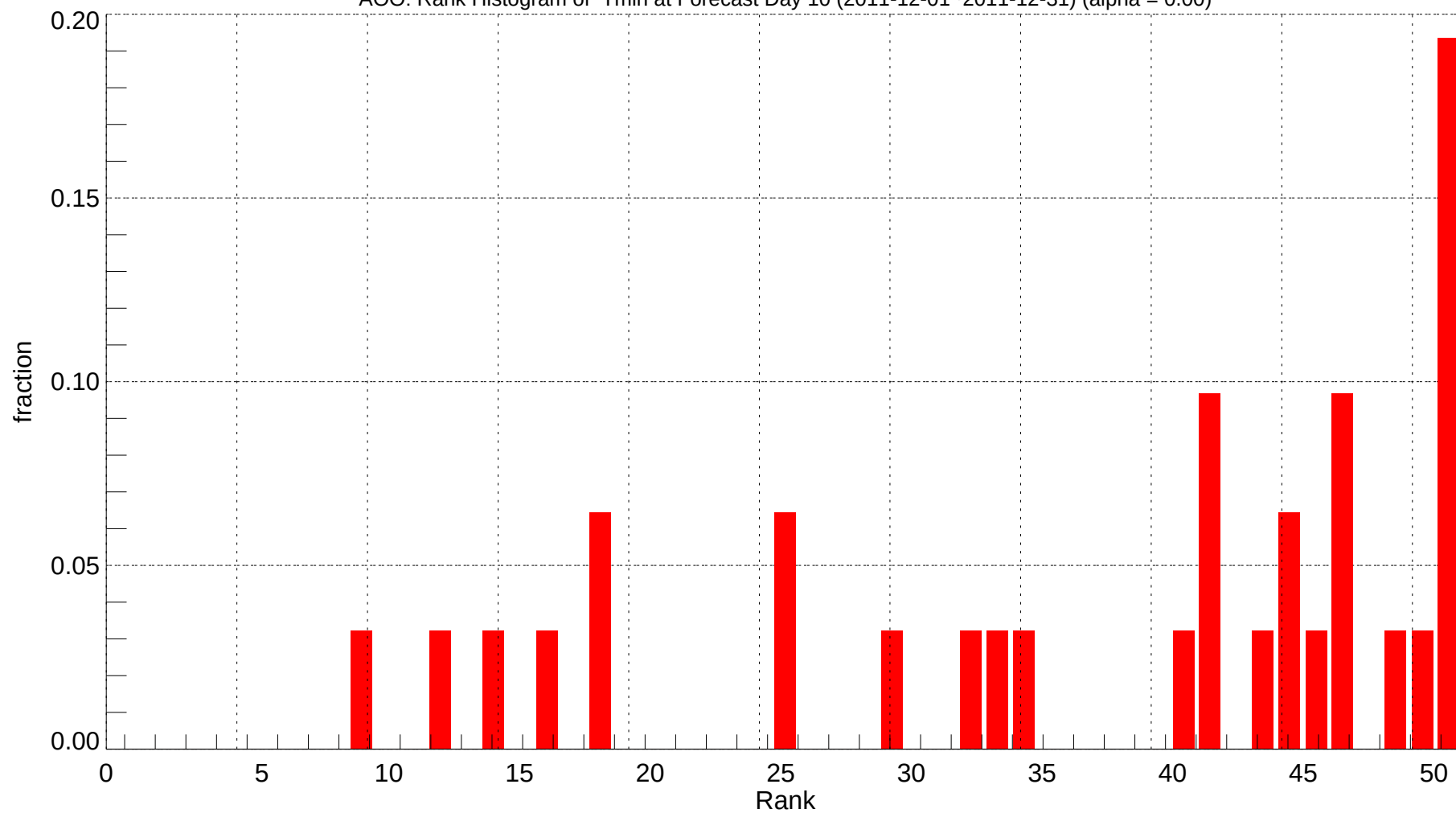
AOO: Rank Histogram of Tmin at Forecast Day 10 (2011-12-01~2011-12-31) (alpha = 0.00)
