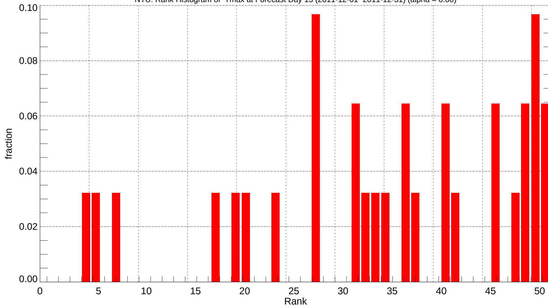
NTU: Rank Histogram of Tmax at Forecast Day 13 (2011-12-01~2011-12-31) (alpha = 0.00)
