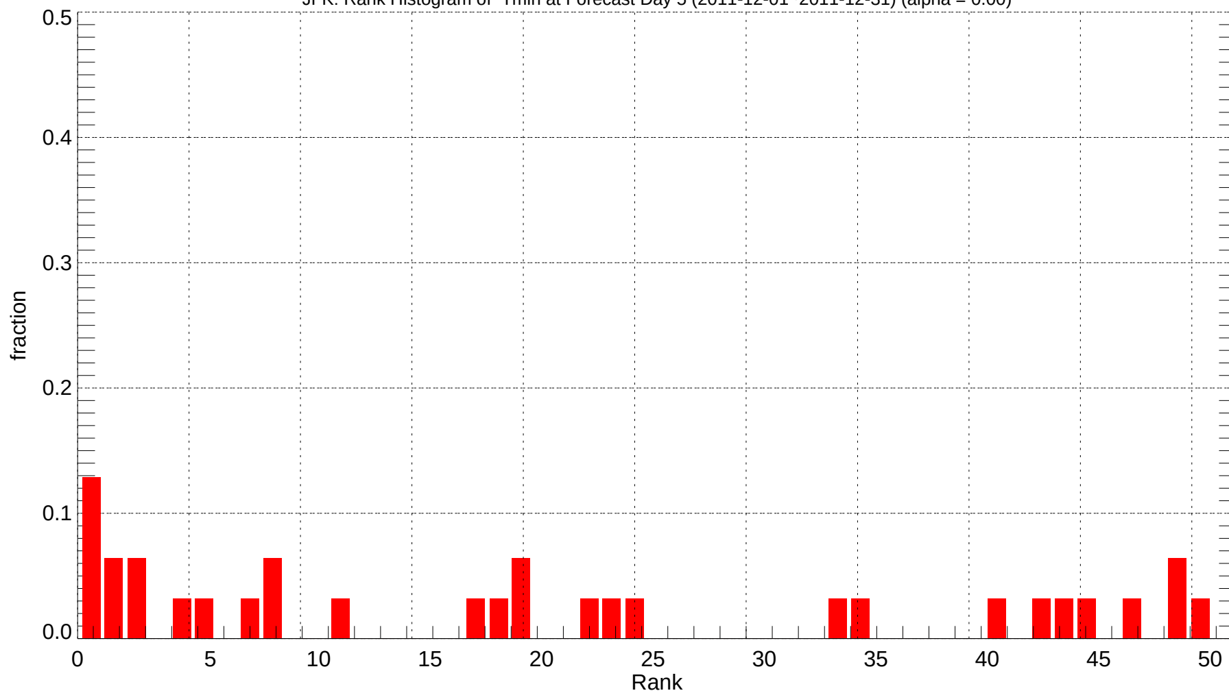
JFK: Rank Histogram of Tmin at Forecast Day 5 (2011-12-01~2011-12-31) (alpha = 0.00)
