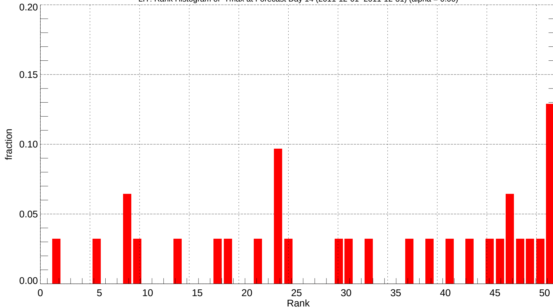
LIT: Rank Histogram of Tmax at Forecast Day 14 (2011-12-01~2011-12-31) (alpha = 0.00)
