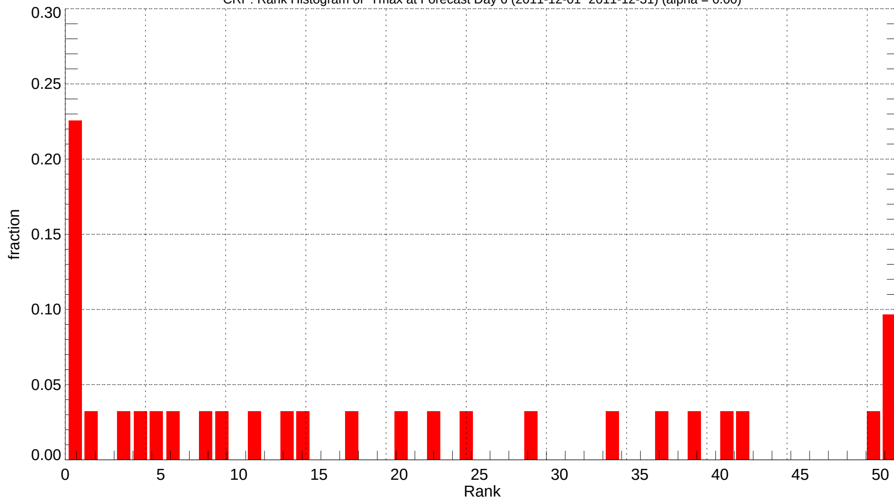
CRP: Rank Histogram of Tmax at Forecast Day 6 (2011-12-01~2011-12-31) (alpha = 0.00)
