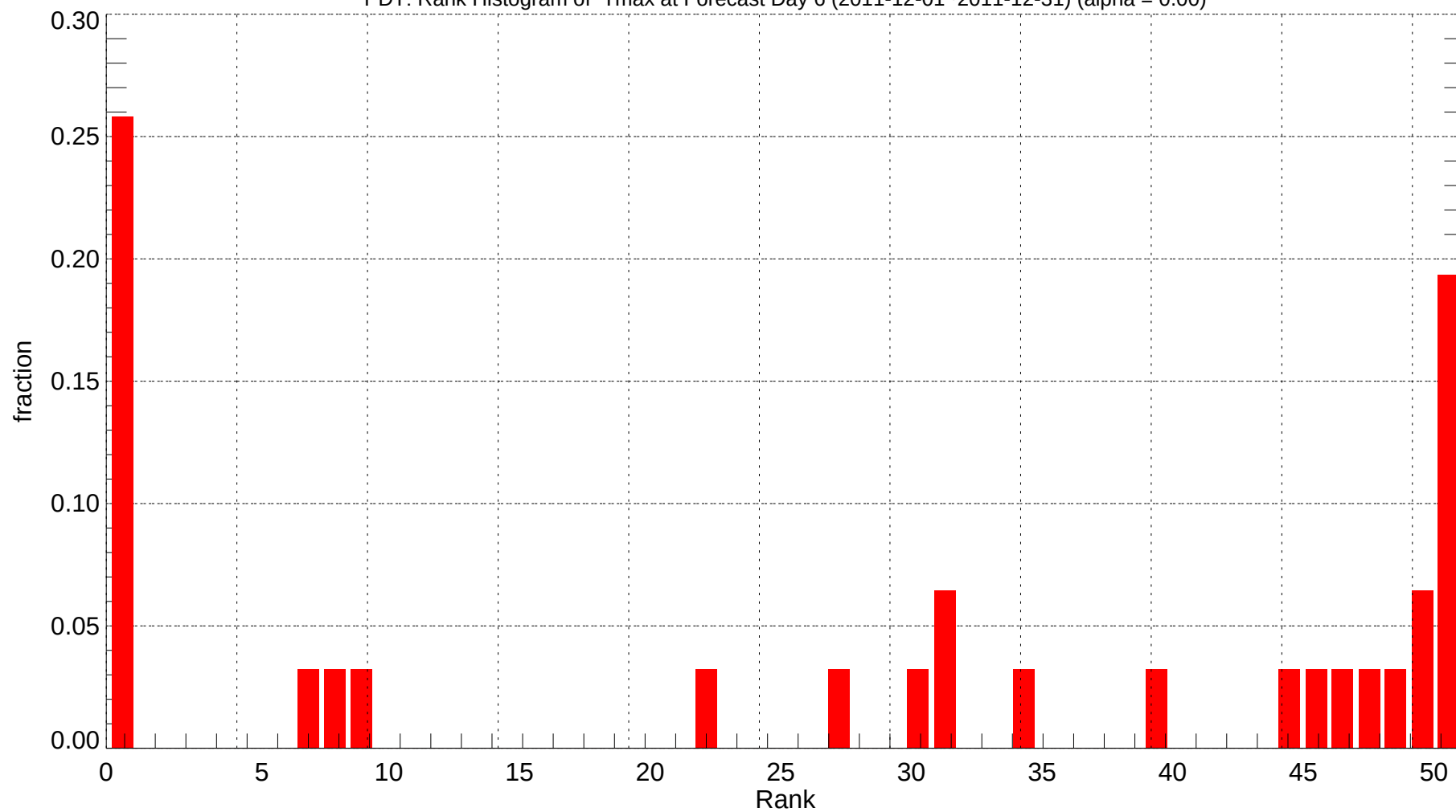
PDT: Rank Histogram of Tmax at Forecast Day 6 (2011-12-01~2011-12-31) (alpha = 0.00)
