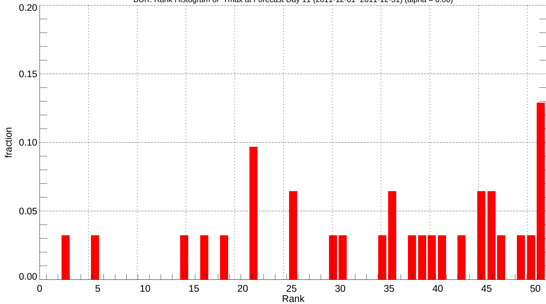
BUR: Rank Histogram of Tmax at Forecast Day 11 (2011-12-01~2011-12-31) (alpha = 0.00)
