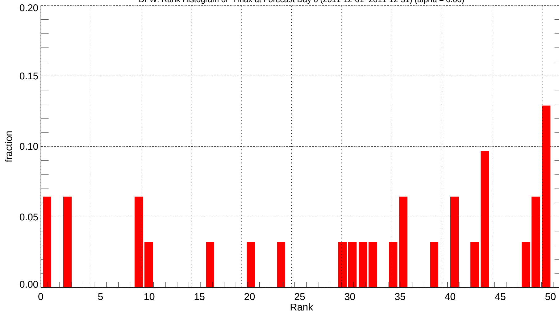
DFW: Rank Histogram of Tmax at Forecast Day 6 (2011-12-01~2011-12-31) (alpha = 0.00)
