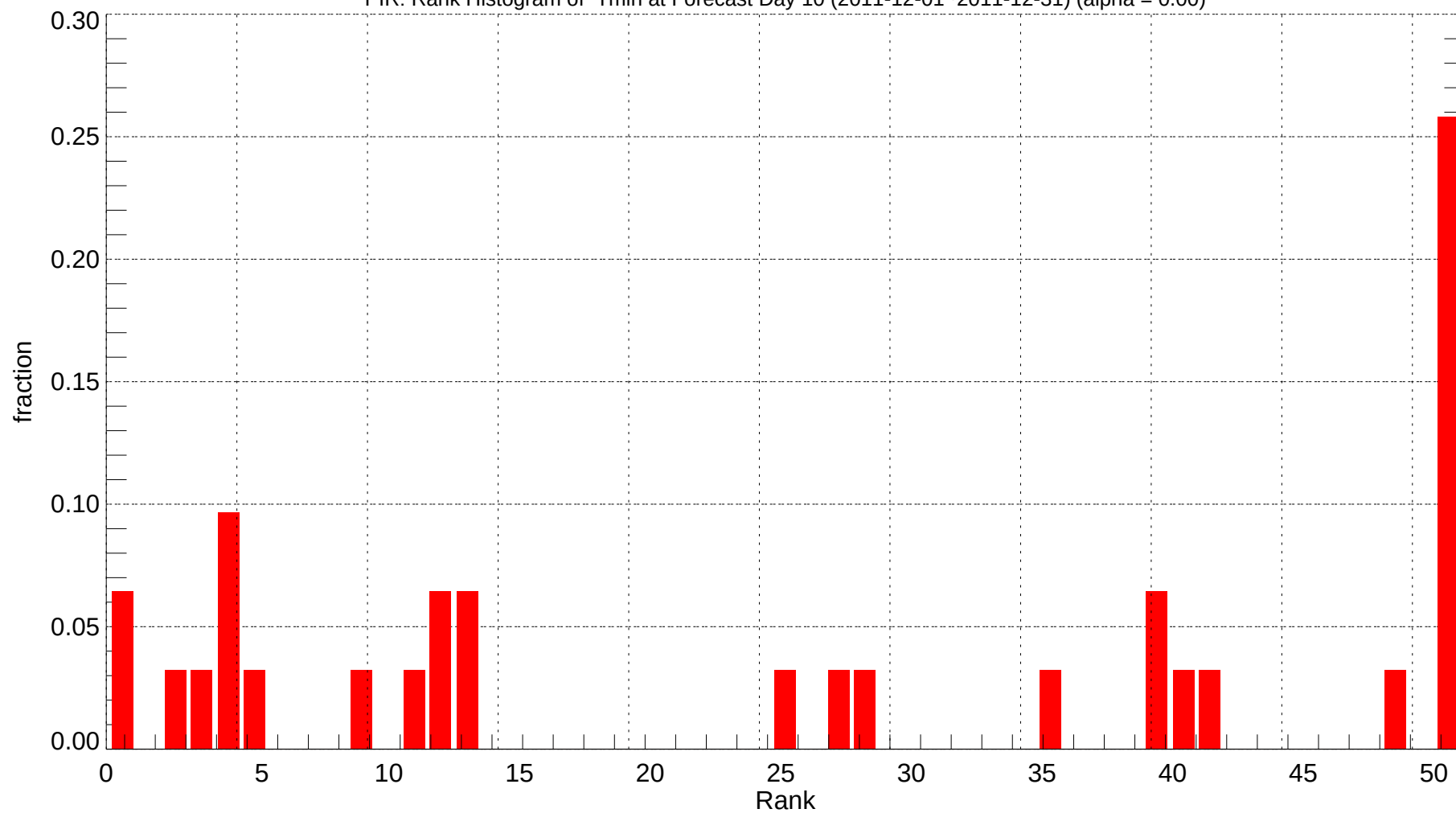
PIR: Rank Histogram of Tmin at Forecast Day 10 (2011-12-01~2011-12-31) (alpha = 0.00)
