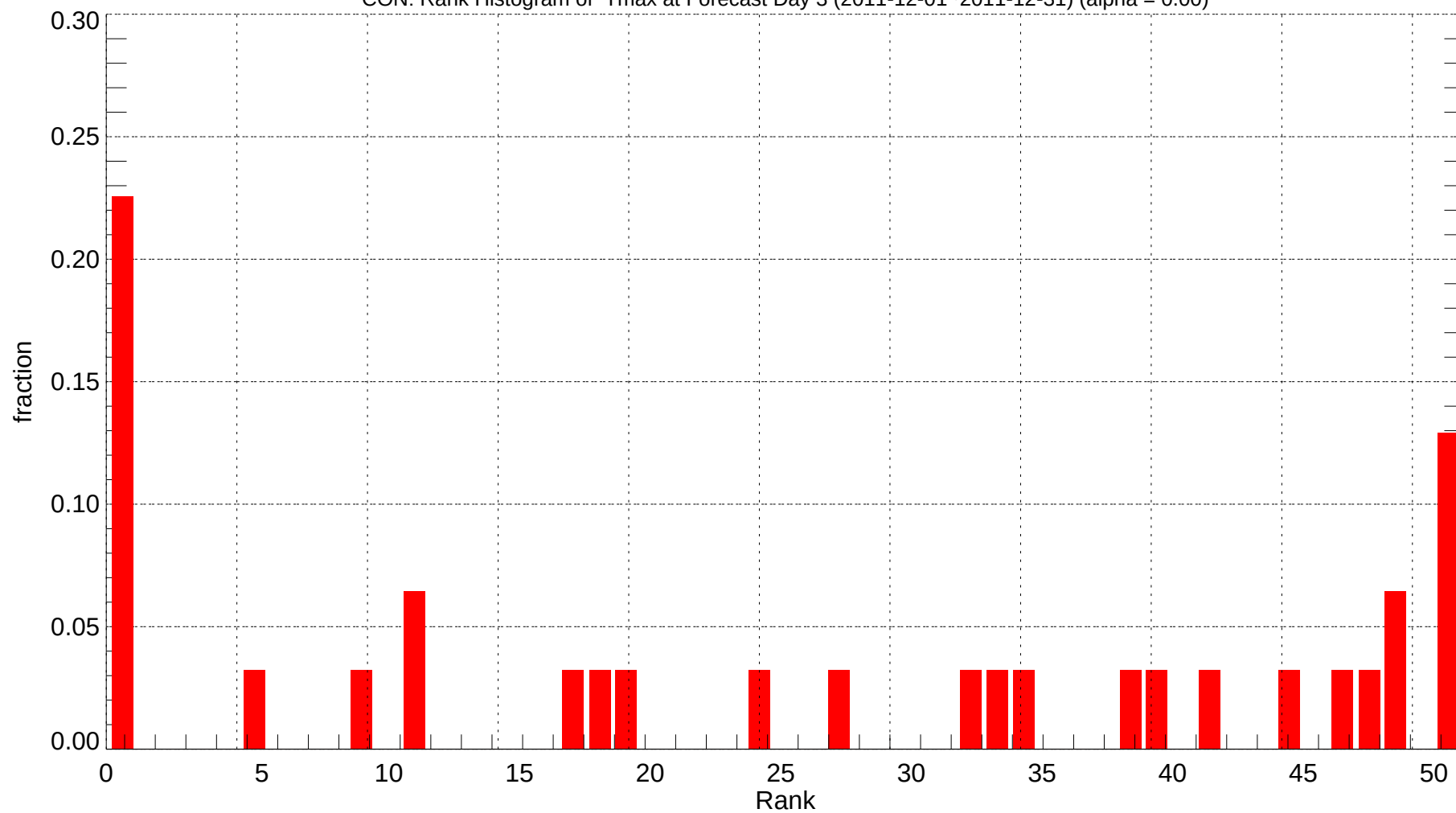
CON: Rank Histogram of Tmax at Forecast Day 3 (2011-12-01~2011-12-31) (alpha = 0.00)
