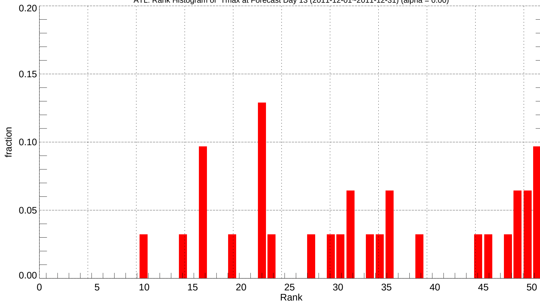
ATL: Rank Histogram of Tmax at Forecast Day 13 (2011-12-01~2011-12-31) (alpha = 0.00)
