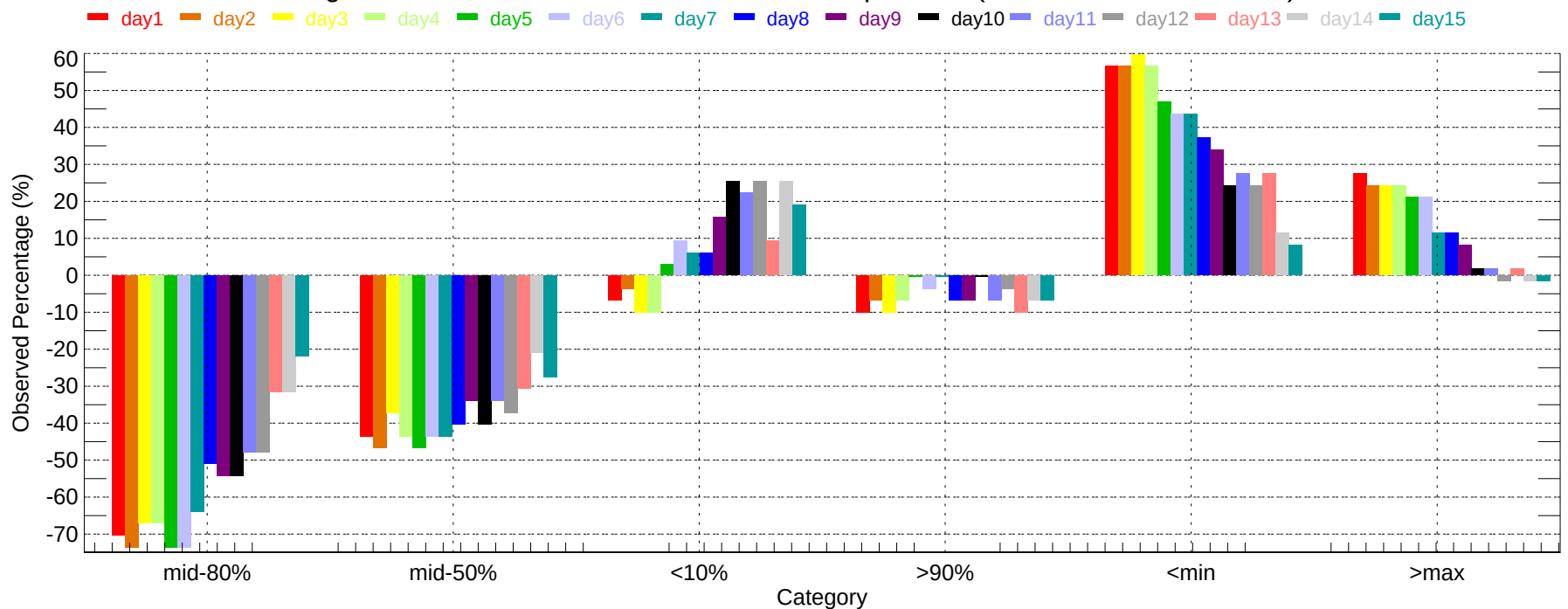
Observed Percentage Deviation of Ensembles - WJF: Min Temperature (2011-12-01~2011-12-31)
