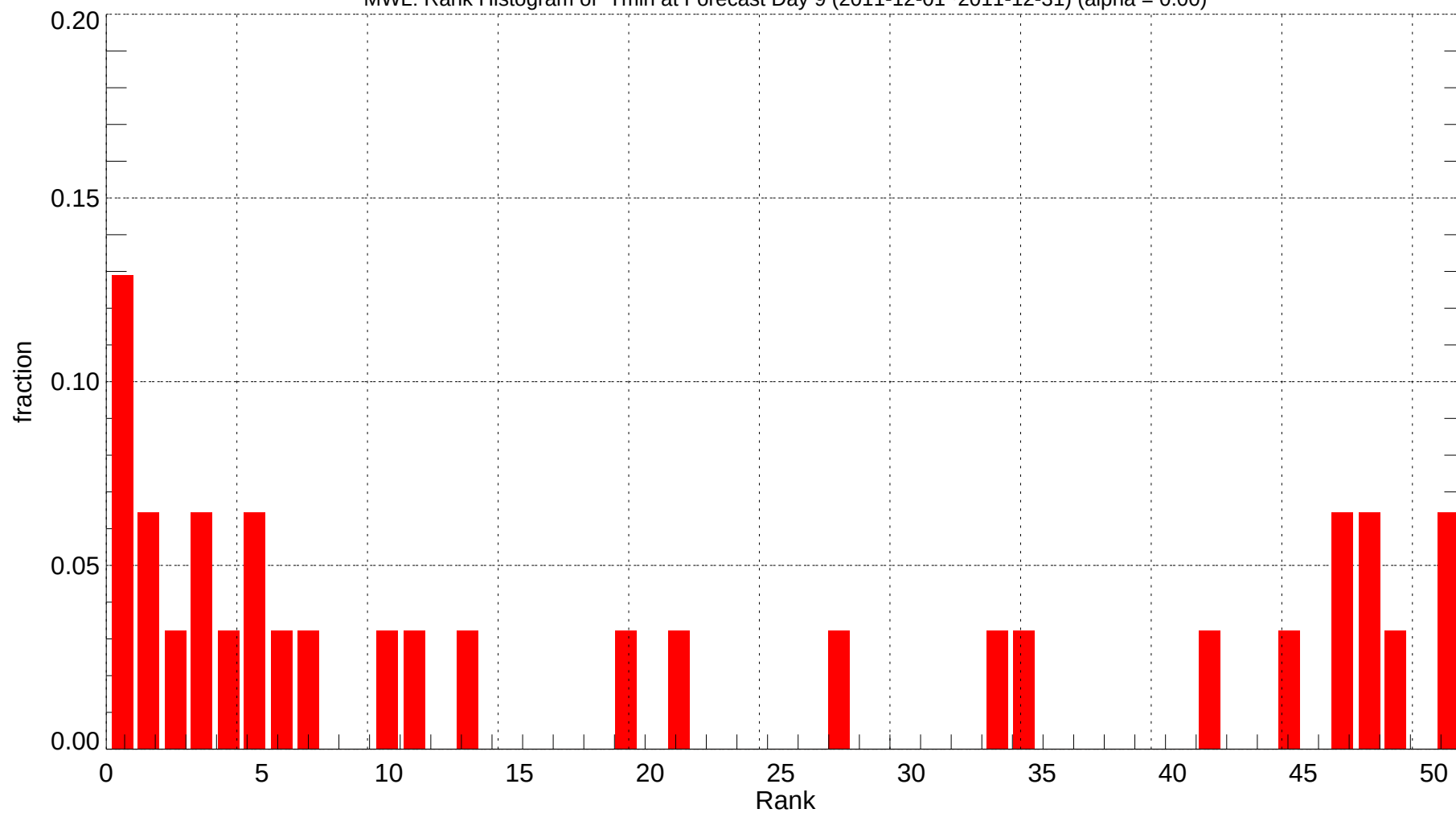
MWL: Rank Histogram of Tmin at Forecast Day 9 (2011-12-01~2011-12-31) (alpha = 0.00)
