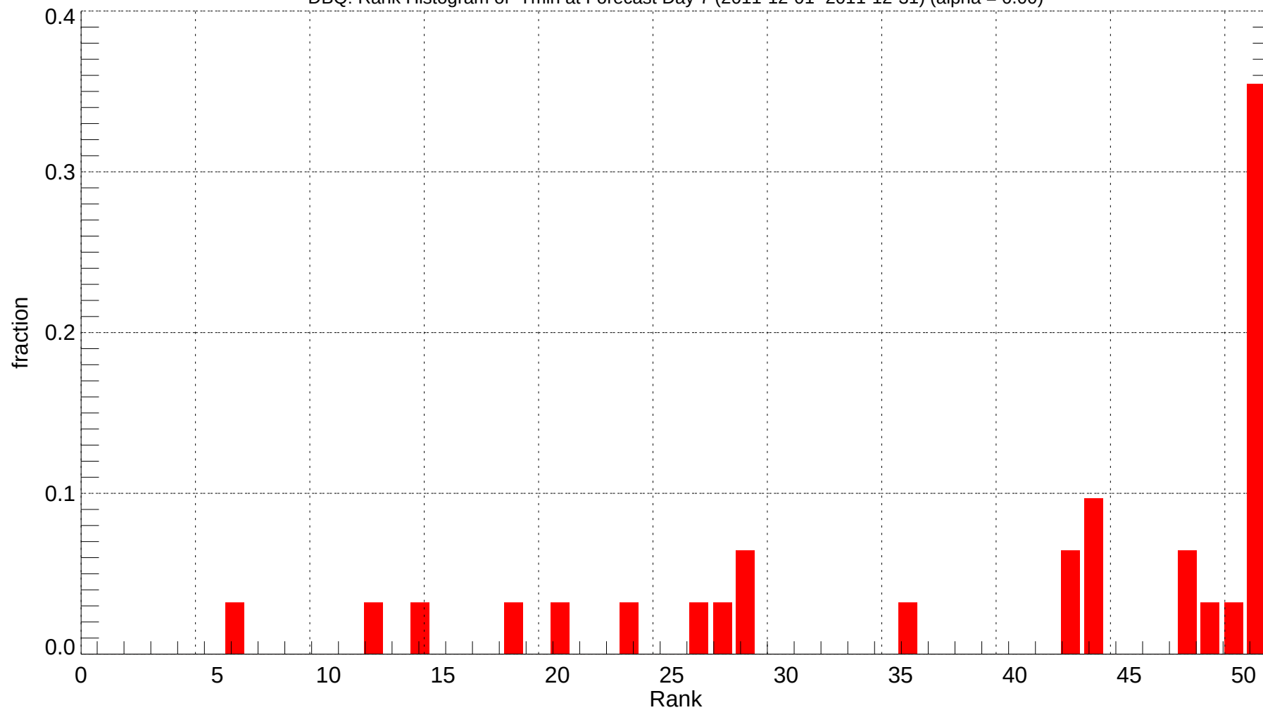
DBQ: Rank Histogram of Tmin at Forecast Day 7 (2011-12-01~2011-12-31) (alpha = 0.00)
