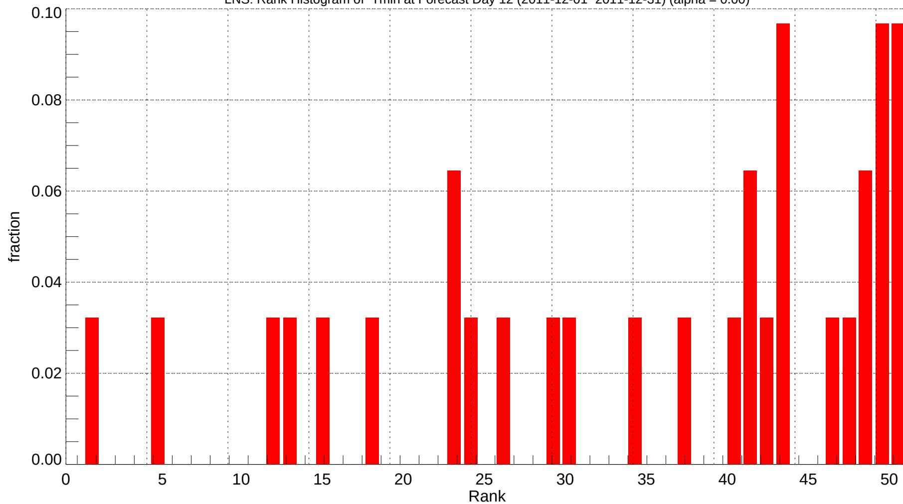
LNS: Rank Histogram of Tmin at Forecast Day 12 (2011-12-01~2011-12-31) (alpha = 0.00)
