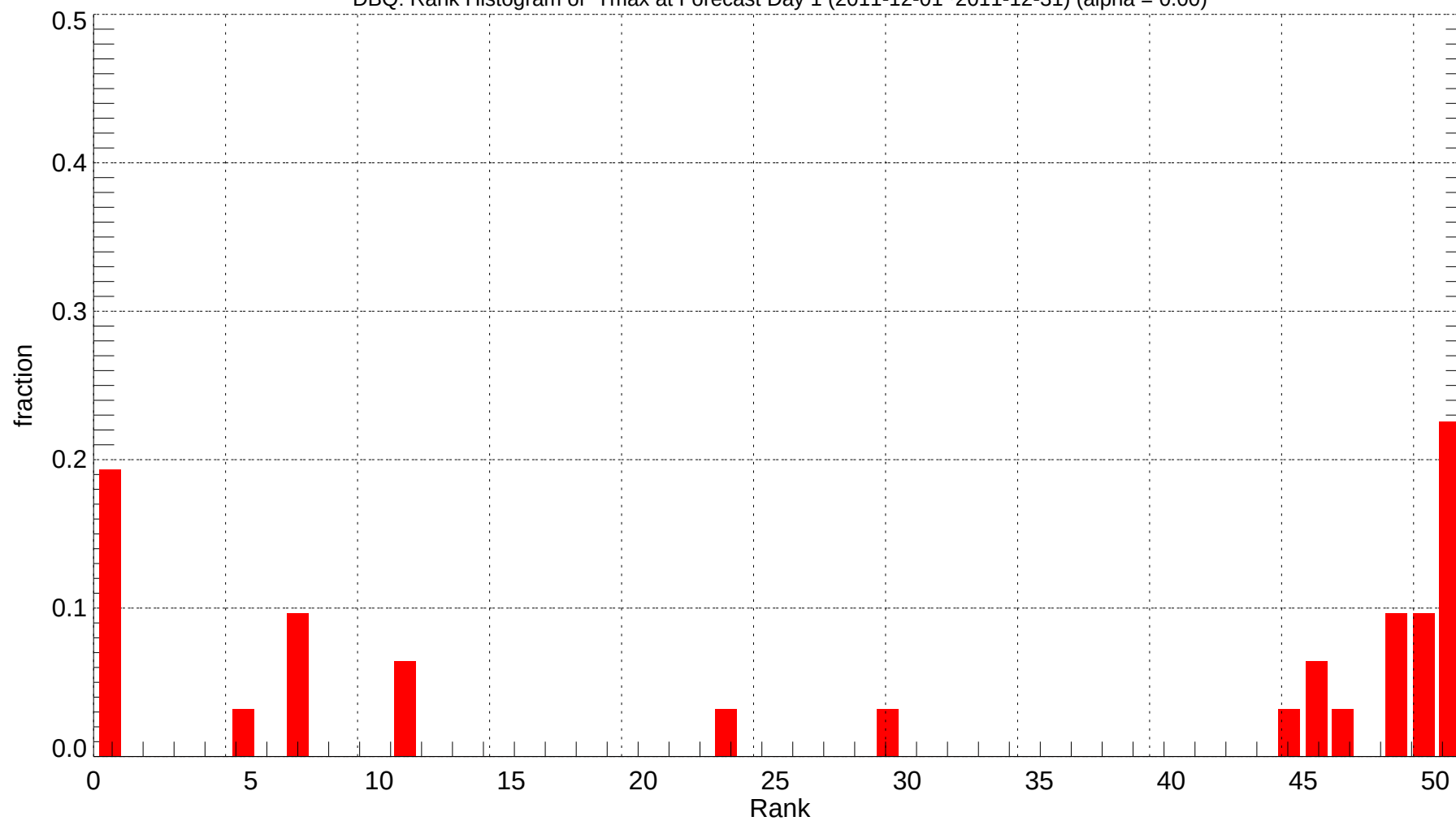
DBQ: Rank Histogram of Tmax at Forecast Day 1 (2011-12-01~2011-12-31) (alpha = 0.00)
