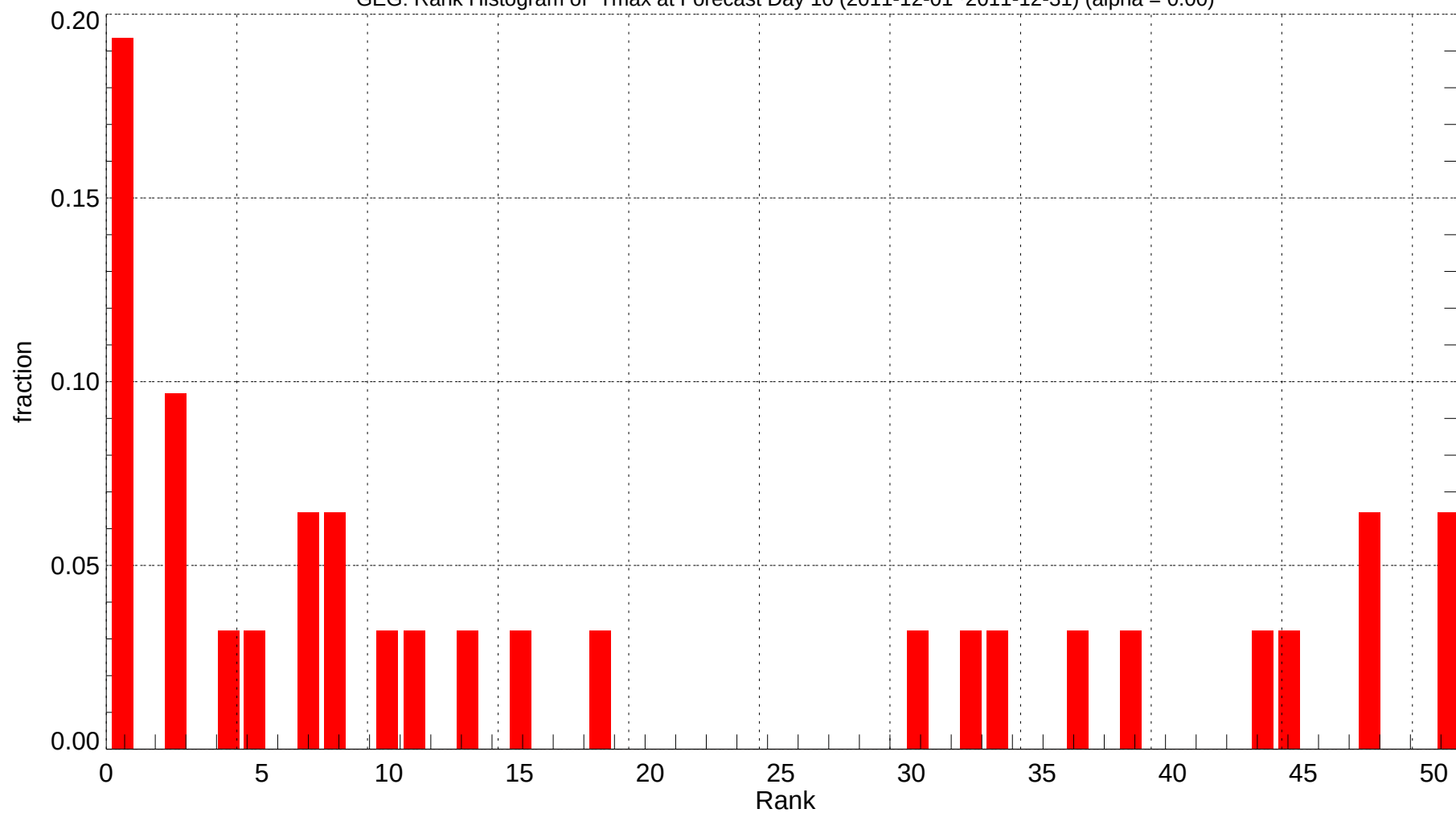
GEG: Rank Histogram of Tmax at Forecast Day 10 (2011-12-01~2011-12-31) (alpha = 0.00)
