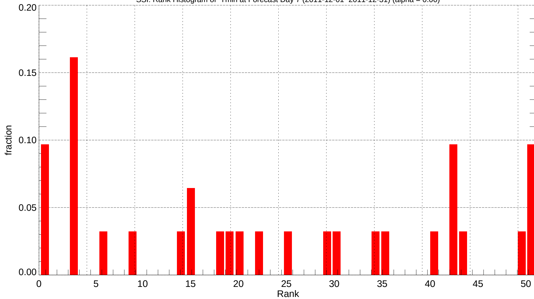
SSI: Rank Histogram of Tmin at Forecast Day 7 (2011-12-01~2011-12-31) (alpha = 0.00)
