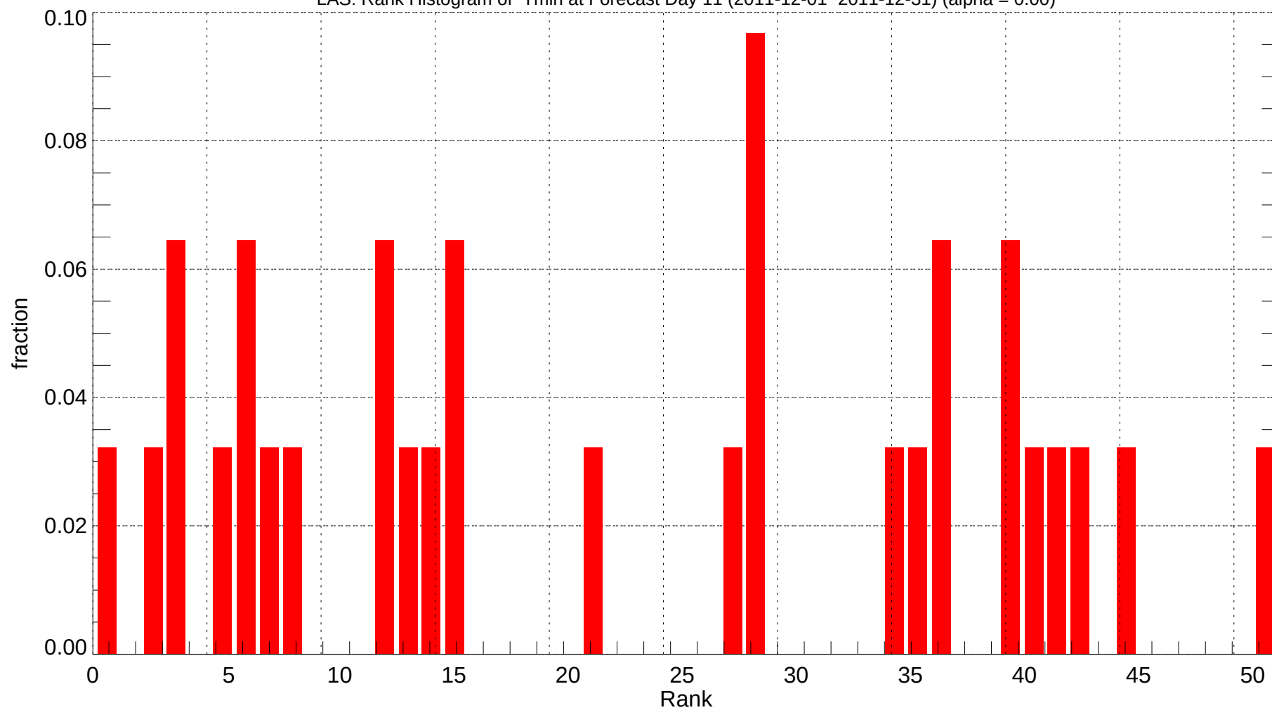
LAS: Rank Histogram of Tmin at Forecast Day 11 (2011-12-01~2011-12-31) (alpha = 0.00)
