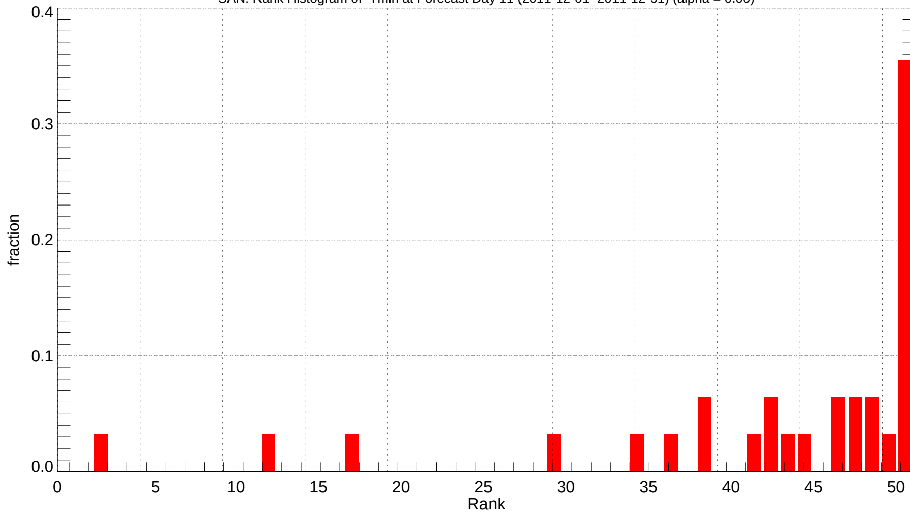
SAN: Rank Histogram of Tmin at Forecast Day 11 (2011-12-01~2011-12-31) (alpha = 0.00)
