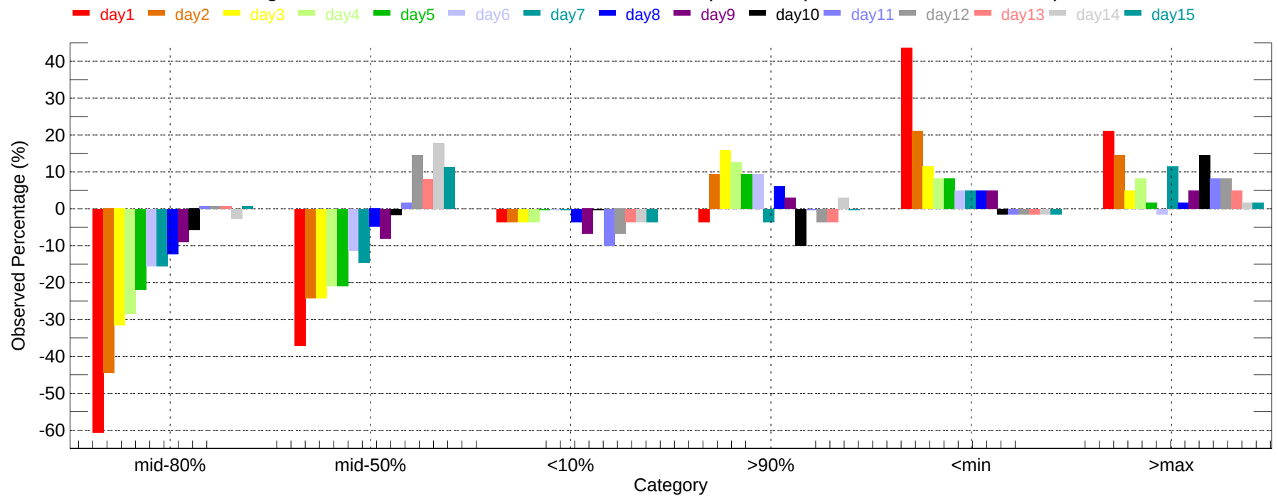
Observed Percentage Deviation of Ensembles - ORH: Min Temperature (2011-12-01~2011-12-31)
