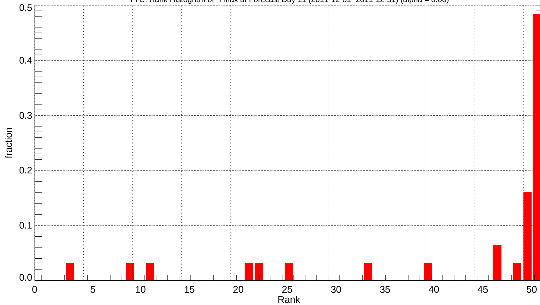
YYC: Rank Histogram of Tmax at Forecast Day 11 (2011-12-01~2011-12-31) (alpha = 0.00)
