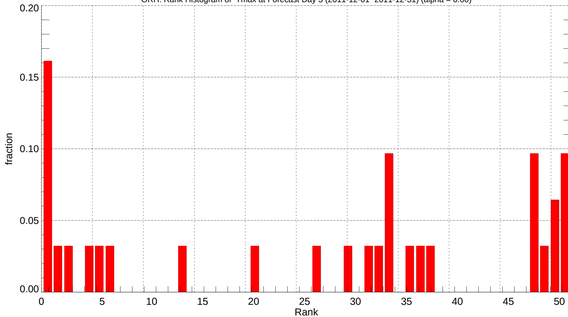
ORH: Rank Histogram of Tmax at Forecast Day 3 (2011-12-01~2011-12-31) (alpha = 0.00)
