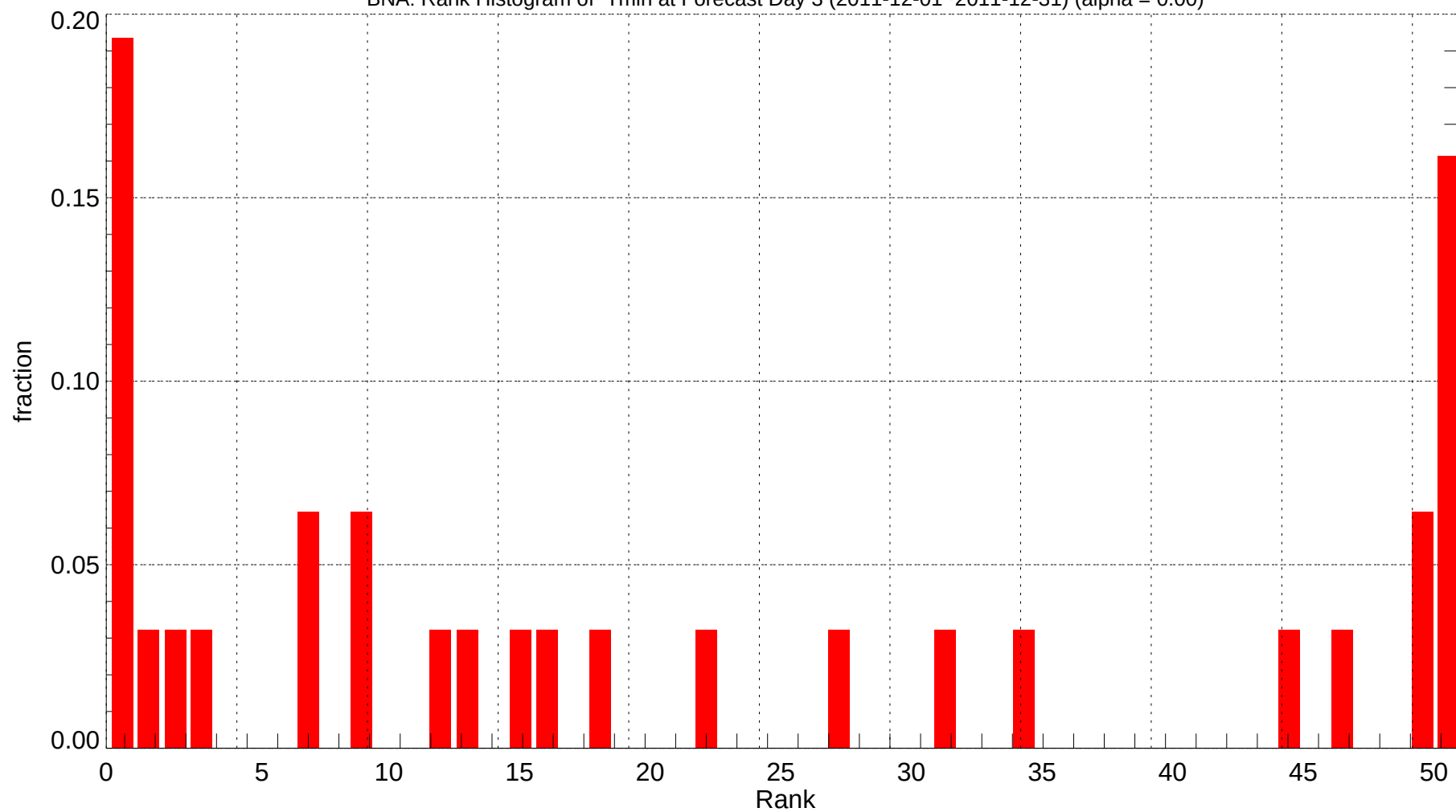
BNA: Rank Histogram of Tmin at Forecast Day 3 (2011-12-01~2011-12-31) (alpha = 0.00)
