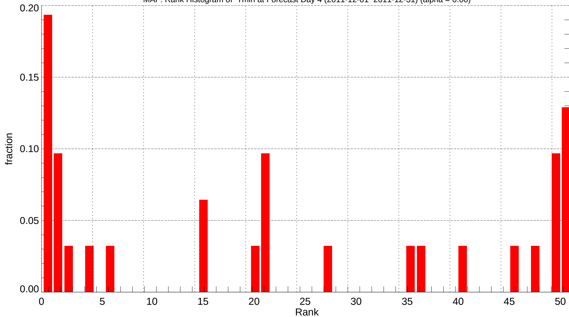
MAF: Rank Histogram of Tmin at Forecast Day 4 (2011-12-01~2011-12-31) (alpha = 0.00)
