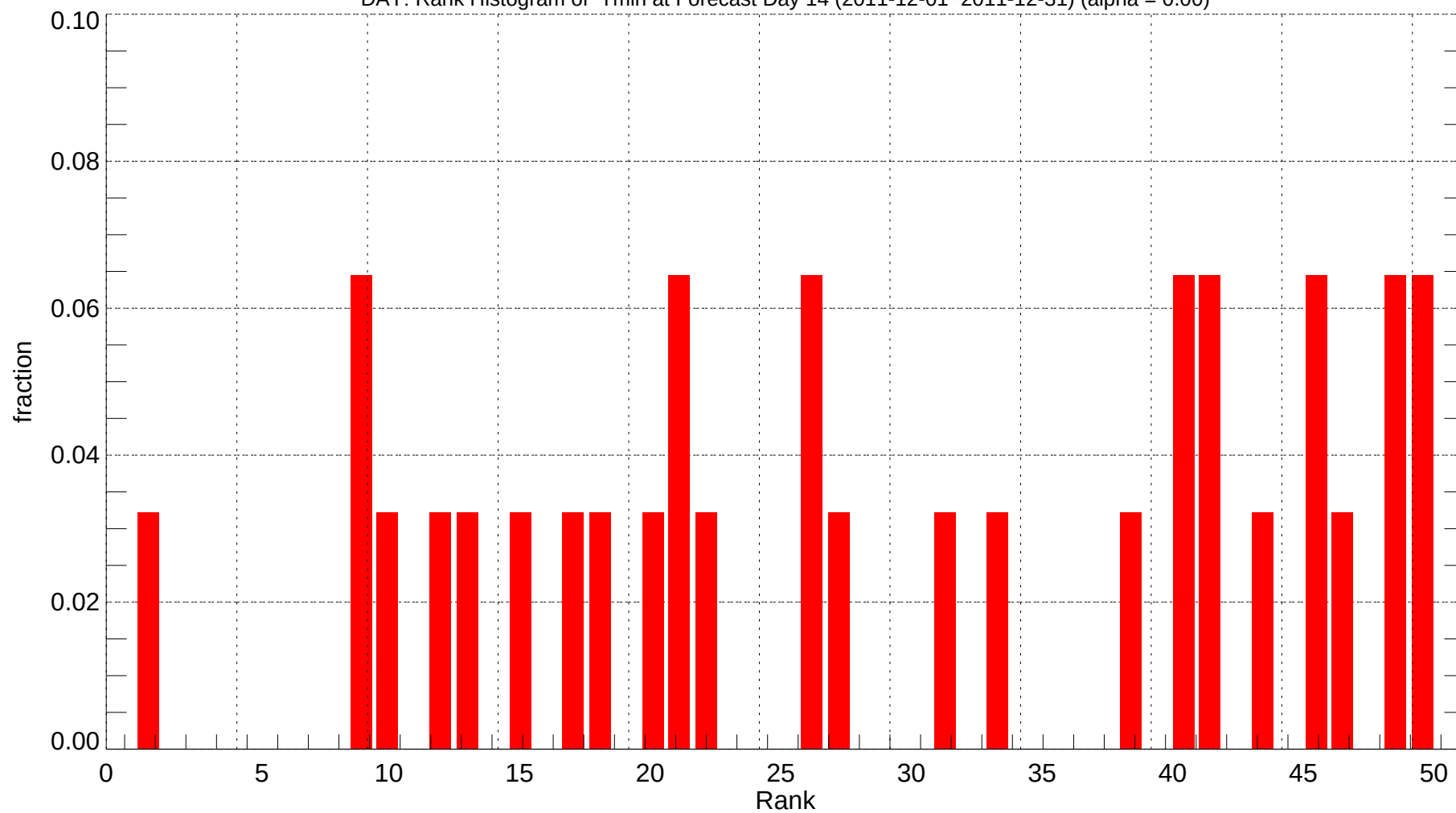
DAY: Rank Histogram of Tmin at Forecast Day 14 (2011-12-01~2011-12-31) (alpha = 0.00)
