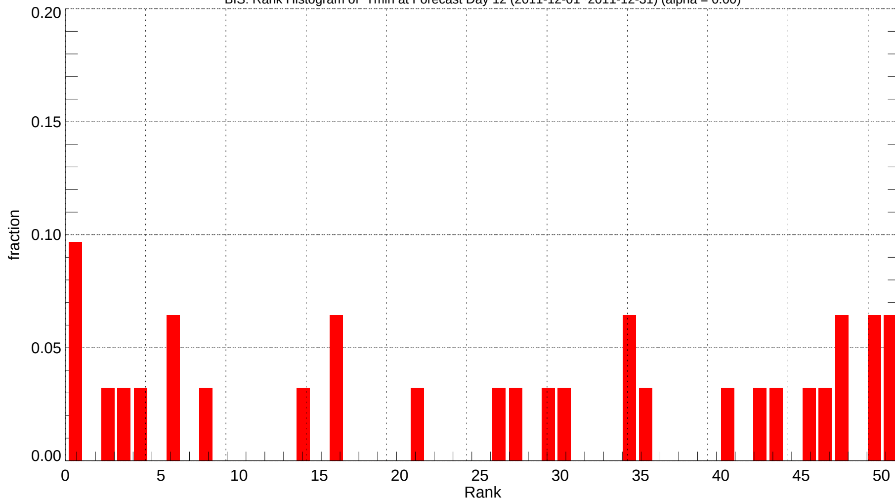
BIS: Rank Histogram of Tmin at Forecast Day 12 (2011-12-01~2011-12-31) (alpha = 0.00)
