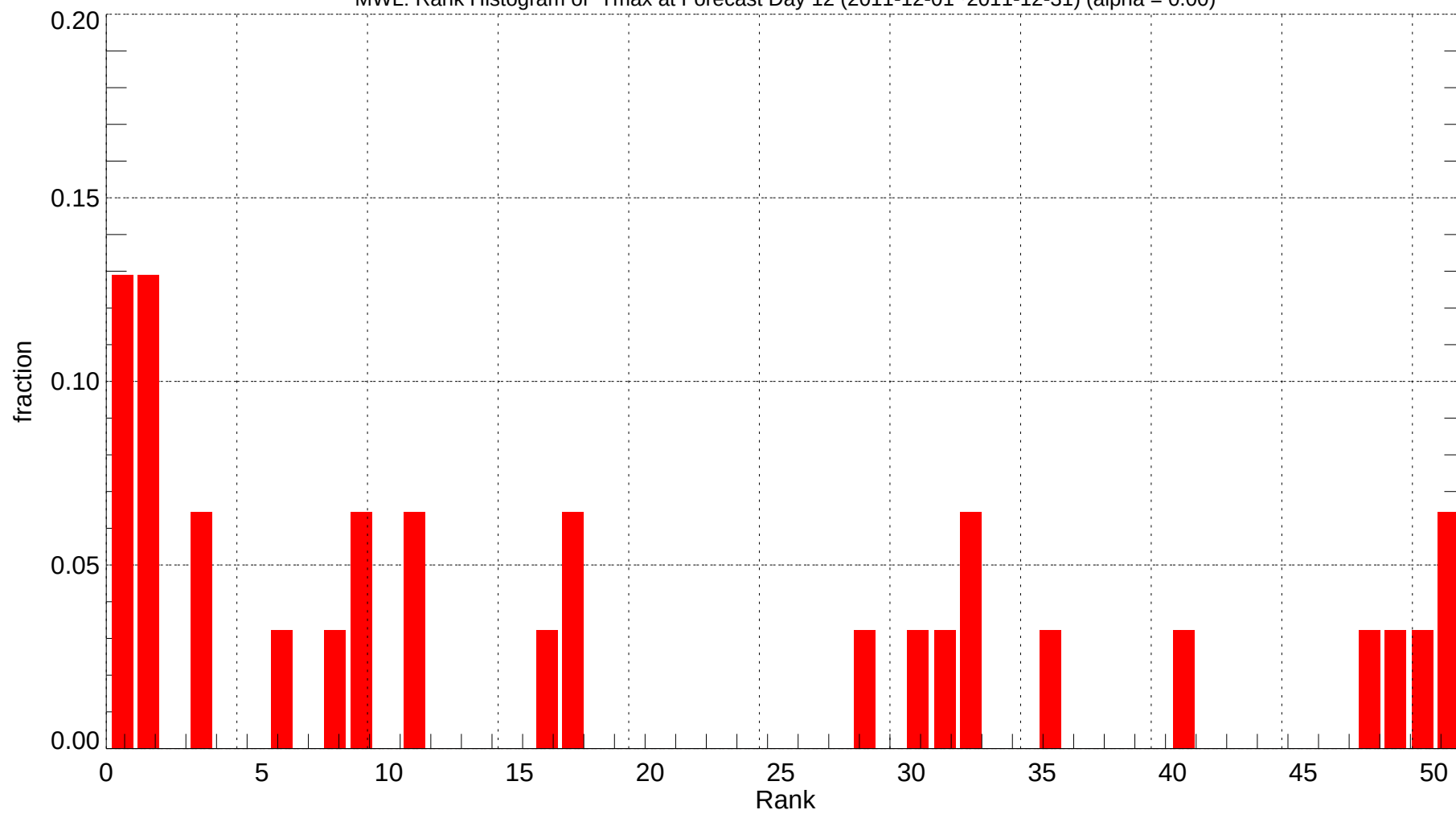
MWL: Rank Histogram of Tmax at Forecast Day 12 (2011-12-01~2011-12-31) (alpha = 0.00)
