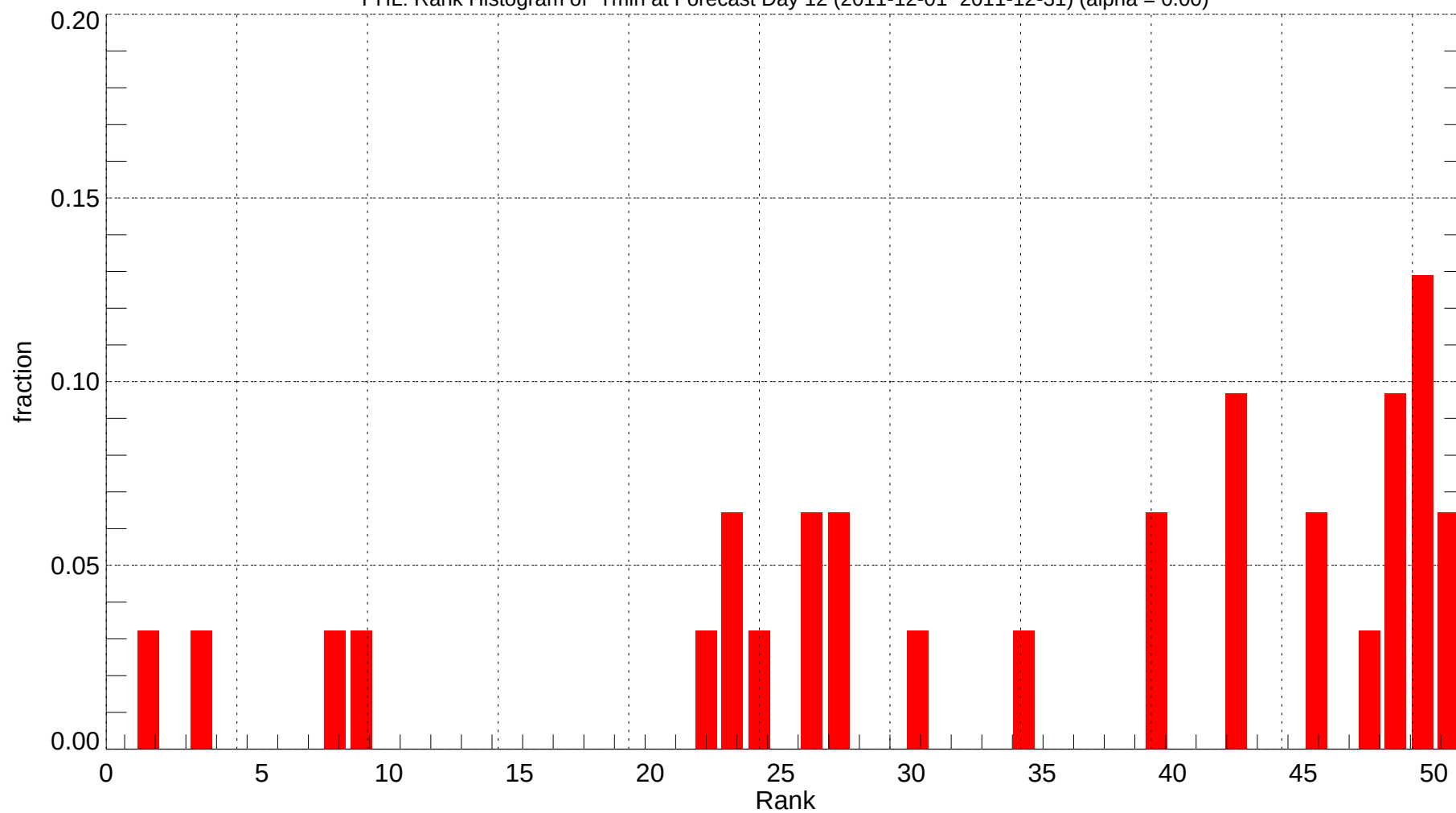
PHL: Rank Histogram of Tmin at Forecast Day 12 (2011-12-01~2011-12-31) (alpha = 0.00)
