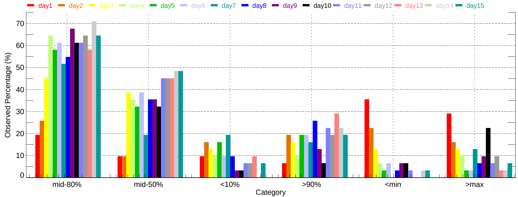
Observed Percentage of Ensembles - ORH: Max Temperature (2011-12-01~2011-12-31)
