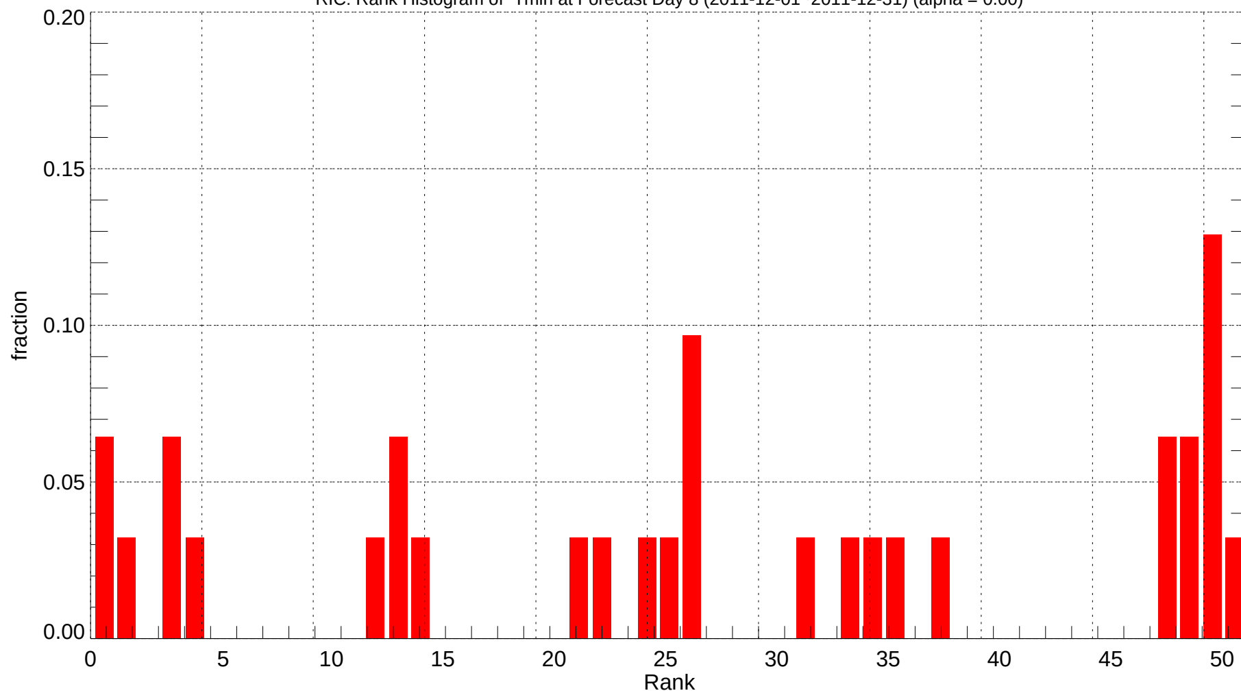
RIC: Rank Histogram of Tmin at Forecast Day 8 (2011-12-01~2011-12-31) (alpha = 0.00)
