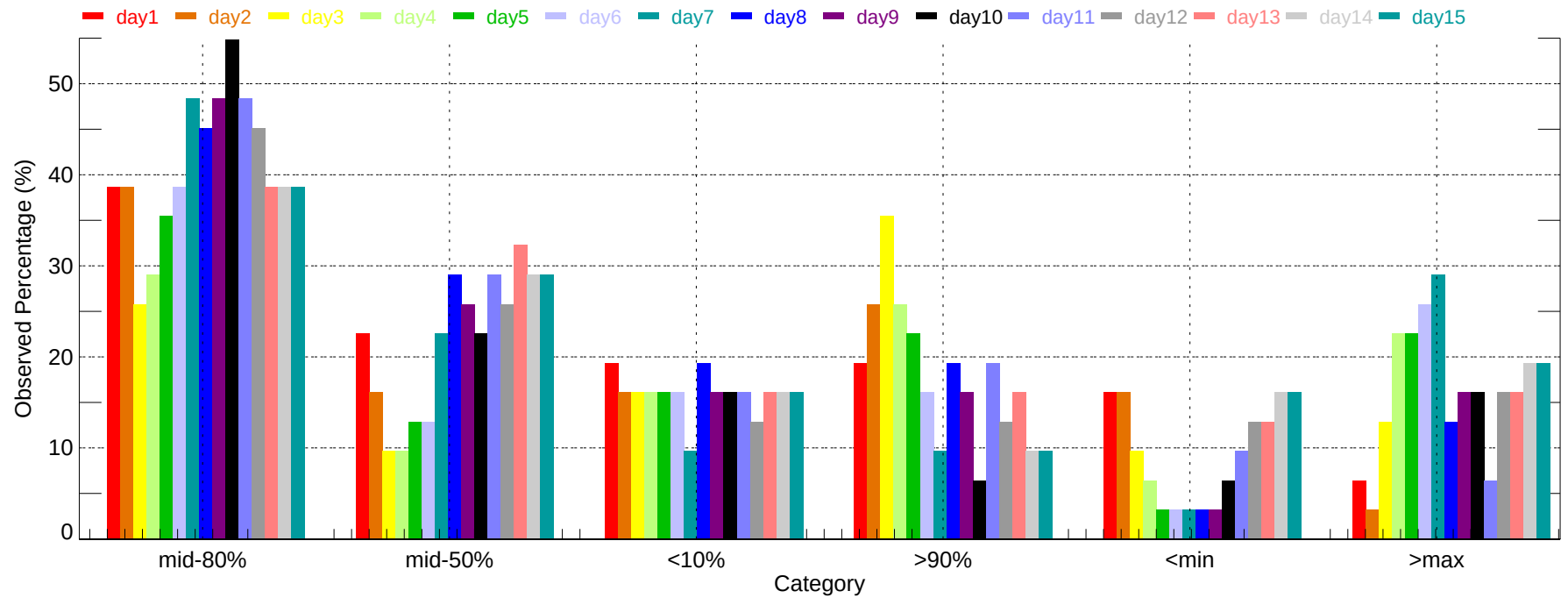
Observed Percentage of Ensembles - TYR: Max Temperature (2011-12-01~2011-12-31)
