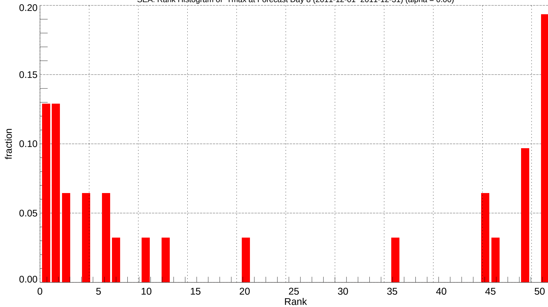
SEA: Rank Histogram of Tmax at Forecast Day 8 (2011-12-01~2011-12-31) (alpha = 0.00)
