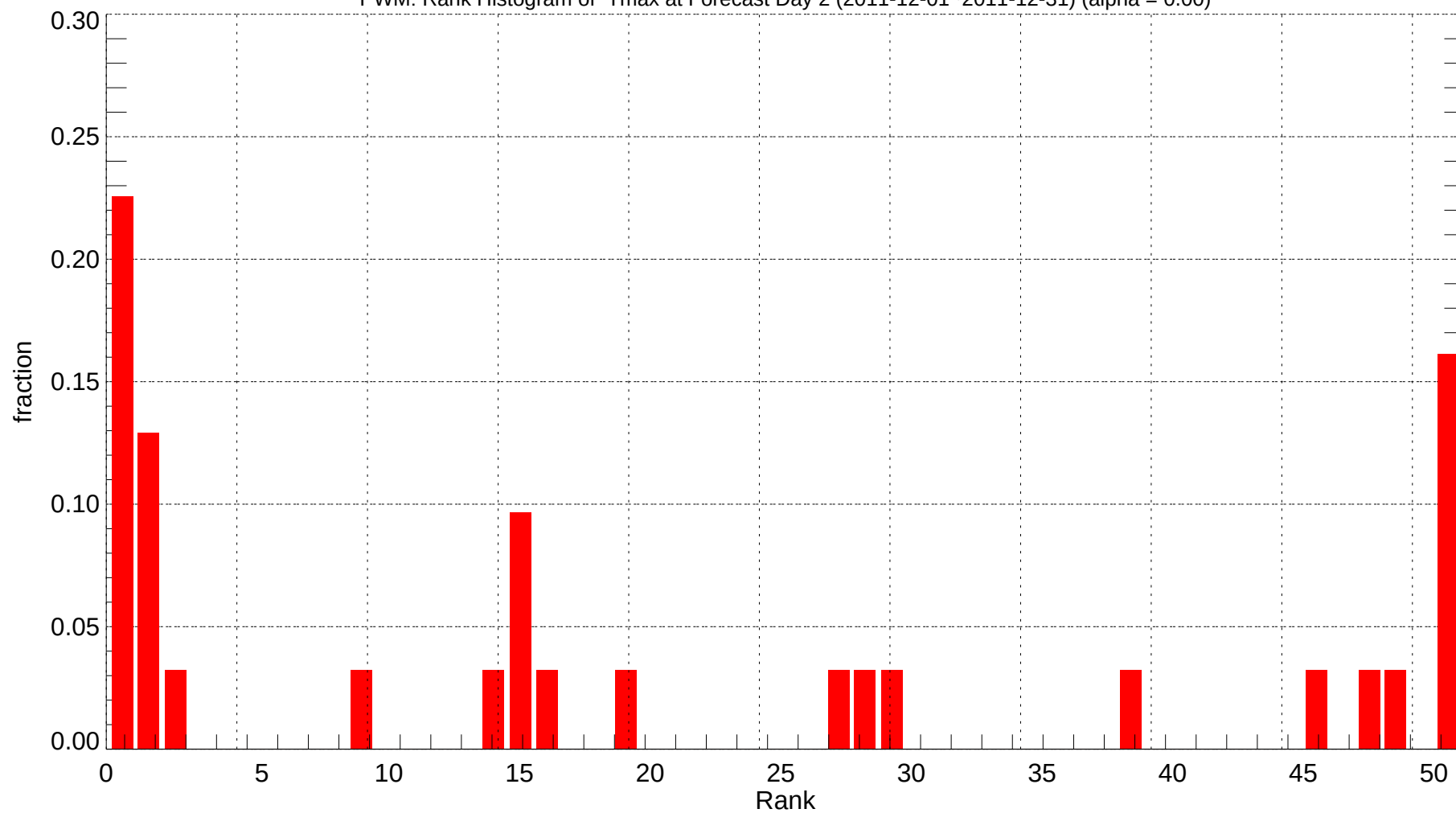
PWM: Rank Histogram of Tmax at Forecast Day 2 (2011-12-01~2011-12-31) (alpha = 0.00)
