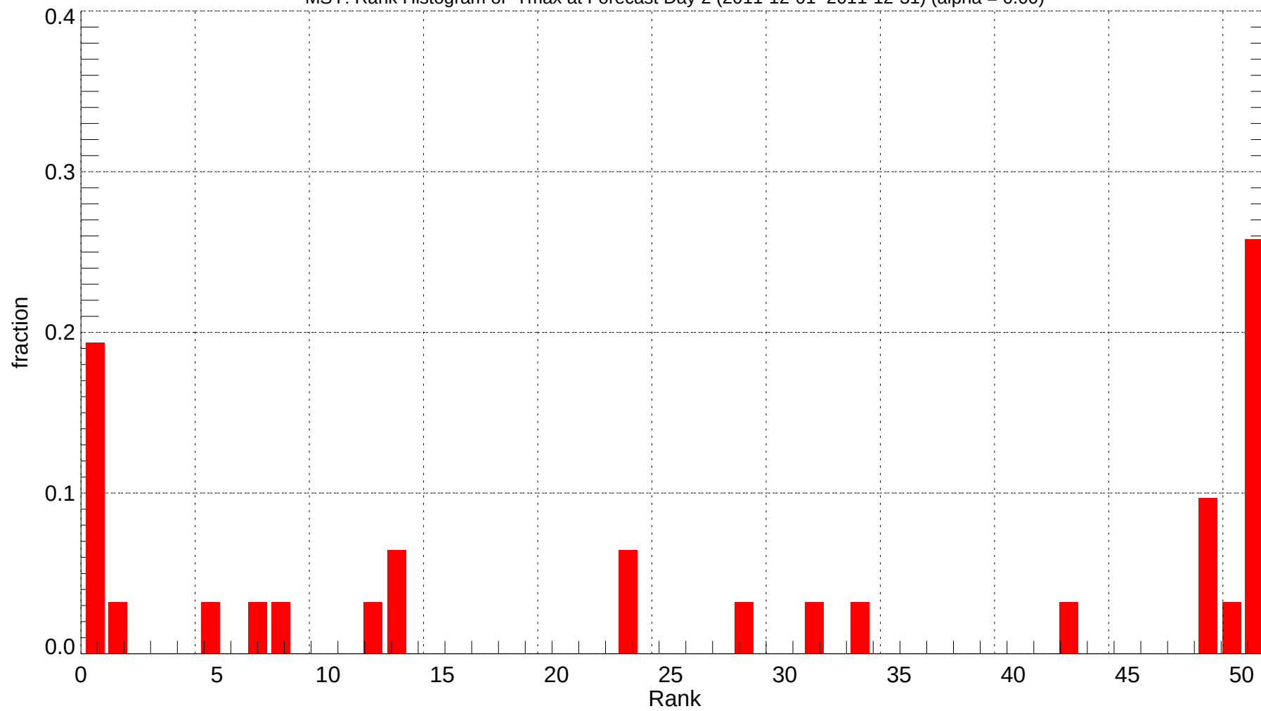
MSY: Rank Histogram of Tmax at Forecast Day 2 (2011-12-01~2011-12-31) (alpha = 0.00)
