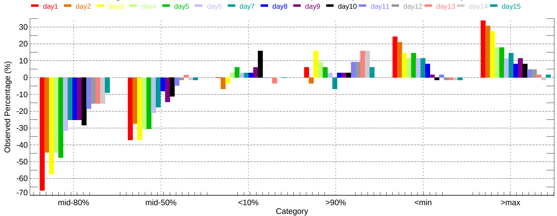
Observed Percentage Deviation of Ensembles - PWM: Min Temperature (2011-12-01~2011-12-31)
