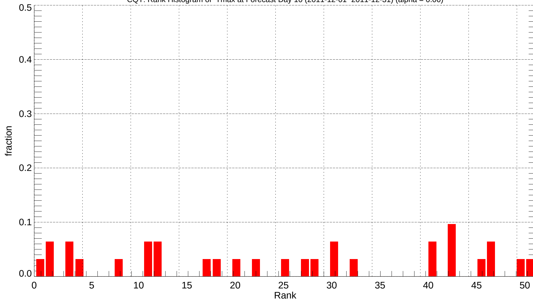
CQT: Rank Histogram of Tmax at Forecast Day 10 (2011-12-01~2011-12-31) (alpha = 0.00)
