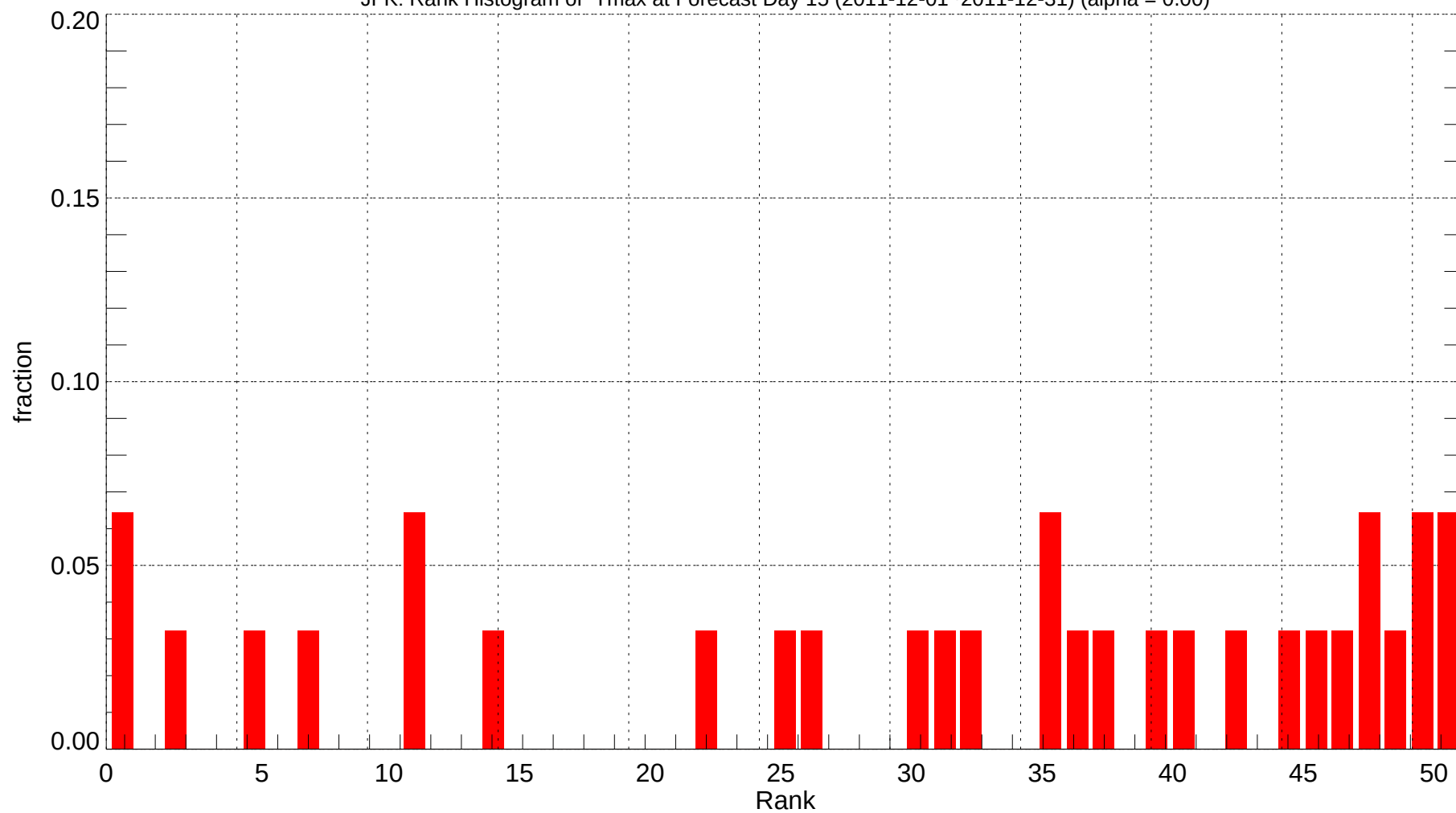
JFK: Rank Histogram of Tmax at Forecast Day 15 (2011-12-01~2011-12-31) (alpha = 0.00)
