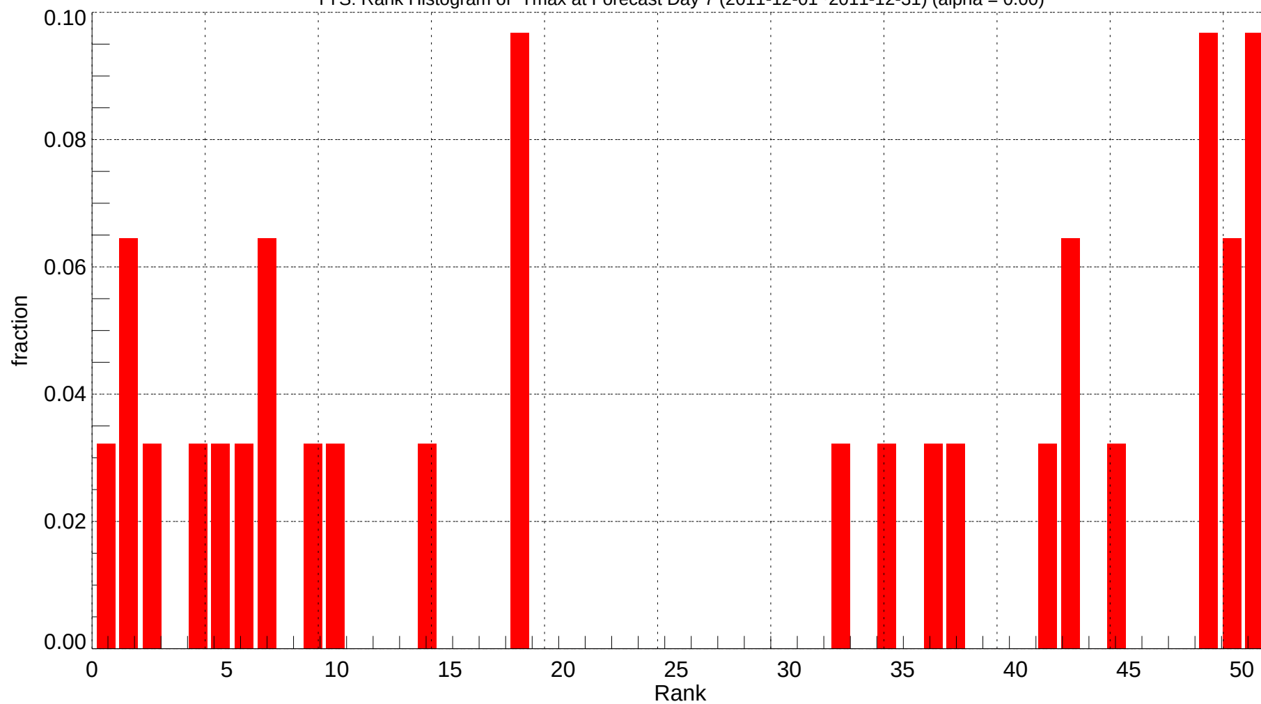
TYS: Rank Histogram of Tmax at Forecast Day 7 (2011-12-01~2011-12-31) (alpha = 0.00)
