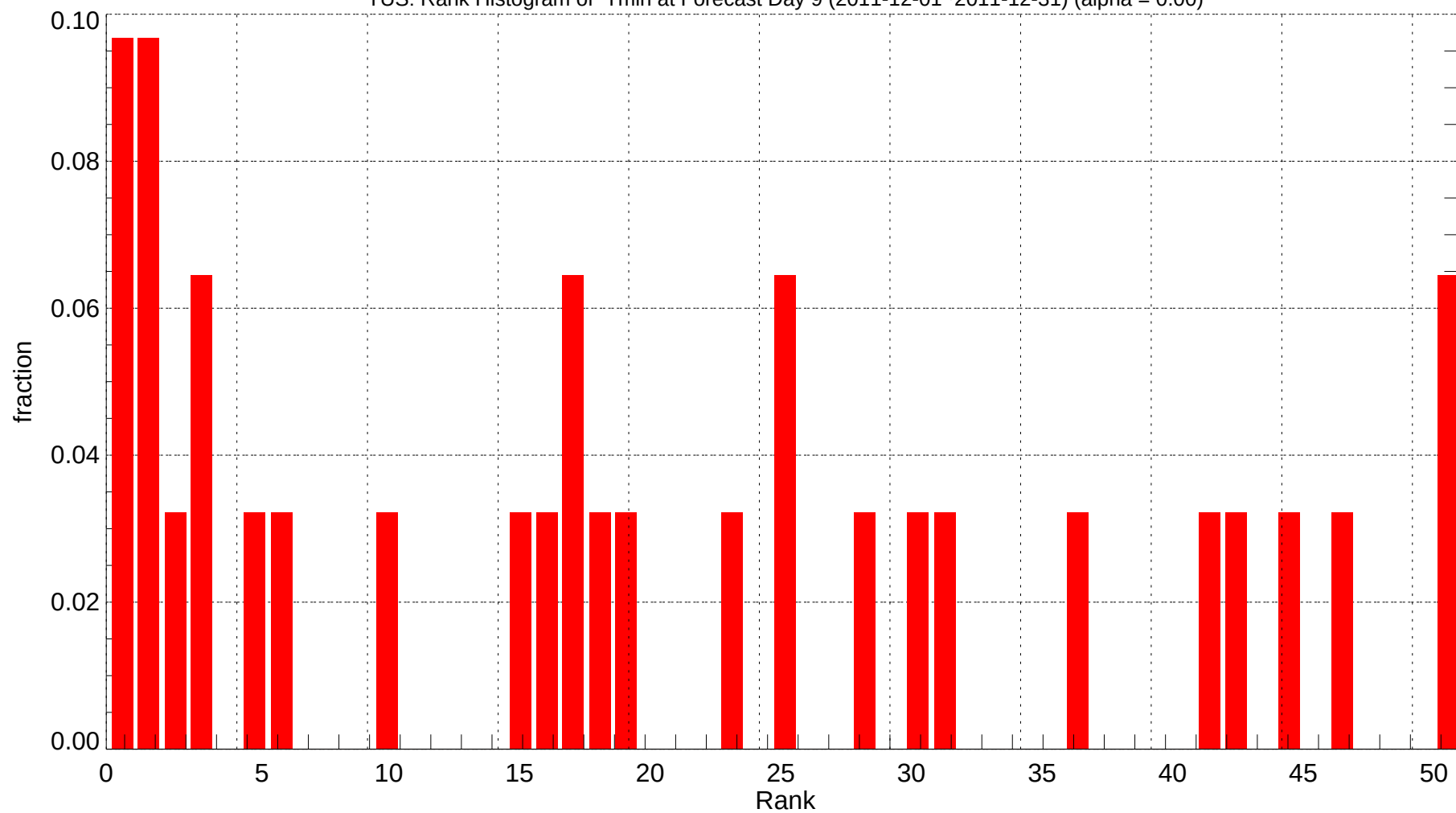
TUS: Rank Histogram of Tmin at Forecast Day 9 (2011-12-01~2011-12-31) (alpha = 0.00)
