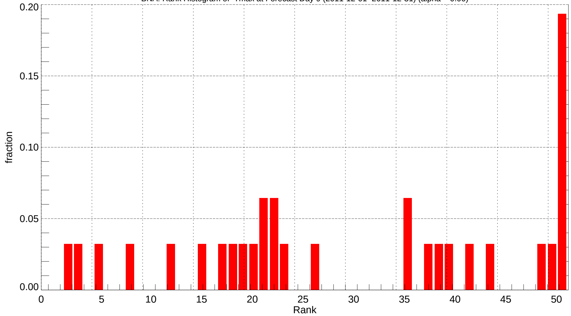
BNA: Rank Histogram of Tmax at Forecast Day 9 (2011-12-01~2011-12-31) (alpha = 0.00)
