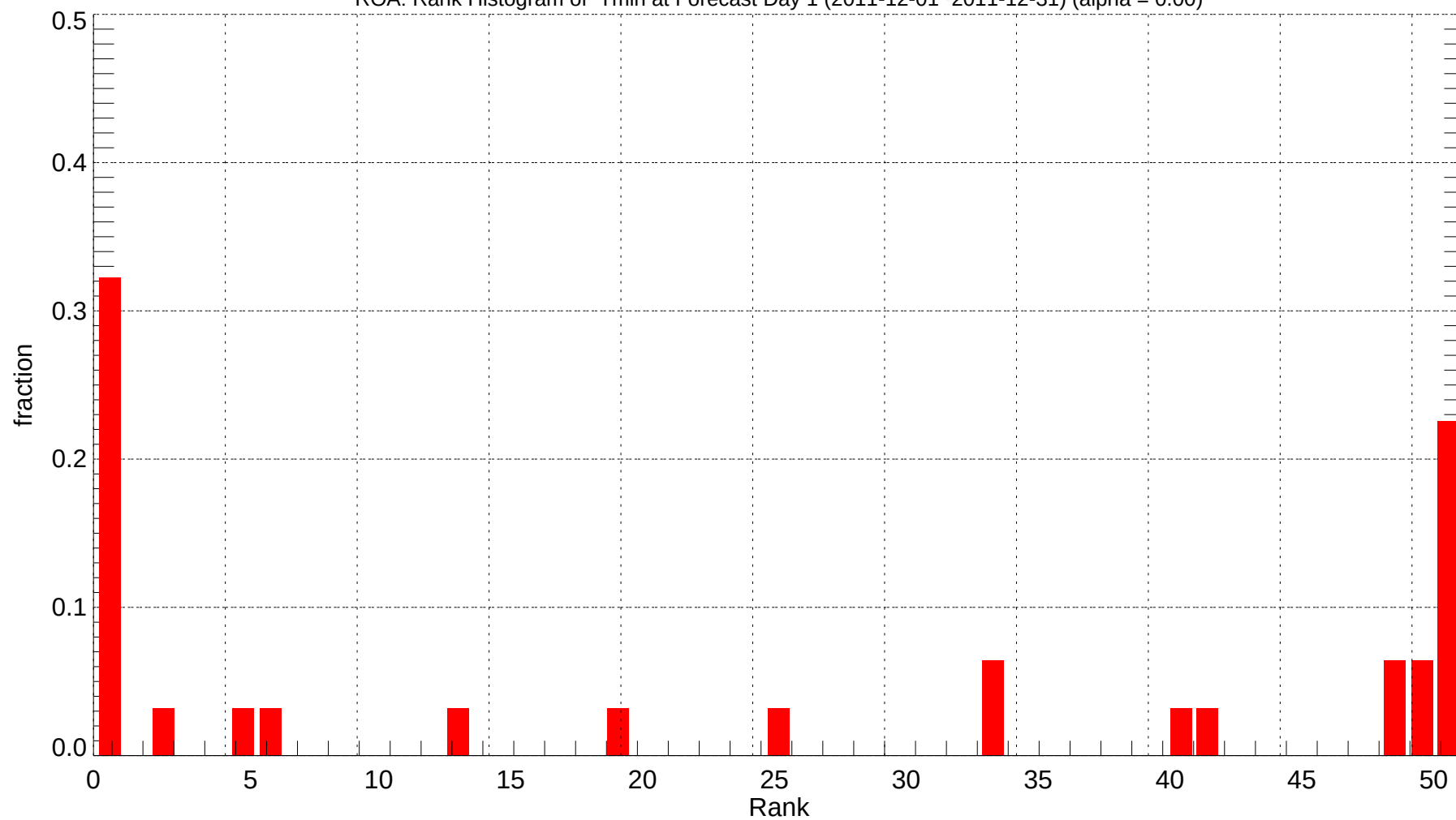
ROA: Rank Histogram of Tmin at Forecast Day 1 (2011-12-01~2011-12-31) (alpha = 0.00)
