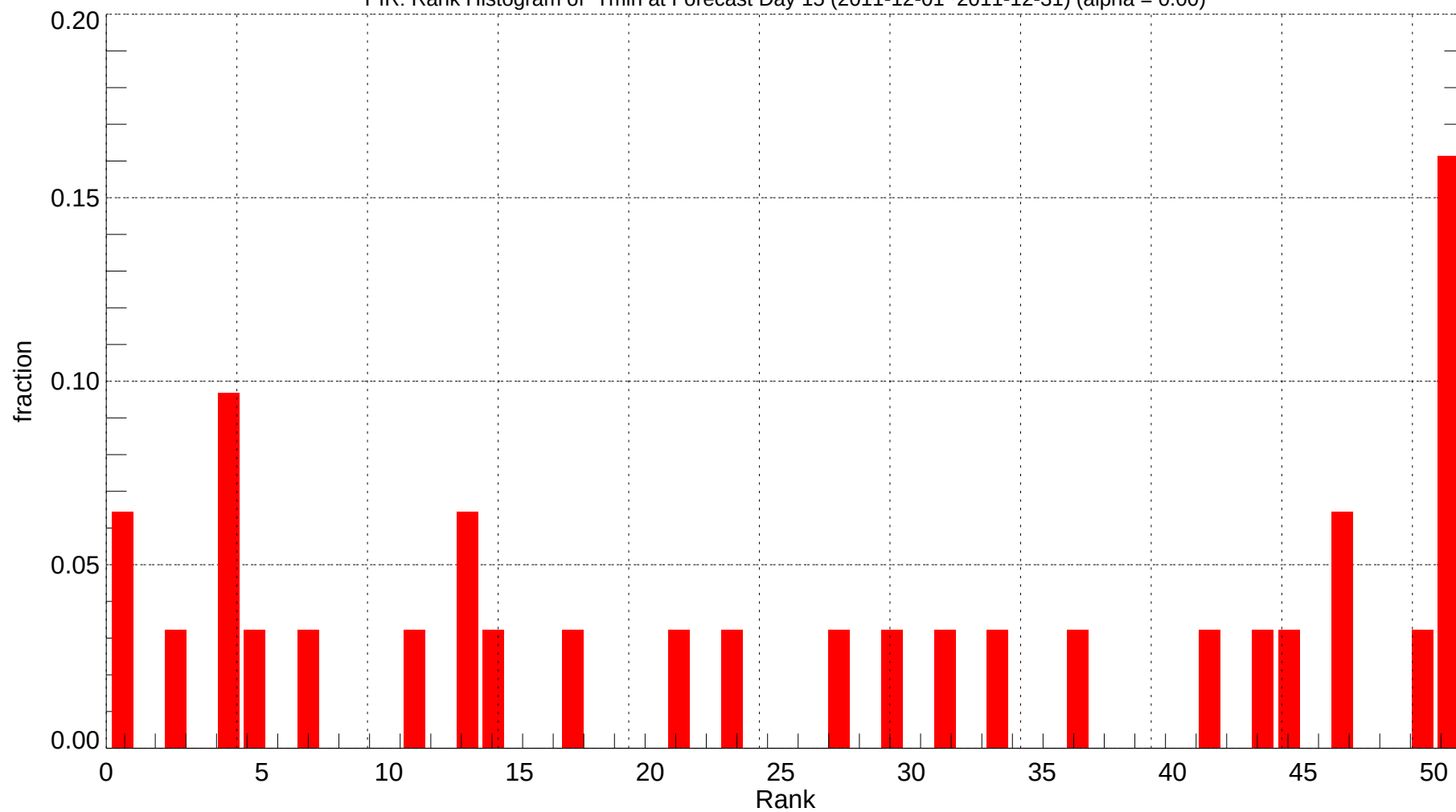
PIR: Rank Histogram of Tmin at Forecast Day 15 (2011-12-01~2011-12-31) (alpha = 0.00)
