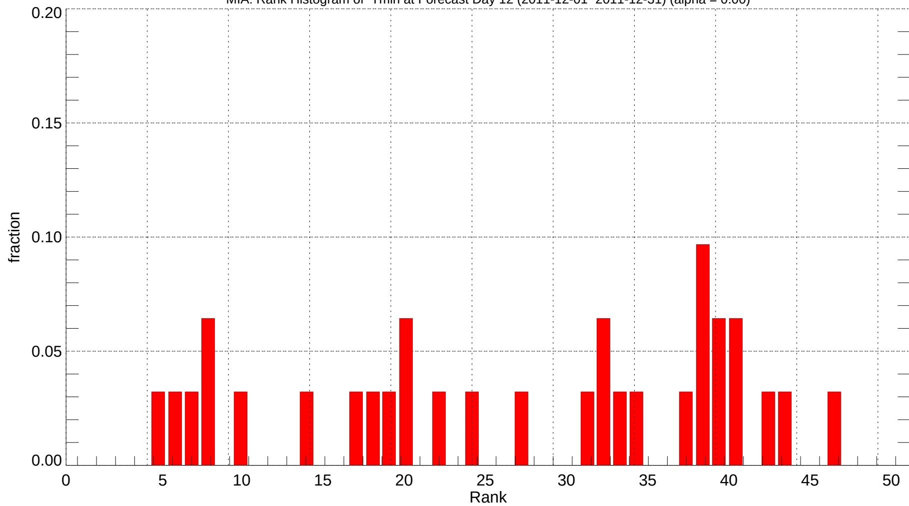
MIA: Rank Histogram of Tmin at Forecast Day 12 (2011-12-01~2011-12-31) (alpha = 0.00)
