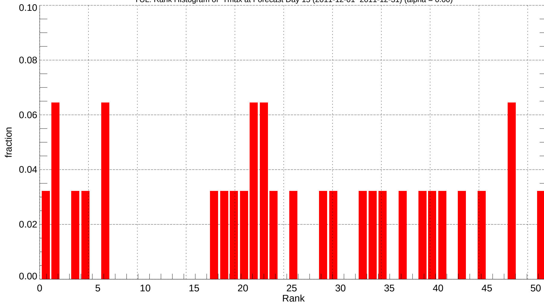
YUL: Rank Histogram of Tmax at Forecast Day 15 (2011-12-01~2011-12-31) (alpha = 0.00)
