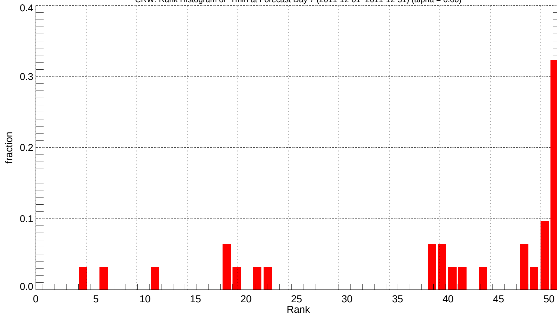
CRW: Rank Histogram of Tmin at Forecast Day 7 (2011-12-01~2011-12-31) (alpha = 0.00)
