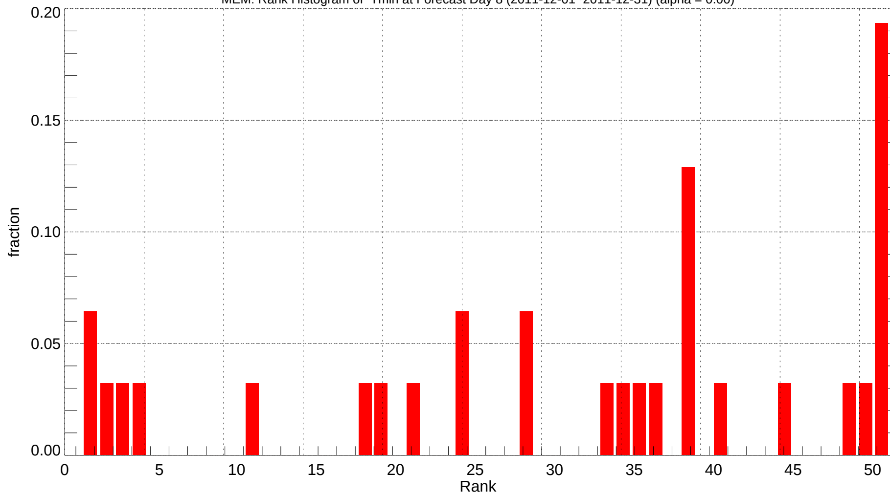
MEM: Rank Histogram of Tmin at Forecast Day 8 (2011-12-01~2011-12-31) (alpha = 0.00)
