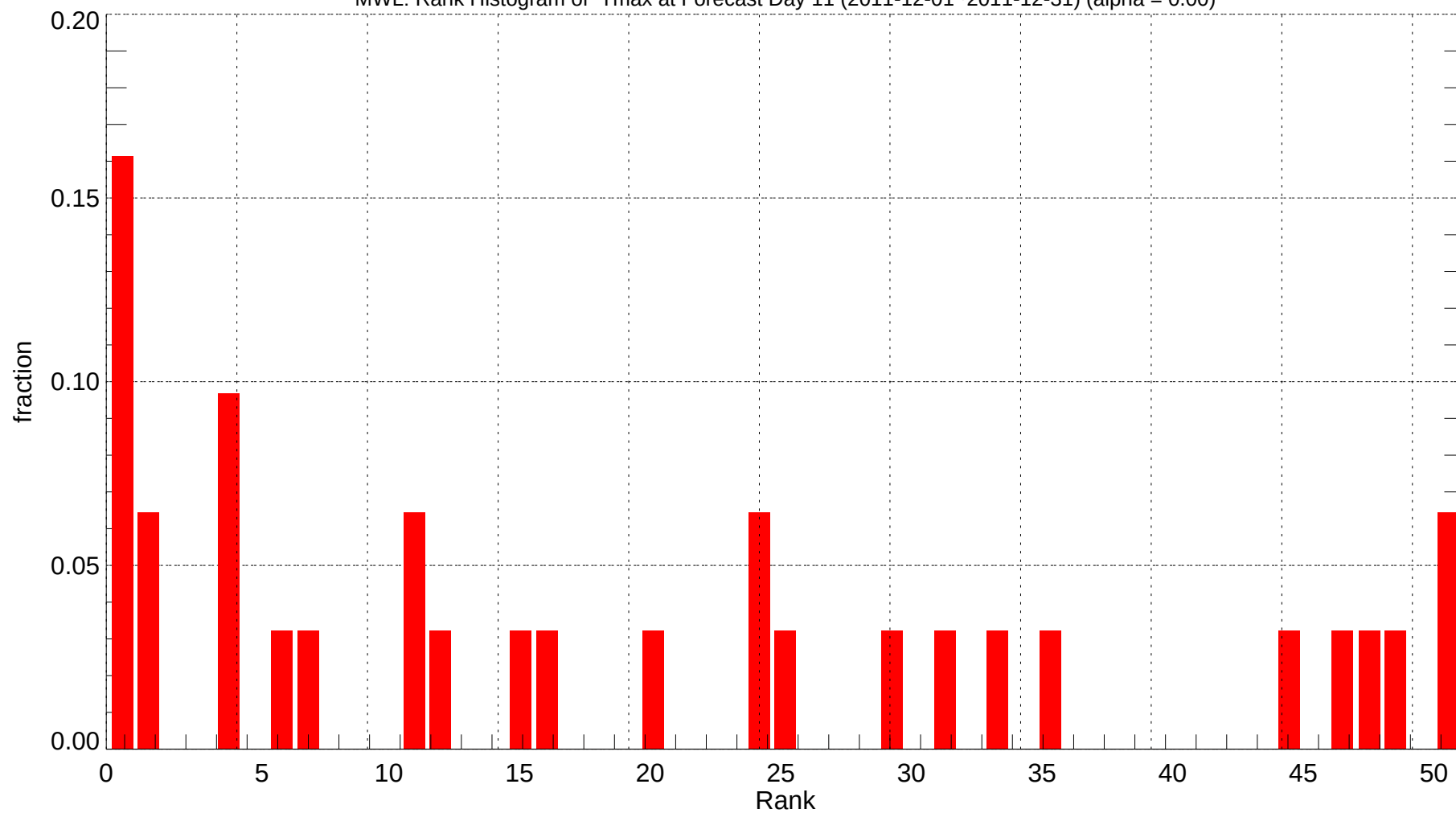
MWL: Rank Histogram of Tmax at Forecast Day 11 (2011-12-01~2011-12-31) (alpha = 0.00)
