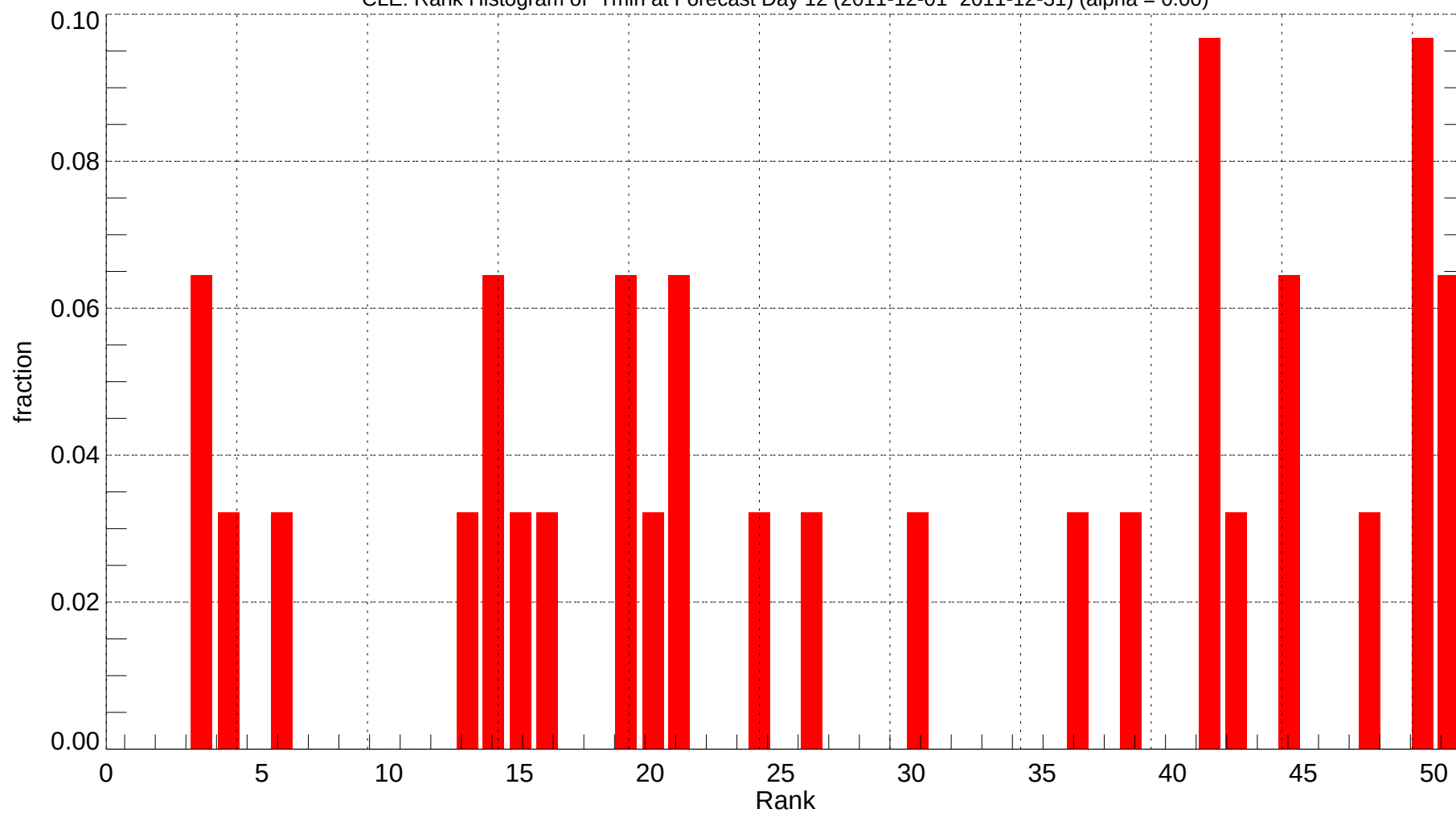
CLE: Rank Histogram of Tmin at Forecast Day 12 (2011-12-01~2011-12-31) (alpha = 0.00)
