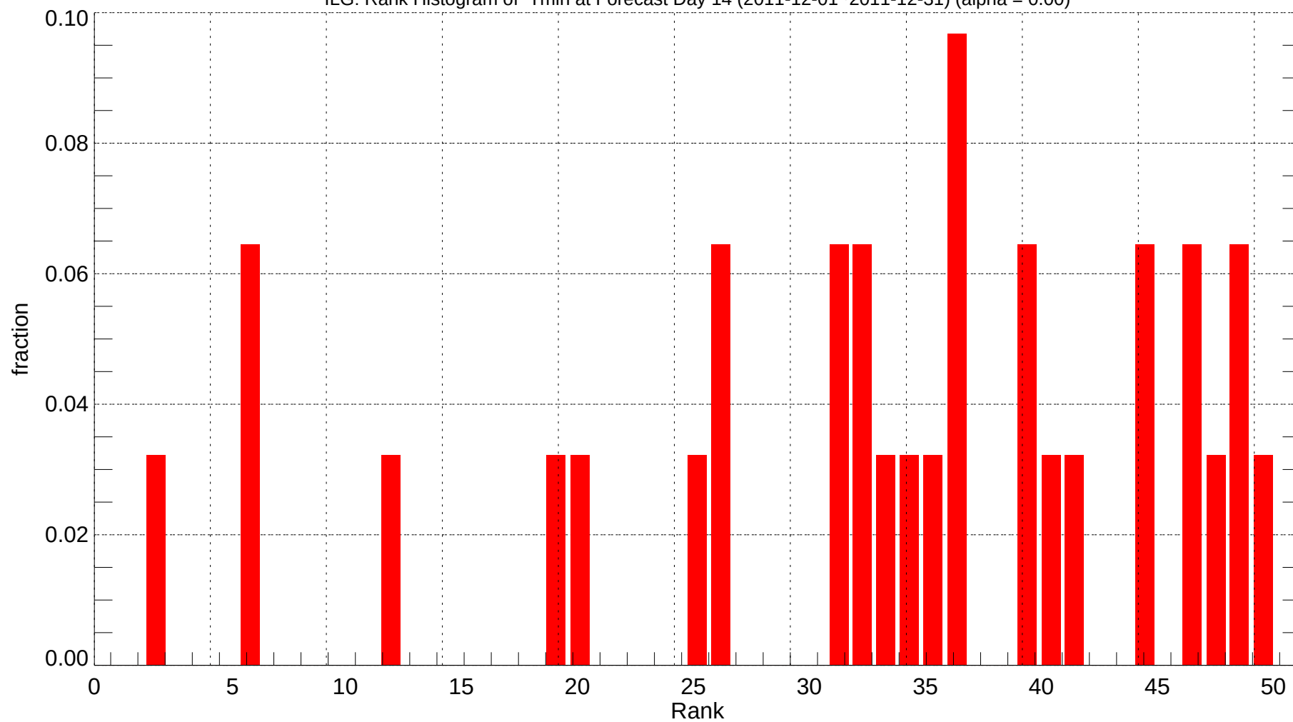
ILG: Rank Histogram of Tmin at Forecast Day 14 (2011-12-01~2011-12-31) (alpha = 0.00)
