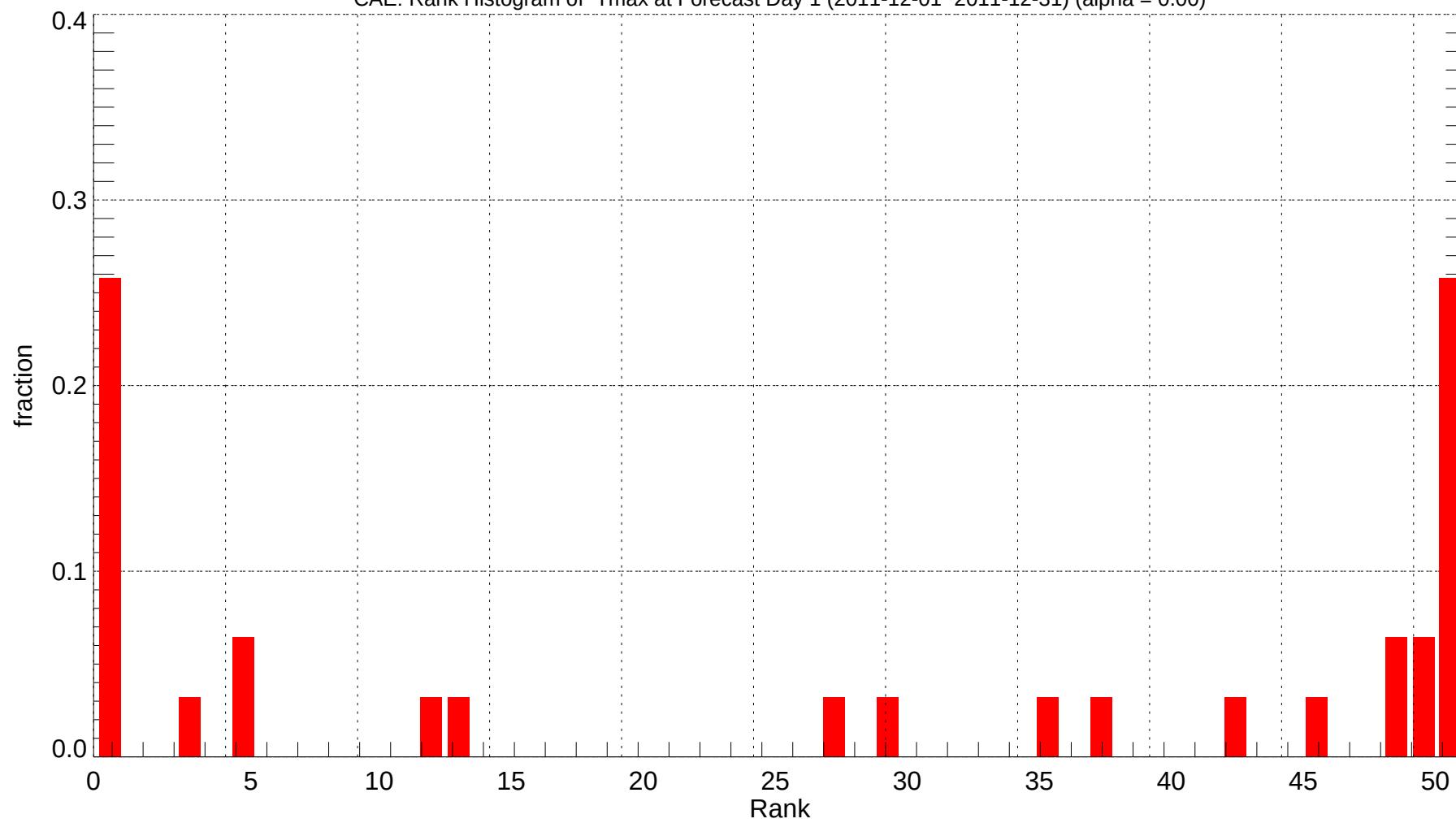
CAE: Rank Histogram of Tmax at Forecast Day 1 (2011-12-01~2011-12-31) (alpha = 0.00)
