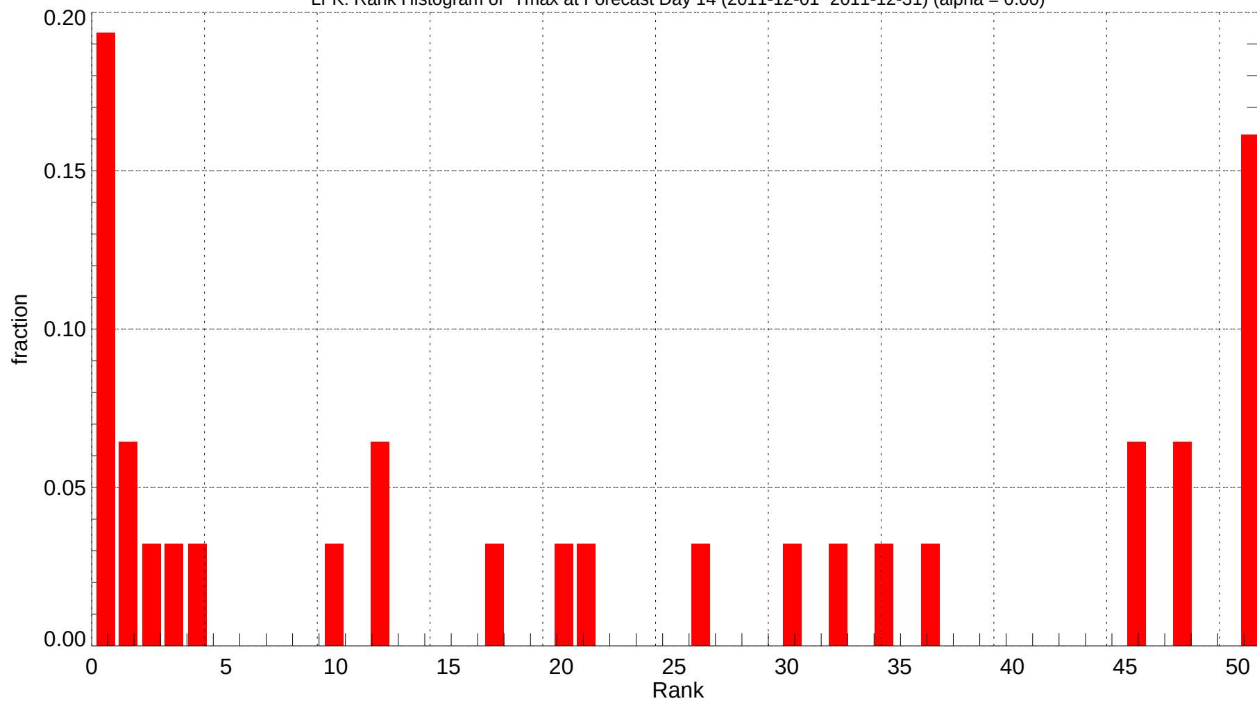
LFK: Rank Histogram of Tmax at Forecast Day 14 (2011-12-01~2011-12-31) (alpha = 0.00)
