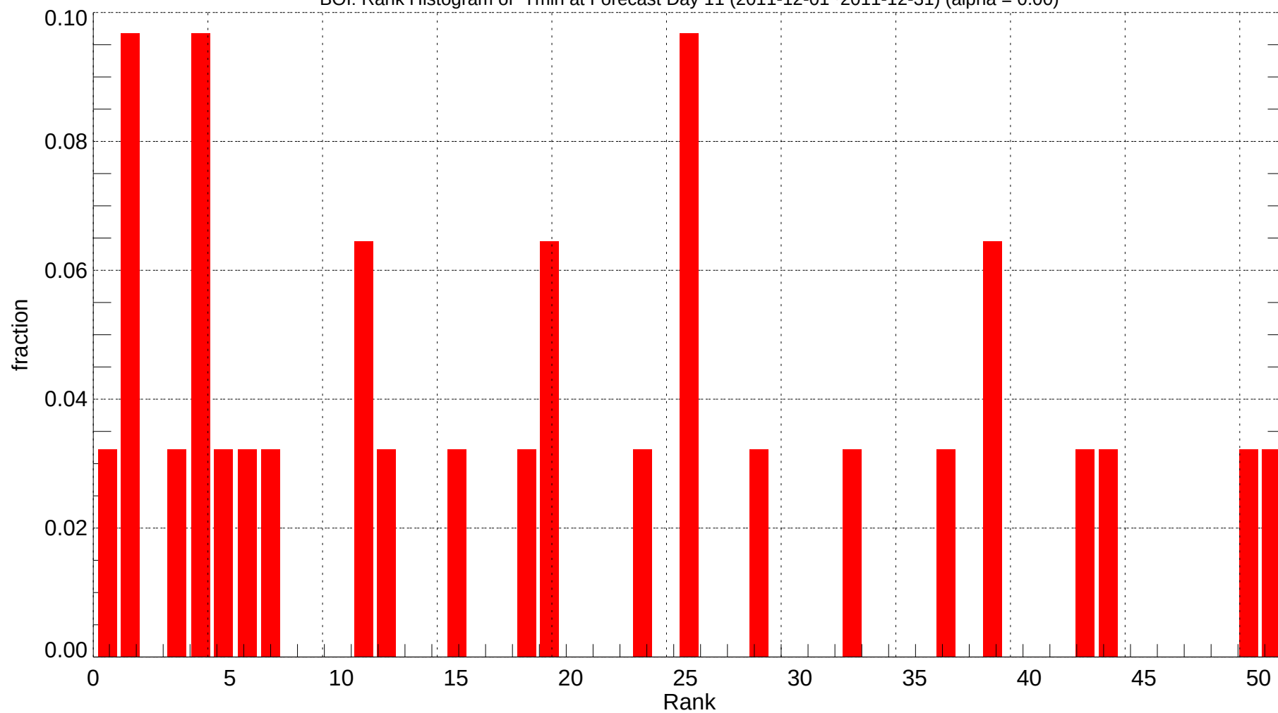
BOI: Rank Histogram of Tmin at Forecast Day 11 (2011-12-01~2011-12-31) (alpha = 0.00)
