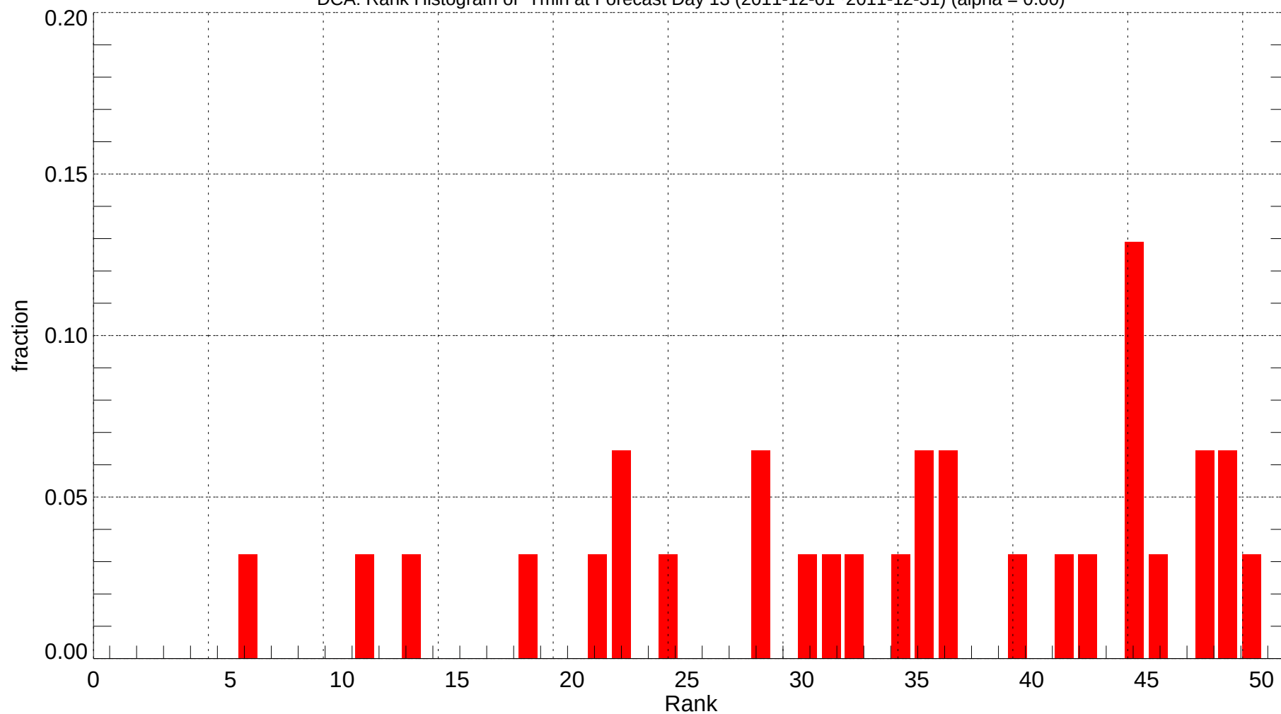
DCA: Rank Histogram of Tmin at Forecast Day 13 (2011-12-01~2011-12-31) (alpha = 0.00)
