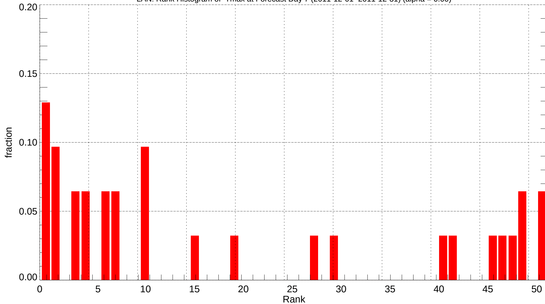
LAN: Rank Histogram of Tmax at Forecast Day 7 (2011-12-01~2011-12-31) (alpha = 0.00)
