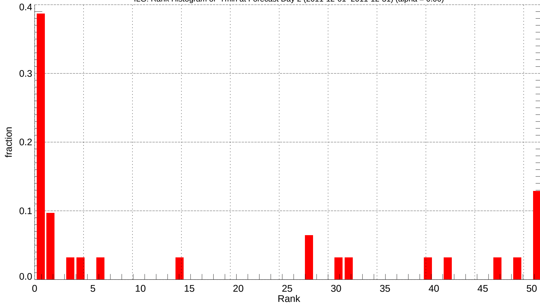
ILG: Rank Histogram of Tmin at Forecast Day 2 (2011-12-01~2011-12-31) (alpha = 0.00)
