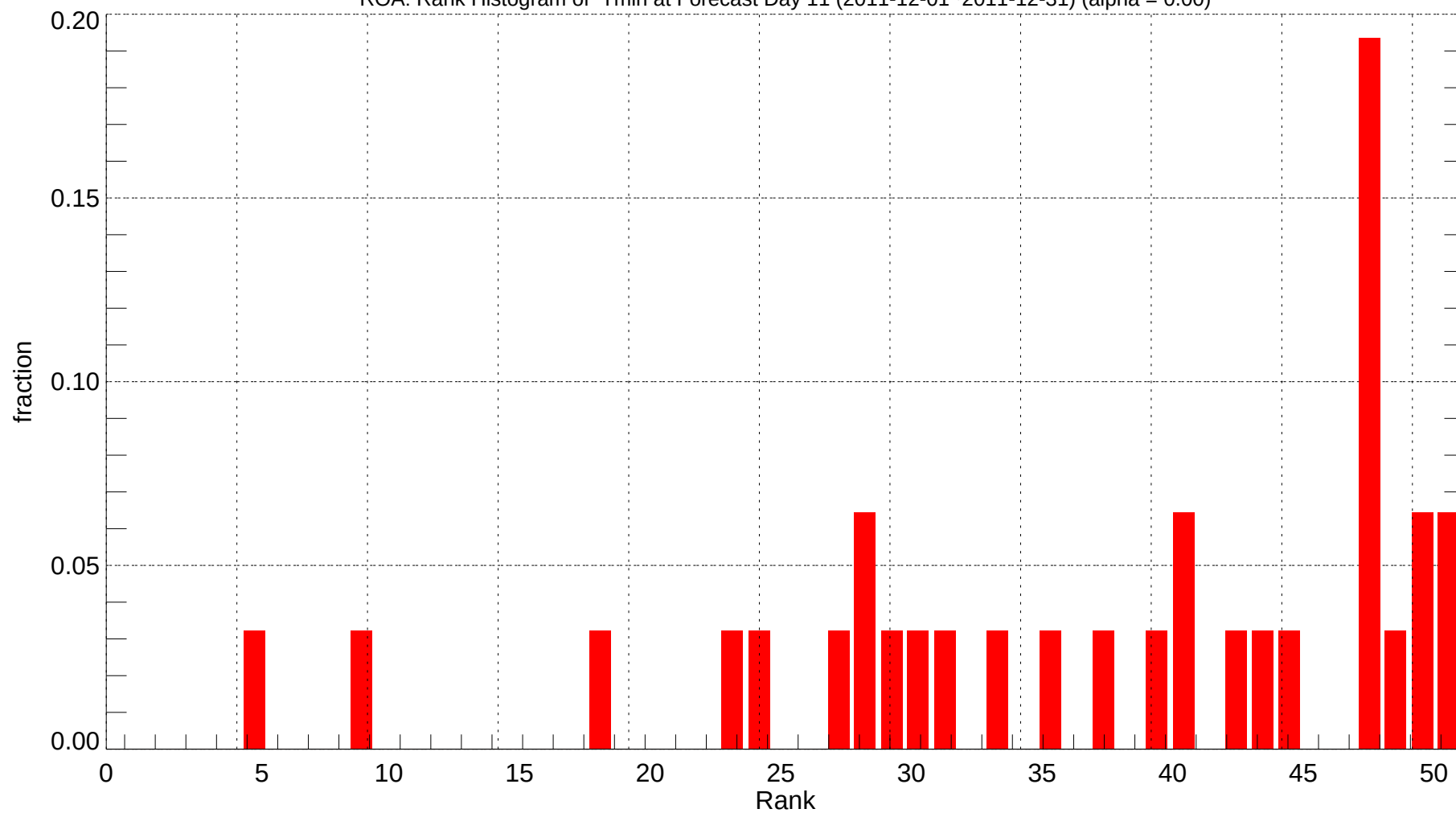
ROA: Rank Histogram of Tmin at Forecast Day 11 (2011-12-01~2011-12-31) (alpha = 0.00)
