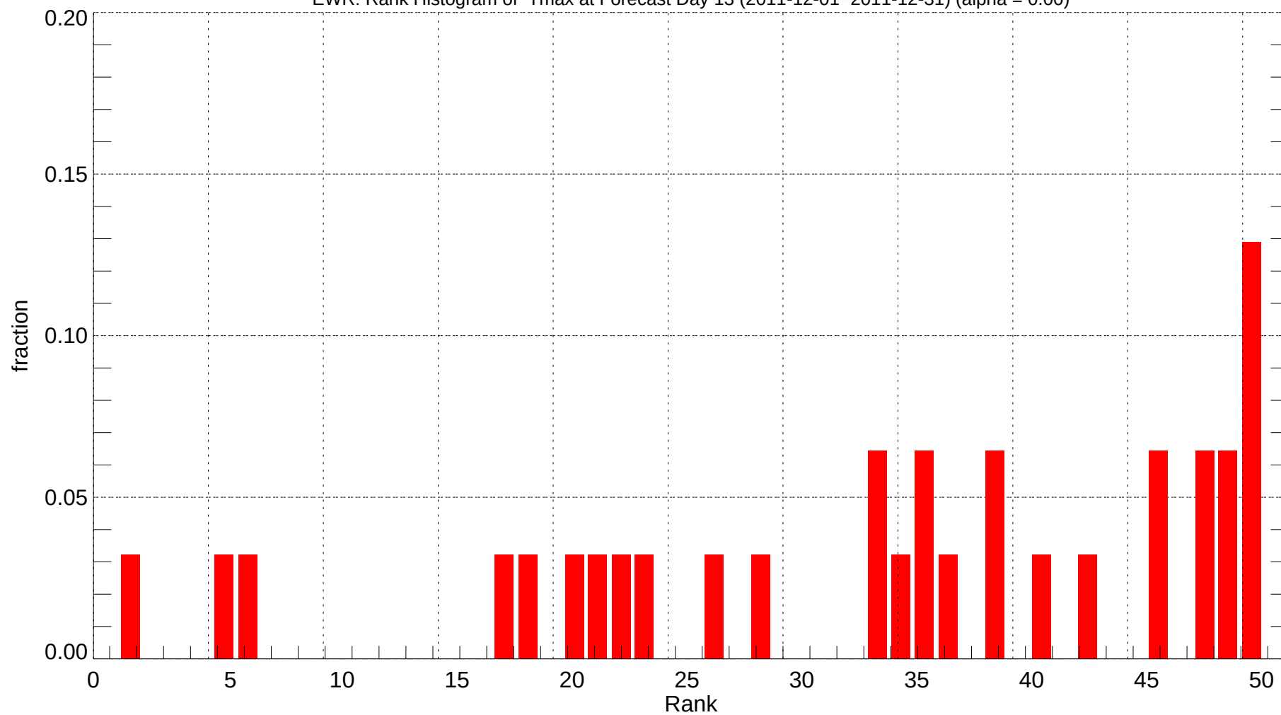
EWR: Rank Histogram of Tmax at Forecast Day 13 (2011-12-01~2011-12-31) (alpha = 0.00)
