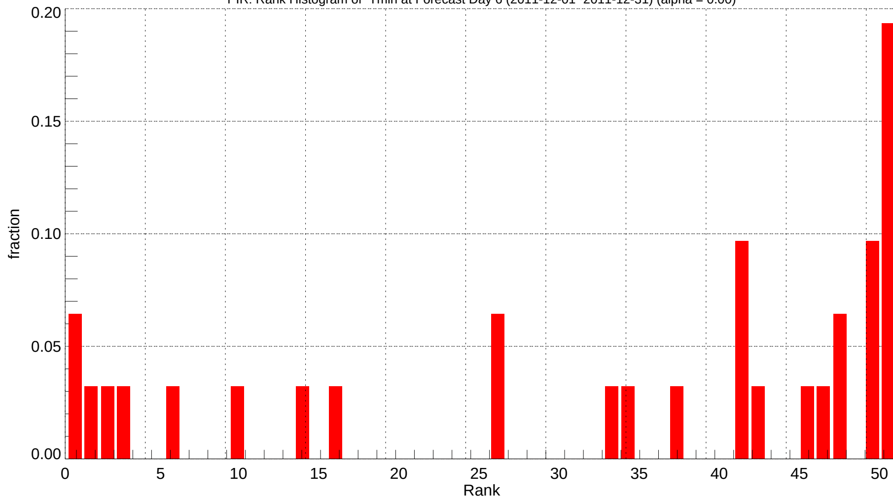
PIR: Rank Histogram of Tmin at Forecast Day 6 (2011-12-01~2011-12-31) (alpha = 0.00)
