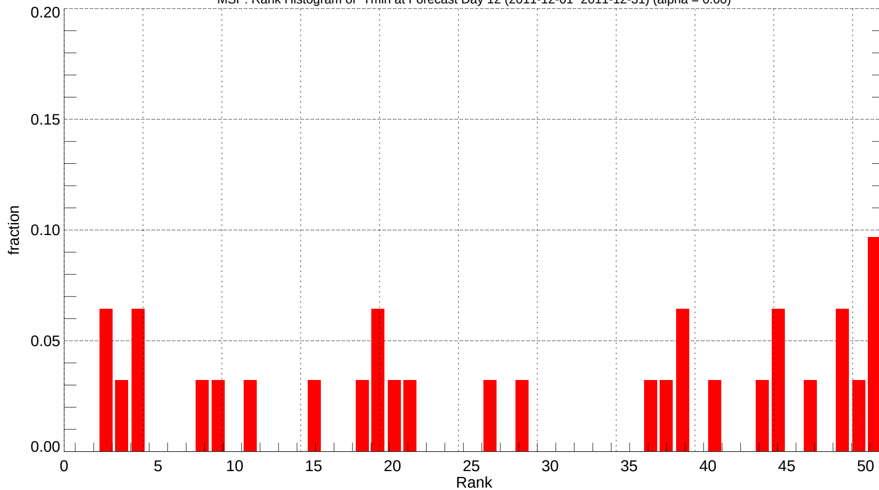
MSP: Rank Histogram of Tmin at Forecast Day 12 (2011-12-01~2011-12-31) (alpha = 0.00)
