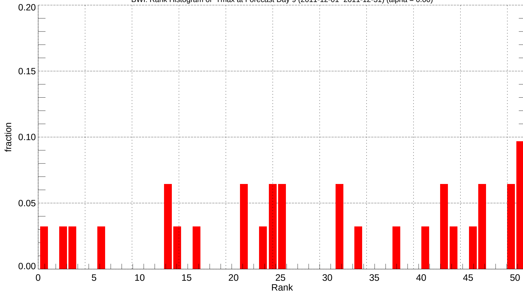
BWI: Rank Histogram of Tmax at Forecast Day 9 (2011-12-01~2011-12-31) (alpha = 0.00)
