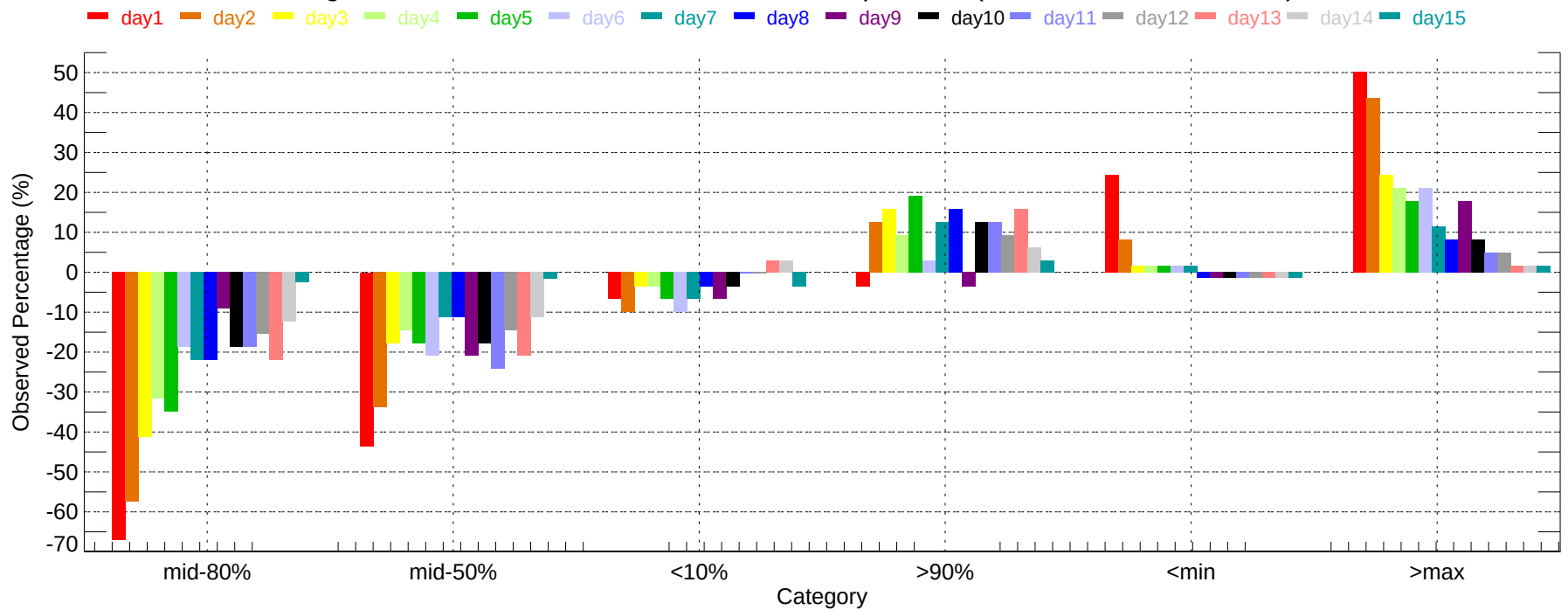
Observed Percentage Deviation of Ensembles - SDF: Min Temperature (2011-12-01~2011-12-31)
