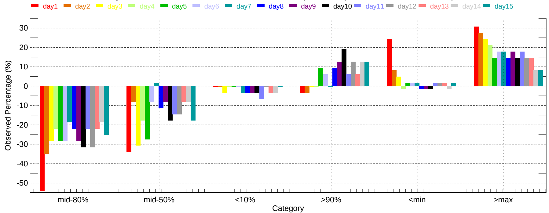
Observed Percentage Deviation of Ensembles - MCI: Max Temperature (2011-12-01~2011-12-31)
