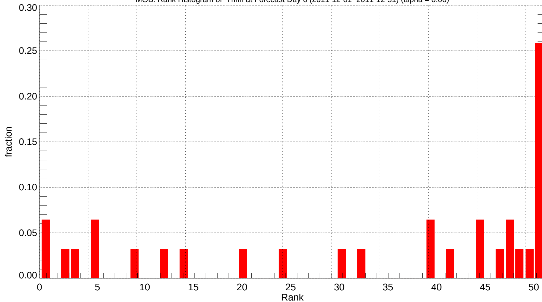
MOB: Rank Histogram of Tmin at Forecast Day 6 (2011-12-01~2011-12-31) (alpha = 0.00)
