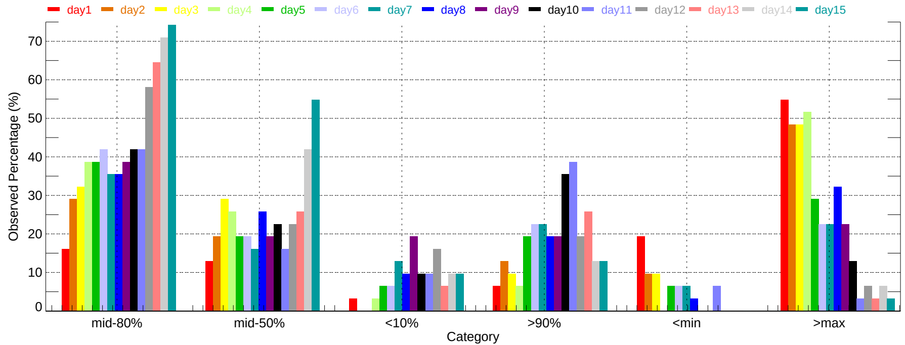
Observed Percentage of Ensembles - AUS: Min Temperature (2011-12-01~2011-12-31)
