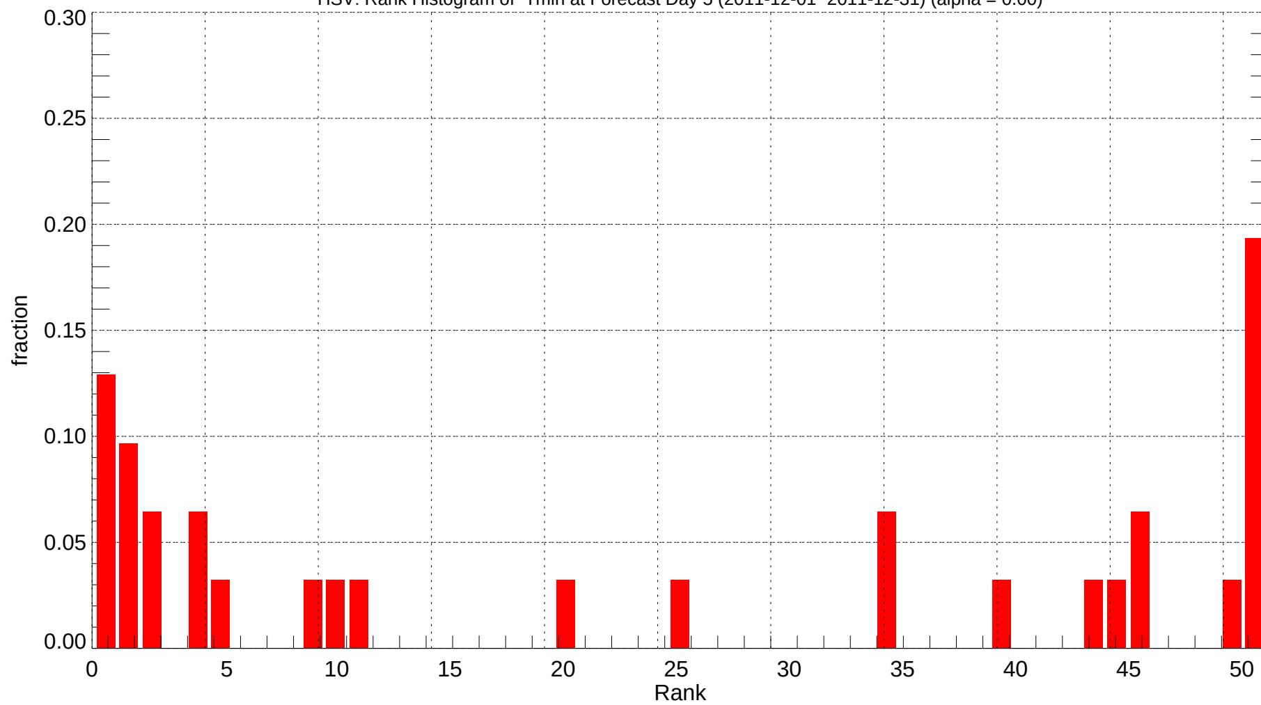
HSV: Rank Histogram of Tmin at Forecast Day 5 (2011-12-01~2011-12-31) (alpha = 0.00)
