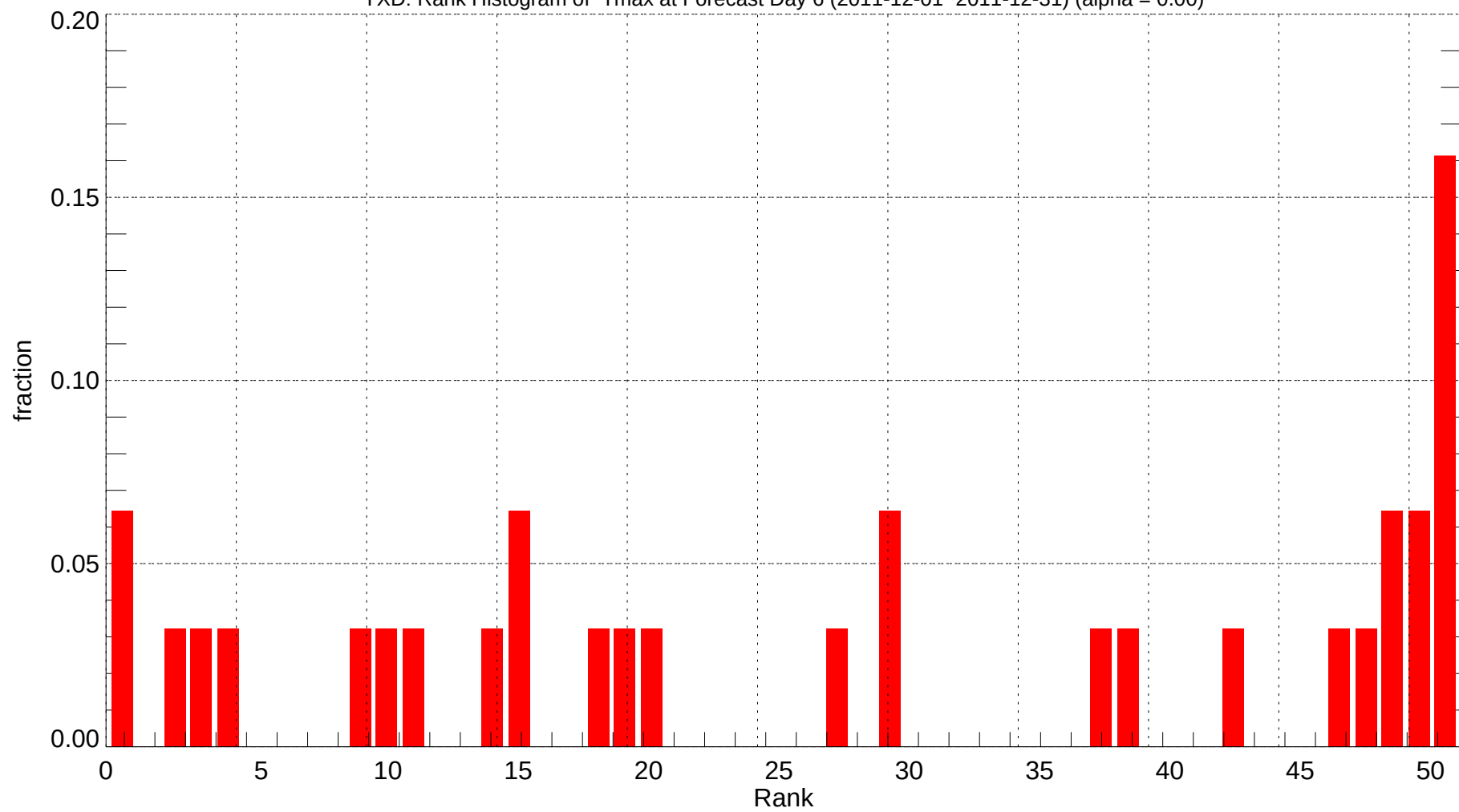
YXD: Rank Histogram of Tmax at Forecast Day 6 (2011-12-01~2011-12-31) (alpha = 0.00)
