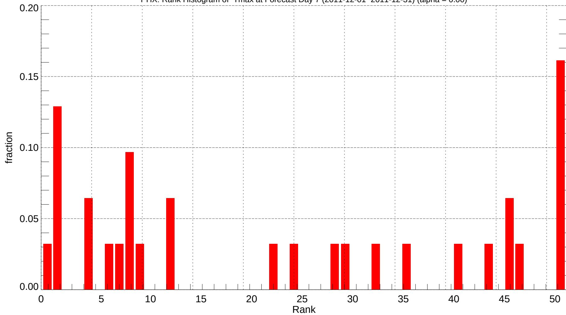
PHX: Rank Histogram of Tmax at Forecast Day 7 (2011-12-01~2011-12-31) (alpha = 0.00)
