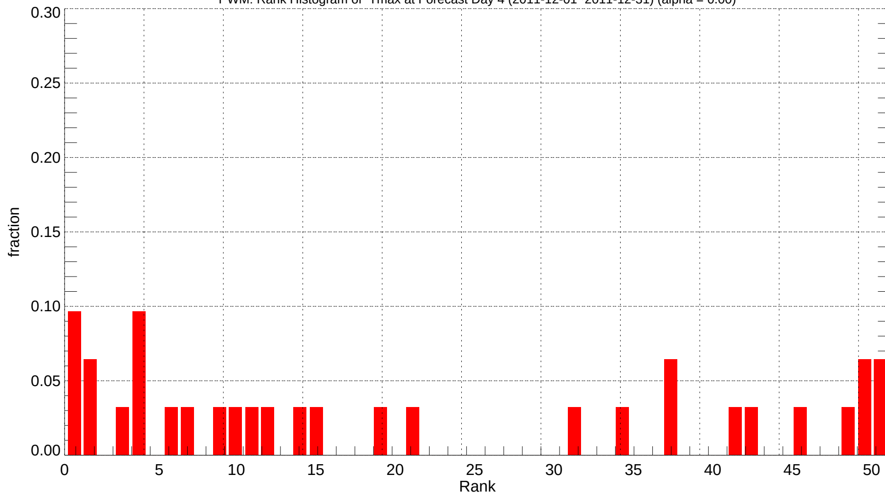
PWM: Rank Histogram of Tmax at Forecast Day 4 (2011-12-01~2011-12-31) (alpha = 0.00)
