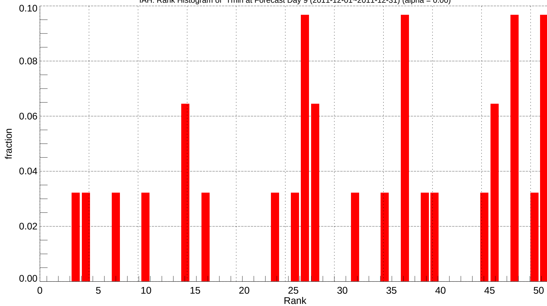
IAH: Rank Histogram of Tmin at Forecast Day 9 (2011-12-01~2011-12-31) (alpha = 0.00)
