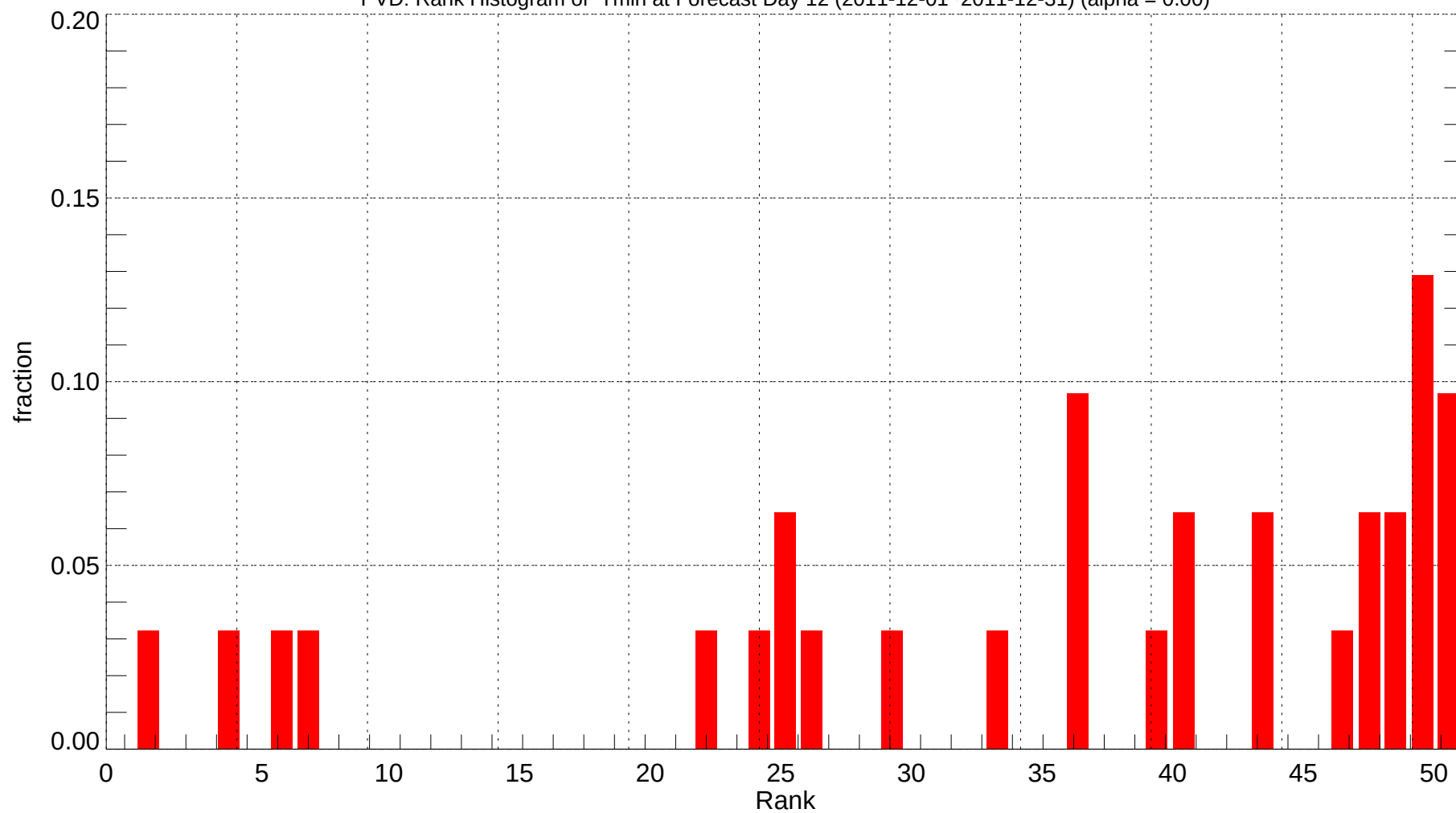
PVD: Rank Histogram of Tmin at Forecast Day 12 (2011-12-01~2011-12-31) (alpha = 0.00)
