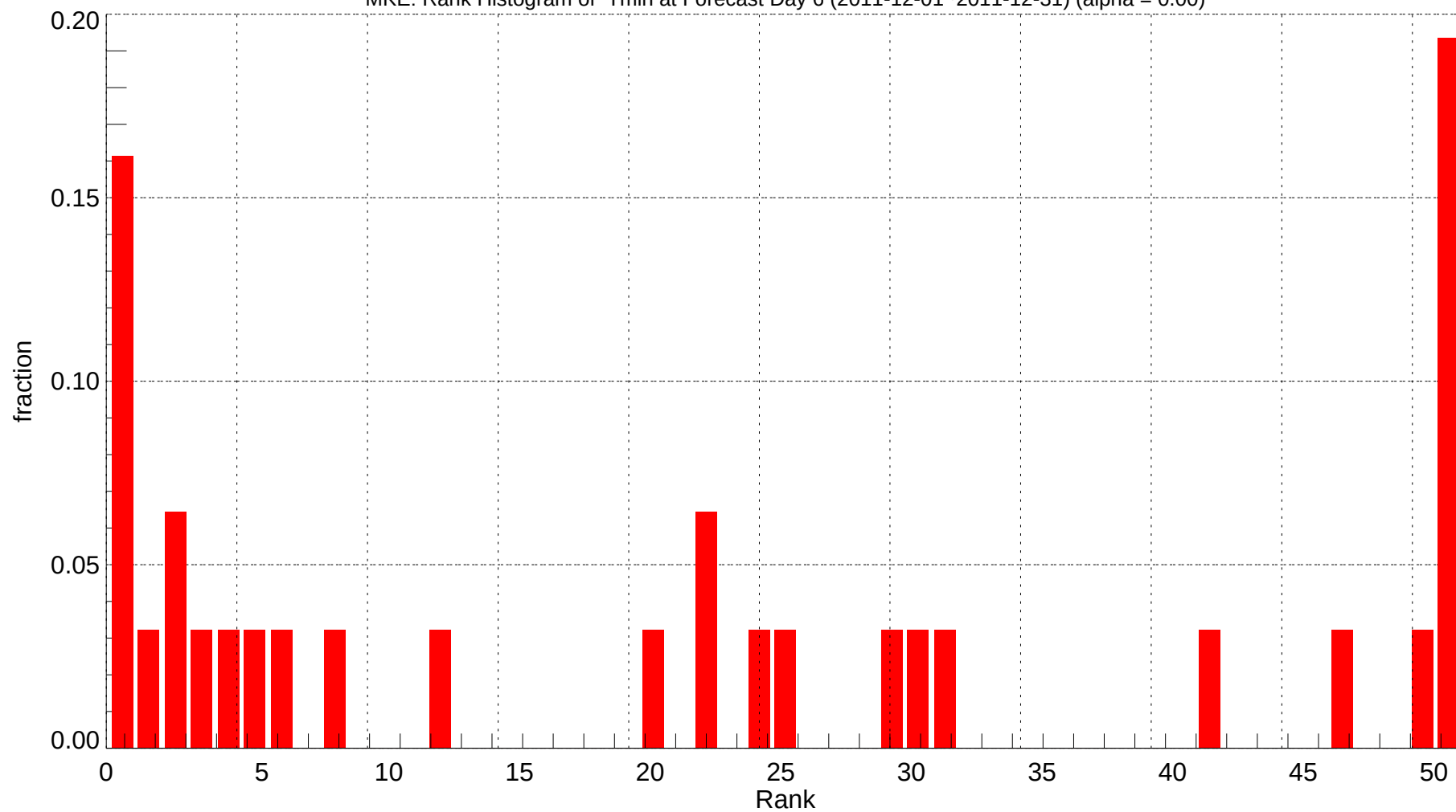
MKE: Rank Histogram of Tmin at Forecast Day 6 (2011-12-01~2011-12-31) (alpha = 0.00)
