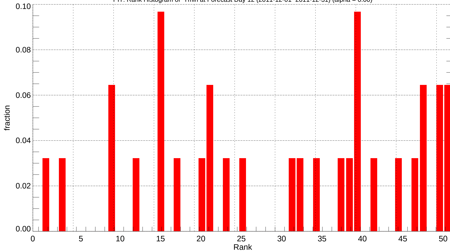
PIT: Rank Histogram of Tmin at Forecast Day 12 (2011-12-01~2011-12-31) (alpha = 0.00)
