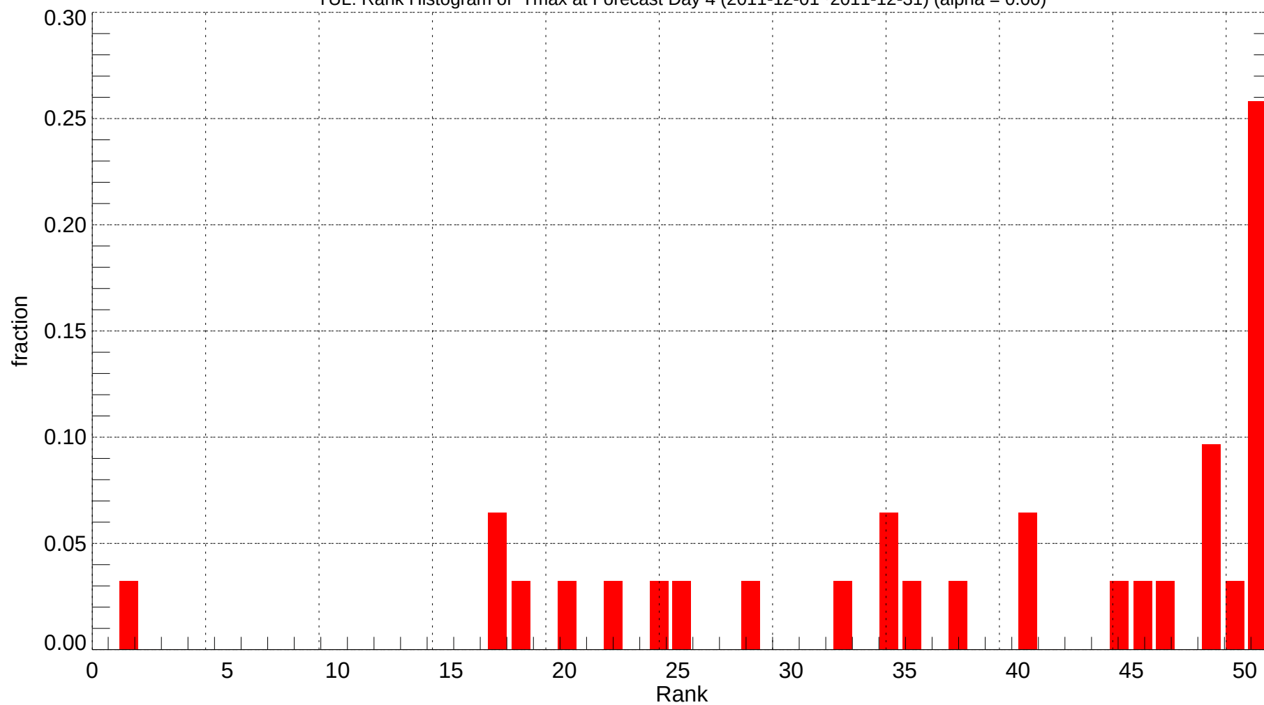
TUL: Rank Histogram of Tmax at Forecast Day 4 (2011-12-01~2011-12-31) (alpha = 0.00)
