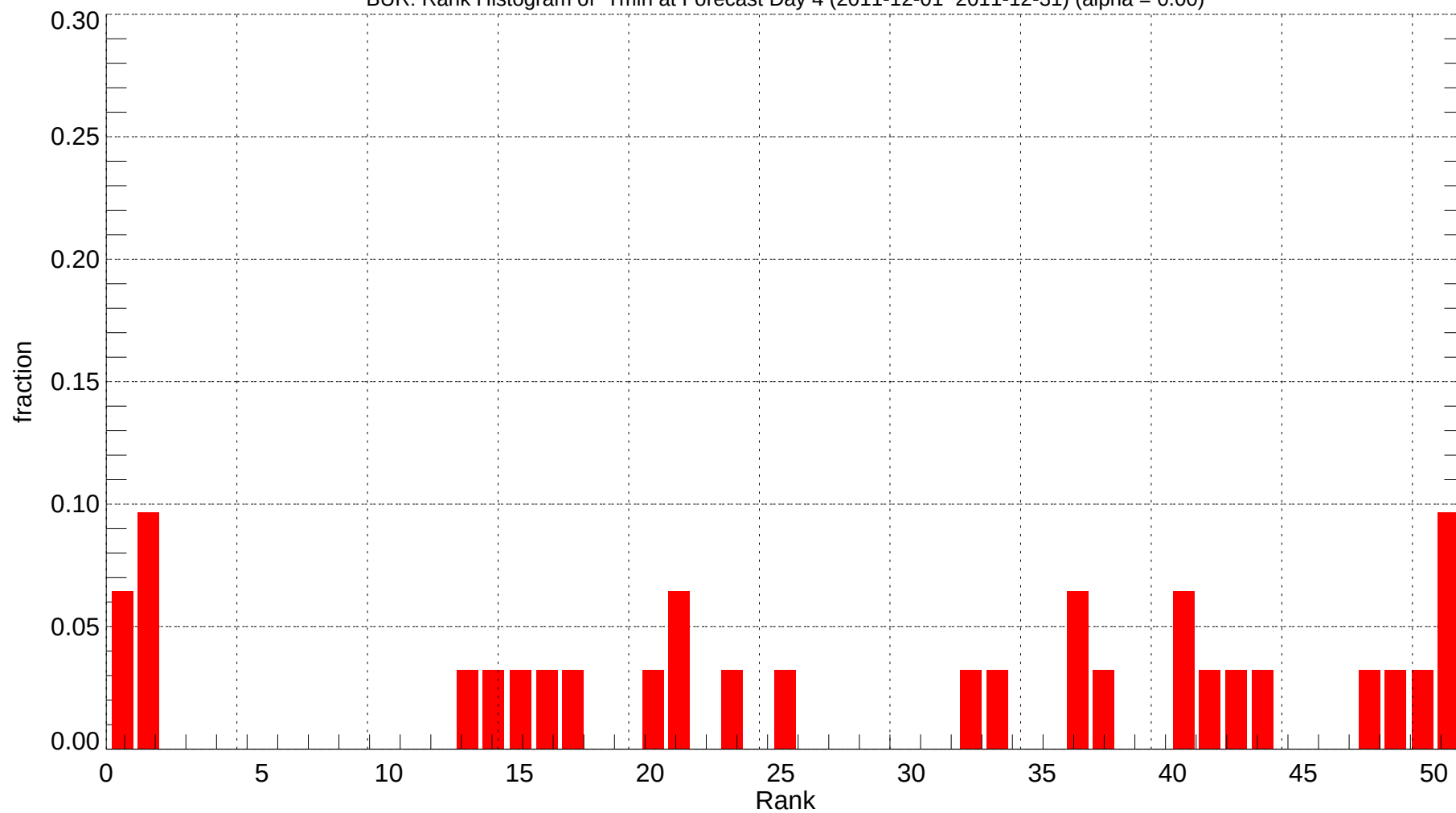
BUR: Rank Histogram of Tmin at Forecast Day 4 (2011-12-01~2011-12-31) (alpha = 0.00)
