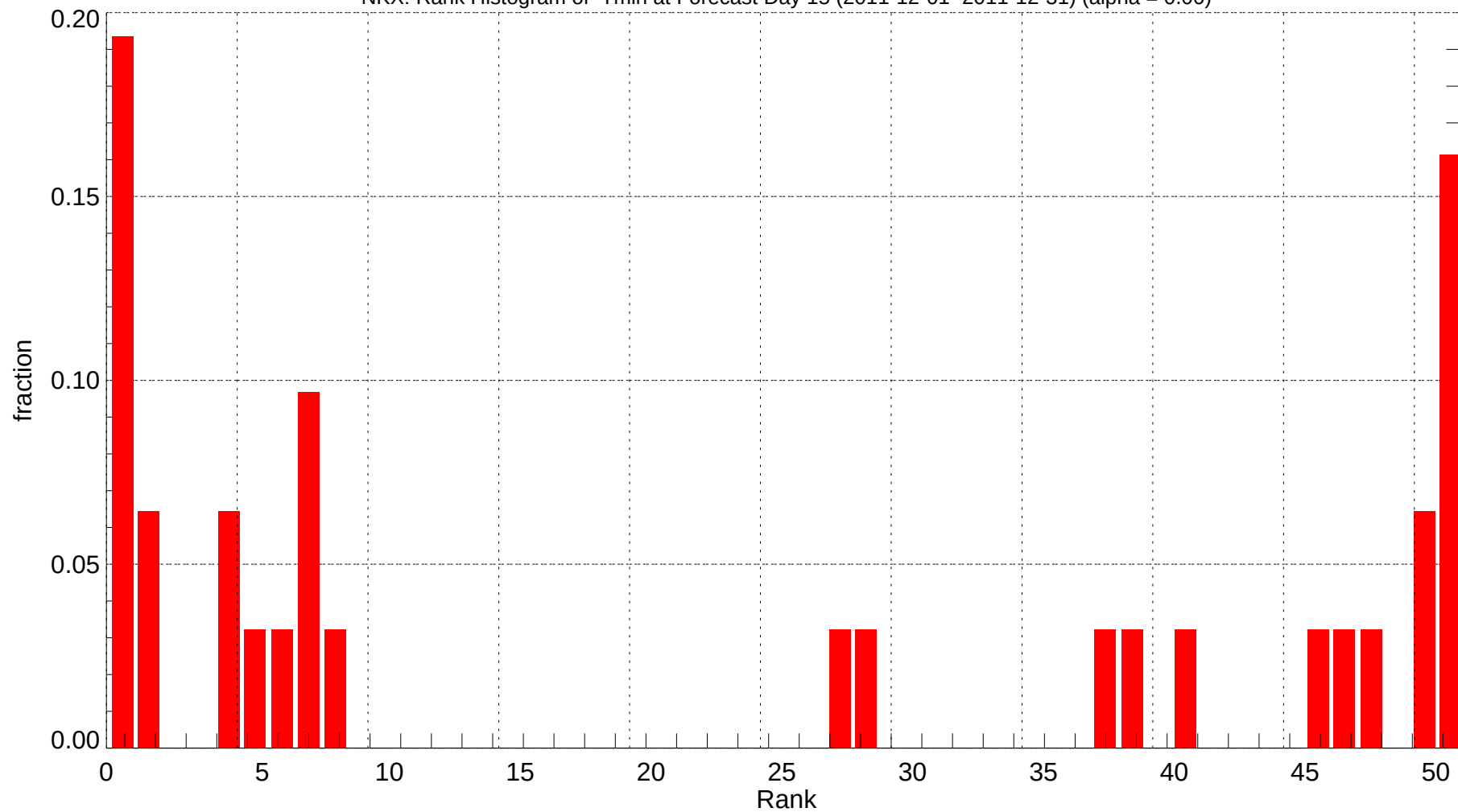
NKX: Rank Histogram of Tmin at Forecast Day 15 (2011-12-01~2011-12-31) (alpha = 0.00)
