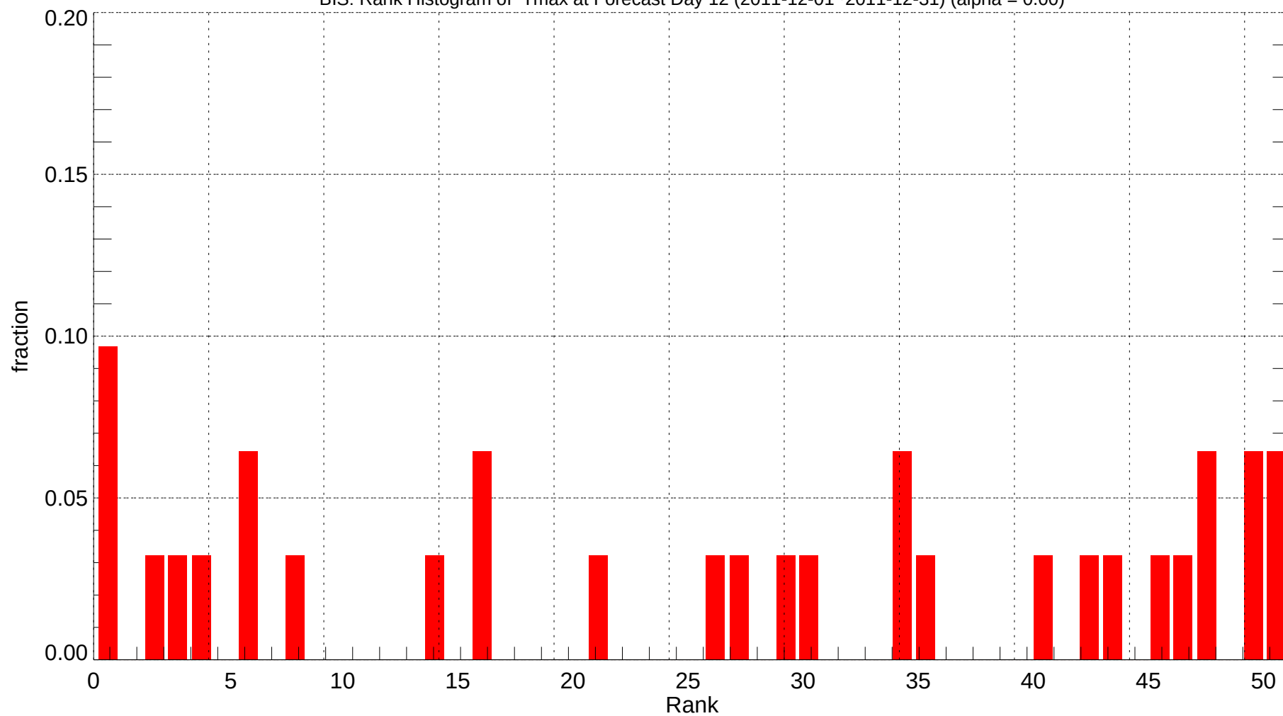
BIS: Rank Histogram of Tmax at Forecast Day 12 (2011-12-01~2011-12-31) (alpha = 0.00)
