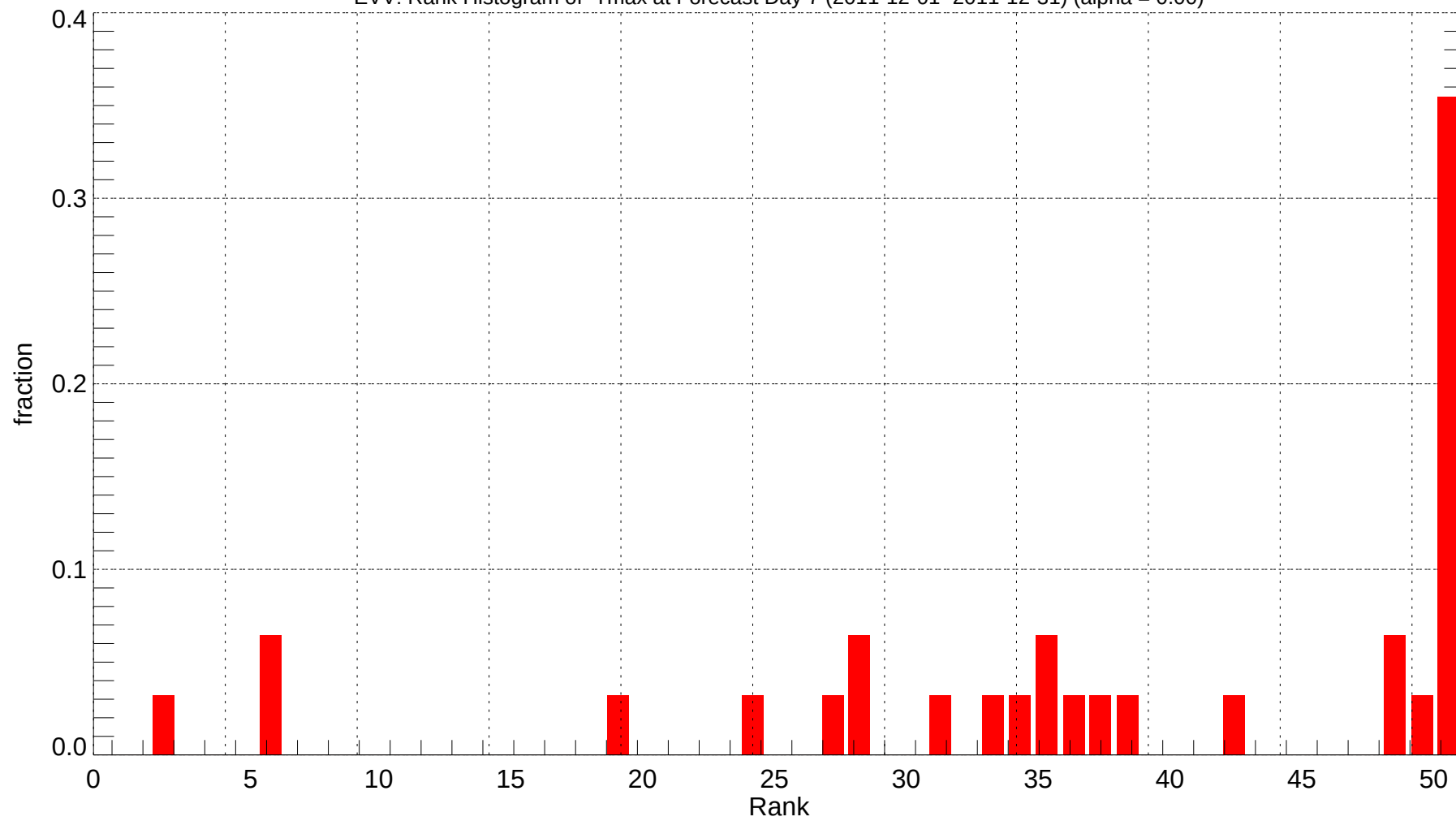
EVV: Rank Histogram of Tmax at Forecast Day 7 (2011-12-01~2011-12-31) (alpha = 0.00)
