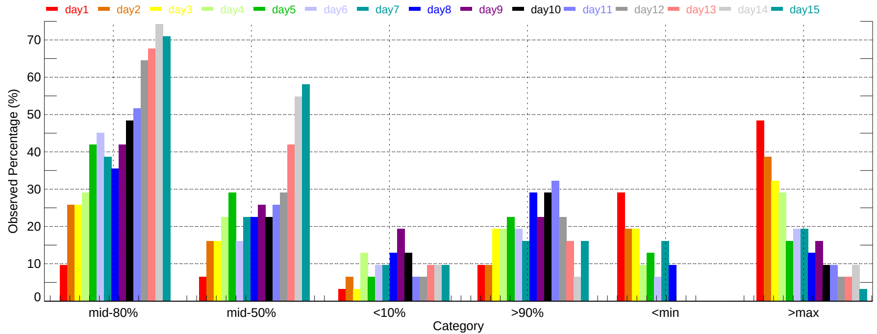
Observed Percentage of Ensembles - SAT: Min Temperature (2011-12-01~2011-12-31)
