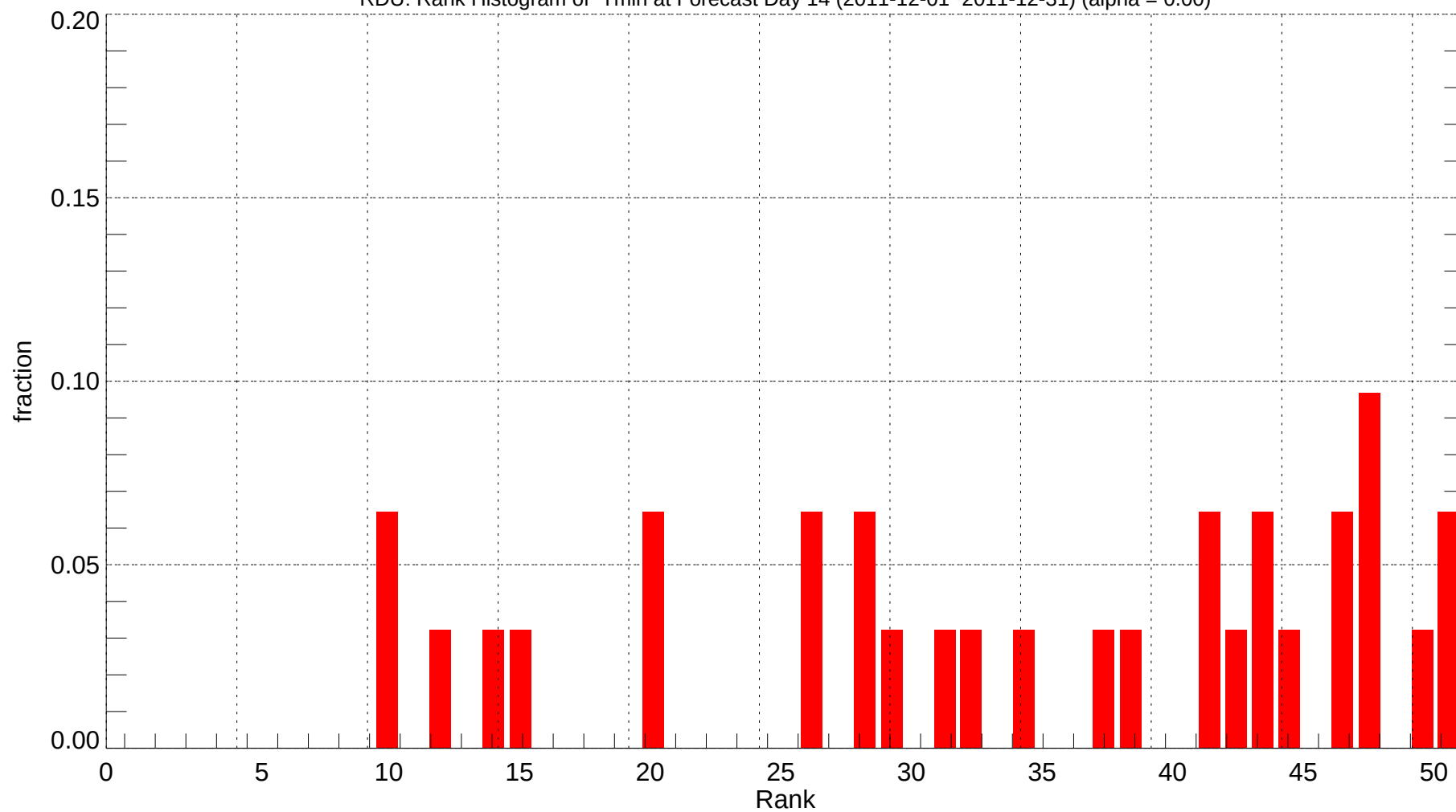
RDU: Rank Histogram of Tmin at Forecast Day 14 (2011-12-01~2011-12-31) (alpha = 0.00)
