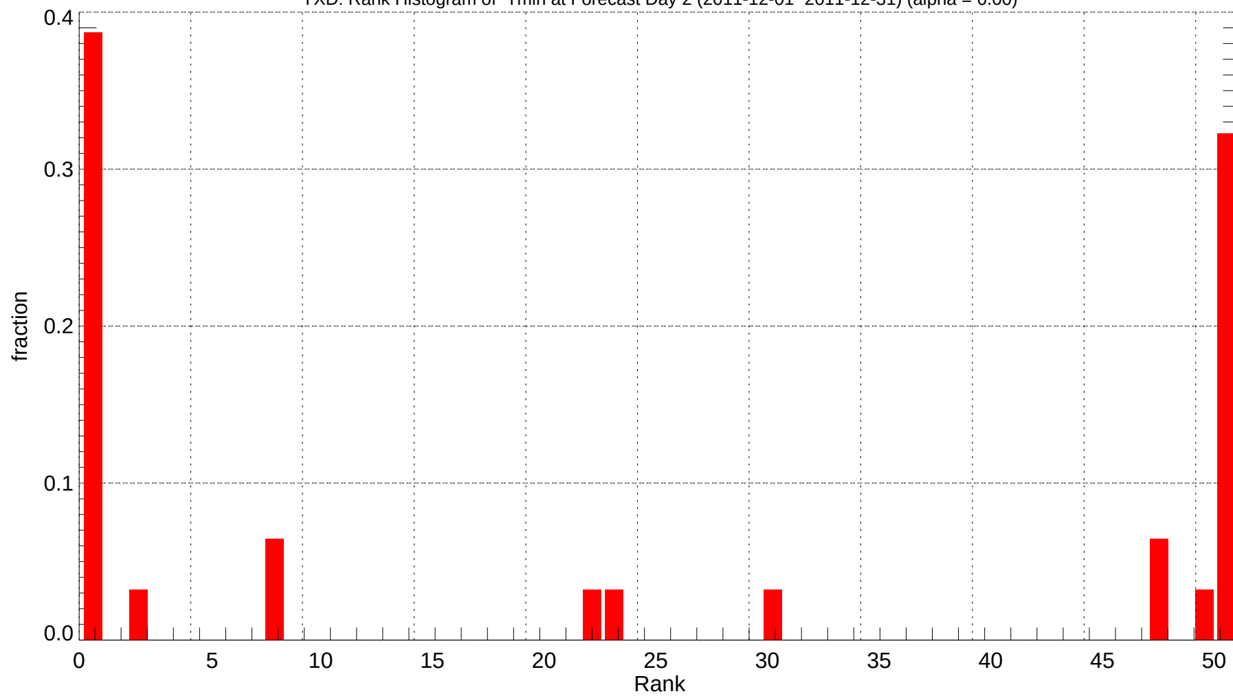
YXD: Rank Histogram of Tmin at Forecast Day 2 (2011-12-01~2011-12-31) (alpha = 0.00)
