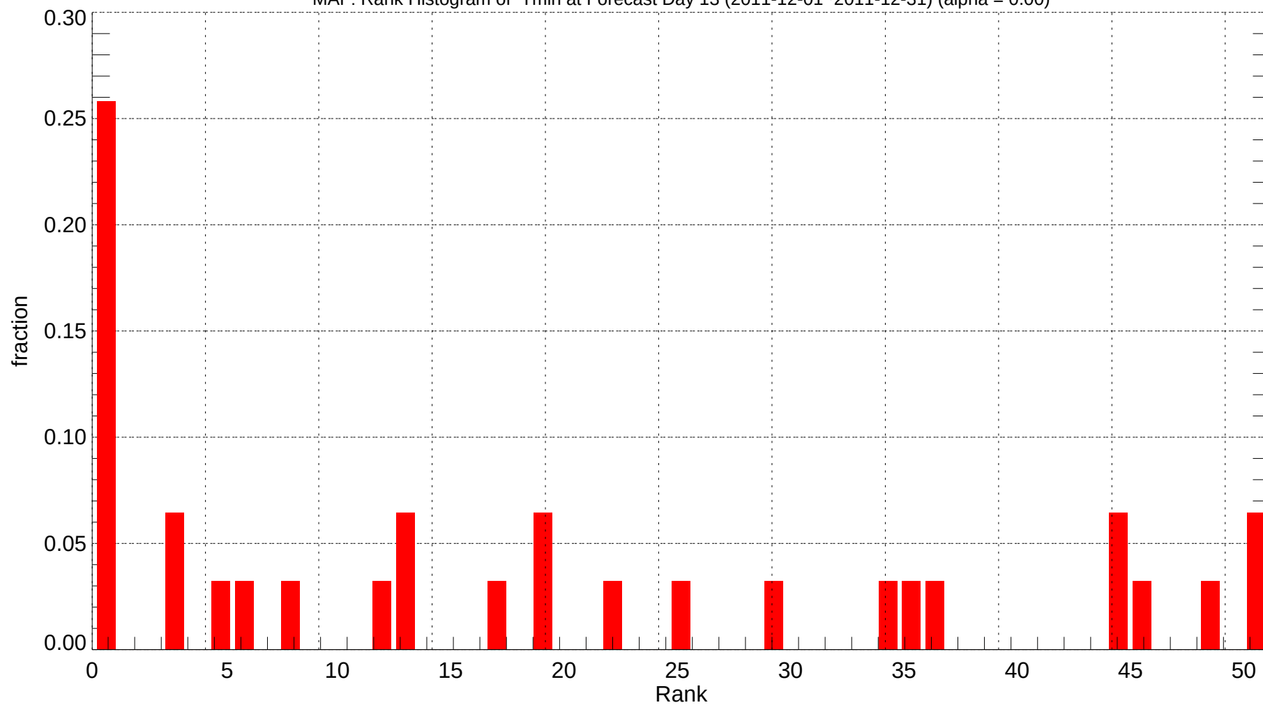
MAF: Rank Histogram of Tmin at Forecast Day 13 (2011-12-01~2011-12-31) (alpha = 0.00)
