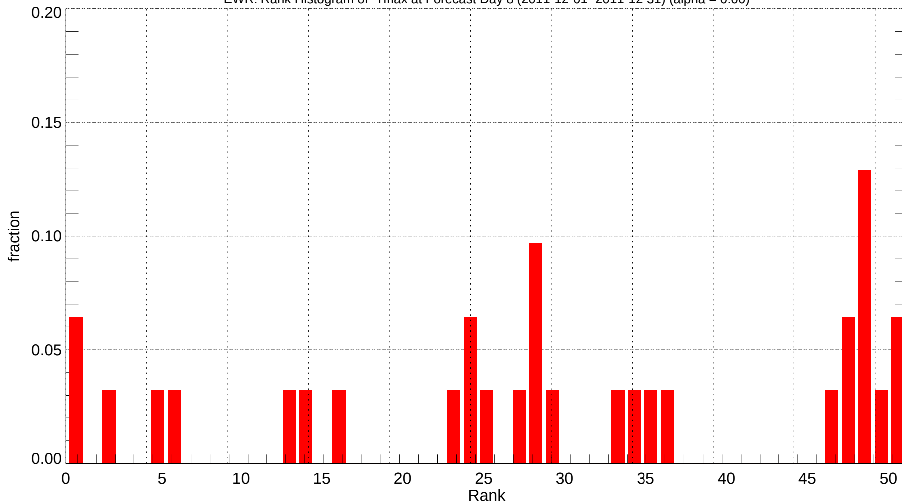
EWR: Rank Histogram of Tmax at Forecast Day 8 (2011-12-01~2011-12-31) (alpha = 0.00)
