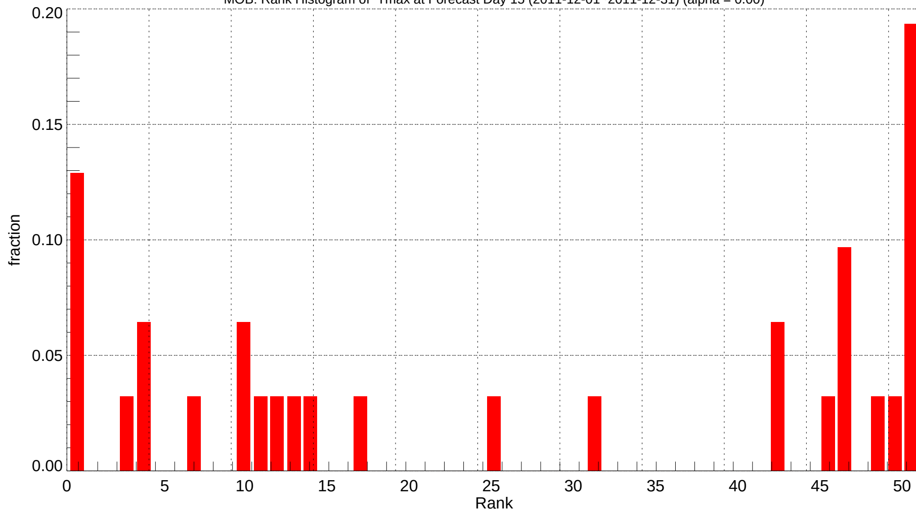
MOB: Rank Histogram of Tmax at Forecast Day 15 (2011-12-01~2011-12-31) (alpha = 0.00)
