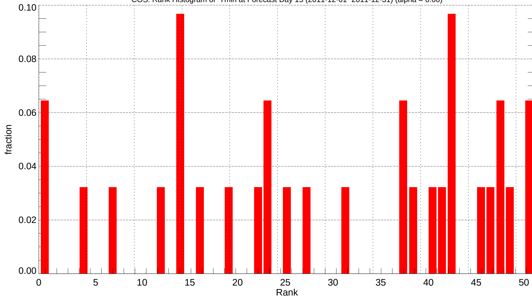
COS: Rank Histogram of Tmin at Forecast Day 15 (2011-12-01~2011-12-31) (alpha = 0.00)
