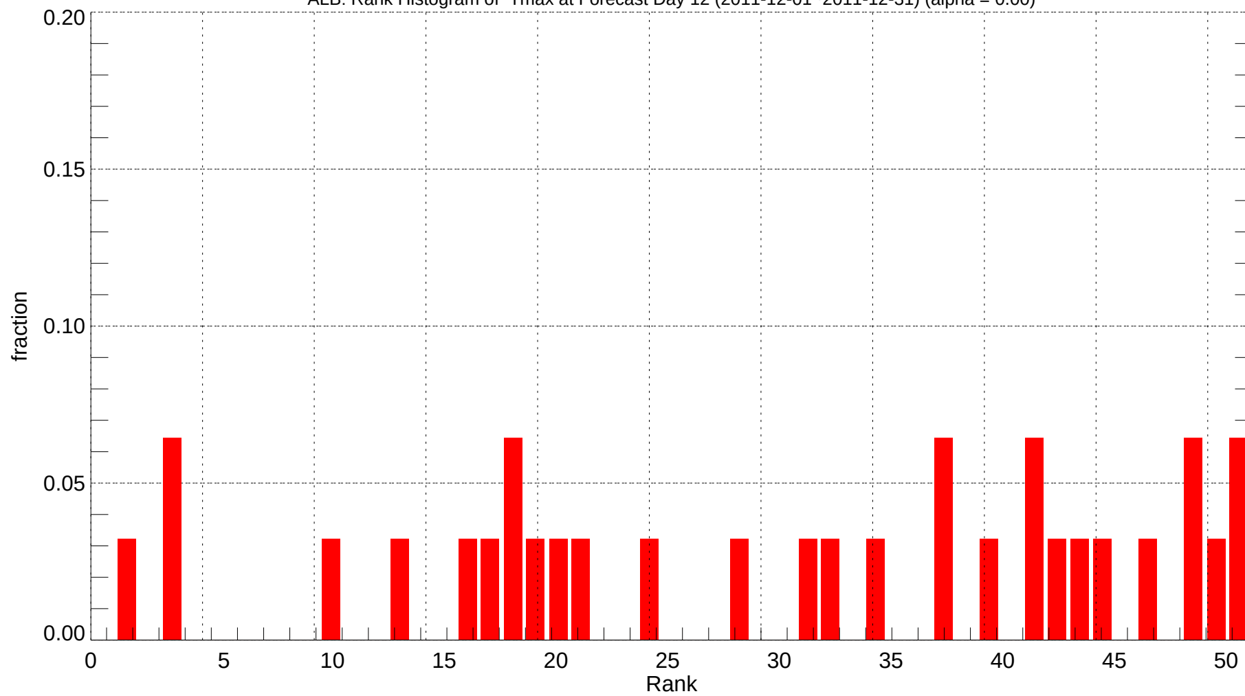
ALB: Rank Histogram of Tmax at Forecast Day 12 (2011-12-01~2011-12-31) (alpha = 0.00)
