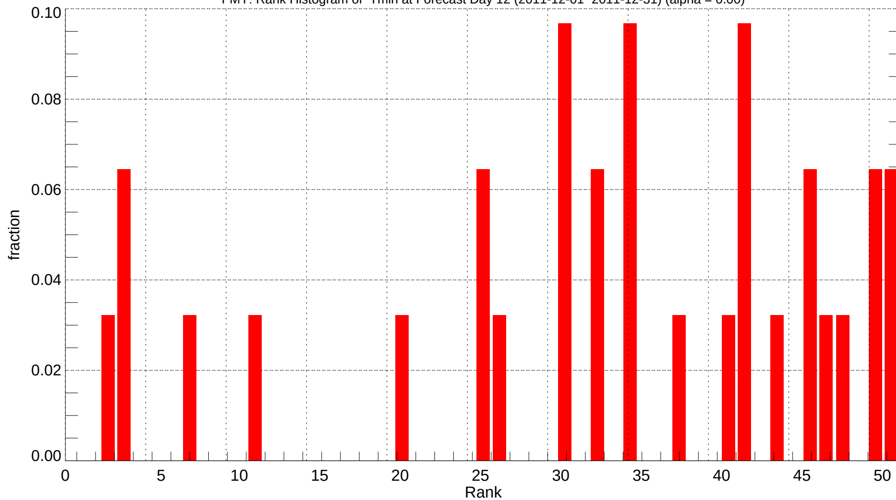
FMY: Rank Histogram of Tmin at Forecast Day 12 (2011-12-01~2011-12-31) (alpha = 0.00)
