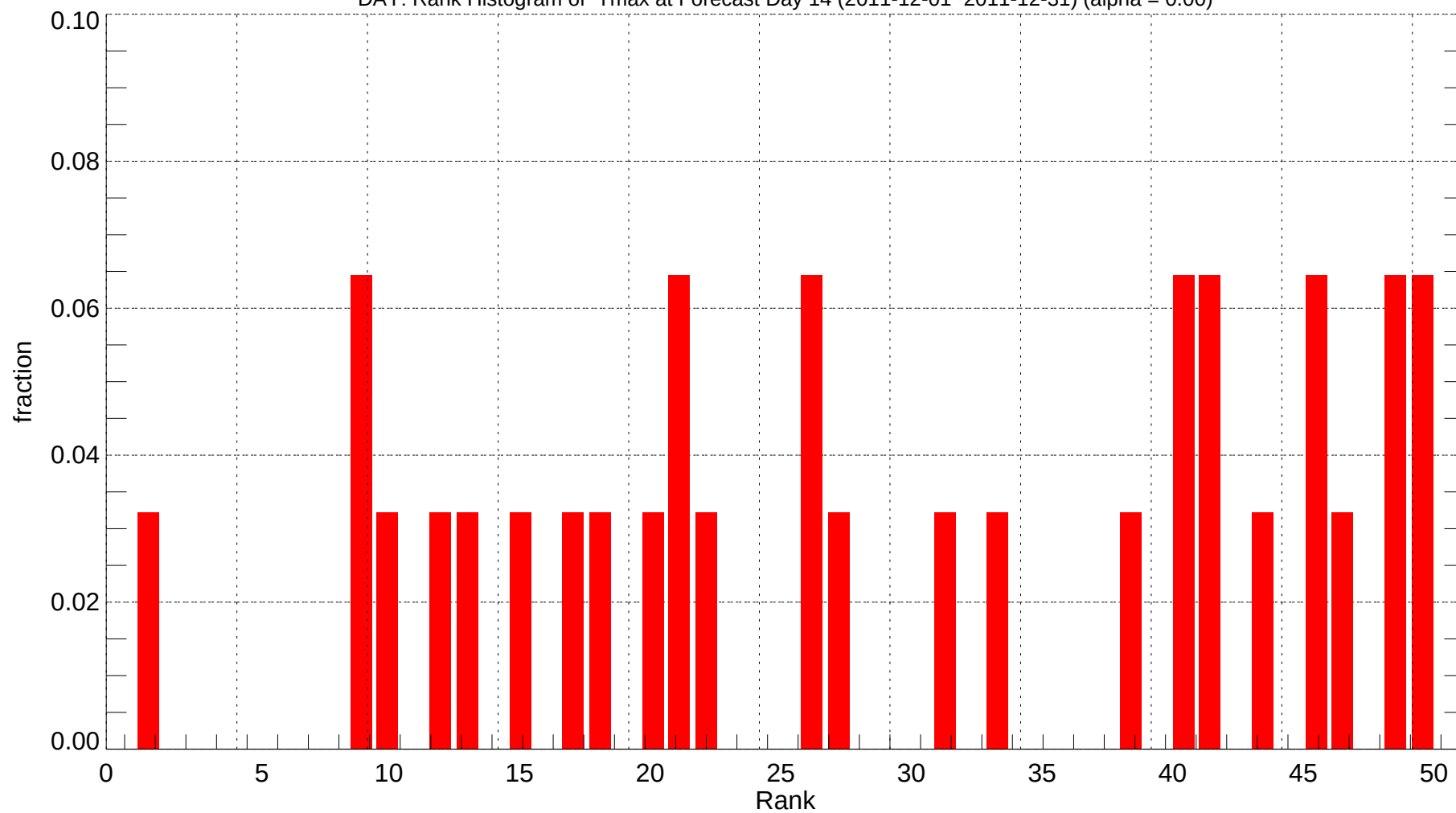
DAY: Rank Histogram of Tmax at Forecast Day 14 (2011-12-01~2011-12-31) (alpha = 0.00)
