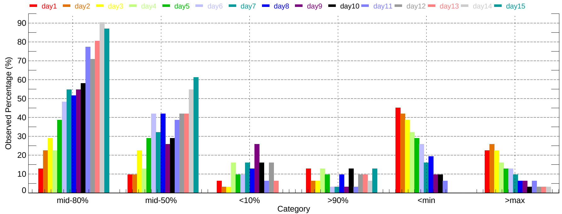
Observed Percentage of Ensembles - LGB: Min Temperature (2011-12-01~2011-12-31)
