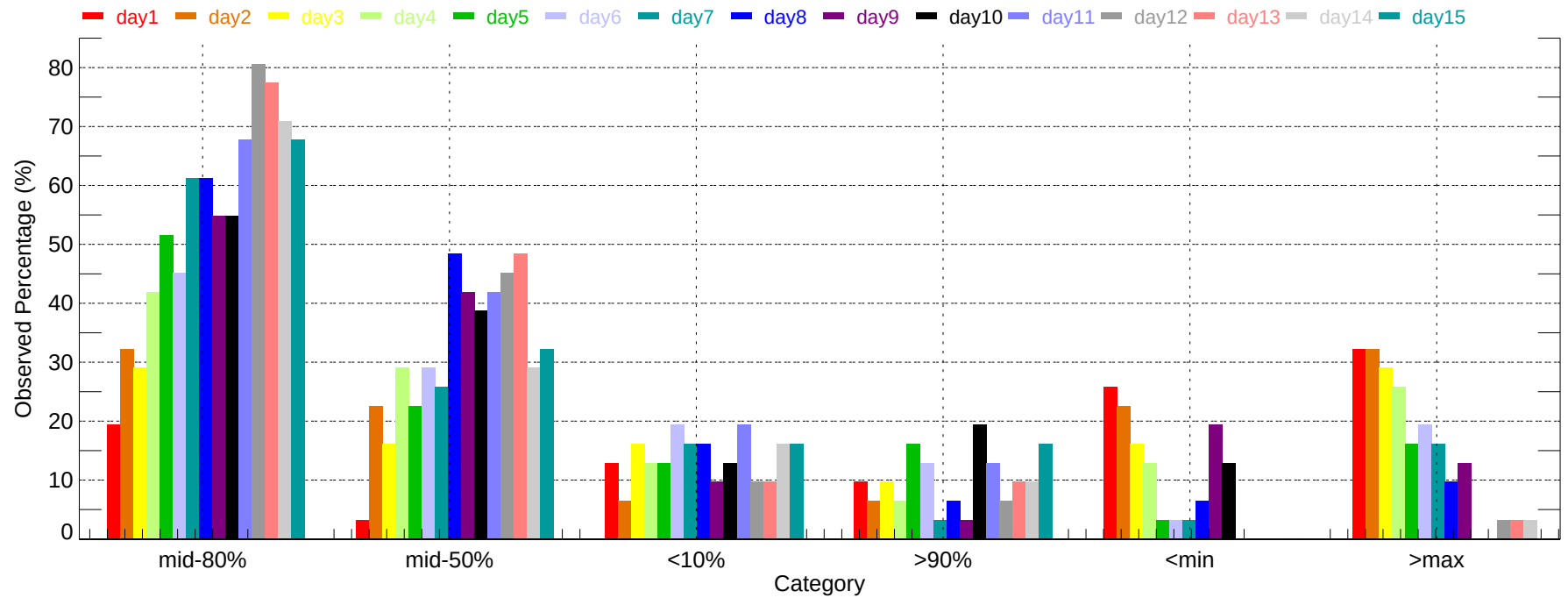
Observed Percentage of Ensembles - PHX: Max Temperature (2011-12-01~2011-12-31)
