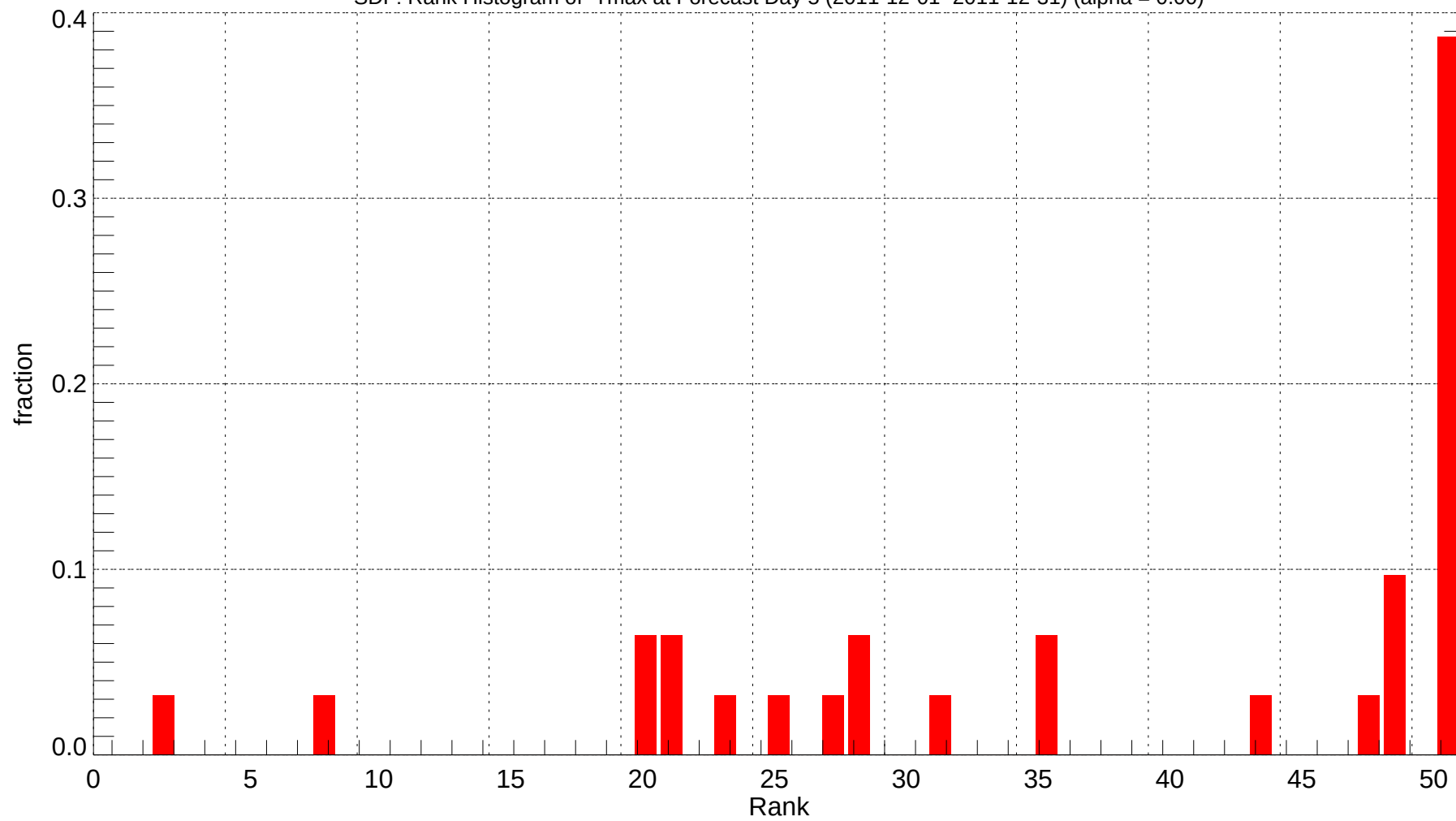
SDF: Rank Histogram of Tmax at Forecast Day 5 (2011-12-01~2011-12-31) (alpha = 0.00)
