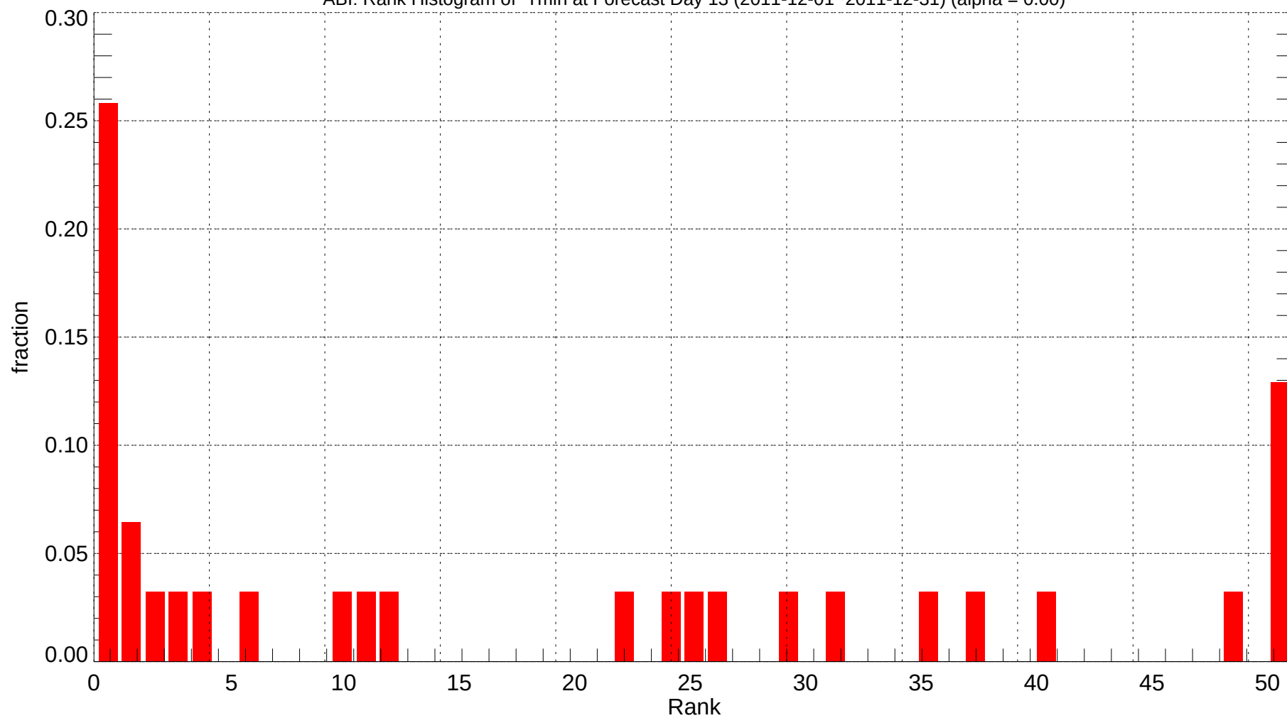
ABI: Rank Histogram of Tmin at Forecast Day 13 (2011-12-01~2011-12-31) (alpha = 0.00)
