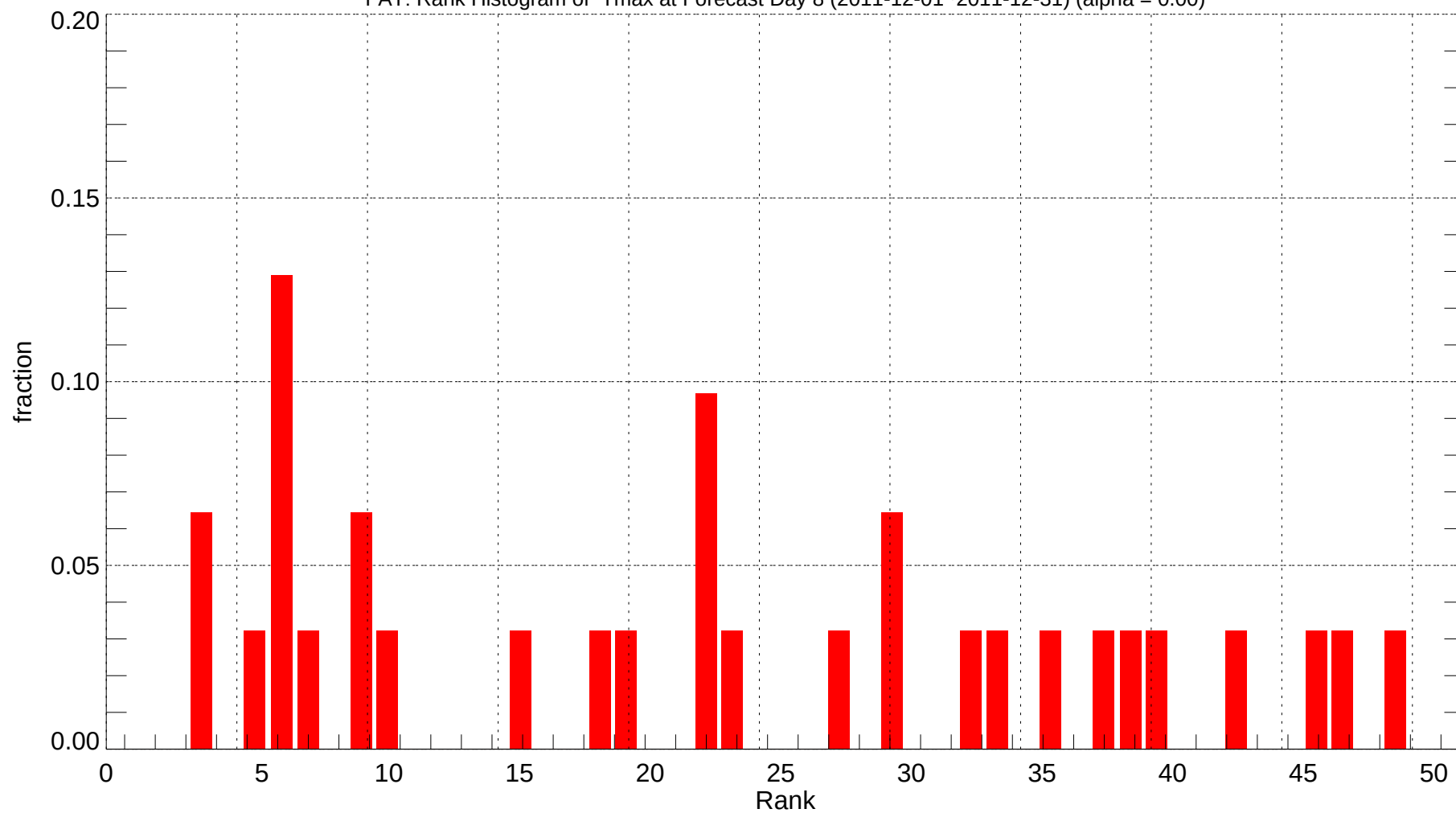
FAT: Rank Histogram of Tmax at Forecast Day 8 (2011-12-01~2011-12-31) (alpha = 0.00)
