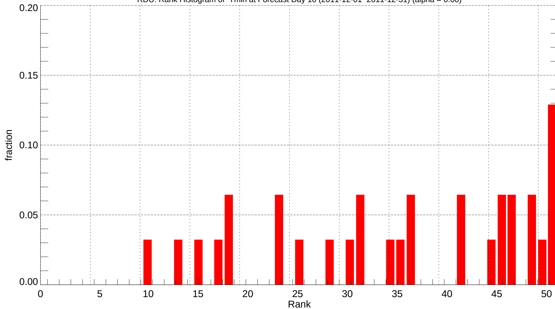
RDU: Rank Histogram of Tmin at Forecast Day 10 (2011-12-01~2011-12-31) (alpha = 0.00)
