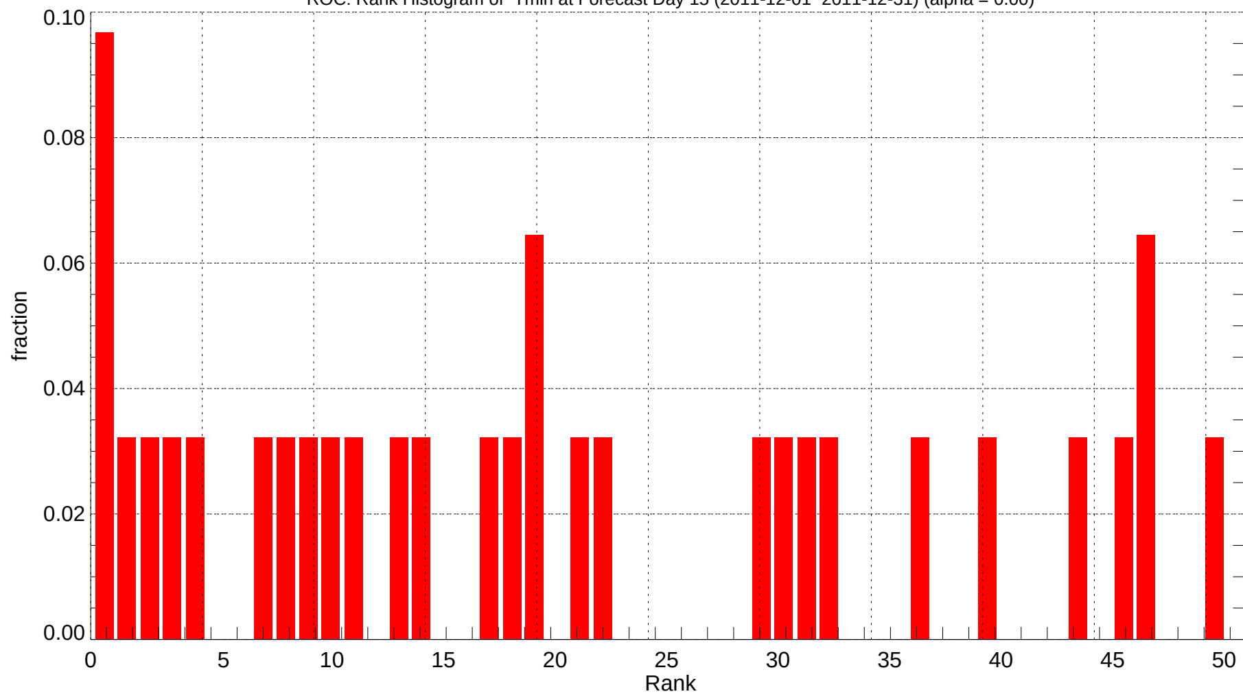
ROC: Rank Histogram of Tmin at Forecast Day 15 (2011-12-01~2011-12-31) (alpha = 0.00)
