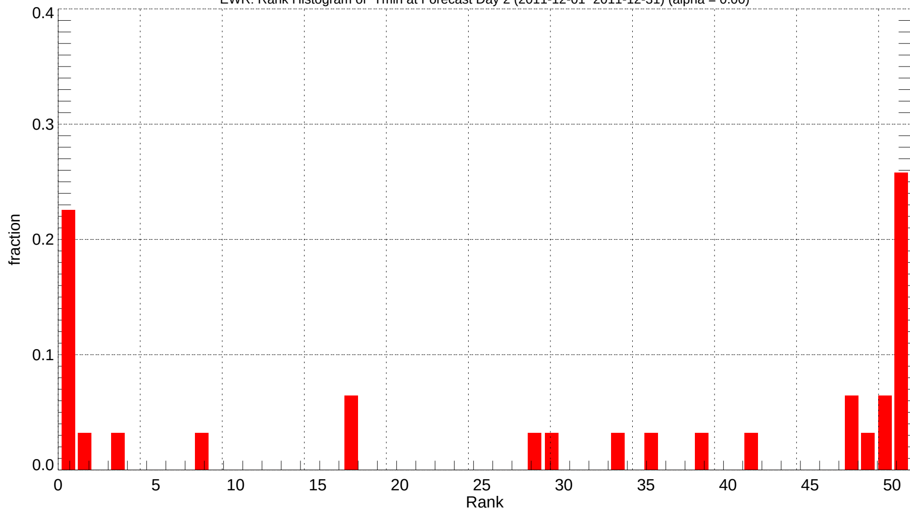
EWR: Rank Histogram of Tmin at Forecast Day 2 (2011-12-01~2011-12-31) (alpha = 0.00)
