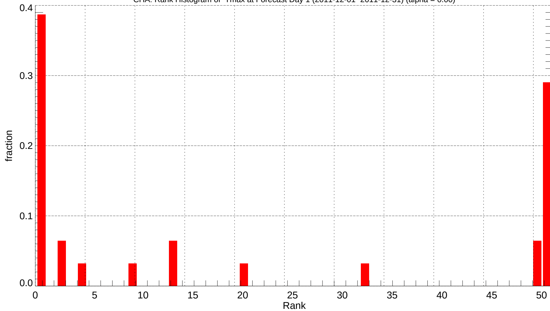
CHA: Rank Histogram of Tmax at Forecast Day 1 (2011-12-01~2011-12-31) (alpha = 0.00)
