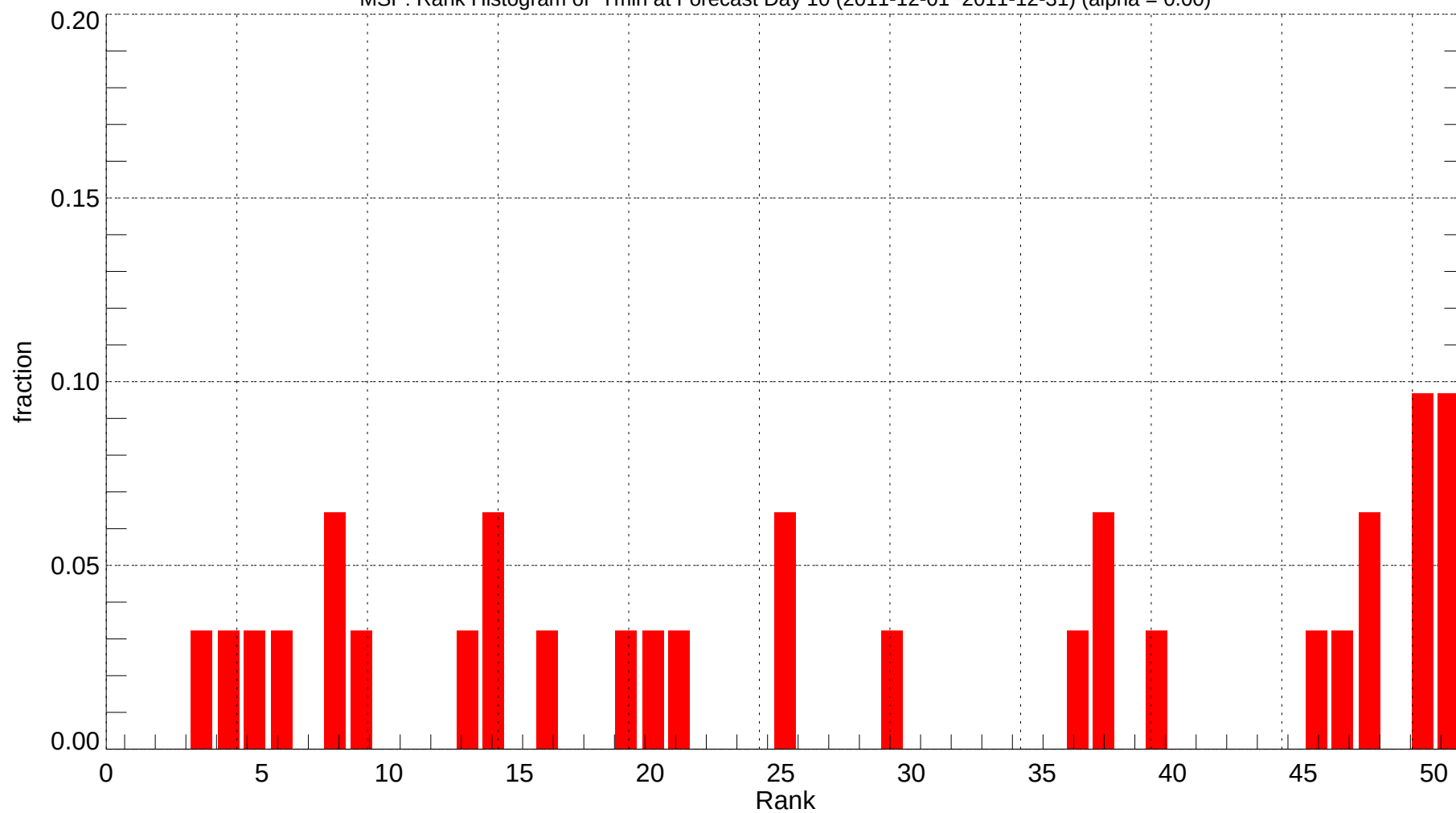
MSP: Rank Histogram of Tmin at Forecast Day 10 (2011-12-01~2011-12-31) (alpha = 0.00)
