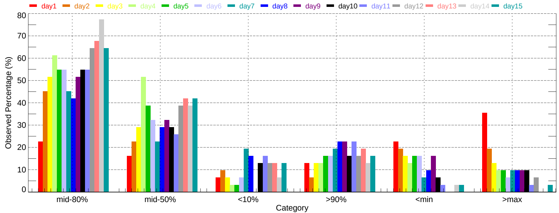
Observed Percentage of Ensembles - CON: Max Temperature (2011-12-01~2011-12-31)
