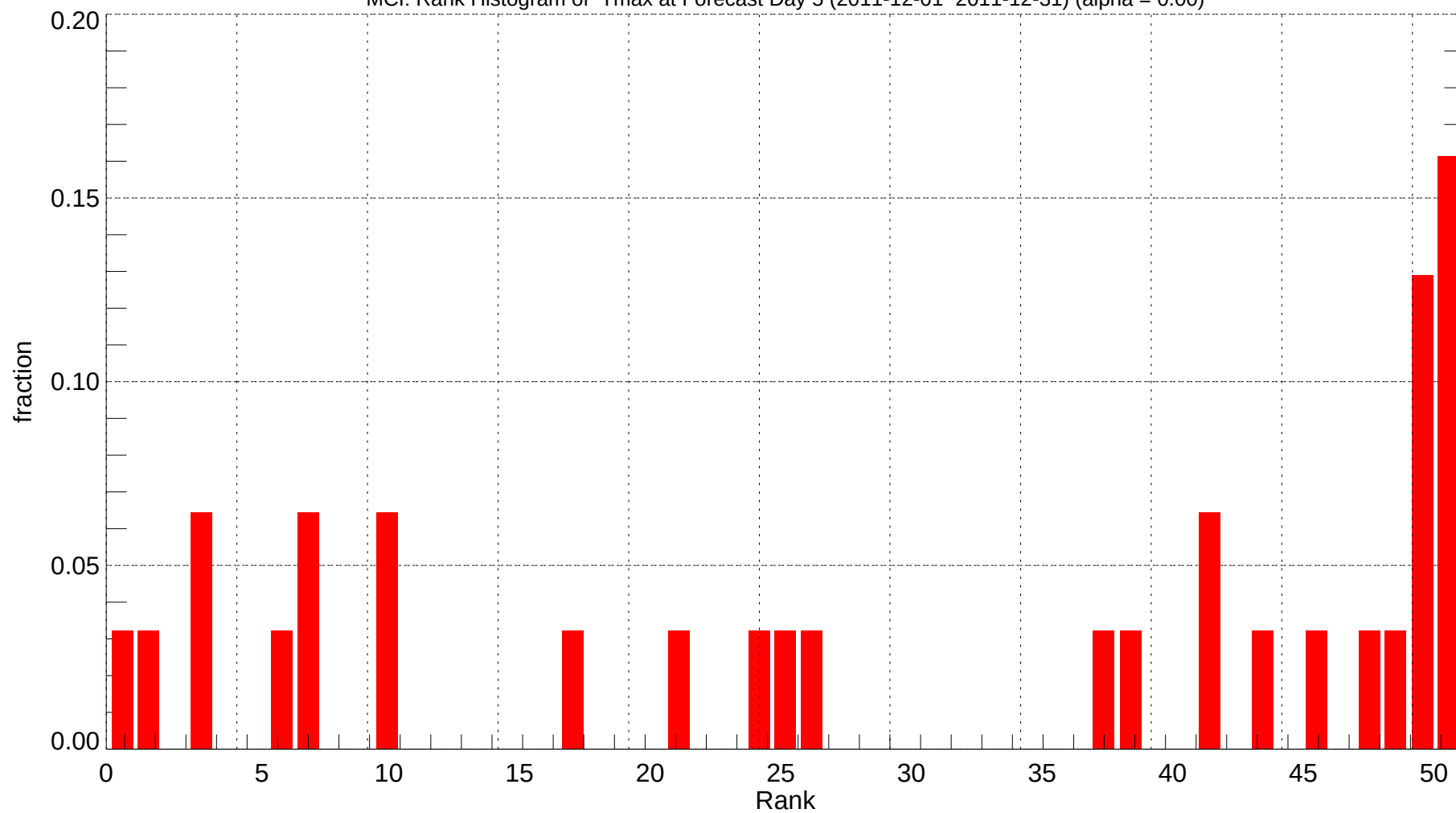
MCI: Rank Histogram of Tmax at Forecast Day 5 (2011-12-01~2011-12-31) (alpha = 0.00)
