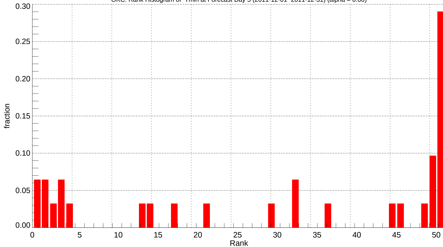
OKC: Rank Histogram of Tmin at Forecast Day 5 (2011-12-01~2011-12-31) (alpha = 0.00)
