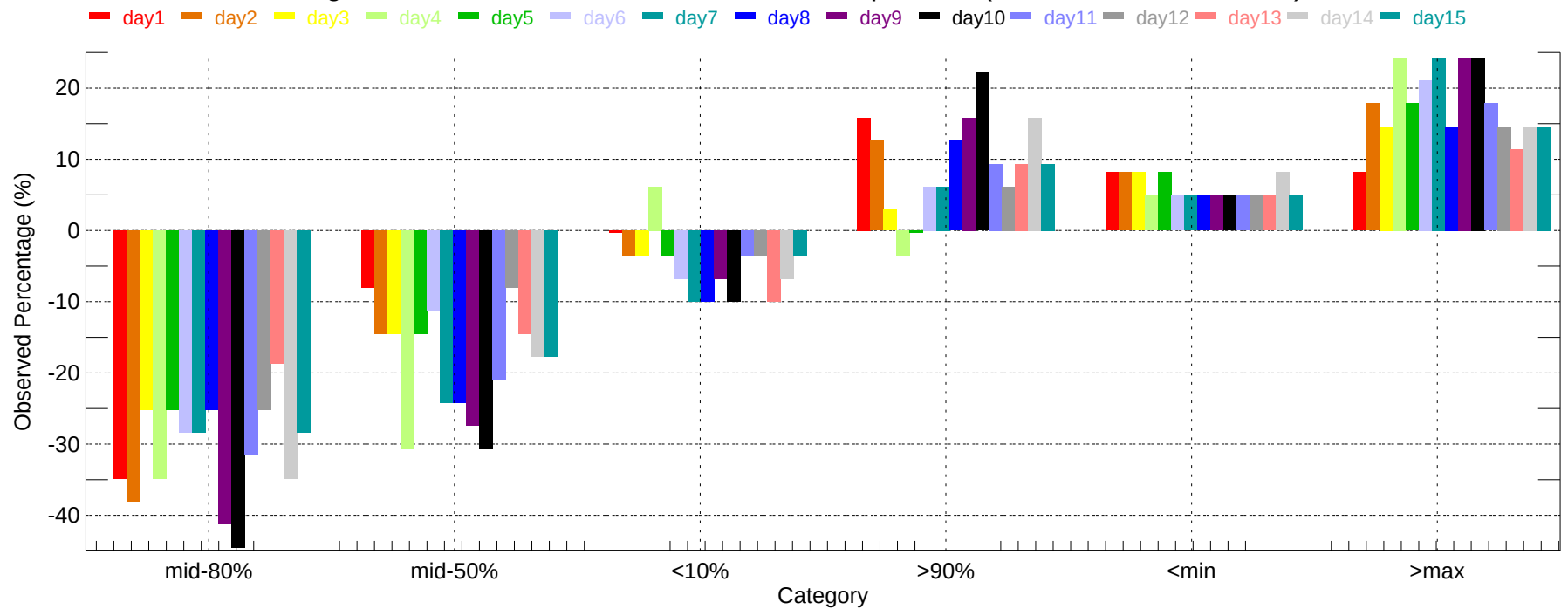
Observed Percentage Deviation of Ensembles - DLH: Max Temperature (2011-12-01~2011-12-31)
