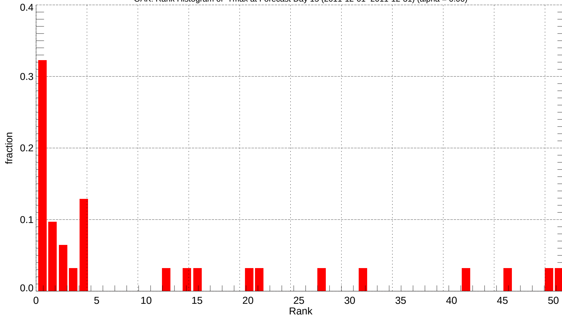
OAK: Rank Histogram of Tmax at Forecast Day 15 (2011-12-01~2011-12-31) (alpha = 0.00)
