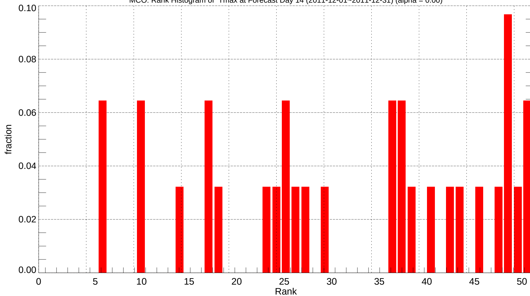
MCO: Rank Histogram of Tmax at Forecast Day 14 (2011-12-01~2011-12-31) (alpha = 0.00)
