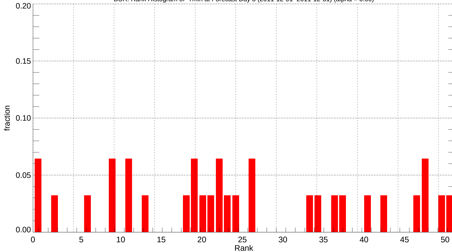
BUR: Rank Histogram of Tmin at Forecast Day 8 (2011-12-01~2011-12-31) (alpha = 0.00)
