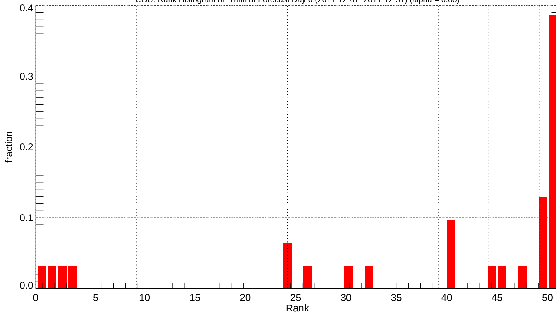
COU: Rank Histogram of Tmin at Forecast Day 6 (2011-12-01~2011-12-31) (alpha = 0.00)
