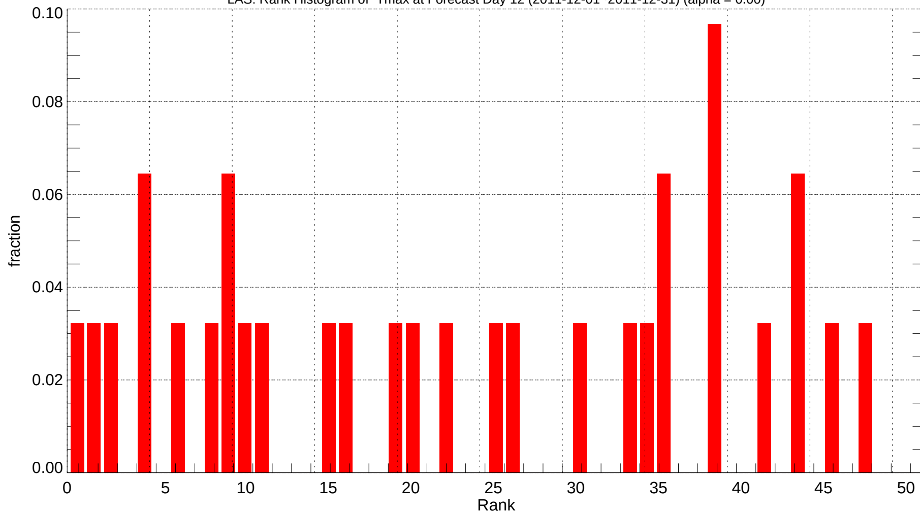
LAS: Rank Histogram of Tmax at Forecast Day 12 (2011-12-01~2011-12-31) (alpha = 0.00)
