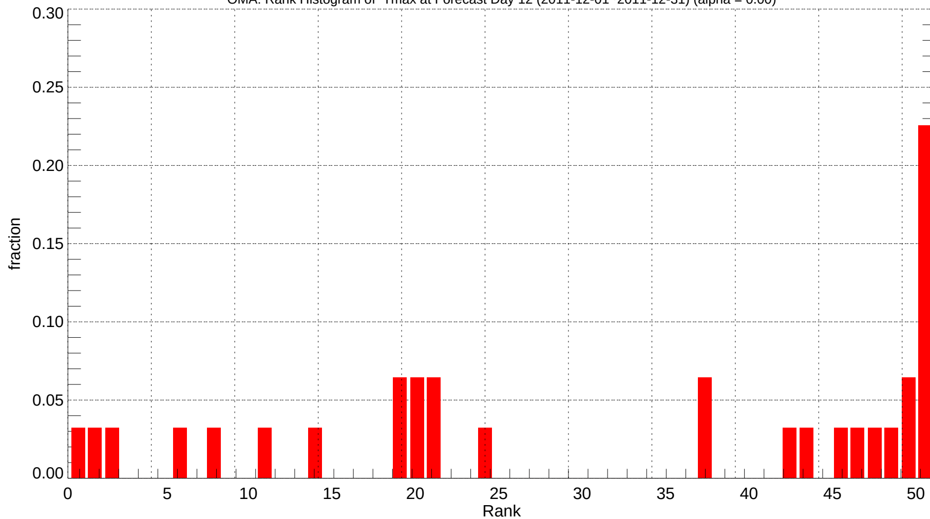
OMA: Rank Histogram of Tmax at Forecast Day 12 (2011-12-01~2011-12-31) (alpha = 0.00)
