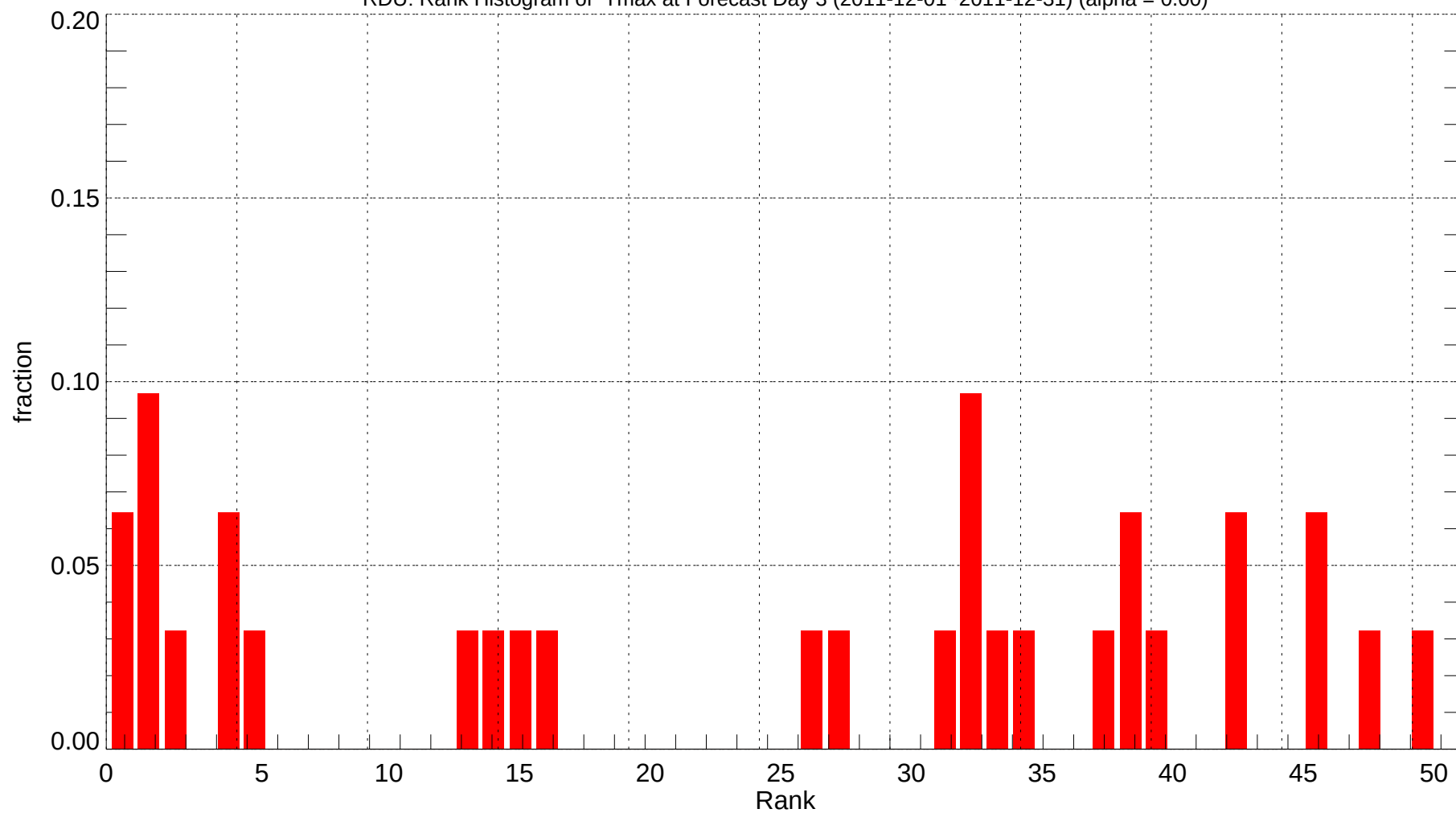
RDU: Rank Histogram of Tmax at Forecast Day 3 (2011-12-01~2011-12-31) (alpha = 0.00)
