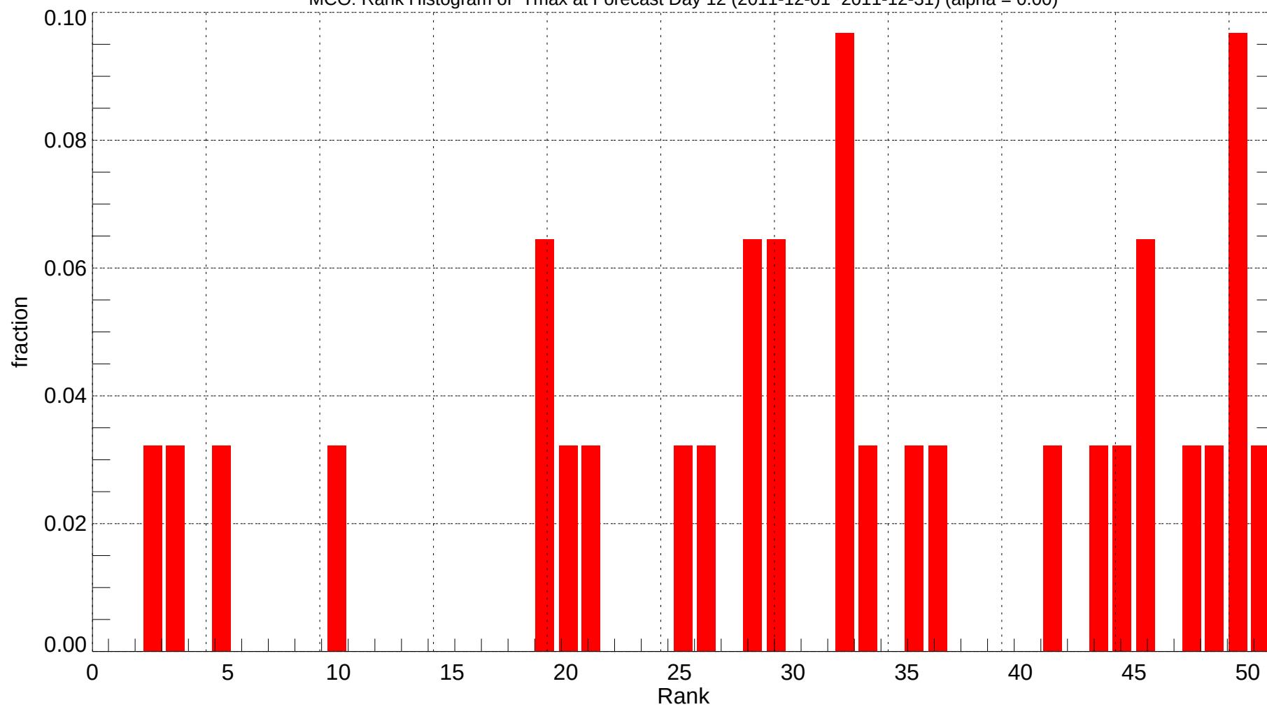
MCO: Rank Histogram of Tmax at Forecast Day 12 (2011-12-01~2011-12-31) (alpha = 0.00)
