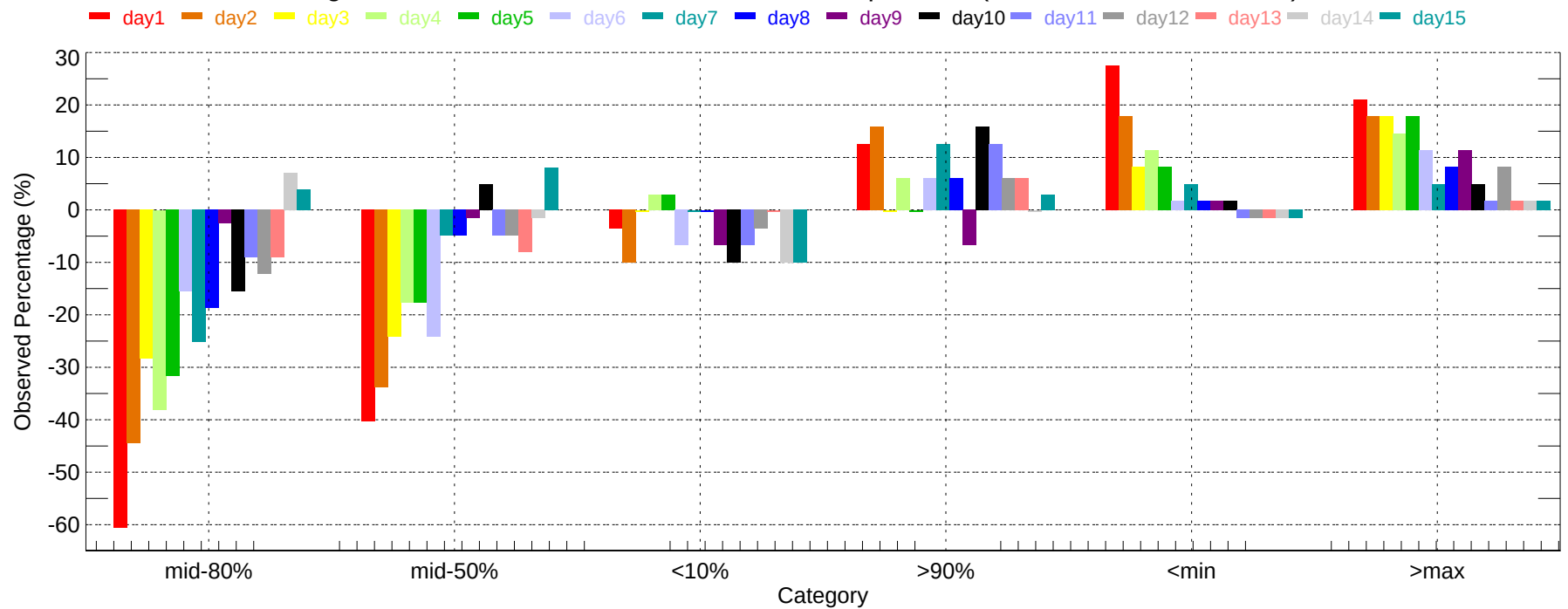
Observed Percentage Deviation of Ensembles - RDU: Min Temperature (2011-12-01~2011-12-31)
