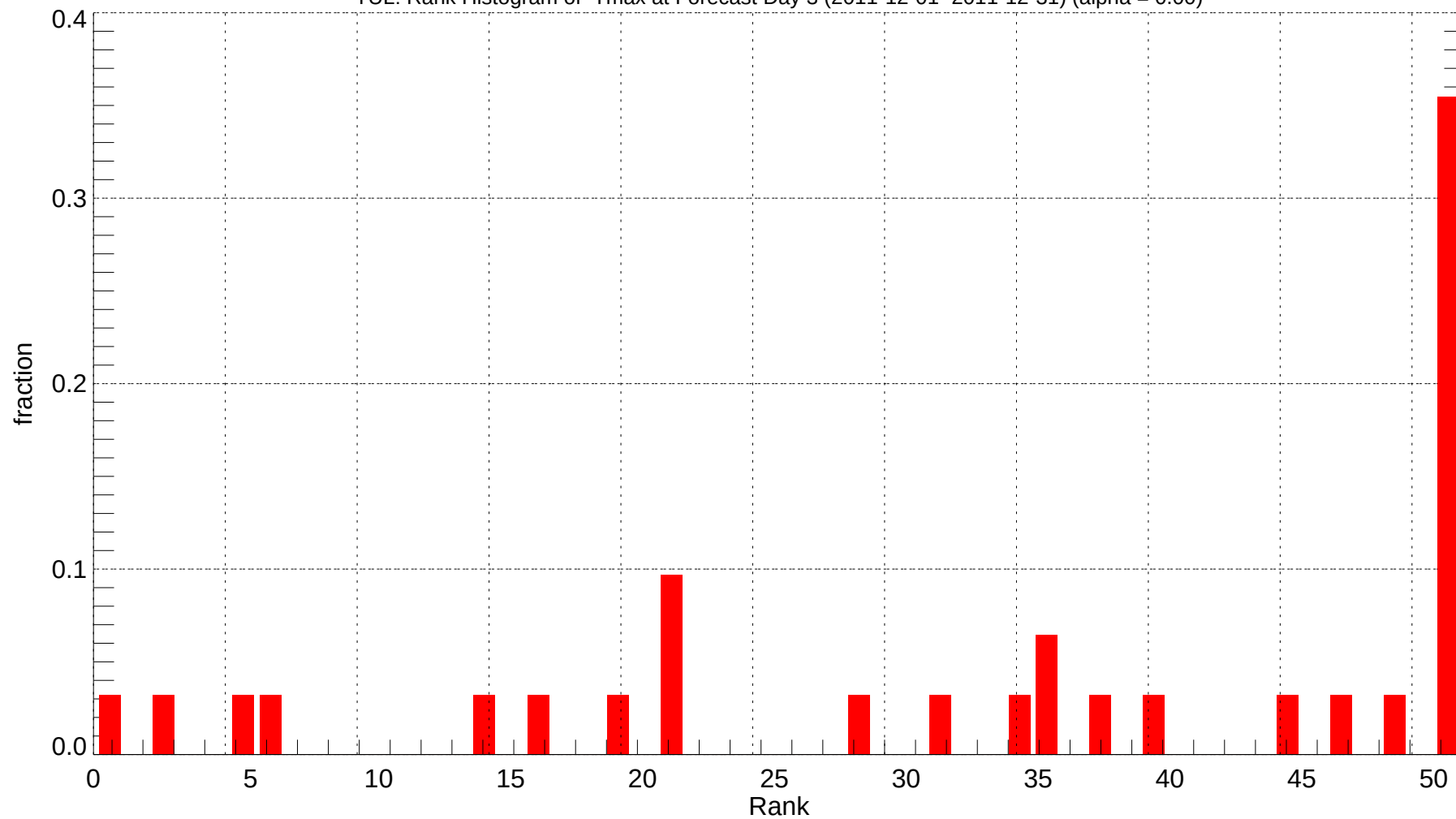
TUL: Rank Histogram of Tmax at Forecast Day 3 (2011-12-01~2011-12-31) (alpha = 0.00)
