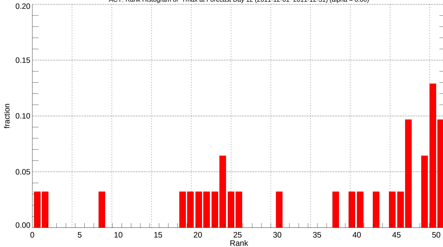
ACY: Rank Histogram of Tmax at Forecast Day 12 (2011-12-01~2011-12-31) (alpha = 0.00)
