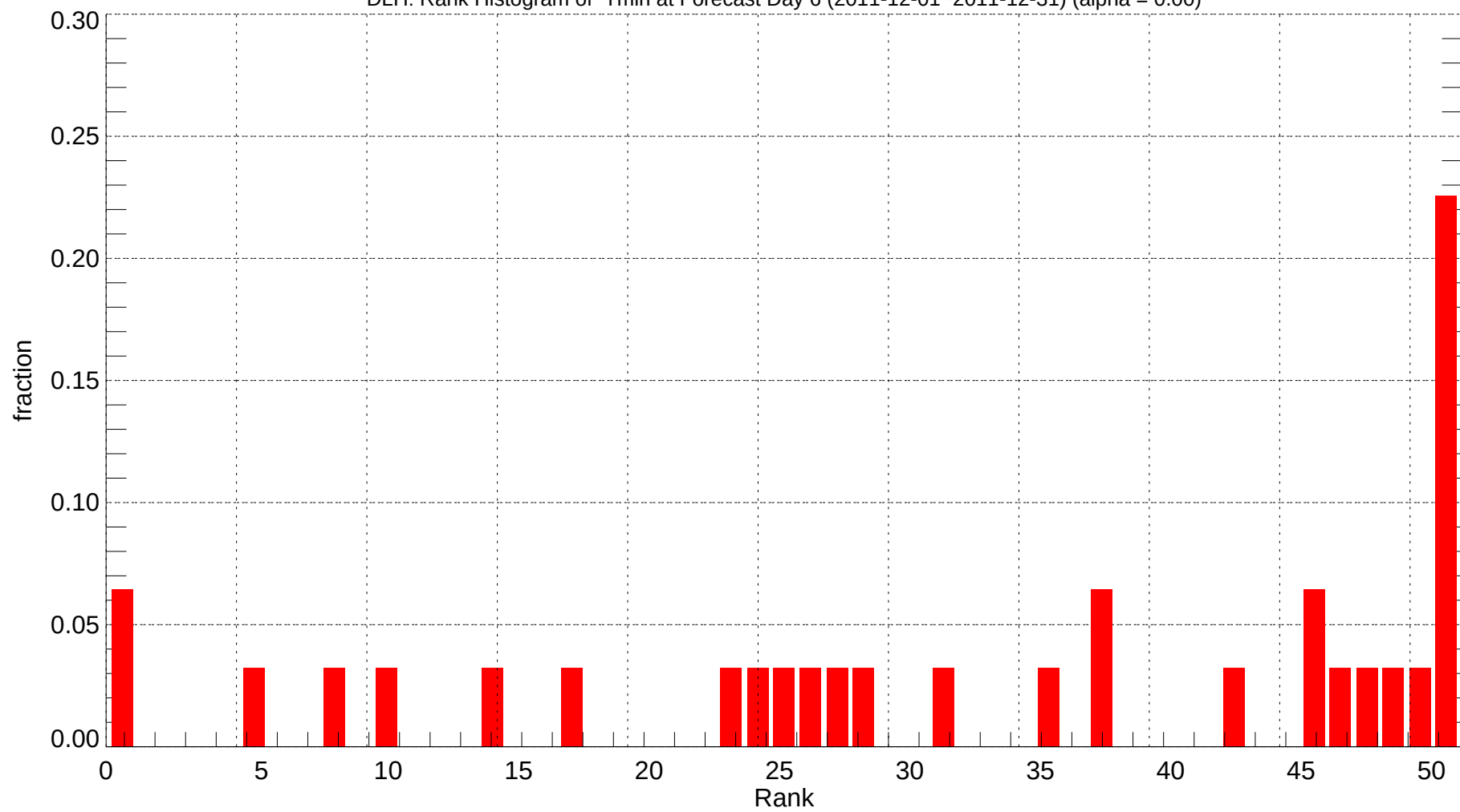
DLH: Rank Histogram of Tmin at Forecast Day 6 (2011-12-01~2011-12-31) (alpha = 0.00)
