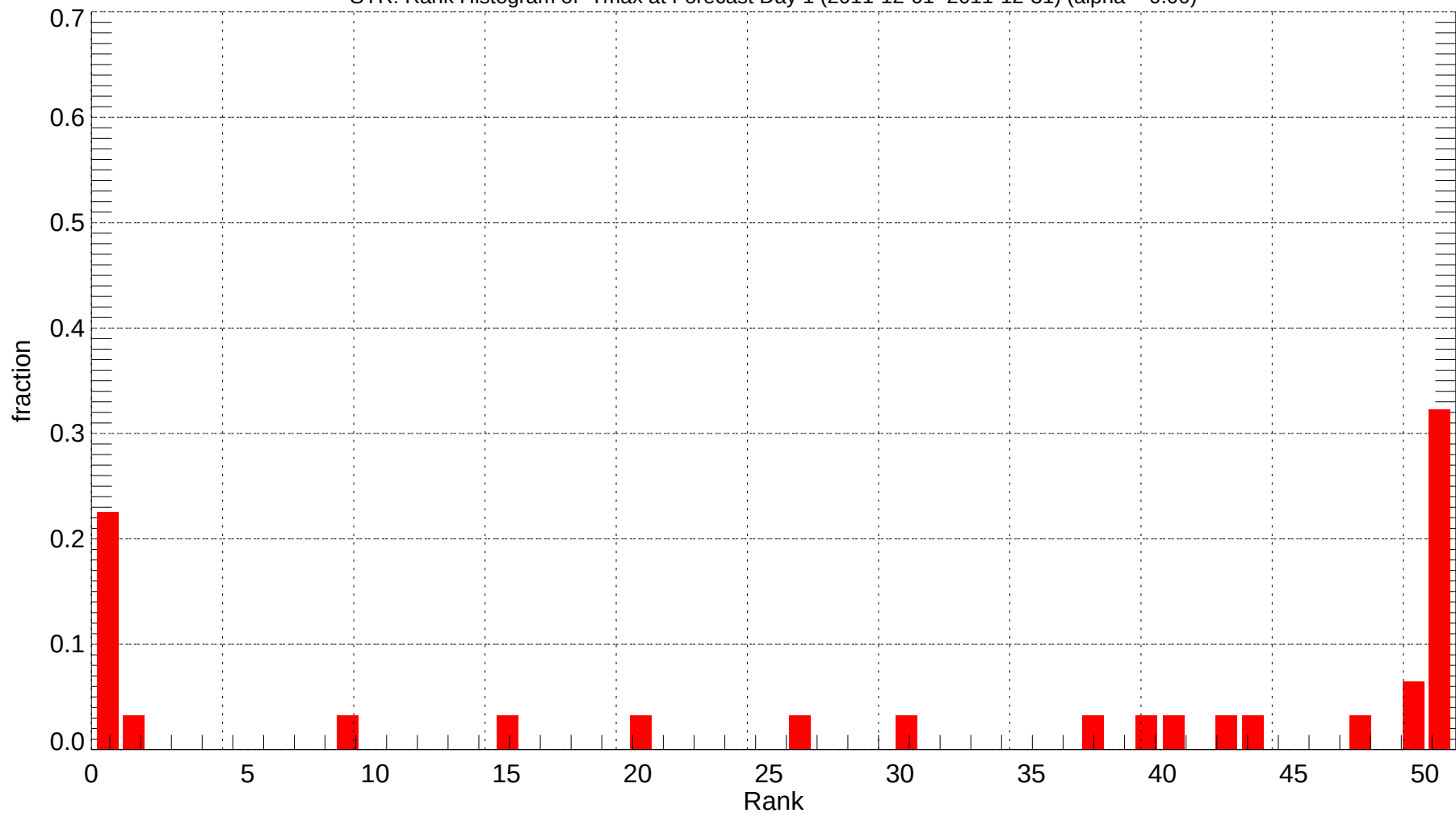
SYR: Rank Histogram of Tmax at Forecast Day 1 (2011-12-01~2011-12-31) (alpha = 0.00)
