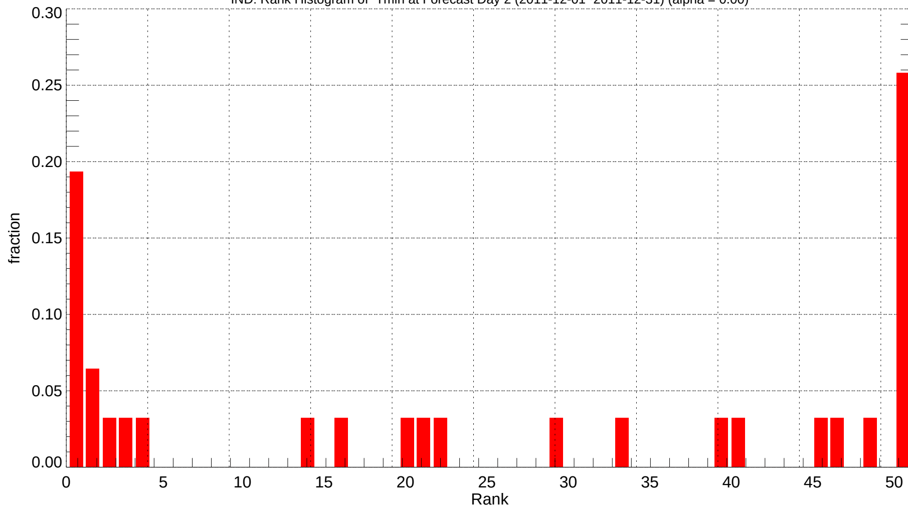
IND: Rank Histogram of Tmin at Forecast Day 2 (2011-12-01~2011-12-31) (alpha = 0.00)
