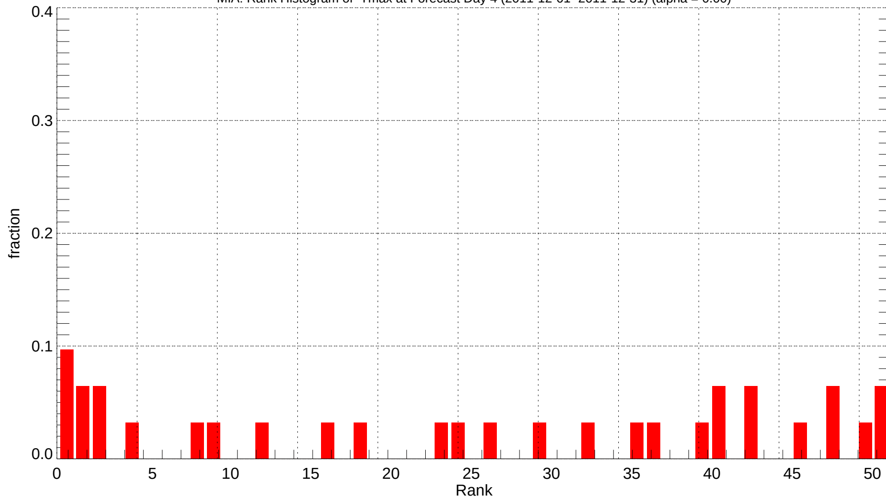
MIA: Rank Histogram of Tmax at Forecast Day 4 (2011-12-01~2011-12-31) (alpha = 0.00)
