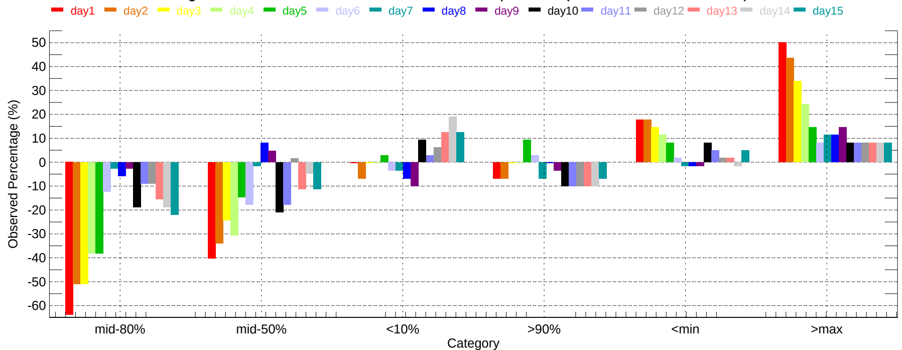
Observed Percentage Deviation of Ensembles - SLC: Max Temperature (2011-12-01~2011-12-31)
