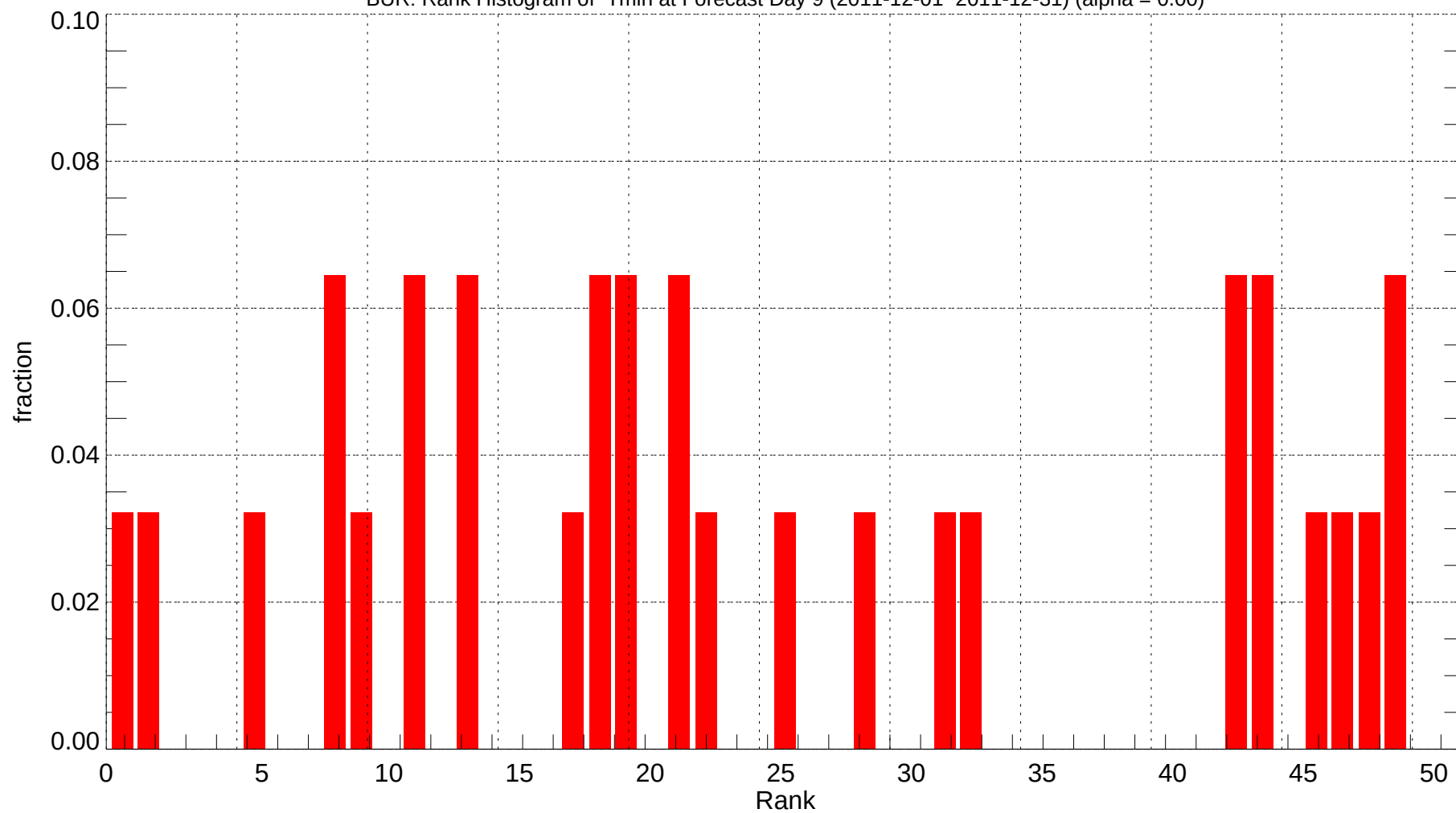
BUR: Rank Histogram of Tmin at Forecast Day 9 (2011-12-01~2011-12-31) (alpha = 0.00)
