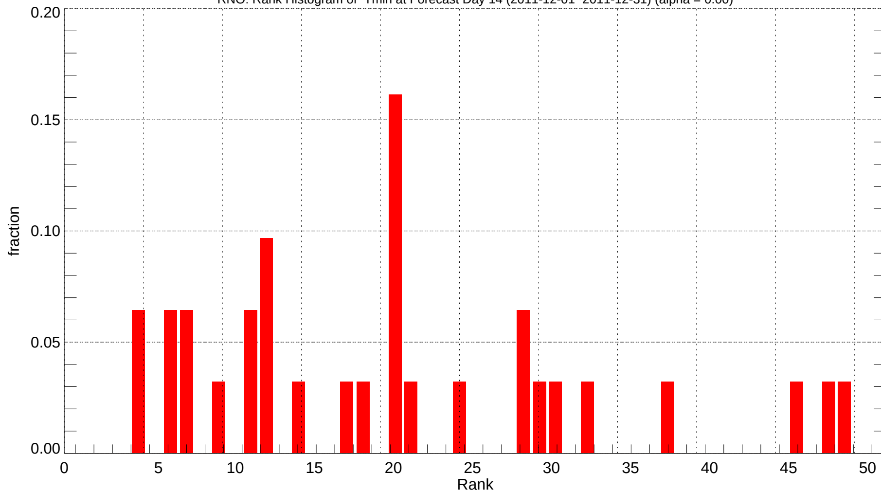
RNO: Rank Histogram of Tmin at Forecast Day 14 (2011-12-01~2011-12-31) (alpha = 0.00)
