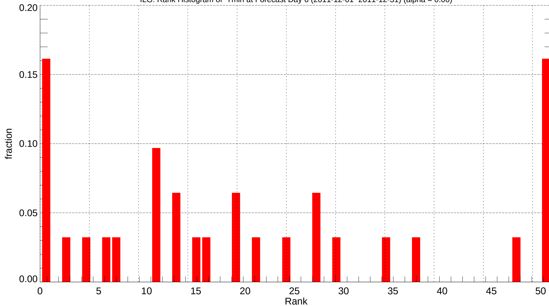
ILG: Rank Histogram of Tmin at Forecast Day 6 (2011-12-01~2011-12-31) (alpha = 0.00)
