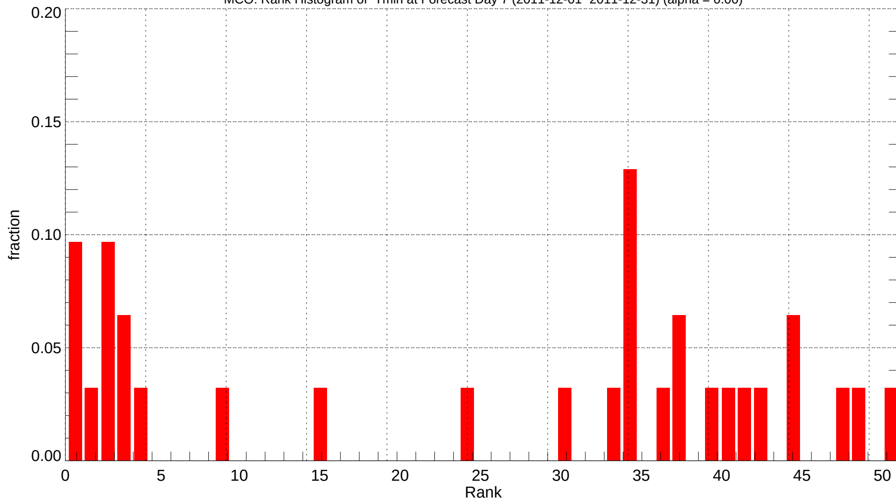
MCO: Rank Histogram of Tmin at Forecast Day 7 (2011-12-01~2011-12-31) (alpha = 0.00)
