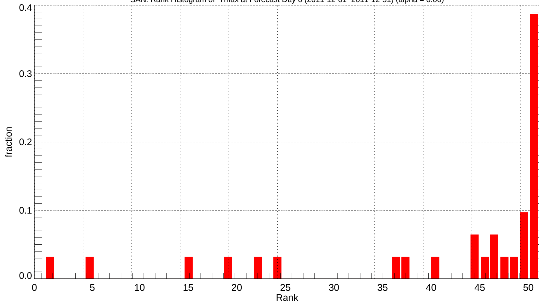
SAN: Rank Histogram of Tmax at Forecast Day 6 (2011-12-01~2011-12-31) (alpha = 0.00)
