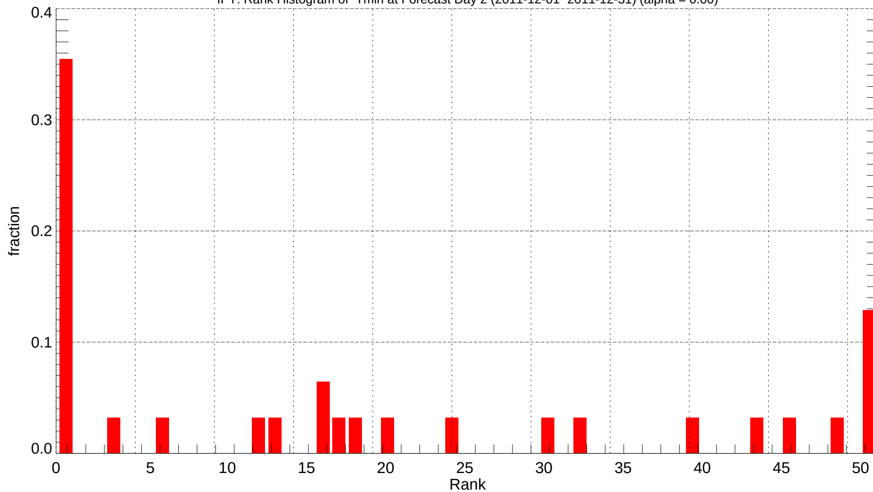
IPT: Rank Histogram of Tmin at Forecast Day 2 (2011-12-01~2011-12-31) (alpha = 0.00)
