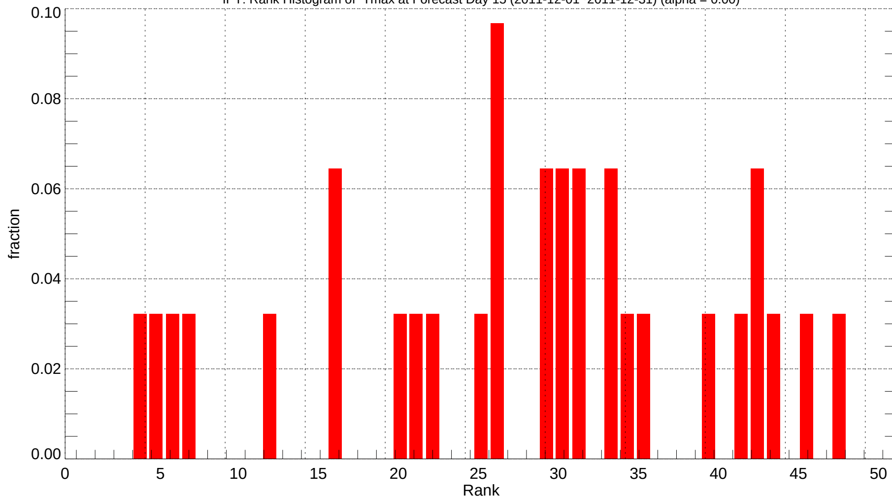
IPT: Rank Histogram of Tmax at Forecast Day 15 (2011-12-01~2011-12-31) (alpha = 0.00)
