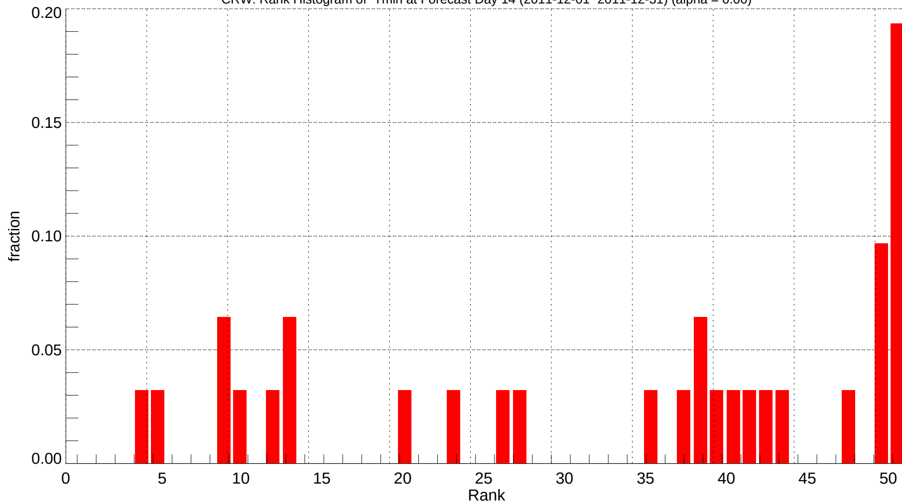
CRW: Rank Histogram of Tmin at Forecast Day 14 (2011-12-01~2011-12-31) (alpha = 0.00)
