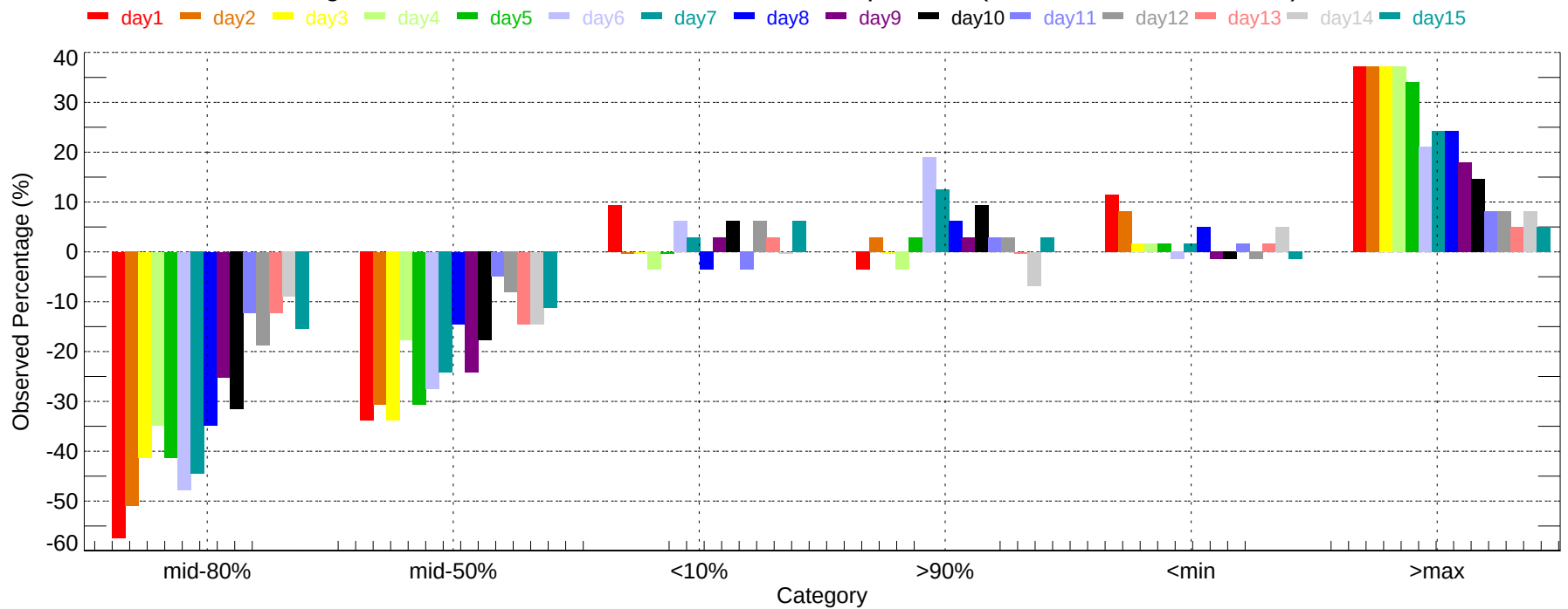
Observed Percentage Deviation of Ensembles - ELP: Max Temperature (2011-12-01~2011-12-31)
