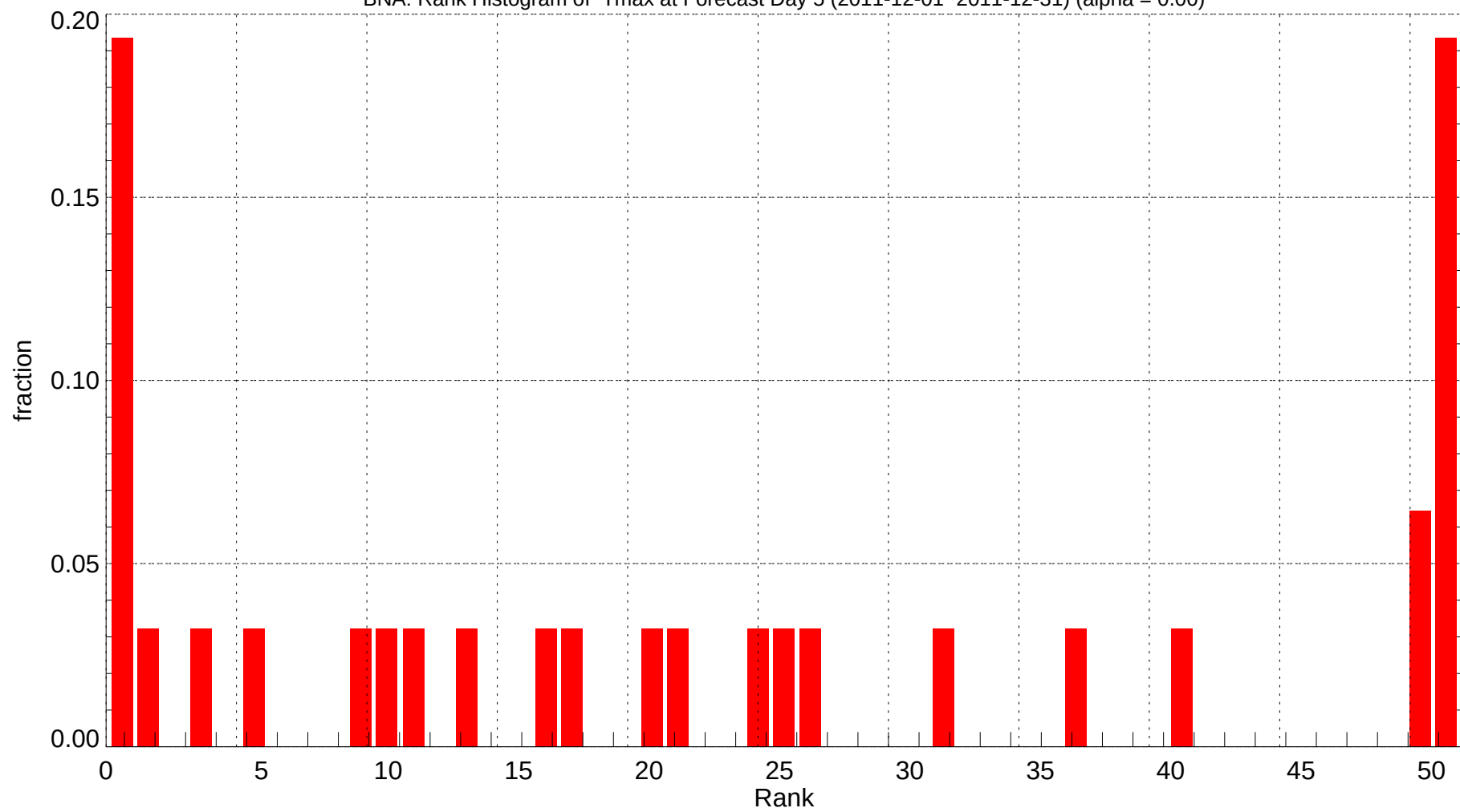
BNA: Rank Histogram of Tmax at Forecast Day 5 (2011-12-01~2011-12-31) (alpha = 0.00)
