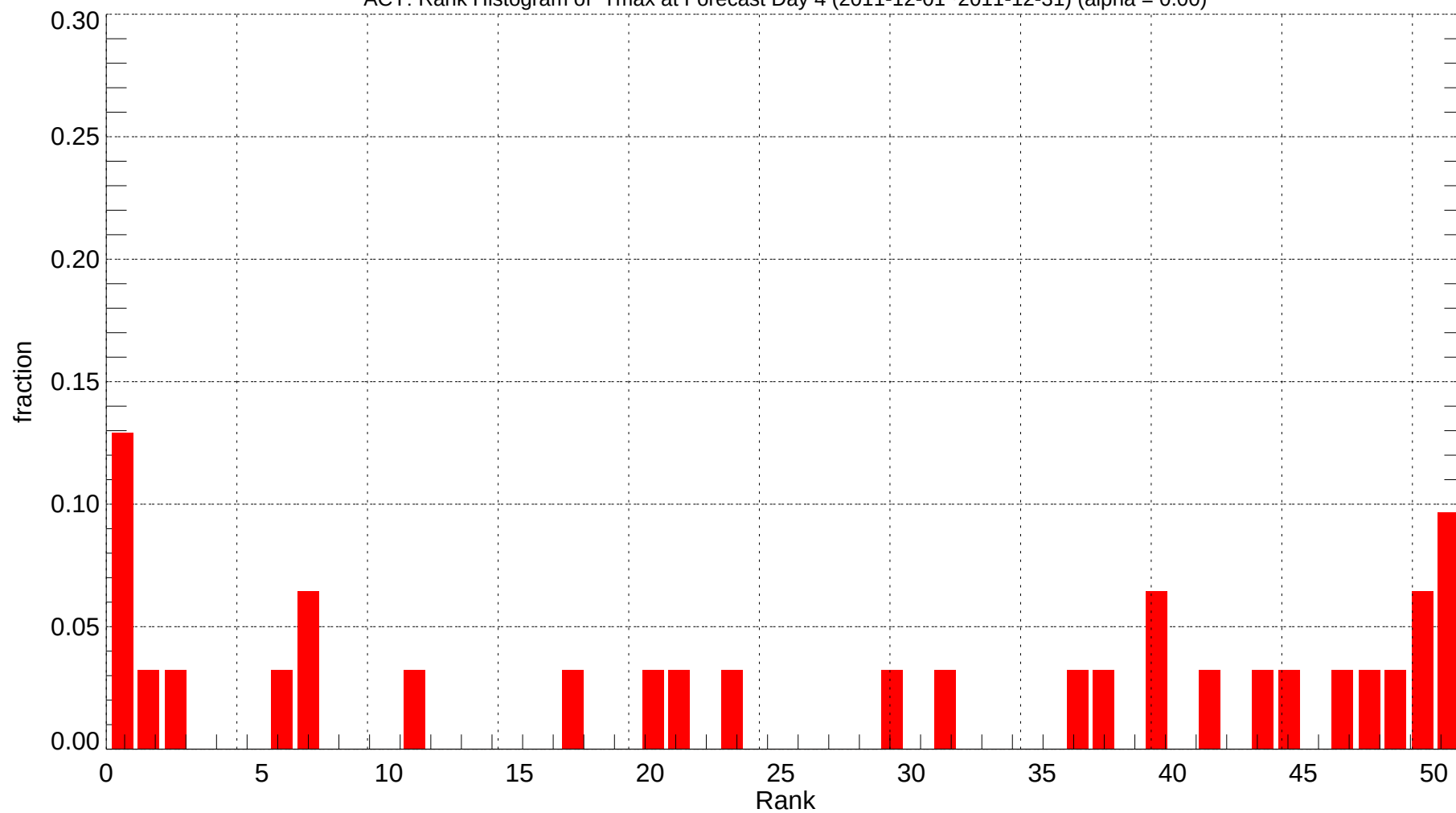
ACY: Rank Histogram of Tmax at Forecast Day 4 (2011-12-01~2011-12-31) (alpha = 0.00)
