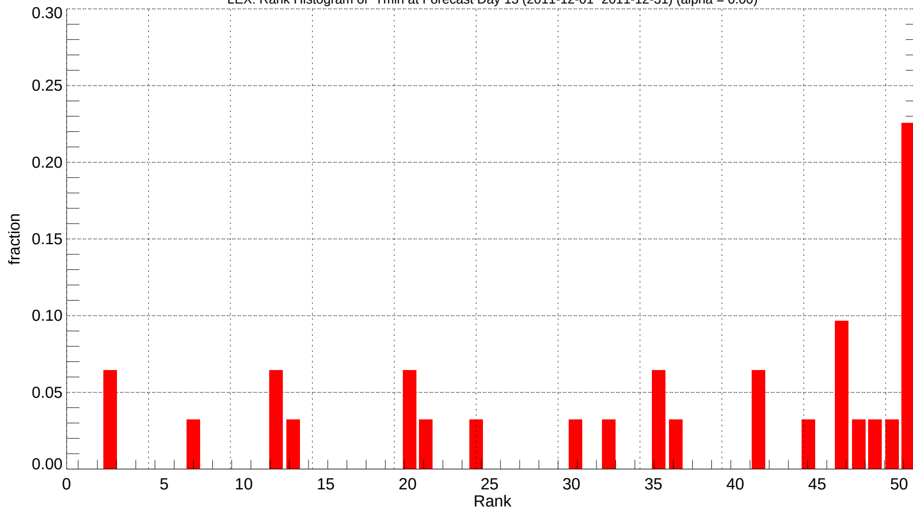
LEX: Rank Histogram of Tmin at Forecast Day 13 (2011-12-01~2011-12-31) (alpha = 0.00)
