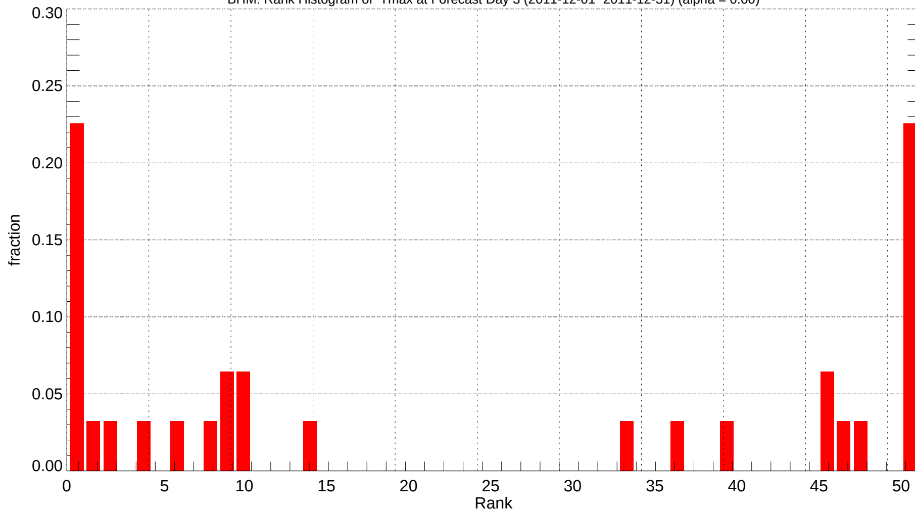
BHM: Rank Histogram of Tmax at Forecast Day 3 (2011-12-01~2011-12-31) (alpha = 0.00)
