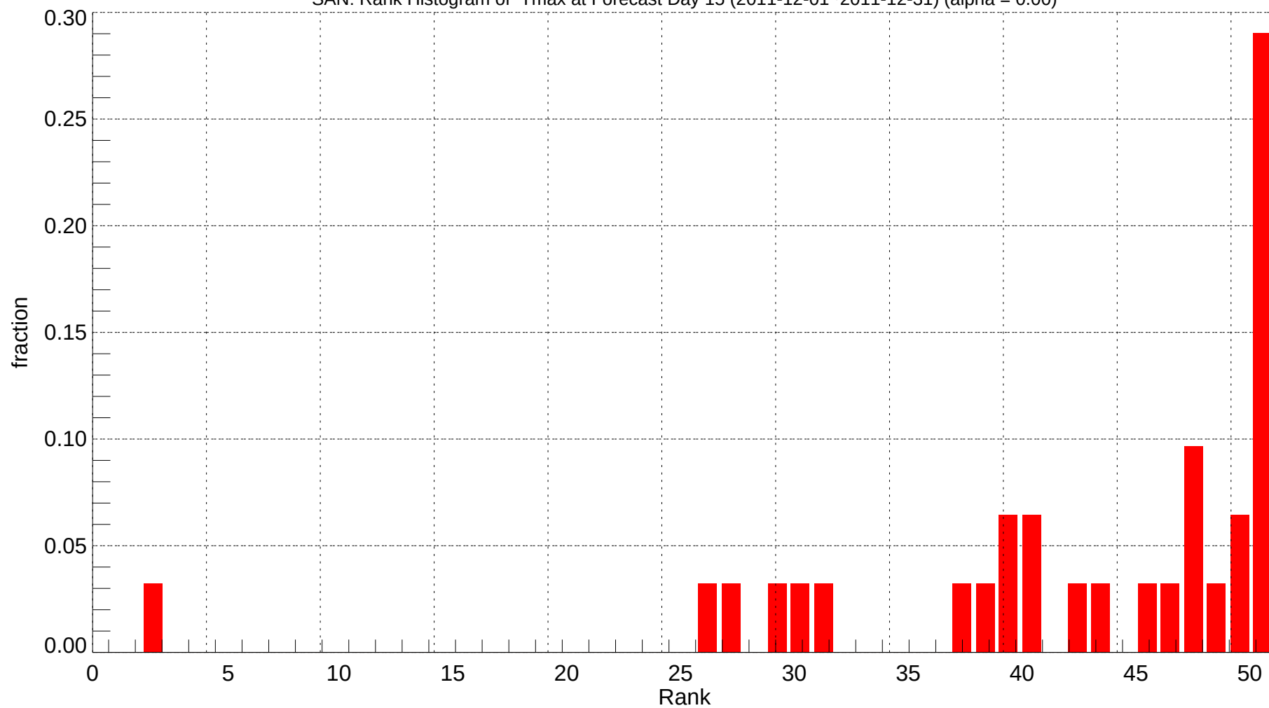
SAN: Rank Histogram of Tmax at Forecast Day 15 (2011-12-01~2011-12-31) (alpha = 0.00)
