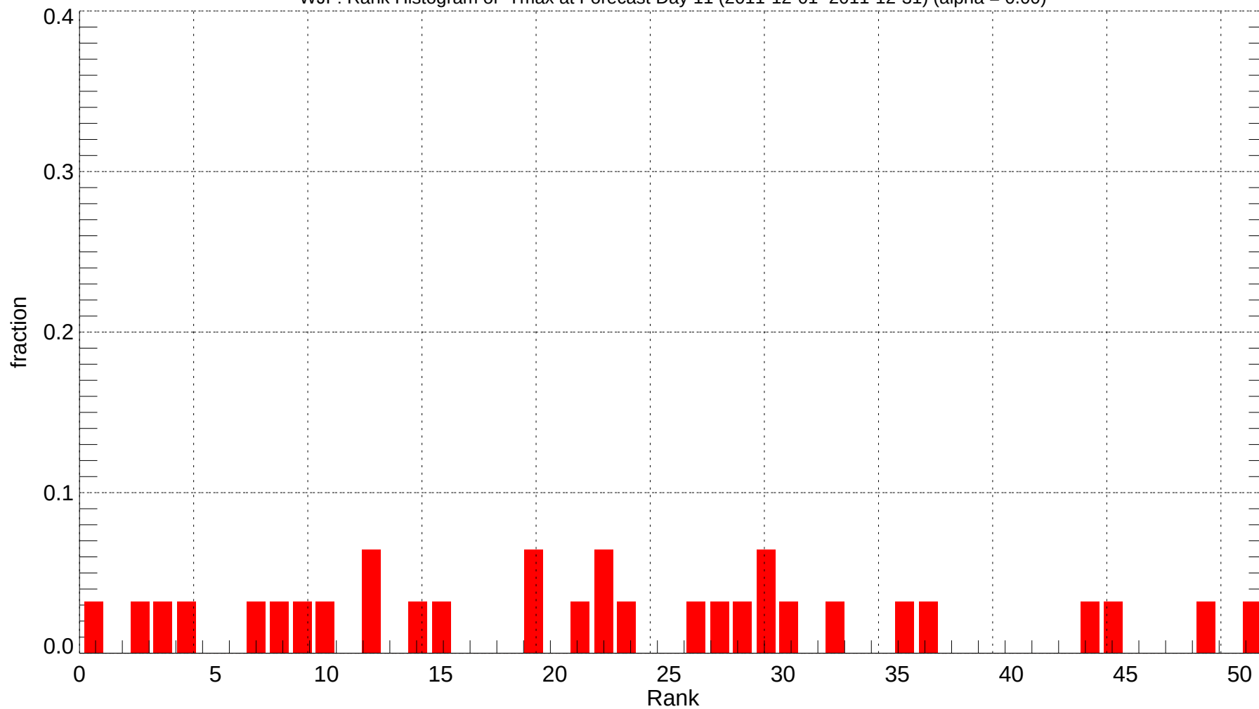
WJF: Rank Histogram of Tmax at Forecast Day 11 (2011-12-01~2011-12-31) (alpha = 0.00)
