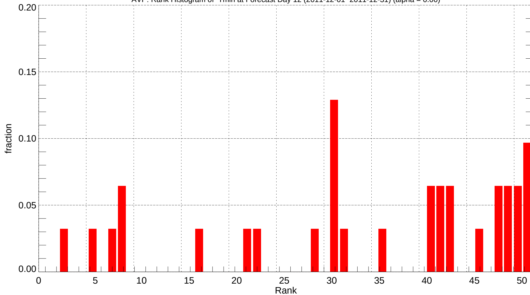
AVP: Rank Histogram of Tmin at Forecast Day 12 (2011-12-01~2011-12-31) (alpha = 0.00)
