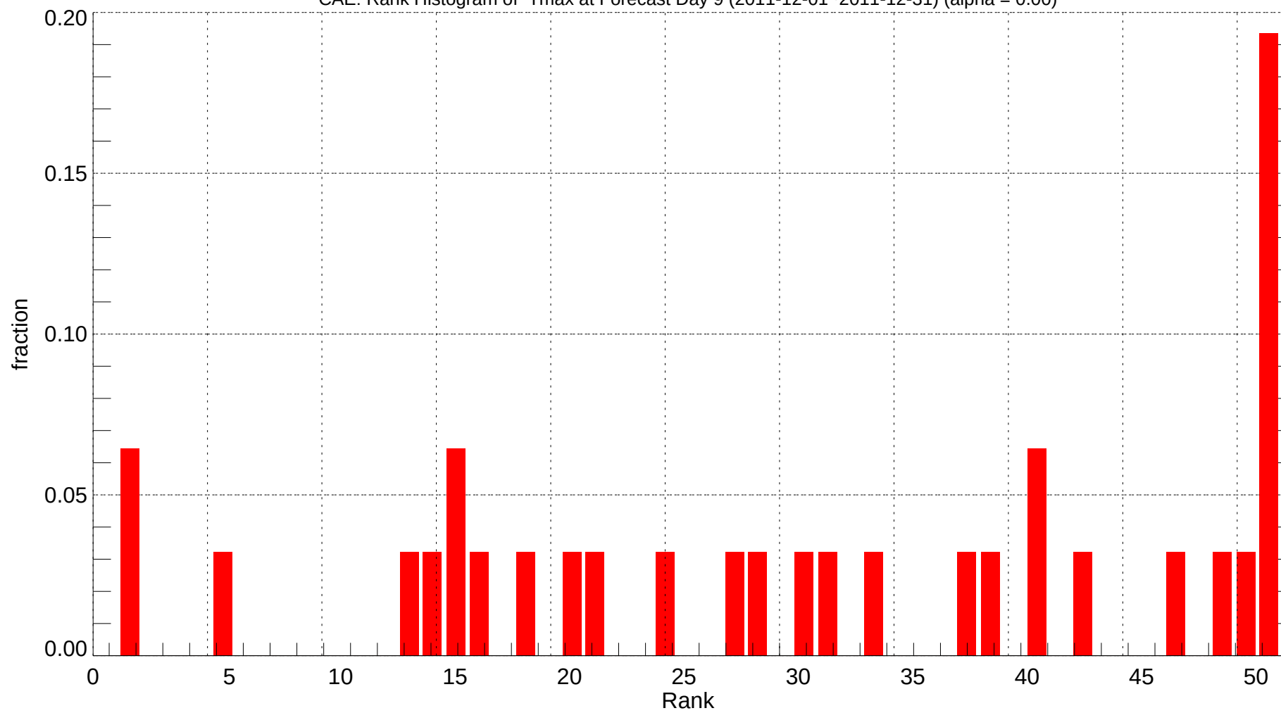
CAE: Rank Histogram of Tmax at Forecast Day 9 (2011-12-01~2011-12-31) (alpha = 0.00)
