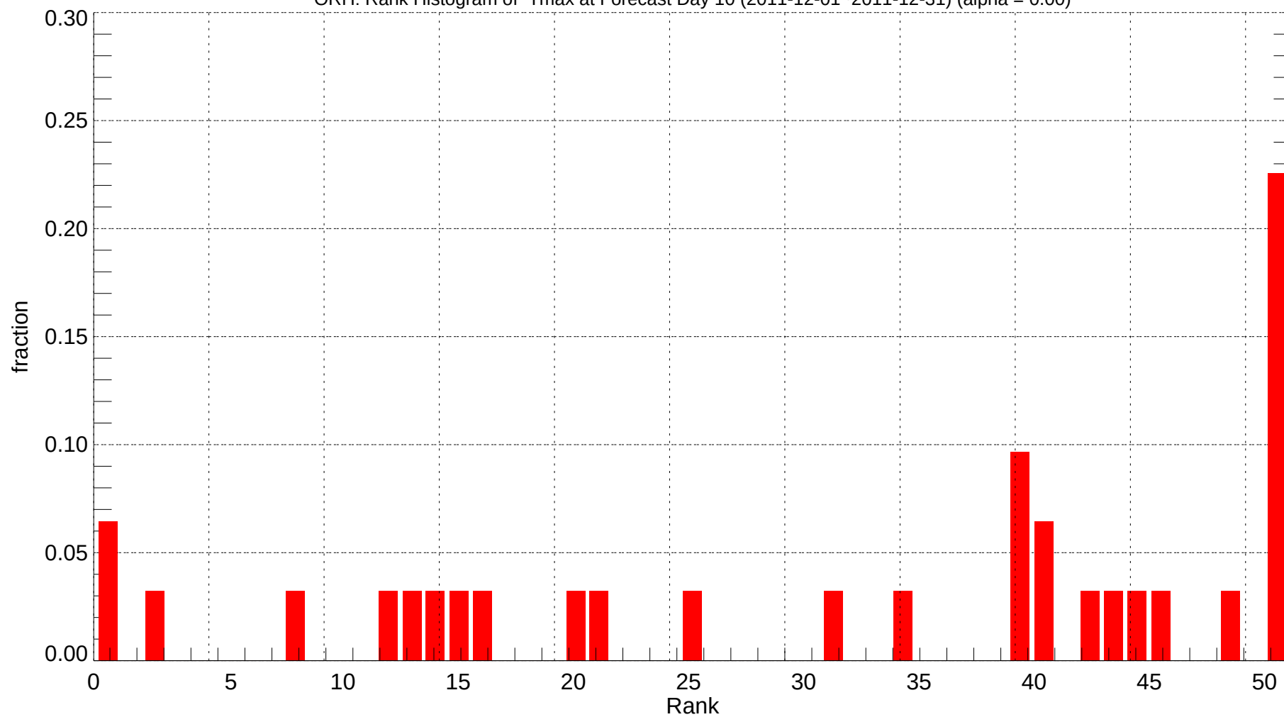
ORH: Rank Histogram of Tmax at Forecast Day 10 (2011-12-01~2011-12-31) (alpha = 0.00)
