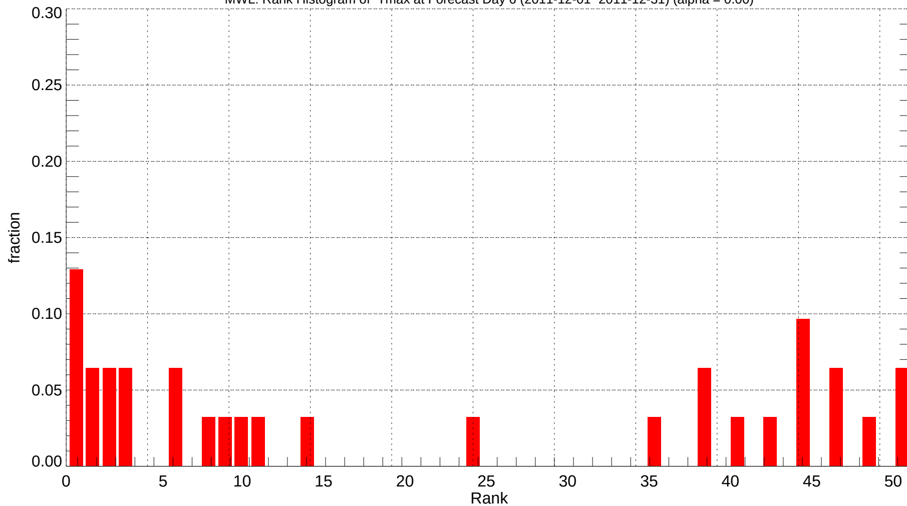
MWL: Rank Histogram of Tmax at Forecast Day 6 (2011-12-01~2011-12-31) (alpha = 0.00)
