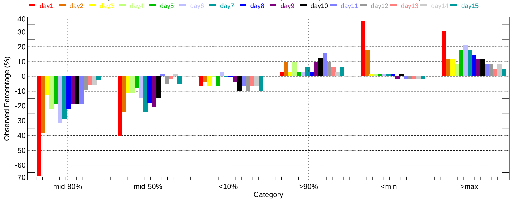
Observed Percentage Deviation of Ensembles - JAN: Min Temperature (2011-12-01~2011-12-31)
