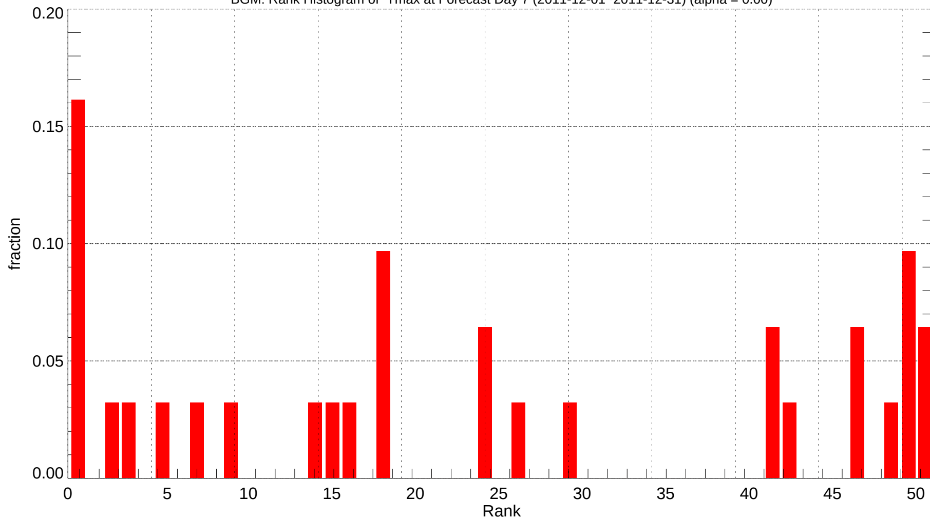
BGM: Rank Histogram of Tmax at Forecast Day 7 (2011-12-01~2011-12-31) (alpha = 0.00)
