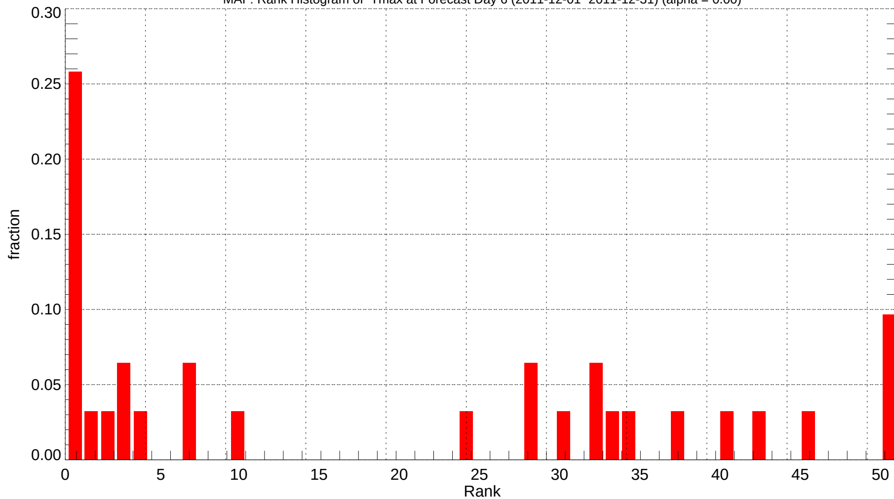
MAF: Rank Histogram of Tmax at Forecast Day 6 (2011-12-01~2011-12-31) (alpha = 0.00)
