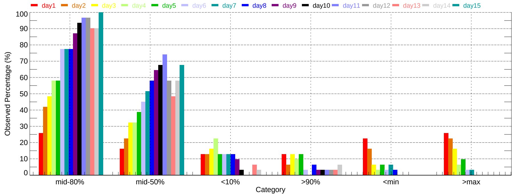
Observed Percentage of Ensembles - MIA: Max Temperature (2011-12-01~2011-12-31)
