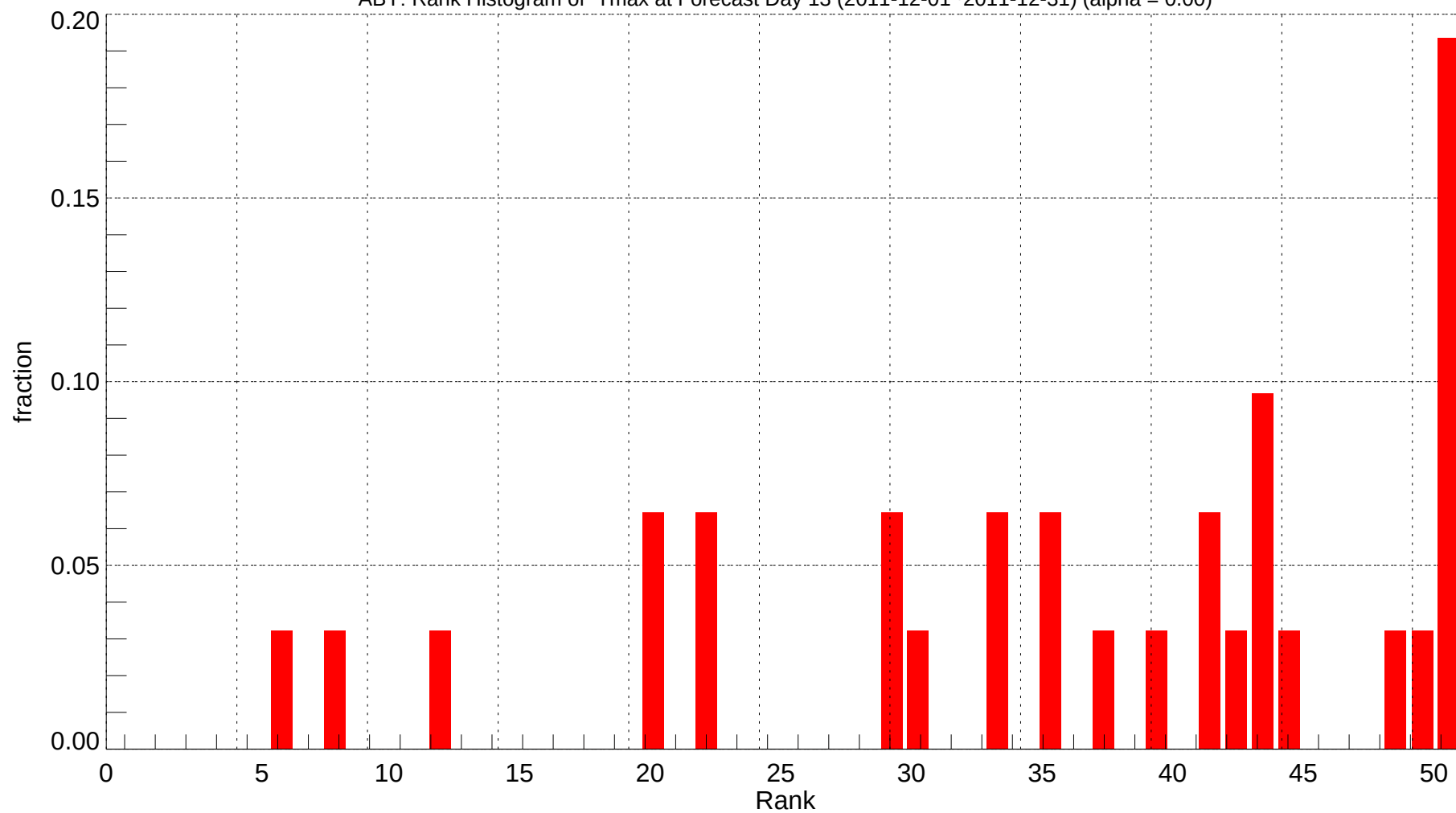
ABY: Rank Histogram of Tmax at Forecast Day 13 (2011-12-01~2011-12-31) (alpha = 0.00)
