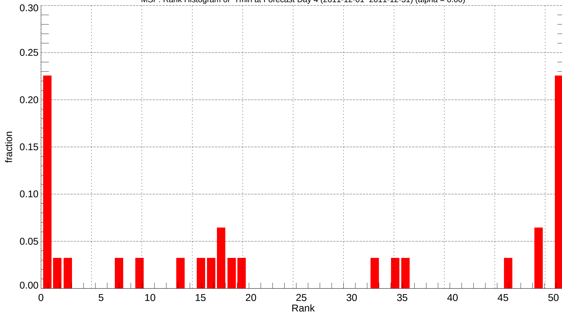
MSP: Rank Histogram of Tmin at Forecast Day 4 (2011-12-01~2011-12-31) (alpha = 0.00)
