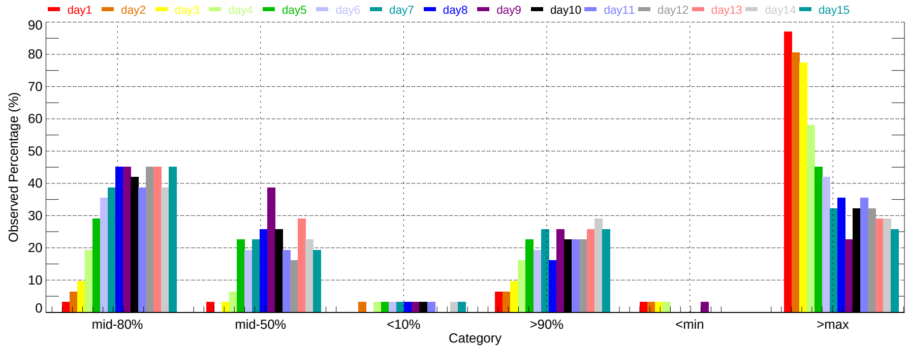
Observed Percentage of Ensembles - SAN: Max Temperature (2011-12-01~2011-12-31)
