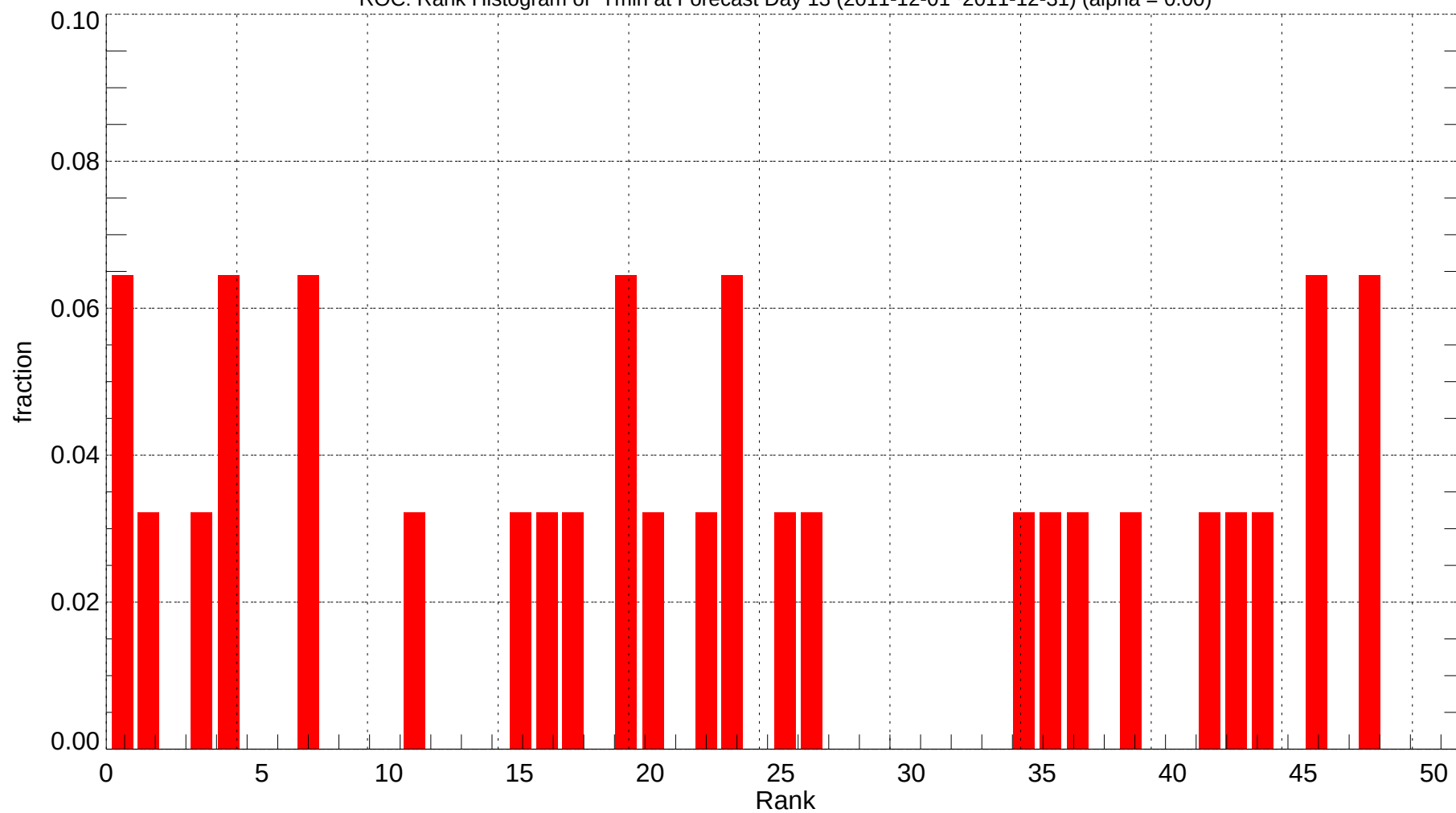
ROC: Rank Histogram of Tmin at Forecast Day 13 (2011-12-01~2011-12-31) (alpha = 0.00)
