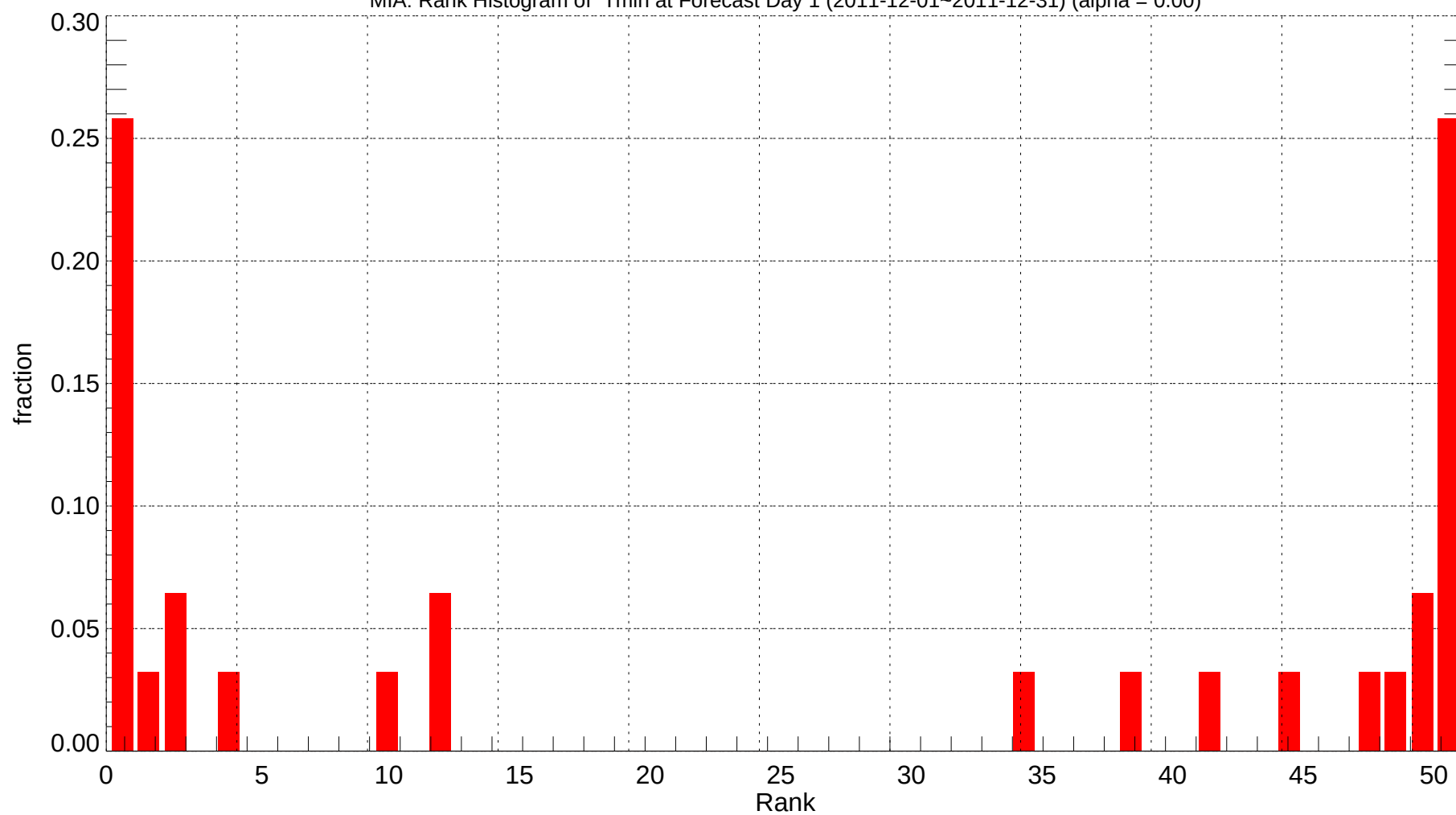
MIA: Rank Histogram of Tmin at Forecast Day 1 (2011-12-01~2011-12-31) (alpha = 0.00)
