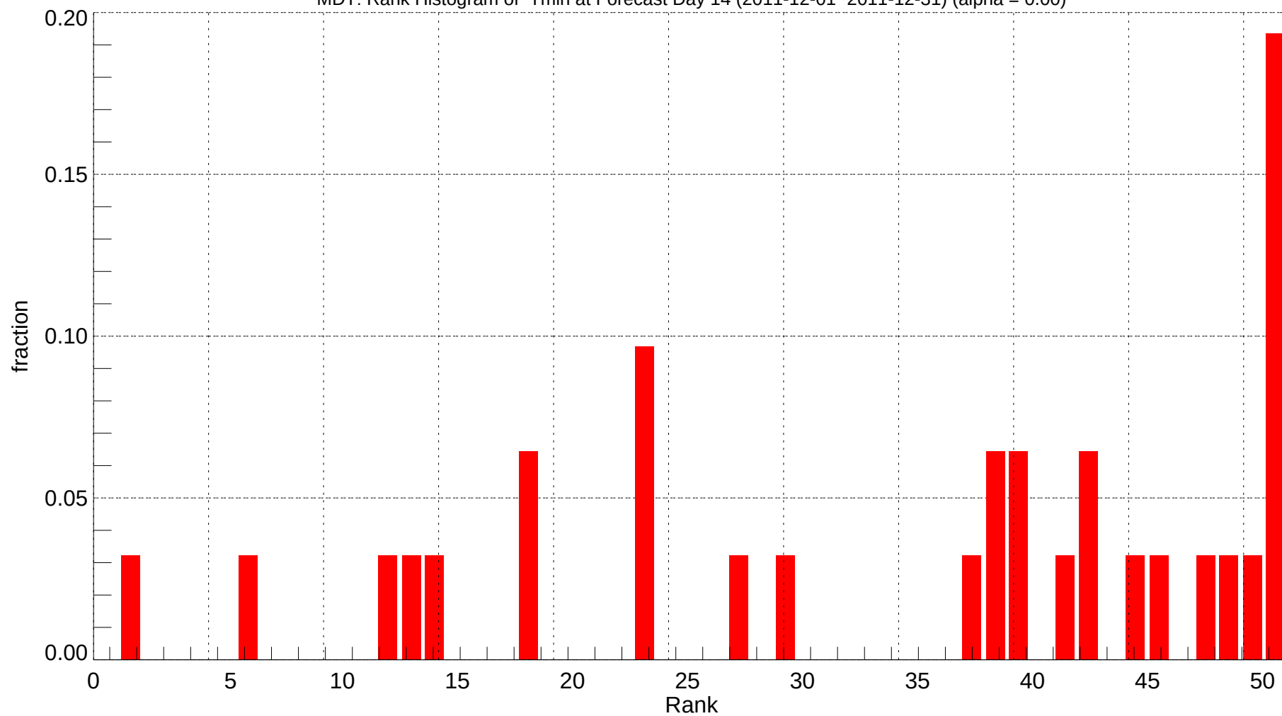
MDT: Rank Histogram of Tmin at Forecast Day 14 (2011-12-01~2011-12-31) (alpha = 0.00)
