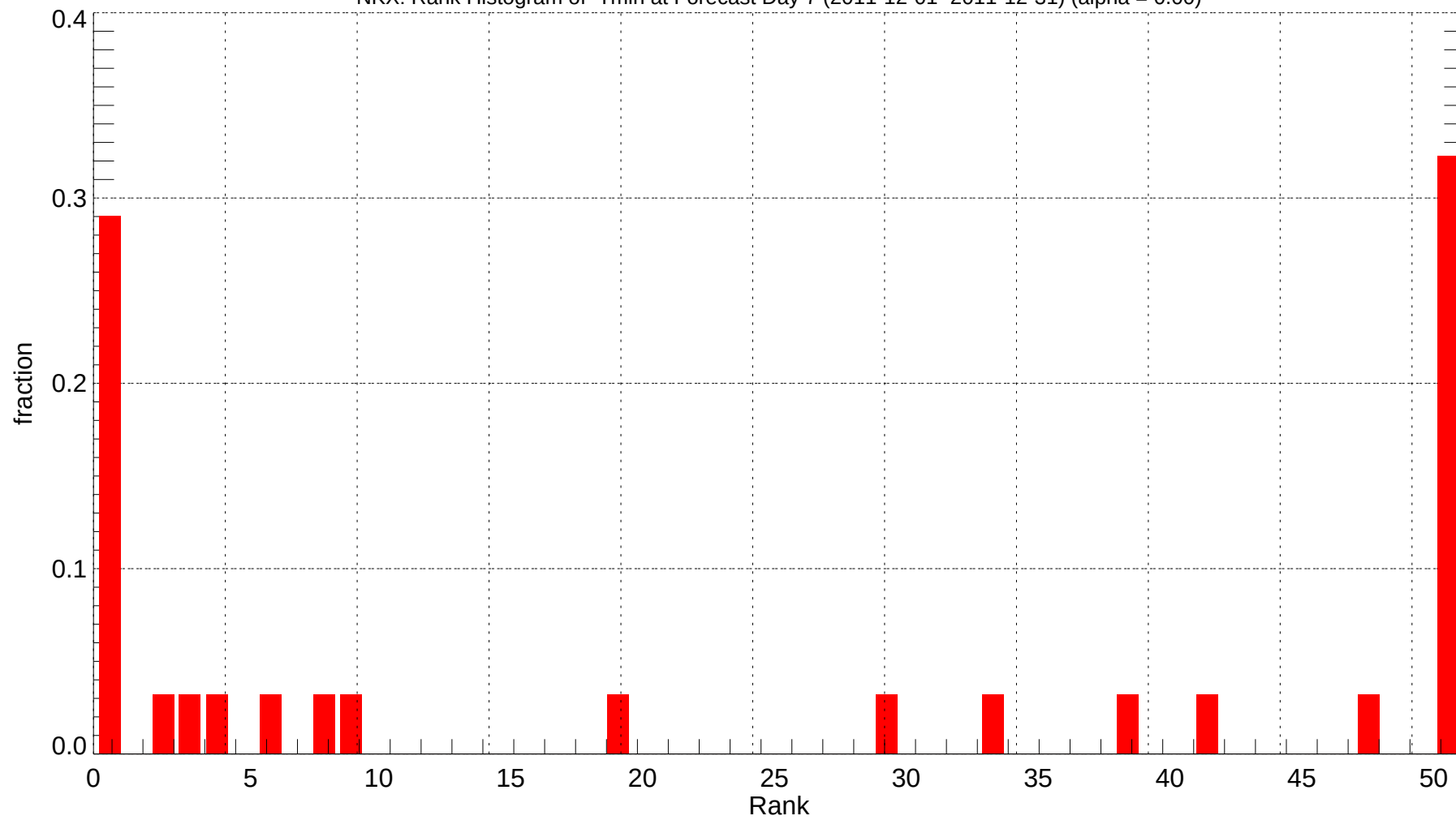
NKX: Rank Histogram of Tmin at Forecast Day 7 (2011-12-01~2011-12-31) (alpha = 0.00)
