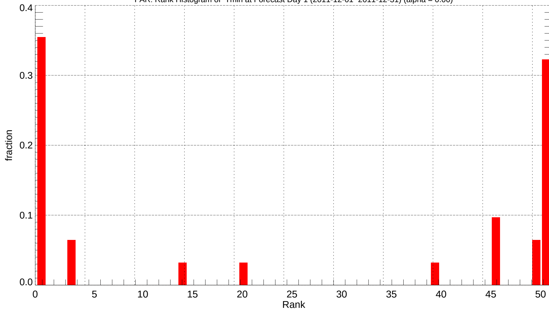
FAR: Rank Histogram of Tmin at Forecast Day 1 (2011-12-01~2011-12-31) (alpha = 0.00)
