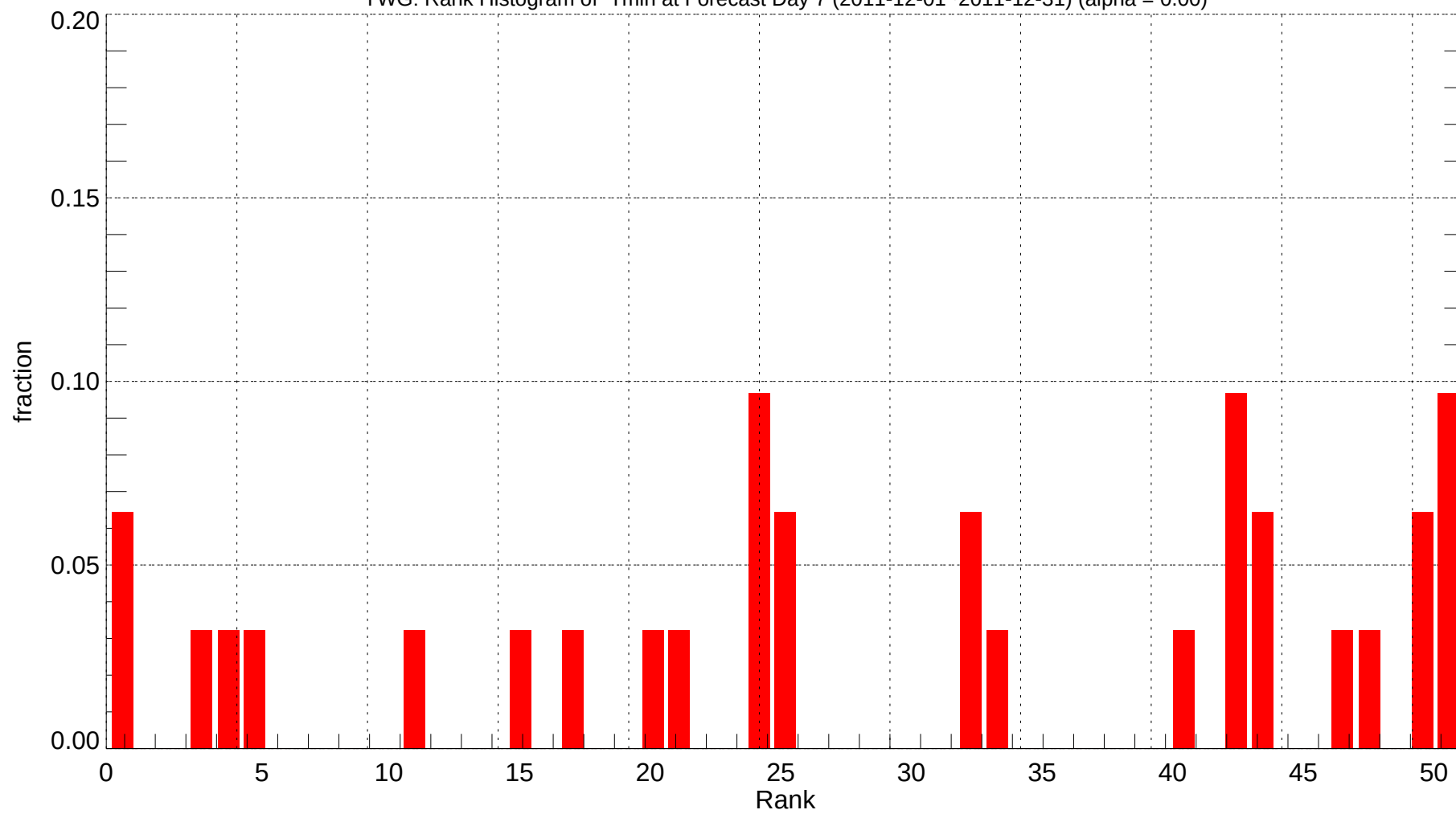
YWG: Rank Histogram of Tmin at Forecast Day 7 (2011-12-01~2011-12-31) (alpha = 0.00)
