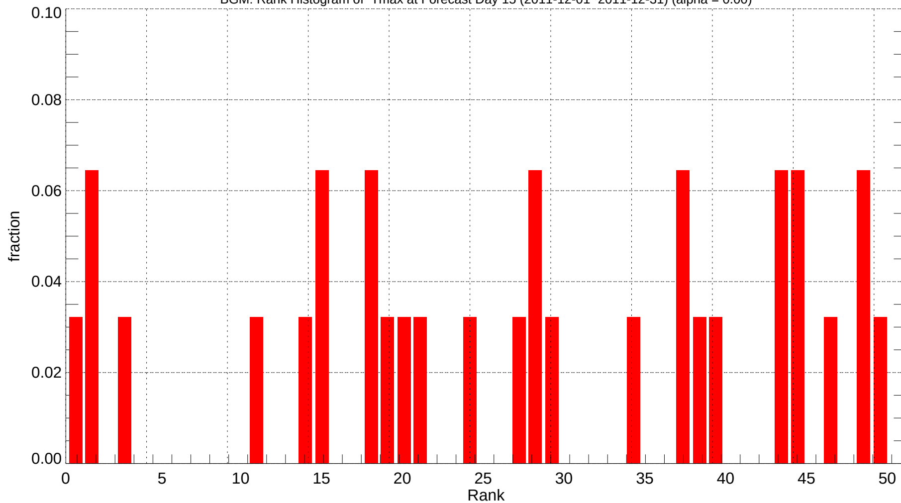
BGM: Rank Histogram of Tmax at Forecast Day 15 (2011-12-01~2011-12-31) (alpha = 0.00)
