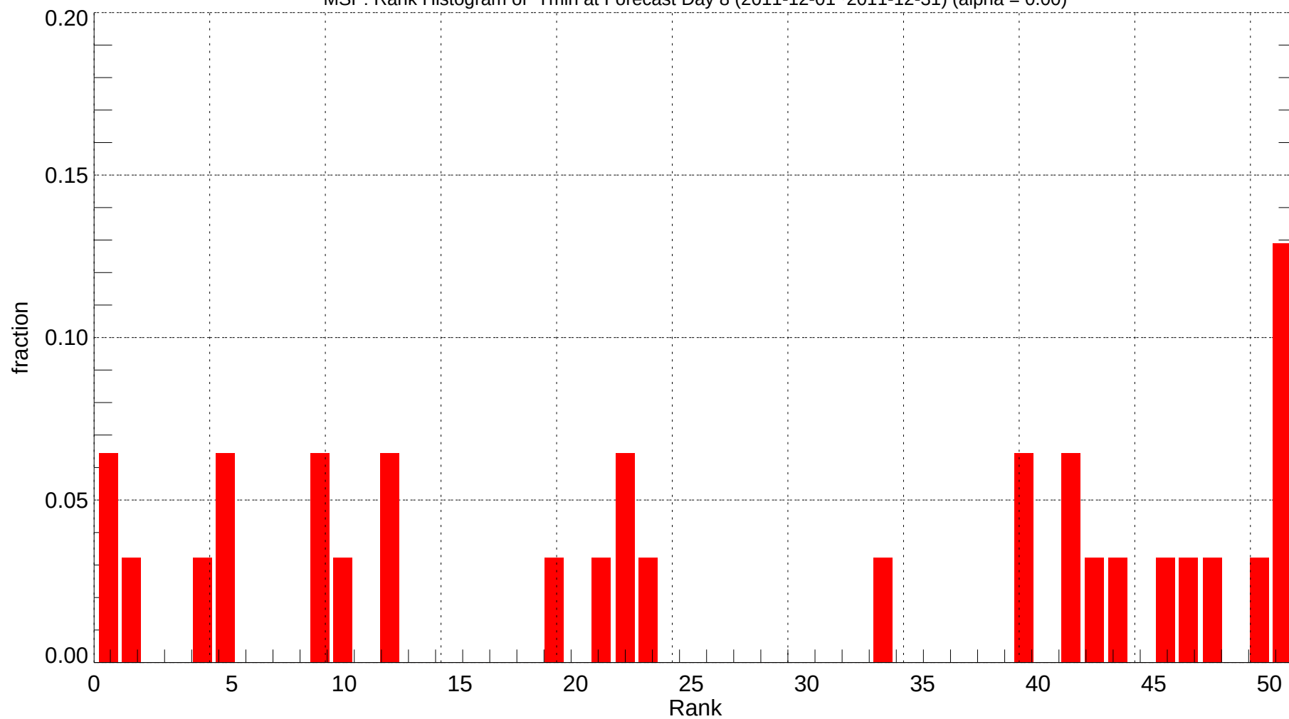
MSP: Rank Histogram of Tmin at Forecast Day 8 (2011-12-01~2011-12-31) (alpha = 0.00)
