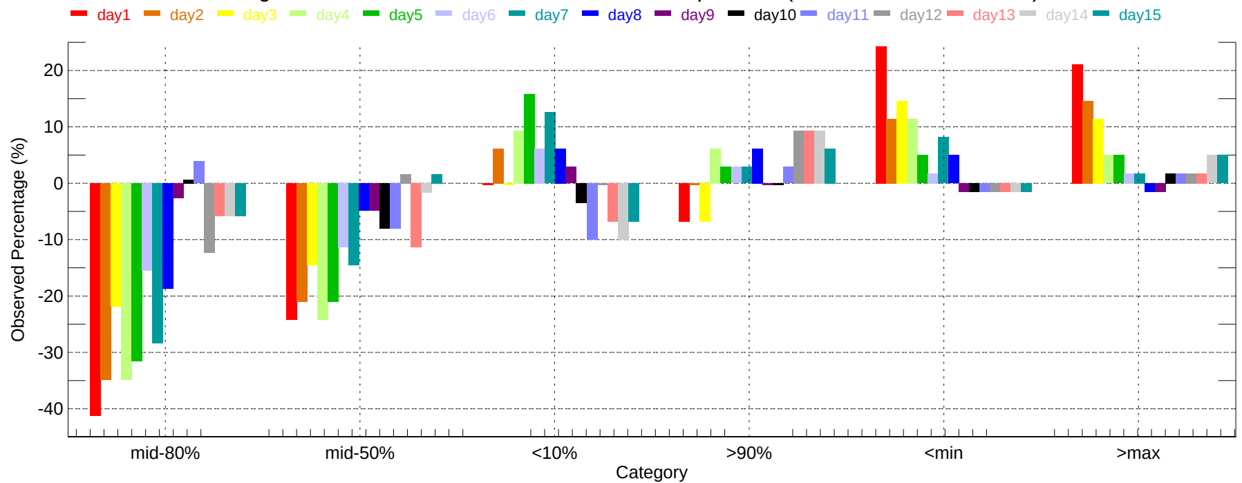
Observed Percentage Deviation of Ensembles - MCO: Max Temperature (2011-12-01~2011-12-31)
