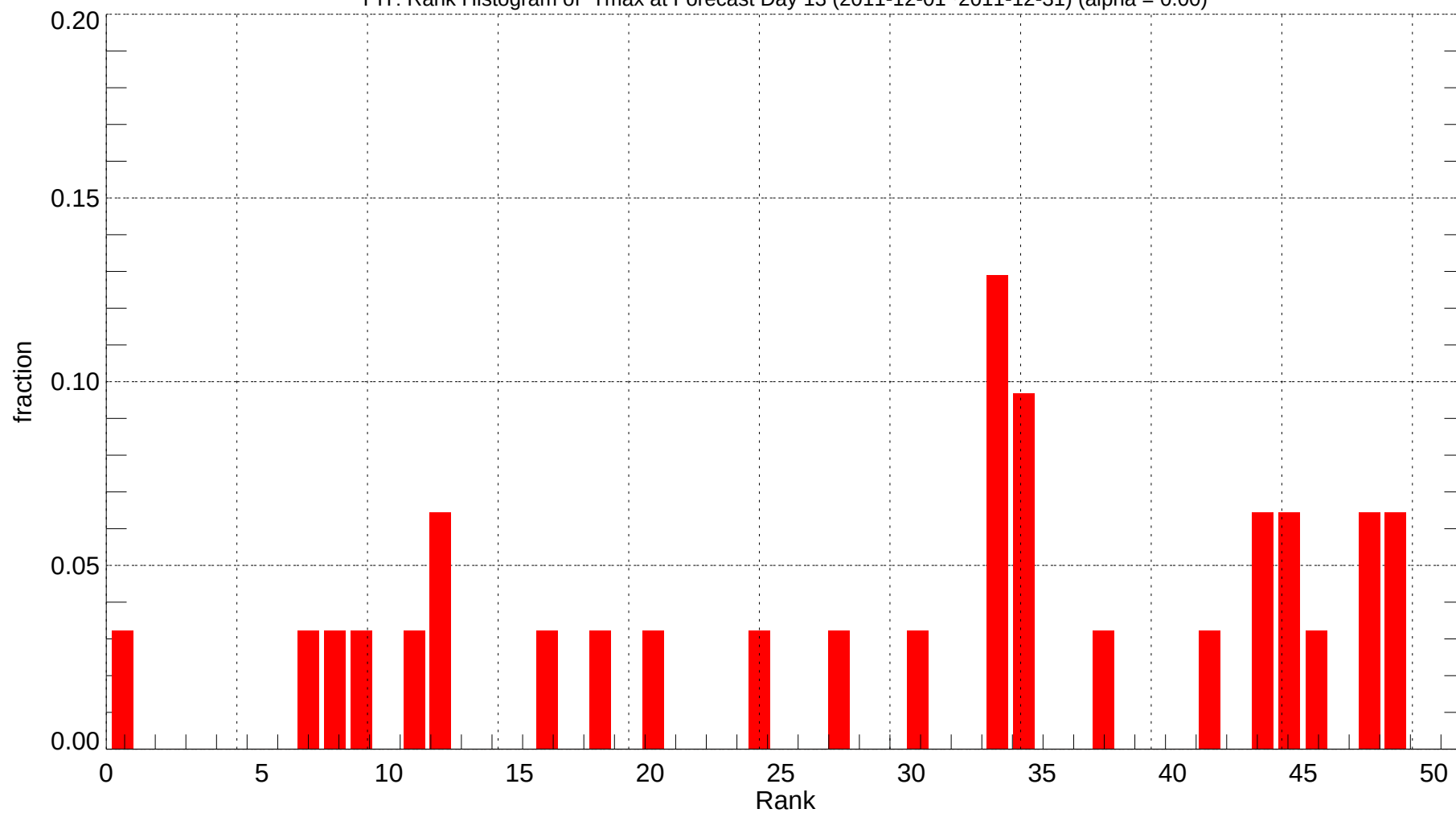
PIT: Rank Histogram of Tmax at Forecast Day 13 (2011-12-01~2011-12-31) (alpha = 0.00)
