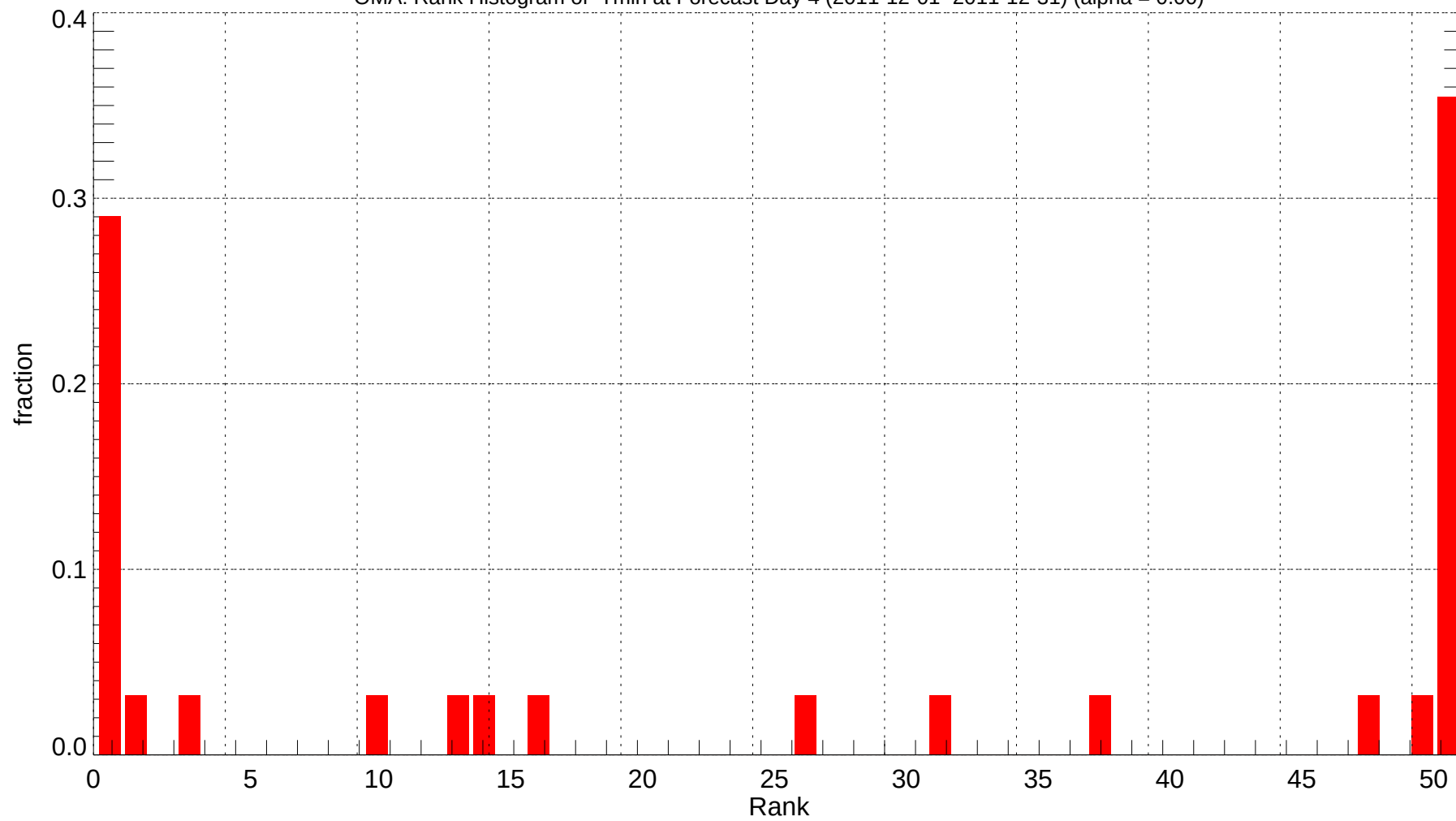
OMA: Rank Histogram of Tmin at Forecast Day 4 (2011-12-01~2011-12-31) (alpha = 0.00)
