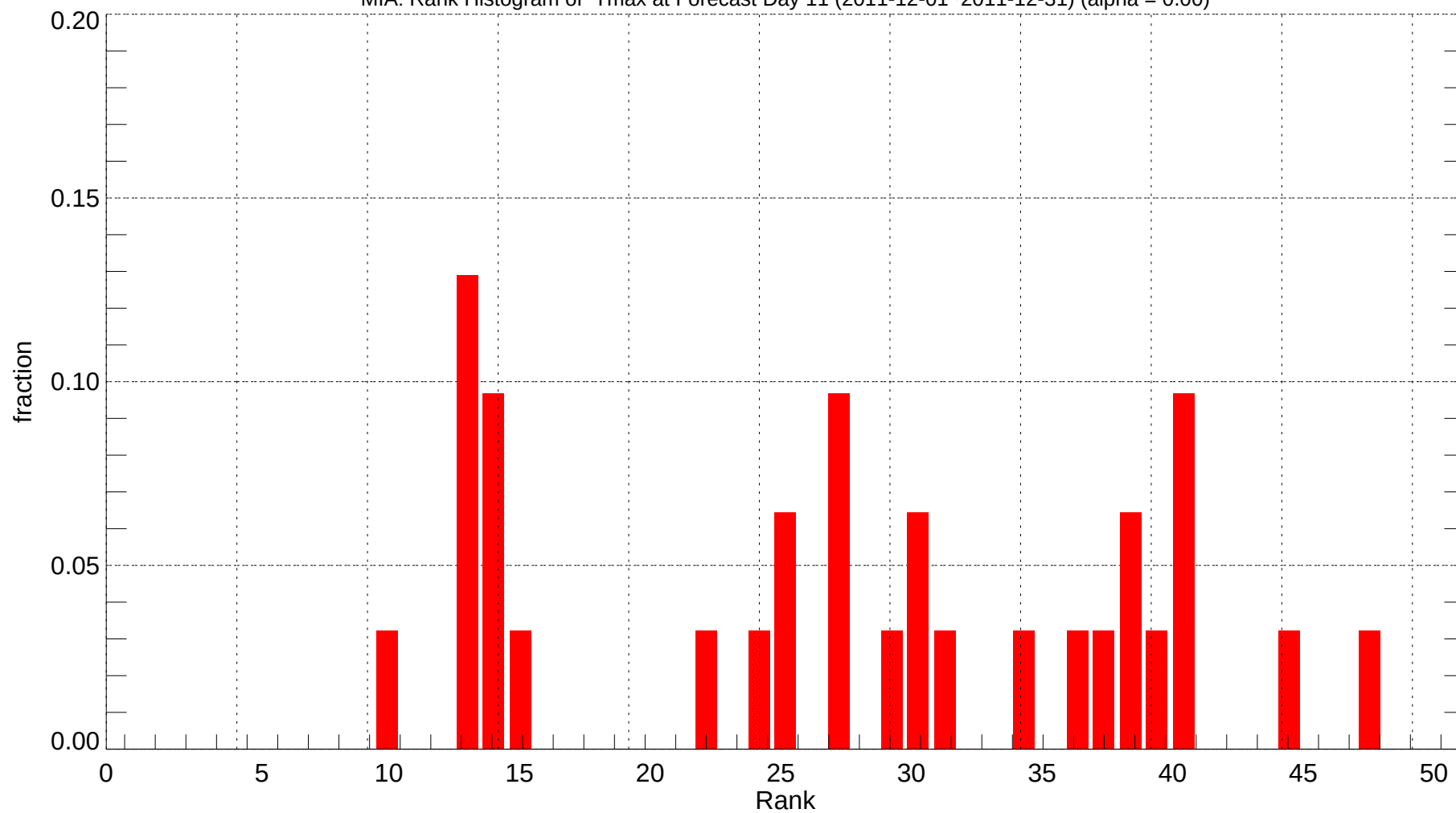
MIA: Rank Histogram of Tmax at Forecast Day 11 (2011-12-01~2011-12-31) (alpha = 0.00)
