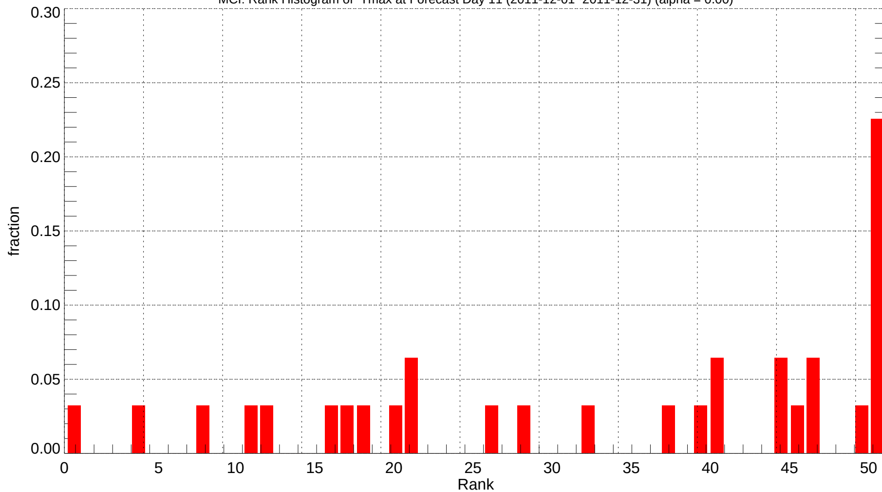
MCI: Rank Histogram of Tmax at Forecast Day 11 (2011-12-01~2011-12-31) (alpha = 0.00)
