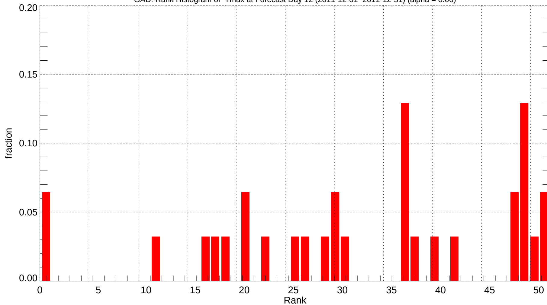
GAD: Rank Histogram of Tmax at Forecast Day 12 (2011-12-01~2011-12-31) (alpha = 0.00)
