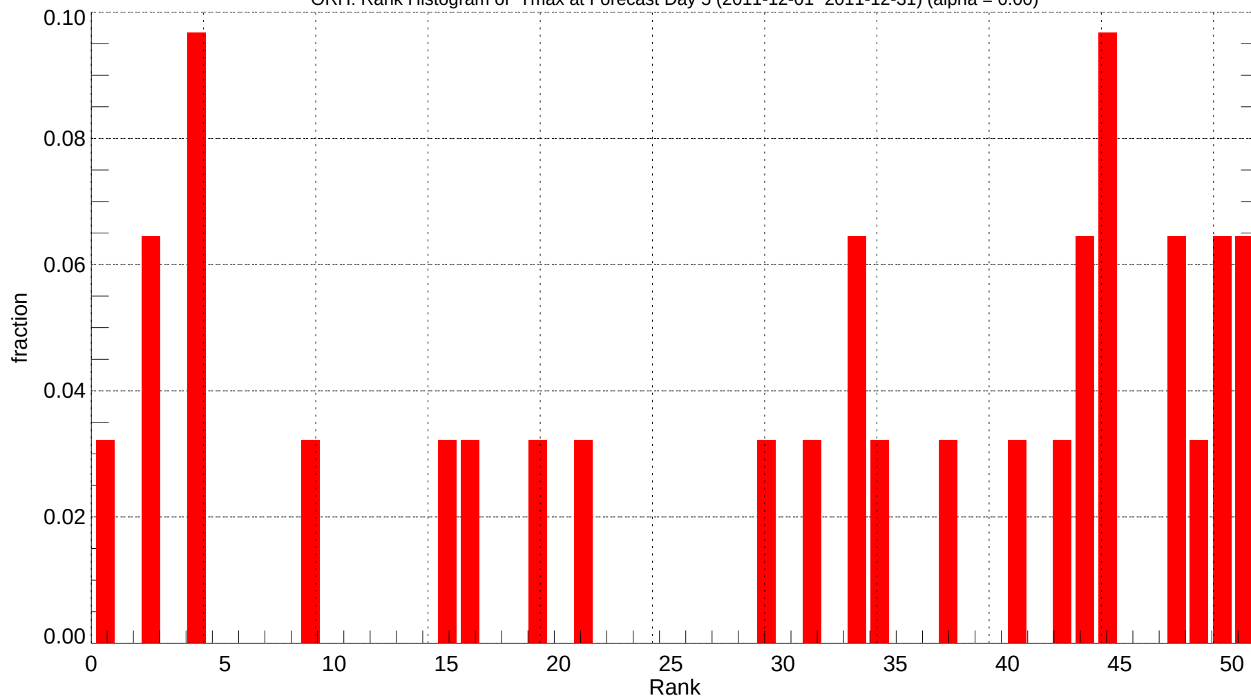
ORH: Rank Histogram of Tmax at Forecast Day 5 (2011-12-01~2011-12-31) (alpha = 0.00)
