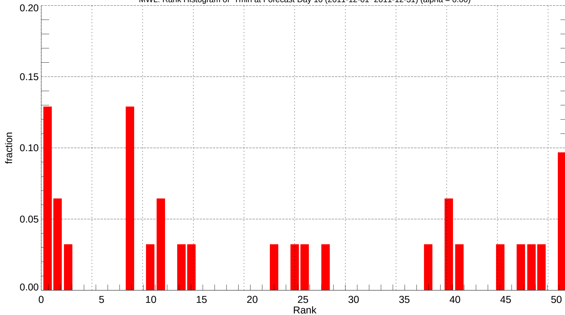
MWL: Rank Histogram of Tmin at Forecast Day 10 (2011-12-01~2011-12-31) (alpha = 0.00)
