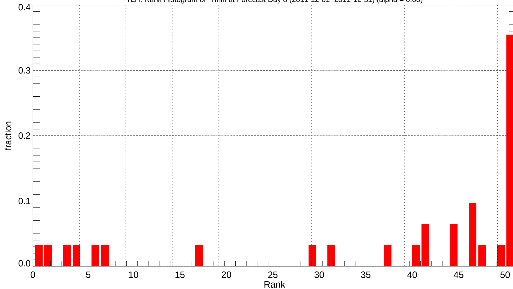
TLH: Rank Histogram of Tmin at Forecast Day 8 (2011-12-01~2011-12-31) (alpha = 0.00)
