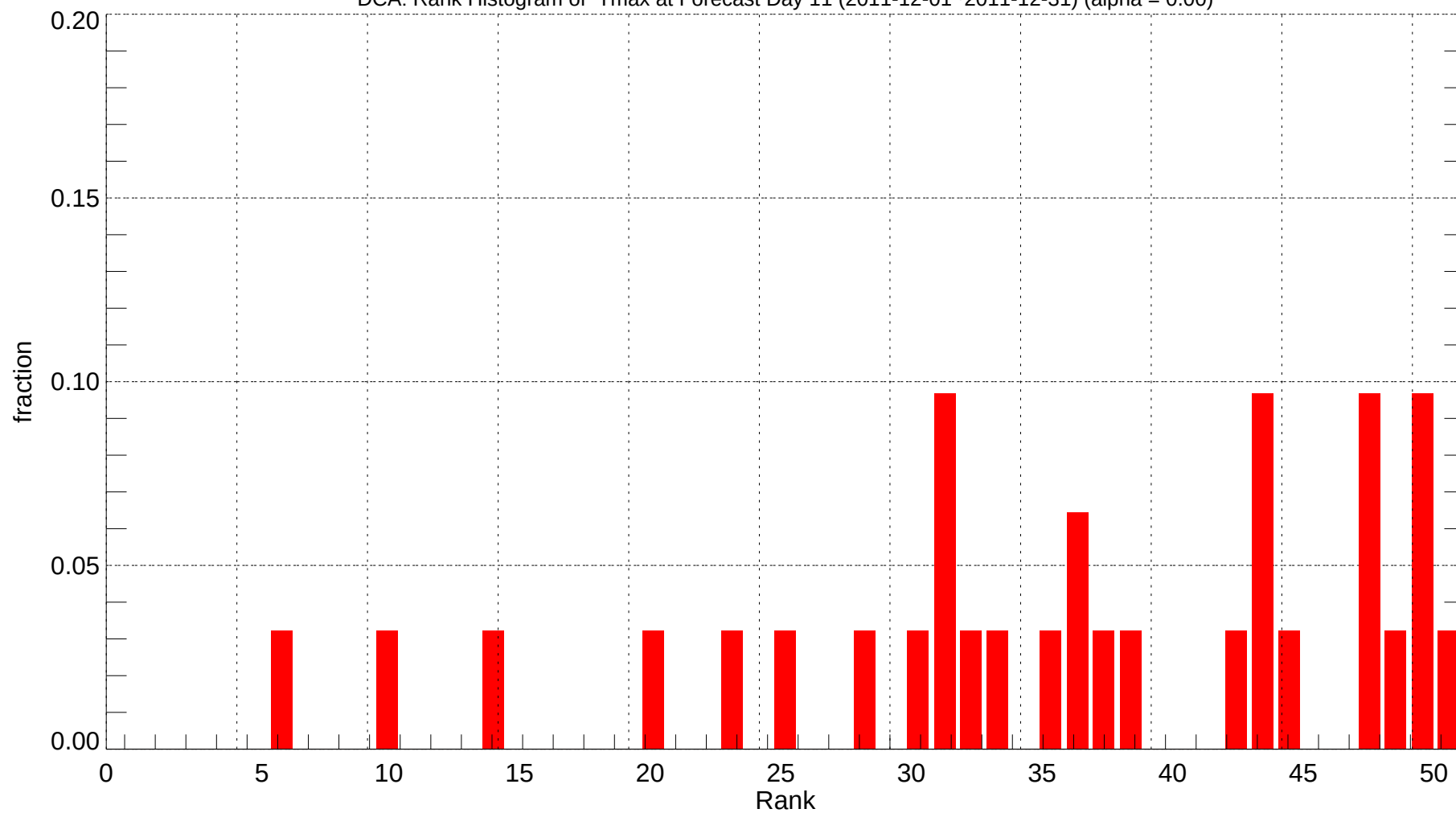
DCA: Rank Histogram of Tmax at Forecast Day 11 (2011-12-01~2011-12-31) (alpha = 0.00)
