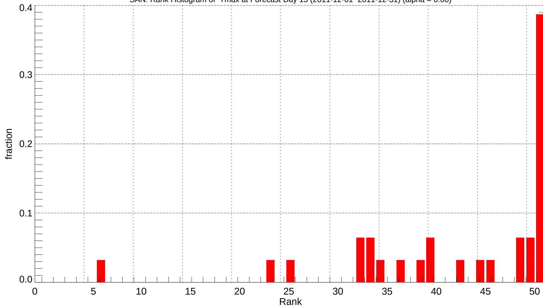
SAN: Rank Histogram of Tmax at Forecast Day 13 (2011-12-01~2011-12-31) (alpha = 0.00)
