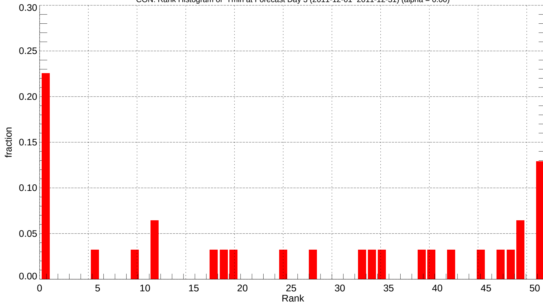
CON: Rank Histogram of Tmin at Forecast Day 3 (2011-12-01~2011-12-31) (alpha = 0.00)
