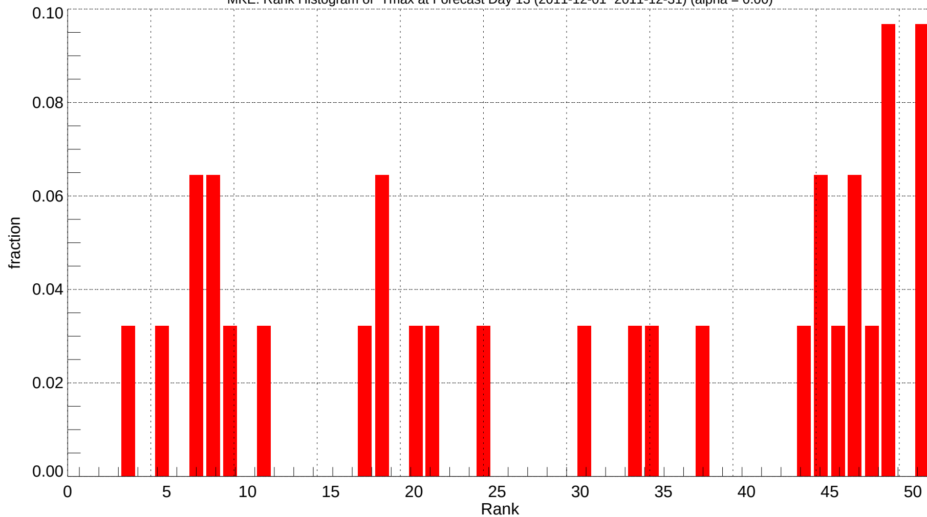
MKE: Rank Histogram of Tmax at Forecast Day 13 (2011-12-01~2011-12-31) (alpha = 0.00)
