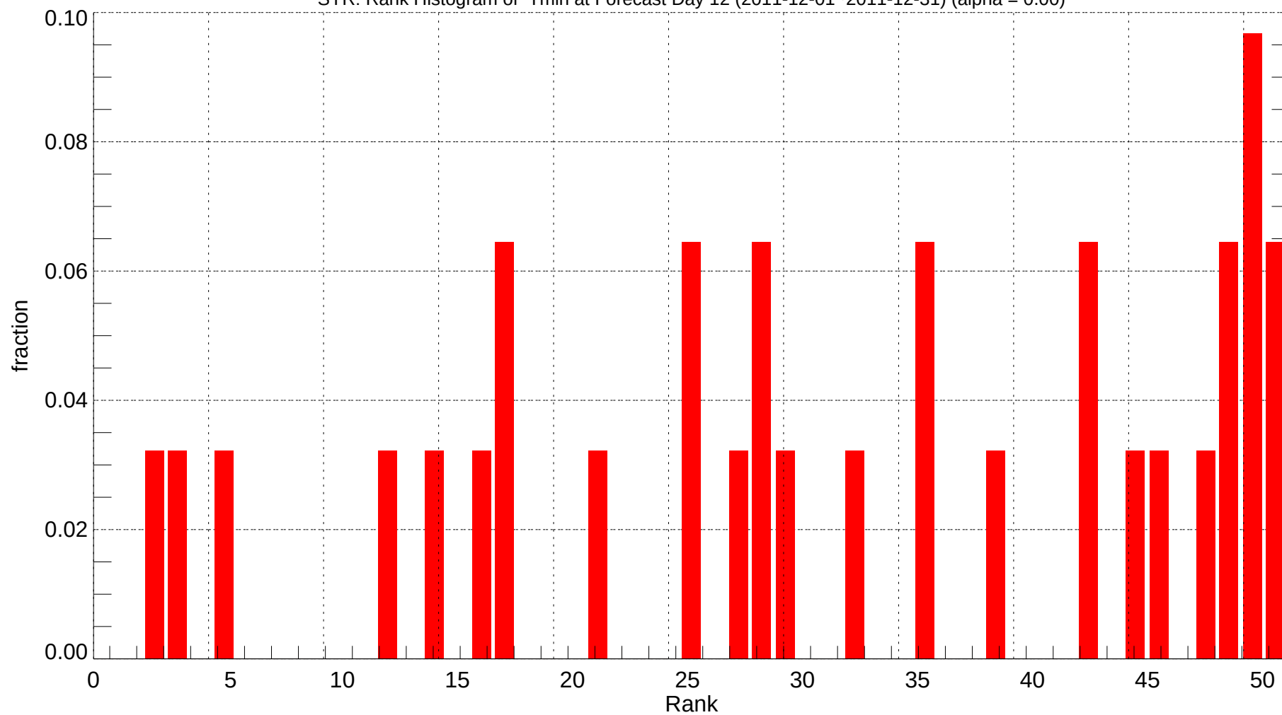
SYR: Rank Histogram of Tmin at Forecast Day 12 (2011-12-01~2011-12-31) (alpha = 0.00)
