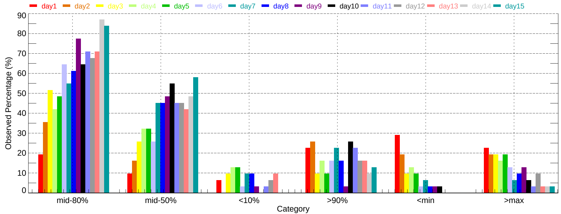
Observed Percentage of Ensembles - RDU: Min Temperature (2011-12-01~2011-12-31)
