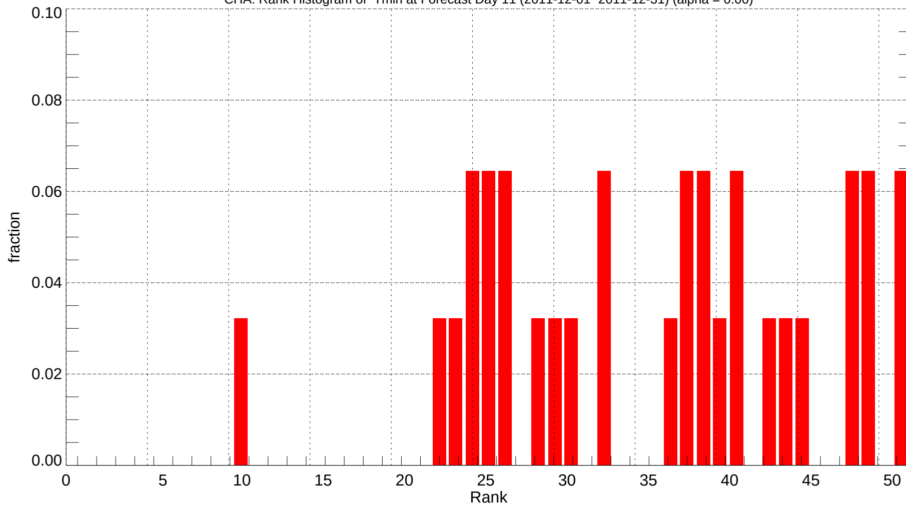
CHA: Rank Histogram of Tmin at Forecast Day 11 (2011-12-01~2011-12-31) (alpha = 0.00)
