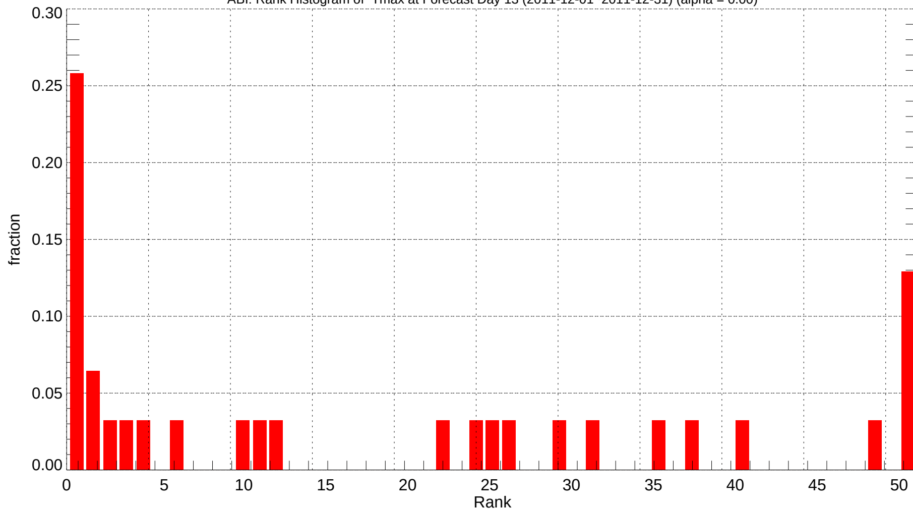
ABI: Rank Histogram of Tmax at Forecast Day 13 (2011-12-01~2011-12-31) (alpha = 0.00)
