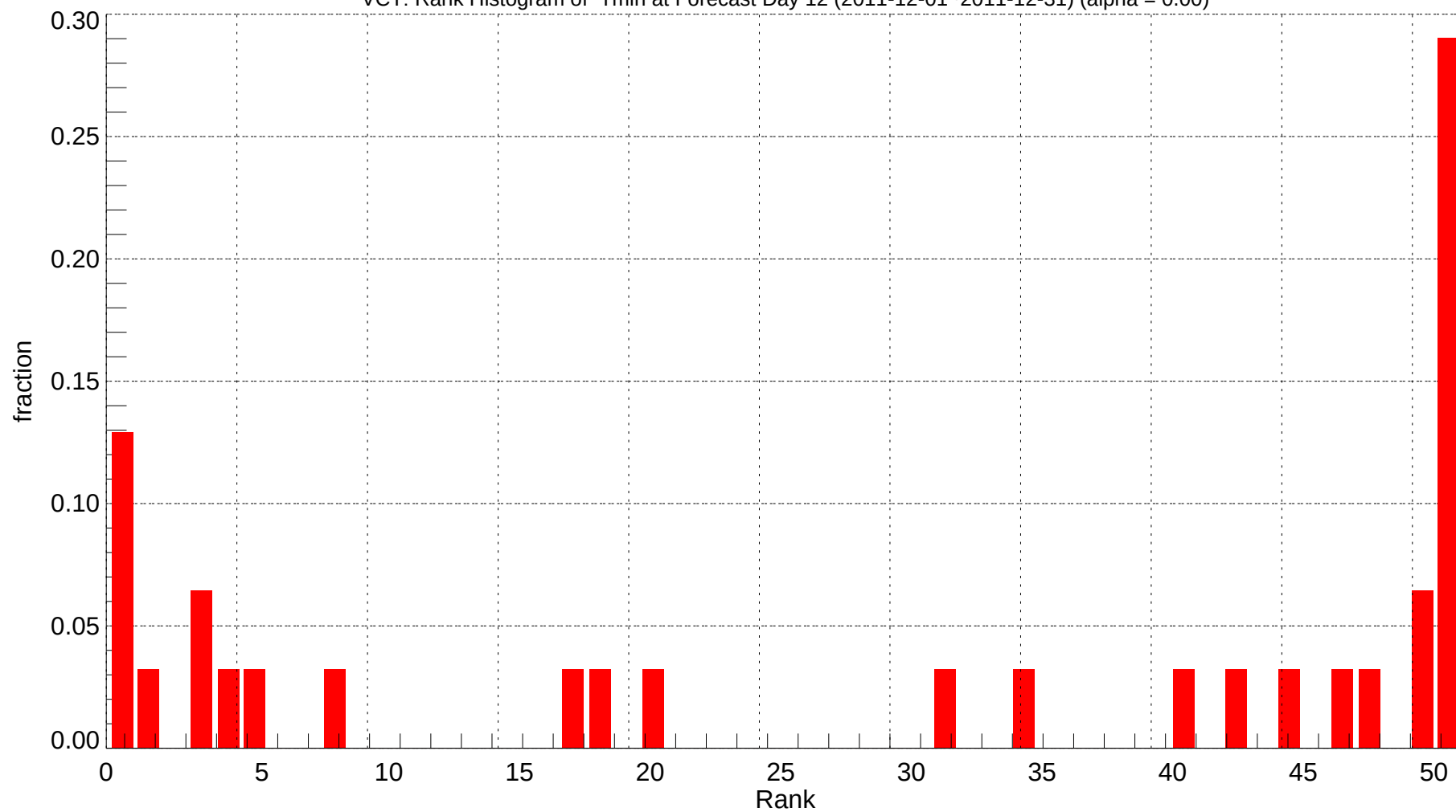
VCT: Rank Histogram of Tmin at Forecast Day 12 (2011-12-01~2011-12-31) (alpha = 0.00)
