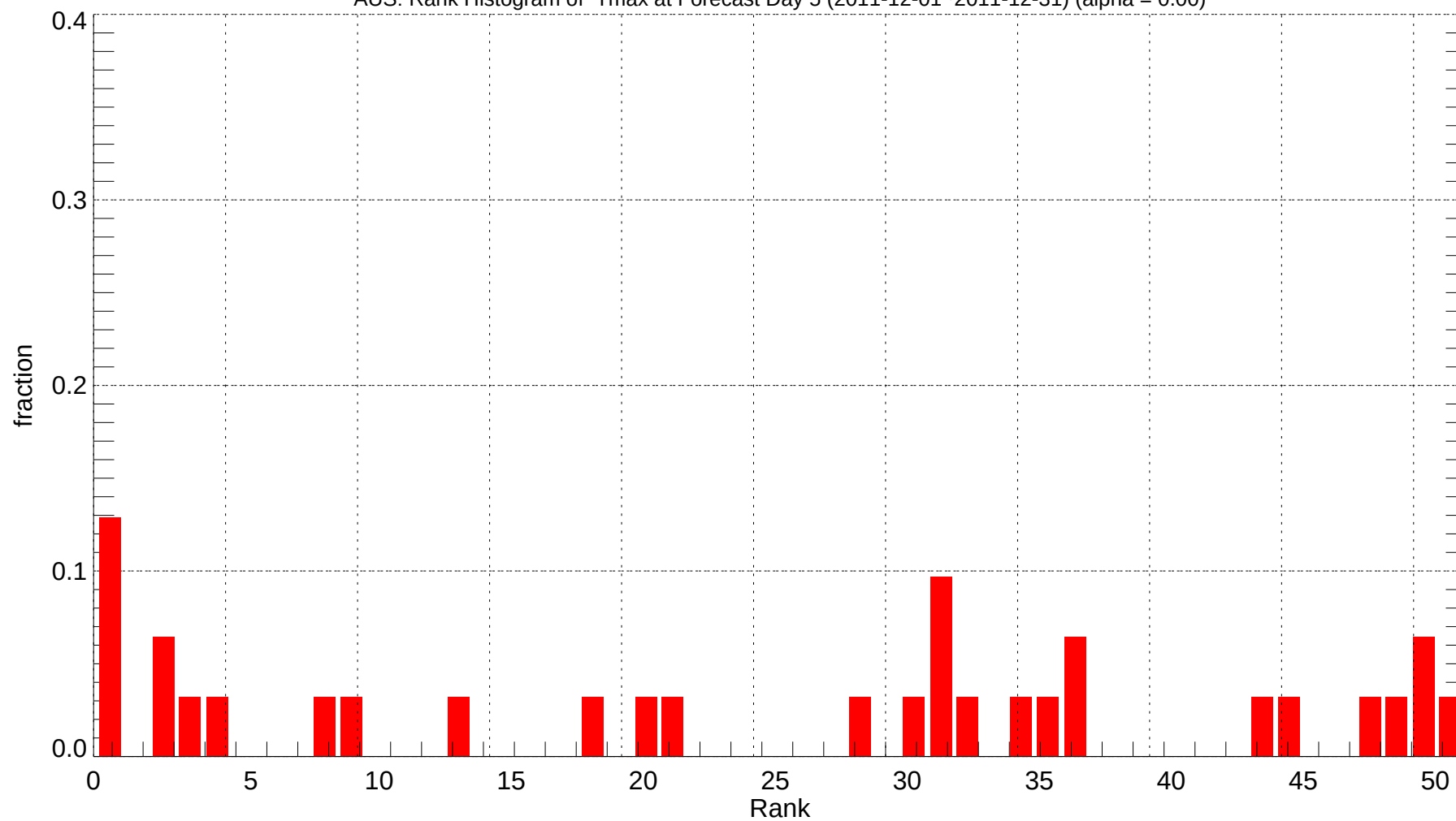
AUS: Rank Histogram of Tmax at Forecast Day 5 (2011-12-01~2011-12-31) (alpha = 0.00)
