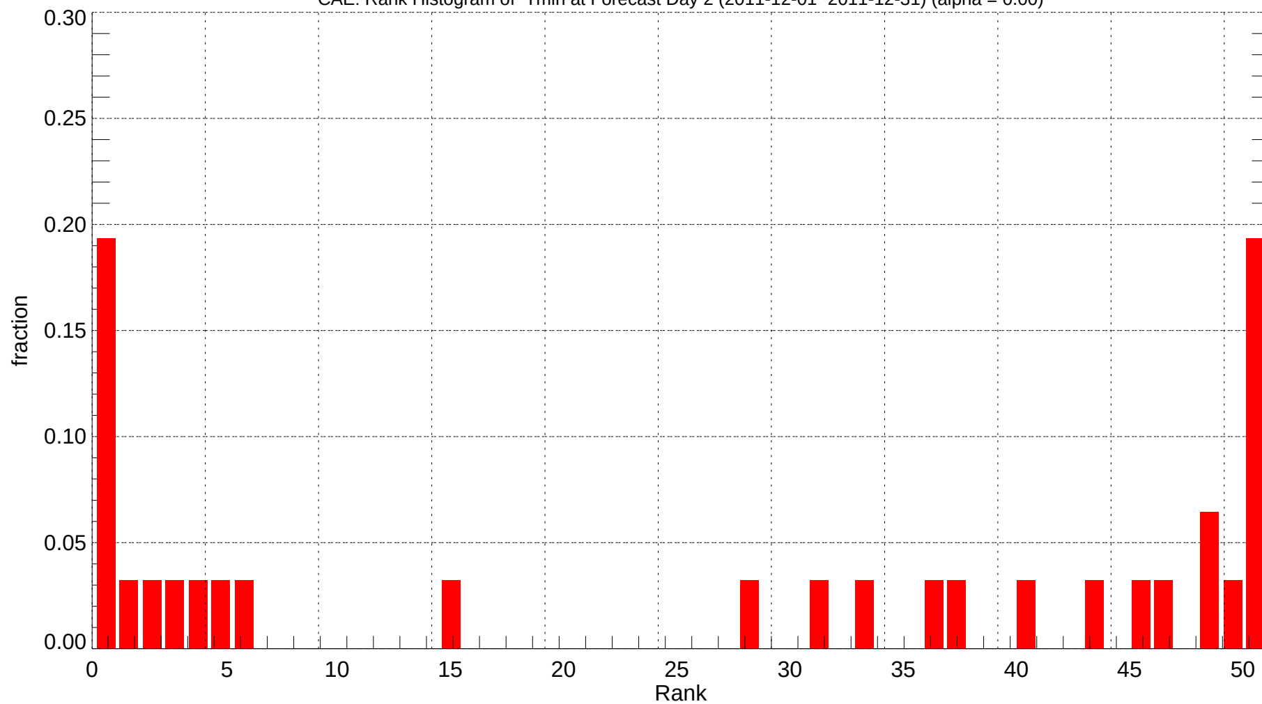
CAE: Rank Histogram of Tmin at Forecast Day 2 (2011-12-01~2011-12-31) (alpha = 0.00)
