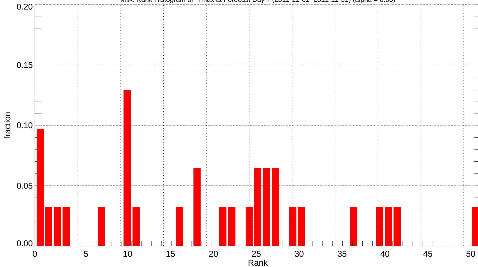
MIA: Rank Histogram of Tmax at Forecast Day 7 (2011-12-01~2011-12-31) (alpha = 0.00)
