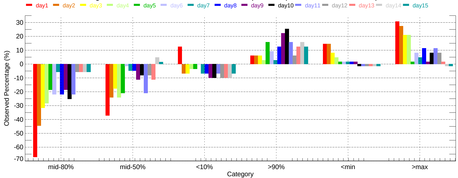
Observed Percentage Deviation of Ensembles - LAN: Min Temperature (2011-12-01~2011-12-31)
