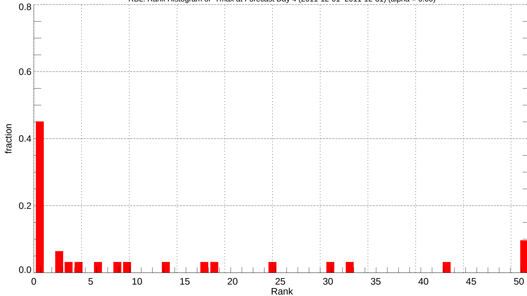
RBL: Rank Histogram of Tmax at Forecast Day 4 (2011-12-01~2011-12-31) (alpha = 0.00)
