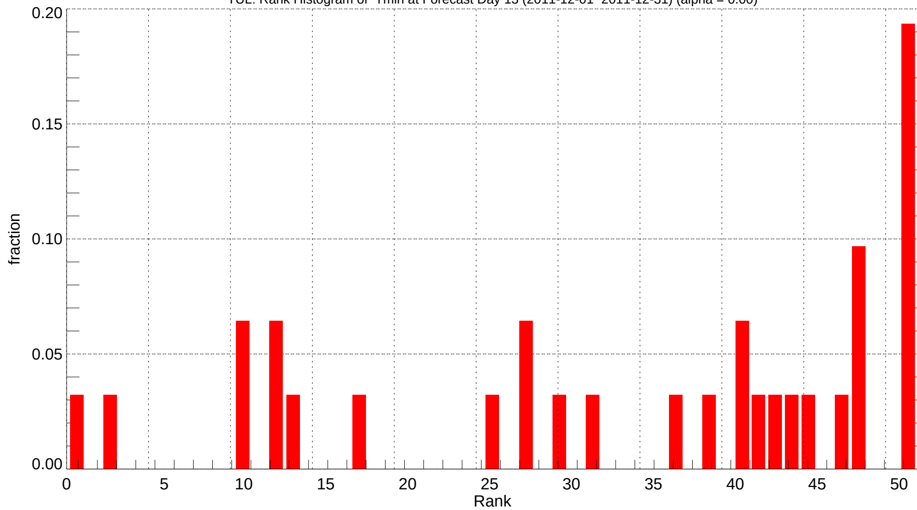
TUL: Rank Histogram of Tmin at Forecast Day 13 (2011-12-01~2011-12-31) (alpha = 0.00)
