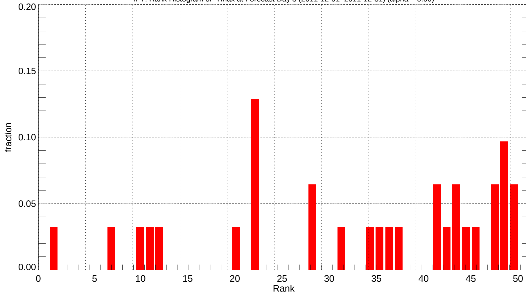
IPT: Rank Histogram of Tmax at Forecast Day 8 (2011-12-01~2011-12-31) (alpha = 0.00)
