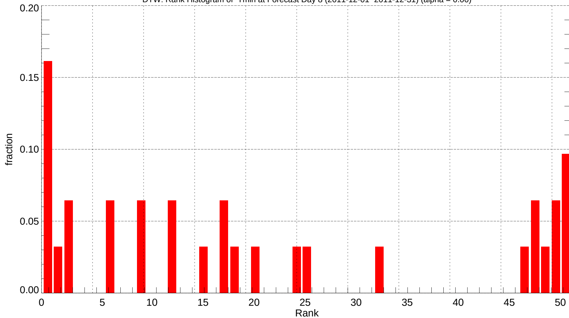
DTW: Rank Histogram of Tmin at Forecast Day 8 (2011-12-01~2011-12-31) (alpha = 0.00)
