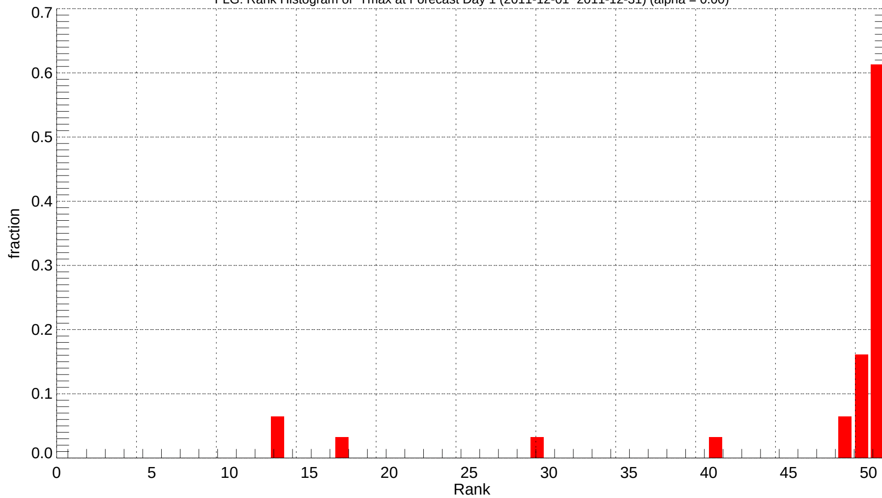
FLG: Rank Histogram of Tmax at Forecast Day 1 (2011-12-01~2011-12-31) (alpha = 0.00)
