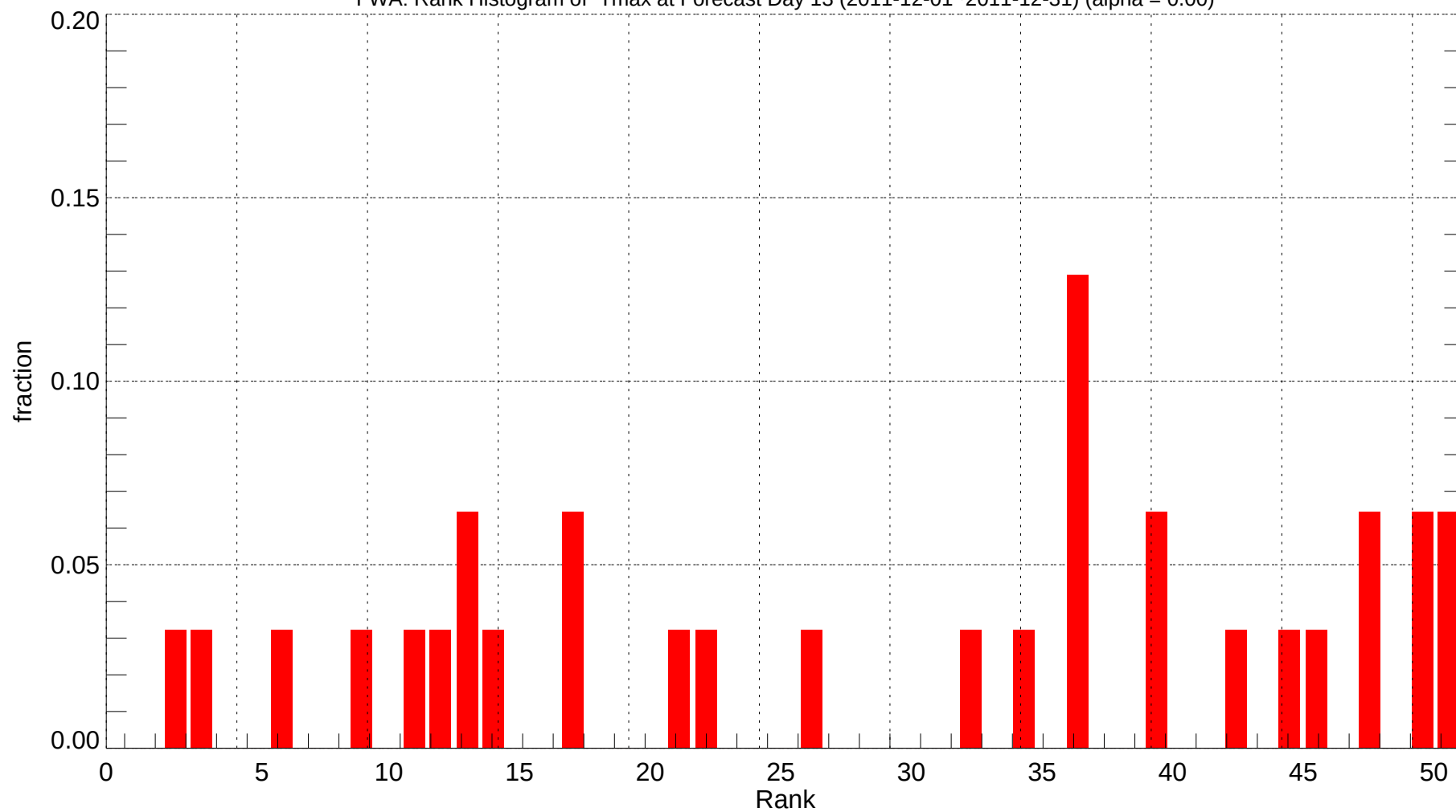
FWA: Rank Histogram of Tmax at Forecast Day 13 (2011-12-01~2011-12-31) (alpha = 0.00)
