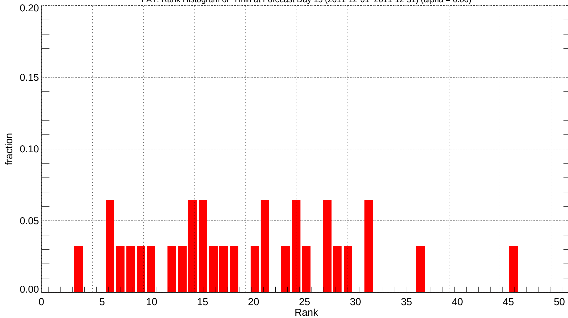
FAT: Rank Histogram of Tmin at Forecast Day 13 (2011-12-01~2011-12-31) (alpha = 0.00)
