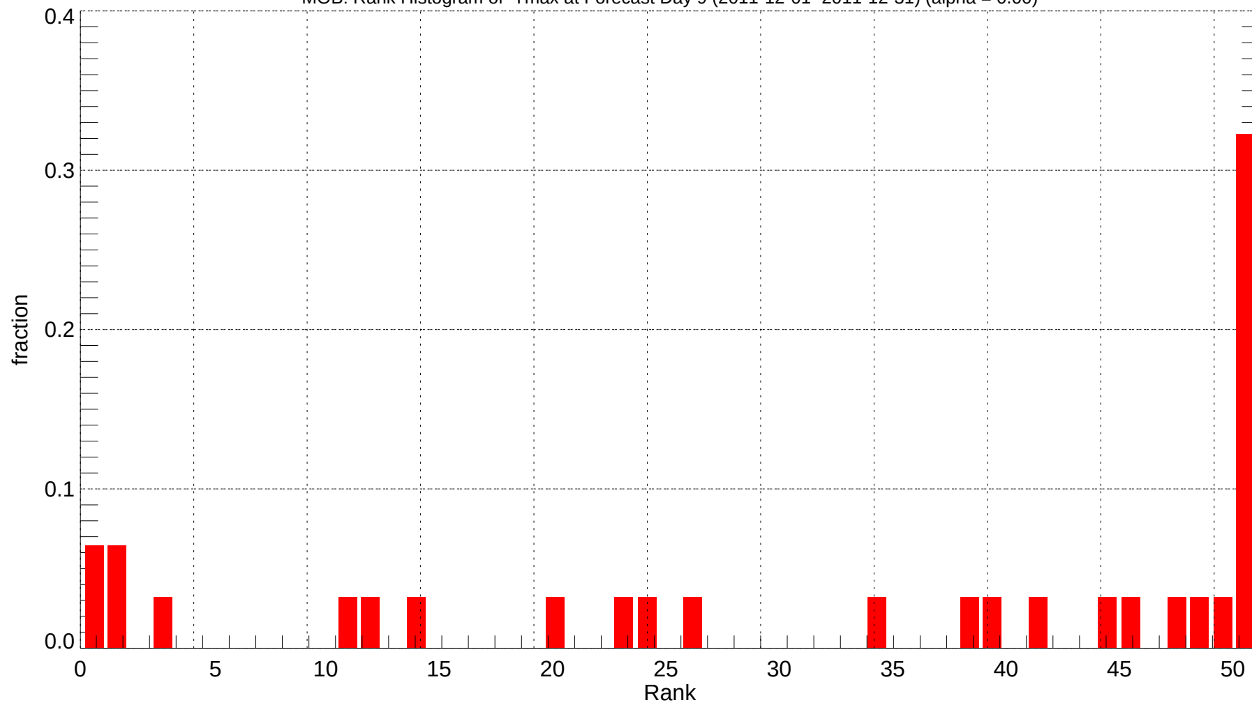
MOB: Rank Histogram of Tmax at Forecast Day 9 (2011-12-01~2011-12-31) (alpha = 0.00)
