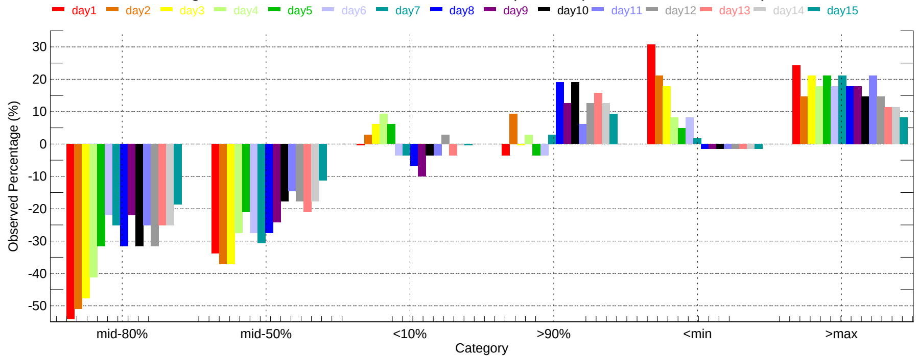
Observed Percentage Deviation of Ensembles - DSM: Max Temperature (2011-12-01~2011-12-31)
