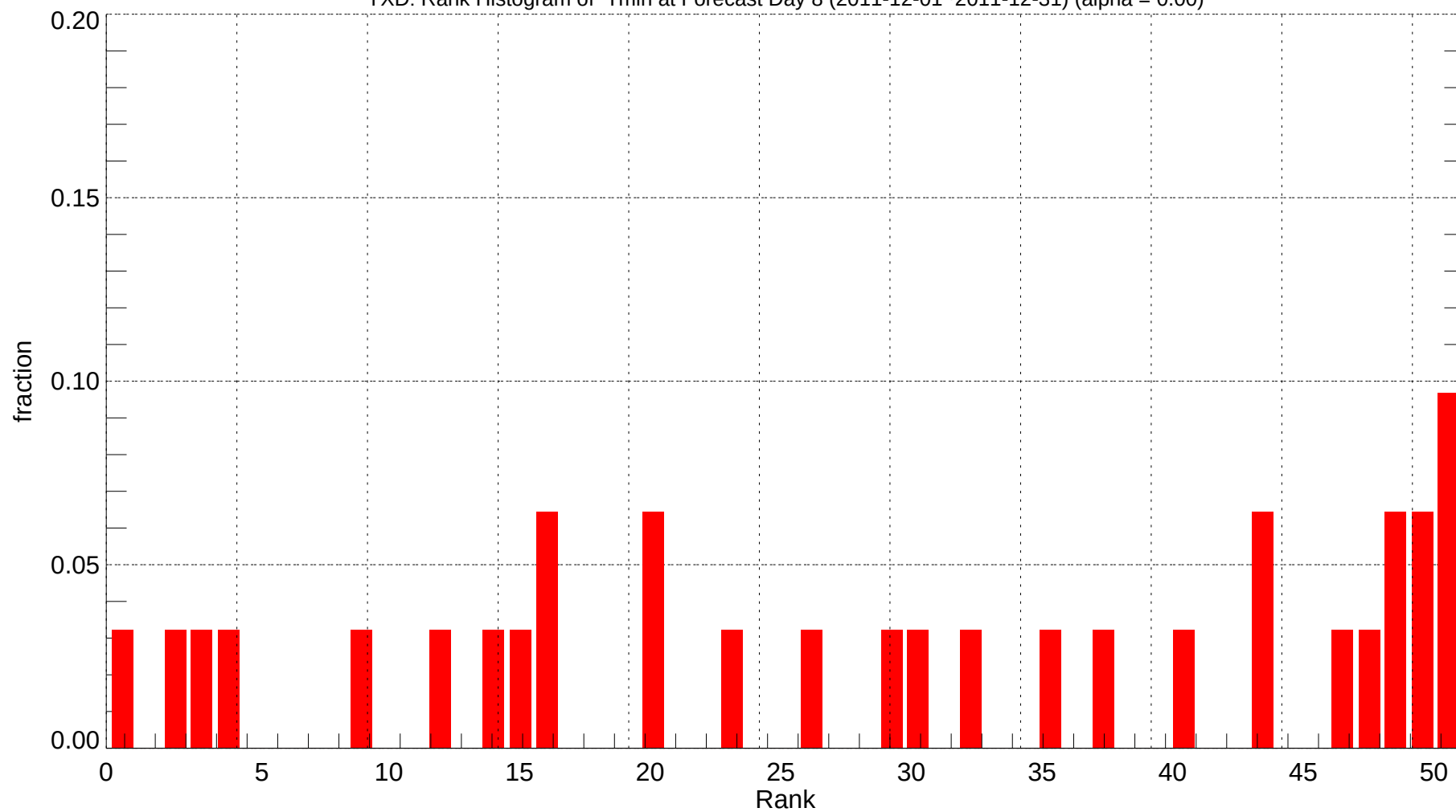
YXD: Rank Histogram of Tmin at Forecast Day 8 (2011-12-01~2011-12-31) (alpha = 0.00)
