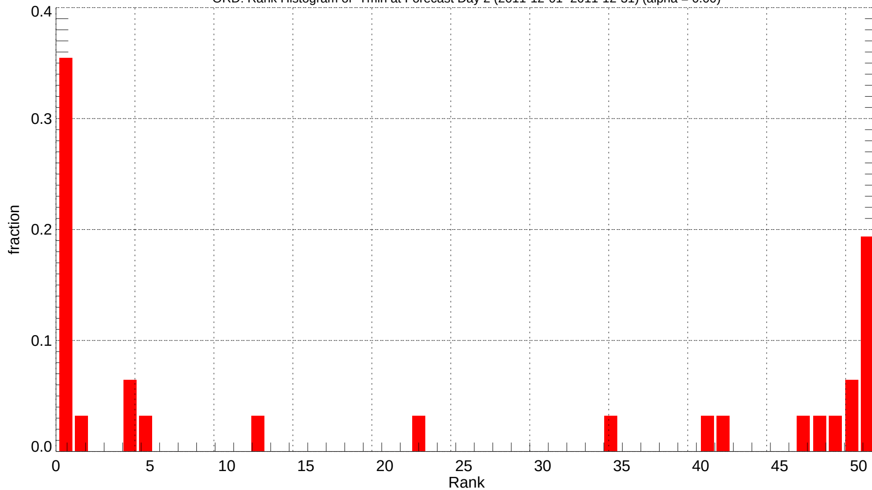
ORD: Rank Histogram of Tmin at Forecast Day 2 (2011-12-01~2011-12-31) (alpha = 0.00)
