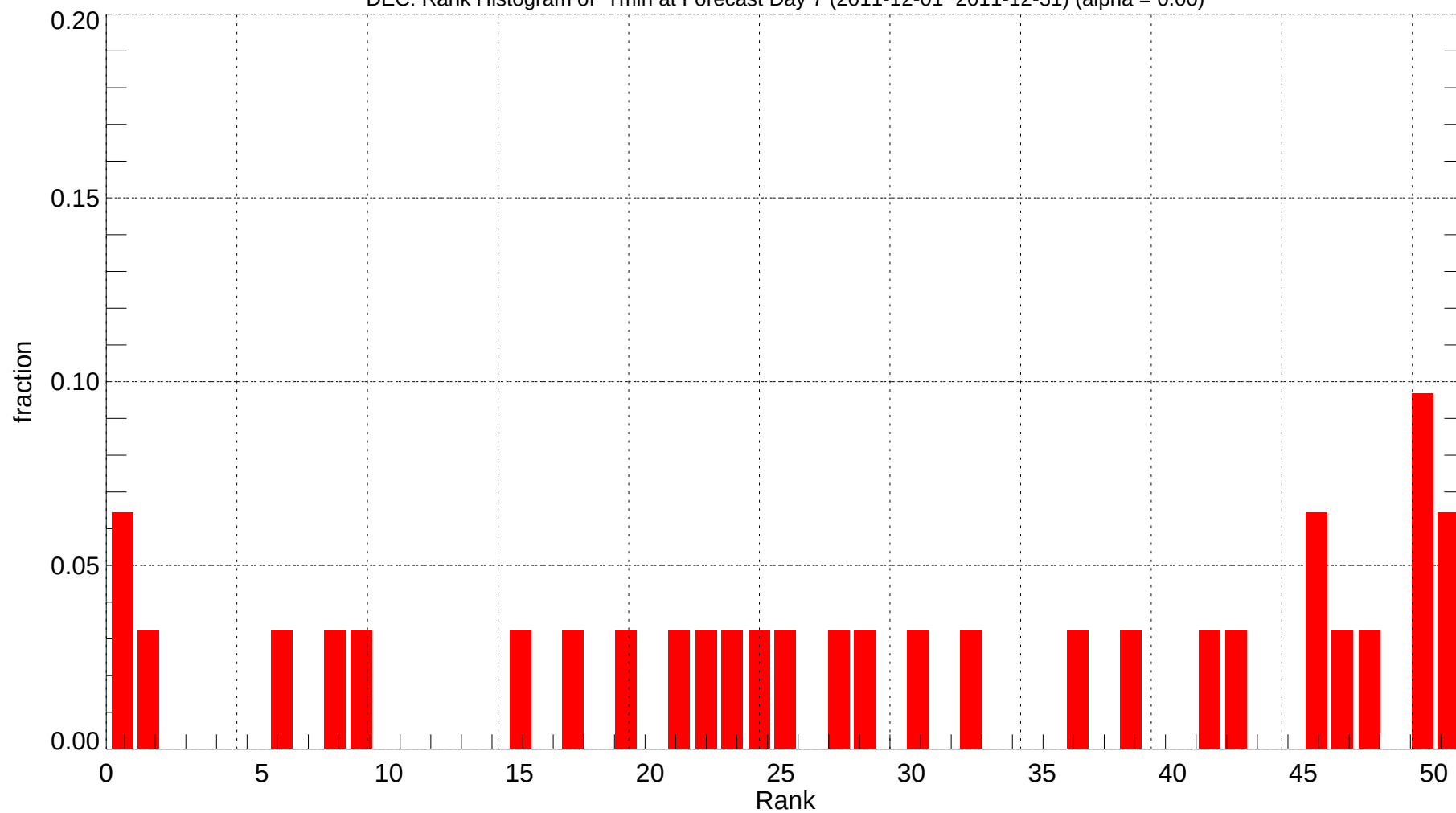
DEC: Rank Histogram of Tmin at Forecast Day 7 (2011-12-01~2011-12-31) (alpha = 0.00)
