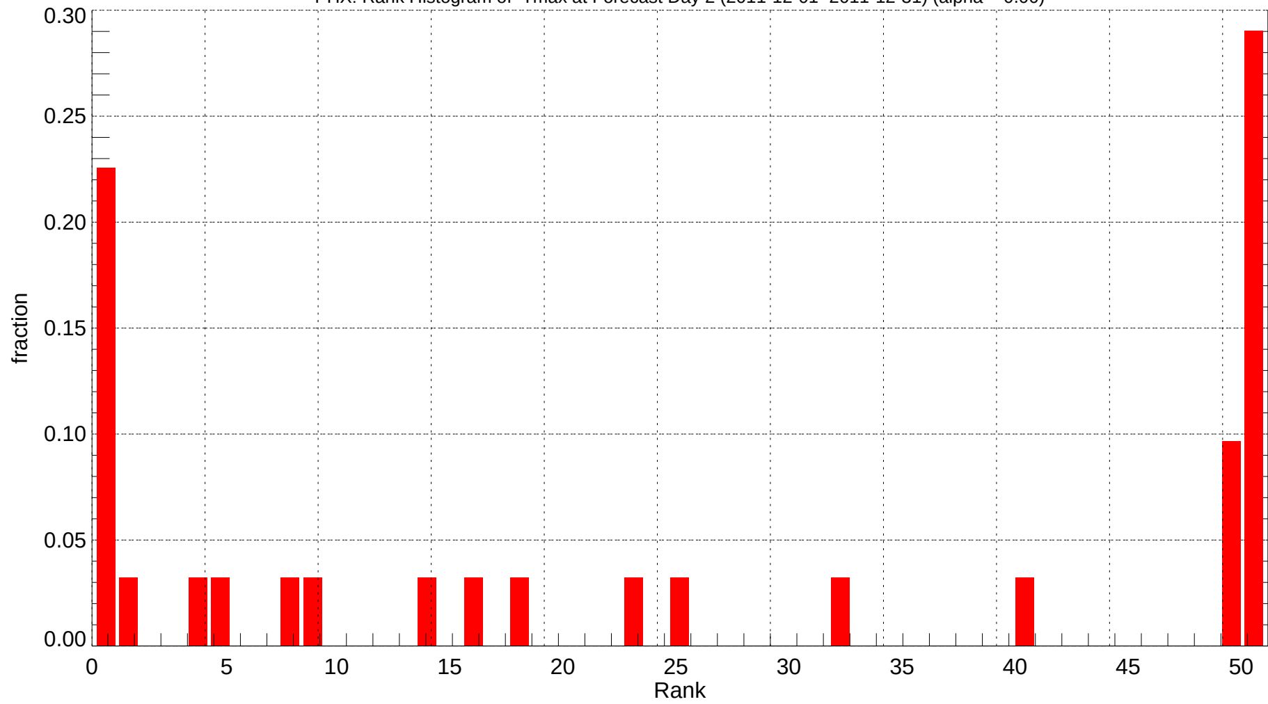
PHX: Rank Histogram of Tmax at Forecast Day 2 (2011-12-01~2011-12-31) (alpha = 0.00)
