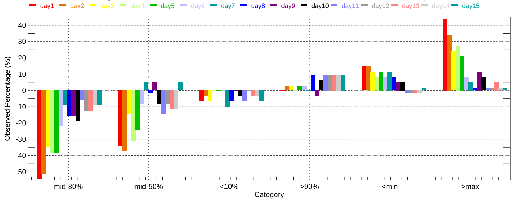
Observed Percentage Deviation of Ensembles - FMY: Max Temperature (2011-12-01~2011-12-31)
