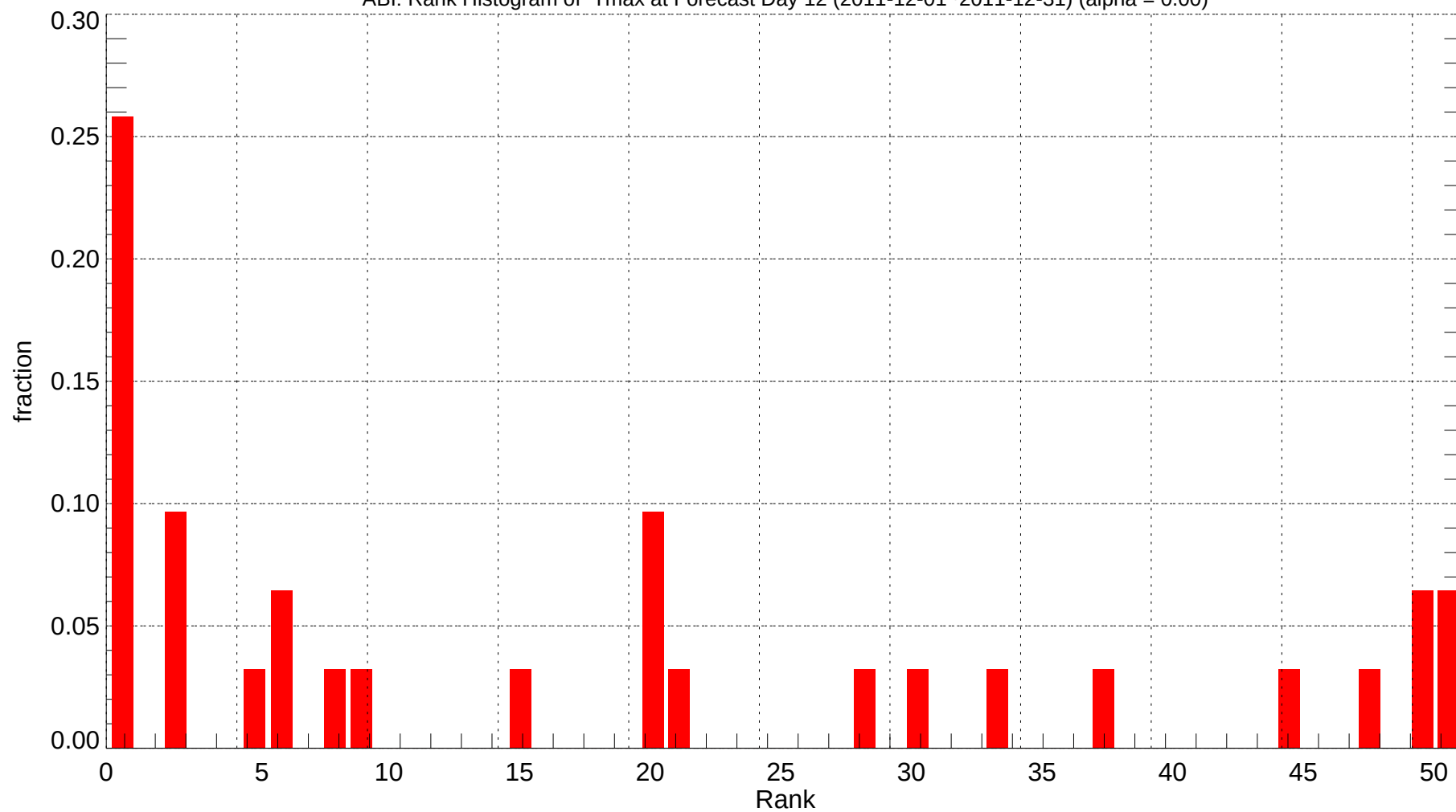
ABI: Rank Histogram of Tmax at Forecast Day 12 (2011-12-01~2011-12-31) (alpha = 0.00)
