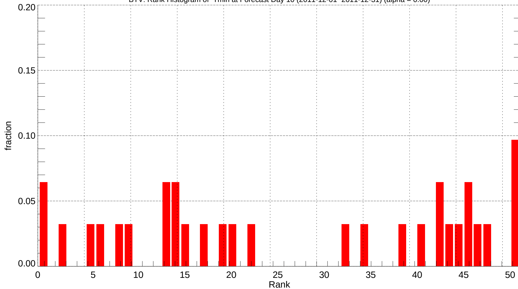
BTV: Rank Histogram of Tmin at Forecast Day 10 (2011-12-01~2011-12-31) (alpha = 0.00)
