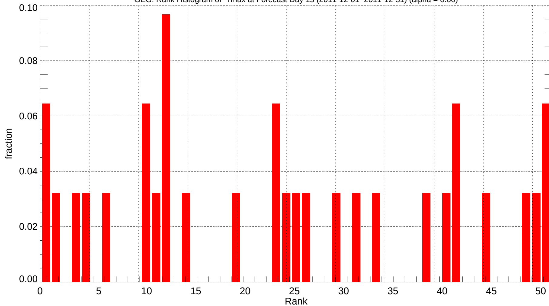
GEG: Rank Histogram of Tmax at Forecast Day 15 (2011-12-01~2011-12-31) (alpha = 0.00)
