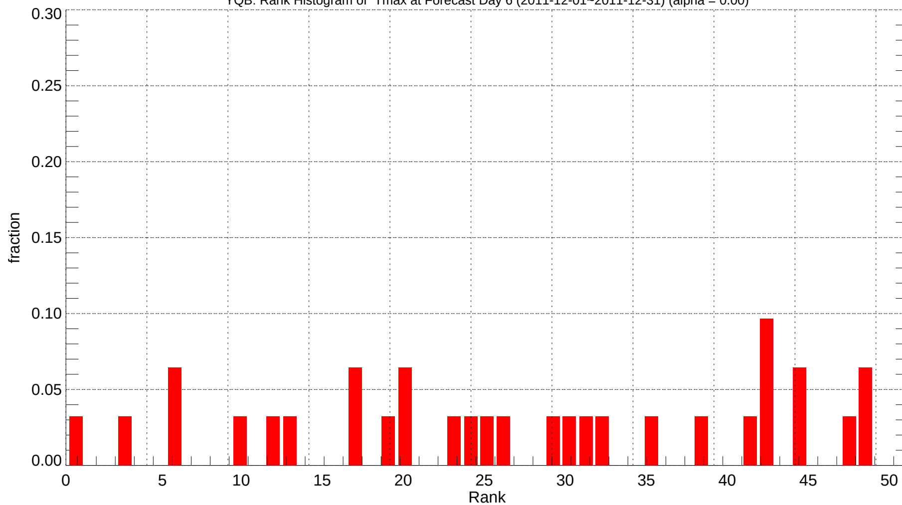
YQB: Rank Histogram of Tmax at Forecast Day 6 (2011-12-01~2011-12-31) (alpha = 0.00)
