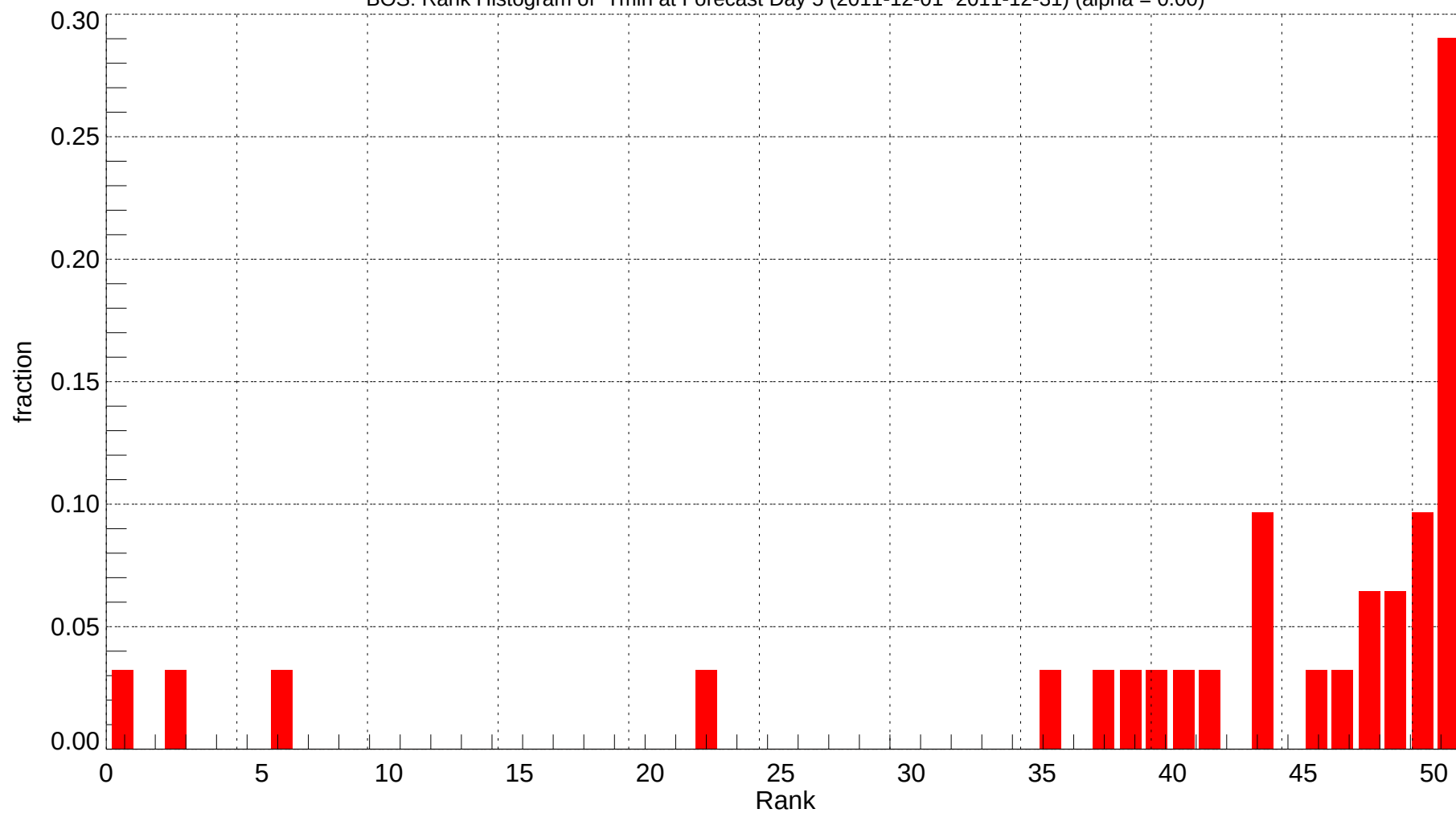
BOS: Rank Histogram of Tmin at Forecast Day 5 (2011-12-01~2011-12-31) (alpha = 0.00)
