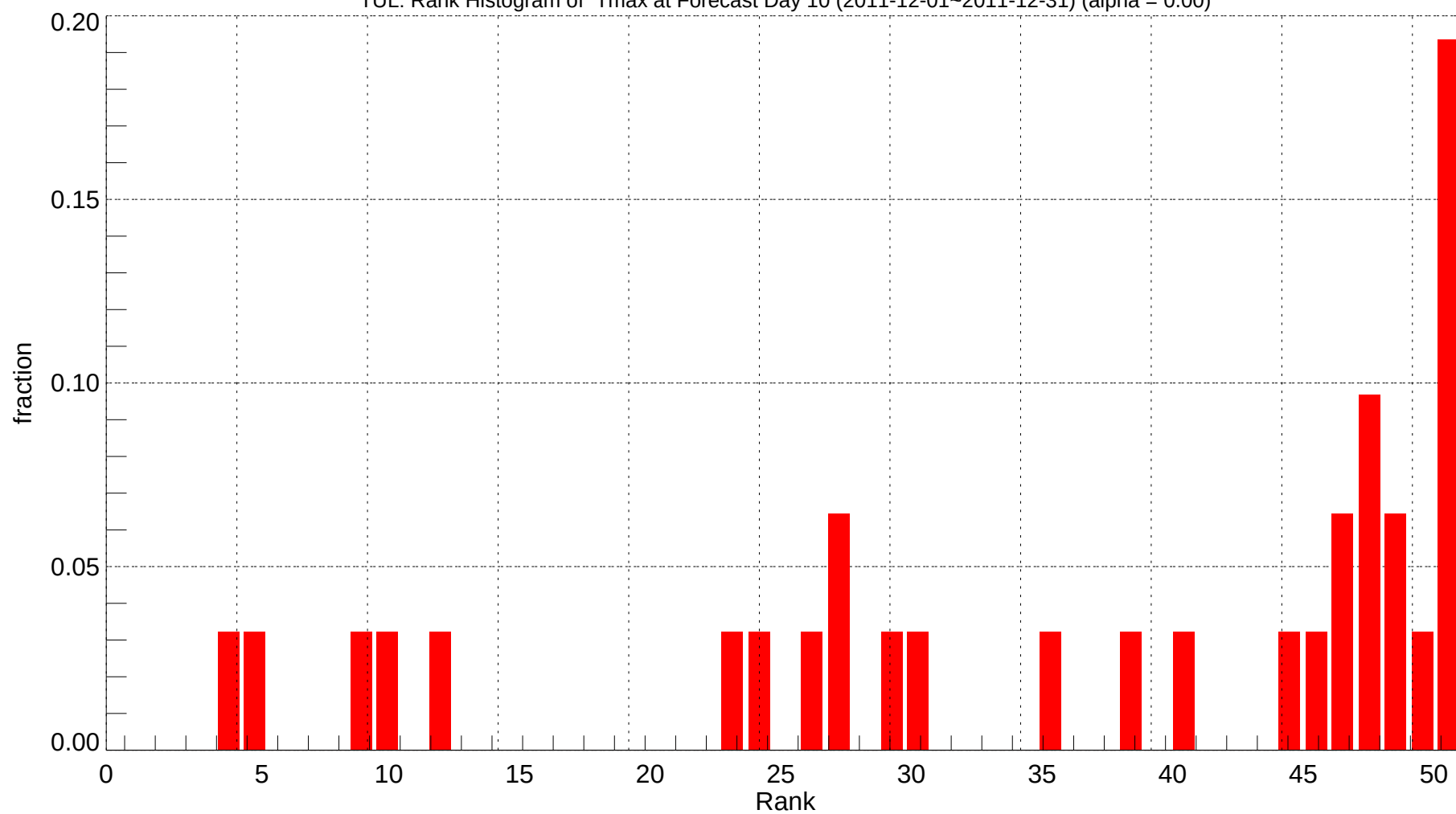
TUL: Rank Histogram of Tmax at Forecast Day 10 (2011-12-01~2011-12-31) (alpha = 0.00)
