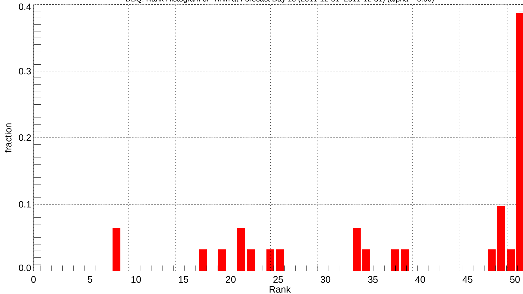
DBQ: Rank Histogram of Tmin at Forecast Day 10 (2011-12-01~2011-12-31) (alpha = 0.00)
