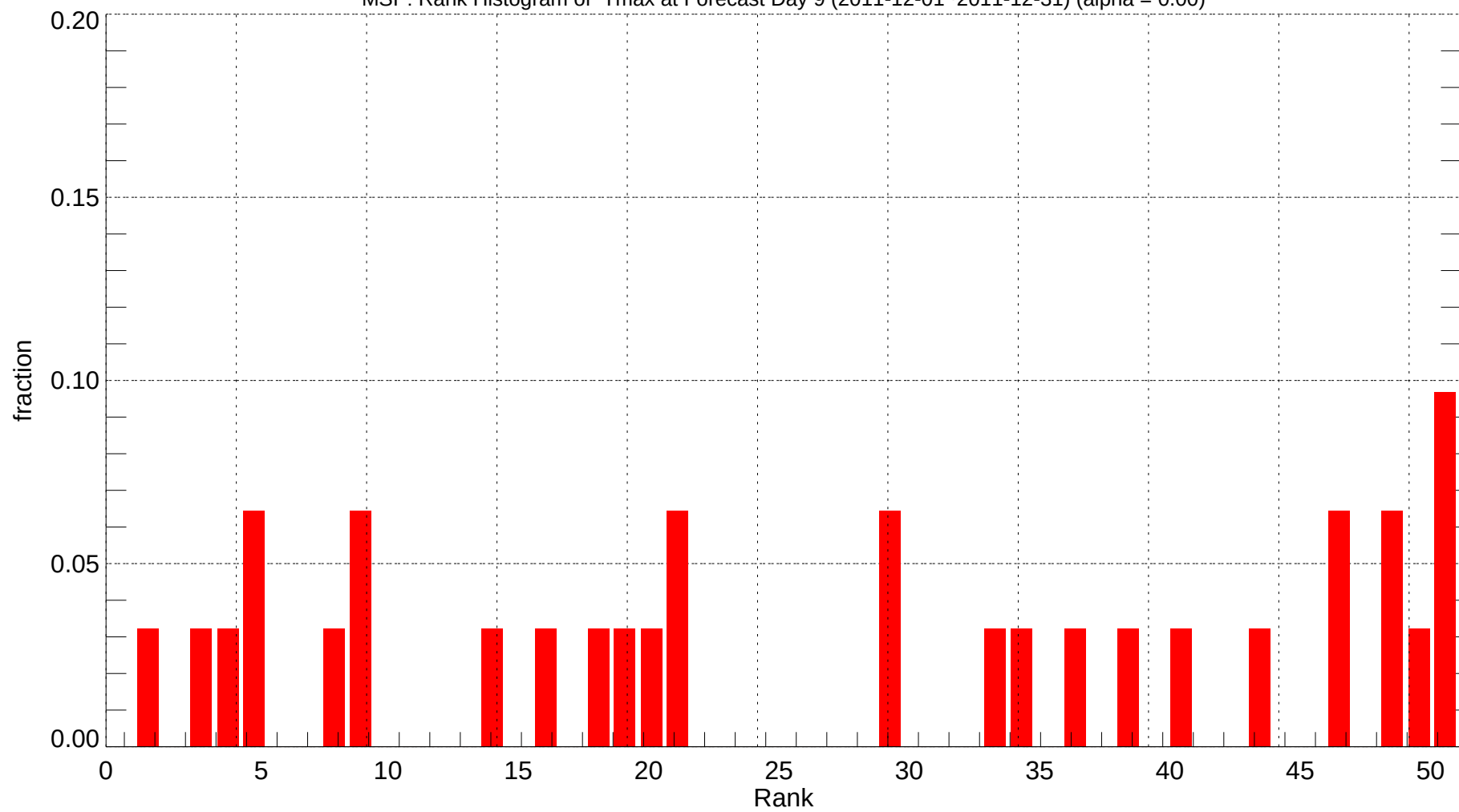
MSP: Rank Histogram of Tmax at Forecast Day 9 (2011-12-01~2011-12-31) (alpha = 0.00)
