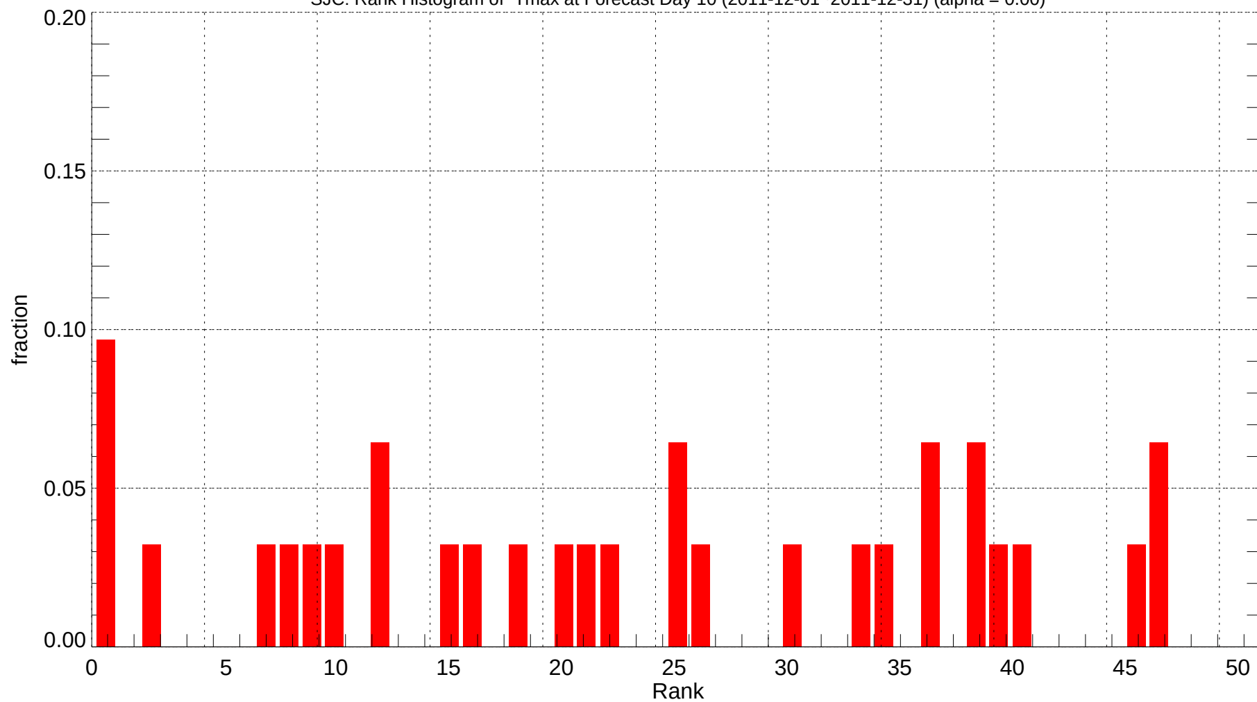
SJC: Rank Histogram of Tmax at Forecast Day 10 (2011-12-01~2011-12-31) (alpha = 0.00)
