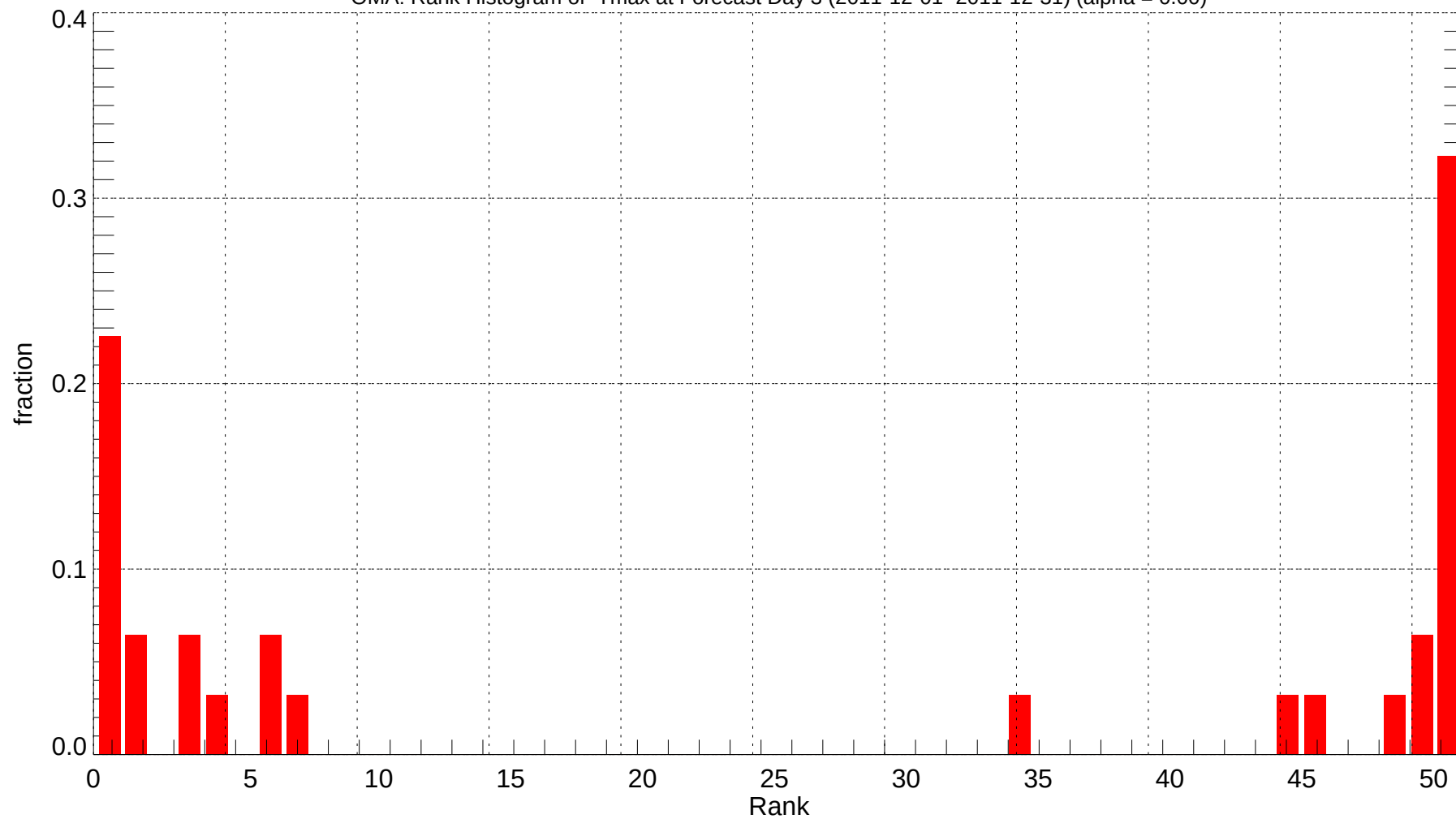
OMA: Rank Histogram of Tmax at Forecast Day 3 (2011-12-01~2011-12-31) (alpha = 0.00)
