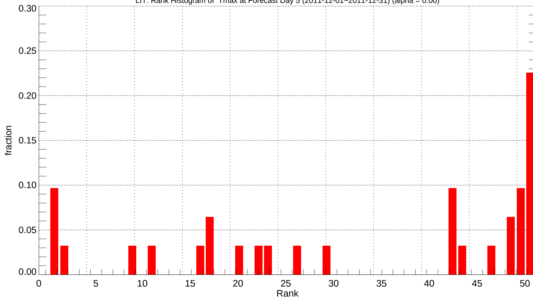
LIT: Rank Histogram of Tmax at Forecast Day 5 (2011-12-01~2011-12-31) (alpha = 0.00)
