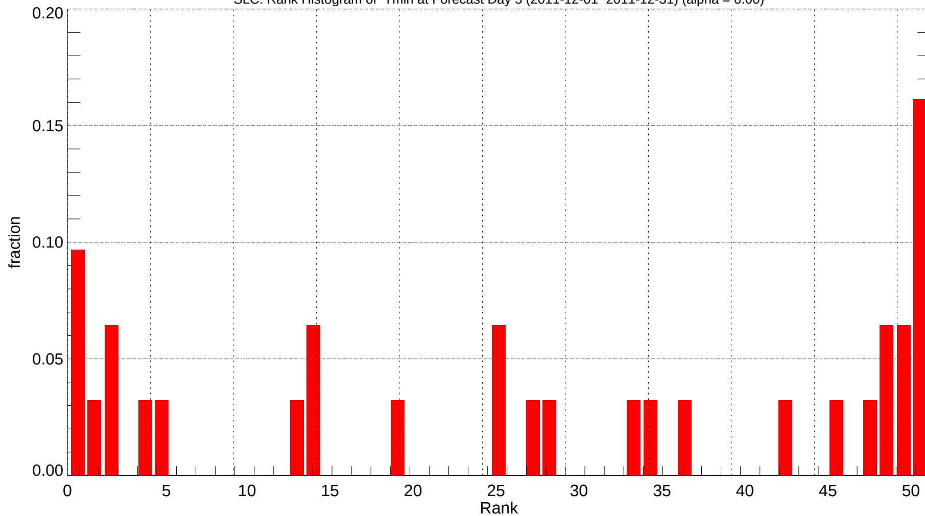
SLC: Rank Histogram of Tmin at Forecast Day 5 (2011-12-01~2011-12-31) (alpha = 0.00)
