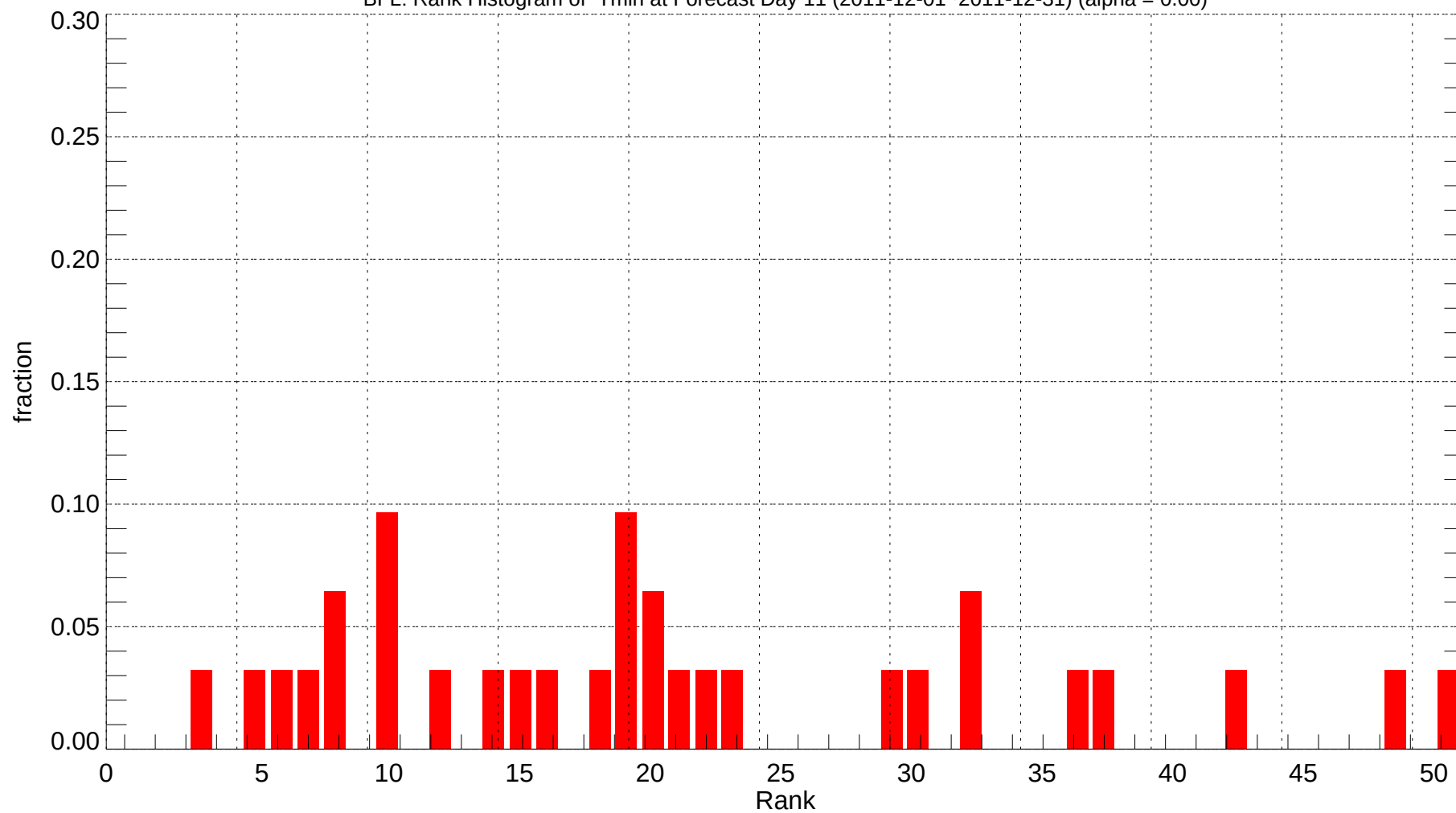
BFL: Rank Histogram of Tmin at Forecast Day 11 (2011-12-01~2011-12-31) (alpha = 0.00)
