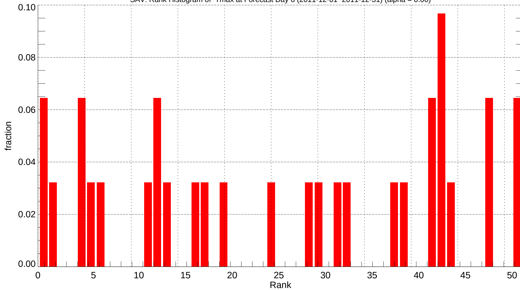
SAV: Rank Histogram of Tmax at Forecast Day 6 (2011-12-01~2011-12-31) (alpha = 0.00)
