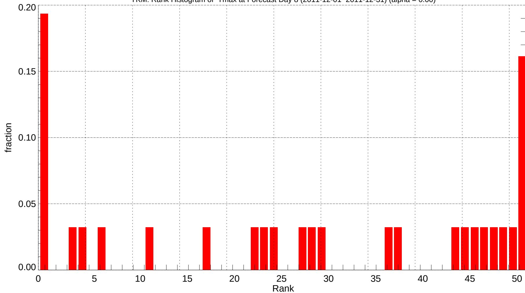
YKM: Rank Histogram of Tmax at Forecast Day 8 (2011-12-01~2011-12-31) (alpha = 0.00)
