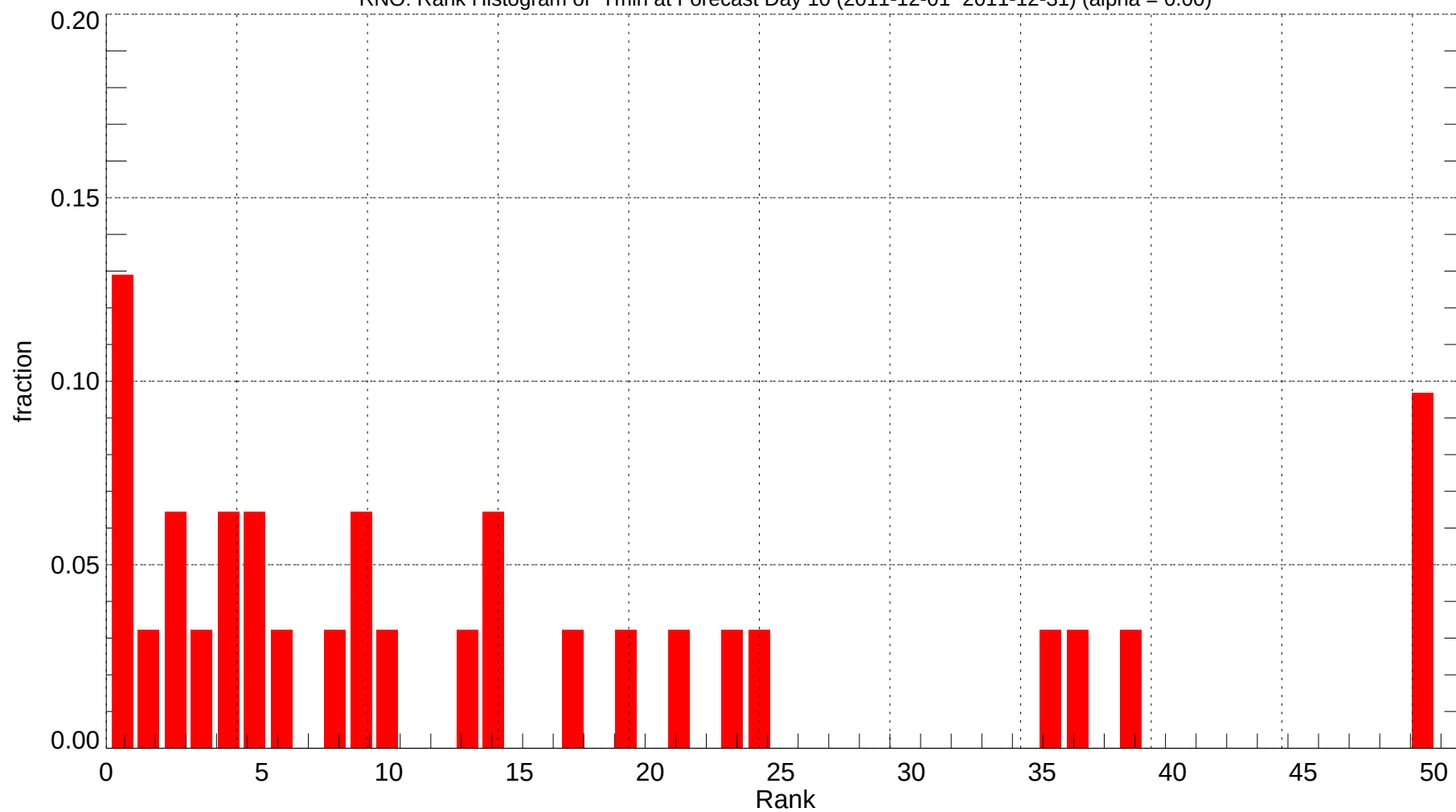
RNO: Rank Histogram of Tmin at Forecast Day 10 (2011-12-01~2011-12-31) (alpha = 0.00)
