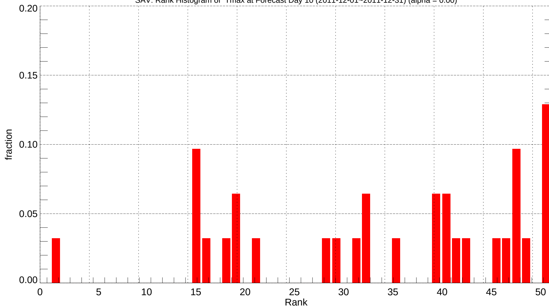
SAV: Rank Histogram of Tmax at Forecast Day 10 (2011-12-01~2011-12-31) (alpha = 0.00)
