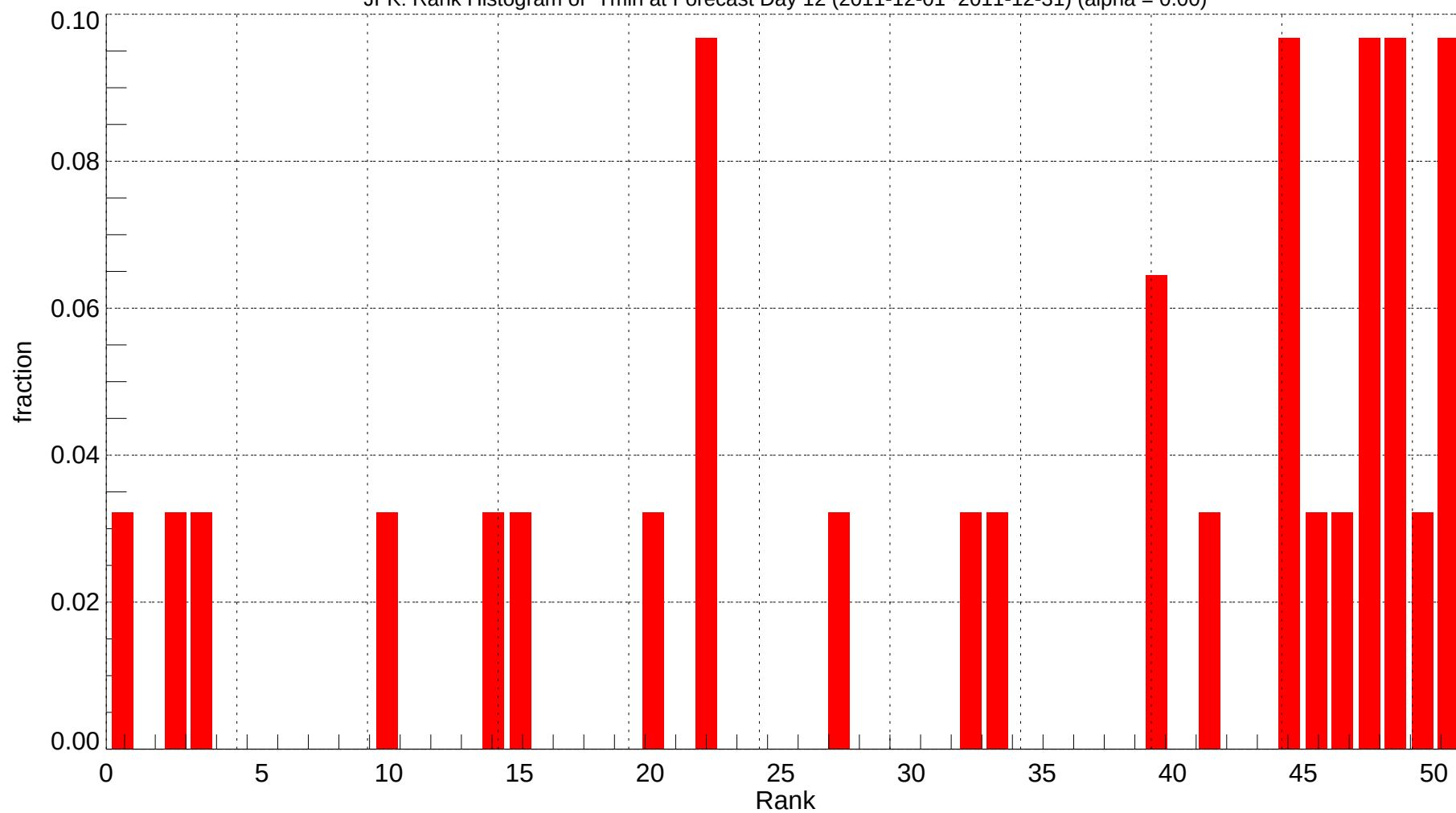
JFK: Rank Histogram of Tmin at Forecast Day 12 (2011-12-01~2011-12-31) (alpha = 0.00)
