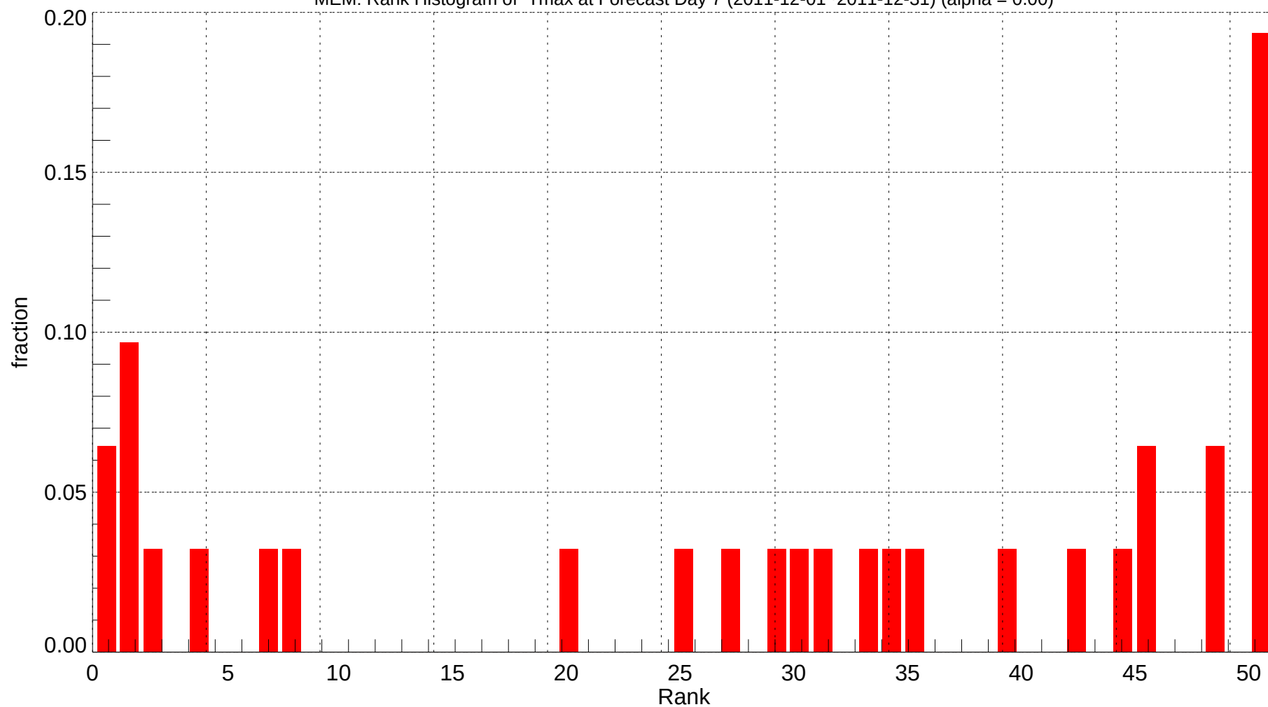
MEM: Rank Histogram of Tmax at Forecast Day 7 (2011-12-01~2011-12-31) (alpha = 0.00)
