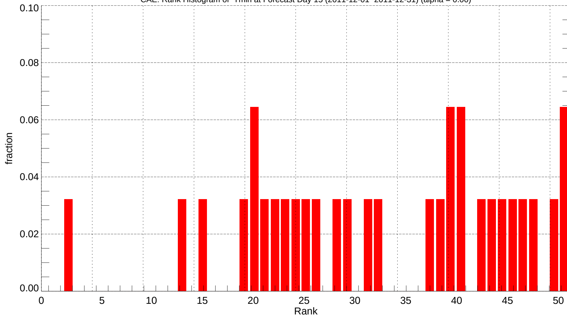
CAE: Rank Histogram of Tmin at Forecast Day 15 (2011-12-01~2011-12-31) (alpha = 0.00)
