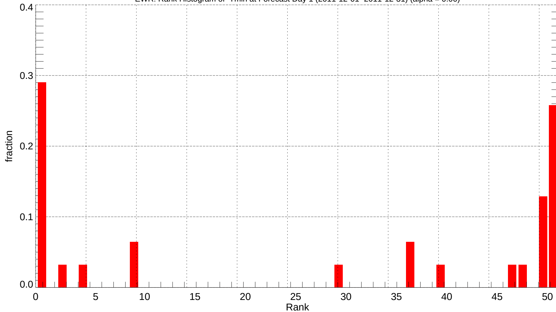
EWR: Rank Histogram of Tmin at Forecast Day 1 (2011-12-01~2011-12-31) (alpha = 0.00)
