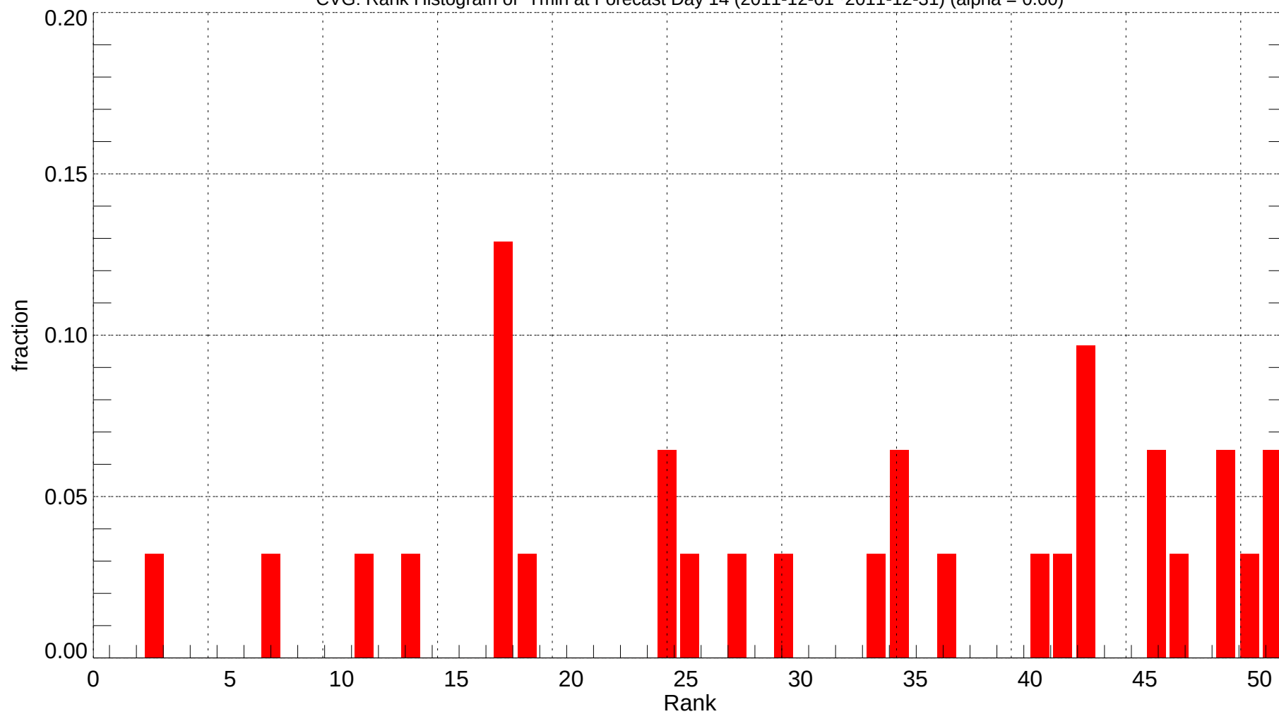
CVG: Rank Histogram of Tmin at Forecast Day 14 (2011-12-01~2011-12-31) (alpha = 0.00)
