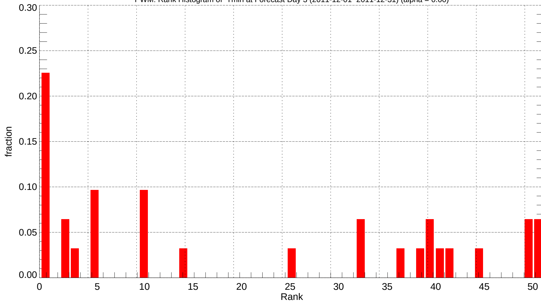
PWM: Rank Histogram of Tmin at Forecast Day 3 (2011-12-01~2011-12-31) (alpha = 0.00)
