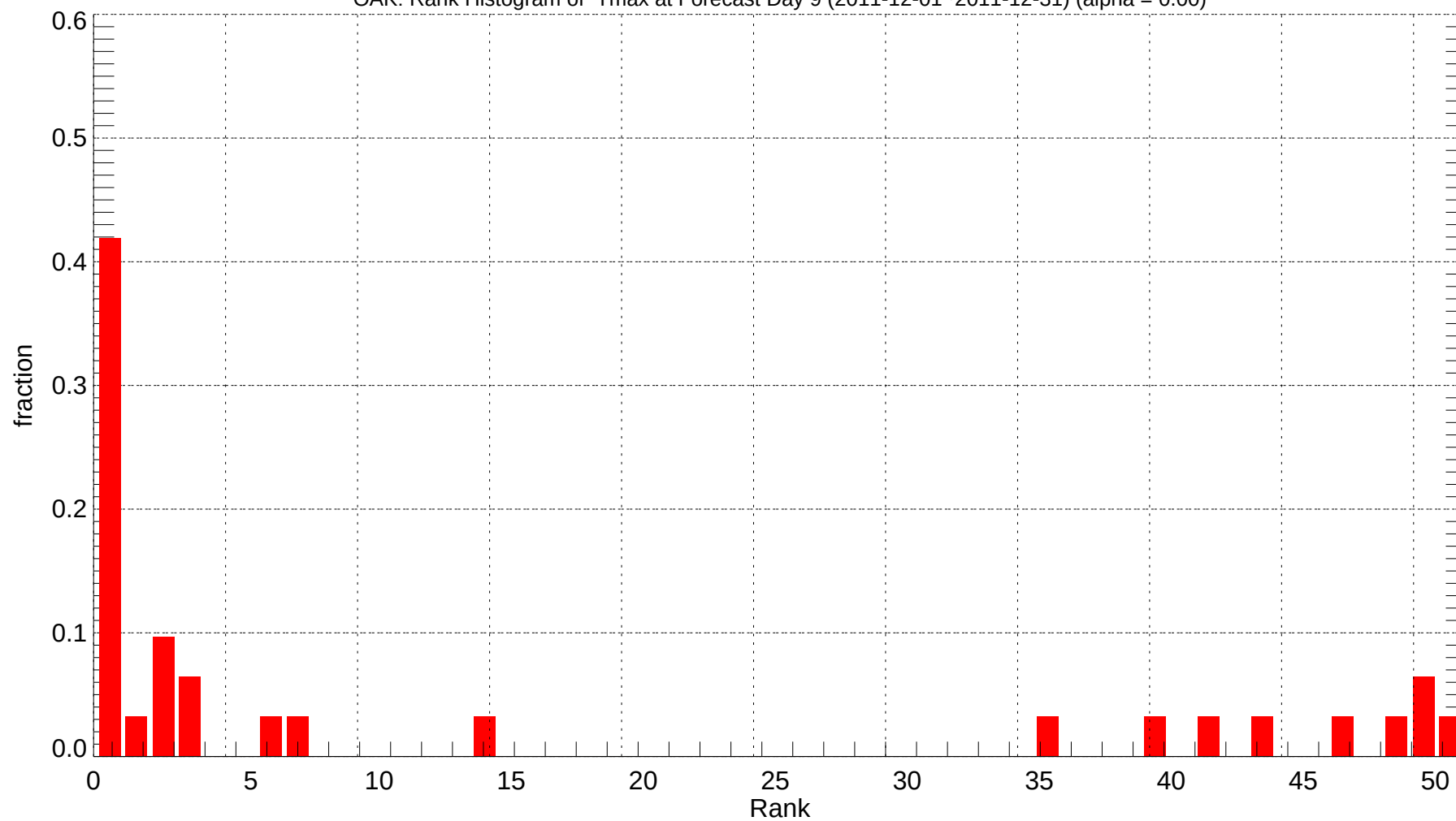
OAK: Rank Histogram of Tmax at Forecast Day 9 (2011-12-01~2011-12-31) (alpha = 0.00)
