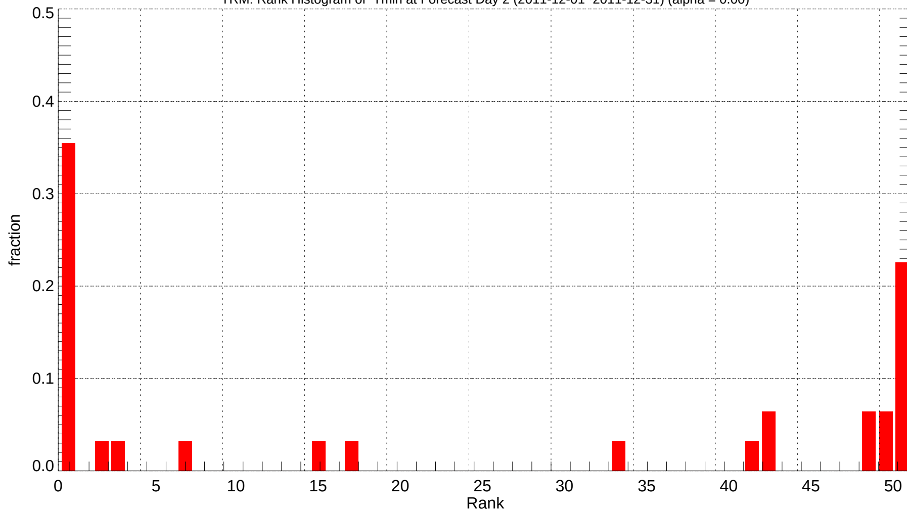
TRM: Rank Histogram of Tmin at Forecast Day 2 (2011-12-01~2011-12-31) (alpha = 0.00)
