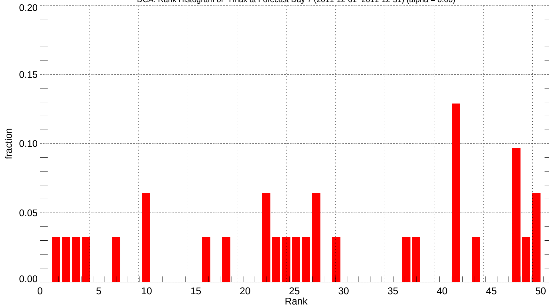
DCA: Rank Histogram of Tmax at Forecast Day 7 (2011-12-01~2011-12-31) (alpha = 0.00)
