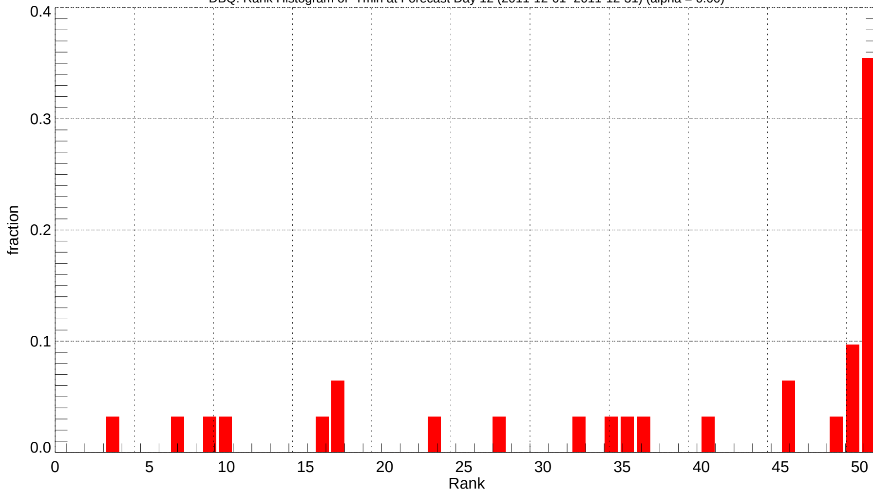
DBQ: Rank Histogram of Tmin at Forecast Day 12 (2011-12-01~2011-12-31) (alpha = 0.00)
