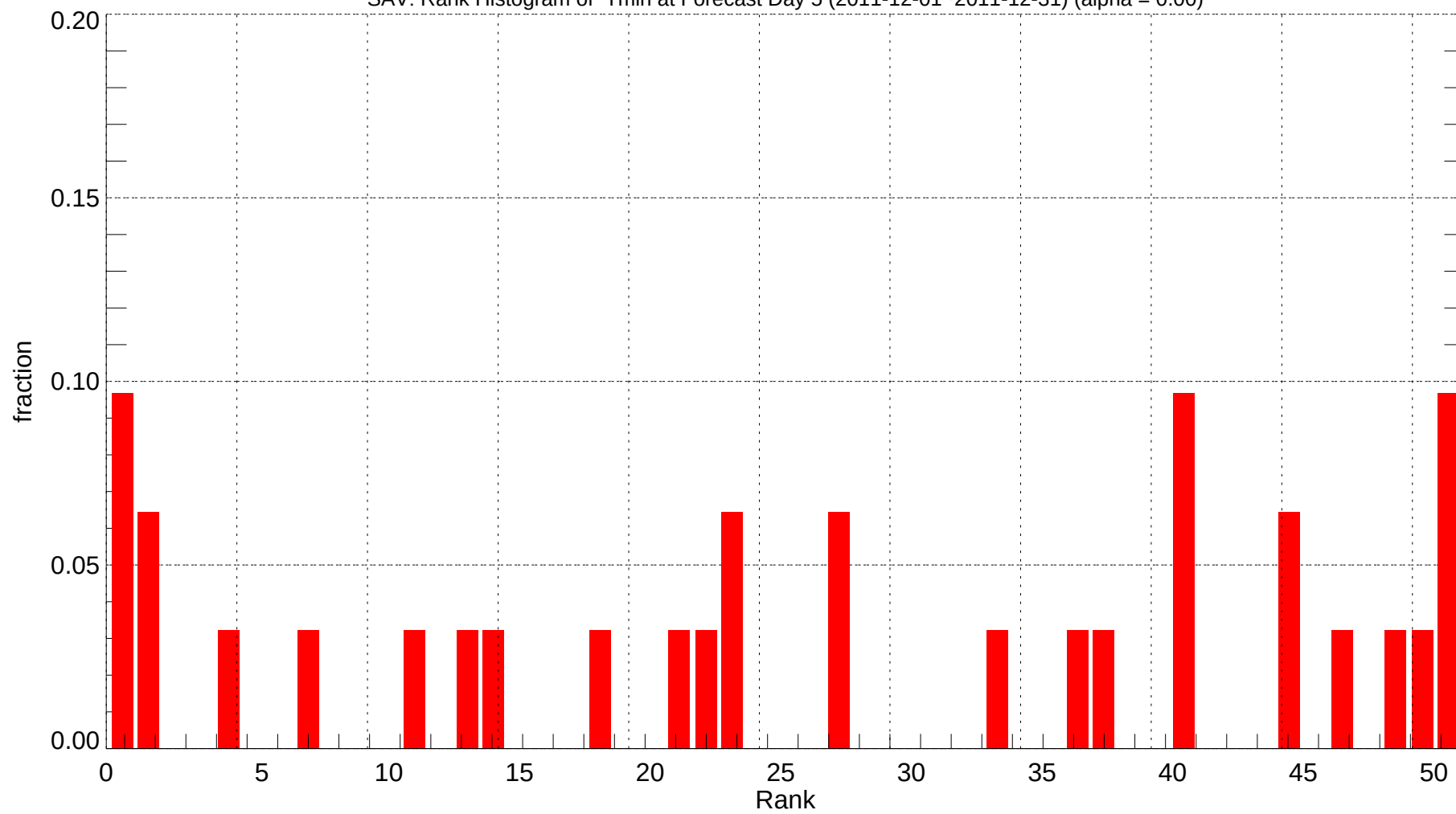
SAV: Rank Histogram of Tmin at Forecast Day 5 (2011-12-01~2011-12-31) (alpha = 0.00)
