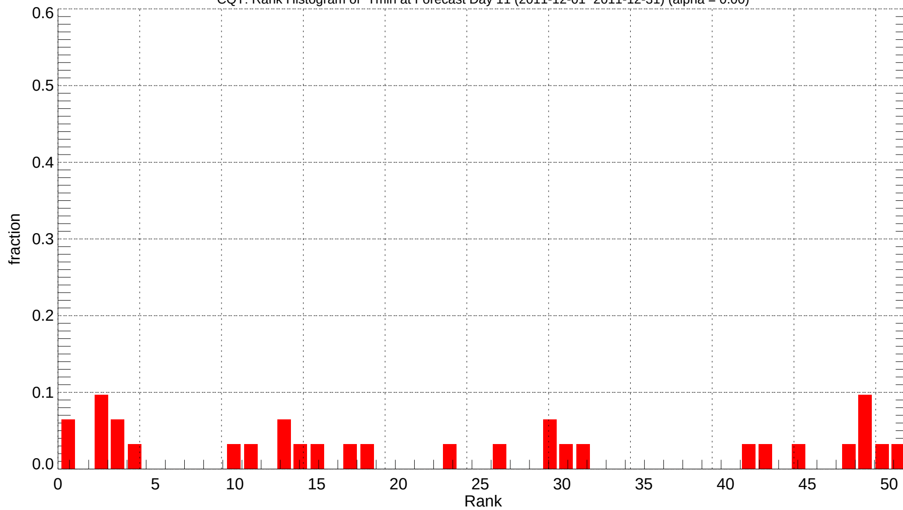
CQT: Rank Histogram of Tmin at Forecast Day 11 (2011-12-01~2011-12-31) (alpha = 0.00)
