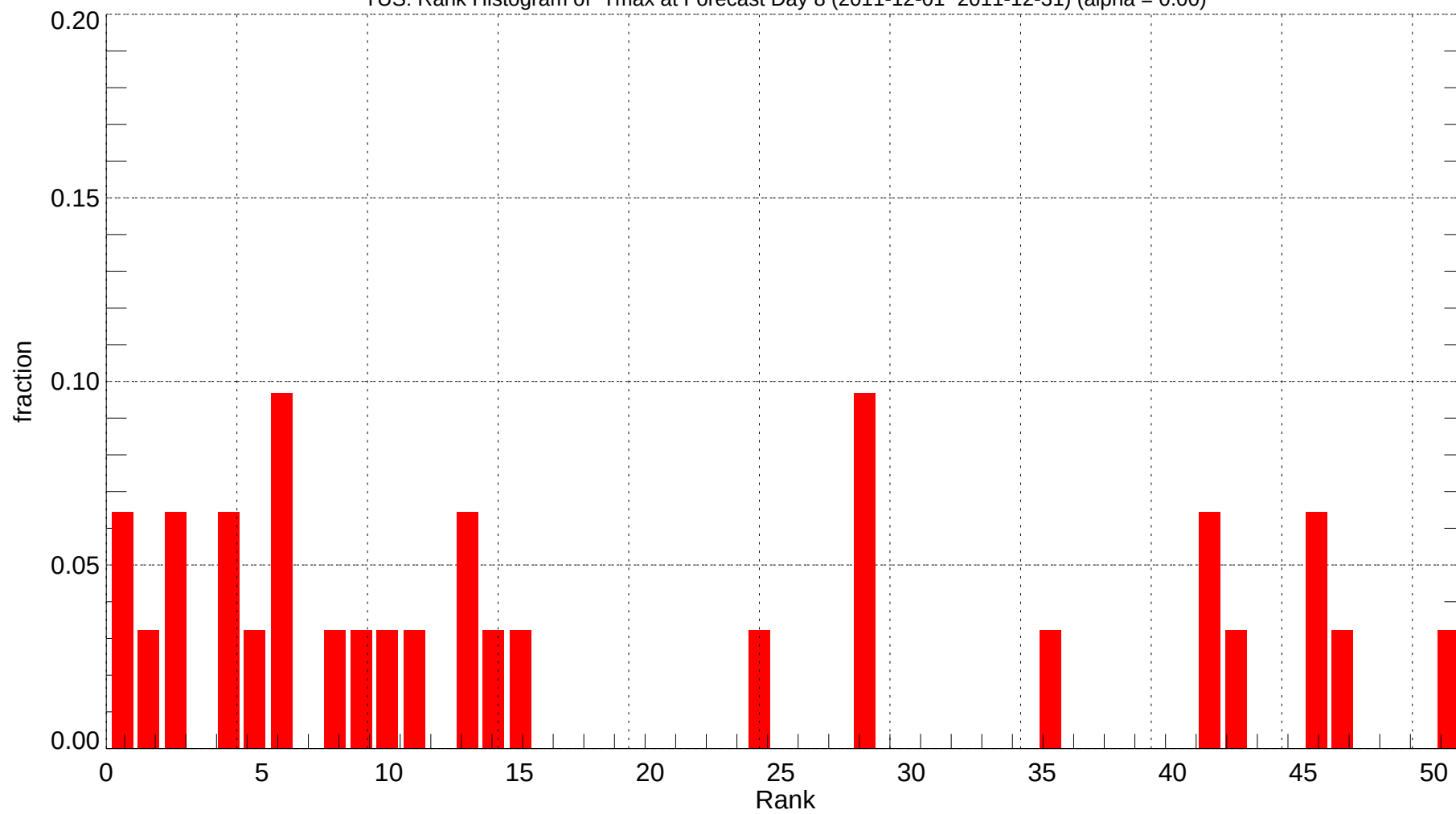
TUS: Rank Histogram of Tmax at Forecast Day 8 (2011-12-01~2011-12-31) (alpha = 0.00)
