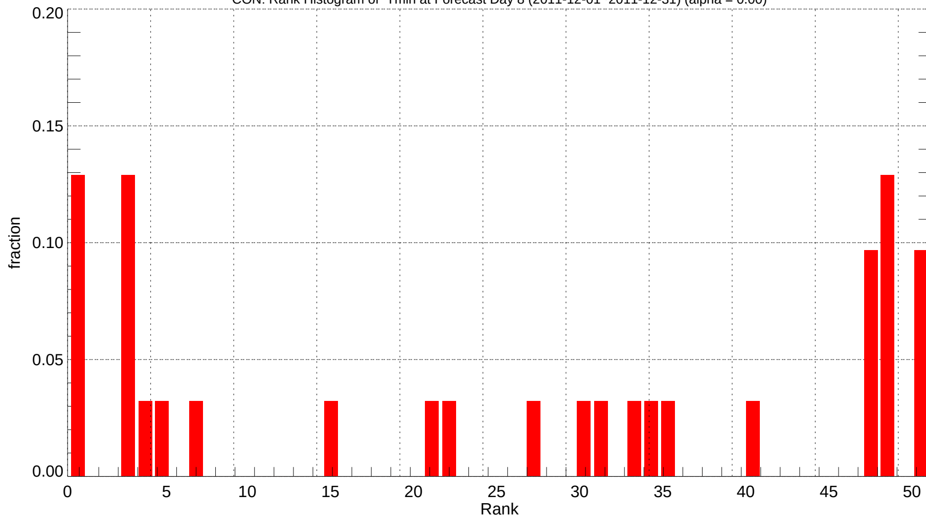
CON: Rank Histogram of Tmin at Forecast Day 8 (2011-12-01~2011-12-31) (alpha = 0.00)
