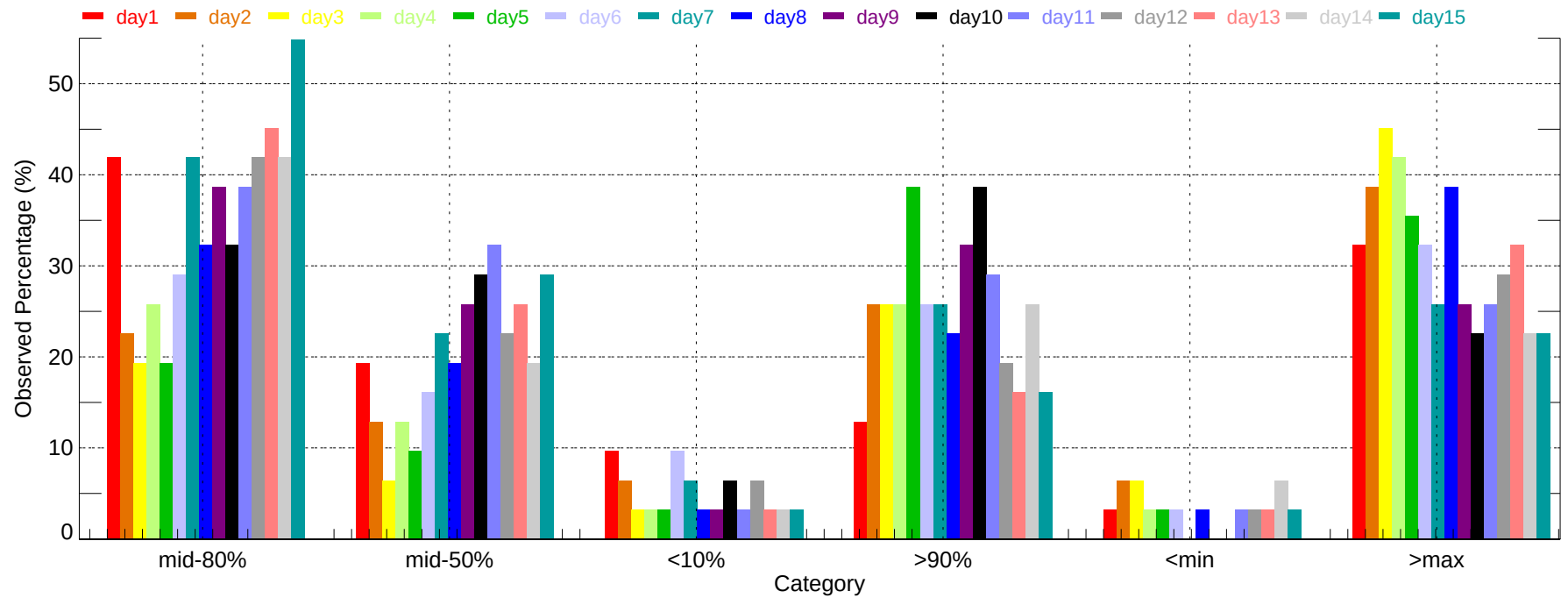
Observed Percentage of Ensembles - COU: Max Temperature (2011-12-01~2011-12-31)
