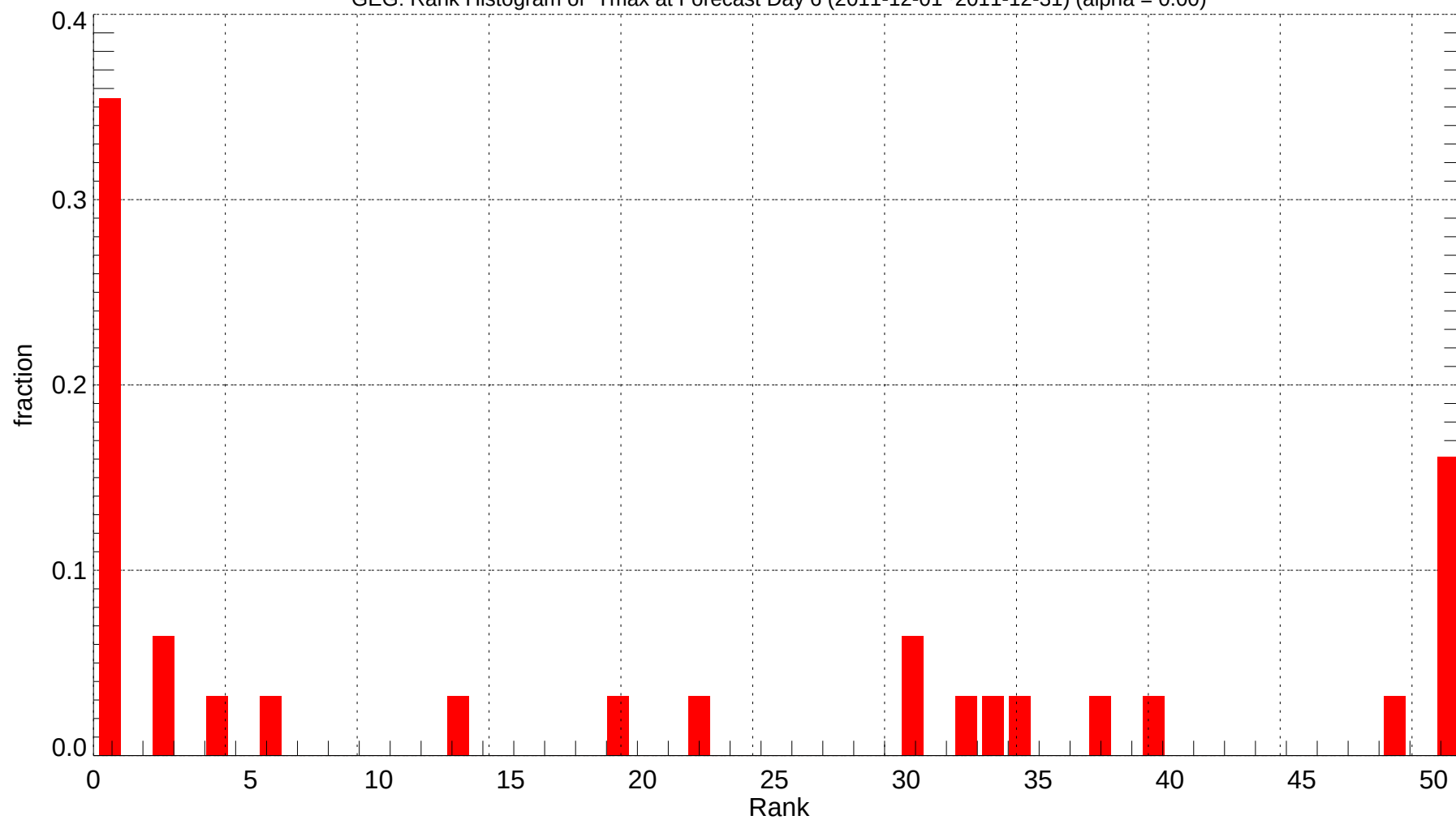
GEG: Rank Histogram of Tmax at Forecast Day 6 (2011-12-01~2011-12-31) (alpha = 0.00)
