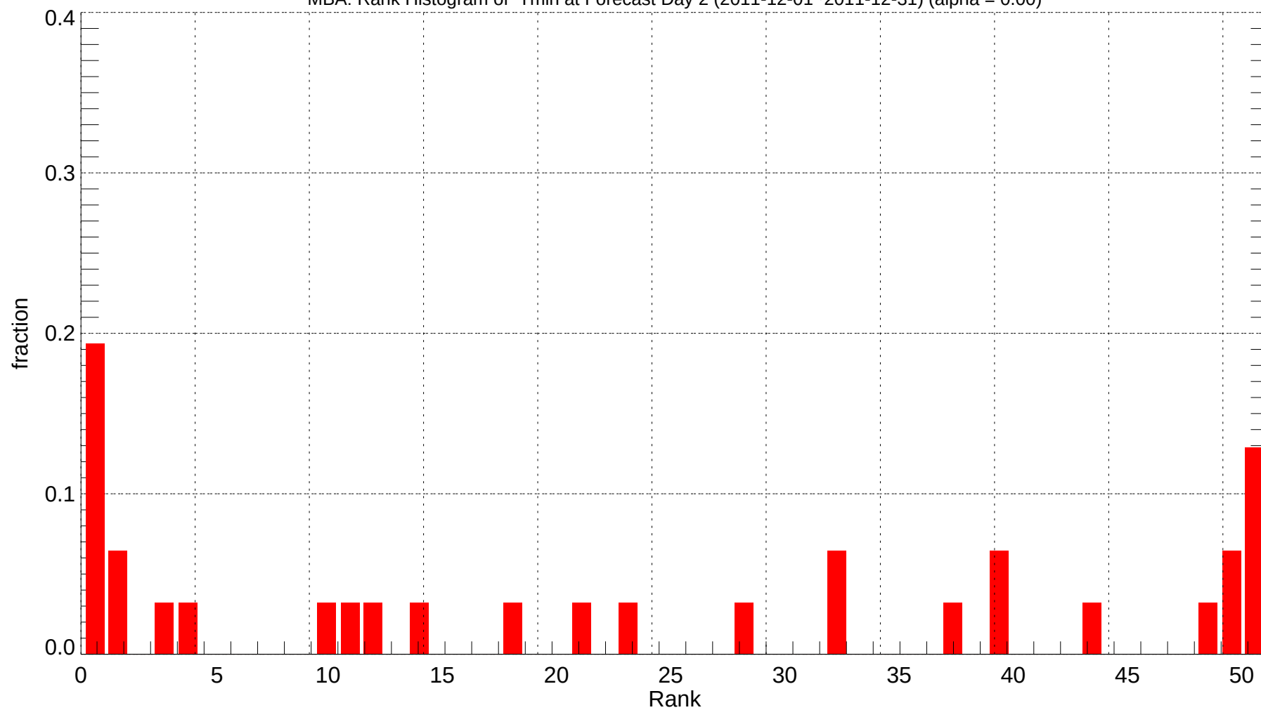
MBA: Rank Histogram of Tmin at Forecast Day 2 (2011-12-01~2011-12-31) (alpha = 0.00)
