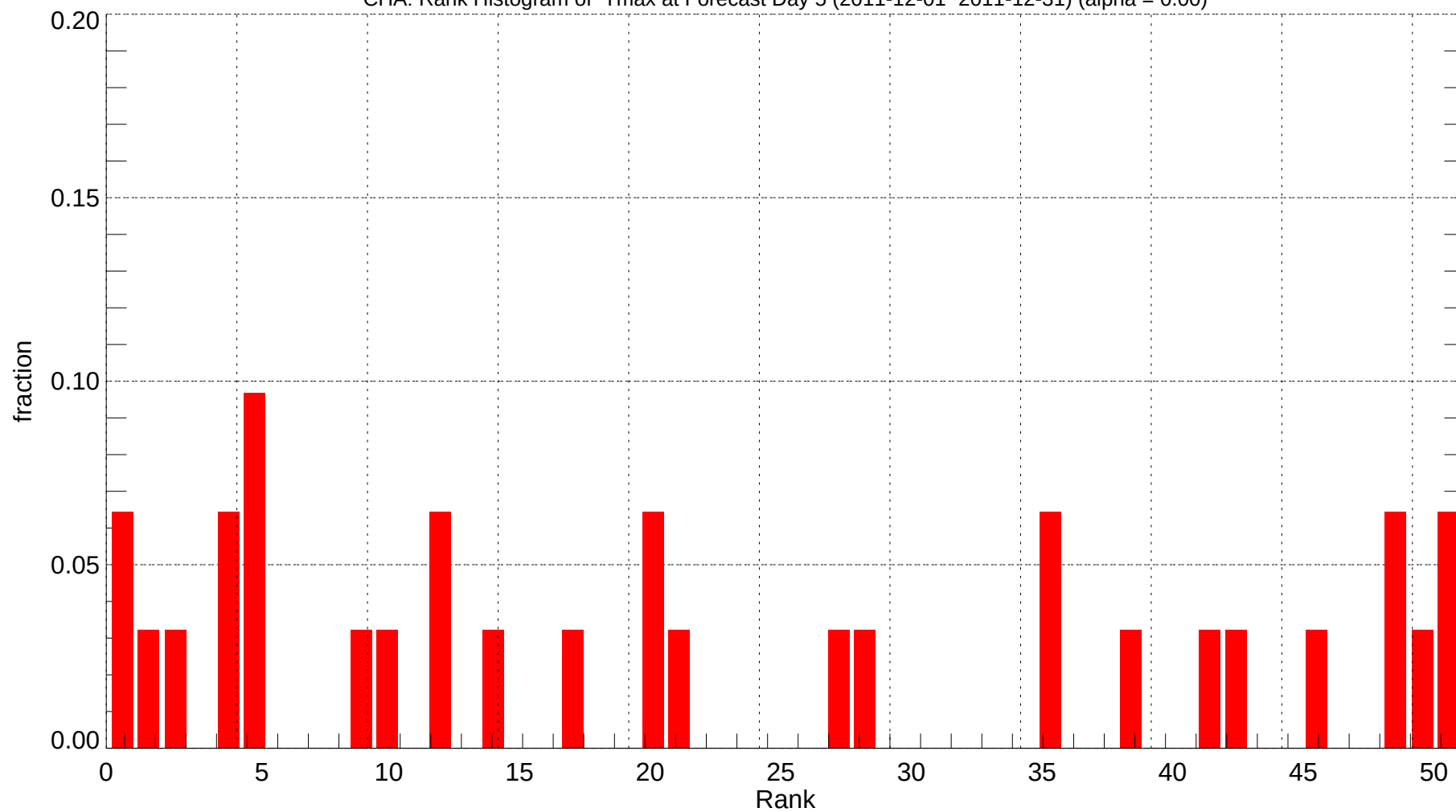
CHA: Rank Histogram of Tmax at Forecast Day 5 (2011-12-01~2011-12-31) (alpha = 0.00)
