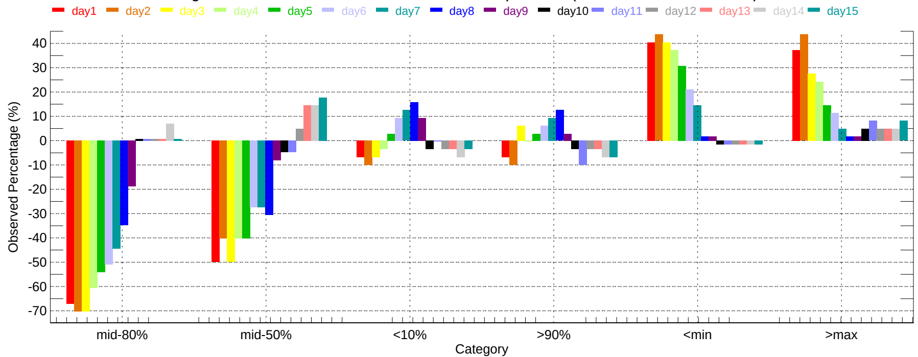
Observed Percentage Deviation of Ensembles - PDT: Min Temperature (2011-12-01~2011-12-31)
