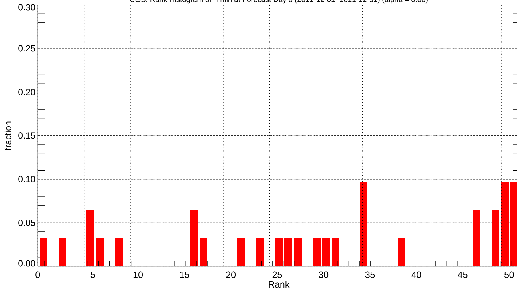
COS: Rank Histogram of Tmin at Forecast Day 8 (2011-12-01~2011-12-31) (alpha = 0.00)
