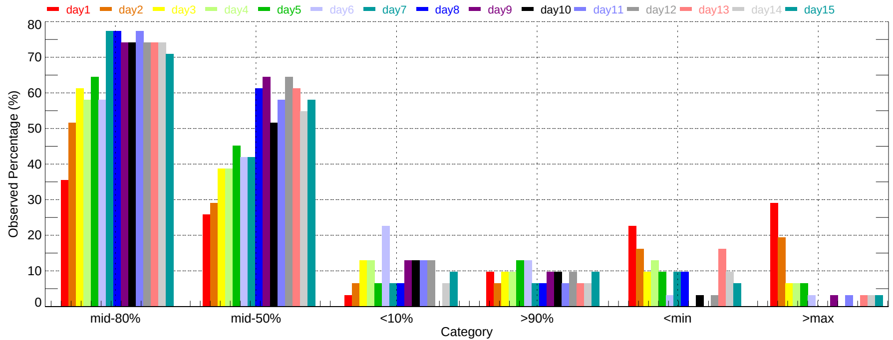
Observed Percentage of Ensembles - TPA: Max Temperature (2011-12-01~2011-12-31)
