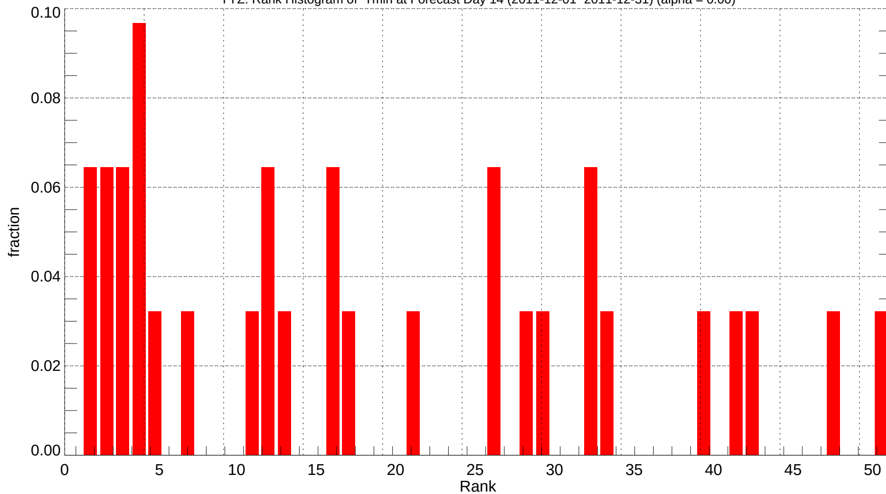
YYZ: Rank Histogram of Tmin at Forecast Day 14 (2011-12-01~2011-12-31) (alpha = 0.00)
