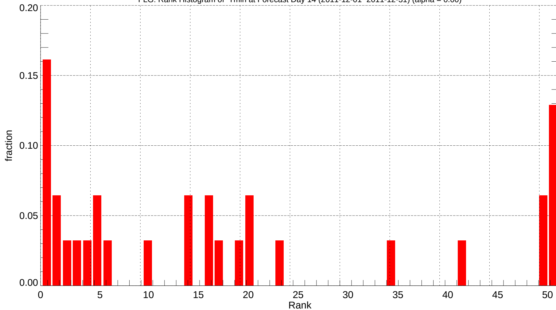
FLG: Rank Histogram of Tmin at Forecast Day 14 (2011-12-01~2011-12-31) (alpha = 0.00)
