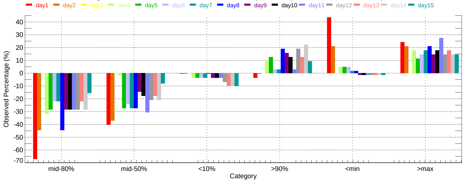
Observed Percentage Deviation of Ensembles - YYC: Min Temperature (2011-12-01~2011-12-31)
