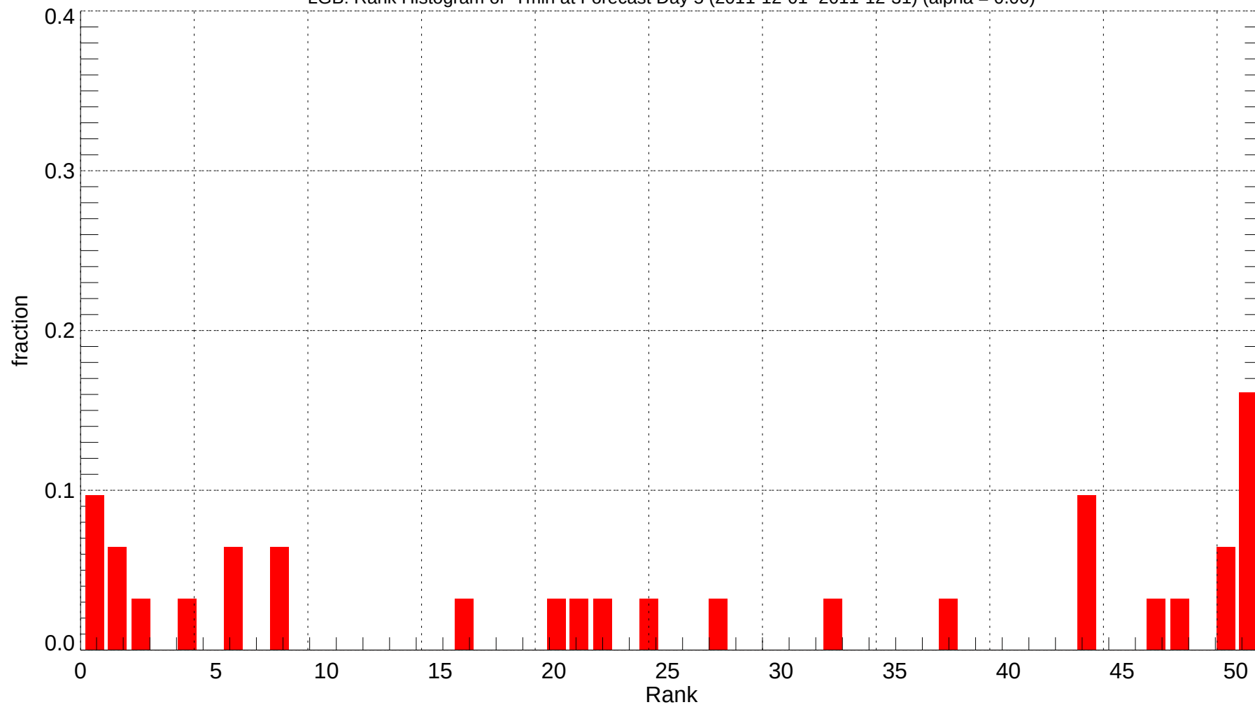
LGB: Rank Histogram of Tmin at Forecast Day 5 (2011-12-01~2011-12-31) (alpha = 0.00)
