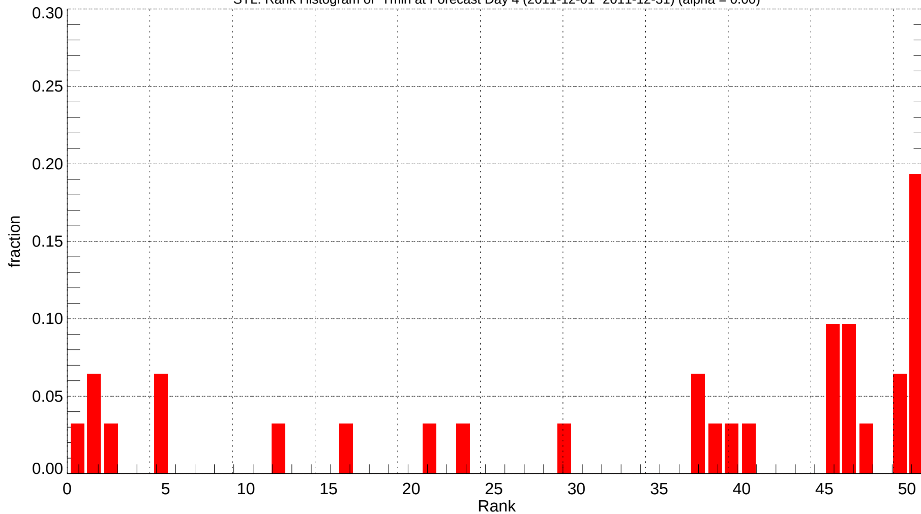
STL: Rank Histogram of Tmin at Forecast Day 4 (2011-12-01~2011-12-31) (alpha = 0.00)
