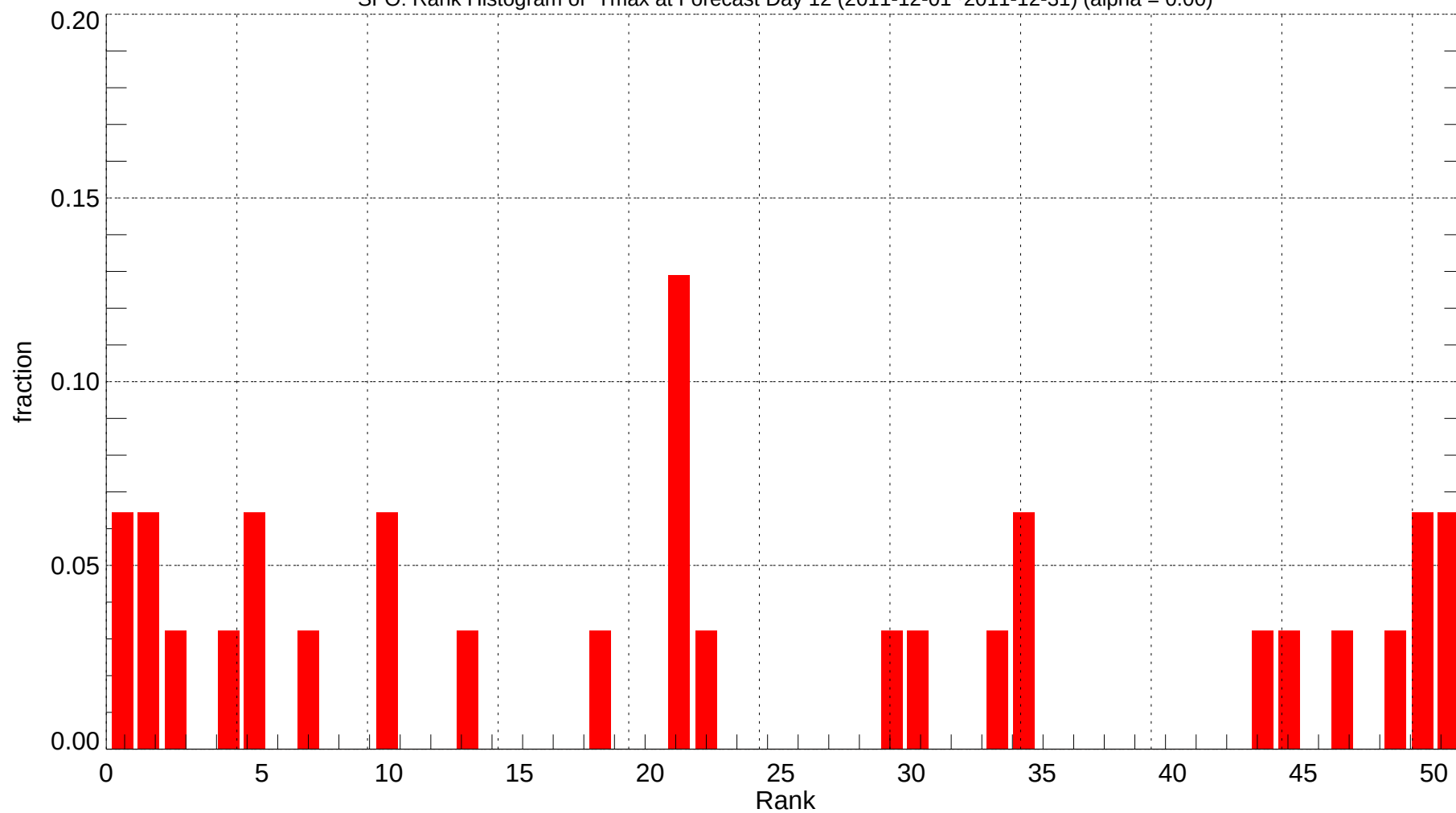
SFO: Rank Histogram of Tmax at Forecast Day 12 (2011-12-01~2011-12-31) (alpha = 0.00)
