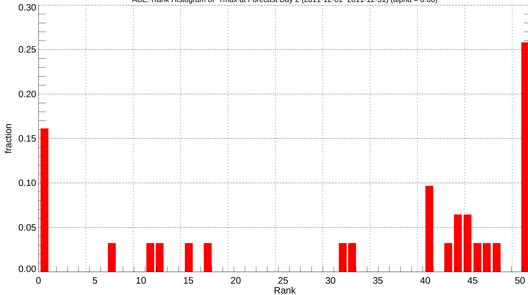
ABE: Rank Histogram of Tmax at Forecast Day 2 (2011-12-01~2011-12-31) (alpha = 0.00)
