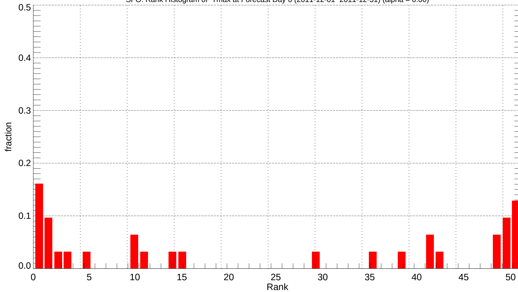
SFO: Rank Histogram of Tmax at Forecast Day 6 (2011-12-01~2011-12-31) (alpha = 0.00)
