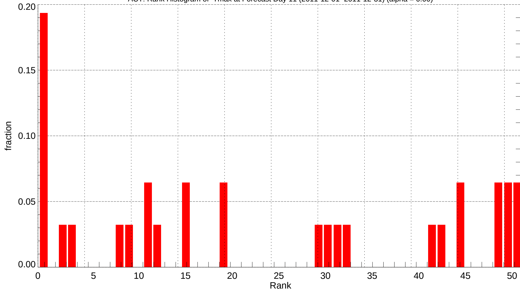
ACT: Rank Histogram of Tmax at Forecast Day 11 (2011-12-01~2011-12-31) (alpha = 0.00)
