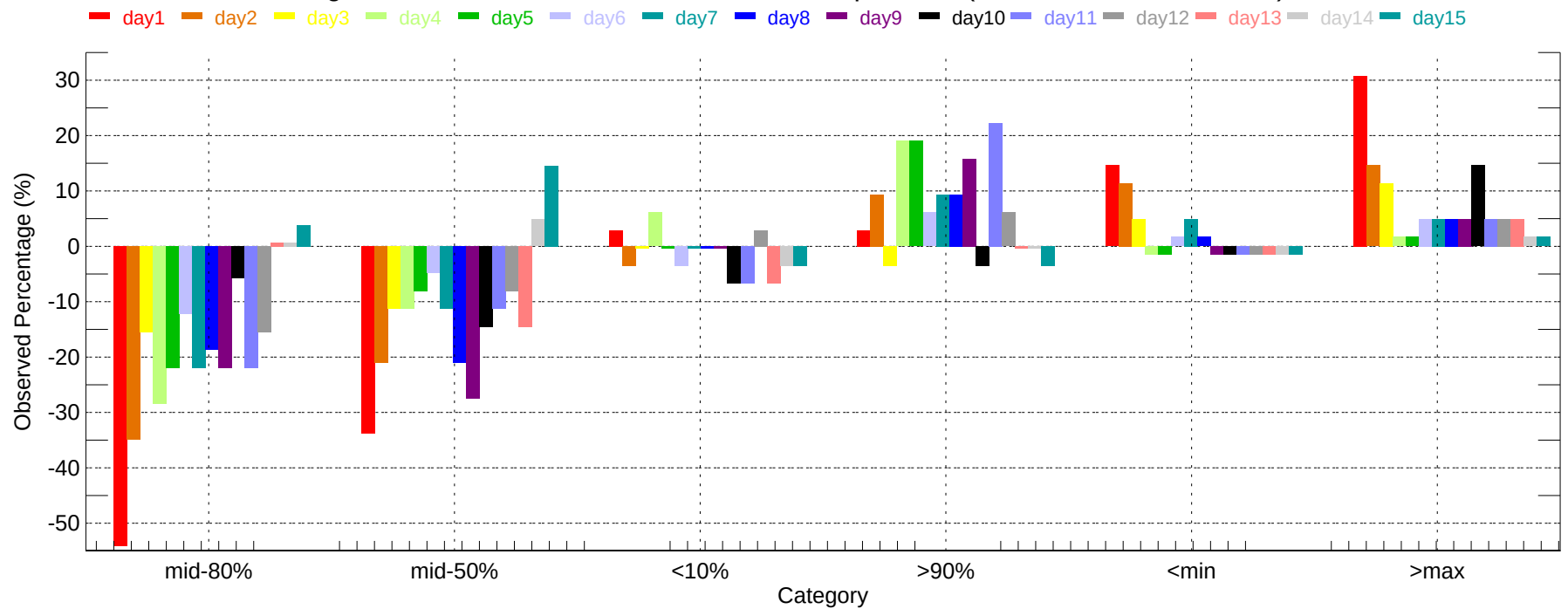
Observed Percentage Deviation of Ensembles - IAH: Min Temperature (2011-12-01~2011-12-31)
