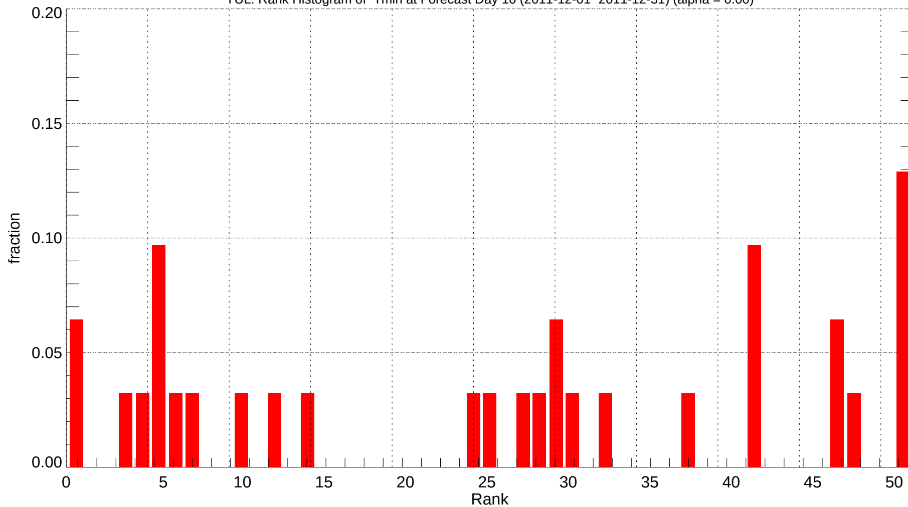
YUL: Rank Histogram of Tmin at Forecast Day 10 (2011-12-01~2011-12-31) (alpha = 0.00)
