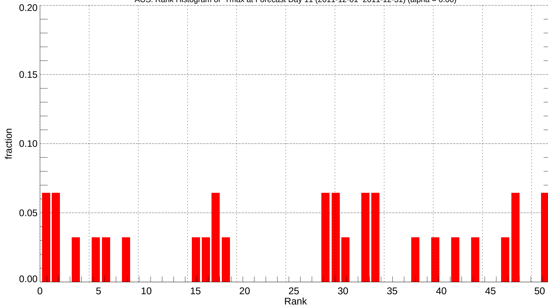
AUS: Rank Histogram of Tmax at Forecast Day 11 (2011-12-01~2011-12-31) (alpha = 0.00)
