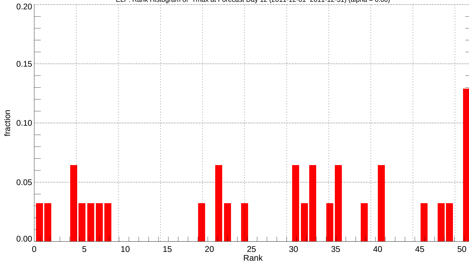
ELP: Rank Histogram of Tmax at Forecast Day 12 (2011-12-01~2011-12-31) (alpha = 0.00)
