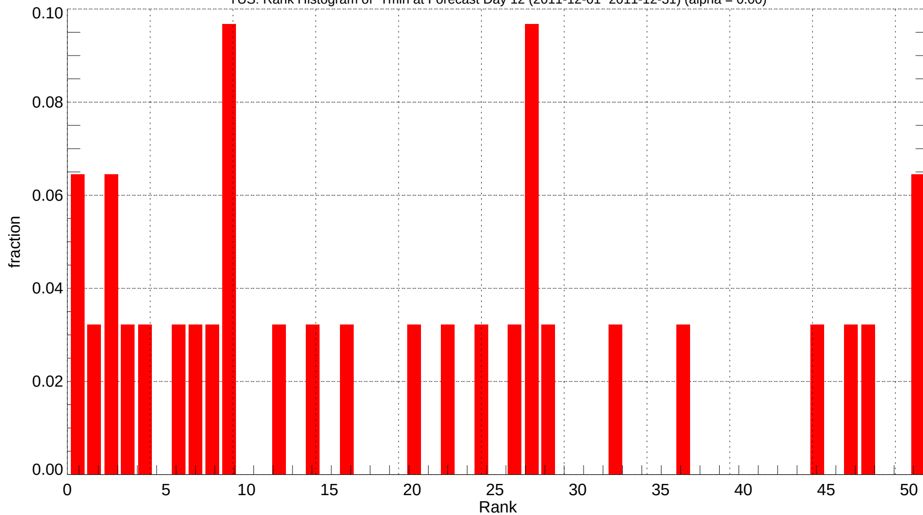
TUS: Rank Histogram of Tmin at Forecast Day 12 (2011-12-01~2011-12-31) (alpha = 0.00)
