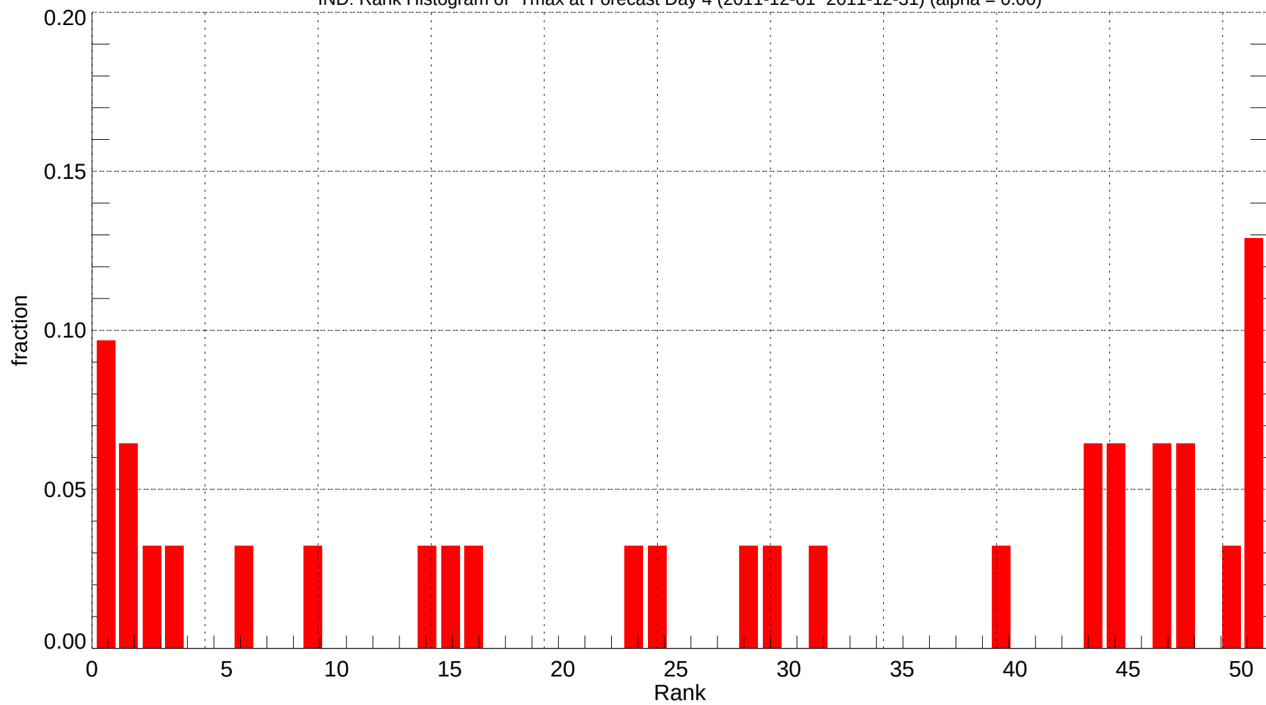
IND: Rank Histogram of Tmax at Forecast Day 4 (2011-12-01~2011-12-31) (alpha = 0.00)
