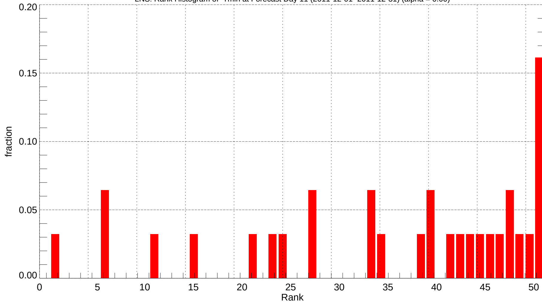
LNS: Rank Histogram of Tmin at Forecast Day 11 (2011-12-01~2011-12-31) (alpha = 0.00)
