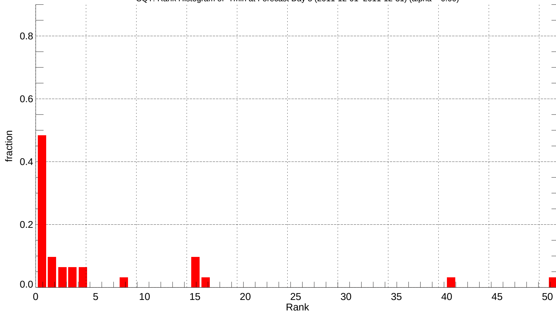
CQT: Rank Histogram of Tmin at Forecast Day 5 (2011-12-01~2011-12-31) (alpha = 0.00)
