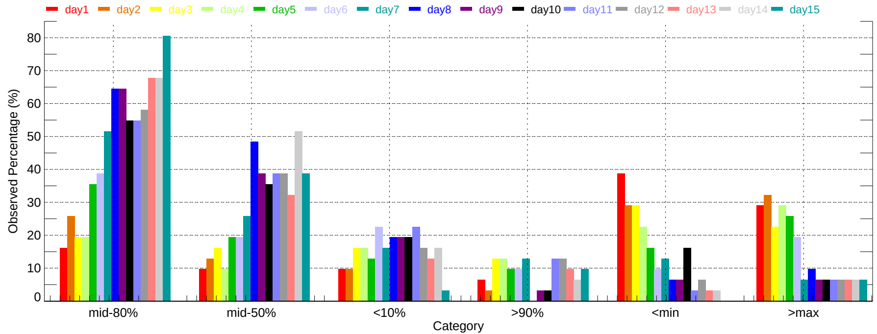
Observed Percentage of Ensembles - SFO: Max Temperature (2011-12-01~2011-12-31)
