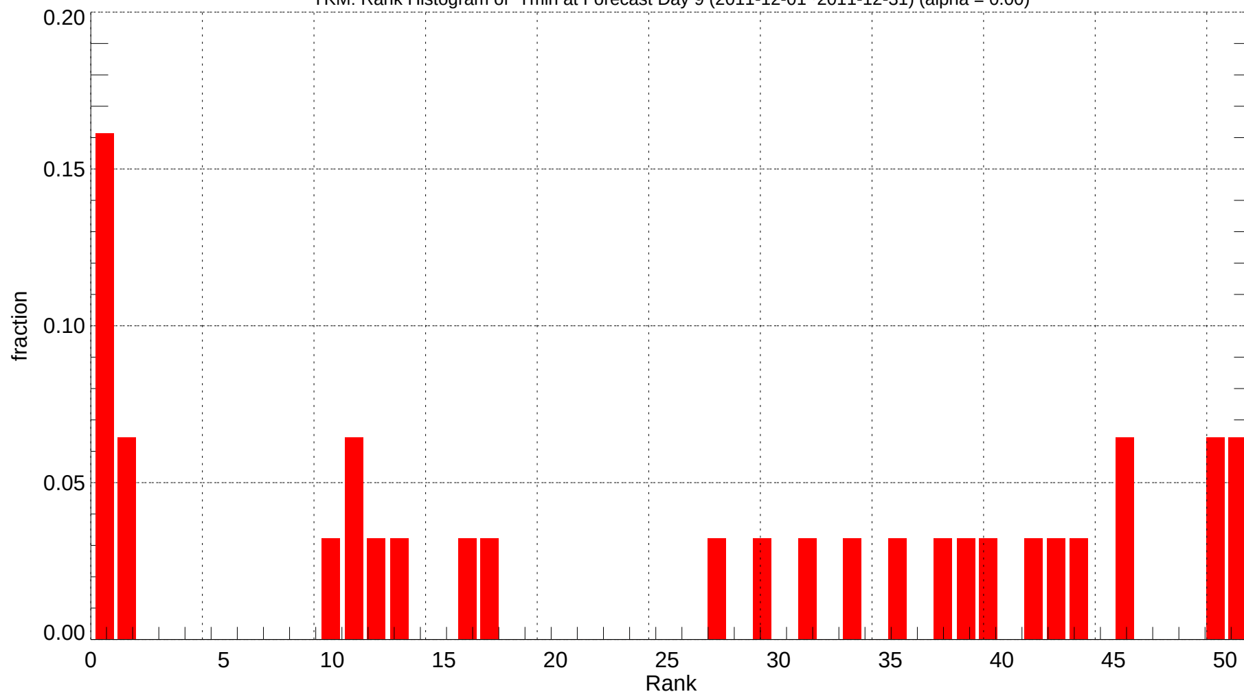
YKM: Rank Histogram of Tmin at Forecast Day 9 (2011-12-01~2011-12-31) (alpha = 0.00)
