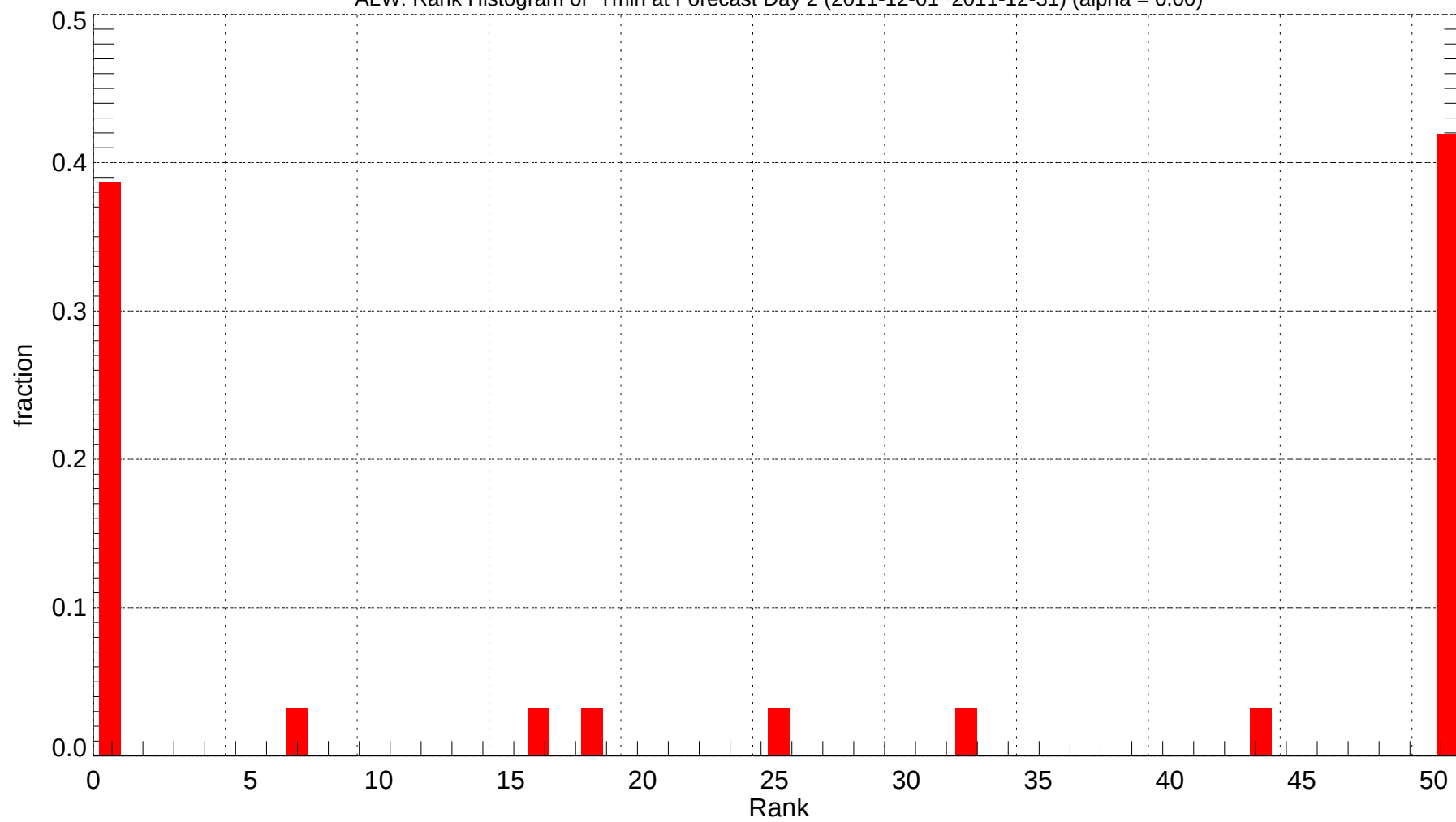
ALW: Rank Histogram of Tmin at Forecast Day 2 (2011-12-01~2011-12-31) (alpha = 0.00)
