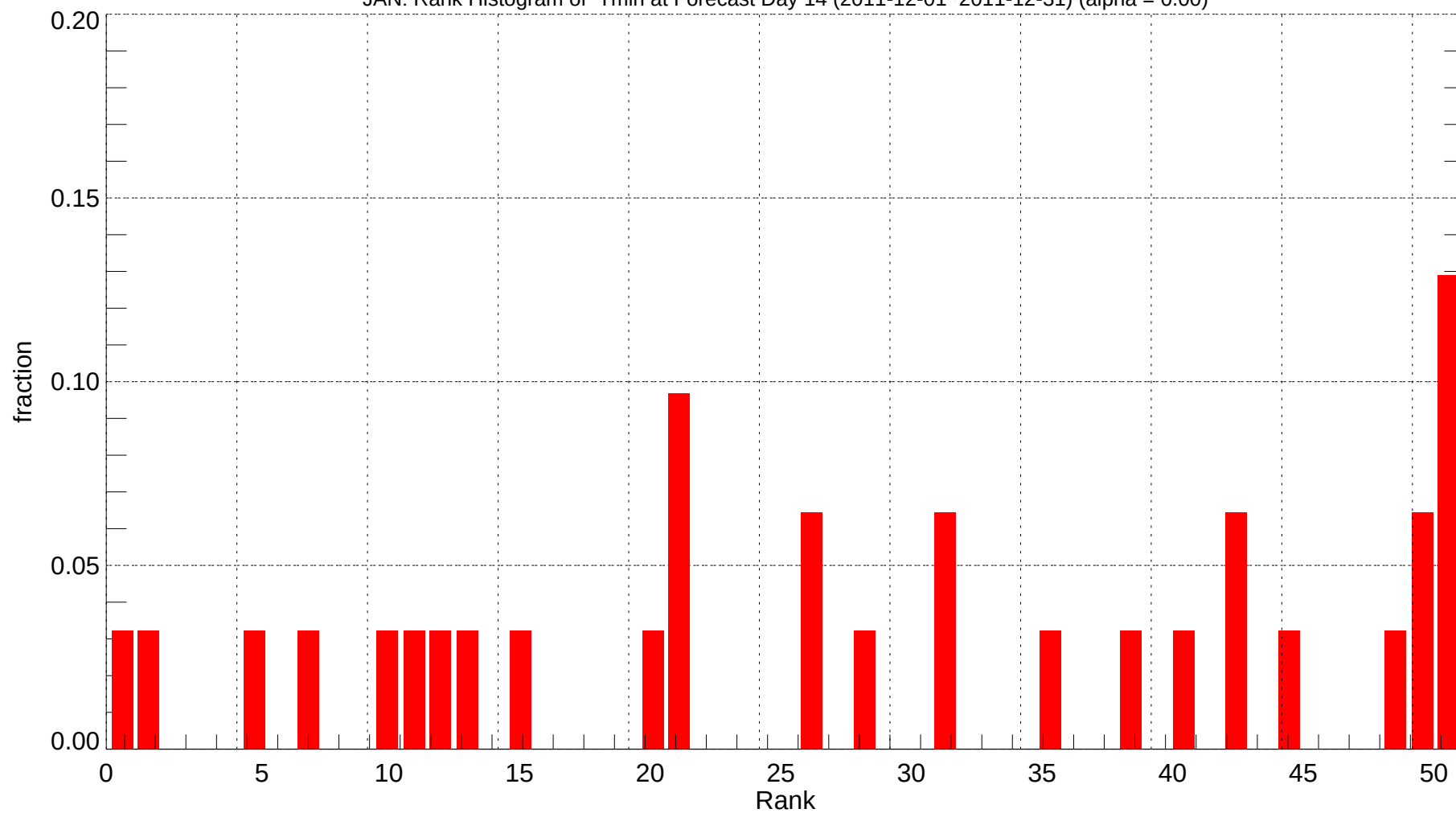
JAN: Rank Histogram of Tmin at Forecast Day 14 (2011-12-01~2011-12-31) (alpha = 0.00)
