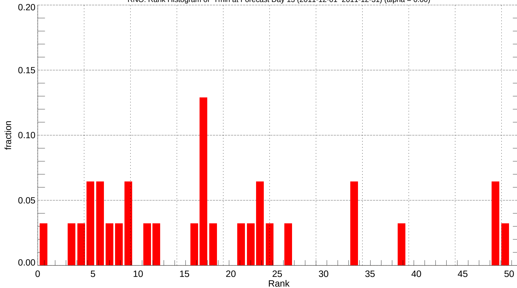
RNO: Rank Histogram of Tmin at Forecast Day 13 (2011-12-01~2011-12-31) (alpha = 0.00)
