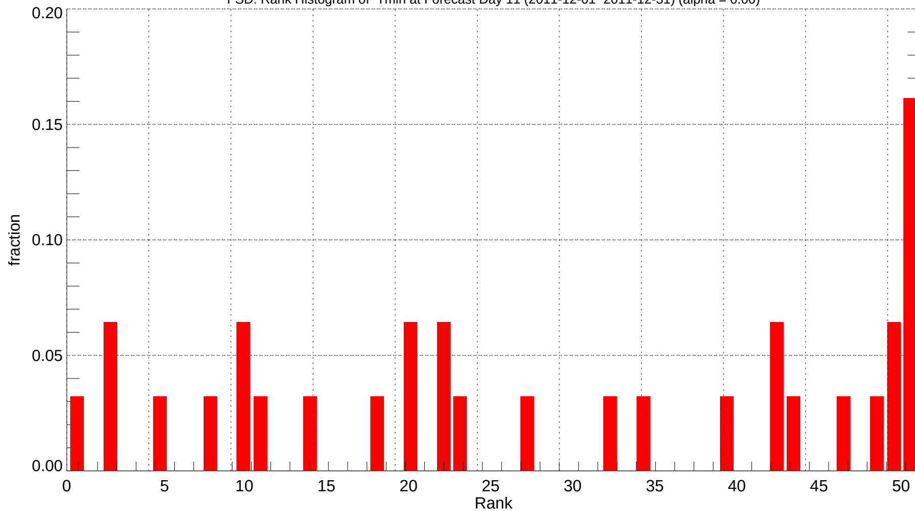
FSD: Rank Histogram of Tmin at Forecast Day 11 (2011-12-01~2011-12-31) (alpha = 0.00)
