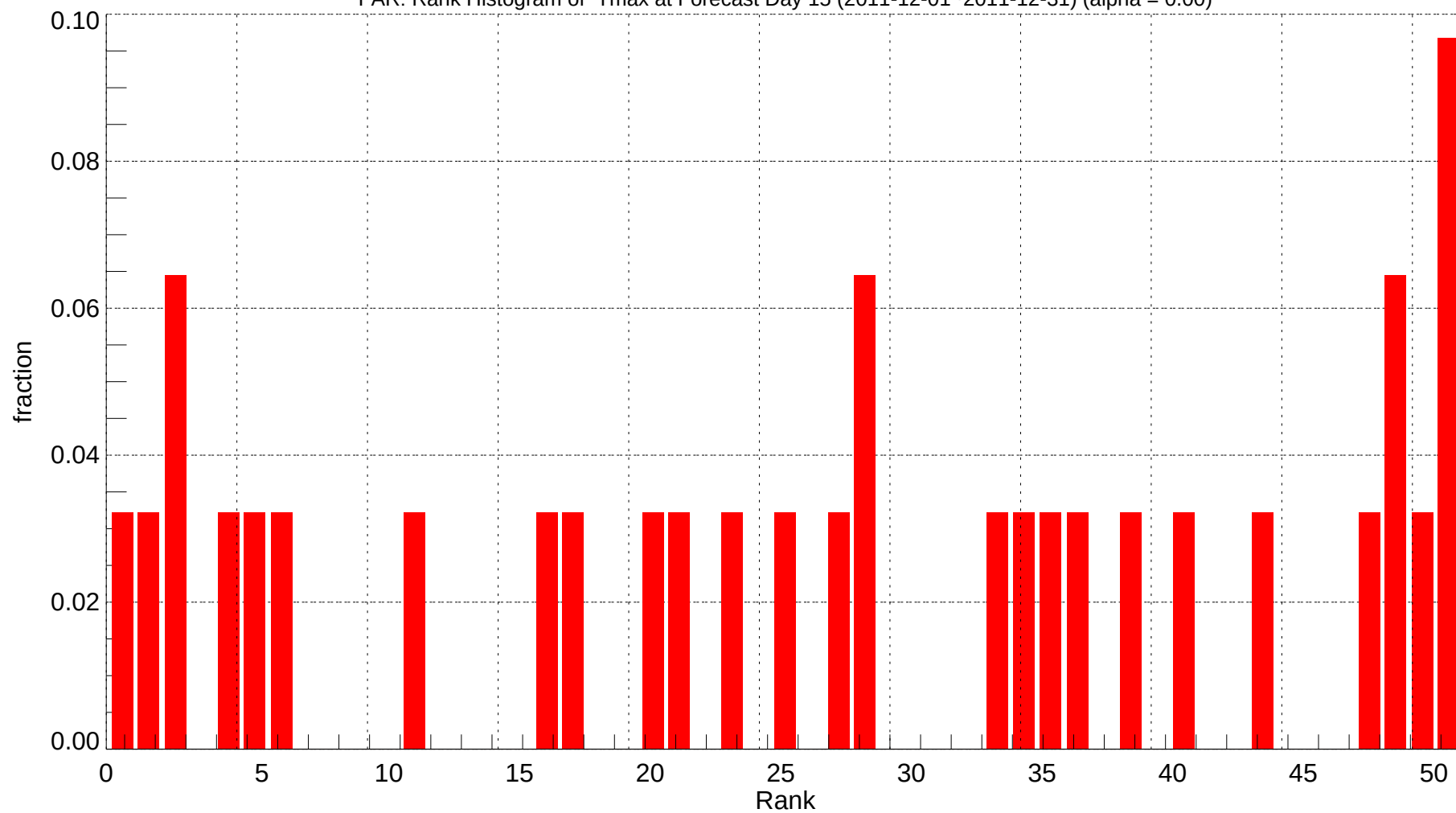
FAR: Rank Histogram of Tmax at Forecast Day 15 (2011-12-01~2011-12-31) (alpha = 0.00)
