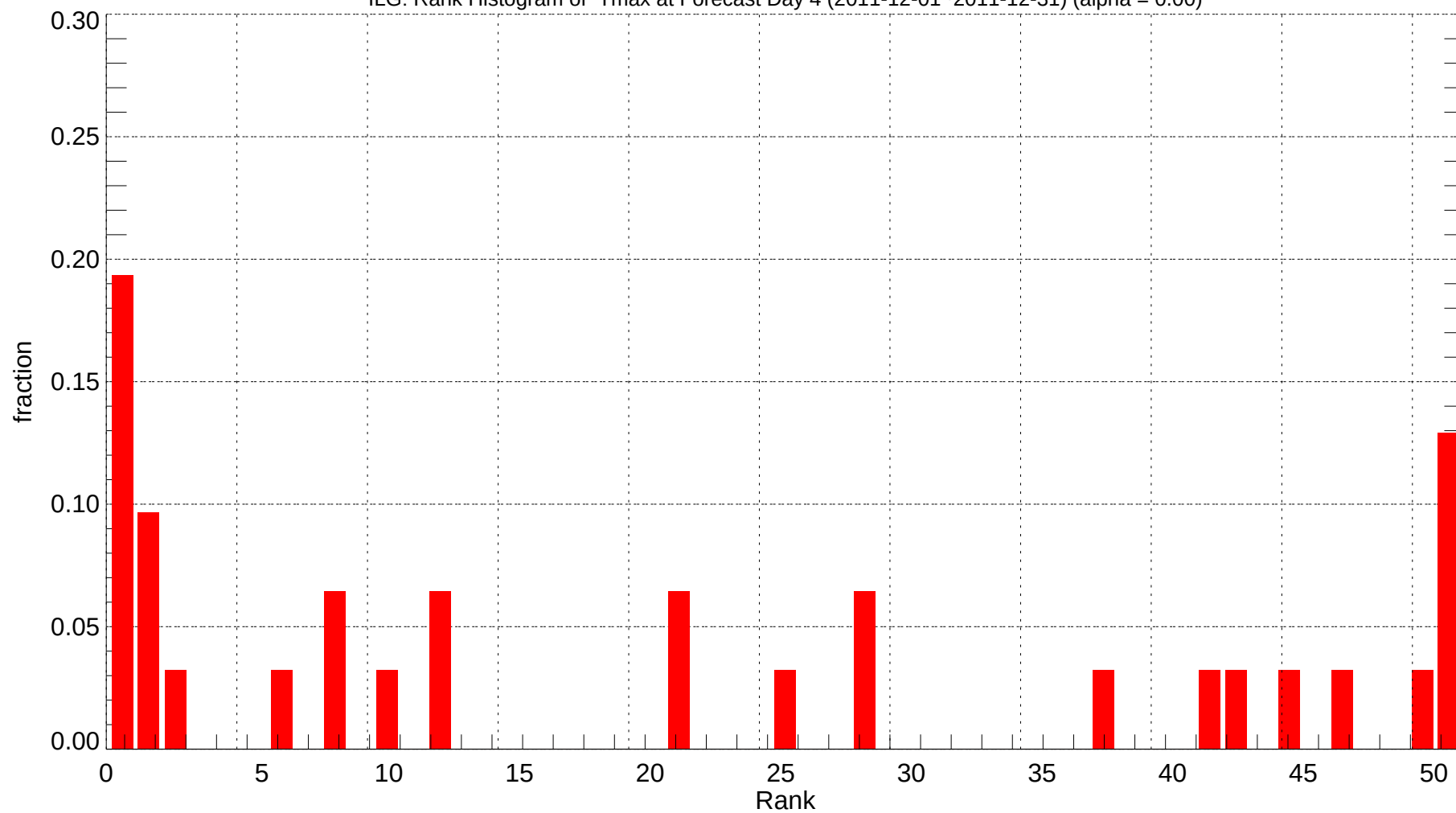
ILG: Rank Histogram of Tmax at Forecast Day 4 (2011-12-01~2011-12-31) (alpha = 0.00)
