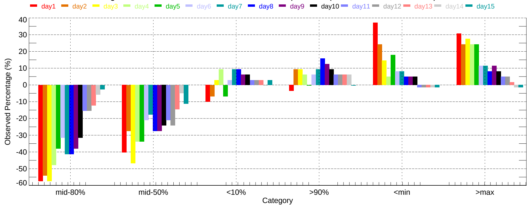
Observed Percentage Deviation of Ensembles - YUL: Min Temperature (2011-12-01~2011-12-31)
