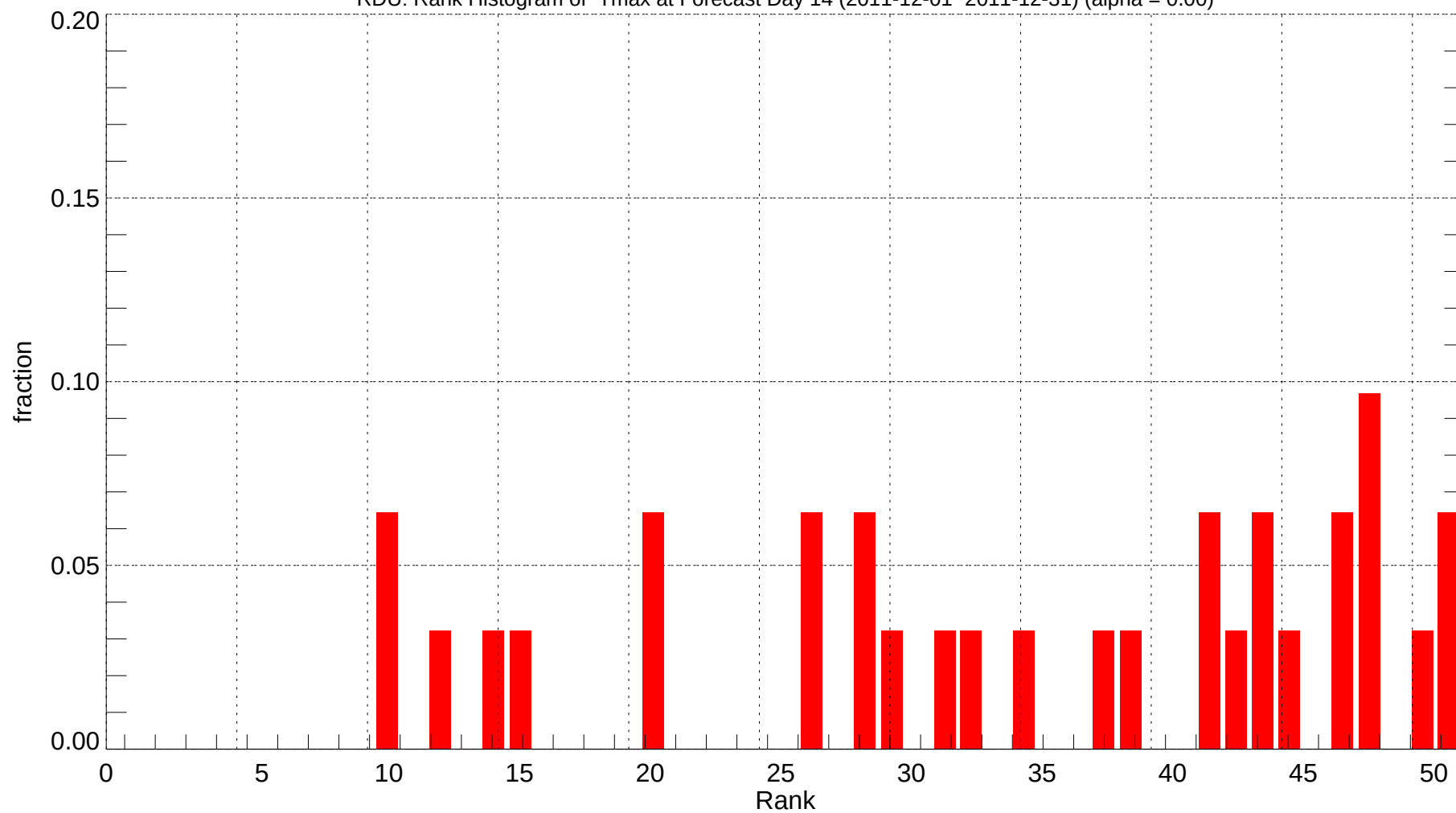
RDU: Rank Histogram of Tmax at Forecast Day 14 (2011-12-01~2011-12-31) (alpha = 0.00)
