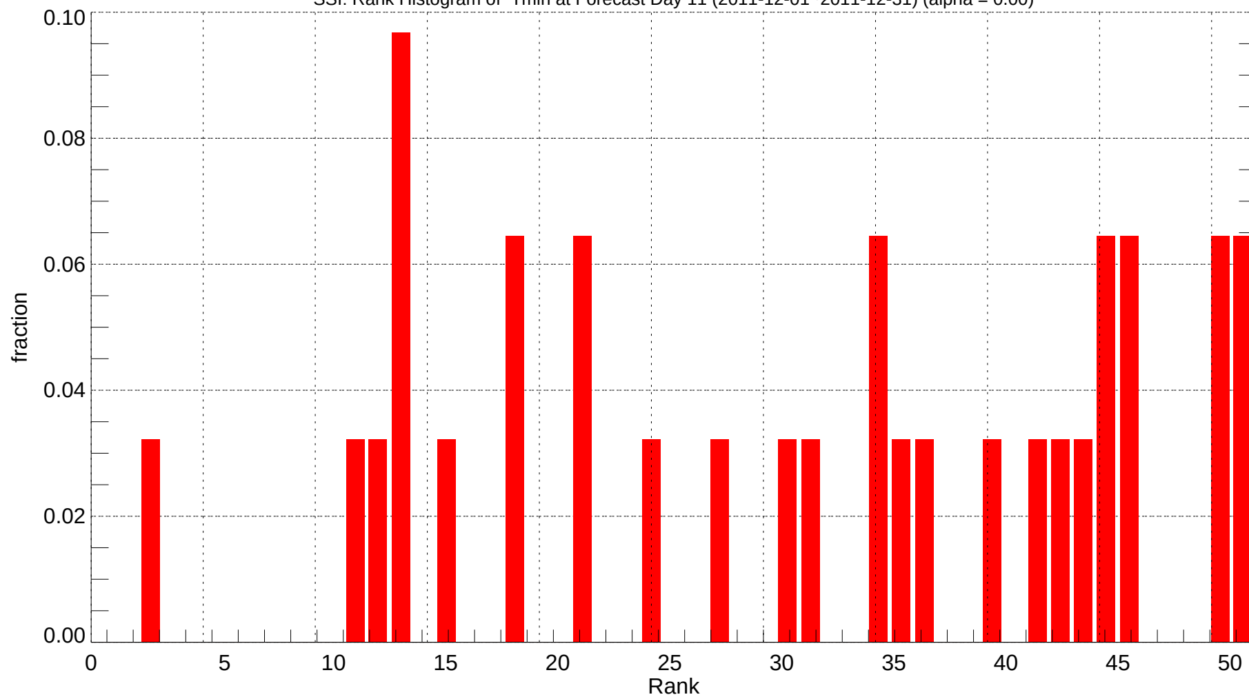
SSI: Rank Histogram of Tmin at Forecast Day 11 (2011-12-01~2011-12-31) (alpha = 0.00)
