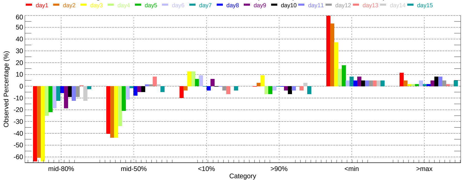
Observed Percentage Deviation of Ensembles - DEN: Max Temperature (2011-12-01~2011-12-31)
