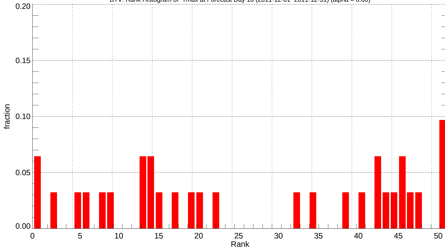
BTV: Rank Histogram of Tmax at Forecast Day 10 (2011-12-01~2011-12-31) (alpha = 0.00)
