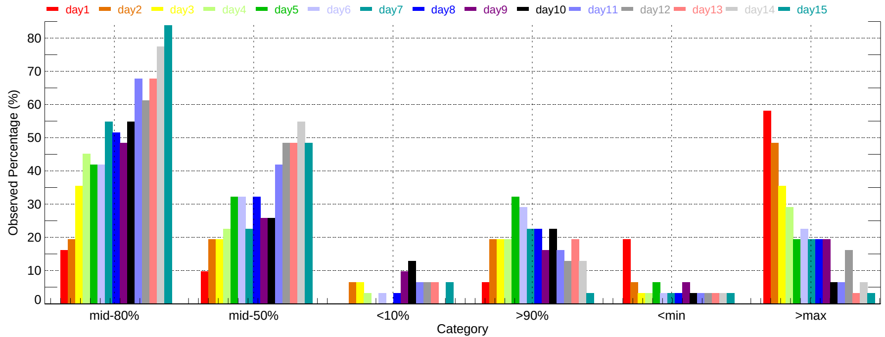
Observed Percentage of Ensembles - COS: Min Temperature (2011-12-01~2011-12-31)
