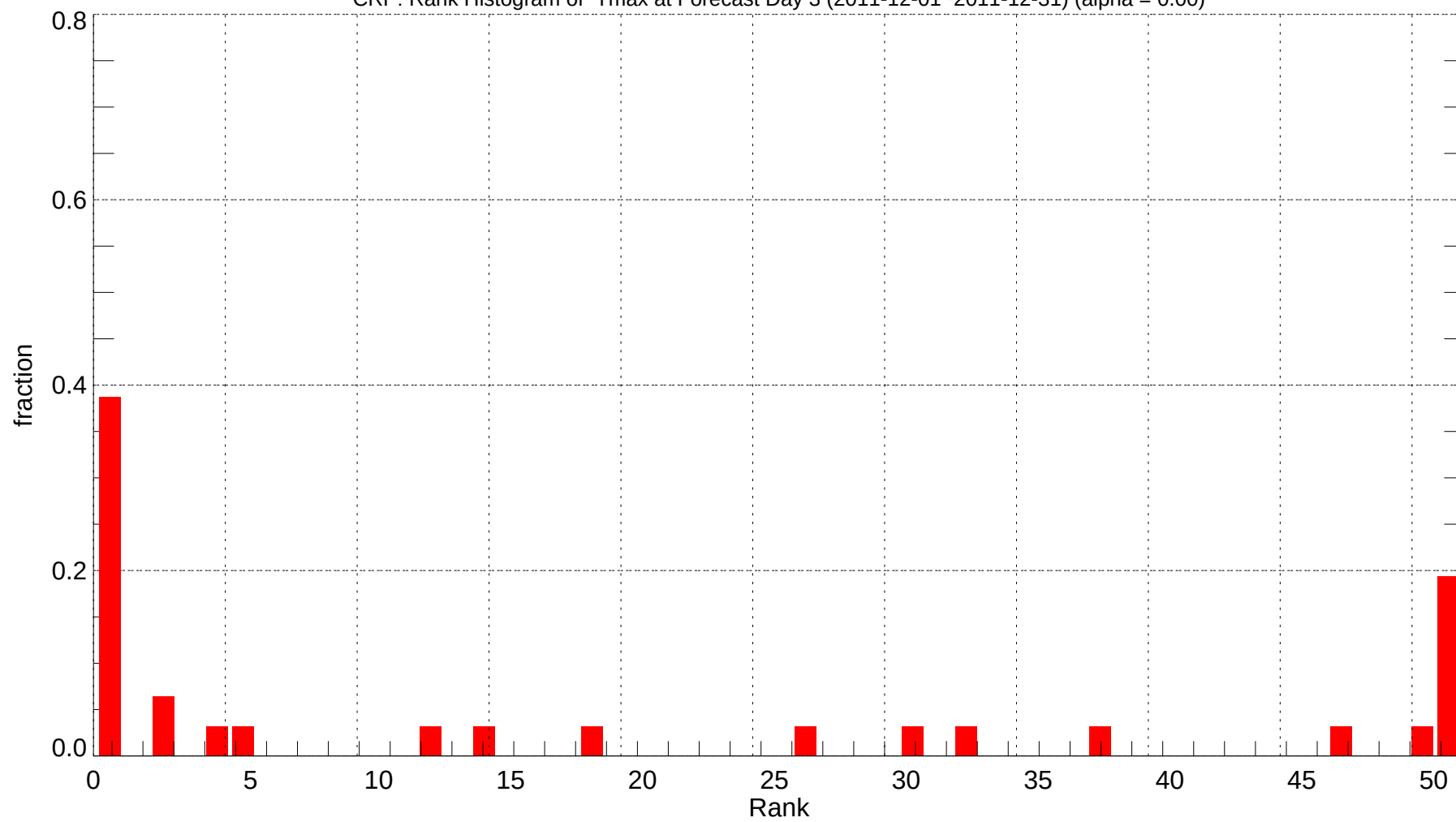
CRP: Rank Histogram of Tmax at Forecast Day 3 (2011-12-01~2011-12-31) (alpha = 0.00)
