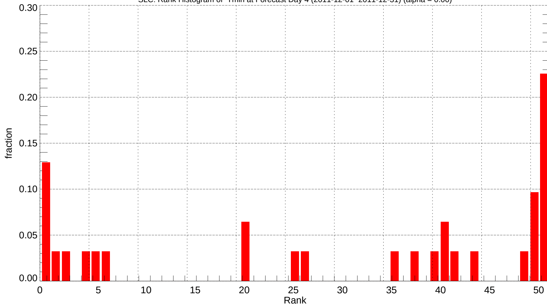
SLC: Rank Histogram of Tmin at Forecast Day 4 (2011-12-01~2011-12-31) (alpha = 0.00)
