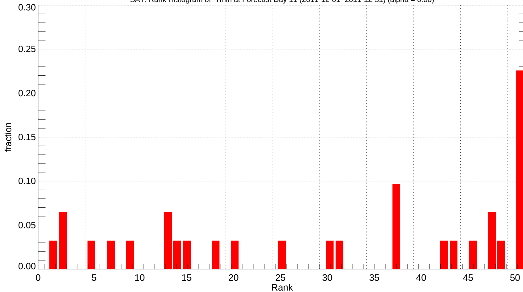
SAT: Rank Histogram of Tmin at Forecast Day 11 (2011-12-01~2011-12-31) (alpha = 0.00)
