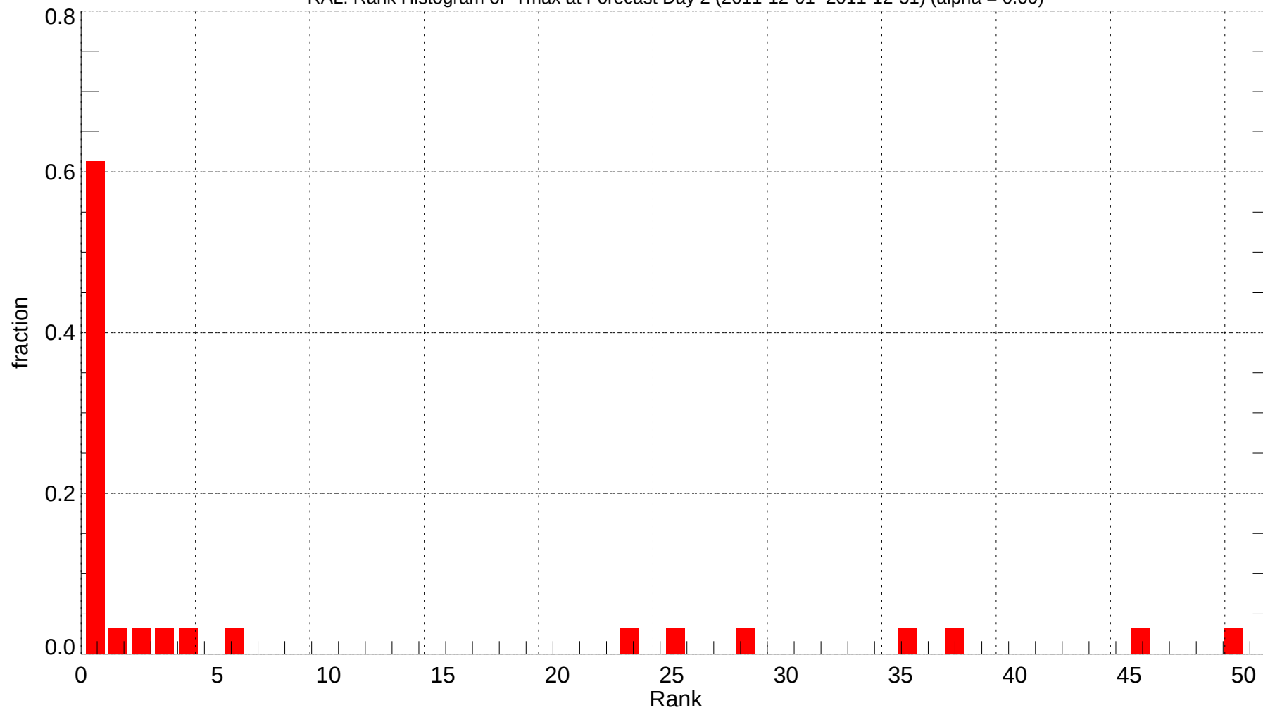
RAL: Rank Histogram of Tmax at Forecast Day 2 (2011-12-01~2011-12-31) (alpha = 0.00)
