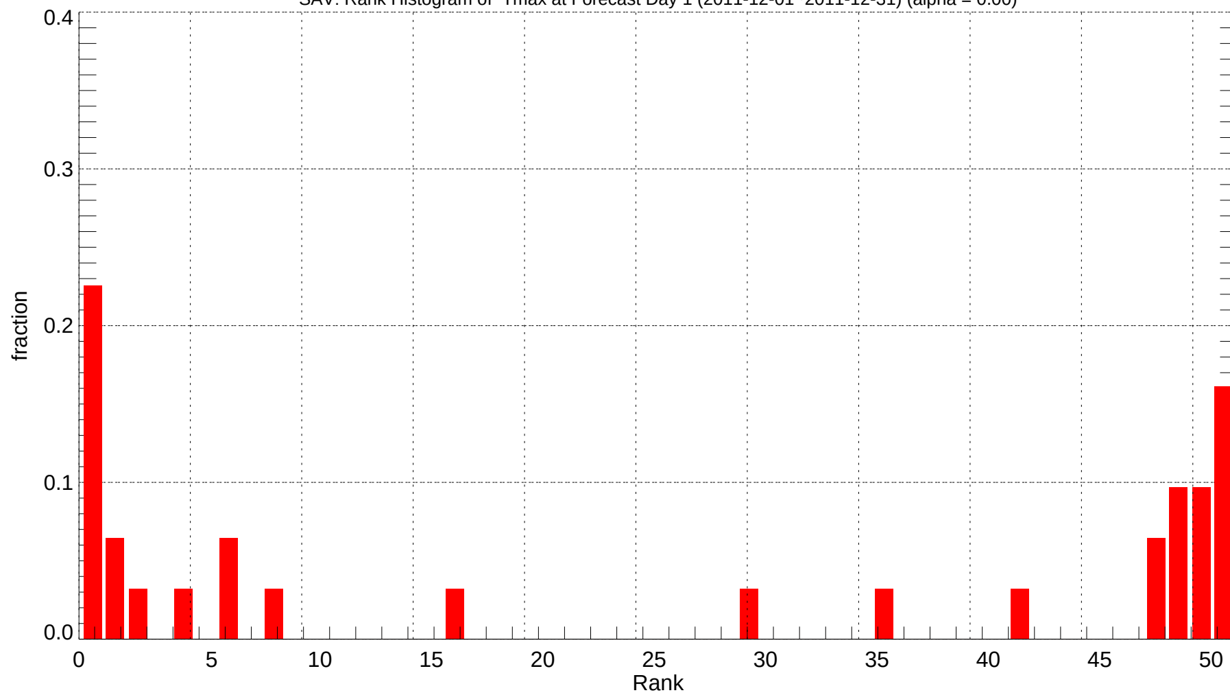
SAV: Rank Histogram of Tmax at Forecast Day 1 (2011-12-01~2011-12-31) (alpha = 0.00)
