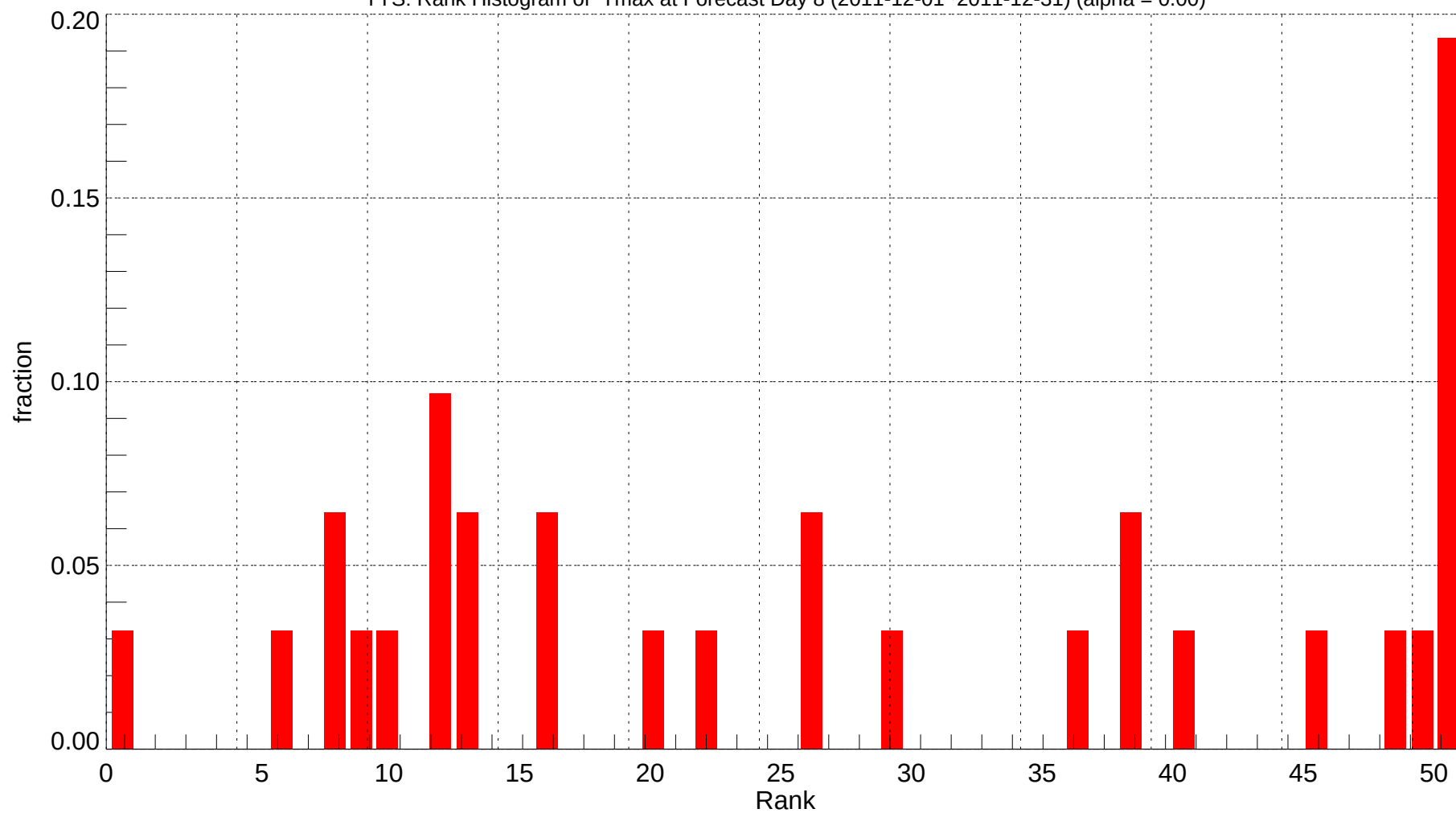
TYS: Rank Histogram of Tmax at Forecast Day 8 (2011-12-01~2011-12-31) (alpha = 0.00)
