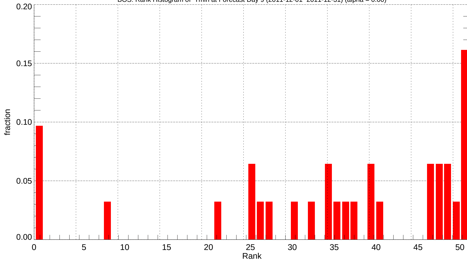
BOS: Rank Histogram of Tmin at Forecast Day 9 (2011-12-01~2011-12-31) (alpha = 0.00)
