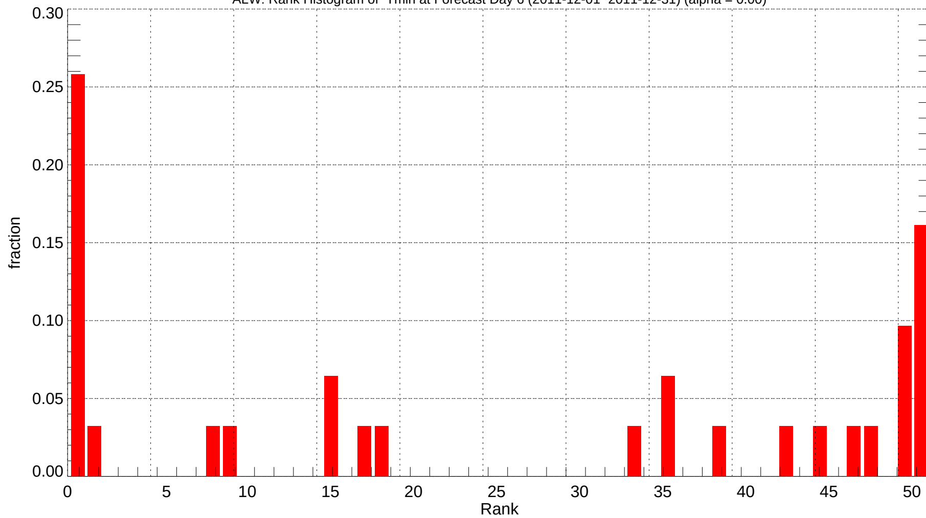
ALW: Rank Histogram of Tmin at Forecast Day 6 (2011-12-01~2011-12-31) (alpha = 0.00)
