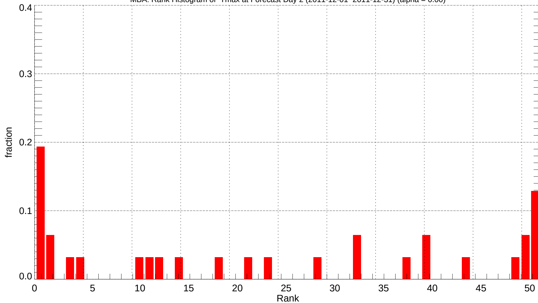
MBA: Rank Histogram of Tmax at Forecast Day 2 (2011-12-01~2011-12-31) (alpha = 0.00)
