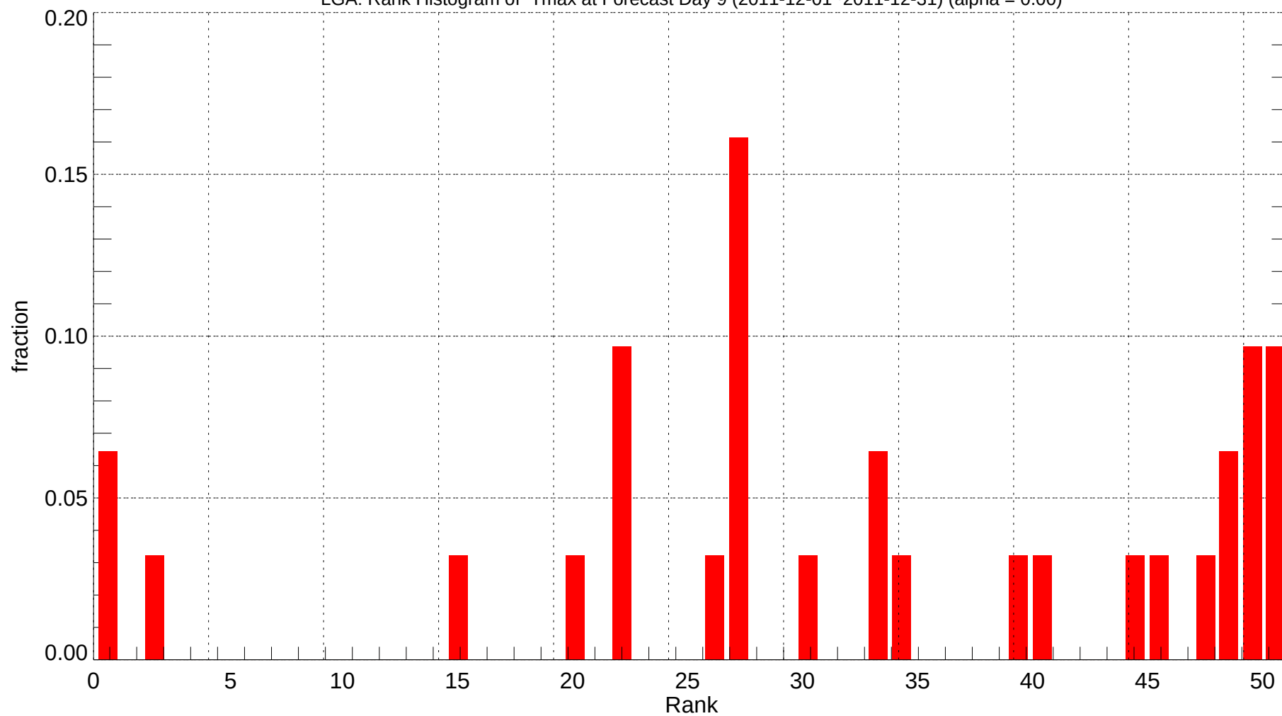
LGA: Rank Histogram of Tmax at Forecast Day 9 (2011-12-01~2011-12-31) (alpha = 0.00)
