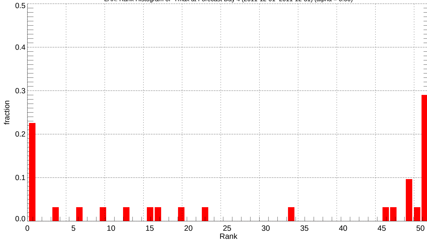
LAX: Rank Histogram of Tmax at Forecast Day 4 (2011-12-01~2011-12-31) (alpha = 0.00)
