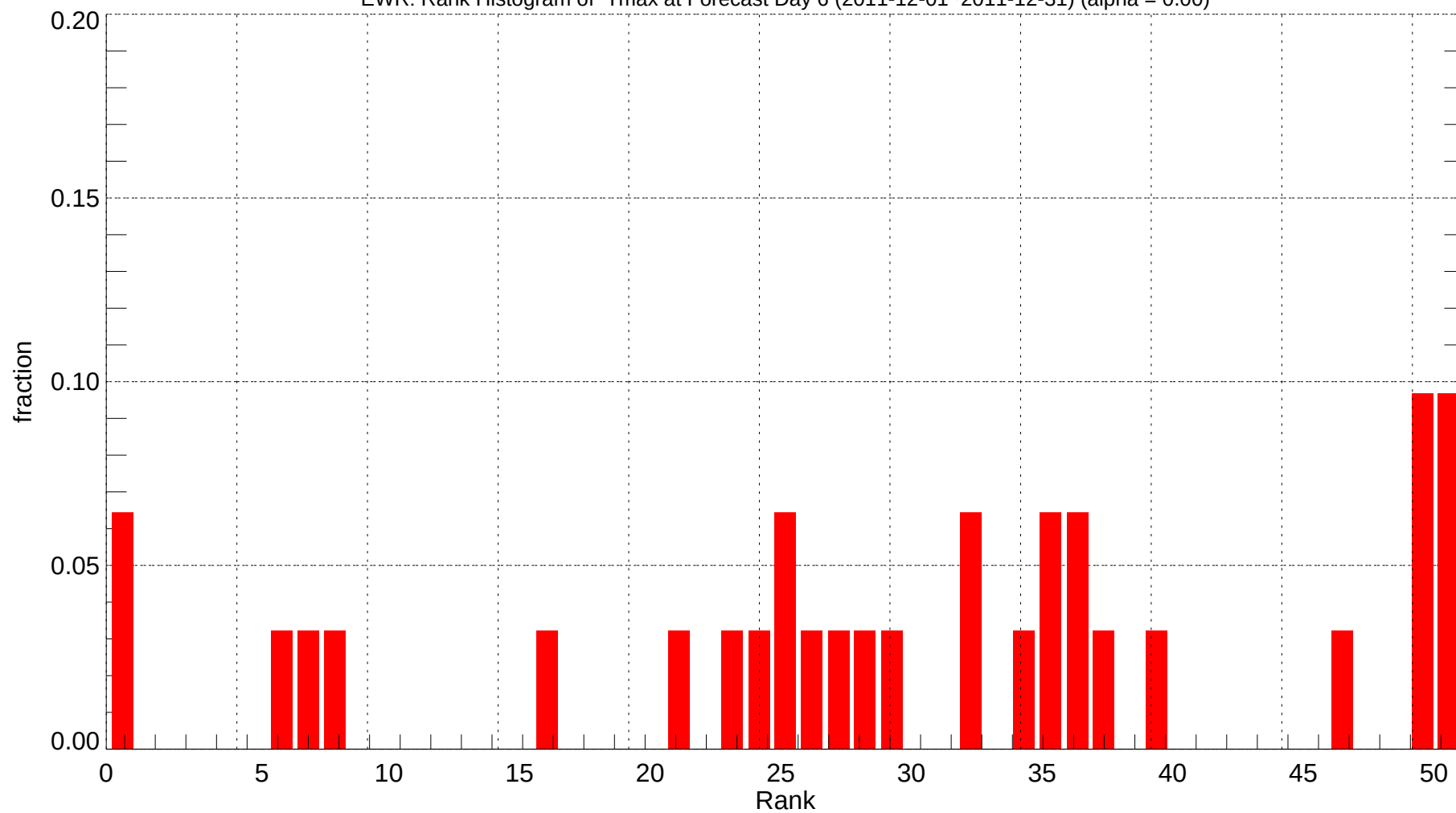
EWR: Rank Histogram of Tmax at Forecast Day 6 (2011-12-01~2011-12-31) (alpha = 0.00)
