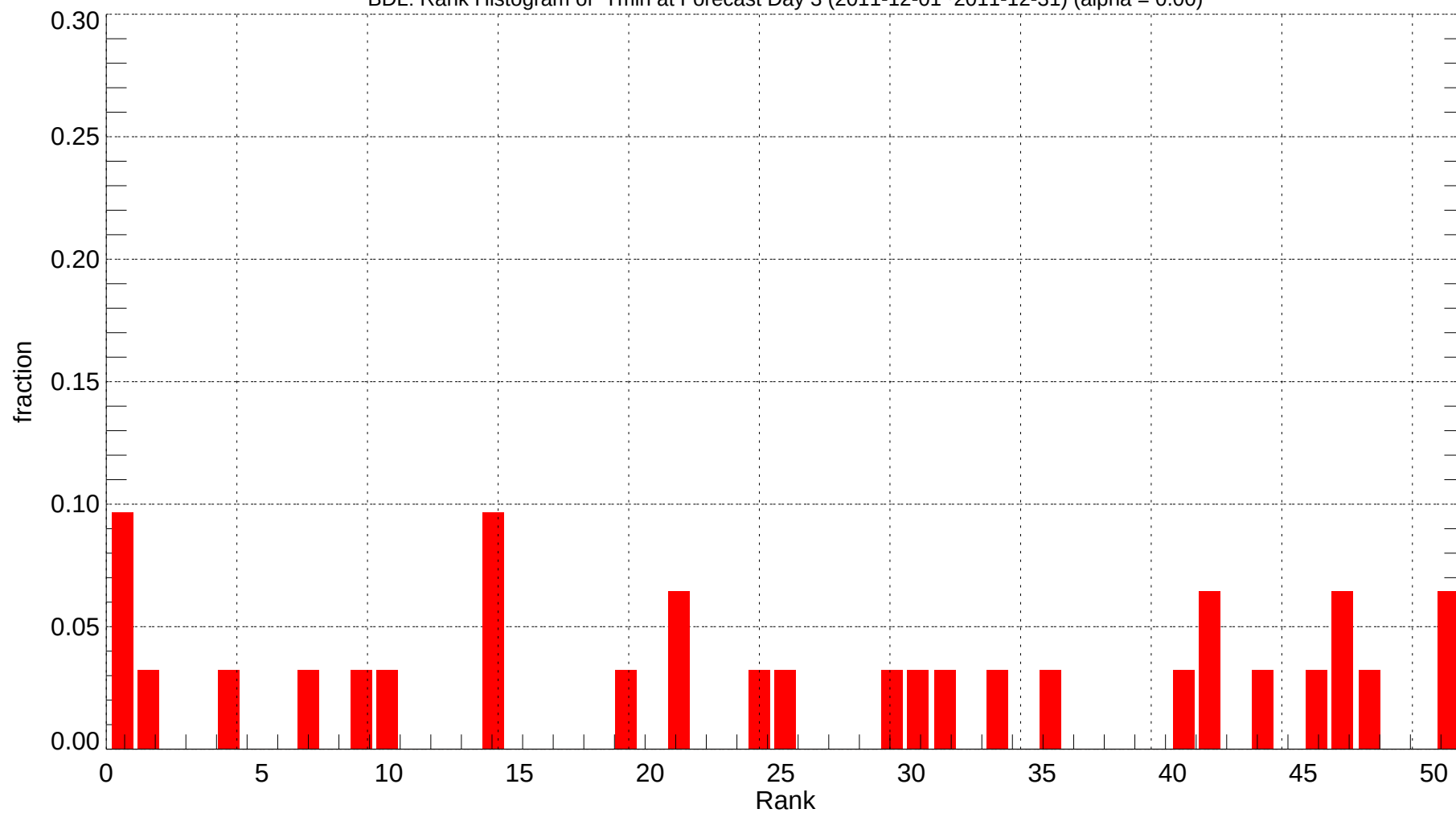
BDL: Rank Histogram of Tmin at Forecast Day 3 (2011-12-01~2011-12-31) (alpha = 0.00)
