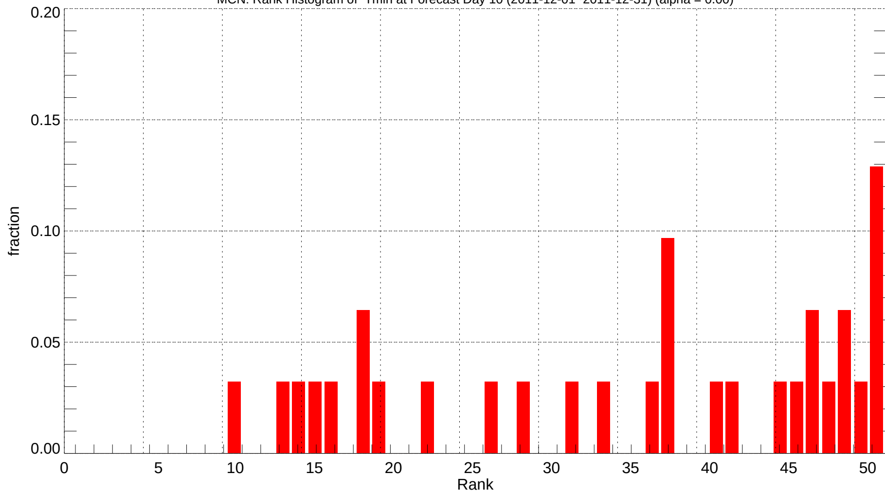
MCN: Rank Histogram of Tmin at Forecast Day 10 (2011-12-01~2011-12-31) (alpha = 0.00)
