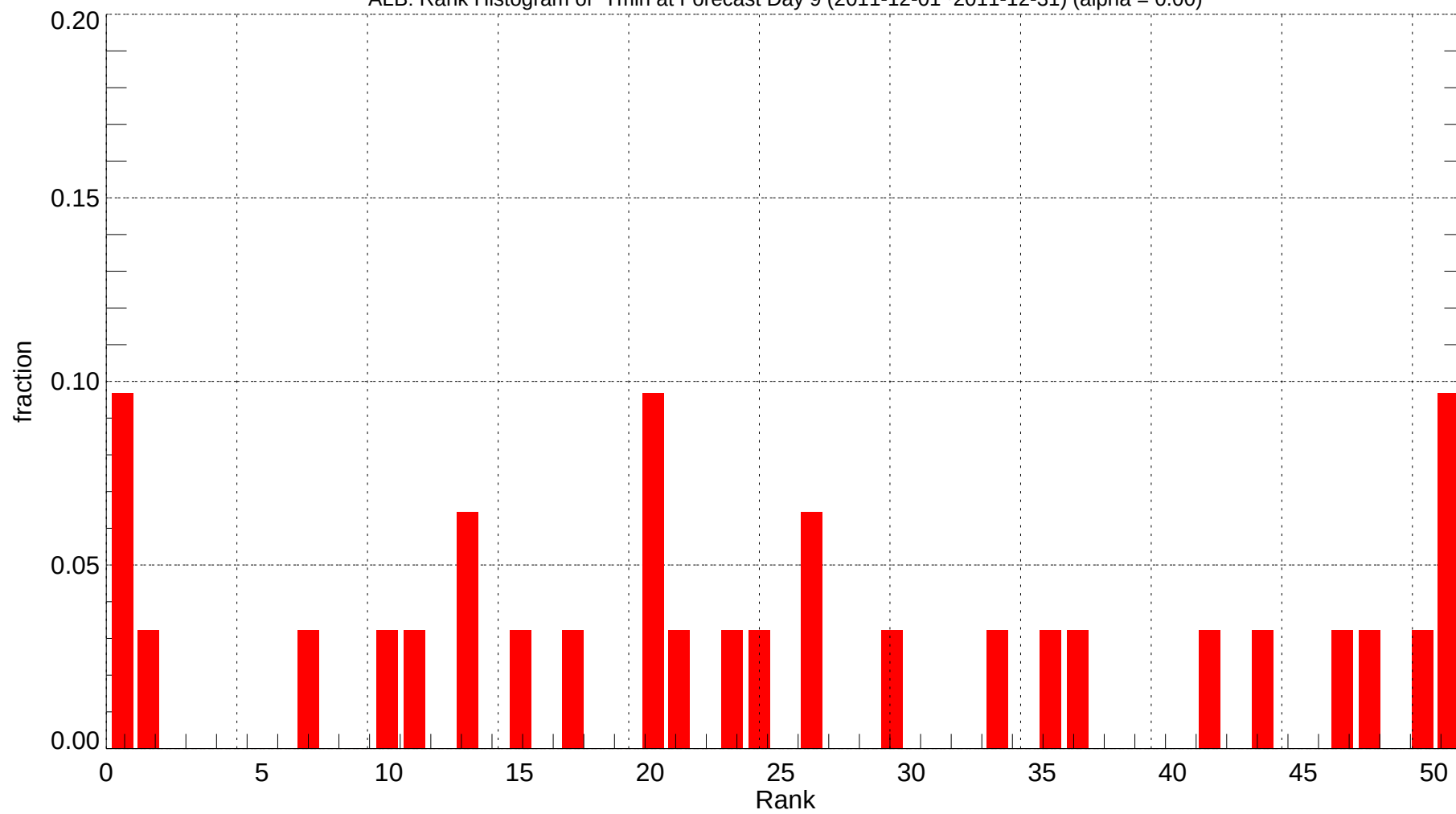
ALB: Rank Histogram of Tmin at Forecast Day 9 (2011-12-01~2011-12-31) (alpha = 0.00)
