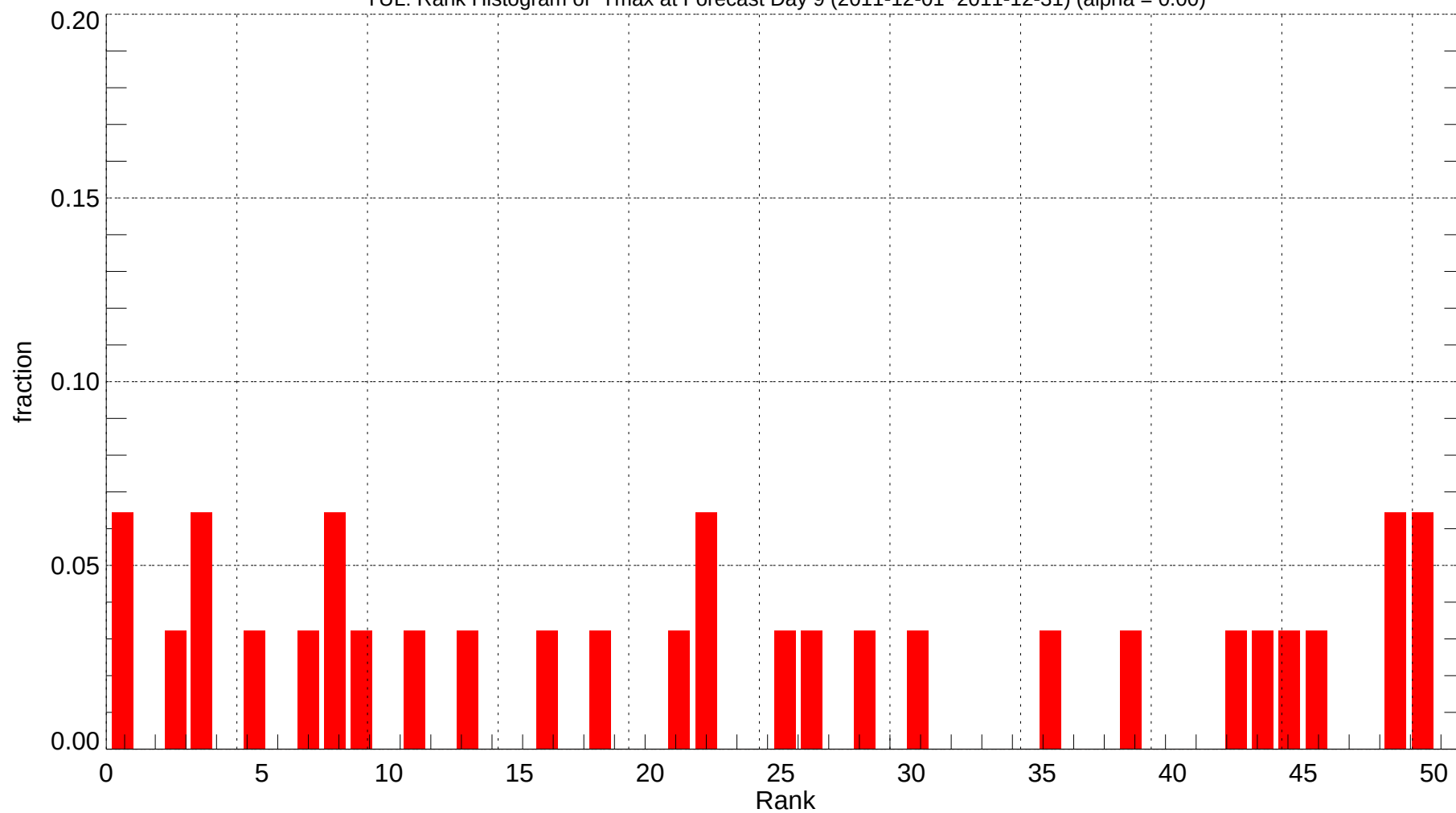
YUL: Rank Histogram of Tmax at Forecast Day 9 (2011-12-01~2011-12-31) (alpha = 0.00)
