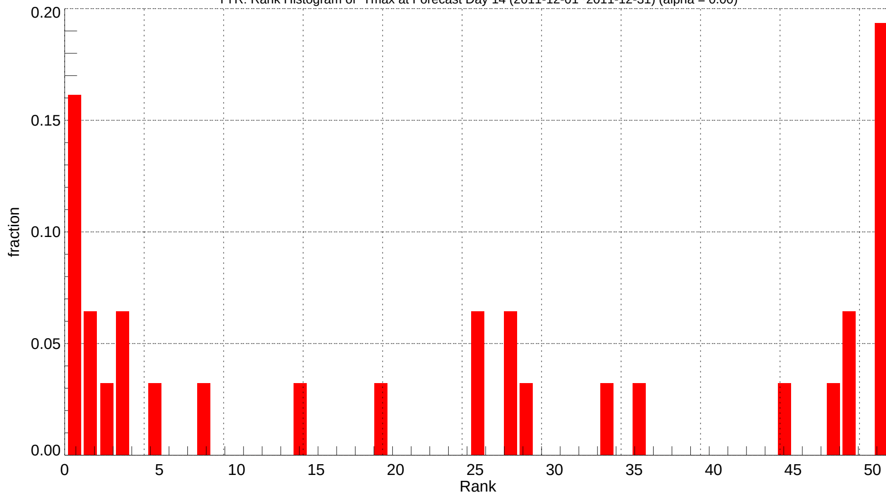
TYR: Rank Histogram of Tmax at Forecast Day 14 (2011-12-01~2011-12-31) (alpha = 0.00)
