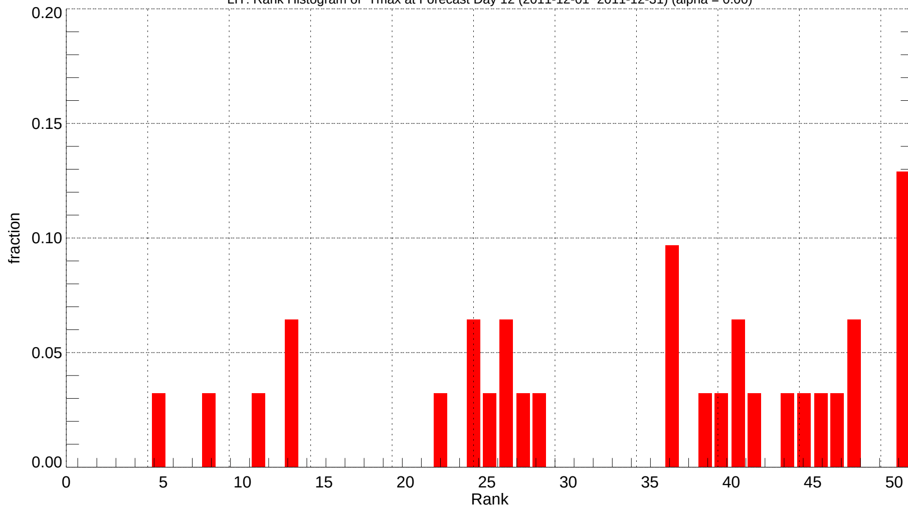
LIT: Rank Histogram of Tmax at Forecast Day 12 (2011-12-01~2011-12-31) (alpha = 0.00)
