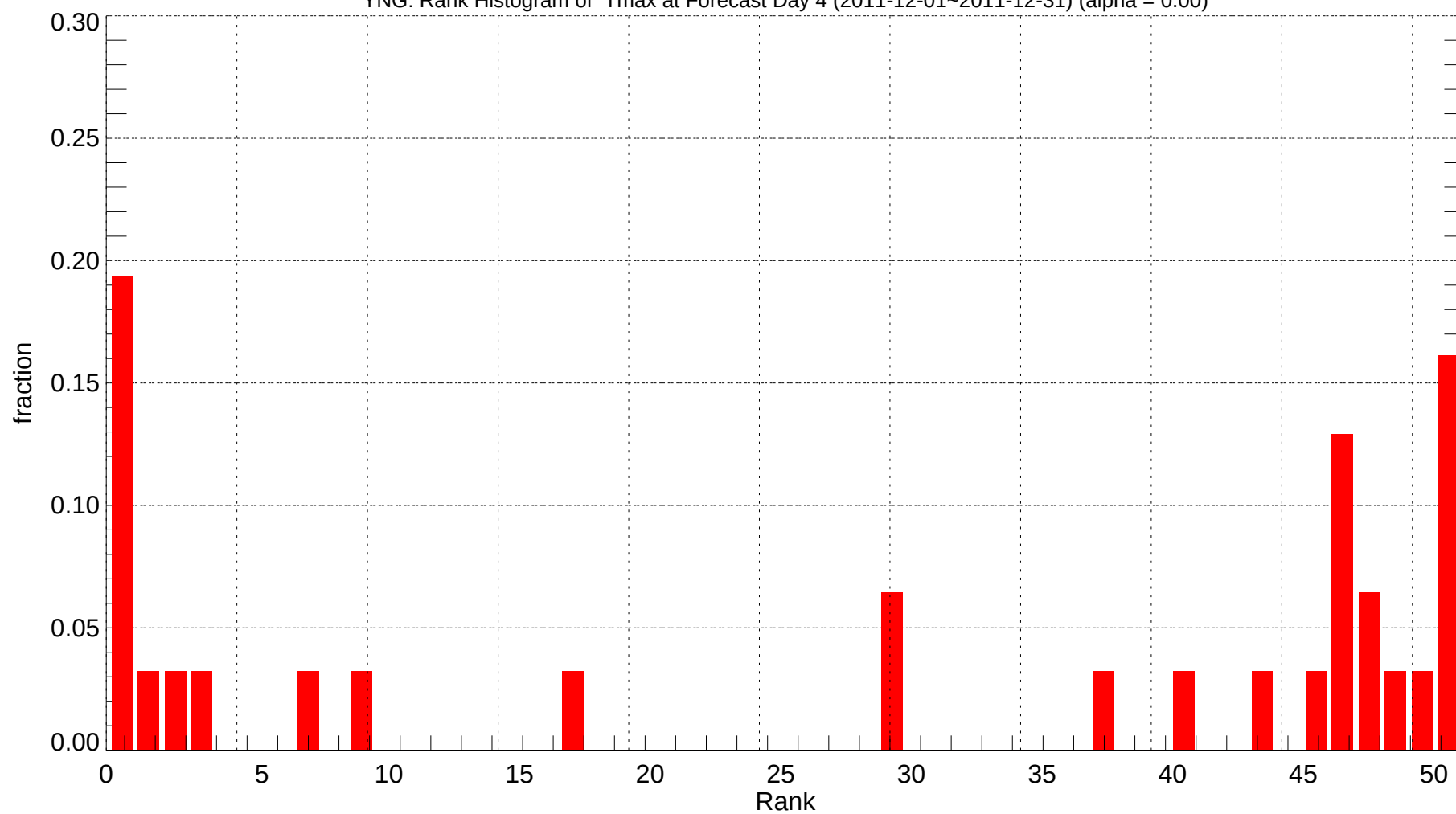
YNG: Rank Histogram of Tmax at Forecast Day 4 (2011-12-01~2011-12-31) (alpha = 0.00)
