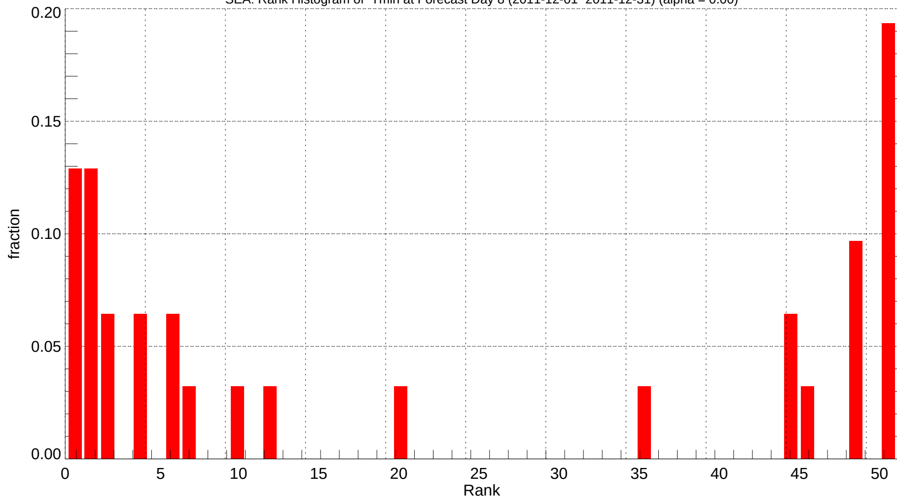
SEA: Rank Histogram of Tmin at Forecast Day 8 (2011-12-01~2011-12-31) (alpha = 0.00)
