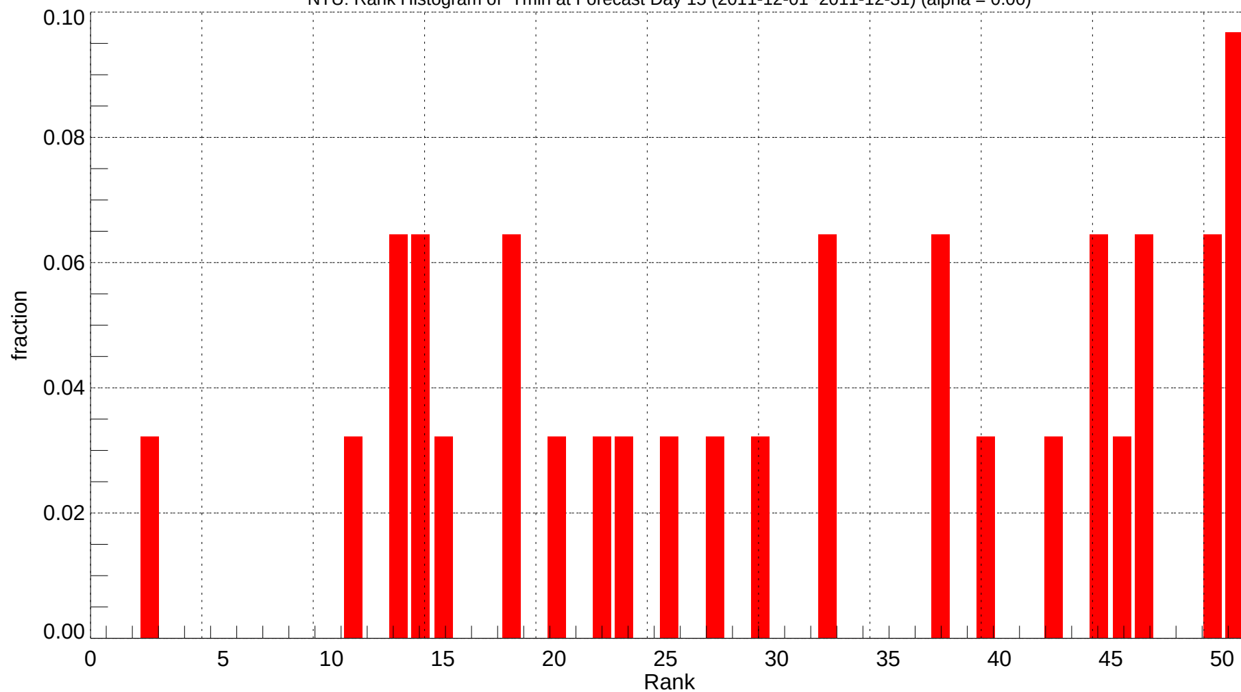
NTU: Rank Histogram of Tmin at Forecast Day 15 (2011-12-01~2011-12-31) (alpha = 0.00)
