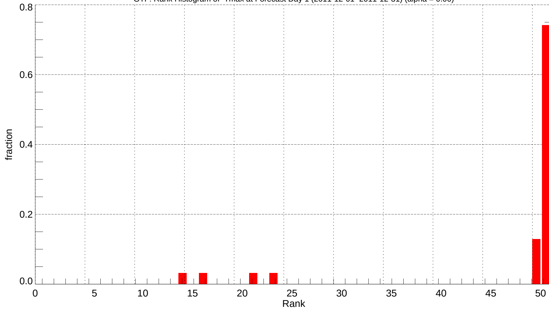
GTF: Rank Histogram of Tmax at Forecast Day 1 (2011-12-01~2011-12-31) (alpha = 0.00)
