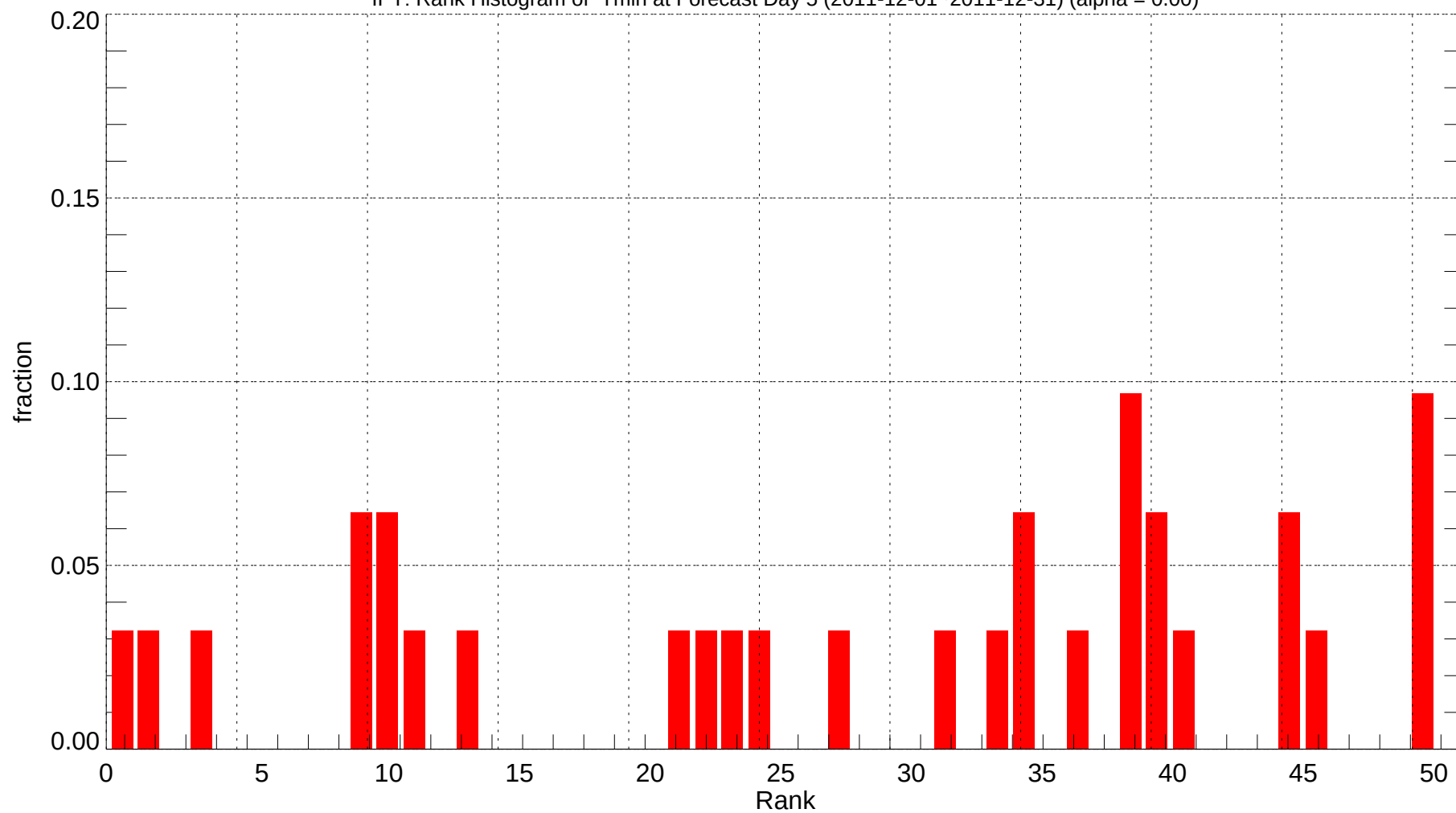
IPT: Rank Histogram of Tmin at Forecast Day 5 (2011-12-01~2011-12-31) (alpha = 0.00)
