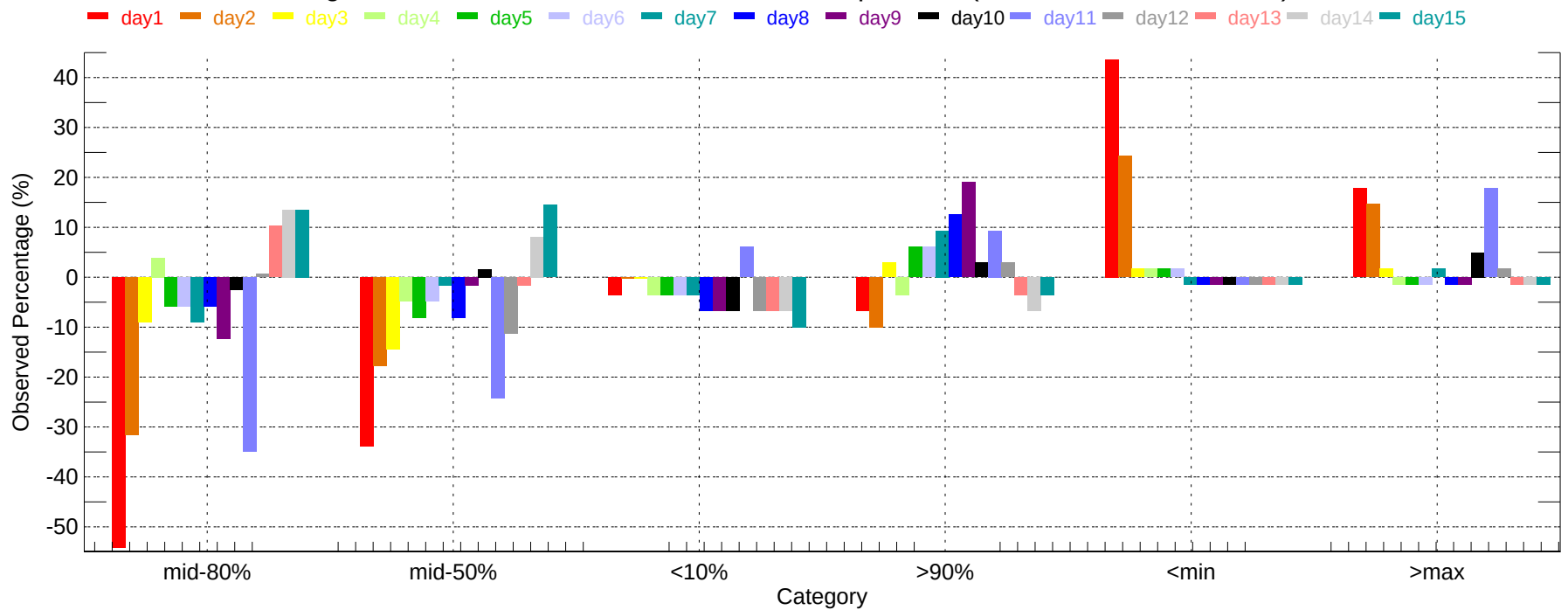
Observed Percentage Deviation of Ensembles - IPT: Max Temperature (2011-12-01~2011-12-31)
