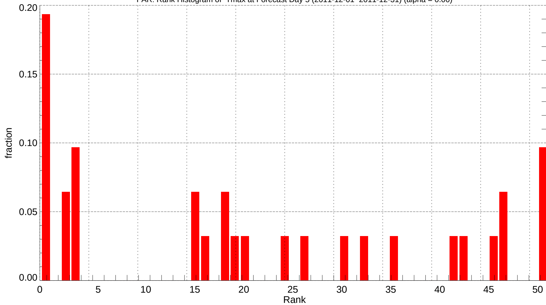
FAR: Rank Histogram of Tmax at Forecast Day 5 (2011-12-01~2011-12-31) (alpha = 0.00)
