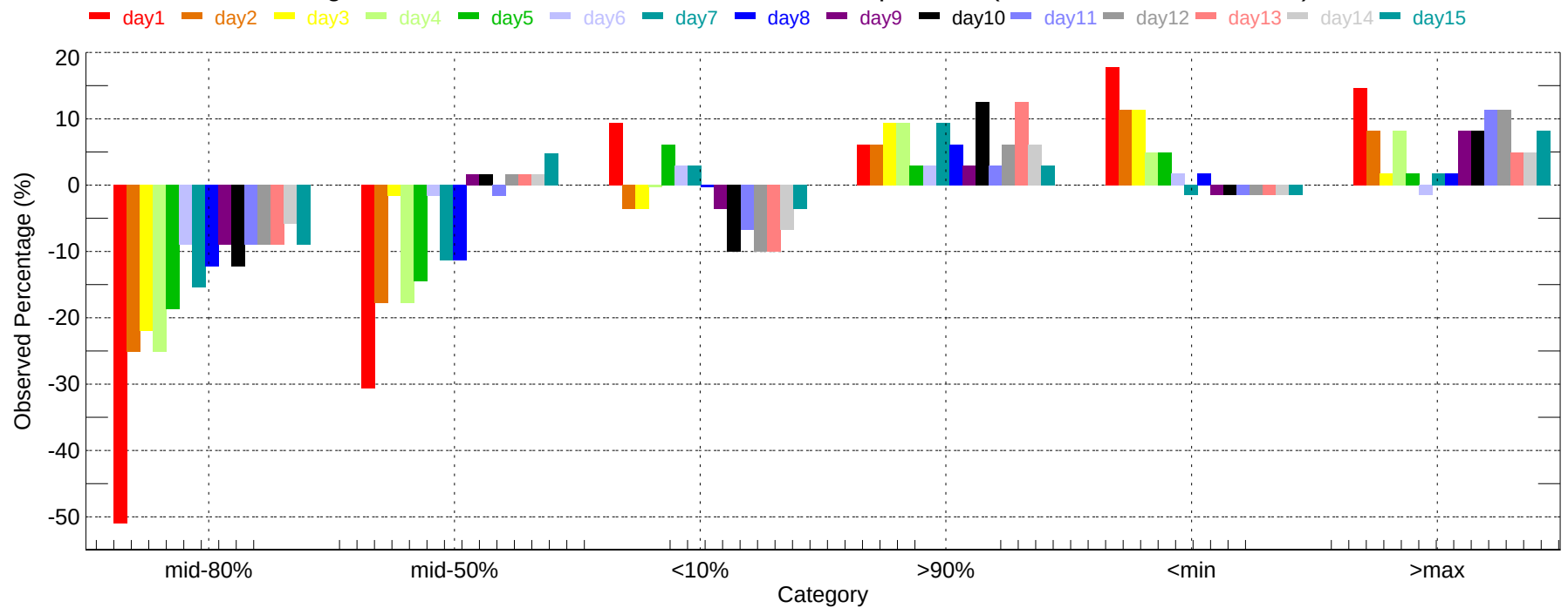
Observed Percentage Deviation of Ensembles - MCN: Max Temperature (2011-12-01~2011-12-31)
