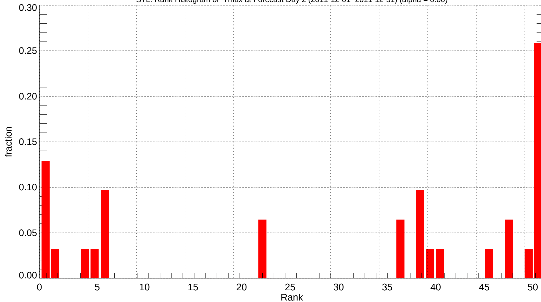
STL: Rank Histogram of Tmax at Forecast Day 2 (2011-12-01~2011-12-31) (alpha = 0.00)
