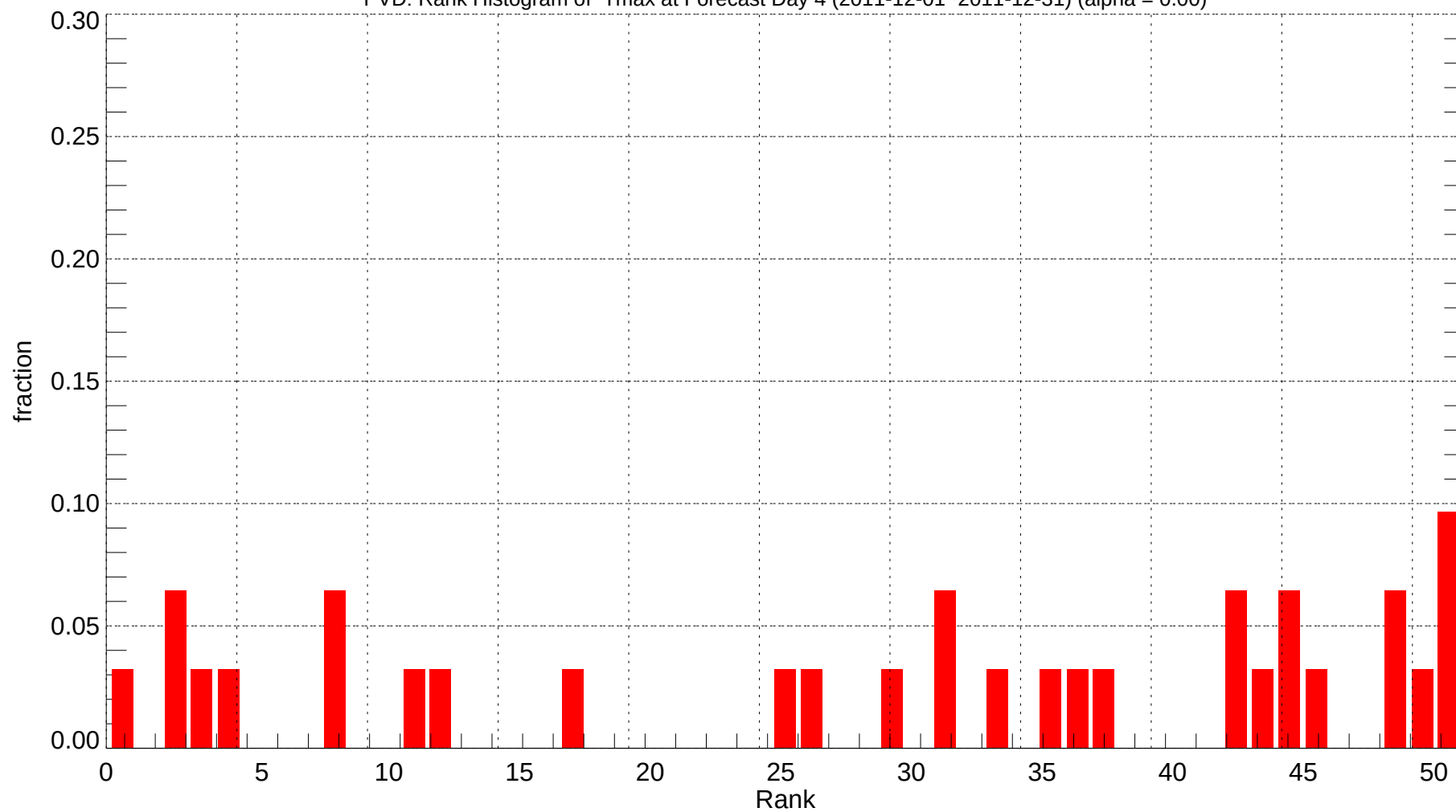
PVD: Rank Histogram of Tmax at Forecast Day 4 (2011-12-01~2011-12-31) (alpha = 0.00)
