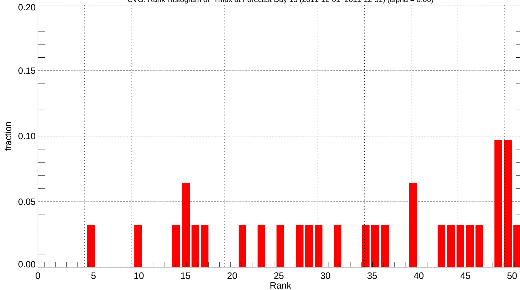
CVG: Rank Histogram of Tmax at Forecast Day 13 (2011-12-01~2011-12-31) (alpha = 0.00)
