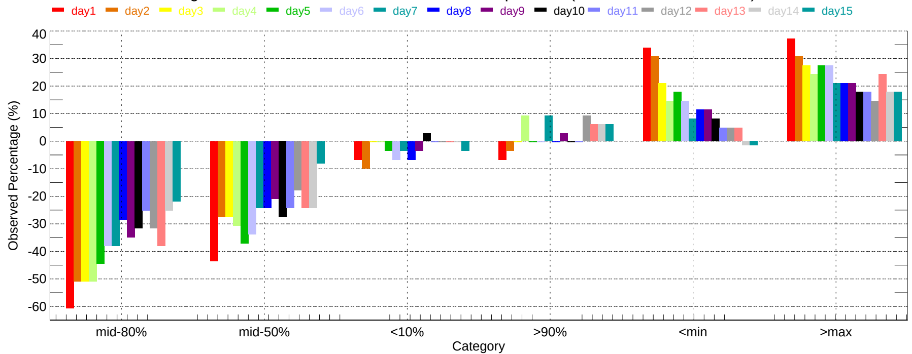
Observed Percentage Deviation of Ensembles - LAX: Max Temperature (2011-12-01~2011-12-31)
