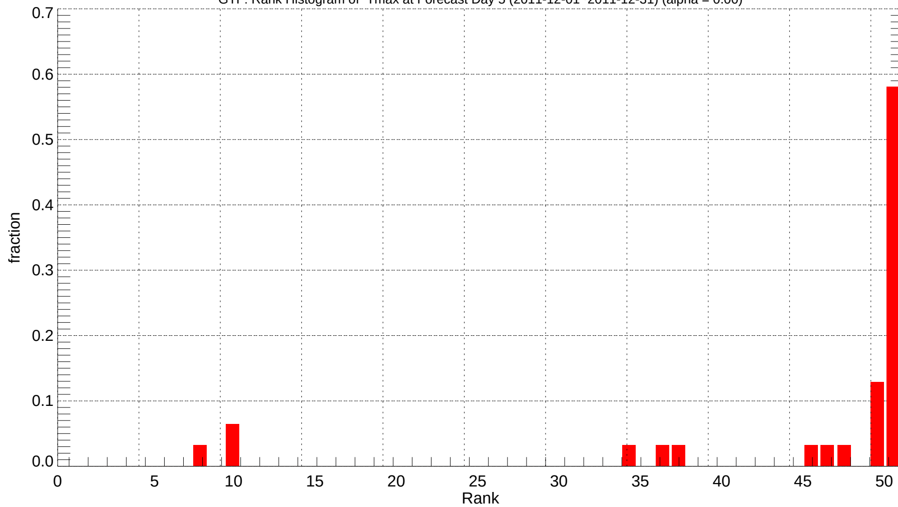
GTF: Rank Histogram of Tmax at Forecast Day 5 (2011-12-01~2011-12-31) (alpha = 0.00)
