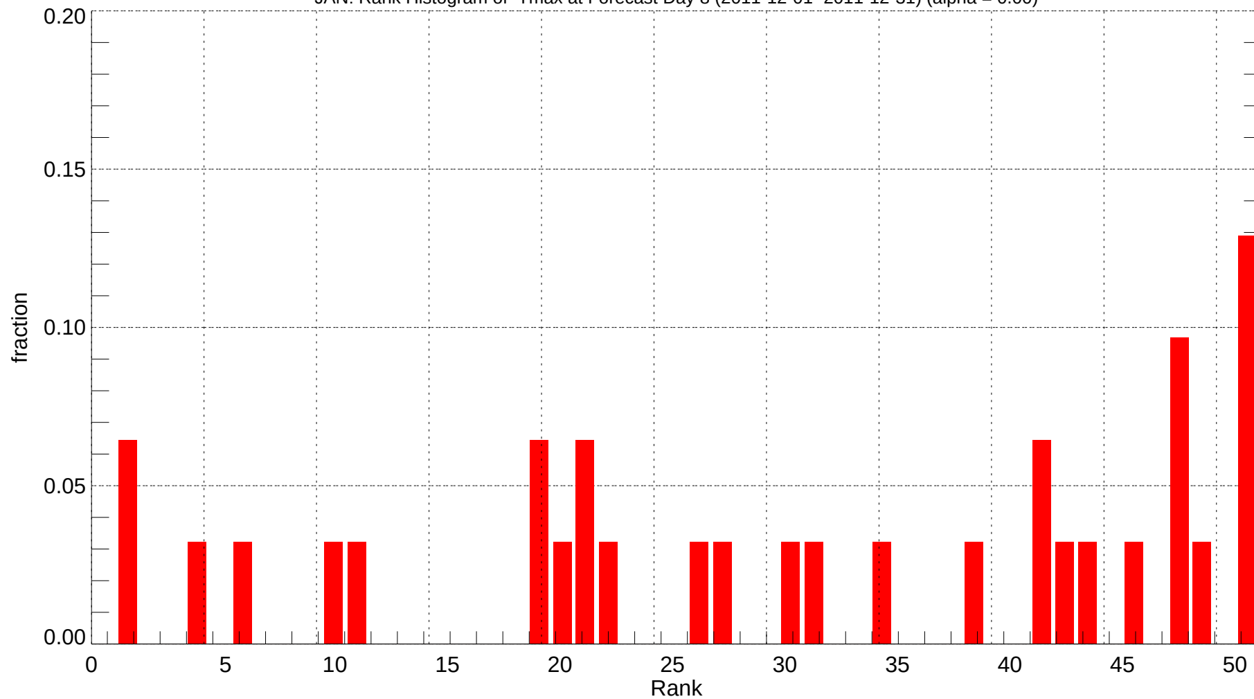
JAN: Rank Histogram of Tmax at Forecast Day 8 (2011-12-01~2011-12-31) (alpha = 0.00)
