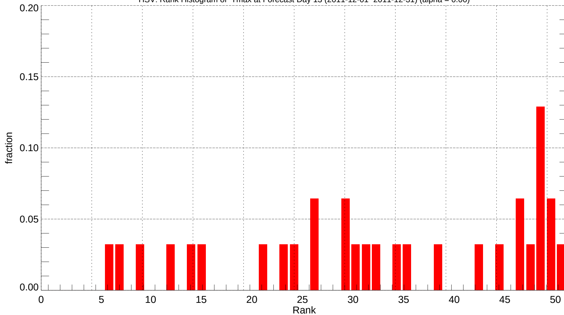
HSV: Rank Histogram of Tmax at Forecast Day 13 (2011-12-01~2011-12-31) (alpha = 0.00)
