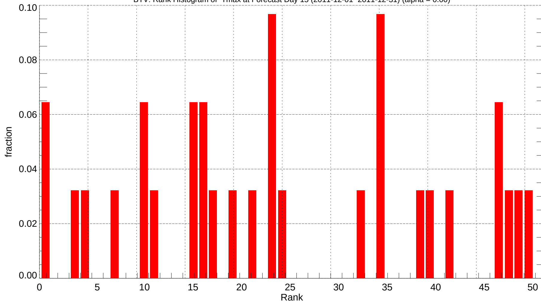
BTV: Rank Histogram of Tmax at Forecast Day 15 (2011-12-01~2011-12-31) (alpha = 0.00)
