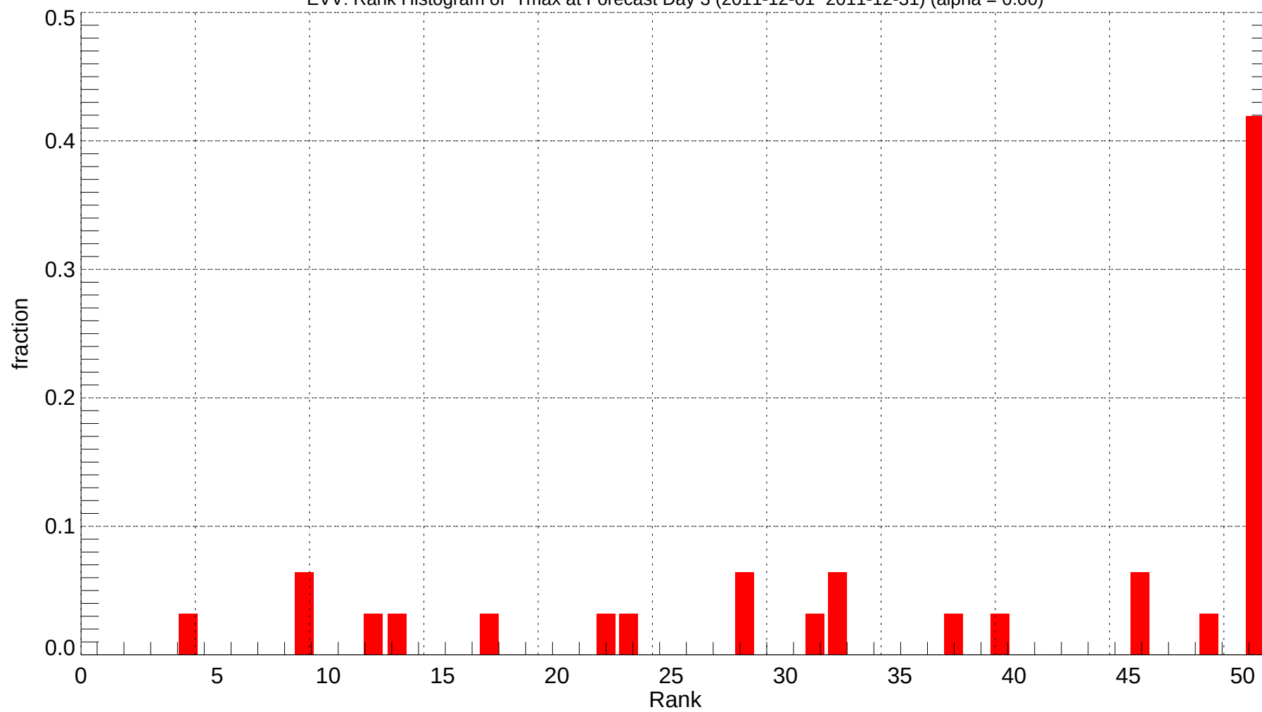
EVV: Rank Histogram of Tmax at Forecast Day 3 (2011-12-01~2011-12-31) (alpha = 0.00)
