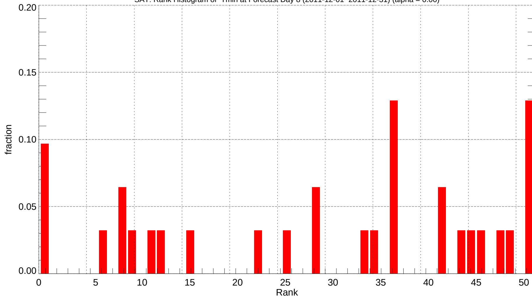
SAT: Rank Histogram of Tmin at Forecast Day 8 (2011-12-01~2011-12-31) (alpha = 0.00)
