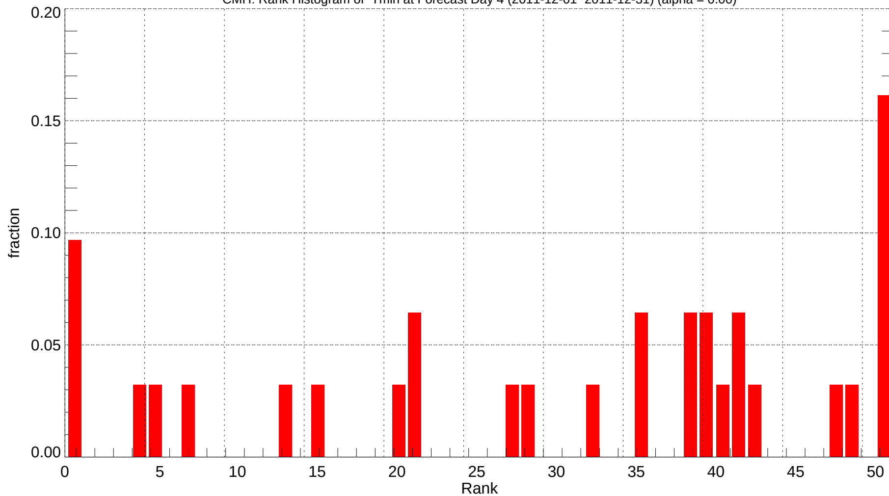
CMH: Rank Histogram of Tmin at Forecast Day 4 (2011-12-01~2011-12-31) (alpha = 0.00)
