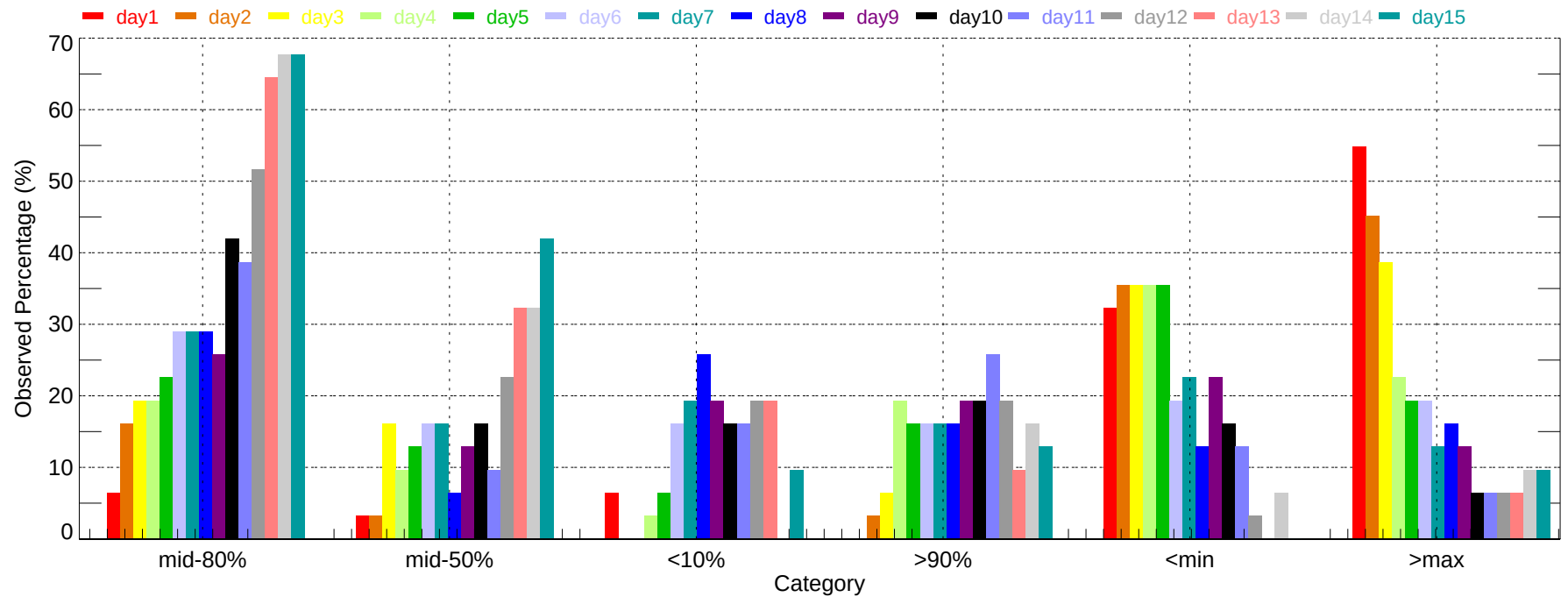
Observed Percentage of Ensembles - SEA: Max Temperature (2011-12-01~2011-12-31)
