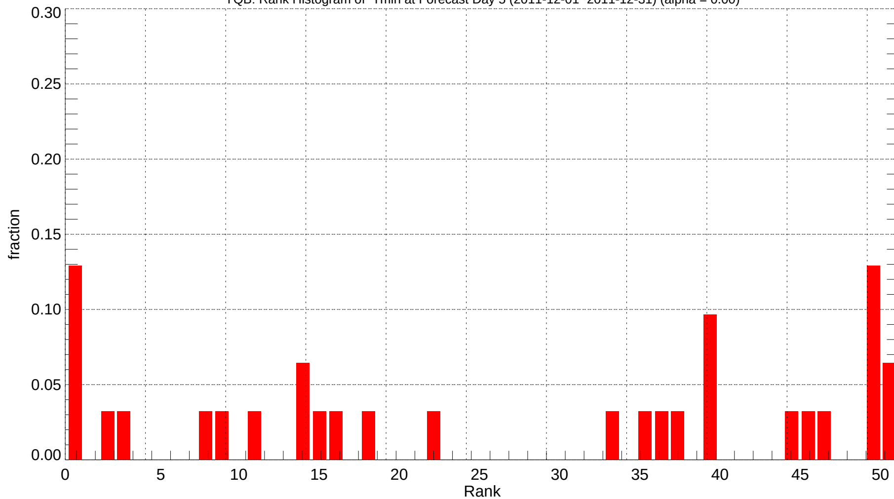
YQB: Rank Histogram of Tmin at Forecast Day 5 (2011-12-01~2011-12-31) (alpha = 0.00)
