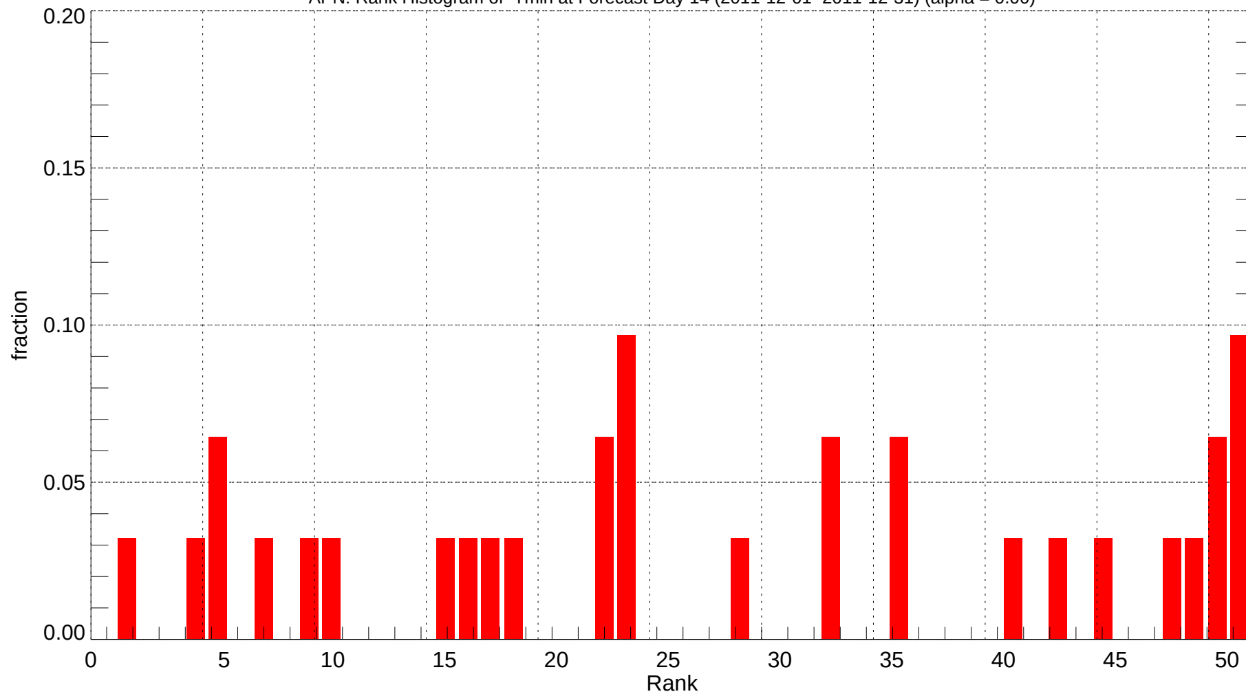
APN: Rank Histogram of Tmin at Forecast Day 14 (2011-12-01~2011-12-31) (alpha = 0.00)
