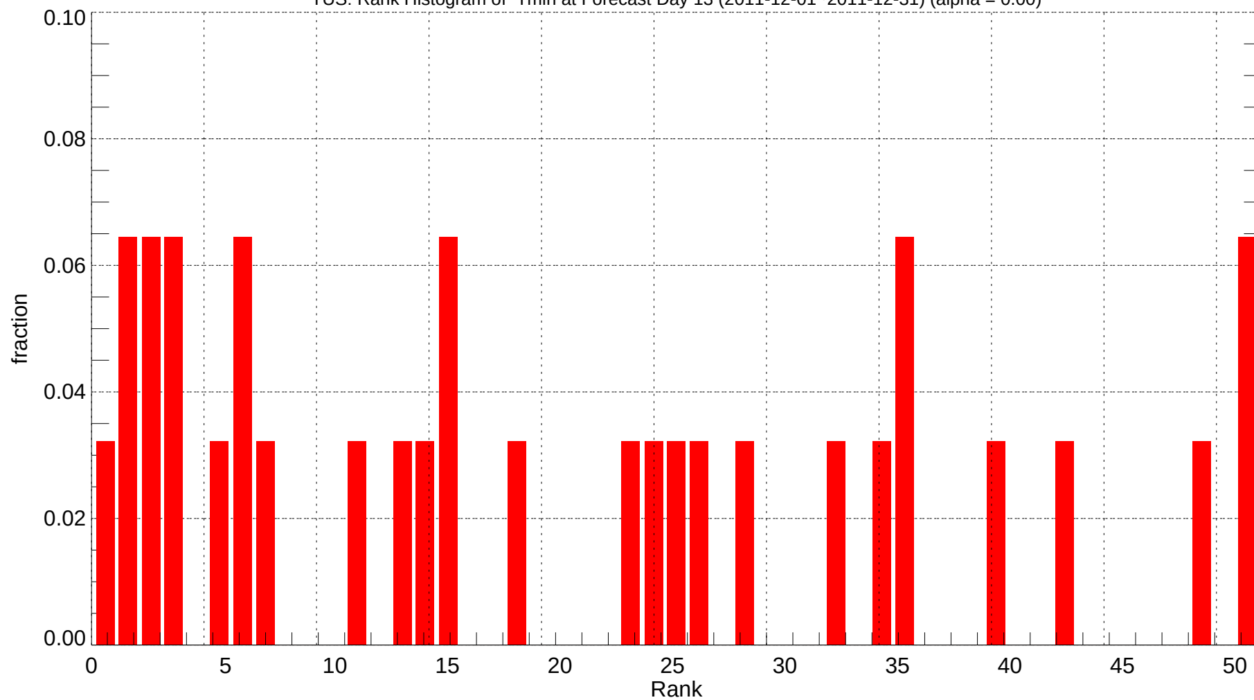
TUS: Rank Histogram of Tmin at Forecast Day 13 (2011-12-01~2011-12-31) (alpha = 0.00)
