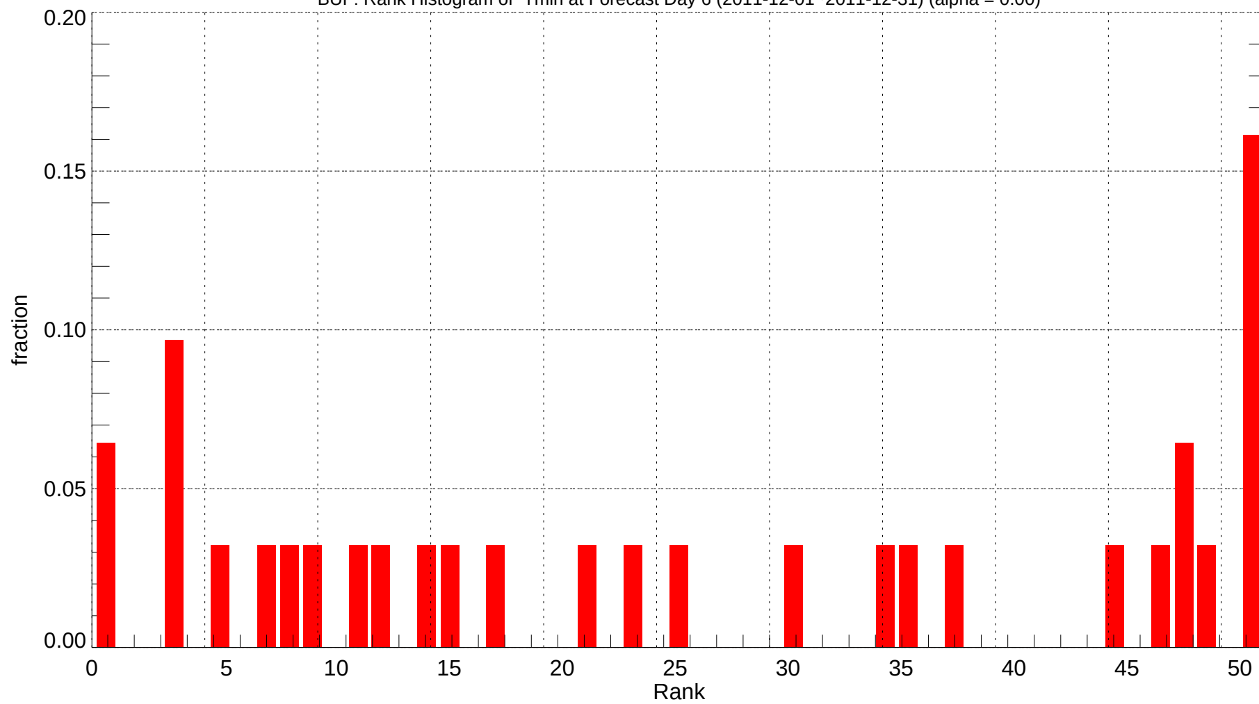
BUF: Rank Histogram of Tmin at Forecast Day 6 (2011-12-01~2011-12-31) (alpha = 0.00)
