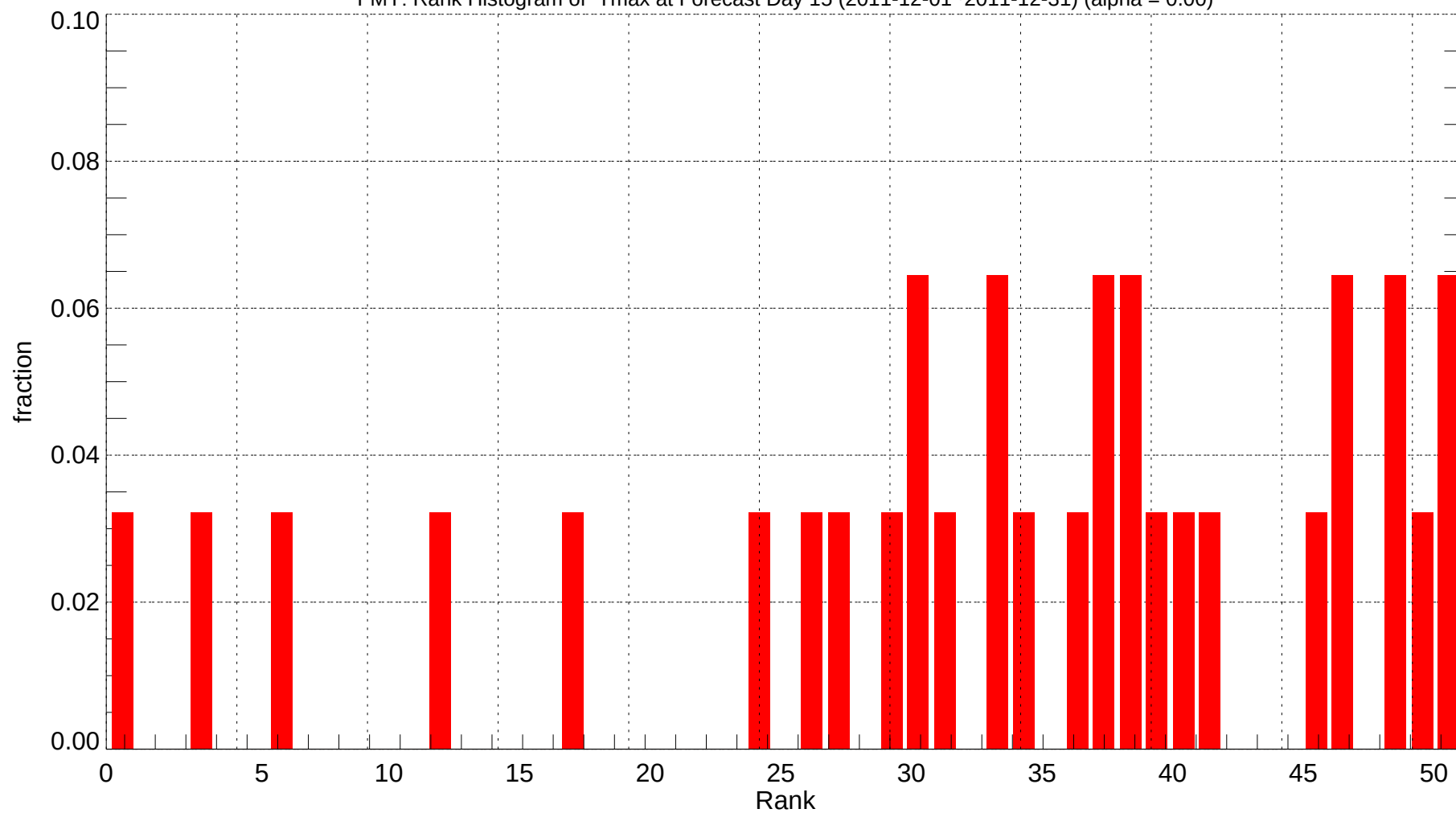
FMY: Rank Histogram of Tmax at Forecast Day 15 (2011-12-01~2011-12-31) (alpha = 0.00)
