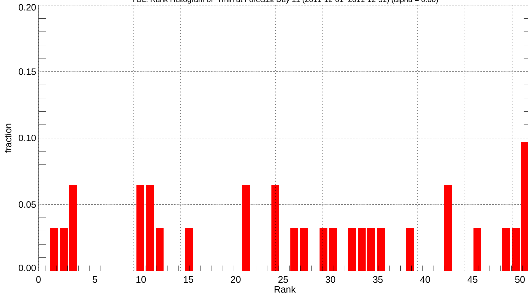
YUL: Rank Histogram of Tmin at Forecast Day 11 (2011-12-01~2011-12-31) (alpha = 0.00)
