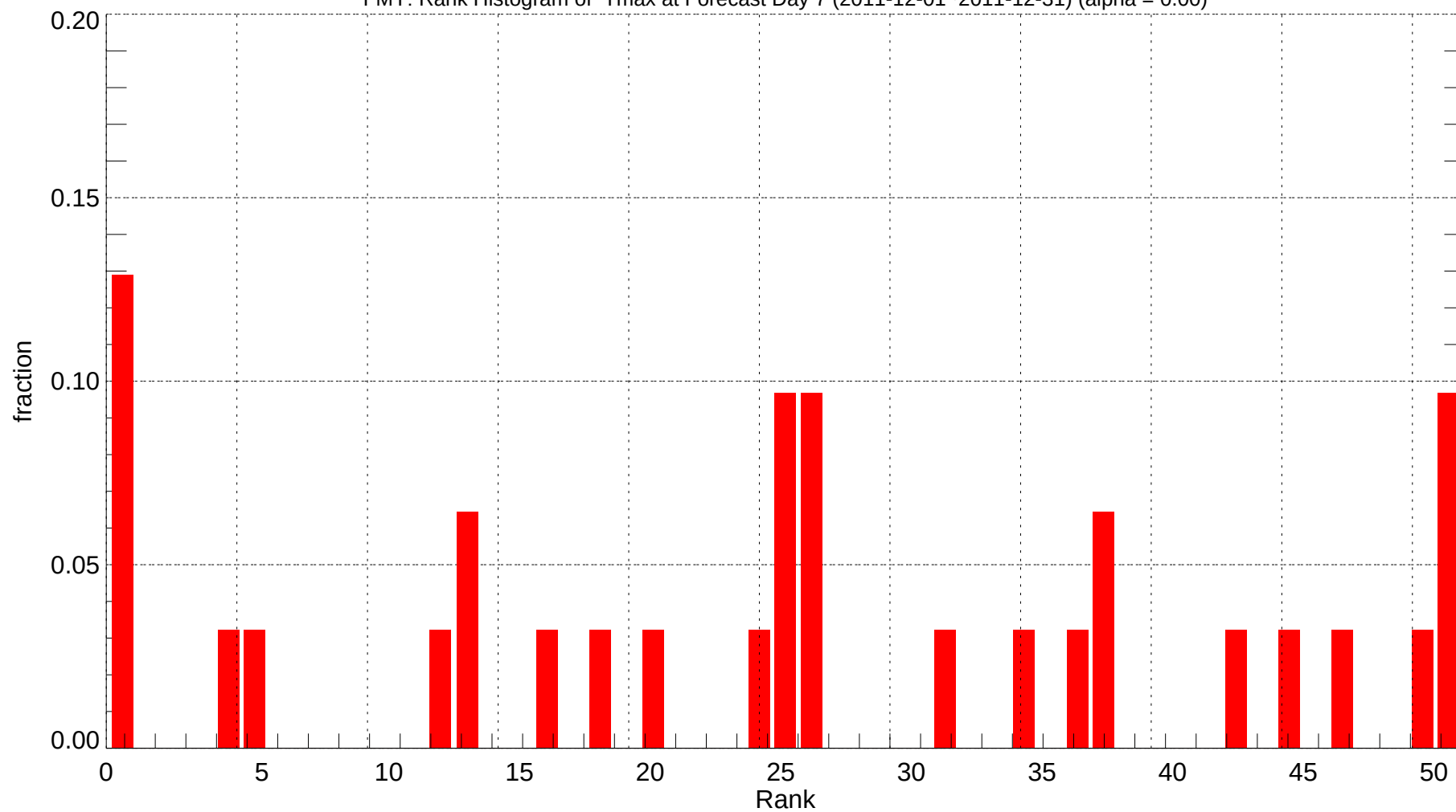
FMY: Rank Histogram of Tmax at Forecast Day 7 (2011-12-01~2011-12-31) (alpha = 0.00)
