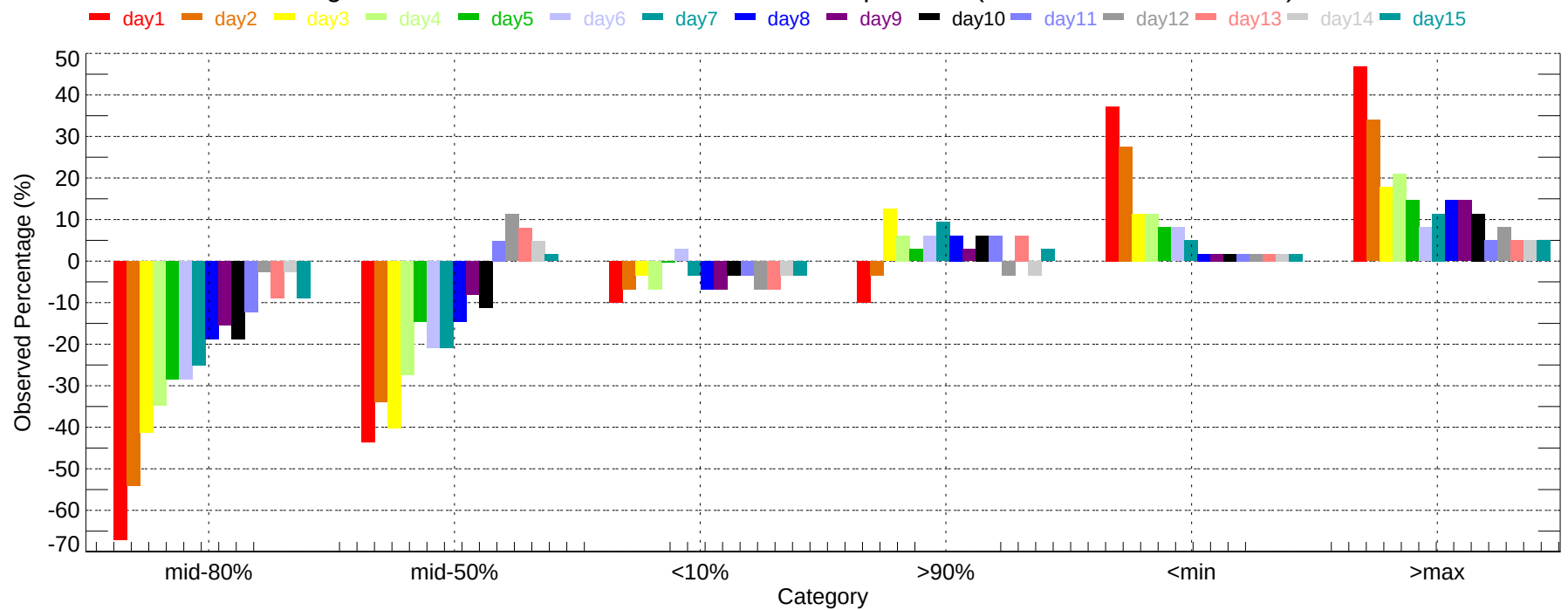
Observed Percentage Deviation of Ensembles - FAR: Min Temperature (2011-12-01~2011-12-31)
