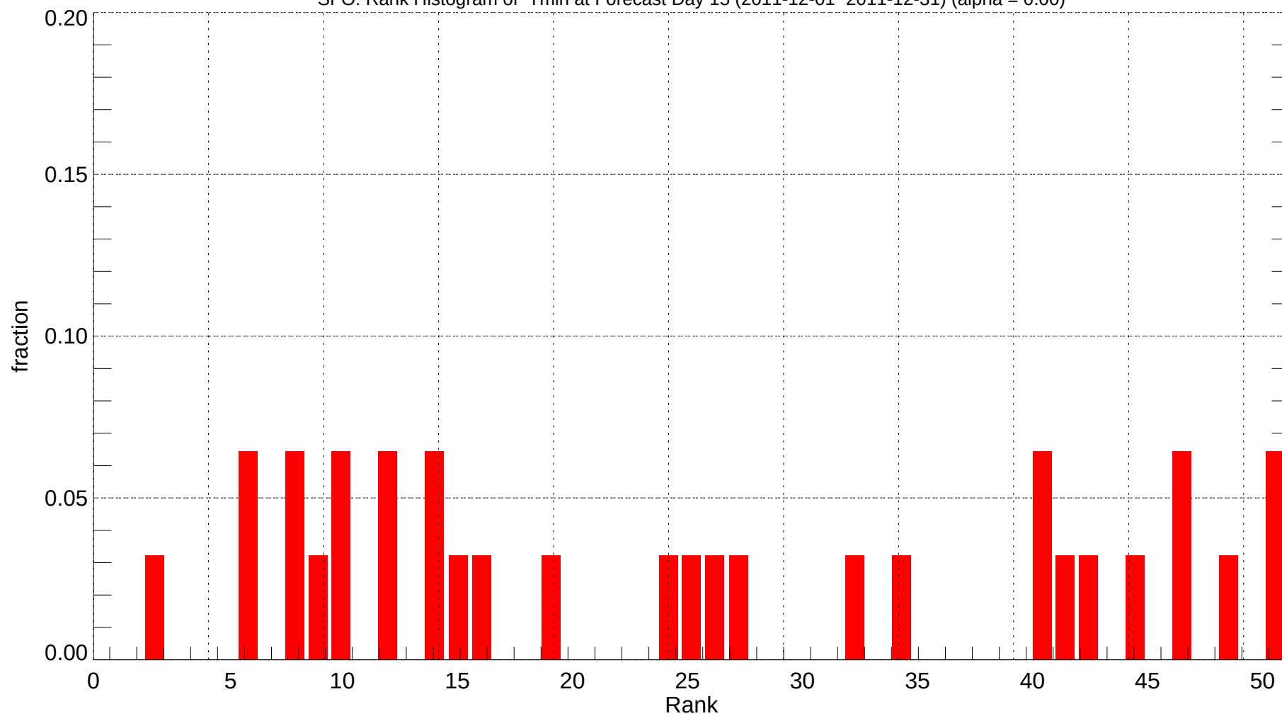
SFO: Rank Histogram of Tmin at Forecast Day 15 (2011-12-01~2011-12-31) (alpha = 0.00)
