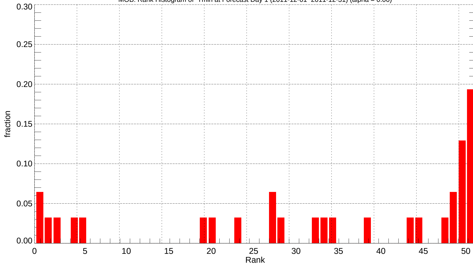
MOB: Rank Histogram of Tmin at Forecast Day 1 (2011-12-01~2011-12-31) (alpha = 0.00)
