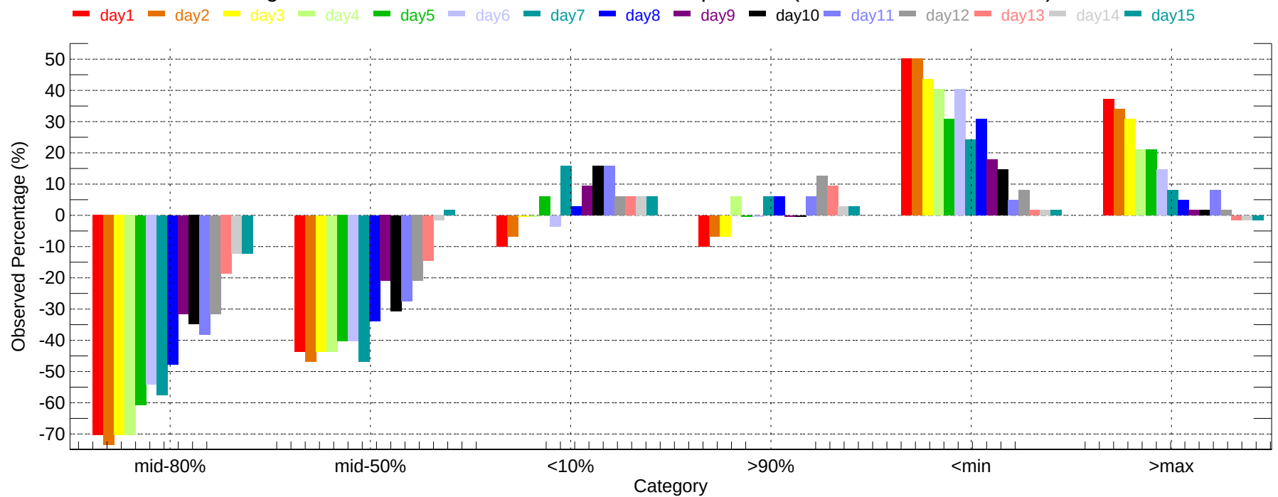
Observed Percentage Deviation of Ensembles - LAX: Min Temperature (2011-12-01~2011-12-31)
