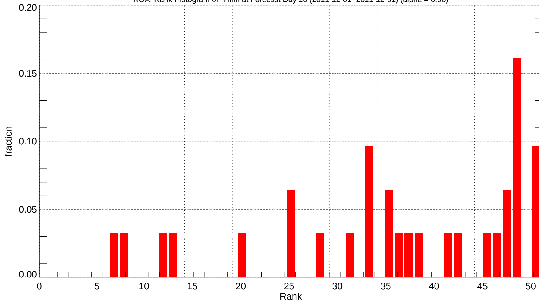
ROA: Rank Histogram of Tmin at Forecast Day 10 (2011-12-01~2011-12-31) (alpha = 0.00)
