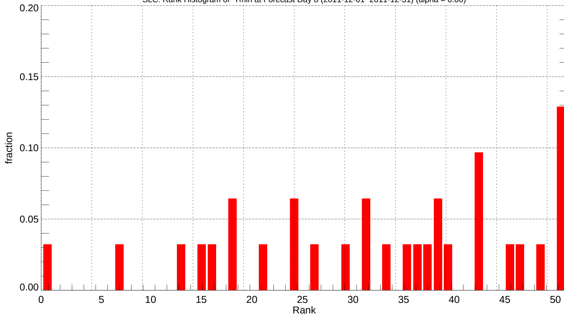
SLC: Rank Histogram of Tmin at Forecast Day 8 (2011-12-01~2011-12-31) (alpha = 0.00)
