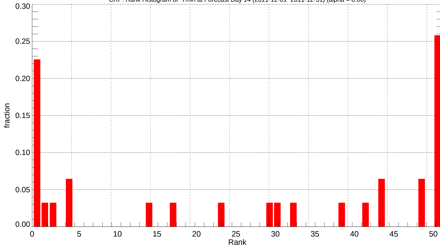
CRP: Rank Histogram of Tmin at Forecast Day 14 (2011-12-01~2011-12-31) (alpha = 0.00)
