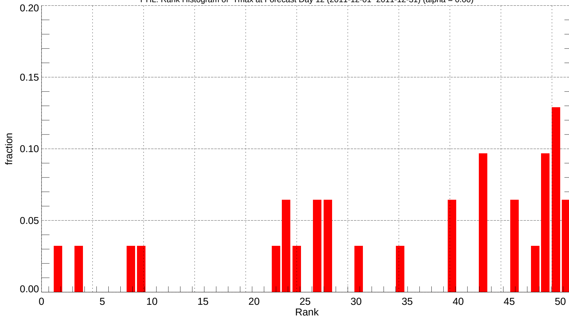
PHL: Rank Histogram of Tmax at Forecast Day 12 (2011-12-01~2011-12-31) (alpha = 0.00)
