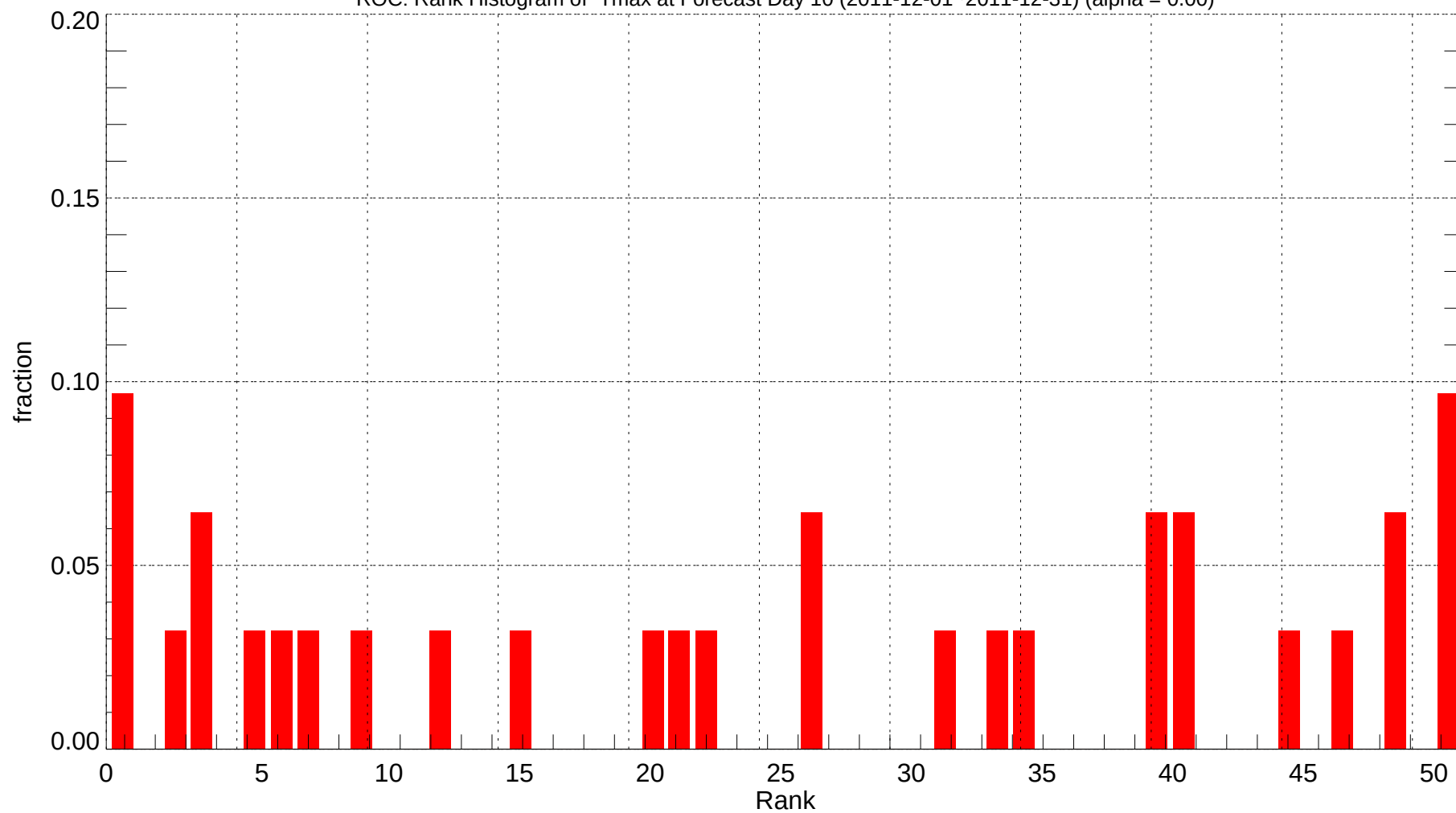
ROC: Rank Histogram of Tmax at Forecast Day 10 (2011-12-01~2011-12-31) (alpha = 0.00)
