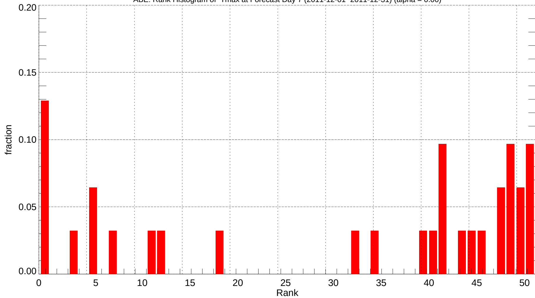
ABE: Rank Histogram of Tmax at Forecast Day 7 (2011-12-01~2011-12-31) (alpha = 0.00)
