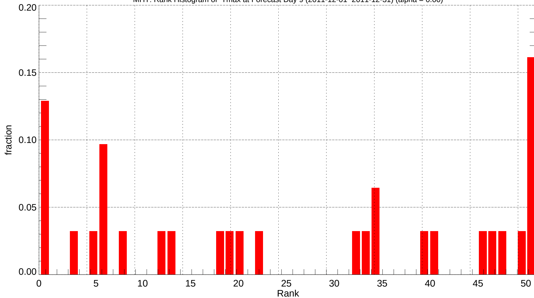
MHT: Rank Histogram of Tmax at Forecast Day 9 (2011-12-01~2011-12-31) (alpha = 0.00)
