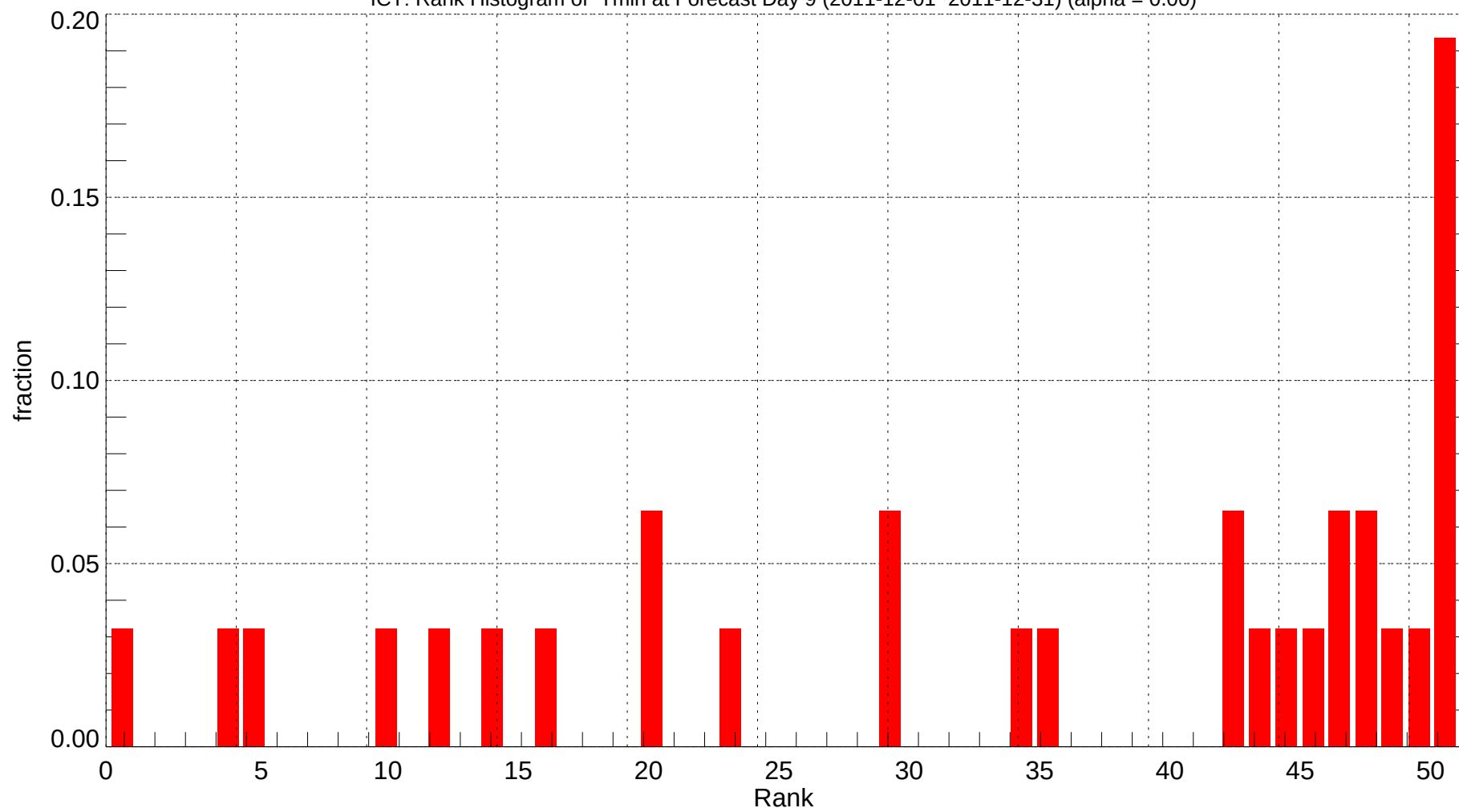
ICT: Rank Histogram of Tmin at Forecast Day 9 (2011-12-01~2011-12-31) (alpha = 0.00)
