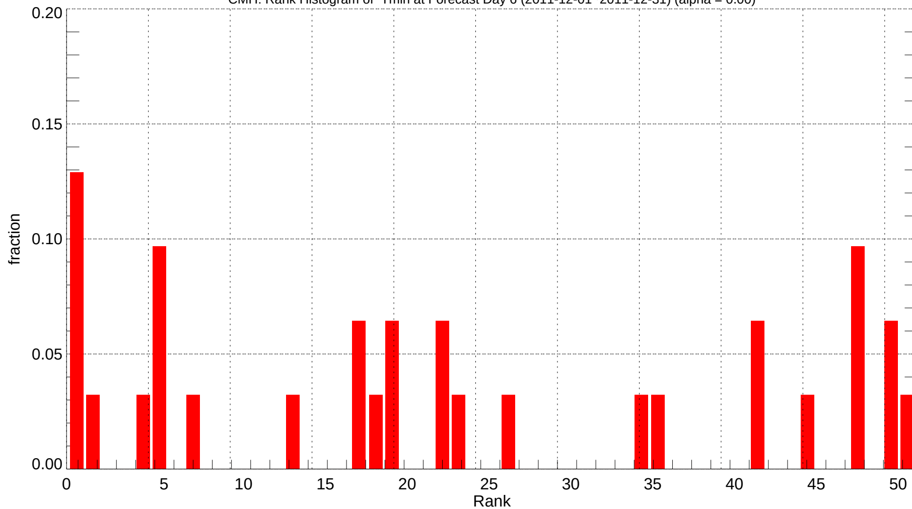
CMH: Rank Histogram of Tmin at Forecast Day 6 (2011-12-01~2011-12-31) (alpha = 0.00)
