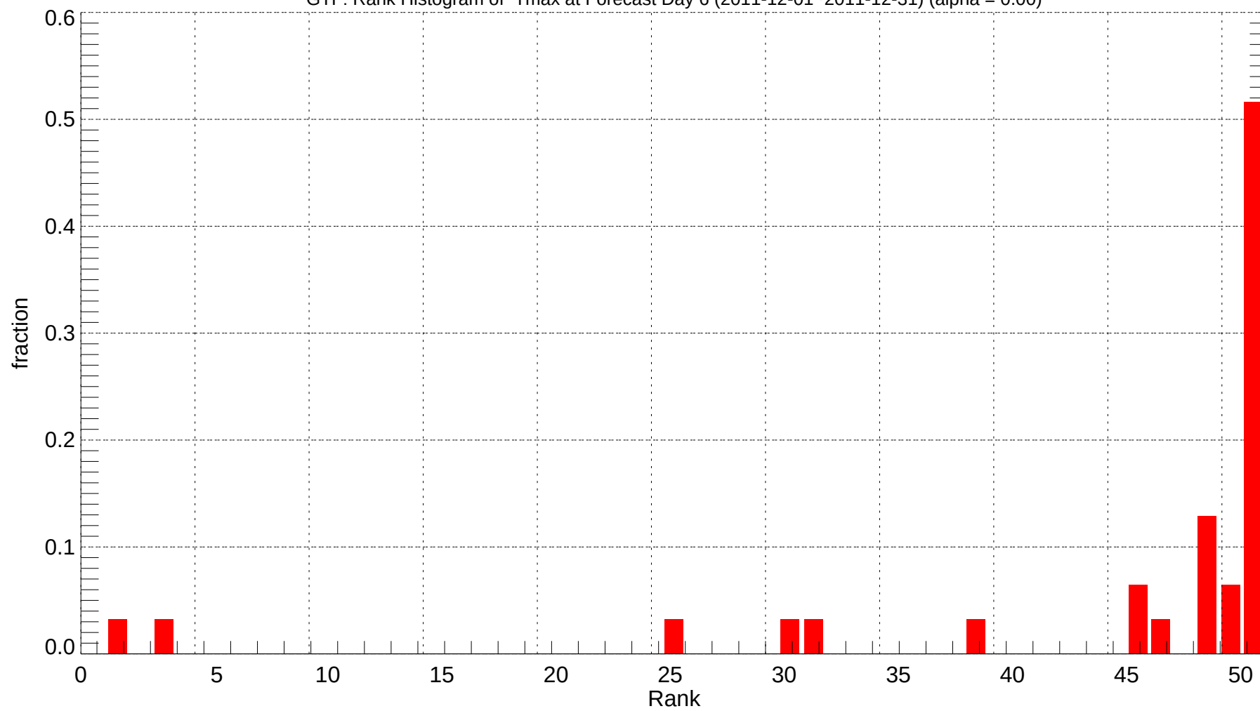
GTF: Rank Histogram of Tmax at Forecast Day 6 (2011-12-01~2011-12-31) (alpha = 0.00)
