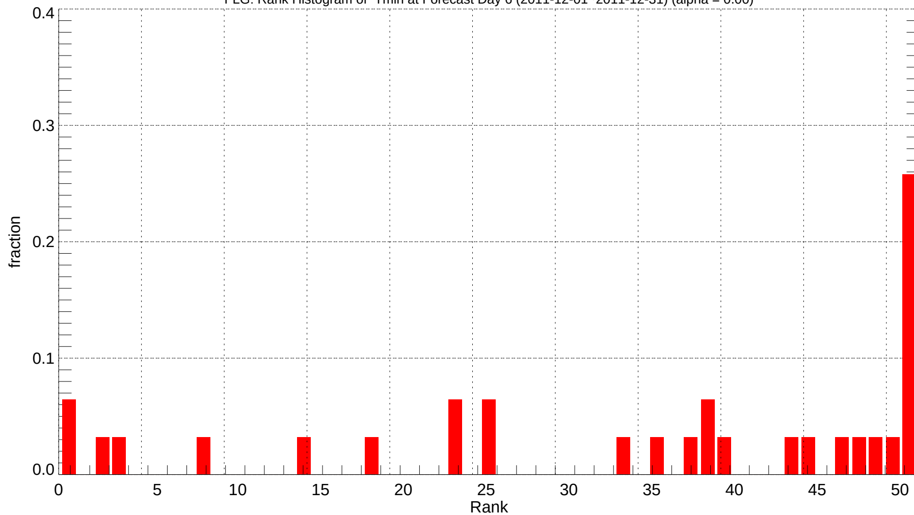
FLG: Rank Histogram of Tmin at Forecast Day 6 (2011-12-01~2011-12-31) (alpha = 0.00)
