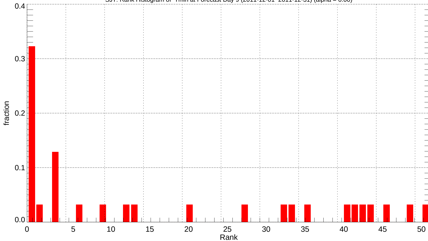
SJT: Rank Histogram of Tmin at Forecast Day 9 (2011-12-01~2011-12-31) (alpha = 0.00)
