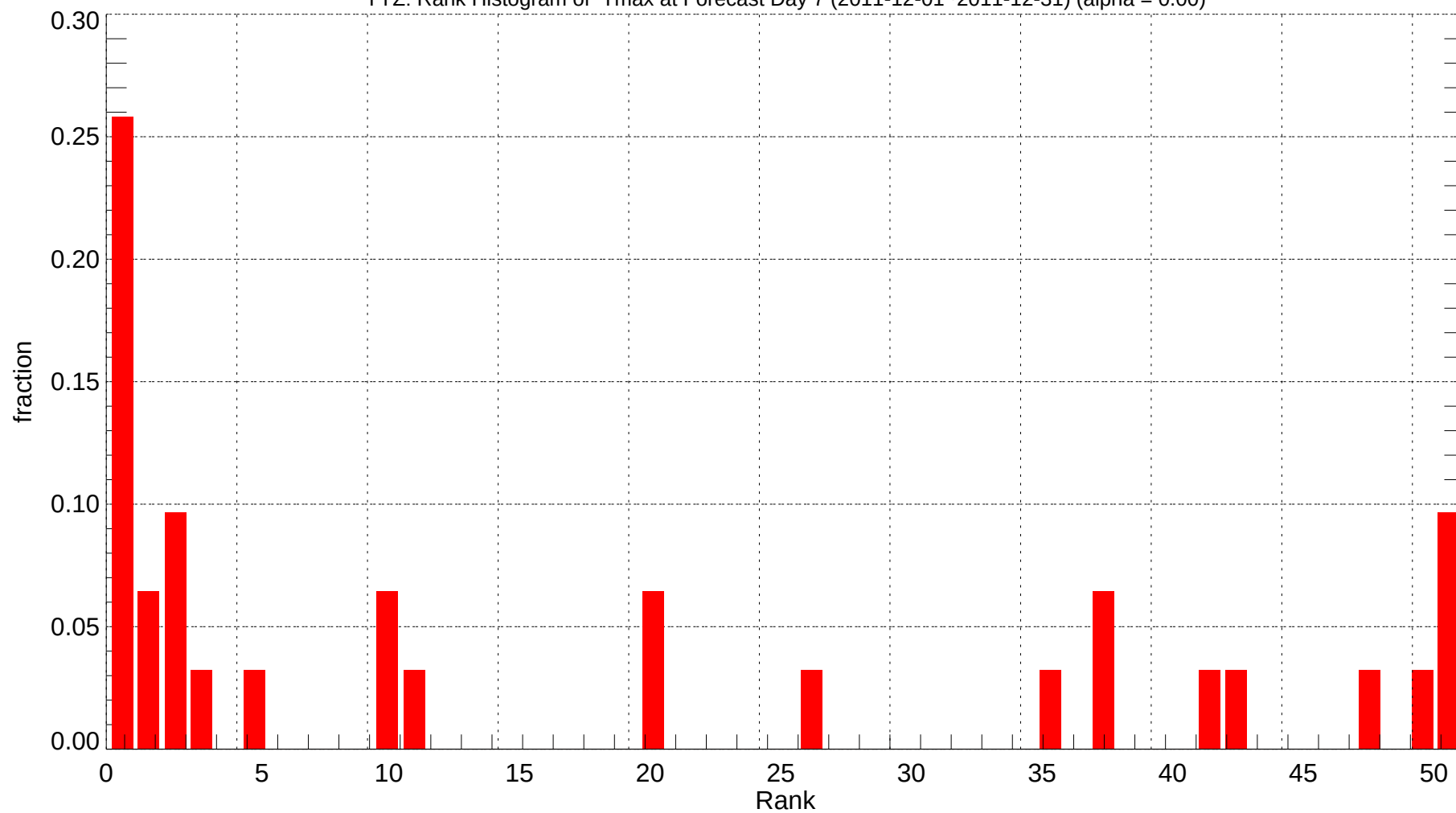
YYZ: Rank Histogram of Tmax at Forecast Day 7 (2011-12-01~2011-12-31) (alpha = 0.00)
