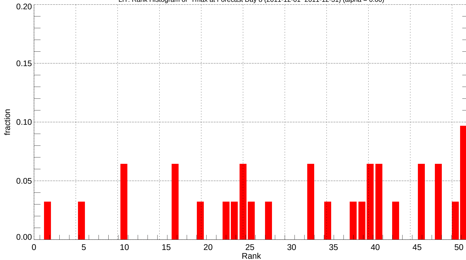
LIT: Rank Histogram of Tmax at Forecast Day 8 (2011-12-01~2011-12-31) (alpha = 0.00)
