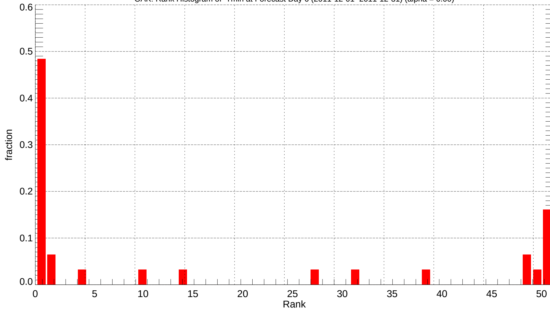
OAK: Rank Histogram of Tmin at Forecast Day 6 (2011-12-01~2011-12-31) (alpha = 0.00)
