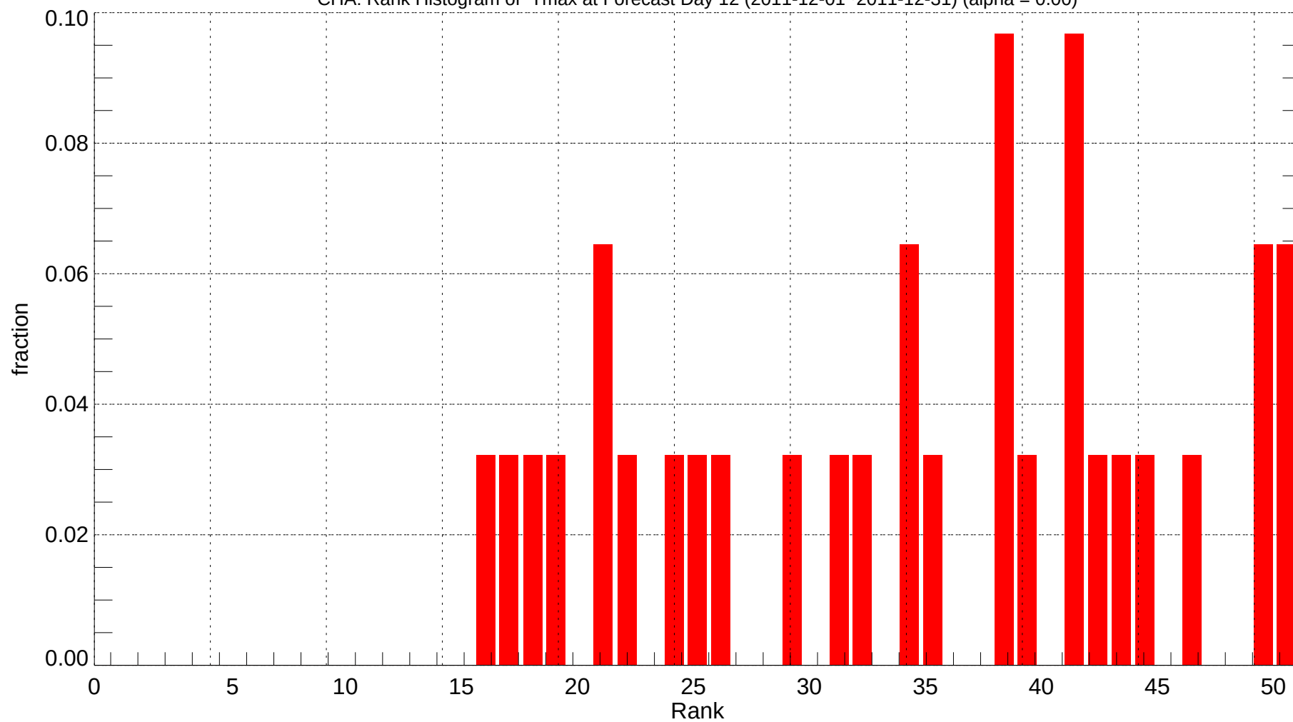
CHA: Rank Histogram of Tmax at Forecast Day 12 (2011-12-01~2011-12-31) (alpha = 0.00)
