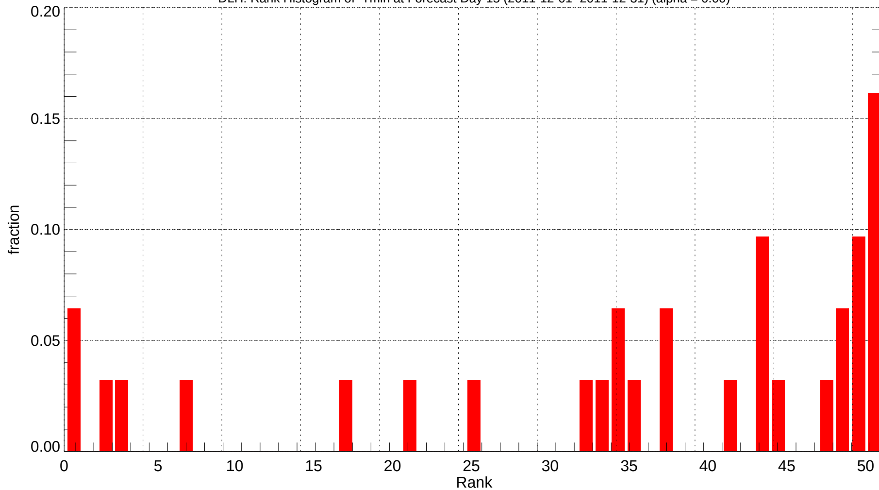
DLH: Rank Histogram of Tmin at Forecast Day 15 (2011-12-01~2011-12-31) (alpha = 0.00)
