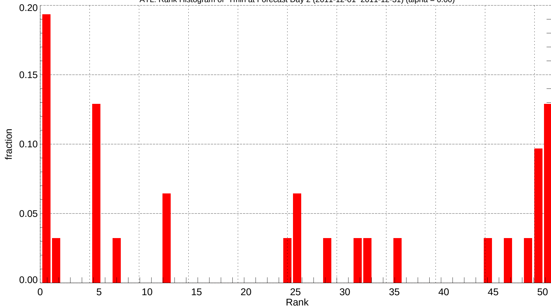
ATL: Rank Histogram of Tmin at Forecast Day 2 (2011-12-01~2011-12-31) (alpha = 0.00)
