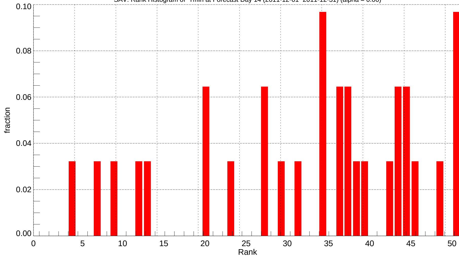
SAV: Rank Histogram of Tmin at Forecast Day 14 (2011-12-01~2011-12-31) (alpha = 0.00)
