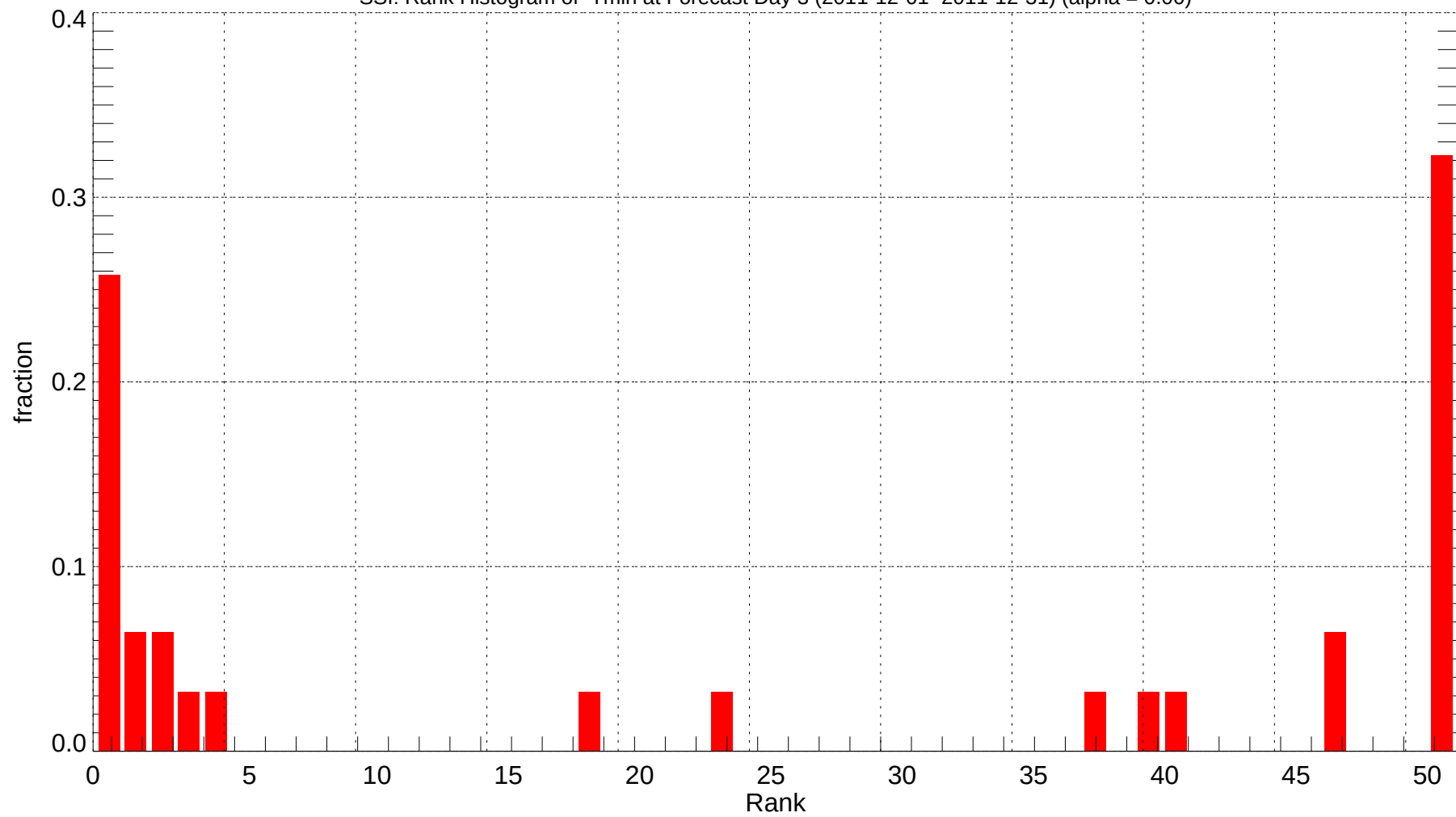
SSI: Rank Histogram of Tmin at Forecast Day 3 (2011-12-01~2011-12-31) (alpha = 0.00)
