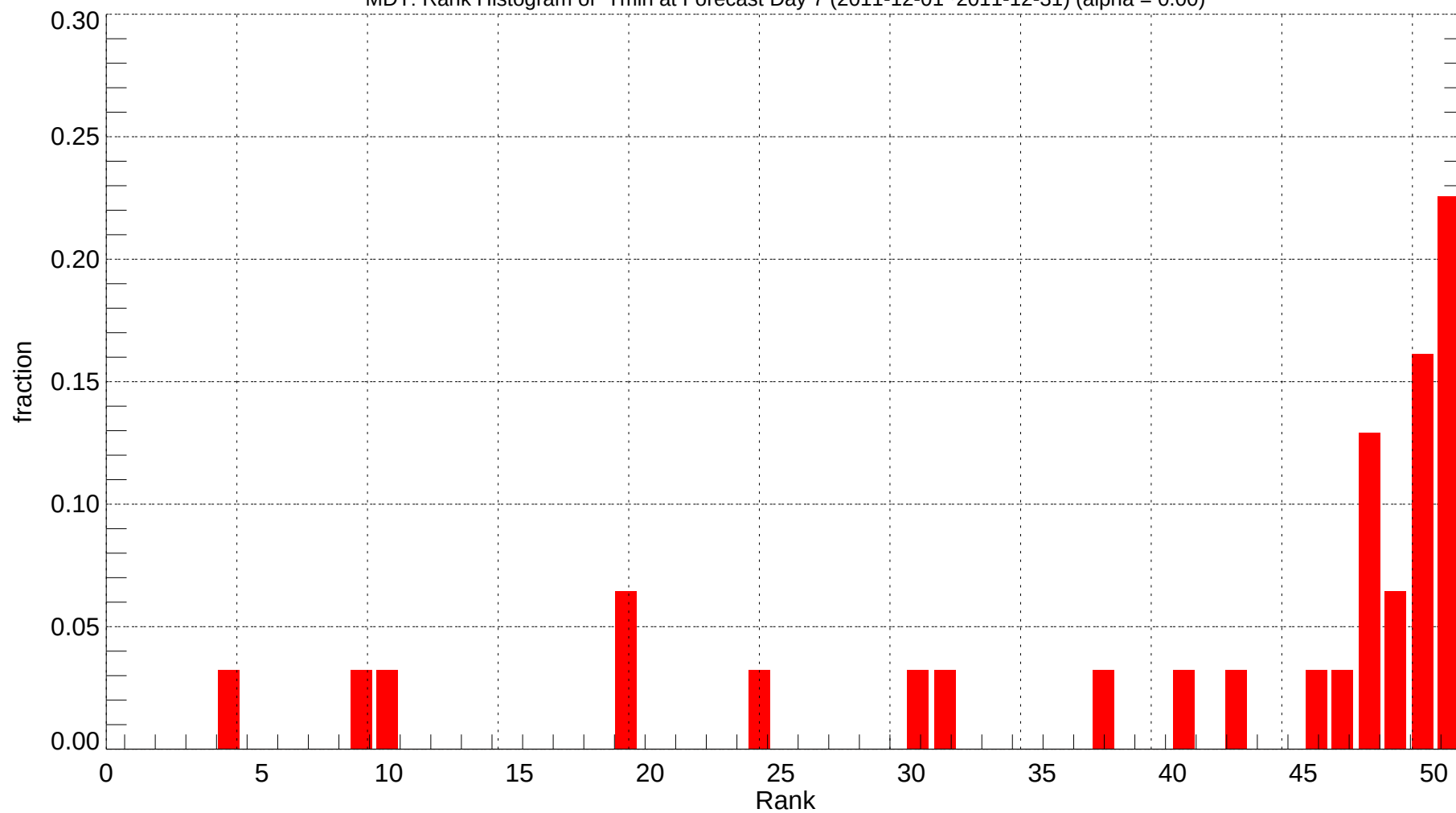
MDT: Rank Histogram of Tmin at Forecast Day 7 (2011-12-01~2011-12-31) (alpha = 0.00)
