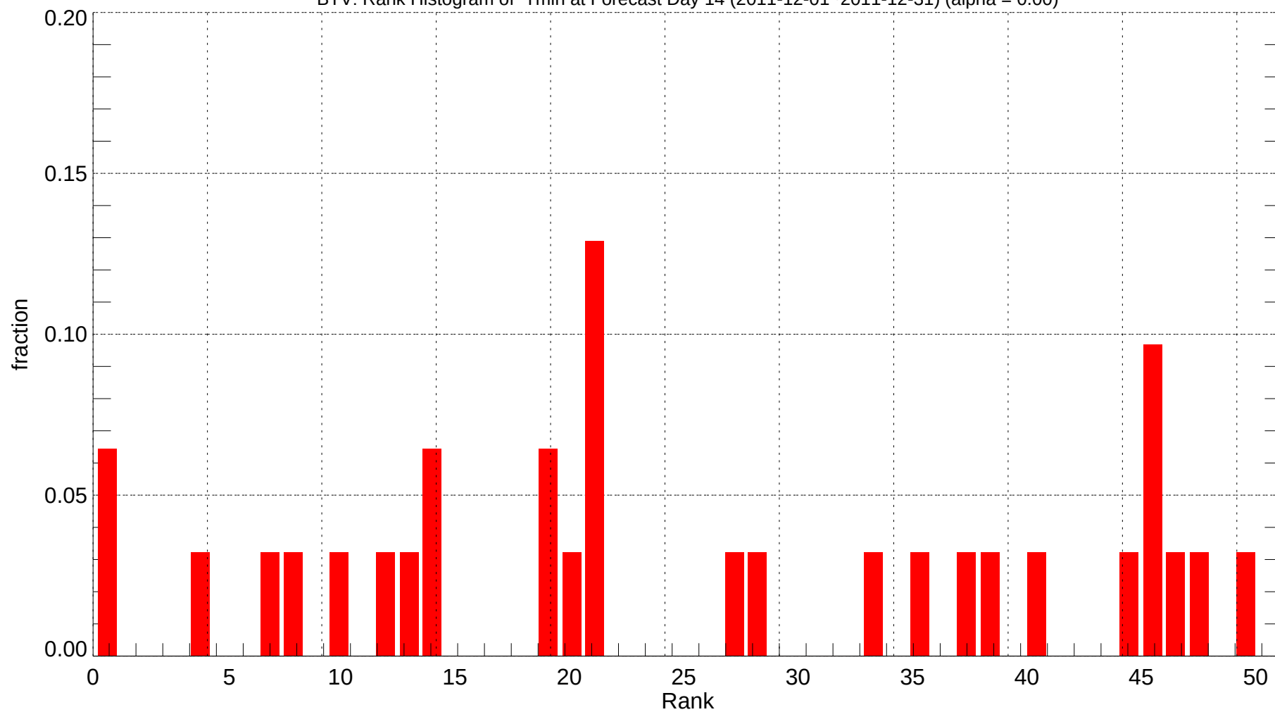
BTV: Rank Histogram of Tmin at Forecast Day 14 (2011-12-01~2011-12-31) (alpha = 0.00)
