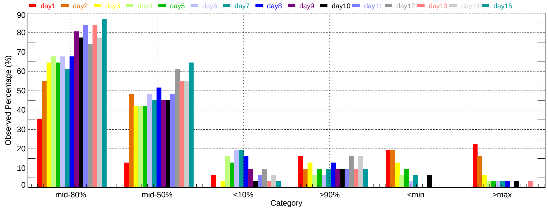
Observed Percentage of Ensembles - NKX: Min Temperature (2011-12-01~2011-12-31)
