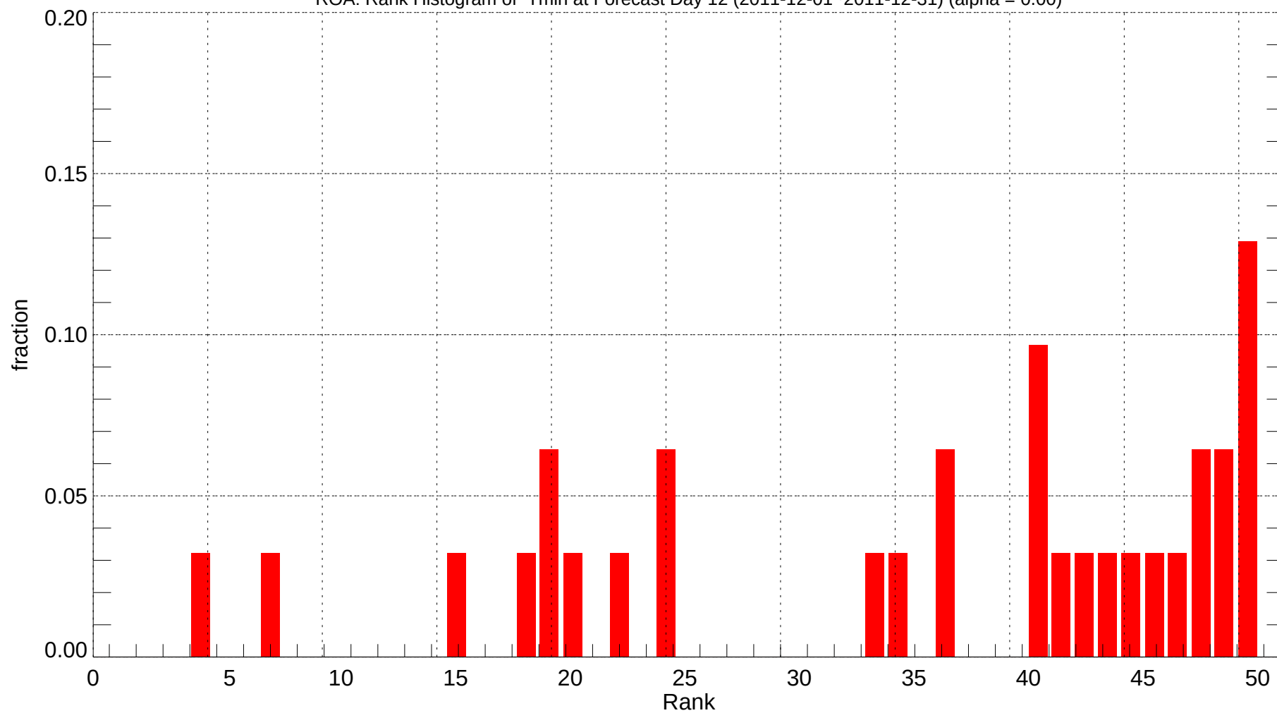
ROA: Rank Histogram of Tmin at Forecast Day 12 (2011-12-01~2011-12-31) (alpha = 0.00)
