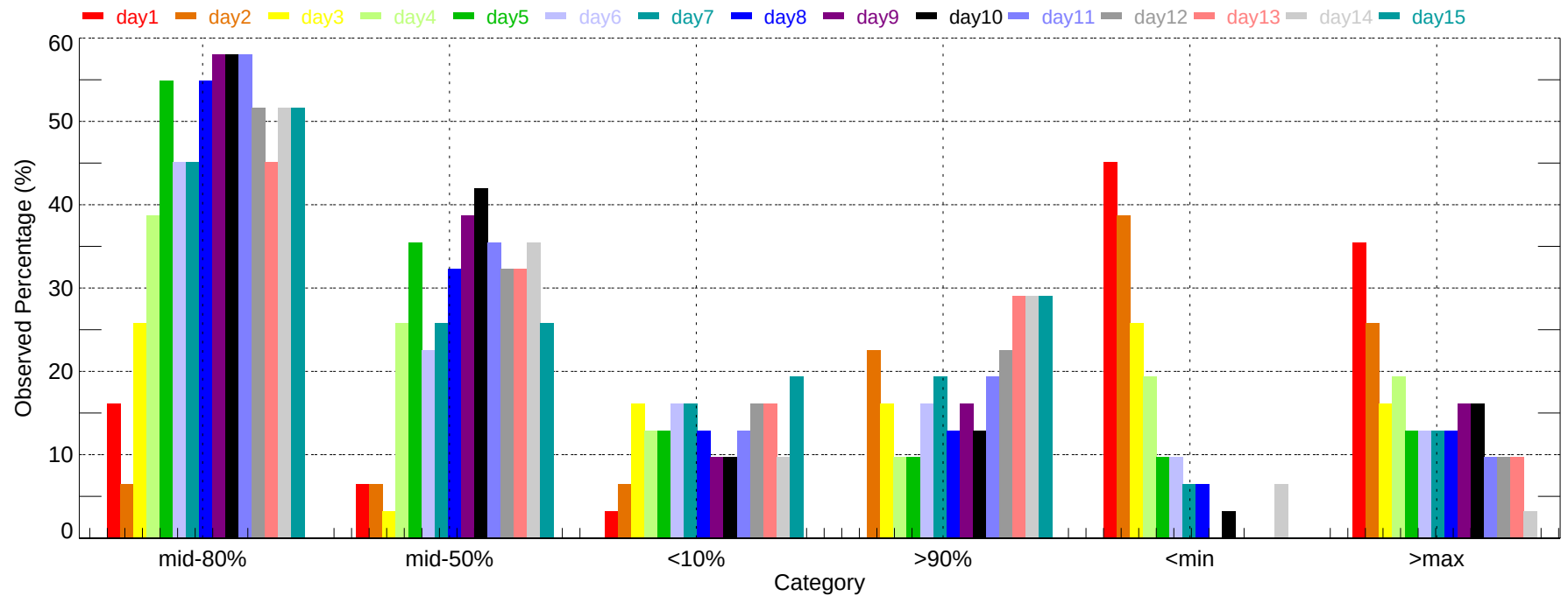
Observed Percentage of Ensembles - DSM: Min Temperature (2011-12-01~2011-12-31)
