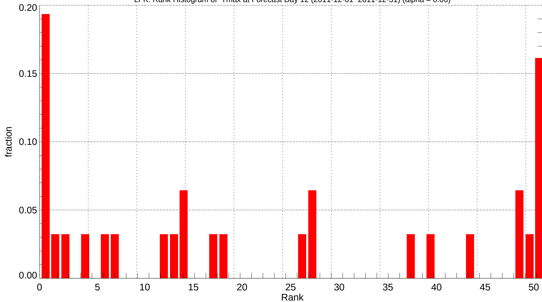
LFK: Rank Histogram of Tmax at Forecast Day 12 (2011-12-01~2011-12-31) (alpha = 0.00)
