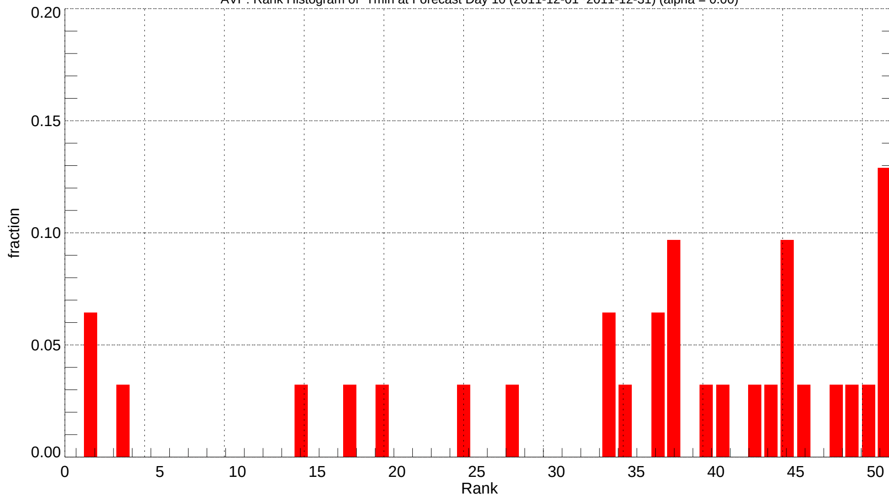
AVP: Rank Histogram of Tmin at Forecast Day 10 (2011-12-01~2011-12-31) (alpha = 0.00)
