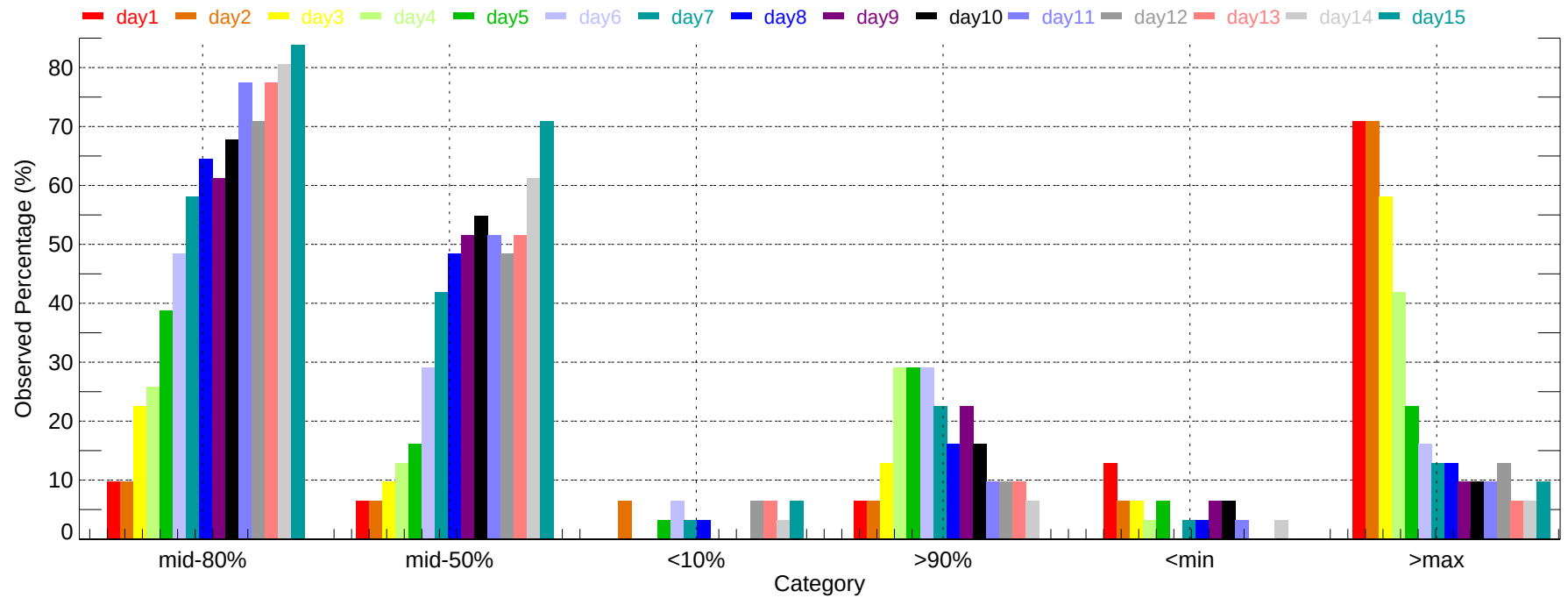
Observed Percentage of Ensembles - EUG: Min Temperature (2011-12-01~2011-12-31)
