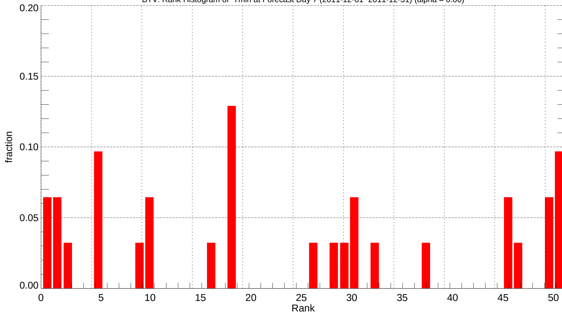
BTV: Rank Histogram of Tmin at Forecast Day 7 (2011-12-01~2011-12-31) (alpha = 0.00)
