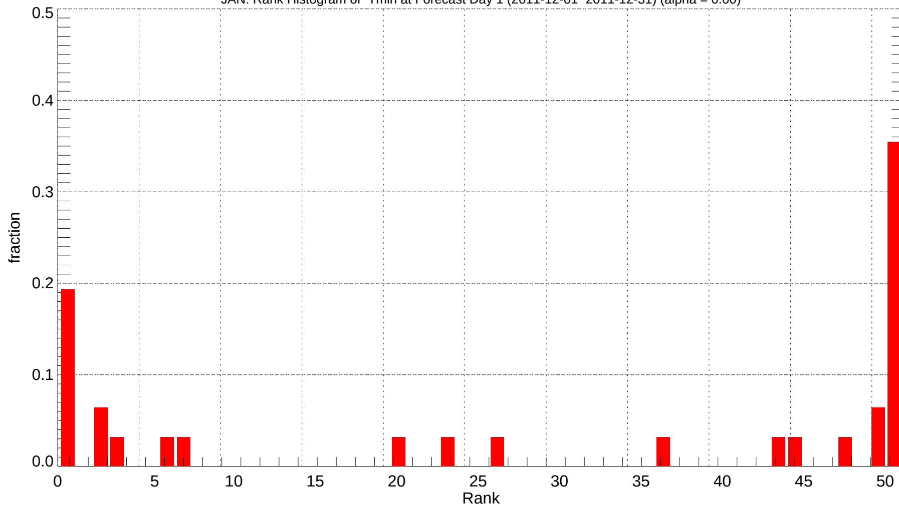
JAN: Rank Histogram of Tmin at Forecast Day 1 (2011-12-01~2011-12-31) (alpha = 0.00)
