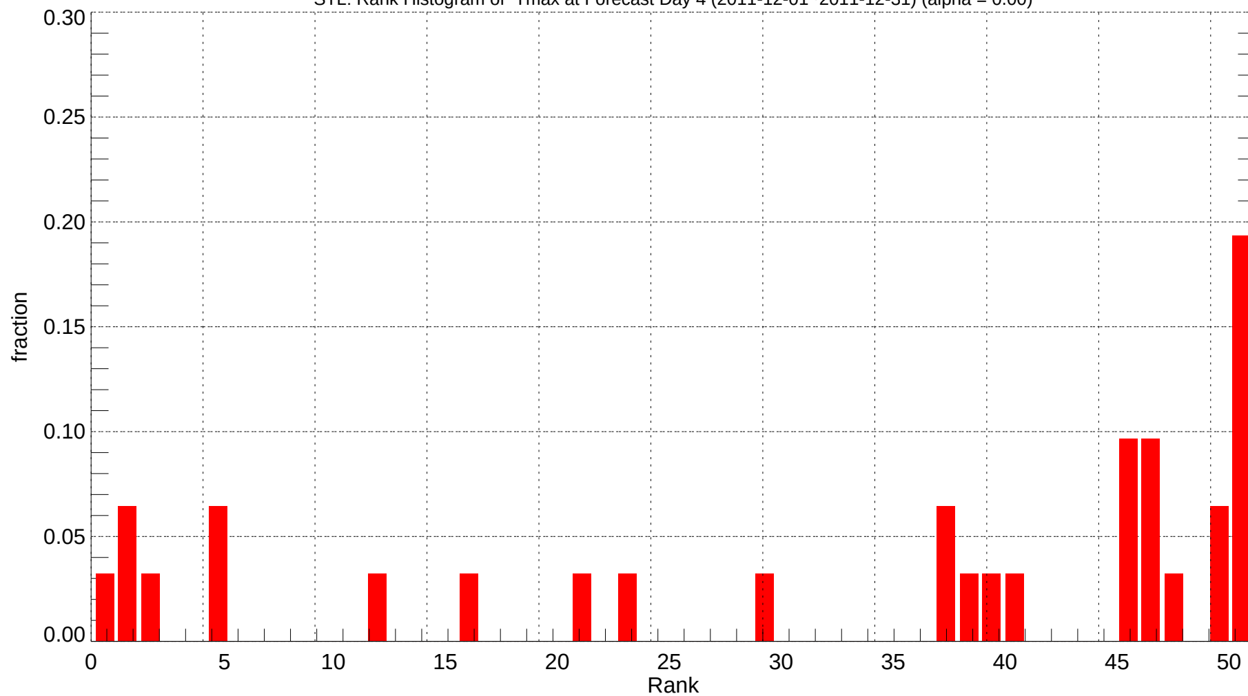
STL: Rank Histogram of Tmax at Forecast Day 4 (2011-12-01~2011-12-31) (alpha = 0.00)
