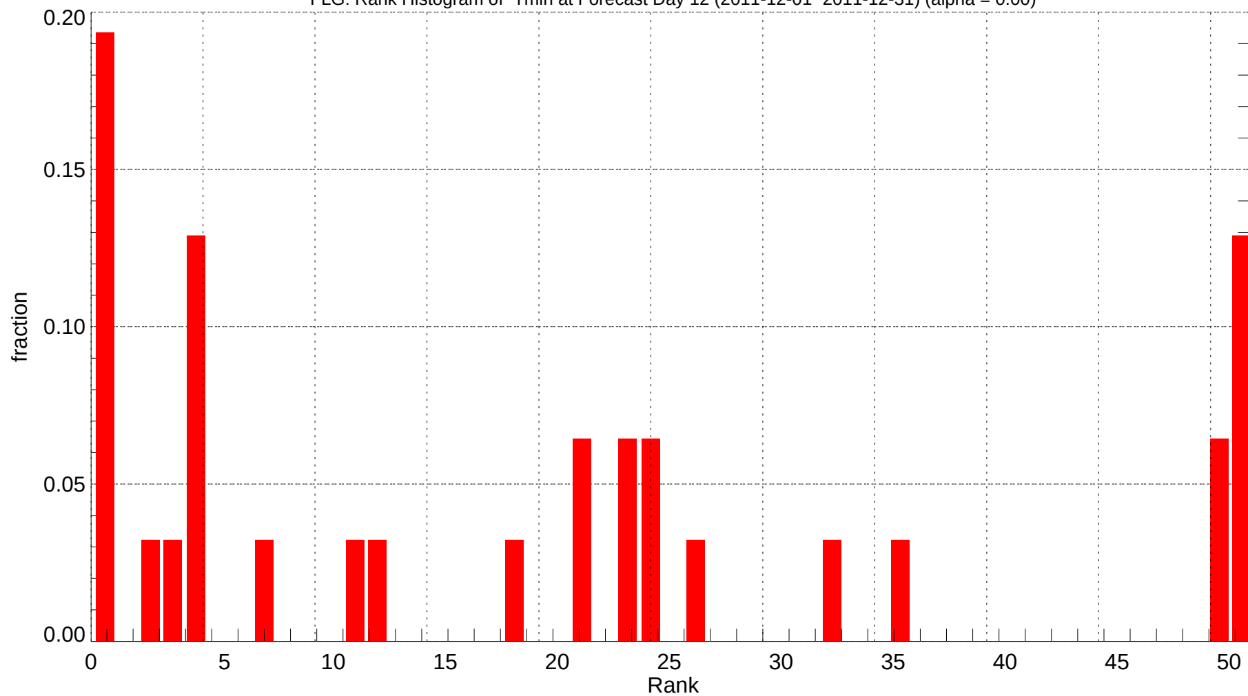
FLG: Rank Histogram of Tmin at Forecast Day 12 (2011-12-01~2011-12-31) (alpha = 0.00)
