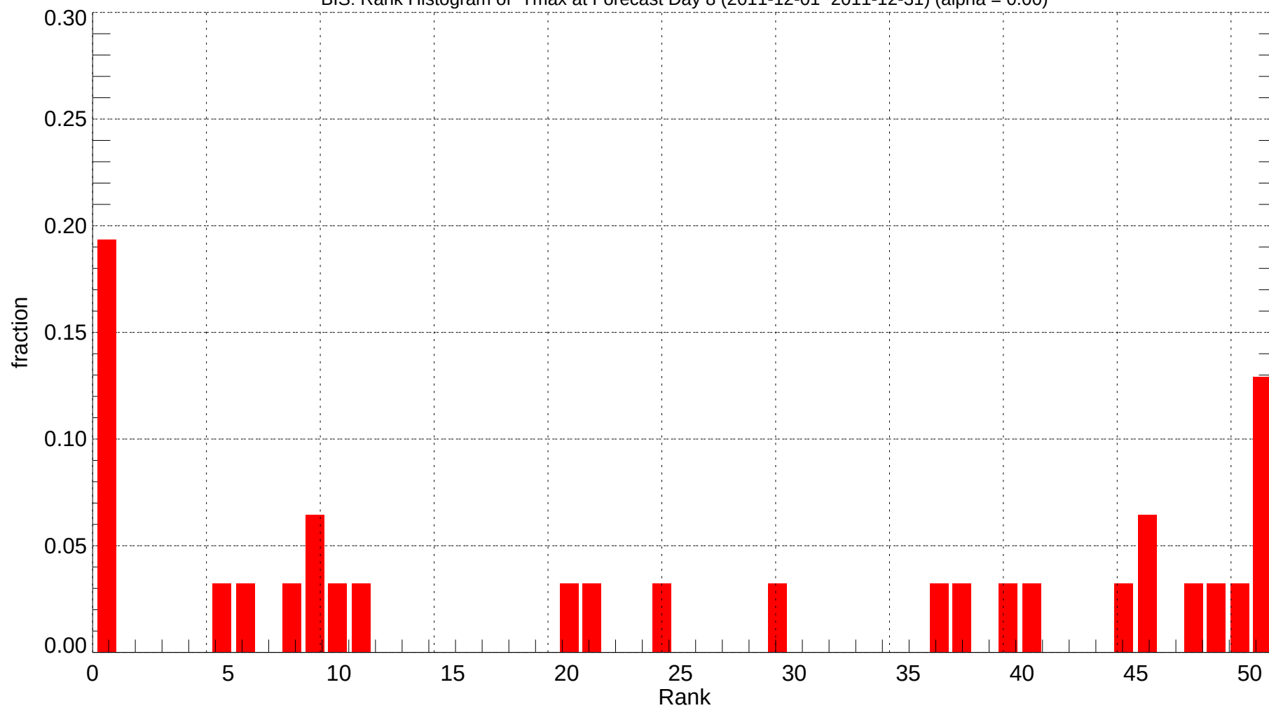
BIS: Rank Histogram of Tmax at Forecast Day 8 (2011-12-01~2011-12-31) (alpha = 0.00)
