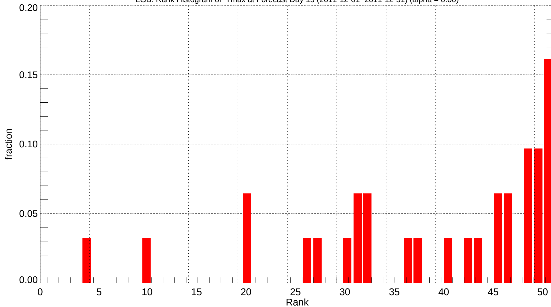
LGB: Rank Histogram of Tmax at Forecast Day 13 (2011-12-01~2011-12-31) (alpha = 0.00)
