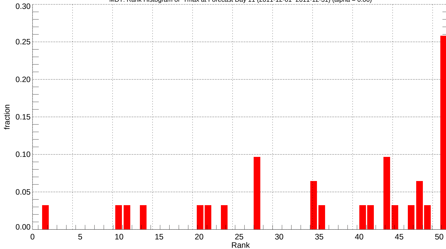
MDT: Rank Histogram of Tmax at Forecast Day 11 (2011-12-01~2011-12-31) (alpha = 0.00)
