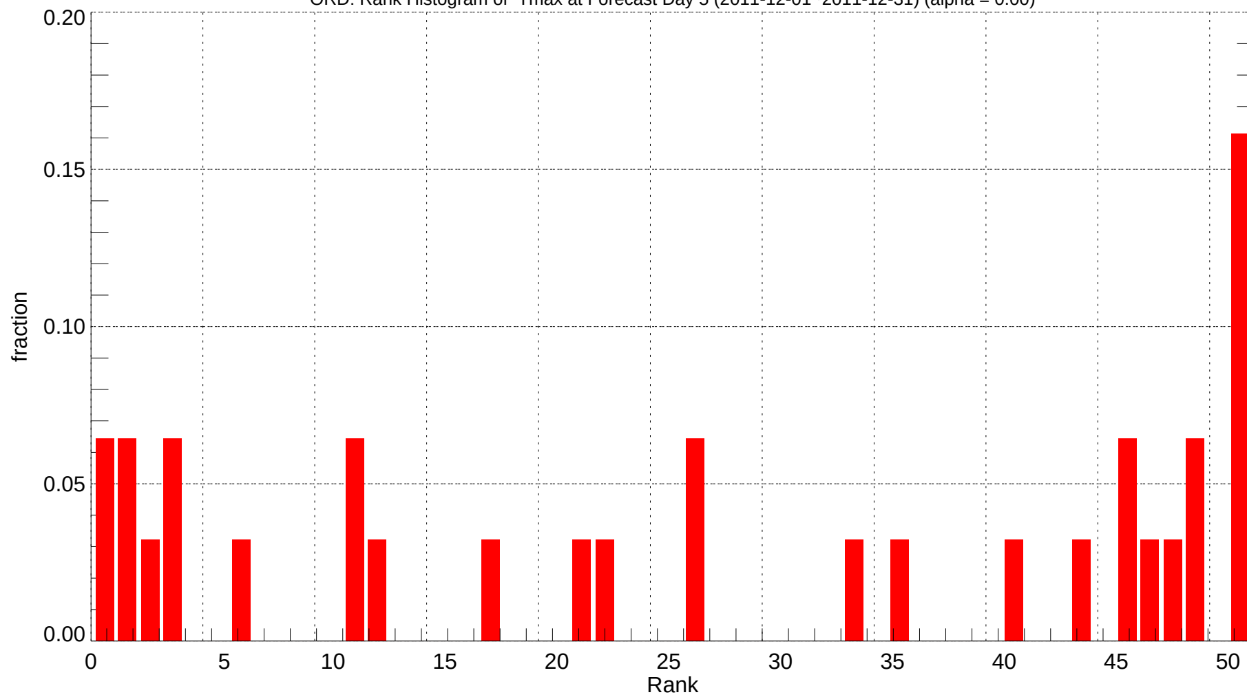
ORD: Rank Histogram of Tmax at Forecast Day 5 (2011-12-01~2011-12-31) (alpha = 0.00)
