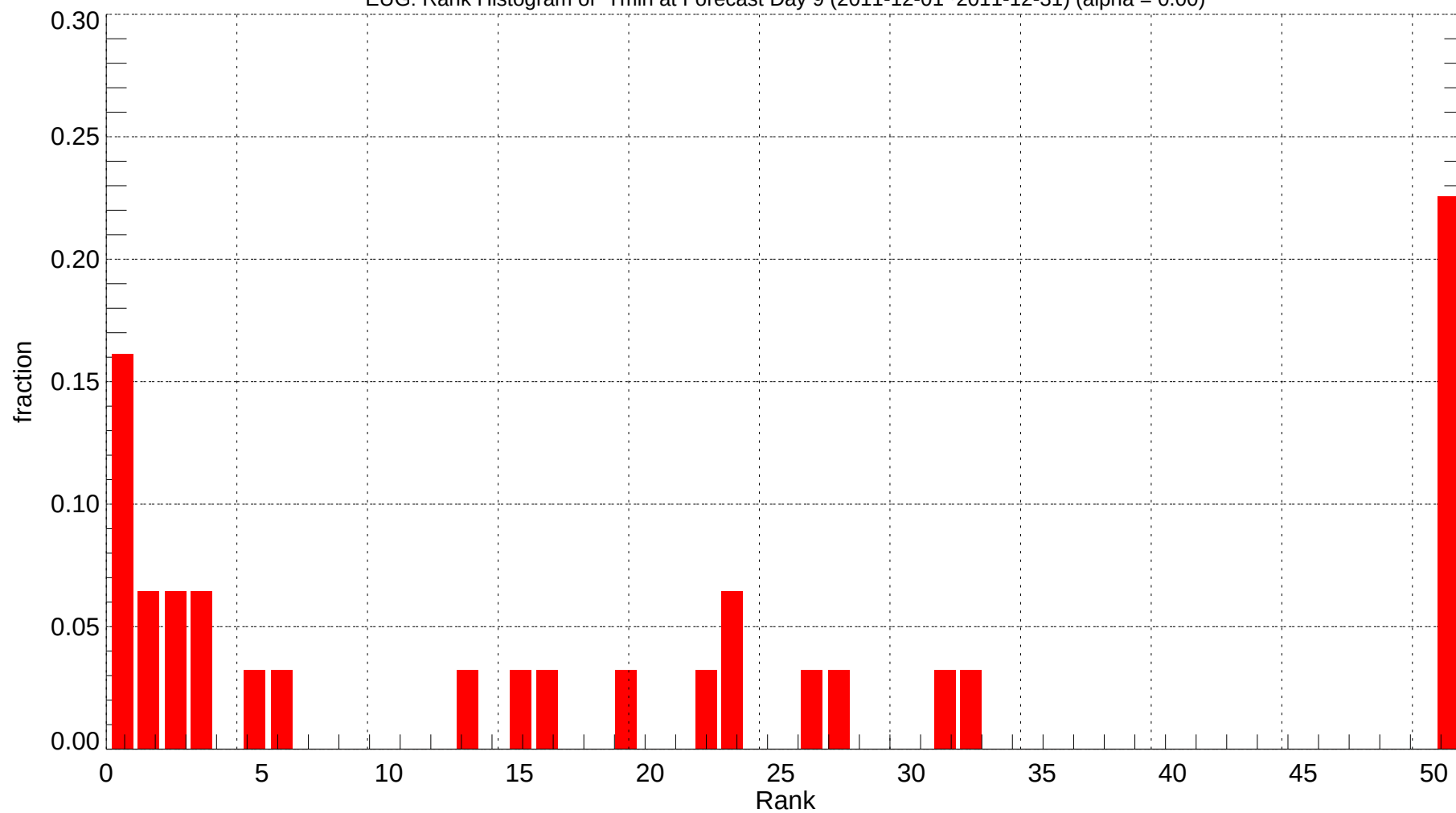
EUG: Rank Histogram of Tmin at Forecast Day 9 (2011-12-01~2011-12-31) (alpha = 0.00)
