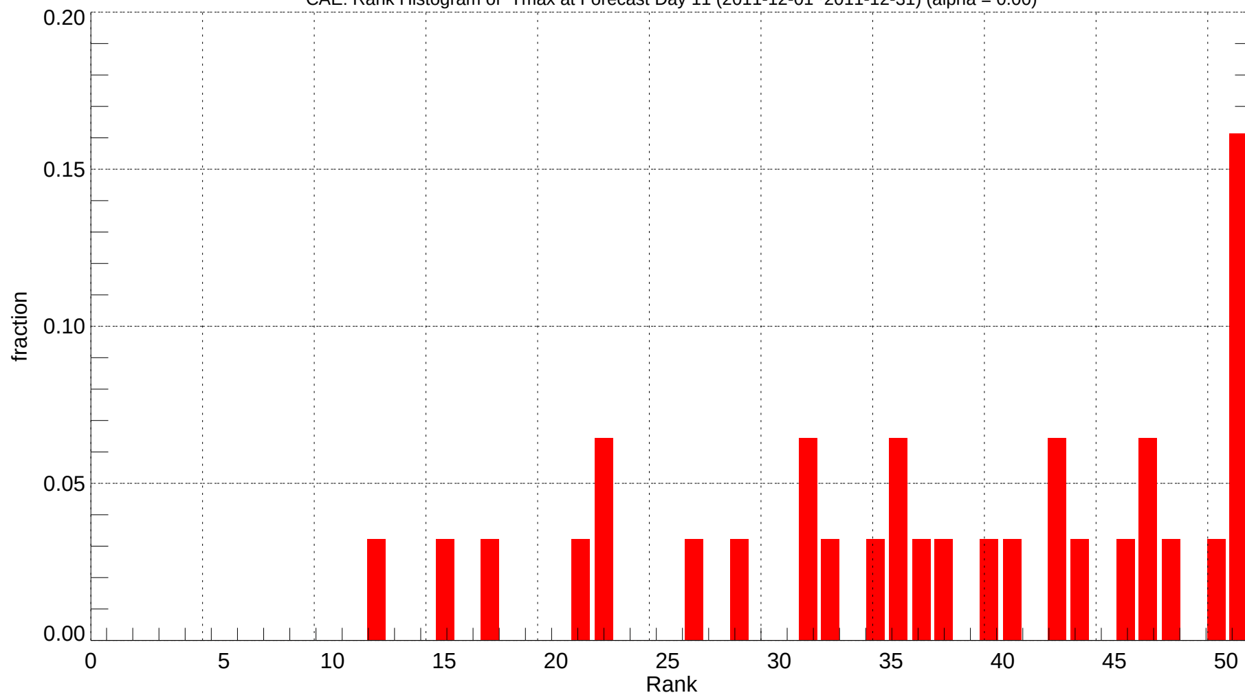
CAE: Rank Histogram of Tmax at Forecast Day 11 (2011-12-01~2011-12-31) (alpha = 0.00)
