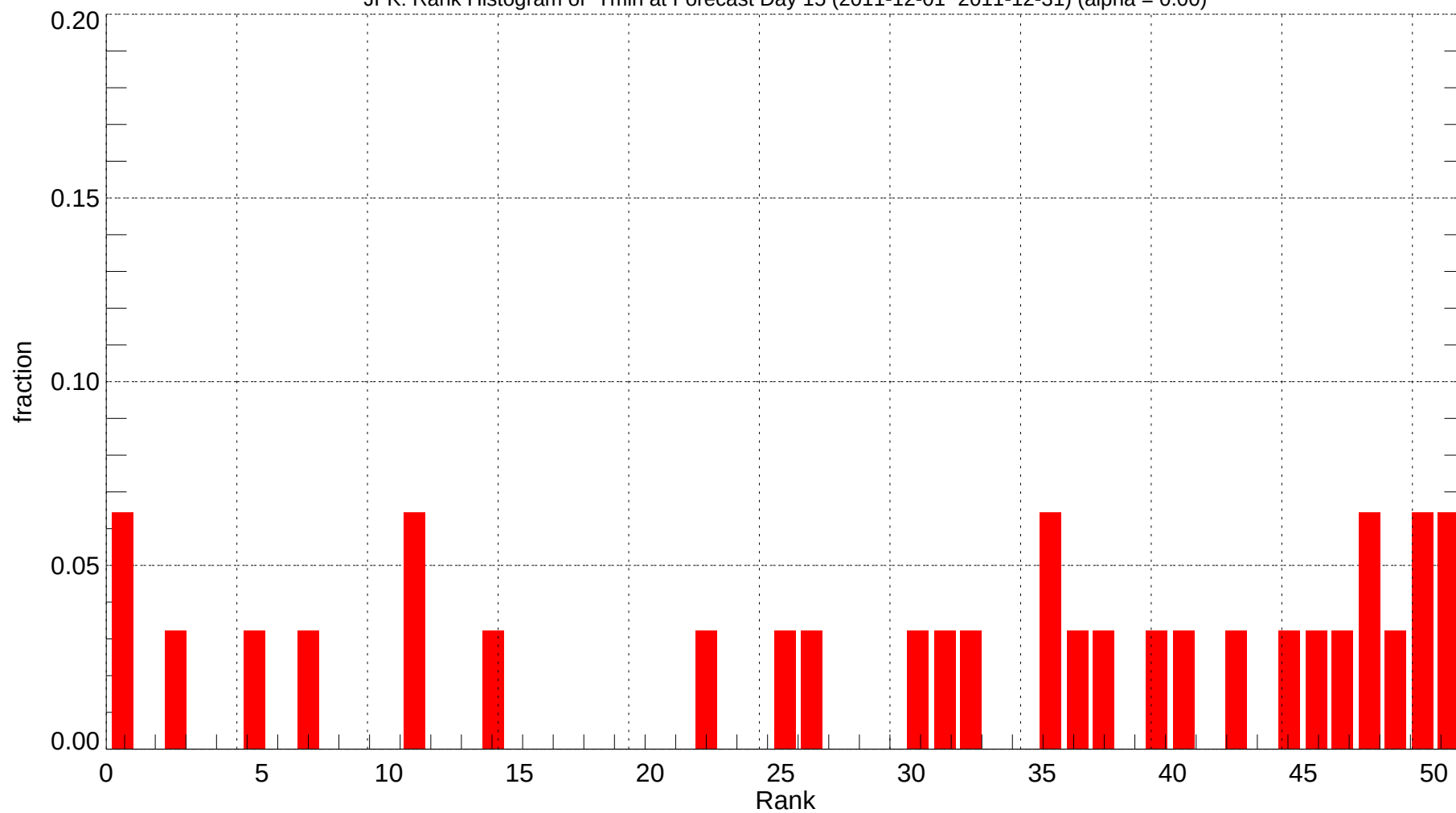
JFK: Rank Histogram of Tmin at Forecast Day 15 (2011-12-01~2011-12-31) (alpha = 0.00)
