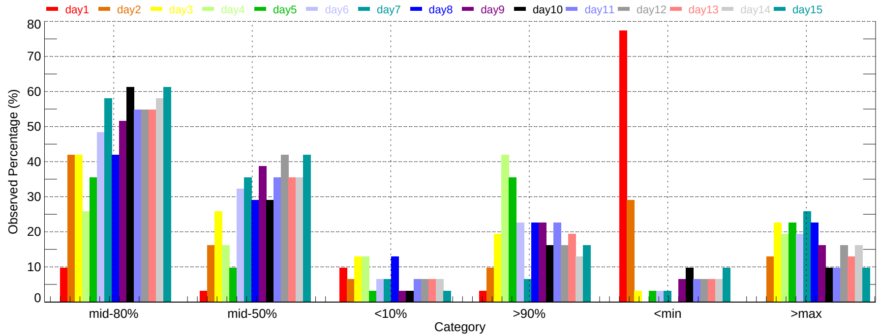
Observed Percentage of Ensembles - BOS: Max Temperature (2011-12-01~2011-12-31)
