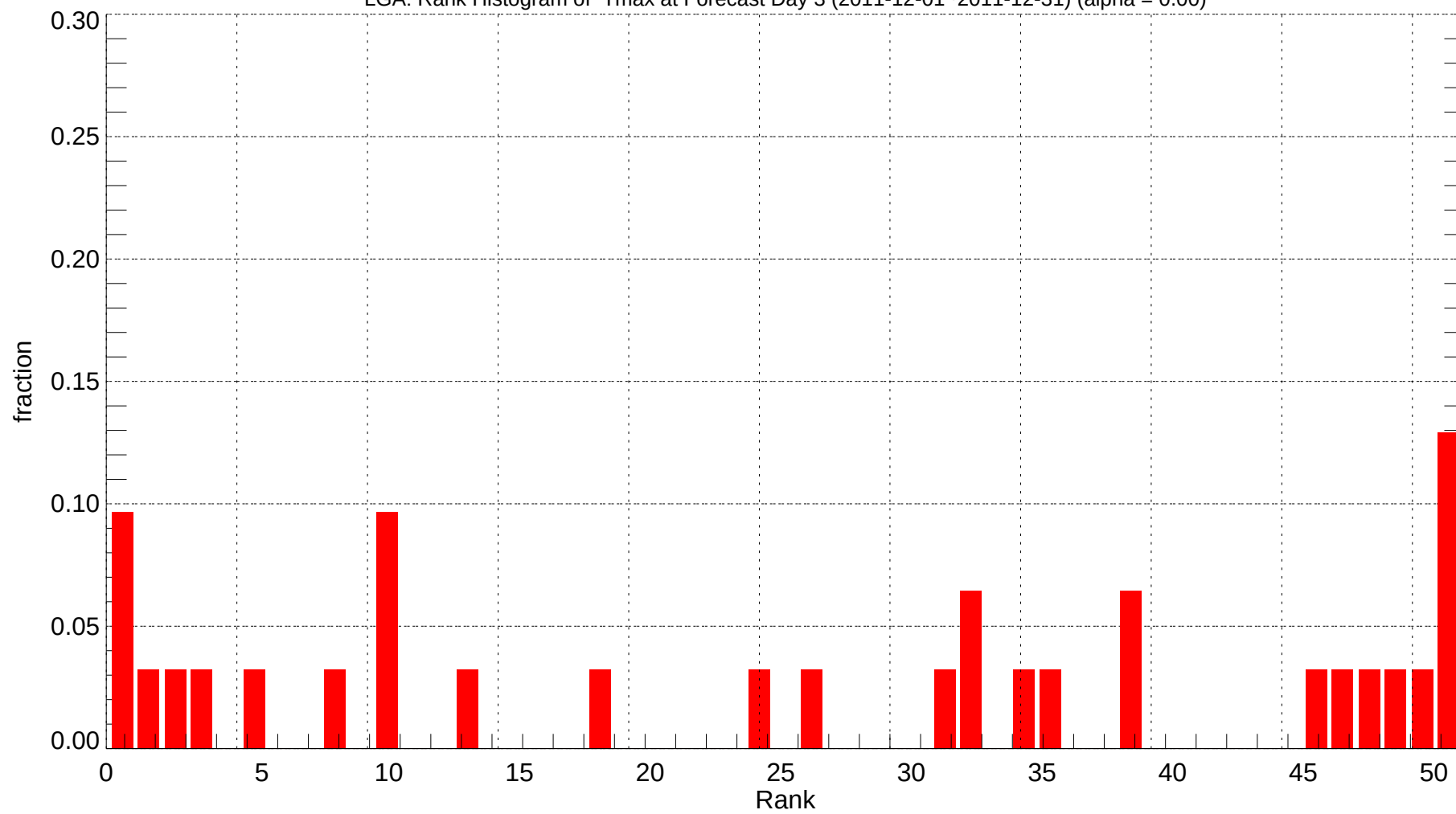
LGA: Rank Histogram of Tmax at Forecast Day 3 (2011-12-01~2011-12-31) (alpha = 0.00)
