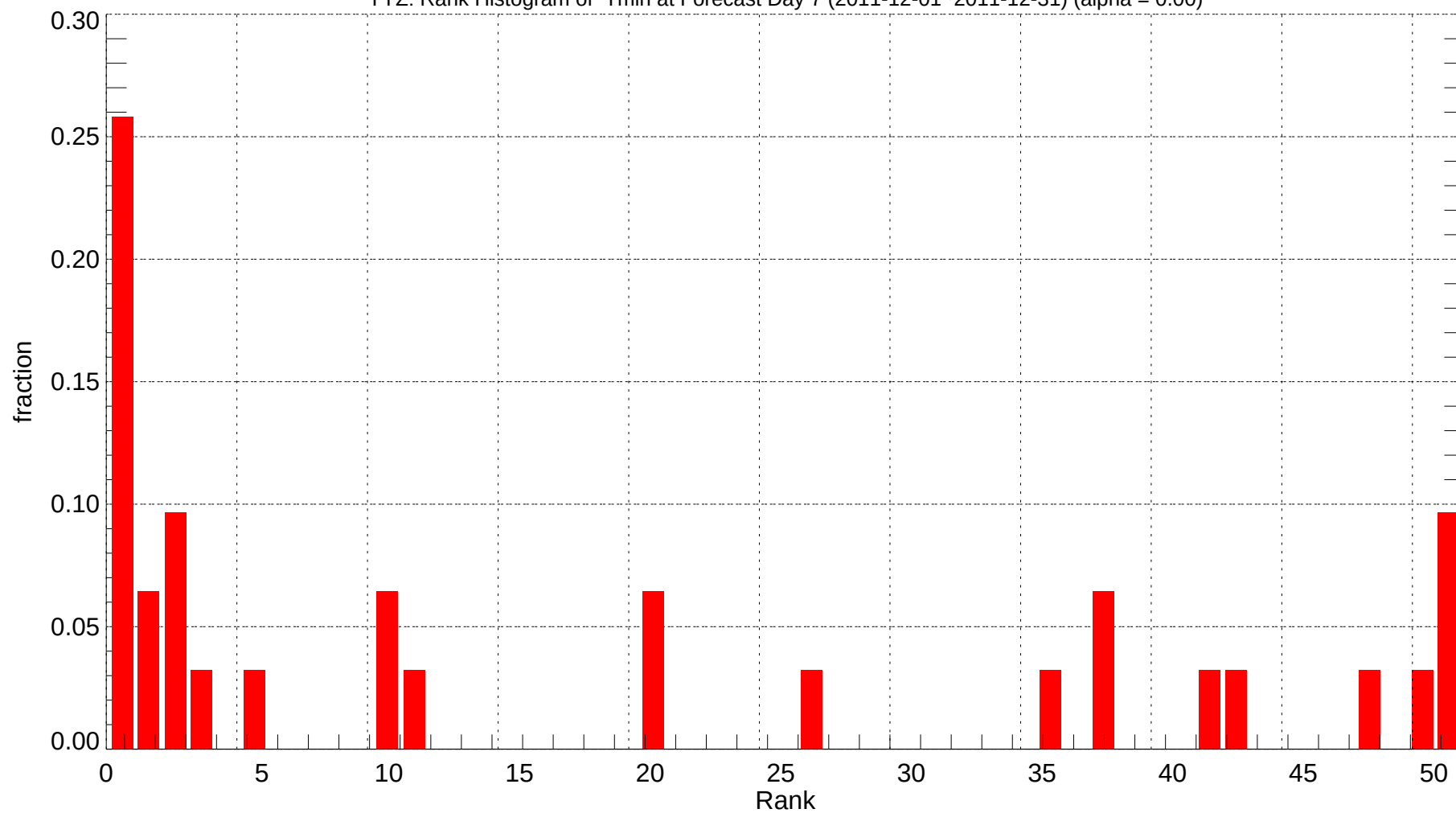
YYZ: Rank Histogram of Tmin at Forecast Day 7 (2011-12-01~2011-12-31) (alpha = 0.00)
