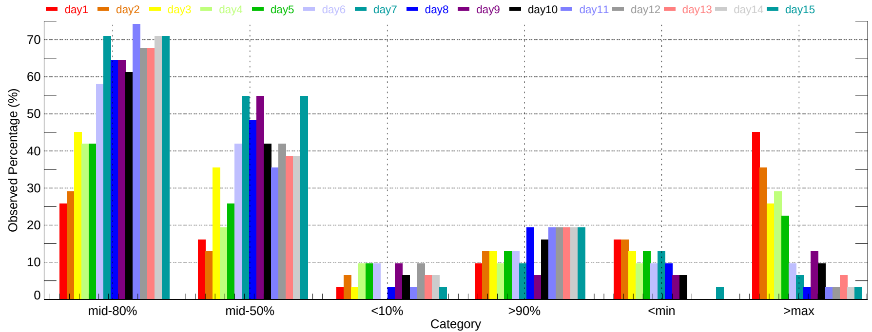
Observed Percentage of Ensembles - FMY: Max Temperature (2011-12-01~2011-12-31)
