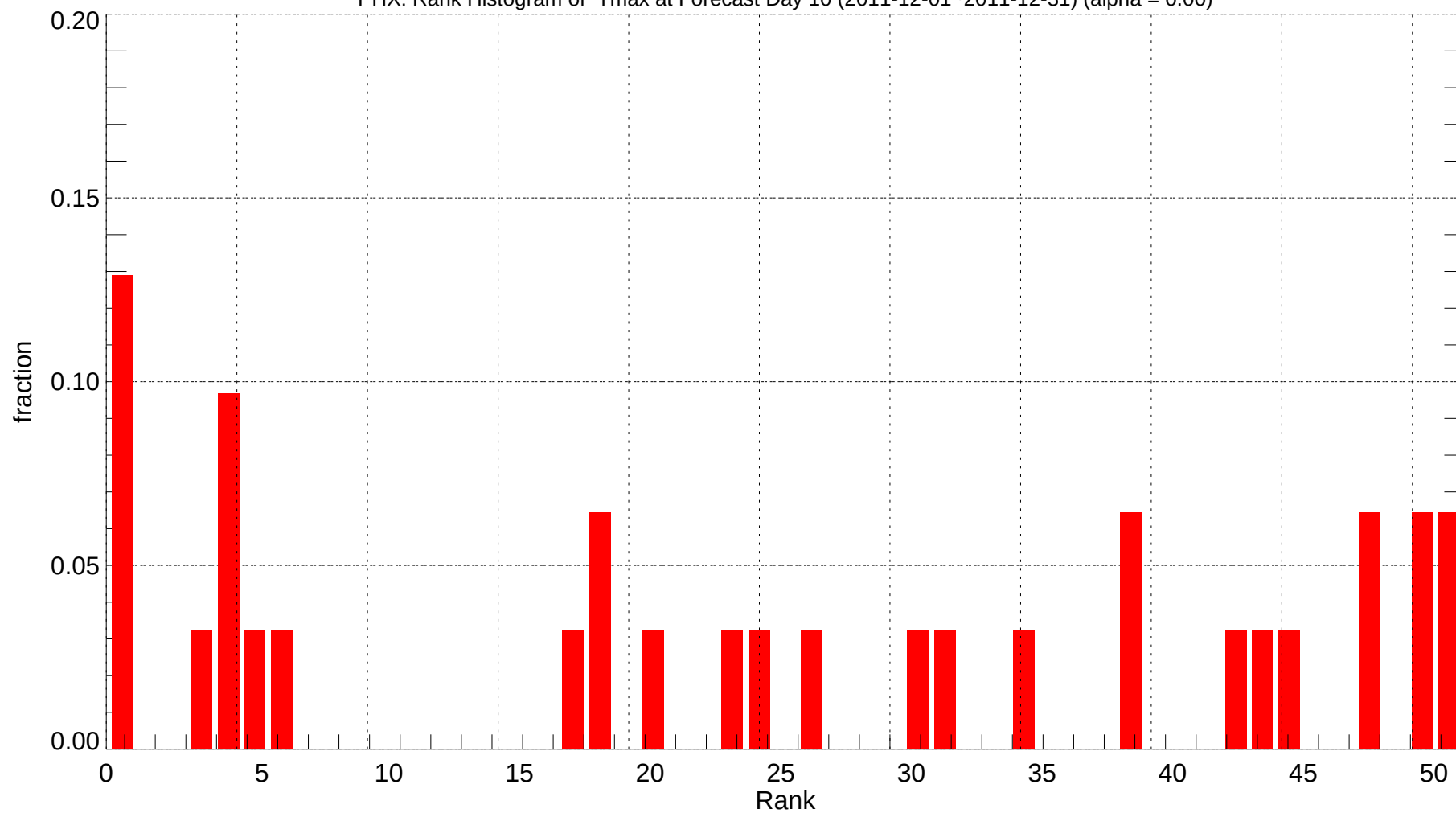
PHX: Rank Histogram of Tmax at Forecast Day 10 (2011-12-01~2011-12-31) (alpha = 0.00)
