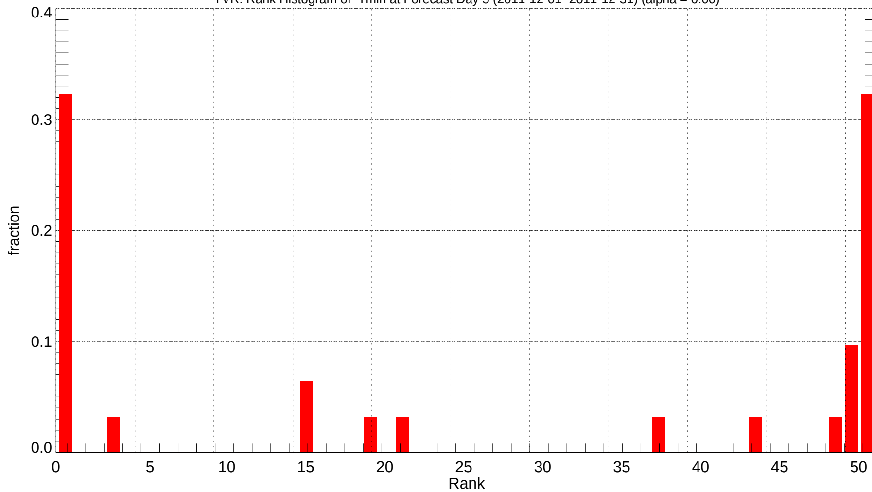
YVR: Rank Histogram of Tmin at Forecast Day 5 (2011-12-01~2011-12-31) (alpha = 0.00)
