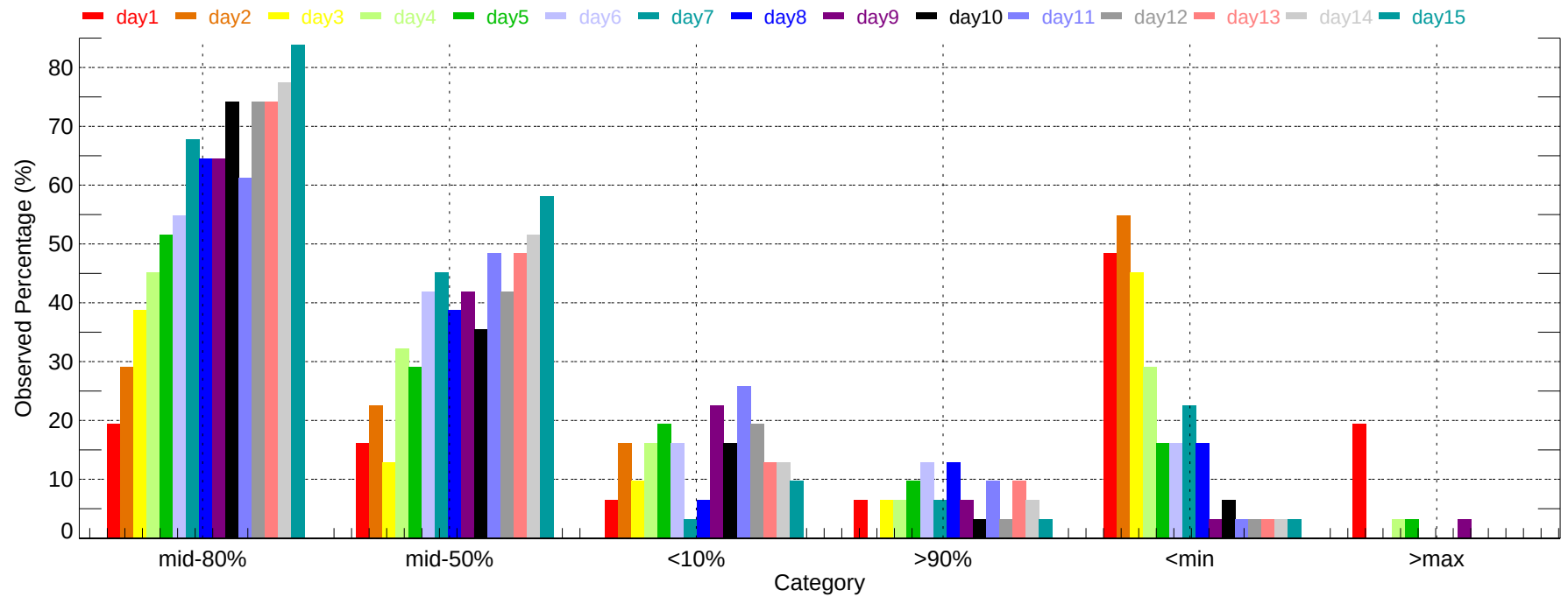
Observed Percentage of Ensembles - SJT: Min Temperature (2011-12-01~2011-12-31)
