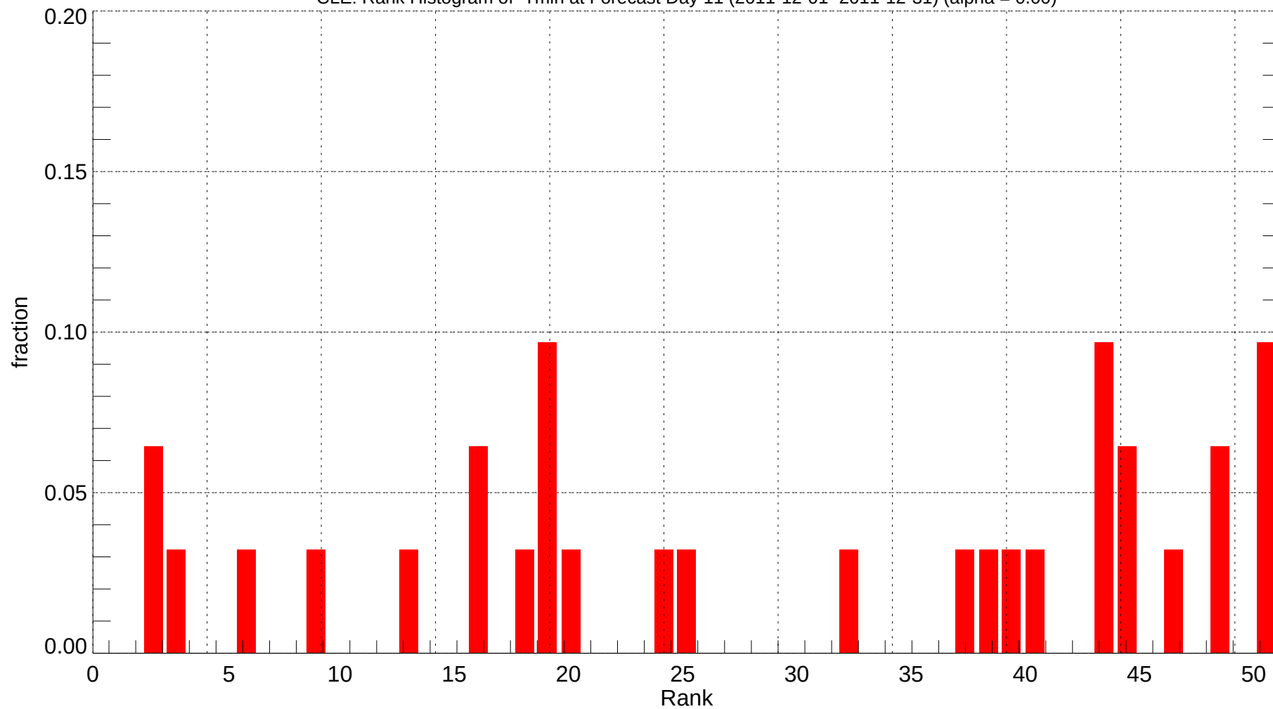
CLE: Rank Histogram of Tmin at Forecast Day 11 (2011-12-01~2011-12-31) (alpha = 0.00)
