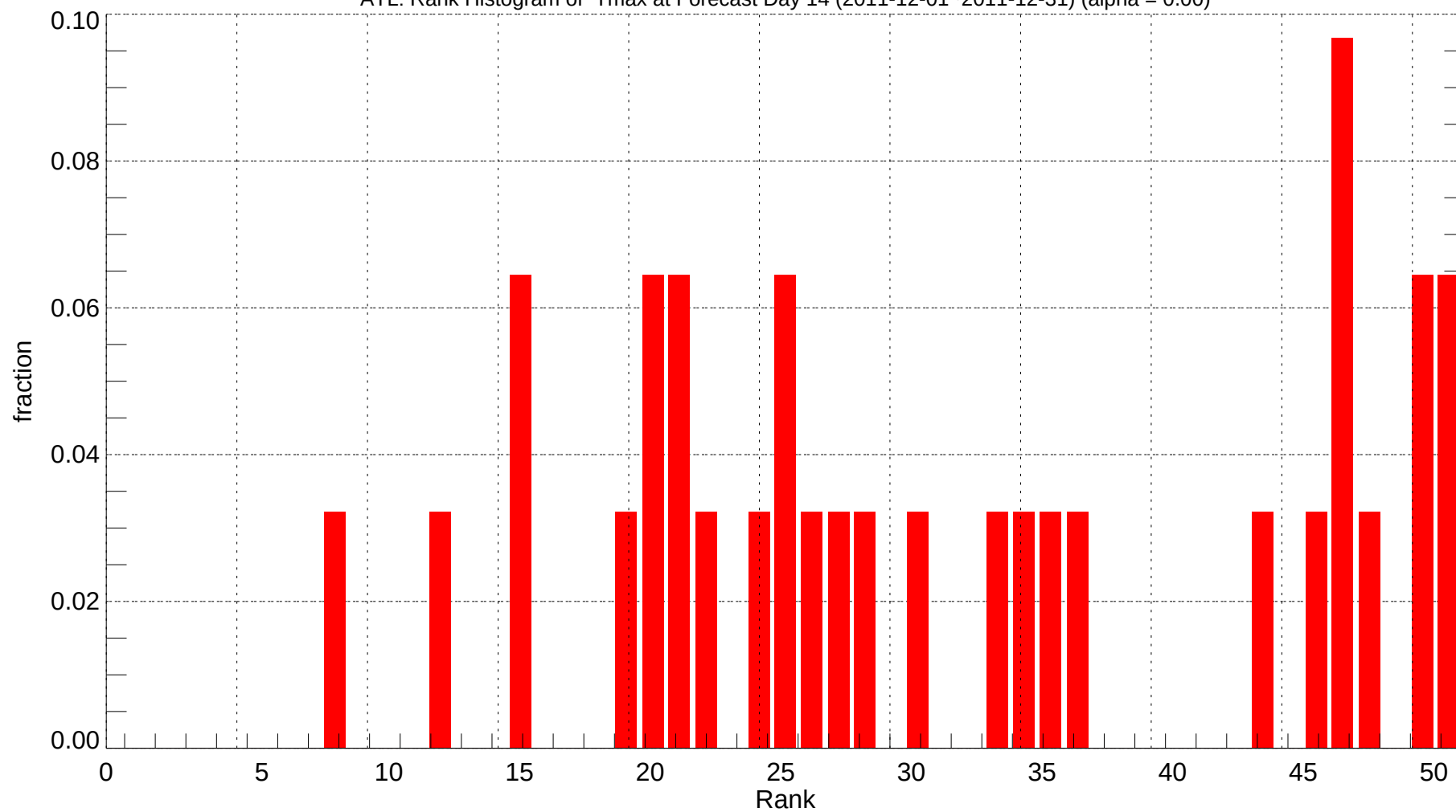
ATL: Rank Histogram of Tmax at Forecast Day 14 (2011-12-01~2011-12-31) (alpha = 0.00)
