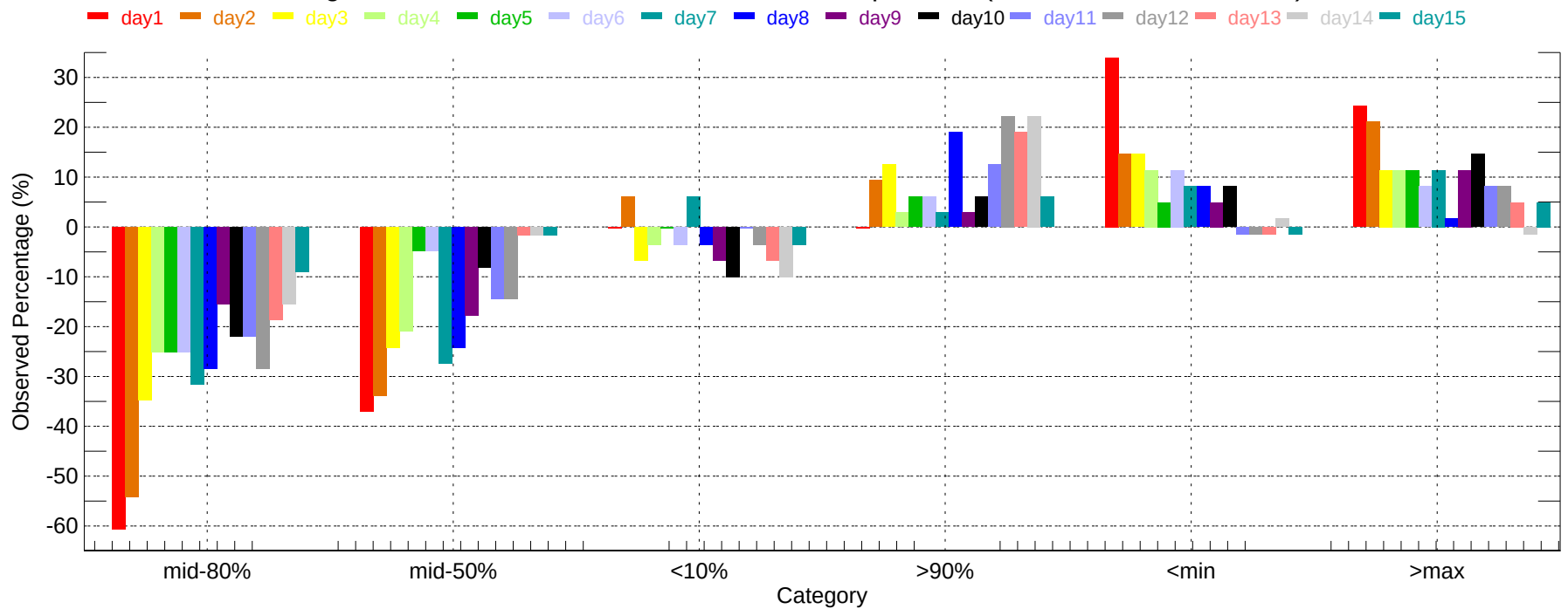
Observed Percentage Deviation of Ensembles - ACY: Max Temperature (2011-12-01~2011-12-31)
