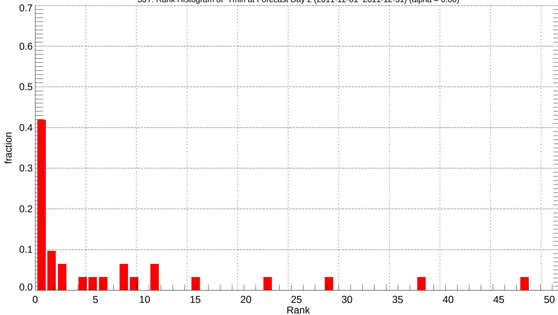
SJT: Rank Histogram of Tmin at Forecast Day 2 (2011-12-01~2011-12-31) (alpha = 0.00)
