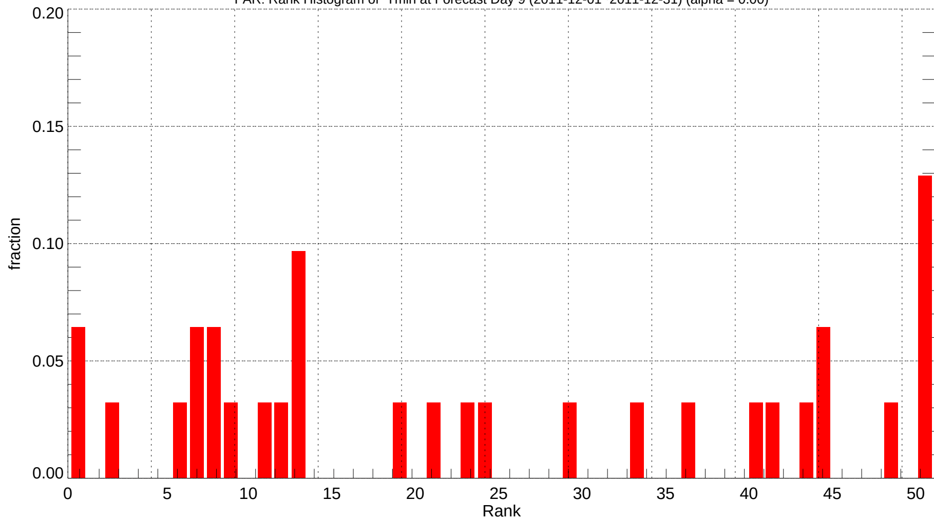
FAR: Rank Histogram of Tmin at Forecast Day 9 (2011-12-01~2011-12-31) (alpha = 0.00)
