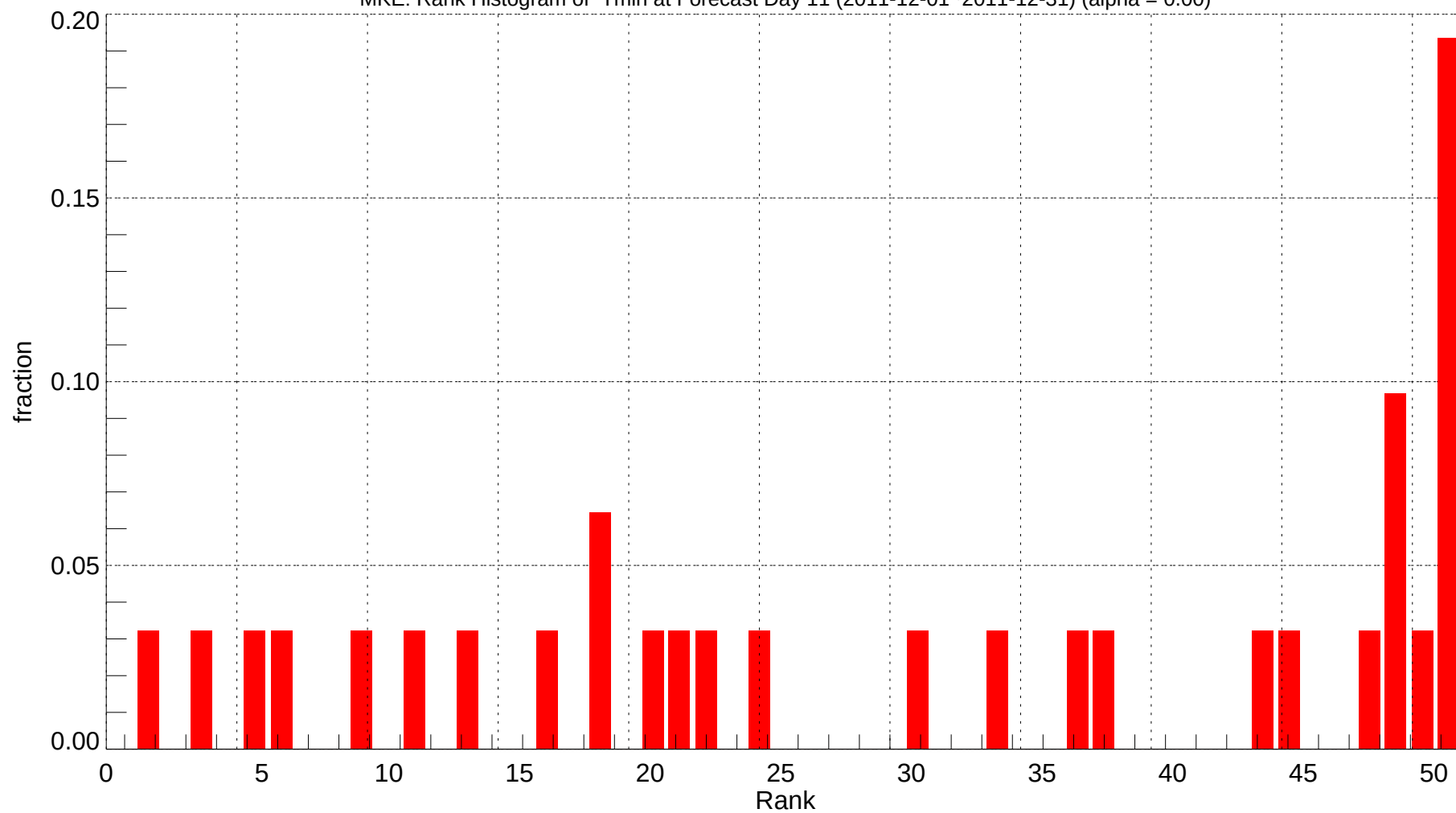
MKE: Rank Histogram of Tmin at Forecast Day 11 (2011-12-01~2011-12-31) (alpha = 0.00)
