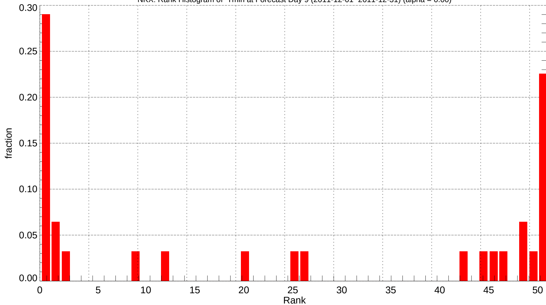
NKX: Rank Histogram of Tmin at Forecast Day 9 (2011-12-01~2011-12-31) (alpha = 0.00)
