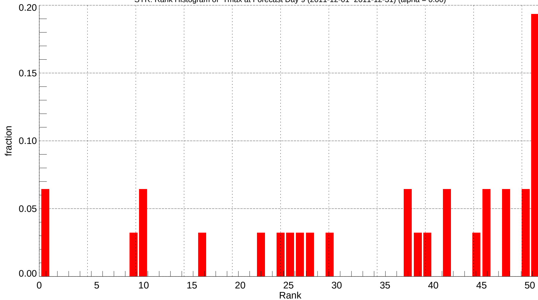
SYR: Rank Histogram of Tmax at Forecast Day 9 (2011-12-01~2011-12-31) (alpha = 0.00)
