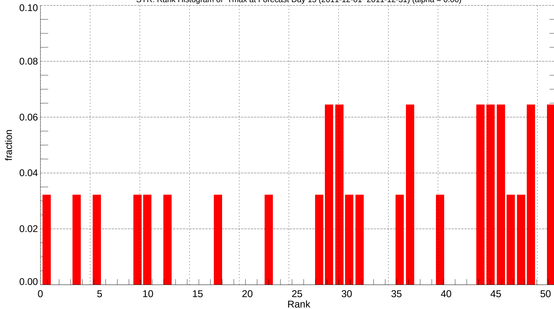
SYR: Rank Histogram of Tmax at Forecast Day 15 (2011-12-01~2011-12-31) (alpha = 0.00)
