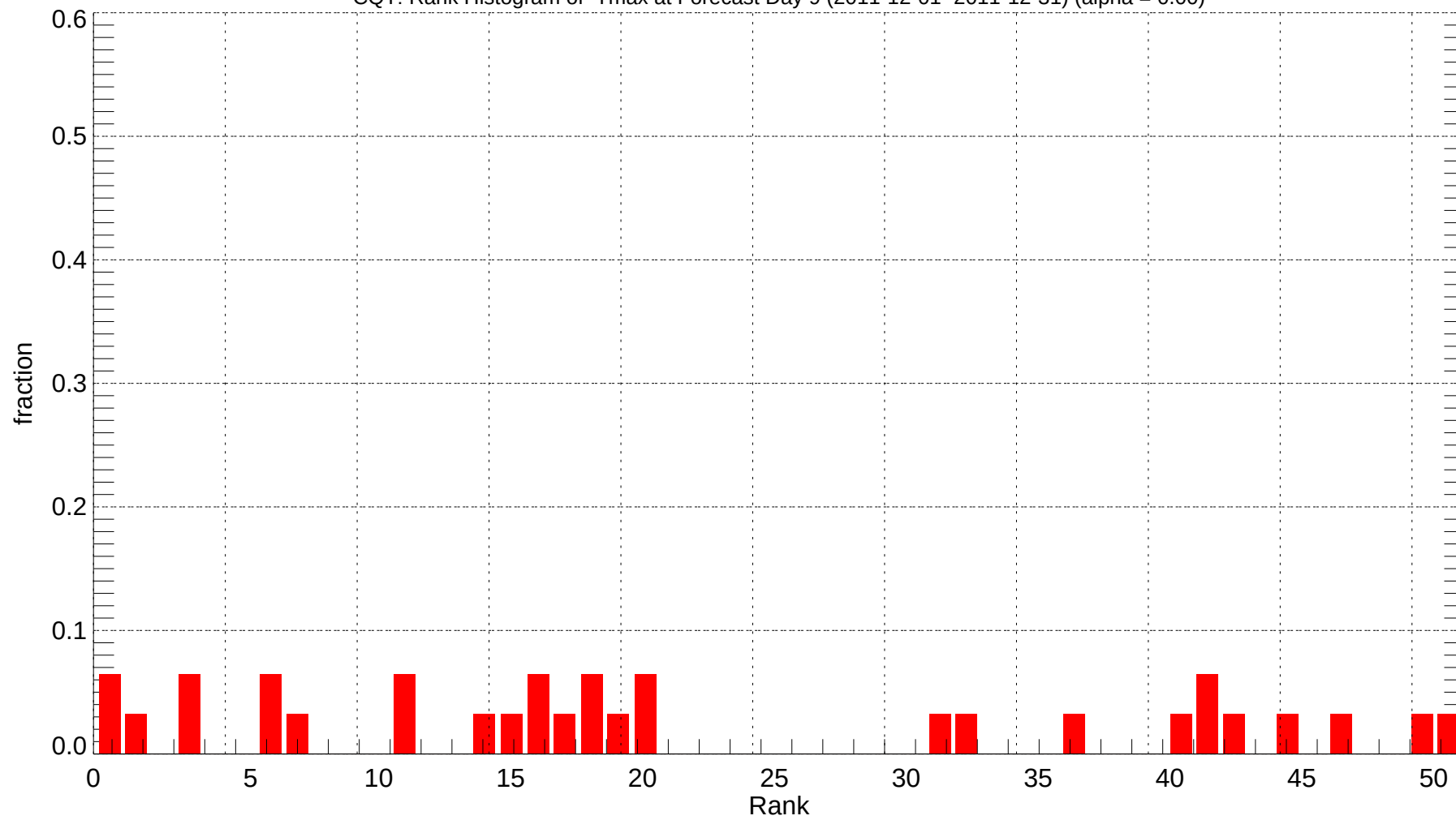
CQT: Rank Histogram of Tmax at Forecast Day 9 (2011-12-01~2011-12-31) (alpha = 0.00)
