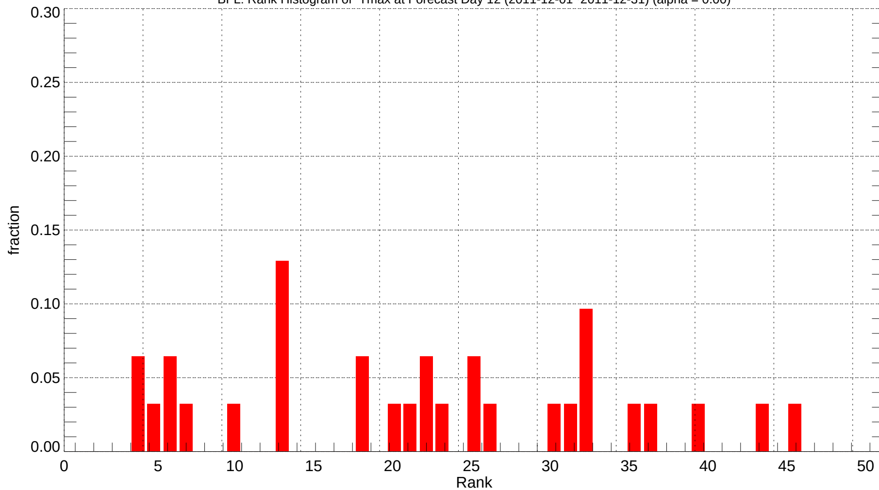
BFL: Rank Histogram of Tmax at Forecast Day 12 (2011-12-01~2011-12-31) (alpha = 0.00)
