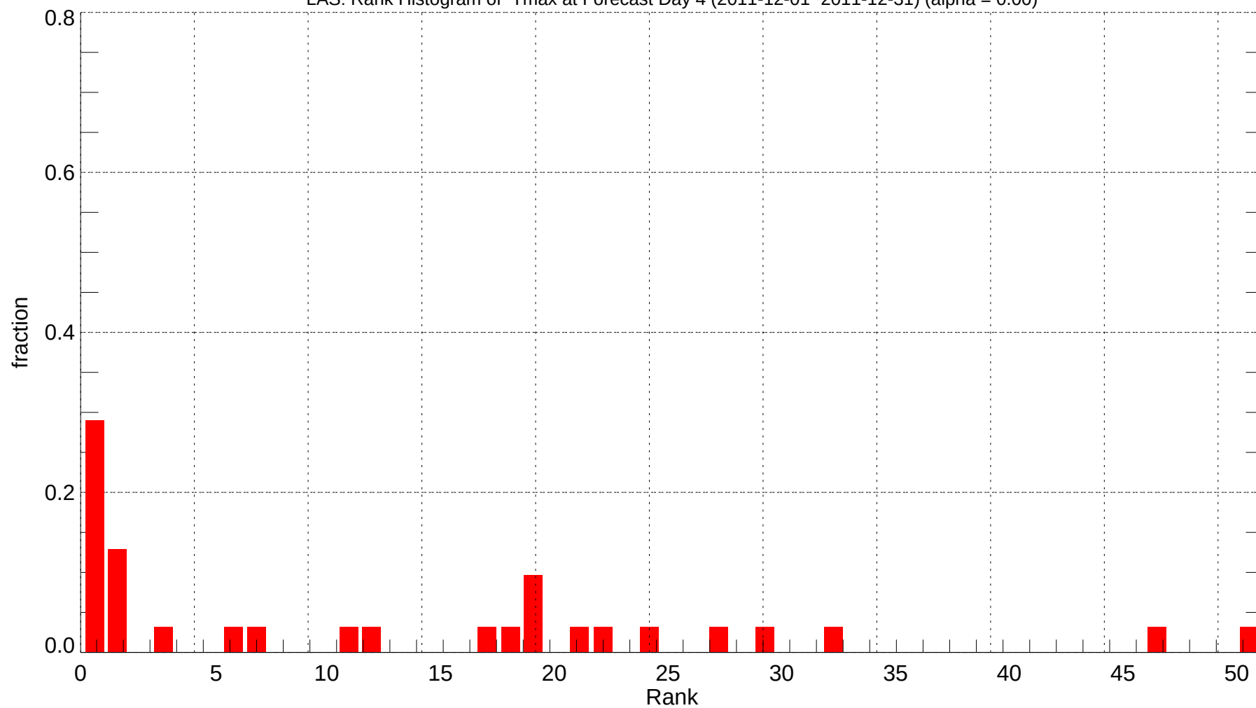
LAS: Rank Histogram of Tmax at Forecast Day 4 (2011-12-01~2011-12-31) (alpha = 0.00)
