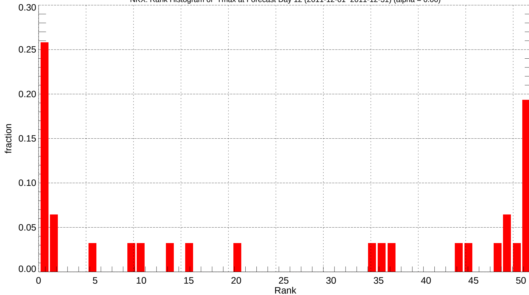
NKX: Rank Histogram of Tmax at Forecast Day 12 (2011-12-01~2011-12-31) (alpha = 0.00)
