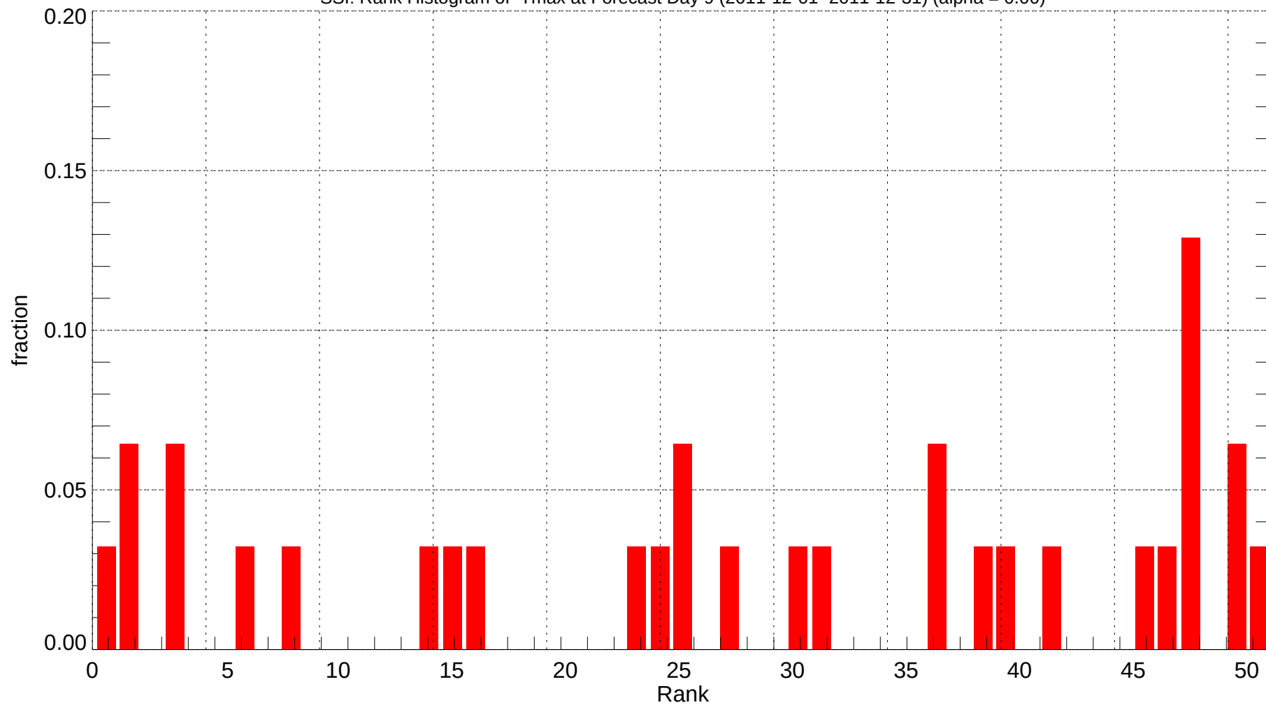
SSI: Rank Histogram of Tmax at Forecast Day 9 (2011-12-01~2011-12-31) (alpha = 0.00)
