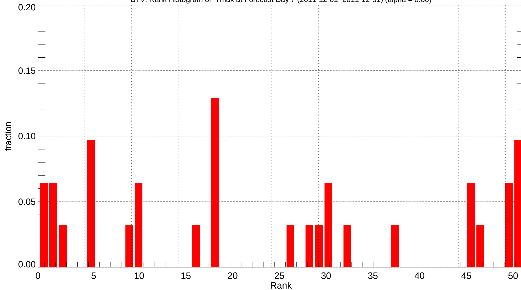
BTV: Rank Histogram of Tmax at Forecast Day 7 (2011-12-01~2011-12-31) (alpha = 0.00)
