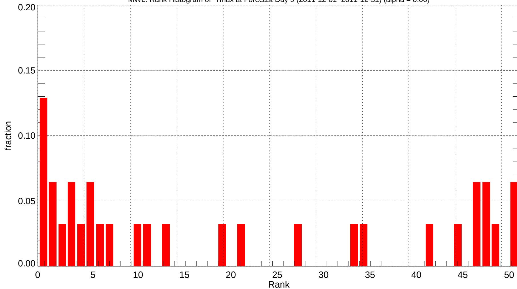
MWL: Rank Histogram of Tmax at Forecast Day 9 (2011-12-01~2011-12-31) (alpha = 0.00)
