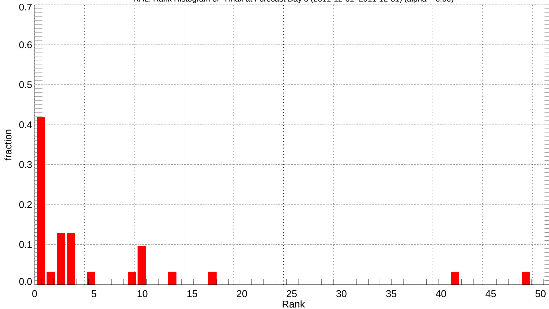
RAL: Rank Histogram of Tmax at Forecast Day 5 (2011-12-01~2011-12-31) (alpha = 0.00)
