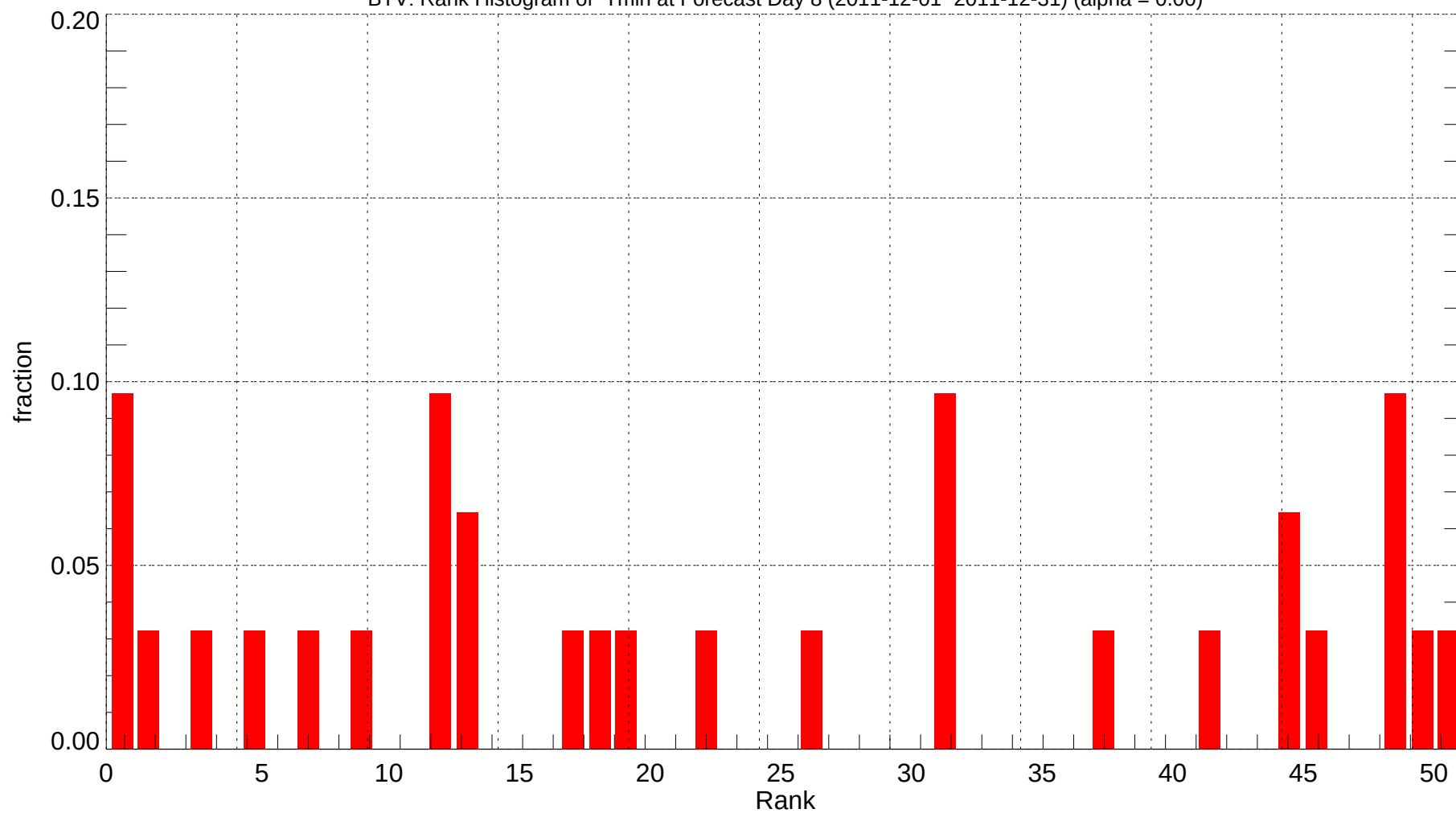
BTV: Rank Histogram of Tmin at Forecast Day 8 (2011-12-01~2011-12-31) (alpha = 0.00)
