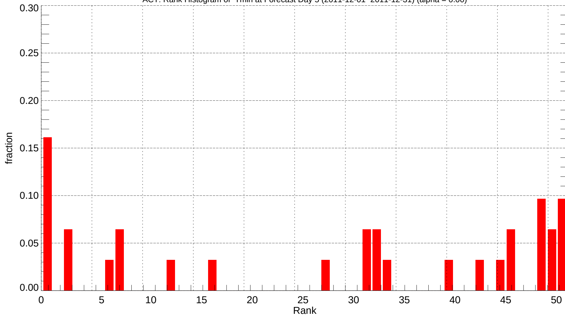
ACT: Rank Histogram of Tmin at Forecast Day 5 (2011-12-01~2011-12-31) (alpha = 0.00)
