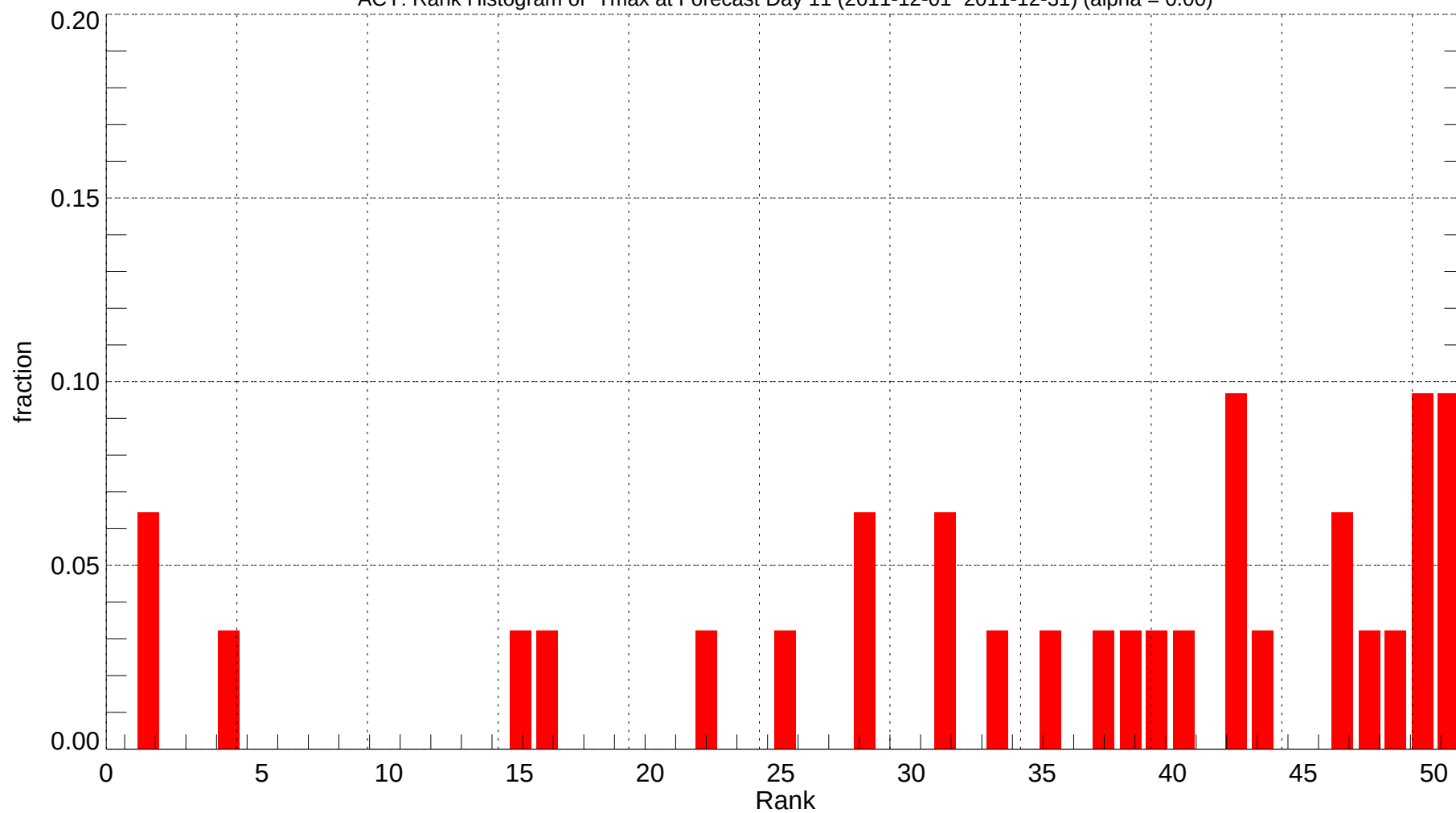
ACY: Rank Histogram of Tmax at Forecast Day 11 (2011-12-01~2011-12-31) (alpha = 0.00)
