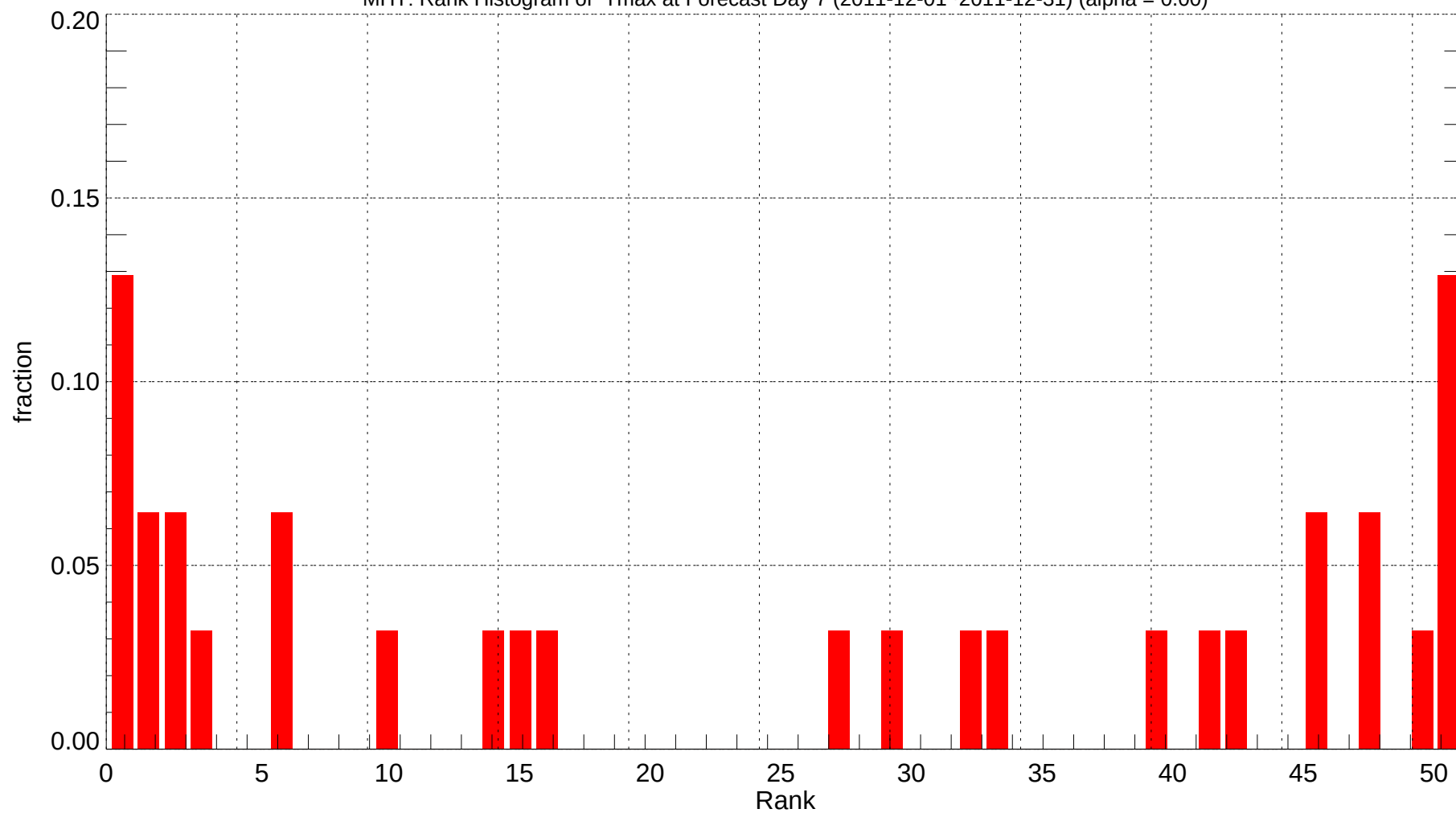
MHT: Rank Histogram of Tmax at Forecast Day 7 (2011-12-01~2011-12-31) (alpha = 0.00)
