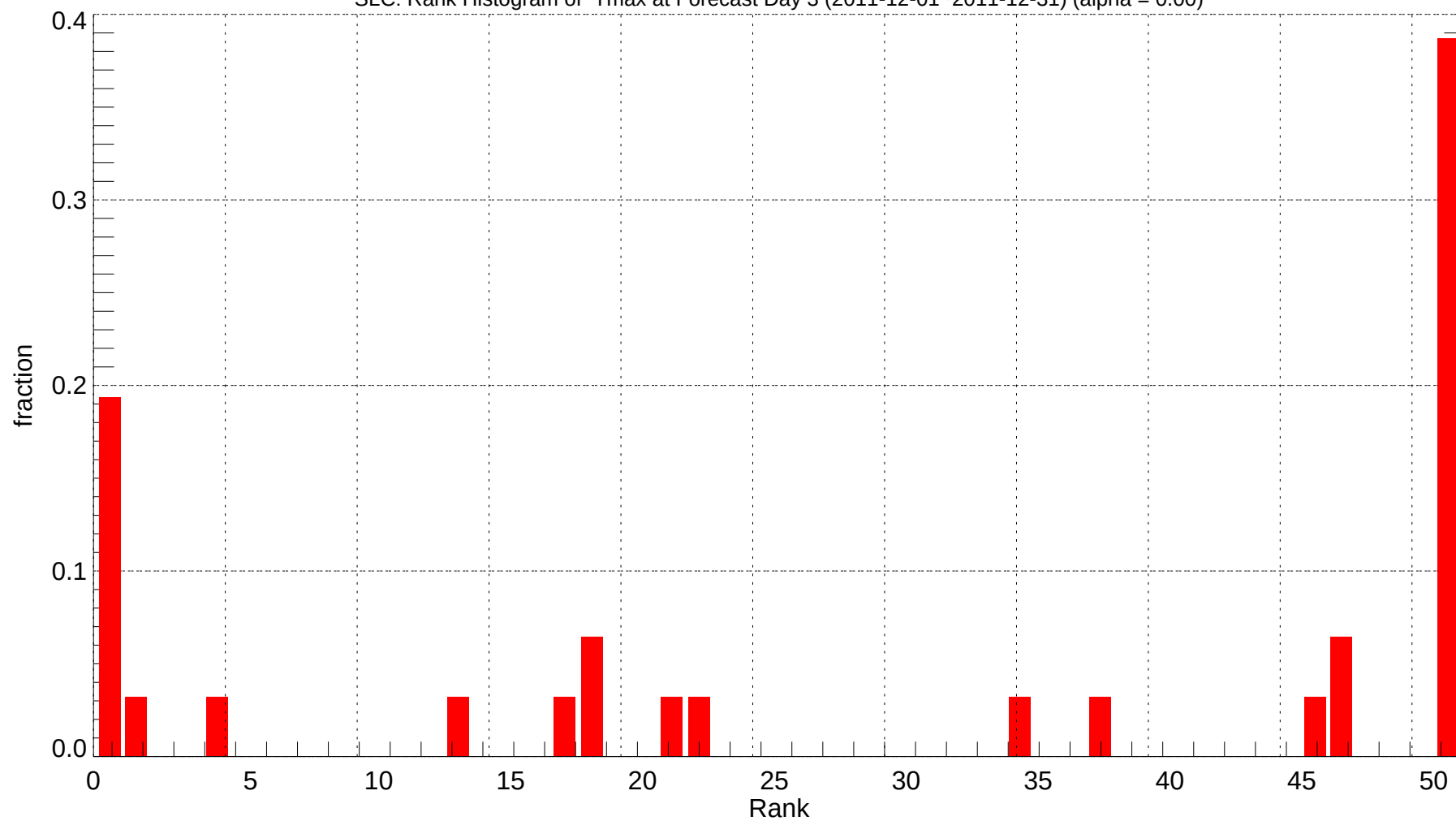
SLC: Rank Histogram of Tmax at Forecast Day 3 (2011-12-01~2011-12-31) (alpha = 0.00)
