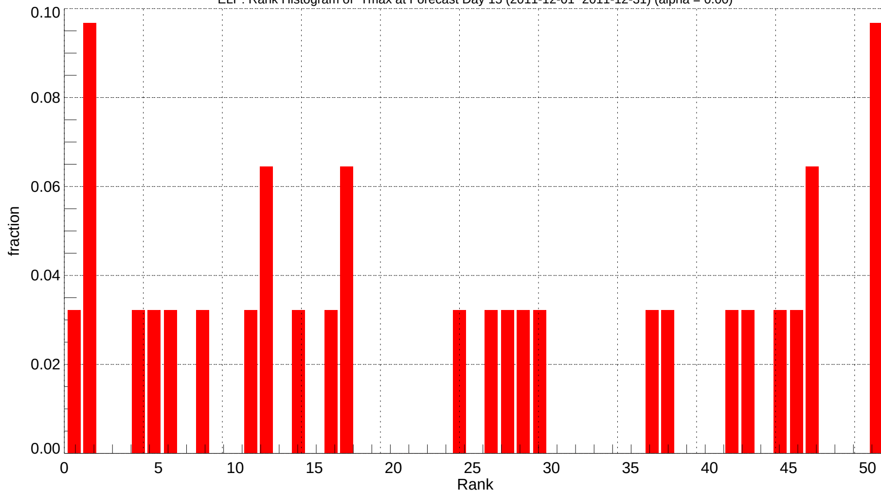
ELP: Rank Histogram of Tmax at Forecast Day 15 (2011-12-01~2011-12-31) (alpha = 0.00)
