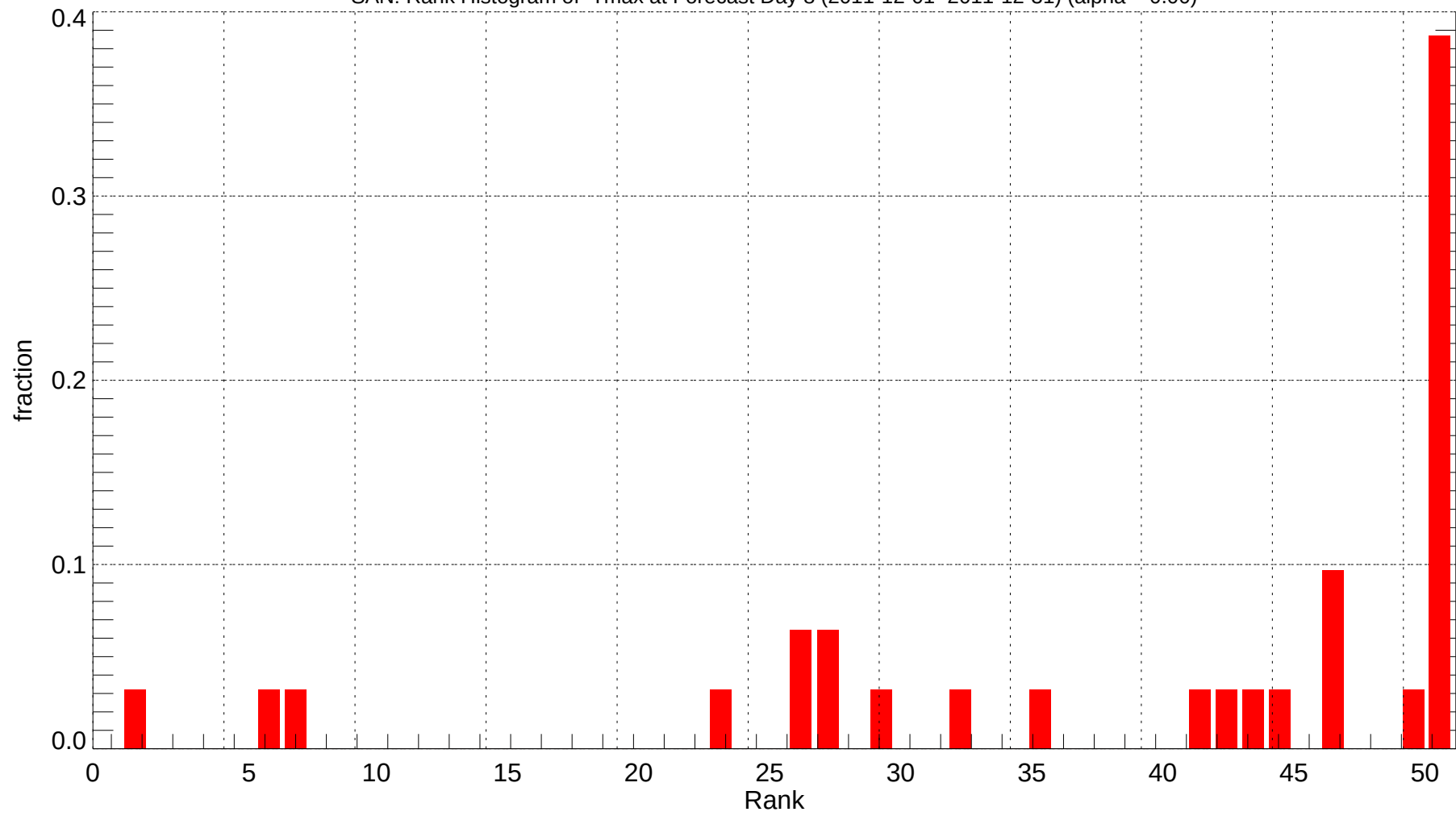
SAN: Rank Histogram of Tmax at Forecast Day 8 (2011-12-01~2011-12-31) (alpha = 0.00)
