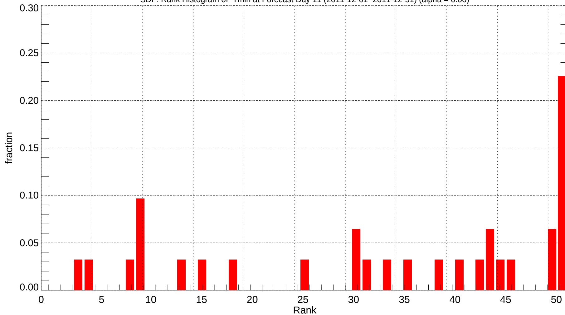
SDF: Rank Histogram of Tmin at Forecast Day 11 (2011-12-01~2011-12-31) (alpha = 0.00)
