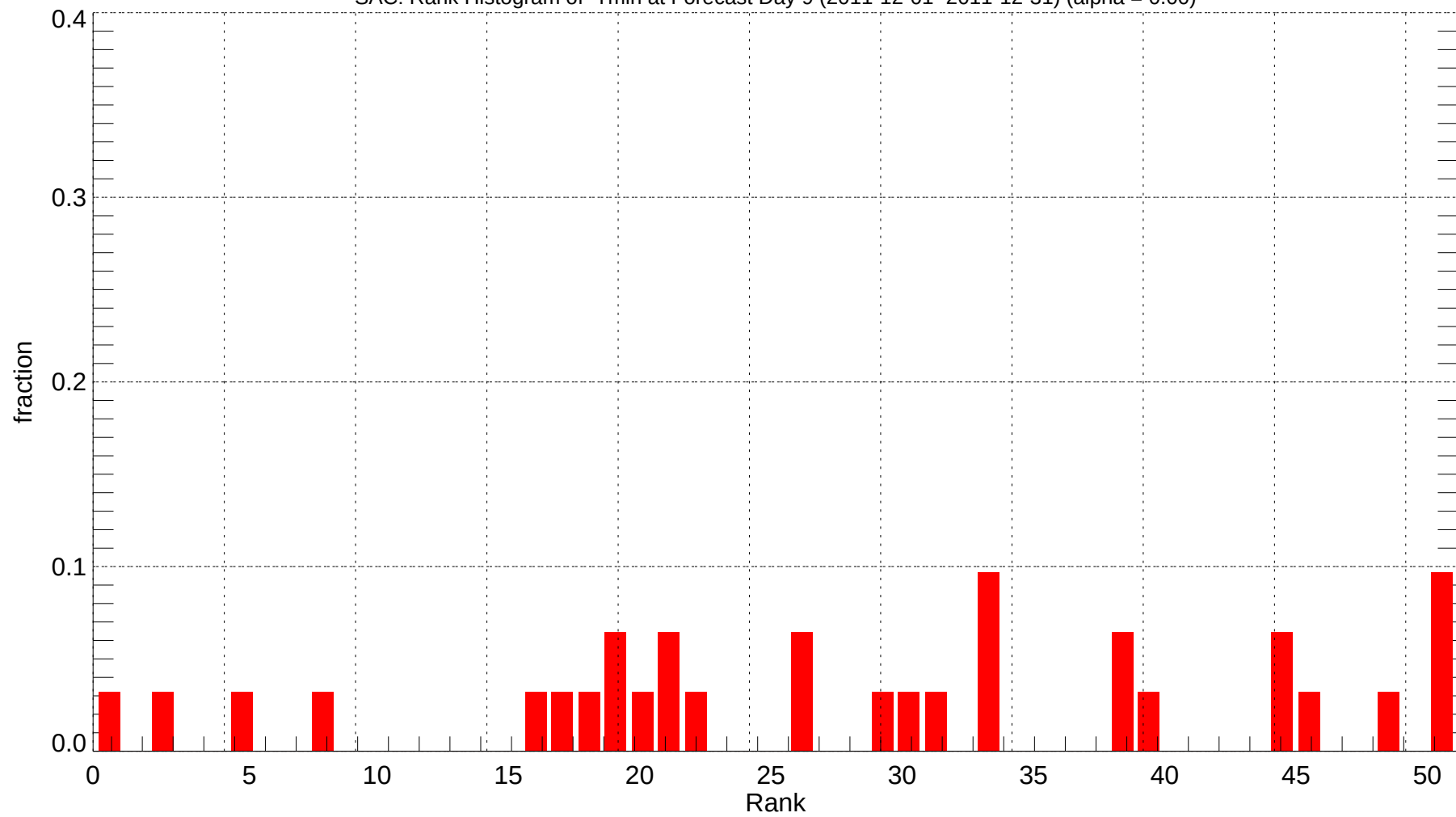
SAC: Rank Histogram of Tmin at Forecast Day 9 (2011-12-01~2011-12-31) (alpha = 0.00)
