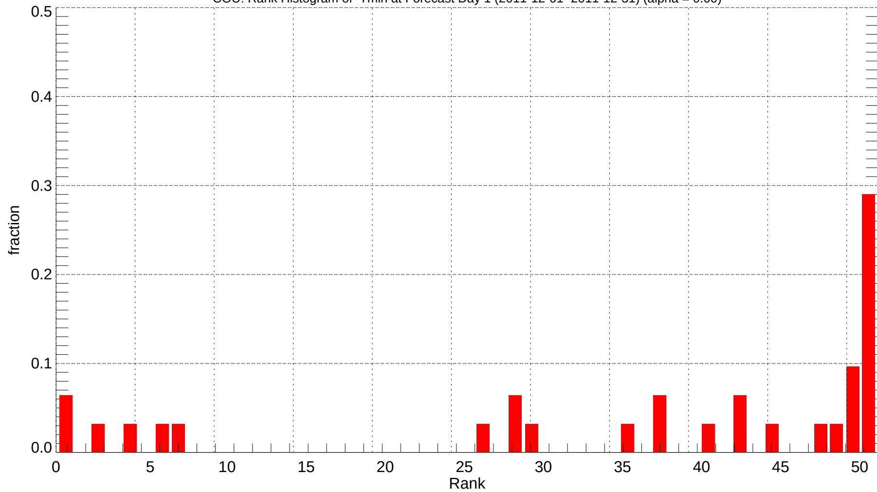
COU: Rank Histogram of Tmin at Forecast Day 1 (2011-12-01~2011-12-31) (alpha = 0.00)
