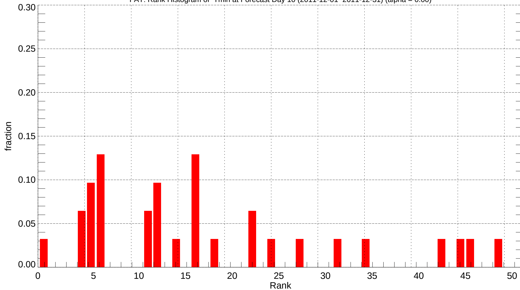
FAT: Rank Histogram of Tmin at Forecast Day 10 (2011-12-01~2011-12-31) (alpha = 0.00)
