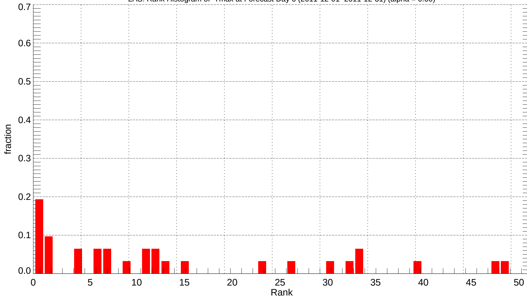
LAS: Rank Histogram of Tmax at Forecast Day 6 (2011-12-01~2011-12-31) (alpha = 0.00)
