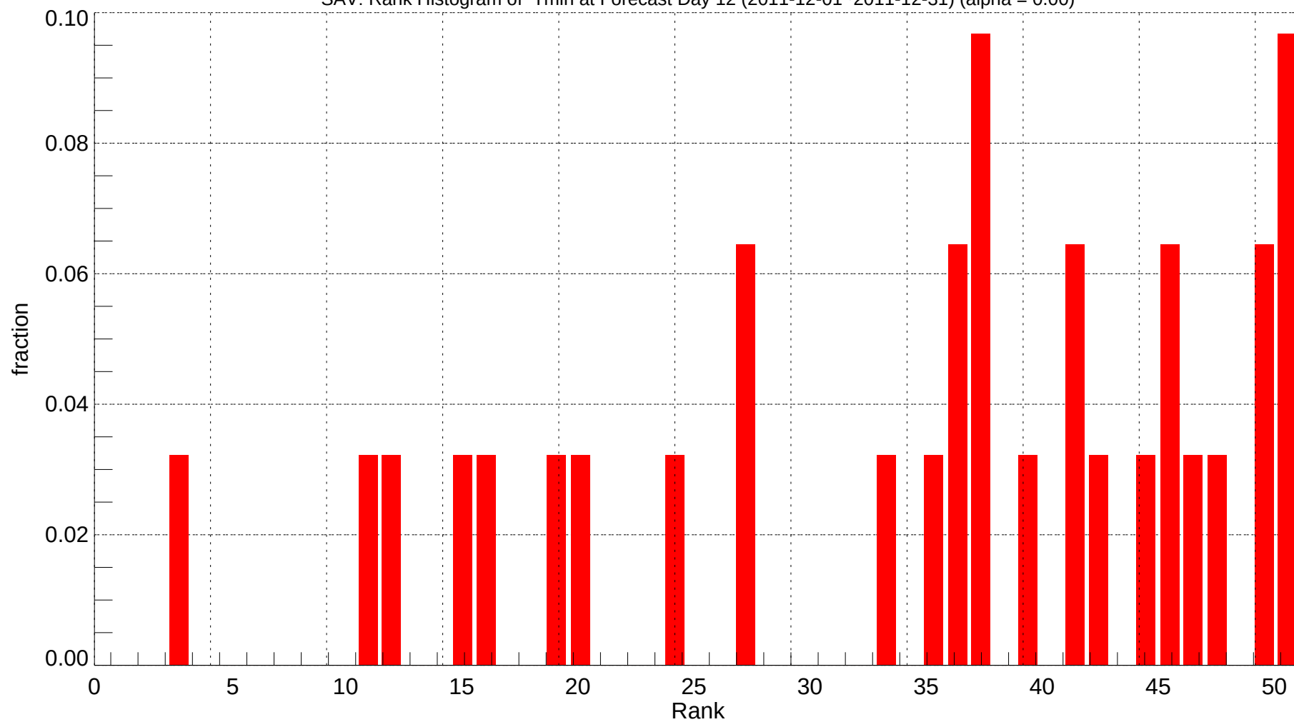
SAV: Rank Histogram of Tmin at Forecast Day 12 (2011-12-01~2011-12-31) (alpha = 0.00)
