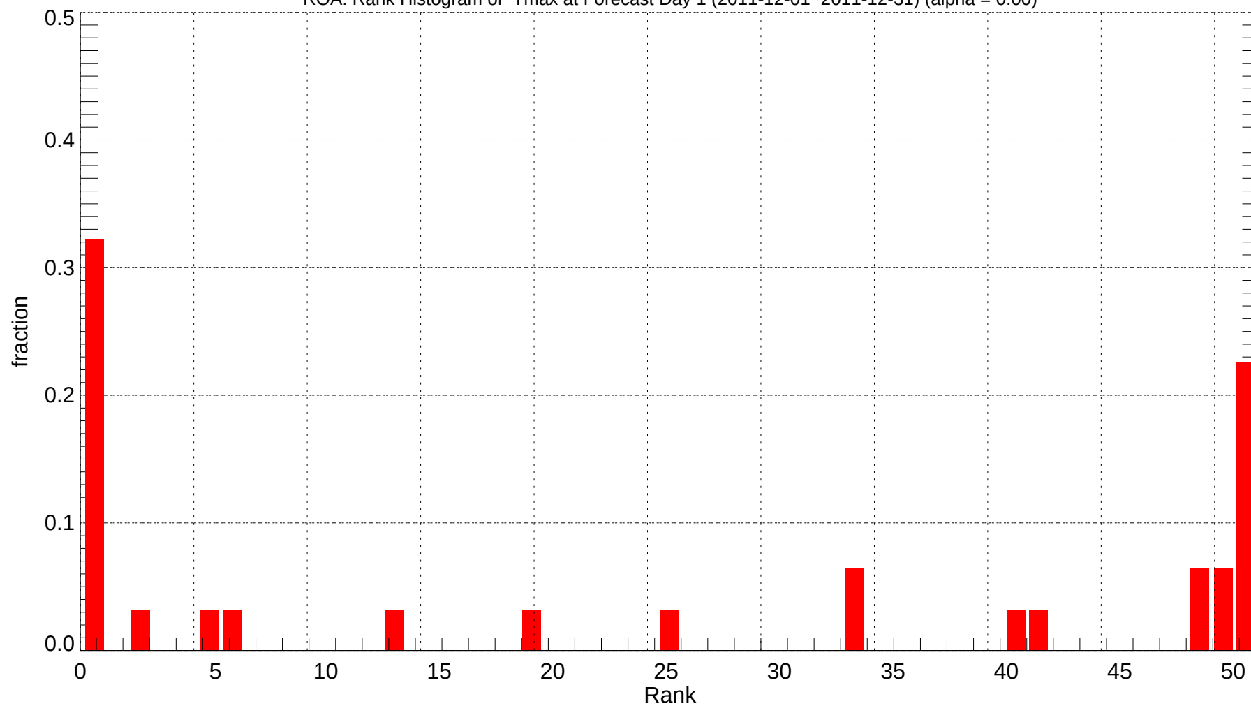
ROA: Rank Histogram of Tmax at Forecast Day 1 (2011-12-01~2011-12-31) (alpha = 0.00)
