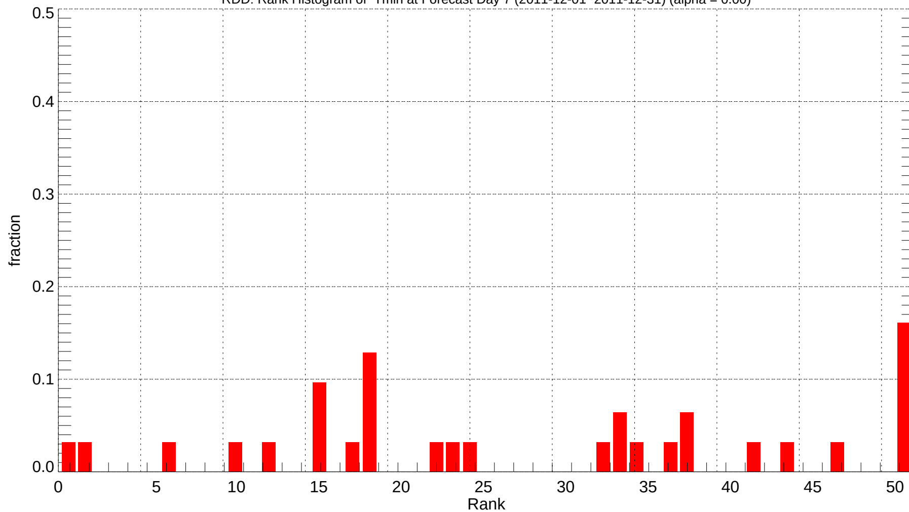
RDD: Rank Histogram of Tmin at Forecast Day 7 (2011-12-01~2011-12-31) (alpha = 0.00)
