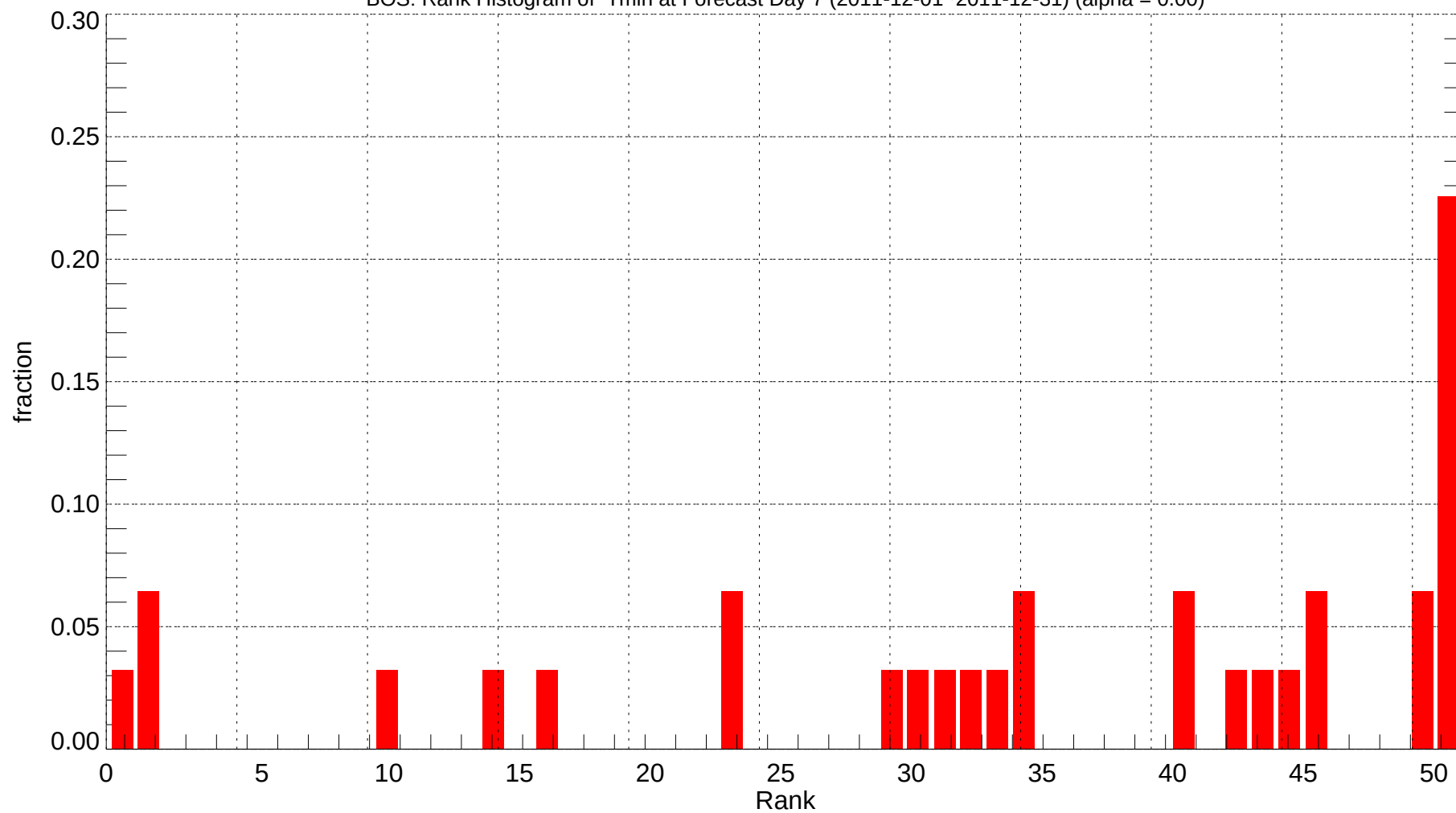
BOS: Rank Histogram of Tmin at Forecast Day 7 (2011-12-01~2011-12-31) (alpha = 0.00)
