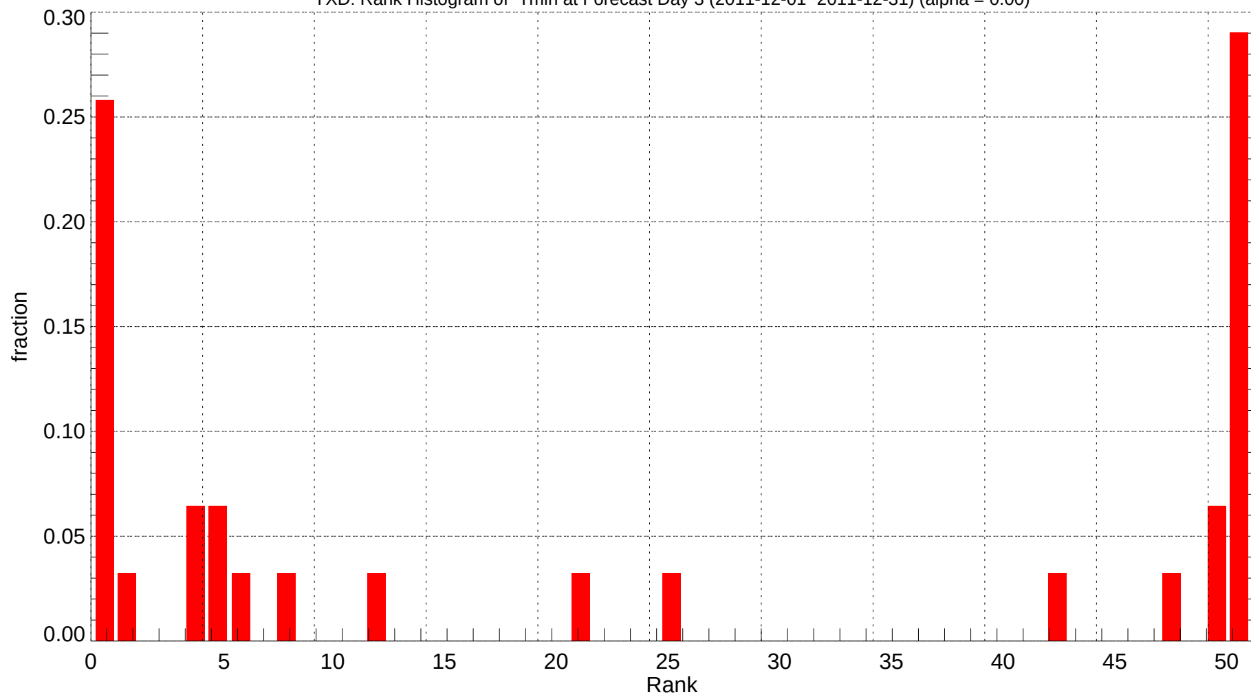
YXD: Rank Histogram of Tmin at Forecast Day 3 (2011-12-01~2011-12-31) (alpha = 0.00)
