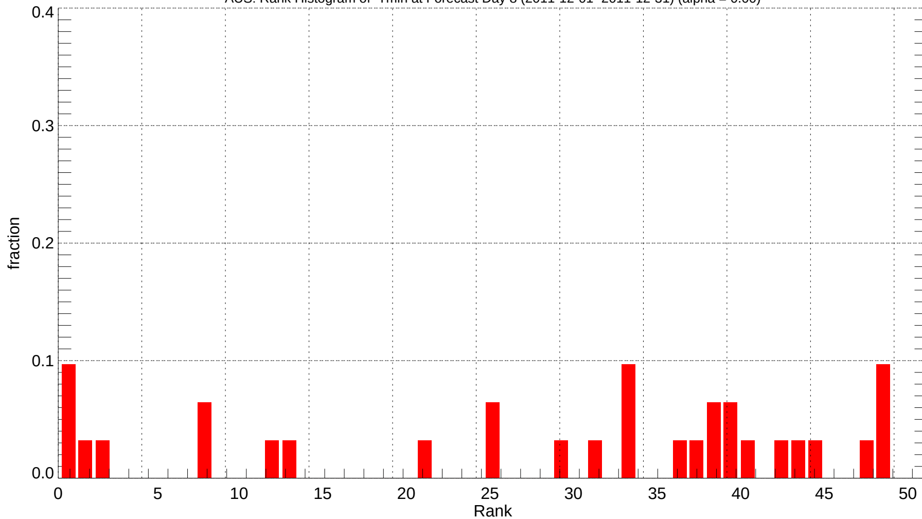
AUS: Rank Histogram of Tmin at Forecast Day 8 (2011-12-01~2011-12-31) (alpha = 0.00)
