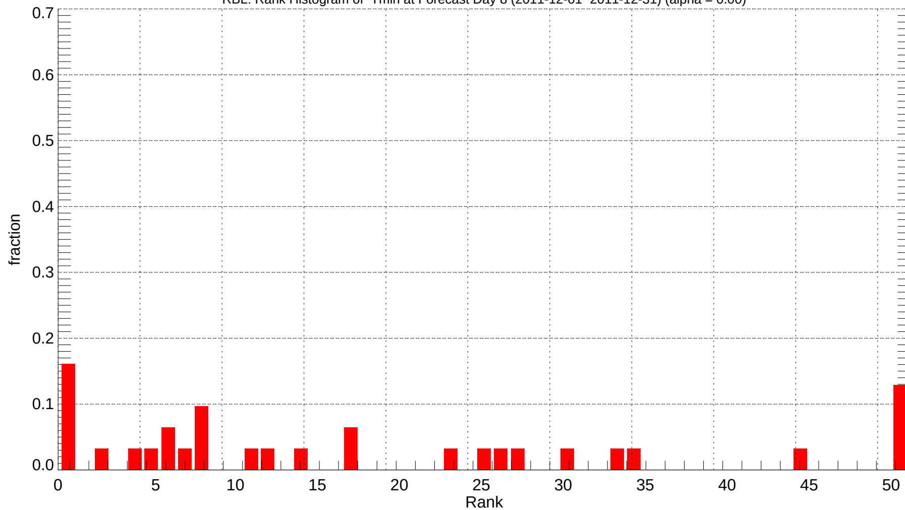
RBL: Rank Histogram of Tmin at Forecast Day 8 (2011-12-01~2011-12-31) (alpha = 0.00)
