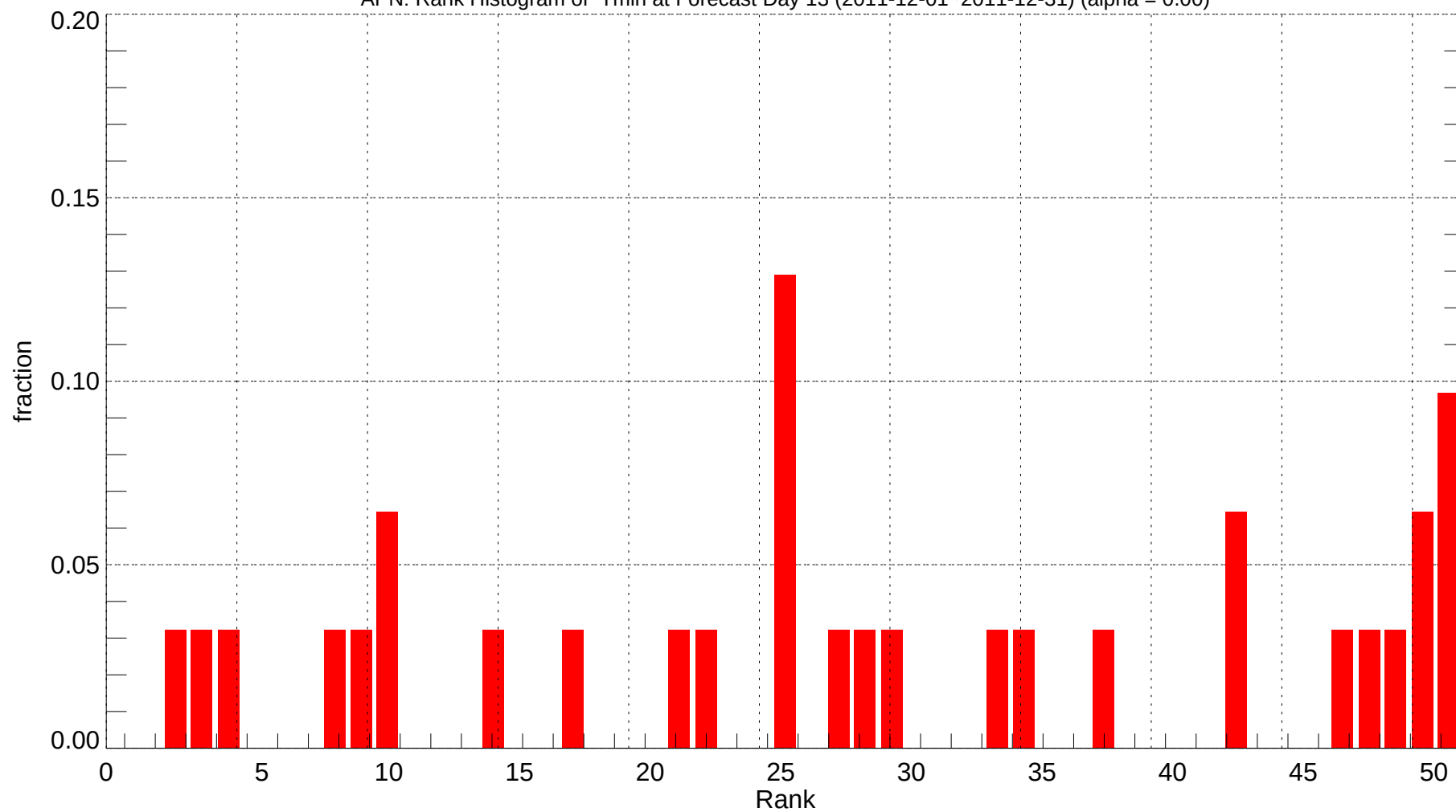
APN: Rank Histogram of Tmin at Forecast Day 13 (2011-12-01~2011-12-31) (alpha = 0.00)
