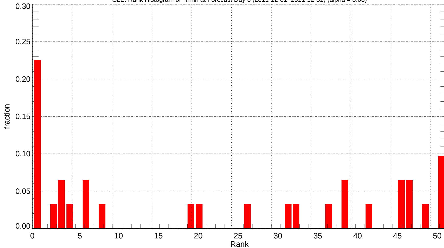
CLE: Rank Histogram of Tmin at Forecast Day 3 (2011-12-01~2011-12-31) (alpha = 0.00)
