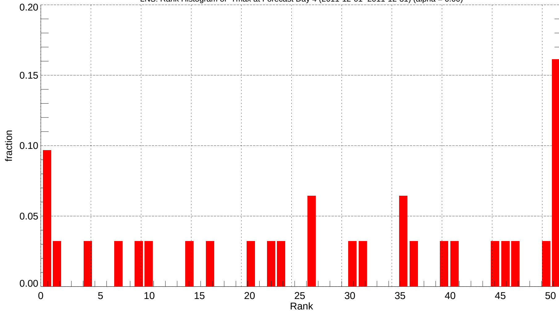
LNS: Rank Histogram of Tmax at Forecast Day 4 (2011-12-01~2011-12-31) (alpha = 0.00)
