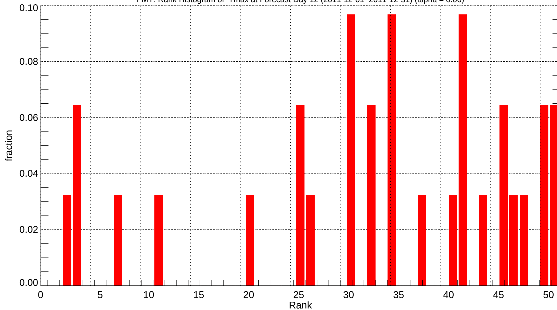
FMY: Rank Histogram of Tmax at Forecast Day 12 (2011-12-01~2011-12-31) (alpha = 0.00)
