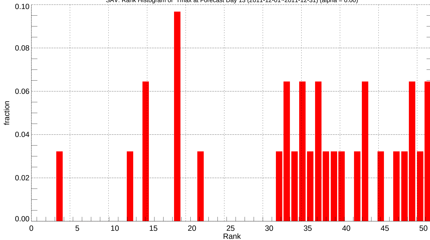
SAV: Rank Histogram of Tmax at Forecast Day 13 (2011-12-01~2011-12-31) (alpha = 0.00)
