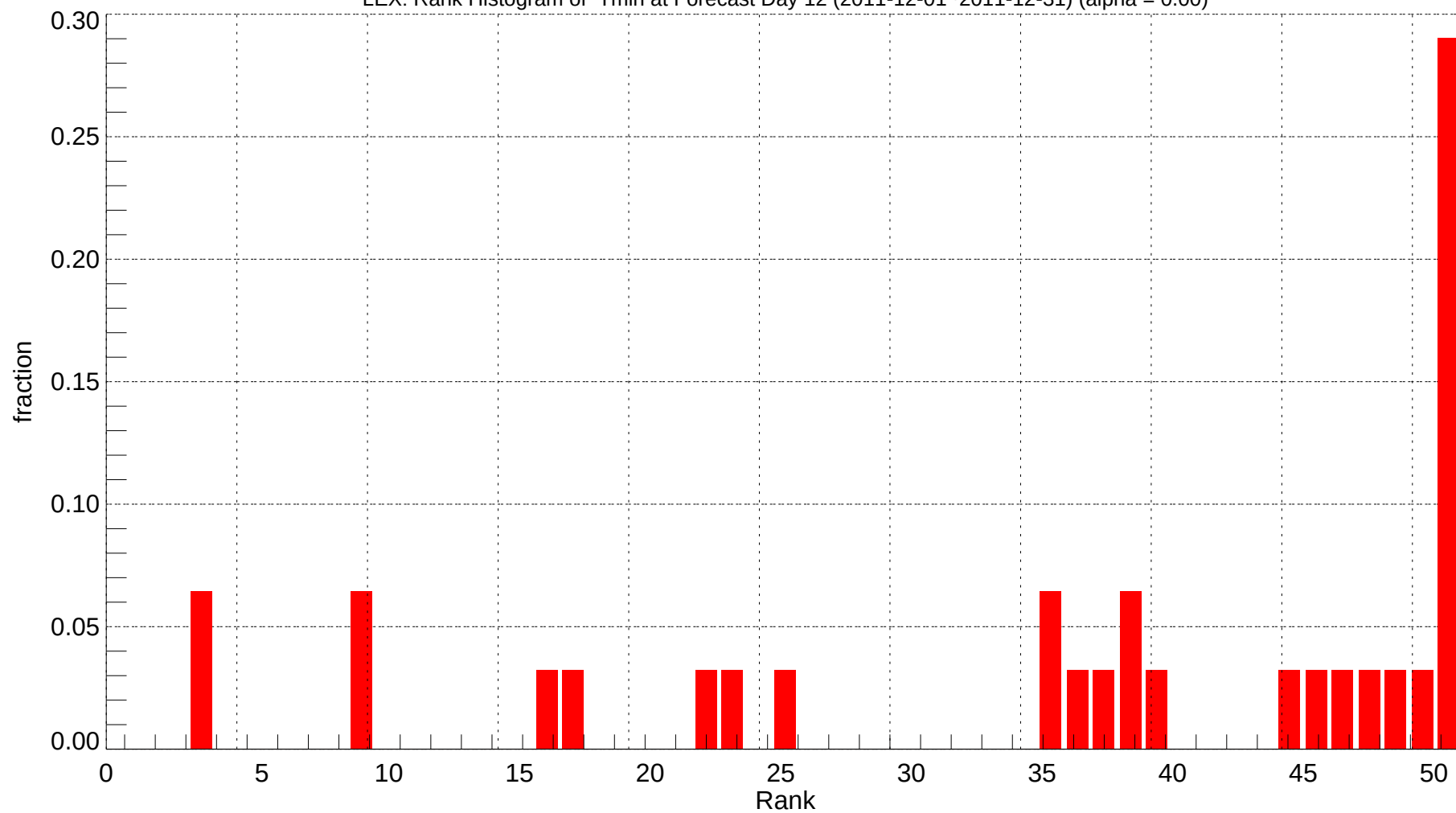
LEX: Rank Histogram of Tmin at Forecast Day 12 (2011-12-01~2011-12-31) (alpha = 0.00)
