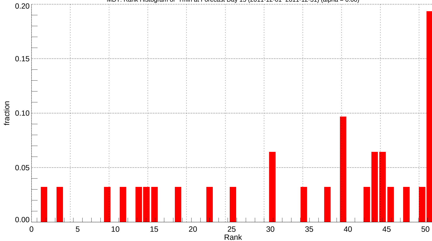
MDT: Rank Histogram of Tmin at Forecast Day 15 (2011-12-01~2011-12-31) (alpha = 0.00)
