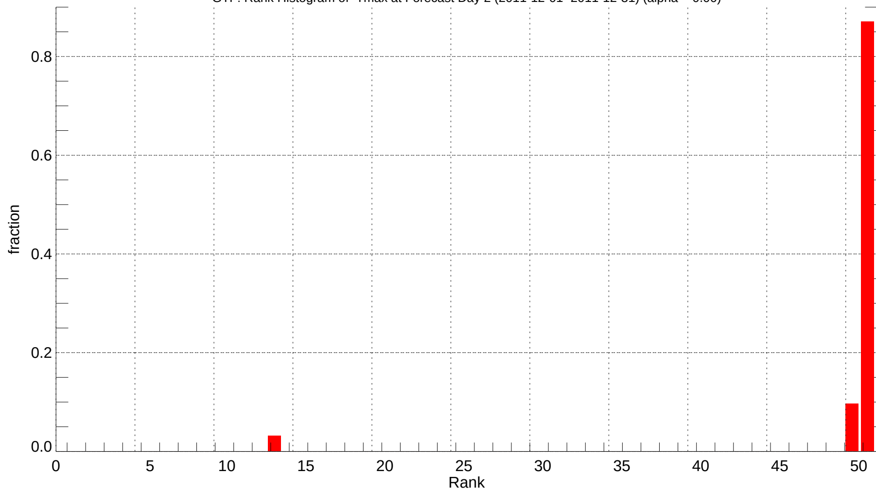
GTF: Rank Histogram of Tmax at Forecast Day 2 (2011-12-01~2011-12-31) (alpha = 0.00)
