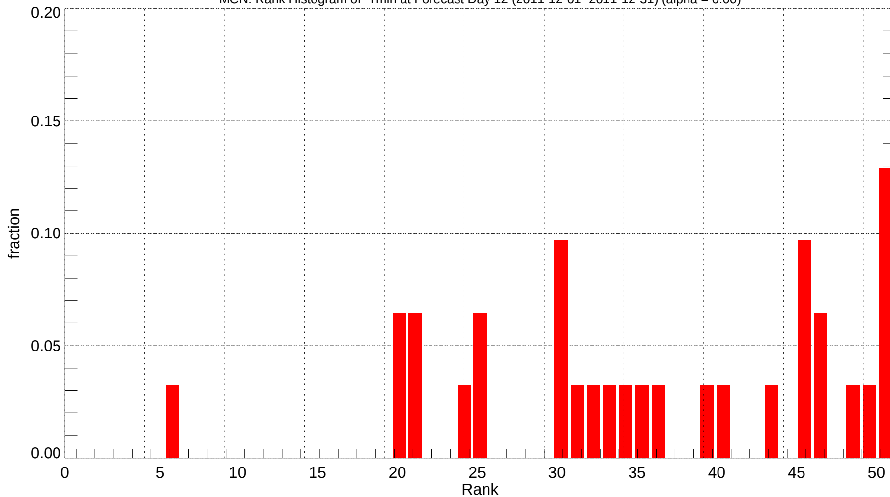
MCN: Rank Histogram of Tmin at Forecast Day 12 (2011-12-01~2011-12-31) (alpha = 0.00)
