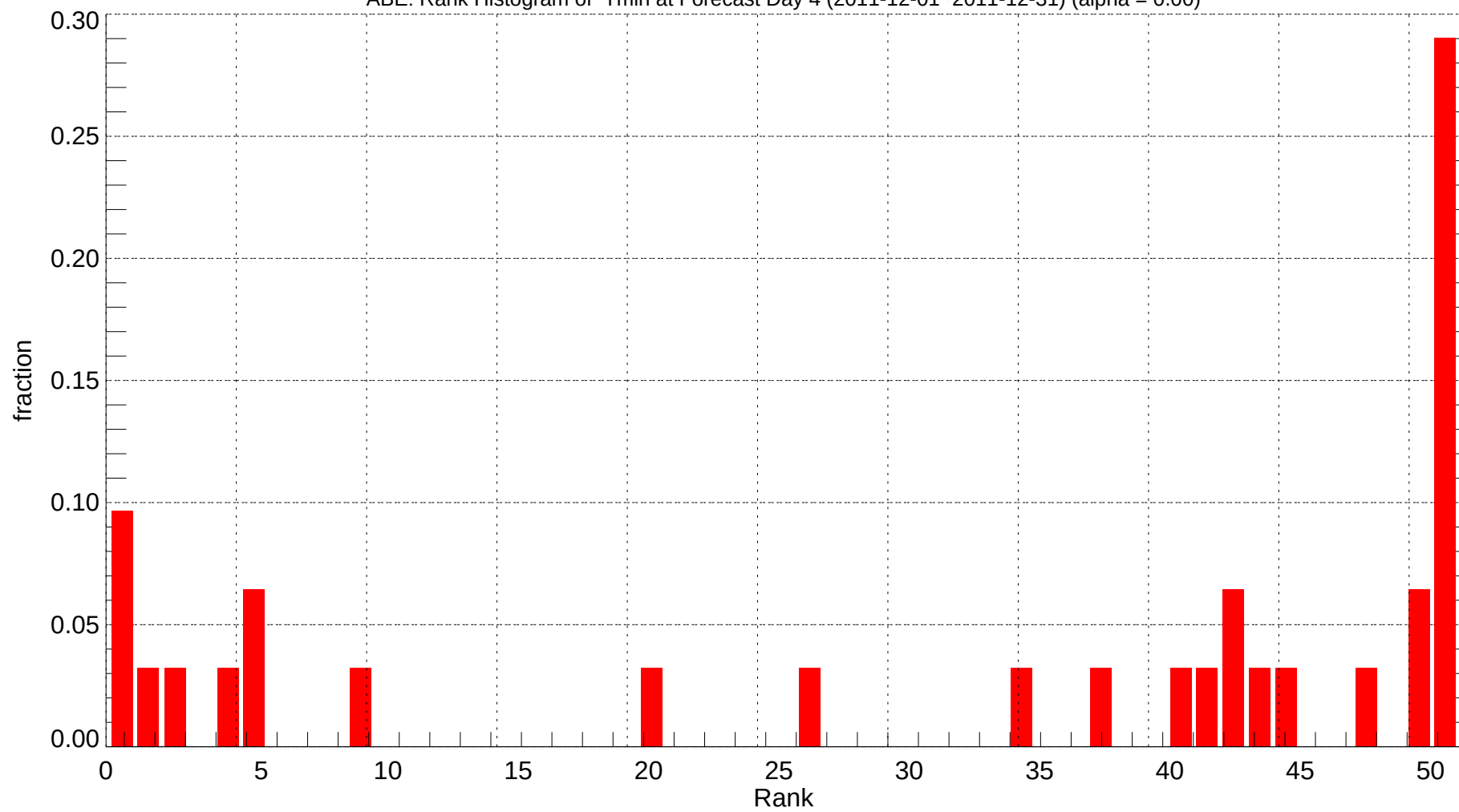
ABE: Rank Histogram of Tmin at Forecast Day 4 (2011-12-01~2011-12-31) (alpha = 0.00)
