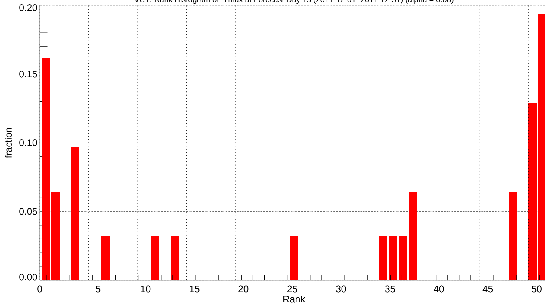
VCT: Rank Histogram of Tmax at Forecast Day 15 (2011-12-01~2011-12-31) (alpha = 0.00)
