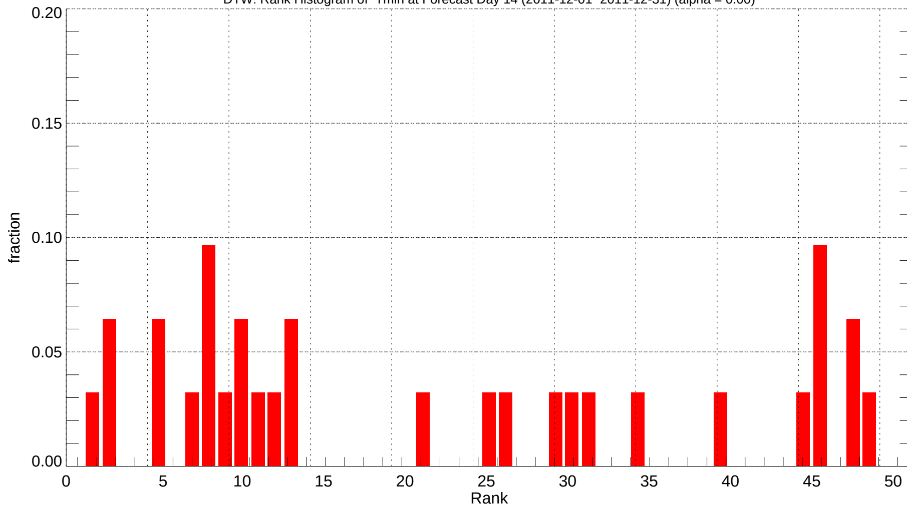
DTW: Rank Histogram of Tmin at Forecast Day 14 (2011-12-01~2011-12-31) (alpha = 0.00)
