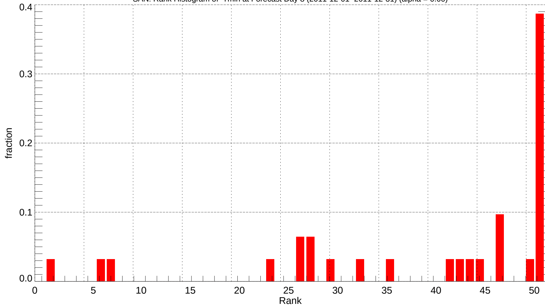
SAN: Rank Histogram of Tmin at Forecast Day 8 (2011-12-01~2011-12-31) (alpha = 0.00)
