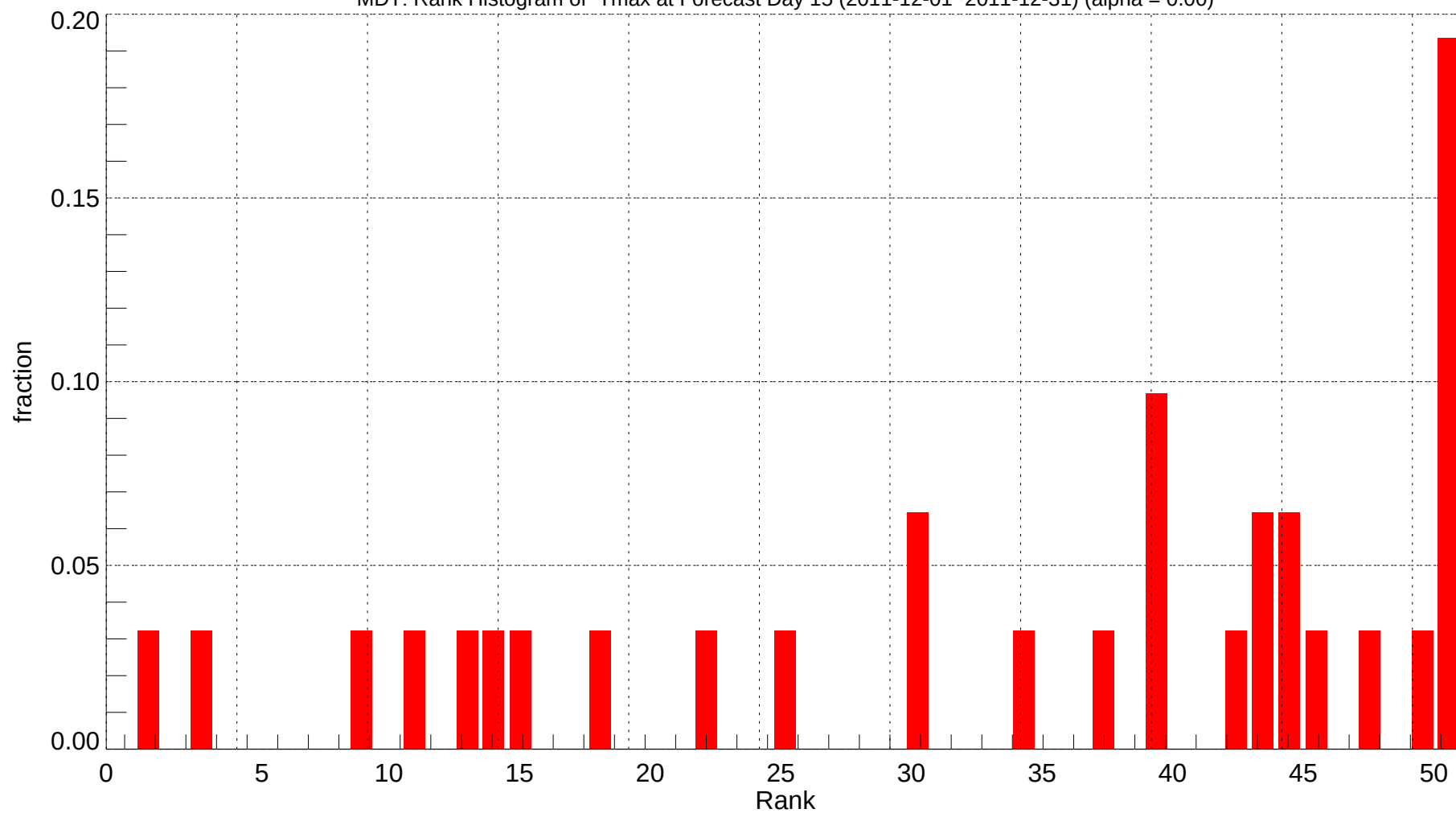
MDT: Rank Histogram of Tmax at Forecast Day 15 (2011-12-01~2011-12-31) (alpha = 0.00)
