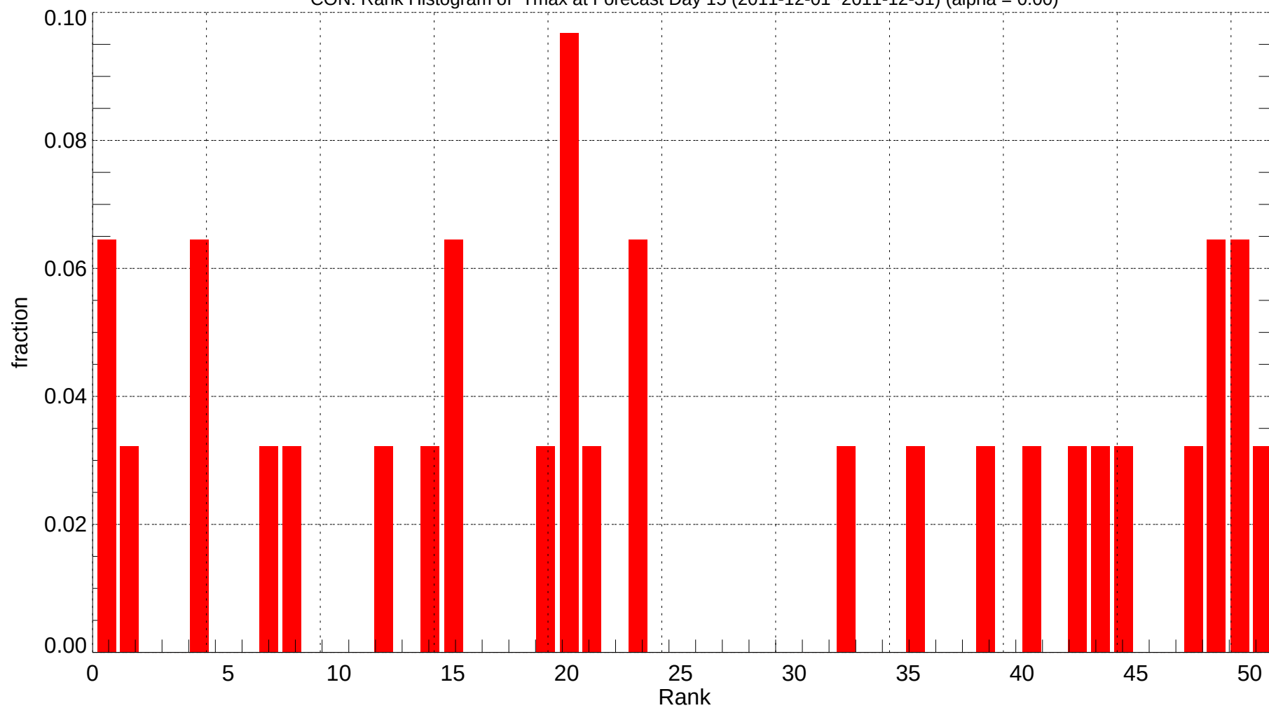
CON: Rank Histogram of Tmax at Forecast Day 15 (2011-12-01~2011-12-31) (alpha = 0.00)
