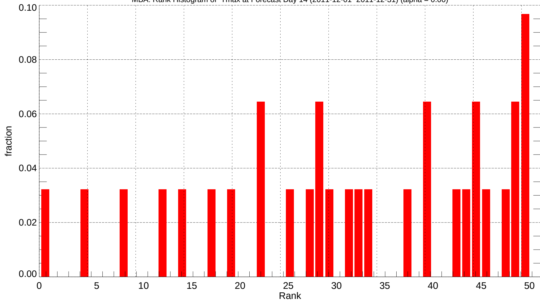
MBA: Rank Histogram of Tmax at Forecast Day 14 (2011-12-01~2011-12-31) (alpha = 0.00)
