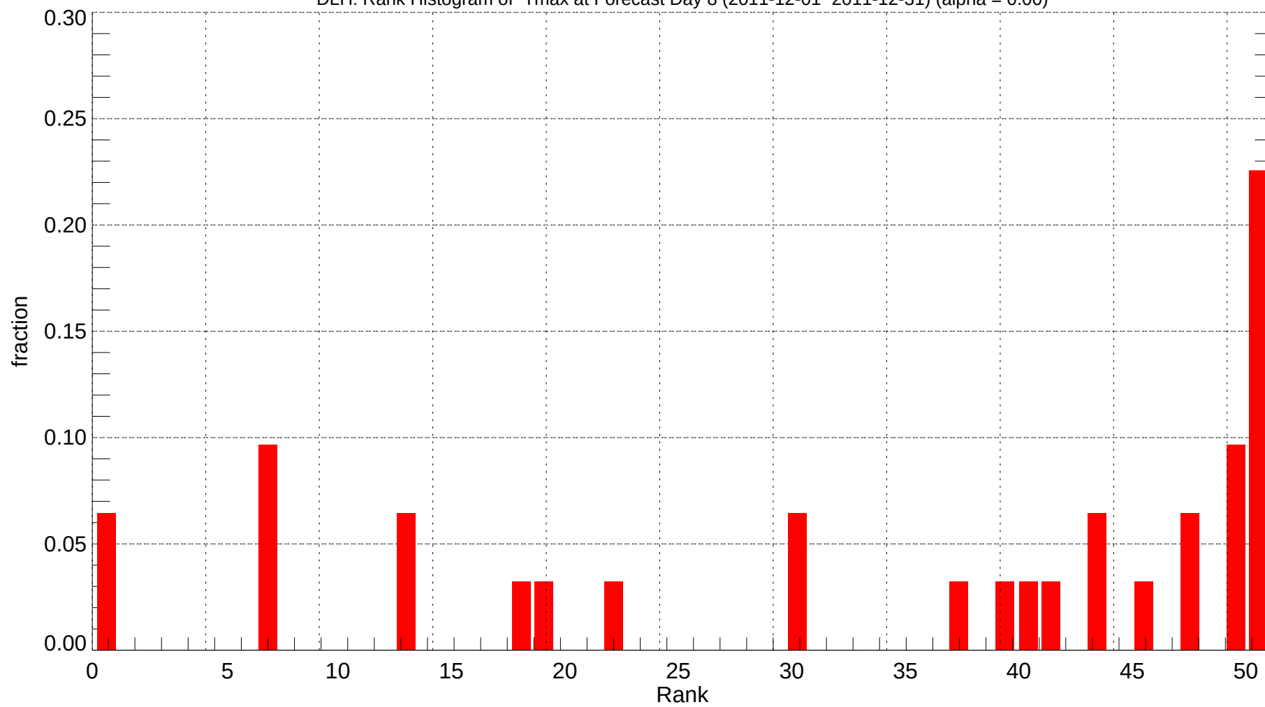
DLH: Rank Histogram of Tmax at Forecast Day 8 (2011-12-01~2011-12-31) (alpha = 0.00)
