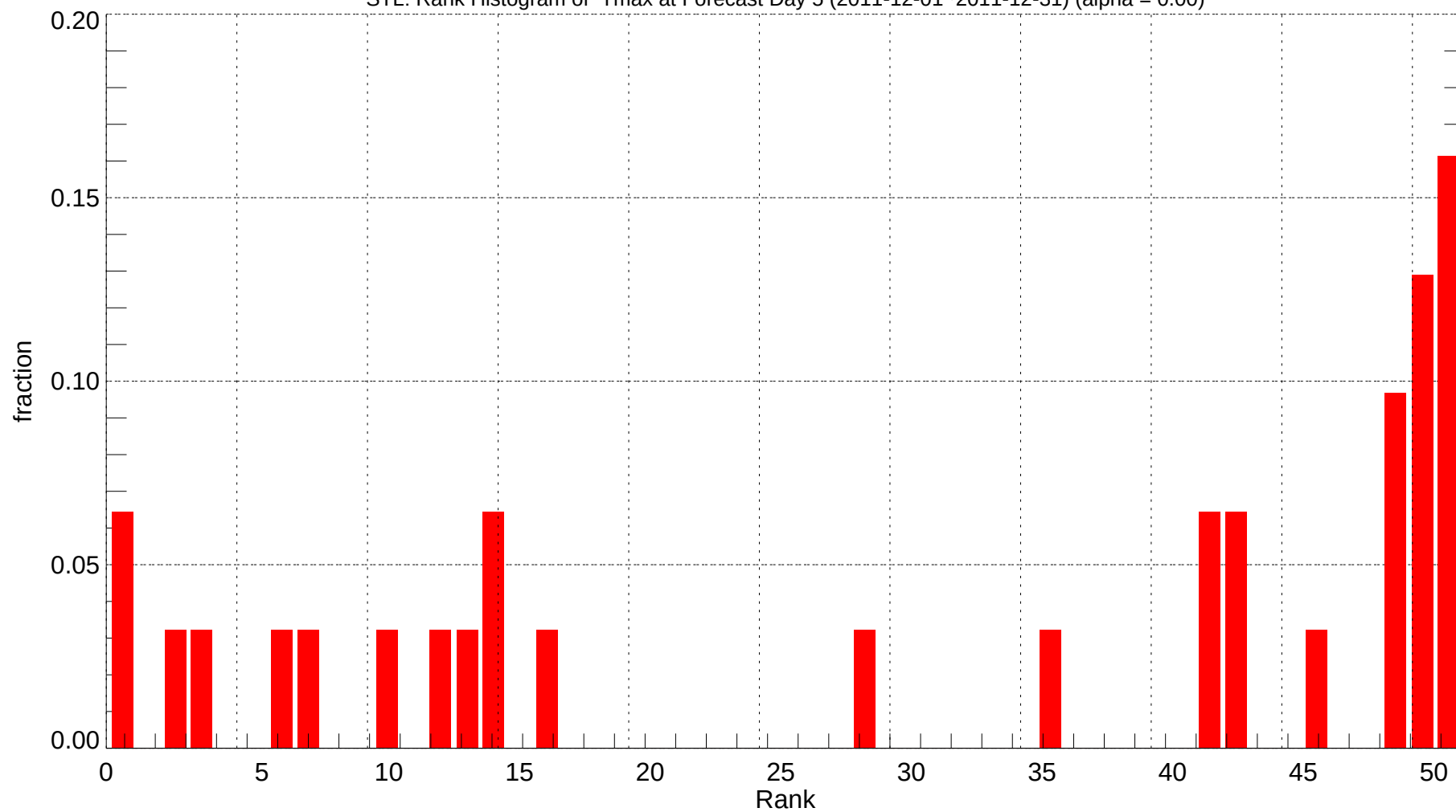
STL: Rank Histogram of Tmax at Forecast Day 5 (2011-12-01~2011-12-31) (alpha = 0.00)
