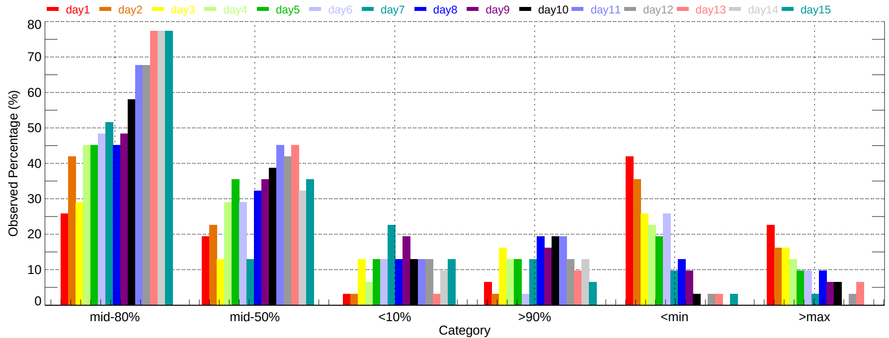
Observed Percentage of Ensembles - DTW: Max Temperature (2011-12-01~2011-12-31)
