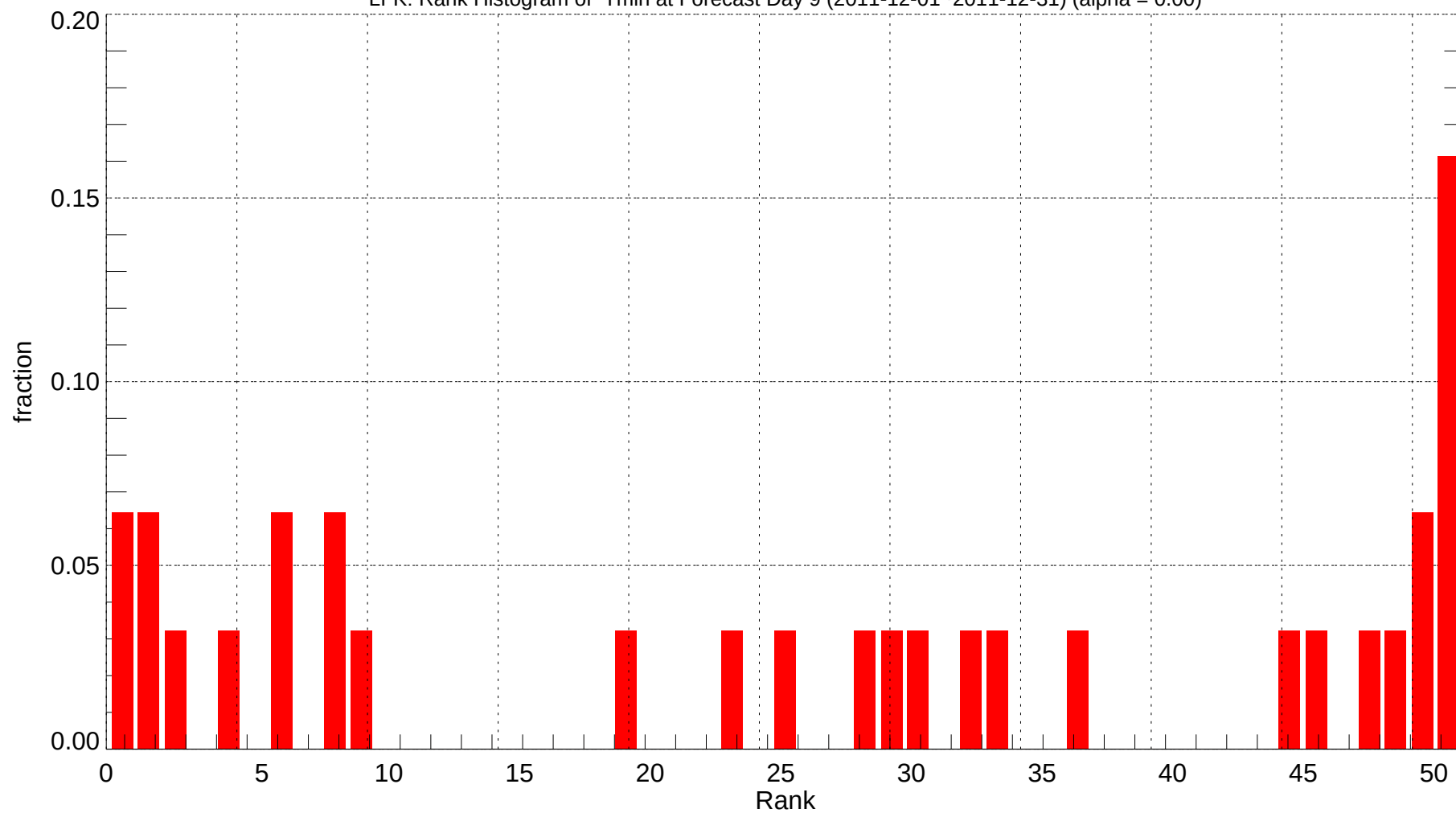
LFK: Rank Histogram of Tmin at Forecast Day 9 (2011-12-01~2011-12-31) (alpha = 0.00)
