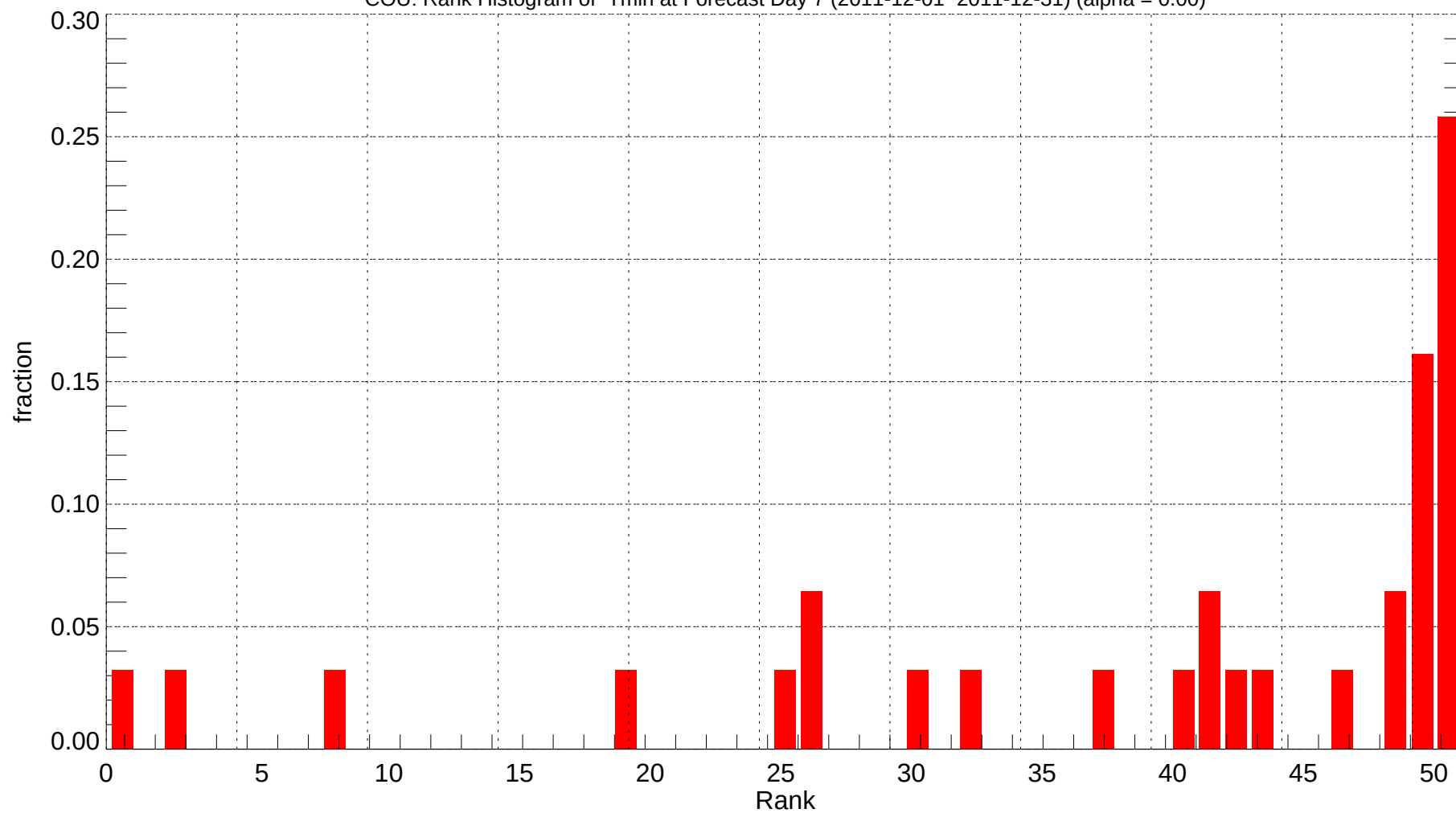
COU: Rank Histogram of Tmin at Forecast Day 7 (2011-12-01~2011-12-31) (alpha = 0.00)
