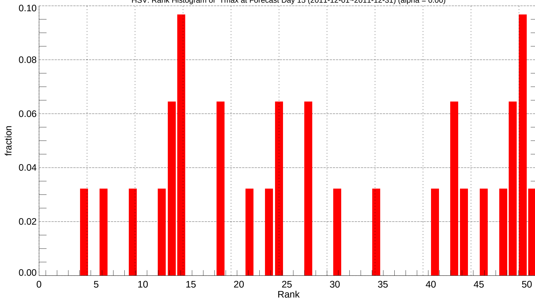
HSV: Rank Histogram of Tmax at Forecast Day 15 (2011-12-01~2011-12-31) (alpha = 0.00)
