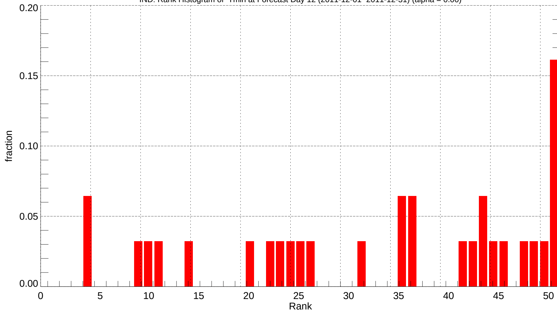
IND: Rank Histogram of Tmin at Forecast Day 12 (2011-12-01~2011-12-31) (alpha = 0.00)
