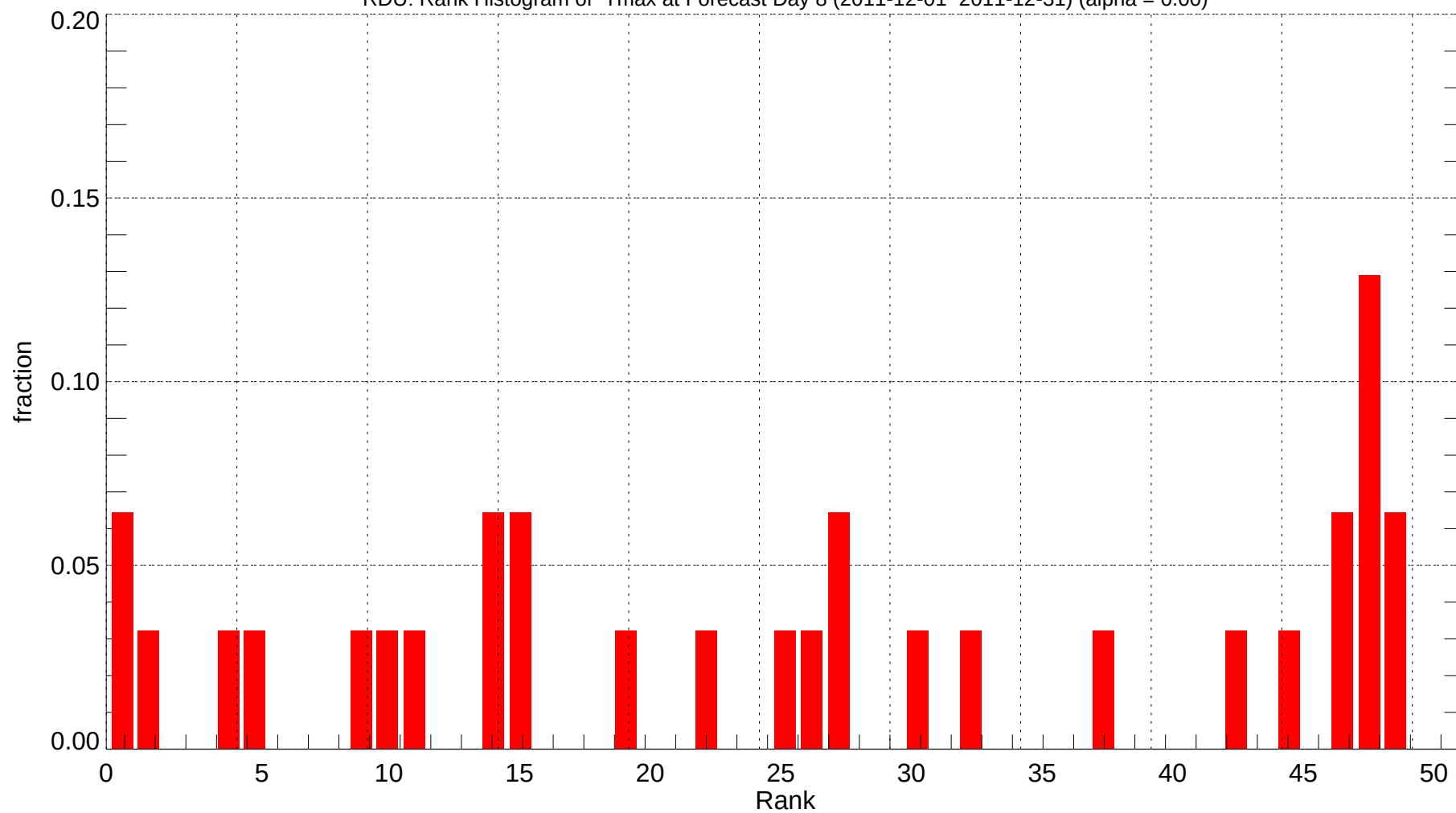
RDU: Rank Histogram of Tmax at Forecast Day 8 (2011-12-01~2011-12-31) (alpha = 0.00)
