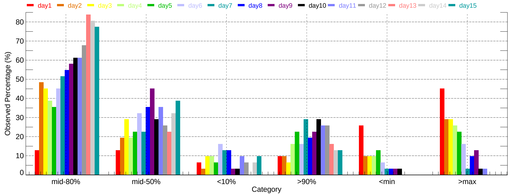
Observed Percentage of Ensembles - ERI: Min Temperature (2011-12-01~2011-12-31)
