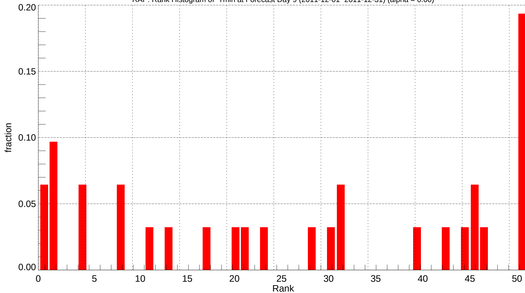
RAP: Rank Histogram of Tmin at Forecast Day 9 (2011-12-01~2011-12-31) (alpha = 0.00)
