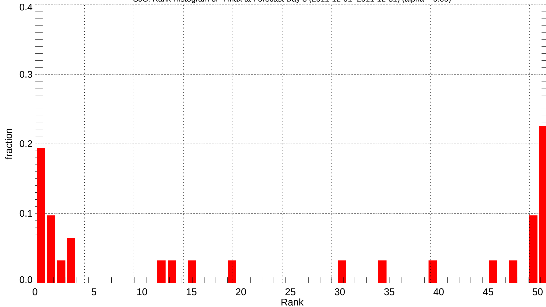
SJC: Rank Histogram of Tmax at Forecast Day 3 (2011-12-01~2011-12-31) (alpha = 0.00)
