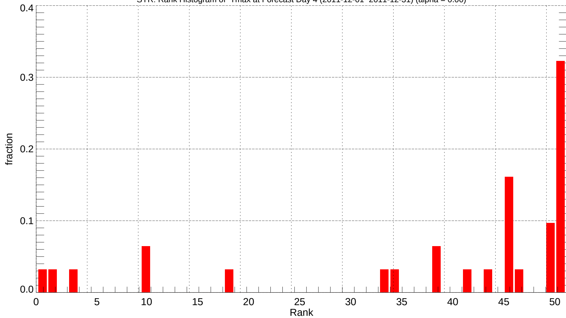
SYR: Rank Histogram of Tmax at Forecast Day 4 (2011-12-01~2011-12-31) (alpha = 0.00)
