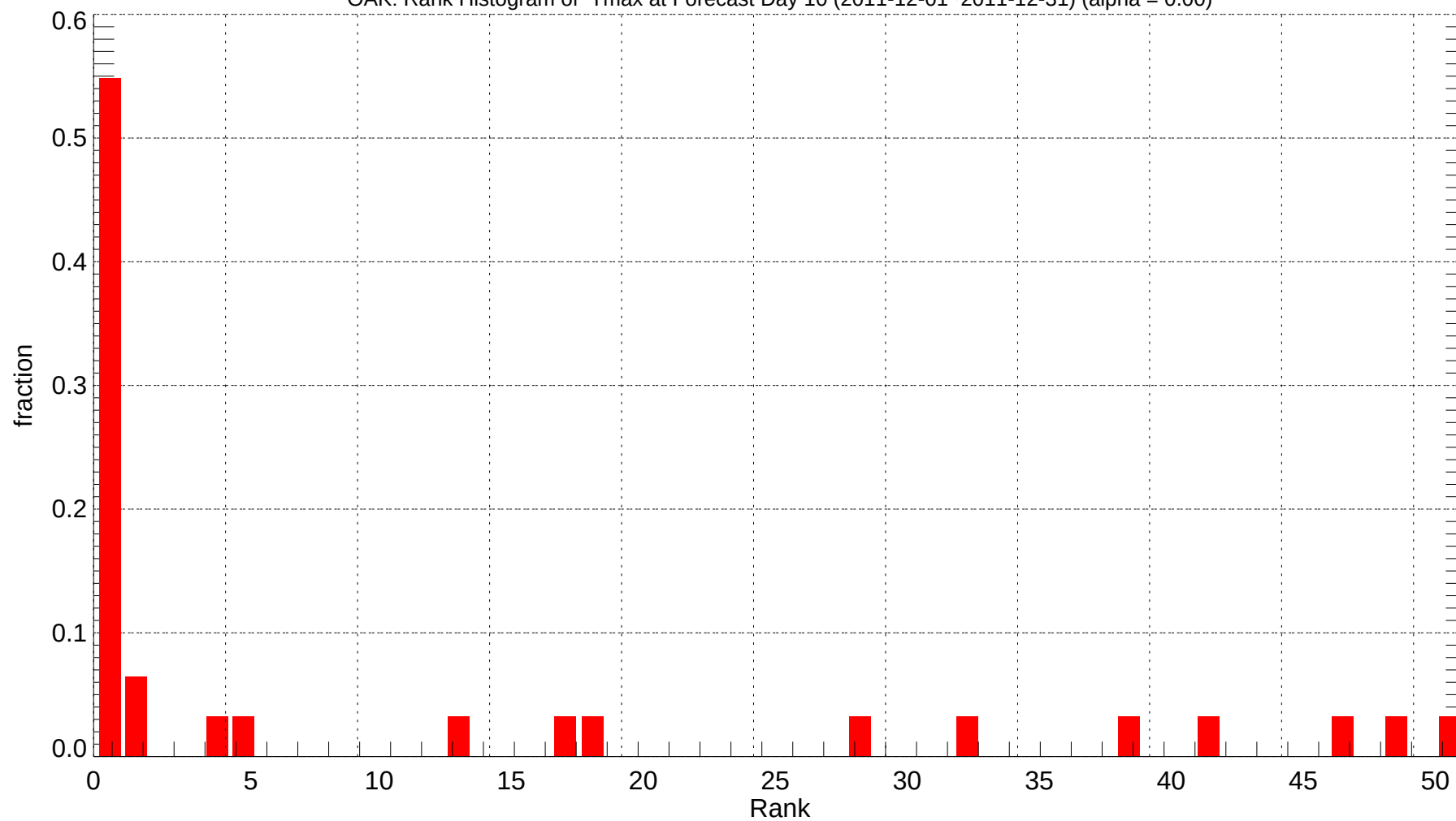
OAK: Rank Histogram of Tmax at Forecast Day 10 (2011-12-01~2011-12-31) (alpha = 0.00)
