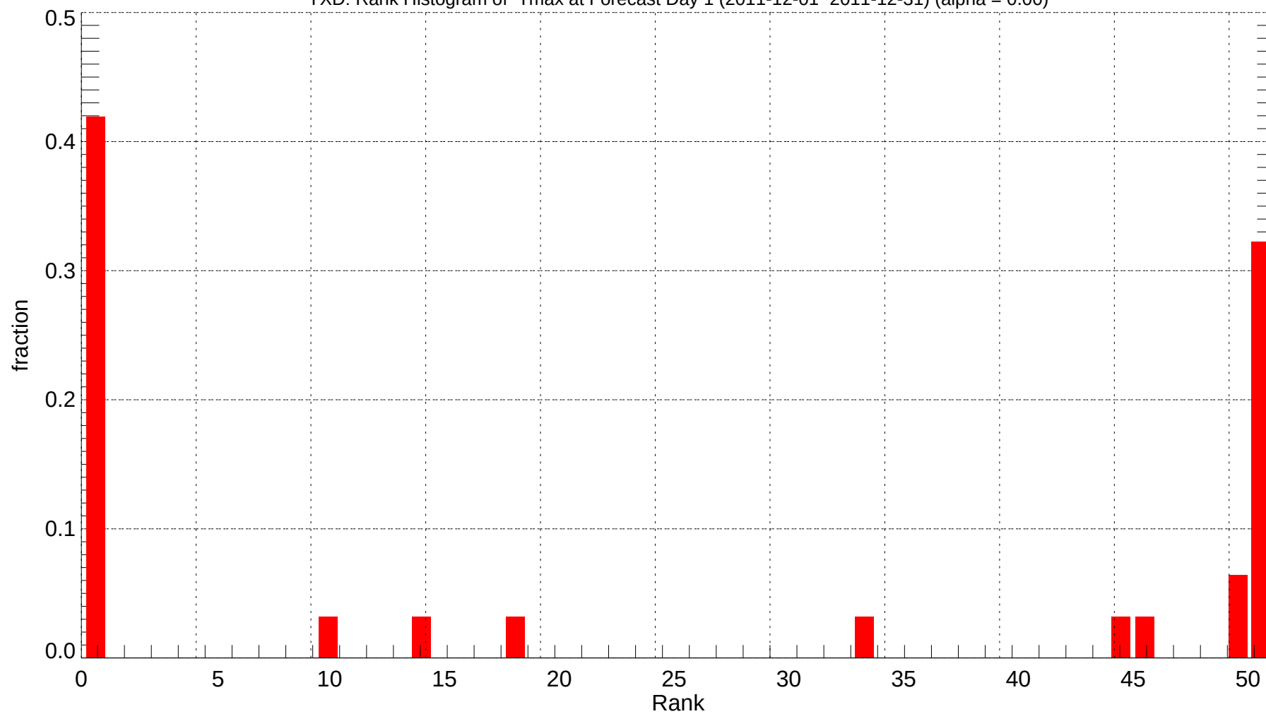
YXD: Rank Histogram of Tmax at Forecast Day 1 (2011-12-01~2011-12-31) (alpha = 0.00)
