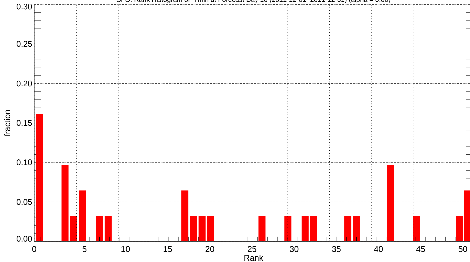
SFO: Rank Histogram of Tmin at Forecast Day 10 (2011-12-01~2011-12-31) (alpha = 0.00)
