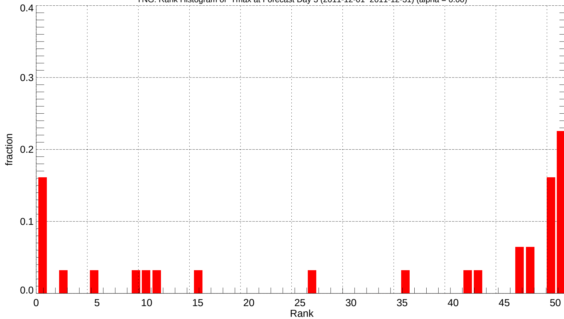
YNG: Rank Histogram of Tmax at Forecast Day 3 (2011-12-01~2011-12-31) (alpha = 0.00)
