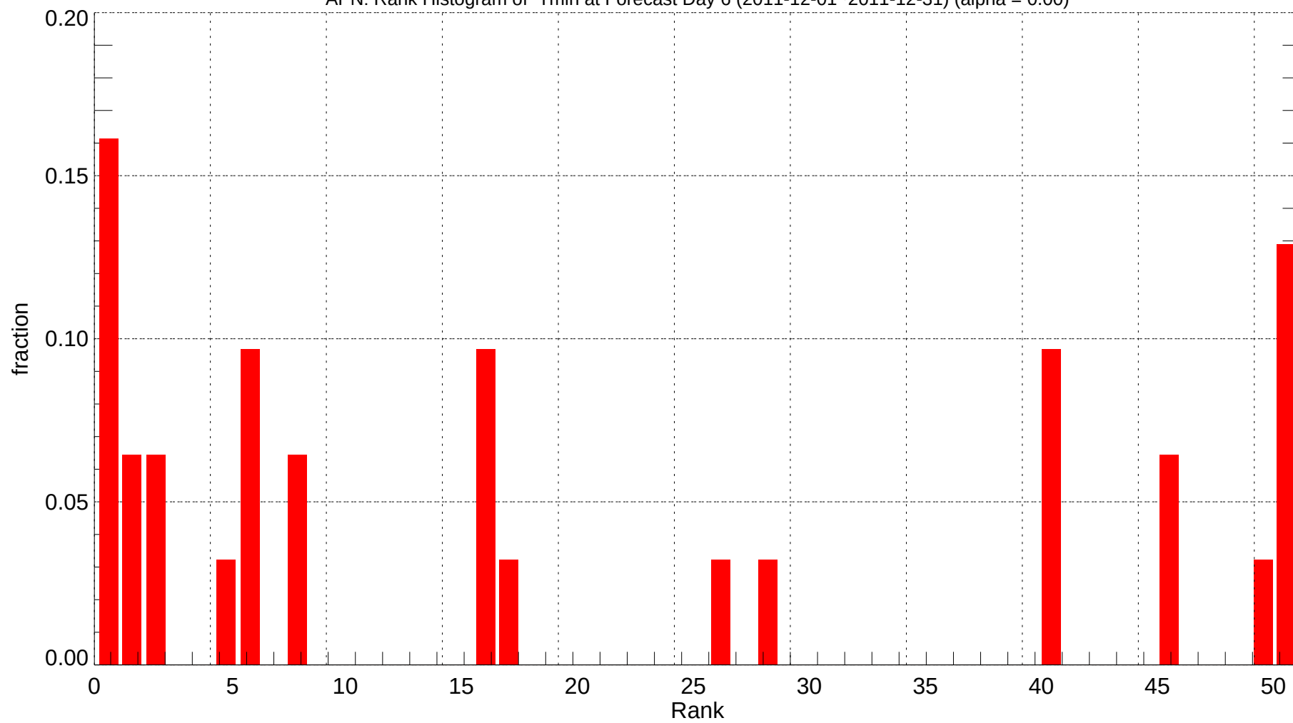
APN: Rank Histogram of Tmin at Forecast Day 6 (2011-12-01~2011-12-31) (alpha = 0.00)
