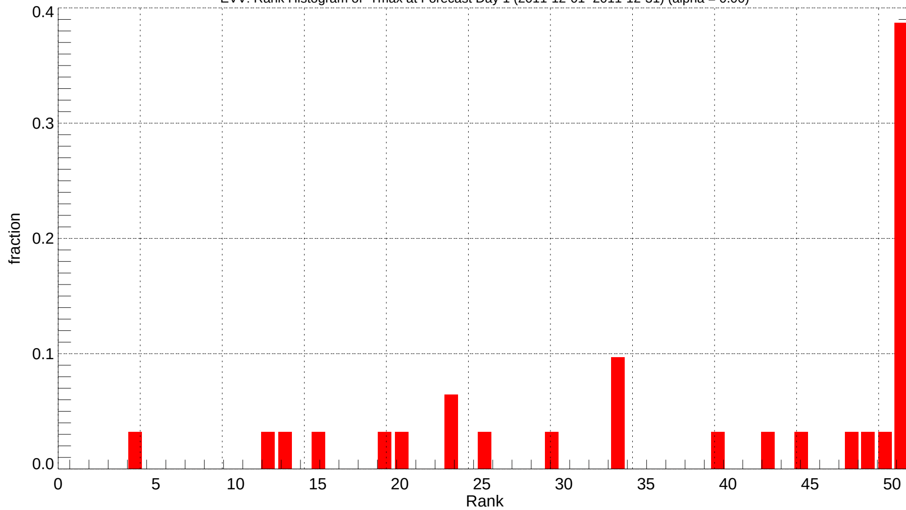
EVV: Rank Histogram of Tmax at Forecast Day 1 (2011-12-01~2011-12-31) (alpha = 0.00)
