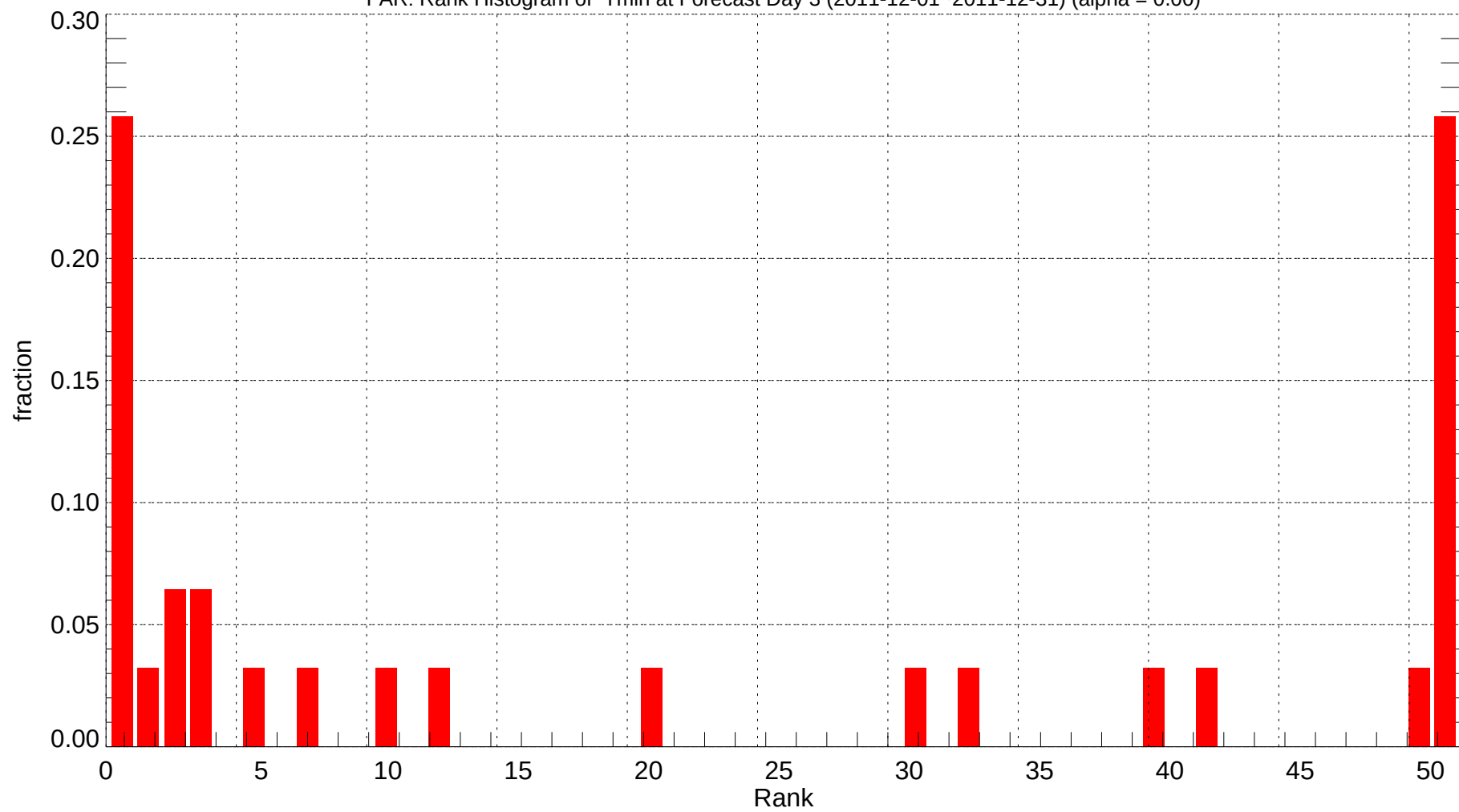
FAR: Rank Histogram of Tmin at Forecast Day 3 (2011-12-01~2011-12-31) (alpha = 0.00)
