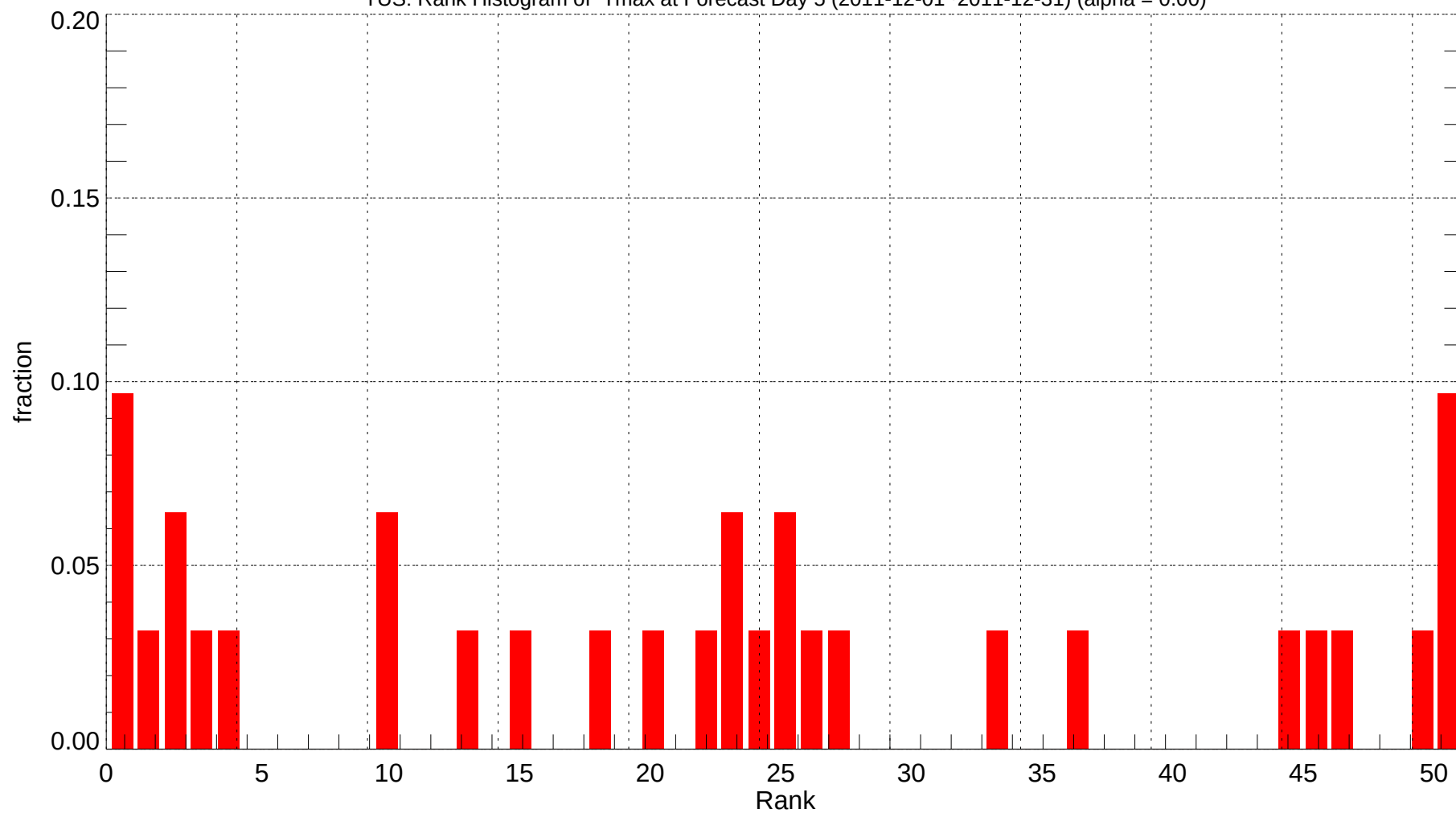
TUS: Rank Histogram of Tmax at Forecast Day 5 (2011-12-01~2011-12-31) (alpha = 0.00)
