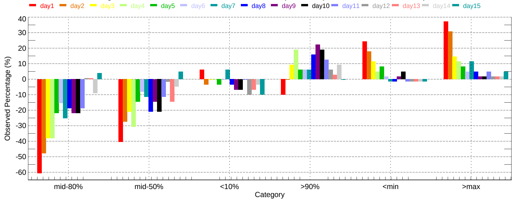
Observed Percentage Deviation of Ensembles - MSY: Min Temperature (2011-12-01~2011-12-31)
