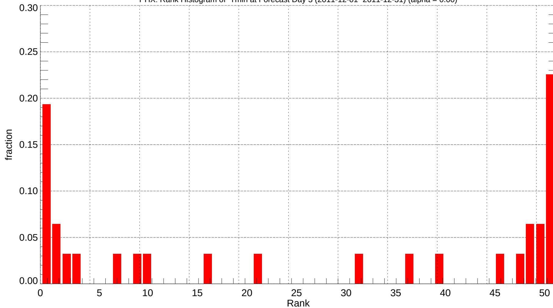
PHX: Rank Histogram of Tmin at Forecast Day 3 (2011-12-01~2011-12-31) (alpha = 0.00)
