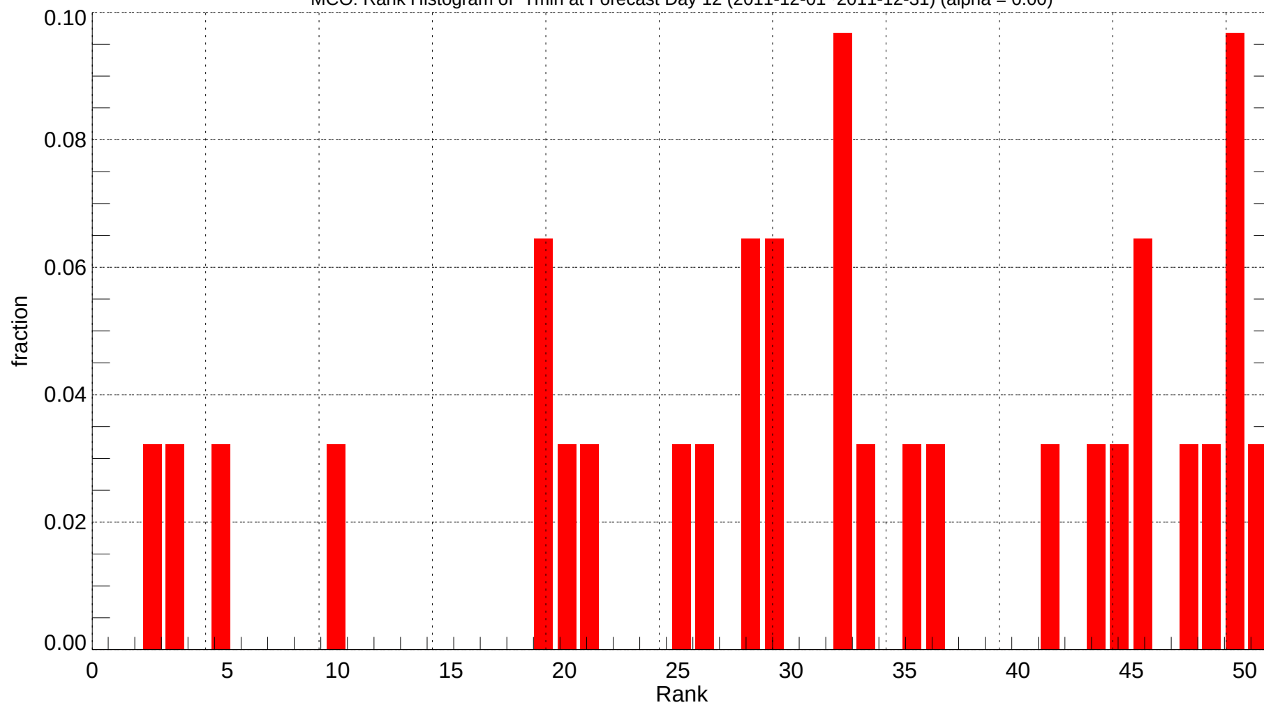
MCO: Rank Histogram of Tmin at Forecast Day 12 (2011-12-01~2011-12-31) (alpha = 0.00)
