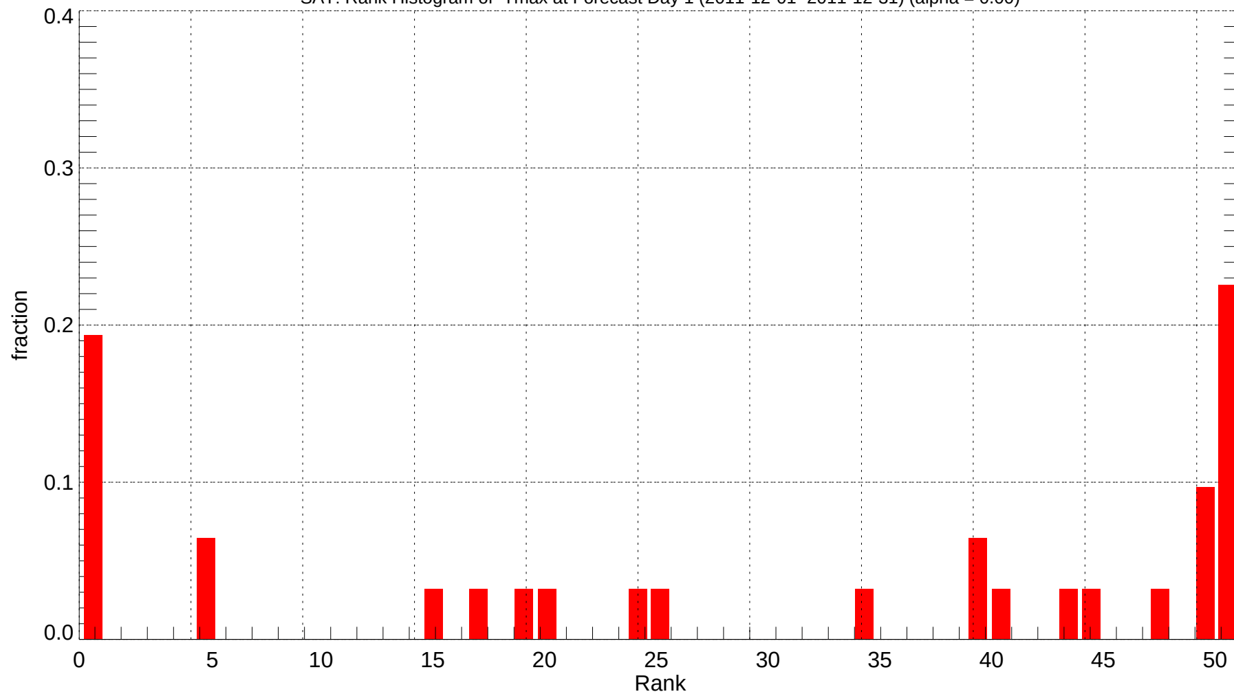
SAT: Rank Histogram of Tmax at Forecast Day 1 (2011-12-01~2011-12-31) (alpha = 0.00)
