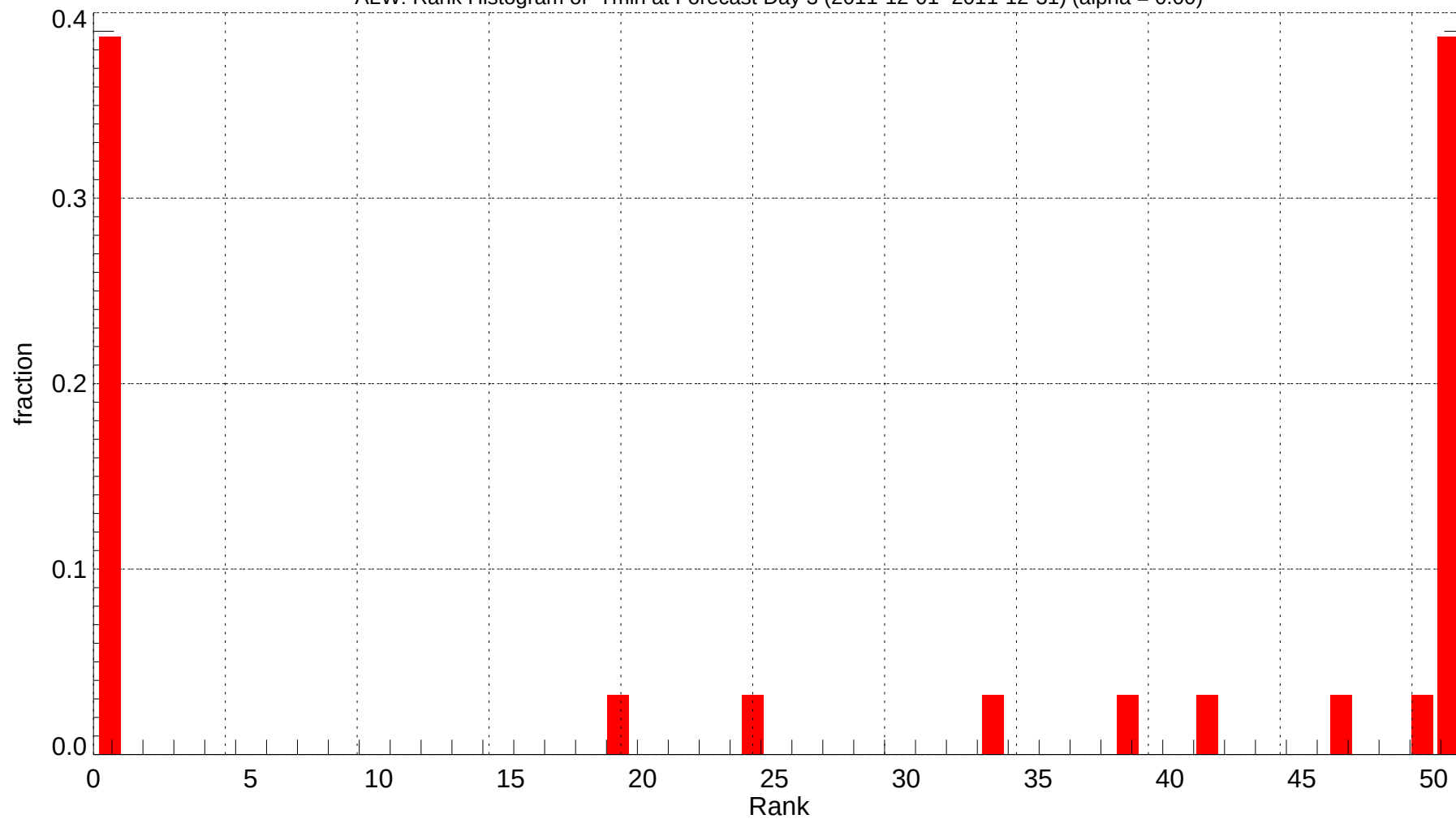
ALW: Rank Histogram of Tmin at Forecast Day 3 (2011-12-01~2011-12-31) (alpha = 0.00)
