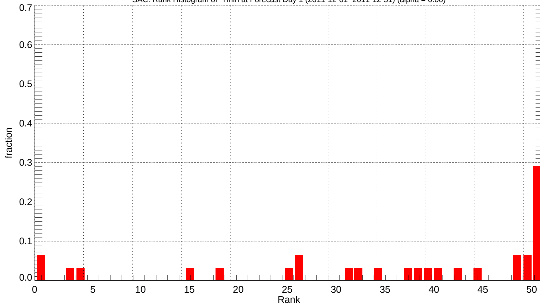
SAC: Rank Histogram of Tmin at Forecast Day 1 (2011-12-01~2011-12-31) (alpha = 0.00)
