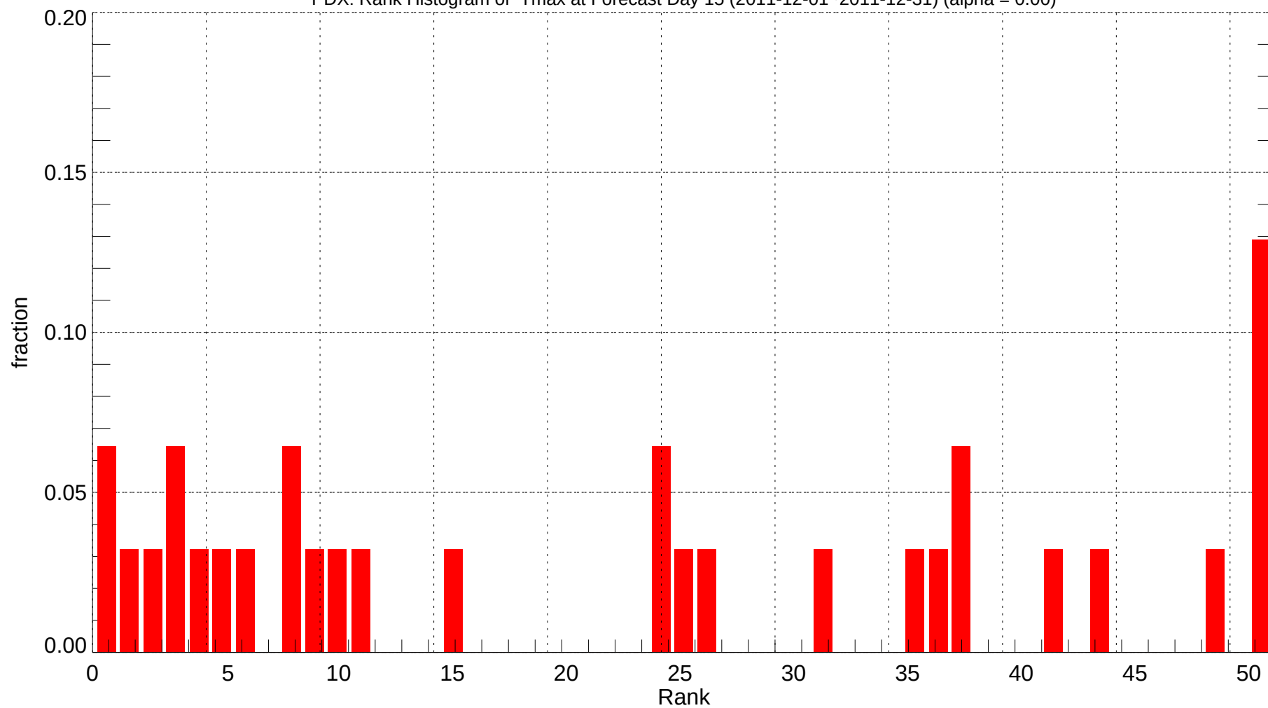
PDX: Rank Histogram of Tmax at Forecast Day 15 (2011-12-01~2011-12-31) (alpha = 0.00)
