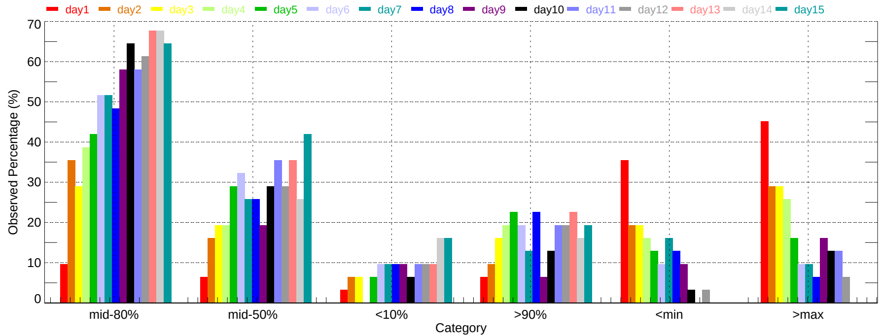
Observed Percentage of Ensembles - ROC: Min Temperature (2011-12-01~2011-12-31)
