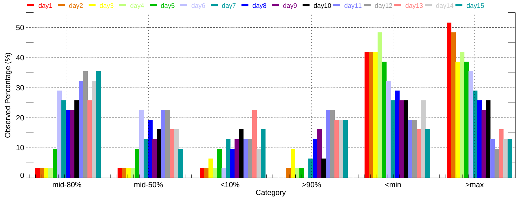
Observed Percentage of Ensembles - NKX: Max Temperature (2011-12-01~2011-12-31)
