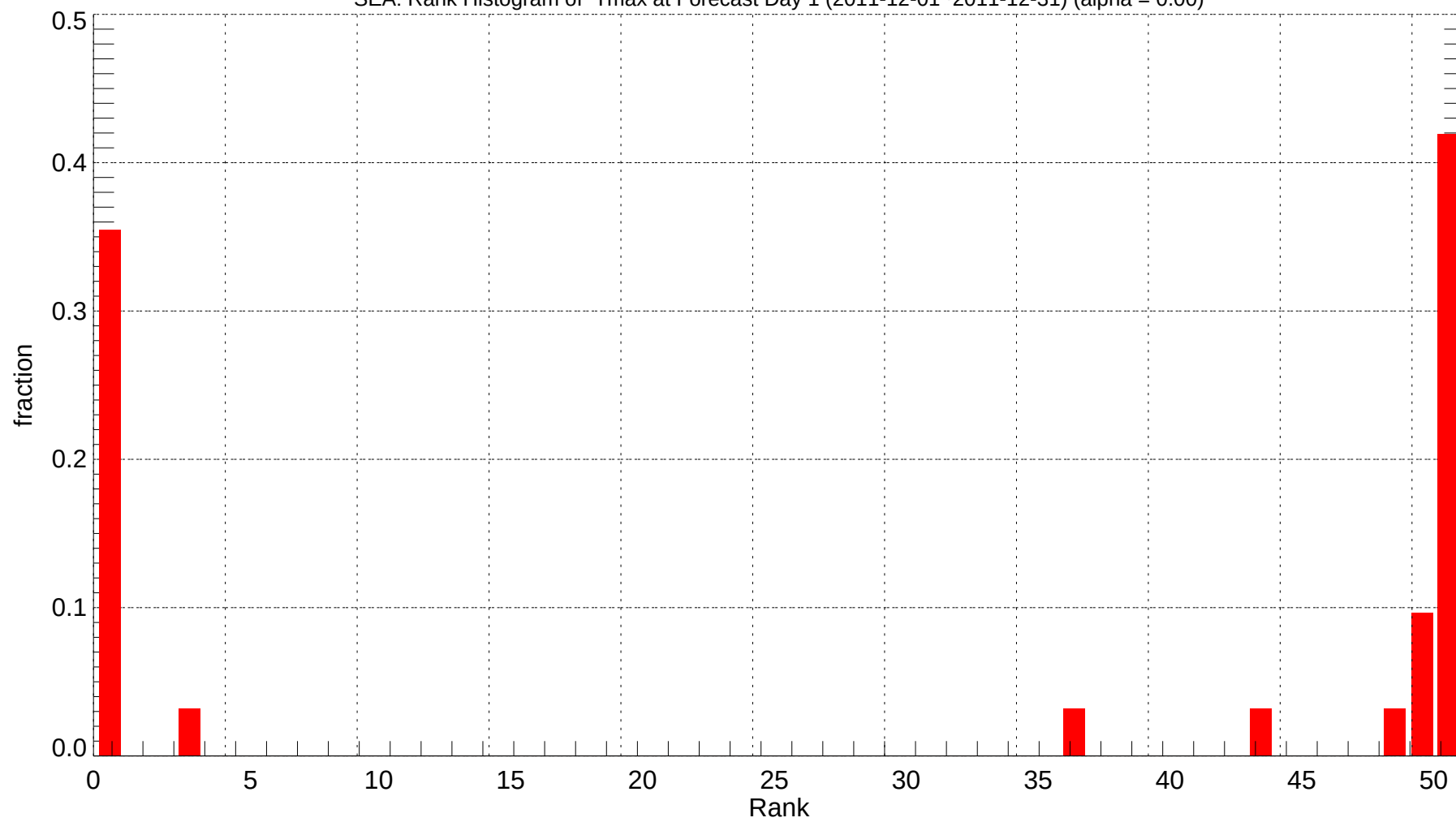
SEA: Rank Histogram of Tmax at Forecast Day 1 (2011-12-01~2011-12-31) (alpha = 0.00)
