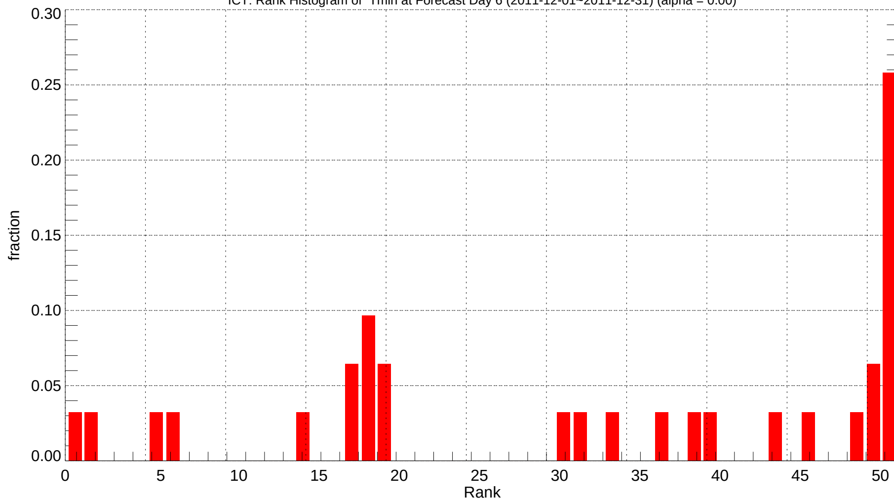
ICT: Rank Histogram of Tmin at Forecast Day 6 (2011-12-01~2011-12-31) (alpha = 0.00)
