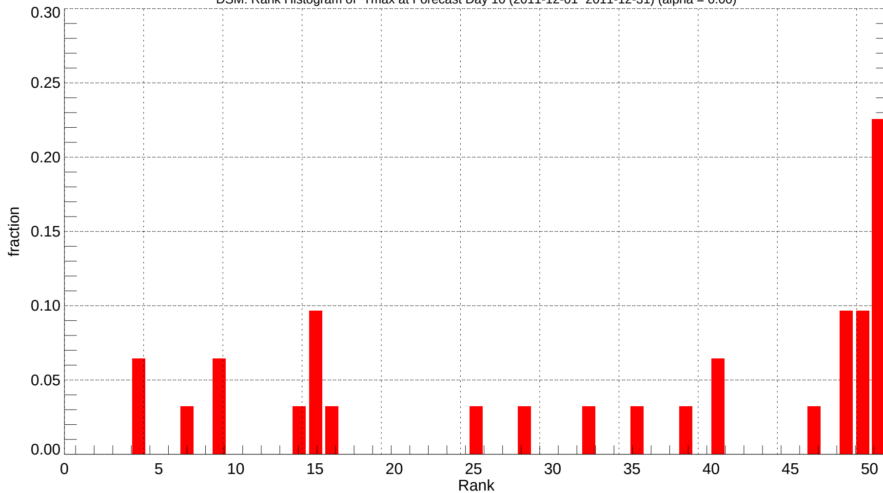
DSM: Rank Histogram of Tmax at Forecast Day 10 (2011-12-01~2011-12-31) (alpha = 0.00)
