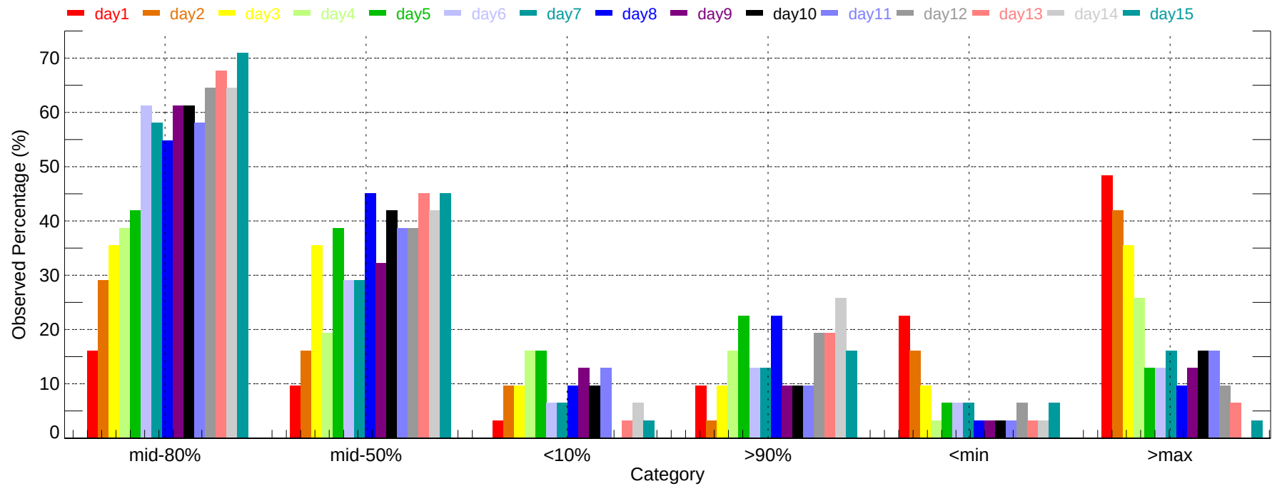
Observed Percentage of Ensembles - COS: Max Temperature (2011-12-01~2011-12-31)
