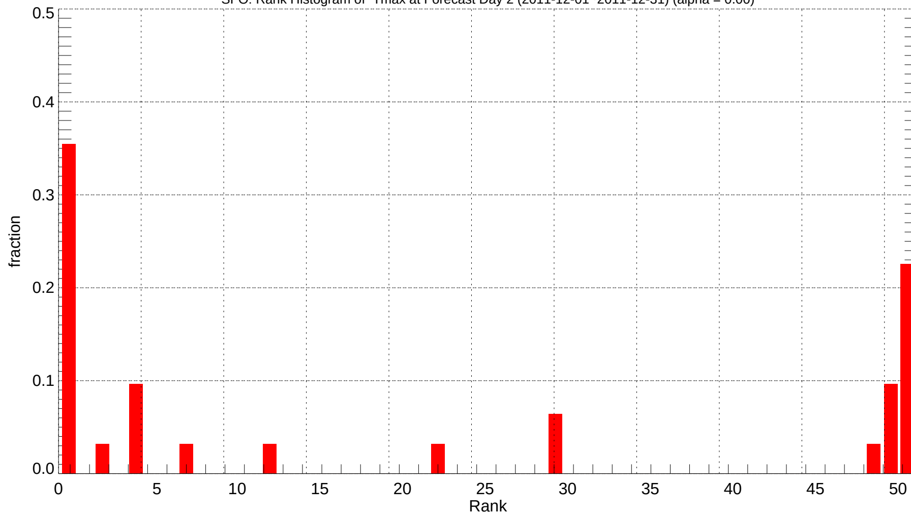
SFO: Rank Histogram of Tmax at Forecast Day 2 (2011-12-01~2011-12-31) (alpha = 0.00)
