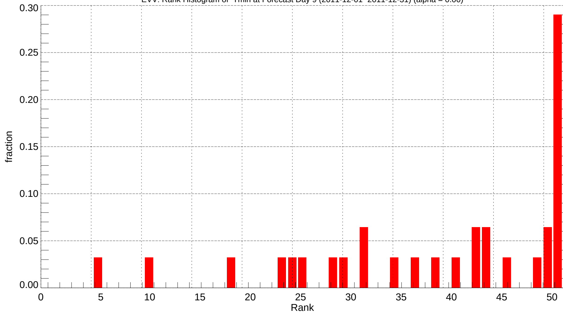
EVV: Rank Histogram of Tmin at Forecast Day 9 (2011-12-01~2011-12-31) (alpha = 0.00)
