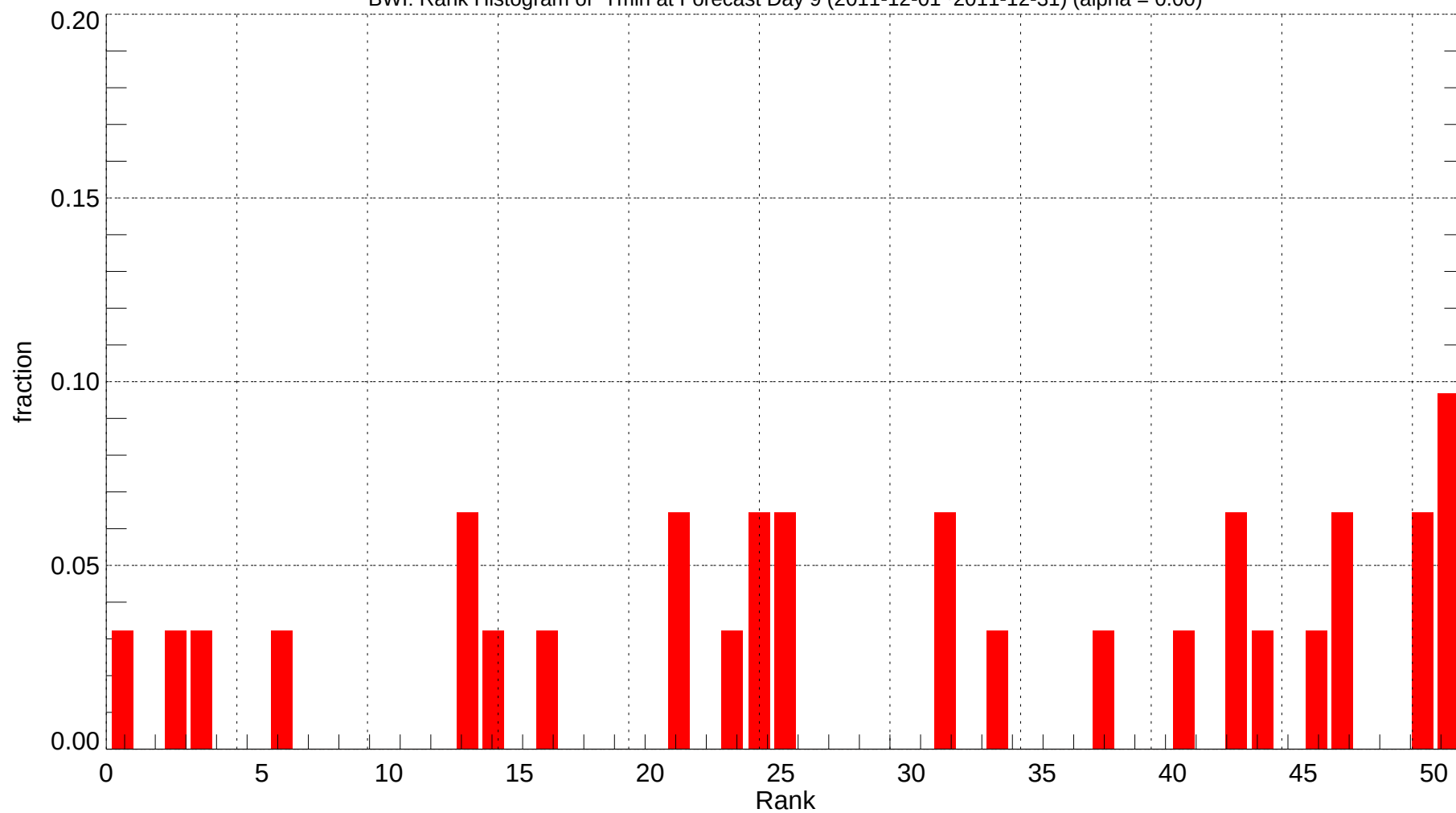
BWI: Rank Histogram of Tmin at Forecast Day 9 (2011-12-01~2011-12-31) (alpha = 0.00)
