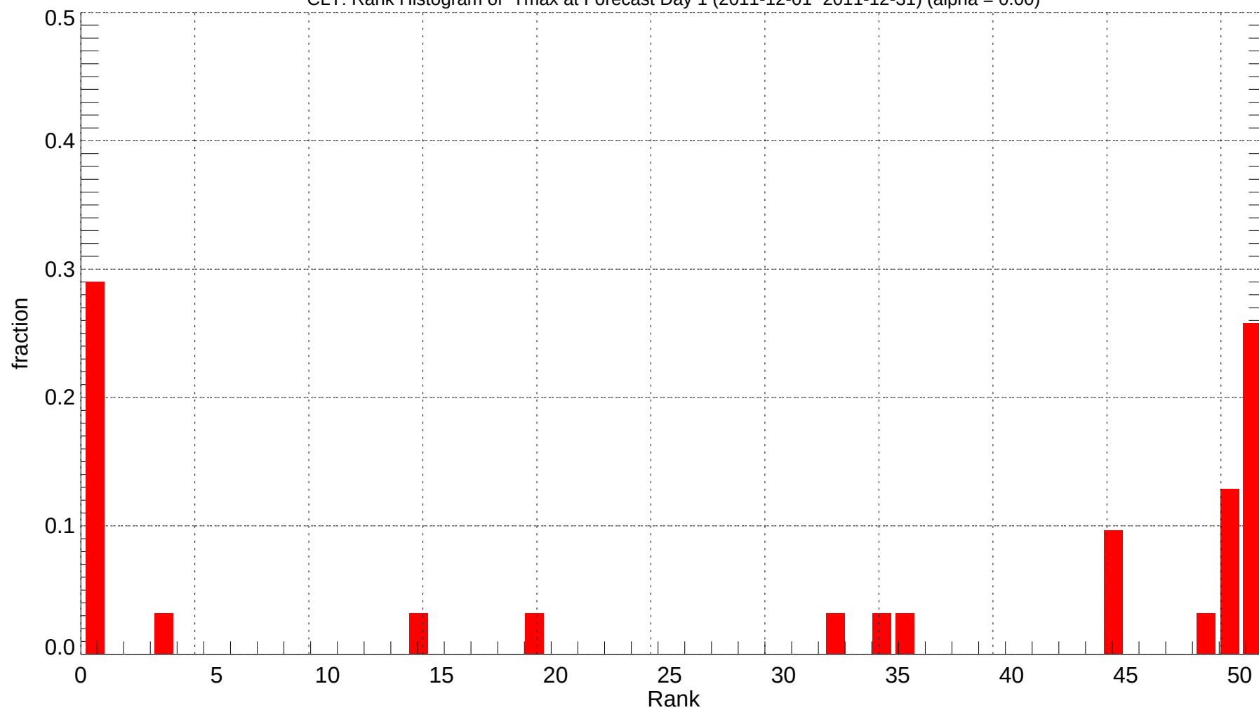
CLT: Rank Histogram of Tmax at Forecast Day 1 (2011-12-01~2011-12-31) (alpha = 0.00)
