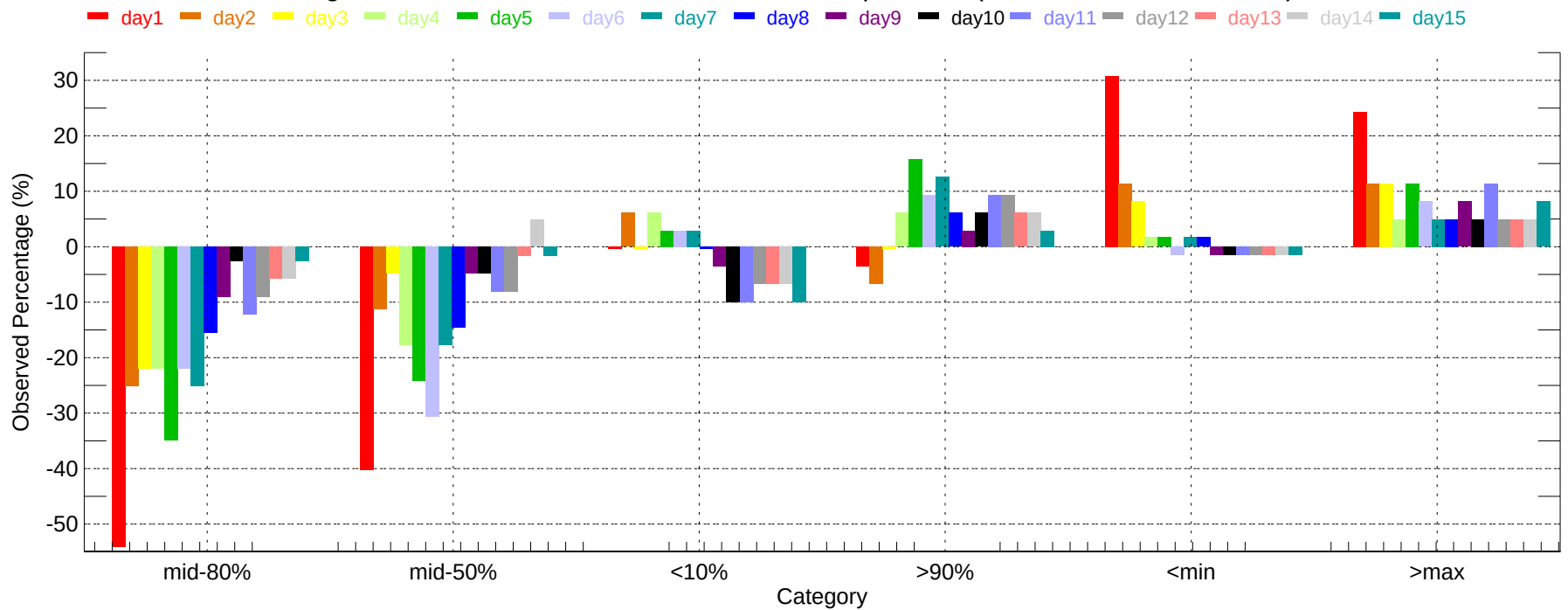
Observed Percentage Deviation of Ensembles - ABY: Min Temperature (2011-12-01~2011-12-31)
