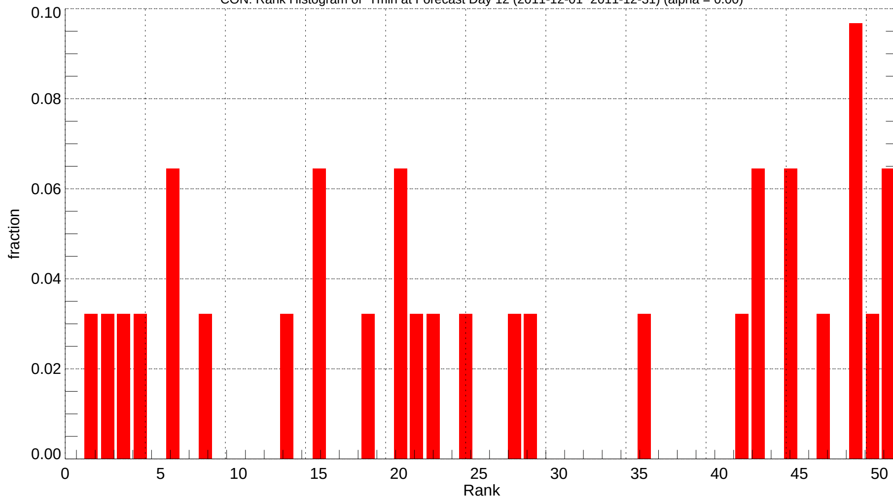
CON: Rank Histogram of Tmin at Forecast Day 12 (2011-12-01~2011-12-31) (alpha = 0.00)
