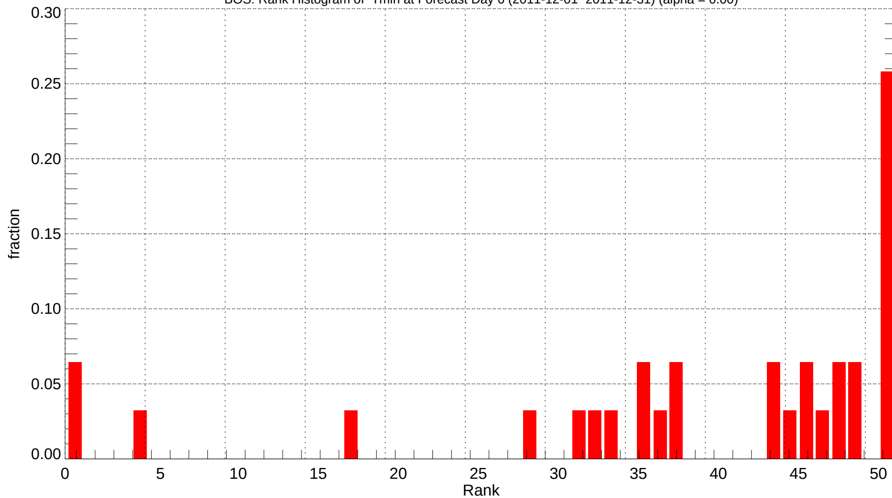
BOS: Rank Histogram of Tmin at Forecast Day 6 (2011-12-01~2011-12-31) (alpha = 0.00)
