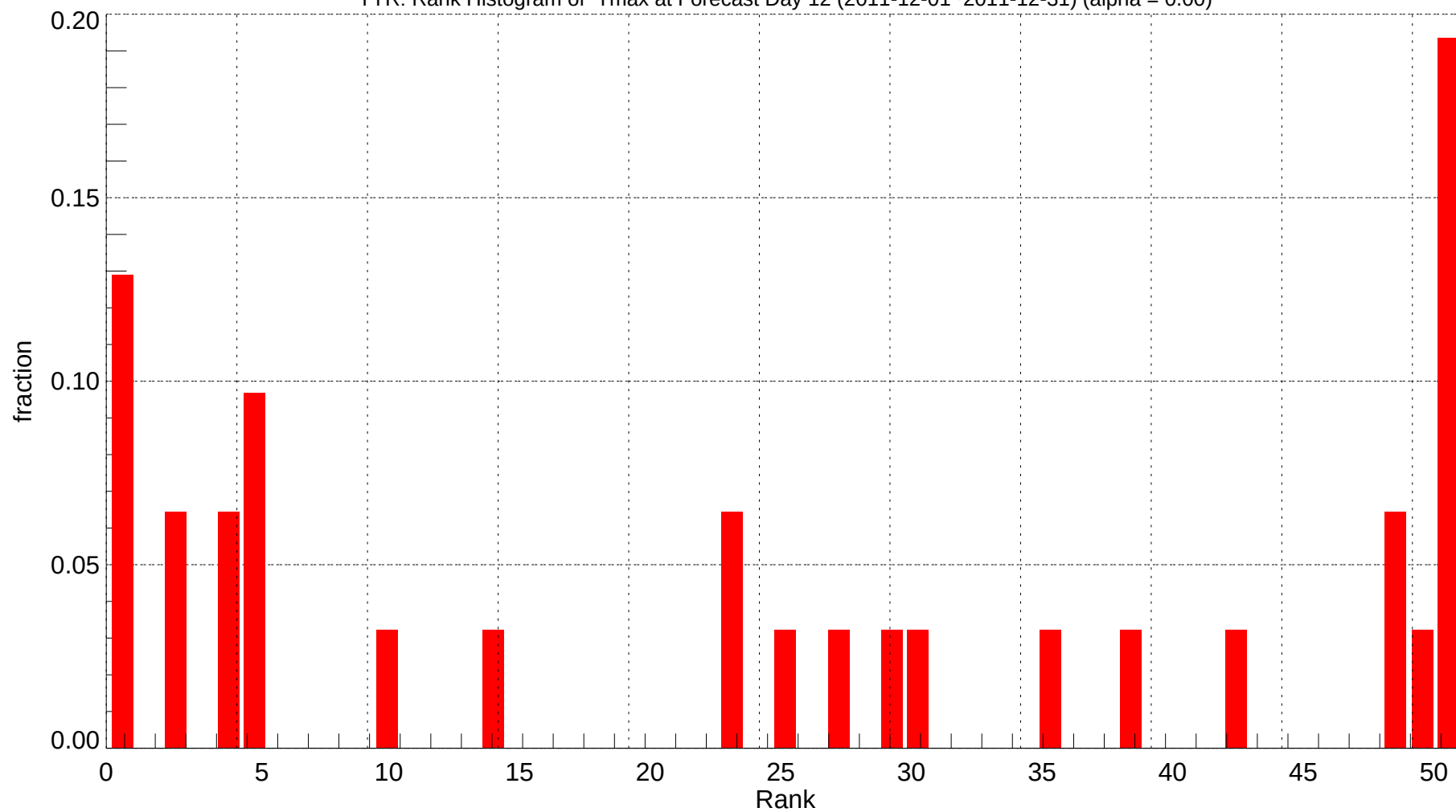
TYR: Rank Histogram of Tmax at Forecast Day 12 (2011-12-01~2011-12-31) (alpha = 0.00)
