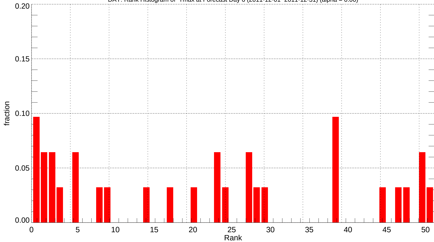
DAY: Rank Histogram of Tmax at Forecast Day 6 (2011-12-01~2011-12-31) (alpha = 0.00)
