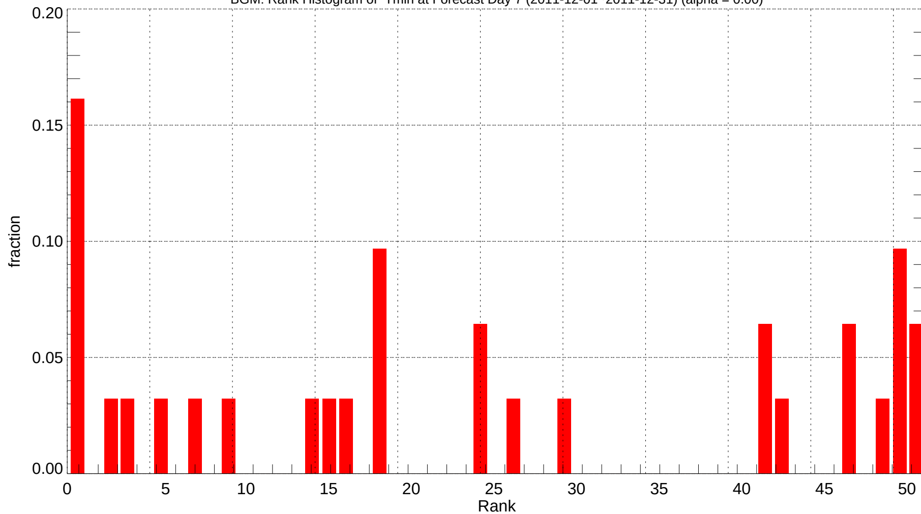
BGM: Rank Histogram of Tmin at Forecast Day 7 (2011-12-01~2011-12-31) (alpha = 0.00)
