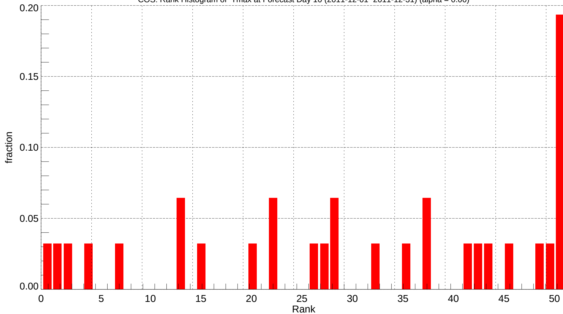
COS: Rank Histogram of Tmax at Forecast Day 10 (2011-12-01~2011-12-31) (alpha = 0.00)
