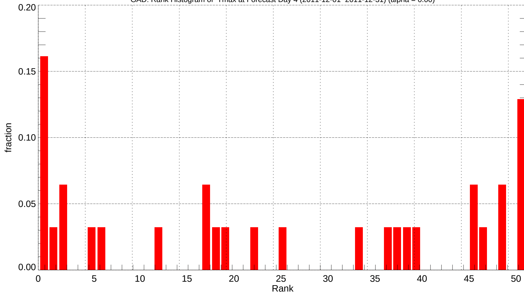
GAD: Rank Histogram of Tmax at Forecast Day 4 (2011-12-01~2011-12-31) (alpha = 0.00)
