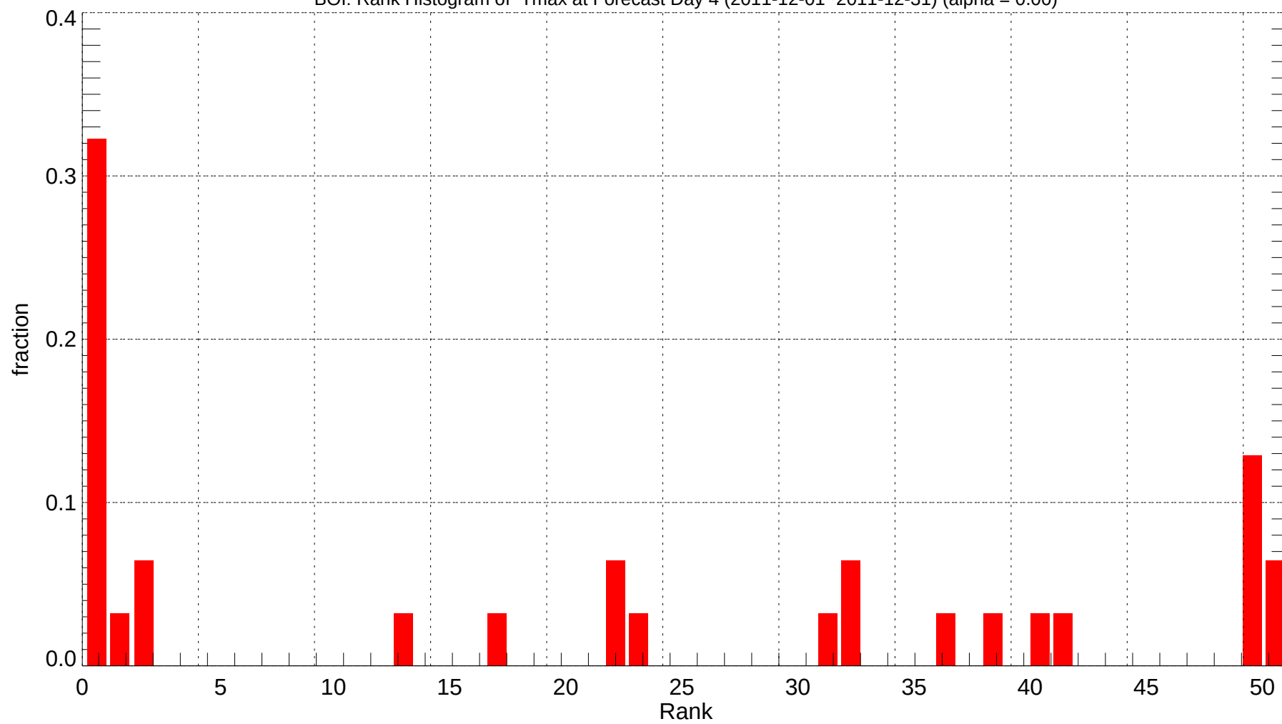
BOI: Rank Histogram of Tmax at Forecast Day 4 (2011-12-01~2011-12-31) (alpha = 0.00)
