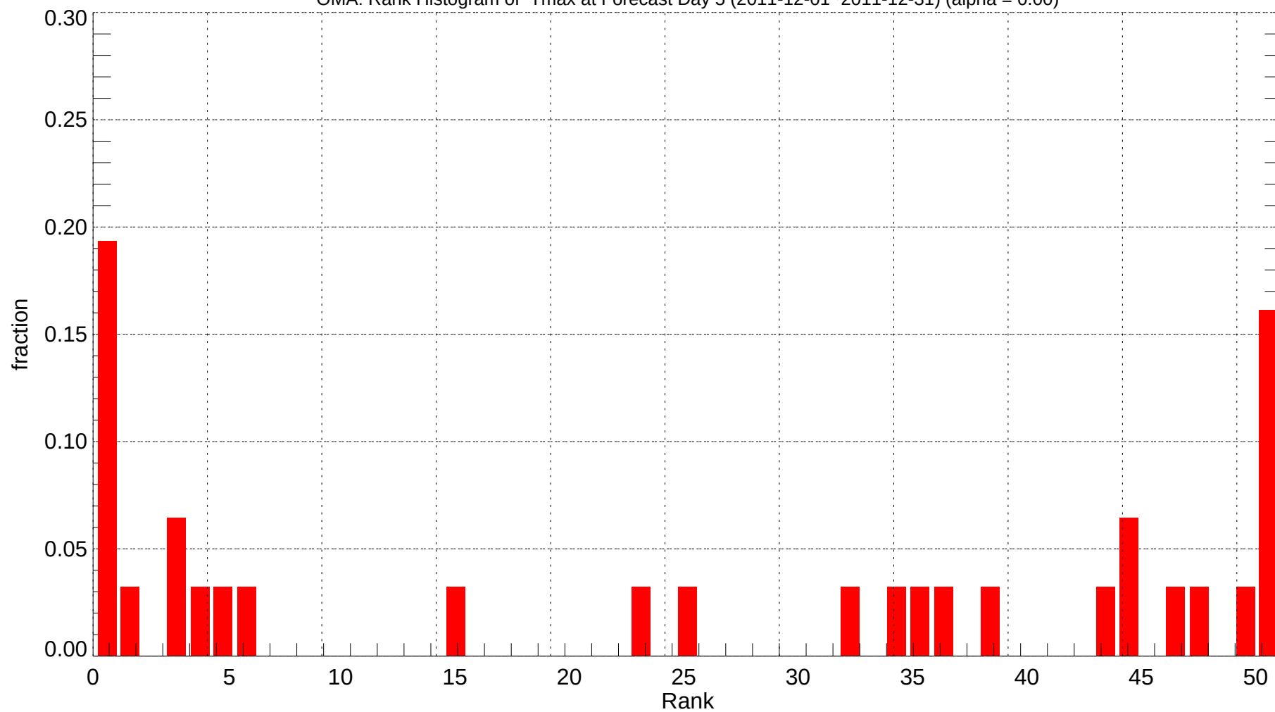
OMA: Rank Histogram of Tmax at Forecast Day 5 (2011-12-01~2011-12-31) (alpha = 0.00)
