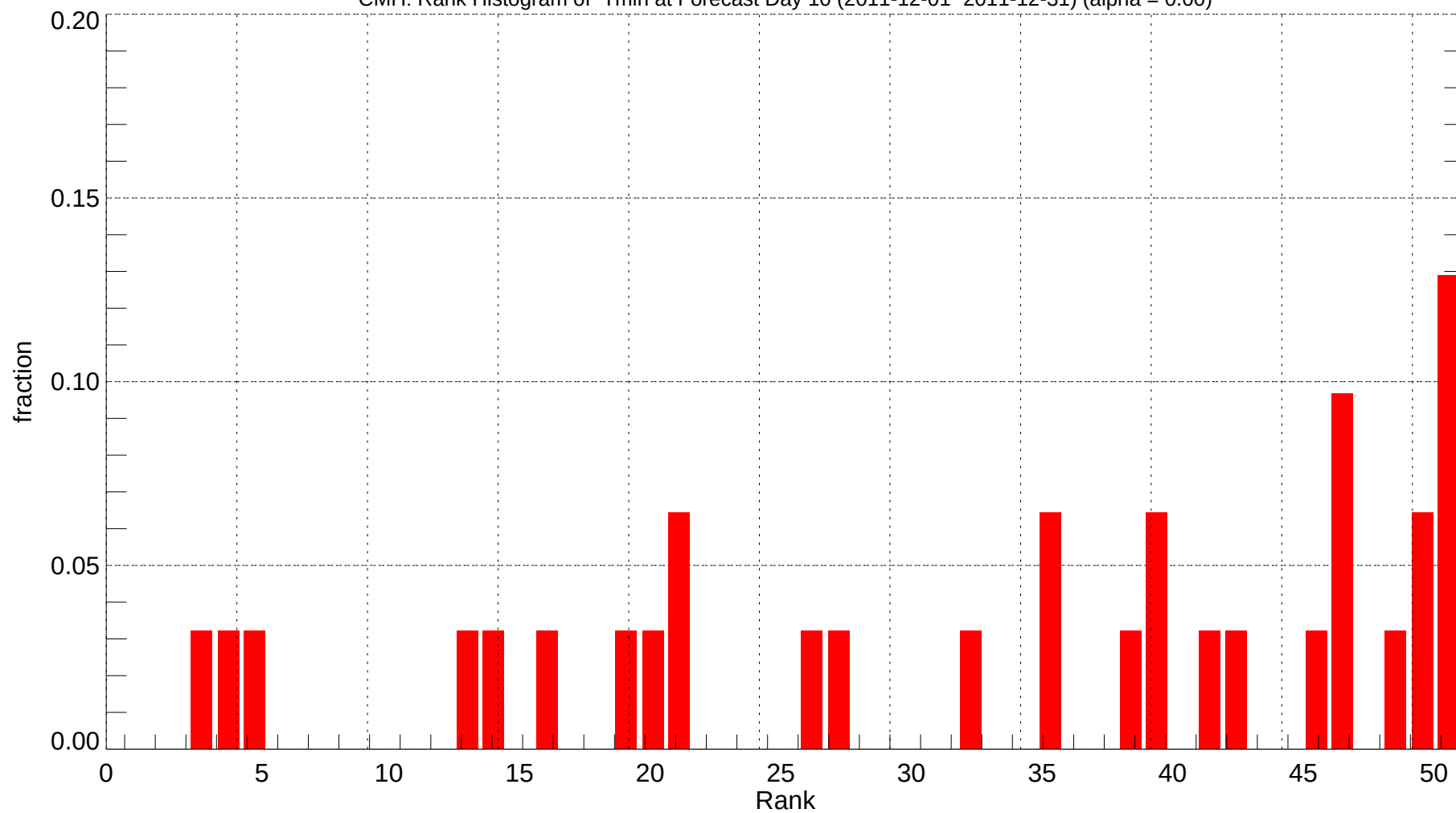
CMH: Rank Histogram of Tmin at Forecast Day 10 (2011-12-01~2011-12-31) (alpha = 0.00)
