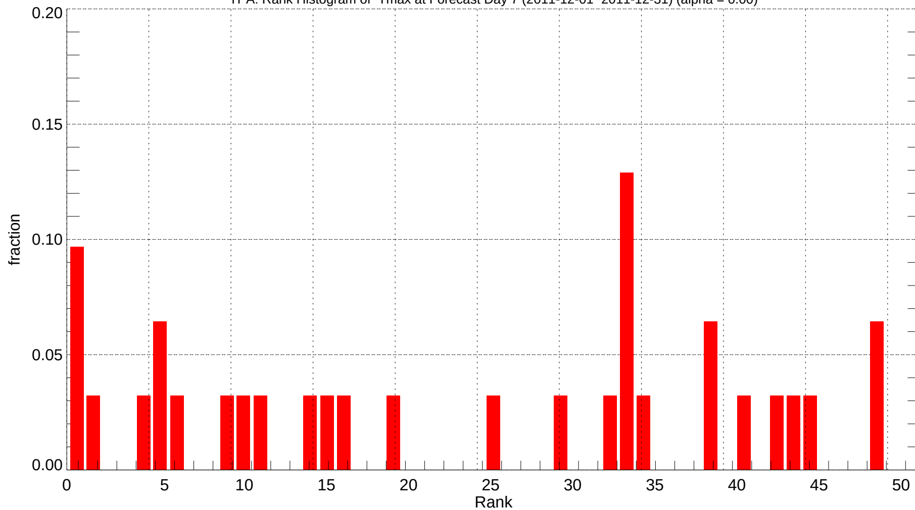
TPA: Rank Histogram of Tmax at Forecast Day 7 (2011-12-01~2011-12-31) (alpha = 0.00)
