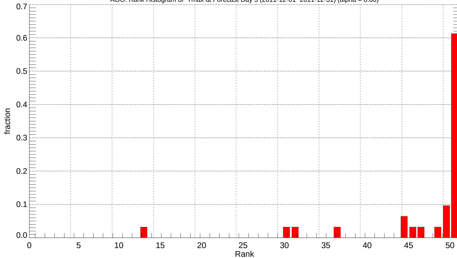
AOO: Rank Histogram of Tmax at Forecast Day 5 (2011-12-01~2011-12-31) (alpha = 0.00)
