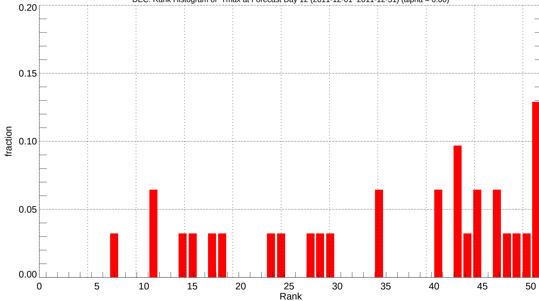
DEC: Rank Histogram of Tmax at Forecast Day 12 (2011-12-01~2011-12-31) (alpha = 0.00)
