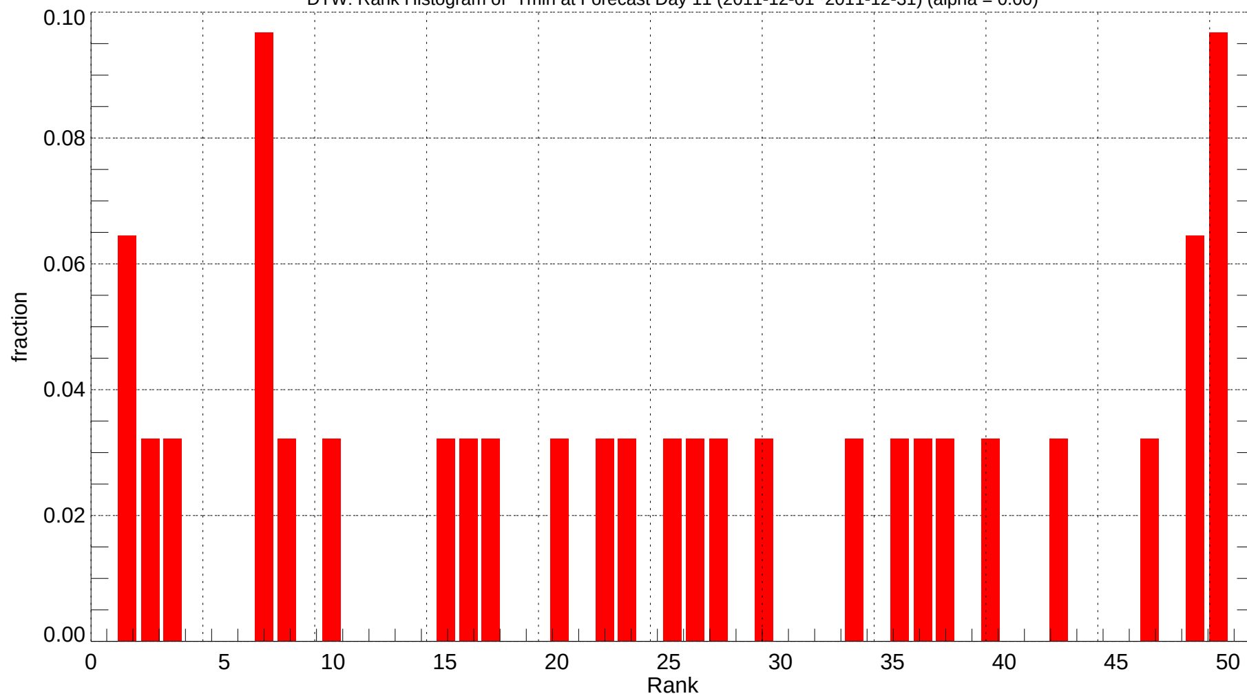
DTW: Rank Histogram of Tmin at Forecast Day 11 (2011-12-01~2011-12-31) (alpha = 0.00)
