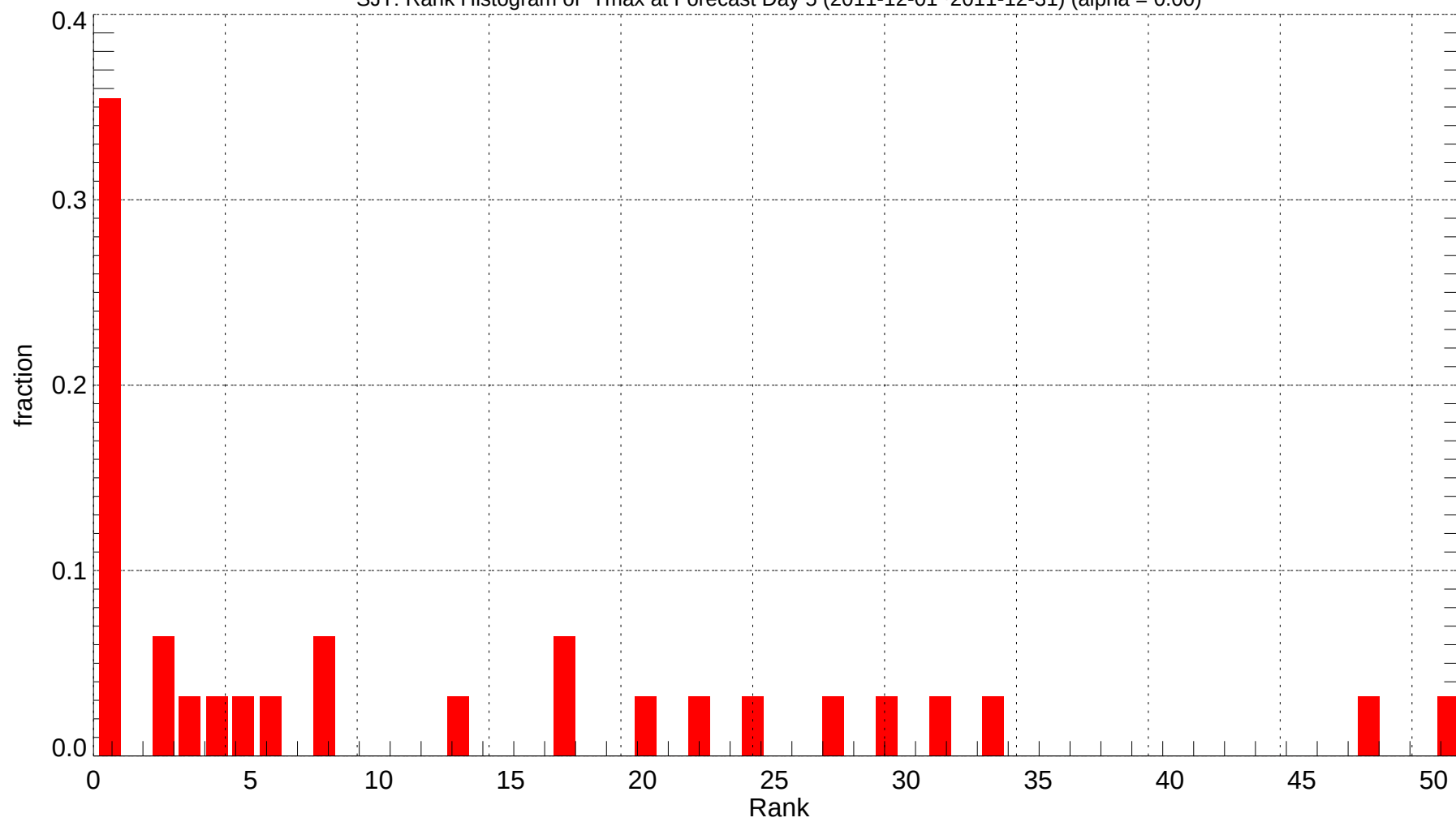
SJT: Rank Histogram of Tmax at Forecast Day 5 (2011-12-01~2011-12-31) (alpha = 0.00)
