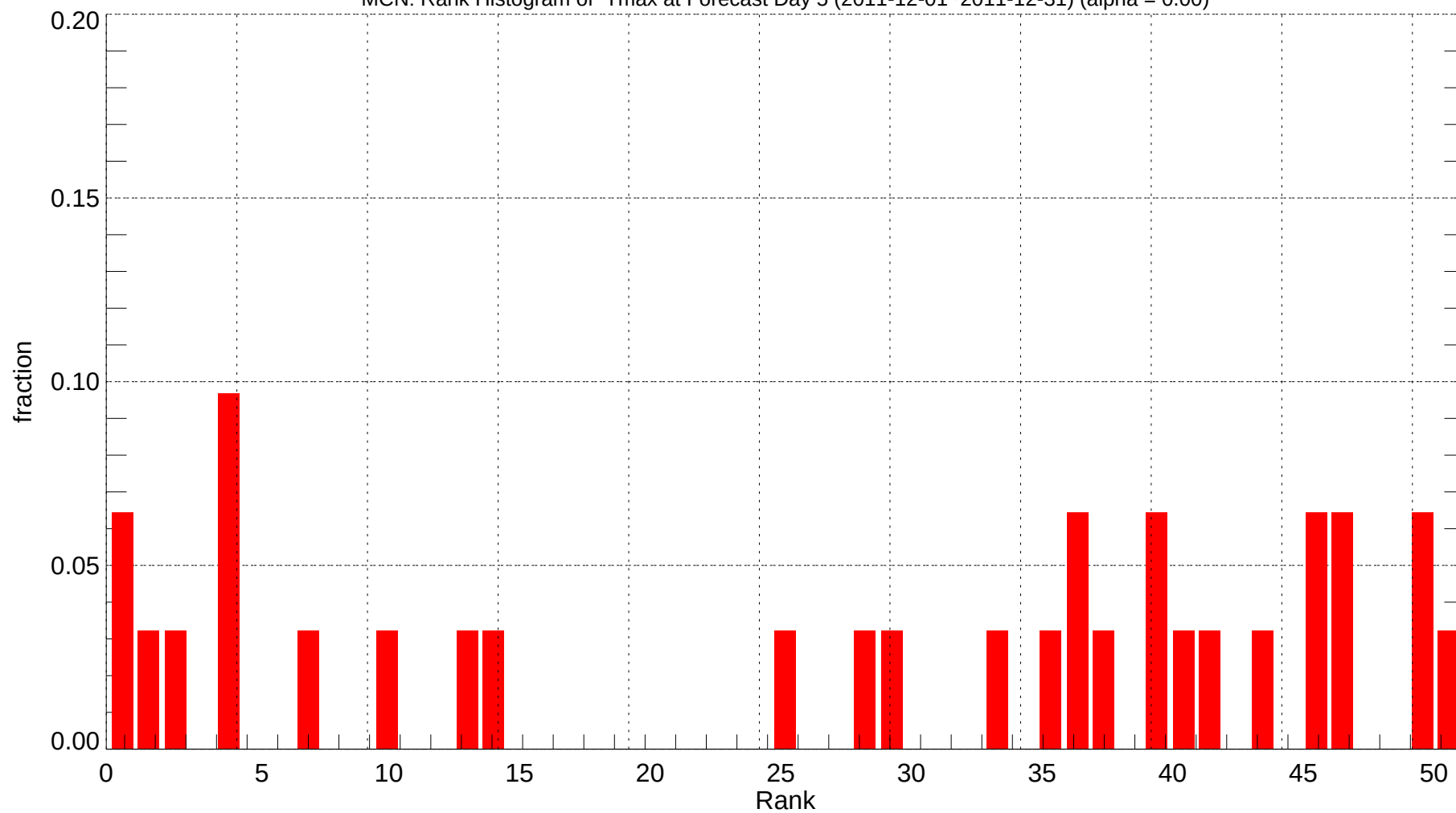
MCN: Rank Histogram of Tmax at Forecast Day 5 (2011-12-01~2011-12-31) (alpha = 0.00)
