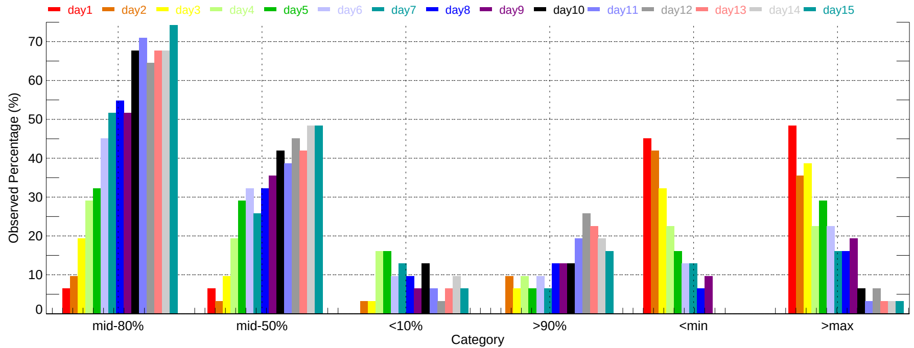
Observed Percentage of Ensembles - BWI: Min Temperature (2011-12-01~2011-12-31)
