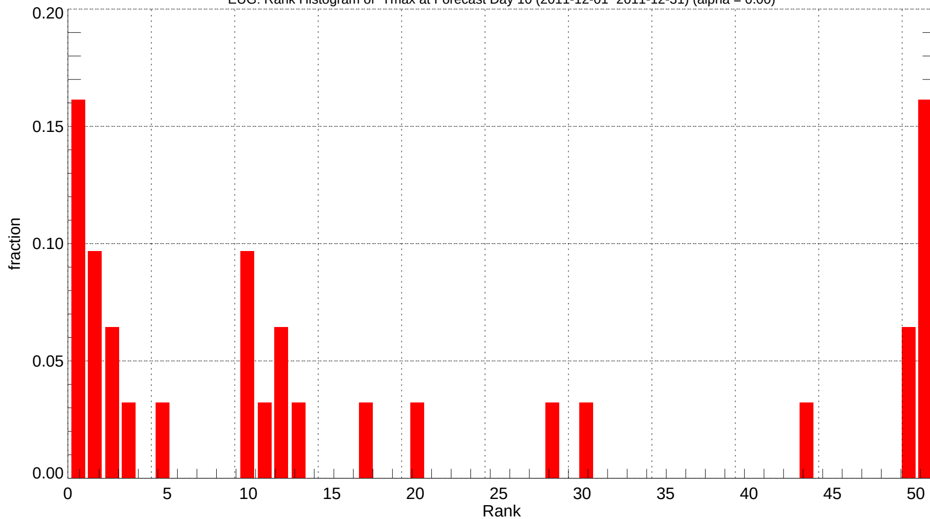
EUG: Rank Histogram of Tmax at Forecast Day 10 (2011-12-01~2011-12-31) (alpha = 0.00)
