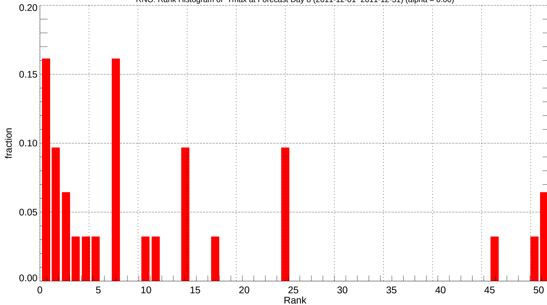
RNO: Rank Histogram of Tmax at Forecast Day 8 (2011-12-01~2011-12-31) (alpha = 0.00)
