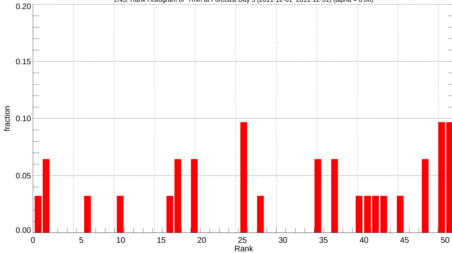
LNS: Rank Histogram of Tmin at Forecast Day 5 (2011-12-01~2011-12-31) (alpha = 0.00)
