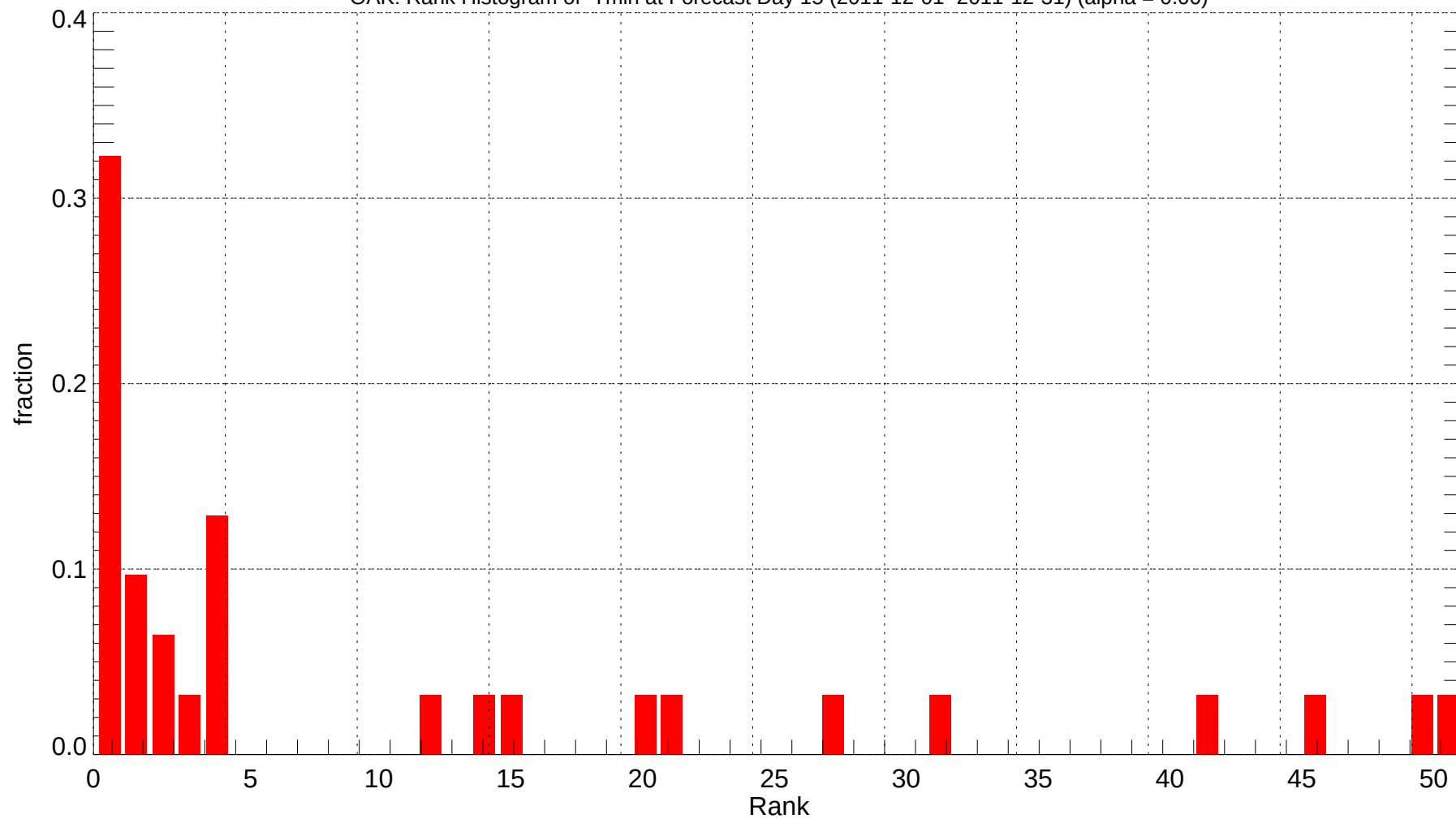
OAK: Rank Histogram of Tmin at Forecast Day 15 (2011-12-01~2011-12-31) (alpha = 0.00)
