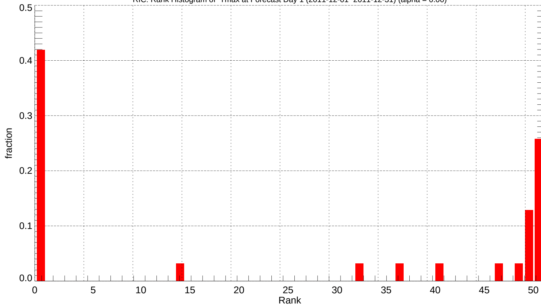
RIC: Rank Histogram of Tmax at Forecast Day 1 (2011-12-01~2011-12-31) (alpha = 0.00)
