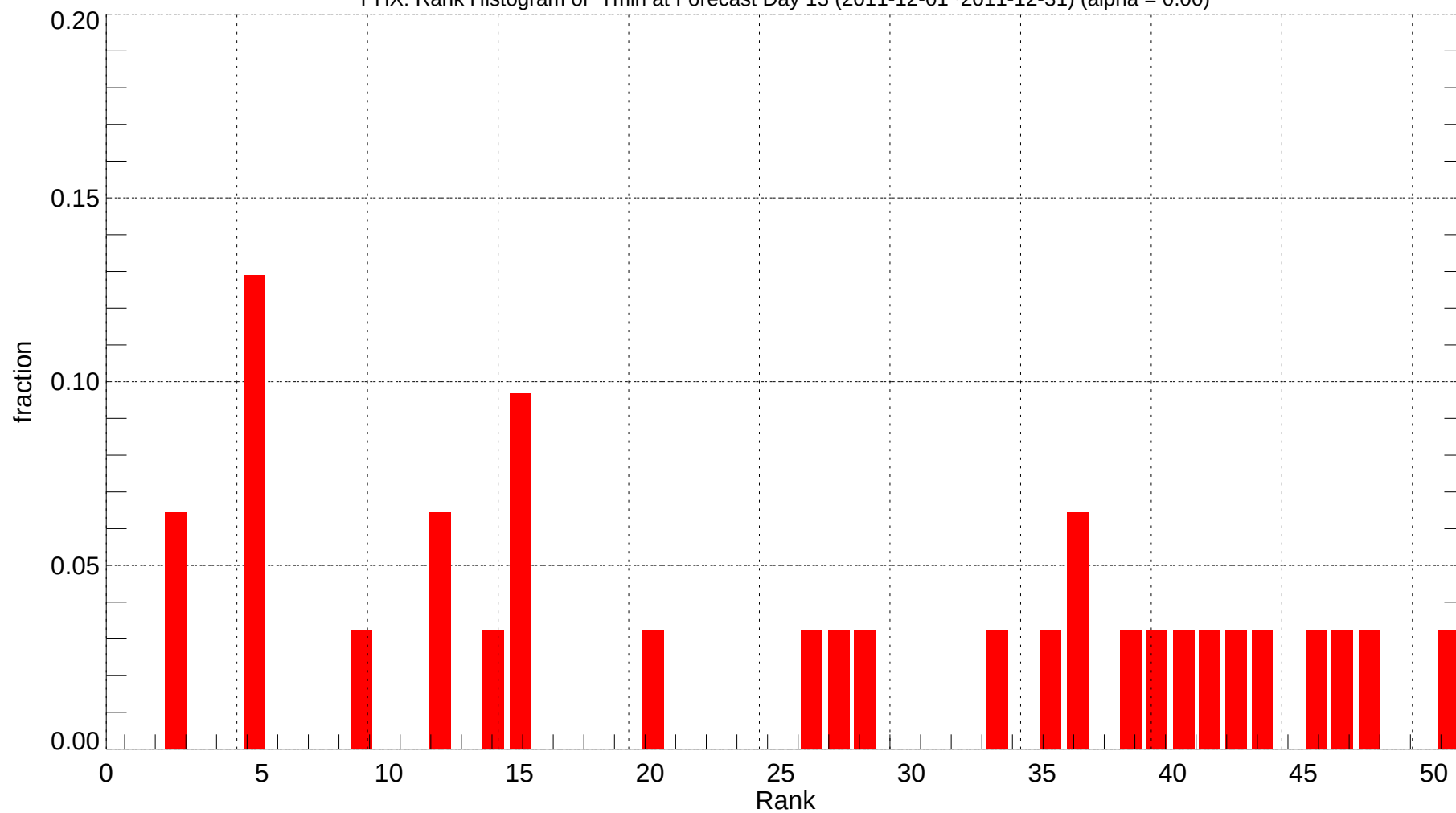
PHX: Rank Histogram of Tmin at Forecast Day 13 (2011-12-01~2011-12-31) (alpha = 0.00)
