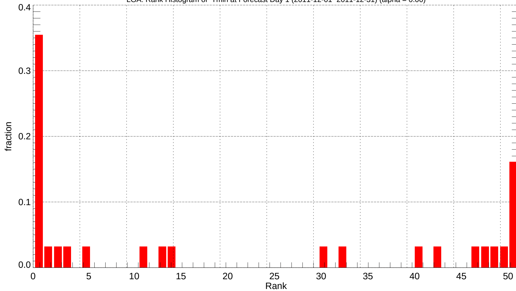
LGA: Rank Histogram of Tmin at Forecast Day 1 (2011-12-01~2011-12-31) (alpha = 0.00)
