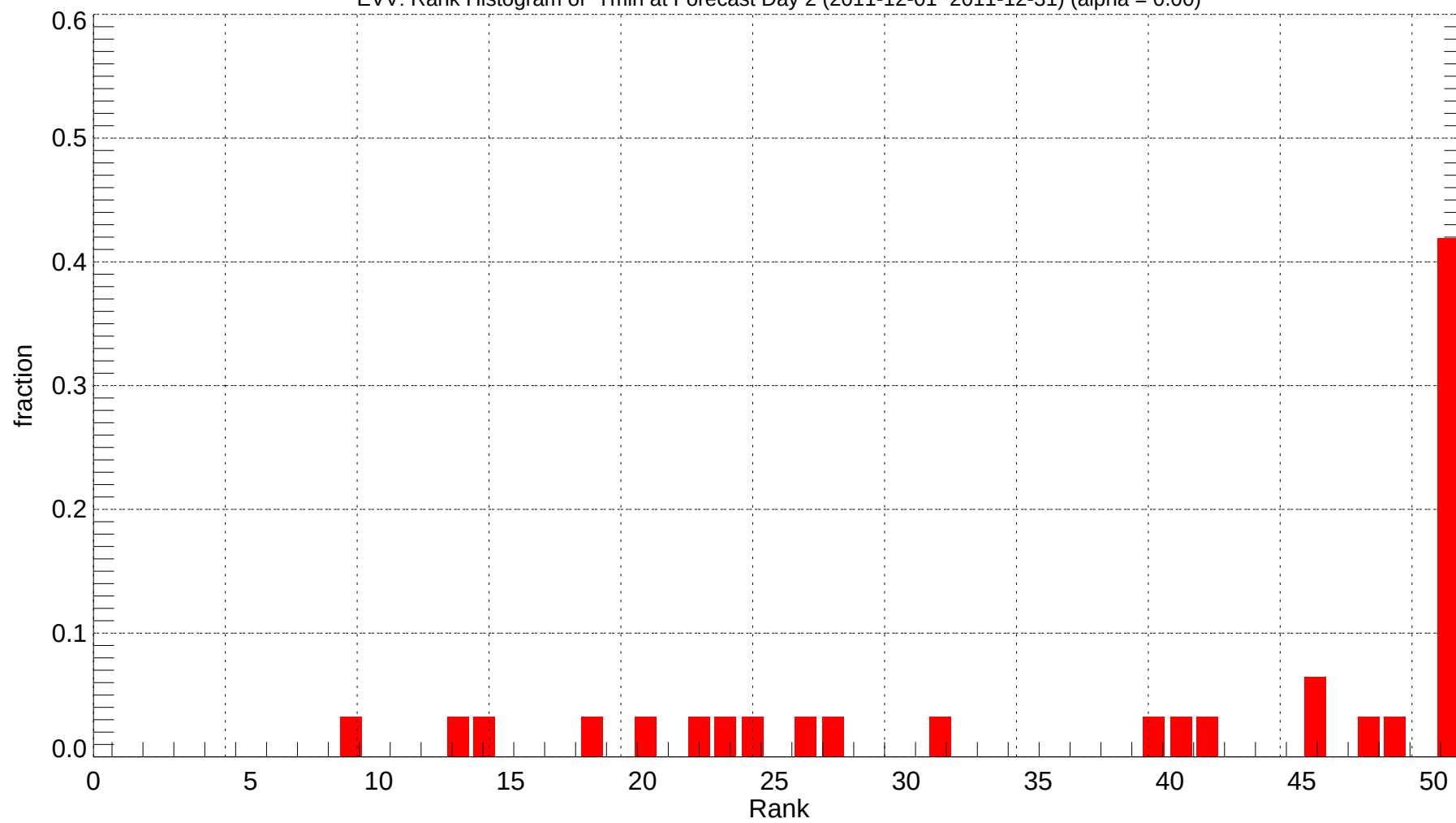
EVV: Rank Histogram of Tmin at Forecast Day 2 (2011-12-01~2011-12-31) (alpha = 0.00)
