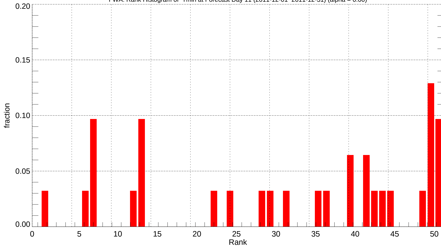
FWA: Rank Histogram of Tmin at Forecast Day 11 (2011-12-01~2011-12-31) (alpha = 0.00)
