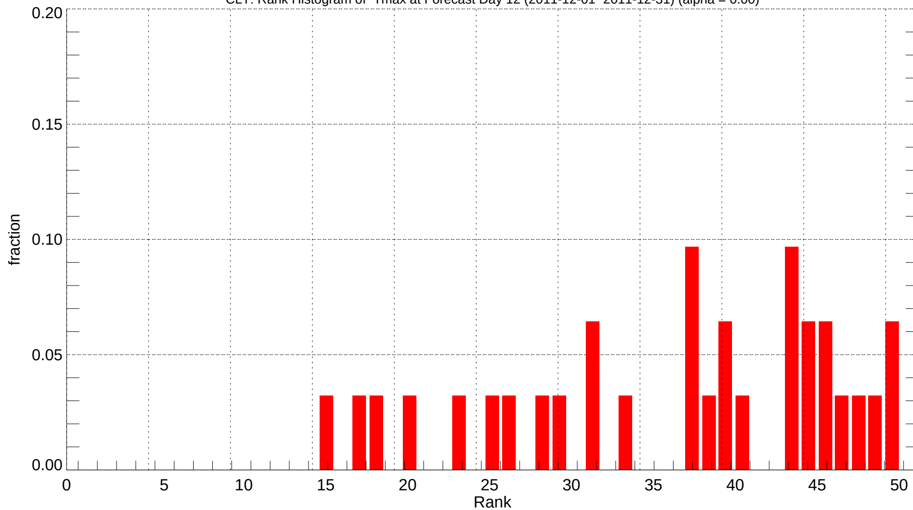
CLT: Rank Histogram of Tmax at Forecast Day 12 (2011-12-01~2011-12-31) (alpha = 0.00)
