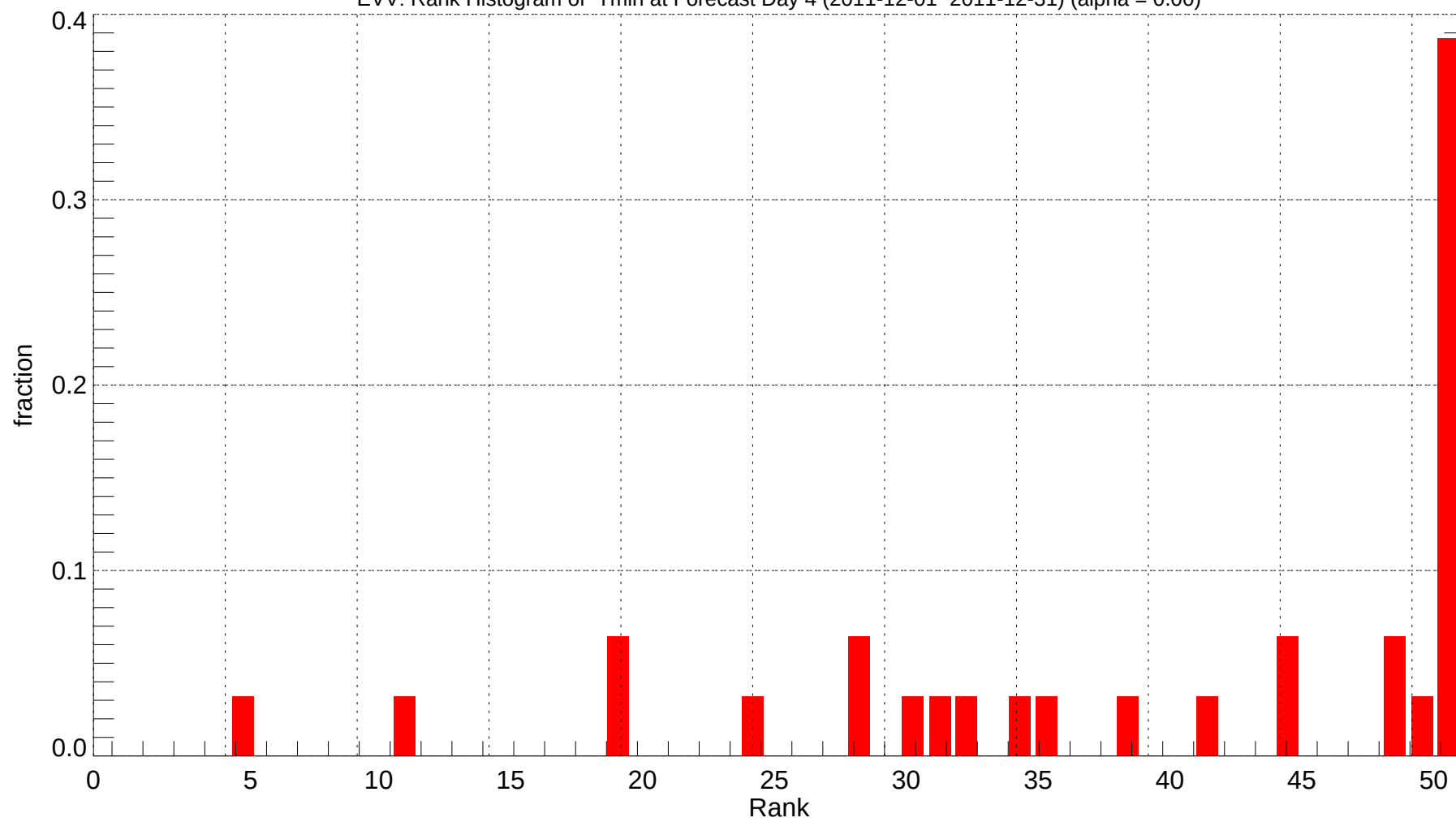
EVV: Rank Histogram of Tmin at Forecast Day 4 (2011-12-01~2011-12-31) (alpha = 0.00)
