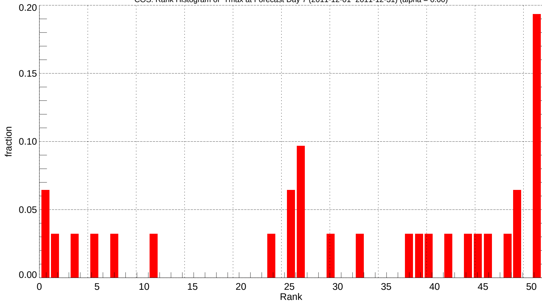
COS: Rank Histogram of Tmax at Forecast Day 7 (2011-12-01~2011-12-31) (alpha = 0.00)
