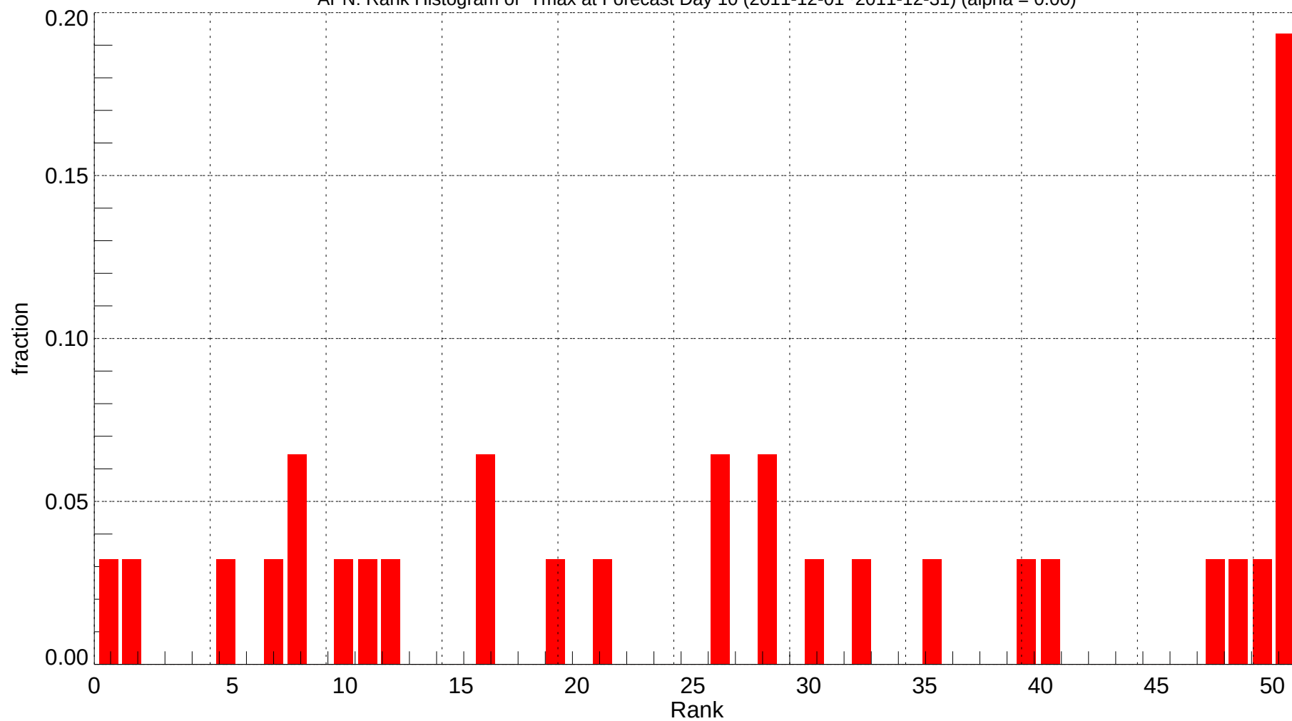
APN: Rank Histogram of Tmax at Forecast Day 10 (2011-12-01~2011-12-31) (alpha = 0.00)
