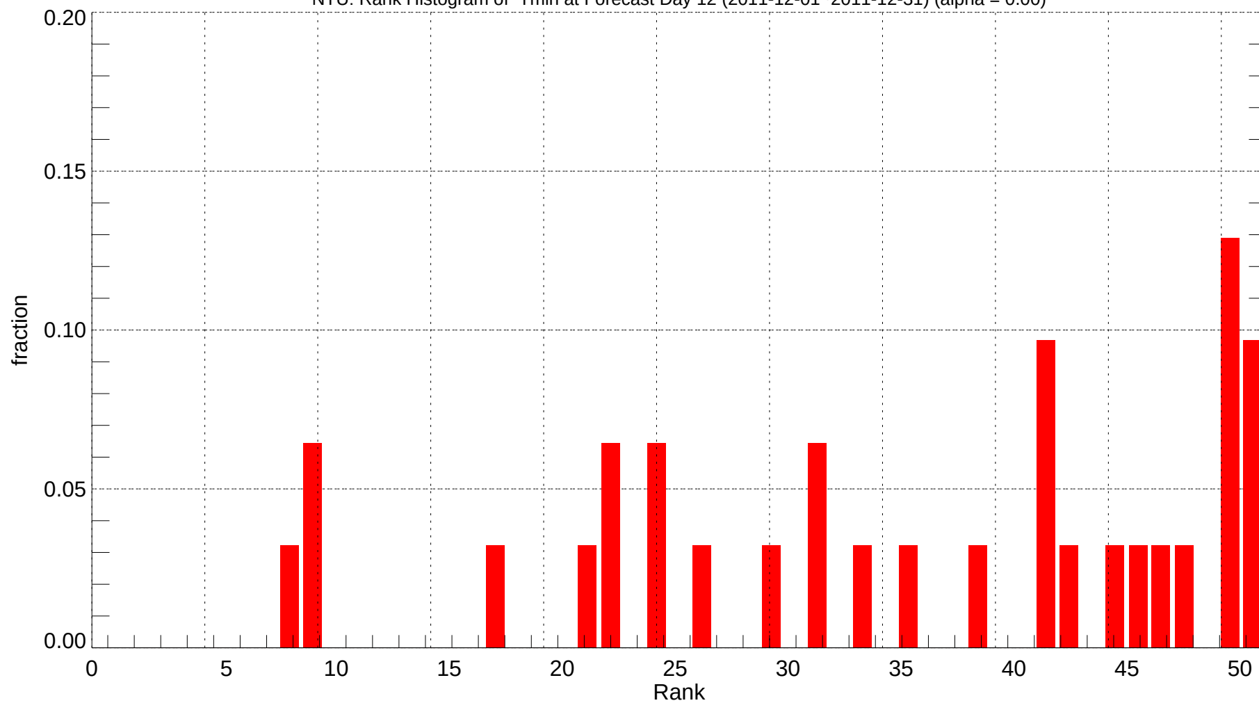
NTU: Rank Histogram of Tmin at Forecast Day 12 (2011-12-01~2011-12-31) (alpha = 0.00)
