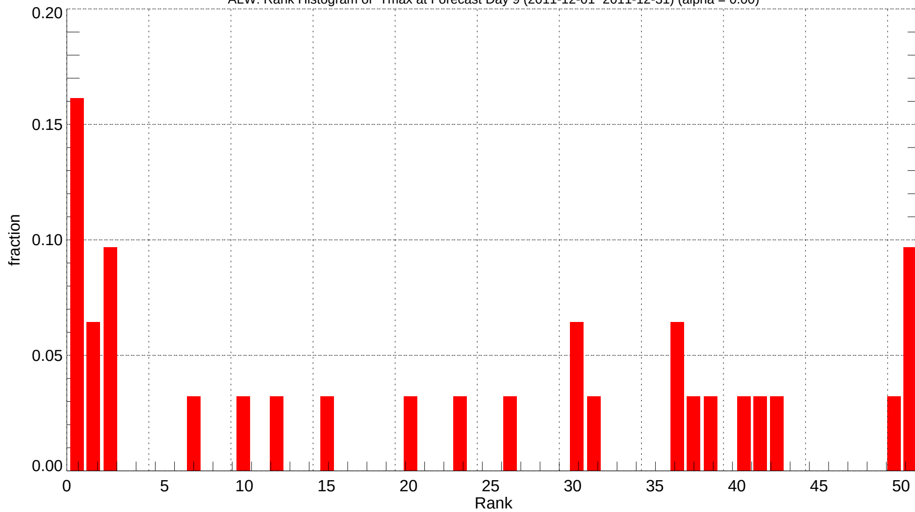
ALW: Rank Histogram of Tmax at Forecast Day 9 (2011-12-01~2011-12-31) (alpha = 0.00)
