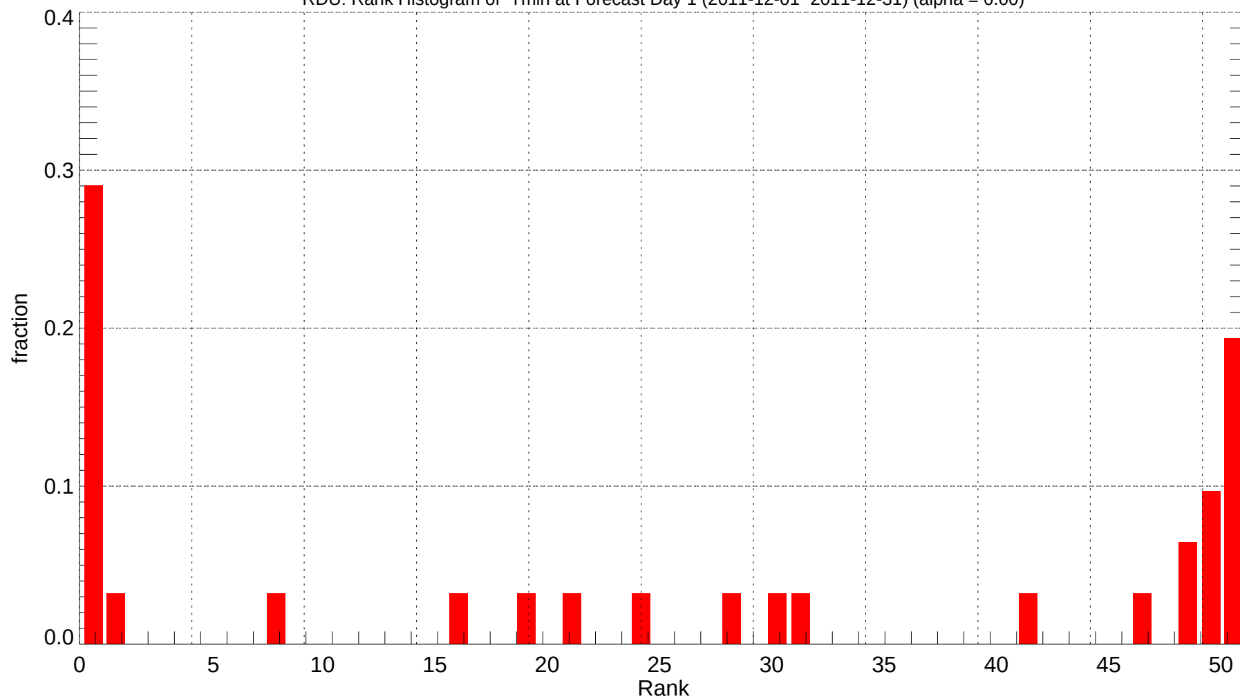
RDU: Rank Histogram of Tmin at Forecast Day 1 (2011-12-01~2011-12-31) (alpha = 0.00)
