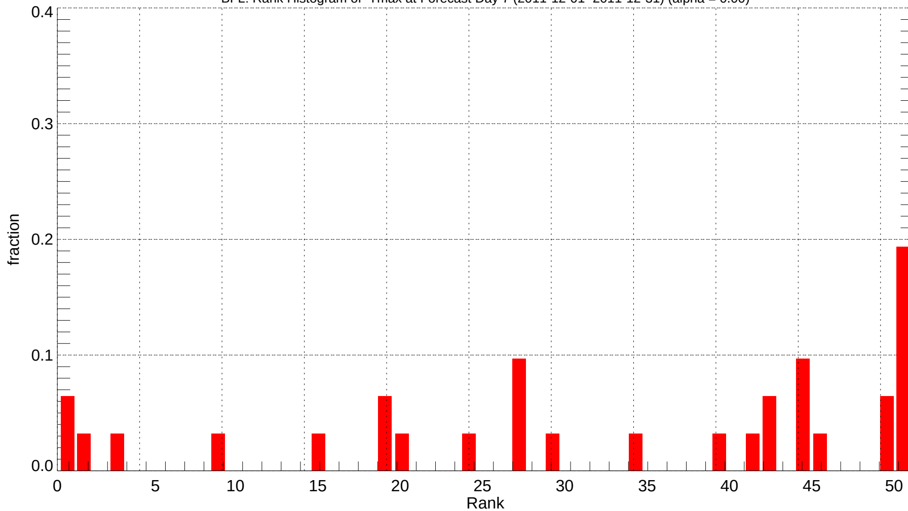
BFL: Rank Histogram of Tmax at Forecast Day 7 (2011-12-01~2011-12-31) (alpha = 0.00)
