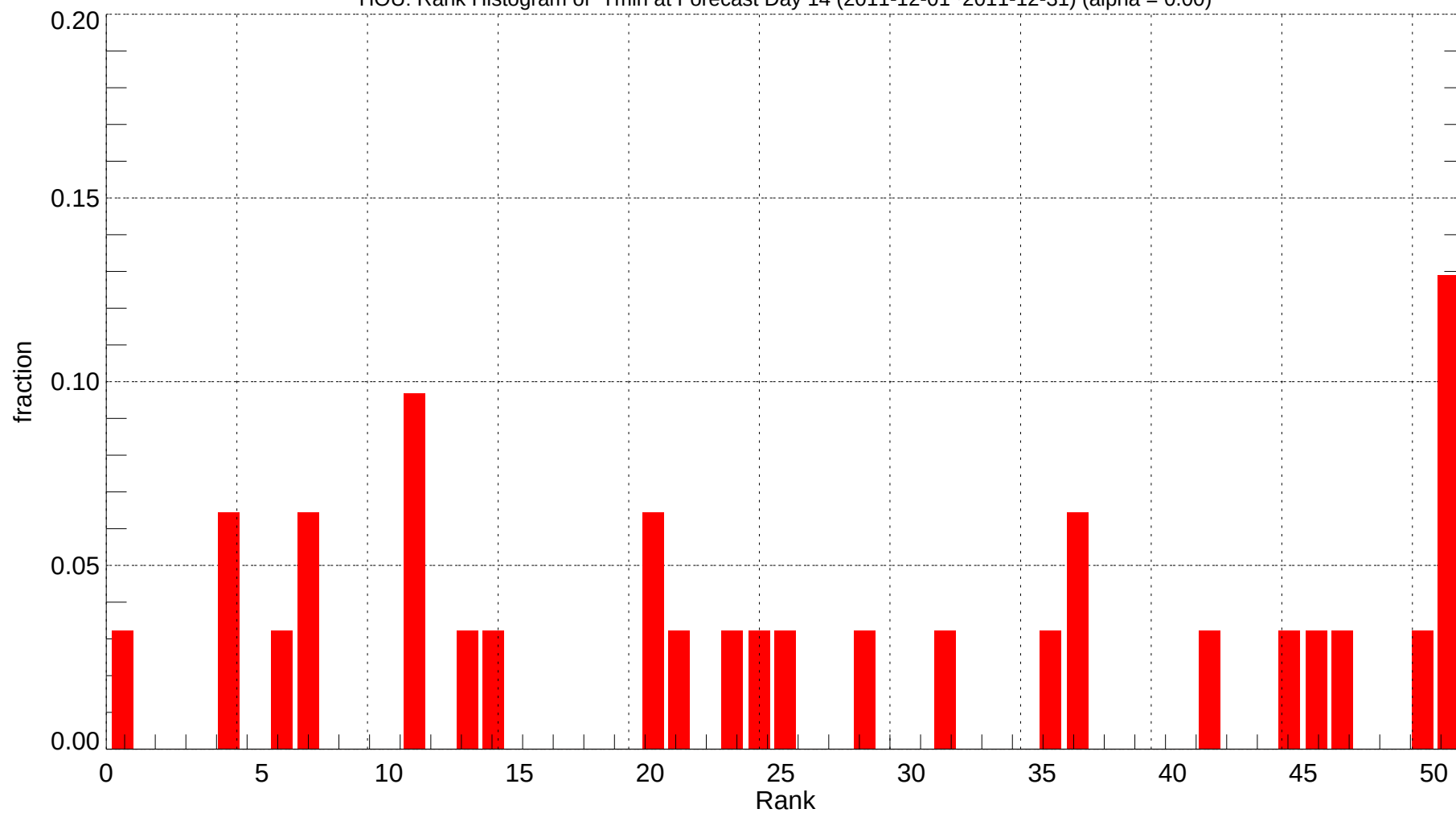
HOU: Rank Histogram of Tmin at Forecast Day 14 (2011-12-01~2011-12-31) (alpha = 0.00)
