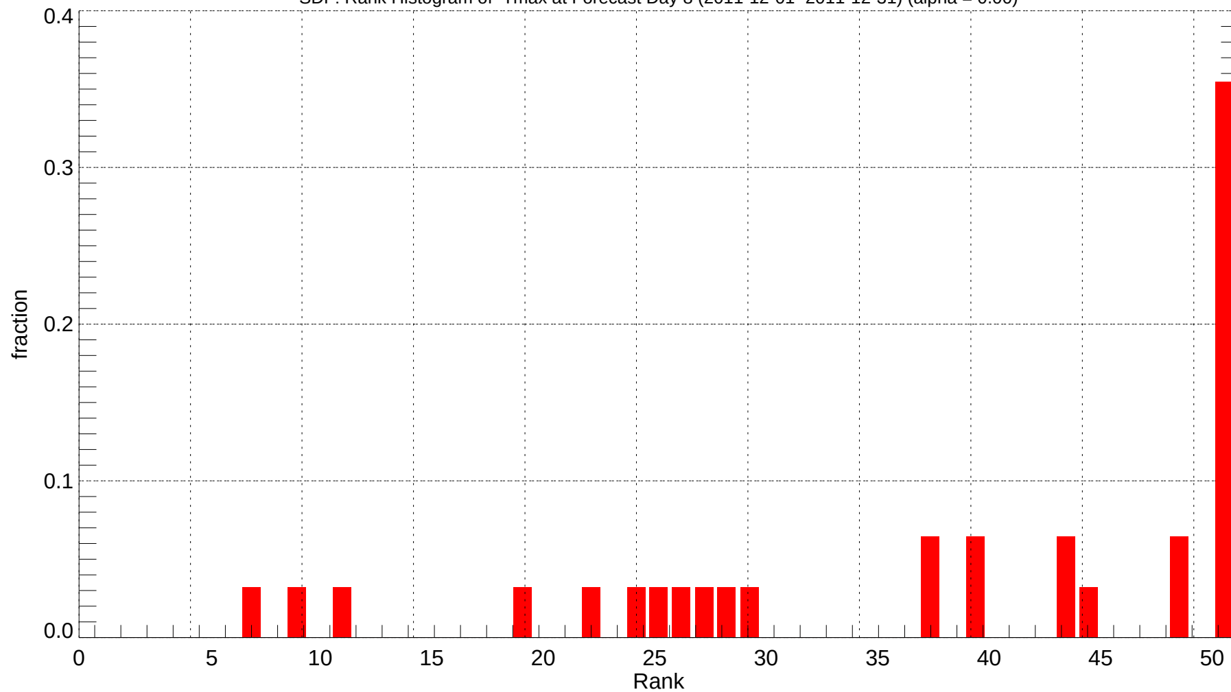
SDF: Rank Histogram of Tmax at Forecast Day 8 (2011-12-01~2011-12-31) (alpha = 0.00)
