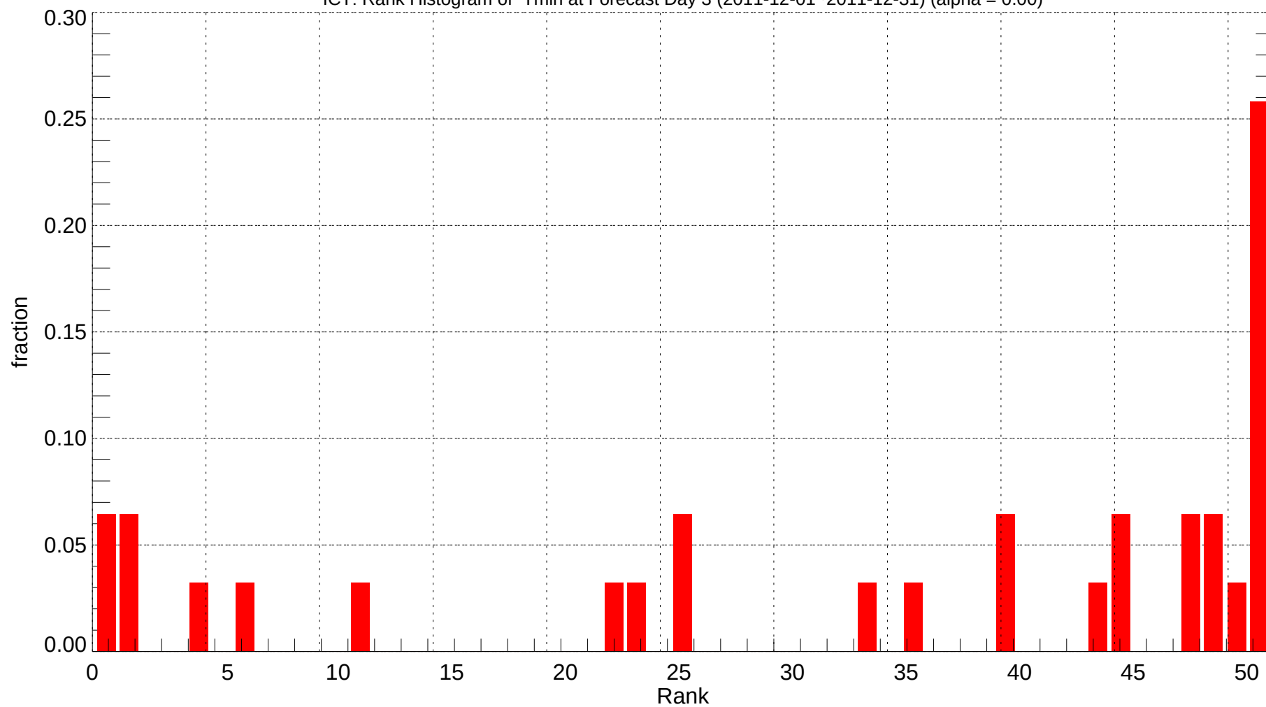
ICT: Rank Histogram of Tmin at Forecast Day 3 (2011-12-01~2011-12-31) (alpha = 0.00)
