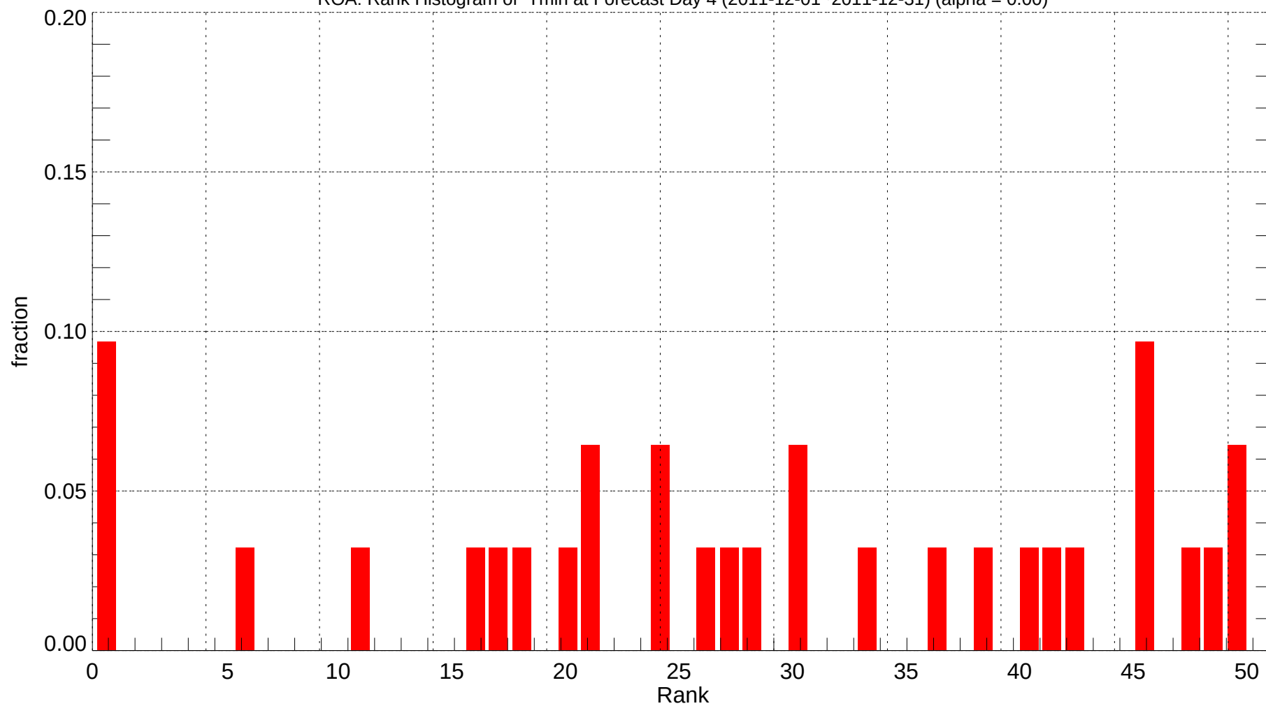
ROA: Rank Histogram of Tmin at Forecast Day 4 (2011-12-01~2011-12-31) (alpha = 0.00)
