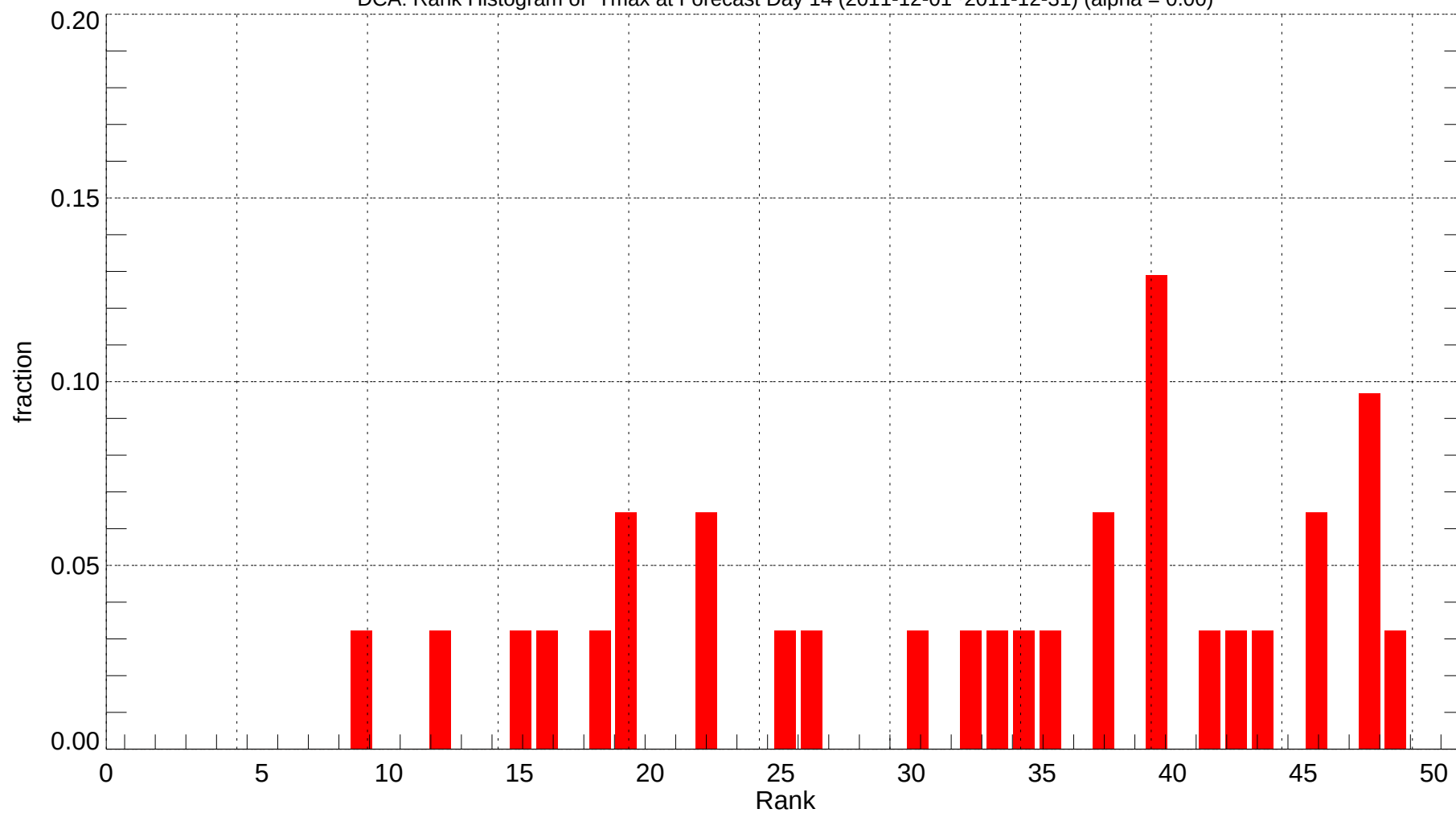
DCA: Rank Histogram of Tmax at Forecast Day 14 (2011-12-01~2011-12-31) (alpha = 0.00)
