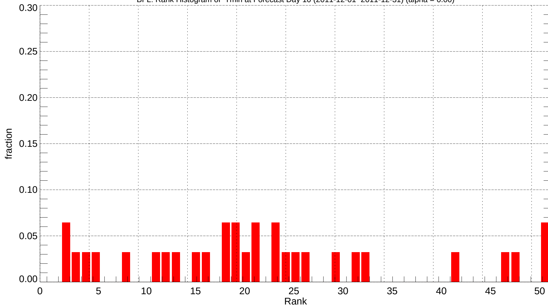
BFL: Rank Histogram of Tmin at Forecast Day 10 (2011-12-01~2011-12-31) (alpha = 0.00)
