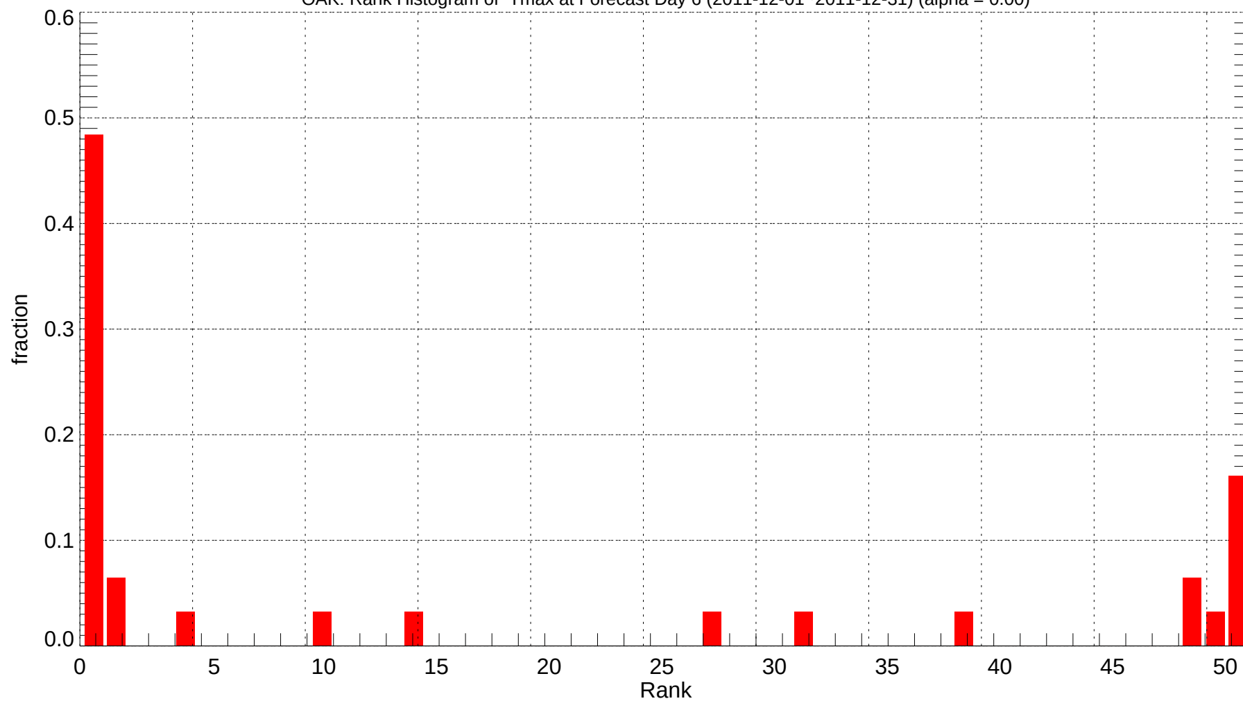
OAK: Rank Histogram of Tmax at Forecast Day 6 (2011-12-01~2011-12-31) (alpha = 0.00)
