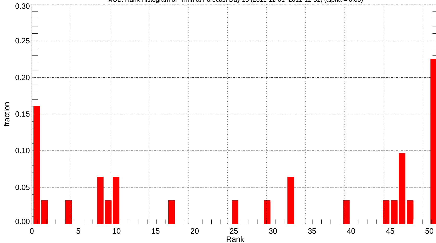
MOB: Rank Histogram of Tmin at Forecast Day 13 (2011-12-01~2011-12-31) (alpha = 0.00)
