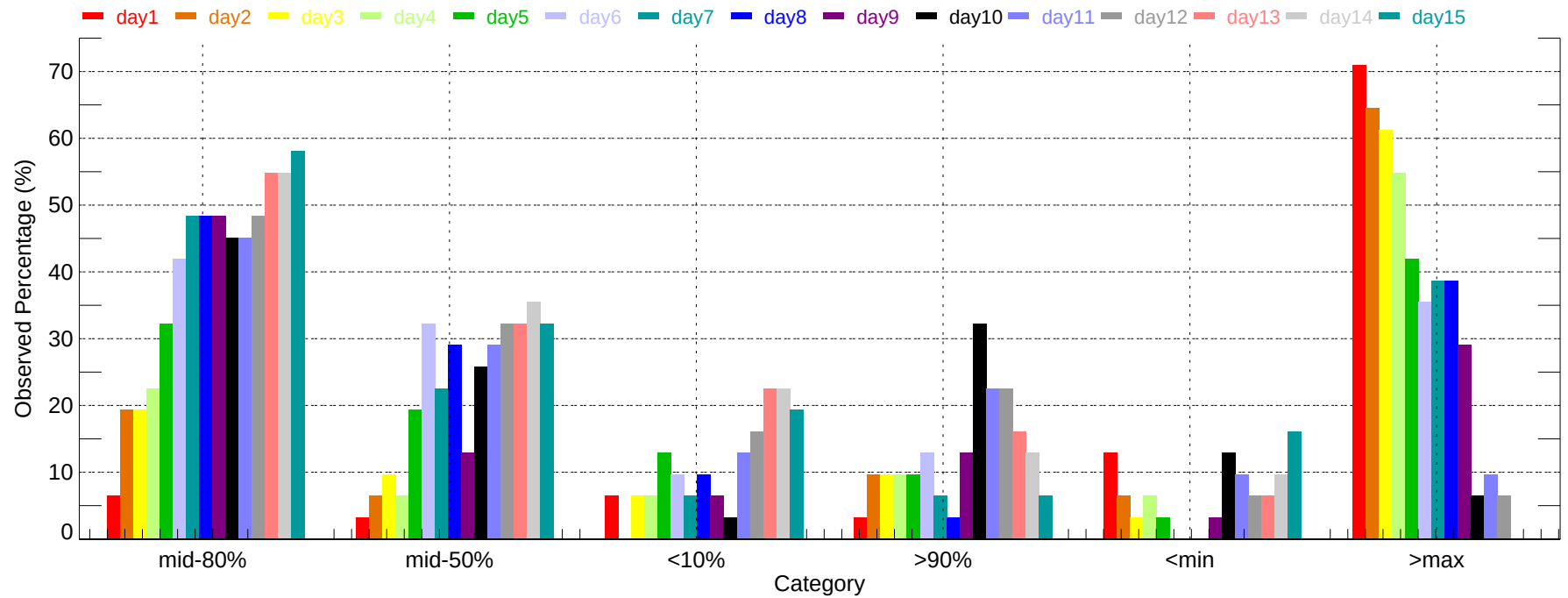
Observed Percentage of Ensembles - FLG: Min Temperature (2011-12-01~2011-12-31)
