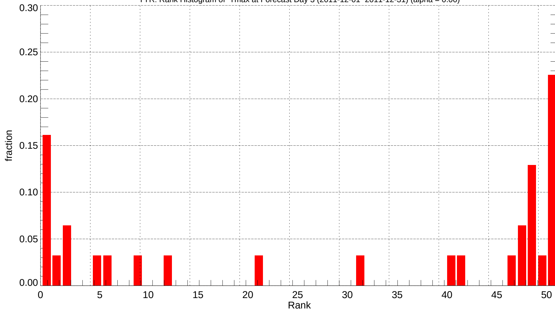
TYR: Rank Histogram of Tmax at Forecast Day 3 (2011-12-01~2011-12-31) (alpha = 0.00)
