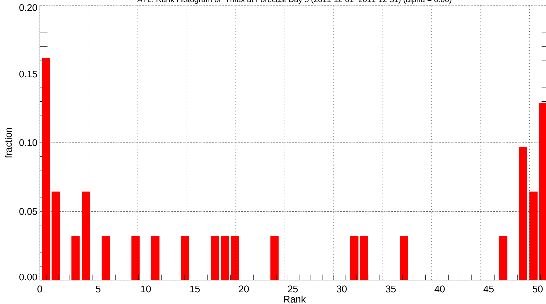
ATL: Rank Histogram of Tmax at Forecast Day 3 (2011-12-01~2011-12-31) (alpha = 0.00)
