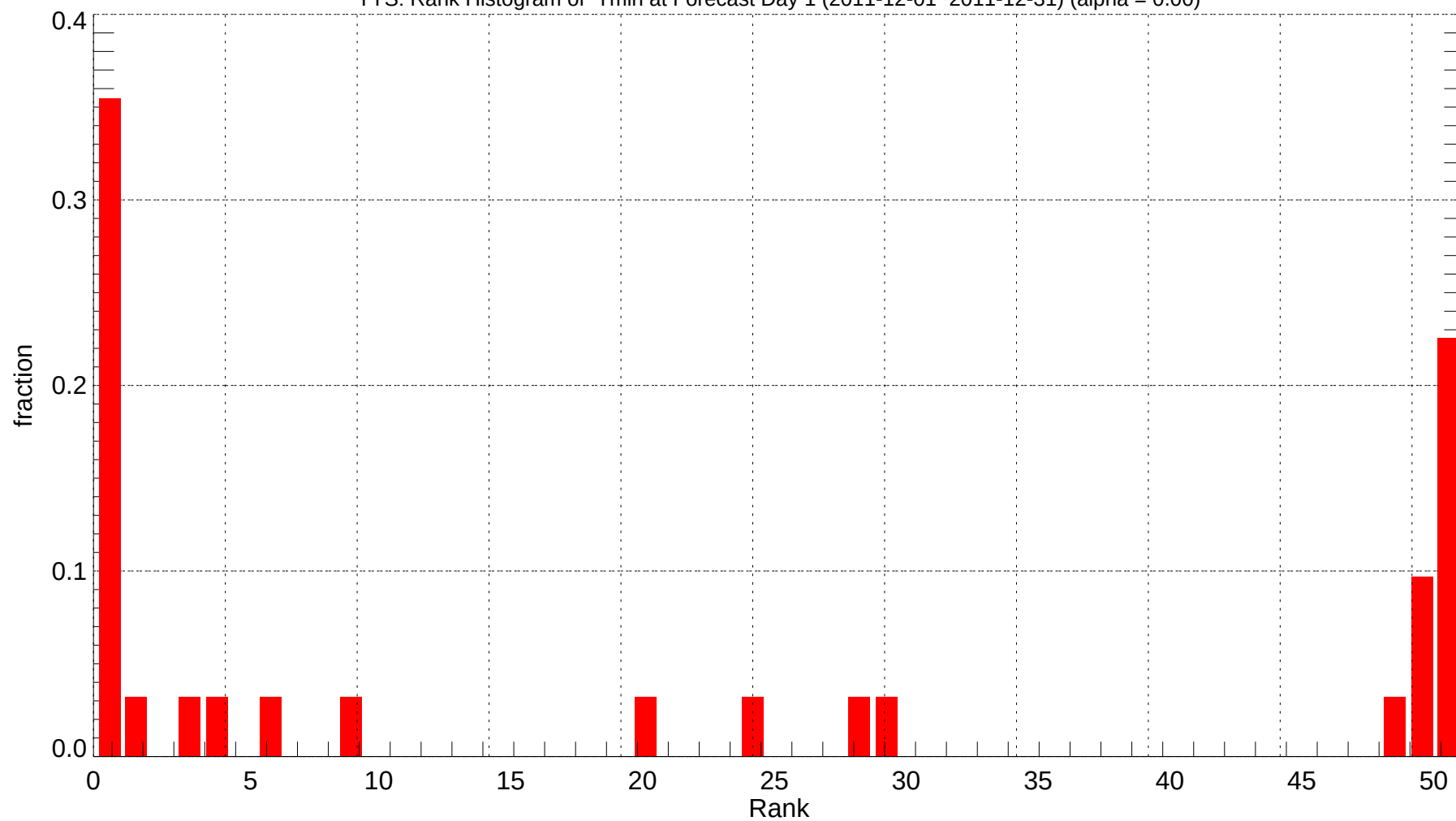
TYS: Rank Histogram of Tmin at Forecast Day 1 (2011-12-01~2011-12-31) (alpha = 0.00)
