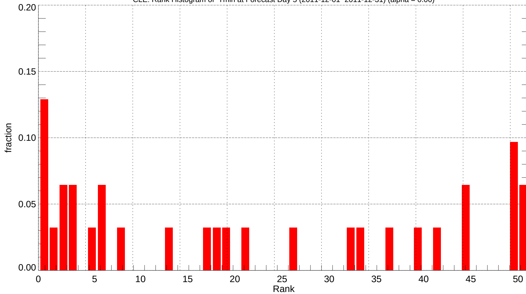
CLE: Rank Histogram of Tmin at Forecast Day 5 (2011-12-01~2011-12-31) (alpha = 0.00)
