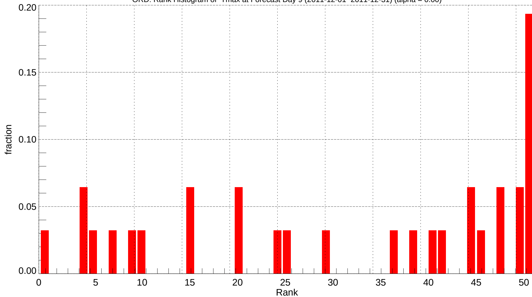
ORD: Rank Histogram of Tmax at Forecast Day 9 (2011-12-01~2011-12-31) (alpha = 0.00)
