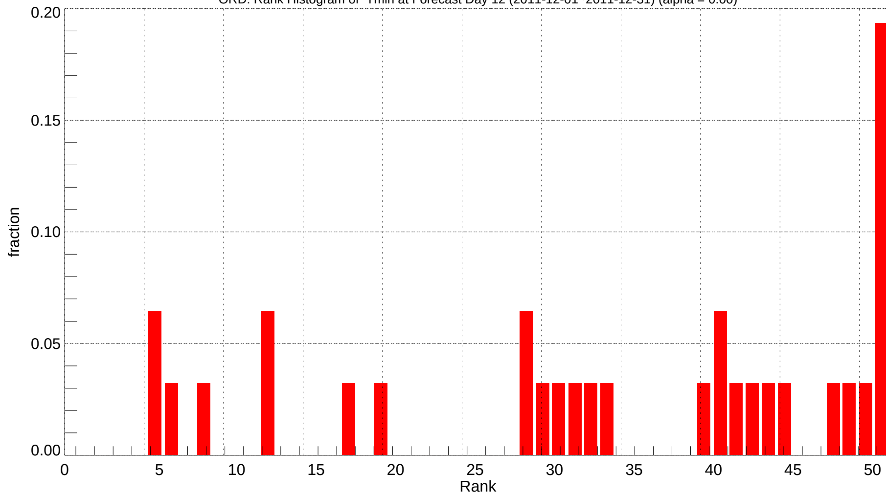
ORD: Rank Histogram of Tmin at Forecast Day 12 (2011-12-01~2011-12-31) (alpha = 0.00)
