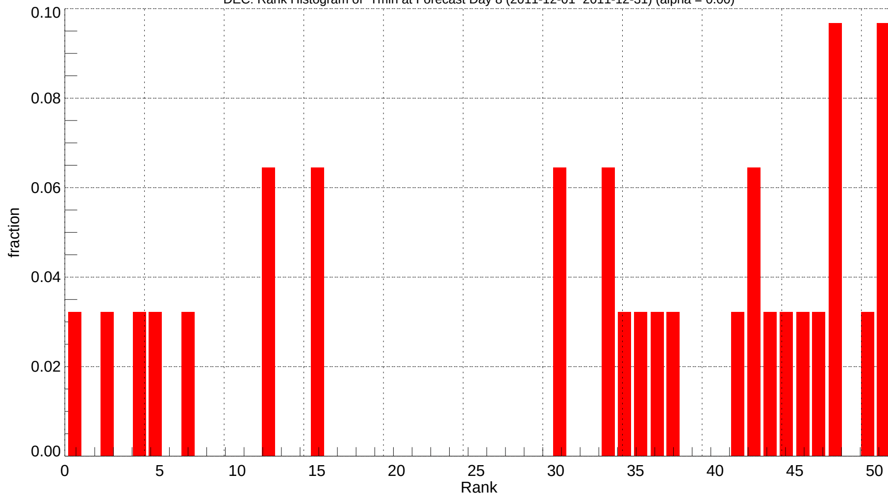
DEC: Rank Histogram of Tmin at Forecast Day 8 (2011-12-01~2011-12-31) (alpha = 0.00)
