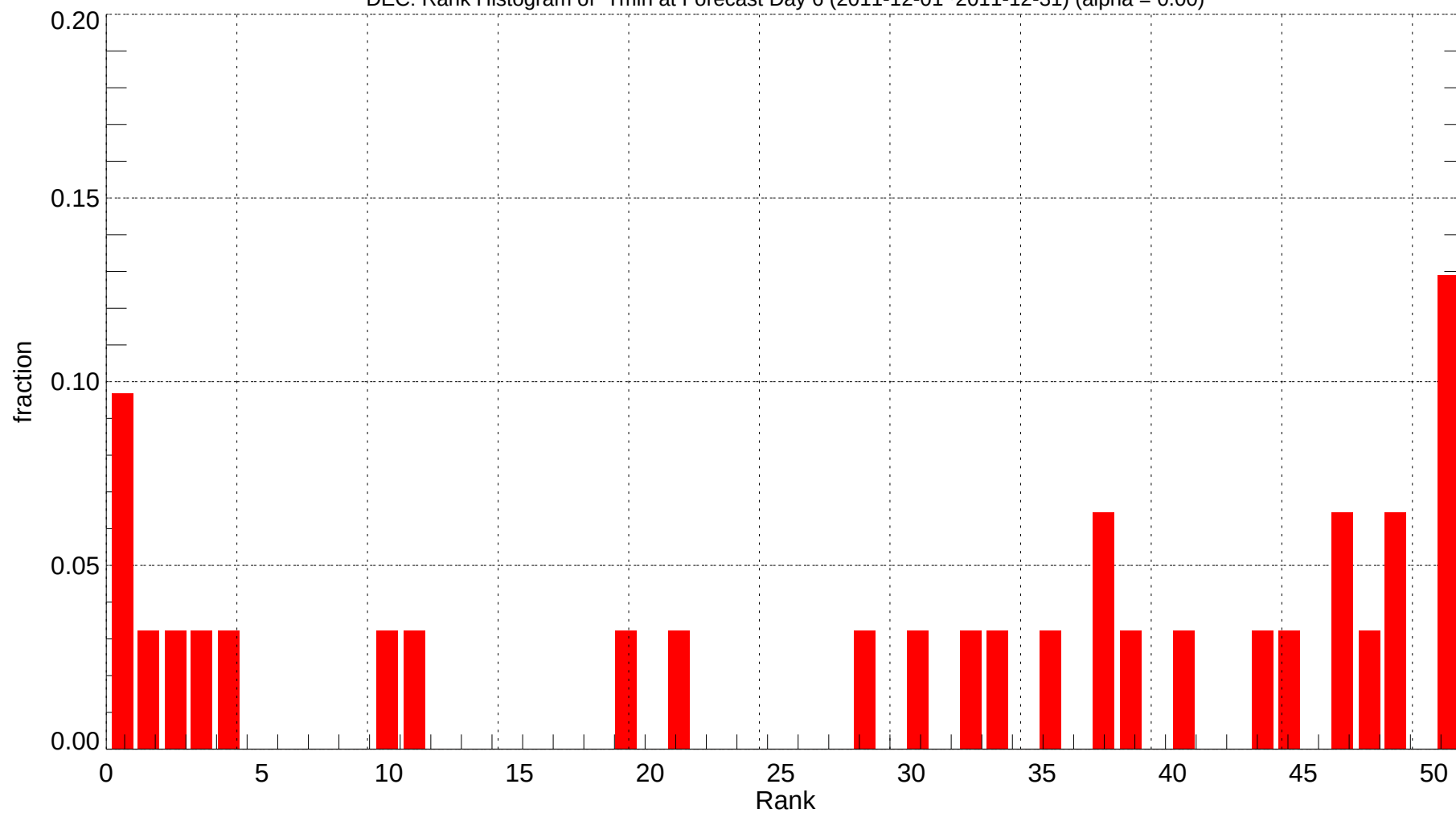
DEC: Rank Histogram of Tmin at Forecast Day 6 (2011-12-01~2011-12-31) (alpha = 0.00)
