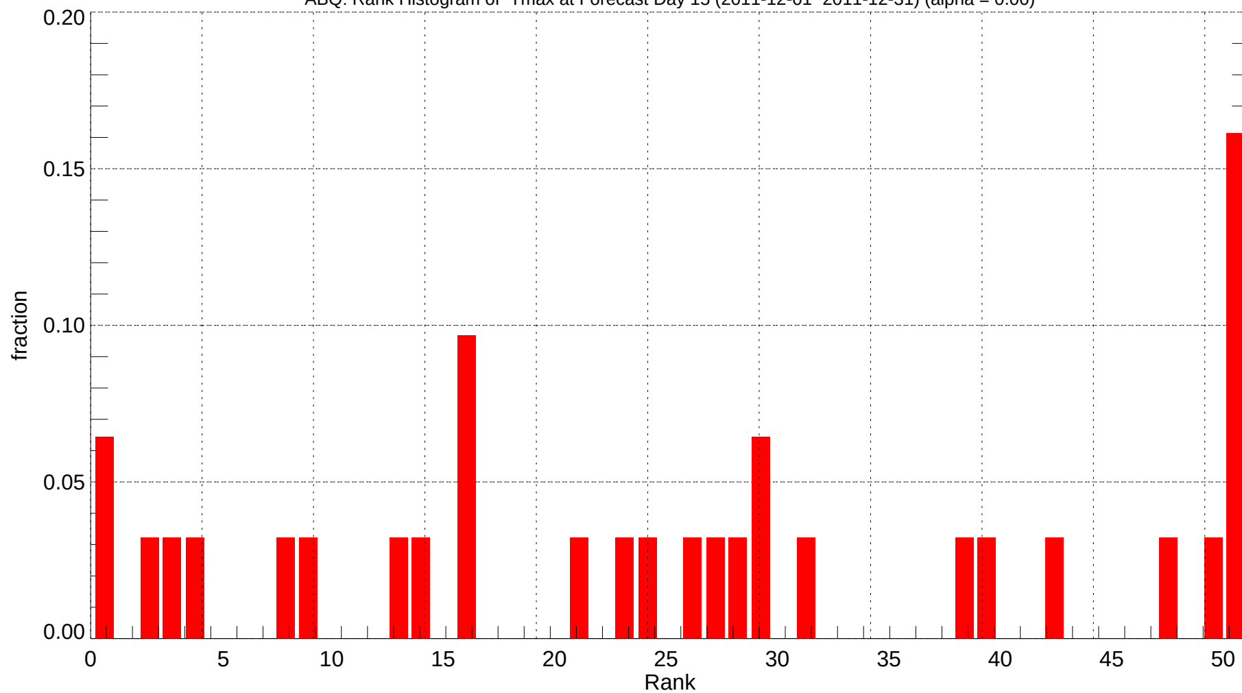
ABQ: Rank Histogram of Tmax at Forecast Day 15 (2011-12-01~2011-12-31) (alpha = 0.00)
