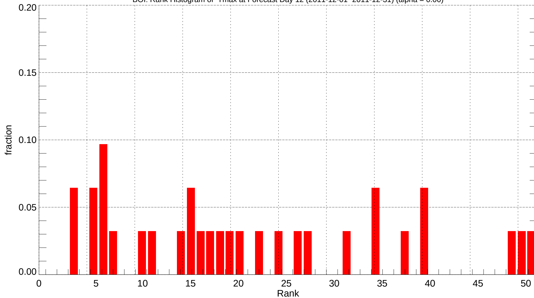
BOI: Rank Histogram of Tmax at Forecast Day 12 (2011-12-01~2011-12-31) (alpha = 0.00)
