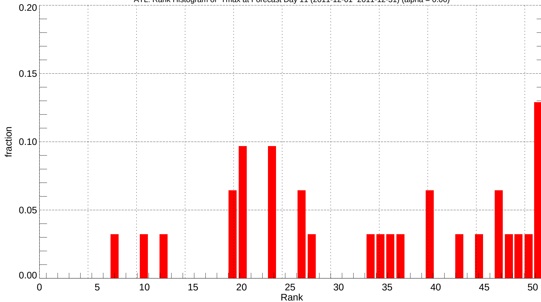
ATL: Rank Histogram of Tmax at Forecast Day 11 (2011-12-01~2011-12-31) (alpha = 0.00)
