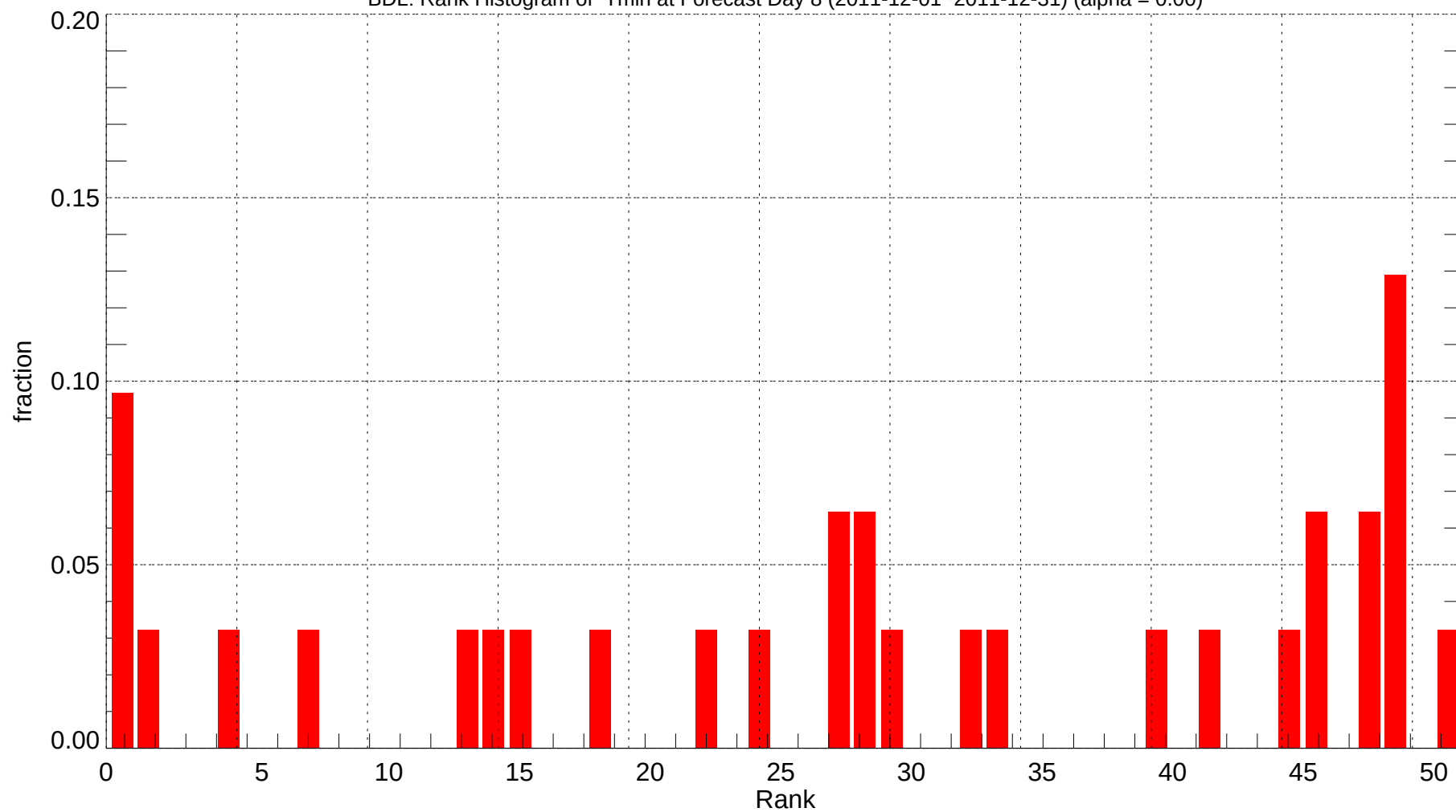
BDL: Rank Histogram of Tmin at Forecast Day 8 (2011-12-01~2011-12-31) (alpha = 0.00)
