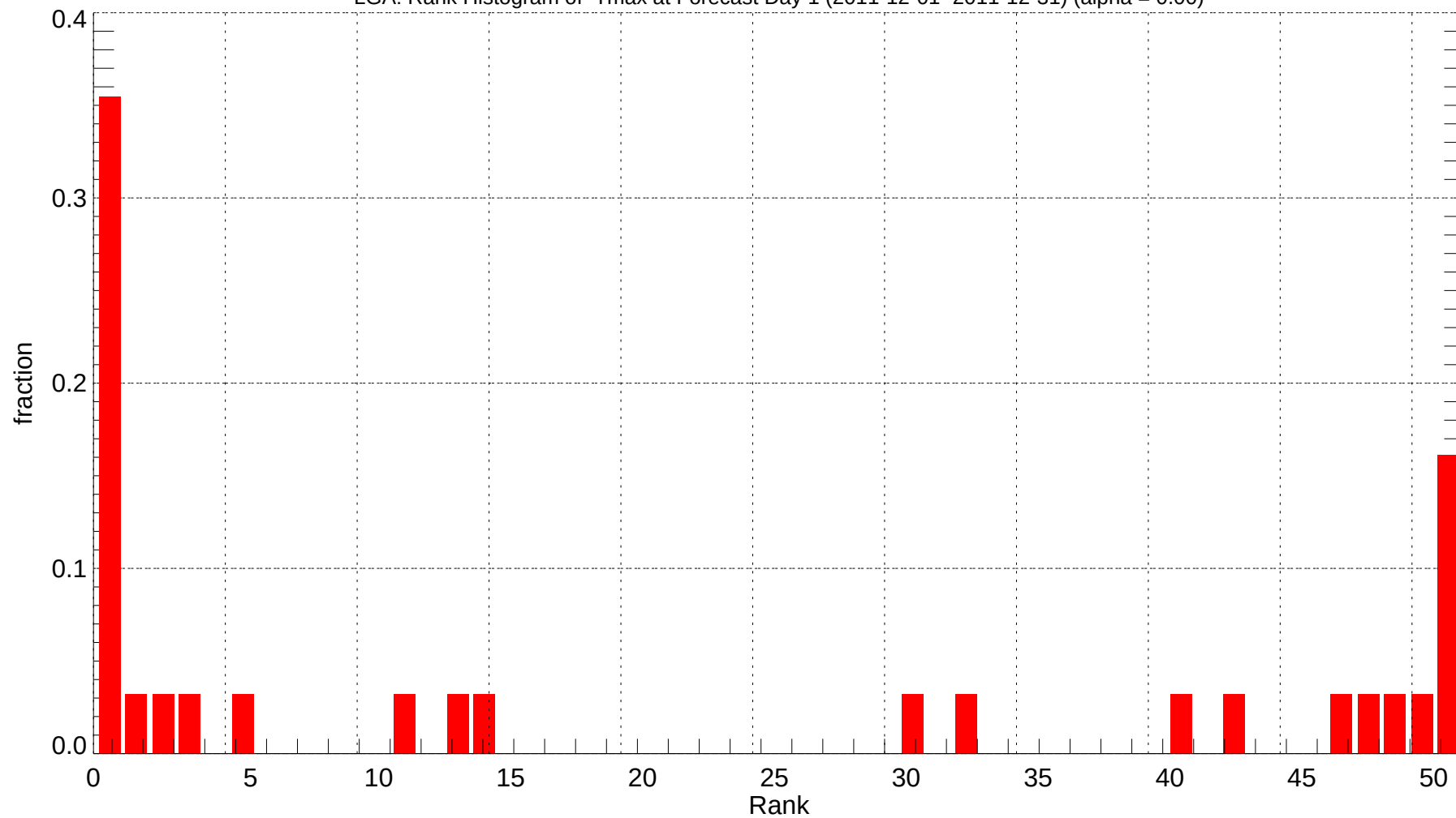
LGA: Rank Histogram of Tmax at Forecast Day 1 (2011-12-01~2011-12-31) (alpha = 0.00)
