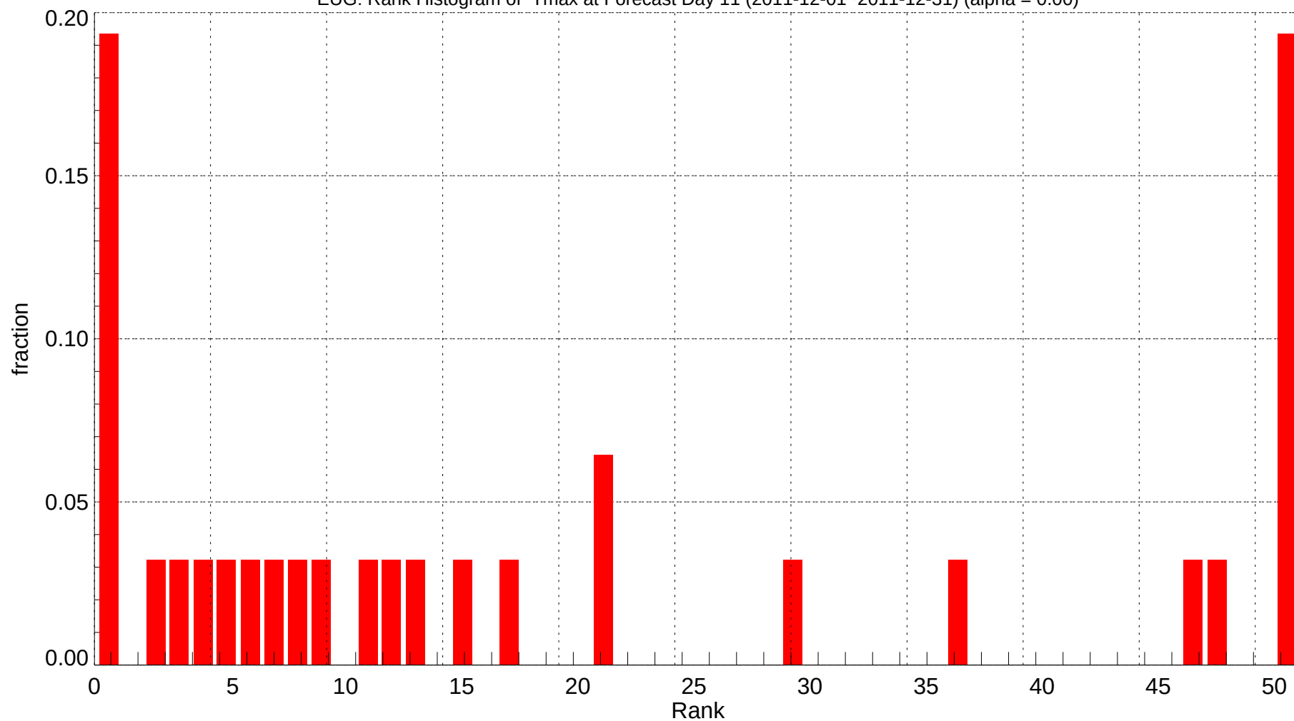
EUG: Rank Histogram of Tmax at Forecast Day 11 (2011-12-01~2011-12-31) (alpha = 0.00)
