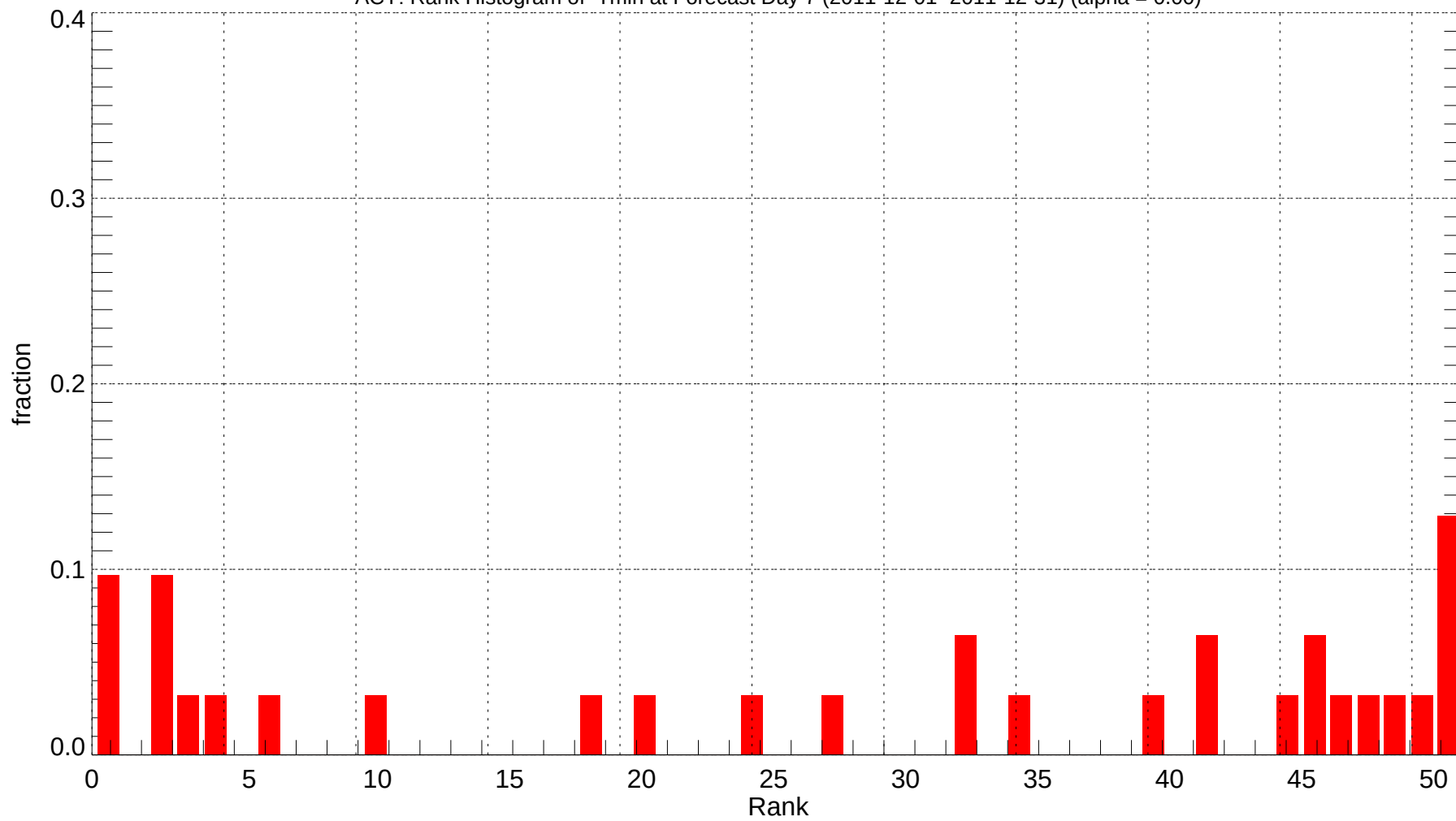
ACY: Rank Histogram of Tmin at Forecast Day 7 (2011-12-01~2011-12-31) (alpha = 0.00)
