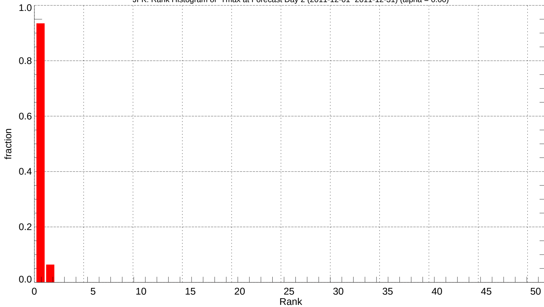
JFK: Rank Histogram of Tmax at Forecast Day 2 (2011-12-01~2011-12-31) (alpha = 0.00)
