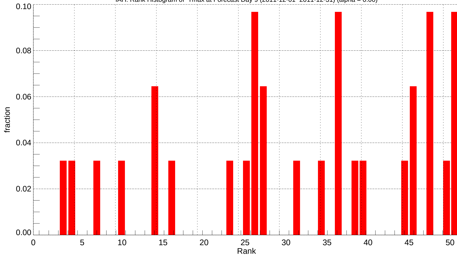
IAH: Rank Histogram of Tmax at Forecast Day 9 (2011-12-01~2011-12-31) (alpha = 0.00)
