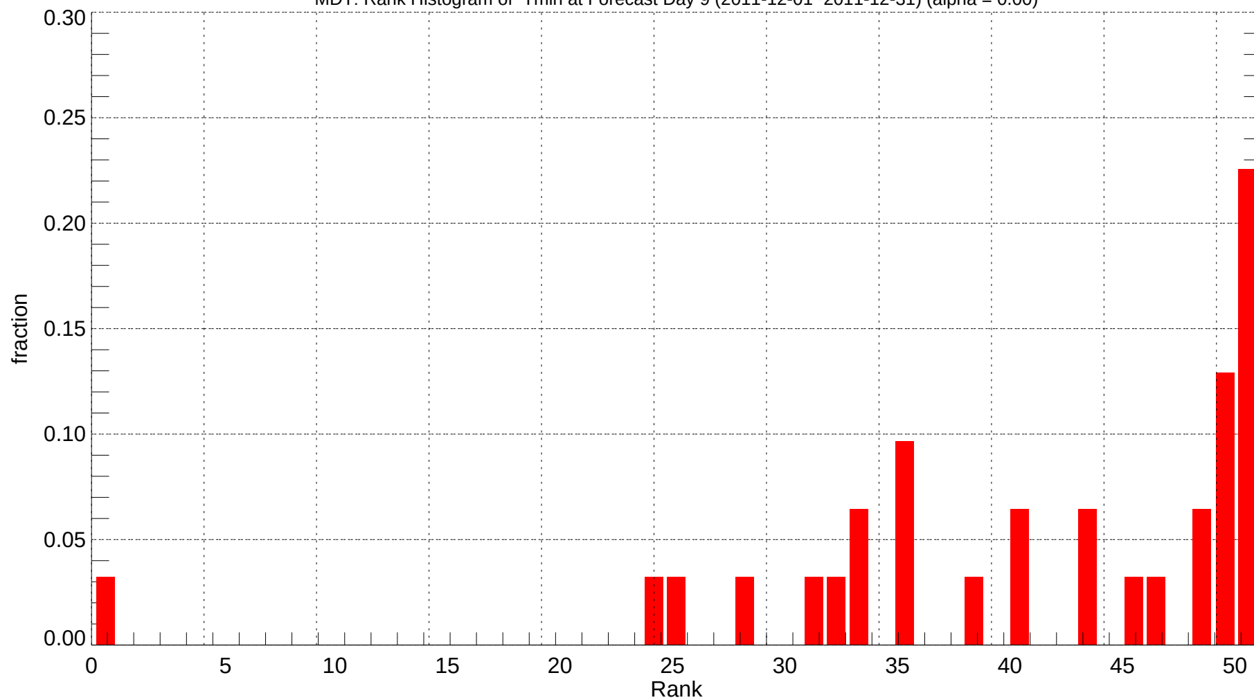
MDT: Rank Histogram of Tmin at Forecast Day 9 (2011-12-01~2011-12-31) (alpha = 0.00)
