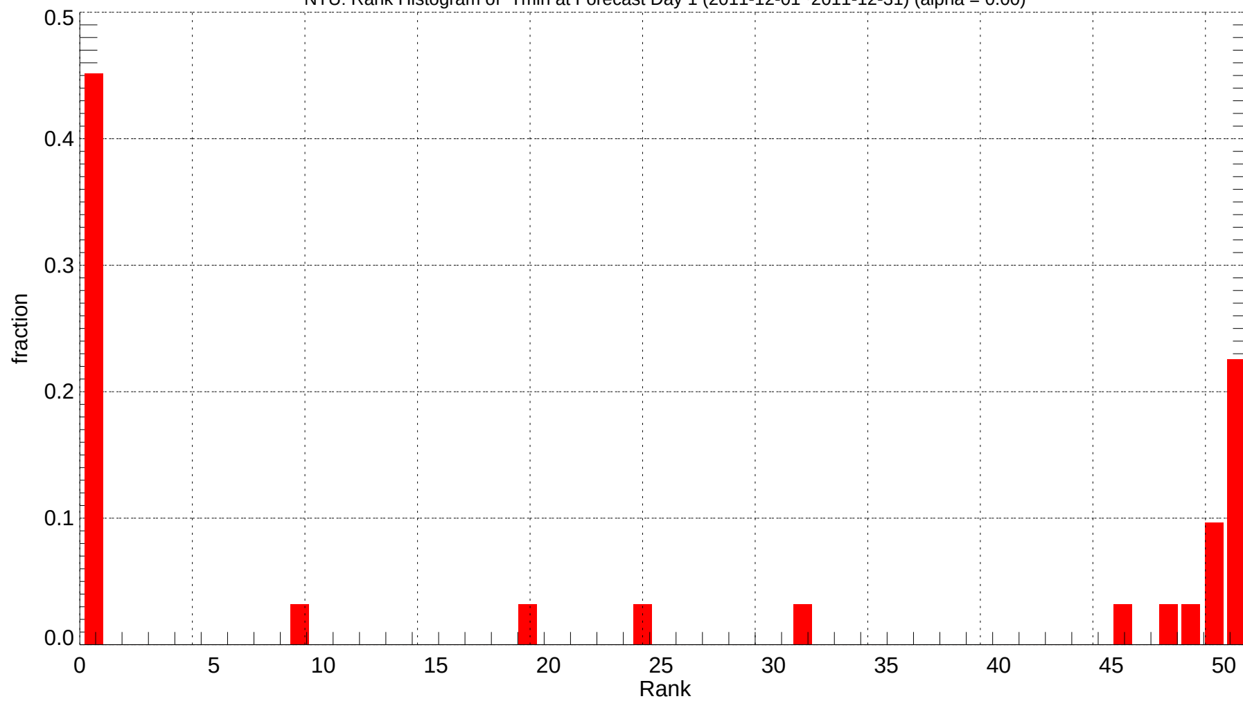
NTU: Rank Histogram of Tmin at Forecast Day 1 (2011-12-01~2011-12-31) (alpha = 0.00)
