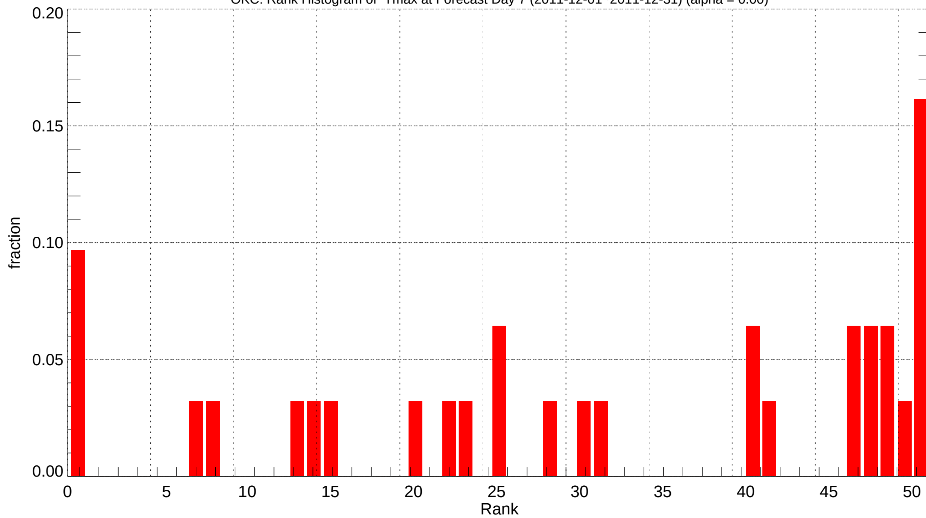
OKC: Rank Histogram of Tmax at Forecast Day 7 (2011-12-01~2011-12-31) (alpha = 0.00)
