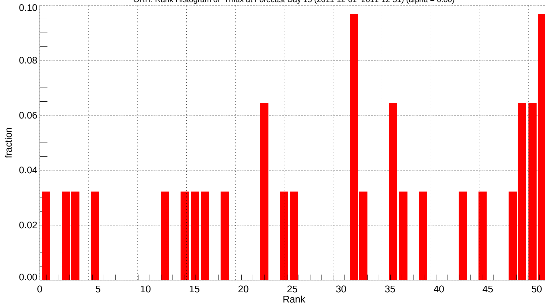
ORH: Rank Histogram of Tmax at Forecast Day 15 (2011-12-01~2011-12-31) (alpha = 0.00)
