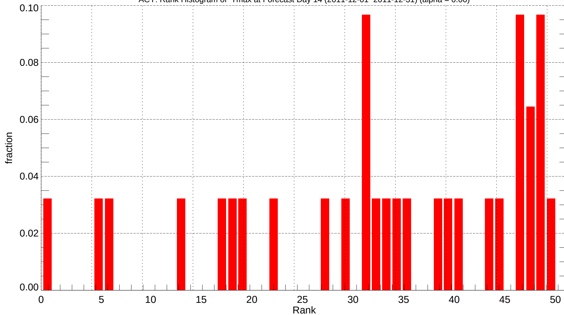
ACY: Rank Histogram of Tmax at Forecast Day 14 (2011-12-01~2011-12-31) (alpha = 0.00)
