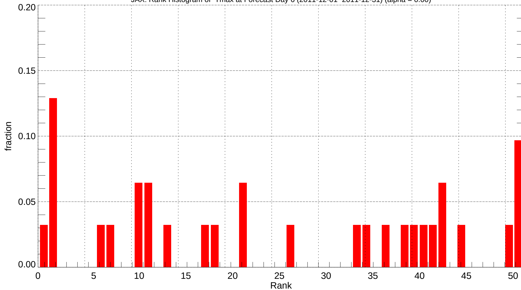
JAX: Rank Histogram of Tmax at Forecast Day 6 (2011-12-01~2011-12-31) (alpha = 0.00)
