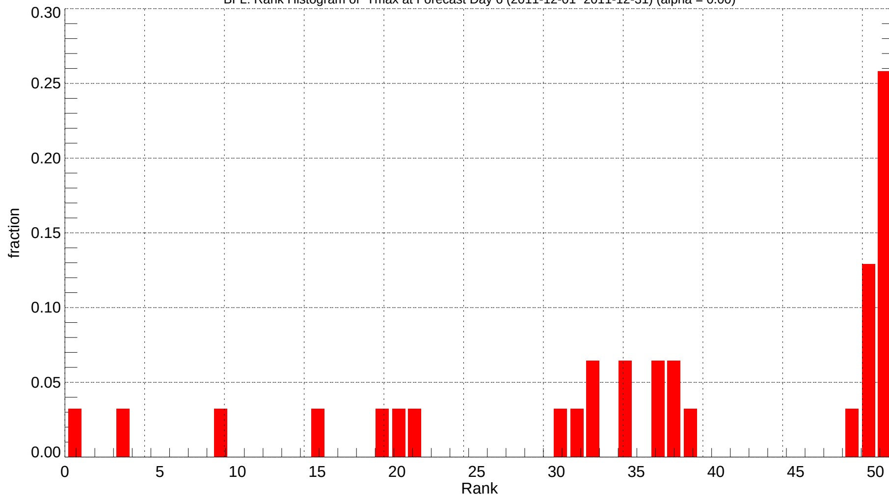
BFL: Rank Histogram of Tmax at Forecast Day 6 (2011-12-01~2011-12-31) (alpha = 0.00)
