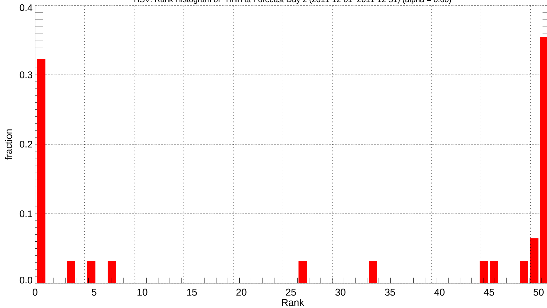
HSV: Rank Histogram of Tmin at Forecast Day 2 (2011-12-01~2011-12-31) (alpha = 0.00)
