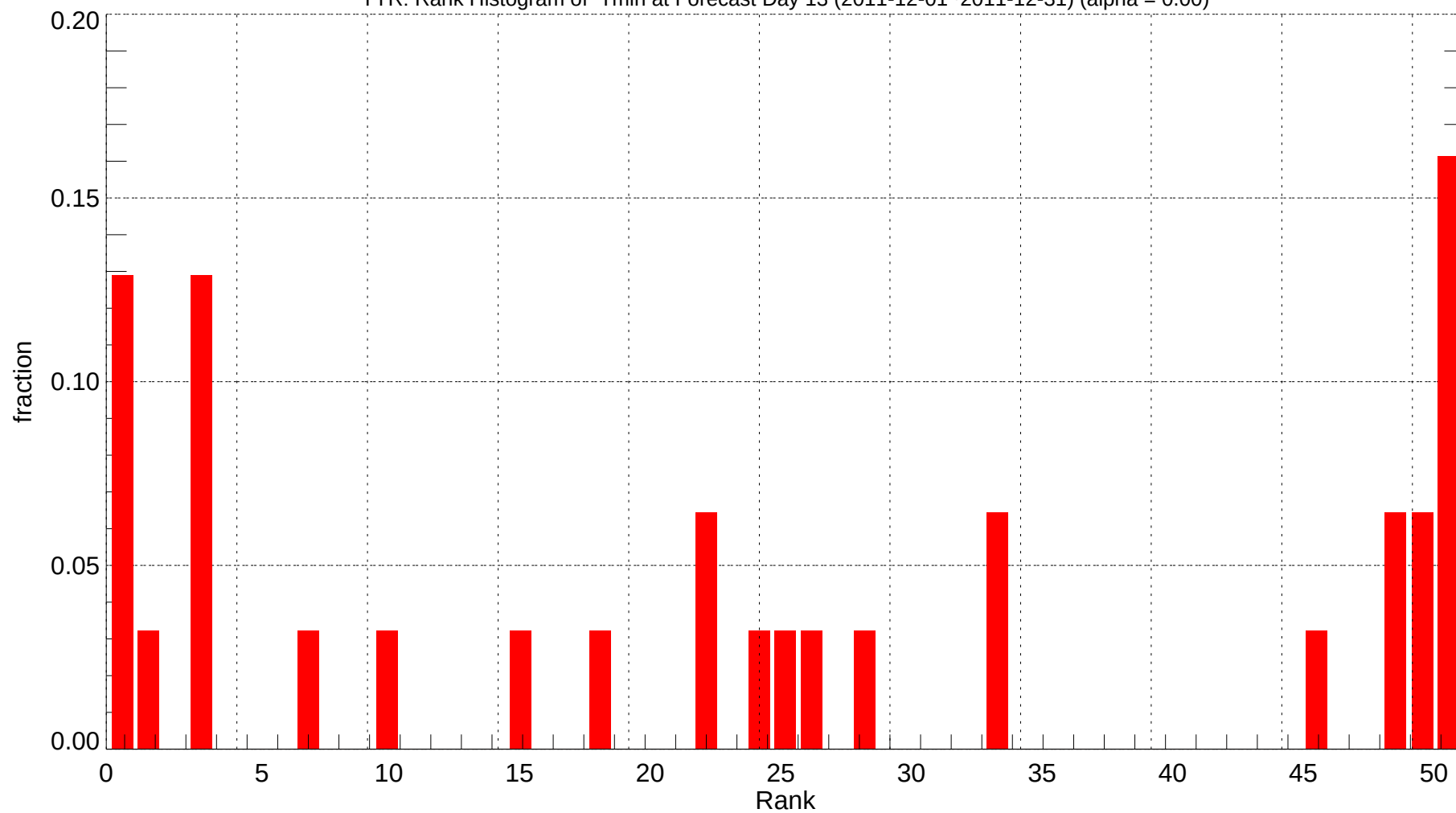
TYR: Rank Histogram of Tmin at Forecast Day 13 (2011-12-01~2011-12-31) (alpha = 0.00)
