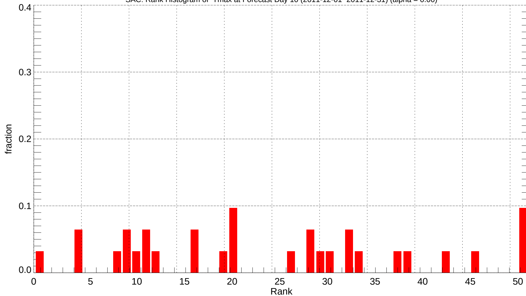
SAC: Rank Histogram of Tmax at Forecast Day 10 (2011-12-01~2011-12-31) (alpha = 0.00)
