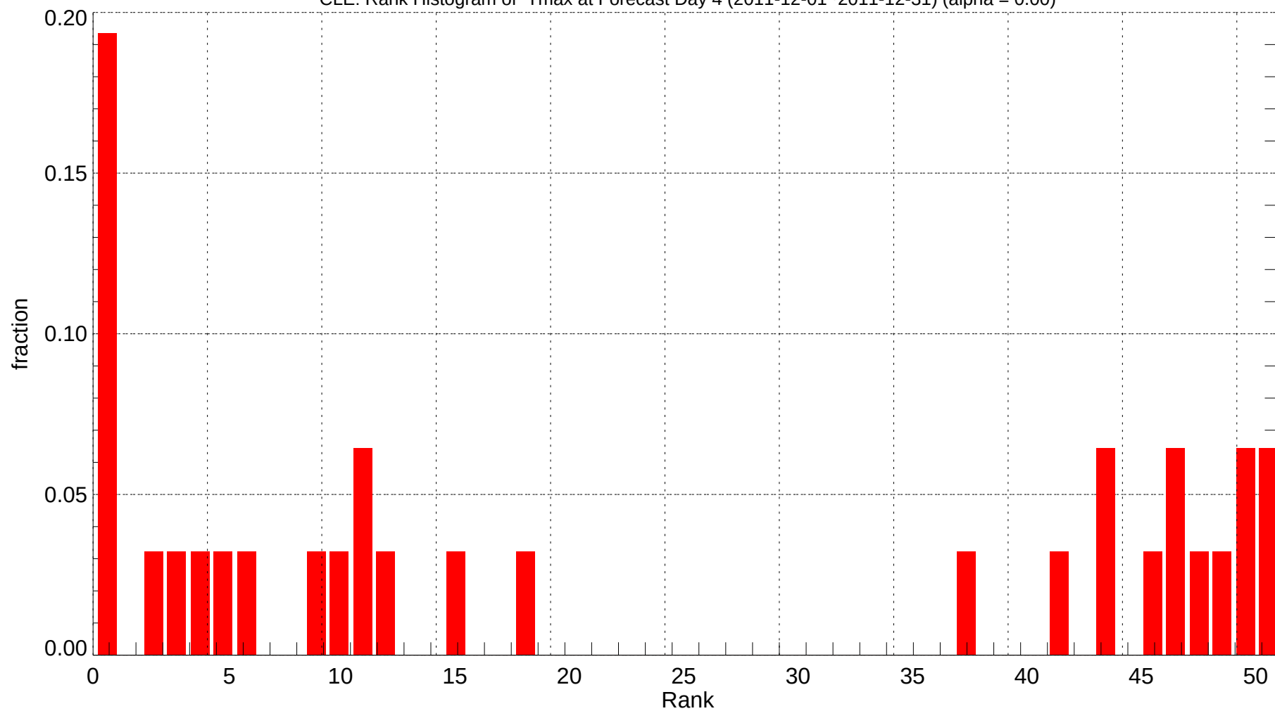
CLE: Rank Histogram of Tmax at Forecast Day 4 (2011-12-01~2011-12-31) (alpha = 0.00)
