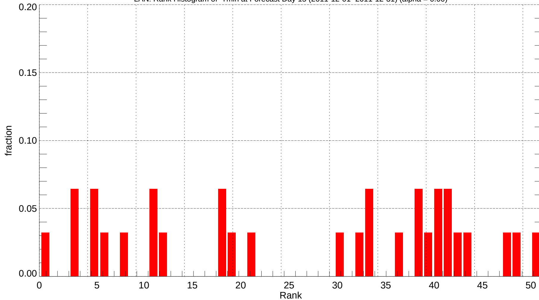
LAN: Rank Histogram of Tmin at Forecast Day 15 (2011-12-01~2011-12-31) (alpha = 0.00)
