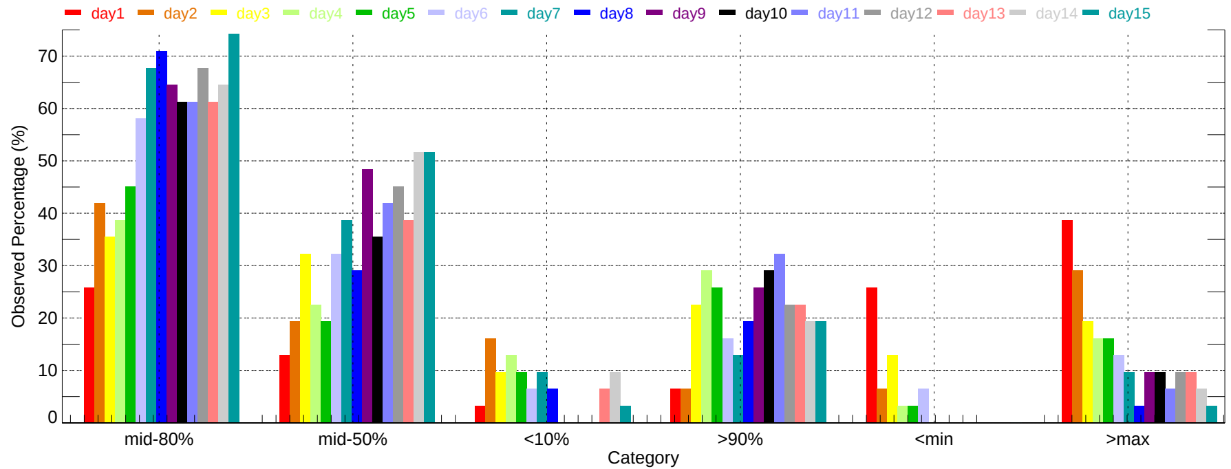
Observed Percentage of Ensembles - STL: Max Temperature (2011-12-01~2011-12-31)
