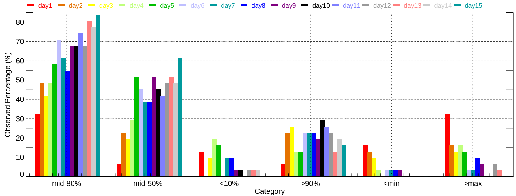
Observed Percentage of Ensembles - TYS: Min Temperature (2011-12-01~2011-12-31)
