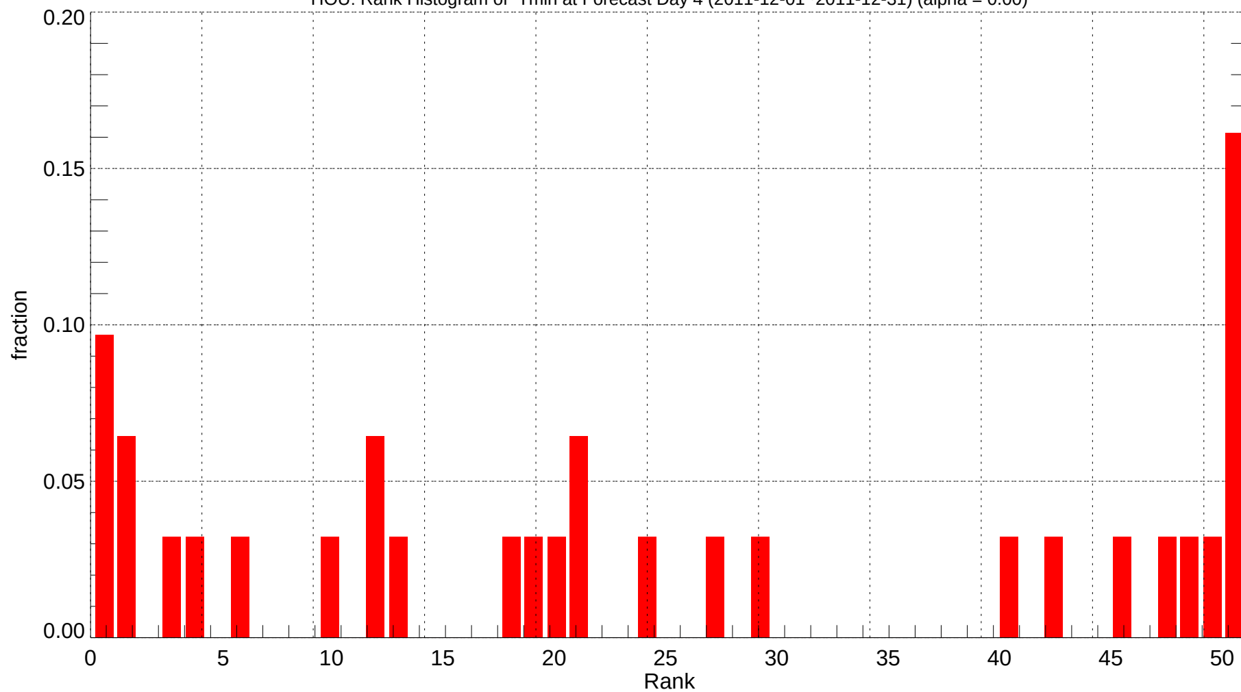
HOU: Rank Histogram of Tmin at Forecast Day 4 (2011-12-01~2011-12-31) (alpha = 0.00)
