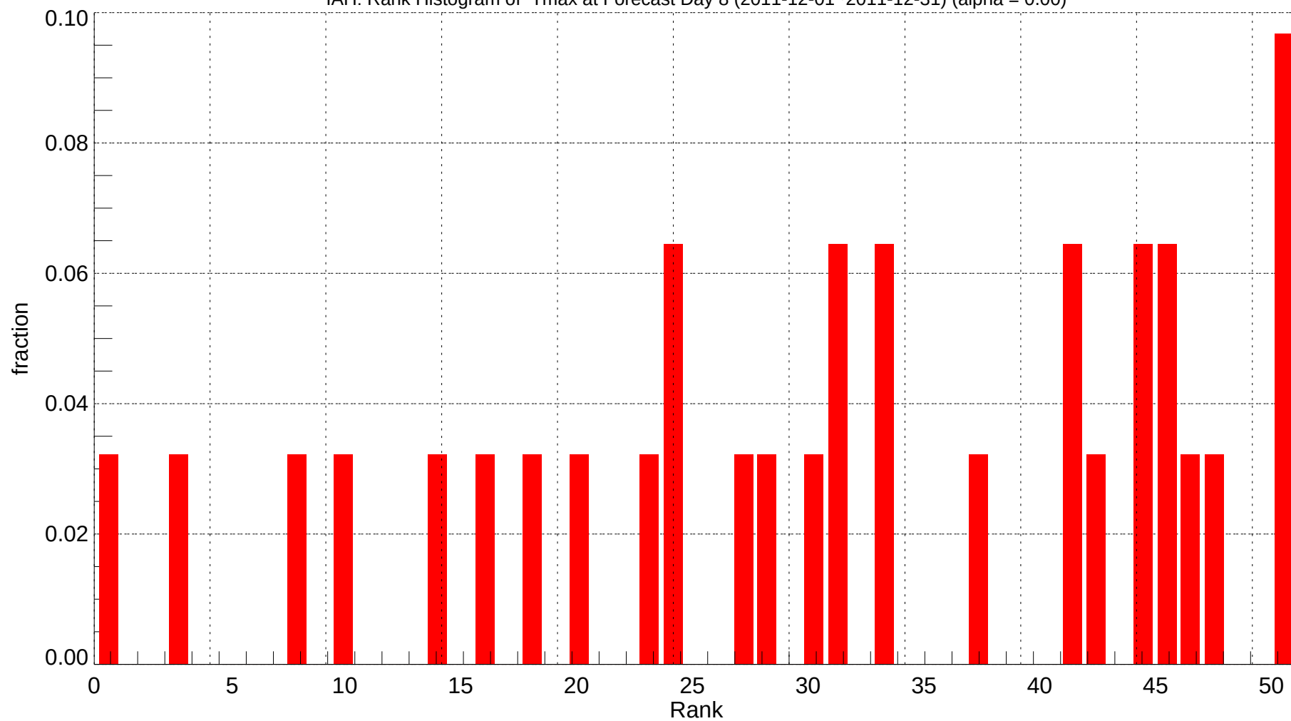
IAH: Rank Histogram of Tmax at Forecast Day 8 (2011-12-01~2011-12-31) (alpha = 0.00)
