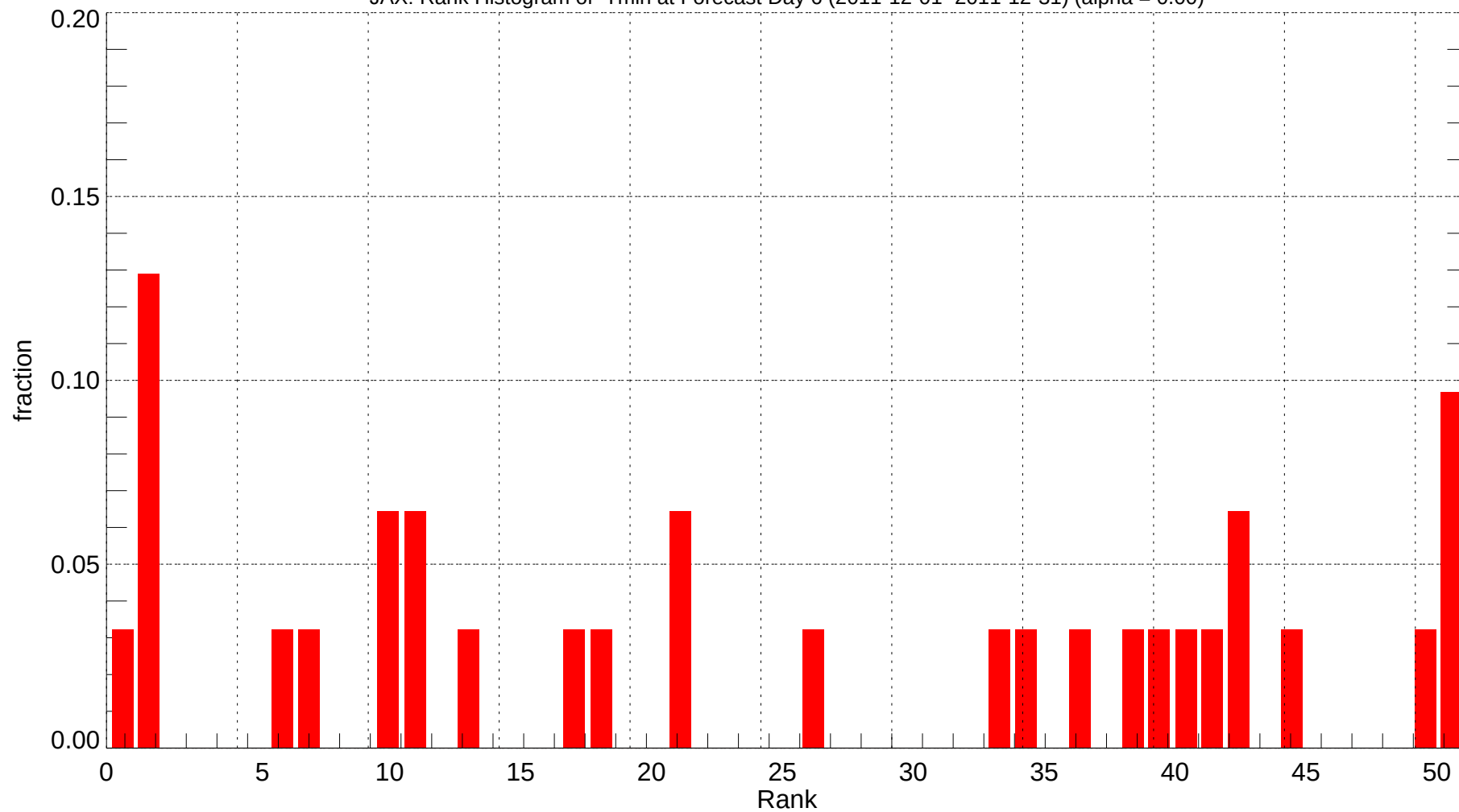
JAX: Rank Histogram of Tmin at Forecast Day 6 (2011-12-01~2011-12-31) (alpha = 0.00)
