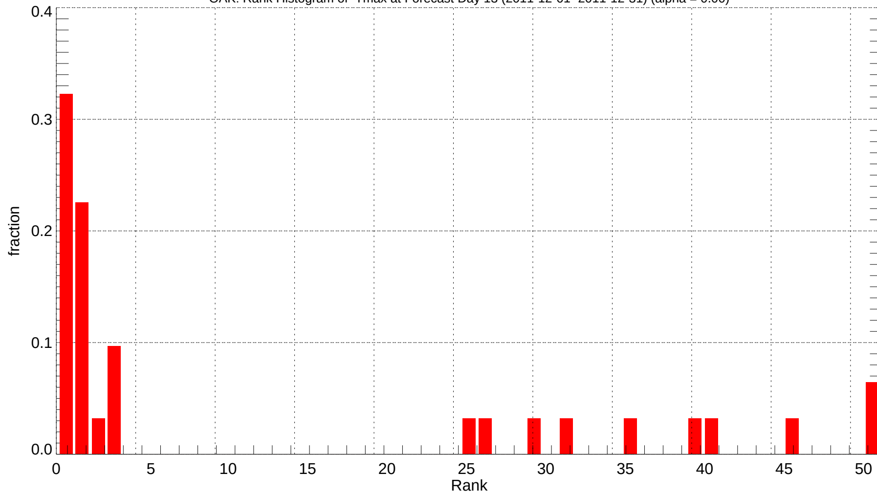
OAK: Rank Histogram of Tmax at Forecast Day 13 (2011-12-01~2011-12-31) (alpha = 0.00)
