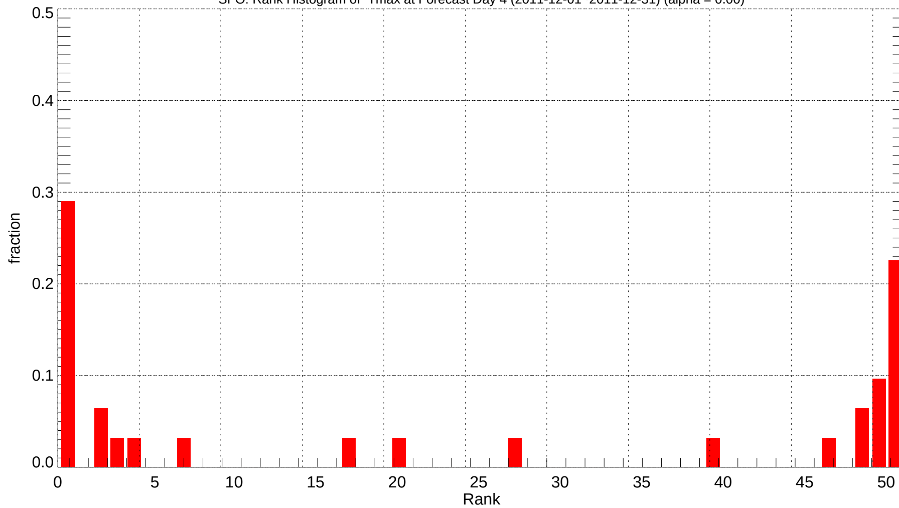
SFO: Rank Histogram of Tmax at Forecast Day 4 (2011-12-01~2011-12-31) (alpha = 0.00)
