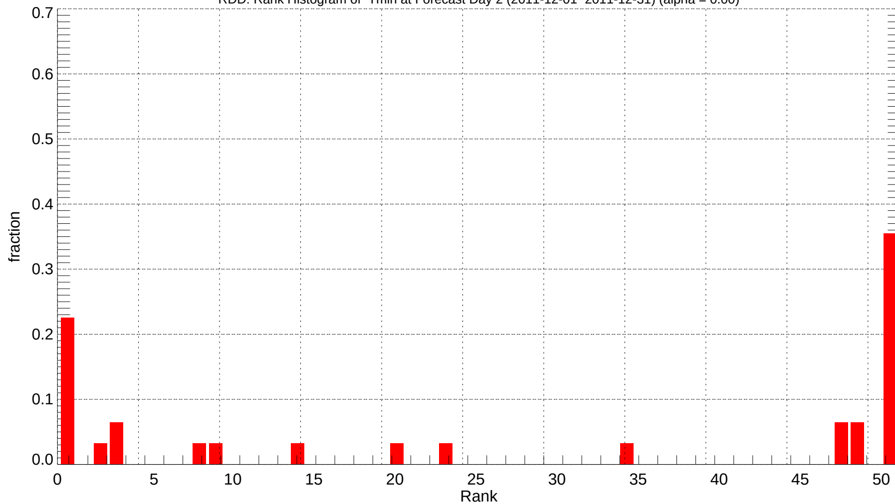
RDD: Rank Histogram of Tmin at Forecast Day 2 (2011-12-01~2011-12-31) (alpha = 0.00)
