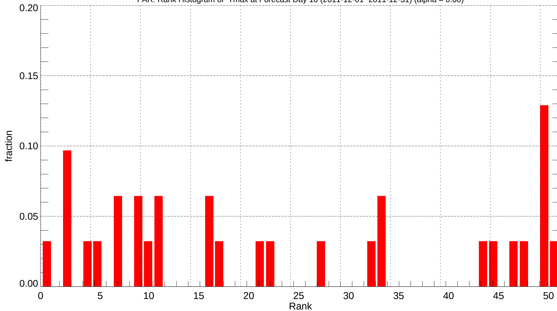
FAR: Rank Histogram of Tmax at Forecast Day 10 (2011-12-01~2011-12-31) (alpha = 0.00)
