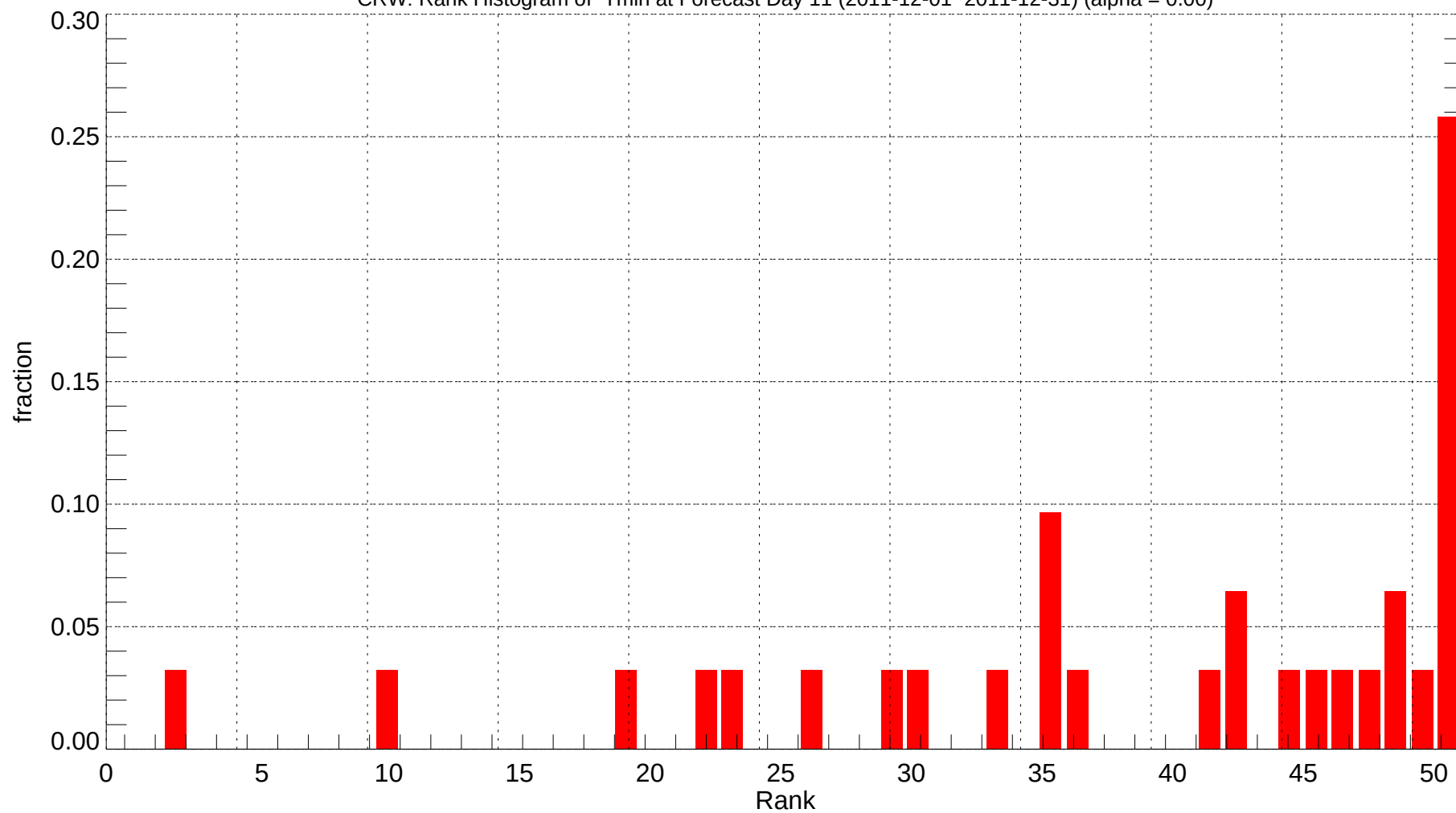
CRW: Rank Histogram of Tmin at Forecast Day 11 (2011-12-01~2011-12-31) (alpha = 0.00)
