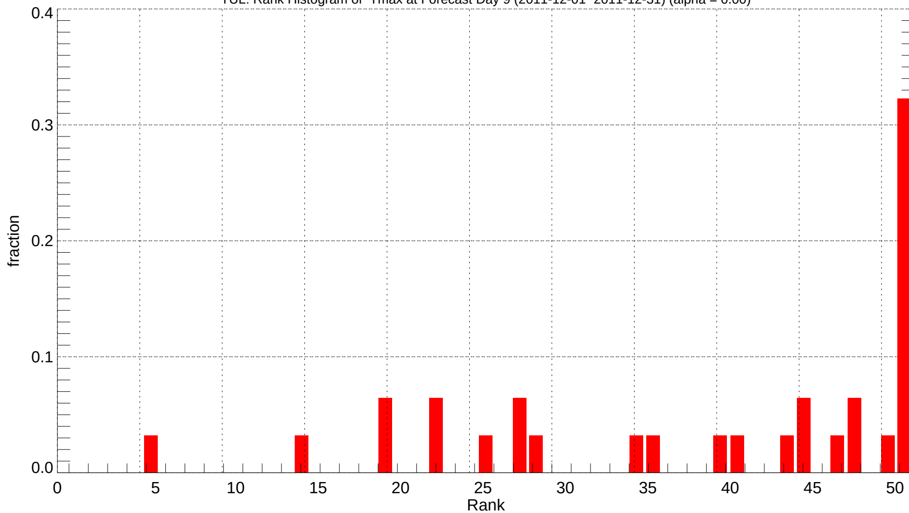
TUL: Rank Histogram of Tmax at Forecast Day 9 (2011-12-01~2011-12-31) (alpha = 0.00)
