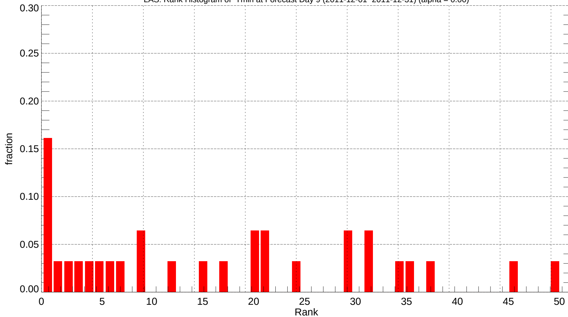
LAS: Rank Histogram of Tmin at Forecast Day 9 (2011-12-01~2011-12-31) (alpha = 0.00)
