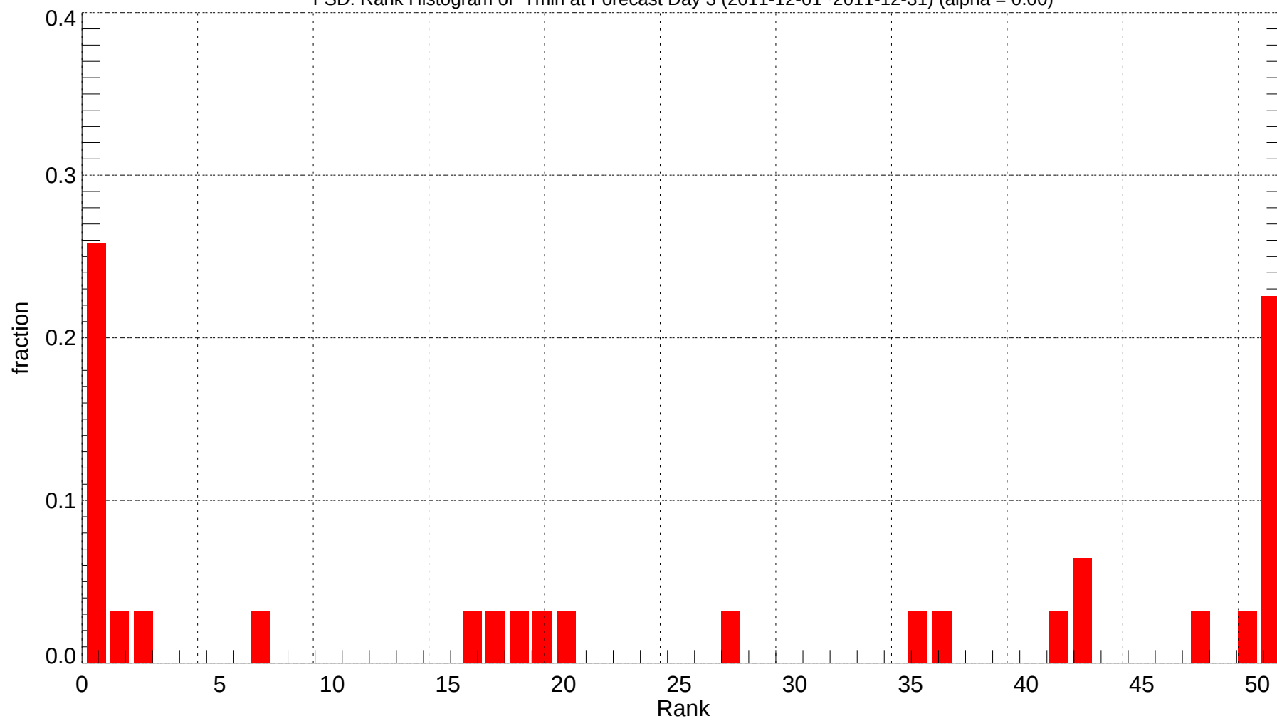
FSD: Rank Histogram of Tmin at Forecast Day 3 (2011-12-01~2011-12-31) (alpha = 0.00)
