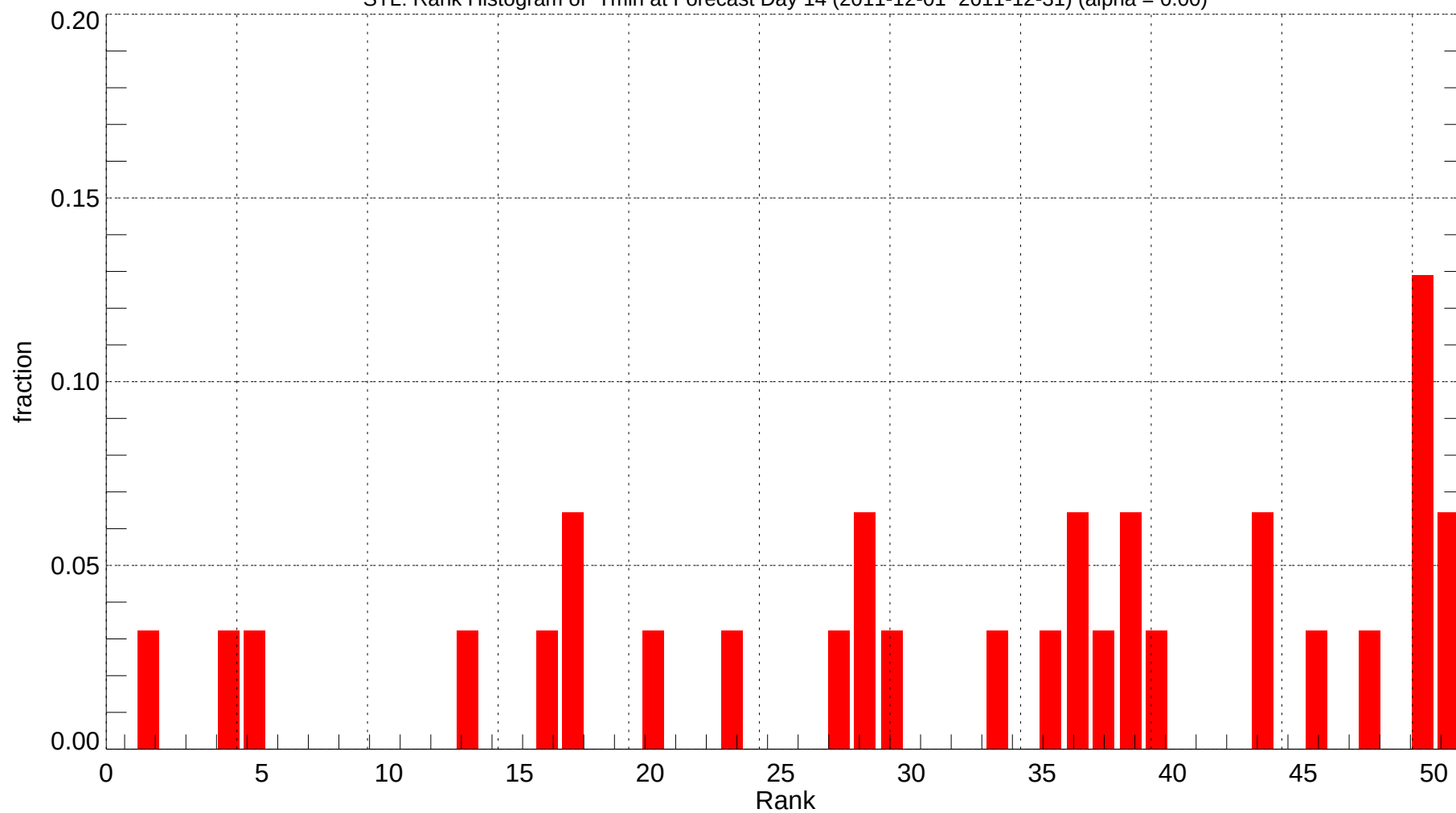
STL: Rank Histogram of Tmin at Forecast Day 14 (2011-12-01~2011-12-31) (alpha = 0.00)
