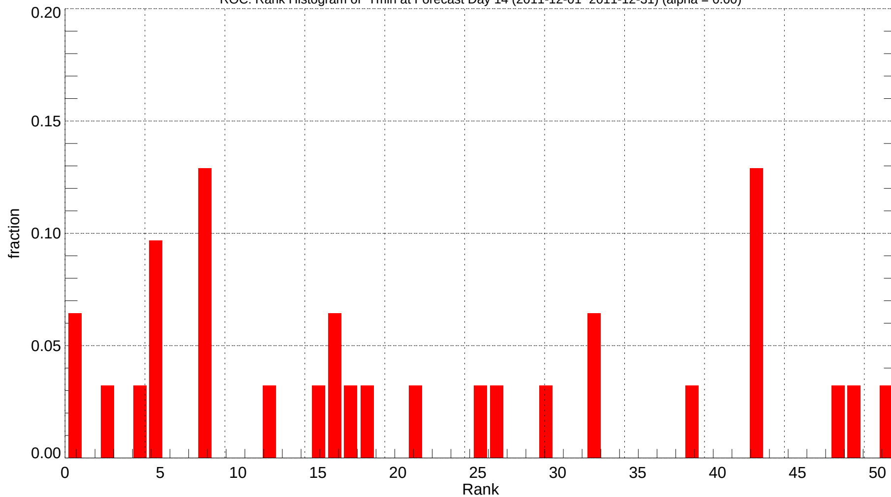
ROC: Rank Histogram of Tmin at Forecast Day 14 (2011-12-01~2011-12-31) (alpha = 0.00)
