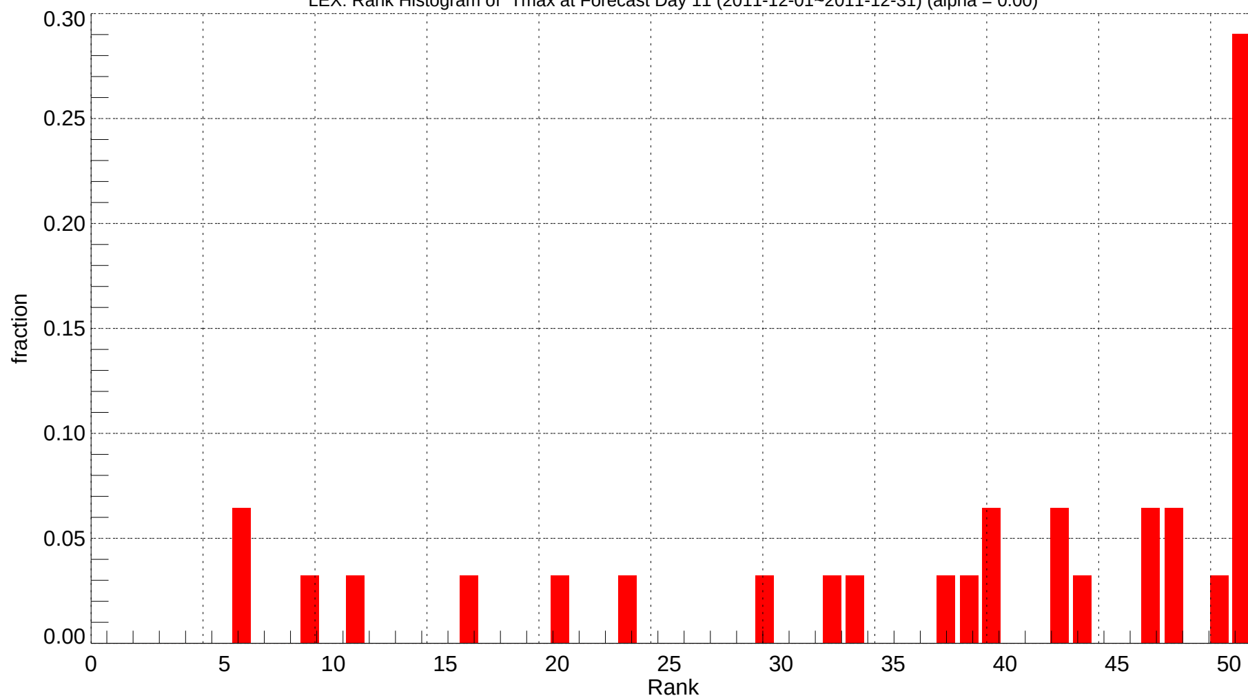
LEX: Rank Histogram of Tmax at Forecast Day 11 (2011-12-01~2011-12-31) (alpha = 0.00)
