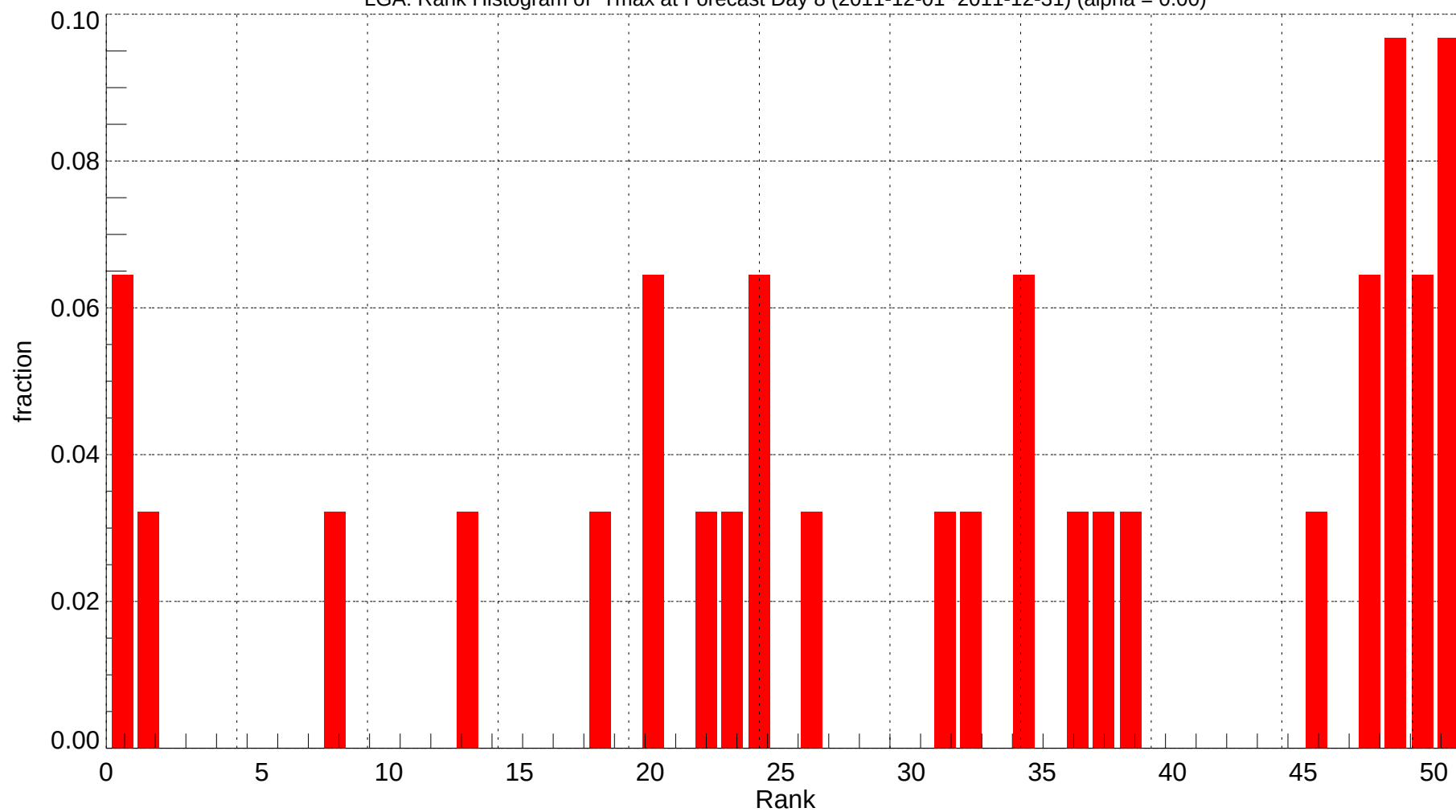
LGA: Rank Histogram of Tmax at Forecast Day 8 (2011-12-01~2011-12-31) (alpha = 0.00)
