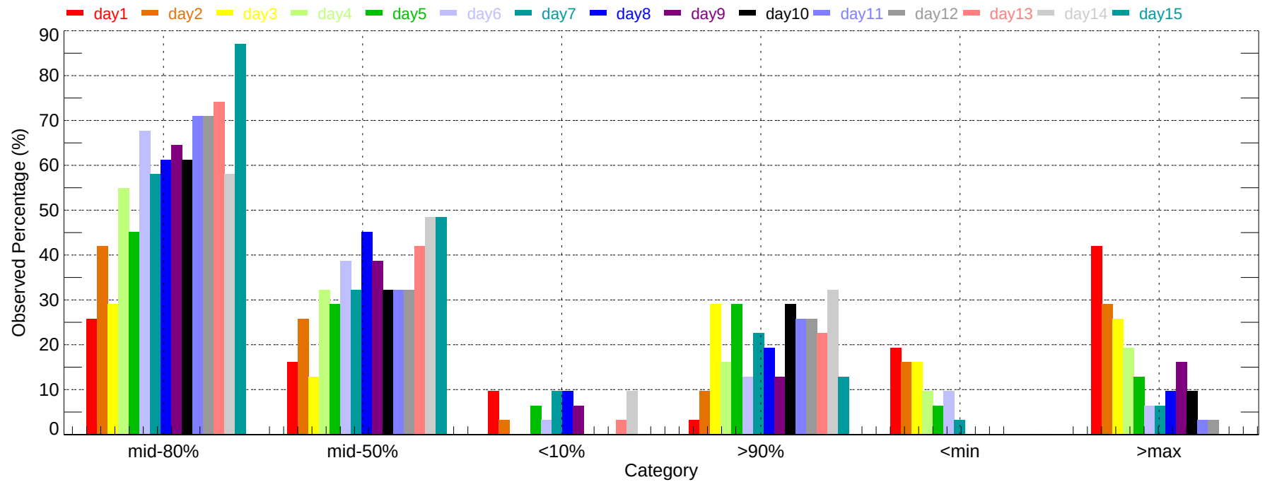
Observed Percentage of Ensembles - CMH: Min Temperature (2011-12-01~2011-12-31)
