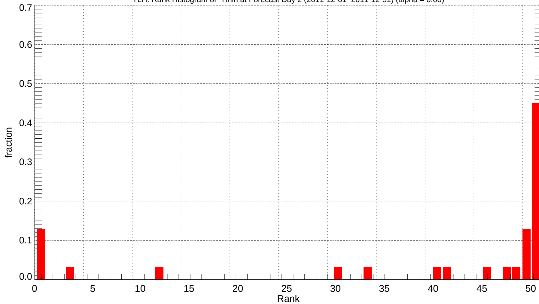
TLH: Rank Histogram of Tmin at Forecast Day 2 (2011-12-01~2011-12-31) (alpha = 0.00)
