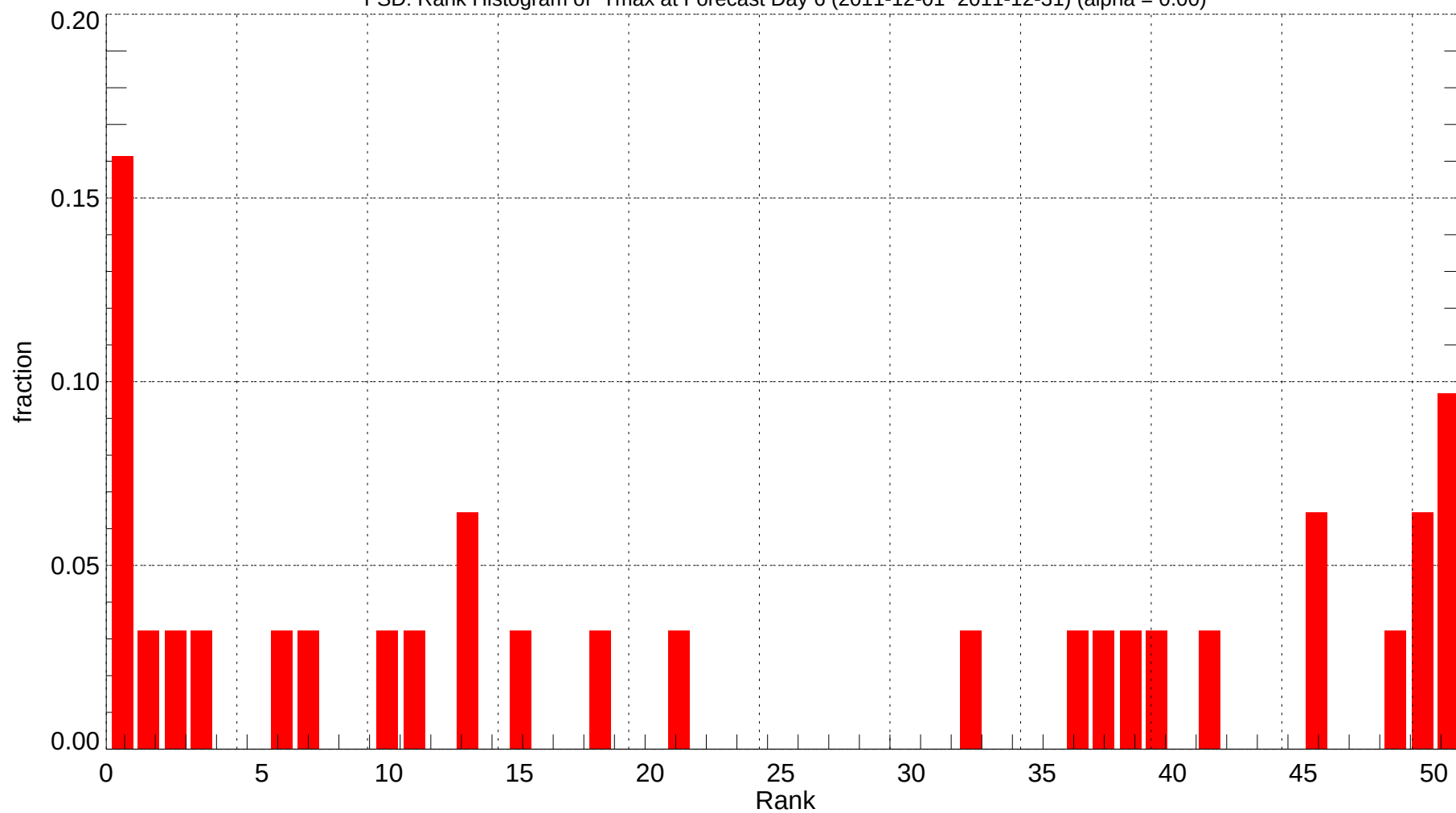
FSD: Rank Histogram of Tmax at Forecast Day 6 (2011-12-01~2011-12-31) (alpha = 0.00)
