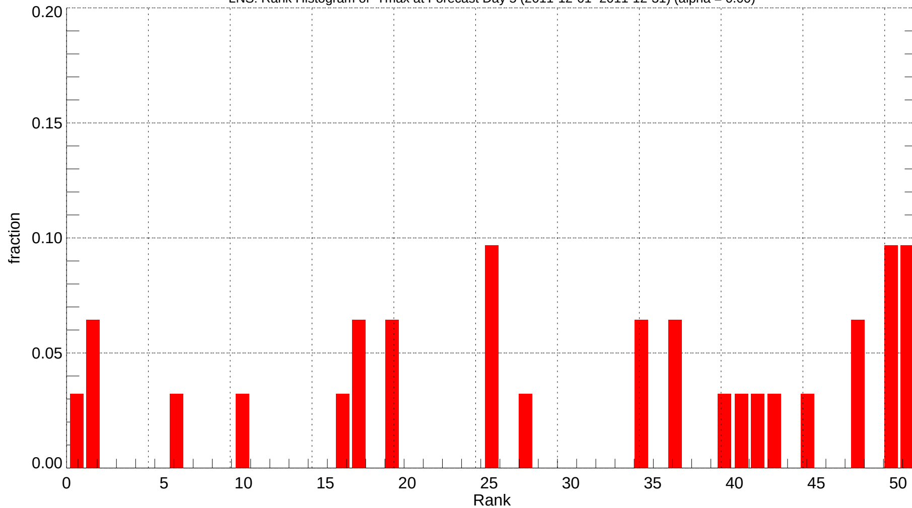
LNS: Rank Histogram of Tmax at Forecast Day 5 (2011-12-01~2011-12-31) (alpha = 0.00)
