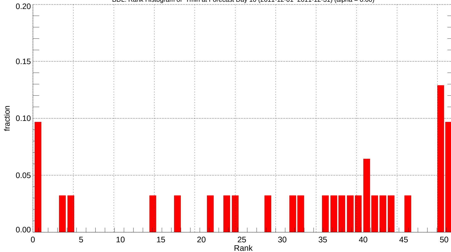
BDL: Rank Histogram of Tmin at Forecast Day 10 (2011-12-01~2011-12-31) (alpha = 0.00)
