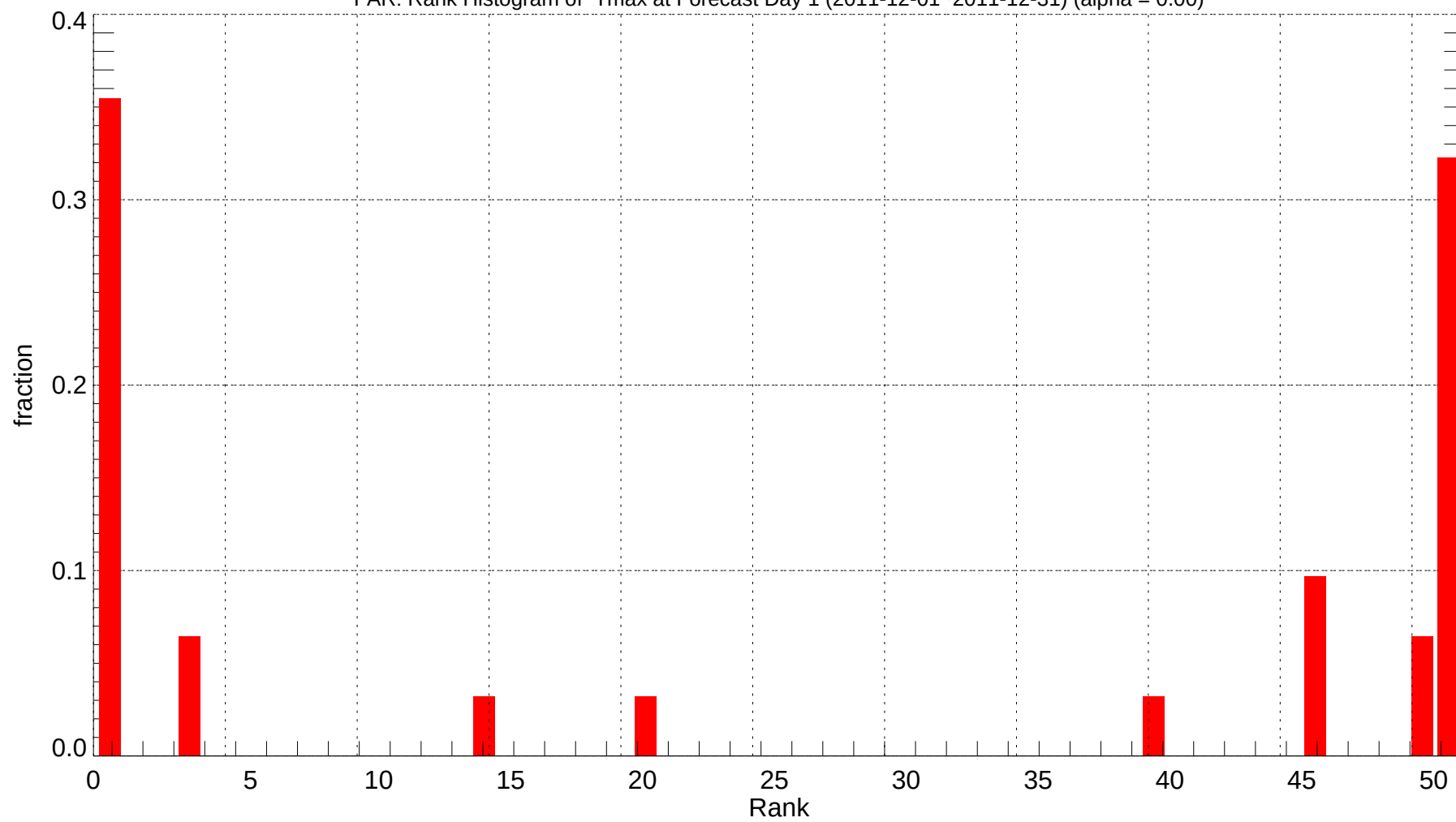
FAR: Rank Histogram of Tmax at Forecast Day 1 (2011-12-01~2011-12-31) (alpha = 0.00)
