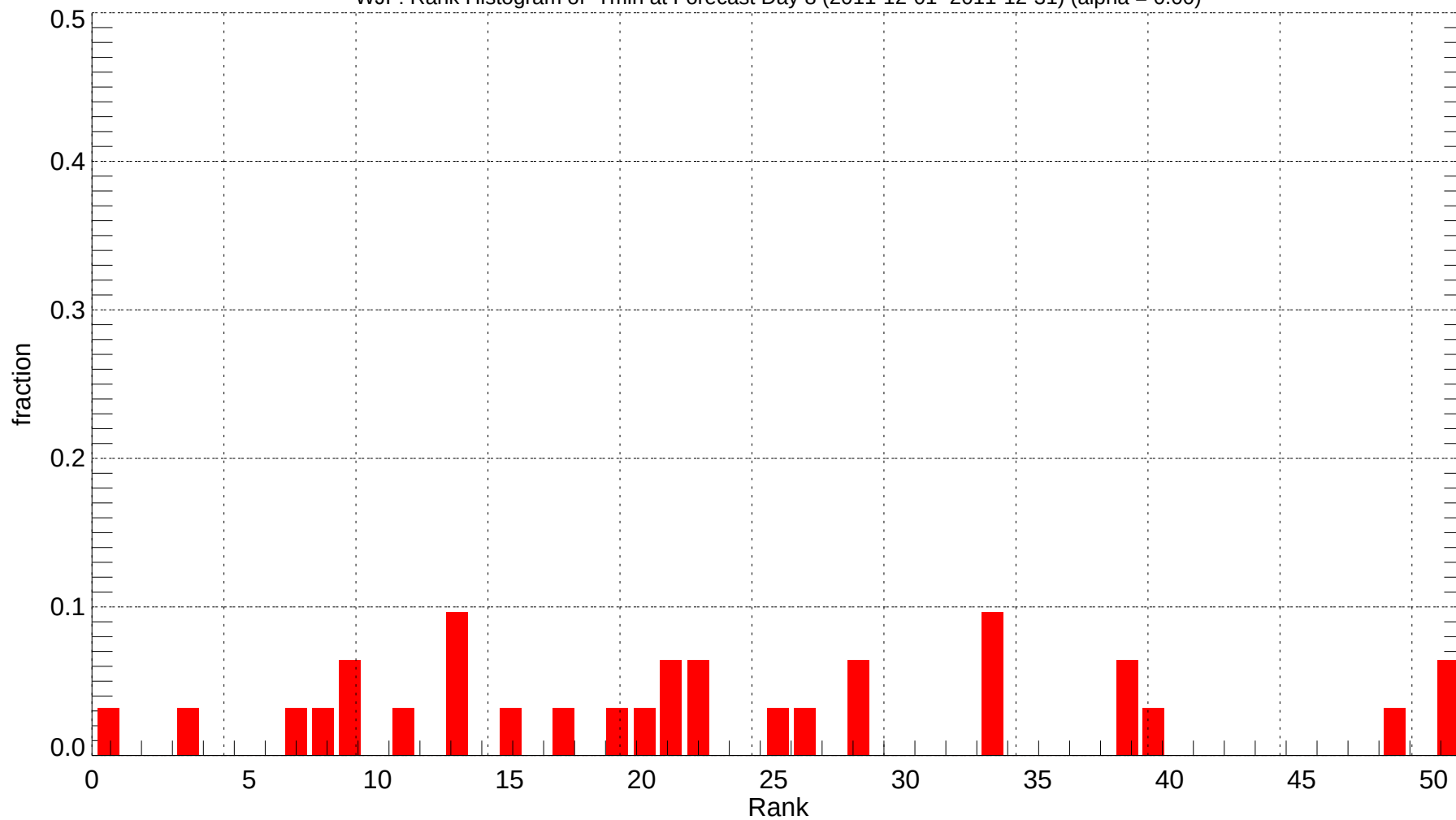
WJF: Rank Histogram of Tmin at Forecast Day 8 (2011-12-01~2011-12-31) (alpha = 0.00)
