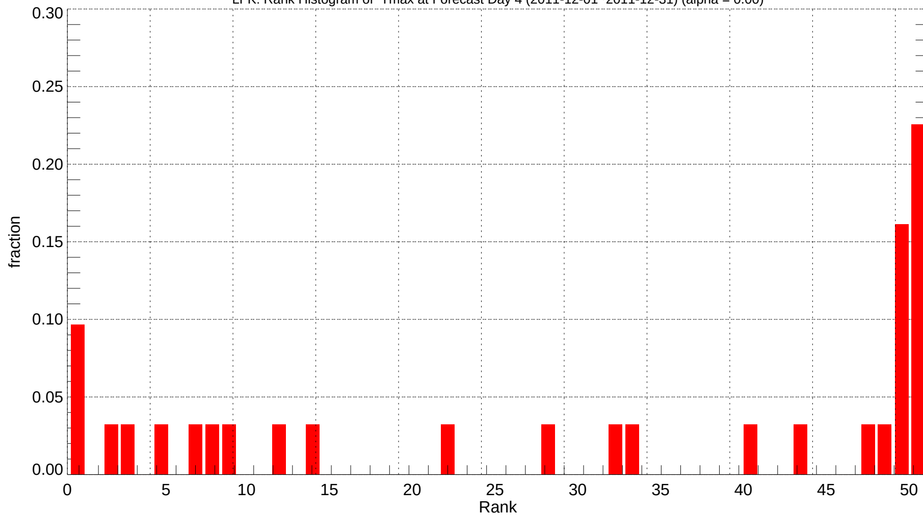
LFK: Rank Histogram of Tmax at Forecast Day 4 (2011-12-01~2011-12-31) (alpha = 0.00)
