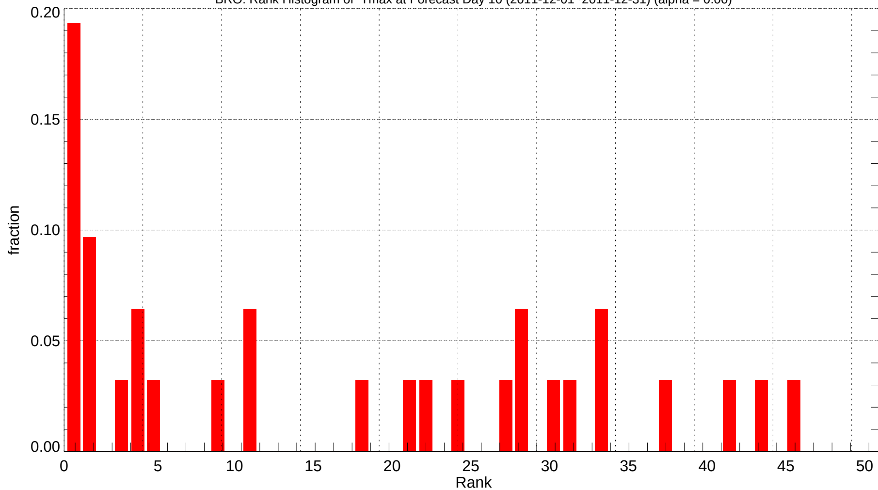
BRO: Rank Histogram of Tmax at Forecast Day 10 (2011-12-01~2011-12-31) (alpha = 0.00)
