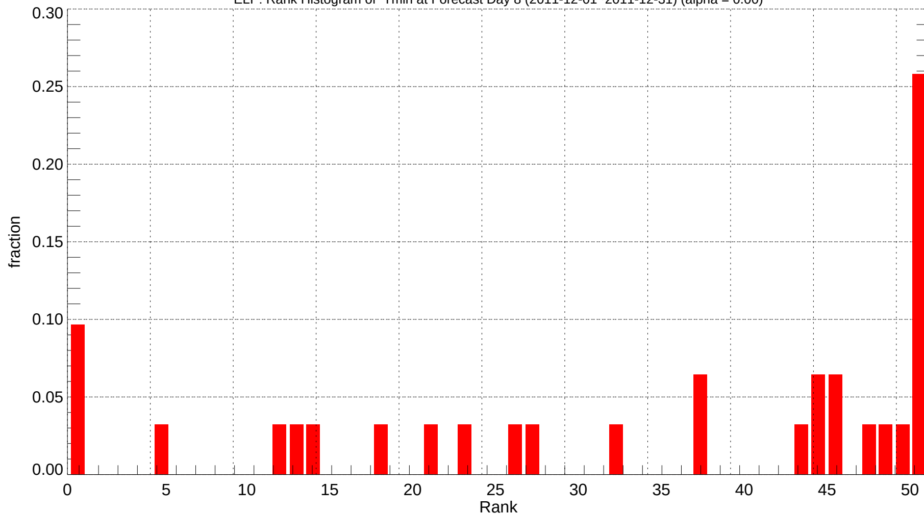
ELP: Rank Histogram of Tmin at Forecast Day 8 (2011-12-01~2011-12-31) (alpha = 0.00)
