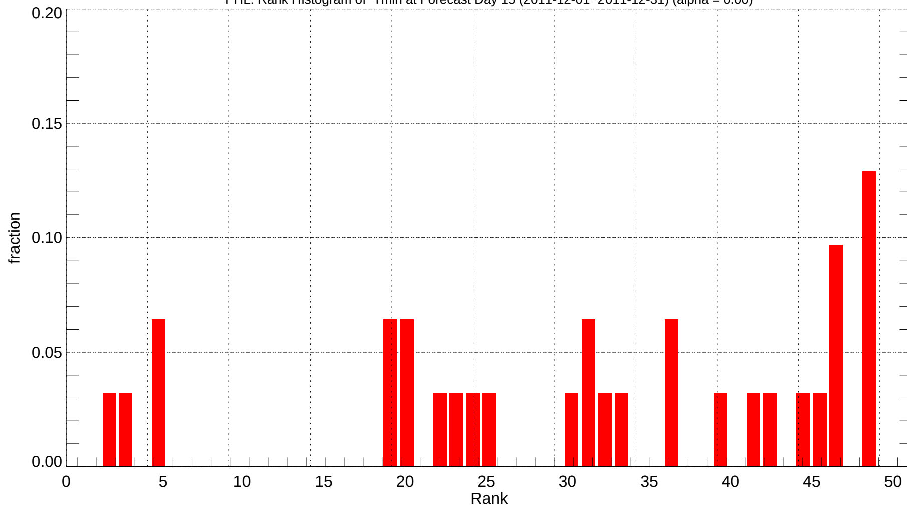
PHL: Rank Histogram of Tmin at Forecast Day 15 (2011-12-01~2011-12-31) (alpha = 0.00)
