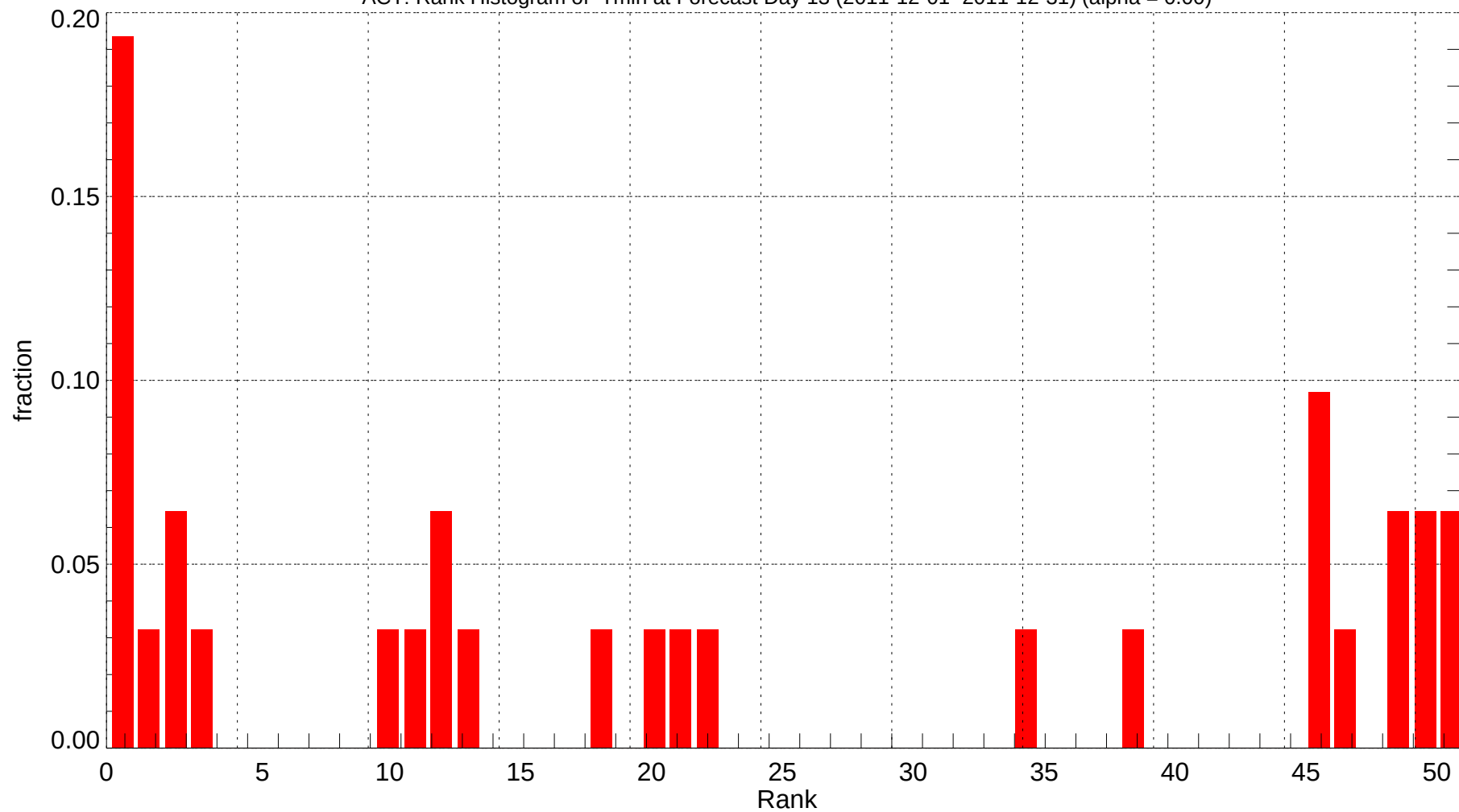
ACT: Rank Histogram of Tmin at Forecast Day 13 (2011-12-01~2011-12-31) (alpha = 0.00)
