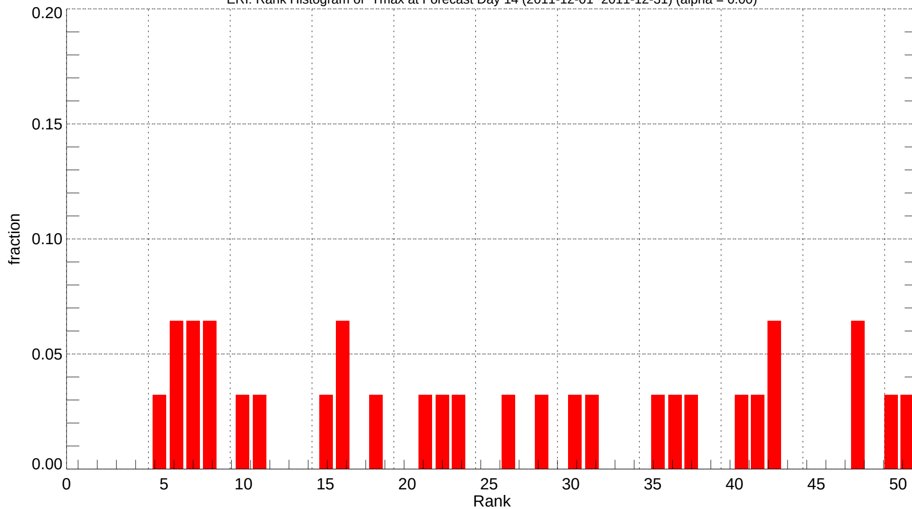
ERI: Rank Histogram of Tmax at Forecast Day 14 (2011-12-01~2011-12-31) (alpha = 0.00)
