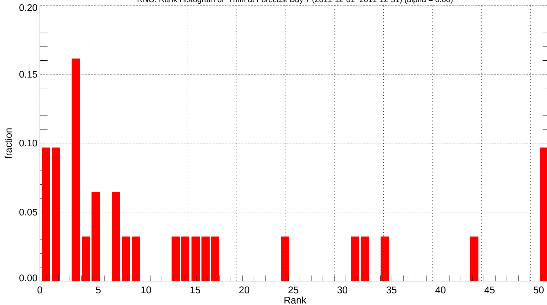
RNO: Rank Histogram of Tmin at Forecast Day 7 (2011-12-01~2011-12-31) (alpha = 0.00)
