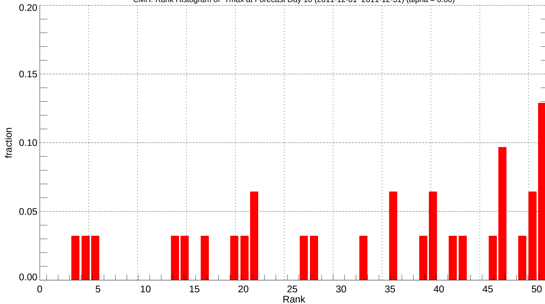
CMH: Rank Histogram of Tmax at Forecast Day 10 (2011-12-01~2011-12-31) (alpha = 0.00)
