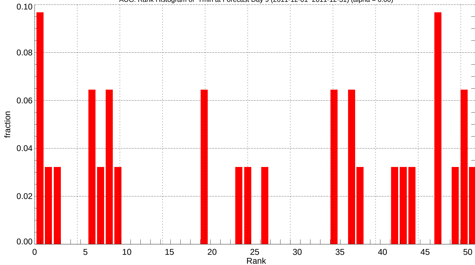
AUG: Rank Histogram of Tmin at Forecast Day 9 (2011-12-01~2011-12-31) (alpha = 0.00)
