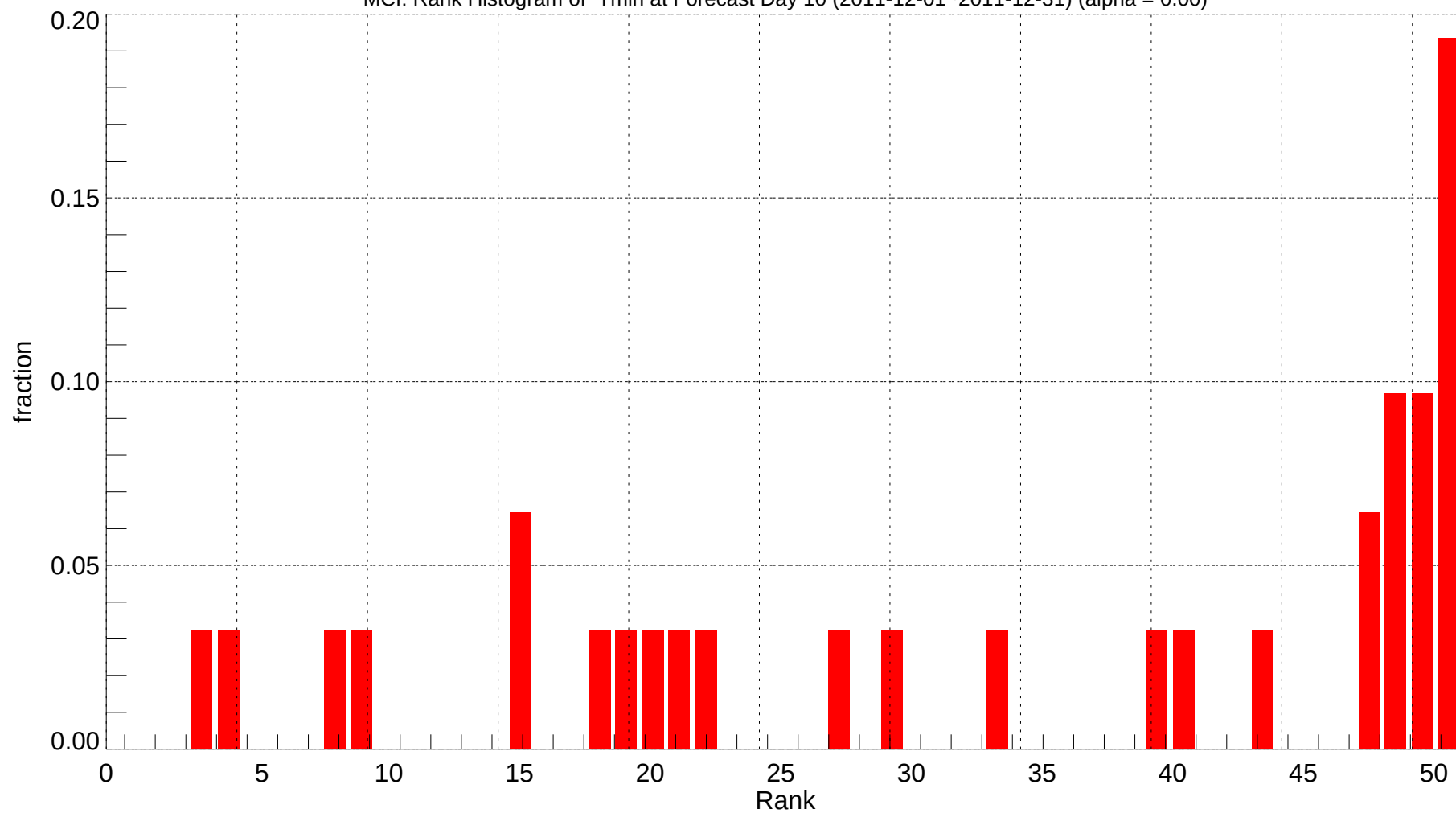
MCI: Rank Histogram of Tmin at Forecast Day 10 (2011-12-01~2011-12-31) (alpha = 0.00)
