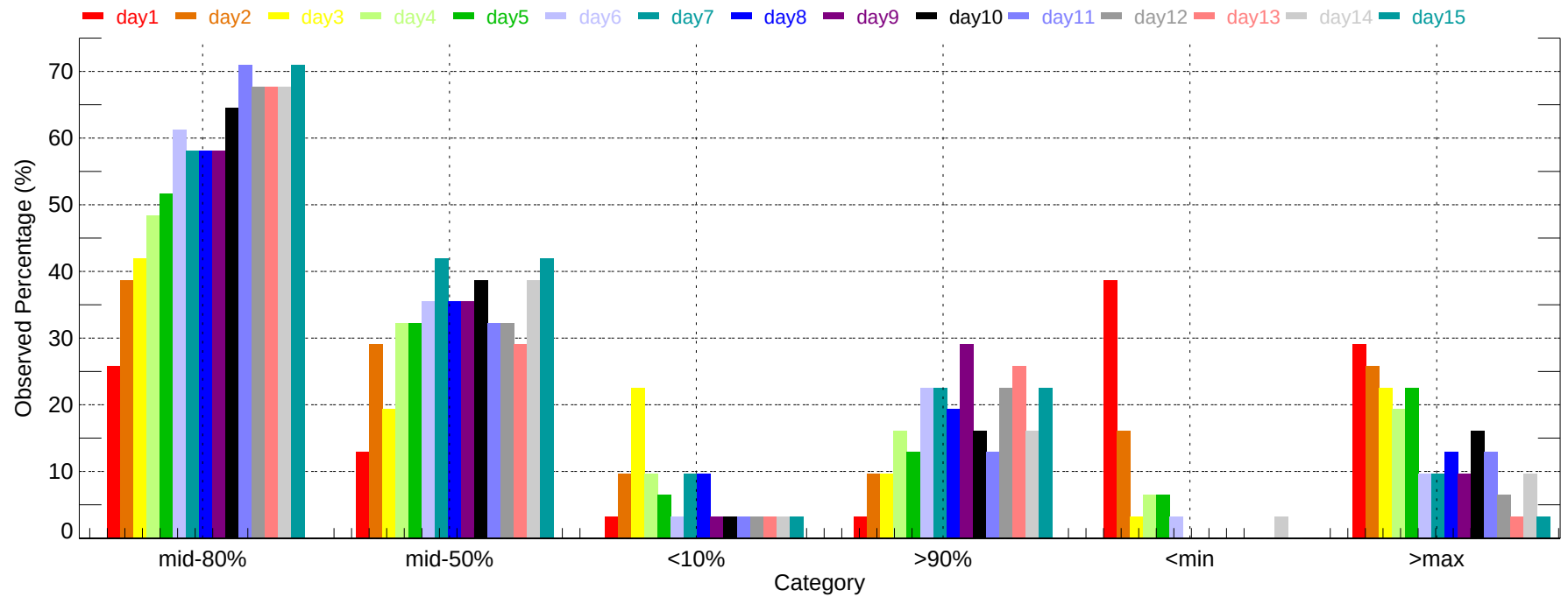
Observed Percentage of Ensembles - MCI: Min Temperature (2011-12-01~2011-12-31)
