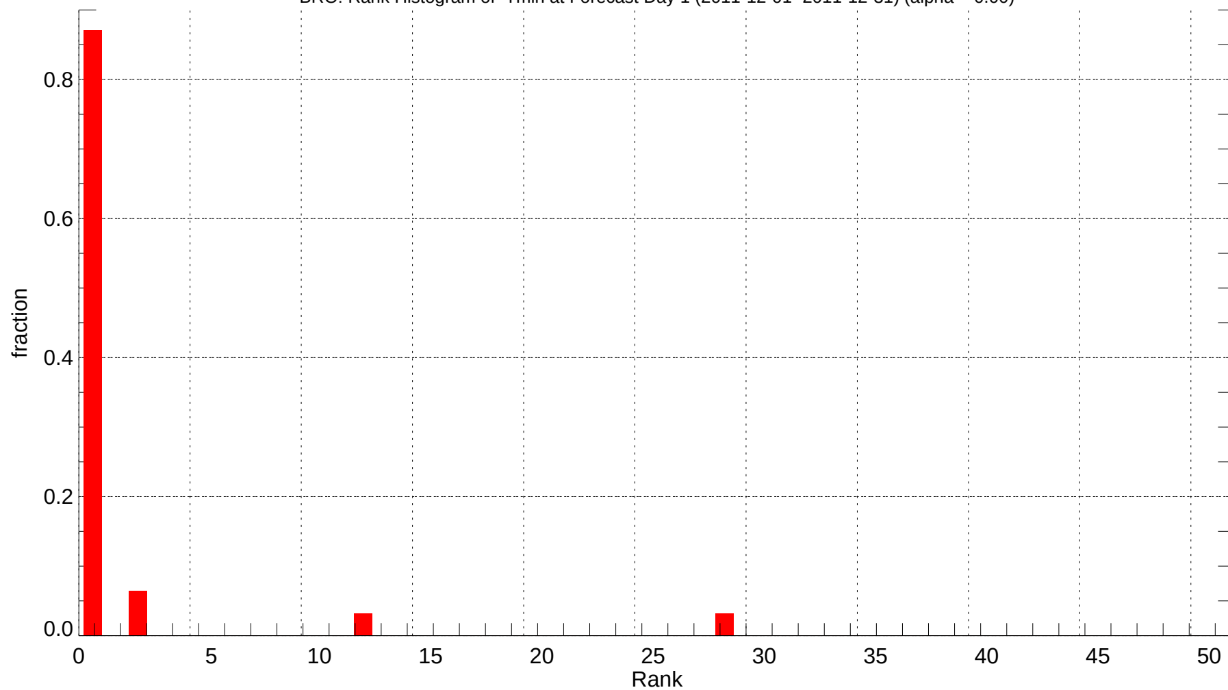
BRO: Rank Histogram of Tmin at Forecast Day 1 (2011-12-01~2011-12-31) (alpha = 0.00)
