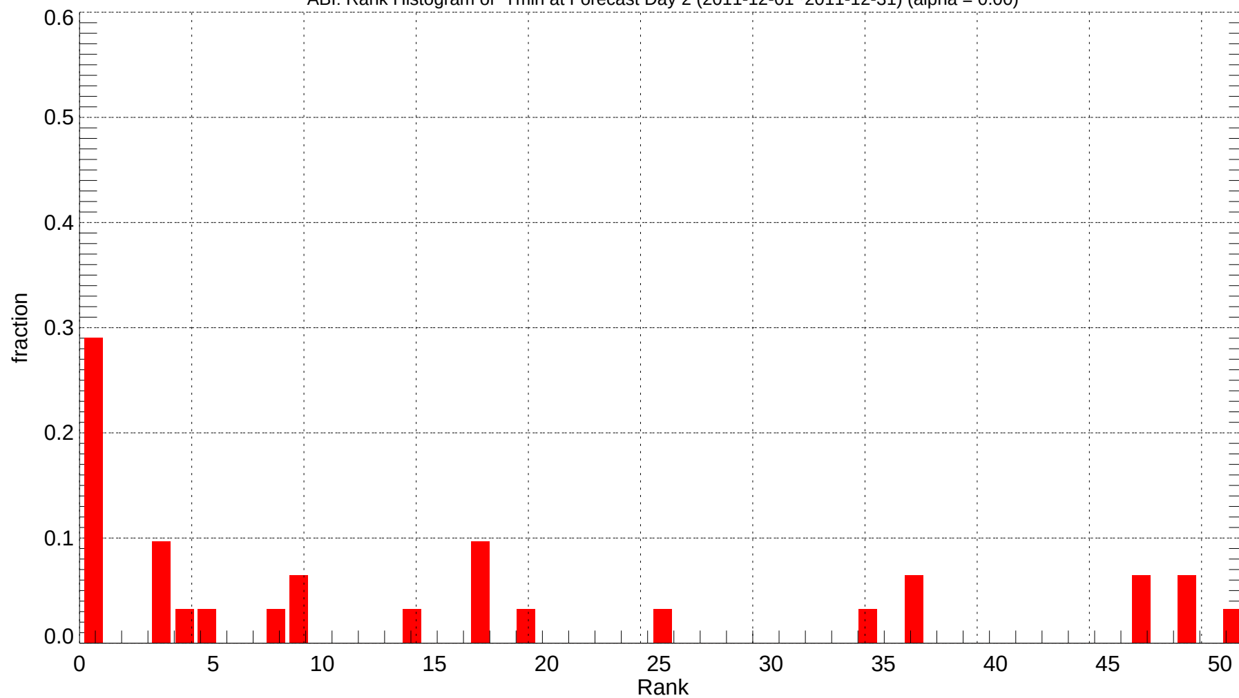
ABI: Rank Histogram of Tmin at Forecast Day 2 (2011-12-01~2011-12-31) (alpha = 0.00)
