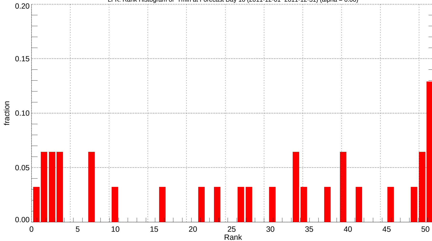
LFK: Rank Histogram of Tmin at Forecast Day 10 (2011-12-01~2011-12-31) (alpha = 0.00)
