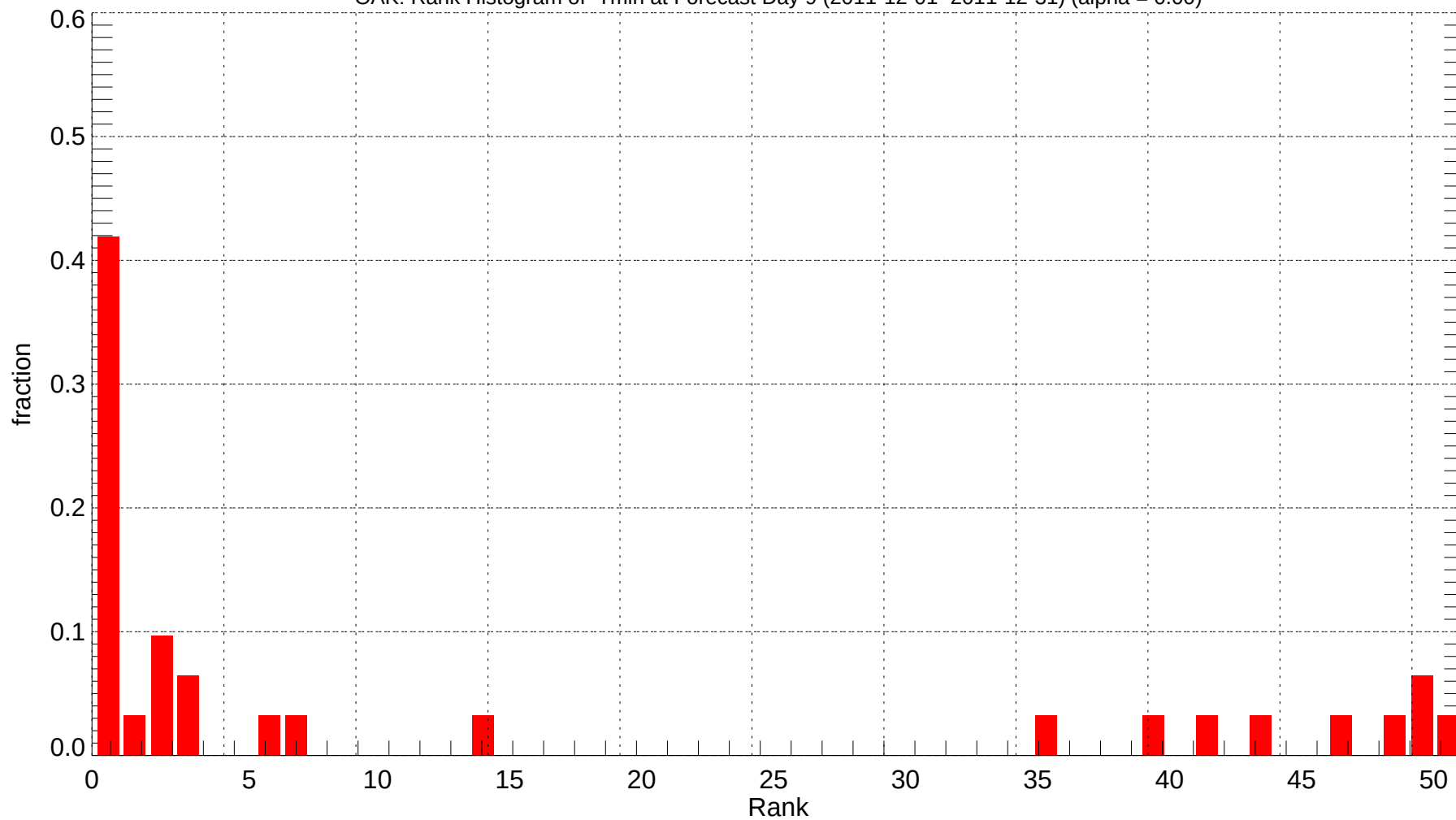
OAK: Rank Histogram of Tmin at Forecast Day 9 (2011-12-01~2011-12-31) (alpha = 0.00)
