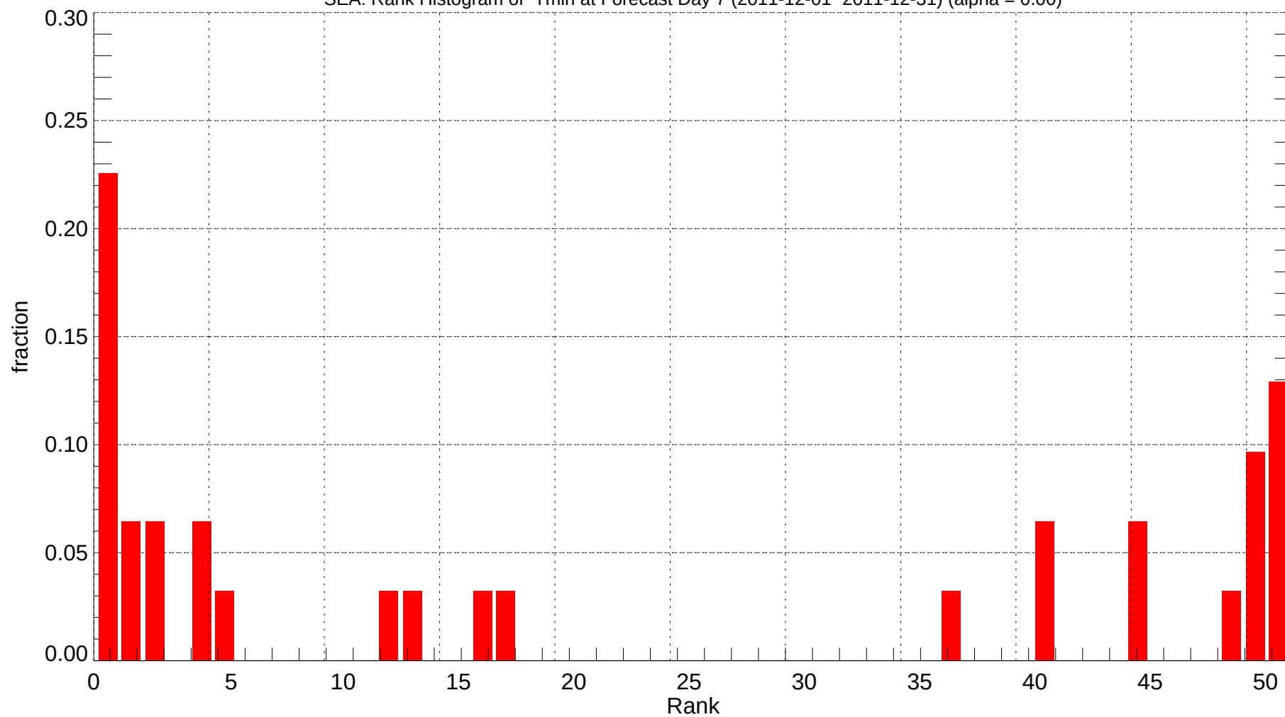
SEA: Rank Histogram of Tmin at Forecast Day 7 (2011-12-01~2011-12-31) (alpha = 0.00)
