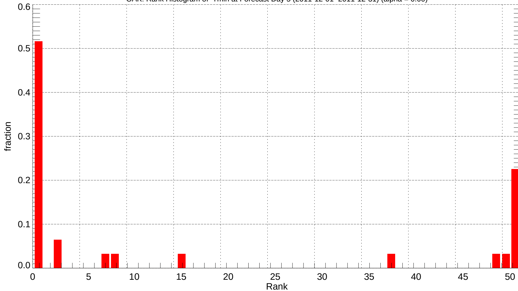
OAK: Rank Histogram of Tmin at Forecast Day 5 (2011-12-01~2011-12-31) (alpha = 0.00)
