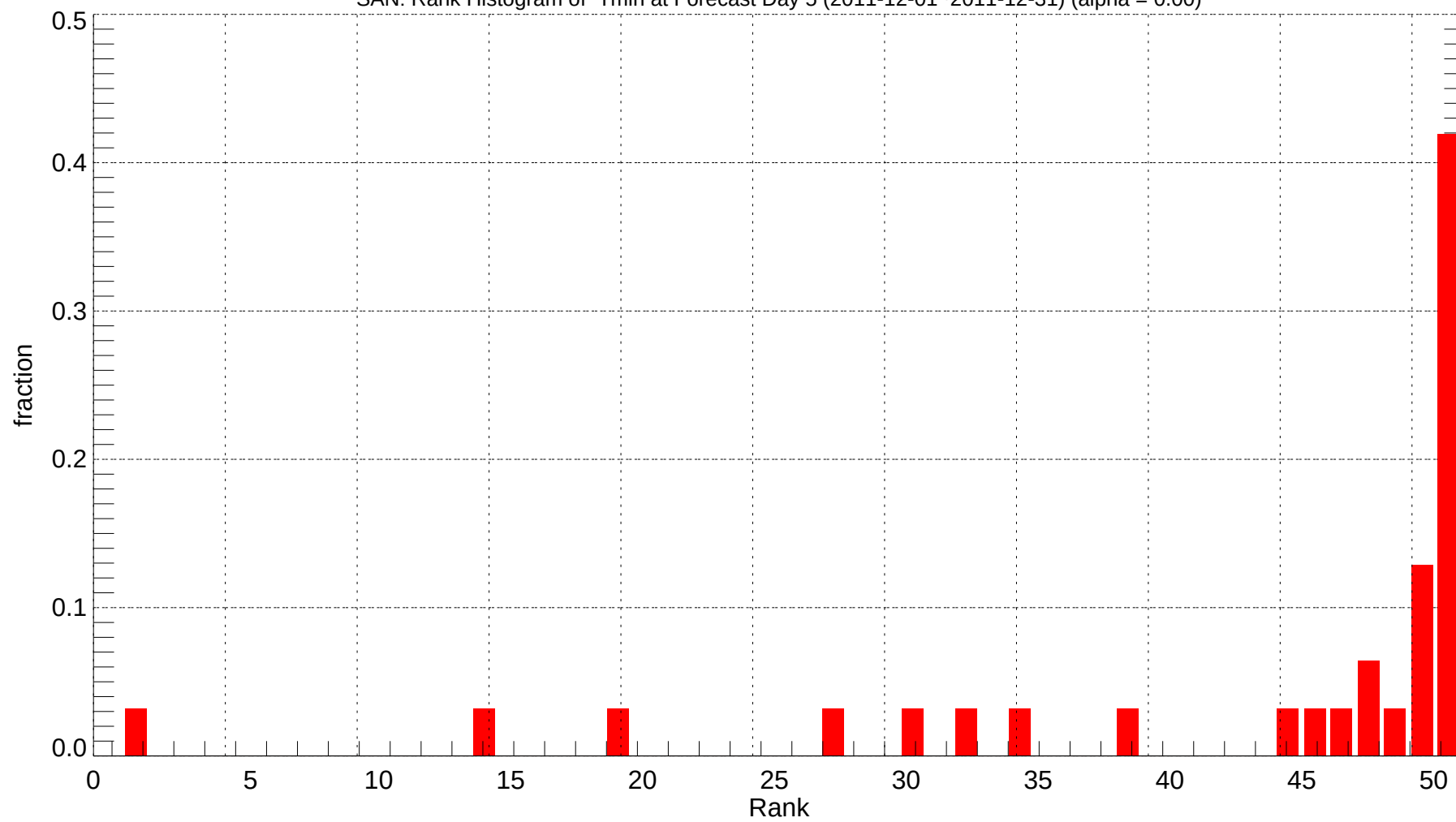
SAN: Rank Histogram of Tmin at Forecast Day 5 (2011-12-01~2011-12-31) (alpha = 0.00)
