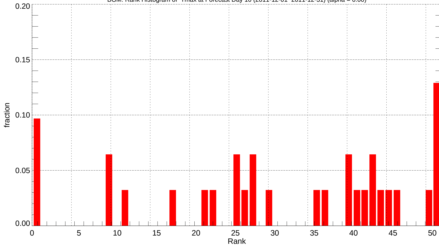
BGM: Rank Histogram of Tmax at Forecast Day 10 (2011-12-01~2011-12-31) (alpha = 0.00)
