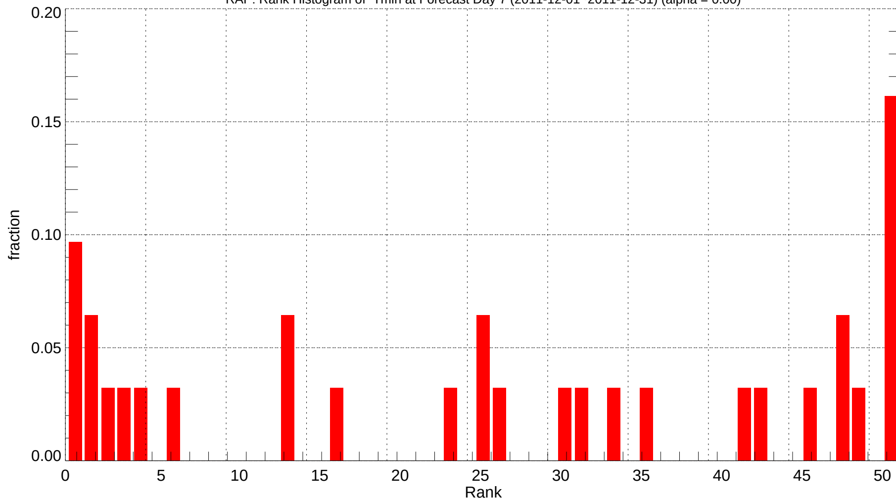
RAP: Rank Histogram of Tmin at Forecast Day 7 (2011-12-01~2011-12-31) (alpha = 0.00)
