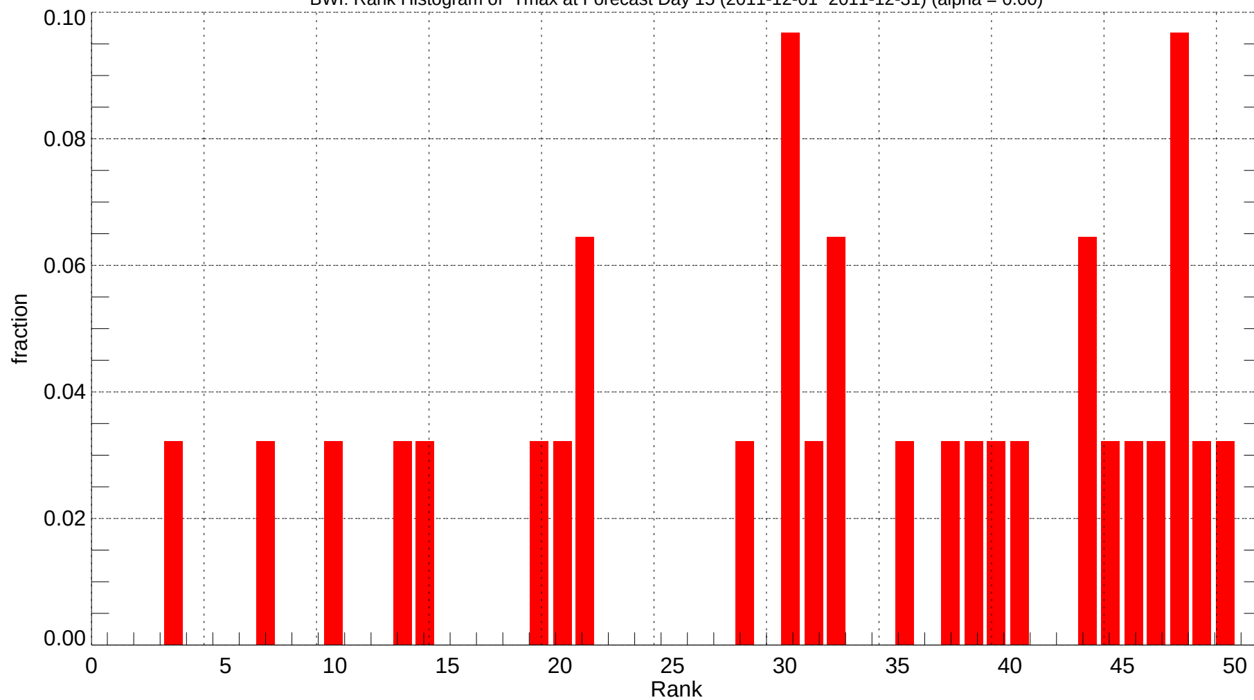
BWI: Rank Histogram of Tmax at Forecast Day 15 (2011-12-01~2011-12-31) (alpha = 0.00)
