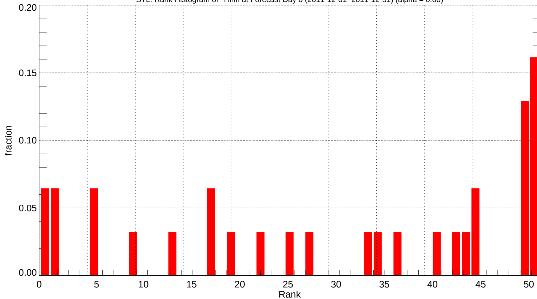
STL: Rank Histogram of Tmin at Forecast Day 6 (2011-12-01~2011-12-31) (alpha = 0.00)
