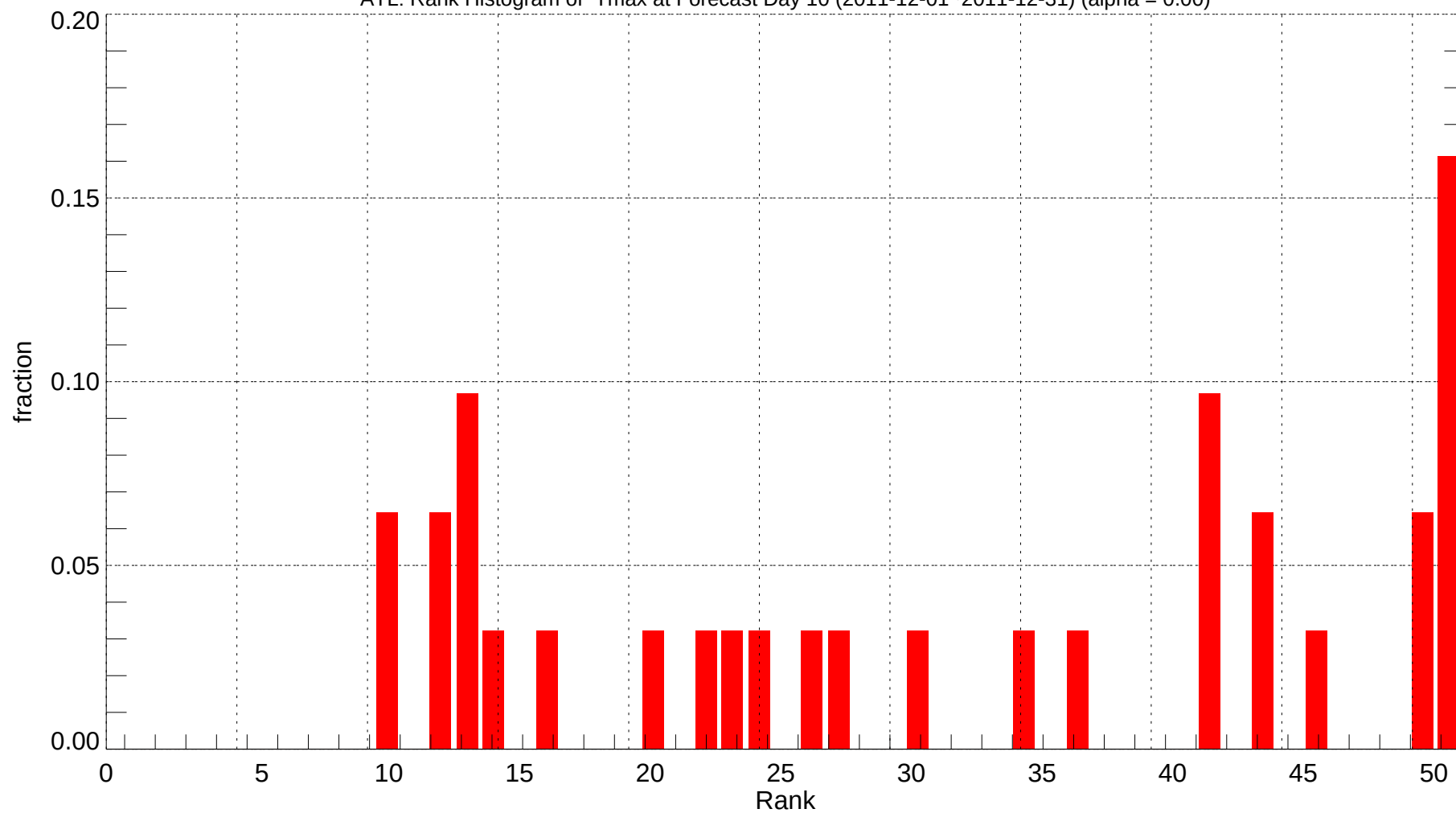
ATL: Rank Histogram of Tmax at Forecast Day 10 (2011-12-01~2011-12-31) (alpha = 0.00)
