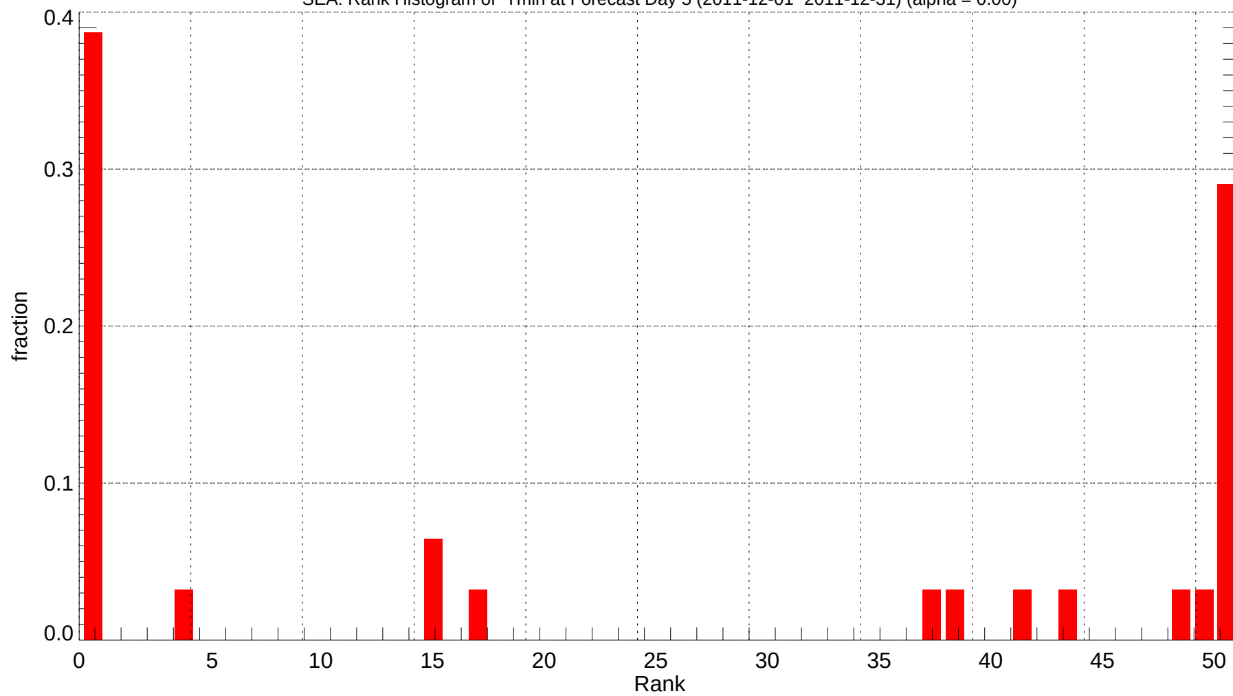
SEA: Rank Histogram of Tmin at Forecast Day 5 (2011-12-01~2011-12-31) (alpha = 0.00)
