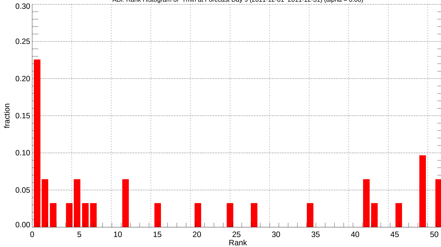
ABI: Rank Histogram of Tmin at Forecast Day 9 (2011-12-01~2011-12-31) (alpha = 0.00)
