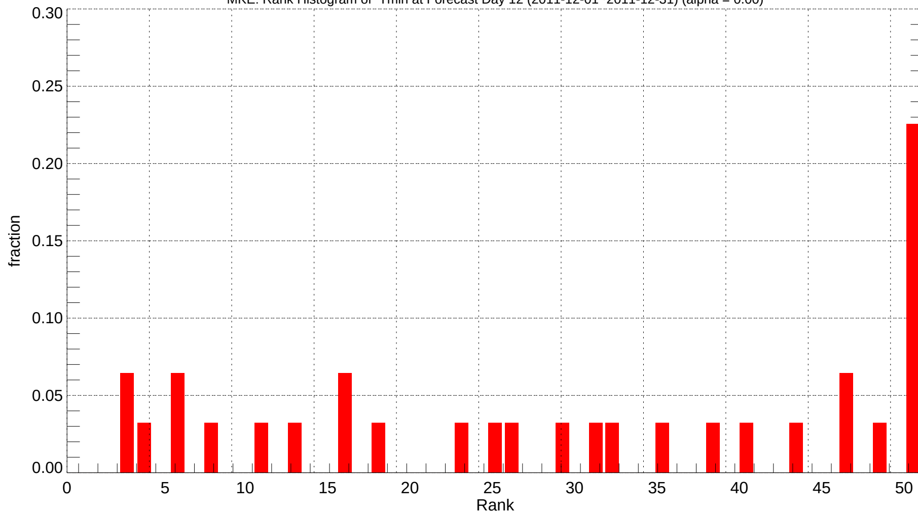
MKE: Rank Histogram of Tmin at Forecast Day 12 (2011-12-01~2011-12-31) (alpha = 0.00)
