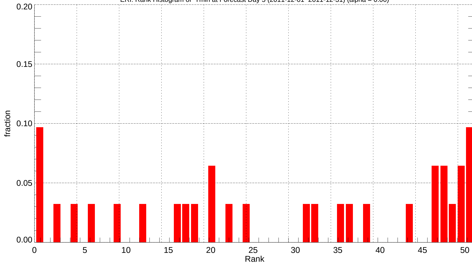
ERI: Rank Histogram of Tmin at Forecast Day 5 (2011-12-01~2011-12-31) (alpha = 0.00)
