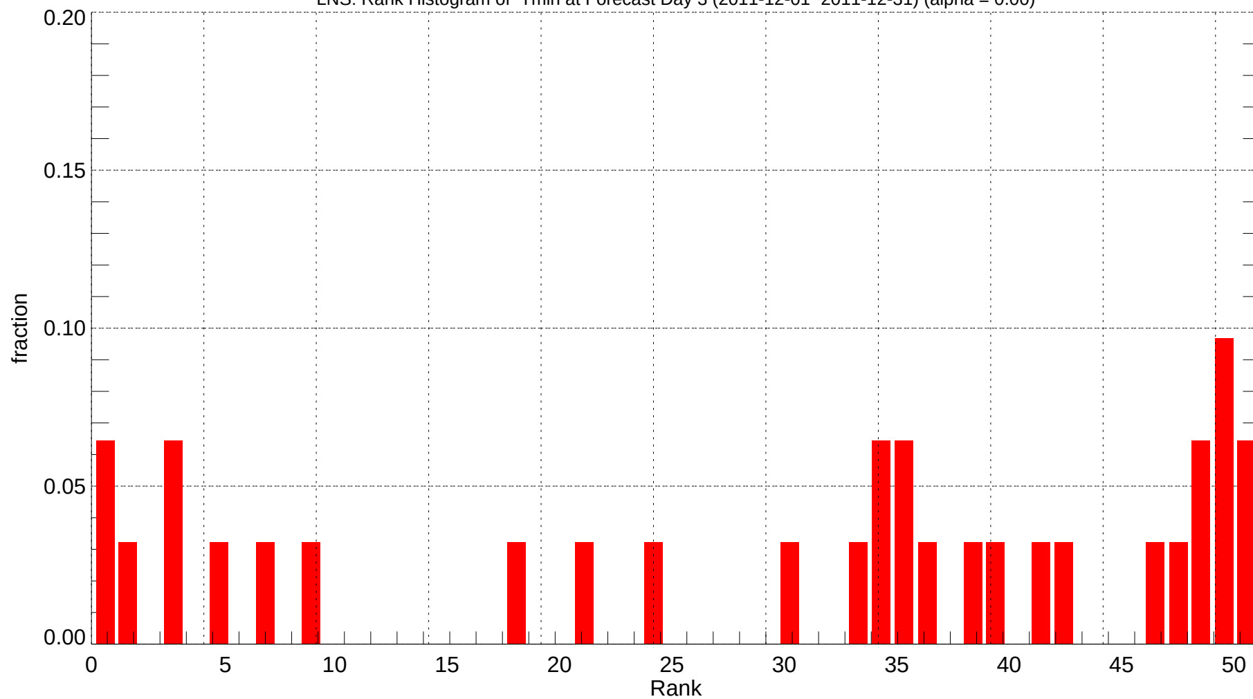
LNS: Rank Histogram of Tmin at Forecast Day 3 (2011-12-01~2011-12-31) (alpha = 0.00)
