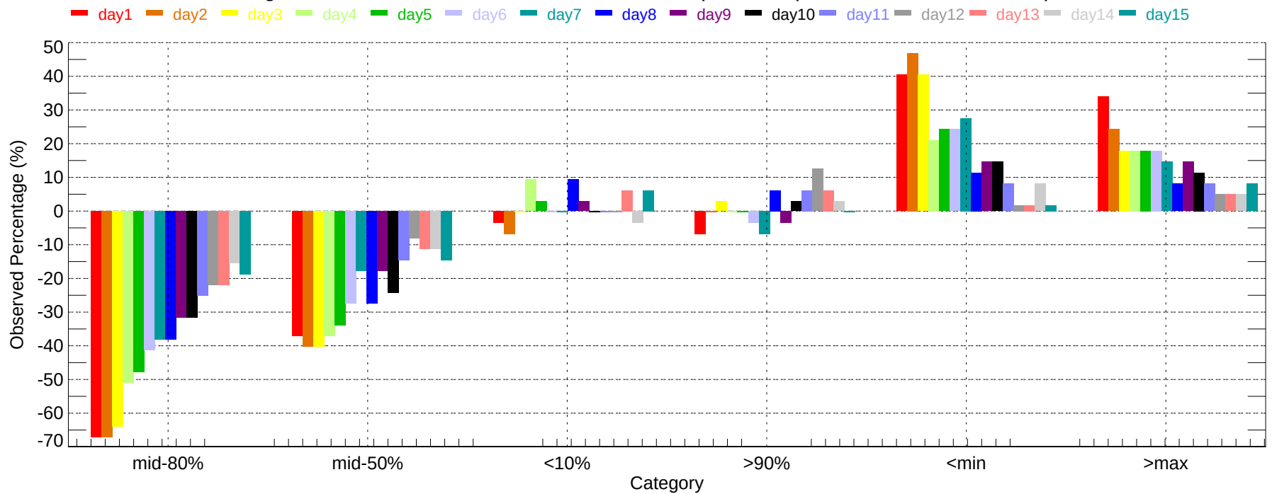
Observed Percentage Deviation of Ensembles - ACY: Min Temperature (2011-12-01~2011-12-31)
