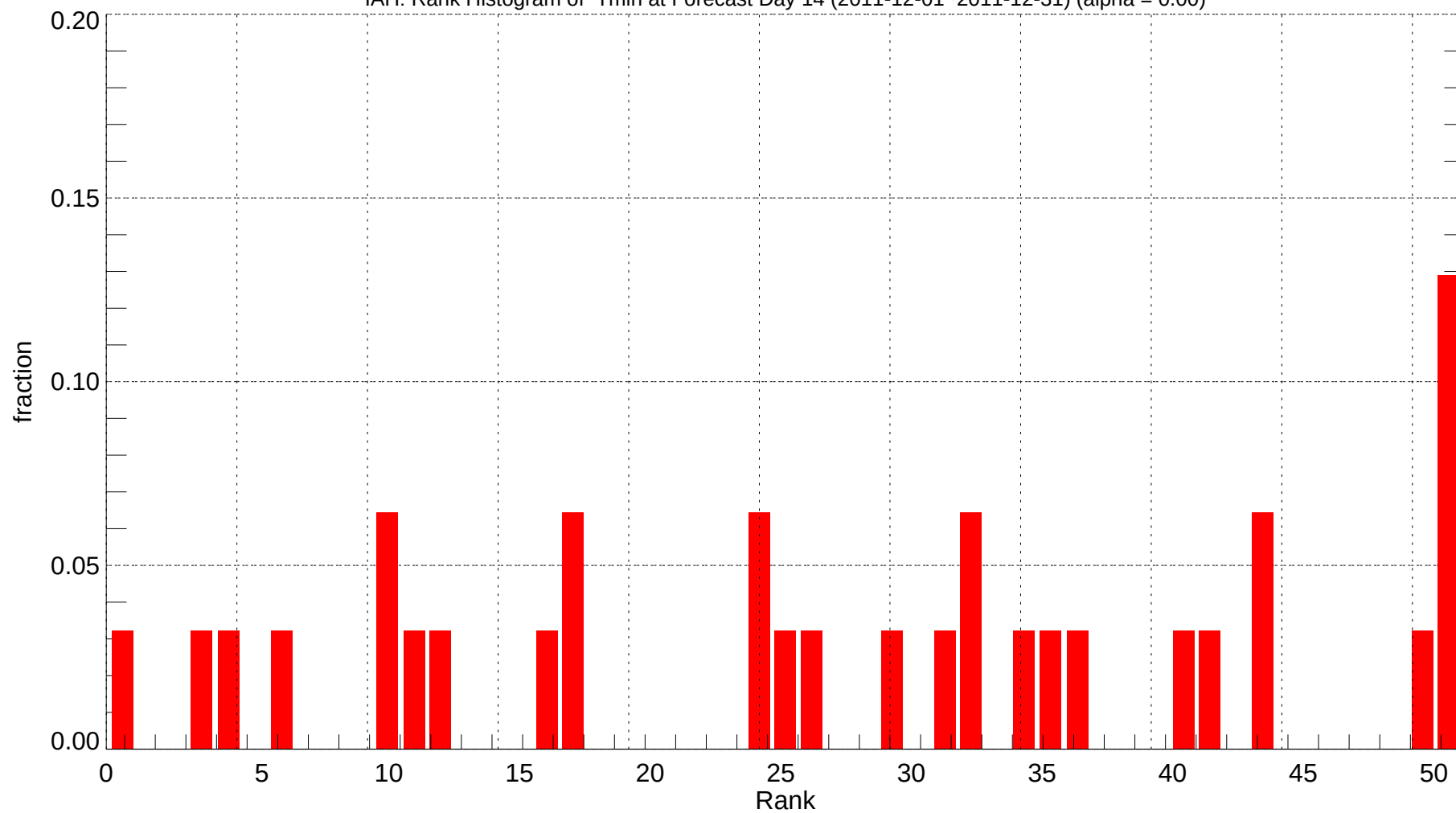
IAH: Rank Histogram of Tmin at Forecast Day 14 (2011-12-01~2011-12-31) (alpha = 0.00)
