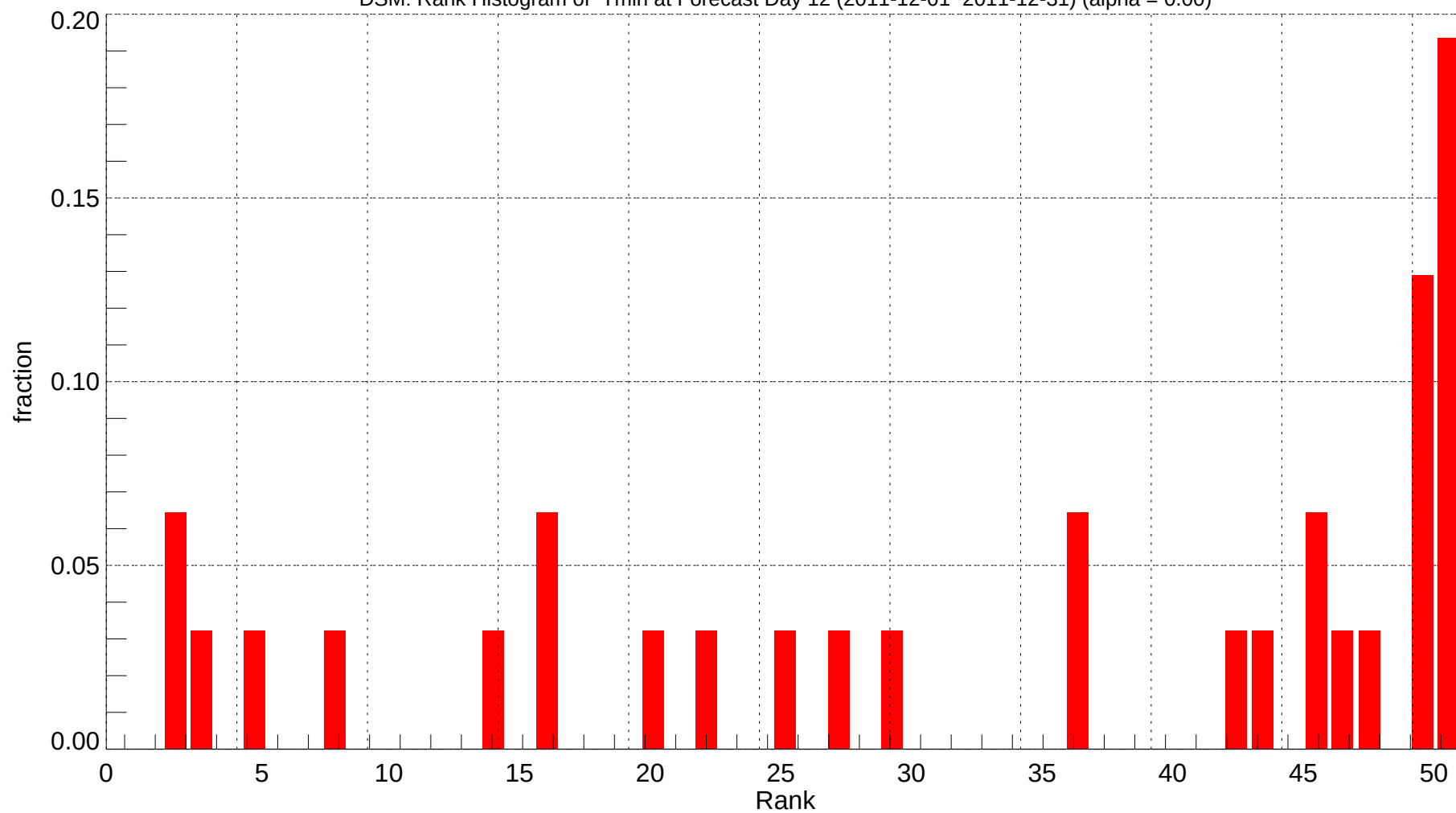
DSM: Rank Histogram of Tmin at Forecast Day 12 (2011-12-01~2011-12-31) (alpha = 0.00)
