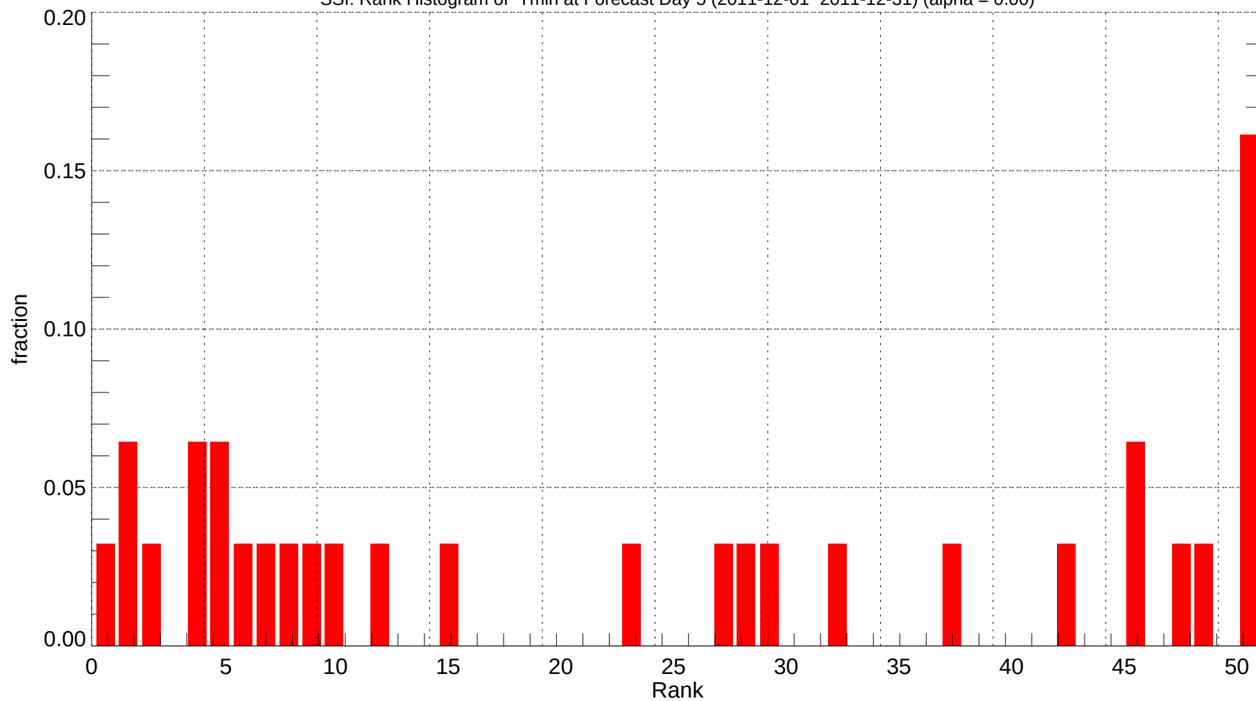
SSI: Rank Histogram of Tmin at Forecast Day 5 (2011-12-01~2011-12-31) (alpha = 0.00)
