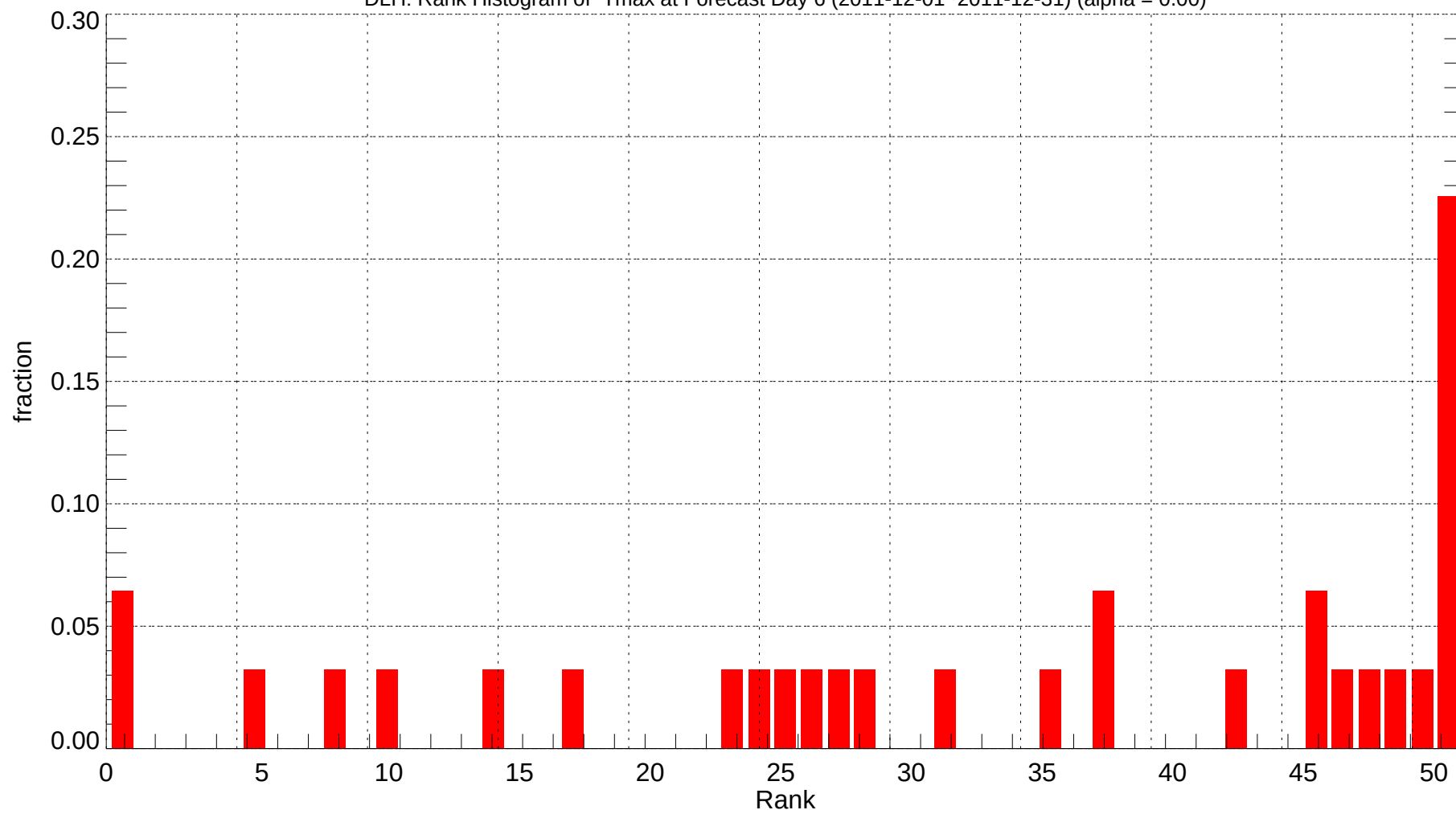
DLH: Rank Histogram of Tmax at Forecast Day 6 (2011-12-01~2011-12-31) (alpha = 0.00)
