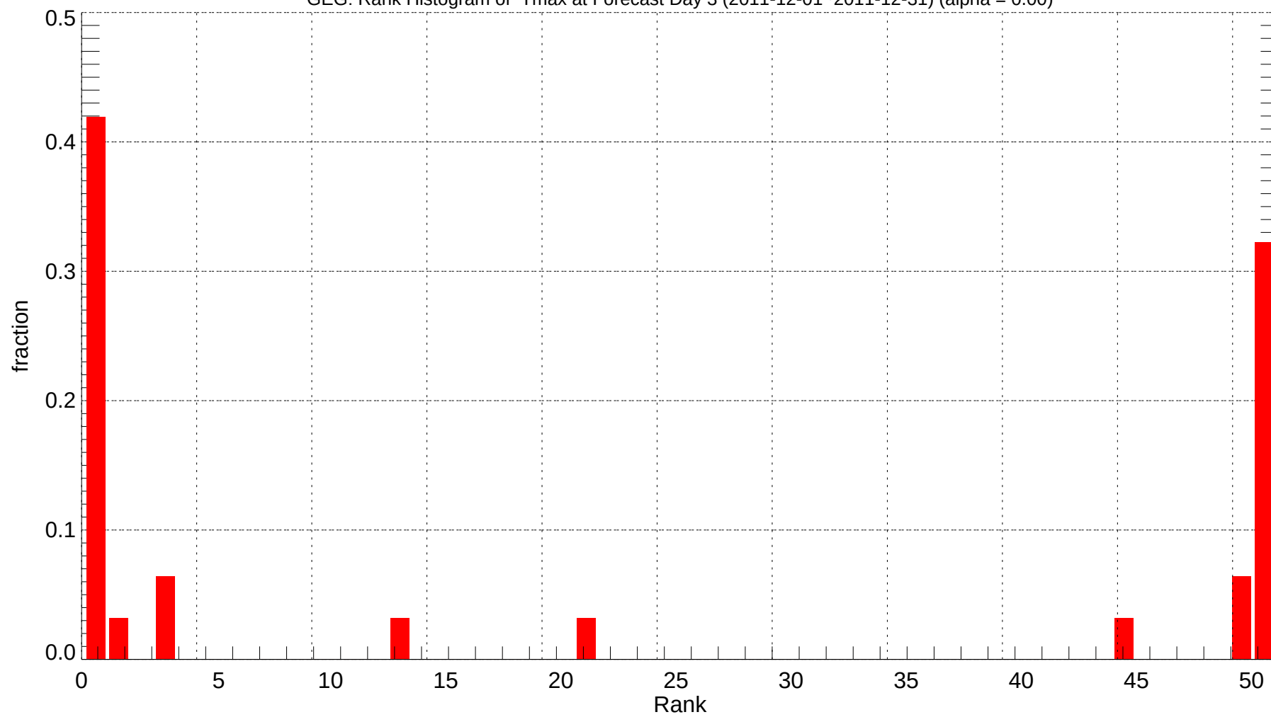
GEG: Rank Histogram of Tmax at Forecast Day 3 (2011-12-01~2011-12-31) (alpha = 0.00)
