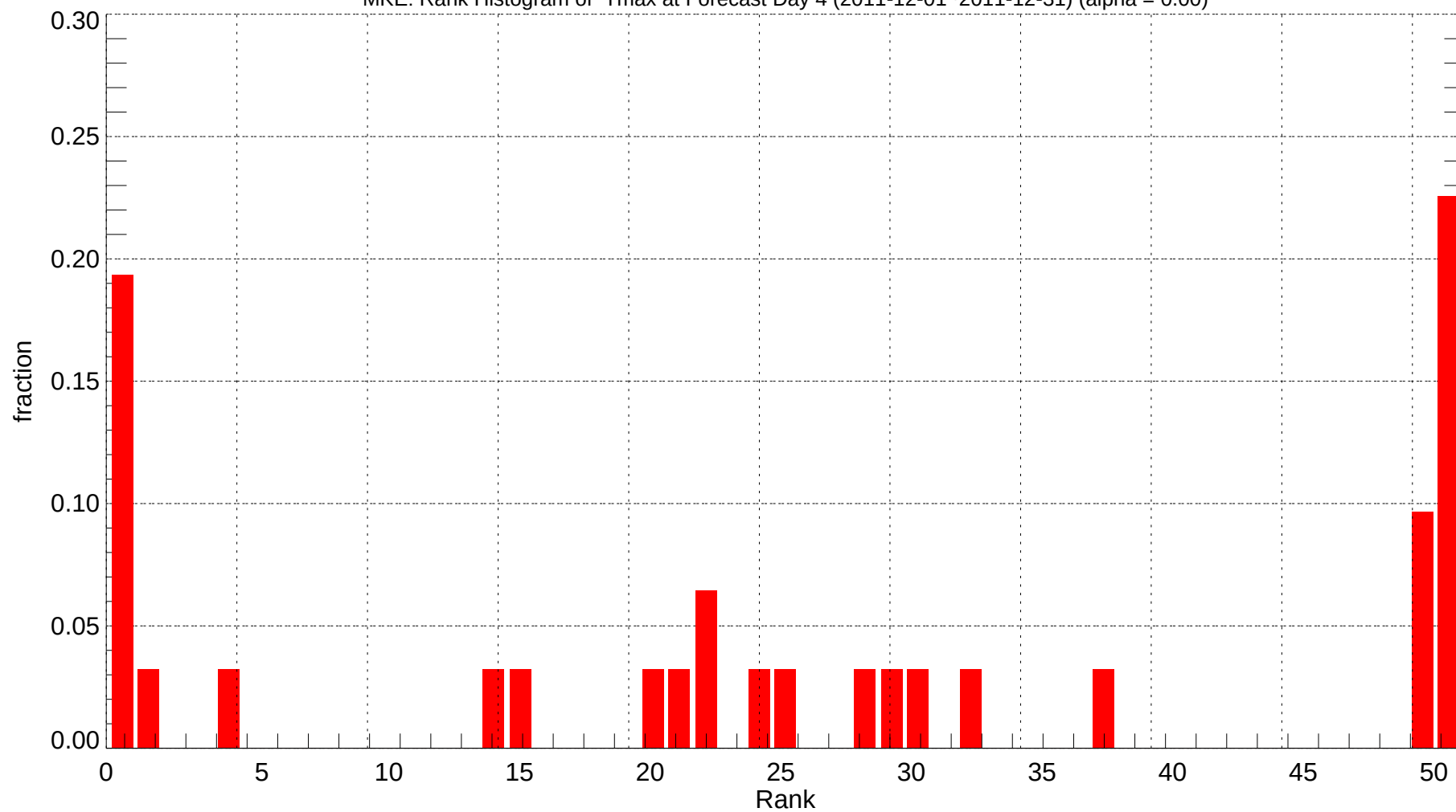
MKE: Rank Histogram of Tmax at Forecast Day 4 (2011-12-01~2011-12-31) (alpha = 0.00)
