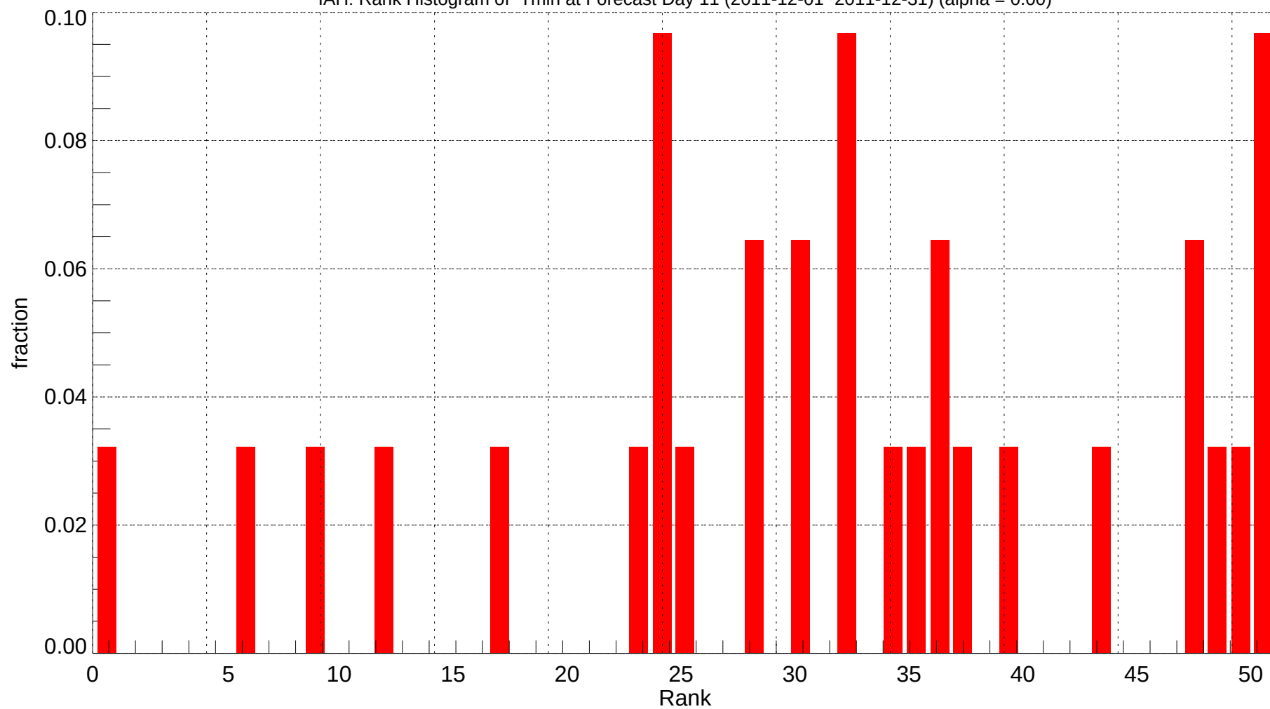
IAH: Rank Histogram of Tmin at Forecast Day 11 (2011-12-01~2011-12-31) (alpha = 0.00)
