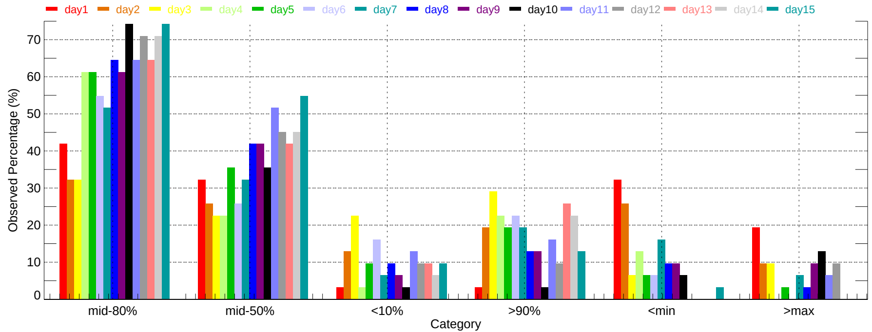
Observed Percentage of Ensembles - BGM: Max Temperature (2011-12-01~2011-12-31)
