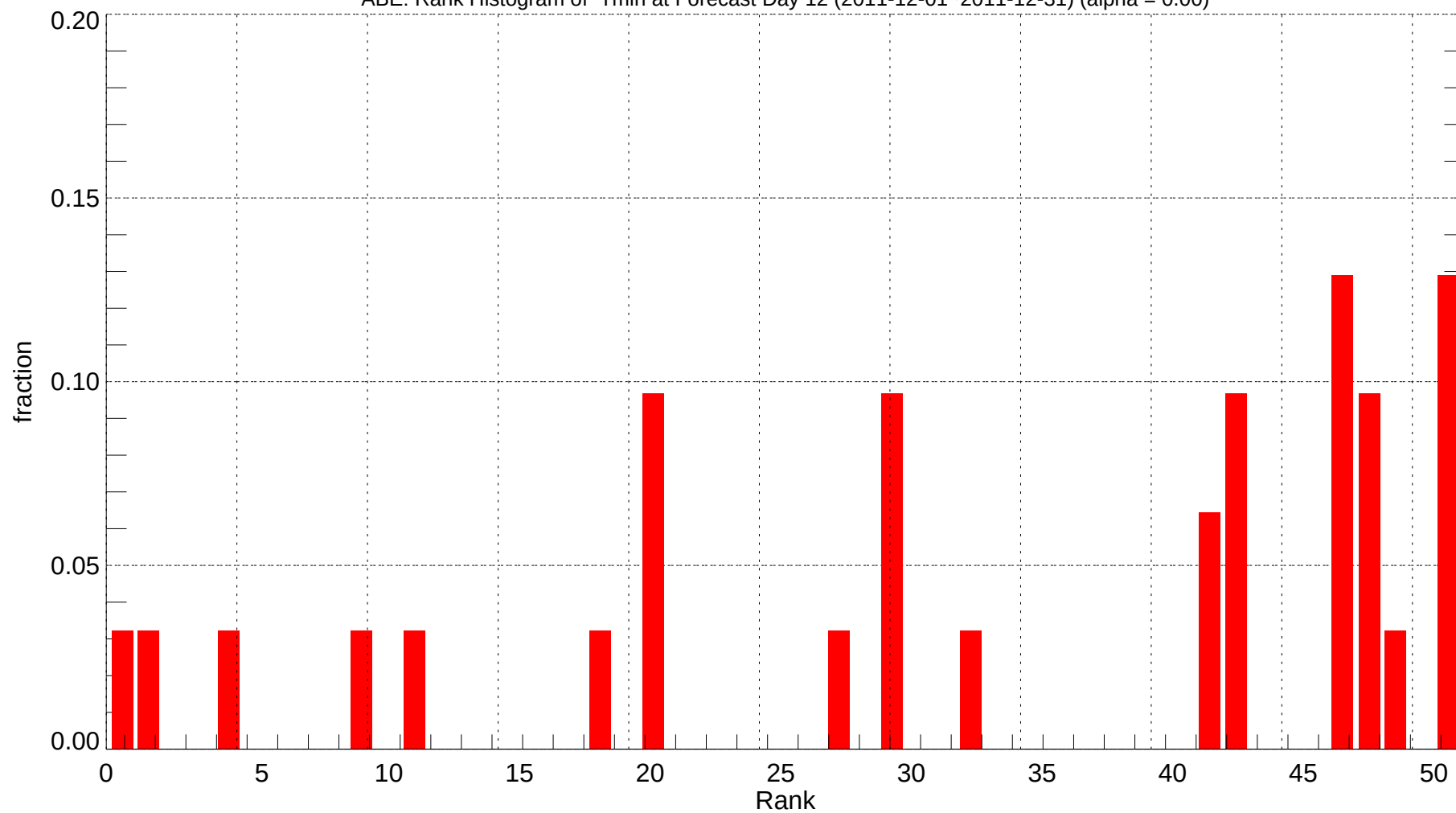
ABE: Rank Histogram of Tmin at Forecast Day 12 (2011-12-01~2011-12-31) (alpha = 0.00)
