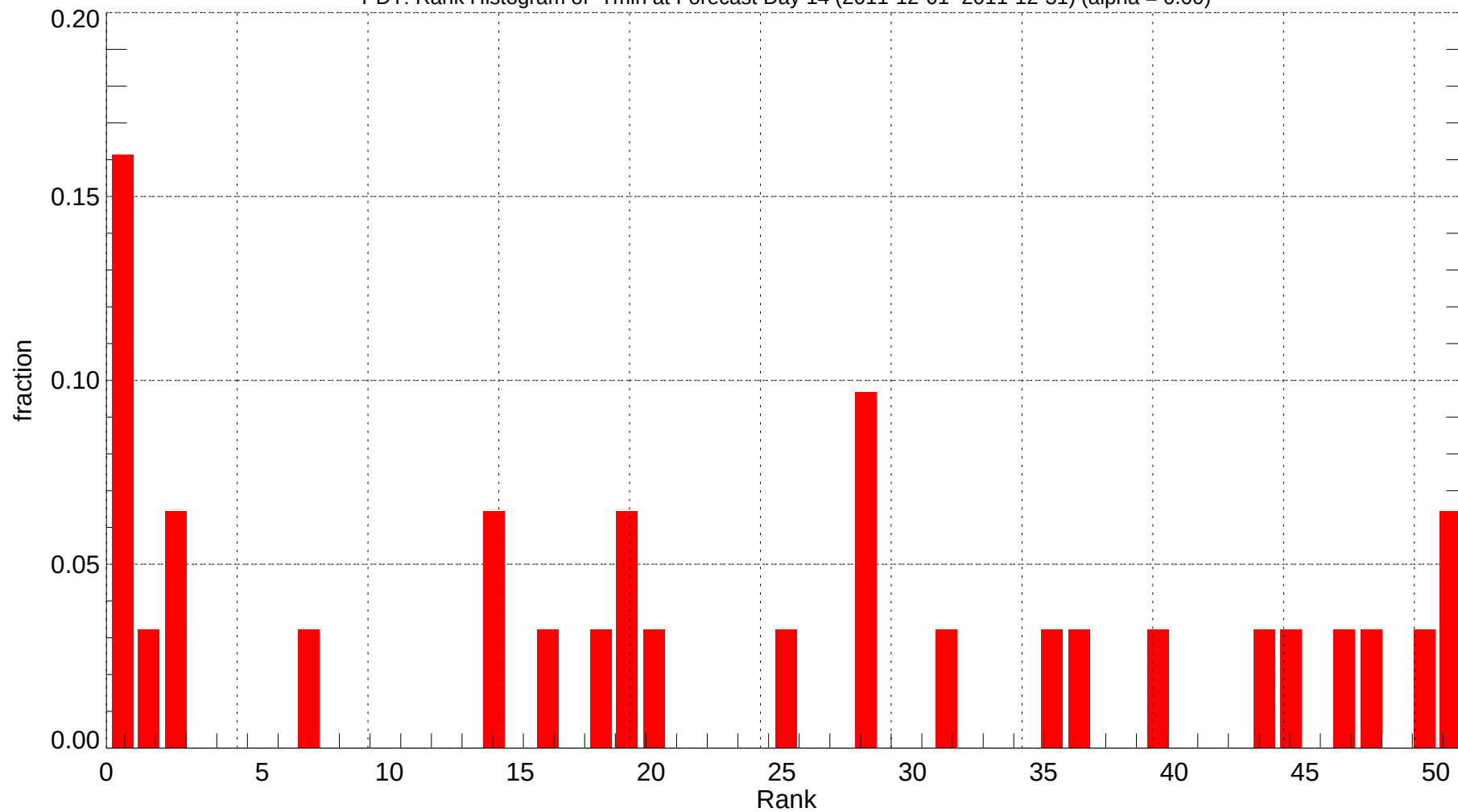
PDT: Rank Histogram of Tmin at Forecast Day 14 (2011-12-01~2011-12-31) (alpha = 0.00)
