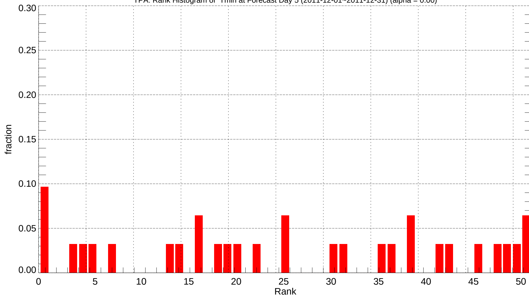
TPA: Rank Histogram of Tmin at Forecast Day 5 (2011-12-01~2011-12-31) (alpha = 0.00)
