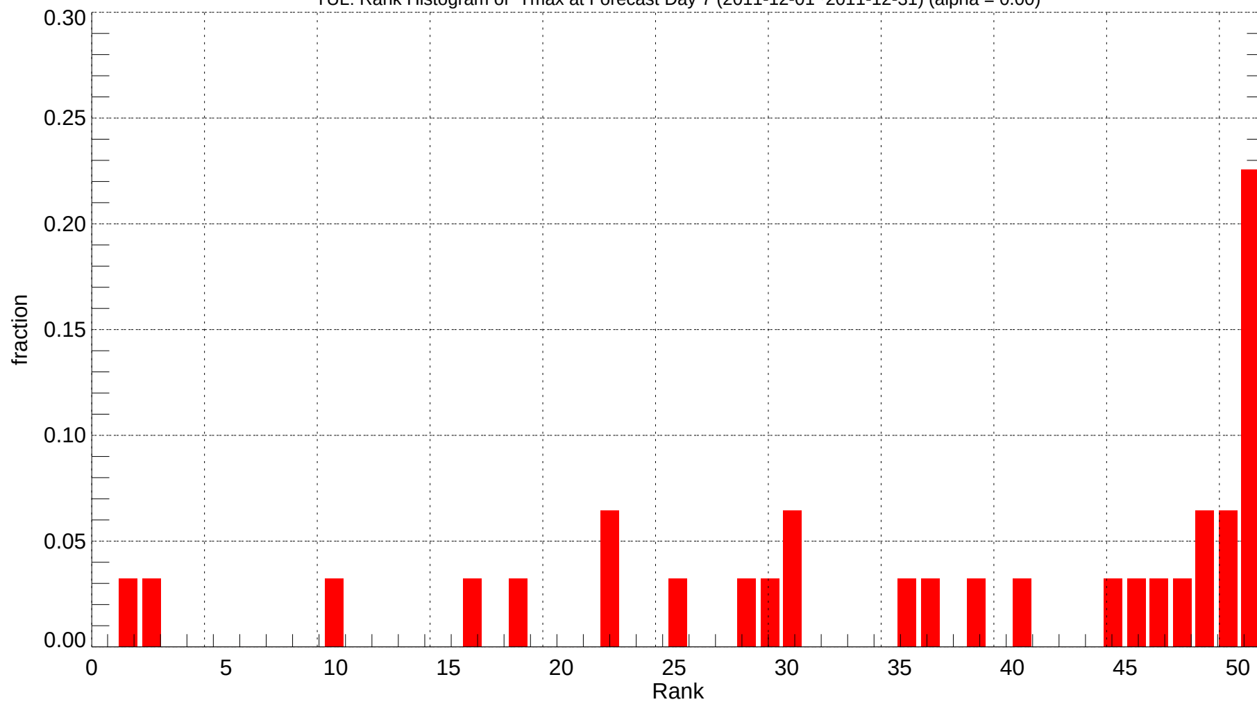
TUL: Rank Histogram of Tmax at Forecast Day 7 (2011-12-01~2011-12-31) (alpha = 0.00)
