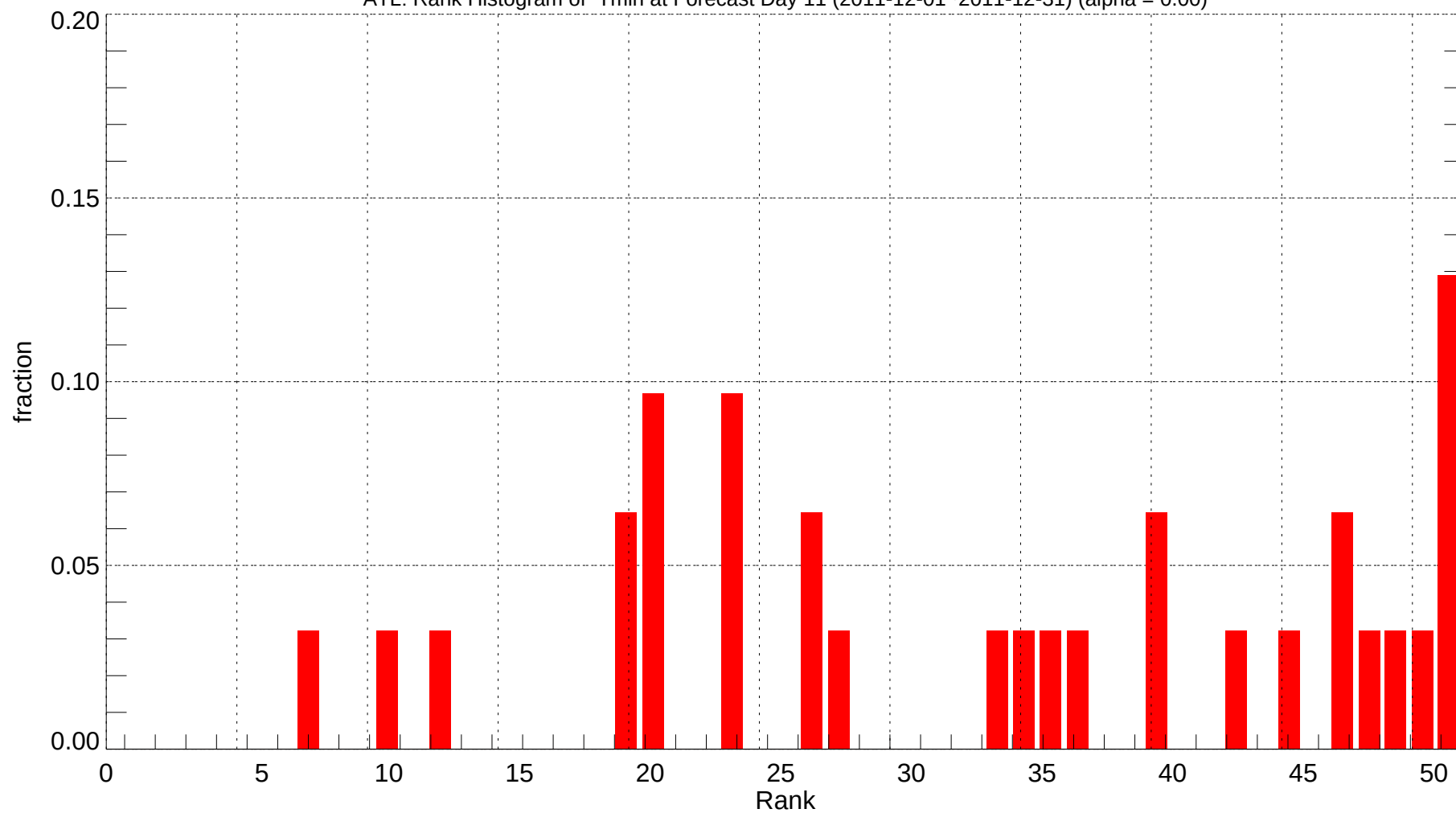
ATL: Rank Histogram of Tmin at Forecast Day 11 (2011-12-01~2011-12-31) (alpha = 0.00)
