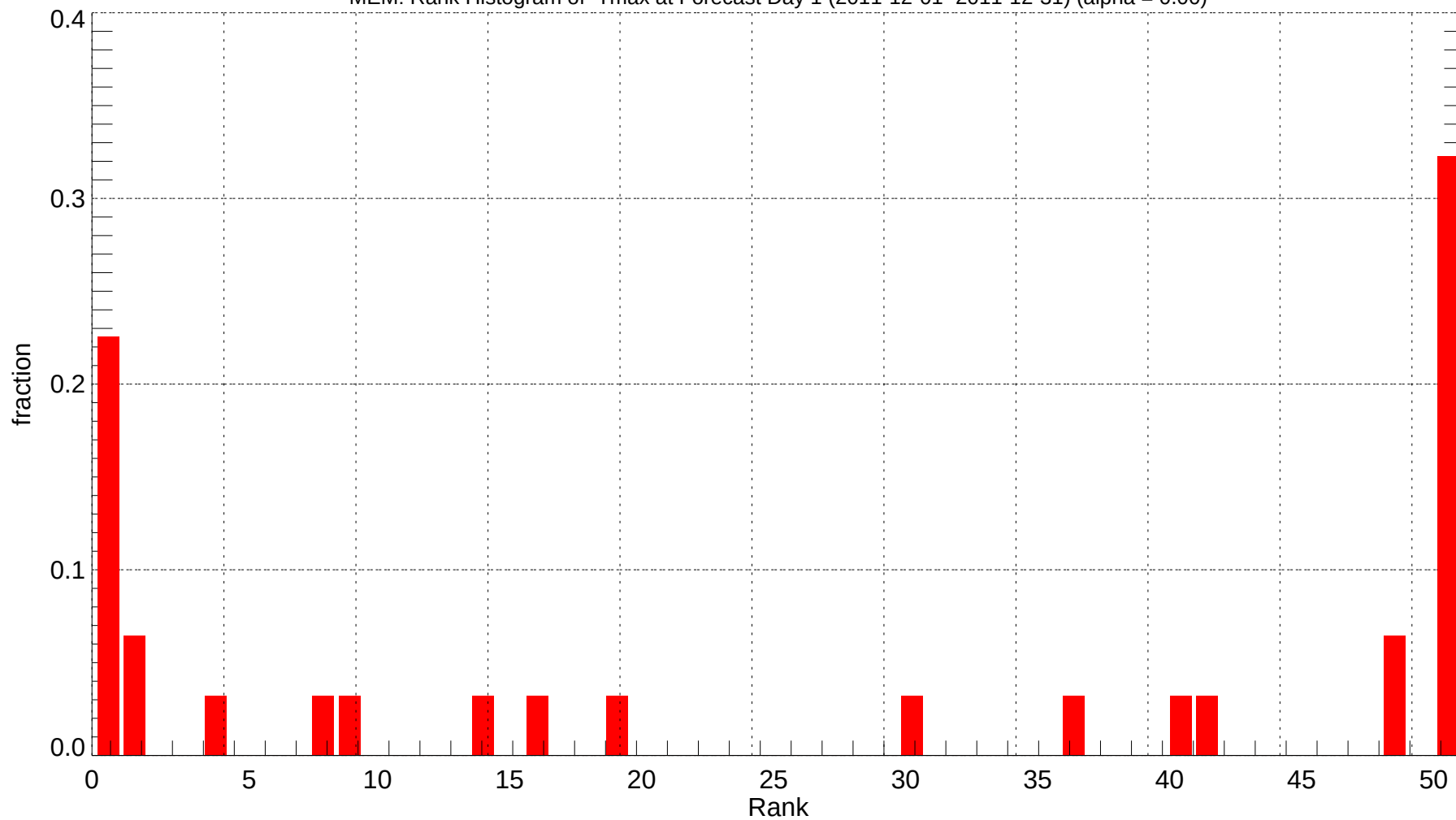
MEM: Rank Histogram of Tmax at Forecast Day 1 (2011-12-01~2011-12-31) (alpha = 0.00)
