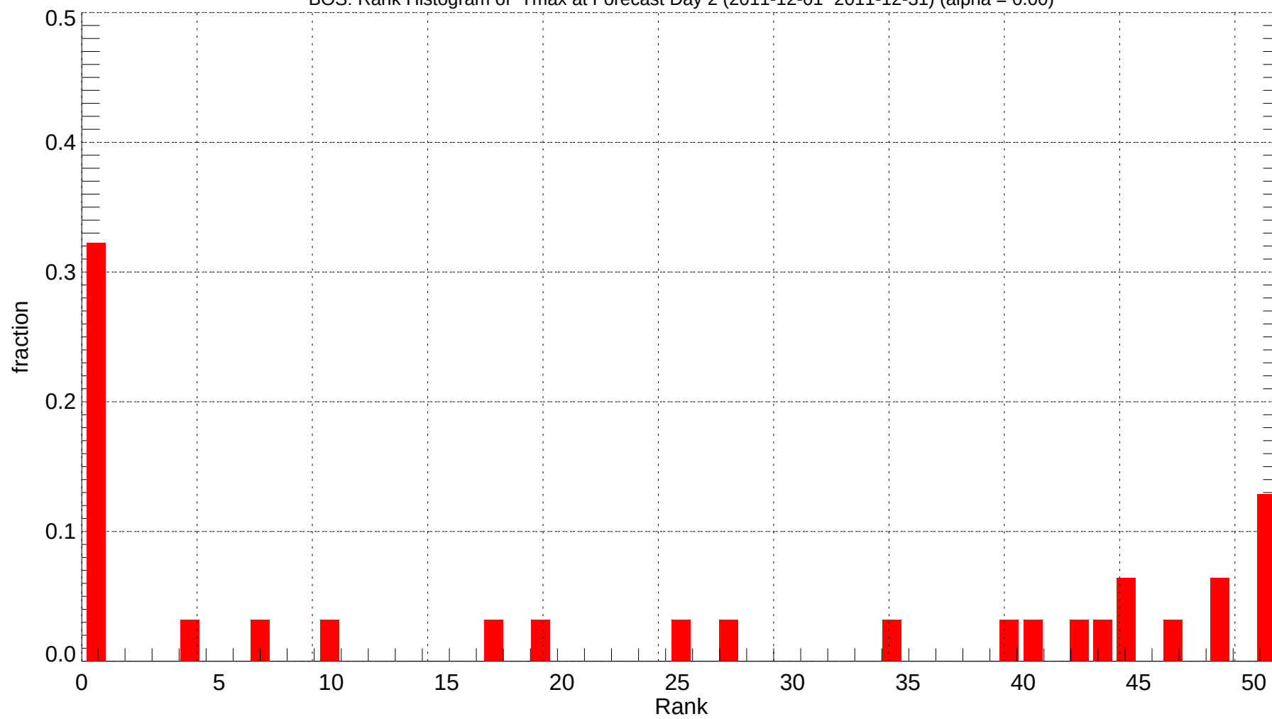
BOS: Rank Histogram of Tmax at Forecast Day 2 (2011-12-01~2011-12-31) (alpha = 0.00)
