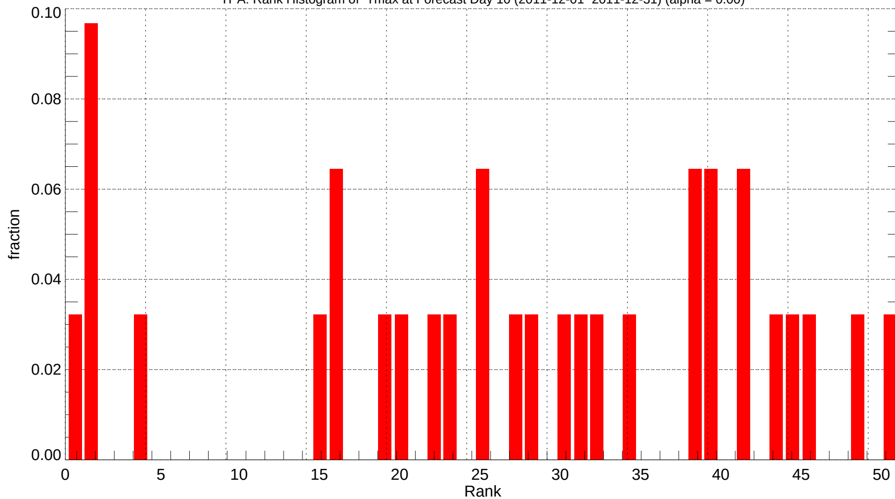
TPA: Rank Histogram of Tmax at Forecast Day 10 (2011-12-01~2011-12-31) (alpha = 0.00)
