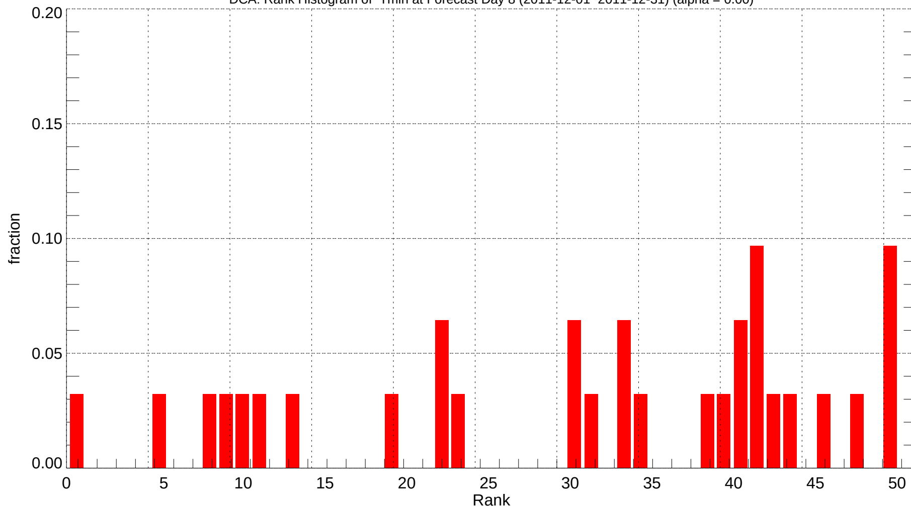
DCA: Rank Histogram of Tmin at Forecast Day 8 (2011-12-01~2011-12-31) (alpha = 0.00)
