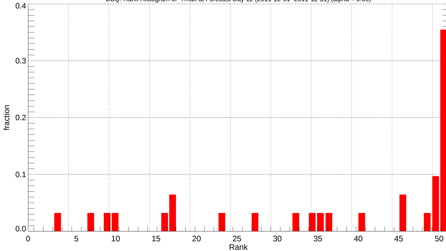
DBQ: Rank Histogram of Tmax at Forecast Day 12 (2011-12-01~2011-12-31) (alpha = 0.00)
