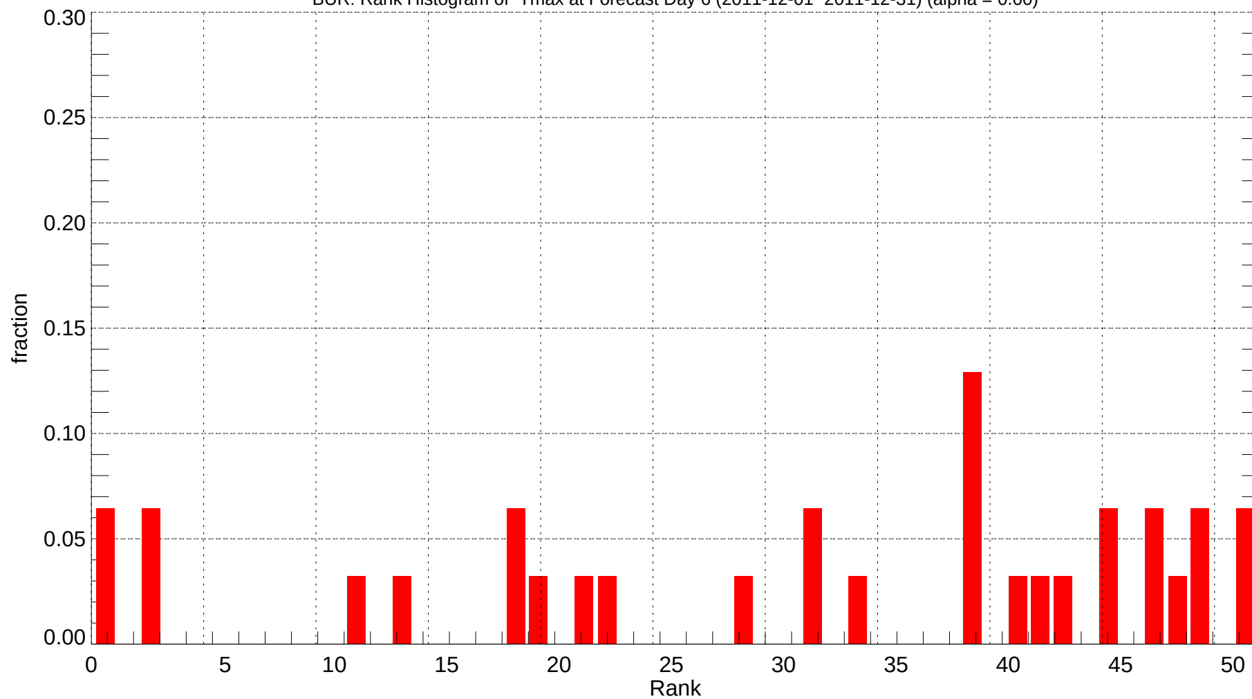
BUR: Rank Histogram of Tmax at Forecast Day 6 (2011-12-01~2011-12-31) (alpha = 0.00)
