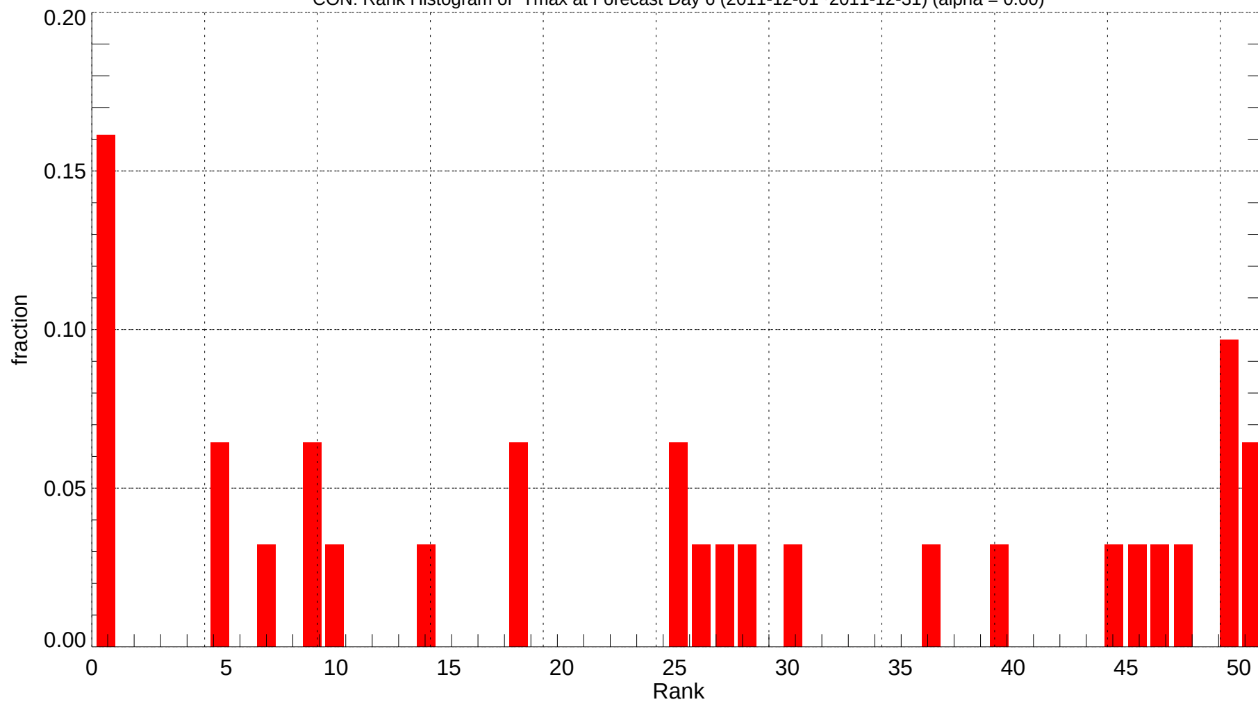
CON: Rank Histogram of Tmax at Forecast Day 6 (2011-12-01~2011-12-31) (alpha = 0.00)
