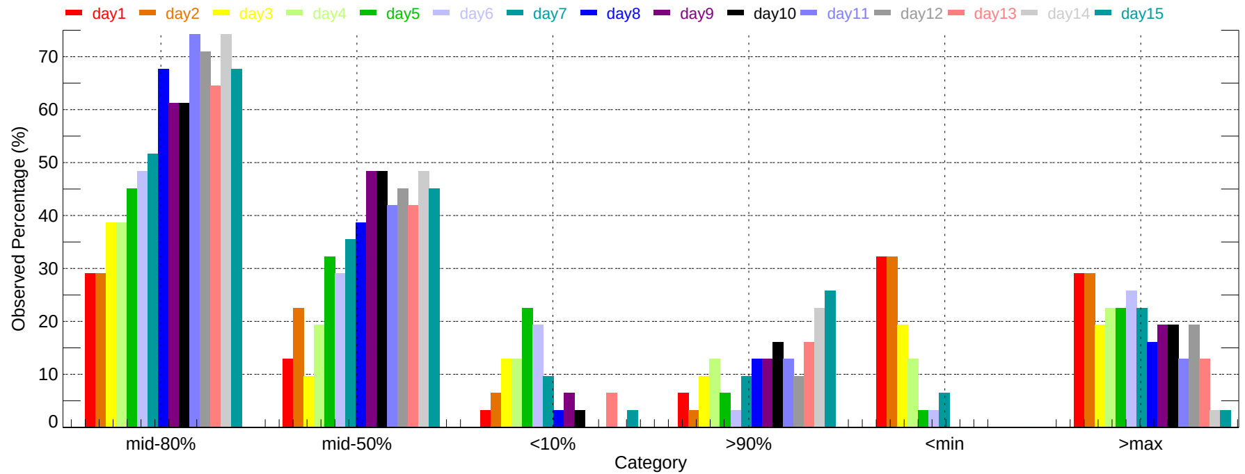
Observed Percentage of Ensembles - BHM: Max Temperature (2011-12-01~2011-12-31)
