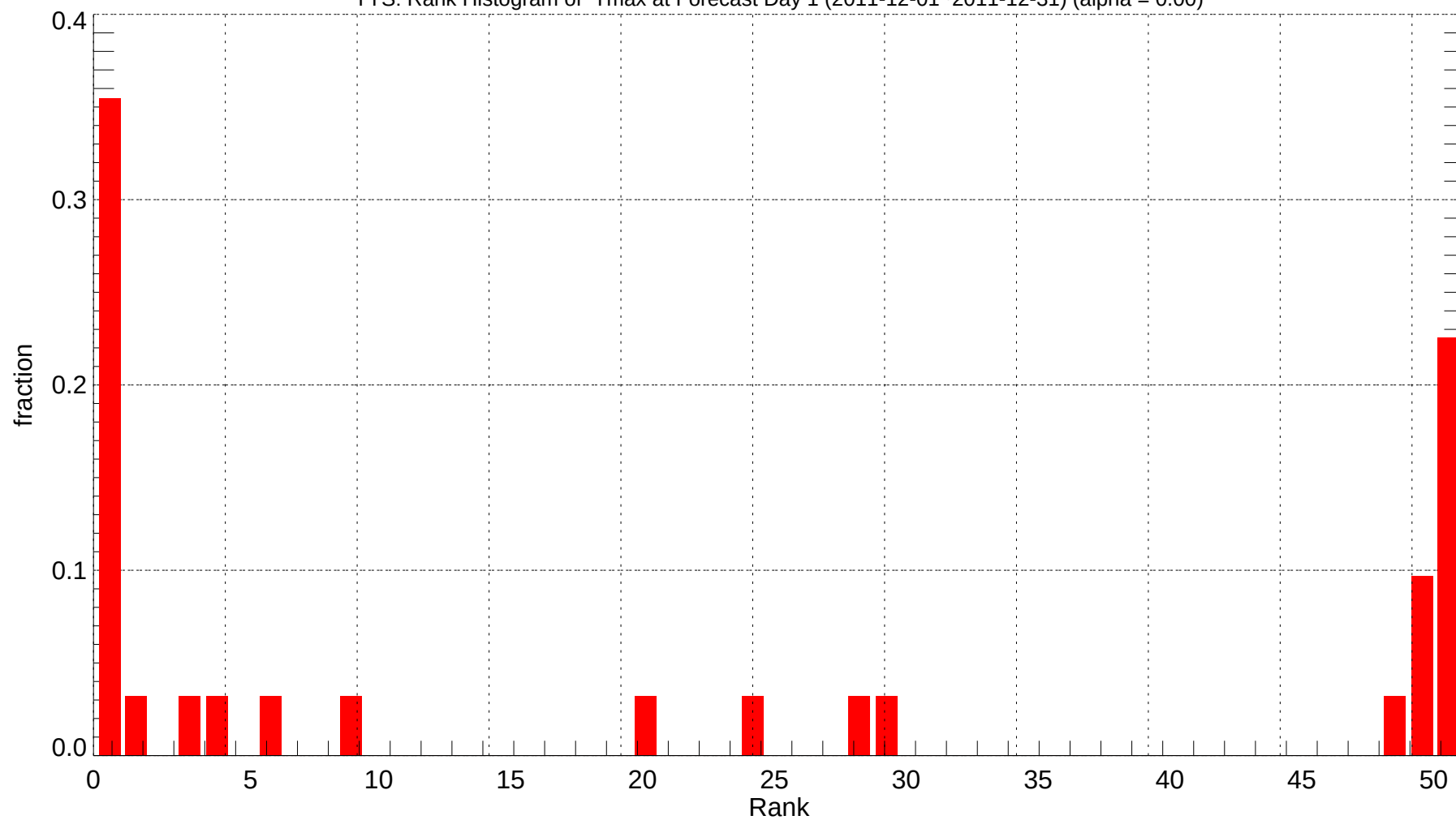
TYS: Rank Histogram of Tmax at Forecast Day 1 (2011-12-01~2011-12-31) (alpha = 0.00)
