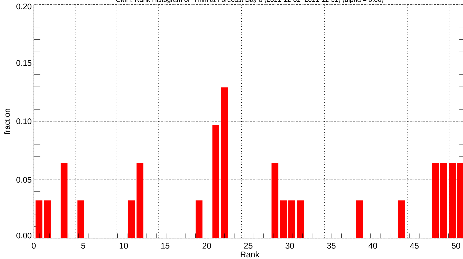
CMH: Rank Histogram of Tmin at Forecast Day 8 (2011-12-01~2011-12-31) (alpha = 0.00)
