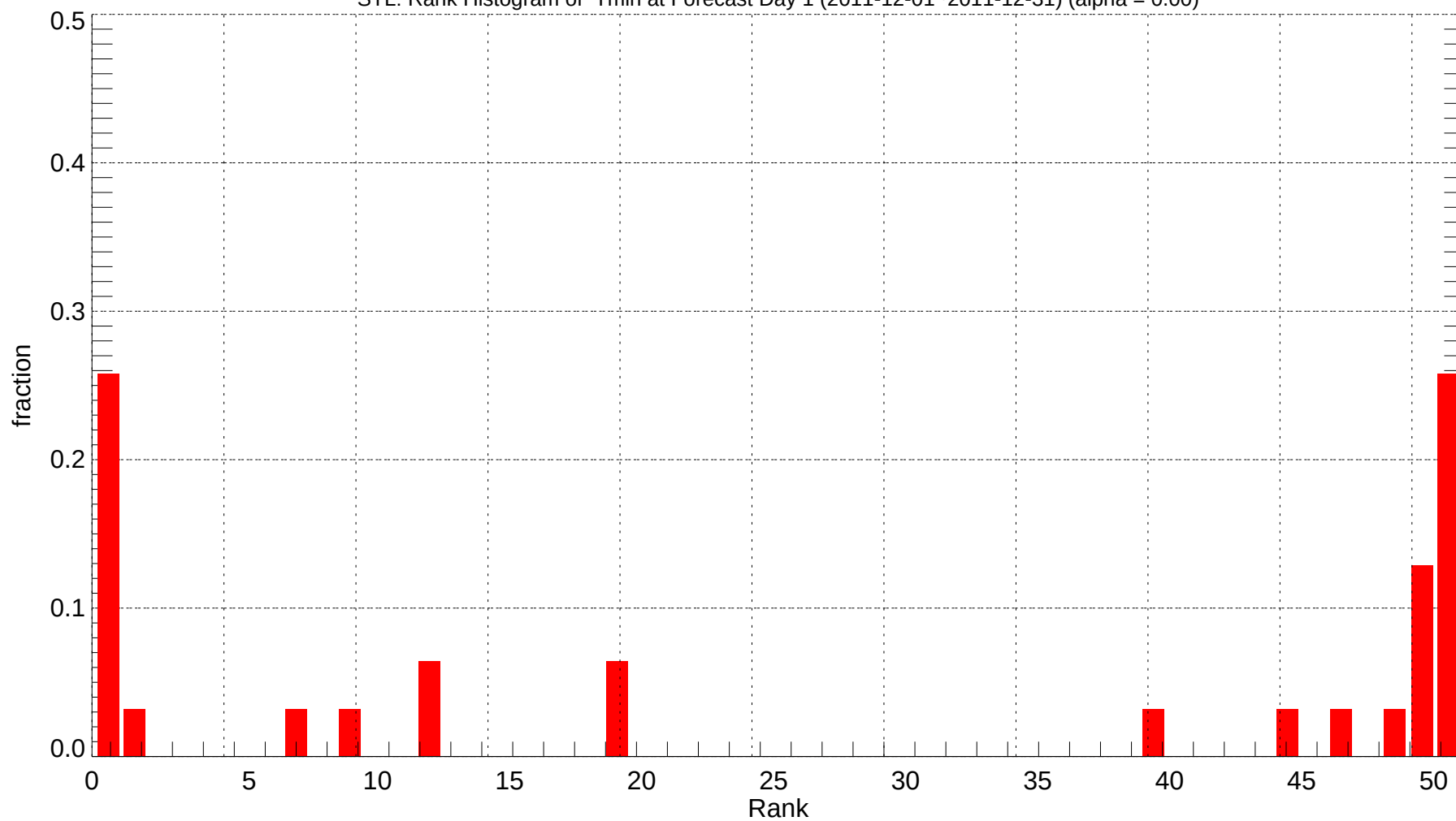
STL: Rank Histogram of Tmin at Forecast Day 1 (2011-12-01~2011-12-31) (alpha = 0.00)
