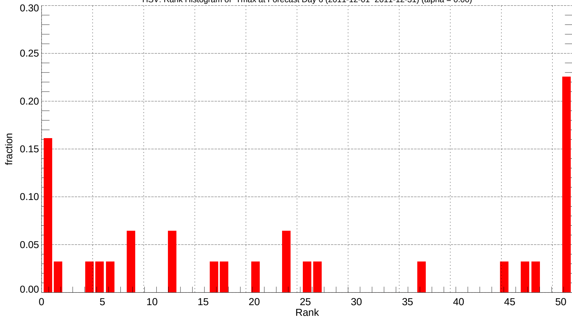
HSV: Rank Histogram of Tmax at Forecast Day 6 (2011-12-01~2011-12-31) (alpha = 0.00)
