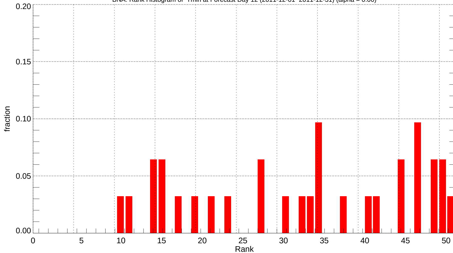
BNA: Rank Histogram of Tmin at Forecast Day 12 (2011-12-01~2011-12-31) (alpha = 0.00)
