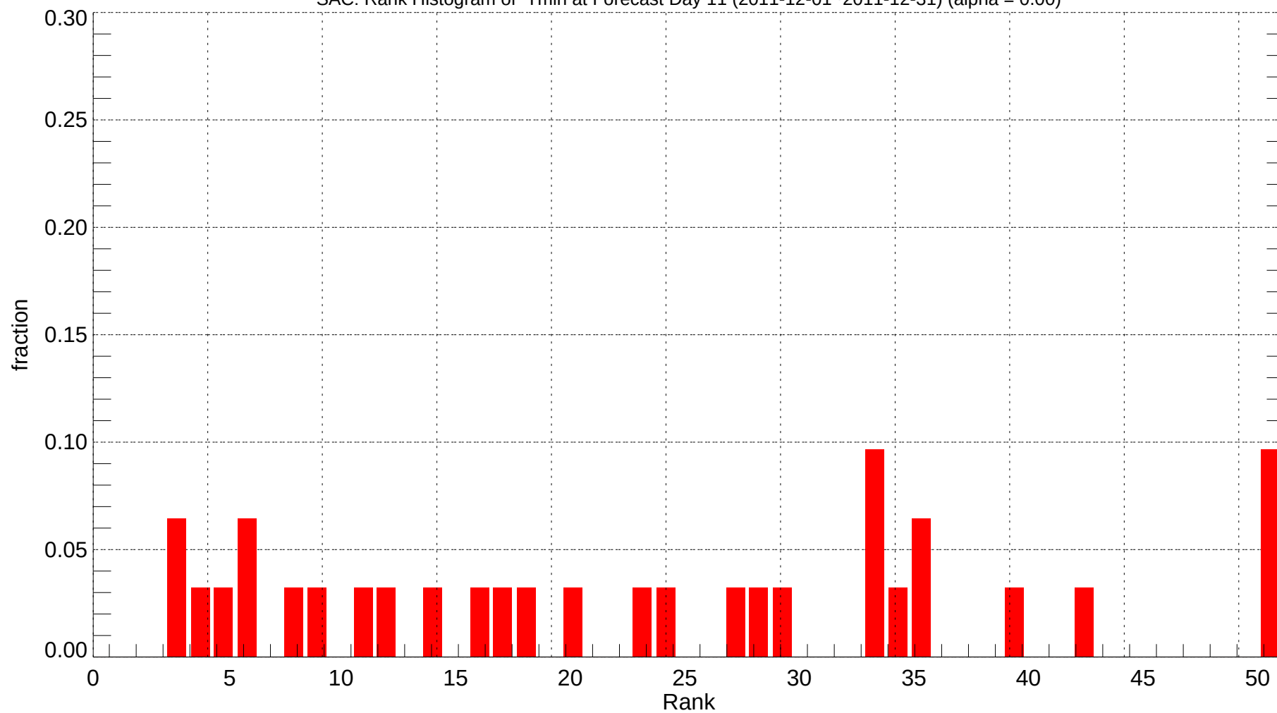
SAC: Rank Histogram of Tmin at Forecast Day 11 (2011-12-01~2011-12-31) (alpha = 0.00)
