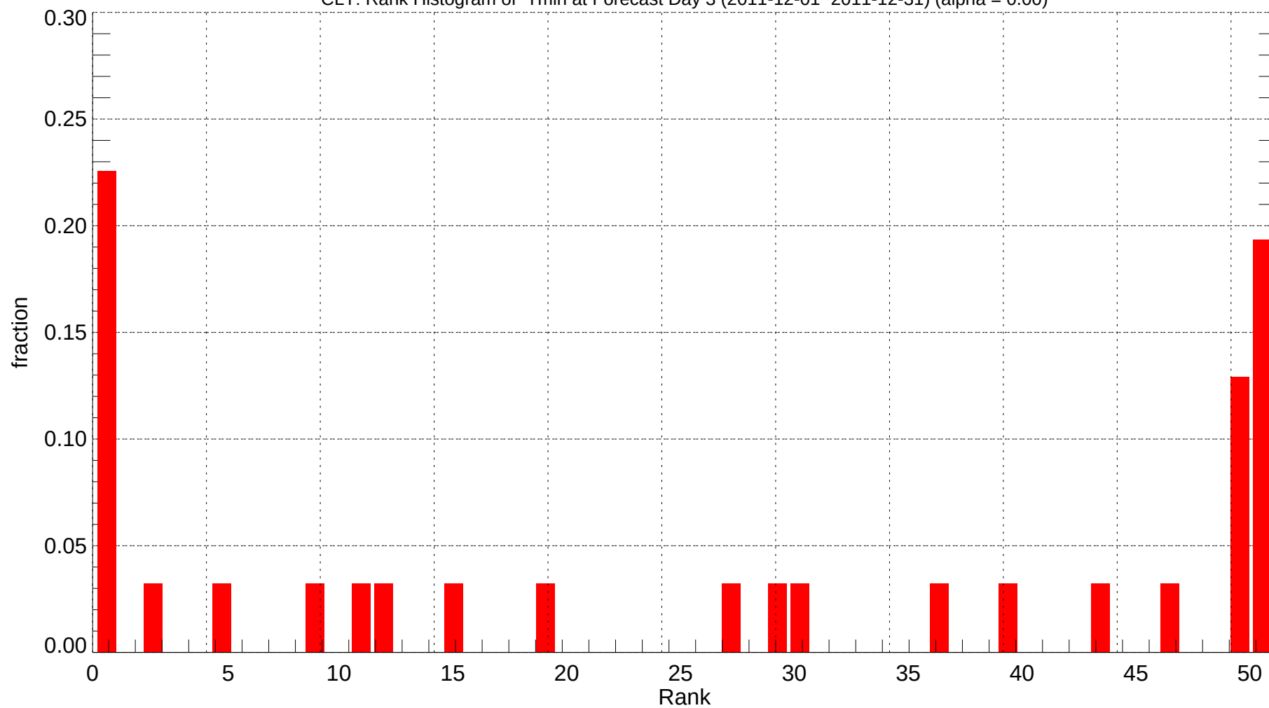
CLT: Rank Histogram of Tmin at Forecast Day 3 (2011-12-01~2011-12-31) (alpha = 0.00)
