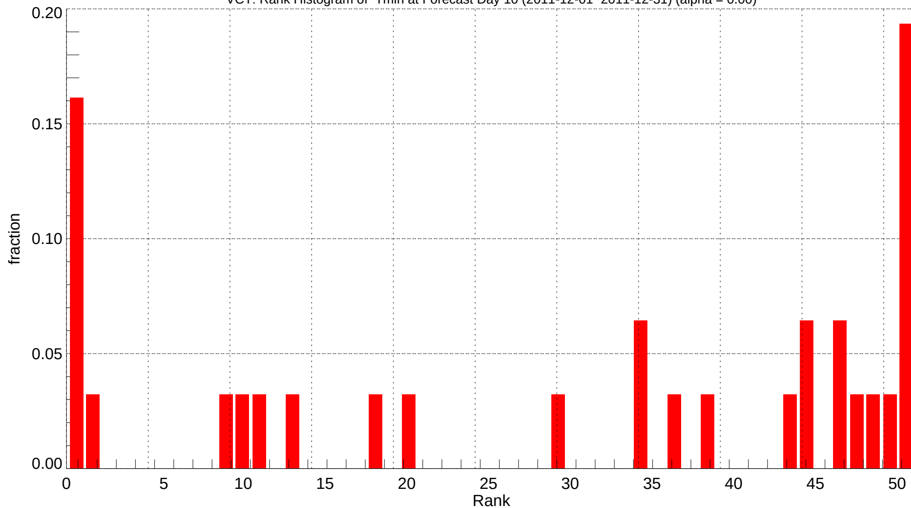
VCT: Rank Histogram of Tmin at Forecast Day 10 (2011-12-01~2011-12-31) (alpha = 0.00)
