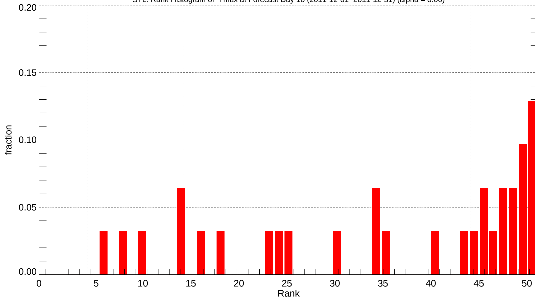
STL: Rank Histogram of Tmax at Forecast Day 10 (2011-12-01~2011-12-31) (alpha = 0.00)
