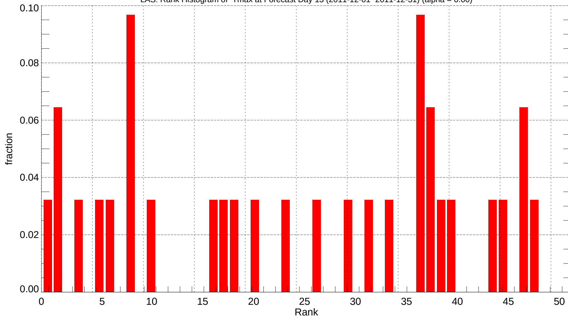
LAS: Rank Histogram of Tmax at Forecast Day 13 (2011-12-01~2011-12-31) (alpha = 0.00)
