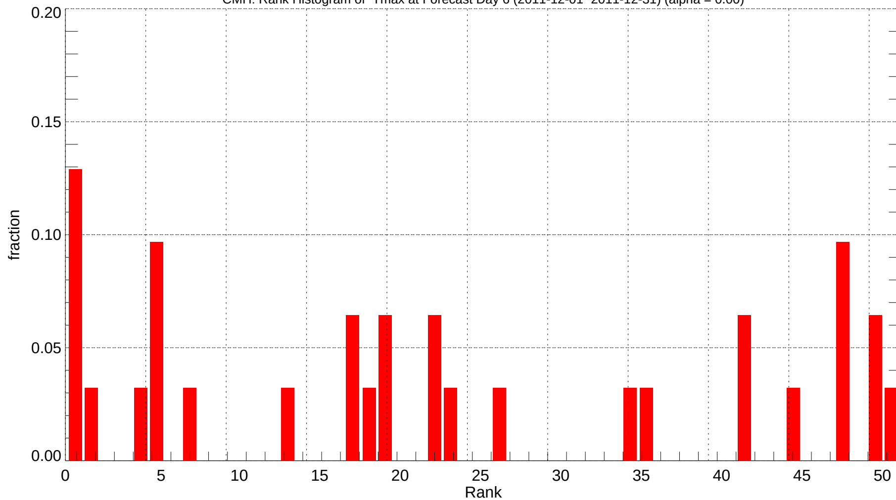
CMH: Rank Histogram of Tmax at Forecast Day 6 (2011-12-01~2011-12-31) (alpha = 0.00)
