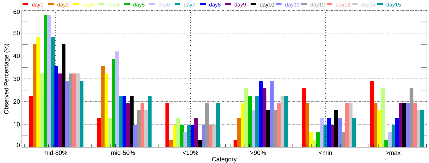
Observed Percentage of Ensembles - VCT: Max Temperature (2011-12-01~2011-12-31)
