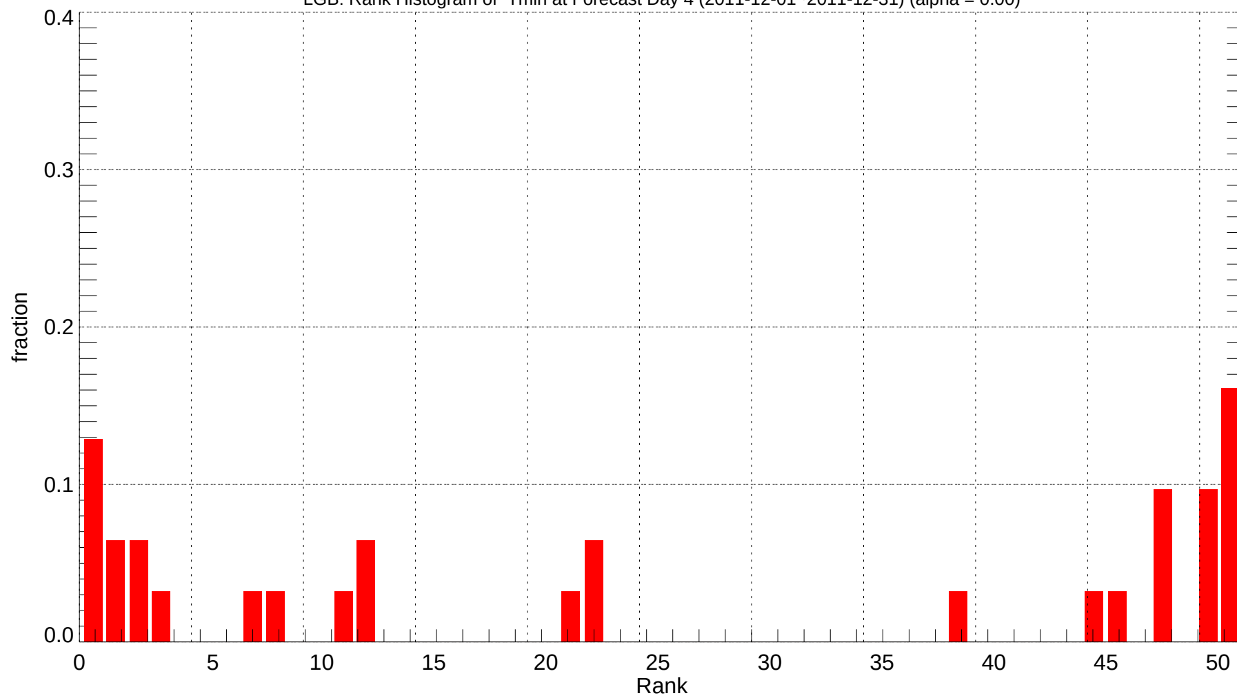
LGB: Rank Histogram of Tmin at Forecast Day 4 (2011-12-01~2011-12-31) (alpha = 0.00)
