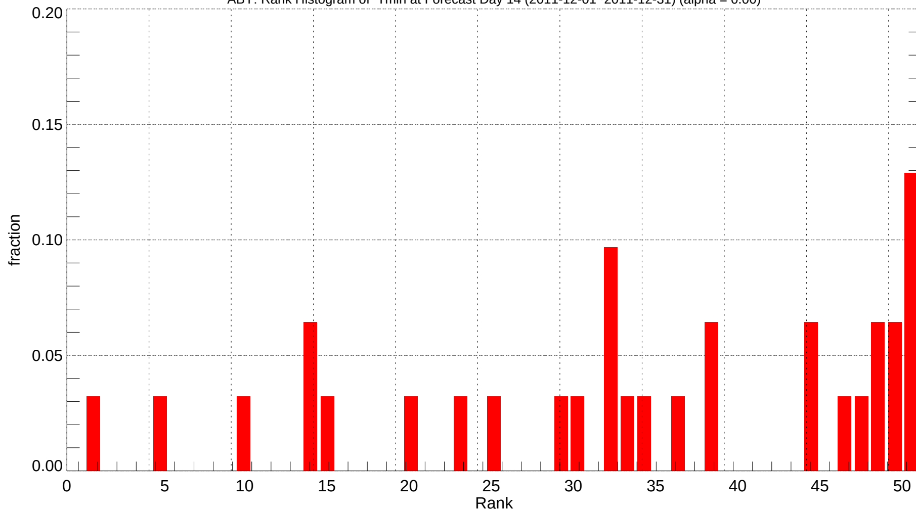
ABY: Rank Histogram of Tmin at Forecast Day 14 (2011-12-01~2011-12-31) (alpha = 0.00)
