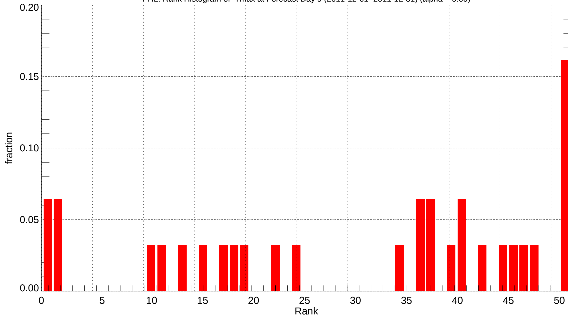
PHL: Rank Histogram of Tmax at Forecast Day 9 (2011-12-01~2011-12-31) (alpha = 0.00)
