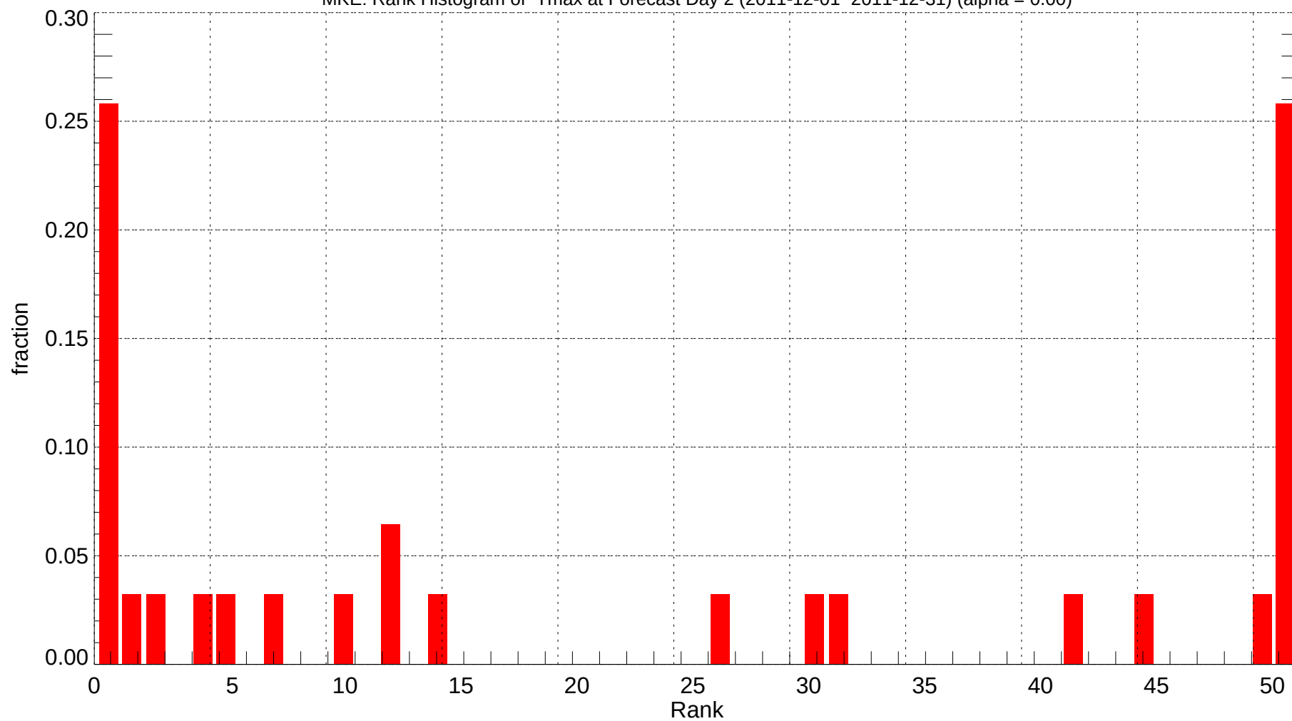
MKE: Rank Histogram of Tmax at Forecast Day 2 (2011-12-01~2011-12-31) (alpha = 0.00)
