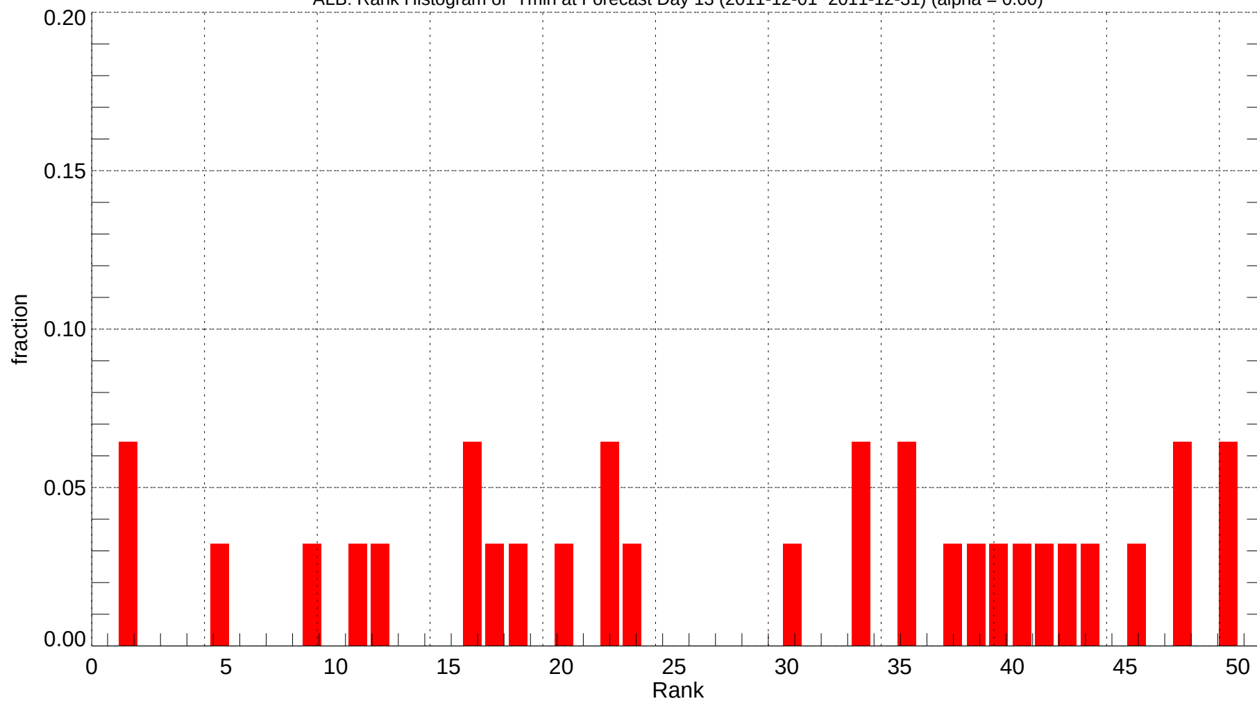
ALB: Rank Histogram of Tmin at Forecast Day 13 (2011-12-01~2011-12-31) (alpha = 0.00)
