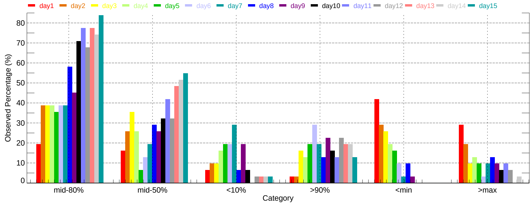
Observed Percentage of Ensembles - HSV: Min Temperature (2011-12-01~2011-12-31)
