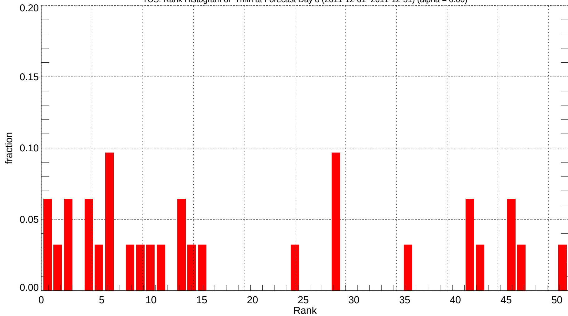
TUS: Rank Histogram of Tmin at Forecast Day 8 (2011-12-01~2011-12-31) (alpha = 0.00)
