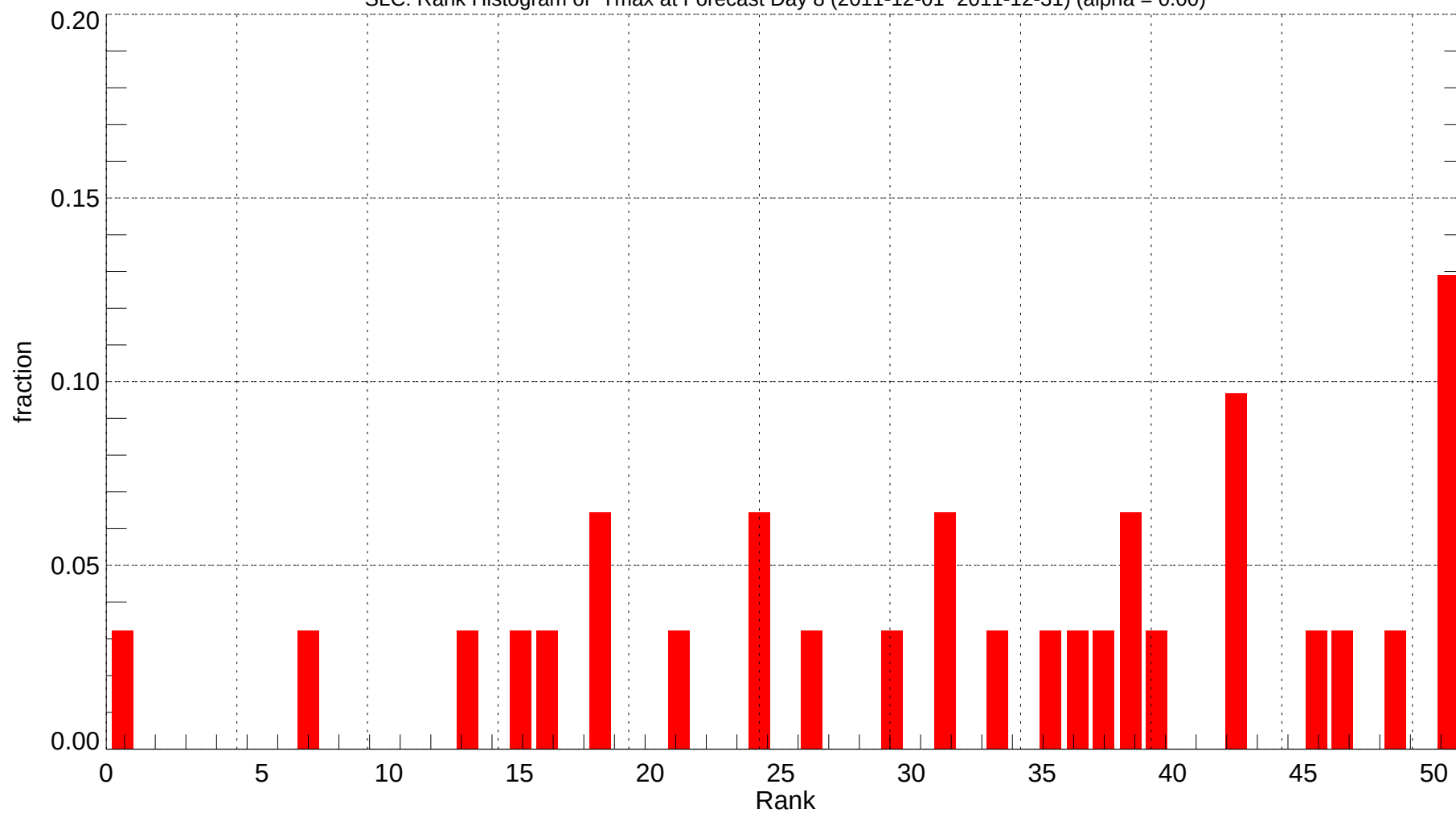
SLC: Rank Histogram of Tmax at Forecast Day 8 (2011-12-01~2011-12-31) (alpha = 0.00)
