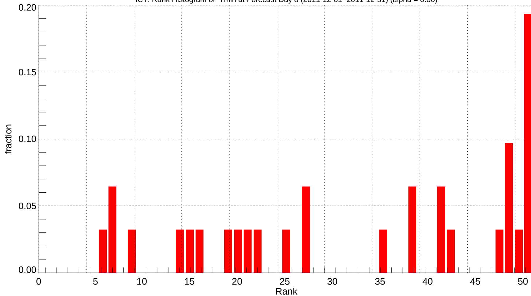
ICT: Rank Histogram of Tmin at Forecast Day 8 (2011-12-01~2011-12-31) (alpha = 0.00)
