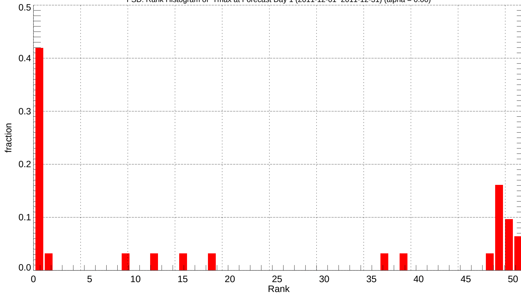
FSD: Rank Histogram of Tmax at Forecast Day 1 (2011-12-01~2011-12-31) (alpha = 0.00)
