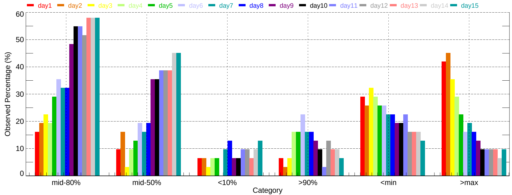
Observed Percentage of Ensembles - PDT: Max Temperature (2011-12-01~2011-12-31)
