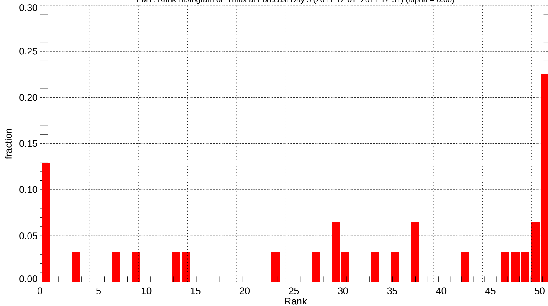
FMY: Rank Histogram of Tmax at Forecast Day 3 (2011-12-01~2011-12-31) (alpha = 0.00)
