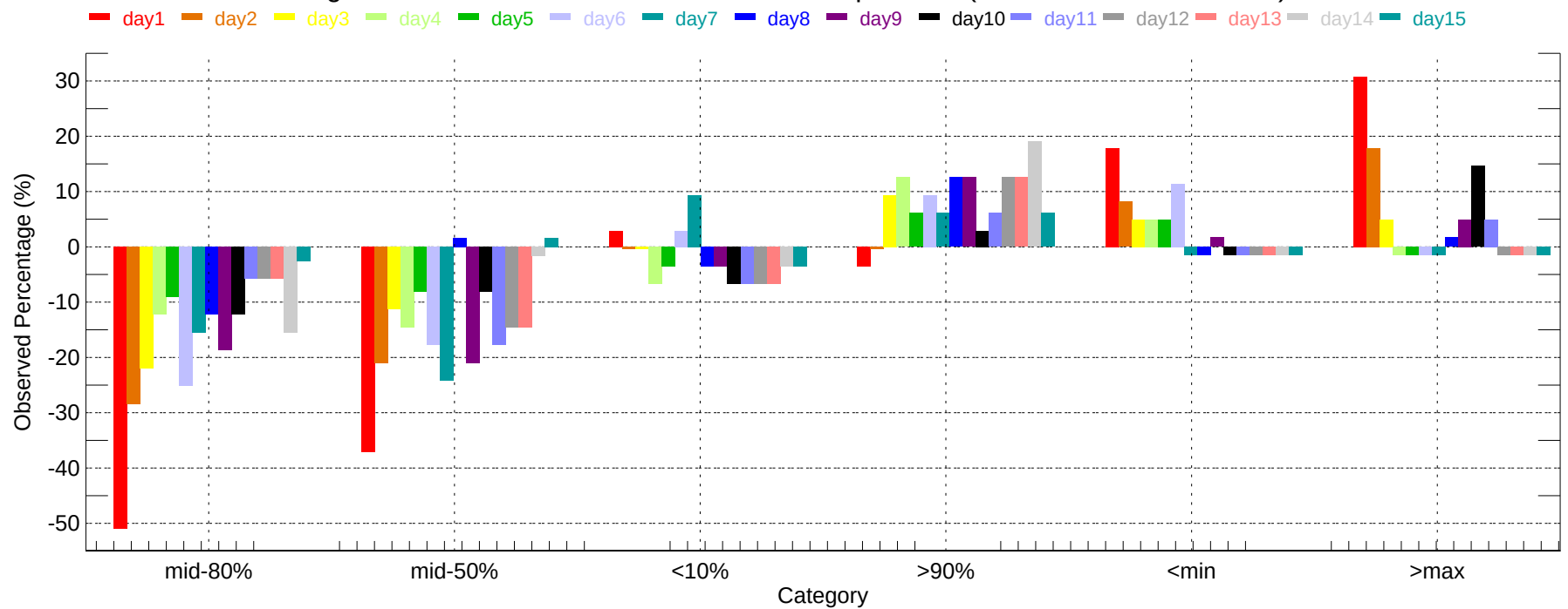
Observed Percentage Deviation of Ensembles - IND: Min Temperature (2011-12-01~2011-12-31)
