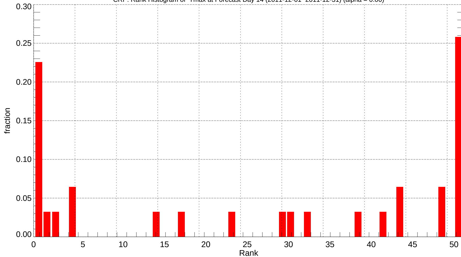
CRP: Rank Histogram of Tmax at Forecast Day 14 (2011-12-01~2011-12-31) (alpha = 0.00)
