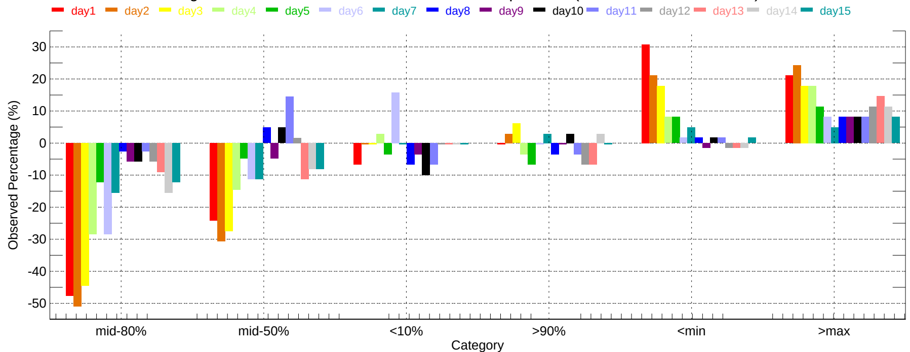
Observed Percentage Deviation of Ensembles - HOU: Max Temperature (2011-12-01~2011-12-31)
