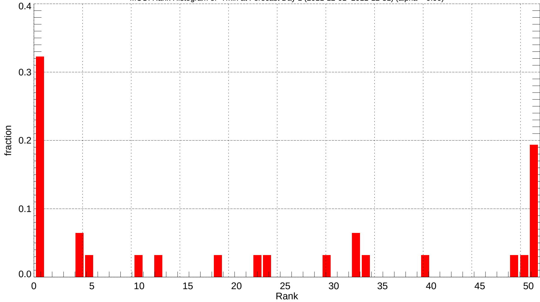
MCO: Rank Histogram of Tmin at Forecast Day 1 (2011-12-01~2011-12-31) (alpha = 0.00)
