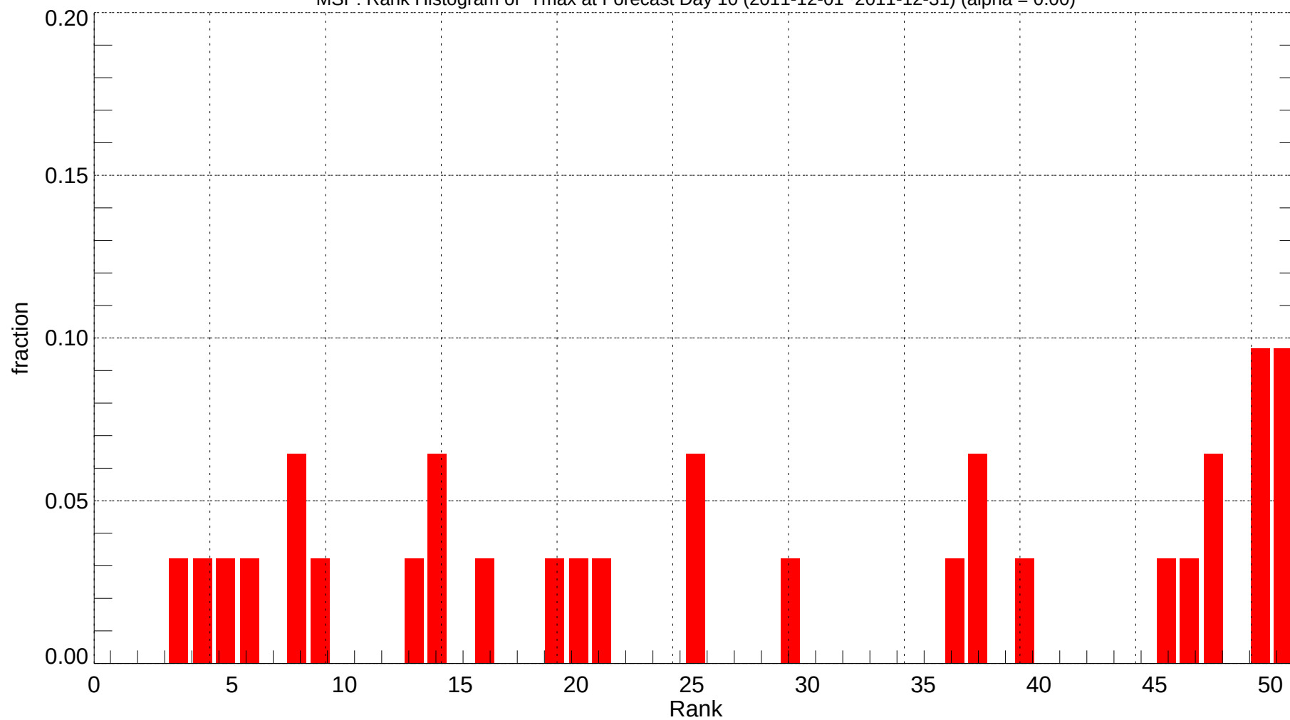
MSP: Rank Histogram of Tmax at Forecast Day 10 (2011-12-01~2011-12-31) (alpha = 0.00)
