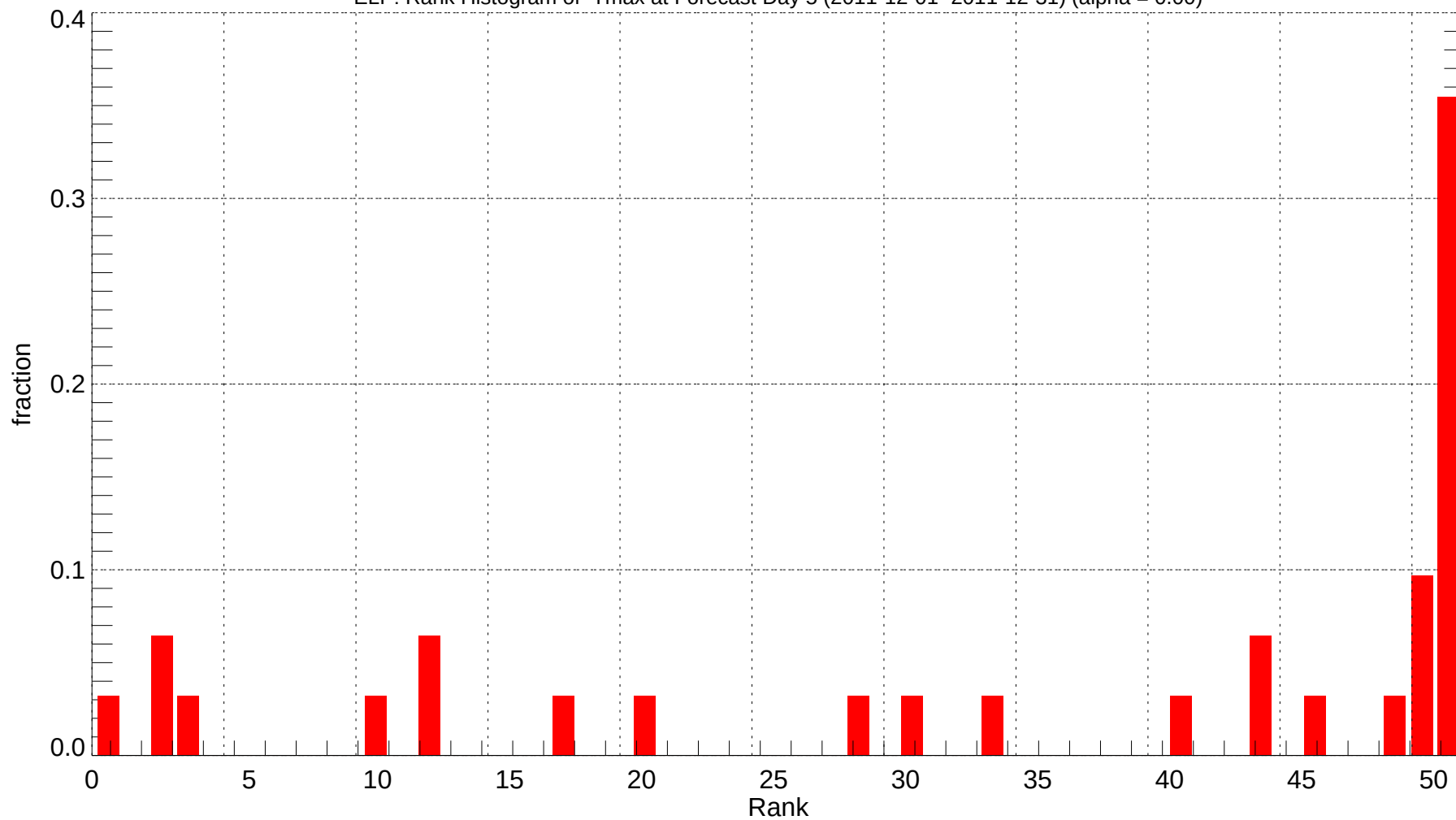
ELP: Rank Histogram of Tmax at Forecast Day 5 (2011-12-01~2011-12-31) (alpha = 0.00)
