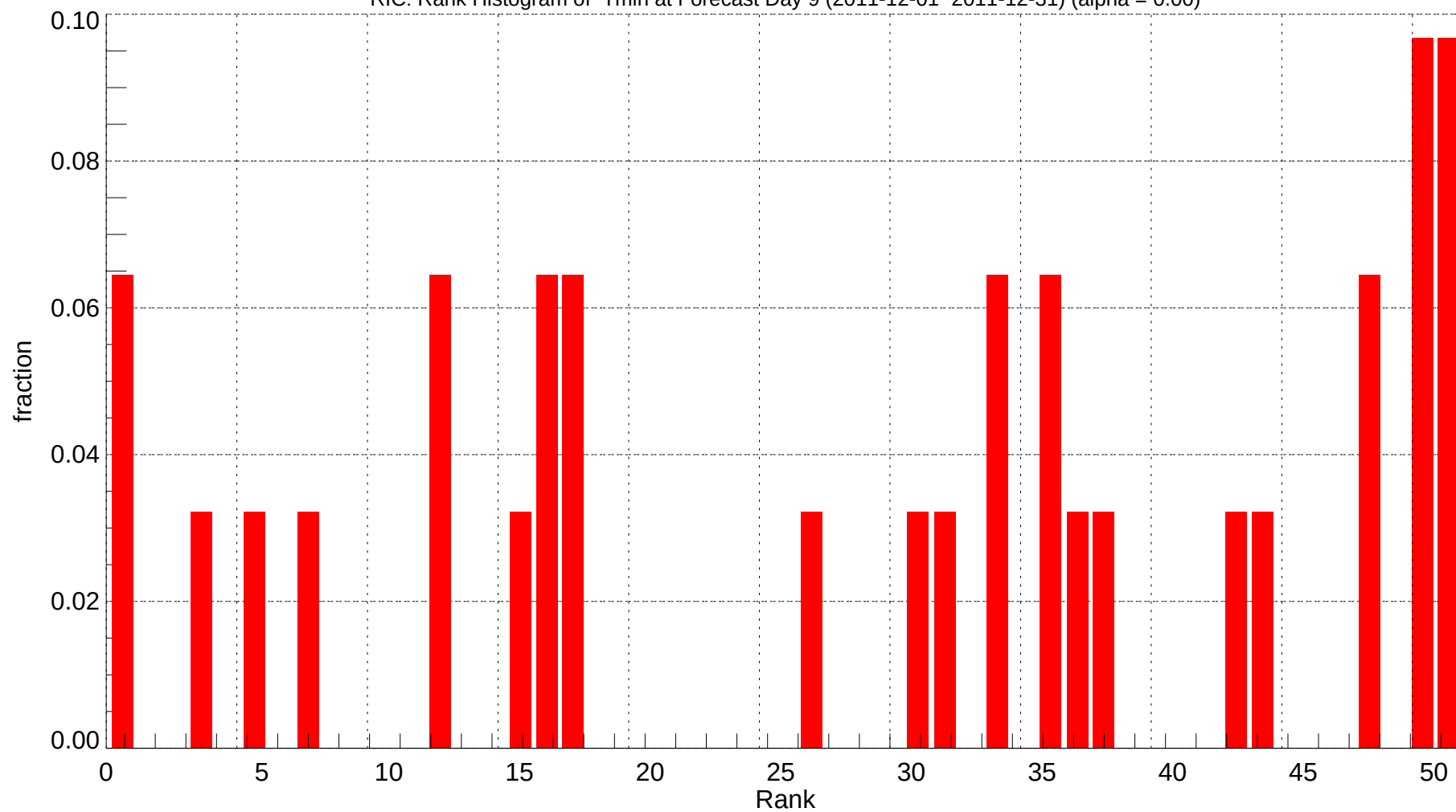
RIC: Rank Histogram of Tmin at Forecast Day 9 (2011-12-01~2011-12-31) (alpha = 0.00)
