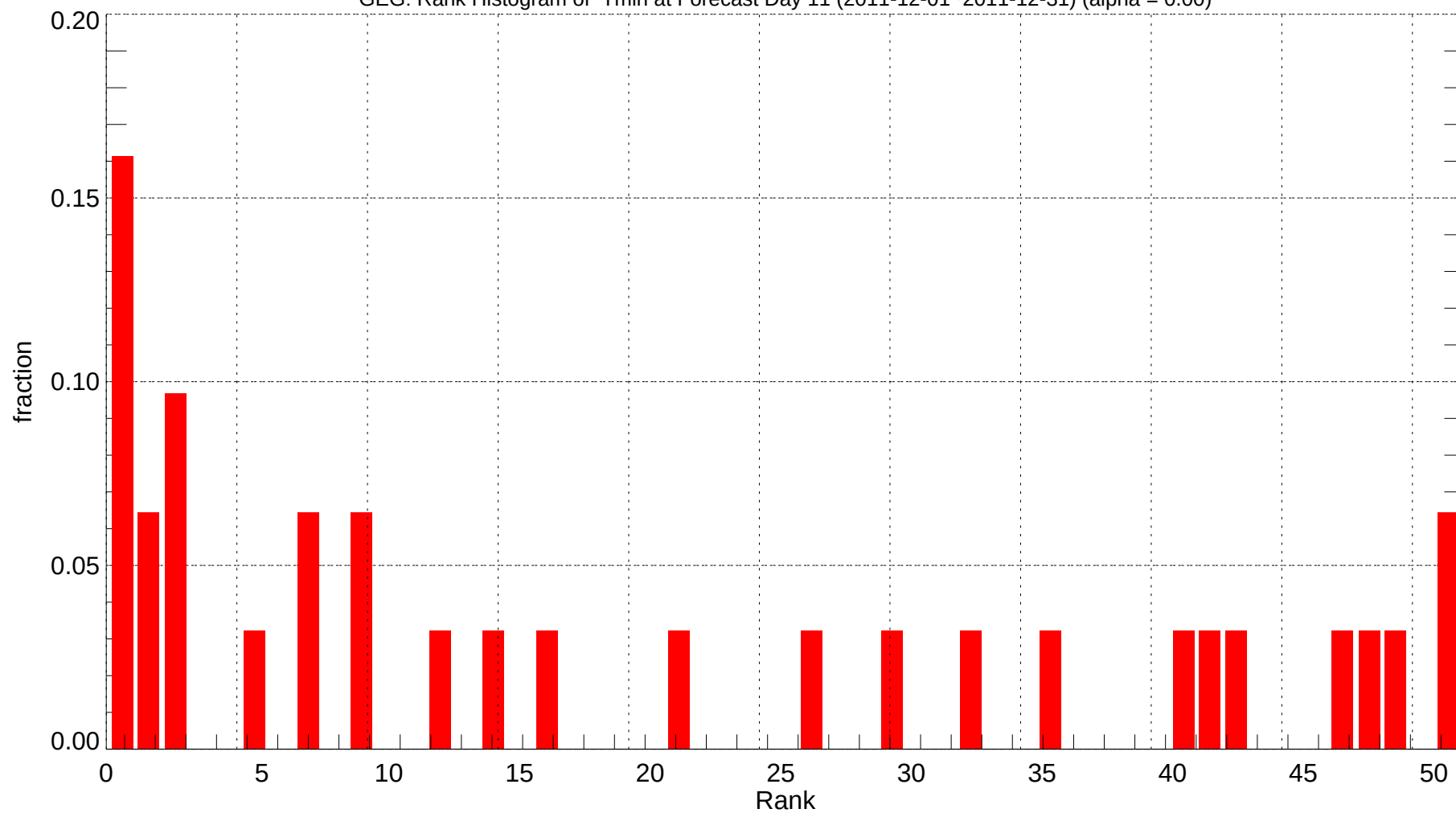
GEG: Rank Histogram of Tmin at Forecast Day 11 (2011-12-01~2011-12-31) (alpha = 0.00)
