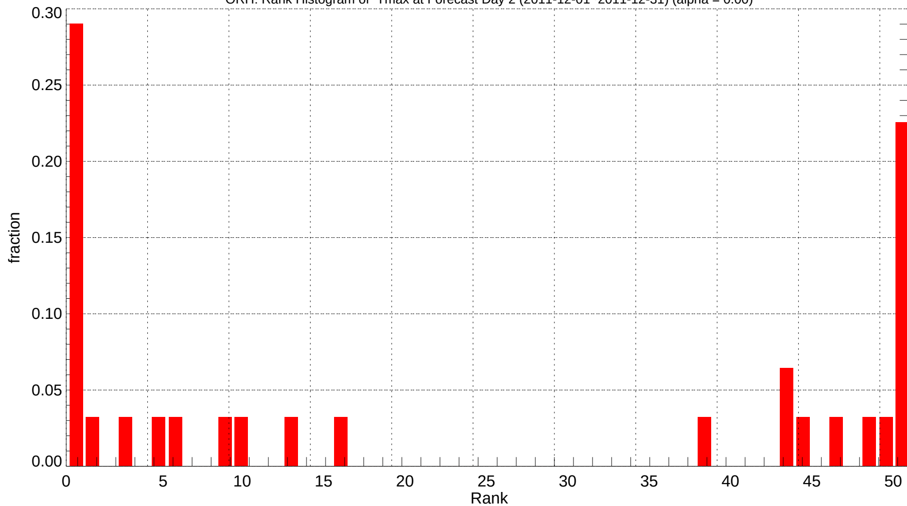
ORH: Rank Histogram of Tmax at Forecast Day 2 (2011-12-01~2011-12-31) (alpha = 0.00)
