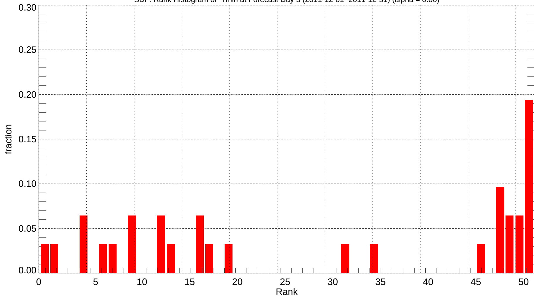
SDF: Rank Histogram of Tmin at Forecast Day 3 (2011-12-01~2011-12-31) (alpha = 0.00)
