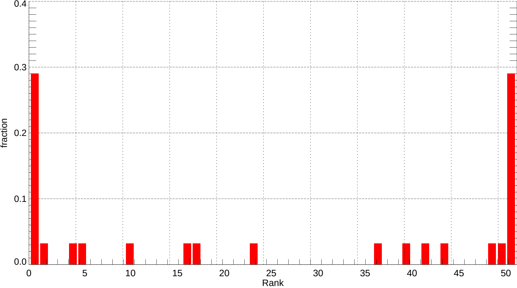
PIT: Rank Histogram of Tmax at Forecast Day 1 (2011-12-01~2011-12-31) (alpha = 0.00)
