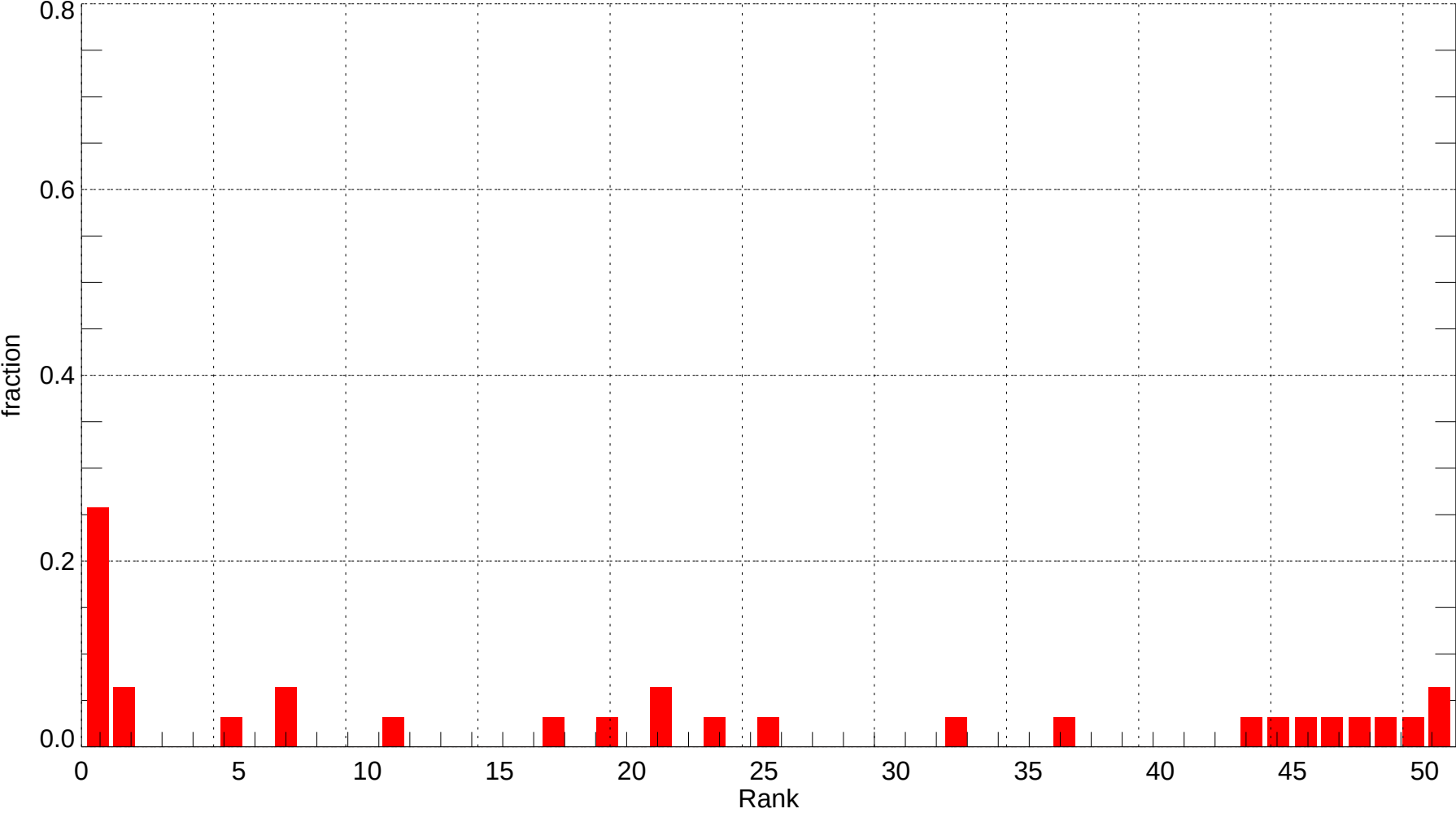
LFK: Rank Histogram of Tmin at Forecast Day 1 (2011-12-01~2011-12-31) (alpha = 0.00)
