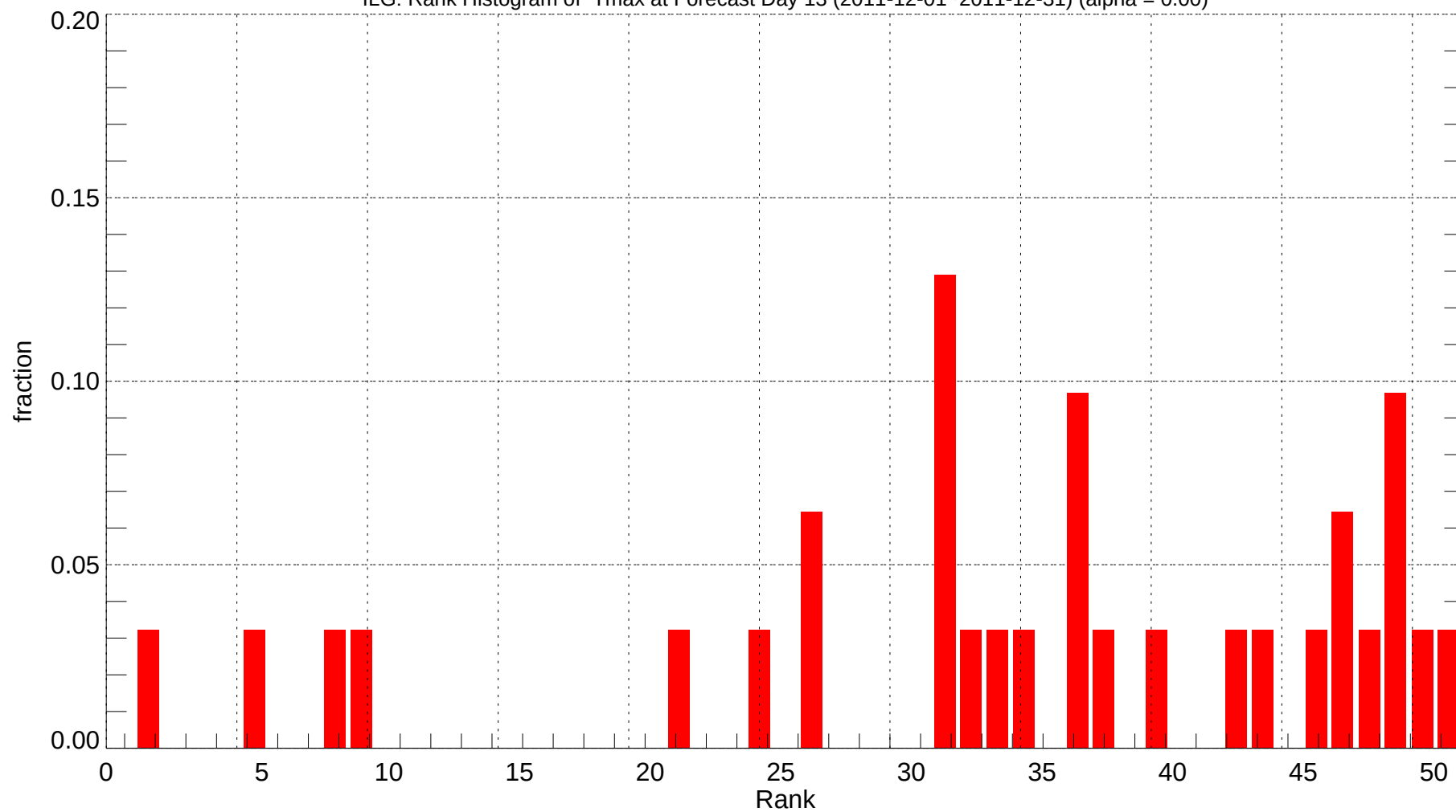
ILG: Rank Histogram of Tmax at Forecast Day 13 (2011-12-01~2011-12-31) (alpha = 0.00)
