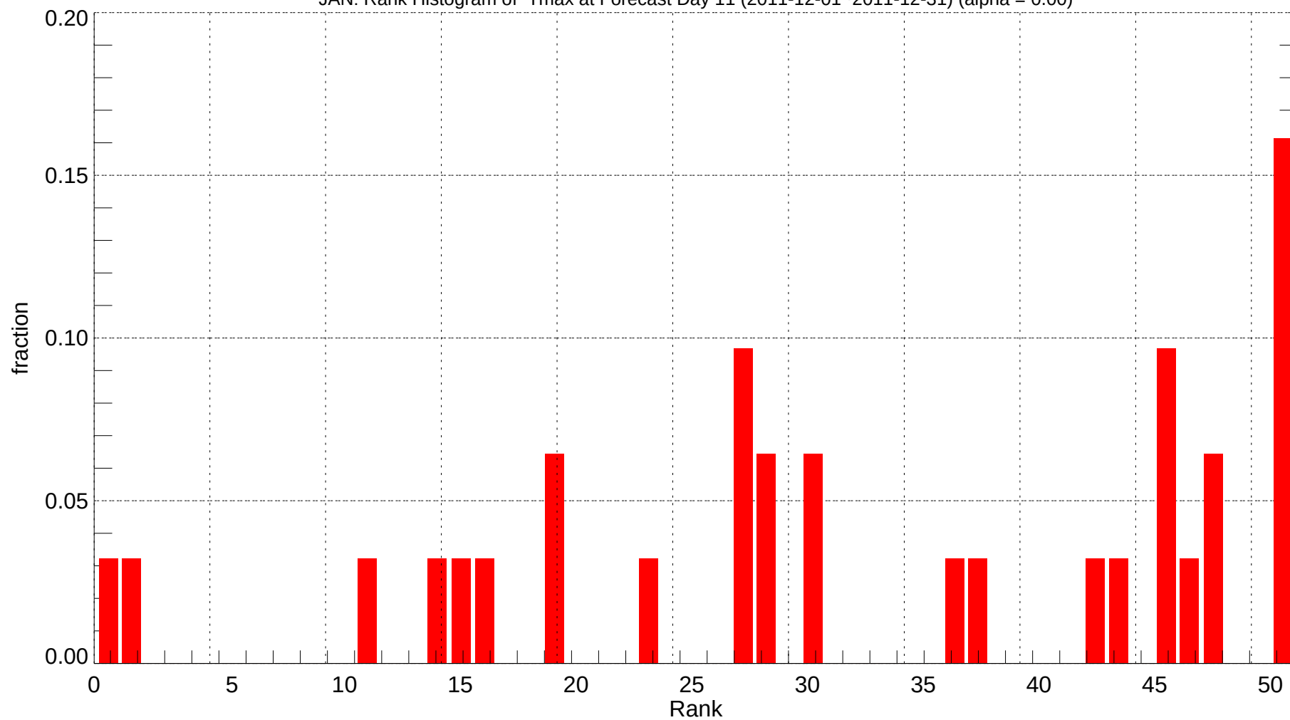
JAN: Rank Histogram of Tmax at Forecast Day 11 (2011-12-01~2011-12-31) (alpha = 0.00)
