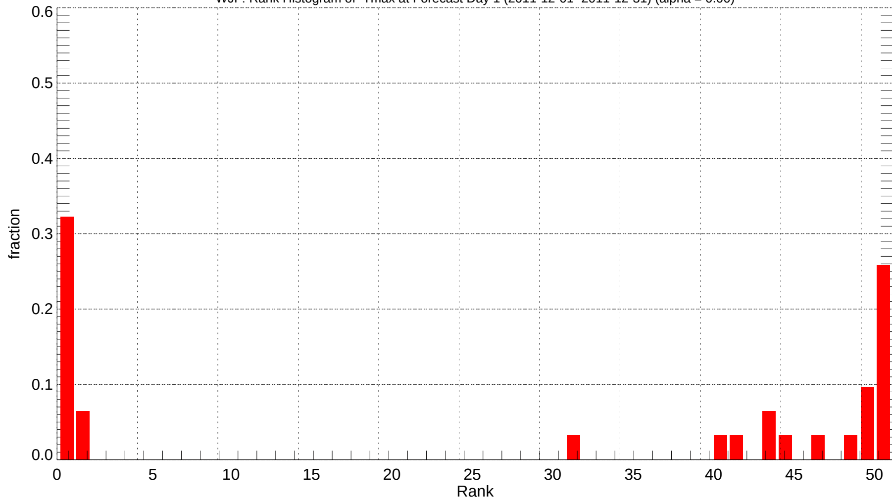
WJF: Rank Histogram of Tmax at Forecast Day 1 (2011-12-01~2011-12-31) (alpha = 0.00)
