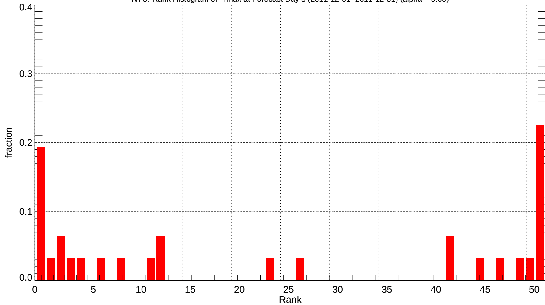
NTU: Rank Histogram of Tmax at Forecast Day 3 (2011-12-01~2011-12-31) (alpha = 0.00)
