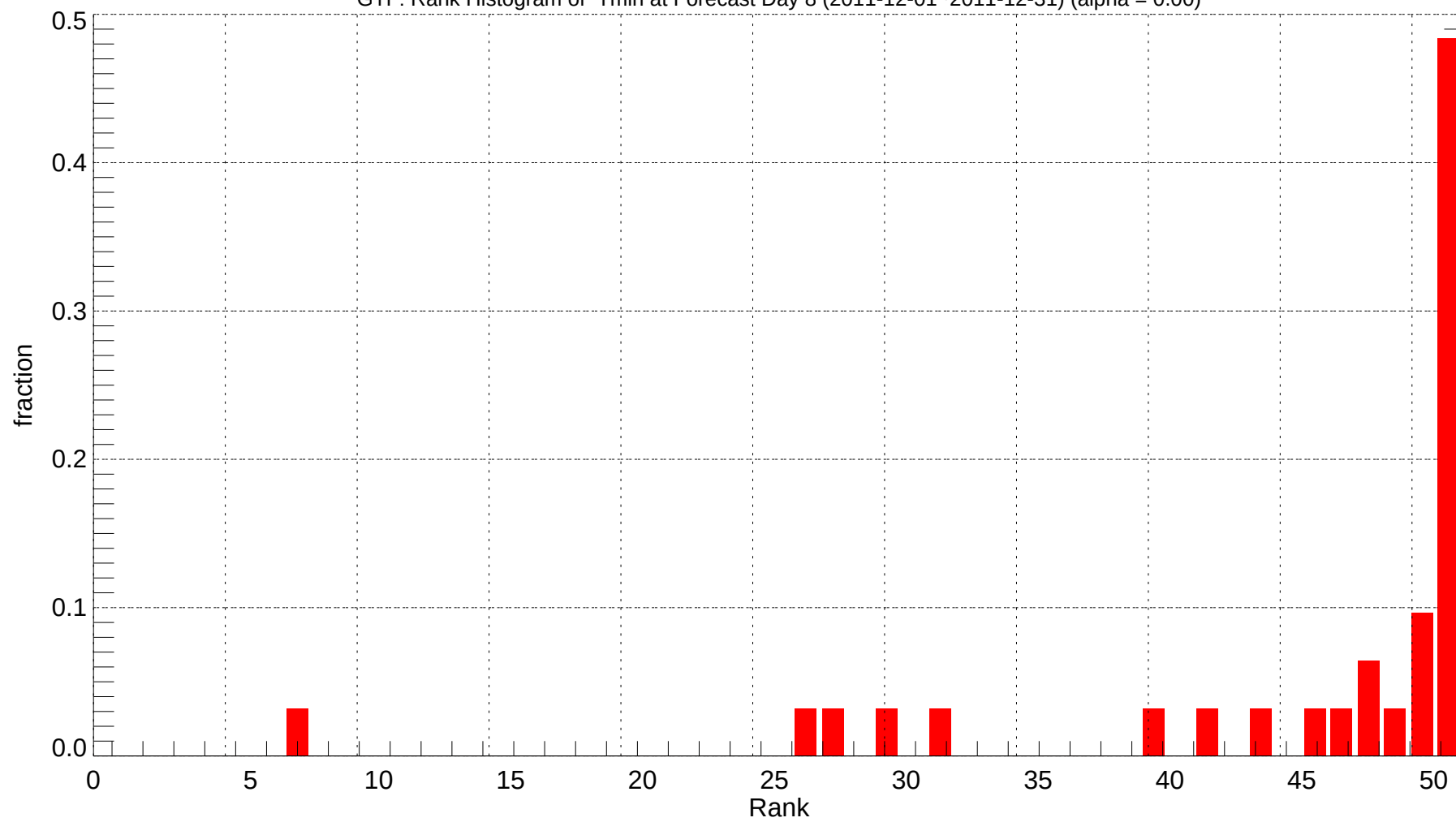
GTF: Rank Histogram of Tmin at Forecast Day 8 (2011-12-01~2011-12-31) (alpha = 0.00)
