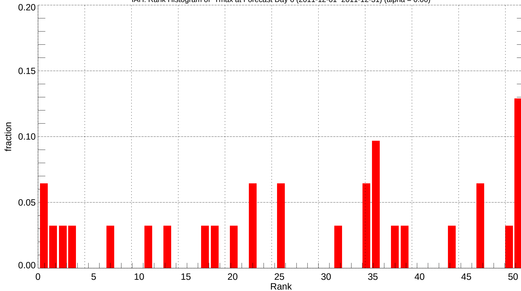
IAH: Rank Histogram of Tmax at Forecast Day 6 (2011-12-01~2011-12-31) (alpha = 0.00)
