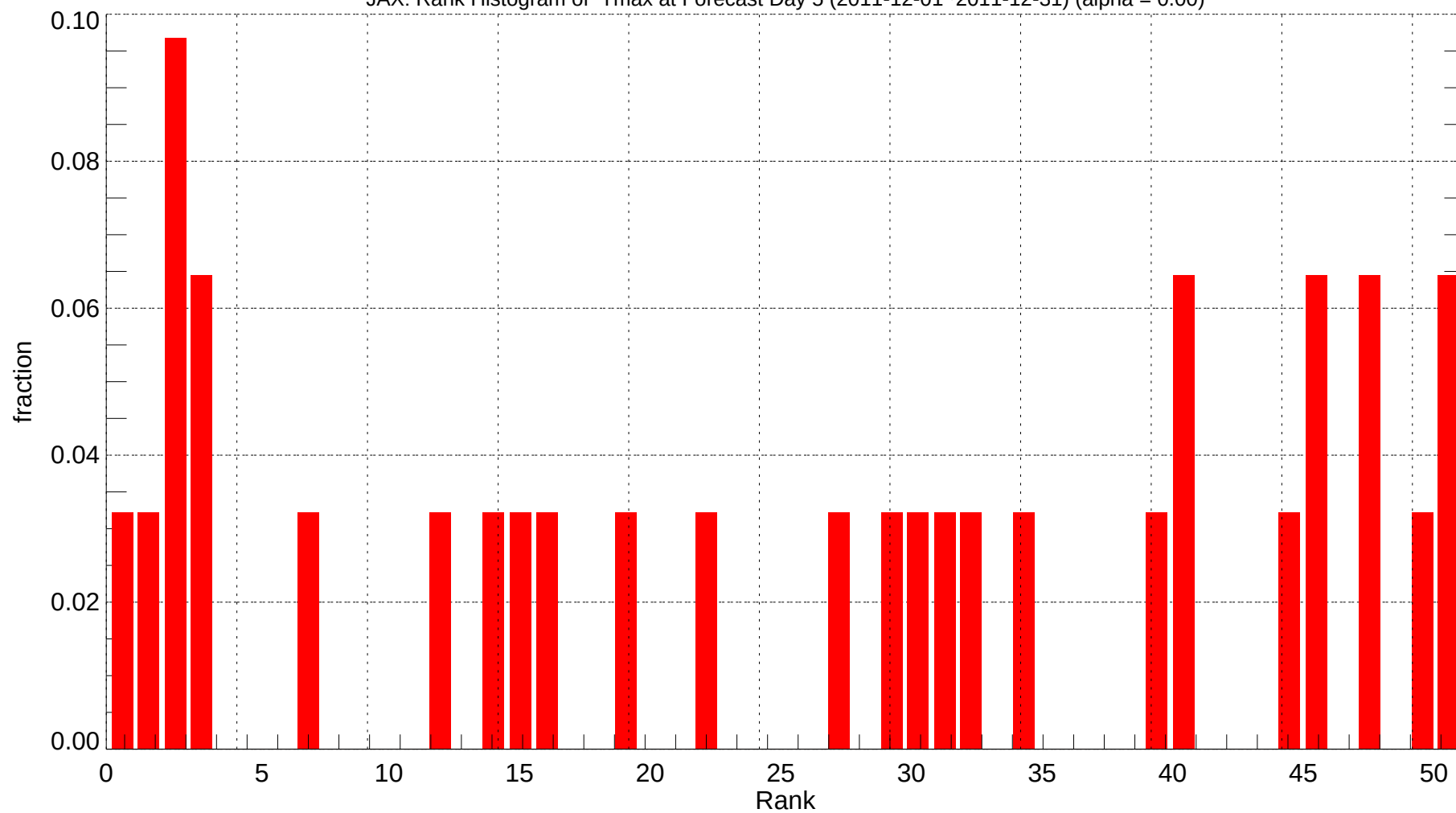
JAX: Rank Histogram of Tmax at Forecast Day 5 (2011-12-01~2011-12-31) (alpha = 0.00)
