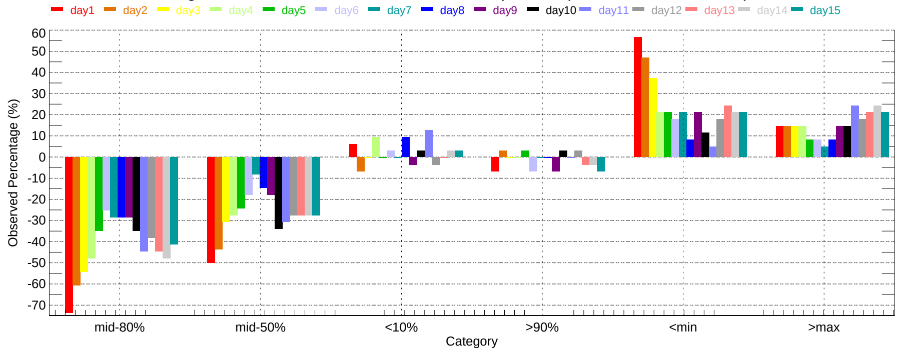
Observed Percentage Deviation of Ensembles - CRP: Max Temperature (2011-12-01~2011-12-31)
