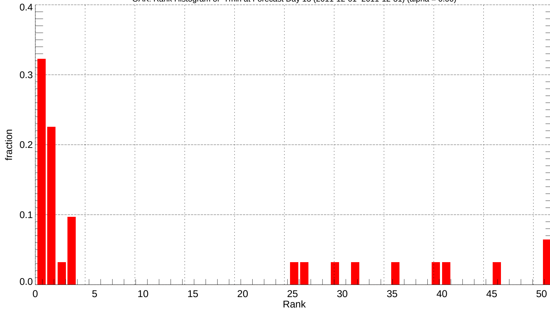
OAK: Rank Histogram of Tmin at Forecast Day 13 (2011-12-01~2011-12-31) (alpha = 0.00)
