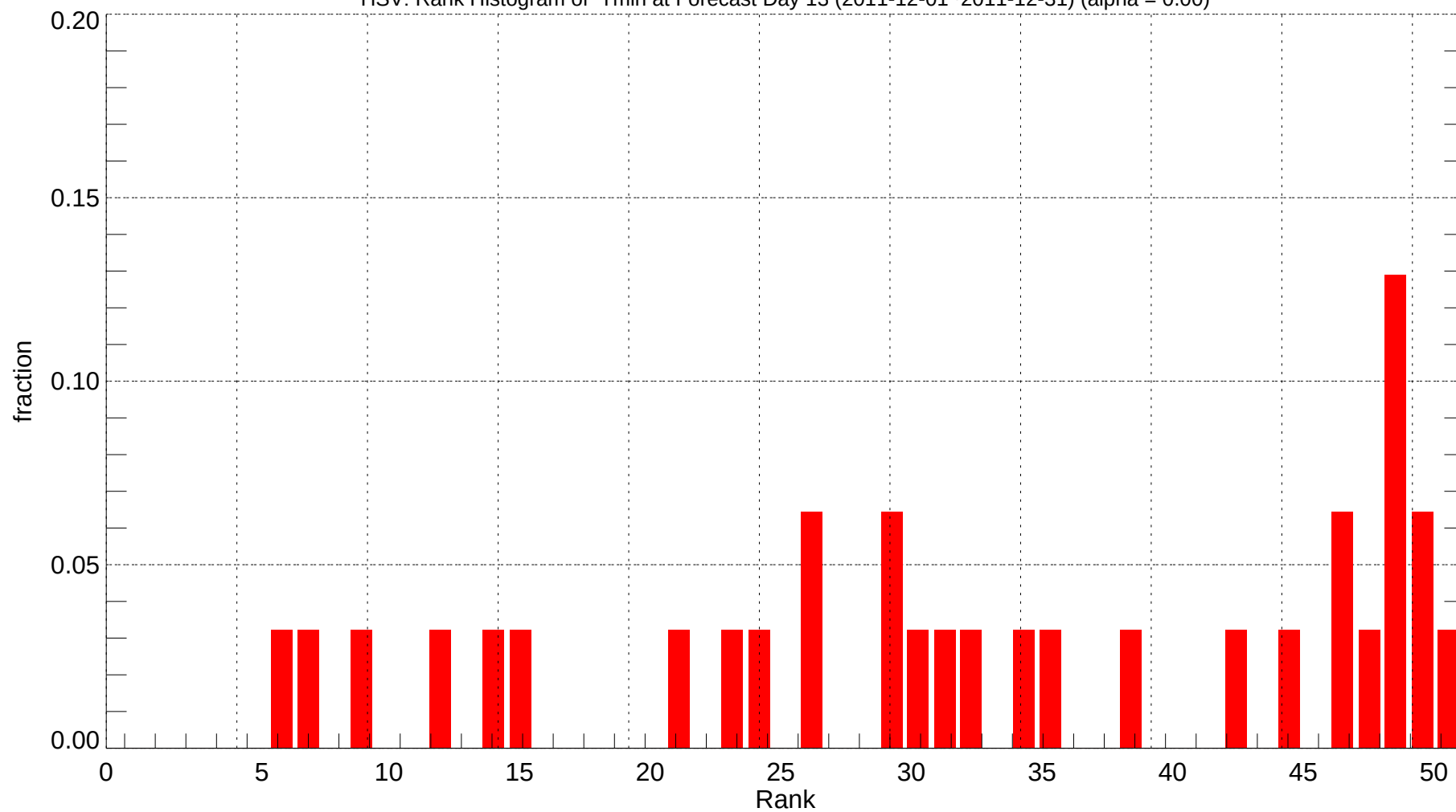
HSV: Rank Histogram of Tmin at Forecast Day 13 (2011-12-01~2011-12-31) (alpha = 0.00)
