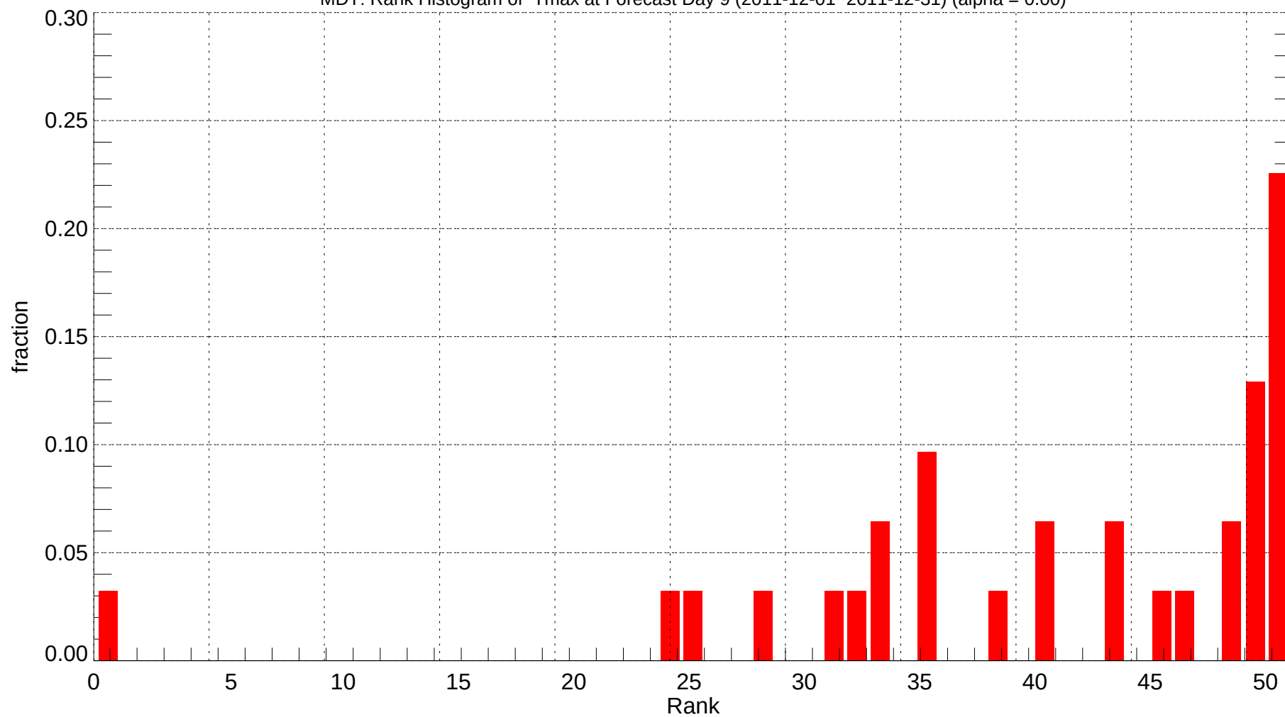
MDT: Rank Histogram of Tmax at Forecast Day 9 (2011-12-01~2011-12-31) (alpha = 0.00)
