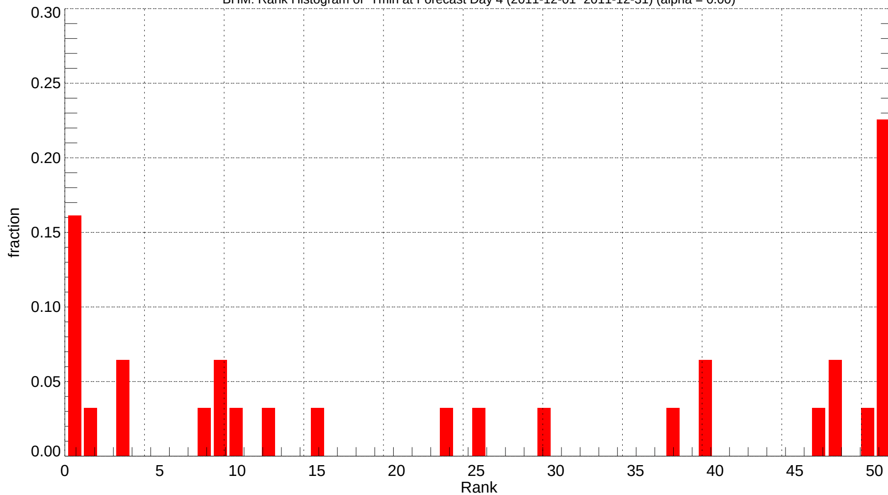
BHM: Rank Histogram of Tmin at Forecast Day 4 (2011-12-01~2011-12-31) (alpha = 0.00)
