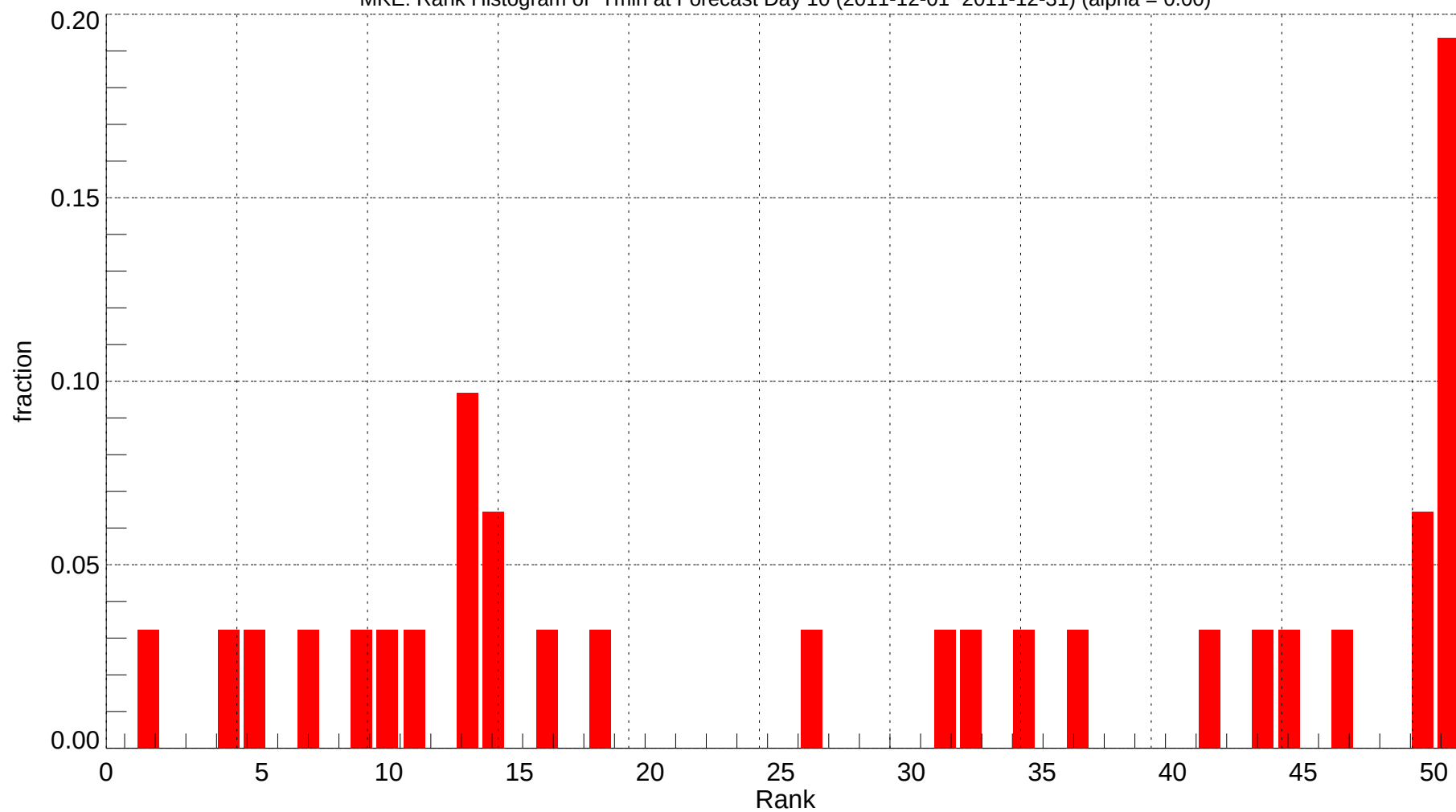
MKE: Rank Histogram of Tmin at Forecast Day 10 (2011-12-01~2011-12-31) (alpha = 0.00)
