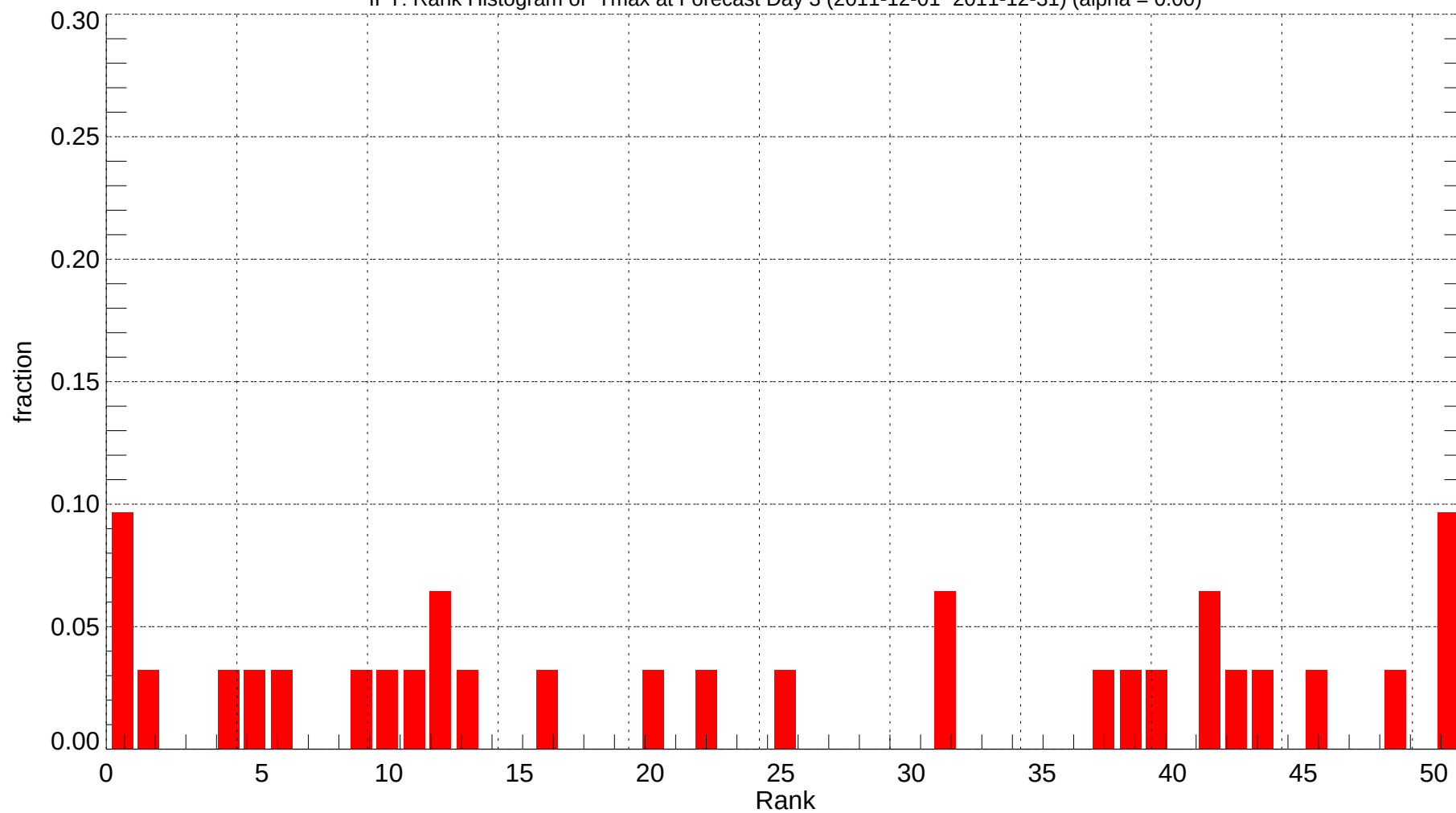
IPT: Rank Histogram of Tmax at Forecast Day 3 (2011-12-01~2011-12-31) (alpha = 0.00)
