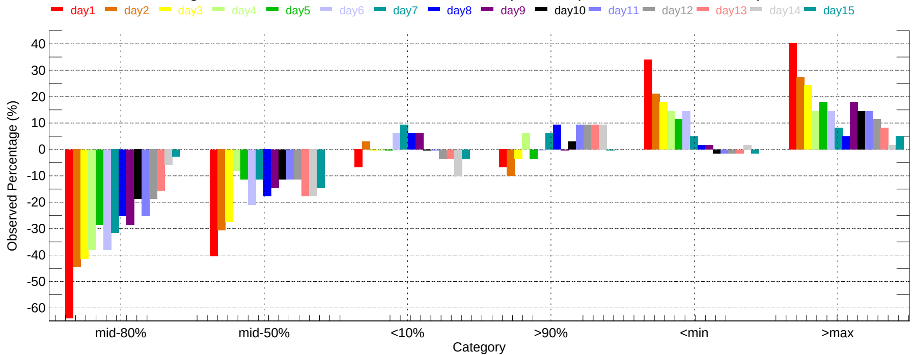
Observed Percentage Deviation of Ensembles - MKE: Max Temperature (2011-12-01~2011-12-31)
