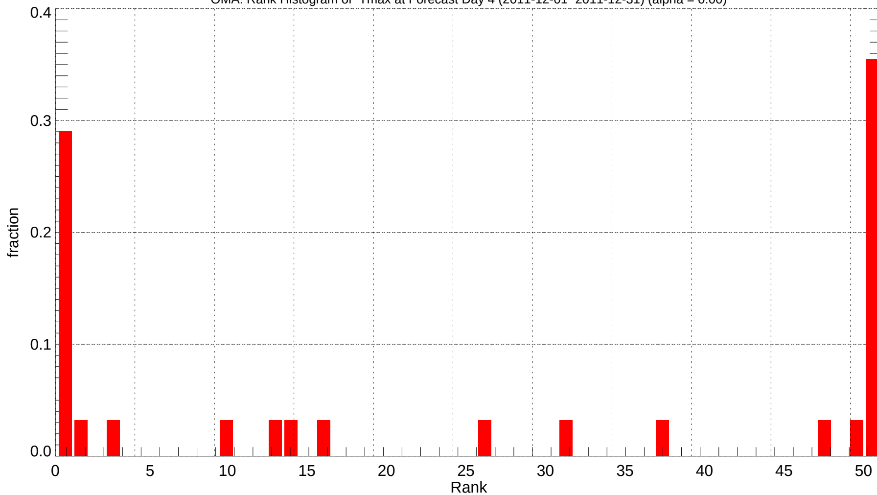
OMA: Rank Histogram of Tmax at Forecast Day 4 (2011-12-01~2011-12-31) (alpha = 0.00)
