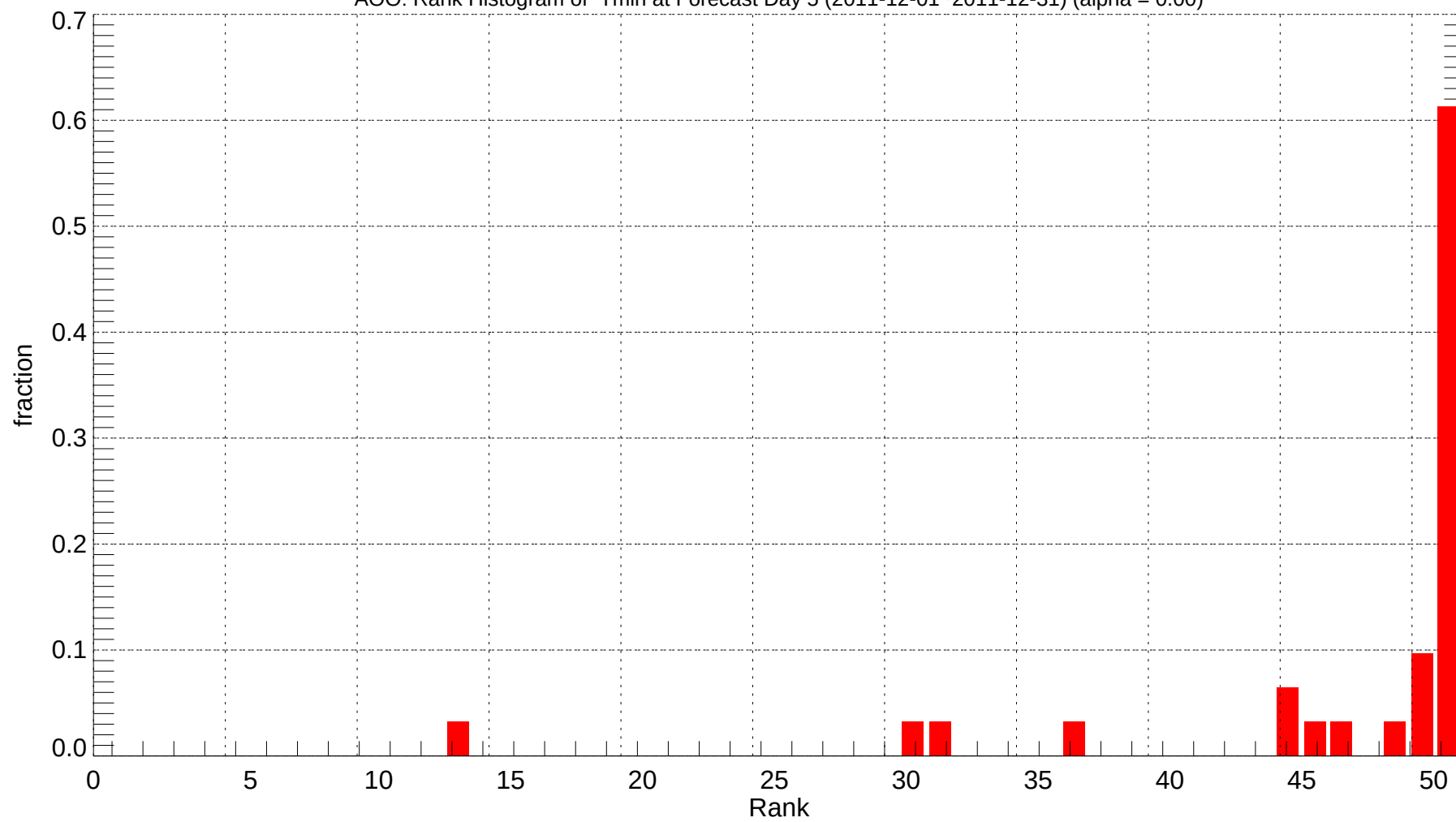
AOO: Rank Histogram of Tmin at Forecast Day 5 (2011-12-01~2011-12-31) (alpha = 0.00)
