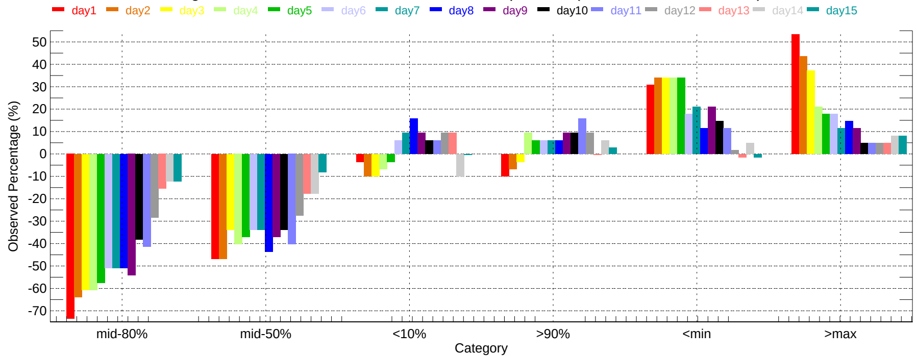
Observed Percentage Deviation of Ensembles - SEA: Max Temperature (2011-12-01~2011-12-31)
