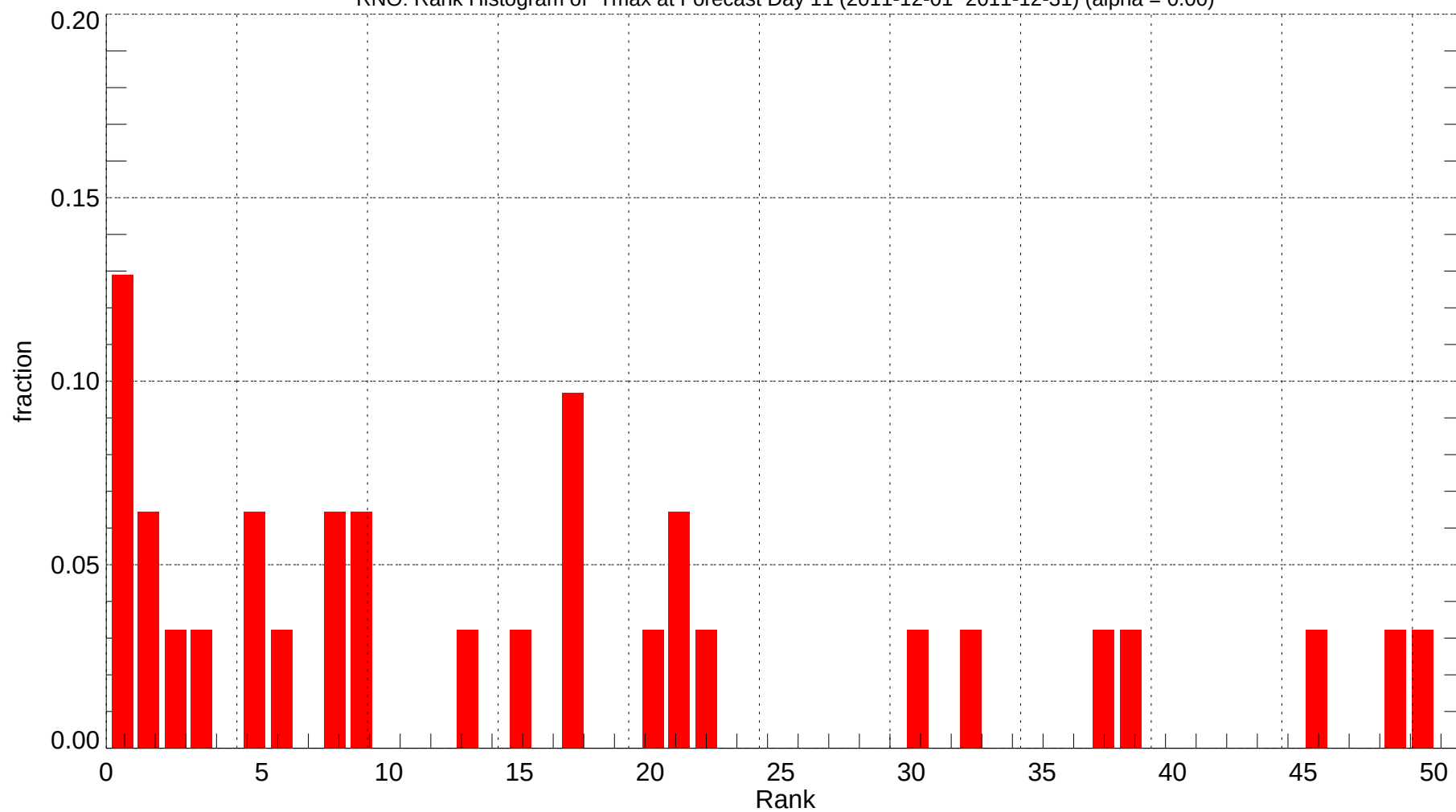
RNO: Rank Histogram of Tmax at Forecast Day 11 (2011-12-01~2011-12-31) (alpha = 0.00)
