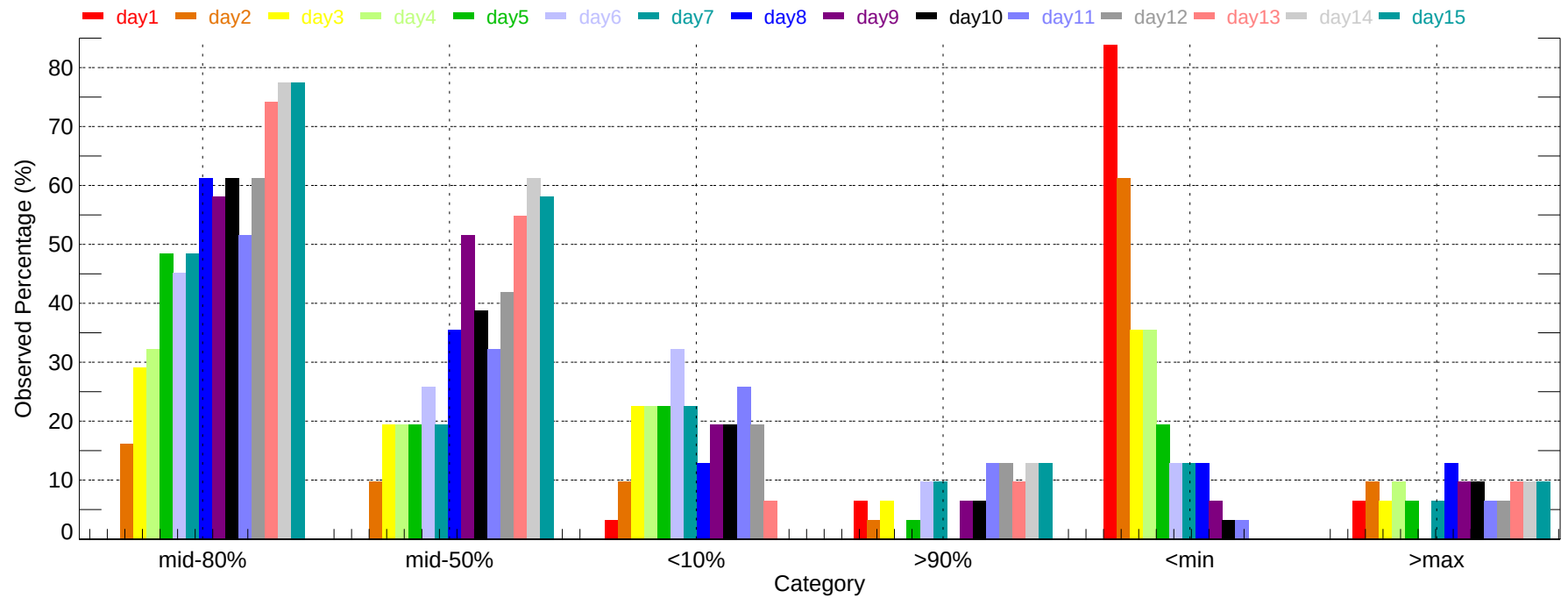
Observed Percentage of Ensembles - RBL: Max Temperature (2011-12-01~2011-12-31)
