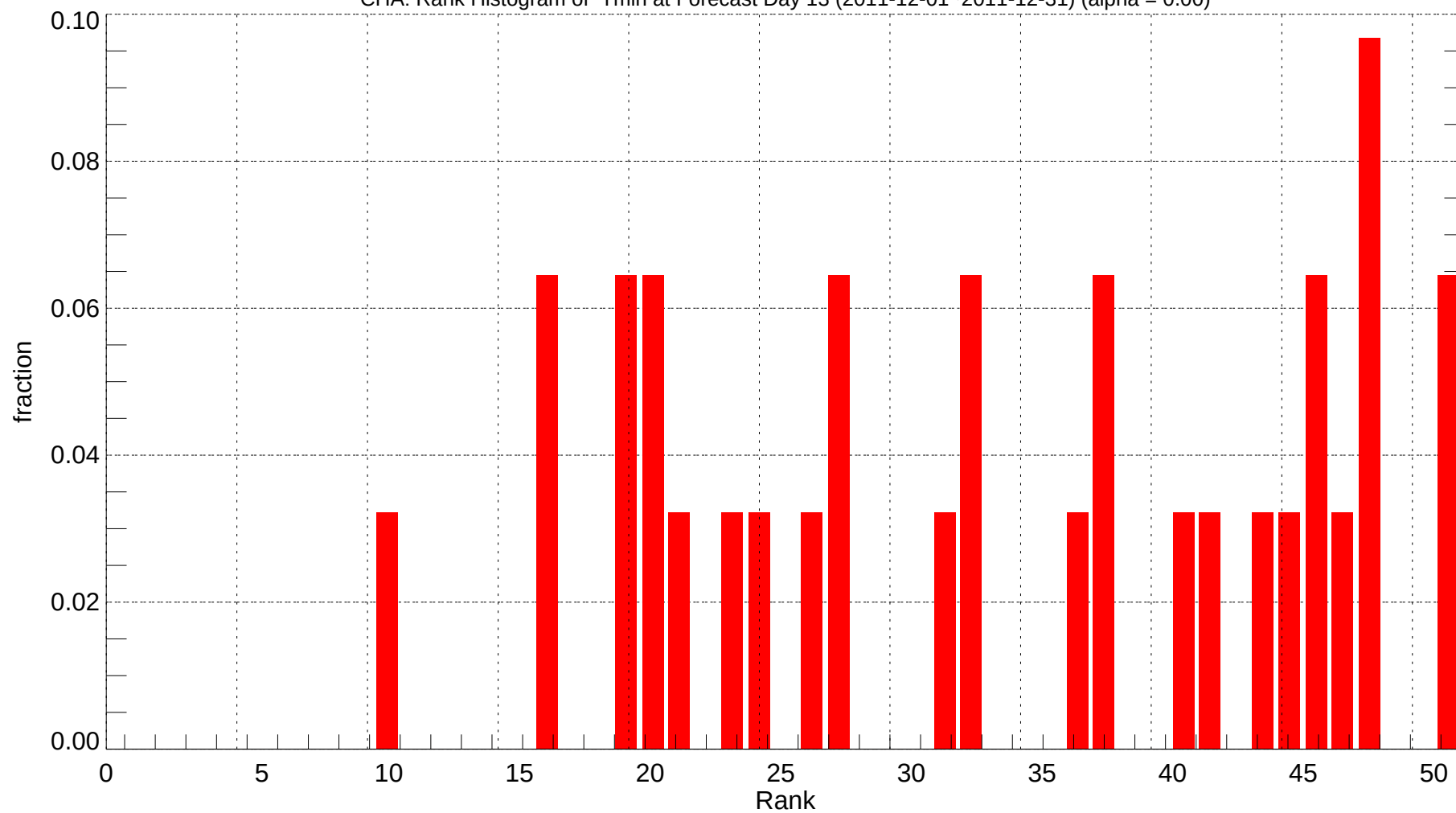
CHA: Rank Histogram of Tmin at Forecast Day 13 (2011-12-01~2011-12-31) (alpha = 0.00)
