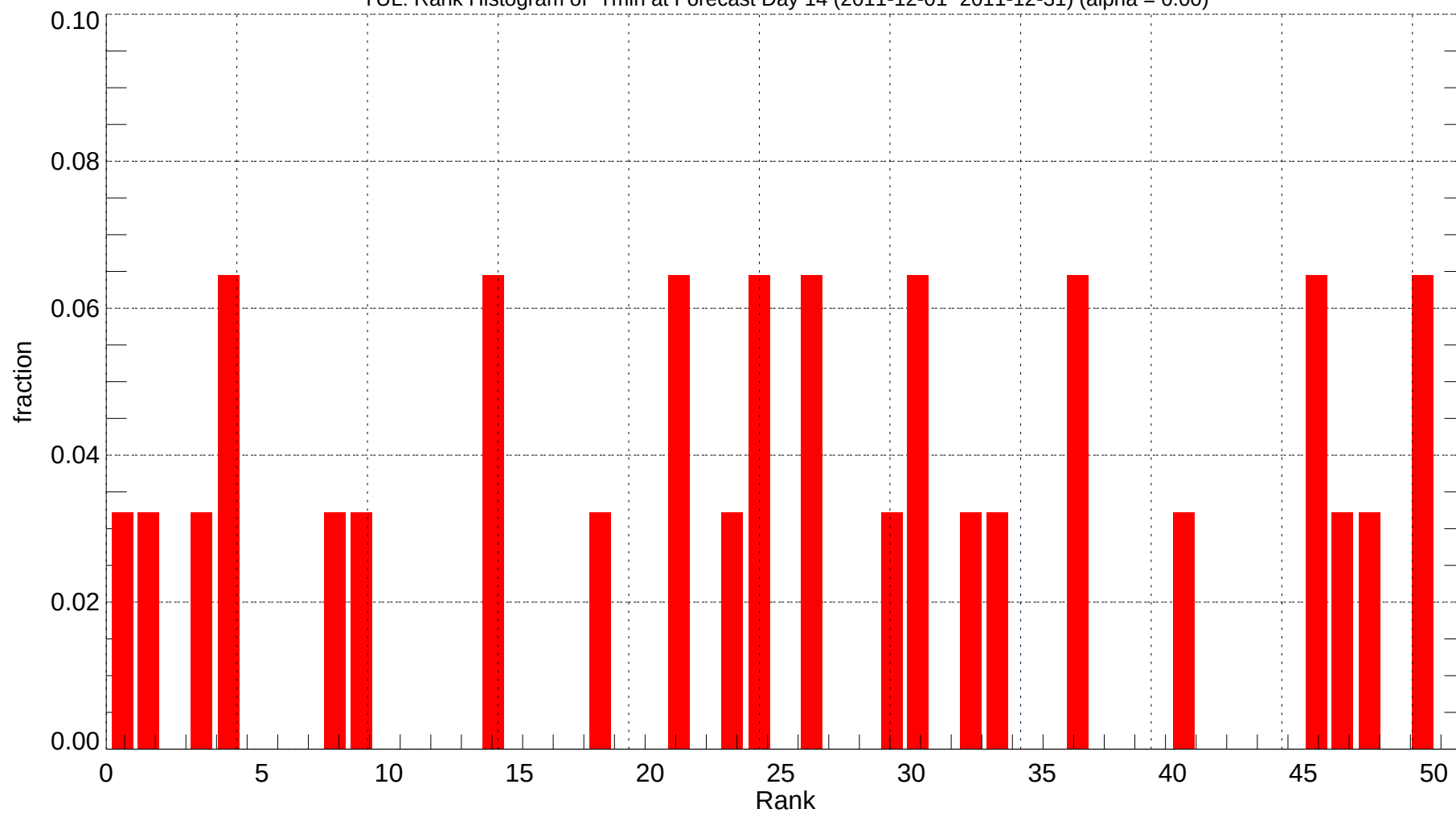
YUL: Rank Histogram of Tmin at Forecast Day 14 (2011-12-01~2011-12-31) (alpha = 0.00)
