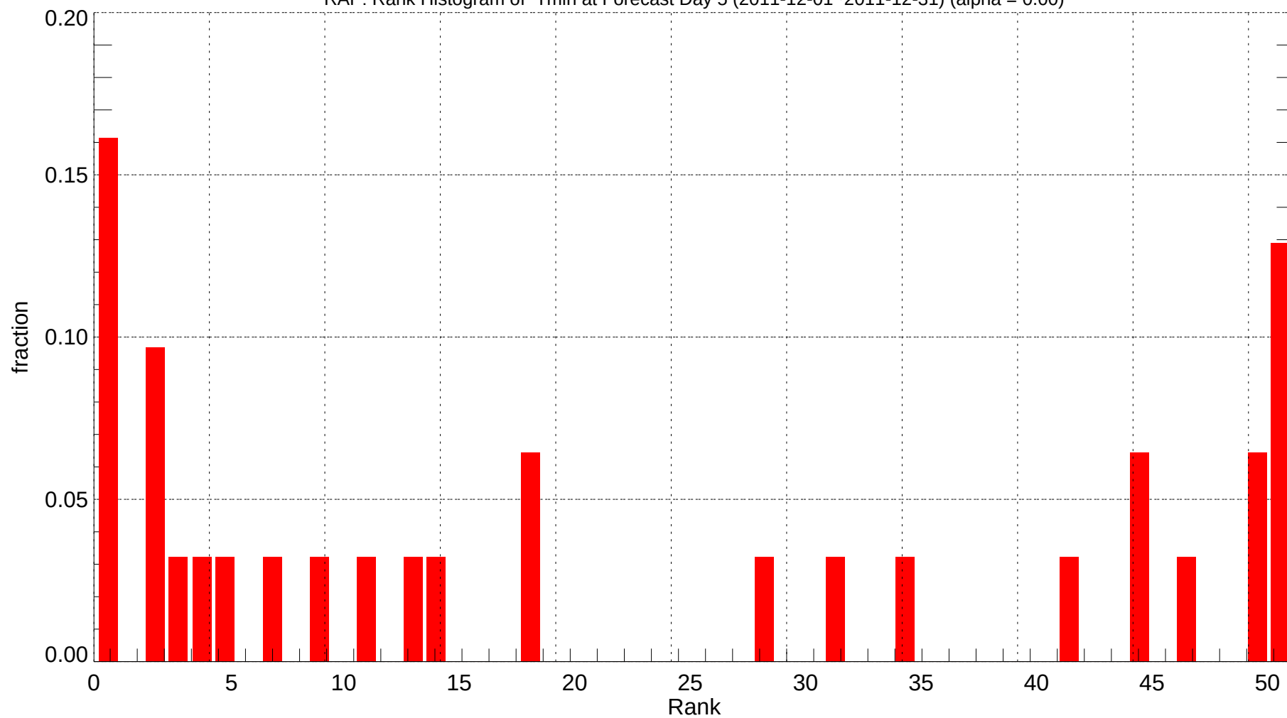
RAP: Rank Histogram of Tmin at Forecast Day 5 (2011-12-01~2011-12-31) (alpha = 0.00)
