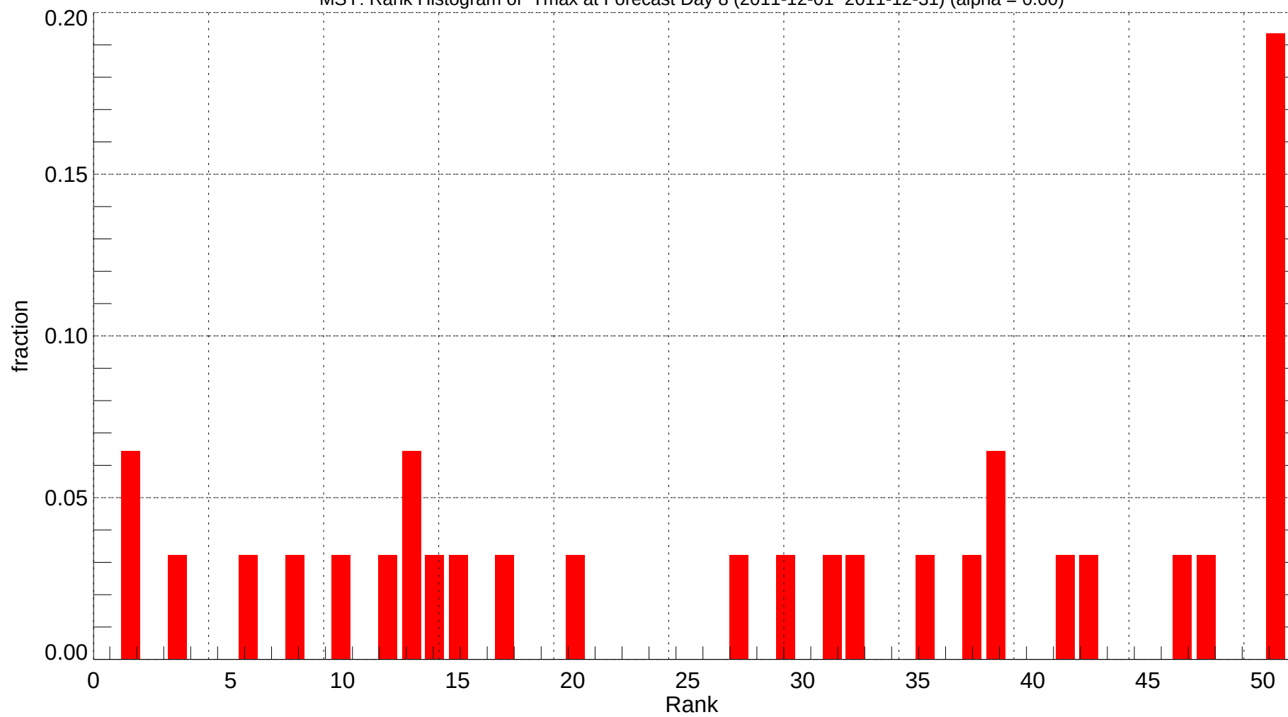
MSY: Rank Histogram of Tmax at Forecast Day 8 (2011-12-01~2011-12-31) (alpha = 0.00)
