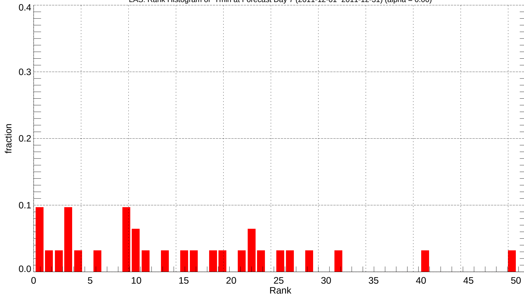
LAS: Rank Histogram of Tmin at Forecast Day 7 (2011-12-01~2011-12-31) (alpha = 0.00)
