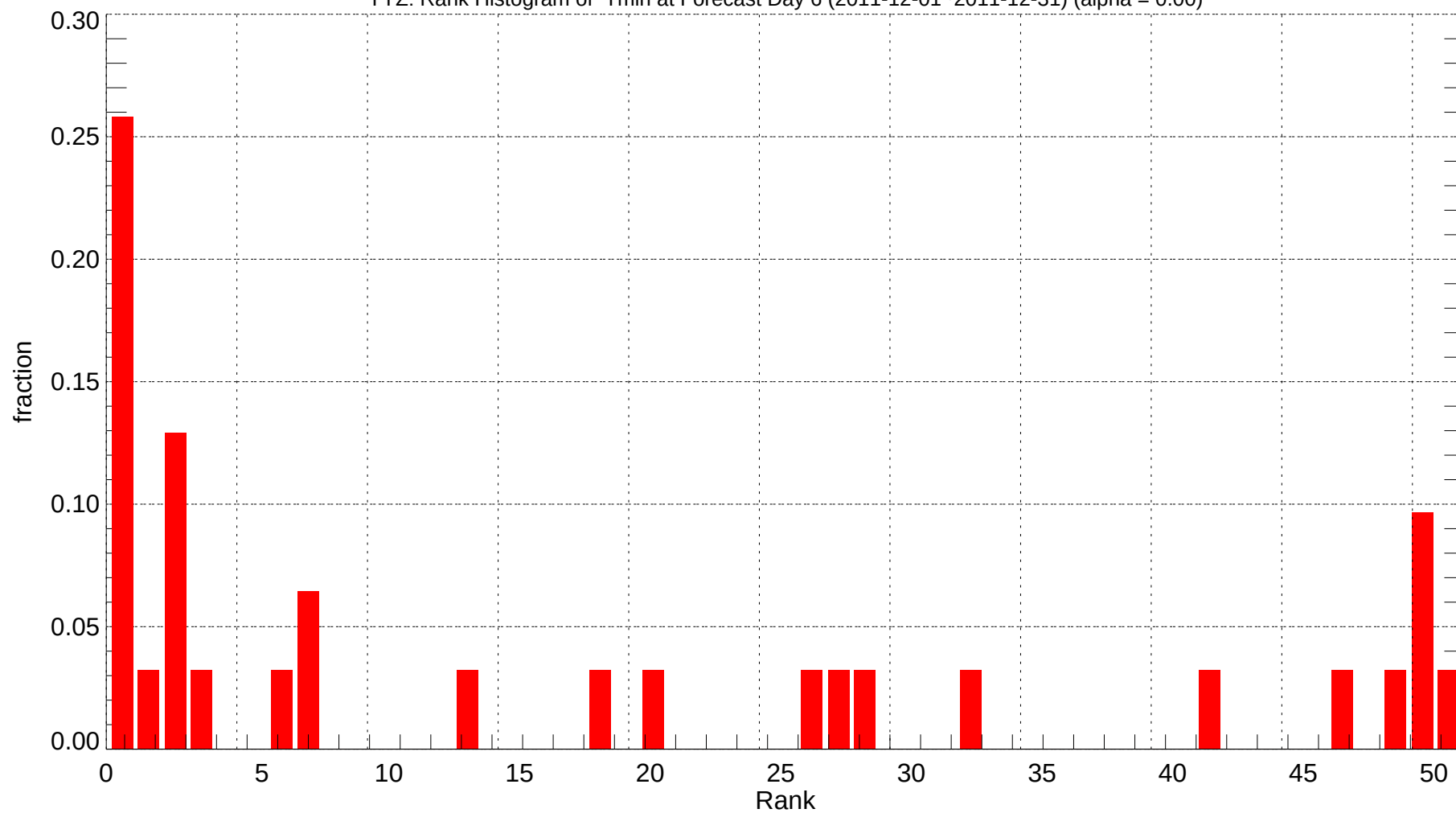
YYZ: Rank Histogram of Tmin at Forecast Day 6 (2011-12-01~2011-12-31) (alpha = 0.00)
