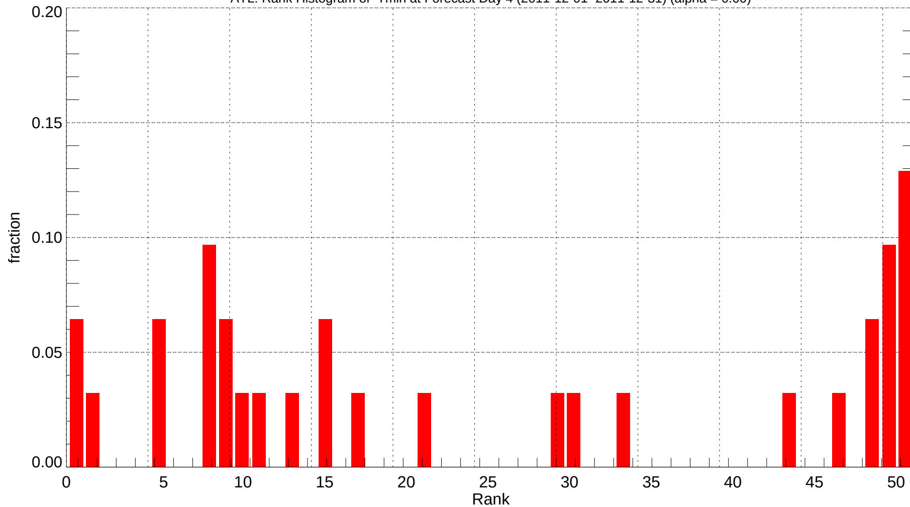
ATL: Rank Histogram of Tmin at Forecast Day 4 (2011-12-01~2011-12-31) (alpha = 0.00)
