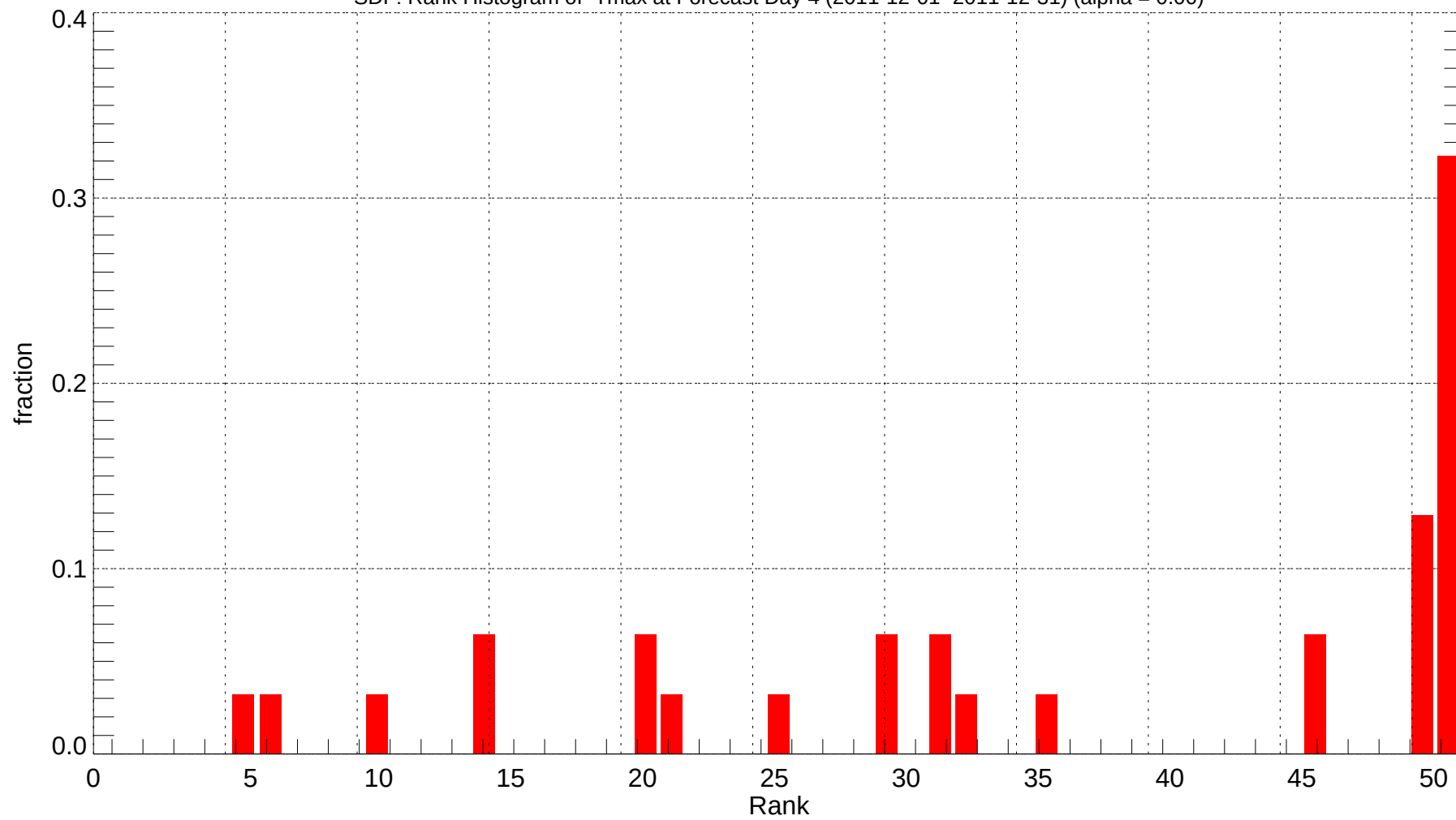
SDF: Rank Histogram of Tmax at Forecast Day 4 (2011-12-01~2011-12-31) (alpha = 0.00)
