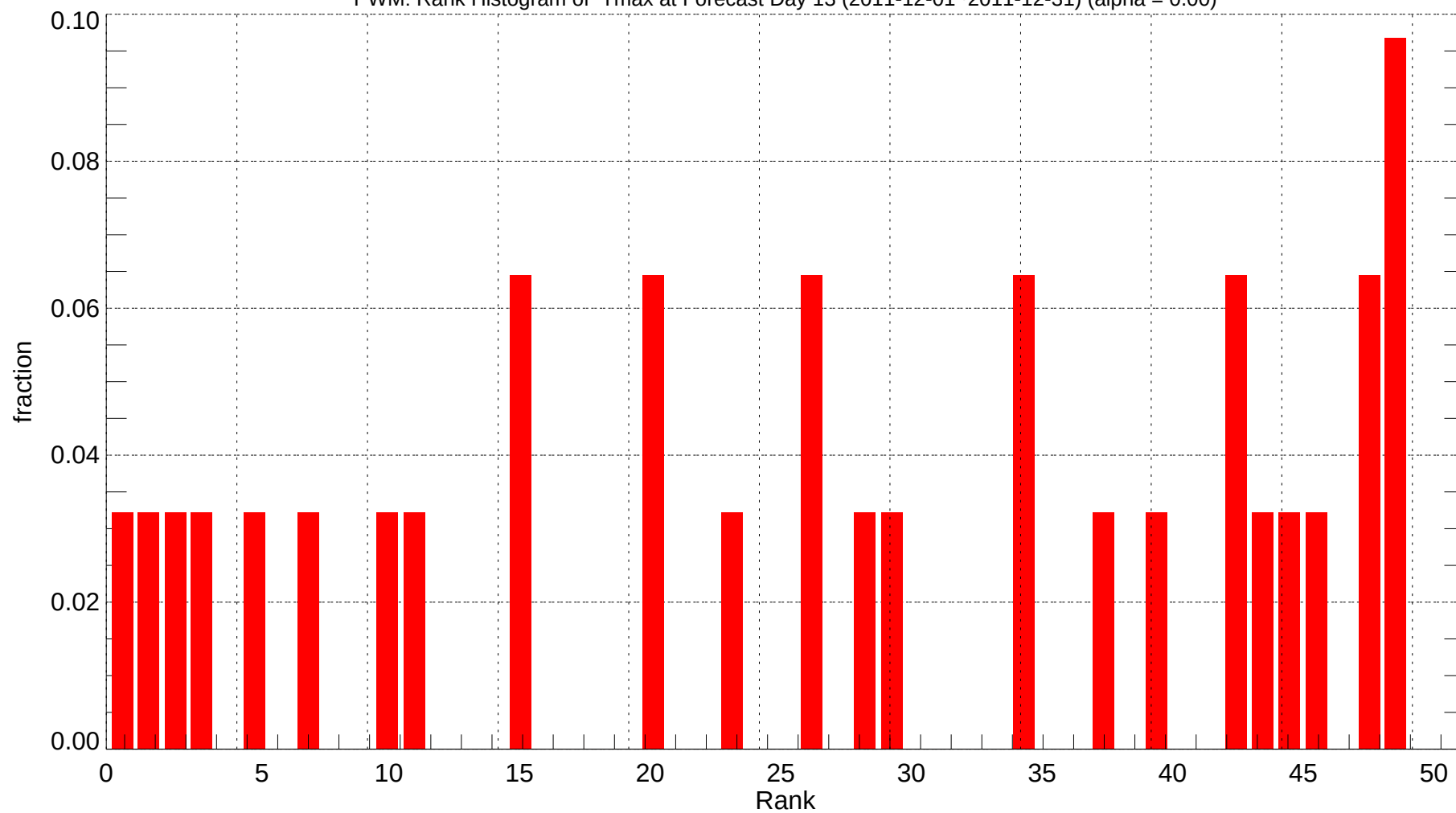
PWM: Rank Histogram of Tmax at Forecast Day 13 (2011-12-01~2011-12-31) (alpha = 0.00)
