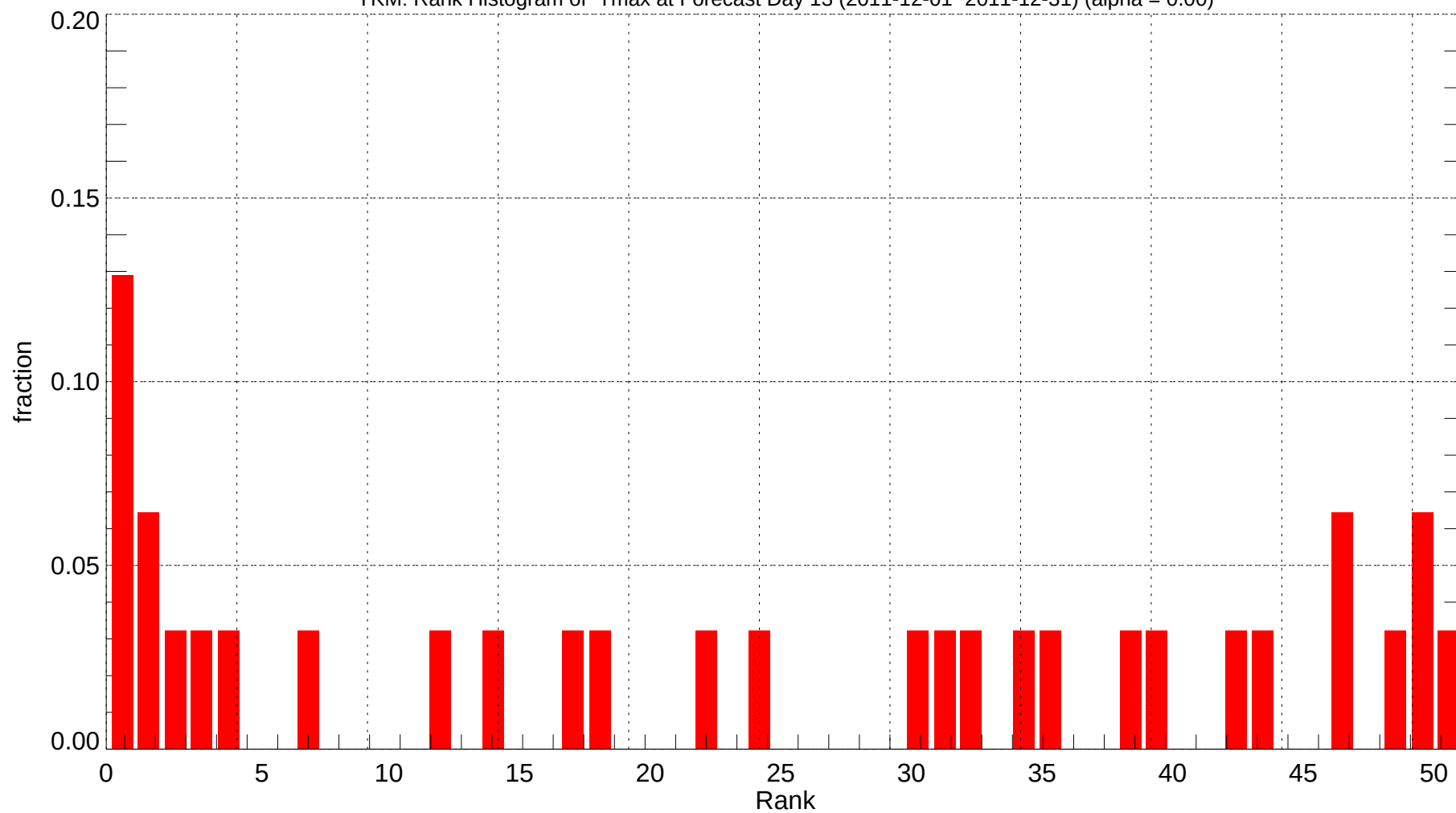
YKM: Rank Histogram of Tmax at Forecast Day 13 (2011-12-01~2011-12-31) (alpha = 0.00)
