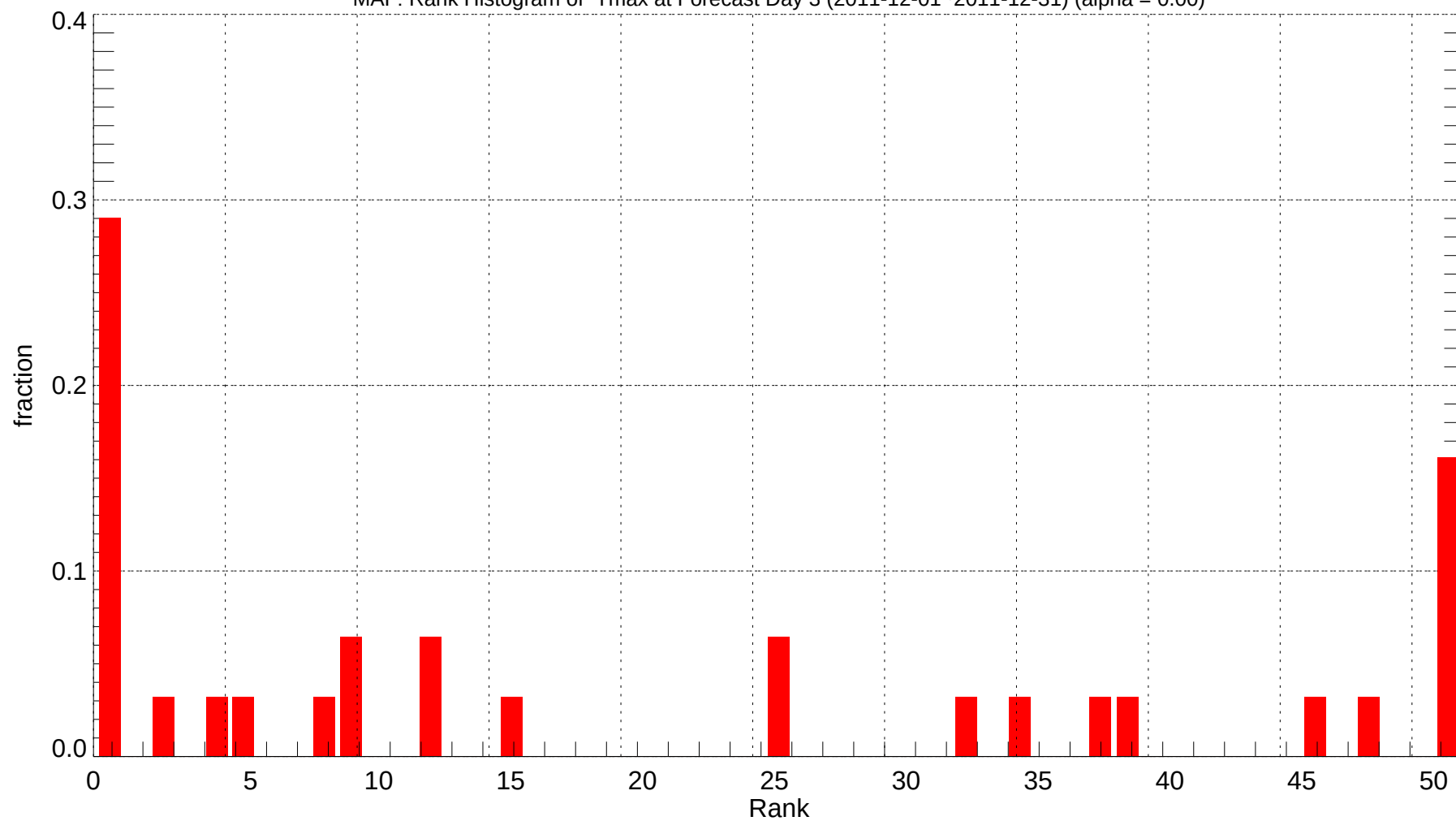
MAF: Rank Histogram of Tmax at Forecast Day 3 (2011-12-01~2011-12-31) (alpha = 0.00)
