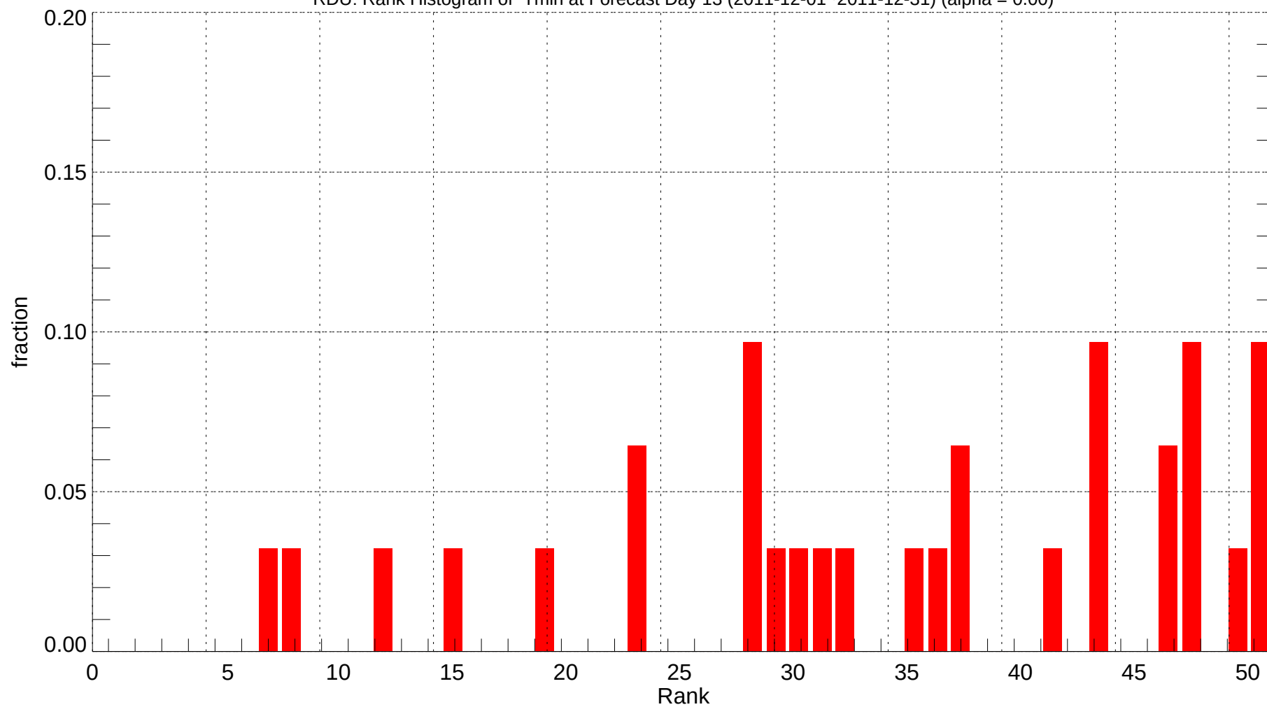
RDU: Rank Histogram of Tmin at Forecast Day 13 (2011-12-01~2011-12-31) (alpha = 0.00)
