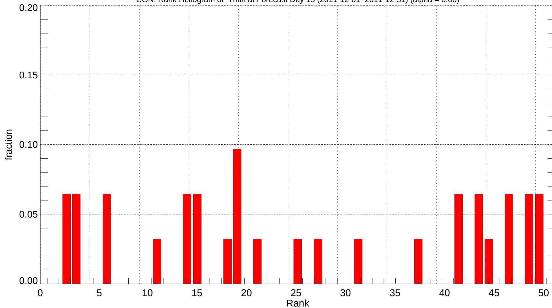
CON: Rank Histogram of Tmin at Forecast Day 13 (2011-12-01~2011-12-31) (alpha = 0.00)
