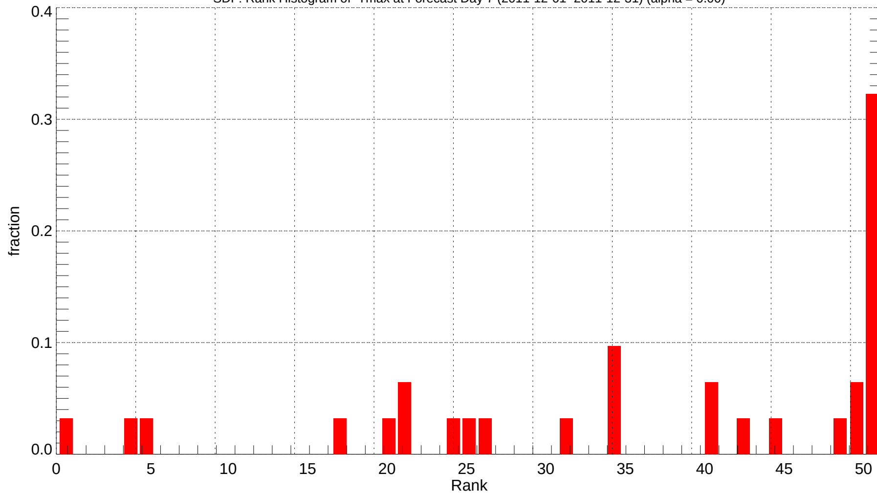
SDF: Rank Histogram of Tmax at Forecast Day 7 (2011-12-01~2011-12-31) (alpha = 0.00)
