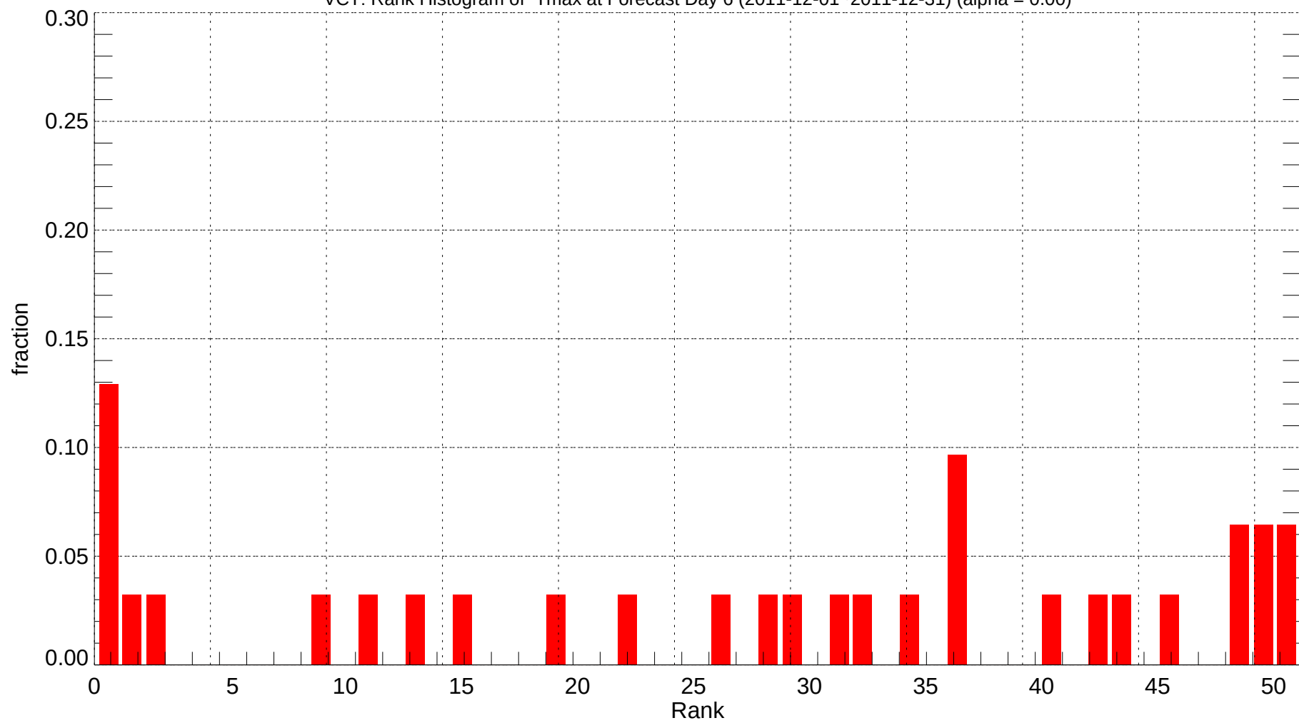
VCT: Rank Histogram of Tmax at Forecast Day 6 (2011-12-01~2011-12-31) (alpha = 0.00)
