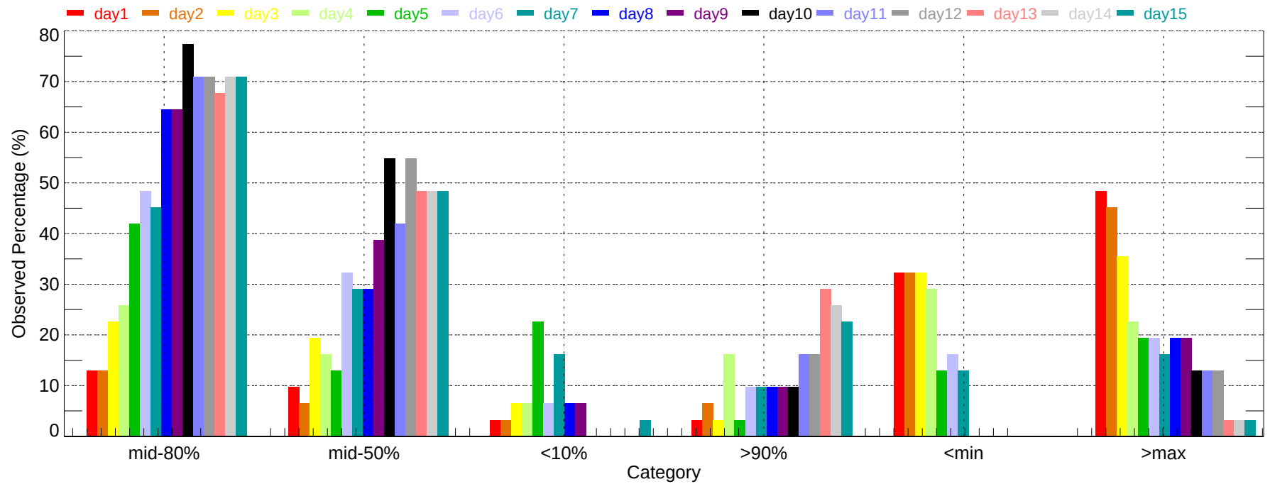
Observed Percentage of Ensembles - HSV: Max Temperature (2011-12-01~2011-12-31)
