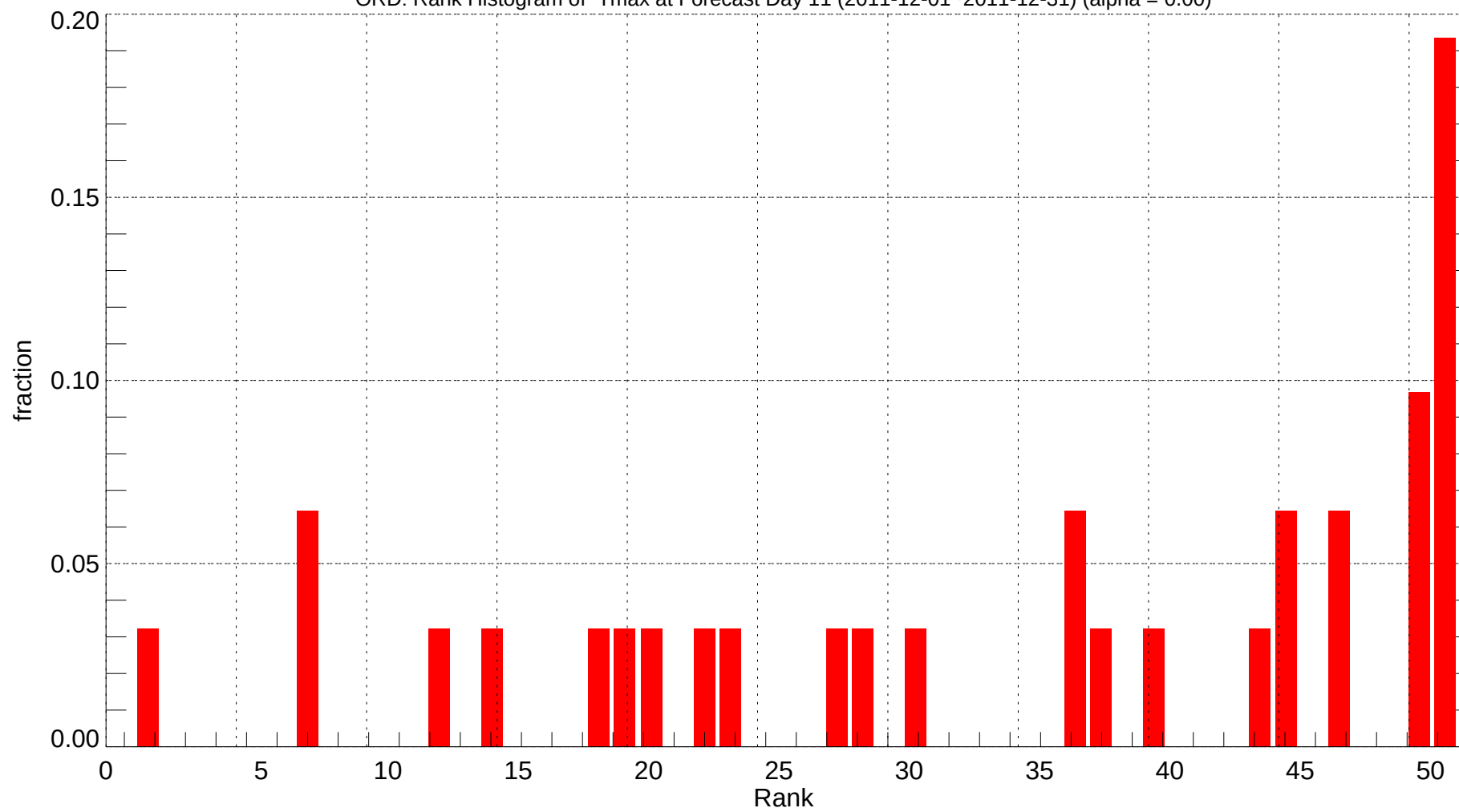
ORD: Rank Histogram of Tmax at Forecast Day 11 (2011-12-01~2011-12-31) (alpha = 0.00)
