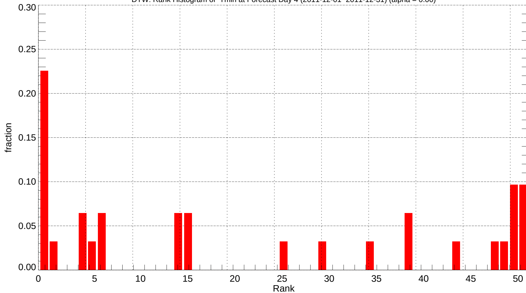
DTW: Rank Histogram of Tmin at Forecast Day 4 (2011-12-01~2011-12-31) (alpha = 0.00)
