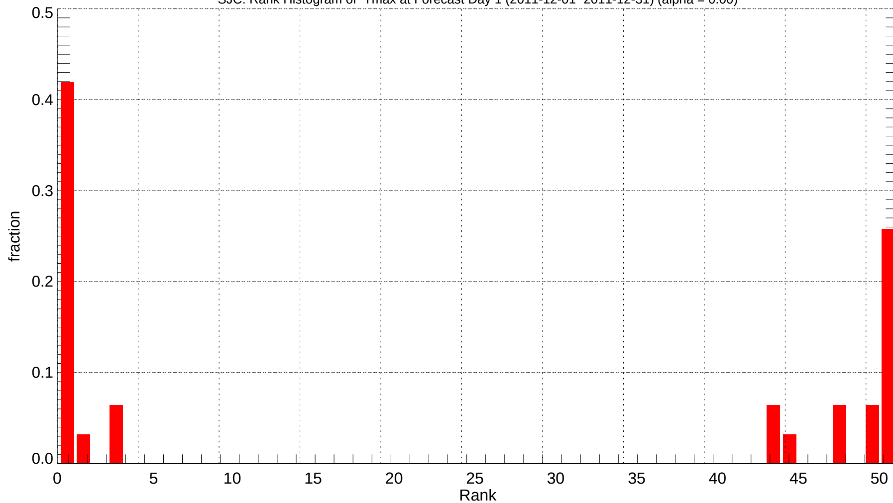
SJC: Rank Histogram of Tmax at Forecast Day 1 (2011-12-01~2011-12-31) (alpha = 0.00)
