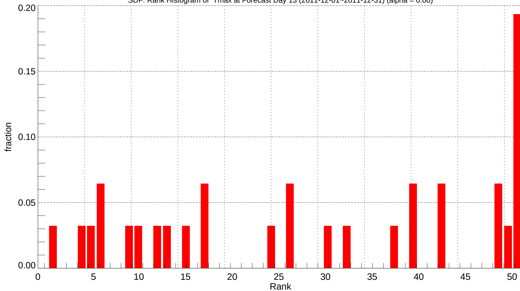
SDF: Rank Histogram of Tmax at Forecast Day 13 (2011-12-01~2011-12-31) (alpha = 0.00)
