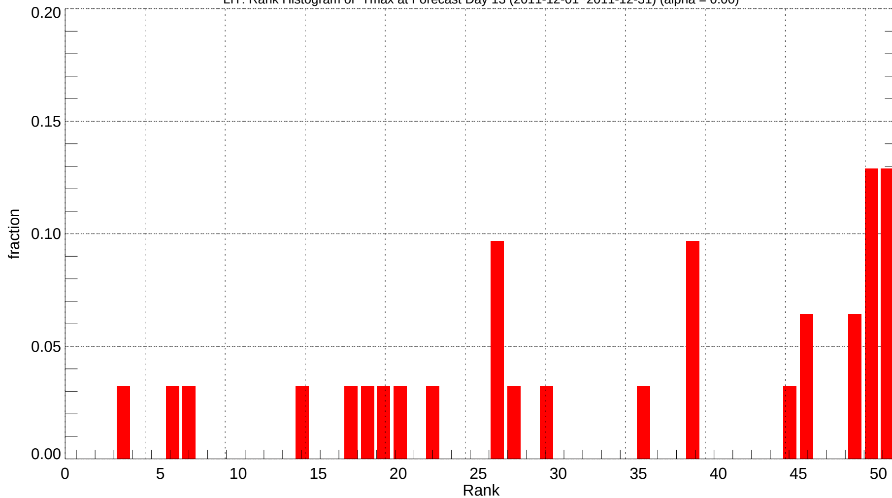
LIT: Rank Histogram of Tmax at Forecast Day 13 (2011-12-01~2011-12-31) (alpha = 0.00)
