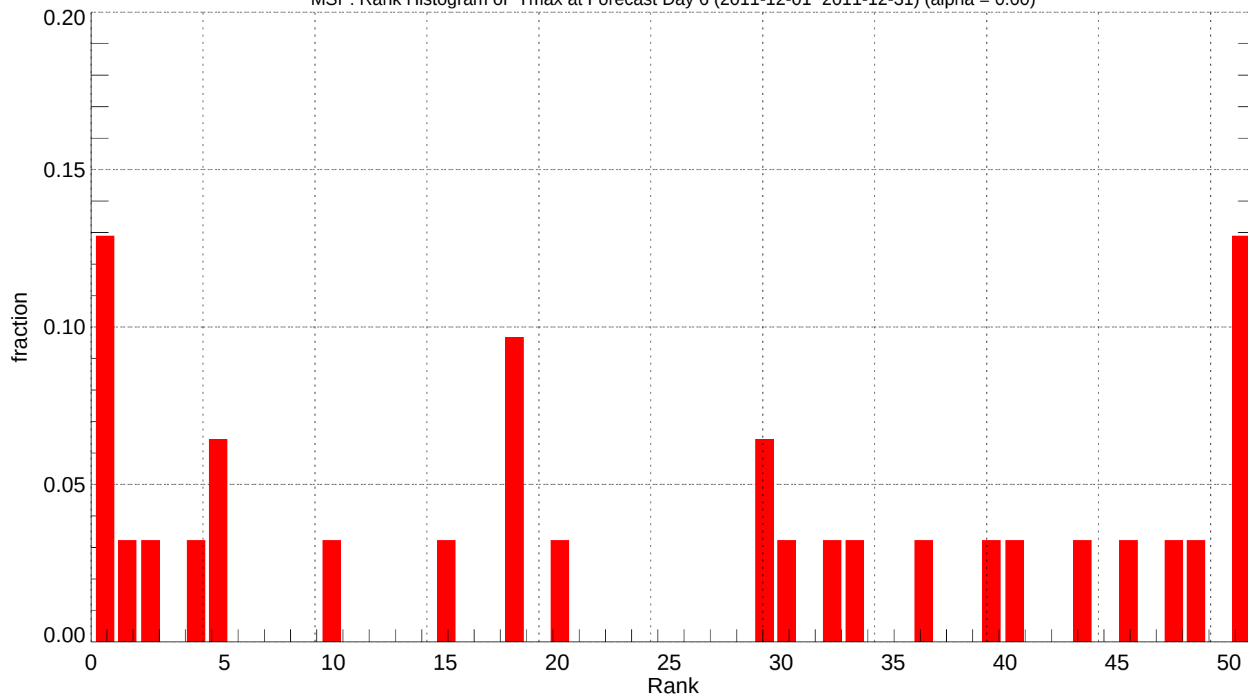
MSP: Rank Histogram of Tmax at Forecast Day 6 (2011-12-01~2011-12-31) (alpha = 0.00)
