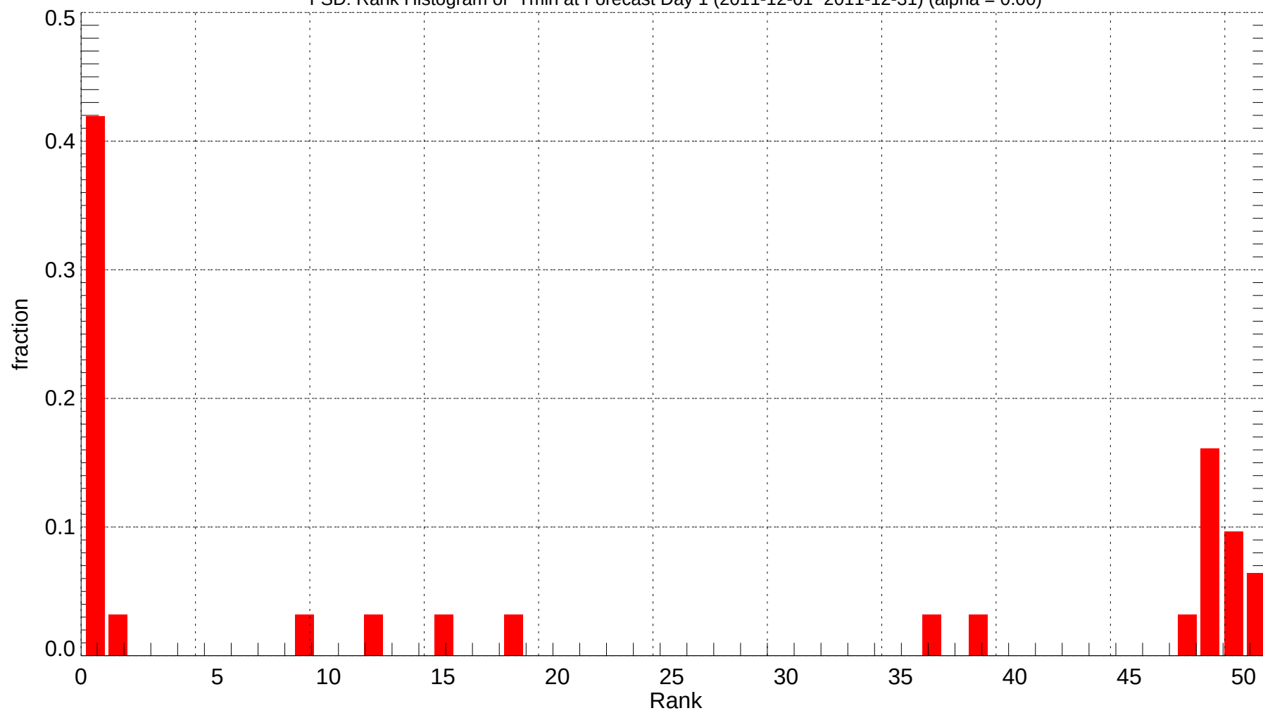
FSD: Rank Histogram of Tmin at Forecast Day 1 (2011-12-01~2011-12-31) (alpha = 0.00)
