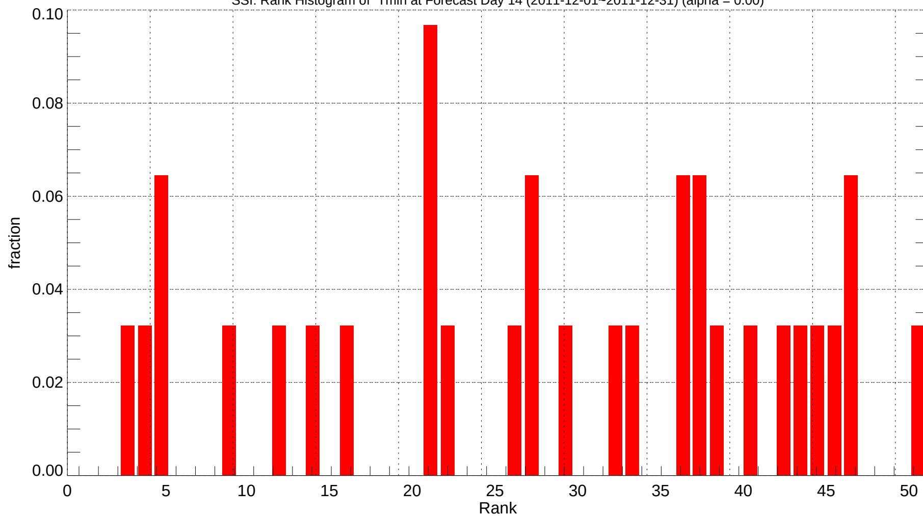
SSI: Rank Histogram of Tmin at Forecast Day 14 (2011-12-01~2011-12-31) (alpha = 0.00)
