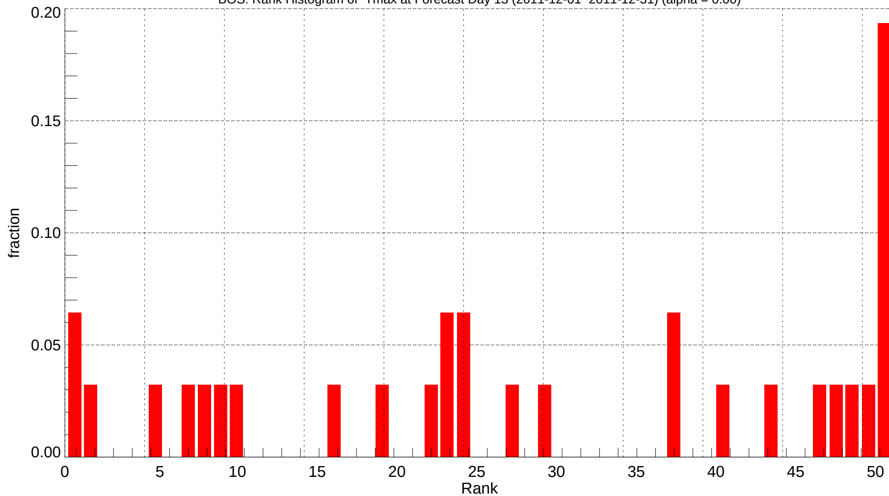
BOS: Rank Histogram of Tmax at Forecast Day 13 (2011-12-01~2011-12-31) (alpha = 0.00)
