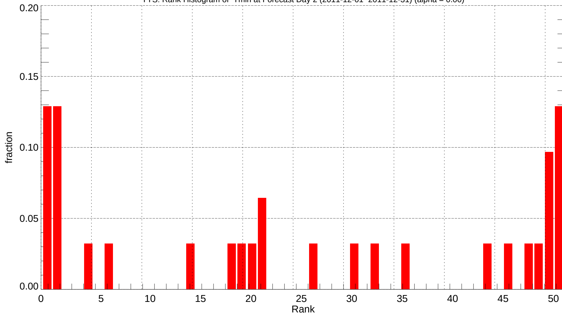
TYS: Rank Histogram of Tmin at Forecast Day 2 (2011-12-01~2011-12-31) (alpha = 0.00)
