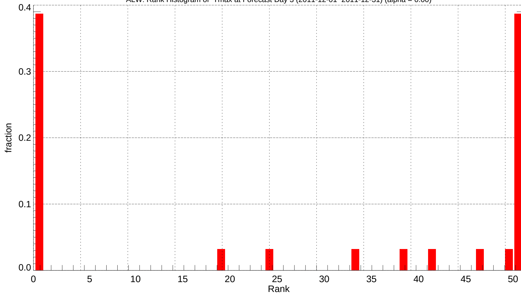
ALW: Rank Histogram of Tmax at Forecast Day 3 (2011-12-01~2011-12-31) (alpha = 0.00)
