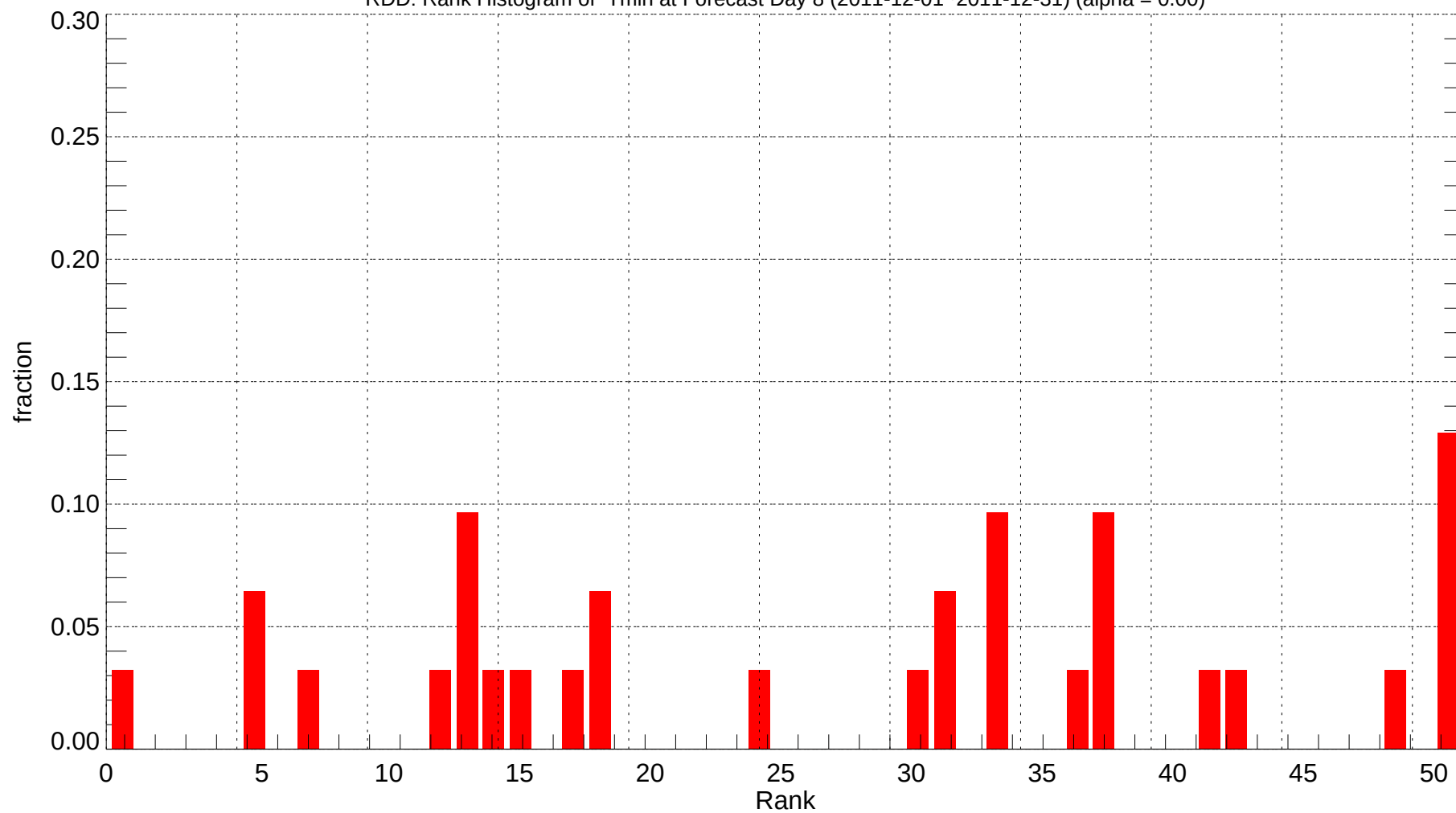
RDD: Rank Histogram of Tmin at Forecast Day 8 (2011-12-01~2011-12-31) (alpha = 0.00)
