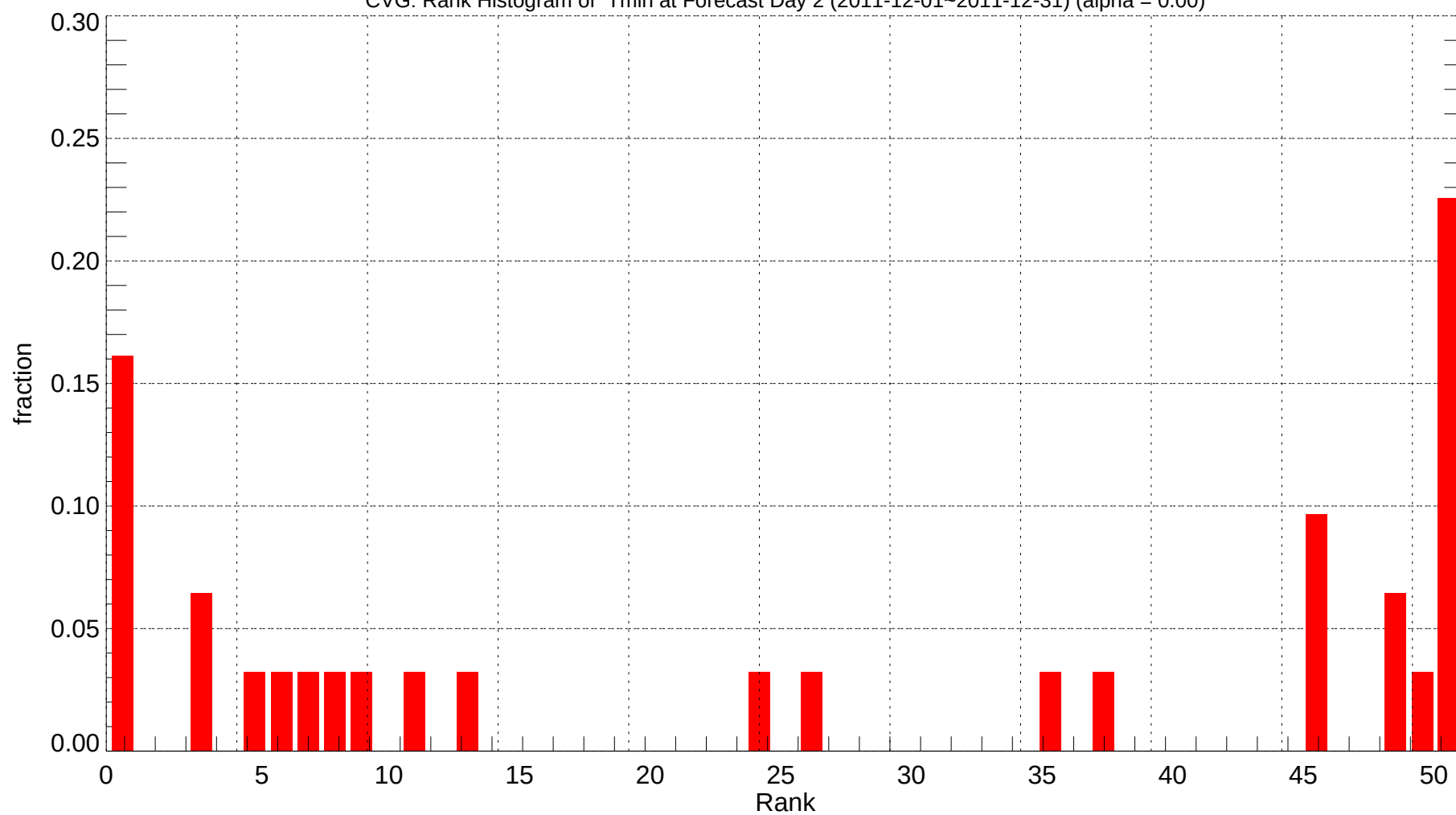
CVG: Rank Histogram of Tmin at Forecast Day 2 (2011-12-01~2011-12-31) (alpha = 0.00)
