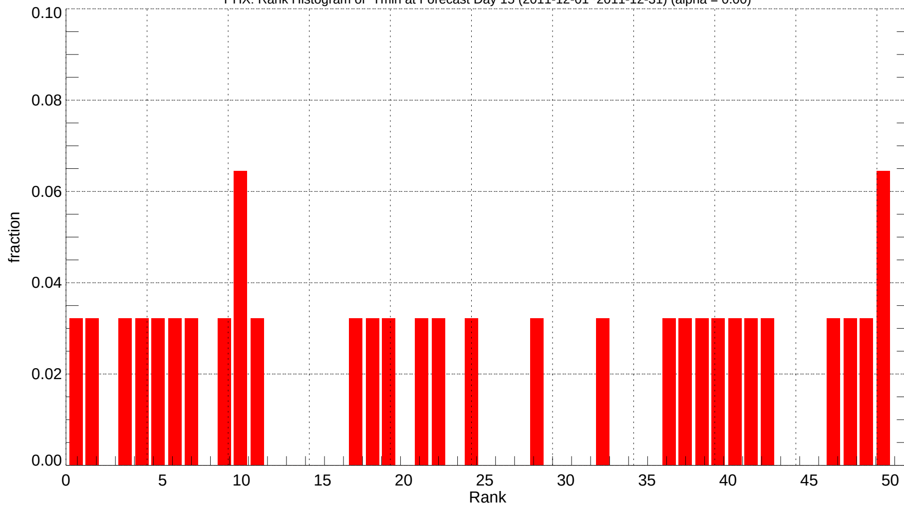
PHX: Rank Histogram of Tmin at Forecast Day 15 (2011-12-01~2011-12-31) (alpha = 0.00)
