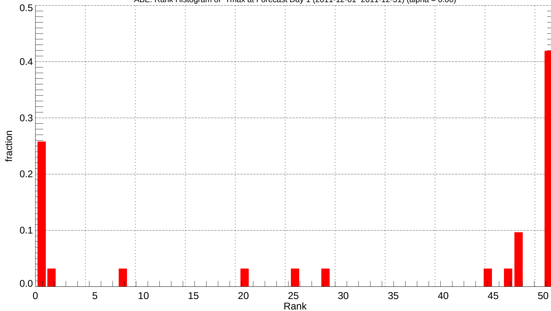
ABE: Rank Histogram of Tmax at Forecast Day 1 (2011-12-01~2011-12-31) (alpha = 0.00)
