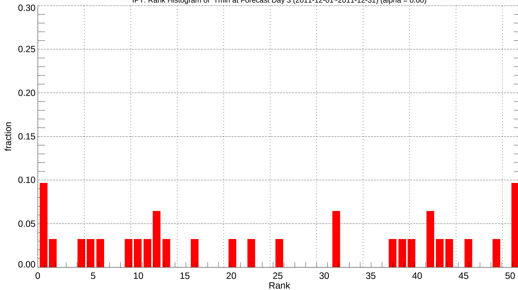
IPT: Rank Histogram of Tmin at Forecast Day 3 (2011-12-01~2011-12-31) (alpha = 0.00)
