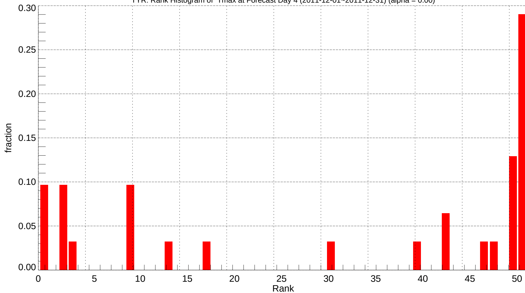
TYR: Rank Histogram of Tmax at Forecast Day 4 (2011-12-01~2011-12-31) (alpha = 0.00)
