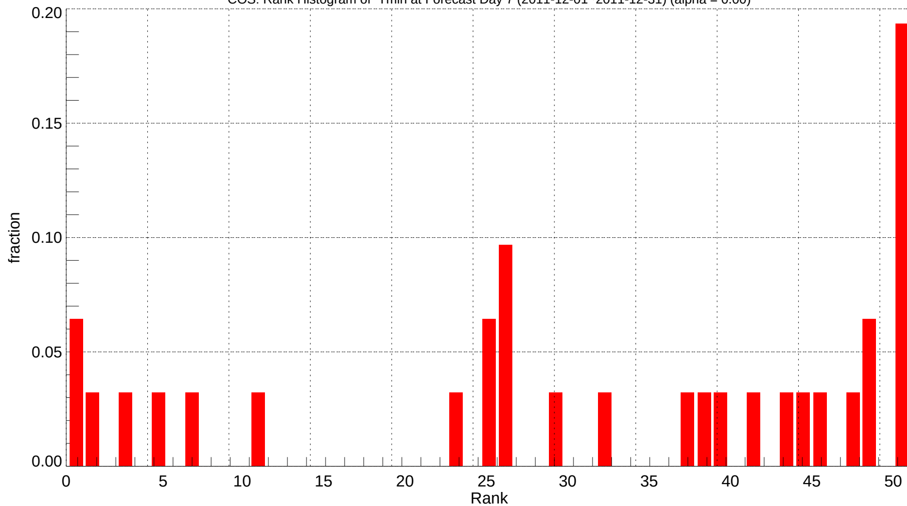
COS: Rank Histogram of Tmin at Forecast Day 7 (2011-12-01~2011-12-31) (alpha = 0.00)
