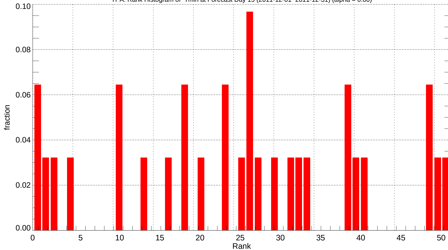
TPA: Rank Histogram of Tmin at Forecast Day 15 (2011-12-01~2011-12-31) (alpha = 0.00)
