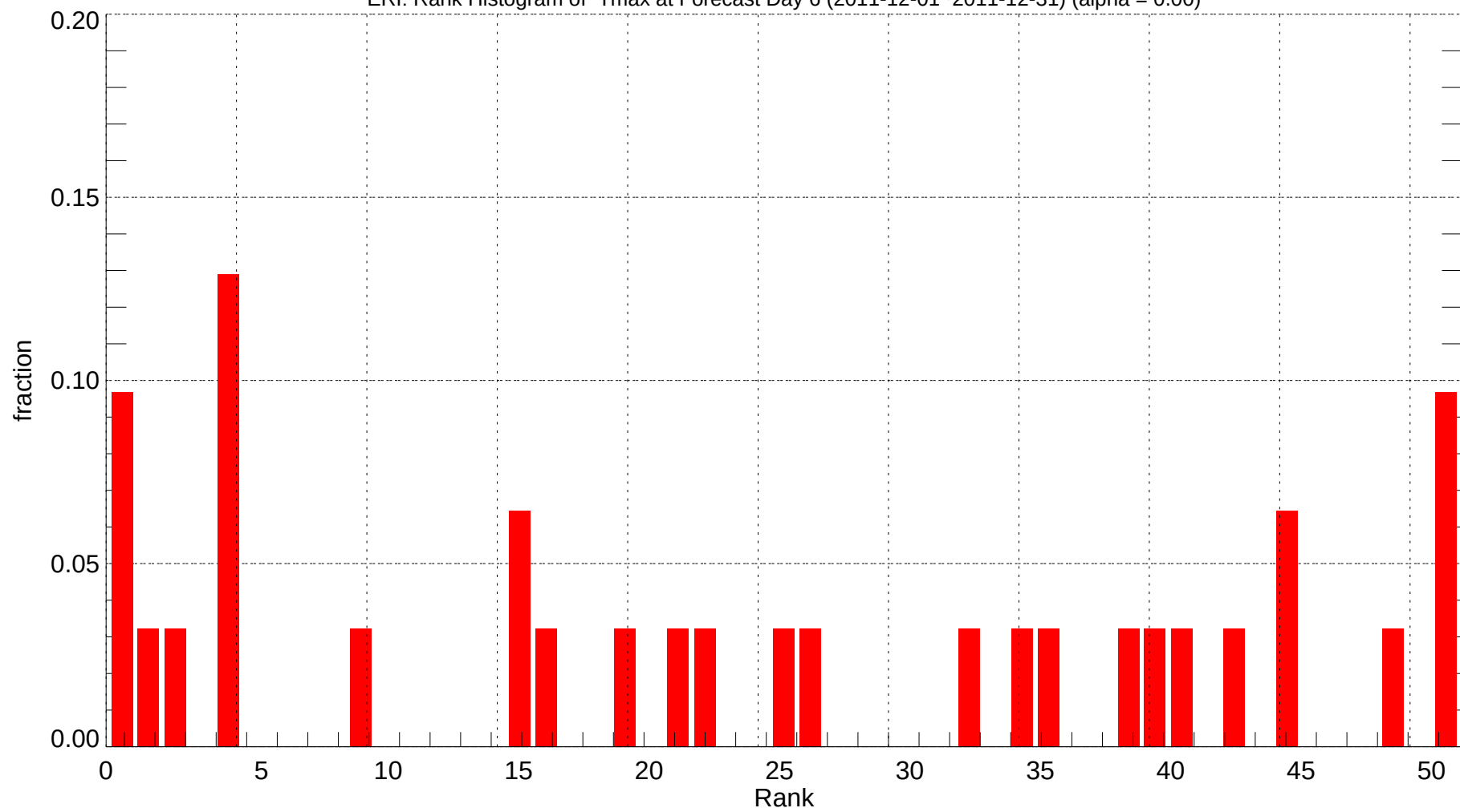
ERI: Rank Histogram of Tmax at Forecast Day 6 (2011-12-01~2011-12-31) (alpha = 0.00)
