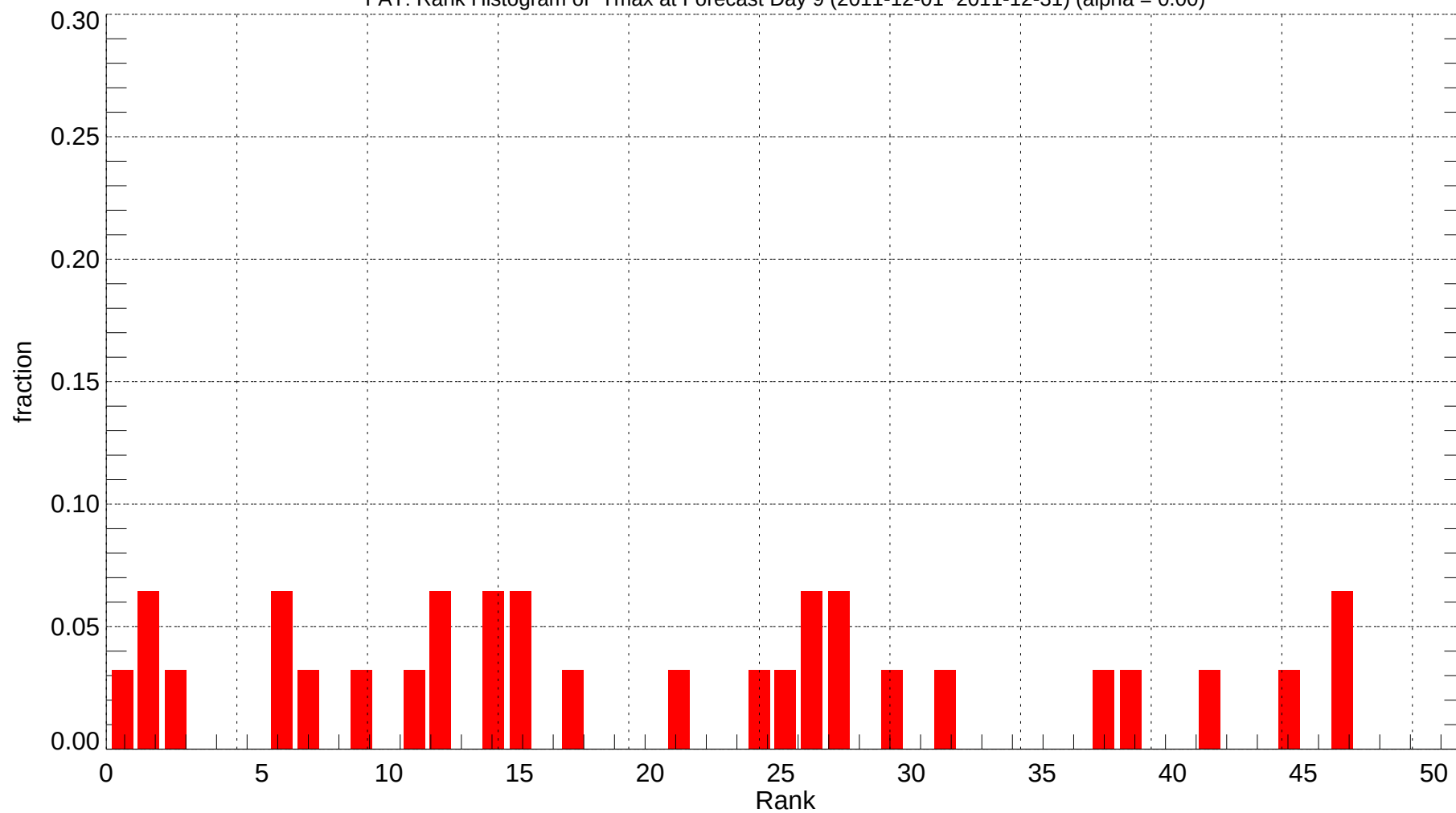
FAT: Rank Histogram of Tmax at Forecast Day 9 (2011-12-01~2011-12-31) (alpha = 0.00)
