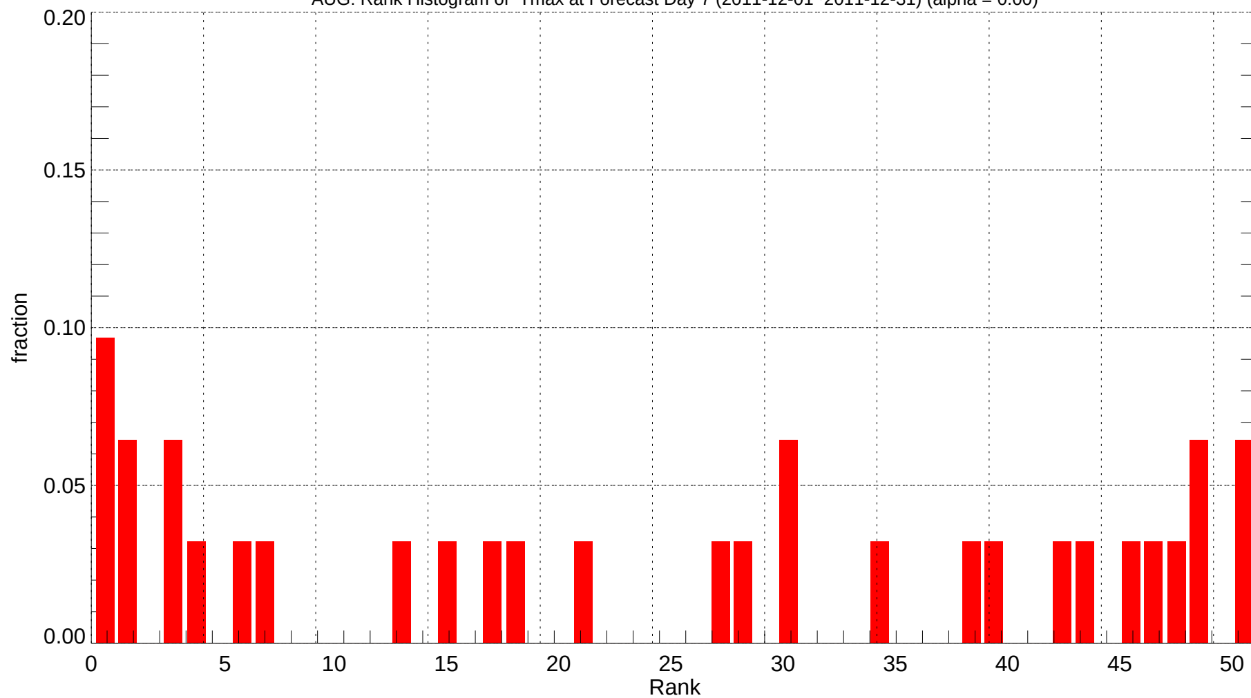
AUG: Rank Histogram of Tmax at Forecast Day 7 (2011-12-01~2011-12-31) (alpha = 0.00)
