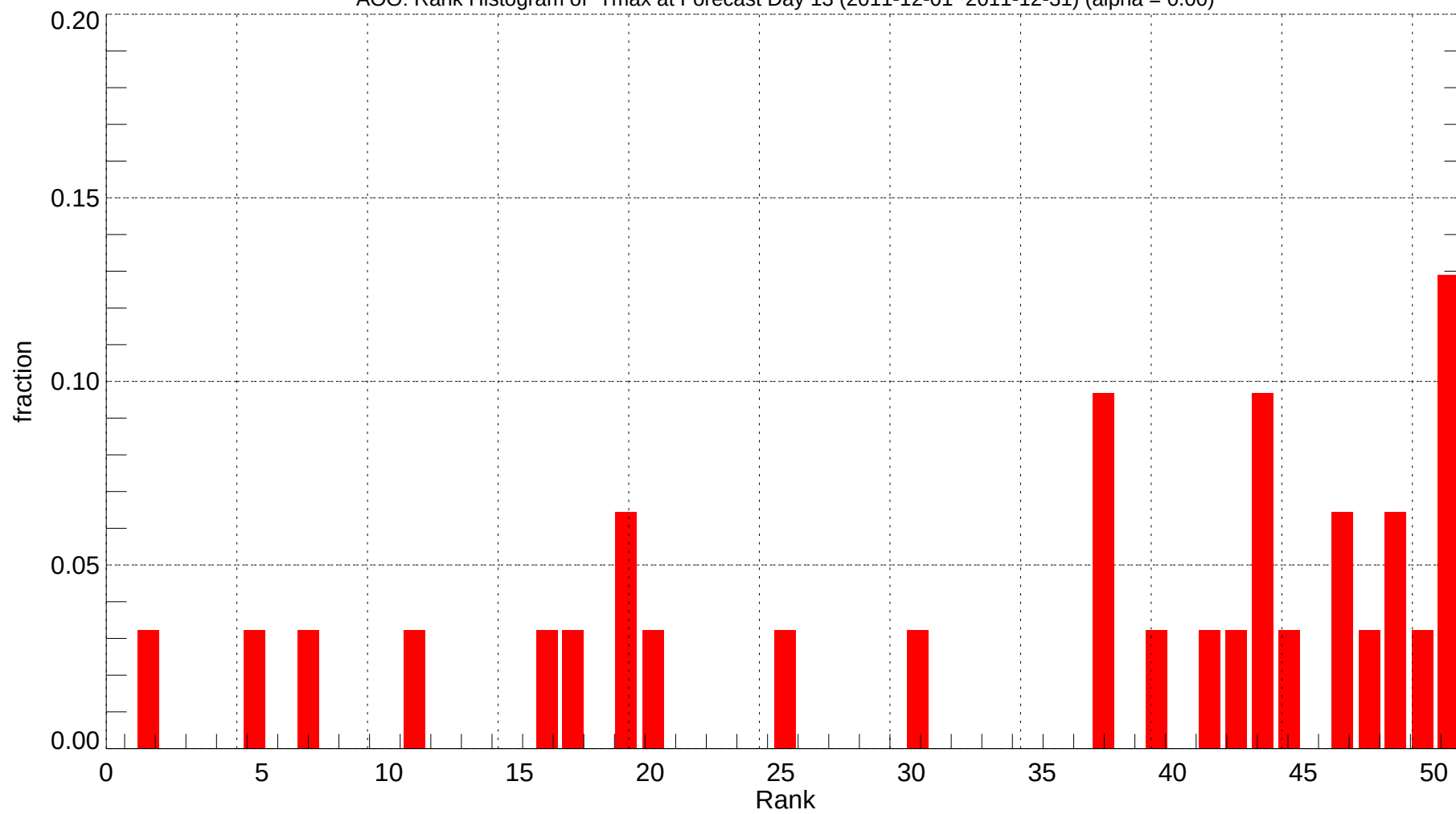
AOO: Rank Histogram of Tmax at Forecast Day 13 (2011-12-01~2011-12-31) (alpha = 0.00)
