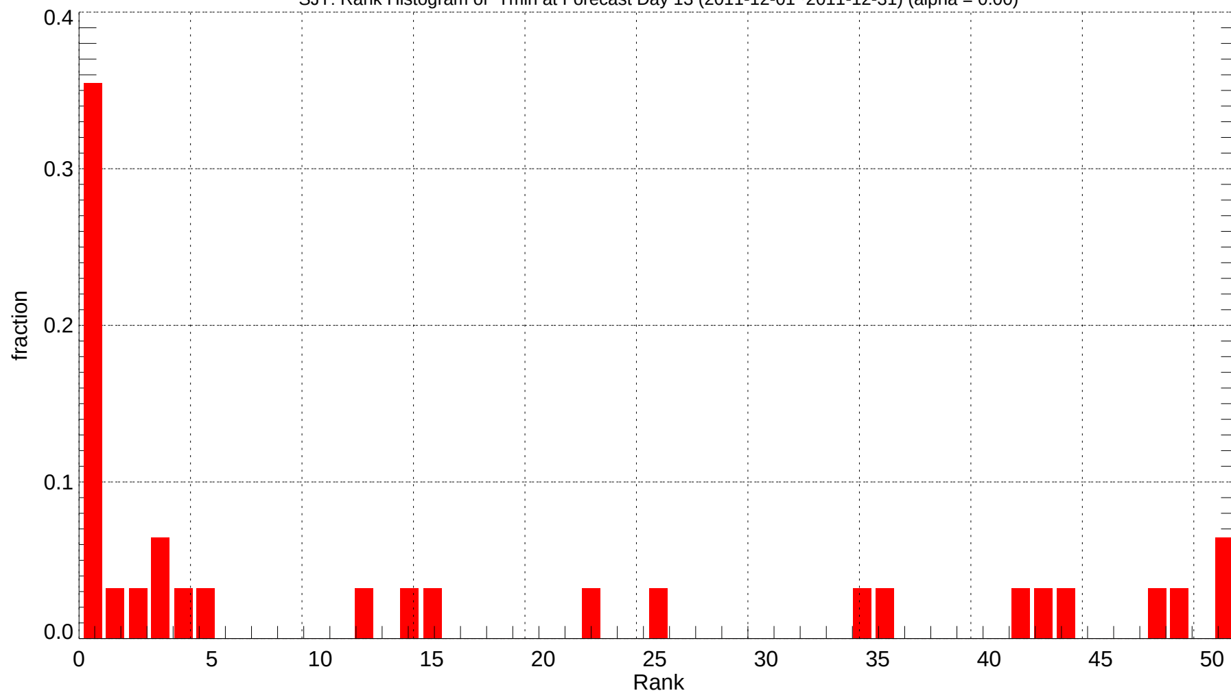
SJT: Rank Histogram of Tmin at Forecast Day 13 (2011-12-01~2011-12-31) (alpha = 0.00)
