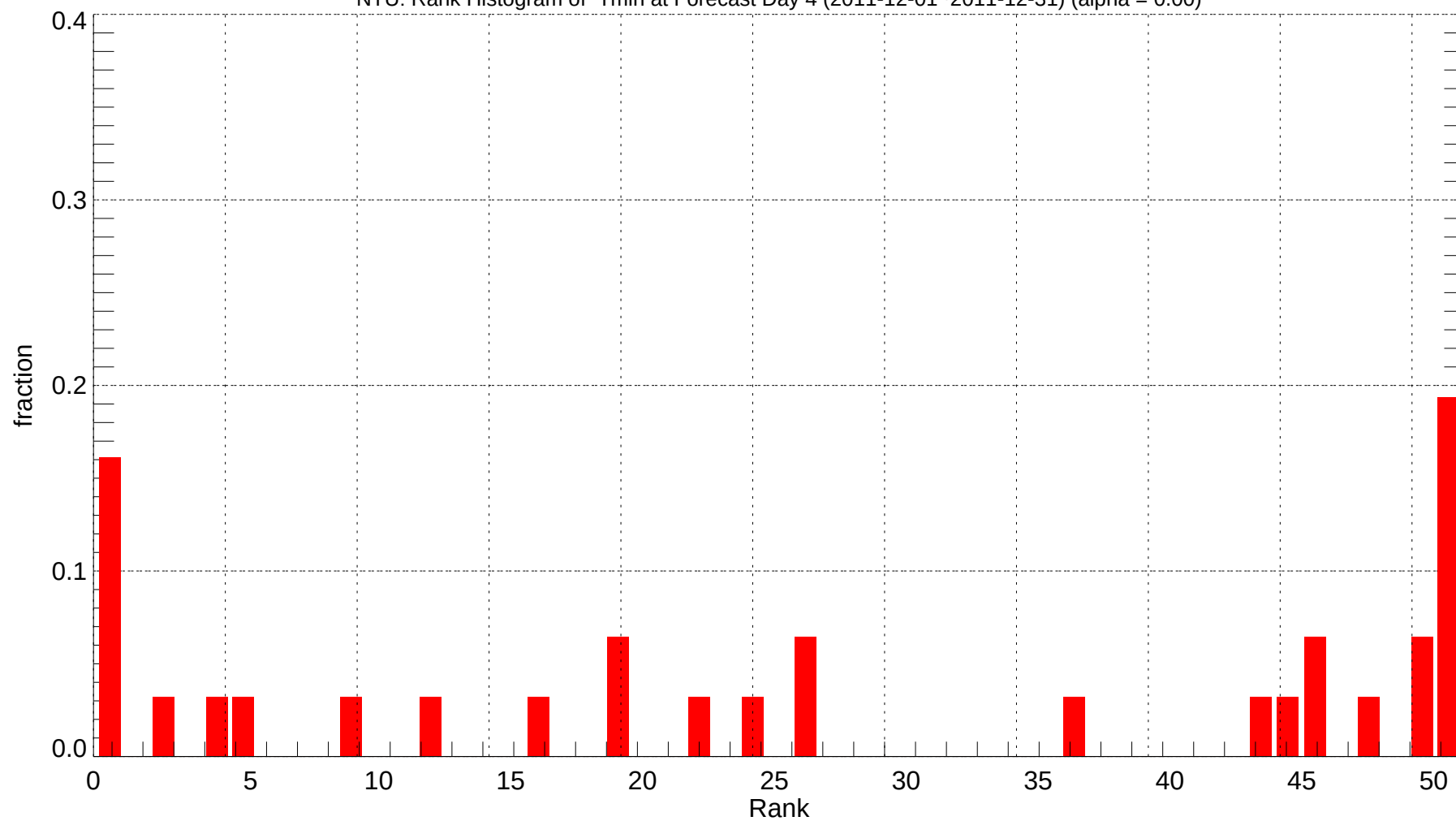
NTU: Rank Histogram of Tmin at Forecast Day 4 (2011-12-01~2011-12-31) (alpha = 0.00)
