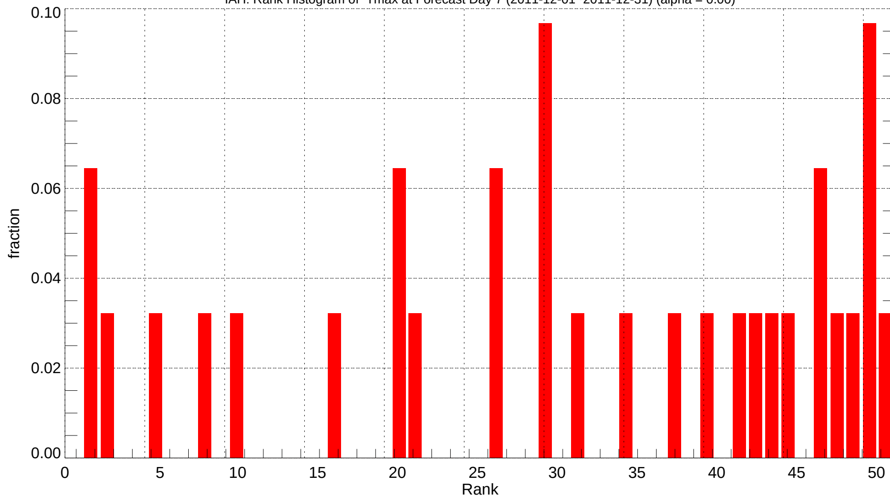
IAH: Rank Histogram of Tmax at Forecast Day 7 (2011-12-01~2011-12-31) (alpha = 0.00)
