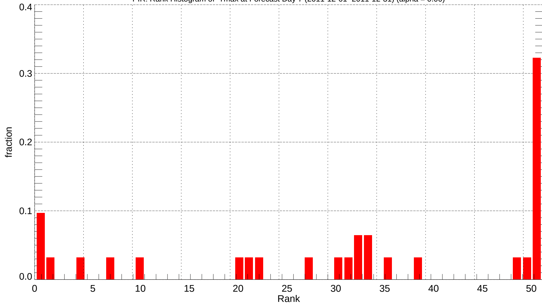
PIR: Rank Histogram of Tmax at Forecast Day 7 (2011-12-01~2011-12-31) (alpha = 0.00)
