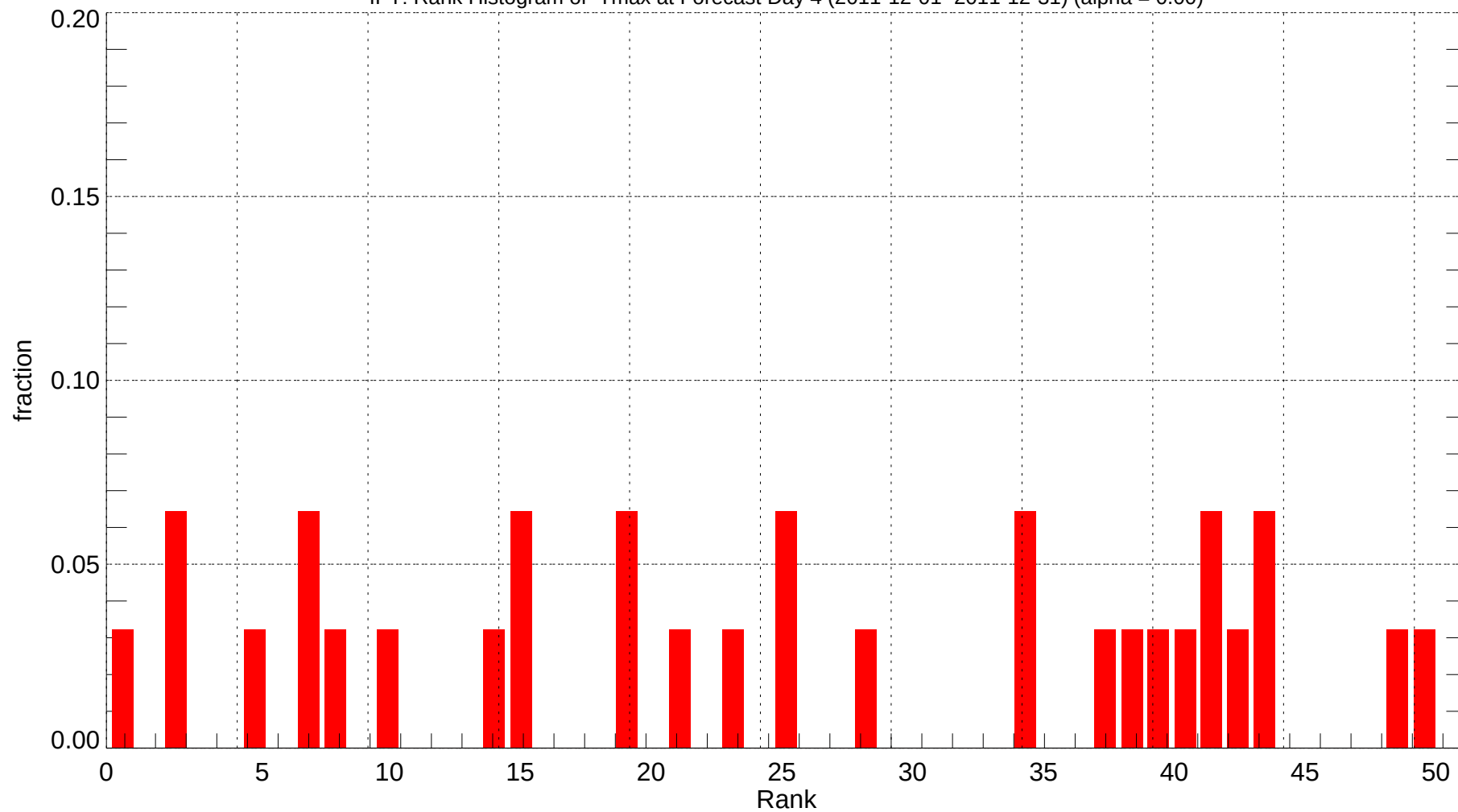
IPT: Rank Histogram of Tmax at Forecast Day 4 (2011-12-01~2011-12-31) (alpha = 0.00)
