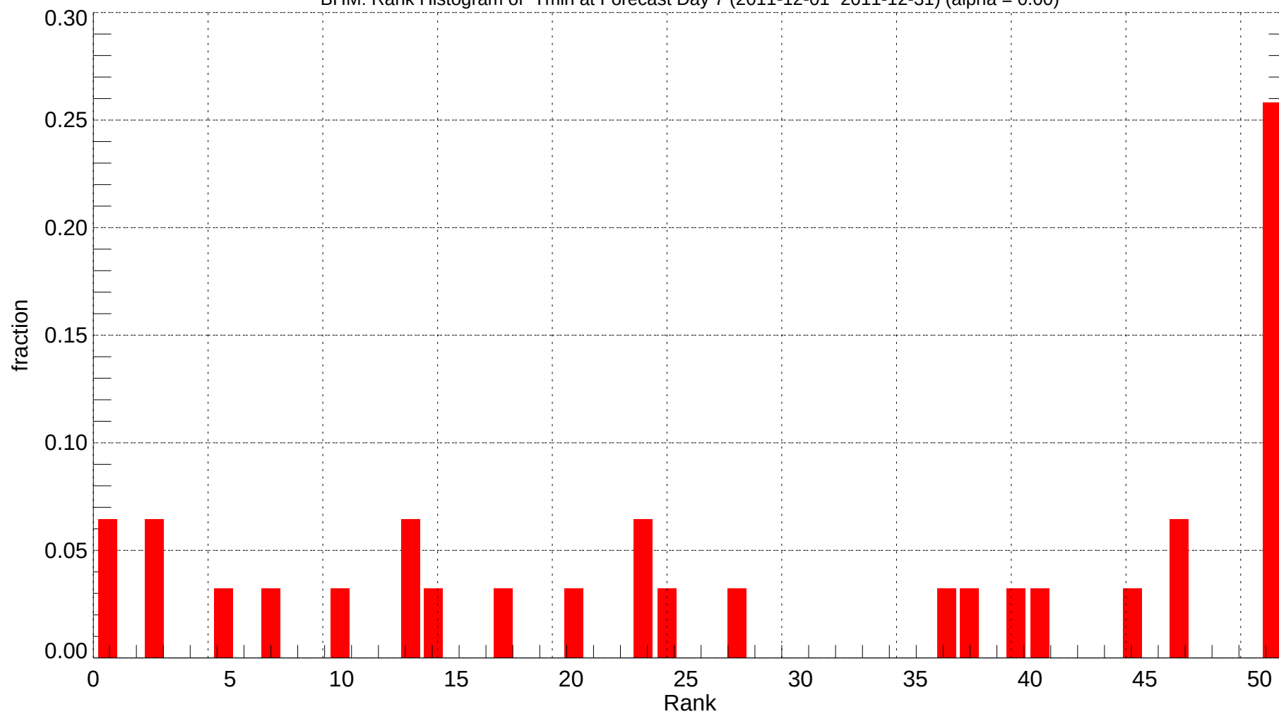
BHM: Rank Histogram of Tmin at Forecast Day 7 (2011-12-01~2011-12-31) (alpha = 0.00)
