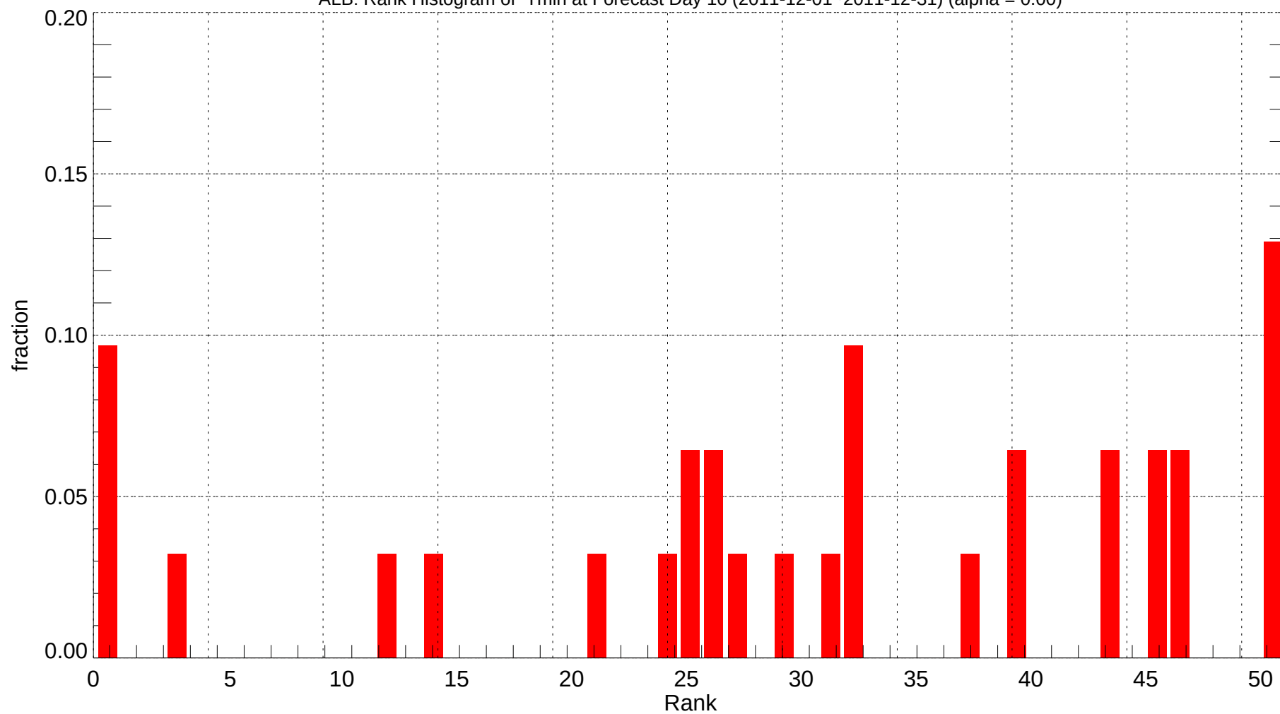
ALB: Rank Histogram of Tmin at Forecast Day 10 (2011-12-01~2011-12-31) (alpha = 0.00)
