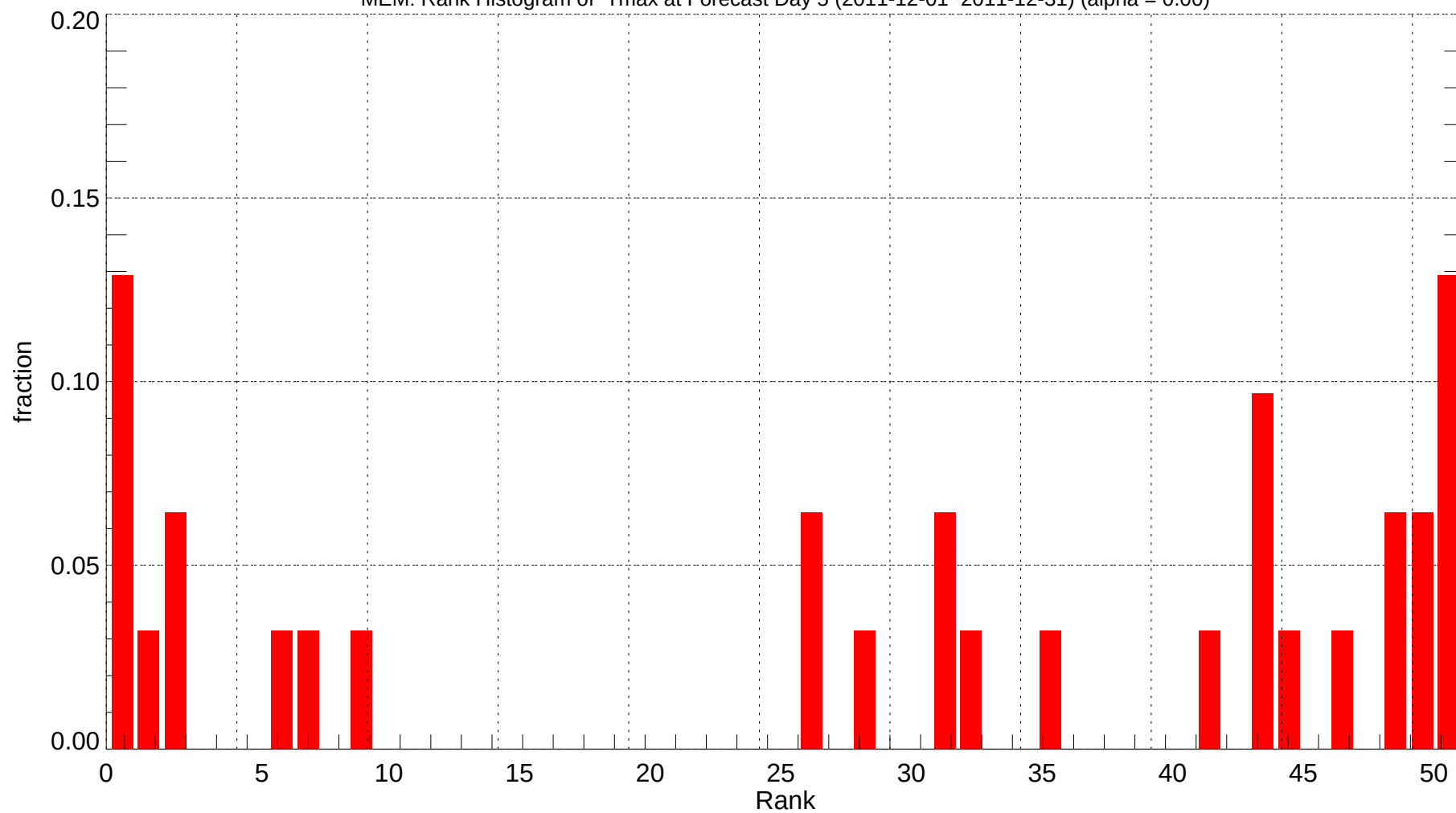
MEM: Rank Histogram of Tmax at Forecast Day 5 (2011-12-01~2011-12-31) (alpha = 0.00)
