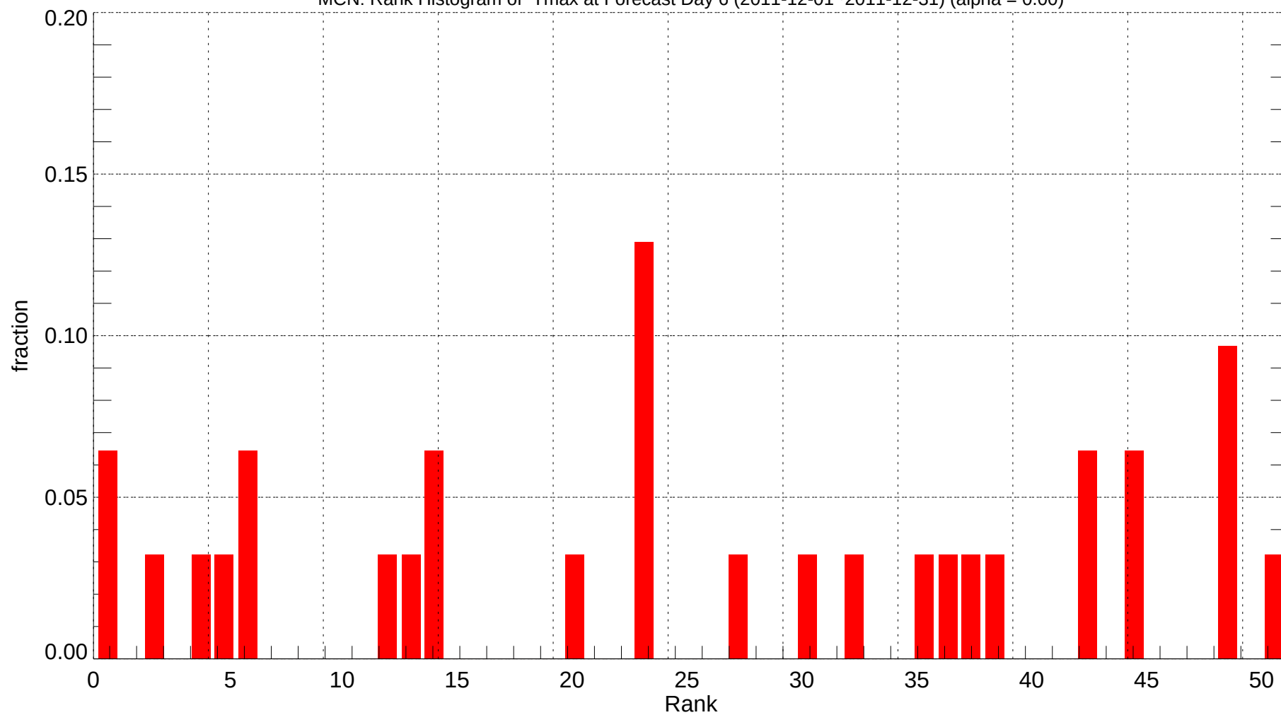
MCN: Rank Histogram of Tmax at Forecast Day 6 (2011-12-01~2011-12-31) (alpha = 0.00)
