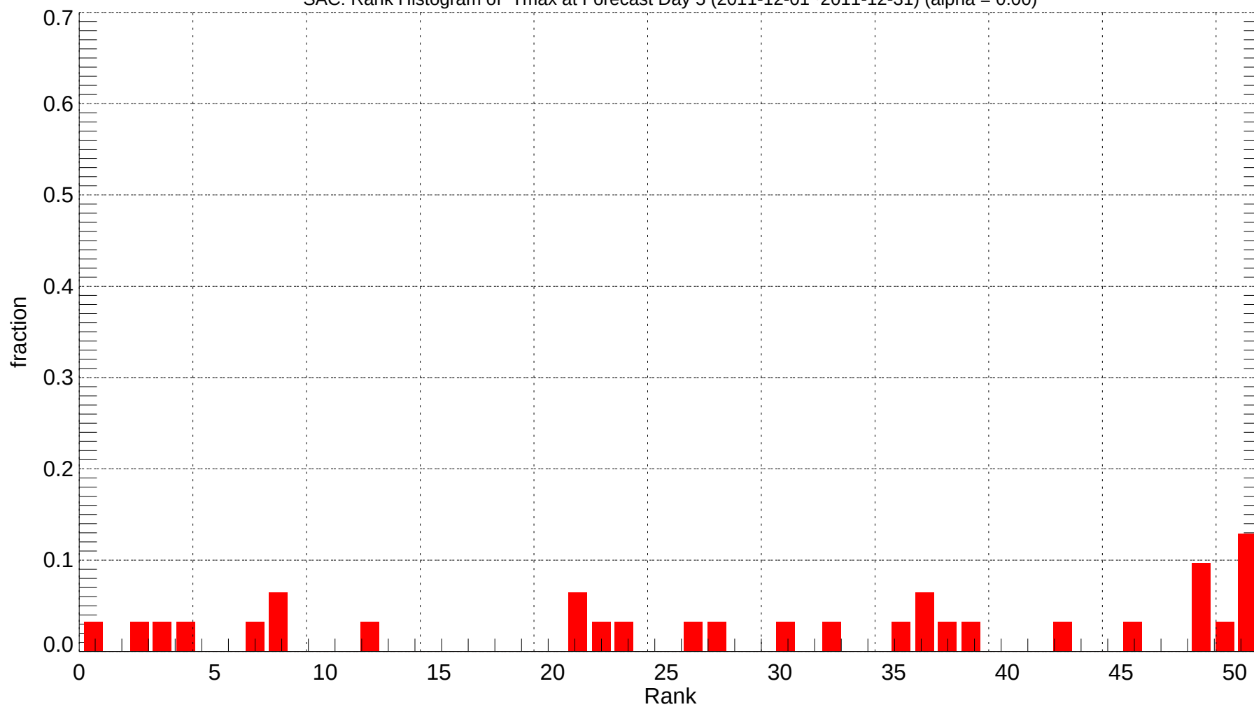
SAC: Rank Histogram of Tmax at Forecast Day 5 (2011-12-01~2011-12-31) (alpha = 0.00)
