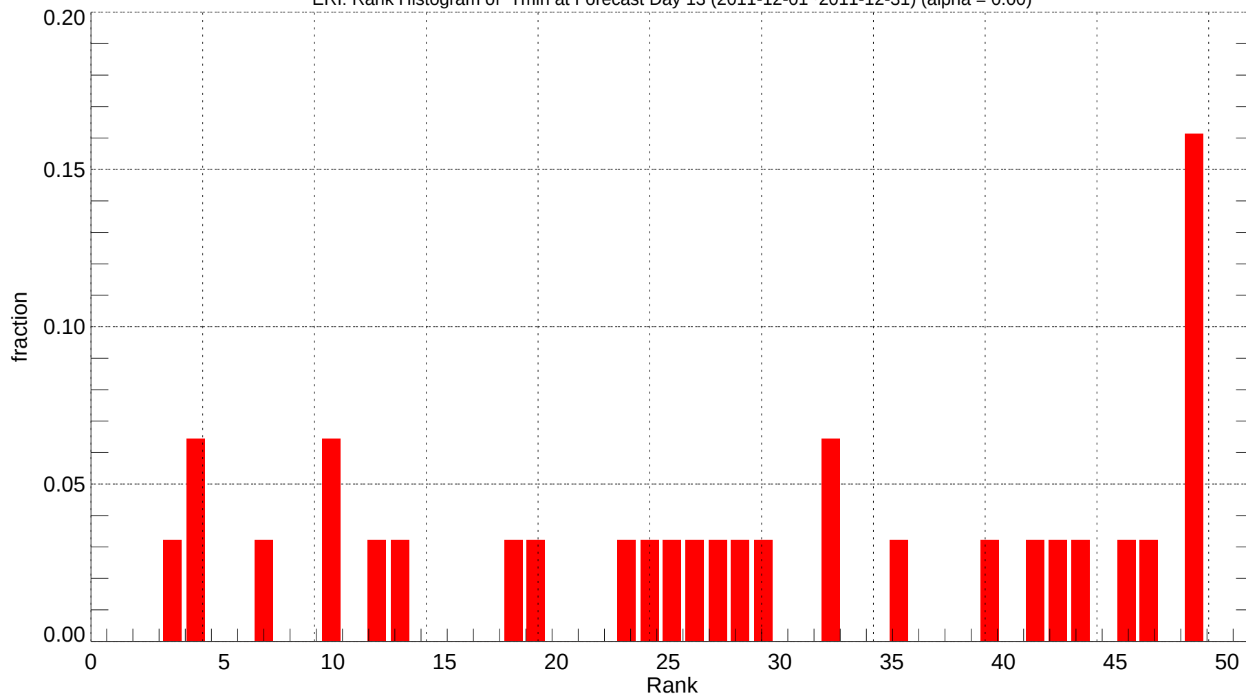
ERI: Rank Histogram of Tmin at Forecast Day 13 (2011-12-01~2011-12-31) (alpha = 0.00)
