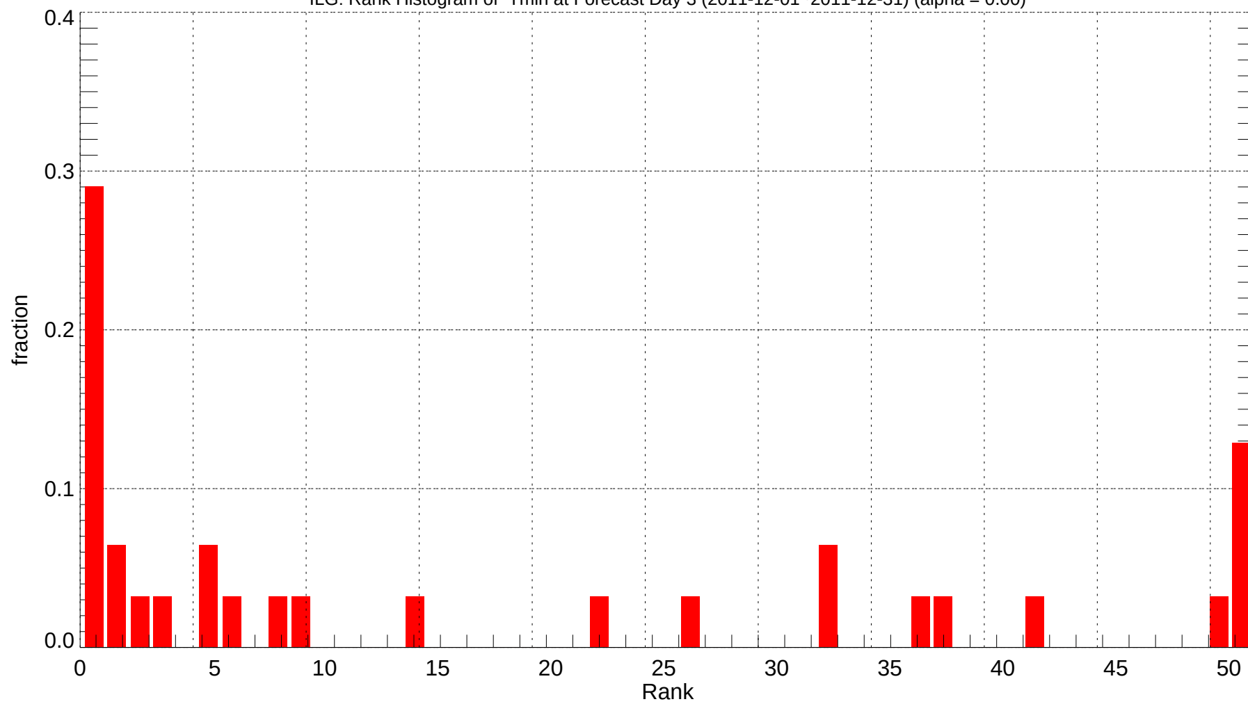
ILG: Rank Histogram of Tmin at Forecast Day 3 (2011-12-01~2011-12-31) (alpha = 0.00)
