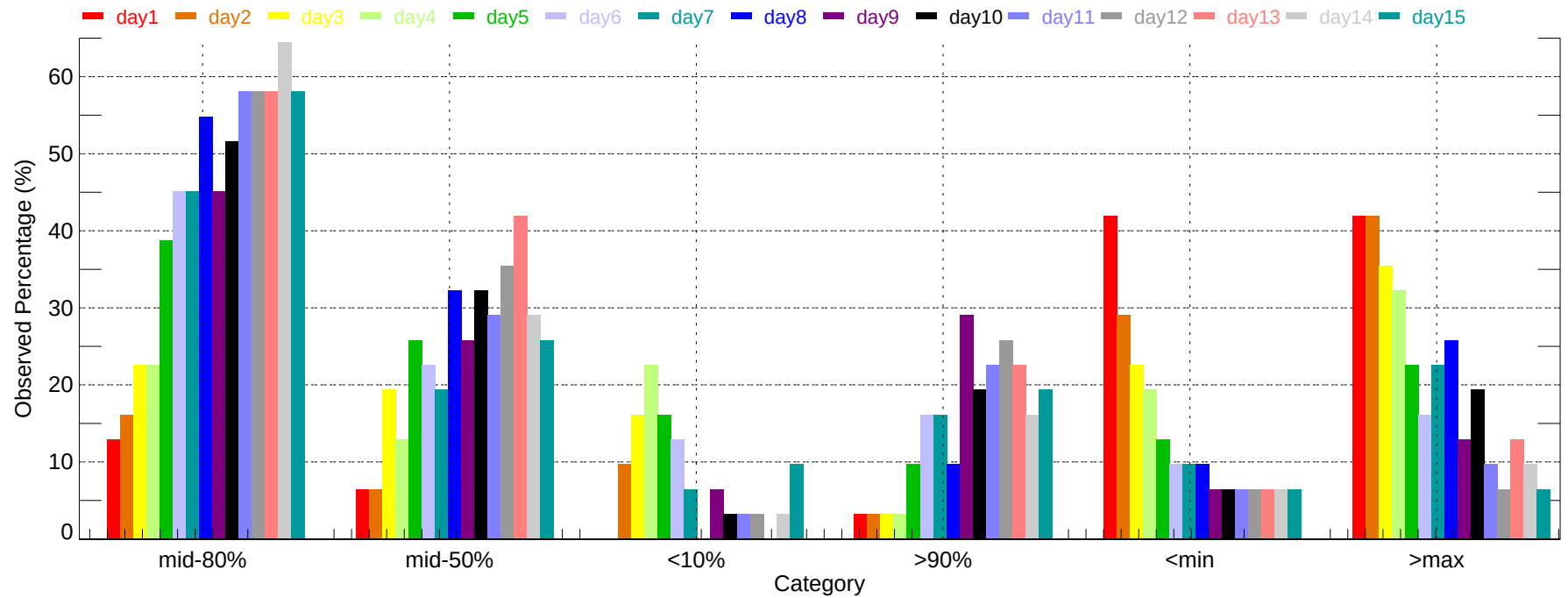
Observed Percentage of Ensembles - PIR: Min Temperature (2011-12-01~2011-12-31)
