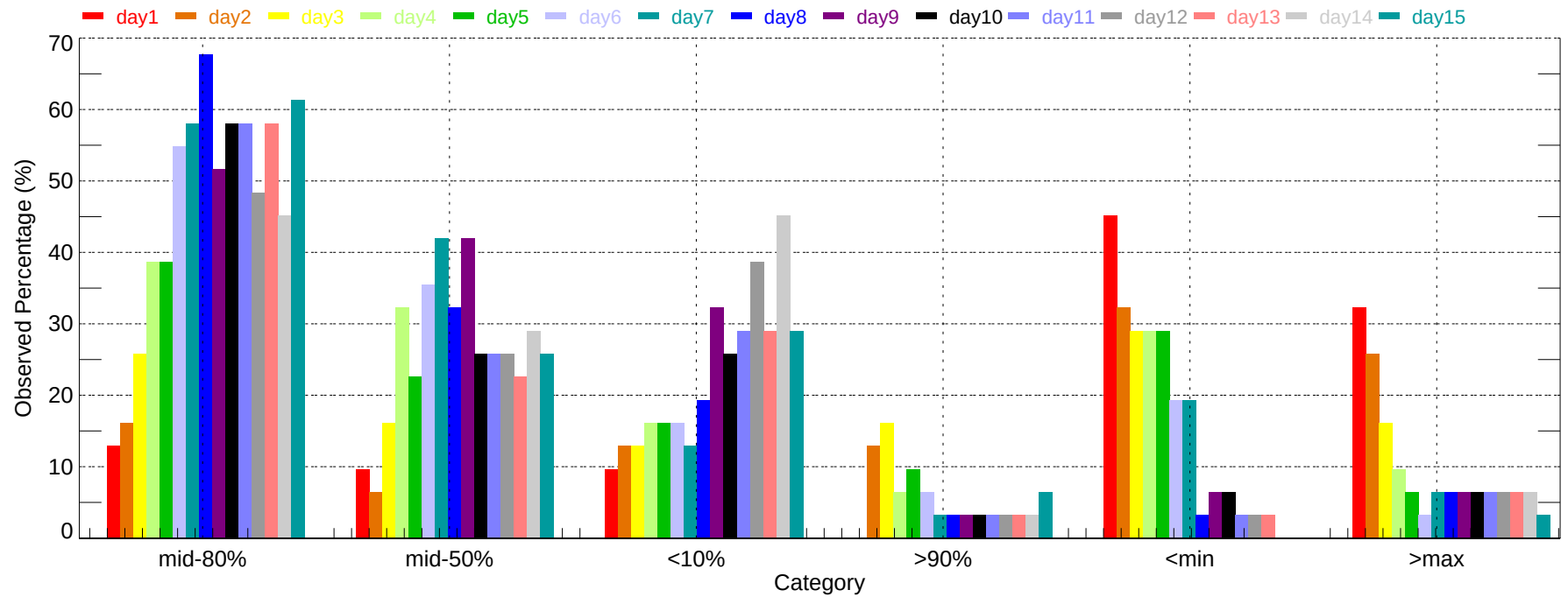
Observed Percentage of Ensembles - BOI: Min Temperature (2011-12-01~2011-12-31)
