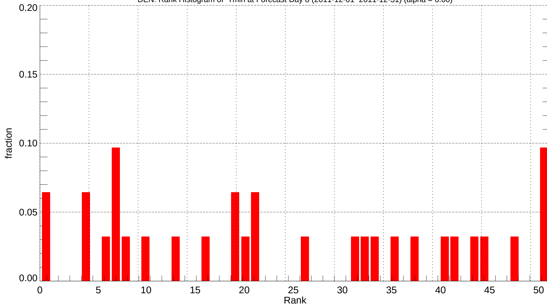
DEN: Rank Histogram of Tmin at Forecast Day 8 (2011-12-01~2011-12-31) (alpha = 0.00)
