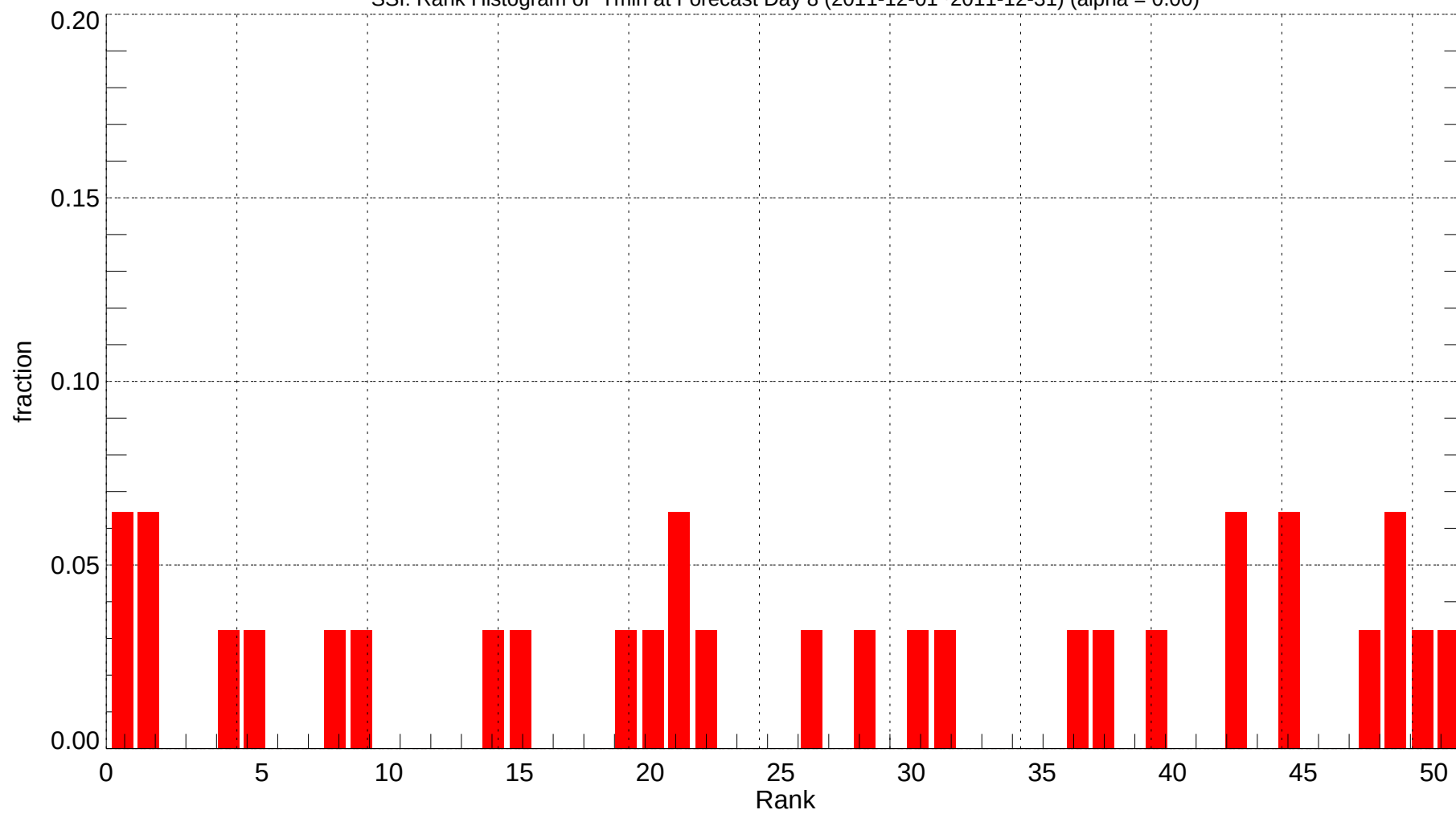
SSI: Rank Histogram of Tmin at Forecast Day 8 (2011-12-01~2011-12-31) (alpha = 0.00)
