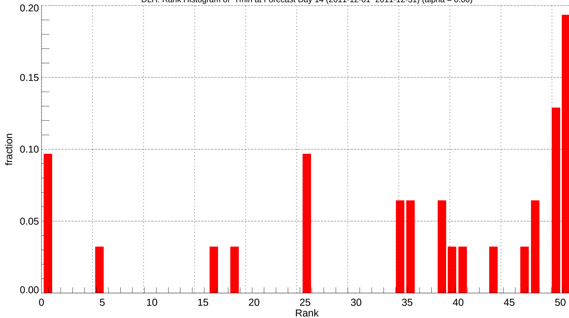
DLH: Rank Histogram of Tmin at Forecast Day 14 (2011-12-01~2011-12-31) (alpha = 0.00)
