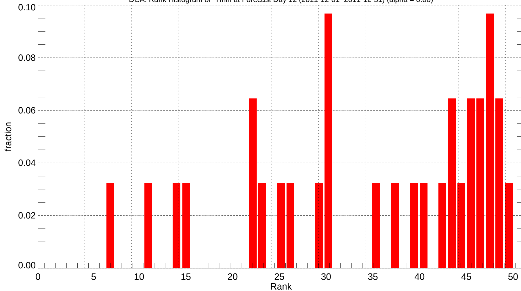
DCA: Rank Histogram of Tmin at Forecast Day 12 (2011-12-01~2011-12-31) (alpha = 0.00)
