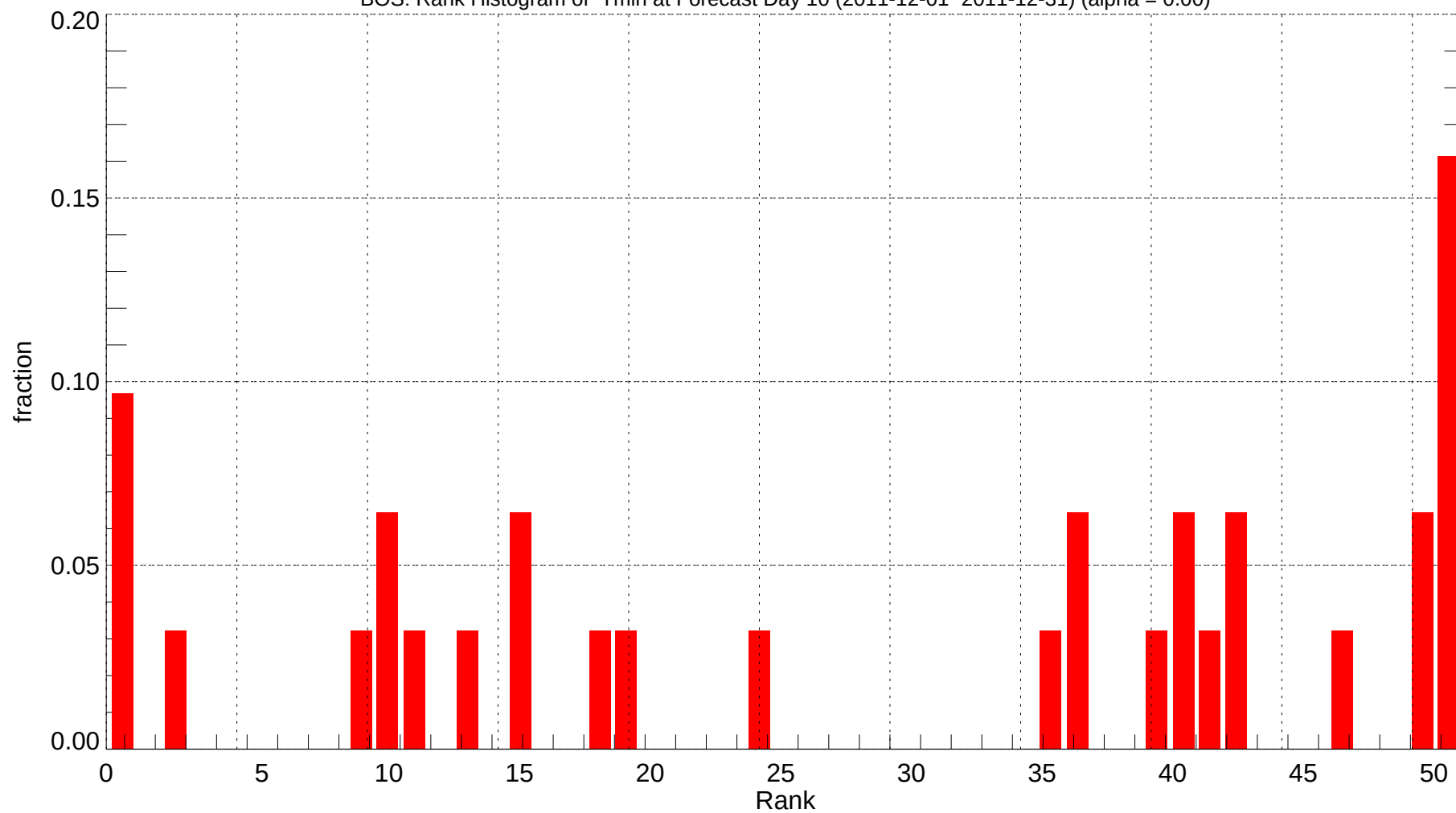
BOS: Rank Histogram of Tmin at Forecast Day 10 (2011-12-01~2011-12-31) (alpha = 0.00)
