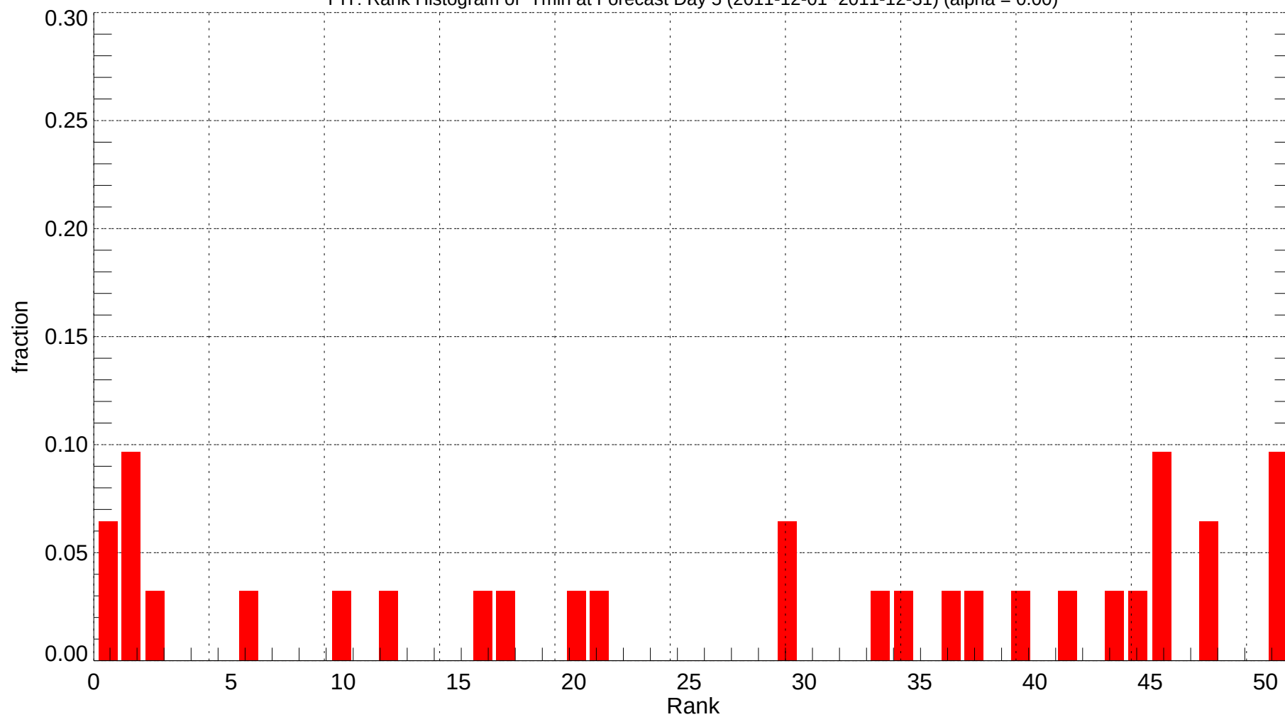
PIT: Rank Histogram of Tmin at Forecast Day 5 (2011-12-01~2011-12-31) (alpha = 0.00)
