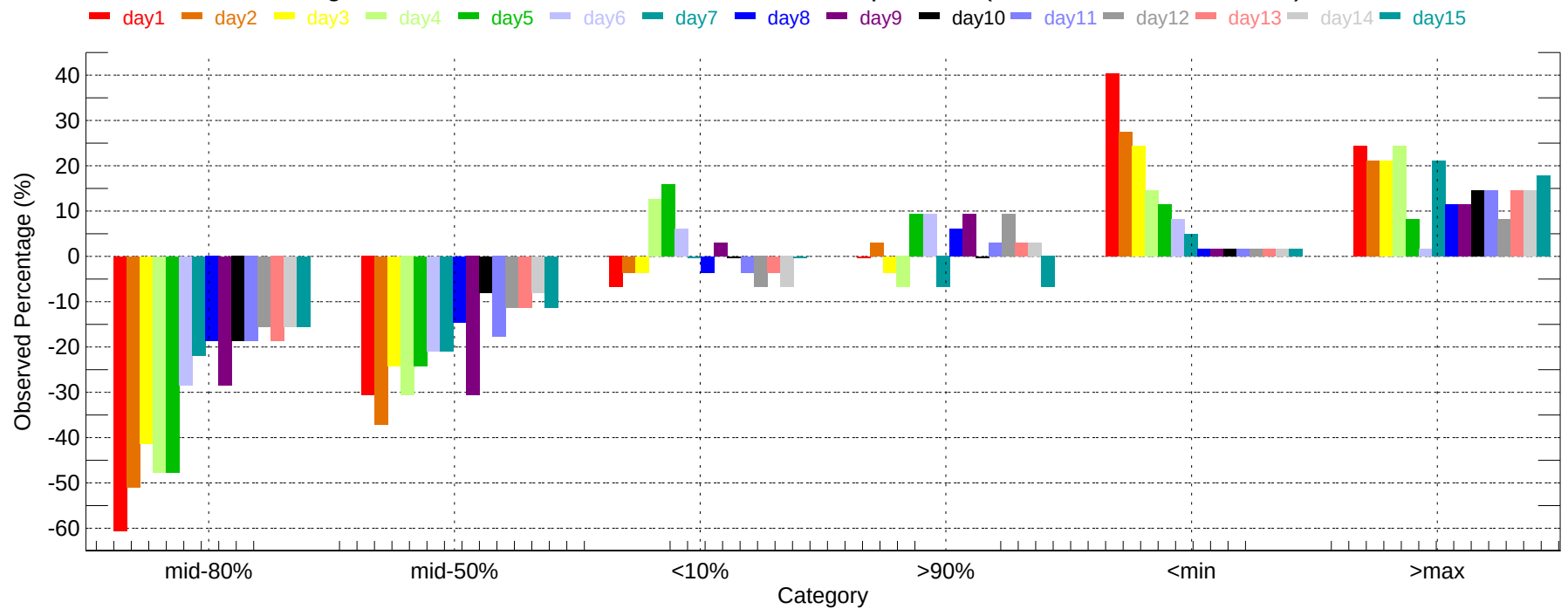
Observed Percentage Deviation of Ensembles - FSD: Max Temperature (2011-12-01~2011-12-31)
