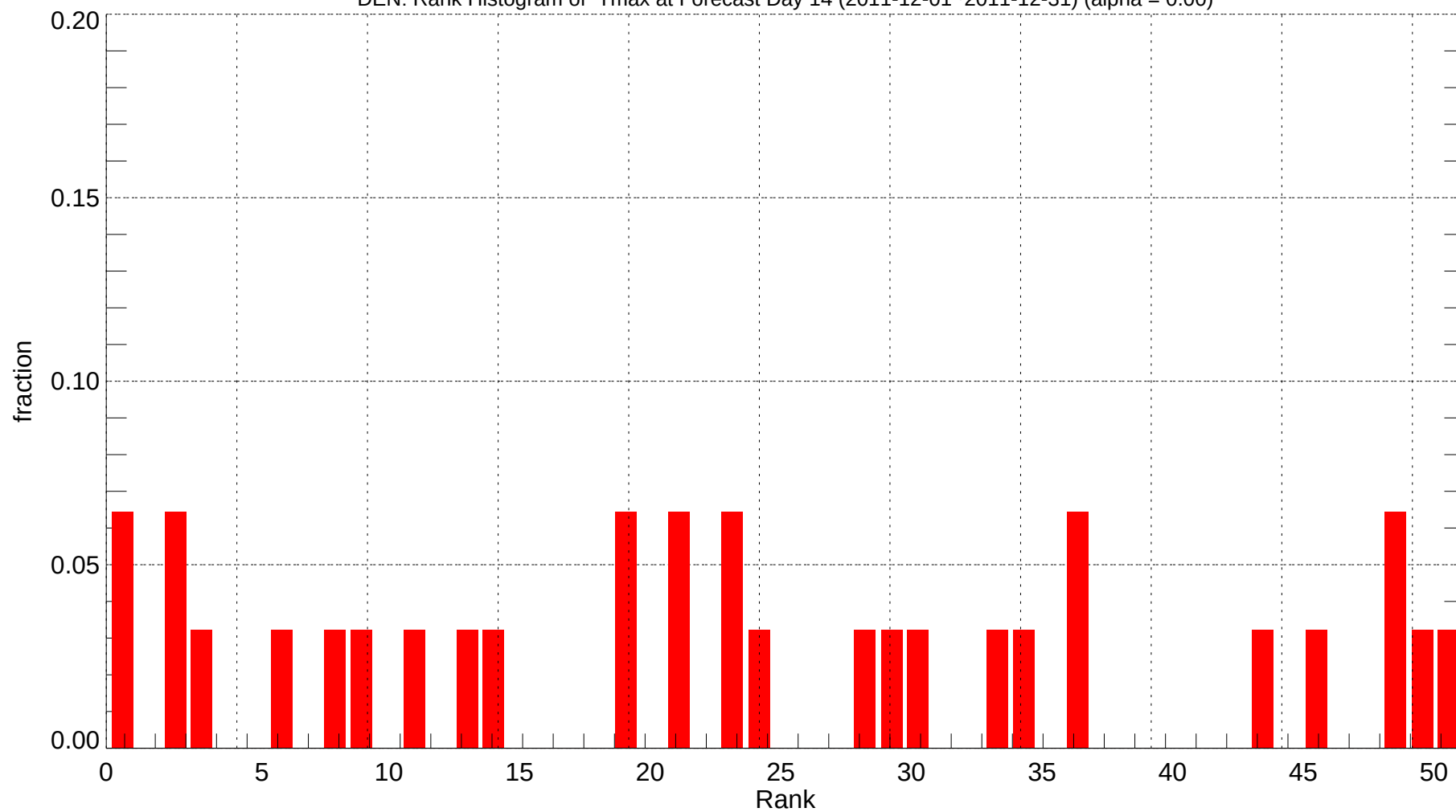
DEN: Rank Histogram of Tmax at Forecast Day 14 (2011-12-01~2011-12-31) (alpha = 0.00)
