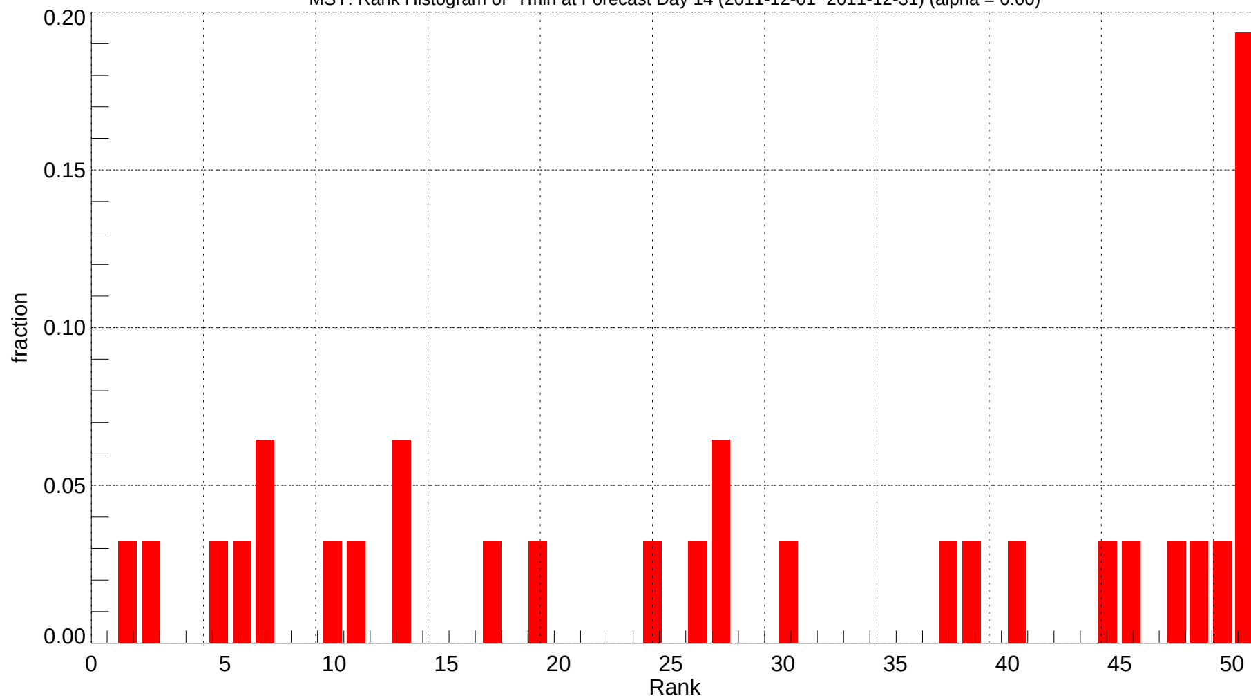
MSY: Rank Histogram of Tmin at Forecast Day 14 (2011-12-01~2011-12-31) (alpha = 0.00)
