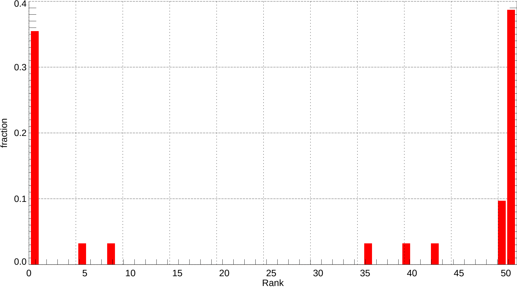
SEA: Rank Histogram of Tmin at Forecast Day 2 (2011-12-01~2011-12-31) (alpha = 0.00)
