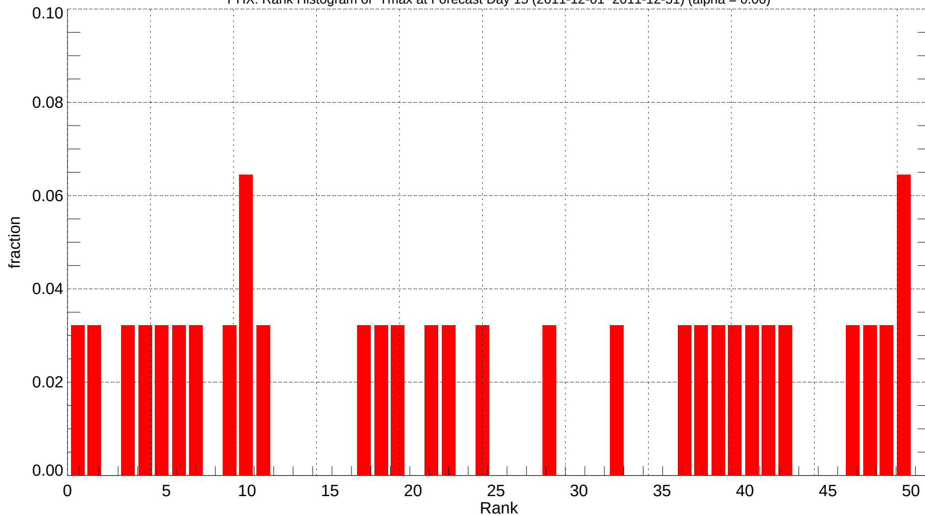
PHX: Rank Histogram of Tmax at Forecast Day 15 (2011-12-01~2011-12-31) (alpha = 0.00)
