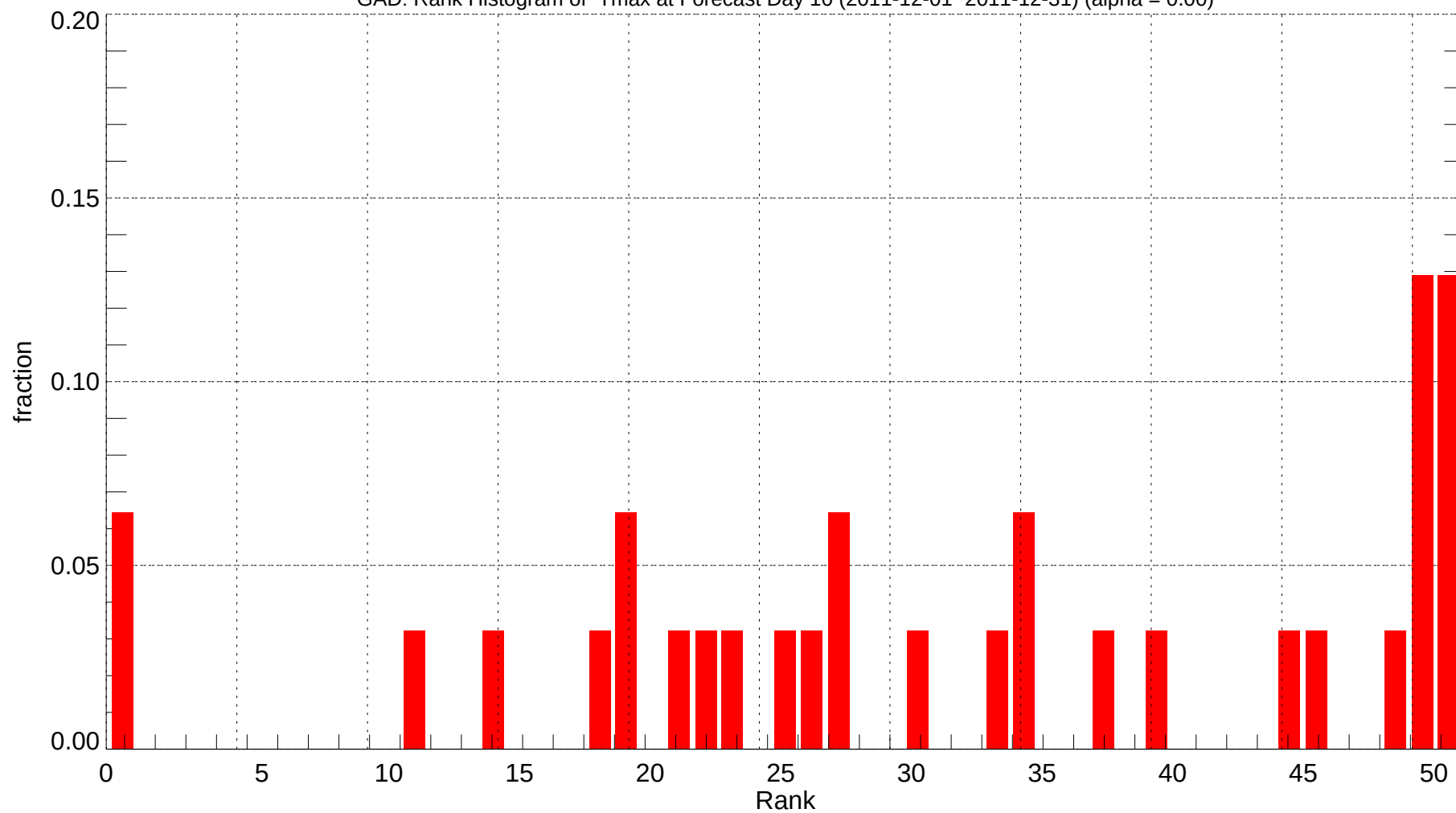
GAD: Rank Histogram of Tmax at Forecast Day 10 (2011-12-01~2011-12-31) (alpha = 0.00)
