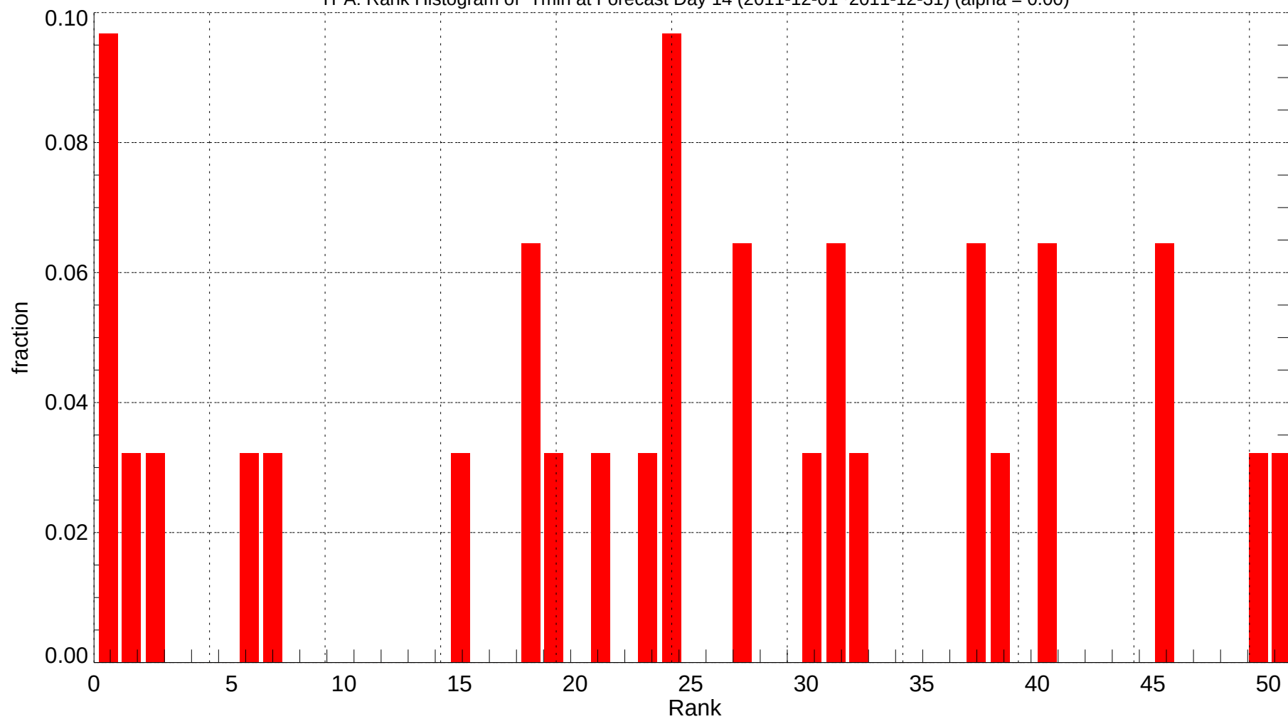
TPA: Rank Histogram of Tmin at Forecast Day 14 (2011-12-01~2011-12-31) (alpha = 0.00)
