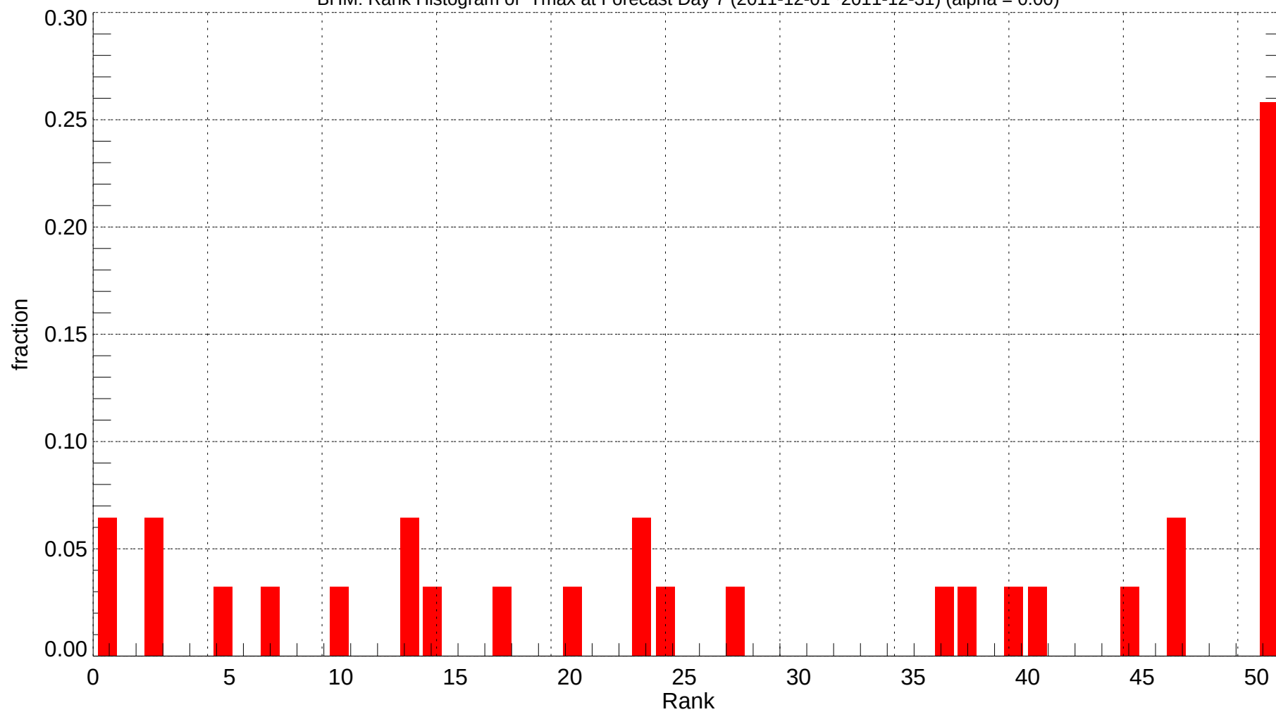
BHM: Rank Histogram of Tmax at Forecast Day 7 (2011-12-01~2011-12-31) (alpha = 0.00)
