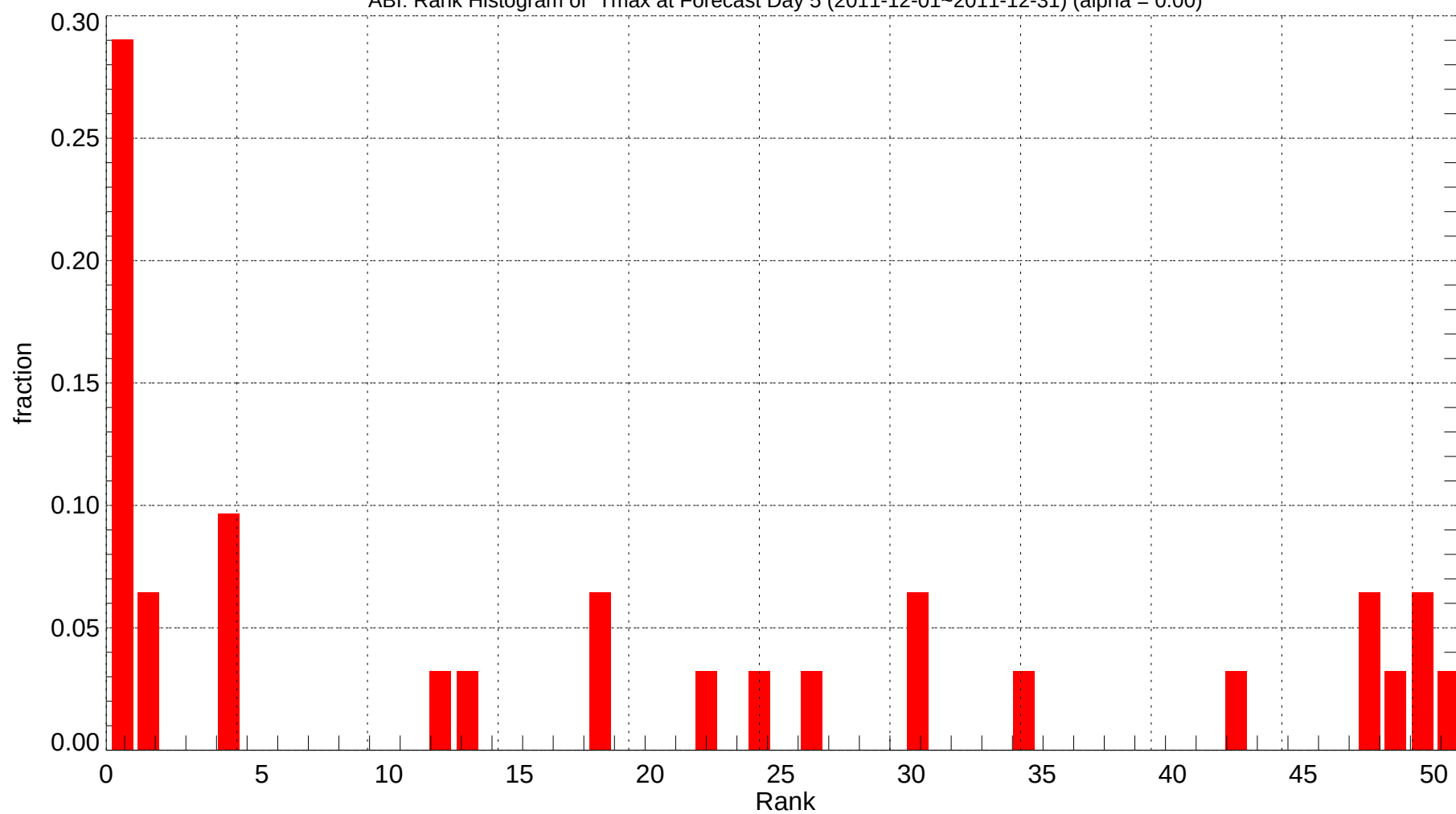
ABI: Rank Histogram of Tmax at Forecast Day 5 (2011-12-01~2011-12-31) (alpha = 0.00)
