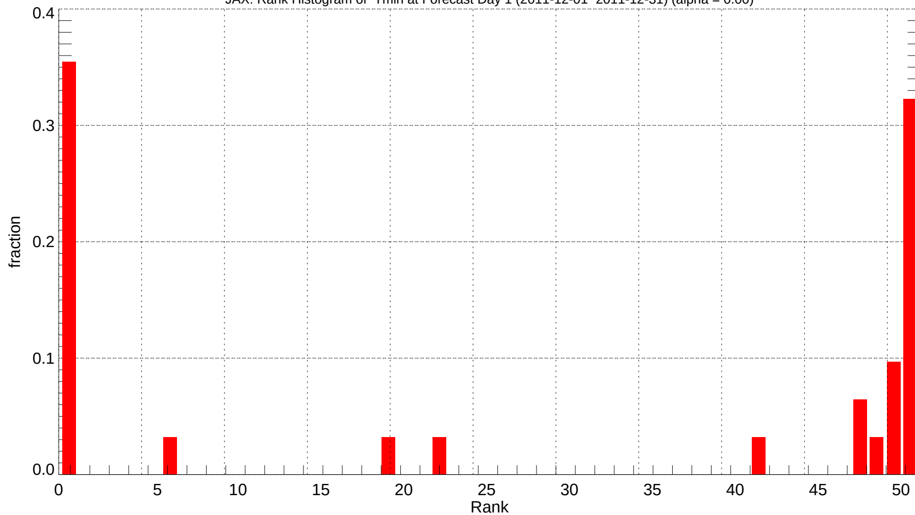
JAX: Rank Histogram of Tmin at Forecast Day 1 (2011-12-01~2011-12-31) (alpha = 0.00)
