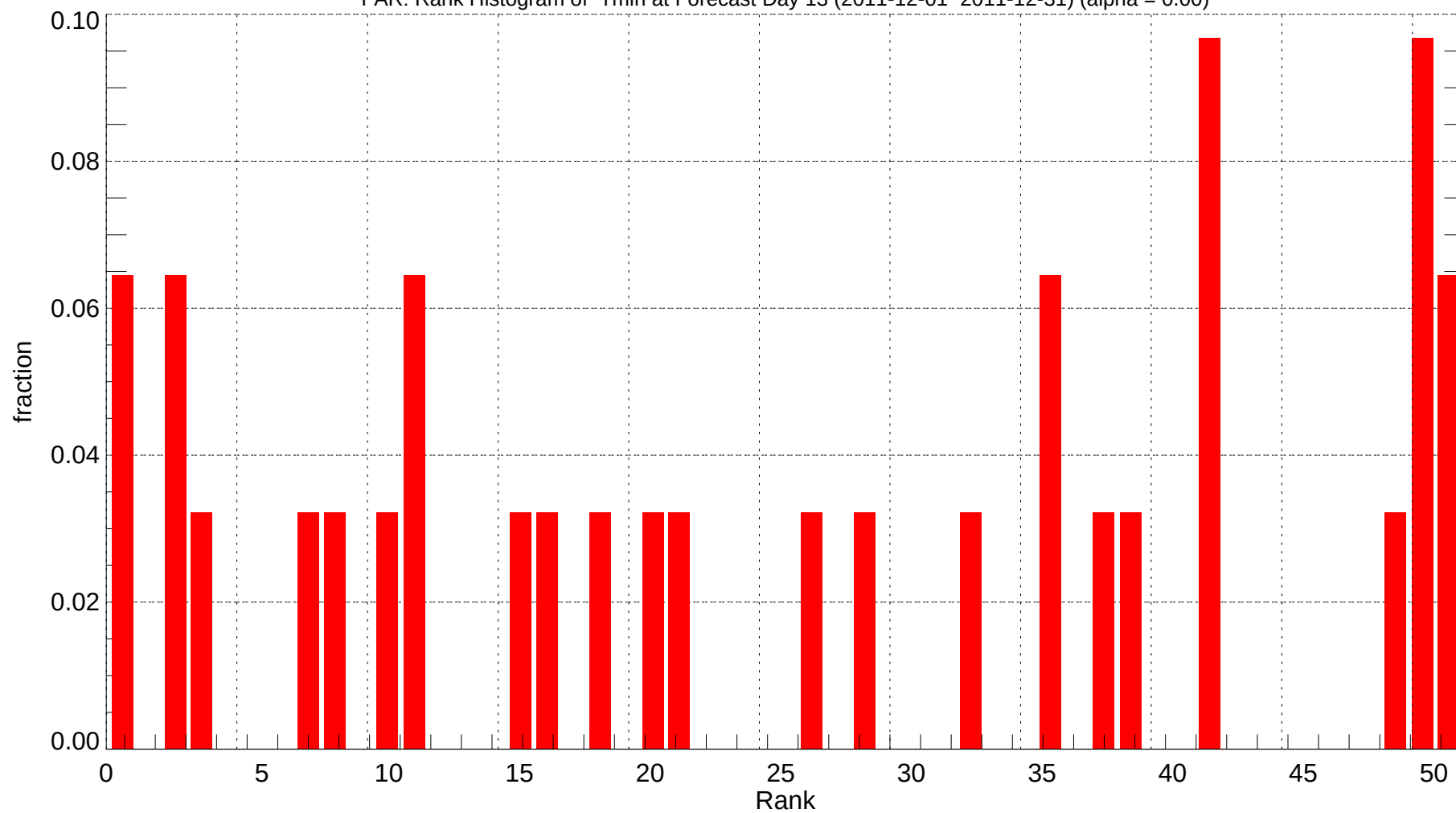
FAR: Rank Histogram of Tmin at Forecast Day 13 (2011-12-01~2011-12-31) (alpha = 0.00)
