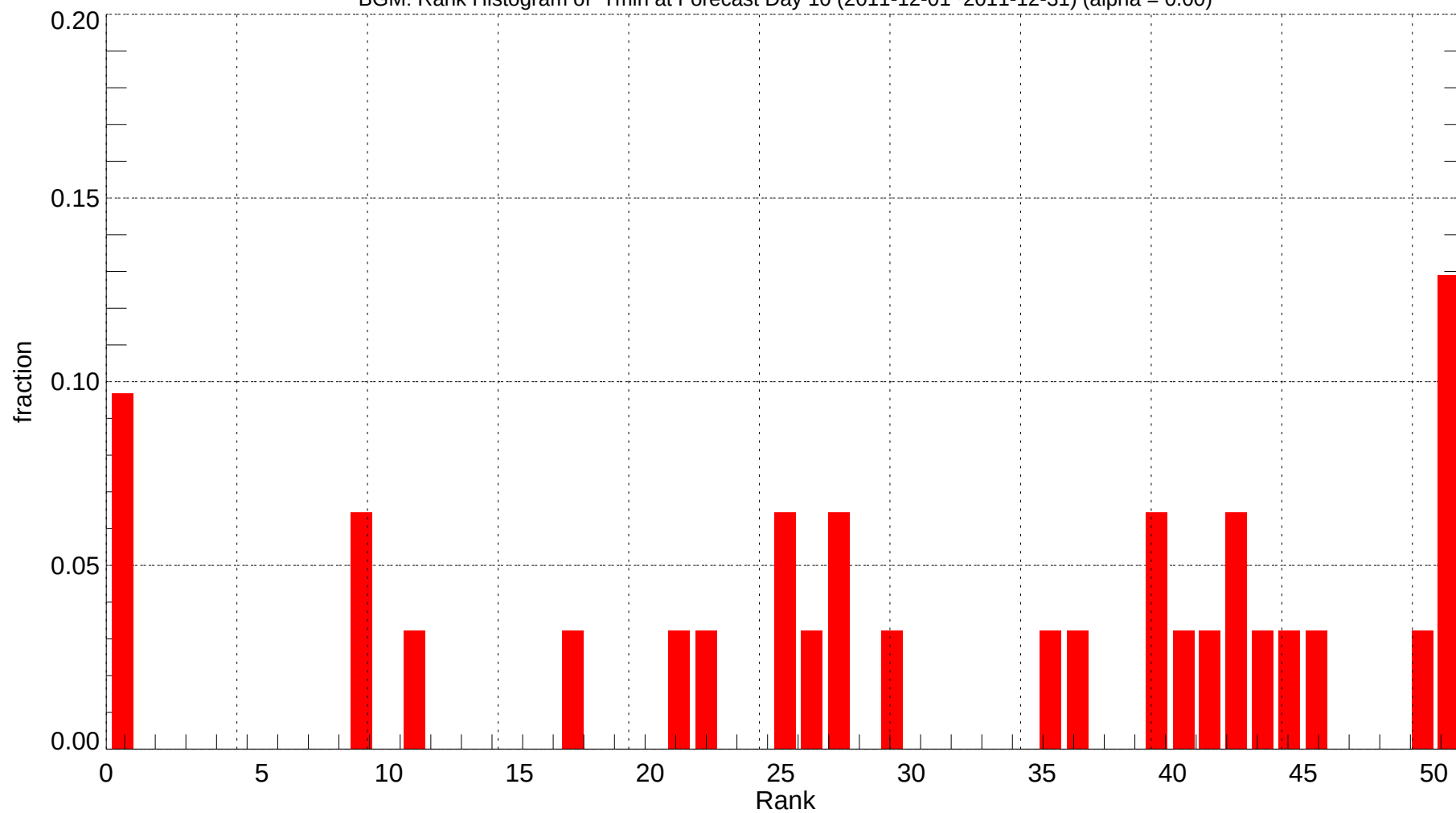
BGM: Rank Histogram of Tmin at Forecast Day 10 (2011-12-01~2011-12-31) (alpha = 0.00)
