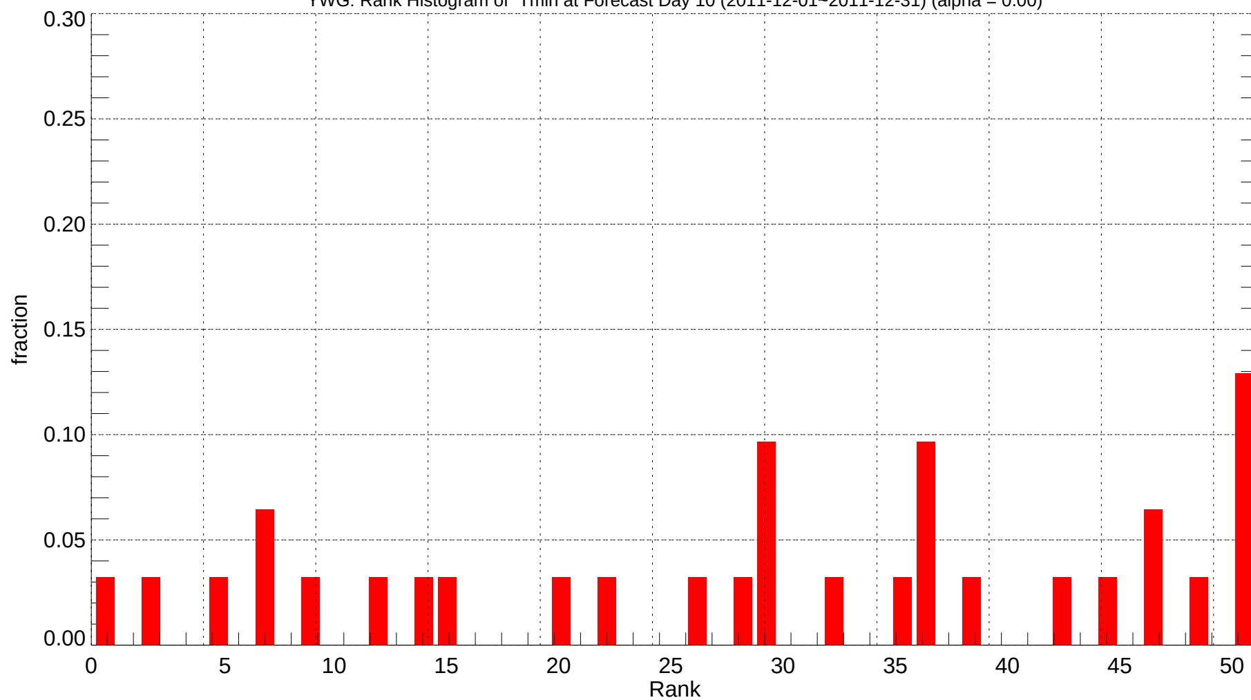
YWG: Rank Histogram of Tmin at Forecast Day 10 (2011-12-01~2011-12-31) (alpha = 0.00)
