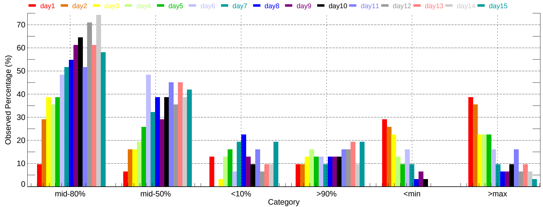
Observed Percentage of Ensembles - EWR: Min Temperature (2011-12-01~2011-12-31)
