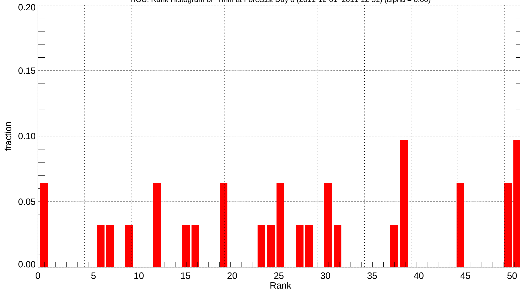
HOU: Rank Histogram of Tmin at Forecast Day 8 (2011-12-01~2011-12-31) (alpha = 0.00)
