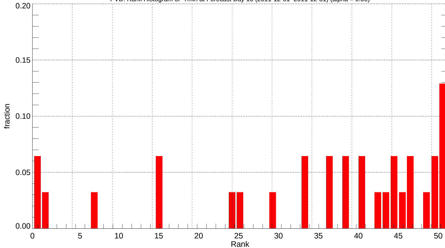
PVD: Rank Histogram of Tmin at Forecast Day 10 (2011-12-01~2011-12-31) (alpha = 0.00)
