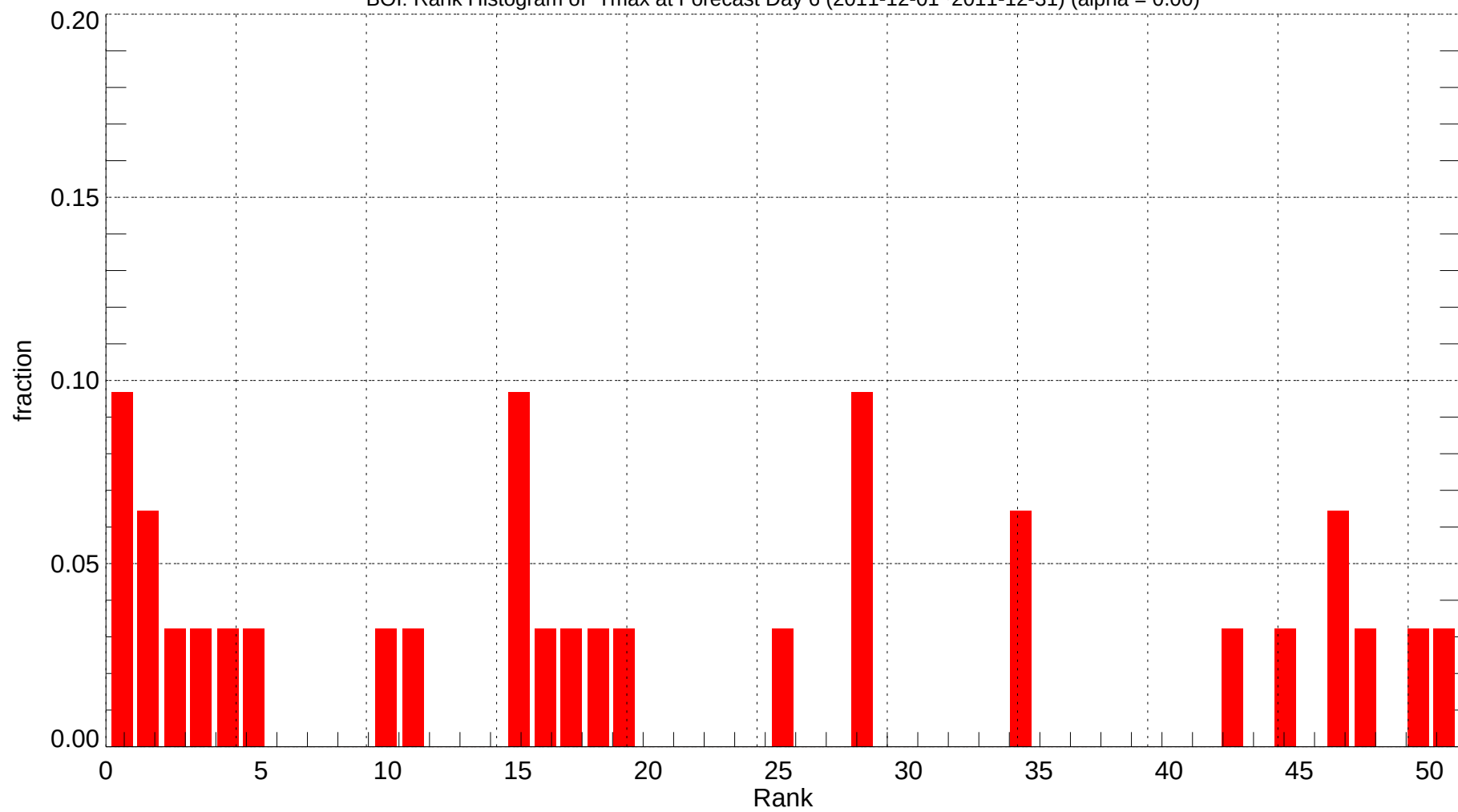
BOI: Rank Histogram of Tmax at Forecast Day 6 (2011-12-01~2011-12-31) (alpha = 0.00)
