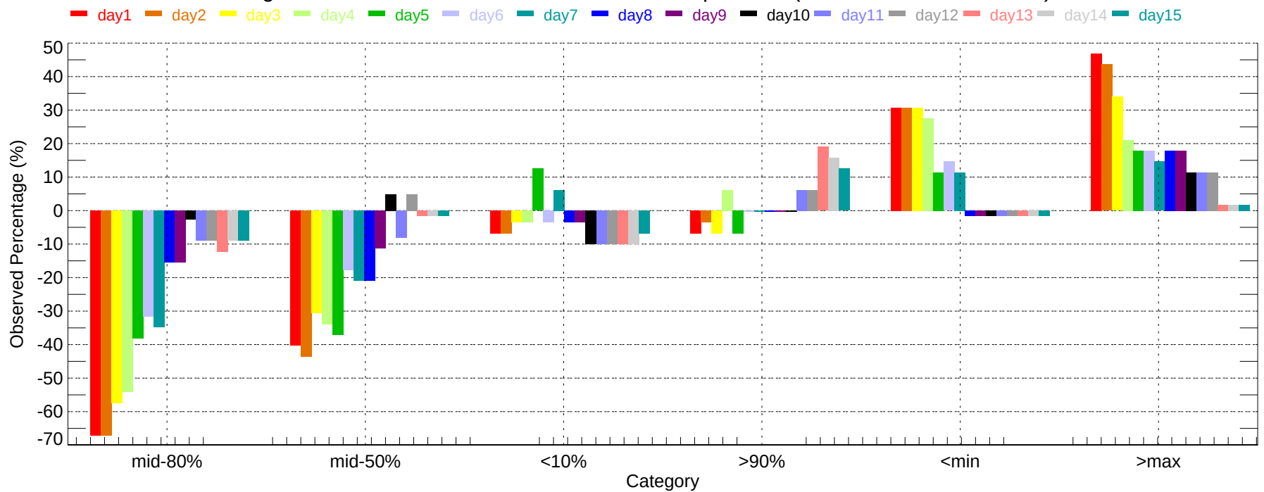
Observed Percentage Deviation of Ensembles - HSV: Max Temperature (2011-12-01~2011-12-31)
