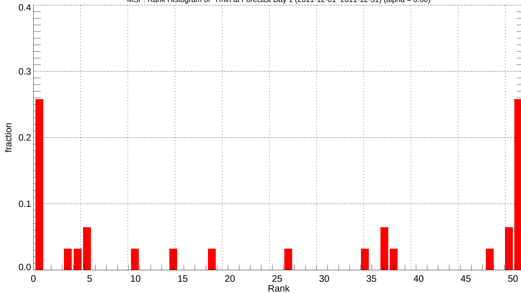
MSP: Rank Histogram of Tmin at Forecast Day 1 (2011-12-01~2011-12-31) (alpha = 0.00)
