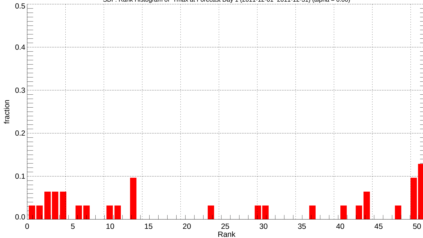
SDF: Rank Histogram of Tmax at Forecast Day 1 (2011-12-01~2011-12-31) (alpha = 0.00)
