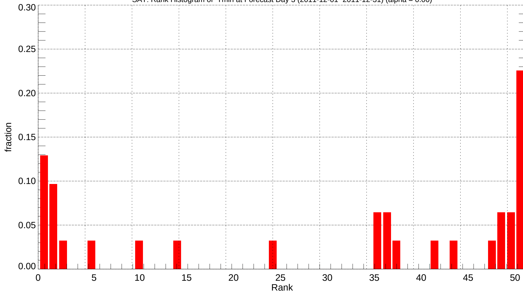
SAT: Rank Histogram of Tmin at Forecast Day 3 (2011-12-01~2011-12-31) (alpha = 0.00)
