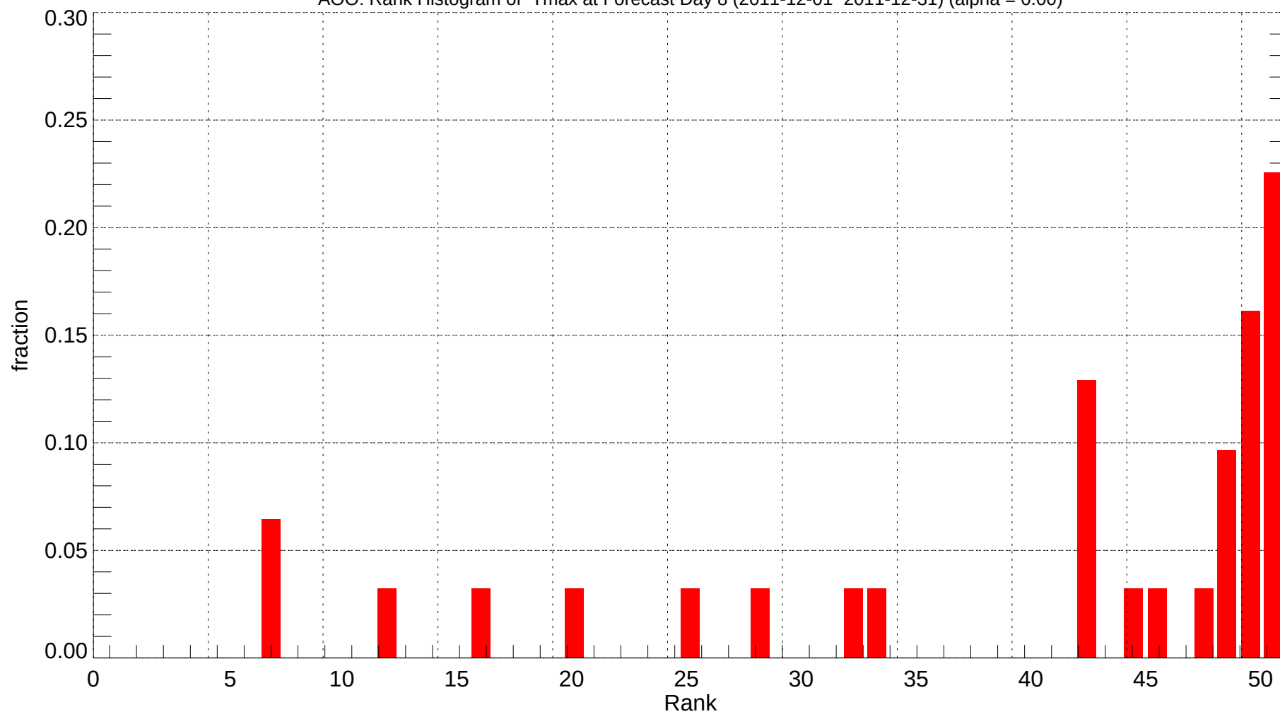
AOO: Rank Histogram of Tmax at Forecast Day 8 (2011-12-01~2011-12-31) (alpha = 0.00)
