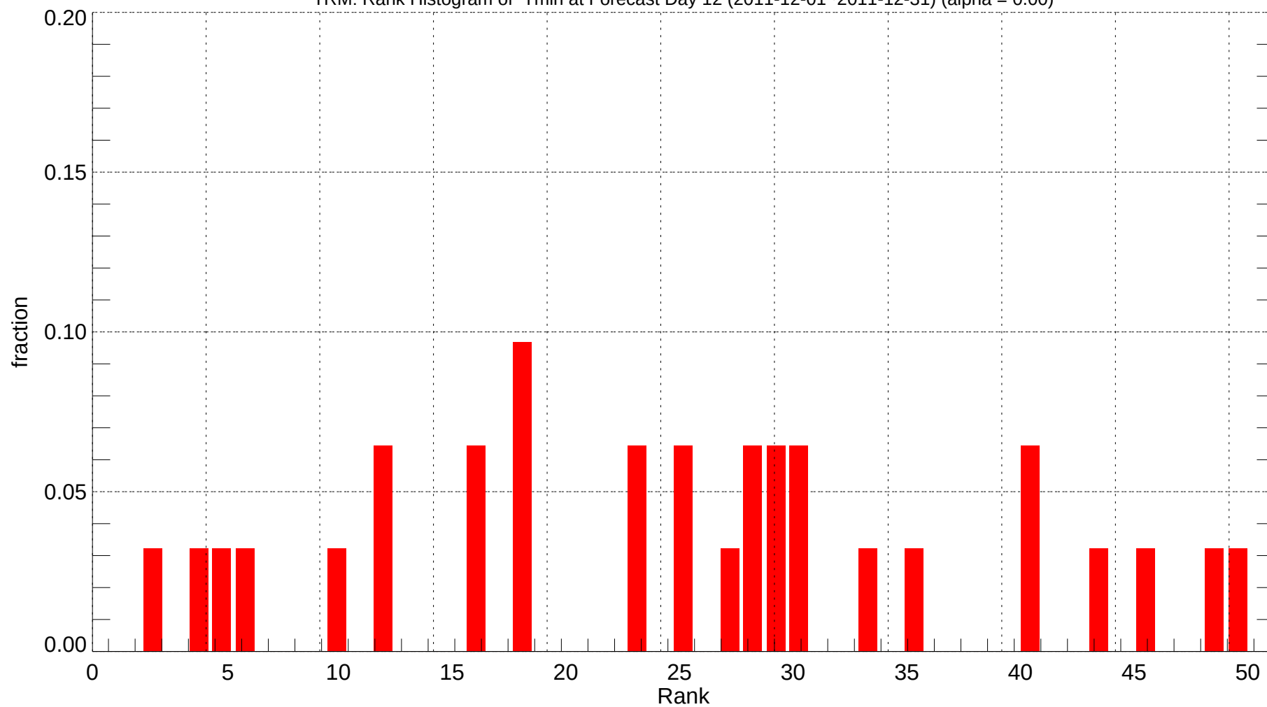
TRM: Rank Histogram of Tmin at Forecast Day 12 (2011-12-01~2011-12-31) (alpha = 0.00)
