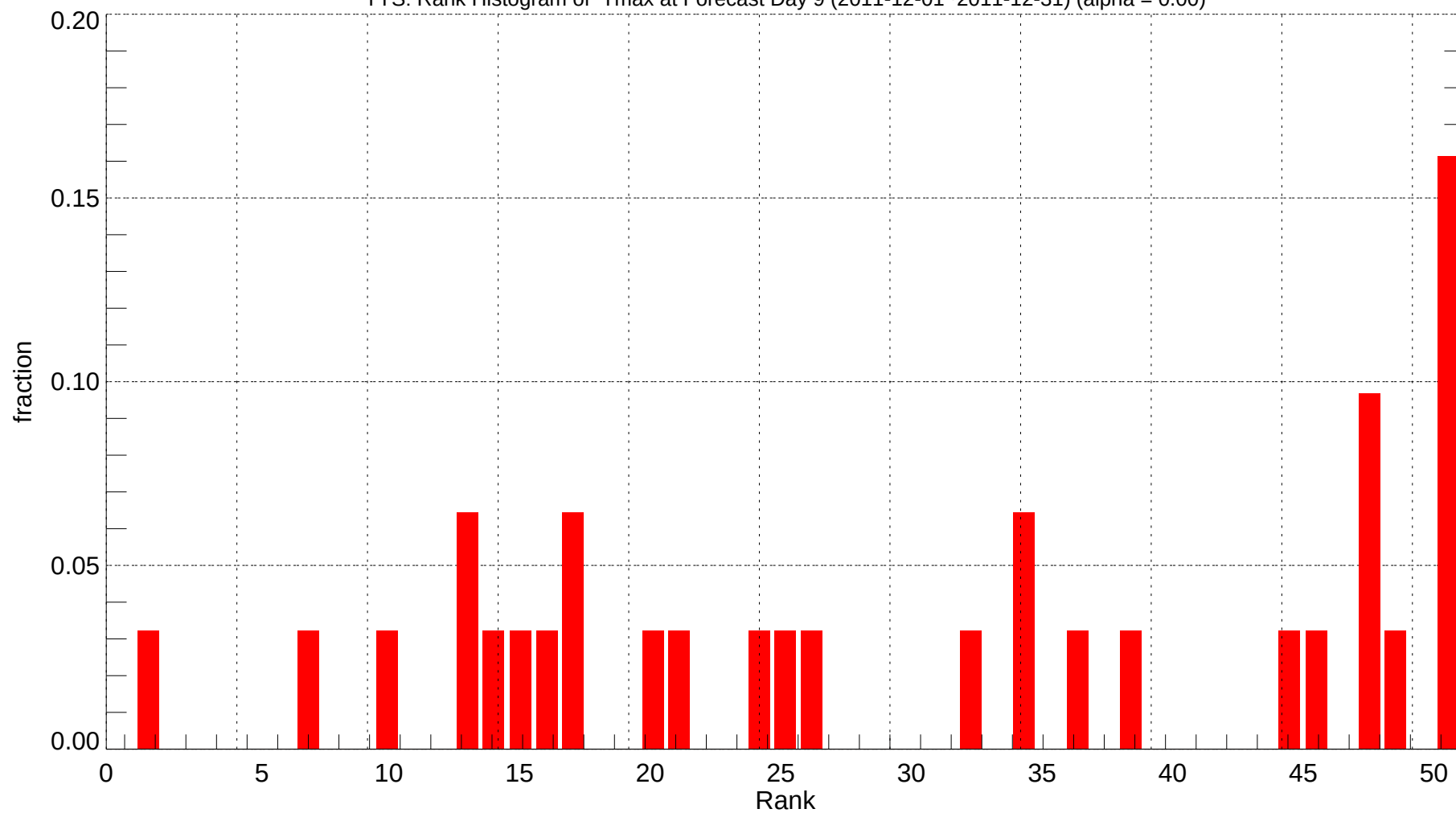
TYS: Rank Histogram of Tmax at Forecast Day 9 (2011-12-01~2011-12-31) (alpha = 0.00)
