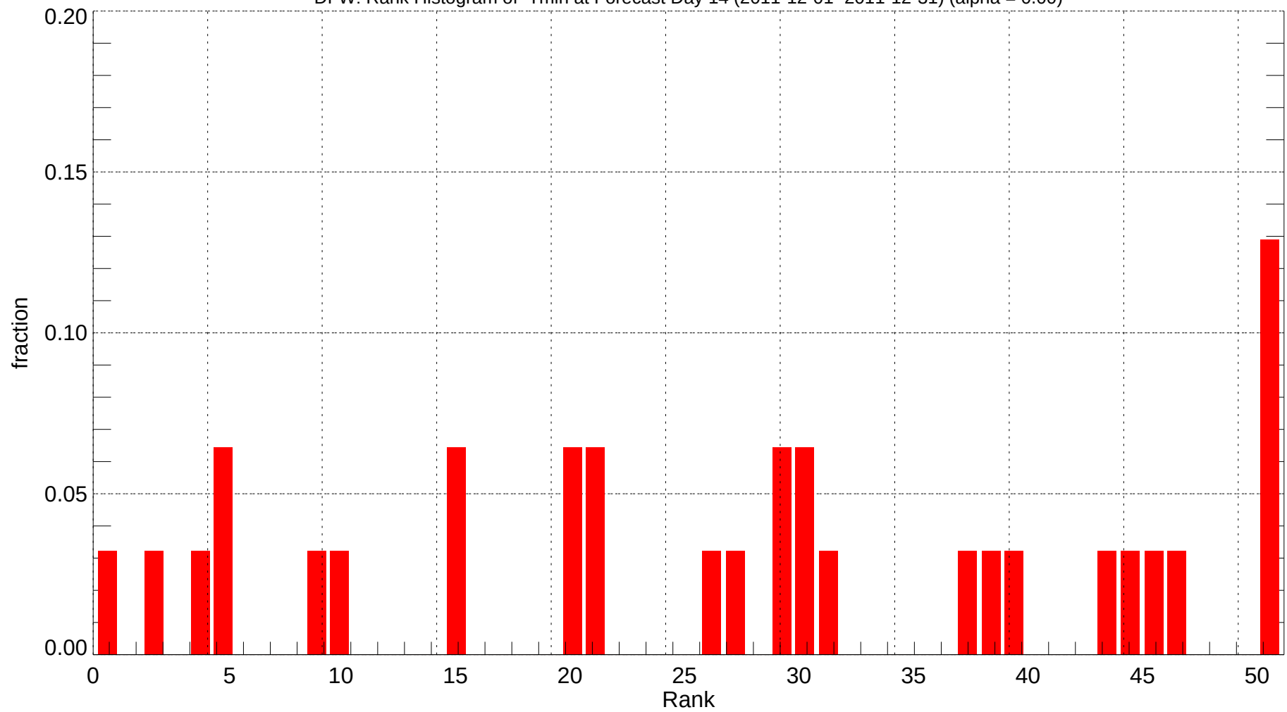
DFW: Rank Histogram of Tmin at Forecast Day 14 (2011-12-01~2011-12-31) (alpha = 0.00)
