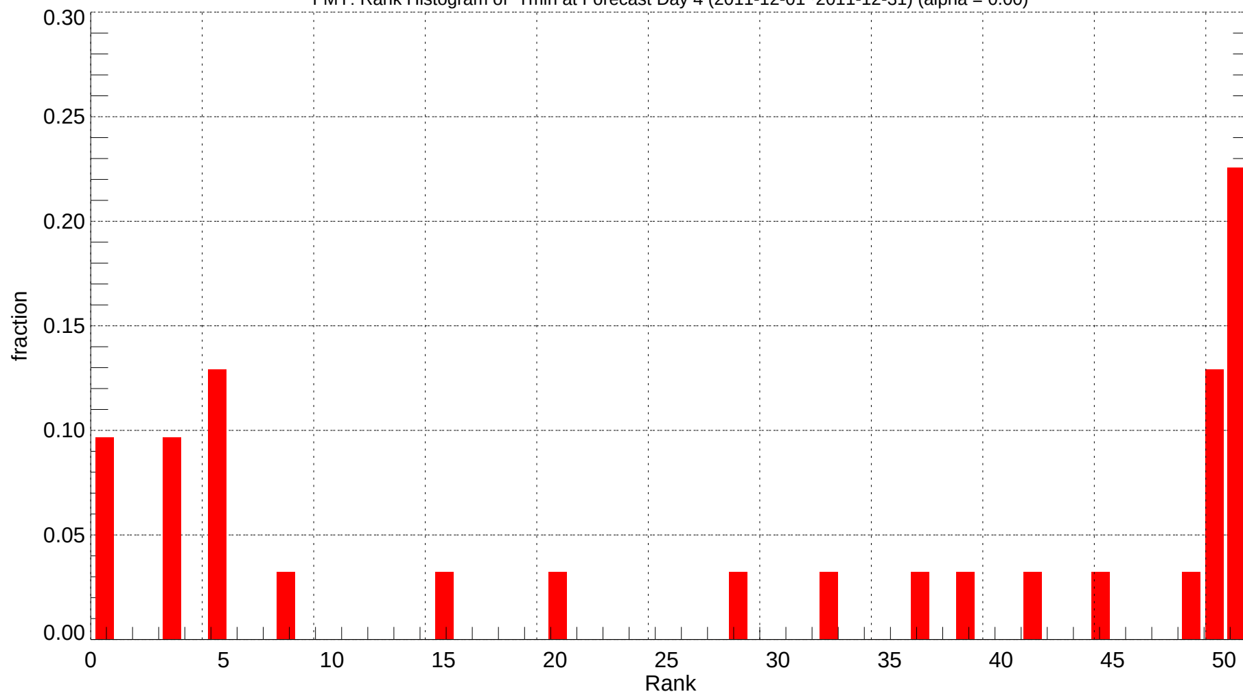
FMY: Rank Histogram of Tmin at Forecast Day 4 (2011-12-01~2011-12-31) (alpha = 0.00)
