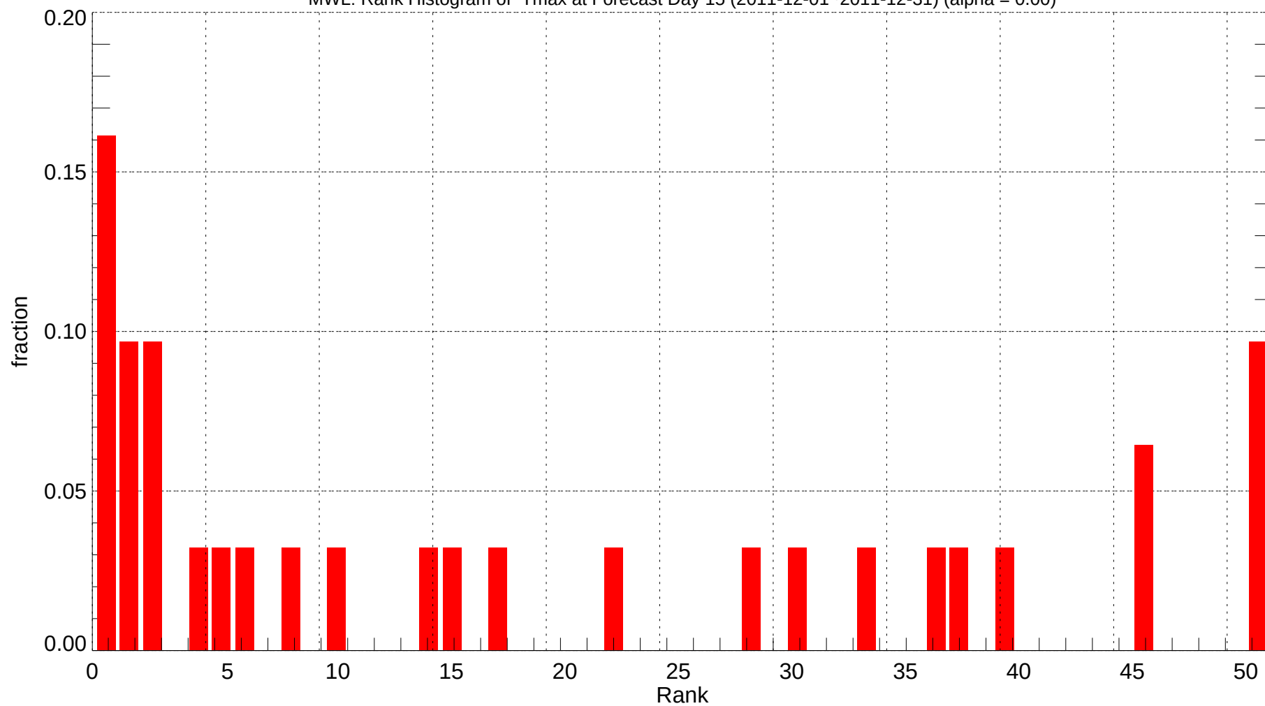
MWL: Rank Histogram of Tmax at Forecast Day 15 (2011-12-01~2011-12-31) (alpha = 0.00)
