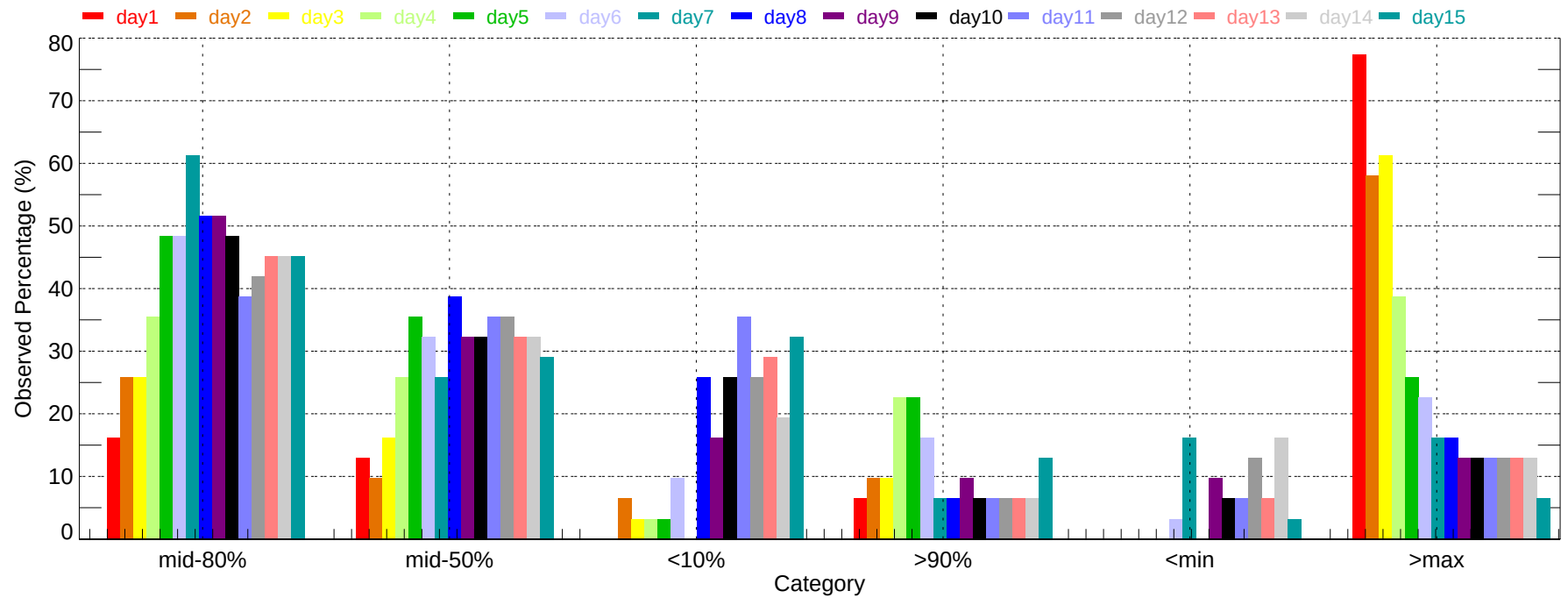
Observed Percentage of Ensembles - FLG: Max Temperature (2011-12-01~2011-12-31)
