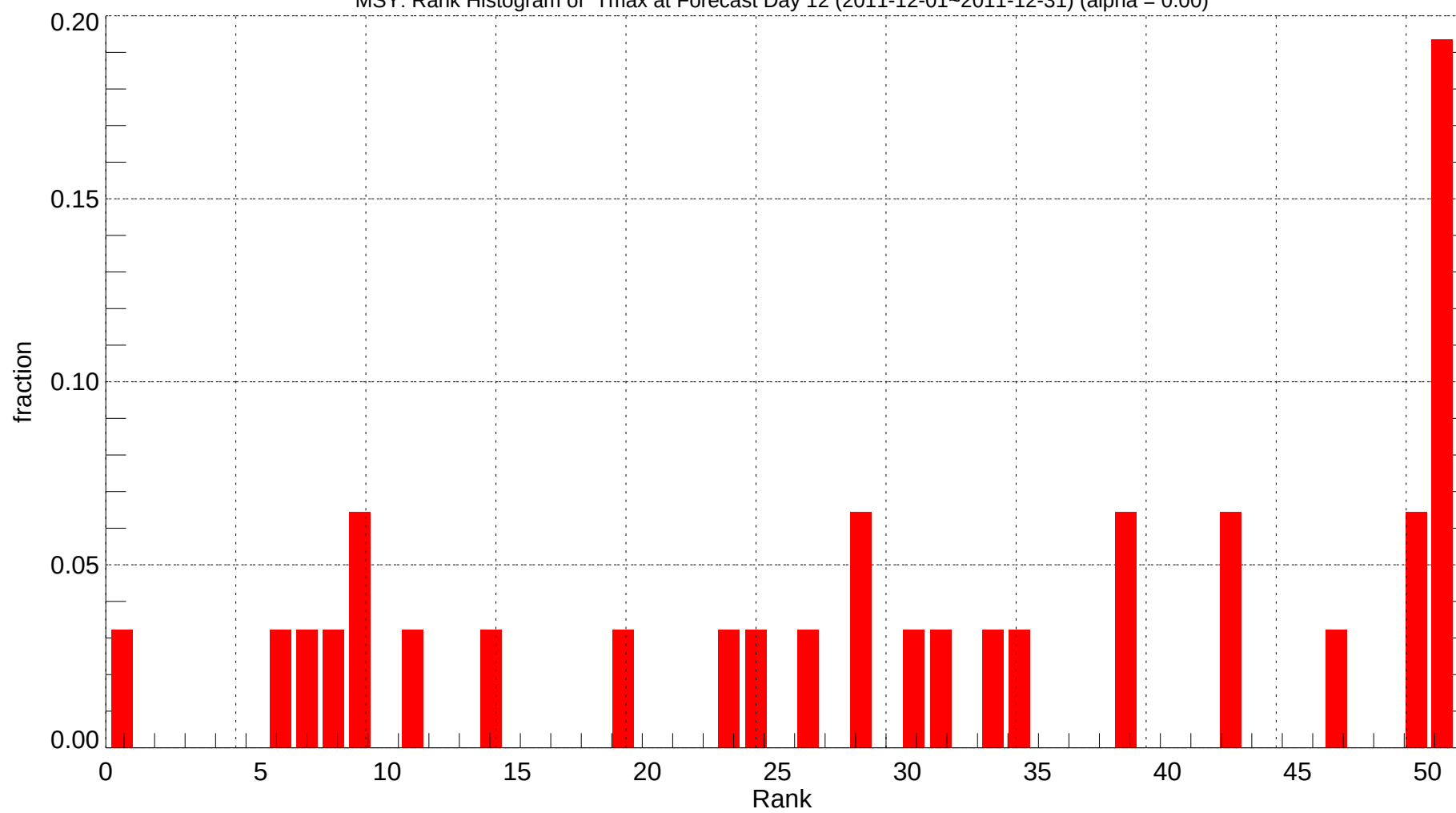
MSY: Rank Histogram of Tmax at Forecast Day 12 (2011-12-01~2011-12-31) (alpha = 0.00)
