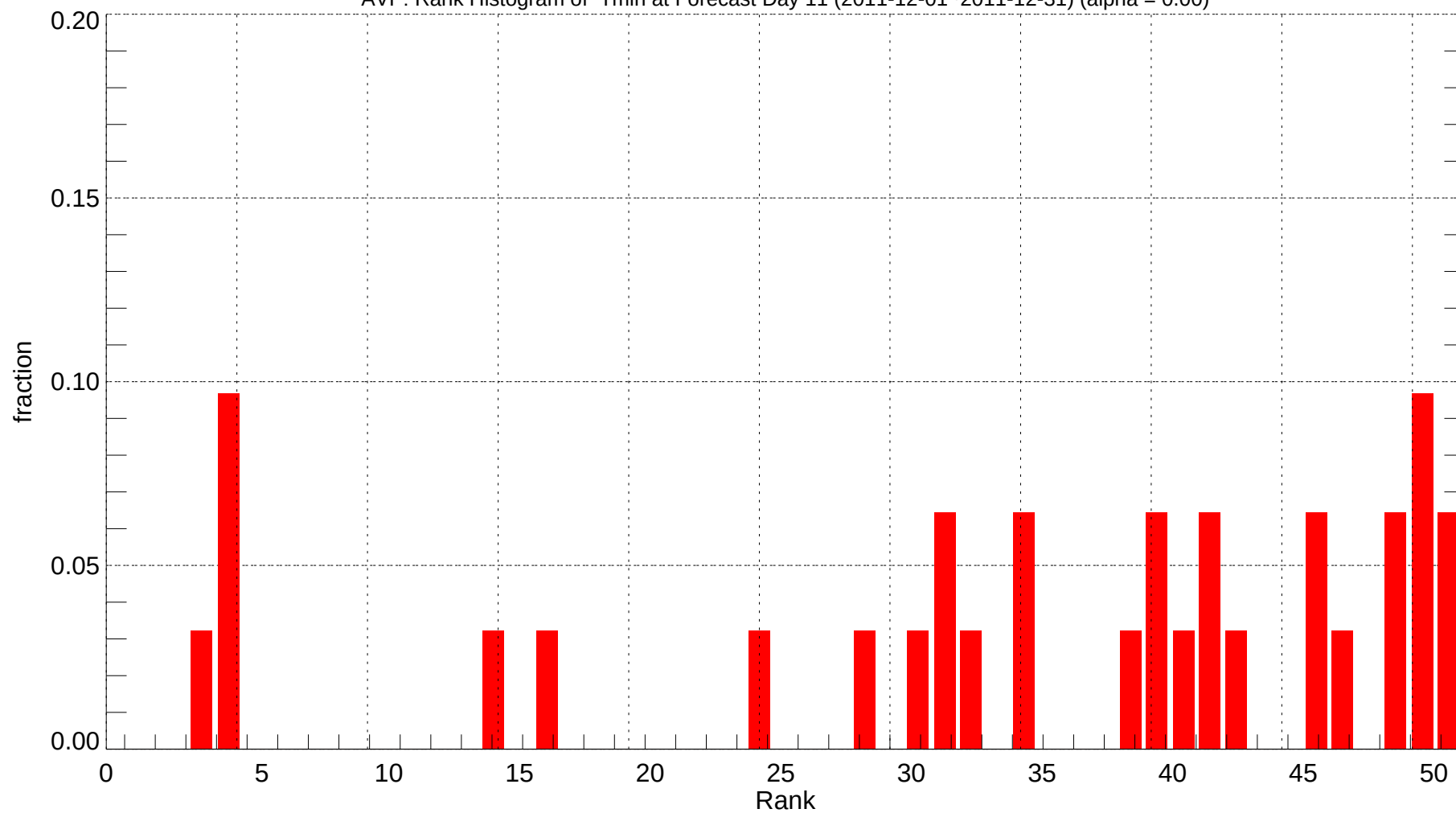
AVP: Rank Histogram of Tmin at Forecast Day 11 (2011-12-01~2011-12-31) (alpha = 0.00)
