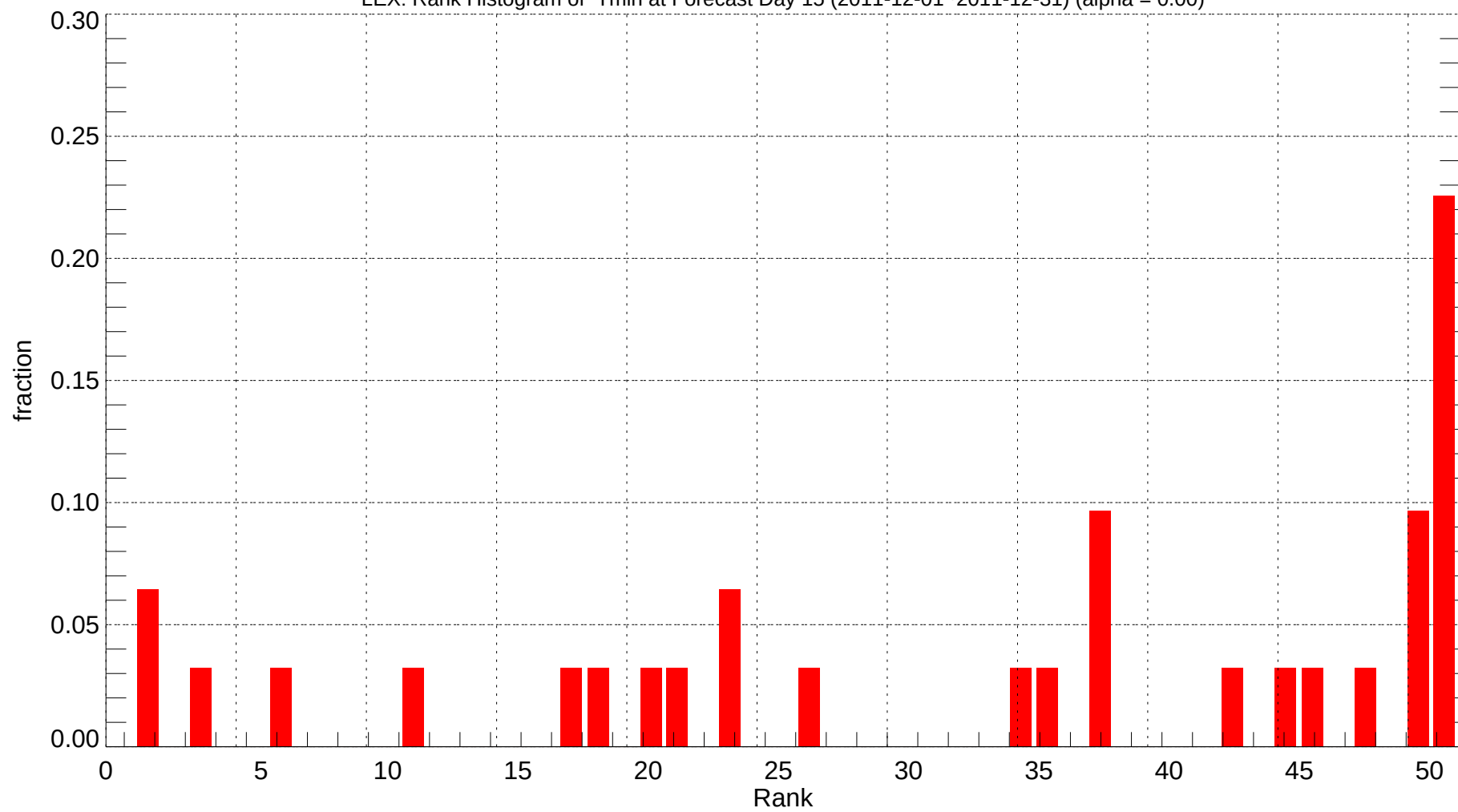
LEX: Rank Histogram of Tmin at Forecast Day 15 (2011-12-01~2011-12-31) (alpha = 0.00)
