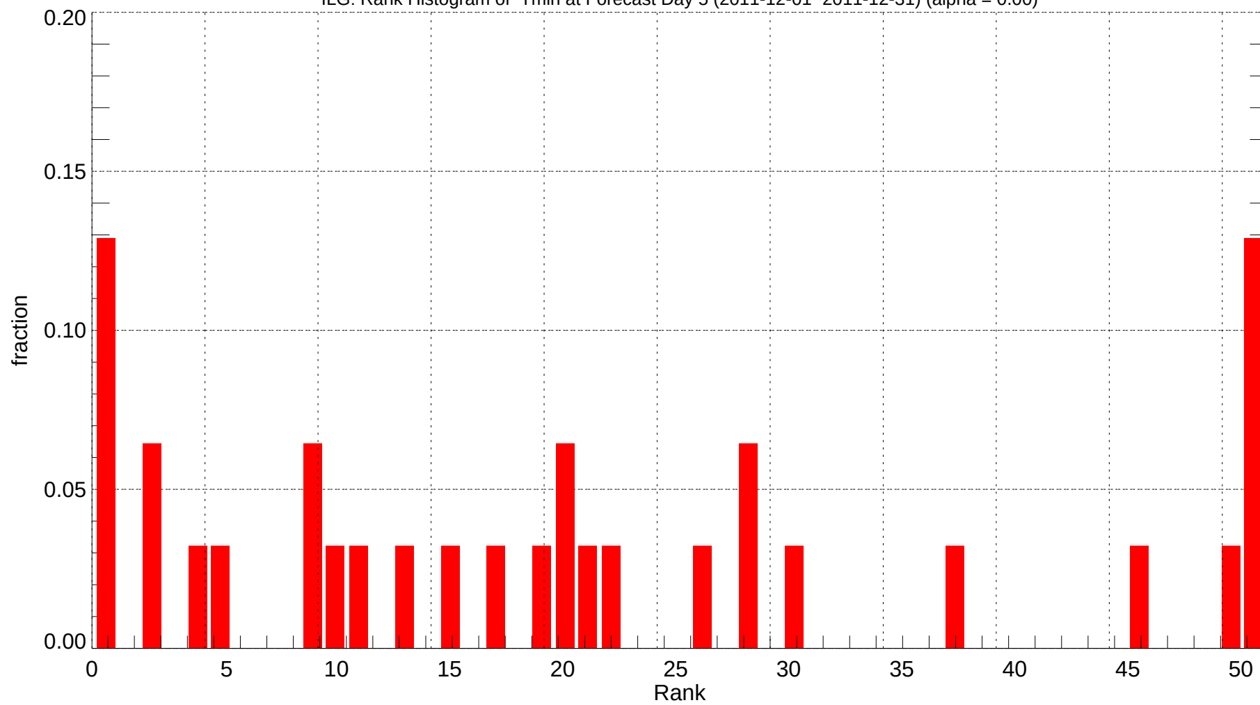
ILG: Rank Histogram of Tmin at Forecast Day 5 (2011-12-01~2011-12-31) (alpha = 0.00)
