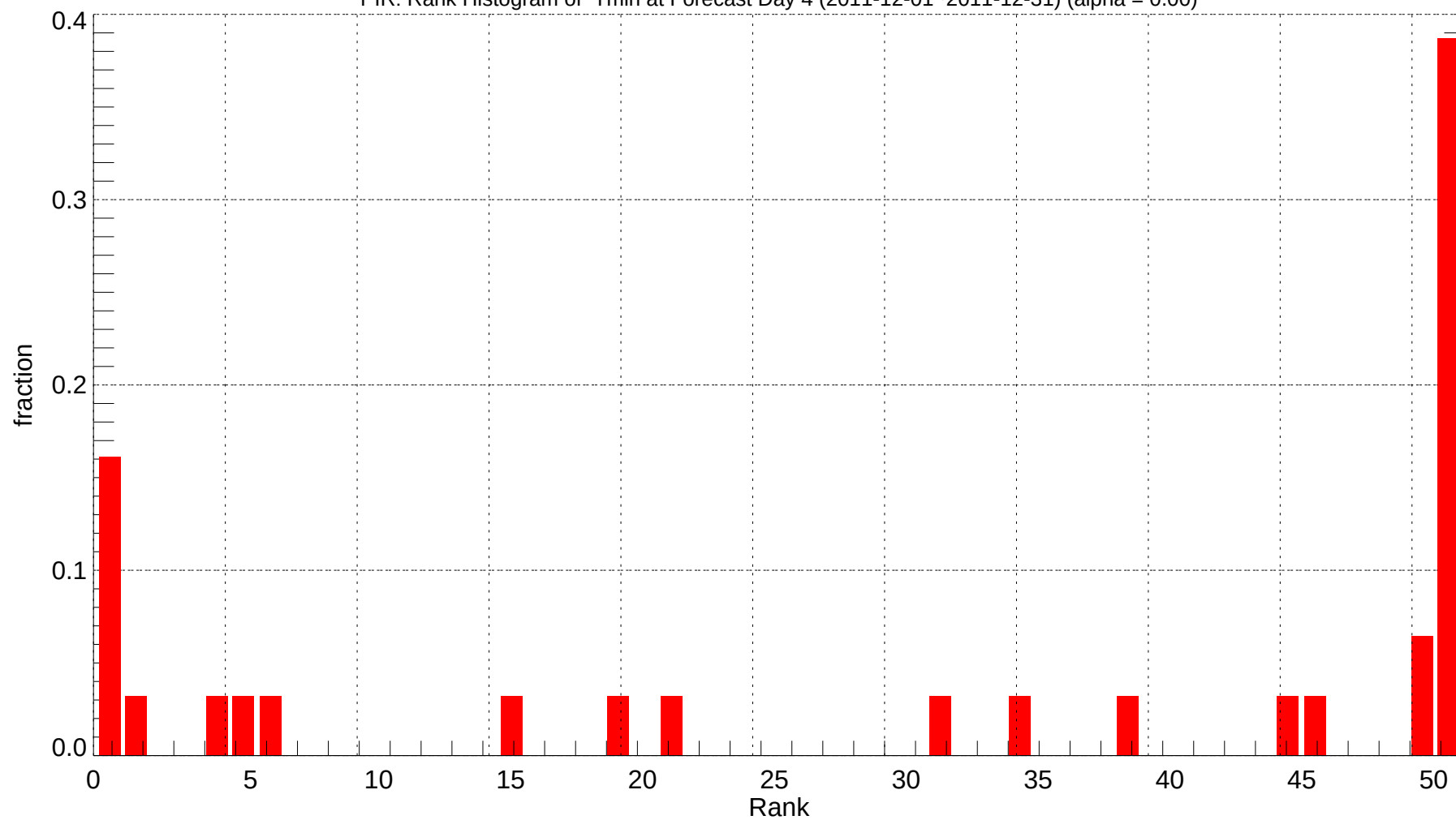
PIR: Rank Histogram of Tmin at Forecast Day 4 (2011-12-01~2011-12-31) (alpha = 0.00)
