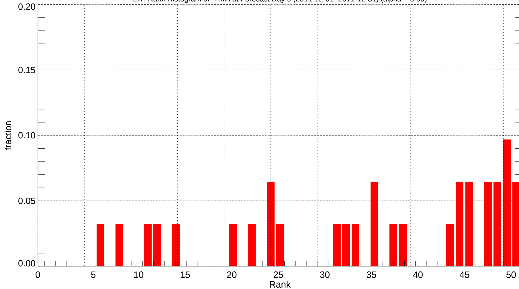
LIT: Rank Histogram of Tmin at Forecast Day 9 (2011-12-01~2011-12-31) (alpha = 0.00)
