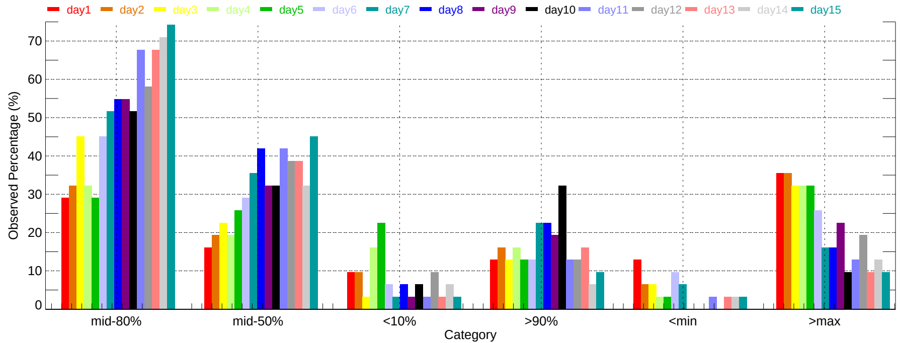
Observed Percentage of Ensembles - OKC: Max Temperature (2011-12-01~2011-12-31)
