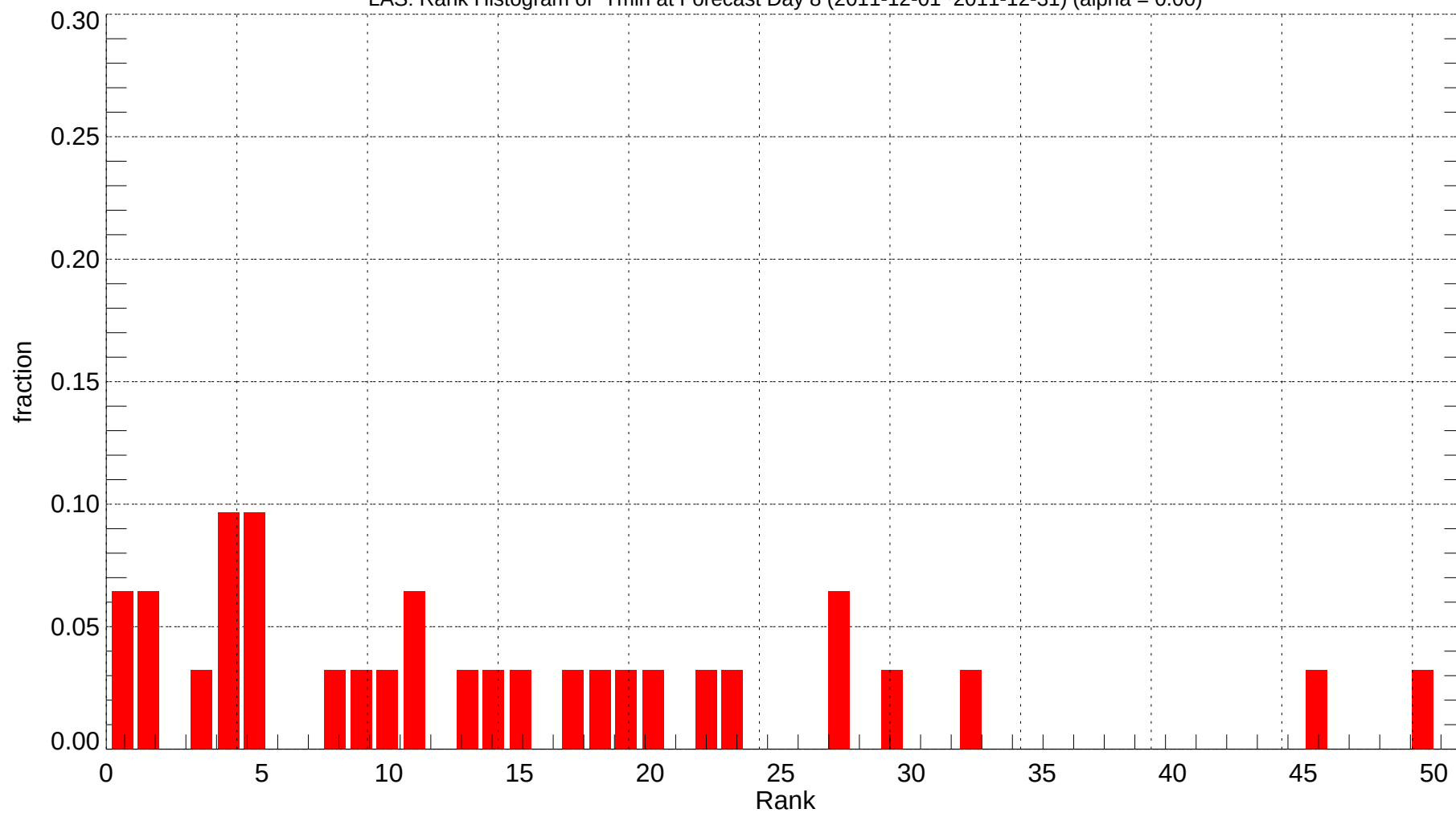
LAS: Rank Histogram of Tmin at Forecast Day 8 (2011-12-01~2011-12-31) (alpha = 0.00)
