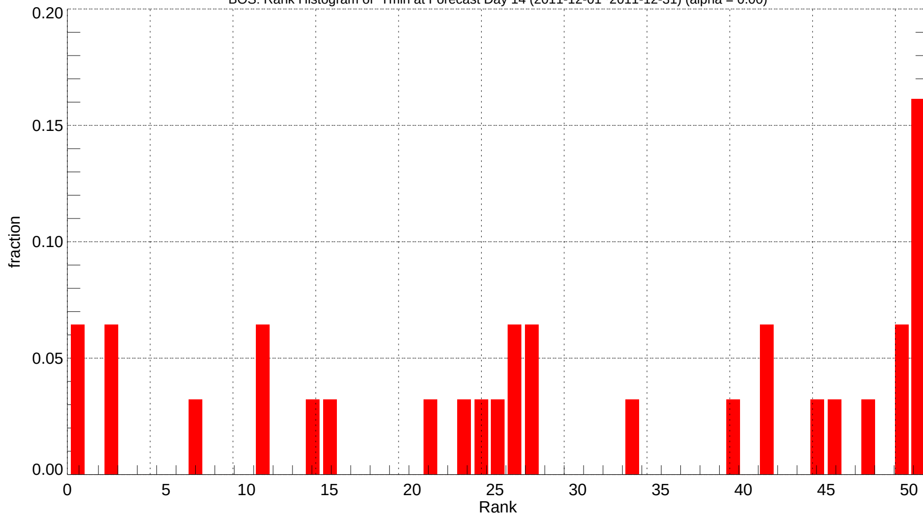
BOS: Rank Histogram of Tmin at Forecast Day 14 (2011-12-01~2011-12-31) (alpha = 0.00)
