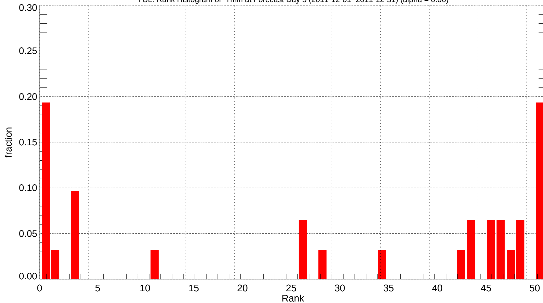
YUL: Rank Histogram of Tmin at Forecast Day 3 (2011-12-01~2011-12-31) (alpha = 0.00)
