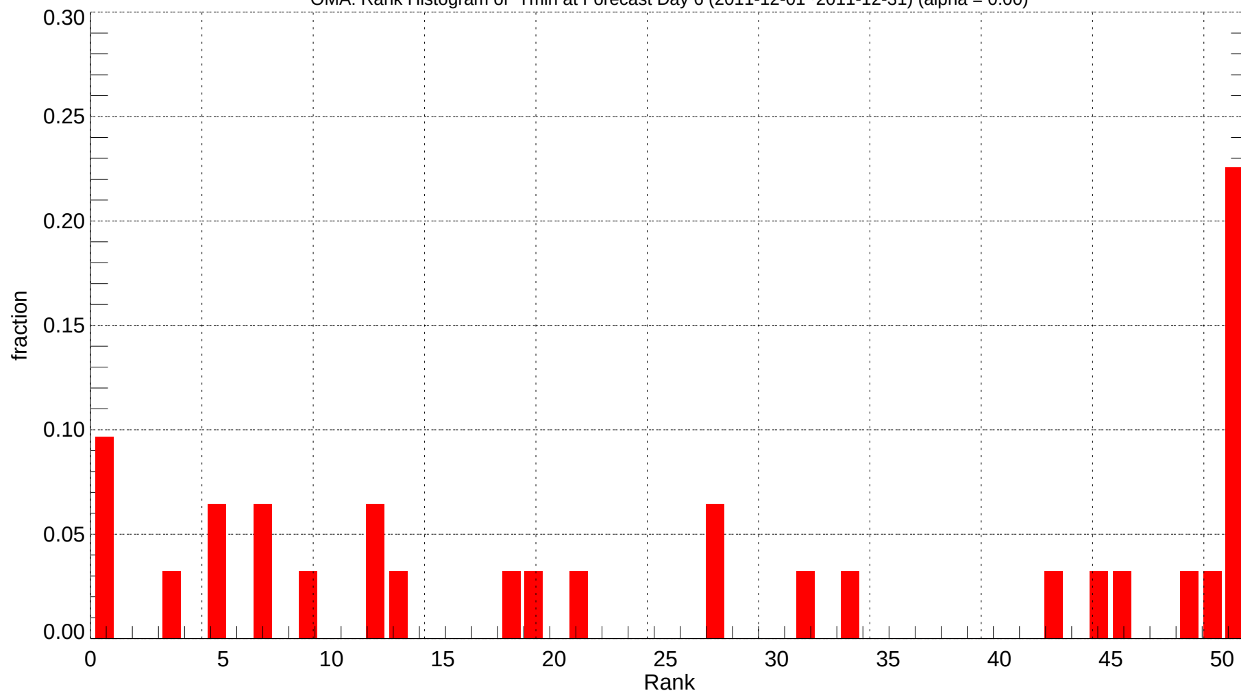
OMA: Rank Histogram of Tmin at Forecast Day 6 (2011-12-01~2011-12-31) (alpha = 0.00)
