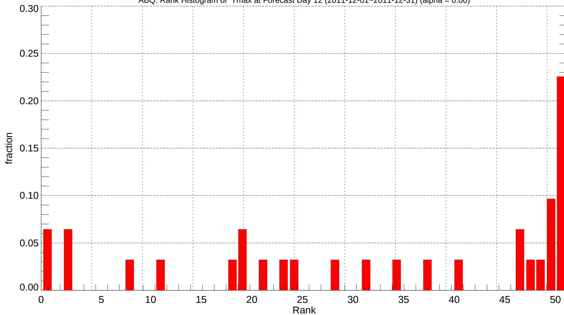
ABQ: Rank Histogram of Tmax at Forecast Day 12 (2011-12-01~2011-12-31) (alpha = 0.00)
