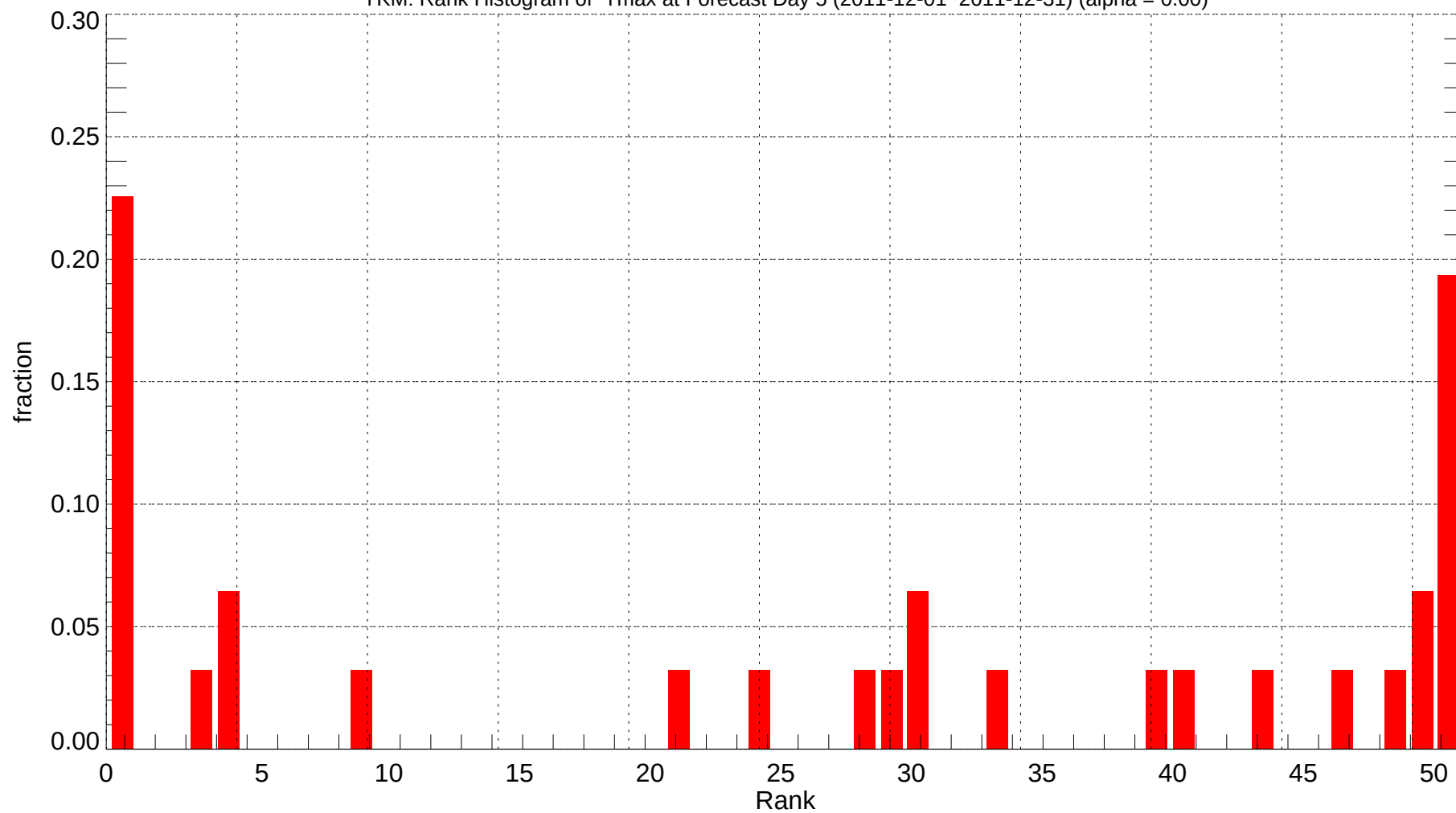
YKM: Rank Histogram of Tmax at Forecast Day 5 (2011-12-01~2011-12-31) (alpha = 0.00)
