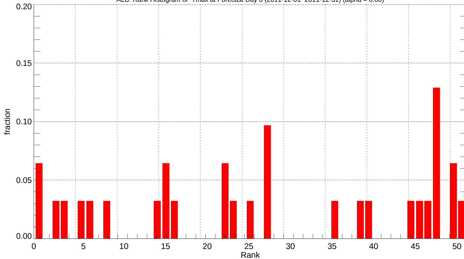
ALB: Rank Histogram of Tmax at Forecast Day 6 (2011-12-01~2011-12-31) (alpha = 0.00)
