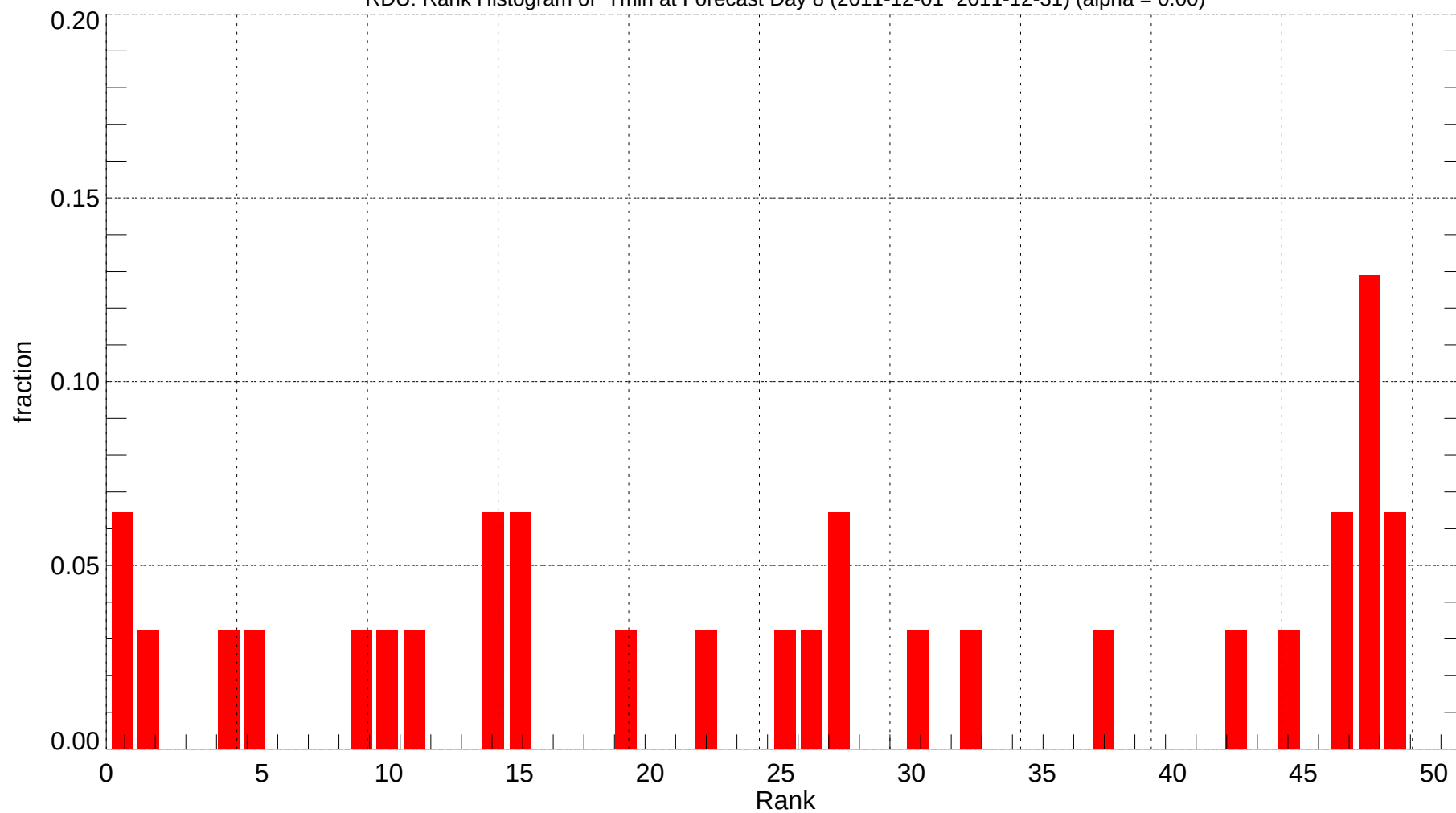
RDU: Rank Histogram of Tmin at Forecast Day 8 (2011-12-01~2011-12-31) (alpha = 0.00)
