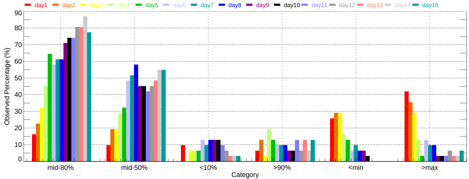
Observed Percentage of Ensembles - SEA: Min Temperature (2011-12-01~2011-12-31)
