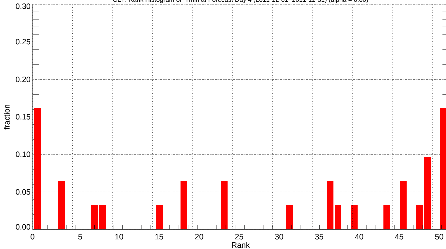
CLT: Rank Histogram of Tmin at Forecast Day 4 (2011-12-01~2011-12-31) (alpha = 0.00)
