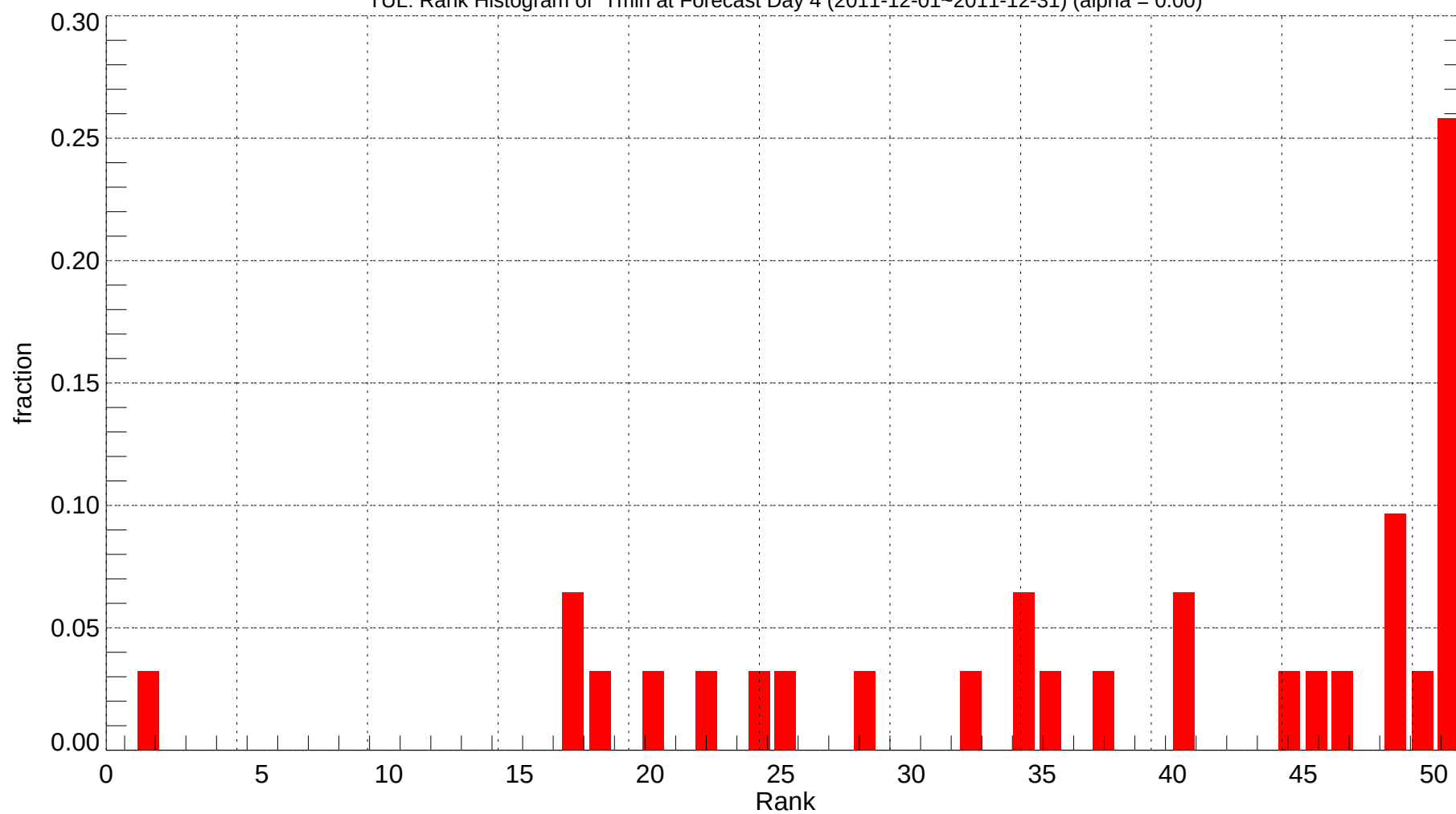
TUL: Rank Histogram of Tmin at Forecast Day 4 (2011-12-01~2011-12-31) (alpha = 0.00)
