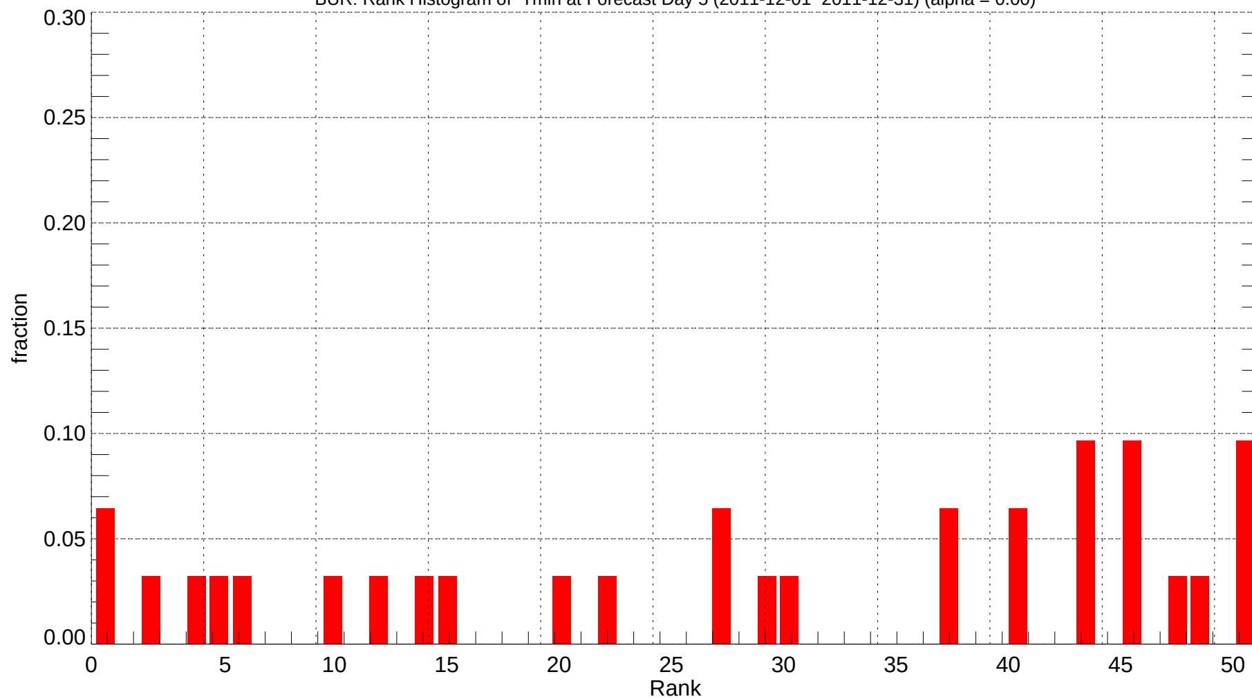
BUR: Rank Histogram of Tmin at Forecast Day 5 (2011-12-01~2011-12-31) (alpha = 0.00)
