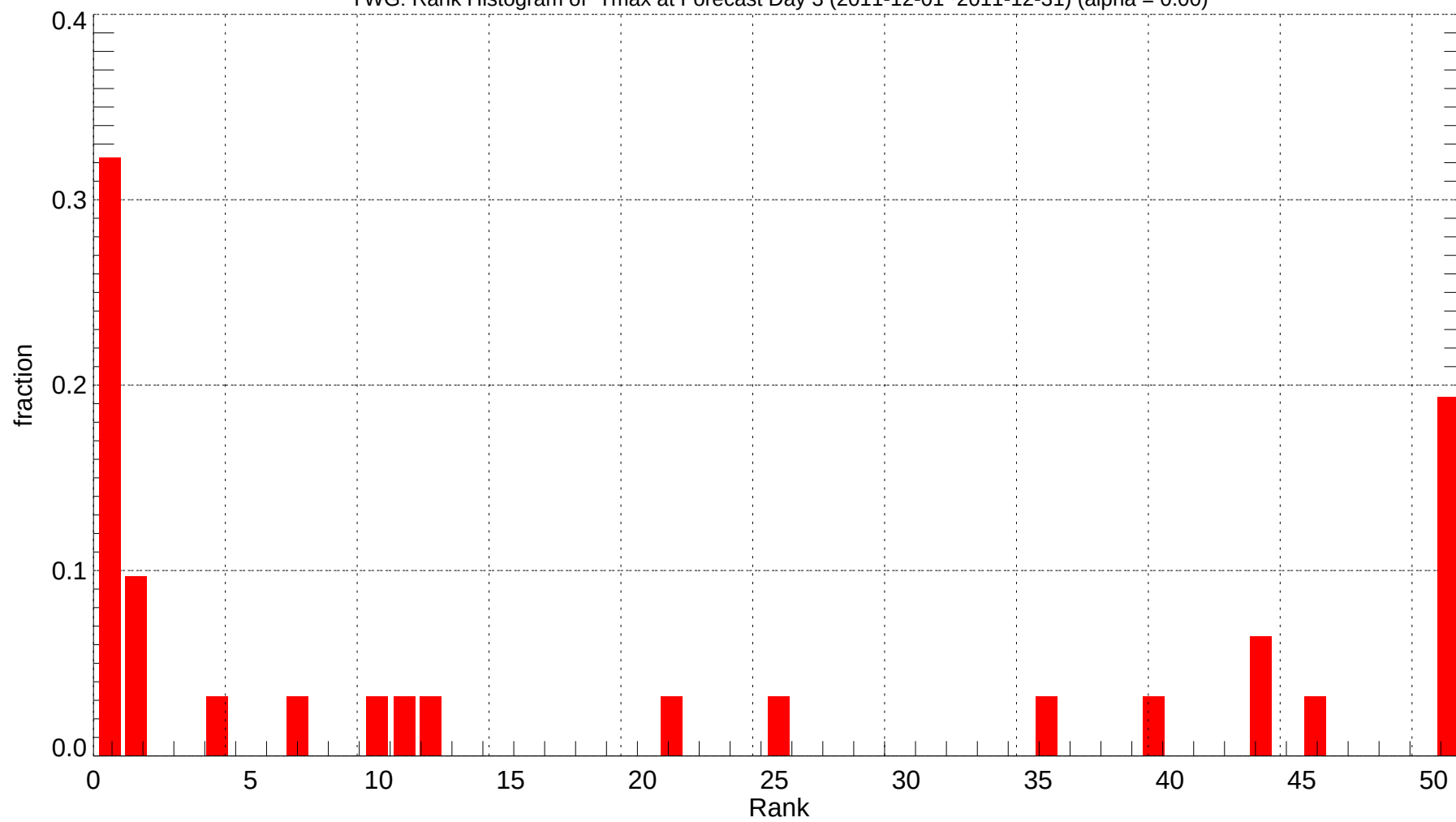
YWG: Rank Histogram of Tmax at Forecast Day 3 (2011-12-01~2011-12-31) (alpha = 0.00)
