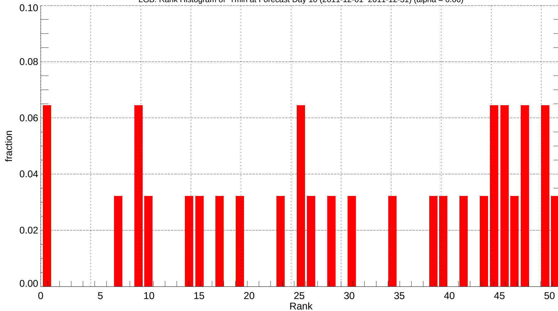
LGB: Rank Histogram of Tmin at Forecast Day 10 (2011-12-01~2011-12-31) (alpha = 0.00)
