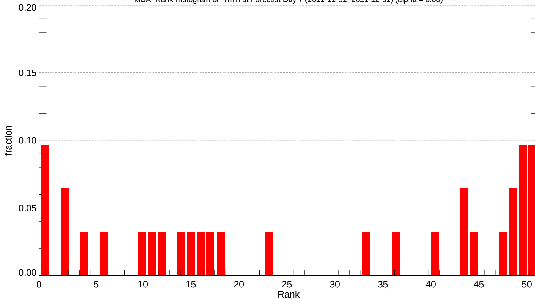
MBA: Rank Histogram of Tmin at Forecast Day 7 (2011-12-01~2011-12-31) (alpha = 0.00)
