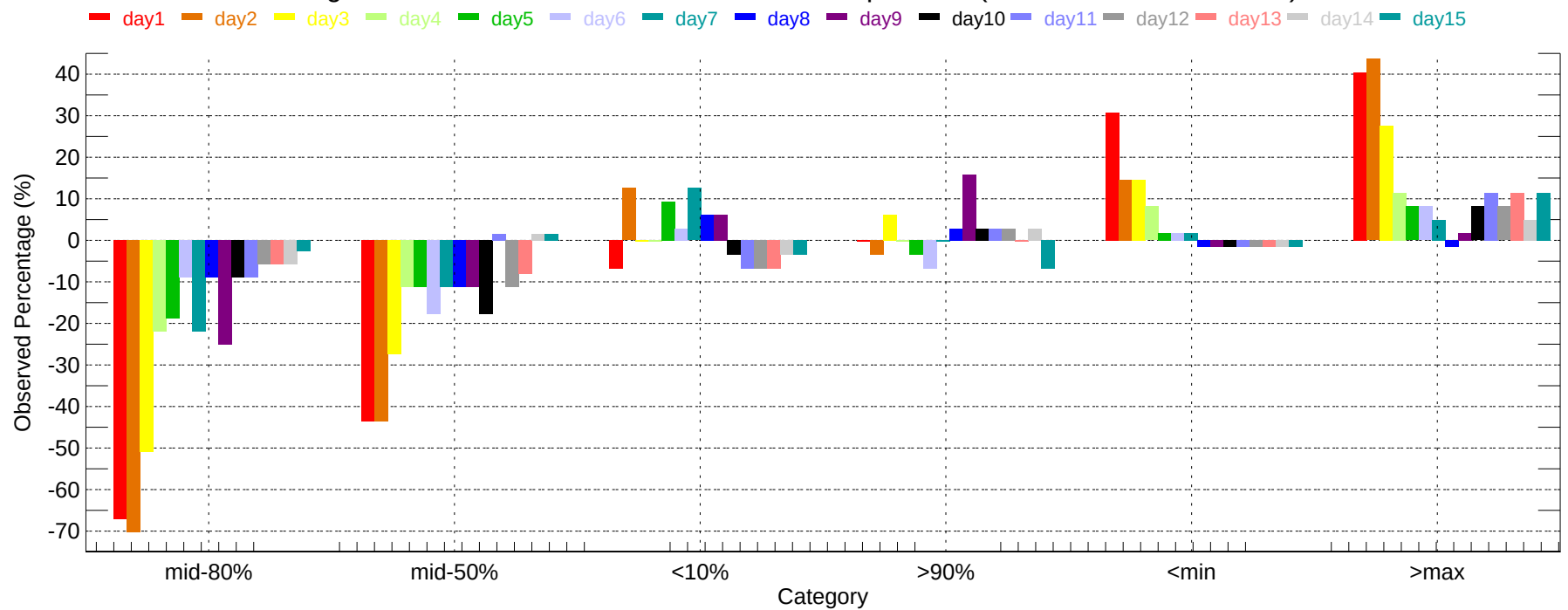
Observed Percentage Deviation of Ensembles - JAX: Max Temperature (2011-12-01~2011-12-31)
