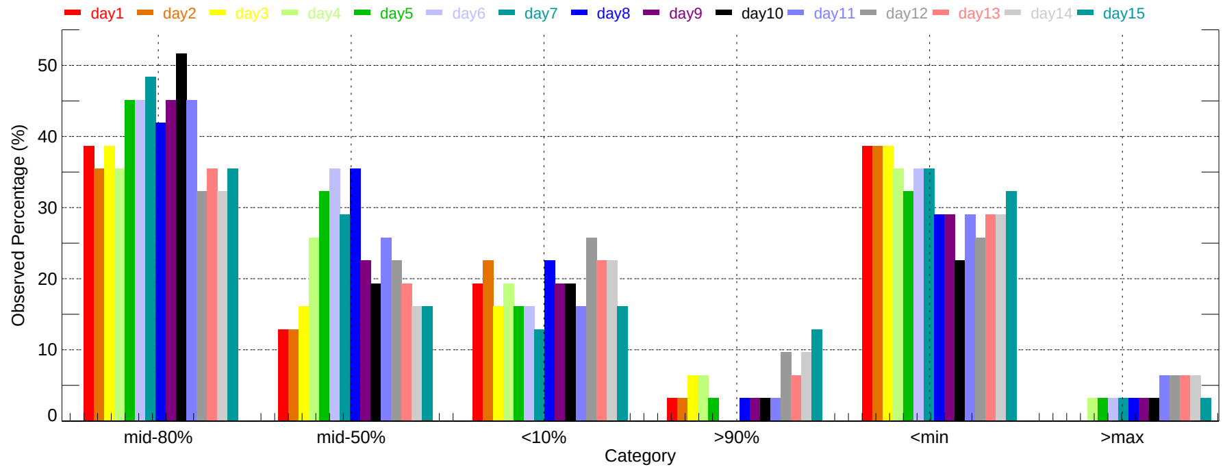
Observed Percentage of Ensembles - SJT: Max Temperature (2011-12-01~2011-12-31)
