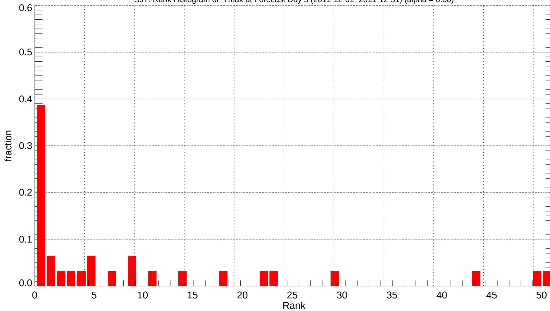
SJT: Rank Histogram of Tmax at Forecast Day 3 (2011-12-01~2011-12-31) (alpha = 0.00)
