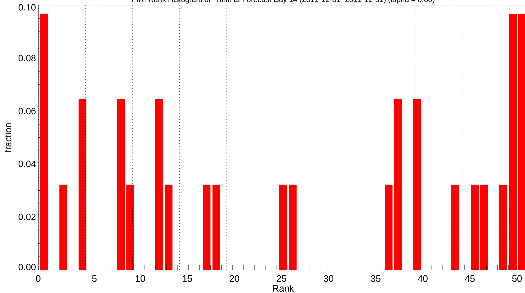
PIR: Rank Histogram of Tmin at Forecast Day 14 (2011-12-01~2011-12-31) (alpha = 0.00)
