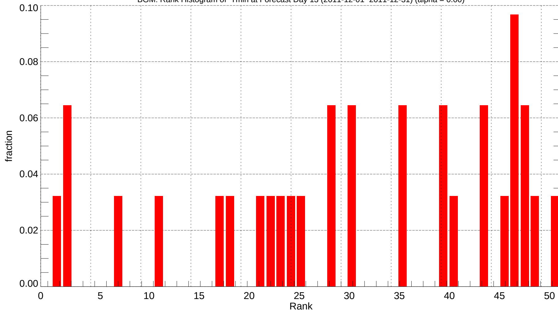
BGM: Rank Histogram of Tmin at Forecast Day 13 (2011-12-01~2011-12-31) (alpha = 0.00)
