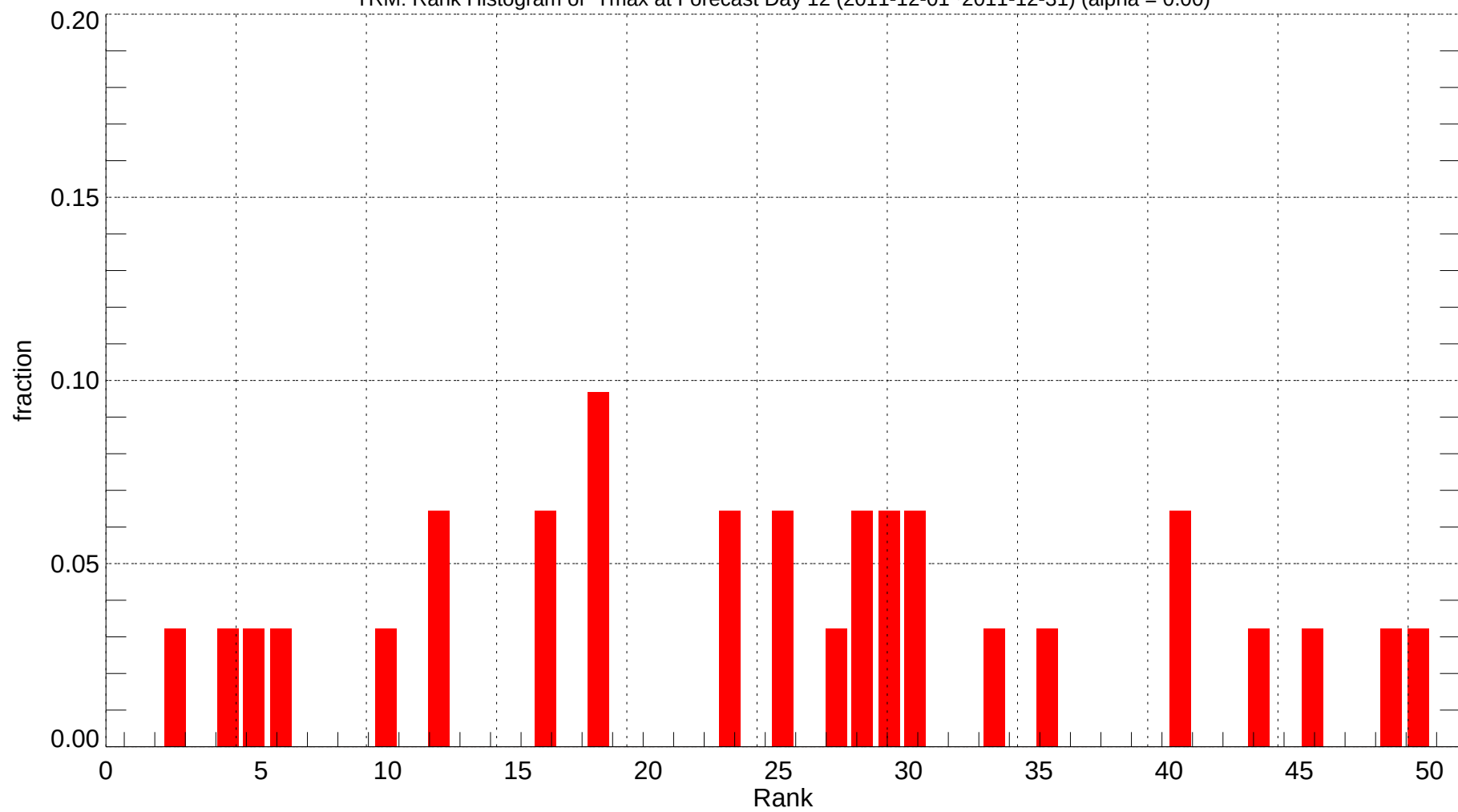
TRM: Rank Histogram of Tmax at Forecast Day 12 (2011-12-01~2011-12-31) (alpha = 0.00)
