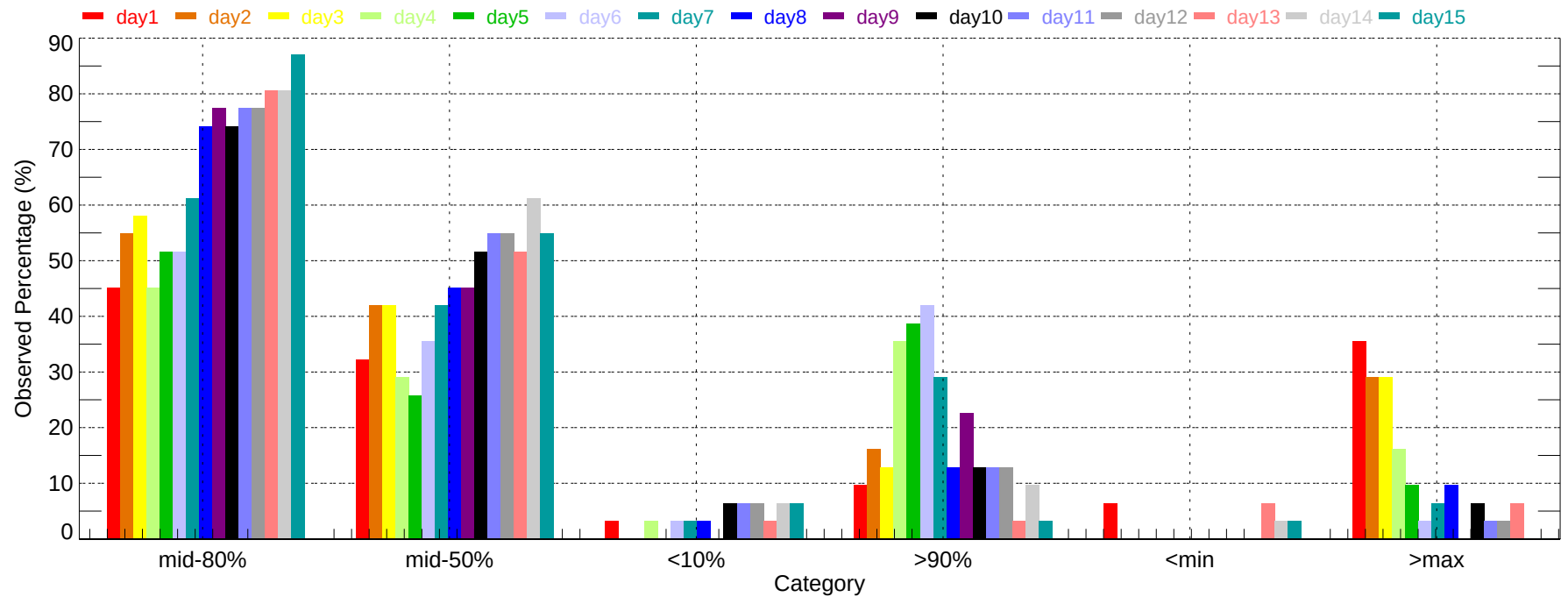
Observed Percentage of Ensembles - ABQ: Min Temperature (2011-12-01~2011-12-31)
