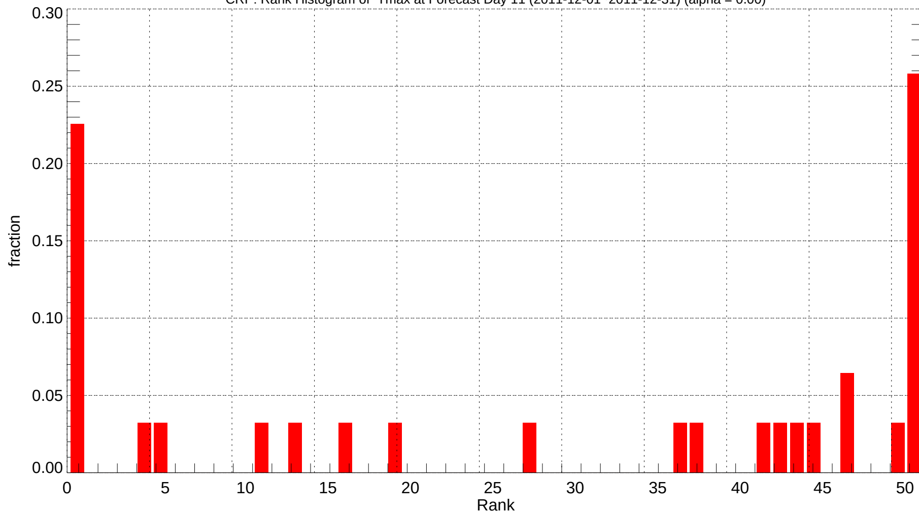
CRP: Rank Histogram of Tmax at Forecast Day 11 (2011-12-01~2011-12-31) (alpha = 0.00)
