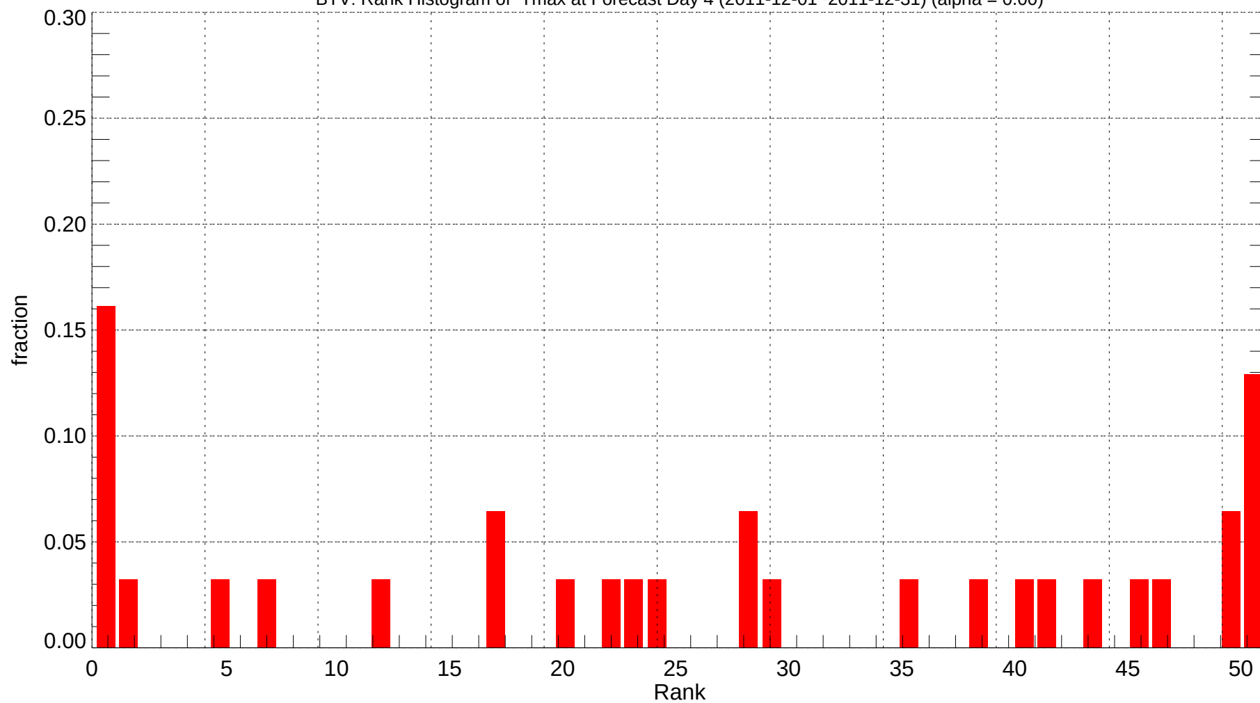
BTV: Rank Histogram of Tmax at Forecast Day 4 (2011-12-01~2011-12-31) (alpha = 0.00)
