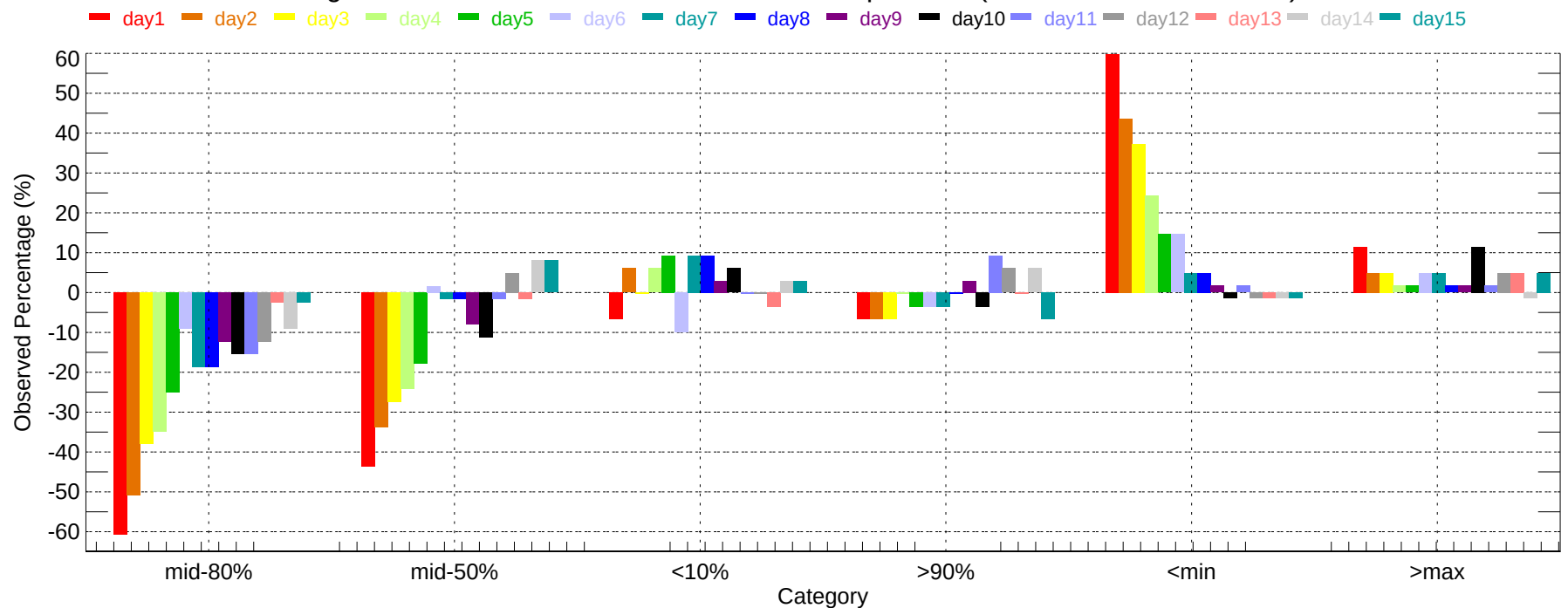
Observed Percentage Deviation of Ensembles - BOS: Min Temperature (2011-12-01~2011-12-31)
