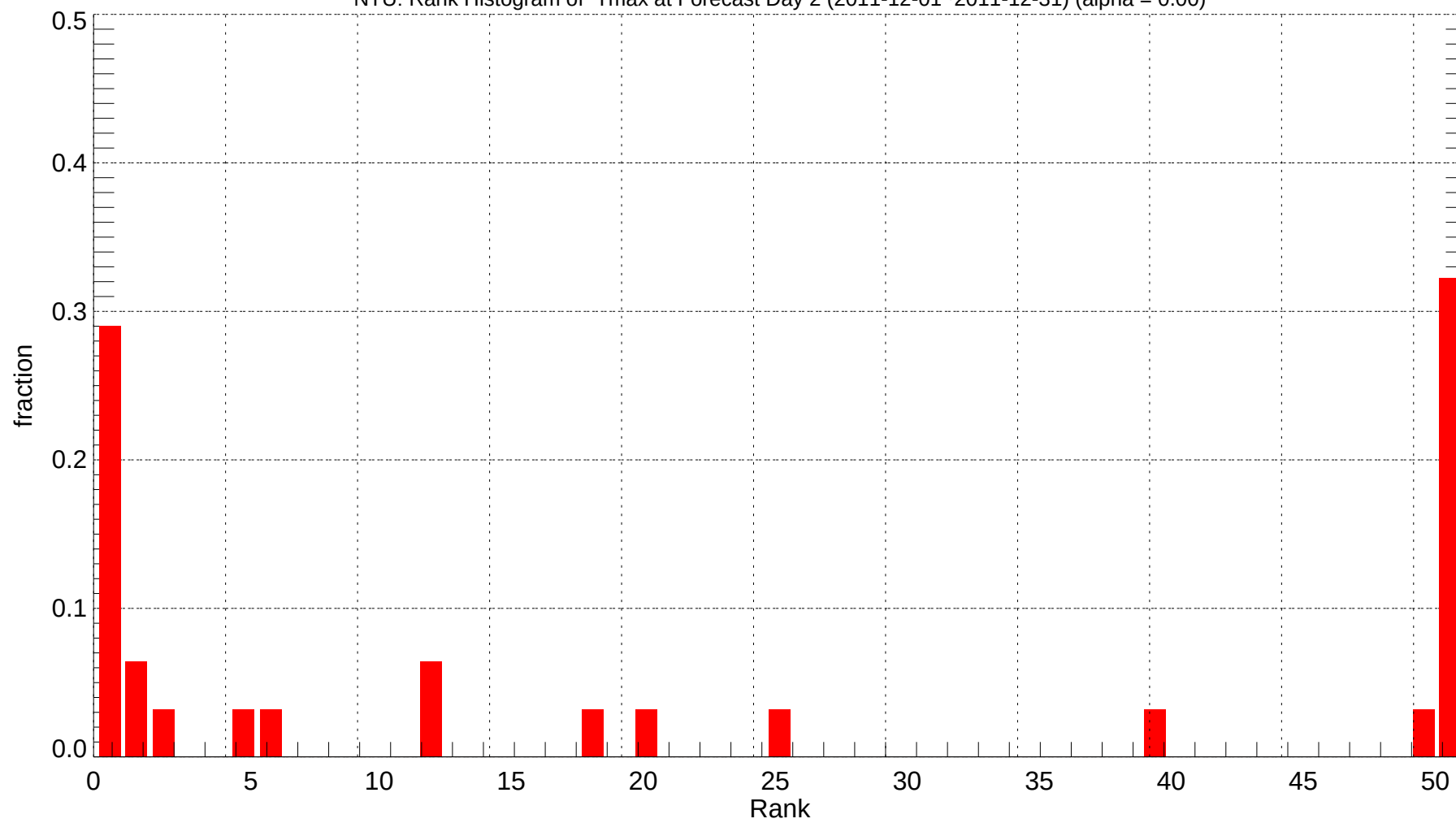
NTU: Rank Histogram of Tmax at Forecast Day 2 (2011-12-01~2011-12-31) (alpha = 0.00)
