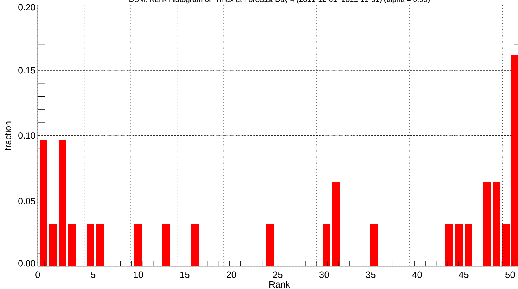
DSM: Rank Histogram of Tmax at Forecast Day 4 (2011-12-01~2011-12-31) (alpha = 0.00)
