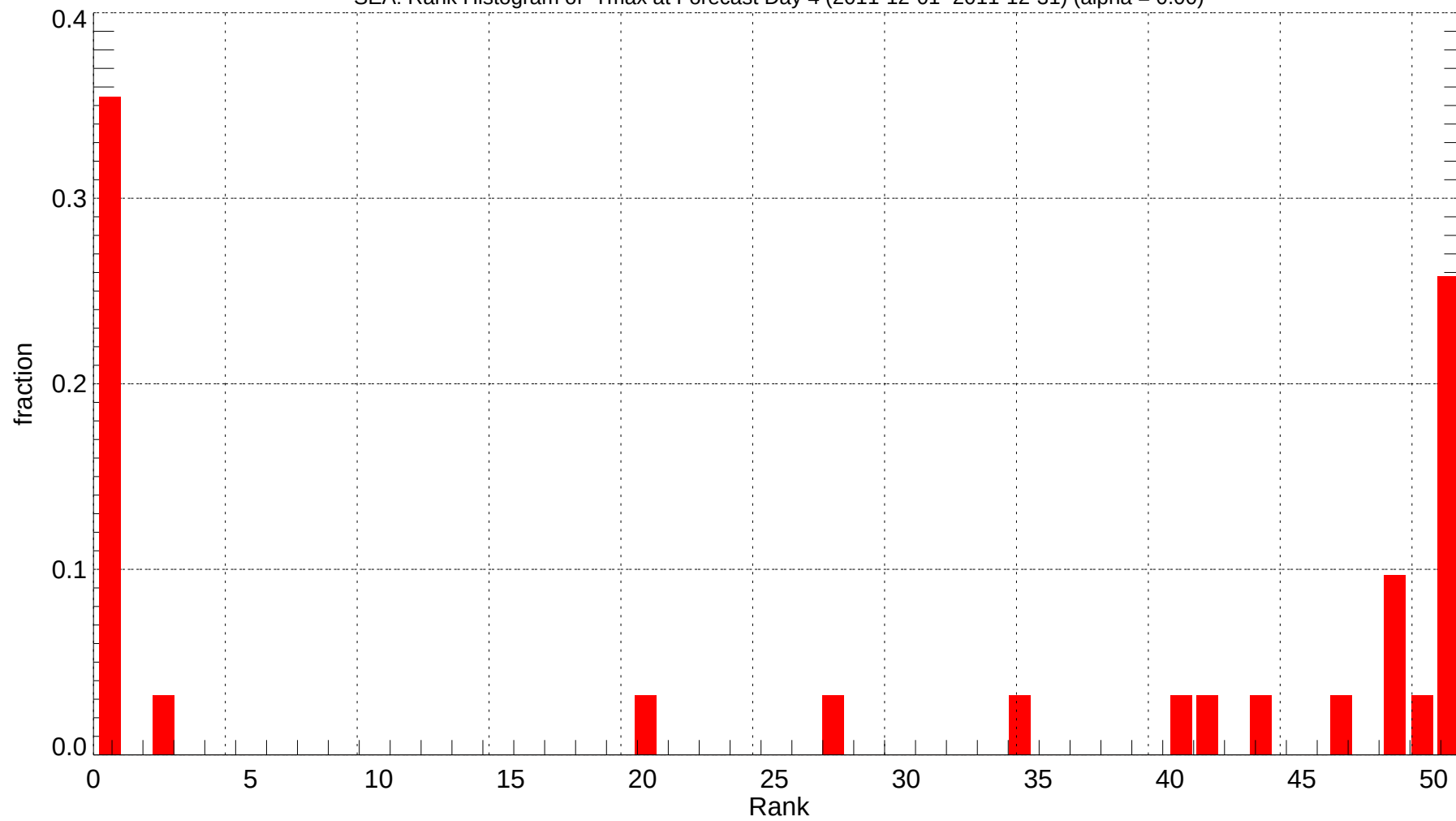
SEA: Rank Histogram of Tmax at Forecast Day 4 (2011-12-01~2011-12-31) (alpha = 0.00)
