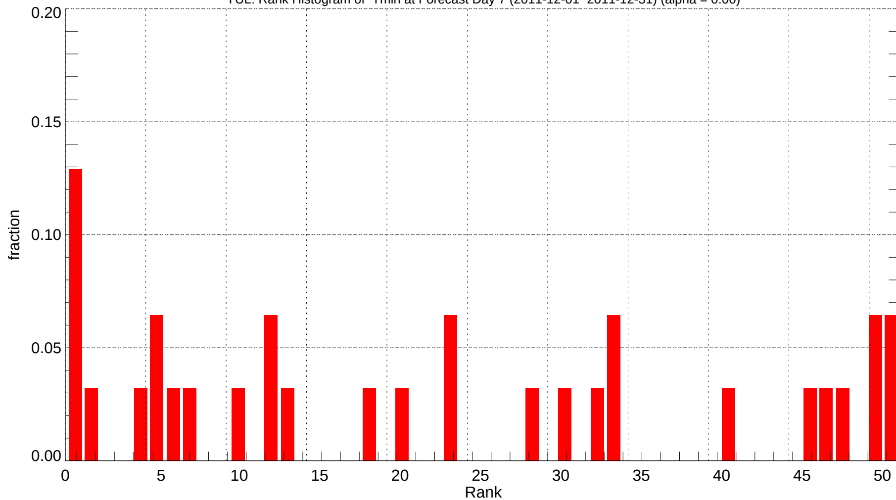
YUL: Rank Histogram of Tmin at Forecast Day 7 (2011-12-01~2011-12-31) (alpha = 0.00)
