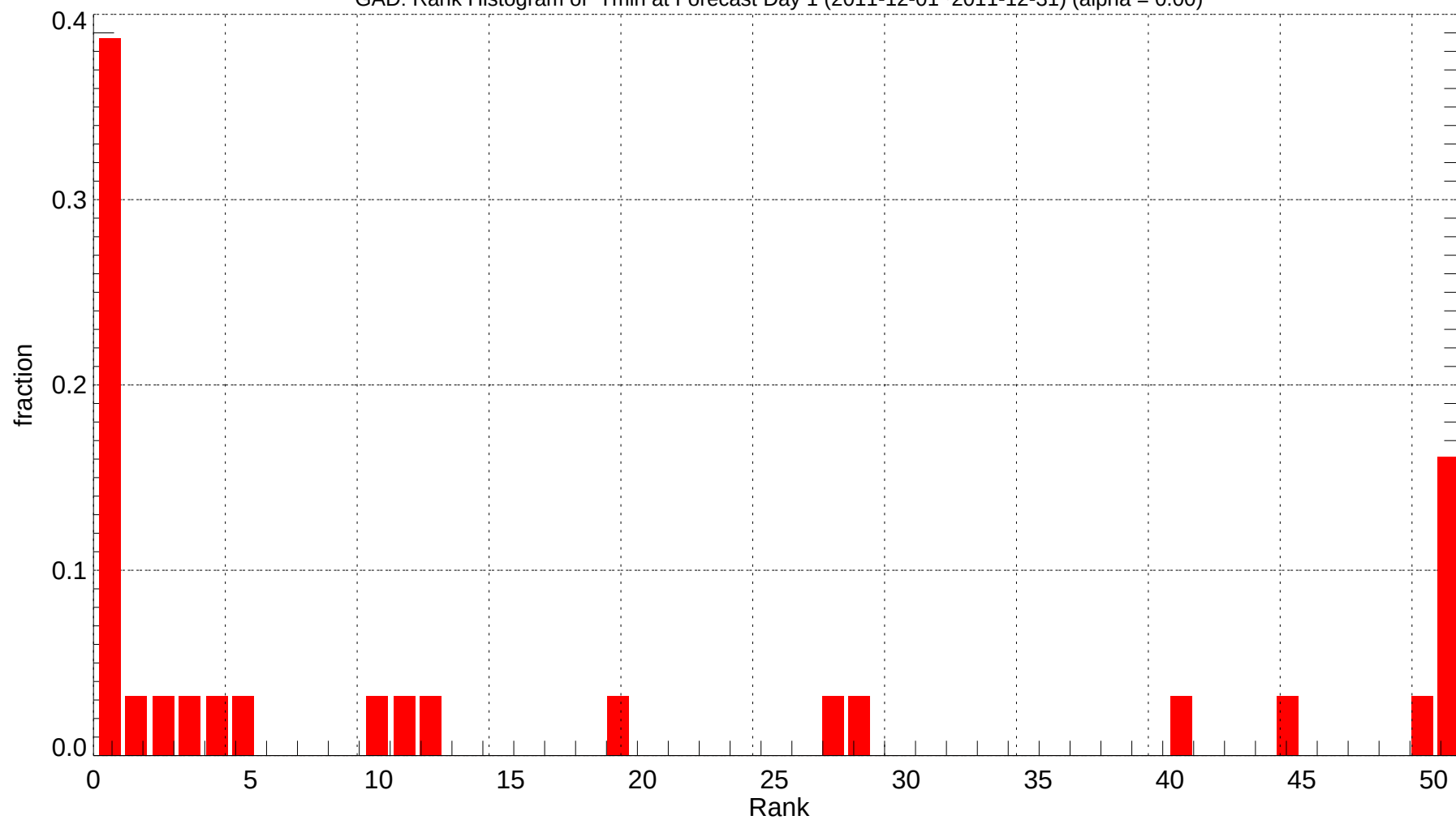
GAD: Rank Histogram of Tmin at Forecast Day 1 (2011-12-01~2011-12-31) (alpha = 0.00)
