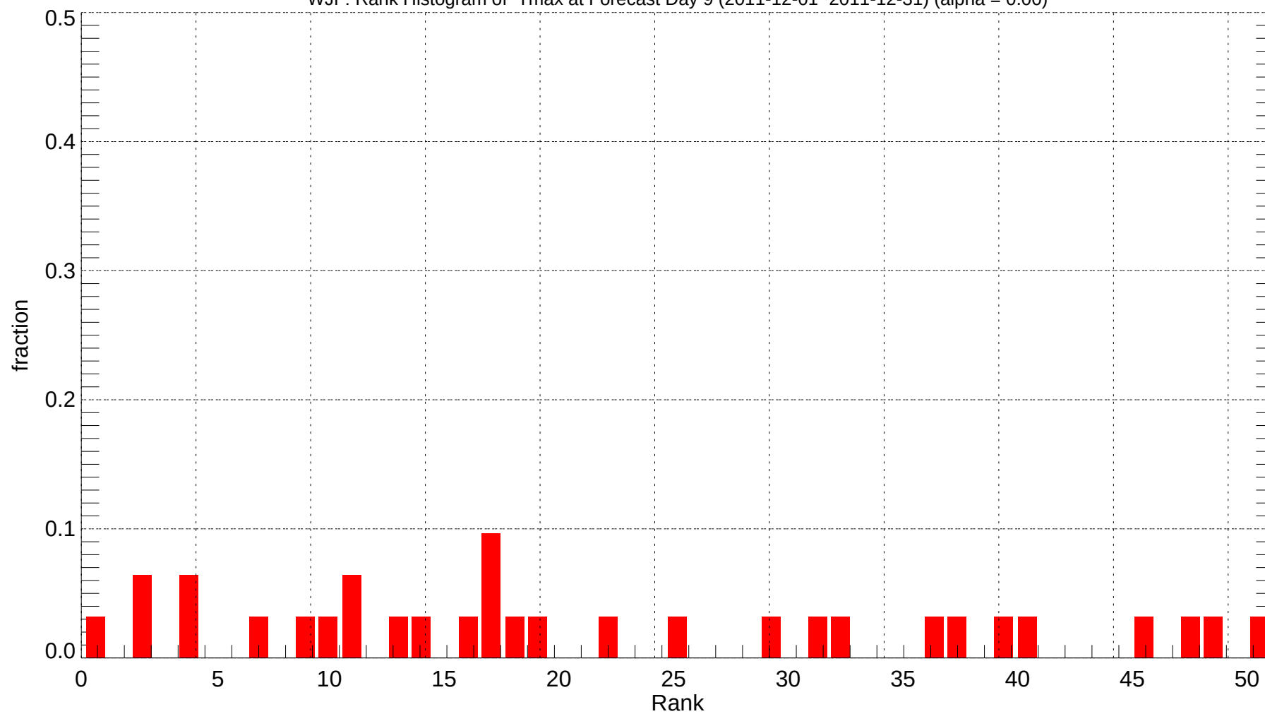
WJF: Rank Histogram of Tmax at Forecast Day 9 (2011-12-01~2011-12-31) (alpha = 0.00)
