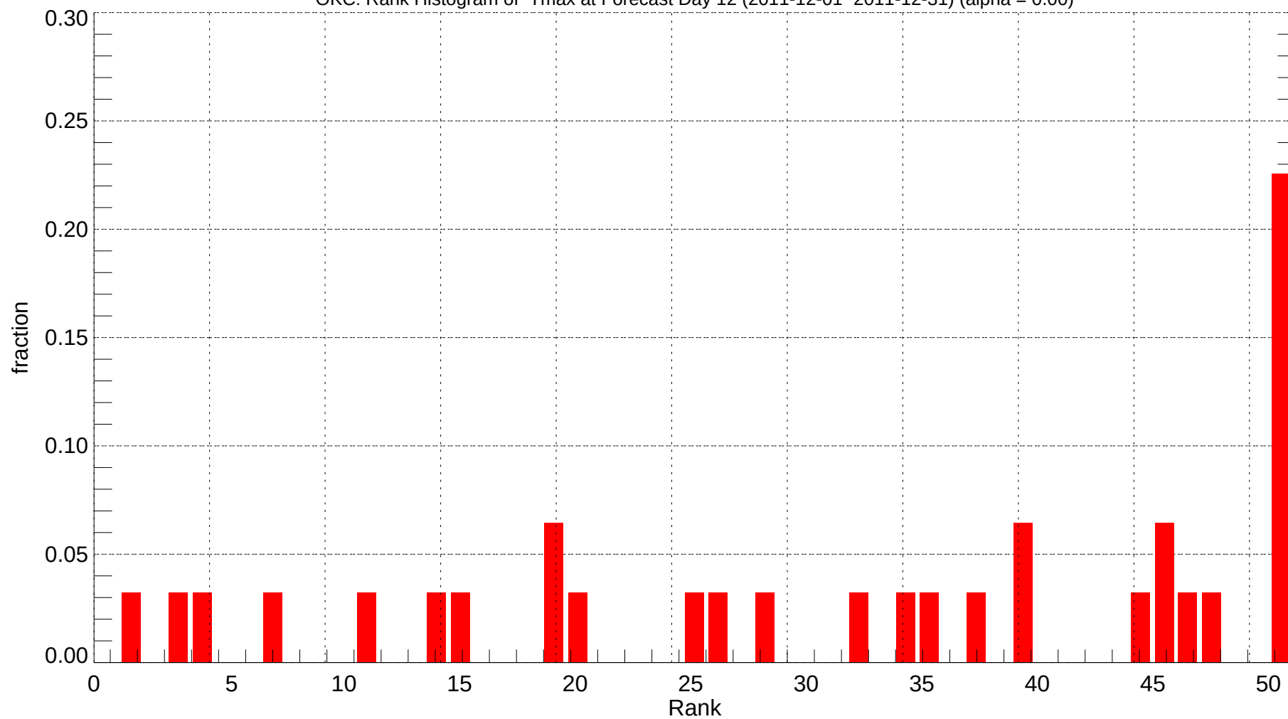
OKC: Rank Histogram of Tmax at Forecast Day 12 (2011-12-01~2011-12-31) (alpha = 0.00)
