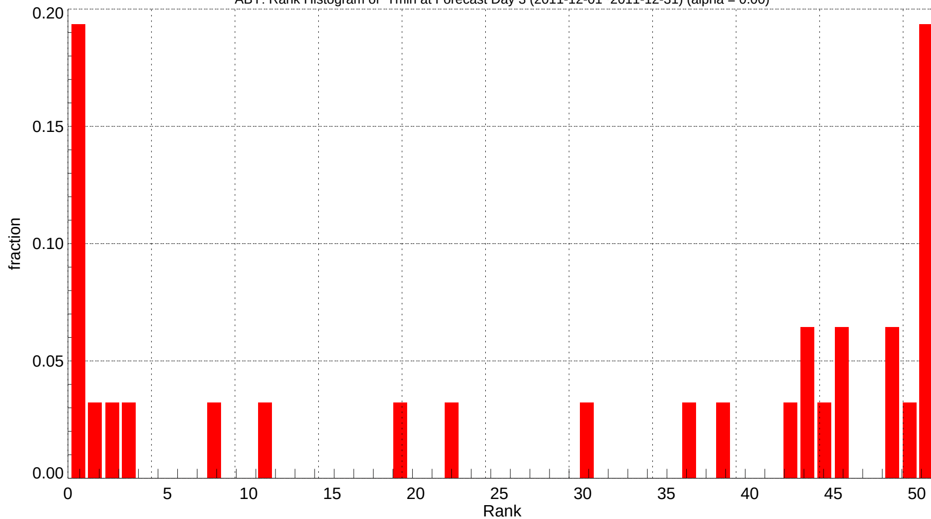
ABY: Rank Histogram of Tmin at Forecast Day 3 (2011-12-01~2011-12-31) (alpha = 0.00)
