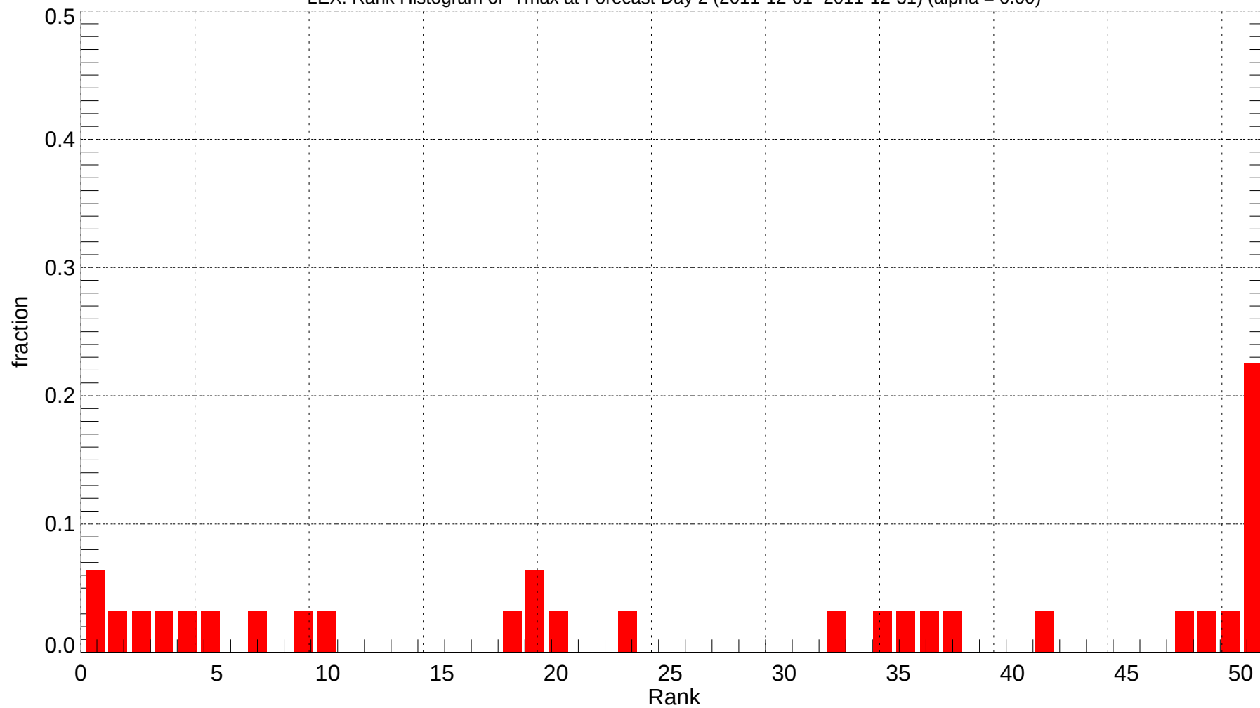
LEX: Rank Histogram of Tmax at Forecast Day 2 (2011-12-01~2011-12-31) (alpha = 0.00)
