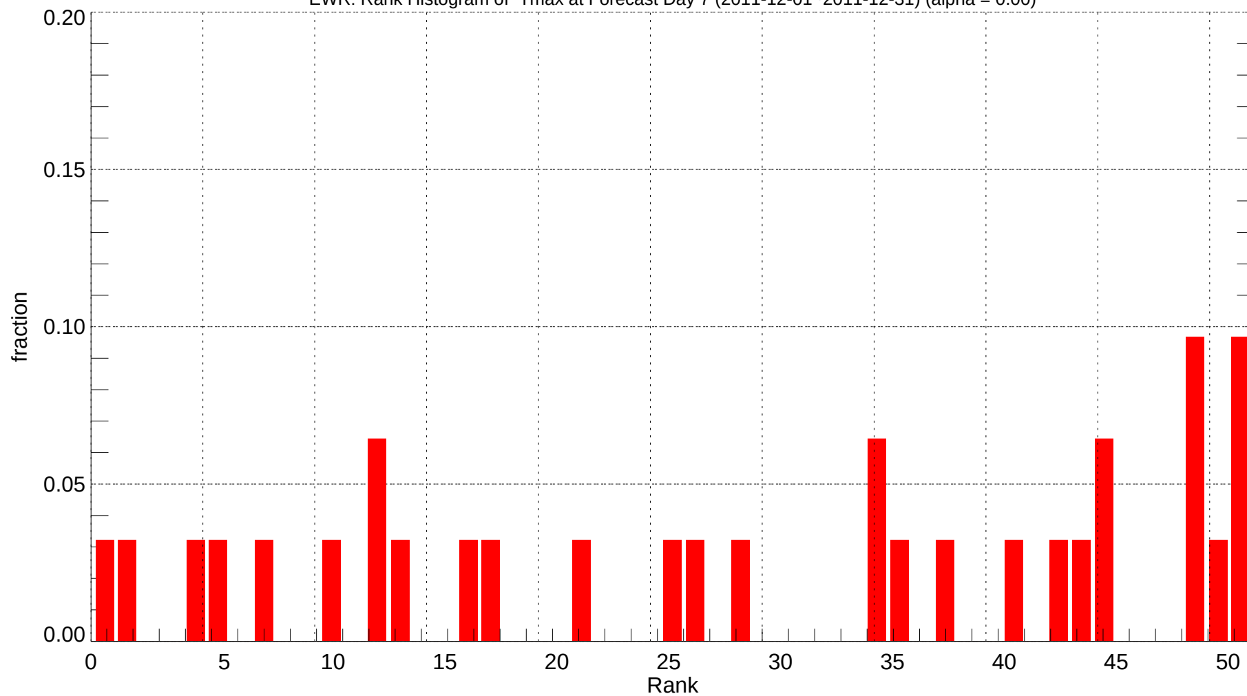
EWR: Rank Histogram of Tmax at Forecast Day 7 (2011-12-01~2011-12-31) (alpha = 0.00)
