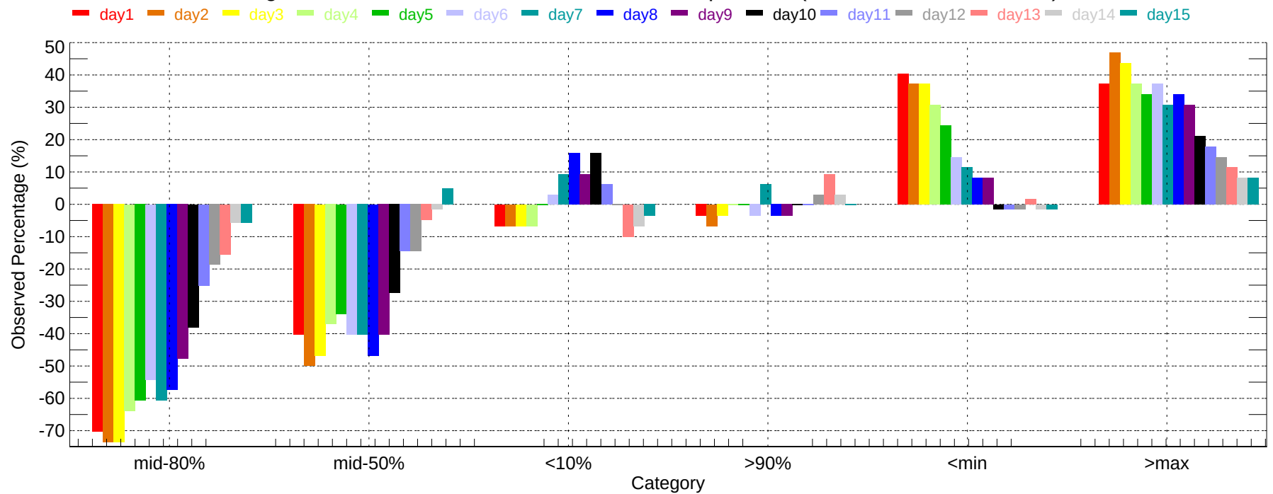
Observed Percentage Deviation of Ensembles - YVR: Max Temperature (2011-12-01~2011-12-31)
