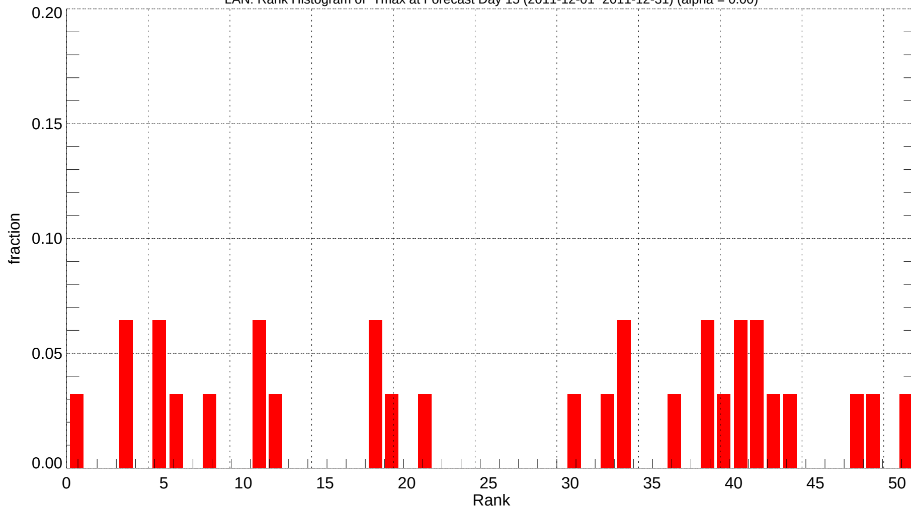
LAN: Rank Histogram of Tmax at Forecast Day 15 (2011-12-01~2011-12-31) (alpha = 0.00)
