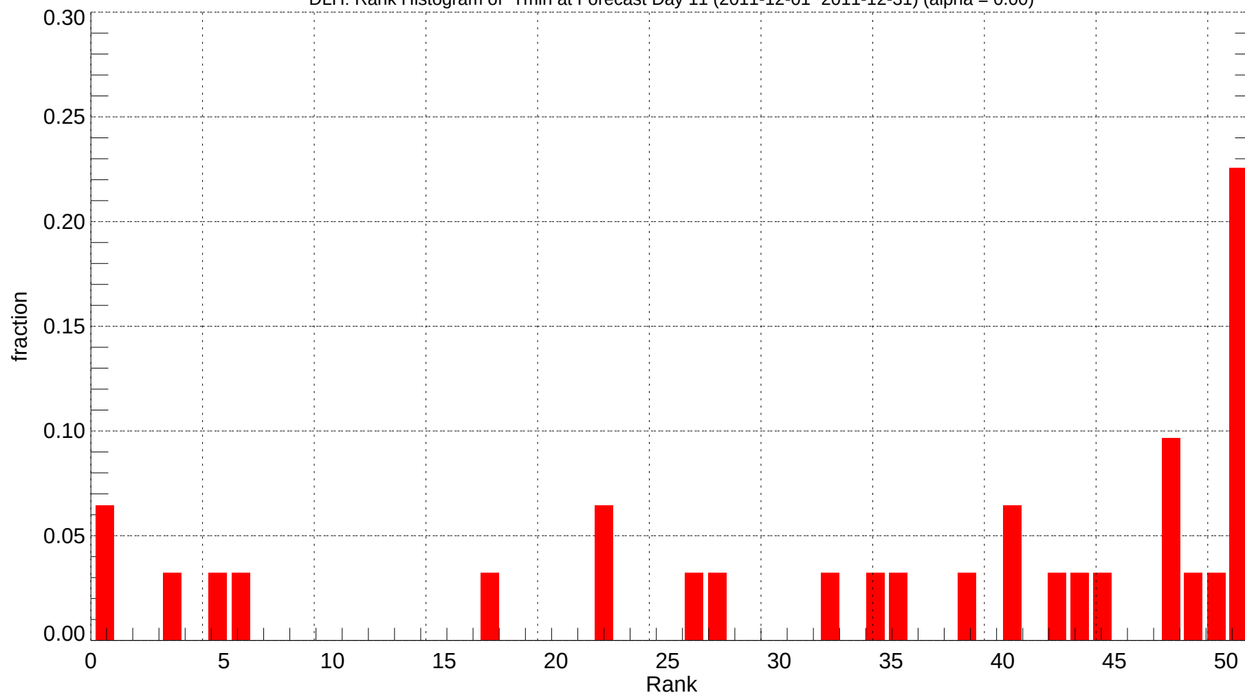
DLH: Rank Histogram of Tmin at Forecast Day 11 (2011-12-01~2011-12-31) (alpha = 0.00)
