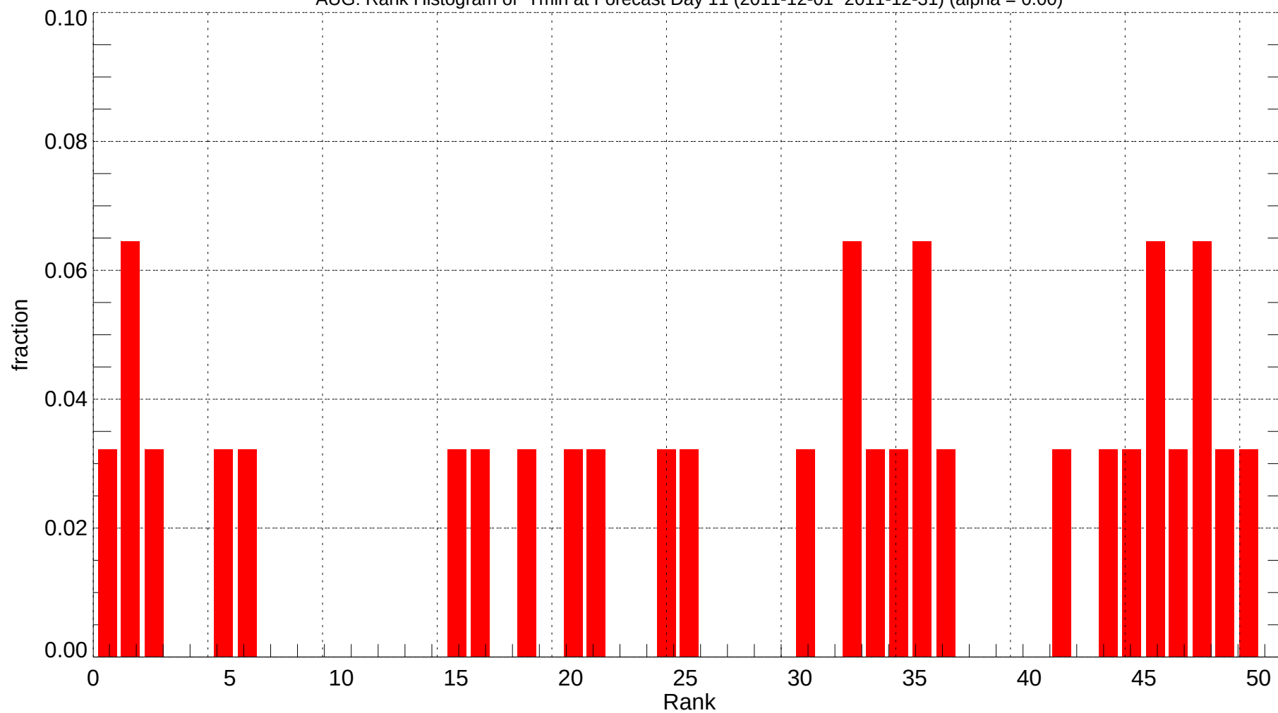
AUG: Rank Histogram of Tmin at Forecast Day 11 (2011-12-01~2011-12-31) (alpha = 0.00)
