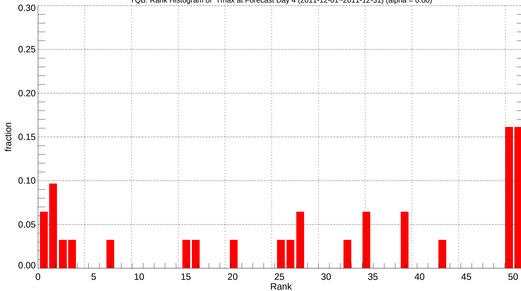
YQB: Rank Histogram of Tmax at Forecast Day 4 (2011-12-01~2011-12-31) (alpha = 0.00)
