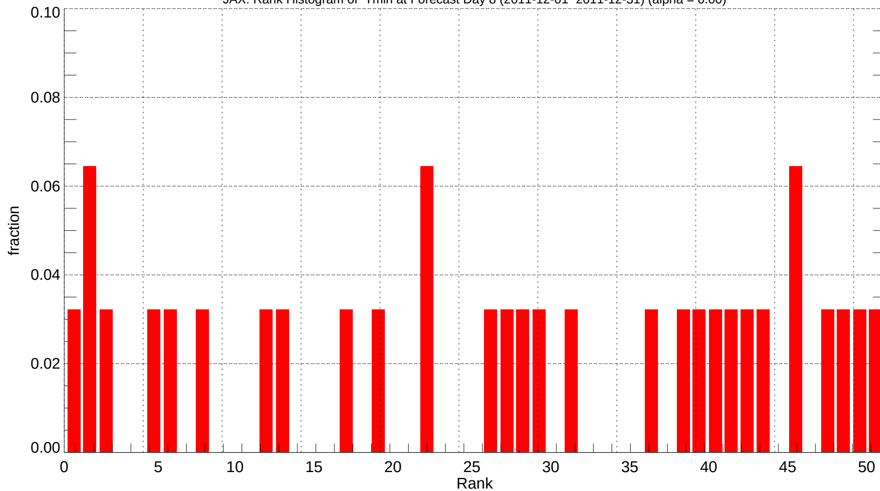
JAX: Rank Histogram of Tmin at Forecast Day 8 (2011-12-01~2011-12-31) (alpha = 0.00)
