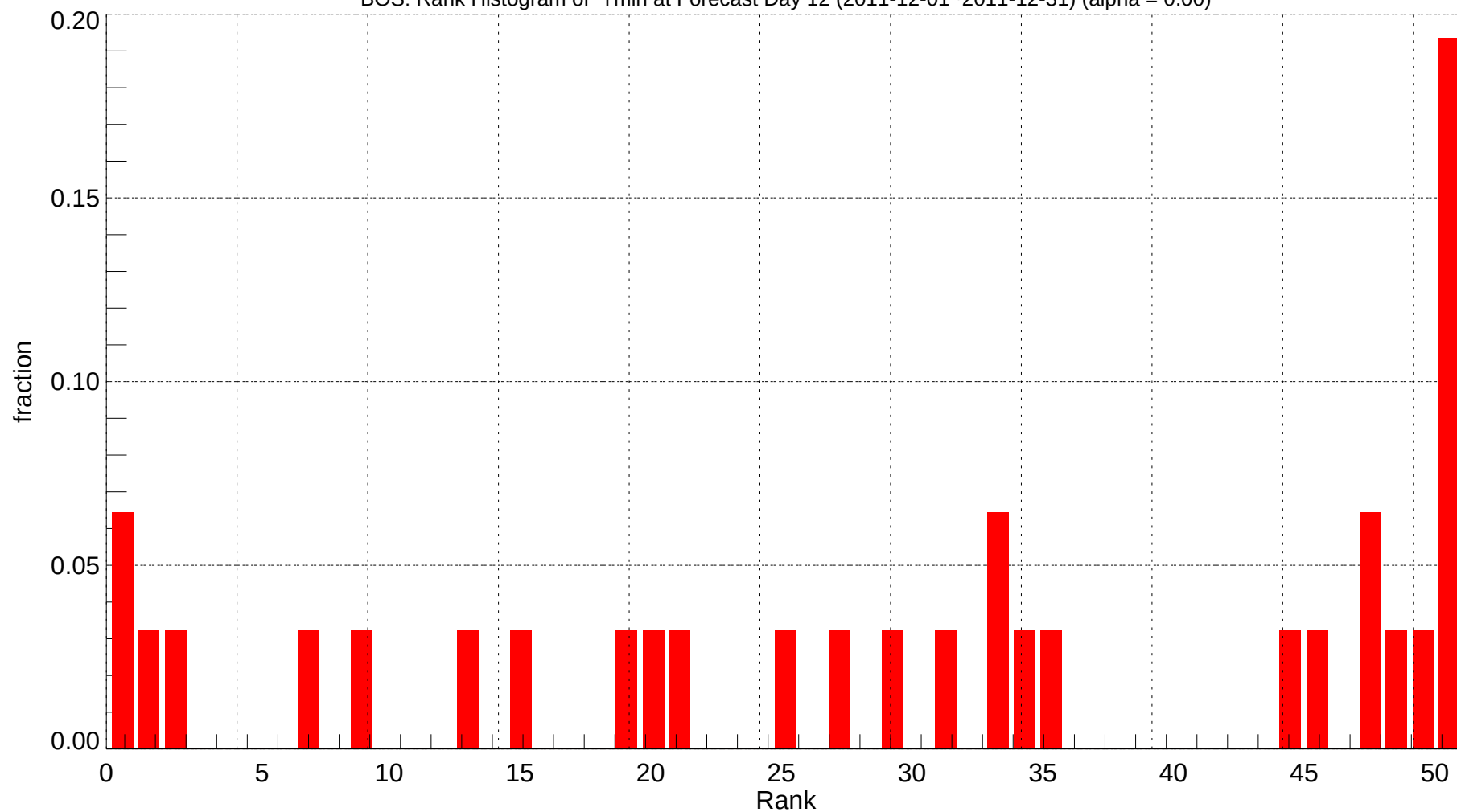
BOS: Rank Histogram of Tmin at Forecast Day 12 (2011-12-01~2011-12-31) (alpha = 0.00)
