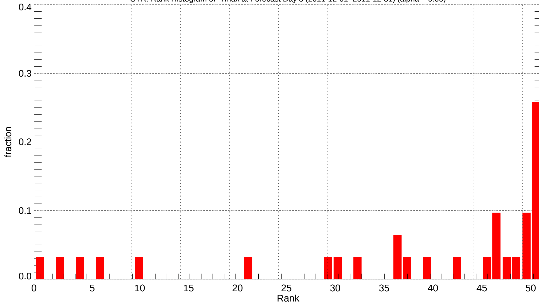
SYR: Rank Histogram of Tmax at Forecast Day 3 (2011-12-01~2011-12-31) (alpha = 0.00)
