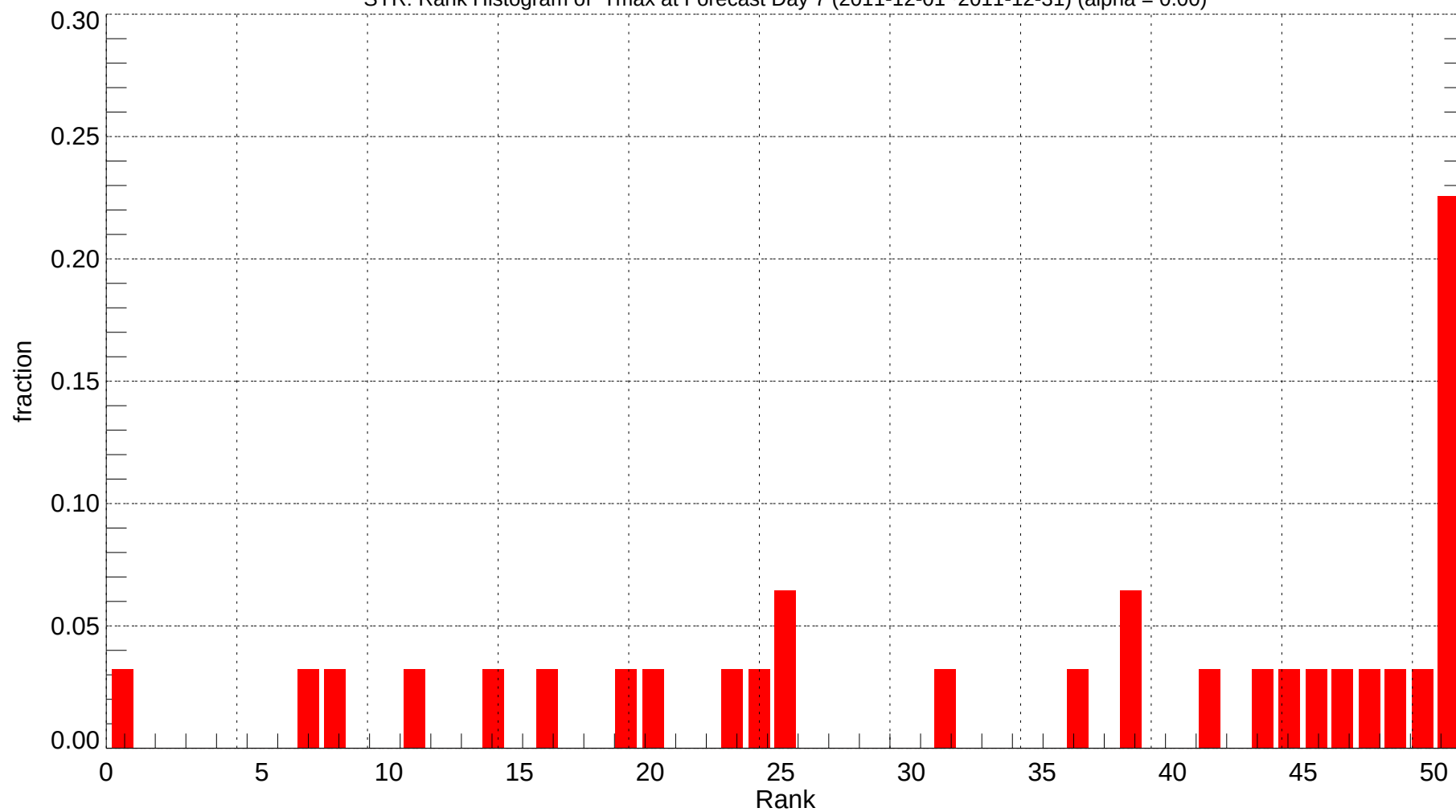
SYR: Rank Histogram of Tmax at Forecast Day 7 (2011-12-01~2011-12-31) (alpha = 0.00)
