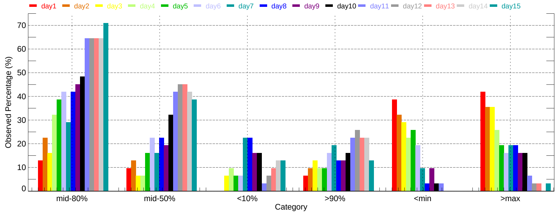
Observed Percentage of Ensembles - YQB: Min Temperature (2011-12-01~2011-12-31)
