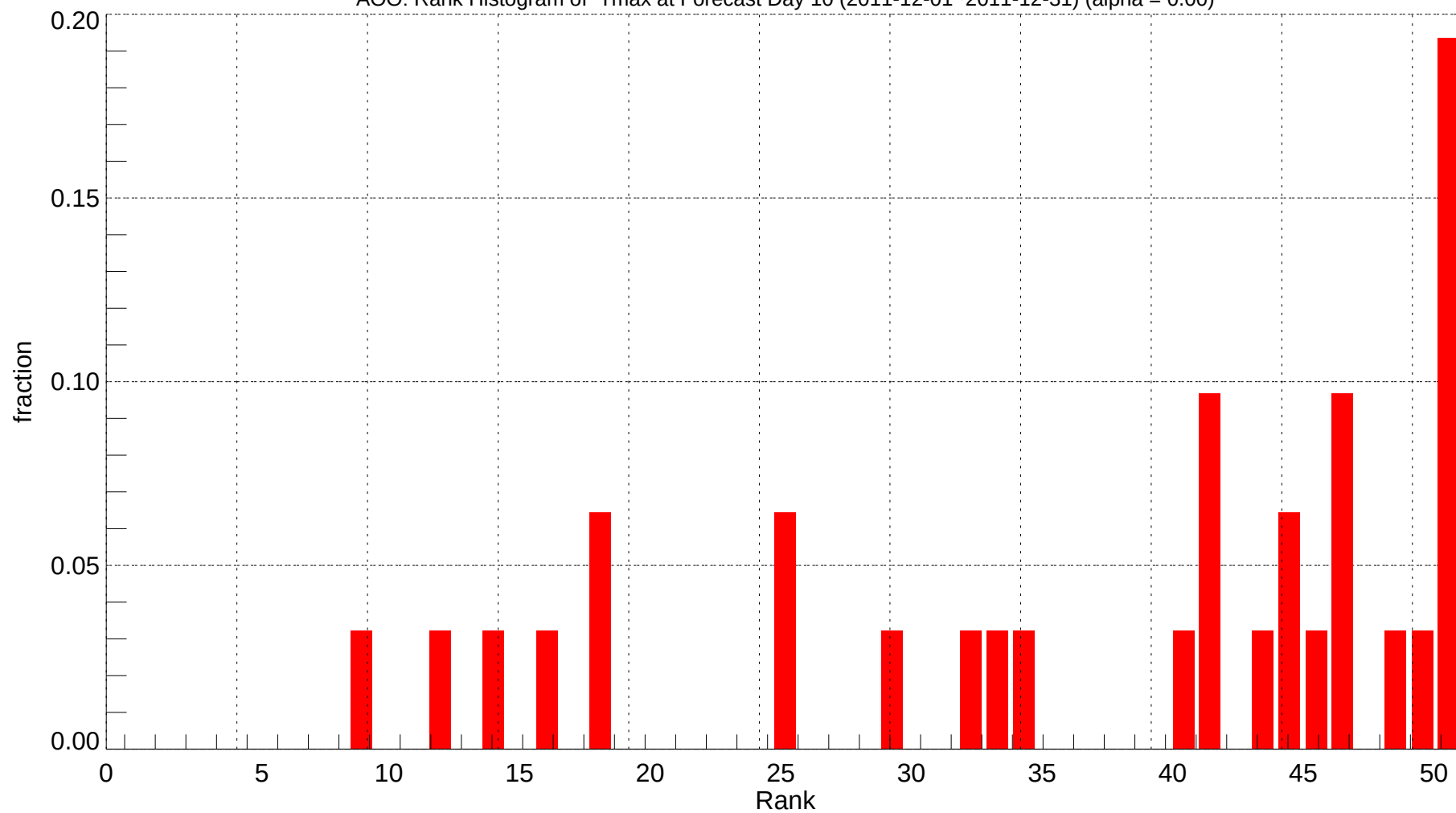
AOO: Rank Histogram of Tmax at Forecast Day 10 (2011-12-01~2011-12-31) (alpha = 0.00)
