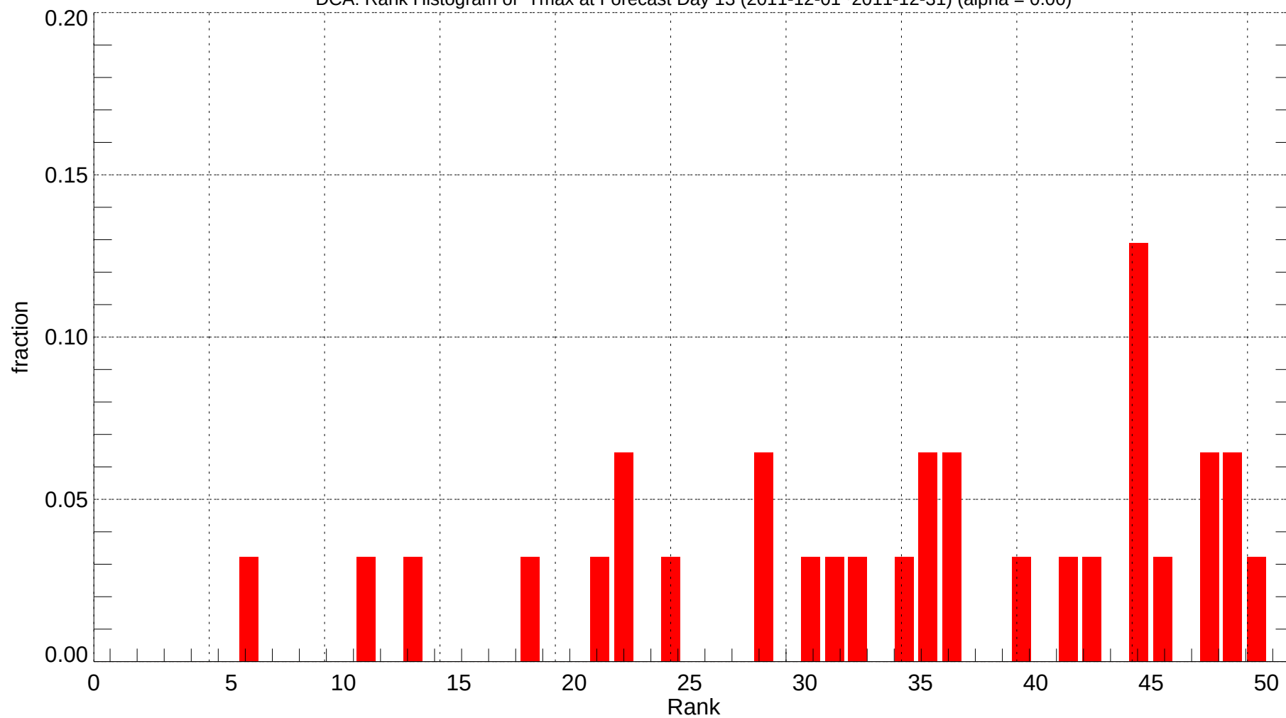
DCA: Rank Histogram of Tmax at Forecast Day 13 (2011-12-01~2011-12-31) (alpha = 0.00)
