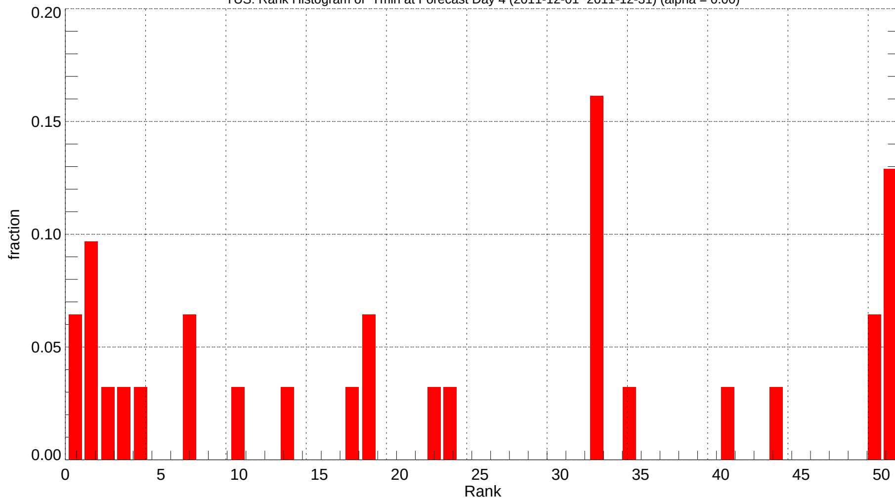
TUS: Rank Histogram of Tmin at Forecast Day 4 (2011-12-01~2011-12-31) (alpha = 0.00)
