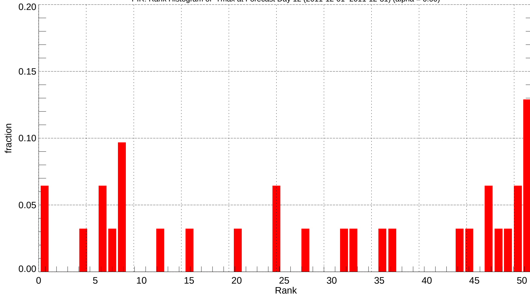
PIR: Rank Histogram of Tmax at Forecast Day 12 (2011-12-01~2011-12-31) (alpha = 0.00)
