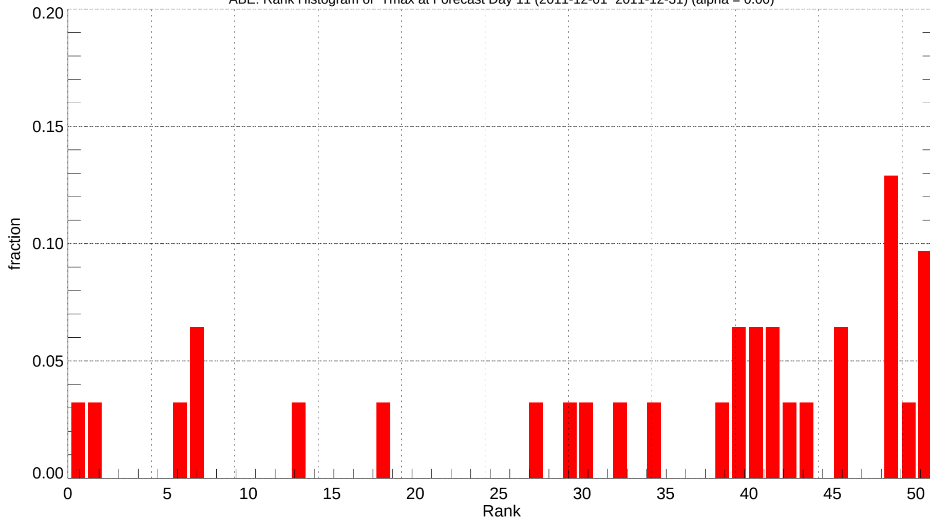
ABE: Rank Histogram of Tmax at Forecast Day 11 (2011-12-01~2011-12-31) (alpha = 0.00)
