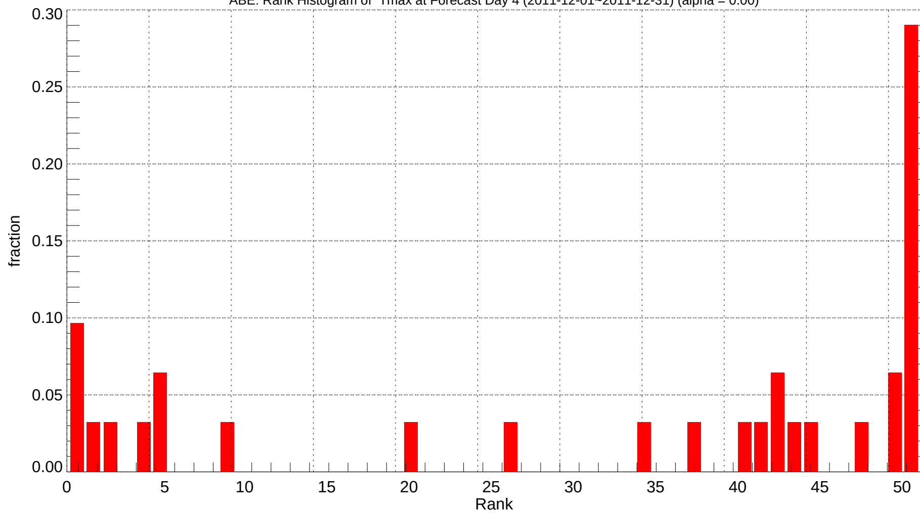
ABE: Rank Histogram of Tmax at Forecast Day 4 (2011-12-01~2011-12-31) (alpha = 0.00)
