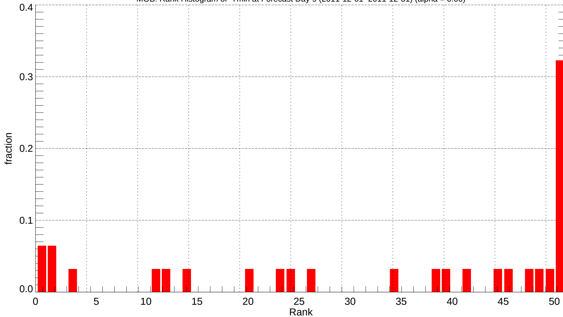
MOB: Rank Histogram of Tmin at Forecast Day 9 (2011-12-01~2011-12-31) (alpha = 0.00)
