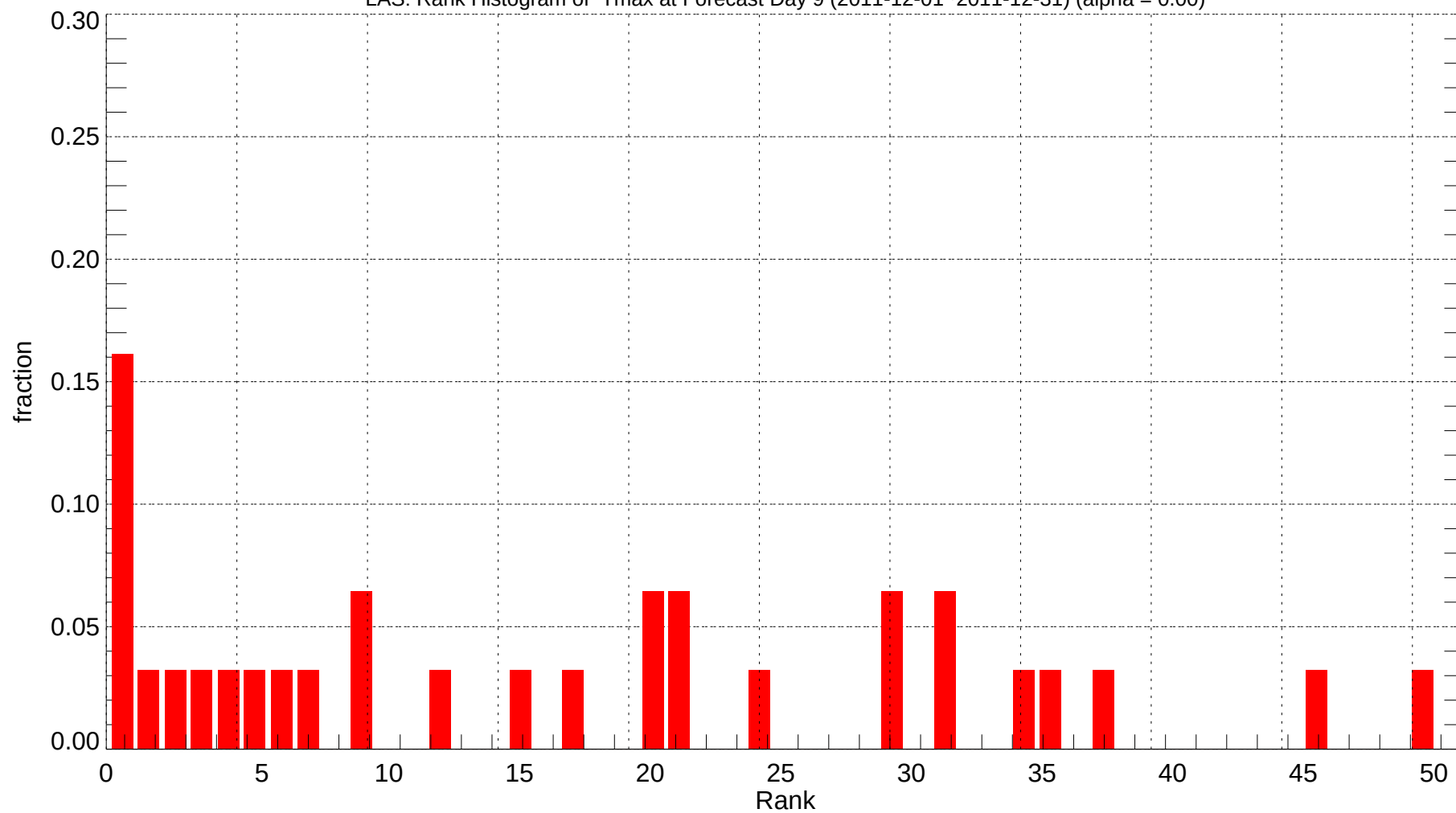
LAS: Rank Histogram of Tmax at Forecast Day 9 (2011-12-01~2011-12-31) (alpha = 0.00)
