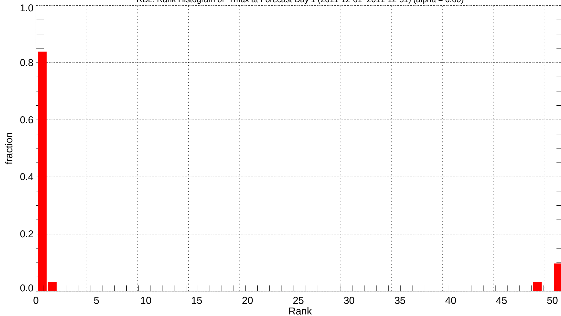
RBL: Rank Histogram of Tmax at Forecast Day 1 (2011-12-01~2011-12-31) (alpha = 0.00)
