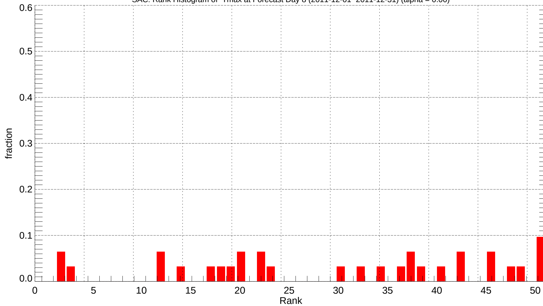
SAC: Rank Histogram of Tmax at Forecast Day 8 (2011-12-01~2011-12-31) (alpha = 0.00)
