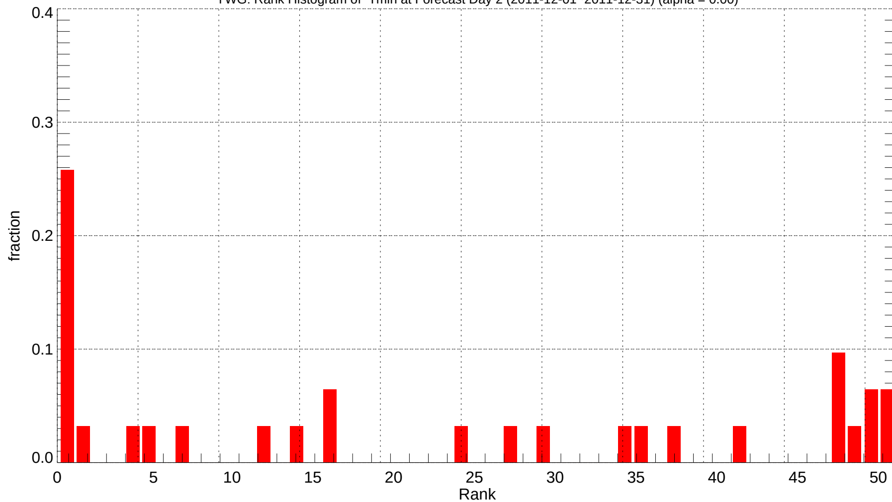
YWG: Rank Histogram of Tmin at Forecast Day 2 (2011-12-01~2011-12-31) (alpha = 0.00)
