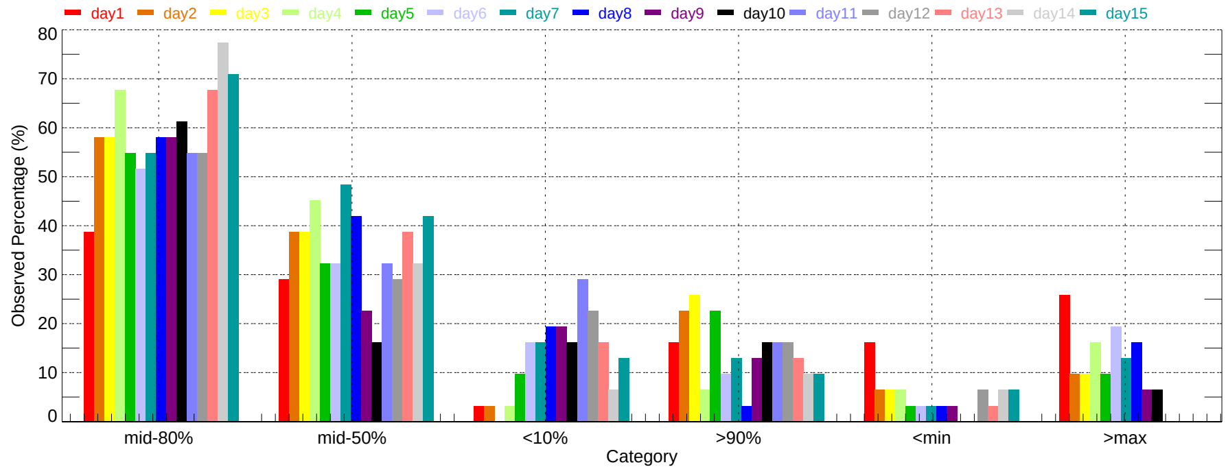
Observed Percentage of Ensembles - TUS: Min Temperature (2011-12-01~2011-12-31)
