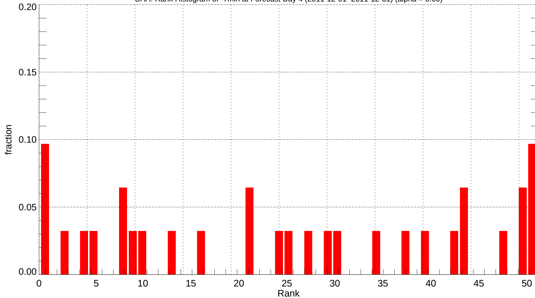
CHA: Rank Histogram of Tmin at Forecast Day 4 (2011-12-01~2011-12-31) (alpha = 0.00)
