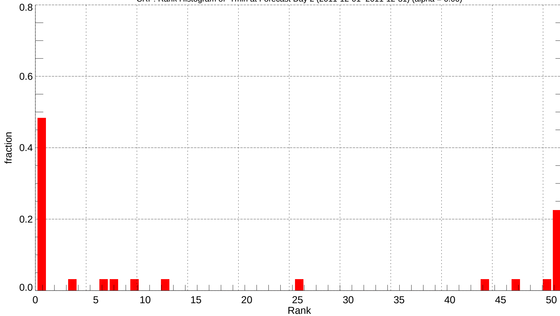
CRP: Rank Histogram of Tmin at Forecast Day 2 (2011-12-01~2011-12-31) (alpha = 0.00)
