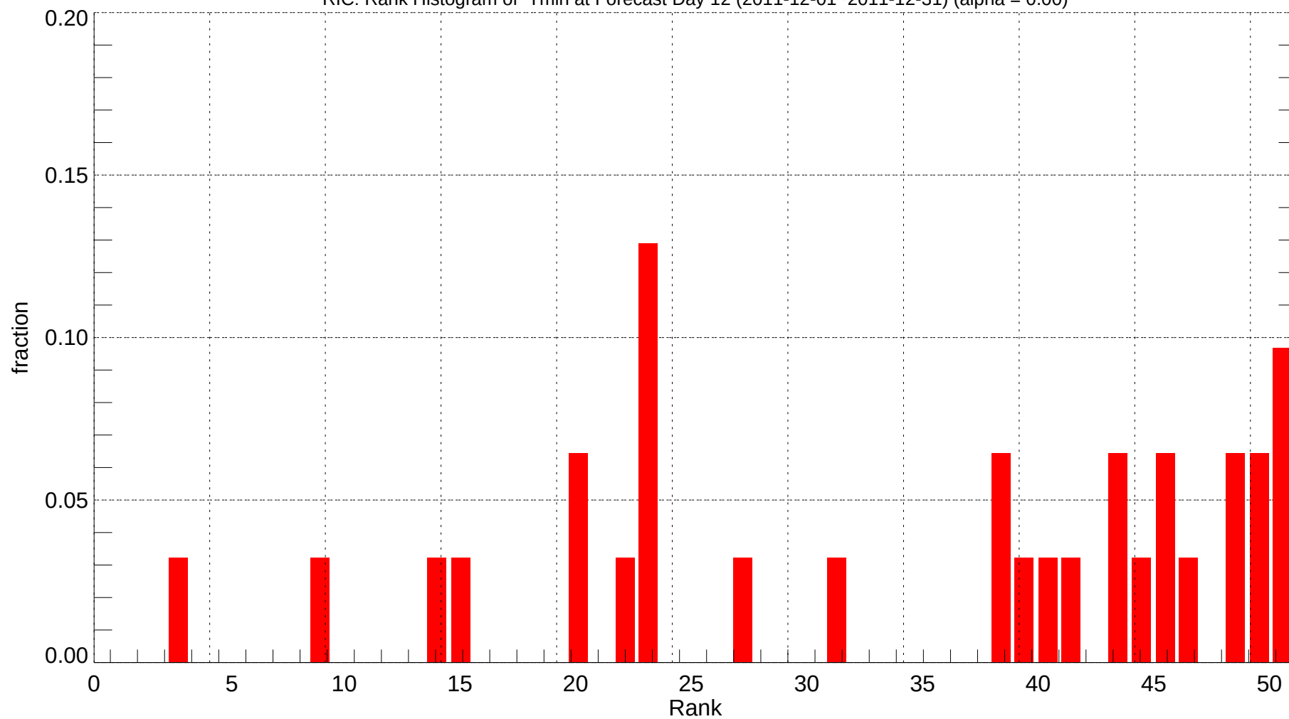
RIC: Rank Histogram of Tmin at Forecast Day 12 (2011-12-01~2011-12-31) (alpha = 0.00)
