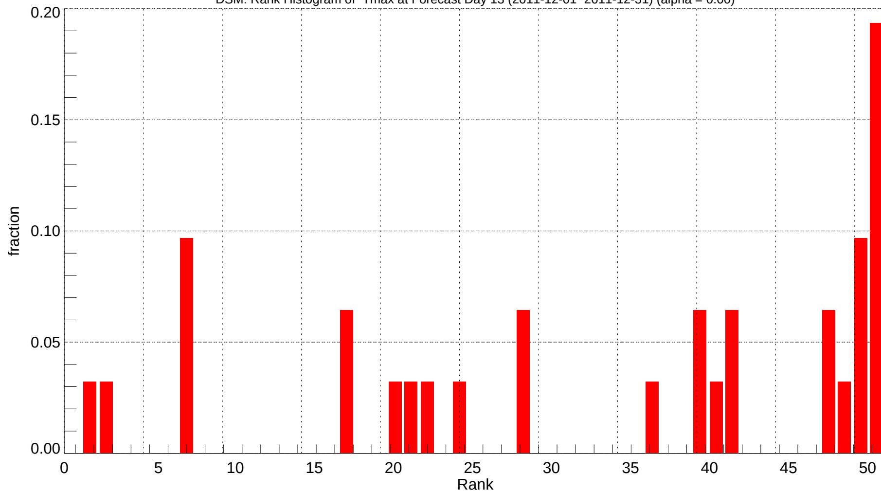
DSM: Rank Histogram of Tmax at Forecast Day 13 (2011-12-01~2011-12-31) (alpha = 0.00)
