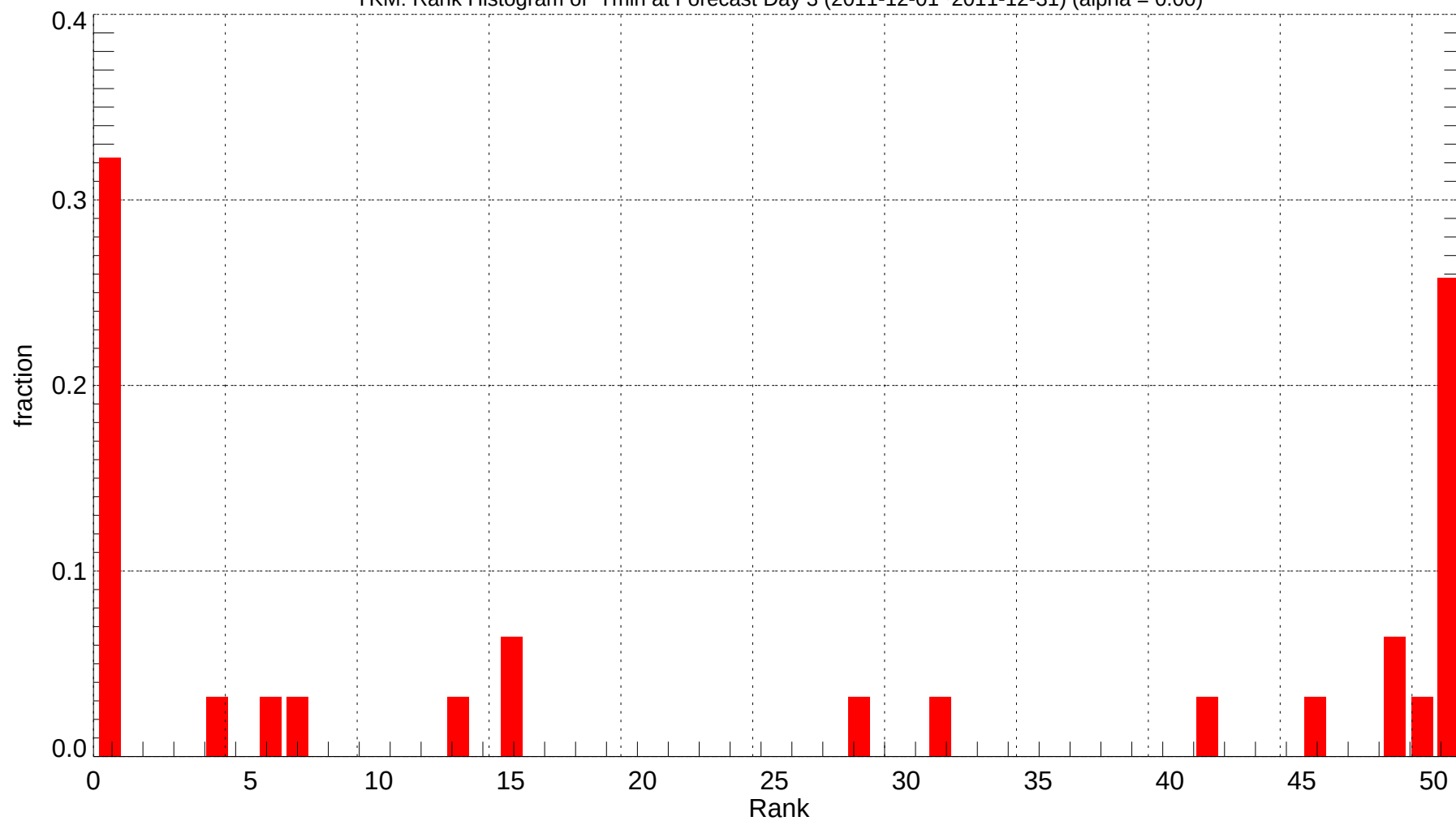
YKM: Rank Histogram of Tmin at Forecast Day 3 (2011-12-01~2011-12-31) (alpha = 0.00)
