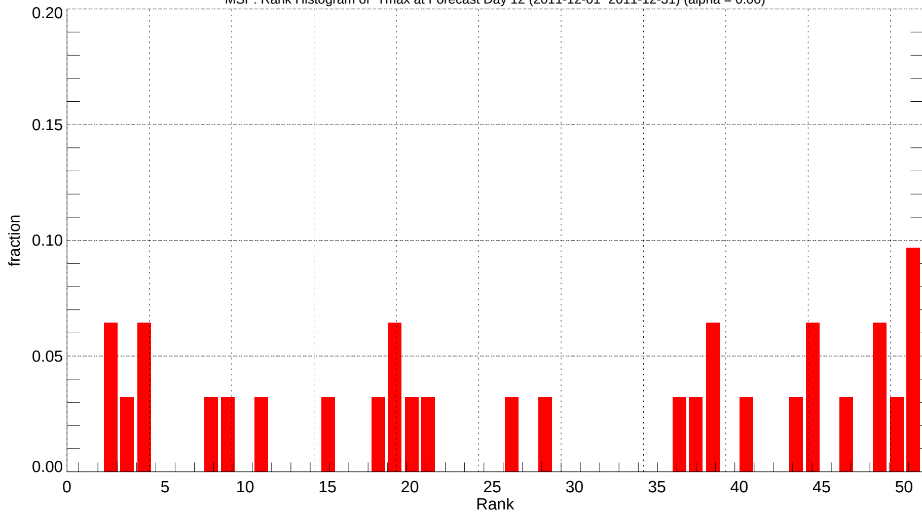
MSP: Rank Histogram of Tmax at Forecast Day 12 (2011-12-01~2011-12-31) (alpha = 0.00)
