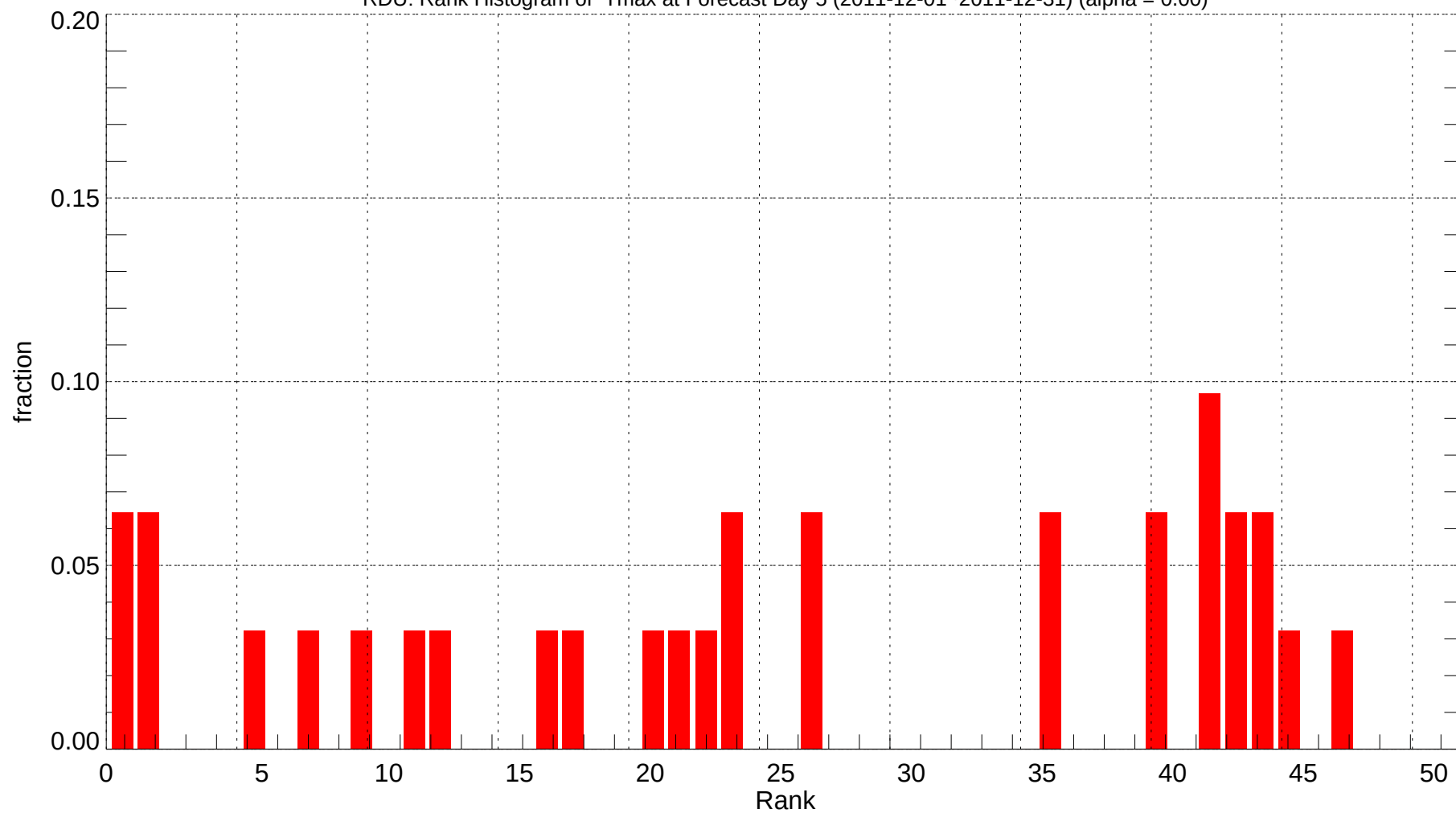
RDU: Rank Histogram of Tmax at Forecast Day 5 (2011-12-01~2011-12-31) (alpha = 0.00)
