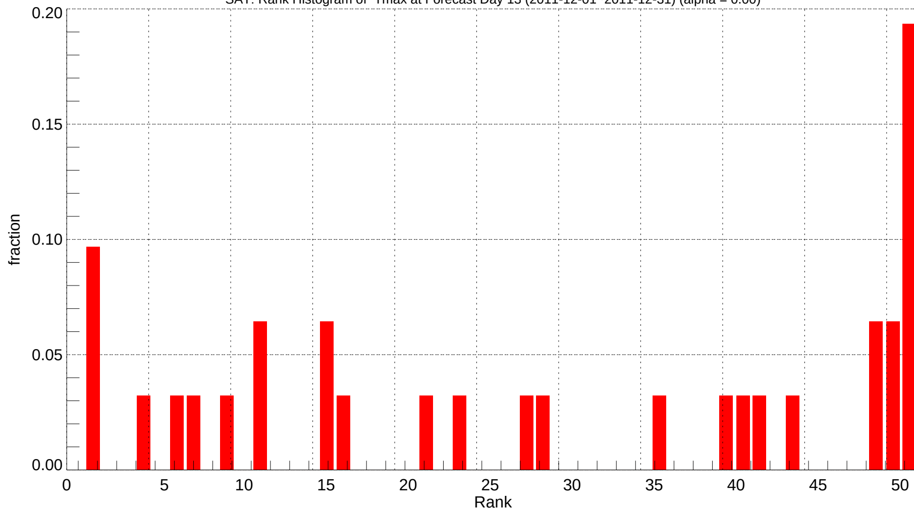
SAT: Rank Histogram of Tmax at Forecast Day 13 (2011-12-01~2011-12-31) (alpha = 0.00)
