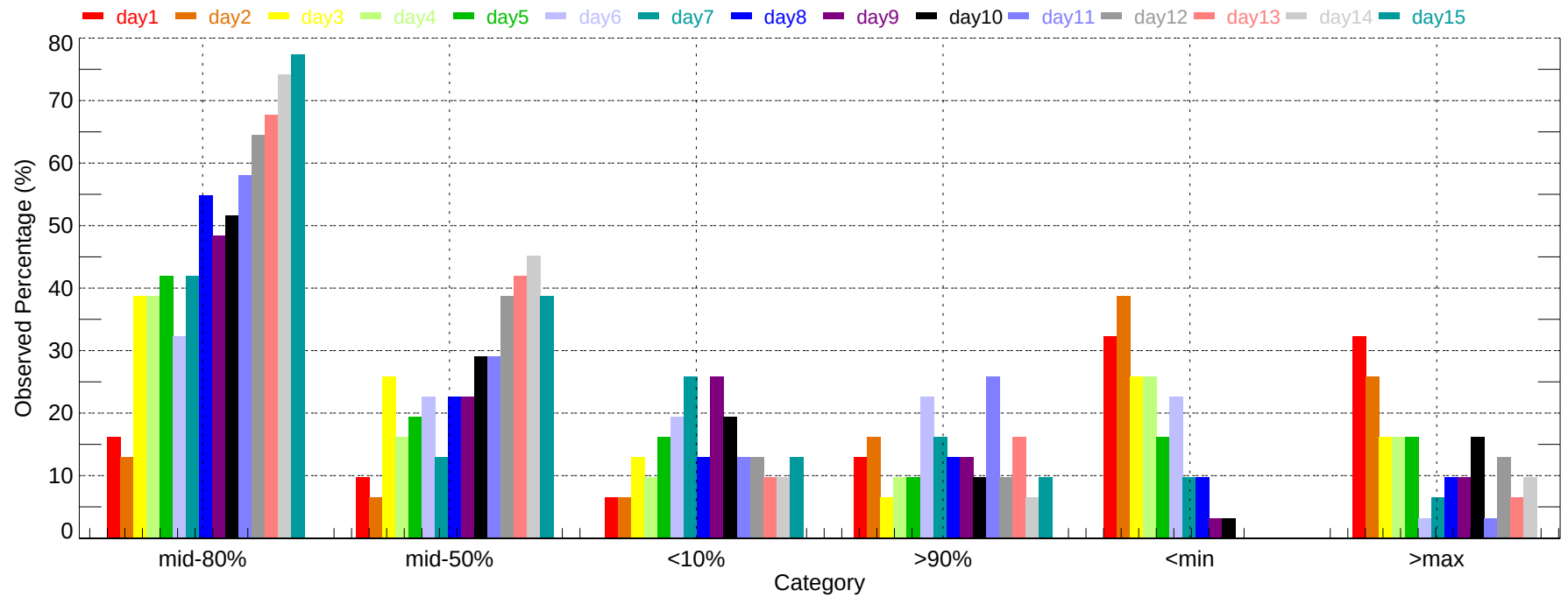
Observed Percentage of Ensembles - LAN: Max Temperature (2011-12-01~2011-12-31)
