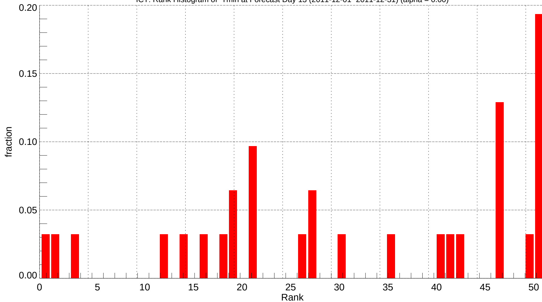
ICT: Rank Histogram of Tmin at Forecast Day 13 (2011-12-01~2011-12-31) (alpha = 0.00)
