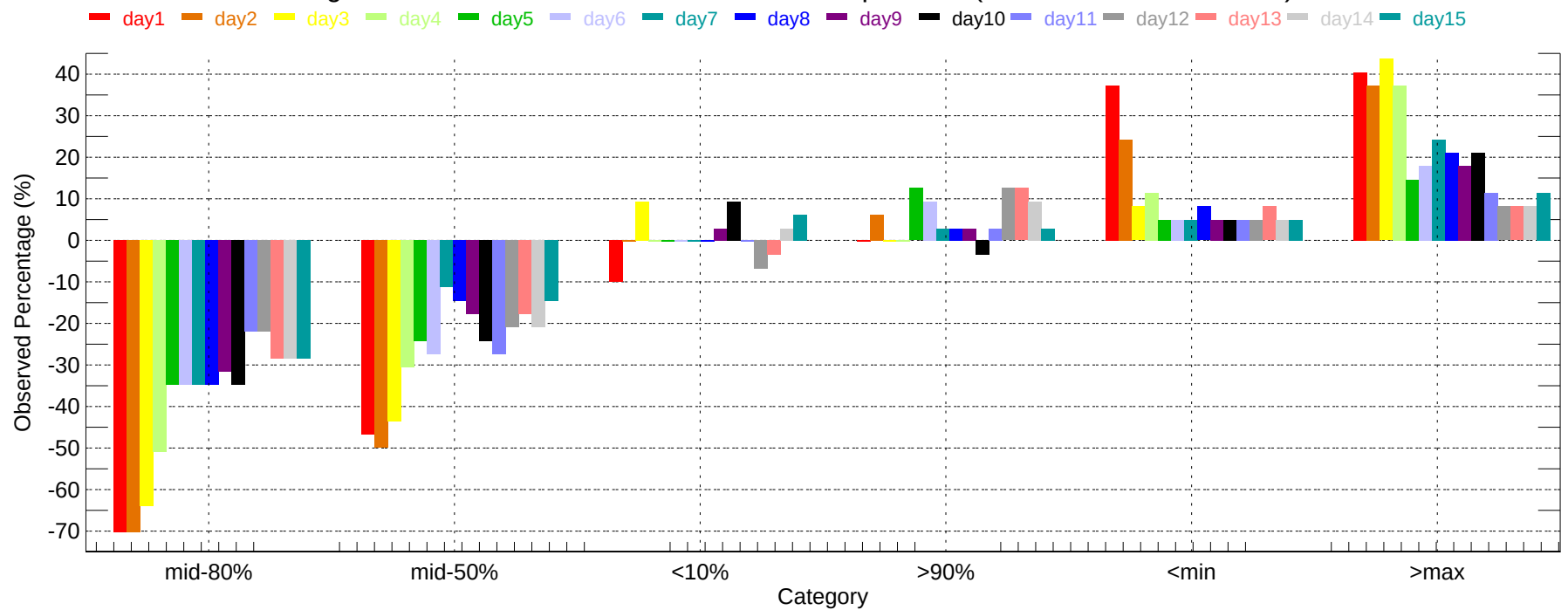
Observed Percentage Deviation of Ensembles - PIR: Max Temperature (2011-12-01~2011-12-31)
