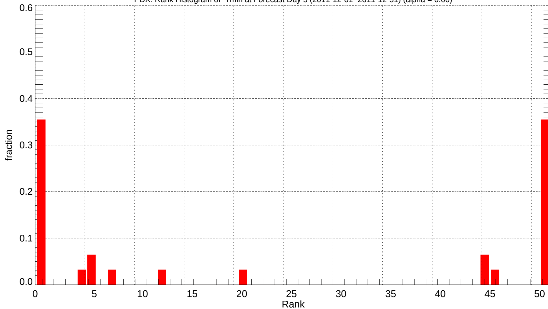
PDX: Rank Histogram of Tmin at Forecast Day 3 (2011-12-01~2011-12-31) (alpha = 0.00)
