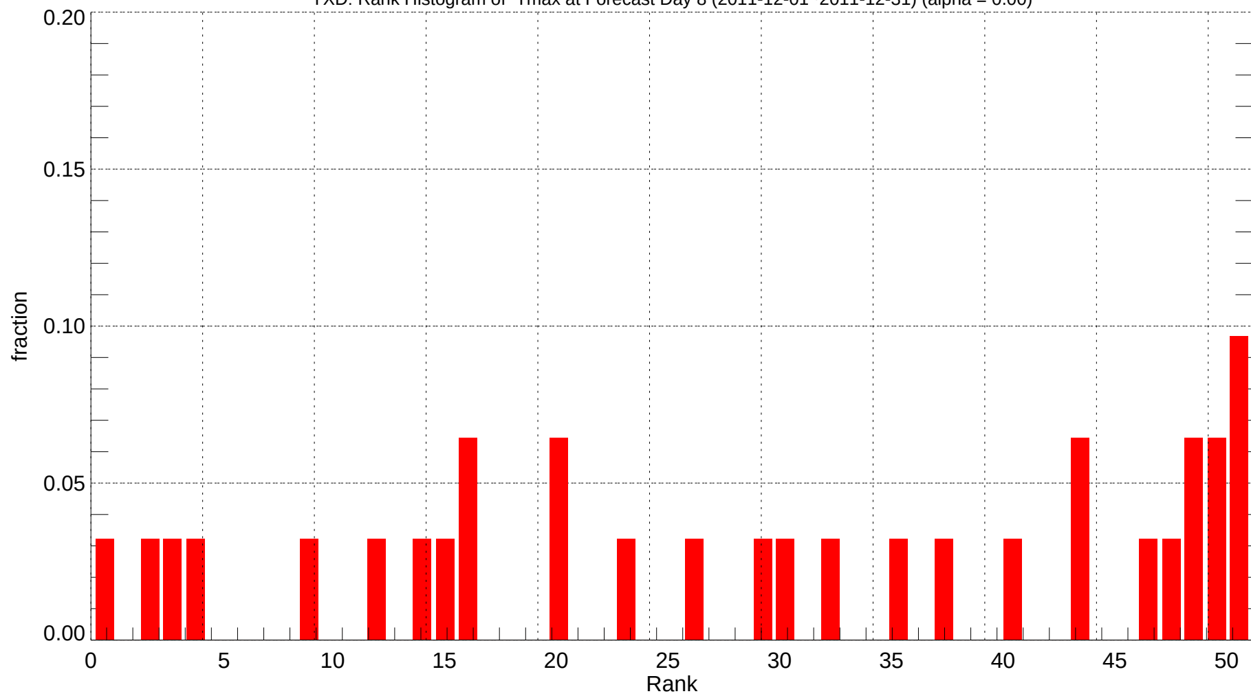
YXD: Rank Histogram of Tmax at Forecast Day 8 (2011-12-01~2011-12-31) (alpha = 0.00)
