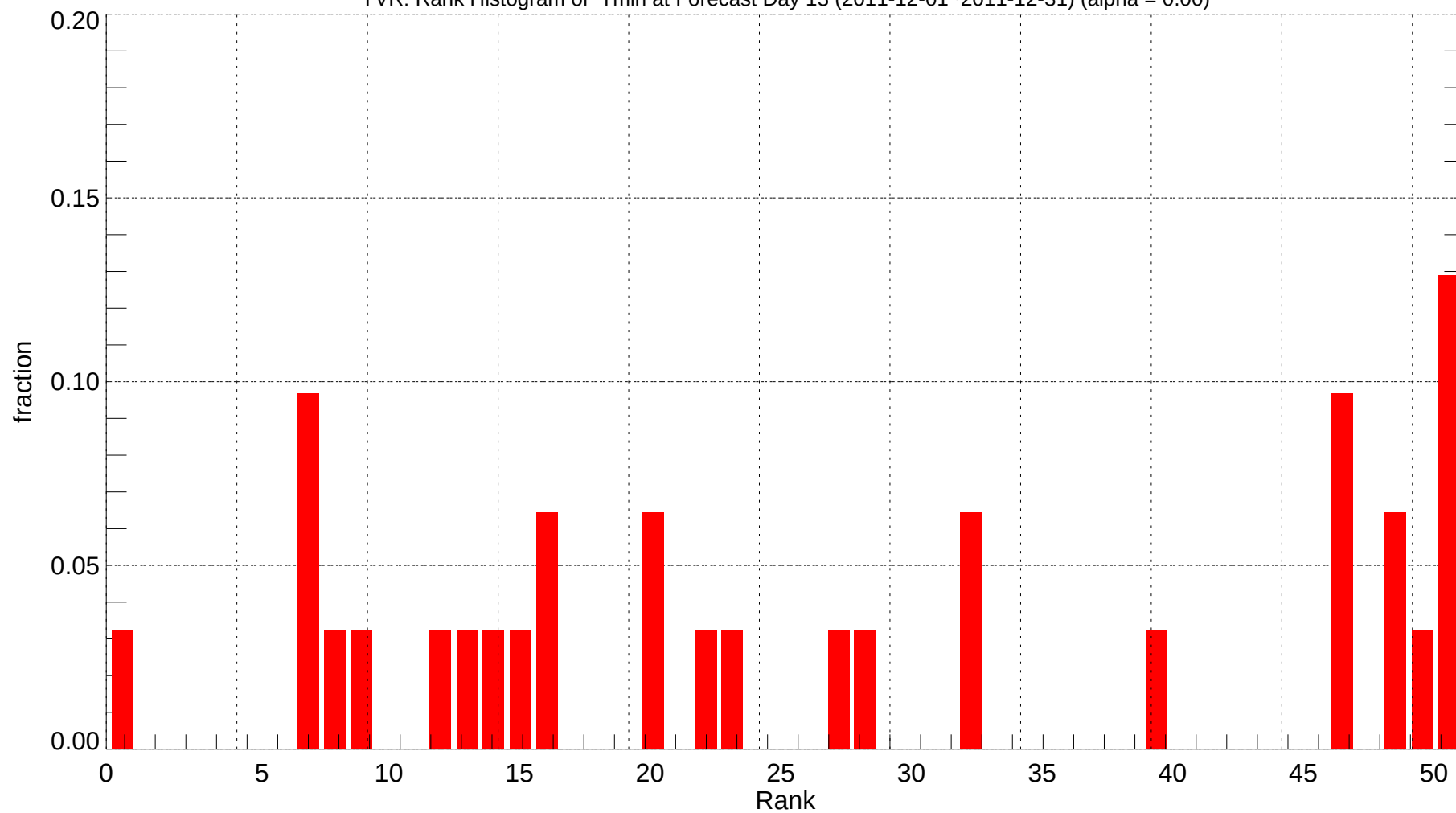
YVR: Rank Histogram of Tmin at Forecast Day 13 (2011-12-01~2011-12-31) (alpha = 0.00)
