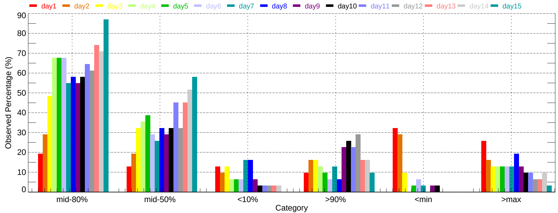
Observed Percentage of Ensembles - BHM: Min Temperature (2011-12-01~2011-12-31)
