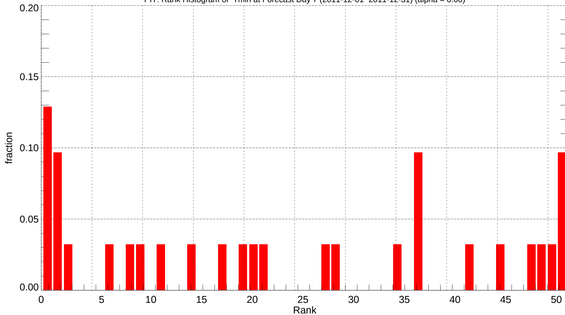
PIT: Rank Histogram of Tmin at Forecast Day 7 (2011-12-01~2011-12-31) (alpha = 0.00)
