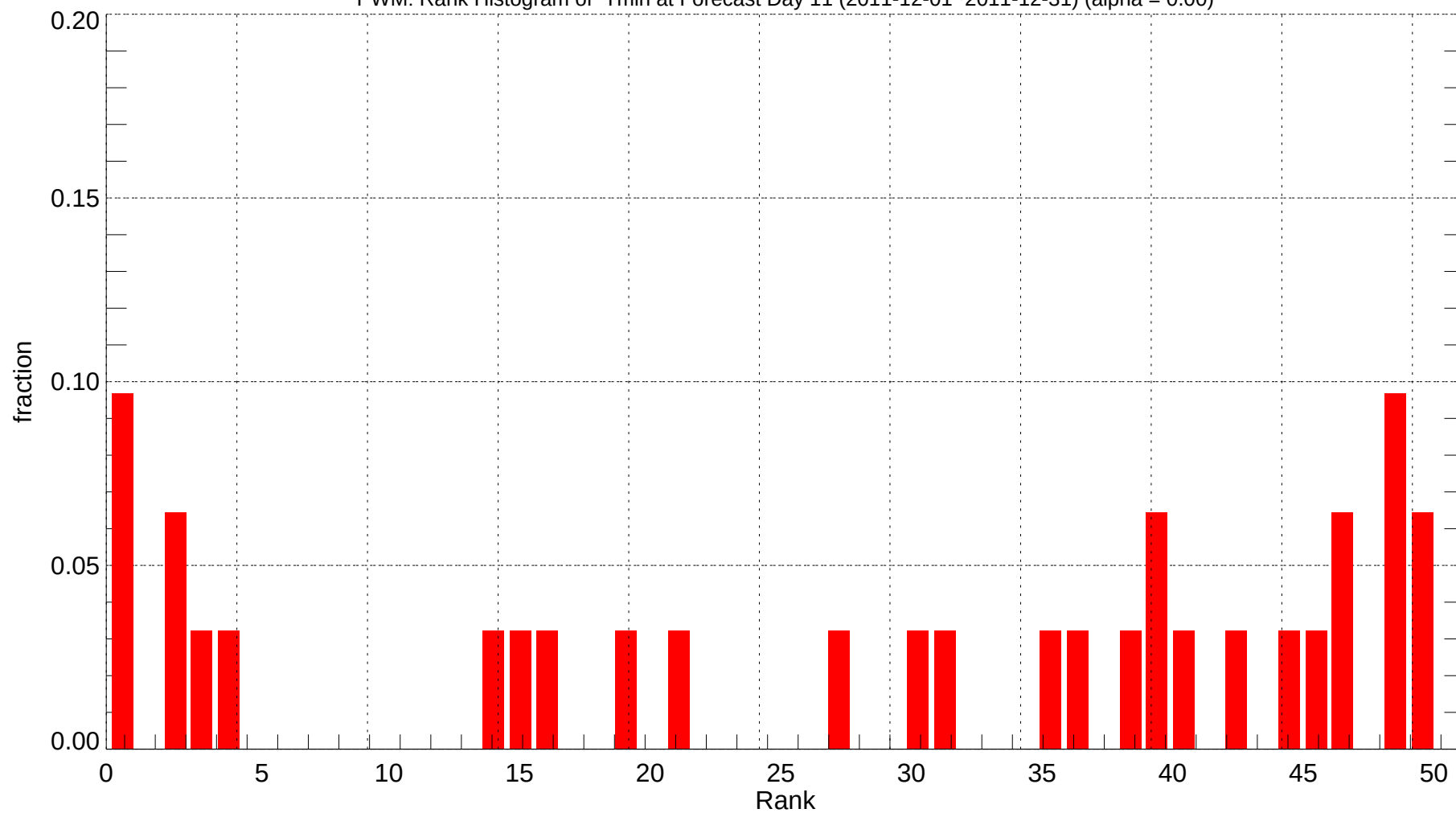
PWM: Rank Histogram of Tmin at Forecast Day 11 (2011-12-01~2011-12-31) (alpha = 0.00)
