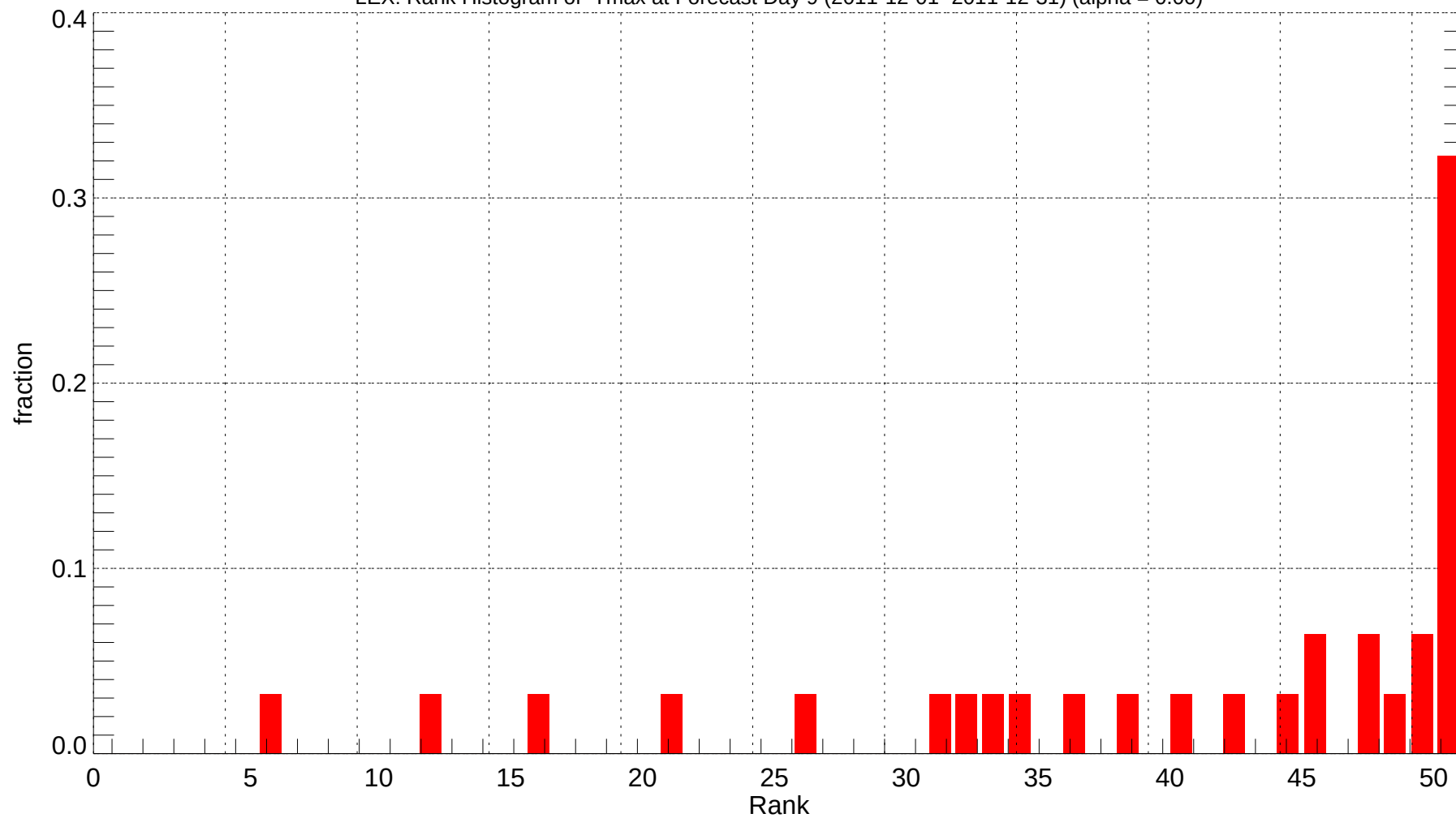
LEX: Rank Histogram of Tmax at Forecast Day 9 (2011-12-01~2011-12-31) (alpha = 0.00)
