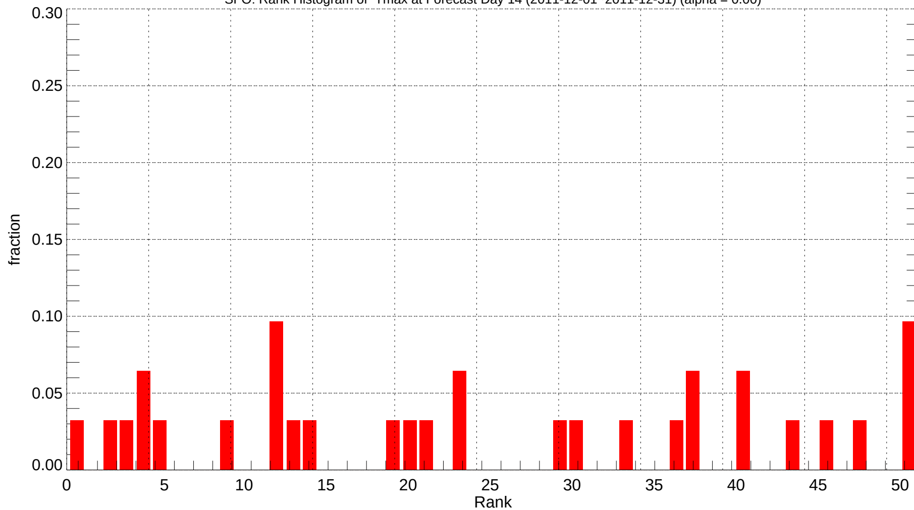
SFO: Rank Histogram of Tmax at Forecast Day 14 (2011-12-01~2011-12-31) (alpha = 0.00)
