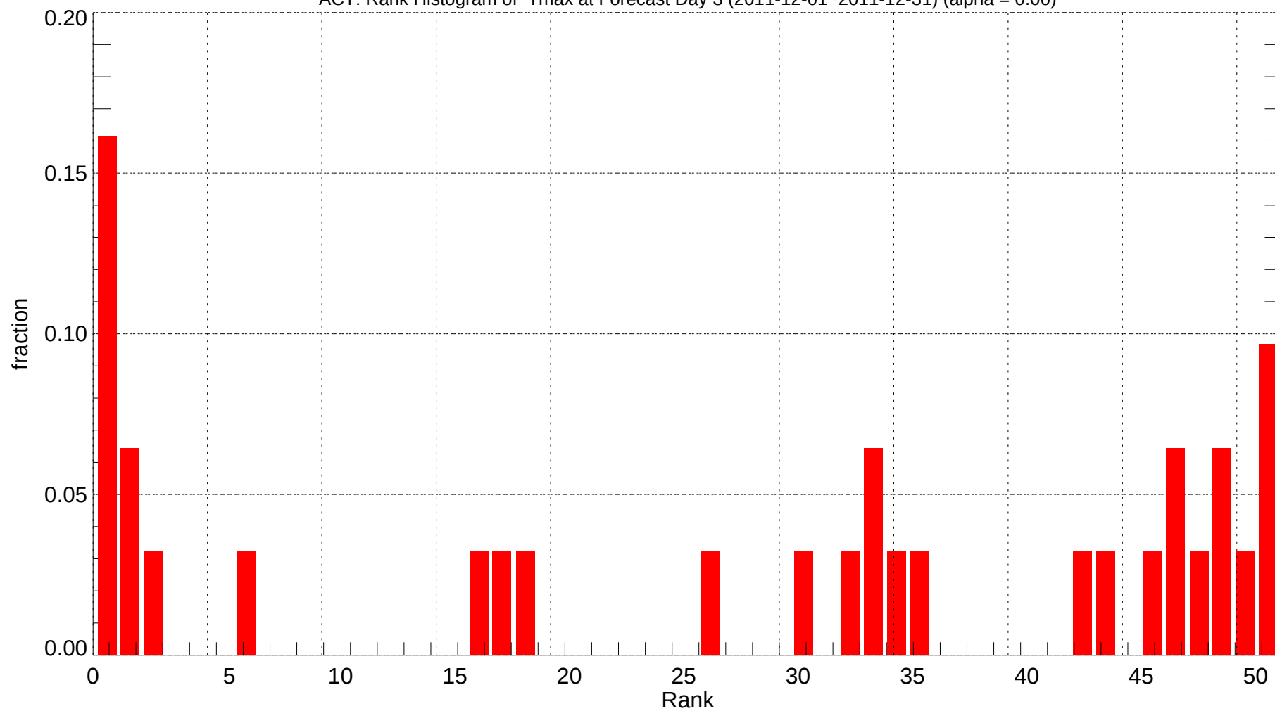
ACT: Rank Histogram of Tmax at Forecast Day 3 (2011-12-01~2011-12-31) (alpha = 0.00)
