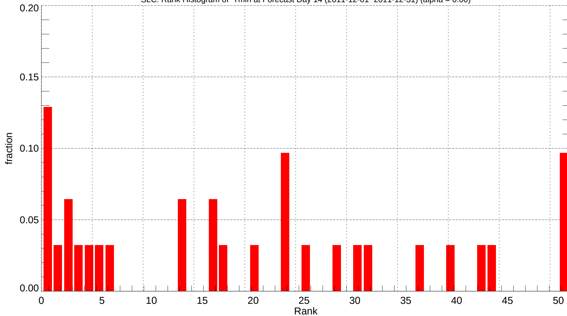
SLC: Rank Histogram of Tmin at Forecast Day 14 (2011-12-01~2011-12-31) (alpha = 0.00)
