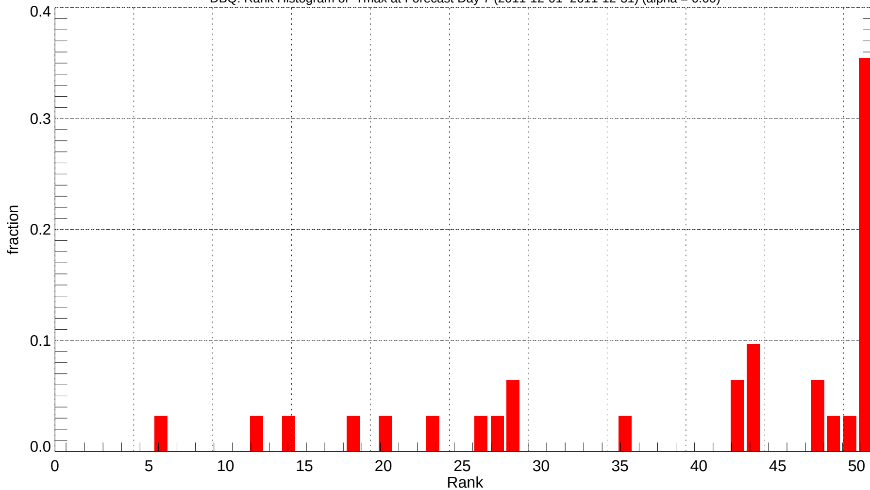
DBQ: Rank Histogram of Tmax at Forecast Day 7 (2011-12-01~2011-12-31) (alpha = 0.00)
