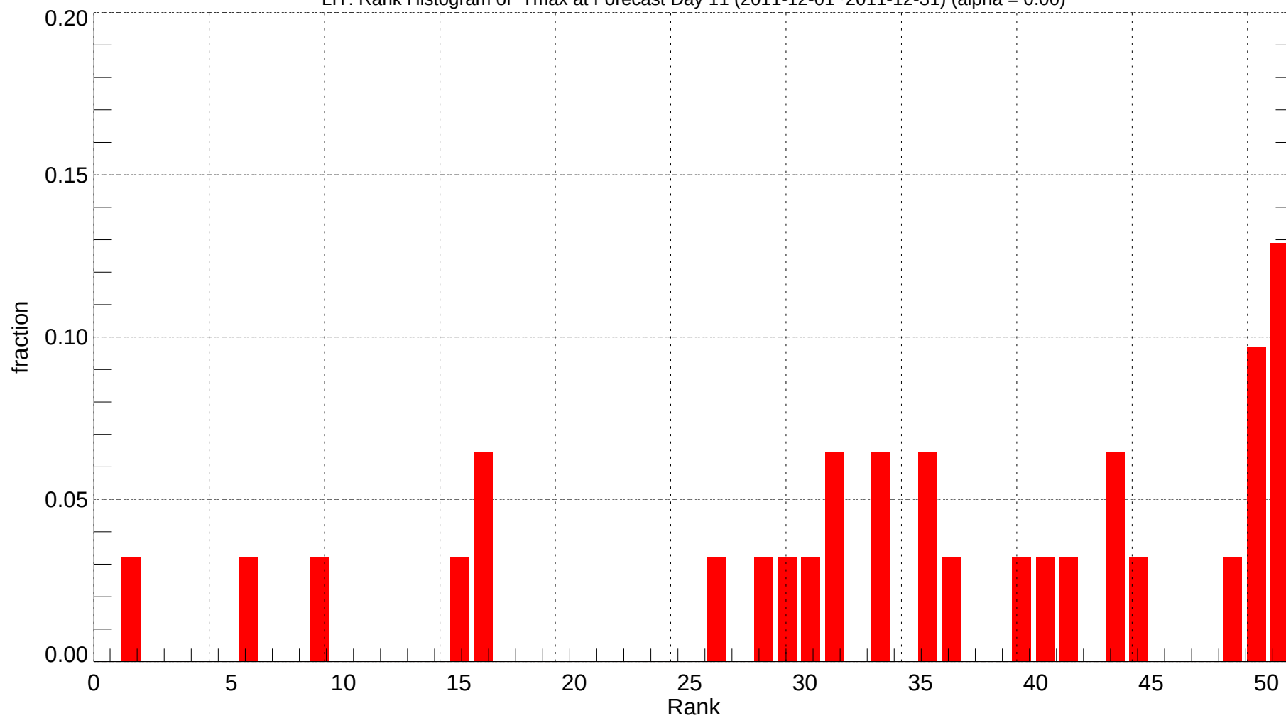
LIT: Rank Histogram of Tmax at Forecast Day 11 (2011-12-01~2011-12-31) (alpha = 0.00)
