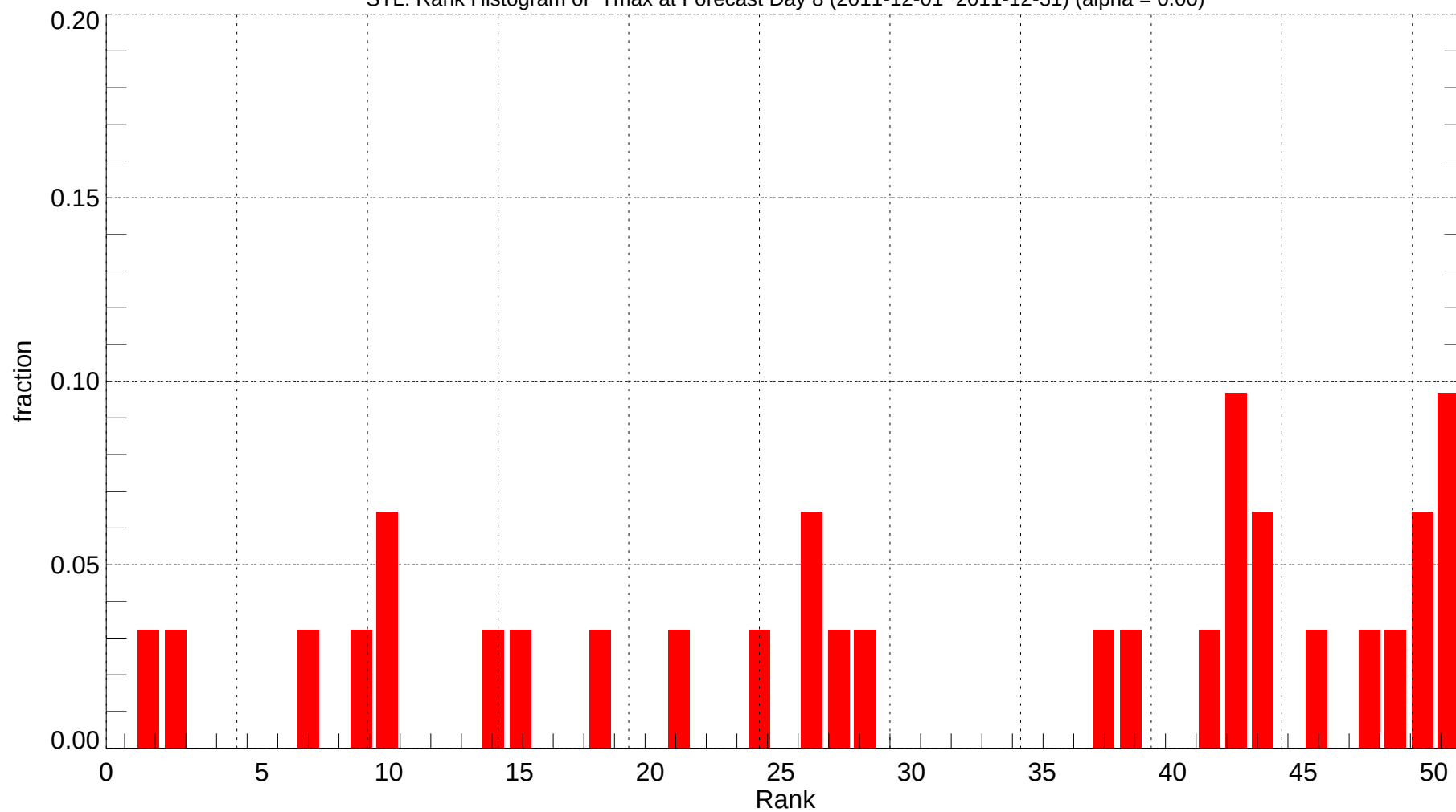
STL: Rank Histogram of Tmax at Forecast Day 8 (2011-12-01~2011-12-31) (alpha = 0.00)
