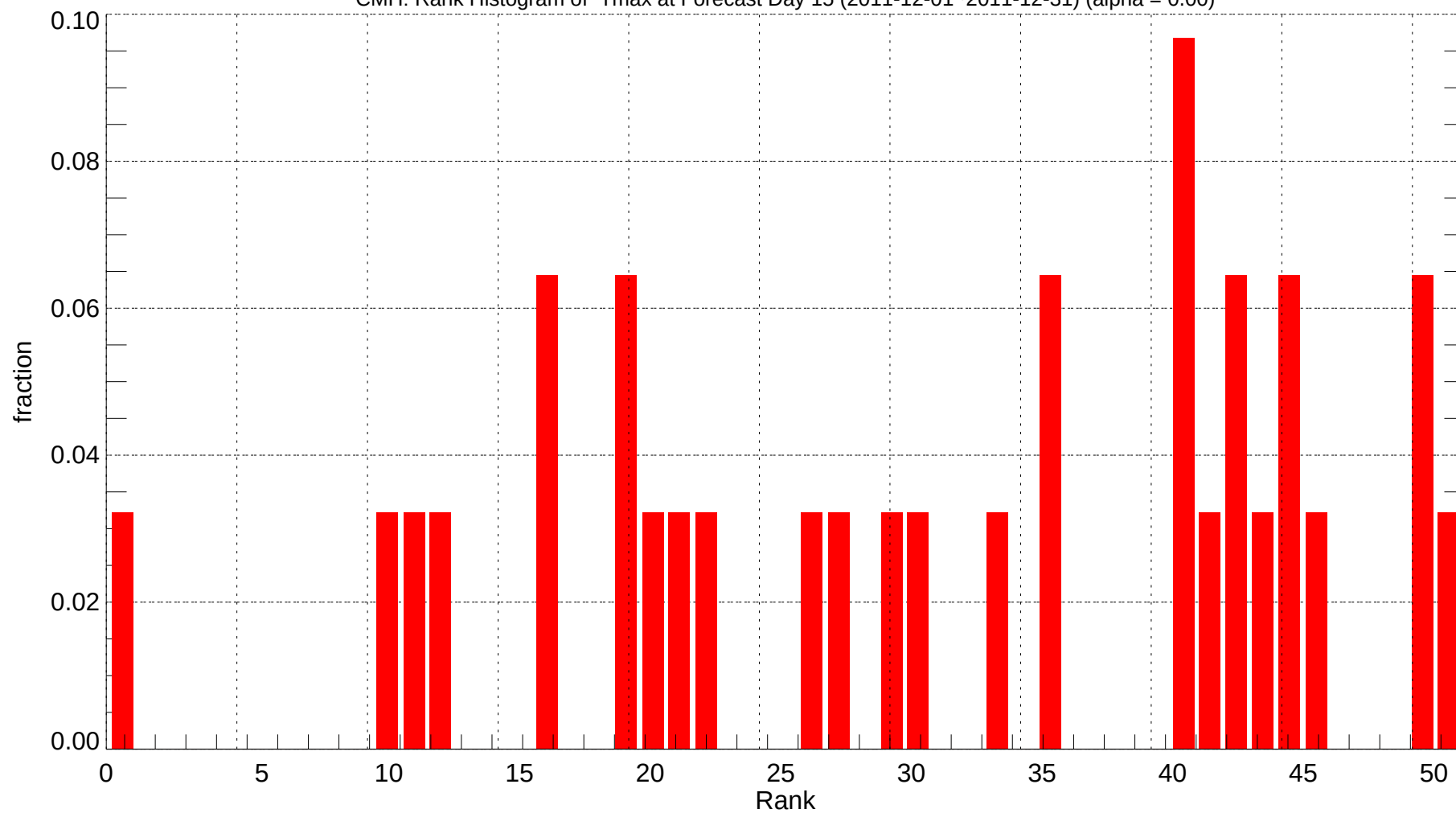
CMH: Rank Histogram of Tmax at Forecast Day 15 (2011-12-01~2011-12-31) (alpha = 0.00)
