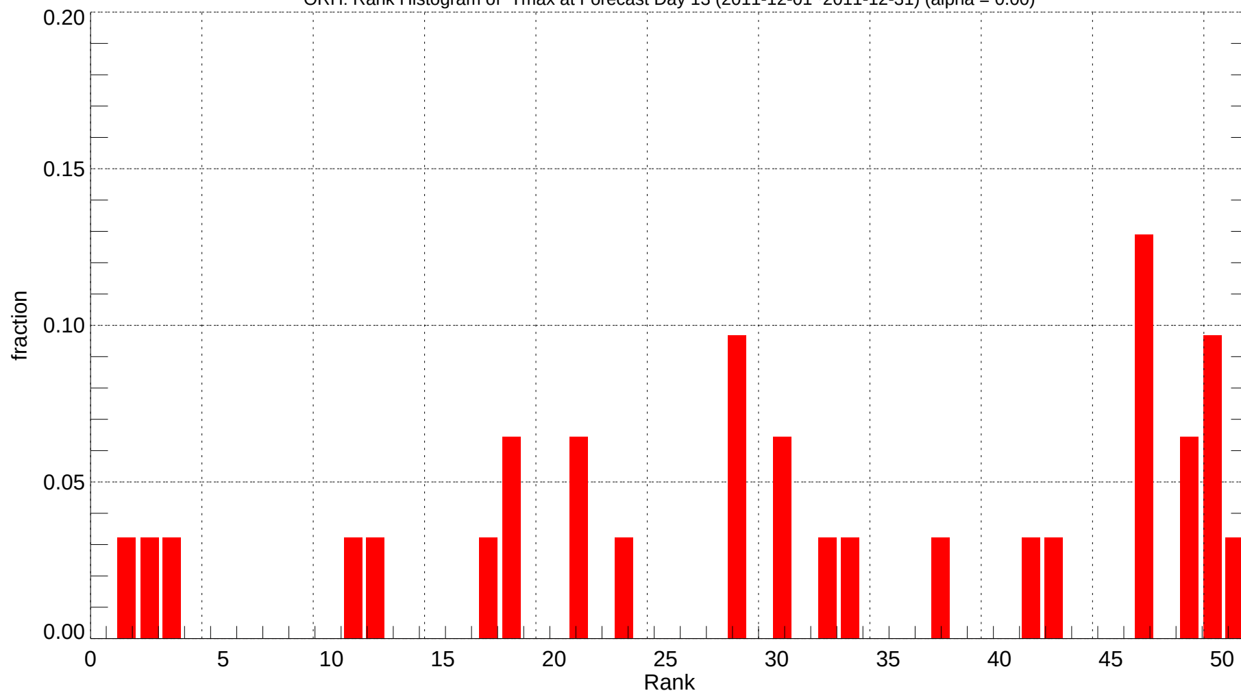
ORH: Rank Histogram of Tmax at Forecast Day 13 (2011-12-01~2011-12-31) (alpha = 0.00)
