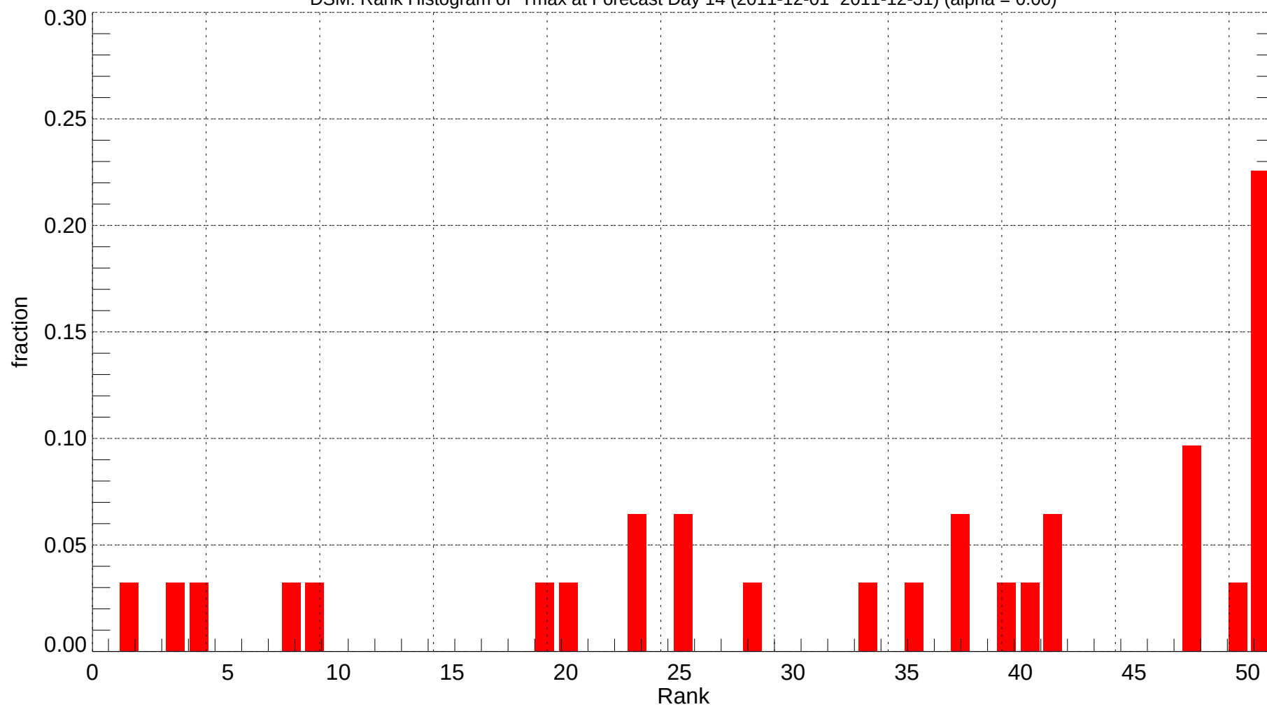
DSM: Rank Histogram of Tmax at Forecast Day 14 (2011-12-01~2011-12-31) (alpha = 0.00)
