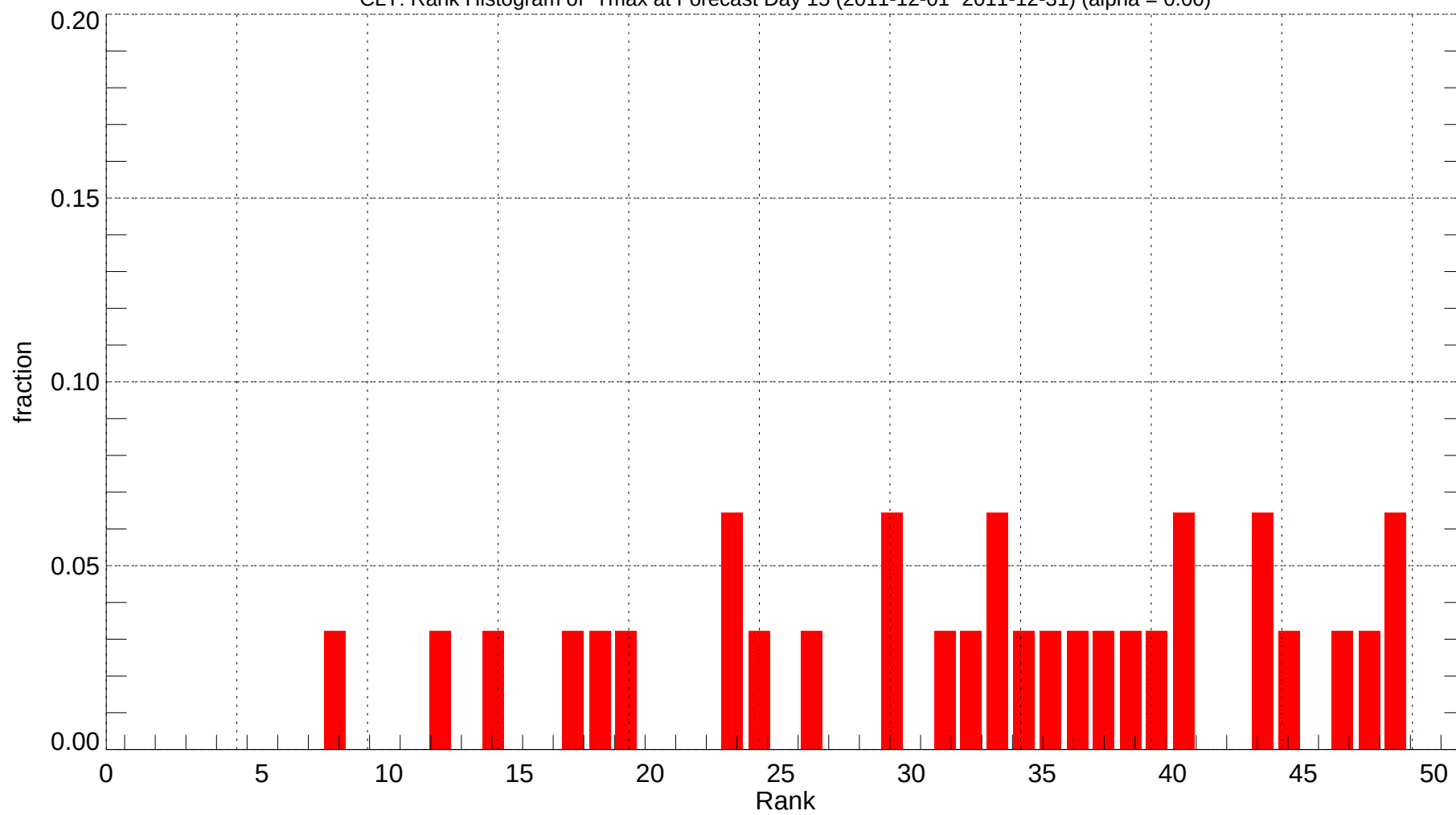
CLT: Rank Histogram of Tmax at Forecast Day 15 (2011-12-01~2011-12-31) (alpha = 0.00)
