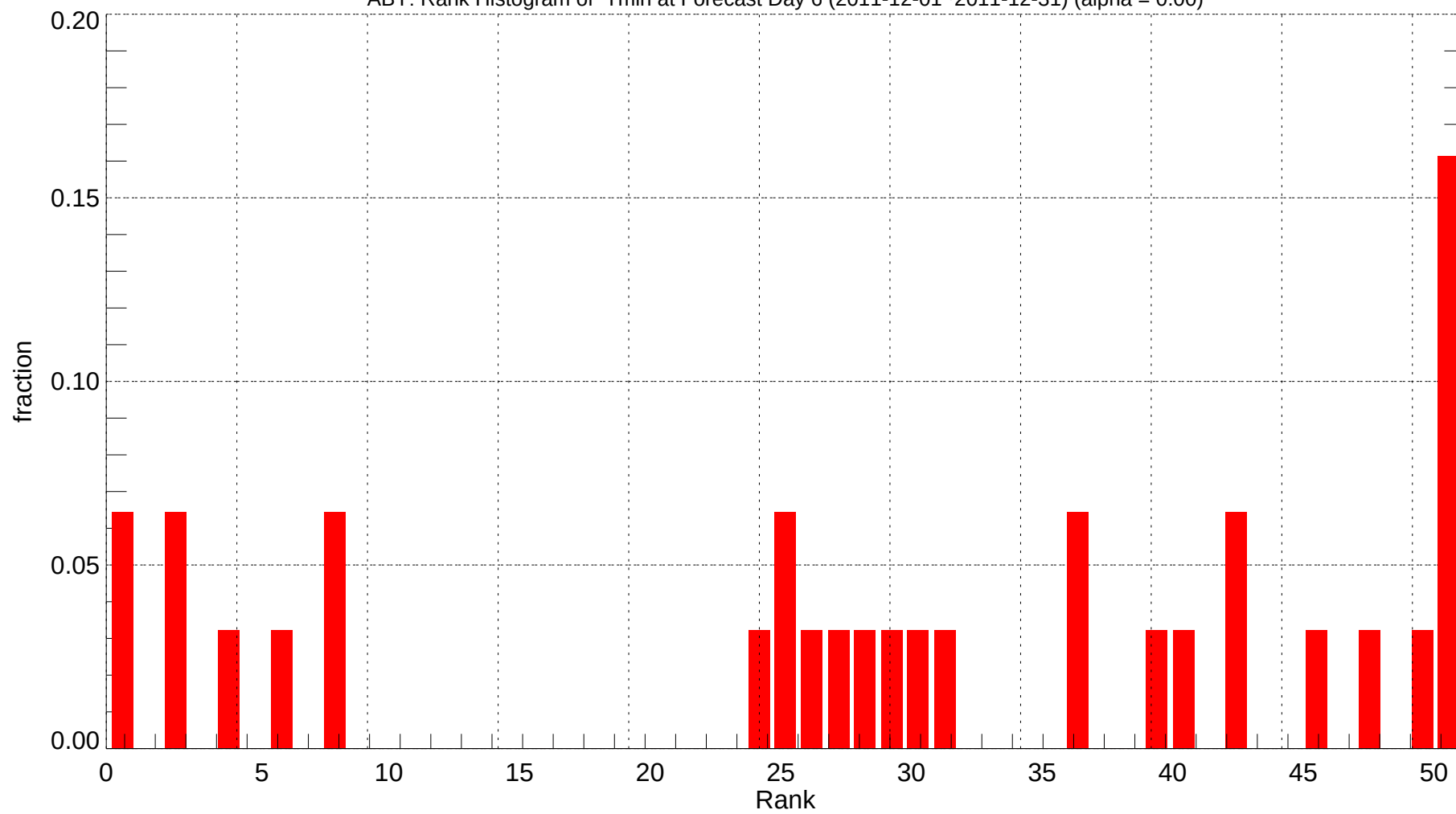
ABY: Rank Histogram of Tmin at Forecast Day 6 (2011-12-01~2011-12-31) (alpha = 0.00)
