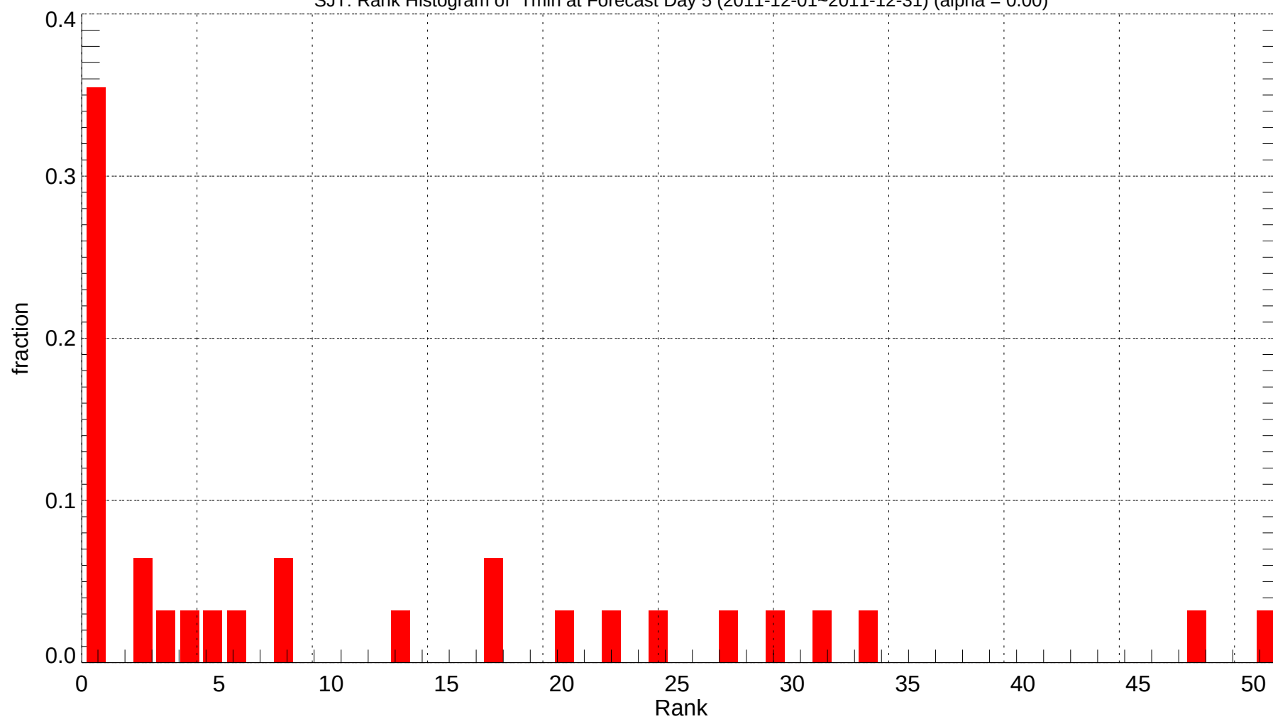
SJT: Rank Histogram of Tmin at Forecast Day 5 (2011-12-01~2011-12-31) (alpha = 0.00)
