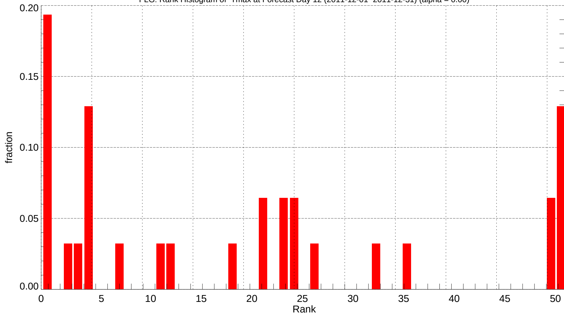
FLG: Rank Histogram of Tmax at Forecast Day 12 (2011-12-01~2011-12-31) (alpha = 0.00)
