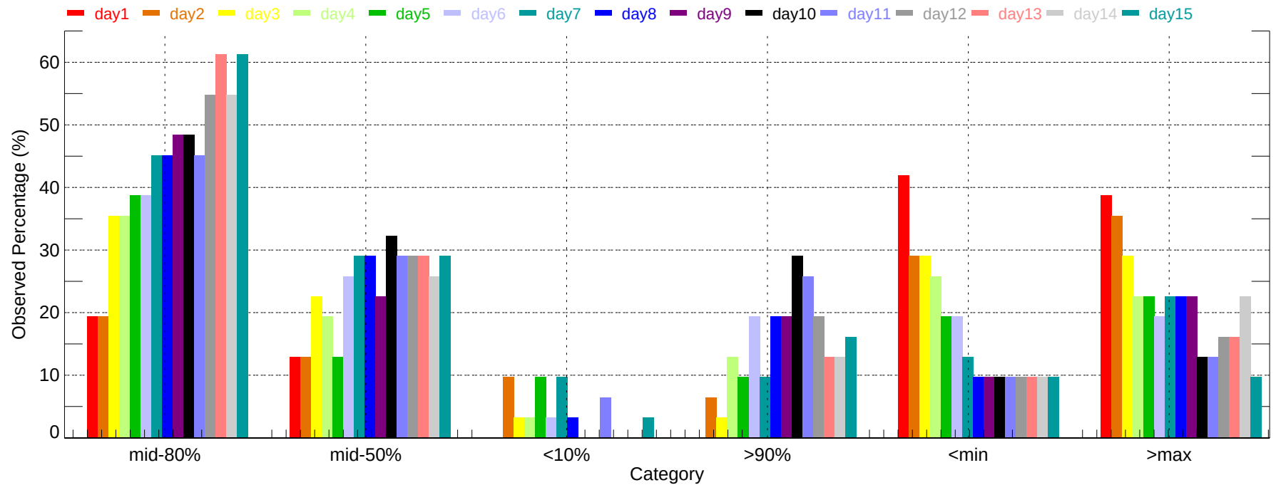
Observed Percentage of Ensembles - BIS: Min Temperature (2011-12-01~2011-12-31)
