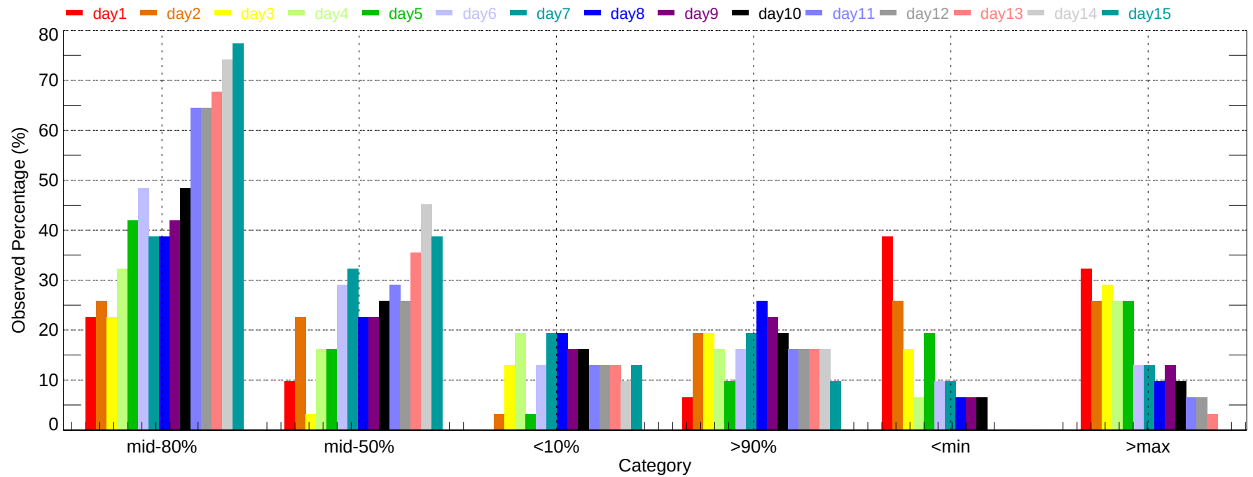
Observed Percentage of Ensembles - YUL: Min Temperature (2011-12-01~2011-12-31)
