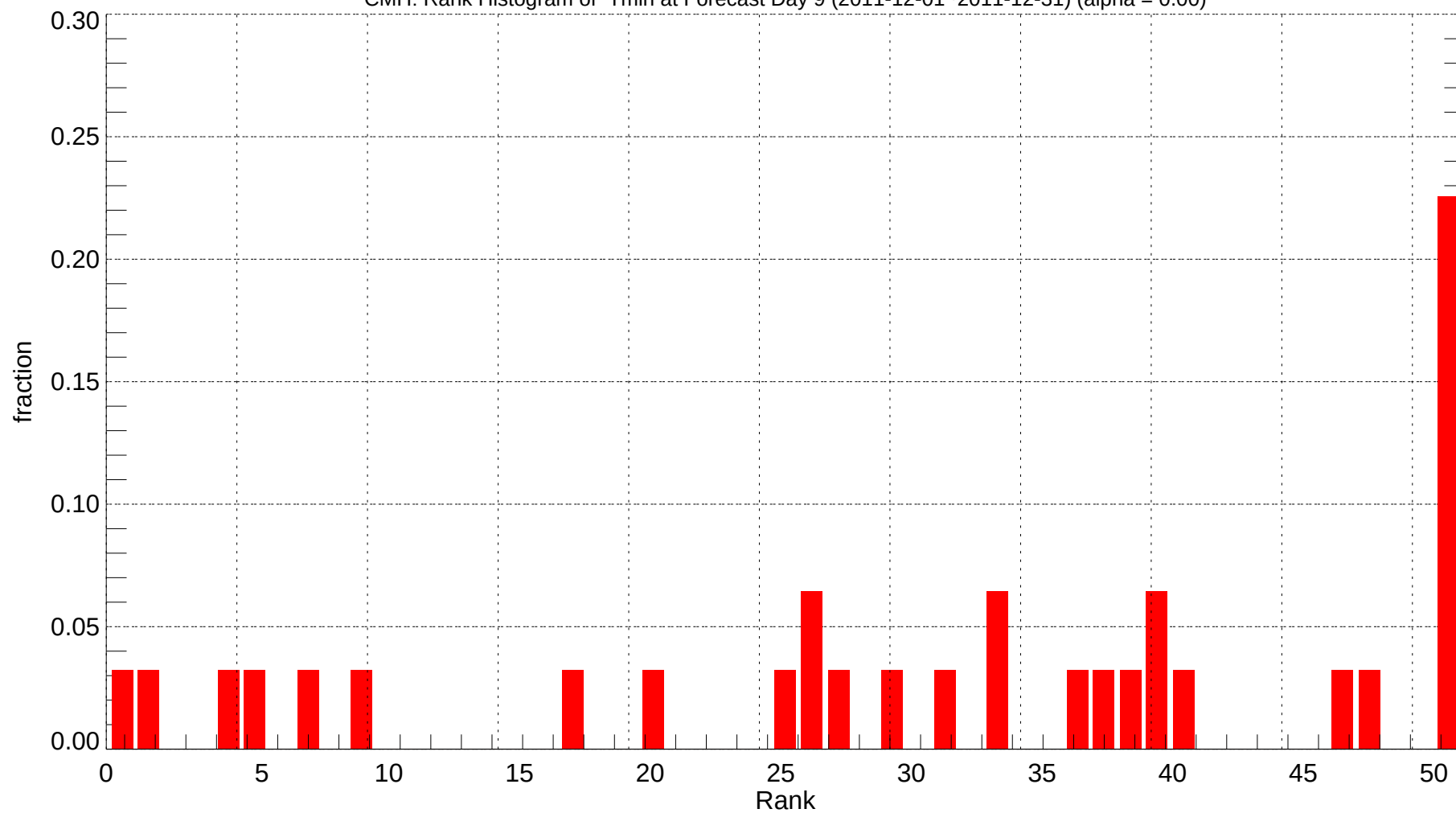
CMH: Rank Histogram of Tmin at Forecast Day 9 (2011-12-01~2011-12-31) (alpha = 0.00)
