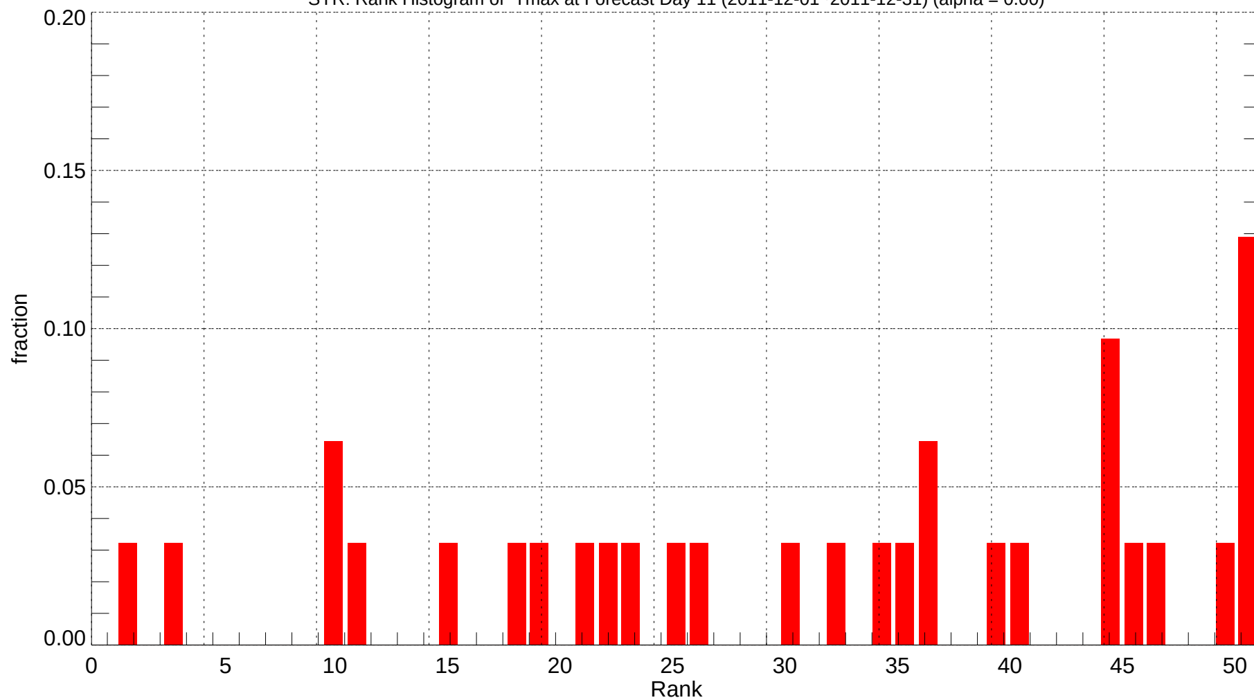
SYR: Rank Histogram of Tmax at Forecast Day 11 (2011-12-01~2011-12-31) (alpha = 0.00)
