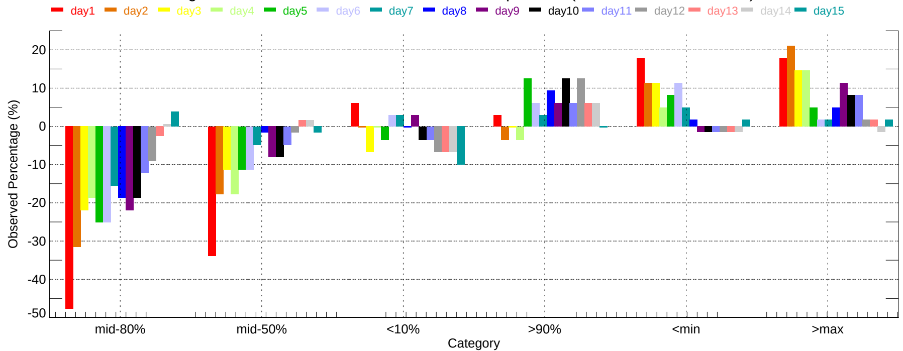
Observed Percentage Deviation of Ensembles - CMH: Max Temperature (2011-12-01~2011-12-31)
