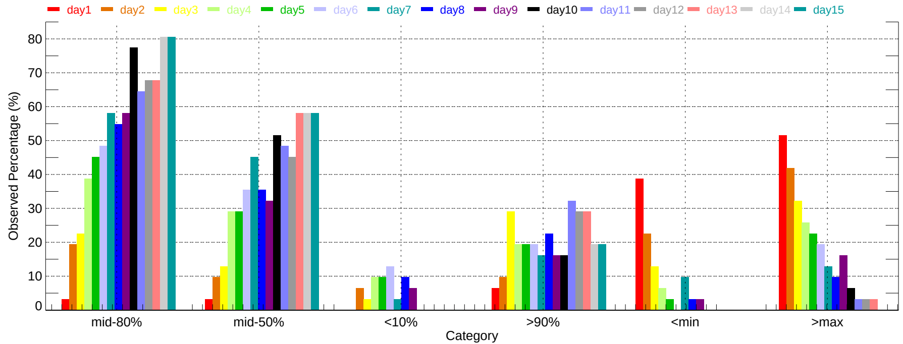
Observed Percentage of Ensembles - DCA: Min Temperature (2011-12-01~2011-12-31)
