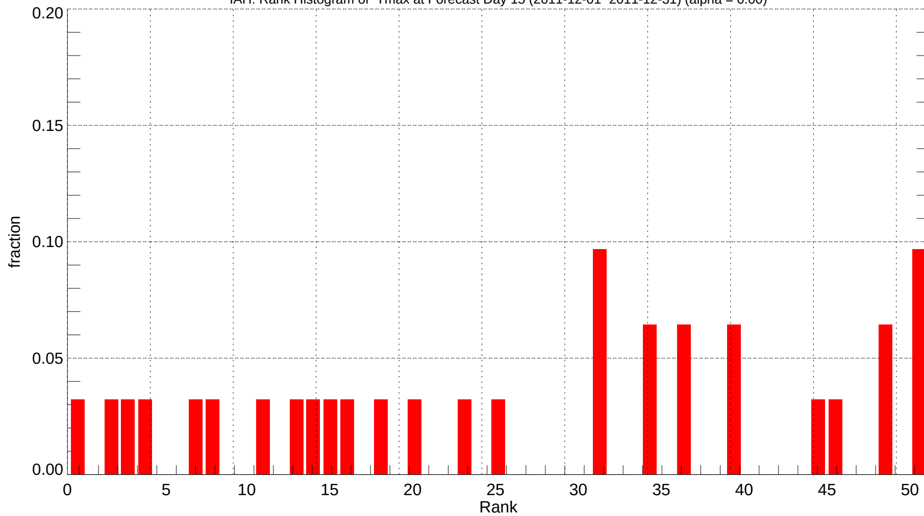
IAH: Rank Histogram of Tmax at Forecast Day 15 (2011-12-01~2011-12-31) (alpha = 0.00)
