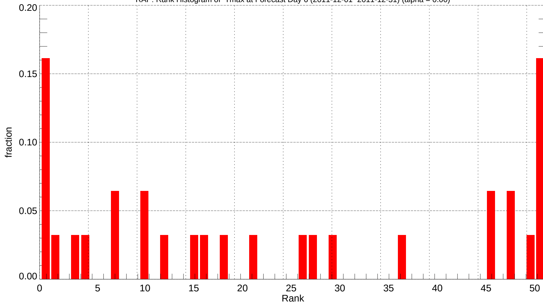
RAP: Rank Histogram of Tmax at Forecast Day 6 (2011-12-01~2011-12-31) (alpha = 0.00)
