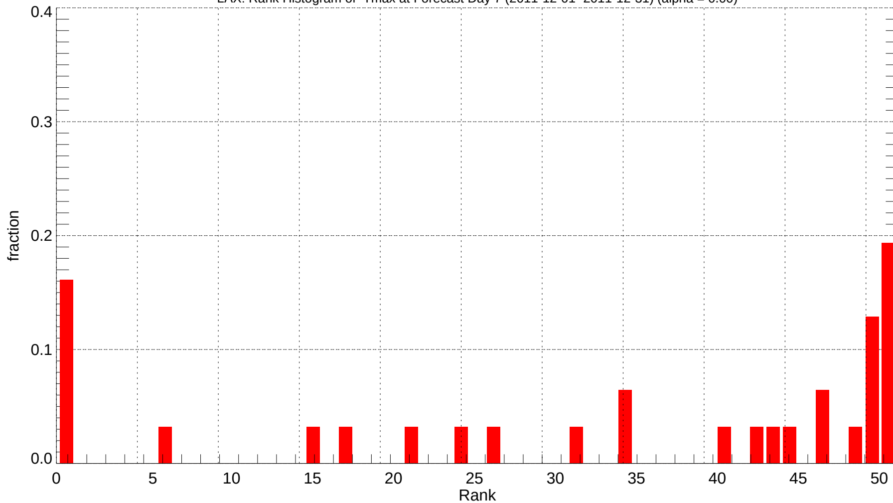
LAX: Rank Histogram of Tmax at Forecast Day 7 (2011-12-01~2011-12-31) (alpha = 0.00)
