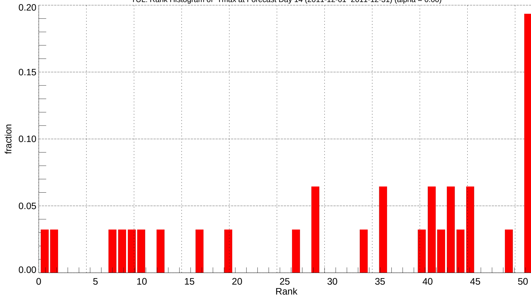
TUL: Rank Histogram of Tmax at Forecast Day 14 (2011-12-01~2011-12-31) (alpha = 0.00)
