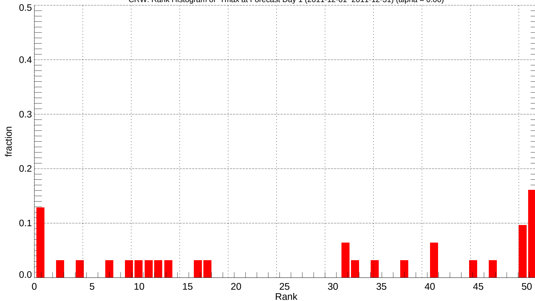
CRW: Rank Histogram of Tmax at Forecast Day 1 (2011-12-01~2011-12-31) (alpha = 0.00)
