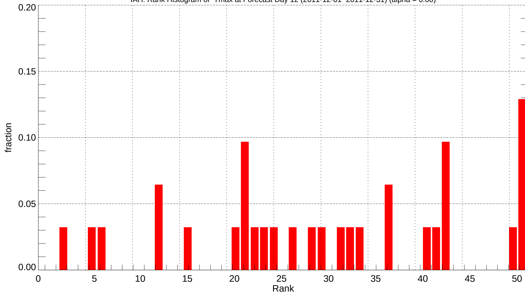
IAH: Rank Histogram of Tmax at Forecast Day 12 (2011-12-01~2011-12-31) (alpha = 0.00)
