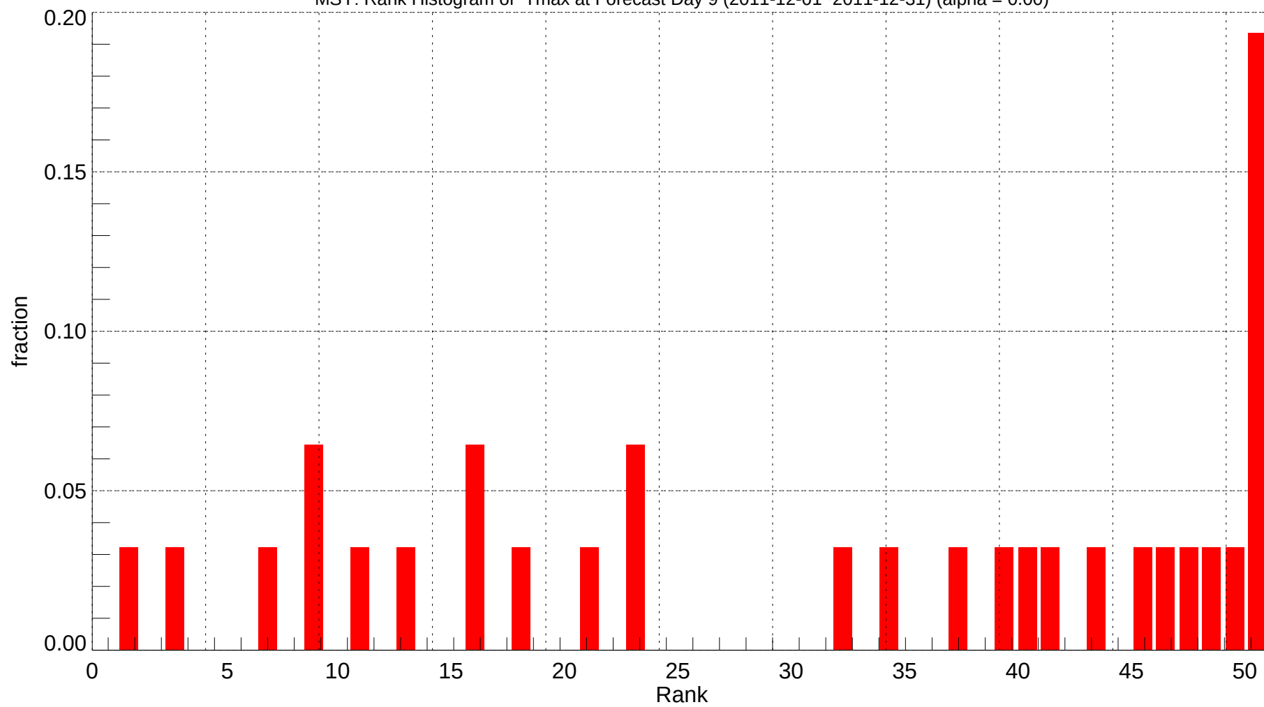
MSY: Rank Histogram of Tmax at Forecast Day 9 (2011-12-01~2011-12-31) (alpha = 0.00)
