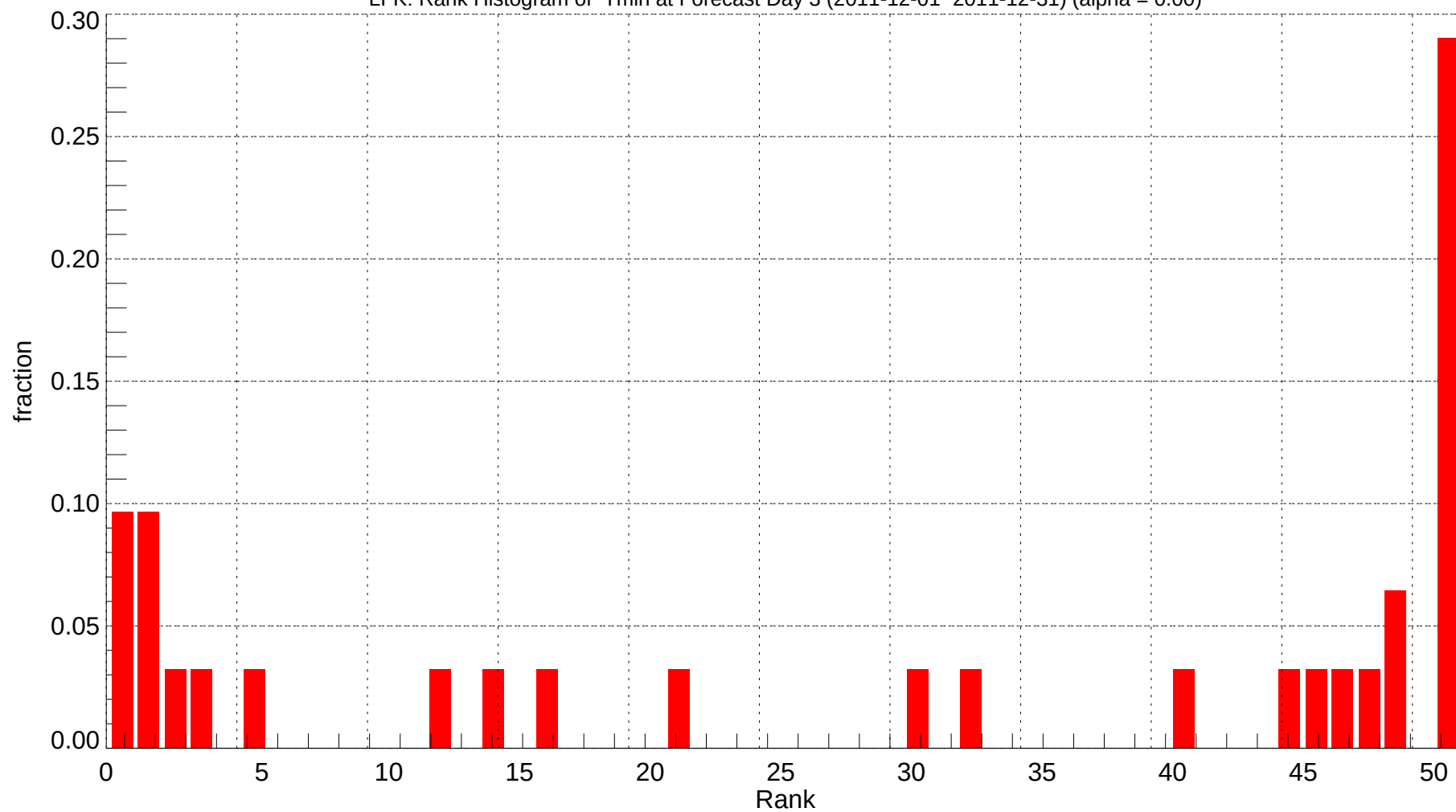
LFK: Rank Histogram of Tmin at Forecast Day 3 (2011-12-01~2011-12-31) (alpha = 0.00)
