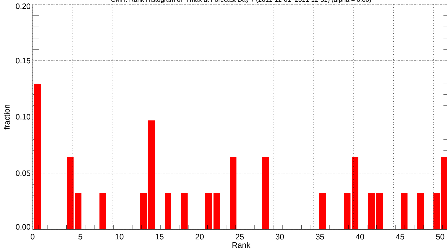
CMH: Rank Histogram of Tmax at Forecast Day 7 (2011-12-01~2011-12-31) (alpha = 0.00)
