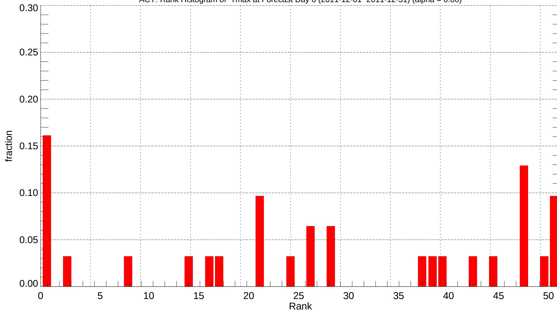
ACY: Rank Histogram of Tmax at Forecast Day 6 (2011-12-01~2011-12-31) (alpha = 0.00)
