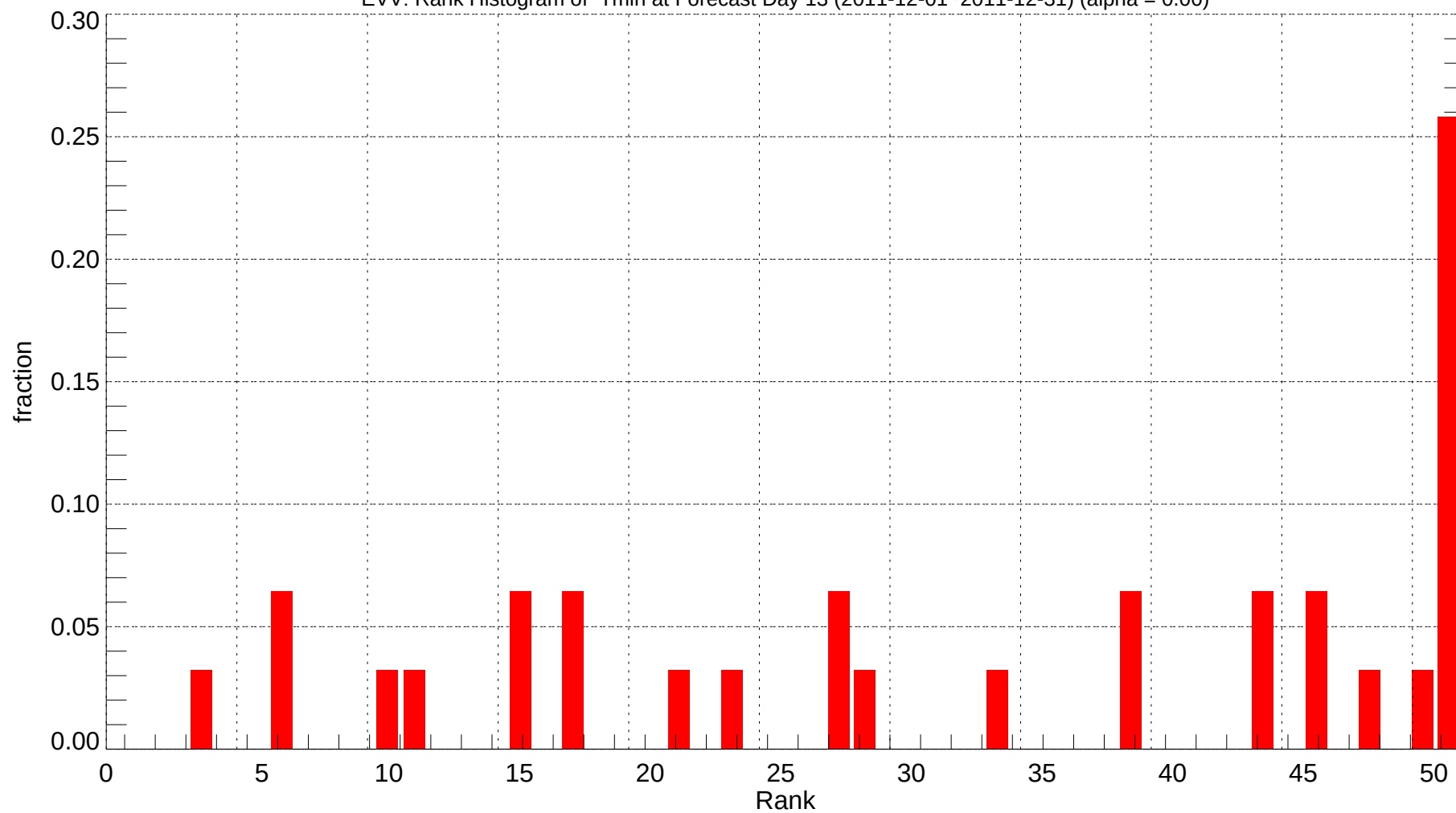
EVV: Rank Histogram of Tmin at Forecast Day 13 (2011-12-01~2011-12-31) (alpha = 0.00)
