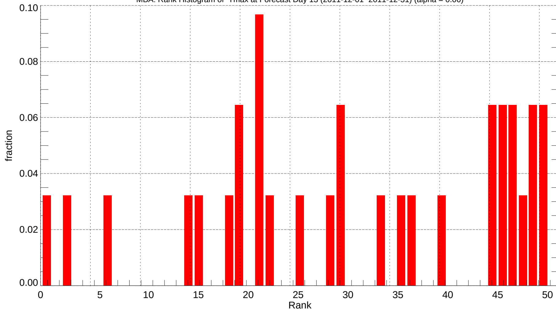
MBA: Rank Histogram of Tmax at Forecast Day 13 (2011-12-01~2011-12-31) (alpha = 0.00)
