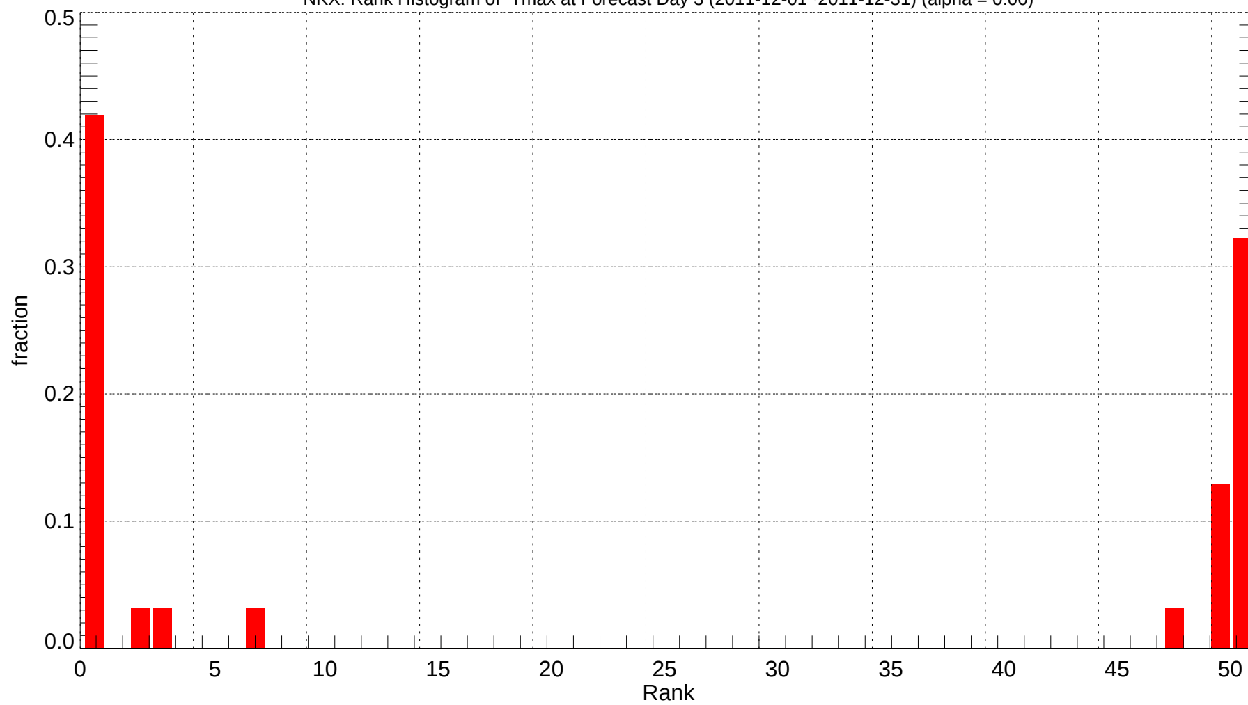
NKX: Rank Histogram of Tmax at Forecast Day 3 (2011-12-01~2011-12-31) (alpha = 0.00)
