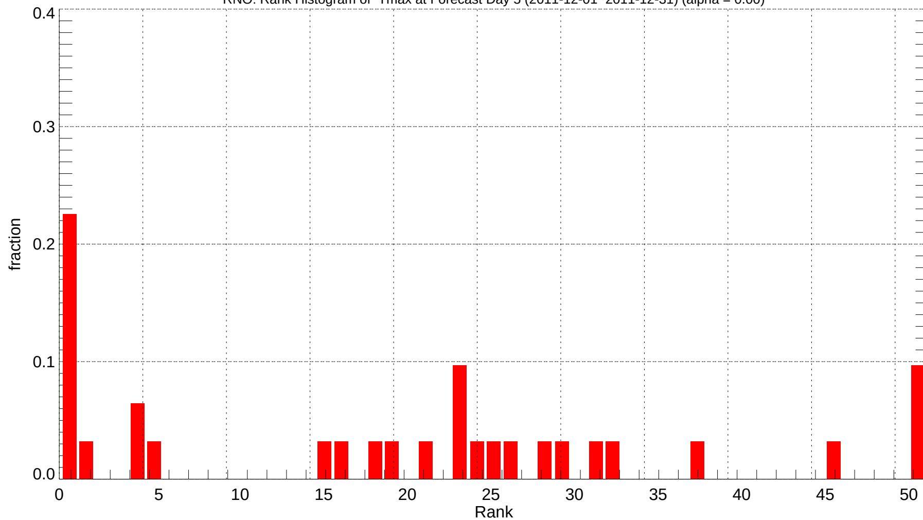
RNO: Rank Histogram of Tmax at Forecast Day 5 (2011-12-01~2011-12-31) (alpha = 0.00)
