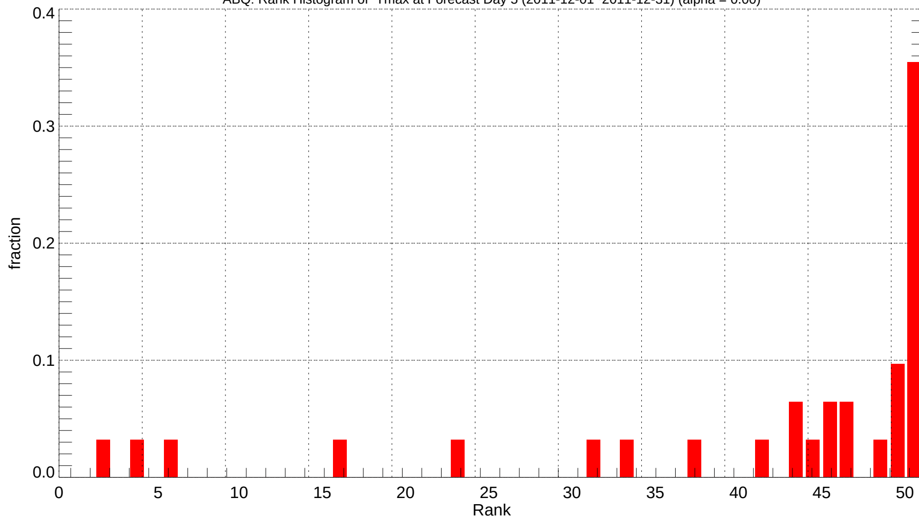
ABQ: Rank Histogram of Tmax at Forecast Day 5 (2011-12-01~2011-12-31) (alpha = 0.00)
