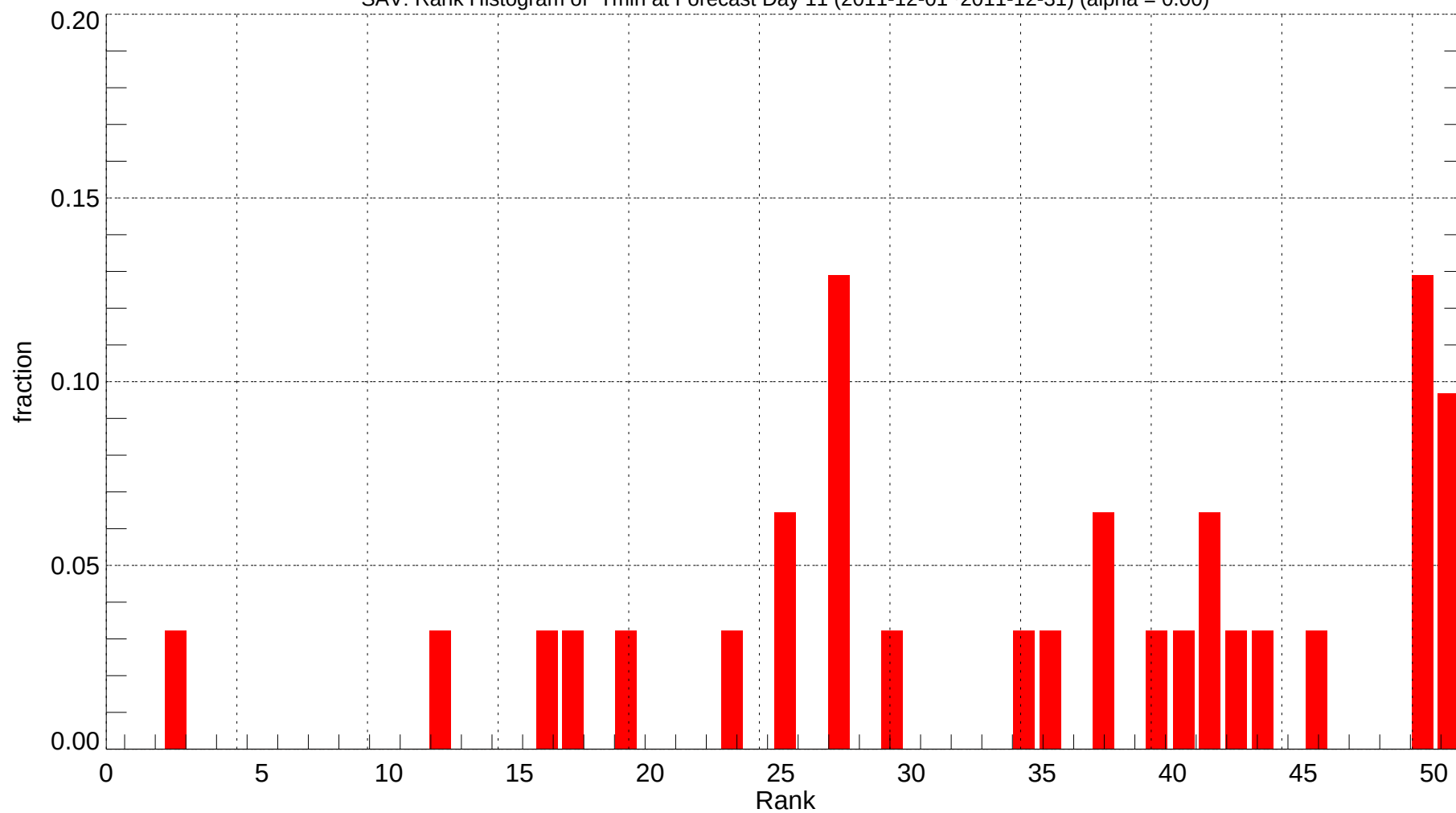
SAV: Rank Histogram of Tmin at Forecast Day 11 (2011-12-01~2011-12-31) (alpha = 0.00)
