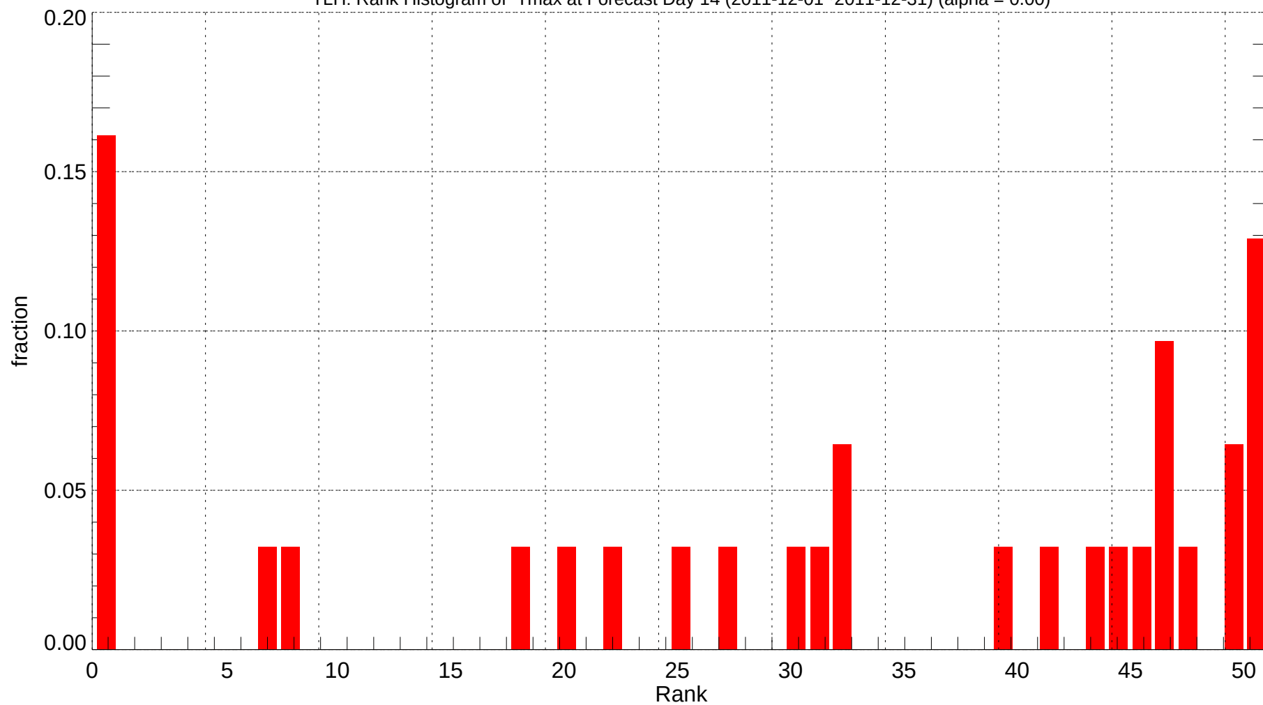
TLH: Rank Histogram of Tmax at Forecast Day 14 (2011-12-01~2011-12-31) (alpha = 0.00)
