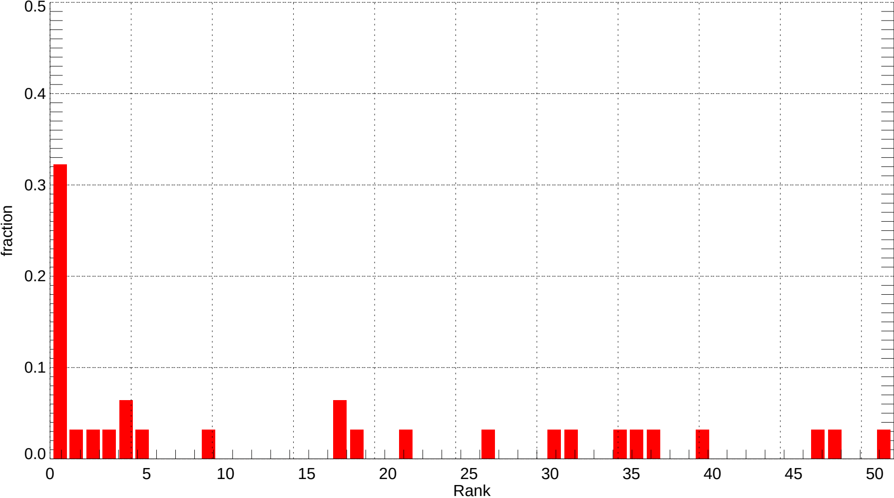
RAL: Rank Histogram of Tmin at Forecast Day 8 (2011-12-01~2011-12-31) (alpha = 0.00)
