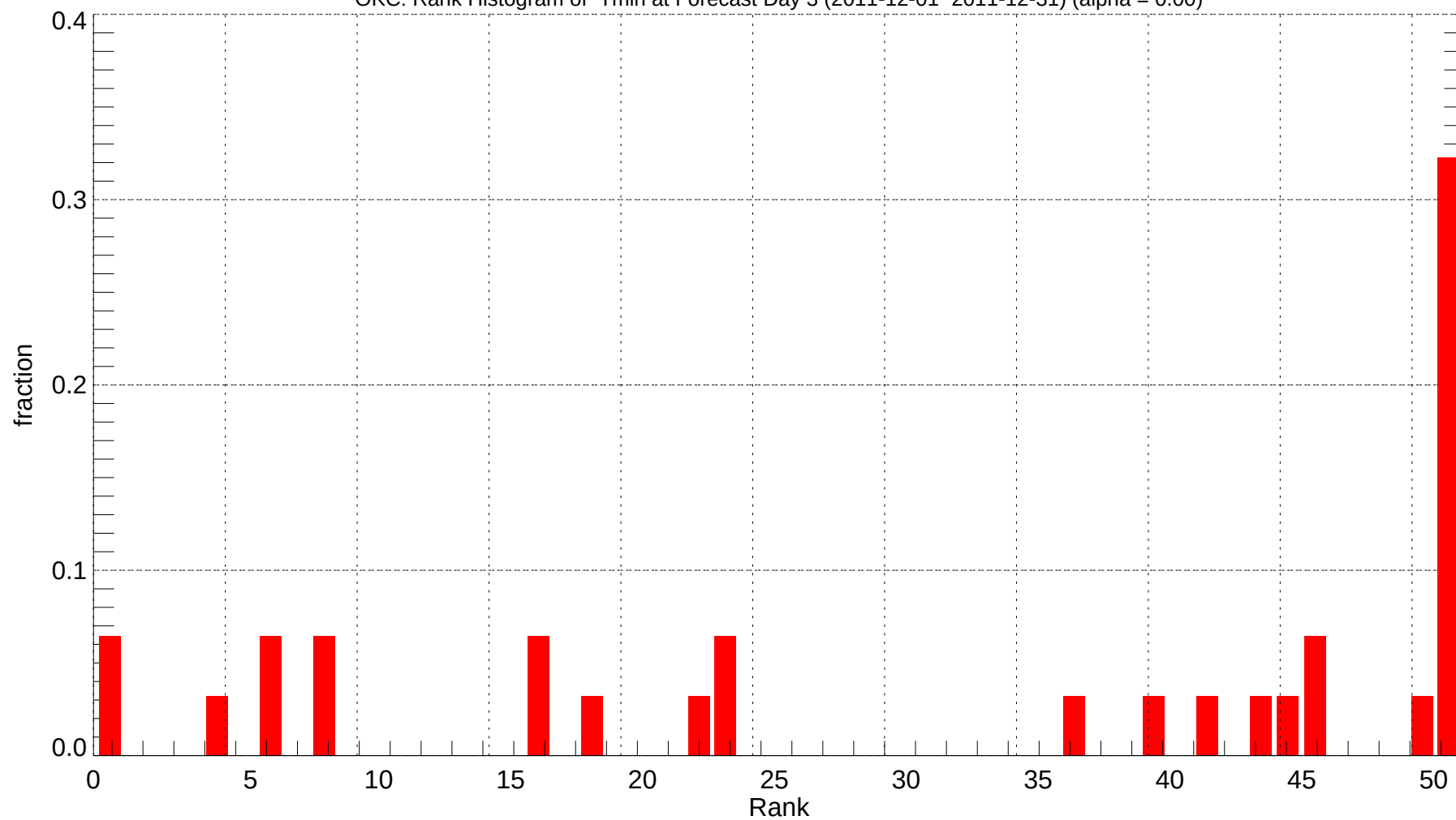
OKC: Rank Histogram of Tmin at Forecast Day 3 (2011-12-01~2011-12-31) (alpha = 0.00)
