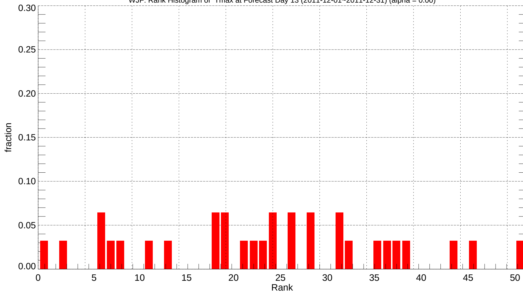
WJF: Rank Histogram of Tmax at Forecast Day 13 (2011-12-01~2011-12-31) (alpha = 0.00)
