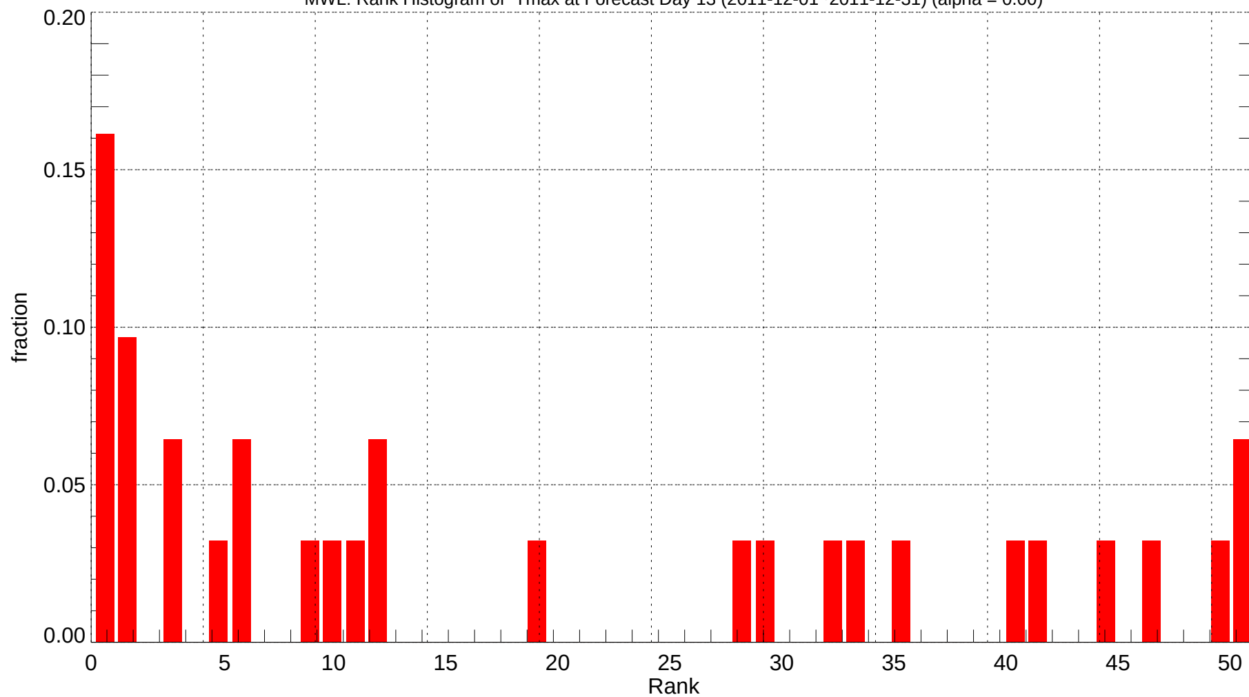
MWL: Rank Histogram of Tmax at Forecast Day 13 (2011-12-01~2011-12-31) (alpha = 0.00)
