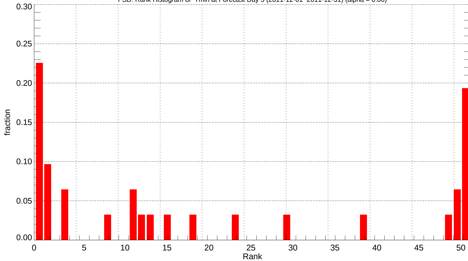
FSD: Rank Histogram of Tmin at Forecast Day 5 (2011-12-01~2011-12-31) (alpha = 0.00)
