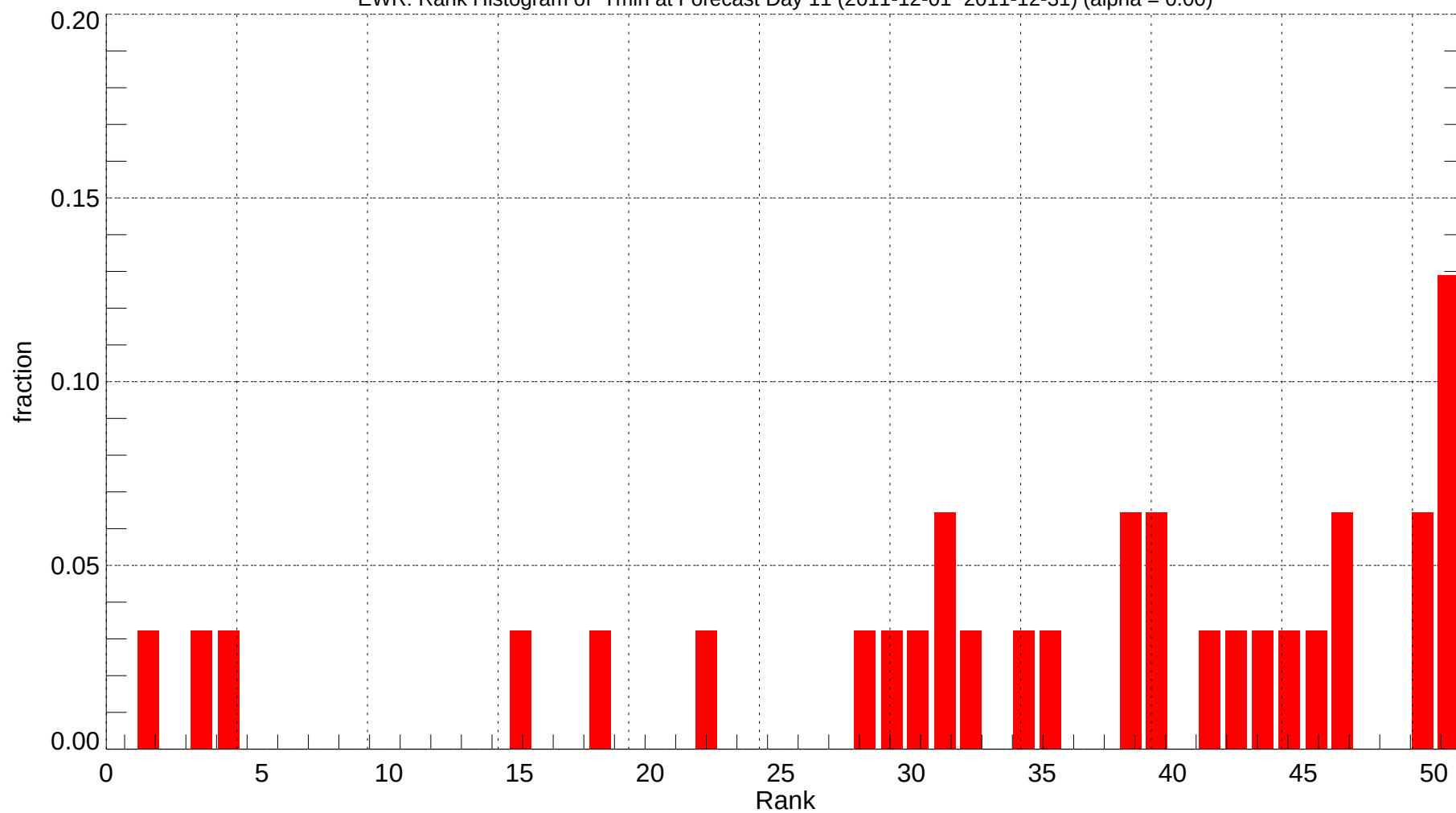
EWR: Rank Histogram of Tmin at Forecast Day 11 (2011-12-01~2011-12-31) (alpha = 0.00)
