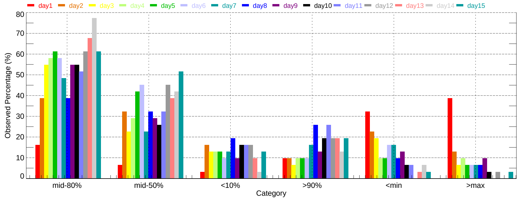
Observed Percentage of Ensembles - PWM: Max Temperature (2011-12-01~2011-12-31)
