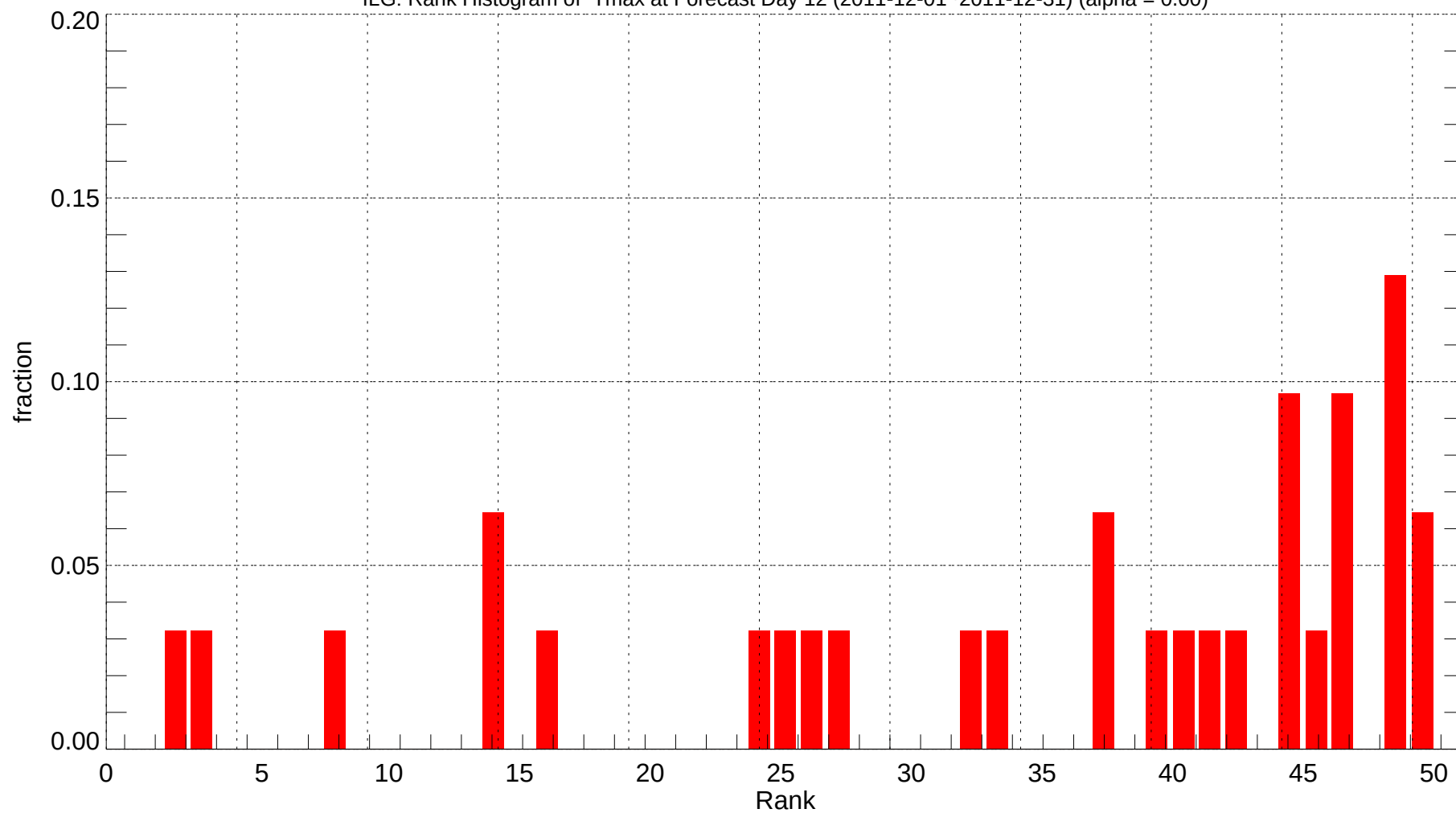
ILG: Rank Histogram of Tmax at Forecast Day 12 (2011-12-01~2011-12-31) (alpha = 0.00)
