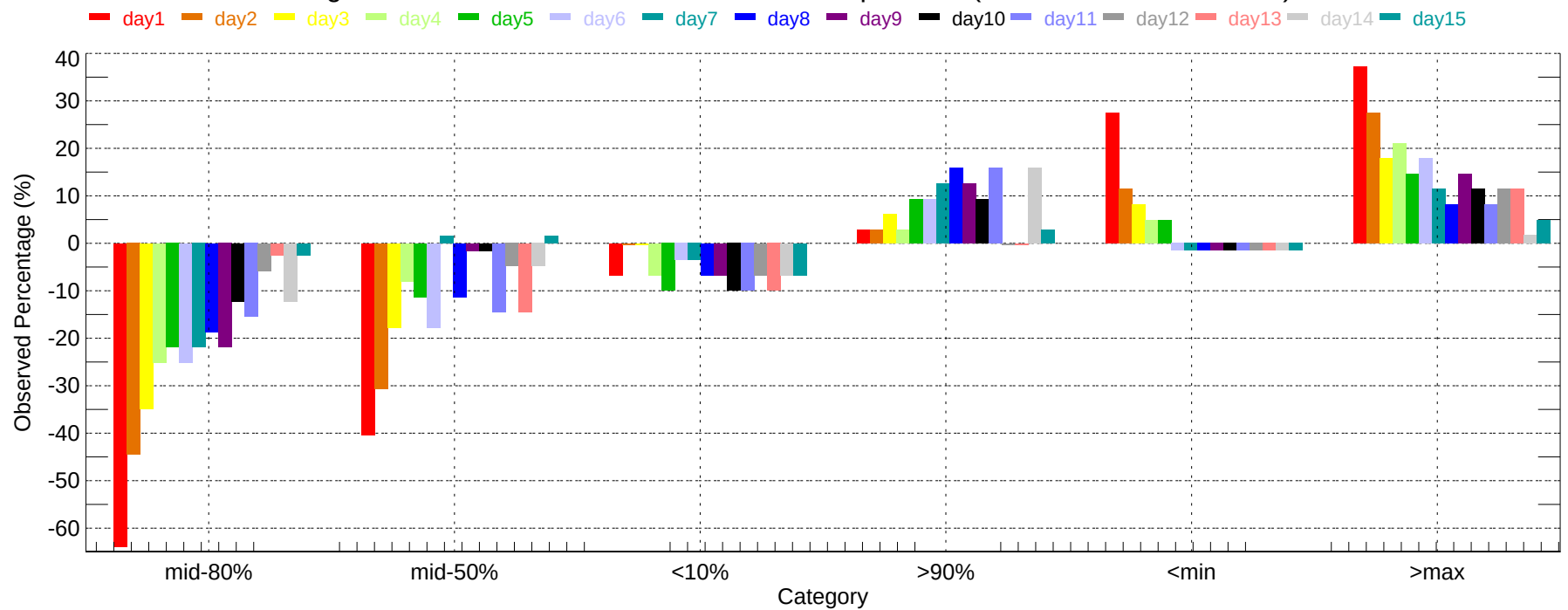
Observed Percentage Deviation of Ensembles - TUL: Min Temperature (2011-12-01~2011-12-31)
