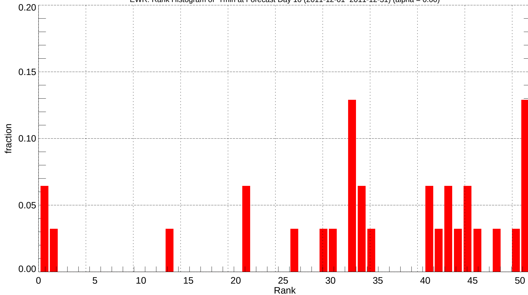
EWR: Rank Histogram of Tmin at Forecast Day 10 (2011-12-01~2011-12-31) (alpha = 0.00)
