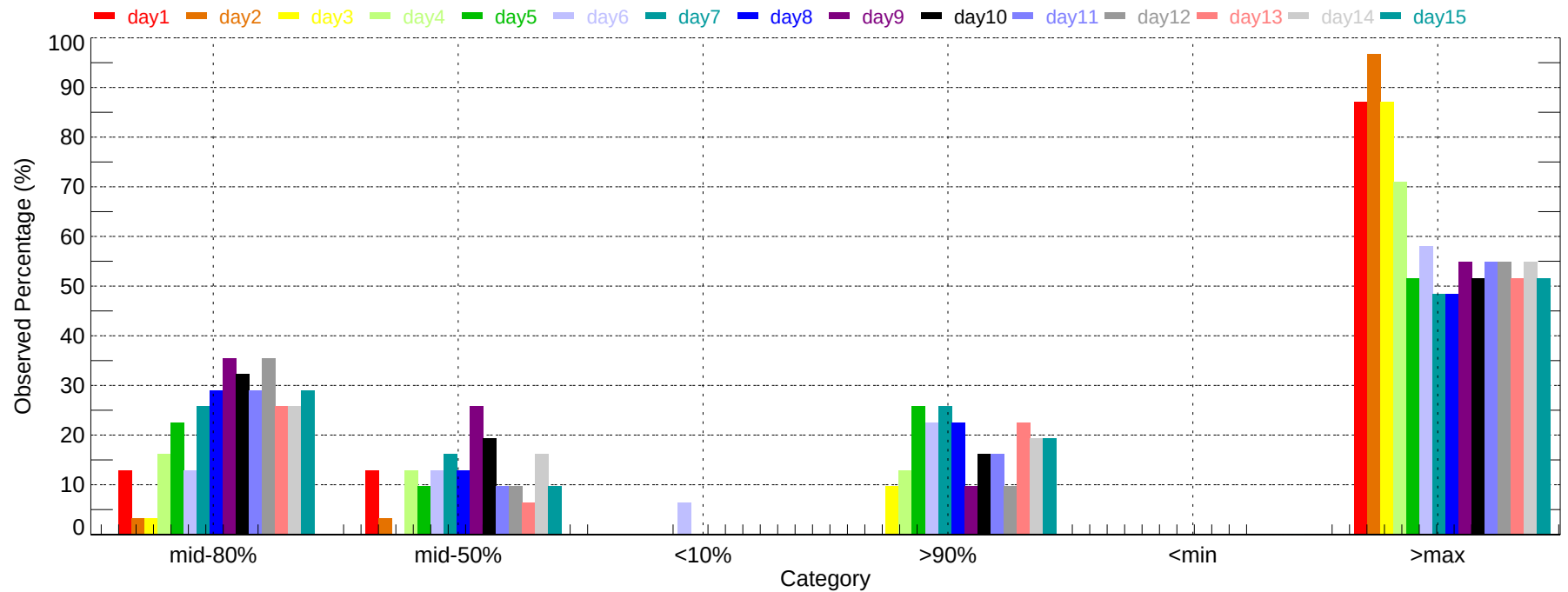
Observed Percentage of Ensembles - GTF: Max Temperature (2011-12-01~2011-12-31)
