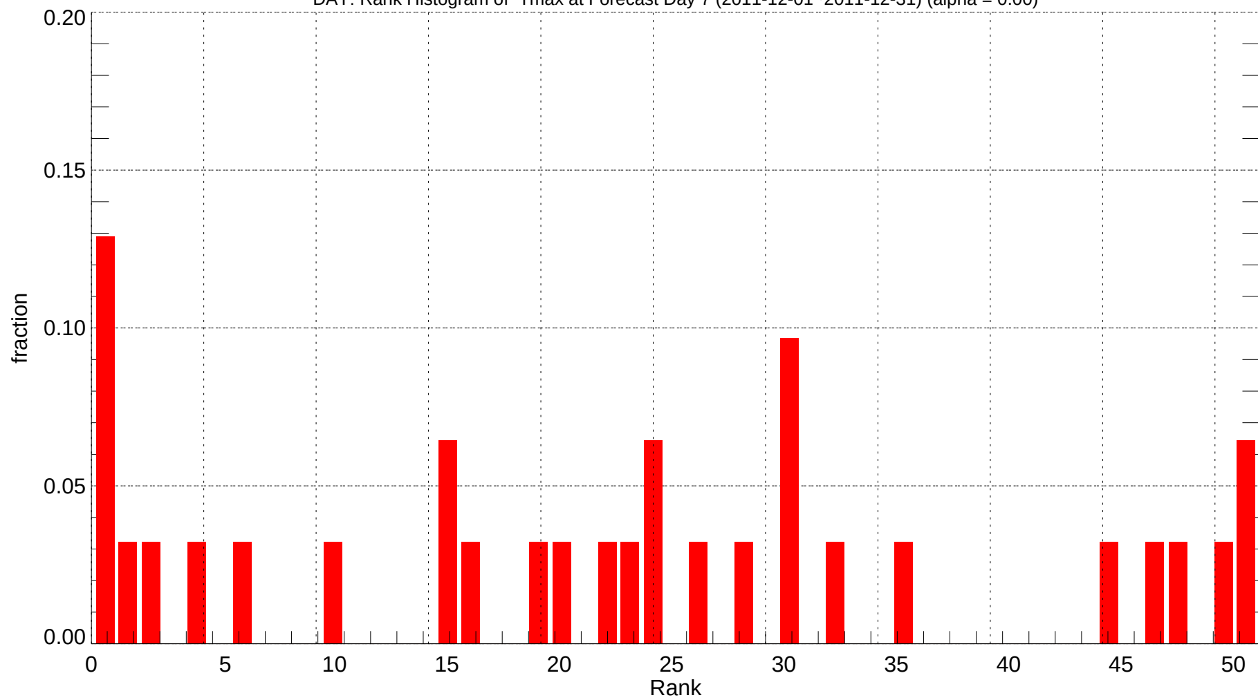
DAY: Rank Histogram of Tmax at Forecast Day 7 (2011-12-01~2011-12-31) (alpha = 0.00)
