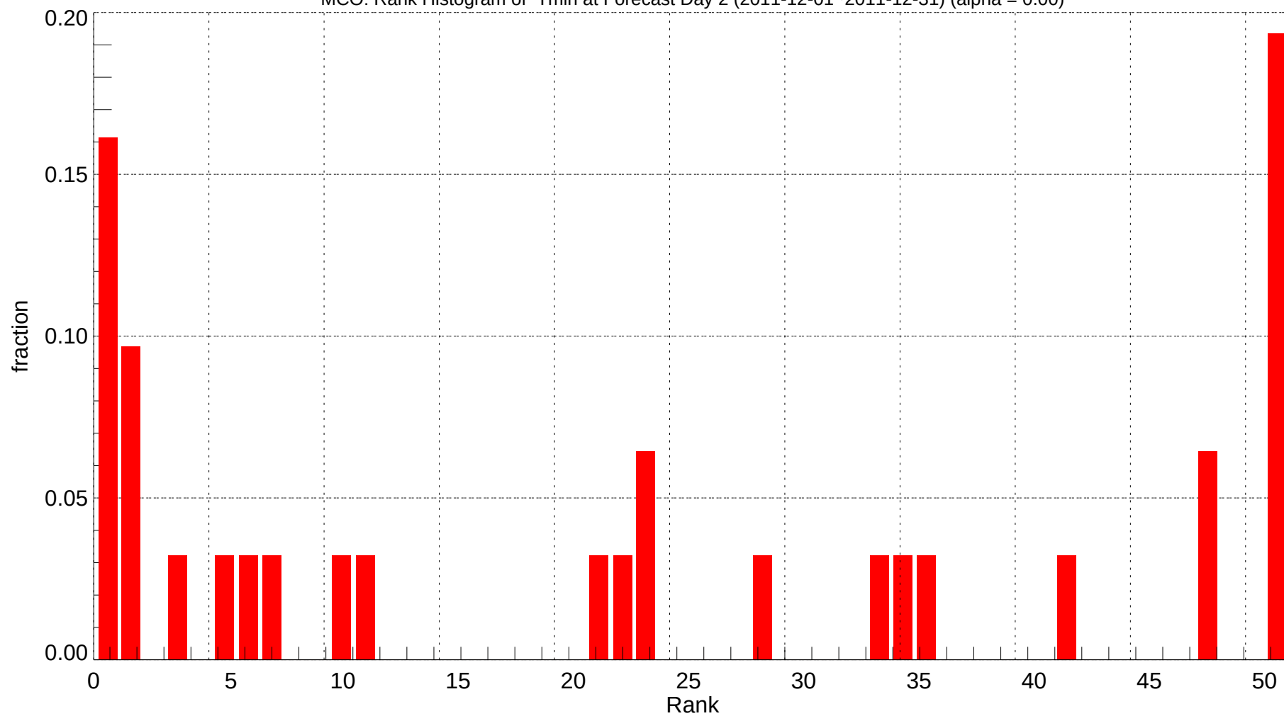
MCO: Rank Histogram of Tmin at Forecast Day 2 (2011-12-01~2011-12-31) (alpha = 0.00)
