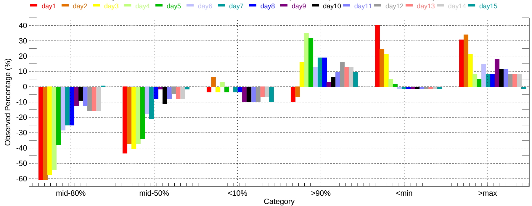
Observed Percentage Deviation of Ensembles - ICT: Min Temperature (2011-12-01~2011-12-31)
