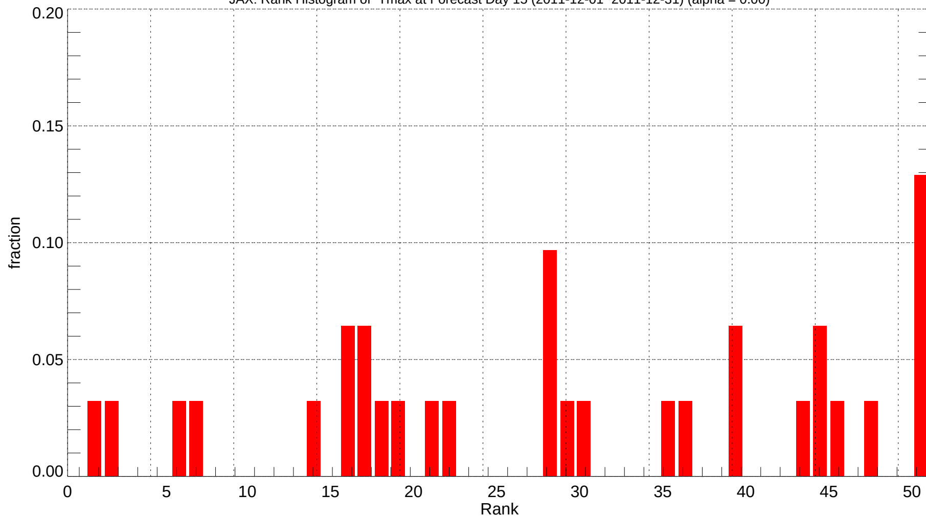
JAX: Rank Histogram of Tmax at Forecast Day 15 (2011-12-01~2011-12-31) (alpha = 0.00)
