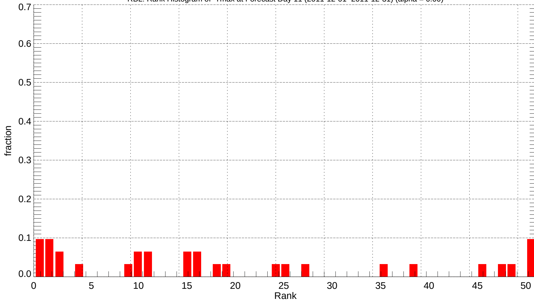
RBL: Rank Histogram of Tmax at Forecast Day 11 (2011-12-01~2011-12-31) (alpha = 0.00)
