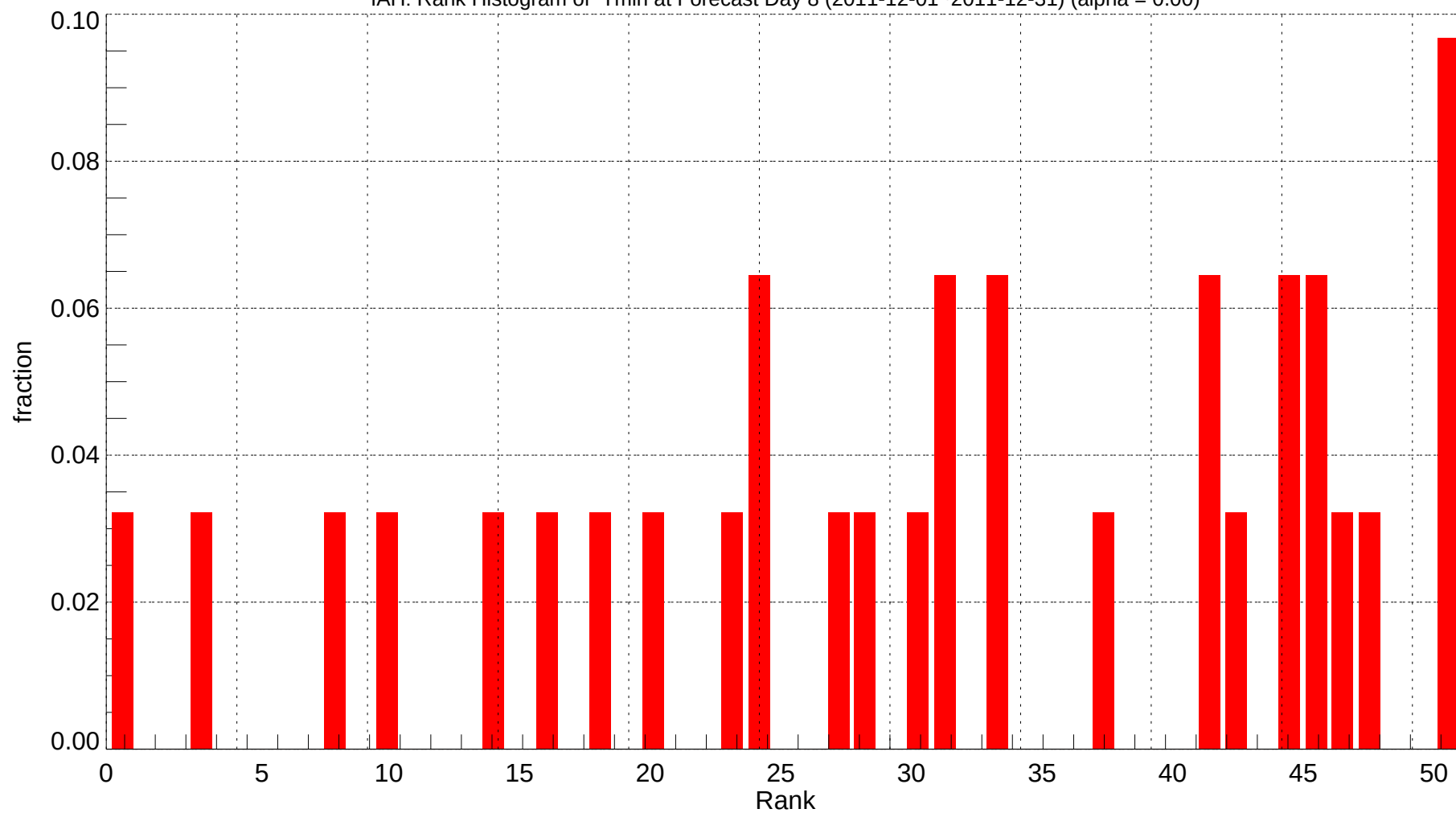
IAH: Rank Histogram of Tmin at Forecast Day 8 (2011-12-01~2011-12-31) (alpha = 0.00)
