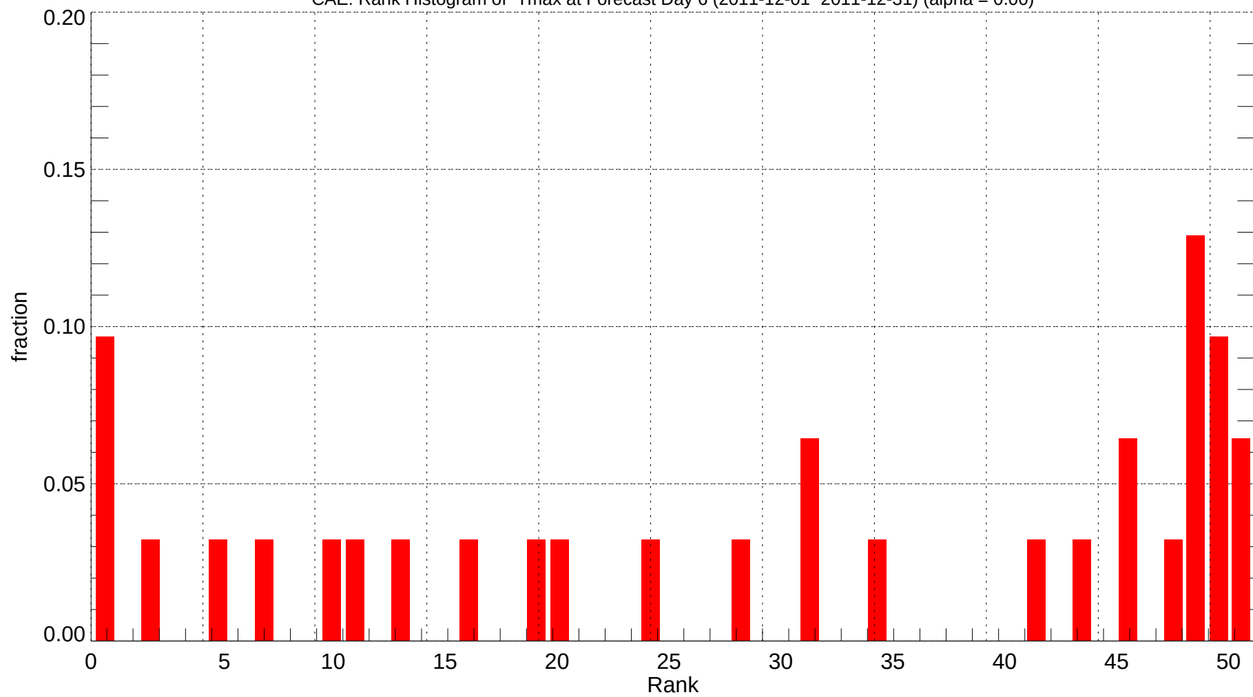
CAE: Rank Histogram of Tmax at Forecast Day 6 (2011-12-01~2011-12-31) (alpha = 0.00)
