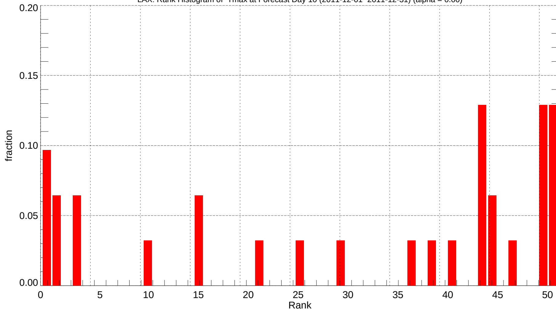
LAX: Rank Histogram of Tmax at Forecast Day 10 (2011-12-01~2011-12-31) (alpha = 0.00)
