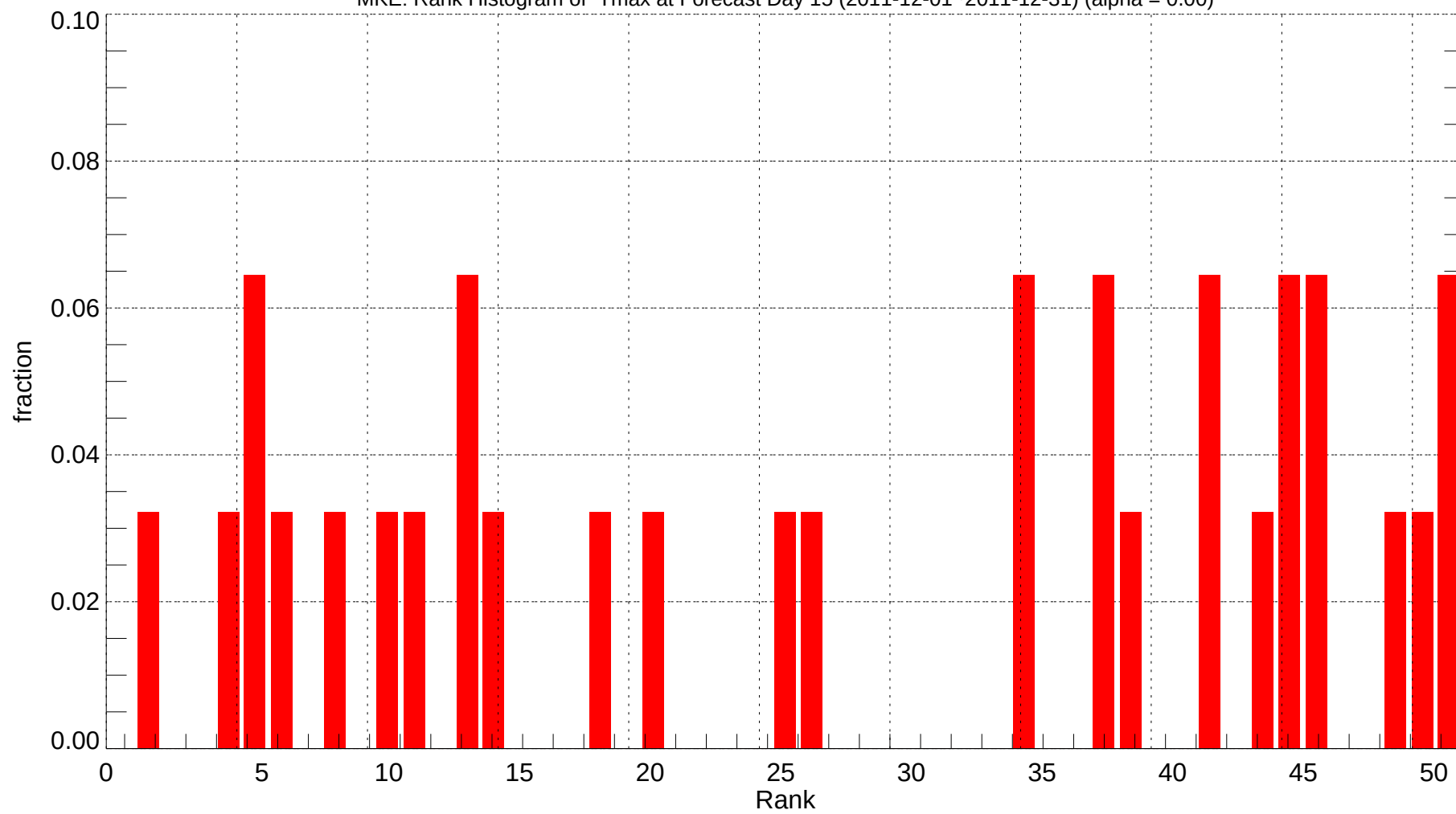
MKE: Rank Histogram of Tmax at Forecast Day 15 (2011-12-01~2011-12-31) (alpha = 0.00)
