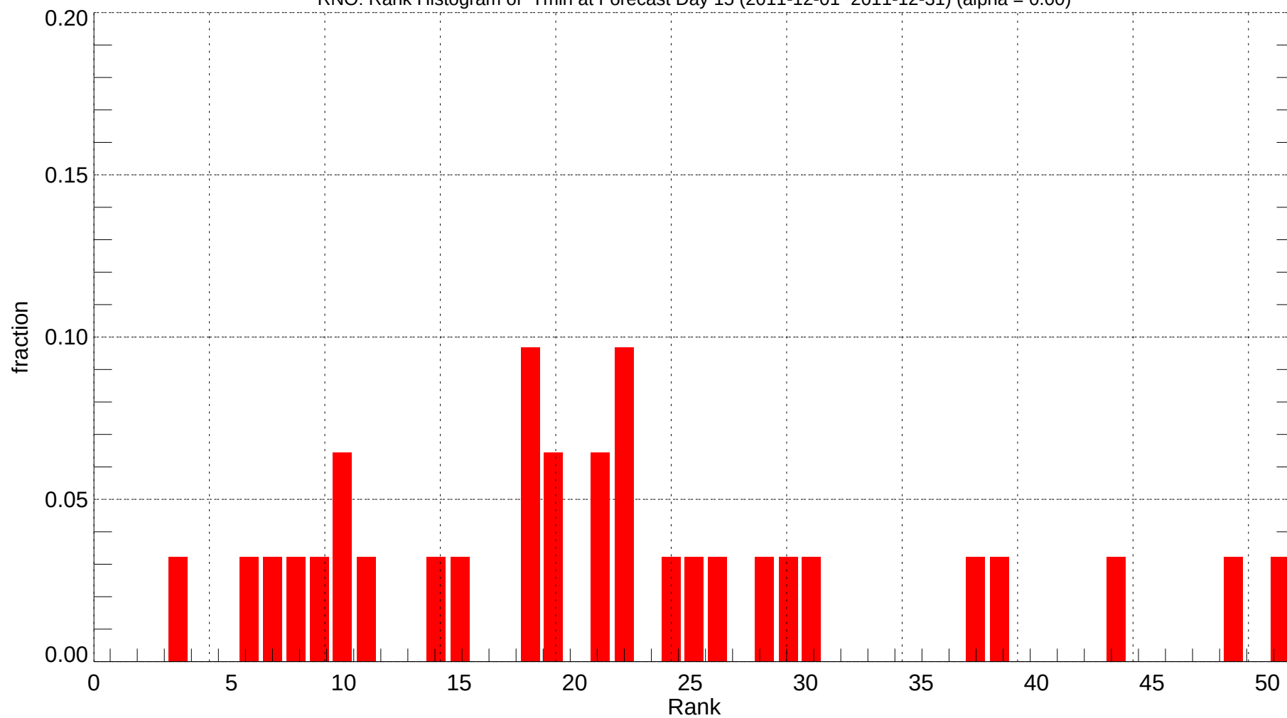
RNO: Rank Histogram of Tmin at Forecast Day 15 (2011-12-01~2011-12-31) (alpha = 0.00)
