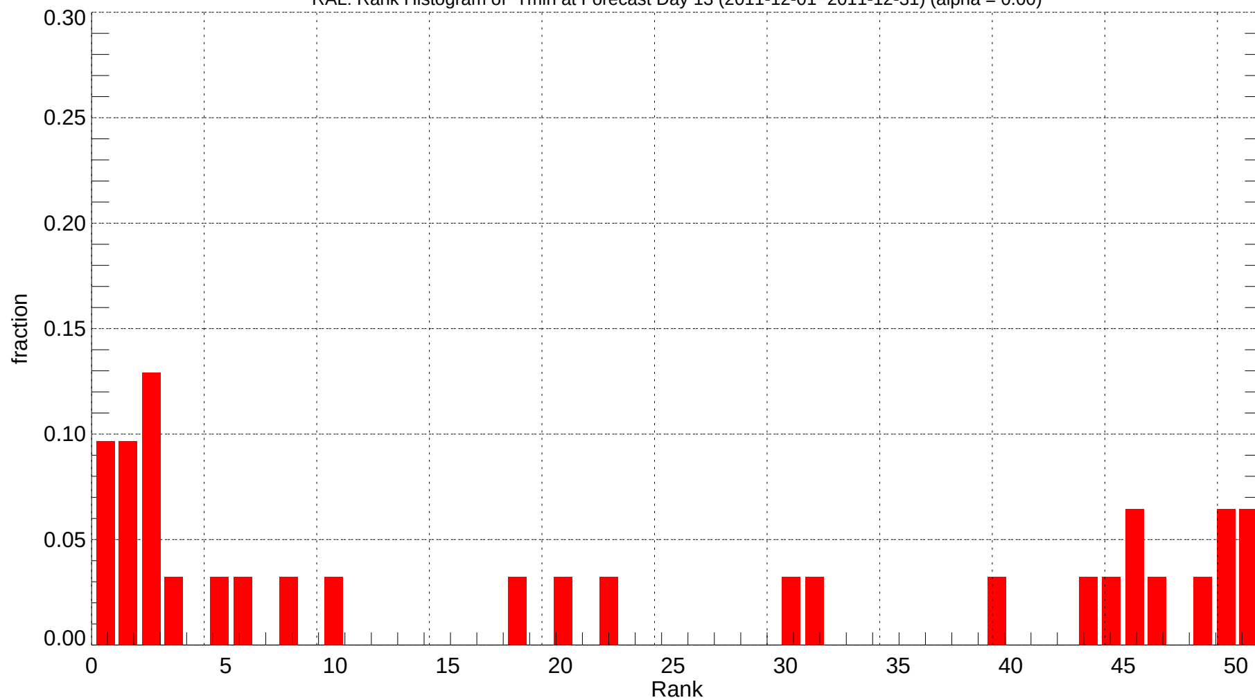
RAL: Rank Histogram of Tmin at Forecast Day 13 (2011-12-01~2011-12-31) (alpha = 0.00)
