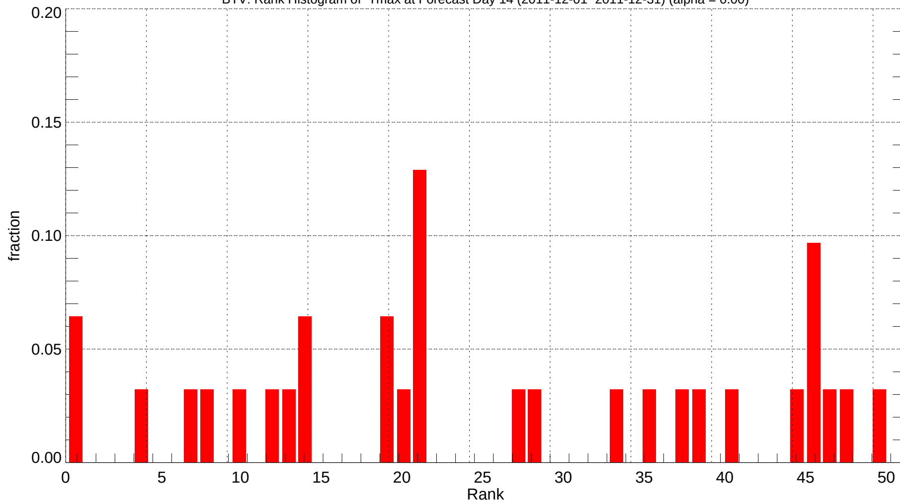
BTV: Rank Histogram of Tmax at Forecast Day 14 (2011-12-01~2011-12-31) (alpha = 0.00)
