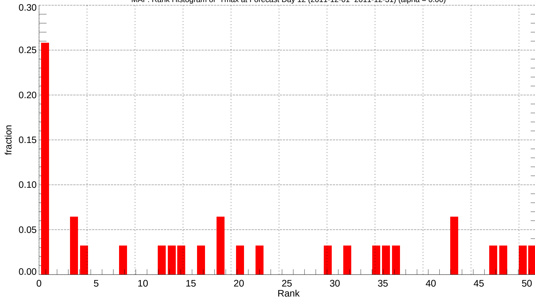
MAF: Rank Histogram of Tmax at Forecast Day 12 (2011-12-01~2011-12-31) (alpha = 0.00)
