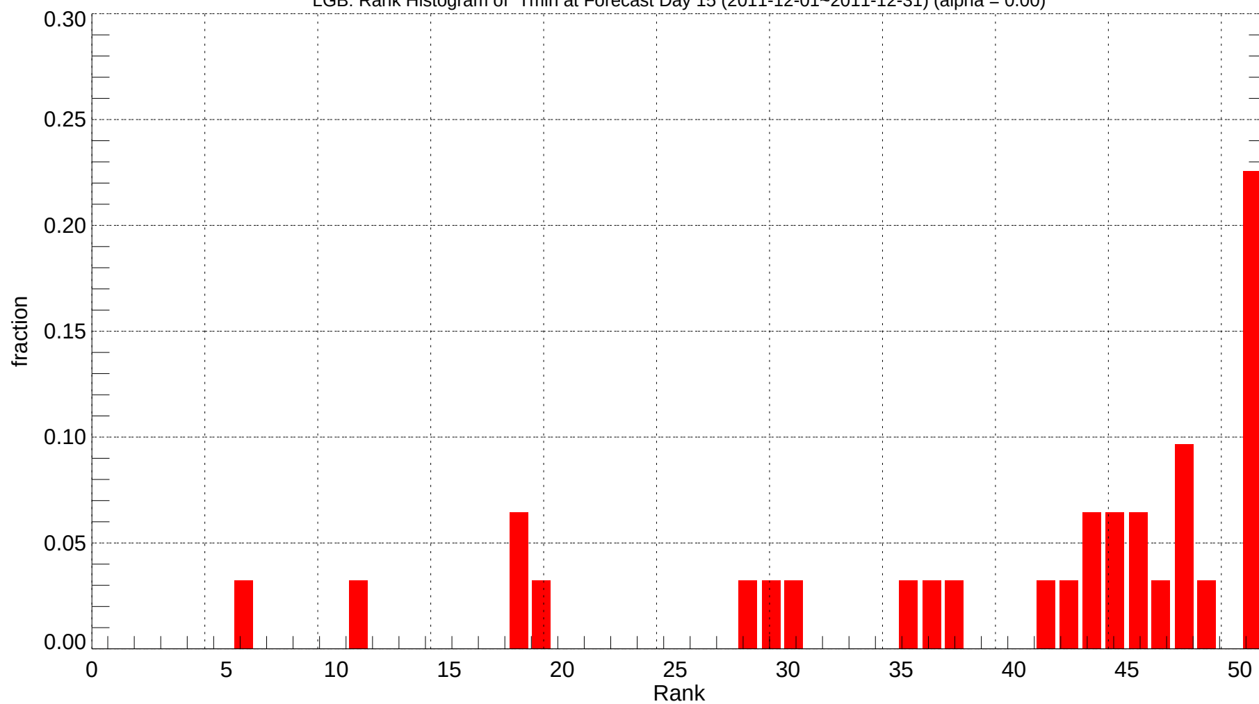
LGB: Rank Histogram of Tmin at Forecast Day 15 (2011-12-01~2011-12-31) (alpha = 0.00)
