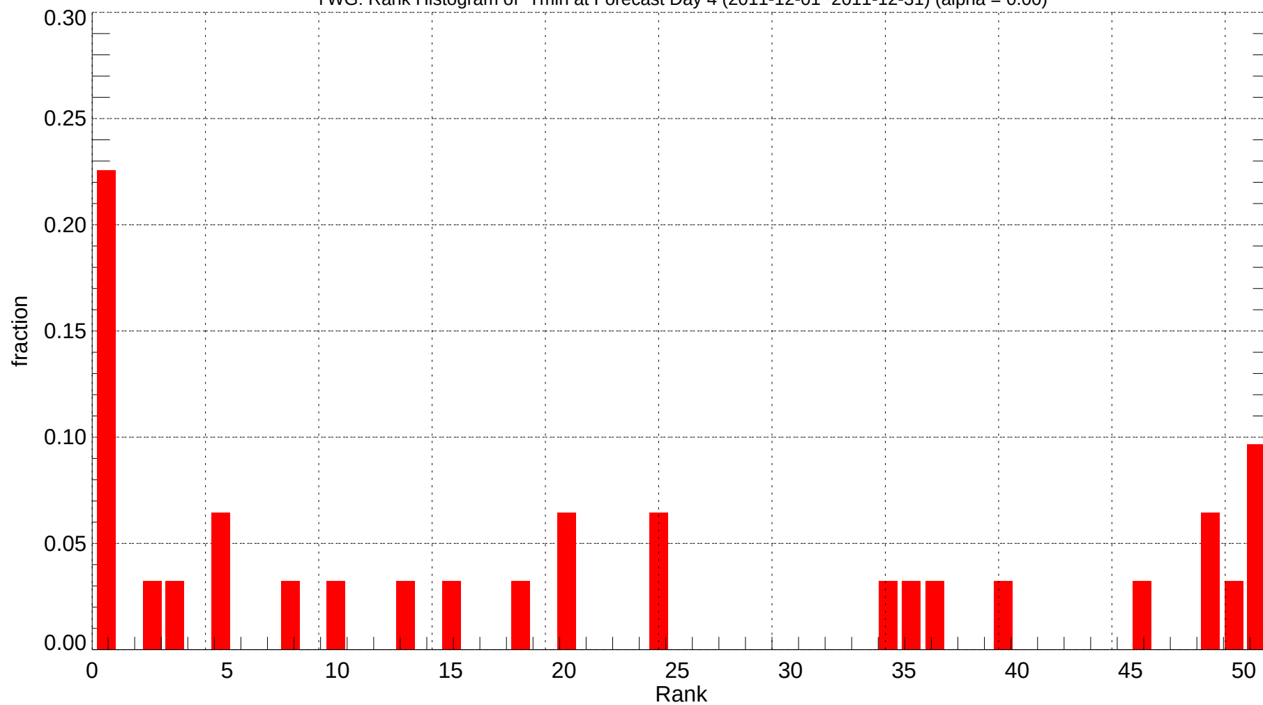
YWG: Rank Histogram of Tmin at Forecast Day 4 (2011-12-01~2011-12-31) (alpha = 0.00)
