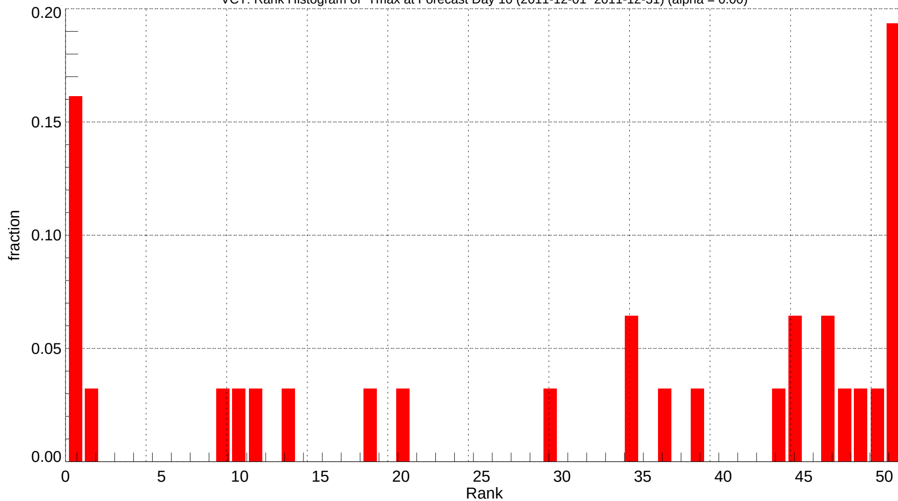
VCT: Rank Histogram of Tmax at Forecast Day 10 (2011-12-01~2011-12-31) (alpha = 0.00)
