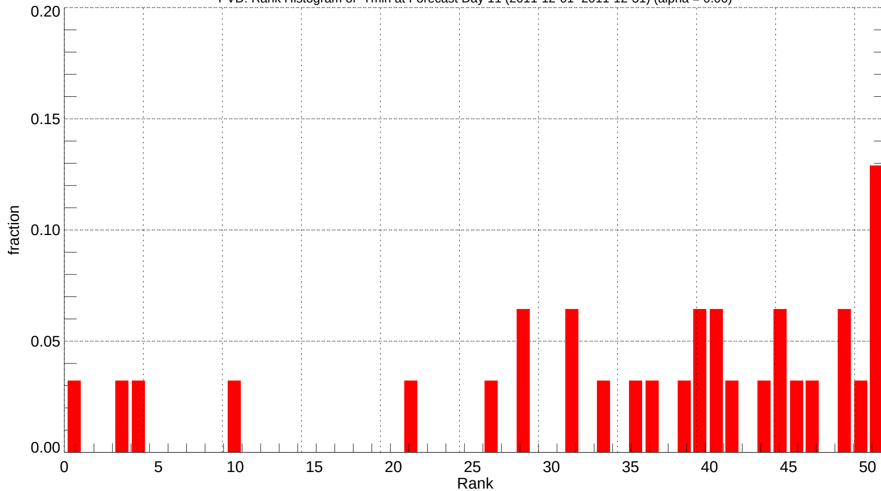
PVD: Rank Histogram of Tmin at Forecast Day 11 (2011-12-01~2011-12-31) (alpha = 0.00)
