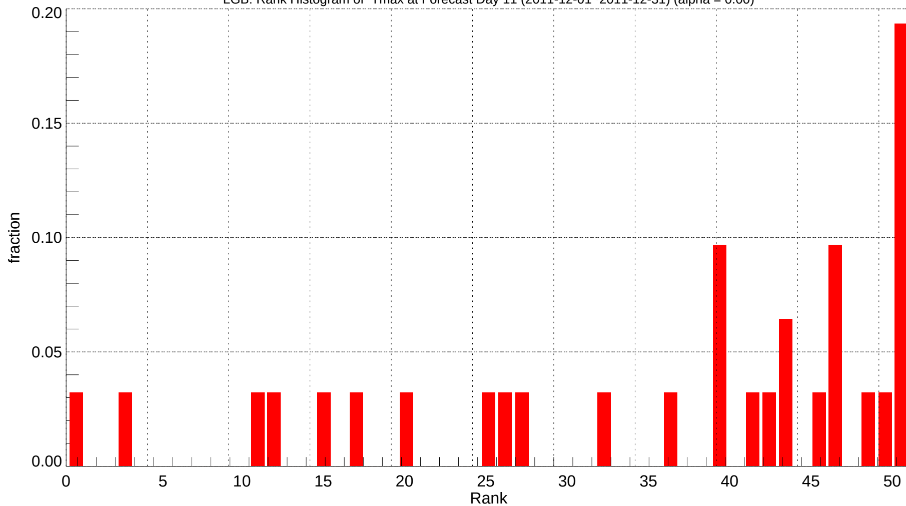
LGB: Rank Histogram of Tmax at Forecast Day 11 (2011-12-01~2011-12-31) (alpha = 0.00)
