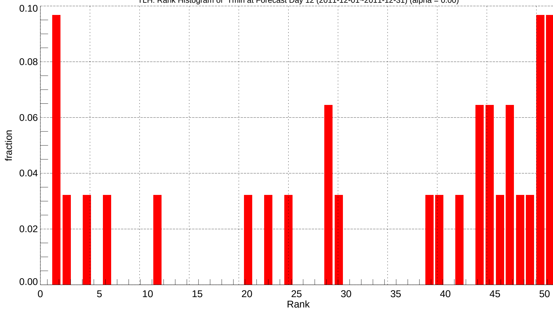
TLH: Rank Histogram of Tmin at Forecast Day 12 (2011-12-01~2011-12-31) (alpha = 0.00)
