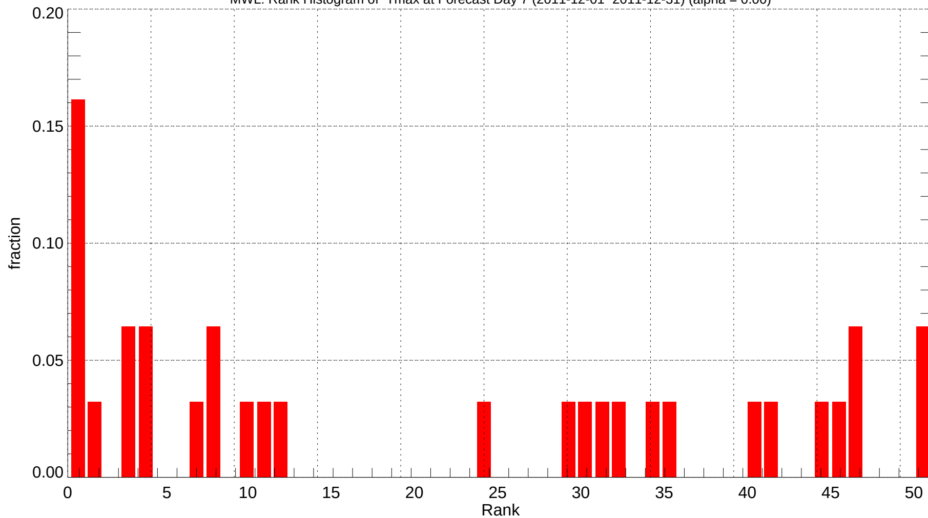
MWL: Rank Histogram of Tmax at Forecast Day 7 (2011-12-01~2011-12-31) (alpha = 0.00)
