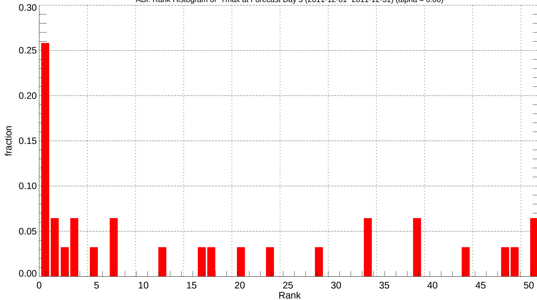
ABI: Rank Histogram of Tmax at Forecast Day 3 (2011-12-01~2011-12-31) (alpha = 0.00)
