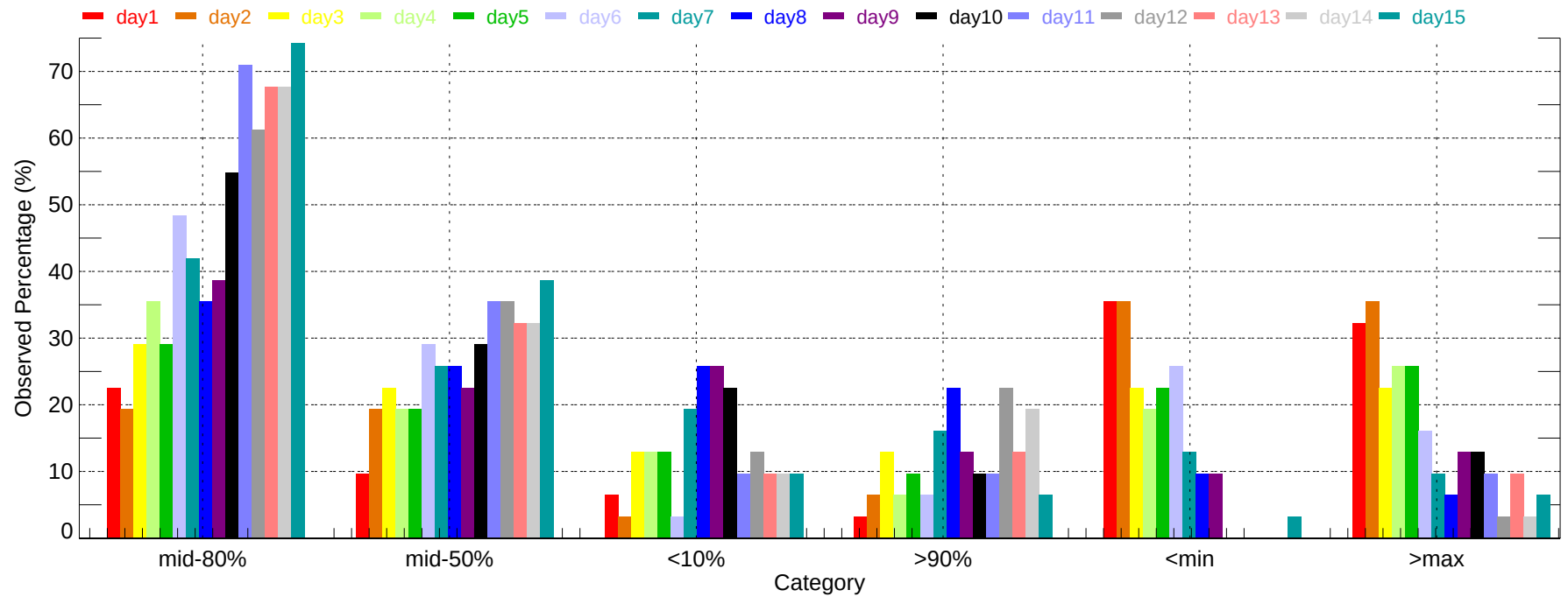
Observed Percentage of Ensembles - BTV: Min Temperature (2011-12-01~2011-12-31)
