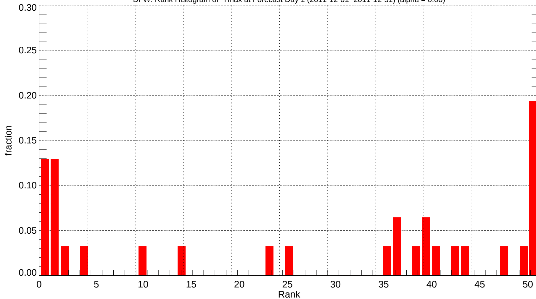
DFW: Rank Histogram of Tmax at Forecast Day 1 (2011-12-01~2011-12-31) (alpha = 0.00)
