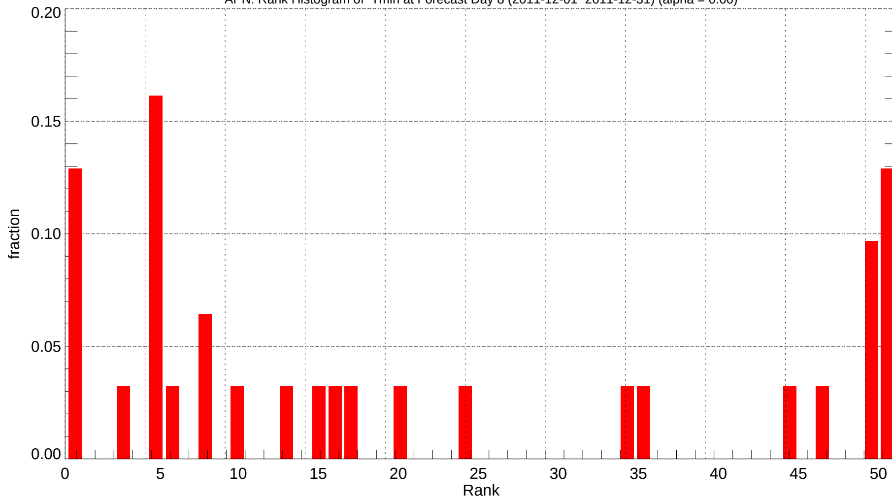
APN: Rank Histogram of Tmin at Forecast Day 8 (2011-12-01~2011-12-31) (alpha = 0.00)
