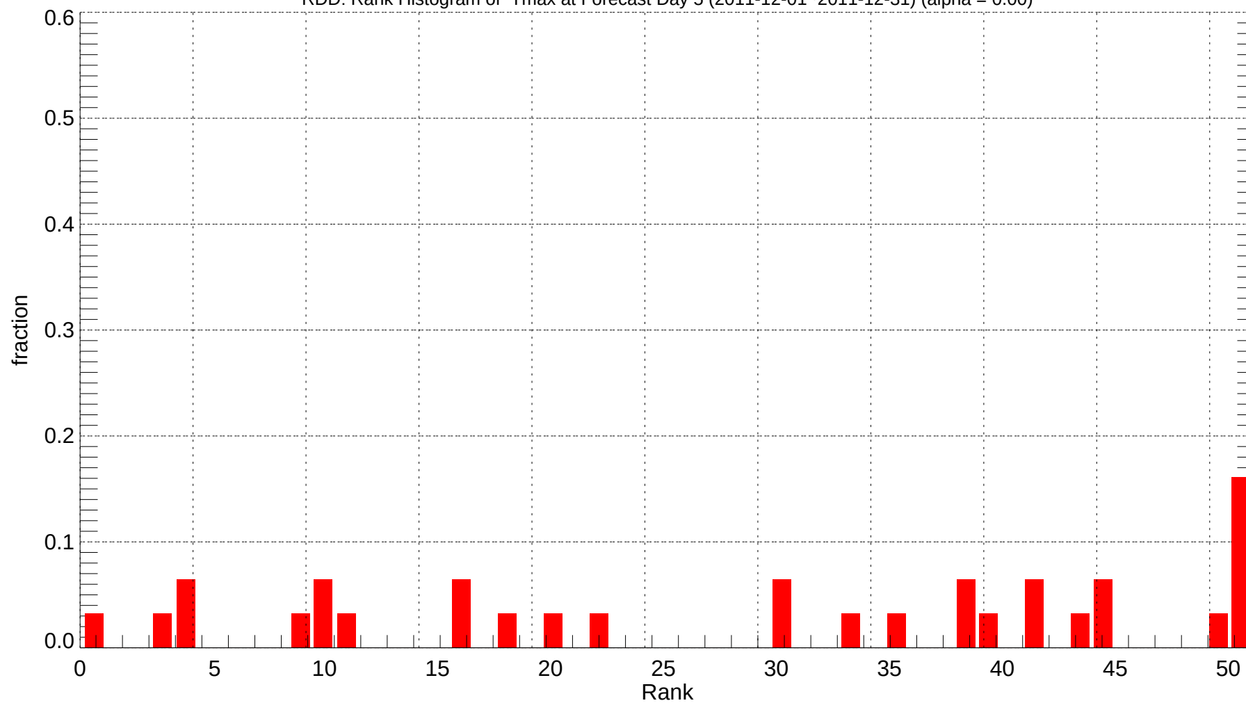
RDD: Rank Histogram of Tmax at Forecast Day 5 (2011-12-01~2011-12-31) (alpha = 0.00)
