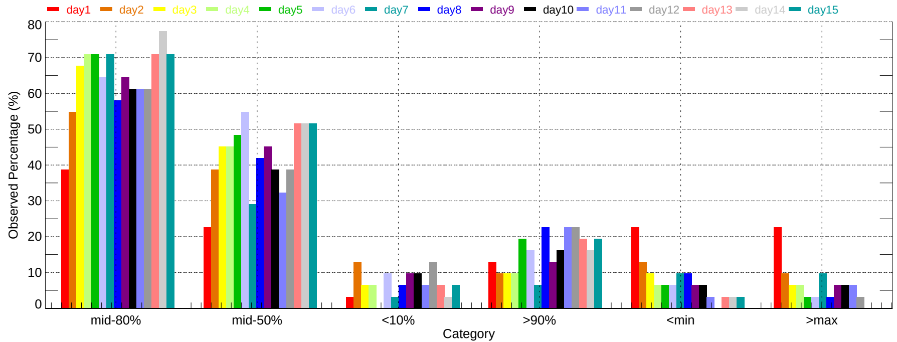
Observed Percentage of Ensembles - BDL: Max Temperature (2011-12-01~2011-12-31)
