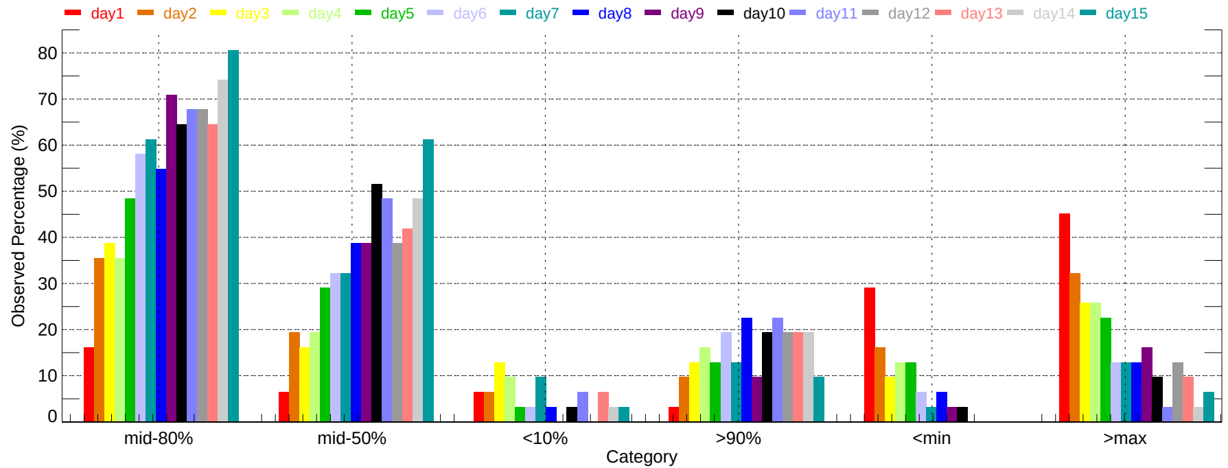
Observed Percentage of Ensembles - CLT: Min Temperature (2011-12-01~2011-12-31)
