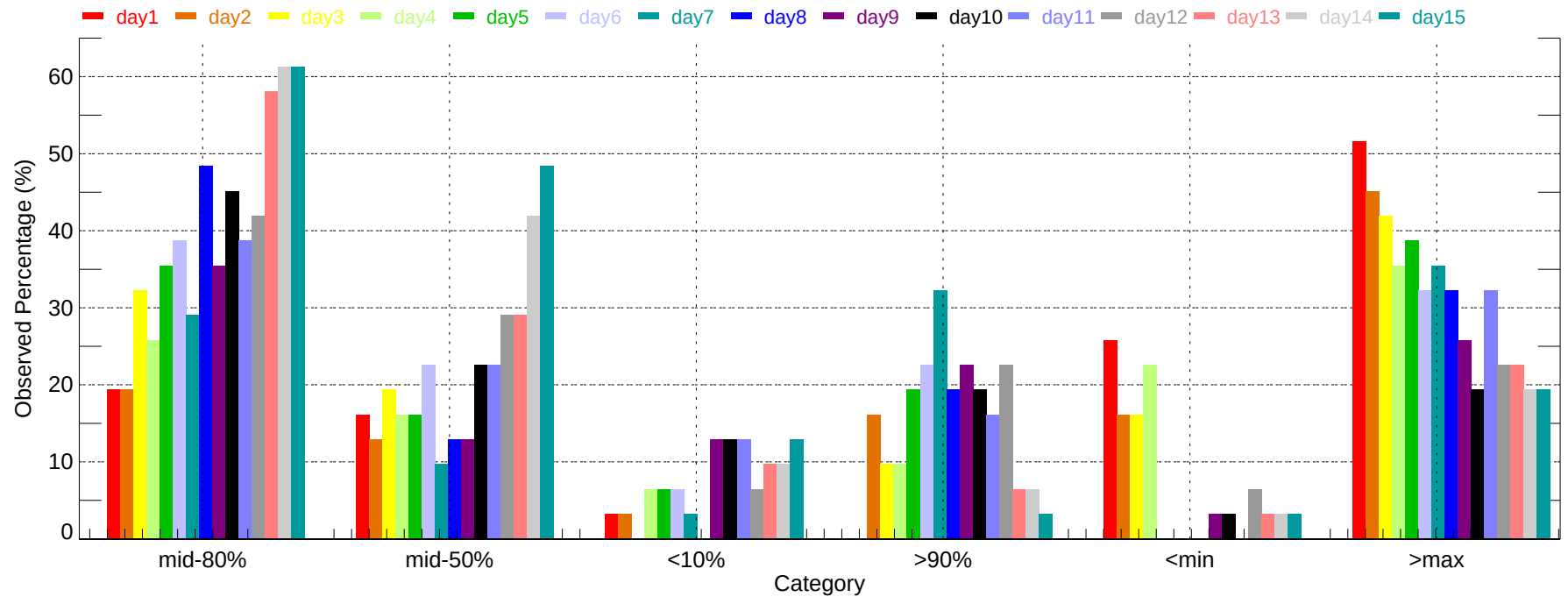
Observed Percentage of Ensembles - ABQ: Max Temperature (2011-12-01~2011-12-31)
