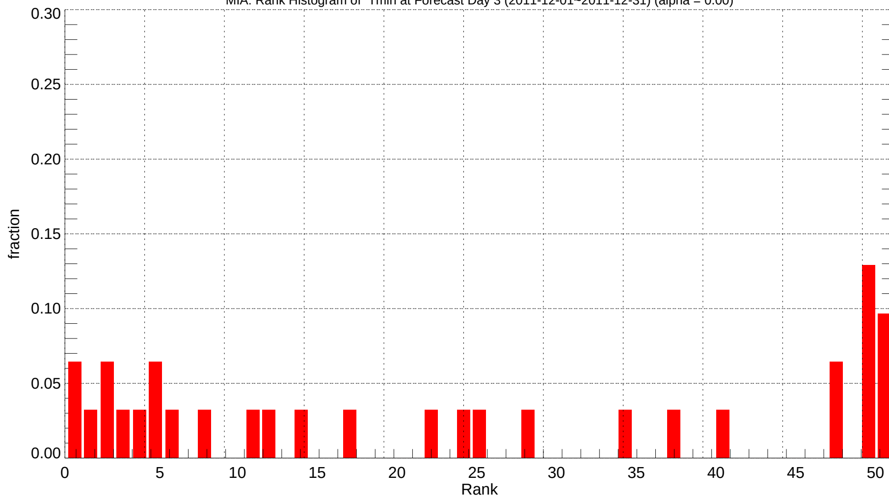
MIA: Rank Histogram of Tmin at Forecast Day 3 (2011-12-01~2011-12-31) (alpha = 0.00)
