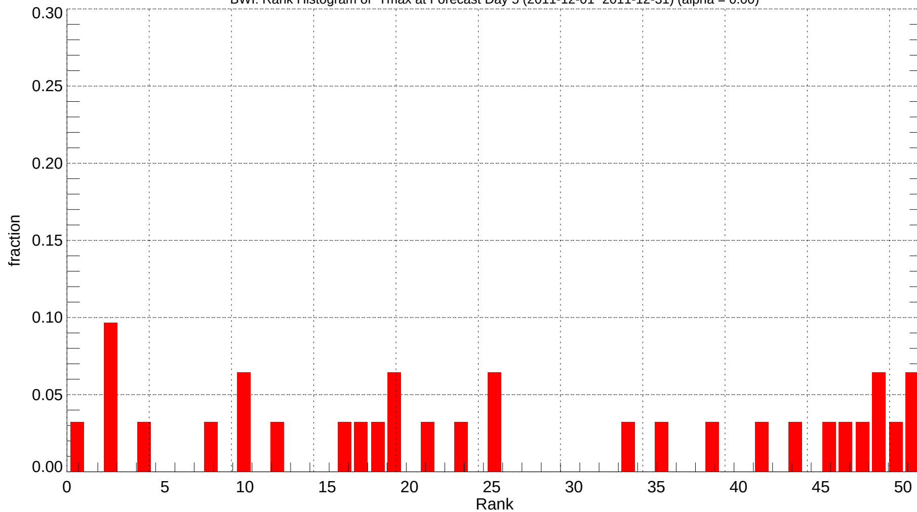
BWI: Rank Histogram of Tmax at Forecast Day 5 (2011-12-01~2011-12-31) (alpha = 0.00)
