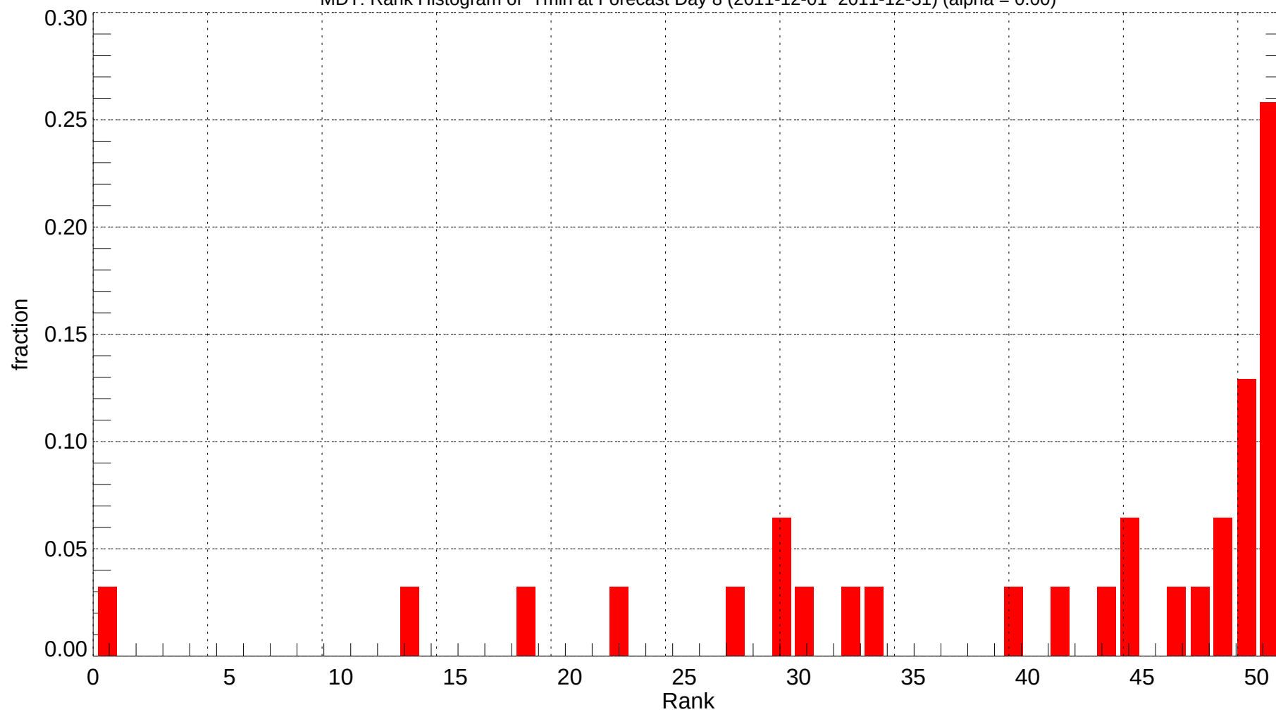
MDT: Rank Histogram of Tmin at Forecast Day 8 (2011-12-01~2011-12-31) (alpha = 0.00)
