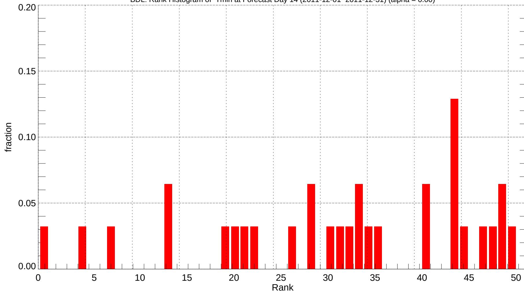
BDL: Rank Histogram of Tmin at Forecast Day 14 (2011-12-01~2011-12-31) (alpha = 0.00)
