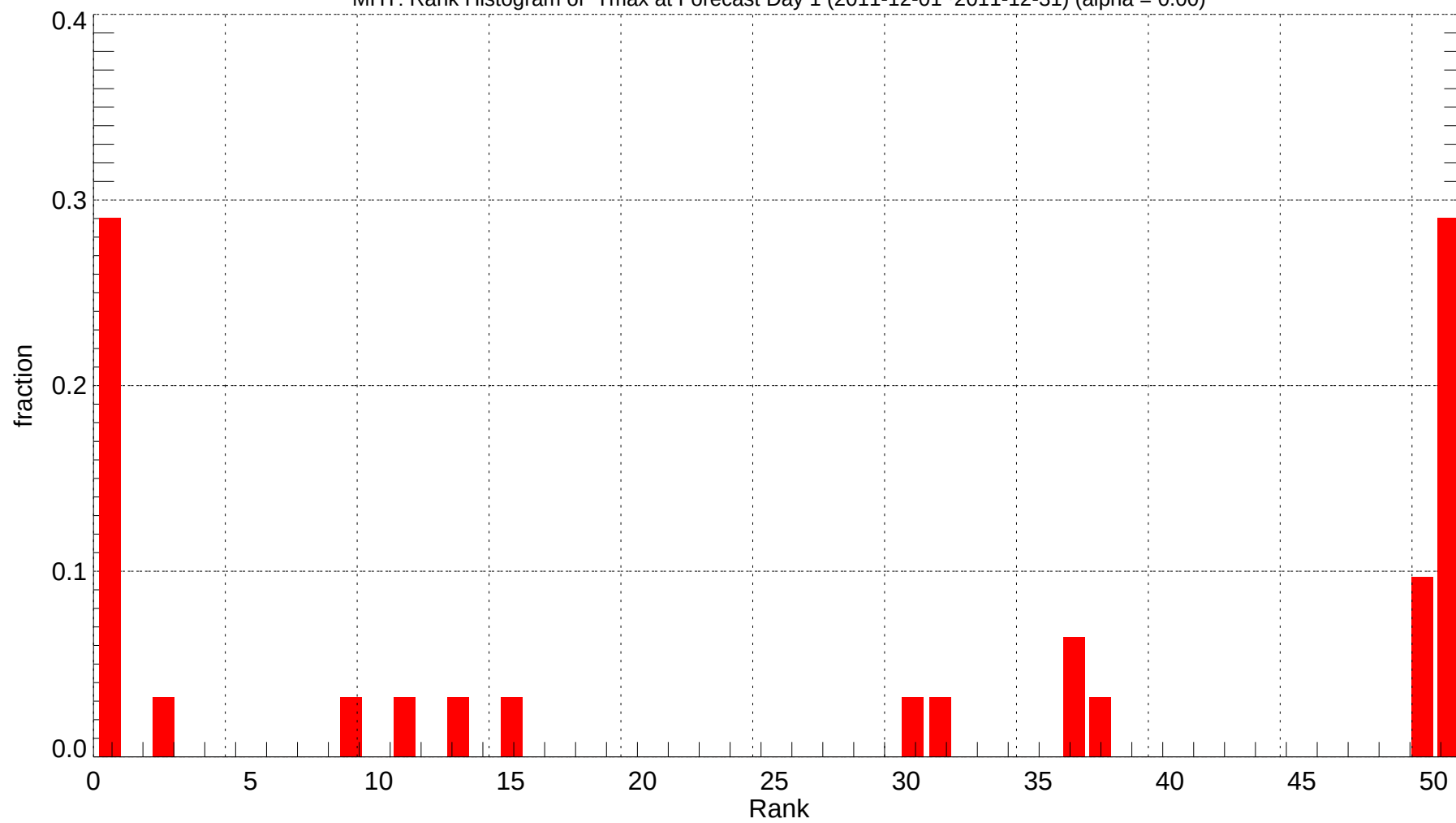
MHT: Rank Histogram of Tmax at Forecast Day 1 (2011-12-01~2011-12-31) (alpha = 0.00)
