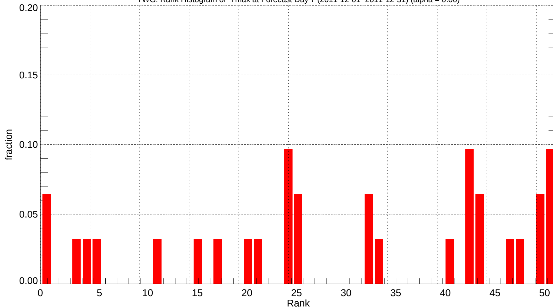
YWG: Rank Histogram of Tmax at Forecast Day 7 (2011-12-01~2011-12-31) (alpha = 0.00)
