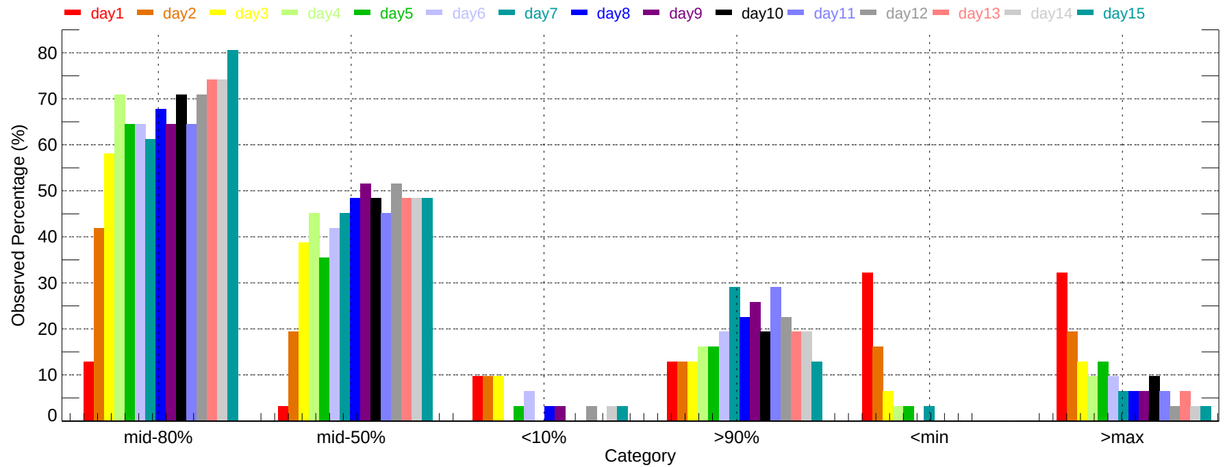
Observed Percentage of Ensembles - OKC: Min Temperature (2011-12-01~2011-12-31)
