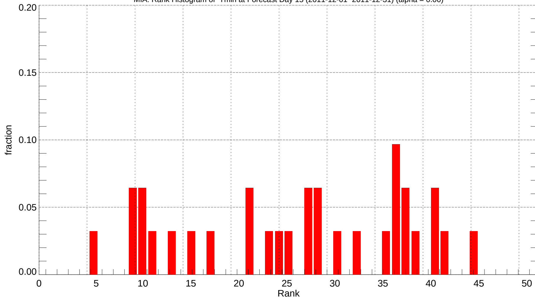
MIA: Rank Histogram of Tmin at Forecast Day 15 (2011-12-01~2011-12-31) (alpha = 0.00)
