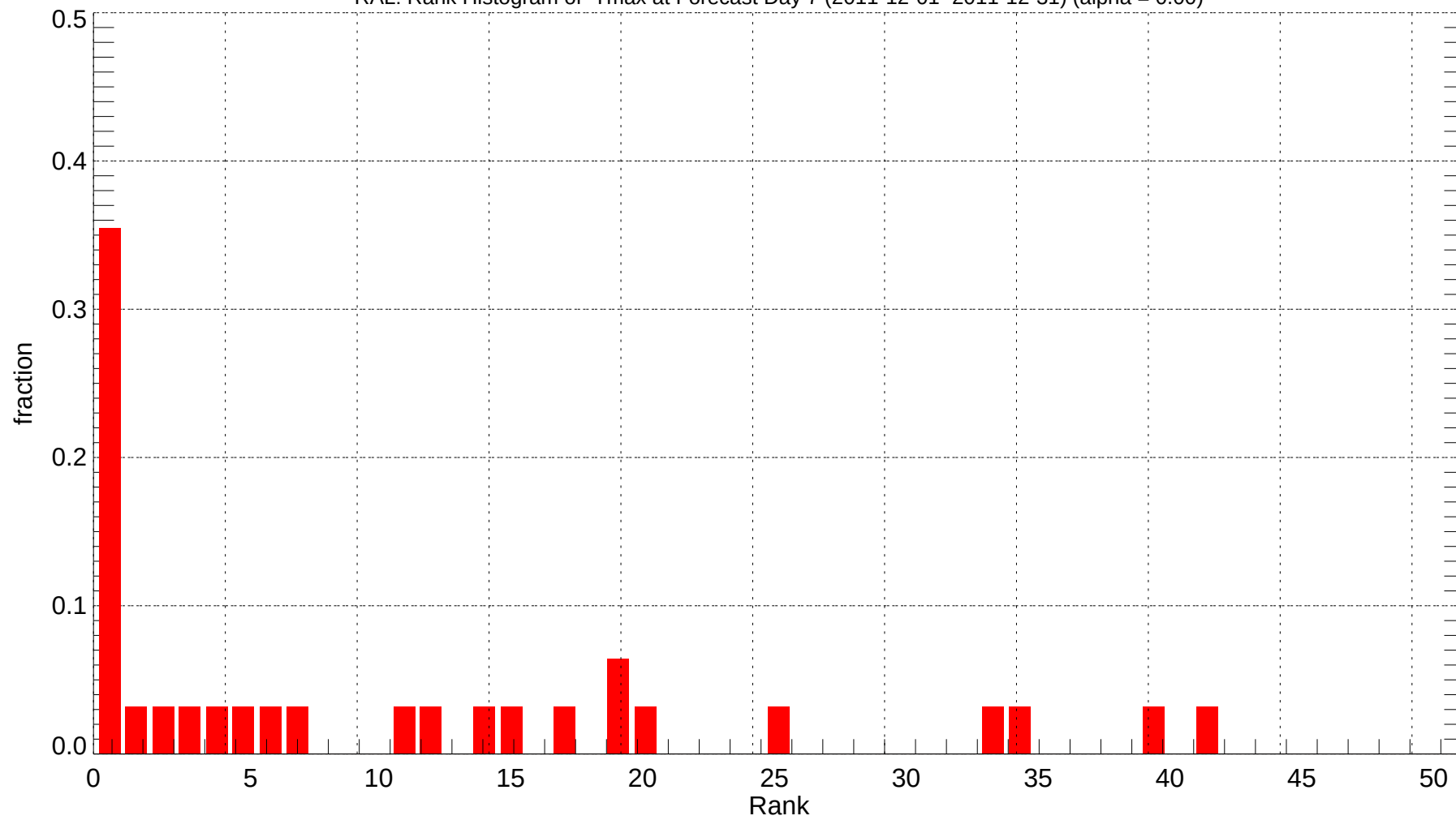
RAL: Rank Histogram of Tmax at Forecast Day 7 (2011-12-01~2011-12-31) (alpha = 0.00)
