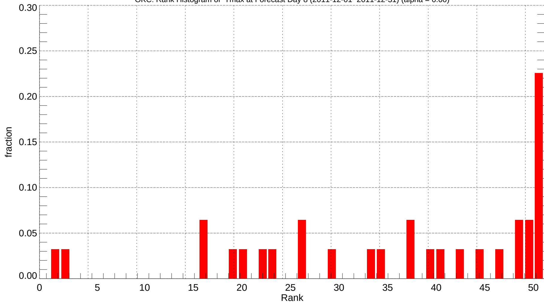
OKC: Rank Histogram of Tmax at Forecast Day 8 (2011-12-01~2011-12-31) (alpha = 0.00)
