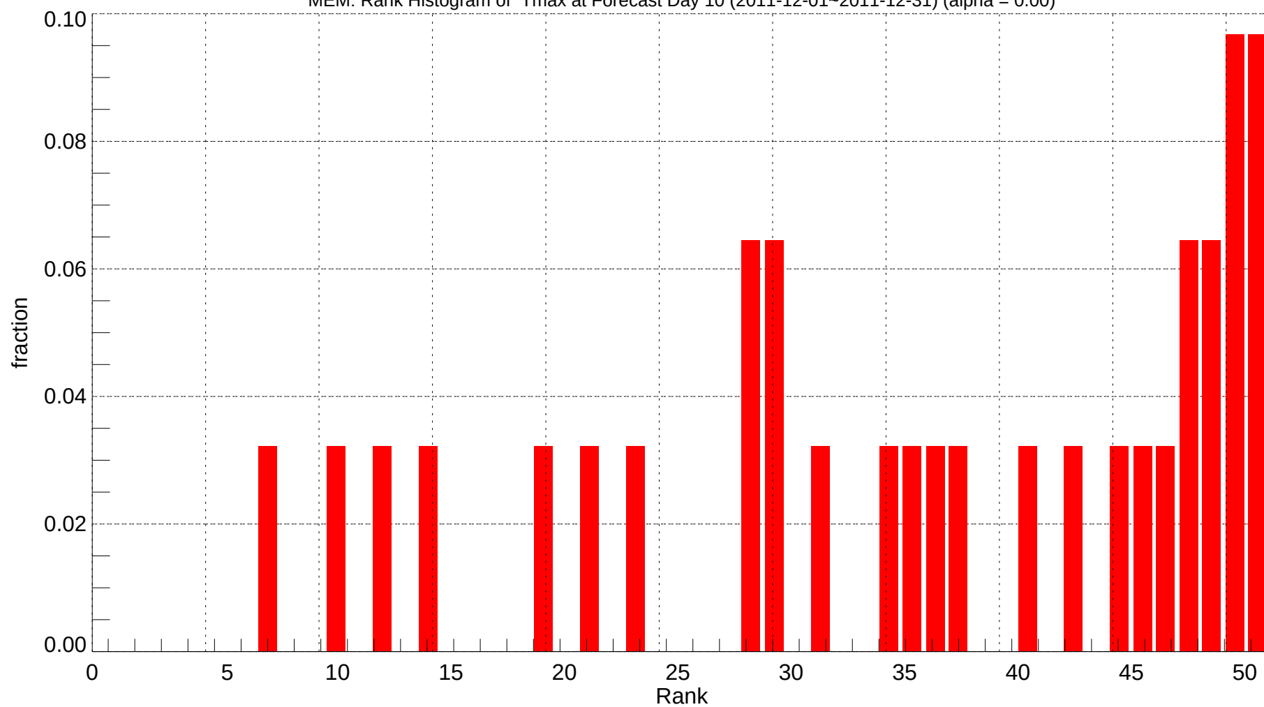
MEM: Rank Histogram of Tmax at Forecast Day 10 (2011-12-01~2011-12-31) (alpha = 0.00)
