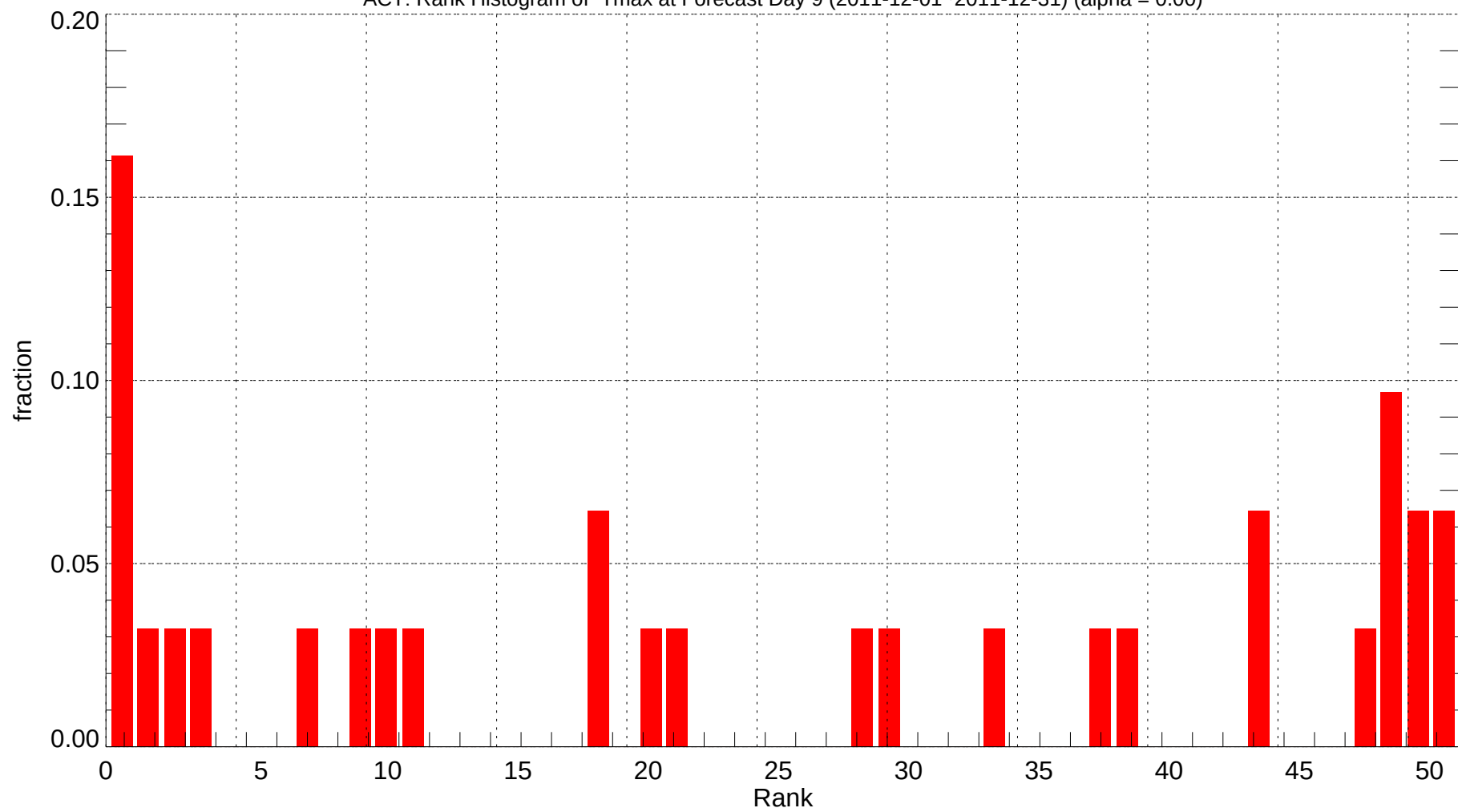
ACT: Rank Histogram of Tmax at Forecast Day 9 (2011-12-01~2011-12-31) (alpha = 0.00)
