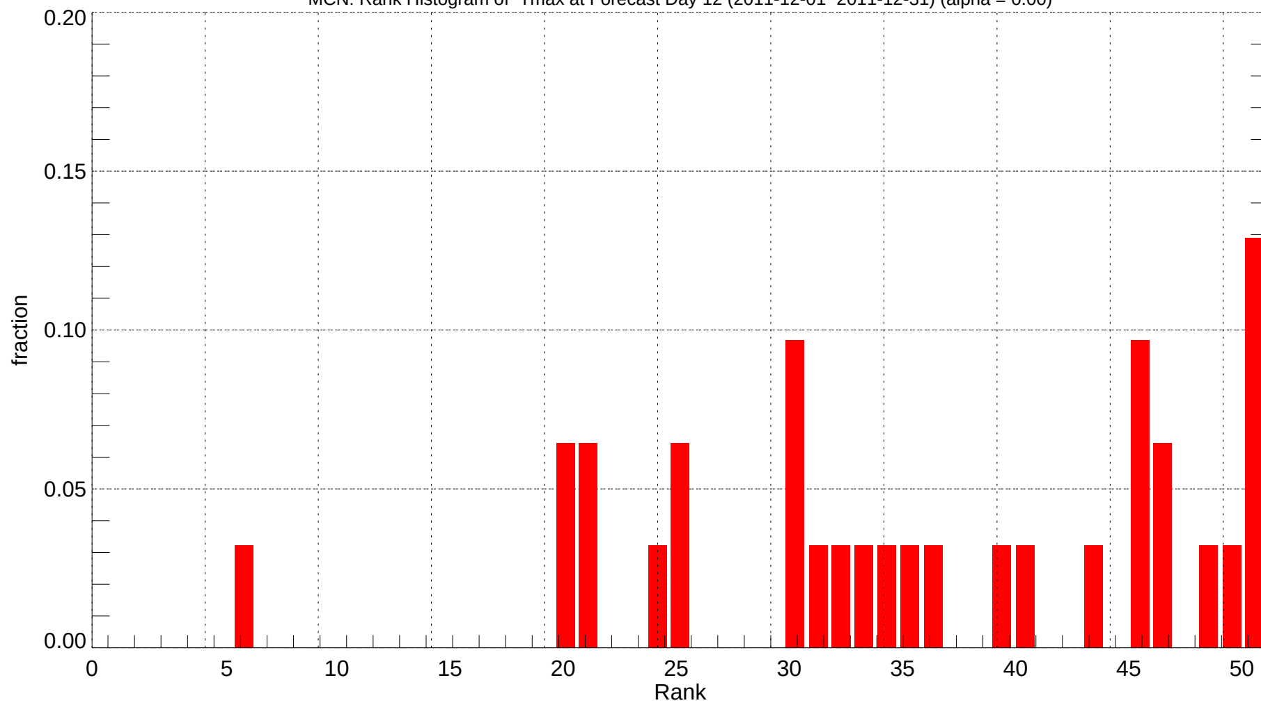
MCN: Rank Histogram of Tmax at Forecast Day 12 (2011-12-01~2011-12-31) (alpha = 0.00)
