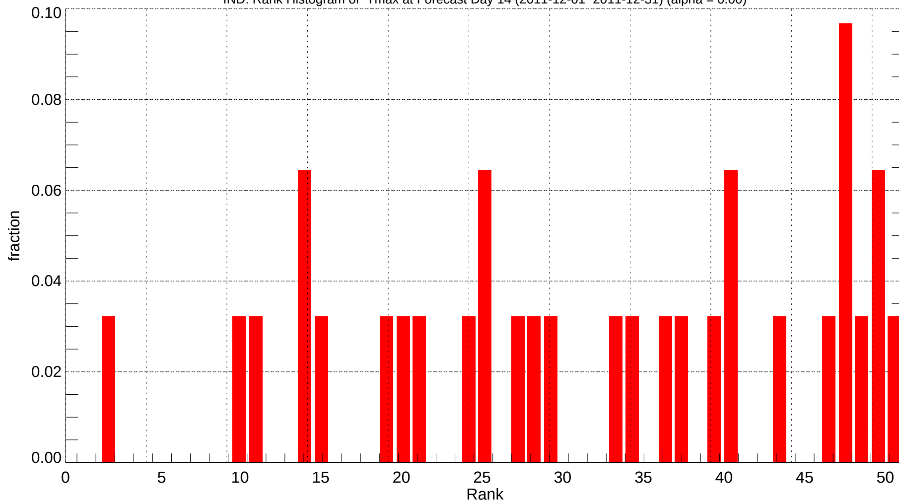
IND: Rank Histogram of Tmax at Forecast Day 14 (2011-12-01~2011-12-31) (alpha = 0.00)
