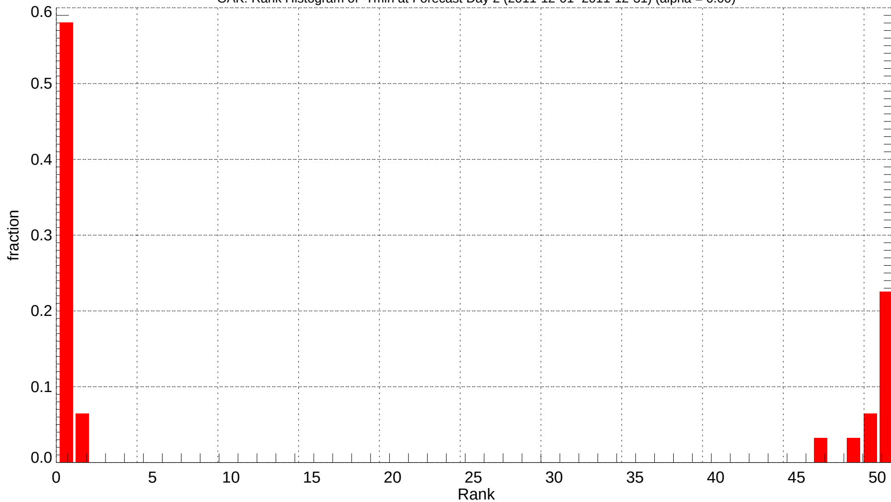
OAK: Rank Histogram of Tmin at Forecast Day 2 (2011-12-01~2011-12-31) (alpha = 0.00)
