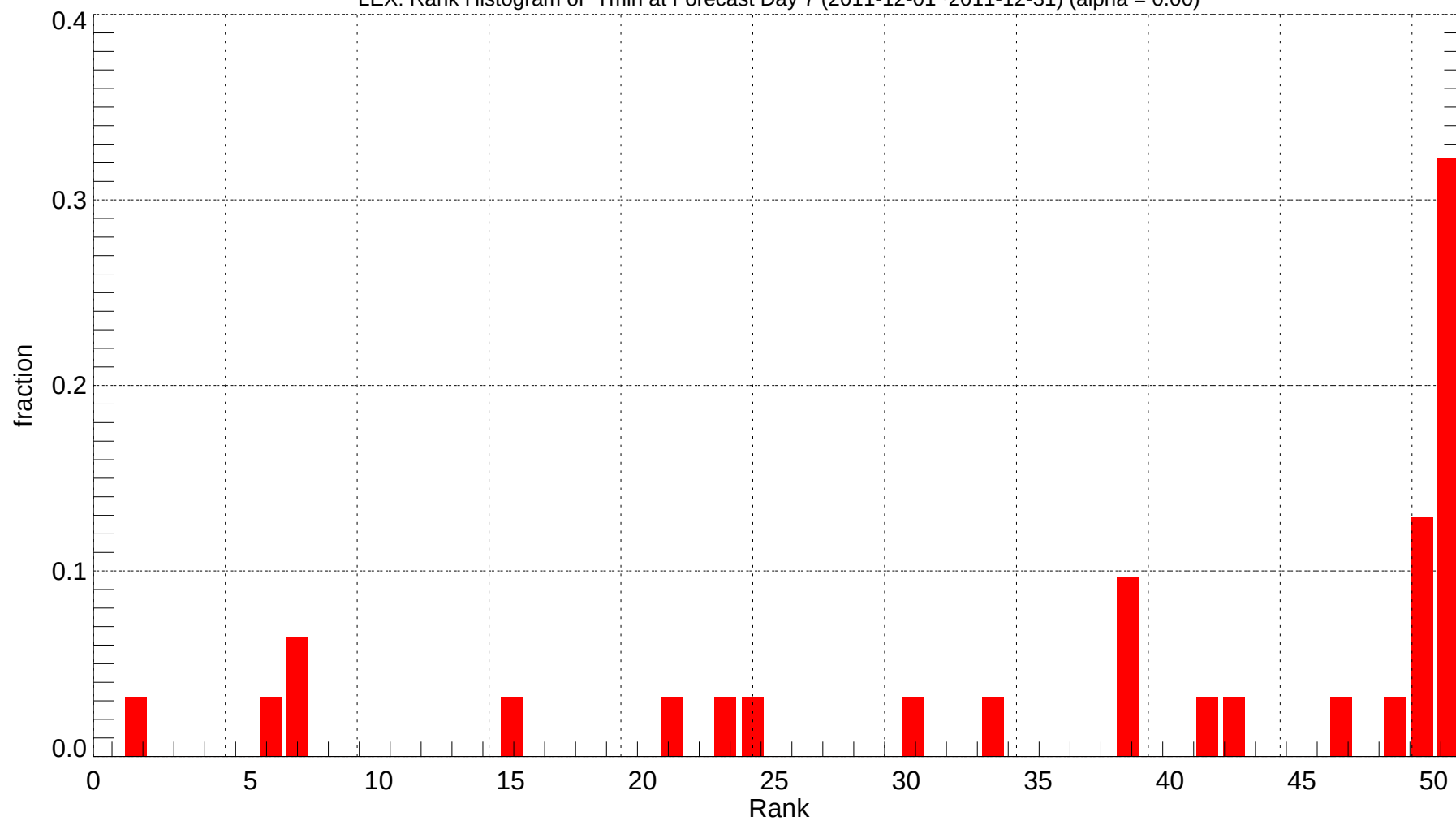
LEX: Rank Histogram of Tmin at Forecast Day 7 (2011-12-01~2011-12-31) (alpha = 0.00)
