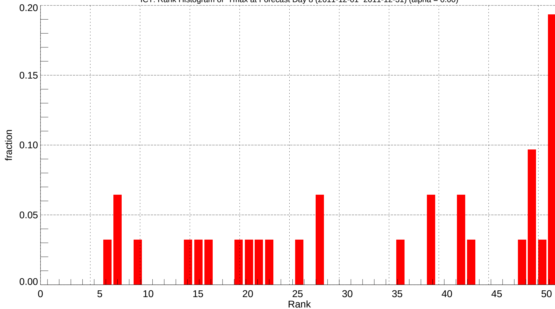
ICT: Rank Histogram of Tmax at Forecast Day 8 (2011-12-01~2011-12-31) (alpha = 0.00)
