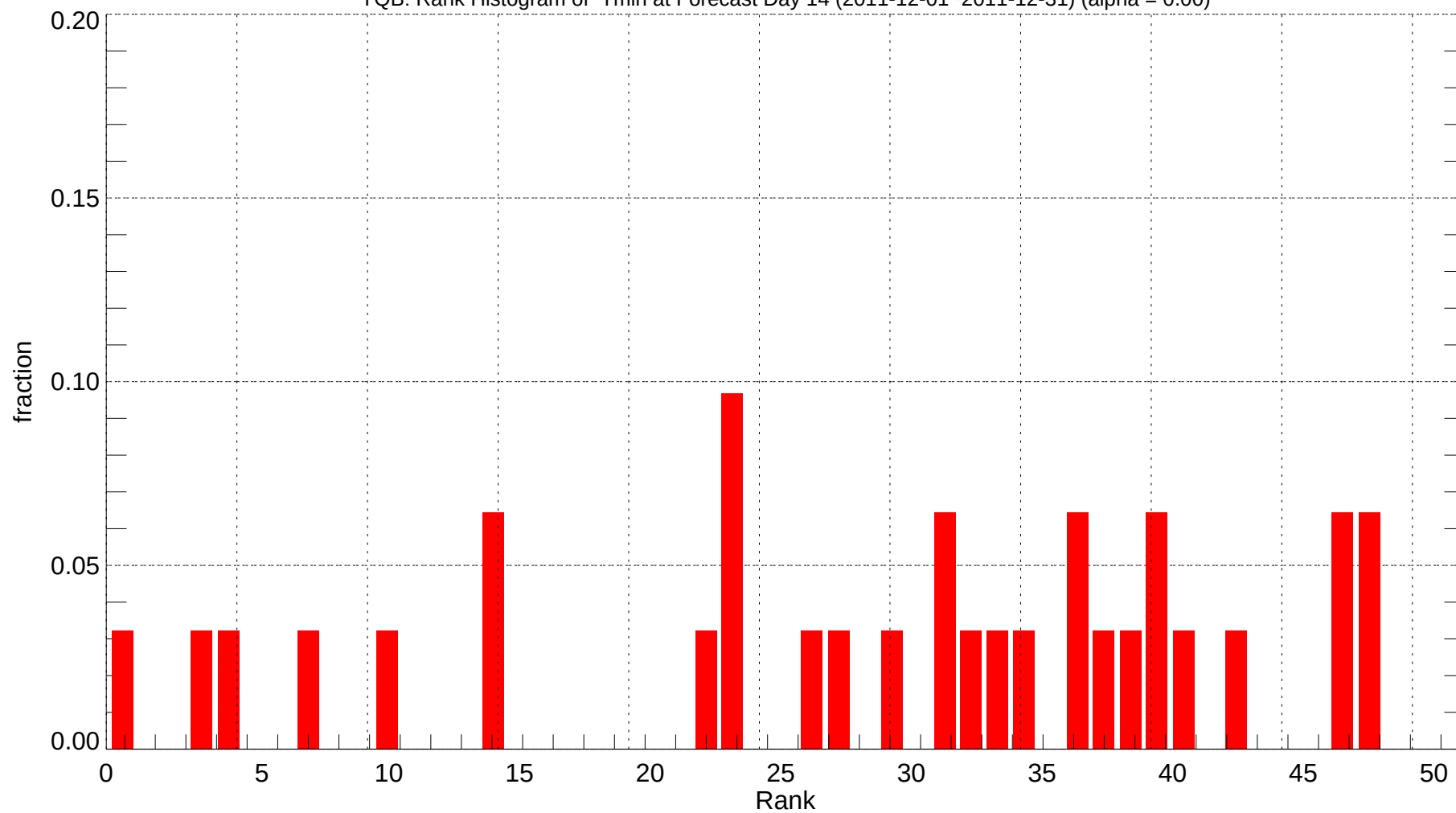
YQB: Rank Histogram of Tmin at Forecast Day 14 (2011-12-01~2011-12-31) (alpha = 0.00)
