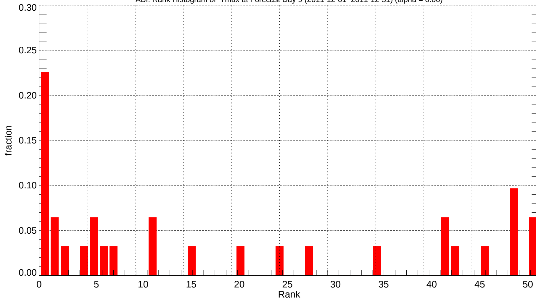
ABI: Rank Histogram of Tmax at Forecast Day 9 (2011-12-01~2011-12-31) (alpha = 0.00)
