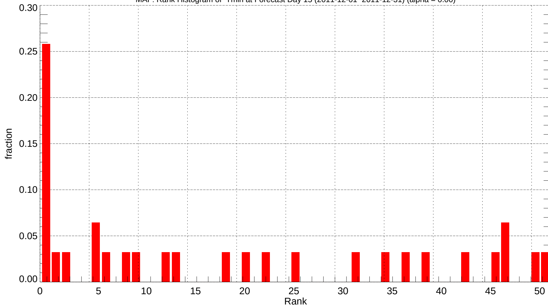
MAF: Rank Histogram of Tmin at Forecast Day 15 (2011-12-01~2011-12-31) (alpha = 0.00)
