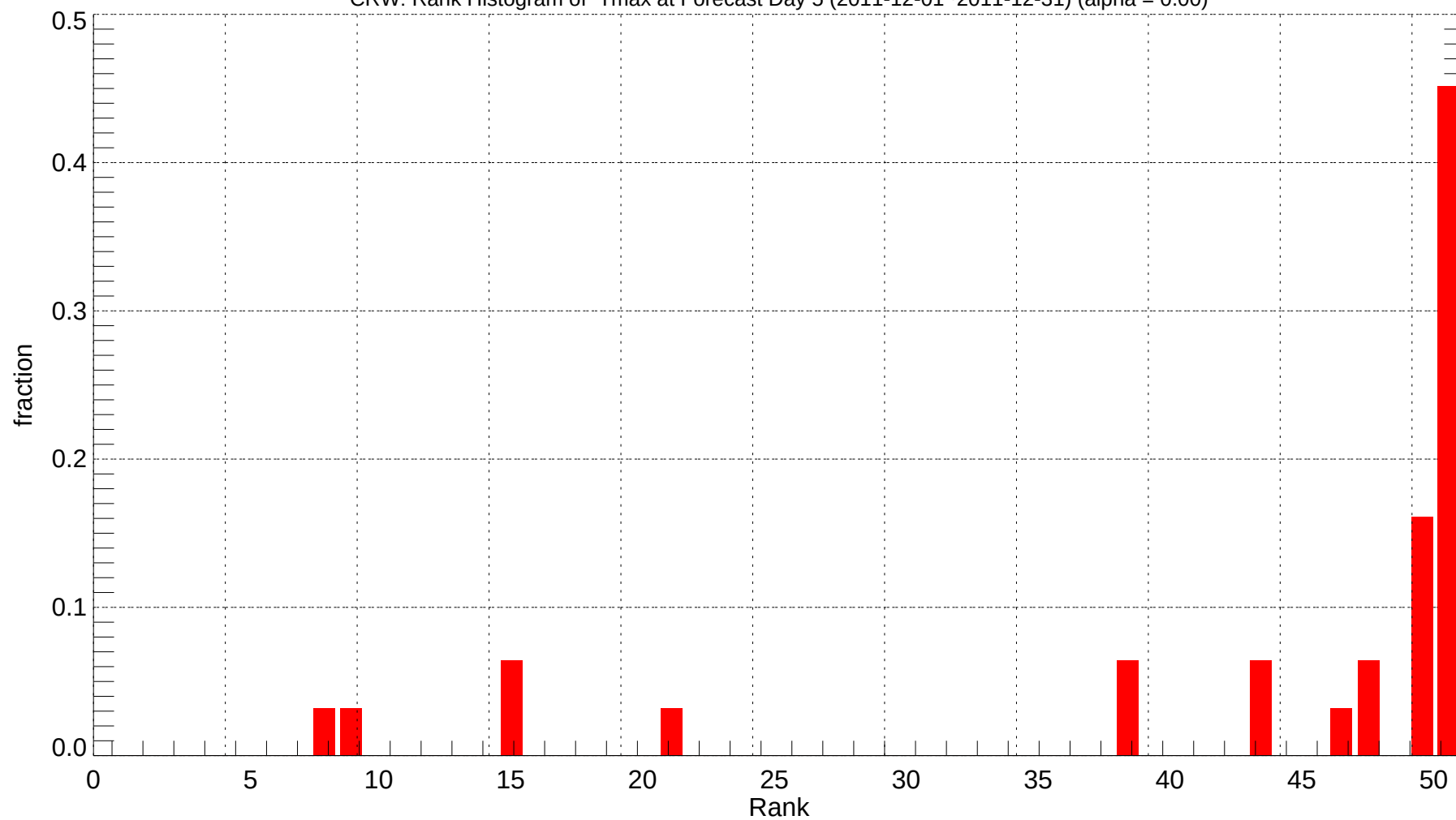
CRW: Rank Histogram of Tmax at Forecast Day 5 (2011-12-01~2011-12-31) (alpha = 0.00)
