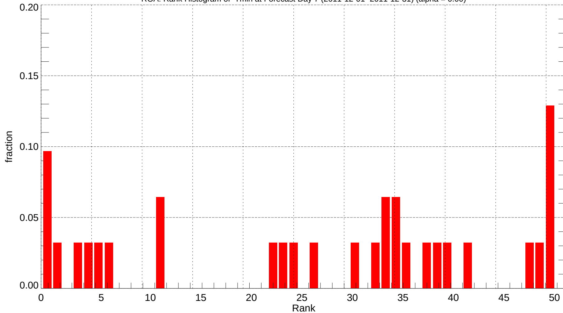
ROA: Rank Histogram of Tmin at Forecast Day 7 (2011-12-01~2011-12-31) (alpha = 0.00)
