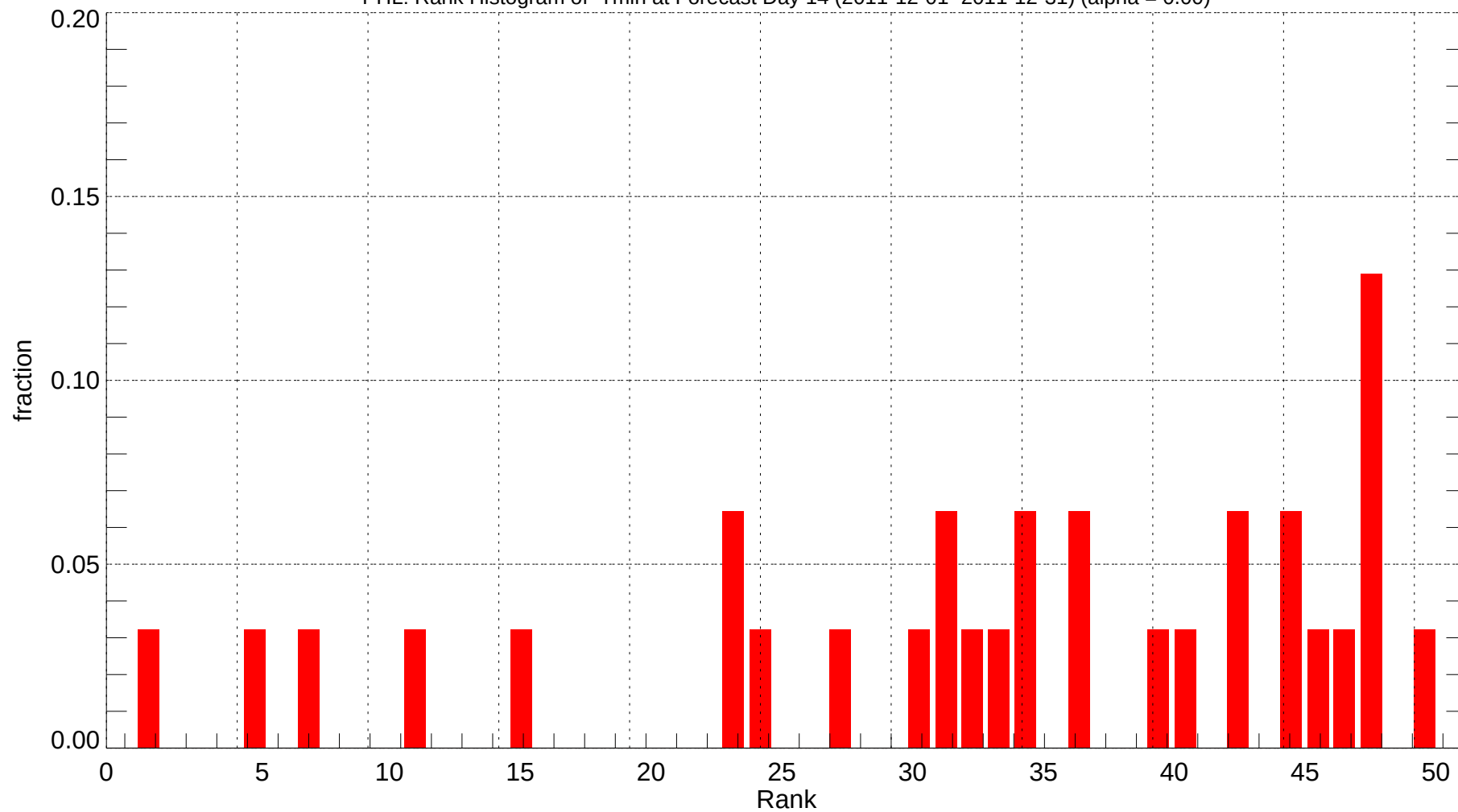
PHL: Rank Histogram of Tmin at Forecast Day 14 (2011-12-01~2011-12-31) (alpha = 0.00)
