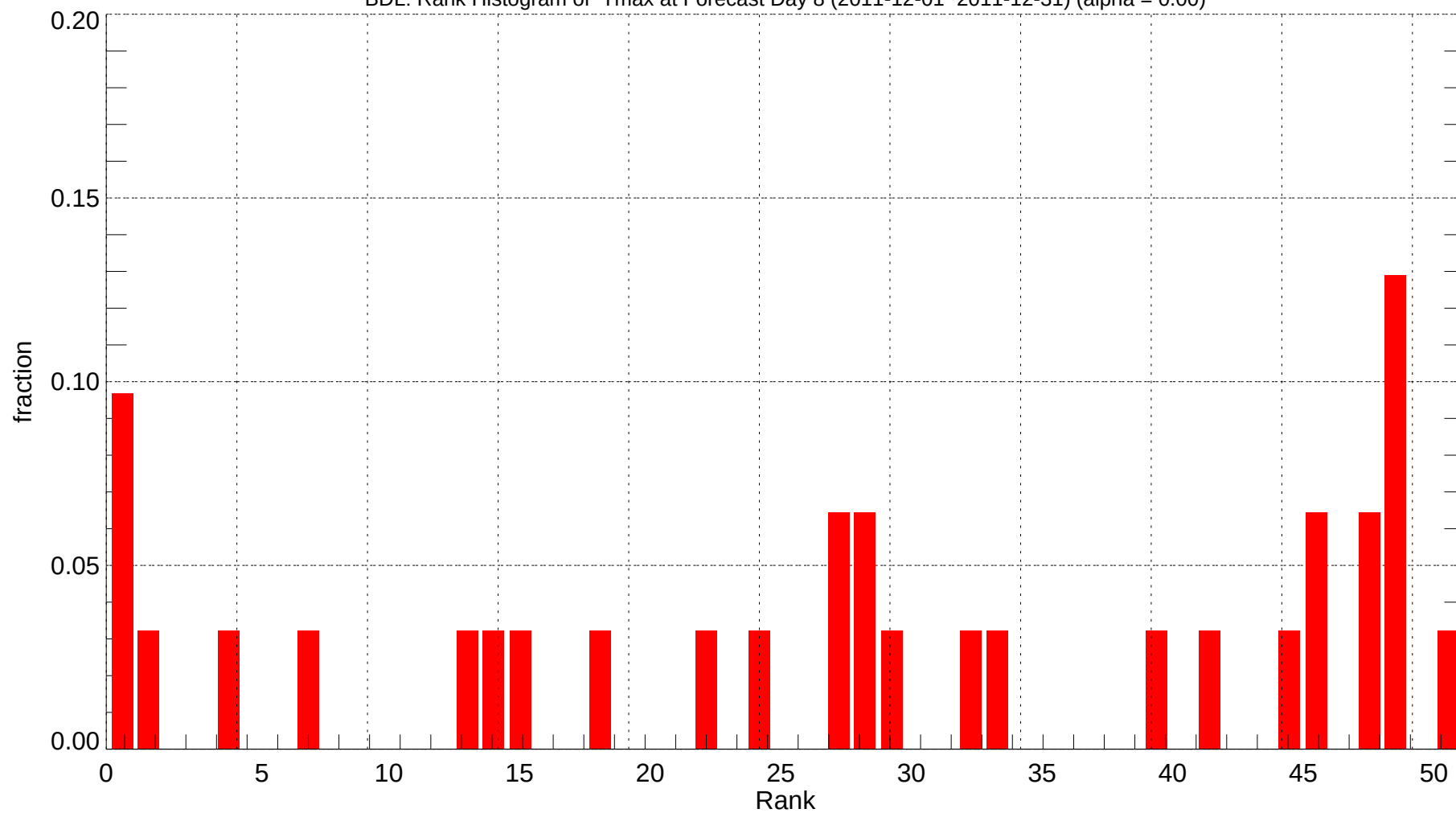
BDL: Rank Histogram of Tmax at Forecast Day 8 (2011-12-01~2011-12-31) (alpha = 0.00)
