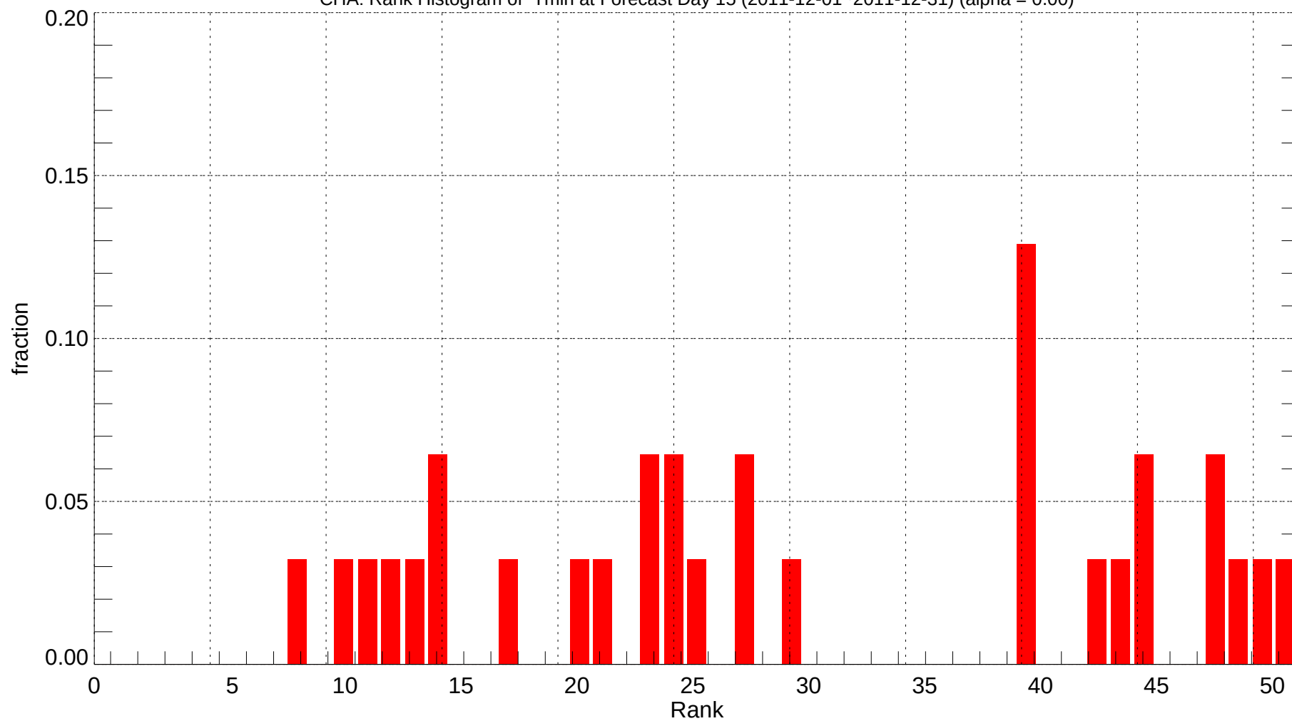
CHA: Rank Histogram of Tmin at Forecast Day 15 (2011-12-01~2011-12-31) (alpha = 0.00)
