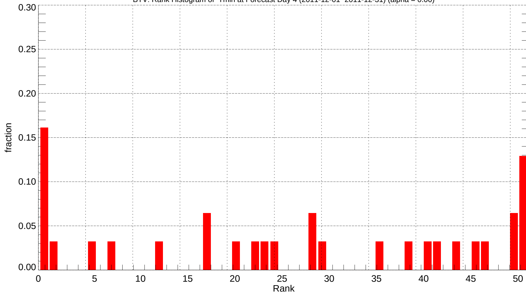
BTV: Rank Histogram of Tmin at Forecast Day 4 (2011-12-01~2011-12-31) (alpha = 0.00)
