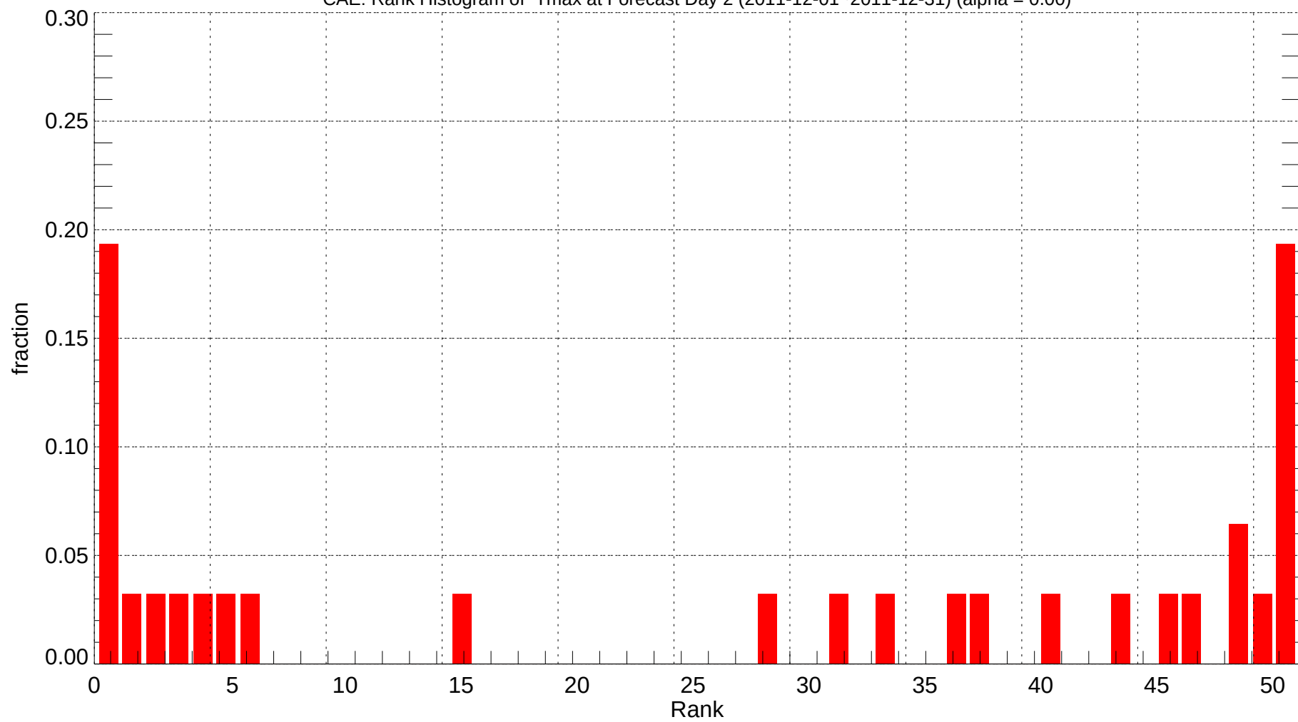
CAE: Rank Histogram of Tmax at Forecast Day 2 (2011-12-01~2011-12-31) (alpha = 0.00)
