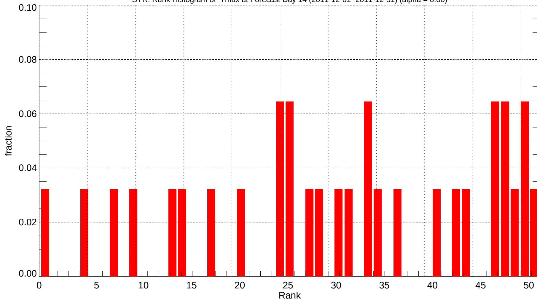
SYR: Rank Histogram of Tmax at Forecast Day 14 (2011-12-01~2011-12-31) (alpha = 0.00)
