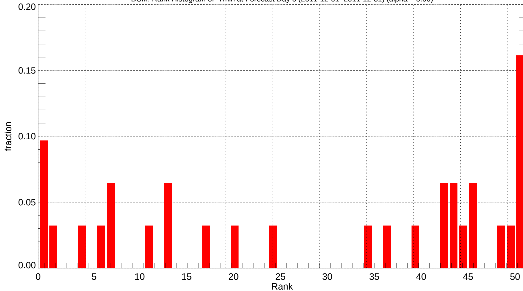
DSM: Rank Histogram of Tmin at Forecast Day 6 (2011-12-01~2011-12-31) (alpha = 0.00)
