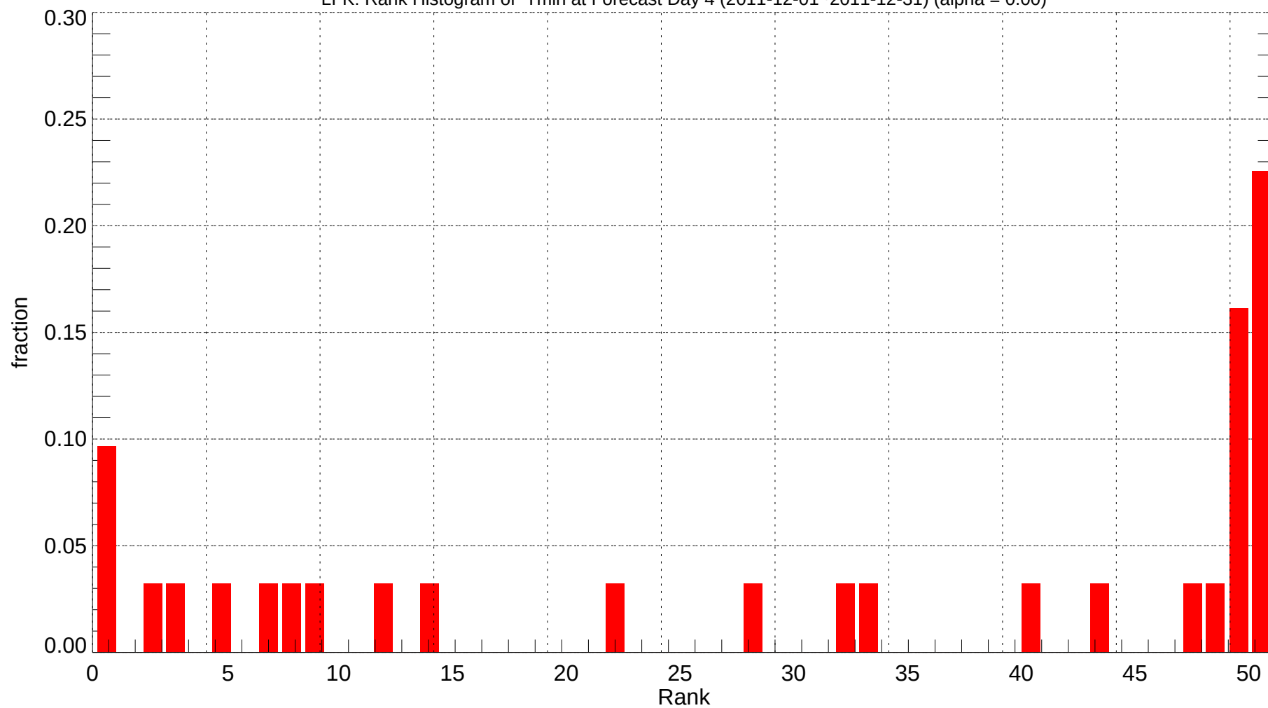
LFK: Rank Histogram of Tmin at Forecast Day 4 (2011-12-01~2011-12-31) (alpha = 0.00)
