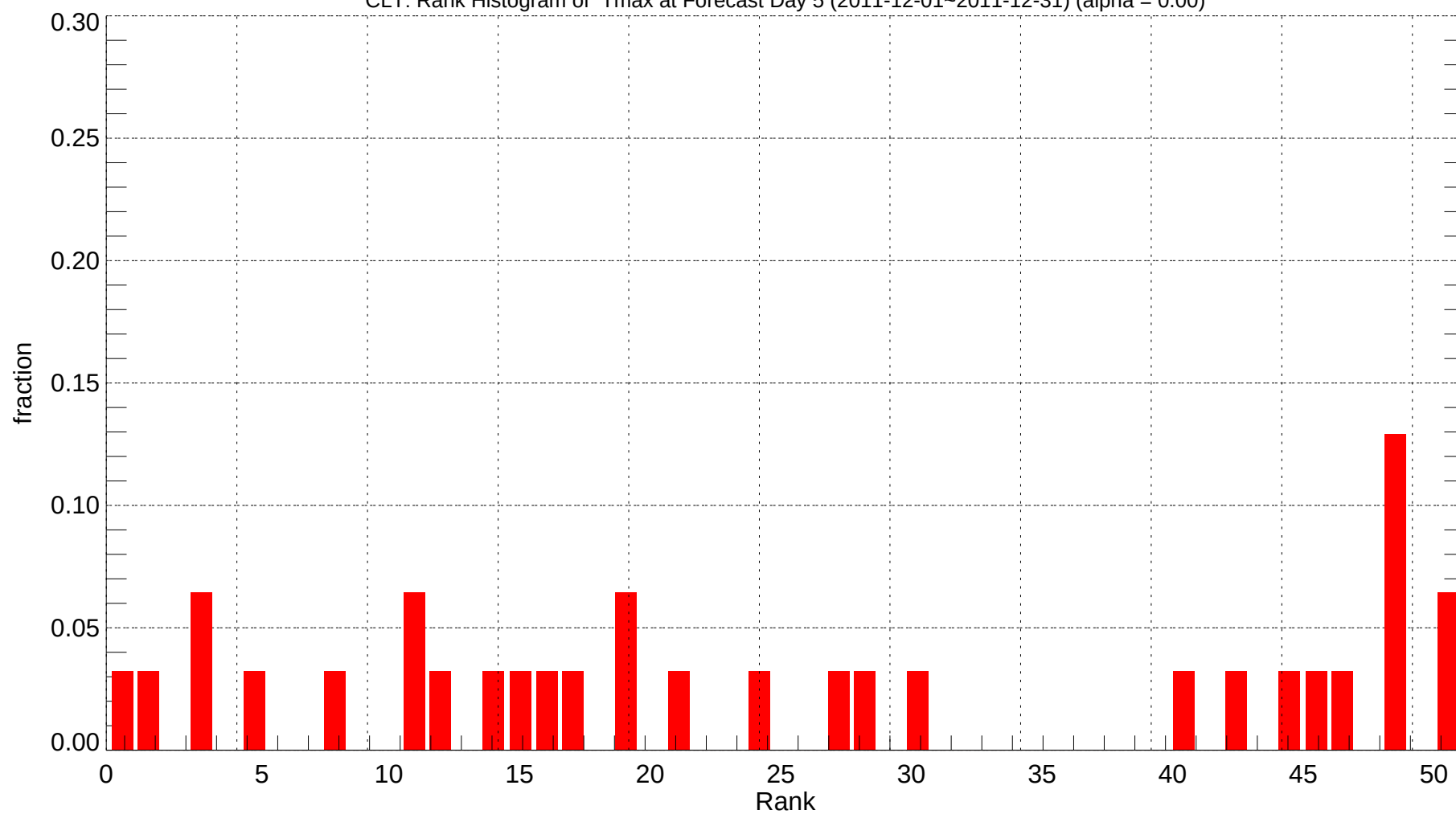
CLT: Rank Histogram of Tmax at Forecast Day 5 (2011-12-01~2011-12-31) (alpha = 0.00)
