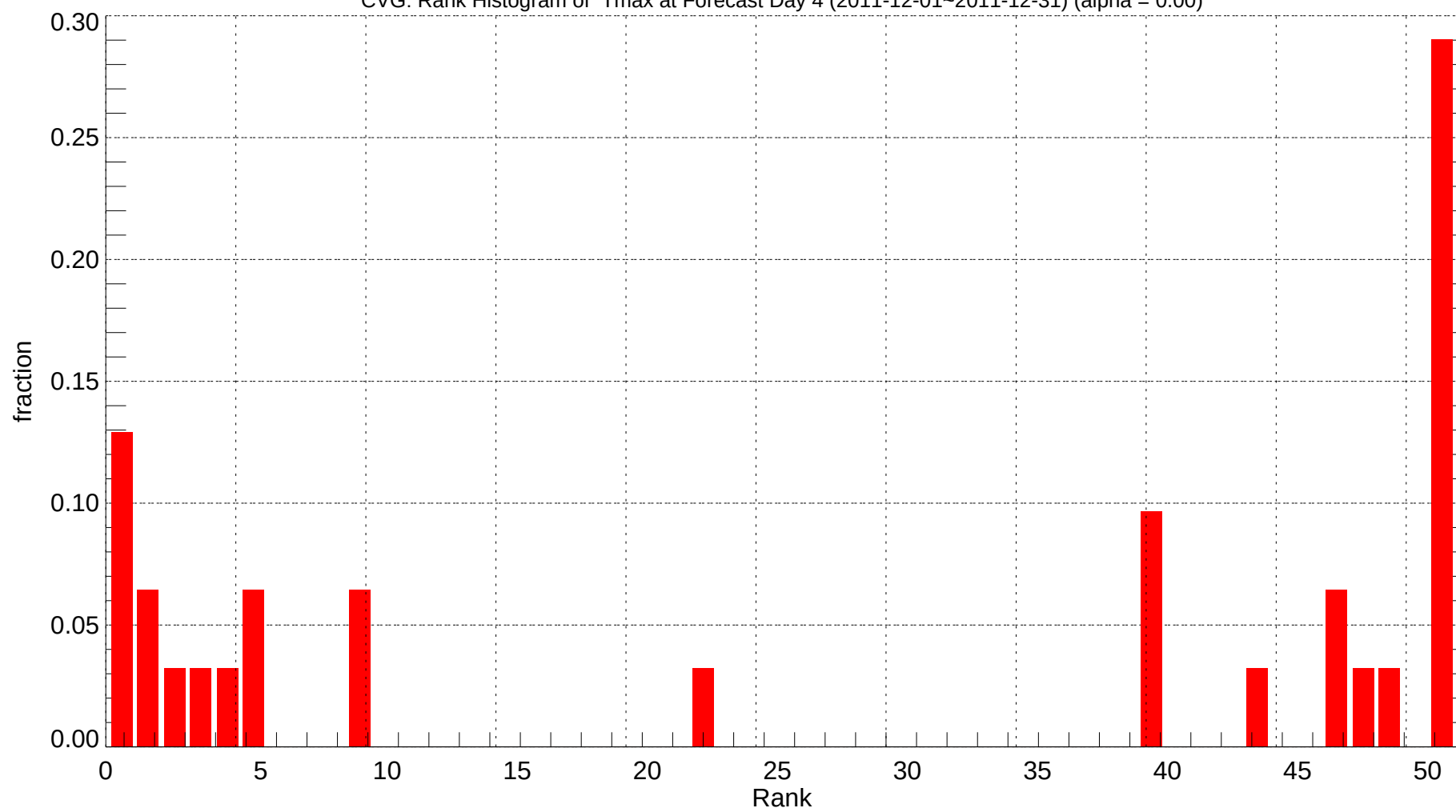
CVG: Rank Histogram of Tmax at Forecast Day 4 (2011-12-01~2011-12-31) (alpha = 0.00)
