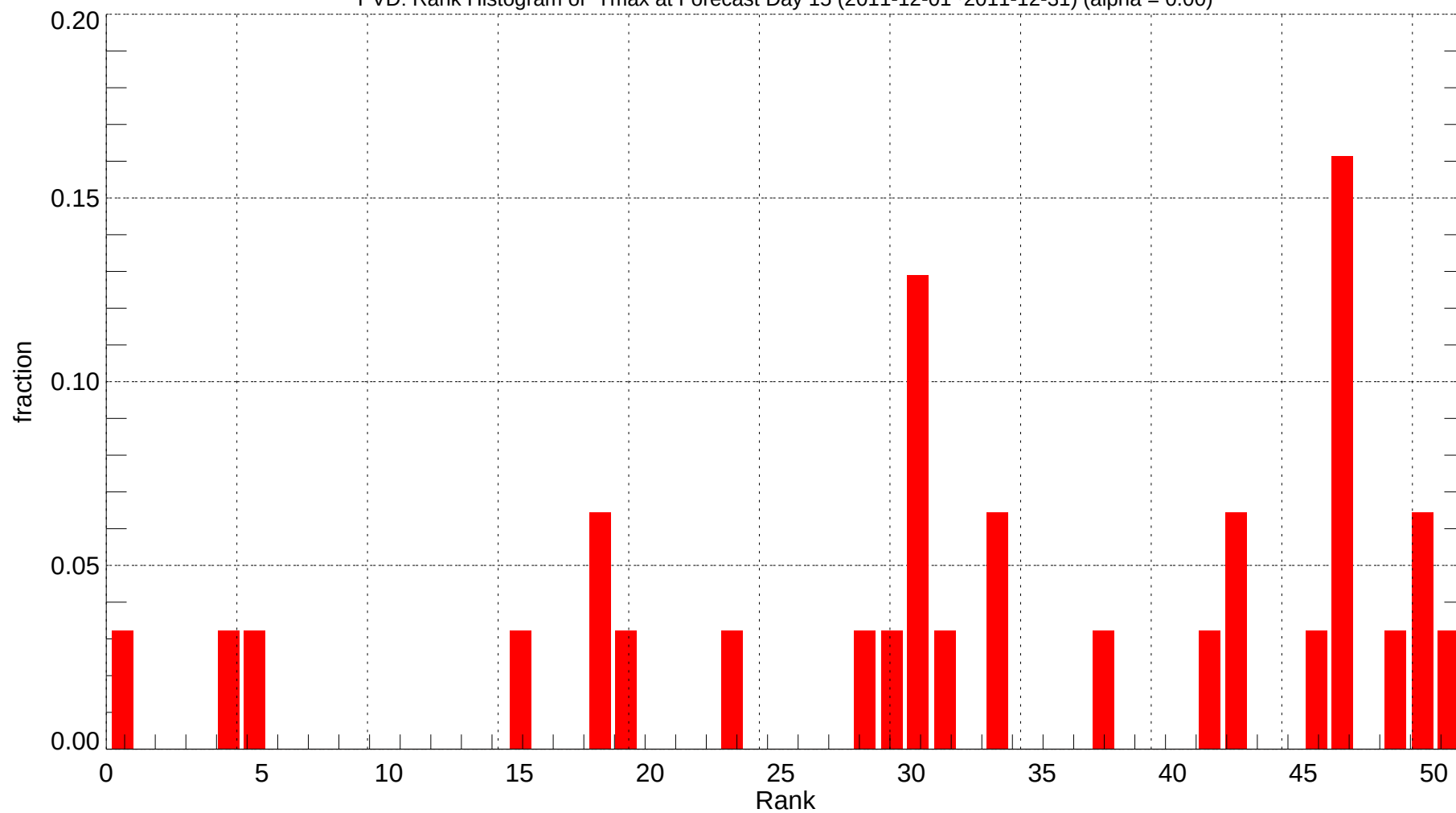
PVD: Rank Histogram of Tmax at Forecast Day 15 (2011-12-01~2011-12-31) (alpha = 0.00)
