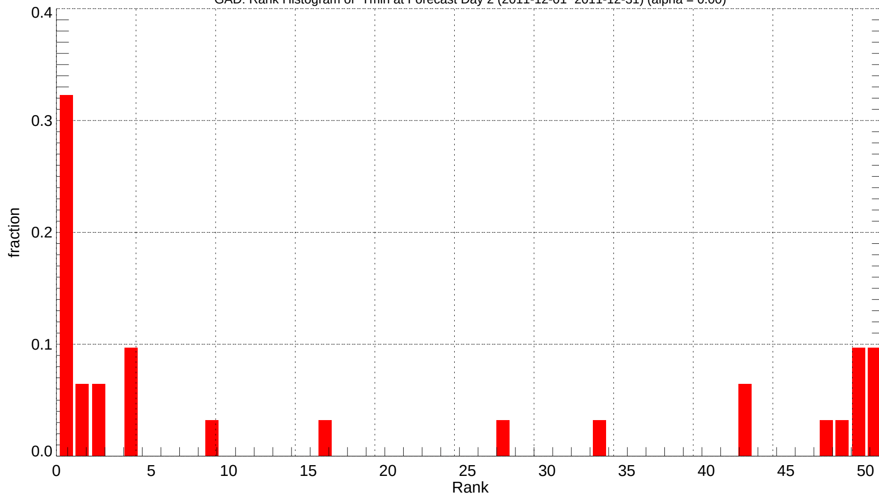
GAD: Rank Histogram of Tmin at Forecast Day 2 (2011-12-01~2011-12-31) (alpha = 0.00)
