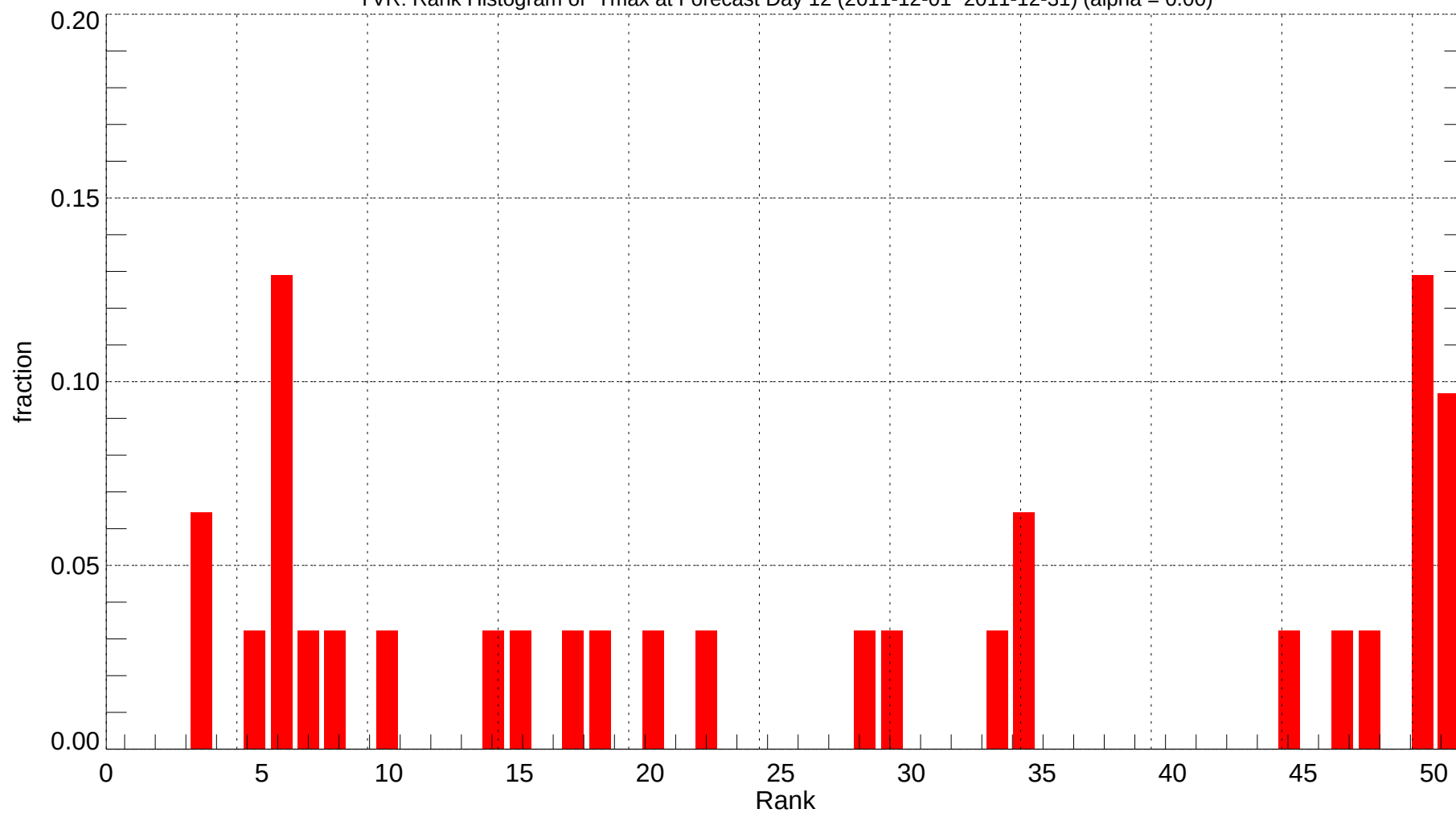
YVR: Rank Histogram of Tmax at Forecast Day 12 (2011-12-01~2011-12-31) (alpha = 0.00)
