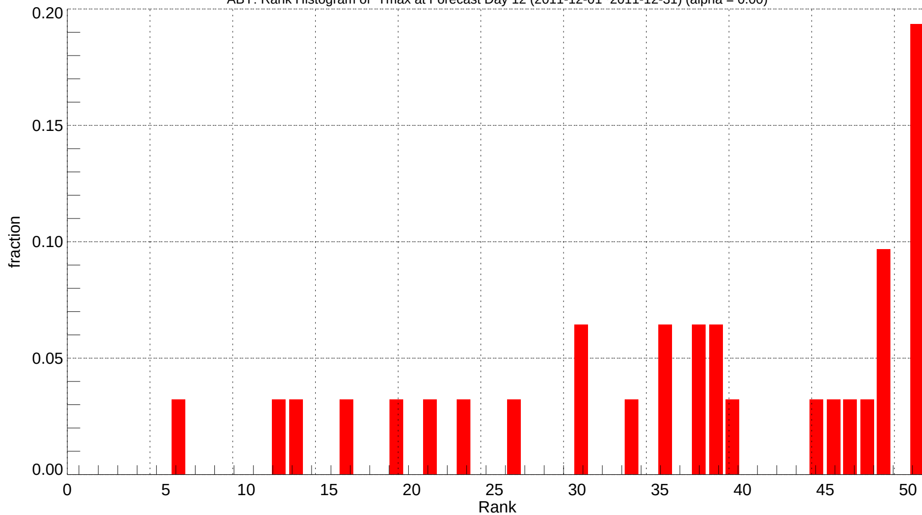
ABY: Rank Histogram of Tmax at Forecast Day 12 (2011-12-01~2011-12-31) (alpha = 0.00)
