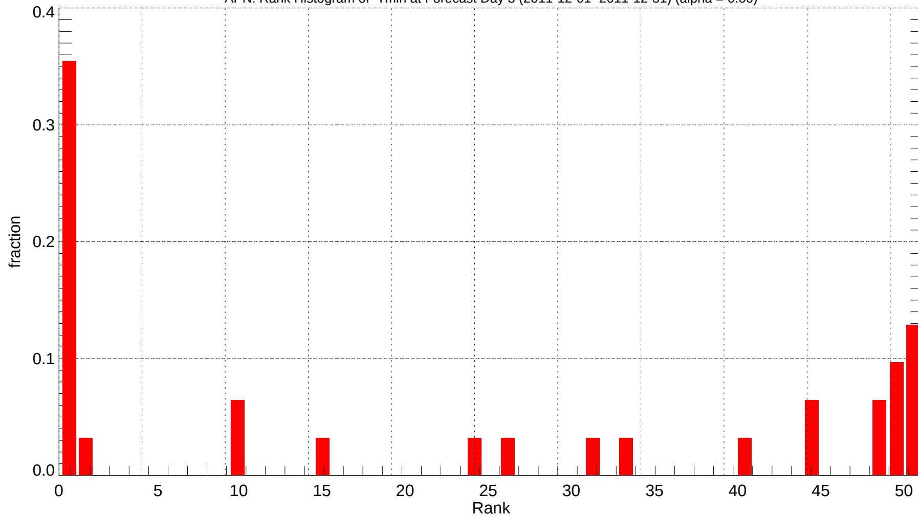
APN: Rank Histogram of Tmin at Forecast Day 3 (2011-12-01~2011-12-31) (alpha = 0.00)
