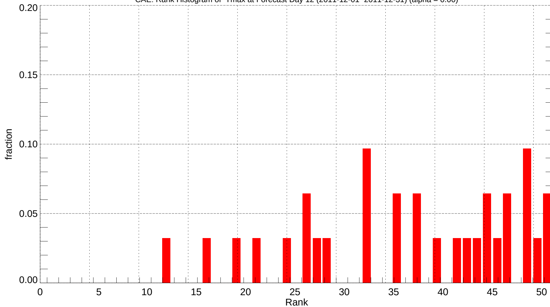
CAE: Rank Histogram of Tmax at Forecast Day 12 (2011-12-01~2011-12-31) (alpha = 0.00)
