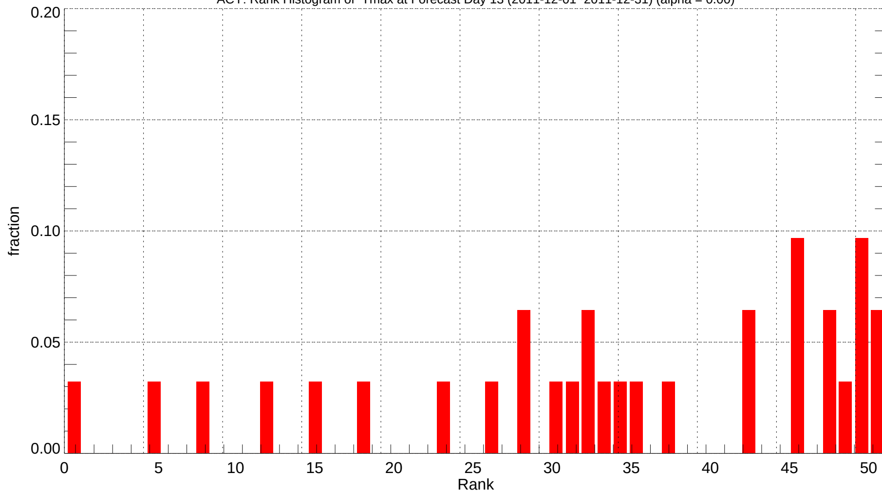
ACY: Rank Histogram of Tmax at Forecast Day 13 (2011-12-01~2011-12-31) (alpha = 0.00)
