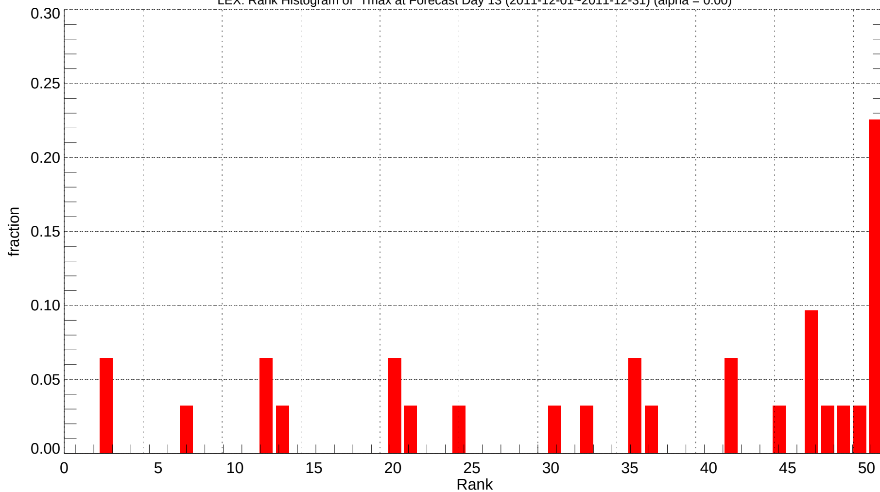
LEX: Rank Histogram of Tmax at Forecast Day 13 (2011-12-01~2011-12-31) (alpha = 0.00)
