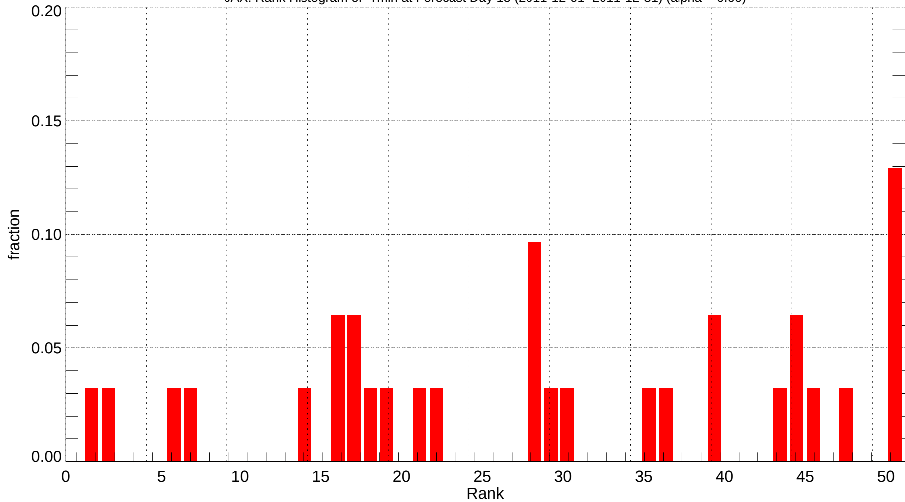
JAX: Rank Histogram of Tmin at Forecast Day 15 (2011-12-01~2011-12-31) (alpha = 0.00)
