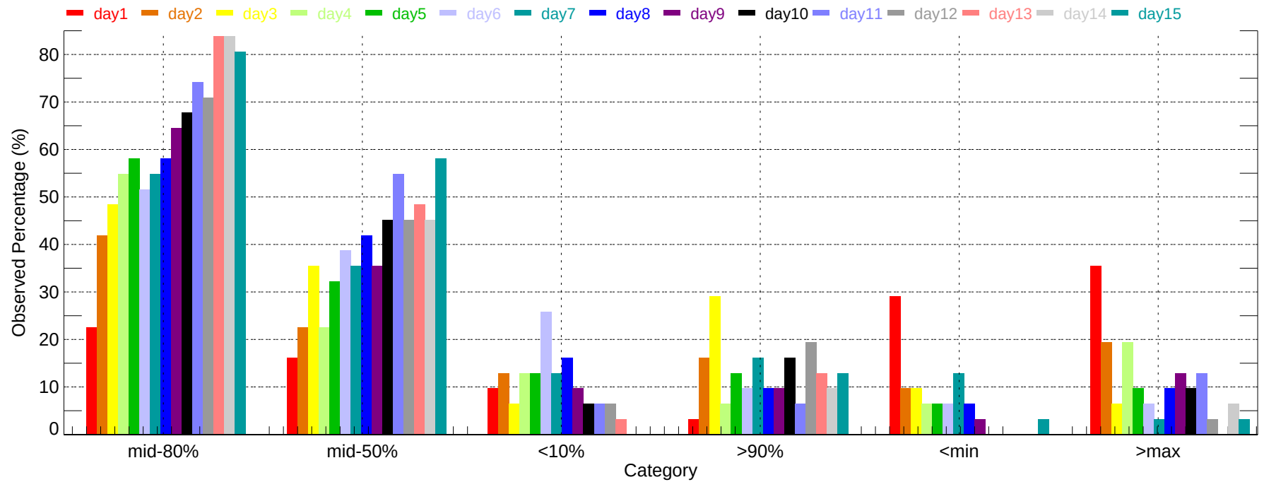
Observed Percentage of Ensembles - PIT: Max Temperature (2011-12-01~2011-12-31)
