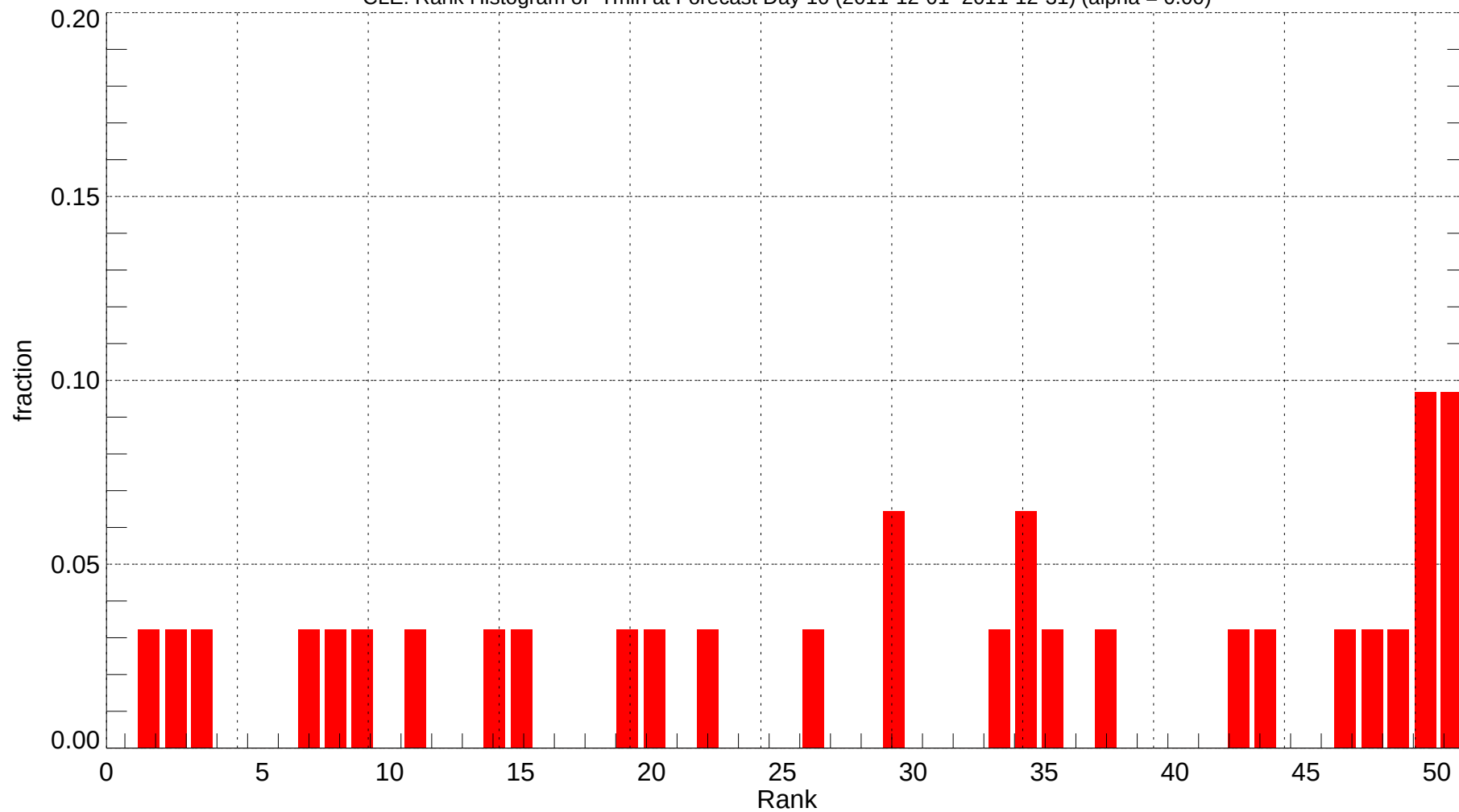
CLE: Rank Histogram of Tmin at Forecast Day 10 (2011-12-01~2011-12-31) (alpha = 0.00)
