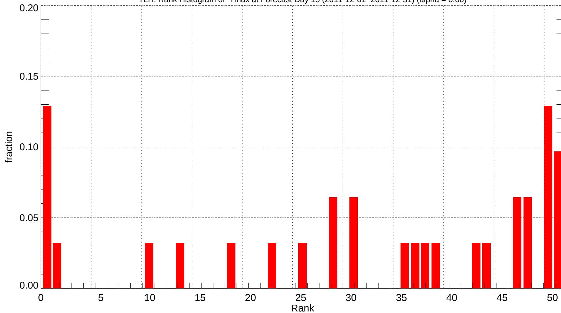
TLH: Rank Histogram of Tmax at Forecast Day 15 (2011-12-01~2011-12-31) (alpha = 0.00)
