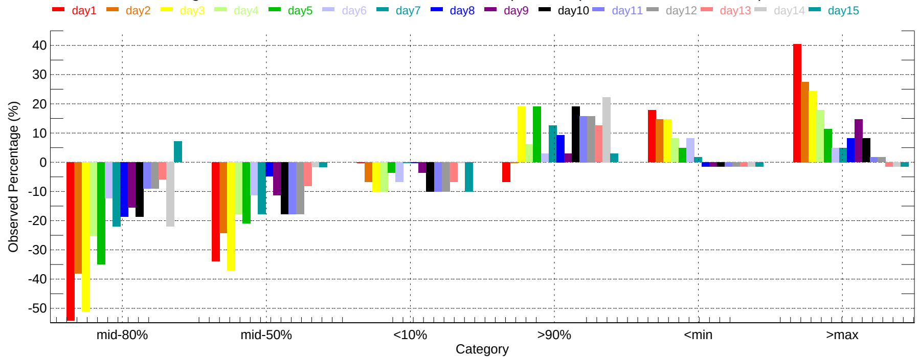
Observed Percentage Deviation of Ensembles - CMH: Min Temperature (2011-12-01~2011-12-31)
