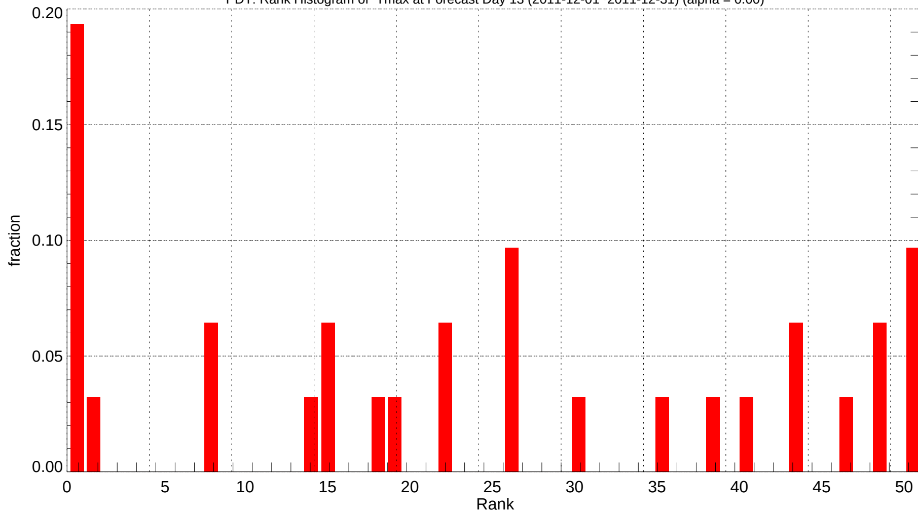
PDT: Rank Histogram of Tmax at Forecast Day 13 (2011-12-01~2011-12-31) (alpha = 0.00)
