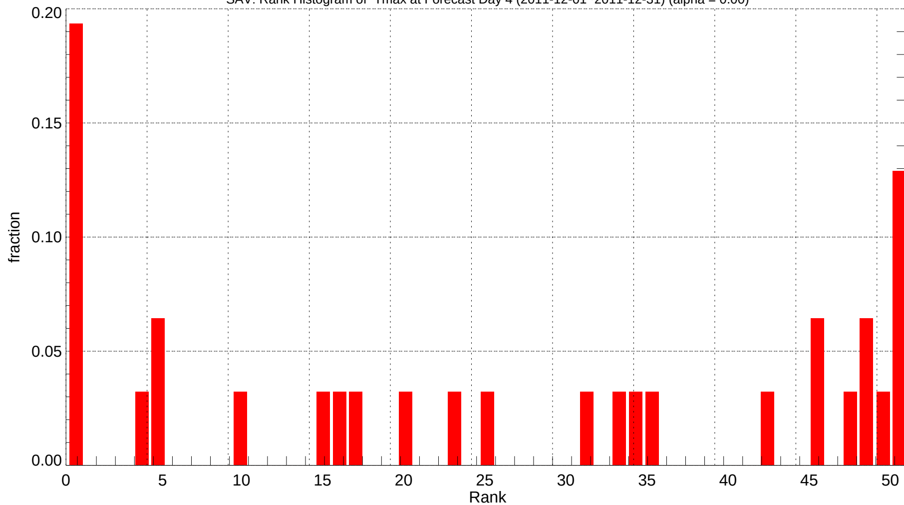
SAV: Rank Histogram of Tmax at Forecast Day 4 (2011-12-01~2011-12-31) (alpha = 0.00)
