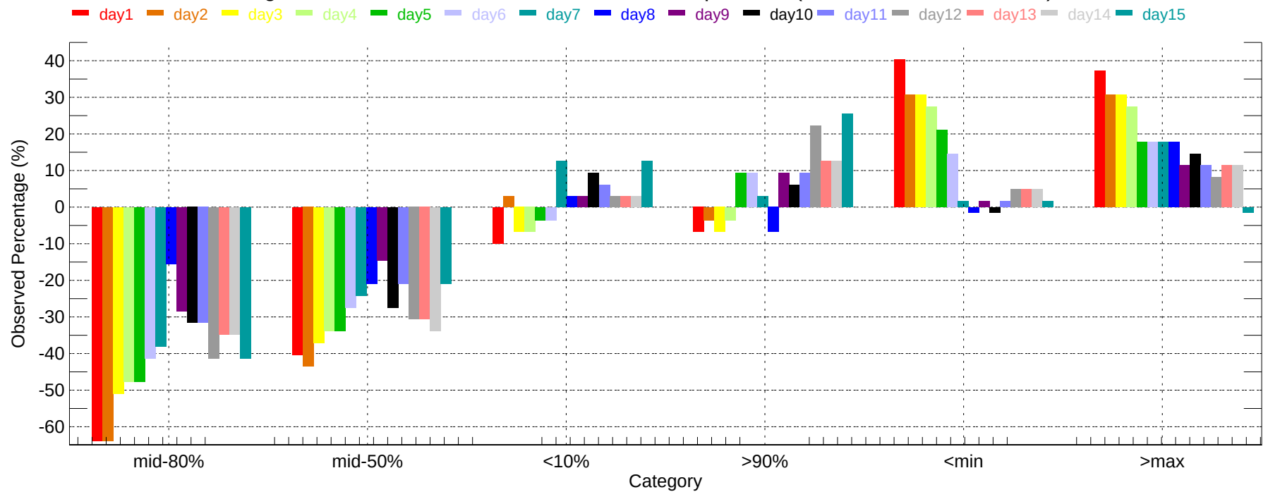
Observed Percentage Deviation of Ensembles - OMA: Min Temperature (2011-12-01~2011-12-31)
