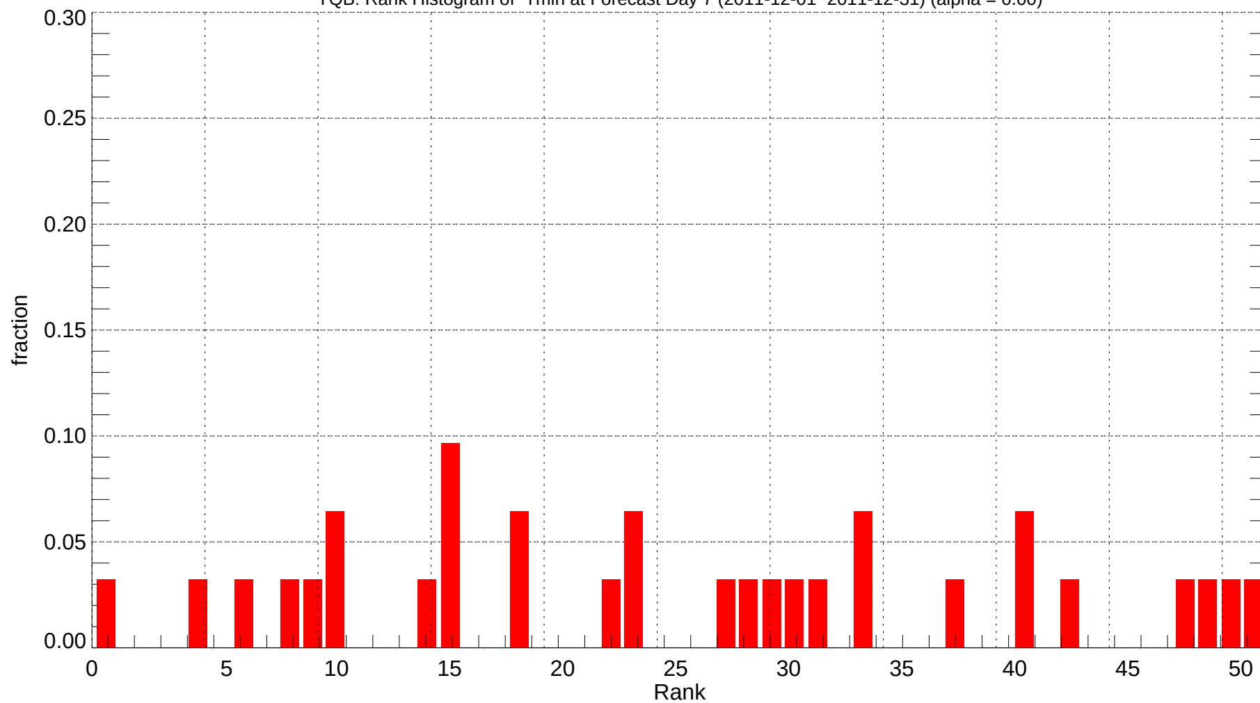
YQB: Rank Histogram of Tmin at Forecast Day 7 (2011-12-01~2011-12-31) (alpha = 0.00)
