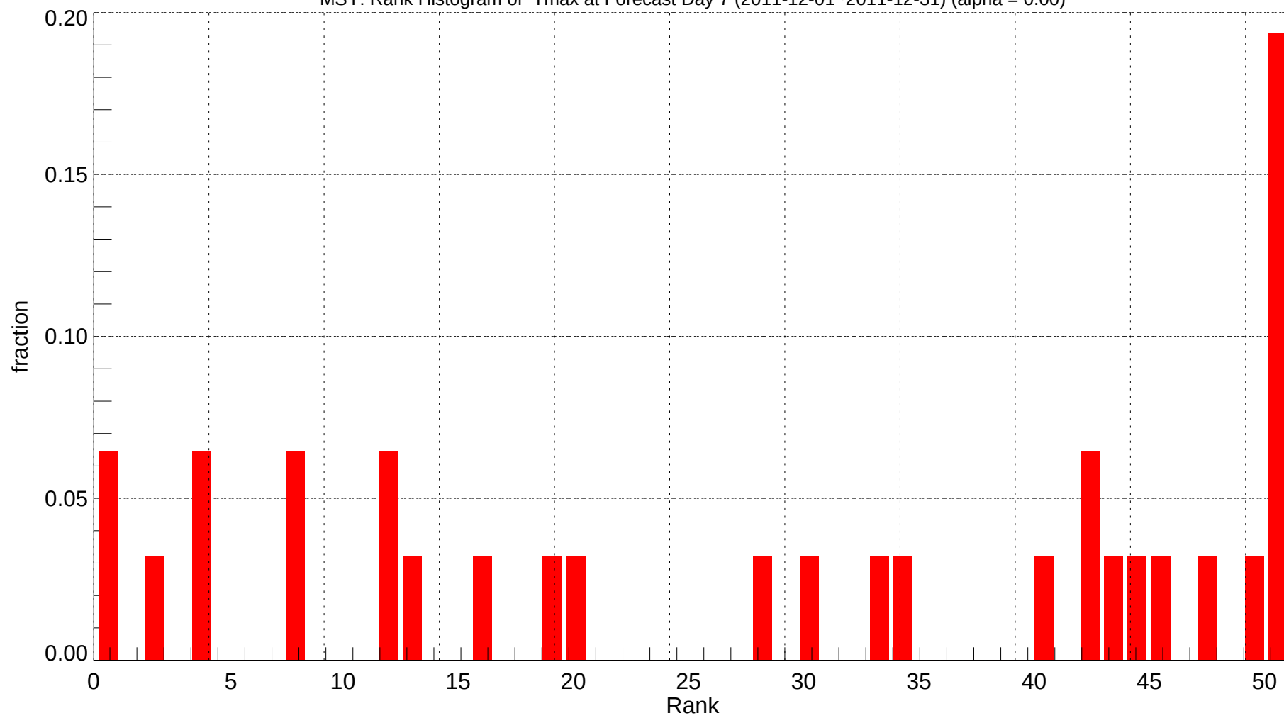
MSY: Rank Histogram of Tmax at Forecast Day 7 (2011-12-01~2011-12-31) (alpha = 0.00)
