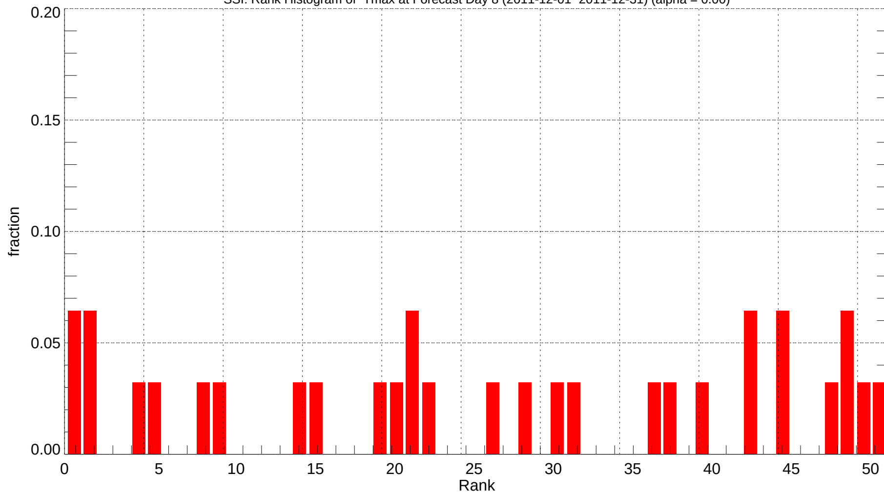
SSI: Rank Histogram of Tmax at Forecast Day 8 (2011-12-01~2011-12-31) (alpha = 0.00)
