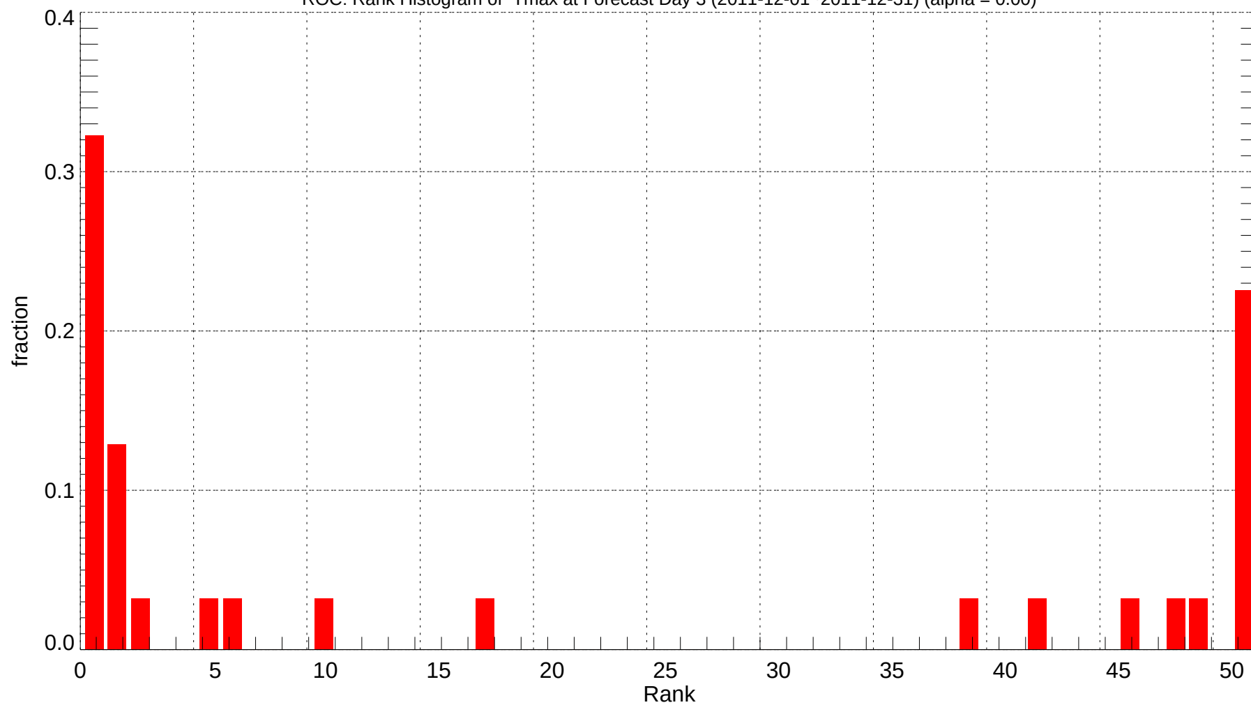
ROC: Rank Histogram of Tmax at Forecast Day 3 (2011-12-01~2011-12-31) (alpha = 0.00)
