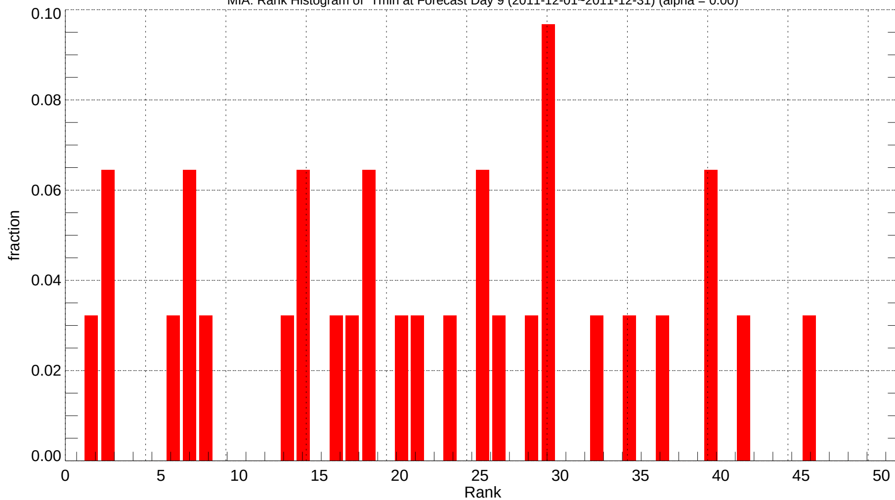
MIA: Rank Histogram of Tmin at Forecast Day 9 (2011-12-01~2011-12-31) (alpha = 0.00)
