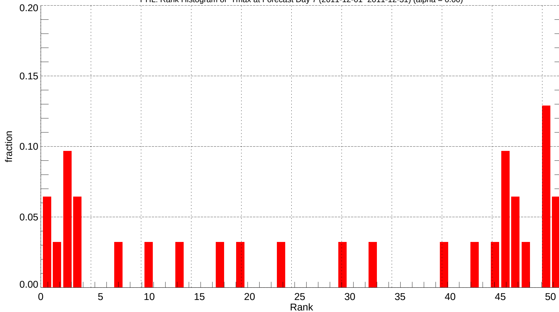
PHL: Rank Histogram of Tmax at Forecast Day 7 (2011-12-01~2011-12-31) (alpha = 0.00)
