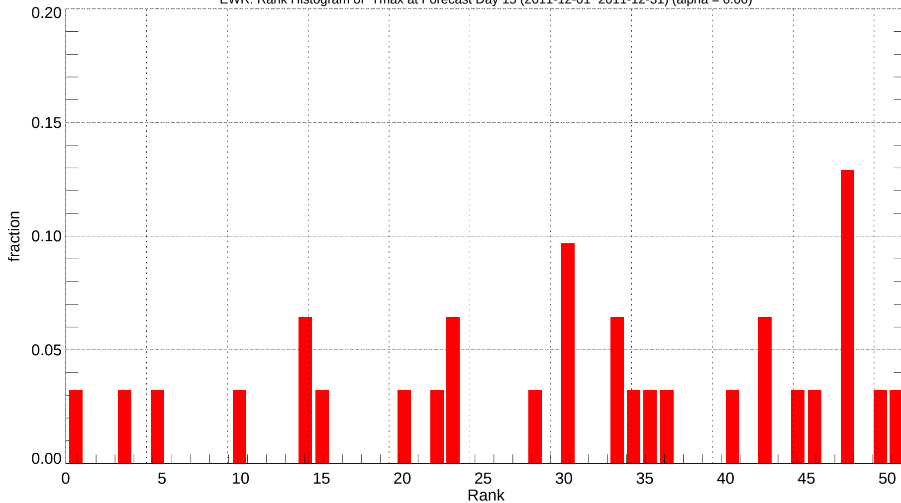
EWR: Rank Histogram of Tmax at Forecast Day 15 (2011-12-01~2011-12-31) (alpha = 0.00)
