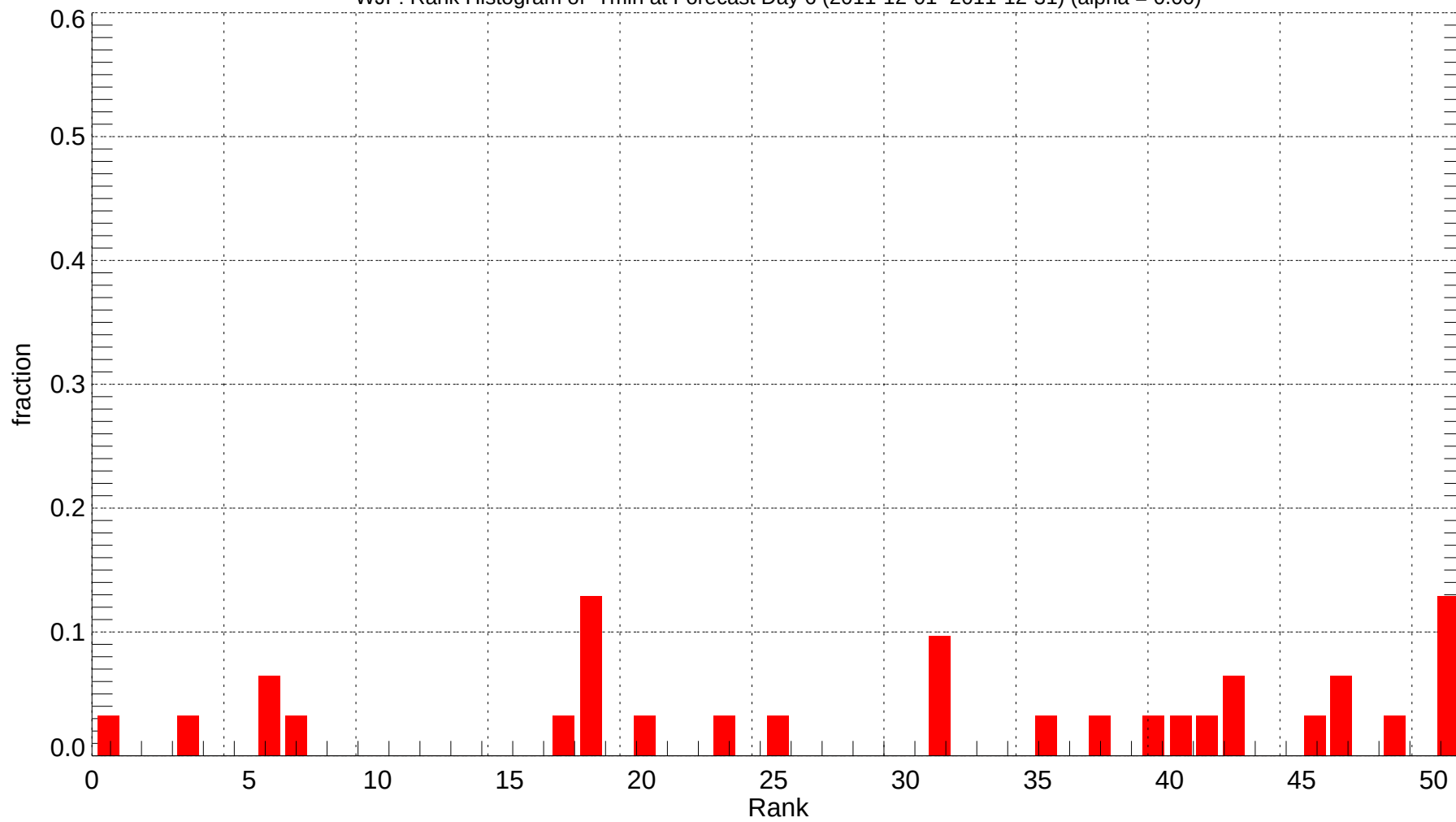
WJF: Rank Histogram of Tmin at Forecast Day 6 (2011-12-01~2011-12-31) (alpha = 0.00)
