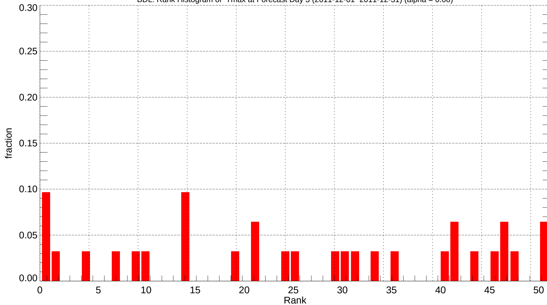
BDL: Rank Histogram of Tmax at Forecast Day 3 (2011-12-01~2011-12-31) (alpha = 0.00)
