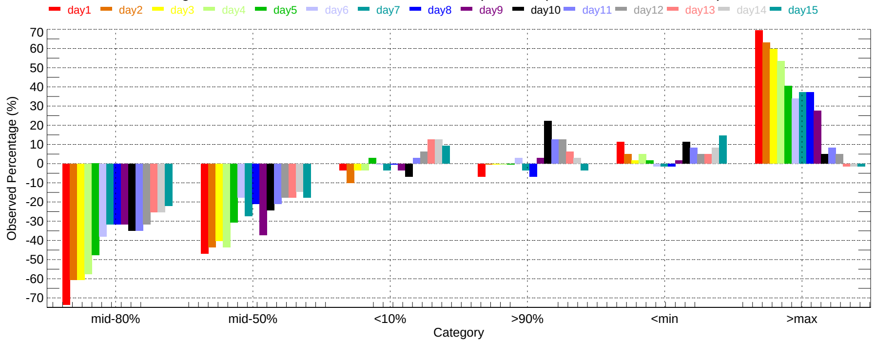
Observed Percentage Deviation of Ensembles - FLG: Min Temperature (2011-12-01~2011-12-31)
