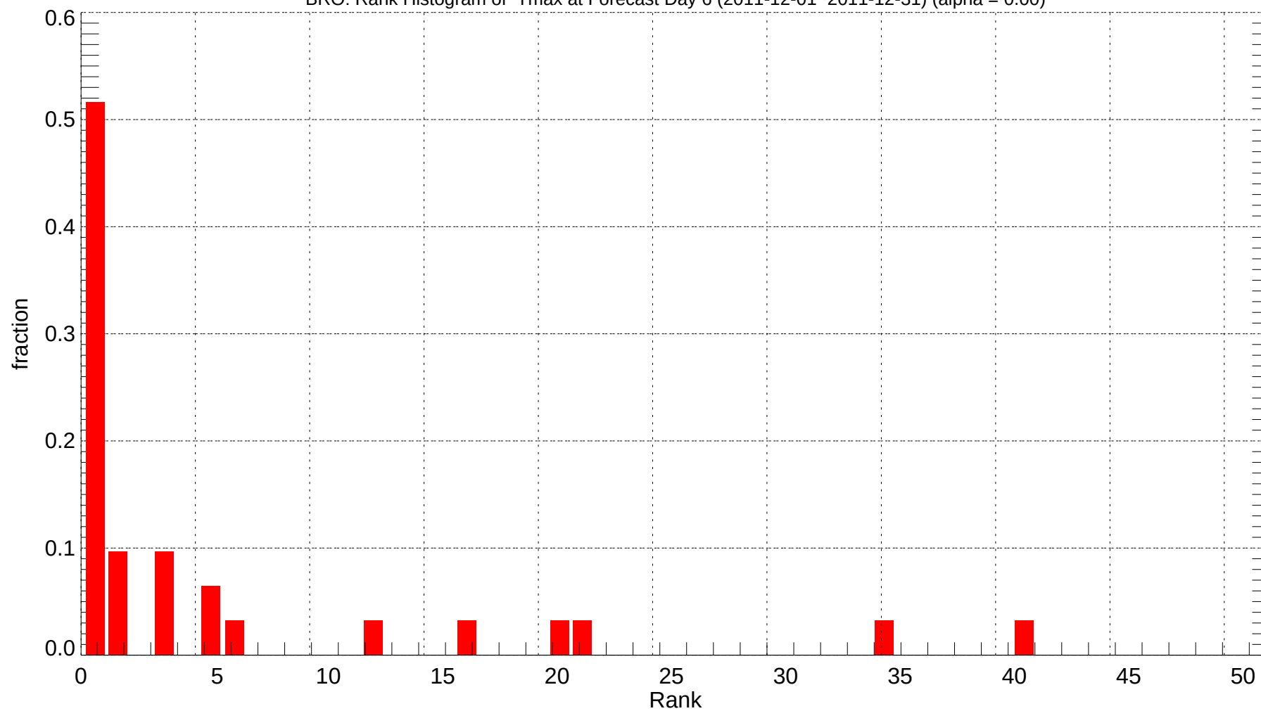
BRO: Rank Histogram of Tmax at Forecast Day 6 (2011-12-01~2011-12-31) (alpha = 0.00)
