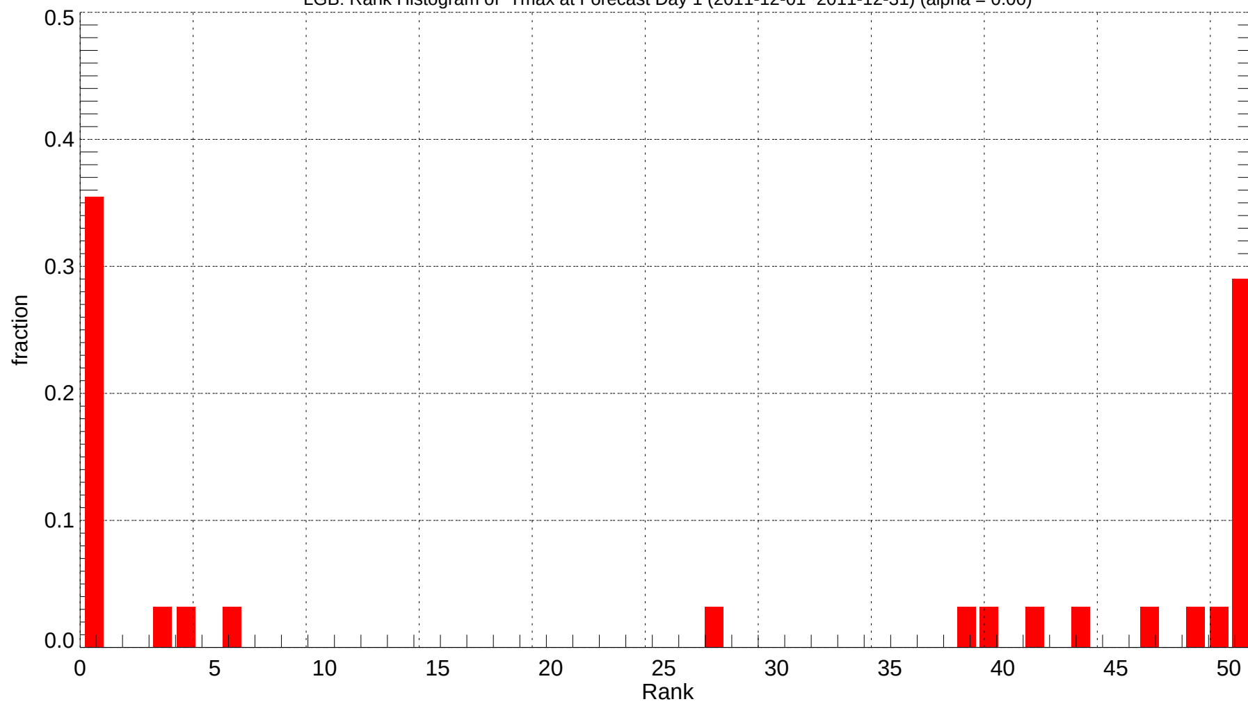
LGB: Rank Histogram of Tmax at Forecast Day 1 (2011-12-01~2011-12-31) (alpha = 0.00)
