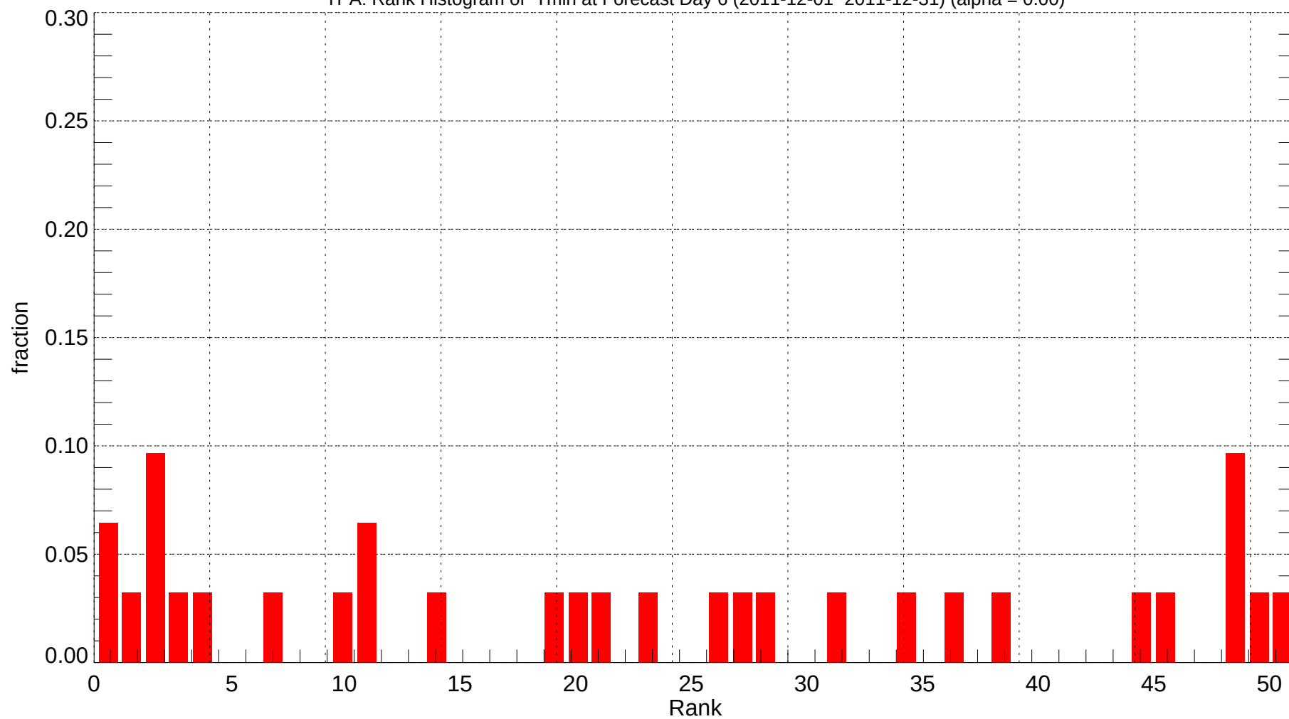
TPA: Rank Histogram of Tmin at Forecast Day 6 (2011-12-01~2011-12-31) (alpha = 0.00)
