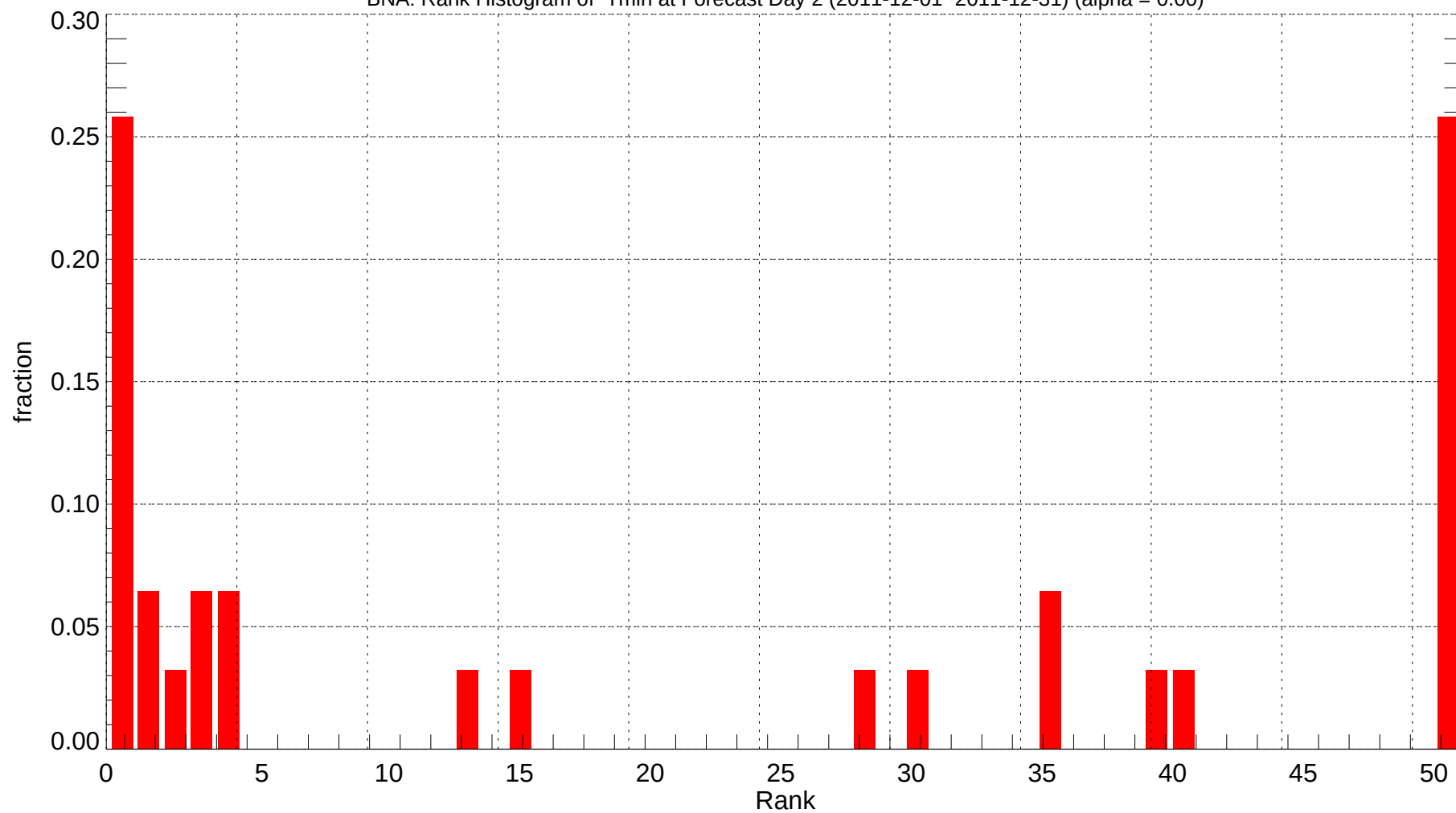
BNA: Rank Histogram of Tmin at Forecast Day 2 (2011-12-01~2011-12-31) (alpha = 0.00)
