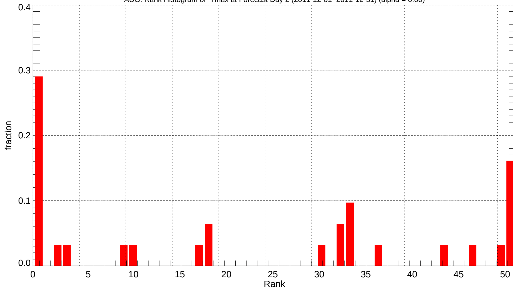
AUG: Rank Histogram of Tmax at Forecast Day 2 (2011-12-01~2011-12-31) (alpha = 0.00)
