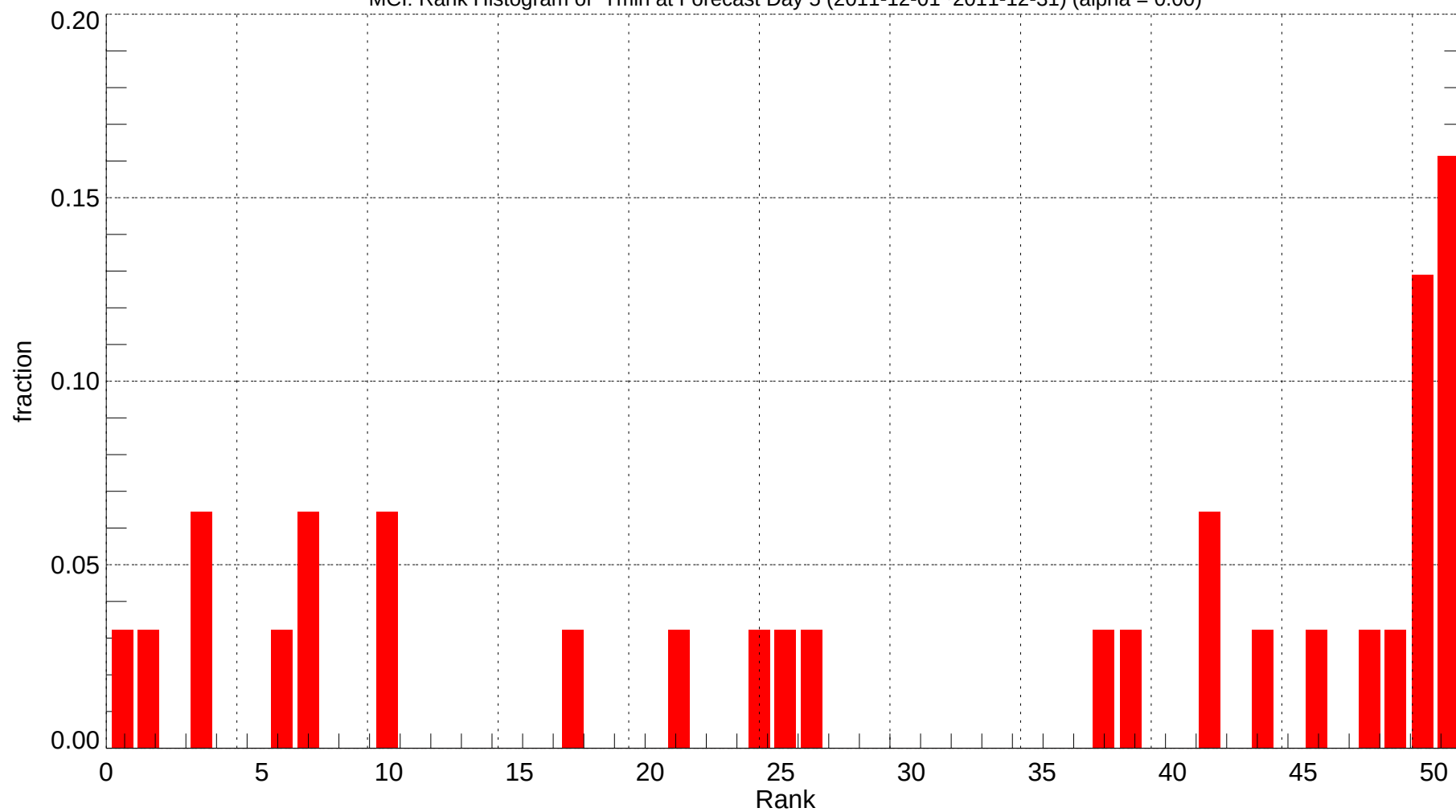
MCI: Rank Histogram of Tmin at Forecast Day 5 (2011-12-01~2011-12-31) (alpha = 0.00)
