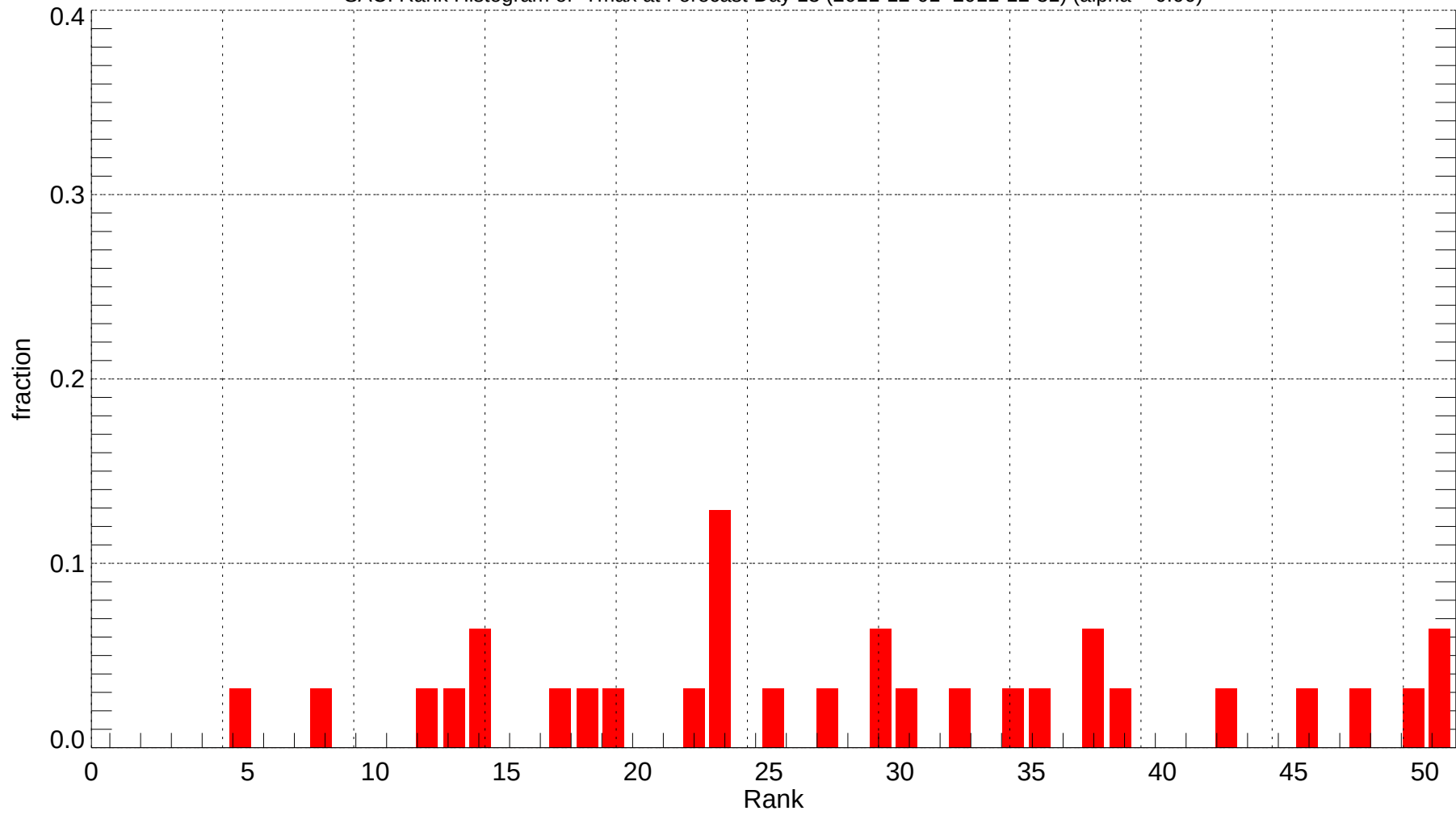
SAC: Rank Histogram of Tmax at Forecast Day 13 (2011-12-01~2011-12-31) (alpha = 0.00)
