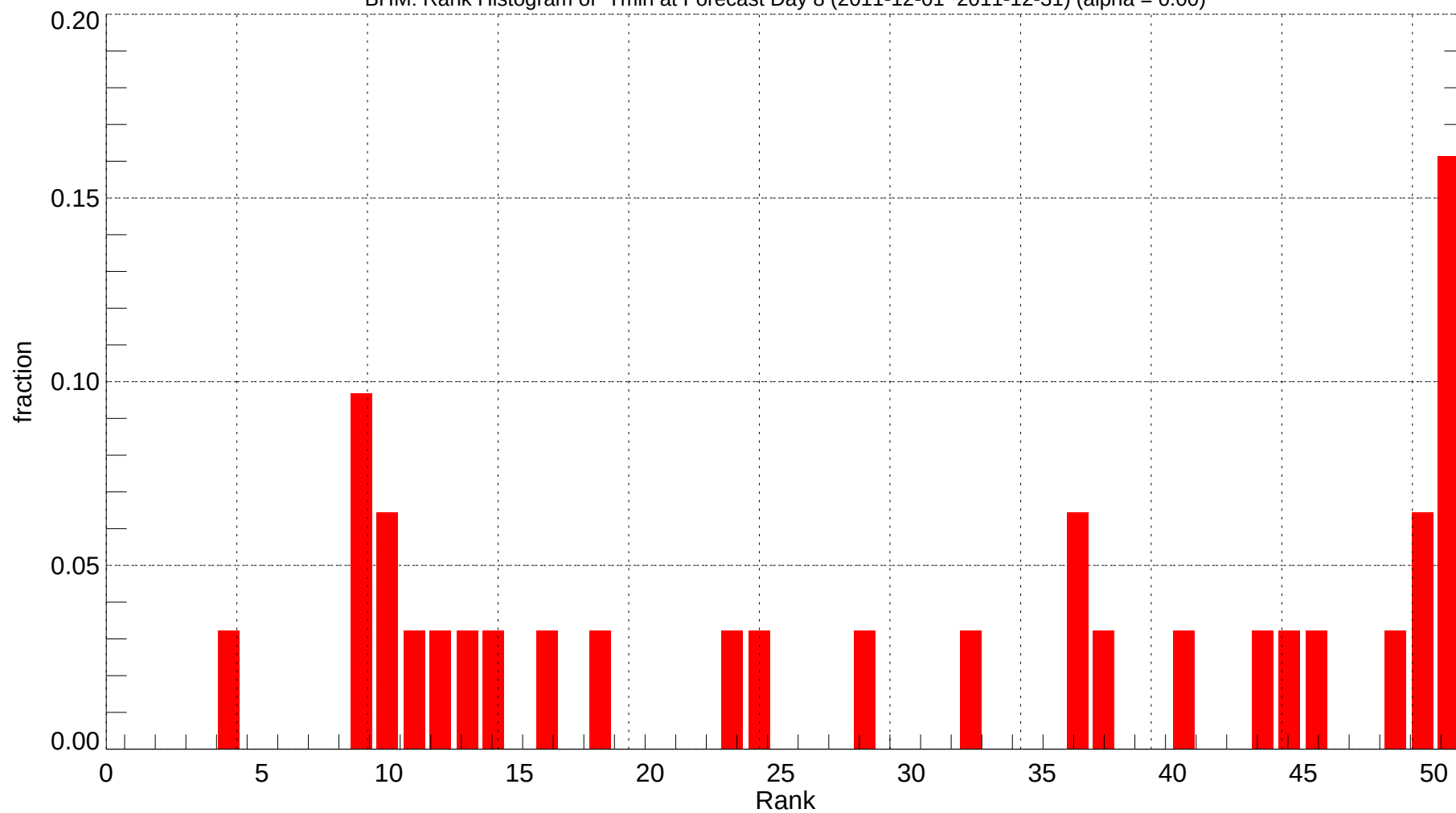
BHM: Rank Histogram of Tmin at Forecast Day 8 (2011-12-01~2011-12-31) (alpha = 0.00)
