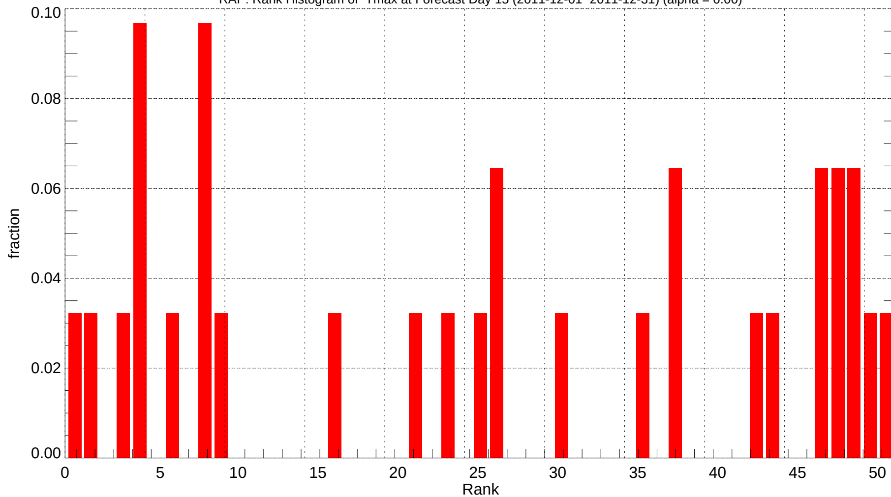
RAP: Rank Histogram of Tmax at Forecast Day 15 (2011-12-01~2011-12-31) (alpha = 0.00)
