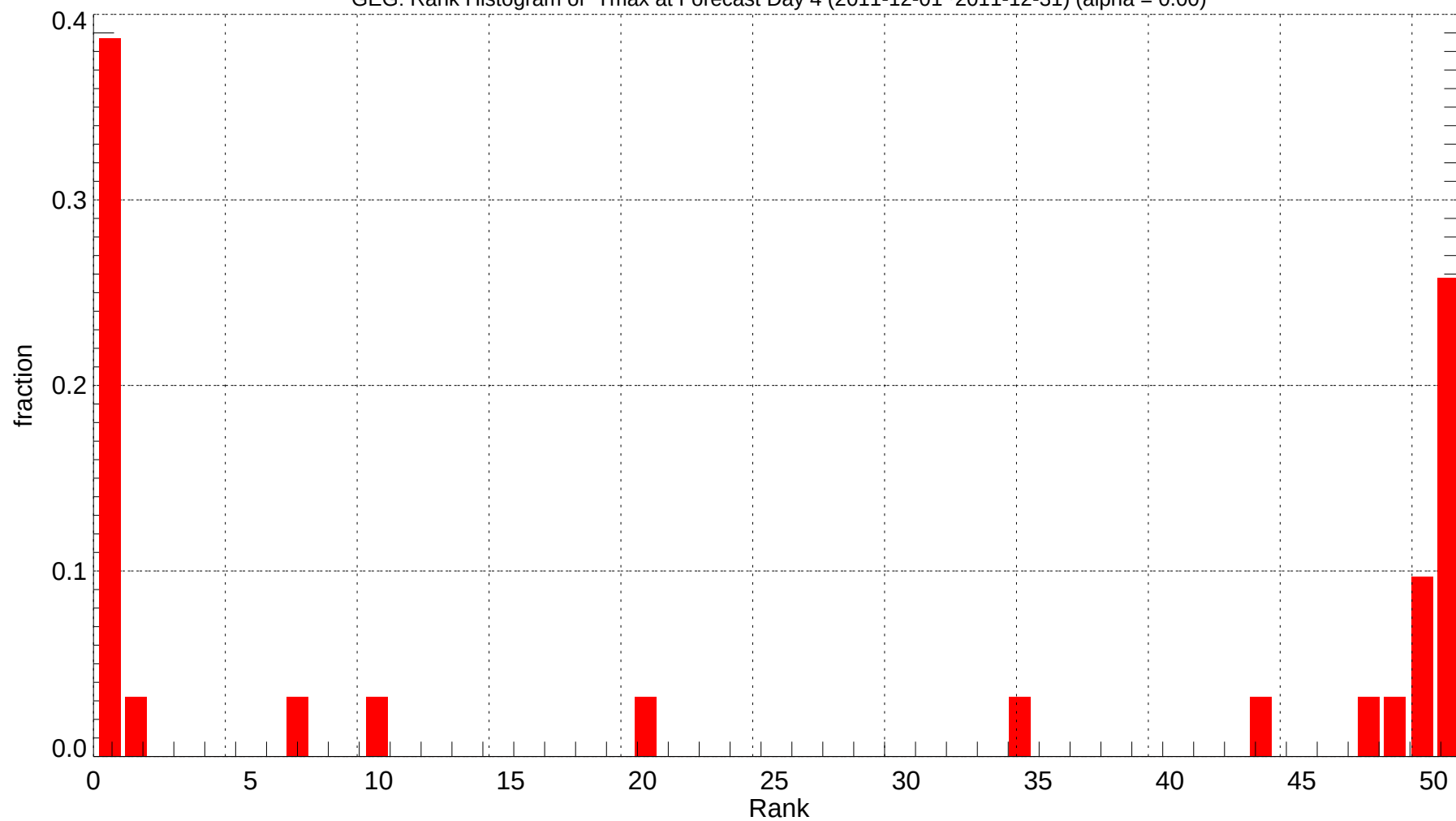
GEG: Rank Histogram of Tmax at Forecast Day 4 (2011-12-01~2011-12-31) (alpha = 0.00)
