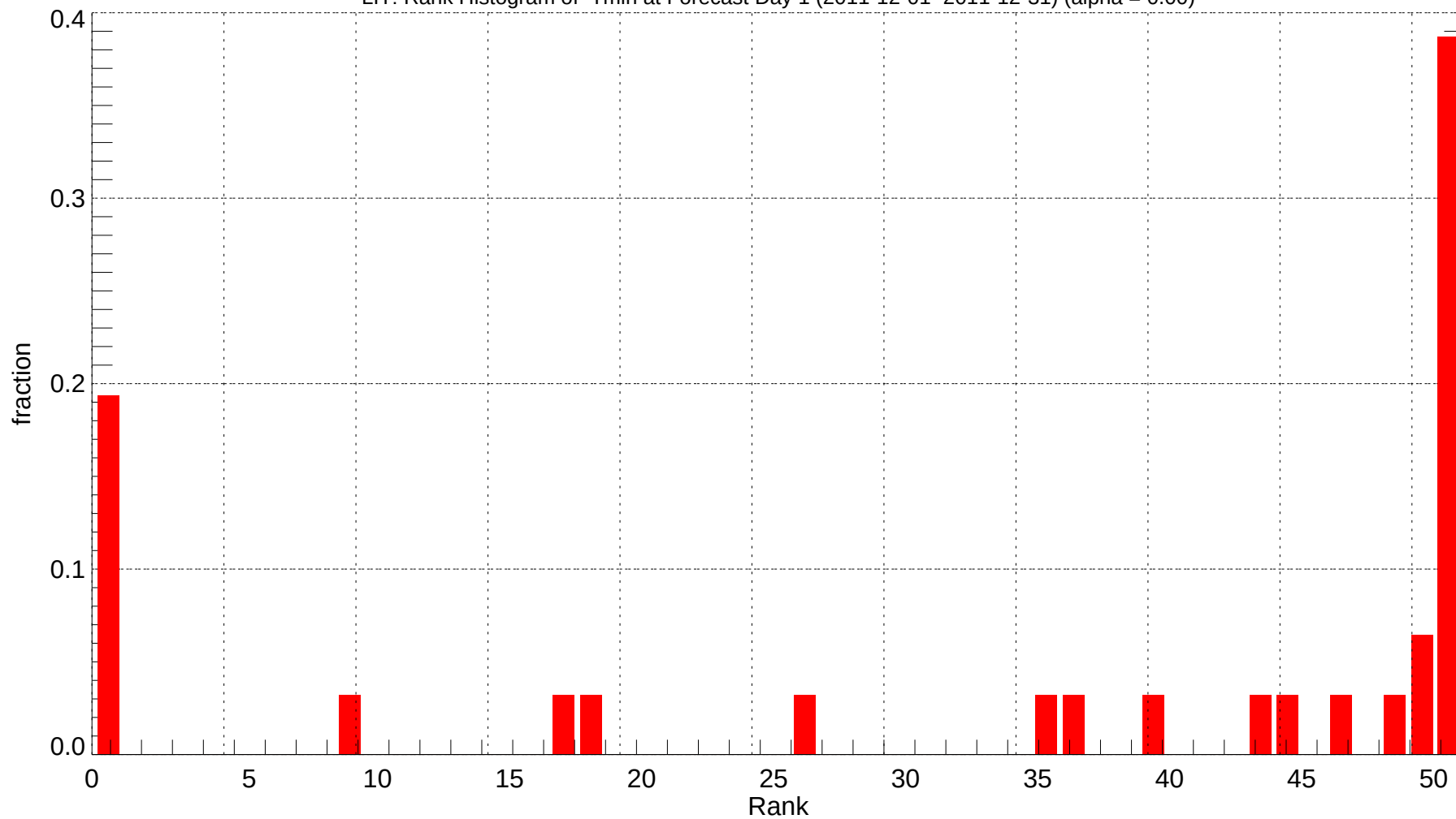
LIT: Rank Histogram of Tmin at Forecast Day 1 (2011-12-01~2011-12-31) (alpha = 0.00)
