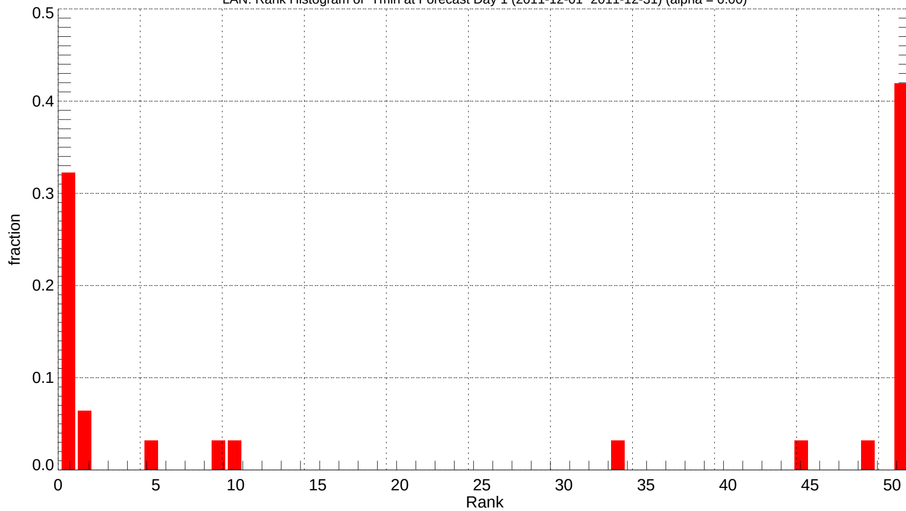
LAN: Rank Histogram of Tmin at Forecast Day 1 (2011-12-01~2011-12-31) (alpha = 0.00)
