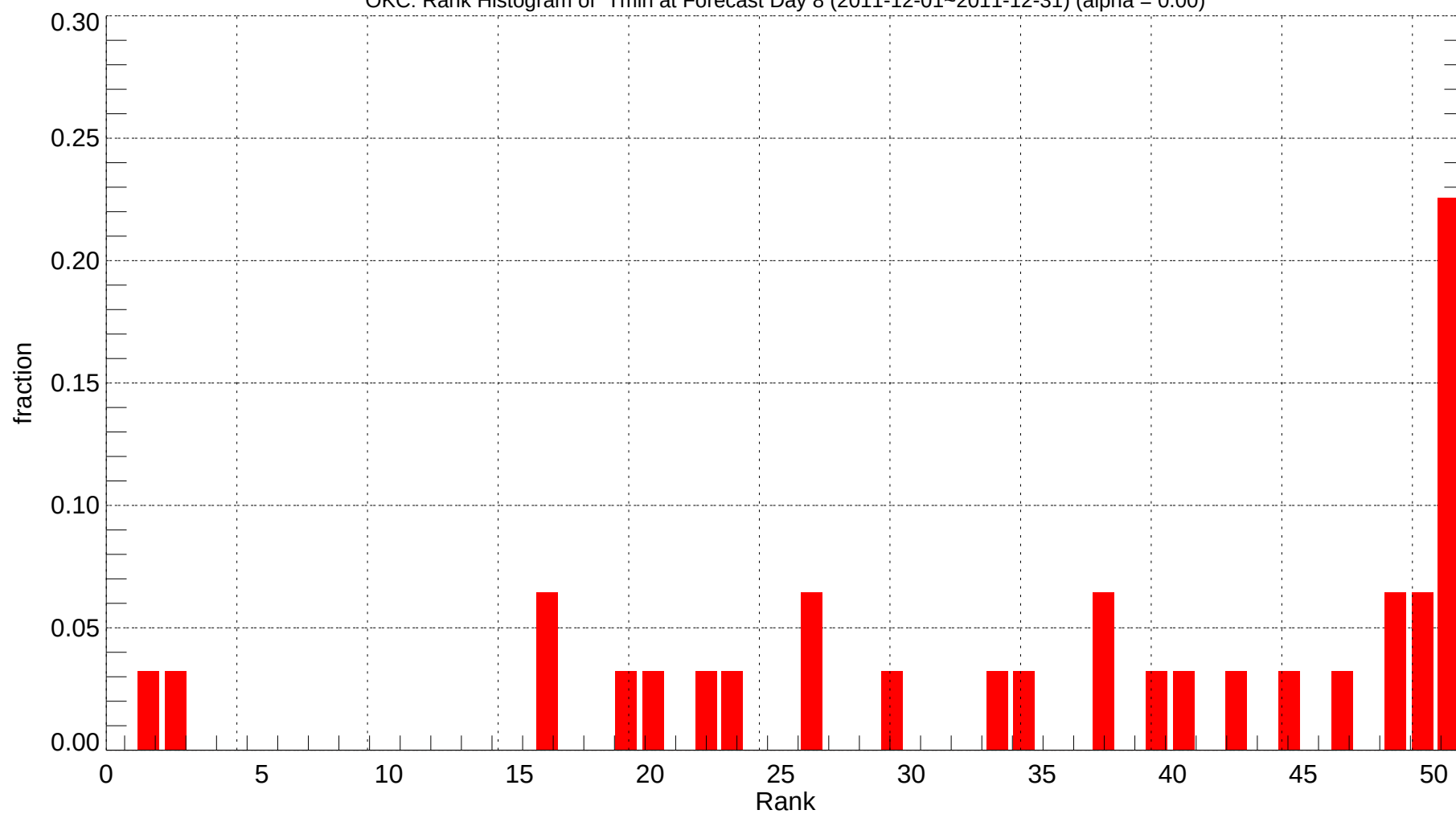
OKC: Rank Histogram of Tmin at Forecast Day 8 (2011-12-01~2011-12-31) (alpha = 0.00)
