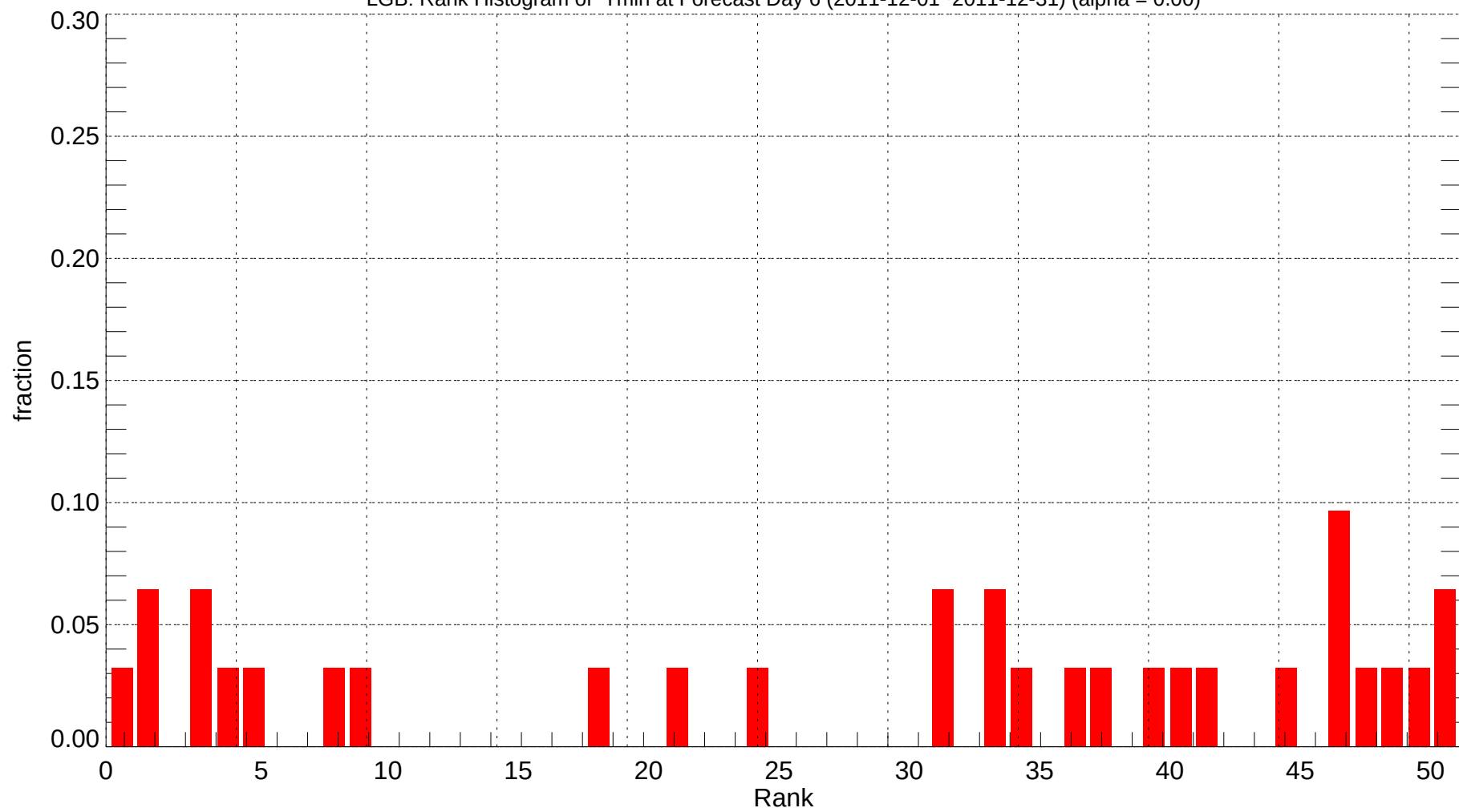
LGB: Rank Histogram of Tmin at Forecast Day 6 (2011-12-01~2011-12-31) (alpha = 0.00)
