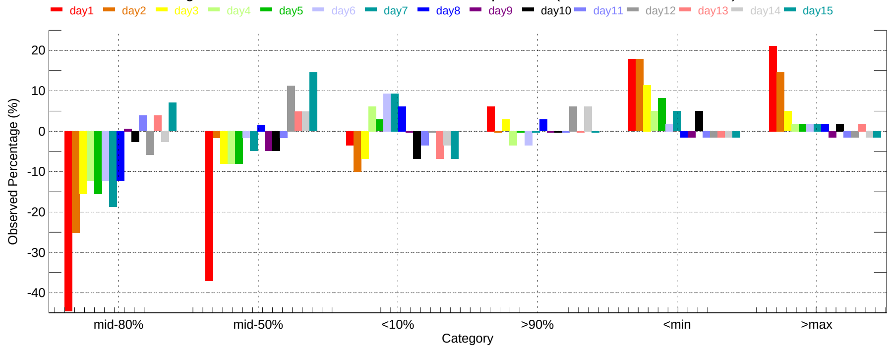
Observed Percentage Deviation of Ensembles - NKX: Min Temperature (2011-12-01~2011-12-31)
