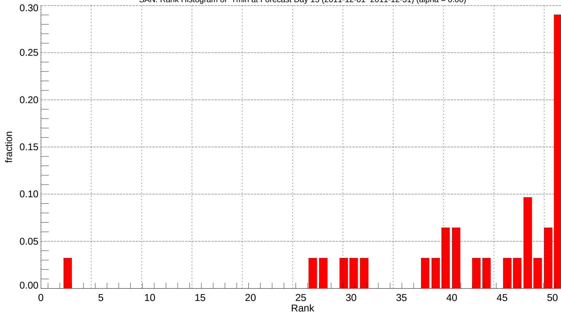
SAN: Rank Histogram of Tmin at Forecast Day 15 (2011-12-01~2011-12-31) (alpha = 0.00)
