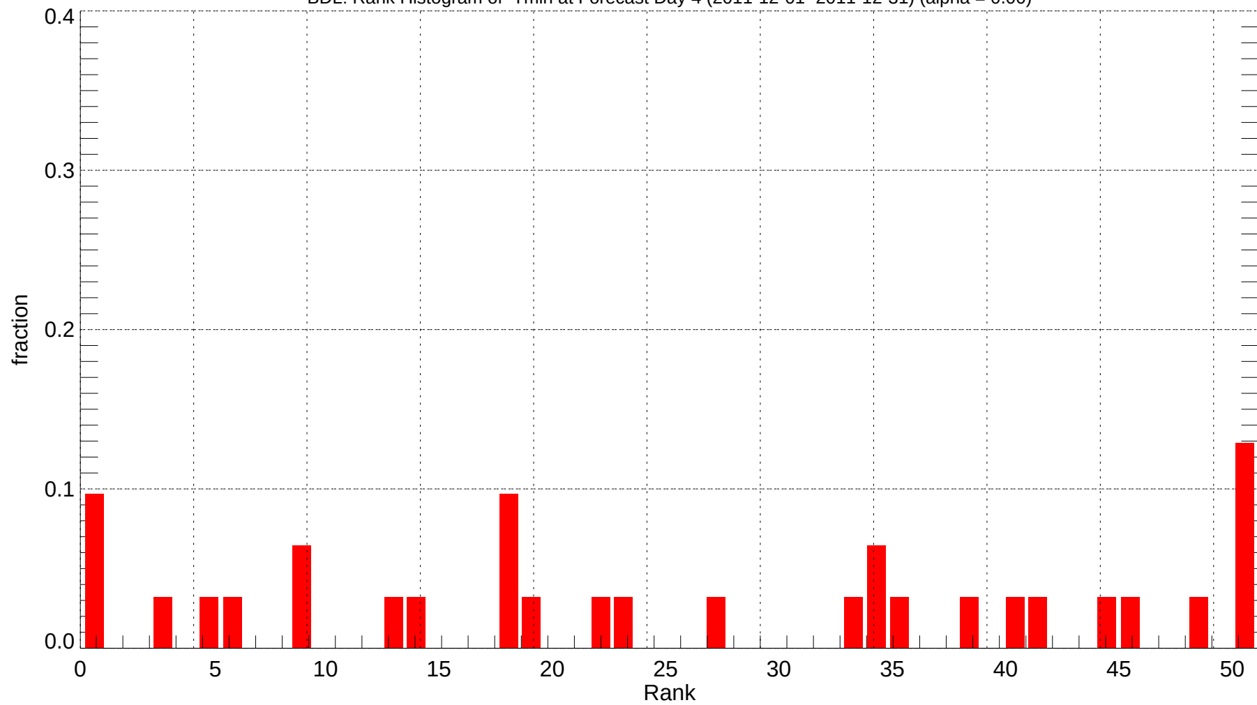
BDL: Rank Histogram of Tmin at Forecast Day 4 (2011-12-01~2011-12-31) (alpha = 0.00)
