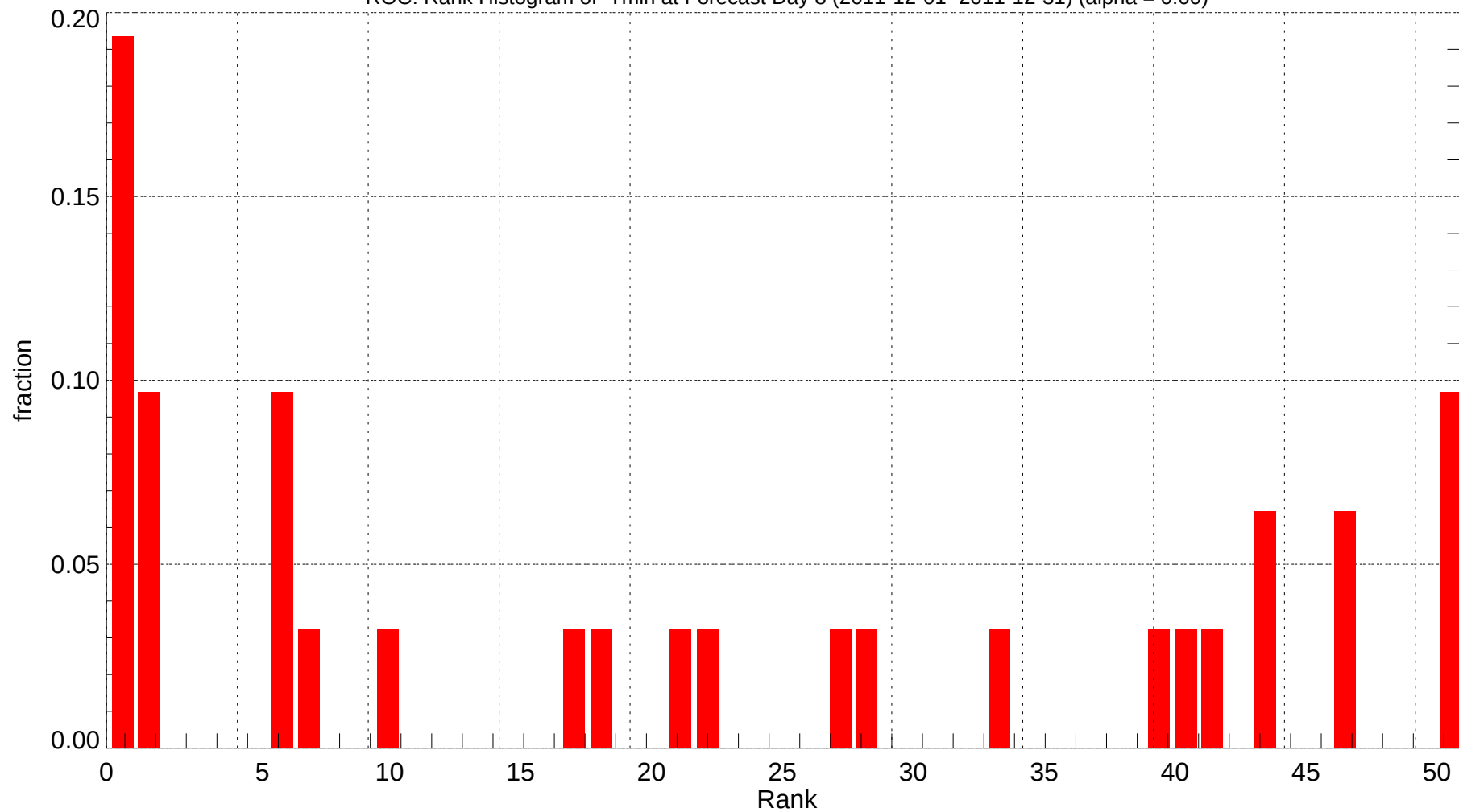
ROC: Rank Histogram of Tmin at Forecast Day 8 (2011-12-01~2011-12-31) (alpha = 0.00)
