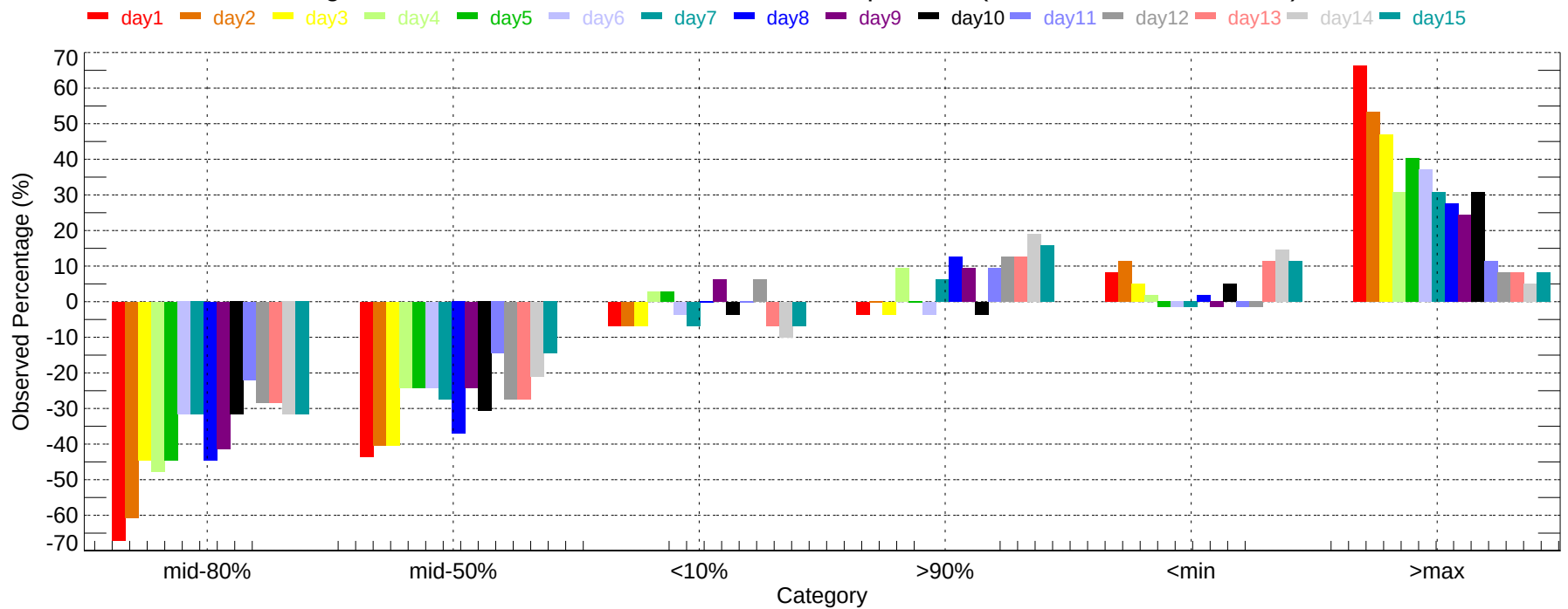
Observed Percentage Deviation of Ensembles - TLH: Max Temperature (2011-12-01~2011-12-31)
