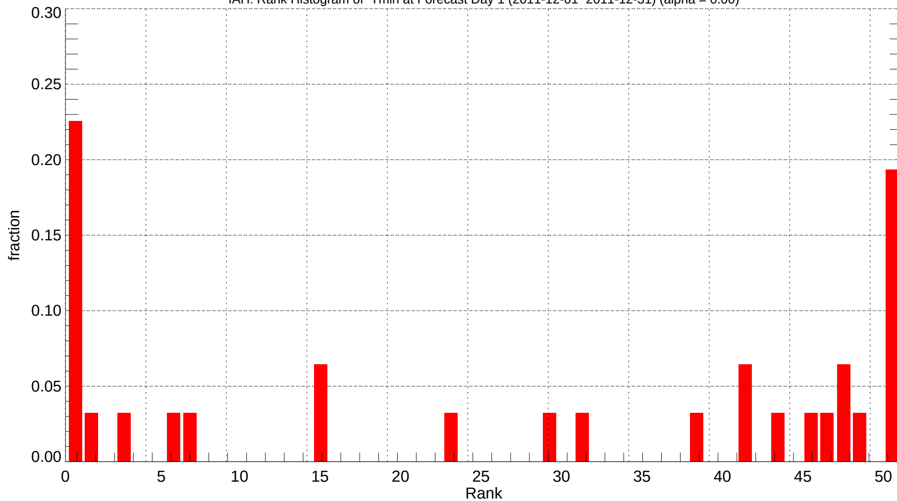
IAH: Rank Histogram of Tmin at Forecast Day 1 (2011-12-01~2011-12-31) (alpha = 0.00)
