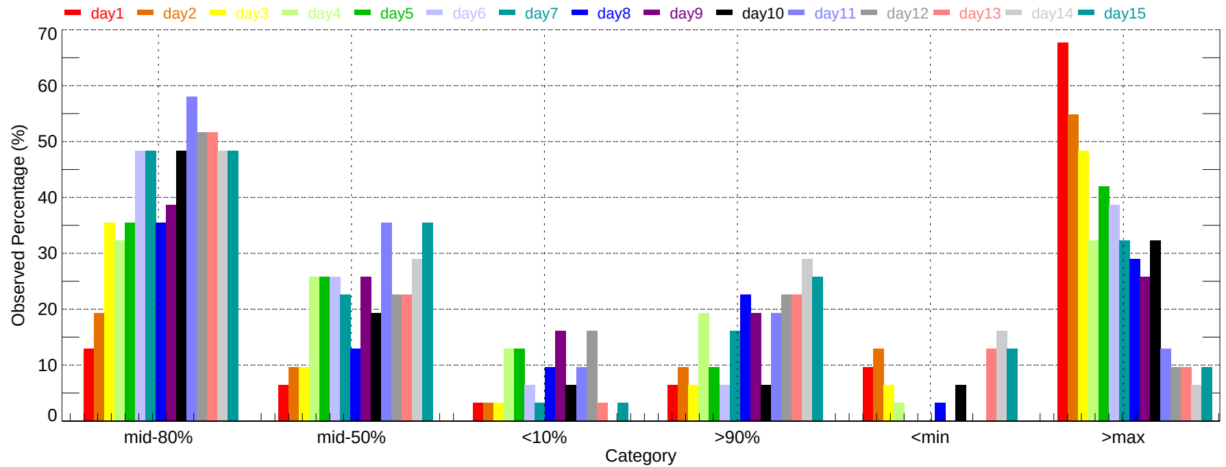
Observed Percentage of Ensembles - TLH: Max Temperature (2011-12-01~2011-12-31)
