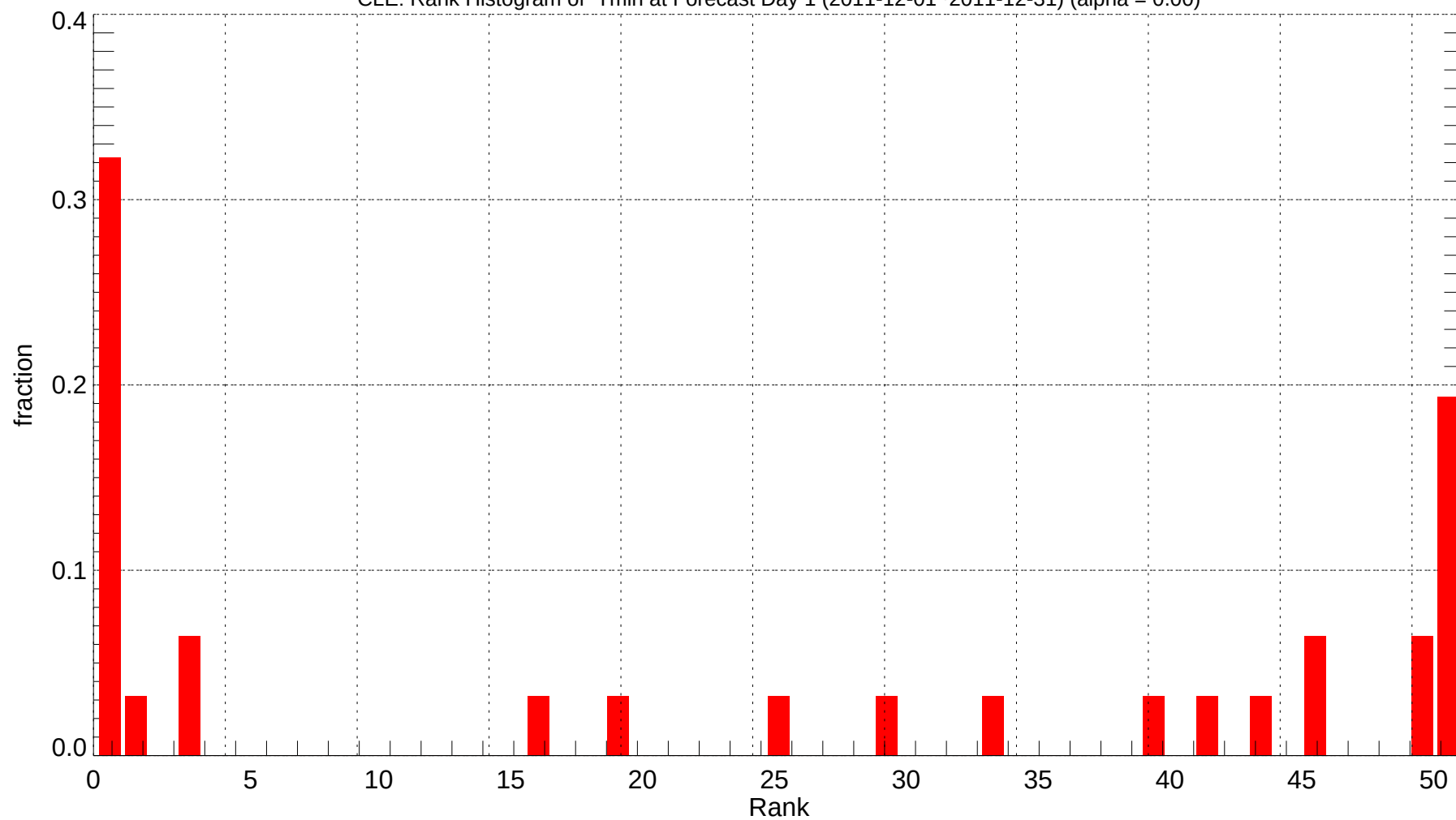
CLE: Rank Histogram of Tmin at Forecast Day 1 (2011-12-01~2011-12-31) (alpha = 0.00)
