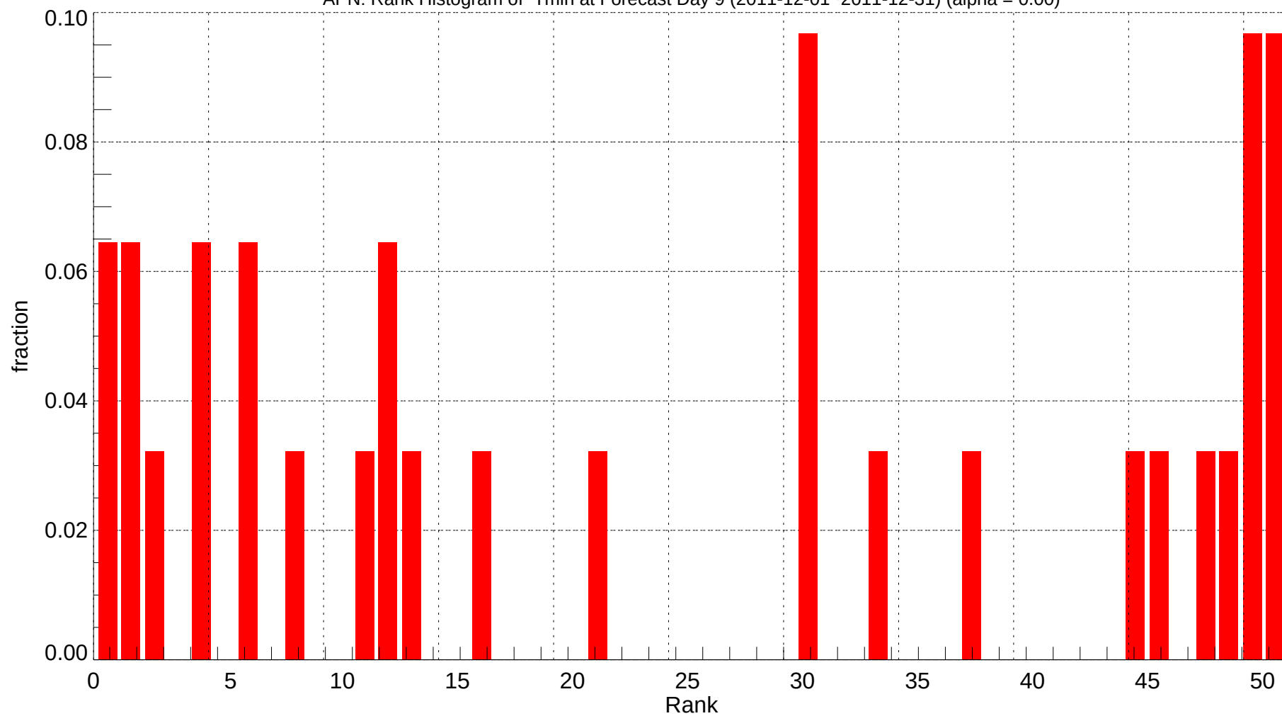
APN: Rank Histogram of Tmin at Forecast Day 9 (2011-12-01~2011-12-31) (alpha = 0.00)
