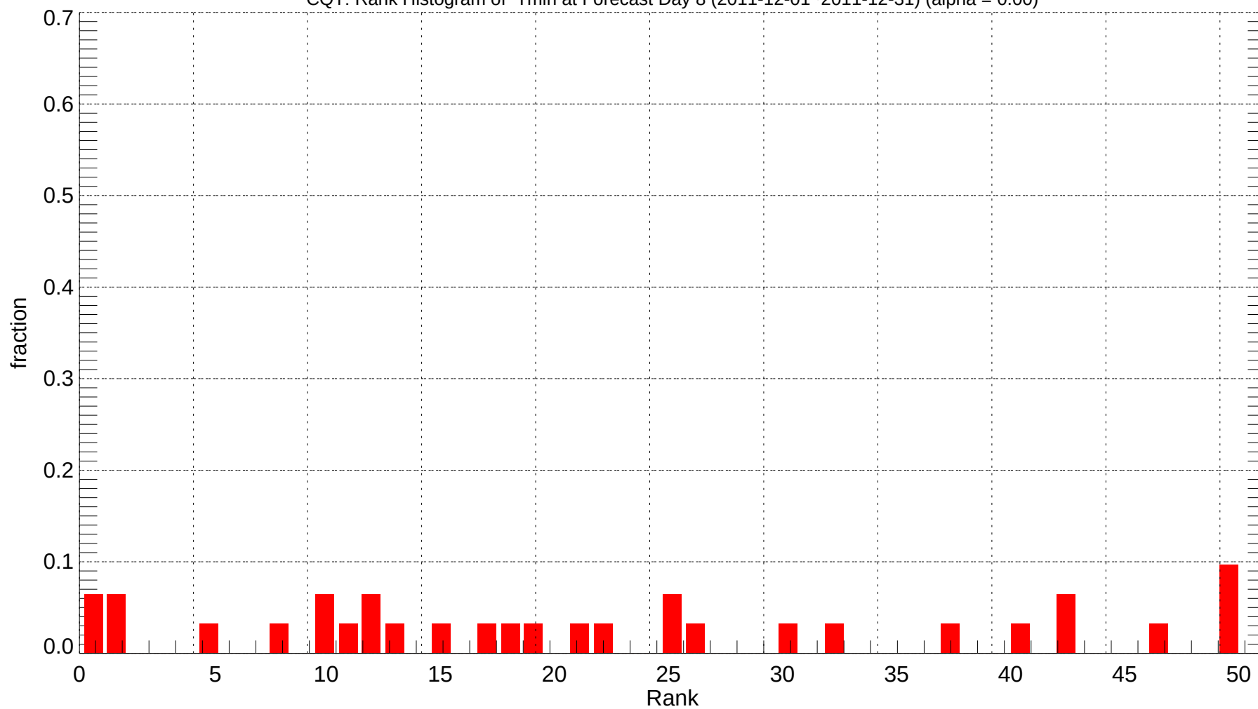
CQT: Rank Histogram of Tmin at Forecast Day 8 (2011-12-01~2011-12-31) (alpha = 0.00)
