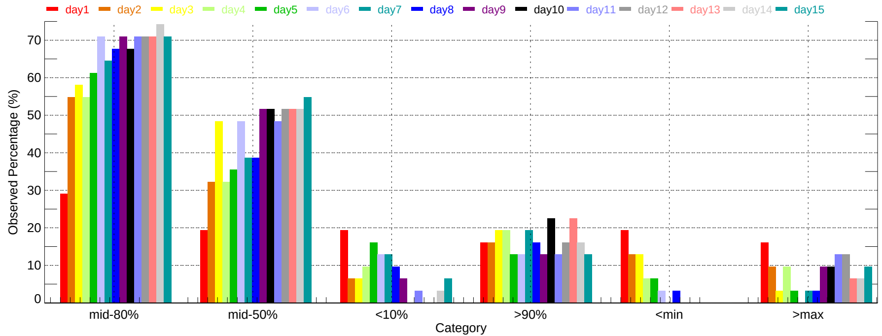
Observed Percentage of Ensembles - MCN: Max Temperature (2011-12-01~2011-12-31)
