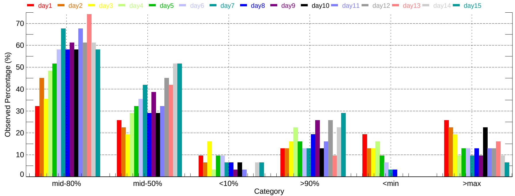
Observed Percentage of Ensembles - ABY: Max Temperature (2011-12-01~2011-12-31)
