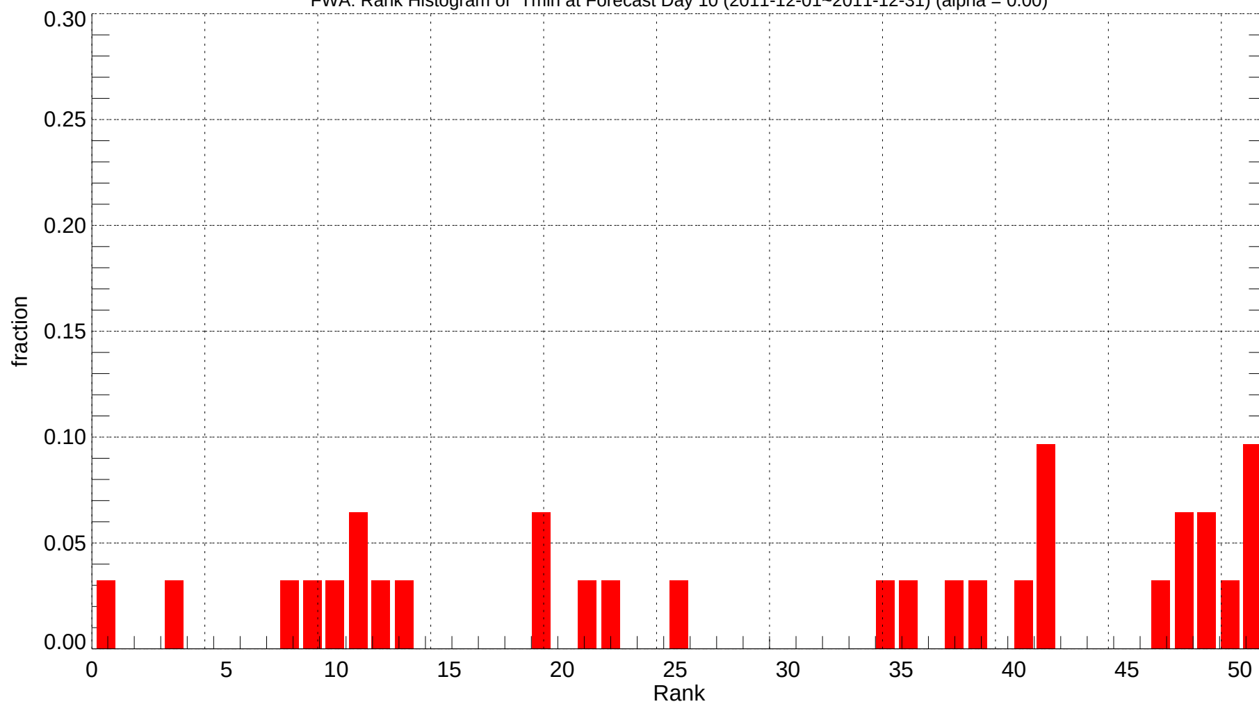
FWA: Rank Histogram of Tmin at Forecast Day 10 (2011-12-01~2011-12-31) (alpha = 0.00)
