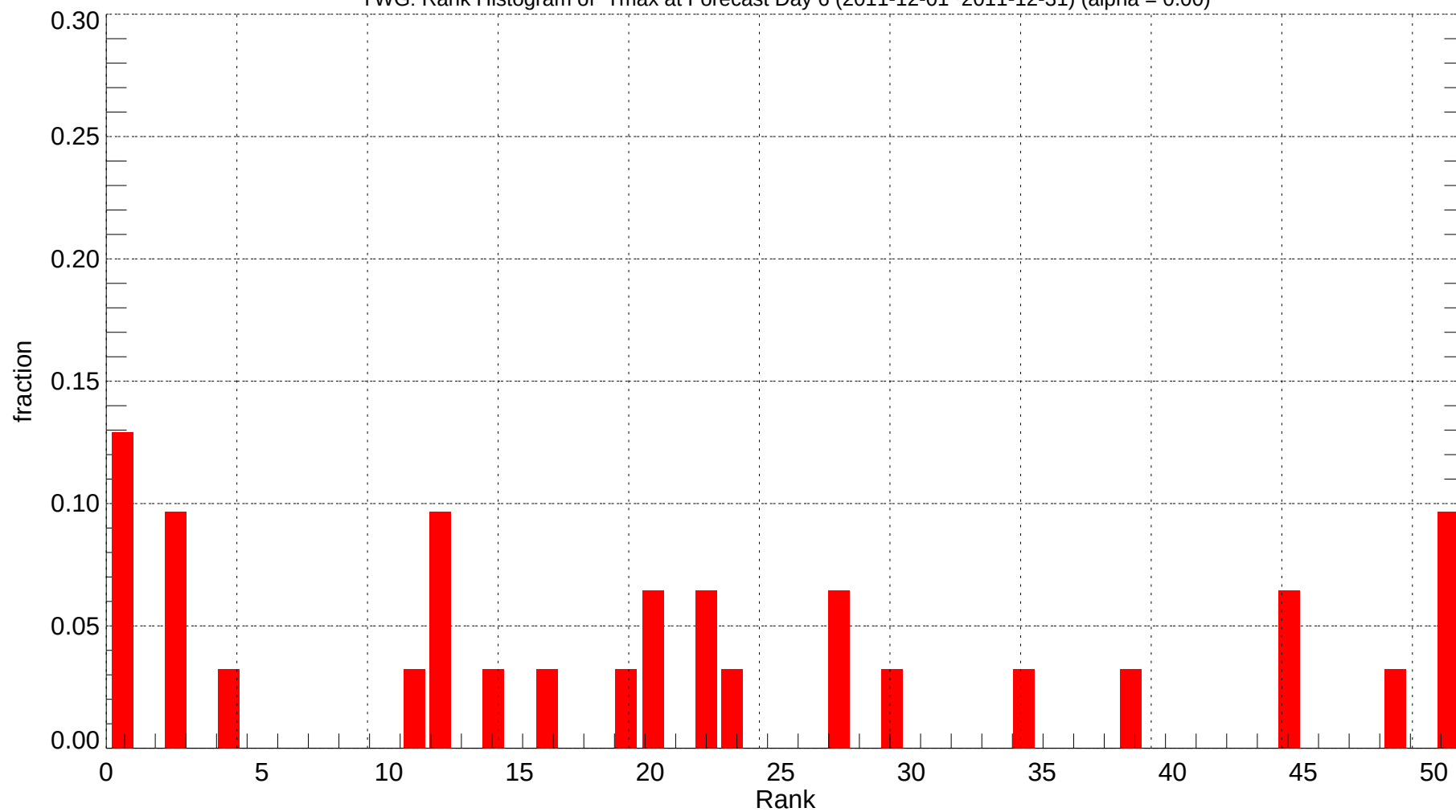
YWG: Rank Histogram of Tmax at Forecast Day 6 (2011-12-01~2011-12-31) (alpha = 0.00)
