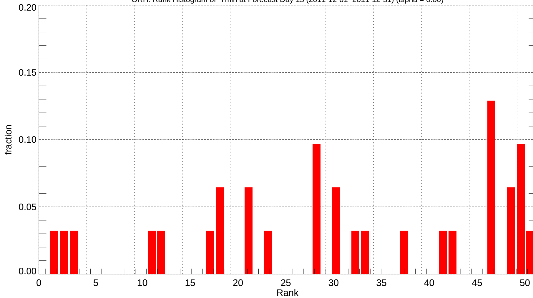
ORH: Rank Histogram of Tmin at Forecast Day 13 (2011-12-01~2011-12-31) (alpha = 0.00)
