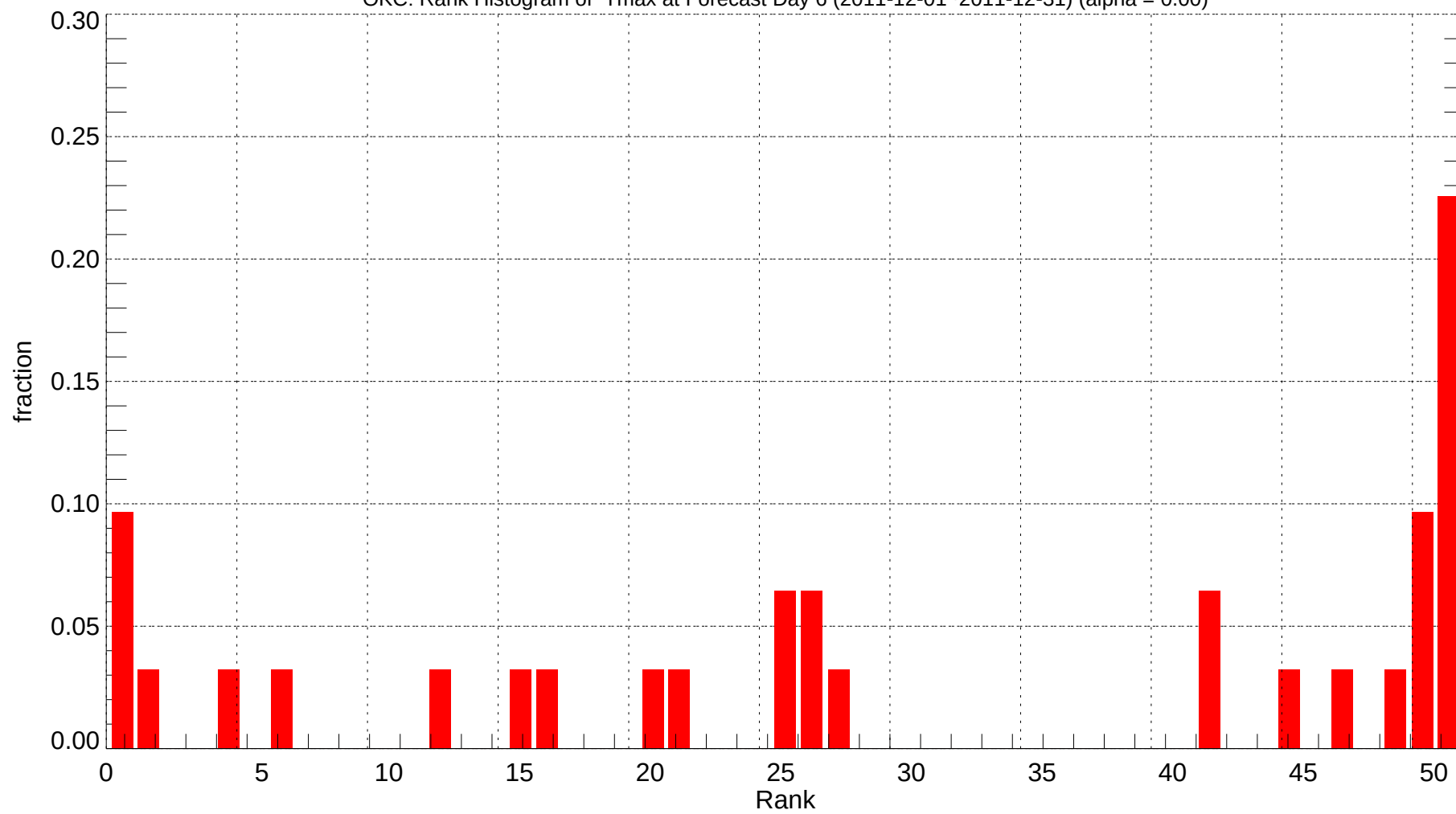
OKC: Rank Histogram of Tmax at Forecast Day 6 (2011-12-01~2011-12-31) (alpha = 0.00)
