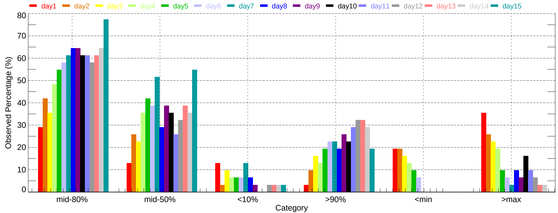
Observed Percentage of Ensembles - FWA: Min Temperature (2011-12-01~2011-12-31)
