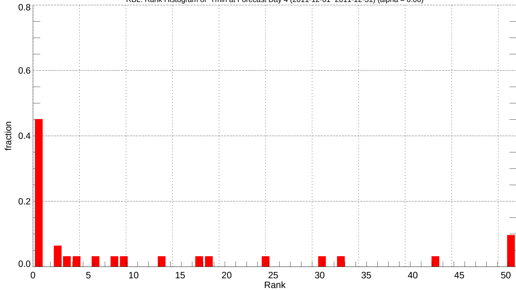
RBL: Rank Histogram of Tmin at Forecast Day 4 (2011-12-01~2011-12-31) (alpha = 0.00)
