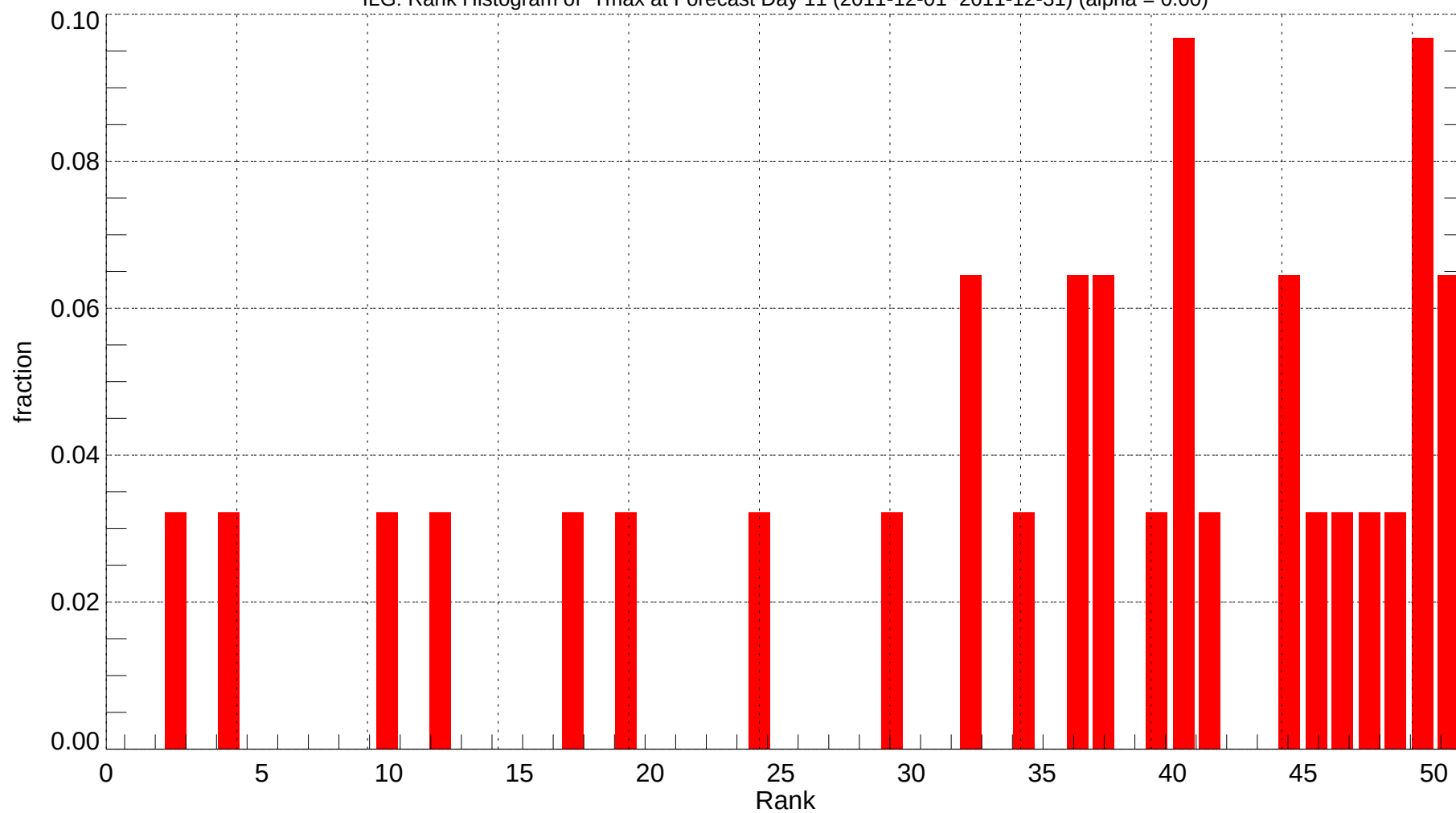
ILG: Rank Histogram of Tmax at Forecast Day 11 (2011-12-01~2011-12-31) (alpha = 0.00)
