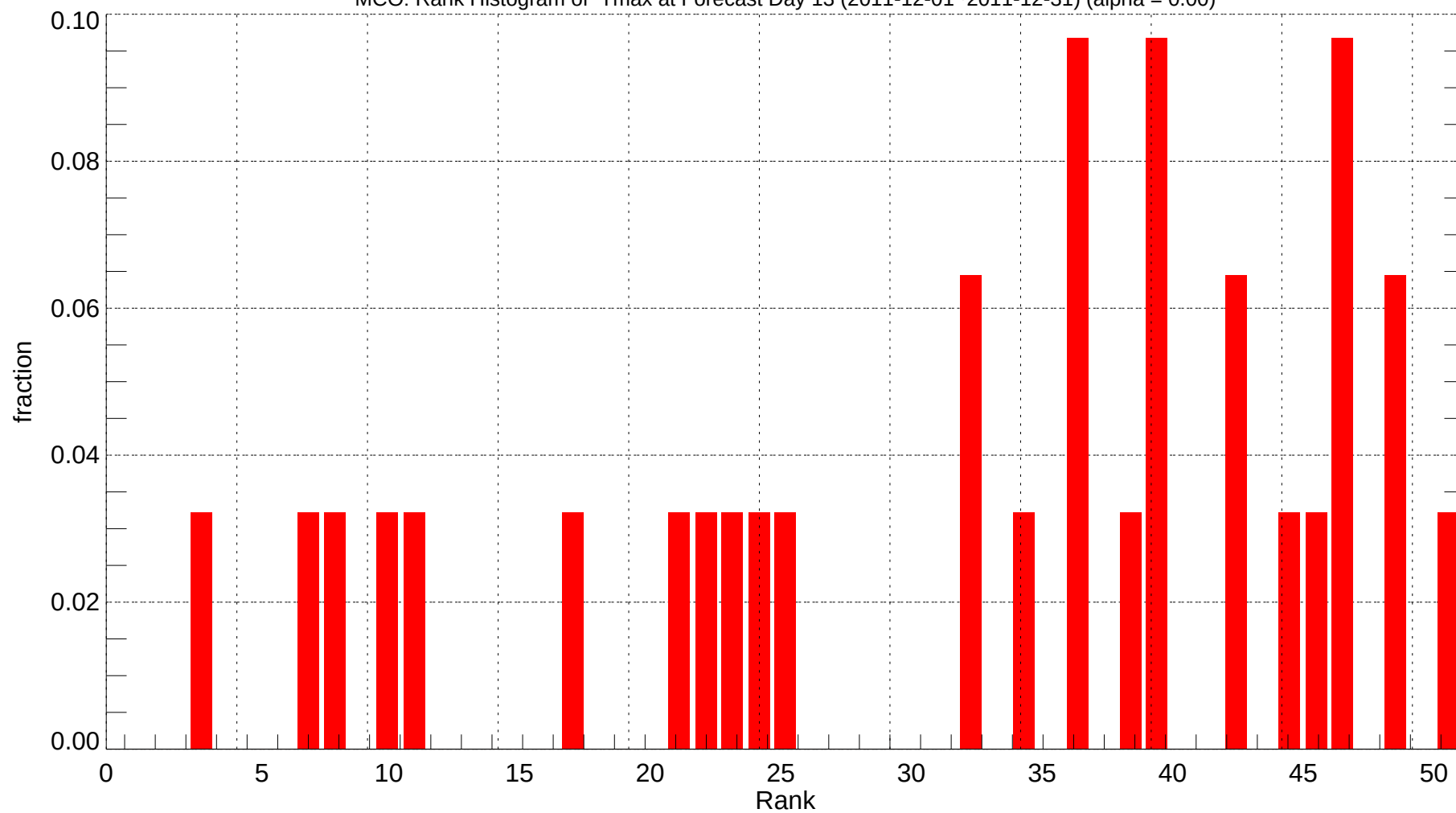
MCO: Rank Histogram of Tmax at Forecast Day 13 (2011-12-01~2011-12-31) (alpha = 0.00)
