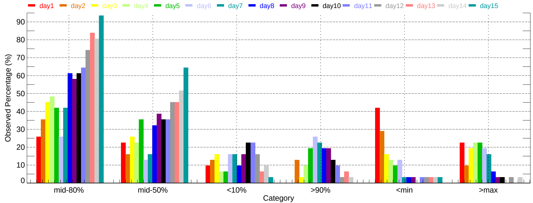
Observed Percentage of Ensembles - ACT: Min Temperature (2011-12-01~2011-12-31)
