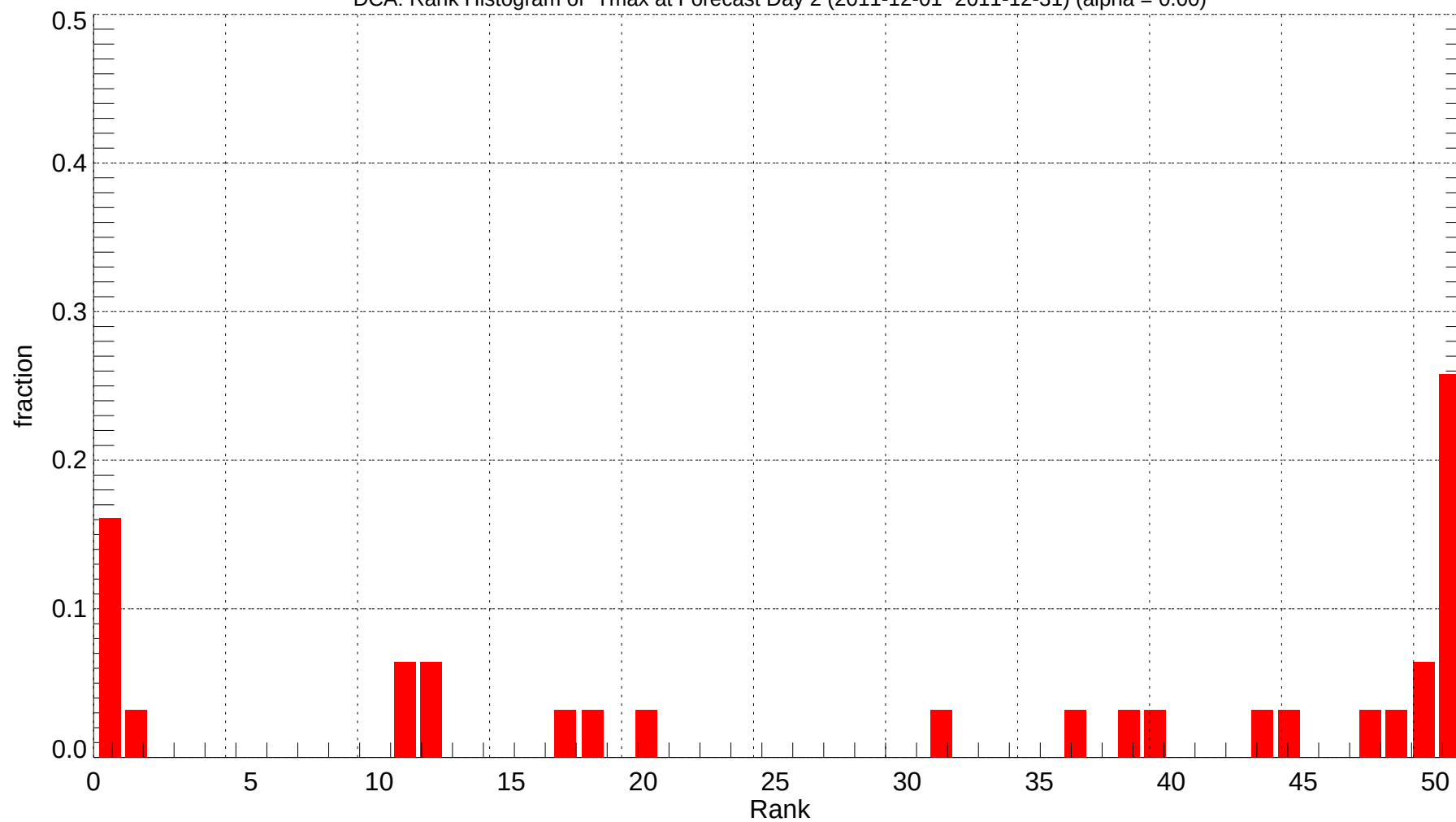
DCA: Rank Histogram of Tmax at Forecast Day 2 (2011-12-01~2011-12-31) (alpha = 0.00)
