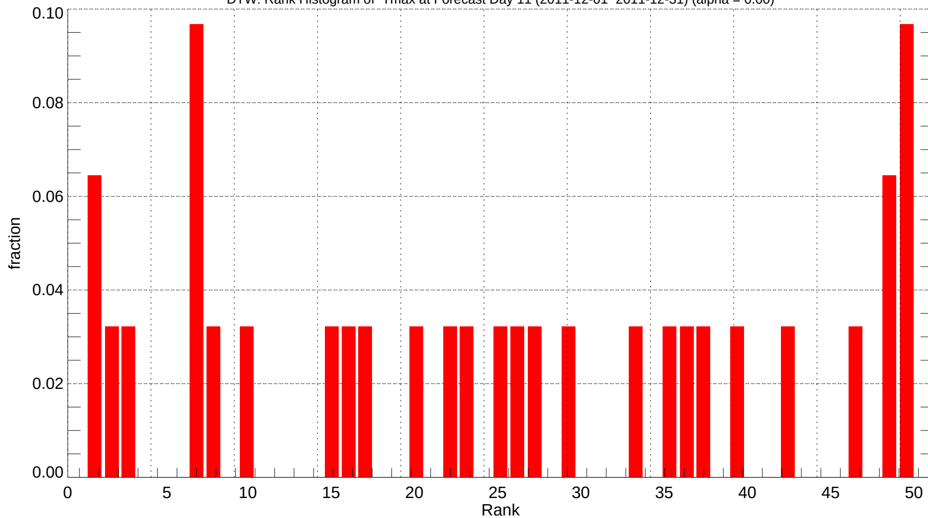
DTW: Rank Histogram of Tmax at Forecast Day 11 (2011-12-01~2011-12-31) (alpha = 0.00)
