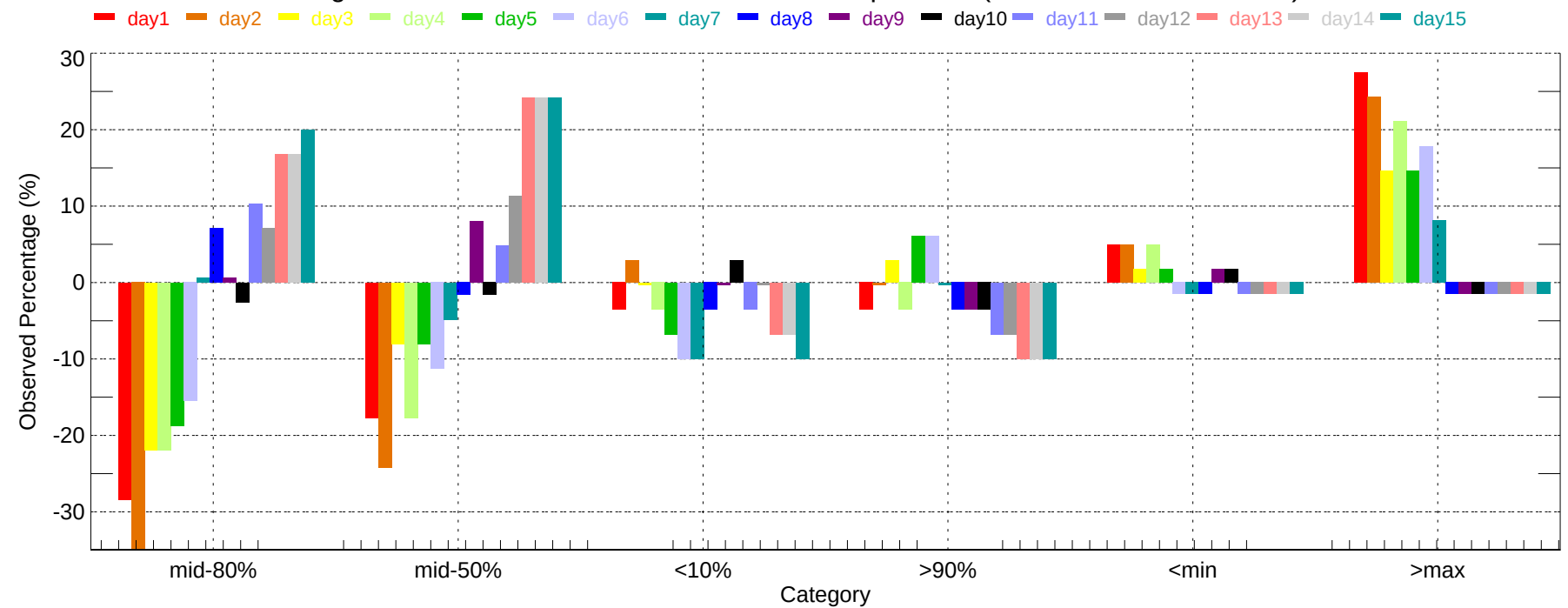
Observed Percentage Deviation of Ensembles - FAT: Max Temperature (2011-12-01~2011-12-31)
