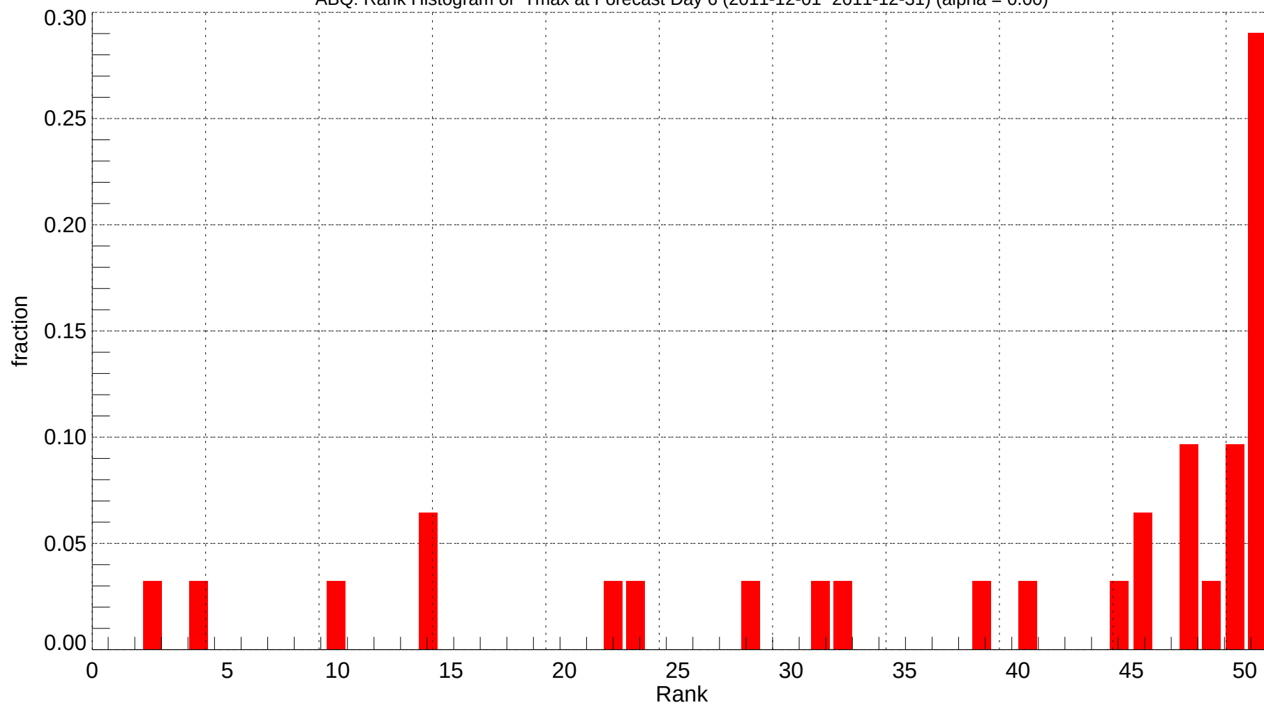
ABQ: Rank Histogram of Tmax at Forecast Day 6 (2011-12-01~2011-12-31) (alpha = 0.00)
