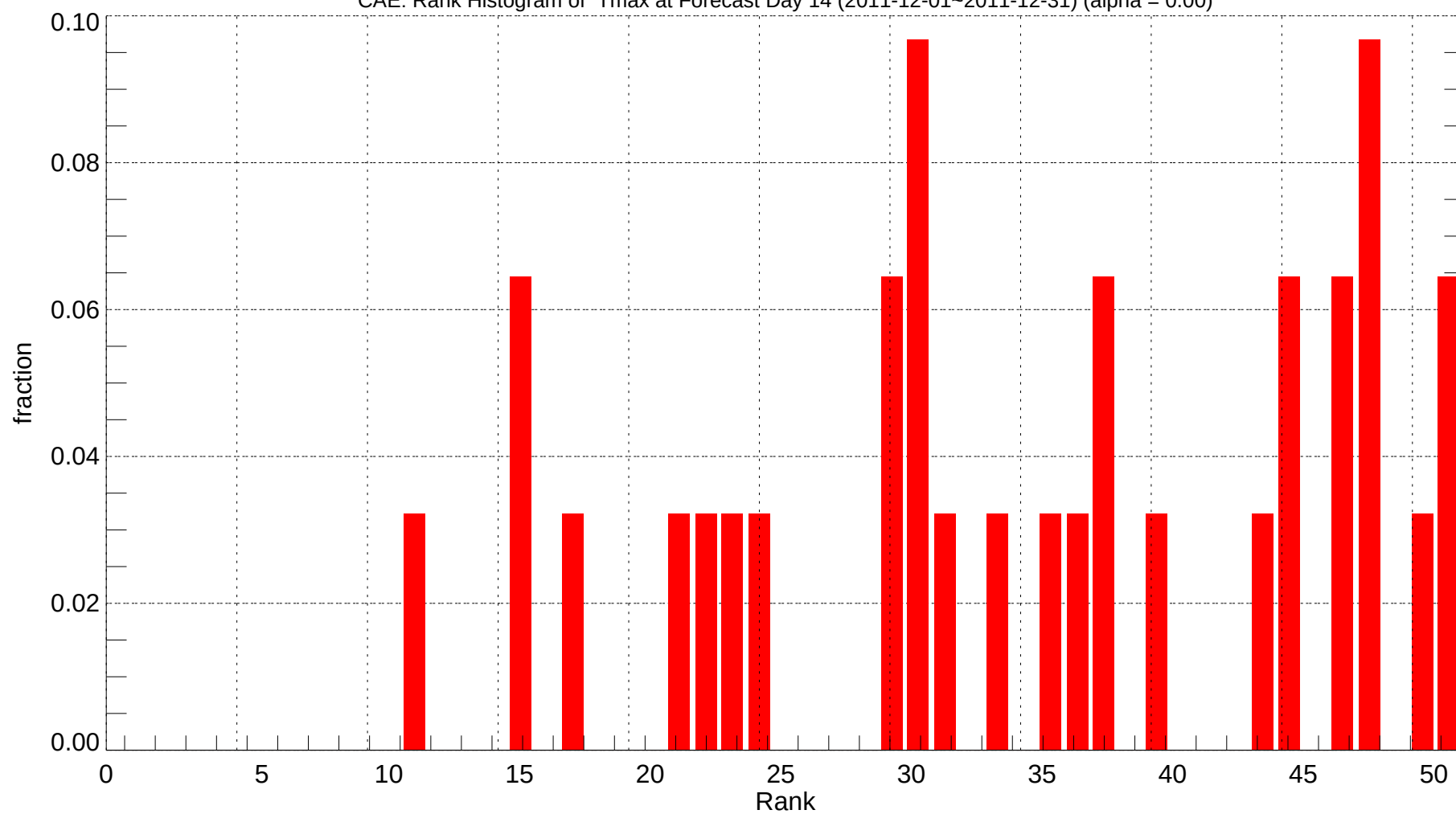
CAE: Rank Histogram of Tmax at Forecast Day 14 (2011-12-01~2011-12-31) (alpha = 0.00)
