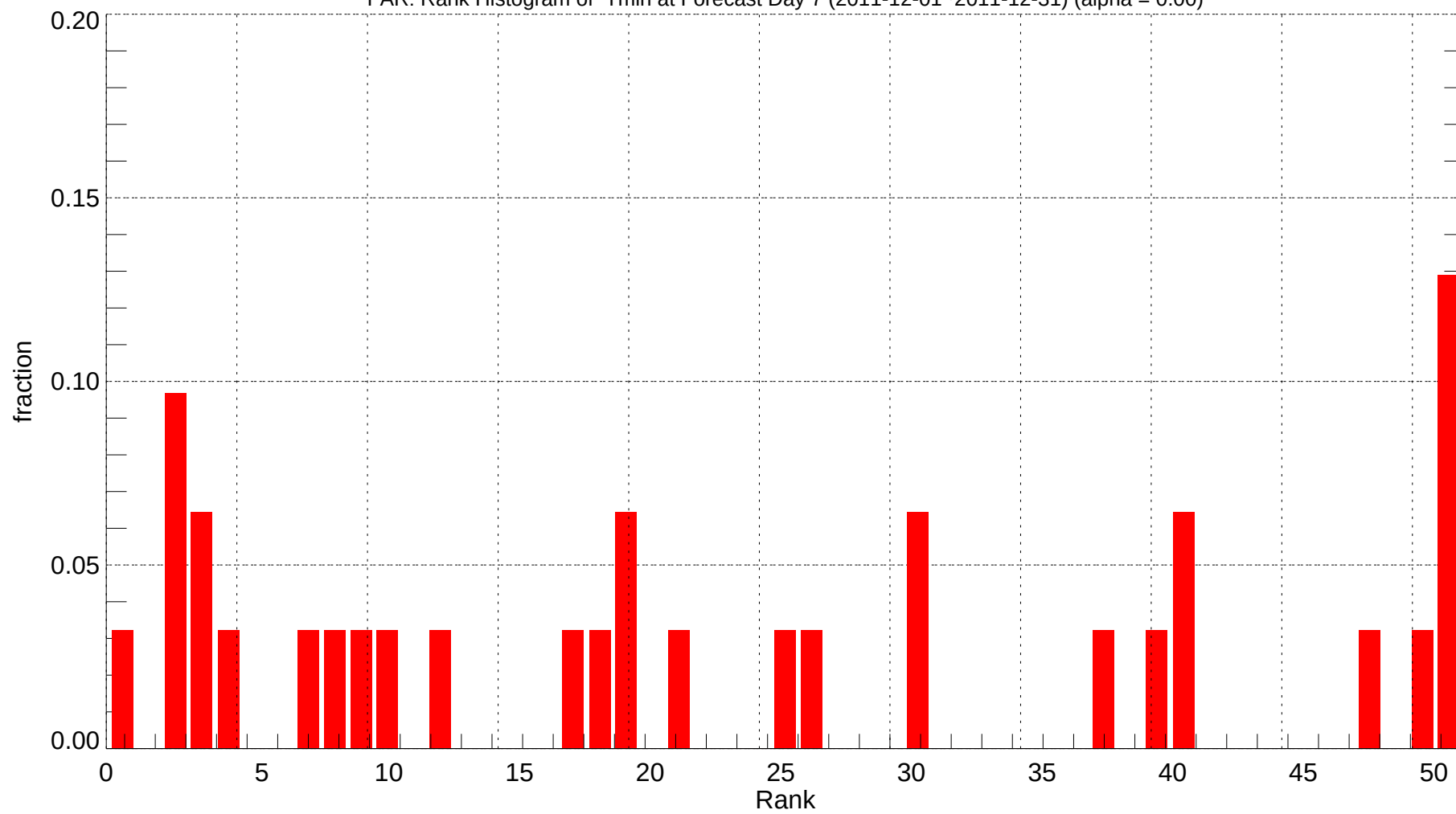
FAR: Rank Histogram of Tmin at Forecast Day 7 (2011-12-01~2011-12-31) (alpha = 0.00)
