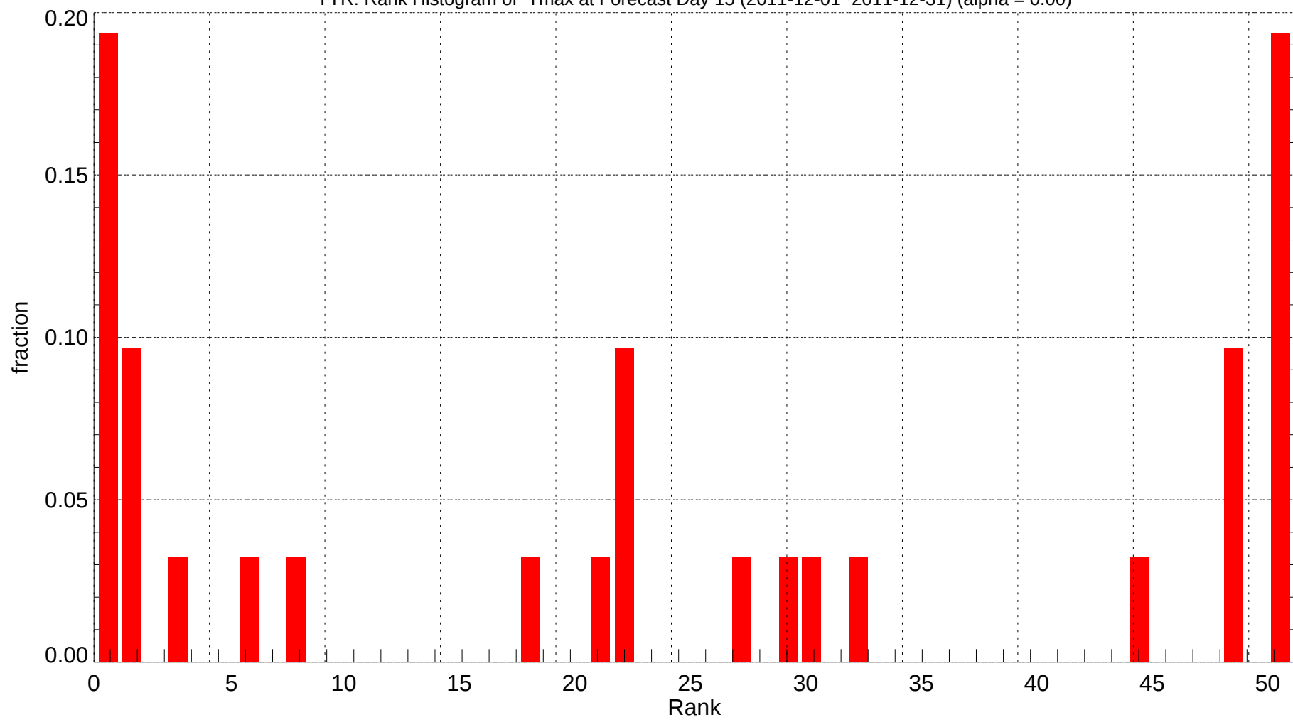
TYR: Rank Histogram of Tmax at Forecast Day 15 (2011-12-01~2011-12-31) (alpha = 0.00)
