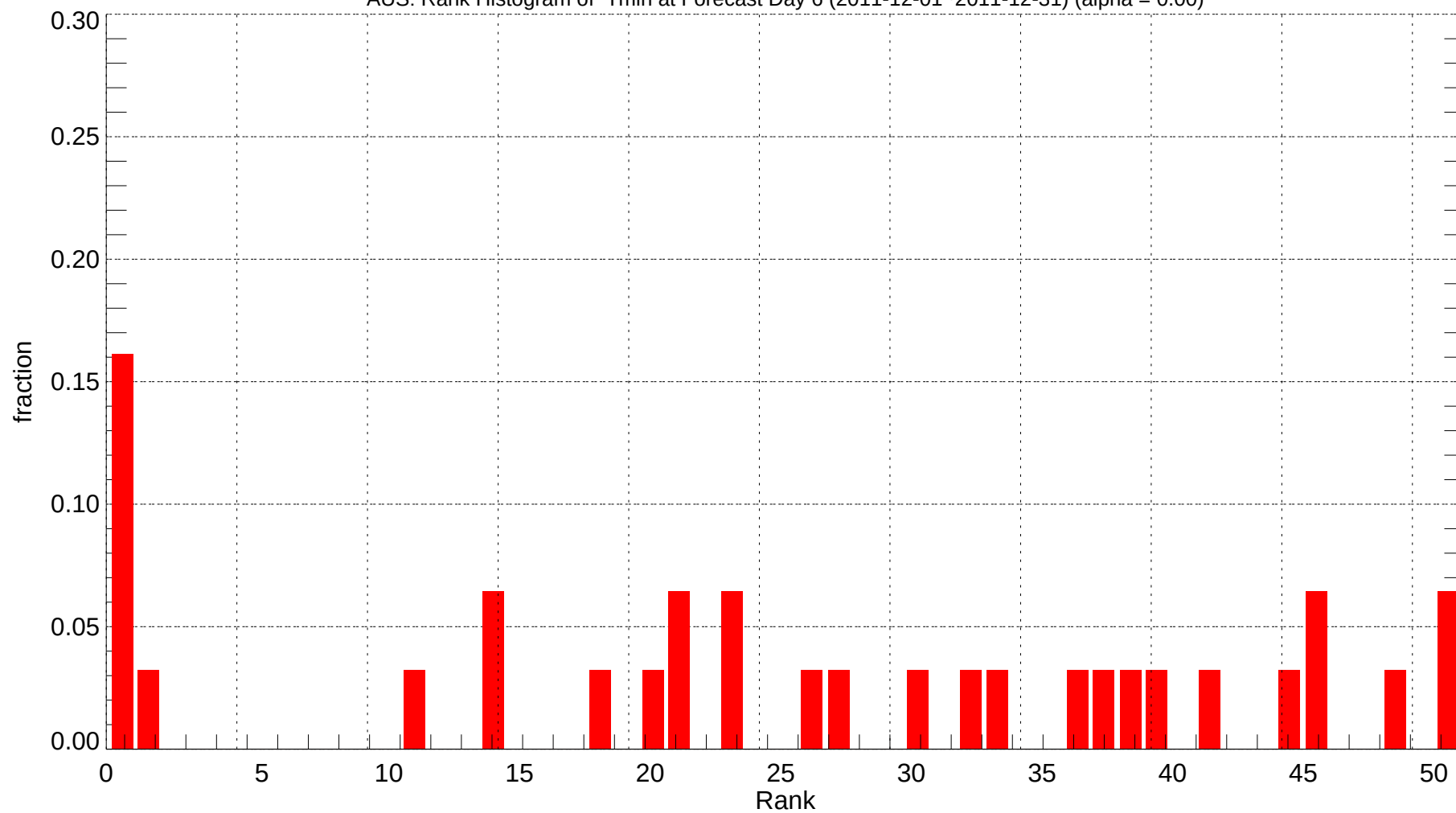
AUS: Rank Histogram of Tmin at Forecast Day 6 (2011-12-01~2011-12-31) (alpha = 0.00)
