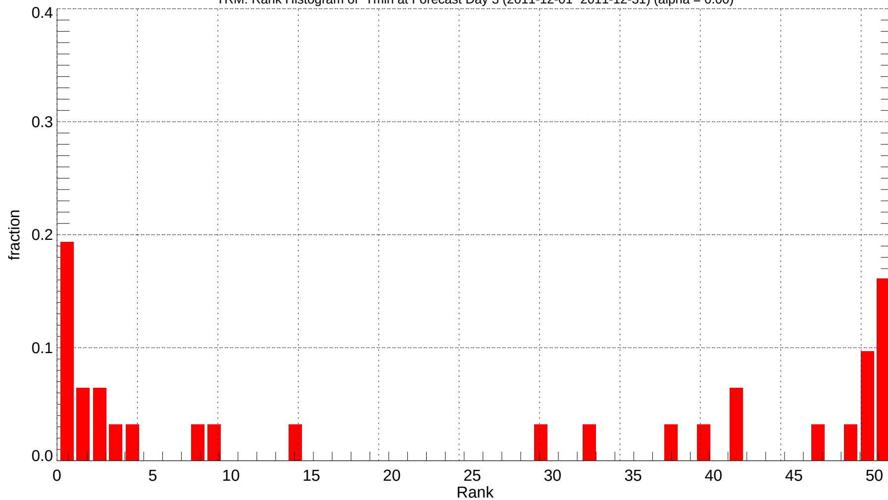
TRM: Rank Histogram of Tmin at Forecast Day 3 (2011-12-01~2011-12-31) (alpha = 0.00)
