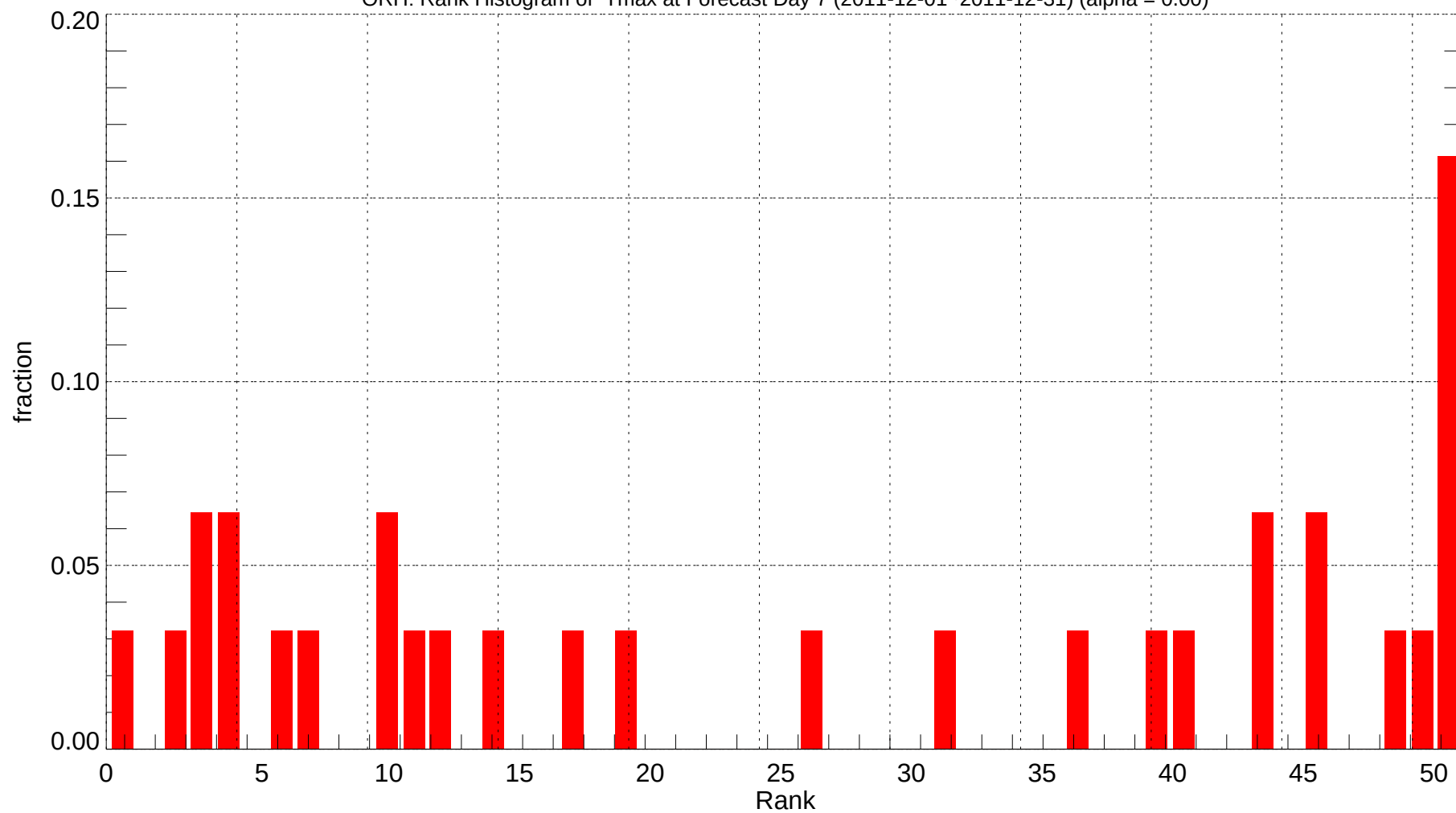
ORH: Rank Histogram of Tmax at Forecast Day 7 (2011-12-01~2011-12-31) (alpha = 0.00)
