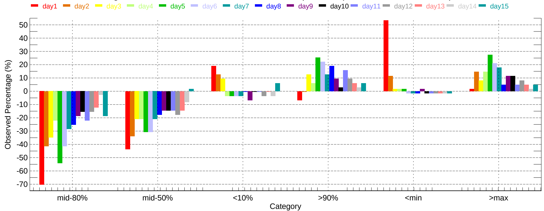
Observed Percentage Deviation of Ensembles - AVP: Max Temperature (2011-12-01~2011-12-31)
