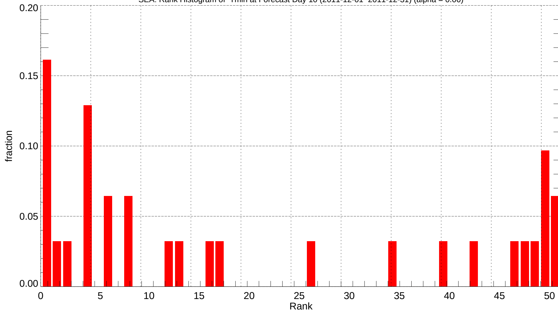
SEA: Rank Histogram of Tmin at Forecast Day 10 (2011-12-01~2011-12-31) (alpha = 0.00)
