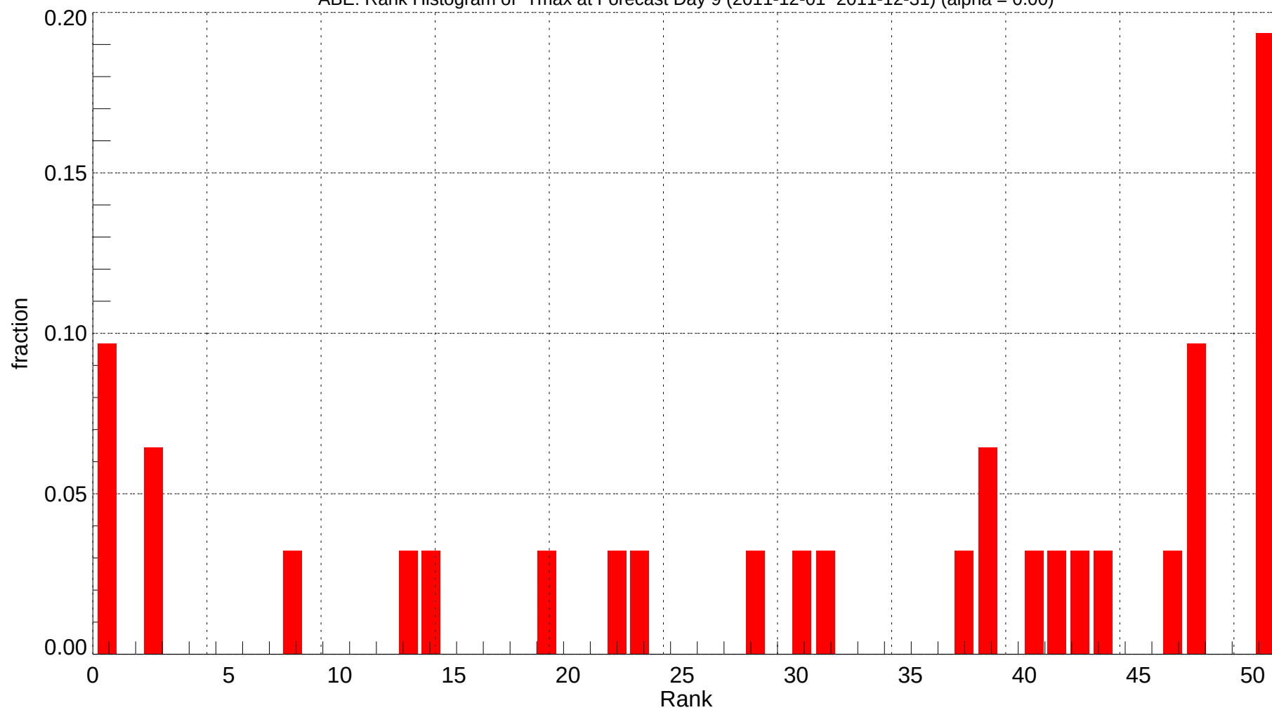
ABE: Rank Histogram of Tmax at Forecast Day 9 (2011-12-01~2011-12-31) (alpha = 0.00)
