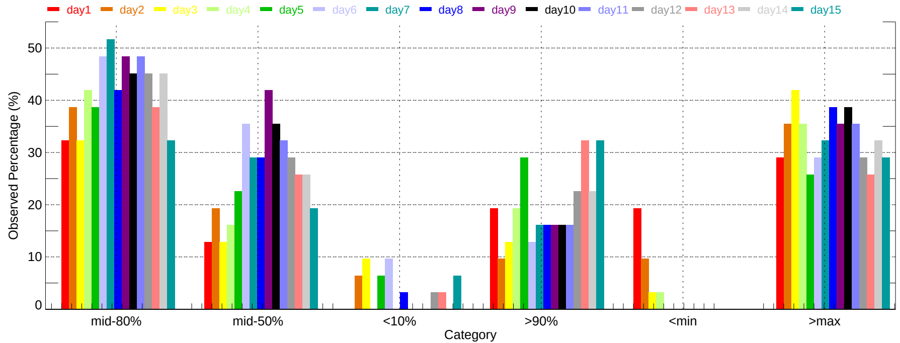
Observed Percentage of Ensembles - DBQ: Max Temperature (2011-12-01~2011-12-31)
