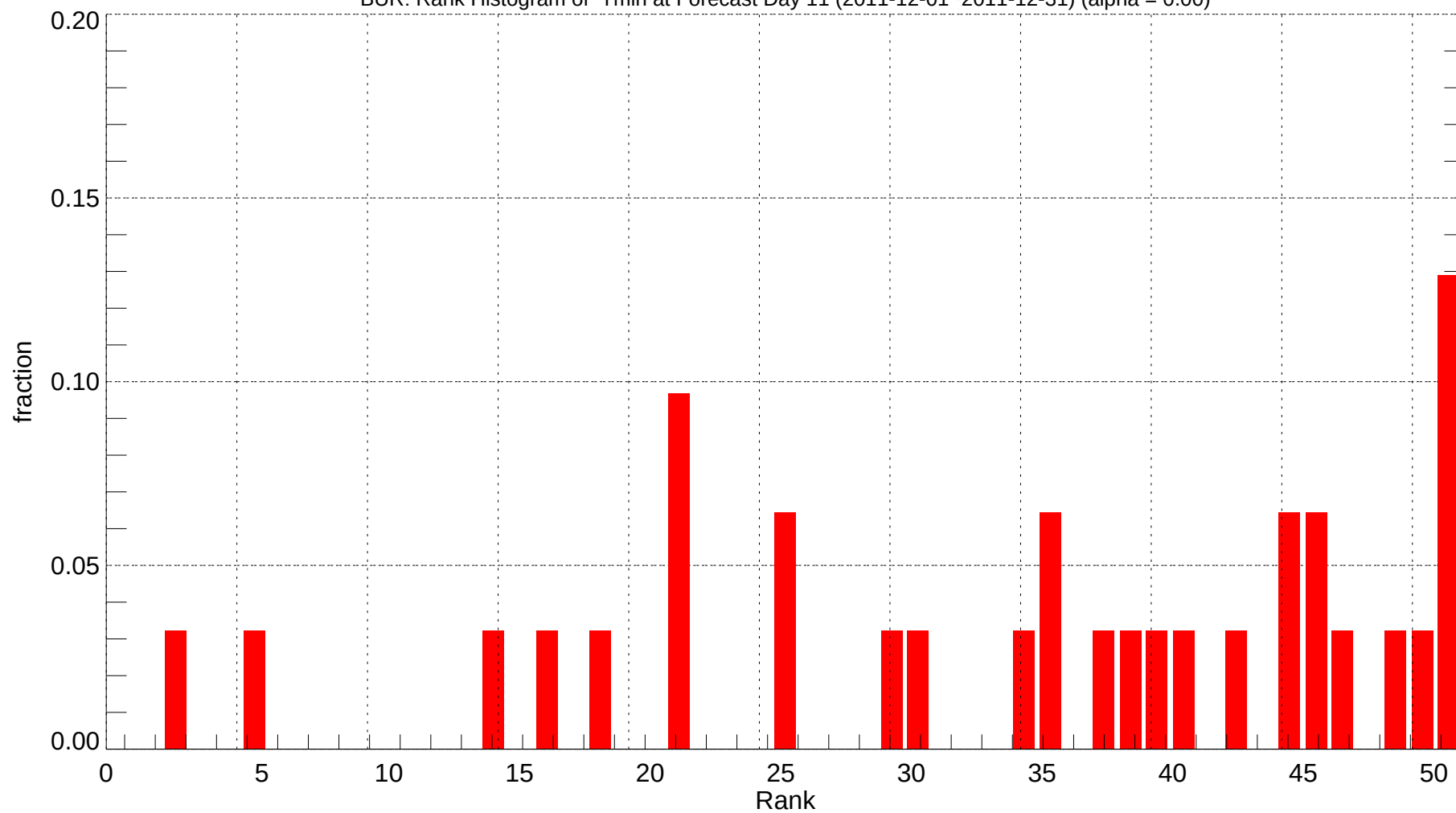
BUR: Rank Histogram of Tmin at Forecast Day 11 (2011-12-01~2011-12-31) (alpha = 0.00)
