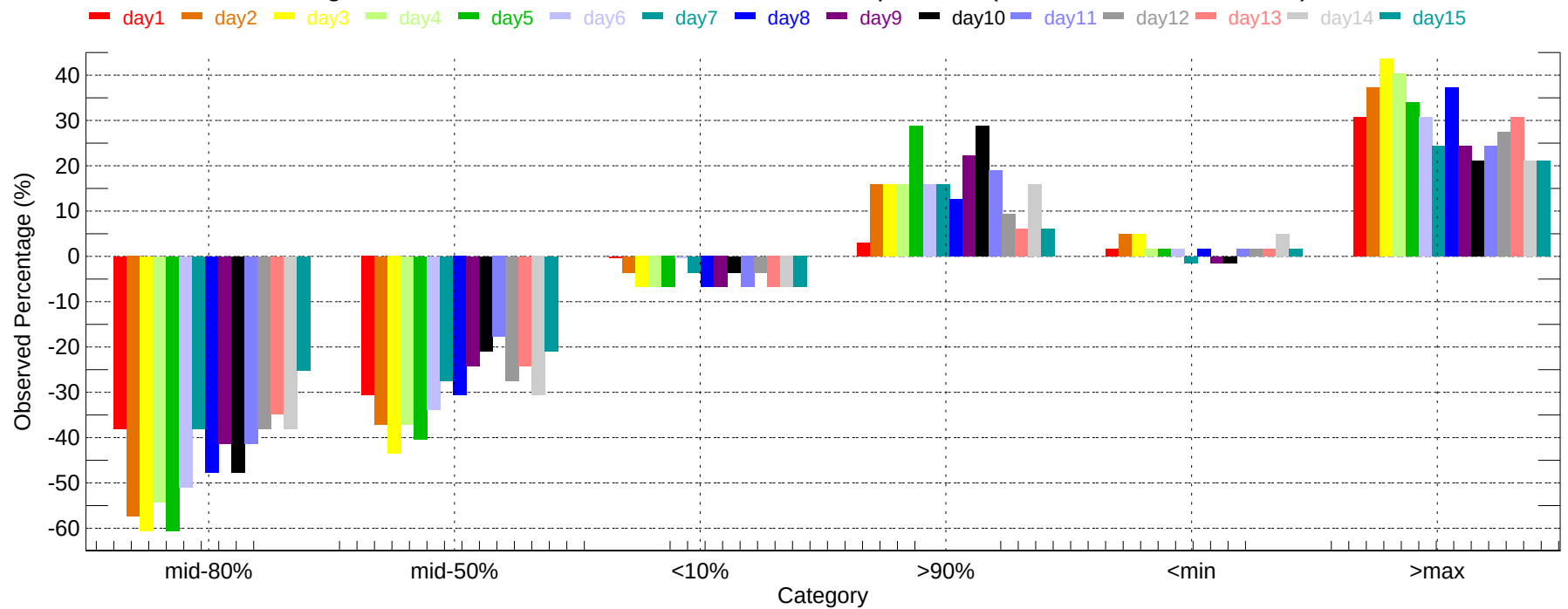
Observed Percentage Deviation of Ensembles - COU: Max Temperature (2011-12-01~2011-12-31)
