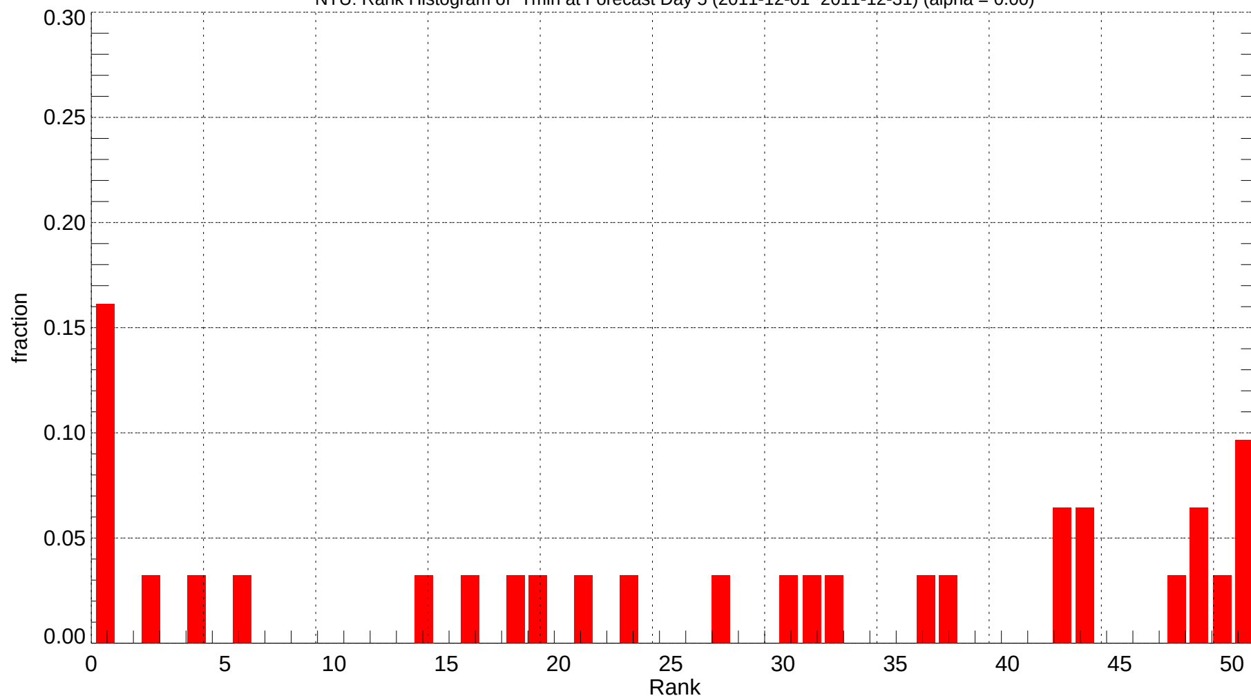
NTU: Rank Histogram of Tmin at Forecast Day 5 (2011-12-01~2011-12-31) (alpha = 0.00)
