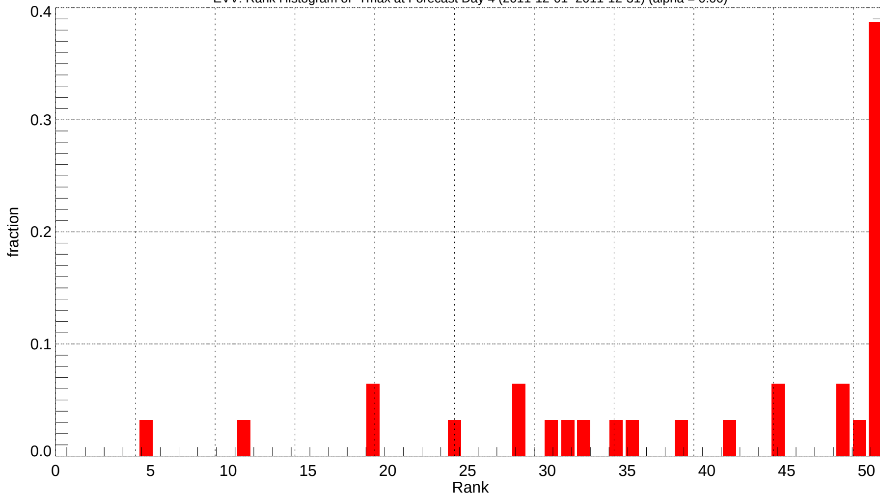
EVV: Rank Histogram of Tmax at Forecast Day 4 (2011-12-01~2011-12-31) (alpha = 0.00)
