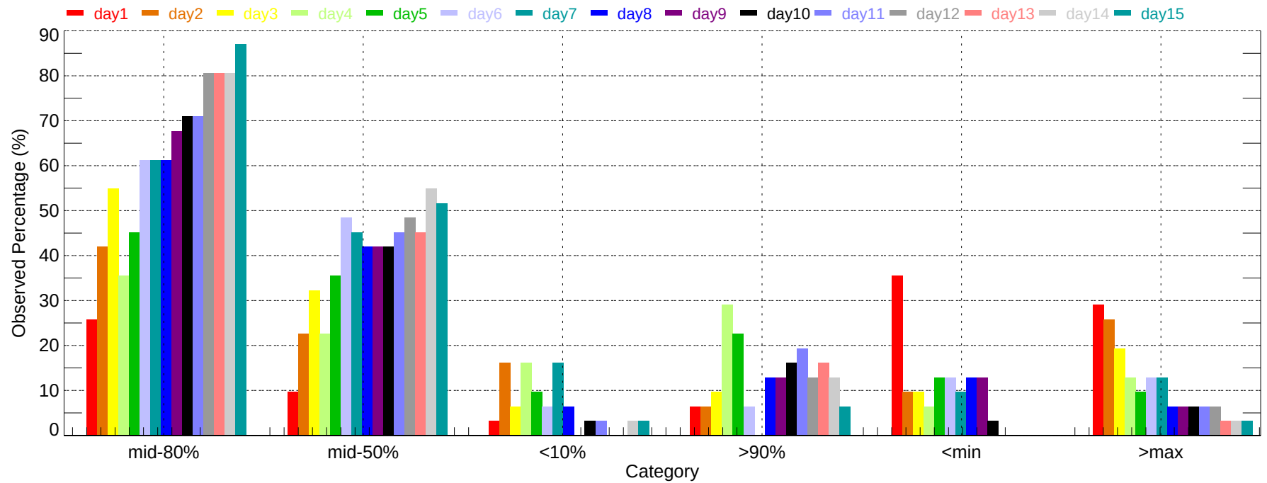
Observed Percentage of Ensembles - PHL: Min Temperature (2011-12-01~2011-12-31)
