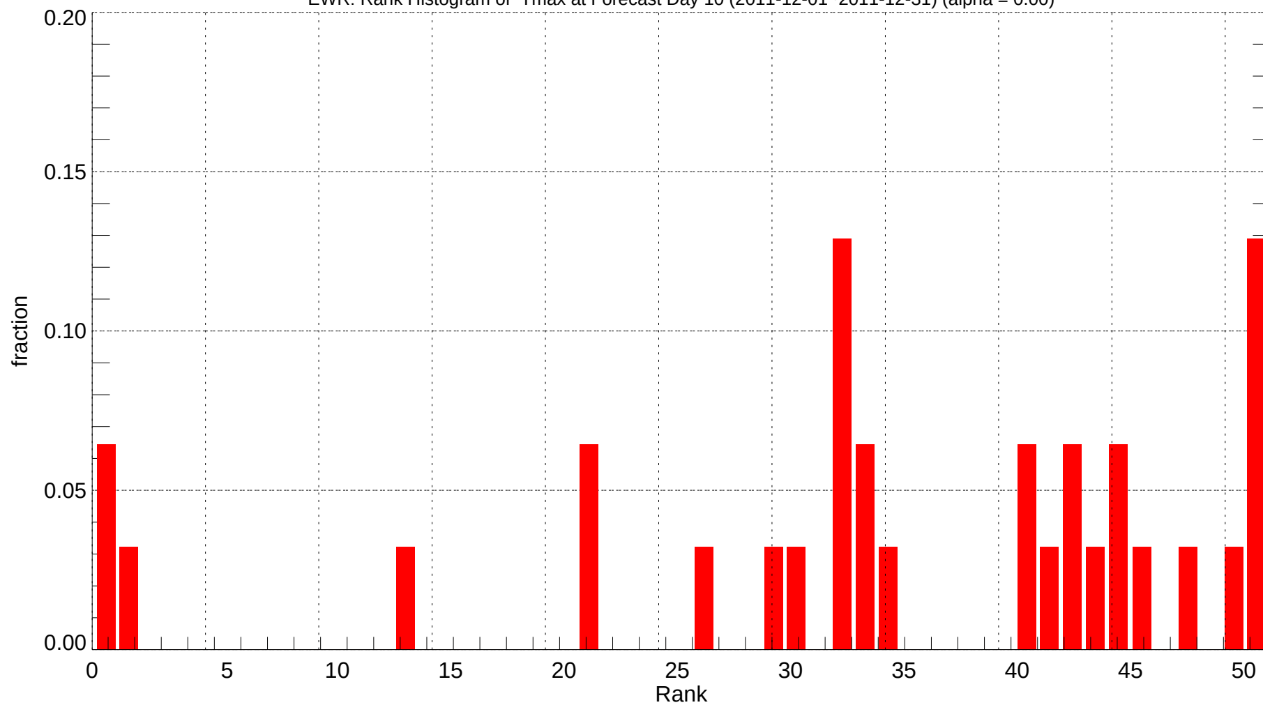
EWR: Rank Histogram of Tmax at Forecast Day 10 (2011-12-01~2011-12-31) (alpha = 0.00)
