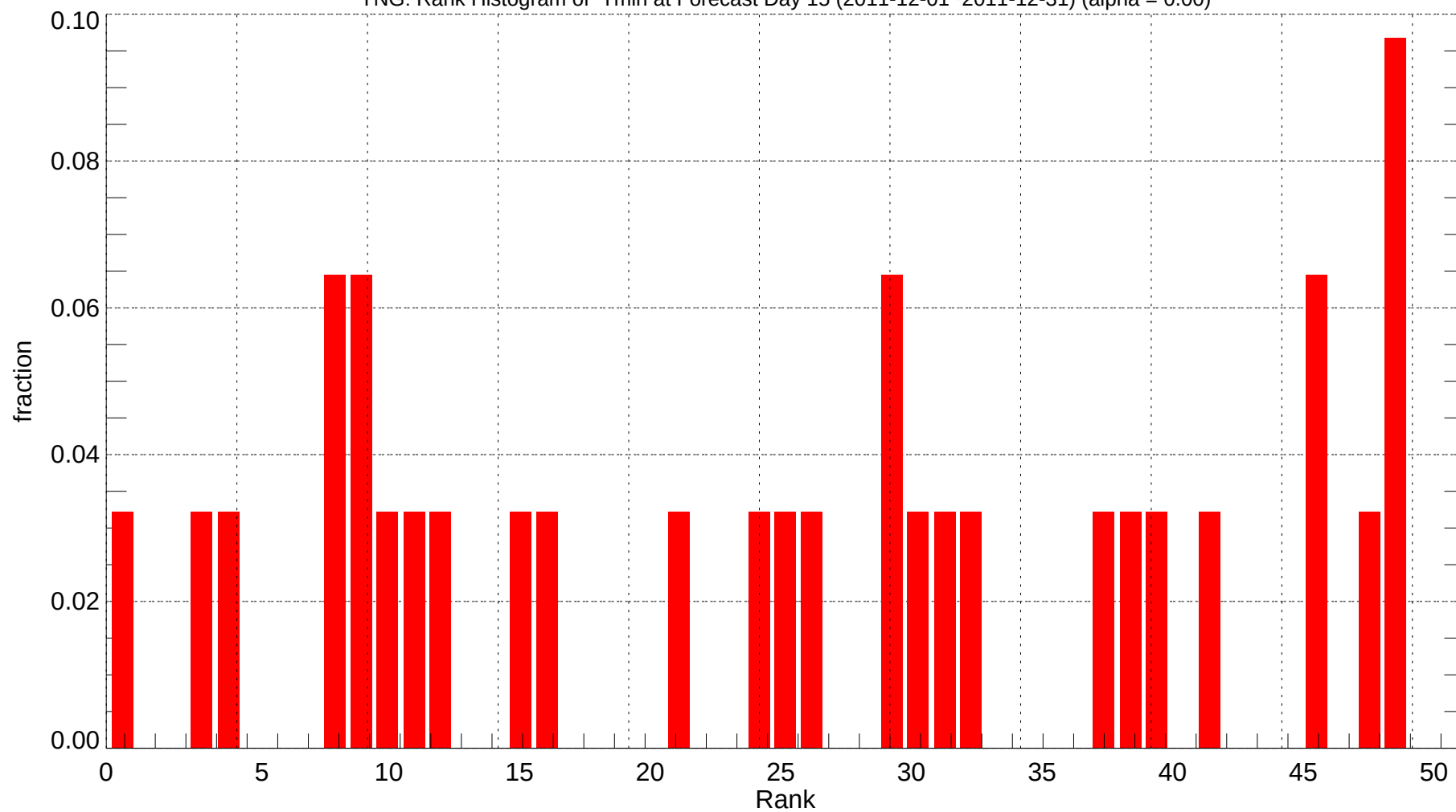
YNG: Rank Histogram of Tmin at Forecast Day 15 (2011-12-01~2011-12-31) (alpha = 0.00)
