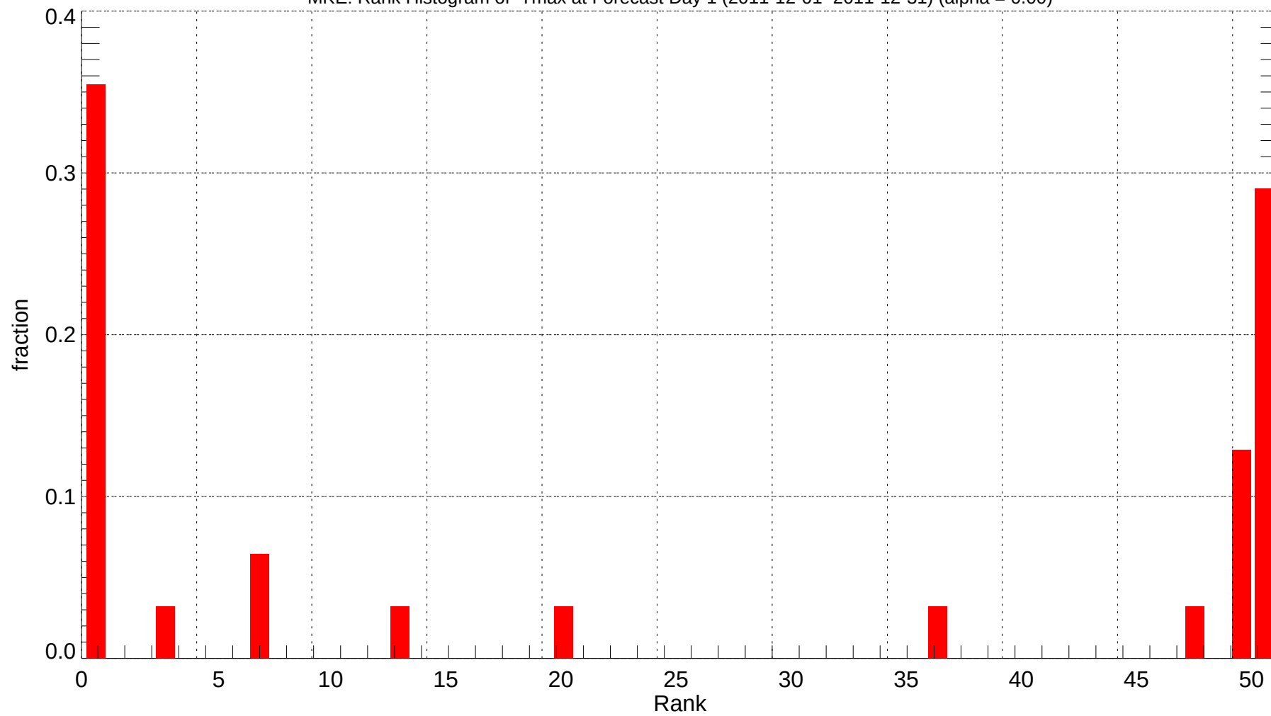
MKE: Rank Histogram of Tmax at Forecast Day 1 (2011-12-01~2011-12-31) (alpha = 0.00)
