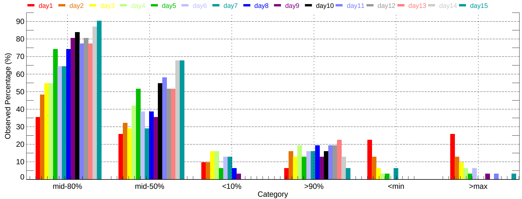
Observed Percentage of Ensembles - JAX: Min Temperature (2011-12-01~2011-12-31)
