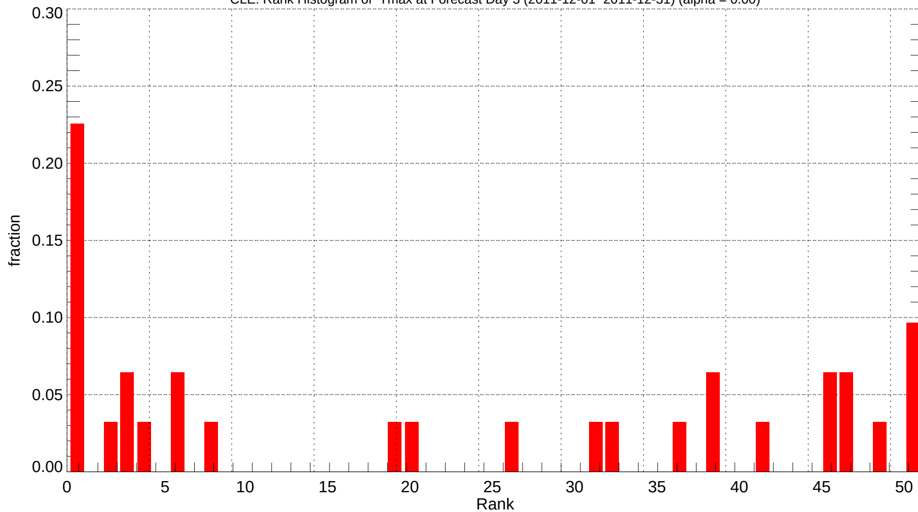
CLE: Rank Histogram of Tmax at Forecast Day 3 (2011-12-01~2011-12-31) (alpha = 0.00)
