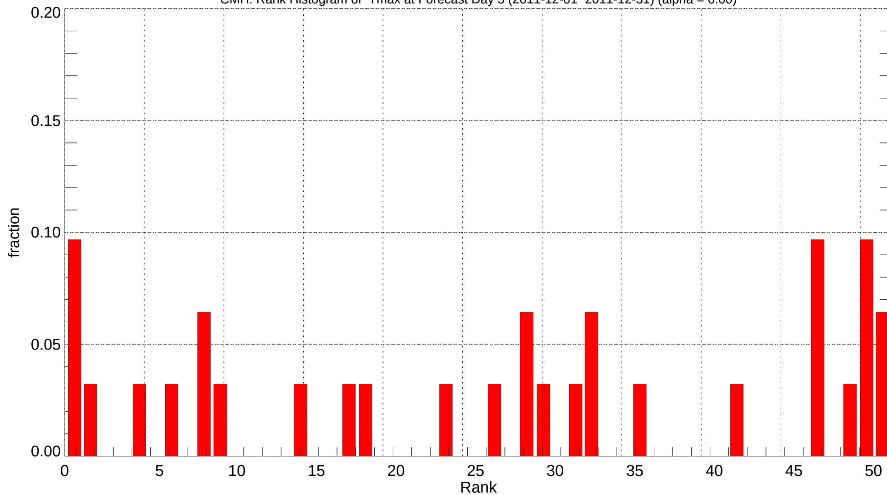
CMH: Rank Histogram of Tmax at Forecast Day 5 (2011-12-01~2011-12-31) (alpha = 0.00)
