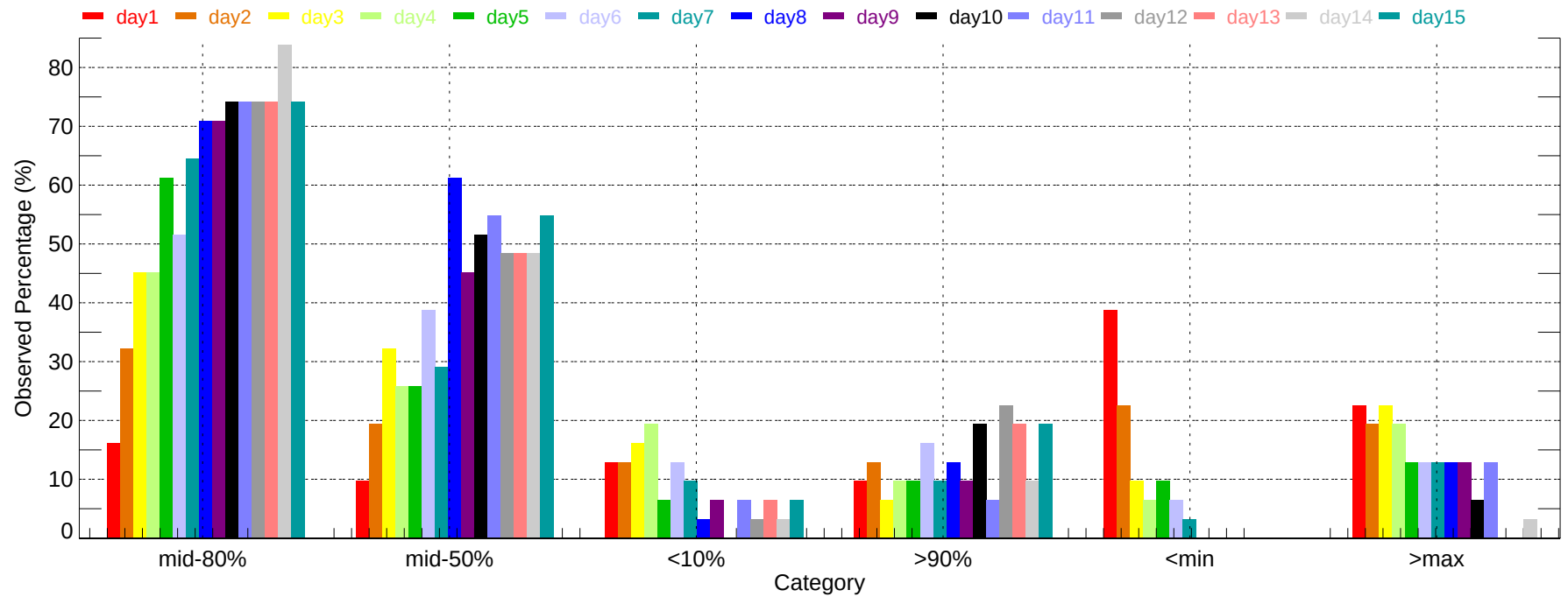
Observed Percentage of Ensembles - BUF: Max Temperature (2011-12-01~2011-12-31)
