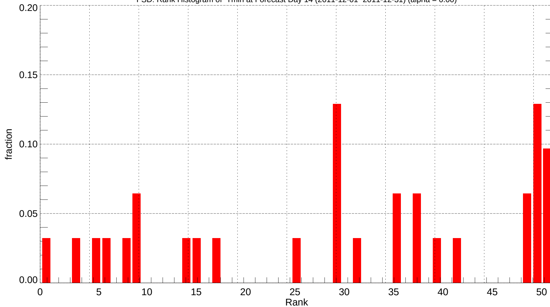
FSD: Rank Histogram of Tmin at Forecast Day 14 (2011-12-01~2011-12-31) (alpha = 0.00)
