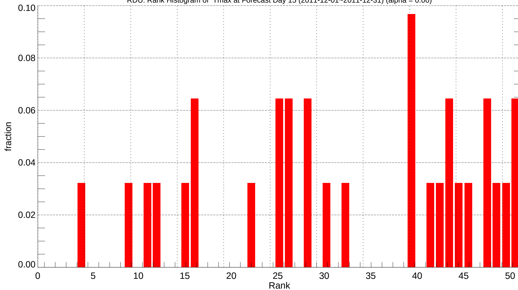
RDU: Rank Histogram of Tmax at Forecast Day 15 (2011-12-01~2011-12-31) (alpha = 0.00)
