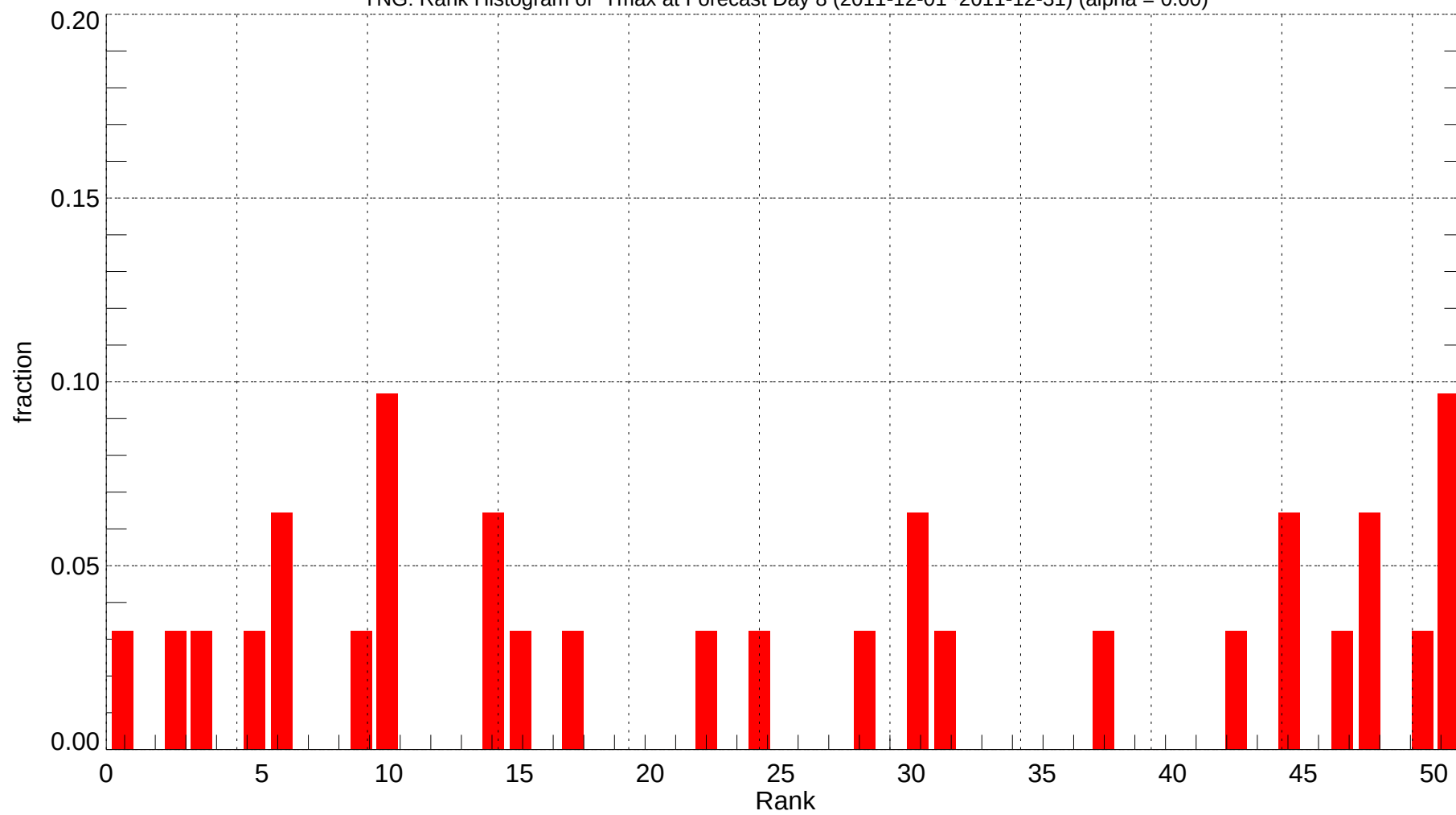
YNG: Rank Histogram of Tmax at Forecast Day 8 (2011-12-01~2011-12-31) (alpha = 0.00)
