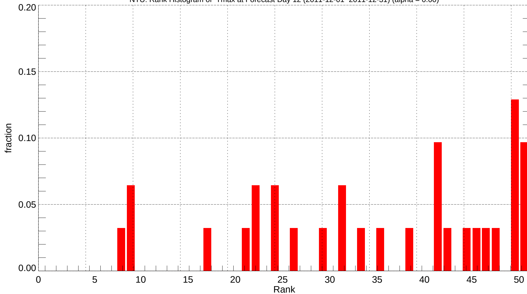
NTU: Rank Histogram of Tmax at Forecast Day 12 (2011-12-01~2011-12-31) (alpha = 0.00)
