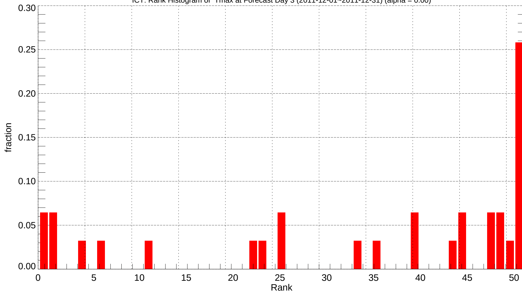
ICT: Rank Histogram of Tmax at Forecast Day 3 (2011-12-01~2011-12-31) (alpha = 0.00)
