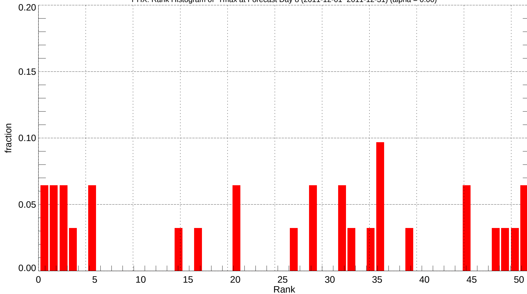
PHX: Rank Histogram of Tmax at Forecast Day 8 (2011-12-01~2011-12-31) (alpha = 0.00)
