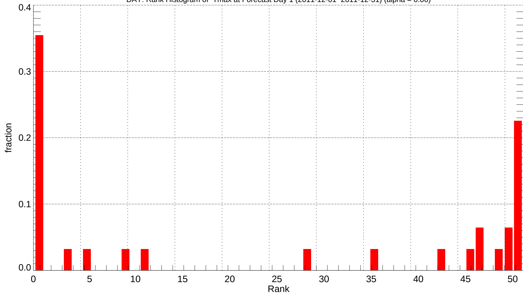
DAY: Rank Histogram of Tmax at Forecast Day 1 (2011-12-01~2011-12-31) (alpha = 0.00)
