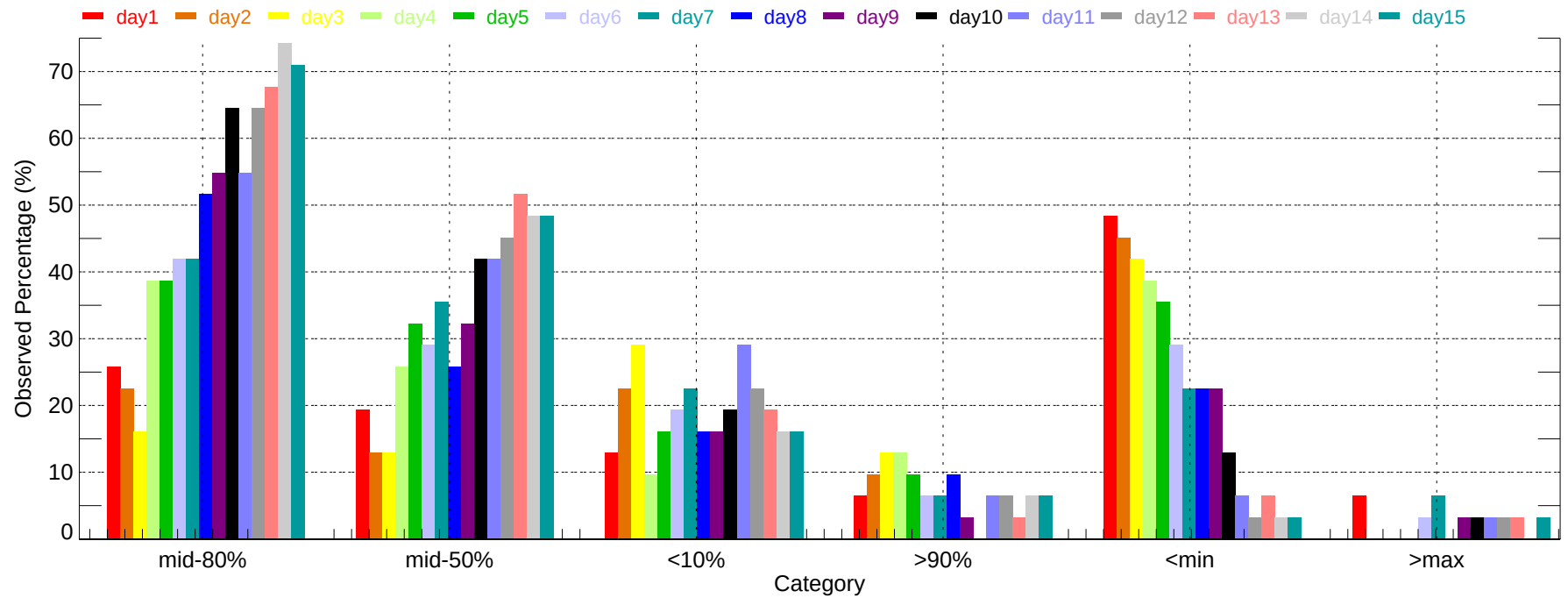
Observed Percentage of Ensembles - PDX: Min Temperature (2011-12-01~2011-12-31)
