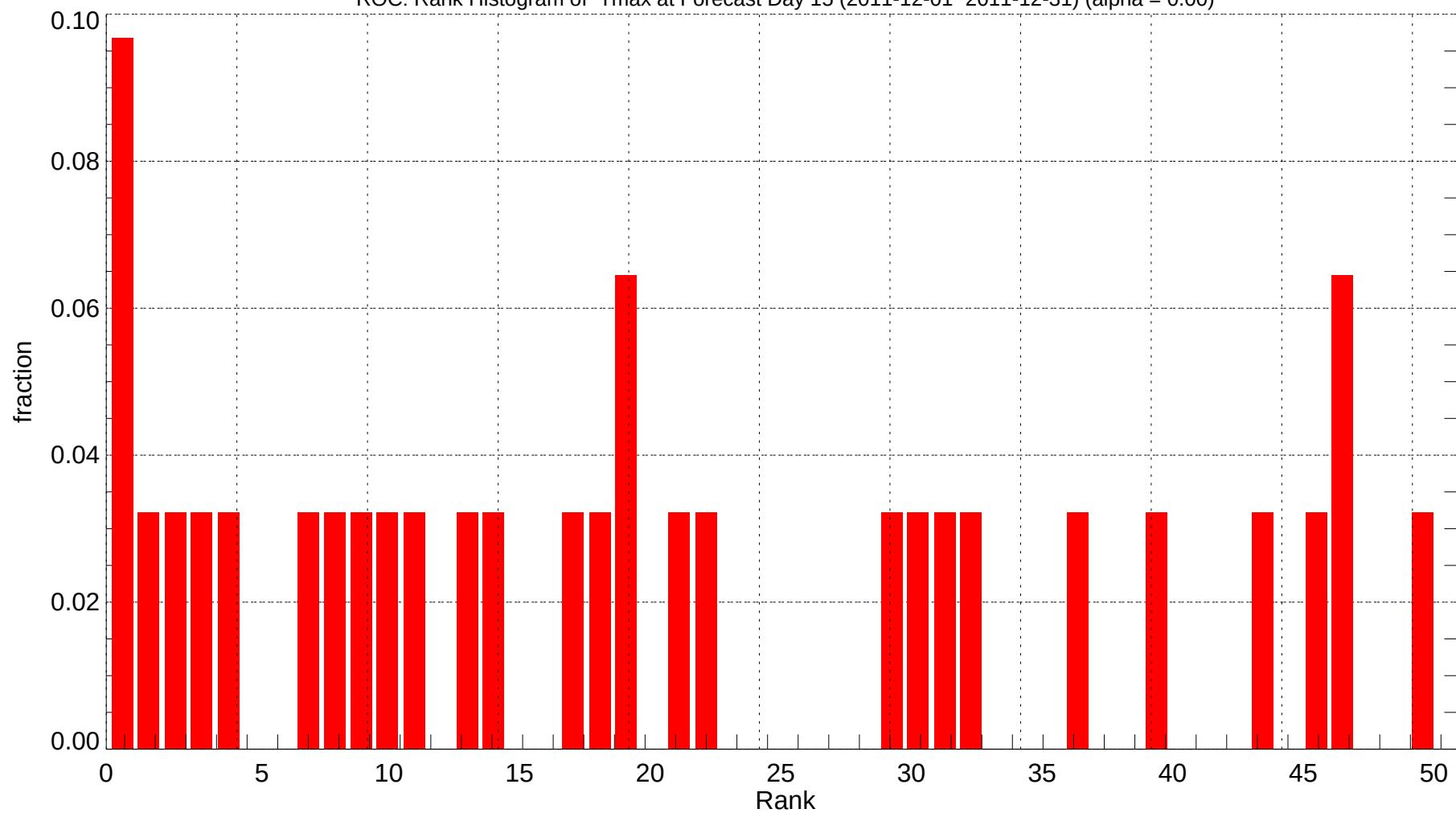
ROC: Rank Histogram of Tmax at Forecast Day 15 (2011-12-01~2011-12-31) (alpha = 0.00)
