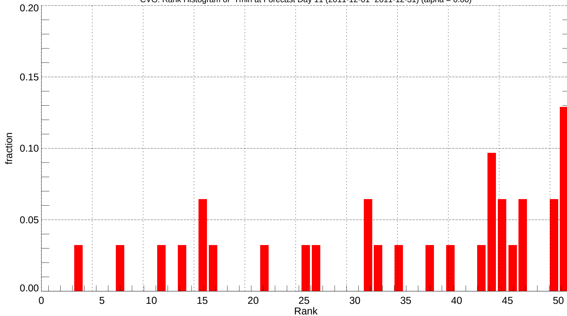
CVG: Rank Histogram of Tmin at Forecast Day 11 (2011-12-01~2011-12-31) (alpha = 0.00)
