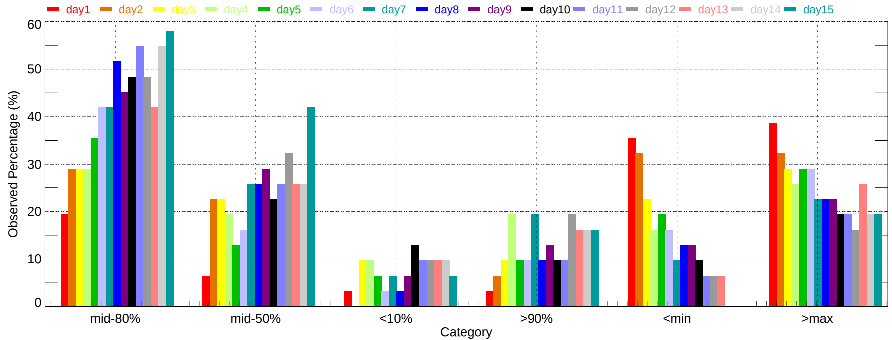
Observed Percentage of Ensembles - LAX: Max Temperature (2011-12-01~2011-12-31)
