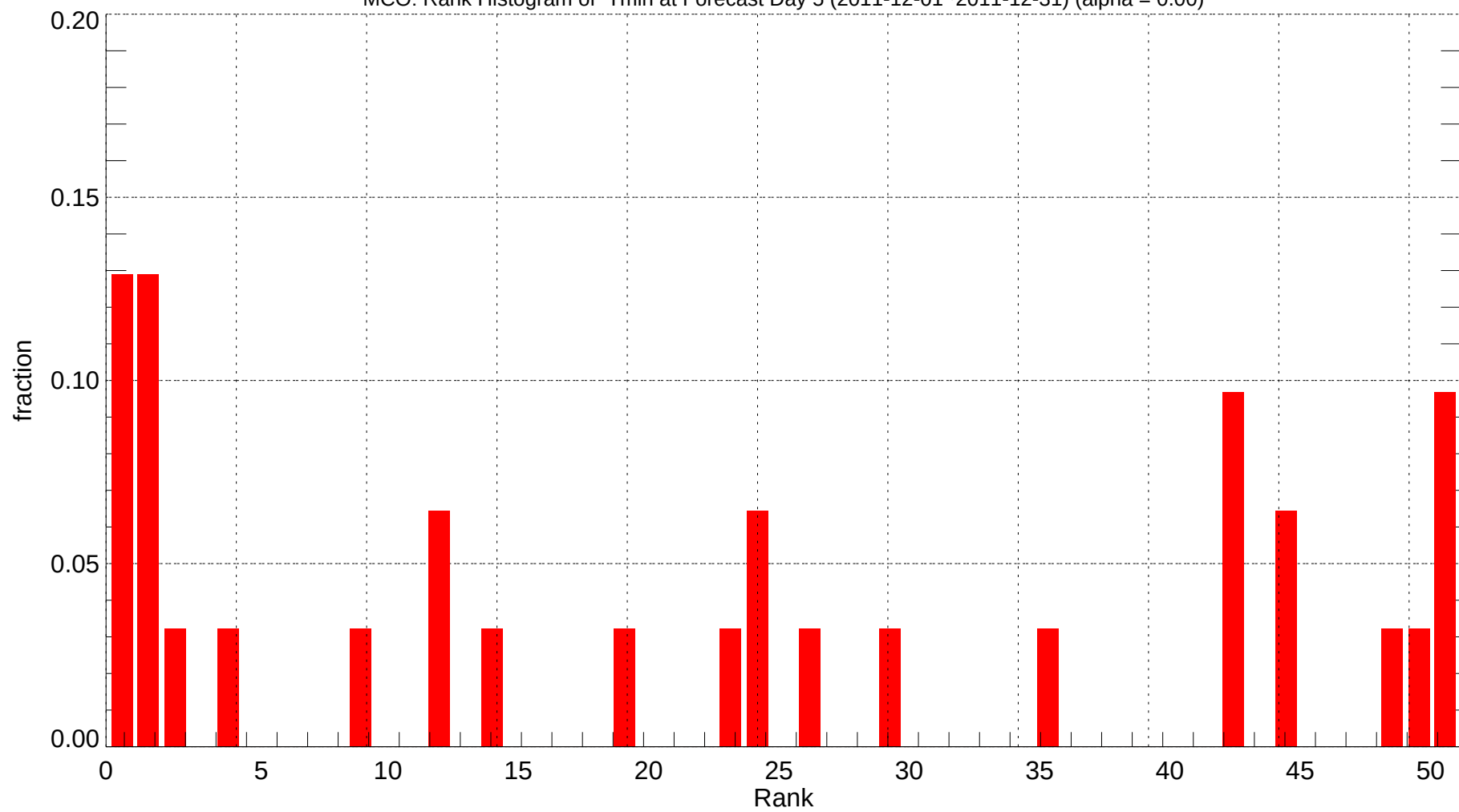
MCO: Rank Histogram of Tmin at Forecast Day 5 (2011-12-01~2011-12-31) (alpha = 0.00)
