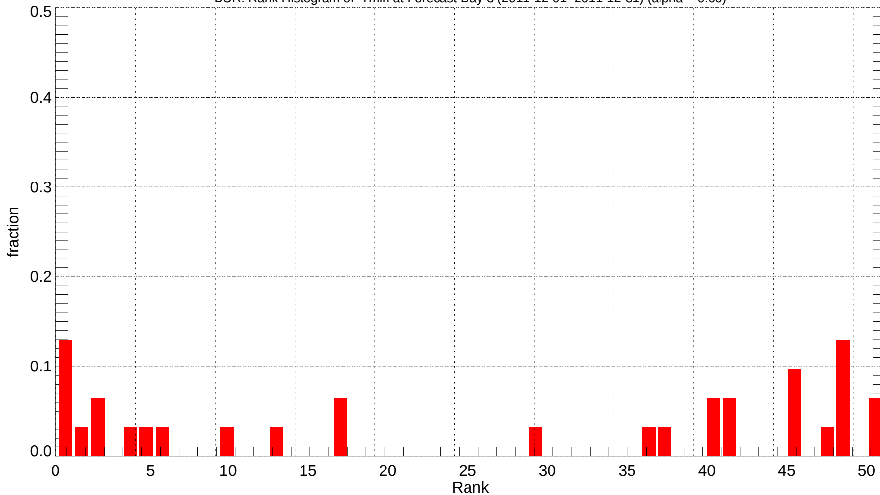
BUR: Rank Histogram of Tmin at Forecast Day 3 (2011-12-01~2011-12-31) (alpha = 0.00)
