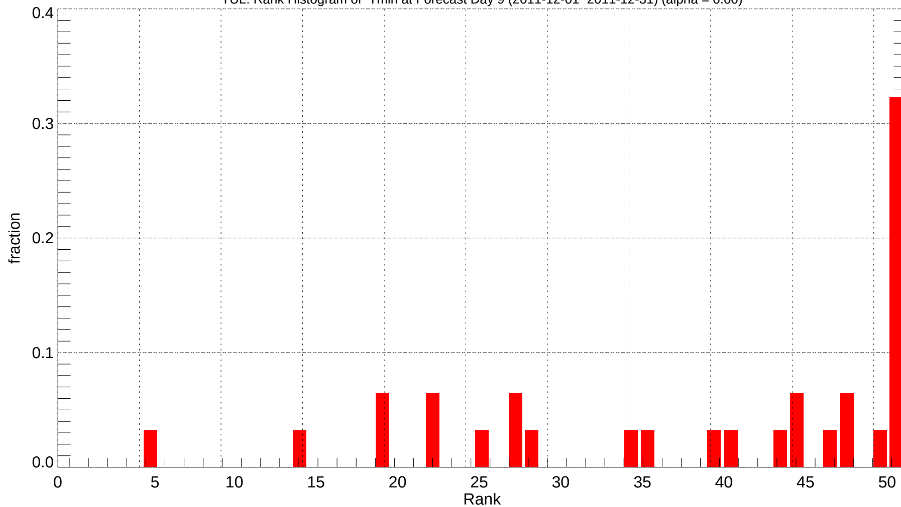
TUL: Rank Histogram of Tmin at Forecast Day 9 (2011-12-01~2011-12-31) (alpha = 0.00)
