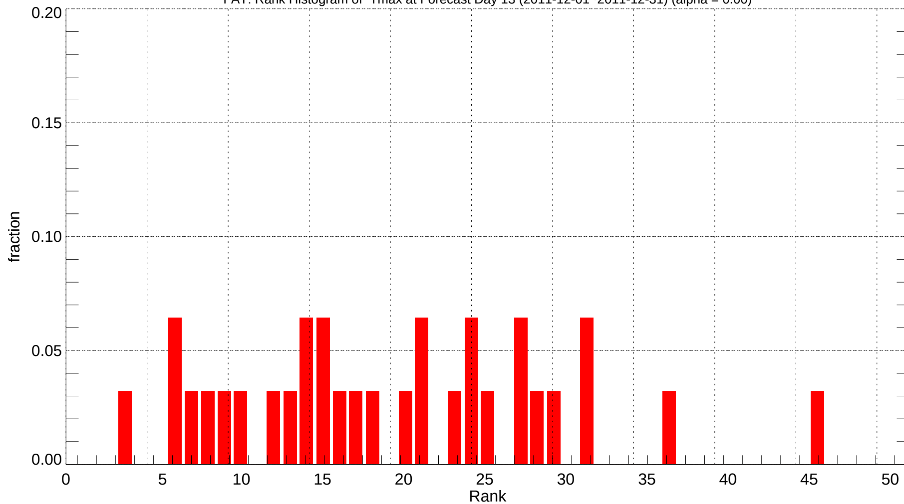
FAT: Rank Histogram of Tmax at Forecast Day 13 (2011-12-01~2011-12-31) (alpha = 0.00)
