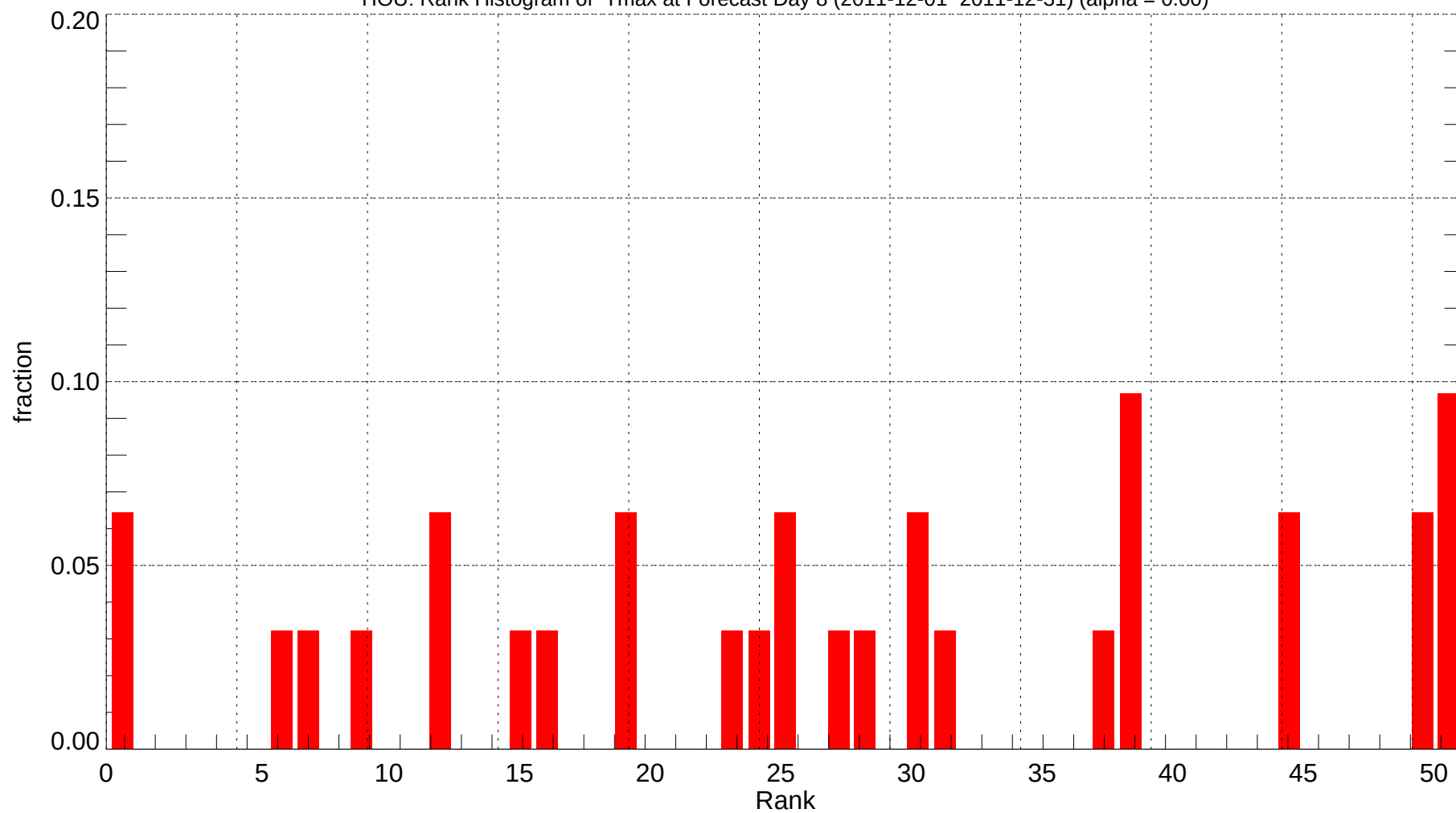
HOU: Rank Histogram of Tmax at Forecast Day 8 (2011-12-01~2011-12-31) (alpha = 0.00)
