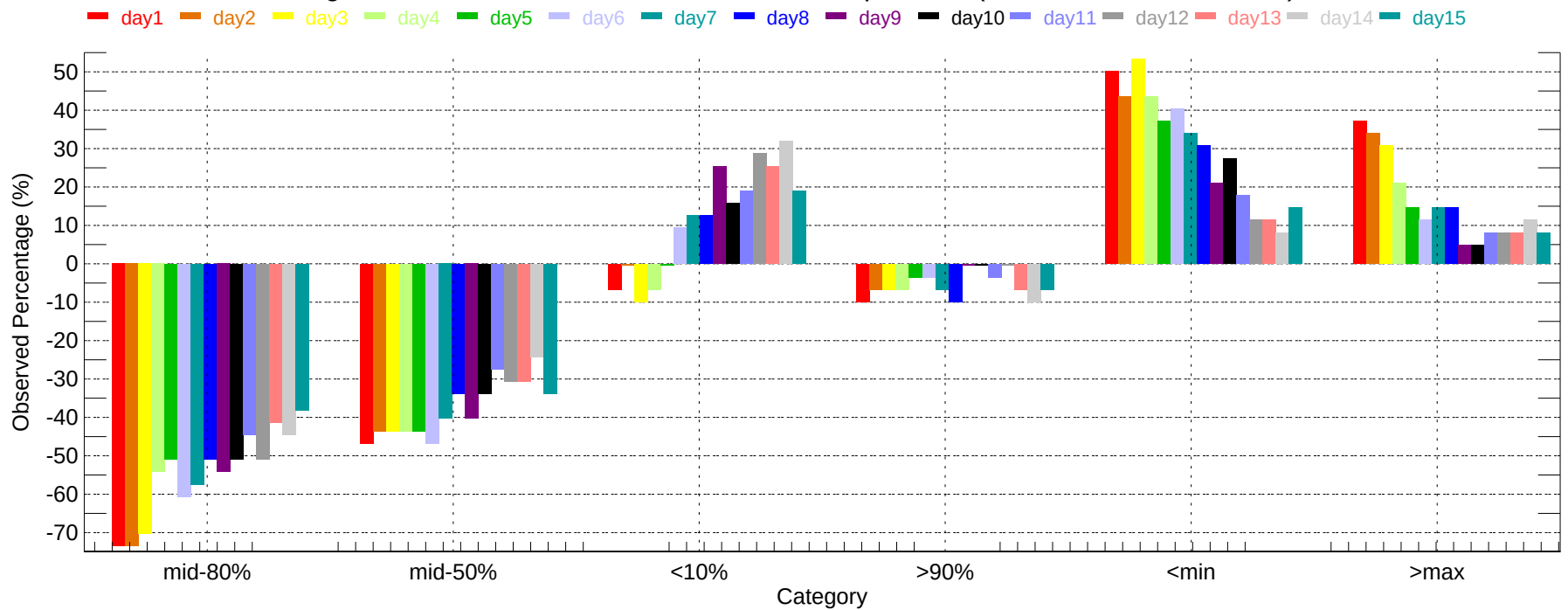
Observed Percentage Deviation of Ensembles - SFO: Min Temperature (2011-12-01~2011-12-31)
