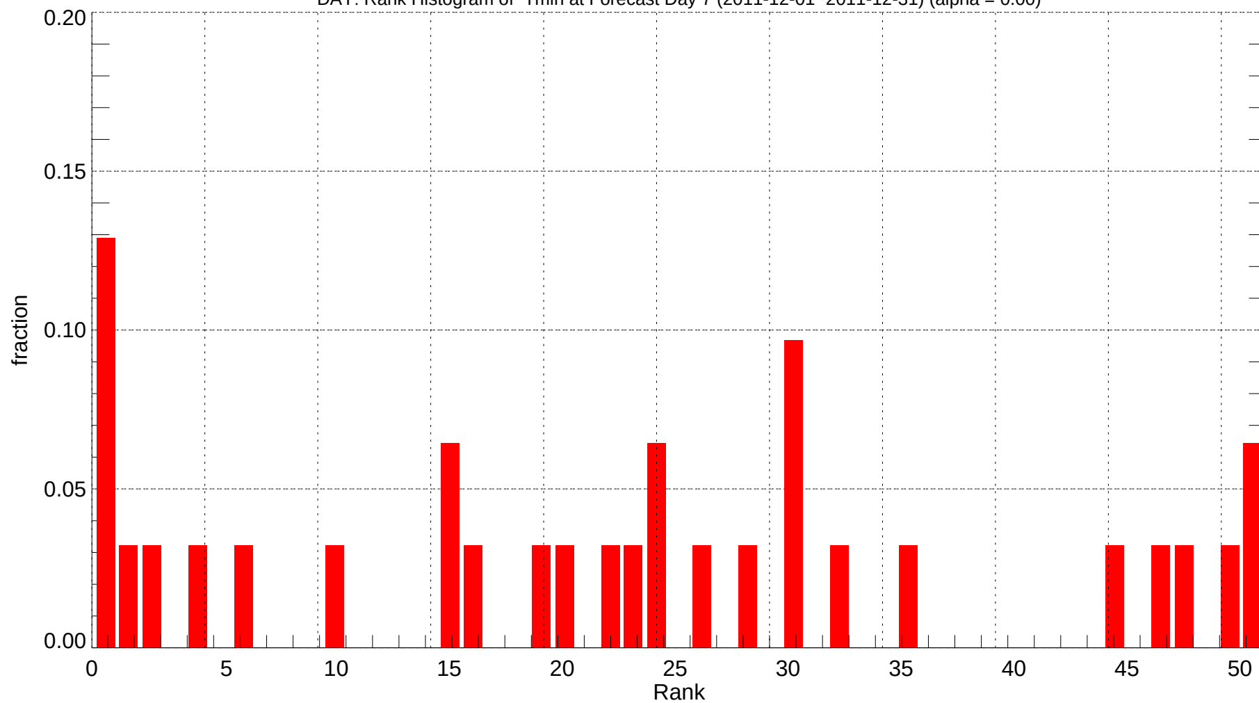
DAY: Rank Histogram of Tmin at Forecast Day 7 (2011-12-01~2011-12-31) (alpha = 0.00)
