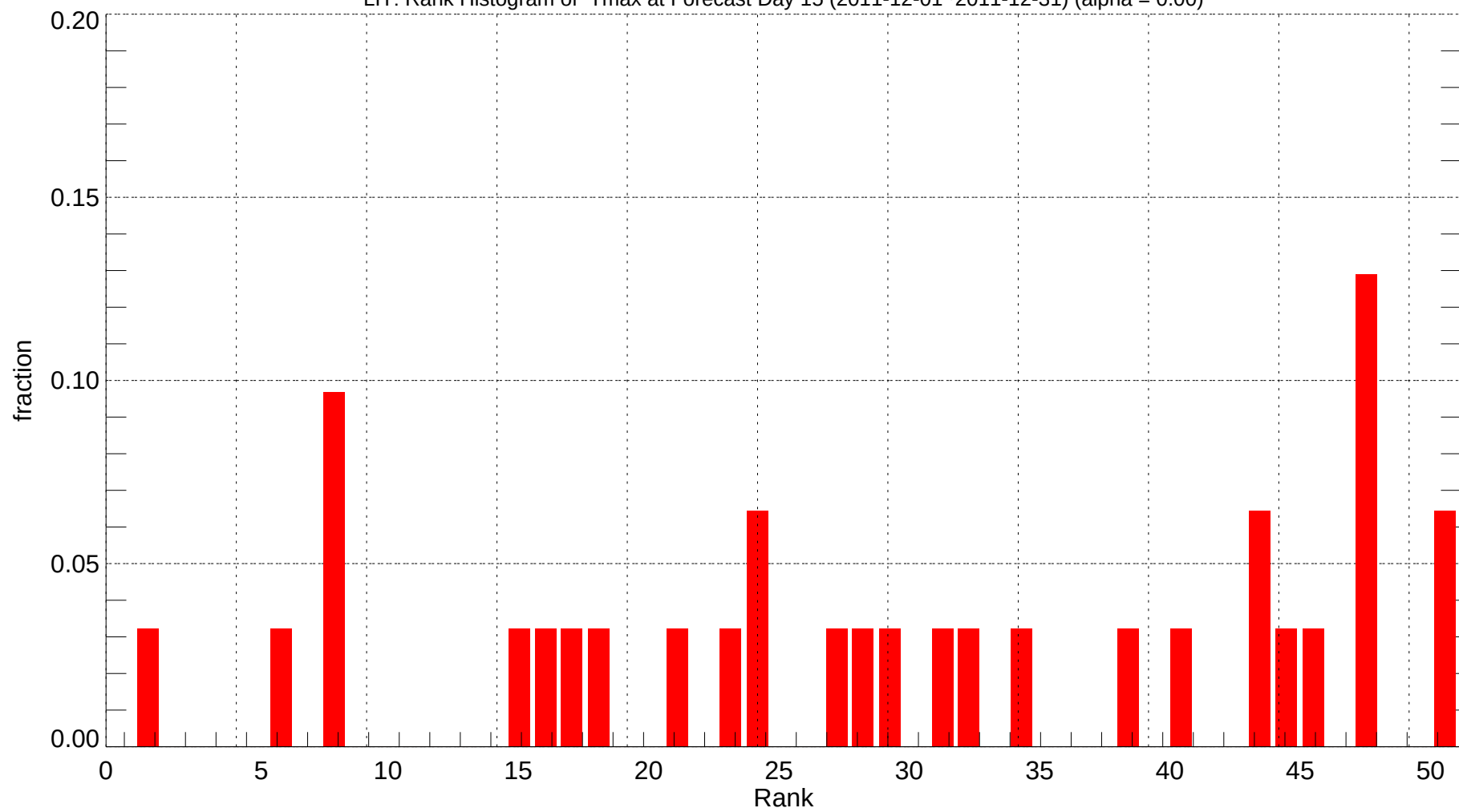
LIT: Rank Histogram of Tmax at Forecast Day 15 (2011-12-01~2011-12-31) (alpha = 0.00)
