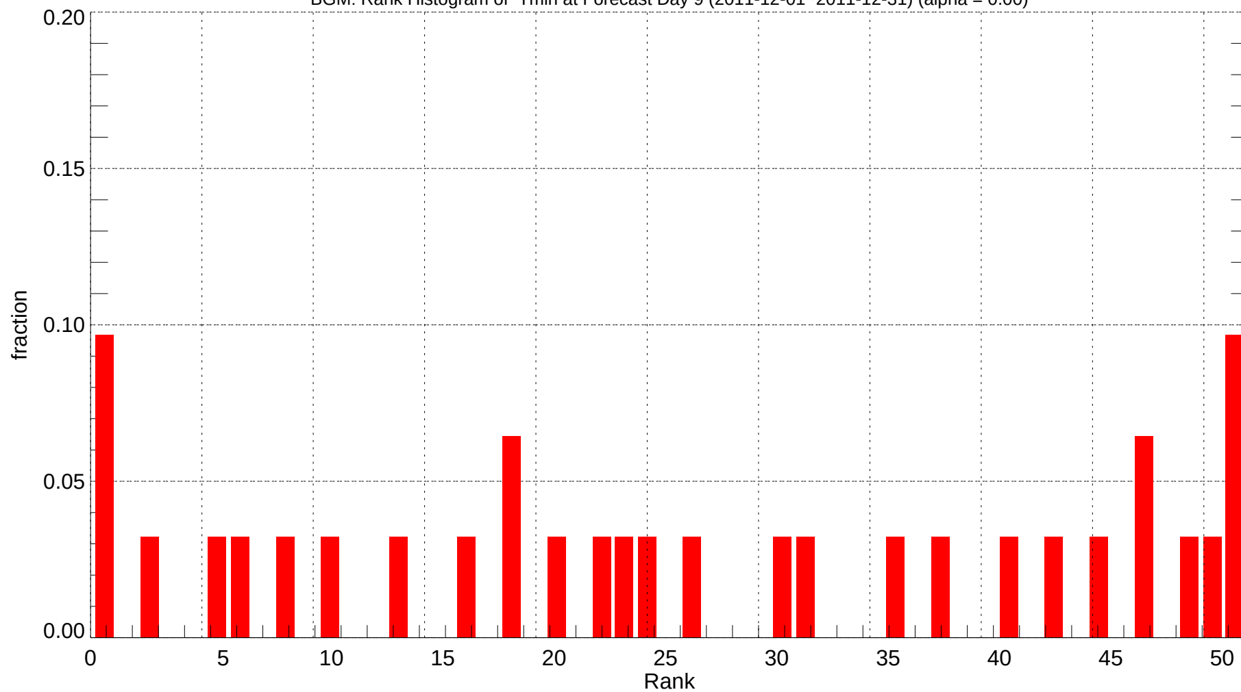
BGM: Rank Histogram of Tmin at Forecast Day 9 (2011-12-01~2011-12-31) (alpha = 0.00)
