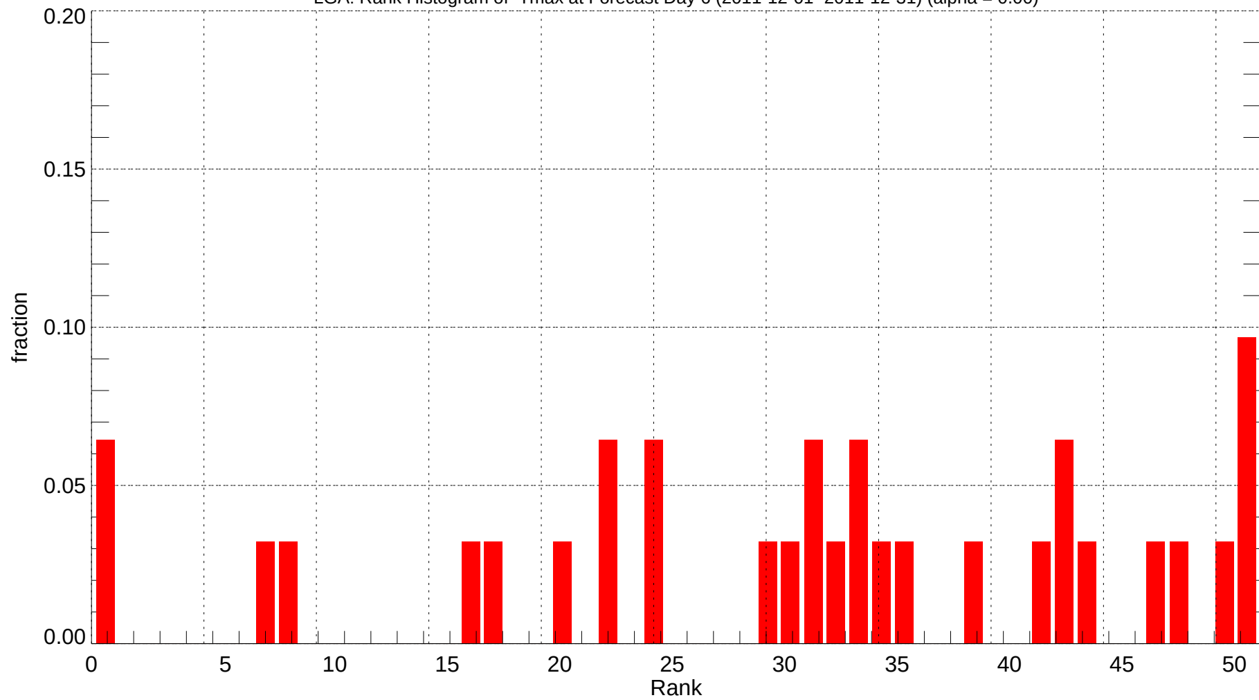
LGA: Rank Histogram of Tmax at Forecast Day 6 (2011-12-01~2011-12-31) (alpha = 0.00)
