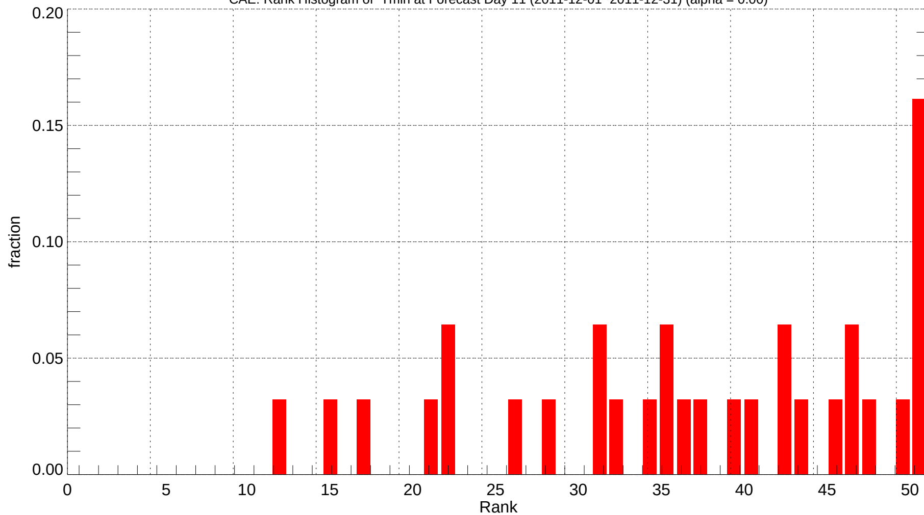
CAE: Rank Histogram of Tmin at Forecast Day 11 (2011-12-01~2011-12-31) (alpha = 0.00)
