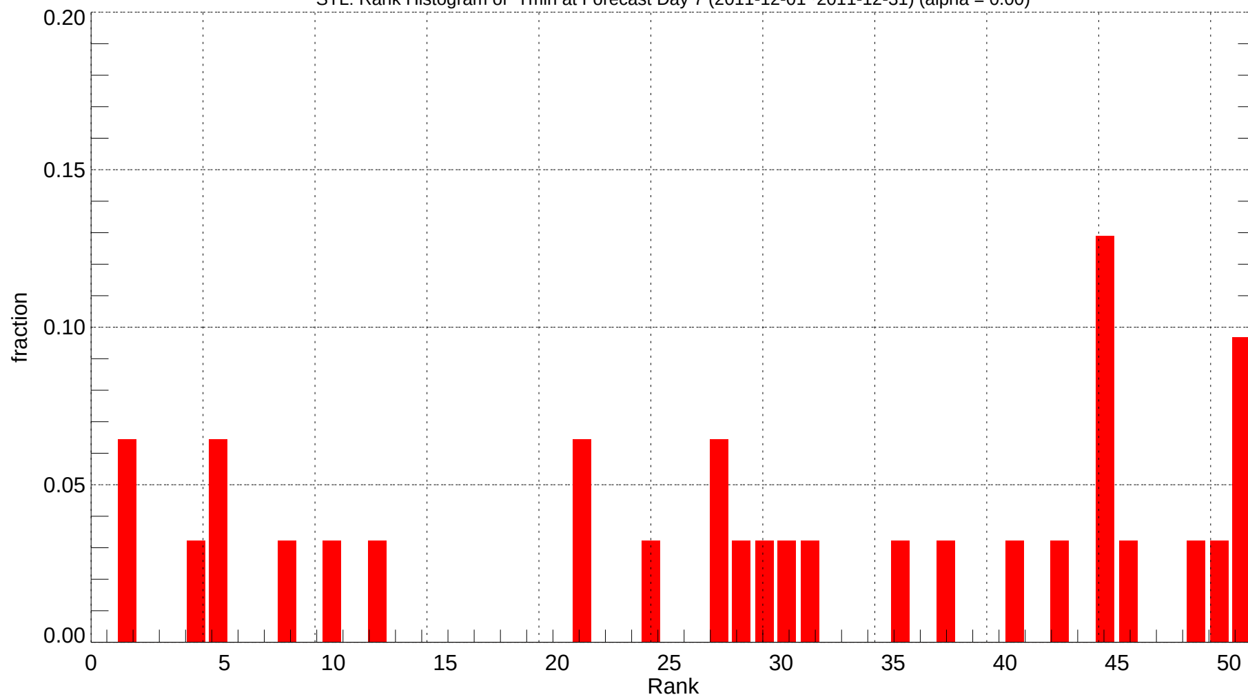
STL: Rank Histogram of Tmin at Forecast Day 7 (2011-12-01~2011-12-31) (alpha = 0.00)
