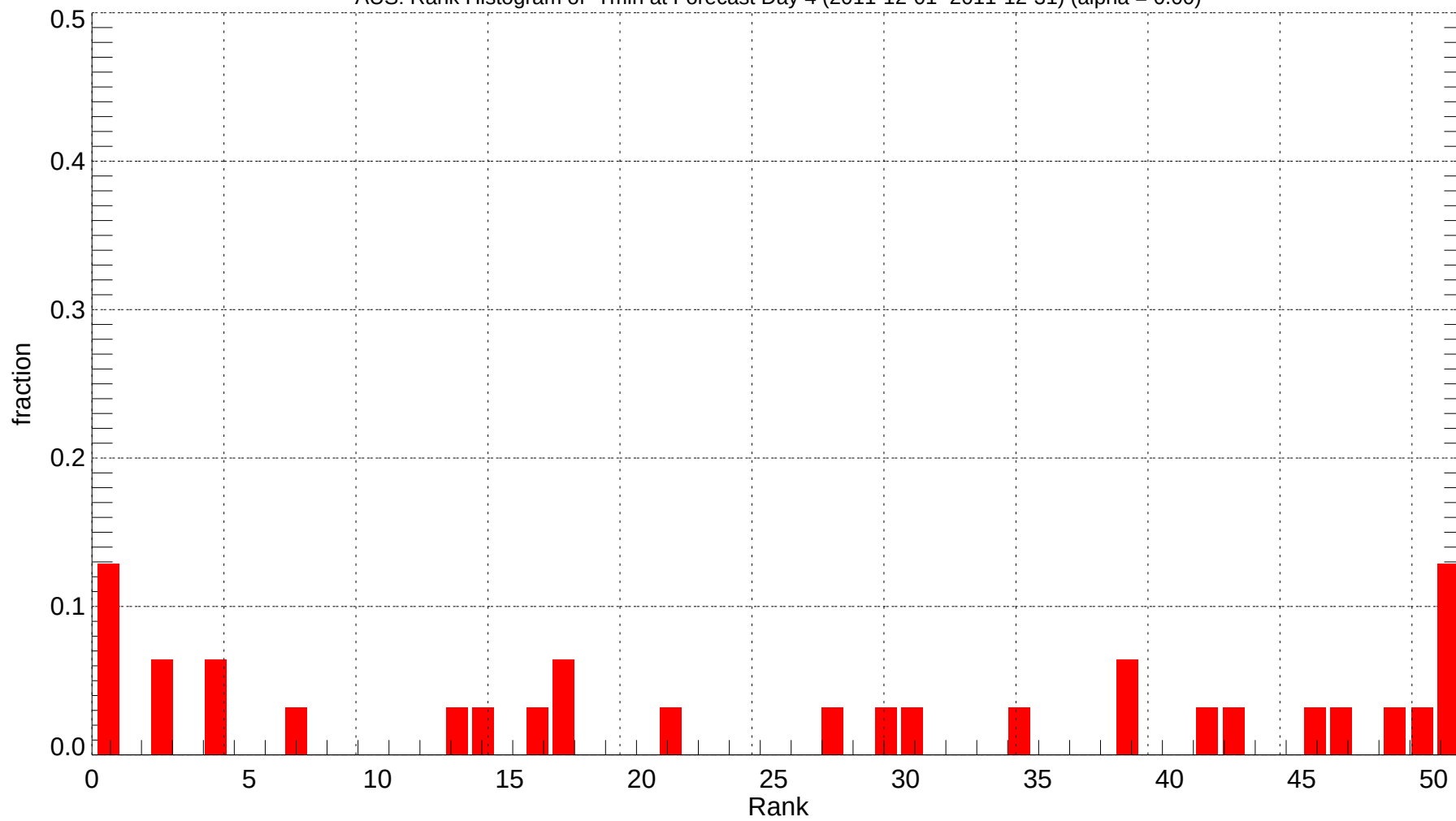
AUS: Rank Histogram of Tmin at Forecast Day 4 (2011-12-01~2011-12-31) (alpha = 0.00)
