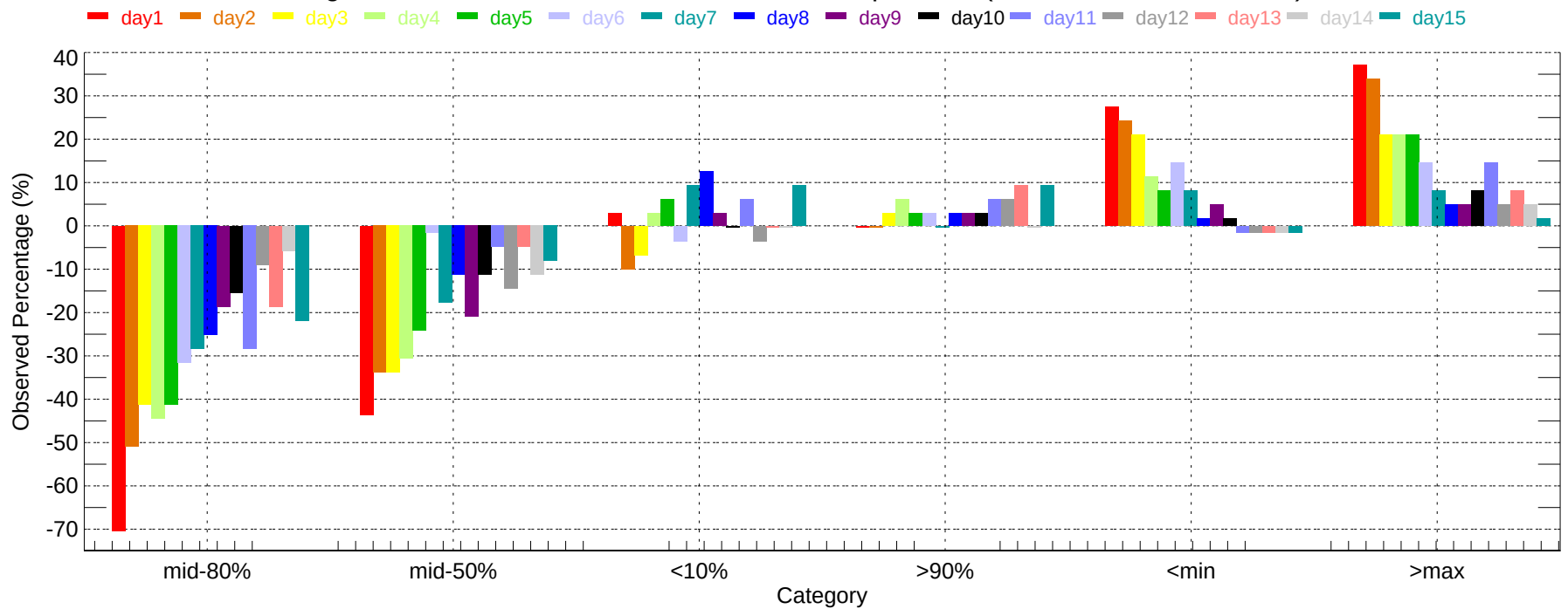
Observed Percentage Deviation of Ensembles - EWR: Min Temperature (2011-12-01~2011-12-31)
