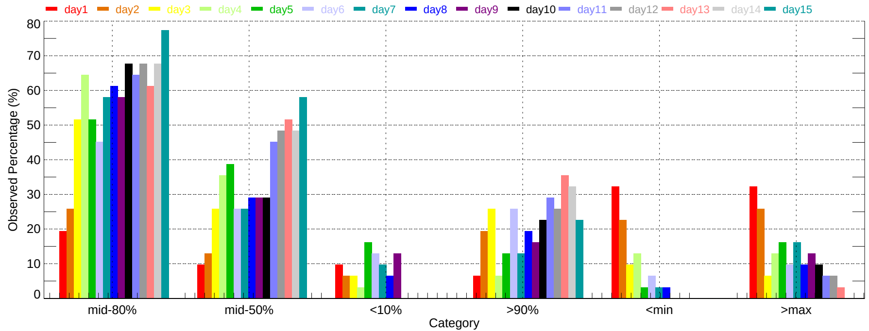
Observed Percentage of Ensembles - LIT: Min Temperature (2011-12-01~2011-12-31)
