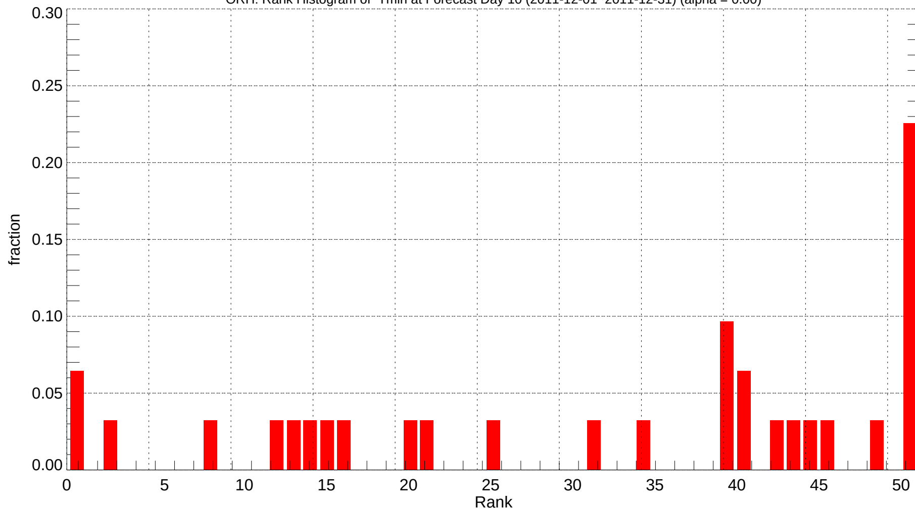
ORH: Rank Histogram of Tmin at Forecast Day 10 (2011-12-01~2011-12-31) (alpha = 0.00)
