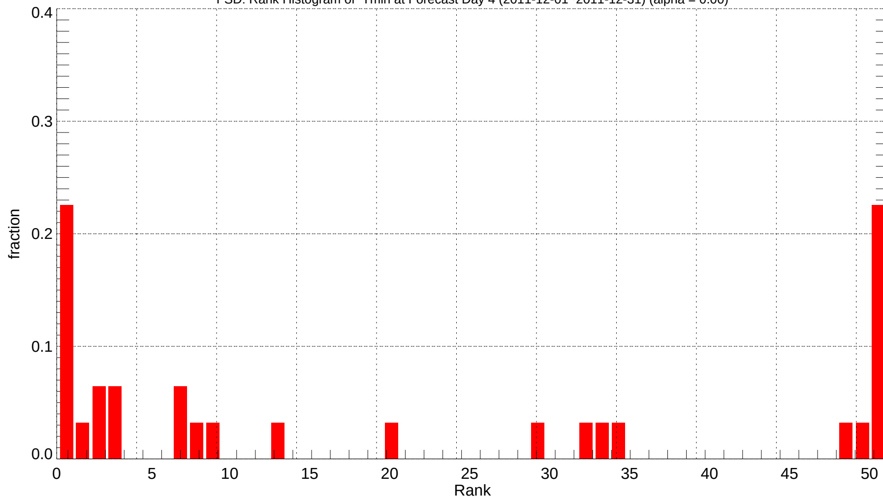
FSD: Rank Histogram of Tmin at Forecast Day 4 (2011-12-01~2011-12-31) (alpha = 0.00)
