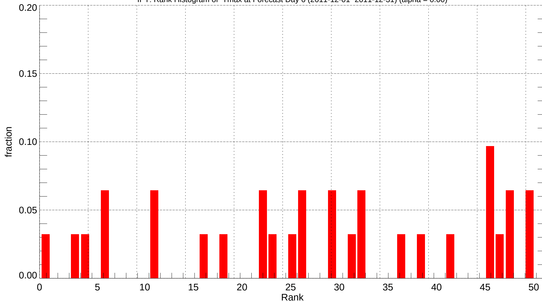
IPT: Rank Histogram of Tmax at Forecast Day 6 (2011-12-01~2011-12-31) (alpha = 0.00)
