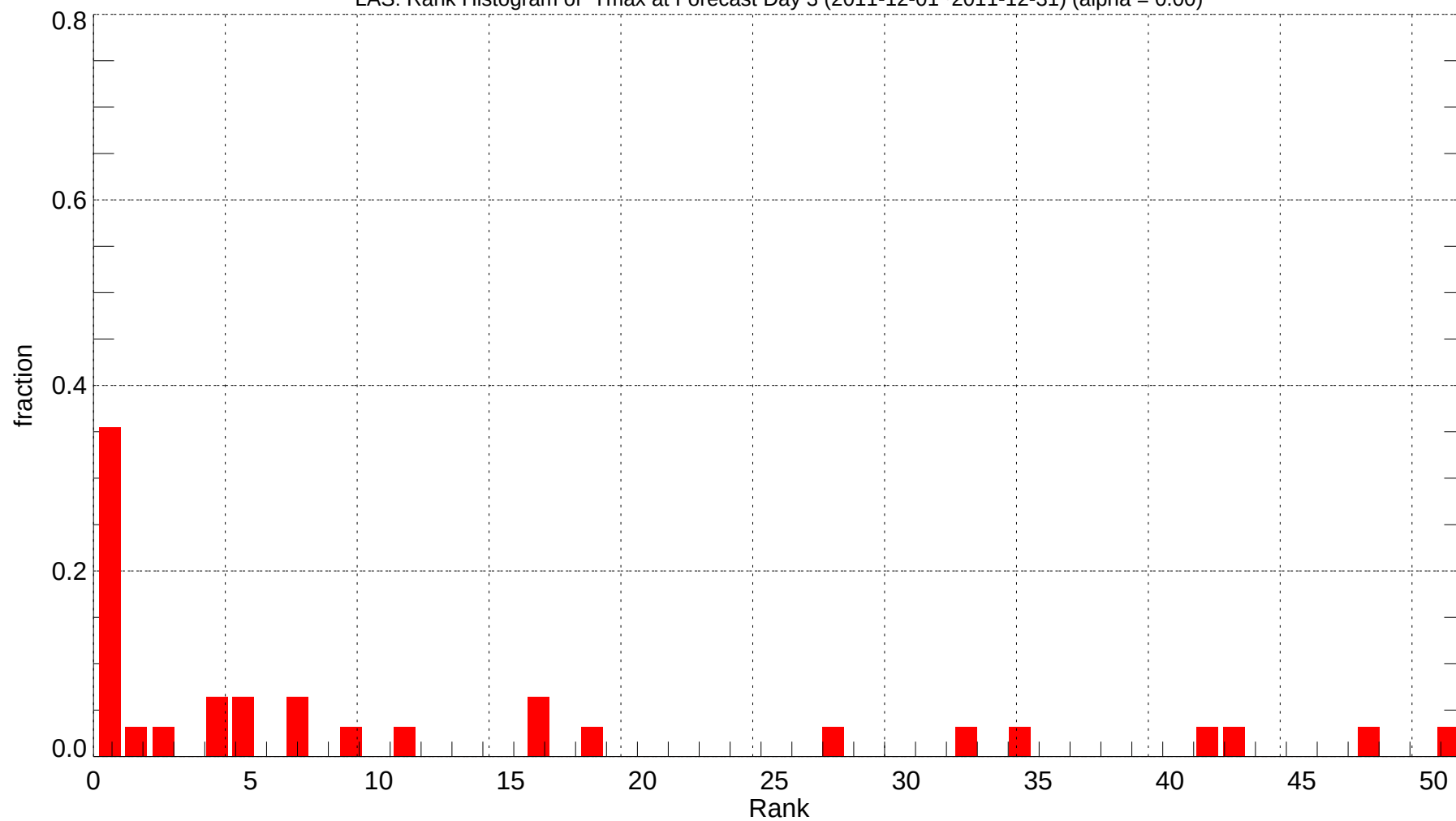
LAS: Rank Histogram of Tmax at Forecast Day 3 (2011-12-01~2011-12-31) (alpha = 0.00)
