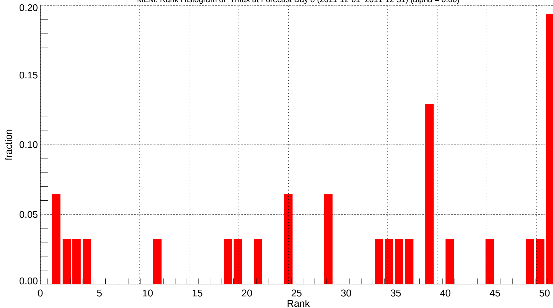
MEM: Rank Histogram of Tmax at Forecast Day 8 (2011-12-01~2011-12-31) (alpha = 0.00)
