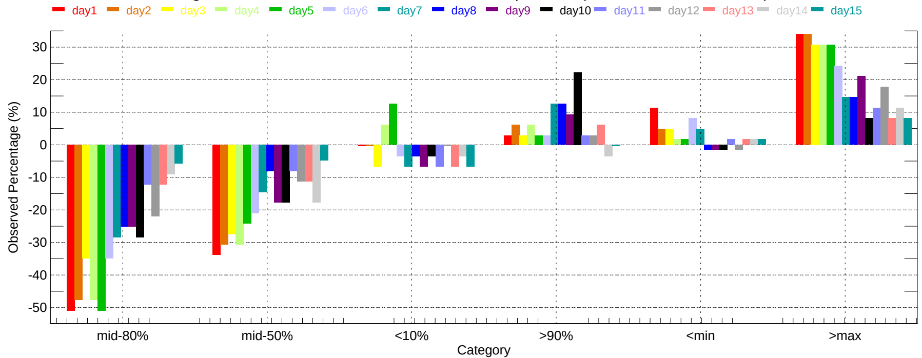
Observed Percentage Deviation of Ensembles - OKC: Max Temperature (2011-12-01~2011-12-31)
