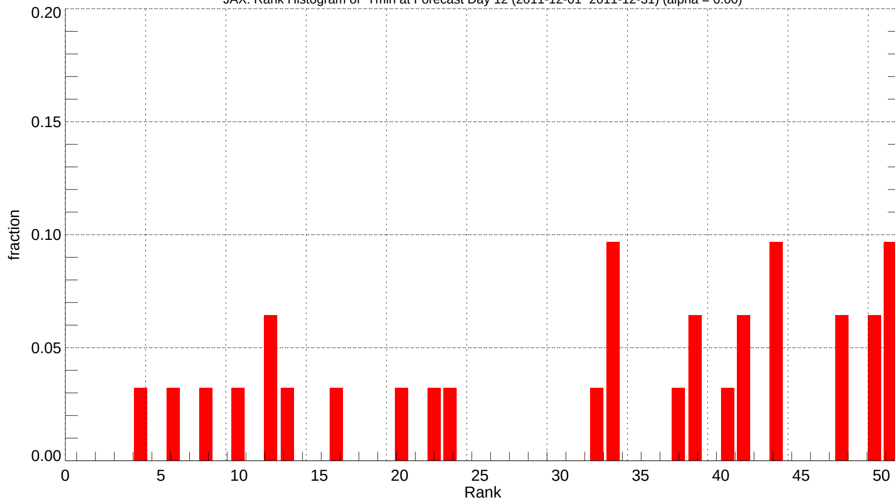
JAX: Rank Histogram of Tmin at Forecast Day 12 (2011-12-01~2011-12-31) (alpha = 0.00)
