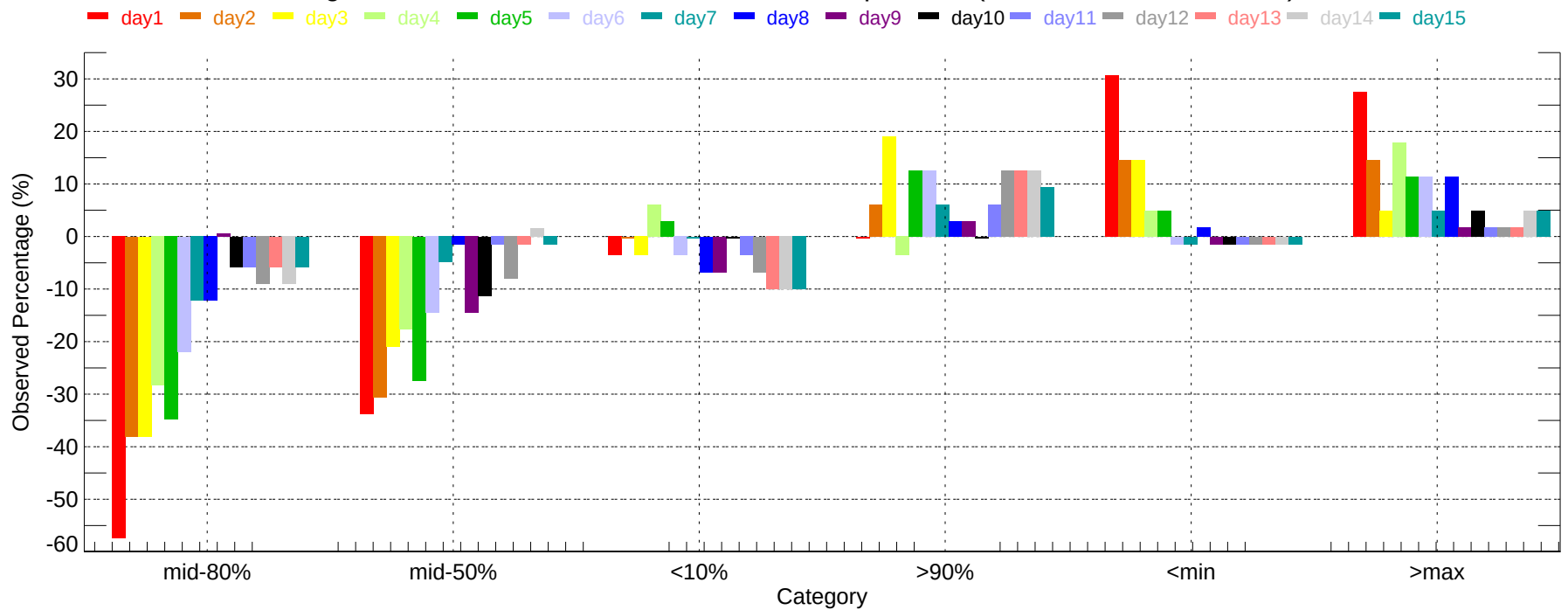
Observed Percentage Deviation of Ensembles - YXD: Min Temperature (2011-12-01~2011-12-31)
