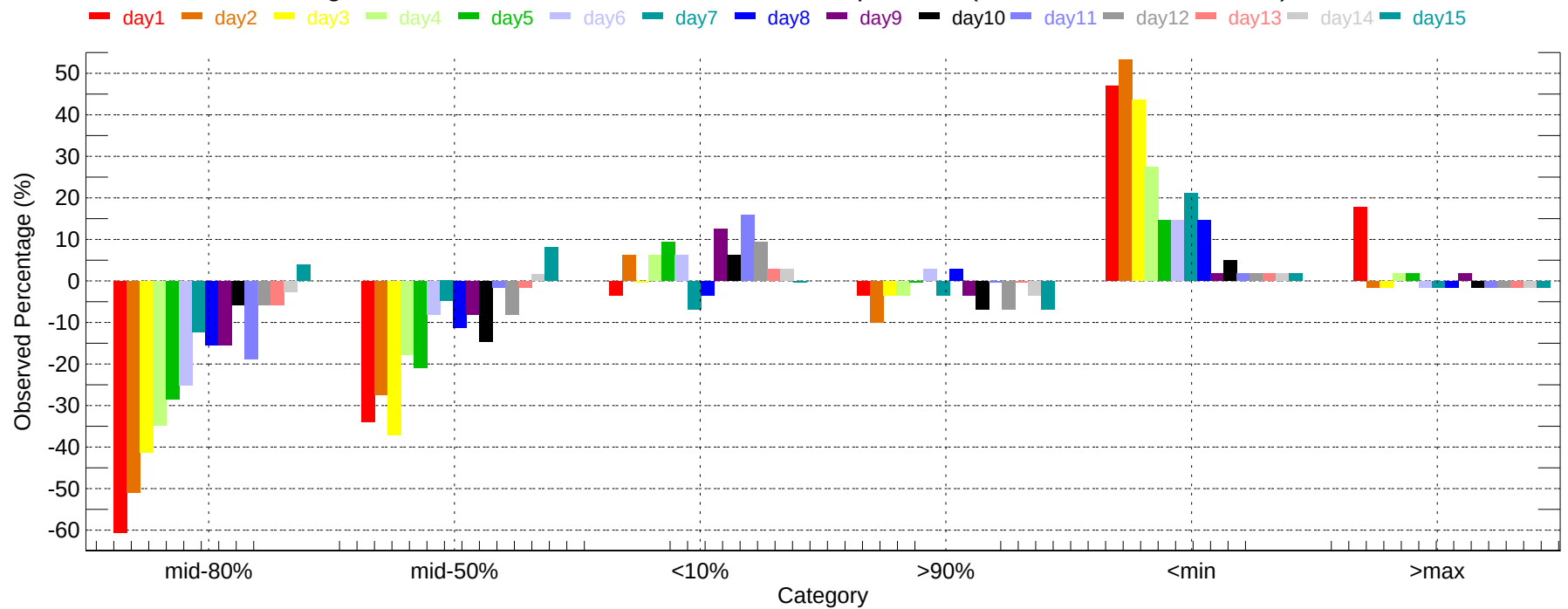
Observed Percentage Deviation of Ensembles - SJT: Min Temperature (2011-12-01~2011-12-31)
