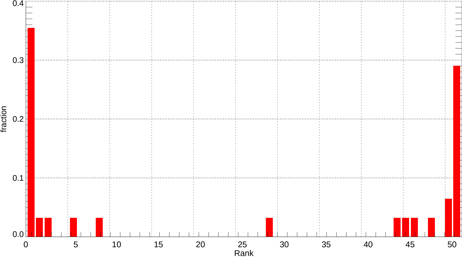
RAP: Rank Histogram of Tmin at Forecast Day 1 (2011-12-01~2011-12-31) (alpha = 0.00)
