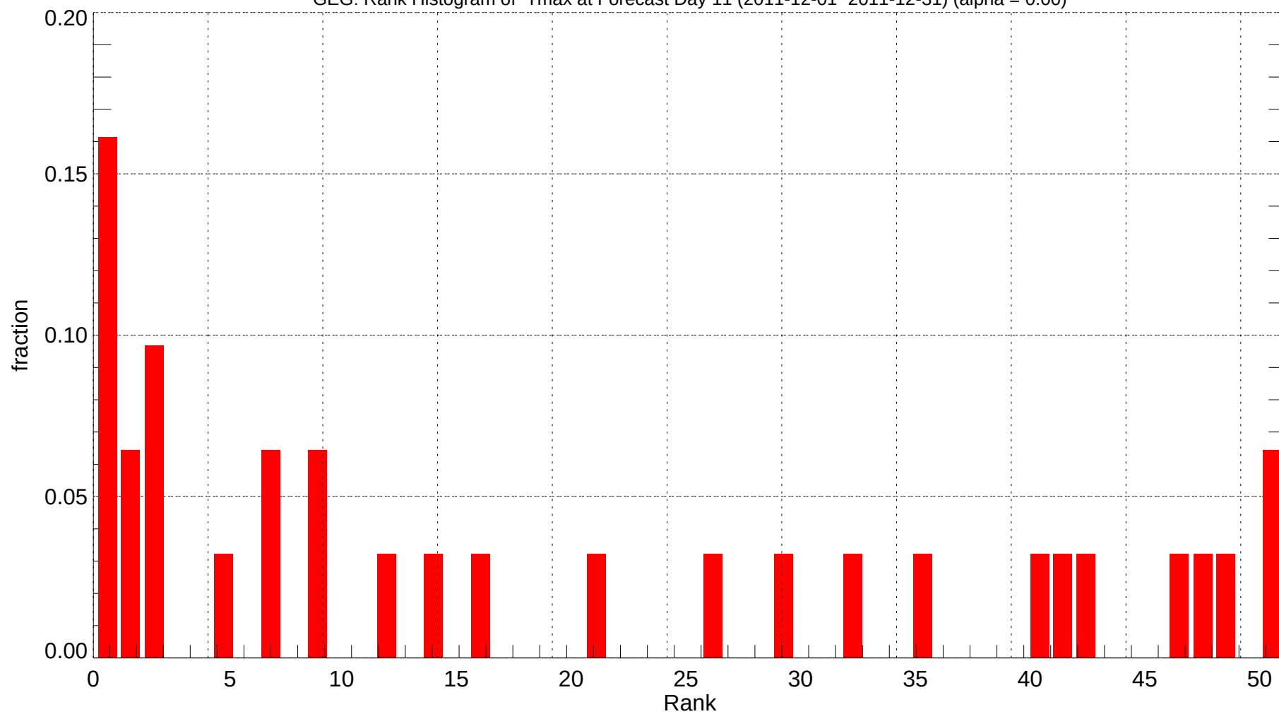
GEG: Rank Histogram of Tmax at Forecast Day 11 (2011-12-01~2011-12-31) (alpha = 0.00)
