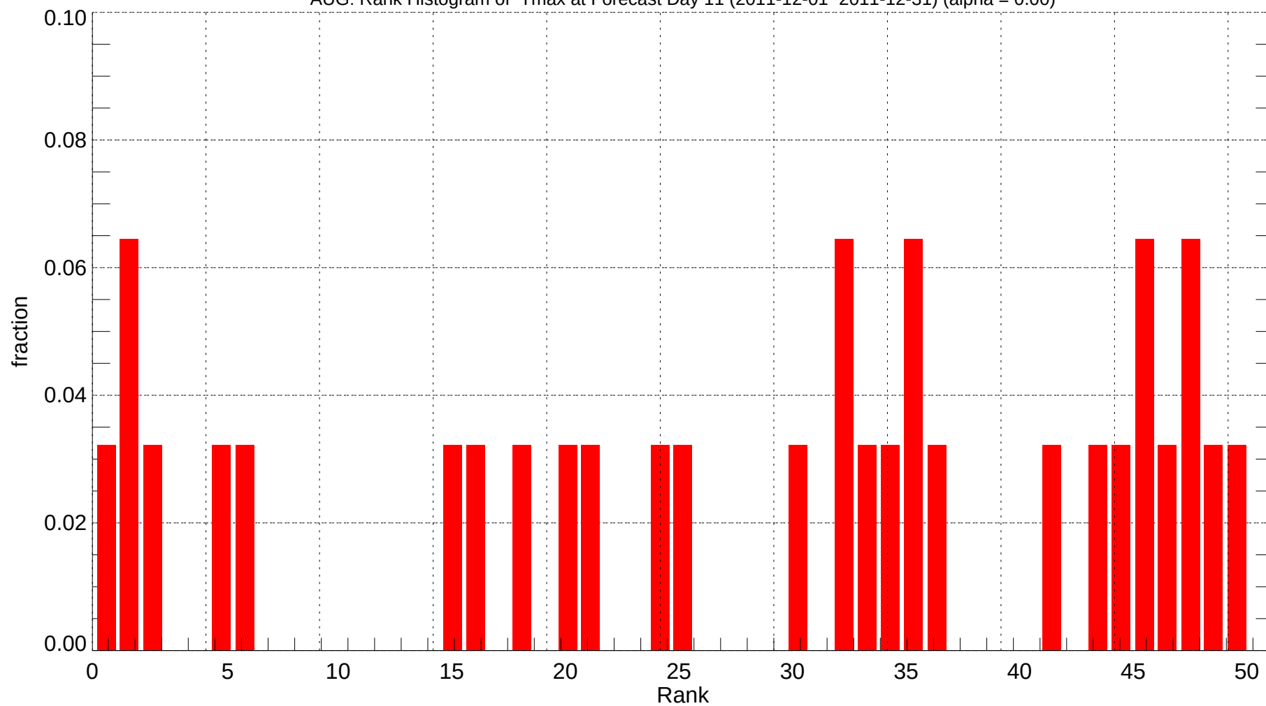
AUG: Rank Histogram of Tmax at Forecast Day 11 (2011-12-01~2011-12-31) (alpha = 0.00)
