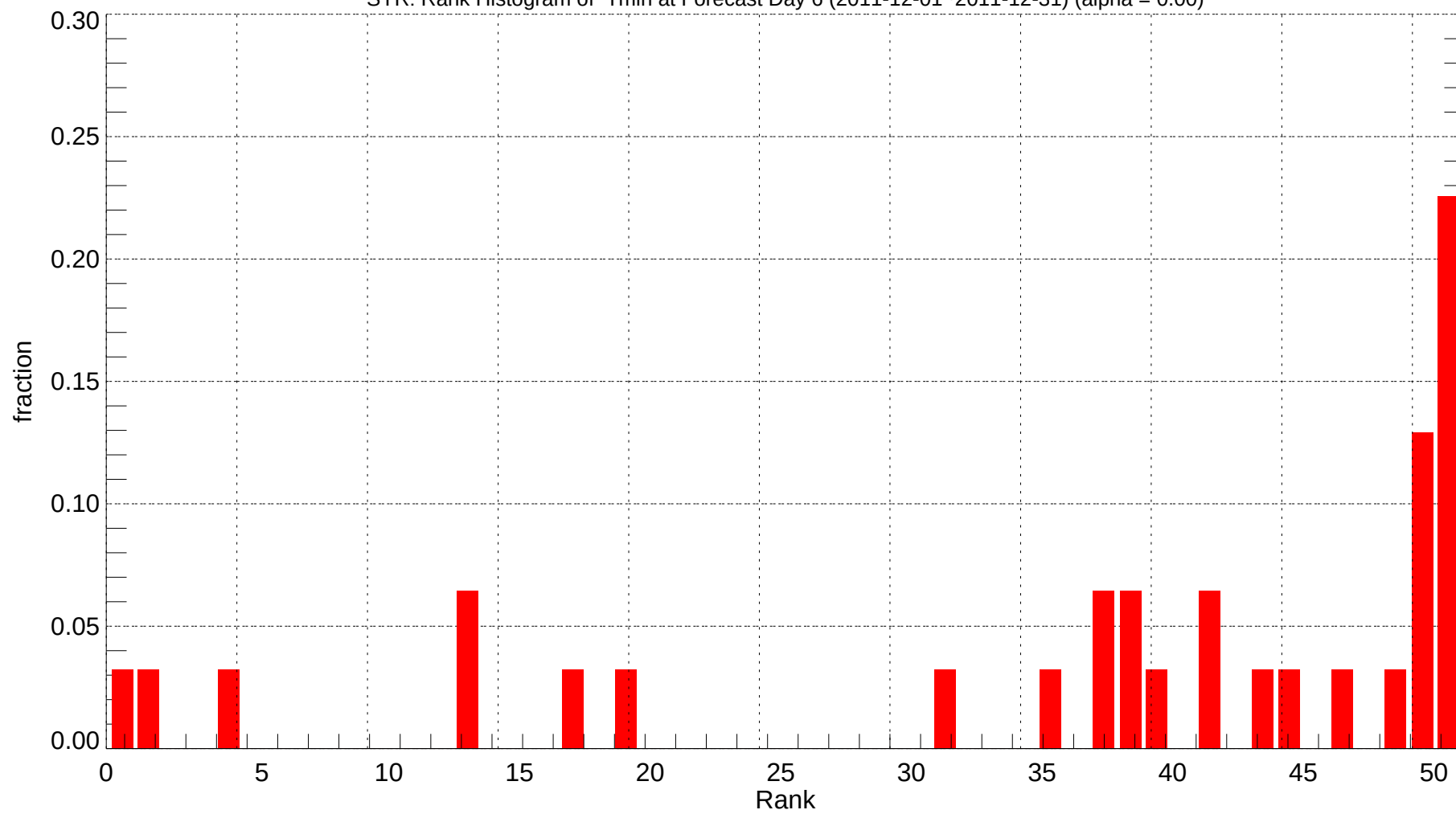
SYR: Rank Histogram of Tmin at Forecast Day 6 (2011-12-01~2011-12-31) (alpha = 0.00)
