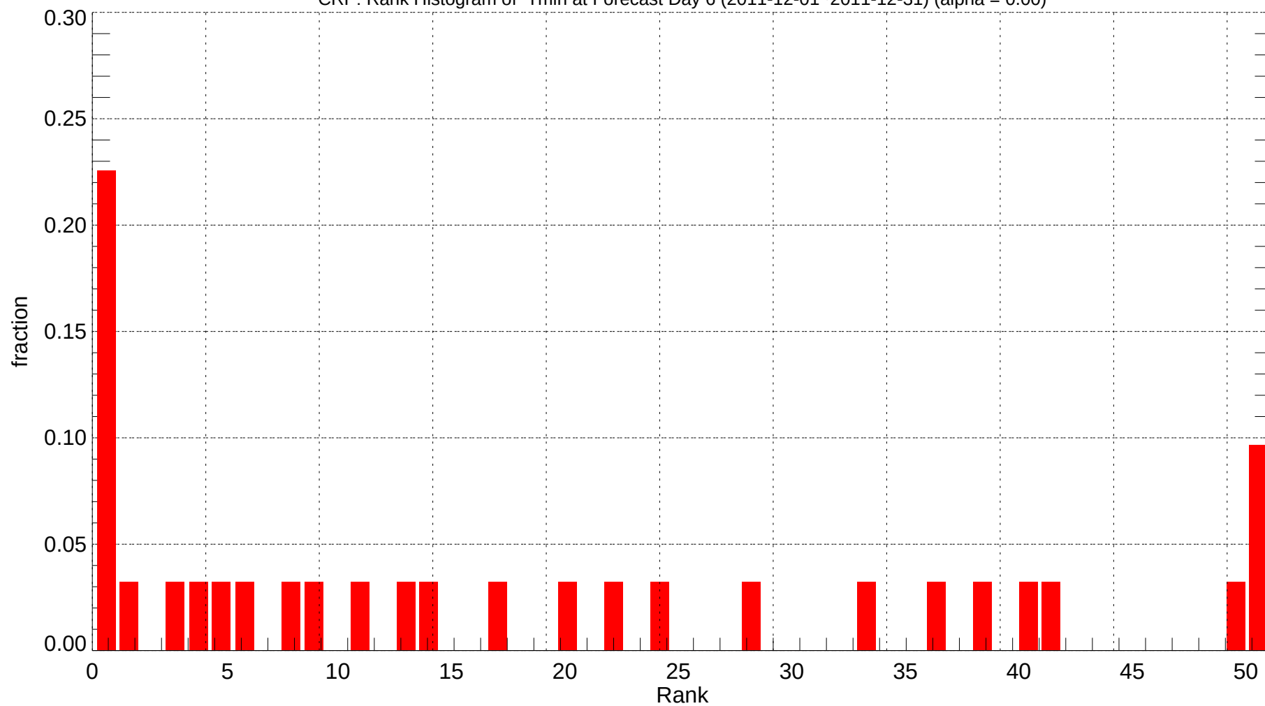
CRP: Rank Histogram of Tmin at Forecast Day 6 (2011-12-01~2011-12-31) (alpha = 0.00)
