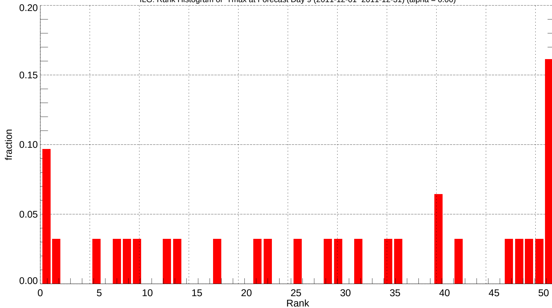
ILG: Rank Histogram of Tmax at Forecast Day 9 (2011-12-01~2011-12-31) (alpha = 0.00)
