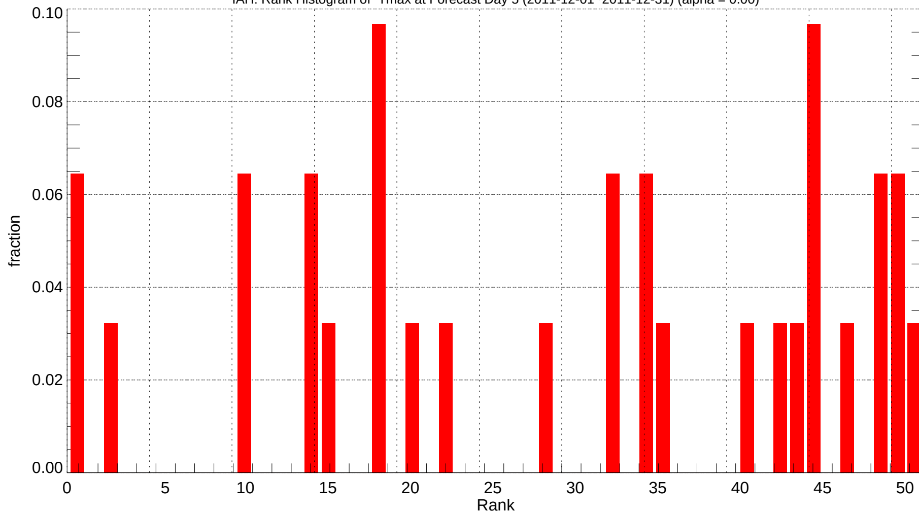
IAH: Rank Histogram of Tmax at Forecast Day 5 (2011-12-01~2011-12-31) (alpha = 0.00)
