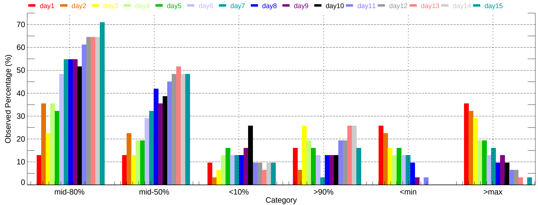
Observed Percentage of Ensembles - PWM: Min Temperature (2011-12-01~2011-12-31)
