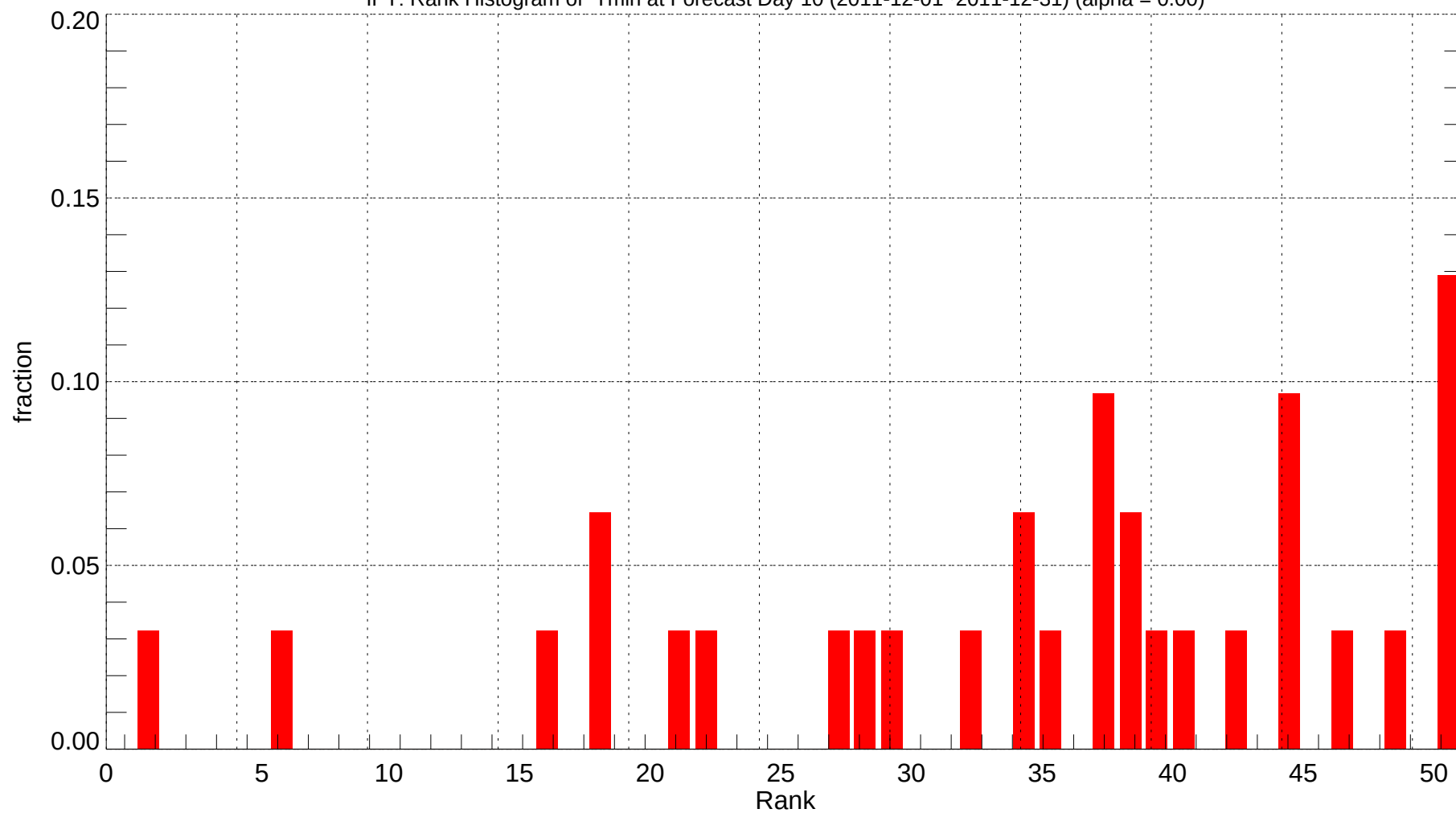
IPT: Rank Histogram of Tmin at Forecast Day 10 (2011-12-01~2011-12-31) (alpha = 0.00)
