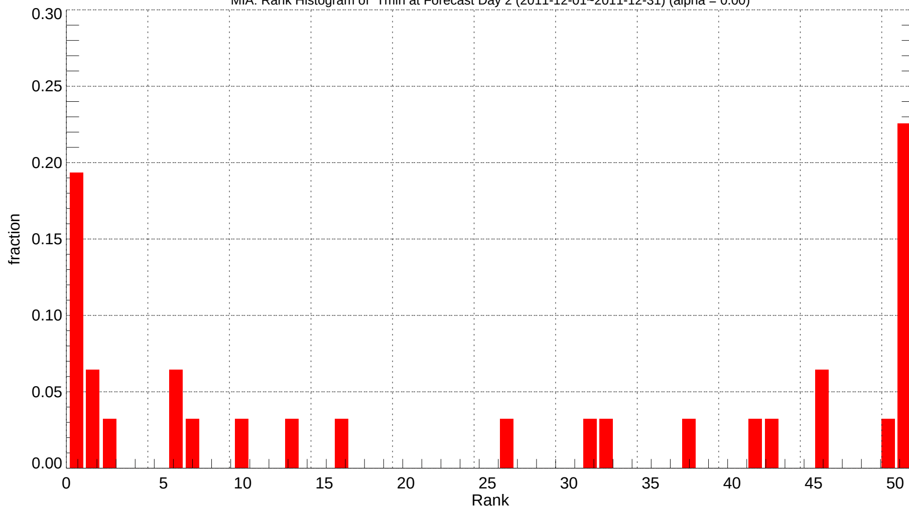
MIA: Rank Histogram of Tmin at Forecast Day 2 (2011-12-01~2011-12-31) (alpha = 0.00)
