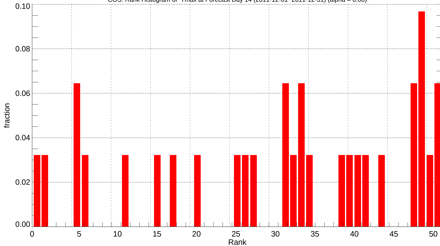
COS: Rank Histogram of Tmax at Forecast Day 14 (2011-12-01~2011-12-31) (alpha = 0.00)
