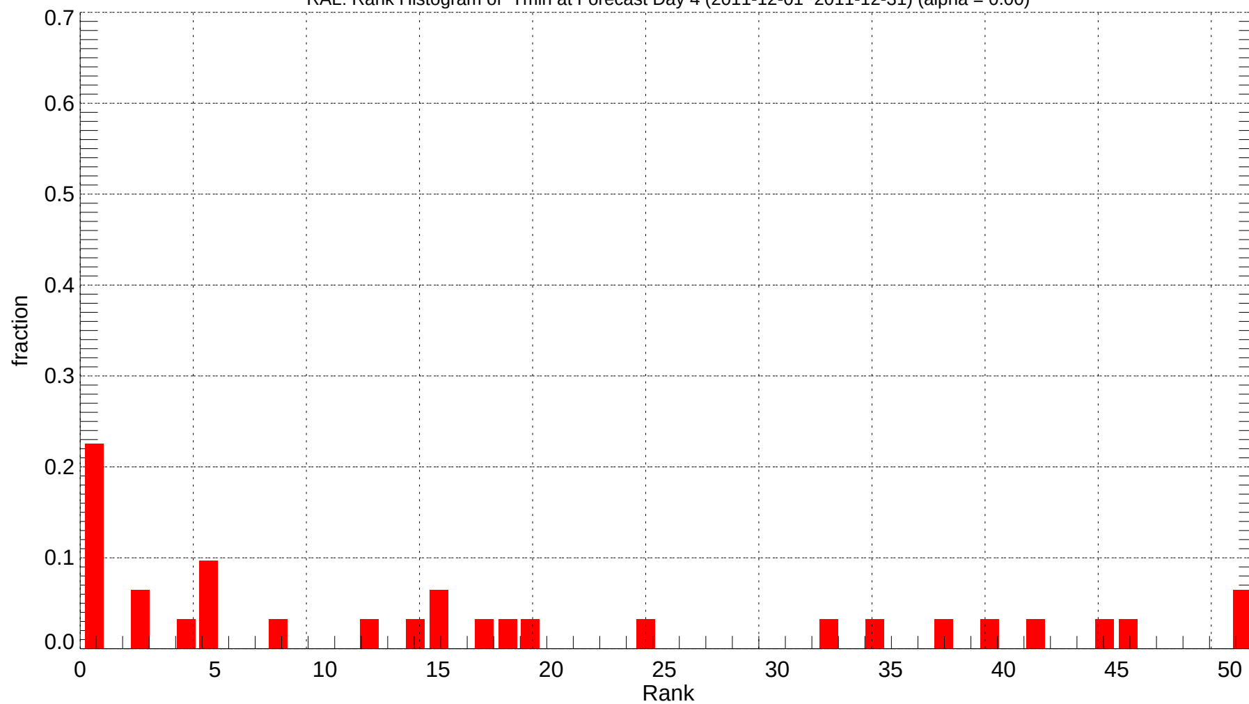
RAL: Rank Histogram of Tmin at Forecast Day 4 (2011-12-01~2011-12-31) (alpha = 0.00)
