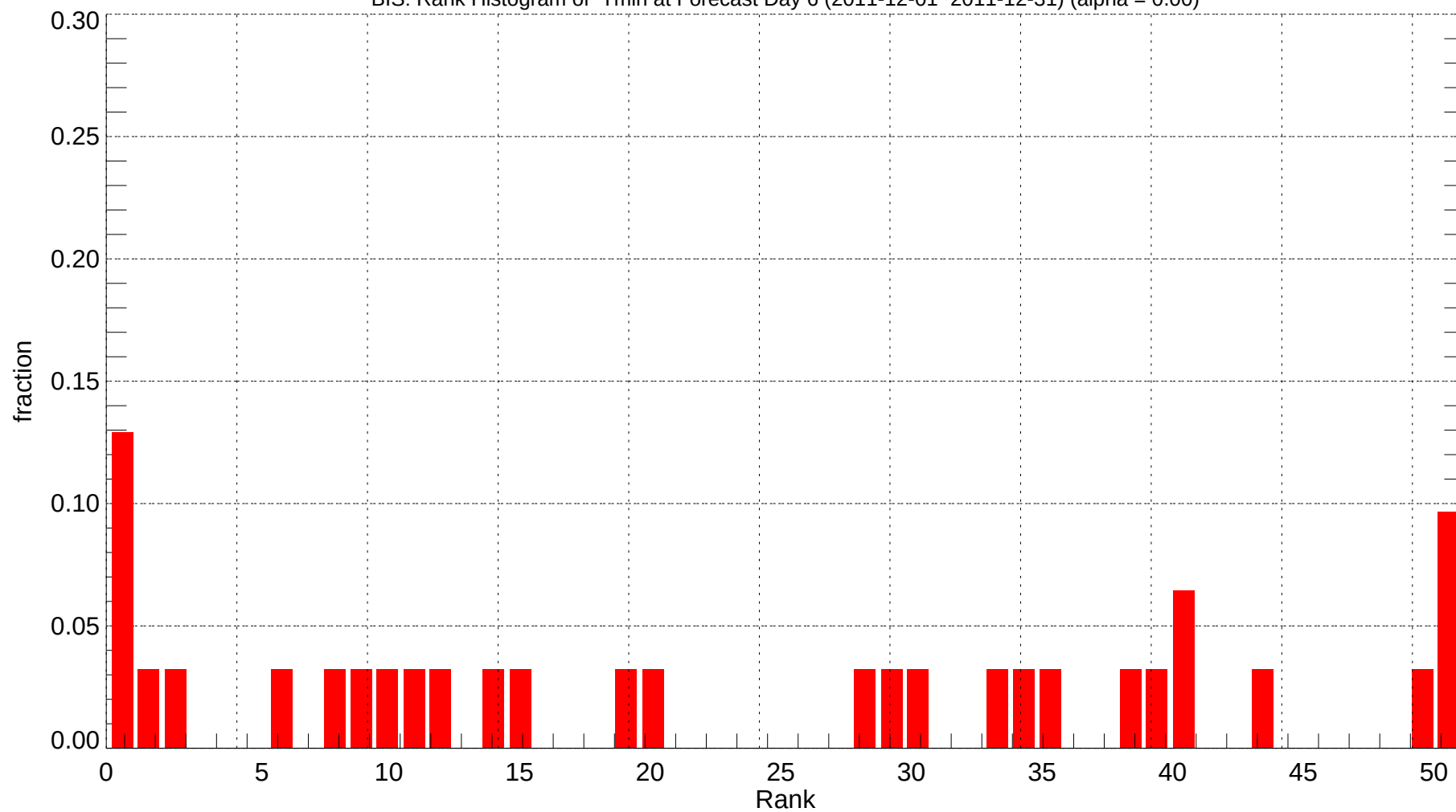
BIS: Rank Histogram of Tmin at Forecast Day 6 (2011-12-01~2011-12-31) (alpha = 0.00)
