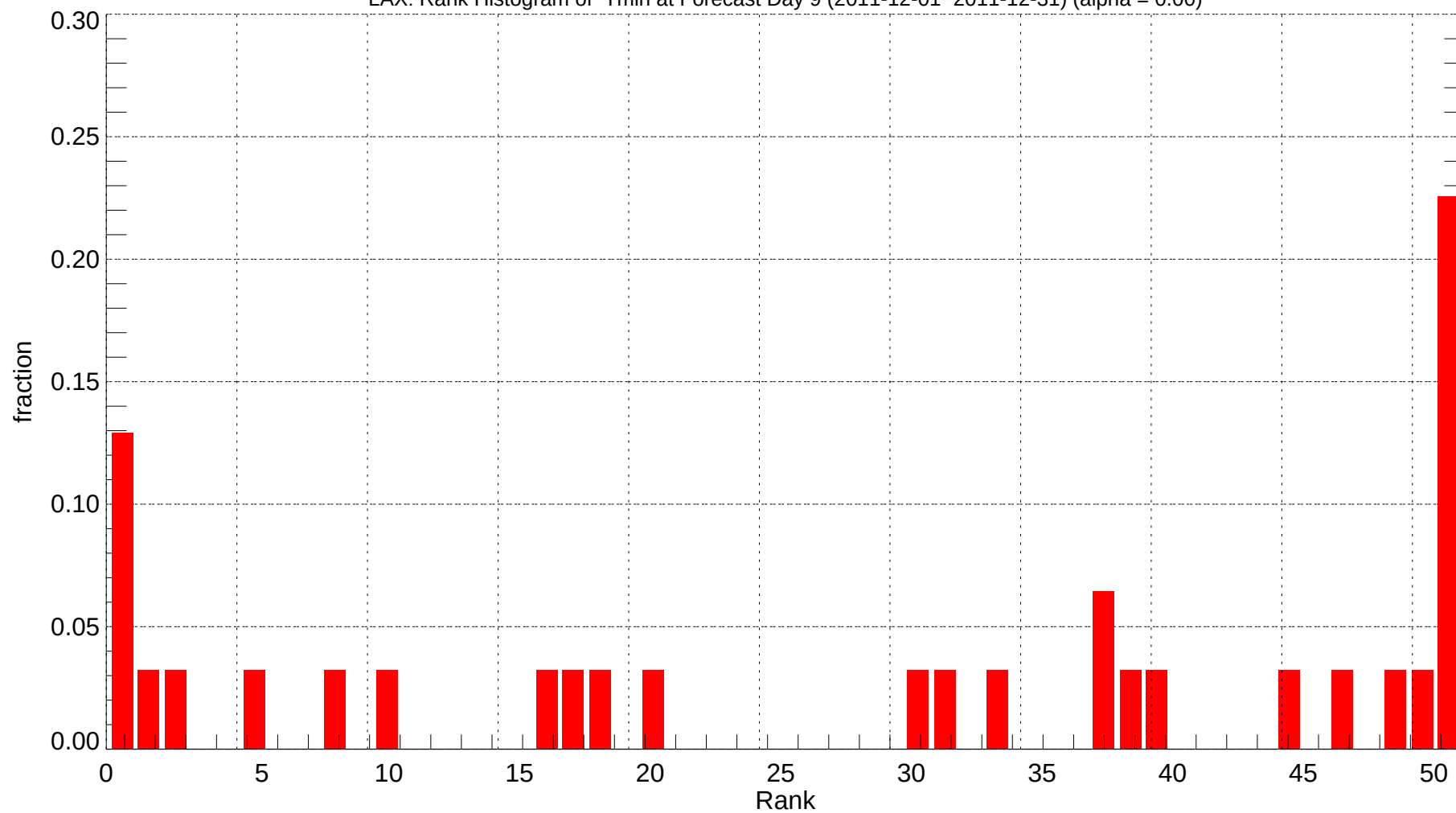
LAX: Rank Histogram of Tmin at Forecast Day 9 (2011-12-01~2011-12-31) (alpha = 0.00)
