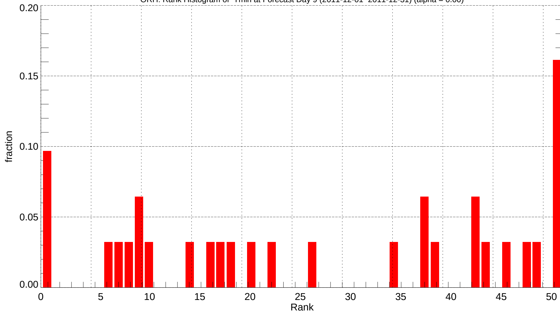
ORH: Rank Histogram of Tmin at Forecast Day 9 (2011-12-01~2011-12-31) (alpha = 0.00)
