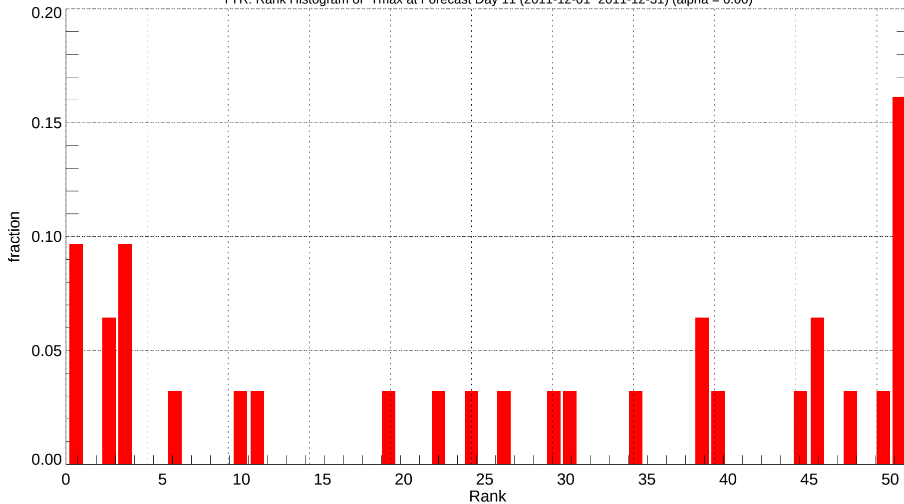
TYR: Rank Histogram of Tmax at Forecast Day 11 (2011-12-01~2011-12-31) (alpha = 0.00)
