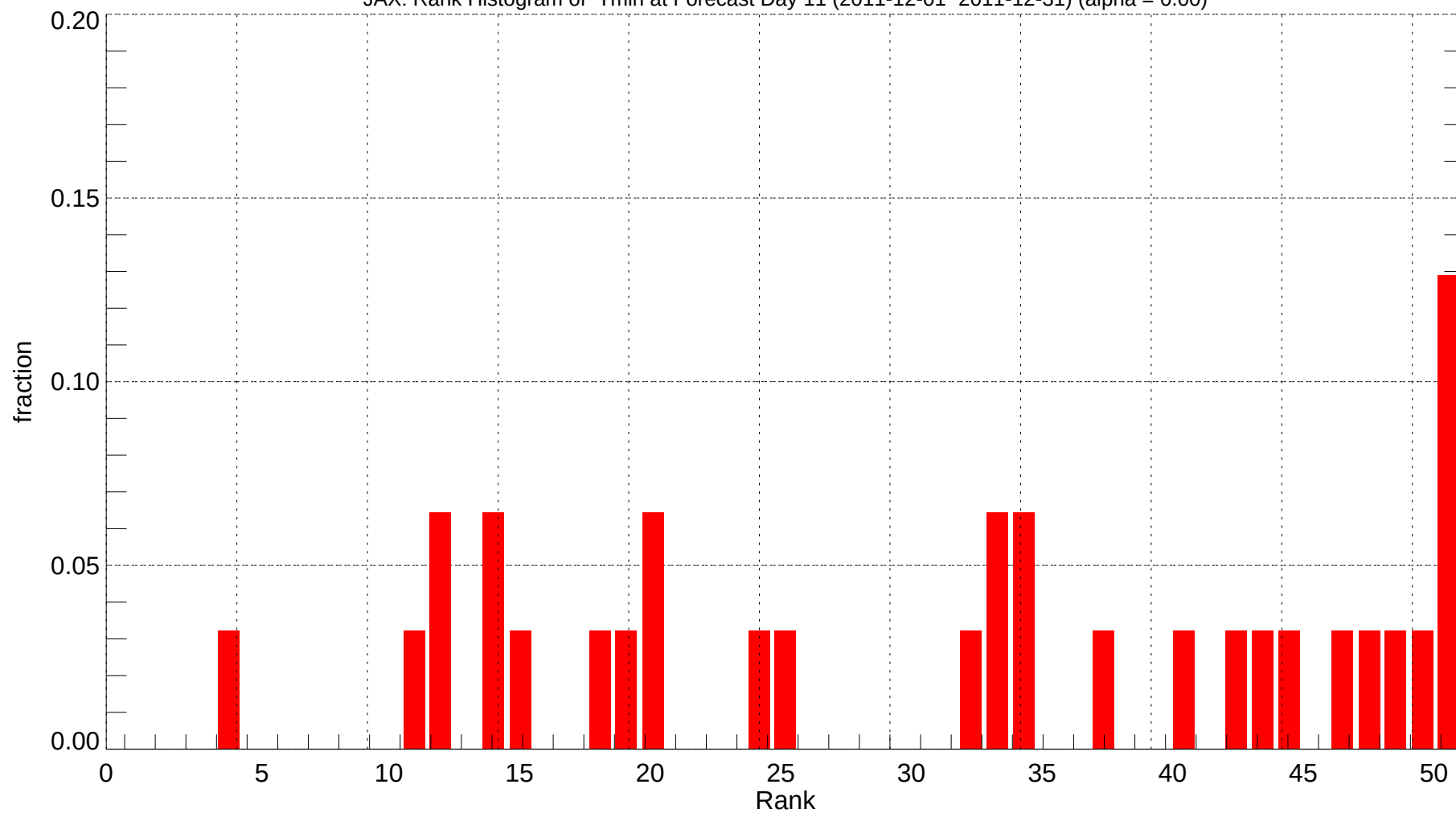
JAX: Rank Histogram of Tmin at Forecast Day 11 (2011-12-01~2011-12-31) (alpha = 0.00)
