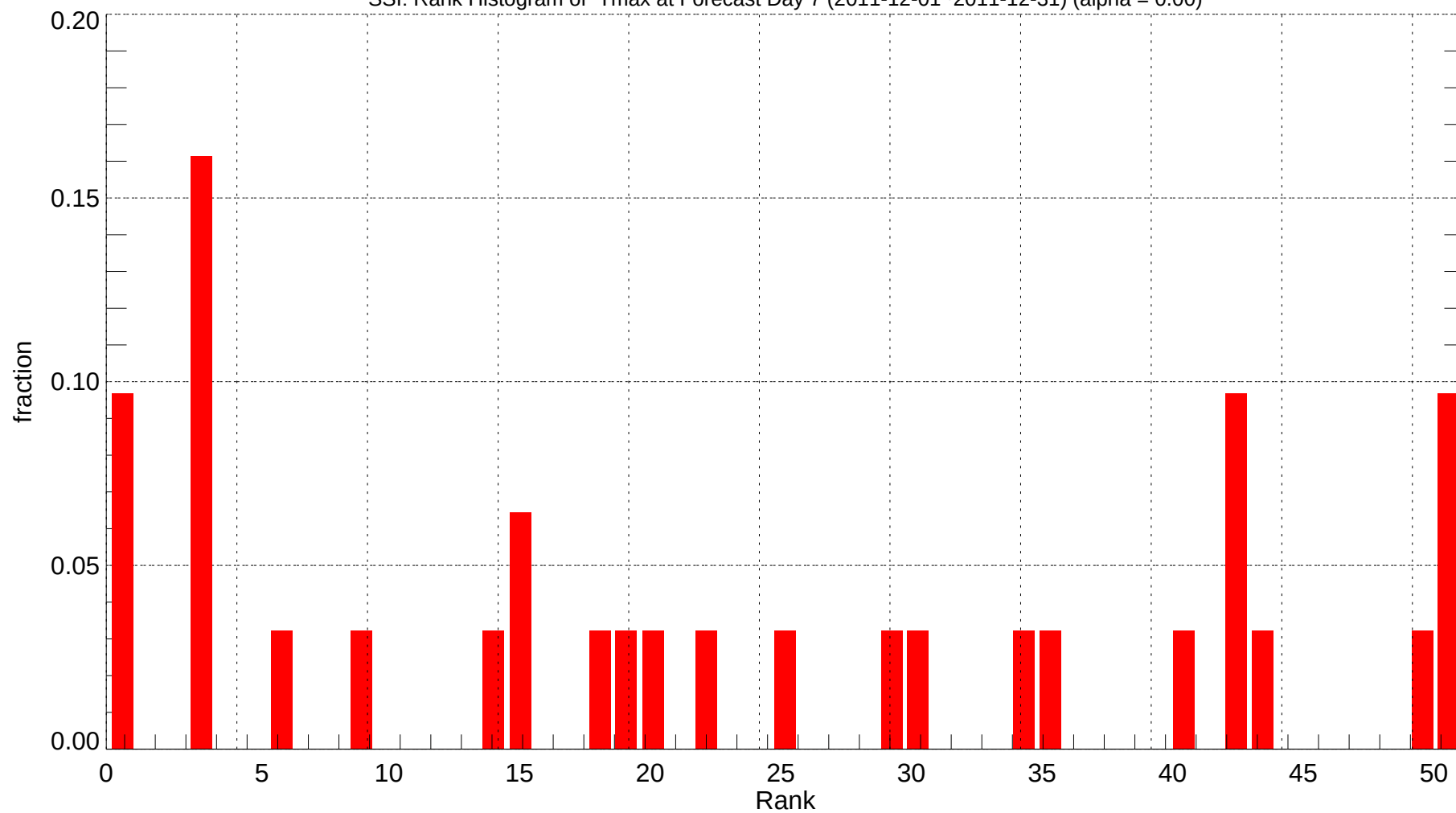
SSI: Rank Histogram of Tmax at Forecast Day 7 (2011-12-01~2011-12-31) (alpha = 0.00)
