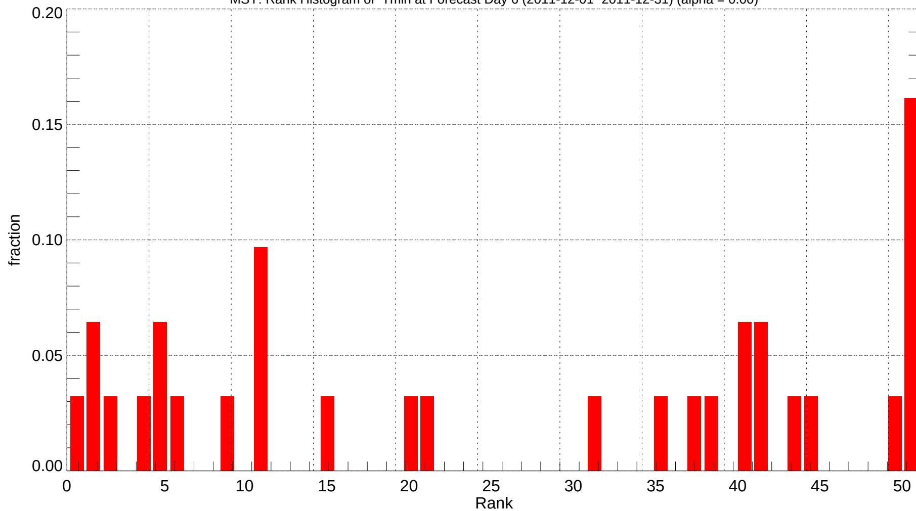
MSY: Rank Histogram of Tmin at Forecast Day 6 (2011-12-01~2011-12-31) (alpha = 0.00)
