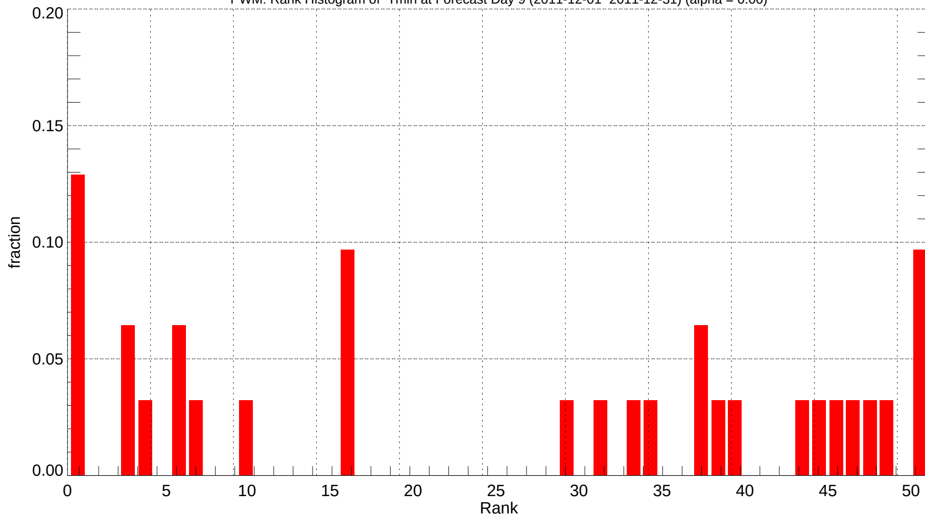
PWM: Rank Histogram of Tmin at Forecast Day 9 (2011-12-01~2011-12-31) (alpha = 0.00)
