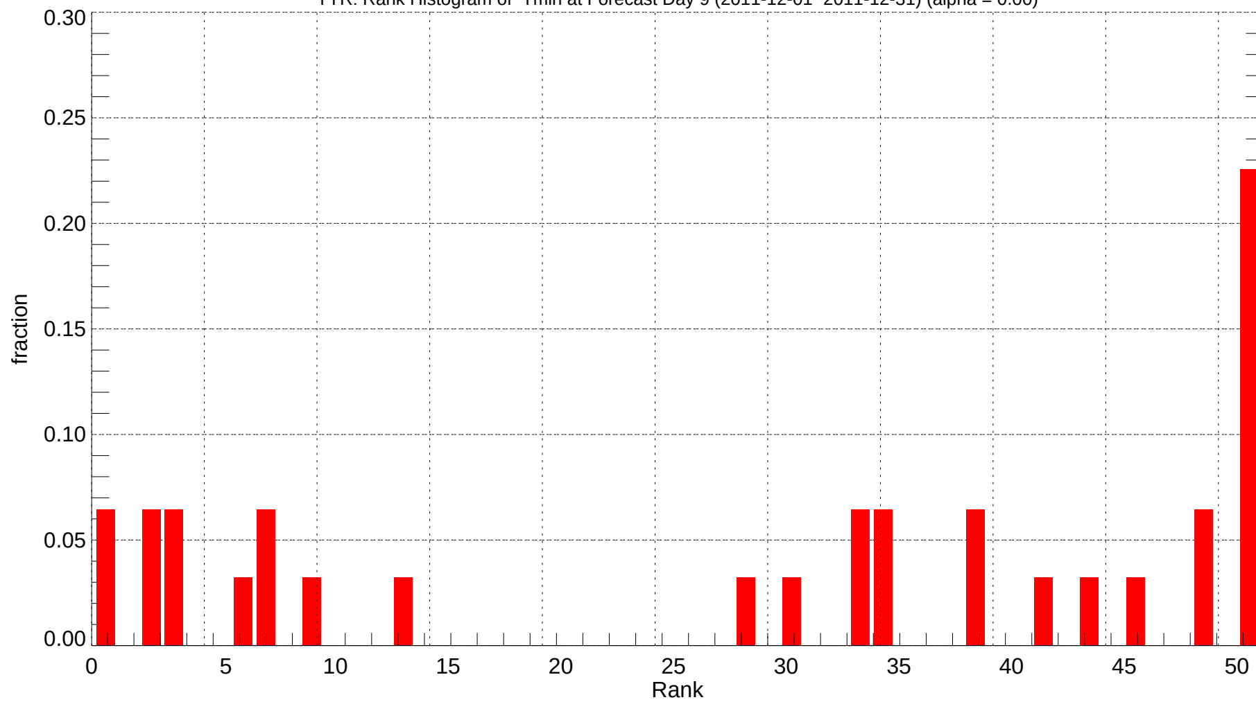
TYR: Rank Histogram of Tmin at Forecast Day 9 (2011-12-01~2011-12-31) (alpha = 0.00)
