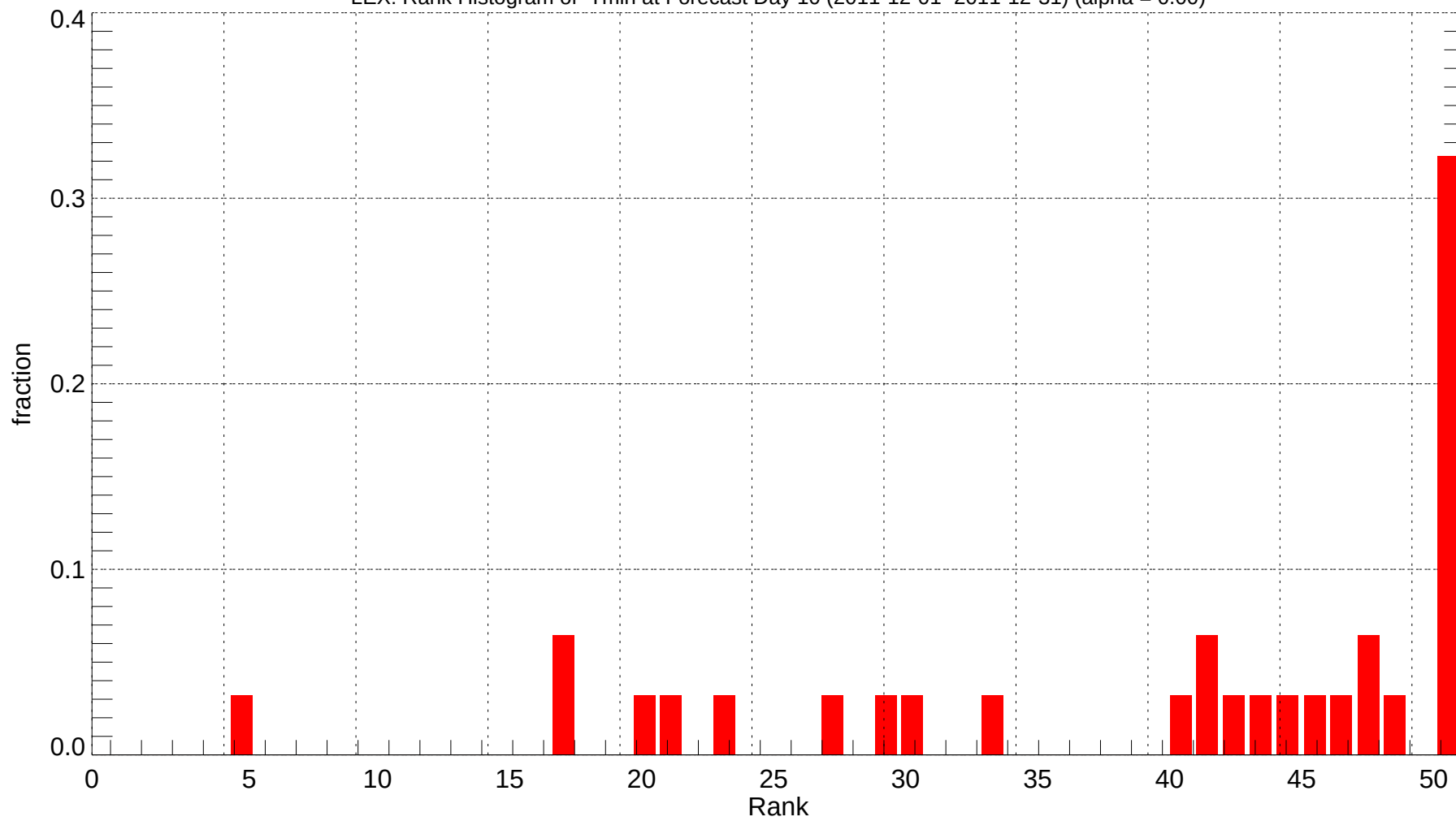
LEX: Rank Histogram of Tmin at Forecast Day 10 (2011-12-01~2011-12-31) (alpha = 0.00)
