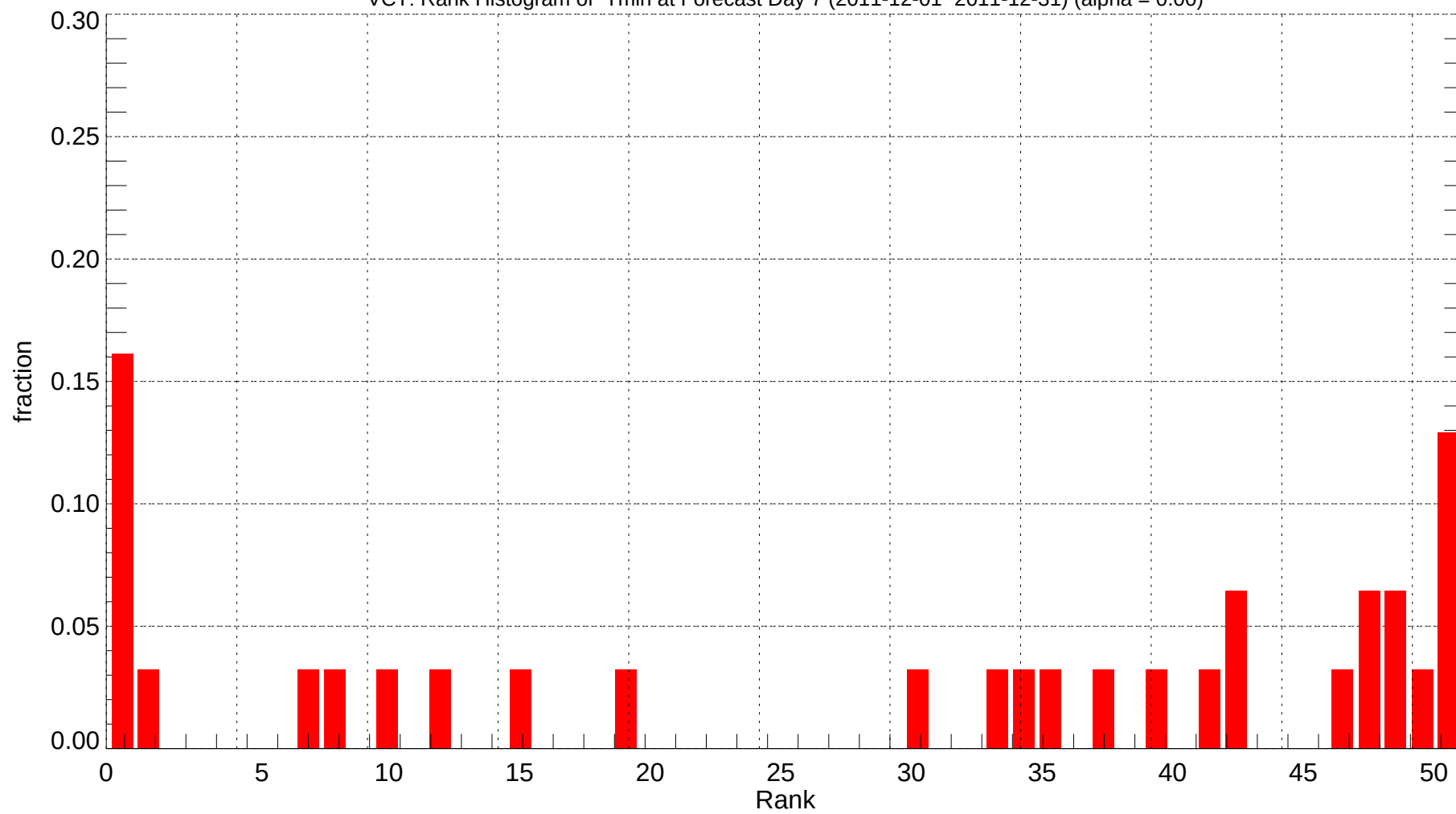
VCT: Rank Histogram of Tmin at Forecast Day 7 (2011-12-01~2011-12-31) (alpha = 0.00)
