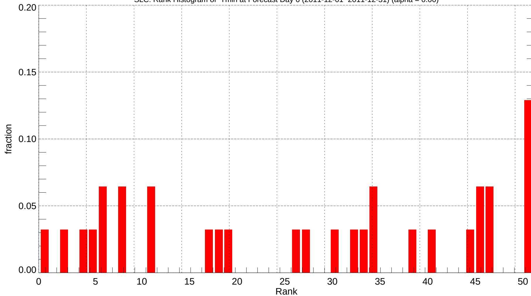
SLC: Rank Histogram of Tmin at Forecast Day 6 (2011-12-01~2011-12-31) (alpha = 0.00)
