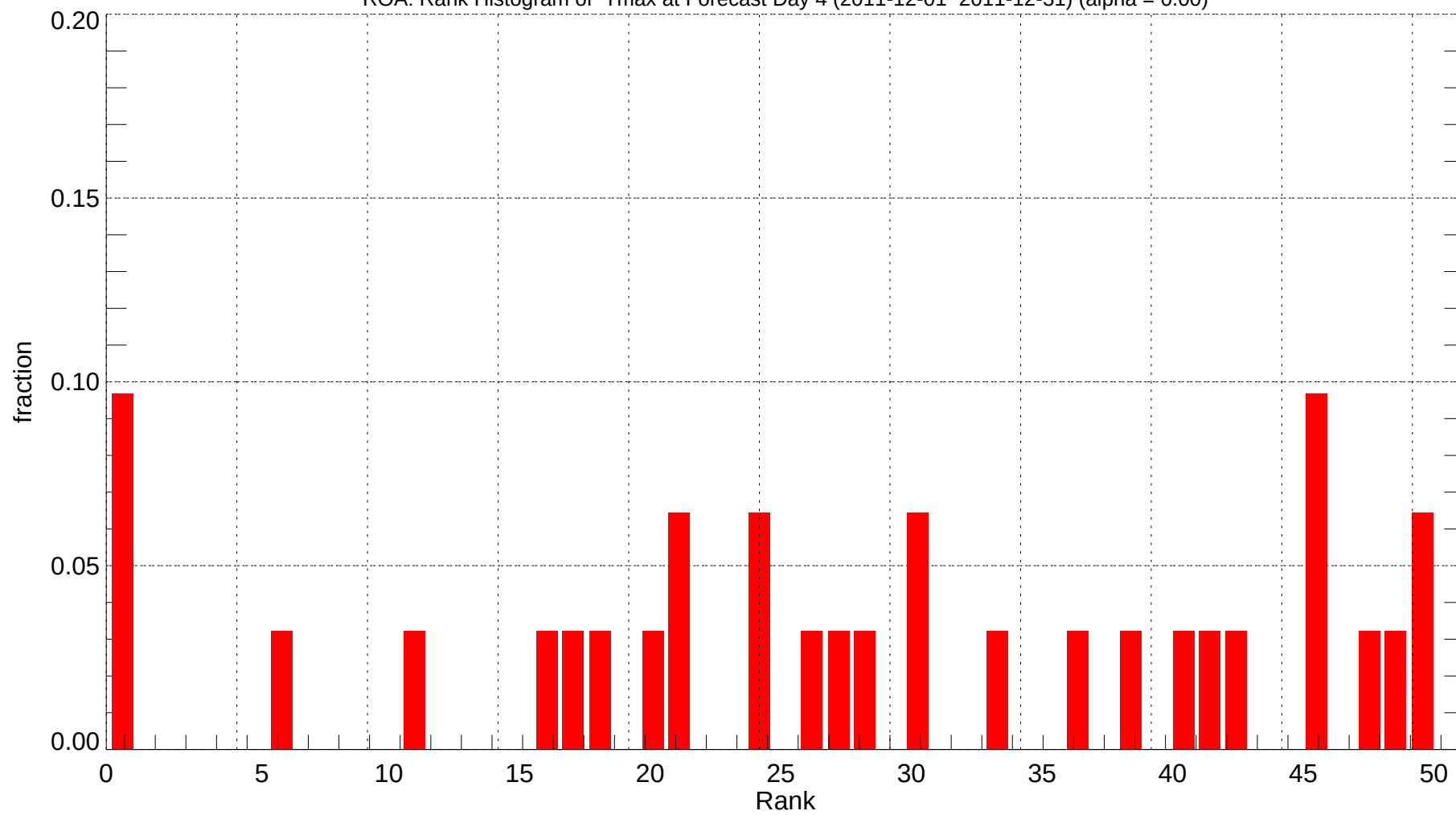
ROA: Rank Histogram of Tmax at Forecast Day 4 (2011-12-01~2011-12-31) (alpha = 0.00)
