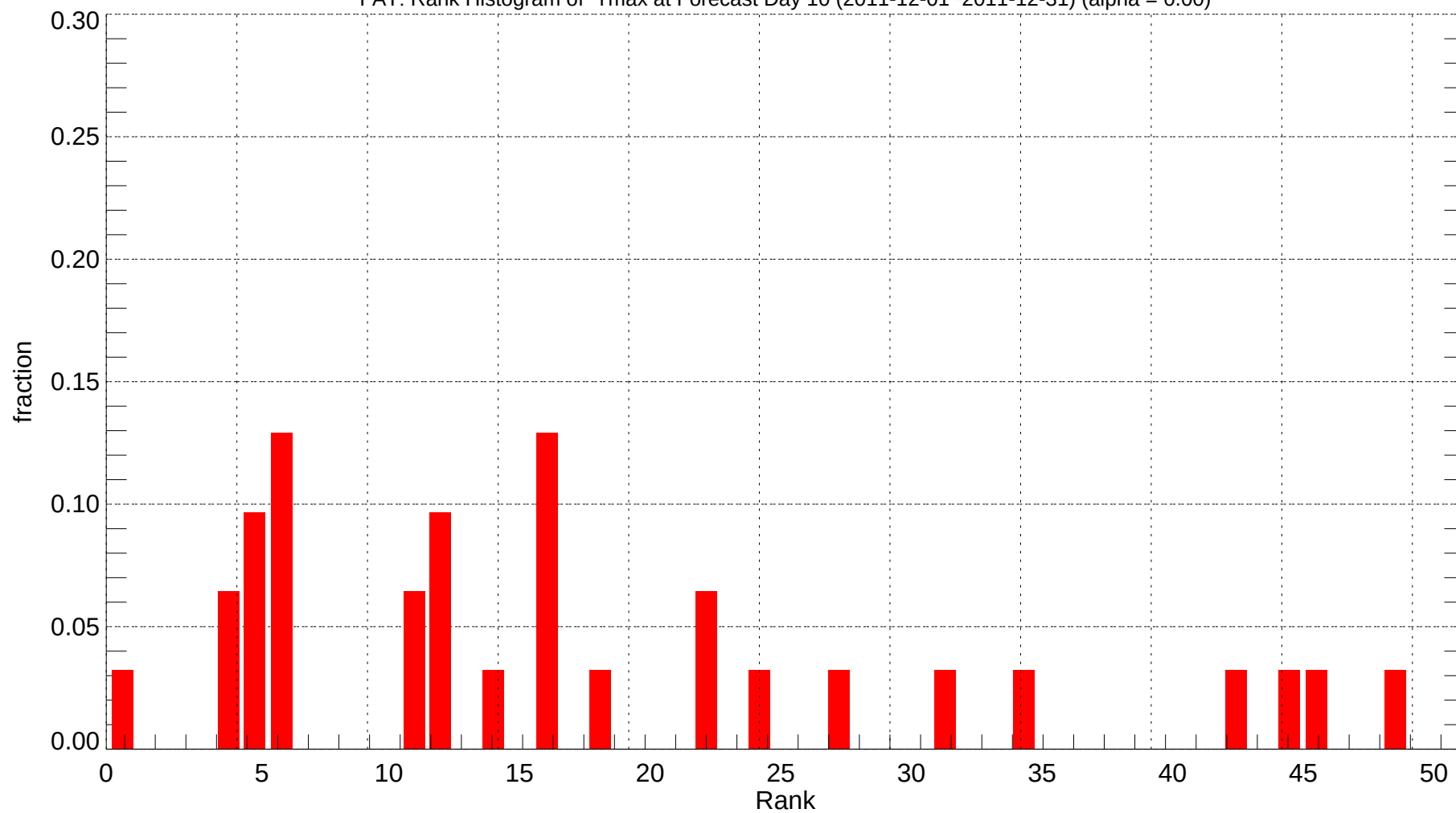
FAT: Rank Histogram of Tmax at Forecast Day 10 (2011-12-01~2011-12-31) (alpha = 0.00)
