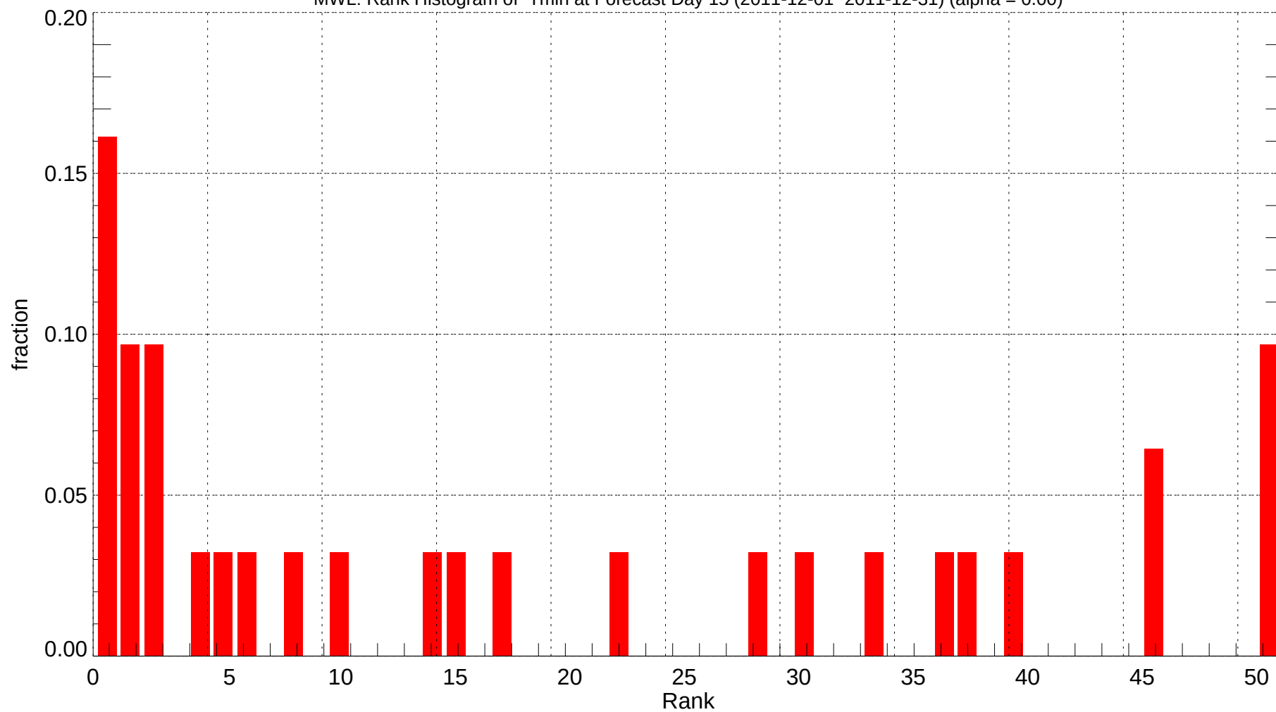
MWL: Rank Histogram of Tmin at Forecast Day 15 (2011-12-01~2011-12-31) (alpha = 0.00)
