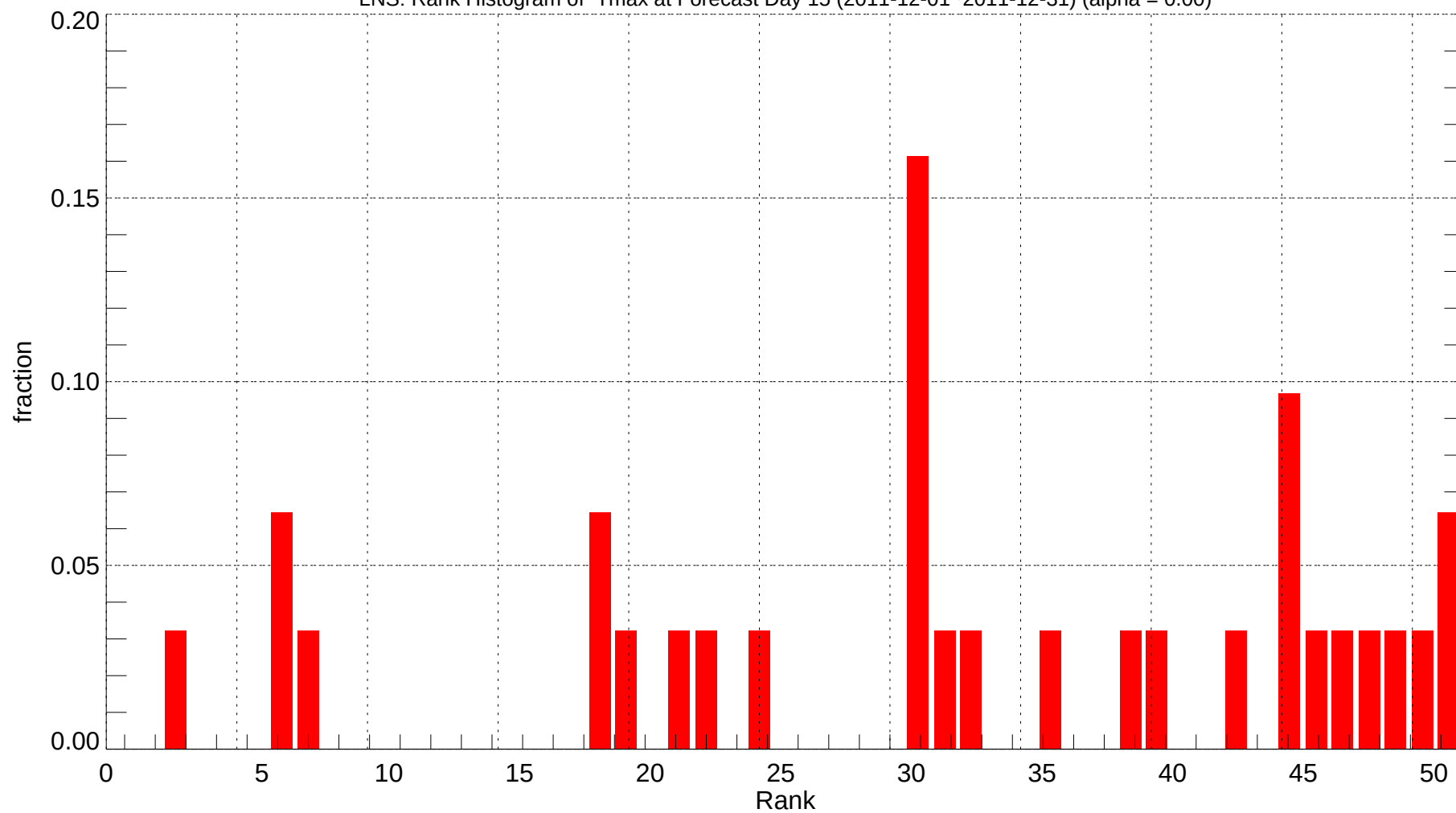
LNS: Rank Histogram of Tmax at Forecast Day 15 (2011-12-01~2011-12-31) (alpha = 0.00)
