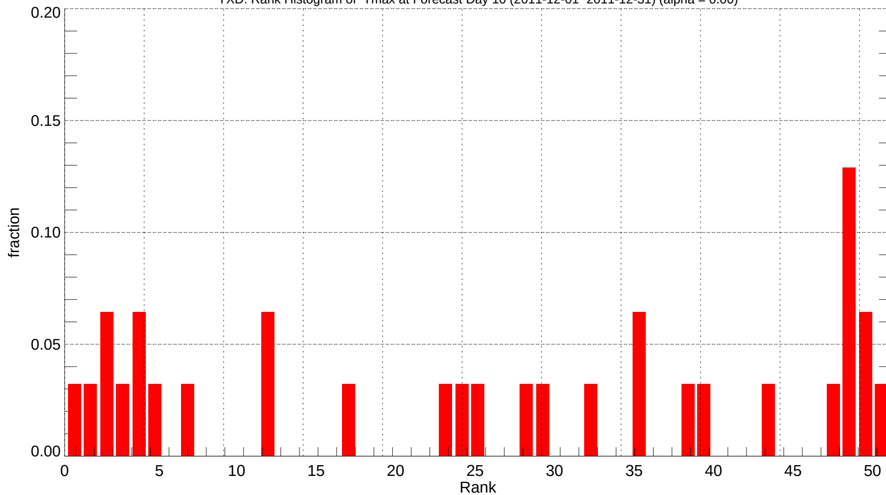
YXD: Rank Histogram of Tmax at Forecast Day 10 (2011-12-01~2011-12-31) (alpha = 0.00)
