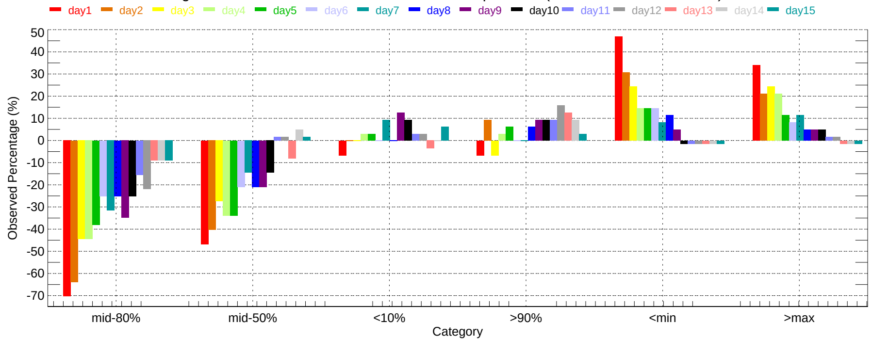
Observed Percentage Deviation of Ensembles - AUG: Min Temperature (2011-12-01~2011-12-31)
