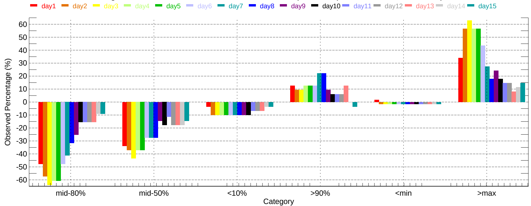
Observed Percentage Deviation of Ensembles - AOO: Max Temperature (2011-12-01~2011-12-31)
