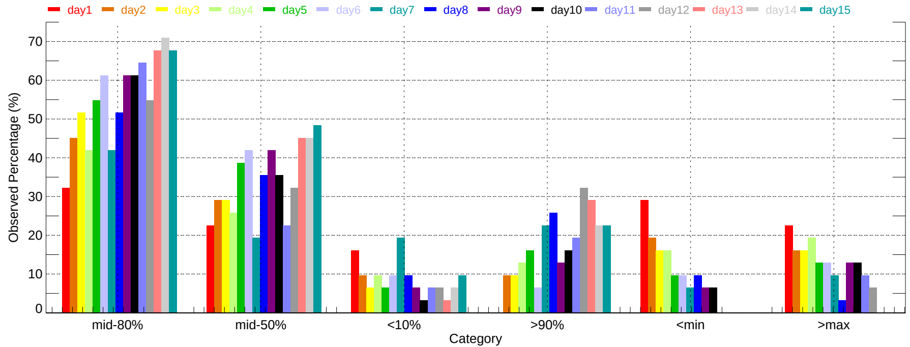
Observed Percentage of Ensembles - PHL: Max Temperature (2011-12-01~2011-12-31)
