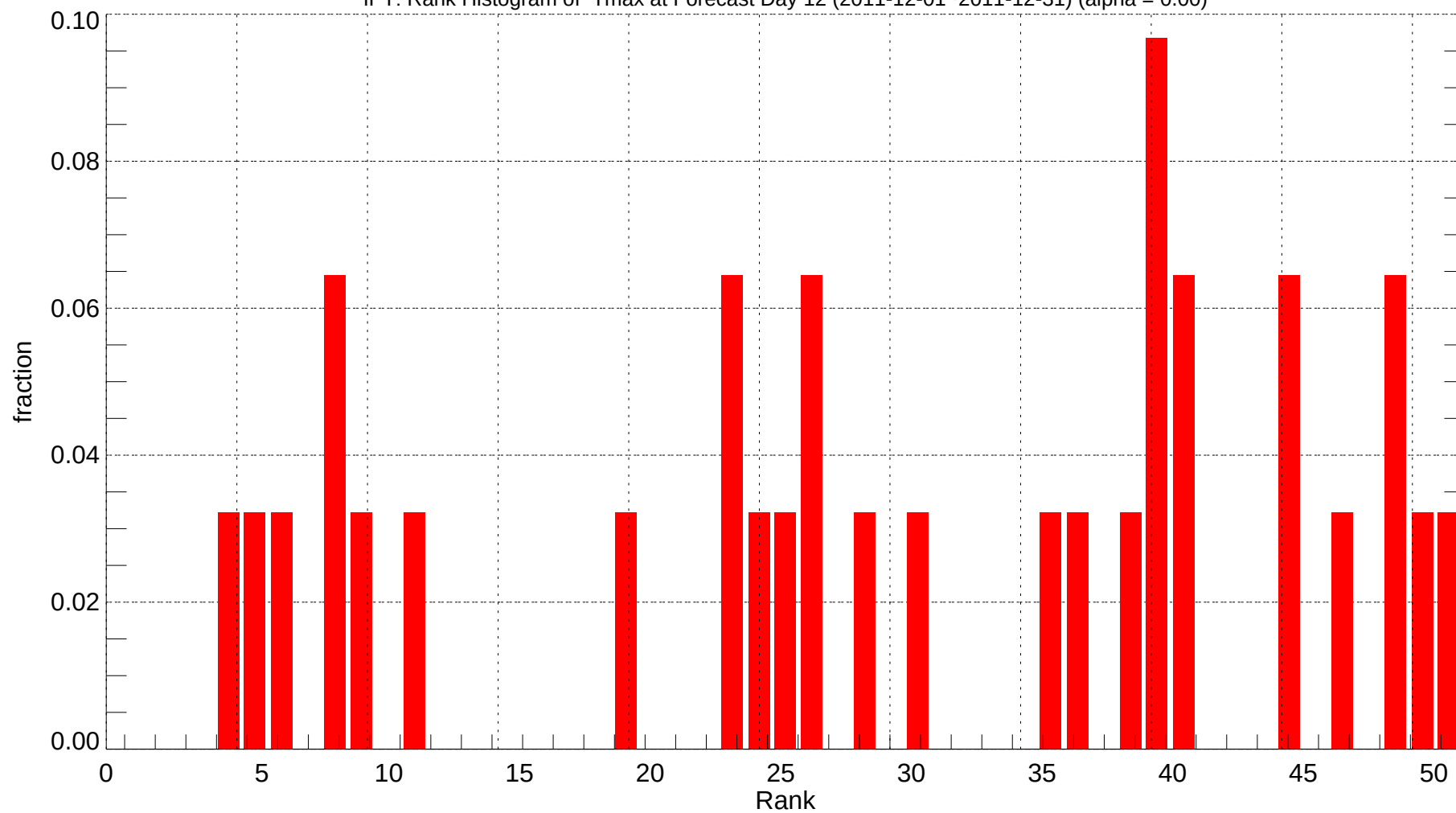
IPT: Rank Histogram of Tmax at Forecast Day 12 (2011-12-01~2011-12-31) (alpha = 0.00)
