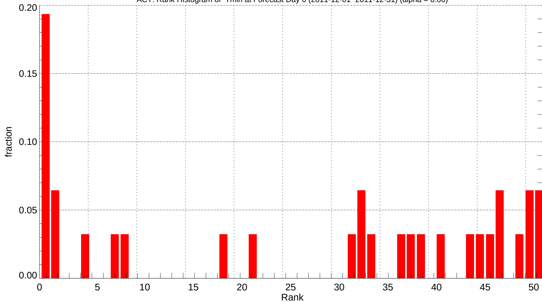
ACT: Rank Histogram of Tmin at Forecast Day 6 (2011-12-01~2011-12-31) (alpha = 0.00)
