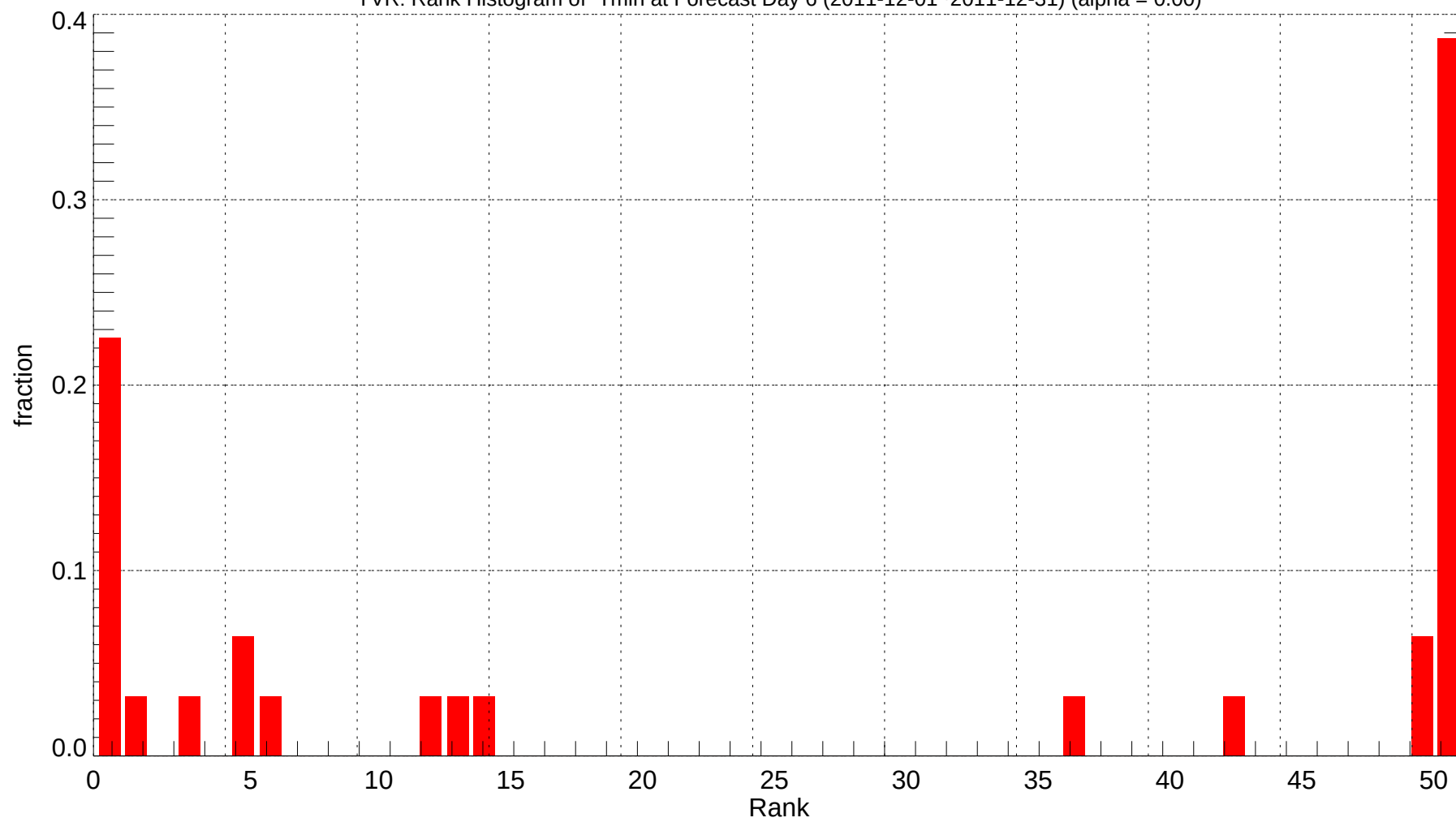
YVR: Rank Histogram of Tmin at Forecast Day 6 (2011-12-01~2011-12-31) (alpha = 0.00)
