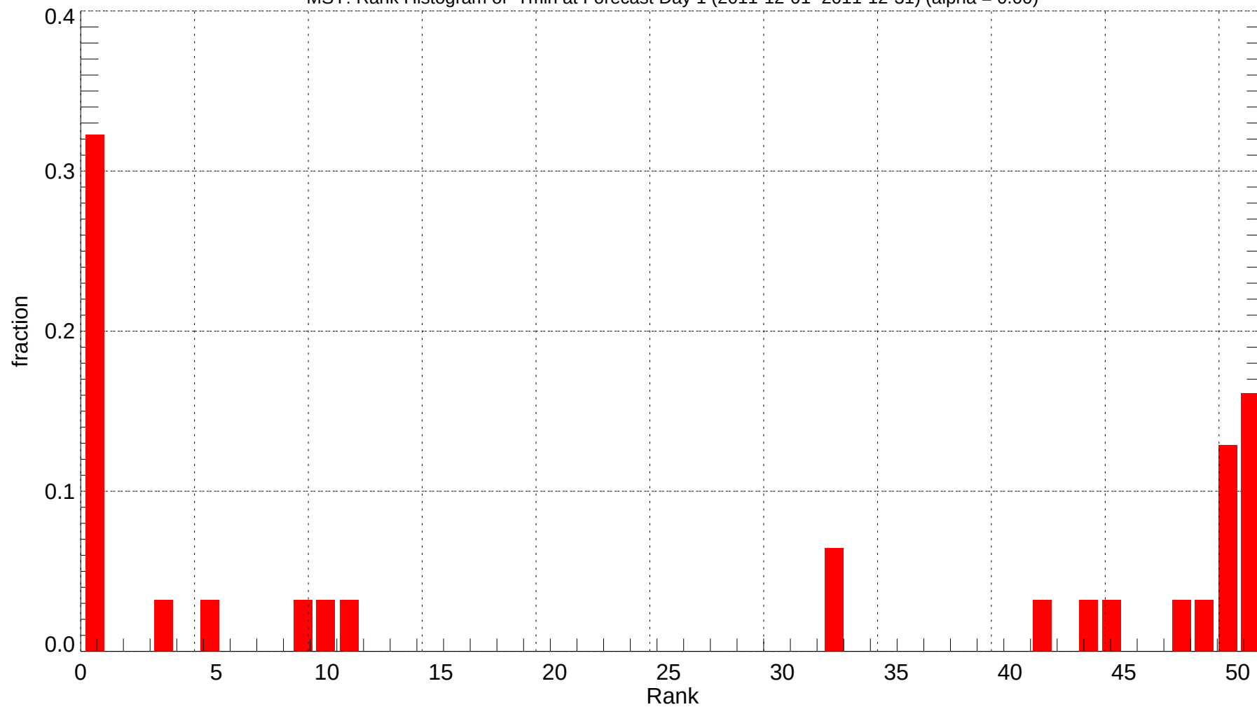
MSY: Rank Histogram of Tmin at Forecast Day 1 (2011-12-01~2011-12-31) (alpha = 0.00)
