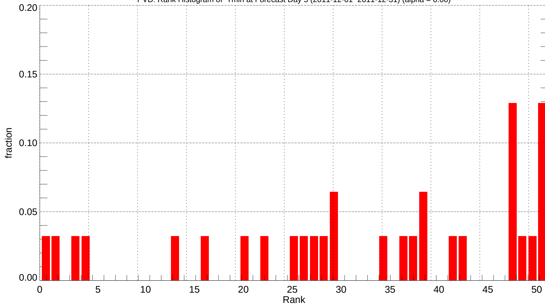
PVD: Rank Histogram of Tmin at Forecast Day 5 (2011-12-01~2011-12-31) (alpha = 0.00)
