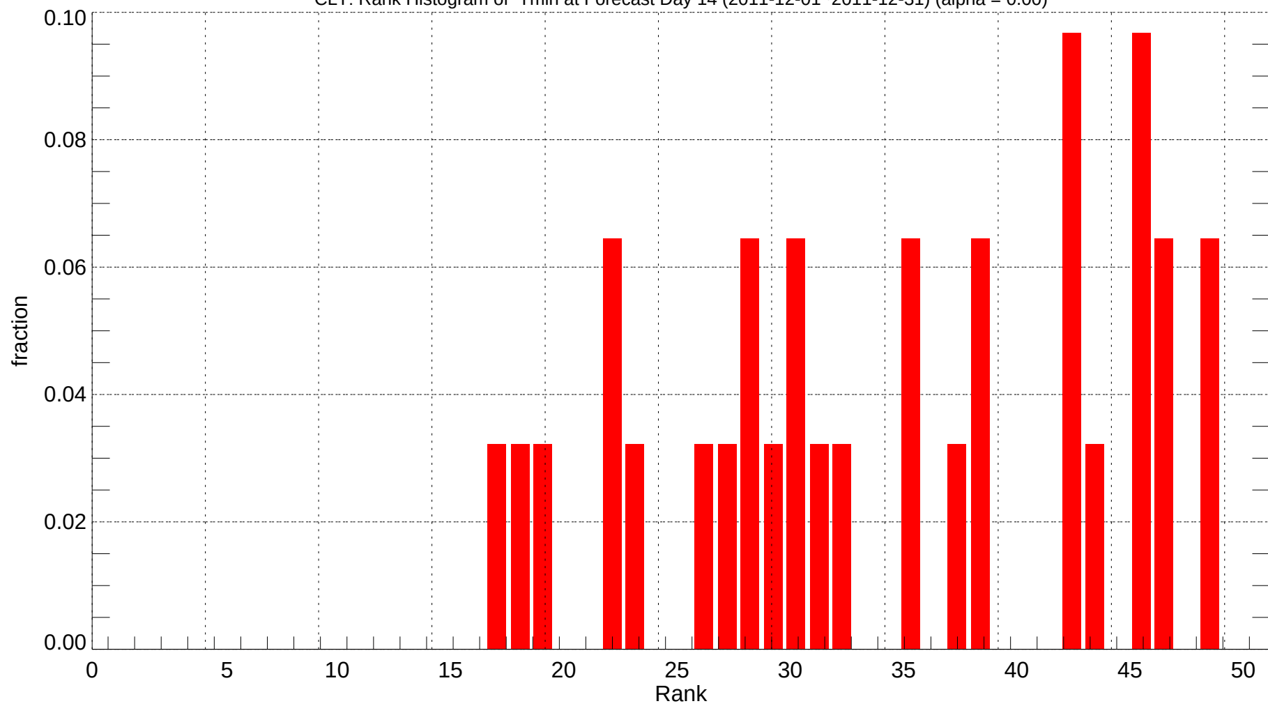
CLT: Rank Histogram of Tmin at Forecast Day 14 (2011-12-01~2011-12-31) (alpha = 0.00)
