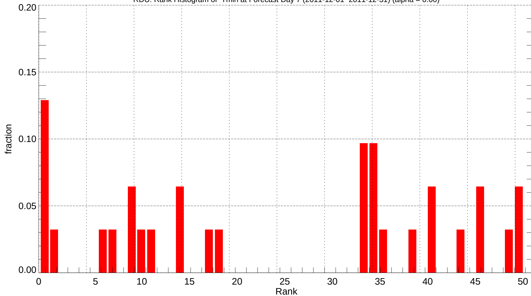
RDU: Rank Histogram of Tmin at Forecast Day 7 (2011-12-01~2011-12-31) (alpha = 0.00)
