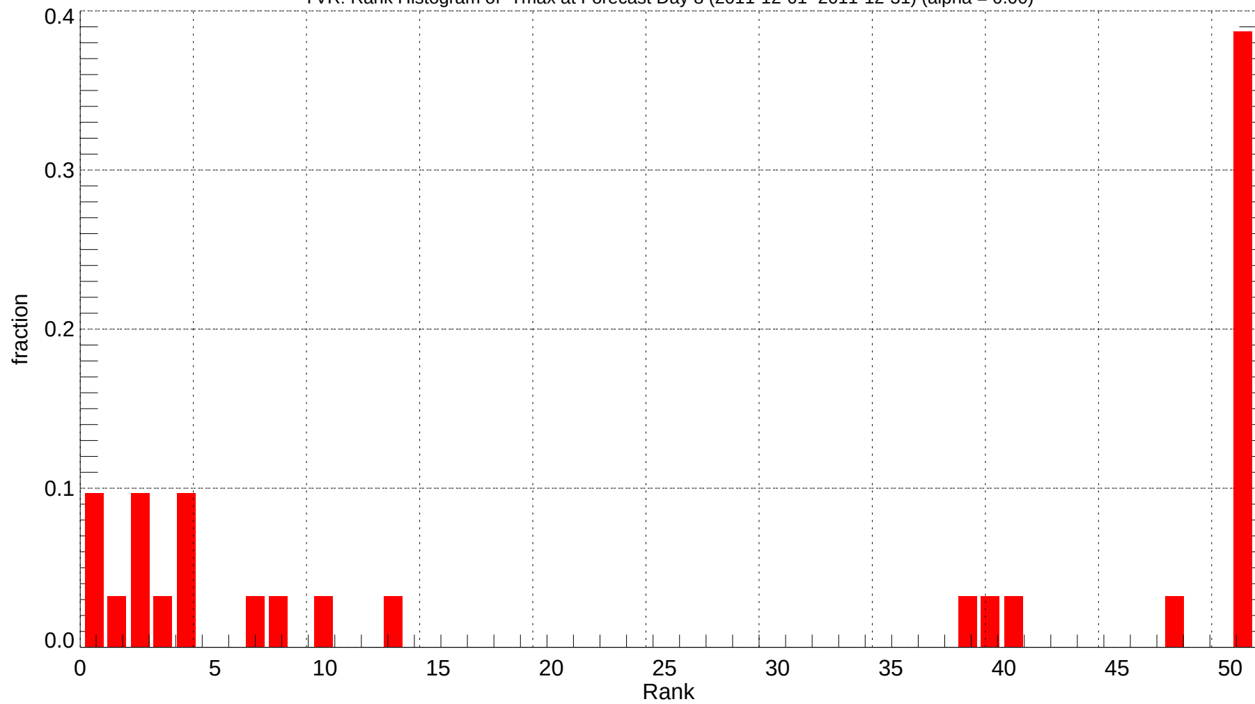
YVR: Rank Histogram of Tmax at Forecast Day 8 (2011-12-01~2011-12-31) (alpha = 0.00)
