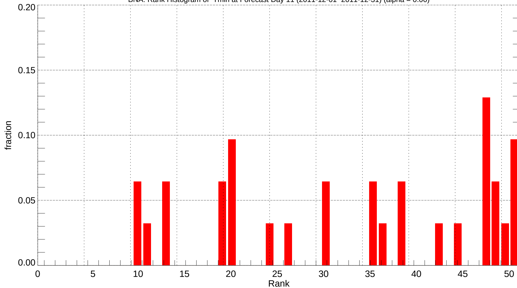
BNA: Rank Histogram of Tmin at Forecast Day 11 (2011-12-01~2011-12-31) (alpha = 0.00)
