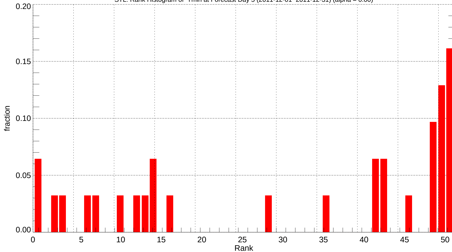
STL: Rank Histogram of Tmin at Forecast Day 5 (2011-12-01~2011-12-31) (alpha = 0.00)
