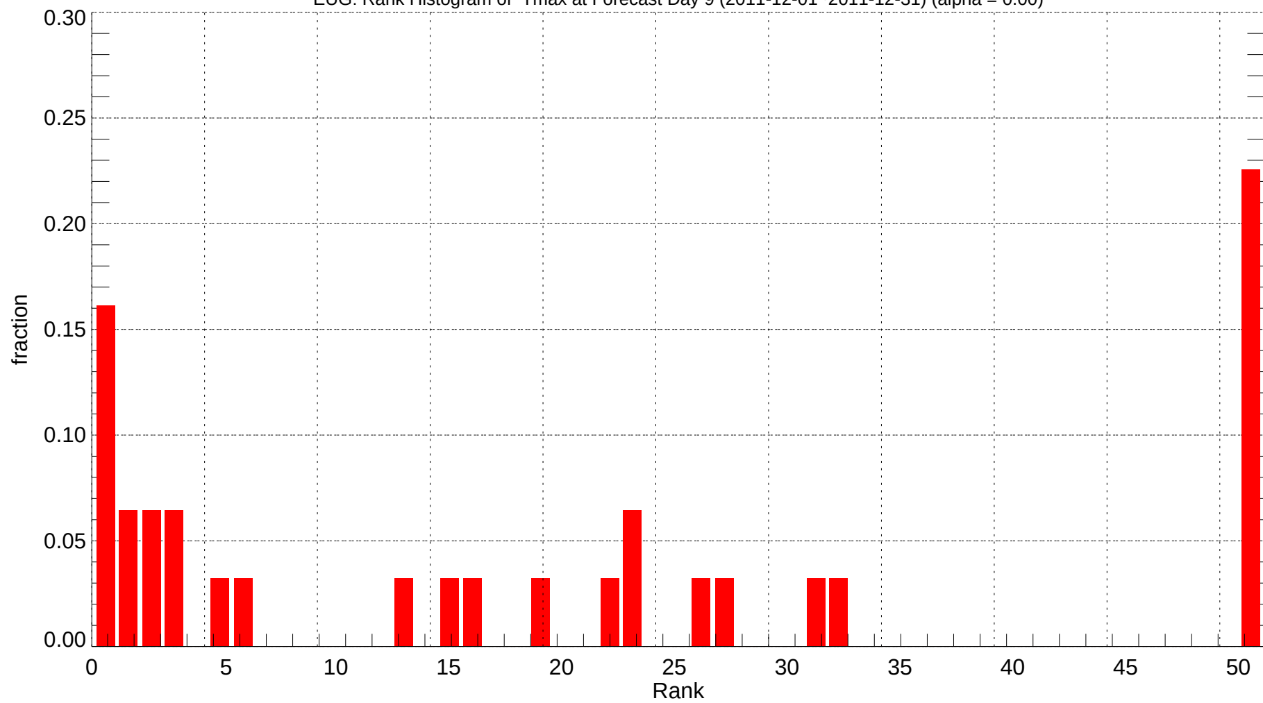
EUG: Rank Histogram of Tmax at Forecast Day 9 (2011-12-01~2011-12-31) (alpha = 0.00)
