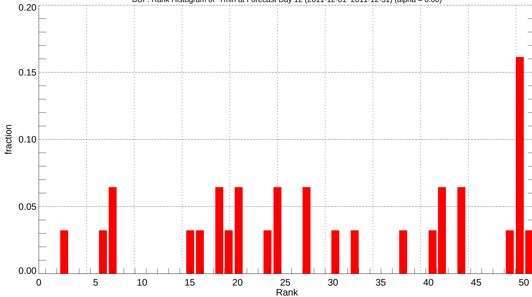
BUF: Rank Histogram of Tmin at Forecast Day 12 (2011-12-01~2011-12-31) (alpha = 0.00)
