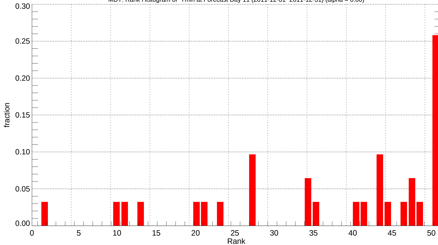
MDT: Rank Histogram of Tmin at Forecast Day 11 (2011-12-01~2011-12-31) (alpha = 0.00)
