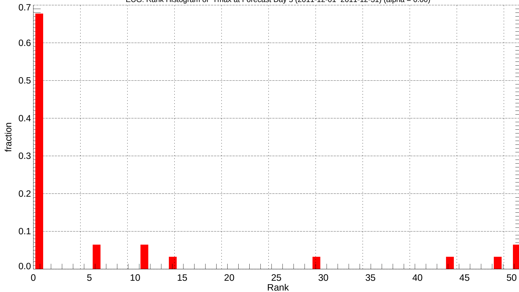
EUG: Rank Histogram of Tmax at Forecast Day 5 (2011-12-01~2011-12-31) (alpha = 0.00)
