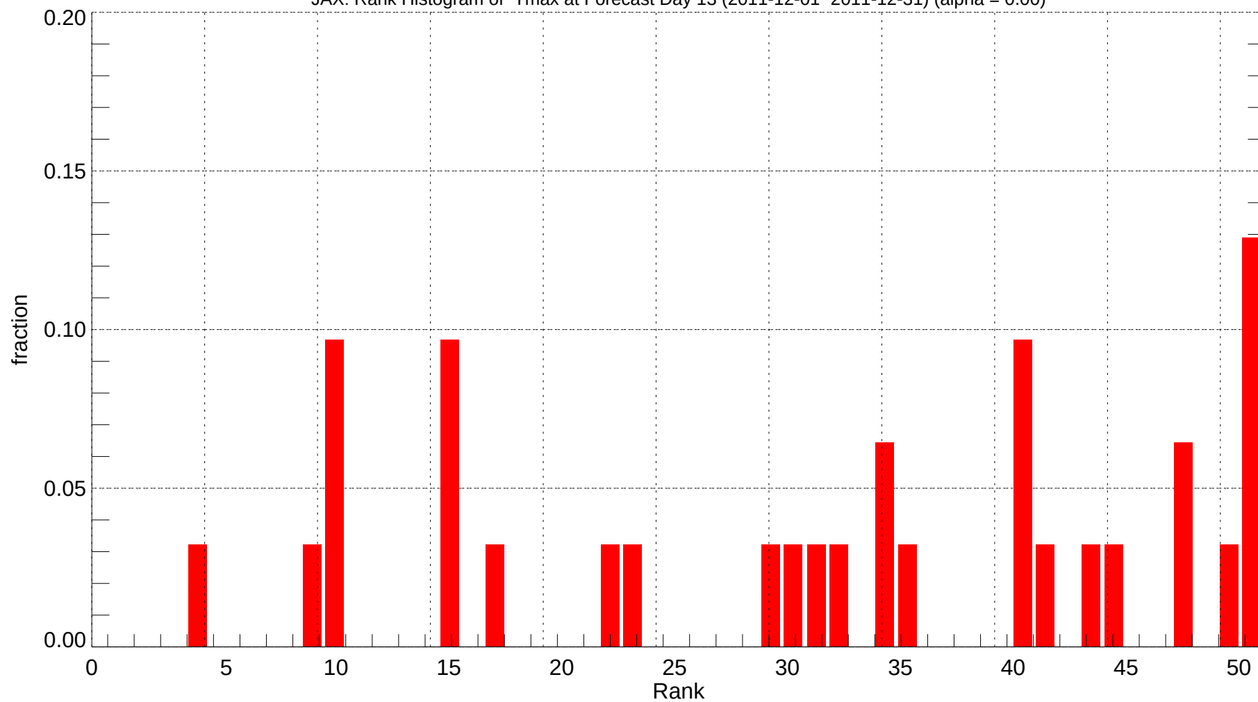
JAX: Rank Histogram of Tmax at Forecast Day 13 (2011-12-01~2011-12-31) (alpha = 0.00)
