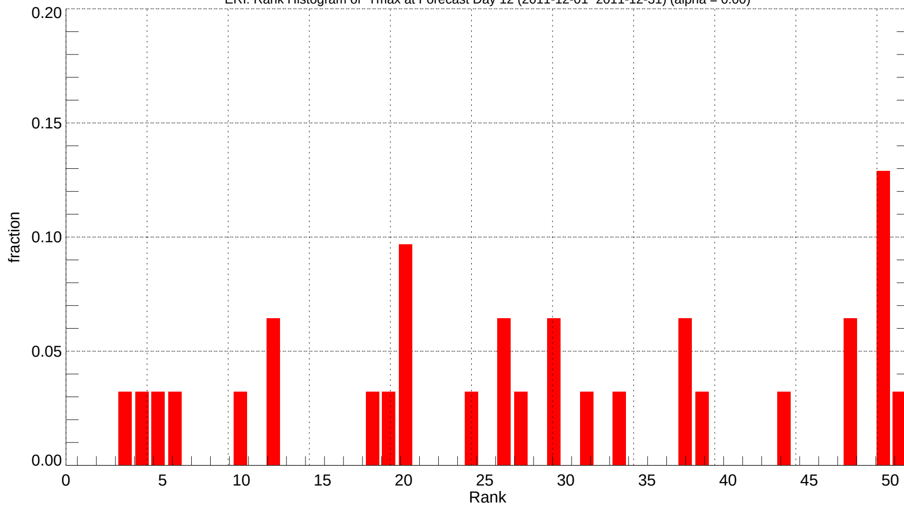
ERI: Rank Histogram of Tmax at Forecast Day 12 (2011-12-01~2011-12-31) (alpha = 0.00)
