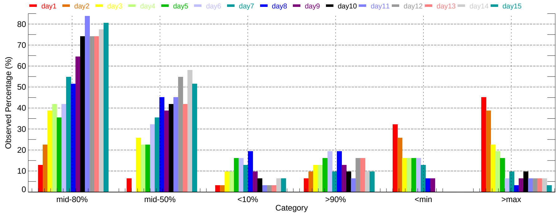
Observed Percentage of Ensembles - CON: Min Temperature (2011-12-01~2011-12-31)
