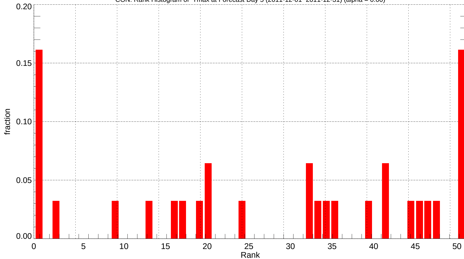
CON: Rank Histogram of Tmax at Forecast Day 5 (2011-12-01~2011-12-31) (alpha = 0.00)
