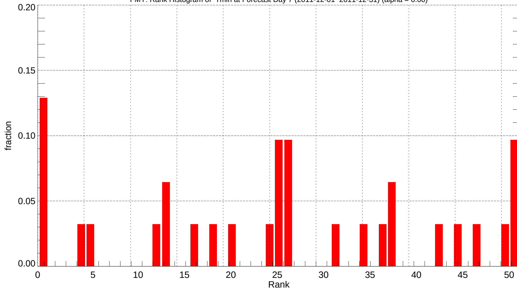
FMY: Rank Histogram of Tmin at Forecast Day 7 (2011-12-01~2011-12-31) (alpha = 0.00)
