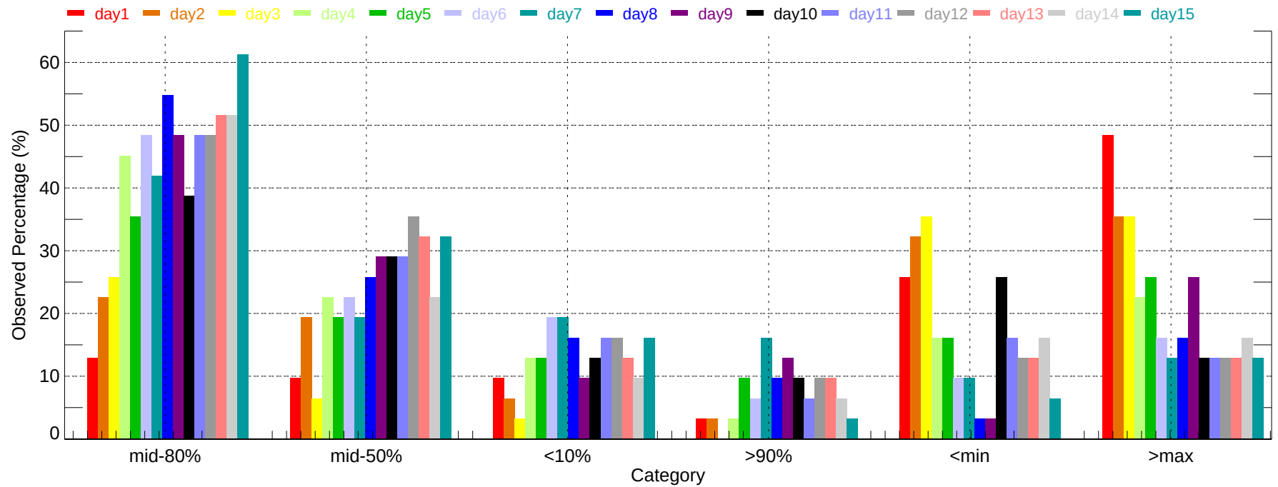
Observed Percentage of Ensembles - PDX: Max Temperature (2011-12-01~2011-12-31)
