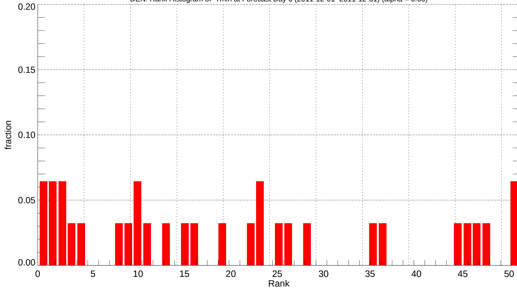
DEN: Rank Histogram of Tmin at Forecast Day 6 (2011-12-01~2011-12-31) (alpha = 0.00)
