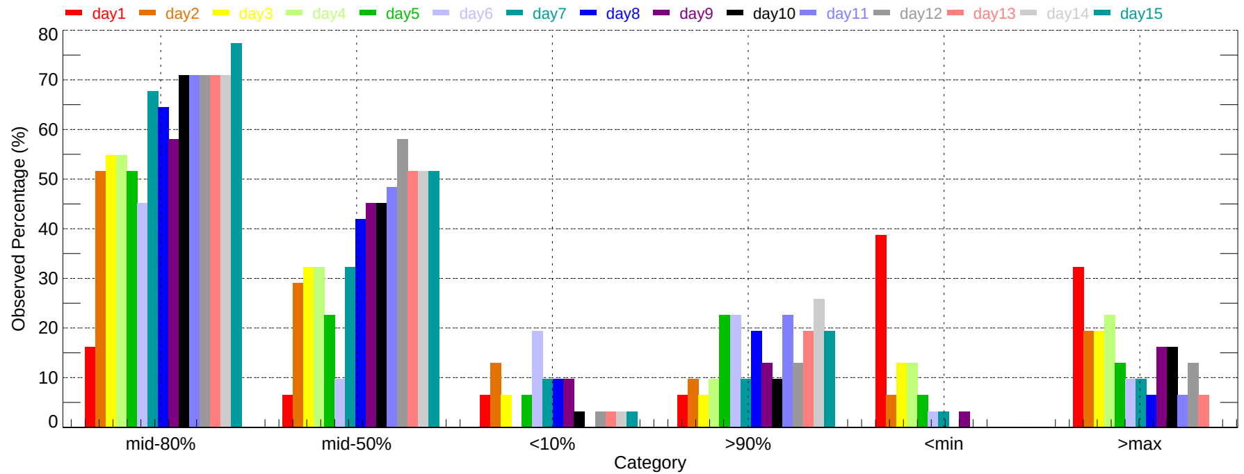
Observed Percentage of Ensembles - STL: Min Temperature (2011-12-01~2011-12-31)
