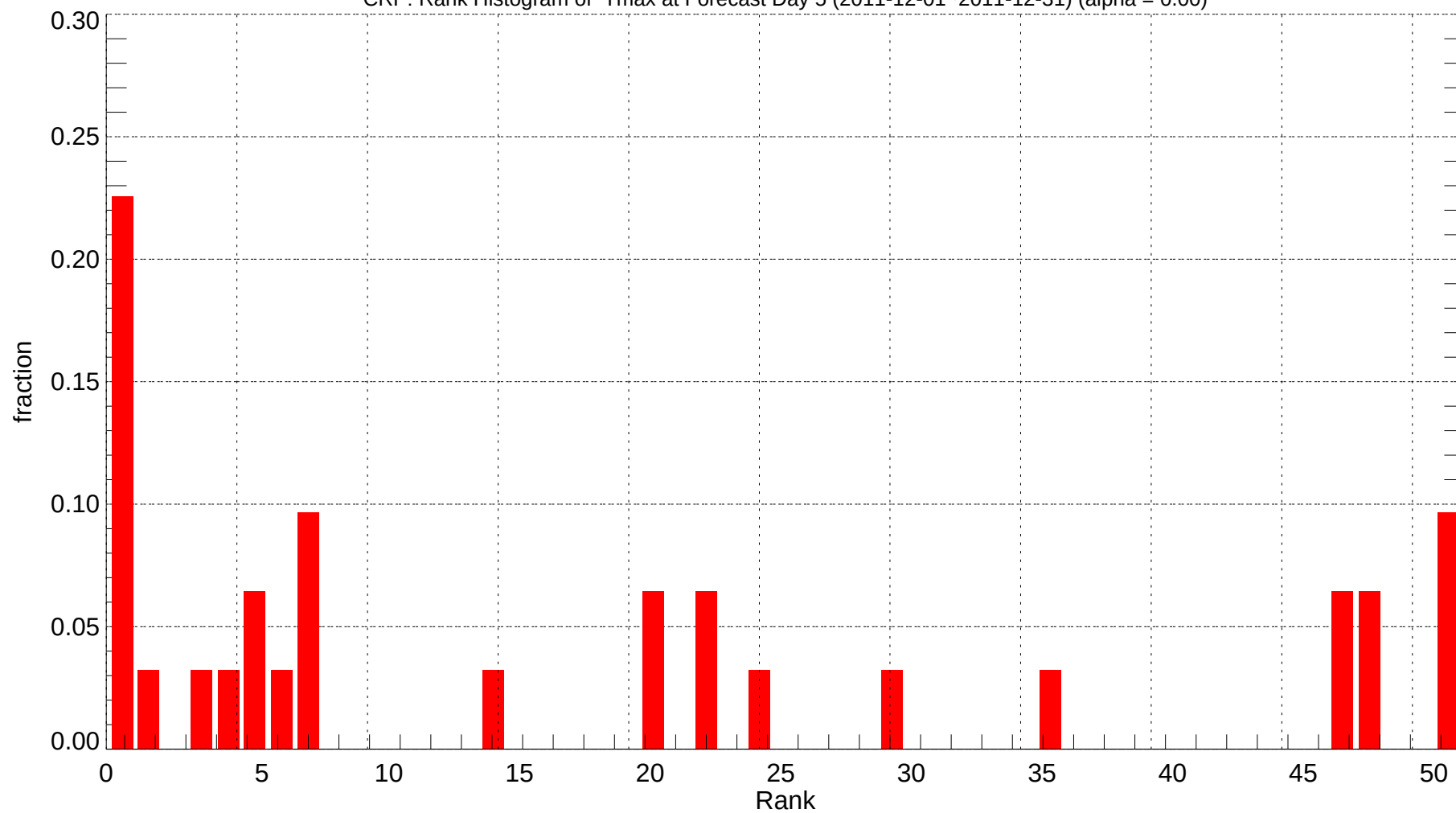
CRP: Rank Histogram of Tmax at Forecast Day 5 (2011-12-01~2011-12-31) (alpha = 0.00)
