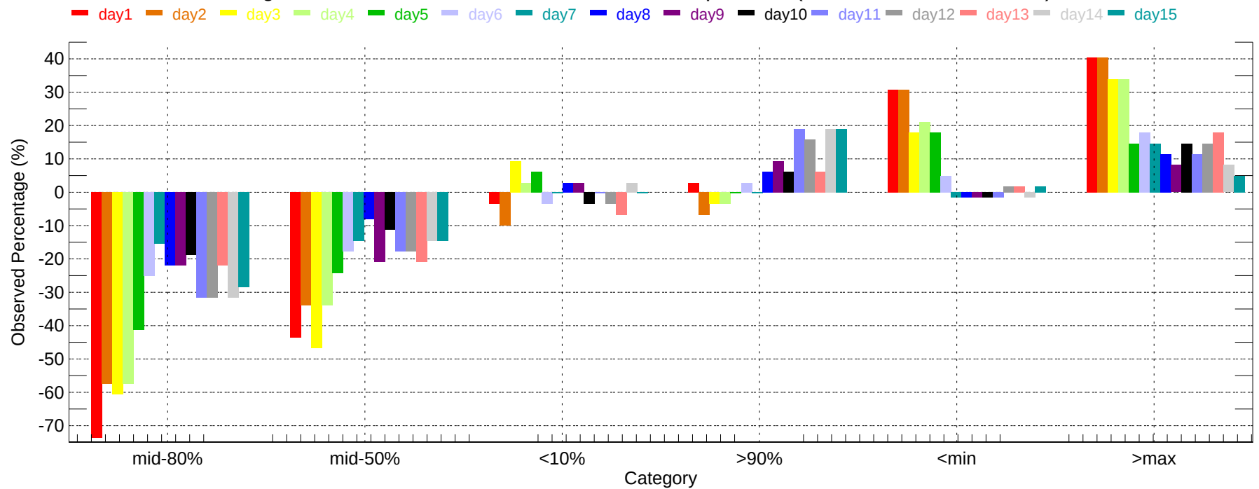
Observed Percentage Deviation of Ensembles - OMA: Max Temperature (2011-12-01~2011-12-31)
