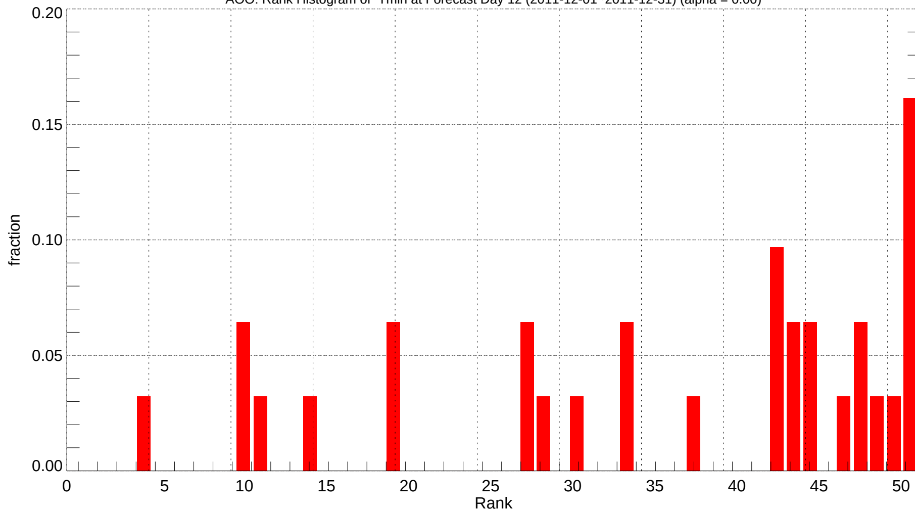
AOO: Rank Histogram of Tmin at Forecast Day 12 (2011-12-01~2011-12-31) (alpha = 0.00)
