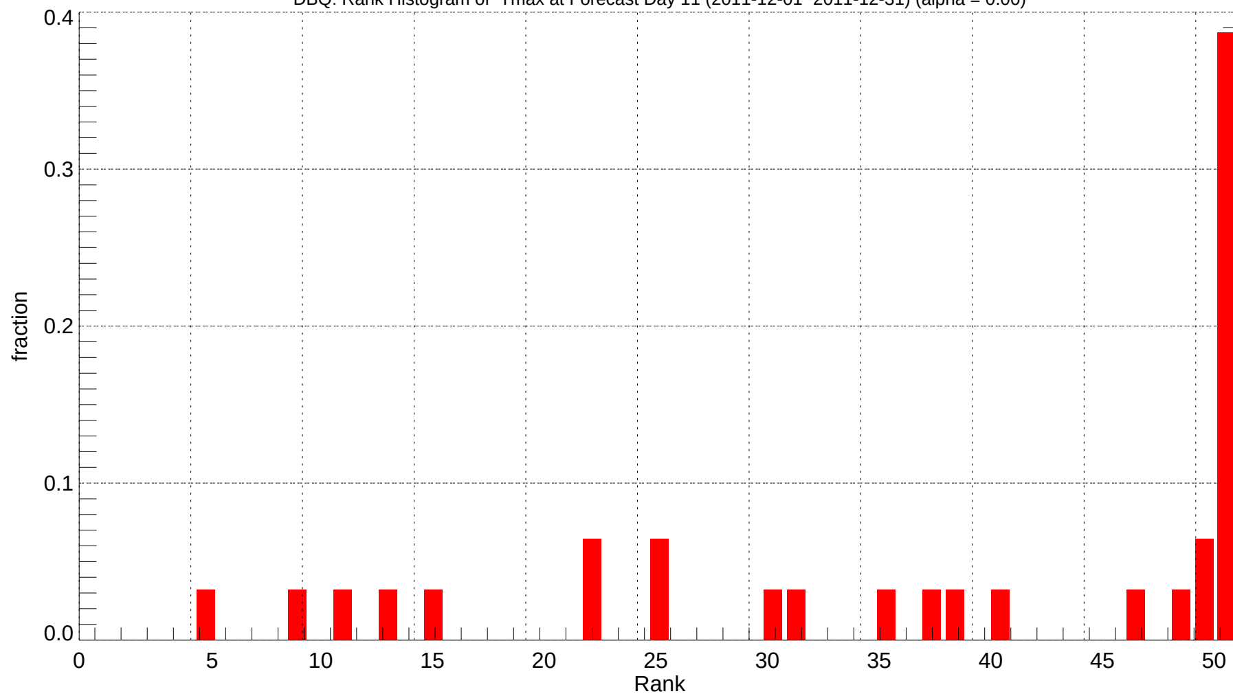
DBQ: Rank Histogram of Tmax at Forecast Day 11 (2011-12-01~2011-12-31) (alpha = 0.00)
