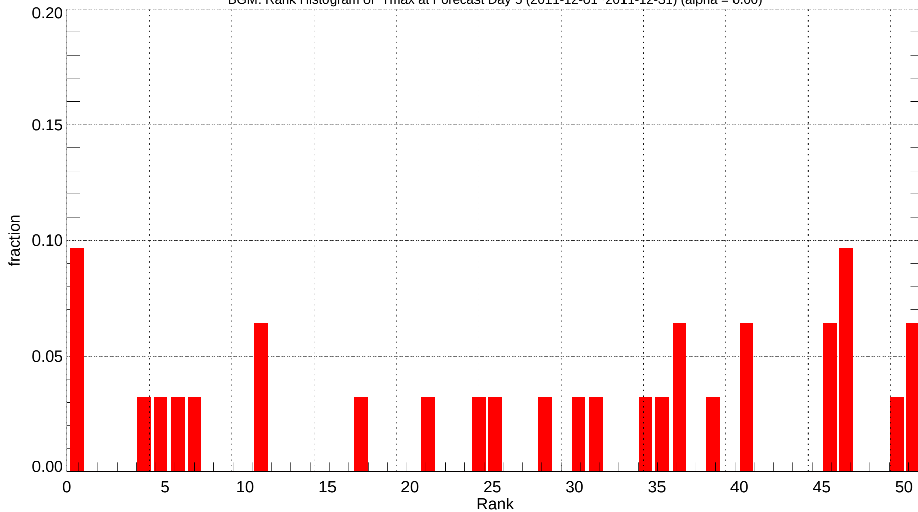
BGM: Rank Histogram of Tmax at Forecast Day 5 (2011-12-01~2011-12-31) (alpha = 0.00)
