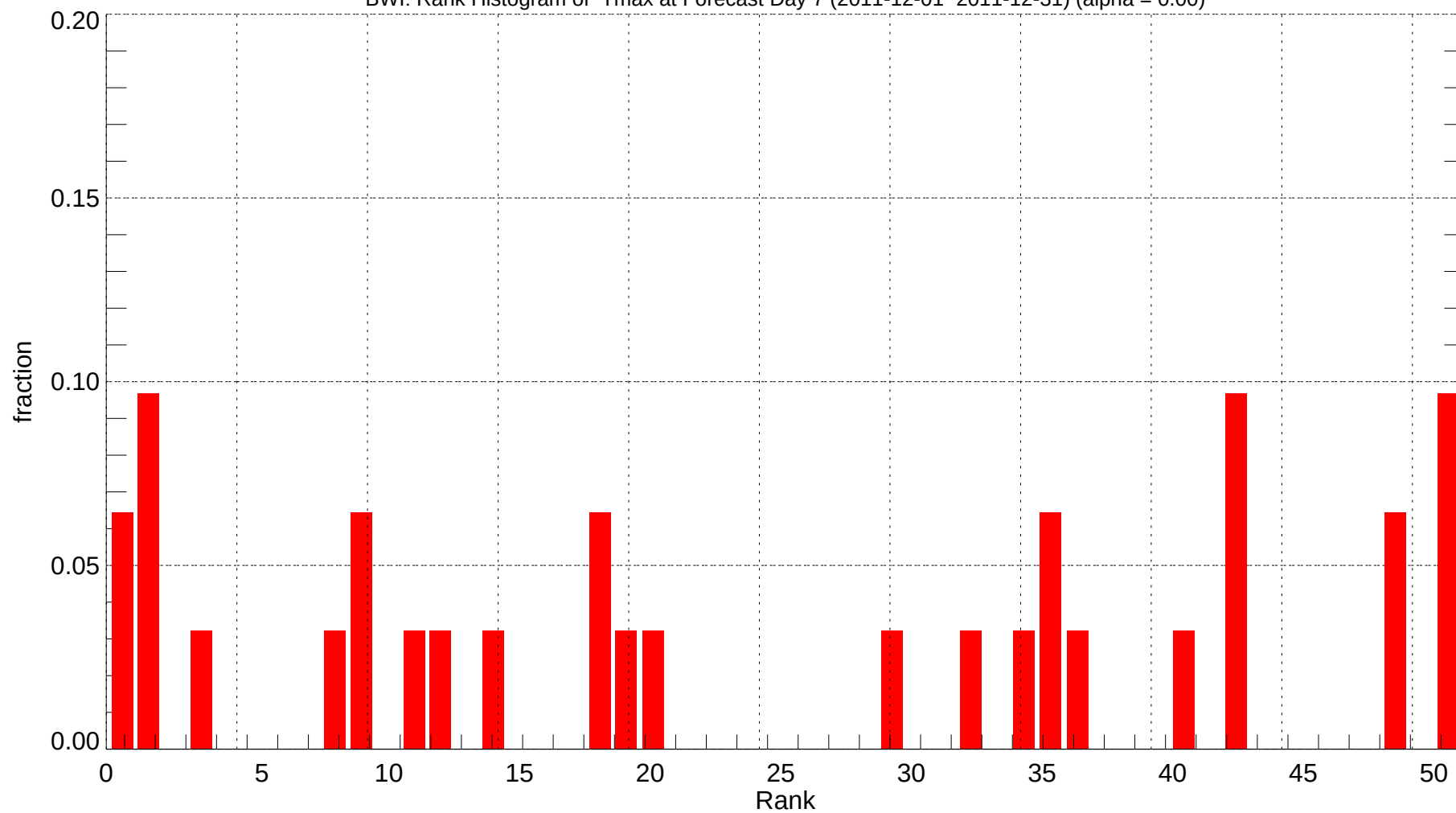
BWI: Rank Histogram of Tmax at Forecast Day 7 (2011-12-01~2011-12-31) (alpha = 0.00)
