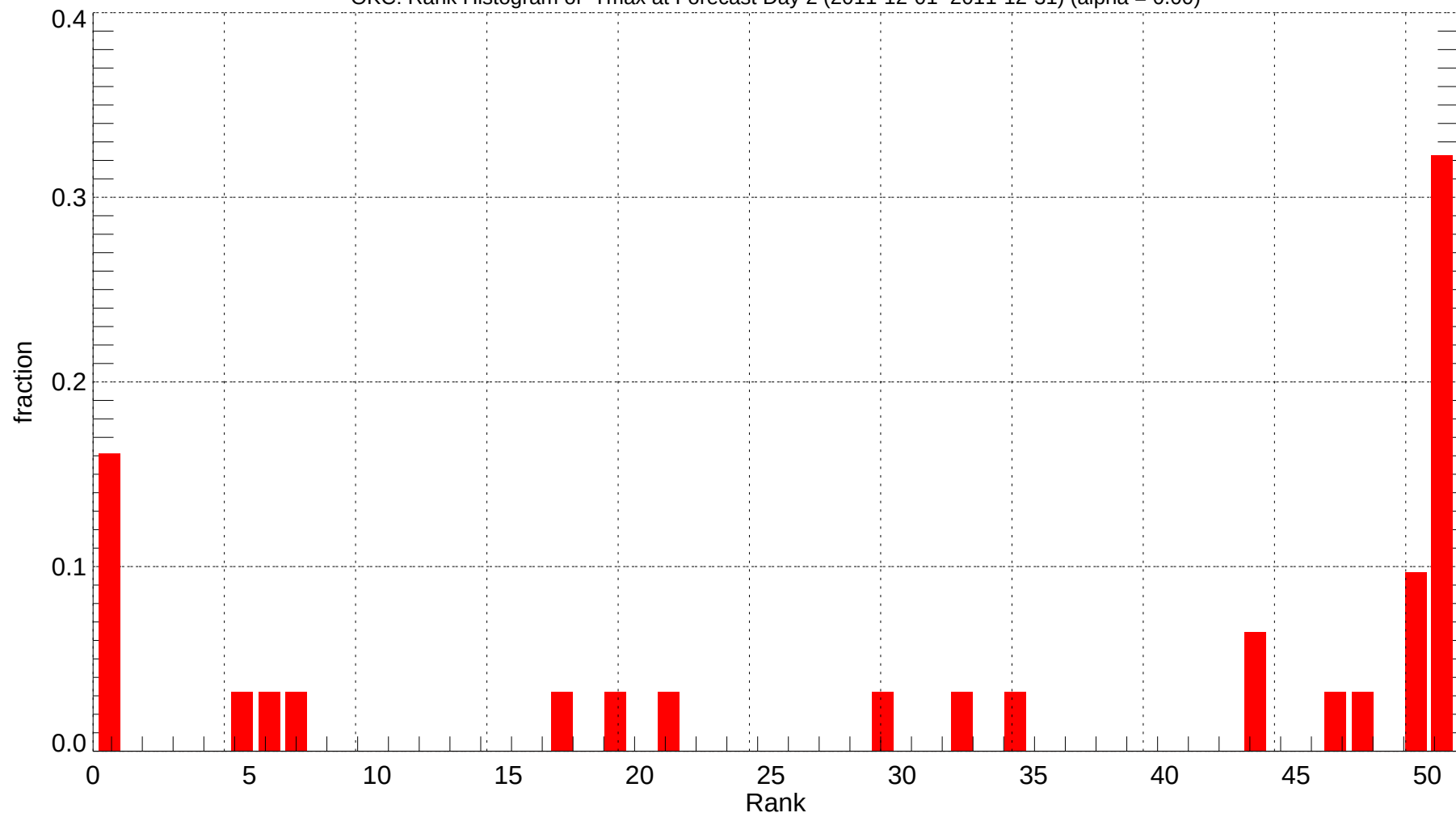
OKC: Rank Histogram of Tmax at Forecast Day 2 (2011-12-01~2011-12-31) (alpha = 0.00)
