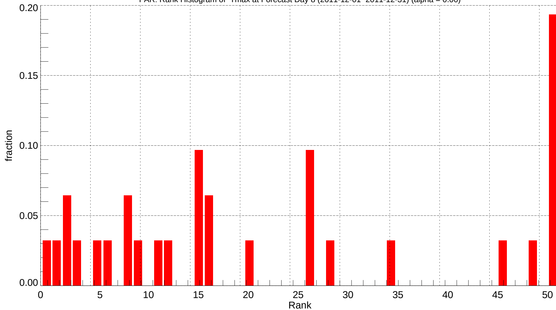
FAR: Rank Histogram of Tmax at Forecast Day 8 (2011-12-01~2011-12-31) (alpha = 0.00)
