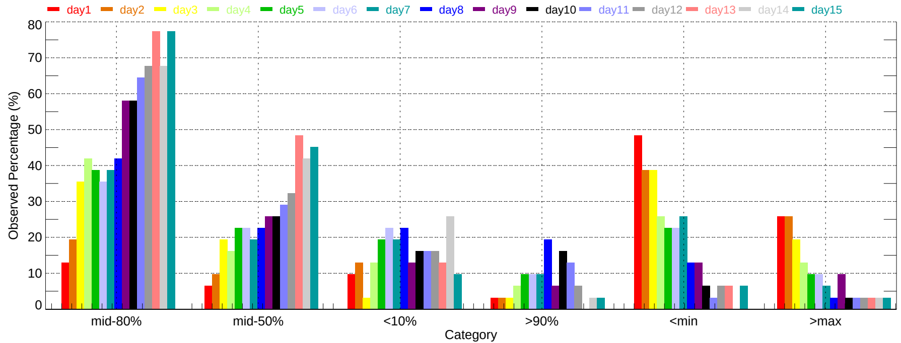
Observed Percentage of Ensembles - YYZ: Max Temperature (2011-12-01~2011-12-31)
