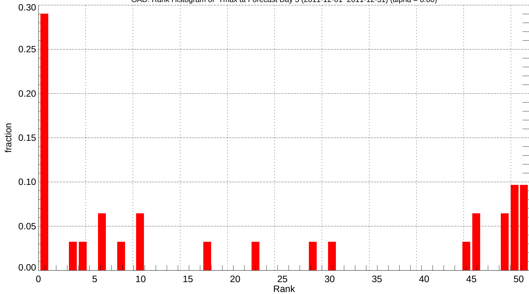
GAD: Rank Histogram of Tmax at Forecast Day 3 (2011-12-01~2011-12-31) (alpha = 0.00)
