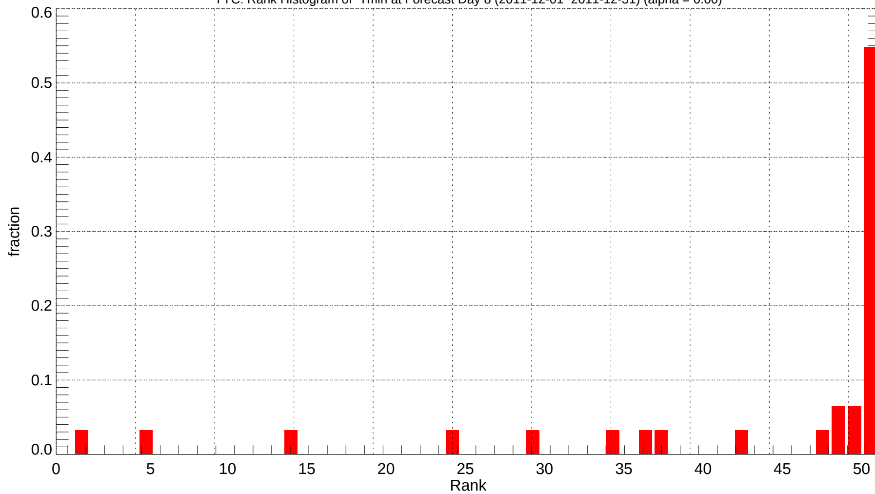
YYC: Rank Histogram of Tmin at Forecast Day 8 (2011-12-01~2011-12-31) (alpha = 0.00)
