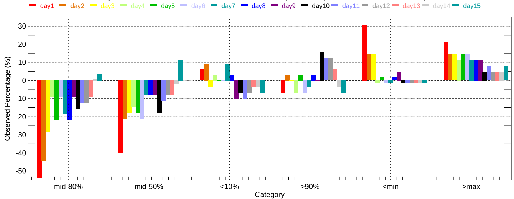
Observed Percentage Deviation of Ensembles - MCN: Min Temperature (2011-12-01~2011-12-31)
