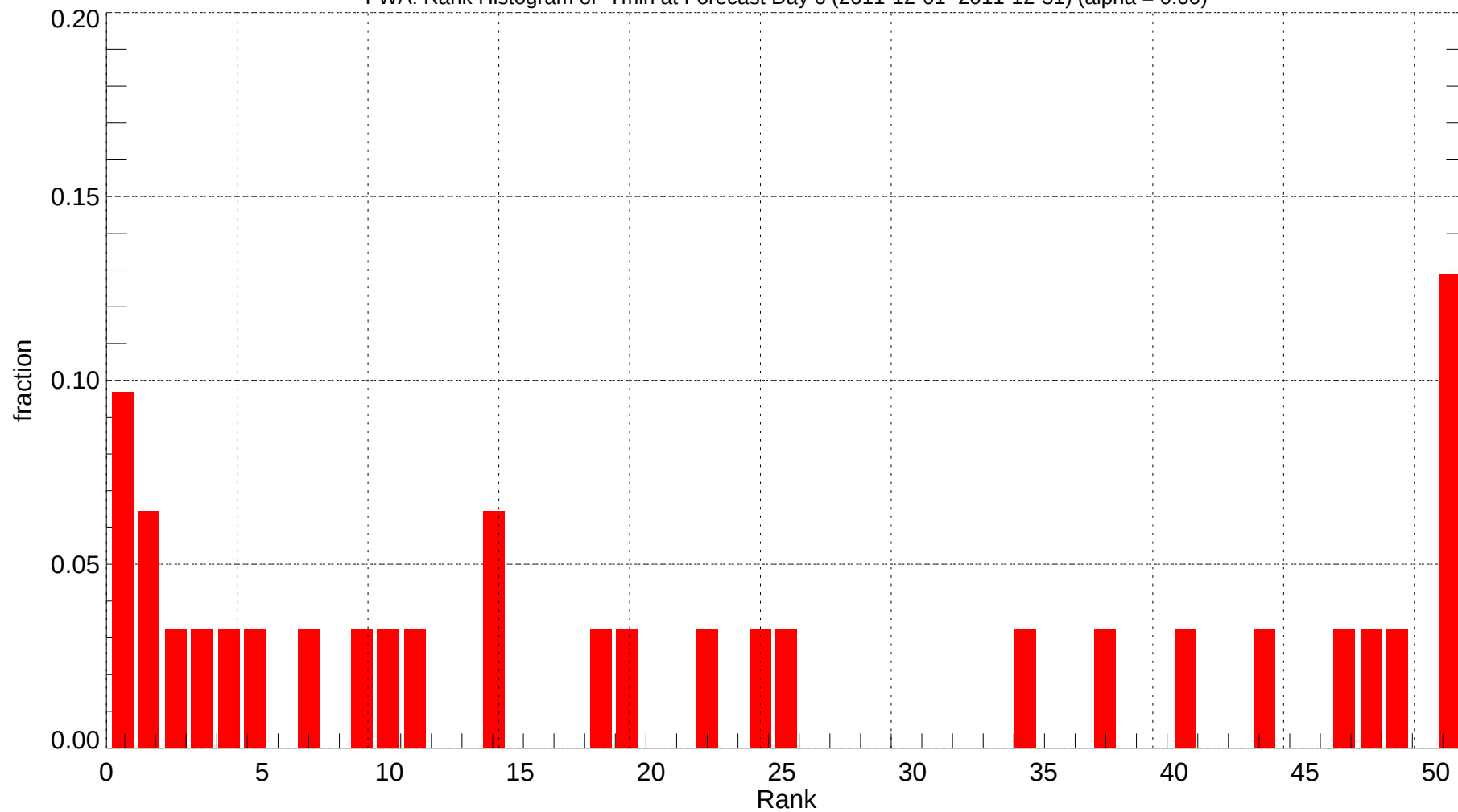
FWA: Rank Histogram of Tmin at Forecast Day 6 (2011-12-01~2011-12-31) (alpha = 0.00)
