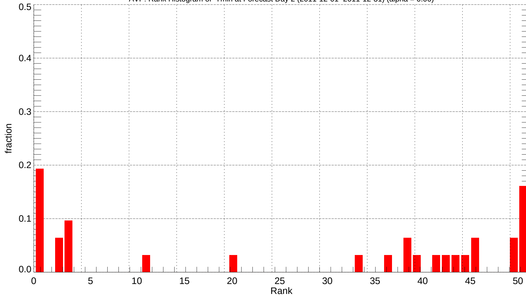
AVP: Rank Histogram of Tmin at Forecast Day 2 (2011-12-01~2011-12-31) (alpha = 0.00)
