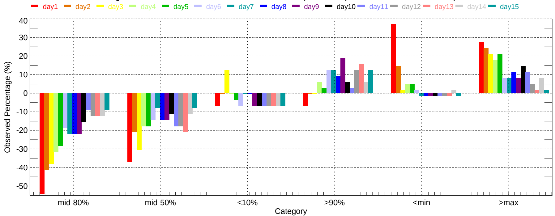
Observed Percentage Deviation of Ensembles - MCI: Min Temperature (2011-12-01~2011-12-31)
