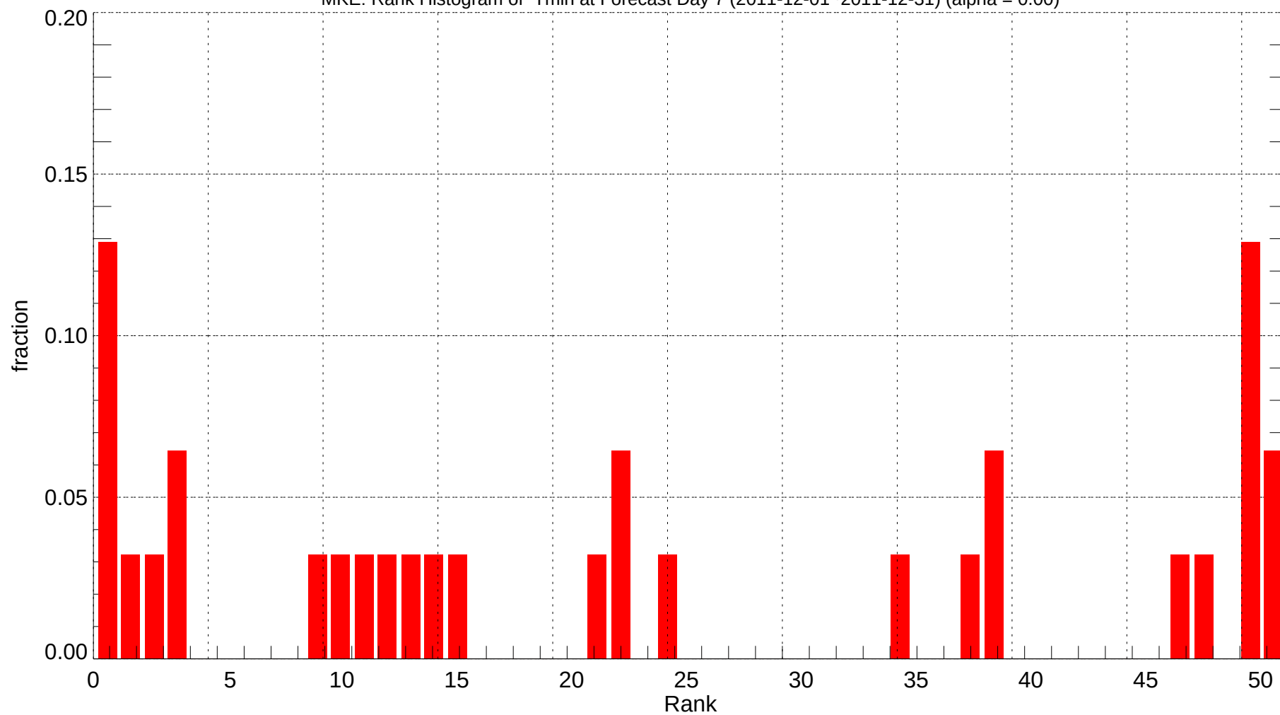
MKE: Rank Histogram of Tmin at Forecast Day 7 (2011-12-01~2011-12-31) (alpha = 0.00)
