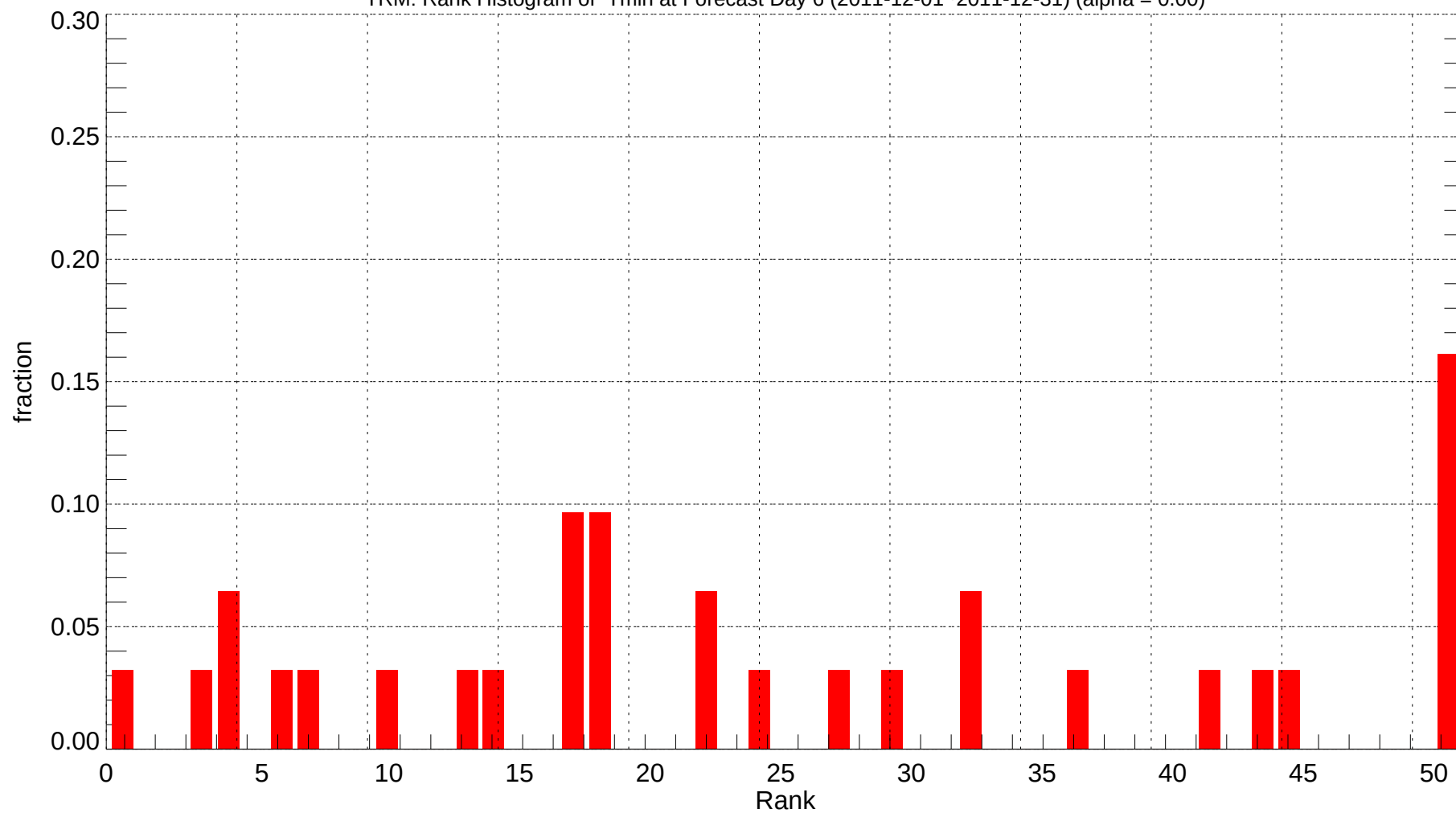
TRM: Rank Histogram of Tmin at Forecast Day 6 (2011-12-01~2011-12-31) (alpha = 0.00)
