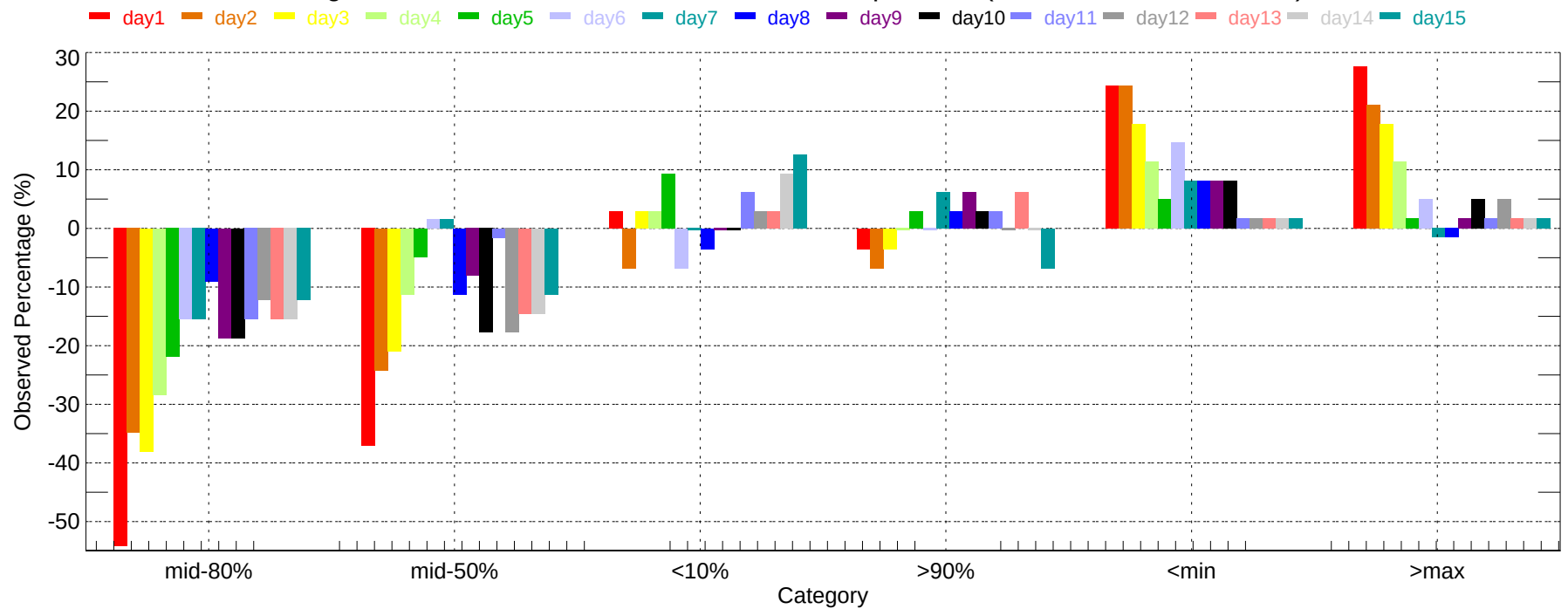
Observed Percentage Deviation of Ensembles - AUS: Max Temperature (2011-12-01~2011-12-31)
