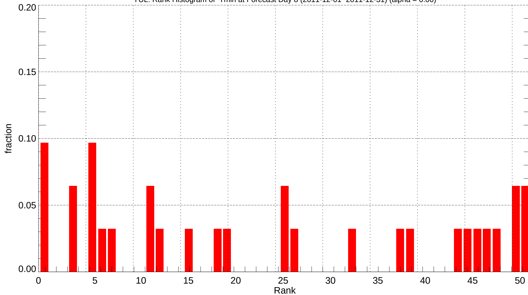
YUL: Rank Histogram of Tmin at Forecast Day 8 (2011-12-01~2011-12-31) (alpha = 0.00)
