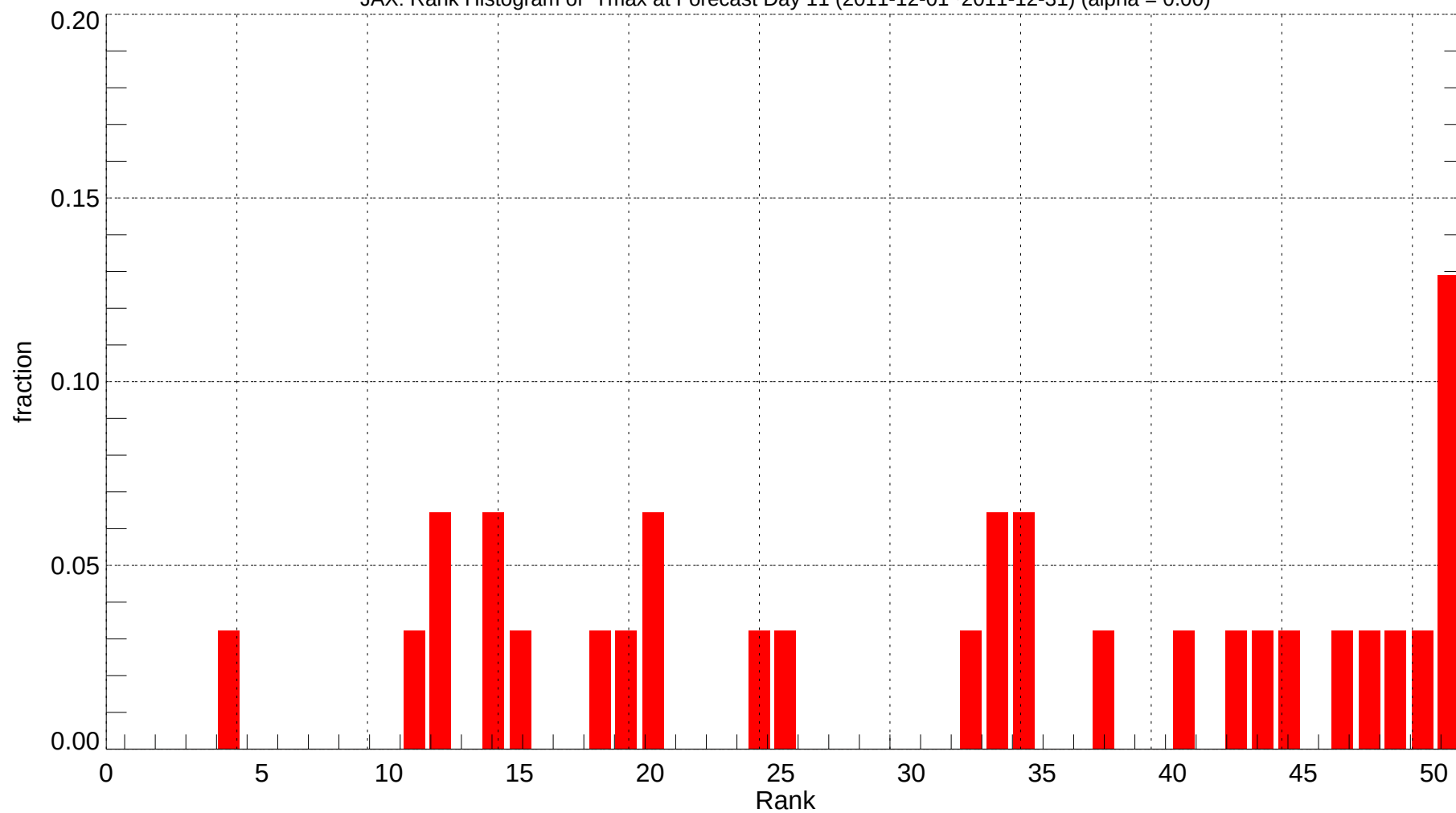
JAX: Rank Histogram of Tmax at Forecast Day 11 (2011-12-01~2011-12-31) (alpha = 0.00)
