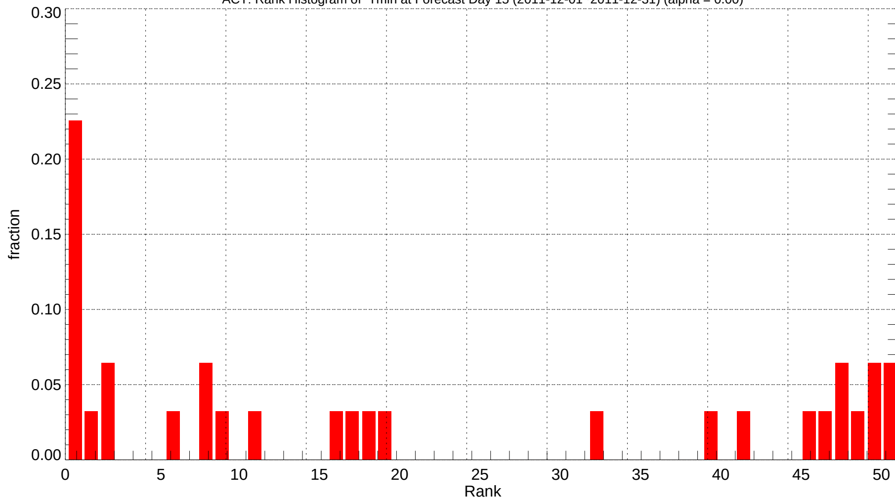
ACT: Rank Histogram of Tmin at Forecast Day 15 (2011-12-01~2011-12-31) (alpha = 0.00)
