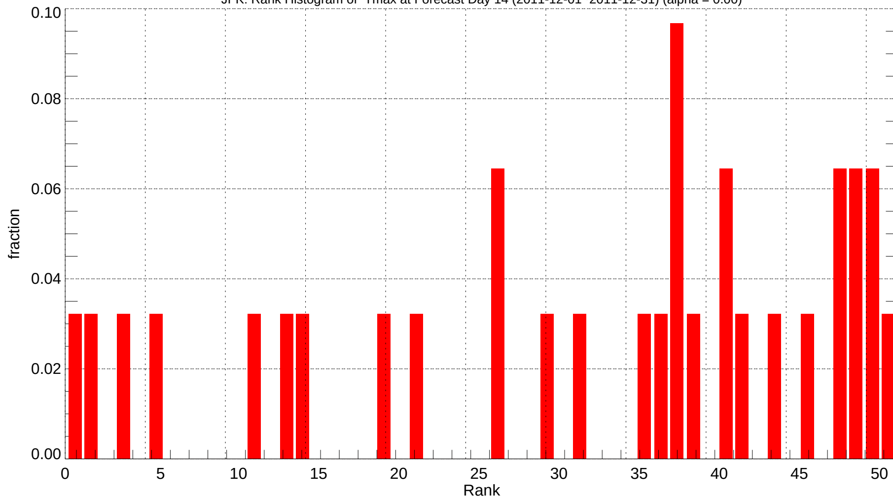
JFK: Rank Histogram of Tmax at Forecast Day 14 (2011-12-01~2011-12-31) (alpha = 0.00)
