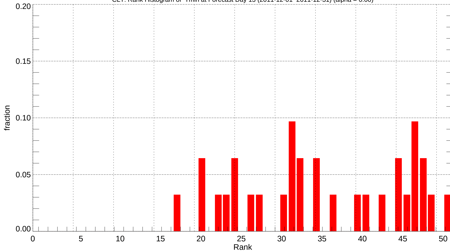
CLT: Rank Histogram of Tmin at Forecast Day 13 (2011-12-01~2011-12-31) (alpha = 0.00)
