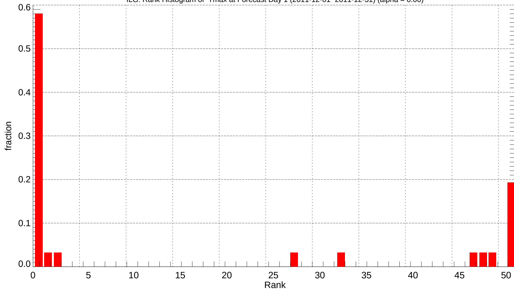
ILG: Rank Histogram of Tmax at Forecast Day 1 (2011-12-01~2011-12-31) (alpha = 0.00)
