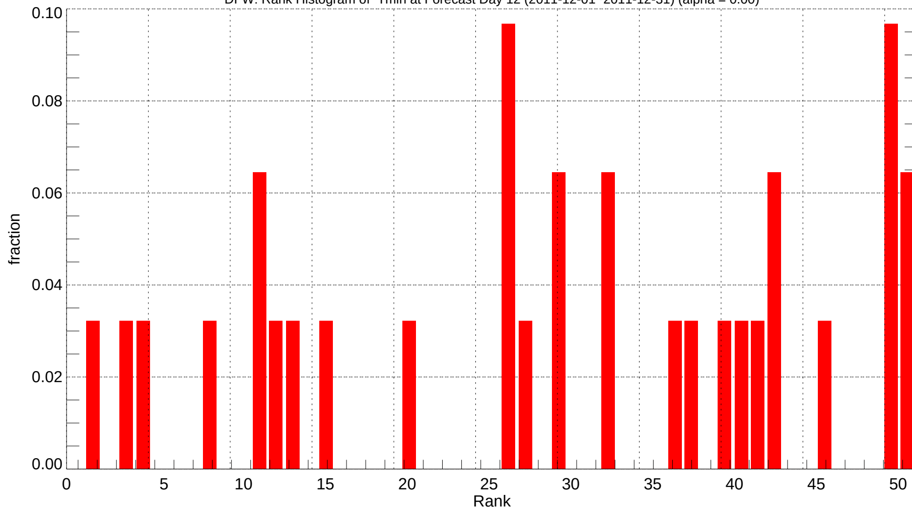
DFW: Rank Histogram of Tmin at Forecast Day 12 (2011-12-01~2011-12-31) (alpha = 0.00)
