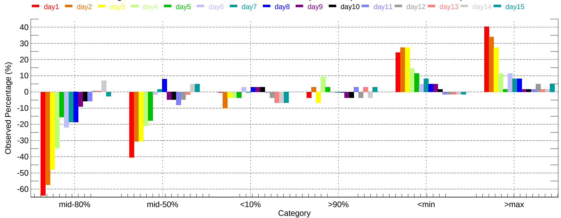
Observed Percentage Deviation of Ensembles - SEA: Min Temperature (2011-12-01~2011-12-31)
