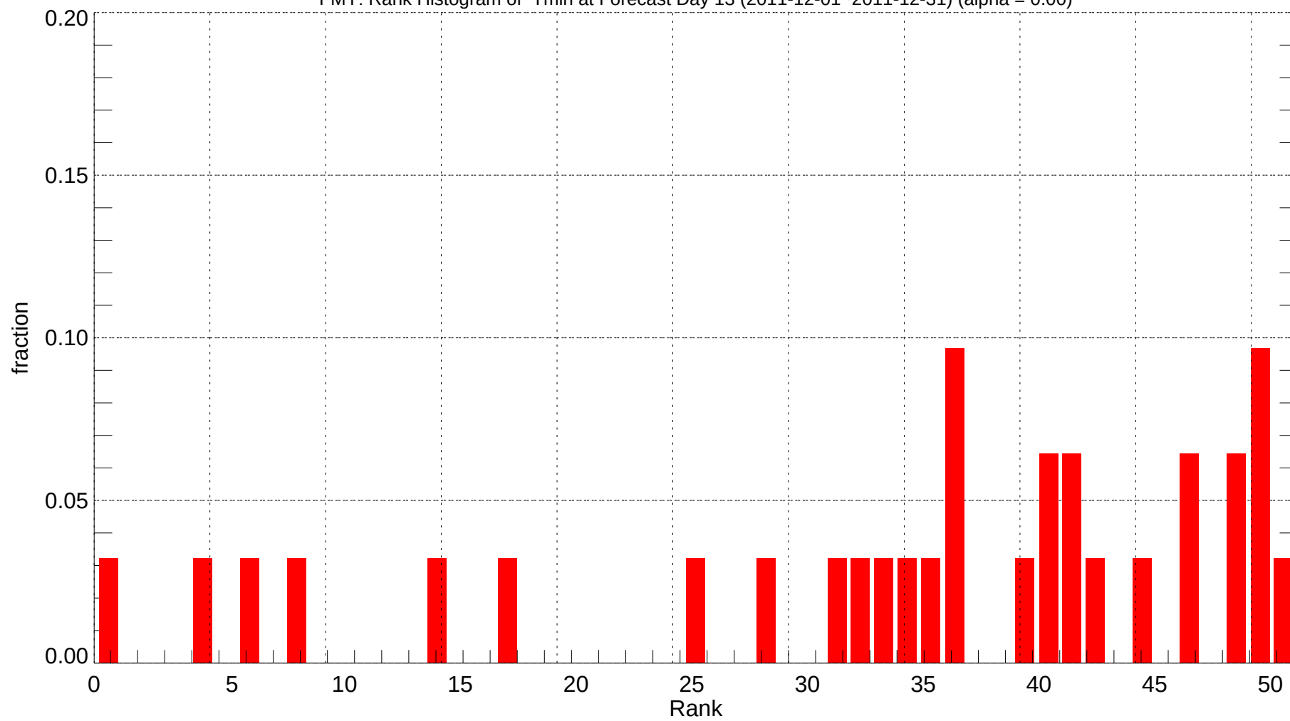
FMY: Rank Histogram of Tmin at Forecast Day 13 (2011-12-01~2011-12-31) (alpha = 0.00)
