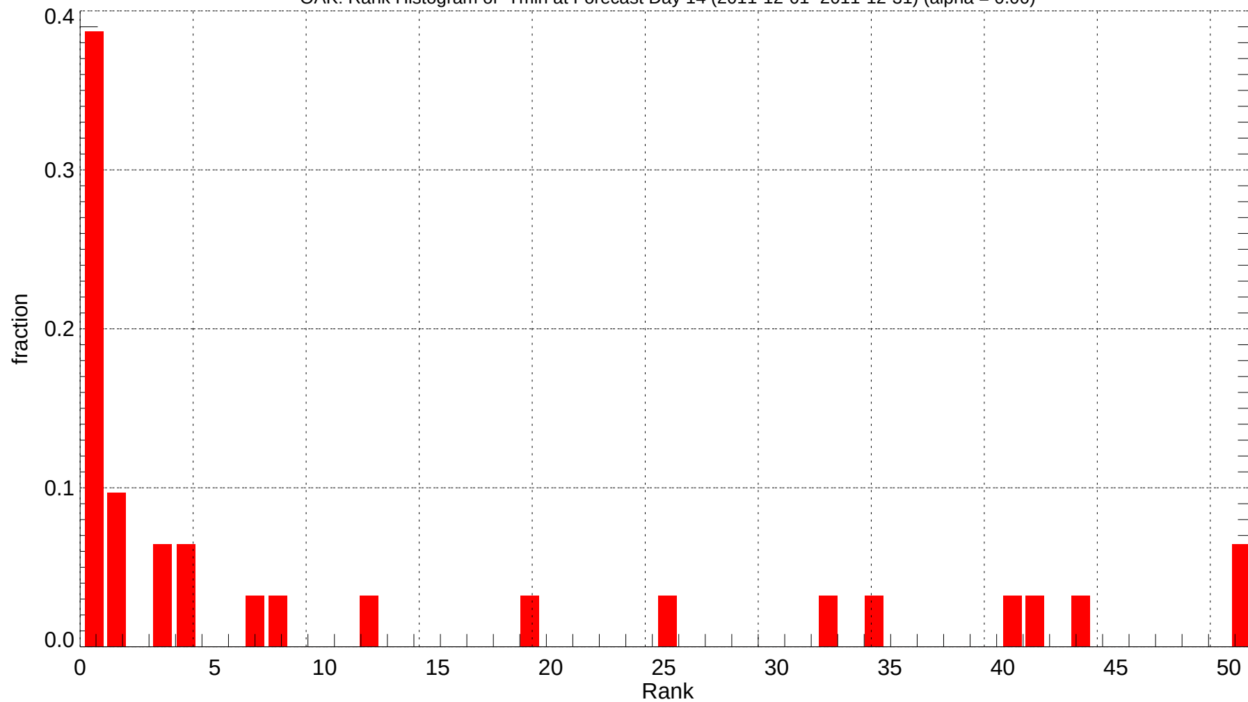
OAK: Rank Histogram of Tmin at Forecast Day 14 (2011-12-01~2011-12-31) (alpha = 0.00)
