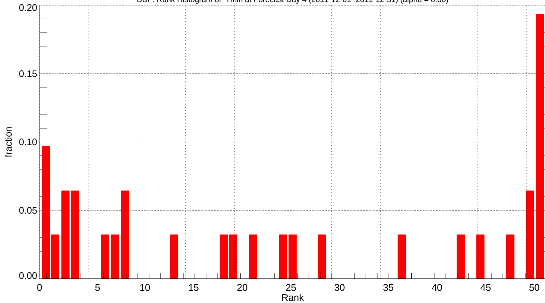
BUF: Rank Histogram of Tmin at Forecast Day 4 (2011-12-01~2011-12-31) (alpha = 0.00)
