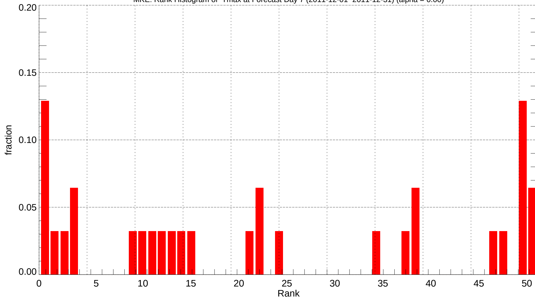
MKE: Rank Histogram of Tmax at Forecast Day 7 (2011-12-01~2011-12-31) (alpha = 0.00)
