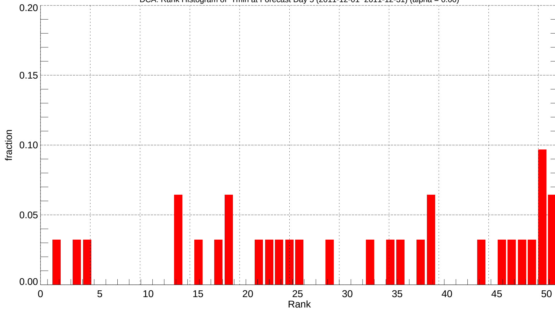
DCA: Rank Histogram of Tmin at Forecast Day 5 (2011-12-01~2011-12-31) (alpha = 0.00)
