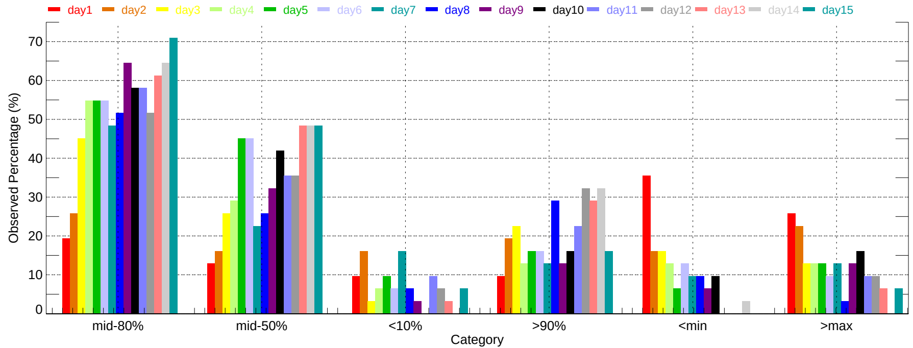
Observed Percentage of Ensembles - ACY: Max Temperature (2011-12-01~2011-12-31)
