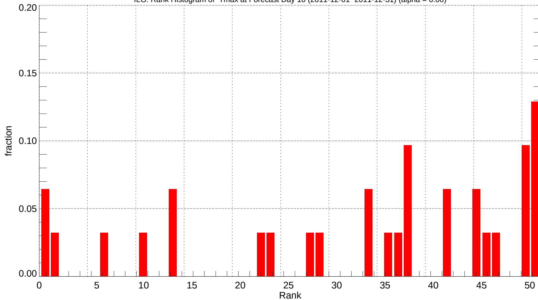
ILG: Rank Histogram of Tmax at Forecast Day 10 (2011-12-01~2011-12-31) (alpha = 0.00)
