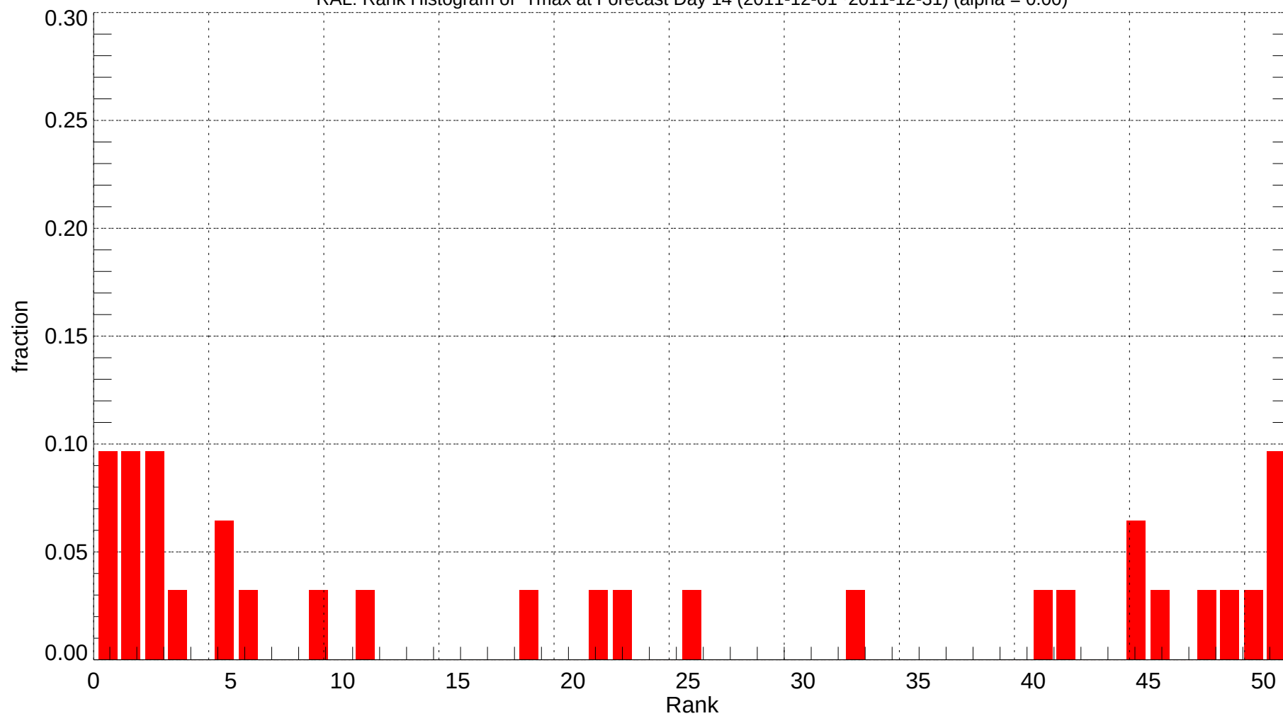
RAL: Rank Histogram of Tmax at Forecast Day 14 (2011-12-01~2011-12-31) (alpha = 0.00)
