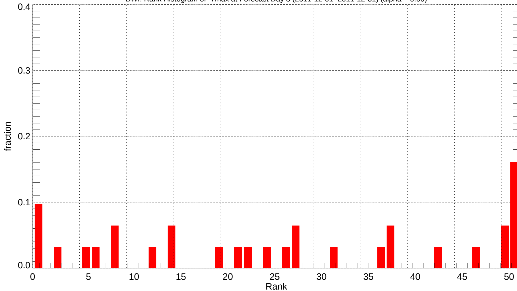
BWI: Rank Histogram of Tmax at Forecast Day 3 (2011-12-01~2011-12-31) (alpha = 0.00)
