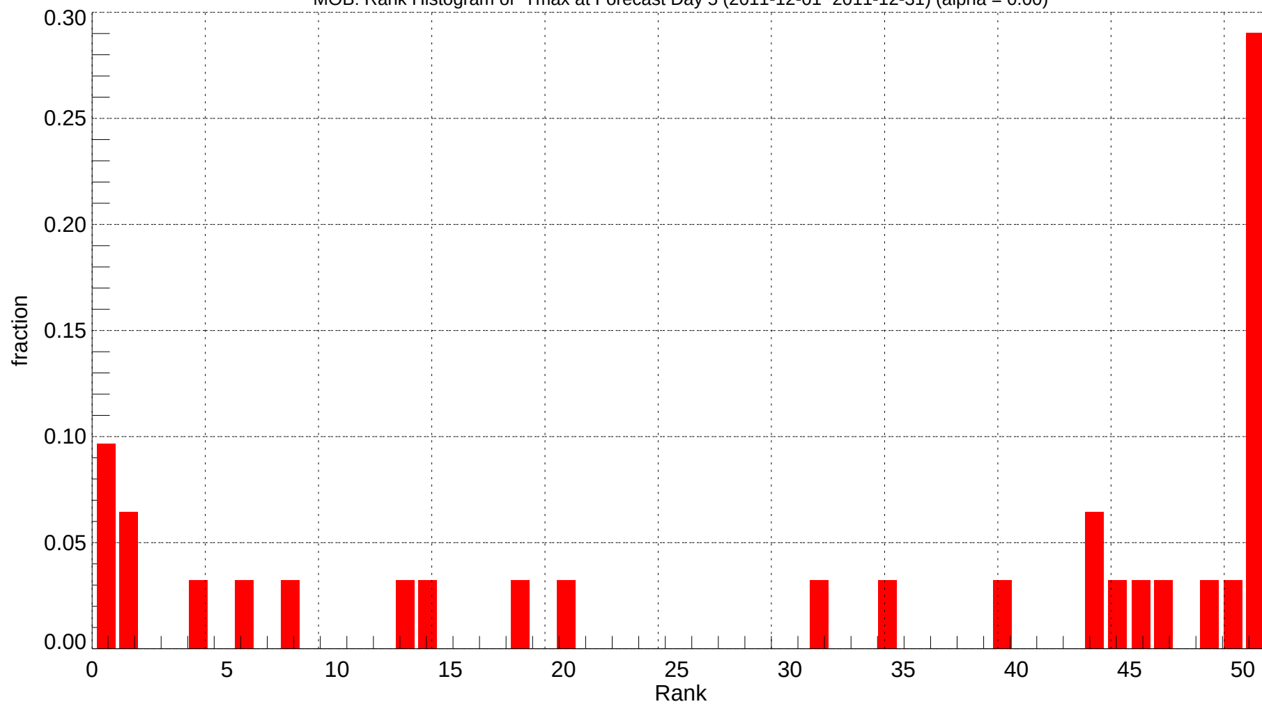
MOB: Rank Histogram of Tmax at Forecast Day 5 (2011-12-01~2011-12-31) (alpha = 0.00)
