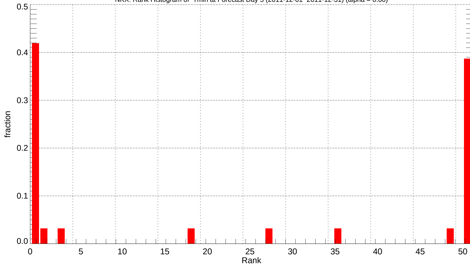
NKX: Rank Histogram of Tmin at Forecast Day 5 (2011-12-01~2011-12-31) (alpha = 0.00)
