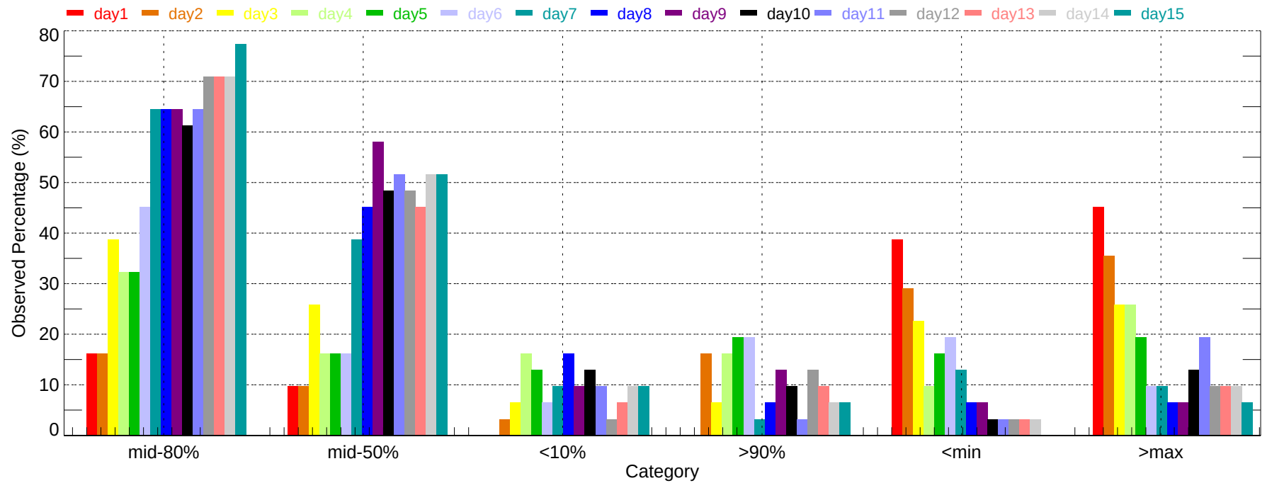
Observed Percentage of Ensembles - PVD: Min Temperature (2011-12-01~2011-12-31)
