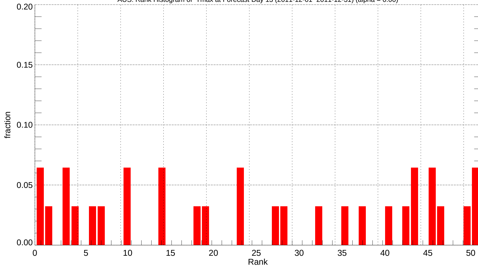
AUS: Rank Histogram of Tmax at Forecast Day 13 (2011-12-01~2011-12-31) (alpha = 0.00)
