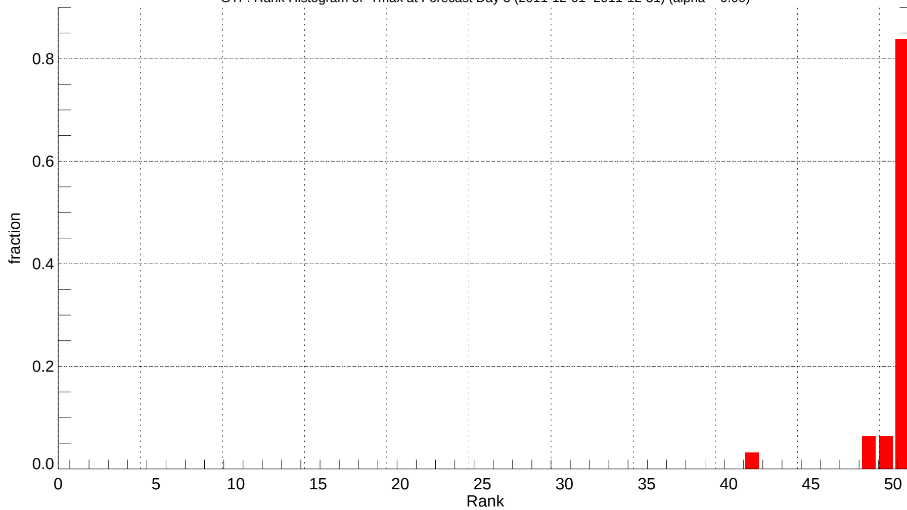
GTF: Rank Histogram of Tmax at Forecast Day 3 (2011-12-01~2011-12-31) (alpha = 0.00)
