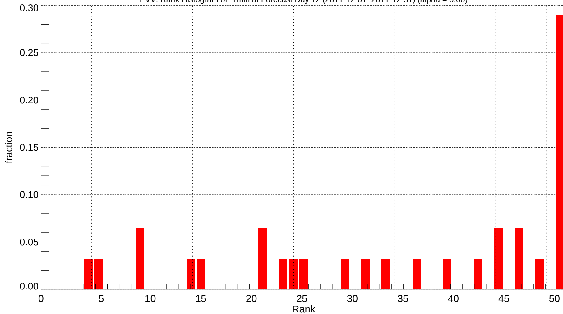
EVV: Rank Histogram of Tmin at Forecast Day 12 (2011-12-01~2011-12-31) (alpha = 0.00)
