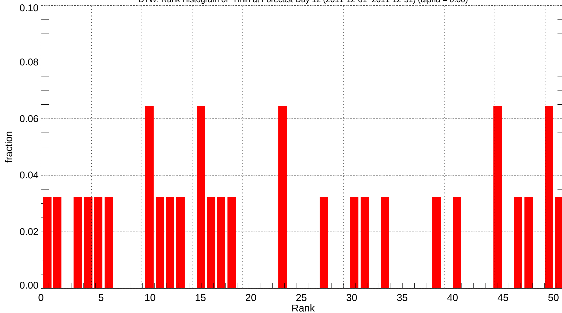
DTW: Rank Histogram of Tmin at Forecast Day 12 (2011-12-01~2011-12-31) (alpha = 0.00)
