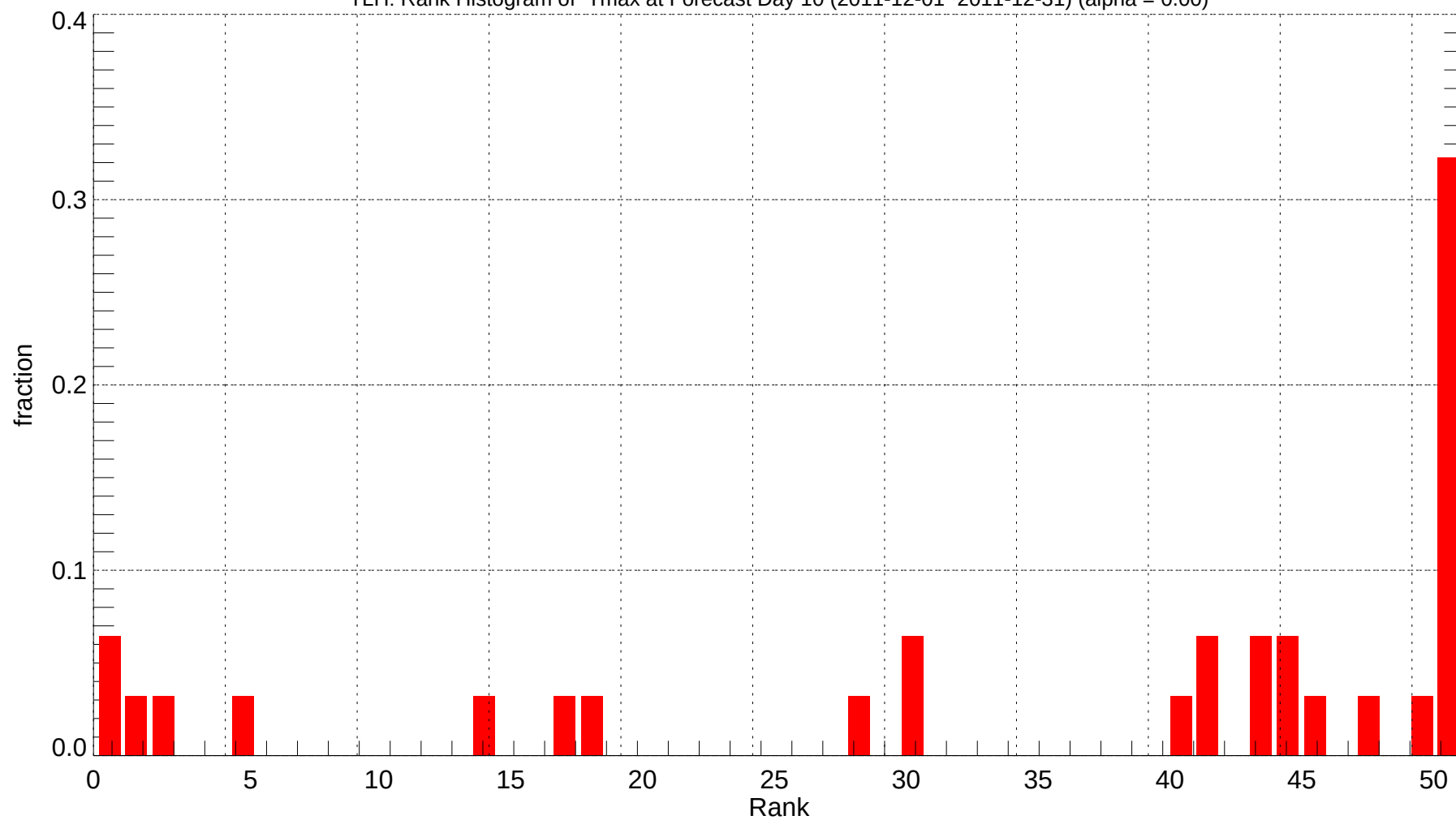
TLH: Rank Histogram of Tmax at Forecast Day 10 (2011-12-01~2011-12-31) (alpha = 0.00)
