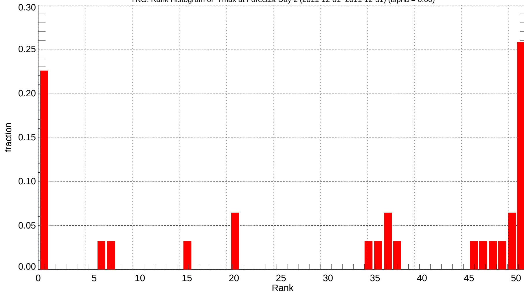
YNG: Rank Histogram of Tmax at Forecast Day 2 (2011-12-01~2011-12-31) (alpha = 0.00)
