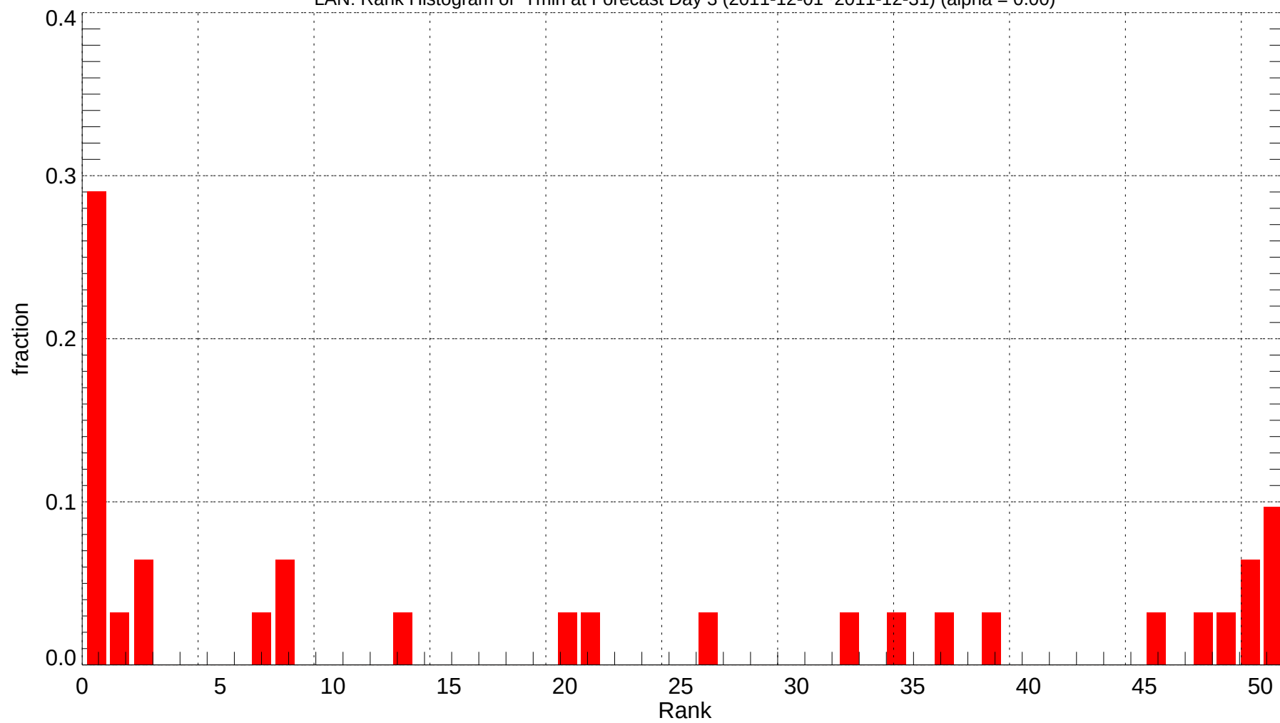
LAN: Rank Histogram of Tmin at Forecast Day 3 (2011-12-01~2011-12-31) (alpha = 0.00)
