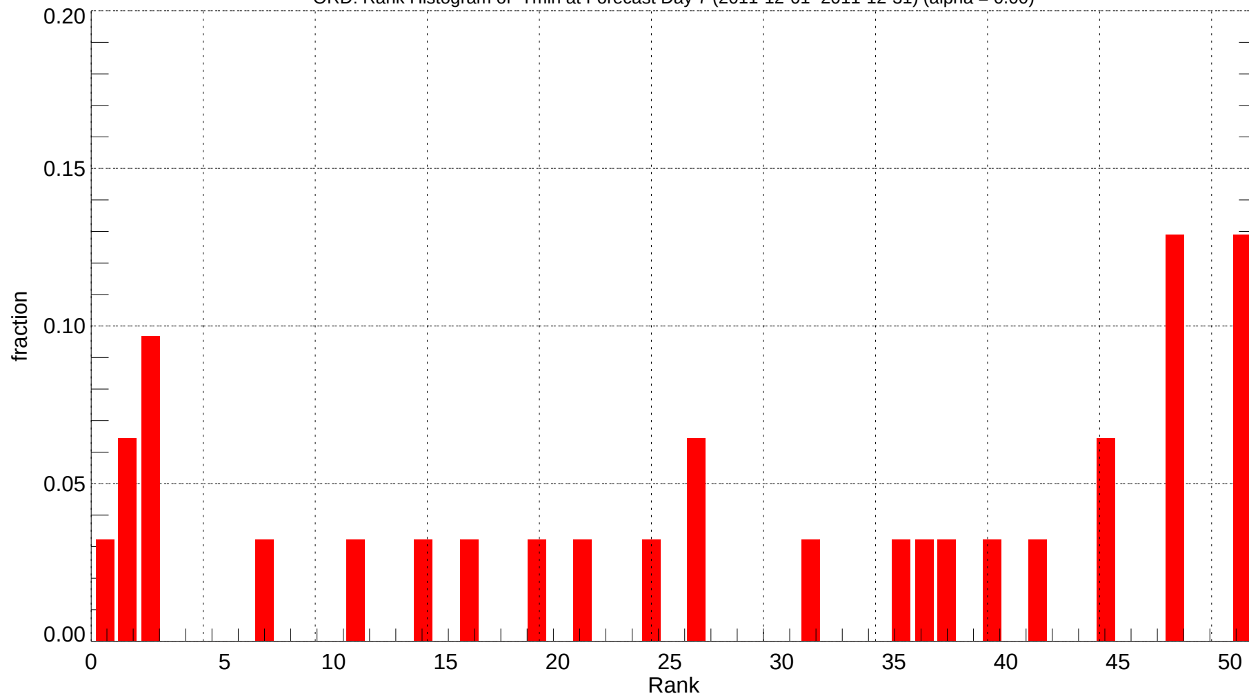
ORD: Rank Histogram of Tmin at Forecast Day 7 (2011-12-01~2011-12-31) (alpha = 0.00)
