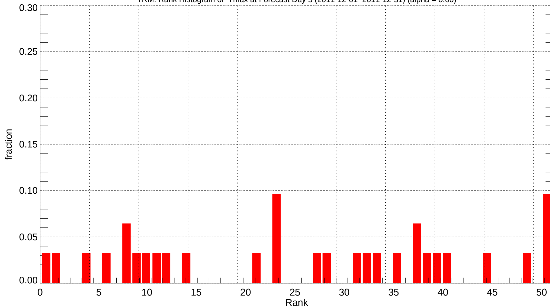
TRM: Rank Histogram of Tmax at Forecast Day 5 (2011-12-01~2011-12-31) (alpha = 0.00)
