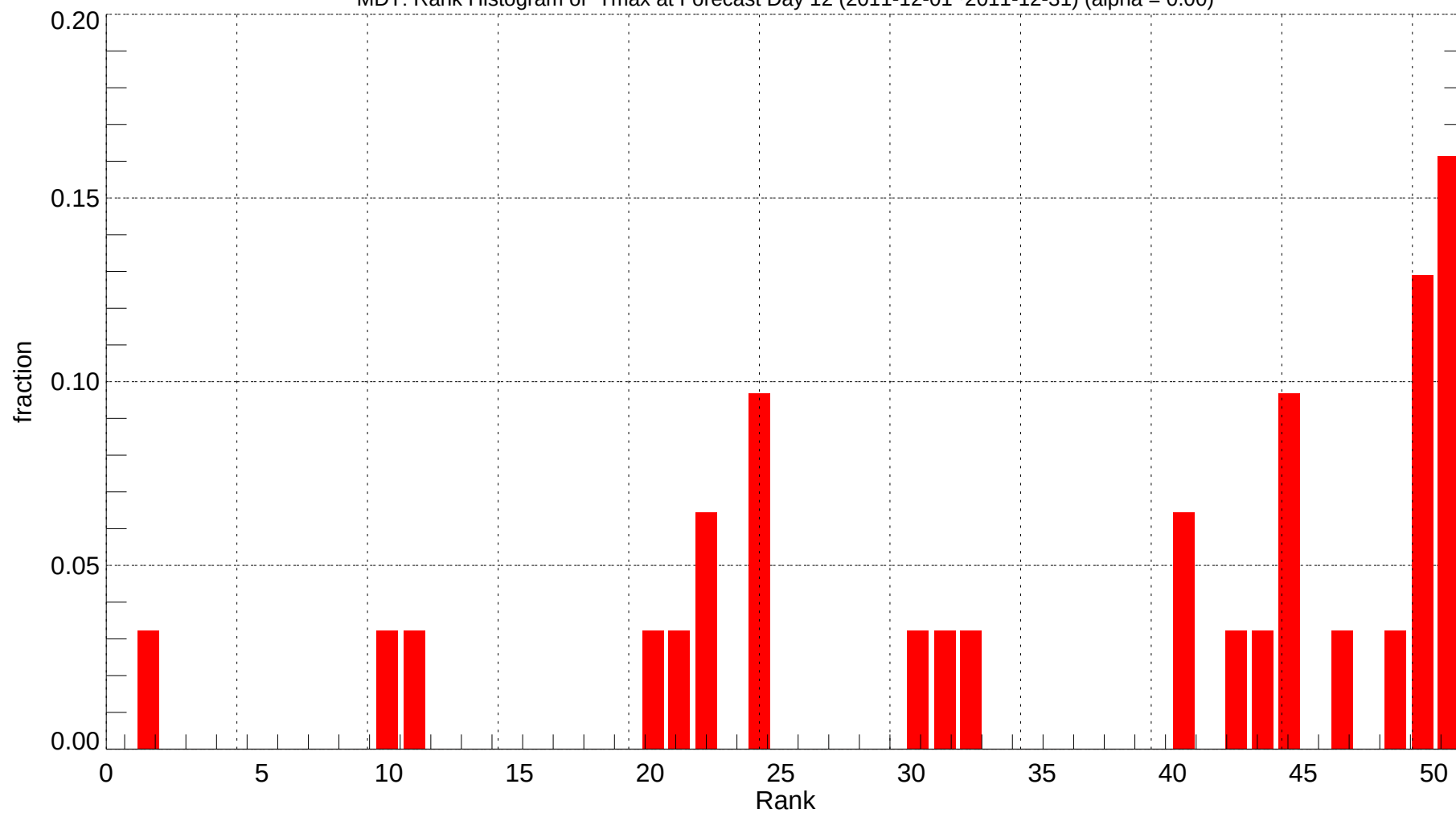
MDT: Rank Histogram of Tmax at Forecast Day 12 (2011-12-01~2011-12-31) (alpha = 0.00)
