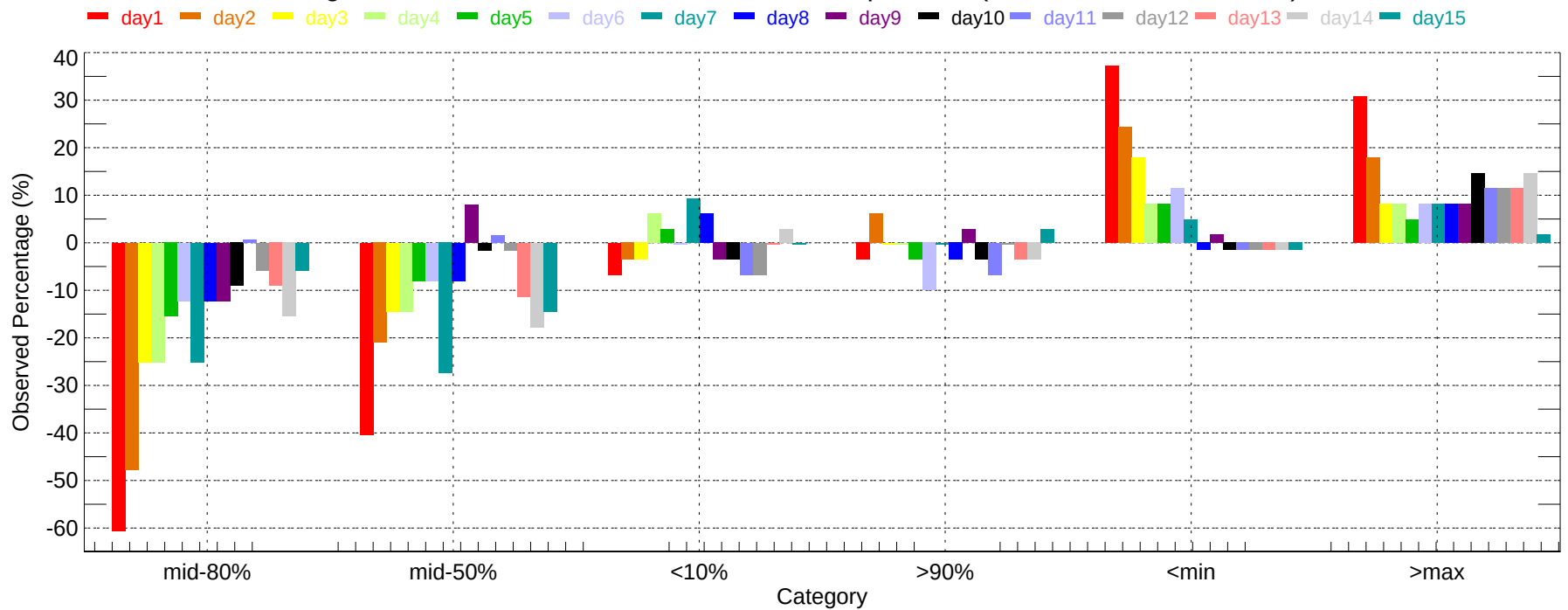
Observed Percentage Deviation of Ensembles - MSP: Min Temperature (2011-12-01~2011-12-31)
