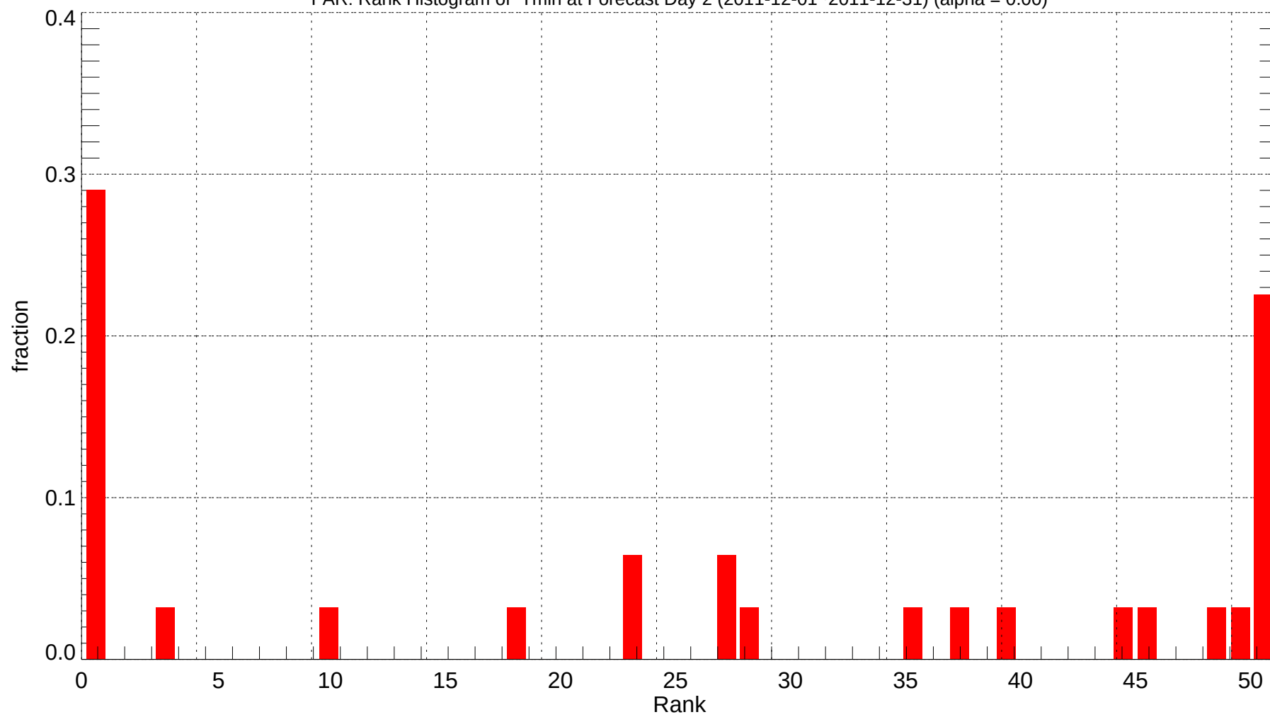
FAR: Rank Histogram of Tmin at Forecast Day 2 (2011-12-01~2011-12-31) (alpha = 0.00)
