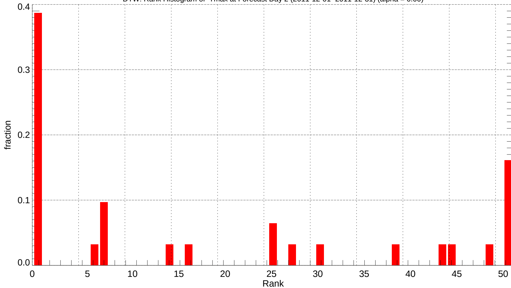
DTW: Rank Histogram of Tmax at Forecast Day 2 (2011-12-01~2011-12-31) (alpha = 0.00)
