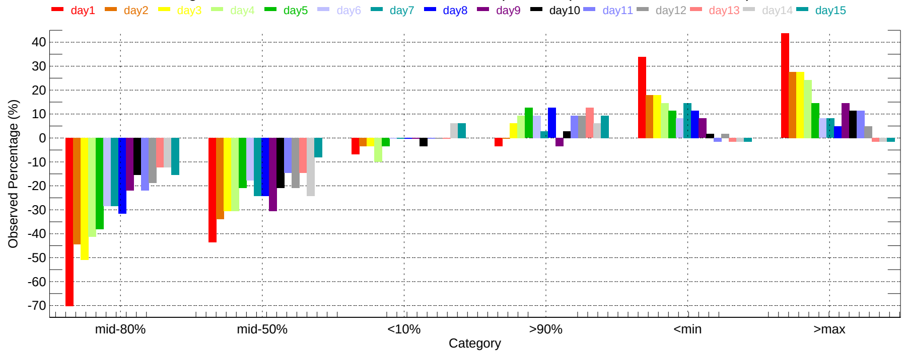
Observed Percentage Deviation of Ensembles - ROC: Min Temperature (2011-12-01~2011-12-31)
