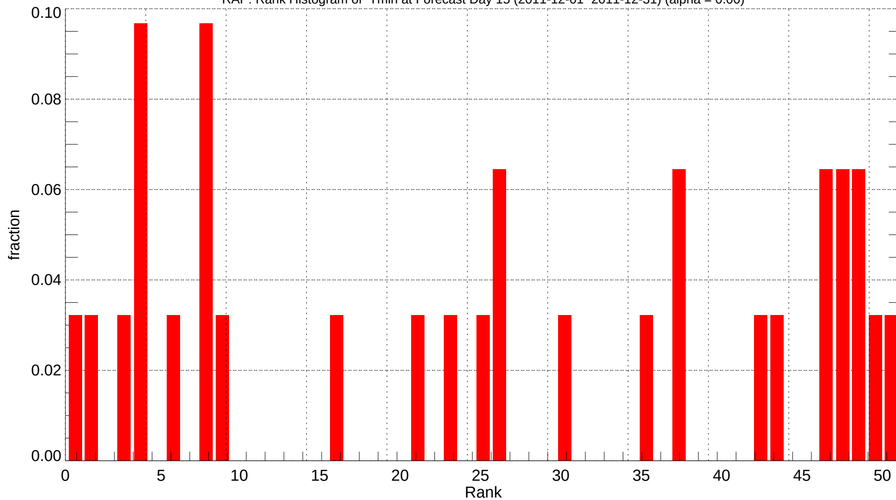
RAP: Rank Histogram of Tmin at Forecast Day 15 (2011-12-01~2011-12-31) (alpha = 0.00)
