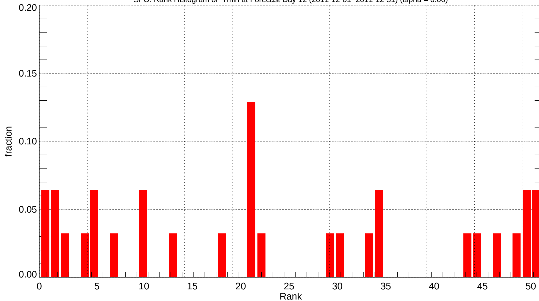
SFO: Rank Histogram of Tmin at Forecast Day 12 (2011-12-01~2011-12-31) (alpha = 0.00)
