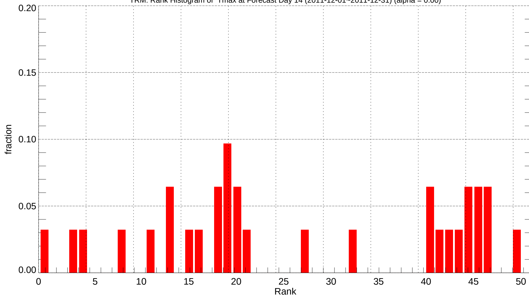
TRM: Rank Histogram of Tmax at Forecast Day 14 (2011-12-01~2011-12-31) (alpha = 0.00)
