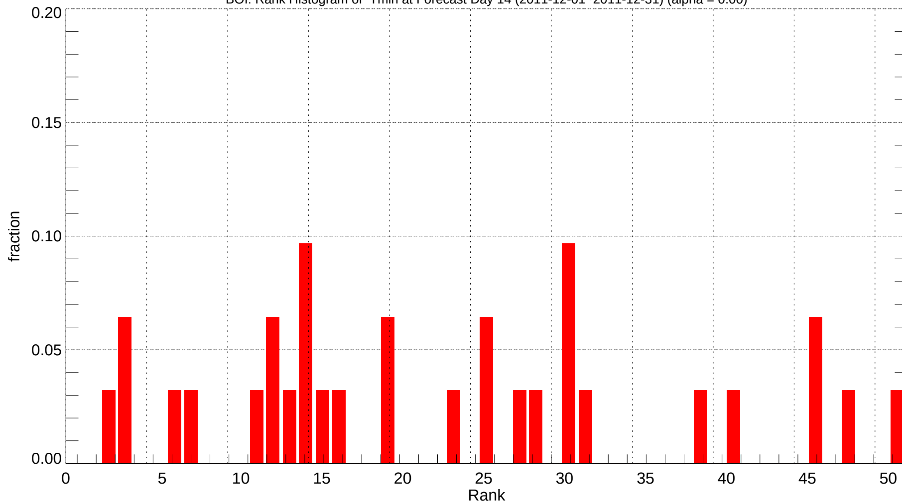
BOI: Rank Histogram of Tmin at Forecast Day 14 (2011-12-01~2011-12-31) (alpha = 0.00)
