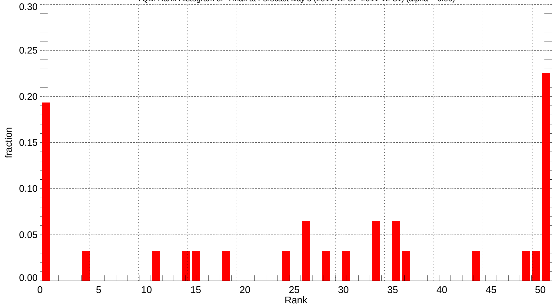
YQB: Rank Histogram of Tmax at Forecast Day 3 (2011-12-01~2011-12-31) (alpha = 0.00)
