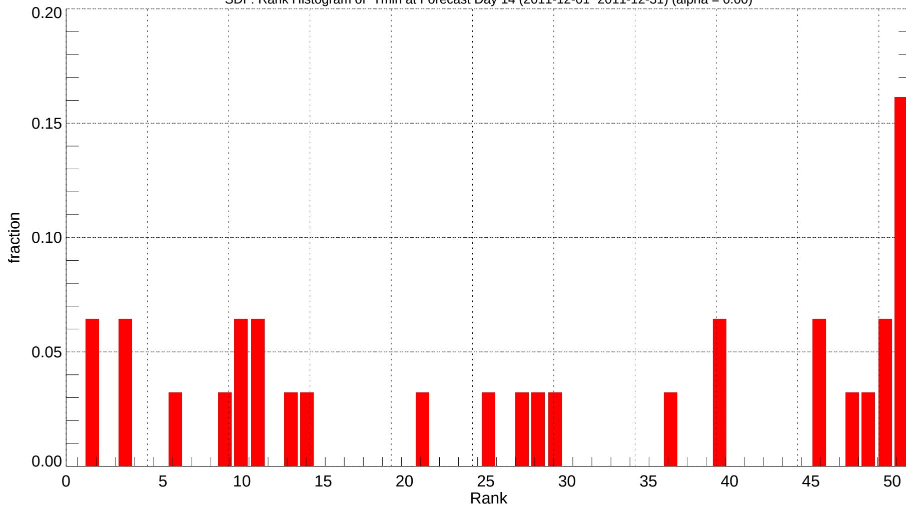
SDF: Rank Histogram of Tmin at Forecast Day 14 (2011-12-01~2011-12-31) (alpha = 0.00)
