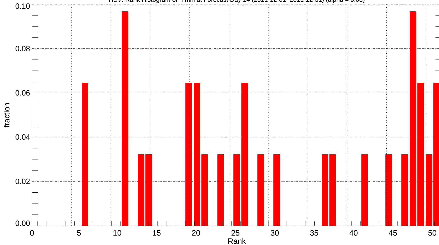
HSV: Rank Histogram of Tmin at Forecast Day 14 (2011-12-01~2011-12-31) (alpha = 0.00)
