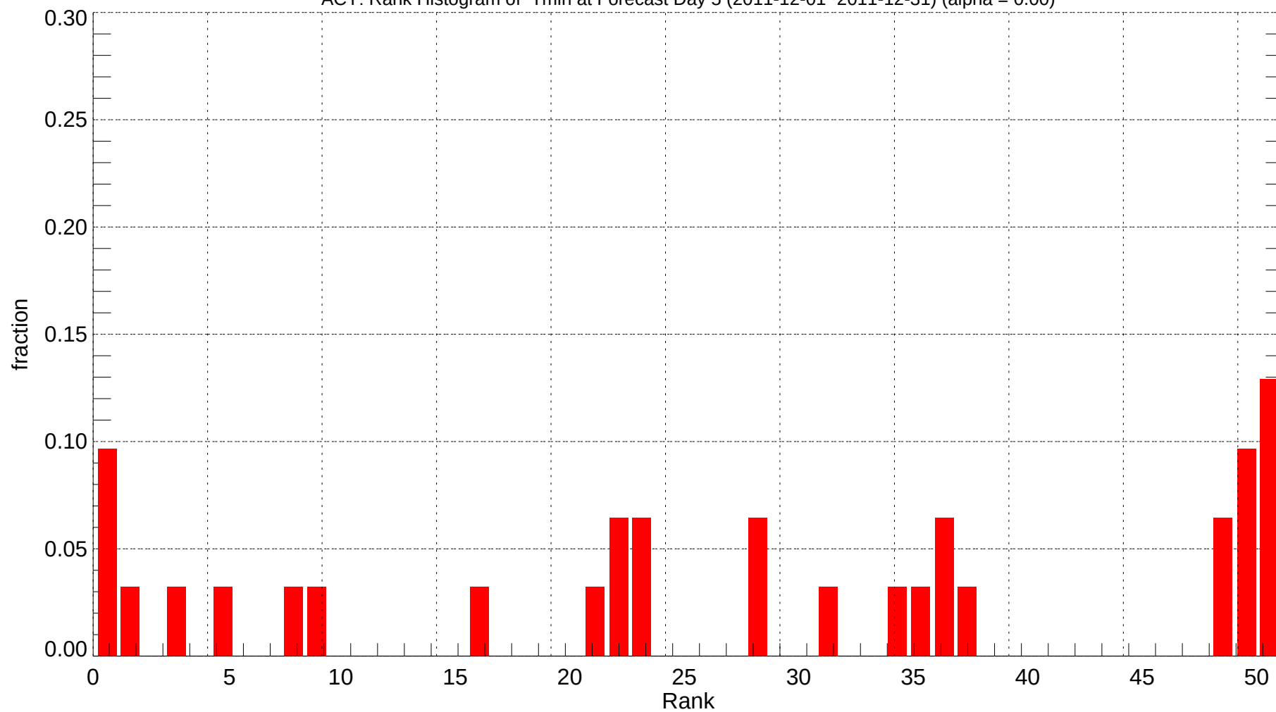
ACY: Rank Histogram of Tmin at Forecast Day 5 (2011-12-01~2011-12-31) (alpha = 0.00)
