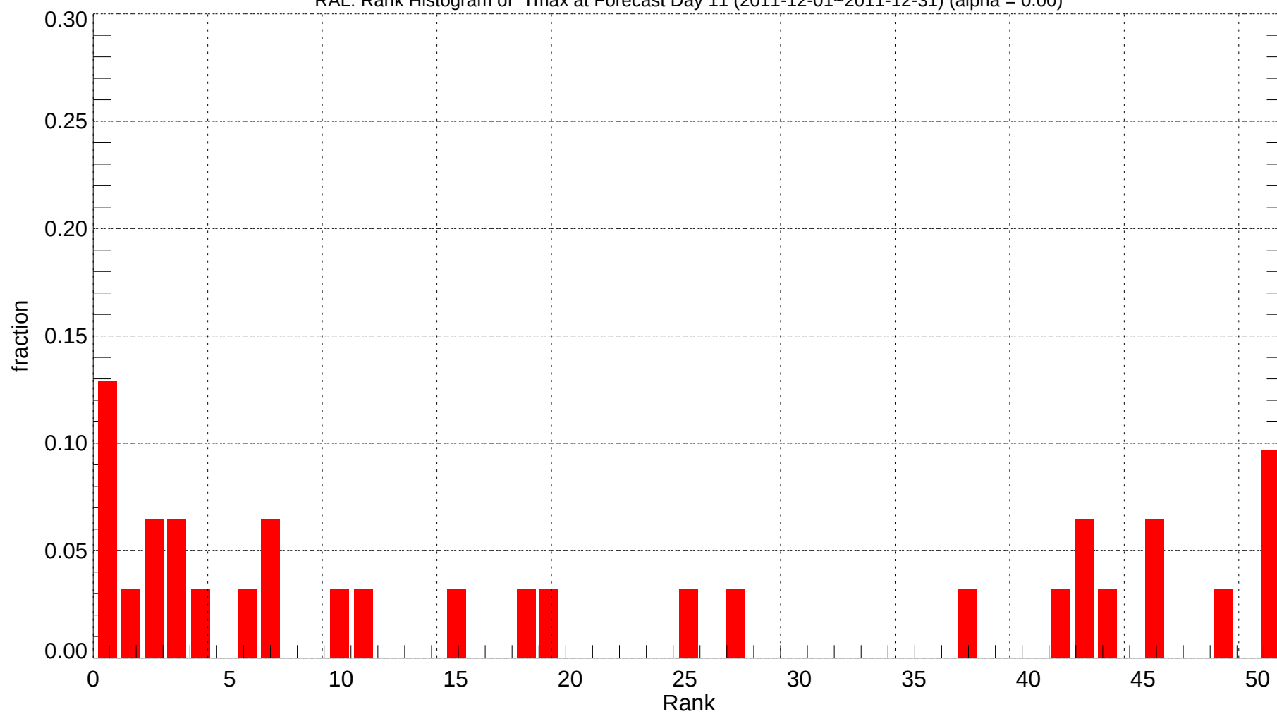
RAL: Rank Histogram of Tmax at Forecast Day 11 (2011-12-01~2011-12-31) (alpha = 0.00)
