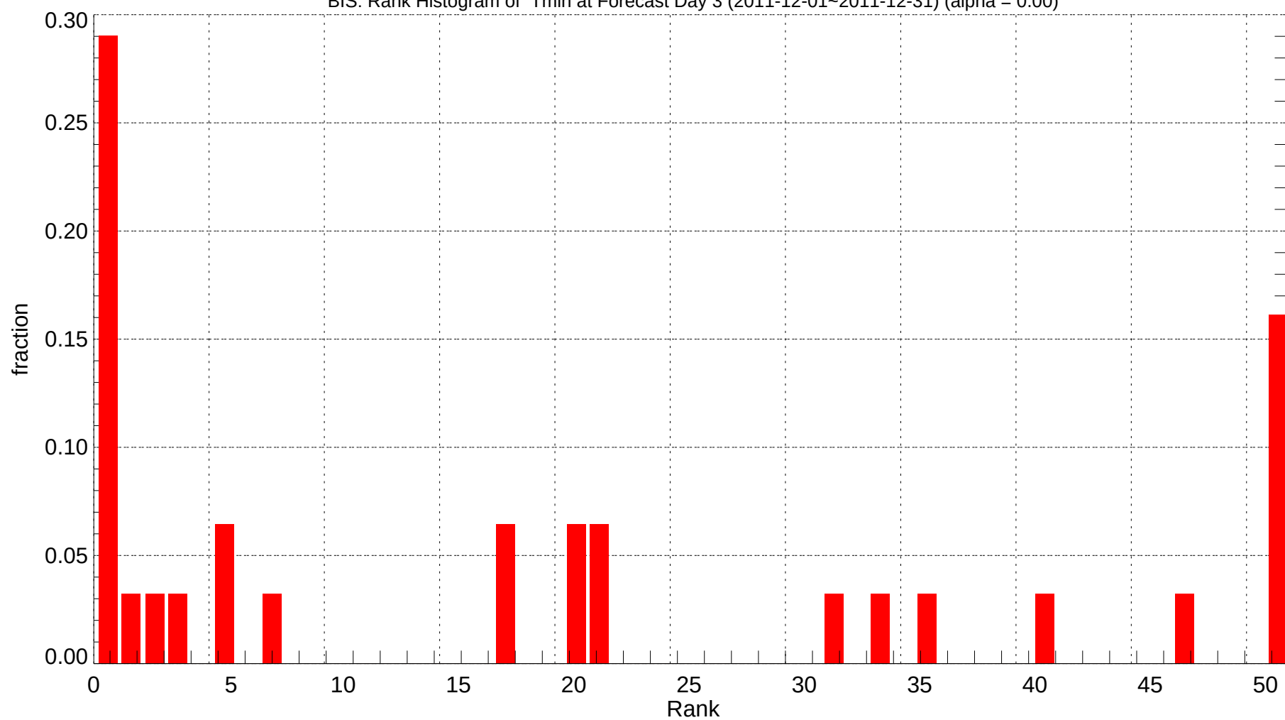
BIS: Rank Histogram of Tmin at Forecast Day 3 (2011-12-01~2011-12-31) (alpha = 0.00)
