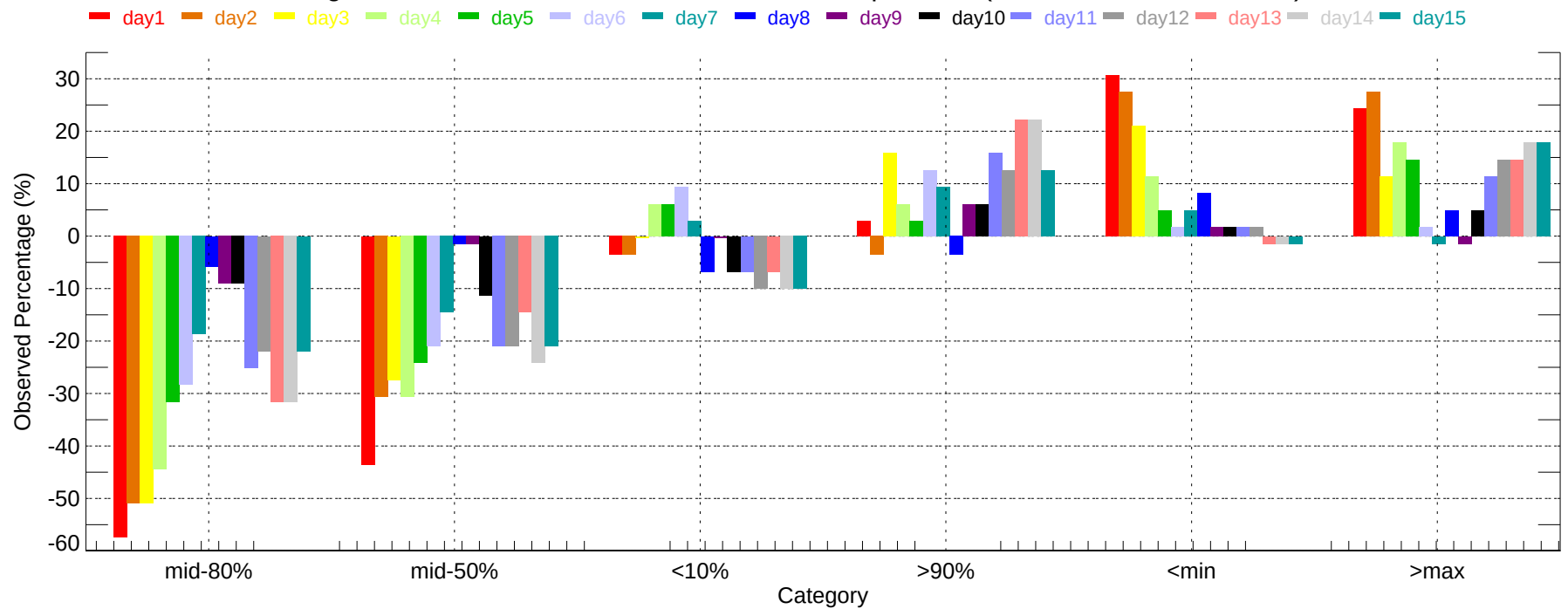
Observed Percentage Deviation of Ensembles - LGB: Max Temperature (2011-12-01~2011-12-31)
