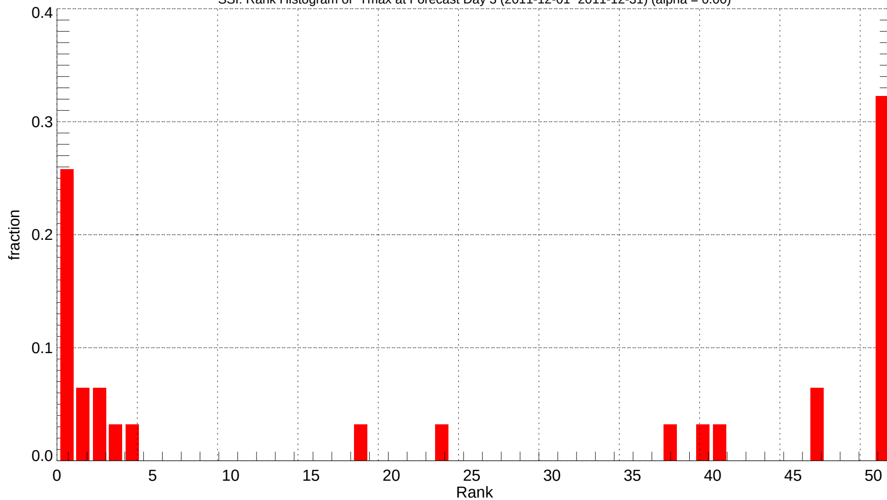
SSI: Rank Histogram of Tmax at Forecast Day 3 (2011-12-01~2011-12-31) (alpha = 0.00)
