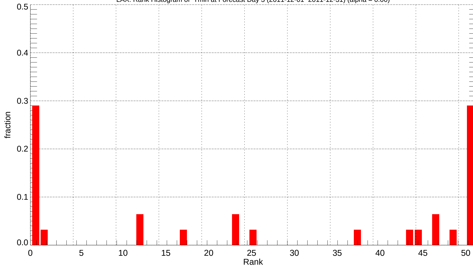
LAX: Rank Histogram of Tmin at Forecast Day 3 (2011-12-01~2011-12-31) (alpha = 0.00)
