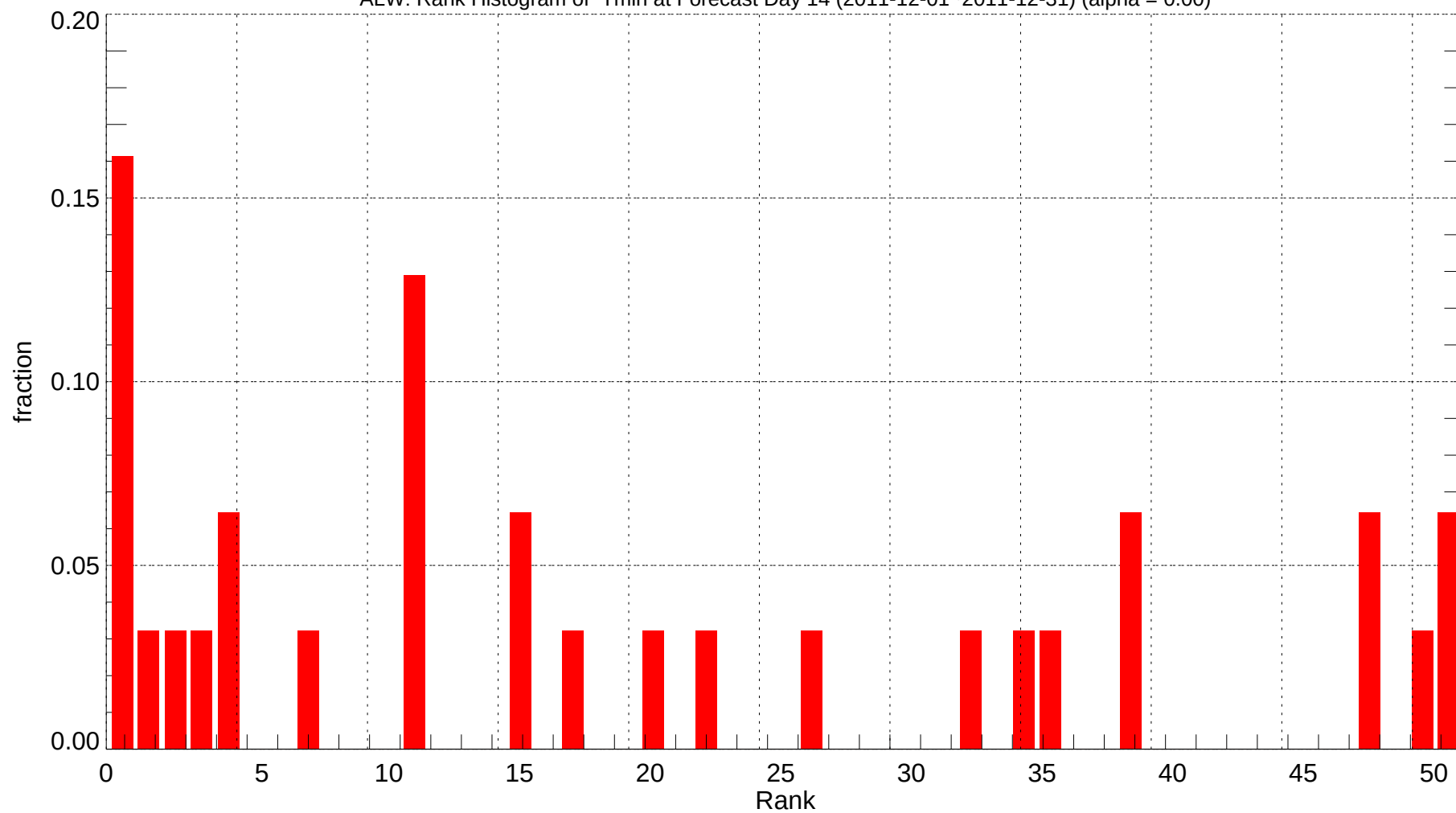
ALW: Rank Histogram of Tmin at Forecast Day 14 (2011-12-01~2011-12-31) (alpha = 0.00)
