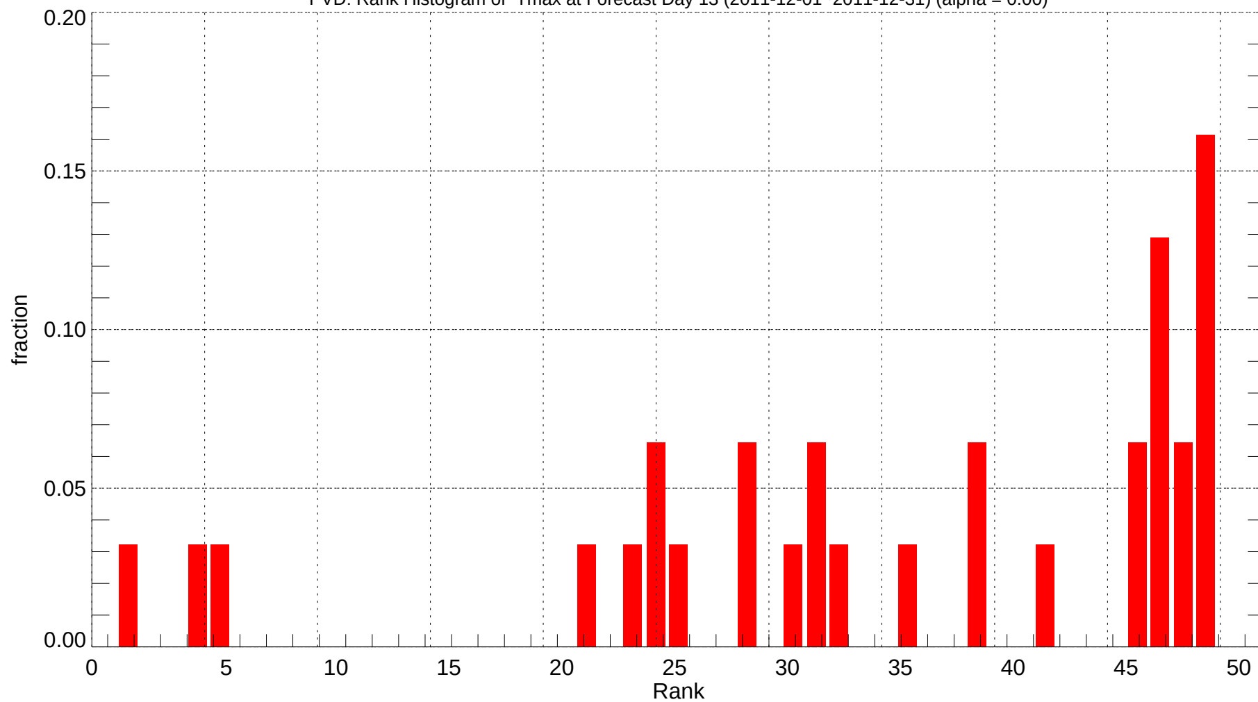
PVD: Rank Histogram of Tmax at Forecast Day 13 (2011-12-01~2011-12-31) (alpha = 0.00)
