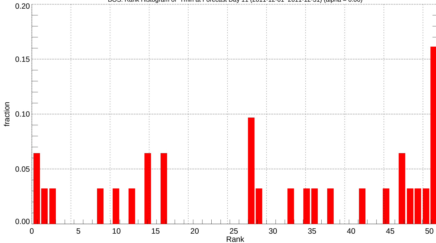
BOS: Rank Histogram of Tmin at Forecast Day 11 (2011-12-01~2011-12-31) (alpha = 0.00)
