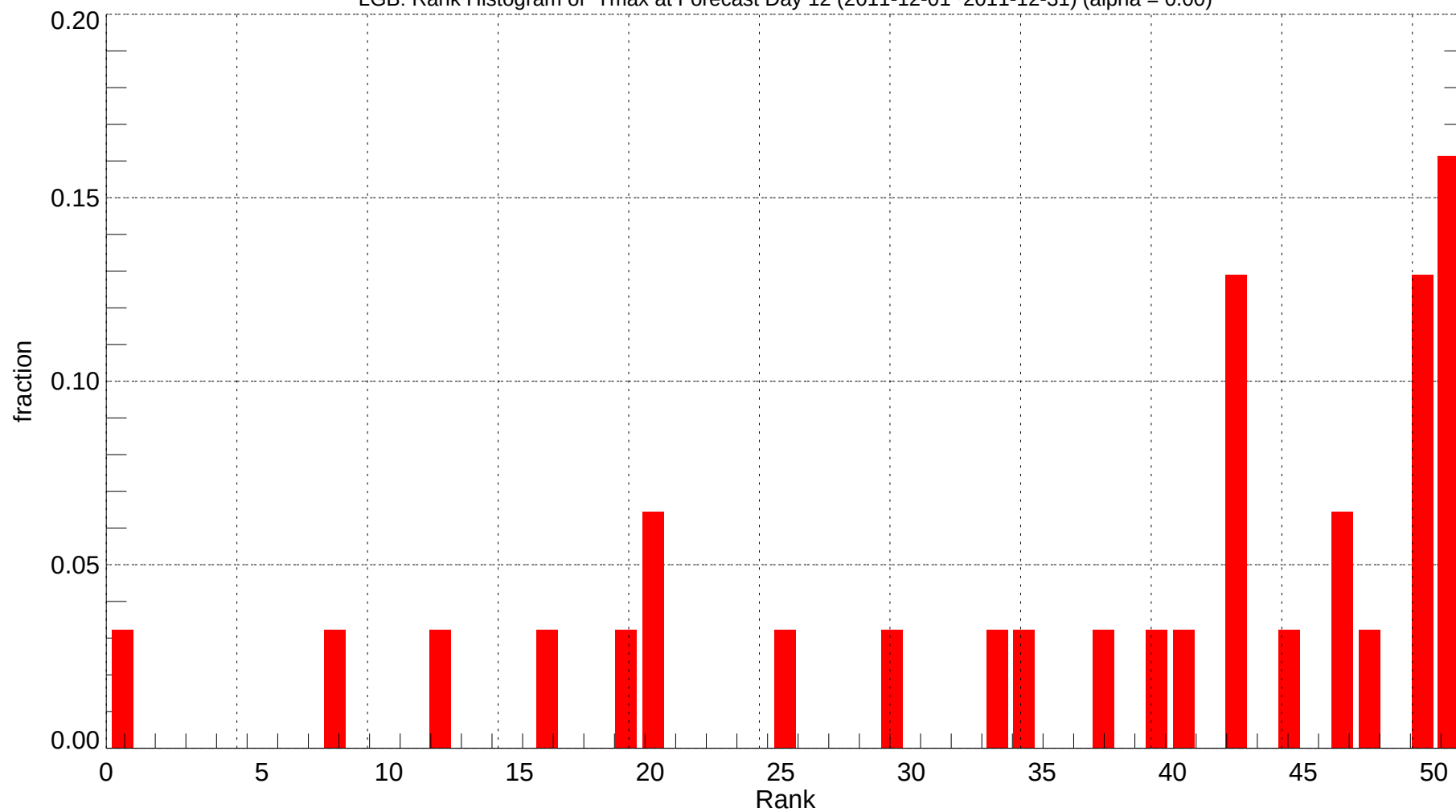
LGB: Rank Histogram of Tmax at Forecast Day 12 (2011-12-01~2011-12-31) (alpha = 0.00)
