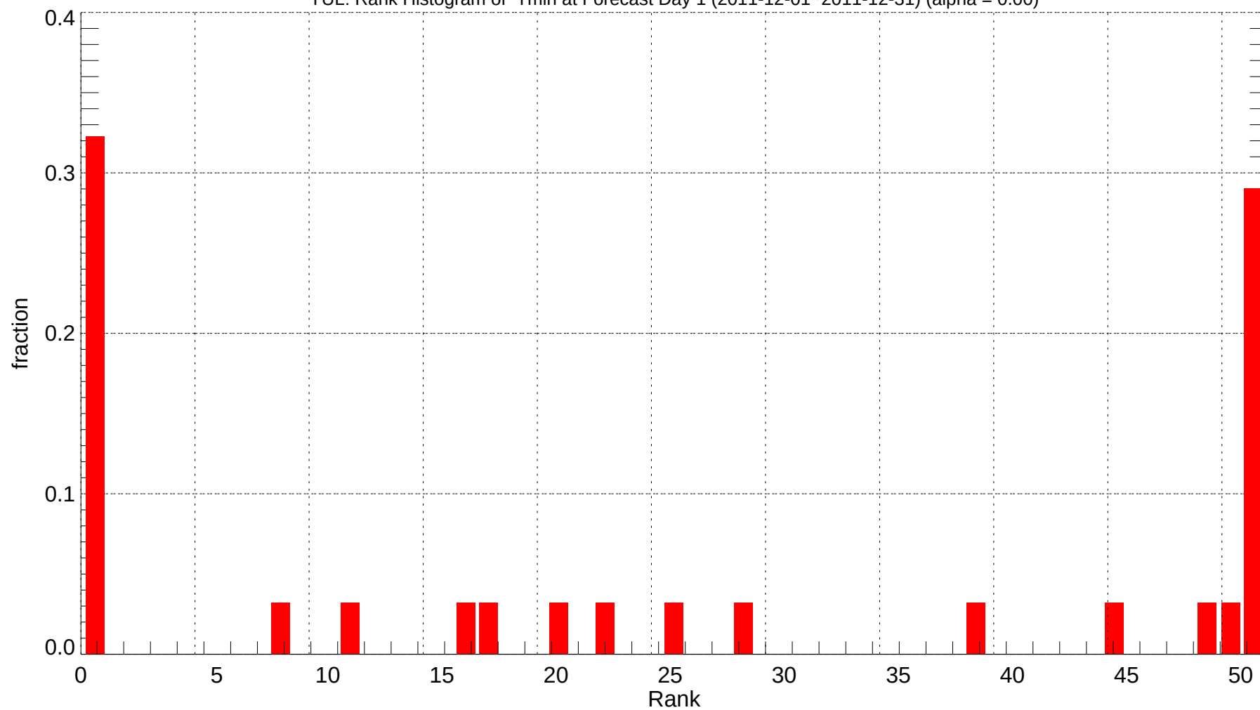
YUL: Rank Histogram of Tmin at Forecast Day 1 (2011-12-01~2011-12-31) (alpha = 0.00)
