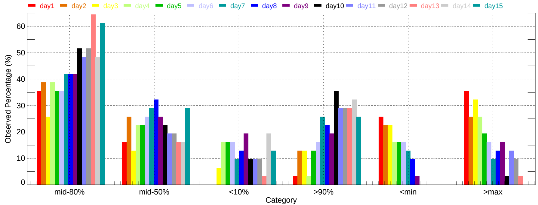
Observed Percentage of Ensembles - YNG: Min Temperature (2011-12-01~2011-12-31)
