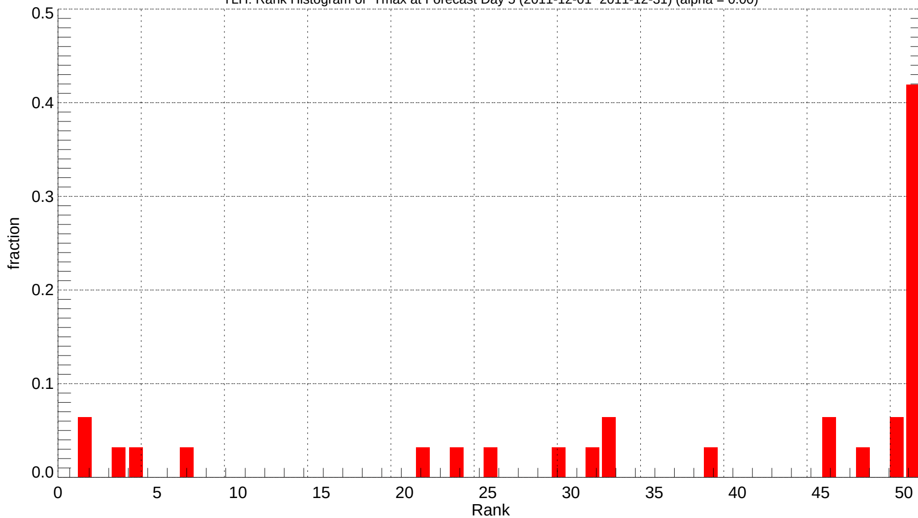
TLH: Rank Histogram of Tmax at Forecast Day 5 (2011-12-01~2011-12-31) (alpha = 0.00)
