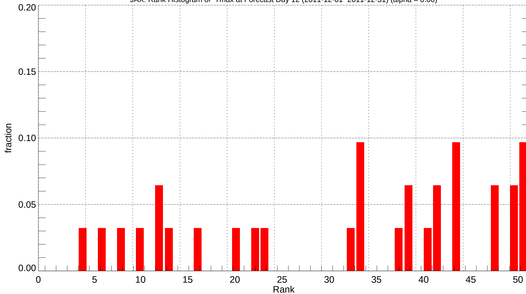
JAX: Rank Histogram of Tmax at Forecast Day 12 (2011-12-01~2011-12-31) (alpha = 0.00)
