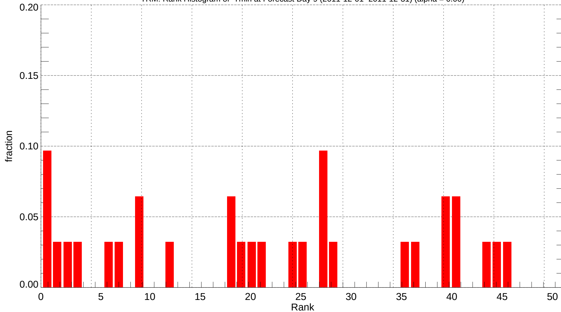
TRM: Rank Histogram of Tmin at Forecast Day 9 (2011-12-01~2011-12-31) (alpha = 0.00)
