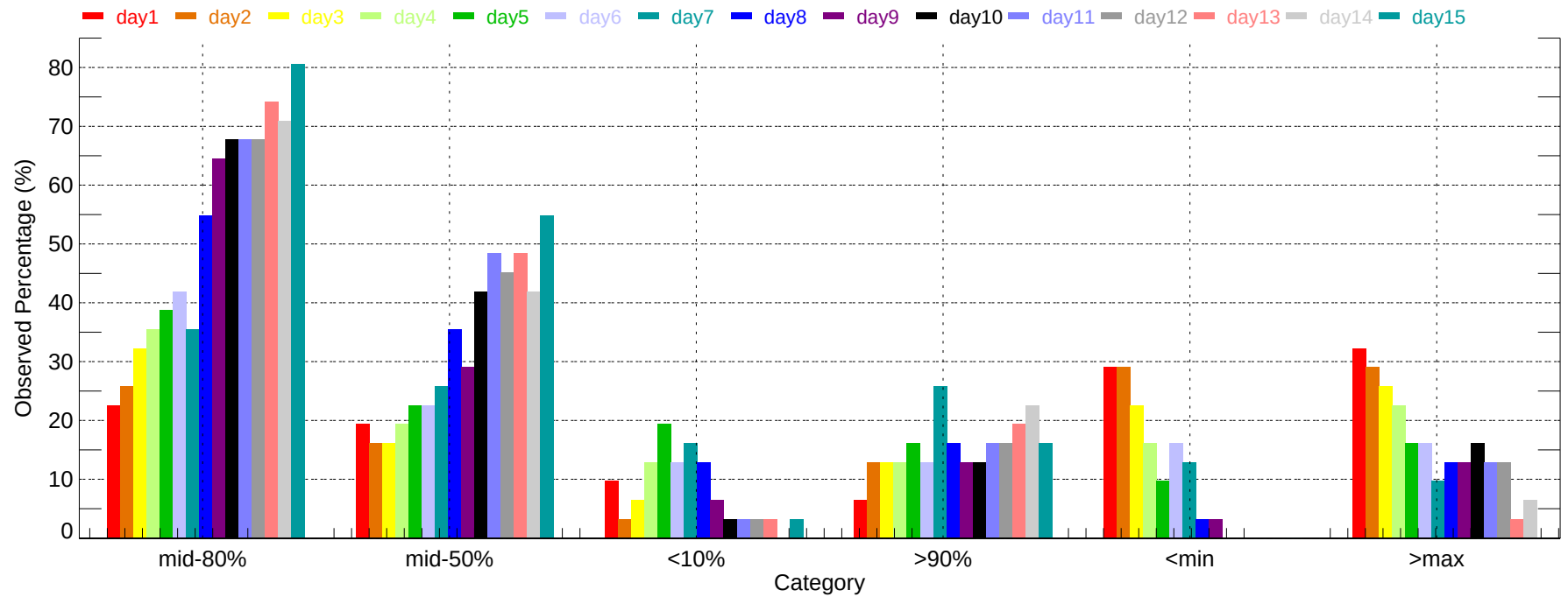
Observed Percentage of Ensembles - ORD: Min Temperature (2011-12-01~2011-12-31)
