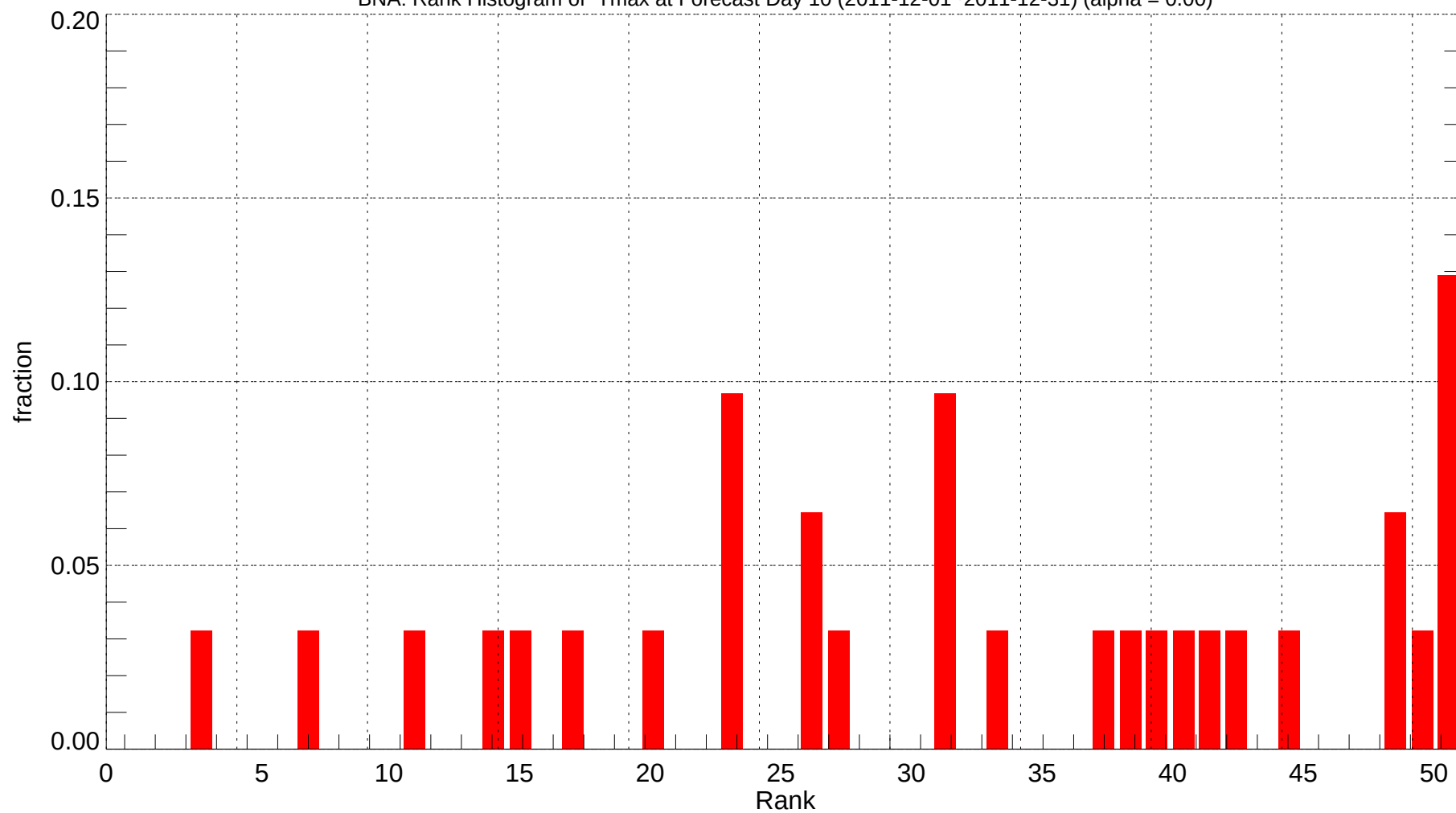
BNA: Rank Histogram of Tmax at Forecast Day 10 (2011-12-01~2011-12-31) (alpha = 0.00)
