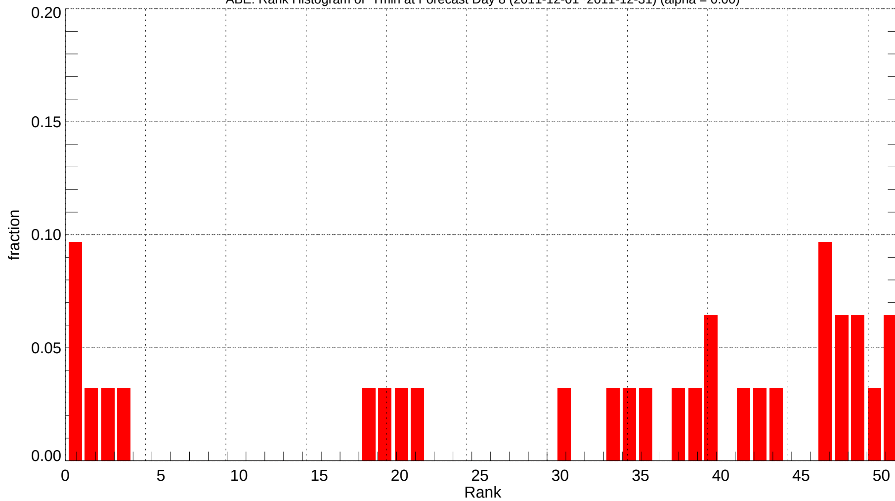
ABE: Rank Histogram of Tmin at Forecast Day 8 (2011-12-01~2011-12-31) (alpha = 0.00)
