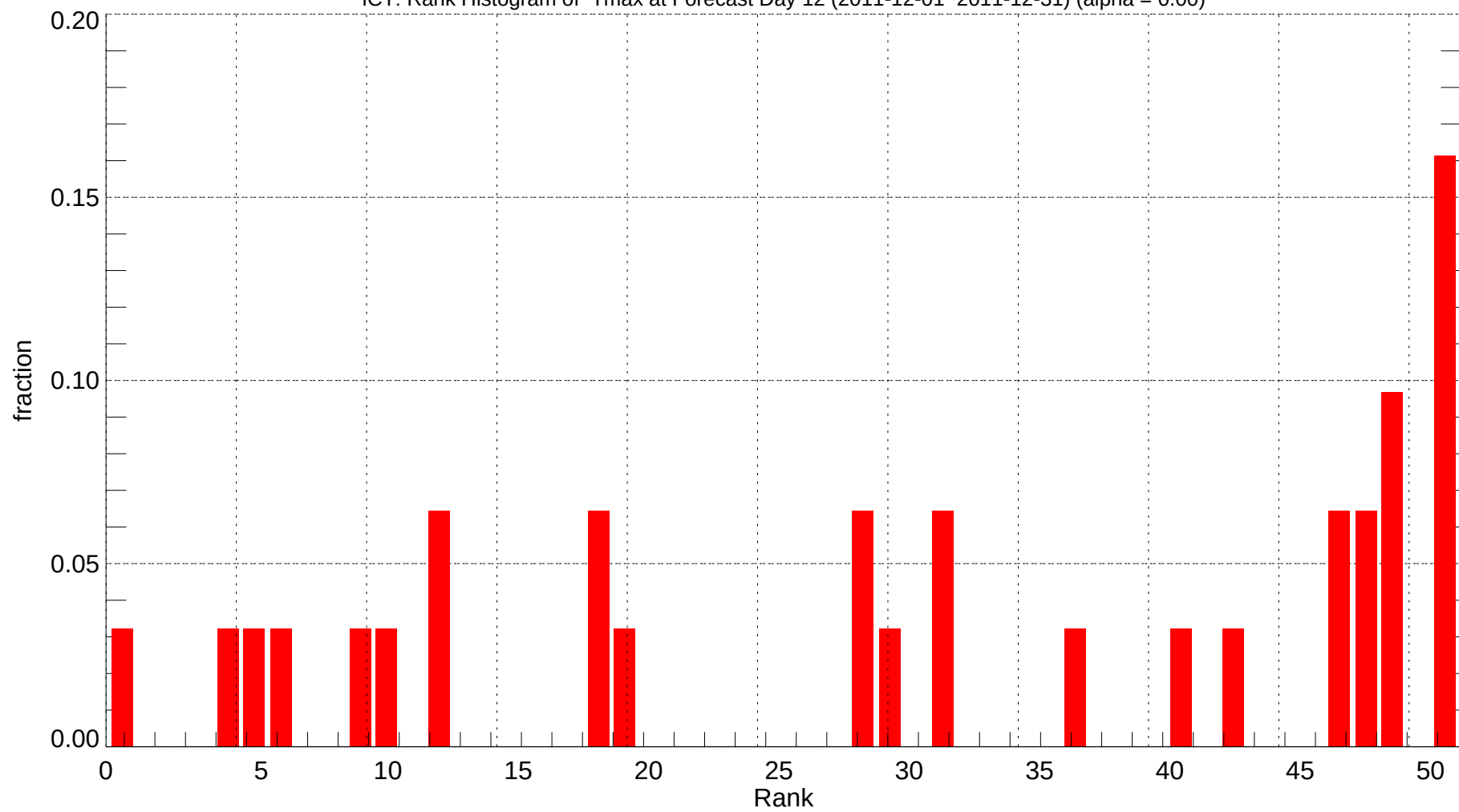
ICT: Rank Histogram of Tmax at Forecast Day 12 (2011-12-01~2011-12-31) (alpha = 0.00)
