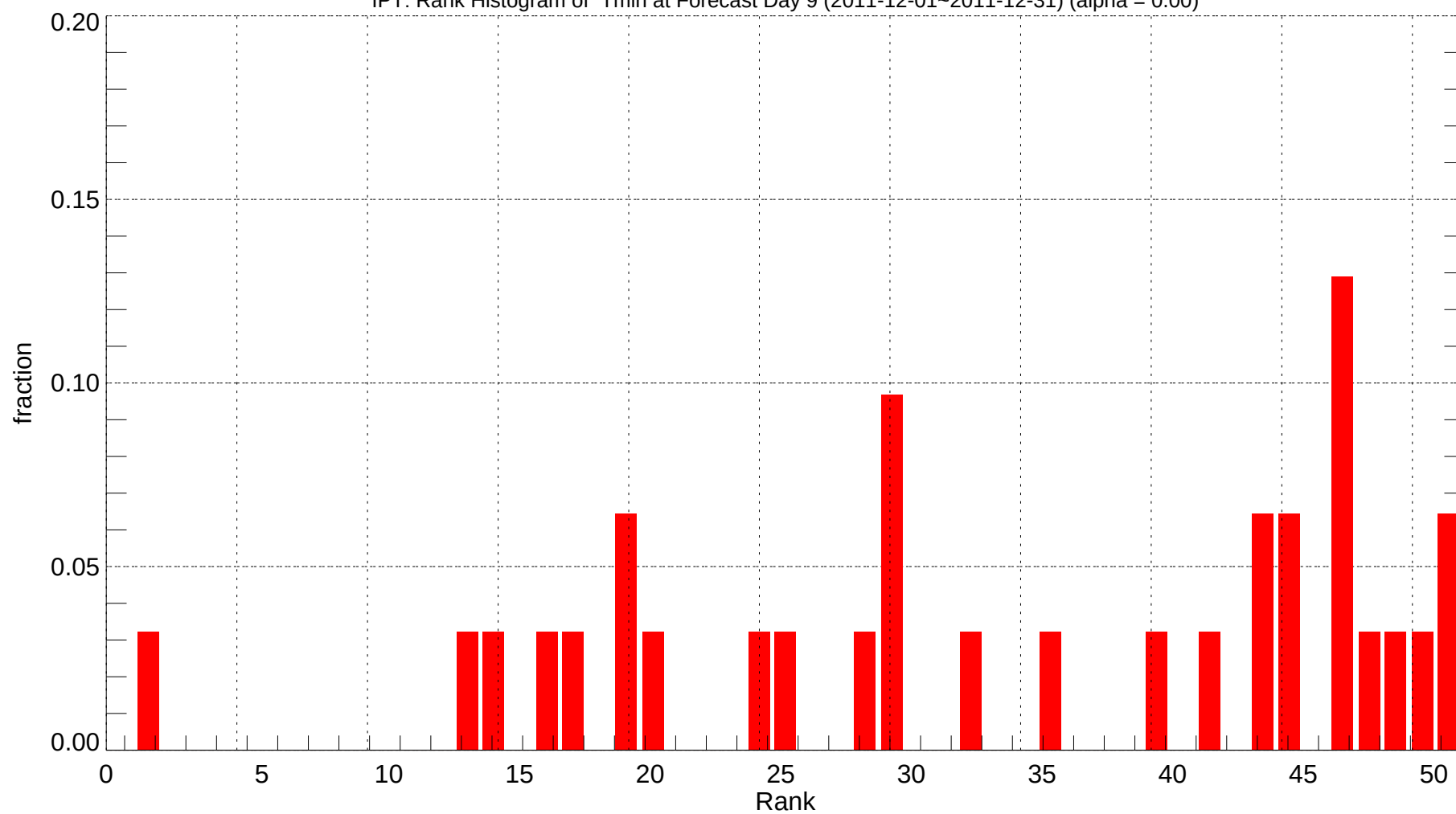
IPT: Rank Histogram of Tmin at Forecast Day 9 (2011-12-01~2011-12-31) (alpha = 0.00)
