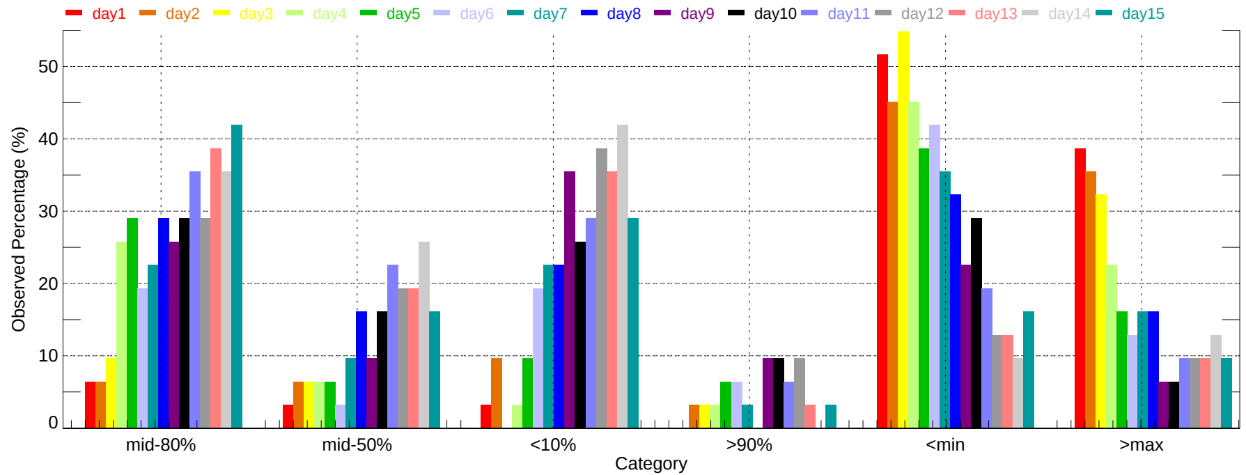
Observed Percentage of Ensembles - SFO: Min Temperature (2011-12-01~2011-12-31)
