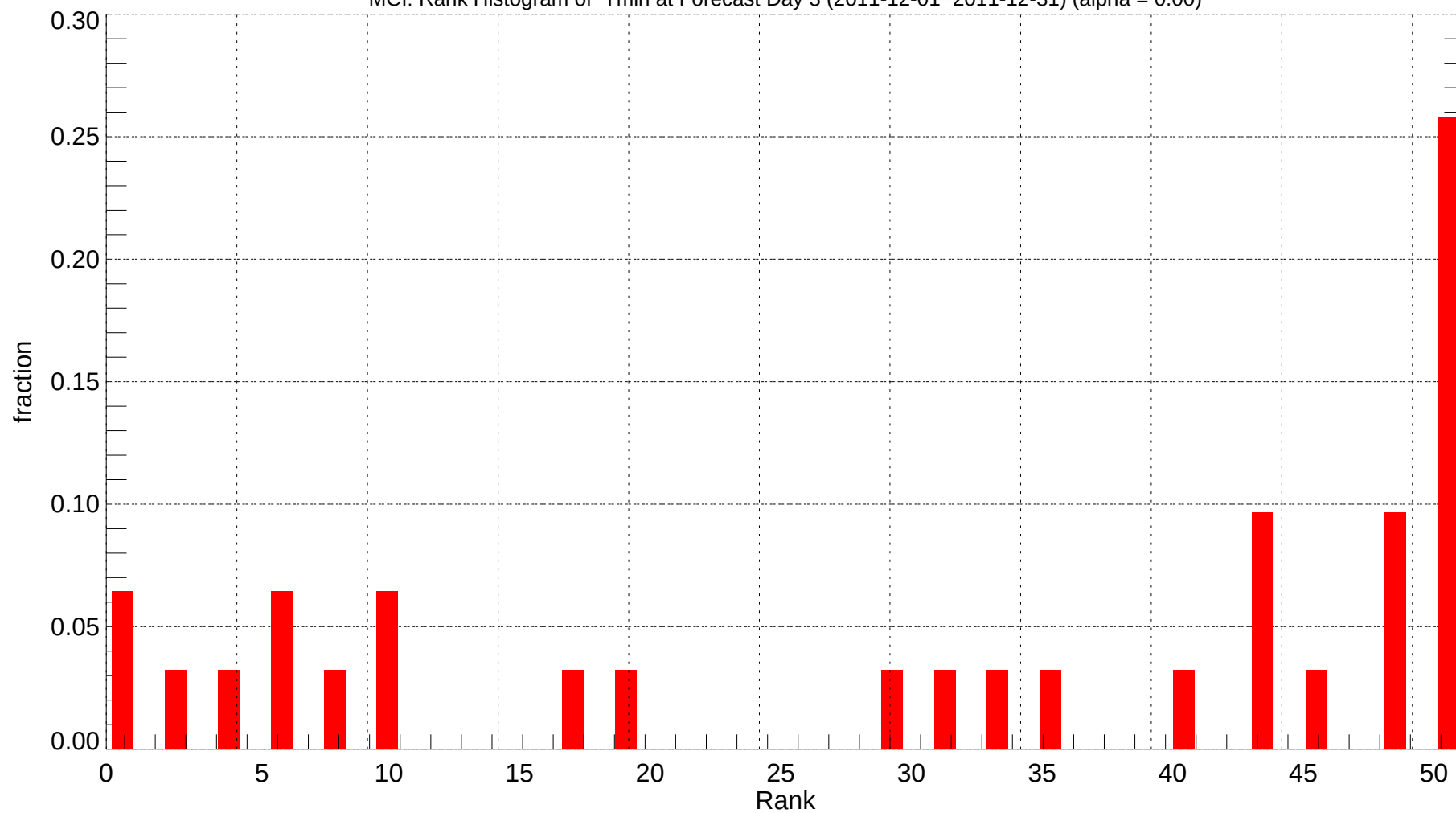
MCI: Rank Histogram of Tmin at Forecast Day 3 (2011-12-01~2011-12-31) (alpha = 0.00)
