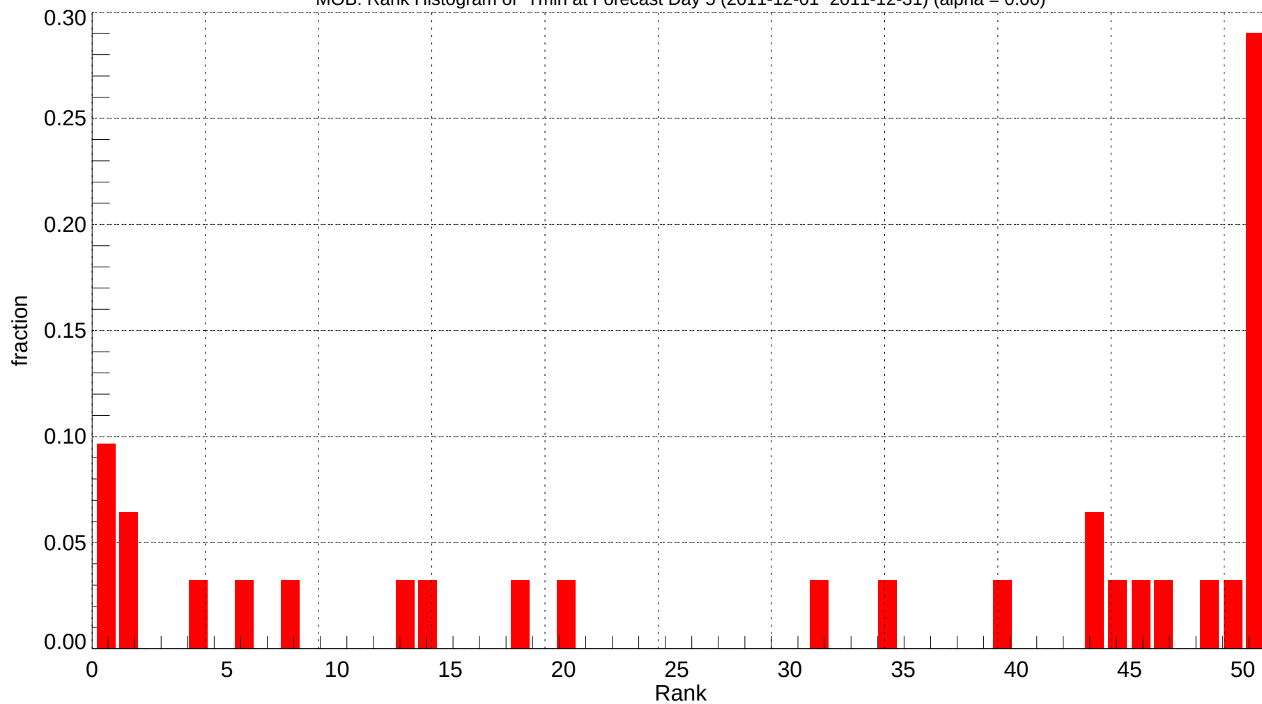
MOB: Rank Histogram of Tmin at Forecast Day 5 (2011-12-01~2011-12-31) (alpha = 0.00)
