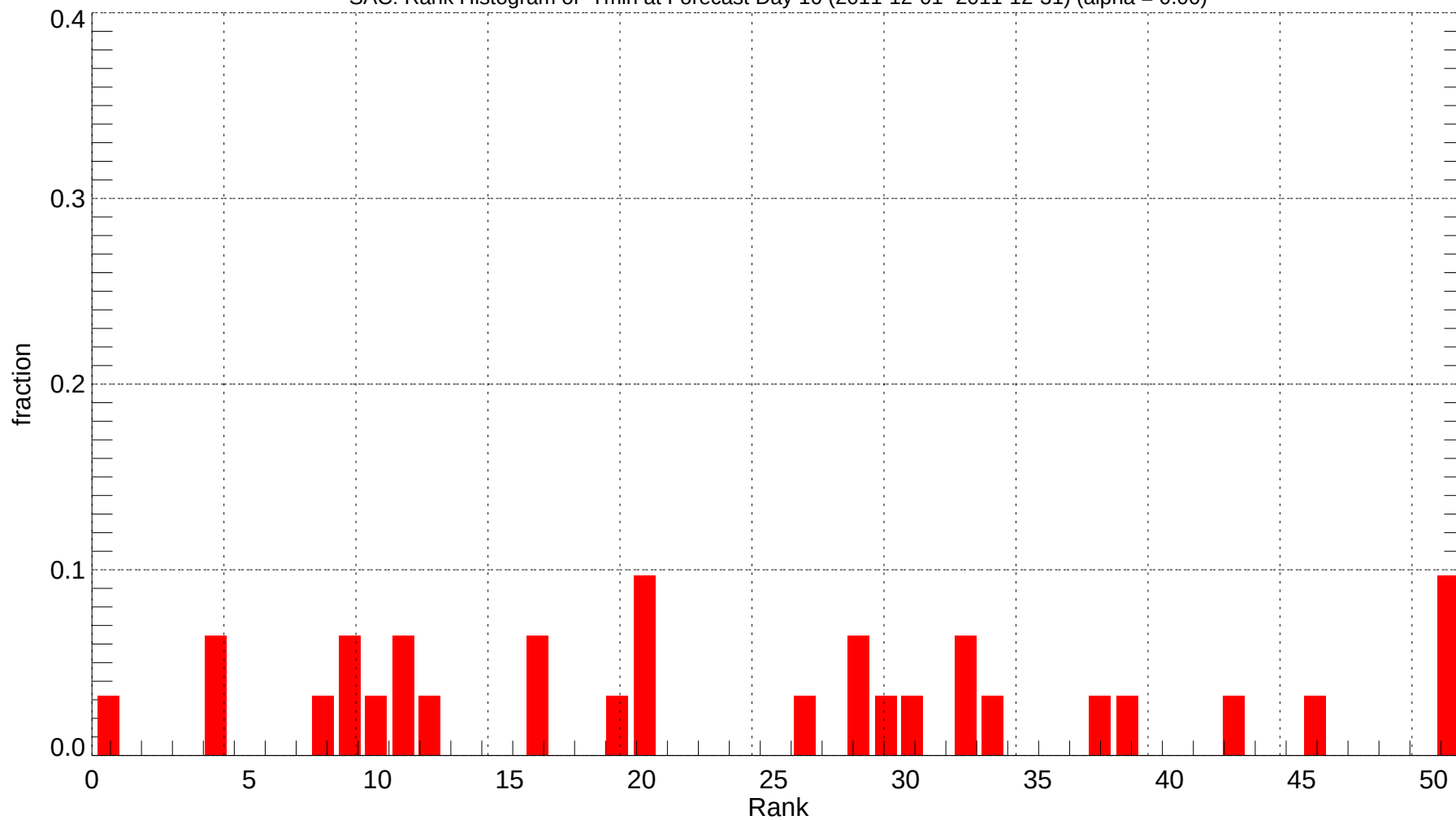
SAC: Rank Histogram of Tmin at Forecast Day 10 (2011-12-01~2011-12-31) (alpha = 0.00)
