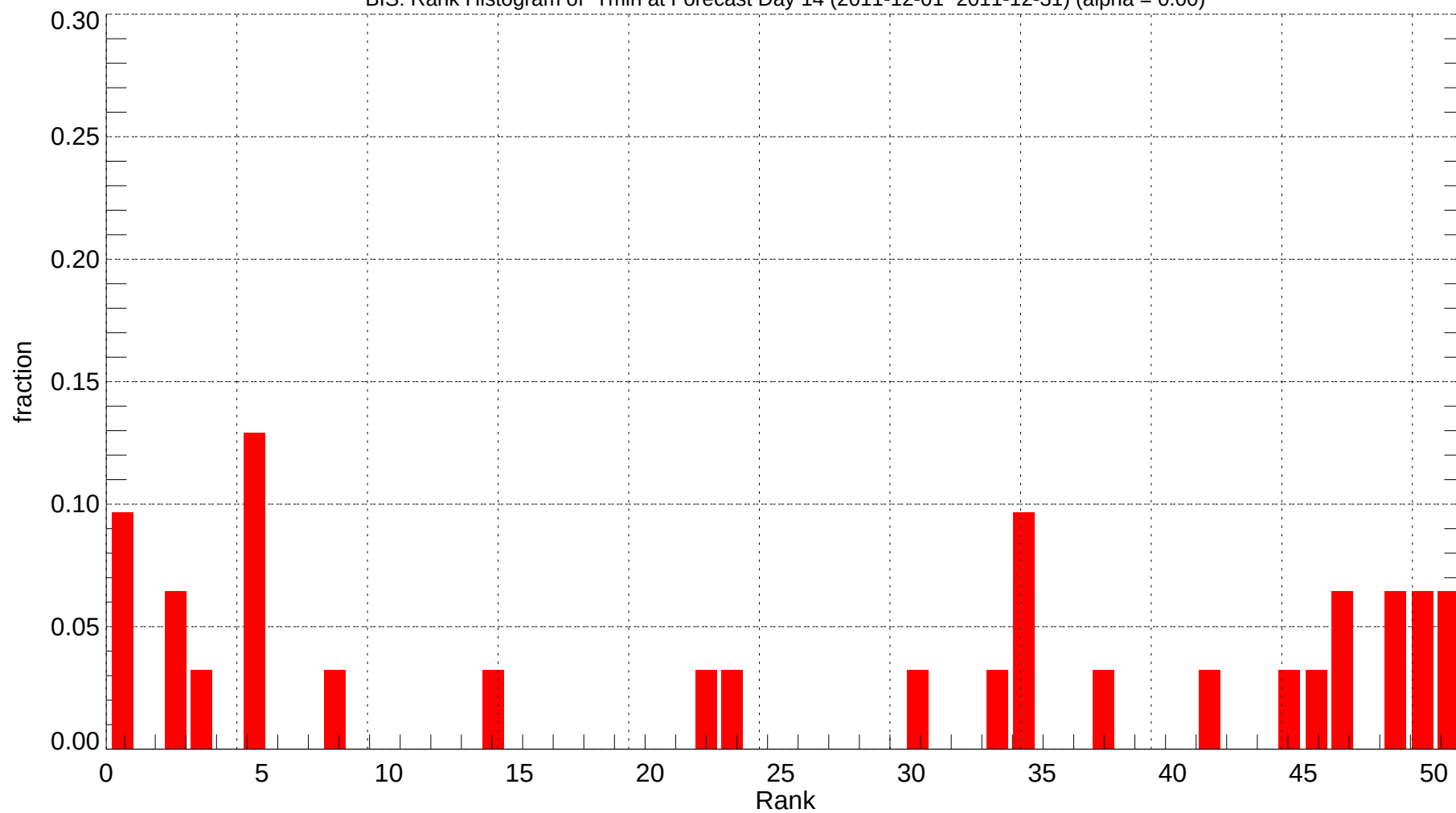
BIS: Rank Histogram of Tmin at Forecast Day 14 (2011-12-01~2011-12-31) (alpha = 0.00)
