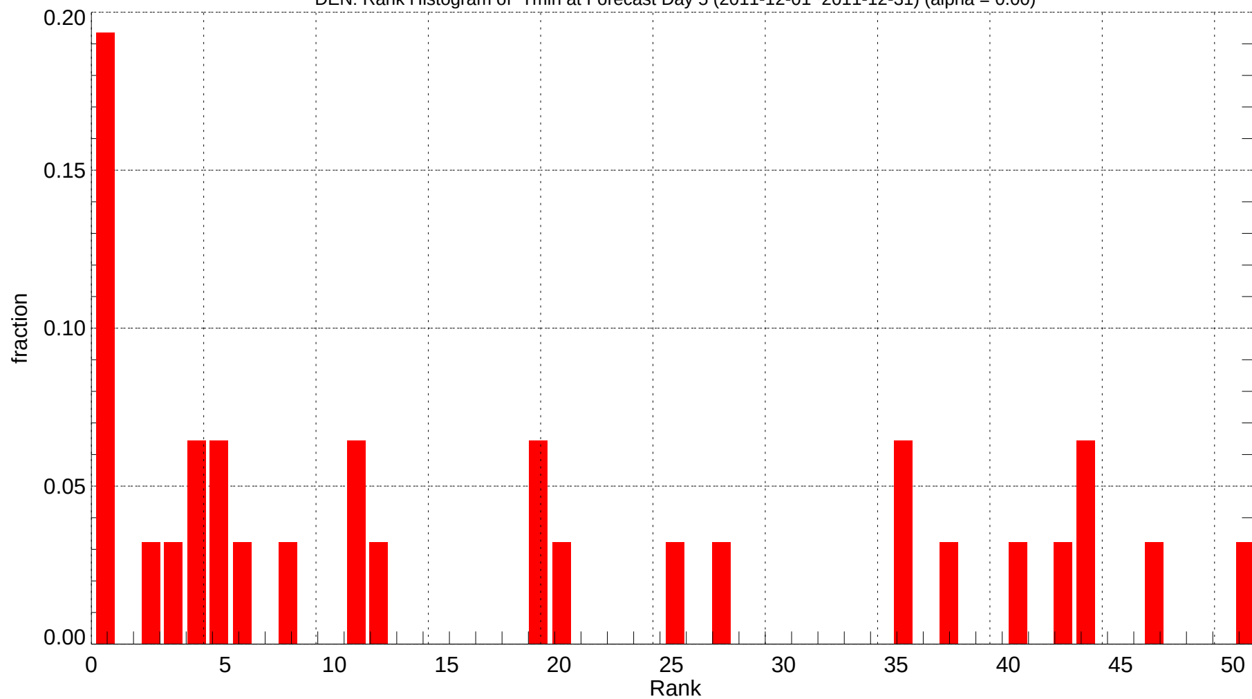
DEN: Rank Histogram of Tmin at Forecast Day 5 (2011-12-01~2011-12-31) (alpha = 0.00)
