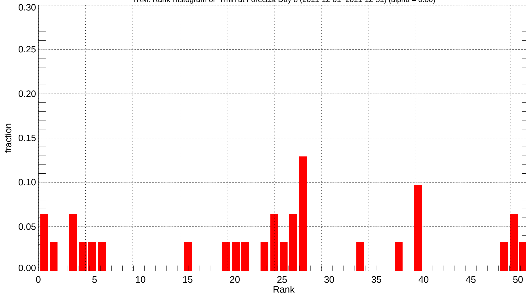
TRM: Rank Histogram of Tmin at Forecast Day 8 (2011-12-01~2011-12-31) (alpha = 0.00)
