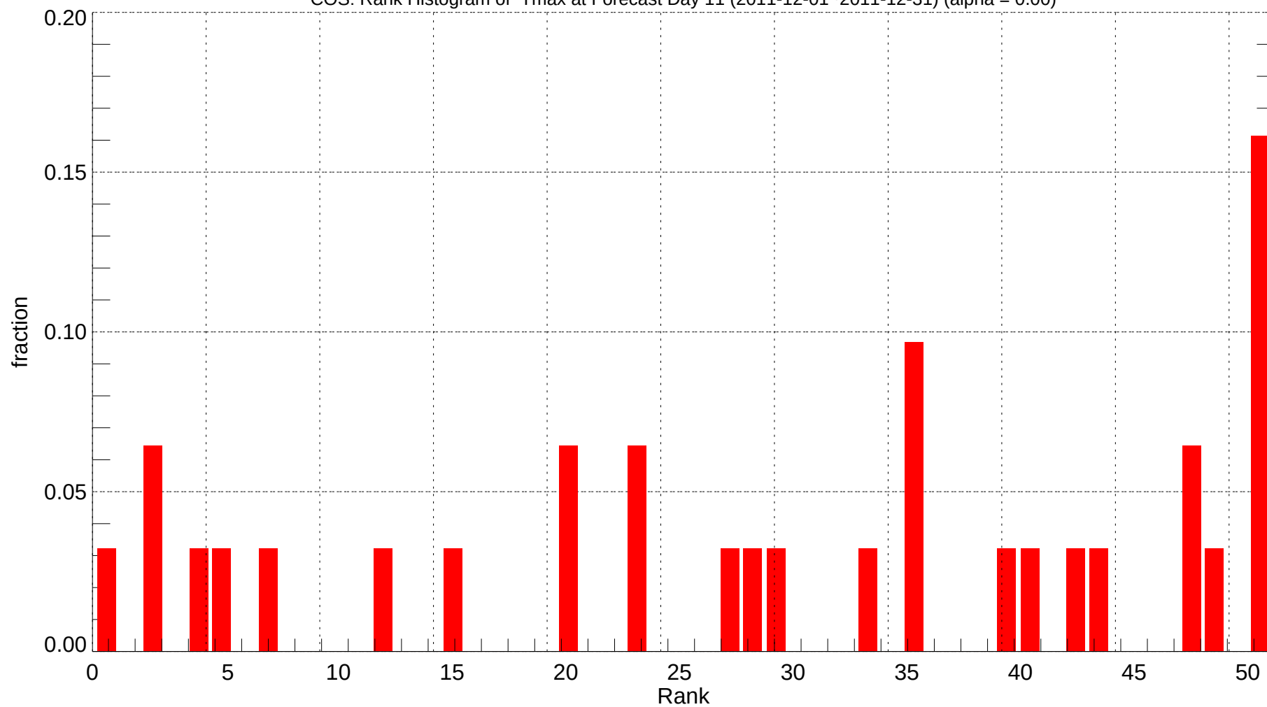
COS: Rank Histogram of Tmax at Forecast Day 11 (2011-12-01~2011-12-31) (alpha = 0.00)
