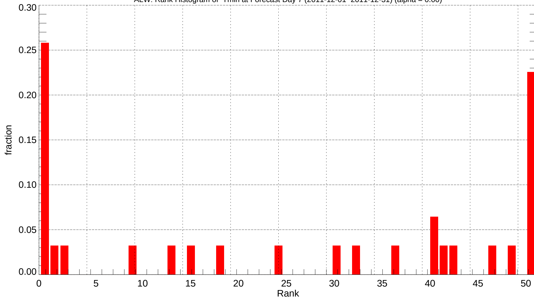
ALW: Rank Histogram of Tmin at Forecast Day 7 (2011-12-01~2011-12-31) (alpha = 0.00)
