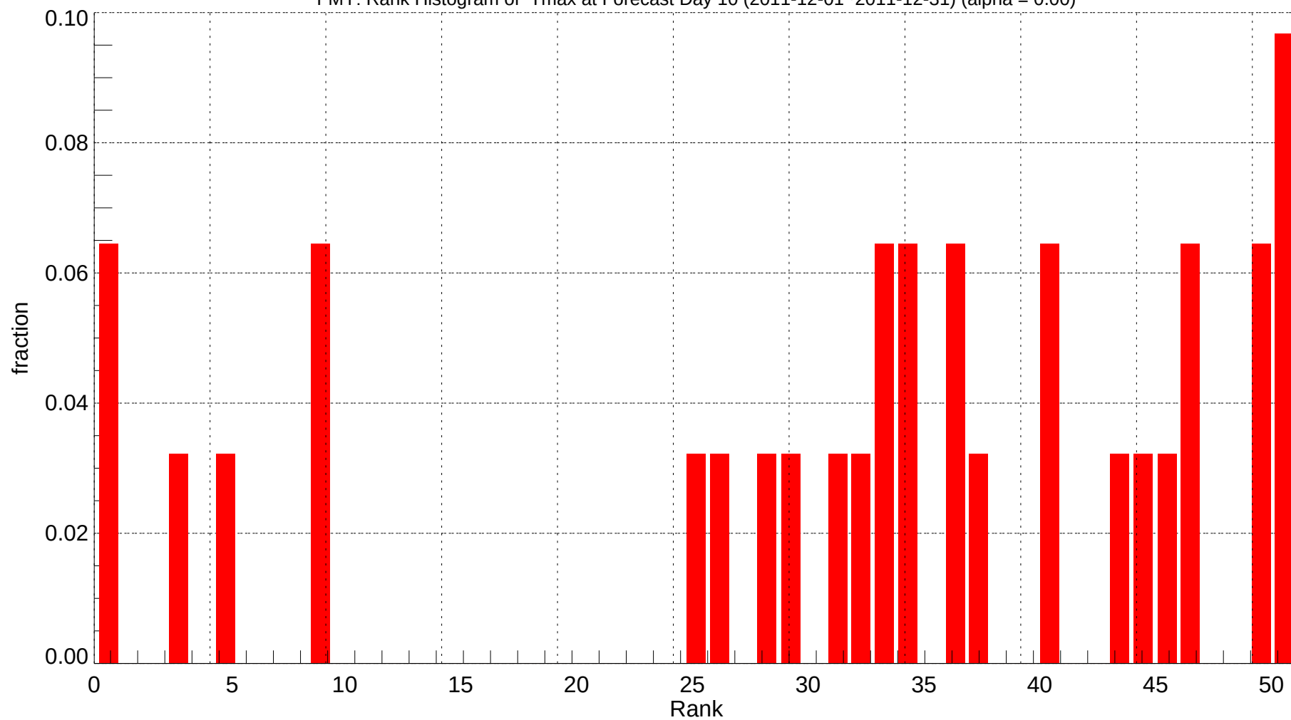
FMY: Rank Histogram of Tmax at Forecast Day 10 (2011-12-01~2011-12-31) (alpha = 0.00)
