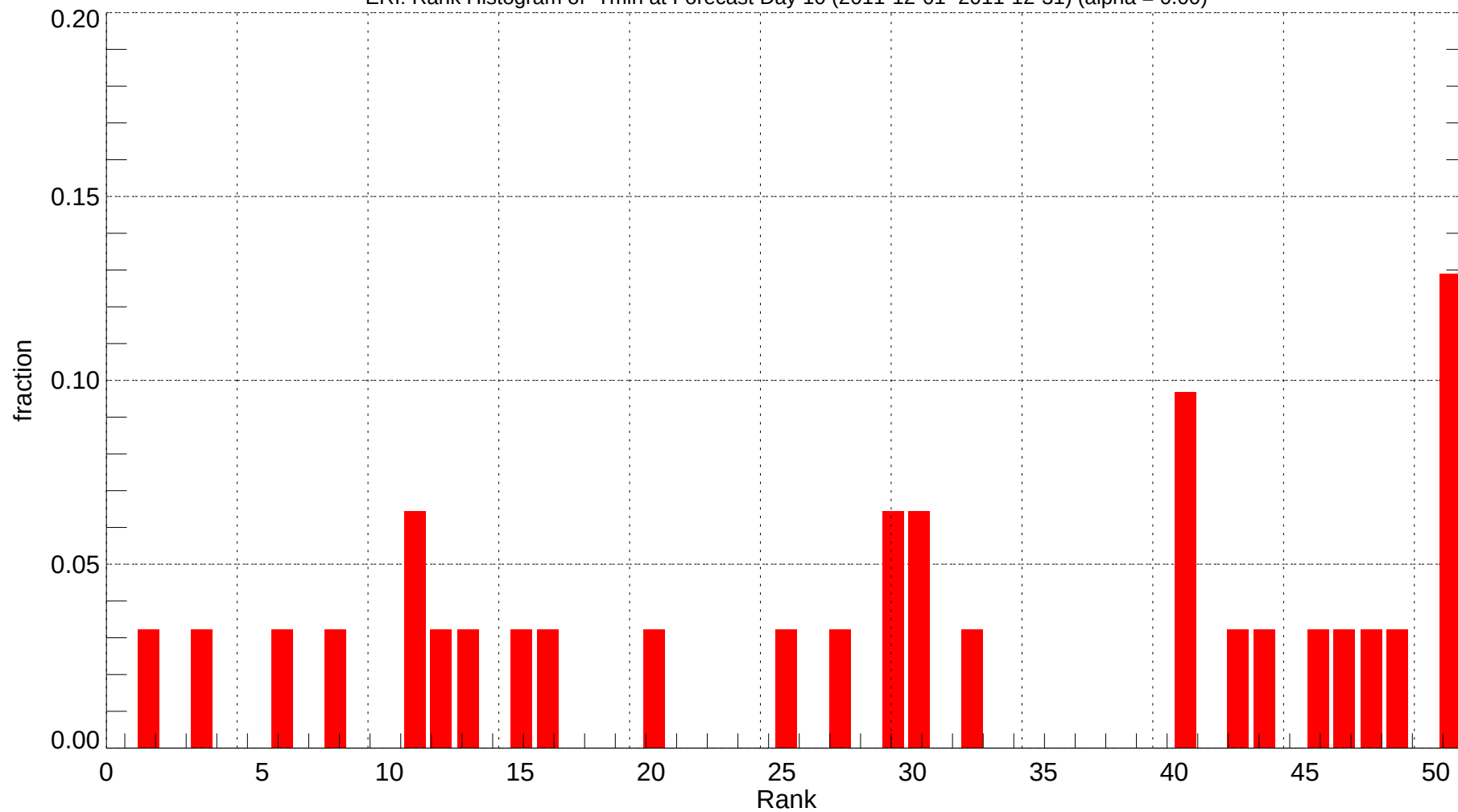
ERI: Rank Histogram of Tmin at Forecast Day 10 (2011-12-01~2011-12-31) (alpha = 0.00)
