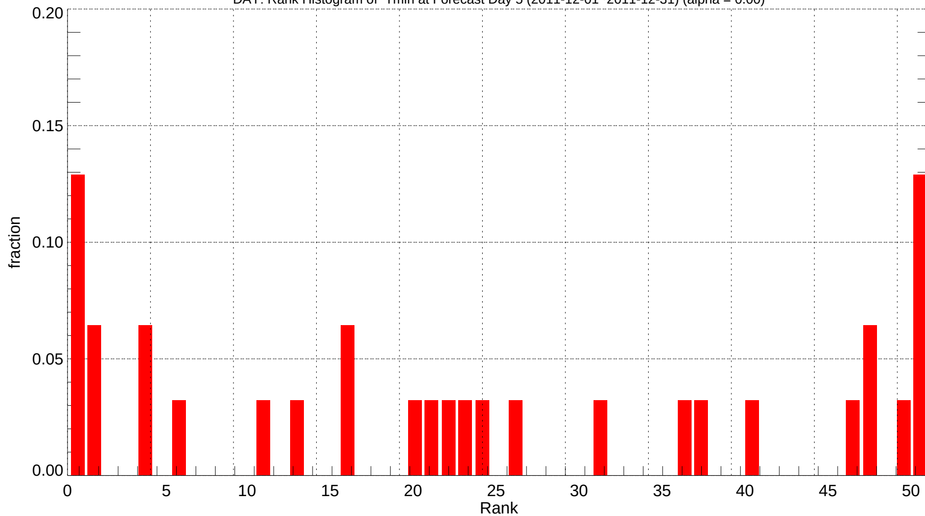
DAY: Rank Histogram of Tmin at Forecast Day 5 (2011-12-01~2011-12-31) (alpha = 0.00)
