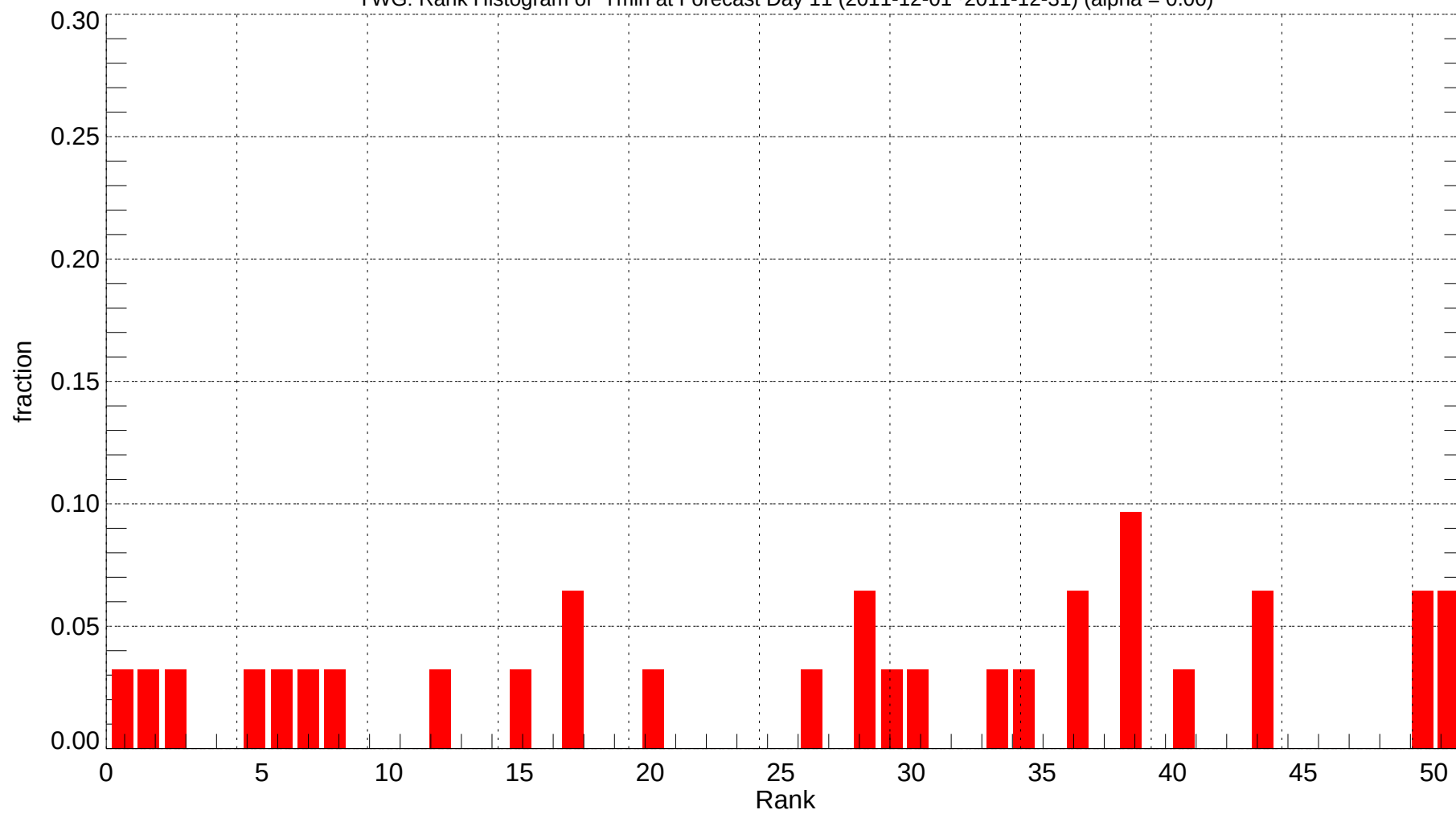
YWG: Rank Histogram of Tmin at Forecast Day 11 (2011-12-01~2011-12-31) (alpha = 0.00)
