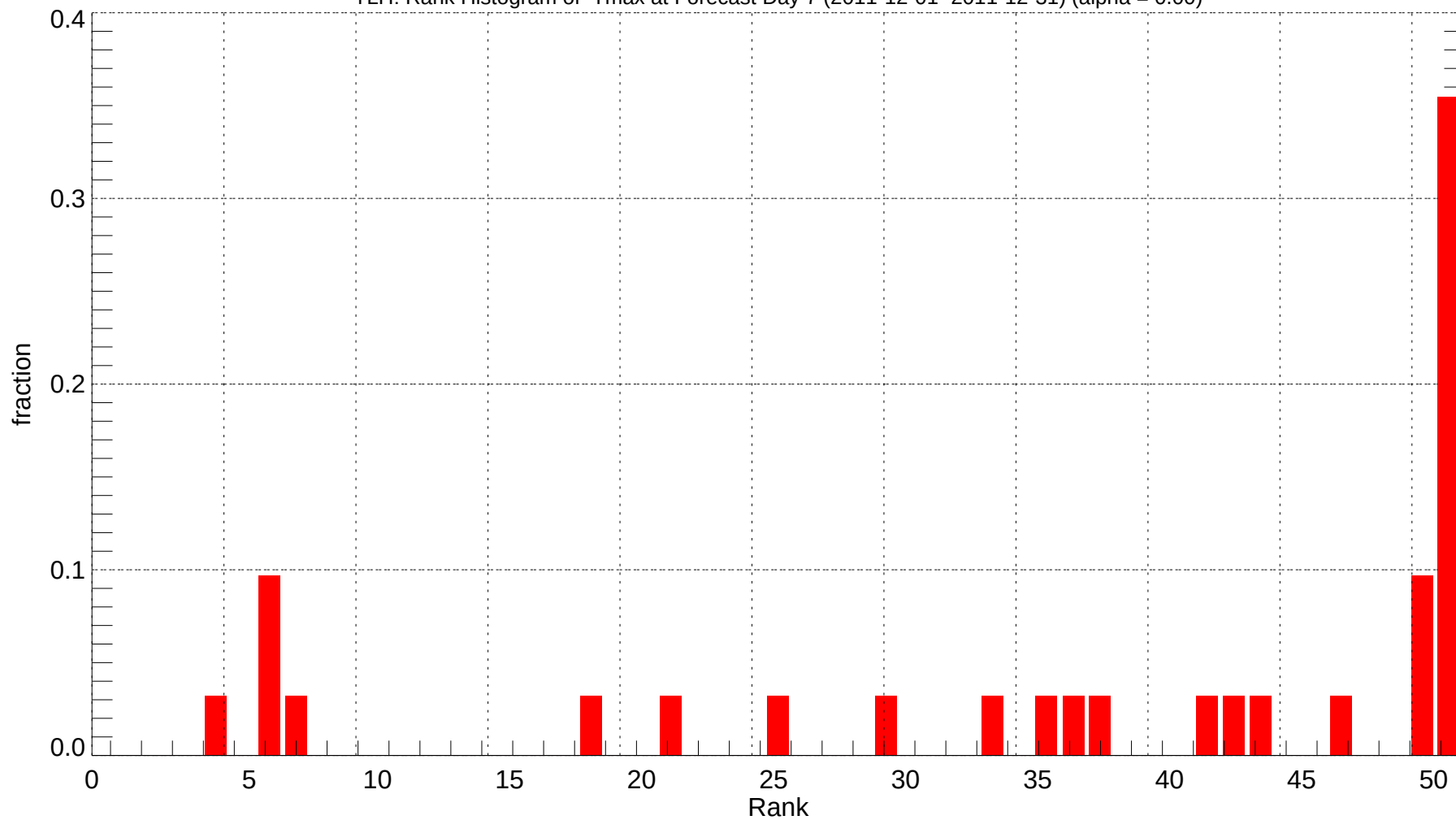
TLH: Rank Histogram of Tmax at Forecast Day 7 (2011-12-01~2011-12-31) (alpha = 0.00)
