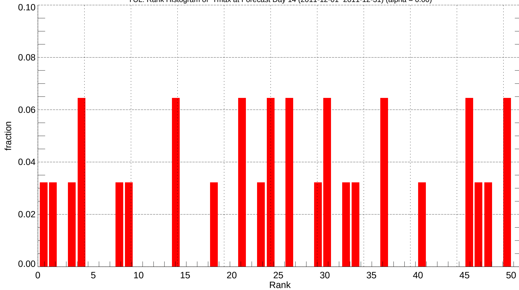
YUL: Rank Histogram of Tmax at Forecast Day 14 (2011-12-01~2011-12-31) (alpha = 0.00)
