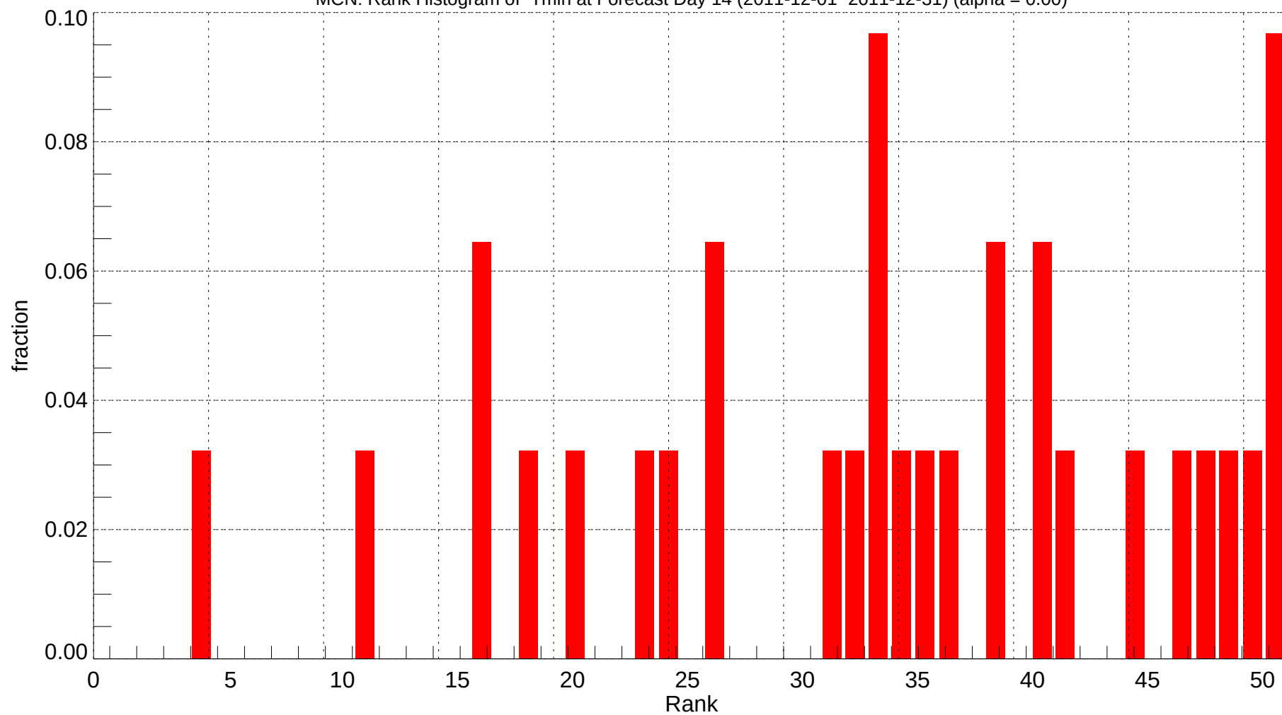
MCN: Rank Histogram of Tmin at Forecast Day 14 (2011-12-01~2011-12-31) (alpha = 0.00)
