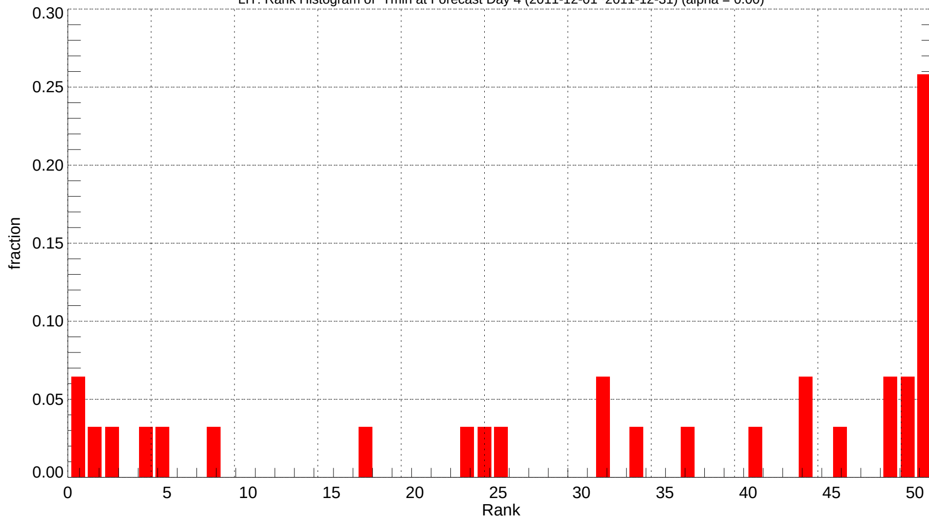
LIT: Rank Histogram of Tmin at Forecast Day 4 (2011-12-01~2011-12-31) (alpha = 0.00)
