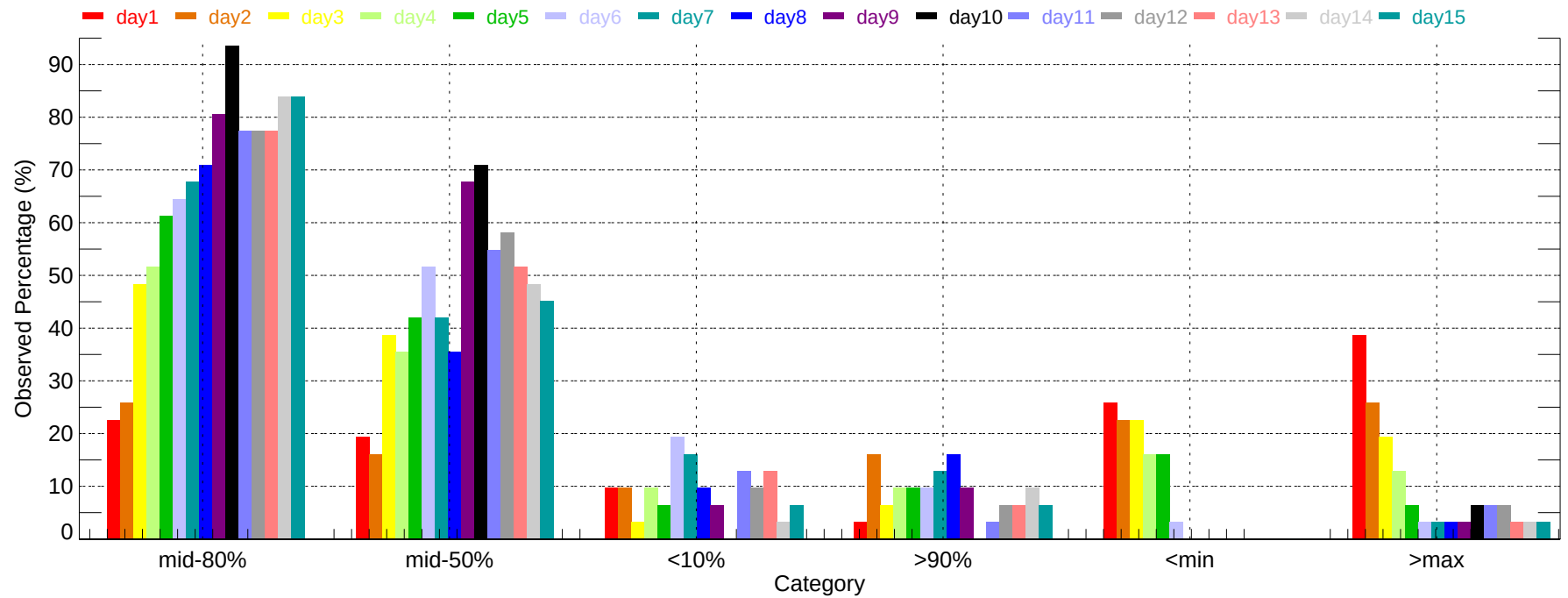
Observed Percentage of Ensembles - ALW: Min Temperature (2011-12-01~2011-12-31)
