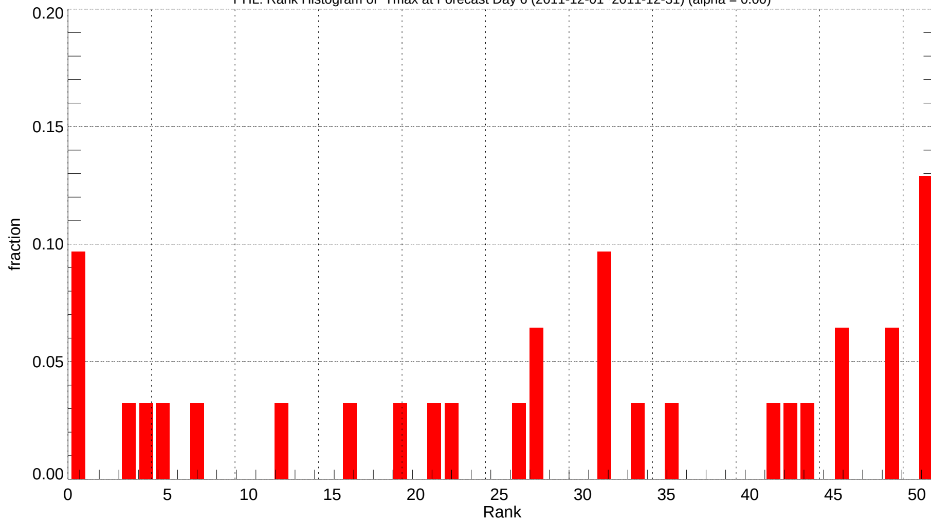
PHL: Rank Histogram of Tmax at Forecast Day 6 (2011-12-01~2011-12-31) (alpha = 0.00)
