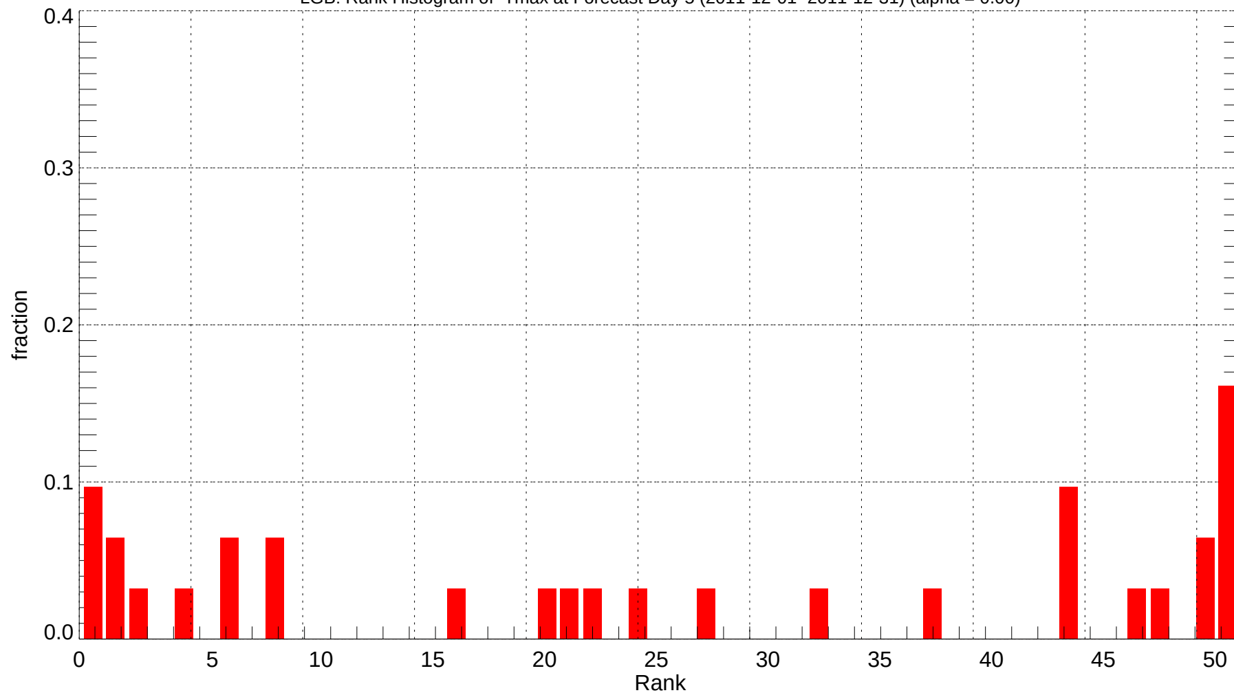
LGB: Rank Histogram of Tmax at Forecast Day 5 (2011-12-01~2011-12-31) (alpha = 0.00)
