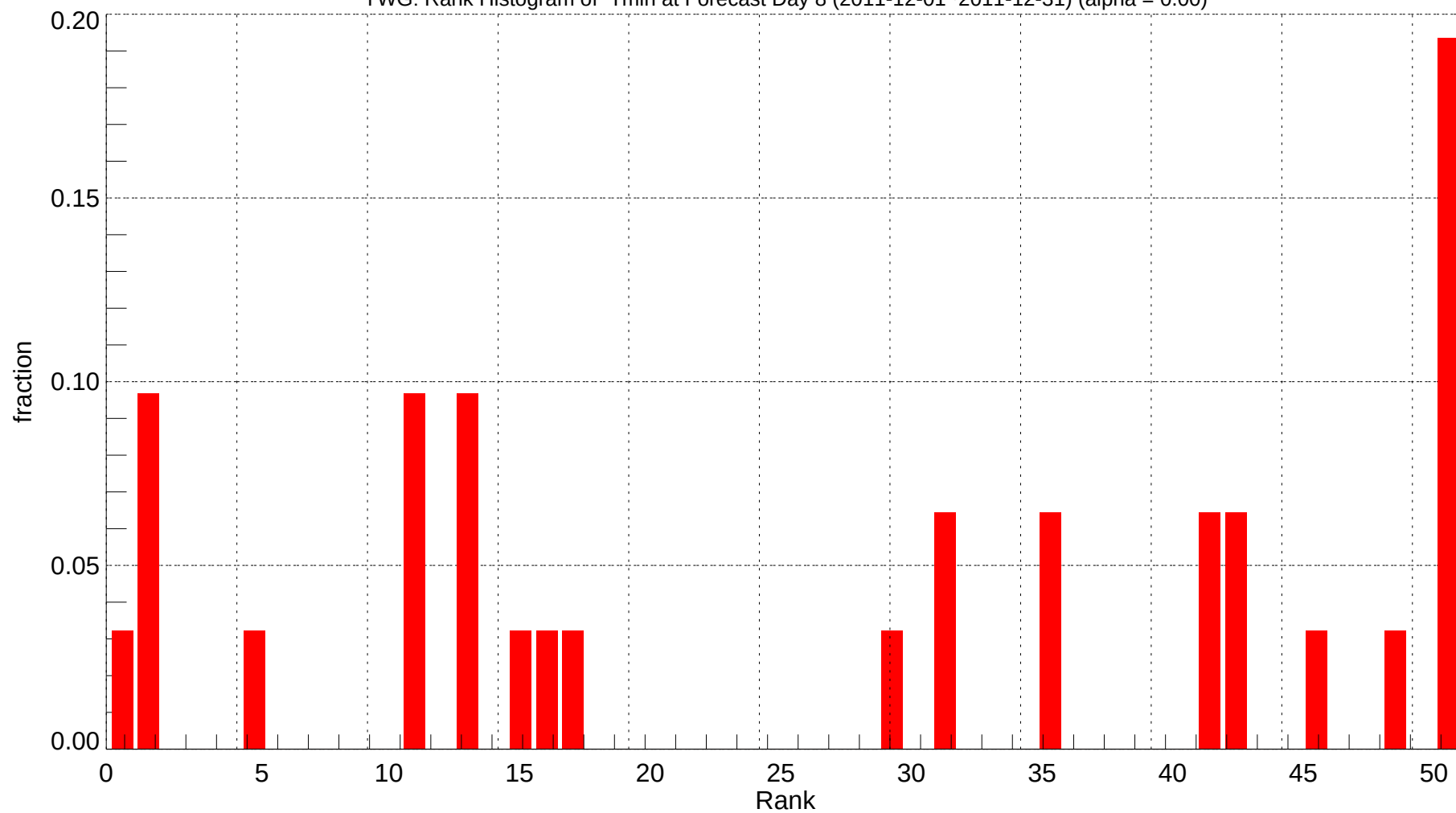
YWG: Rank Histogram of Tmin at Forecast Day 8 (2011-12-01~2011-12-31) (alpha = 0.00)
