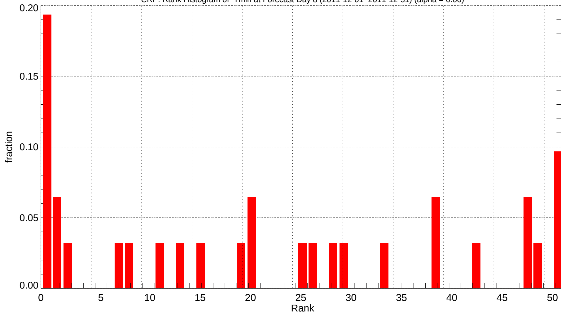
CRP: Rank Histogram of Tmin at Forecast Day 8 (2011-12-01~2011-12-31) (alpha = 0.00)
