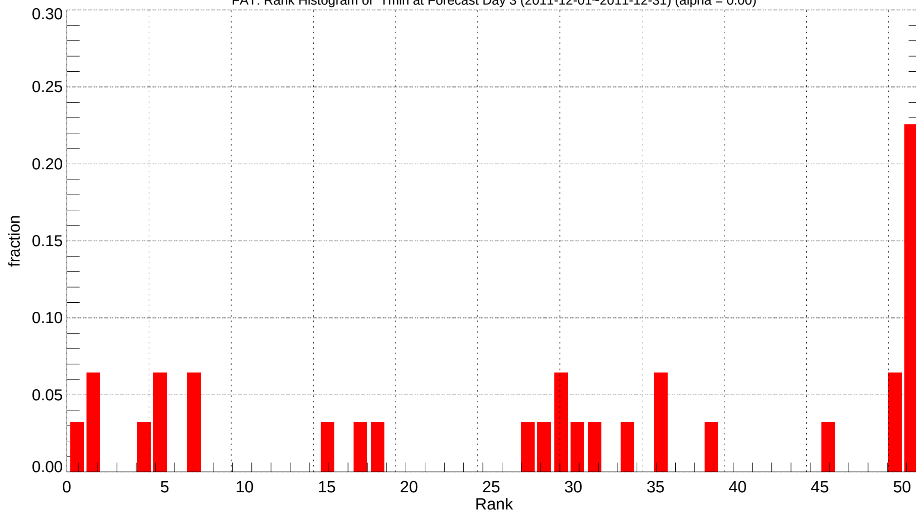
FAT: Rank Histogram of Tmin at Forecast Day 3 (2011-12-01~2011-12-31) (alpha = 0.00)
