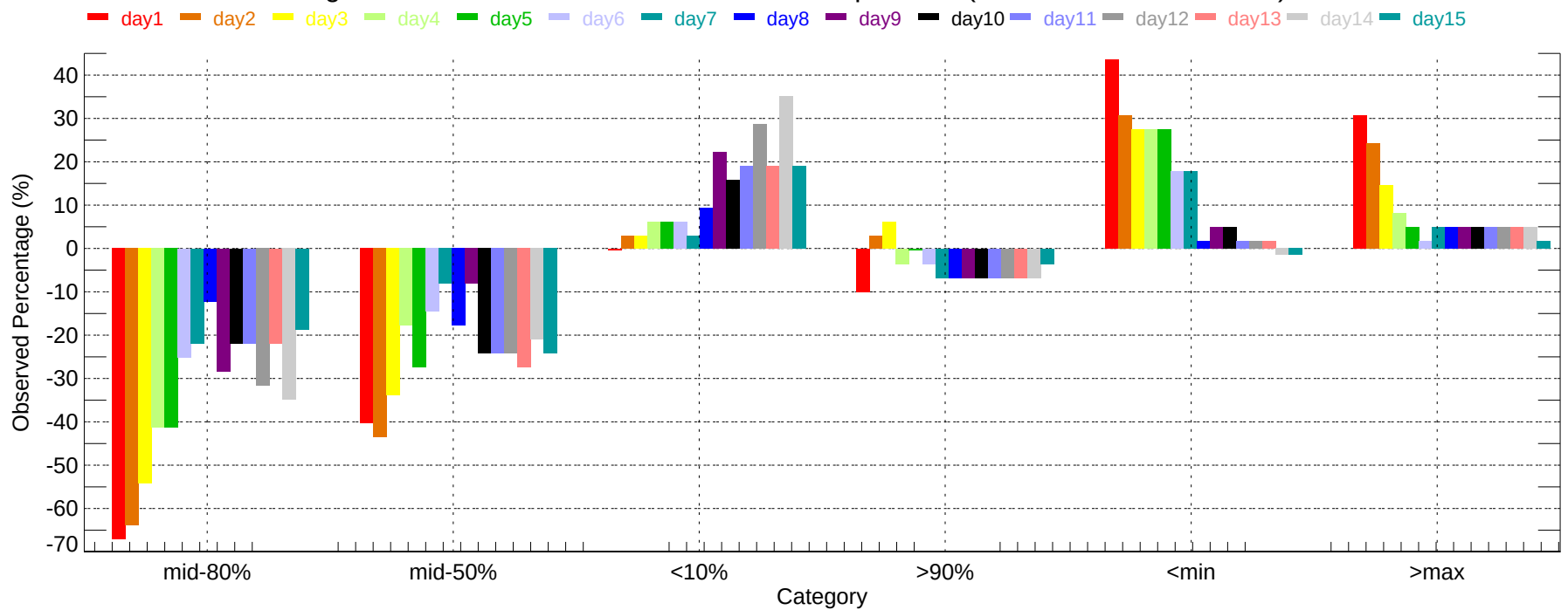
Observed Percentage Deviation of Ensembles - BOI: Min Temperature (2011-12-01~2011-12-31)
