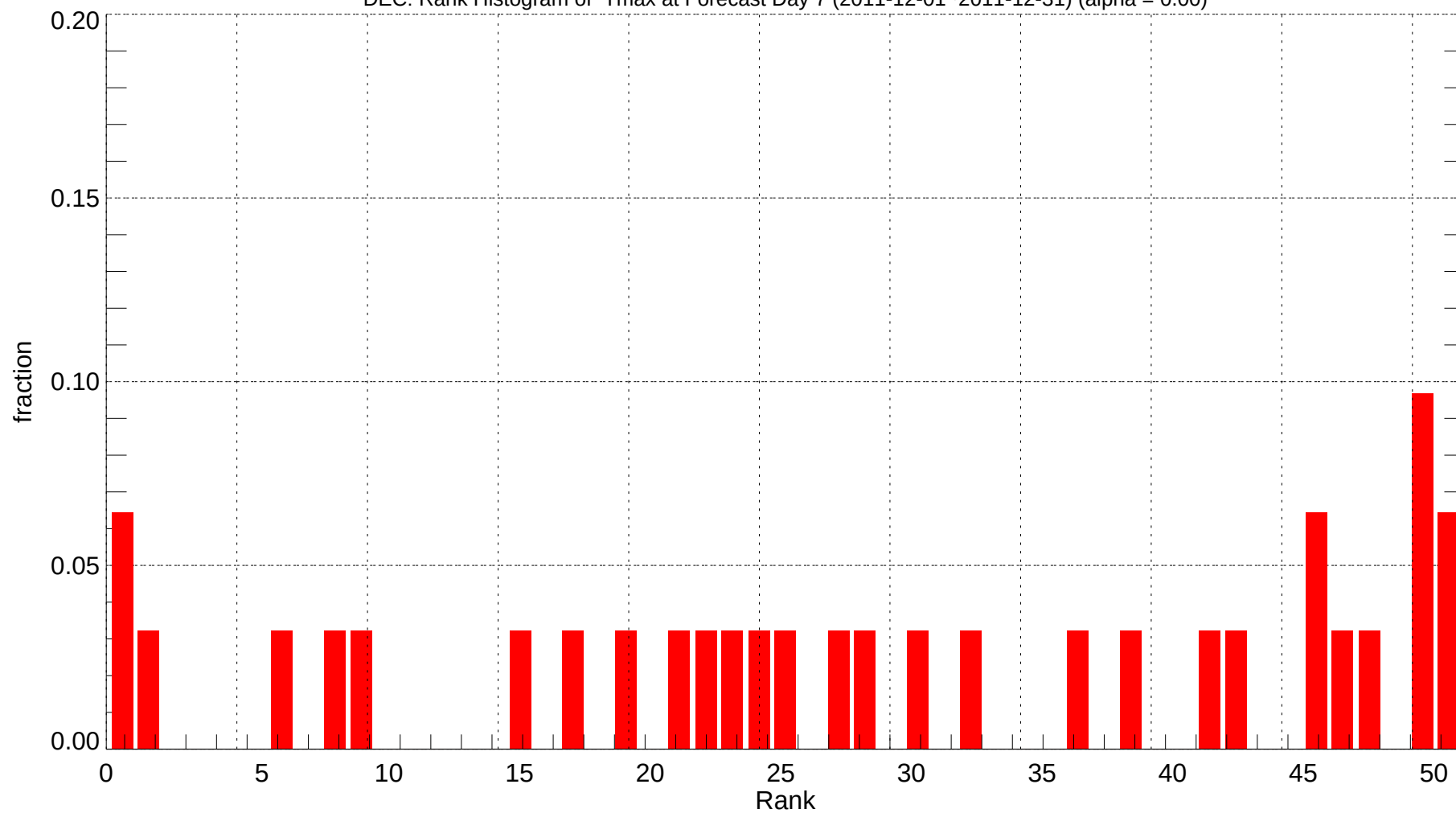
DEC: Rank Histogram of Tmax at Forecast Day 7 (2011-12-01~2011-12-31) (alpha = 0.00)
