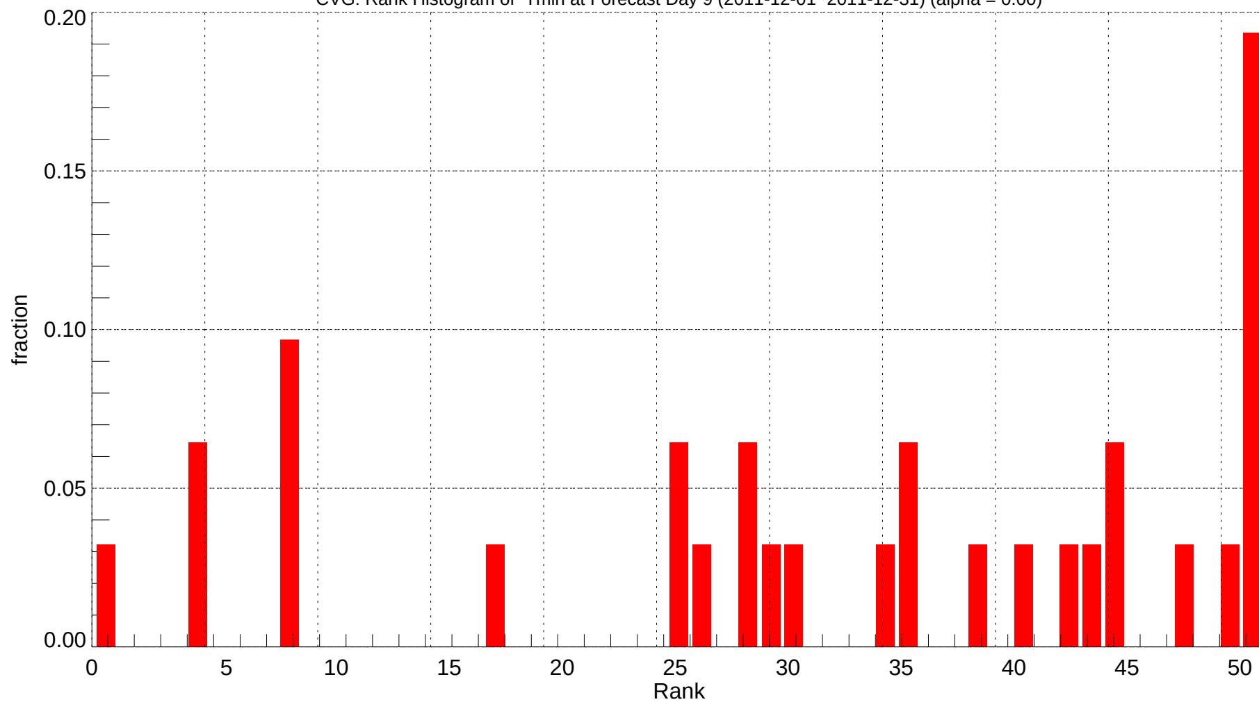
CVG: Rank Histogram of Tmin at Forecast Day 9 (2011-12-01~2011-12-31) (alpha = 0.00)
