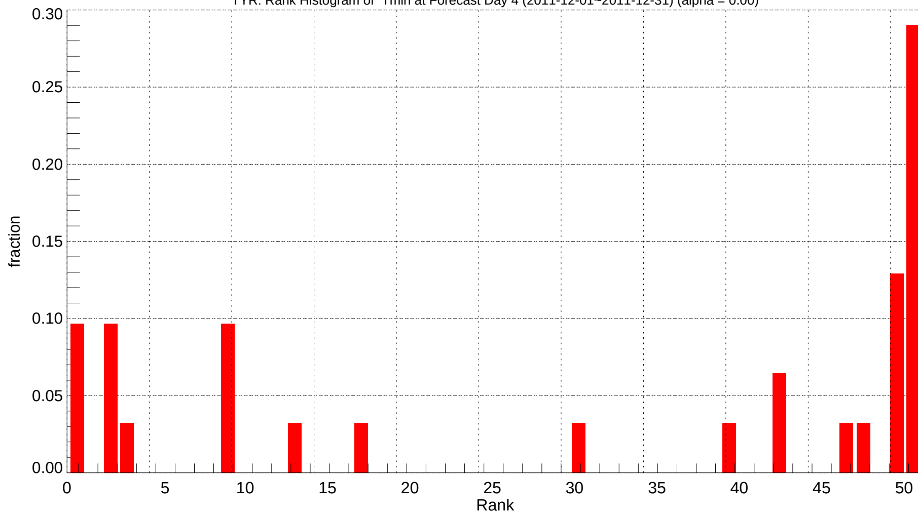
TYR: Rank Histogram of Tmin at Forecast Day 4 (2011-12-01~2011-12-31) (alpha = 0.00)
