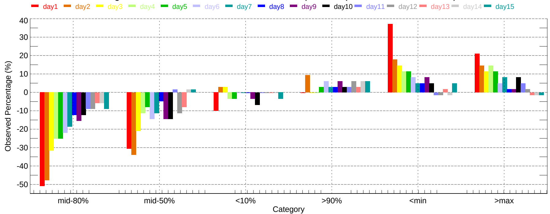
Observed Percentage Deviation of Ensembles - BTV: Max Temperature (2011-12-01~2011-12-31)
