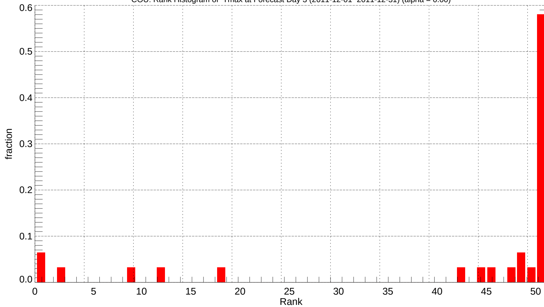
COU: Rank Histogram of Tmax at Forecast Day 3 (2011-12-01~2011-12-31) (alpha = 0.00)
