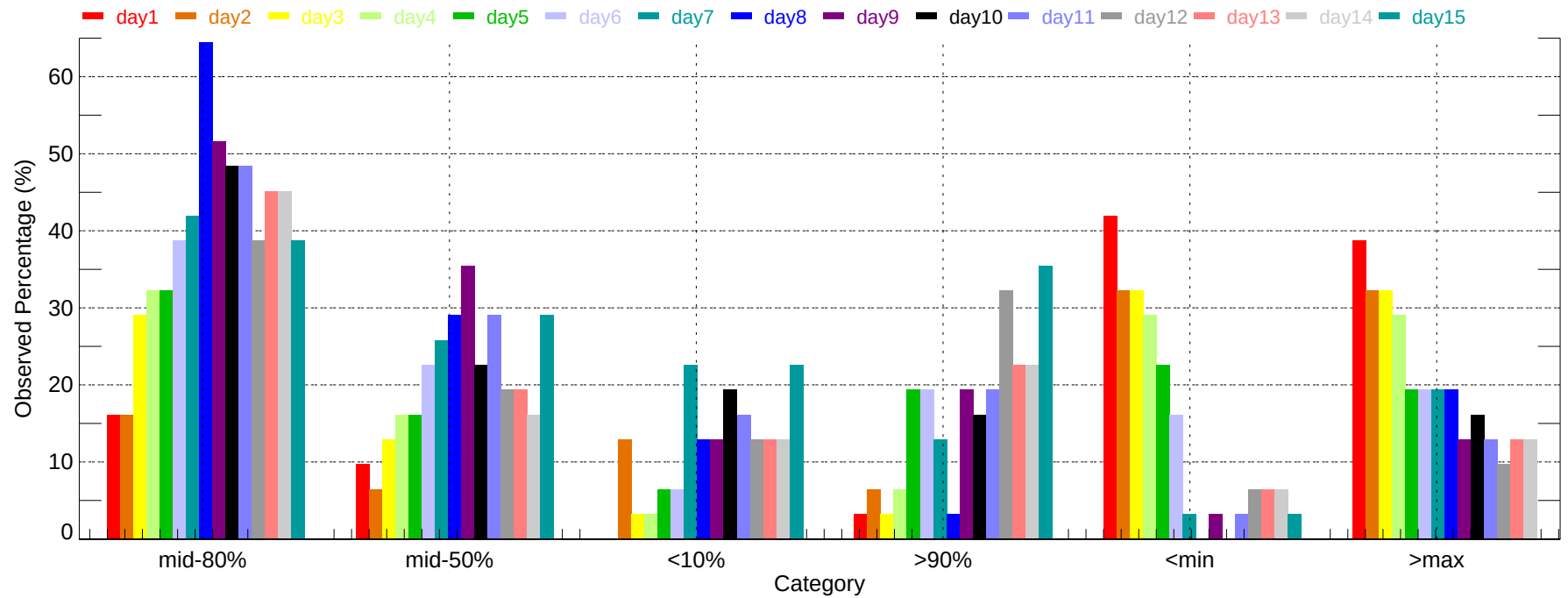
Observed Percentage of Ensembles - OMA: Min Temperature (2011-12-01~2011-12-31)
