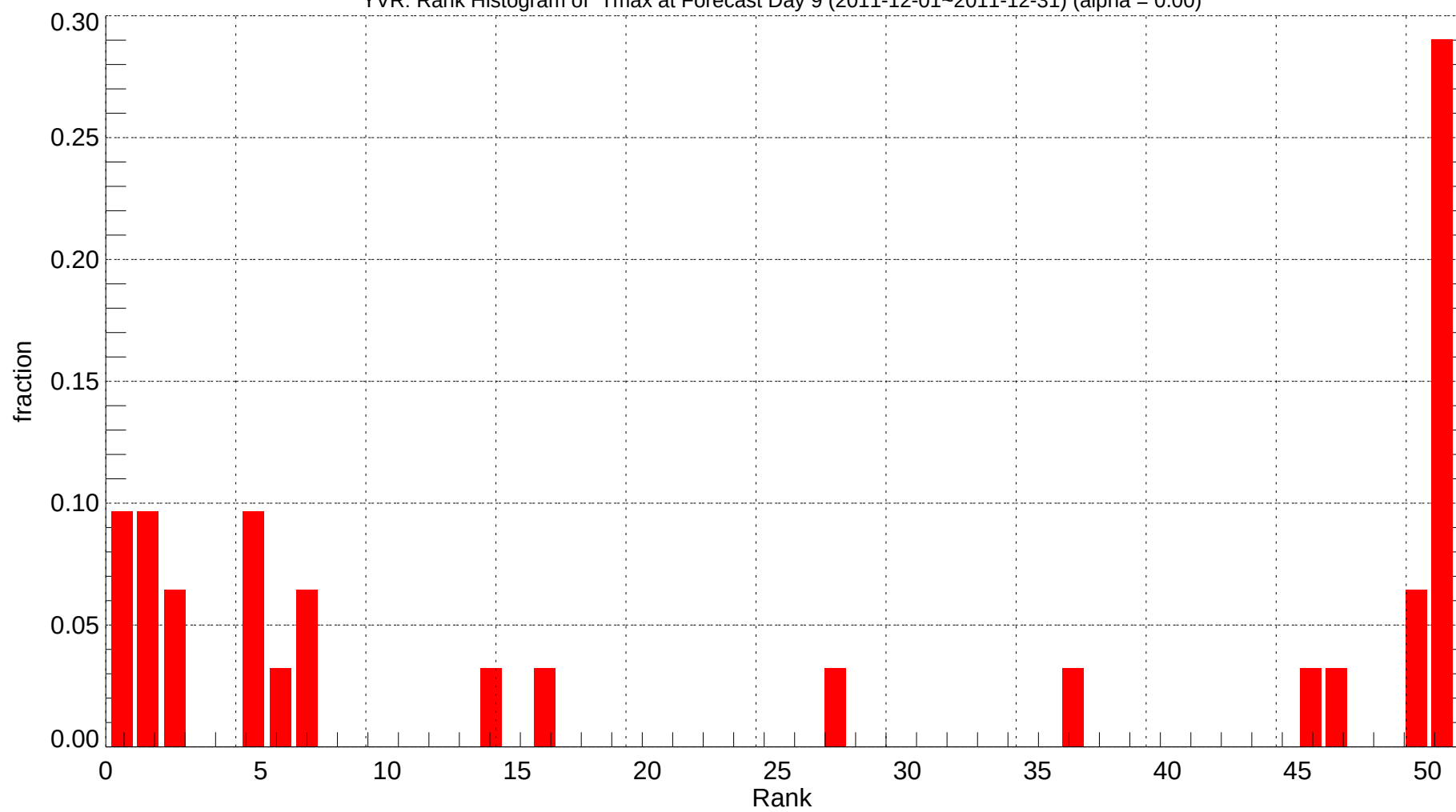
YVR: Rank Histogram of Tmax at Forecast Day 9 (2011-12-01~2011-12-31) (alpha = 0.00)
