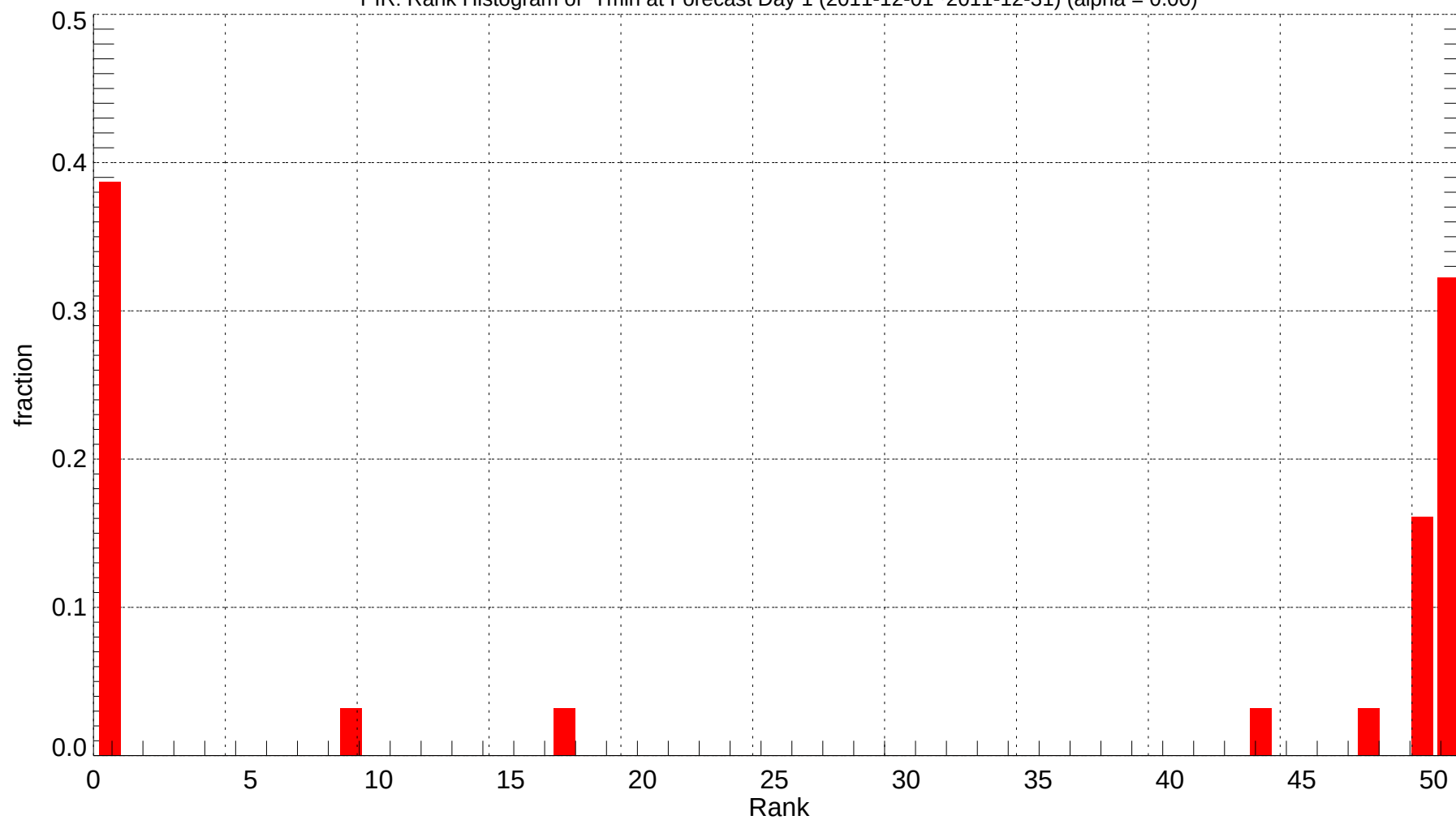
PIR: Rank Histogram of Tmin at Forecast Day 1 (2011-12-01~2011-12-31) (alpha = 0.00)
