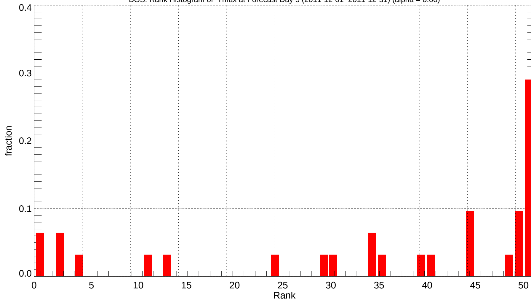
BOS: Rank Histogram of Tmax at Forecast Day 3 (2011-12-01~2011-12-31) (alpha = 0.00)
