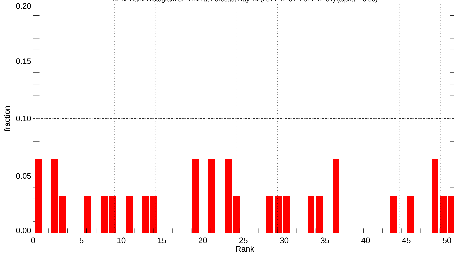
DEN: Rank Histogram of Tmin at Forecast Day 14 (2011-12-01~2011-12-31) (alpha = 0.00)
