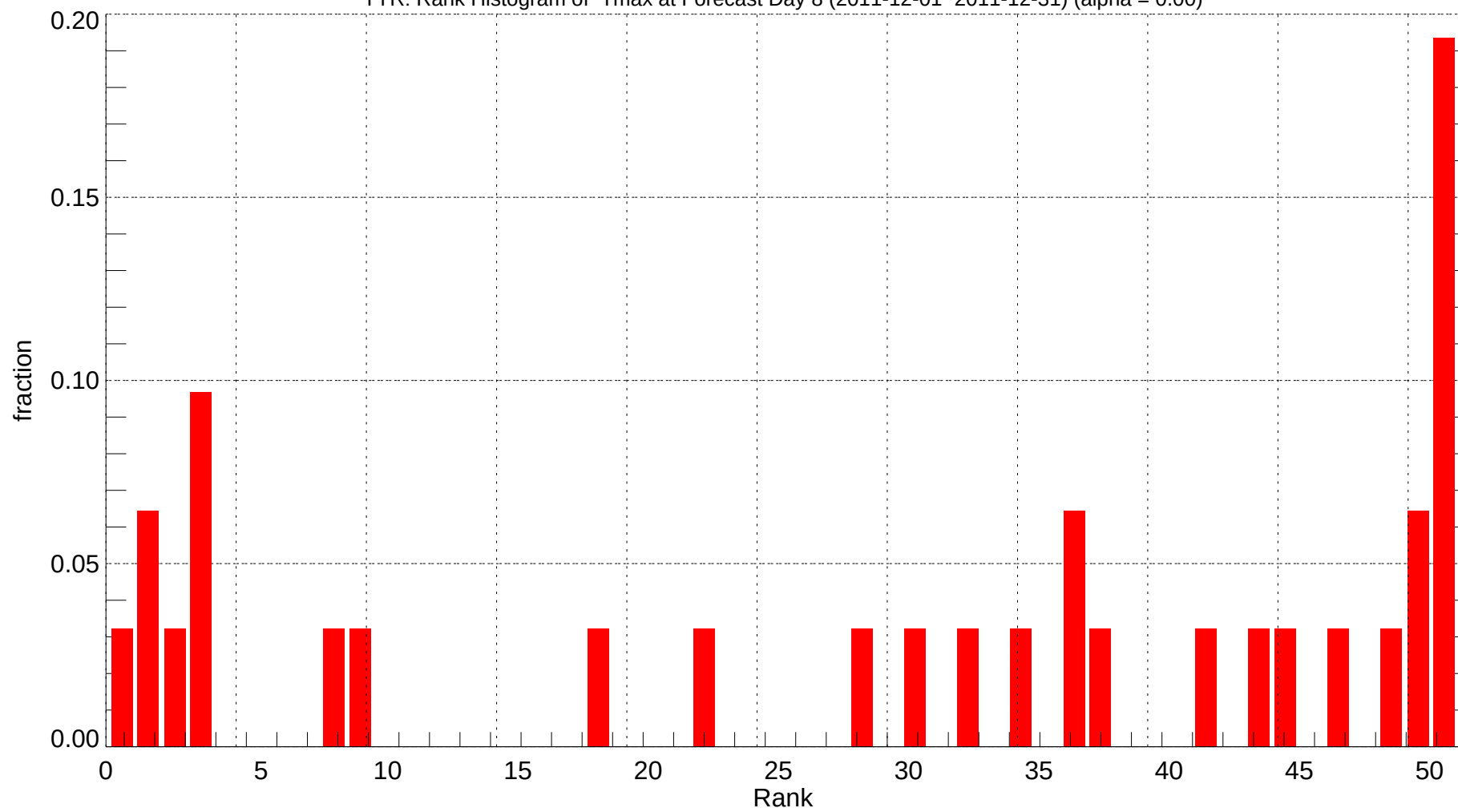
TYR: Rank Histogram of Tmax at Forecast Day 8 (2011-12-01~2011-12-31) (alpha = 0.00)
