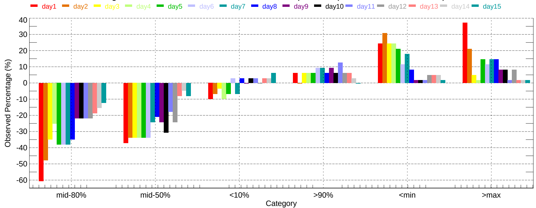
Observed Percentage Deviation of Ensembles - MOB: Min Temperature (2011-12-01~2011-12-31)
