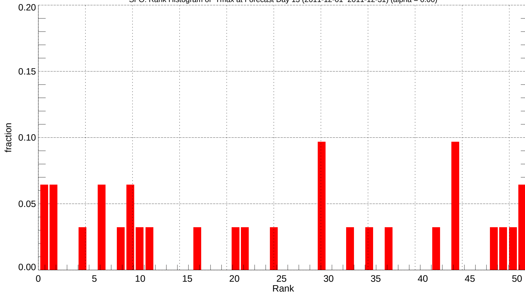
SFO: Rank Histogram of Tmax at Forecast Day 13 (2011-12-01~2011-12-31) (alpha = 0.00)
