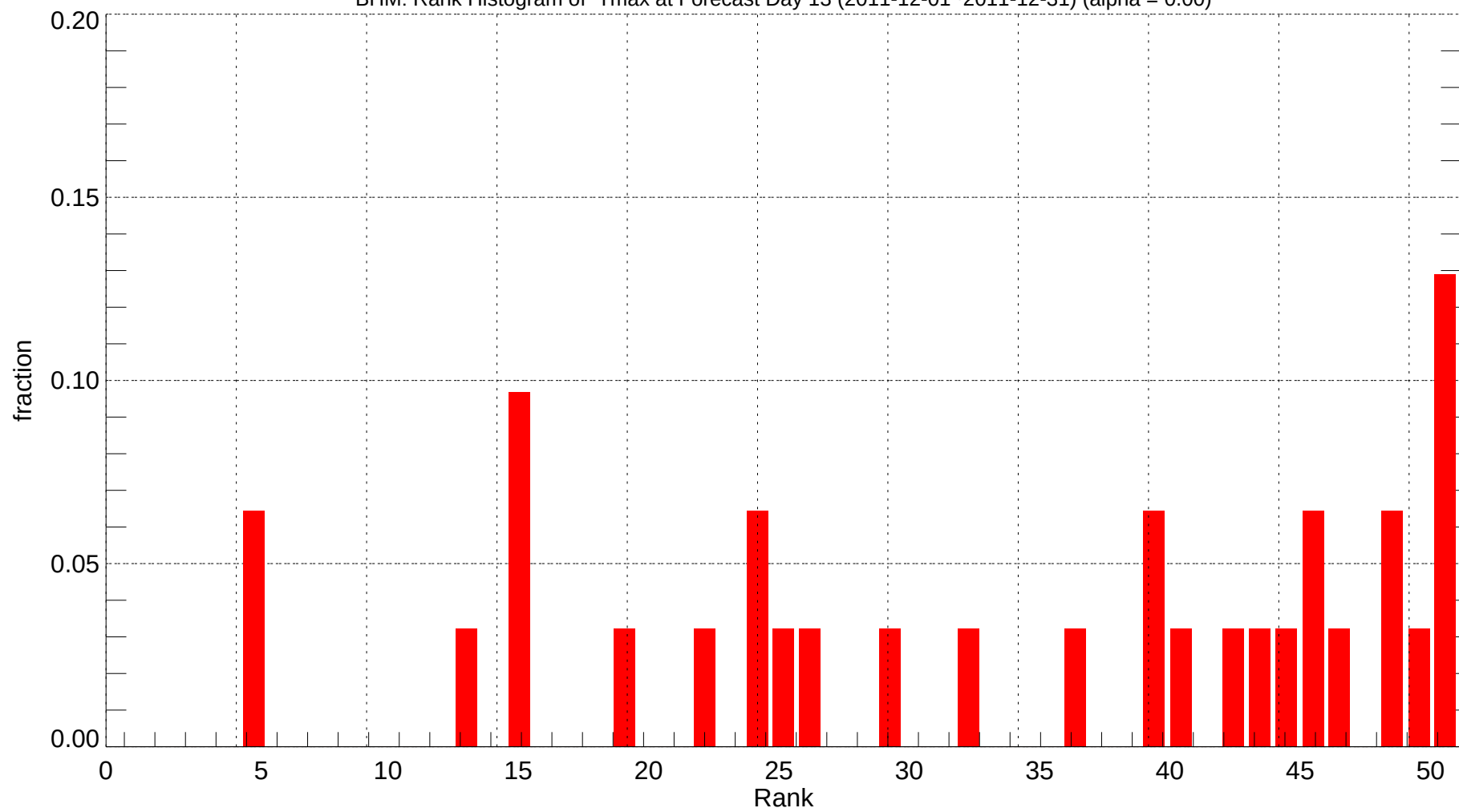
BHM: Rank Histogram of Tmax at Forecast Day 13 (2011-12-01~2011-12-31) (alpha = 0.00)
