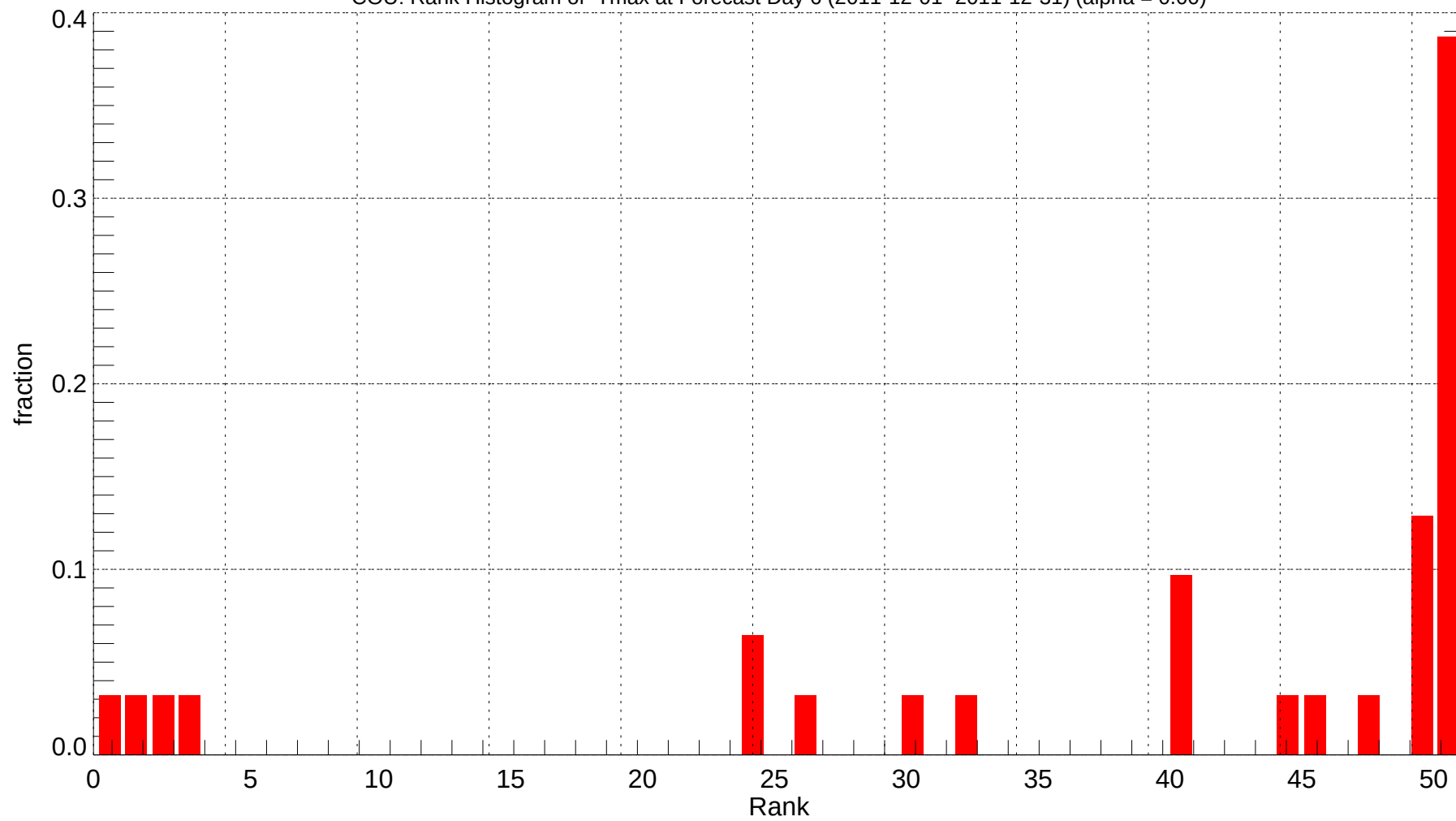
COU: Rank Histogram of Tmax at Forecast Day 6 (2011-12-01~2011-12-31) (alpha = 0.00)
