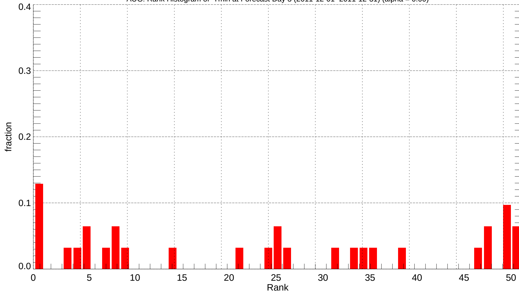
AUG: Rank Histogram of Tmin at Forecast Day 3 (2011-12-01~2011-12-31) (alpha = 0.00)
