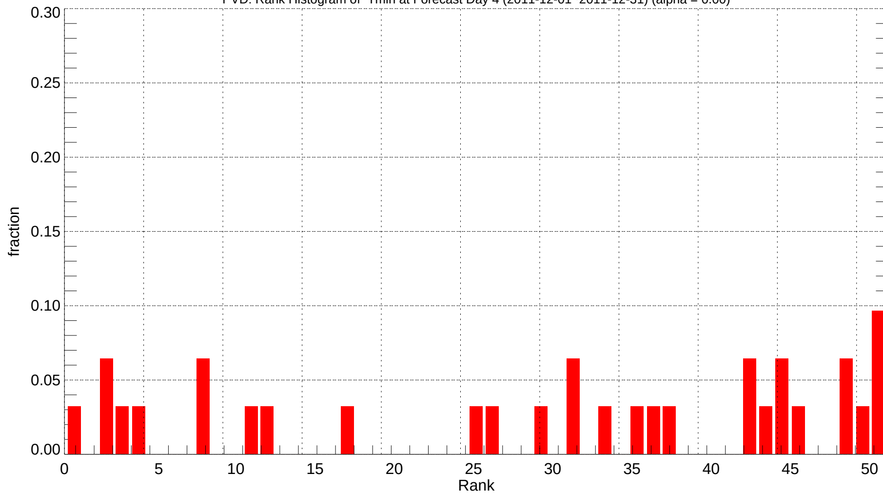
PVD: Rank Histogram of Tmin at Forecast Day 4 (2011-12-01~2011-12-31) (alpha = 0.00)
