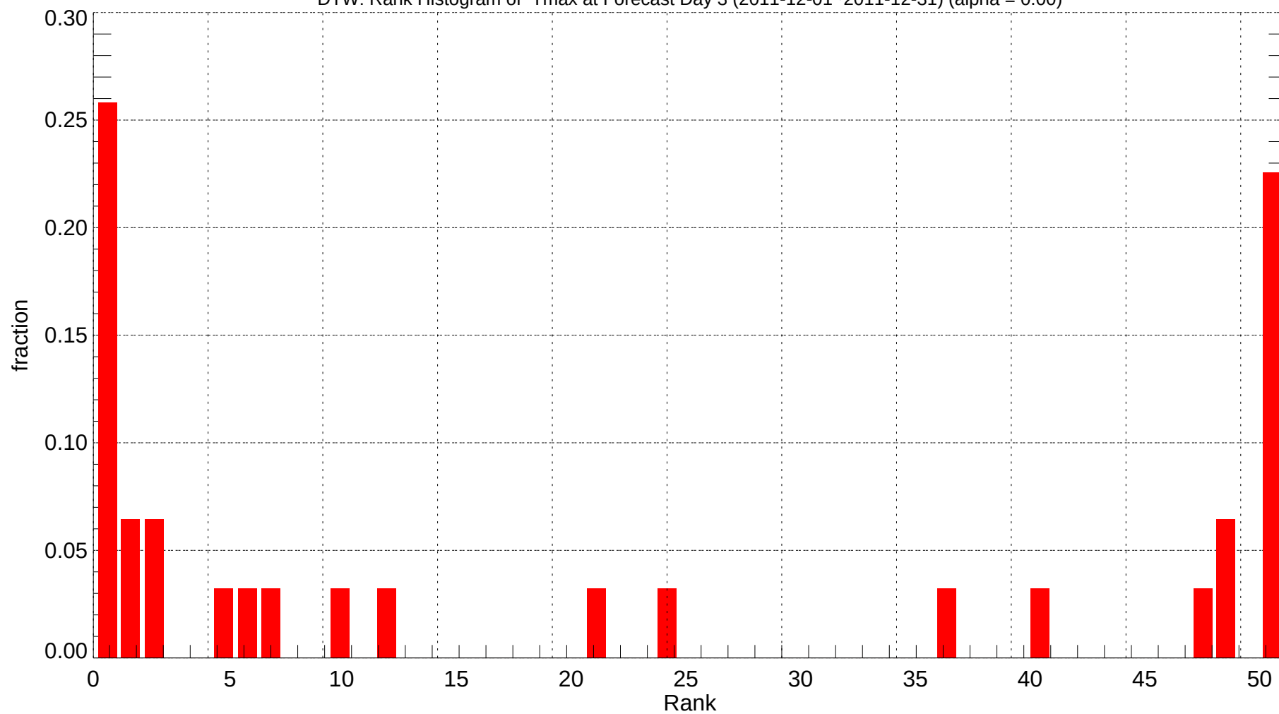
DTW: Rank Histogram of Tmax at Forecast Day 3 (2011-12-01~2011-12-31) (alpha = 0.00)
