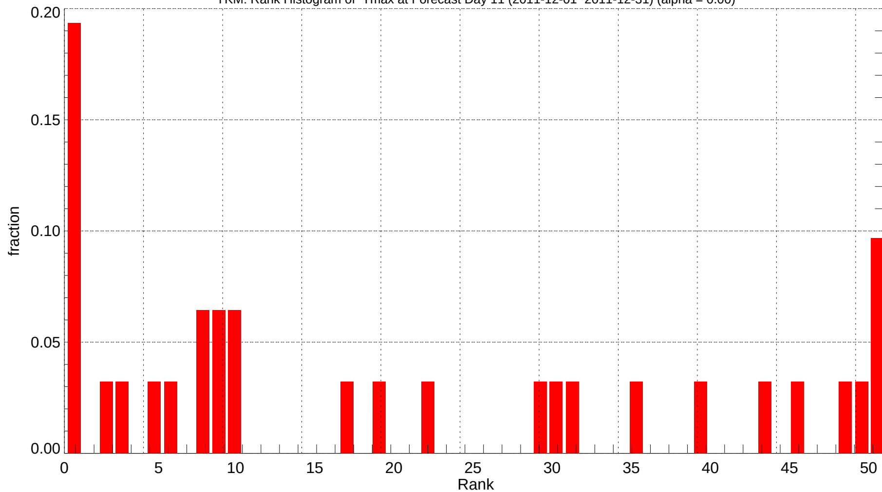
YKM: Rank Histogram of Tmax at Forecast Day 11 (2011-12-01~2011-12-31) (alpha = 0.00)
