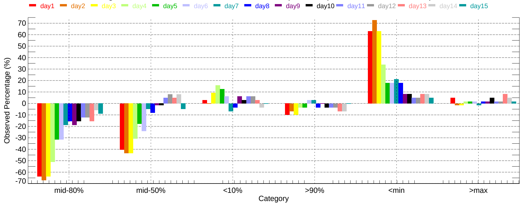
Observed Percentage Deviation of Ensembles - CRP: Min Temperature (2011-12-01~2011-12-31)
