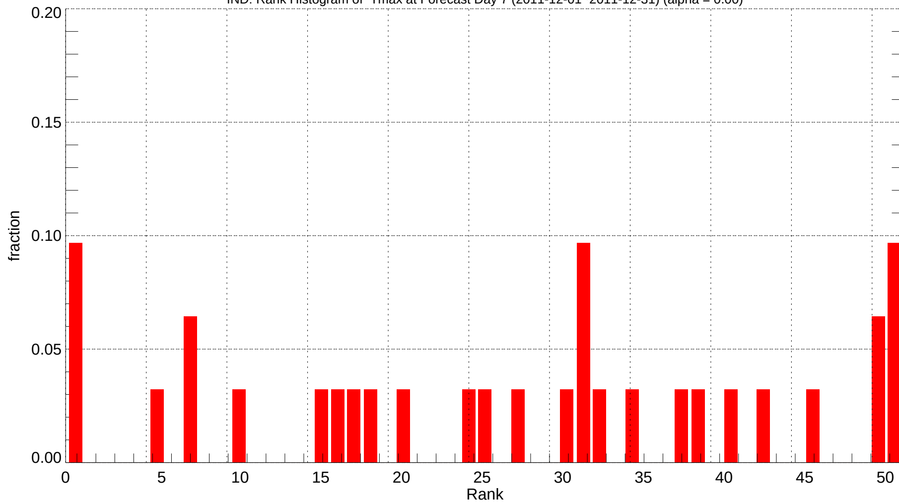
IND: Rank Histogram of Tmax at Forecast Day 7 (2011-12-01~2011-12-31) (alpha = 0.00)
