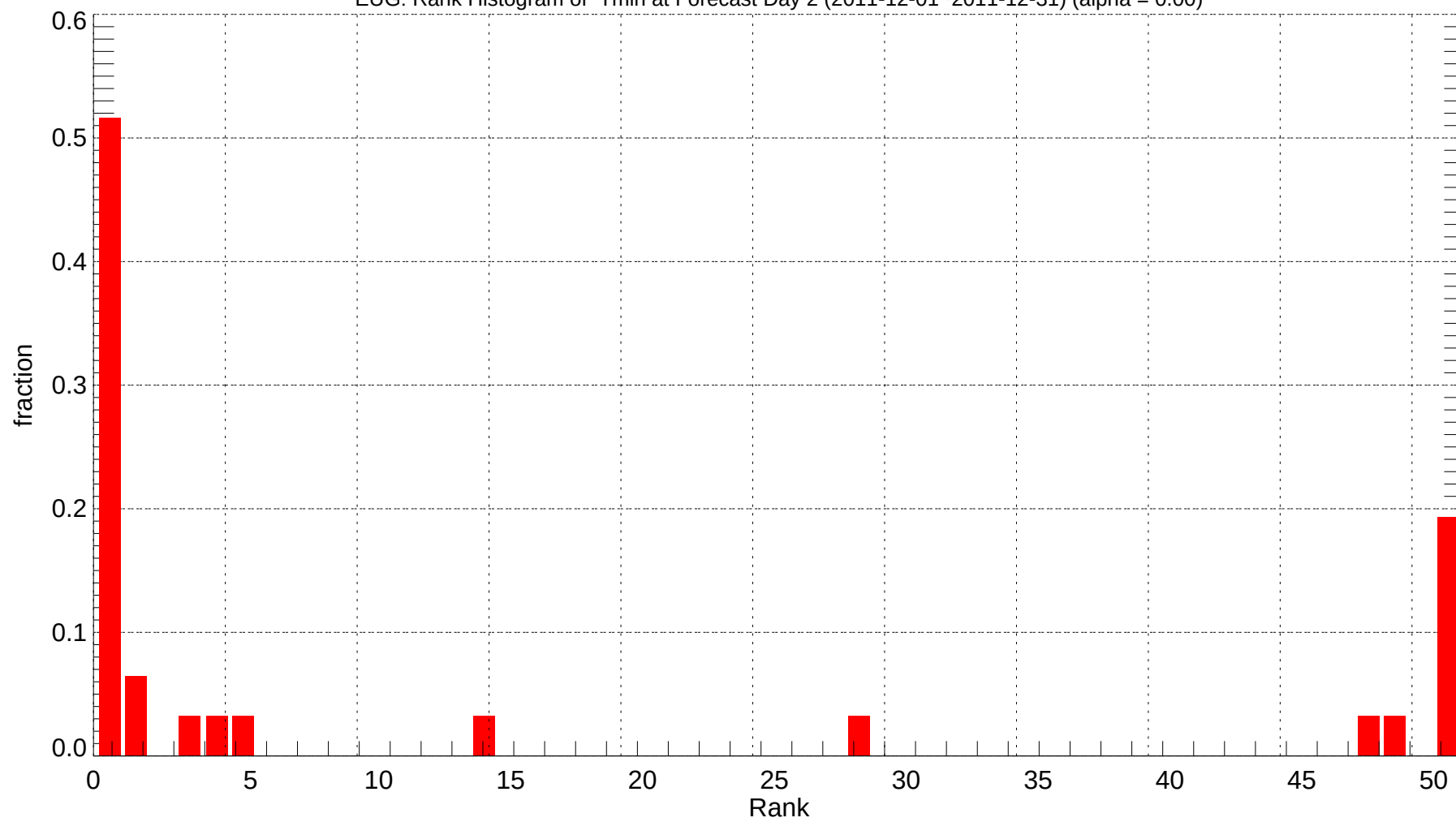
EUG: Rank Histogram of Tmin at Forecast Day 2 (2011-12-01~2011-12-31) (alpha = 0.00)
