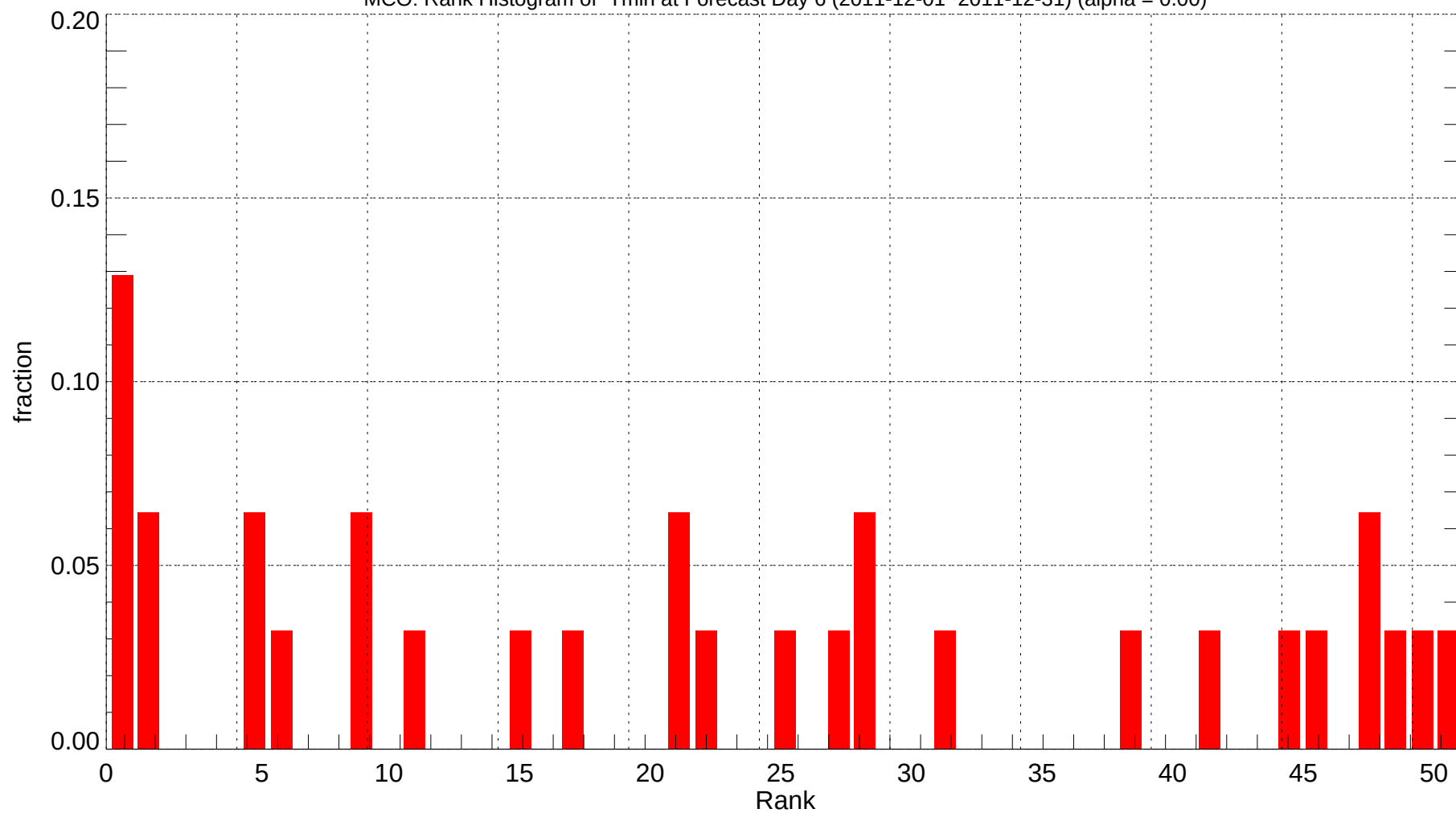
MCO: Rank Histogram of Tmin at Forecast Day 6 (2011-12-01~2011-12-31) (alpha = 0.00)
