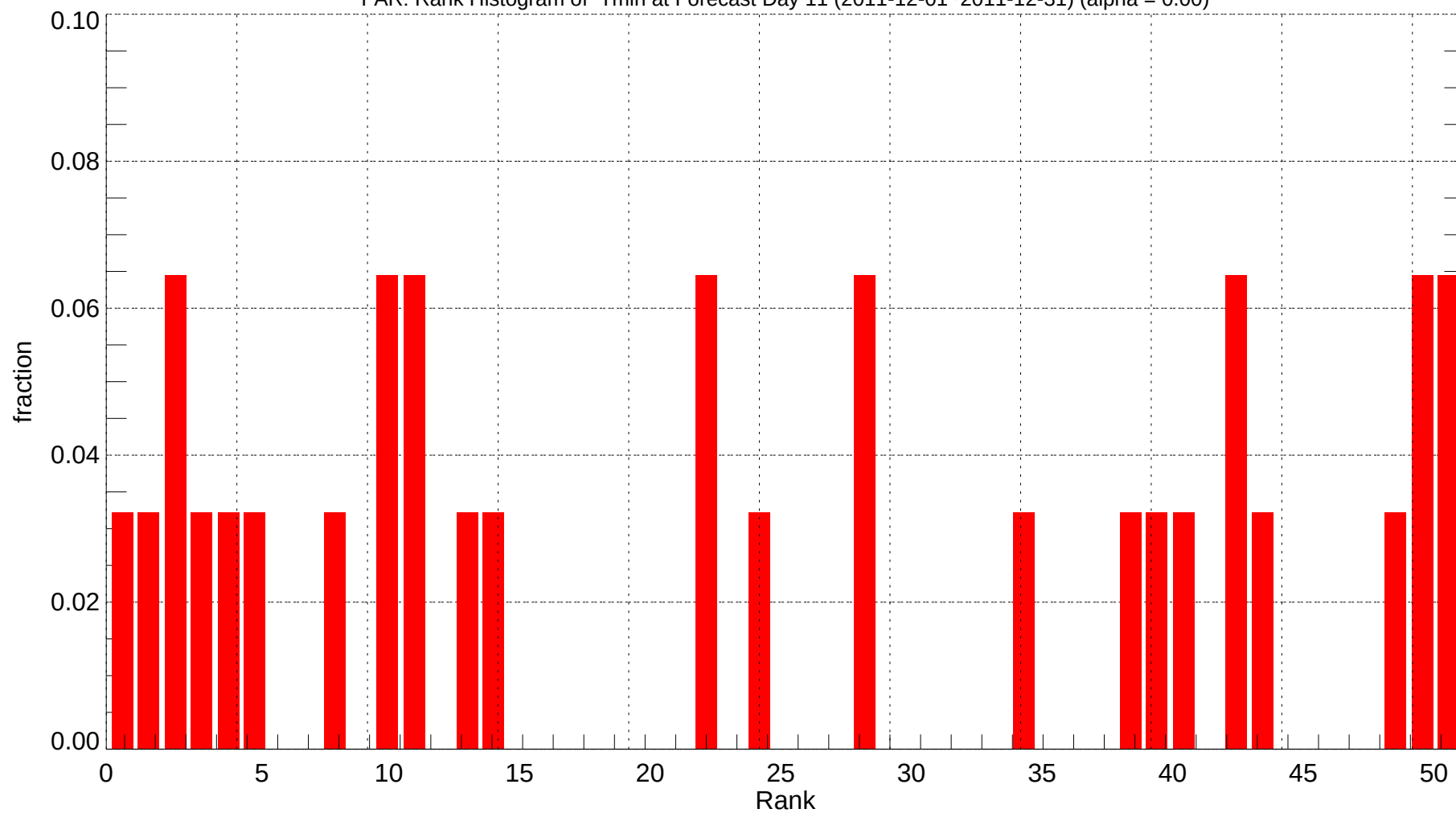
FAR: Rank Histogram of Tmin at Forecast Day 11 (2011-12-01~2011-12-31) (alpha = 0.00)
