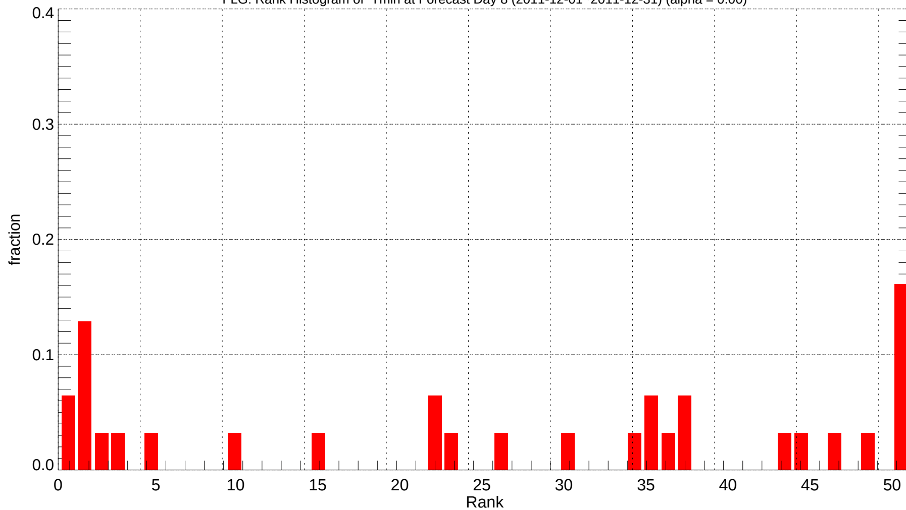
FLG: Rank Histogram of Tmin at Forecast Day 8 (2011-12-01~2011-12-31) (alpha = 0.00)
