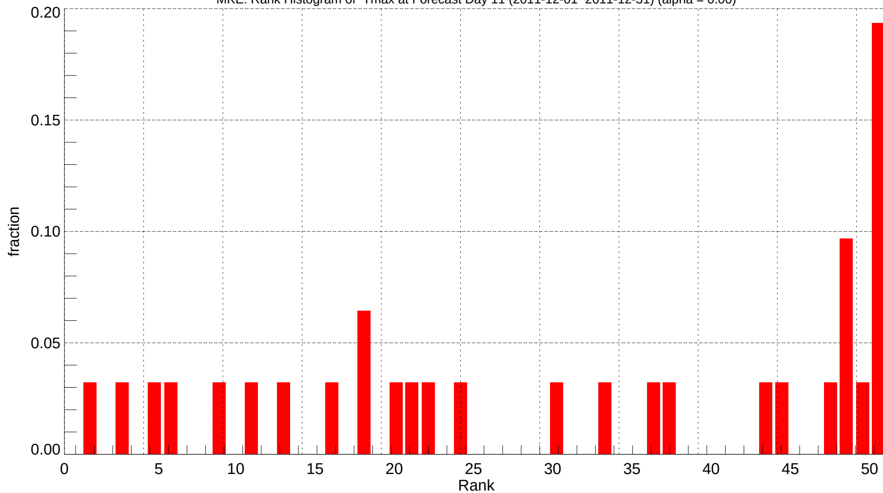
MKE: Rank Histogram of Tmax at Forecast Day 11 (2011-12-01~2011-12-31) (alpha = 0.00)
