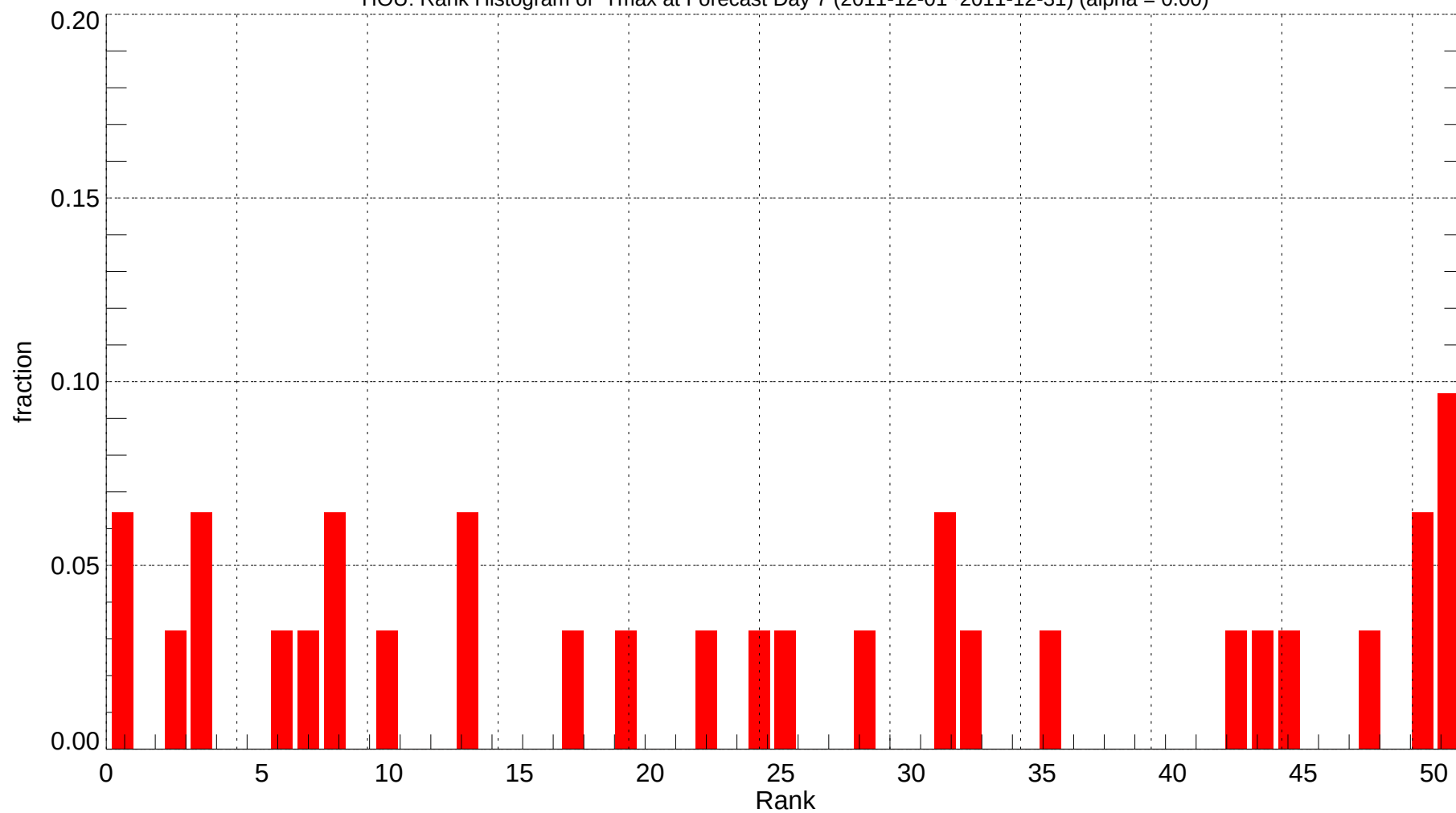
HOU: Rank Histogram of Tmax at Forecast Day 7 (2011-12-01~2011-12-31) (alpha = 0.00)
