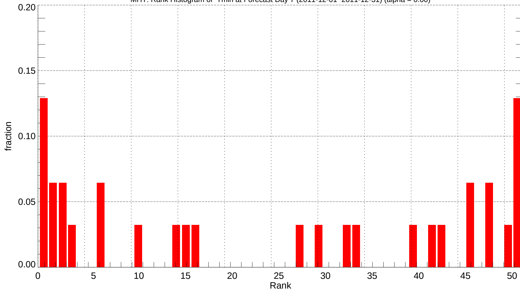
MHT: Rank Histogram of Tmin at Forecast Day 7 (2011-12-01~2011-12-31) (alpha = 0.00)
