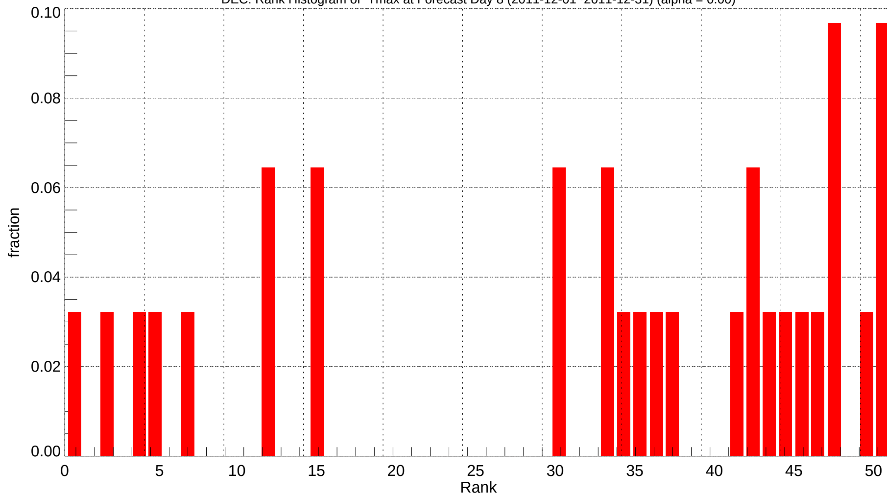
DEC: Rank Histogram of Tmax at Forecast Day 8 (2011-12-01~2011-12-31) (alpha = 0.00)
