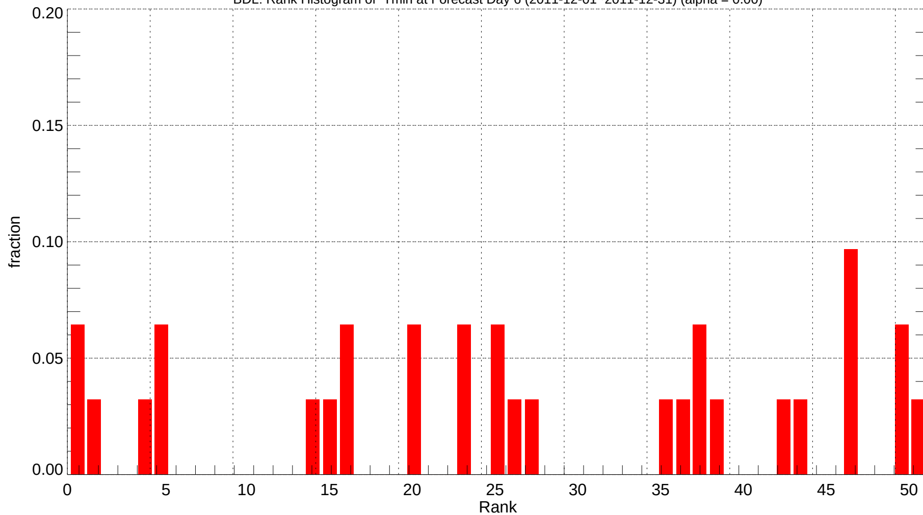
BDL: Rank Histogram of Tmin at Forecast Day 6 (2011-12-01~2011-12-31) (alpha = 0.00)
