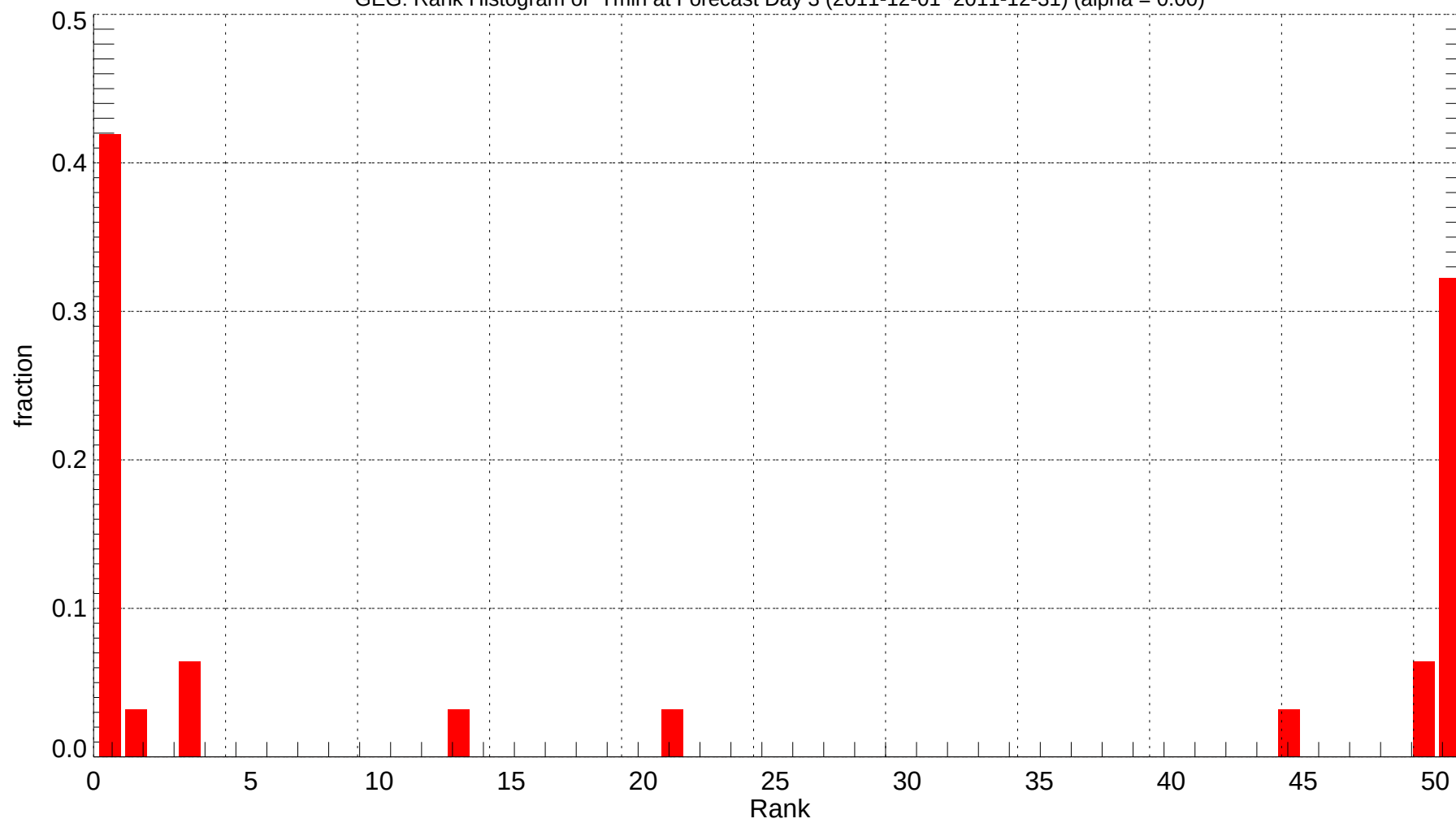
GEG: Rank Histogram of Tmin at Forecast Day 3 (2011-12-01~2011-12-31) (alpha = 0.00)
