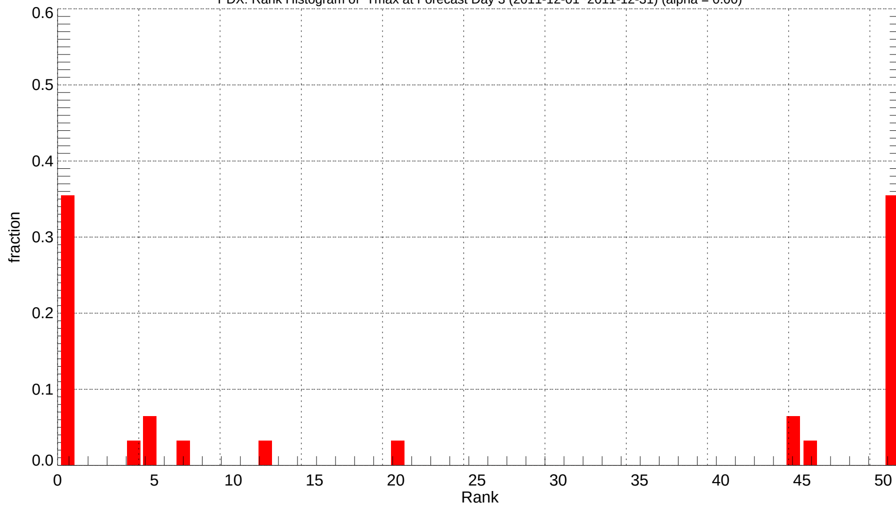
PDX: Rank Histogram of Tmax at Forecast Day 3 (2011-12-01~2011-12-31) (alpha = 0.00)
