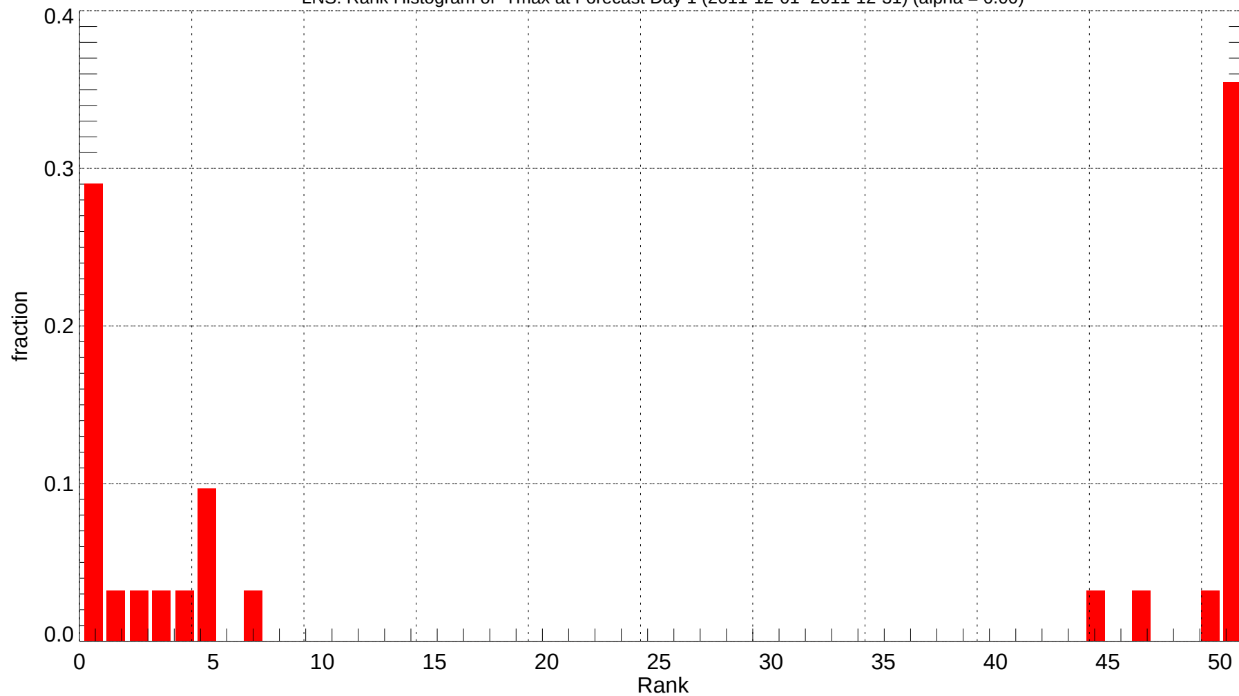
LNS: Rank Histogram of Tmax at Forecast Day 1 (2011-12-01~2011-12-31) (alpha = 0.00)
