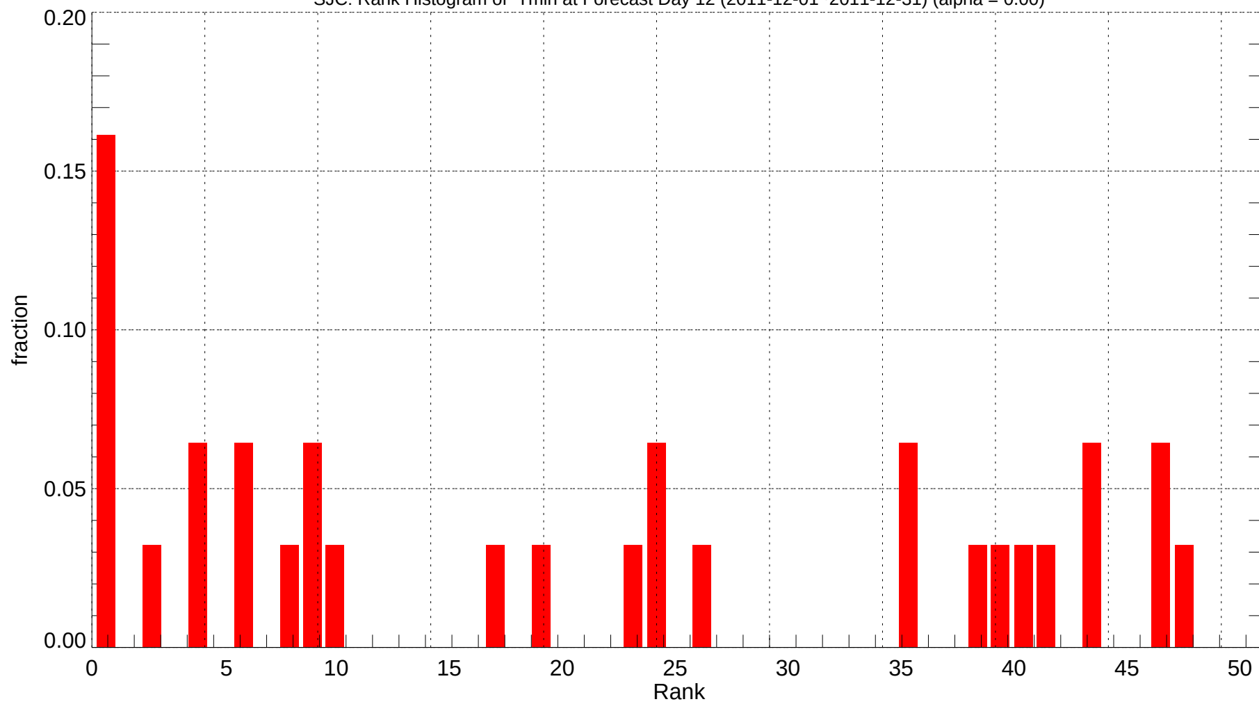
SJC: Rank Histogram of Tmin at Forecast Day 12 (2011-12-01~2011-12-31) (alpha = 0.00)
