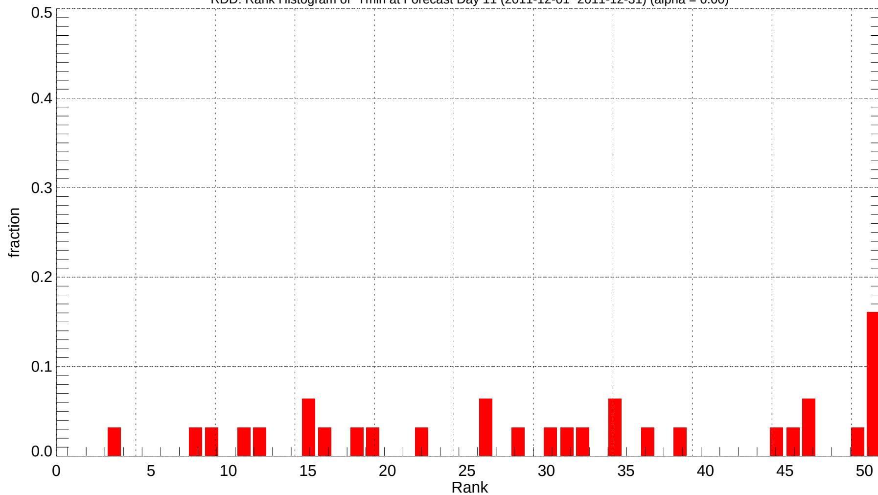
RDD: Rank Histogram of Tmin at Forecast Day 11 (2011-12-01~2011-12-31) (alpha = 0.00)
