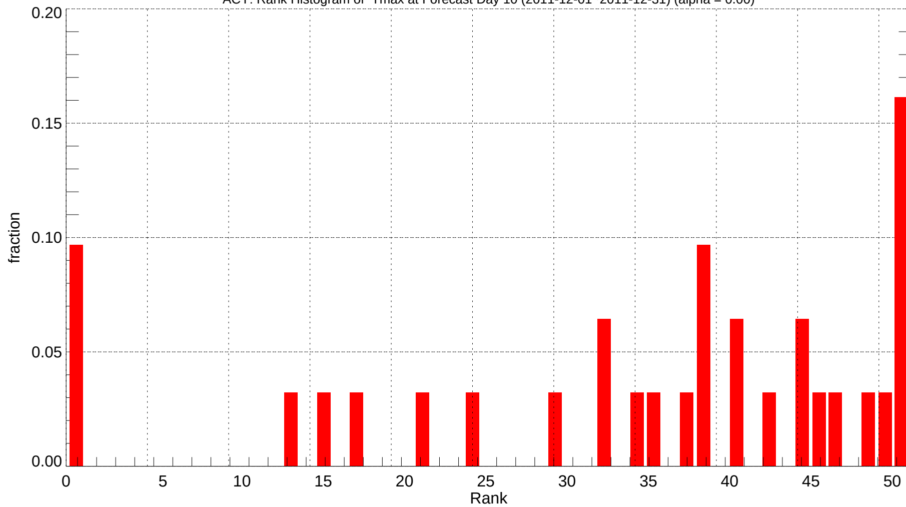
ACY: Rank Histogram of Tmax at Forecast Day 10 (2011-12-01~2011-12-31) (alpha = 0.00)
