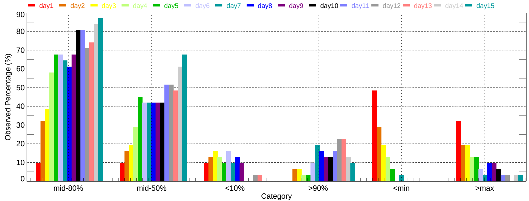
Observed Percentage of Ensembles - SSI: Min Temperature (2011-12-01~2011-12-31)
