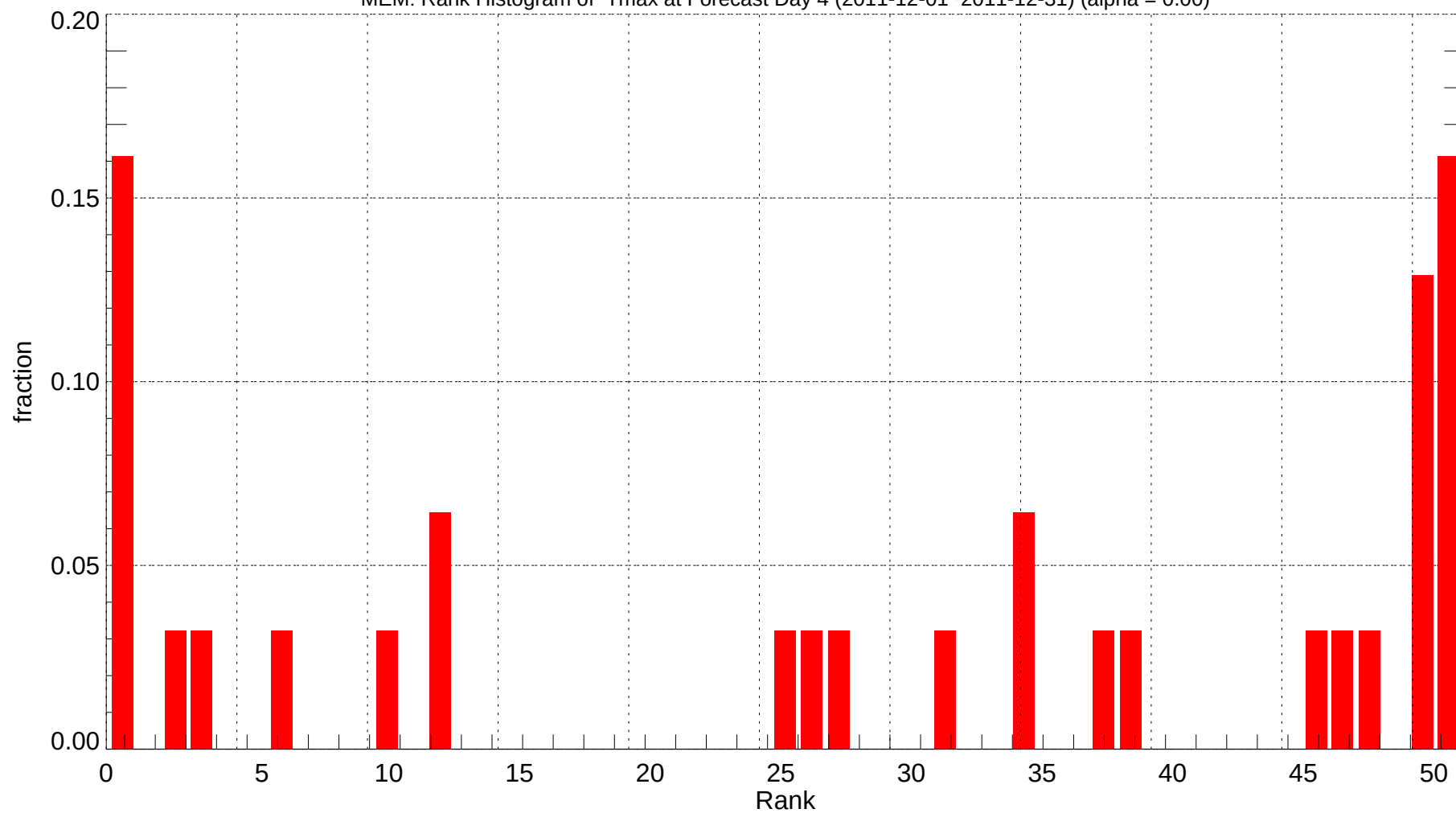
MEM: Rank Histogram of Tmax at Forecast Day 4 (2011-12-01~2011-12-31) (alpha = 0.00)
