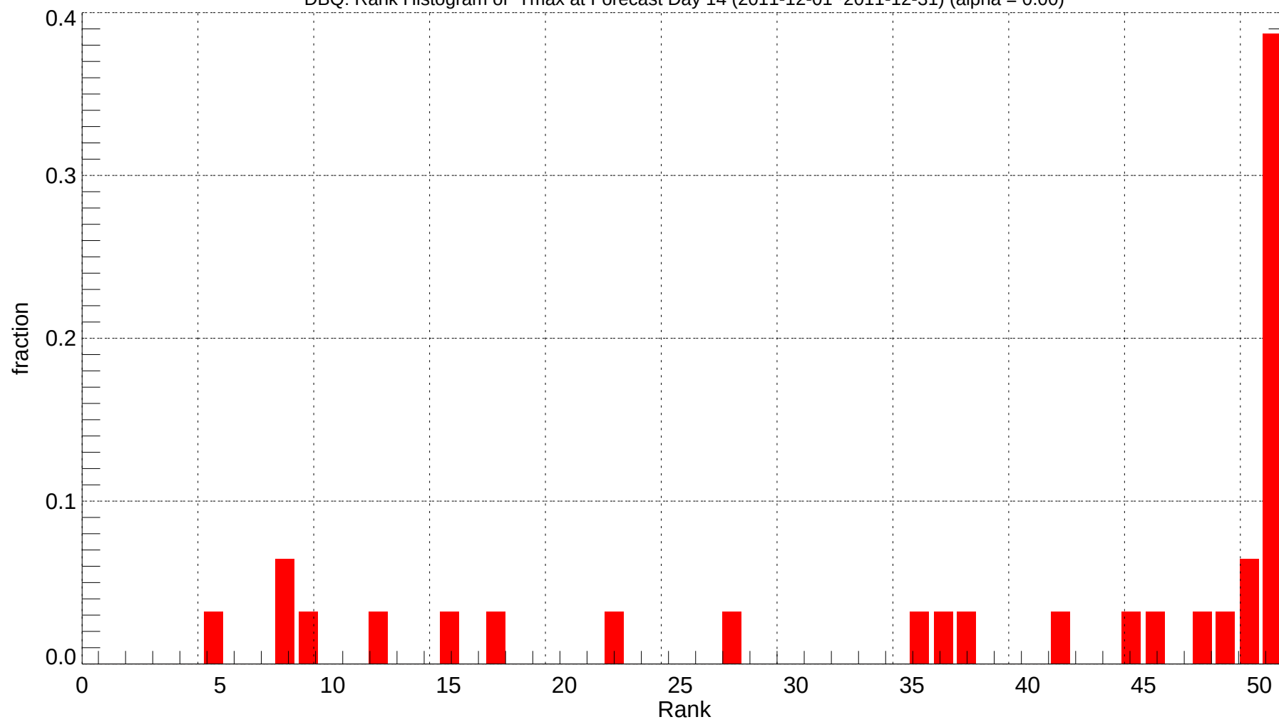
DBQ: Rank Histogram of Tmax at Forecast Day 14 (2011-12-01~2011-12-31) (alpha = 0.00)
