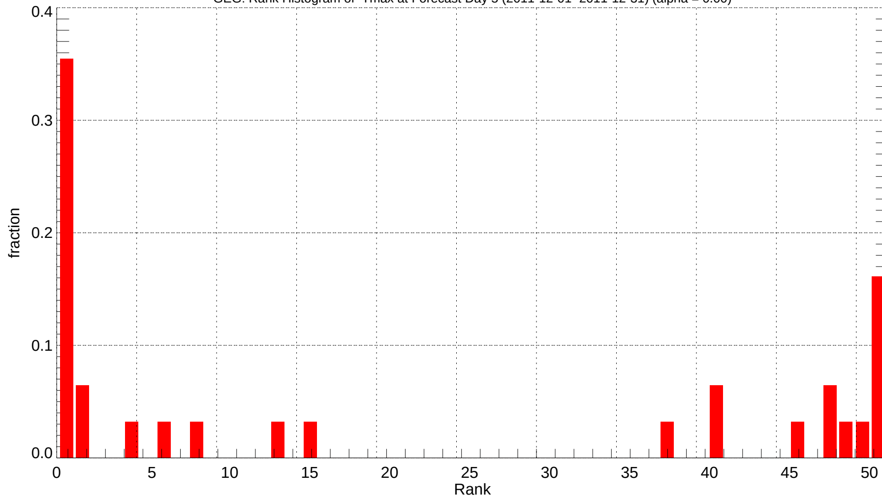
GEG: Rank Histogram of Tmax at Forecast Day 5 (2011-12-01~2011-12-31) (alpha = 0.00)
