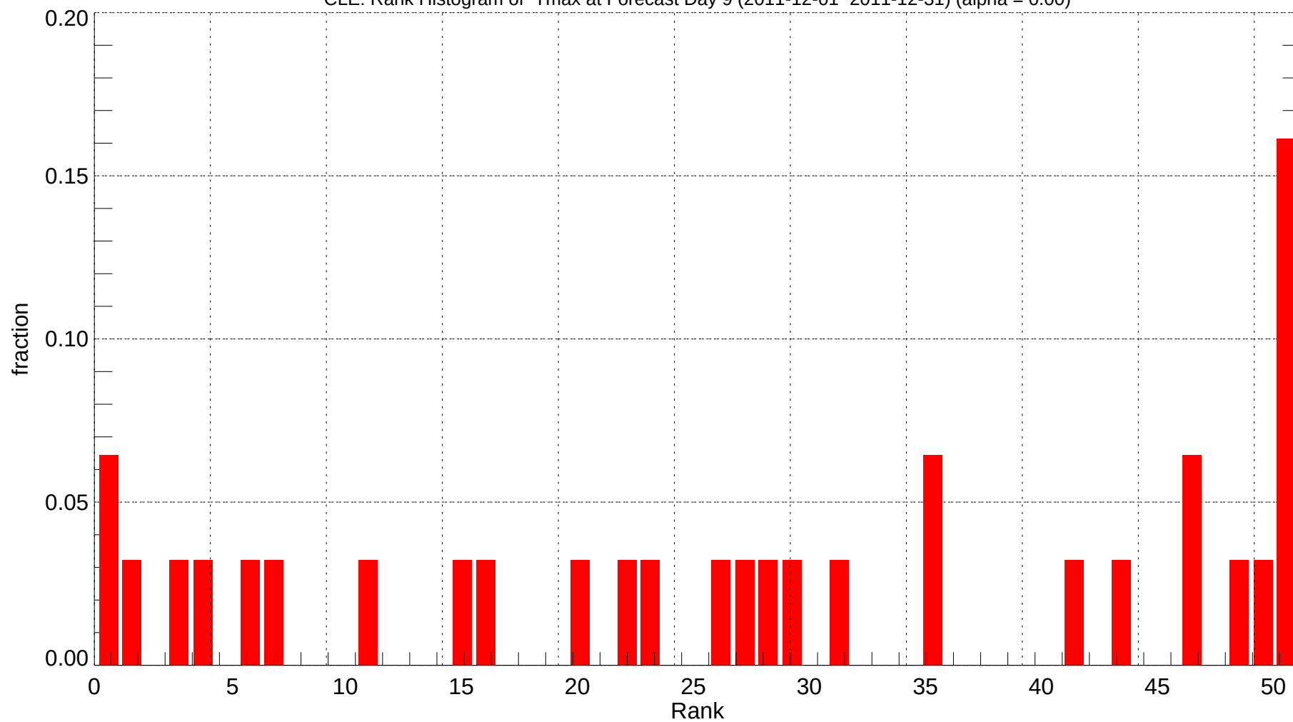
CLE: Rank Histogram of Tmax at Forecast Day 9 (2011-12-01~2011-12-31) (alpha = 0.00)
