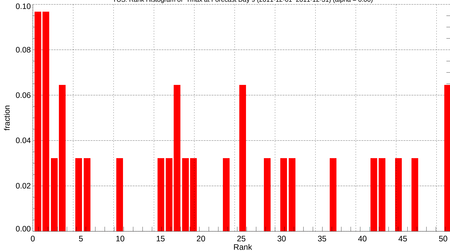
TUS: Rank Histogram of Tmax at Forecast Day 9 (2011-12-01~2011-12-31) (alpha = 0.00)
