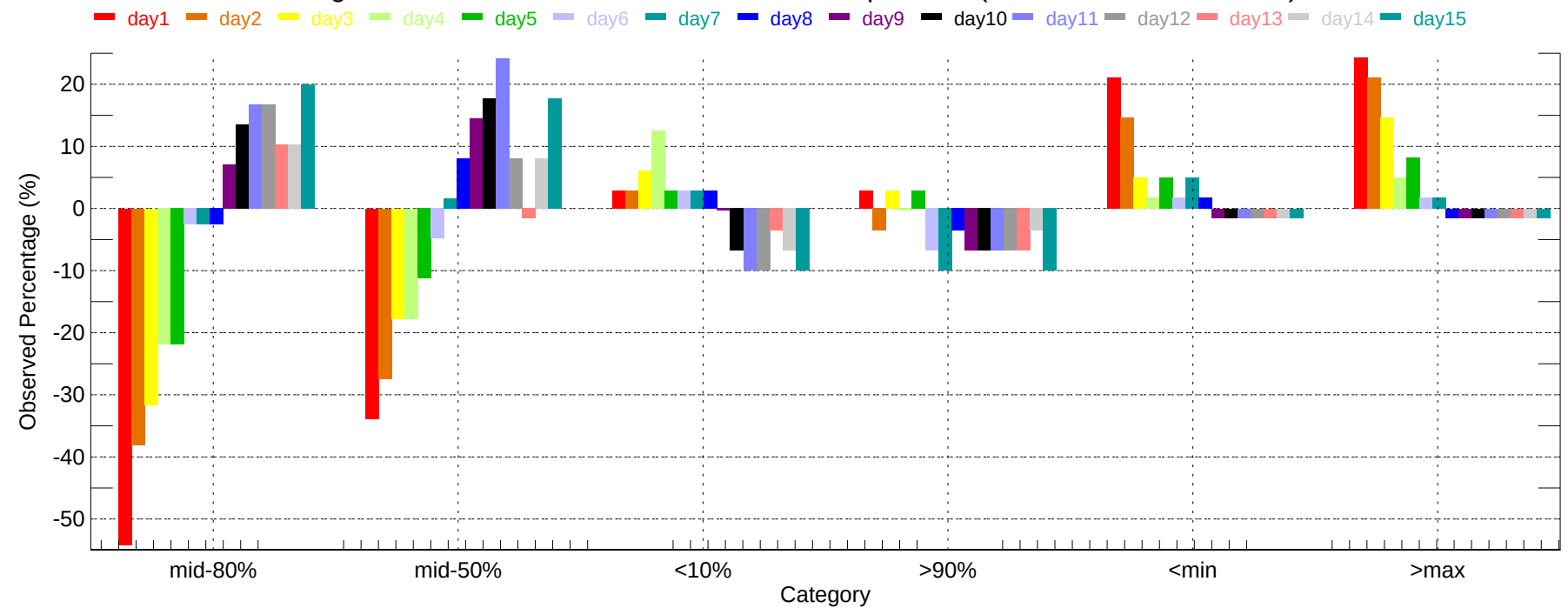
Observed Percentage Deviation of Ensembles - MIA: Max Temperature (2011-12-01~2011-12-31)
