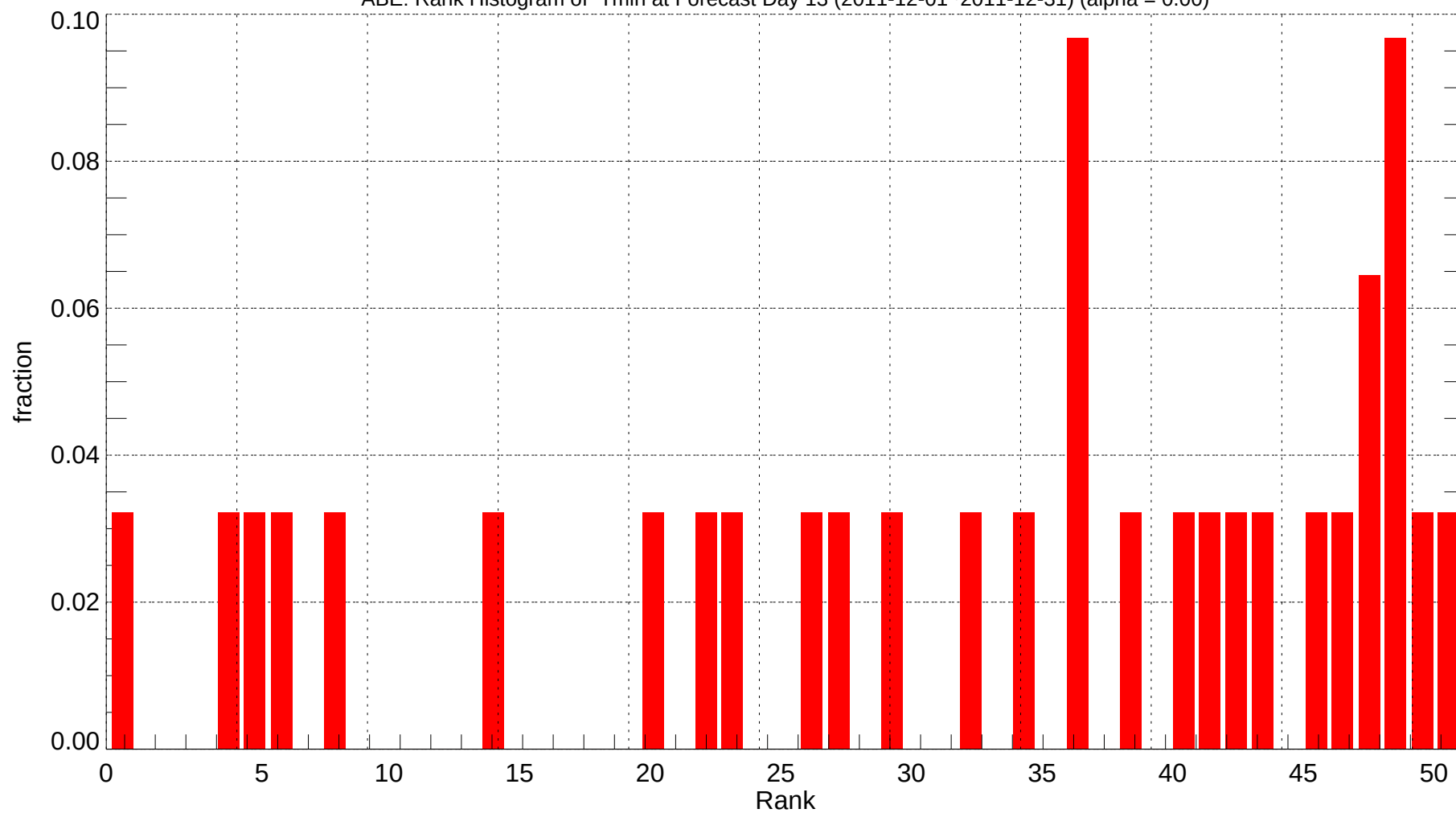
ABE: Rank Histogram of Tmin at Forecast Day 13 (2011-12-01~2011-12-31) (alpha = 0.00)
