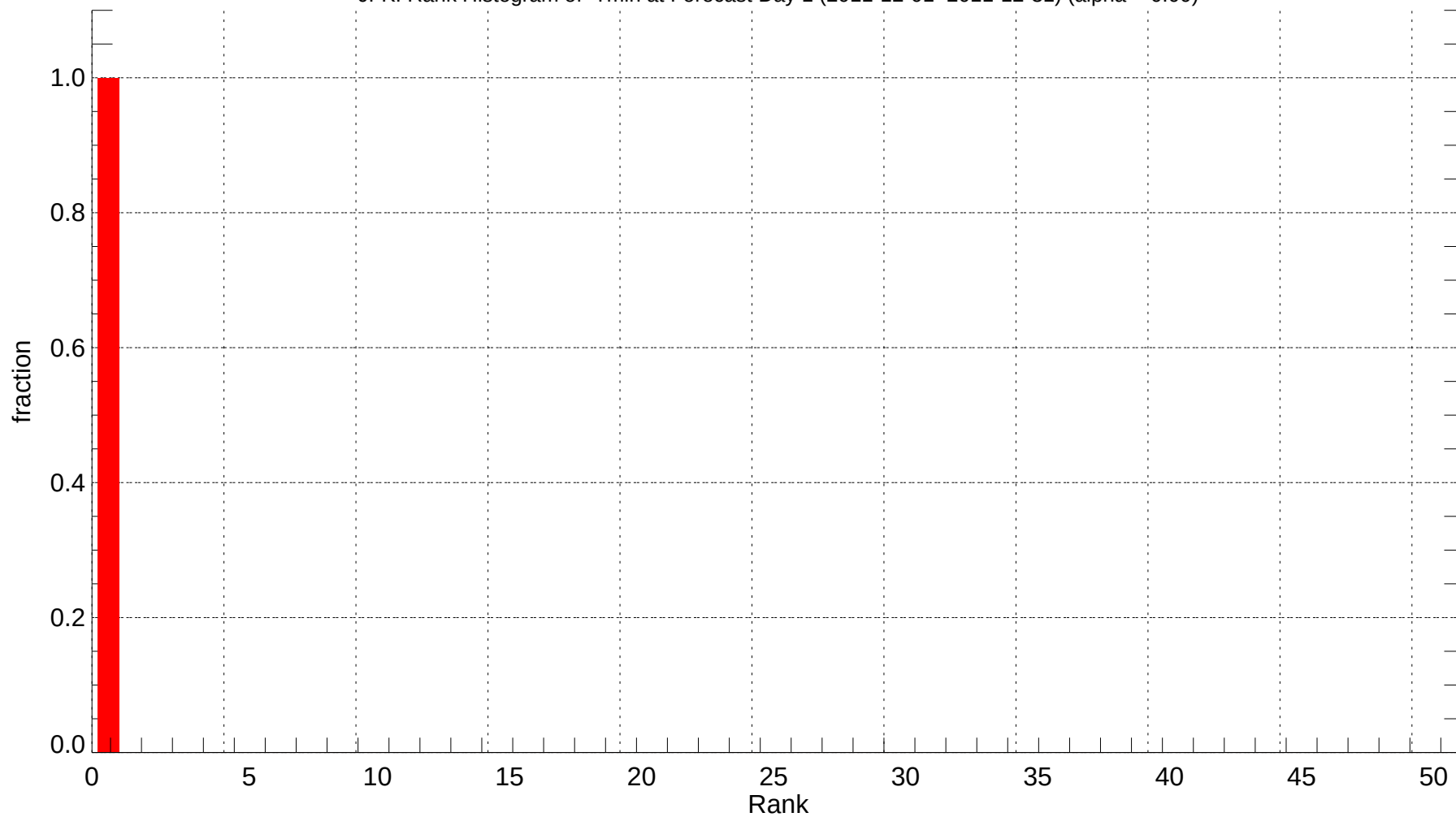
JFK: Rank Histogram of Tmin at Forecast Day 1 (2011-12-01~2011-12-31) (alpha = 0.00)
