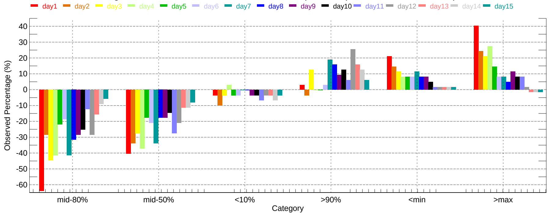
Observed Percentage Deviation of Ensembles - ABE: Max Temperature (2011-12-01~2011-12-31)
