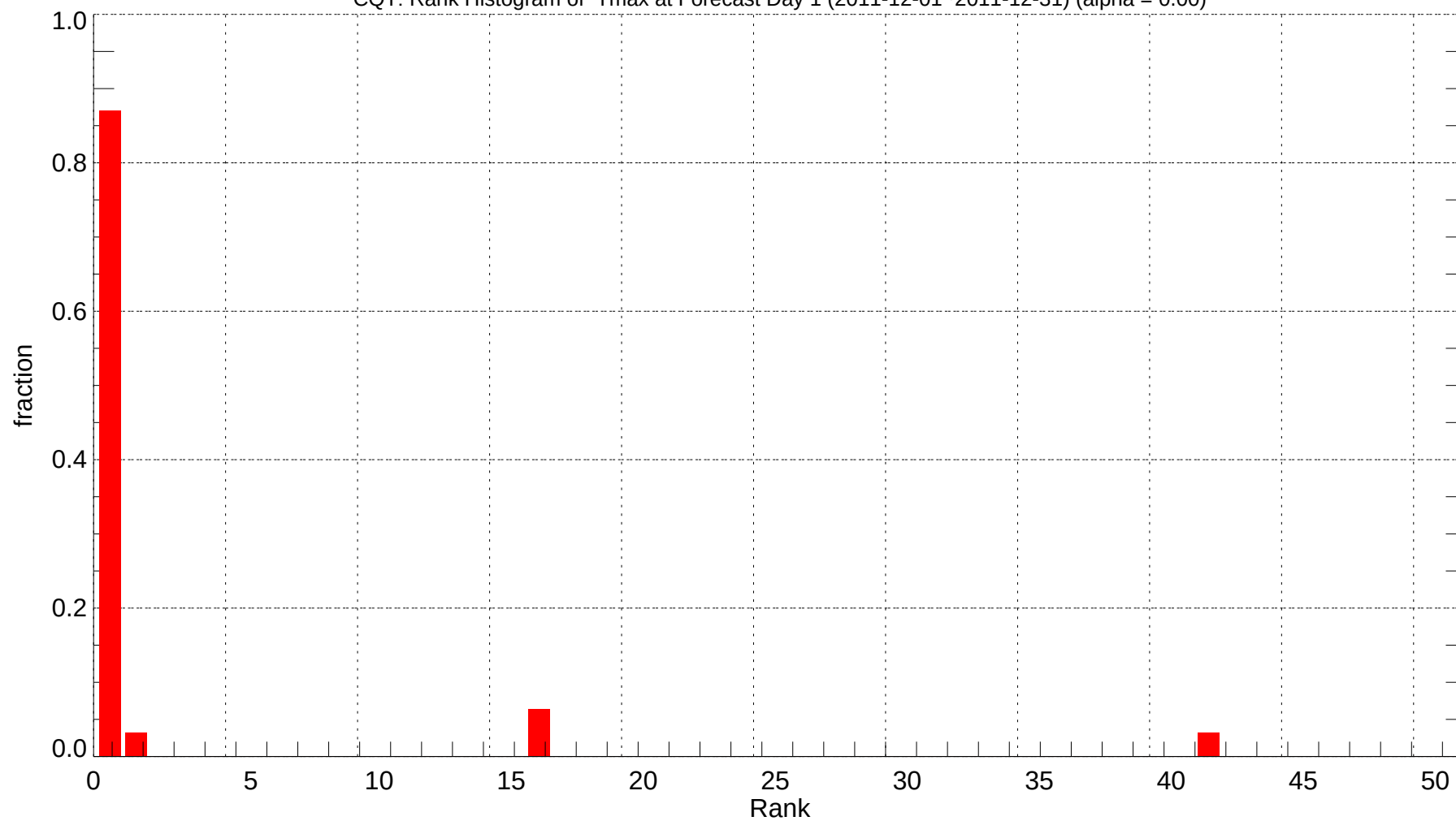
CQT: Rank Histogram of Tmax at Forecast Day 1 (2011-12-01~2011-12-31) (alpha = 0.00)
