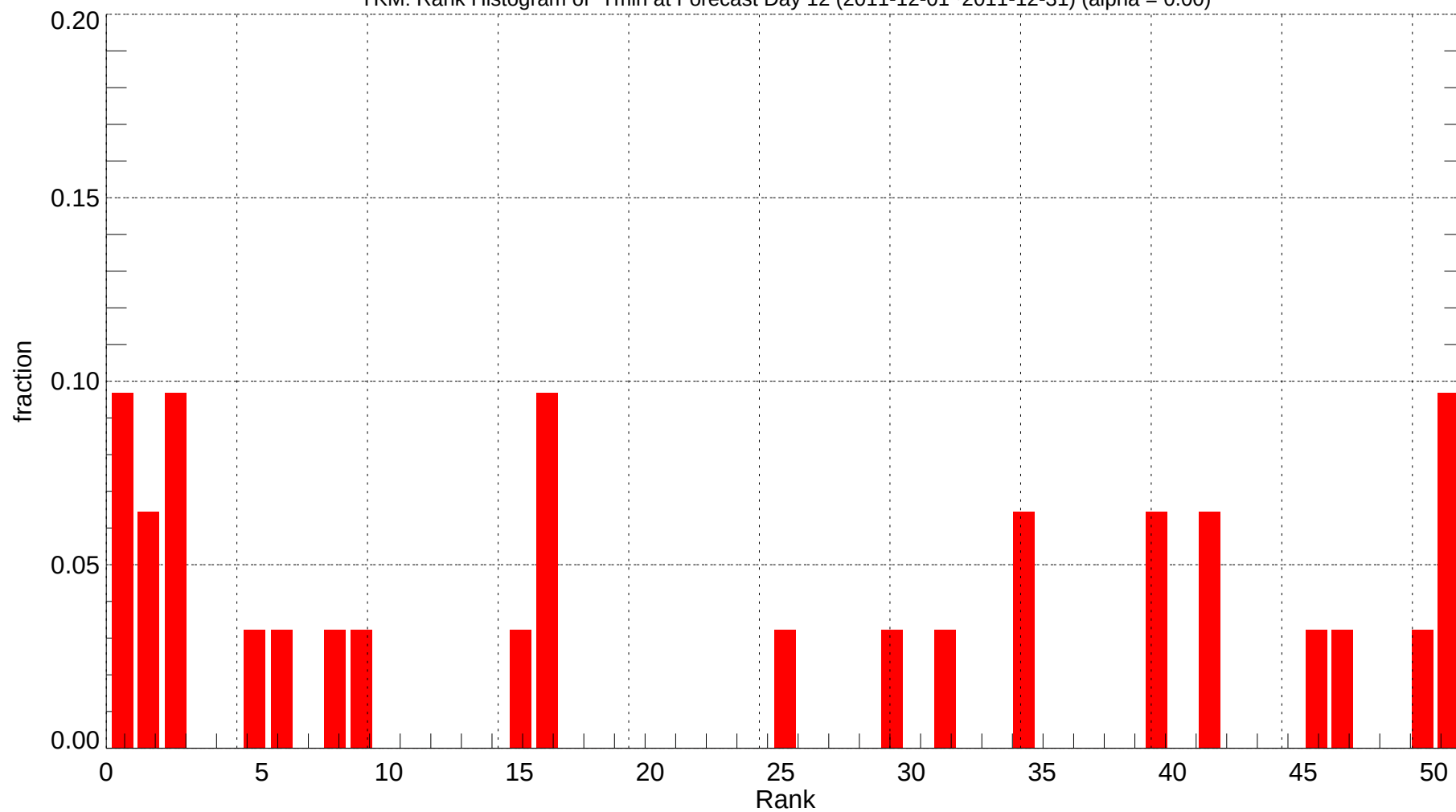
YKM: Rank Histogram of Tmin at Forecast Day 12 (2011-12-01~2011-12-31) (alpha = 0.00)
