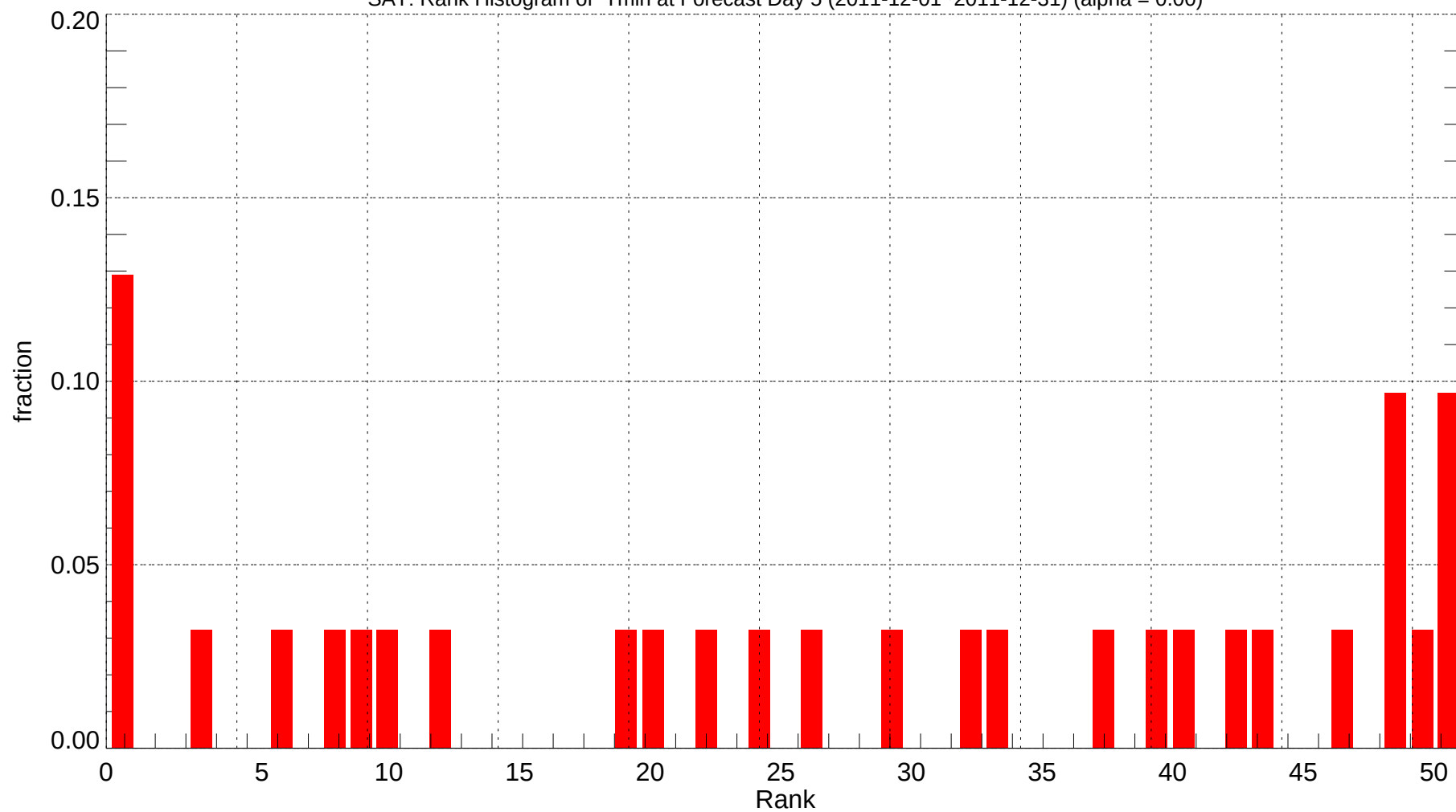
SAT: Rank Histogram of Tmin at Forecast Day 5 (2011-12-01~2011-12-31) (alpha = 0.00)
