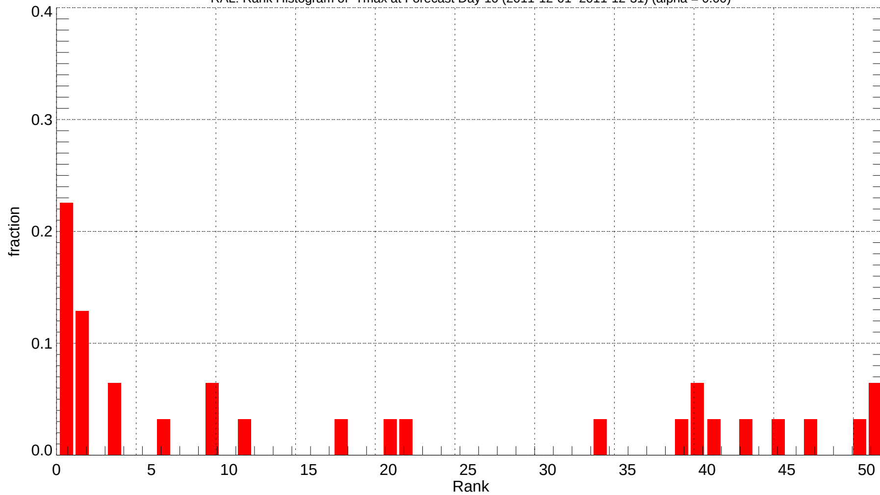
RAL: Rank Histogram of Tmax at Forecast Day 10 (2011-12-01~2011-12-31) (alpha = 0.00)
