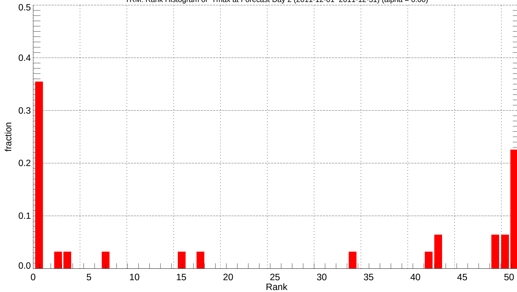
TRM: Rank Histogram of Tmax at Forecast Day 2 (2011-12-01~2011-12-31) (alpha = 0.00)
