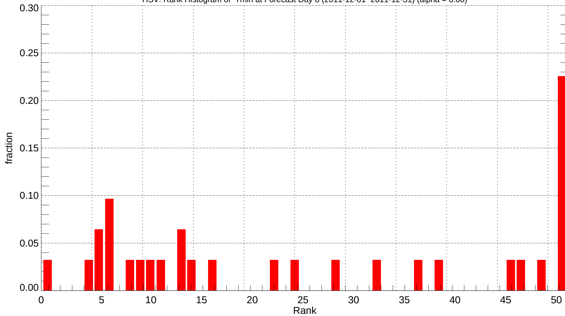
HSV: Rank Histogram of Tmin at Forecast Day 8 (2011-12-01~2011-12-31) (alpha = 0.00)
