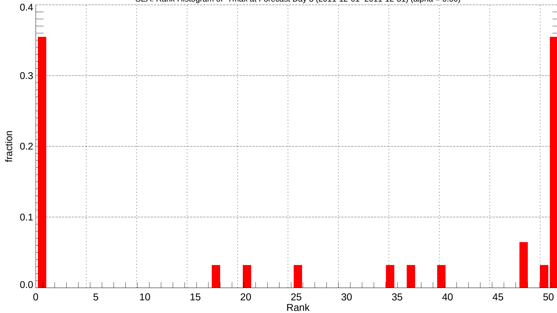
SEA: Rank Histogram of Tmax at Forecast Day 3 (2011-12-01~2011-12-31) (alpha = 0.00)
