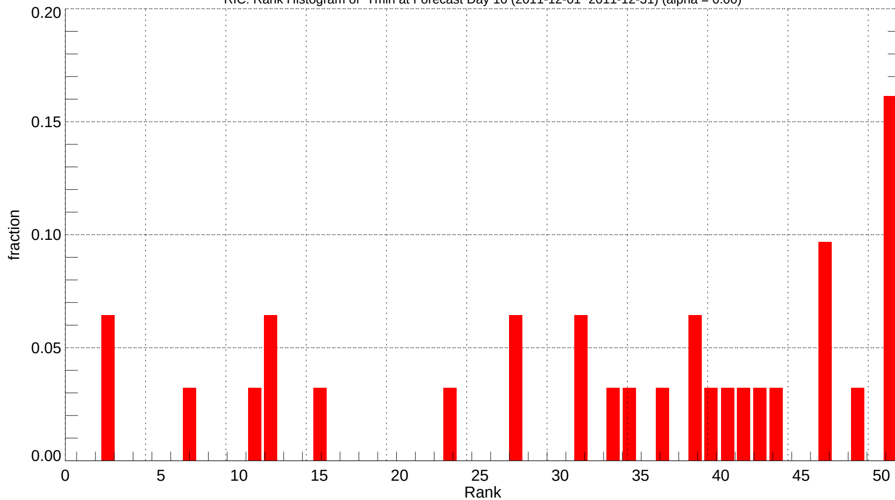
RIC: Rank Histogram of Tmin at Forecast Day 10 (2011-12-01~2011-12-31) (alpha = 0.00)
