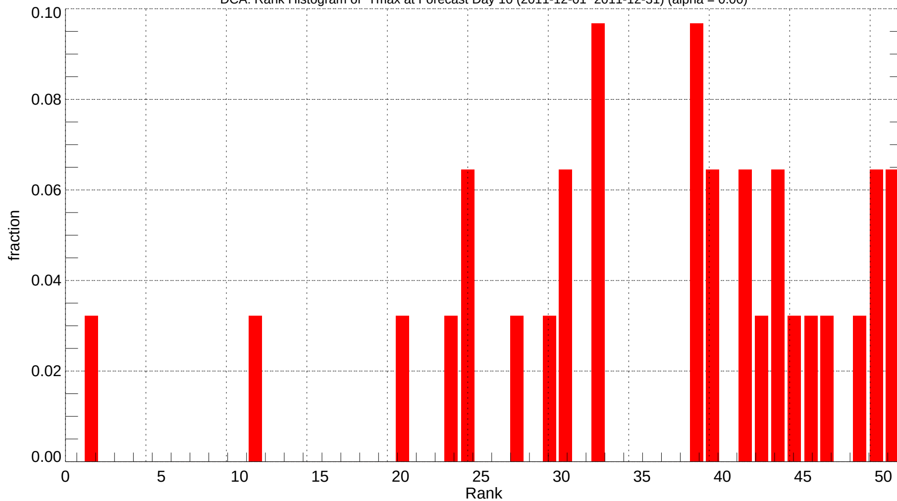
DCA: Rank Histogram of Tmax at Forecast Day 10 (2011-12-01~2011-12-31) (alpha = 0.00)
