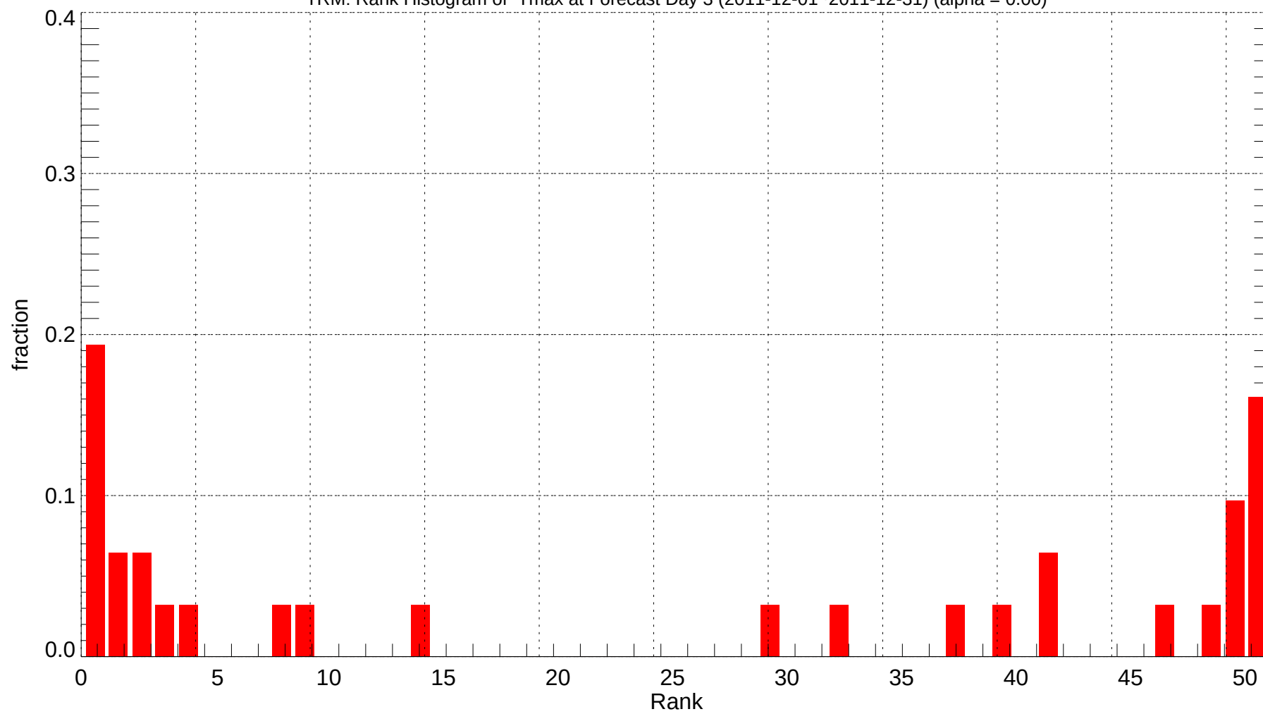
TRM: Rank Histogram of Tmax at Forecast Day 3 (2011-12-01~2011-12-31) (alpha = 0.00)
