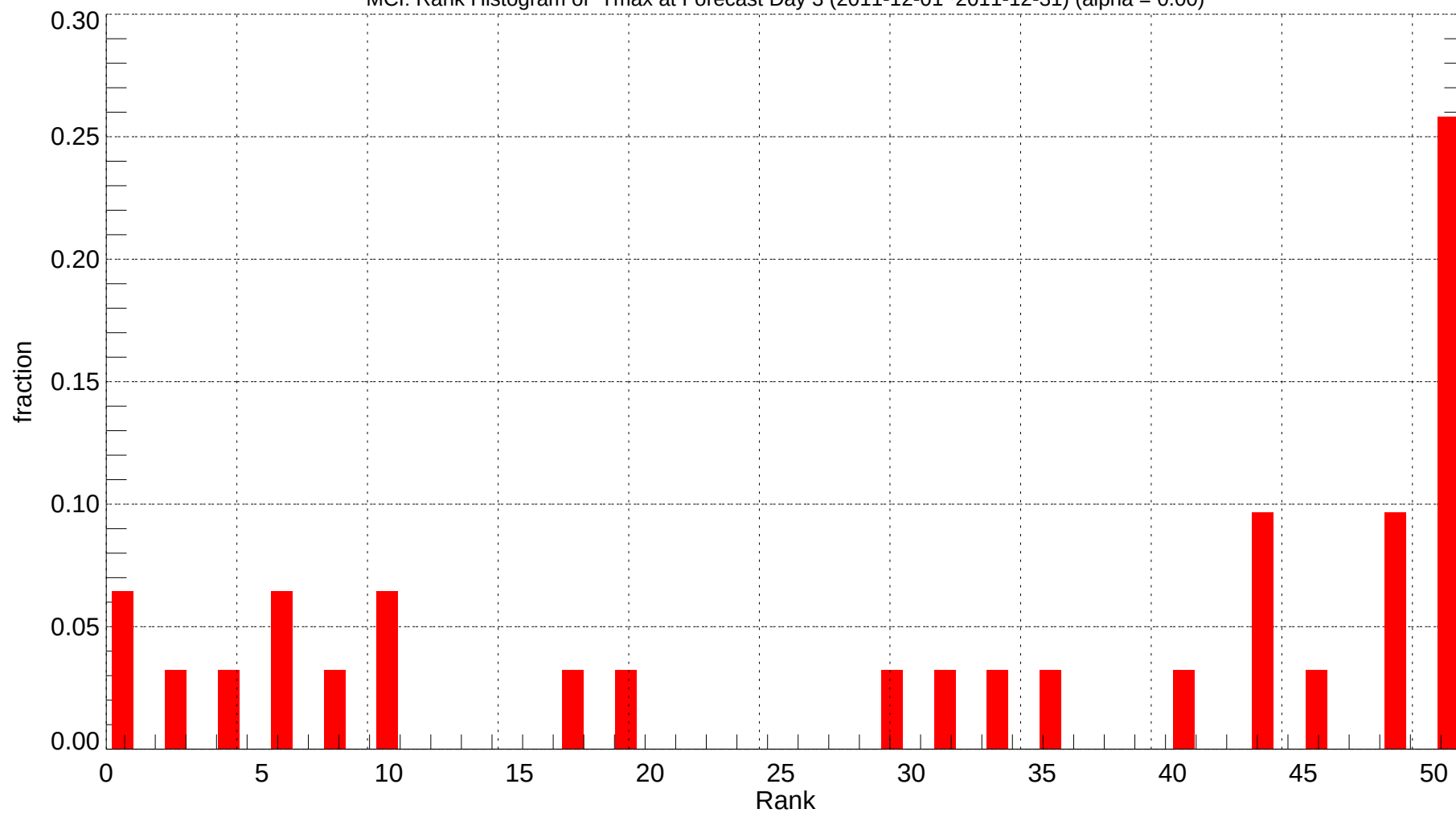
MCI: Rank Histogram of Tmax at Forecast Day 3 (2011-12-01~2011-12-31) (alpha = 0.00)
