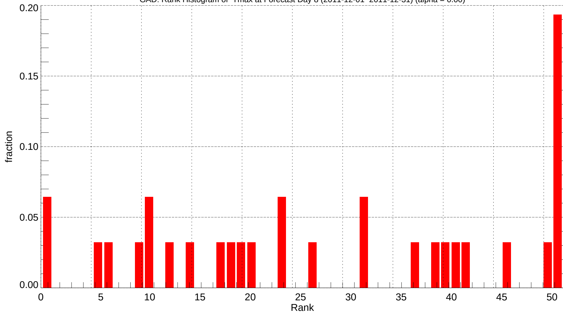
GAD: Rank Histogram of Tmax at Forecast Day 8 (2011-12-01~2011-12-31) (alpha = 0.00)
