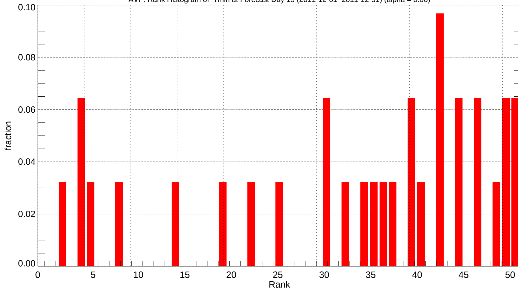
AVP: Rank Histogram of Tmin at Forecast Day 13 (2011-12-01~2011-12-31) (alpha = 0.00)
