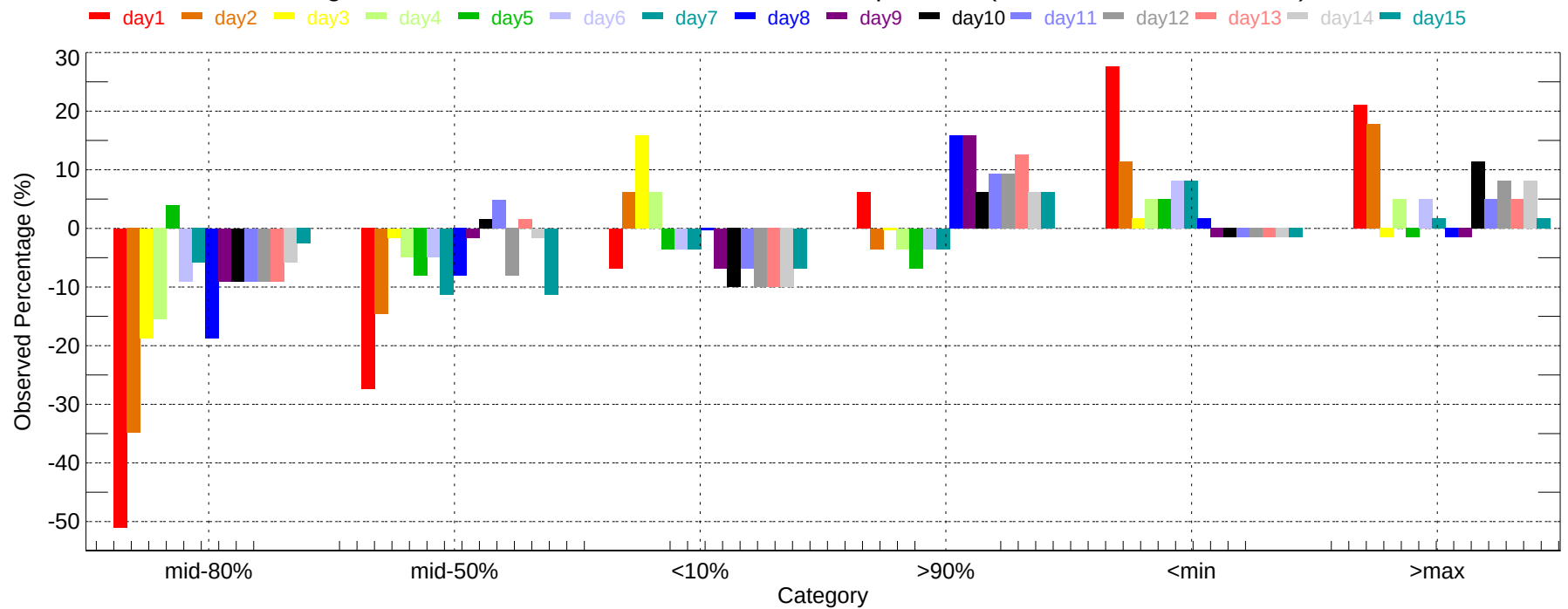
Observed Percentage Deviation of Ensembles - RDU: Max Temperature (2011-12-01~2011-12-31)
