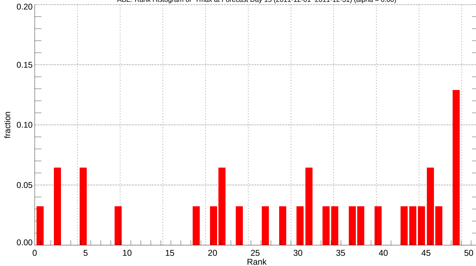
ABE: Rank Histogram of Tmax at Forecast Day 15 (2011-12-01~2011-12-31) (alpha = 0.00)
