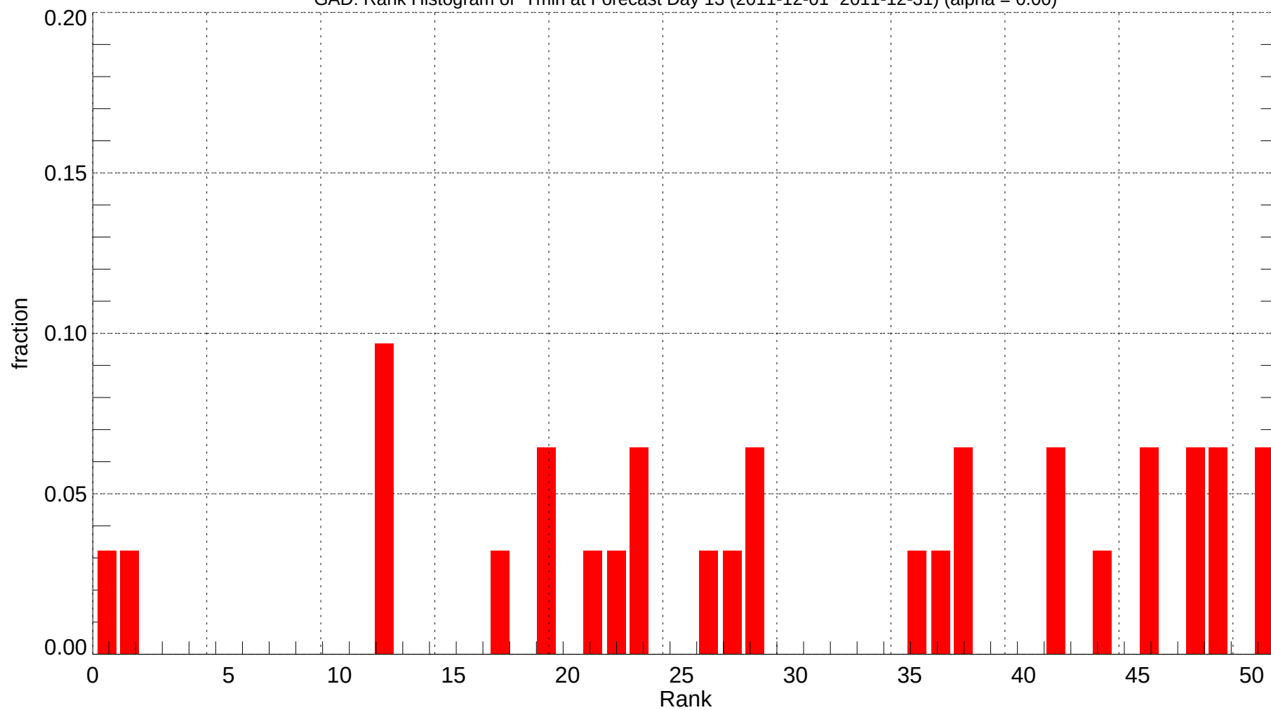
GAD: Rank Histogram of Tmin at Forecast Day 13 (2011-12-01~2011-12-31) (alpha = 0.00)
