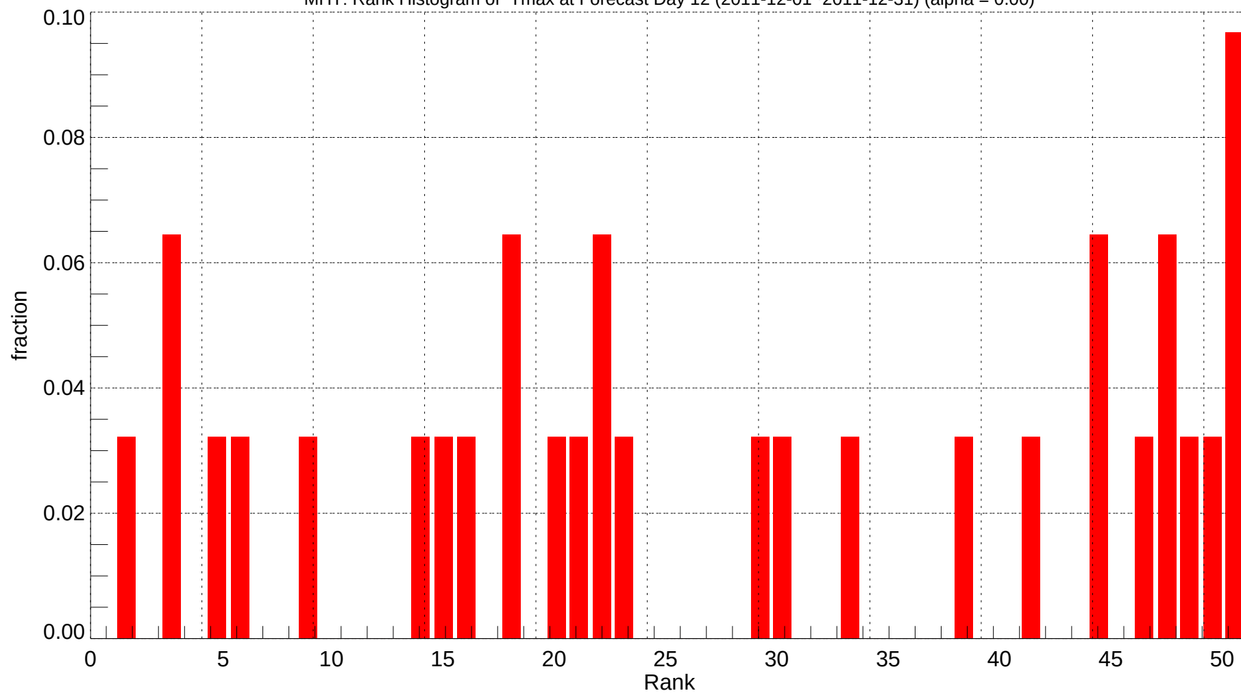
MHT: Rank Histogram of Tmax at Forecast Day 12 (2011-12-01~2011-12-31) (alpha = 0.00)
