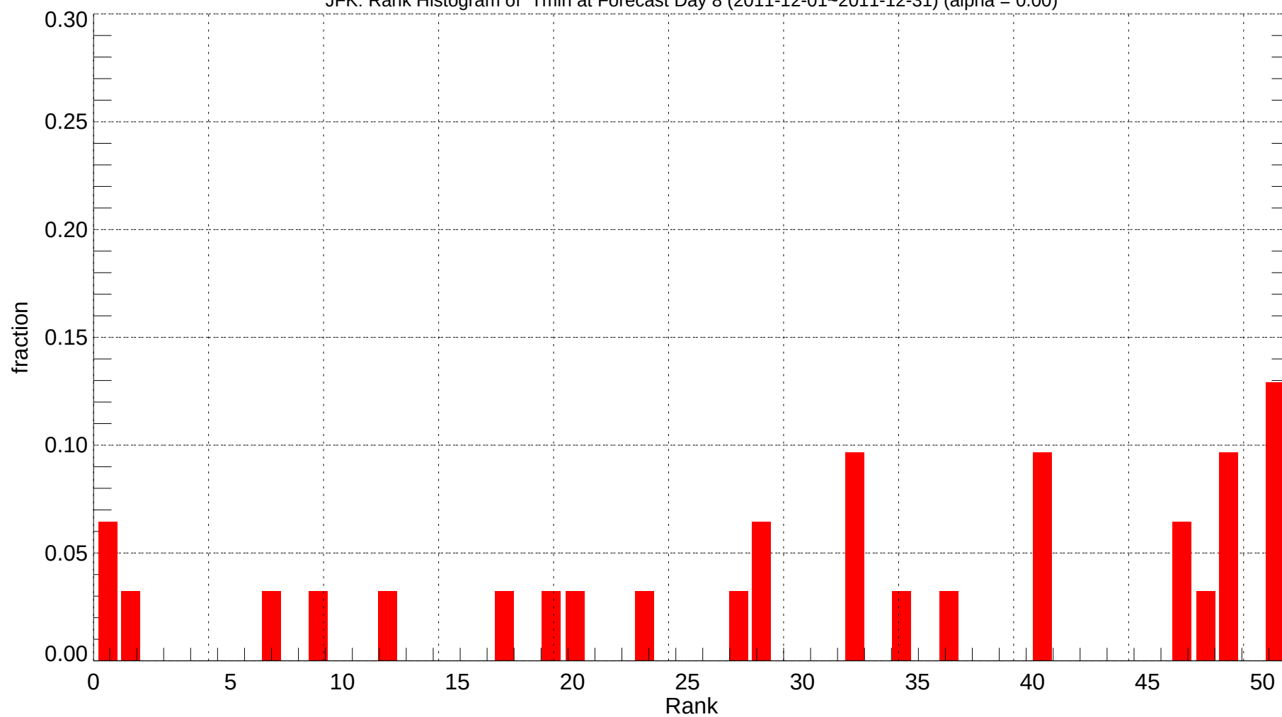
JFK: Rank Histogram of Tmin at Forecast Day 8 (2011-12-01~2011-12-31) (alpha = 0.00)
