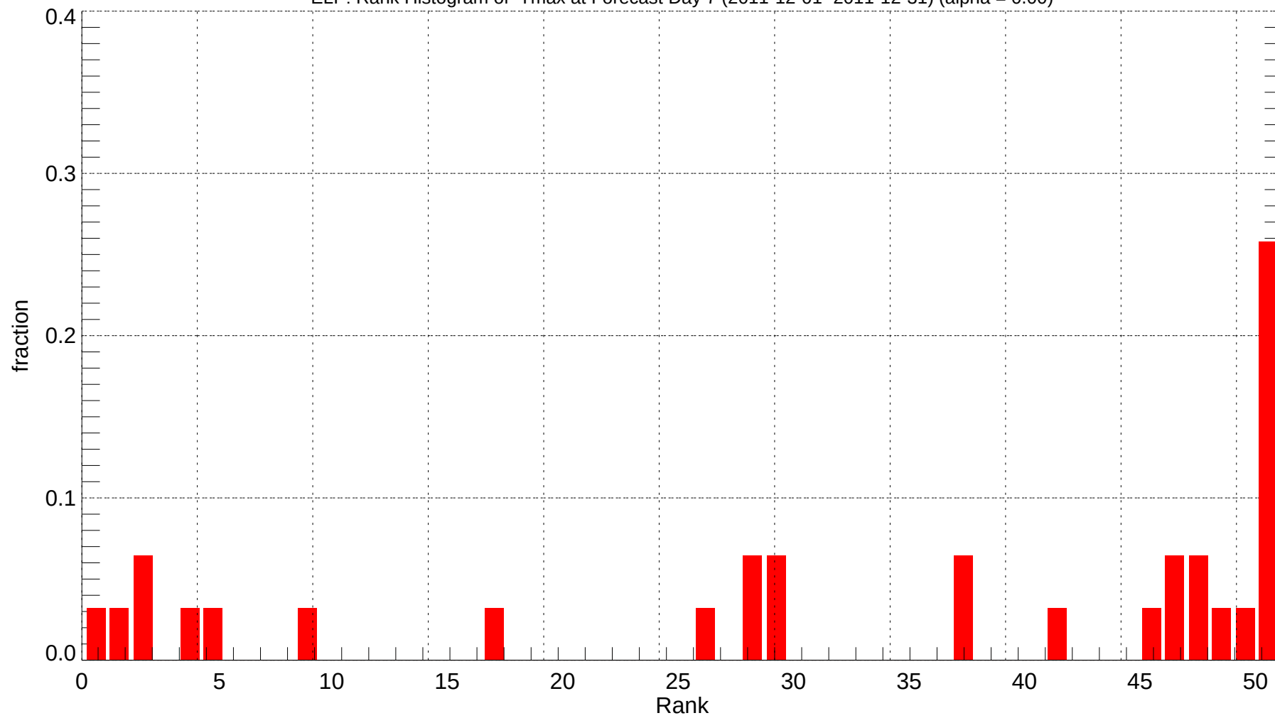
ELP: Rank Histogram of Tmax at Forecast Day 7 (2011-12-01~2011-12-31) (alpha = 0.00)
