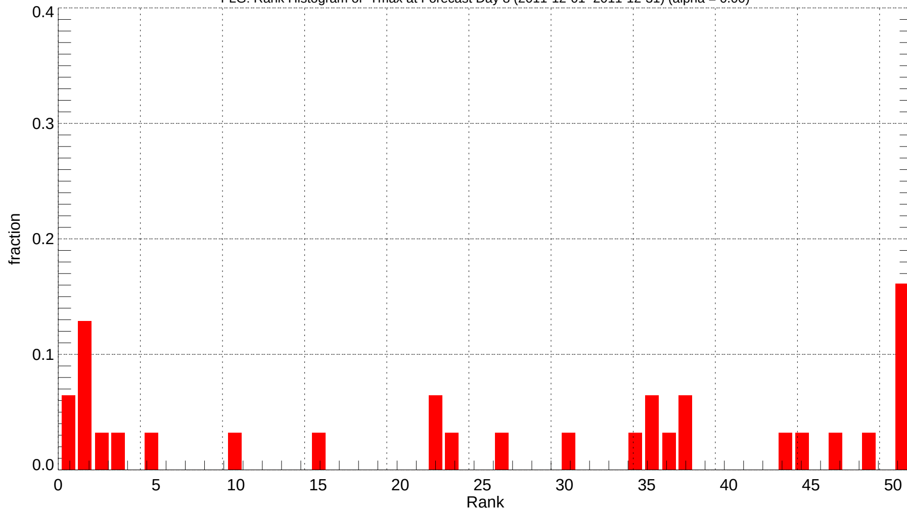
FLG: Rank Histogram of Tmax at Forecast Day 8 (2011-12-01~2011-12-31) (alpha = 0.00)
