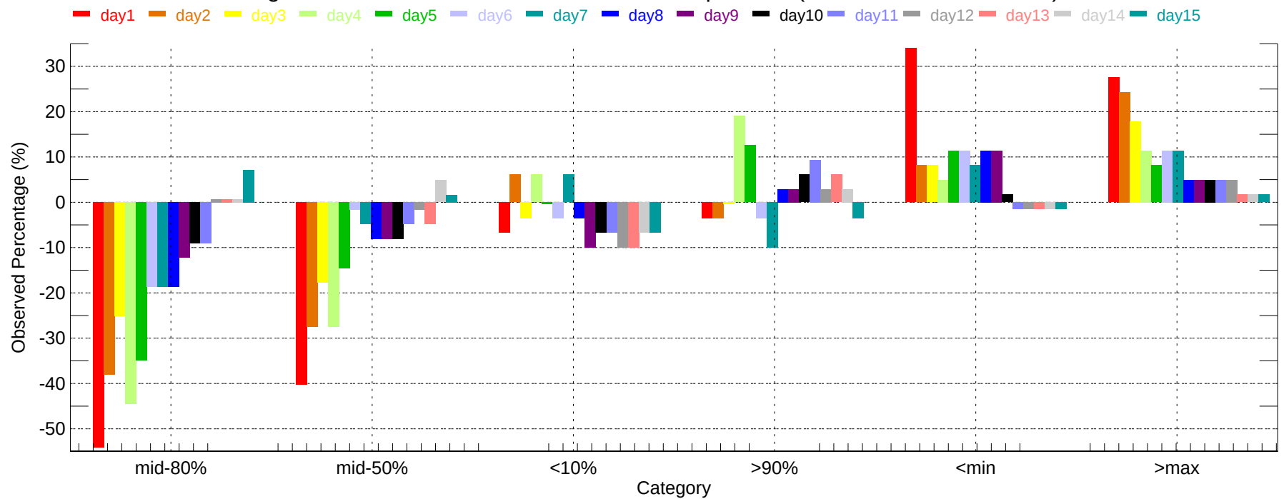
Observed Percentage Deviation of Ensembles - PHL: Min Temperature (2011-12-01~2011-12-31)
