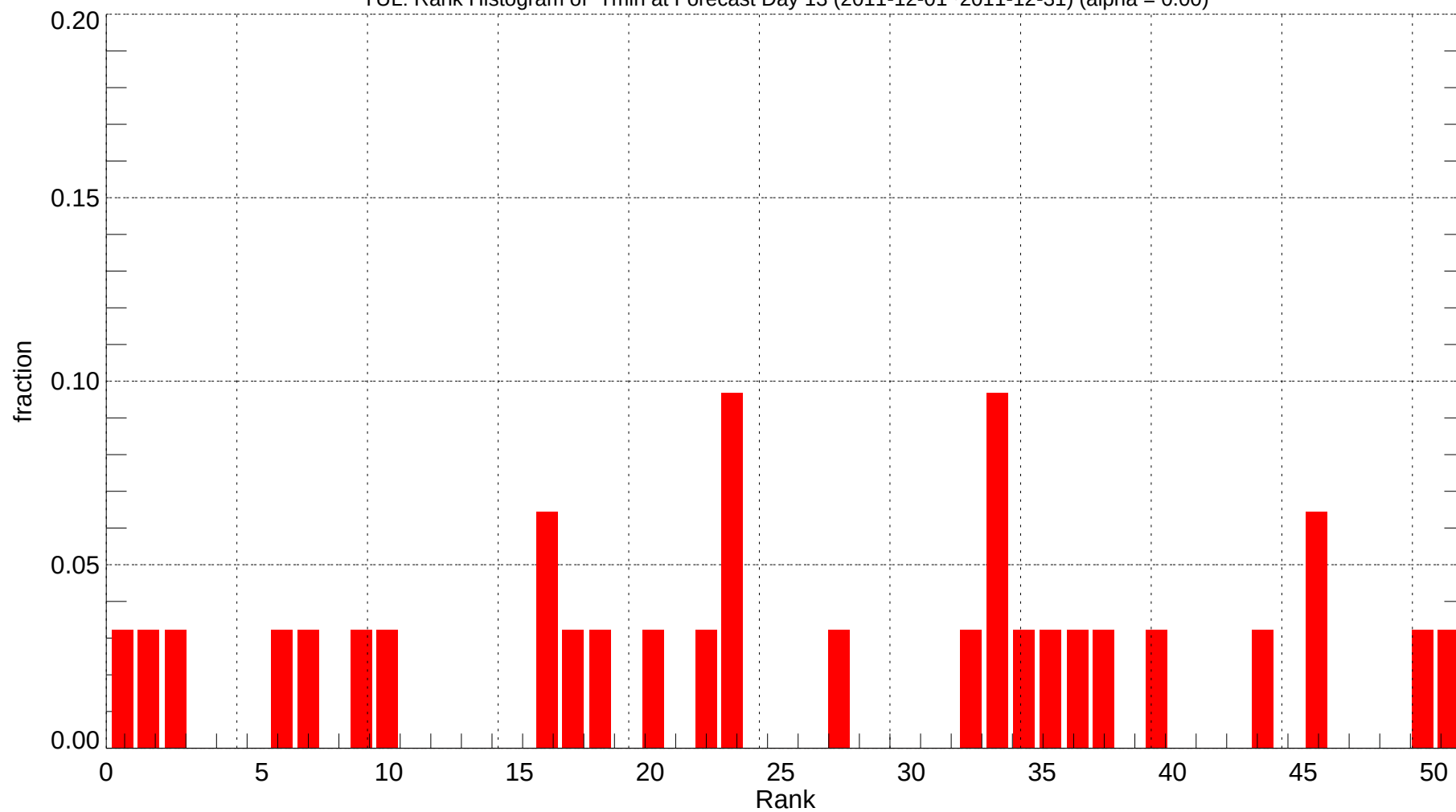
YUL: Rank Histogram of Tmin at Forecast Day 13 (2011-12-01~2011-12-31) (alpha = 0.00)
