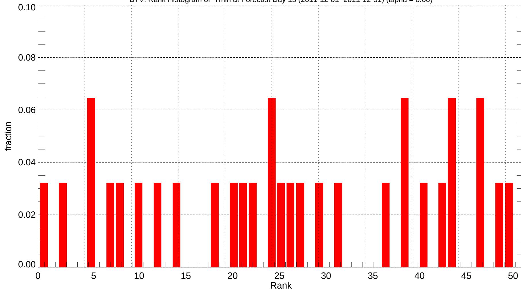
BTV: Rank Histogram of Tmin at Forecast Day 13 (2011-12-01~2011-12-31) (alpha = 0.00)
