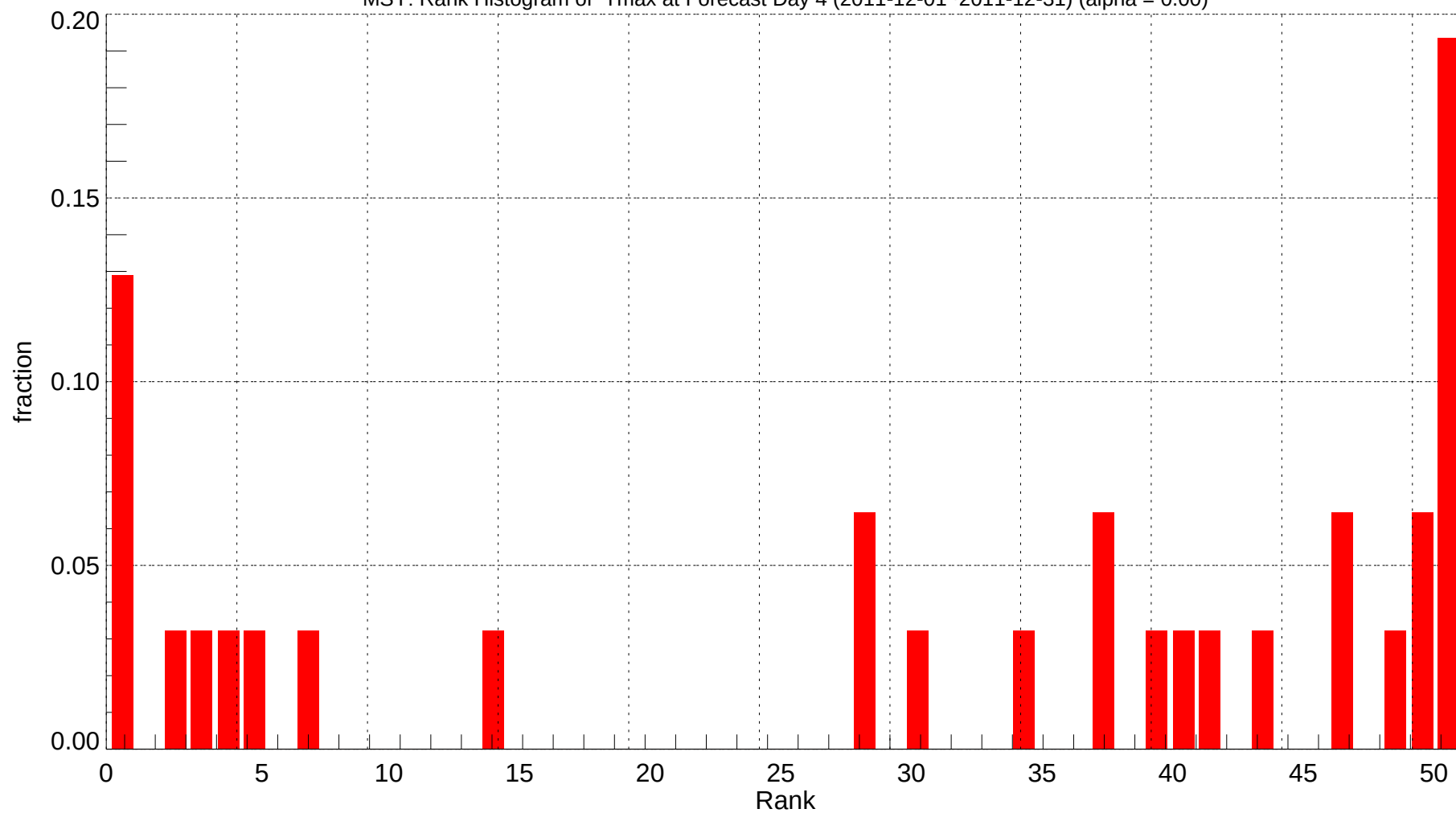
MSY: Rank Histogram of Tmax at Forecast Day 4 (2011-12-01~2011-12-31) (alpha = 0.00)
