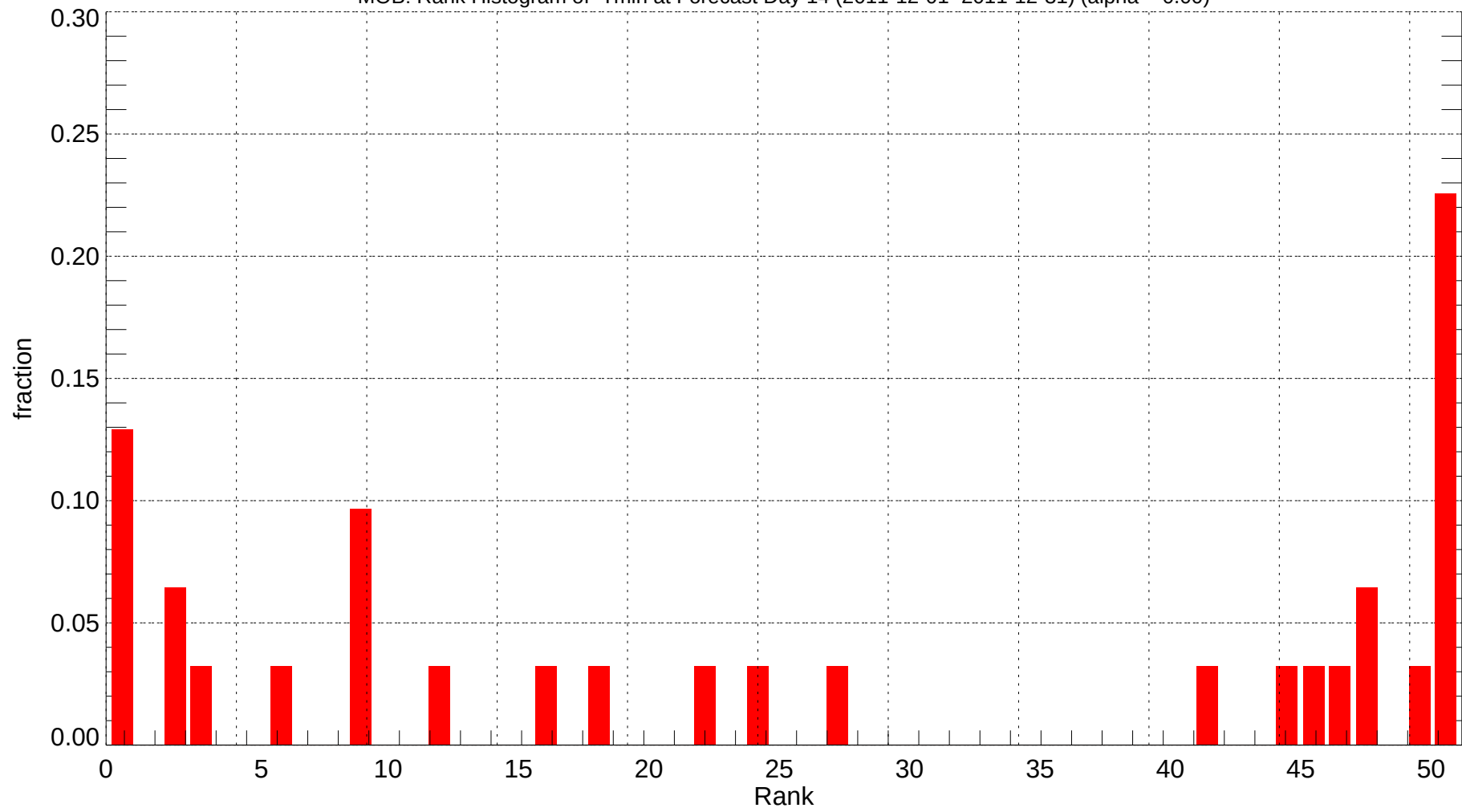
MOB: Rank Histogram of Tmin at Forecast Day 14 (2011-12-01~2011-12-31) (alpha = 0.00)
