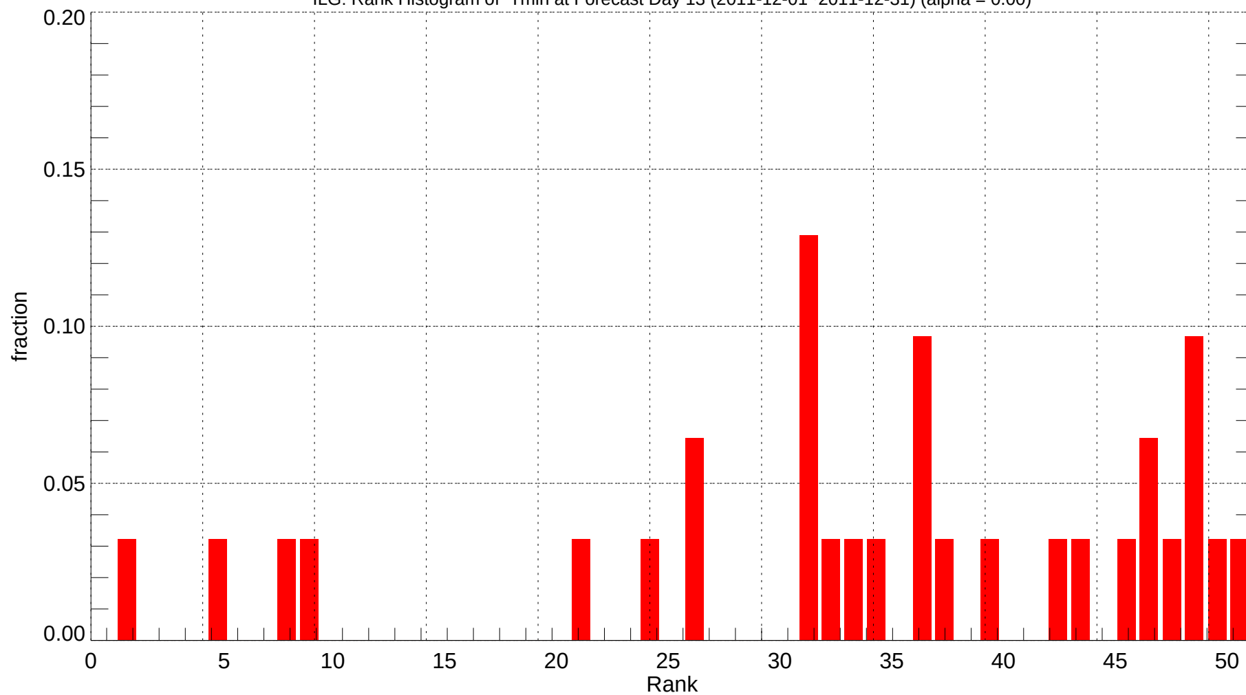
ILG: Rank Histogram of Tmin at Forecast Day 13 (2011-12-01~2011-12-31) (alpha = 0.00)
