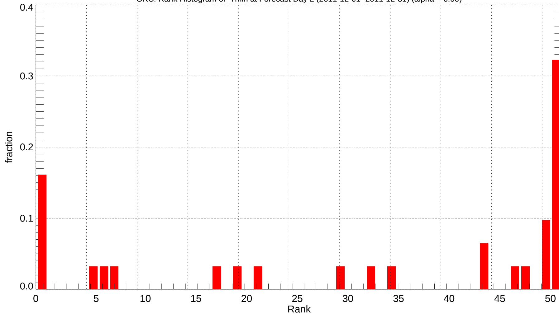
OKC: Rank Histogram of Tmin at Forecast Day 2 (2011-12-01~2011-12-31) (alpha = 0.00)
