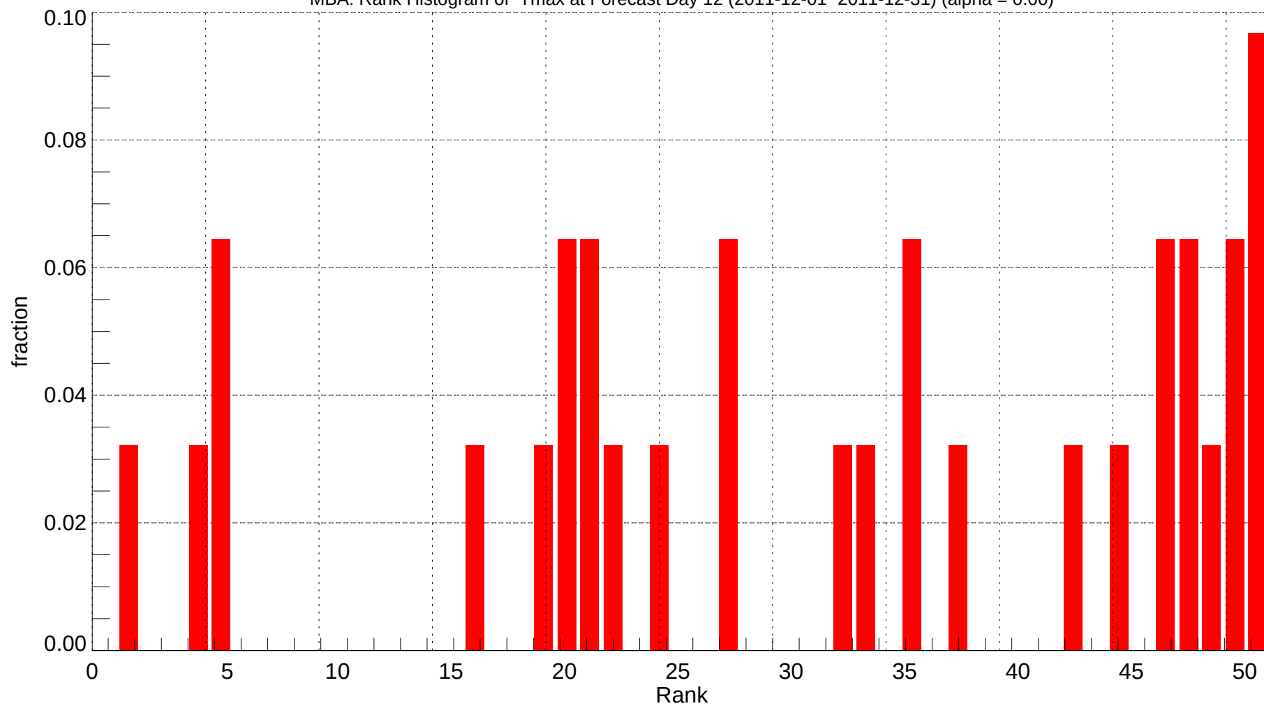
MBA: Rank Histogram of Tmax at Forecast Day 12 (2011-12-01~2011-12-31) (alpha = 0.00)
