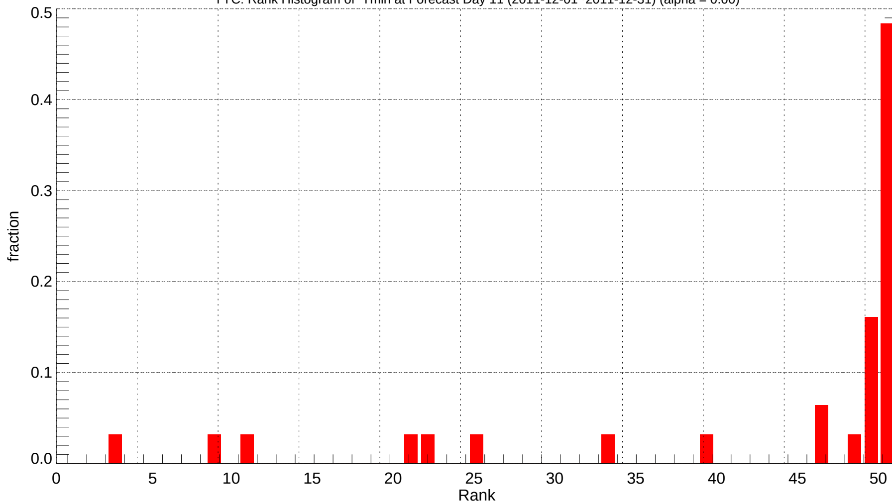
YYC: Rank Histogram of Tmin at Forecast Day 11 (2011-12-01~2011-12-31) (alpha = 0.00)
