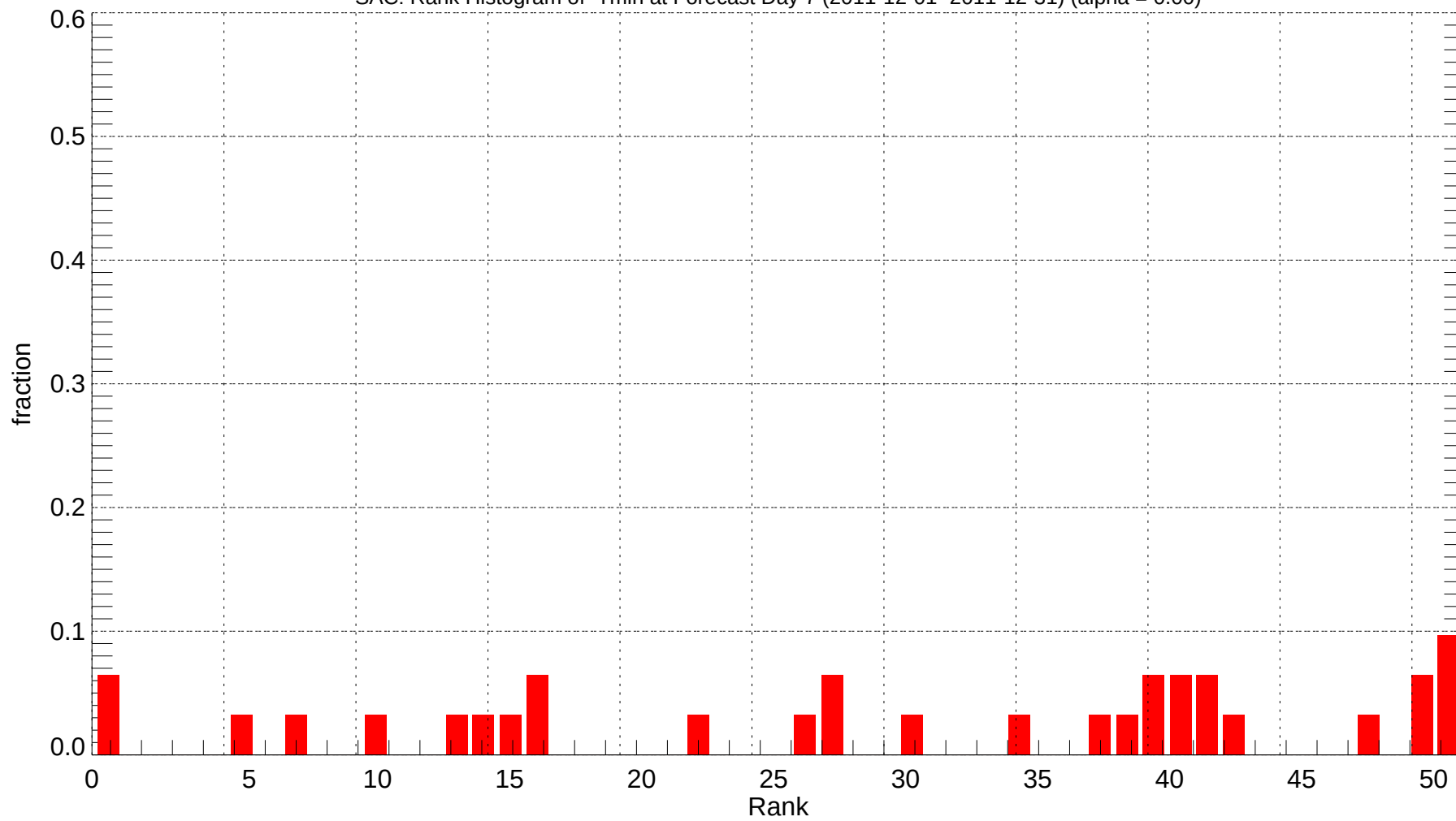
SAC: Rank Histogram of Tmin at Forecast Day 7 (2011-12-01~2011-12-31) (alpha = 0.00)
