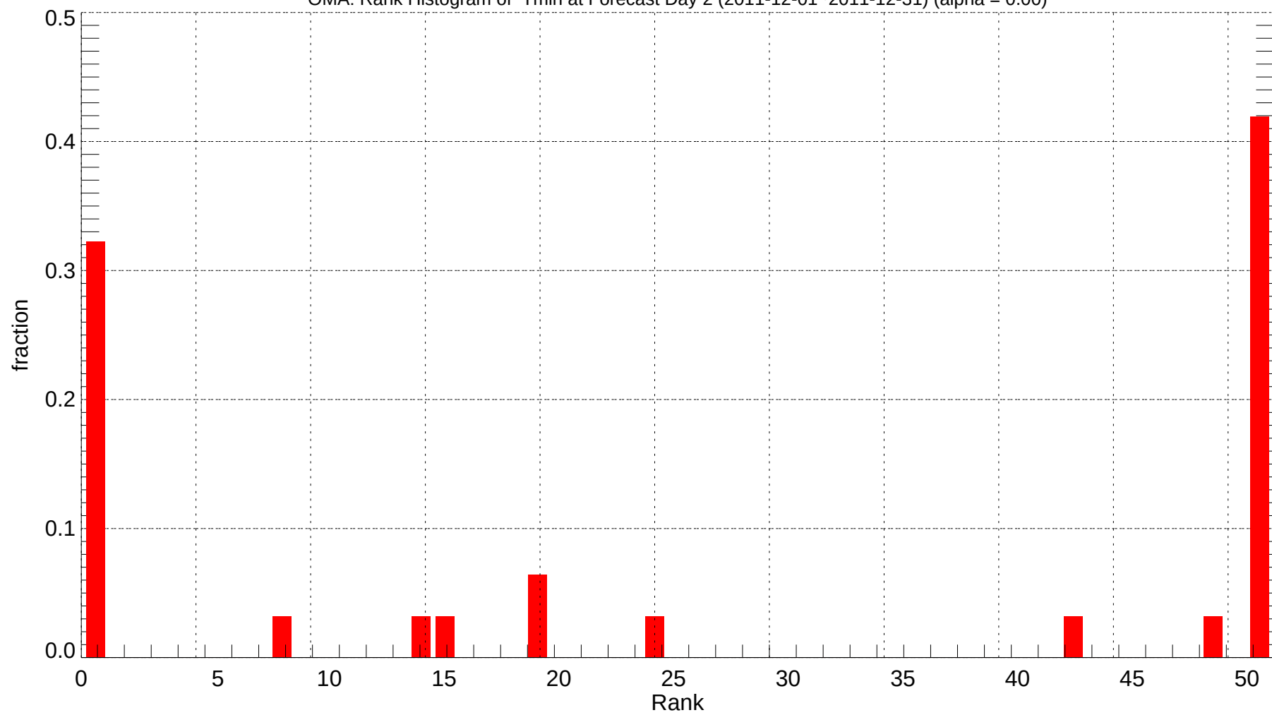
OMA: Rank Histogram of Tmin at Forecast Day 2 (2011-12-01~2011-12-31) (alpha = 0.00)
