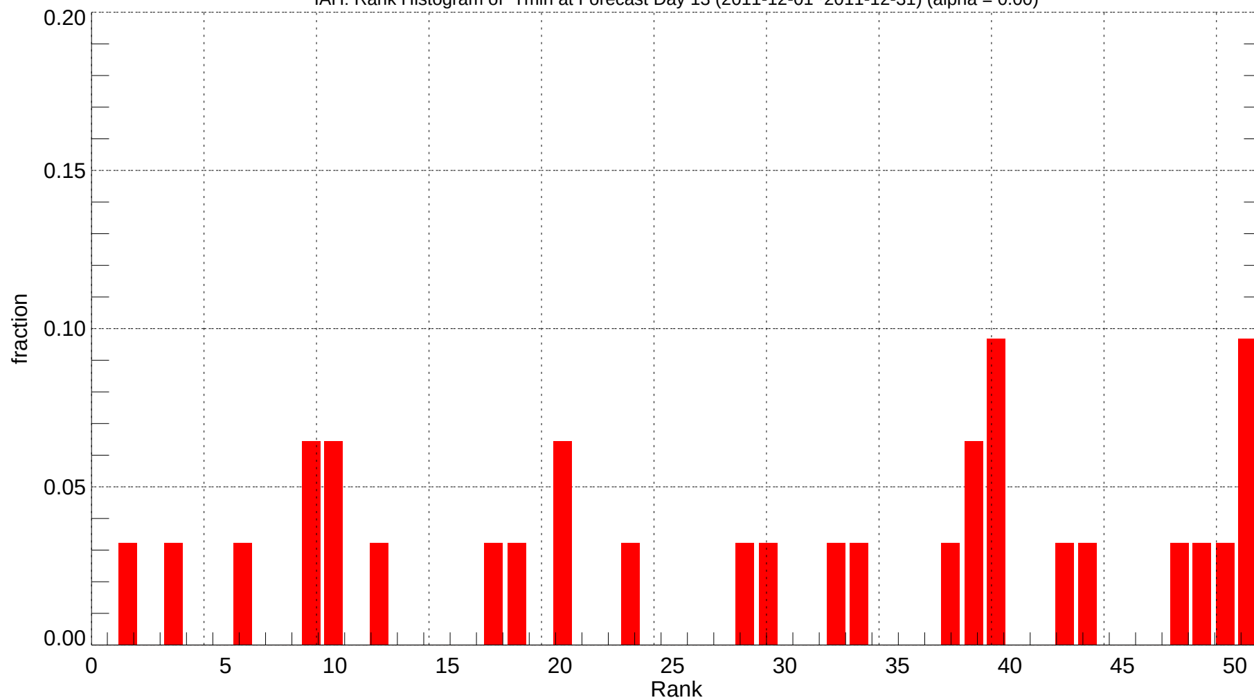
IAH: Rank Histogram of Tmin at Forecast Day 13 (2011-12-01~2011-12-31) (alpha = 0.00)
