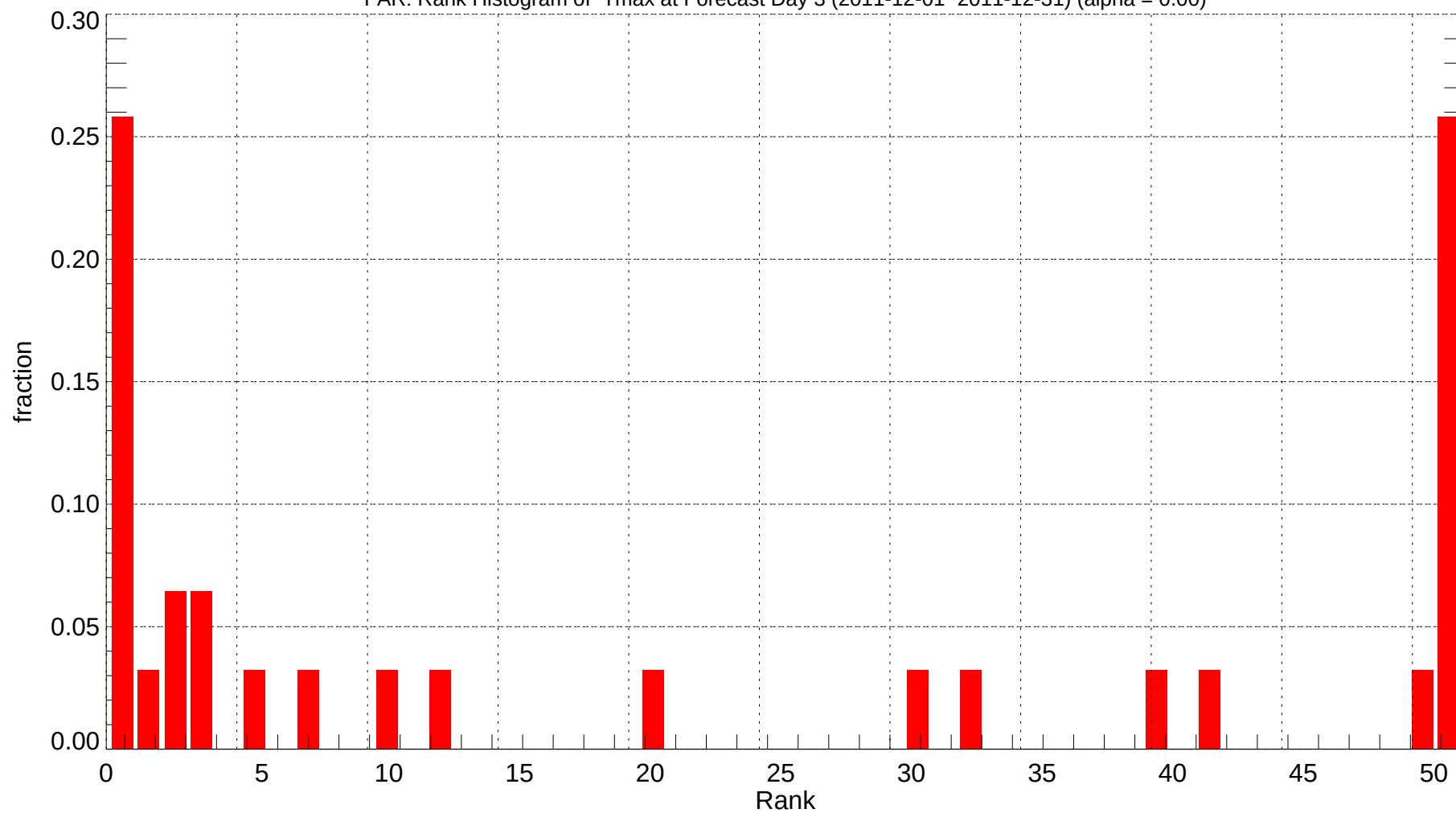
FAR: Rank Histogram of Tmax at Forecast Day 3 (2011-12-01~2011-12-31) (alpha = 0.00)
