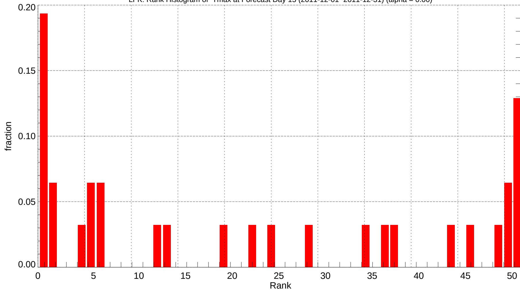
LFK: Rank Histogram of Tmax at Forecast Day 15 (2011-12-01~2011-12-31) (alpha = 0.00)
