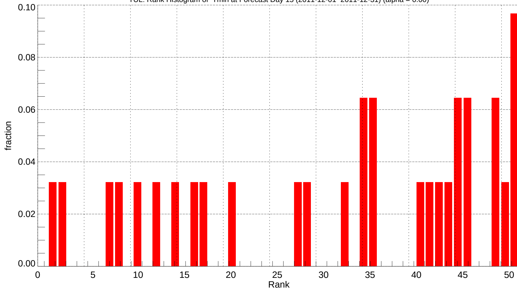
TUL: Rank Histogram of Tmin at Forecast Day 15 (2011-12-01~2011-12-31) (alpha = 0.00)
