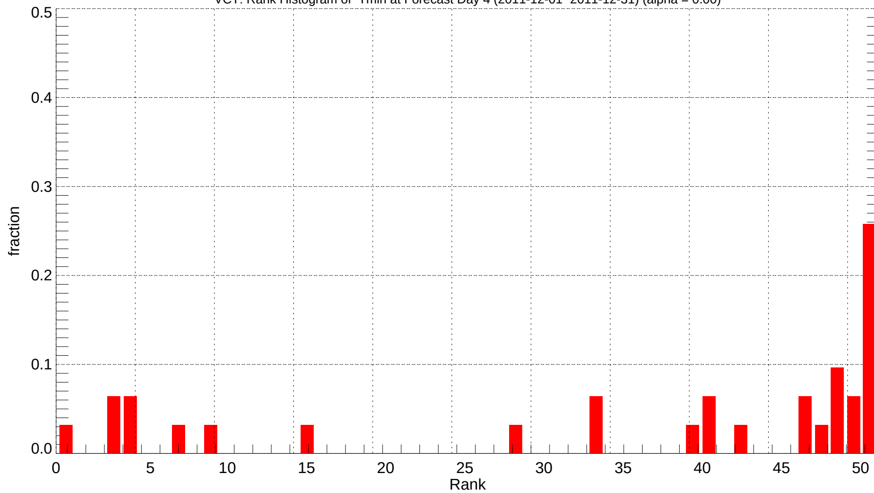
VCT: Rank Histogram of Tmin at Forecast Day 4 (2011-12-01~2011-12-31) (alpha = 0.00)
