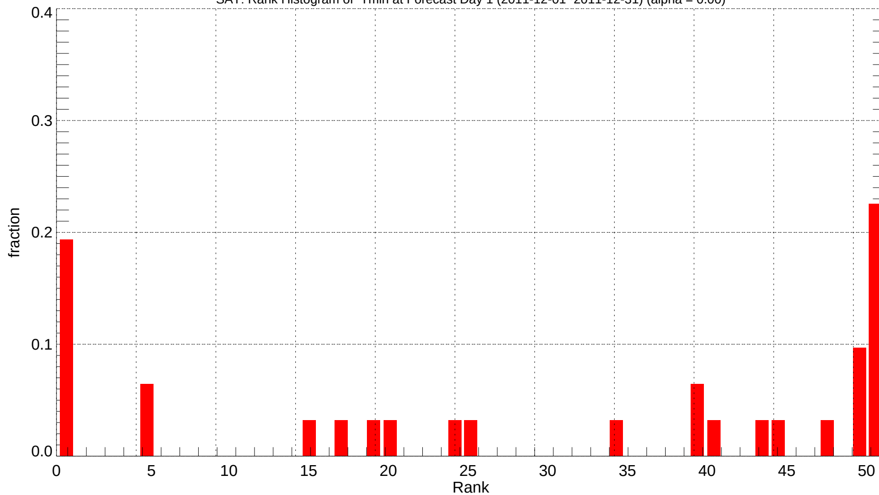
SAT: Rank Histogram of Tmin at Forecast Day 1 (2011-12-01~2011-12-31) (alpha = 0.00)
