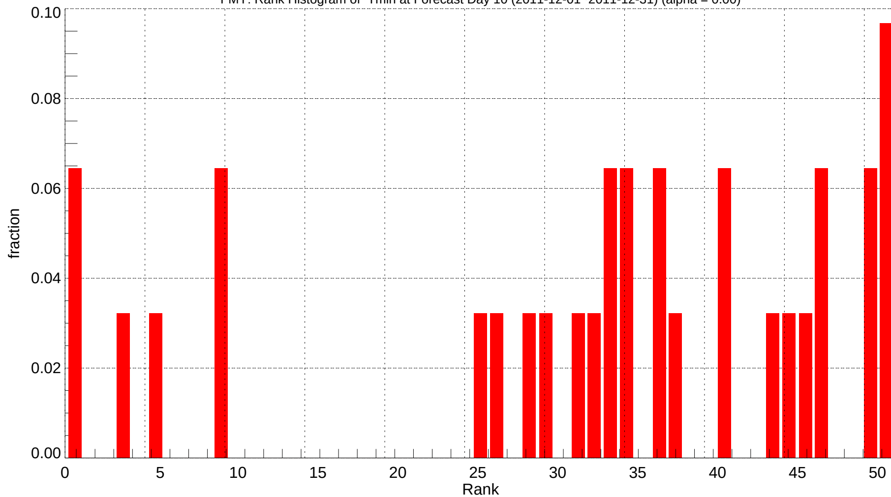
FMY: Rank Histogram of Tmin at Forecast Day 10 (2011-12-01~2011-12-31) (alpha = 0.00)
