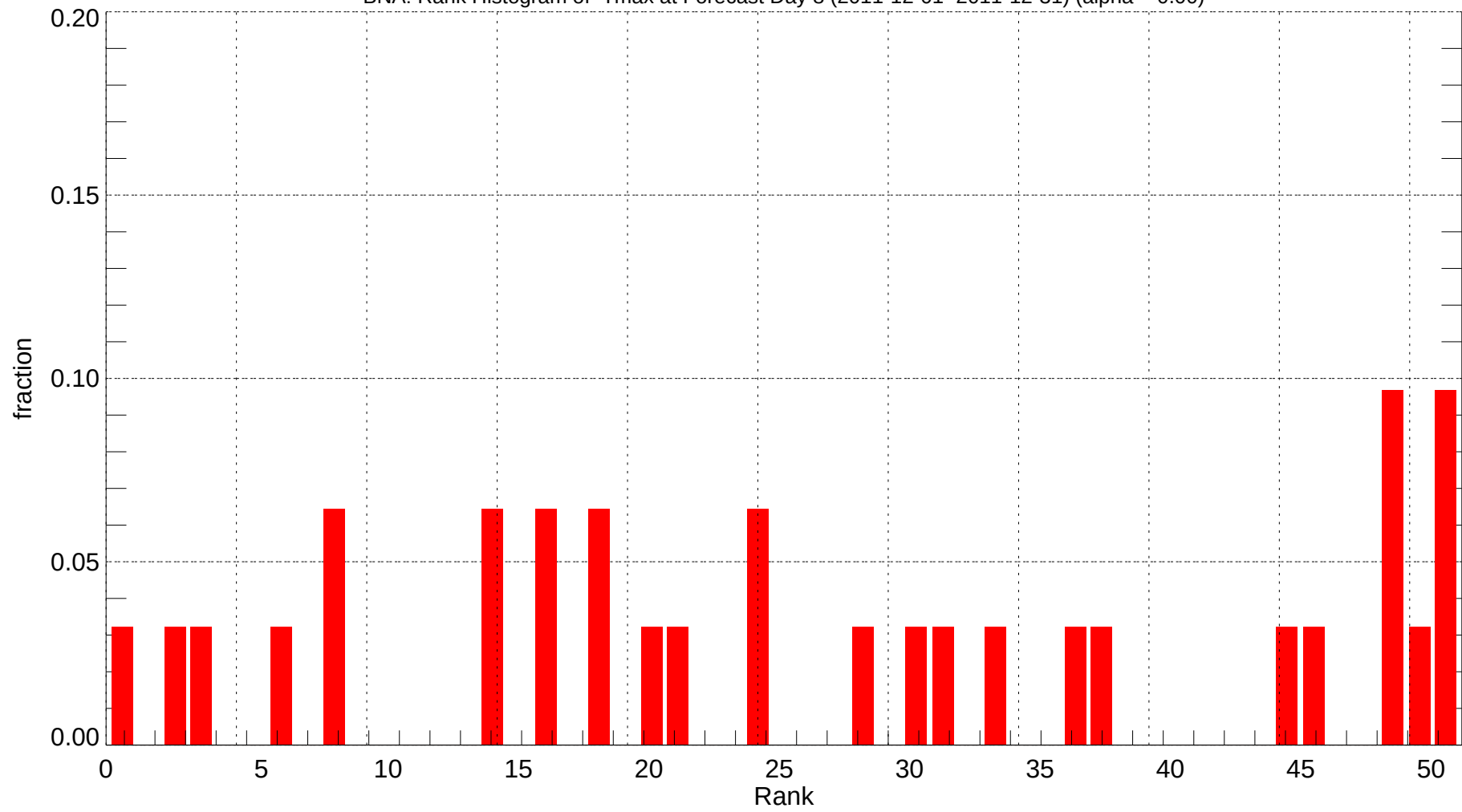
BNA: Rank Histogram of Tmax at Forecast Day 8 (2011-12-01~2011-12-31) (alpha = 0.00)
