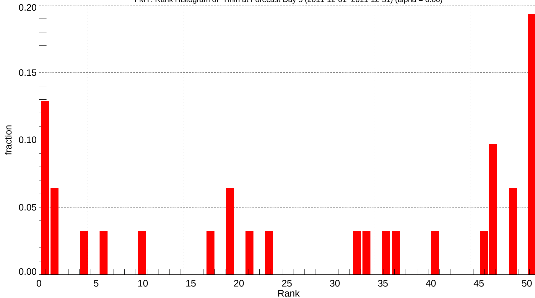
FMY: Rank Histogram of Tmin at Forecast Day 5 (2011-12-01~2011-12-31) (alpha = 0.00)
