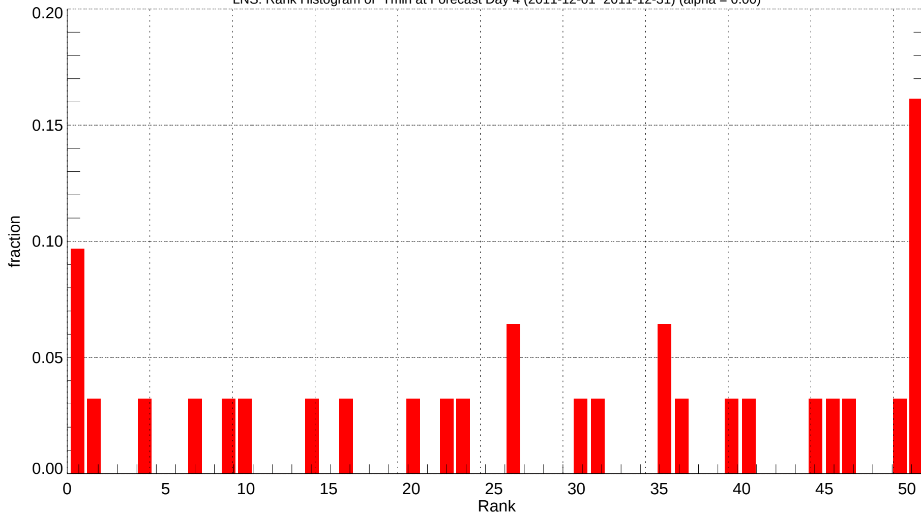
LNS: Rank Histogram of Tmin at Forecast Day 4 (2011-12-01~2011-12-31) (alpha = 0.00)
