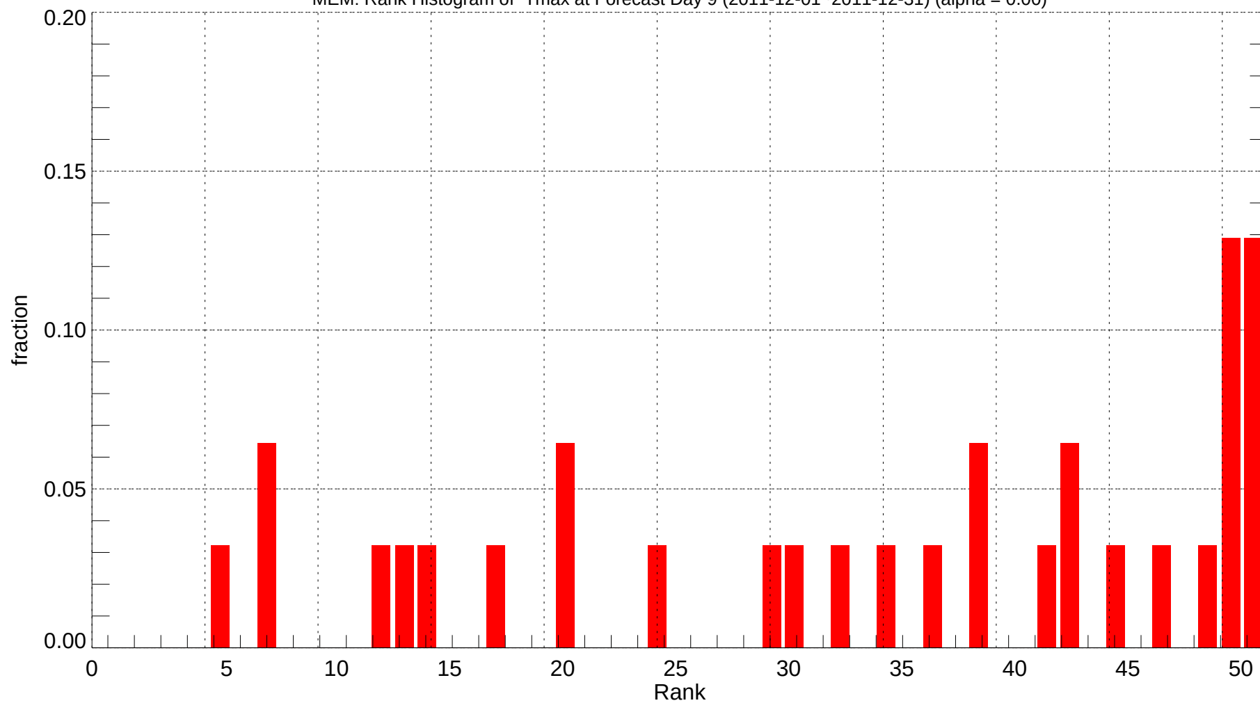
MEM: Rank Histogram of Tmax at Forecast Day 9 (2011-12-01~2011-12-31) (alpha = 0.00)
