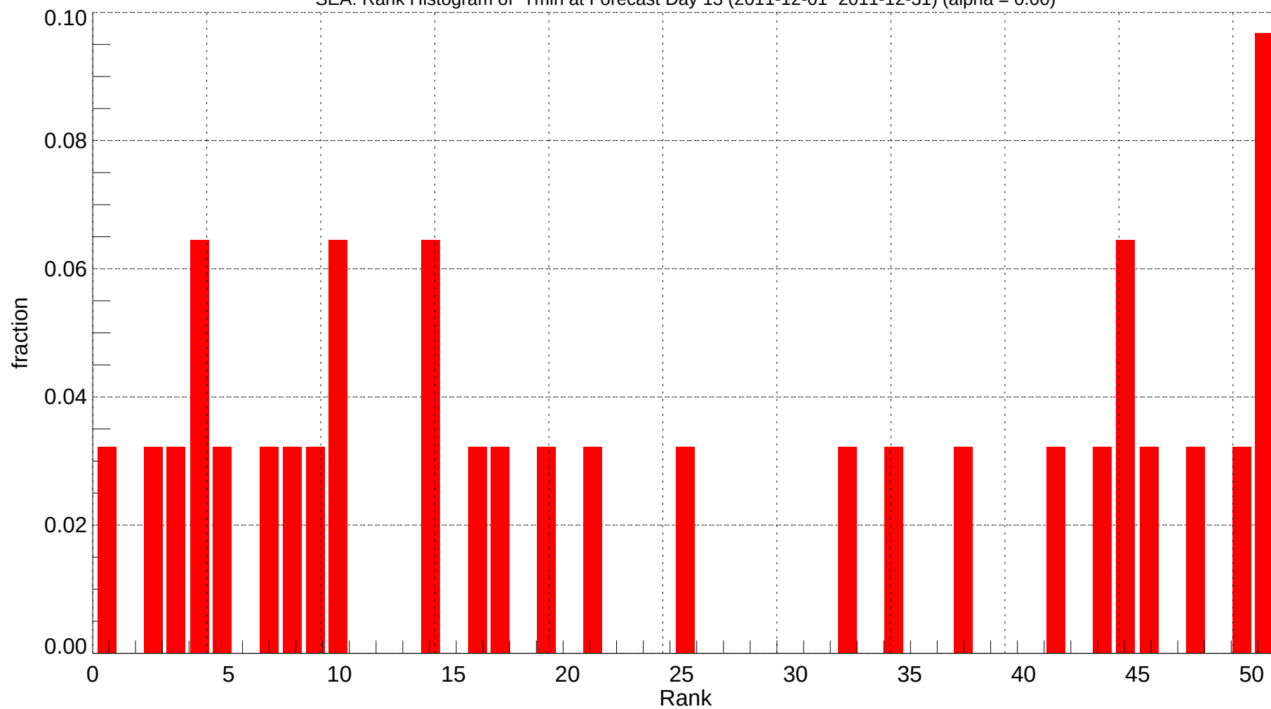
SEA: Rank Histogram of Tmin at Forecast Day 13 (2011-12-01~2011-12-31) (alpha = 0.00)
