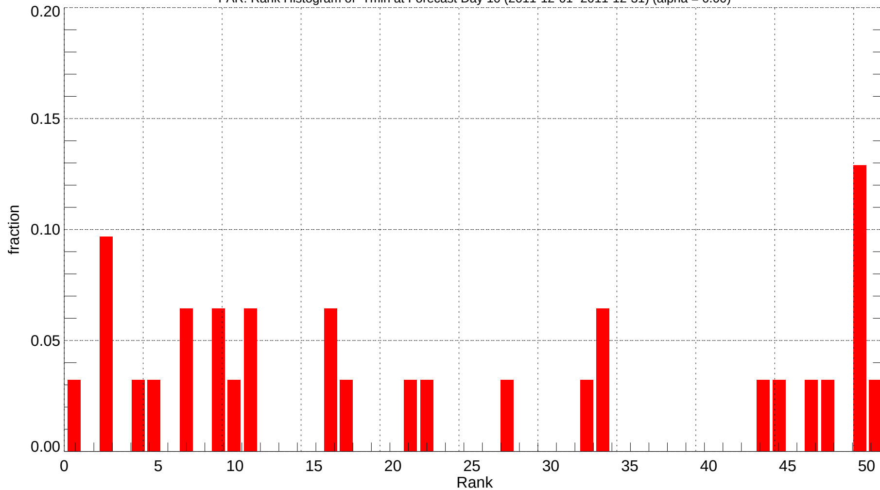
FAR: Rank Histogram of Tmin at Forecast Day 10 (2011-12-01~2011-12-31) (alpha = 0.00)
