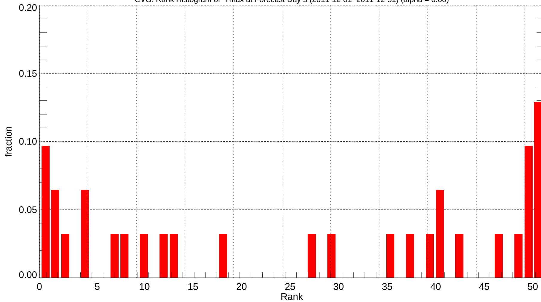
CVG: Rank Histogram of Tmax at Forecast Day 5 (2011-12-01~2011-12-31) (alpha = 0.00)
