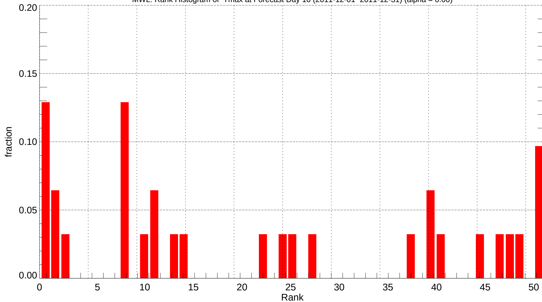
MWL: Rank Histogram of Tmax at Forecast Day 10 (2011-12-01~2011-12-31) (alpha = 0.00)
