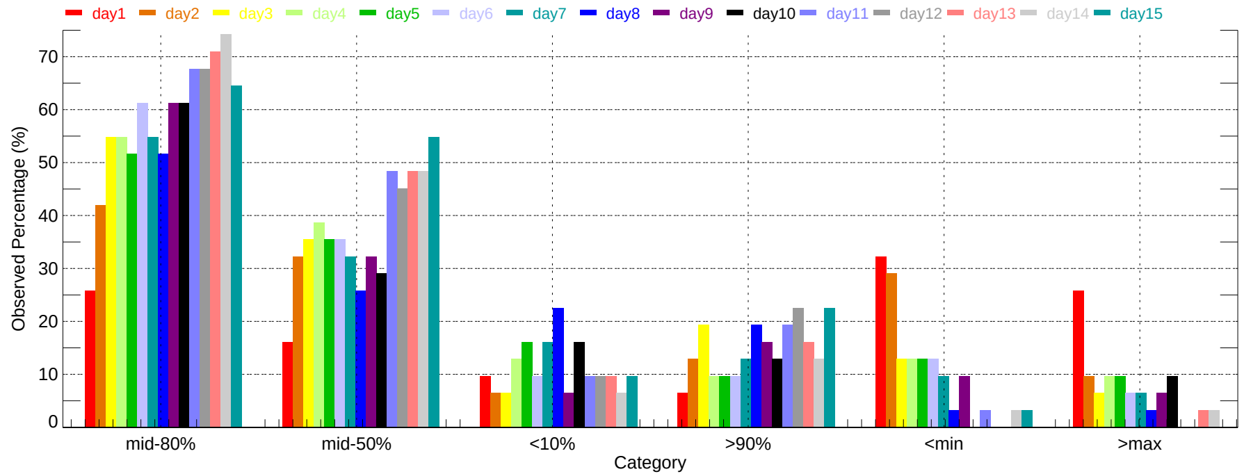
Observed Percentage of Ensembles - AUG: Max Temperature (2011-12-01~2011-12-31)
