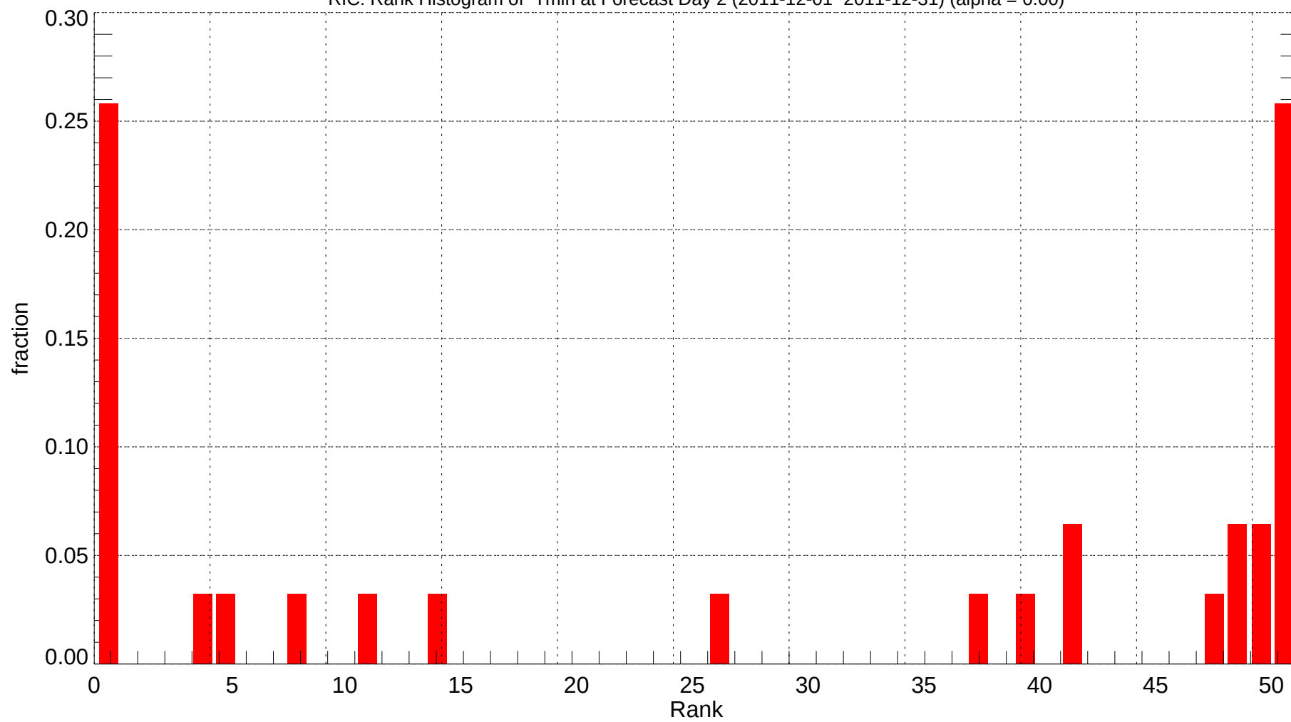
RIC: Rank Histogram of Tmin at Forecast Day 2 (2011-12-01~2011-12-31) (alpha = 0.00)
