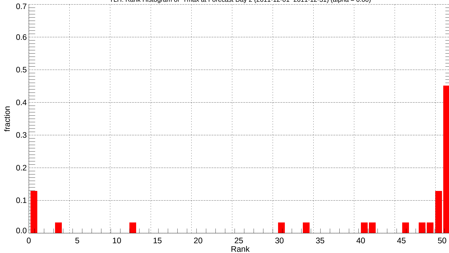
TLH: Rank Histogram of Tmax at Forecast Day 2 (2011-12-01~2011-12-31) (alpha = 0.00)
