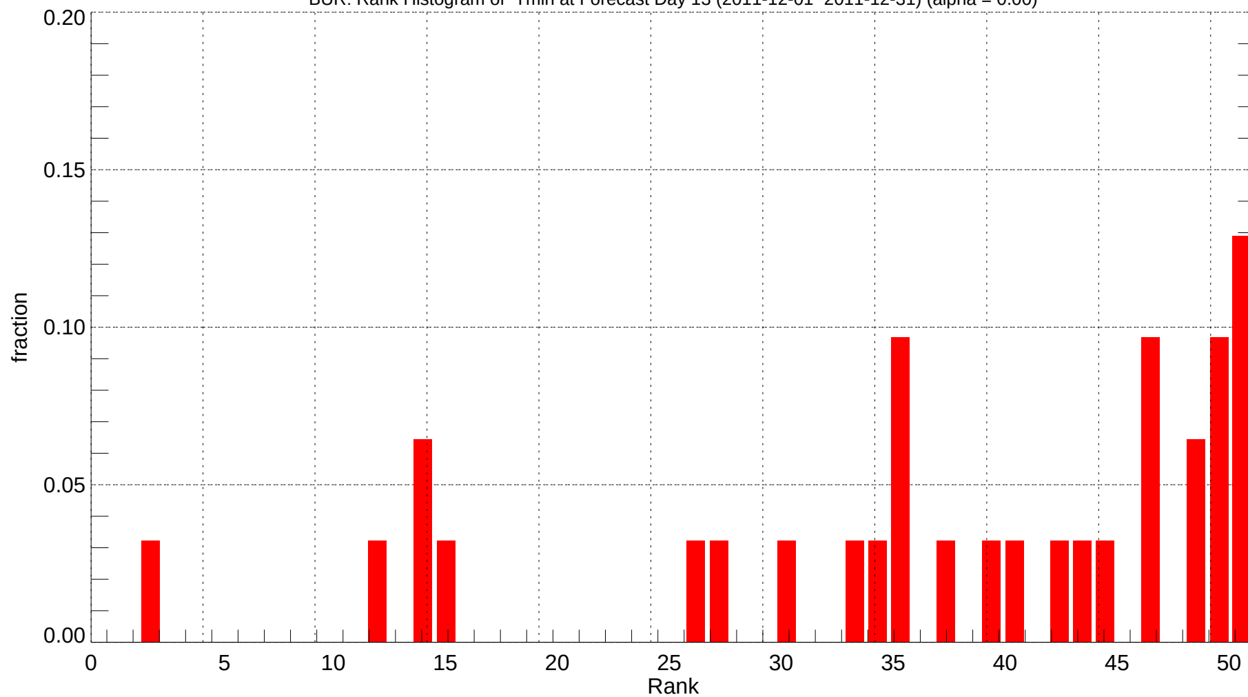
BUR: Rank Histogram of Tmin at Forecast Day 13 (2011-12-01~2011-12-31) (alpha = 0.00)
