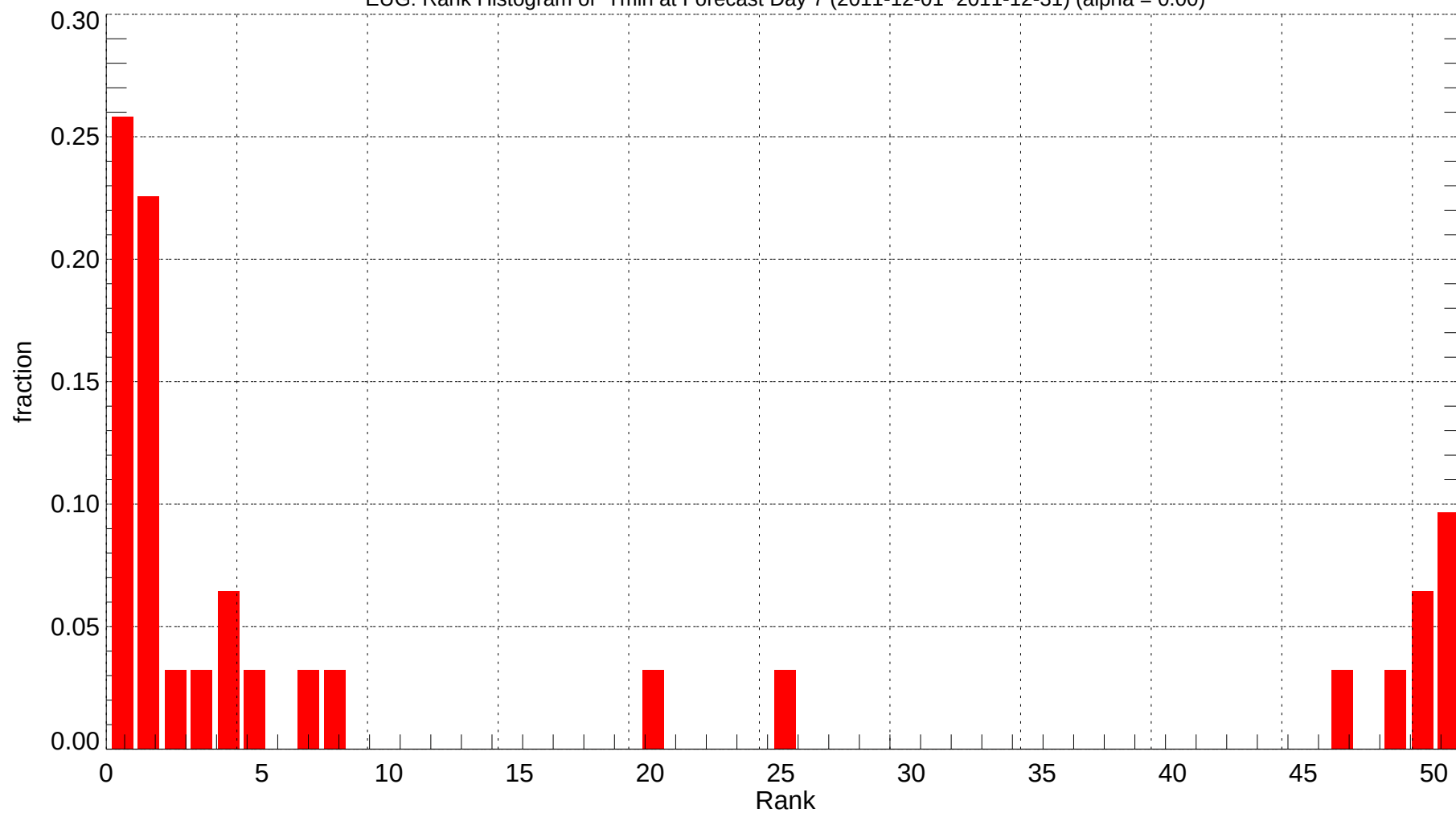
EUG: Rank Histogram of Tmin at Forecast Day 7 (2011-12-01~2011-12-31) (alpha = 0.00)
