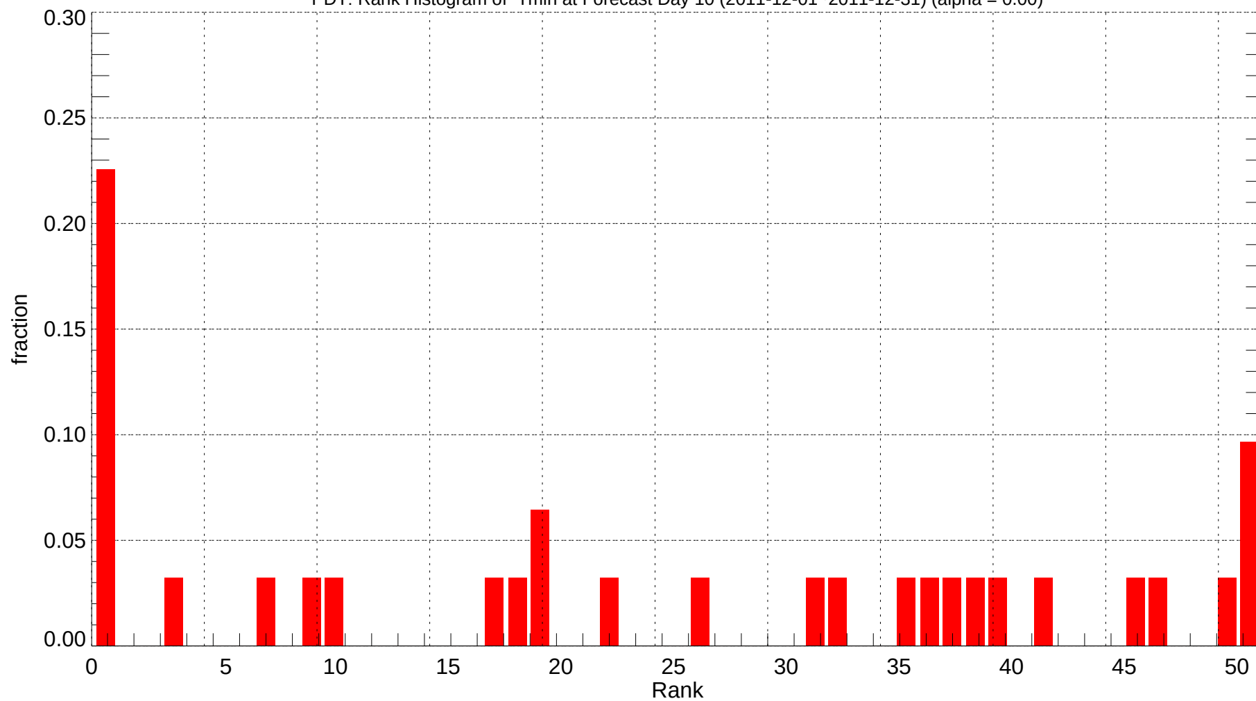
PDT: Rank Histogram of Tmin at Forecast Day 10 (2011-12-01~2011-12-31) (alpha = 0.00)
