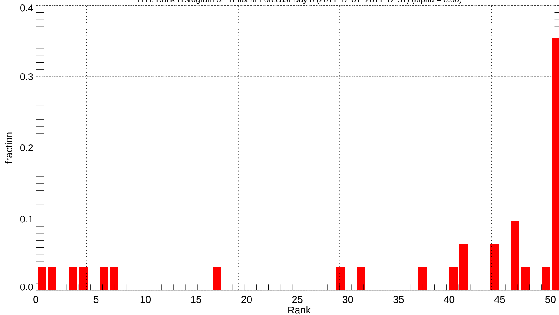
TLH: Rank Histogram of Tmax at Forecast Day 8 (2011-12-01~2011-12-31) (alpha = 0.00)
