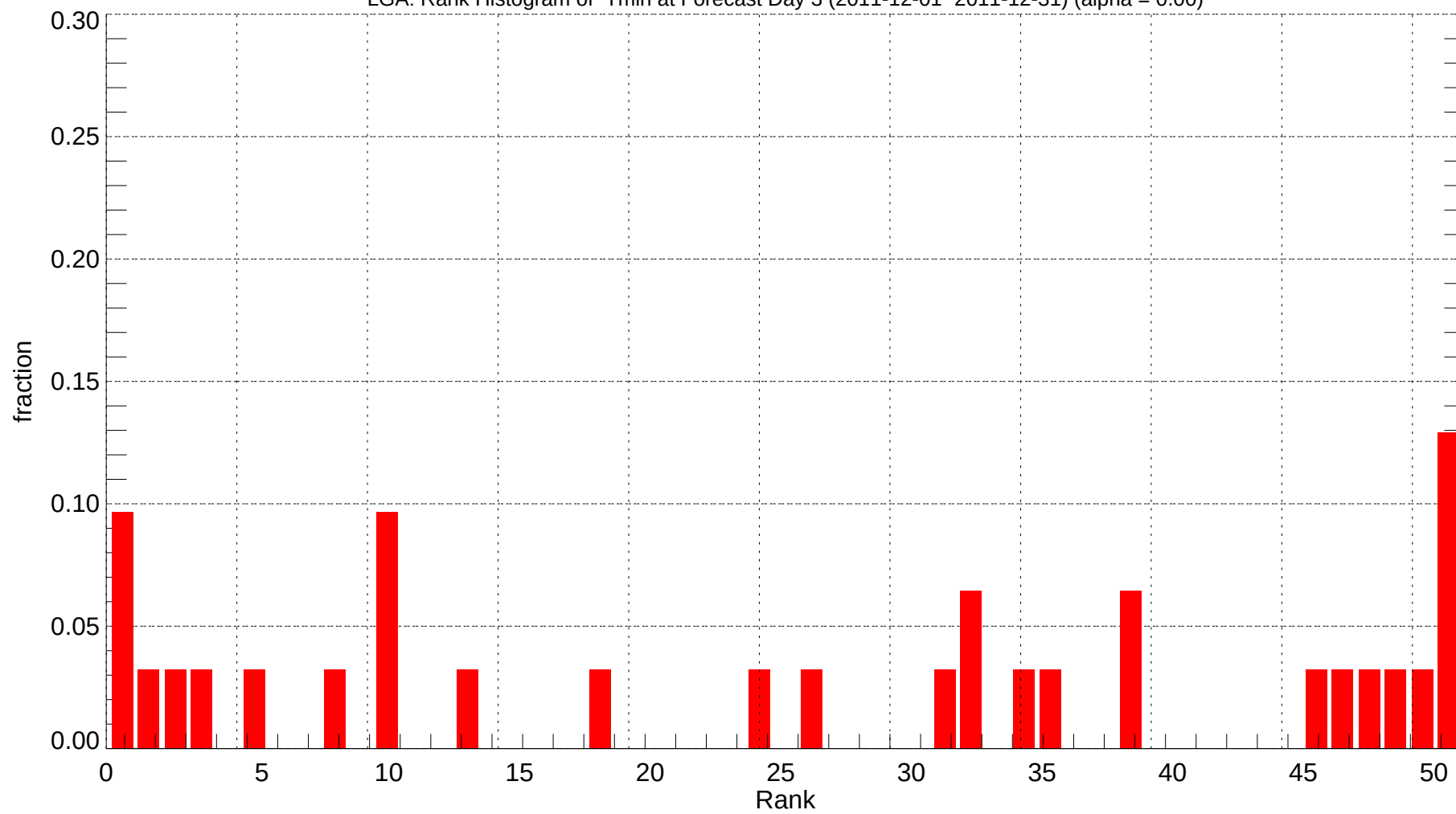
LGA: Rank Histogram of Tmin at Forecast Day 3 (2011-12-01~2011-12-31) (alpha = 0.00)
