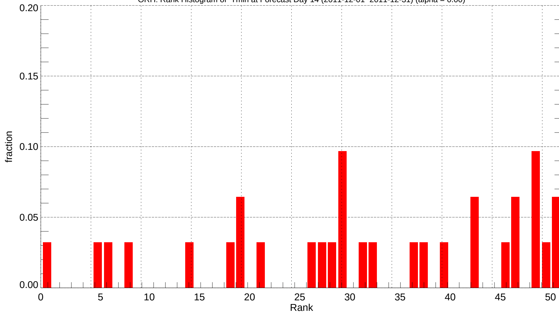
ORH: Rank Histogram of Tmin at Forecast Day 14 (2011-12-01~2011-12-31) (alpha = 0.00)
