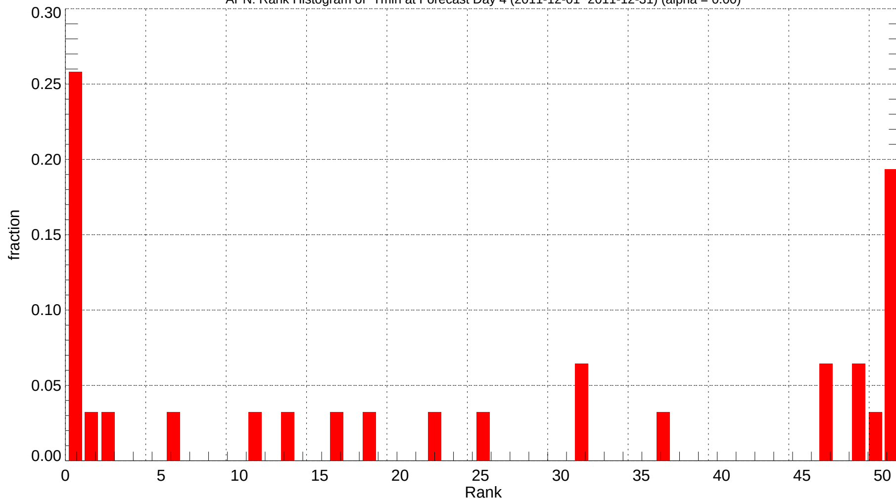
APN: Rank Histogram of Tmin at Forecast Day 4 (2011-12-01~2011-12-31) (alpha = 0.00)
