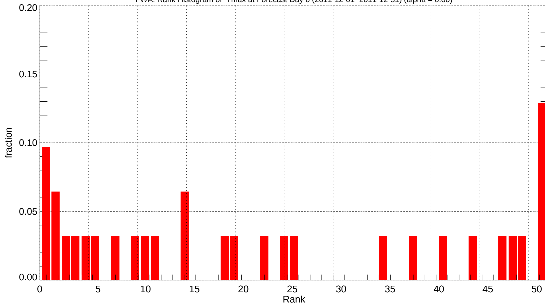
FWA: Rank Histogram of Tmax at Forecast Day 6 (2011-12-01~2011-12-31) (alpha = 0.00)
