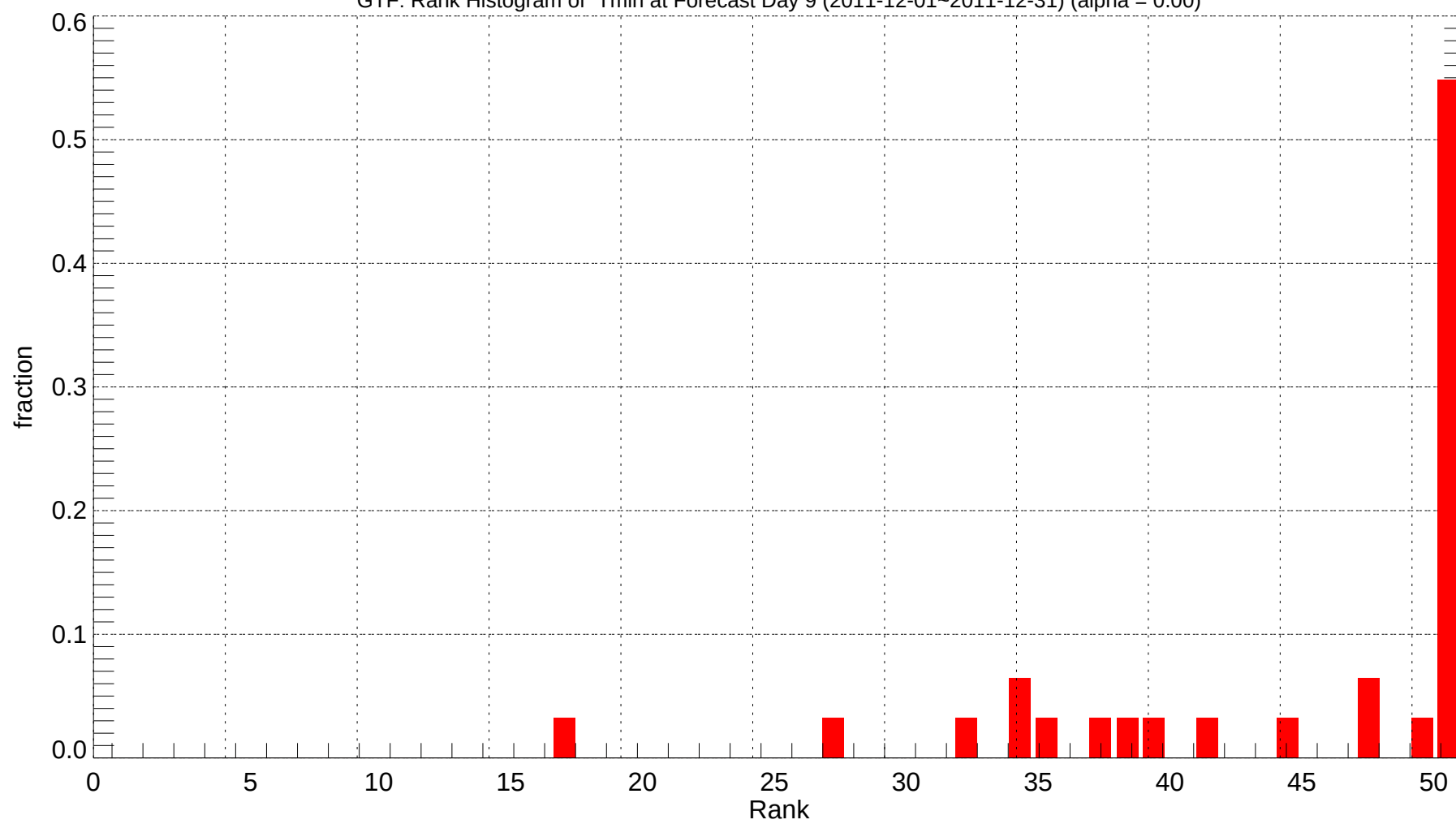
GTF: Rank Histogram of Tmin at Forecast Day 9 (2011-12-01~2011-12-31) (alpha = 0.00)
