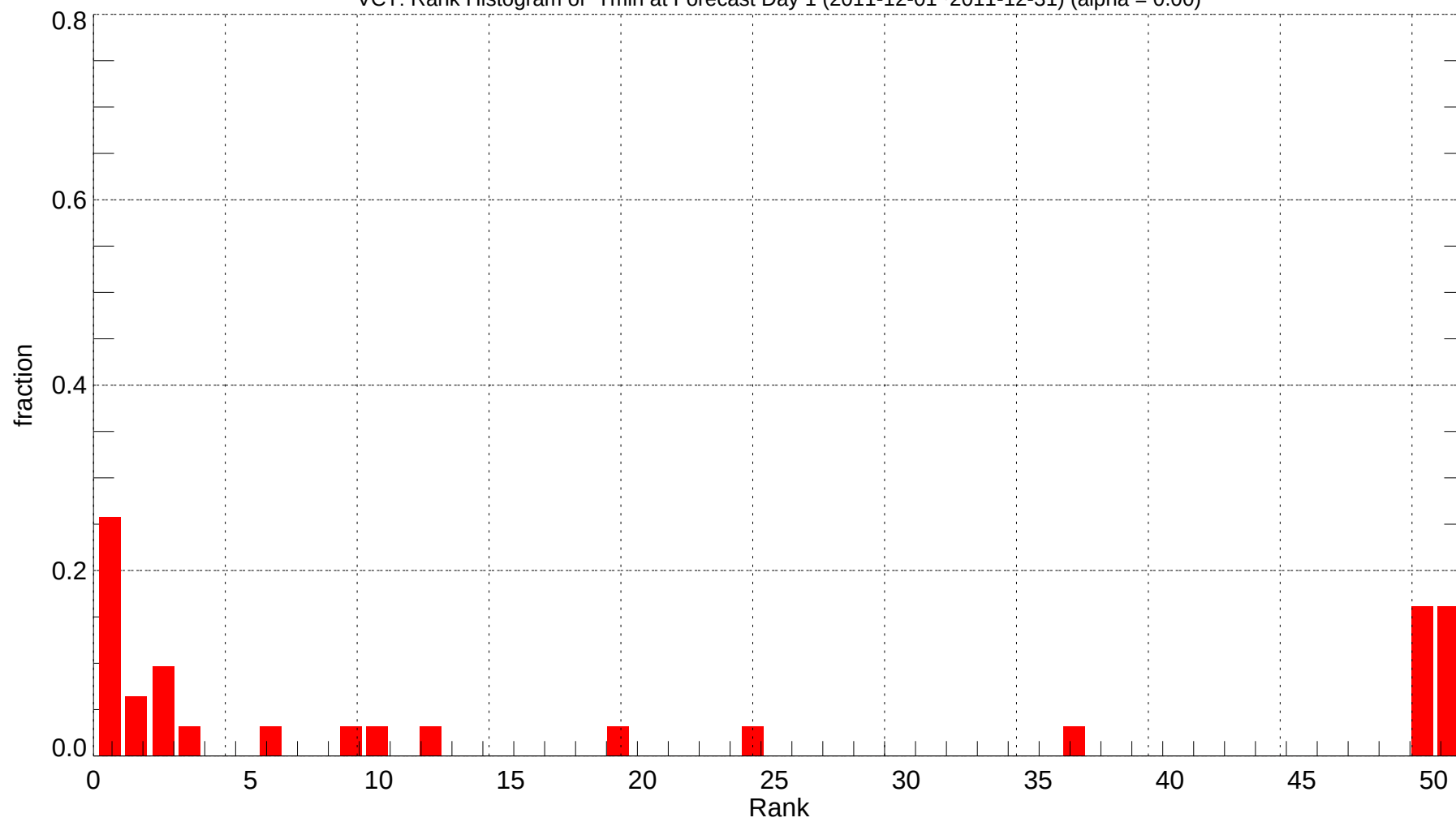
VCT: Rank Histogram of Tmin at Forecast Day 1 (2011-12-01~2011-12-31) (alpha = 0.00)
