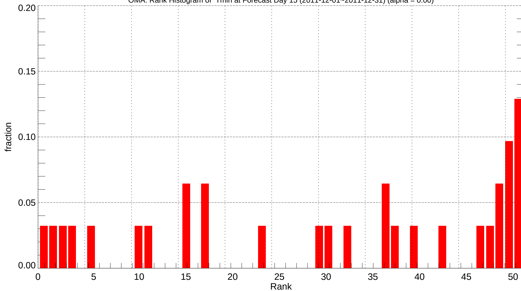
OMA: Rank Histogram of Tmin at Forecast Day 15 (2011-12-01~2011-12-31) (alpha = 0.00)
