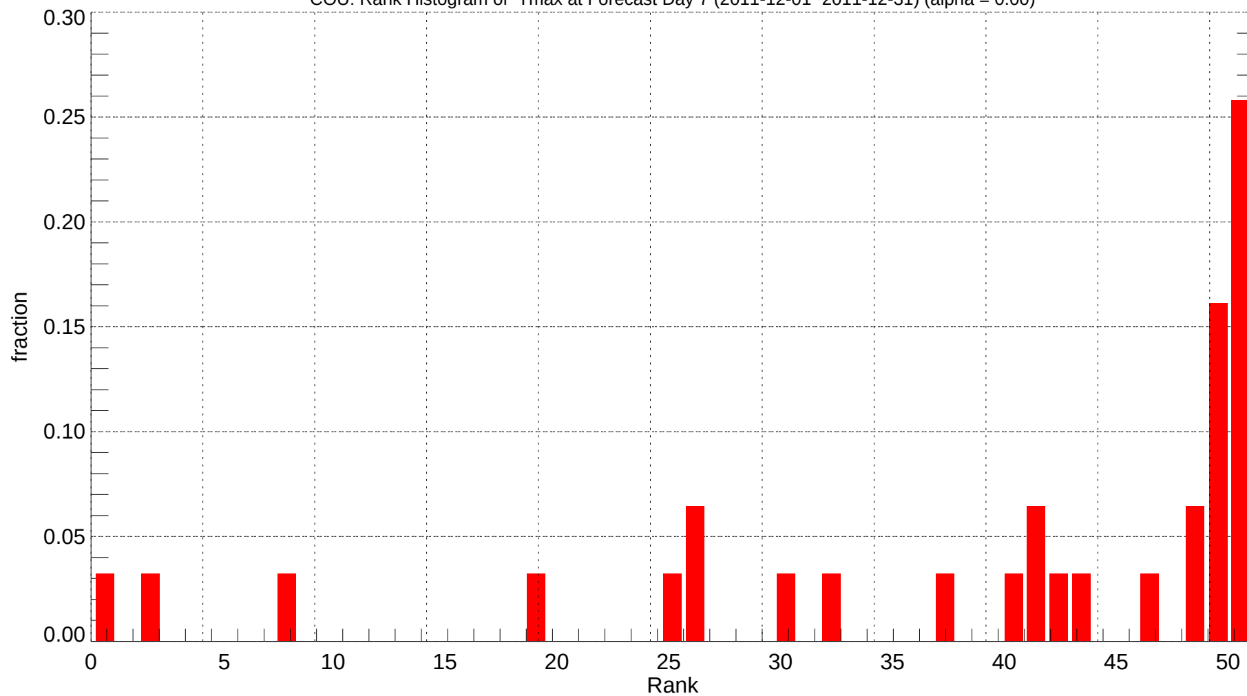
COU: Rank Histogram of Tmax at Forecast Day 7 (2011-12-01~2011-12-31) (alpha = 0.00)
