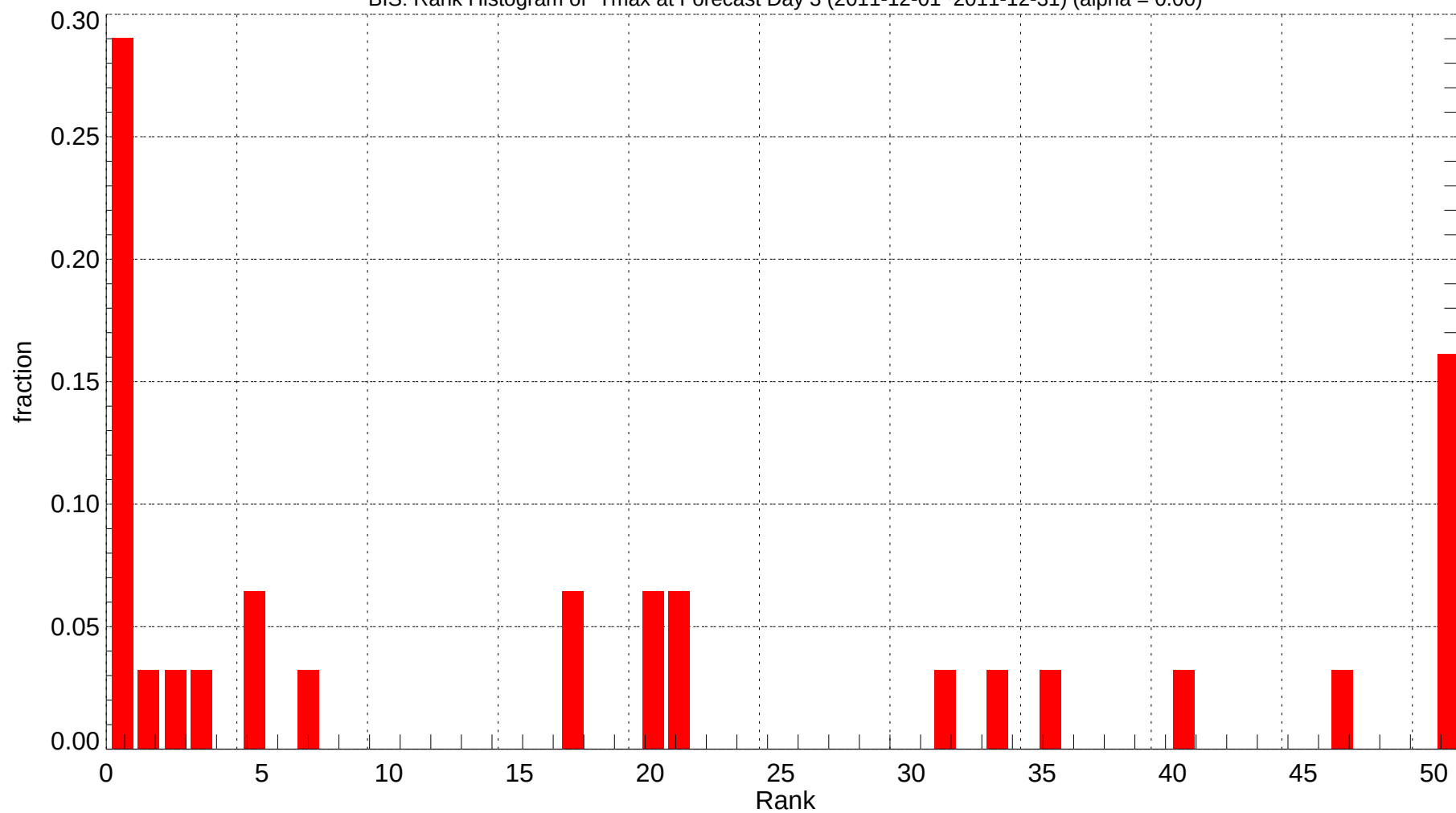
BIS: Rank Histogram of Tmax at Forecast Day 3 (2011-12-01~2011-12-31) (alpha = 0.00)
