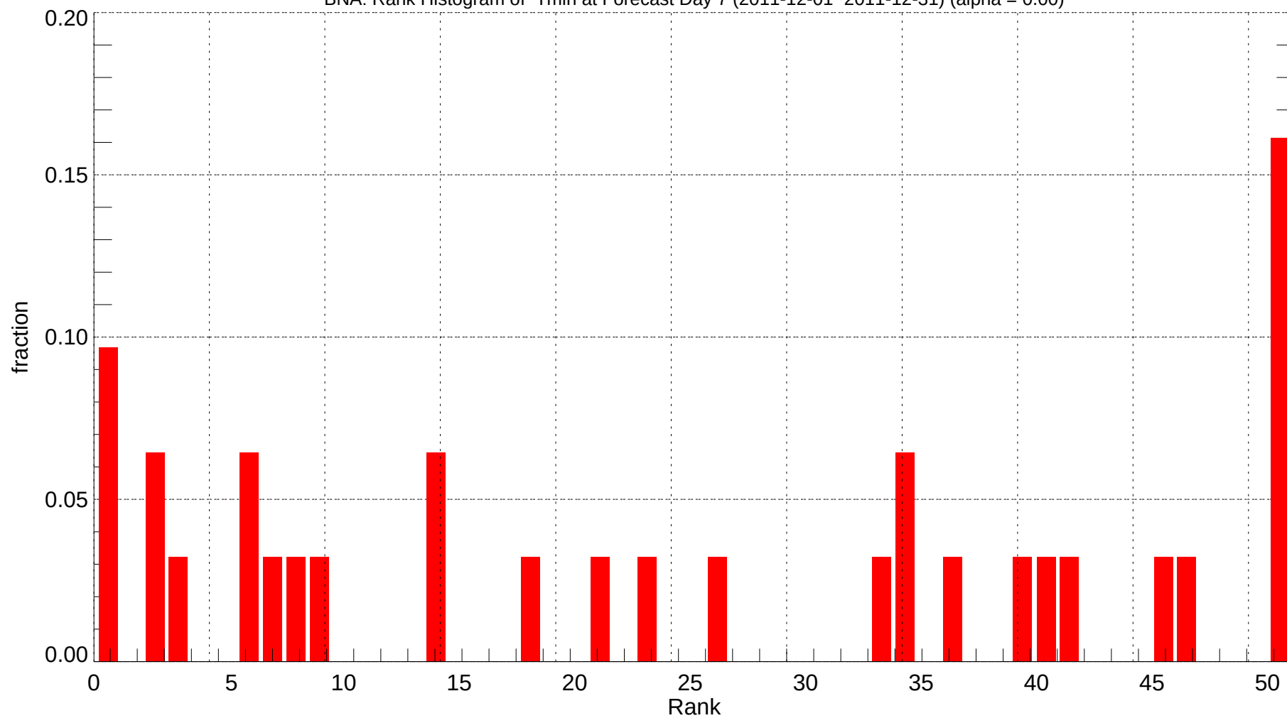
BNA: Rank Histogram of Tmin at Forecast Day 7 (2011-12-01~2011-12-31) (alpha = 0.00)
