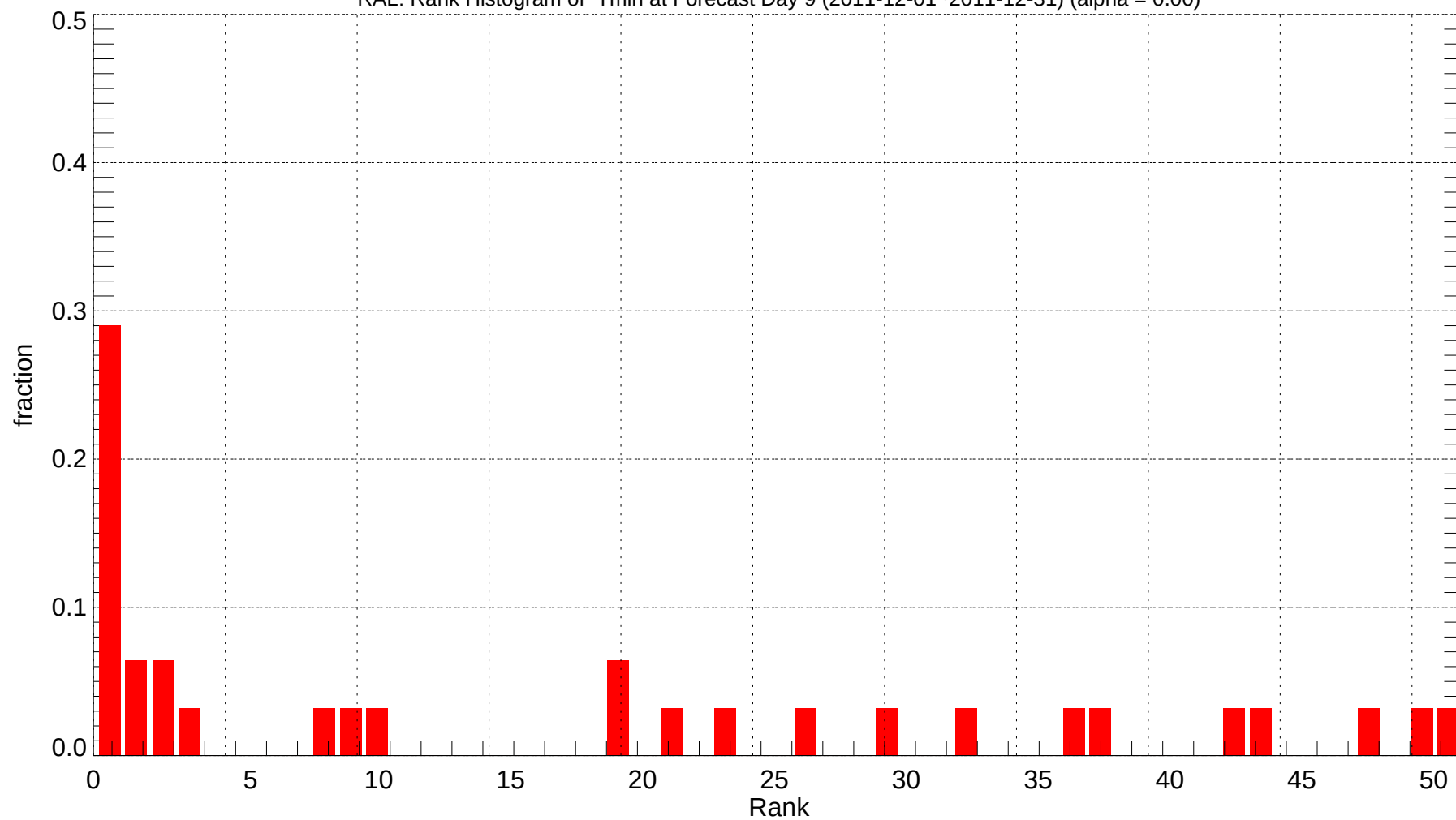
RAL: Rank Histogram of Tmin at Forecast Day 9 (2011-12-01~2011-12-31) (alpha = 0.00)
