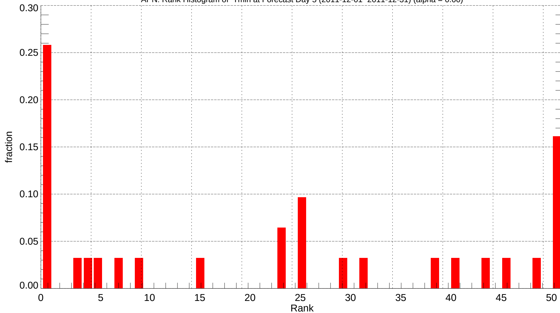
APN: Rank Histogram of Tmin at Forecast Day 5 (2011-12-01~2011-12-31) (alpha = 0.00)
