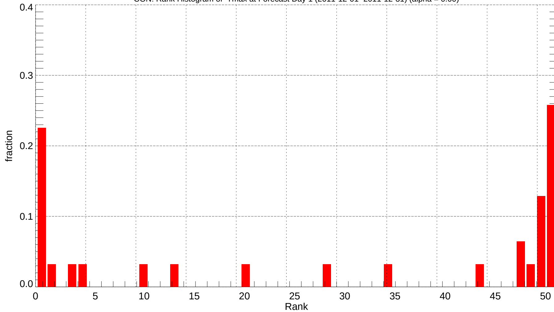
CON: Rank Histogram of Tmax at Forecast Day 1 (2011-12-01~2011-12-31) (alpha = 0.00)
