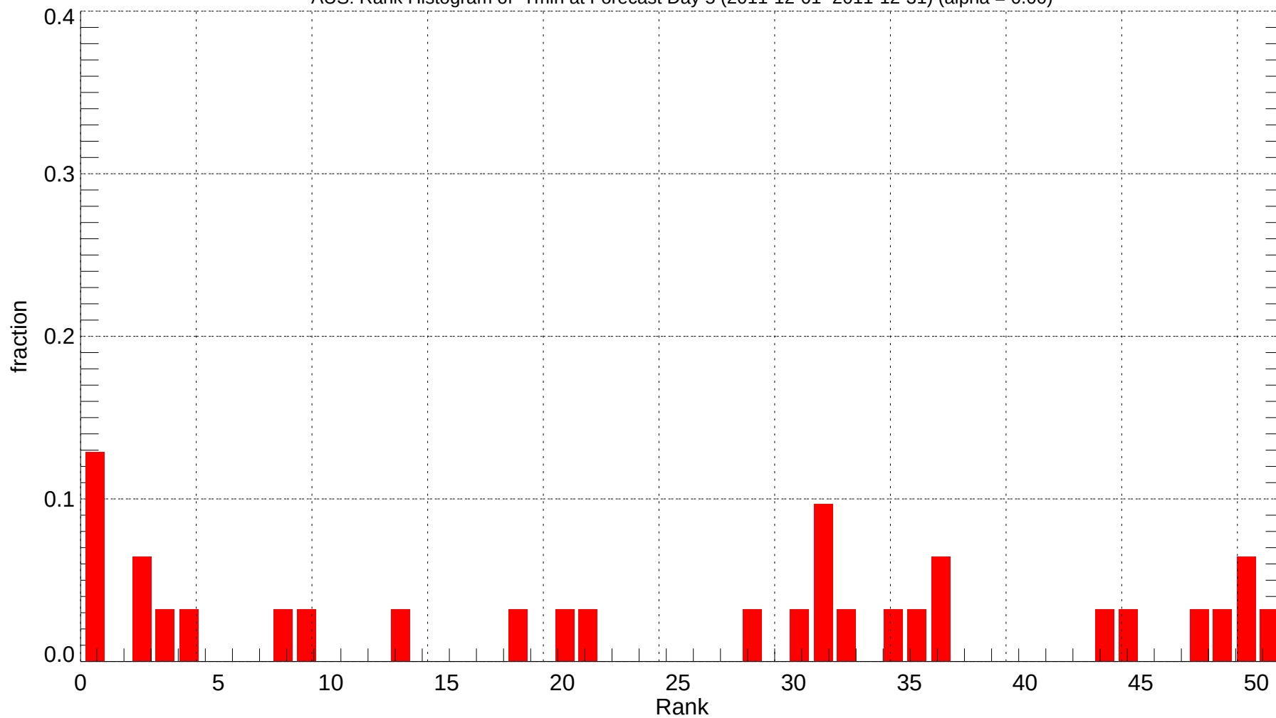
AUS: Rank Histogram of Tmin at Forecast Day 5 (2011-12-01~2011-12-31) (alpha = 0.00)
