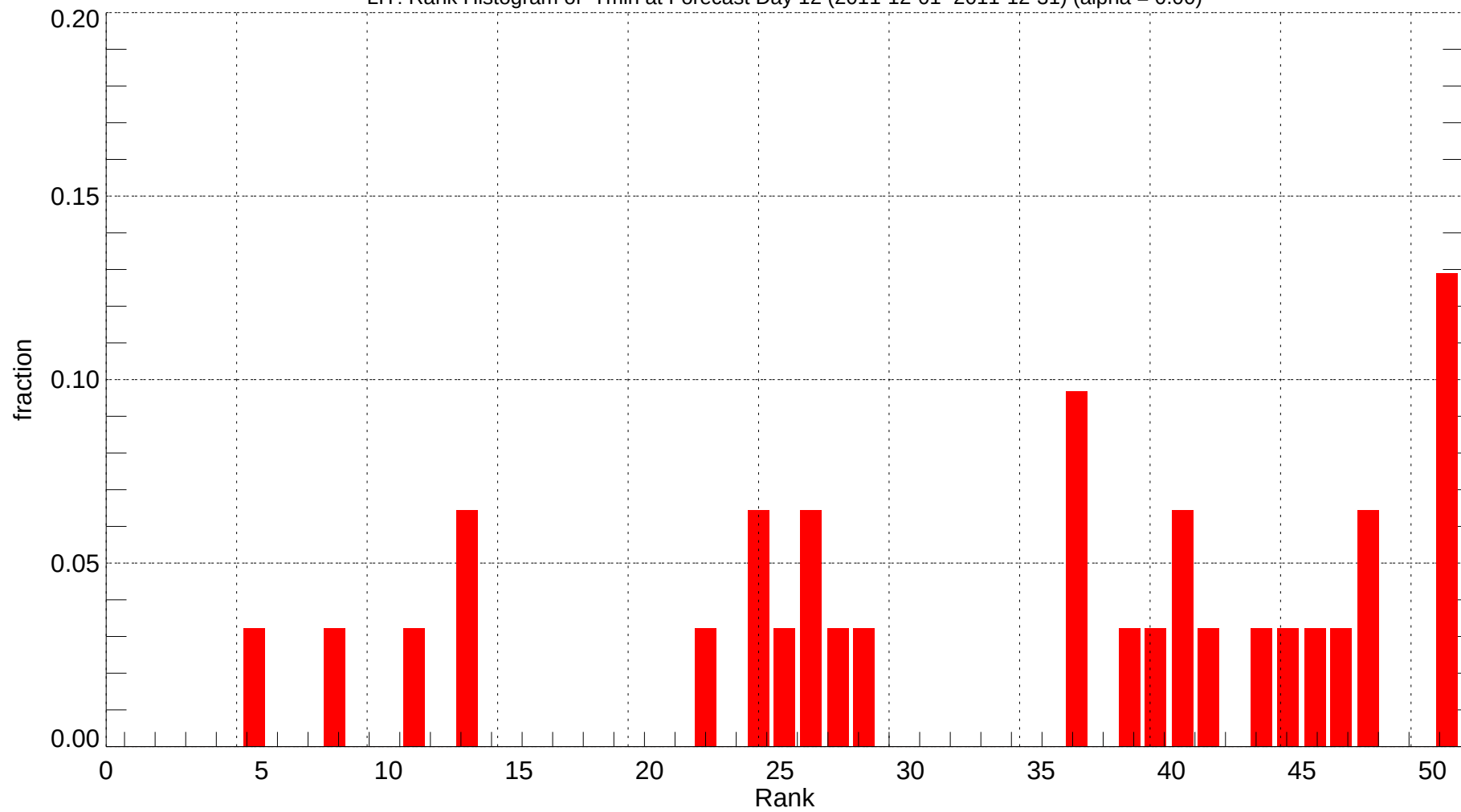
LIT: Rank Histogram of Tmin at Forecast Day 12 (2011-12-01~2011-12-31) (alpha = 0.00)
