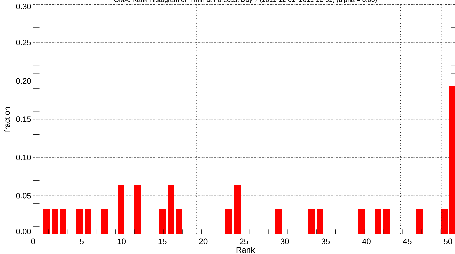
OMA: Rank Histogram of Tmin at Forecast Day 7 (2011-12-01~2011-12-31) (alpha = 0.00)
