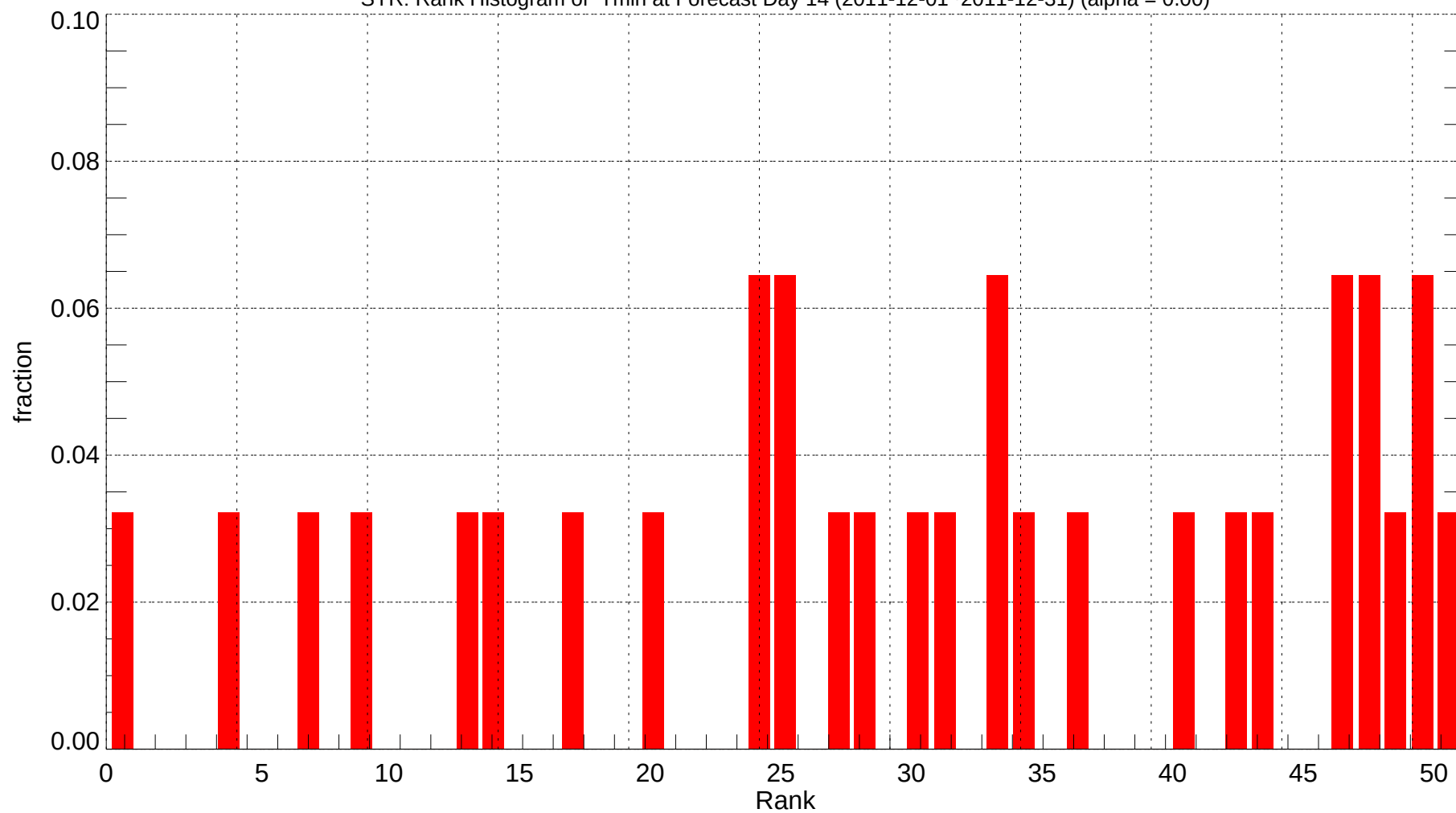
SYR: Rank Histogram of Tmin at Forecast Day 14 (2011-12-01~2011-12-31) (alpha = 0.00)
