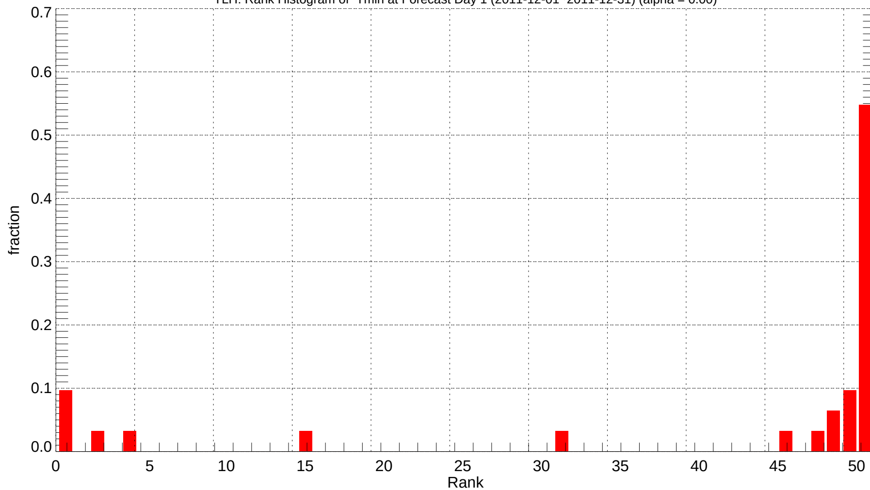
TLH: Rank Histogram of Tmin at Forecast Day 1 (2011-12-01~2011-12-31) (alpha = 0.00)
