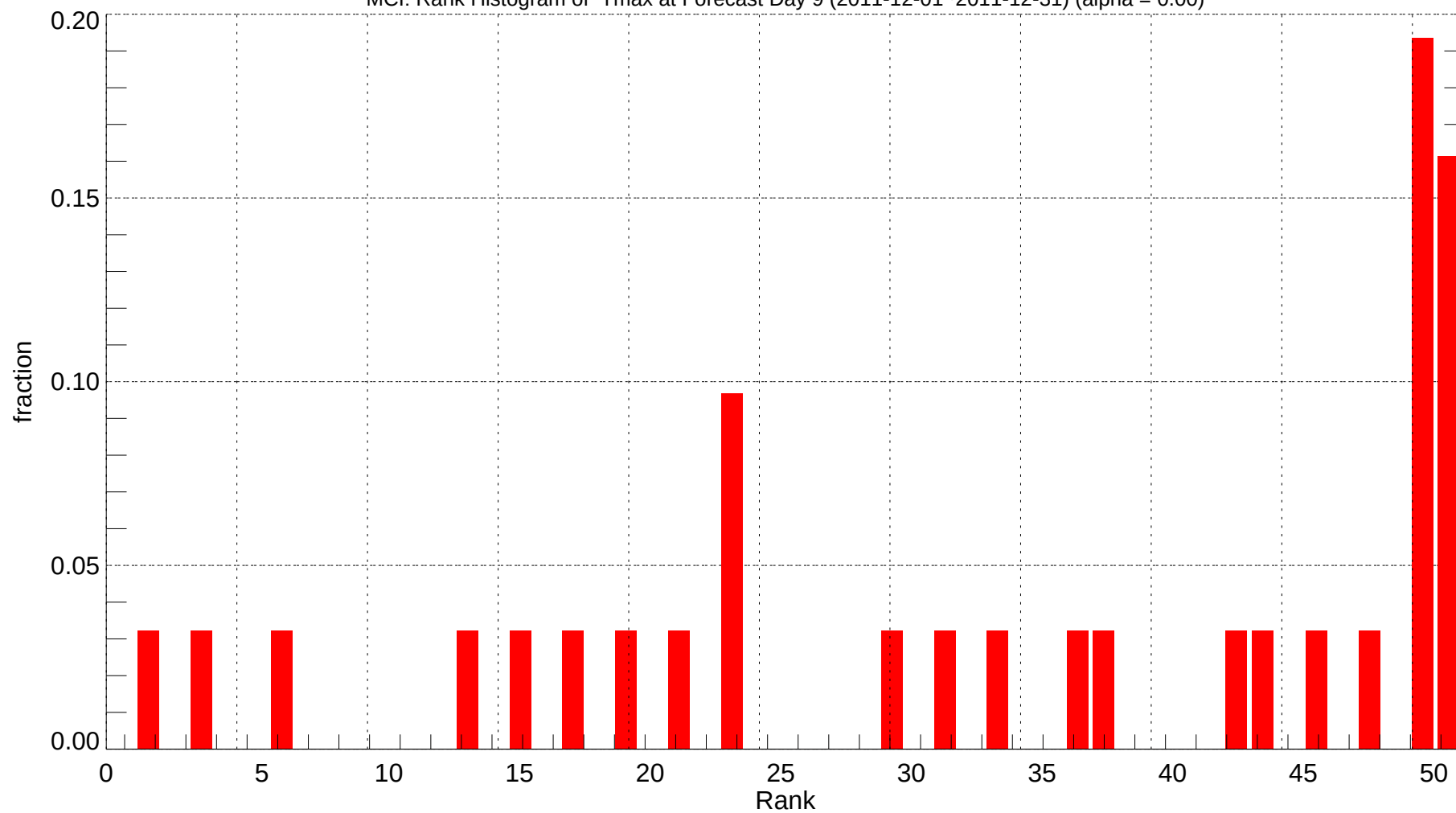
MCI: Rank Histogram of Tmax at Forecast Day 9 (2011-12-01~2011-12-31) (alpha = 0.00)
