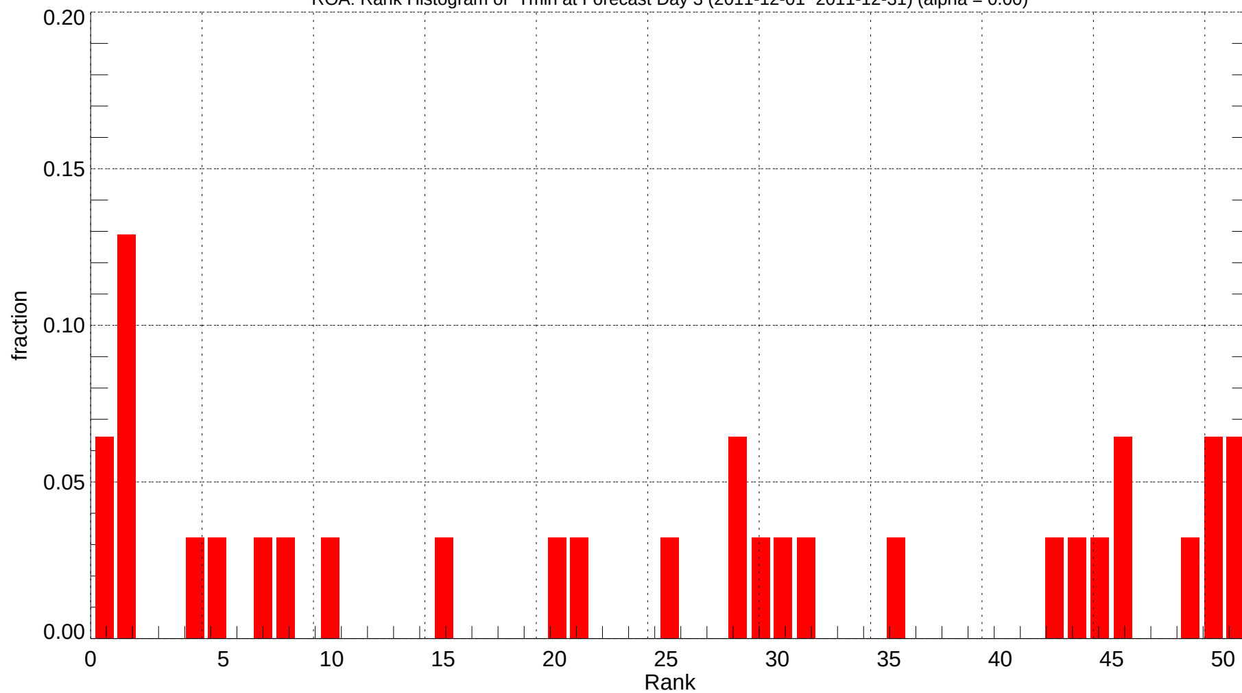
ROA: Rank Histogram of Tmin at Forecast Day 3 (2011-12-01~2011-12-31) (alpha = 0.00)
