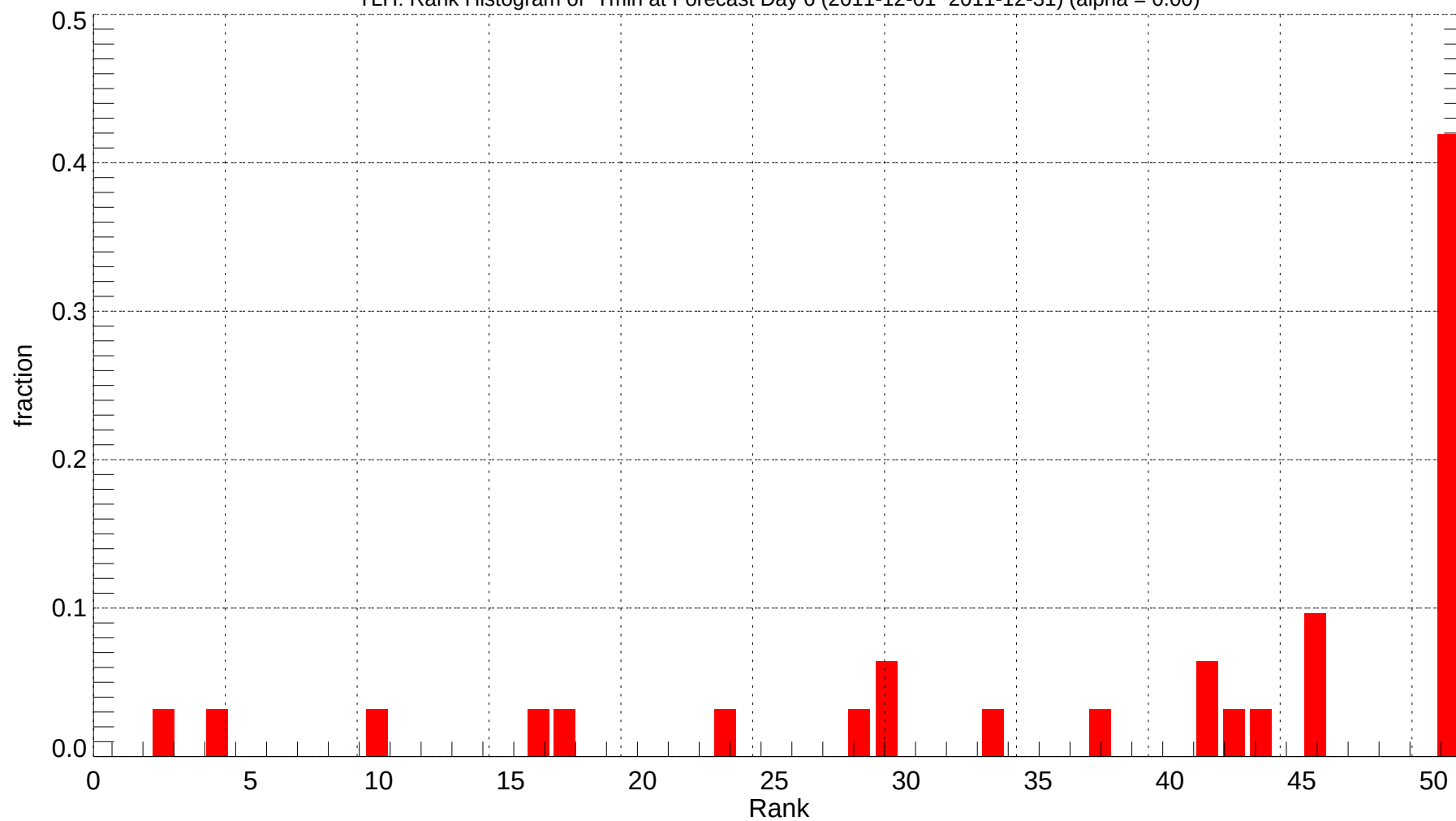
TLH: Rank Histogram of Tmin at Forecast Day 6 (2011-12-01~2011-12-31) (alpha = 0.00)
