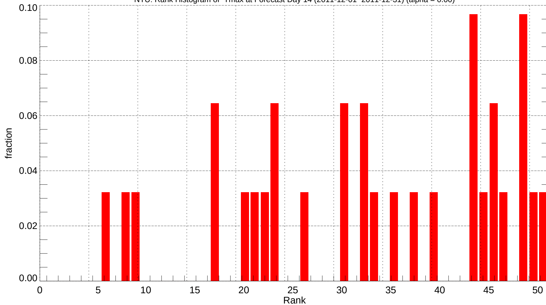
NTU: Rank Histogram of Tmax at Forecast Day 14 (2011-12-01~2011-12-31) (alpha = 0.00)
