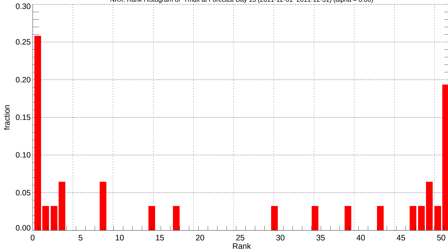
NKX: Rank Histogram of Tmax at Forecast Day 13 (2011-12-01~2011-12-31) (alpha = 0.00)
