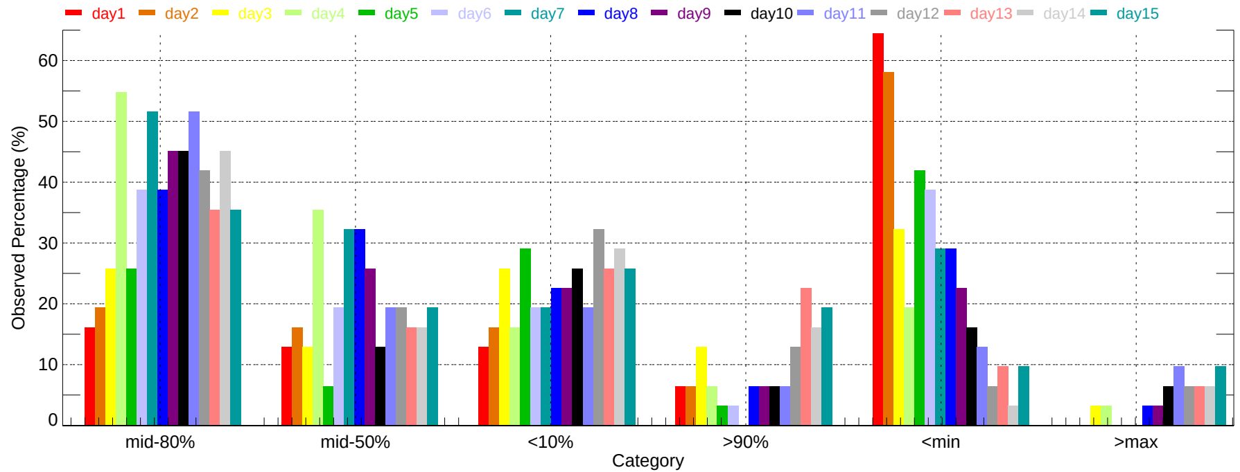
Observed Percentage of Ensembles - RAL: Max Temperature (2011-12-01~2011-12-31)
