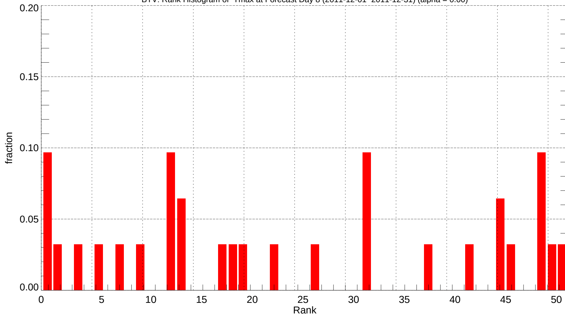
BTV: Rank Histogram of Tmax at Forecast Day 8 (2011-12-01~2011-12-31) (alpha = 0.00)
