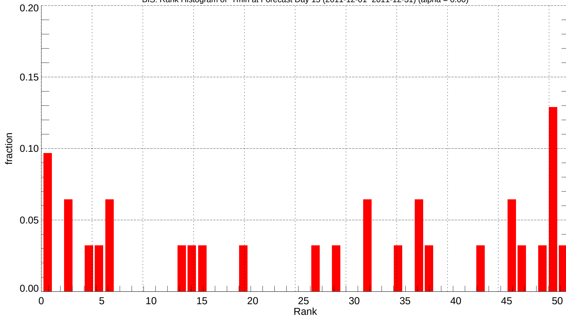
BIS: Rank Histogram of Tmin at Forecast Day 15 (2011-12-01~2011-12-31) (alpha = 0.00)
