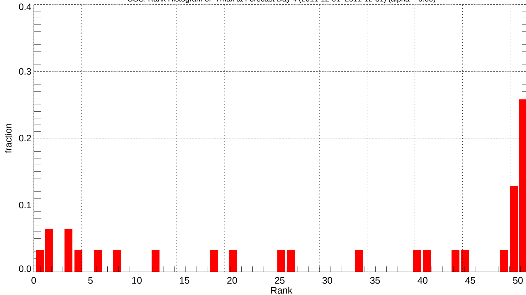
COS: Rank Histogram of Tmax at Forecast Day 4 (2011-12-01~2011-12-31) (alpha = 0.00)
