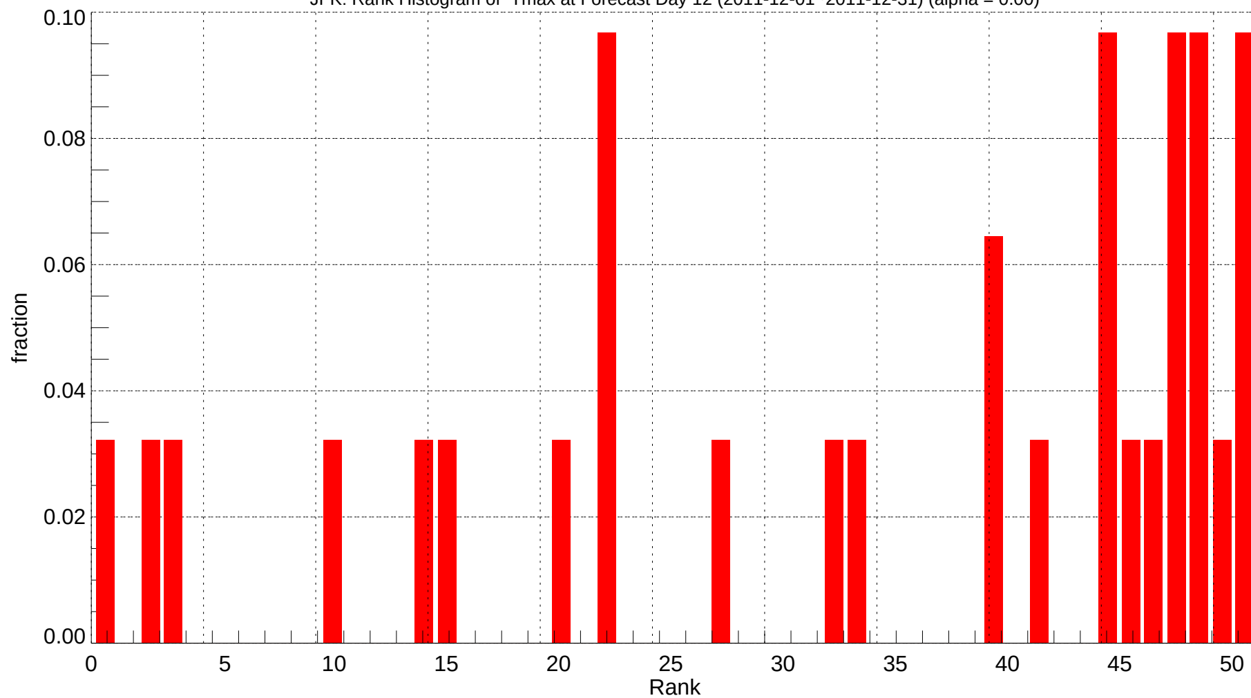
JFK: Rank Histogram of Tmax at Forecast Day 12 (2011-12-01~2011-12-31) (alpha = 0.00)
