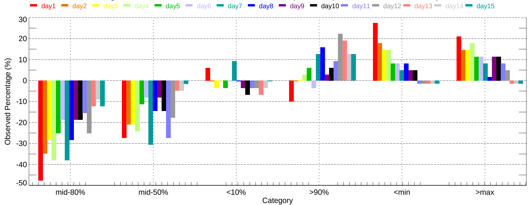
Observed Percentage Deviation of Ensembles - PHL: Max Temperature (2011-12-01~2011-12-31)
