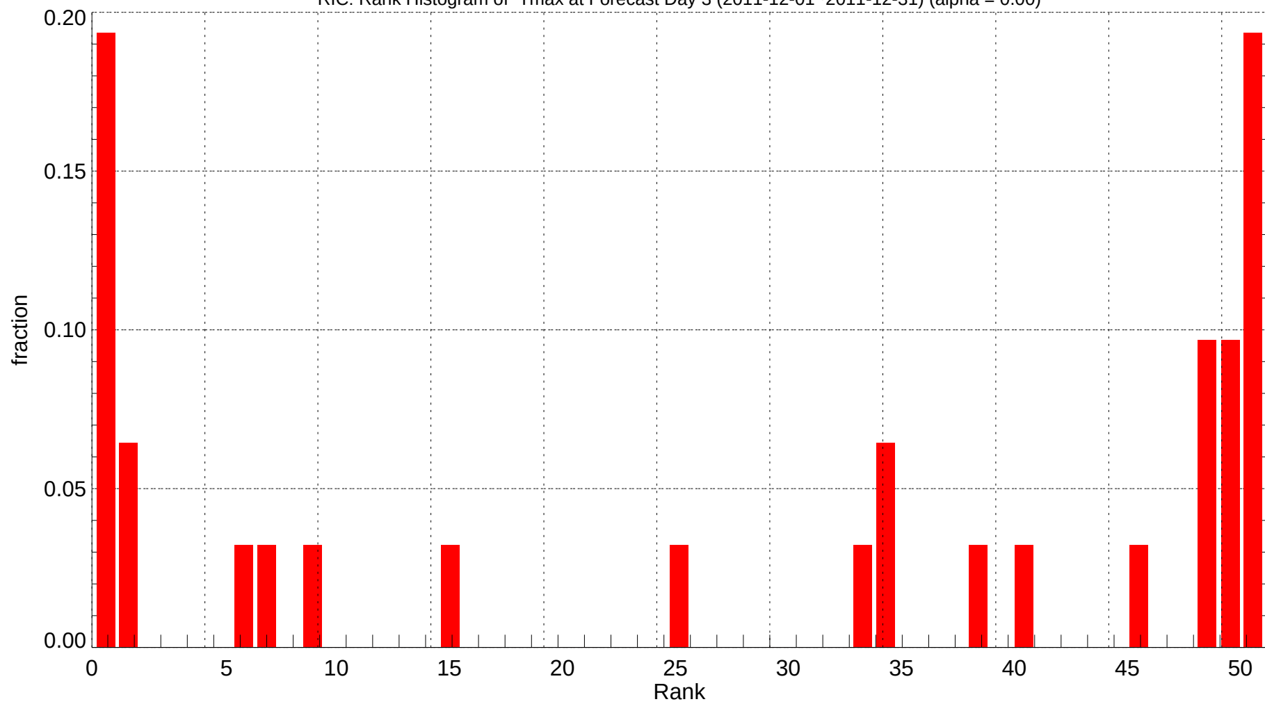
RIC: Rank Histogram of Tmax at Forecast Day 3 (2011-12-01~2011-12-31) (alpha = 0.00)
