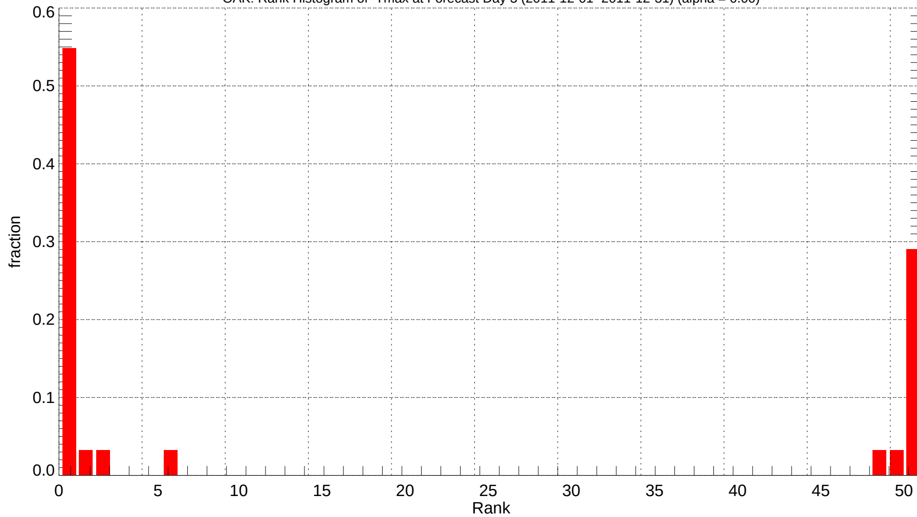
OAK: Rank Histogram of Tmax at Forecast Day 3 (2011-12-01~2011-12-31) (alpha = 0.00)
