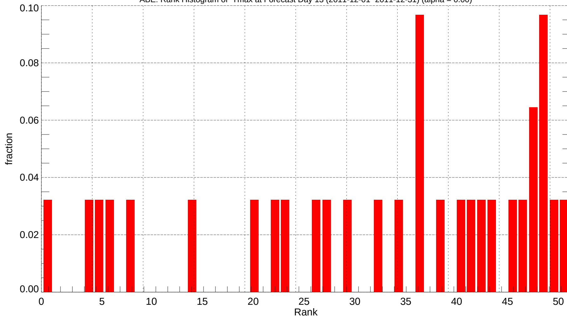
ABE: Rank Histogram of Tmax at Forecast Day 13 (2011-12-01~2011-12-31) (alpha = 0.00)
