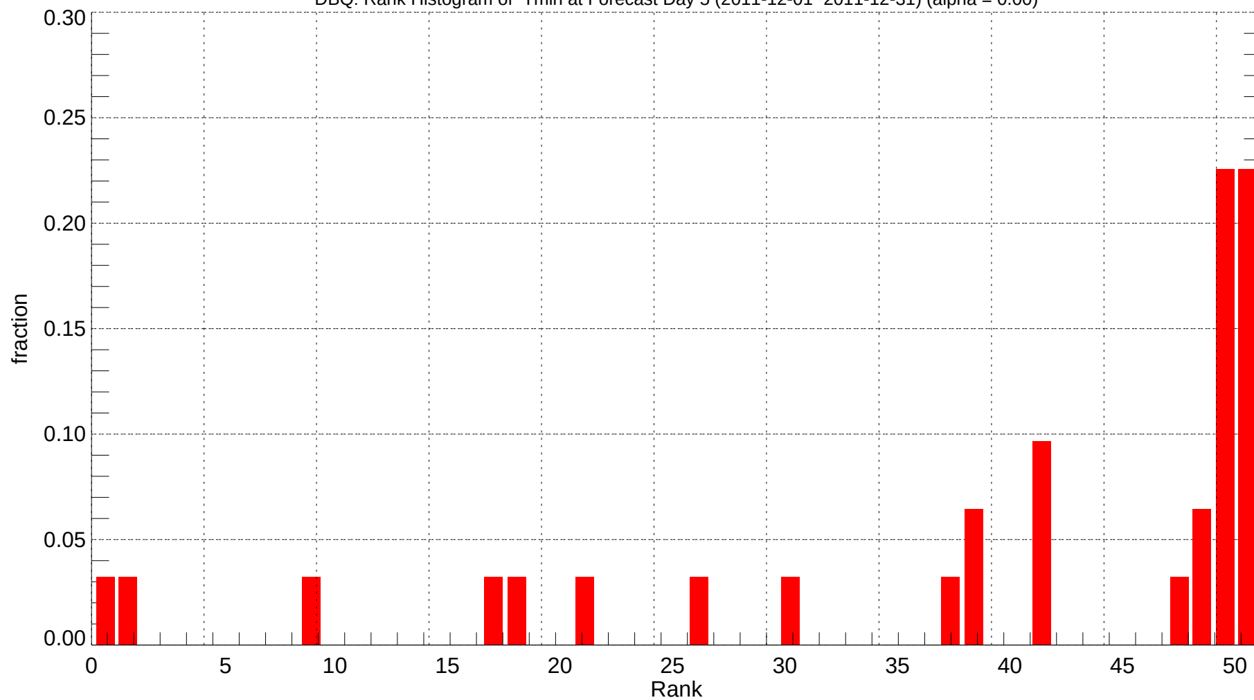
DBQ: Rank Histogram of Tmin at Forecast Day 5 (2011-12-01~2011-12-31) (alpha = 0.00)
