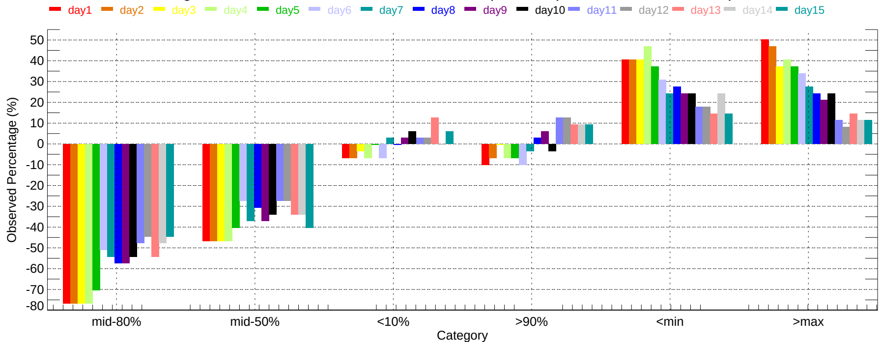
Observed Percentage Deviation of Ensembles - NKX: Max Temperature (2011-12-01~2011-12-31)
