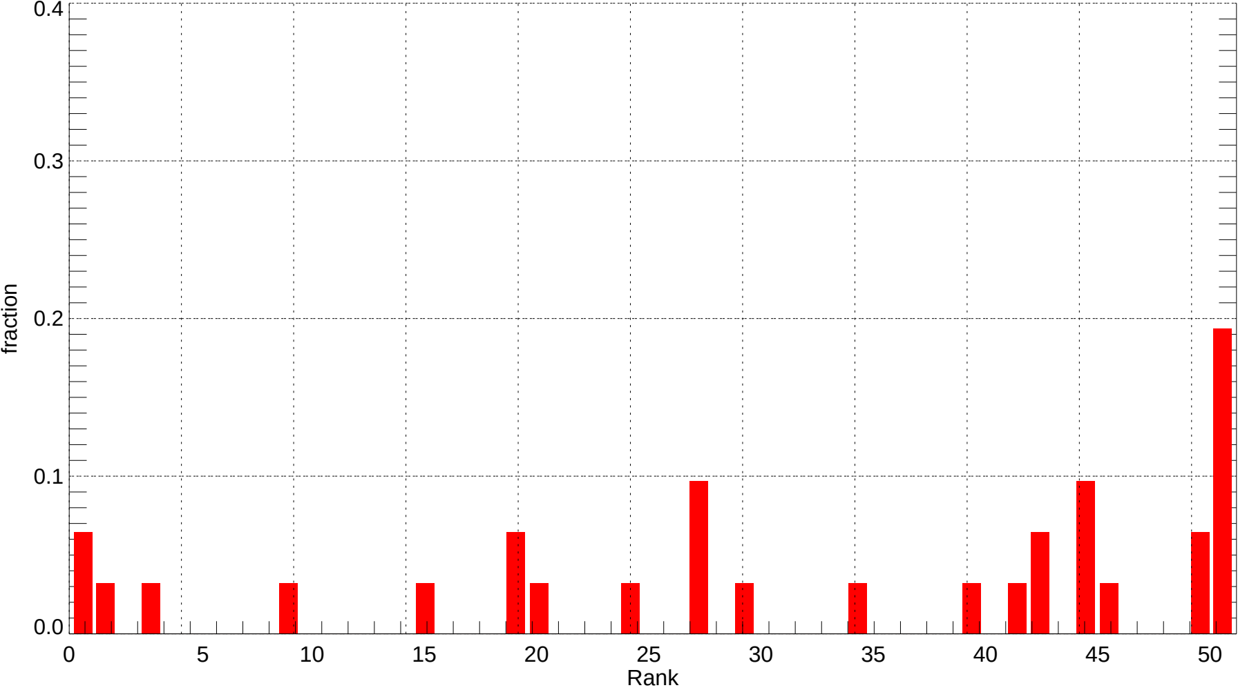
BFL: Rank Histogram of Tmin at Forecast Day 7 (2011-12-01~2011-12-31) (alpha = 0.00)
