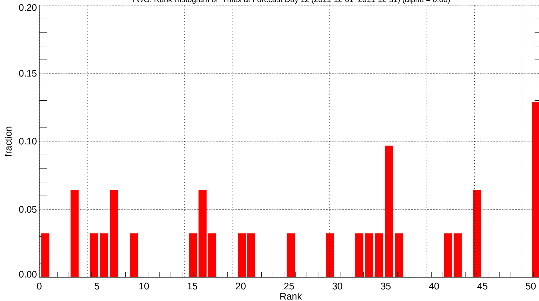
YWG: Rank Histogram of Tmax at Forecast Day 12 (2011-12-01~2011-12-31) (alpha = 0.00)
