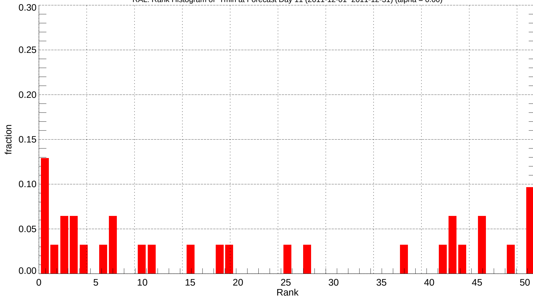
RAL: Rank Histogram of Tmin at Forecast Day 11 (2011-12-01~2011-12-31) (alpha = 0.00)
