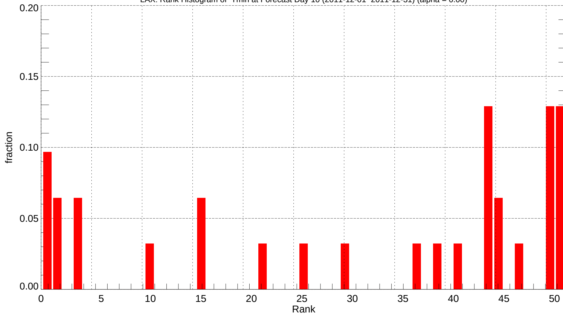
LAX: Rank Histogram of Tmin at Forecast Day 10 (2011-12-01~2011-12-31) (alpha = 0.00)
