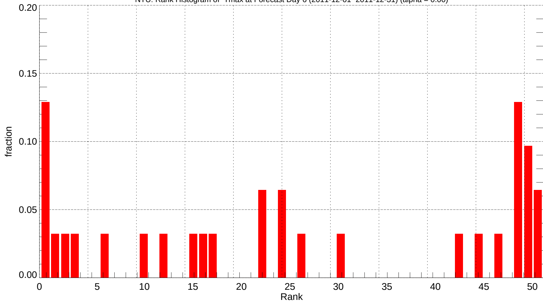
NTU: Rank Histogram of Tmax at Forecast Day 6 (2011-12-01~2011-12-31) (alpha = 0.00)
