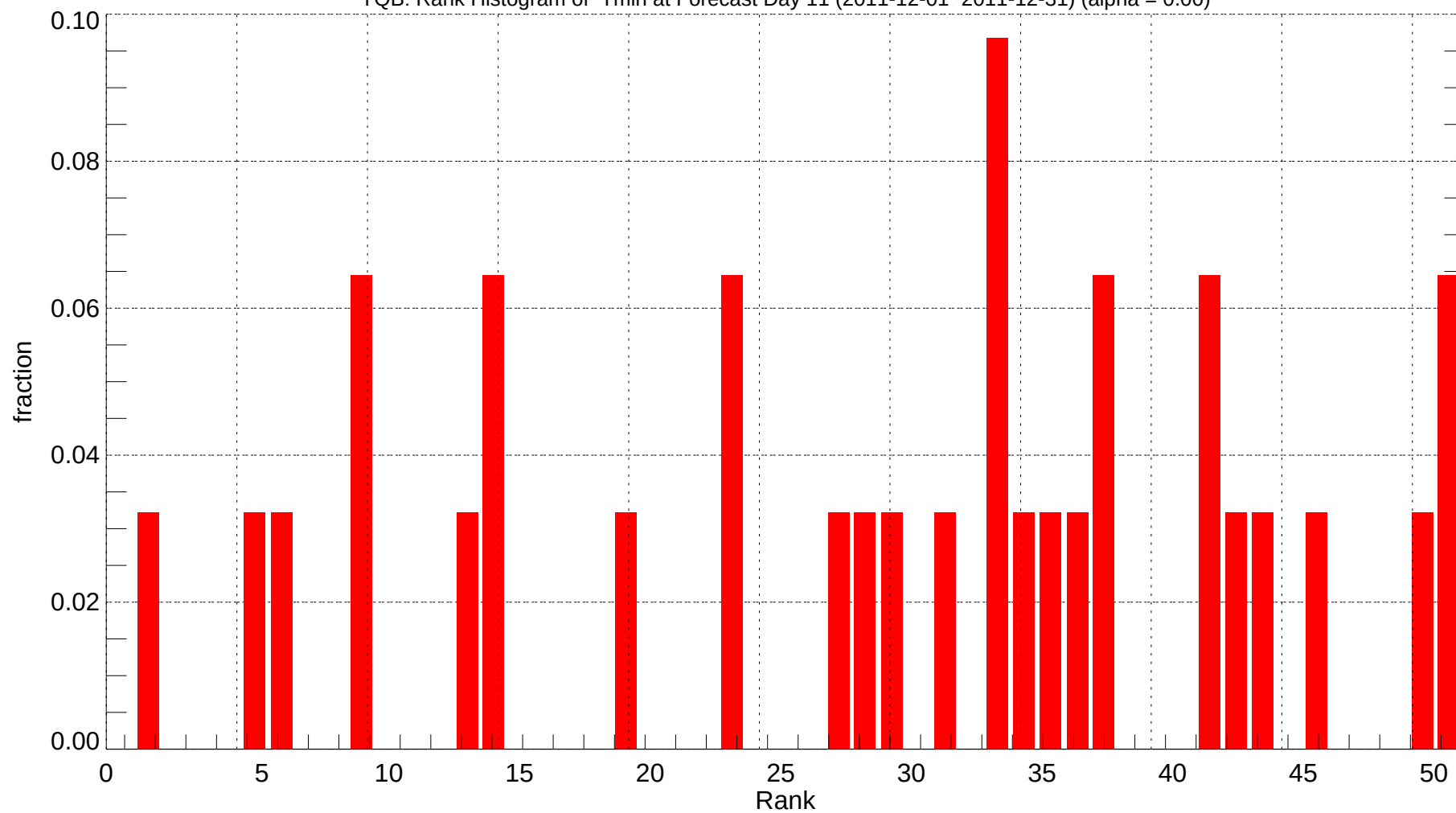
YQB: Rank Histogram of Tmin at Forecast Day 11 (2011-12-01~2011-12-31) (alpha = 0.00)
