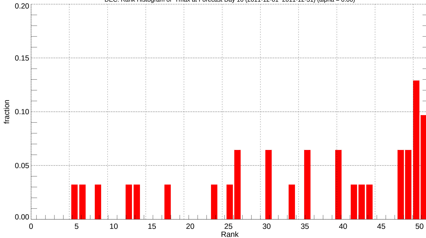
DEC: Rank Histogram of Tmax at Forecast Day 10 (2011-12-01~2011-12-31) (alpha = 0.00)
