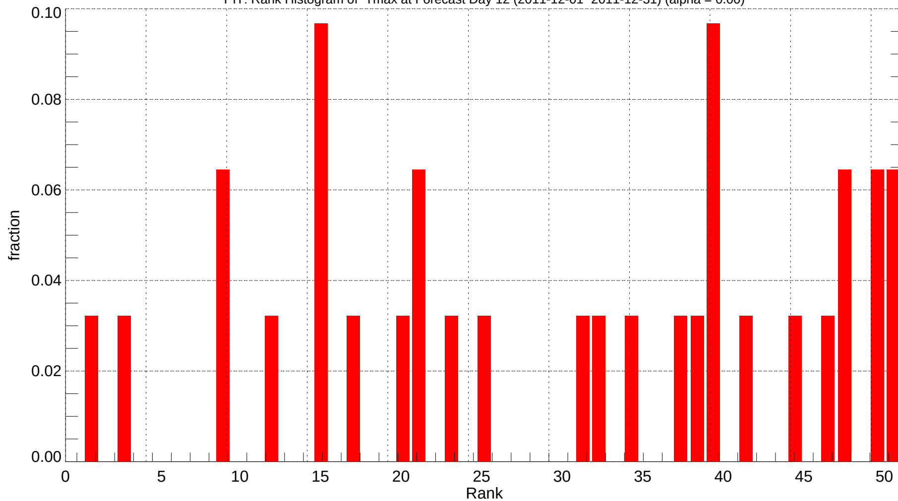
PIT: Rank Histogram of Tmax at Forecast Day 12 (2011-12-01~2011-12-31) (alpha = 0.00)
