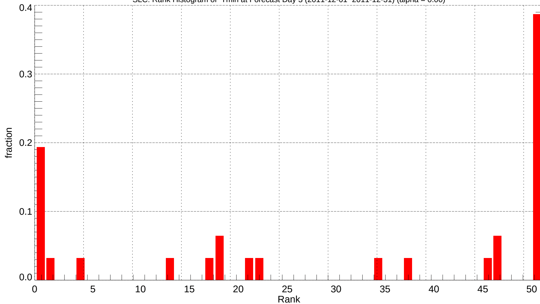
SLC: Rank Histogram of Tmin at Forecast Day 3 (2011-12-01~2011-12-31) (alpha = 0.00)
