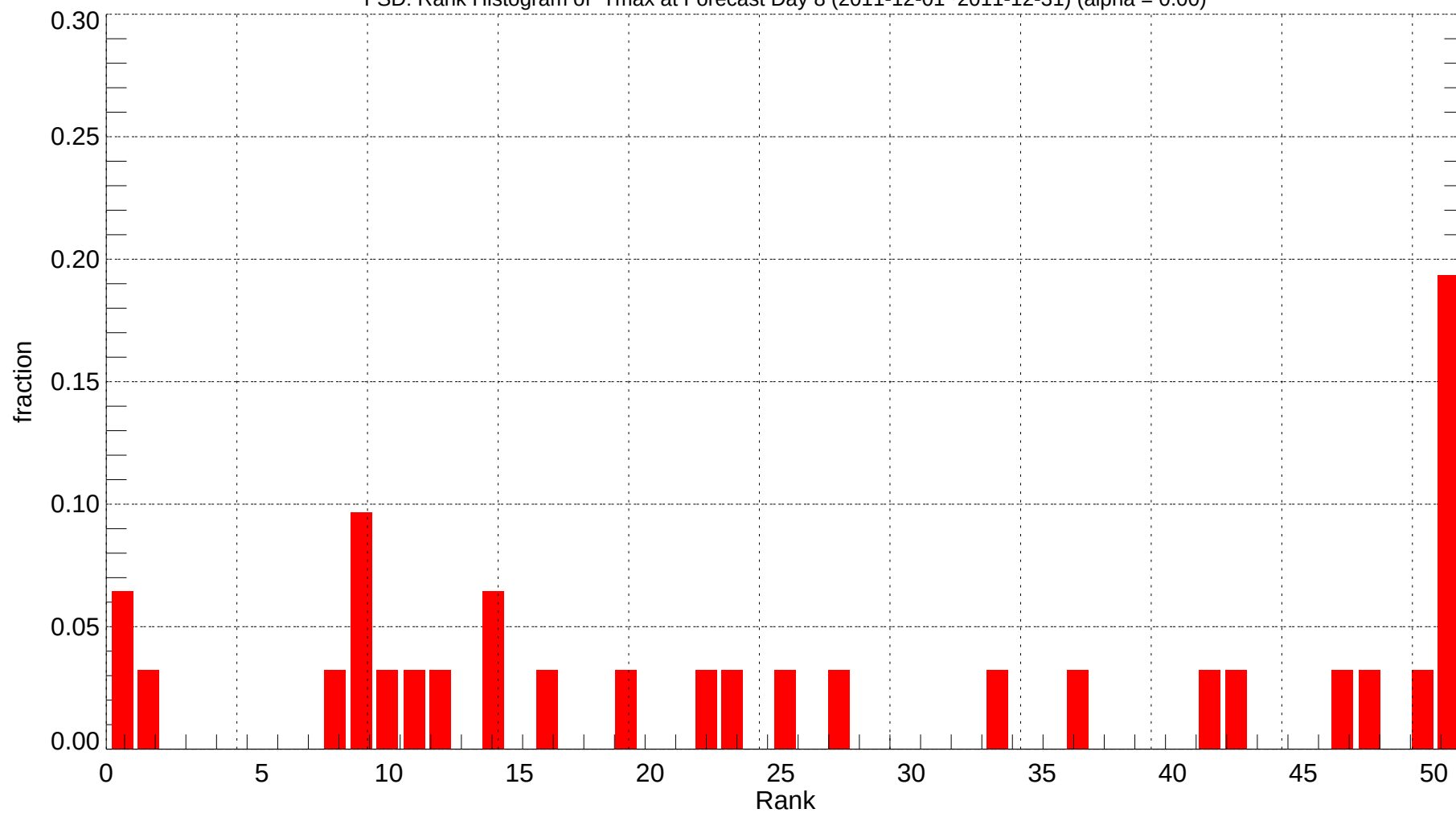
FSD: Rank Histogram of Tmax at Forecast Day 8 (2011-12-01~2011-12-31) (alpha = 0.00)
