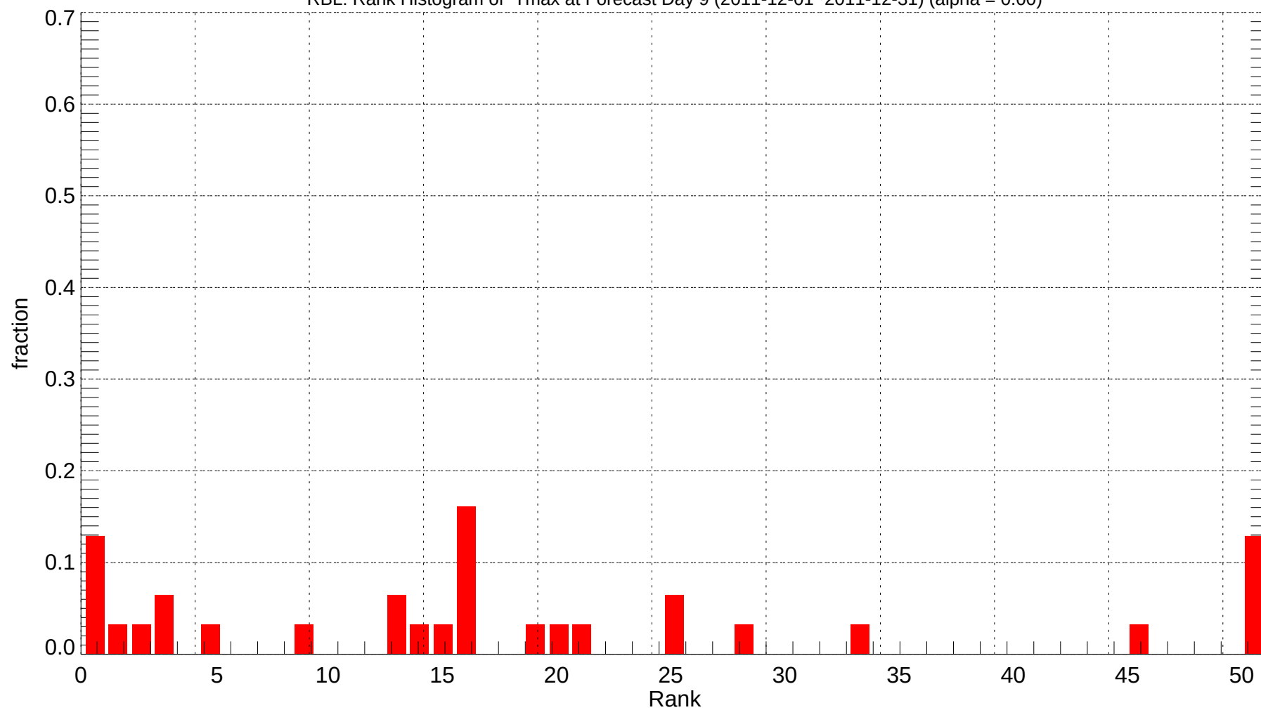
RBL: Rank Histogram of Tmax at Forecast Day 9 (2011-12-01~2011-12-31) (alpha = 0.00)
