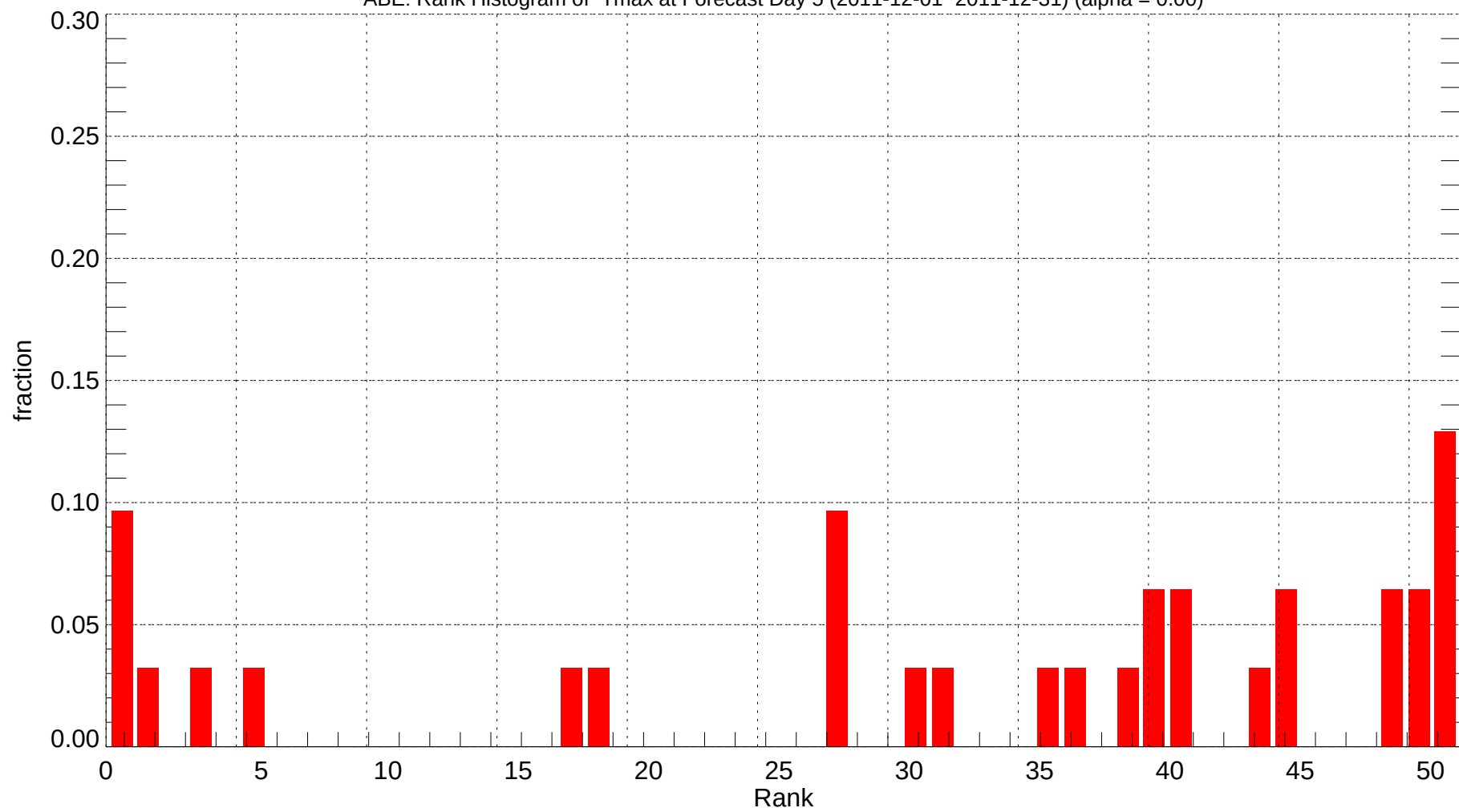
ABE: Rank Histogram of Tmax at Forecast Day 5 (2011-12-01~2011-12-31) (alpha = 0.00)
