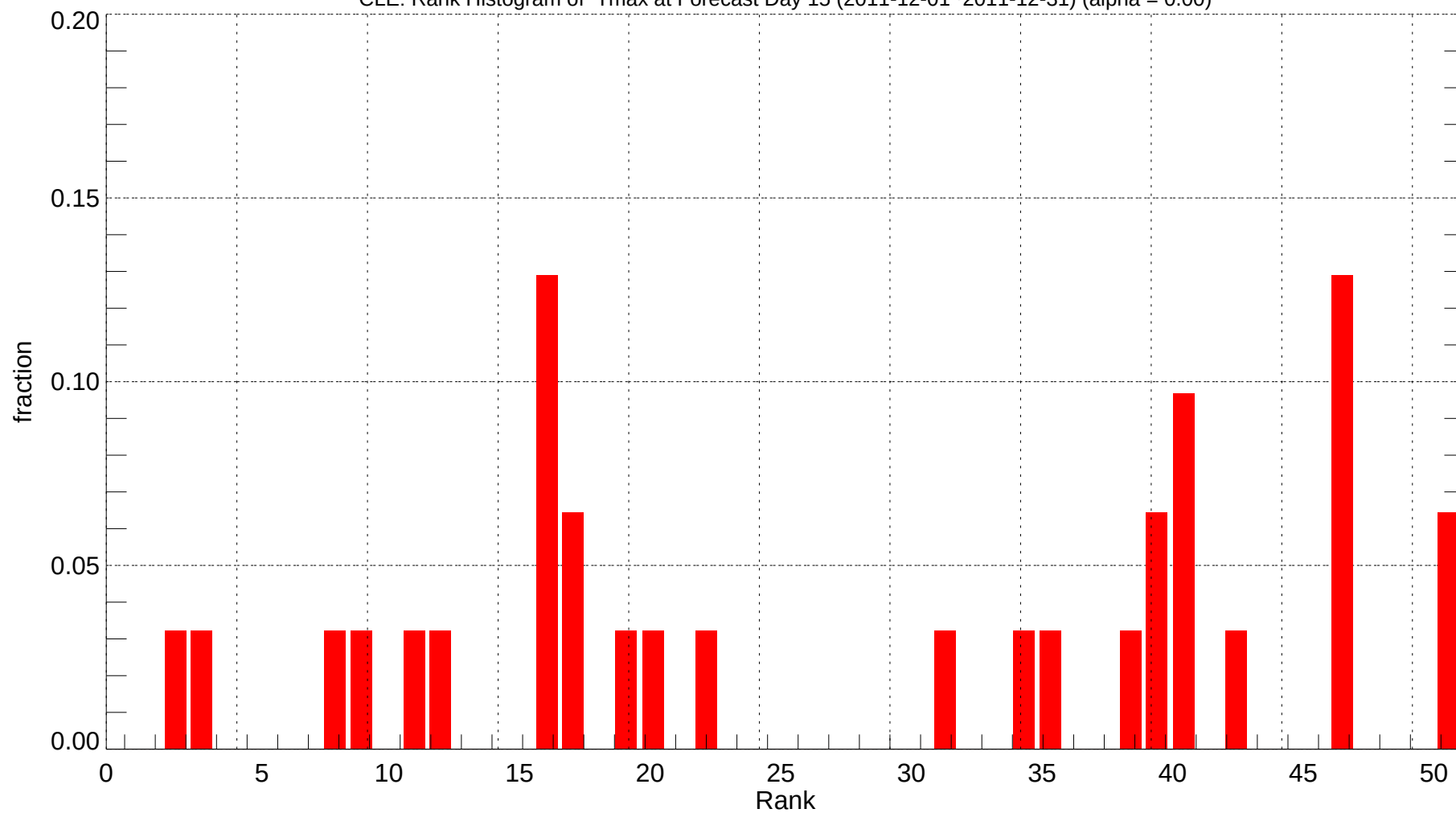
CLE: Rank Histogram of Tmax at Forecast Day 15 (2011-12-01~2011-12-31) (alpha = 0.00)
