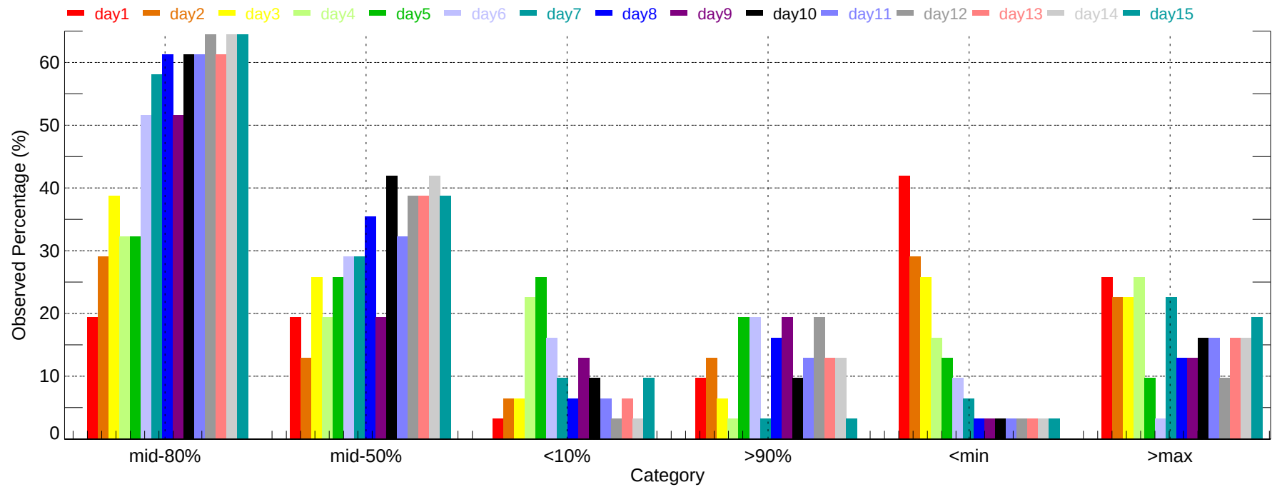
Observed Percentage of Ensembles - FSD: Max Temperature (2011-12-01~2011-12-31)
