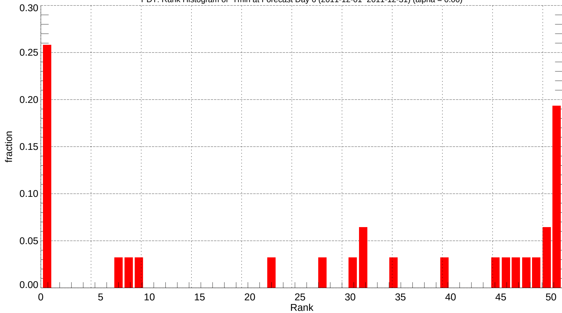
PDT: Rank Histogram of Tmin at Forecast Day 6 (2011-12-01~2011-12-31) (alpha = 0.00)
