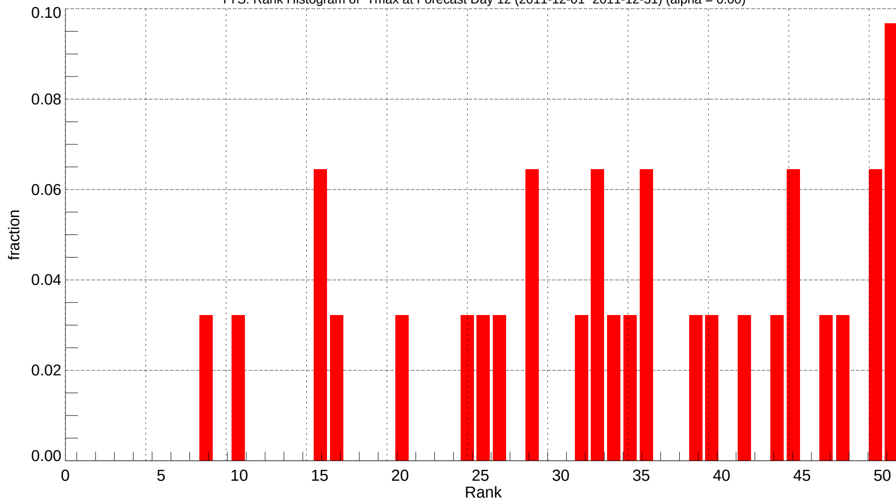
TYS: Rank Histogram of Tmax at Forecast Day 12 (2011-12-01~2011-12-31) (alpha = 0.00)
