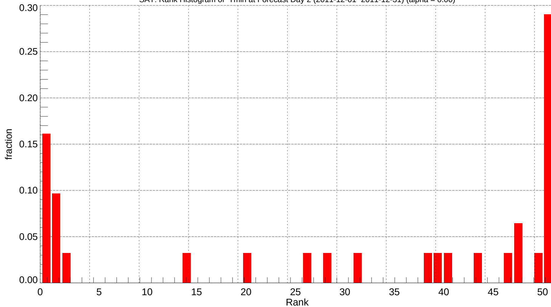
SAT: Rank Histogram of Tmin at Forecast Day 2 (2011-12-01~2011-12-31) (alpha = 0.00)
