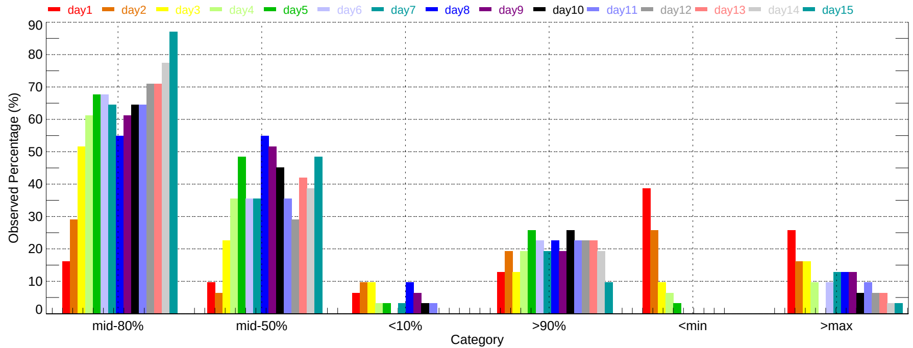
Observed Percentage of Ensembles - AOO: Min Temperature (2011-12-01~2011-12-31)
