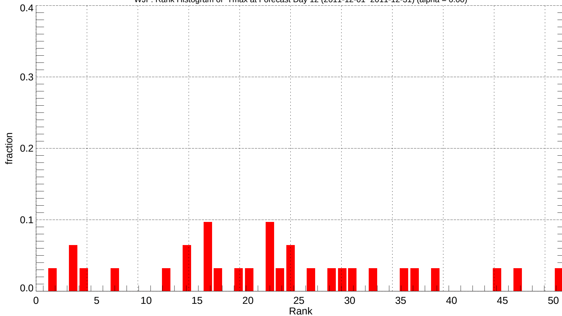
WJF: Rank Histogram of Tmax at Forecast Day 12 (2011-12-01~2011-12-31) (alpha = 0.00)
