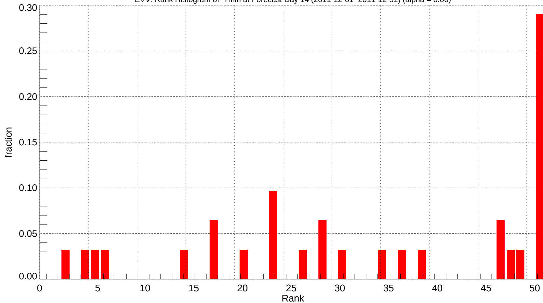
EVV: Rank Histogram of Tmin at Forecast Day 14 (2011-12-01~2011-12-31) (alpha = 0.00)
