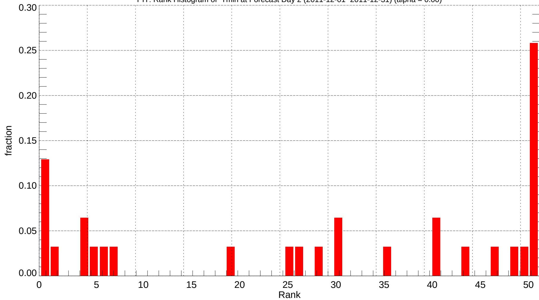
PIT: Rank Histogram of Tmin at Forecast Day 2 (2011-12-01~2011-12-31) (alpha = 0.00)
