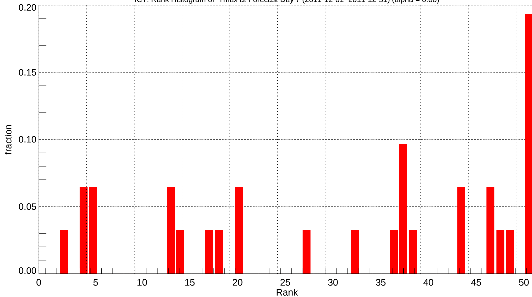
ICT: Rank Histogram of Tmax at Forecast Day 7 (2011-12-01~2011-12-31) (alpha = 0.00)
