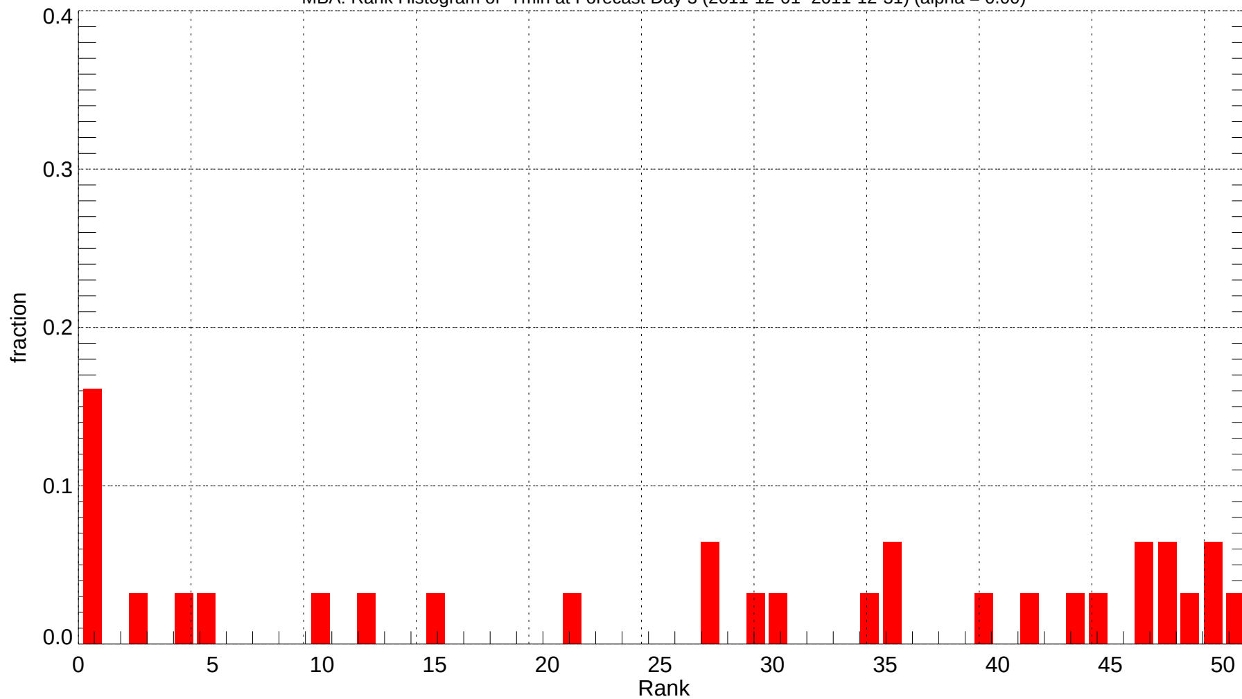
MBA: Rank Histogram of Tmin at Forecast Day 3 (2011-12-01~2011-12-31) (alpha = 0.00)
