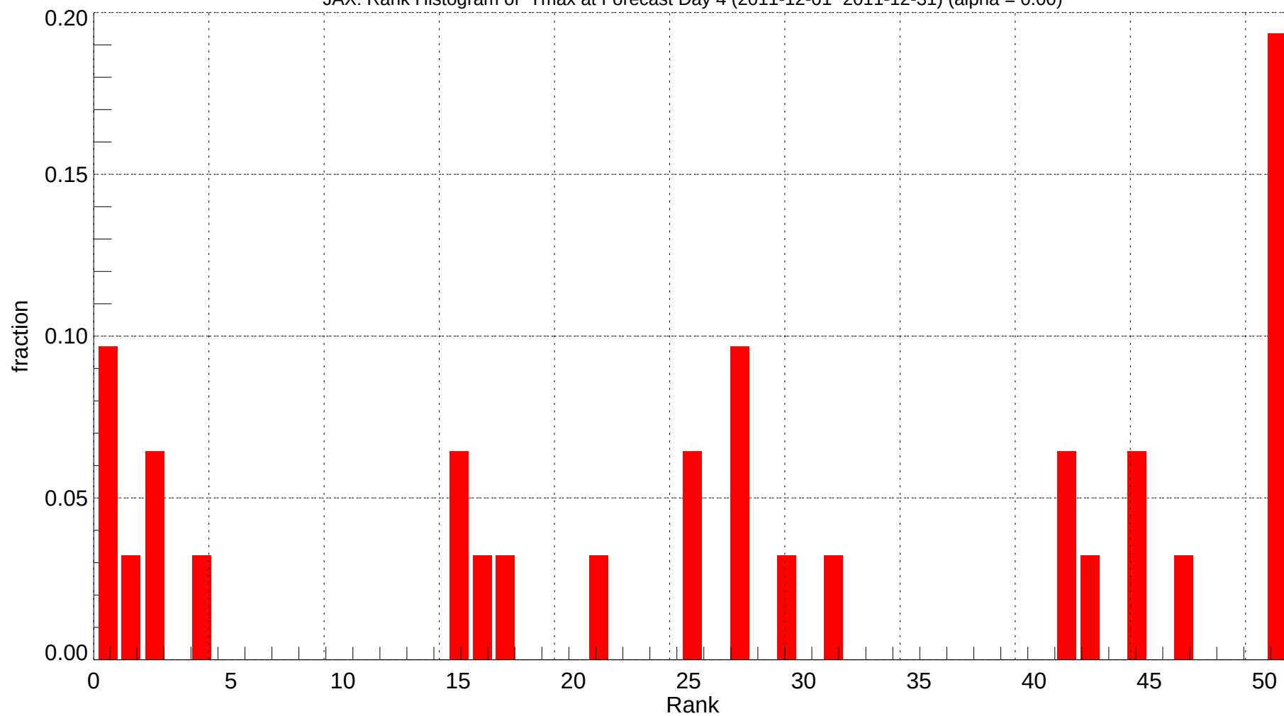
JAX: Rank Histogram of Tmax at Forecast Day 4 (2011-12-01~2011-12-31) (alpha = 0.00)
