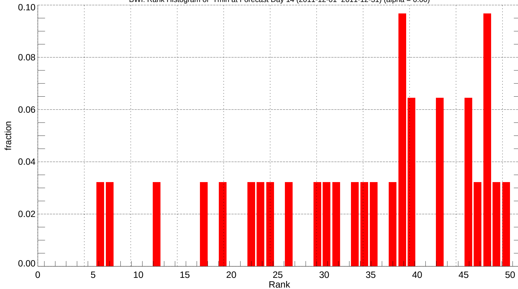
BWI: Rank Histogram of Tmin at Forecast Day 14 (2011-12-01~2011-12-31) (alpha = 0.00)
