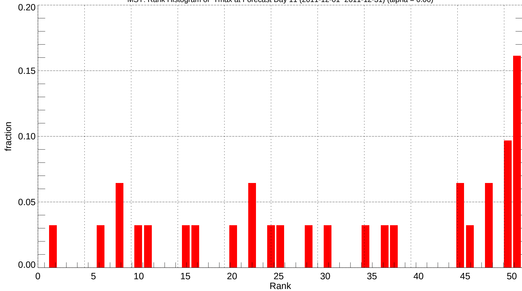
MSY: Rank Histogram of Tmax at Forecast Day 11 (2011-12-01~2011-12-31) (alpha = 0.00)
