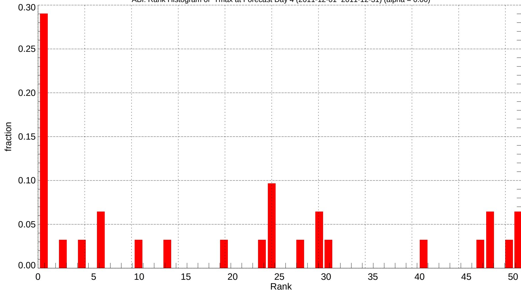
ABI: Rank Histogram of Tmax at Forecast Day 4 (2011-12-01~2011-12-31) (alpha = 0.00)
