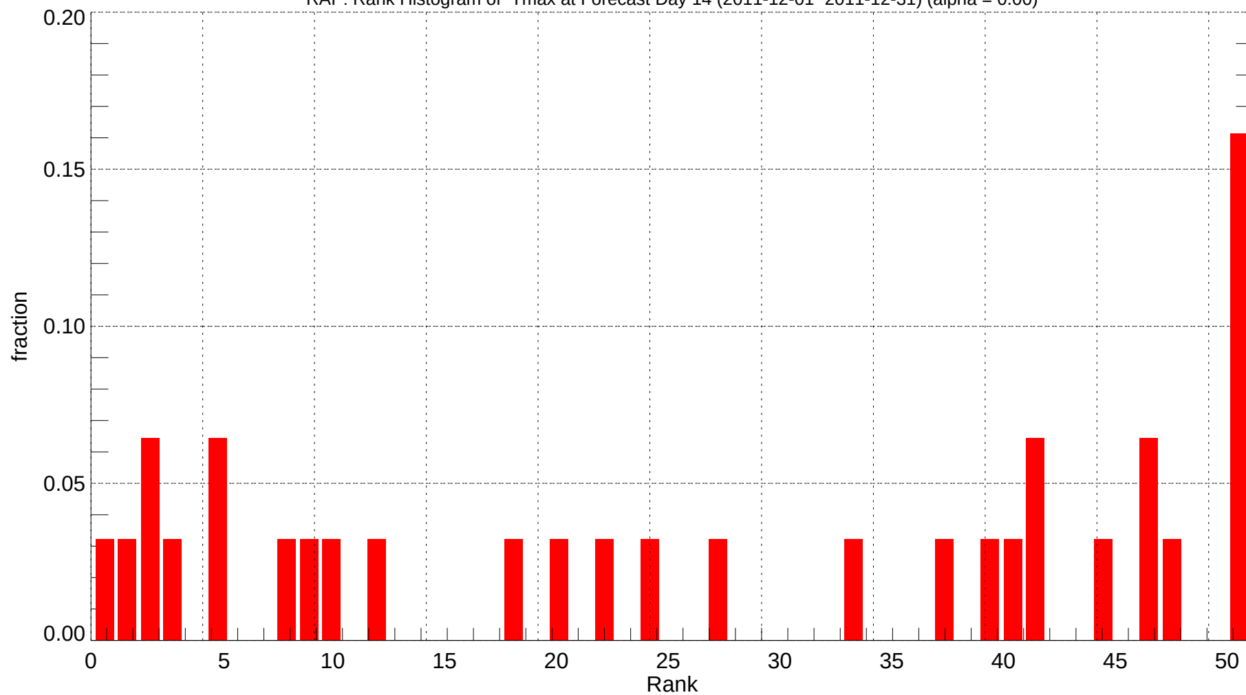
RAP: Rank Histogram of Tmax at Forecast Day 14 (2011-12-01~2011-12-31) (alpha = 0.00)
