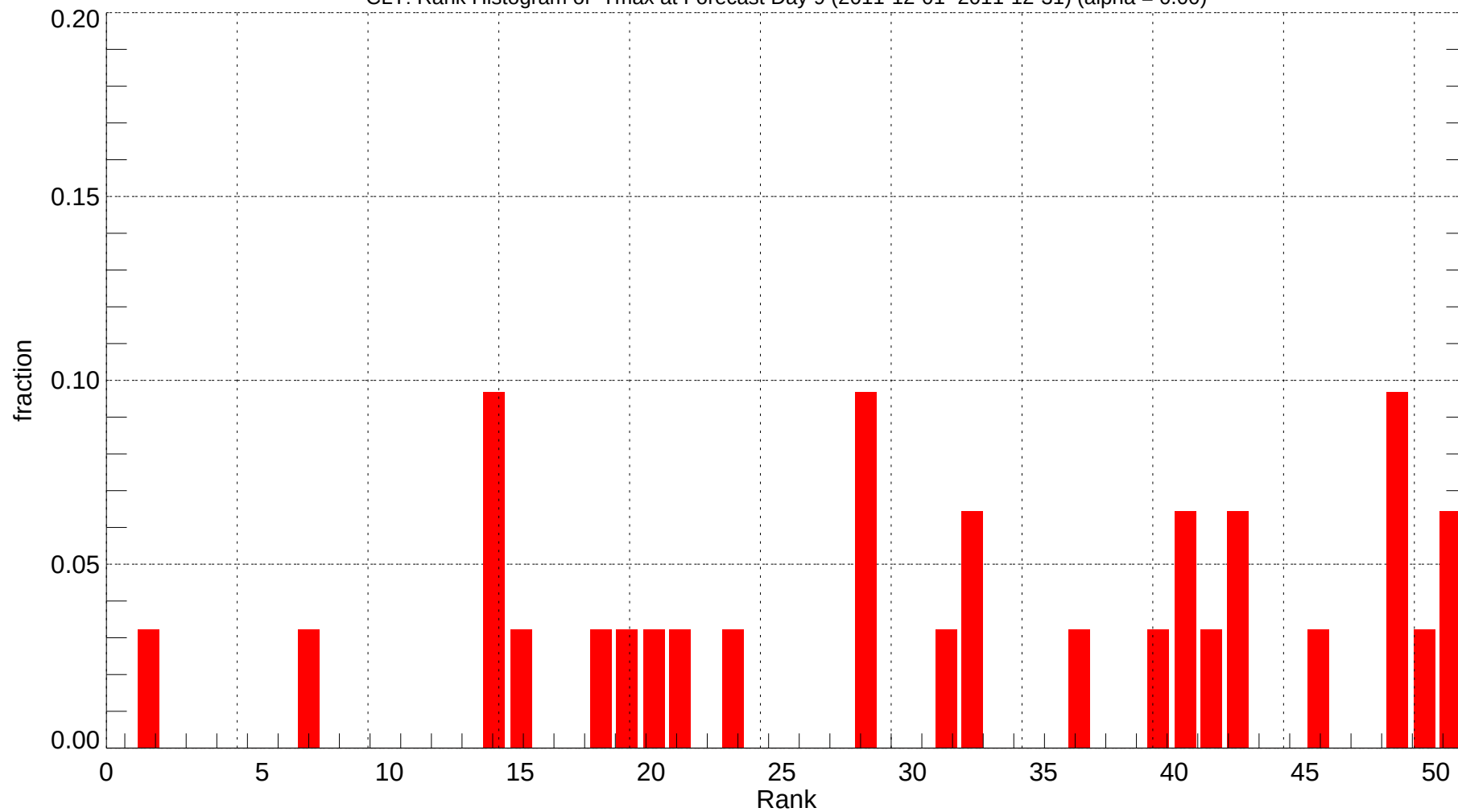
CLT: Rank Histogram of Tmax at Forecast Day 9 (2011-12-01~2011-12-31) (alpha = 0.00)
