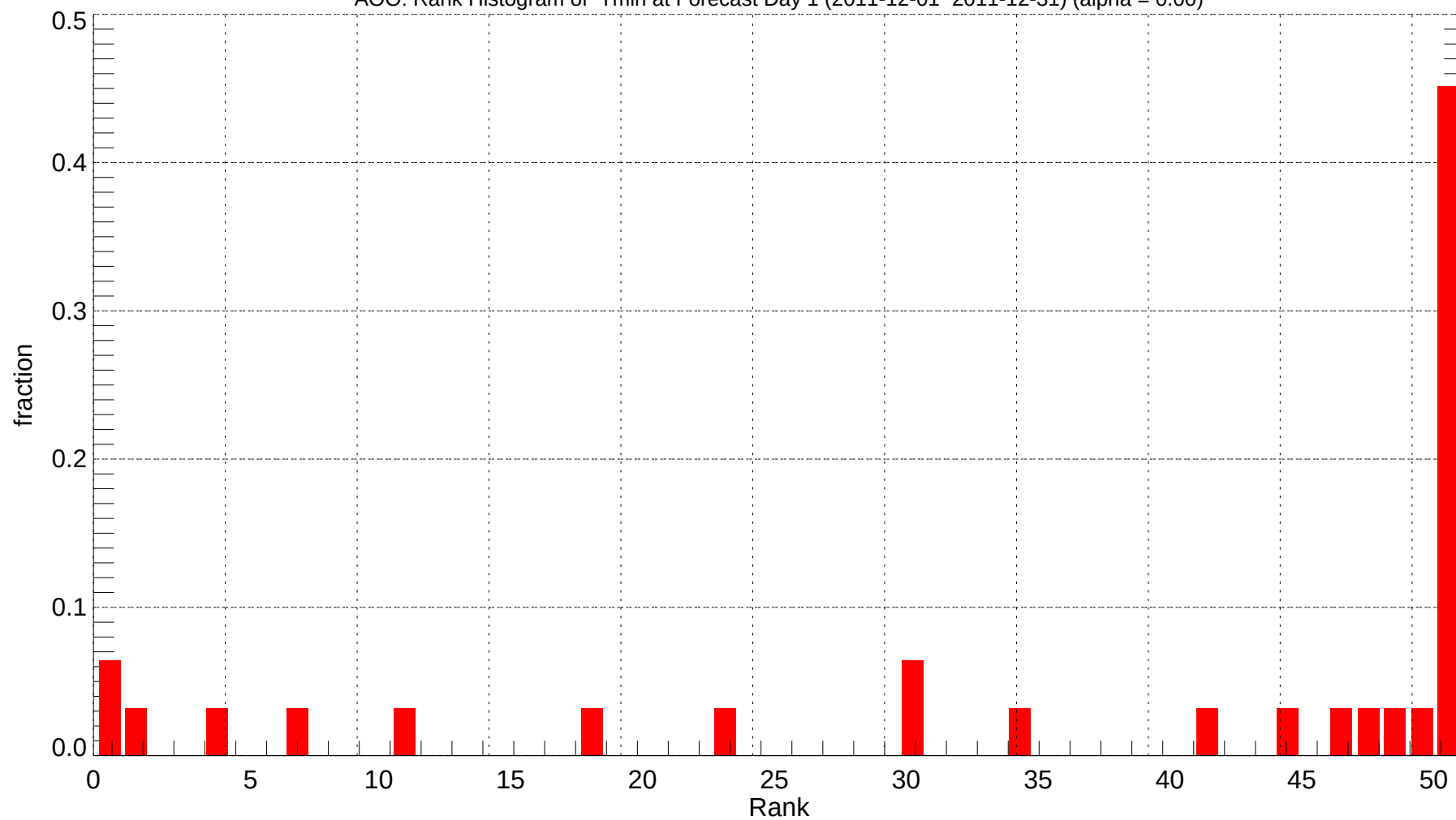
AOO: Rank Histogram of Tmin at Forecast Day 1 (2011-12-01~2011-12-31) (alpha = 0.00)
