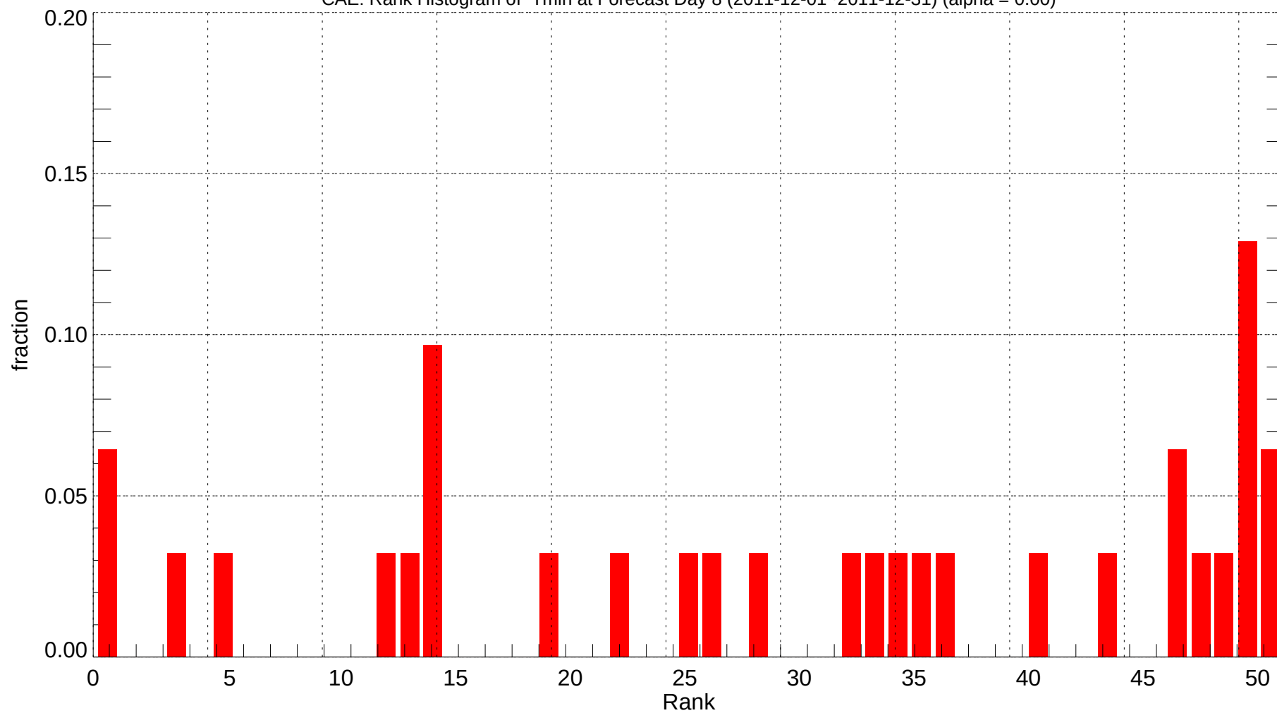
CAE: Rank Histogram of Tmin at Forecast Day 8 (2011-12-01~2011-12-31) (alpha = 0.00)
