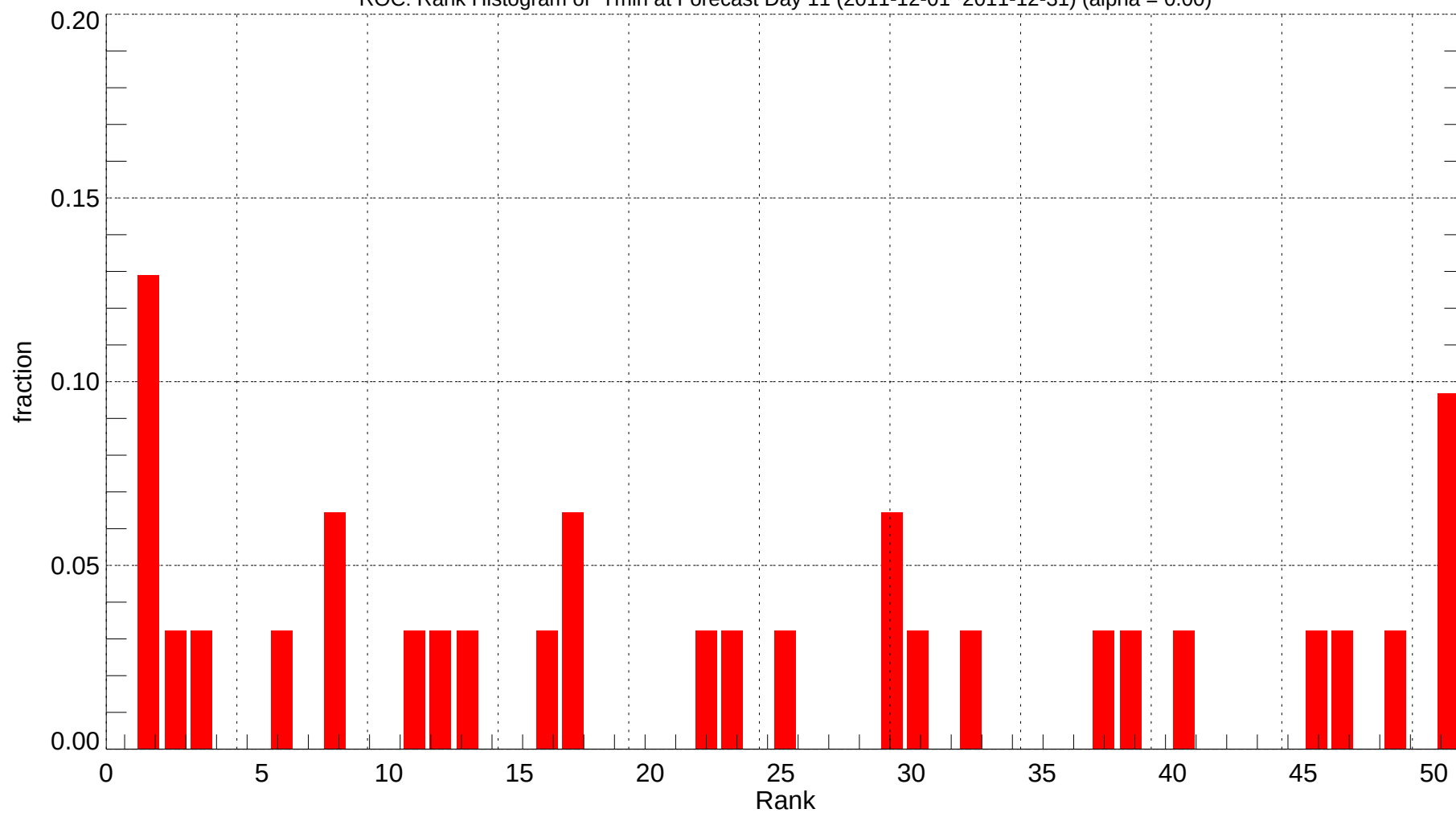
ROC: Rank Histogram of Tmin at Forecast Day 11 (2011-12-01~2011-12-31) (alpha = 0.00)
