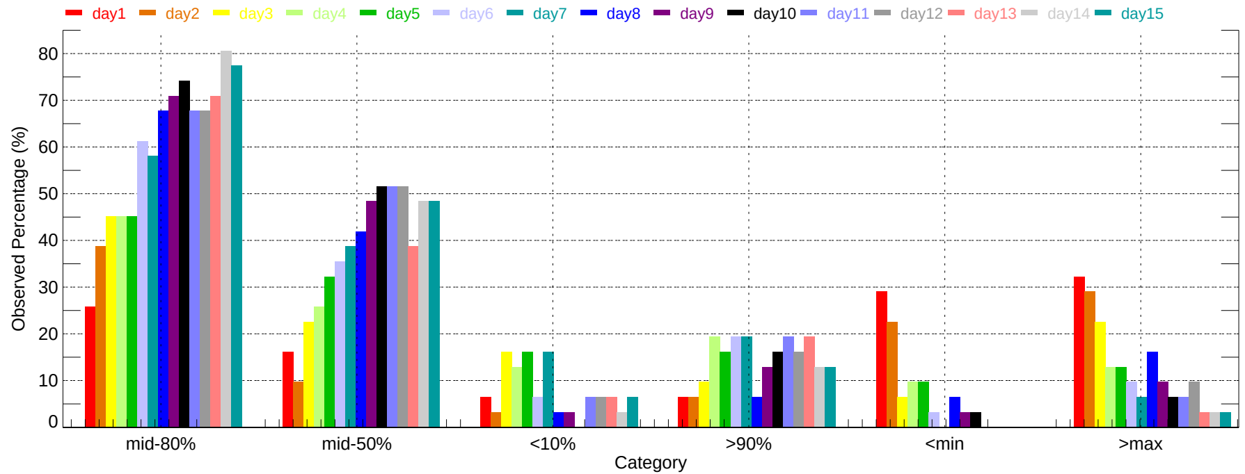
Observed Percentage of Ensembles - RIC: Min Temperature (2011-12-01~2011-12-31)
