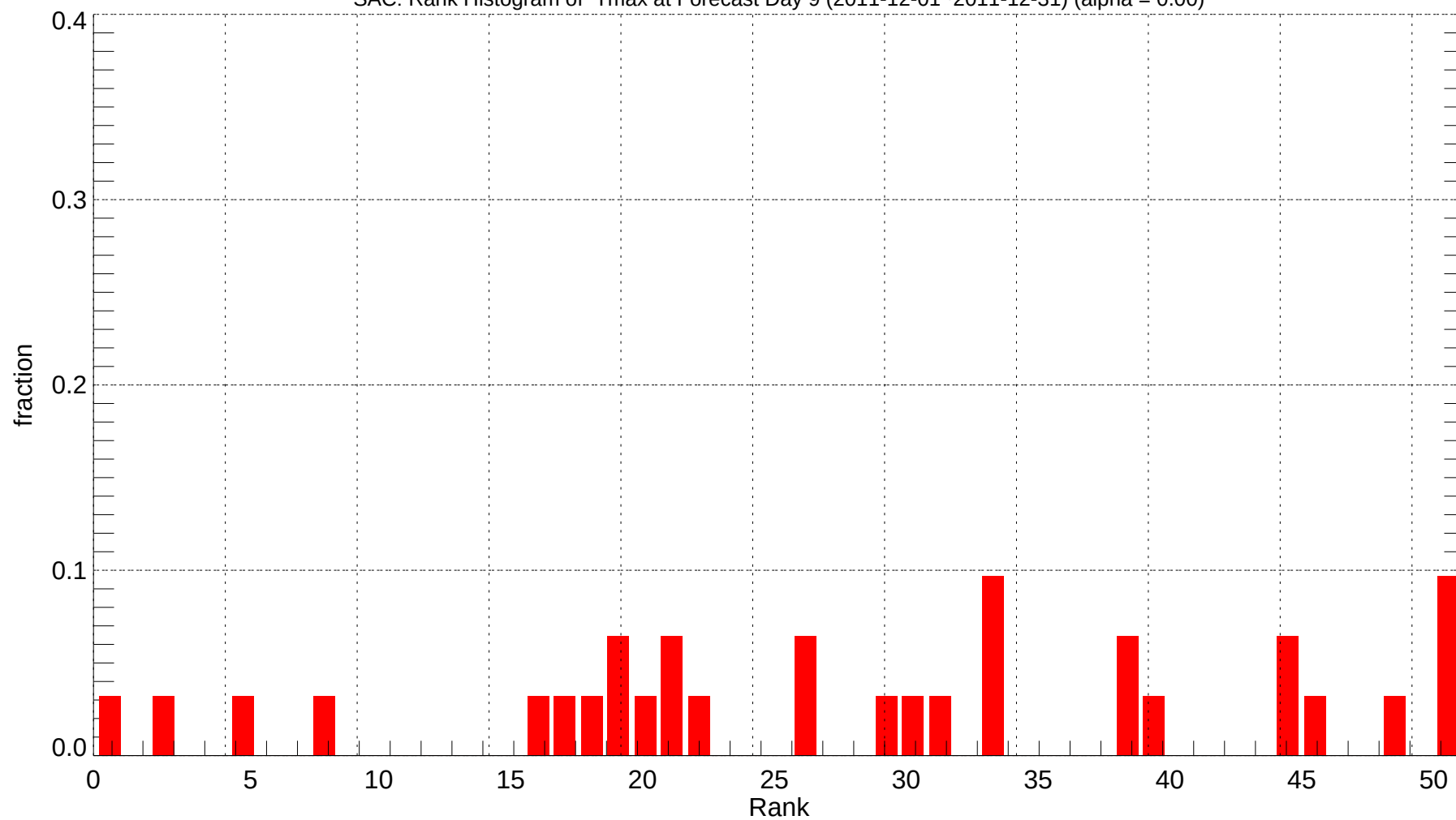
SAC: Rank Histogram of Tmax at Forecast Day 9 (2011-12-01~2011-12-31) (alpha = 0.00)
