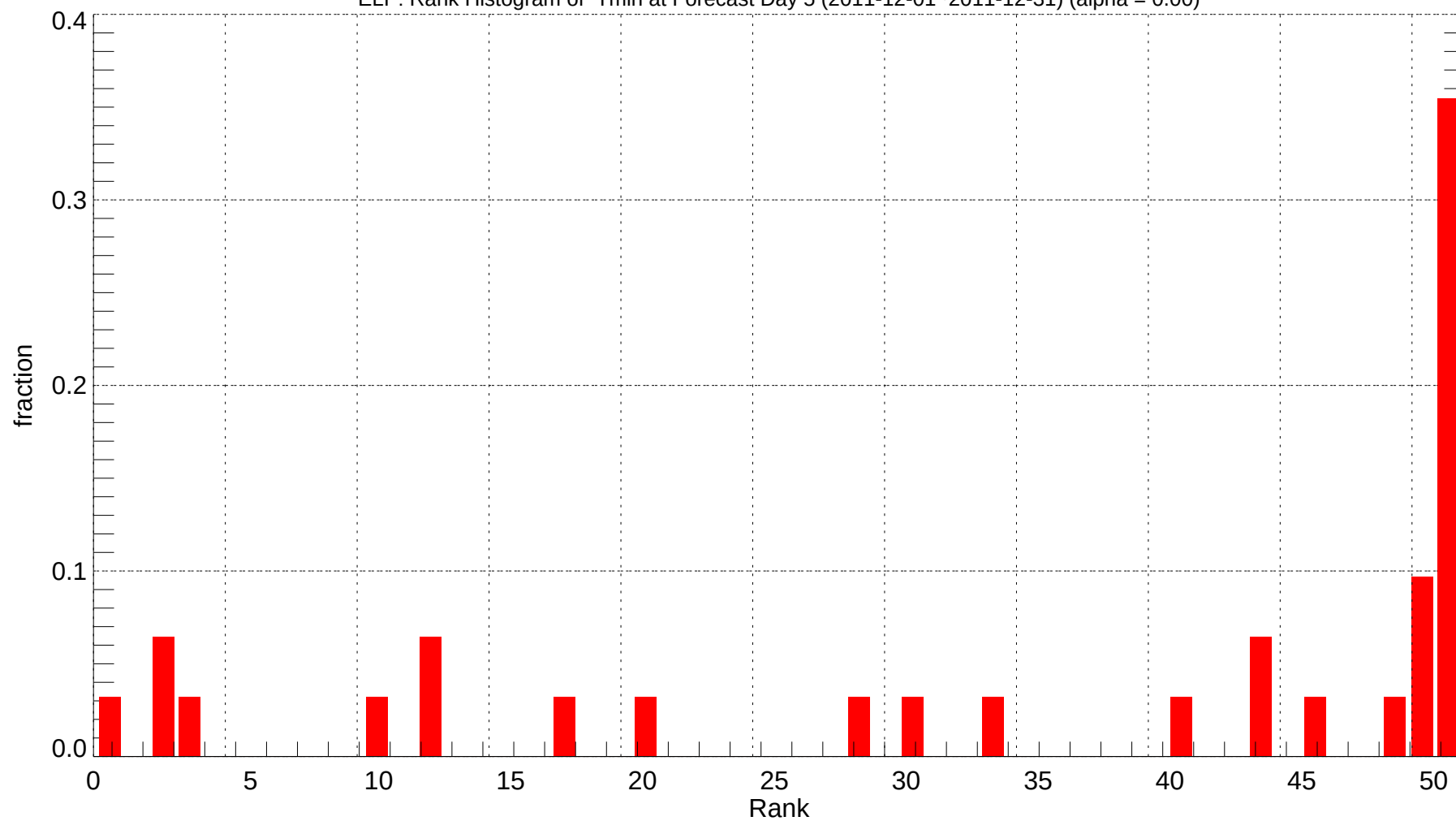
ELP: Rank Histogram of Tmin at Forecast Day 5 (2011-12-01~2011-12-31) (alpha = 0.00)
