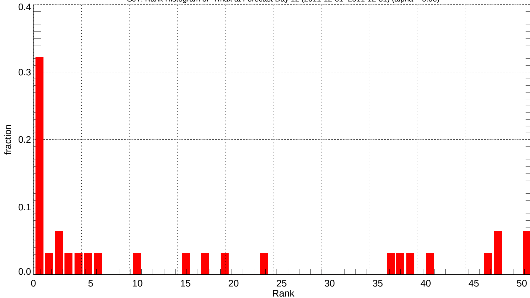
SJT: Rank Histogram of Tmax at Forecast Day 12 (2011-12-01~2011-12-31) (alpha = 0.00)
