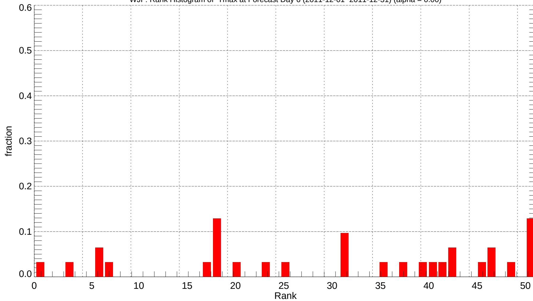
WJF: Rank Histogram of Tmax at Forecast Day 6 (2011-12-01~2011-12-31) (alpha = 0.00)
