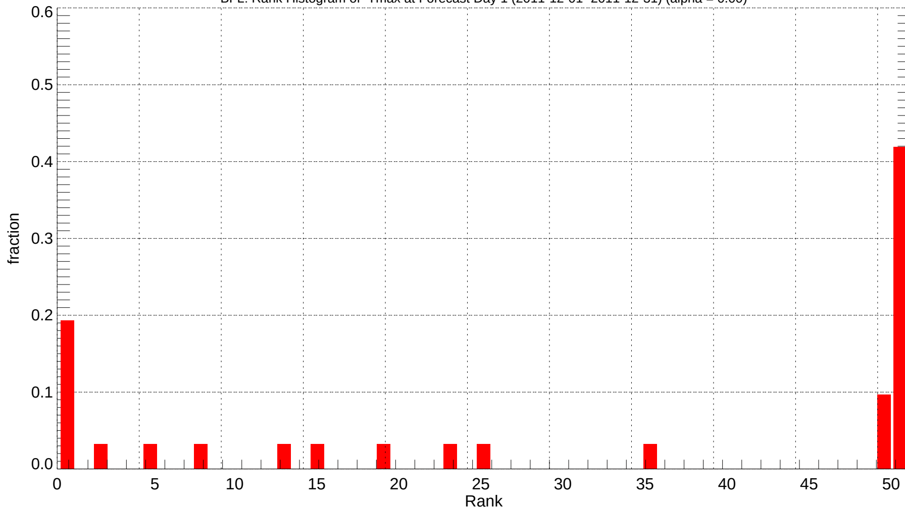
BFL: Rank Histogram of Tmax at Forecast Day 1 (2011-12-01~2011-12-31) (alpha = 0.00)
