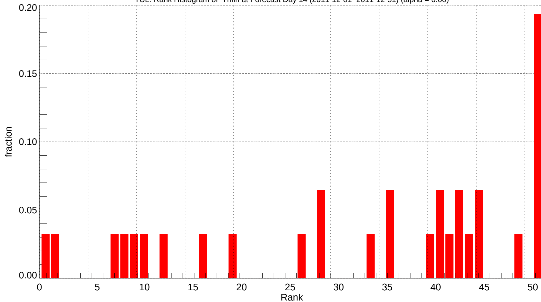
TUL: Rank Histogram of Tmin at Forecast Day 14 (2011-12-01~2011-12-31) (alpha = 0.00)
