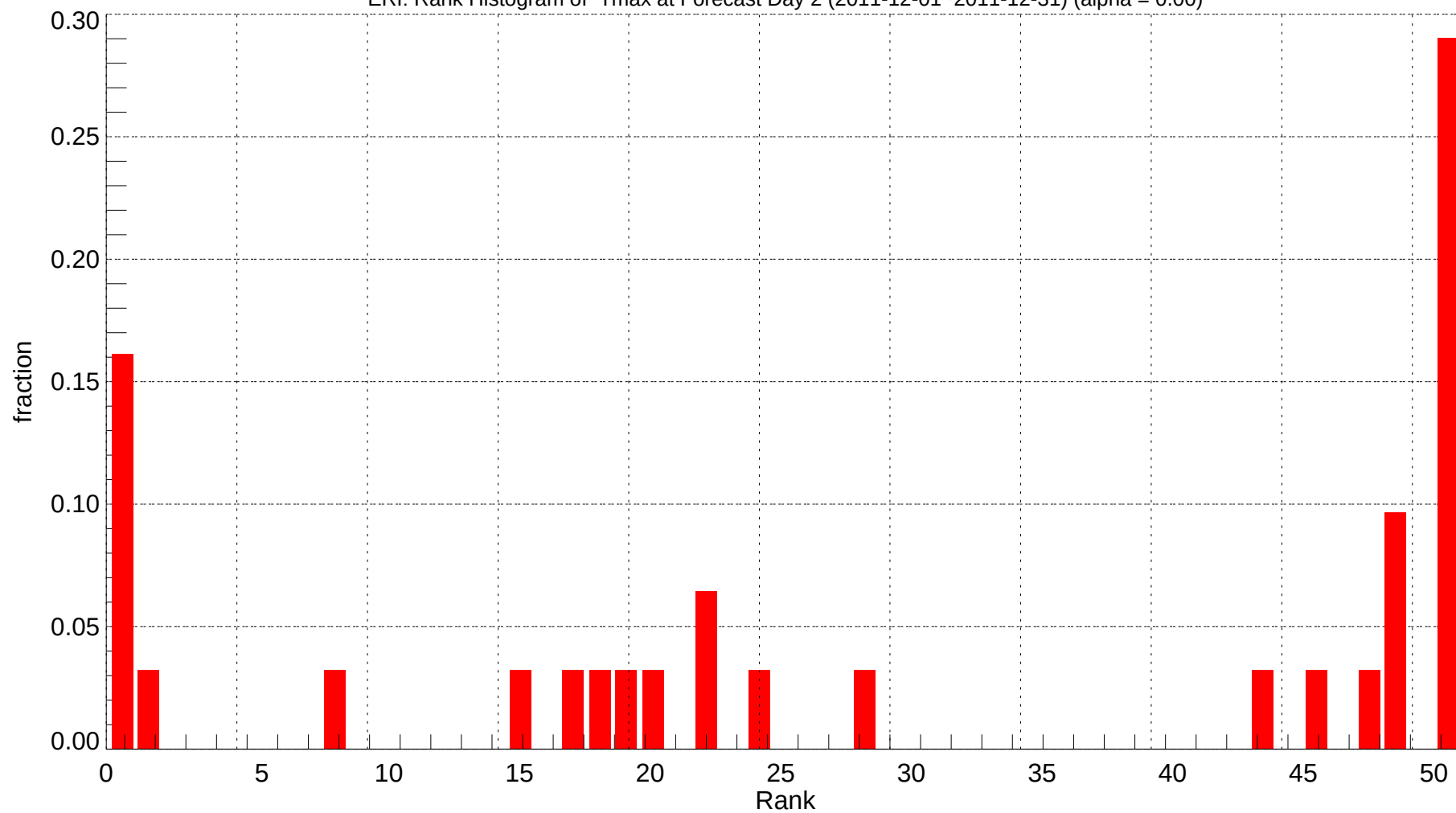
ERI: Rank Histogram of Tmax at Forecast Day 2 (2011-12-01~2011-12-31) (alpha = 0.00)
