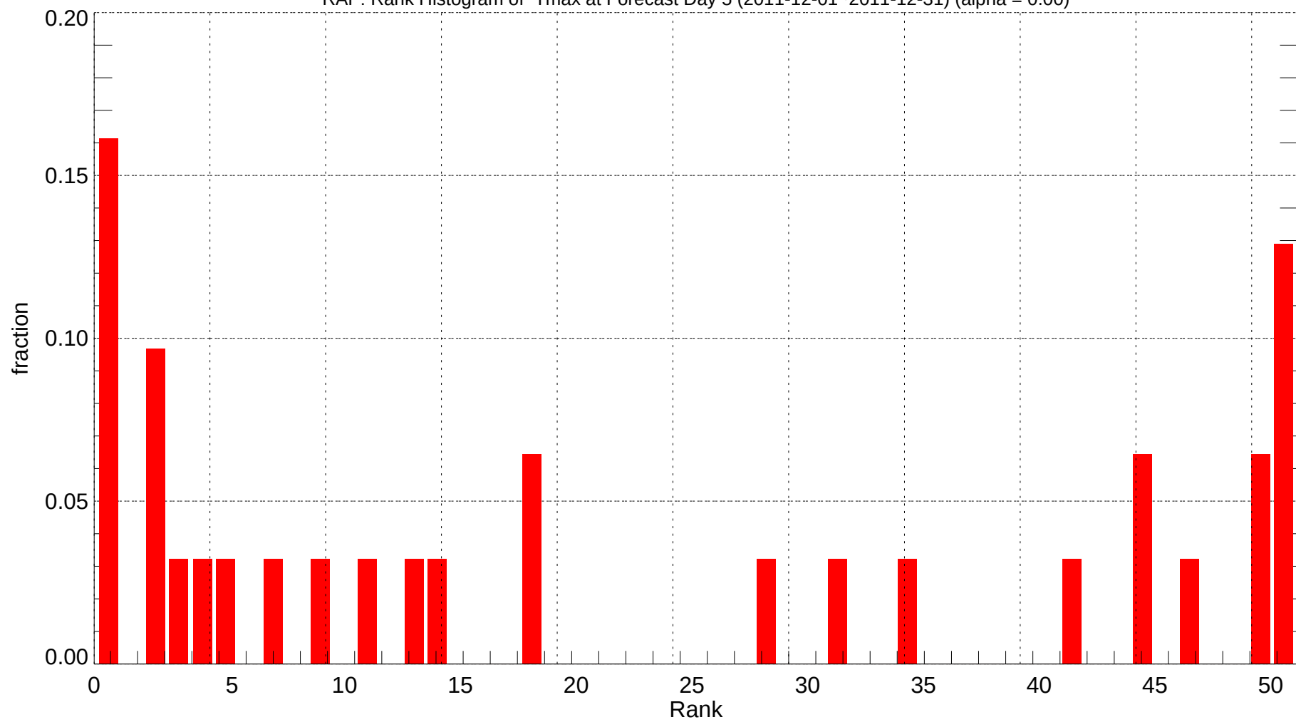
RAP: Rank Histogram of Tmax at Forecast Day 5 (2011-12-01~2011-12-31) (alpha = 0.00)
