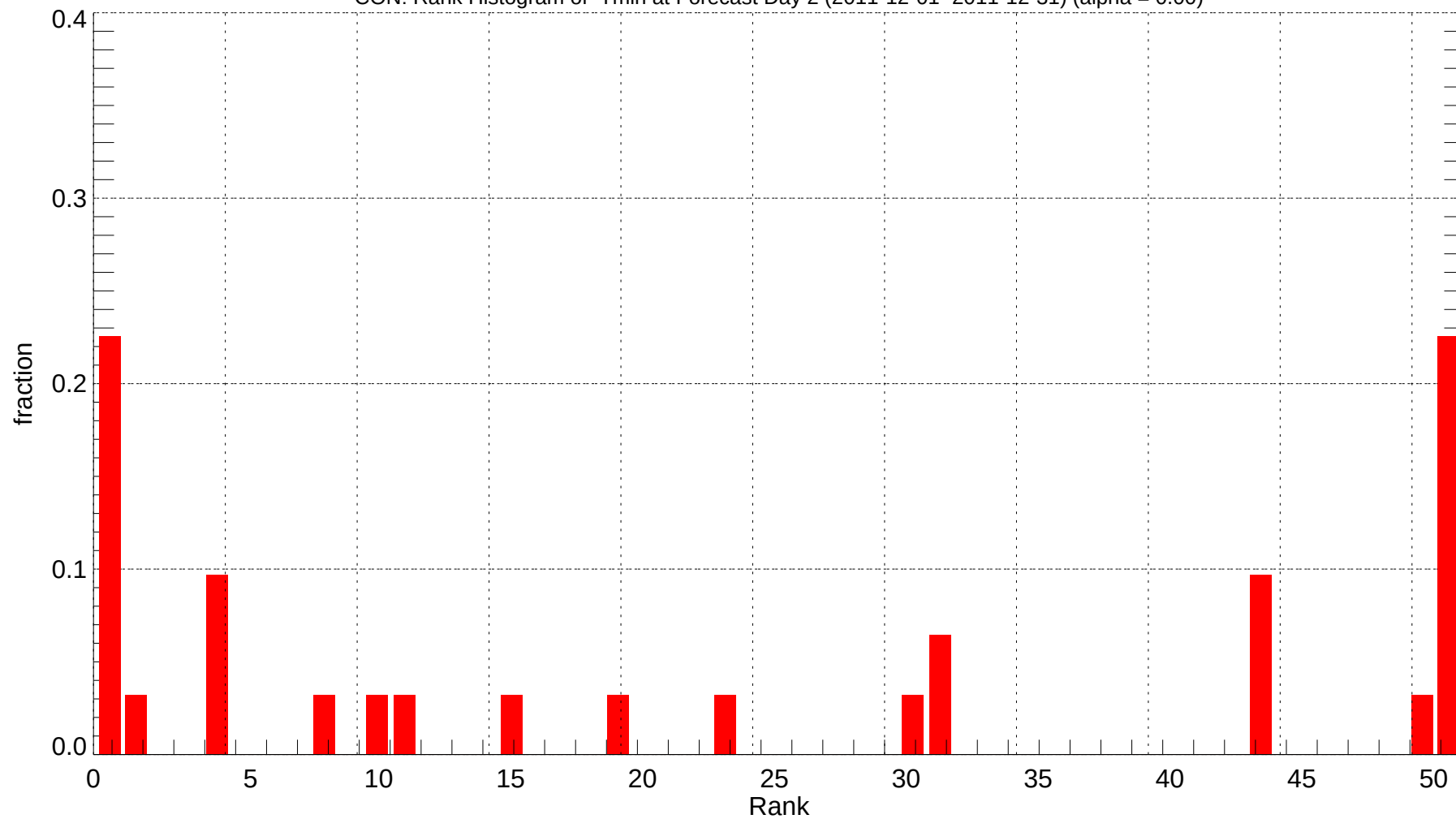
CON: Rank Histogram of Tmin at Forecast Day 2 (2011-12-01~2011-12-31) (alpha = 0.00)
