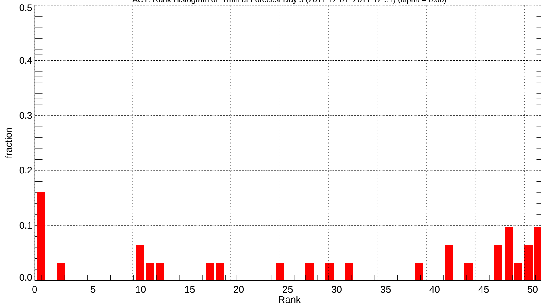
ACY: Rank Histogram of Tmin at Forecast Day 3 (2011-12-01~2011-12-31) (alpha = 0.00)
