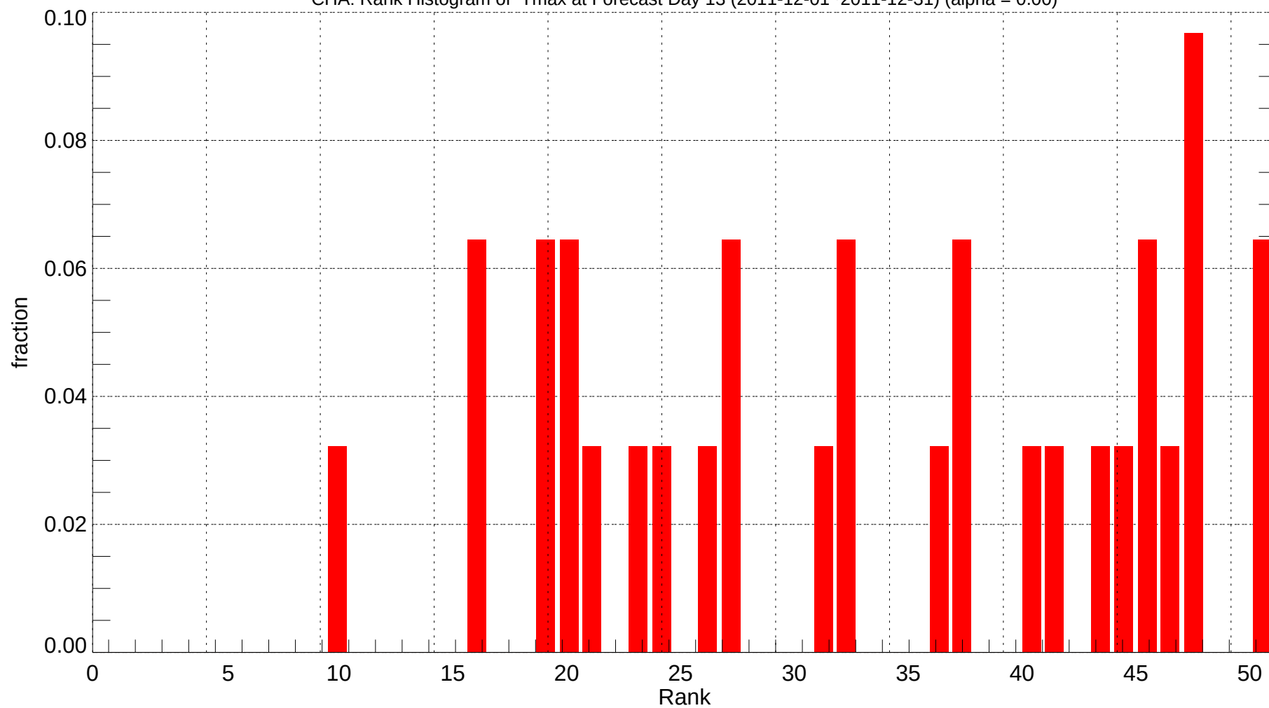
CHA: Rank Histogram of Tmax at Forecast Day 13 (2011-12-01~2011-12-31) (alpha = 0.00)
