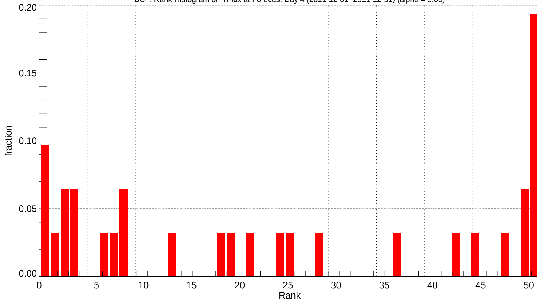
BUF: Rank Histogram of Tmax at Forecast Day 4 (2011-12-01~2011-12-31) (alpha = 0.00)
