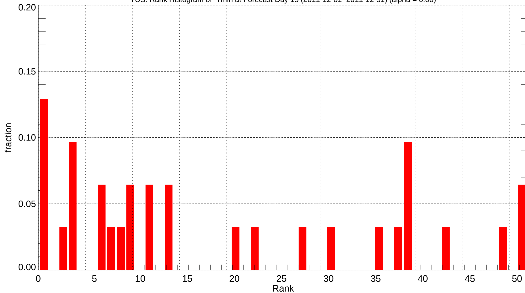
TUS: Rank Histogram of Tmin at Forecast Day 15 (2011-12-01~2011-12-31) (alpha = 0.00)
