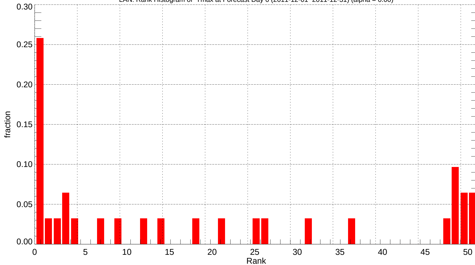
LAN: Rank Histogram of Tmax at Forecast Day 6 (2011-12-01~2011-12-31) (alpha = 0.00)
