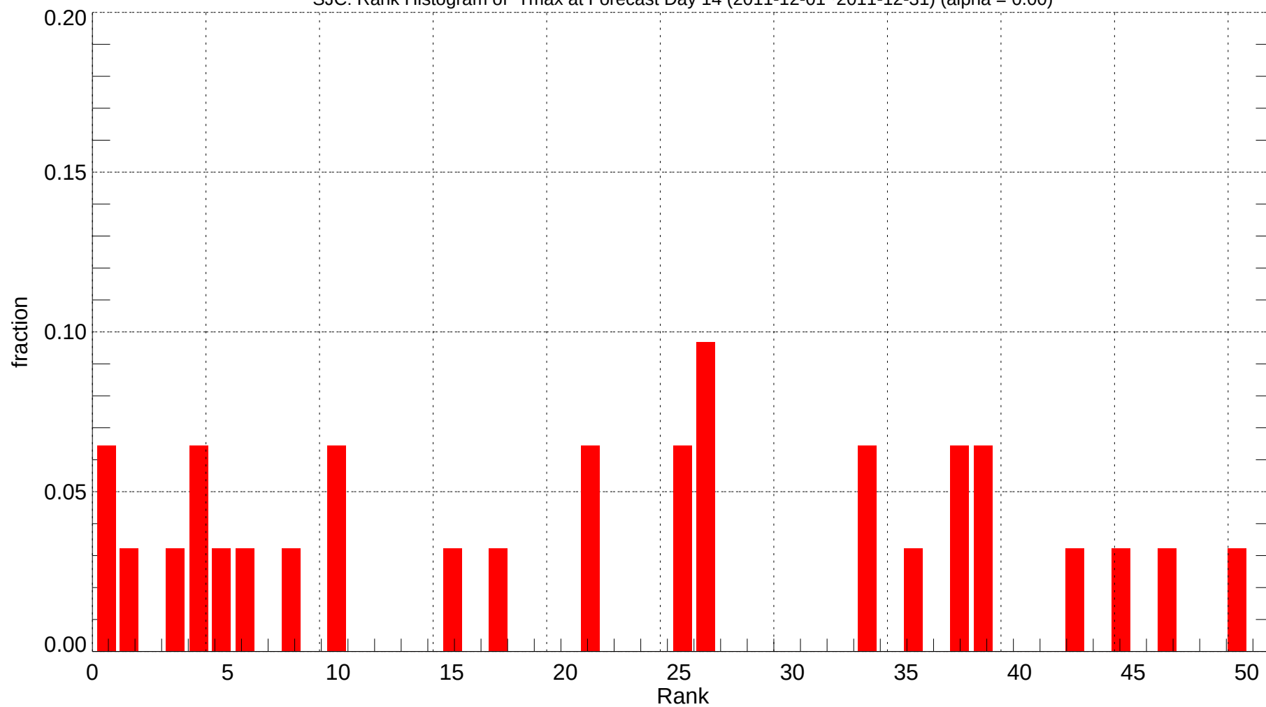
SJC: Rank Histogram of Tmax at Forecast Day 14 (2011-12-01~2011-12-31) (alpha = 0.00)
