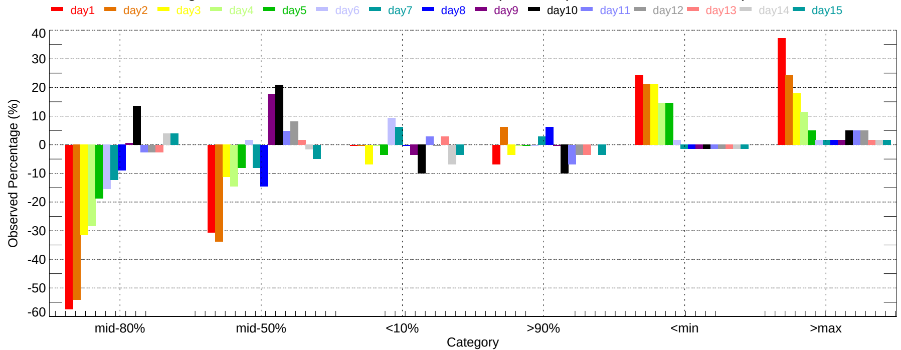
Observed Percentage Deviation of Ensembles - ALW: Min Temperature (2011-12-01~2011-12-31)
