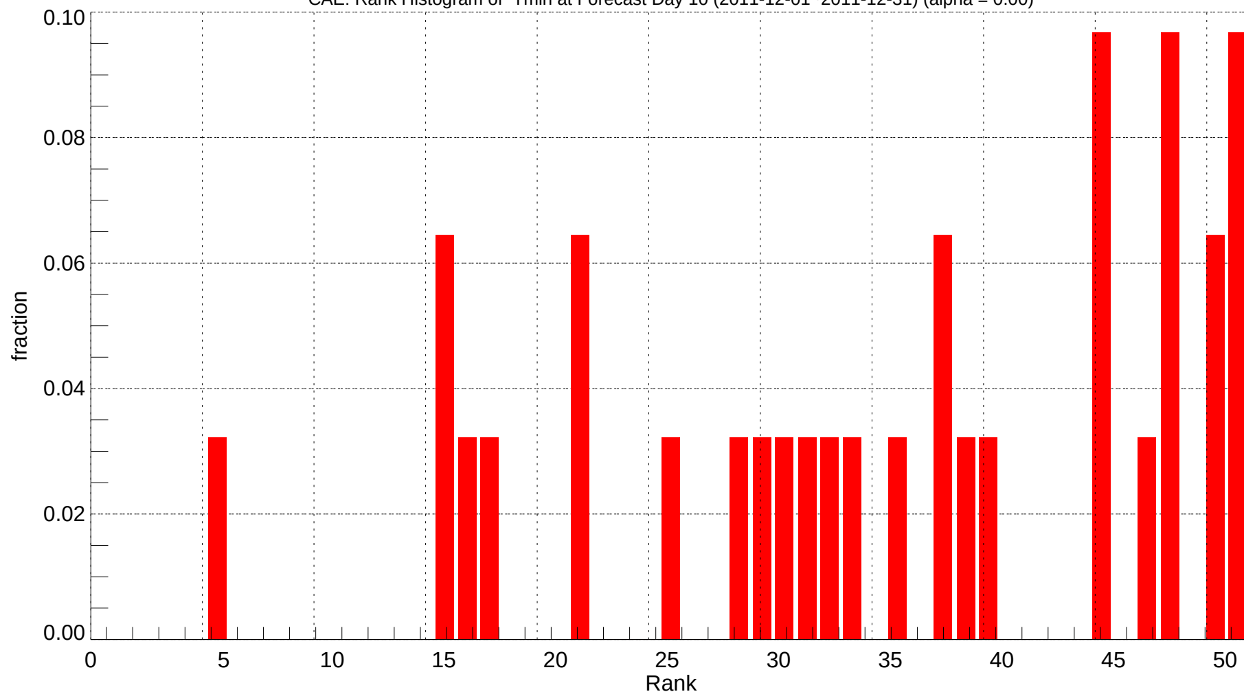
CAE: Rank Histogram of Tmin at Forecast Day 10 (2011-12-01~2011-12-31) (alpha = 0.00)
