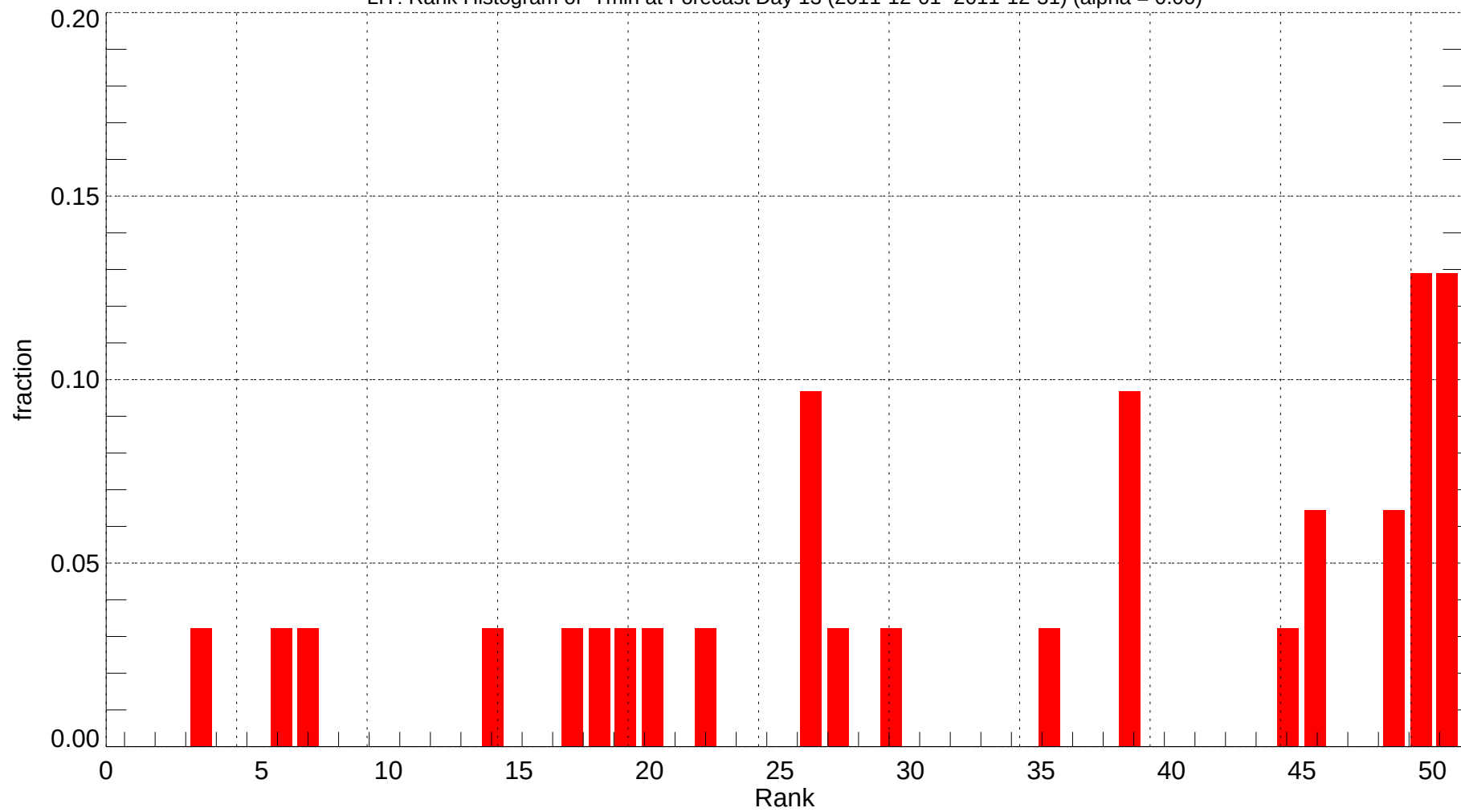
LIT: Rank Histogram of Tmin at Forecast Day 13 (2011-12-01~2011-12-31) (alpha = 0.00)
