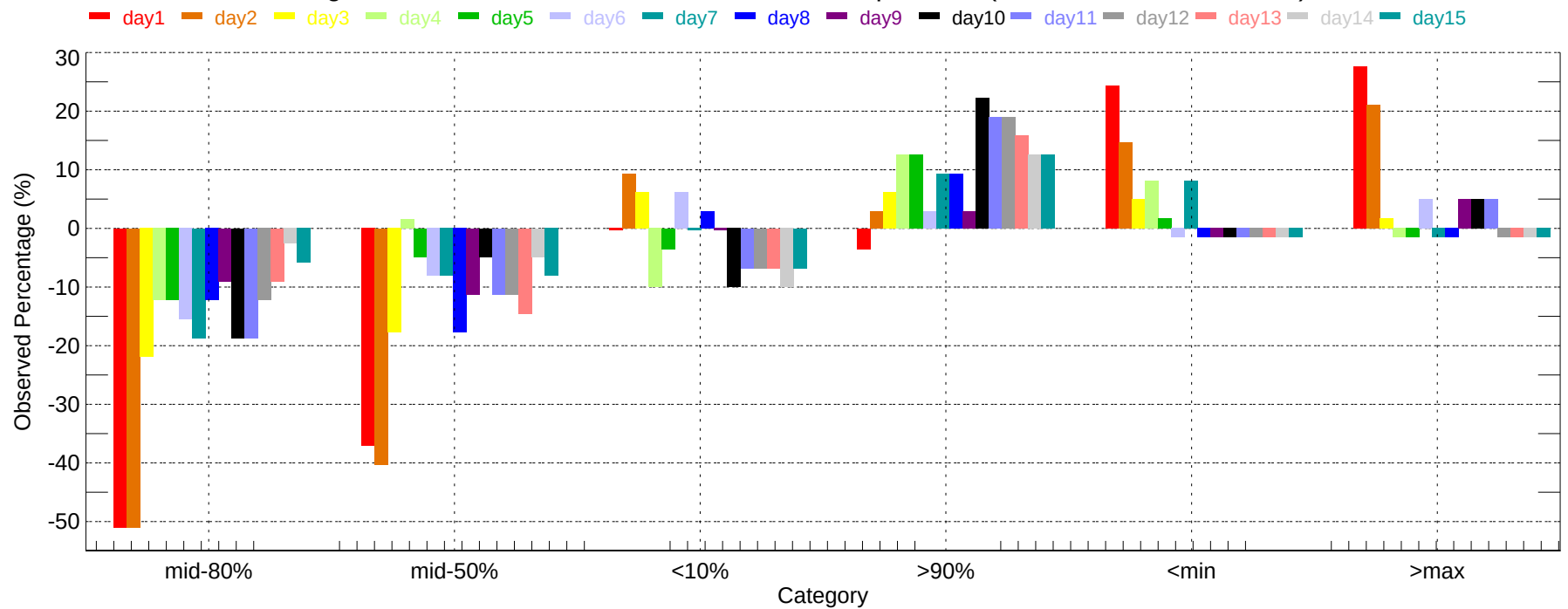
Observed Percentage Deviation of Ensembles - ROA: Max Temperature (2011-12-01~2011-12-31)
