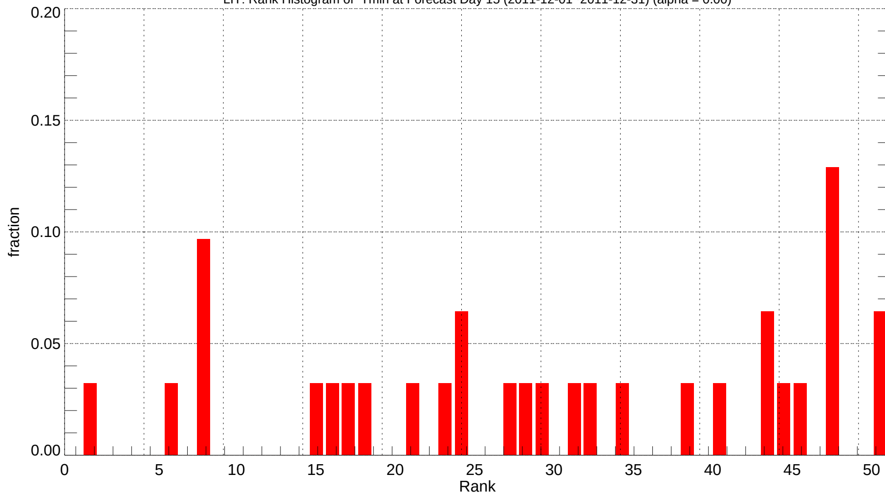
LIT: Rank Histogram of Tmin at Forecast Day 15 (2011-12-01~2011-12-31) (alpha = 0.00)
