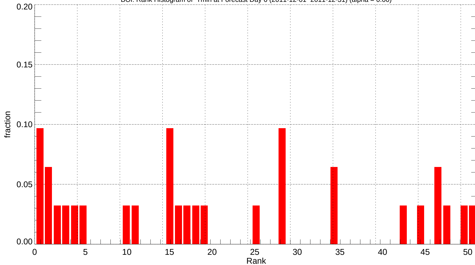
BOI: Rank Histogram of Tmin at Forecast Day 6 (2011-12-01~2011-12-31) (alpha = 0.00)
