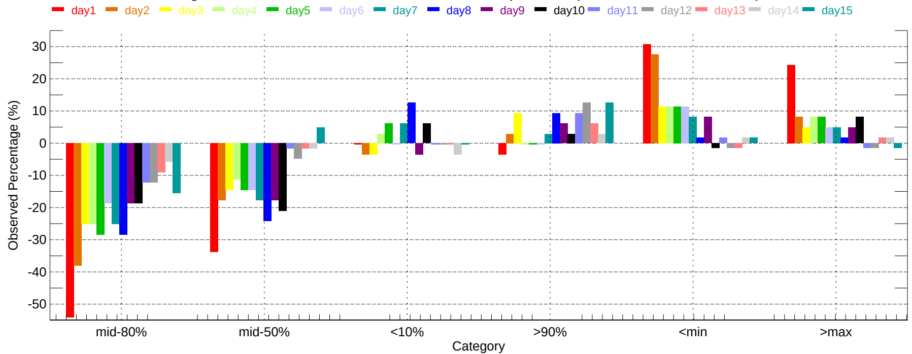
Observed Percentage Deviation of Ensembles - AUG: Max Temperature (2011-12-01~2011-12-31)
