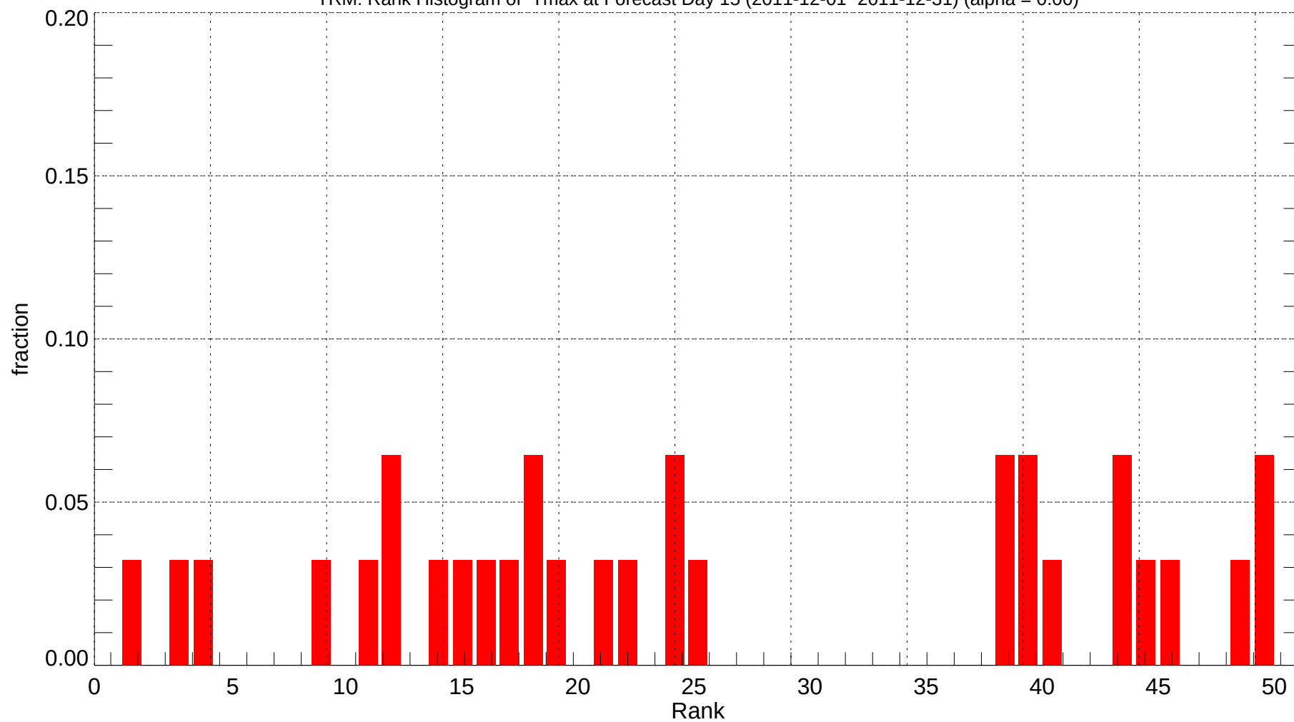
TRM: Rank Histogram of Tmax at Forecast Day 15 (2011-12-01~2011-12-31) (alpha = 0.00)
