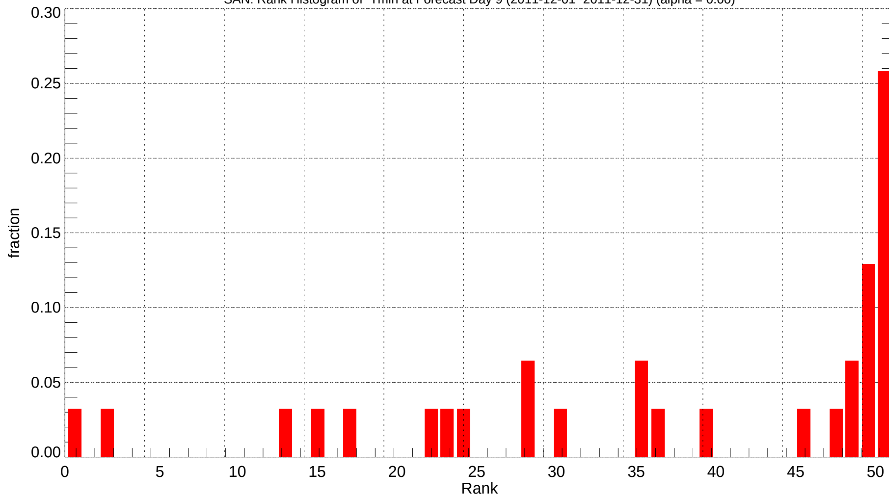
SAN: Rank Histogram of Tmin at Forecast Day 9 (2011-12-01~2011-12-31) (alpha = 0.00)
