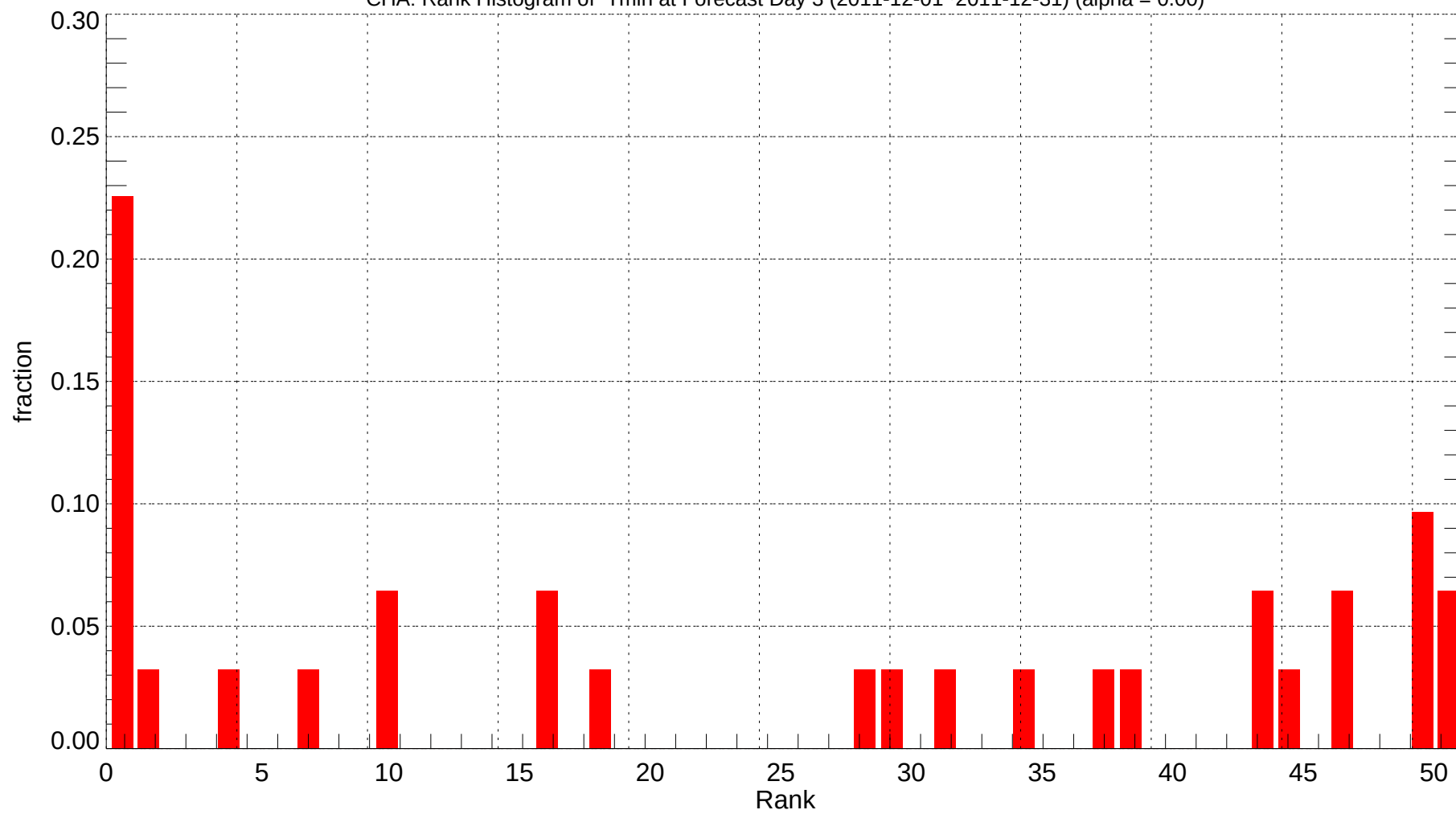
CHA: Rank Histogram of Tmin at Forecast Day 3 (2011-12-01~2011-12-31) (alpha = 0.00)
