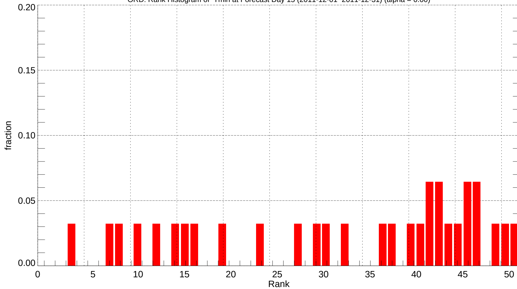
ORD: Rank Histogram of Tmin at Forecast Day 15 (2011-12-01~2011-12-31) (alpha = 0.00)
