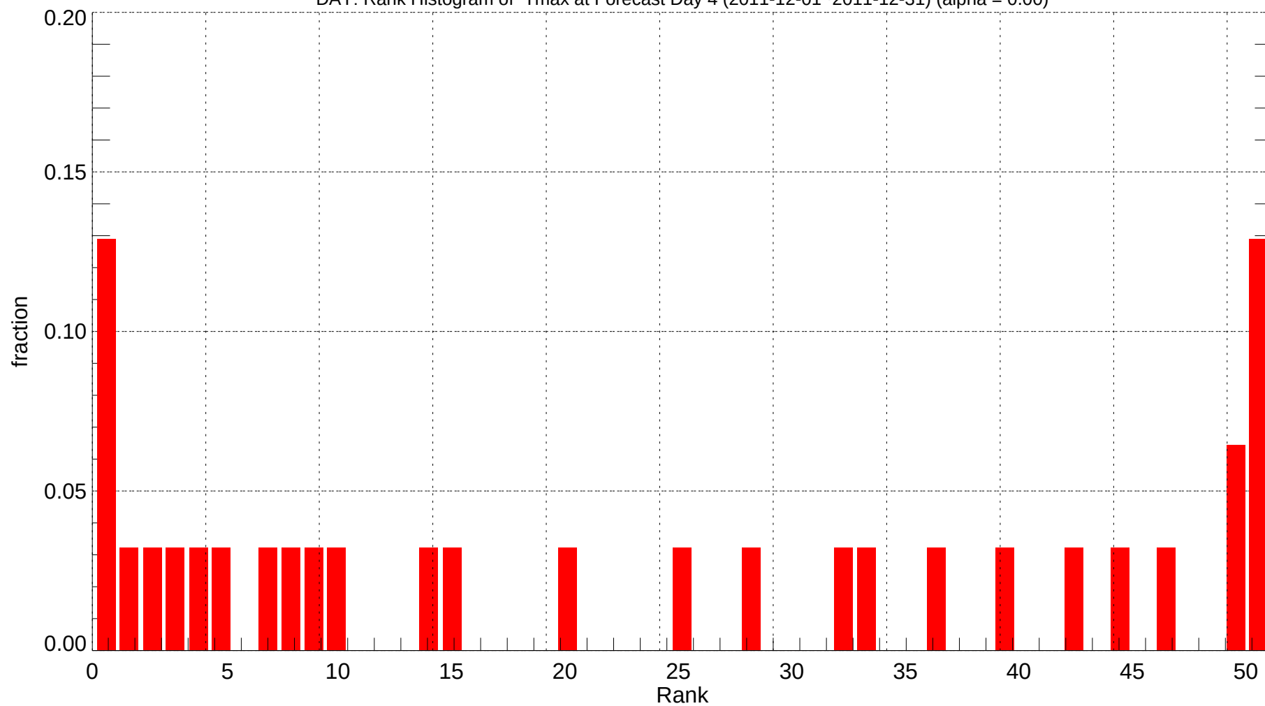
DAY: Rank Histogram of Tmax at Forecast Day 4 (2011-12-01~2011-12-31) (alpha = 0.00)
