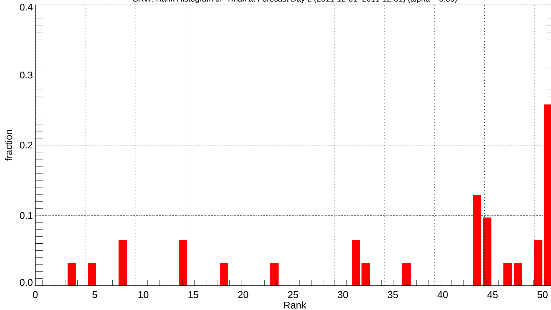
CRW: Rank Histogram of Tmax at Forecast Day 2 (2011-12-01~2011-12-31) (alpha = 0.00)
