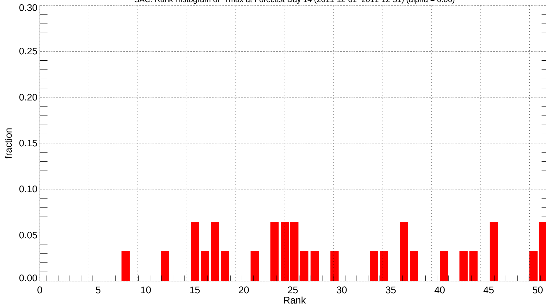
SAC: Rank Histogram of Tmax at Forecast Day 14 (2011-12-01~2011-12-31) (alpha = 0.00)
