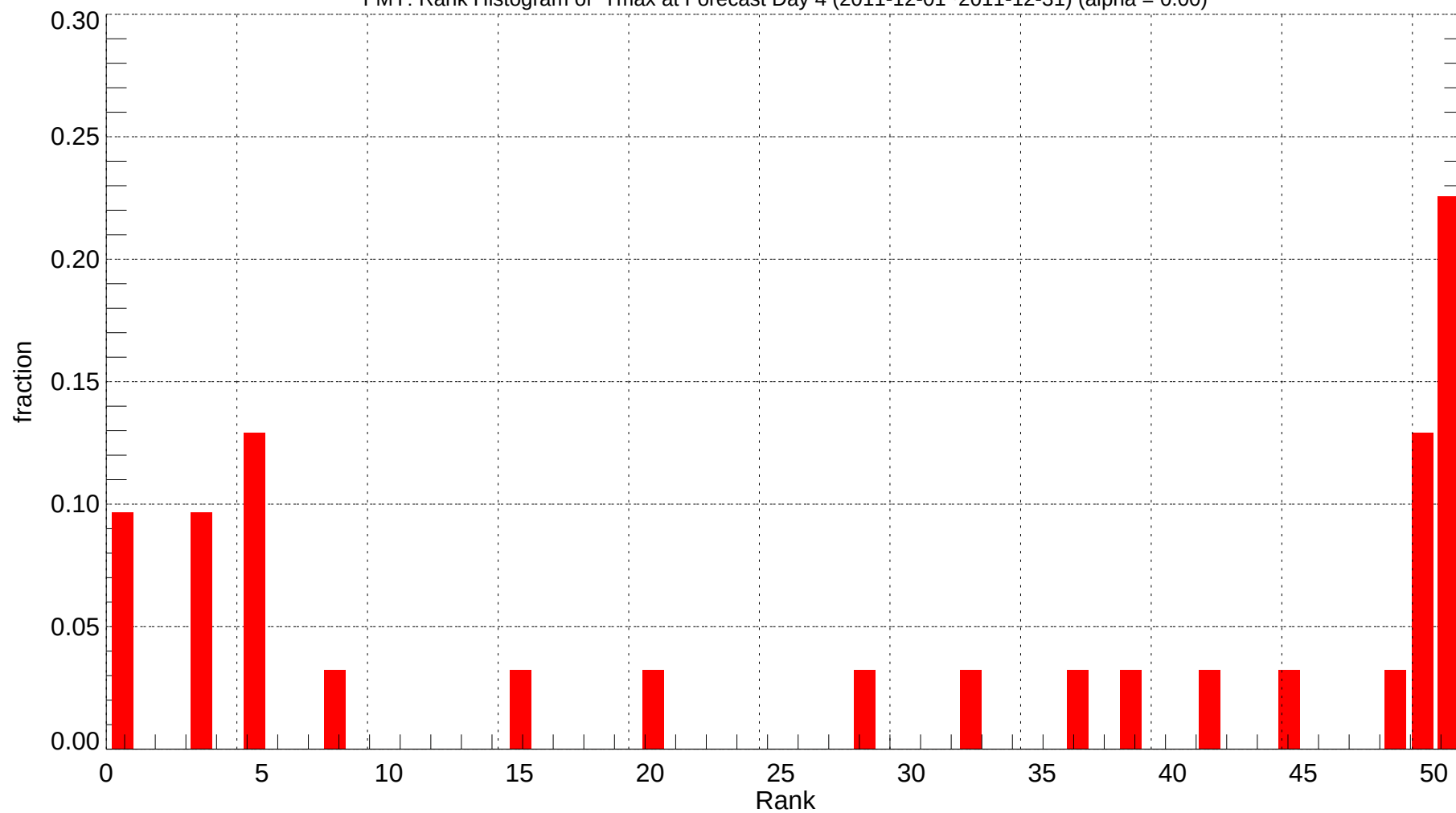
FMY: Rank Histogram of Tmax at Forecast Day 4 (2011-12-01~2011-12-31) (alpha = 0.00)
