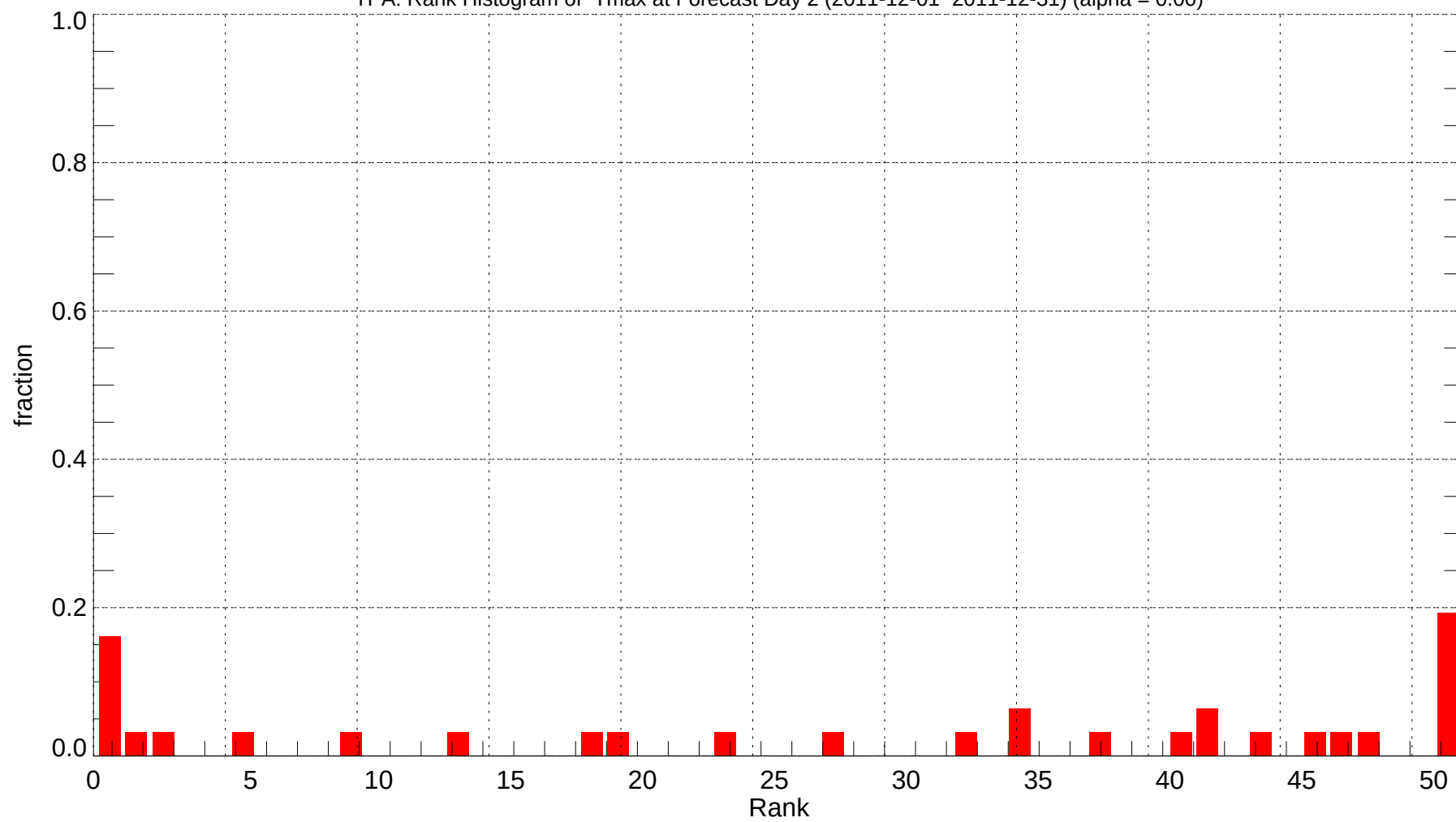
TPA: Rank Histogram of Tmax at Forecast Day 2 (2011-12-01~2011-12-31) (alpha = 0.00)
