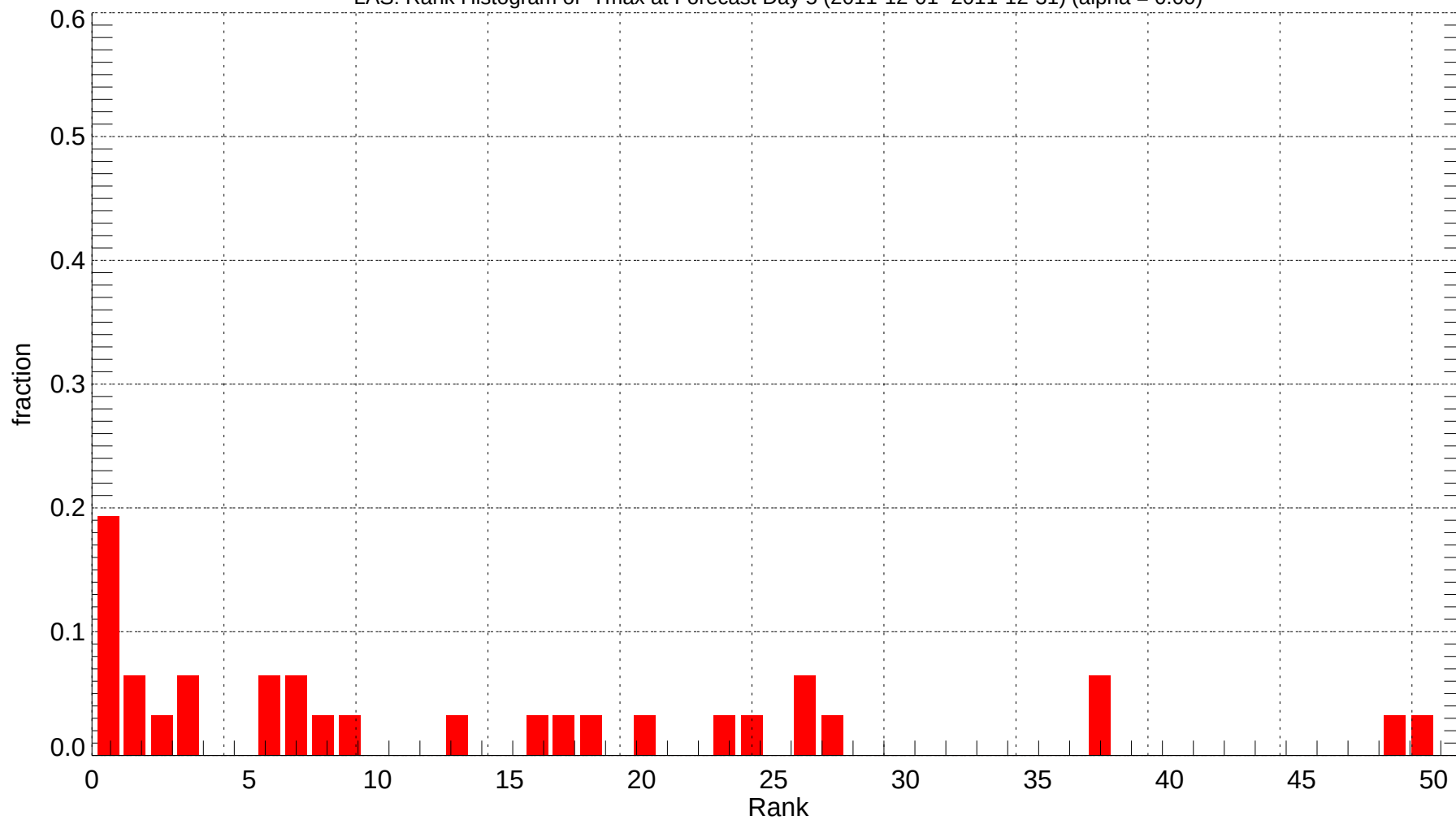
LAS: Rank Histogram of Tmax at Forecast Day 5 (2011-12-01~2011-12-31) (alpha = 0.00)
