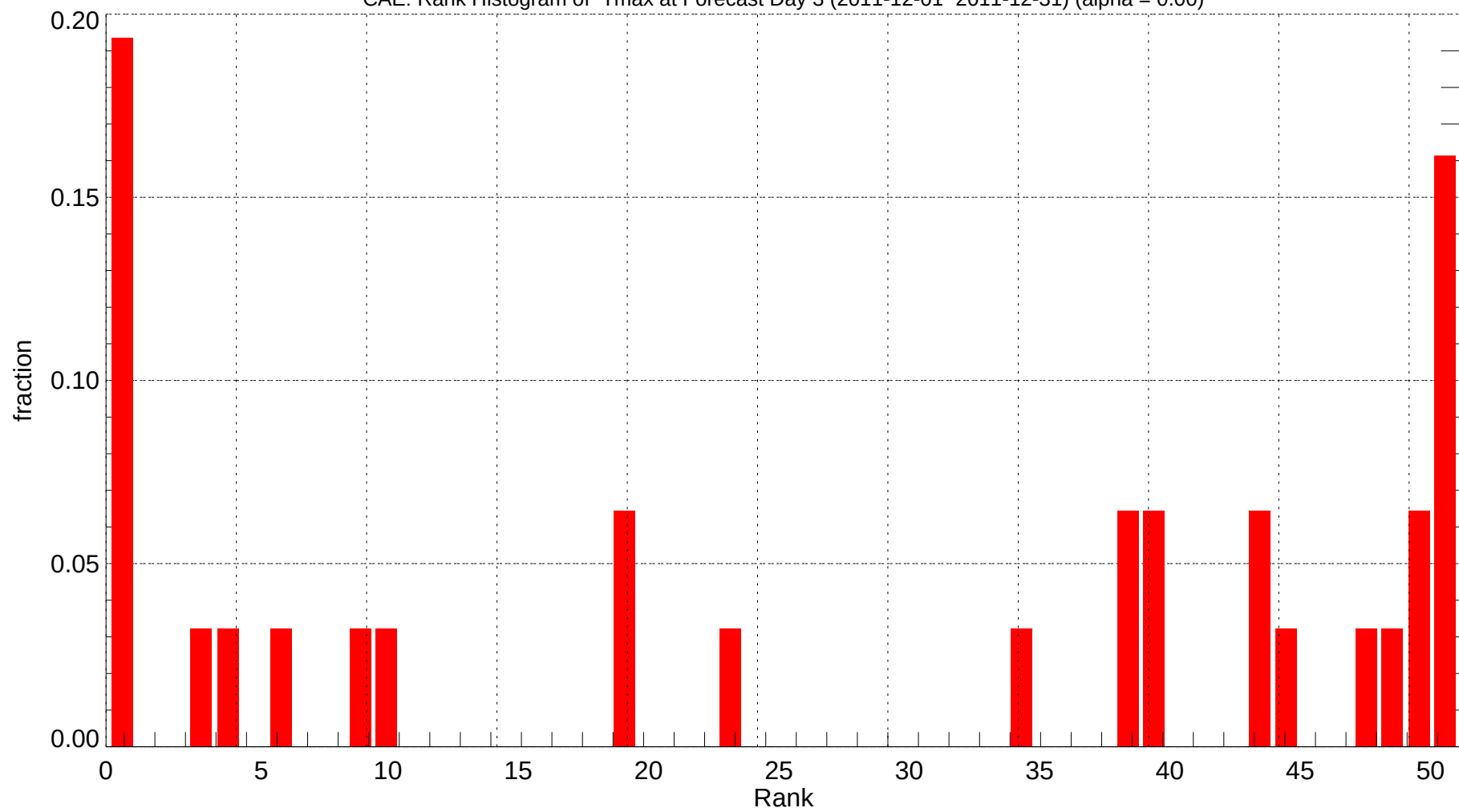
CAE: Rank Histogram of Tmax at Forecast Day 3 (2011-12-01~2011-12-31) (alpha = 0.00)
