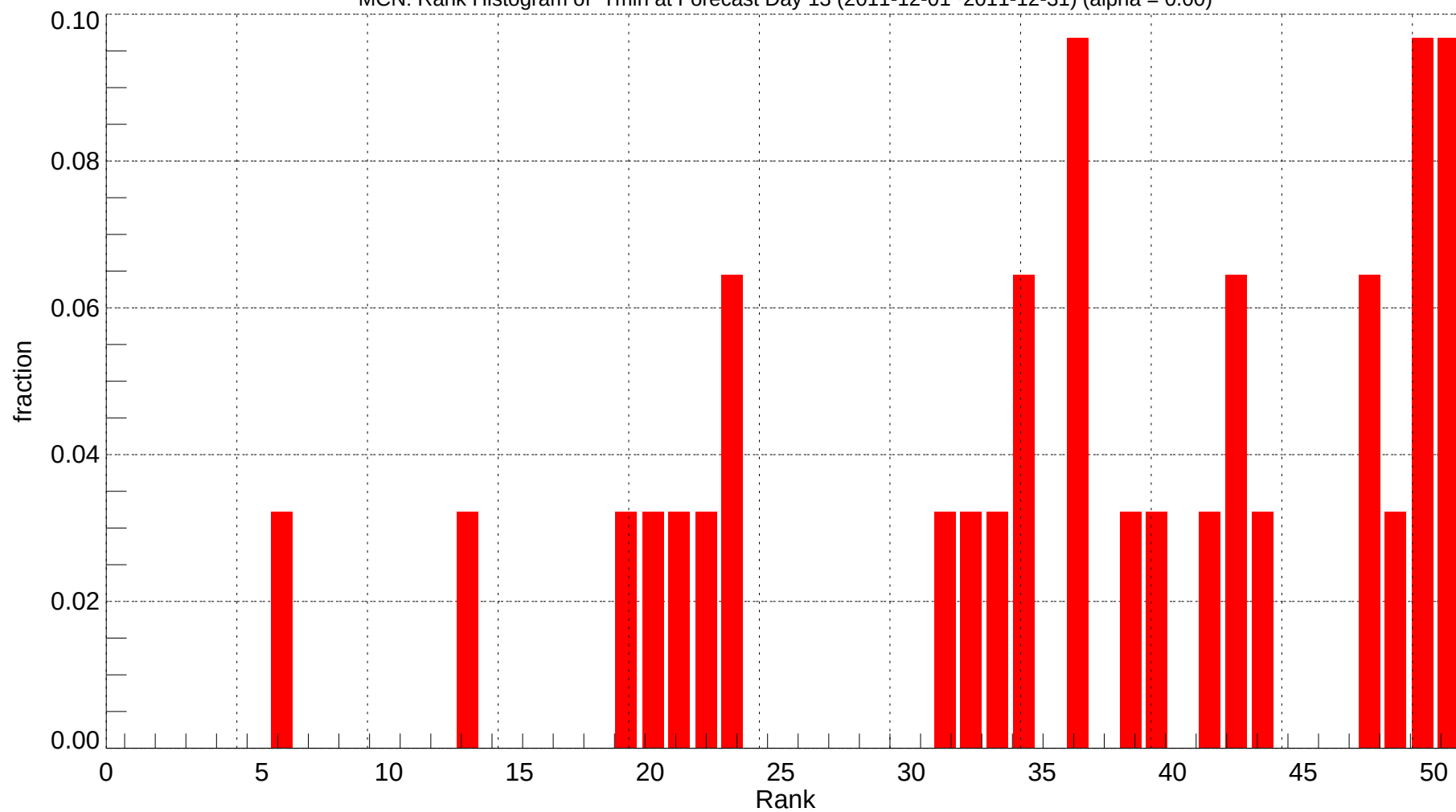
MCN: Rank Histogram of Tmin at Forecast Day 13 (2011-12-01~2011-12-31) (alpha = 0.00)
