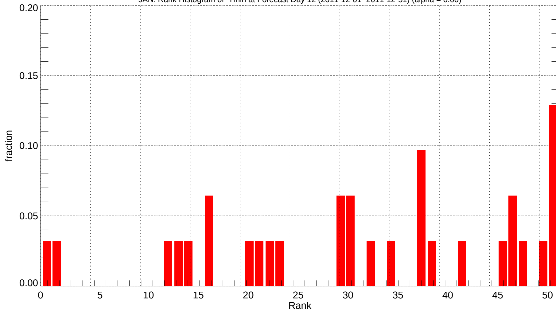
JAN: Rank Histogram of Tmin at Forecast Day 12 (2011-12-01~2011-12-31) (alpha = 0.00)
