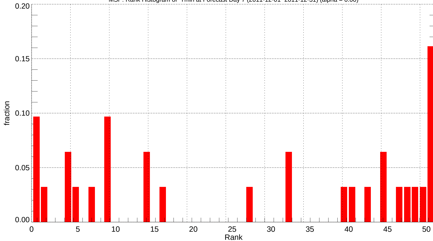
MSP: Rank Histogram of Tmin at Forecast Day 7 (2011-12-01~2011-12-31) (alpha = 0.00)
