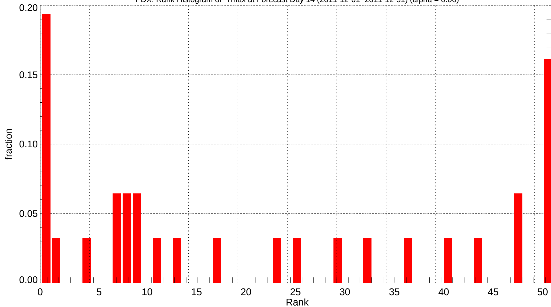
PDX: Rank Histogram of Tmax at Forecast Day 14 (2011-12-01~2011-12-31) (alpha = 0.00)
