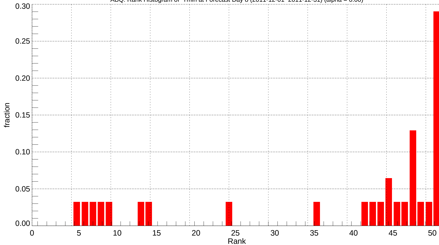
ABQ: Rank Histogram of Tmin at Forecast Day 8 (2011-12-01~2011-12-31) (alpha = 0.00)
