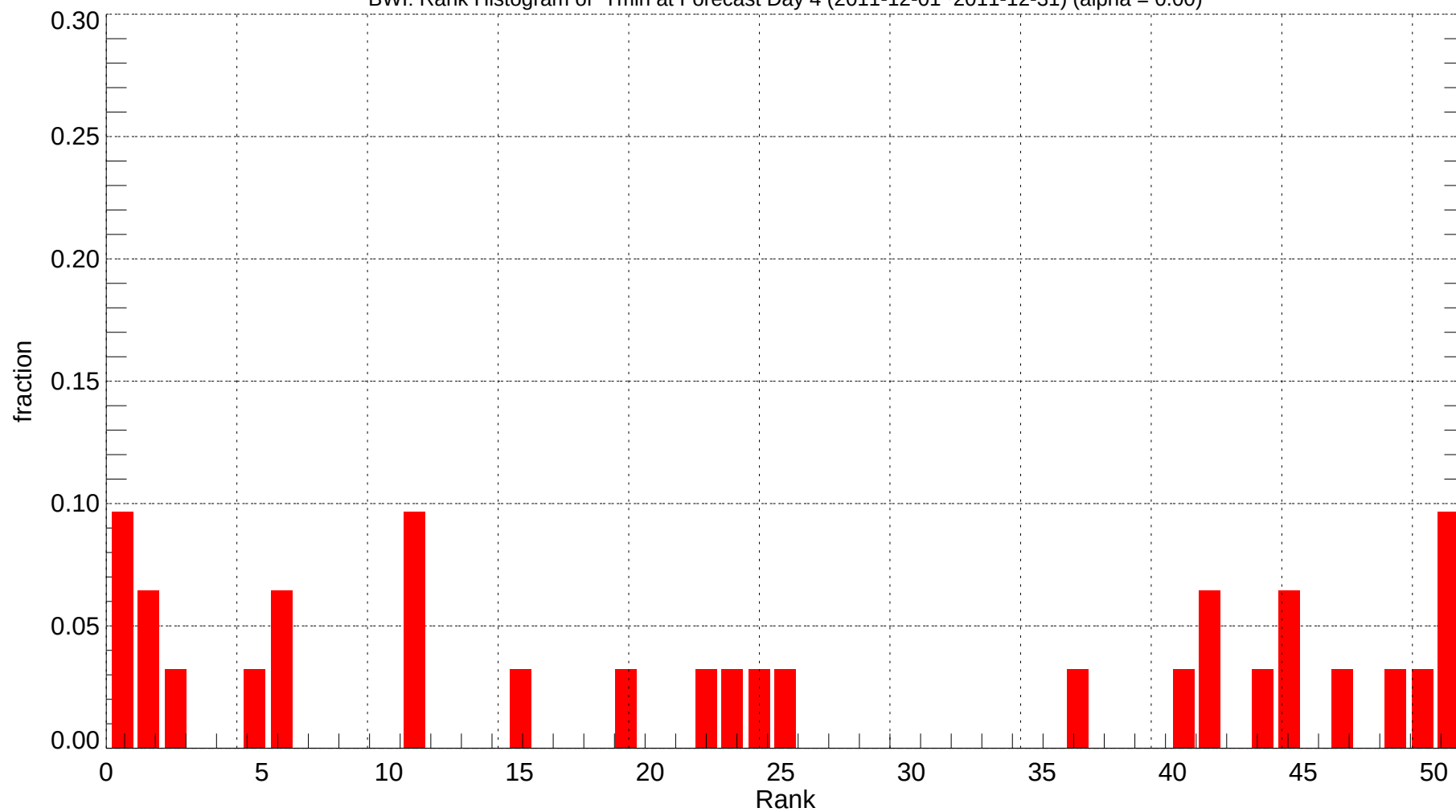
BWI: Rank Histogram of Tmin at Forecast Day 4 (2011-12-01~2011-12-31) (alpha = 0.00)
