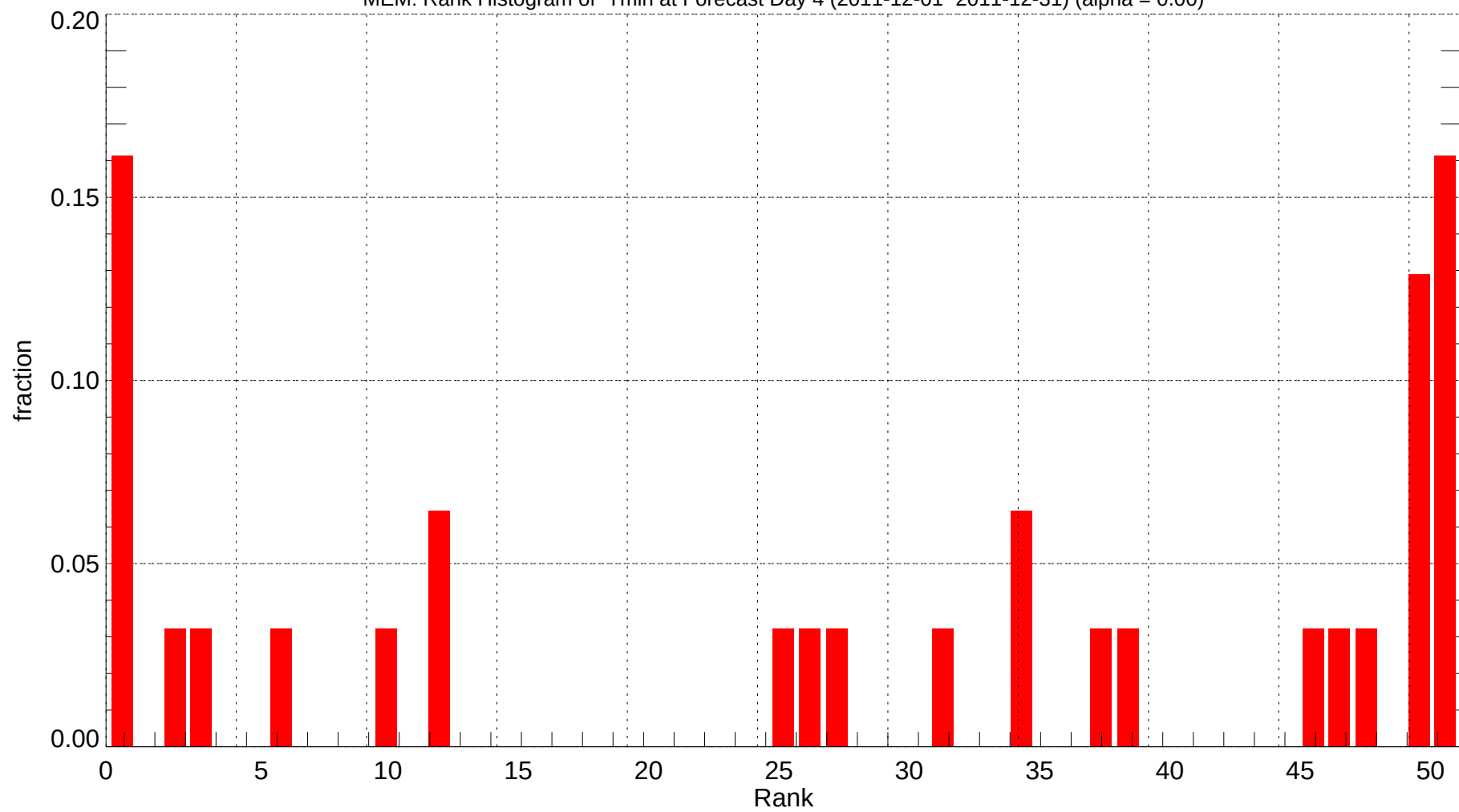
MEM: Rank Histogram of Tmin at Forecast Day 4 (2011-12-01~2011-12-31) (alpha = 0.00)
