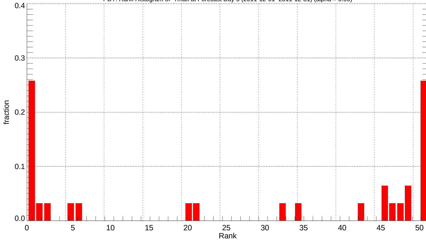
PDT: Rank Histogram of Tmax at Forecast Day 5 (2011-12-01~2011-12-31) (alpha = 0.00)
