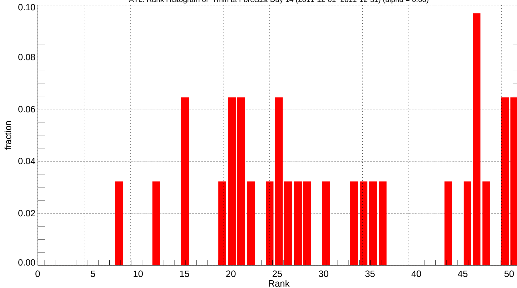
ATL: Rank Histogram of Tmin at Forecast Day 14 (2011-12-01~2011-12-31) (alpha = 0.00)
