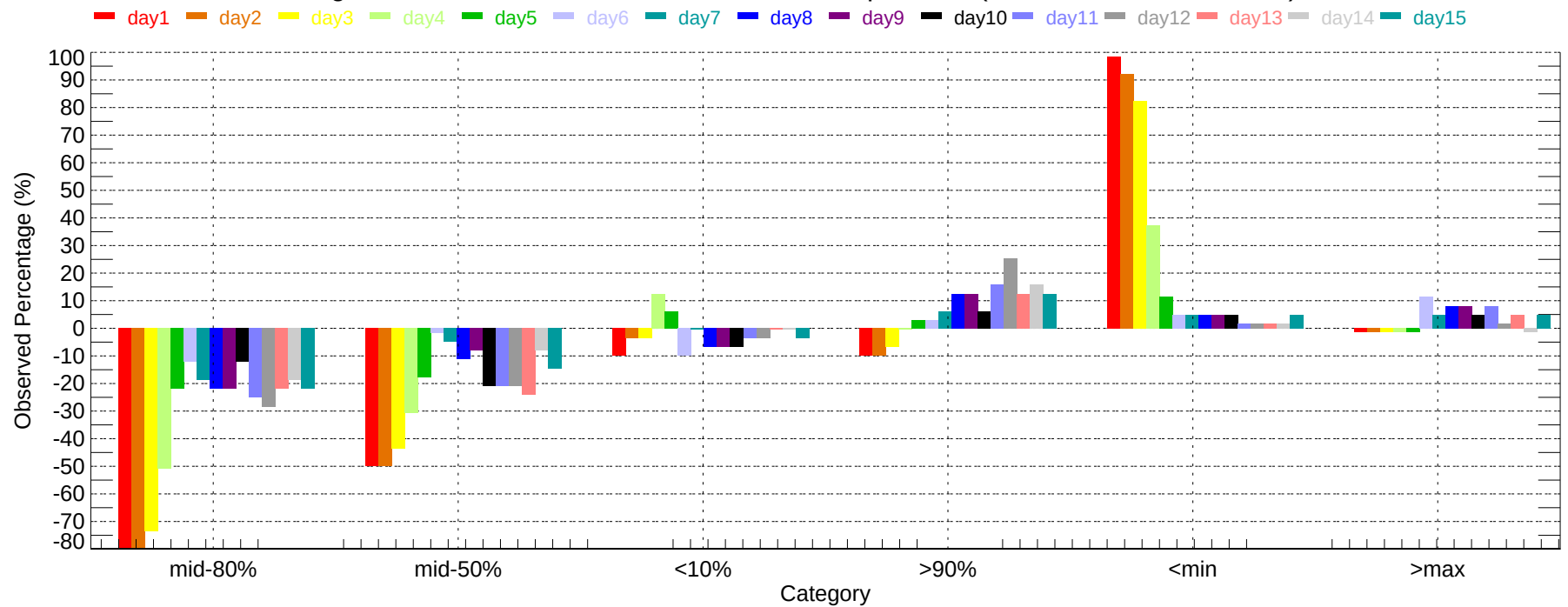
Observed Percentage Deviation of Ensembles - JFK: Max Temperature (2011-12-01~2011-12-31)
