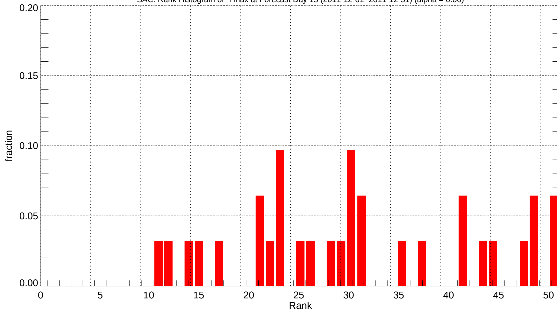
SAC: Rank Histogram of Tmax at Forecast Day 15 (2011-12-01~2011-12-31) (alpha = 0.00)
