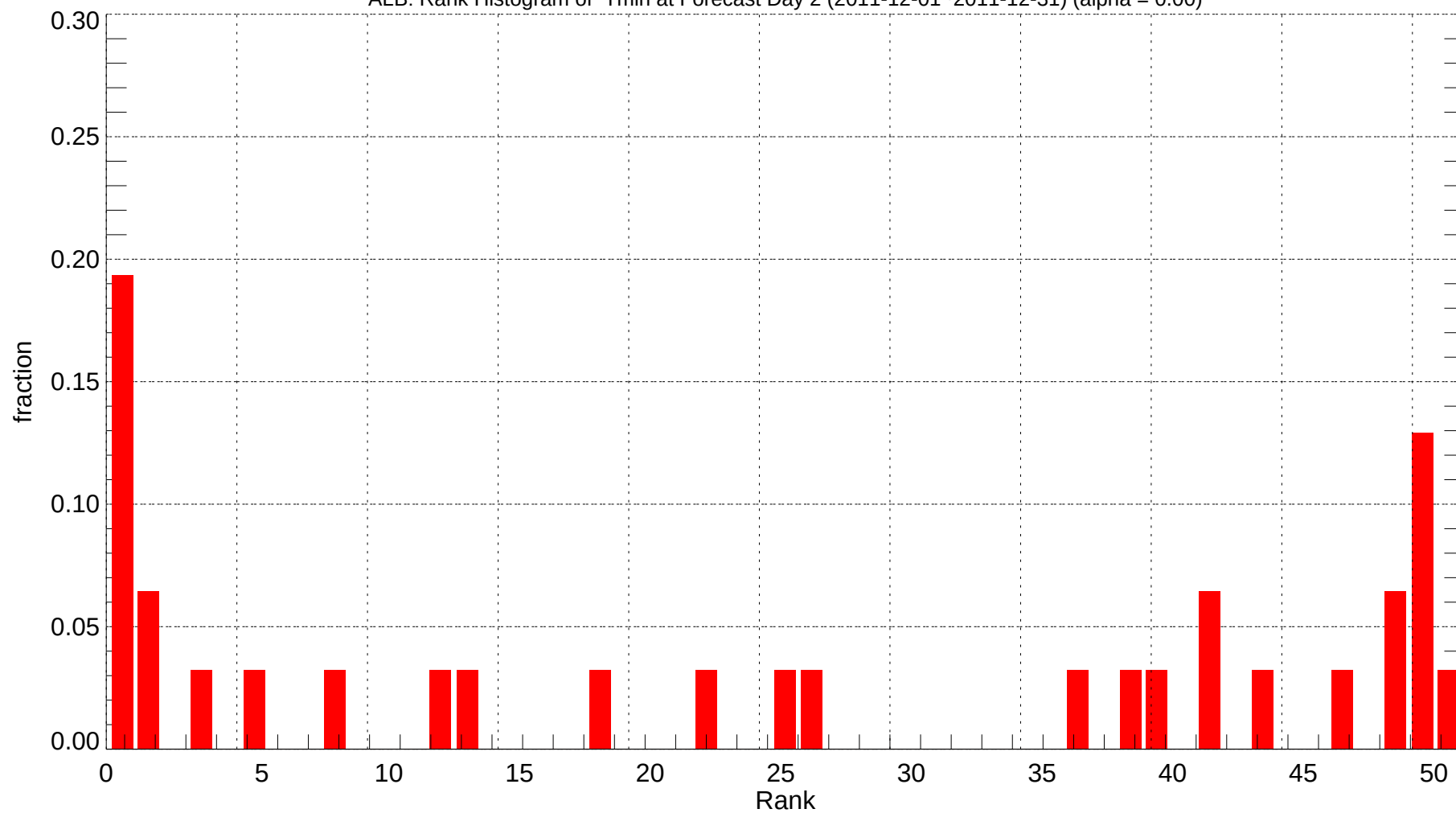
ALB: Rank Histogram of Tmin at Forecast Day 2 (2011-12-01~2011-12-31) (alpha = 0.00)
