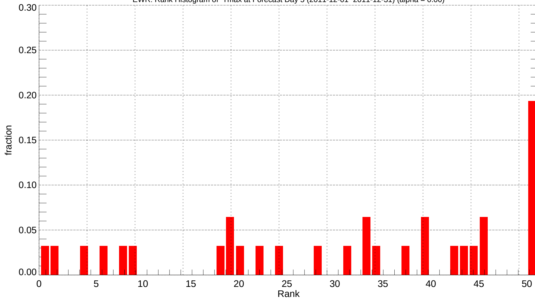
EWR: Rank Histogram of Tmax at Forecast Day 5 (2011-12-01~2011-12-31) (alpha = 0.00)
