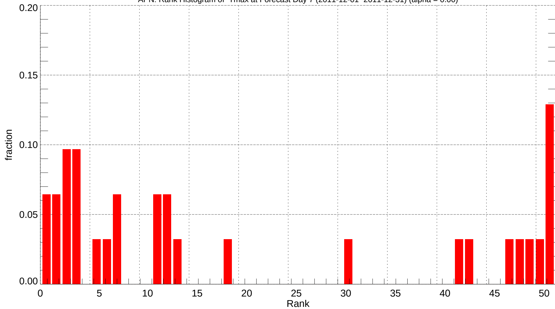
APN: Rank Histogram of Tmax at Forecast Day 7 (2011-12-01~2011-12-31) (alpha = 0.00)
