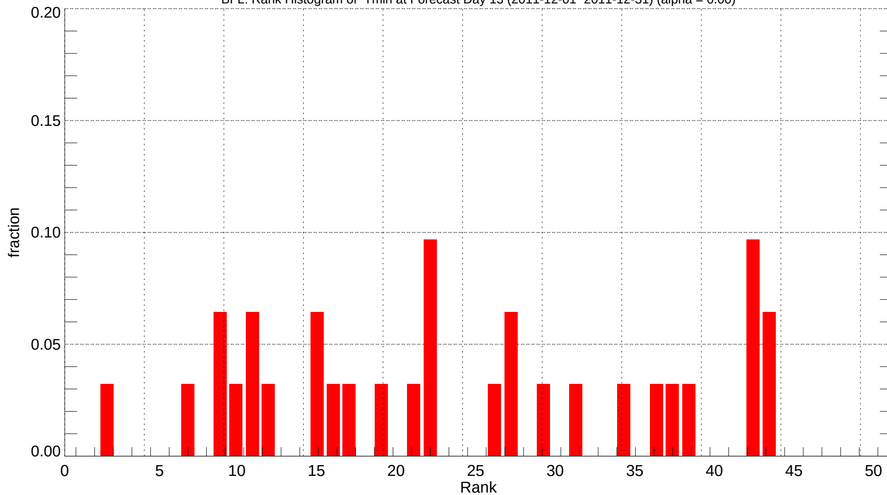
BFL: Rank Histogram of Tmin at Forecast Day 13 (2011-12-01~2011-12-31) (alpha = 0.00)
