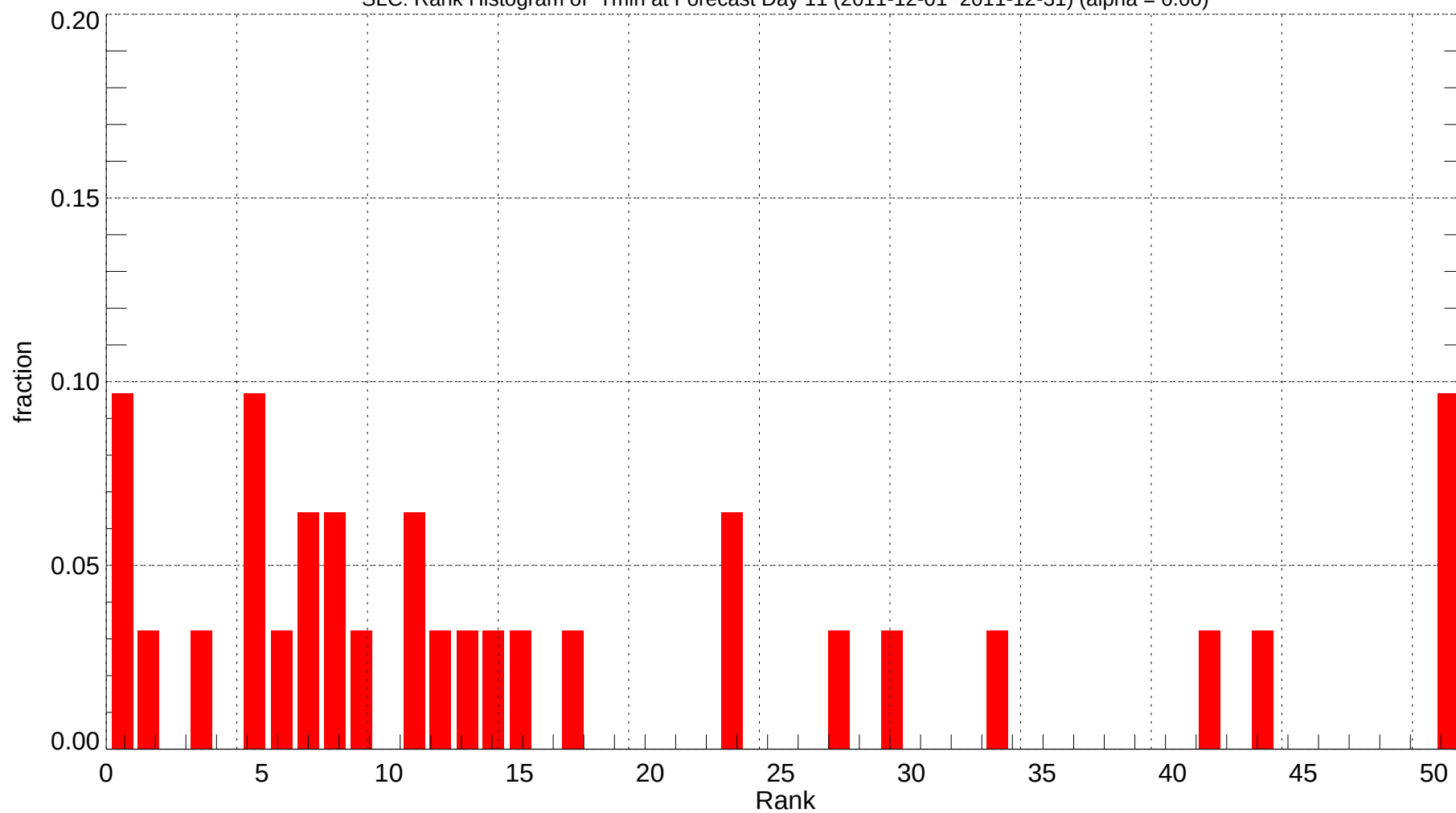
SLC: Rank Histogram of Tmin at Forecast Day 11 (2011-12-01~2011-12-31) (alpha = 0.00)
