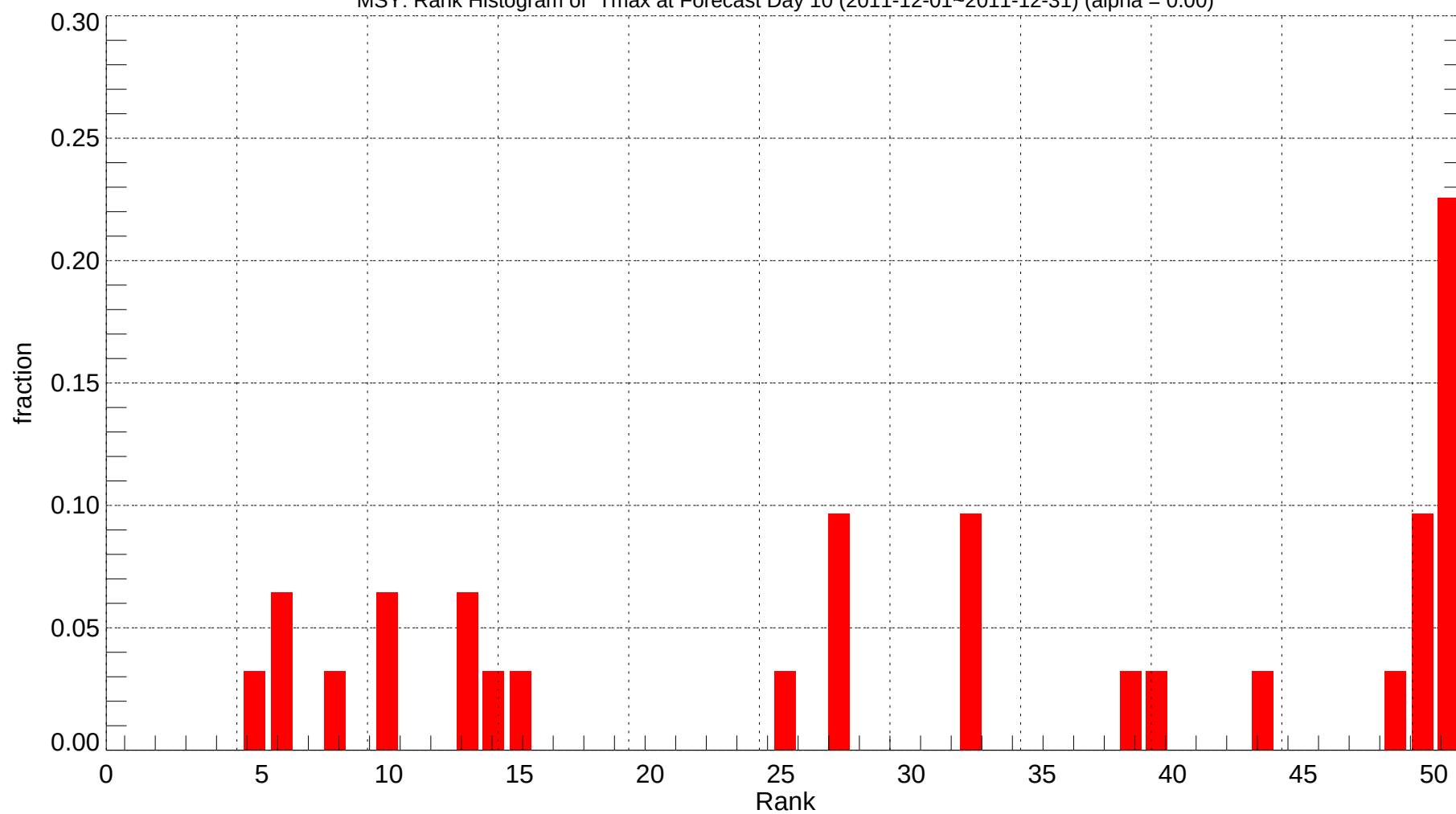
MSY: Rank Histogram of Tmax at Forecast Day 10 (2011-12-01~2011-12-31) (alpha = 0.00)
