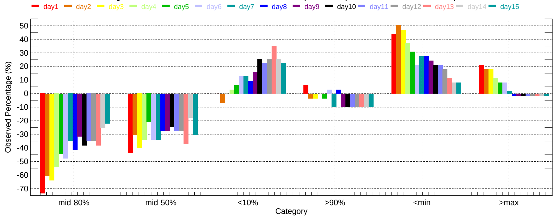
Observed Percentage Deviation of Ensembles - BFL: Min Temperature (2011-12-01~2011-12-31)
