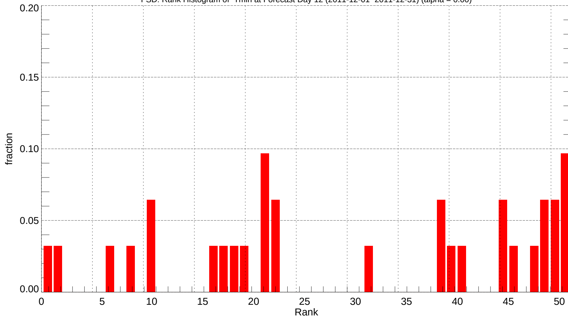
FSD: Rank Histogram of Tmin at Forecast Day 12 (2011-12-01~2011-12-31) (alpha = 0.00)
