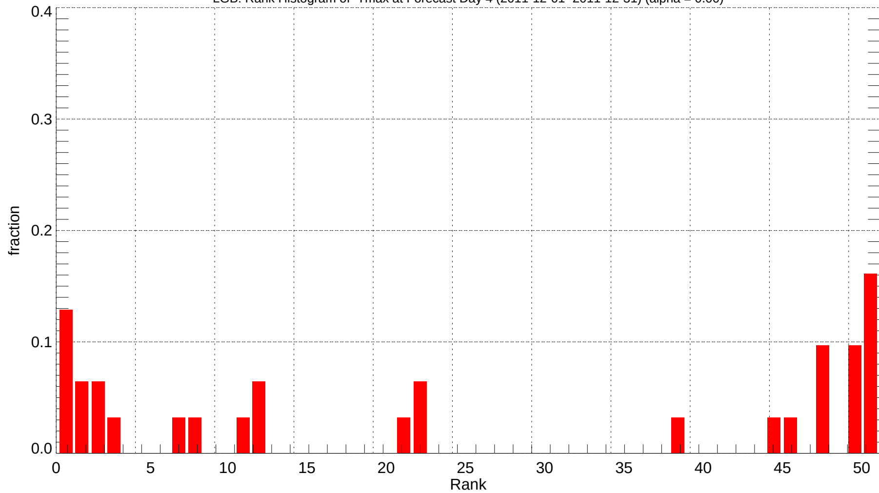
LGB: Rank Histogram of Tmax at Forecast Day 4 (2011-12-01~2011-12-31) (alpha = 0.00)
