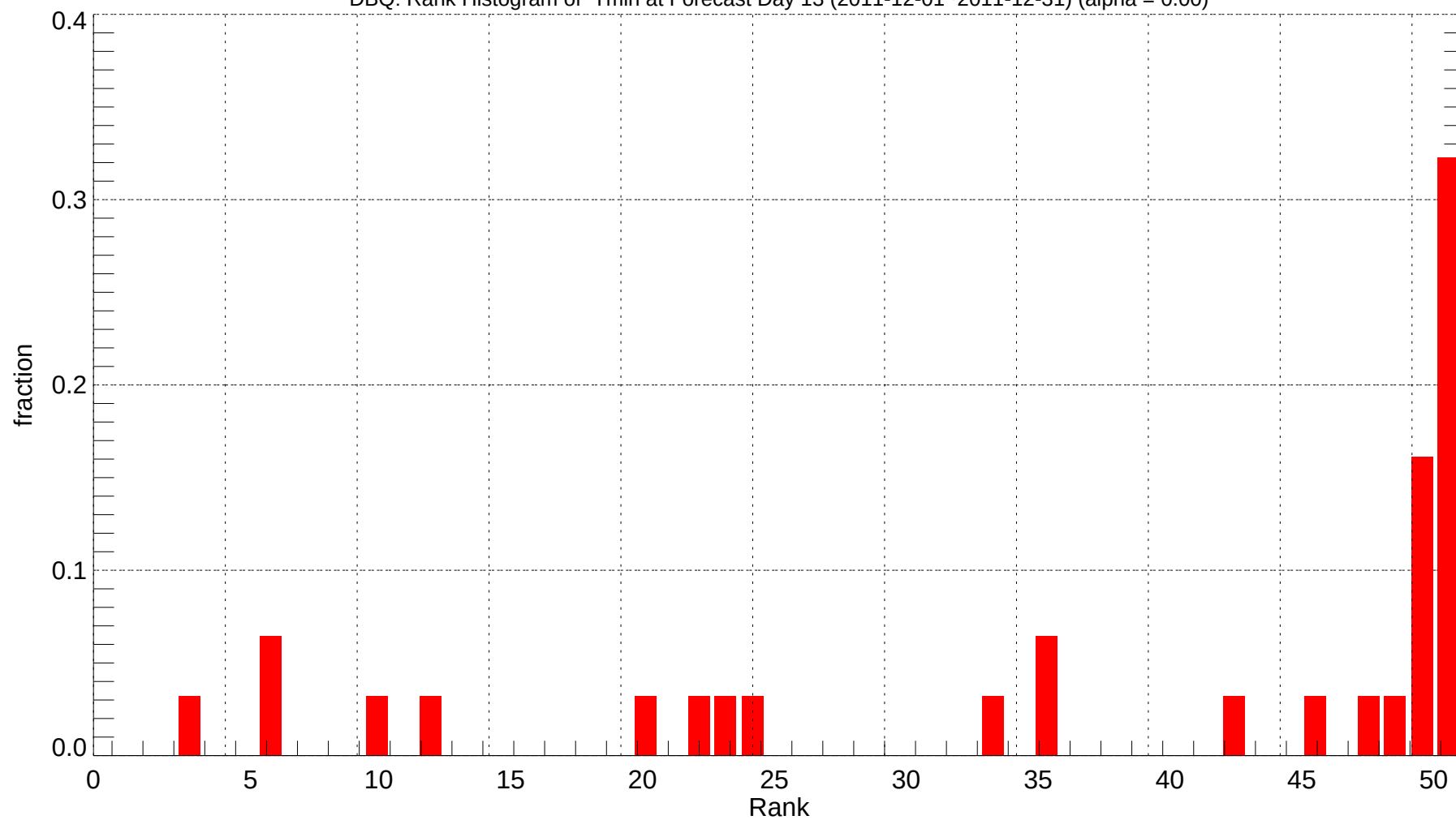
DBQ: Rank Histogram of Tmin at Forecast Day 13 (2011-12-01~2011-12-31) (alpha = 0.00)
