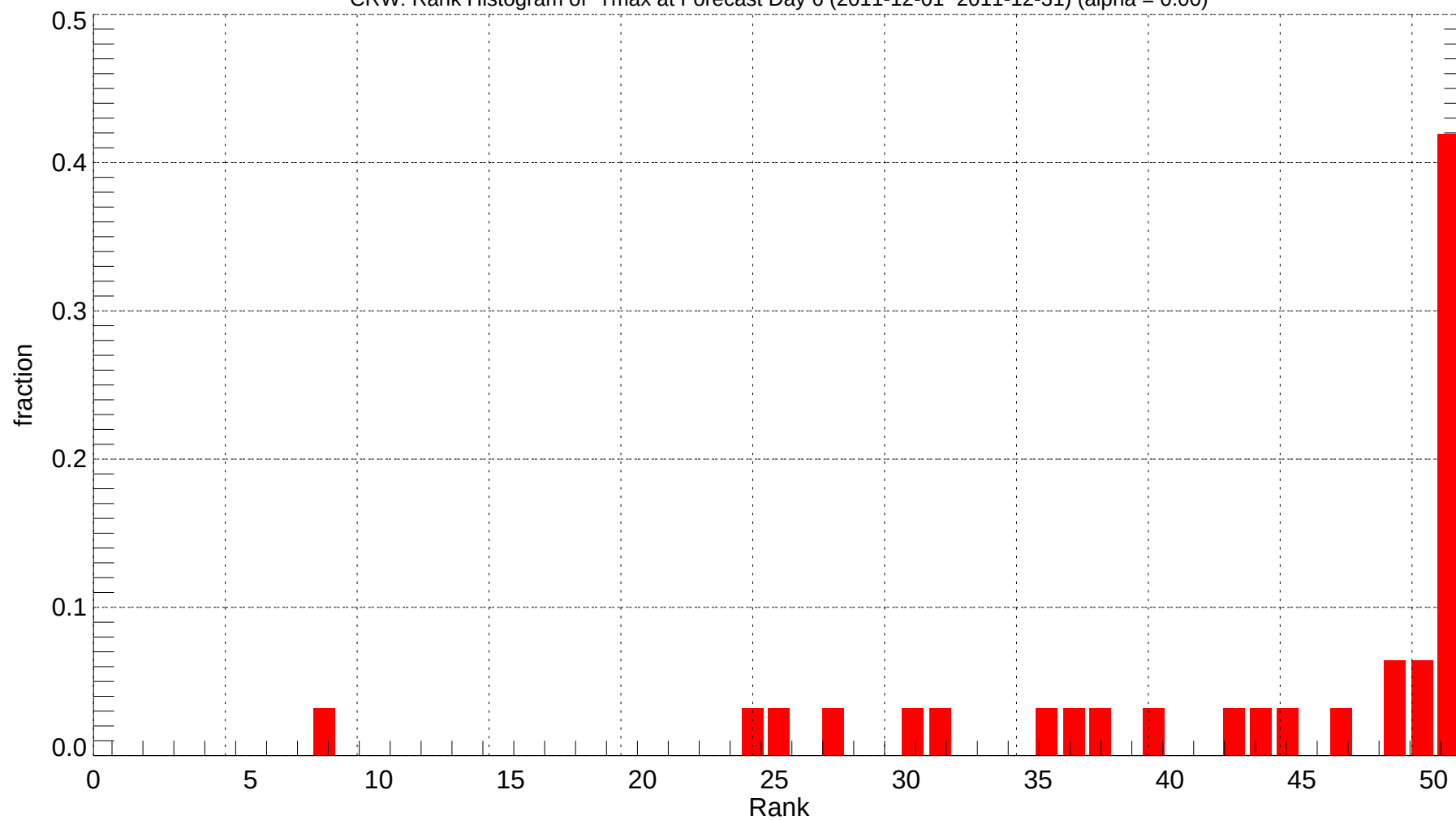
CRW: Rank Histogram of Tmax at Forecast Day 6 (2011-12-01~2011-12-31) (alpha = 0.00)
