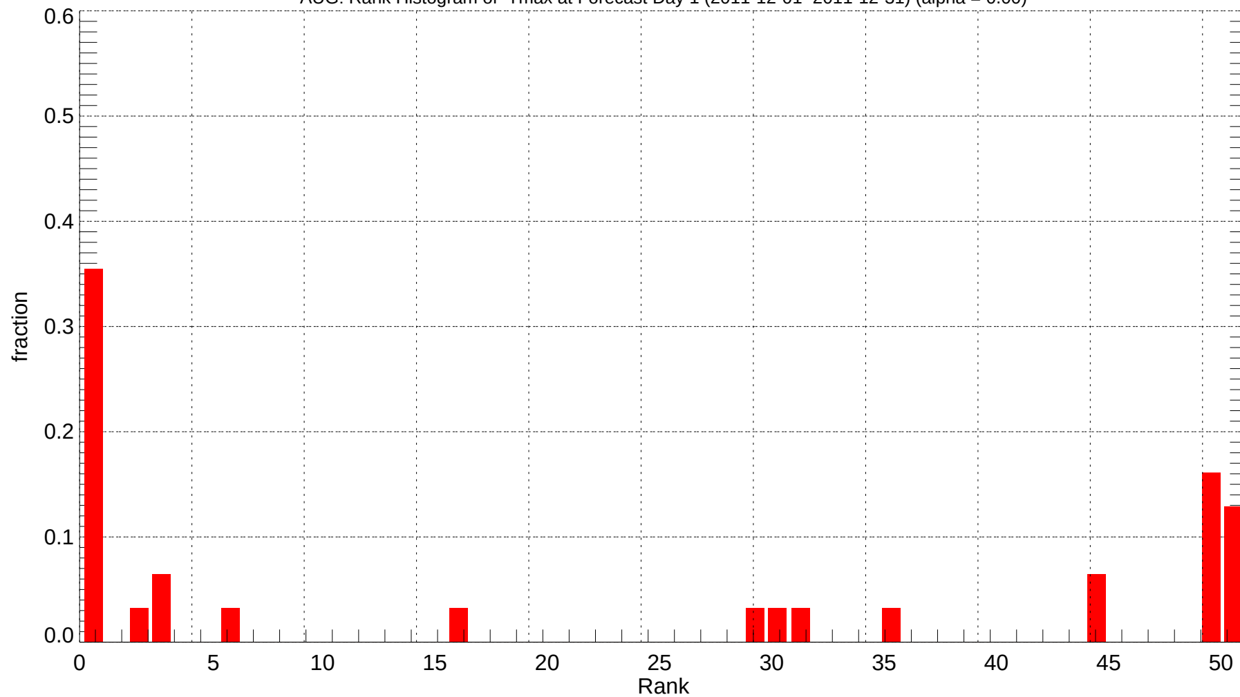
AUG: Rank Histogram of Tmax at Forecast Day 1 (2011-12-01~2011-12-31) (alpha = 0.00)
