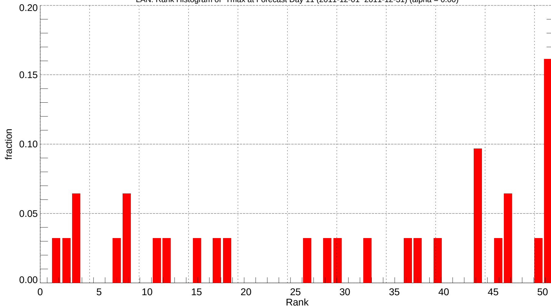
LAN: Rank Histogram of Tmax at Forecast Day 11 (2011-12-01~2011-12-31) (alpha = 0.00)
