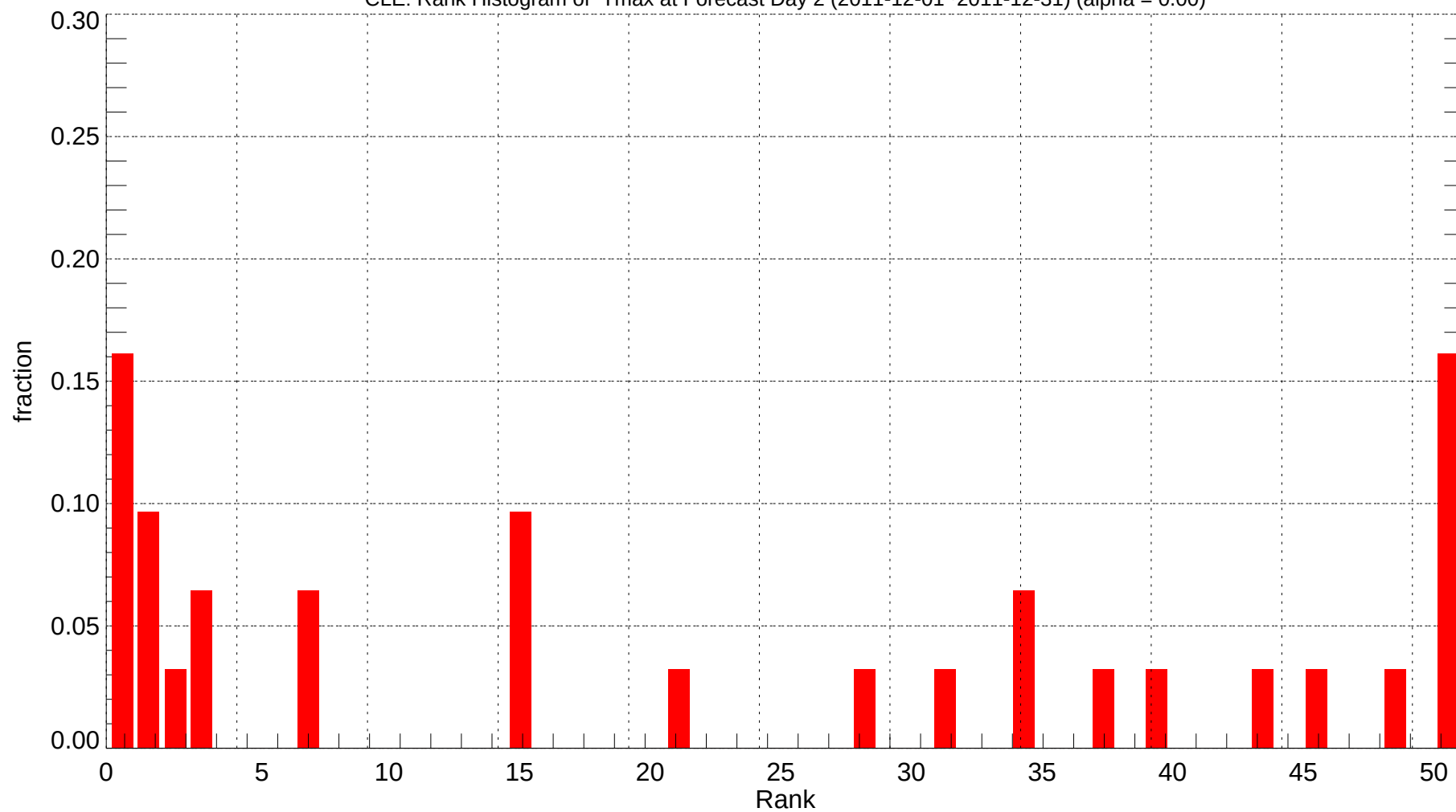
CLE: Rank Histogram of Tmax at Forecast Day 2 (2011-12-01~2011-12-31) (alpha = 0.00)
