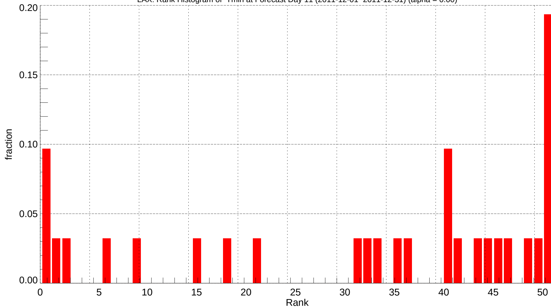
LAX: Rank Histogram of Tmin at Forecast Day 11 (2011-12-01~2011-12-31) (alpha = 0.00)
