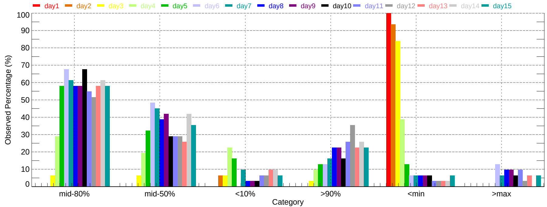
Observed Percentage of Ensembles - JFK: Max Temperature (2011-12-01~2011-12-31)
