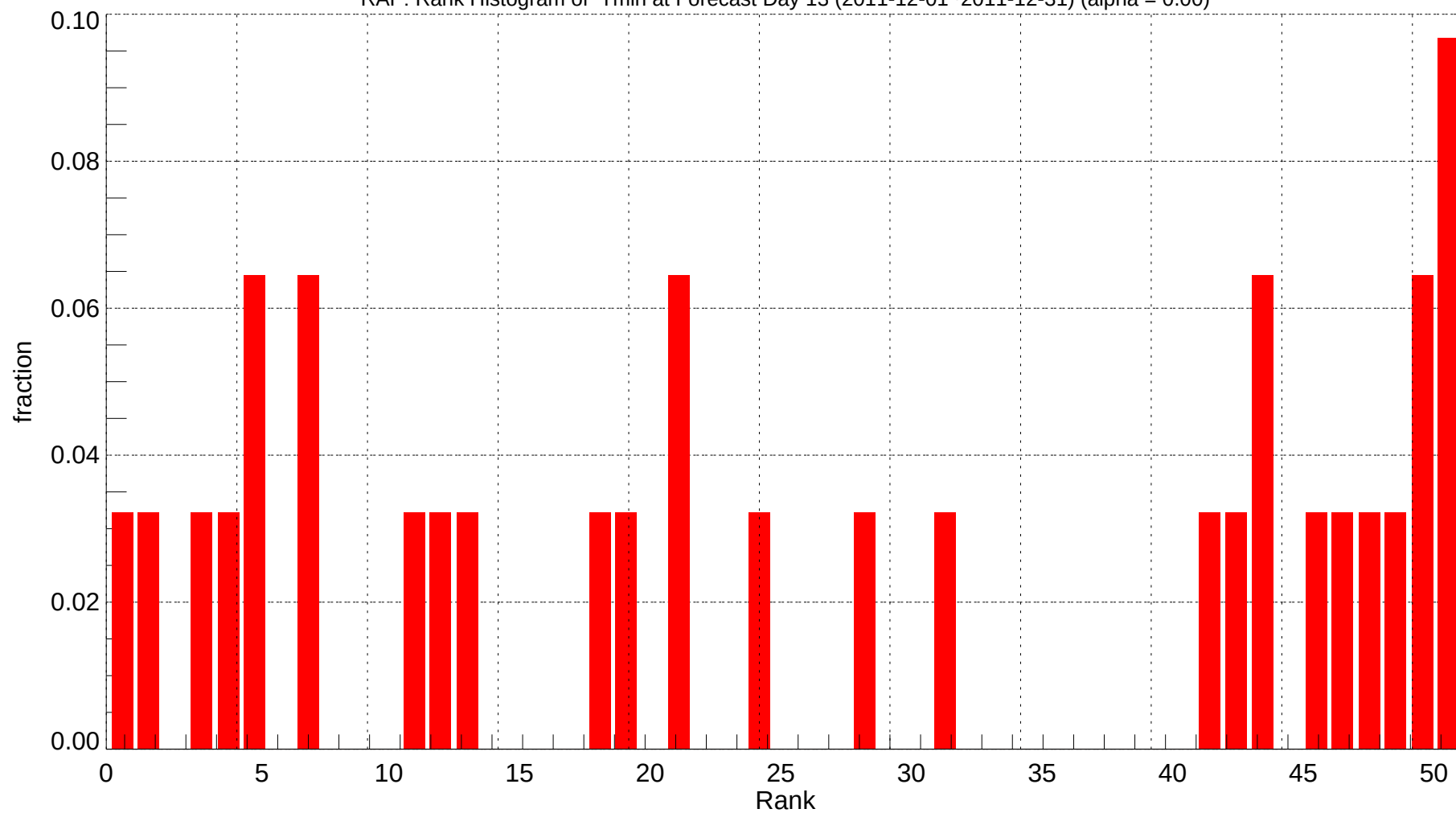
RAP: Rank Histogram of Tmin at Forecast Day 13 (2011-12-01~2011-12-31) (alpha = 0.00)
