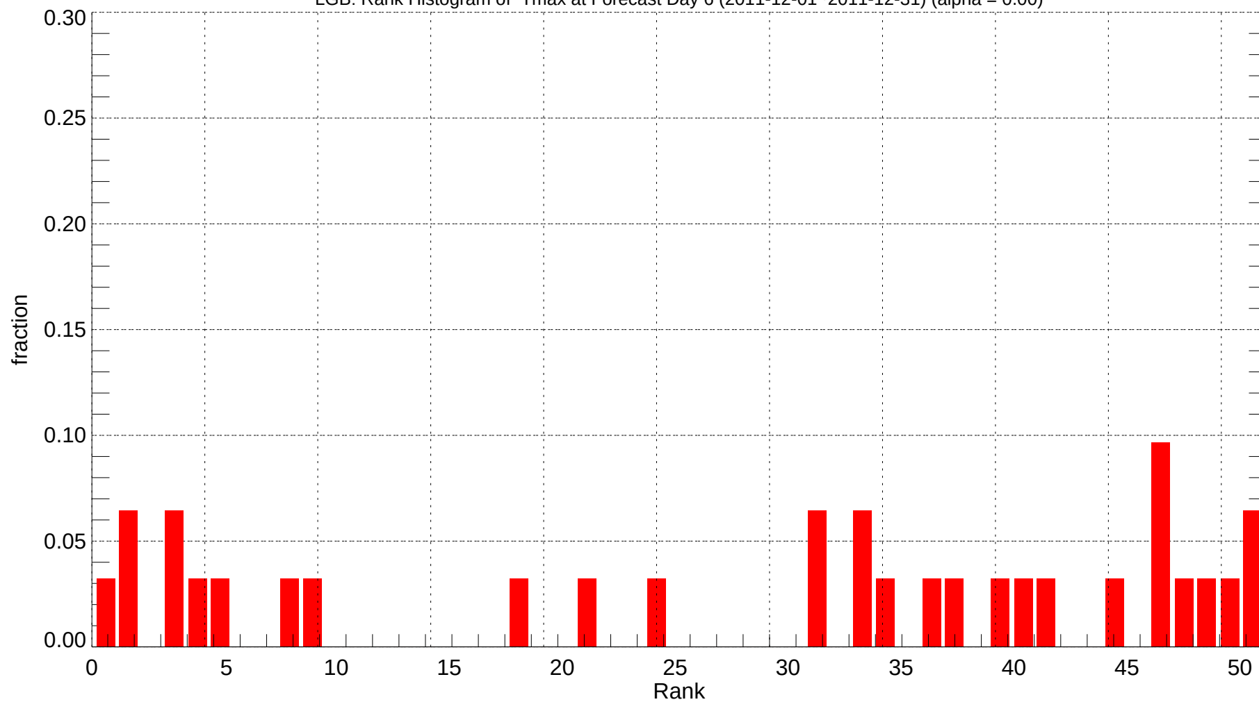
LGB: Rank Histogram of Tmax at Forecast Day 6 (2011-12-01~2011-12-31) (alpha = 0.00)
