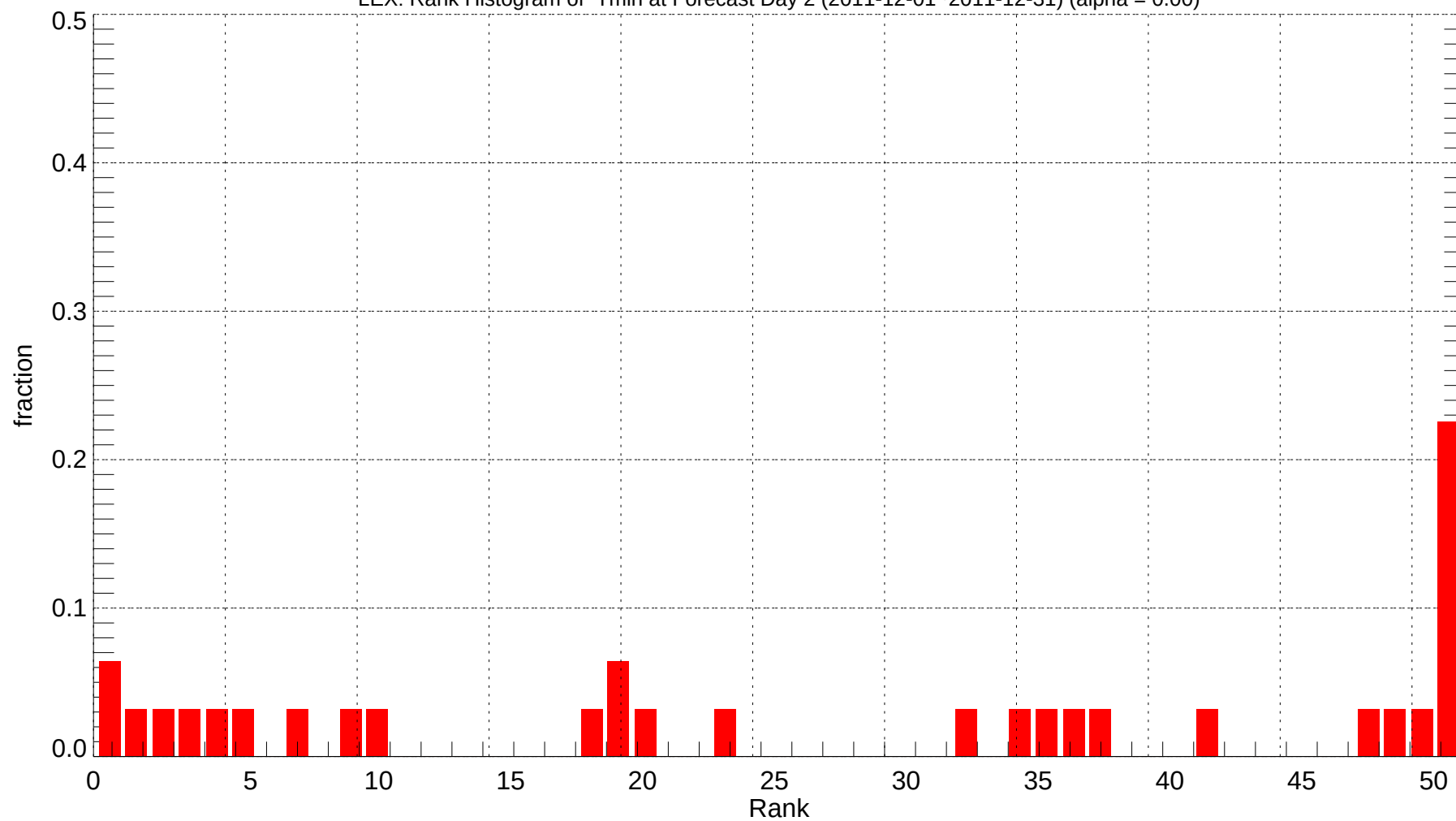
LEX: Rank Histogram of Tmin at Forecast Day 2 (2011-12-01~2011-12-31) (alpha = 0.00)
