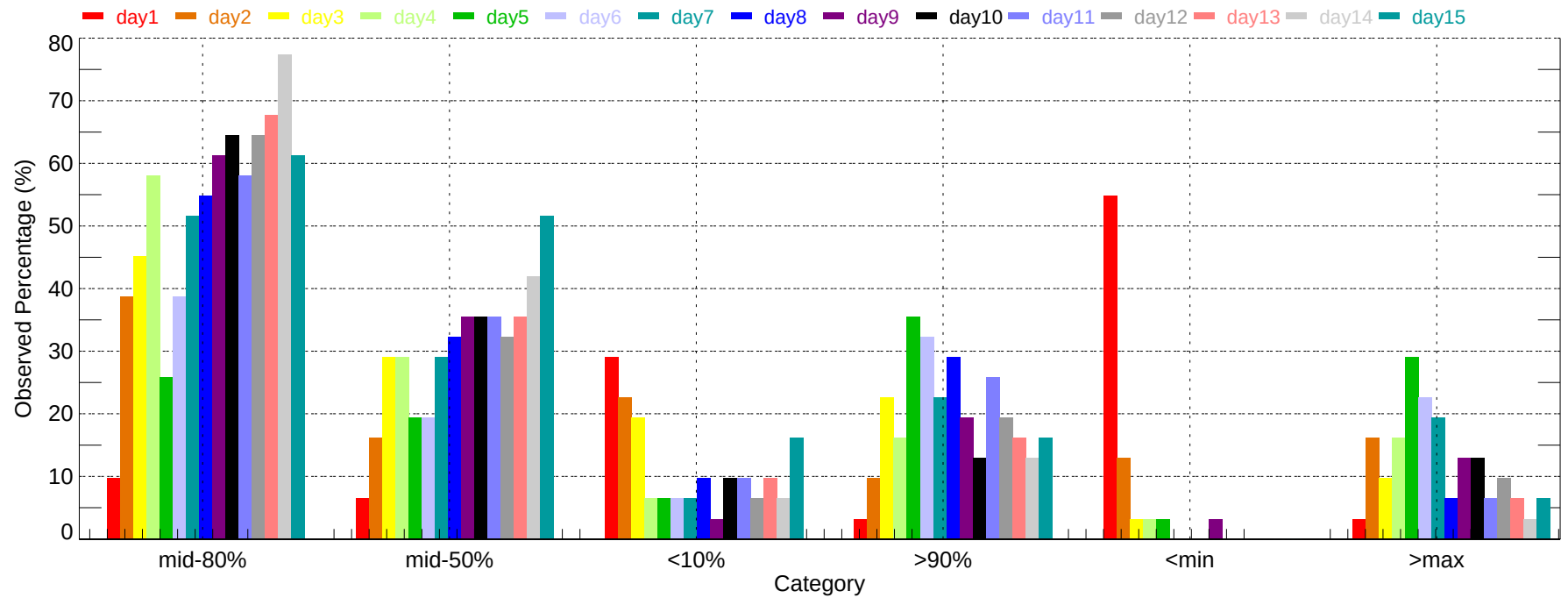
Observed Percentage of Ensembles - AVP: Max Temperature (2011-12-01~2011-12-31)
