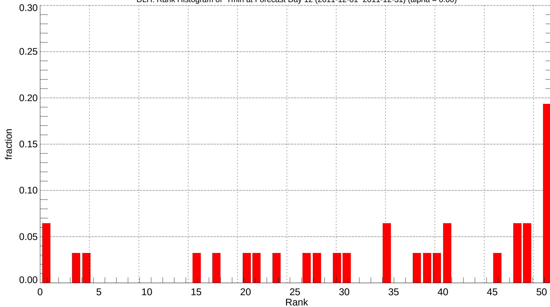
DLH: Rank Histogram of Tmin at Forecast Day 12 (2011-12-01~2011-12-31) (alpha = 0.00)
