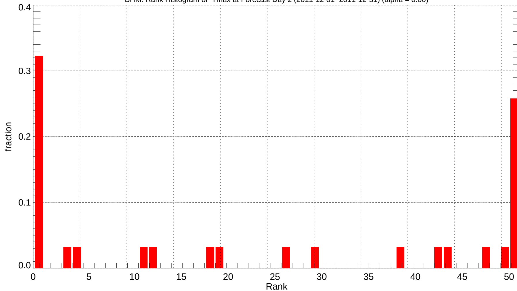
BHM: Rank Histogram of Tmax at Forecast Day 2 (2011-12-01~2011-12-31) (alpha = 0.00)
