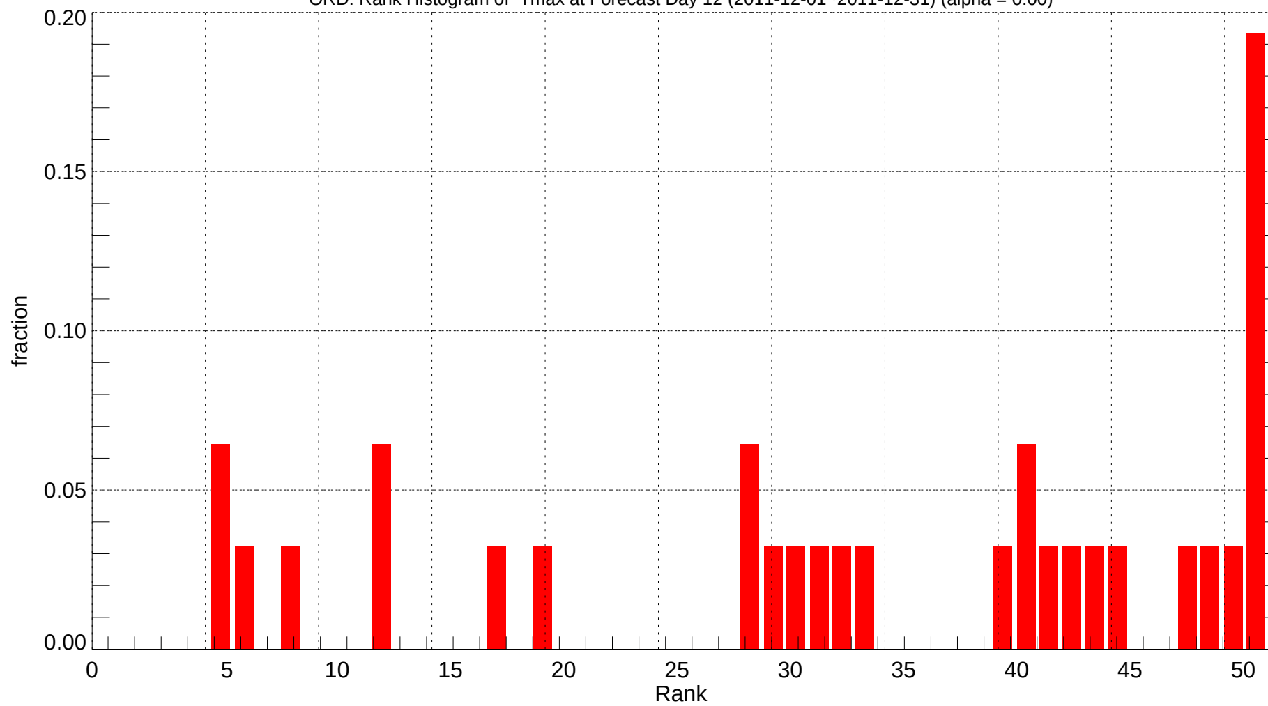
ORD: Rank Histogram of Tmax at Forecast Day 12 (2011-12-01~2011-12-31) (alpha = 0.00)
