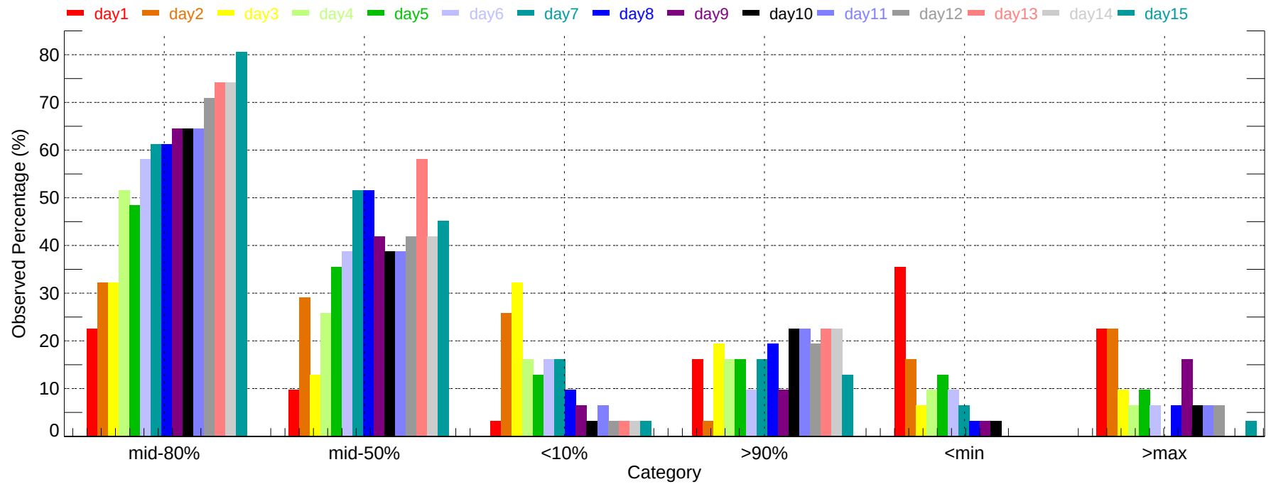
Observed Percentage of Ensembles - DAY: Max Temperature (2011-12-01~2011-12-31)
