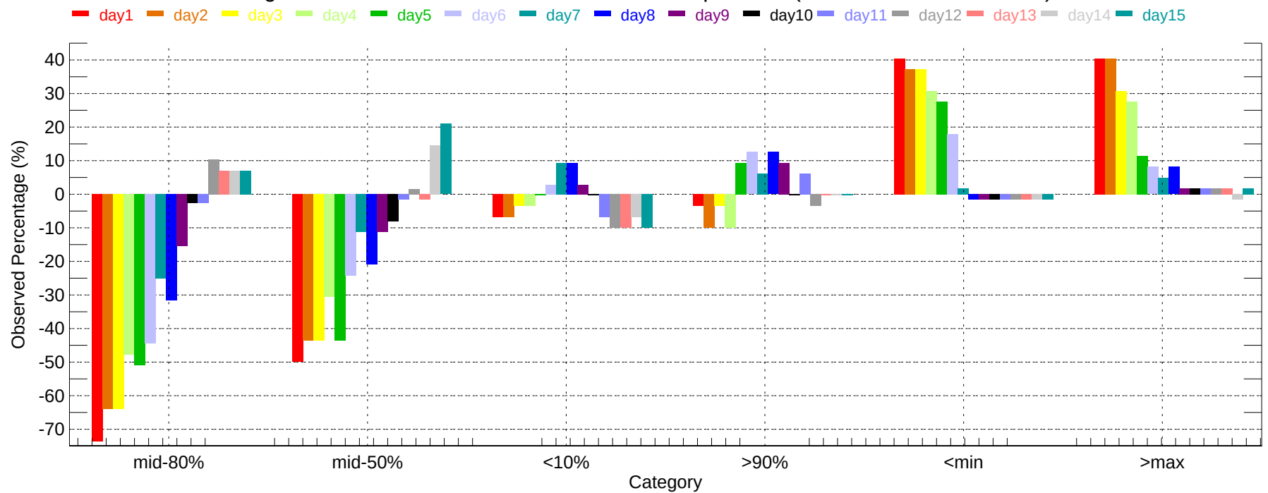
Observed Percentage Deviation of Ensembles - GEG: Min Temperature (2011-12-01~2011-12-31)
