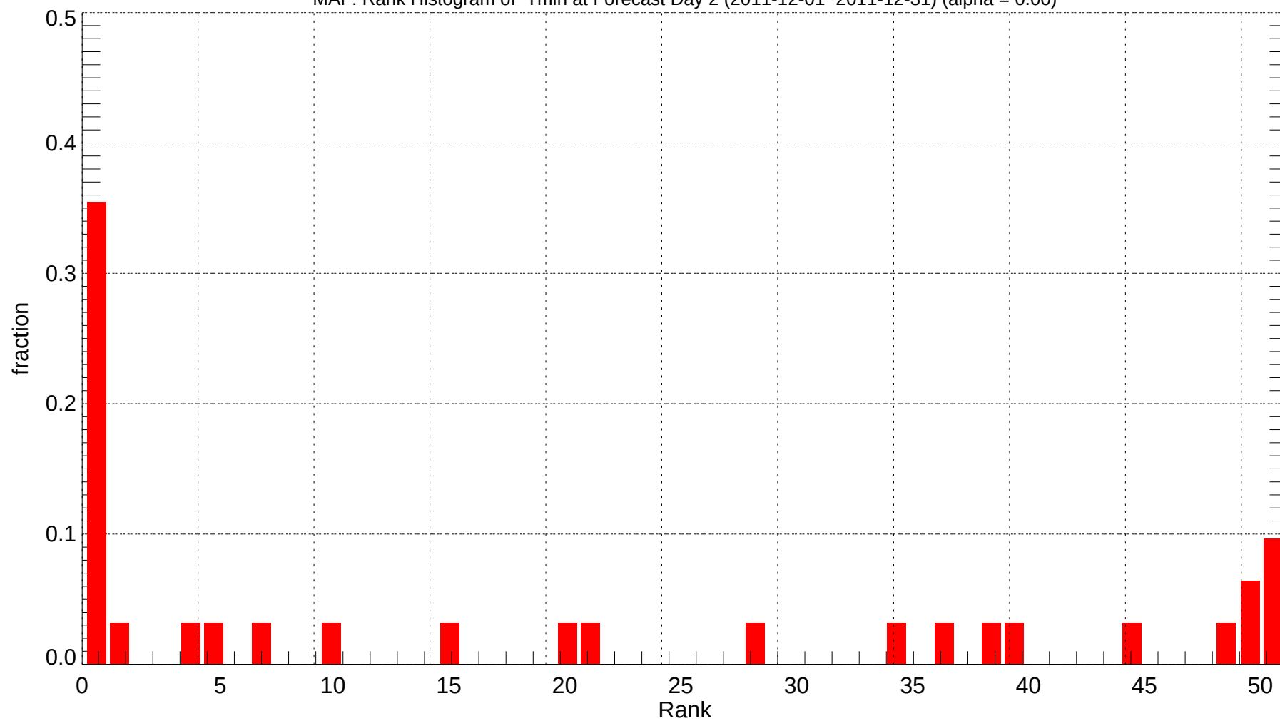
MAF: Rank Histogram of Tmin at Forecast Day 2 (2011-12-01~2011-12-31) (alpha = 0.00)
