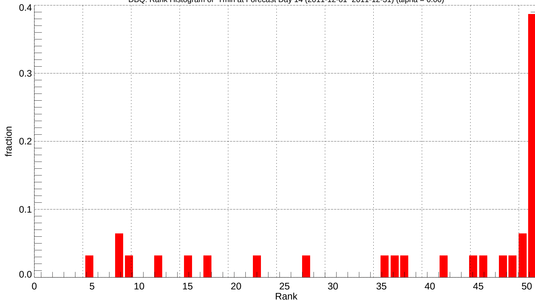
DBQ: Rank Histogram of Tmin at Forecast Day 14 (2011-12-01~2011-12-31) (alpha = 0.00)
