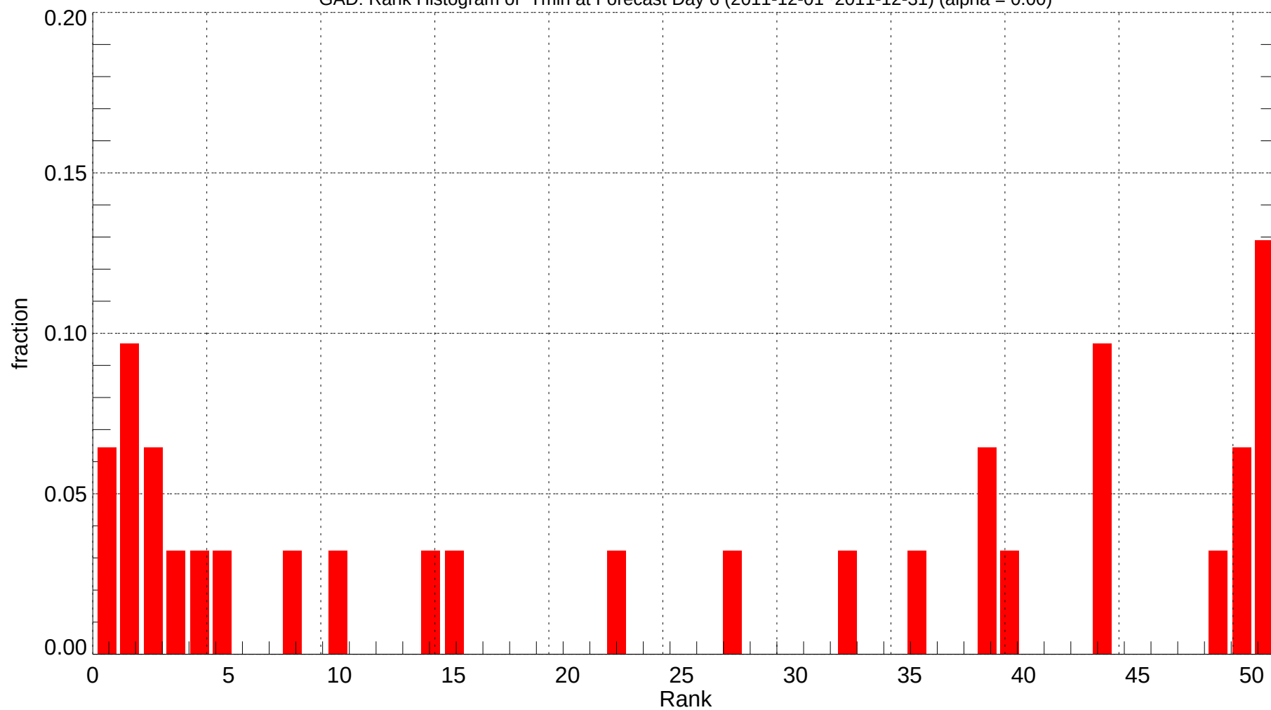
GAD: Rank Histogram of Tmin at Forecast Day 6 (2011-12-01~2011-12-31) (alpha = 0.00)
