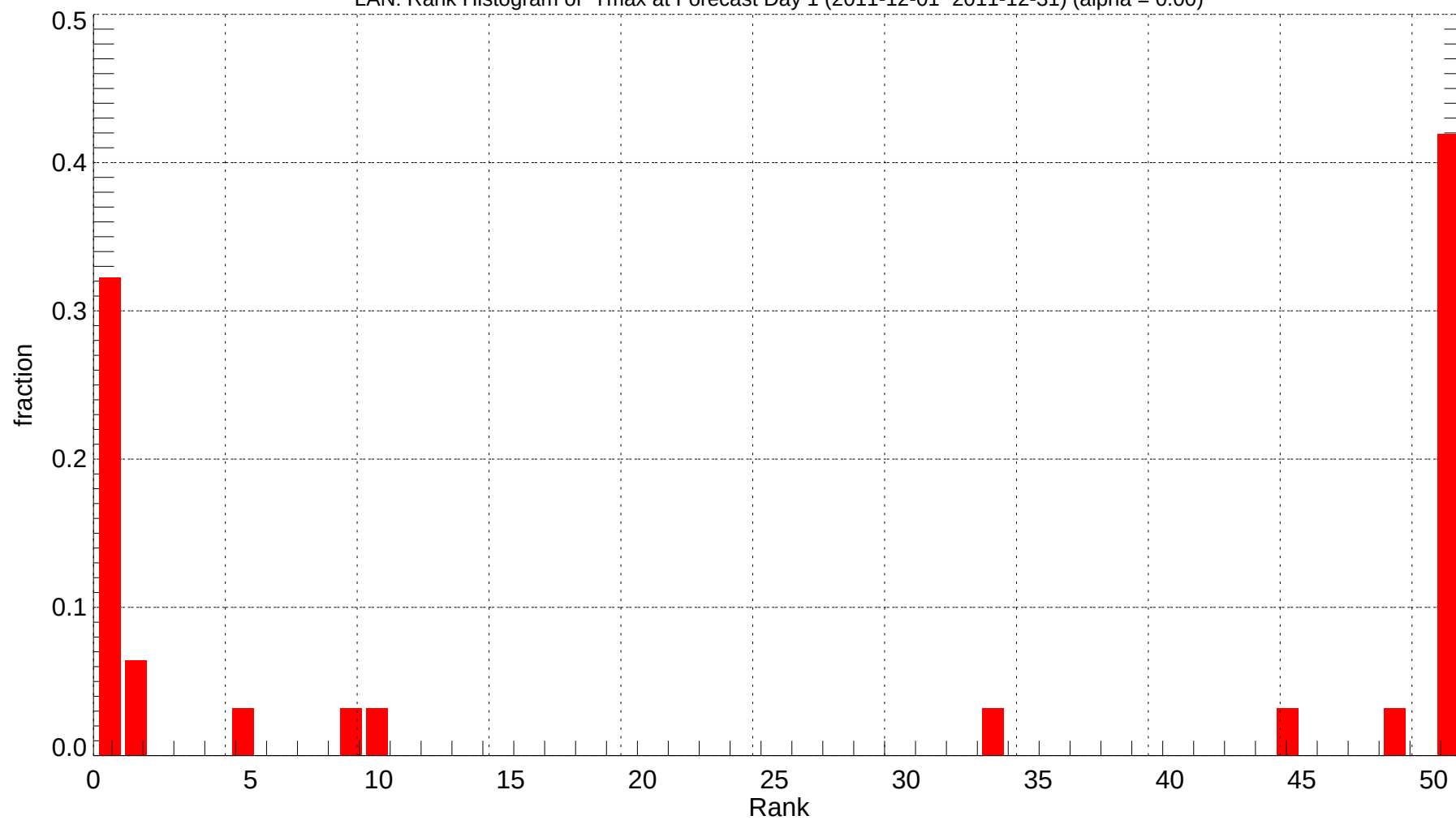
LAN: Rank Histogram of Tmax at Forecast Day 1 (2011-12-01~2011-12-31) (alpha = 0.00)
