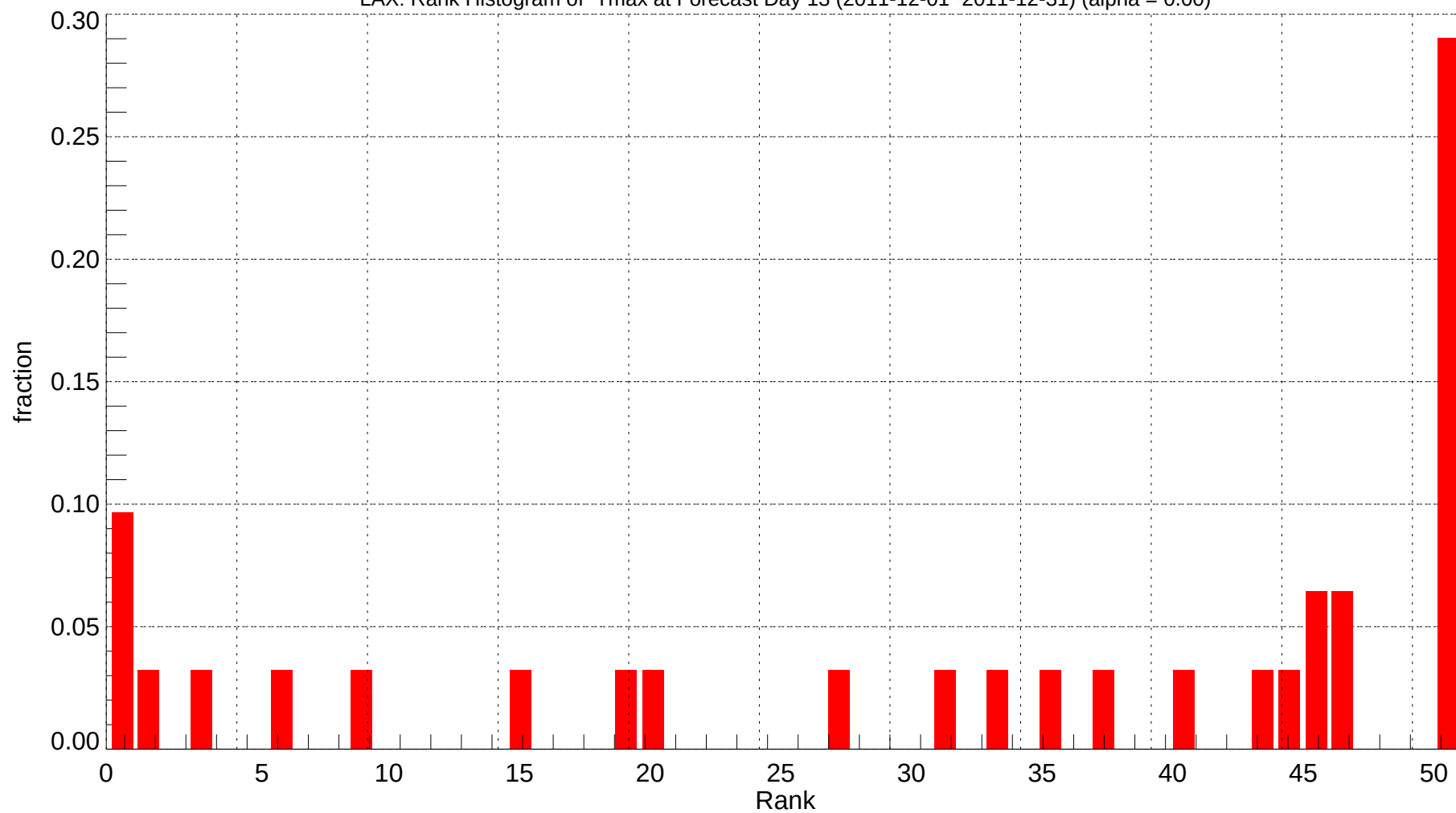
LAX: Rank Histogram of Tmax at Forecast Day 13 (2011-12-01~2011-12-31) (alpha = 0.00)
