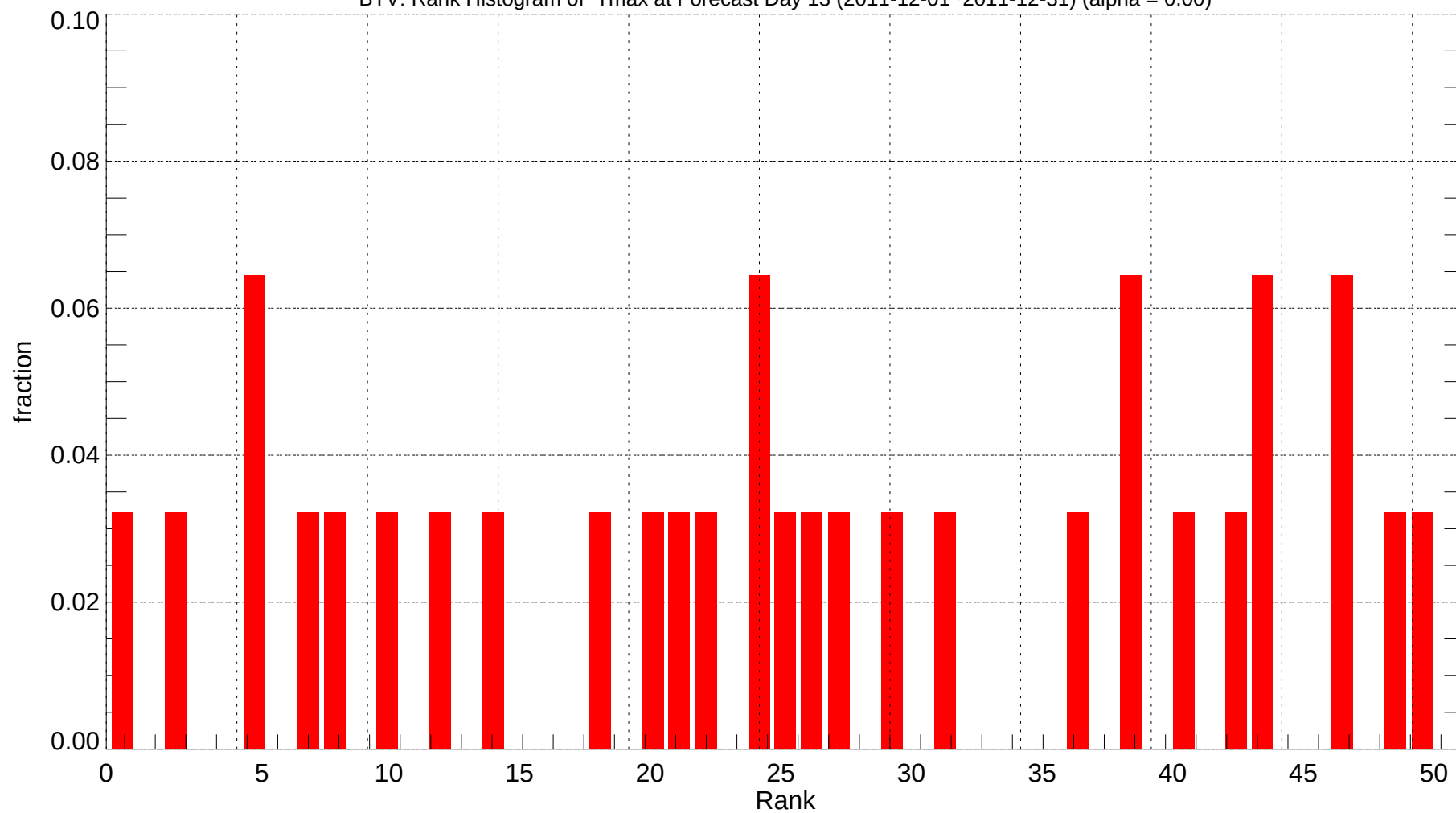
BTV: Rank Histogram of Tmax at Forecast Day 13 (2011-12-01~2011-12-31) (alpha = 0.00)
