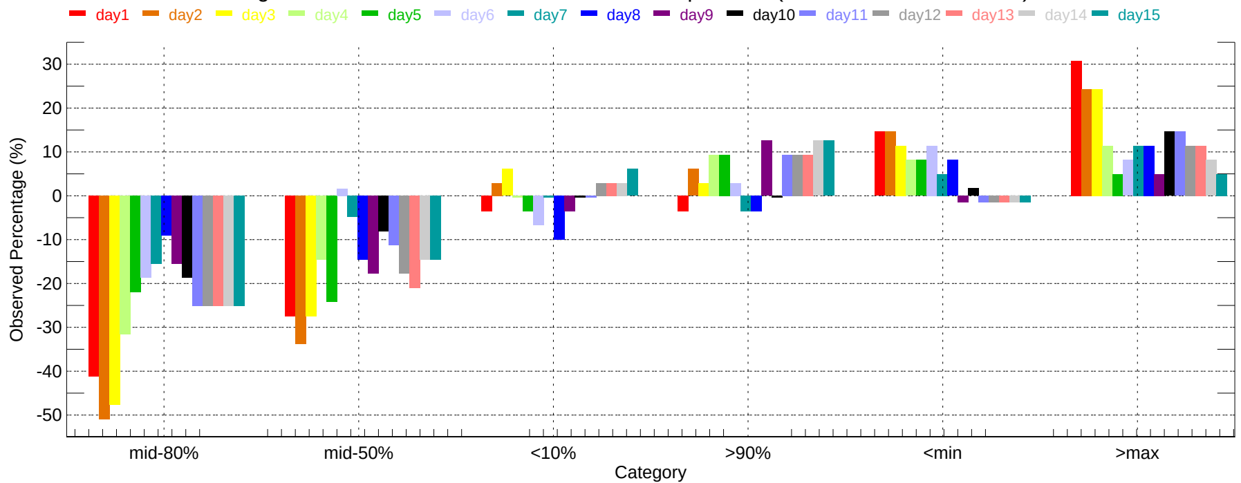
Observed Percentage Deviation of Ensembles - SAT: Max Temperature (2011-12-01~2011-12-31)
