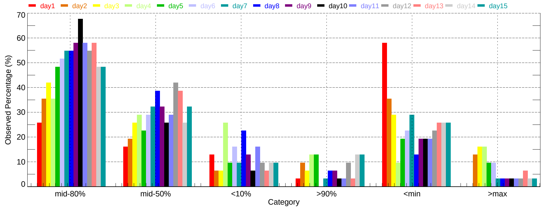
Observed Percentage of Ensembles - MAF: Max Temperature (2011-12-01~2011-12-31)
