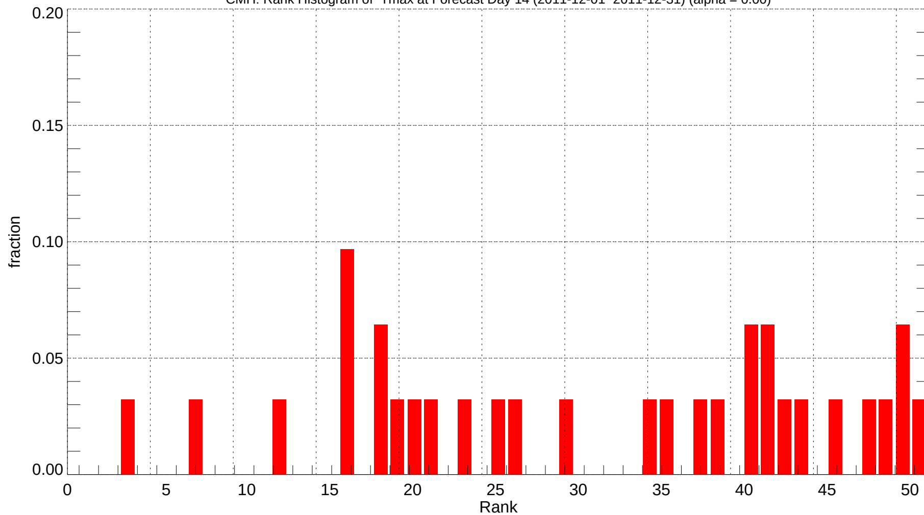
CMH: Rank Histogram of Tmax at Forecast Day 14 (2011-12-01~2011-12-31) (alpha = 0.00)
