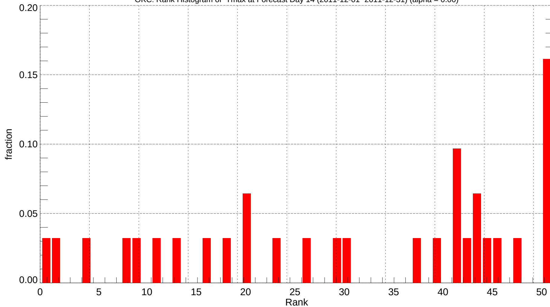
OKC: Rank Histogram of Tmax at Forecast Day 14 (2011-12-01~2011-12-31) (alpha = 0.00)
