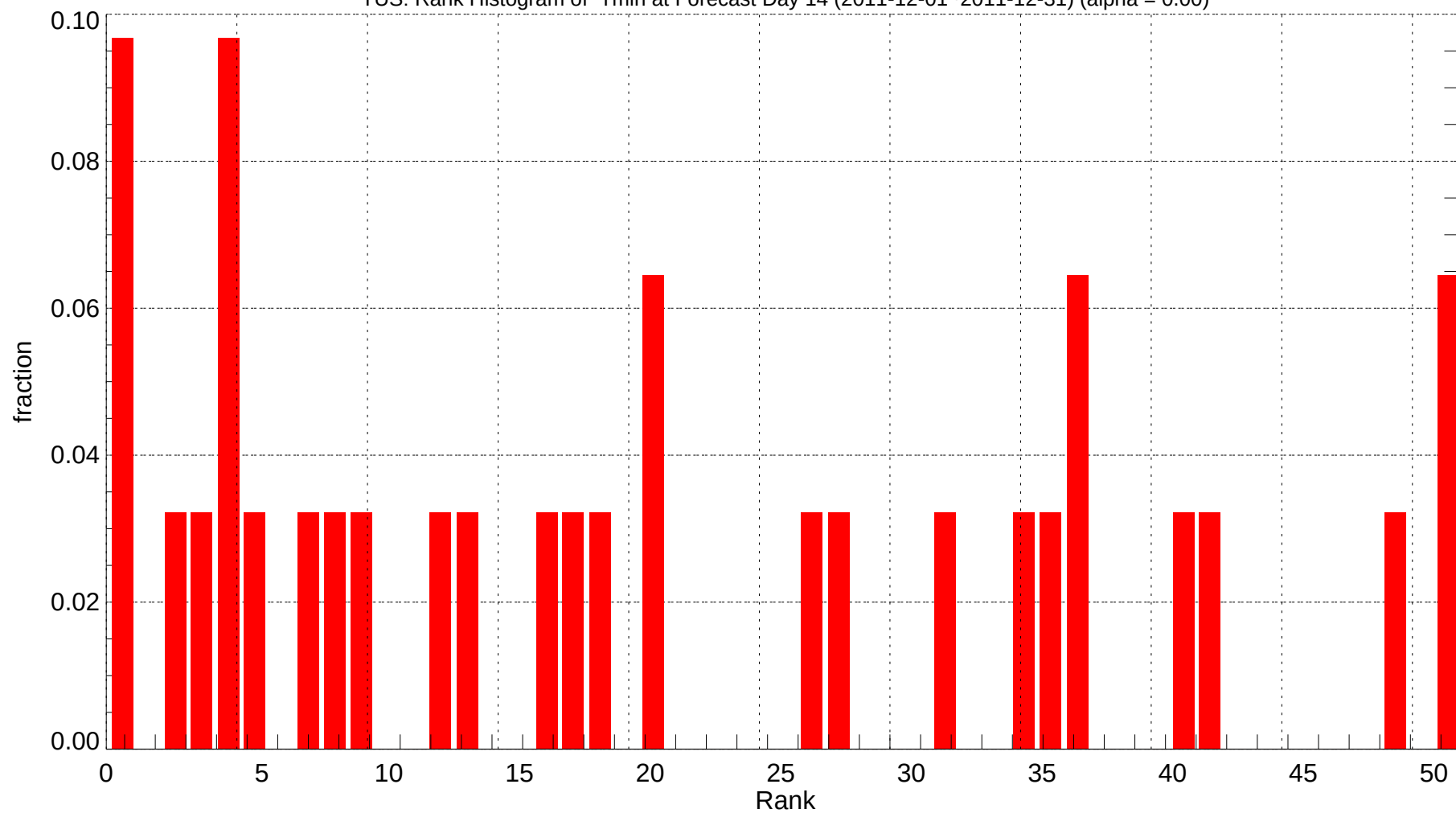
TUS: Rank Histogram of Tmin at Forecast Day 14 (2011-12-01~2011-12-31) (alpha = 0.00)
