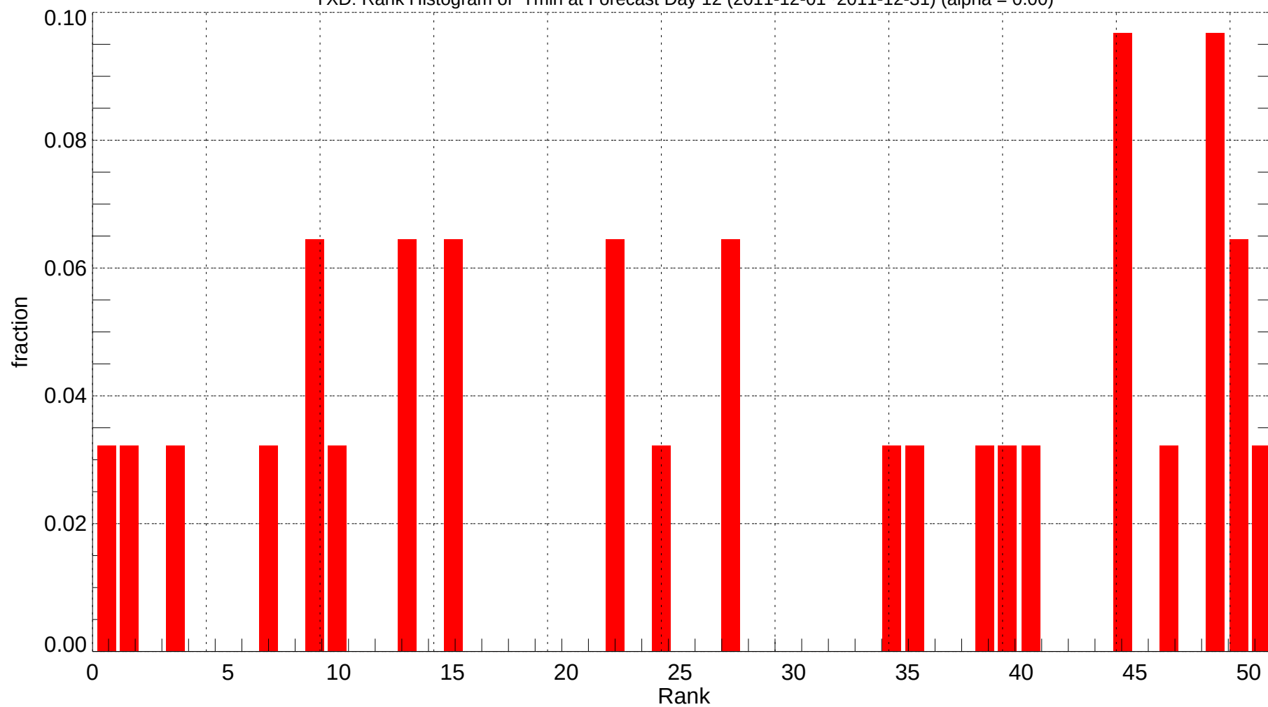
YXD: Rank Histogram of Tmin at Forecast Day 12 (2011-12-01~2011-12-31) (alpha = 0.00)
