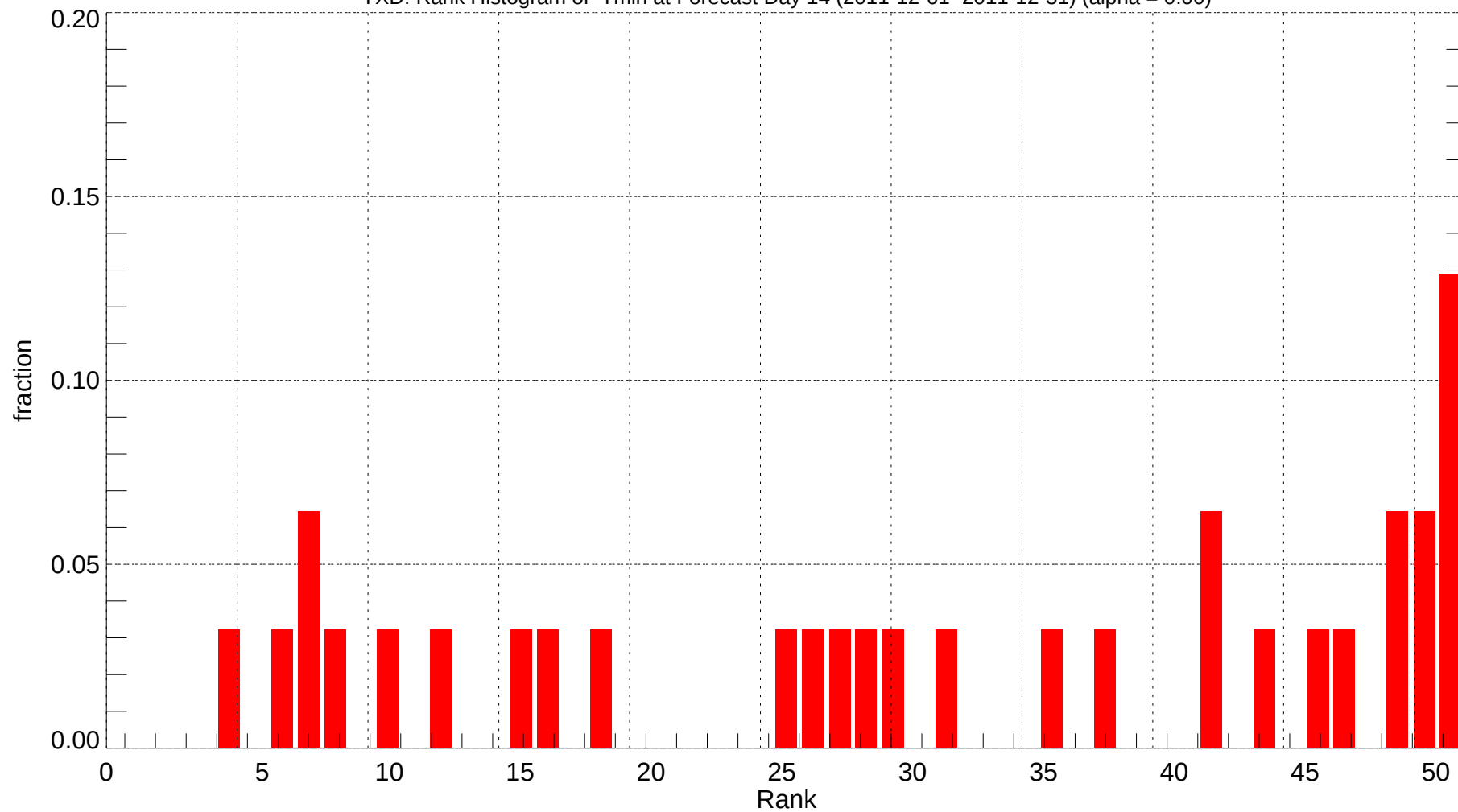
YXD: Rank Histogram of Tmin at Forecast Day 14 (2011-12-01~2011-12-31) (alpha = 0.00)
