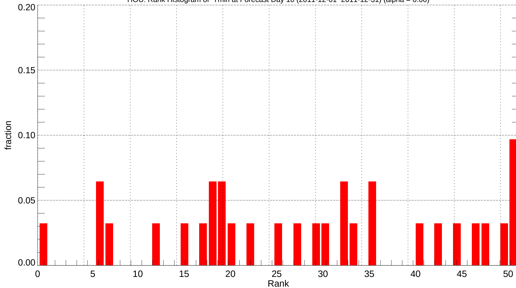
HOU: Rank Histogram of Tmin at Forecast Day 10 (2011-12-01~2011-12-31) (alpha = 0.00)
