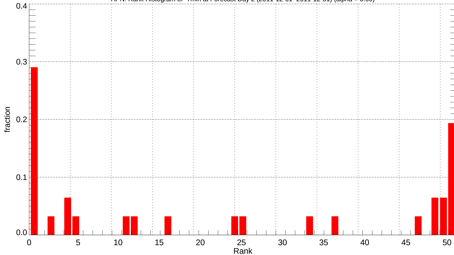
APN: Rank Histogram of Tmin at Forecast Day 2 (2011-12-01~2011-12-31) (alpha = 0.00)
