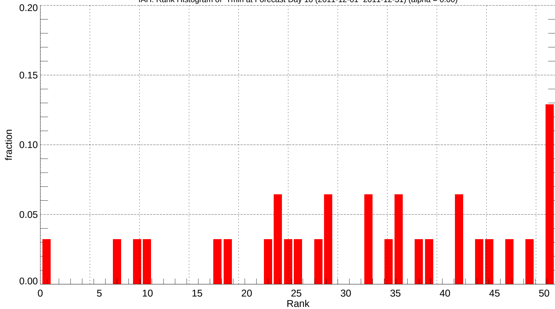
IAH: Rank Histogram of Tmin at Forecast Day 10 (2011-12-01~2011-12-31) (alpha = 0.00)
