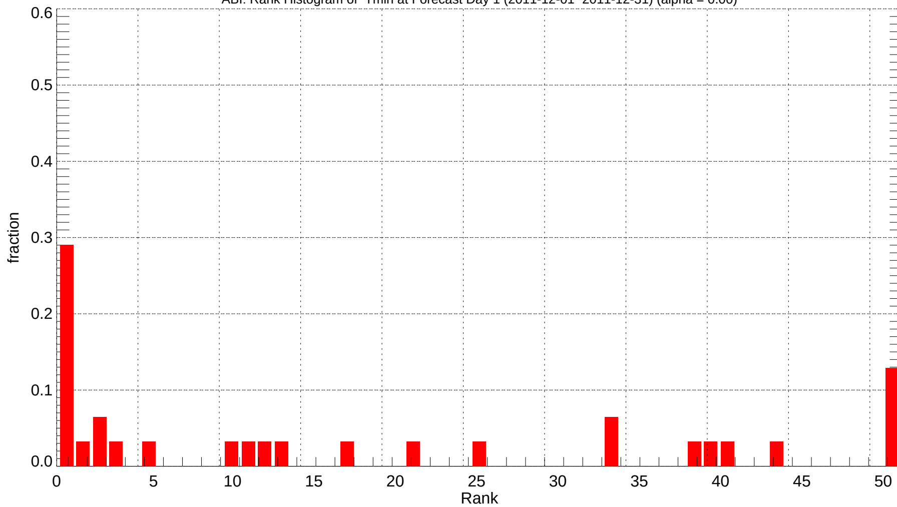
ABI: Rank Histogram of Tmin at Forecast Day 1 (2011-12-01~2011-12-31) (alpha = 0.00)
