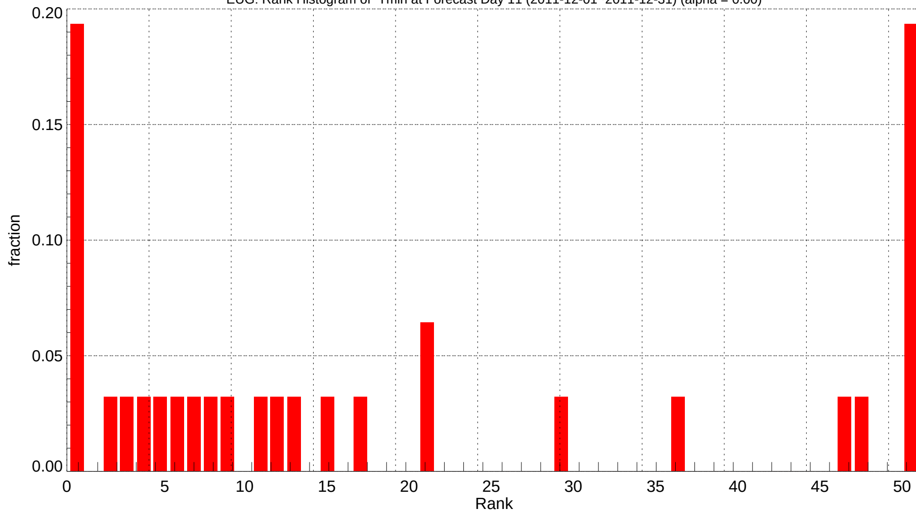
EUG: Rank Histogram of Tmin at Forecast Day 11 (2011-12-01~2011-12-31) (alpha = 0.00)
