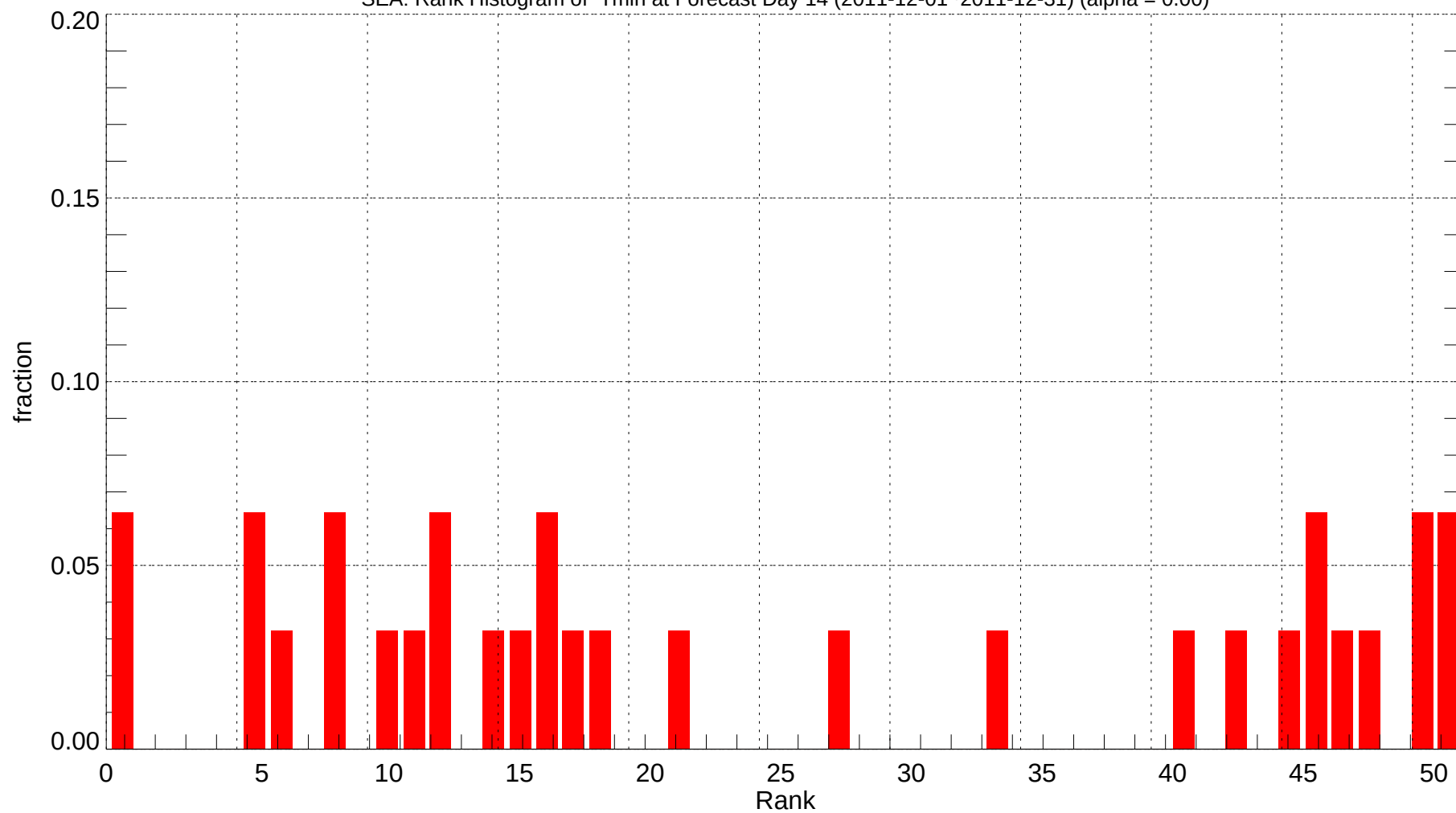
SEA: Rank Histogram of Tmin at Forecast Day 14 (2011-12-01~2011-12-31) (alpha = 0.00)
