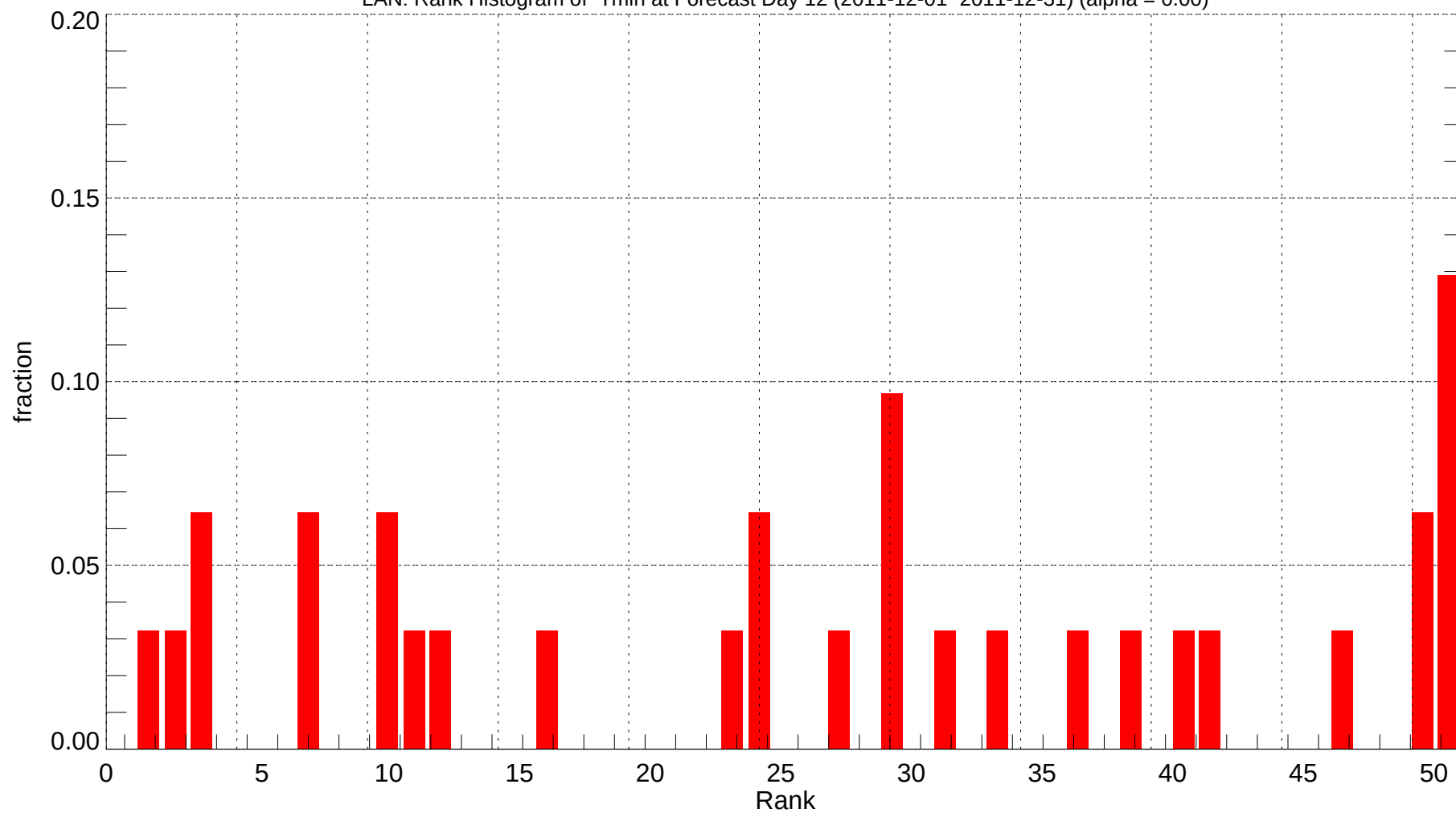
LAN: Rank Histogram of Tmin at Forecast Day 12 (2011-12-01~2011-12-31) (alpha = 0.00)
