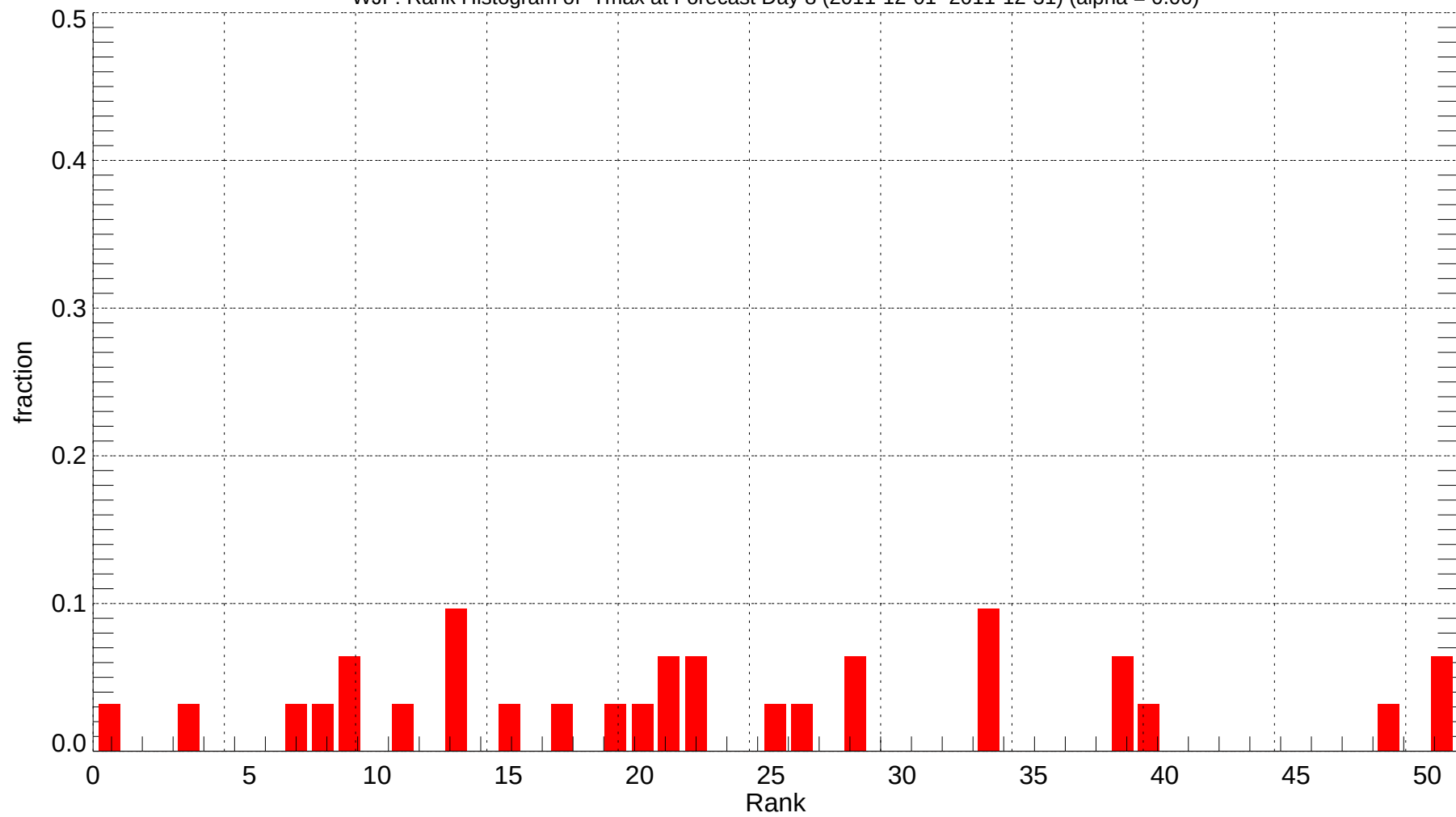
WJF: Rank Histogram of Tmax at Forecast Day 8 (2011-12-01~2011-12-31) (alpha = 0.00)
