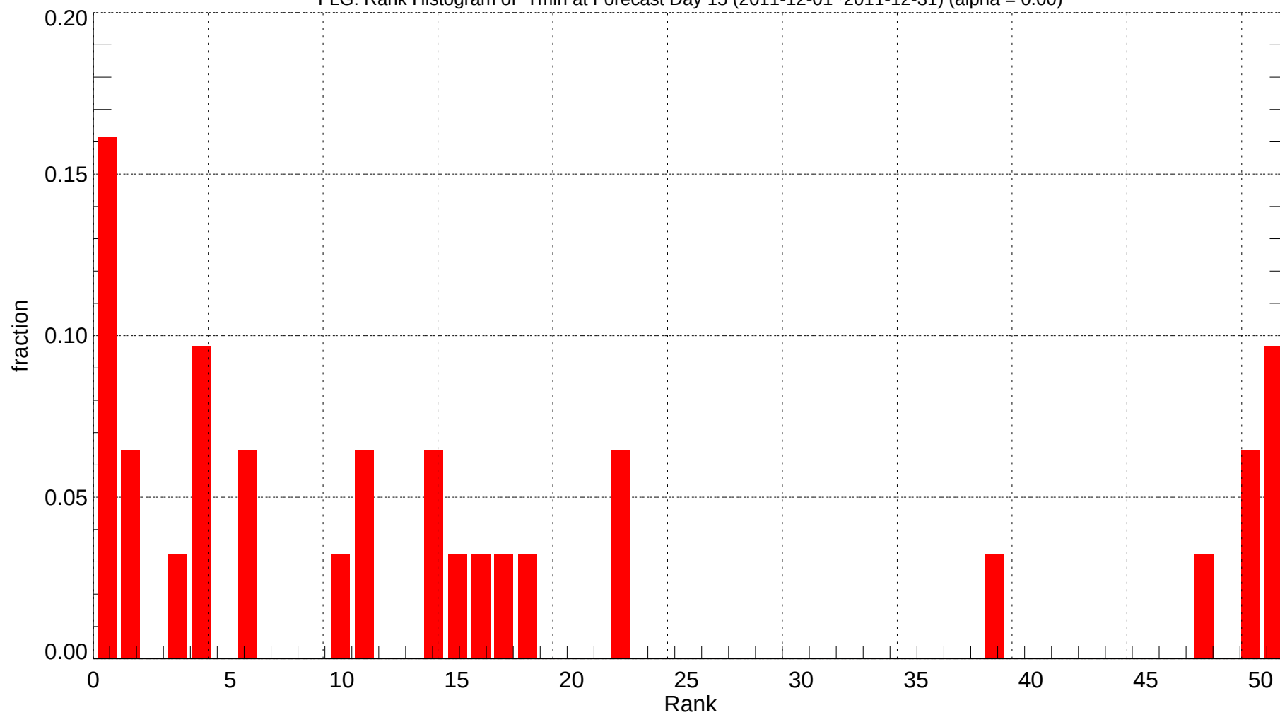
FLG: Rank Histogram of Tmin at Forecast Day 15 (2011-12-01~2011-12-31) (alpha = 0.00)
