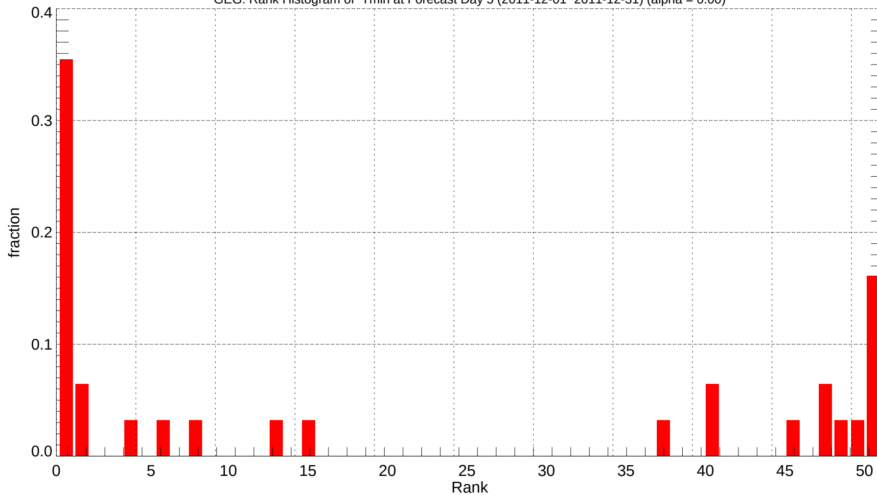
GEG: Rank Histogram of Tmin at Forecast Day 5 (2011-12-01~2011-12-31) (alpha = 0.00)
