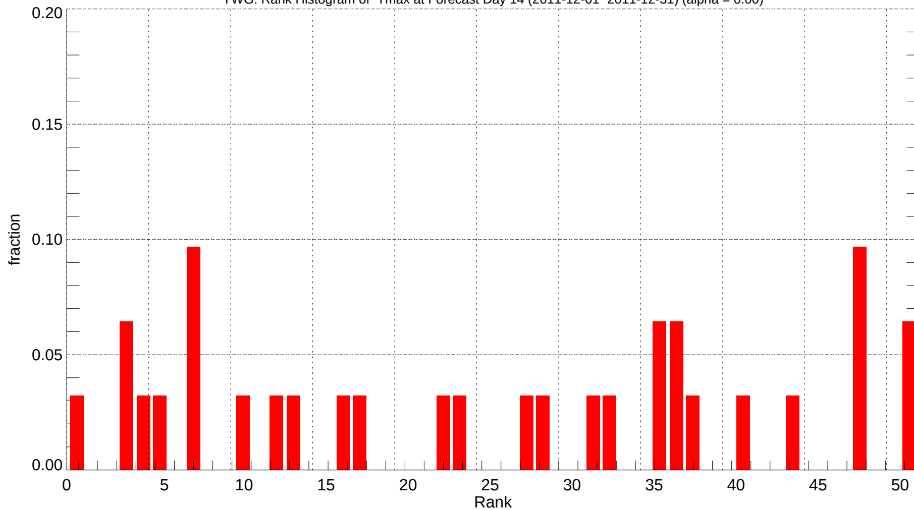
YWG: Rank Histogram of Tmax at Forecast Day 14 (2011-12-01~2011-12-31) (alpha = 0.00)
