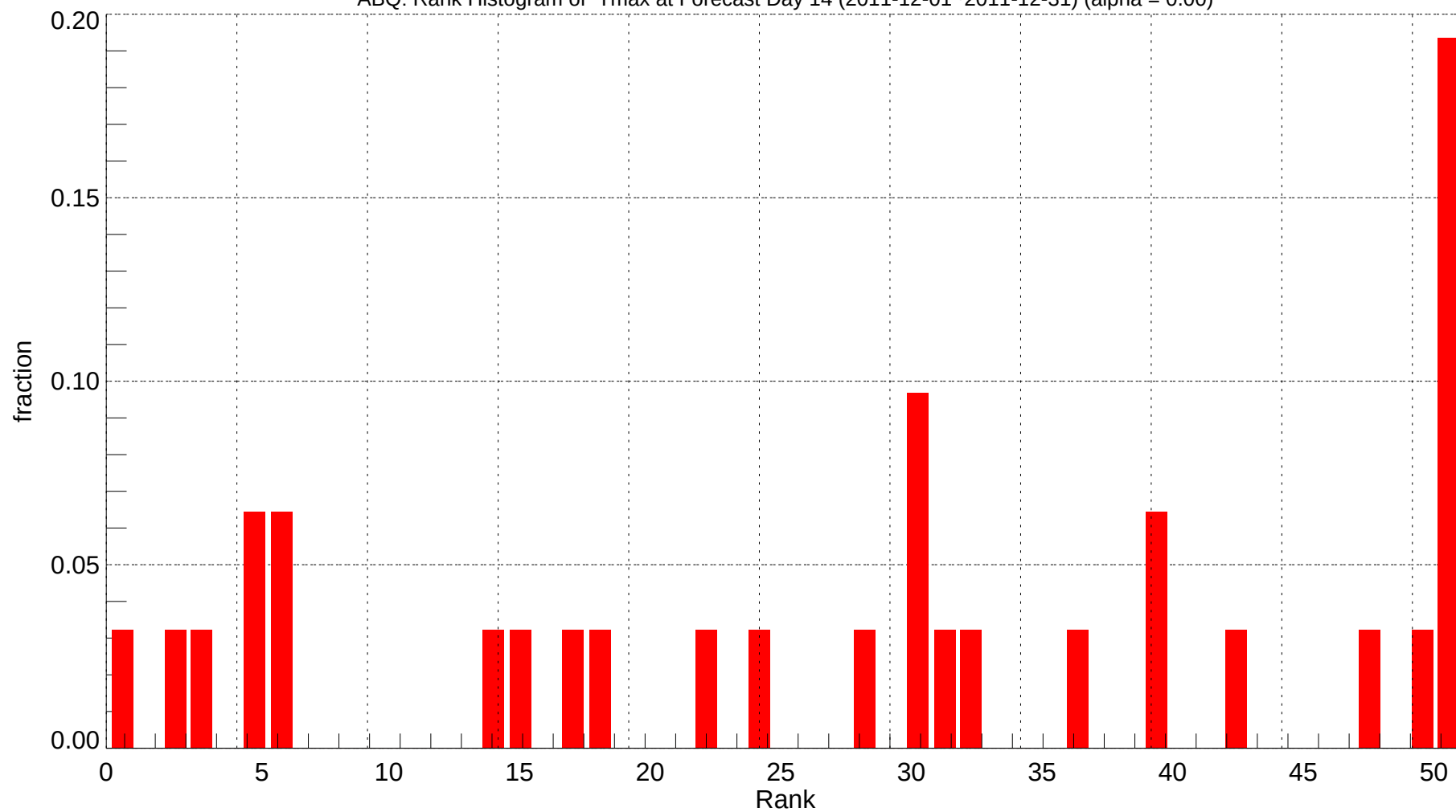
ABQ: Rank Histogram of Tmax at Forecast Day 14 (2011-12-01~2011-12-31) (alpha = 0.00)
