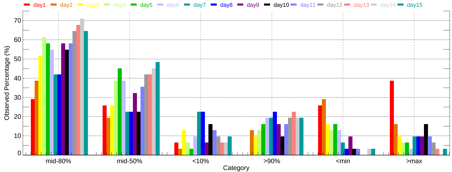
Observed Percentage of Ensembles - MHT: Max Temperature (2011-12-01~2011-12-31)
