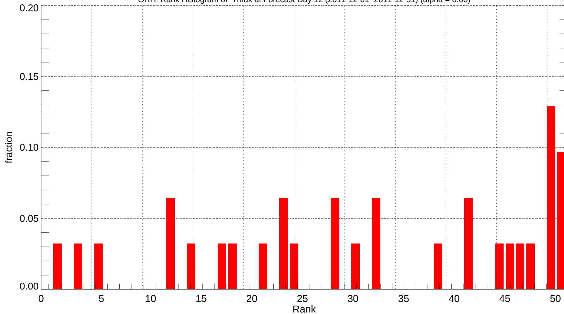
ORH: Rank Histogram of Tmax at Forecast Day 12 (2011-12-01~2011-12-31) (alpha = 0.00)
