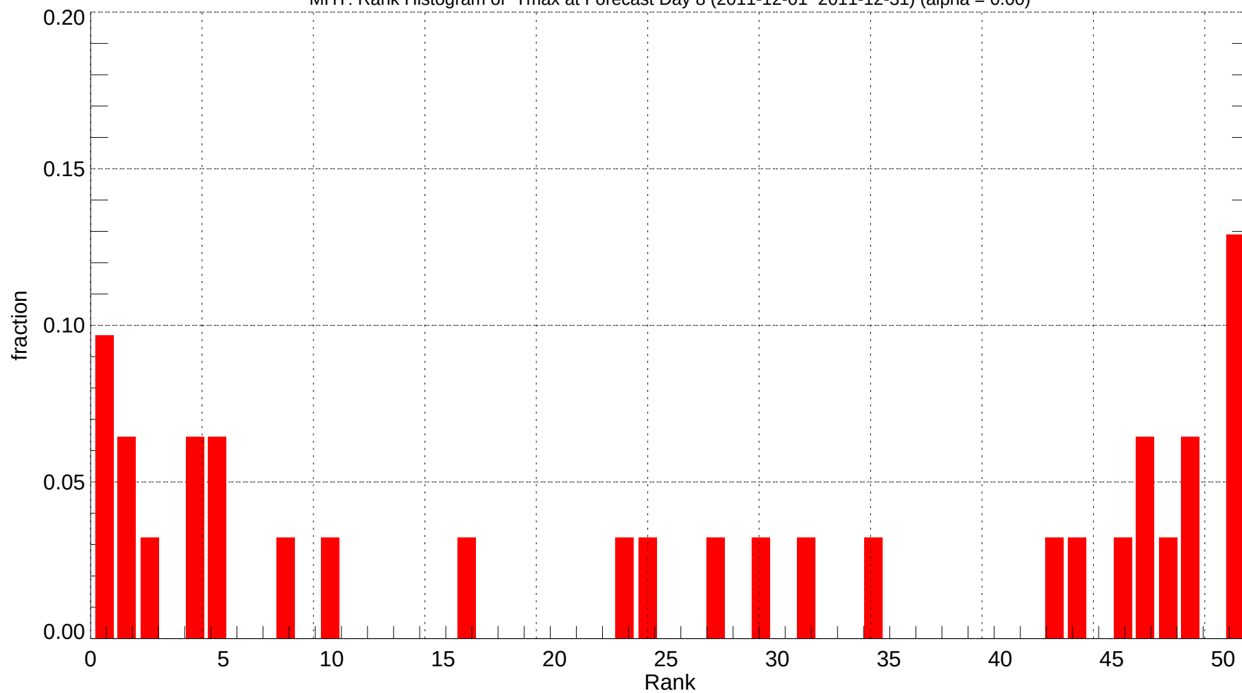
MHT: Rank Histogram of Tmax at Forecast Day 8 (2011-12-01~2011-12-31) (alpha = 0.00)
