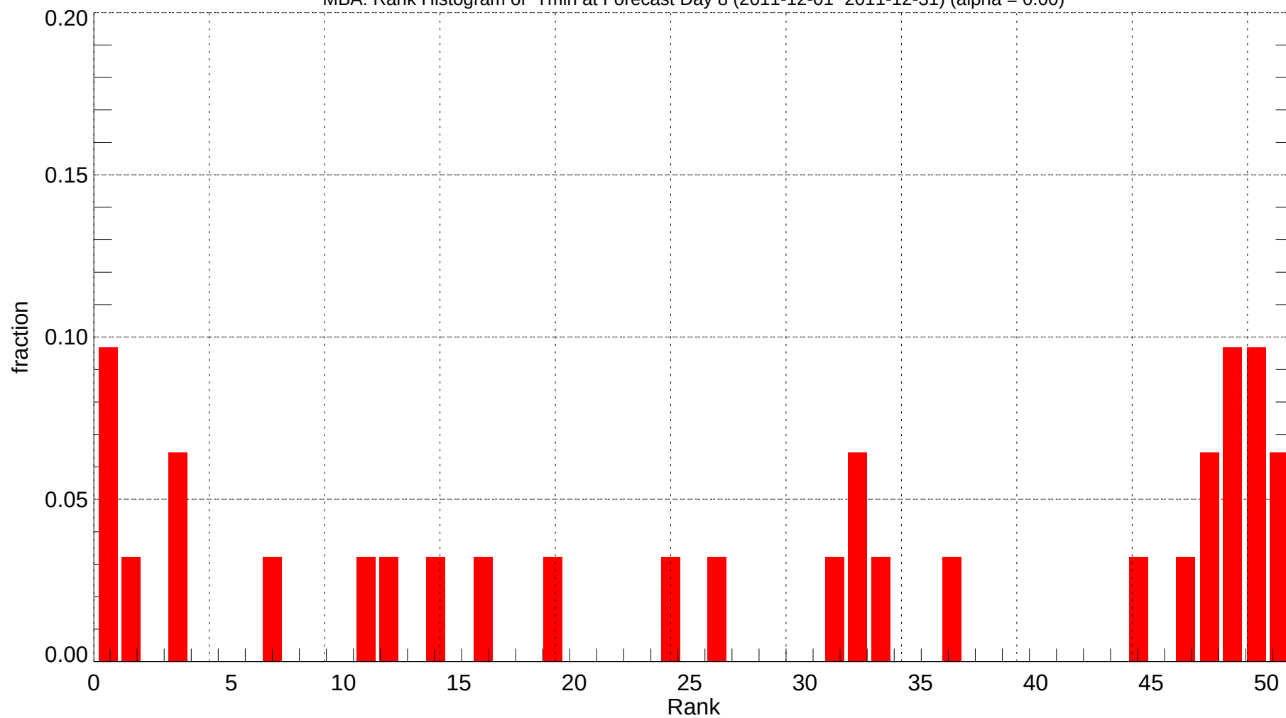
MBA: Rank Histogram of Tmin at Forecast Day 8 (2011-12-01~2011-12-31) (alpha = 0.00)
