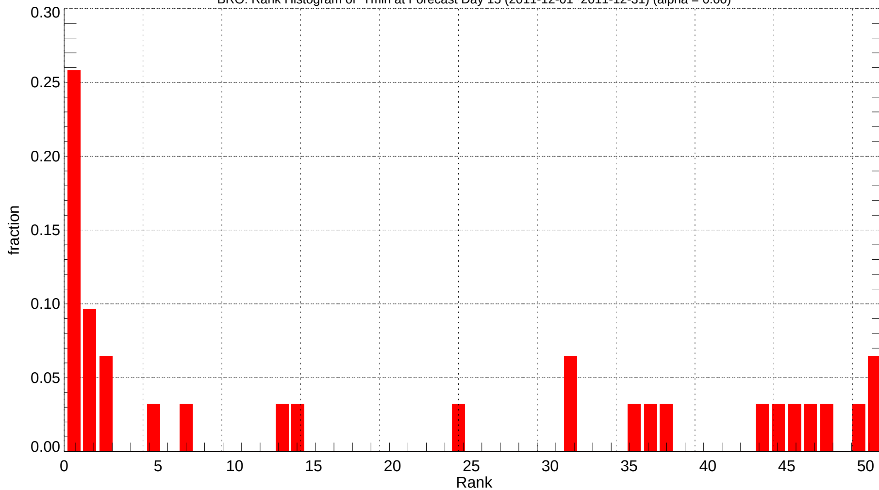
BRO: Rank Histogram of Tmin at Forecast Day 15 (2011-12-01~2011-12-31) (alpha = 0.00)
