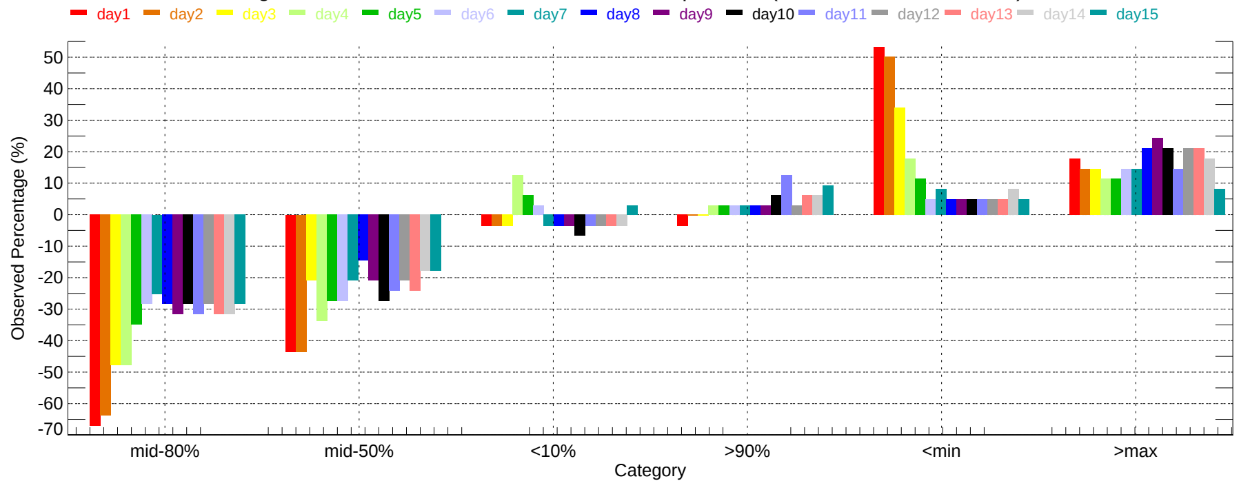
Observed Percentage Deviation of Ensembles - DLH: Min Temperature (2011-12-01~2011-12-31)
