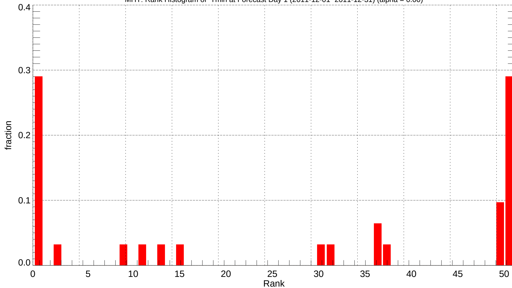
MHT: Rank Histogram of Tmin at Forecast Day 1 (2011-12-01~2011-12-31) (alpha = 0.00)
