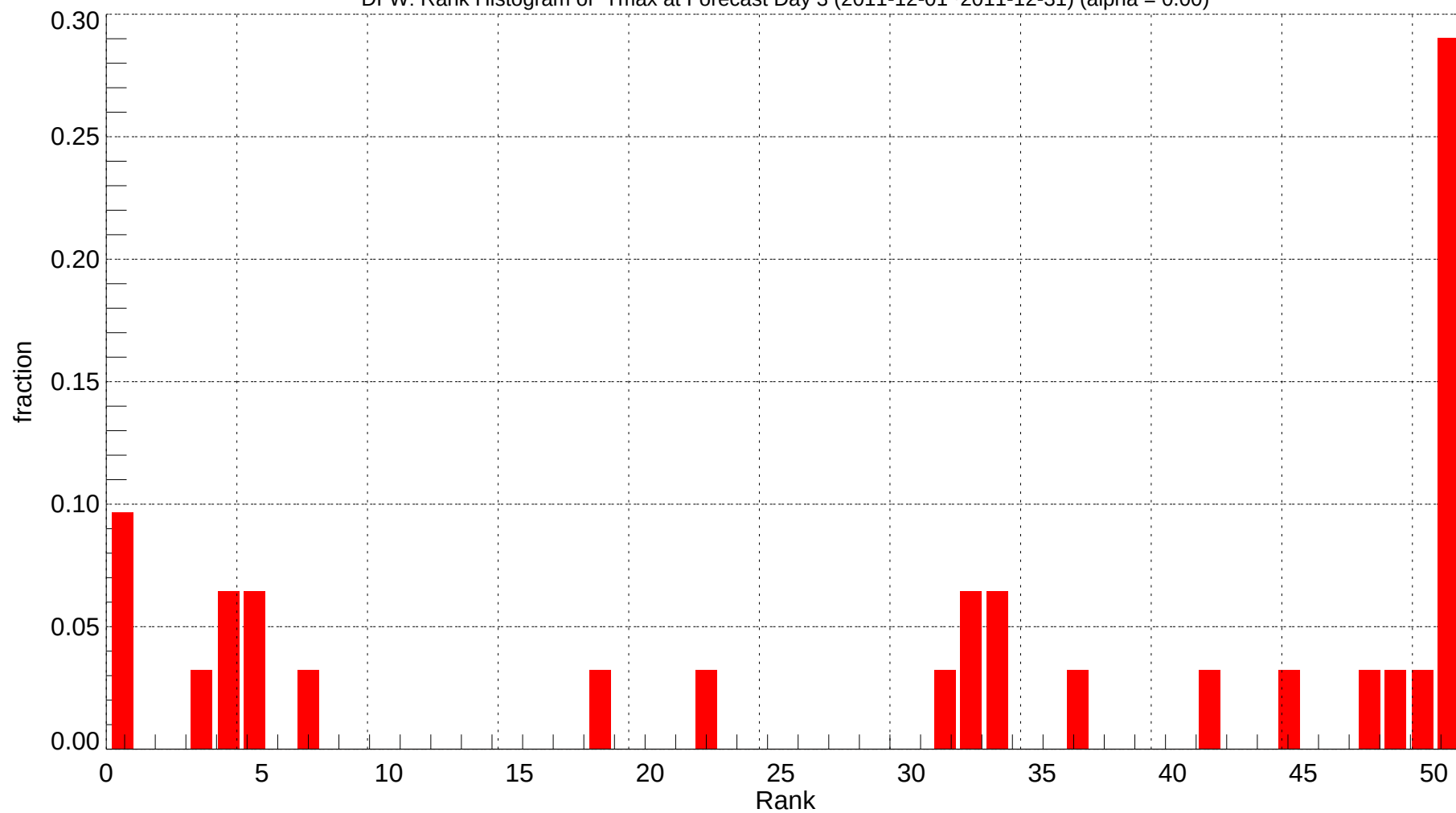
DFW: Rank Histogram of Tmax at Forecast Day 3 (2011-12-01~2011-12-31) (alpha = 0.00)
