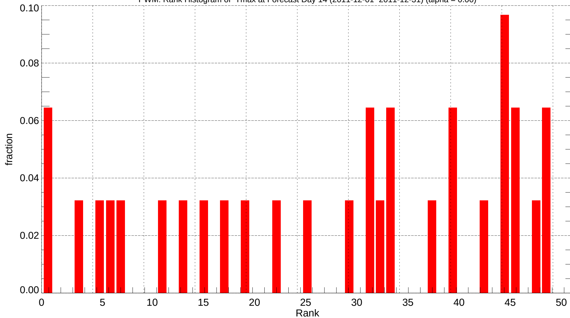
PWM: Rank Histogram of Tmax at Forecast Day 14 (2011-12-01~2011-12-31) (alpha = 0.00)
