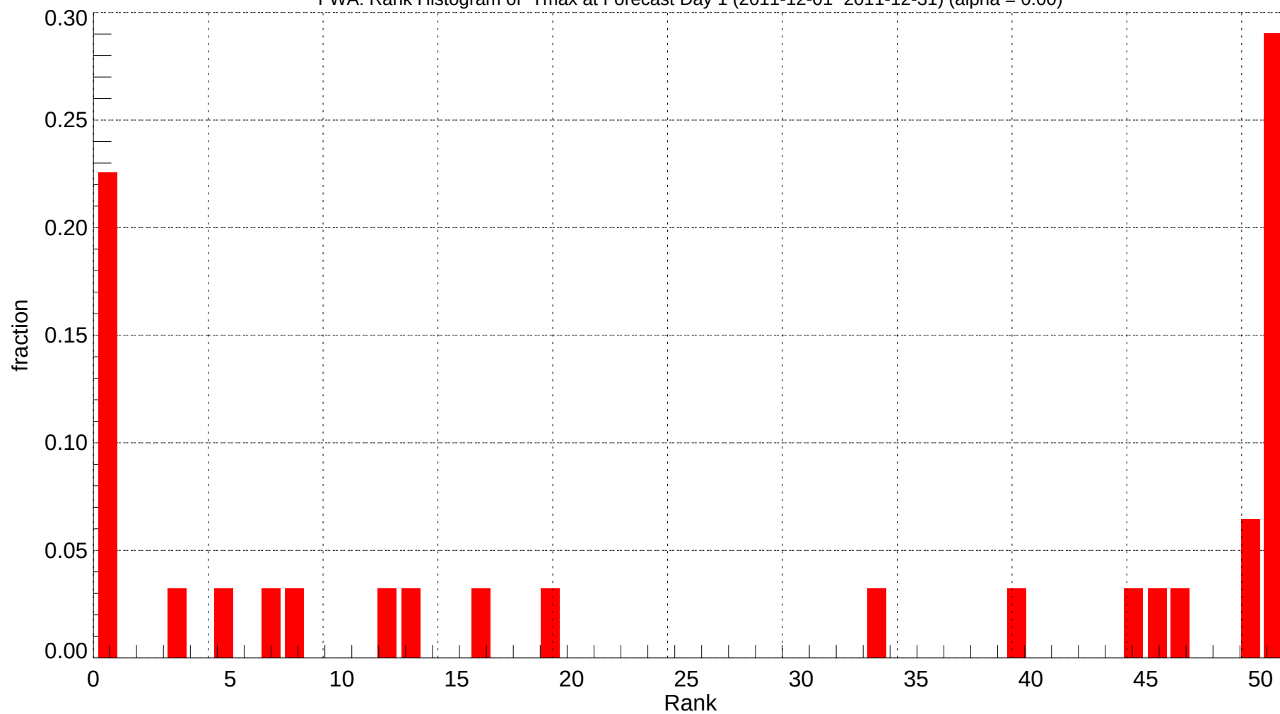
FWA: Rank Histogram of Tmax at Forecast Day 1 (2011-12-01~2011-12-31) (alpha = 0.00)
