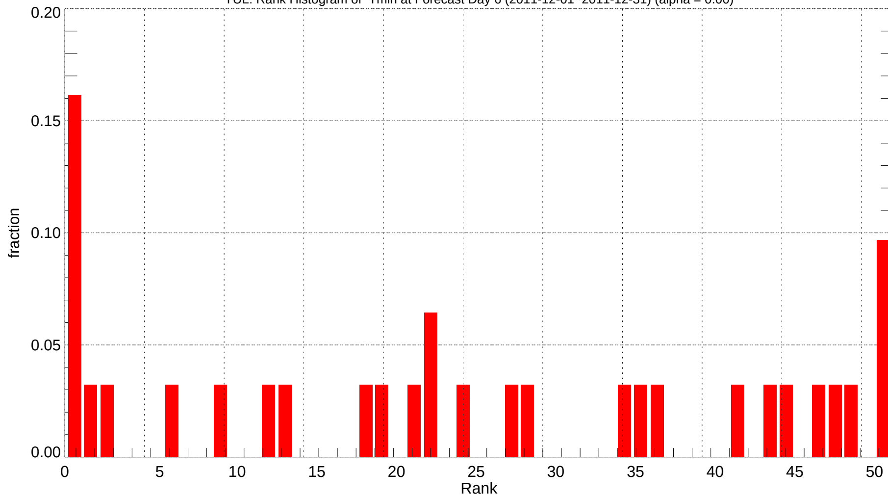
YUL: Rank Histogram of Tmin at Forecast Day 6 (2011-12-01~2011-12-31) (alpha = 0.00)
