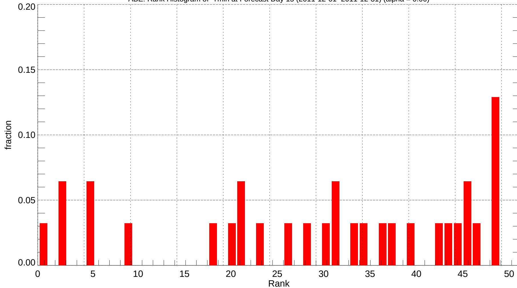
ABE: Rank Histogram of Tmin at Forecast Day 15 (2011-12-01~2011-12-31) (alpha = 0.00)
