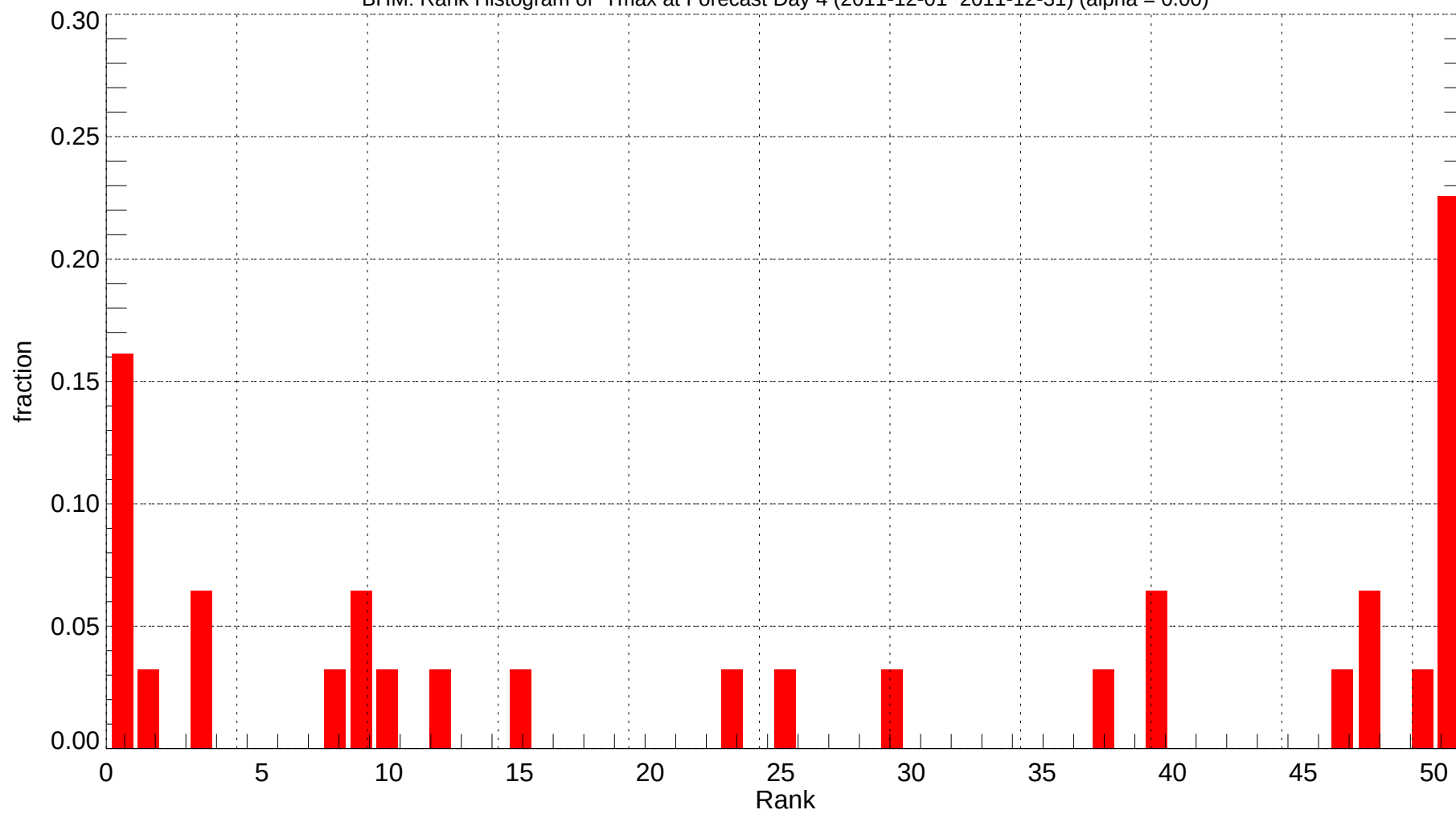
BHM: Rank Histogram of Tmax at Forecast Day 4 (2011-12-01~2011-12-31) (alpha = 0.00)
