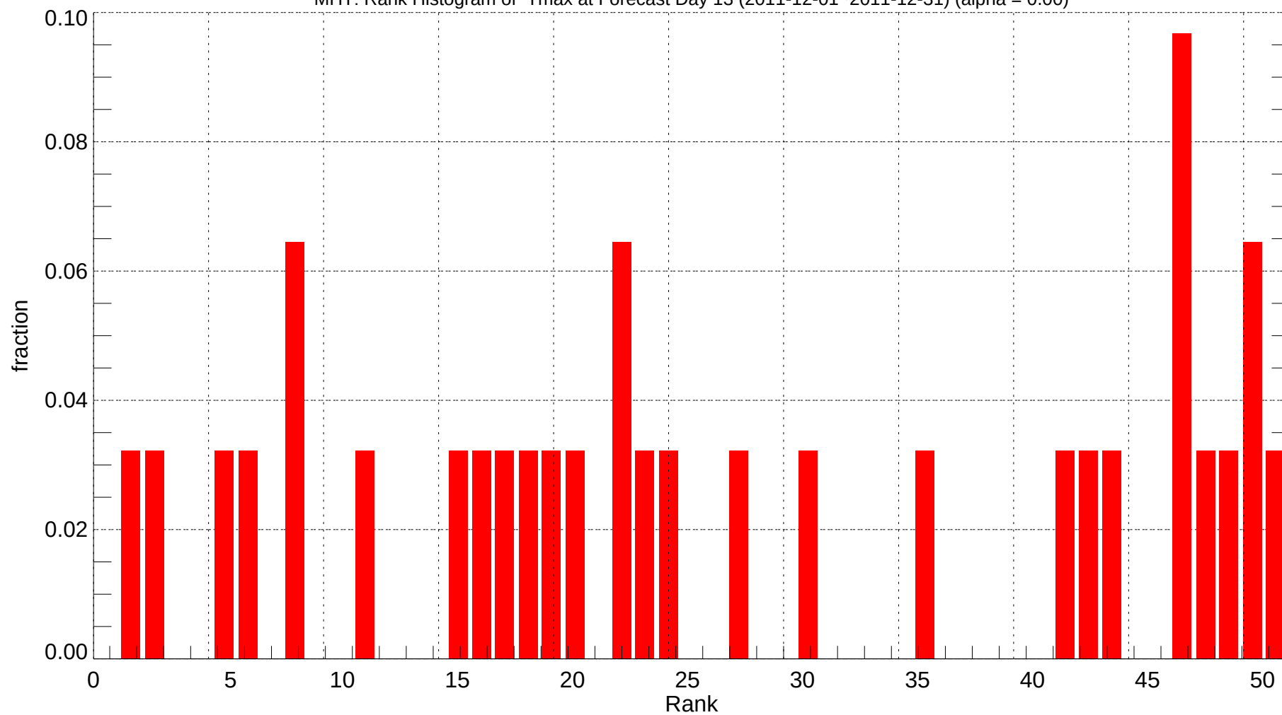
MHT: Rank Histogram of Tmax at Forecast Day 13 (2011-12-01~2011-12-31) (alpha = 0.00)
