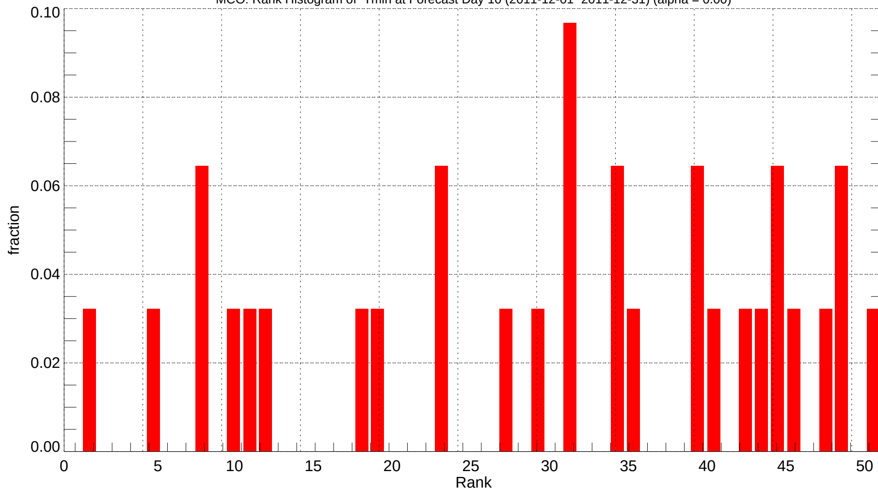
MCO: Rank Histogram of Tmin at Forecast Day 10 (2011-12-01~2011-12-31) (alpha = 0.00)
