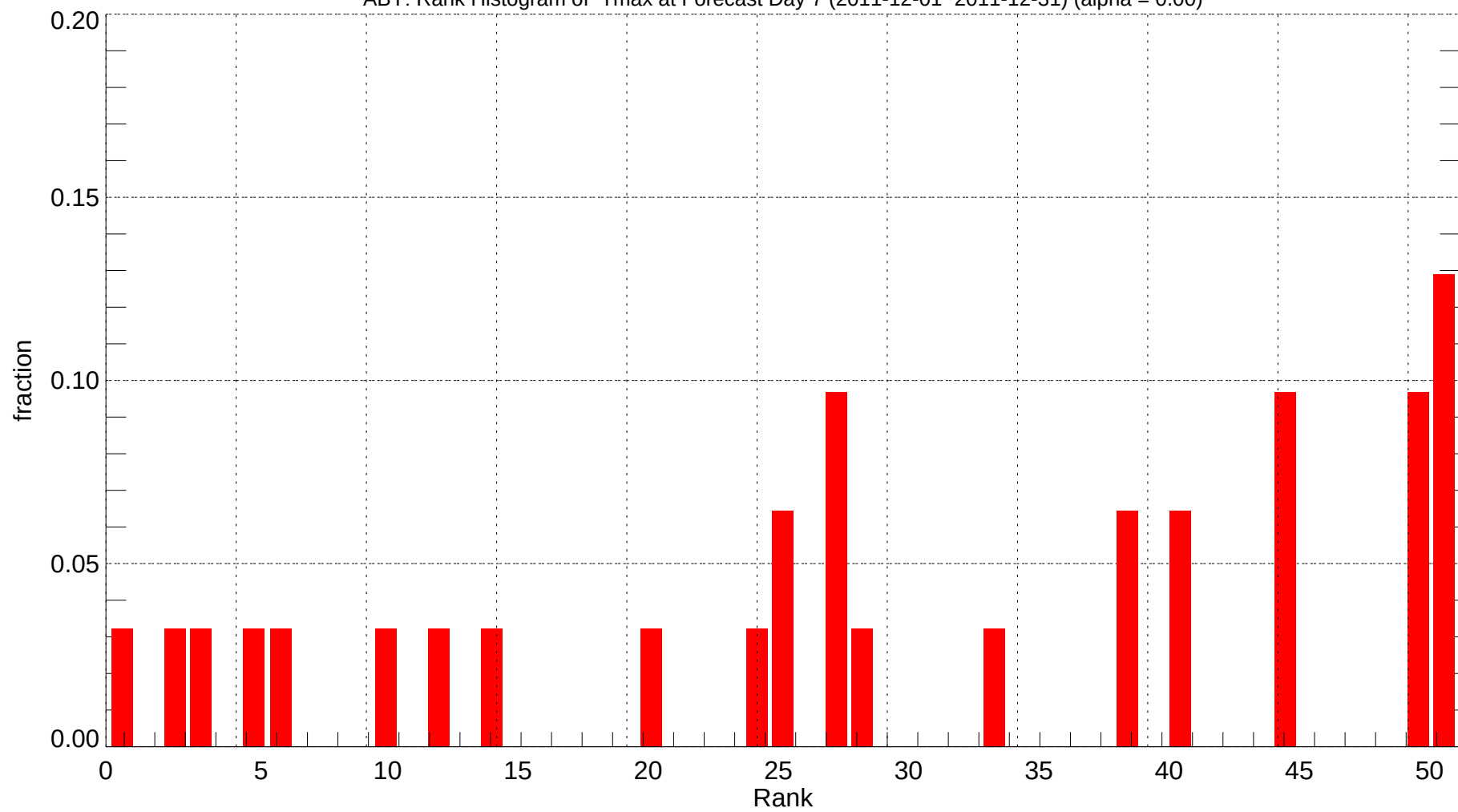
ABY: Rank Histogram of Tmax at Forecast Day 7 (2011-12-01~2011-12-31) (alpha = 0.00)
