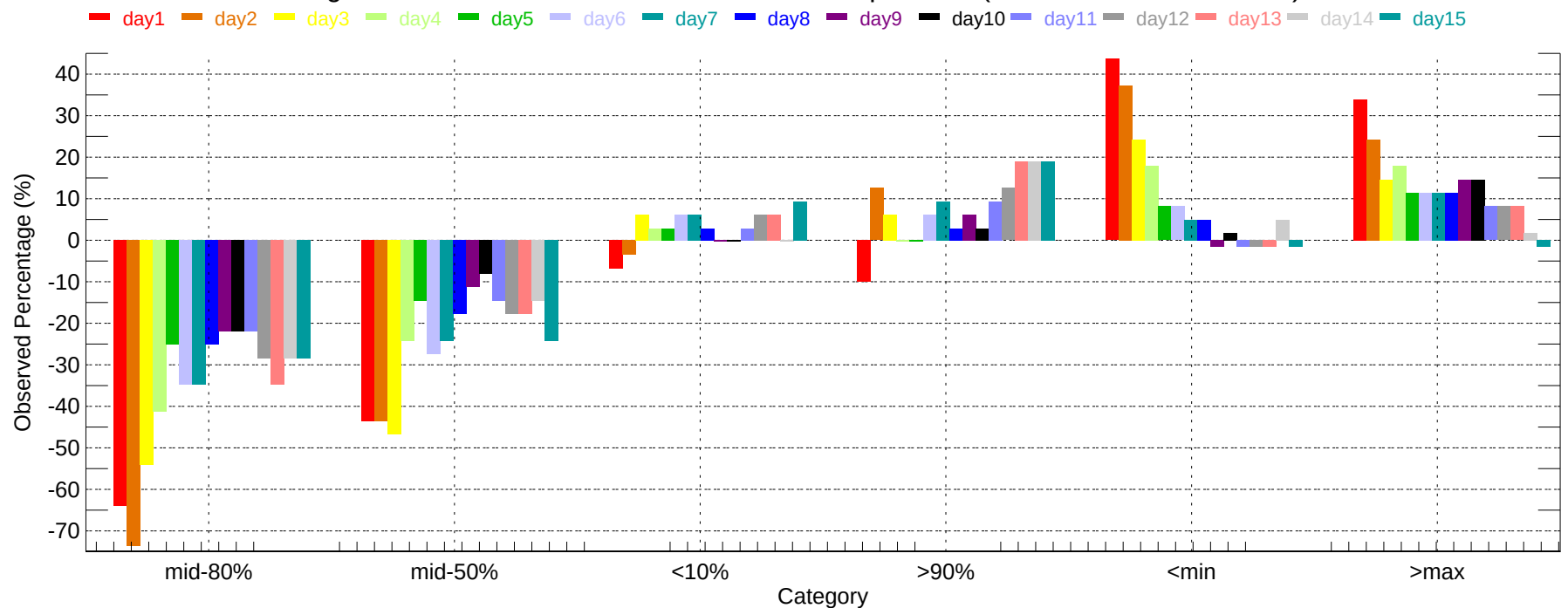
Observed Percentage Deviation of Ensembles - DSM: Min Temperature (2011-12-01~2011-12-31)
