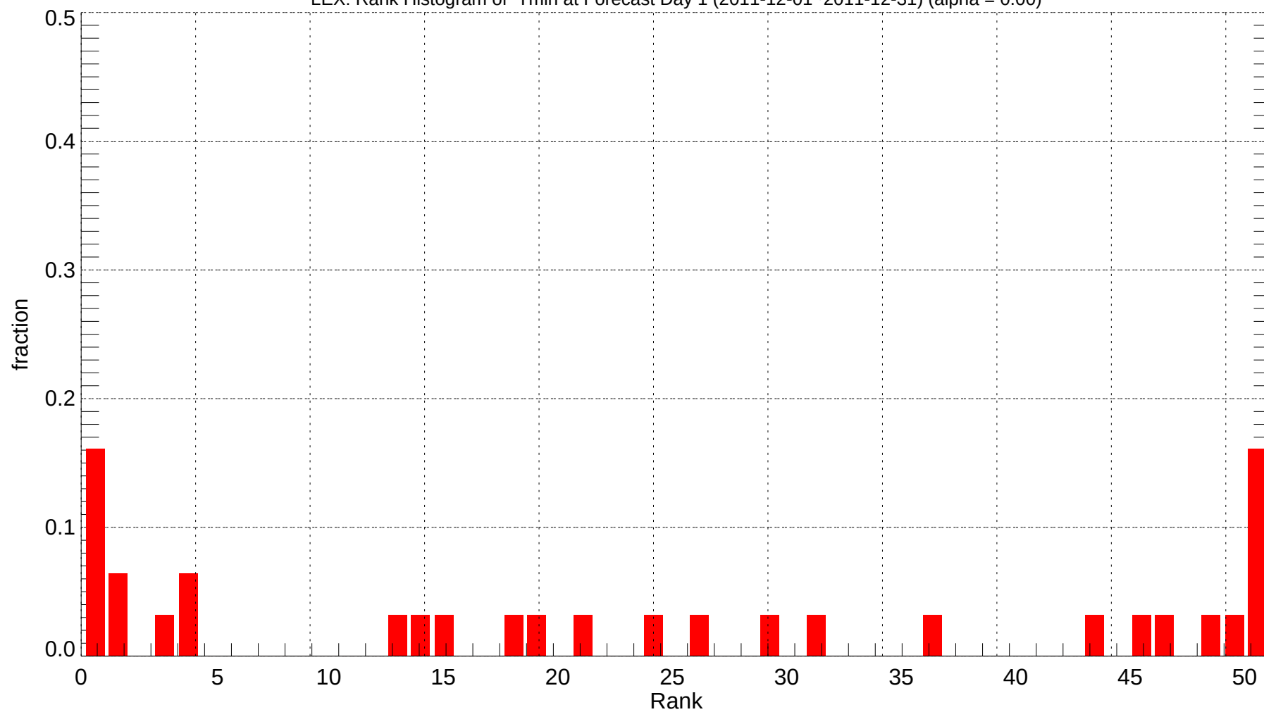
LEX: Rank Histogram of Tmin at Forecast Day 1 (2011-12-01~2011-12-31) (alpha = 0.00)
