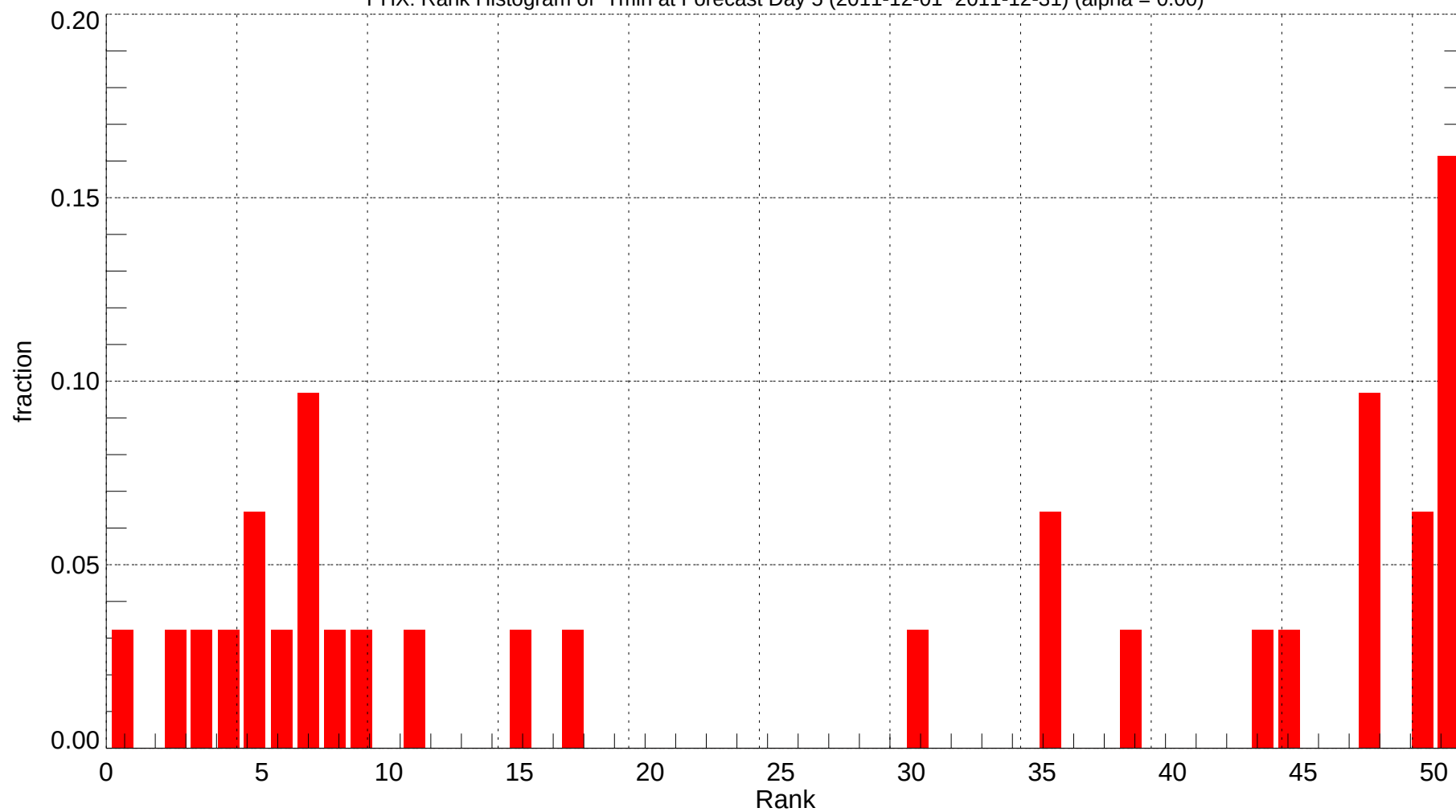
PHX: Rank Histogram of Tmin at Forecast Day 5 (2011-12-01~2011-12-31) (alpha = 0.00)
