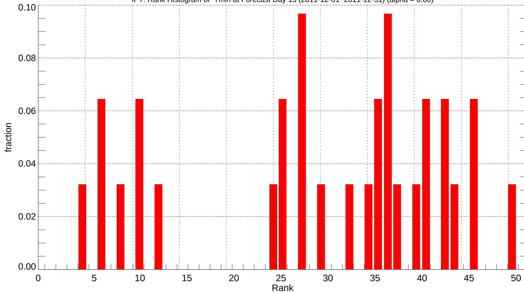
IPT: Rank Histogram of Tmin at Forecast Day 13 (2011-12-01~2011-12-31) (alpha = 0.00)
