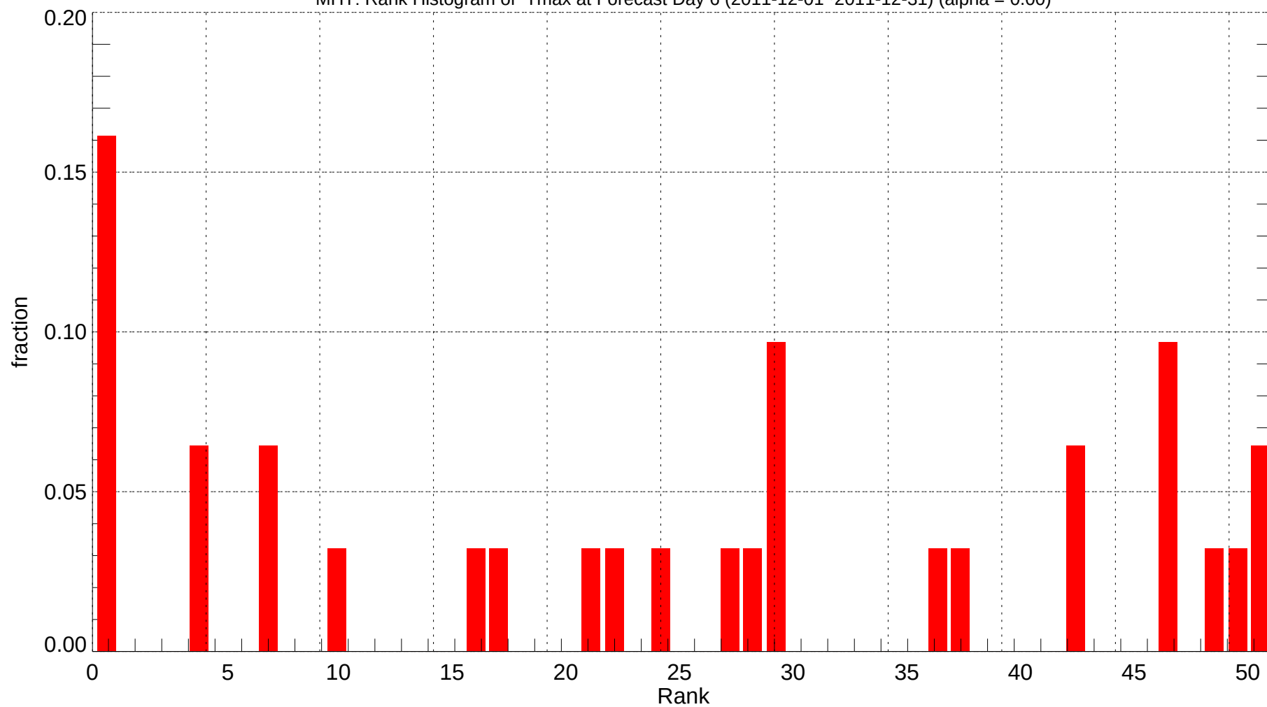
MHT: Rank Histogram of Tmax at Forecast Day 6 (2011-12-01~2011-12-31) (alpha = 0.00)
