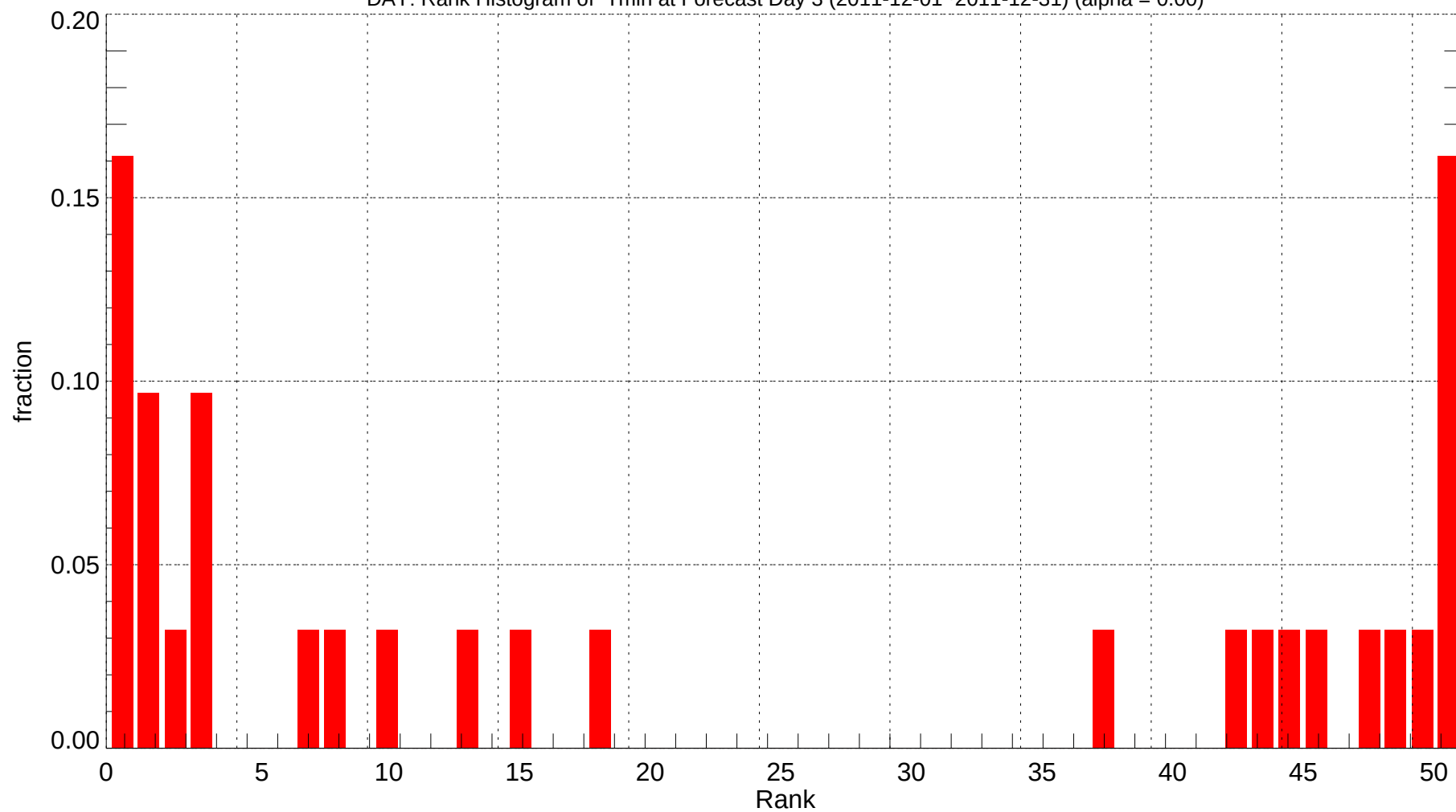
DAY: Rank Histogram of Tmin at Forecast Day 3 (2011-12-01~2011-12-31) (alpha = 0.00)
