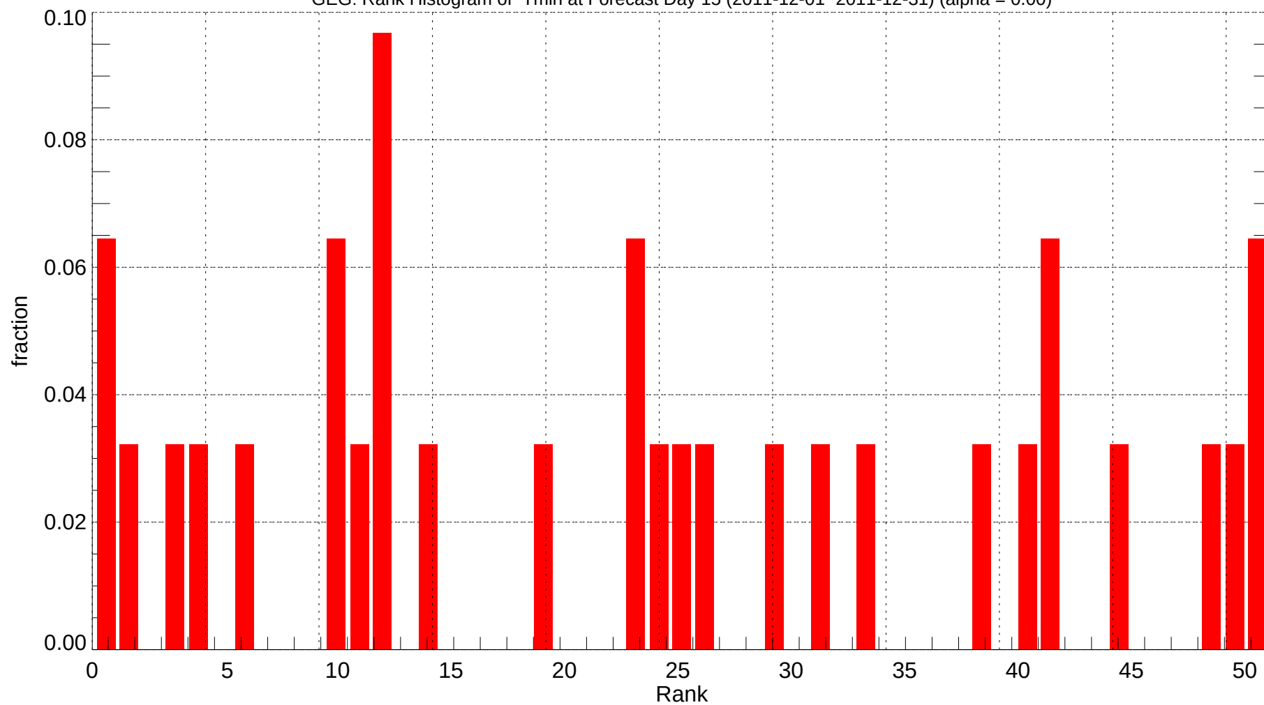
GEG: Rank Histogram of Tmin at Forecast Day 15 (2011-12-01~2011-12-31) (alpha = 0.00)
