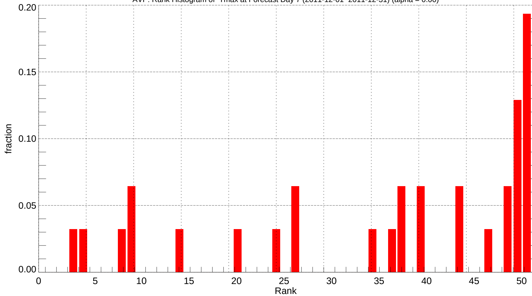
AVP: Rank Histogram of Tmax at Forecast Day 7 (2011-12-01~2011-12-31) (alpha = 0.00)
