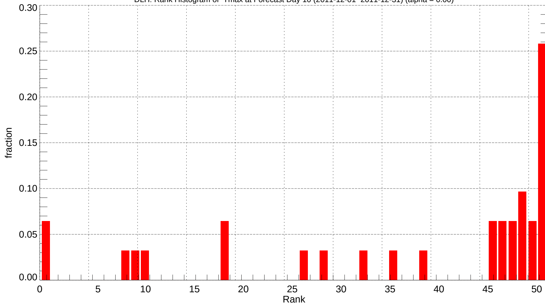
DLH: Rank Histogram of Tmax at Forecast Day 10 (2011-12-01~2011-12-31) (alpha = 0.00)
