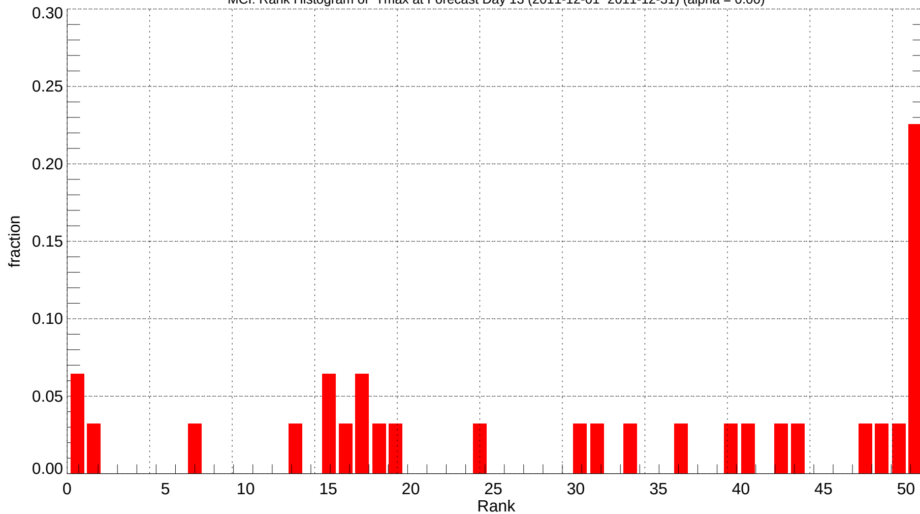
MCI: Rank Histogram of Tmax at Forecast Day 13 (2011-12-01~2011-12-31) (alpha = 0.00)
