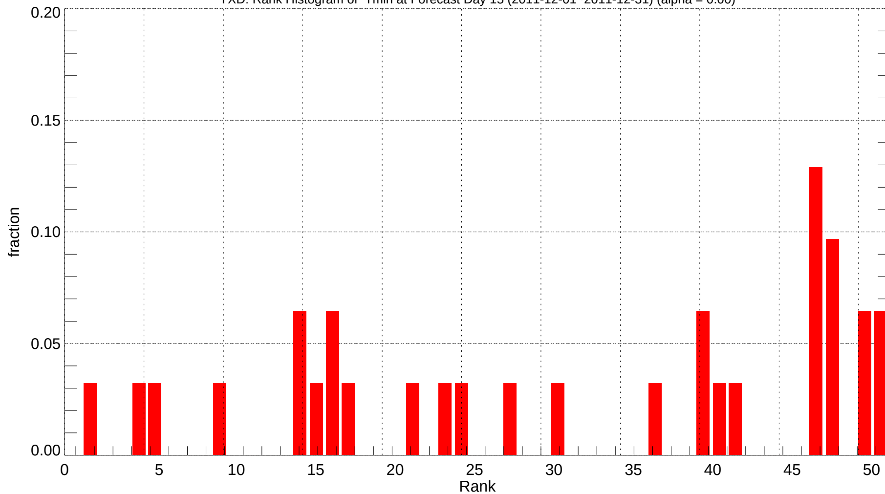
YXD: Rank Histogram of Tmin at Forecast Day 15 (2011-12-01~2011-12-31) (alpha = 0.00)
