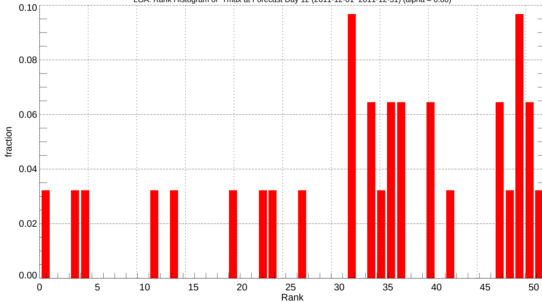
LGA: Rank Histogram of Tmax at Forecast Day 12 (2011-12-01~2011-12-31) (alpha = 0.00)
