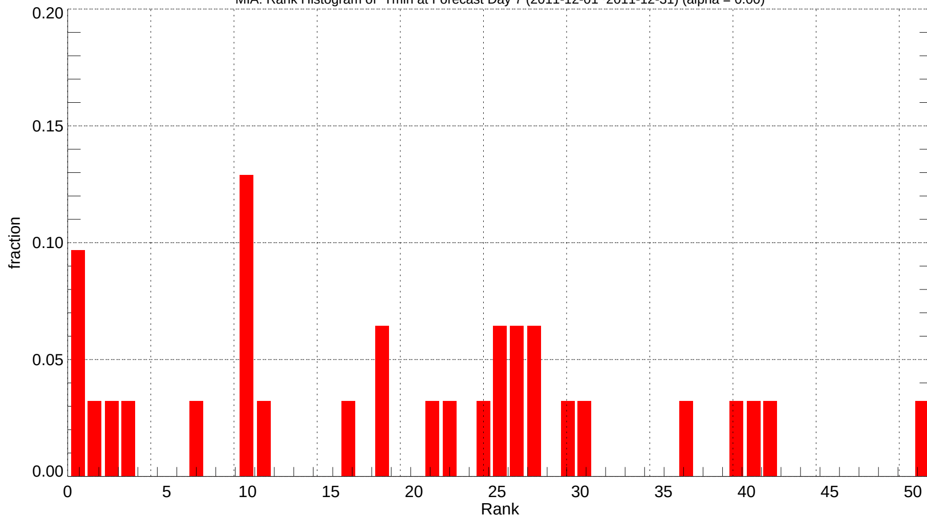
MIA: Rank Histogram of Tmin at Forecast Day 7 (2011-12-01~2011-12-31) (alpha = 0.00)
