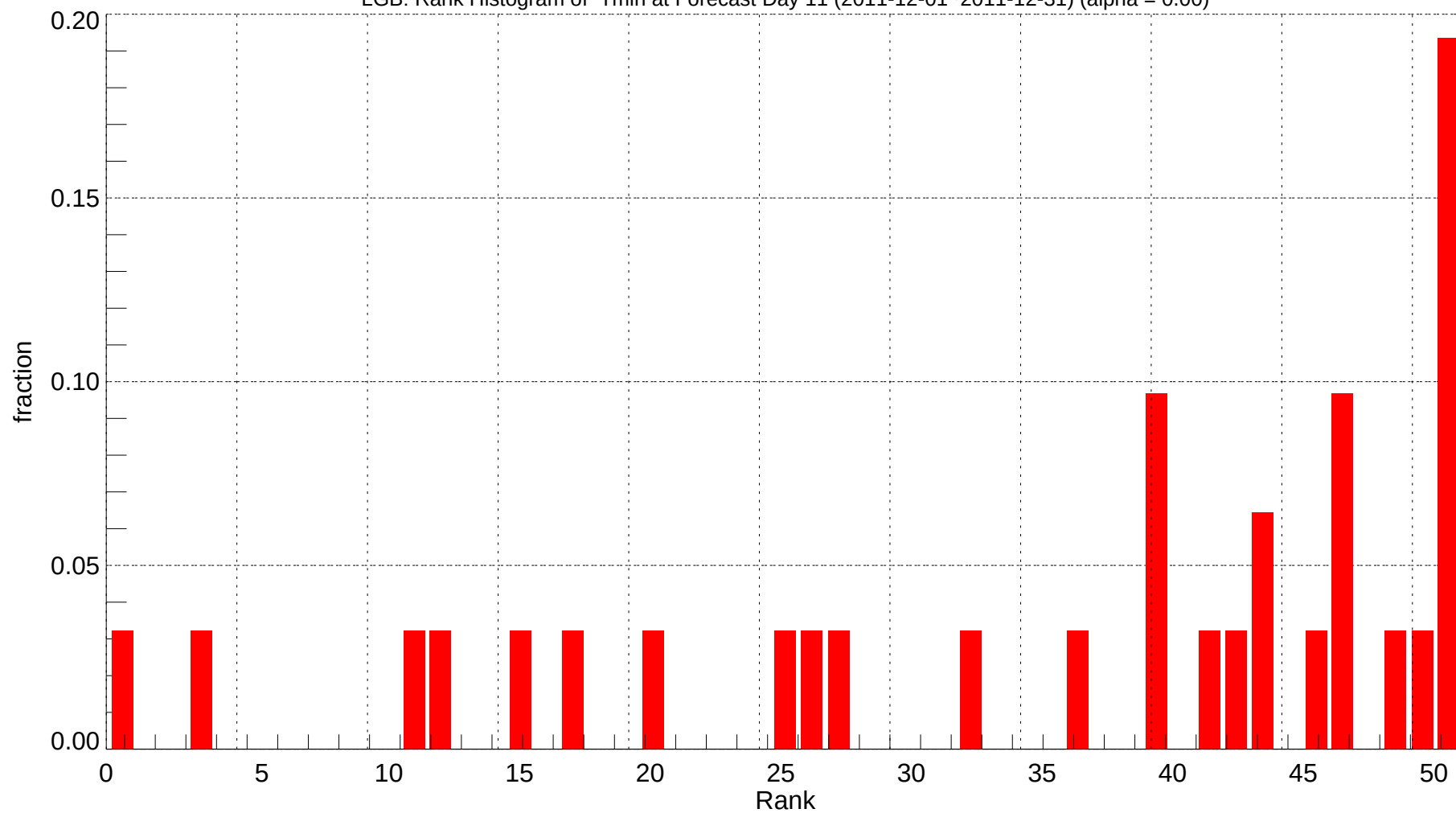
LGB: Rank Histogram of Tmin at Forecast Day 11 (2011-12-01~2011-12-31) (alpha = 0.00)
