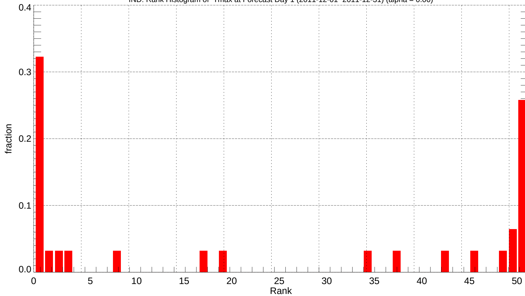
IND: Rank Histogram of Tmax at Forecast Day 1 (2011-12-01~2011-12-31) (alpha = 0.00)
