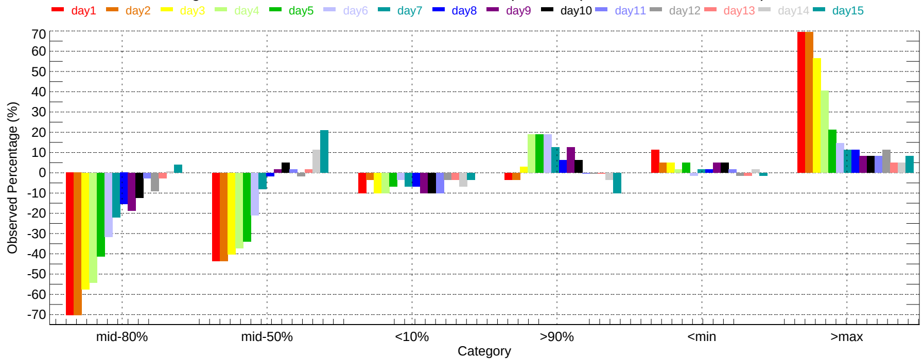
Observed Percentage Deviation of Ensembles - EUG: Min Temperature (2011-12-01~2011-12-31)
