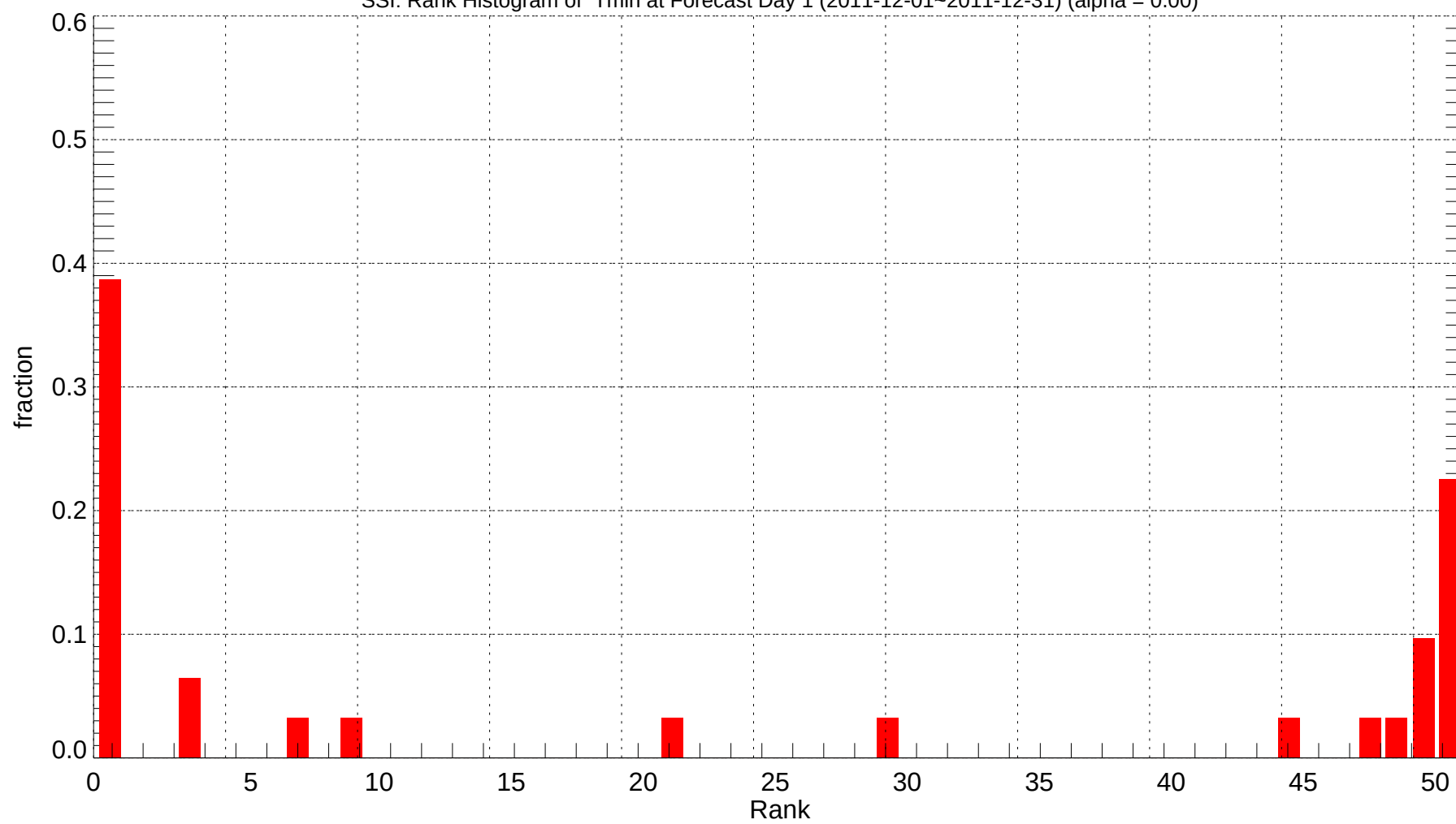
SSI: Rank Histogram of Tmin at Forecast Day 1 (2011-12-01~2011-12-31) (alpha = 0.00)
