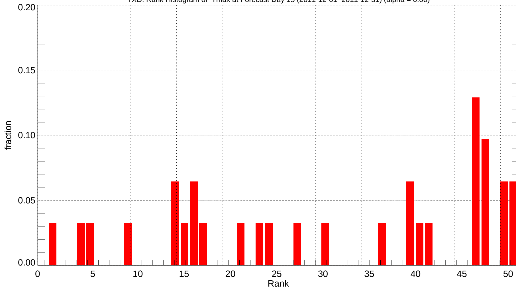
YXD: Rank Histogram of Tmax at Forecast Day 15 (2011-12-01~2011-12-31) (alpha = 0.00)
