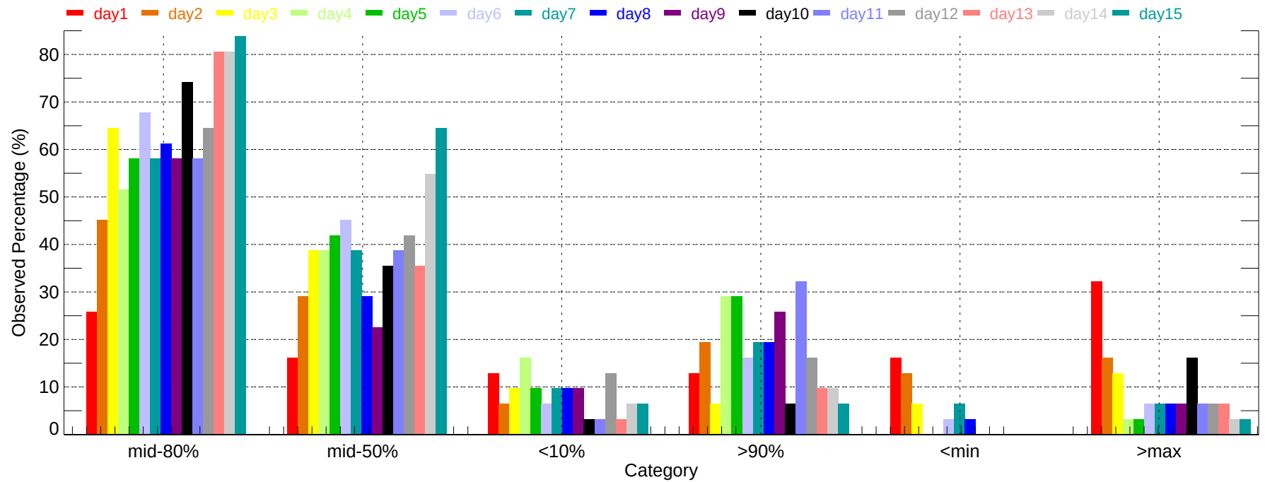
Observed Percentage of Ensembles - IAH: Min Temperature (2011-12-01~2011-12-31)
