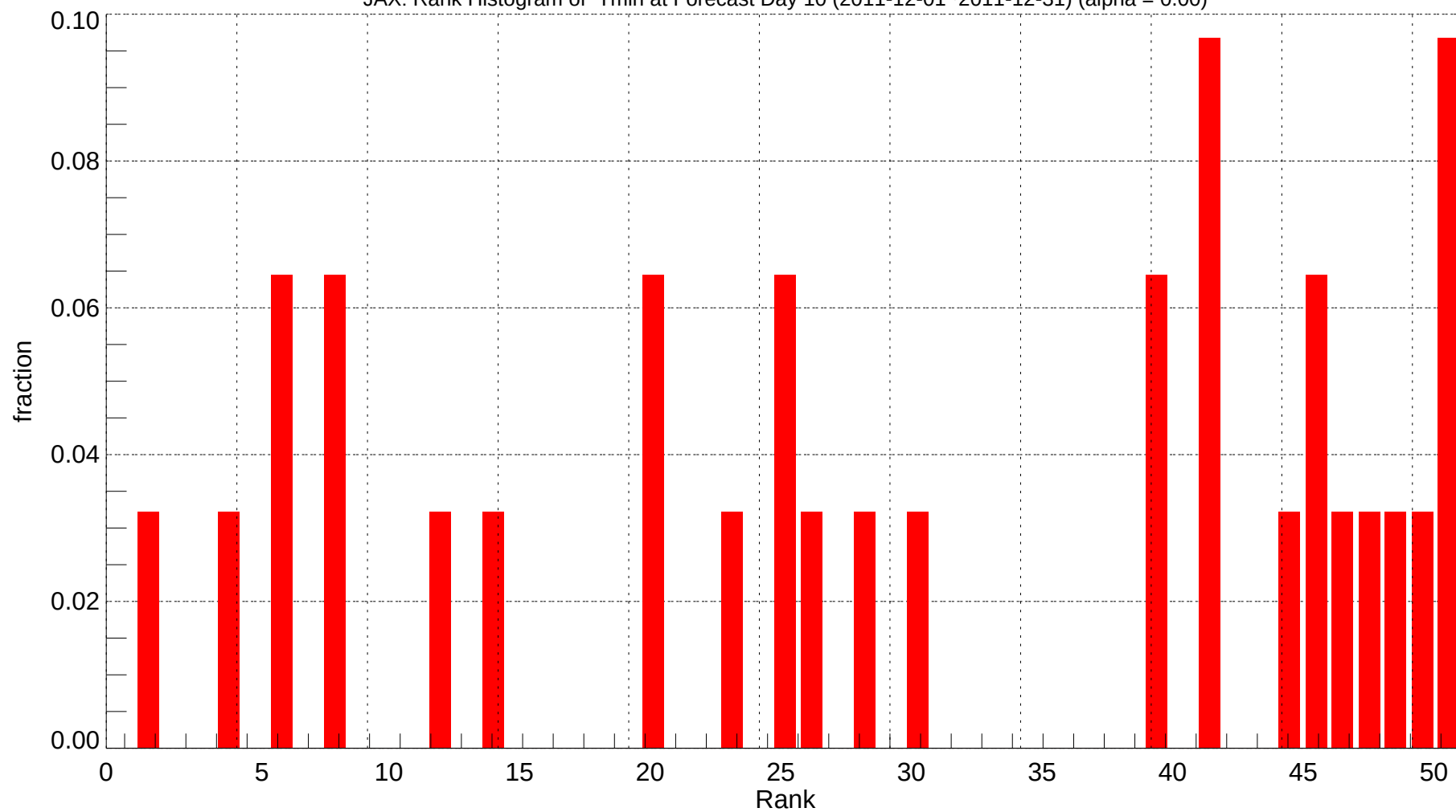
JAX: Rank Histogram of Tmin at Forecast Day 10 (2011-12-01~2011-12-31) (alpha = 0.00)
