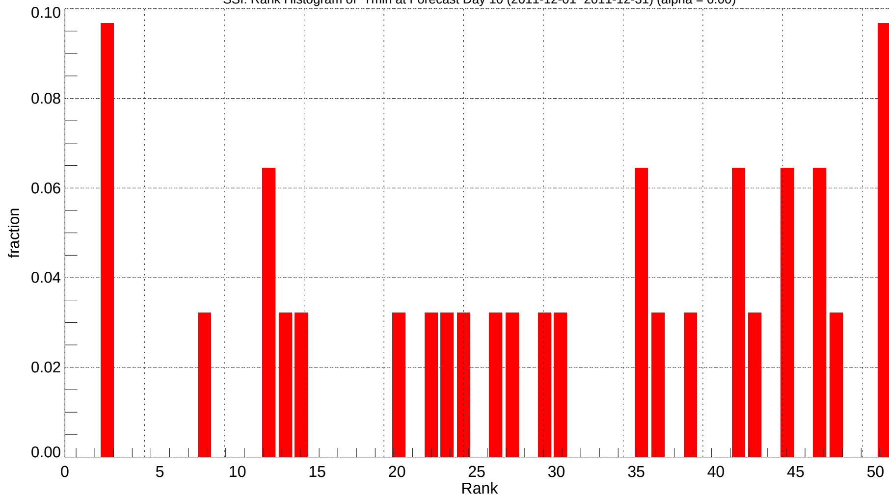
SSI: Rank Histogram of Tmin at Forecast Day 10 (2011-12-01~2011-12-31) (alpha = 0.00)
