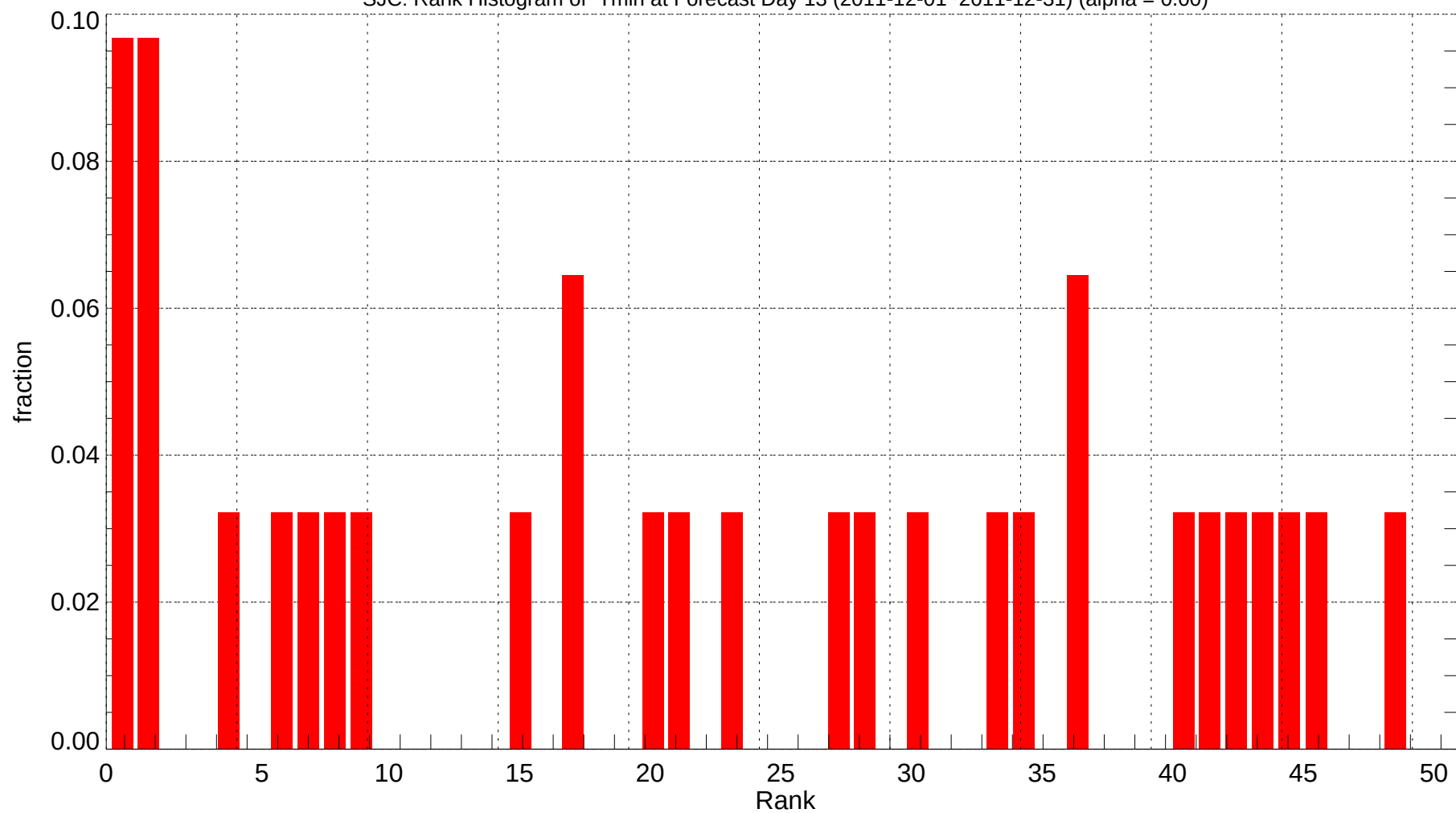
SJC: Rank Histogram of Tmin at Forecast Day 13 (2011-12-01~2011-12-31) (alpha = 0.00)
