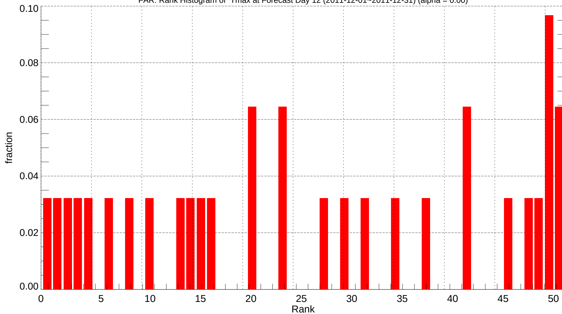
FAR: Rank Histogram of Tmax at Forecast Day 12 (2011-12-01~2011-12-31) (alpha = 0.00)
