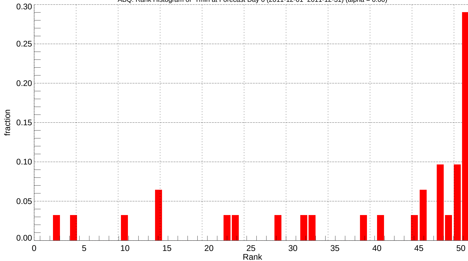
ABQ: Rank Histogram of Tmin at Forecast Day 6 (2011-12-01~2011-12-31) (alpha = 0.00)
