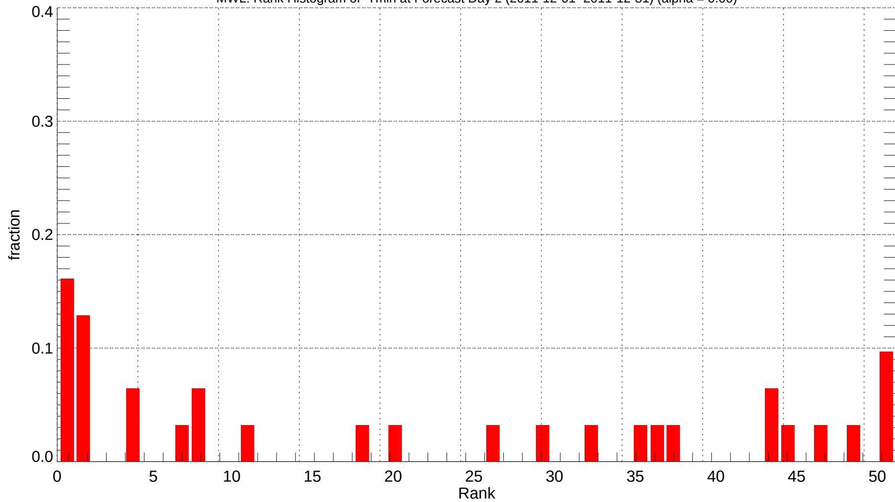
MWL: Rank Histogram of Tmin at Forecast Day 2 (2011-12-01~2011-12-31) (alpha = 0.00)
