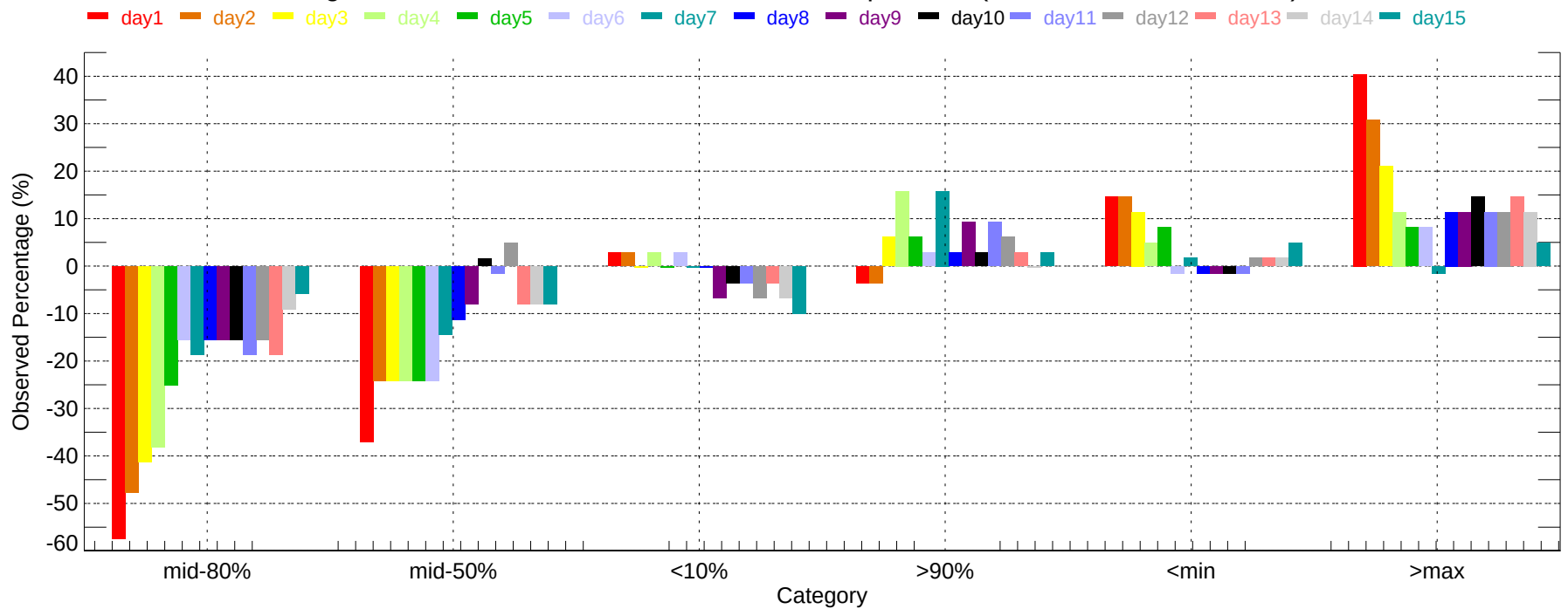
Observed Percentage Deviation of Ensembles - JAN: Max Temperature (2011-12-01~2011-12-31)
