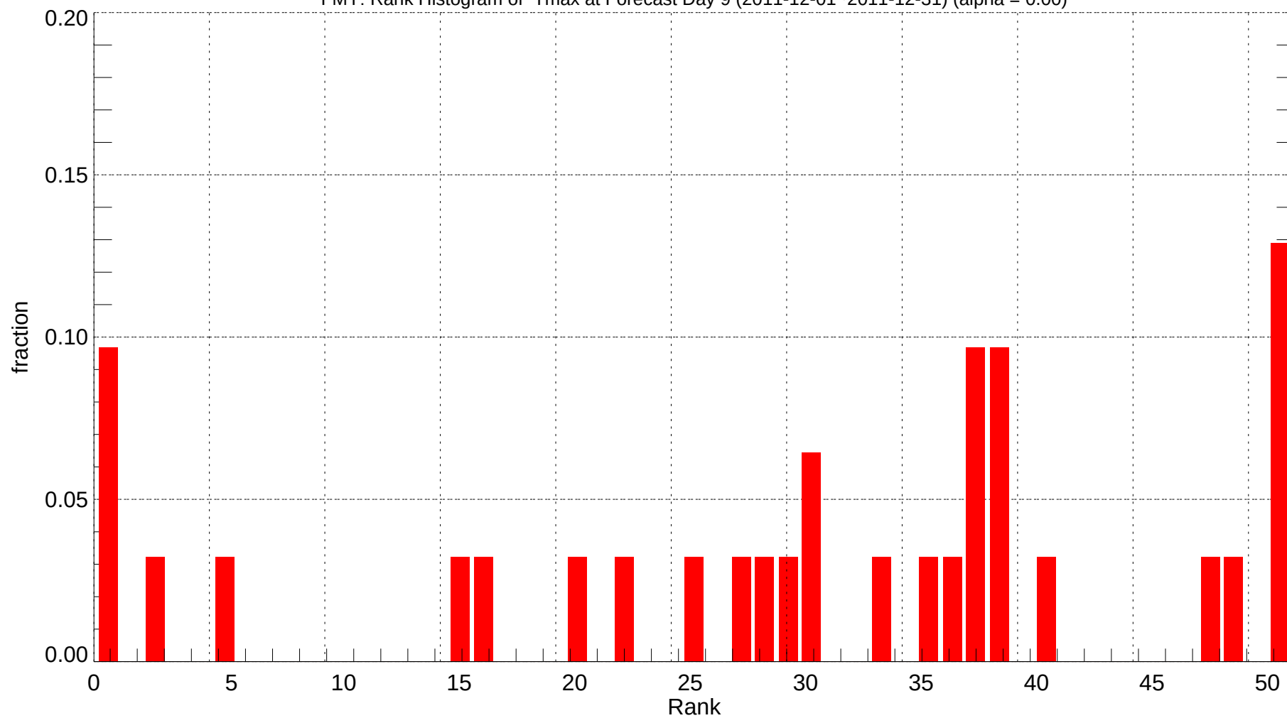
FMY: Rank Histogram of Tmax at Forecast Day 9 (2011-12-01~2011-12-31) (alpha = 0.00)
