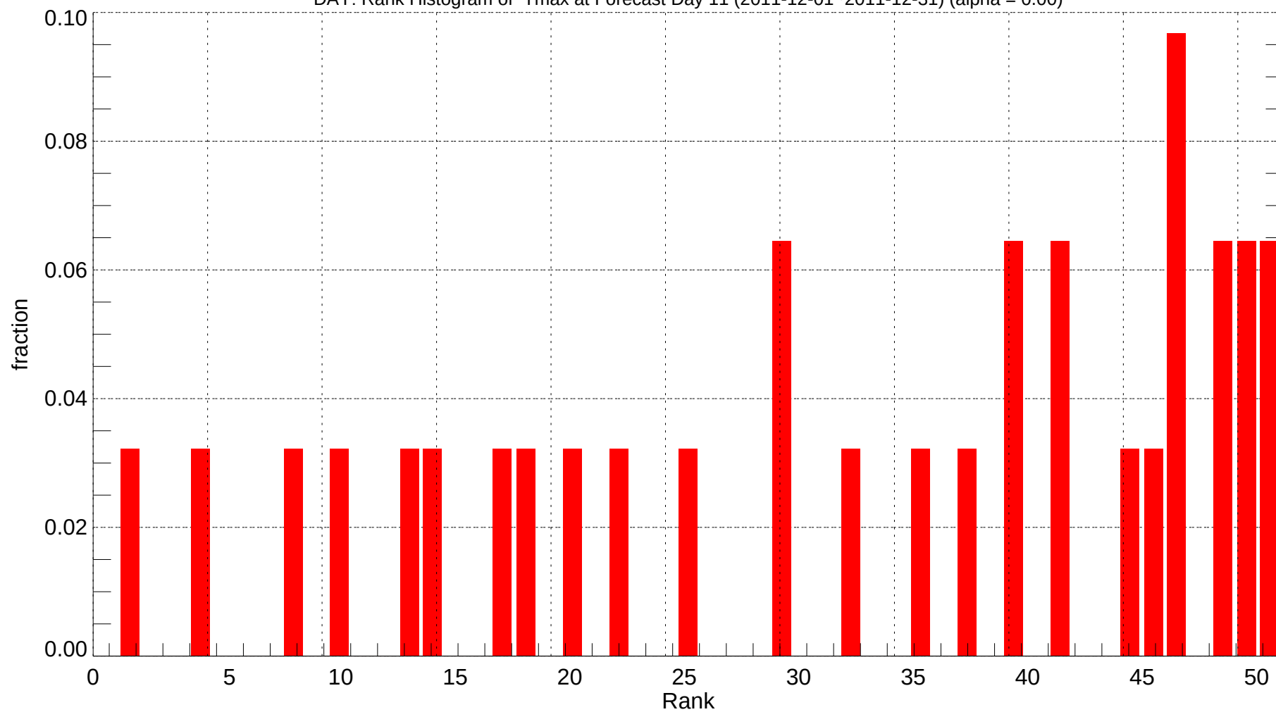
DAY: Rank Histogram of Tmax at Forecast Day 11 (2011-12-01~2011-12-31) (alpha = 0.00)
