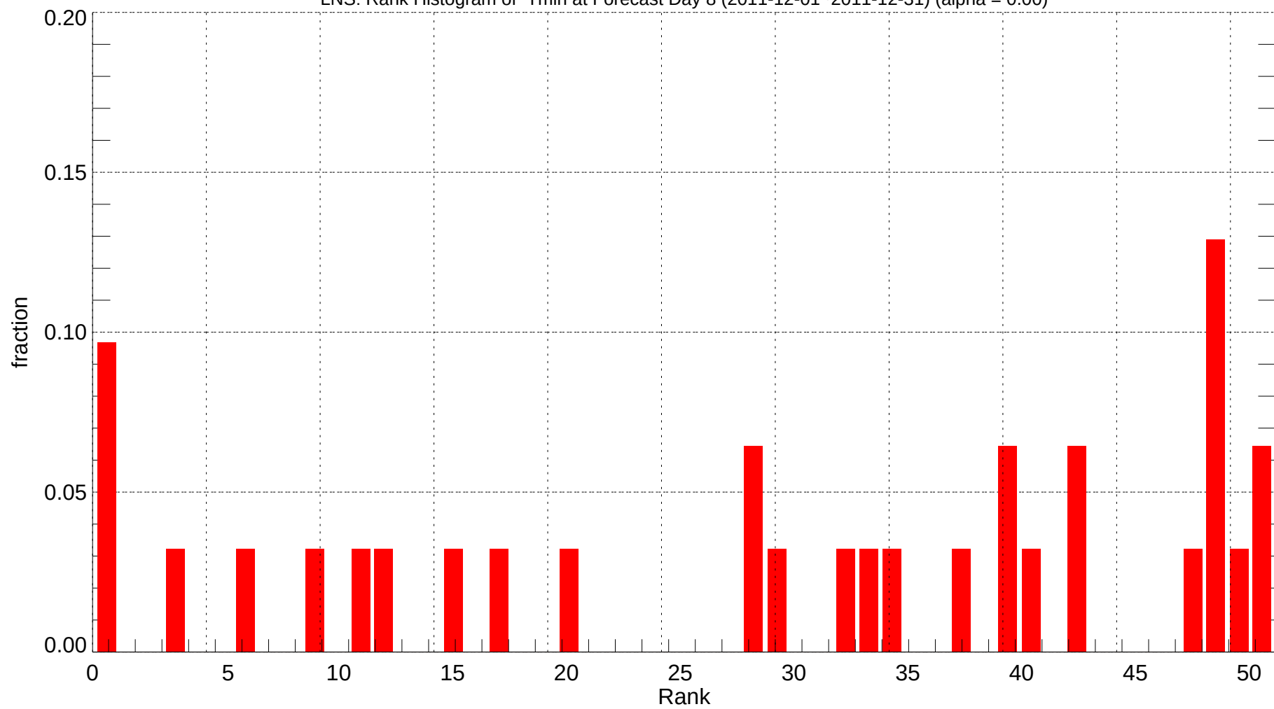
LNS: Rank Histogram of Tmin at Forecast Day 8 (2011-12-01~2011-12-31) (alpha = 0.00)
