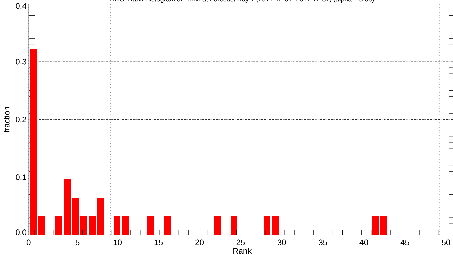
BRO: Rank Histogram of Tmin at Forecast Day 7 (2011-12-01~2011-12-31) (alpha = 0.00)
