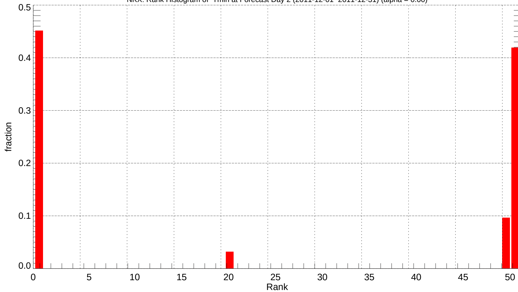
NKX: Rank Histogram of Tmin at Forecast Day 2 (2011-12-01~2011-12-31) (alpha = 0.00)
