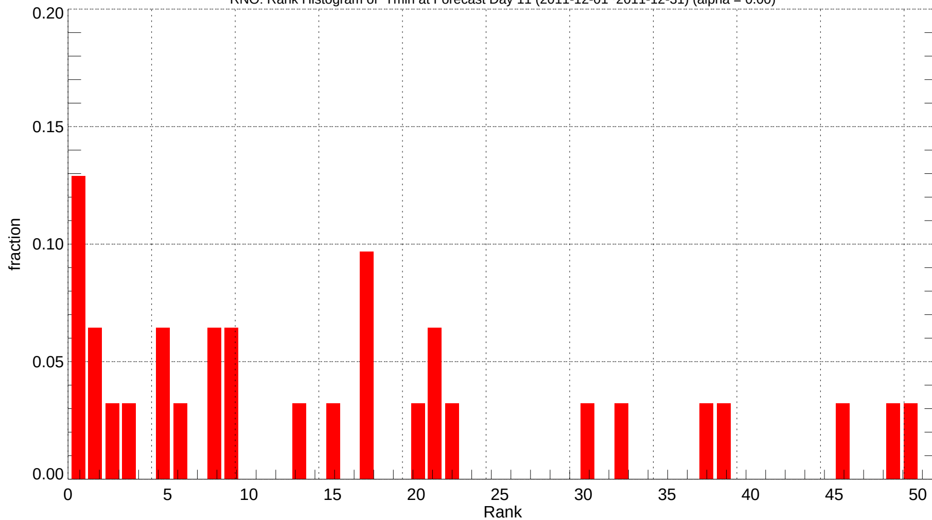
RNO: Rank Histogram of Tmin at Forecast Day 11 (2011-12-01~2011-12-31) (alpha = 0.00)
