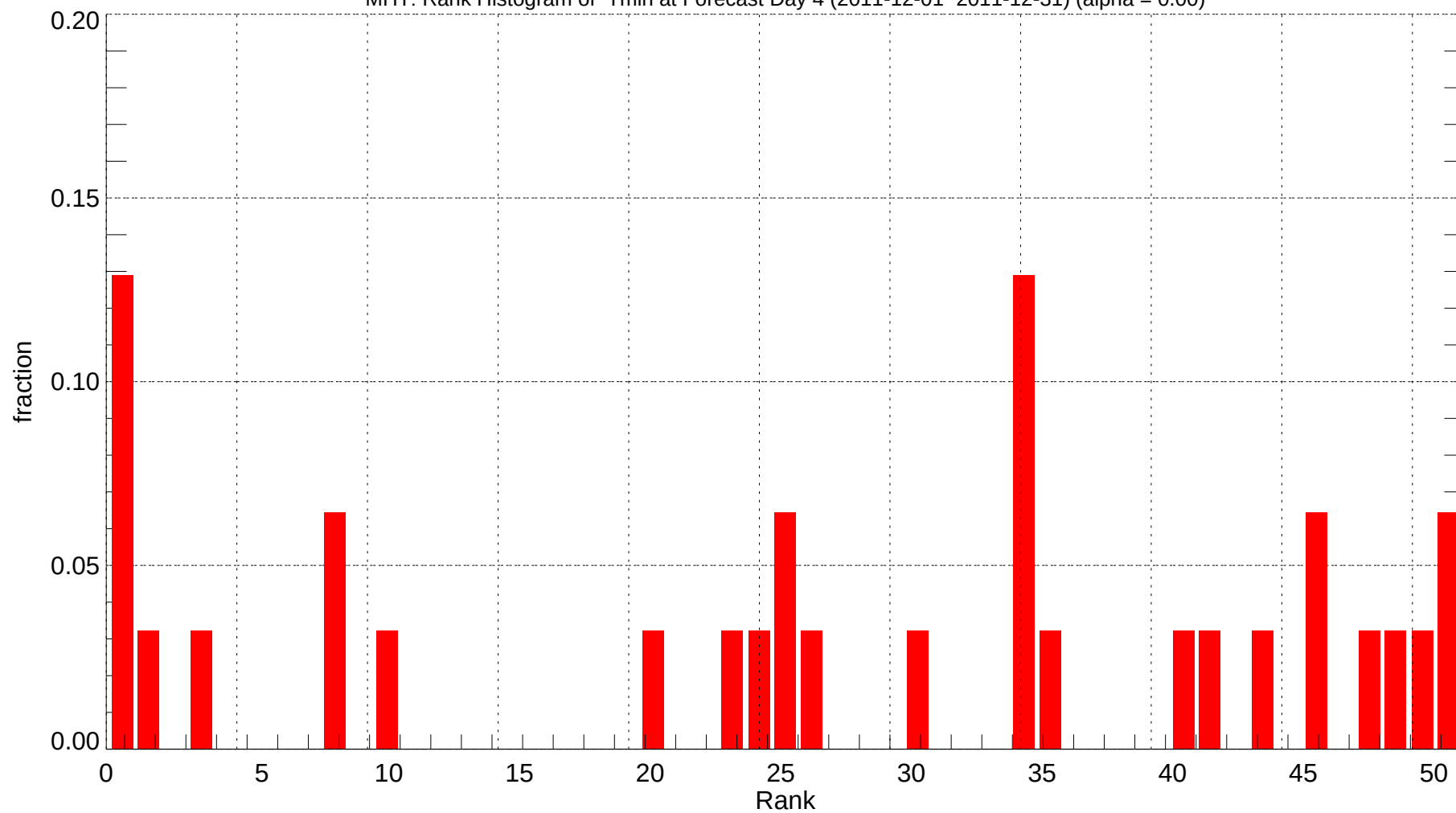
MHT: Rank Histogram of Tmin at Forecast Day 4 (2011-12-01~2011-12-31) (alpha = 0.00)
