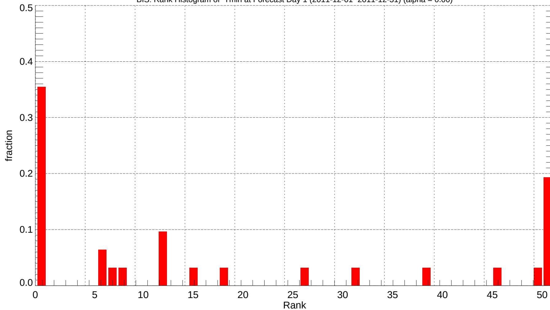
BIS: Rank Histogram of Tmin at Forecast Day 1 (2011-12-01~2011-12-31) (alpha = 0.00)
