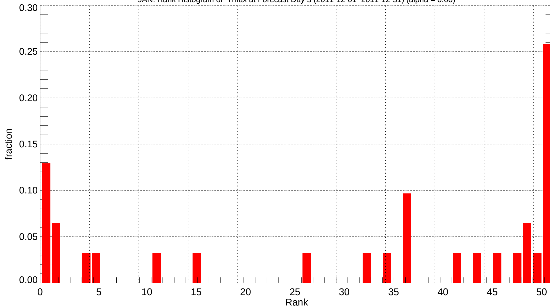
JAN: Rank Histogram of Tmax at Forecast Day 3 (2011-12-01~2011-12-31) (alpha = 0.00)
