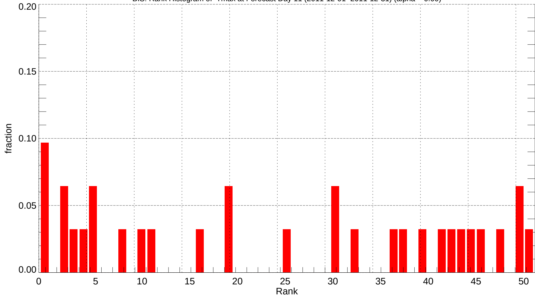
BIS: Rank Histogram of Tmax at Forecast Day 11 (2011-12-01~2011-12-31) (alpha = 0.00)
