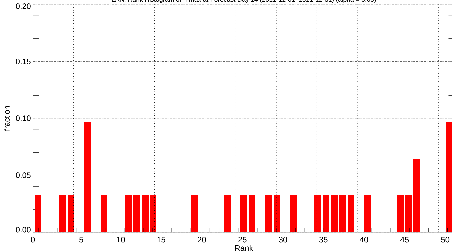
LAN: Rank Histogram of Tmax at Forecast Day 14 (2011-12-01~2011-12-31) (alpha = 0.00)
