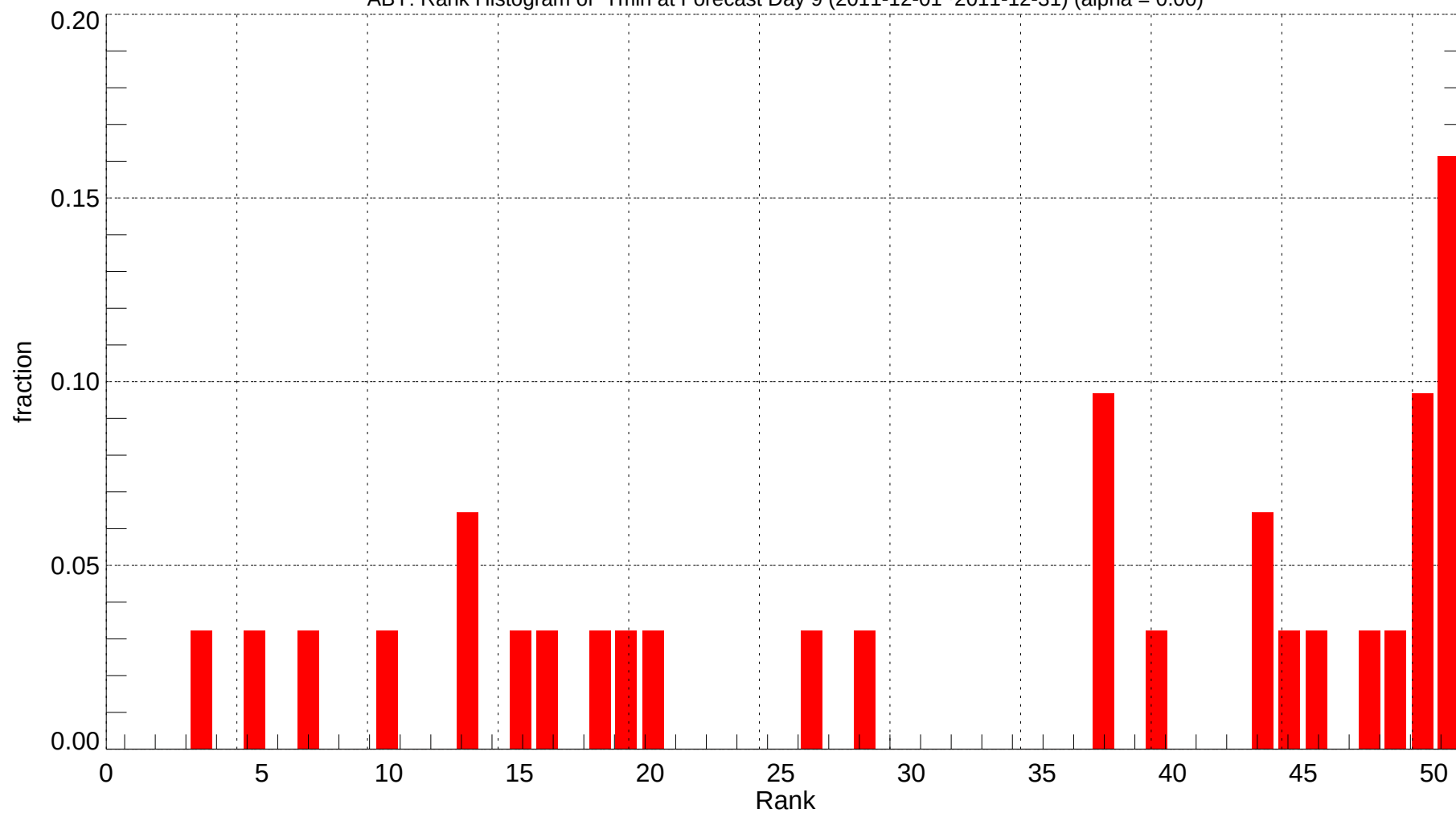
ABY: Rank Histogram of Tmin at Forecast Day 9 (2011-12-01~2011-12-31) (alpha = 0.00)
