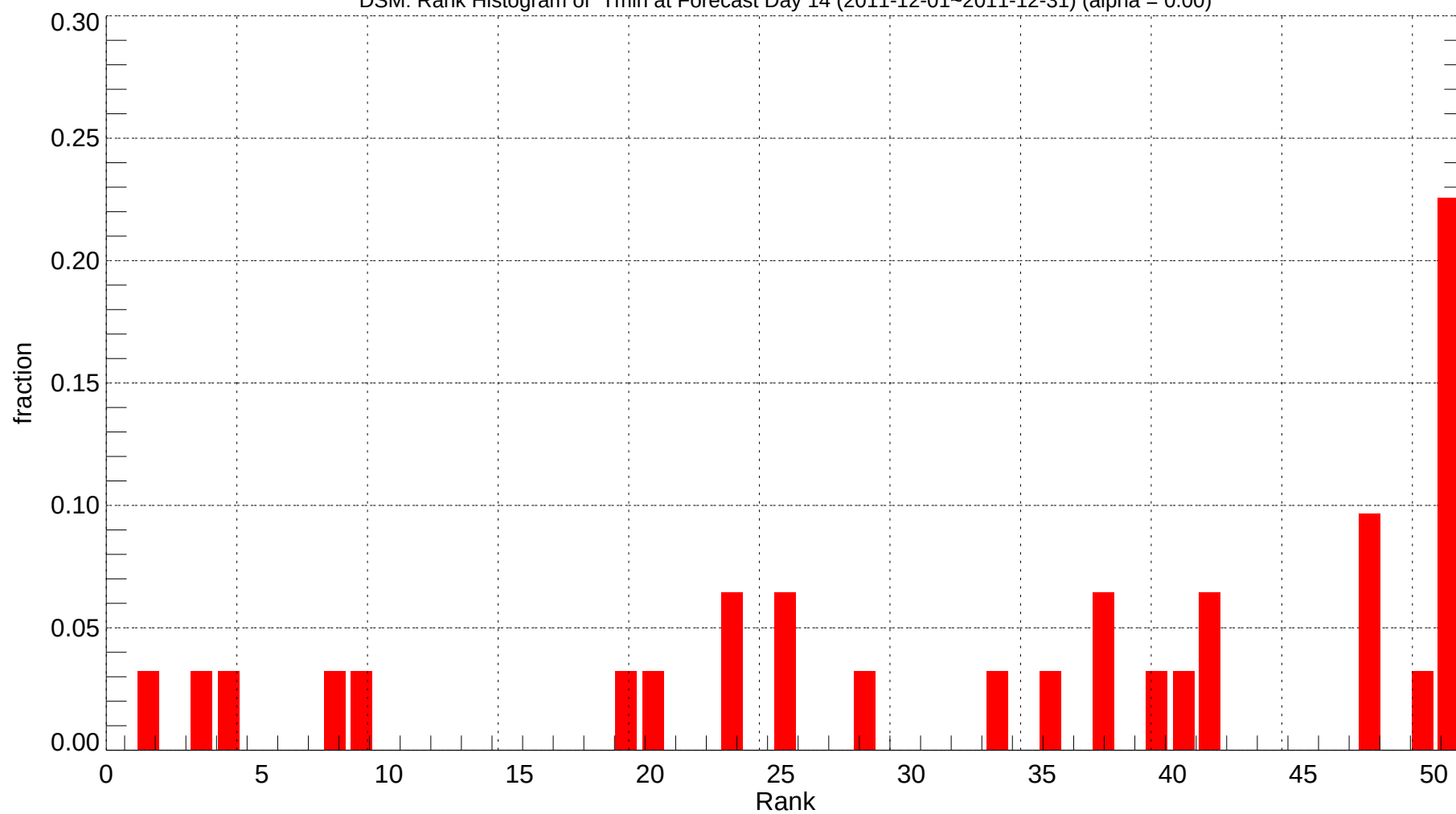
DSM: Rank Histogram of Tmin at Forecast Day 14 (2011-12-01~2011-12-31) (alpha = 0.00)
