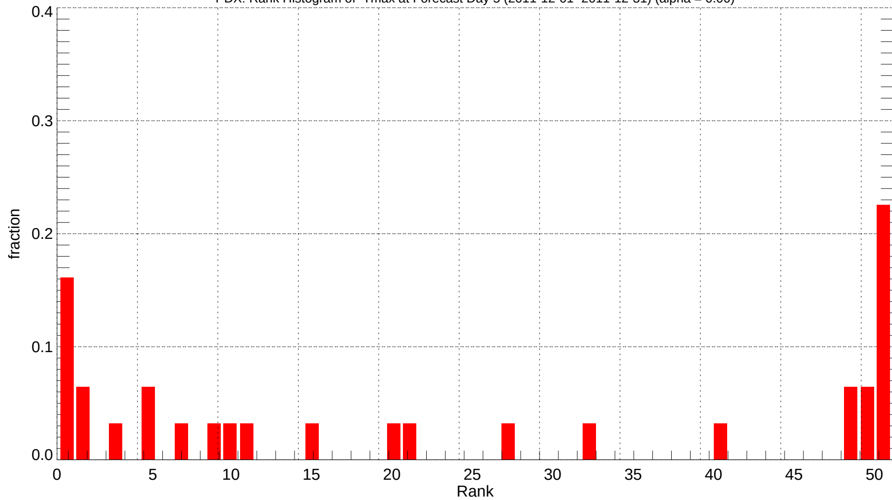
PDX: Rank Histogram of Tmax at Forecast Day 5 (2011-12-01~2011-12-31) (alpha = 0.00)
