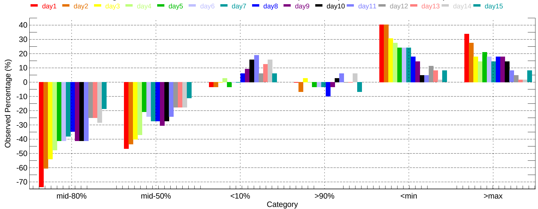
Observed Percentage Deviation of Ensembles - TRM: Min Temperature (2011-12-01~2011-12-31)
