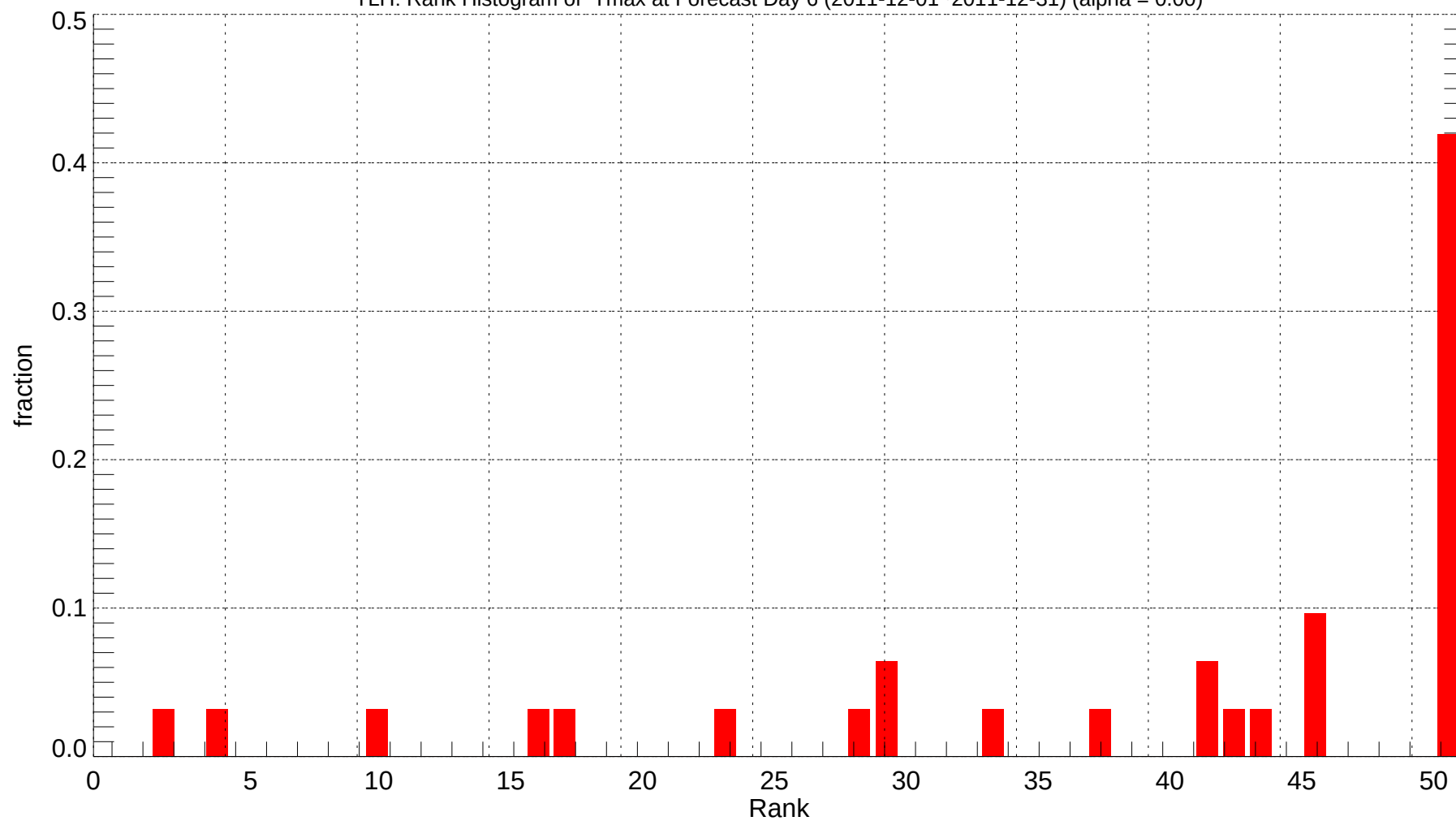
TLH: Rank Histogram of Tmax at Forecast Day 6 (2011-12-01~2011-12-31) (alpha = 0.00)
