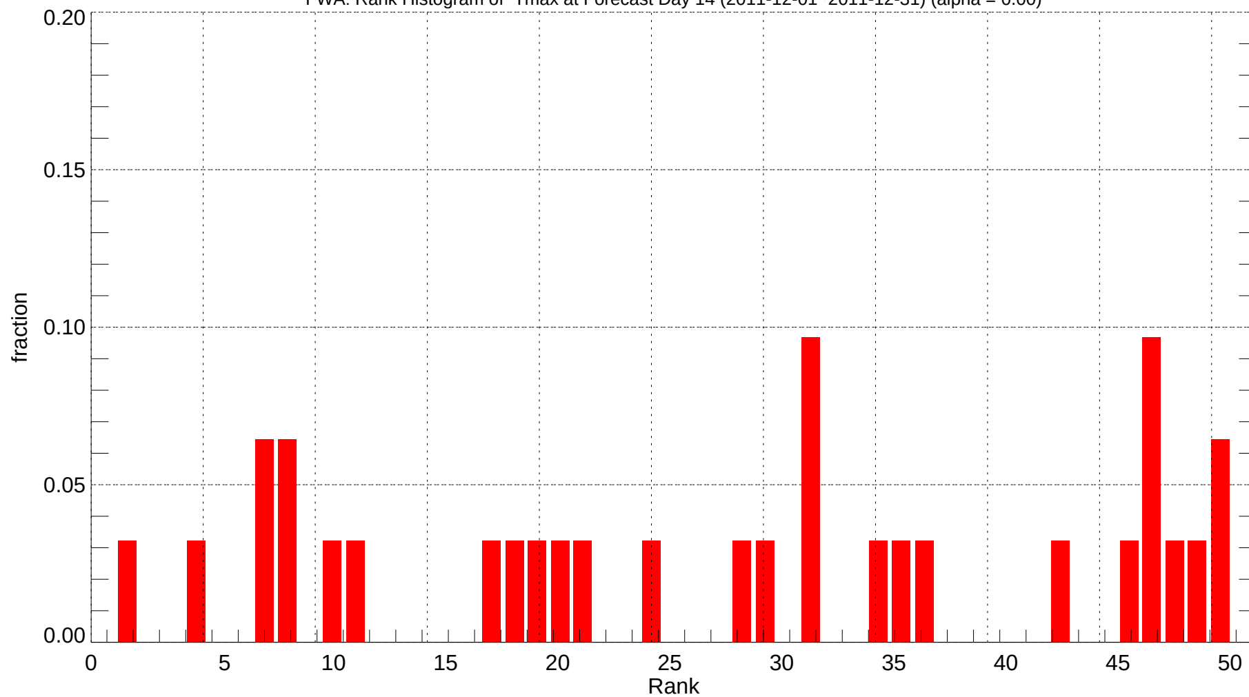
FWA: Rank Histogram of Tmax at Forecast Day 14 (2011-12-01~2011-12-31) (alpha = 0.00)
