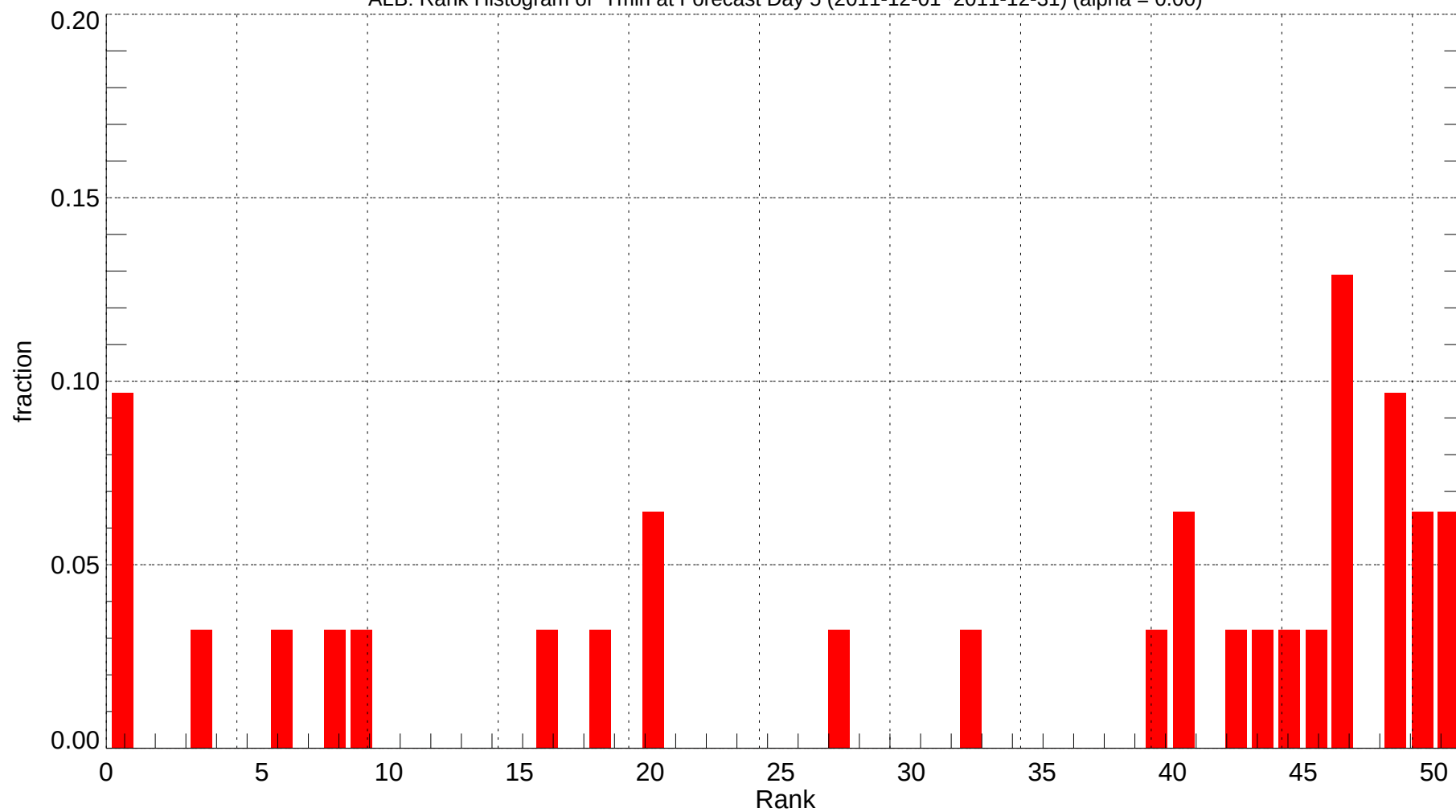
ALB: Rank Histogram of Tmin at Forecast Day 5 (2011-12-01~2011-12-31) (alpha = 0.00)
