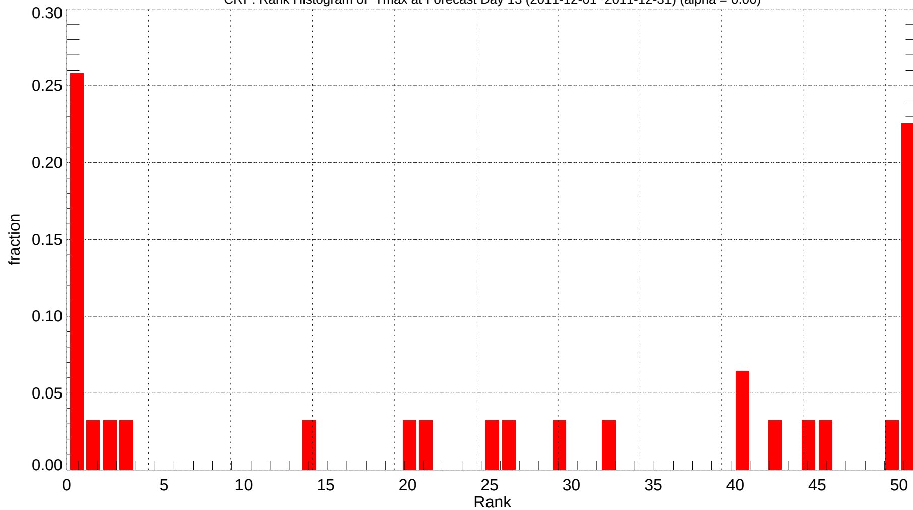
CRP: Rank Histogram of Tmax at Forecast Day 13 (2011-12-01~2011-12-31) (alpha = 0.00)
