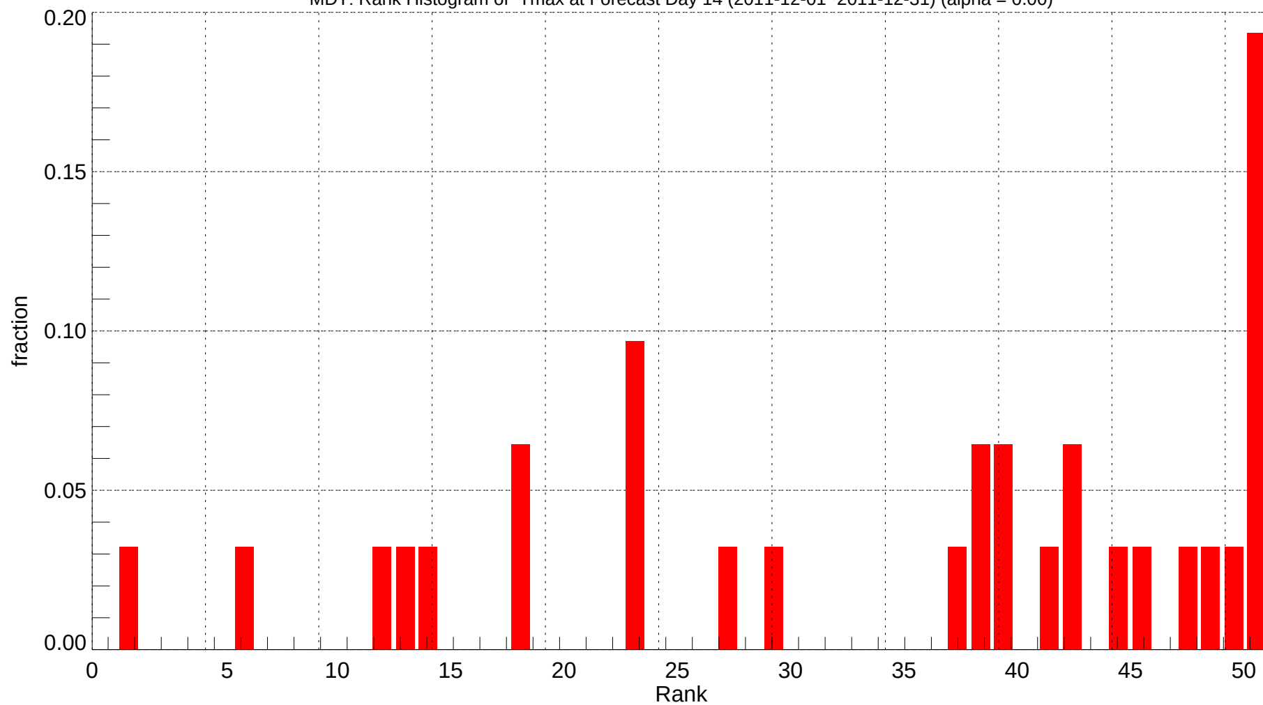
MDT: Rank Histogram of Tmax at Forecast Day 14 (2011-12-01~2011-12-31) (alpha = 0.00)
