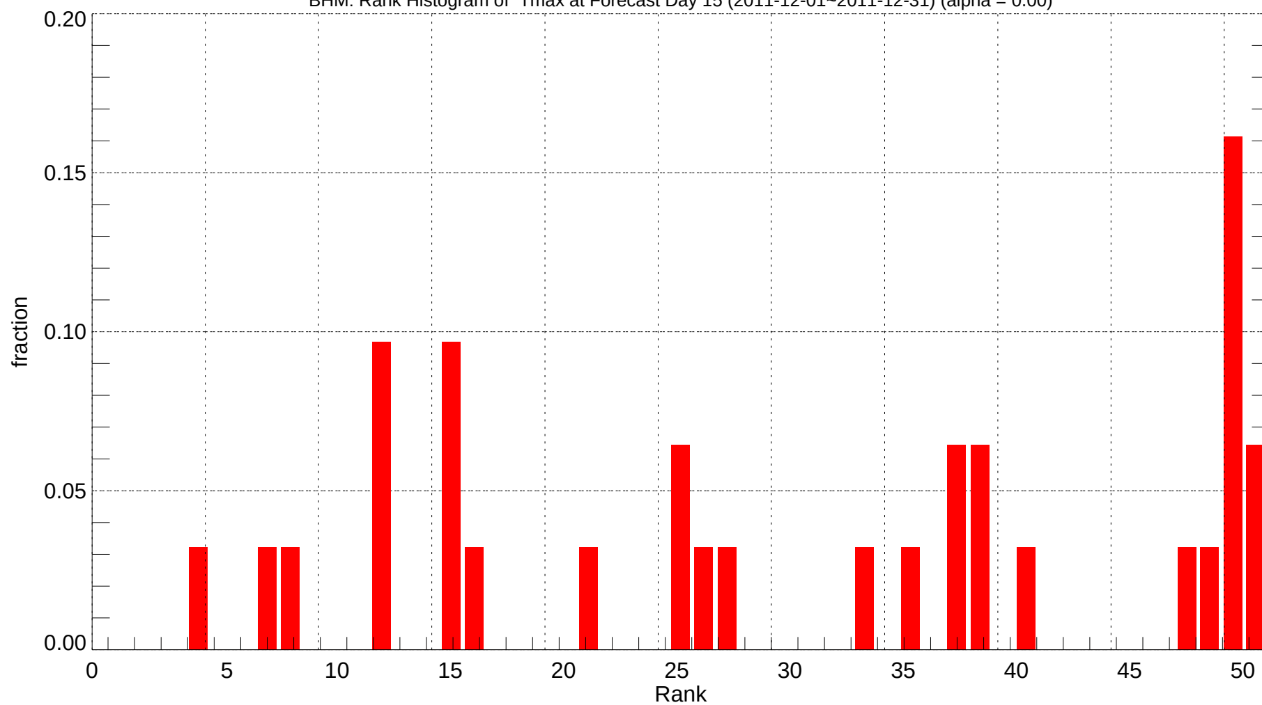
BHM: Rank Histogram of Tmax at Forecast Day 15 (2011-12-01~2011-12-31) (alpha = 0.00)
