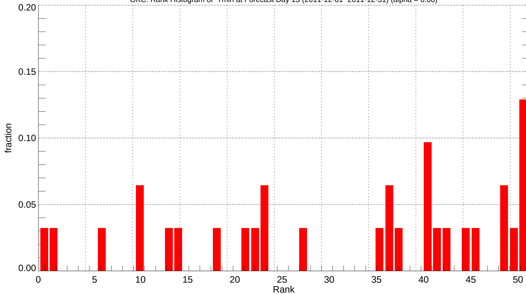
OKC: Rank Histogram of Tmin at Forecast Day 13 (2011-12-01~2011-12-31) (alpha = 0.00)
