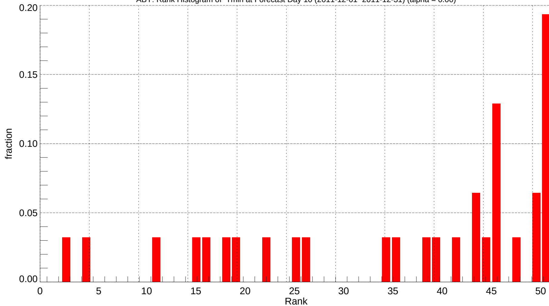
ABY: Rank Histogram of Tmin at Forecast Day 10 (2011-12-01~2011-12-31) (alpha = 0.00)
