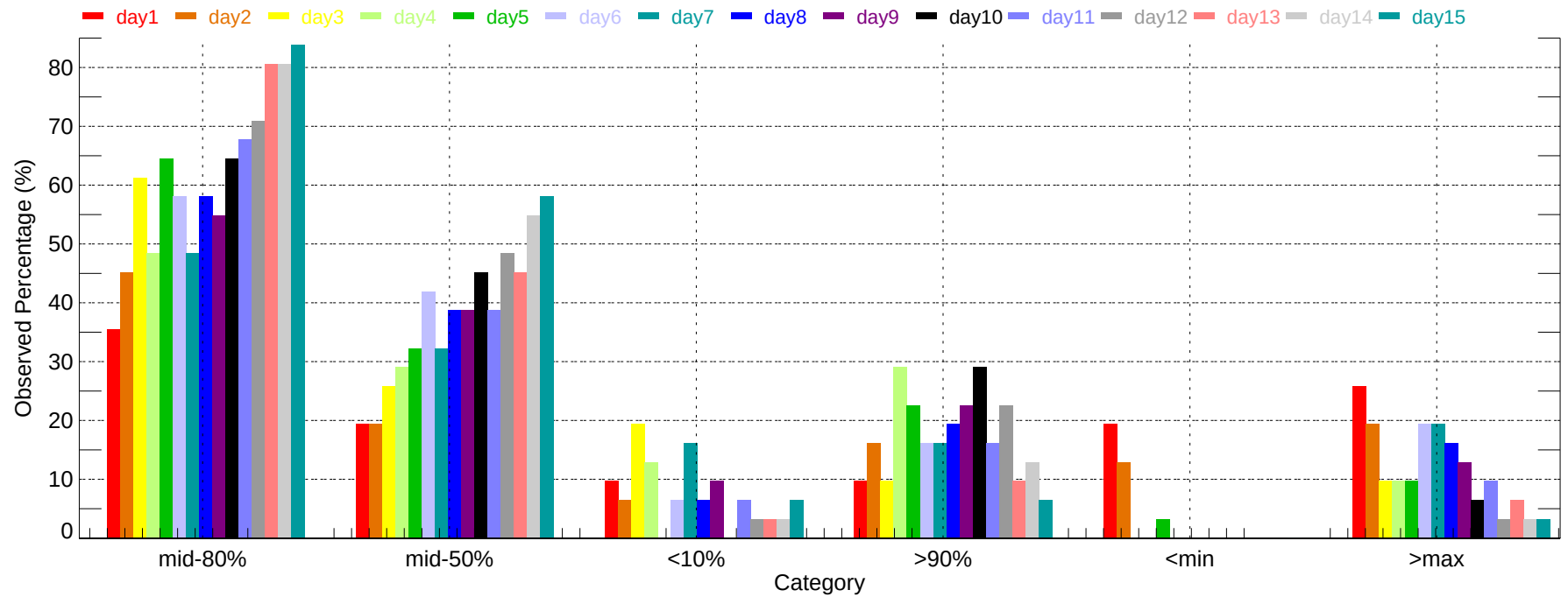
Observed Percentage of Ensembles - DFW: Min Temperature (2011-12-01~2011-12-31)
