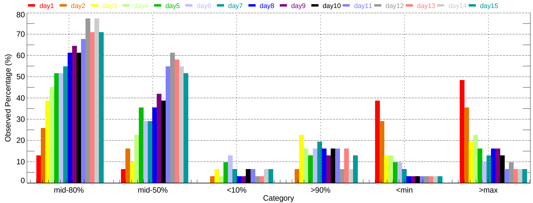
Observed Percentage of Ensembles - FAR: Min Temperature (2011-12-01~2011-12-31)
