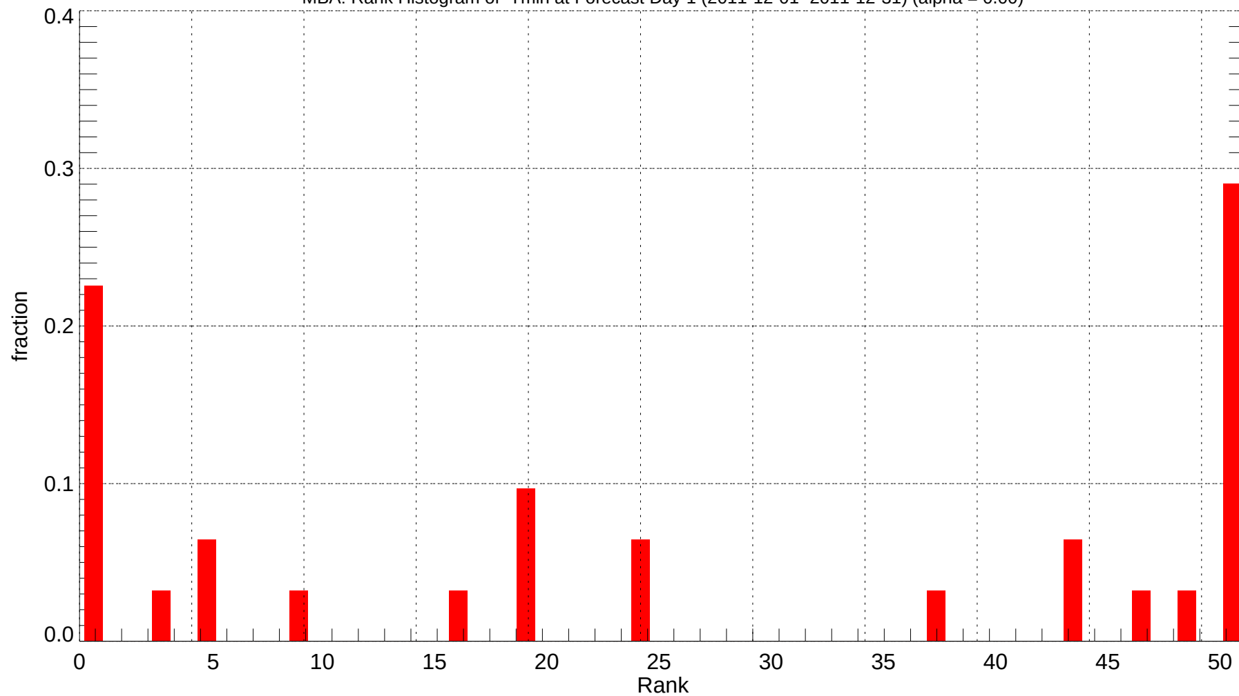
MBA: Rank Histogram of Tmin at Forecast Day 1 (2011-12-01~2011-12-31) (alpha = 0.00)
