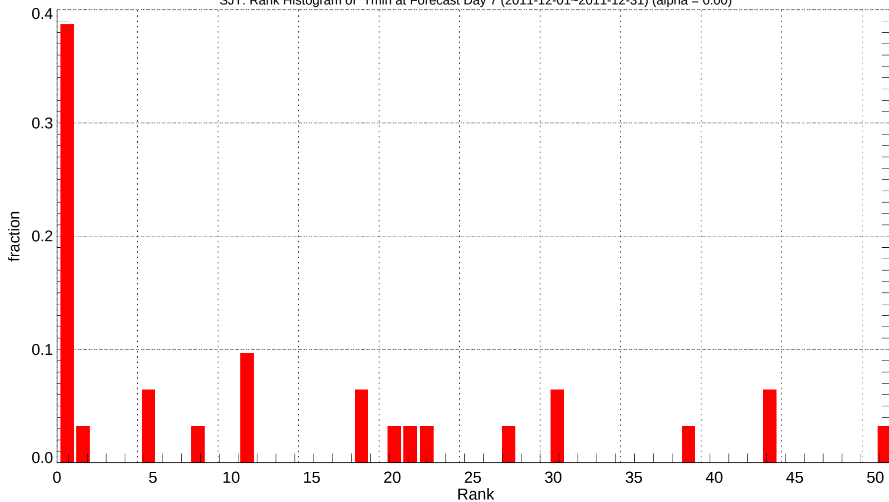
SJT: Rank Histogram of Tmin at Forecast Day 7 (2011-12-01~2011-12-31) (alpha = 0.00)
