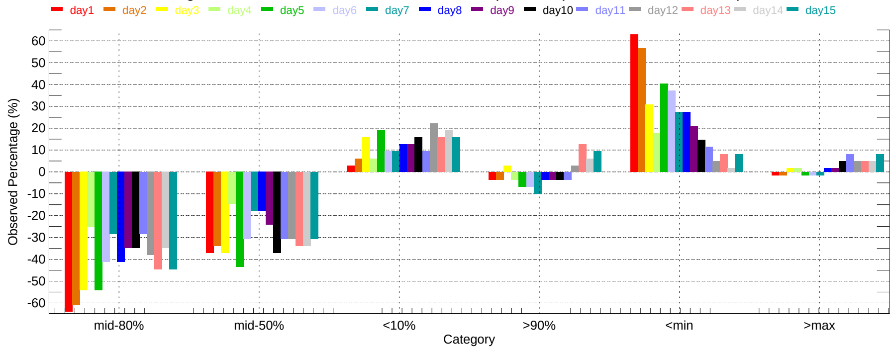
Observed Percentage Deviation of Ensembles - RAL: Max Temperature (2011-12-01~2011-12-31)
