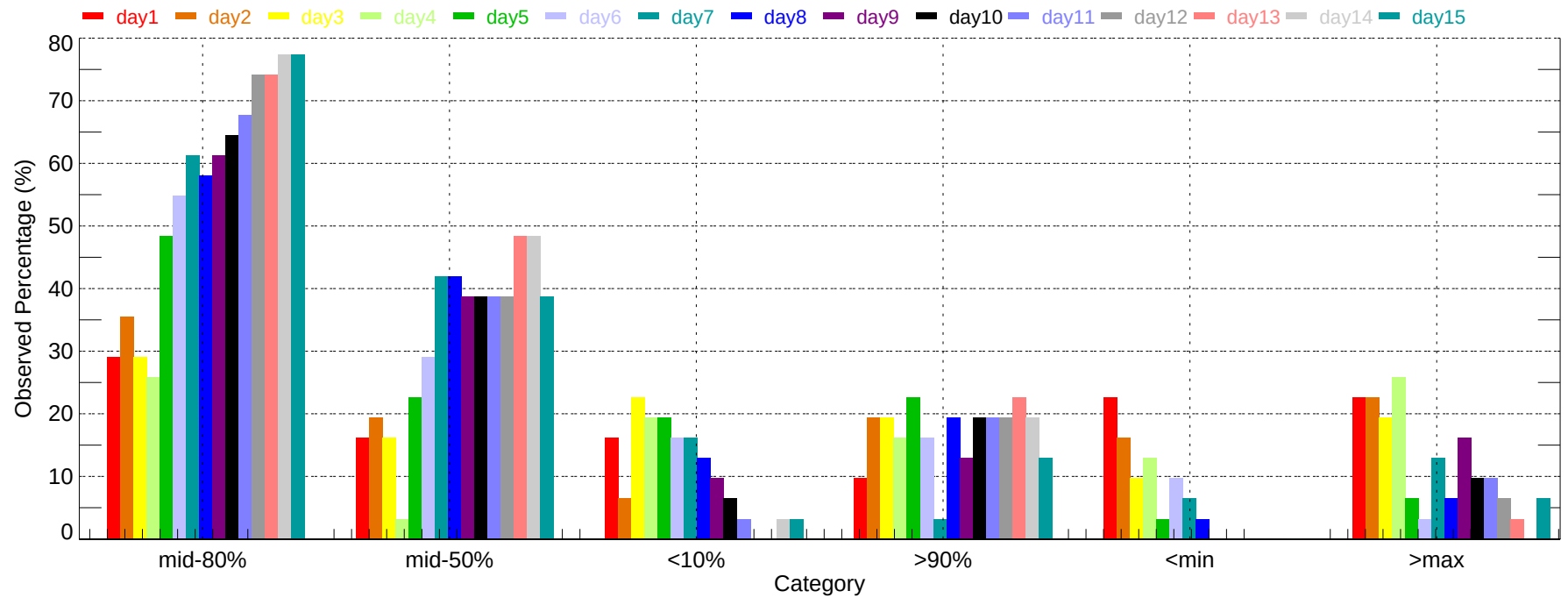
Observed Percentage of Ensembles - CVG: Max Temperature (2011-12-01~2011-12-31)
