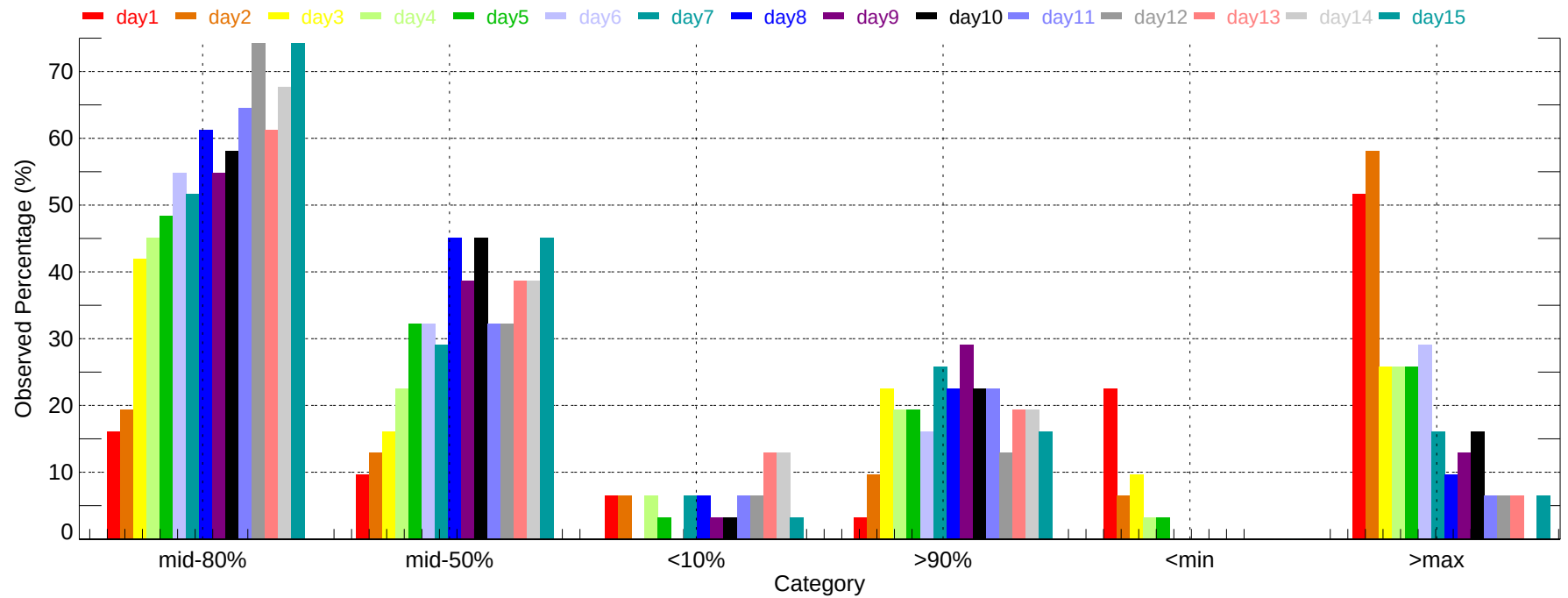
Observed Percentage of Ensembles - EVV: Min Temperature (2011-12-01~2011-12-31)
