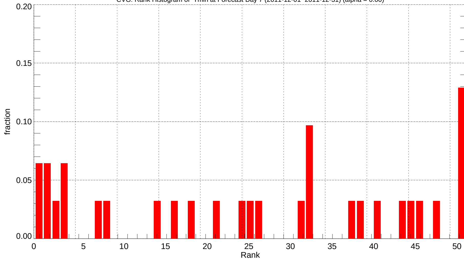
CVG: Rank Histogram of Tmin at Forecast Day 7 (2011-12-01~2011-12-31) (alpha = 0.00)
