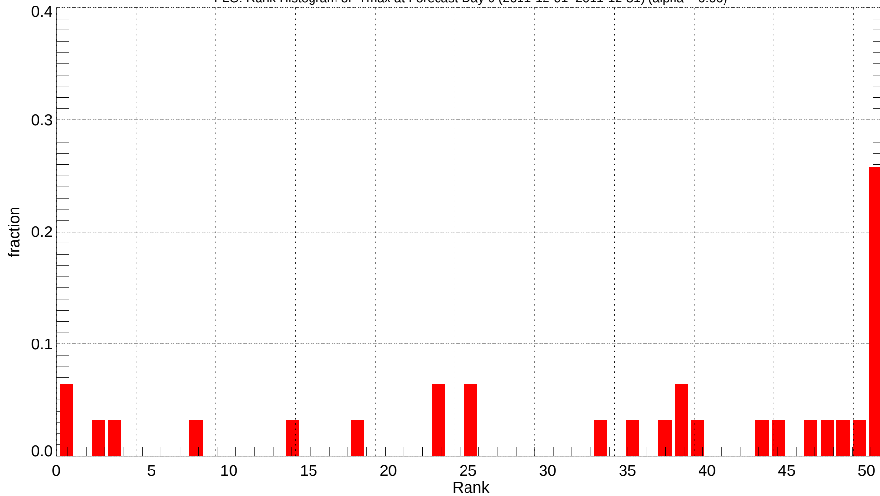
FLG: Rank Histogram of Tmax at Forecast Day 6 (2011-12-01~2011-12-31) (alpha = 0.00)
