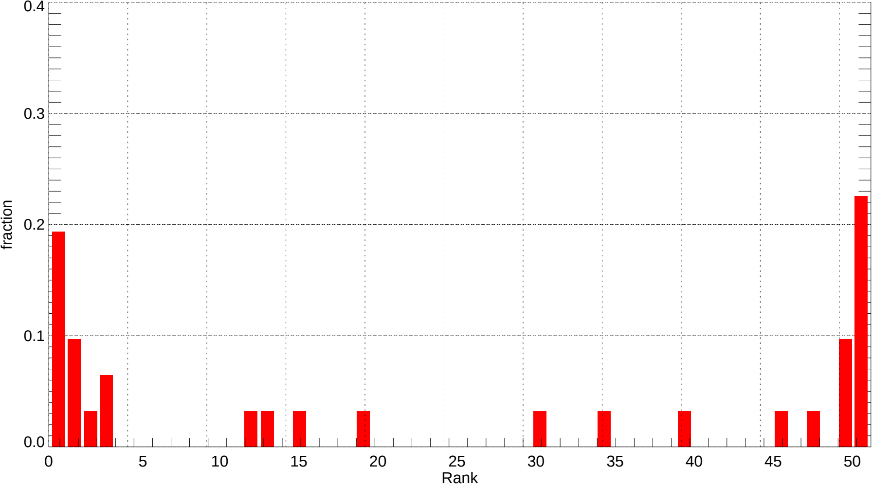
SJC: Rank Histogram of Tmin at Forecast Day 3 (2011-12-01~2011-12-31) (alpha = 0.00)
