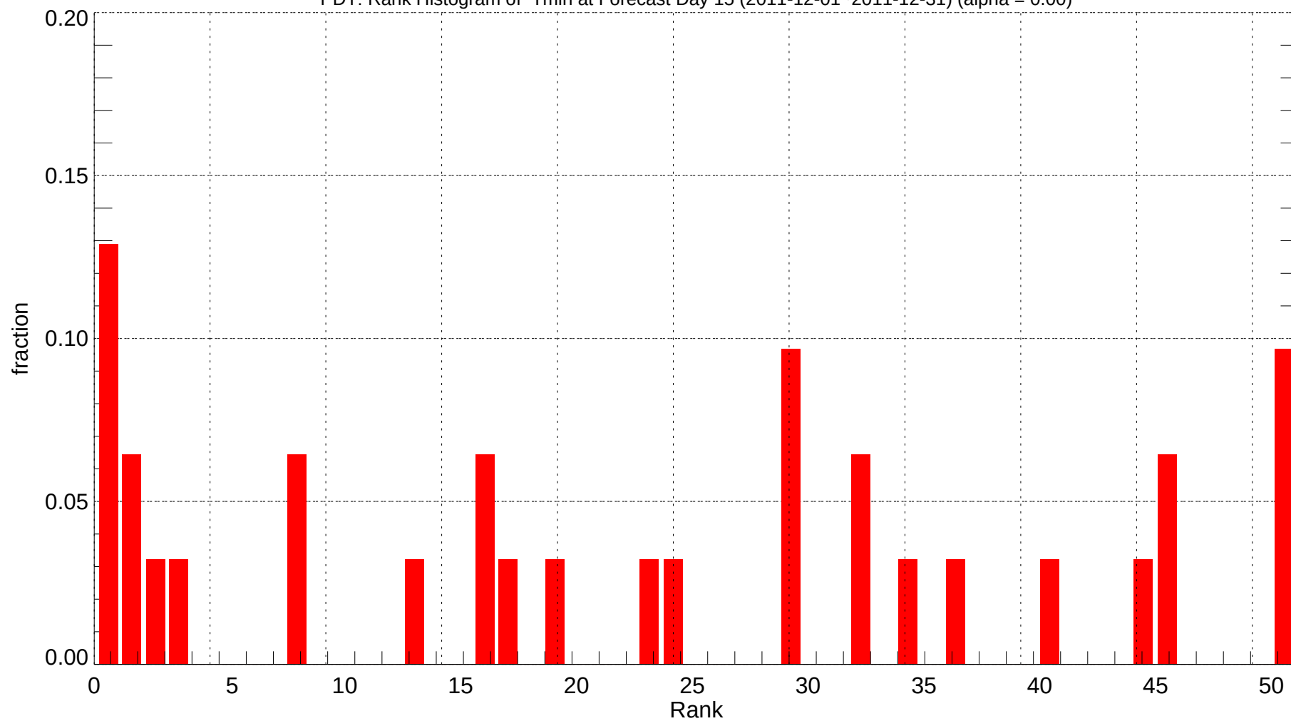
PDT: Rank Histogram of Tmin at Forecast Day 15 (2011-12-01~2011-12-31) (alpha = 0.00)
