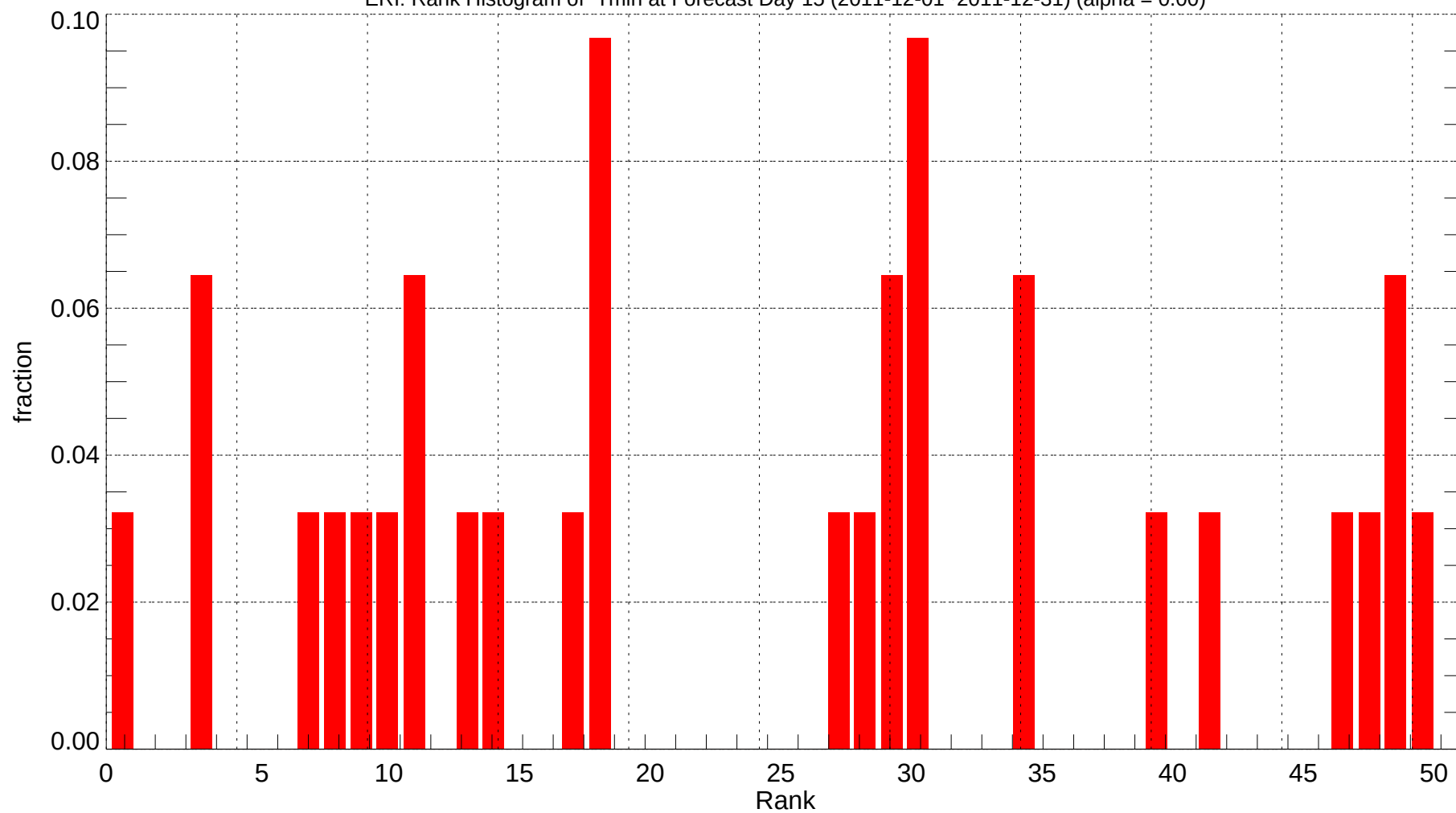
ERI: Rank Histogram of Tmin at Forecast Day 15 (2011-12-01~2011-12-31) (alpha = 0.00)
