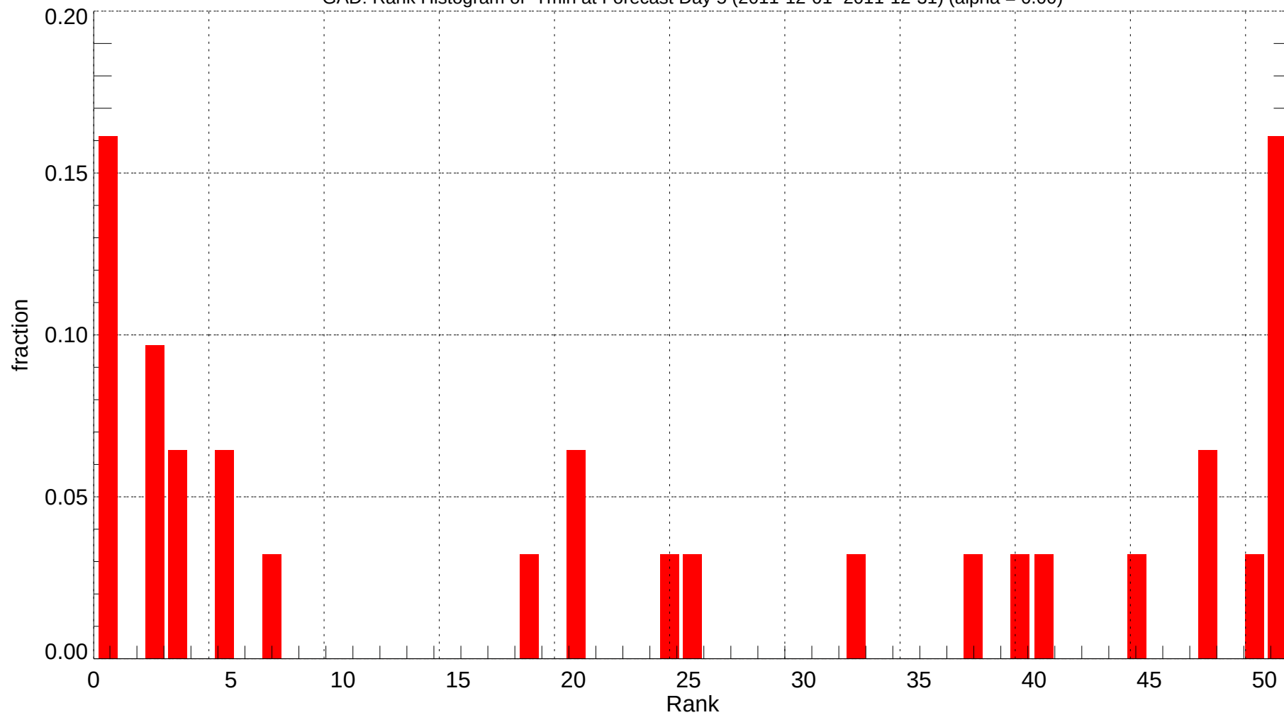
GAD: Rank Histogram of Tmin at Forecast Day 5 (2011-12-01~2011-12-31) (alpha = 0.00)
