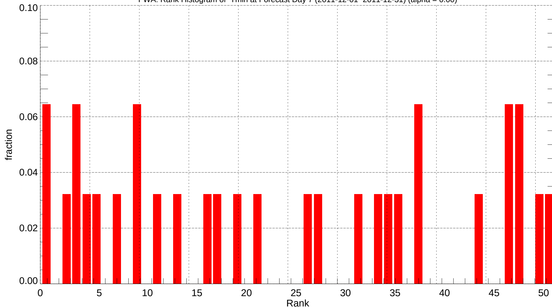
FWA: Rank Histogram of Tmin at Forecast Day 7 (2011-12-01~2011-12-31) (alpha = 0.00)
