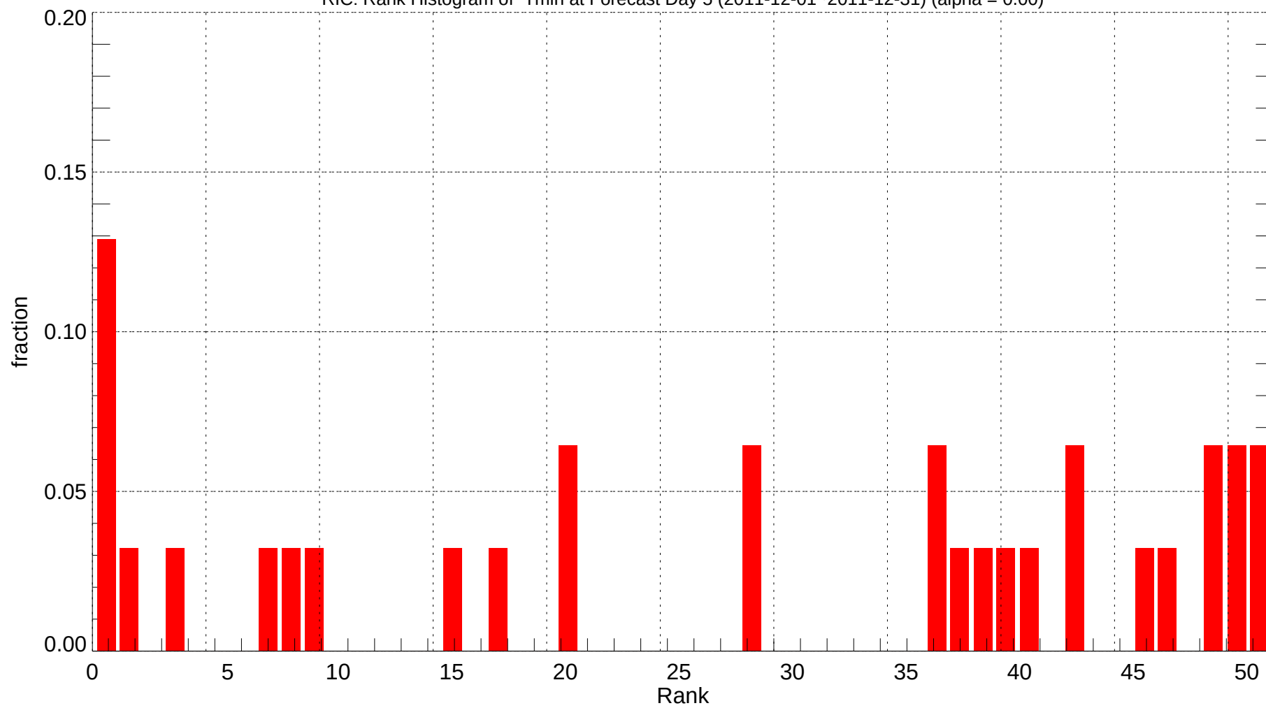
RIC: Rank Histogram of Tmin at Forecast Day 5 (2011-12-01~2011-12-31) (alpha = 0.00)
