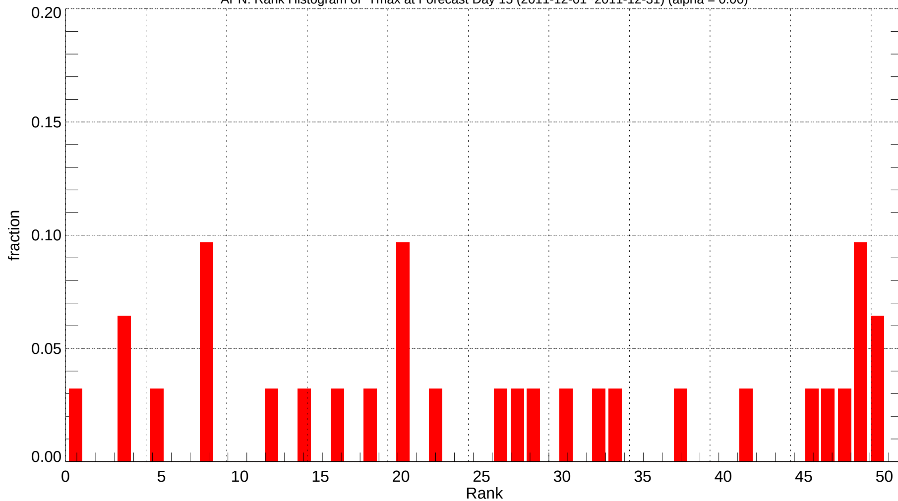
APN: Rank Histogram of Tmax at Forecast Day 15 (2011-12-01~2011-12-31) (alpha = 0.00)
