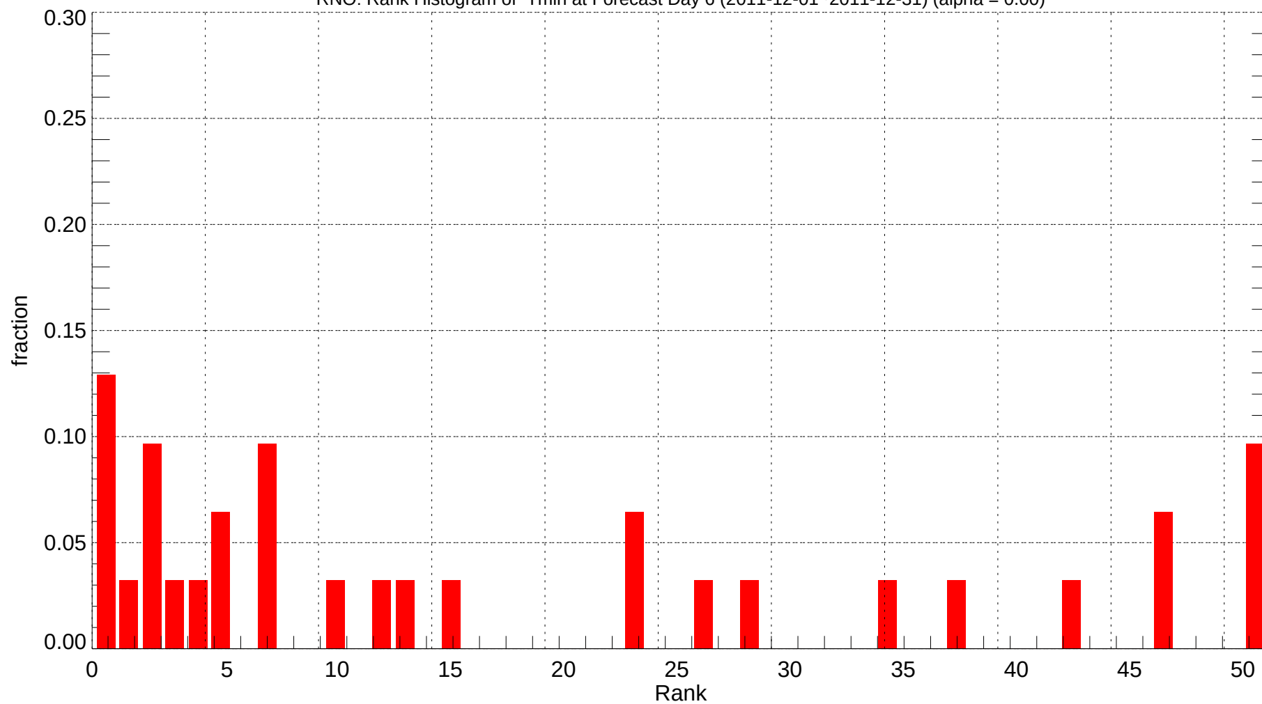
RNO: Rank Histogram of Tmin at Forecast Day 6 (2011-12-01~2011-12-31) (alpha = 0.00)
