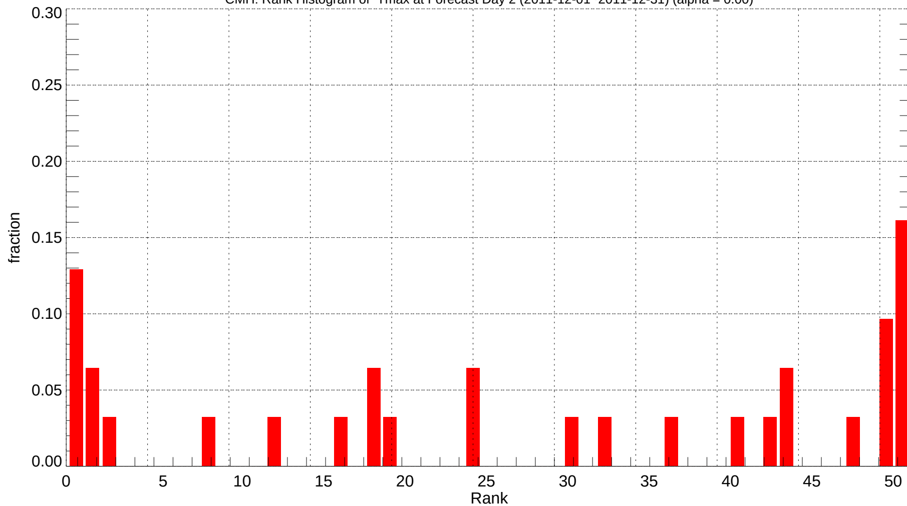
CMH: Rank Histogram of Tmax at Forecast Day 2 (2011-12-01~2011-12-31) (alpha = 0.00)
