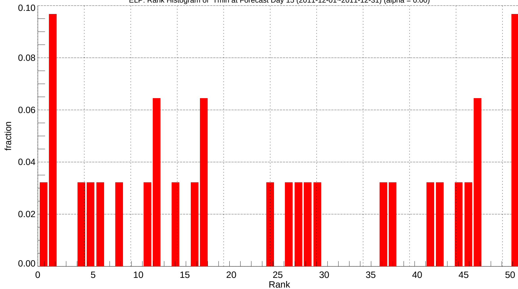
ELP: Rank Histogram of Tmin at Forecast Day 15 (2011-12-01~2011-12-31) (alpha = 0.00)
