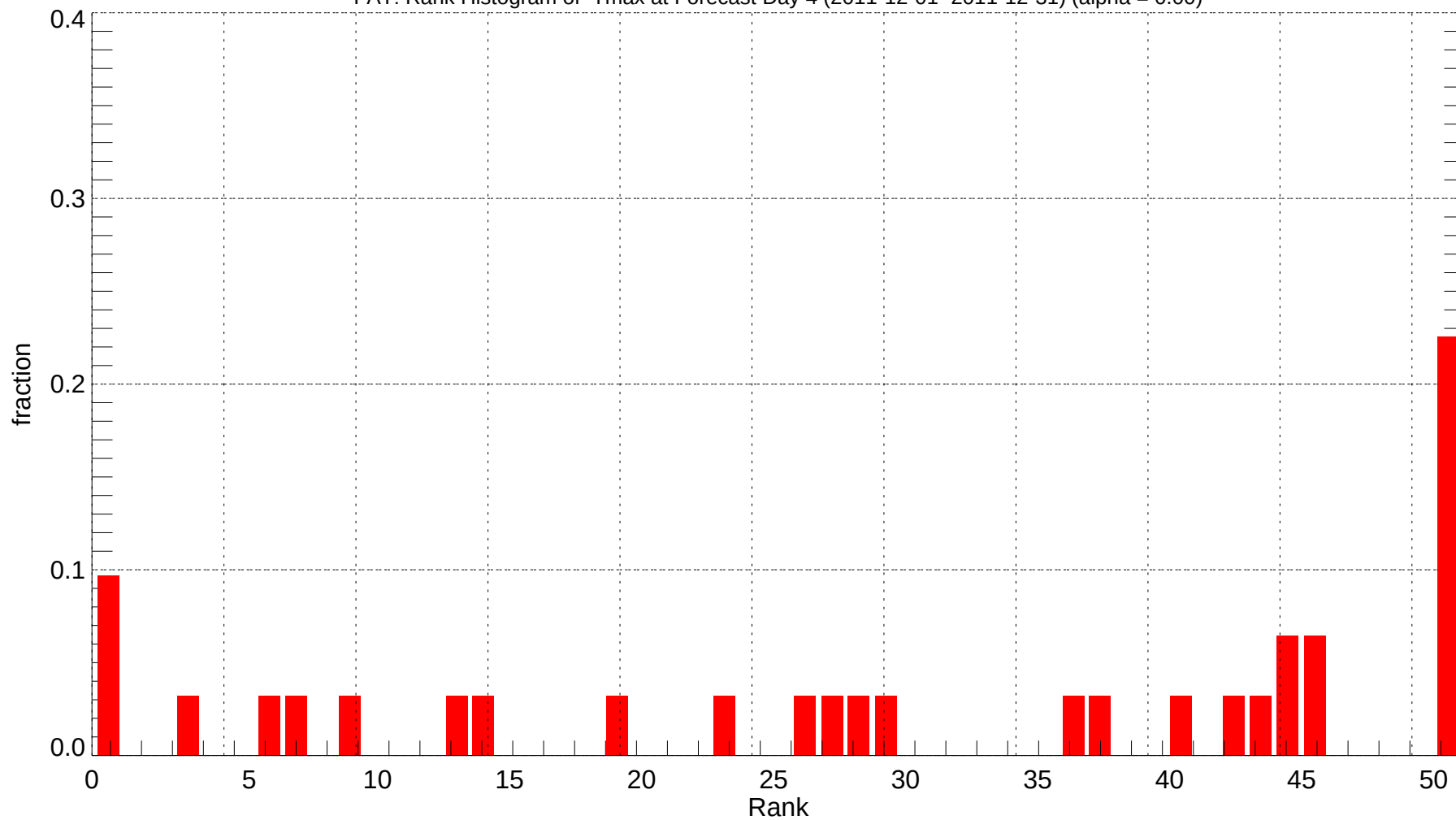
FAT: Rank Histogram of Tmax at Forecast Day 4 (2011-12-01~2011-12-31) (alpha = 0.00)
