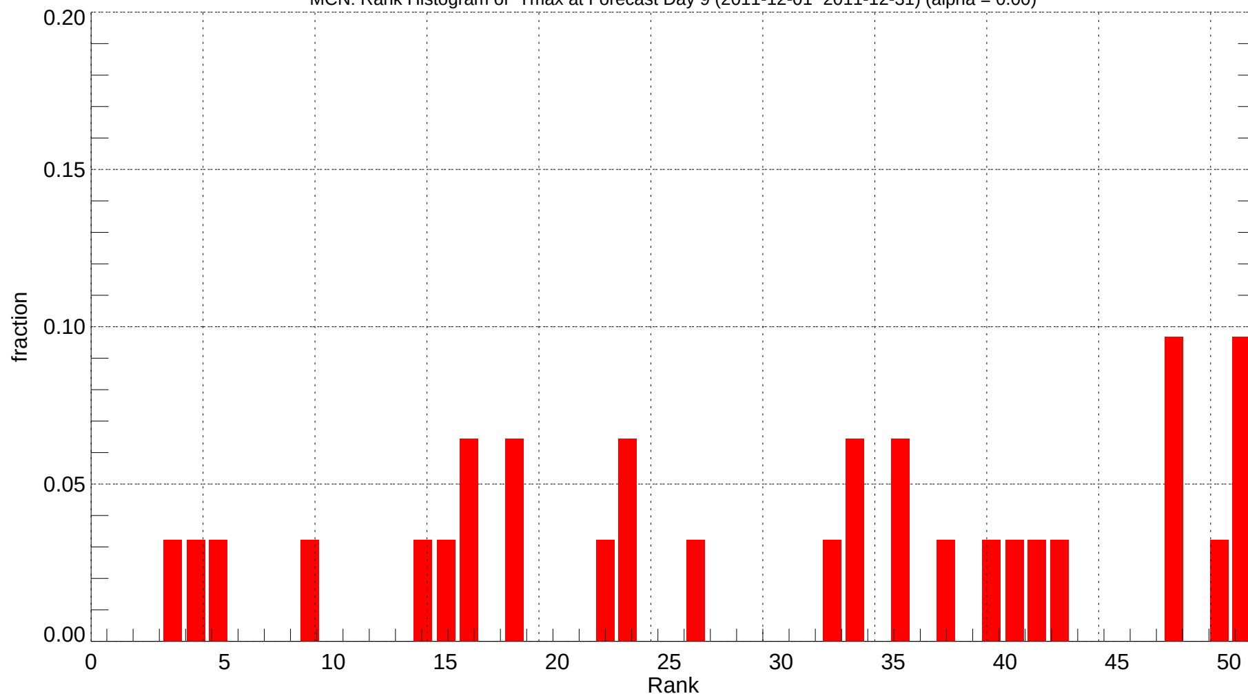
MCN: Rank Histogram of Tmax at Forecast Day 9 (2011-12-01~2011-12-31) (alpha = 0.00)
