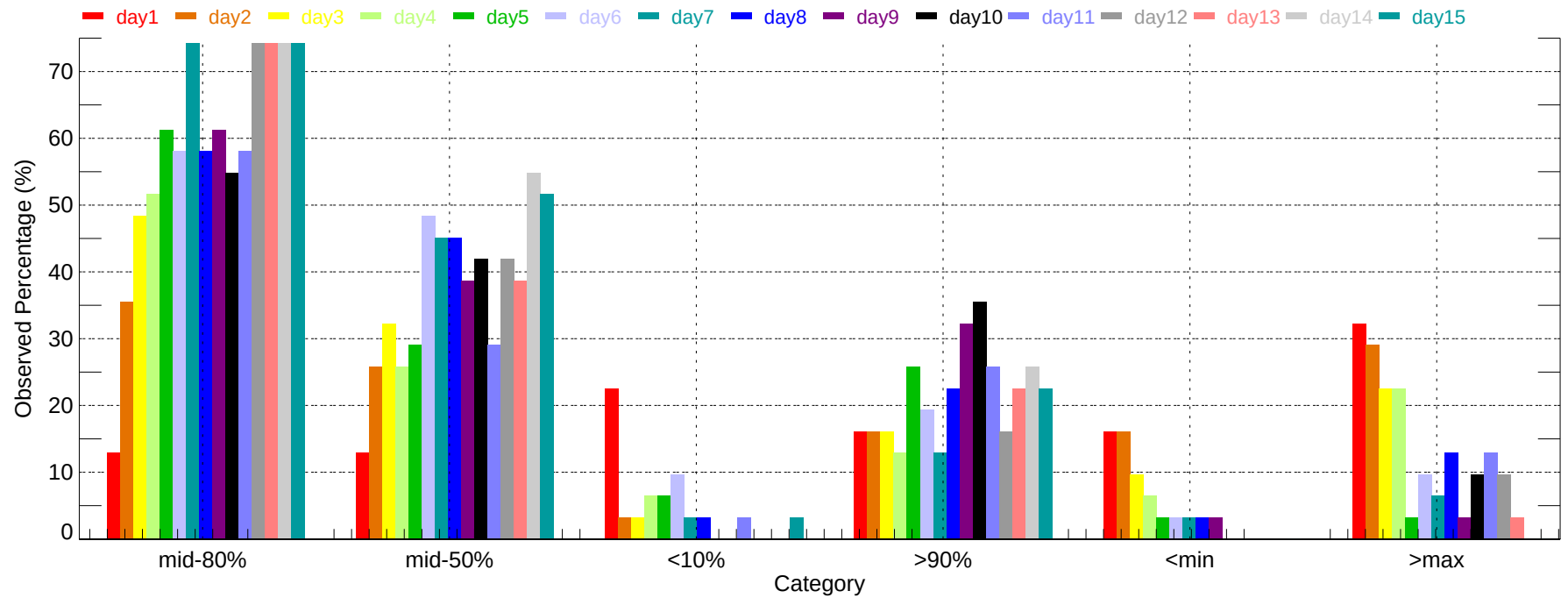
Observed Percentage of Ensembles - LAN: Min Temperature (2011-12-01~2011-12-31)
