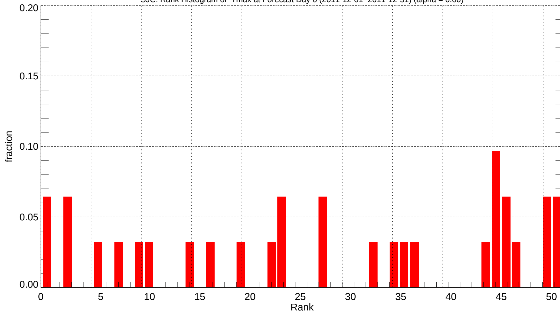
SJC: Rank Histogram of Tmax at Forecast Day 6 (2011-12-01~2011-12-31) (alpha = 0.00)
