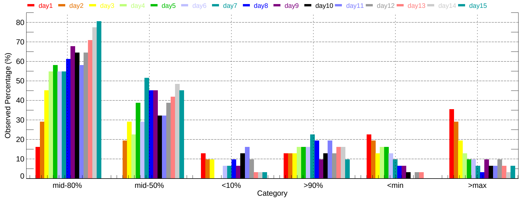
Observed Percentage of Ensembles - YVR: Min Temperature (2011-12-01~2011-12-31)
