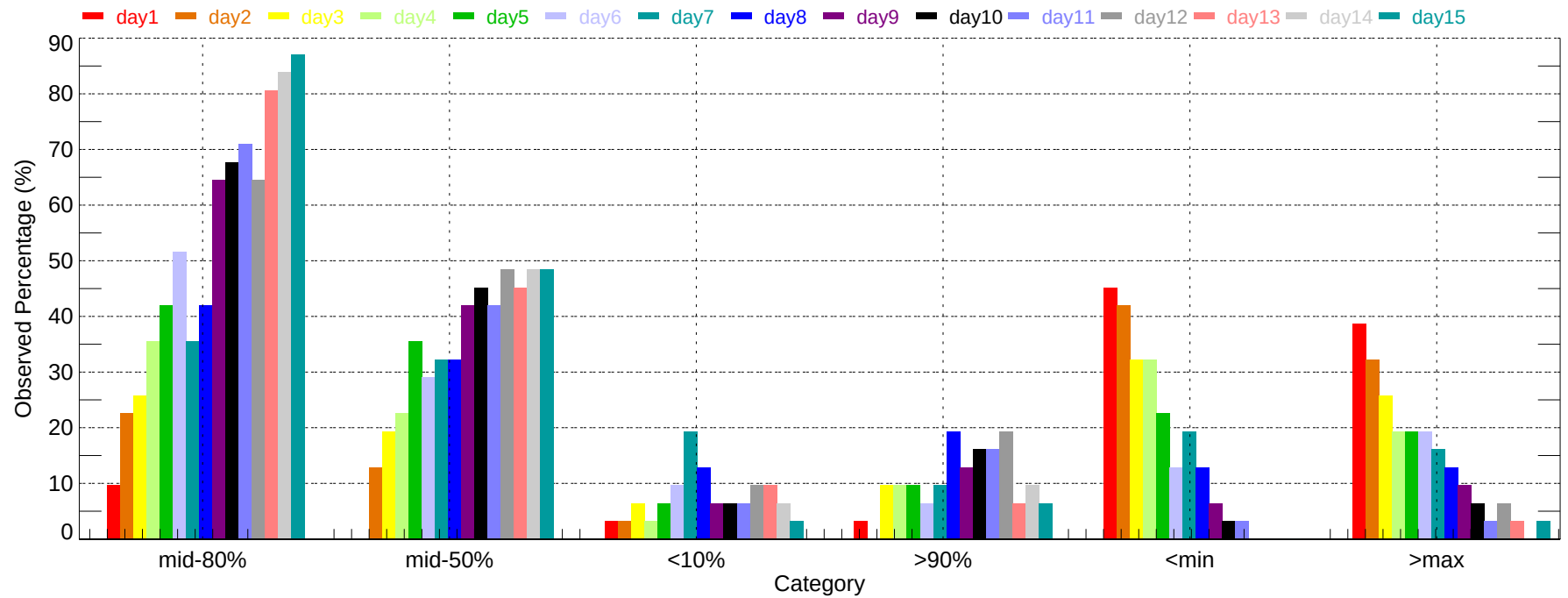
Observed Percentage of Ensembles - NTU: Min Temperature (2011-12-01~2011-12-31)
