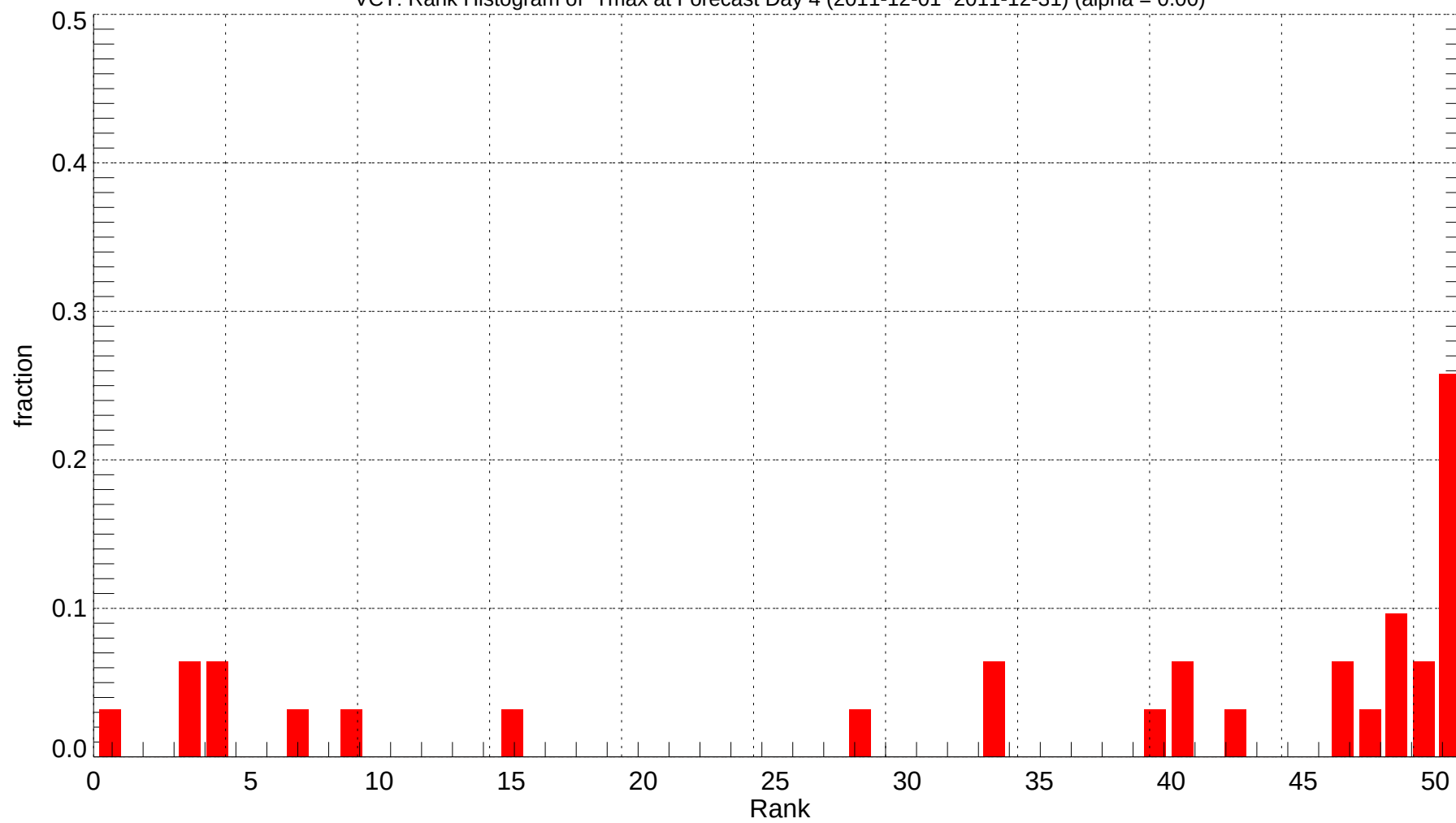
VCT: Rank Histogram of Tmax at Forecast Day 4 (2011-12-01~2011-12-31) (alpha = 0.00)
