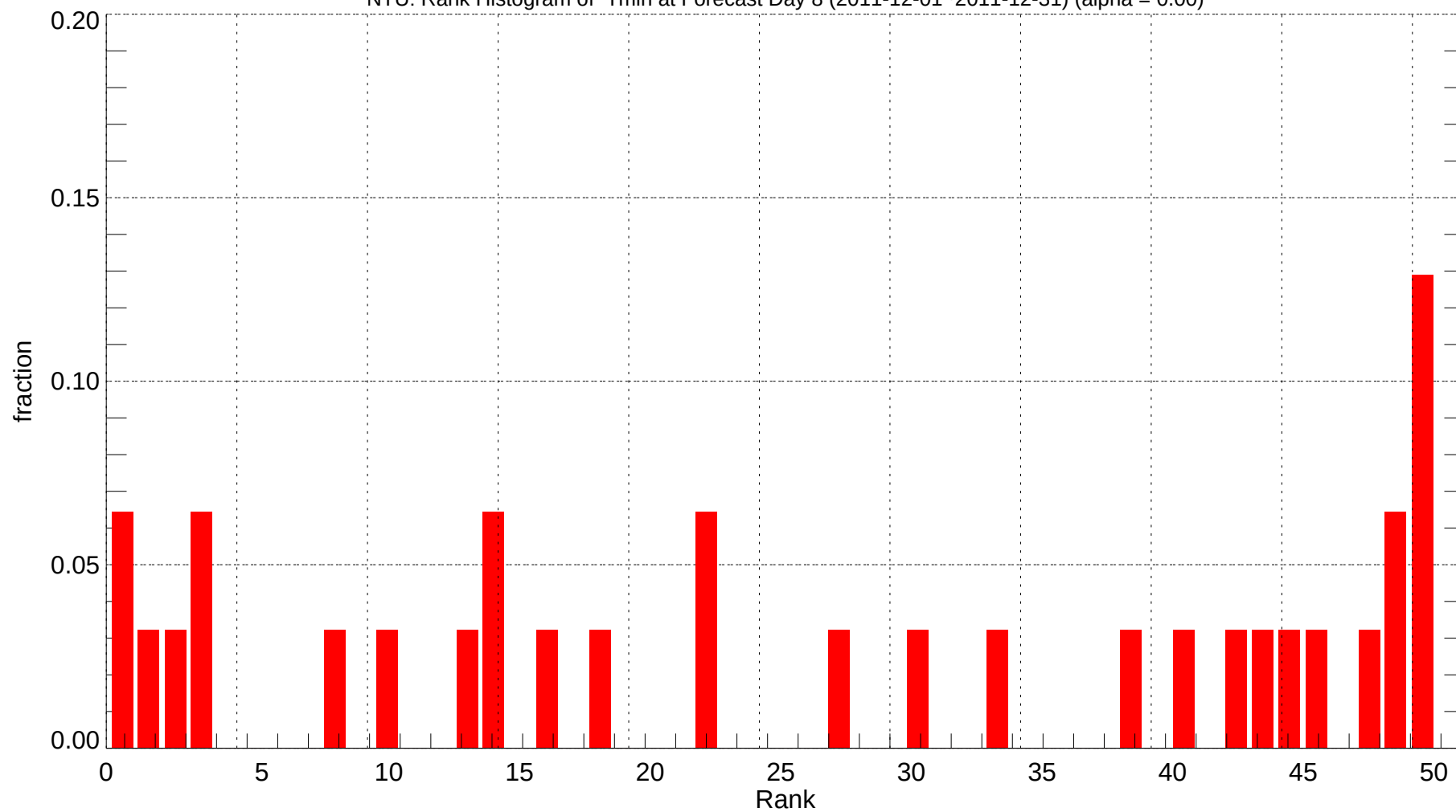
NTU: Rank Histogram of Tmin at Forecast Day 8 (2011-12-01~2011-12-31) (alpha = 0.00)
