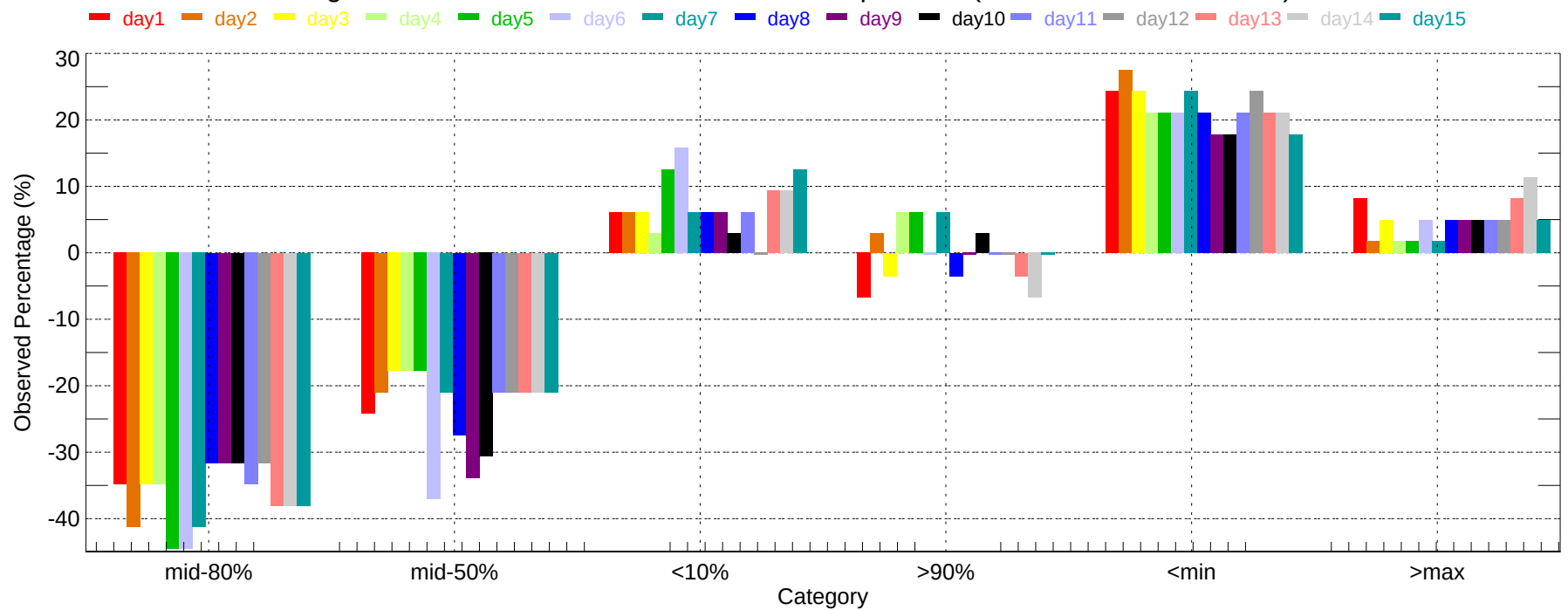
Observed Percentage Deviation of Ensembles - ABI: Max Temperature (2011-12-01~2011-12-31)
