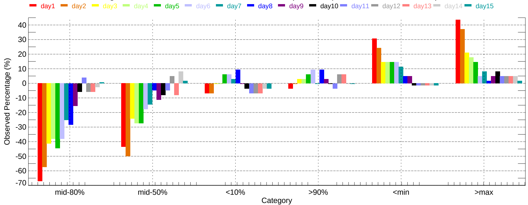
Observed Percentage Deviation of Ensembles - CON: Min Temperature (2011-12-01~2011-12-31)
