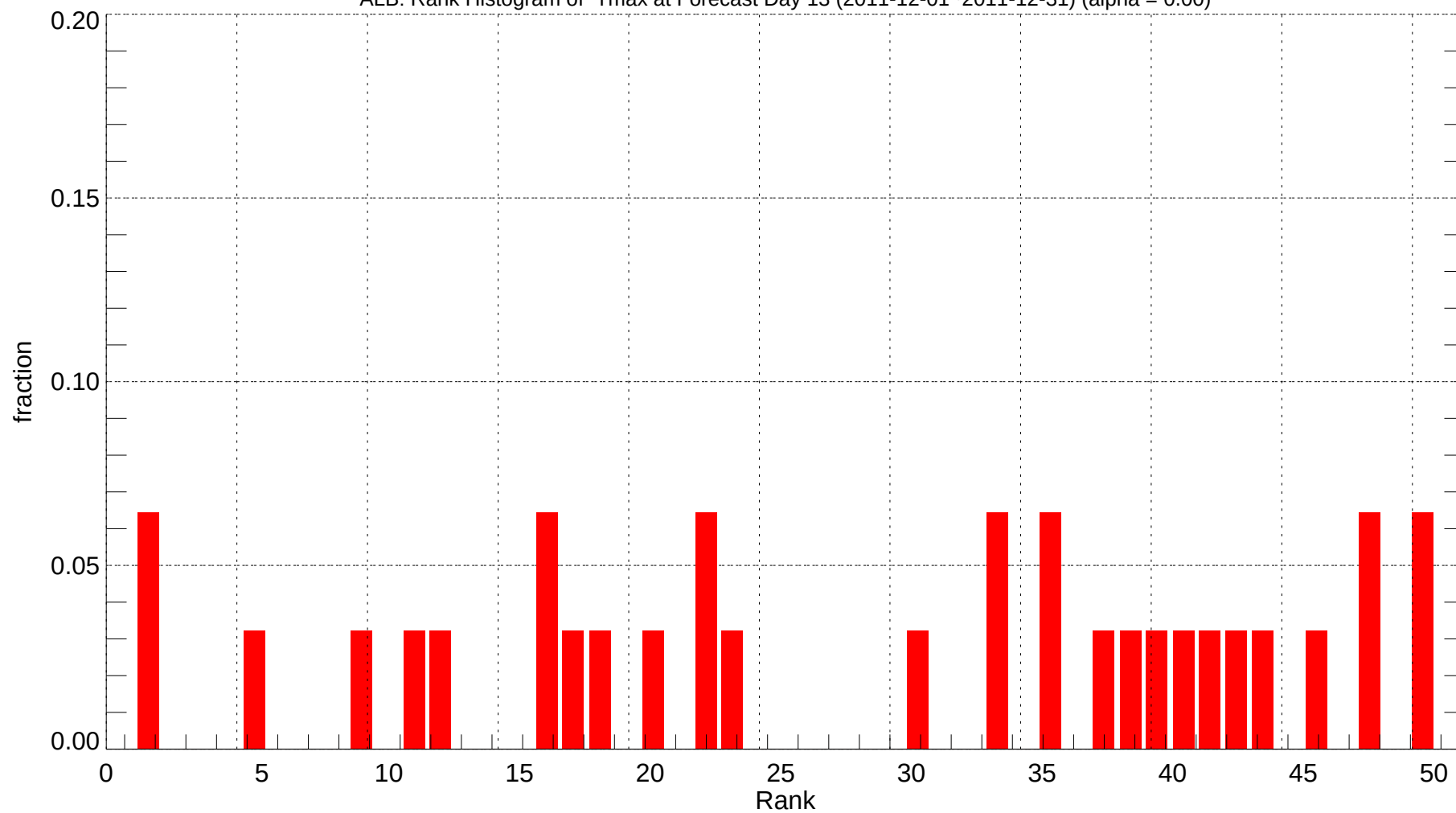
ALB: Rank Histogram of Tmax at Forecast Day 13 (2011-12-01~2011-12-31) (alpha = 0.00)
