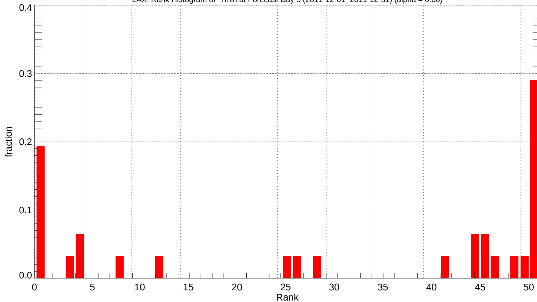
LAX: Rank Histogram of Tmin at Forecast Day 5 (2011-12-01~2011-12-31) (alpha = 0.00)
