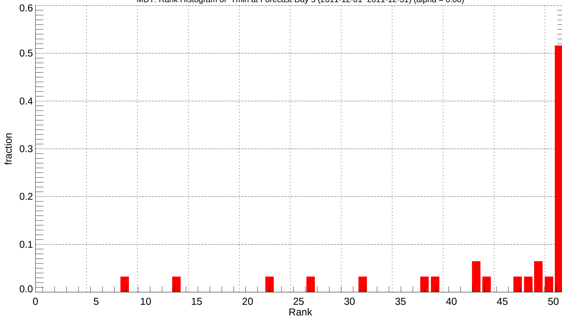
MDT: Rank Histogram of Tmin at Forecast Day 5 (2011-12-01~2011-12-31) (alpha = 0.00)
