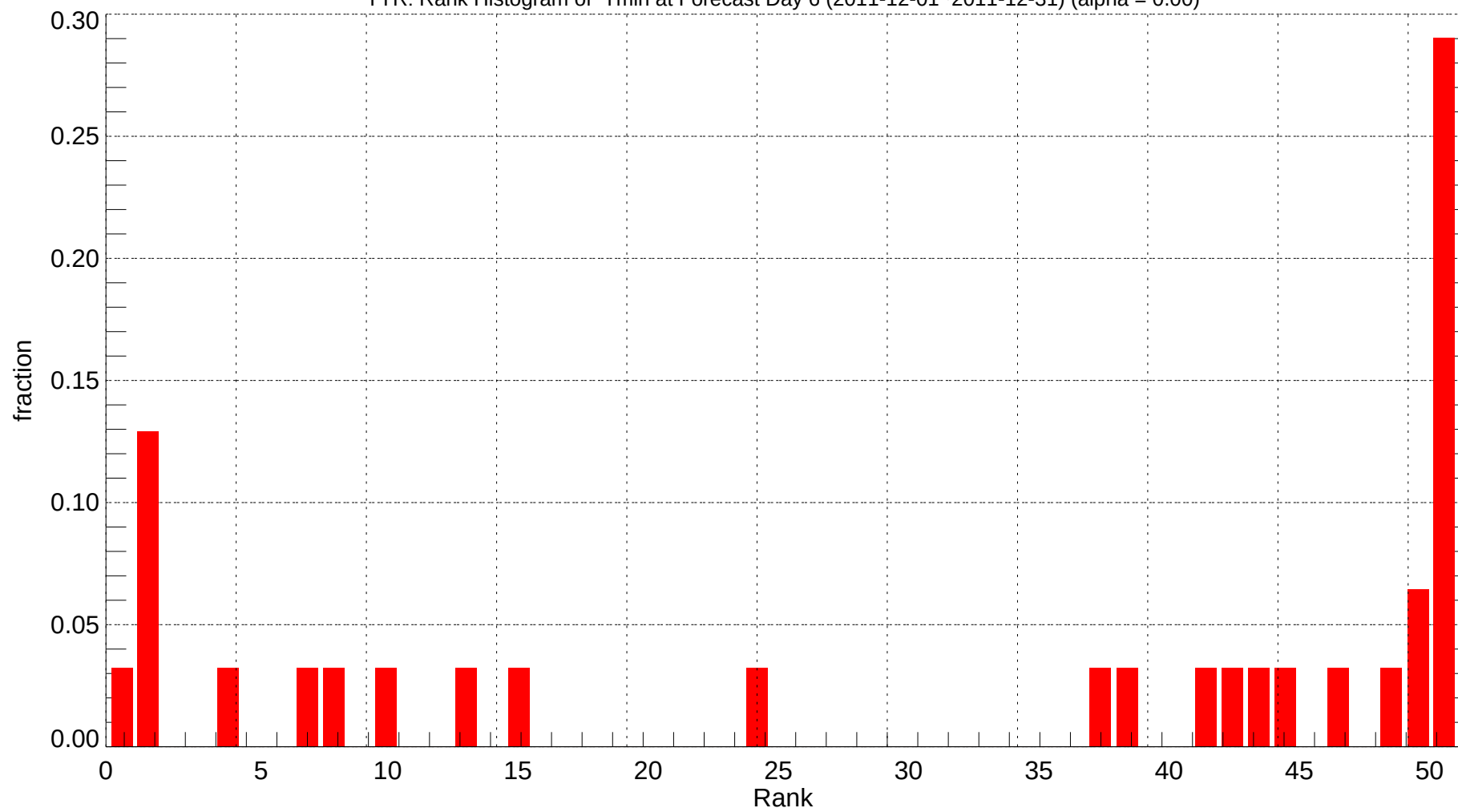
TYR: Rank Histogram of Tmin at Forecast Day 6 (2011-12-01~2011-12-31) (alpha = 0.00)
