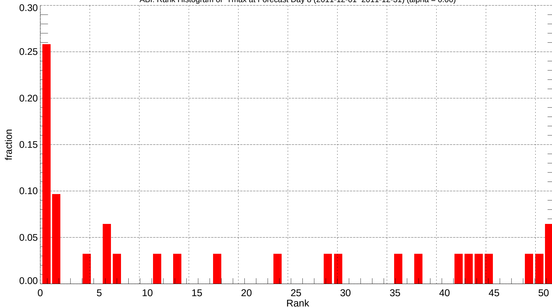
ABI: Rank Histogram of Tmax at Forecast Day 8 (2011-12-01~2011-12-31) (alpha = 0.00)
