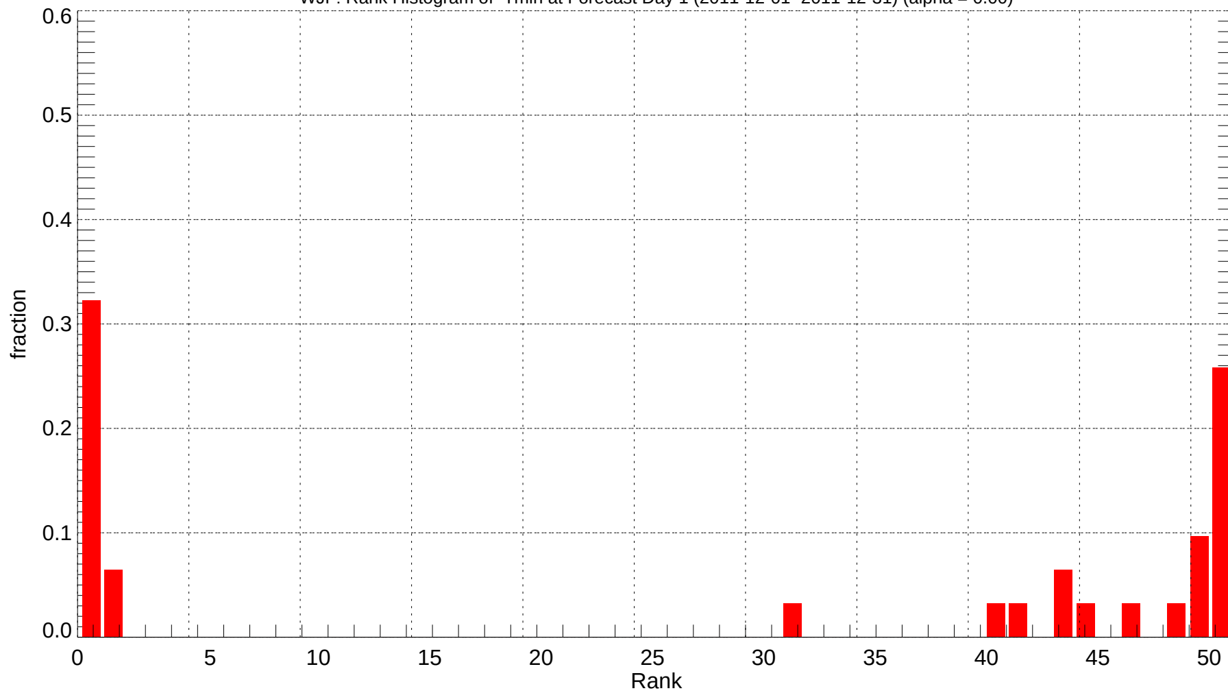
WJF: Rank Histogram of Tmin at Forecast Day 1 (2011-12-01~2011-12-31) (alpha = 0.00)
