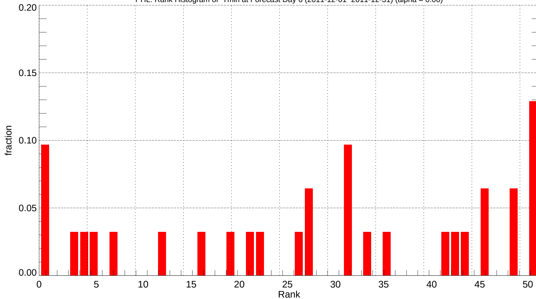
PHL: Rank Histogram of Tmin at Forecast Day 6 (2011-12-01~2011-12-31) (alpha = 0.00)
