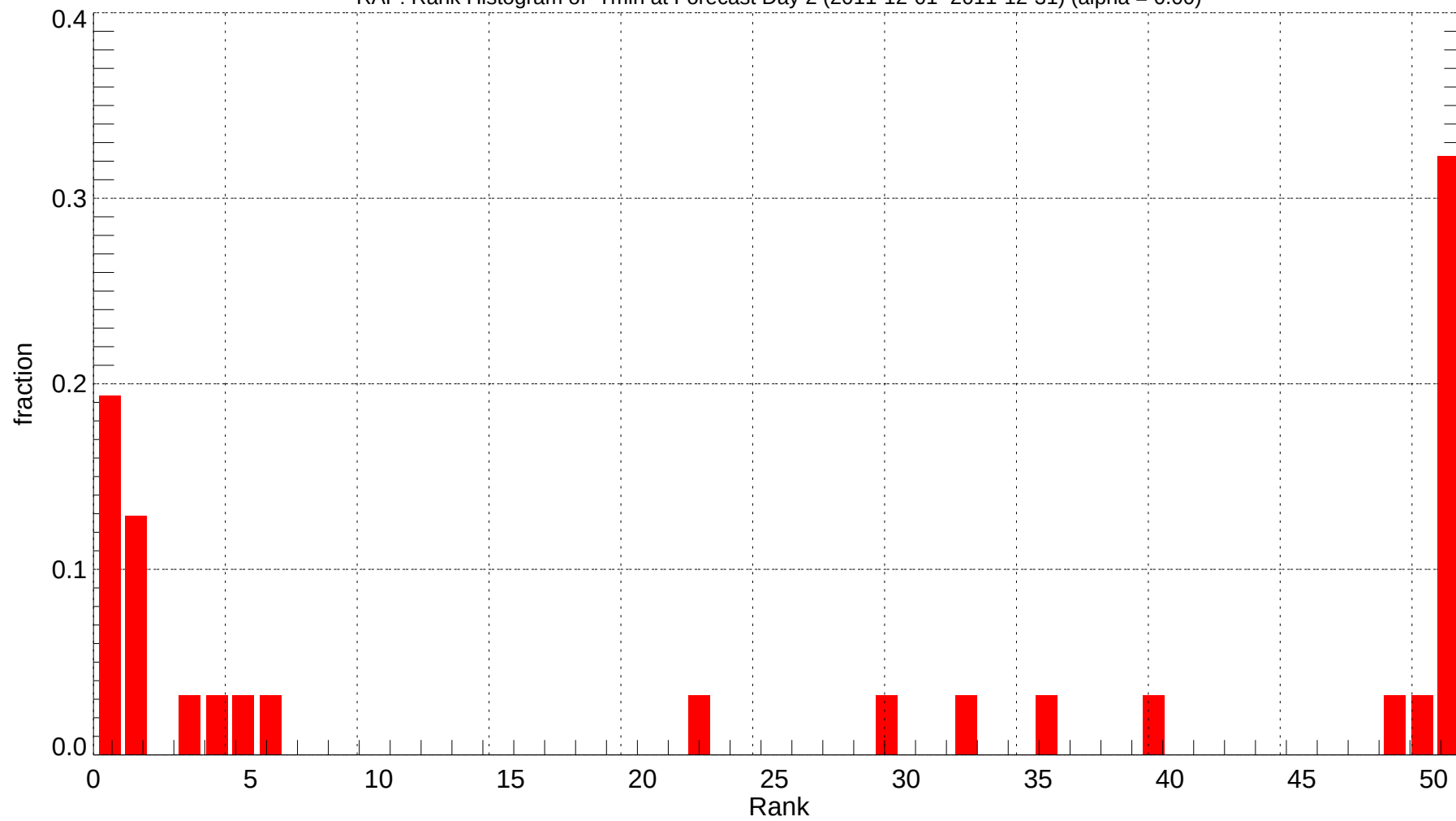
RAP: Rank Histogram of Tmin at Forecast Day 2 (2011-12-01~2011-12-31) (alpha = 0.00)
