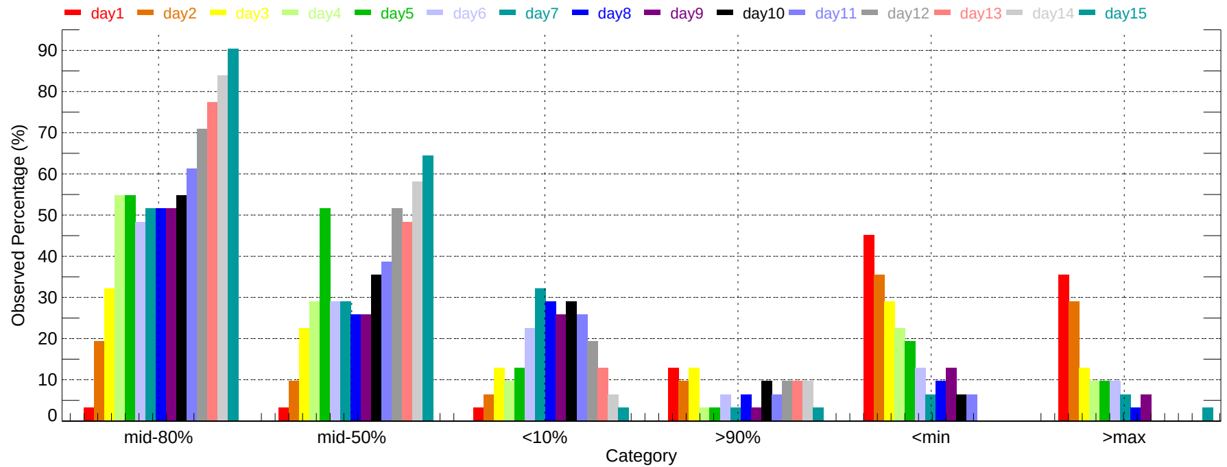
Observed Percentage of Ensembles - RNO: Max Temperature (2011-12-01~2011-12-31)
