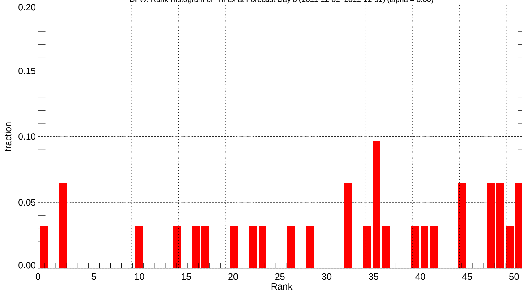
DFW: Rank Histogram of Tmax at Forecast Day 8 (2011-12-01~2011-12-31) (alpha = 0.00)
