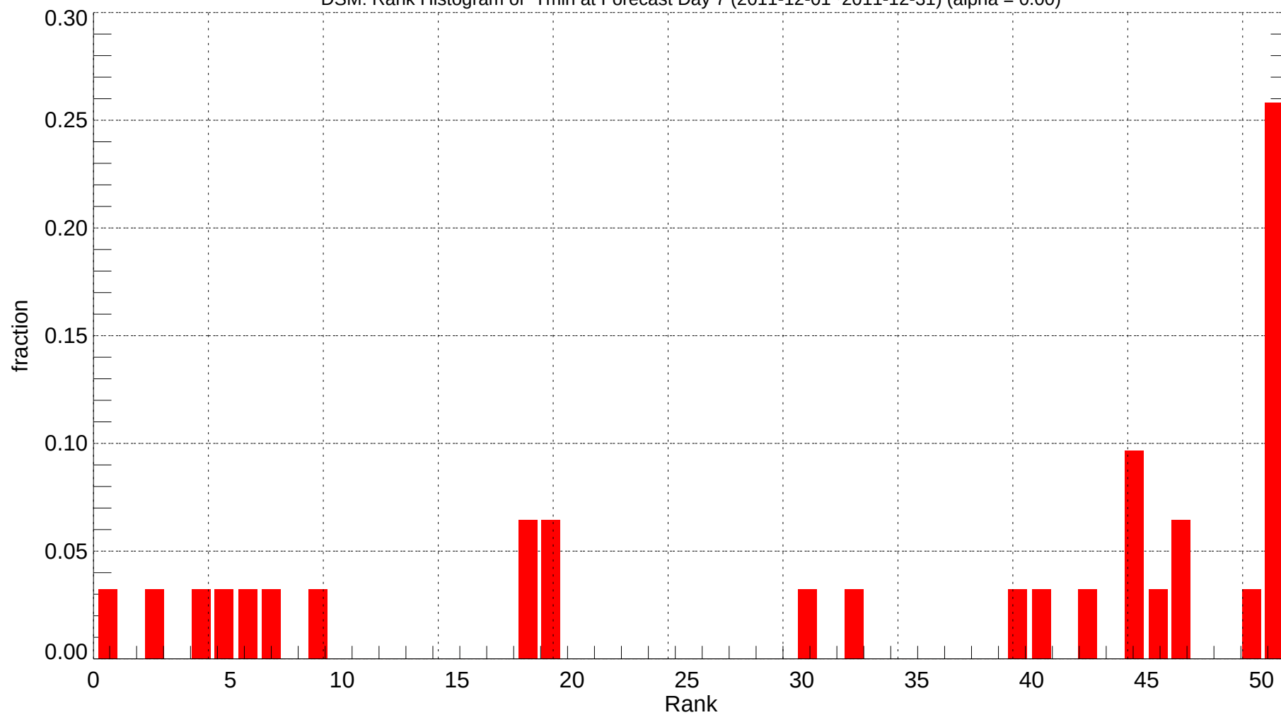
DSM: Rank Histogram of Tmin at Forecast Day 7 (2011-12-01~2011-12-31) (alpha = 0.00)
