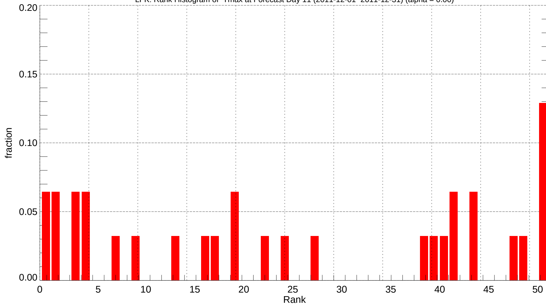
LFK: Rank Histogram of Tmax at Forecast Day 11 (2011-12-01~2011-12-31) (alpha = 0.00)
