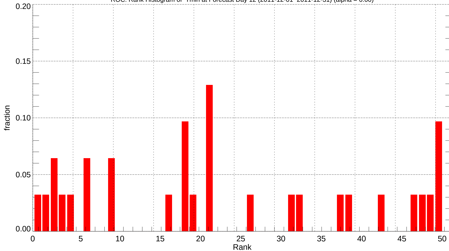
ROC: Rank Histogram of Tmin at Forecast Day 12 (2011-12-01~2011-12-31) (alpha = 0.00)
