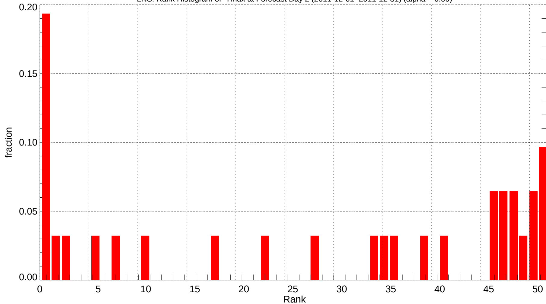
LNS: Rank Histogram of Tmax at Forecast Day 2 (2011-12-01~2011-12-31) (alpha = 0.00)
