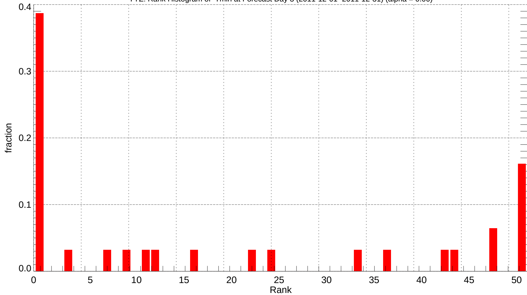
YYZ: Rank Histogram of Tmin at Forecast Day 3 (2011-12-01~2011-12-31) (alpha = 0.00)
