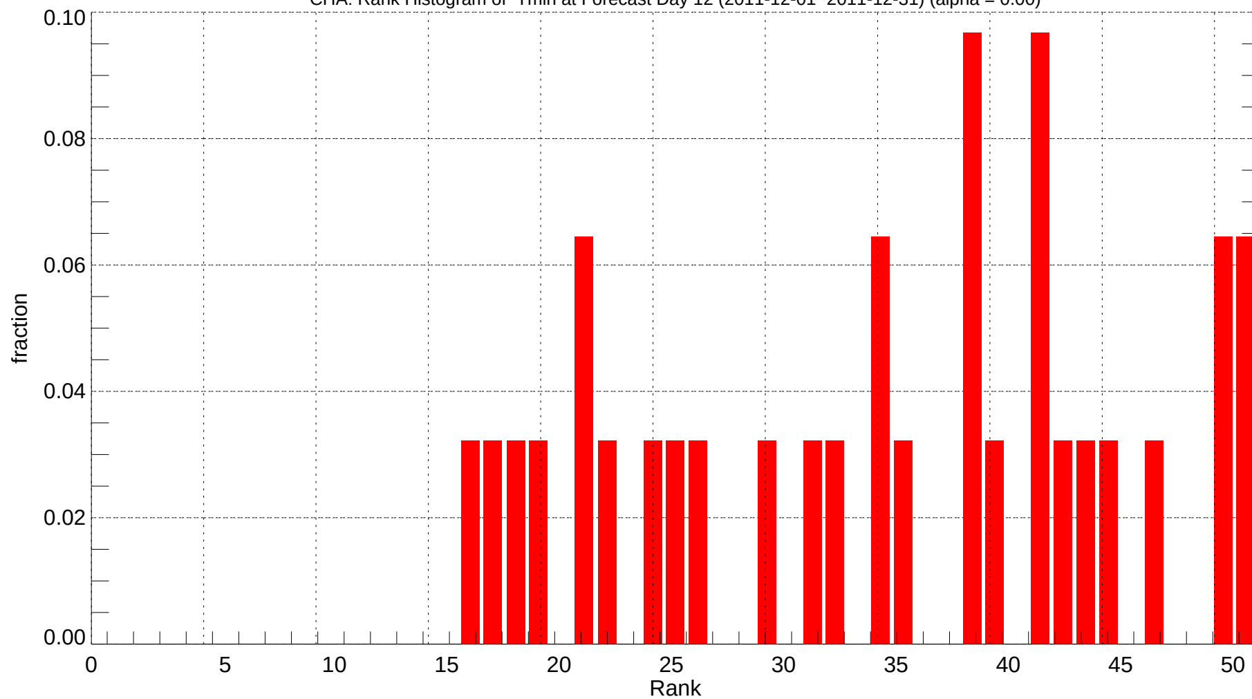
CHA: Rank Histogram of Tmin at Forecast Day 12 (2011-12-01~2011-12-31) (alpha = 0.00)
