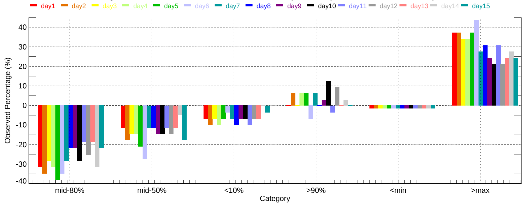
Observed Percentage Deviation of Ensembles - EVV: Max Temperature (2011-12-01~2011-12-31)
