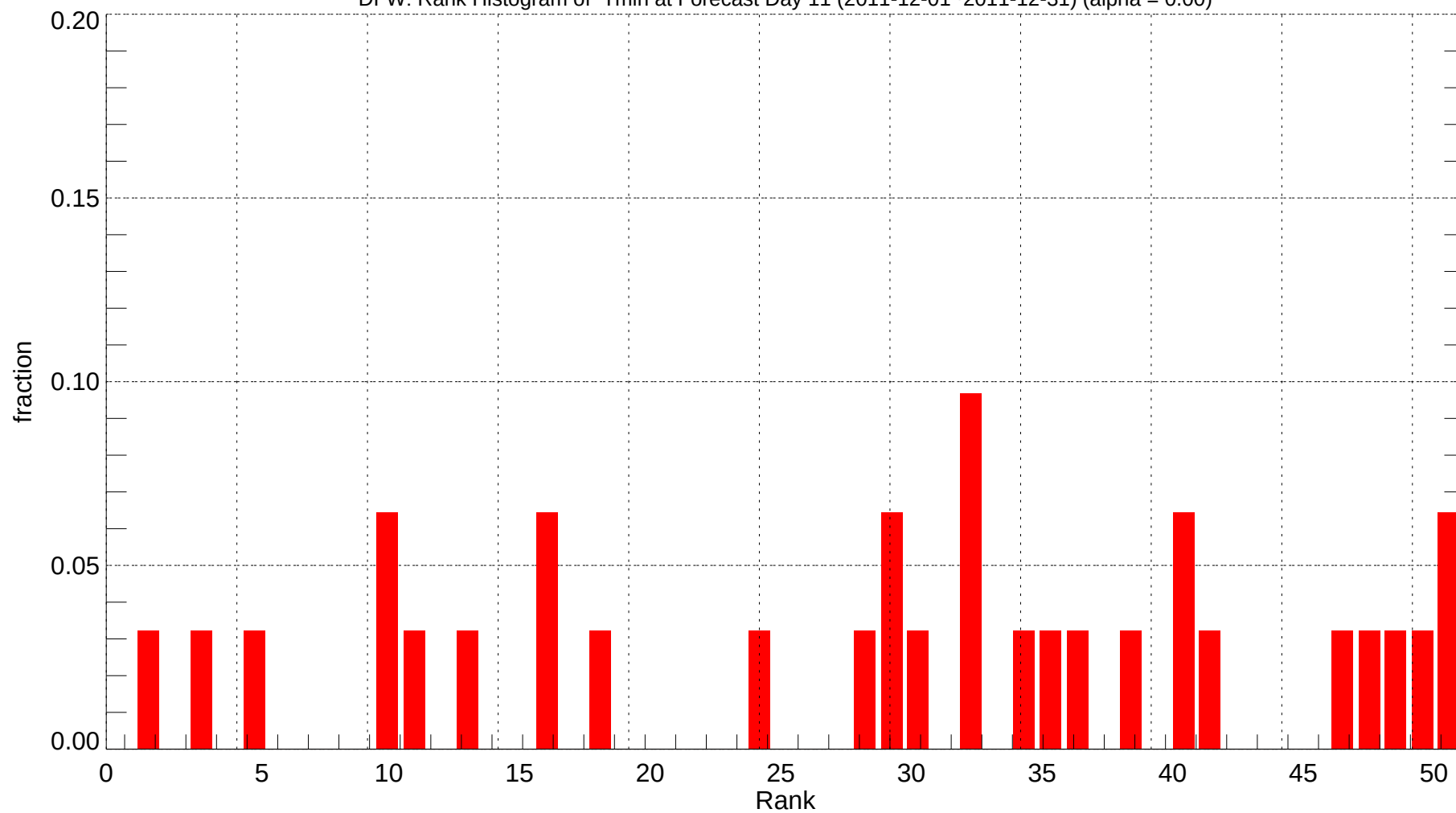
DFW: Rank Histogram of Tmin at Forecast Day 11 (2011-12-01~2011-12-31) (alpha = 0.00)
