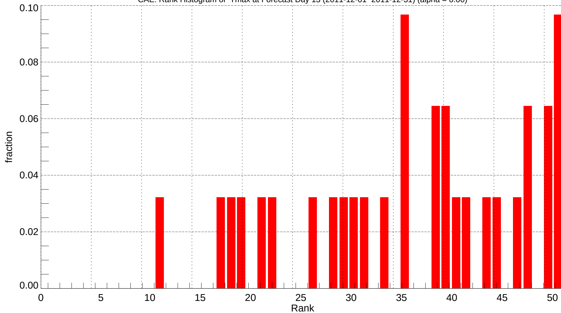
CAE: Rank Histogram of Tmax at Forecast Day 13 (2011-12-01~2011-12-31) (alpha = 0.00)
