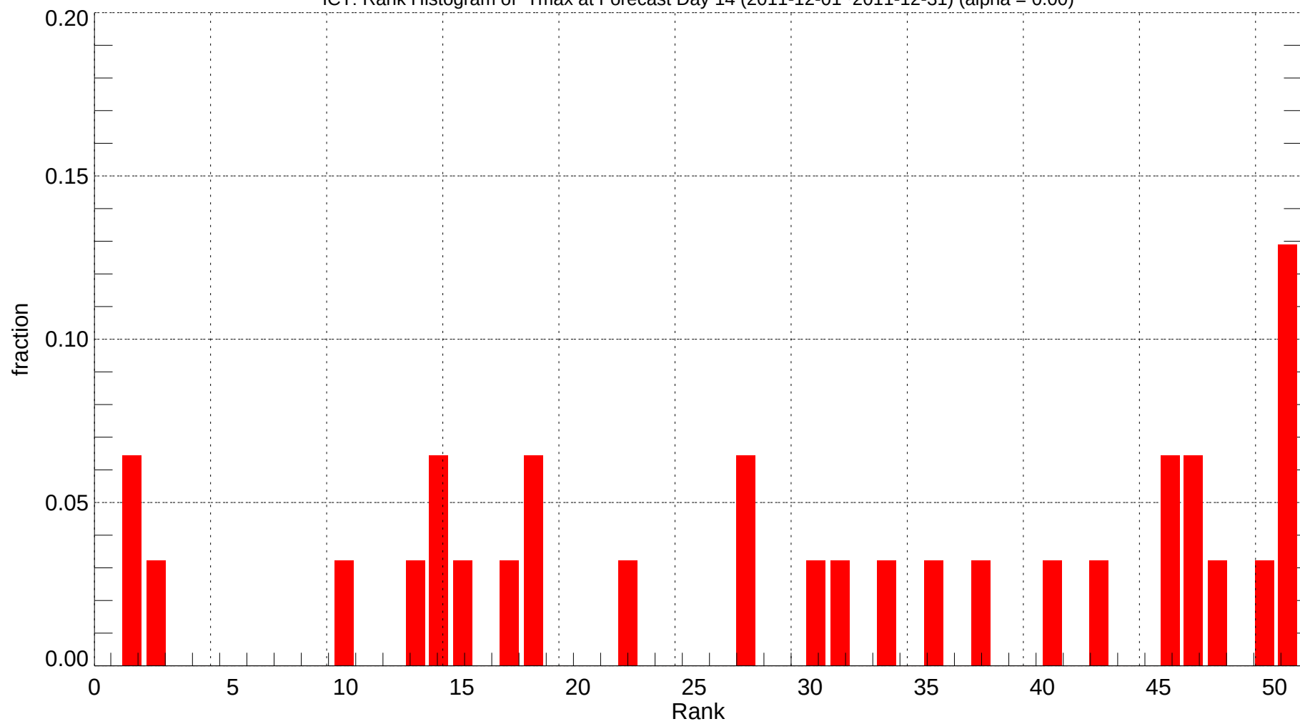
ICT: Rank Histogram of Tmax at Forecast Day 14 (2011-12-01~2011-12-31) (alpha = 0.00)
