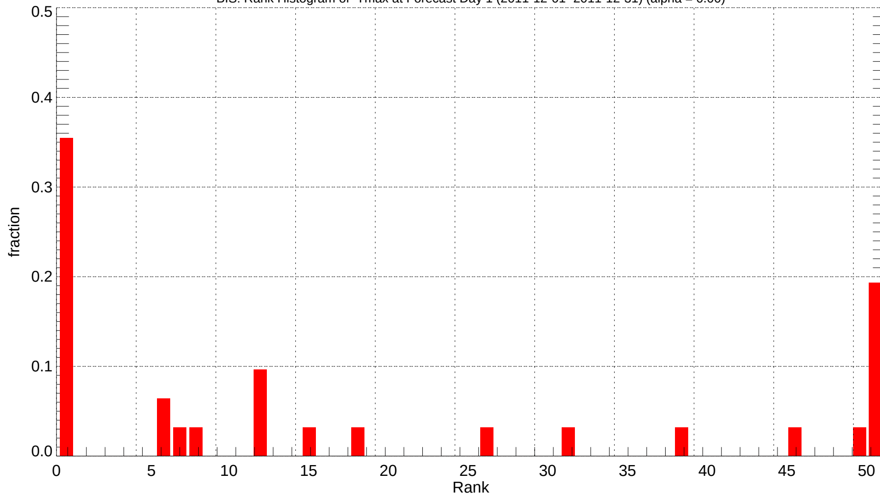
BIS: Rank Histogram of Tmax at Forecast Day 1 (2011-12-01~2011-12-31) (alpha = 0.00)
