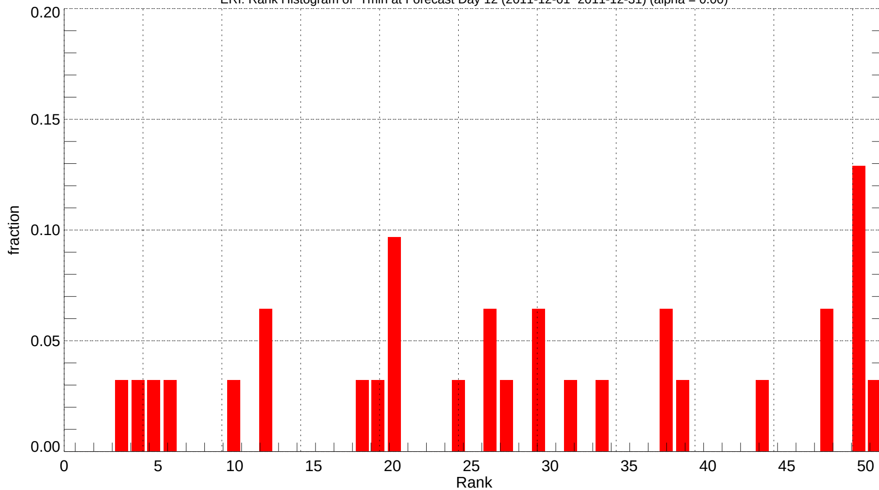
ERI: Rank Histogram of Tmin at Forecast Day 12 (2011-12-01~2011-12-31) (alpha = 0.00)
