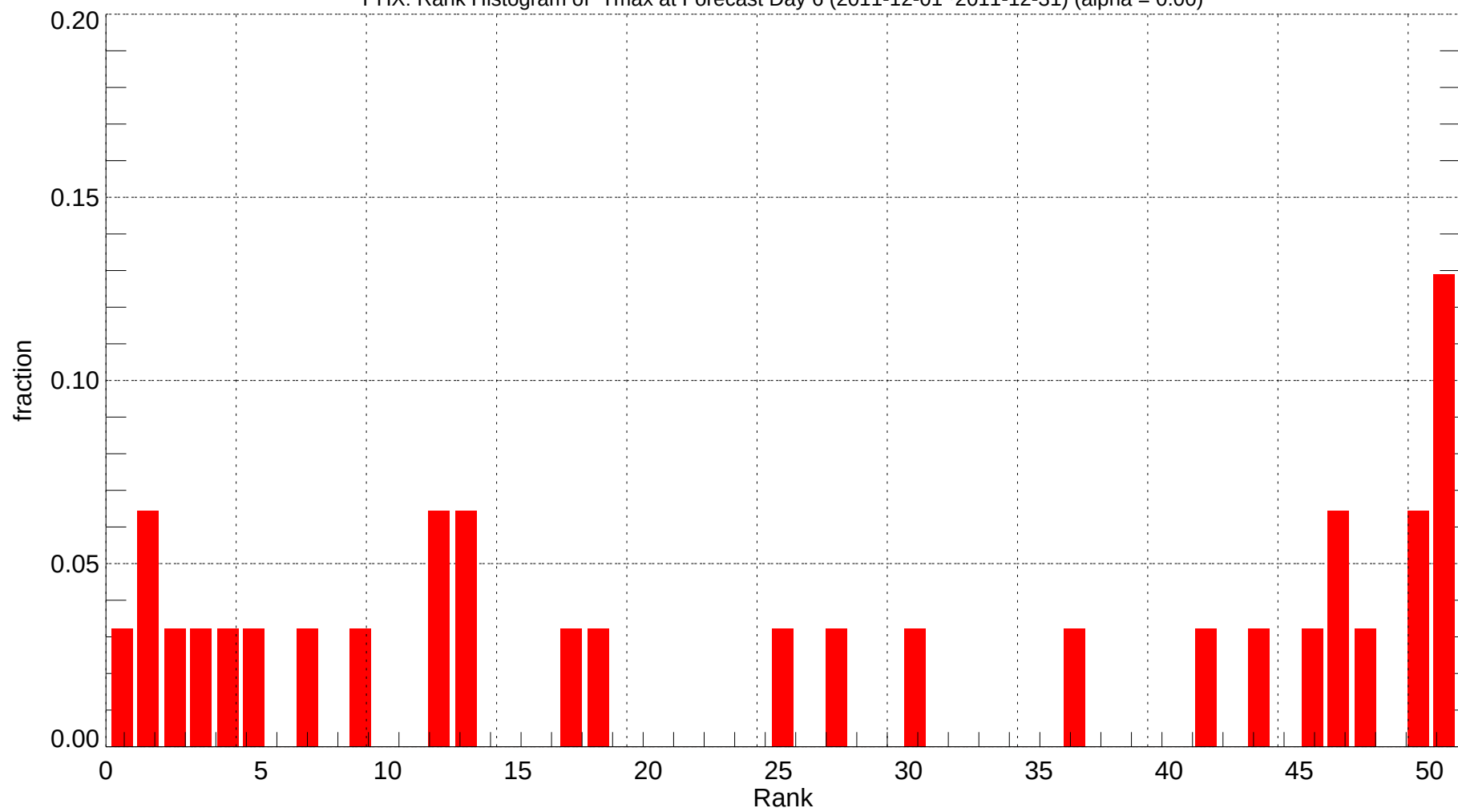
PHX: Rank Histogram of Tmax at Forecast Day 6 (2011-12-01~2011-12-31) (alpha = 0.00)
