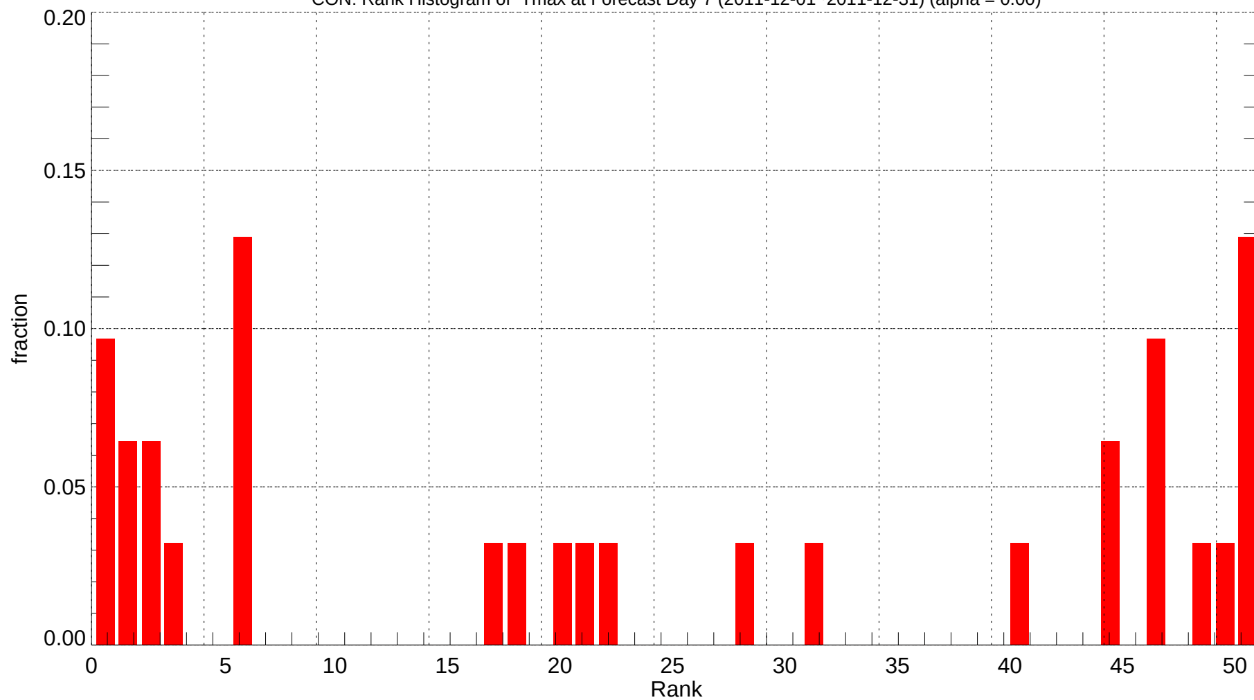
CON: Rank Histogram of Tmax at Forecast Day 7 (2011-12-01~2011-12-31) (alpha = 0.00)
