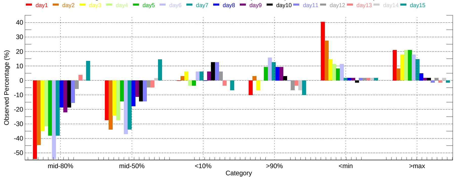
Observed Percentage Deviation of Ensembles - ACT: Min Temperature (2011-12-01~2011-12-31)
