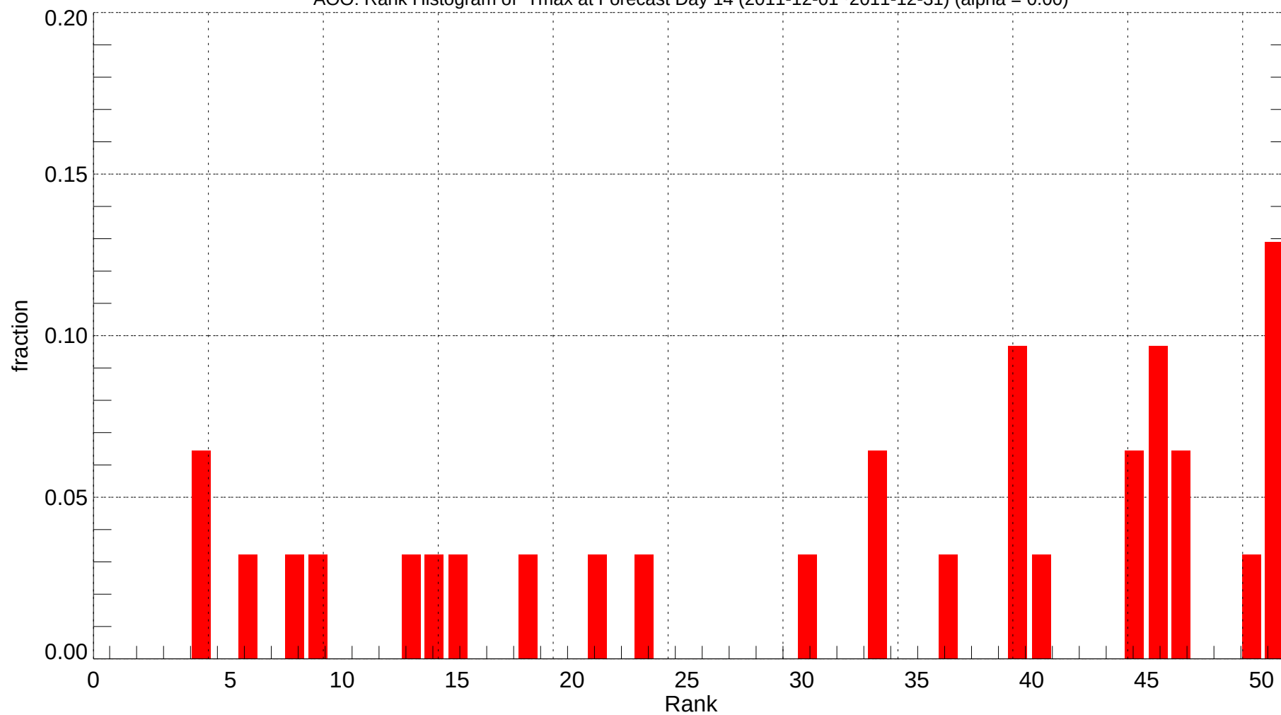
AOO: Rank Histogram of Tmax at Forecast Day 14 (2011-12-01~2011-12-31) (alpha = 0.00)
