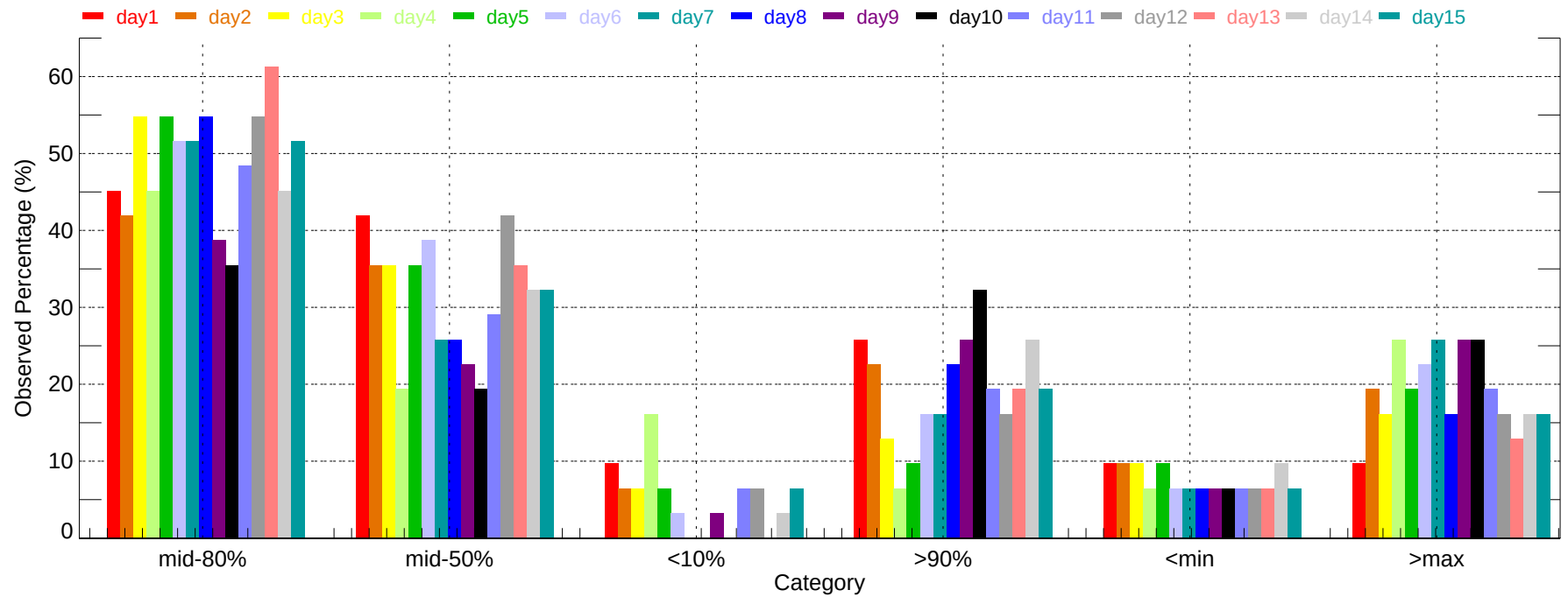
Observed Percentage of Ensembles - DLH: Max Temperature (2011-12-01~2011-12-31)
