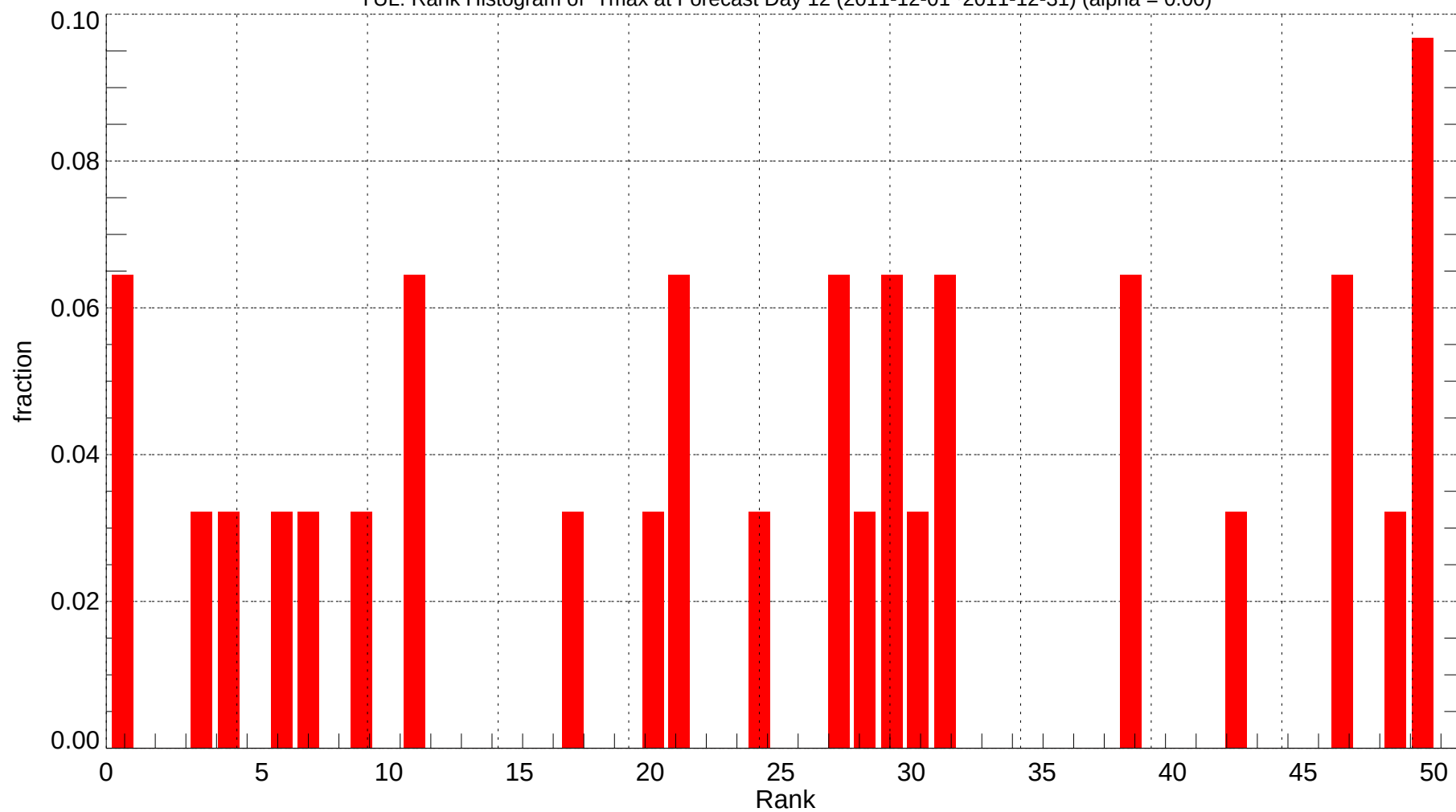
YUL: Rank Histogram of Tmax at Forecast Day 12 (2011-12-01~2011-12-31) (alpha = 0.00)
