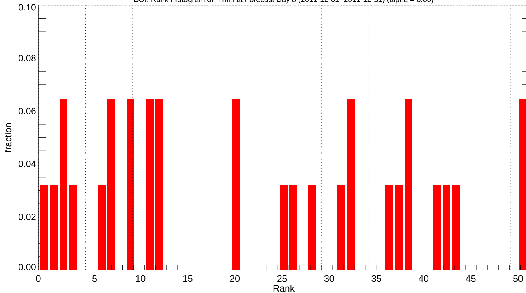
BOI: Rank Histogram of Tmin at Forecast Day 8 (2011-12-01~2011-12-31) (alpha = 0.00)
