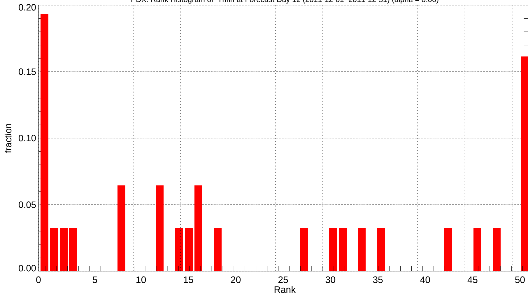
PDX: Rank Histogram of Tmin at Forecast Day 12 (2011-12-01~2011-12-31) (alpha = 0.00)
