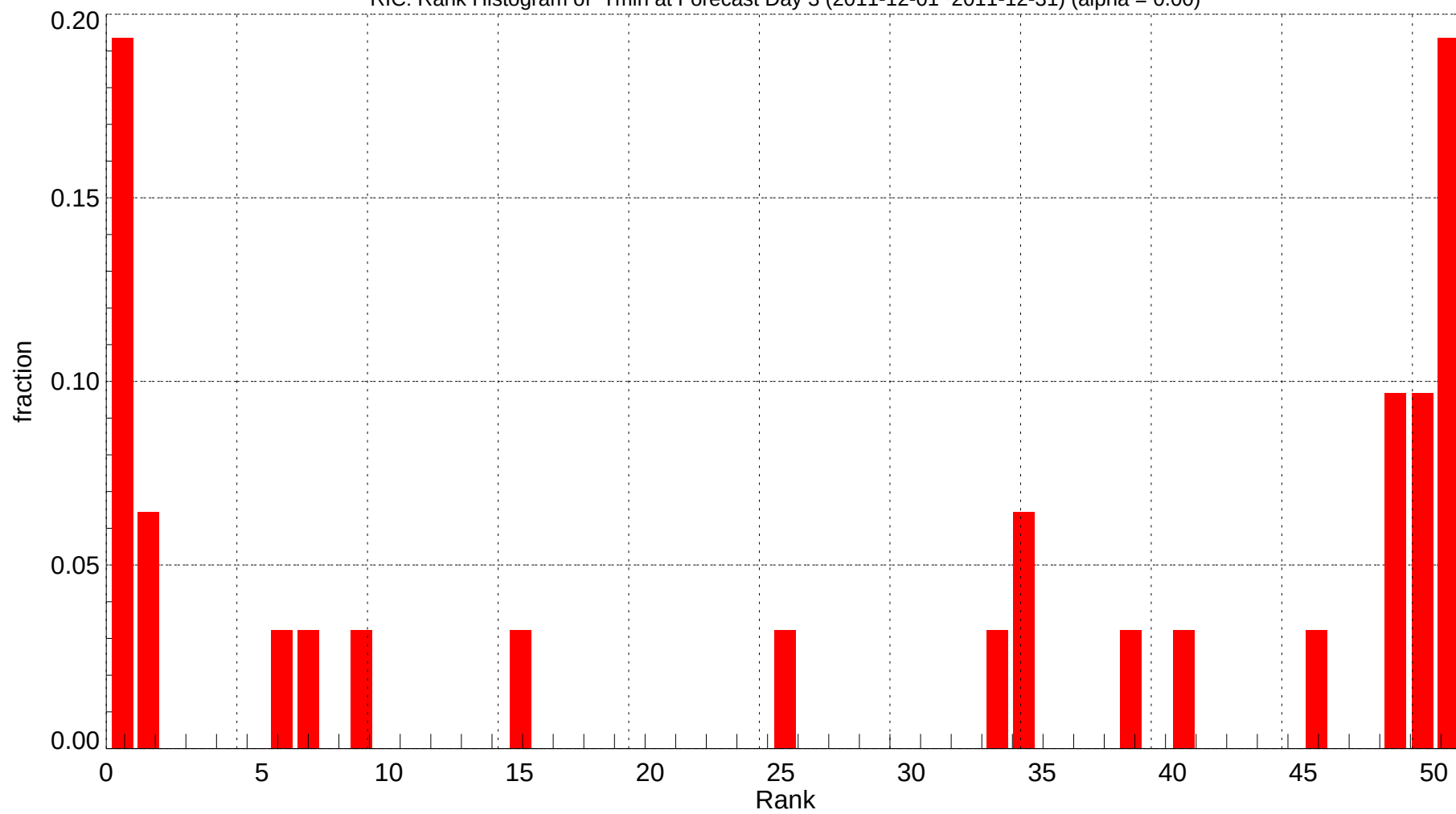
RIC: Rank Histogram of Tmin at Forecast Day 3 (2011-12-01~2011-12-31) (alpha = 0.00)
