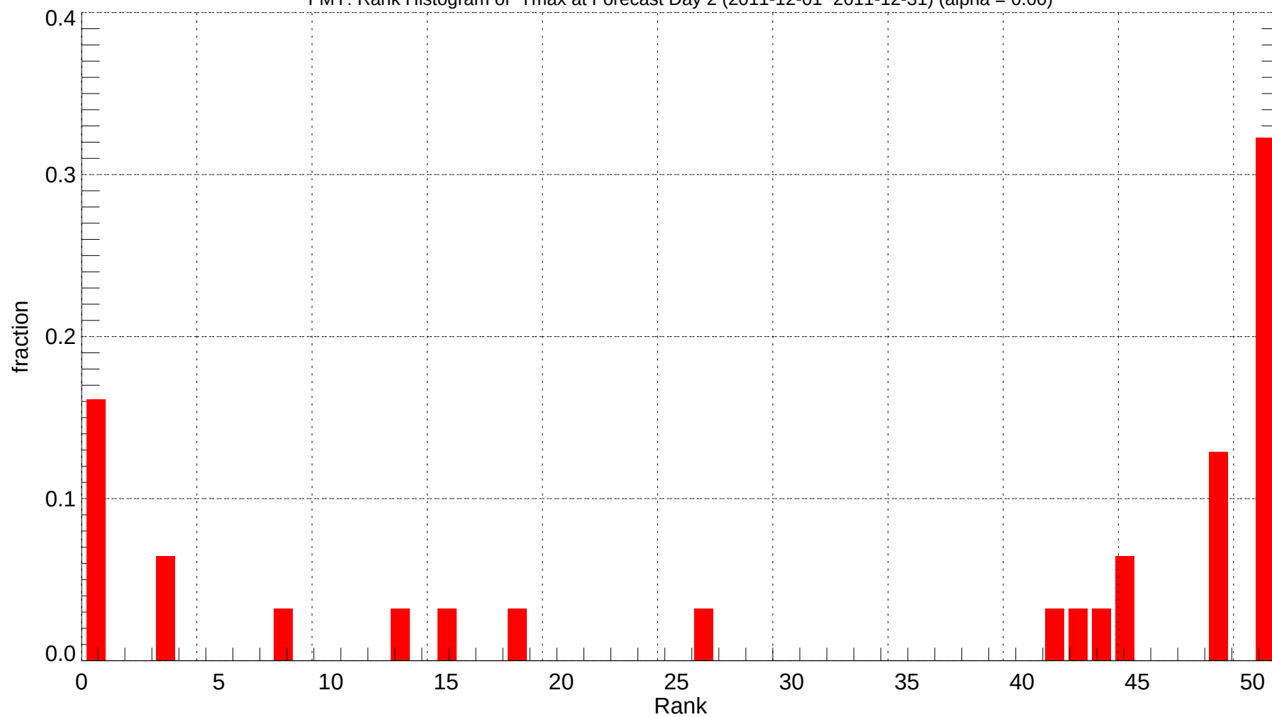
FMY: Rank Histogram of Tmax at Forecast Day 2 (2011-12-01~2011-12-31) (alpha = 0.00)
