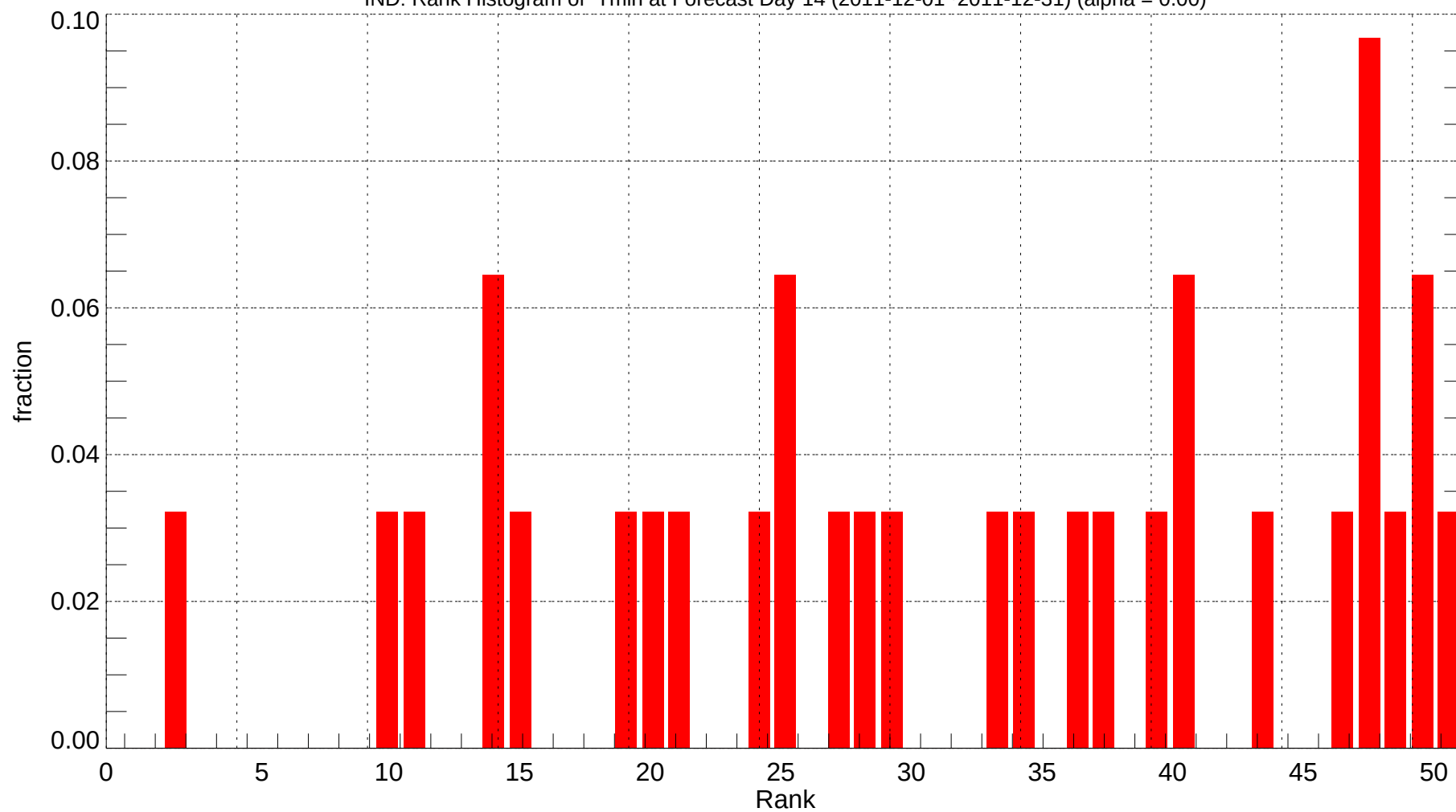
IND: Rank Histogram of Tmin at Forecast Day 14 (2011-12-01~2011-12-31) (alpha = 0.00)
