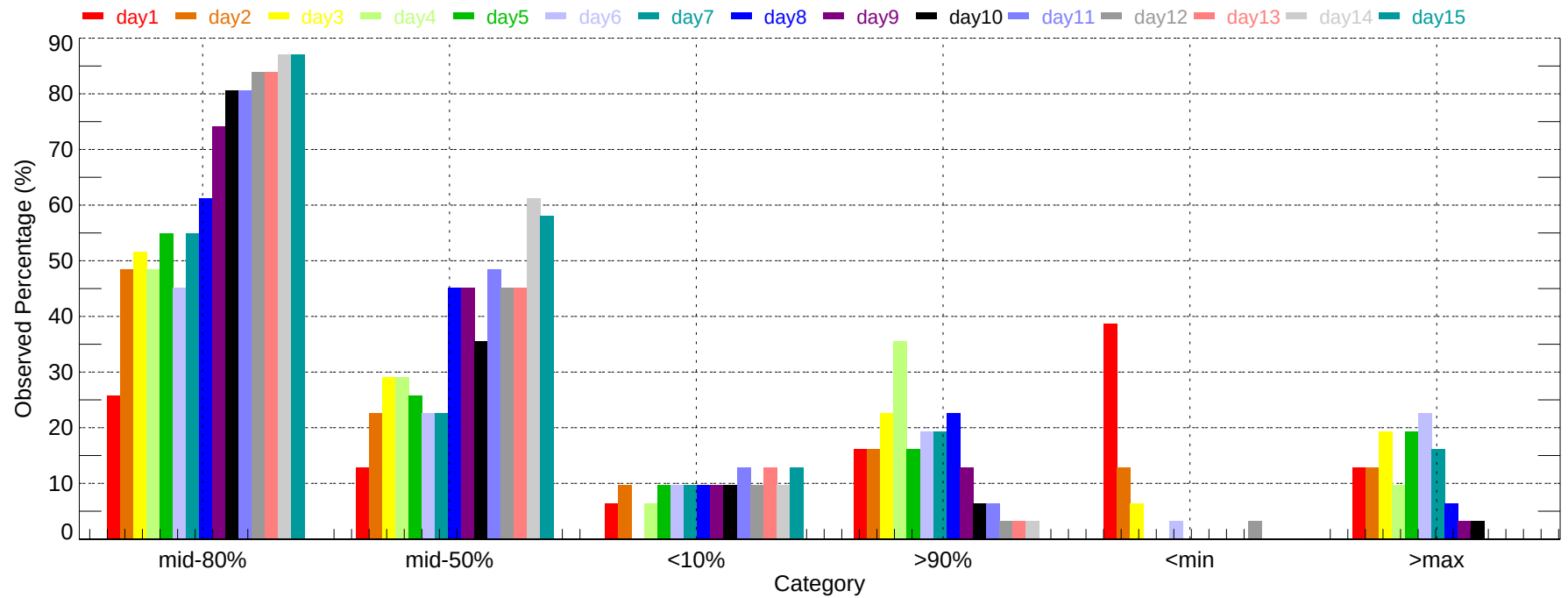
Observed Percentage of Ensembles - TYR: Min Temperature (2011-12-01~2011-12-31)
