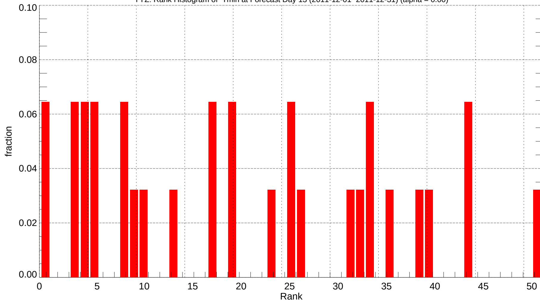
YYZ: Rank Histogram of Tmin at Forecast Day 13 (2011-12-01~2011-12-31) (alpha = 0.00)
