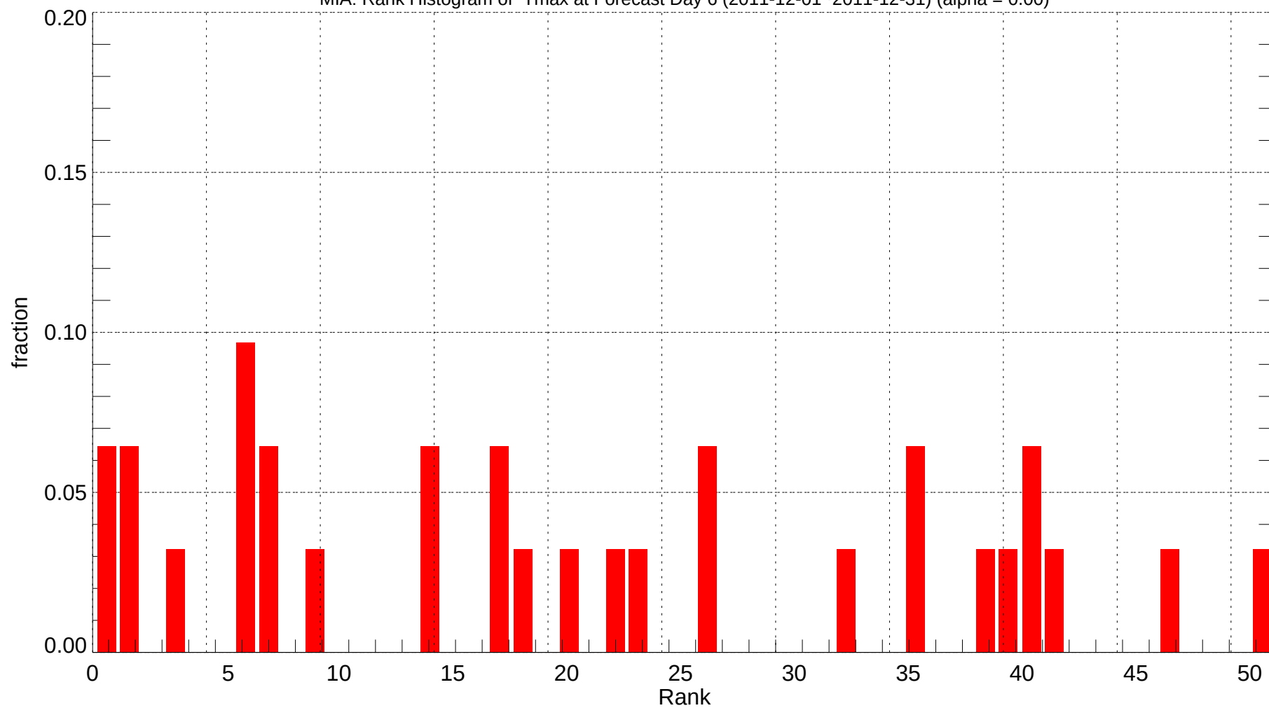
MIA: Rank Histogram of Tmax at Forecast Day 6 (2011-12-01~2011-12-31) (alpha = 0.00)
