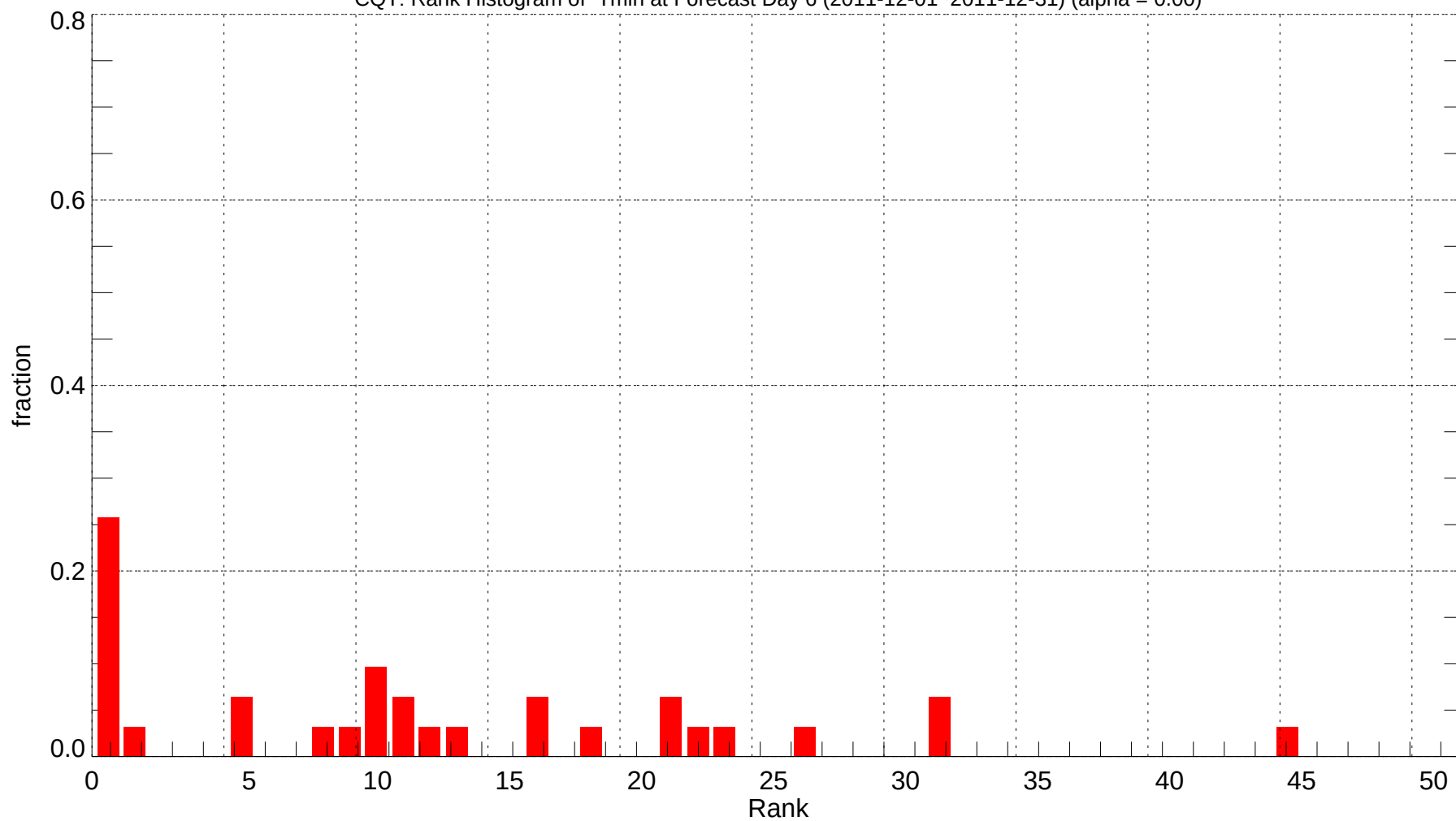
CQT: Rank Histogram of Tmin at Forecast Day 6 (2011-12-01~2011-12-31) (alpha = 0.00)
