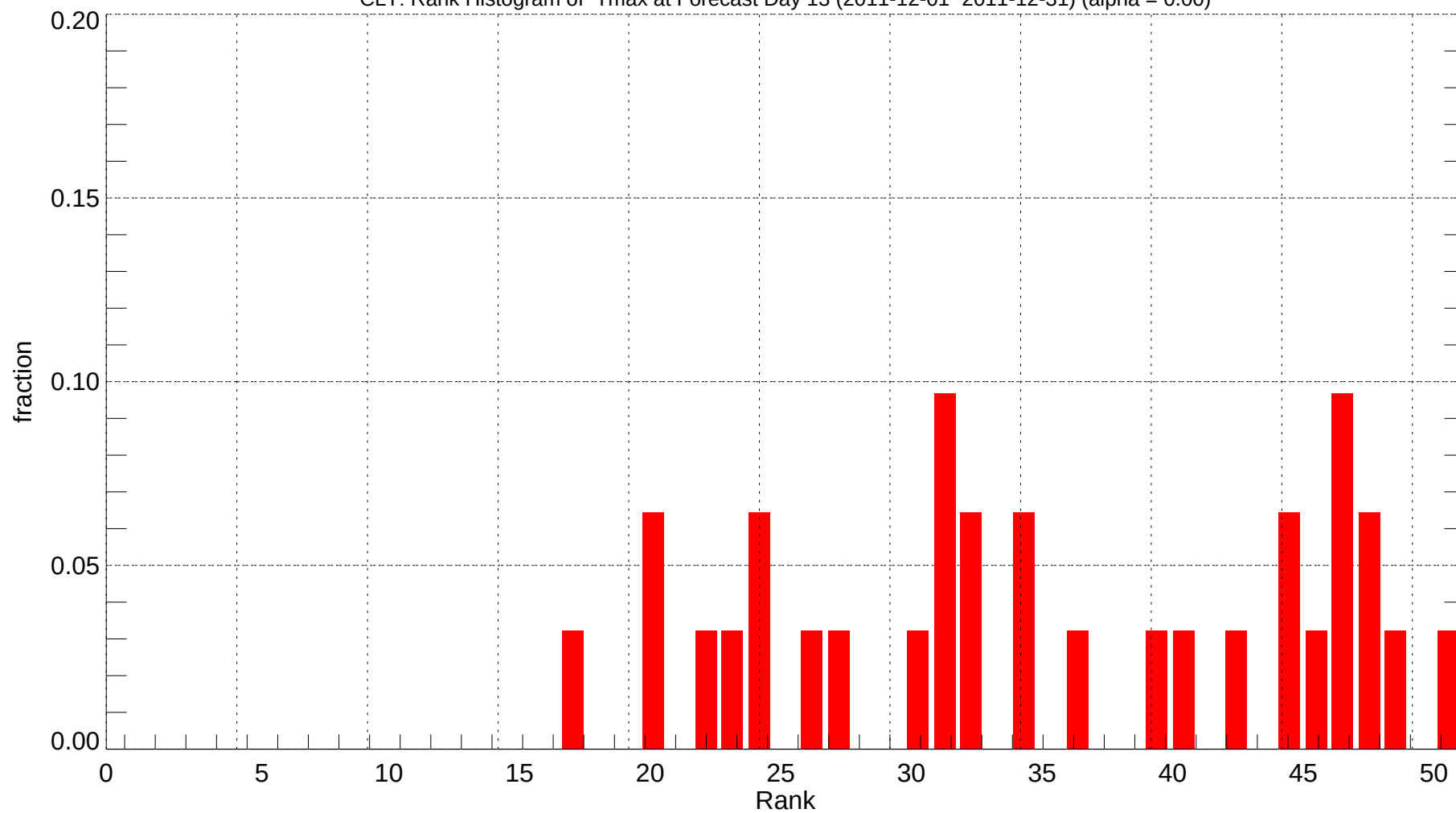
CLT: Rank Histogram of Tmax at Forecast Day 13 (2011-12-01~2011-12-31) (alpha = 0.00)
