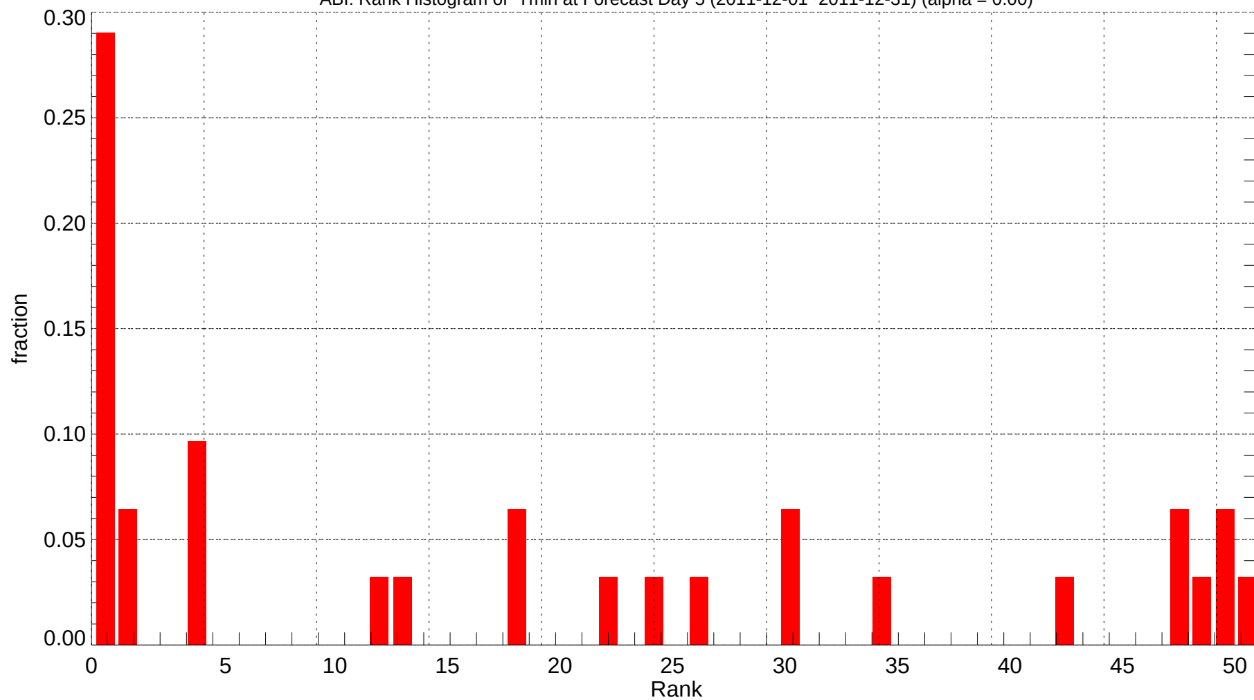
ABI: Rank Histogram of Tmin at Forecast Day 5 (2011-12-01~2011-12-31) (alpha = 0.00)
