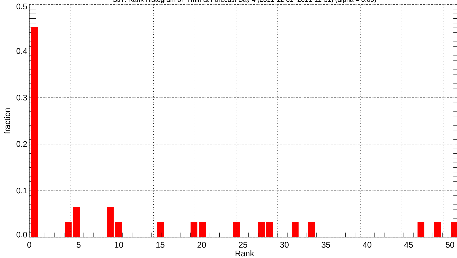
SJT: Rank Histogram of Tmin at Forecast Day 4 (2011-12-01~2011-12-31) (alpha = 0.00)
