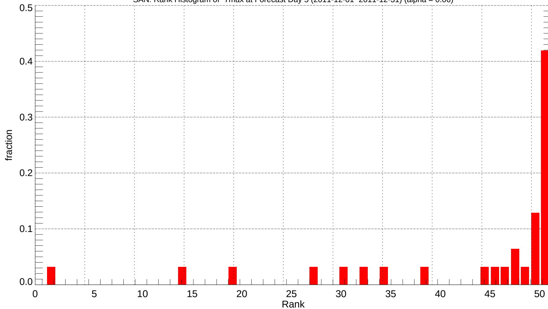
SAN: Rank Histogram of Tmax at Forecast Day 5 (2011-12-01~2011-12-31) (alpha = 0.00)
