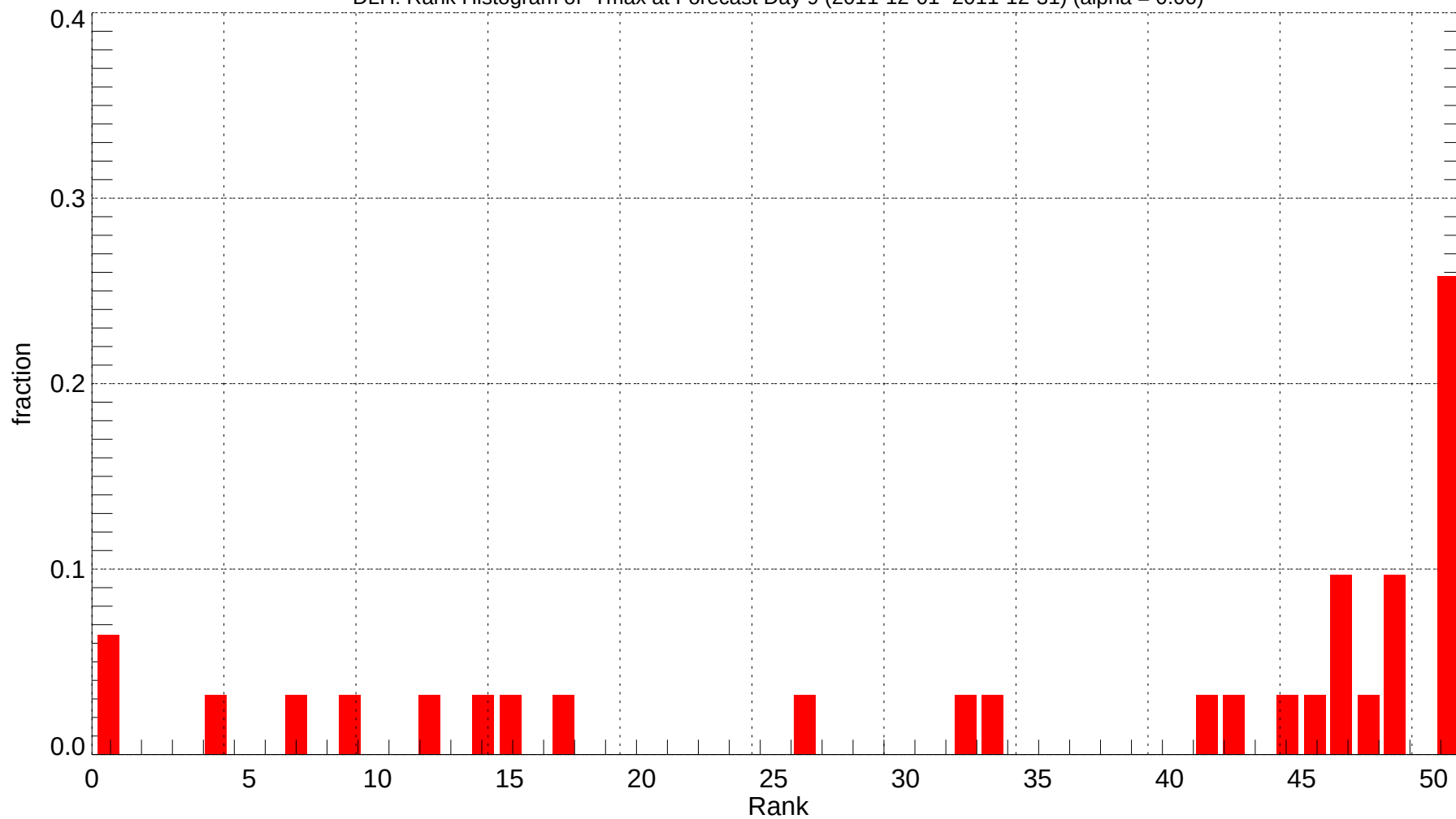
DLH: Rank Histogram of Tmax at Forecast Day 9 (2011-12-01~2011-12-31) (alpha = 0.00)
