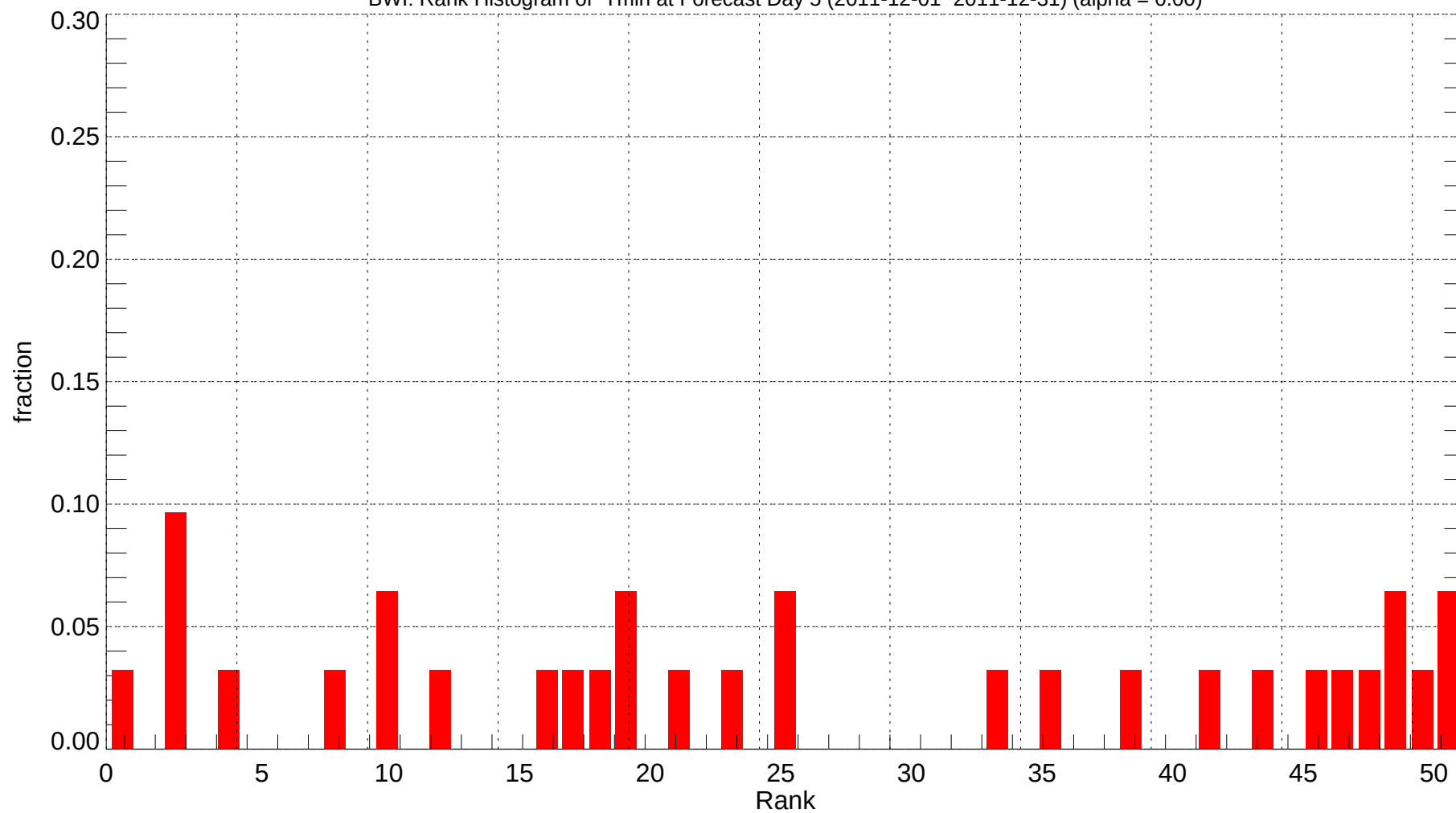
BWI: Rank Histogram of Tmin at Forecast Day 5 (2011-12-01~2011-12-31) (alpha = 0.00)
