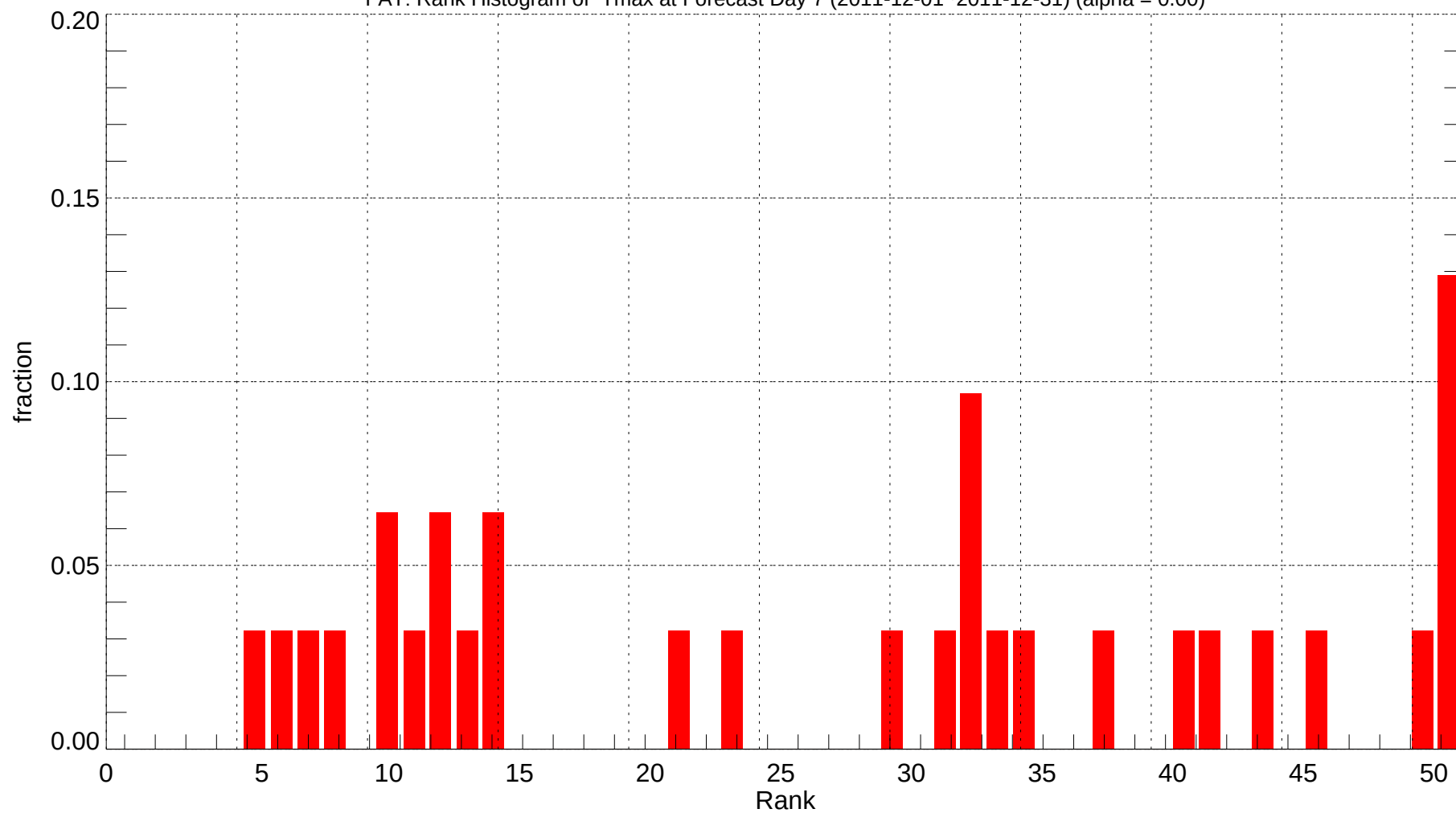
FAT: Rank Histogram of Tmax at Forecast Day 7 (2011-12-01~2011-12-31) (alpha = 0.00)
