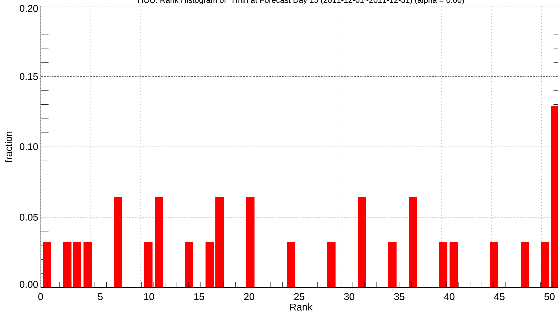
HOU: Rank Histogram of Tmin at Forecast Day 15 (2011-12-01~2011-12-31) (alpha = 0.00)
