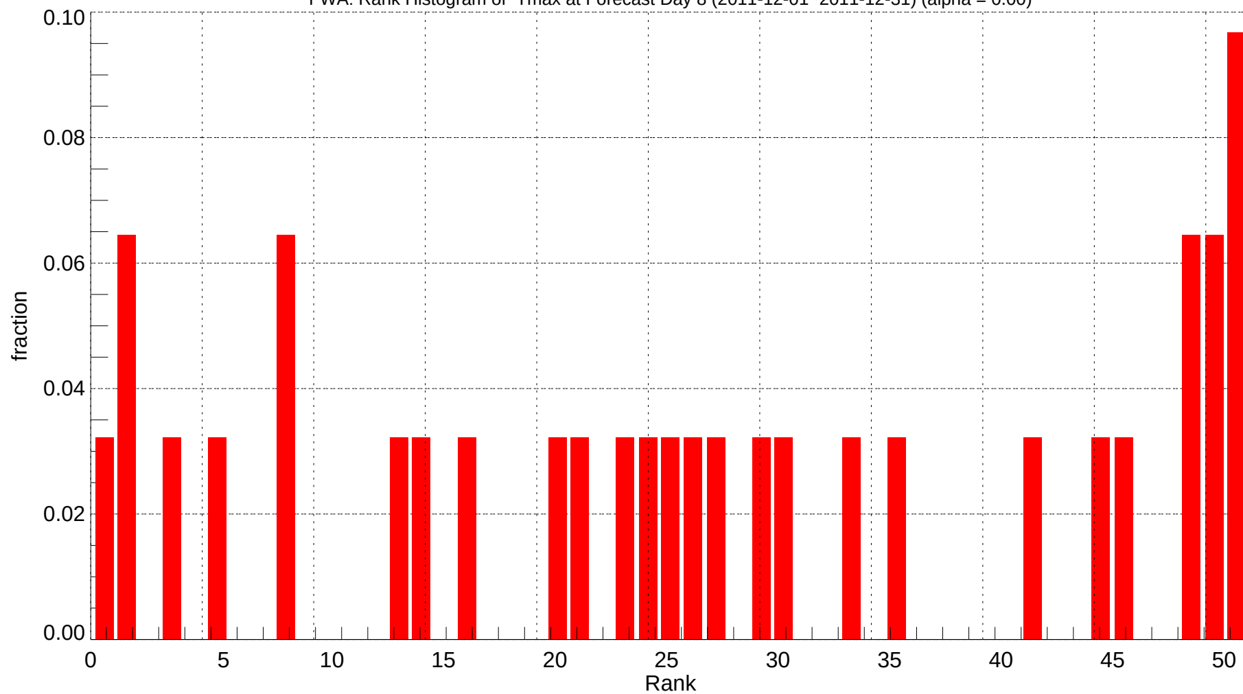
FWA: Rank Histogram of Tmax at Forecast Day 8 (2011-12-01~2011-12-31) (alpha = 0.00)
