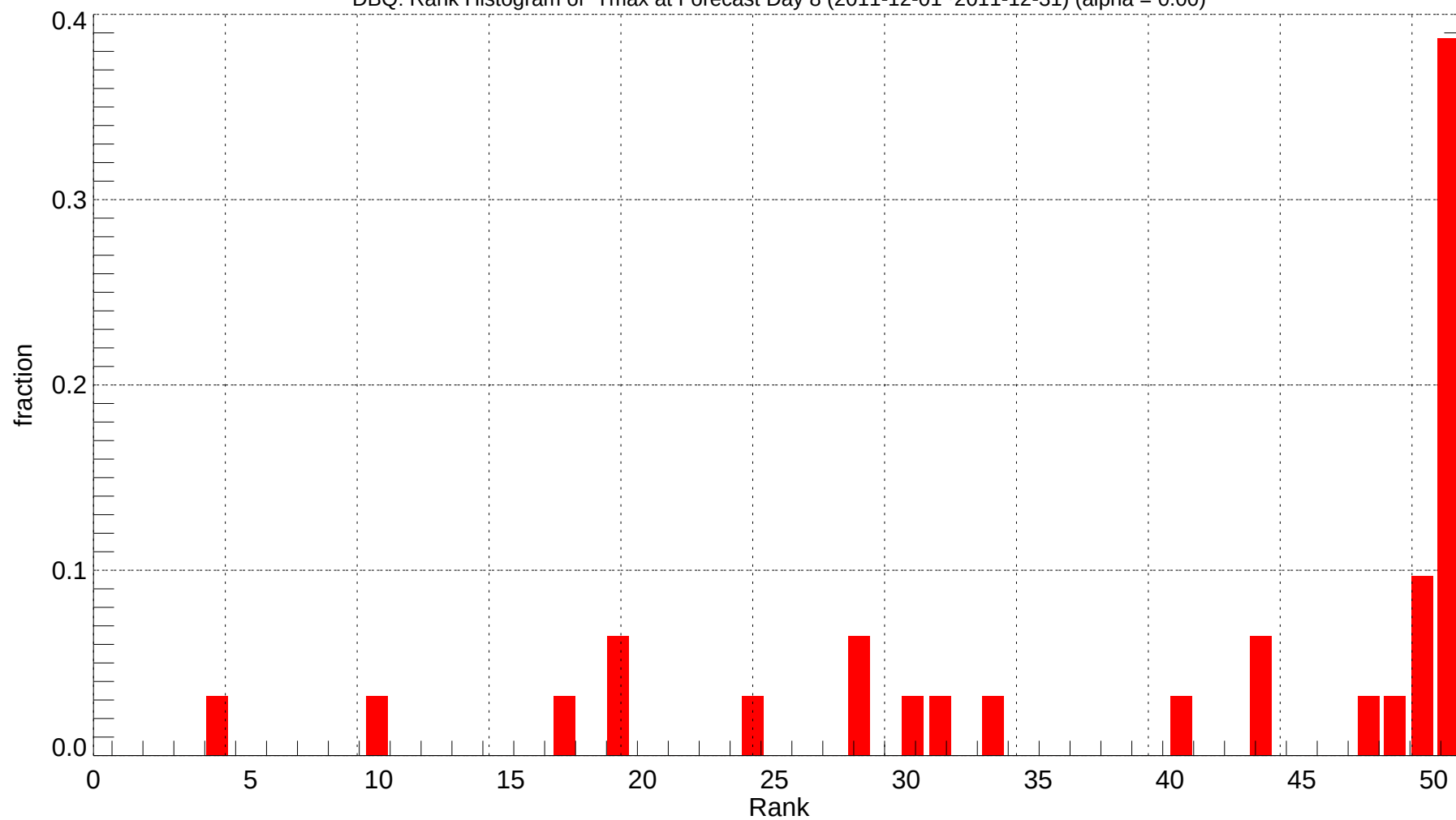
DBQ: Rank Histogram of Tmax at Forecast Day 8 (2011-12-01~2011-12-31) (alpha = 0.00)
