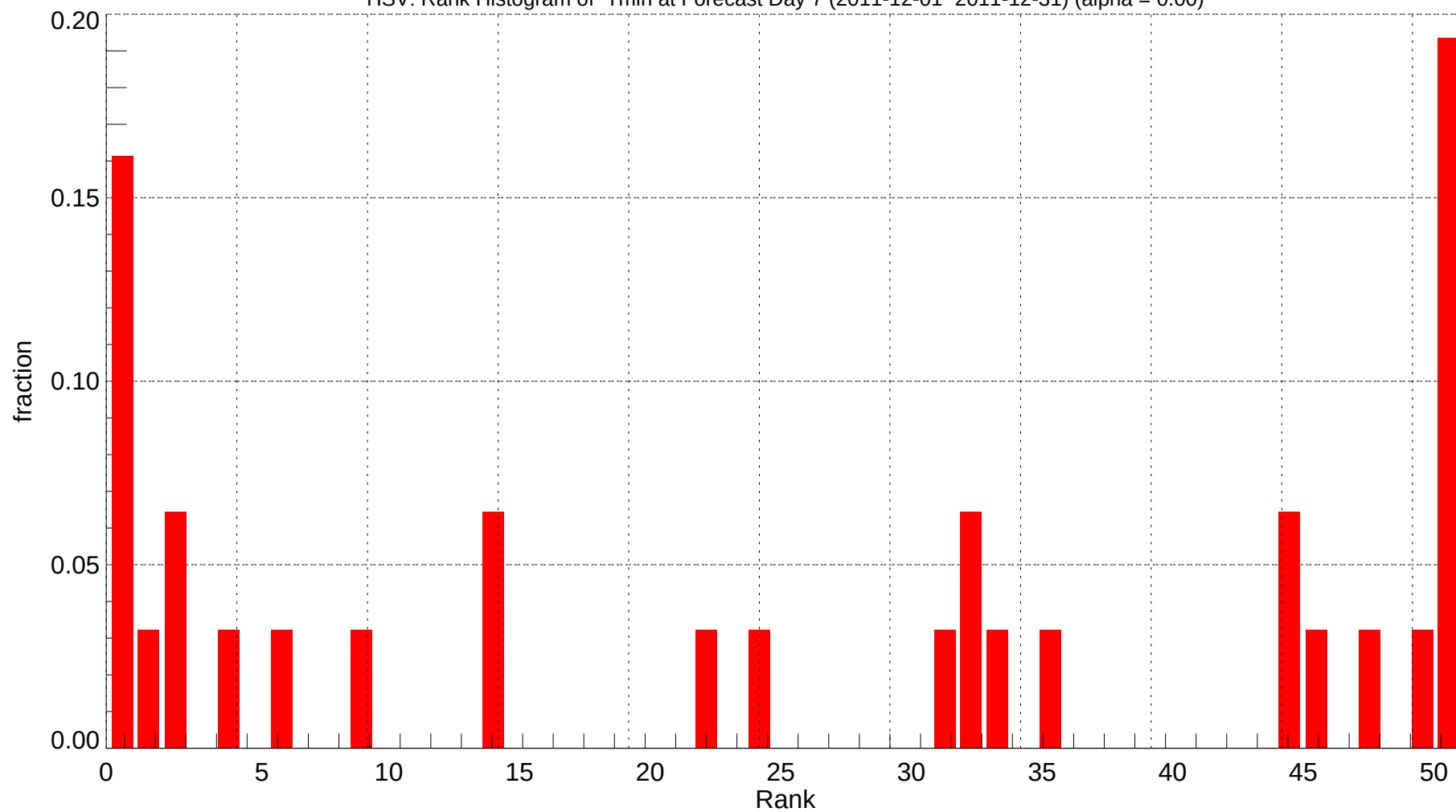
HSV: Rank Histogram of Tmin at Forecast Day 7 (2011-12-01~2011-12-31) (alpha = 0.00)
