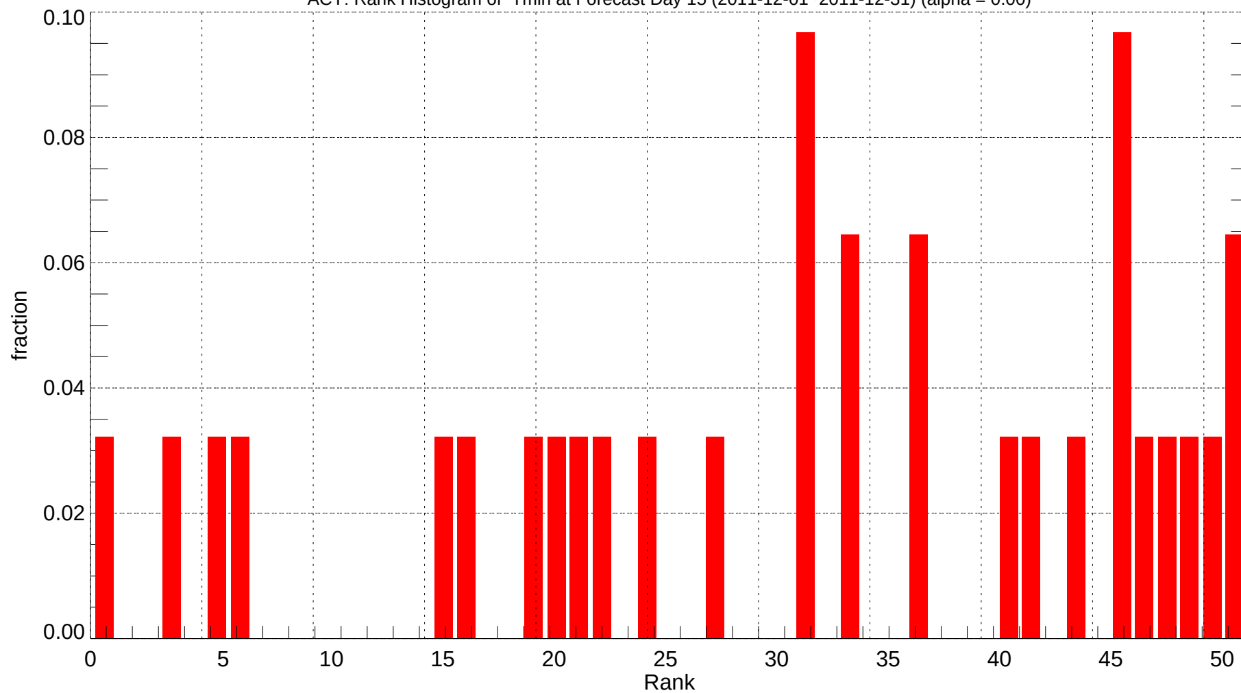
ACY: Rank Histogram of Tmin at Forecast Day 15 (2011-12-01~2011-12-31) (alpha = 0.00)
