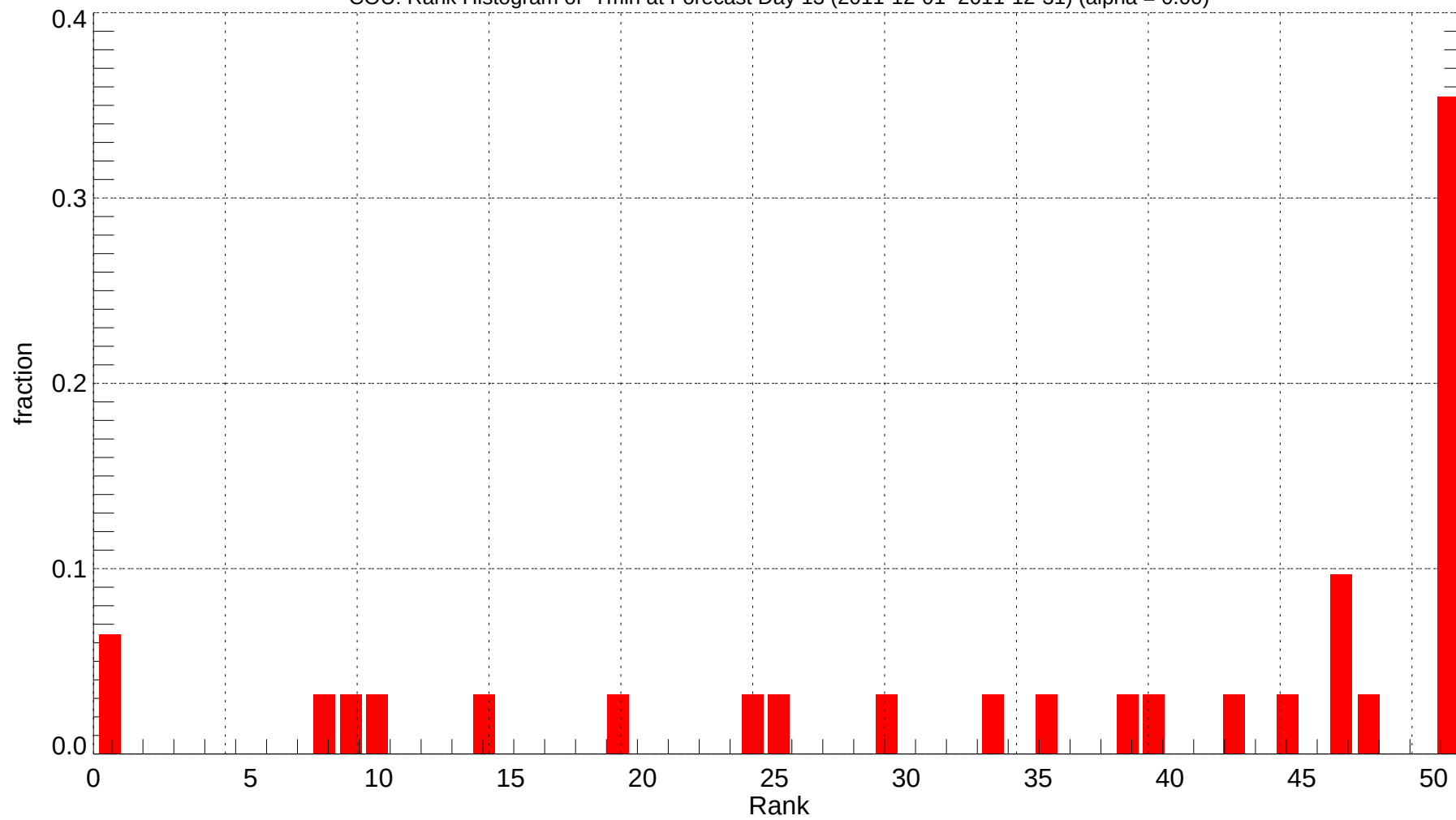
COU: Rank Histogram of Tmin at Forecast Day 13 (2011-12-01~2011-12-31) (alpha = 0.00)
