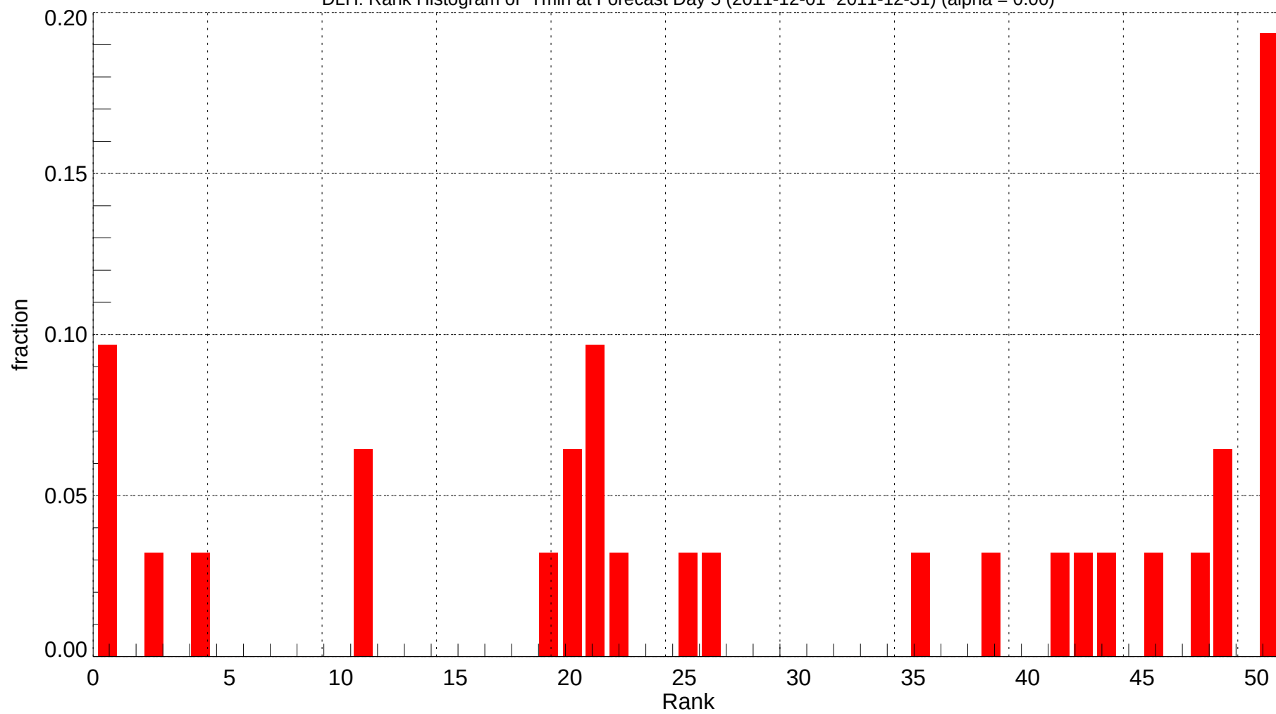
DLH: Rank Histogram of Tmin at Forecast Day 5 (2011-12-01~2011-12-31) (alpha = 0.00)
