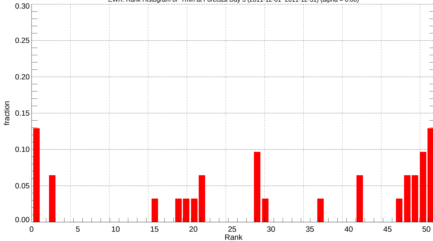
EWR: Rank Histogram of Tmin at Forecast Day 3 (2011-12-01~2011-12-31) (alpha = 0.00)
