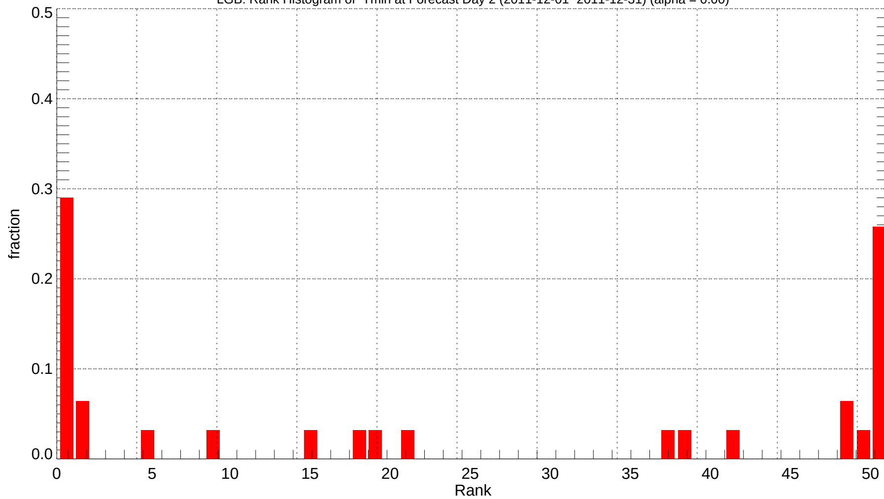
LGB: Rank Histogram of Tmin at Forecast Day 2 (2011-12-01~2011-12-31) (alpha = 0.00)
