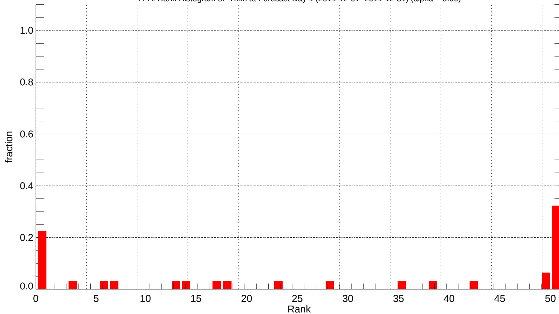
TPA: Rank Histogram of Tmin at Forecast Day 1 (2011-12-01~2011-12-31) (alpha = 0.00)
