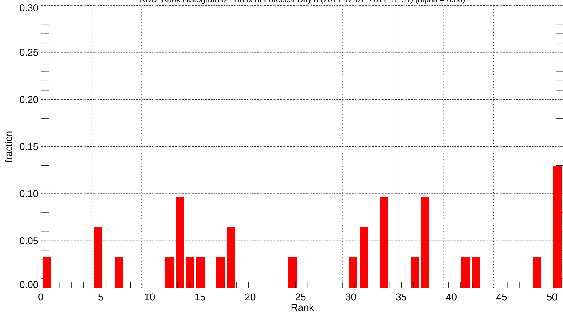
RDD: Rank Histogram of Tmax at Forecast Day 8 (2011-12-01~2011-12-31) (alpha = 0.00)
