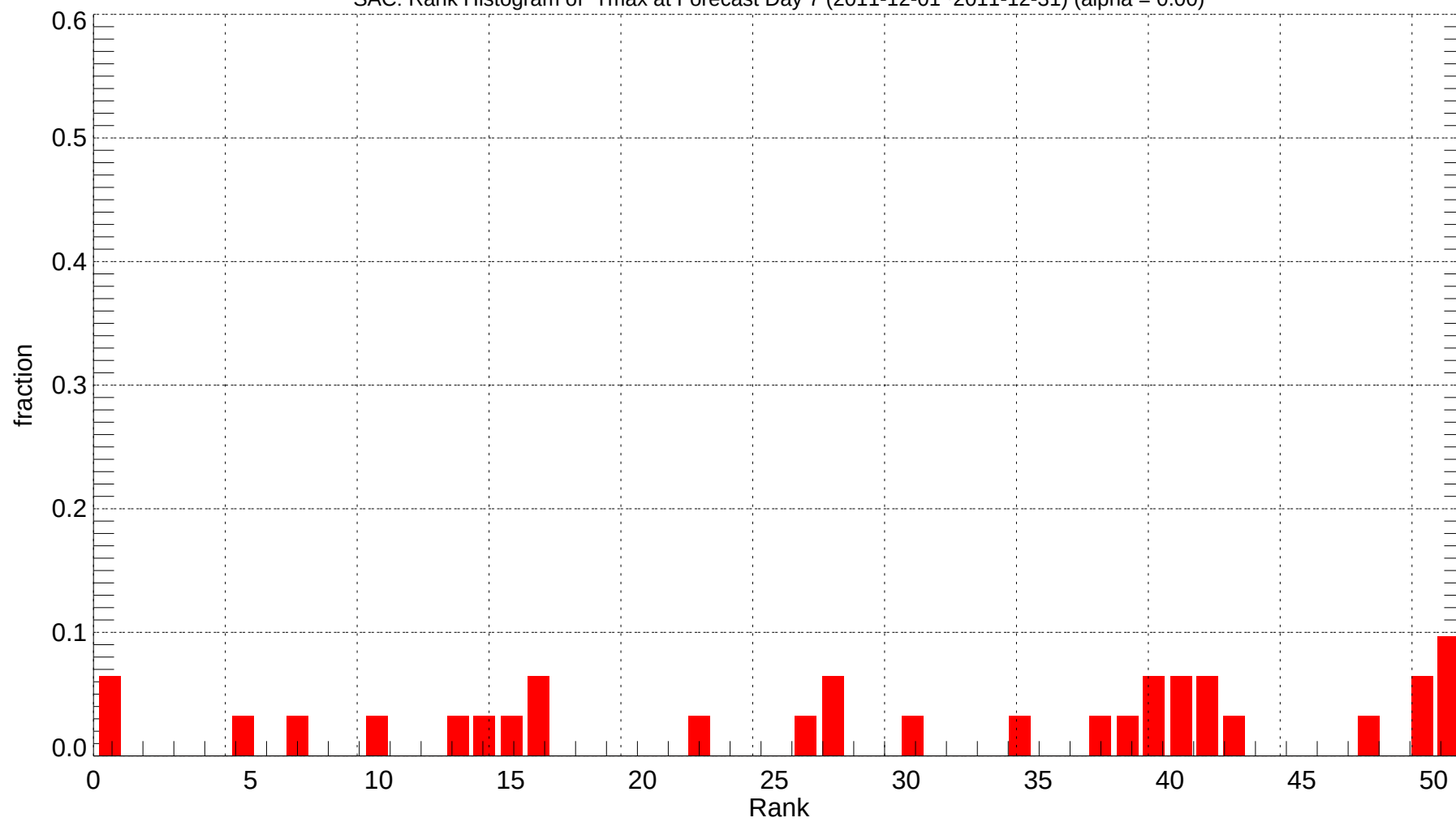
SAC: Rank Histogram of Tmax at Forecast Day 7 (2011-12-01~2011-12-31) (alpha = 0.00)
