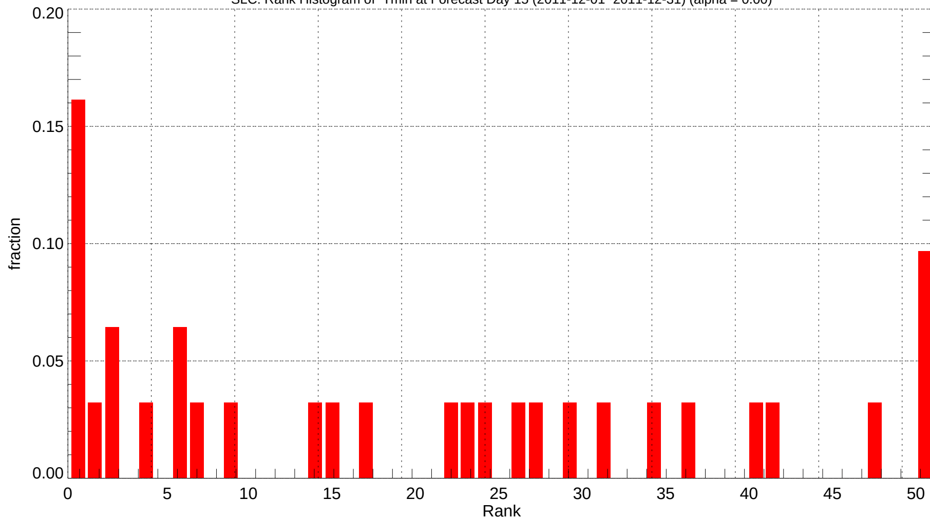
SLC: Rank Histogram of Tmin at Forecast Day 15 (2011-12-01~2011-12-31) (alpha = 0.00)
