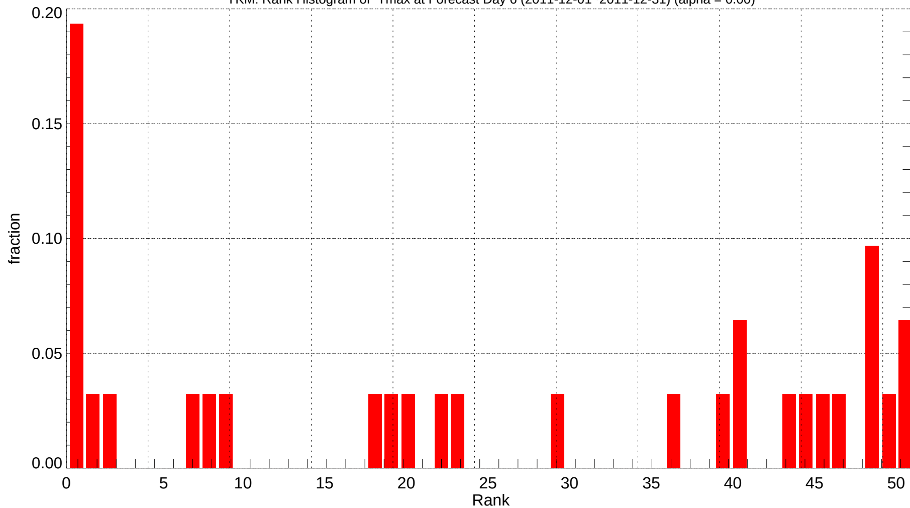
YKM: Rank Histogram of Tmax at Forecast Day 6 (2011-12-01~2011-12-31) (alpha = 0.00)
