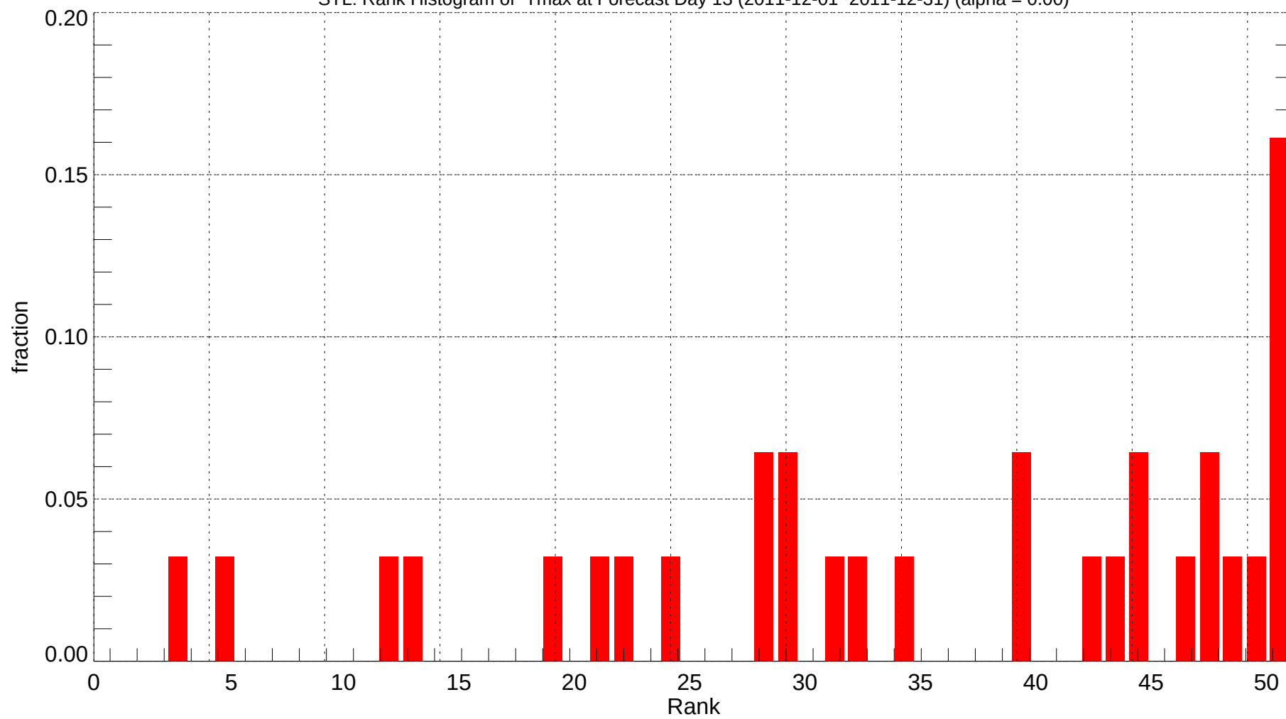
STL: Rank Histogram of Tmax at Forecast Day 13 (2011-12-01~2011-12-31) (alpha = 0.00)
