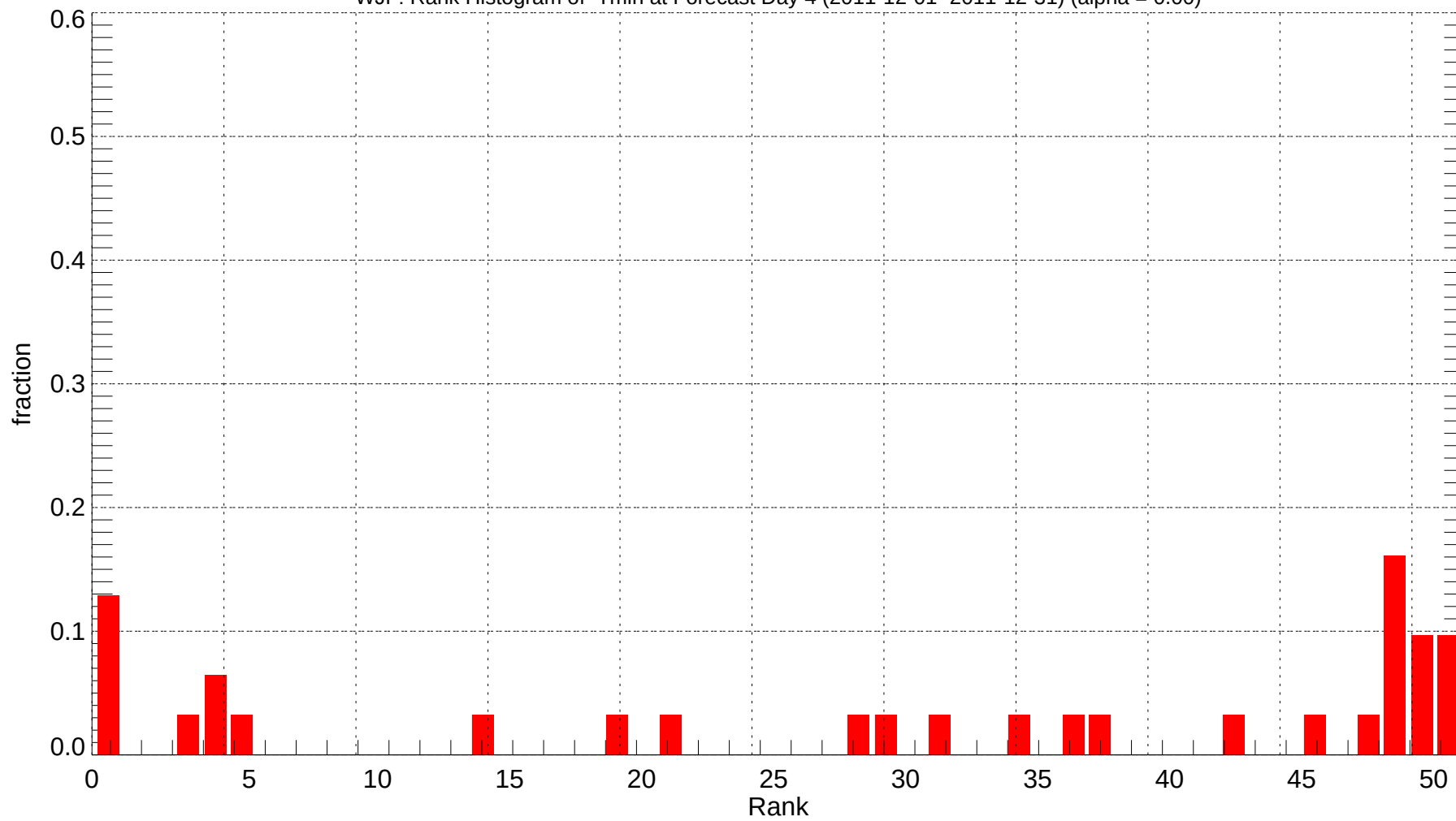
WJF: Rank Histogram of Tmin at Forecast Day 4 (2011-12-01~2011-12-31) (alpha = 0.00)
