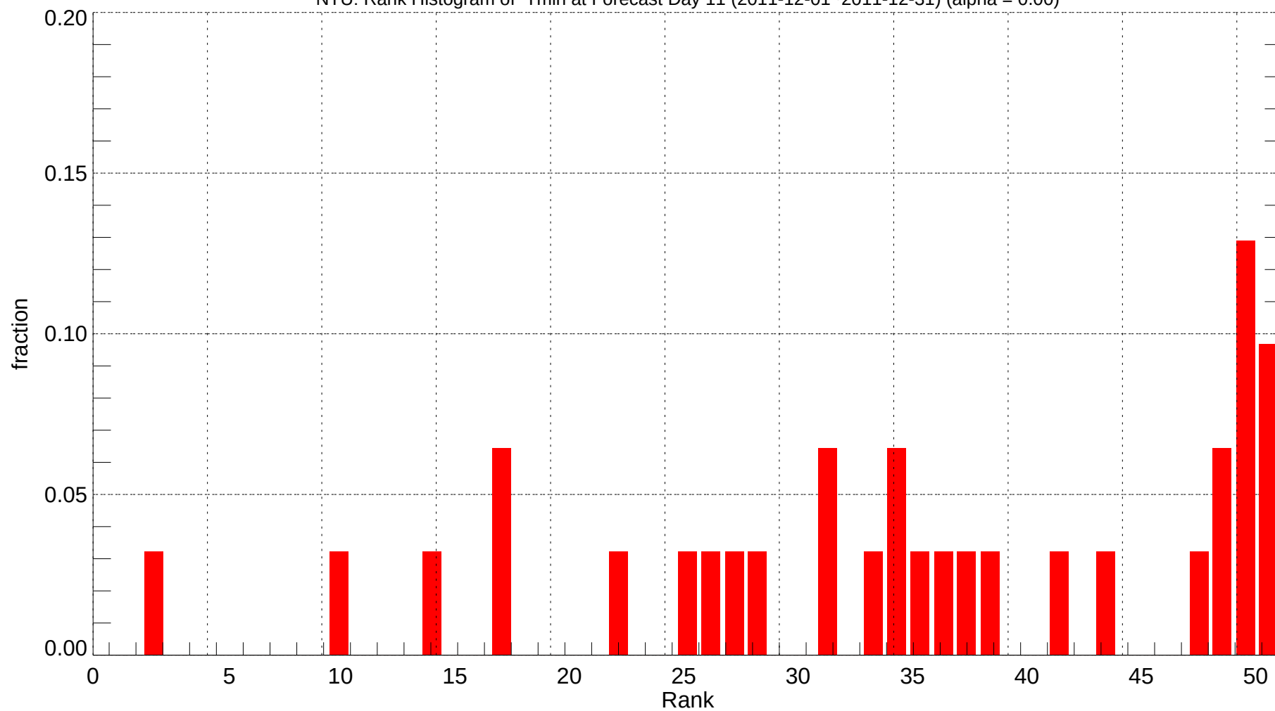
NTU: Rank Histogram of Tmin at Forecast Day 11 (2011-12-01~2011-12-31) (alpha = 0.00)
