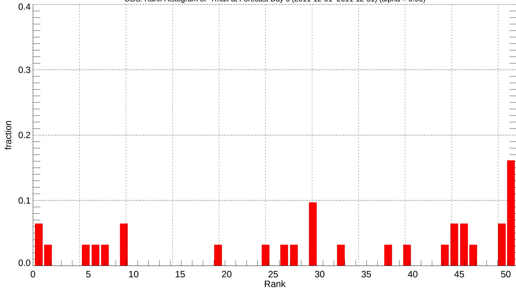
COS: Rank Histogram of Tmax at Forecast Day 6 (2011-12-01~2011-12-31) (alpha = 0.00)
