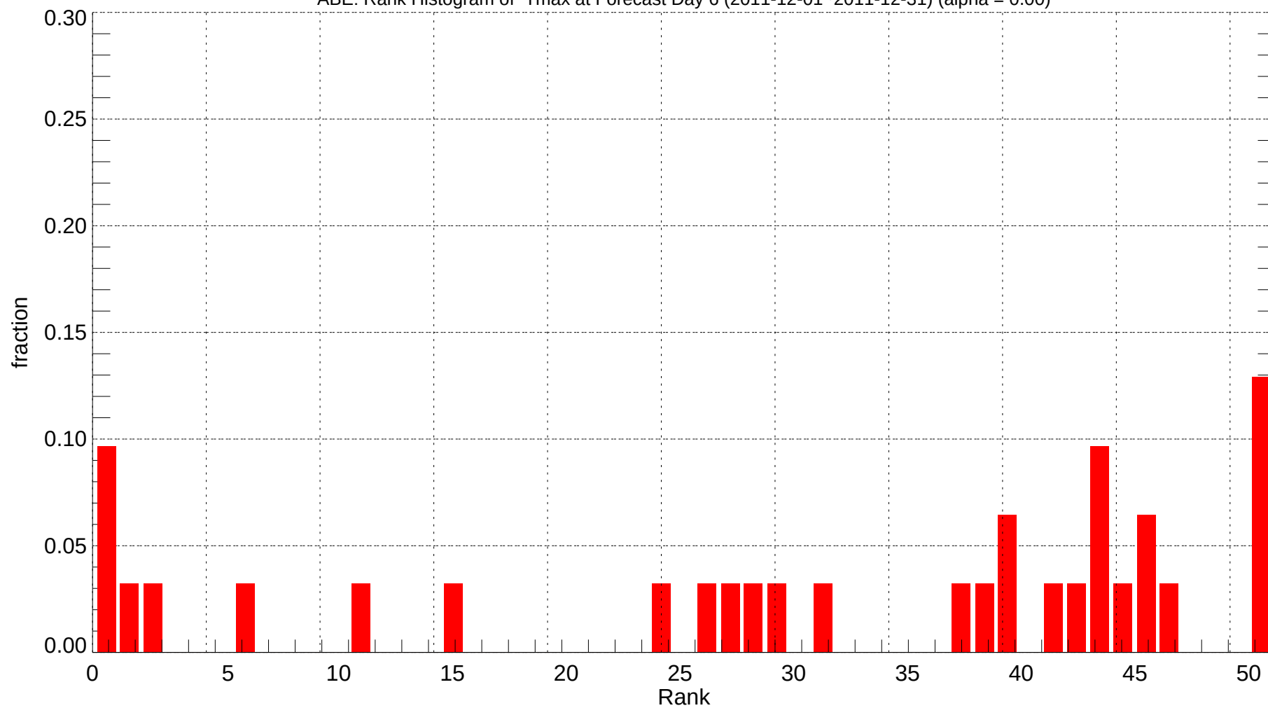
ABE: Rank Histogram of Tmax at Forecast Day 6 (2011-12-01~2011-12-31) (alpha = 0.00)
