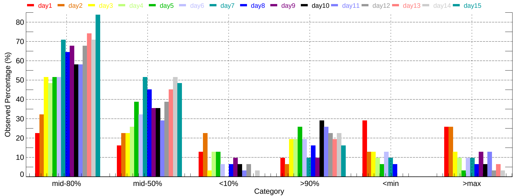
Observed Percentage of Ensembles - IND: Max Temperature (2011-12-01~2011-12-31)
