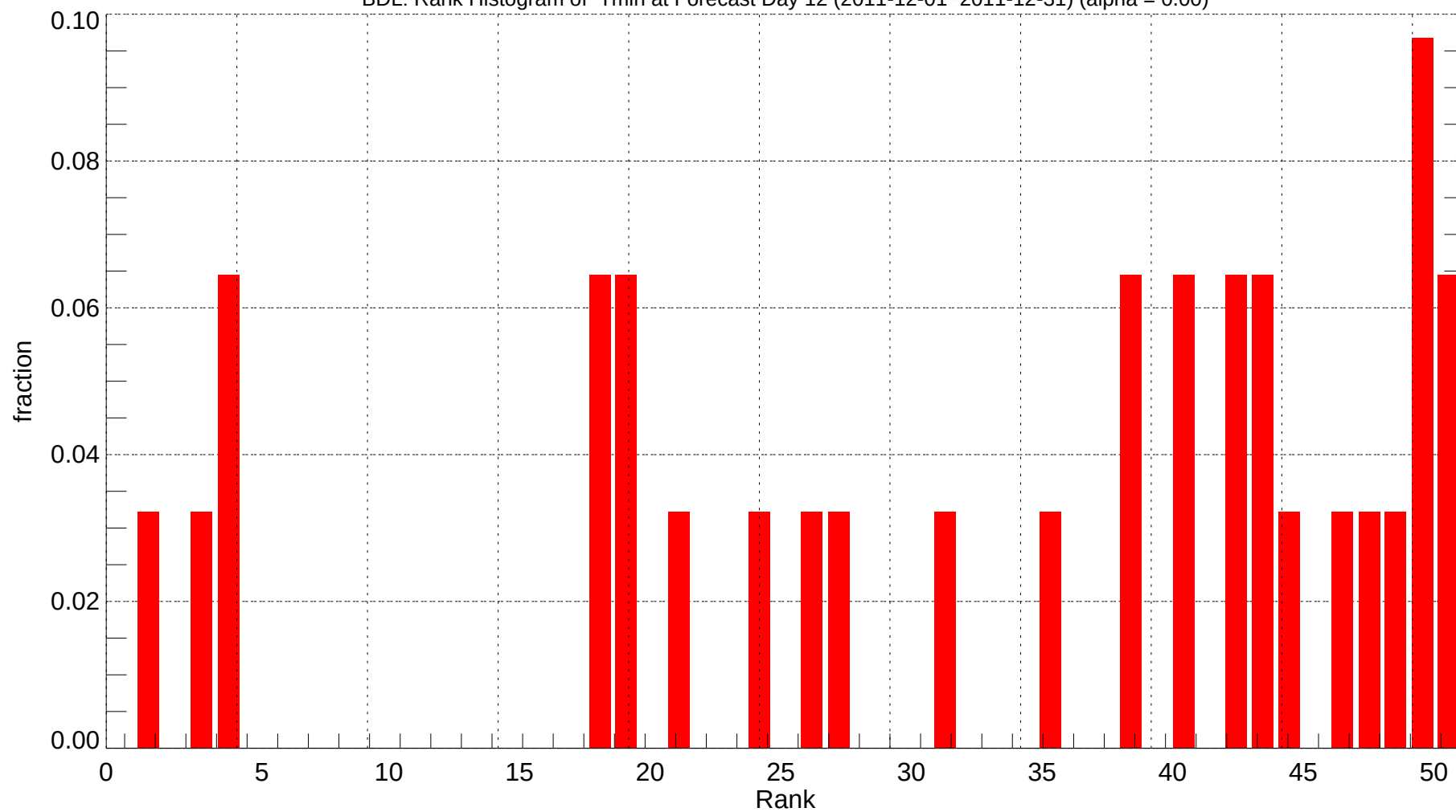
BDL: Rank Histogram of Tmin at Forecast Day 12 (2011-12-01~2011-12-31) (alpha = 0.00)
