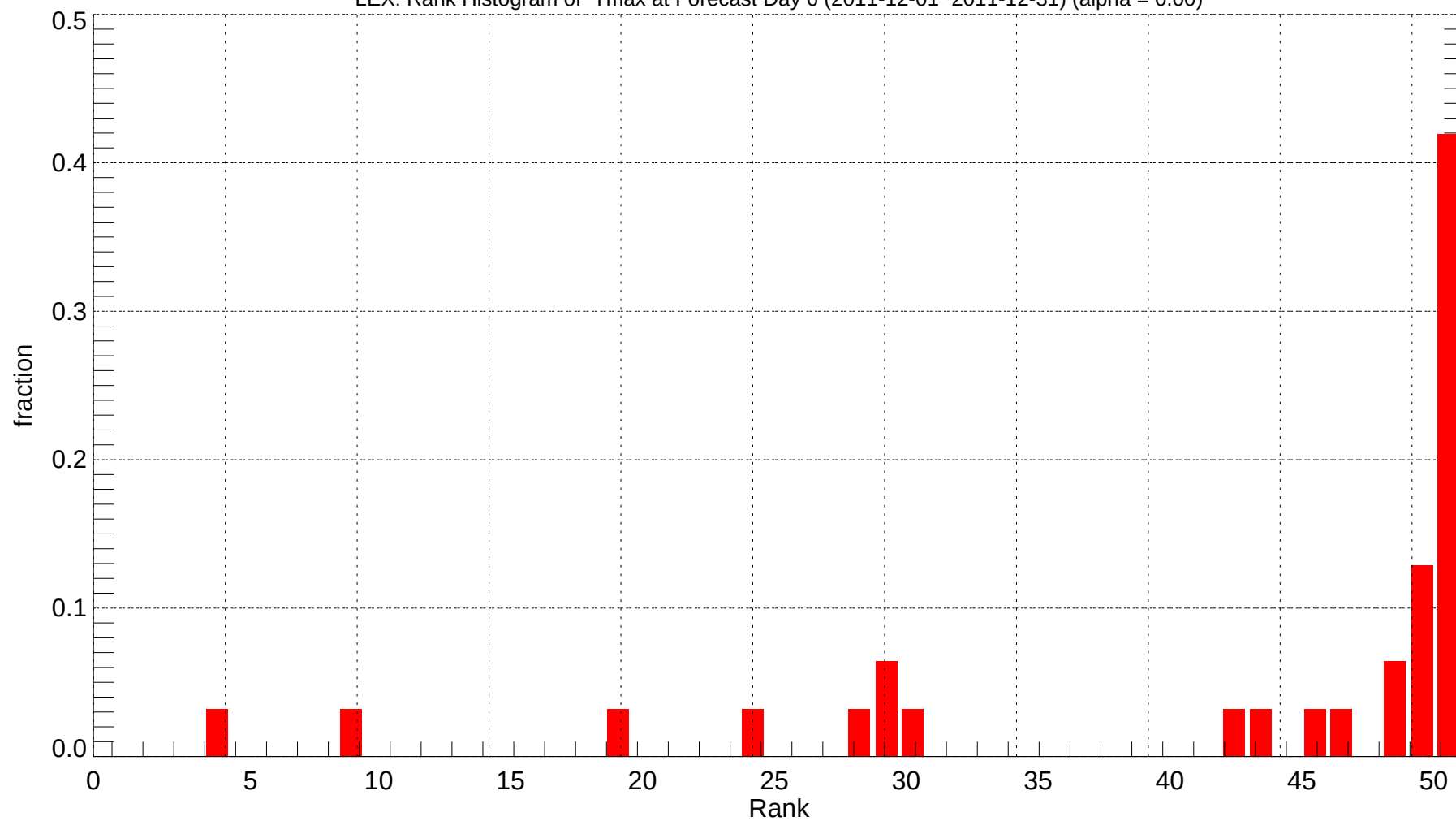
LEX: Rank Histogram of Tmax at Forecast Day 6 (2011-12-01~2011-12-31) (alpha = 0.00)
