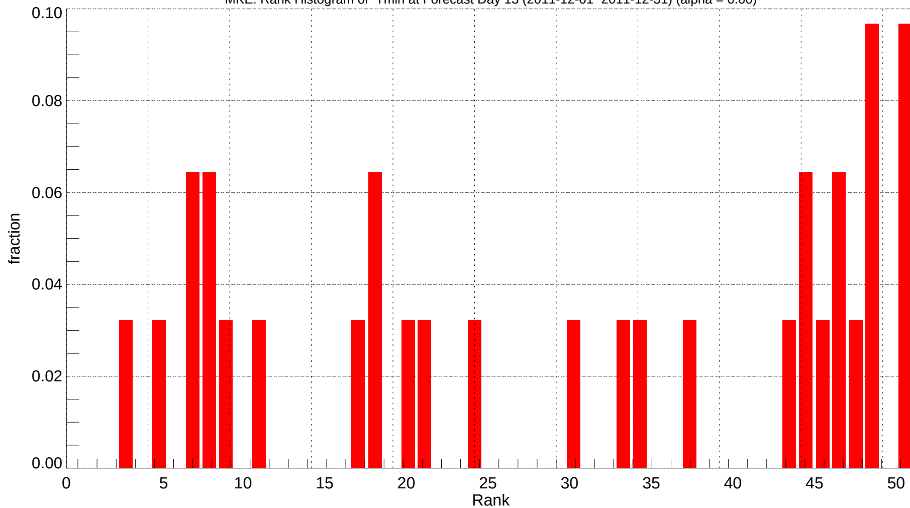
MKE: Rank Histogram of Tmin at Forecast Day 13 (2011-12-01~2011-12-31) (alpha = 0.00)
