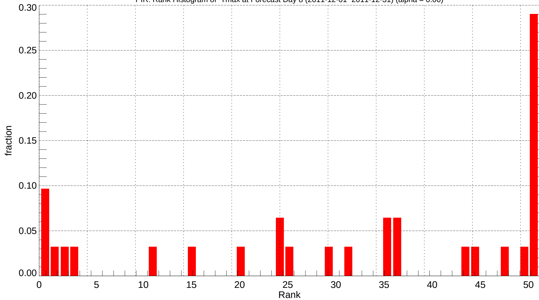
PIR: Rank Histogram of Tmax at Forecast Day 8 (2011-12-01~2011-12-31) (alpha = 0.00)
