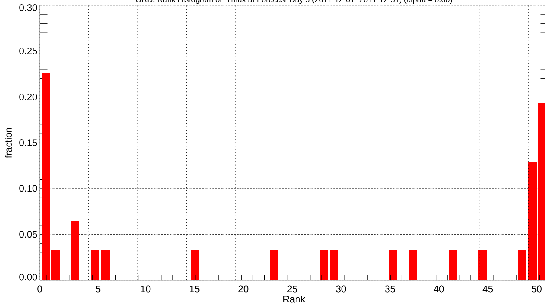
ORD: Rank Histogram of Tmax at Forecast Day 3 (2011-12-01~2011-12-31) (alpha = 0.00)
