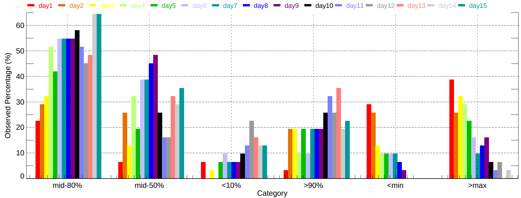
Observed Percentage of Ensembles - PIT: Min Temperature (2011-12-01~2011-12-31)
