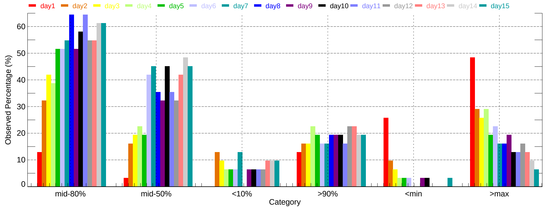
Observed Percentage of Ensembles - ICT: Max Temperature (2011-12-01~2011-12-31)
