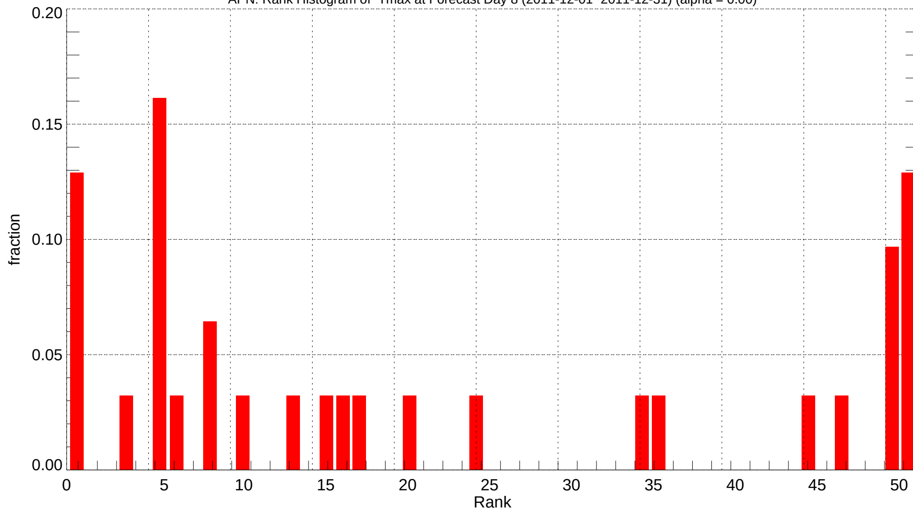
APN: Rank Histogram of Tmax at Forecast Day 8 (2011-12-01~2011-12-31) (alpha = 0.00)
