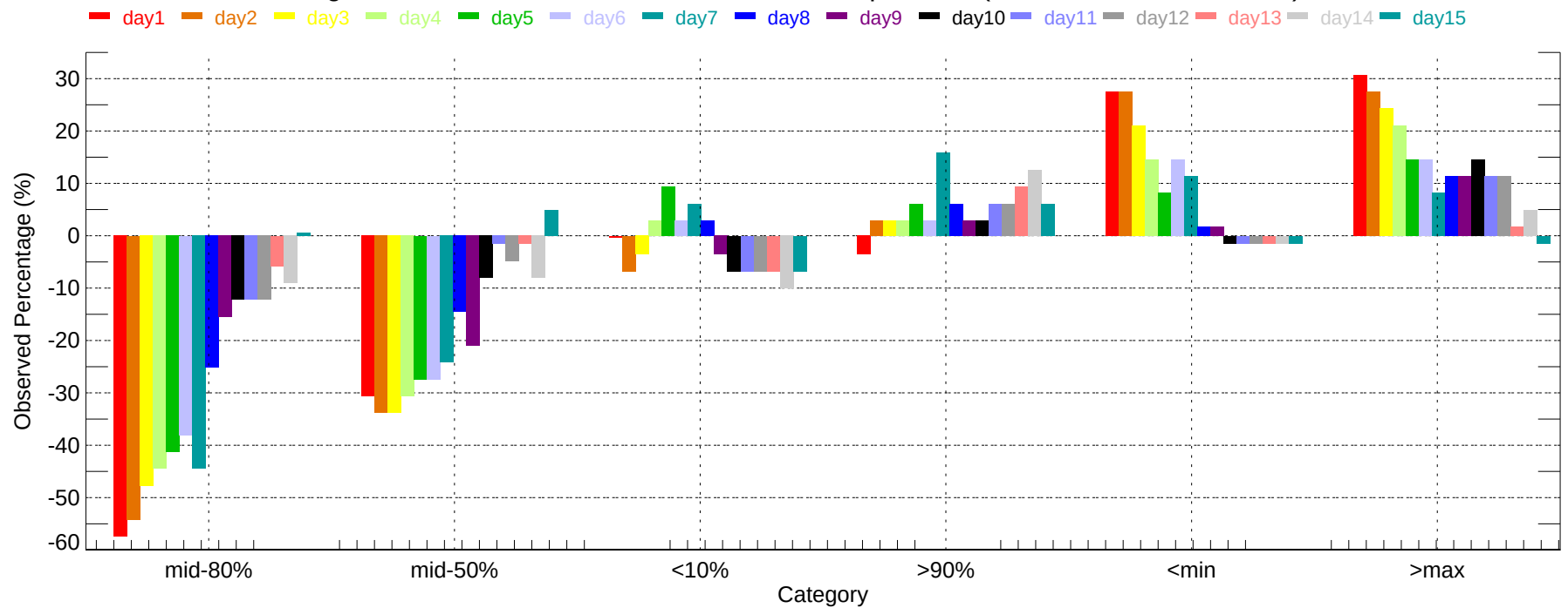
Observed Percentage Deviation of Ensembles - ORD: Min Temperature (2011-12-01~2011-12-31)
