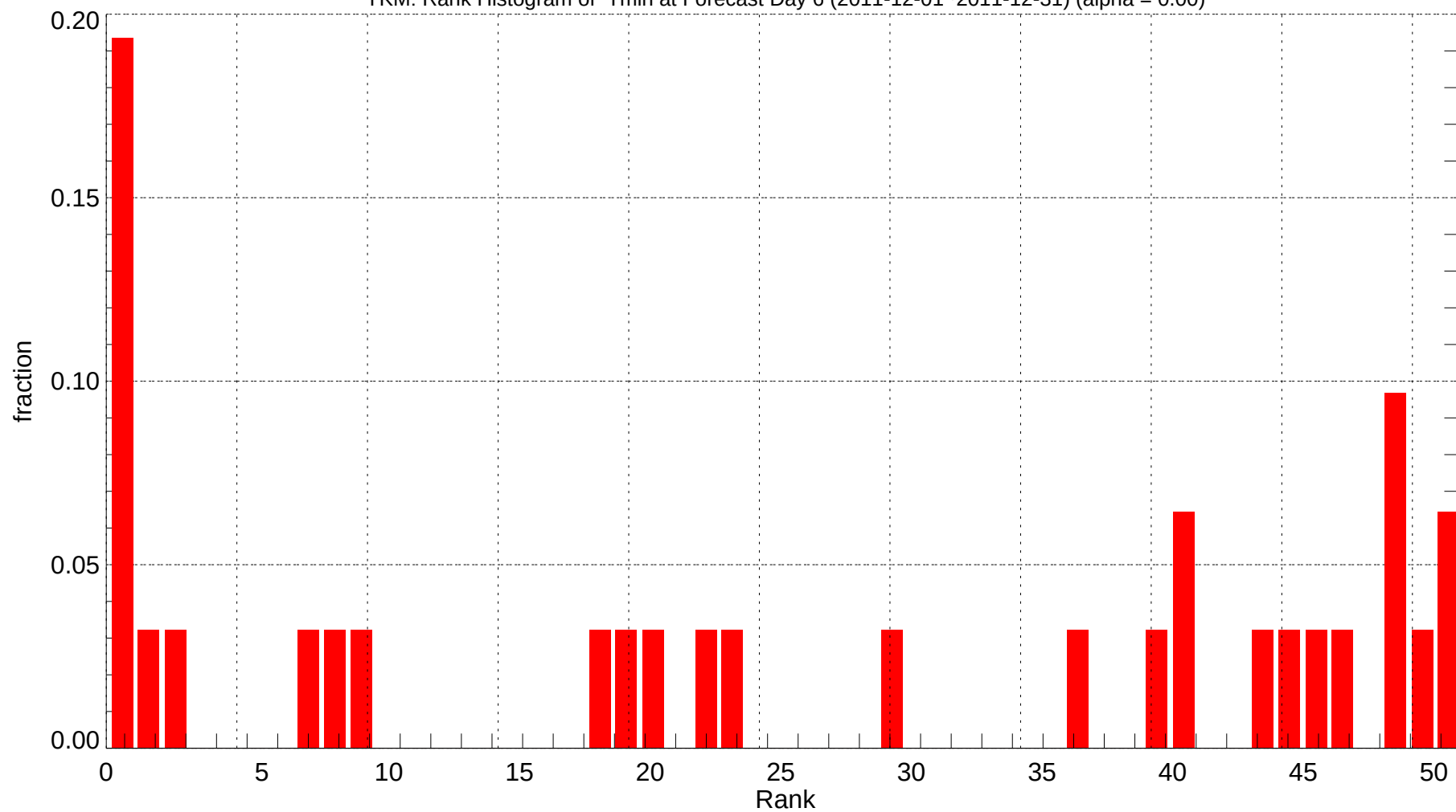
YKM: Rank Histogram of Tmin at Forecast Day 6 (2011-12-01~2011-12-31) (alpha = 0.00)
