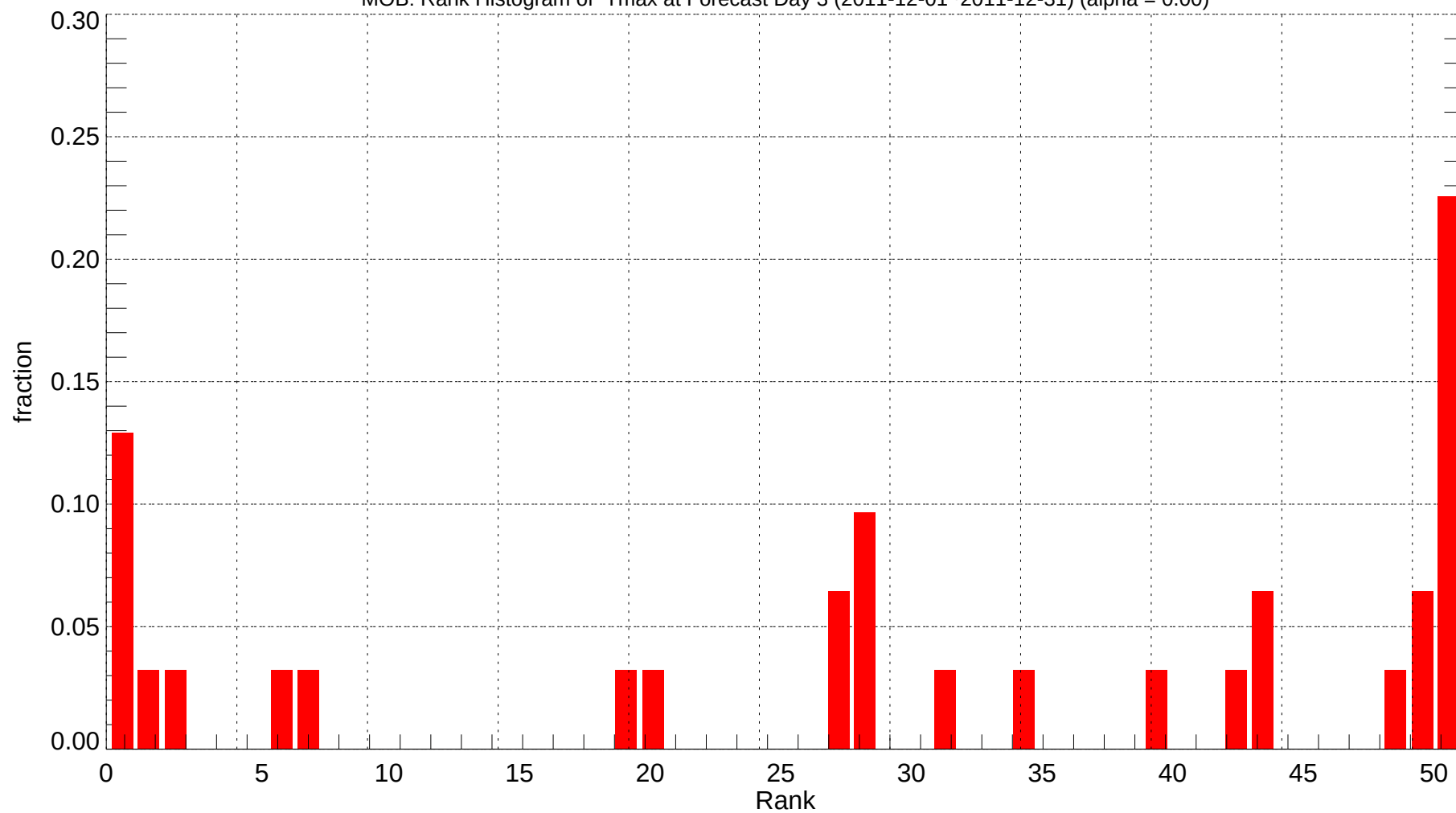
MOB: Rank Histogram of Tmax at Forecast Day 3 (2011-12-01~2011-12-31) (alpha = 0.00)
