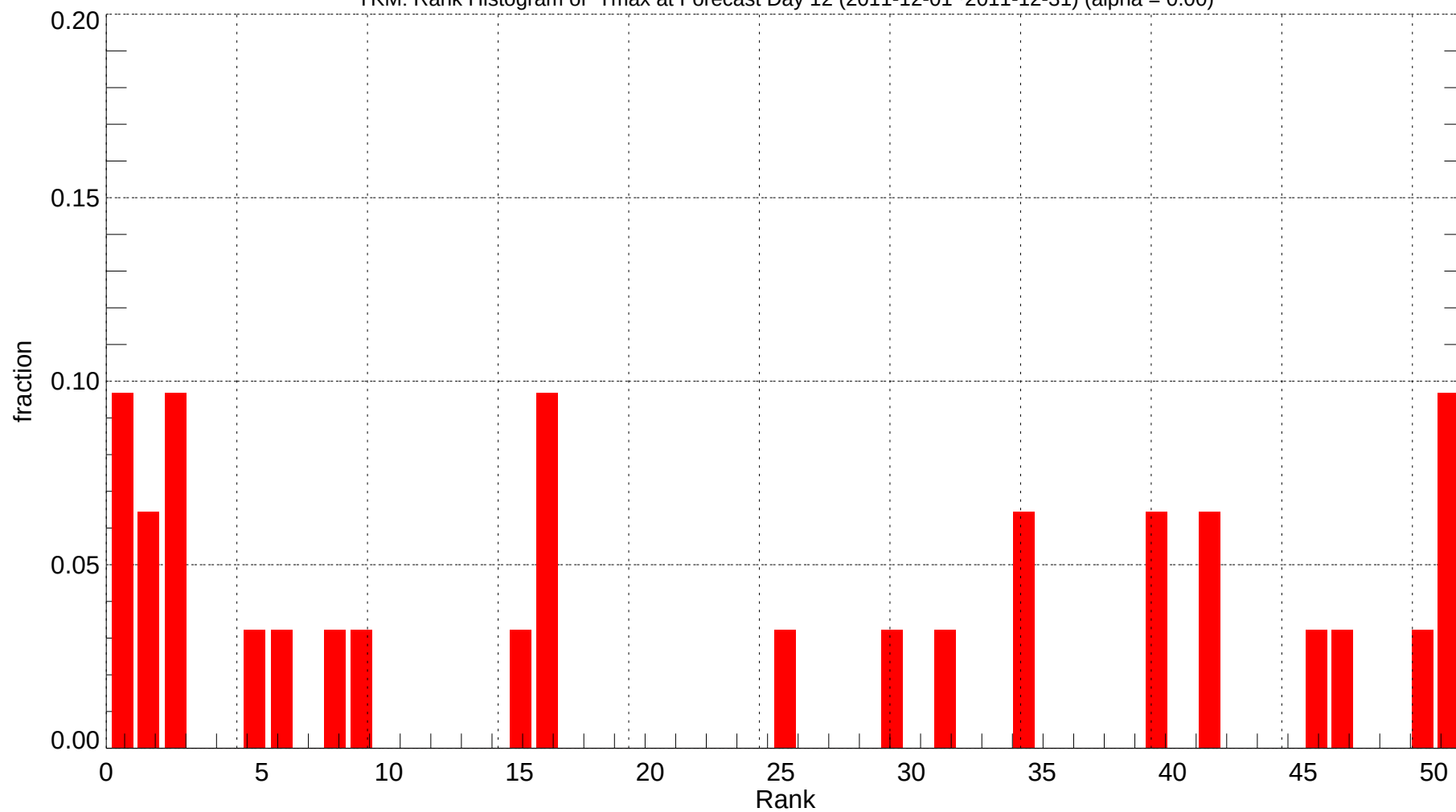
YKM: Rank Histogram of Tmax at Forecast Day 12 (2011-12-01~2011-12-31) (alpha = 0.00)
