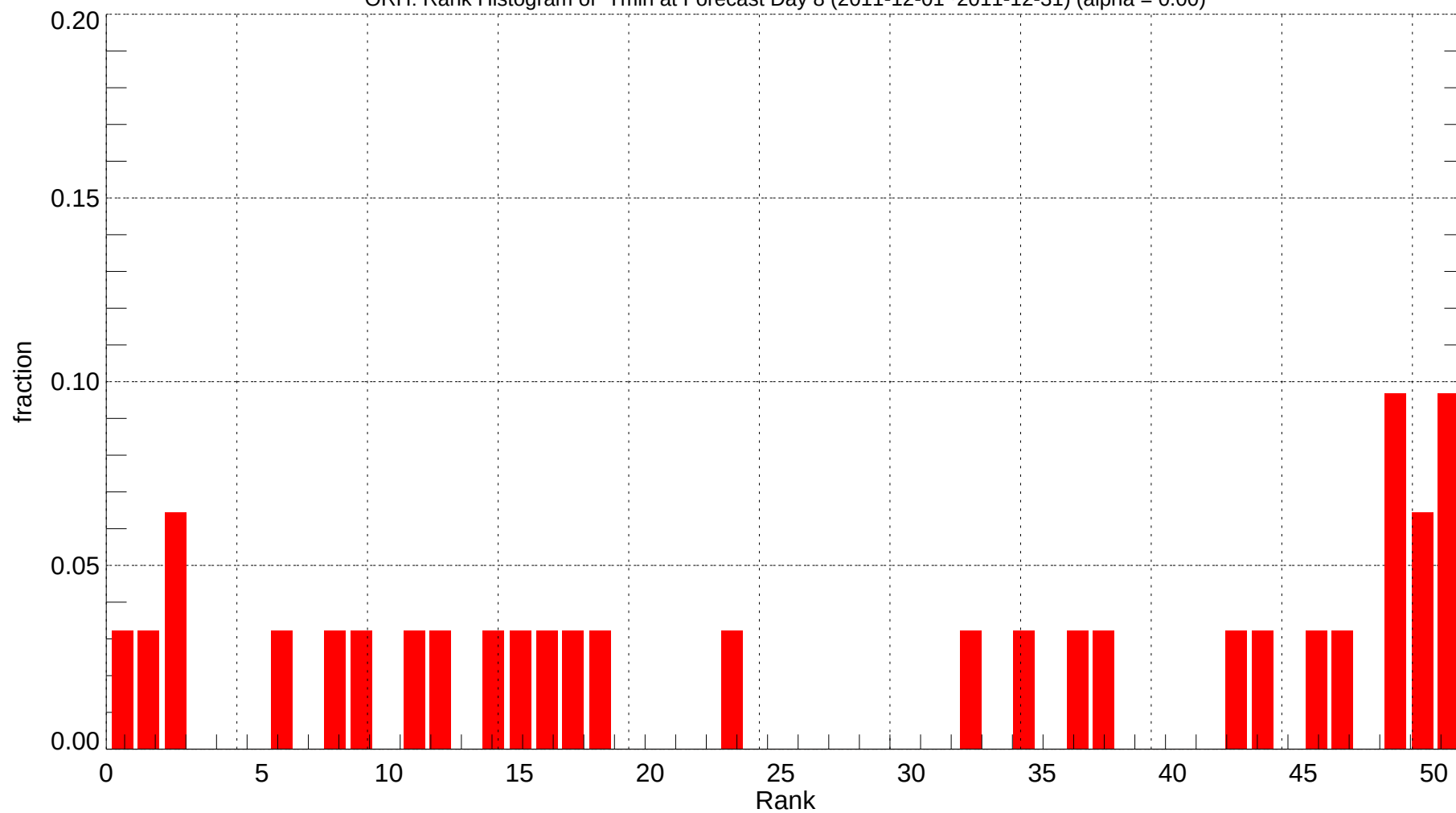
ORH: Rank Histogram of Tmin at Forecast Day 8 (2011-12-01~2011-12-31) (alpha = 0.00)
