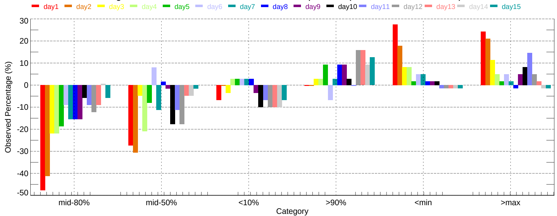
Observed Percentage Deviation of Ensembles - BWI: Max Temperature (2011-12-01~2011-12-31)
