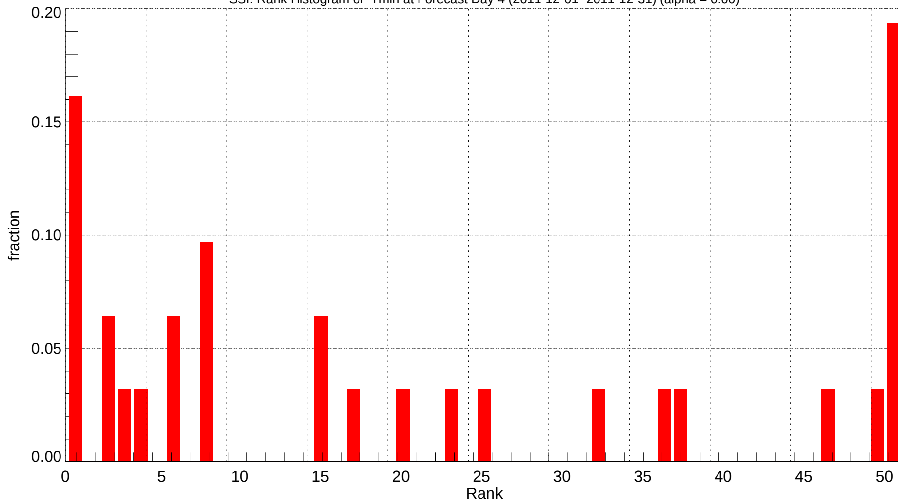
SSI: Rank Histogram of Tmin at Forecast Day 4 (2011-12-01~2011-12-31) (alpha = 0.00)
