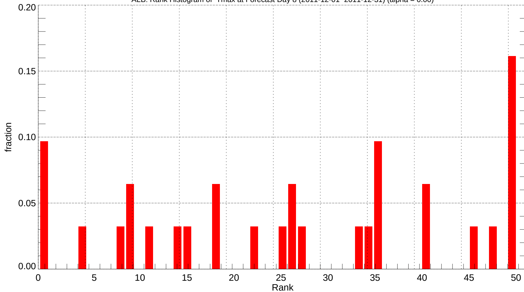
ALB: Rank Histogram of Tmax at Forecast Day 8 (2011-12-01~2011-12-31) (alpha = 0.00)
