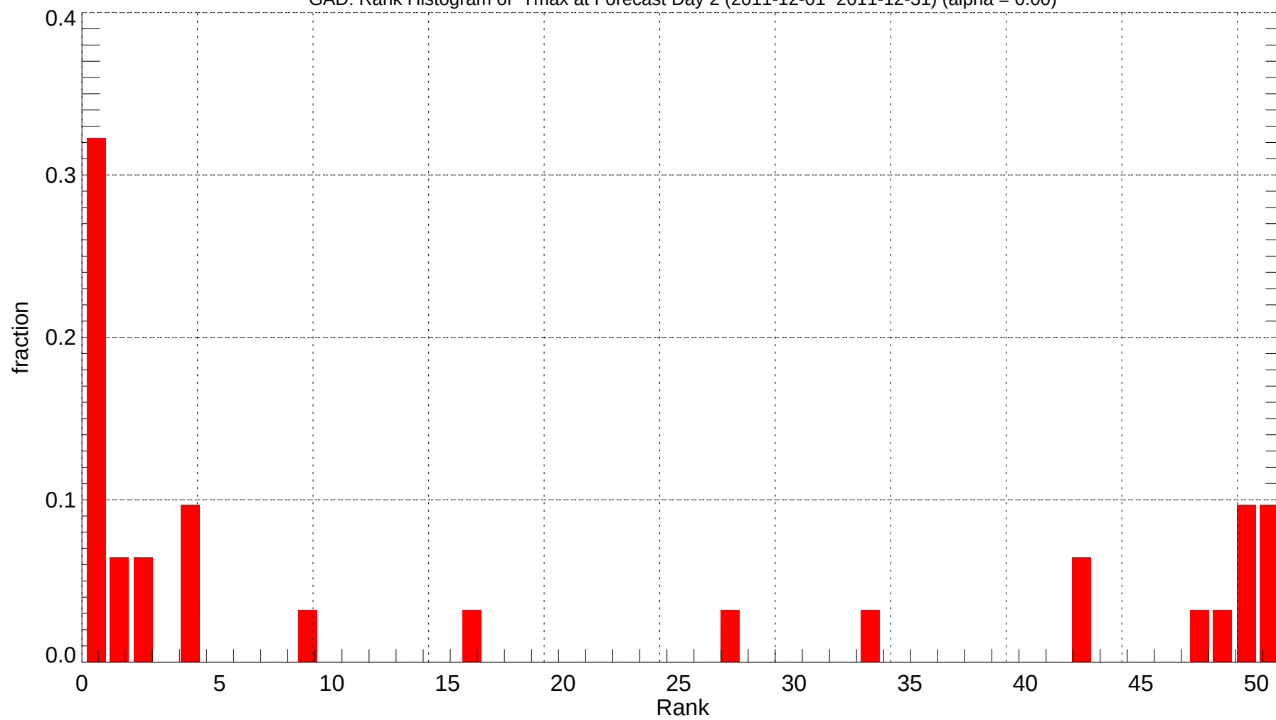
GAD: Rank Histogram of Tmax at Forecast Day 2 (2011-12-01~2011-12-31) (alpha = 0.00)
