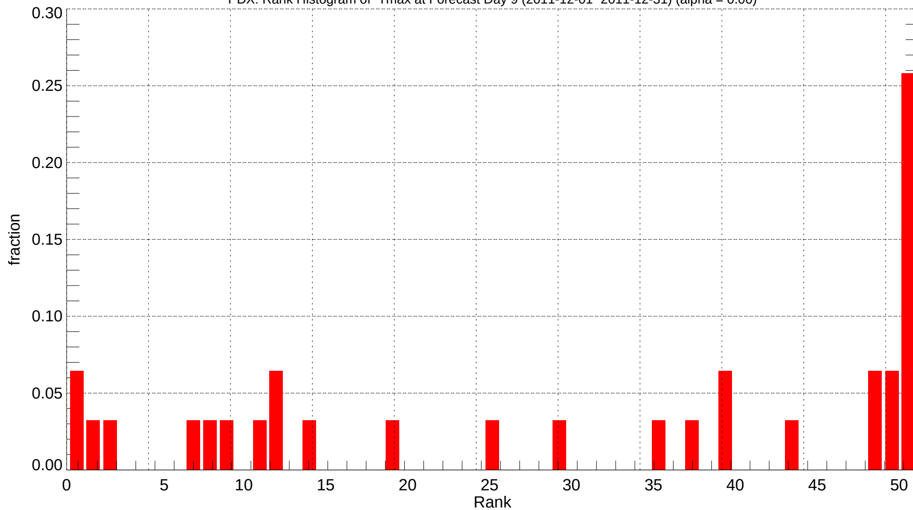
PDX: Rank Histogram of Tmax at Forecast Day 9 (2011-12-01~2011-12-31) (alpha = 0.00)
