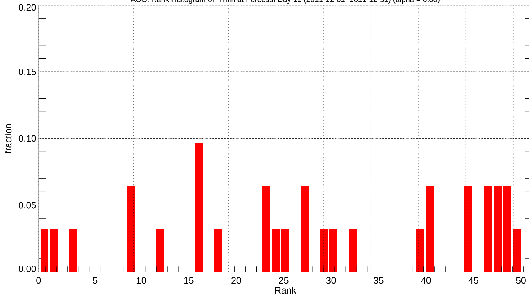
AUG: Rank Histogram of Tmin at Forecast Day 12 (2011-12-01~2011-12-31) (alpha = 0.00)
