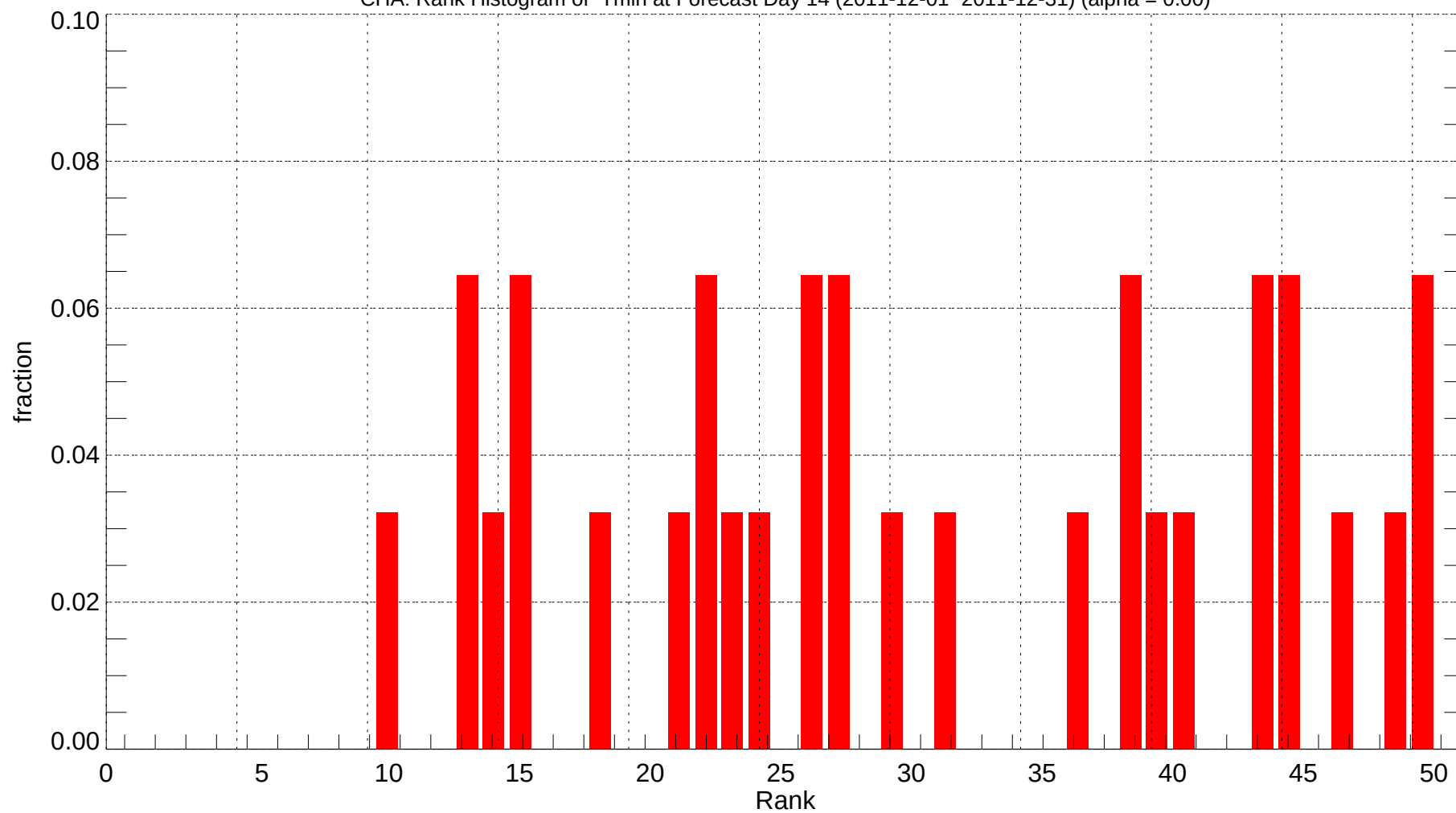
CHA: Rank Histogram of Tmin at Forecast Day 14 (2011-12-01~2011-12-31) (alpha = 0.00)
