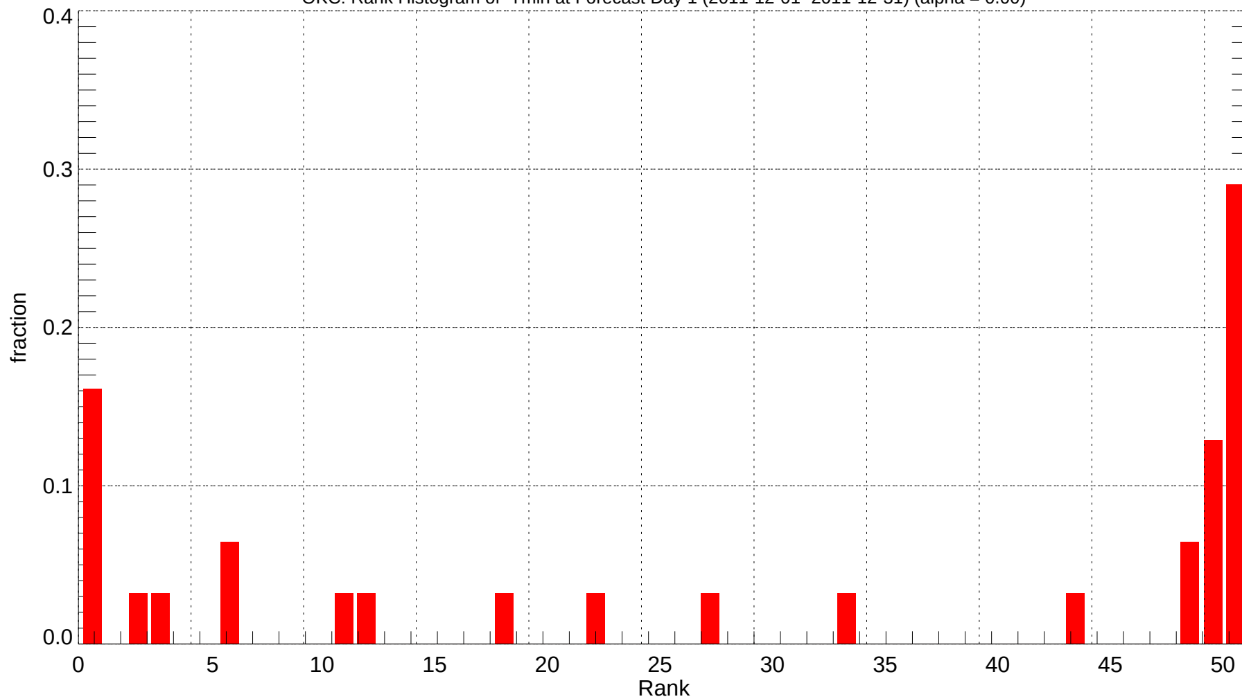
OKC: Rank Histogram of Tmin at Forecast Day 1 (2011-12-01~2011-12-31) (alpha = 0.00)
