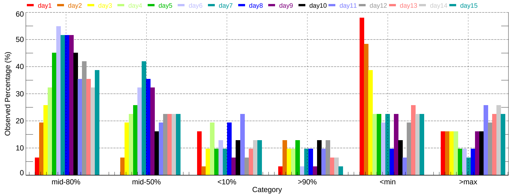
Observed Percentage of Ensembles - CRP: Max Temperature (2011-12-01~2011-12-31)
