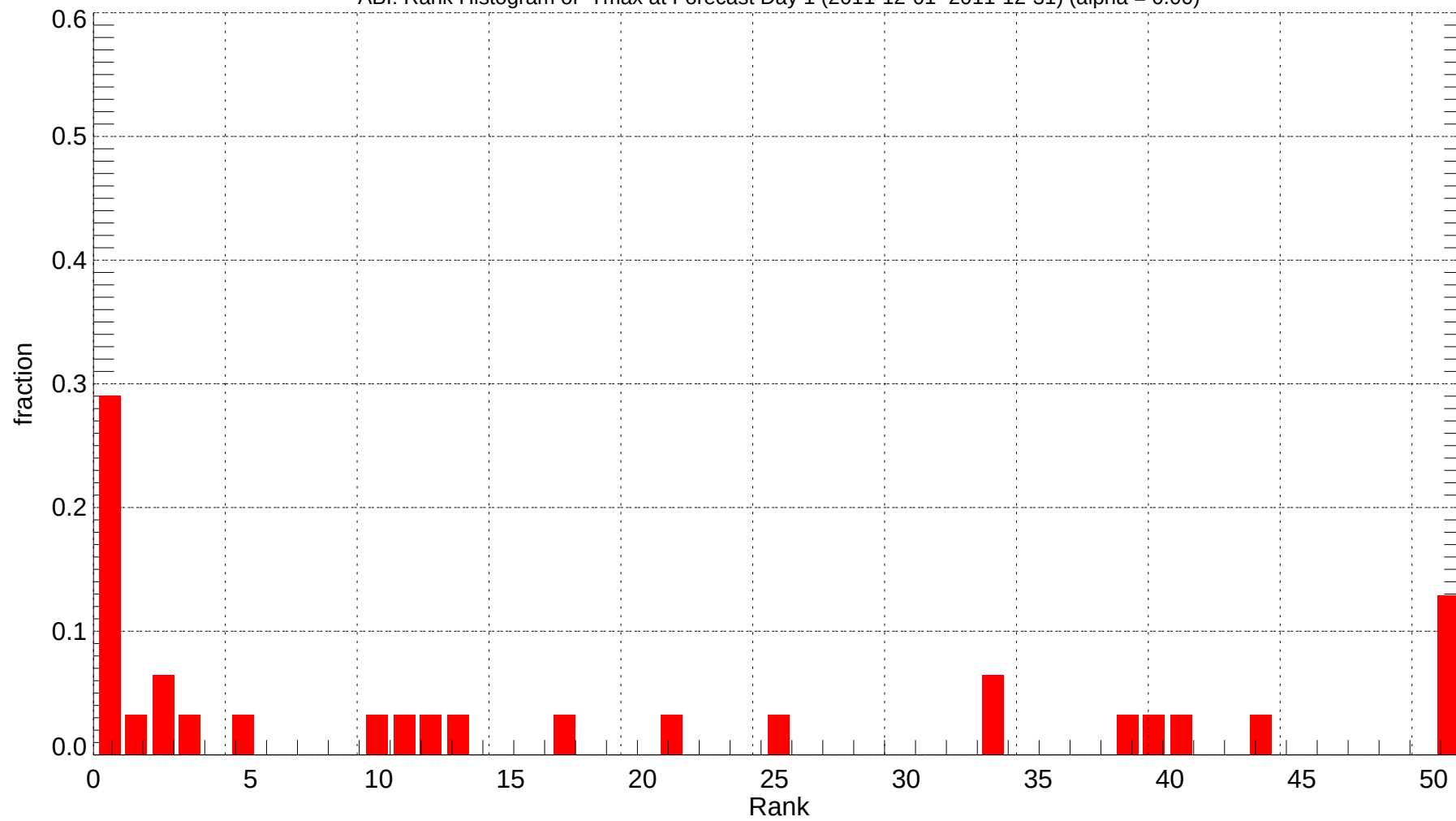
ABI: Rank Histogram of Tmax at Forecast Day 1 (2011-12-01~2011-12-31) (alpha = 0.00)
