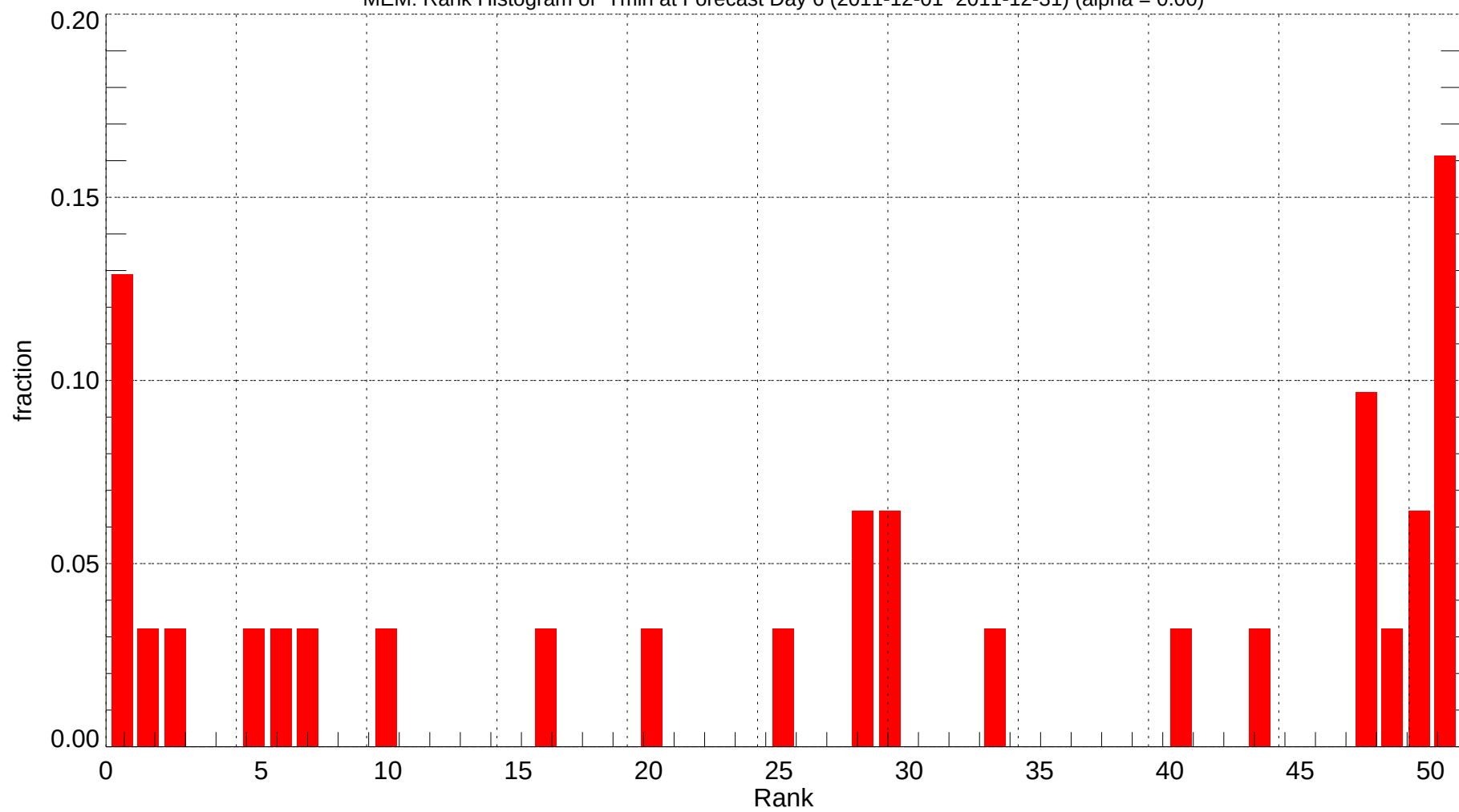
MEM: Rank Histogram of Tmin at Forecast Day 6 (2011-12-01~2011-12-31) (alpha = 0.00)
