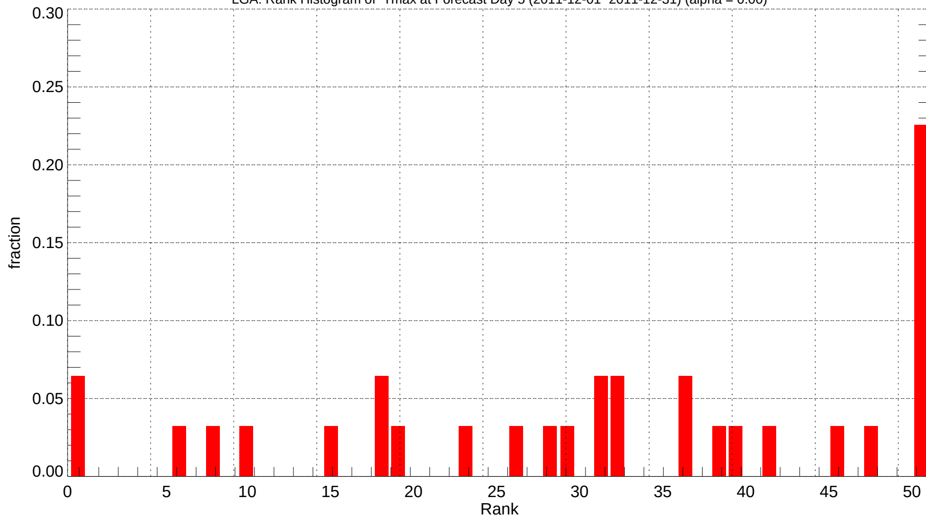
LGA: Rank Histogram of Tmax at Forecast Day 5 (2011-12-01~2011-12-31) (alpha = 0.00)
