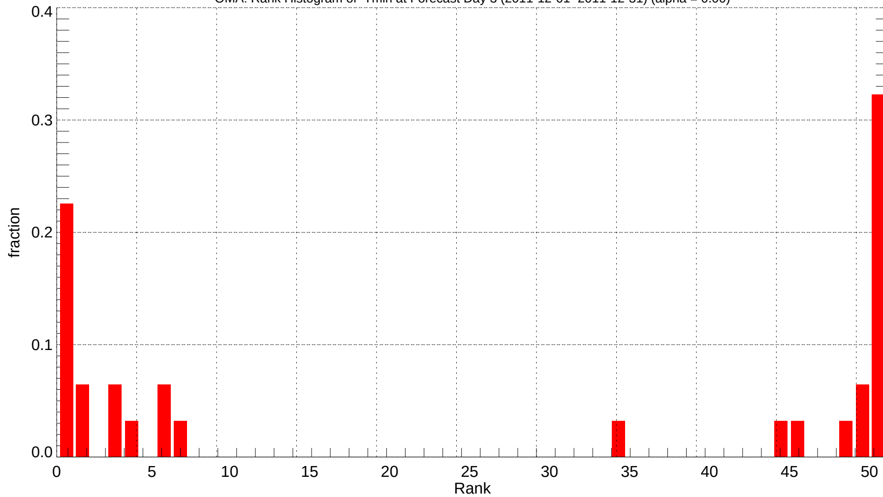
OMA: Rank Histogram of Tmin at Forecast Day 3 (2011-12-01~2011-12-31) (alpha = 0.00)
