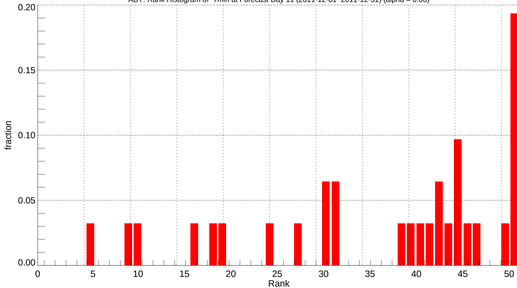
ABY: Rank Histogram of Tmin at Forecast Day 11 (2011-12-01~2011-12-31) (alpha = 0.00)
