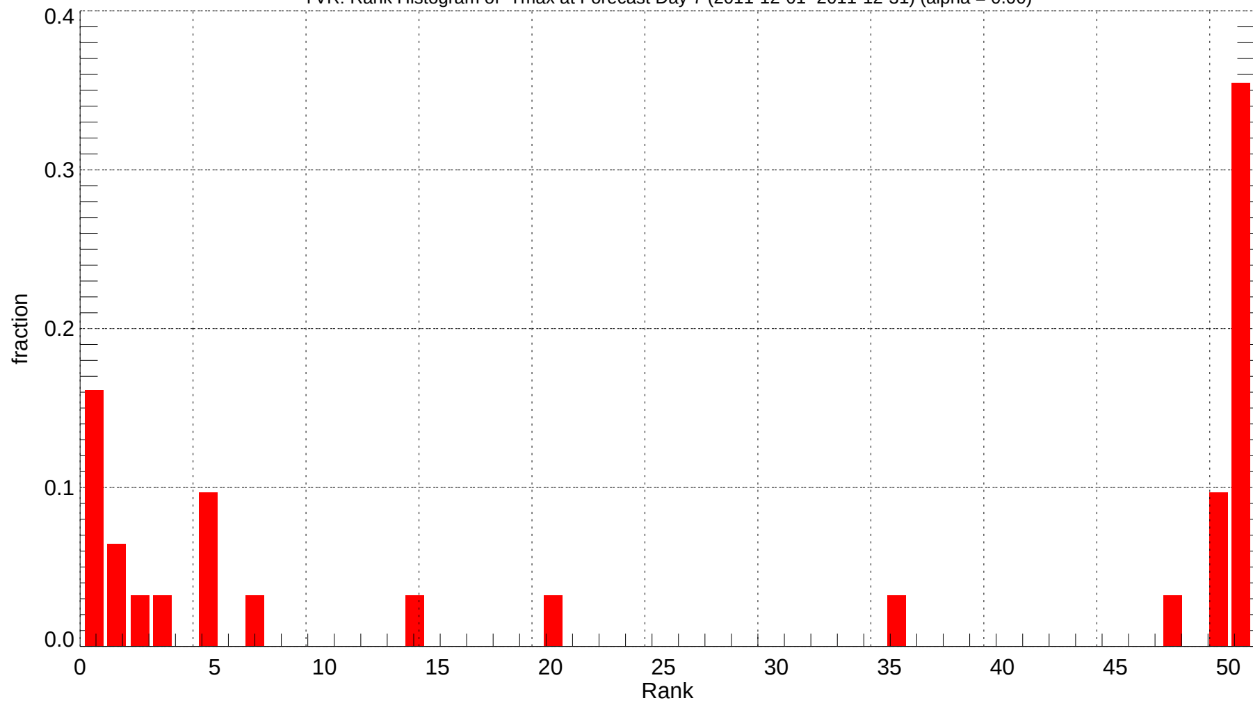
YVR: Rank Histogram of Tmax at Forecast Day 7 (2011-12-01~2011-12-31) (alpha = 0.00)
