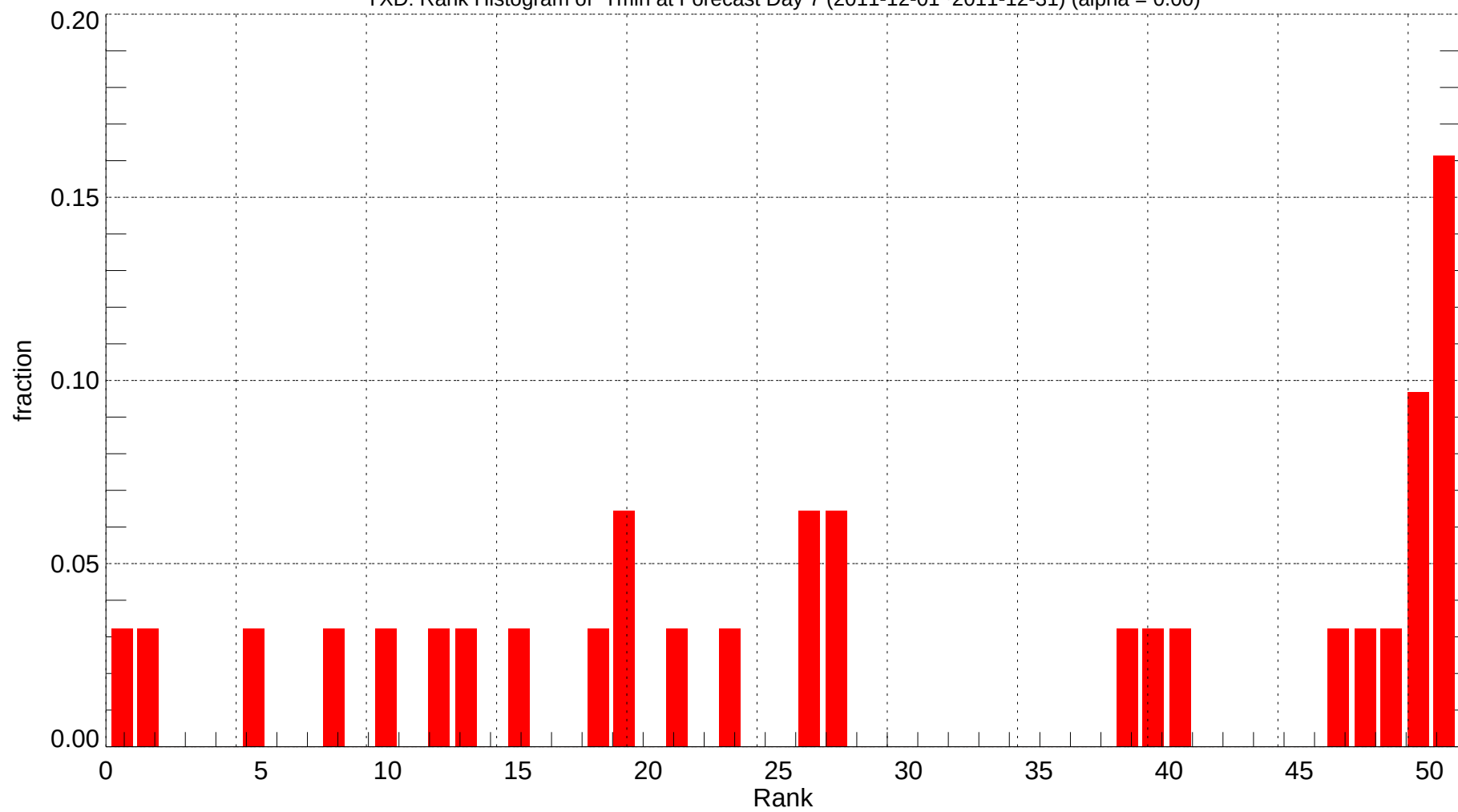
YXD: Rank Histogram of Tmin at Forecast Day 7 (2011-12-01~2011-12-31) (alpha = 0.00)
