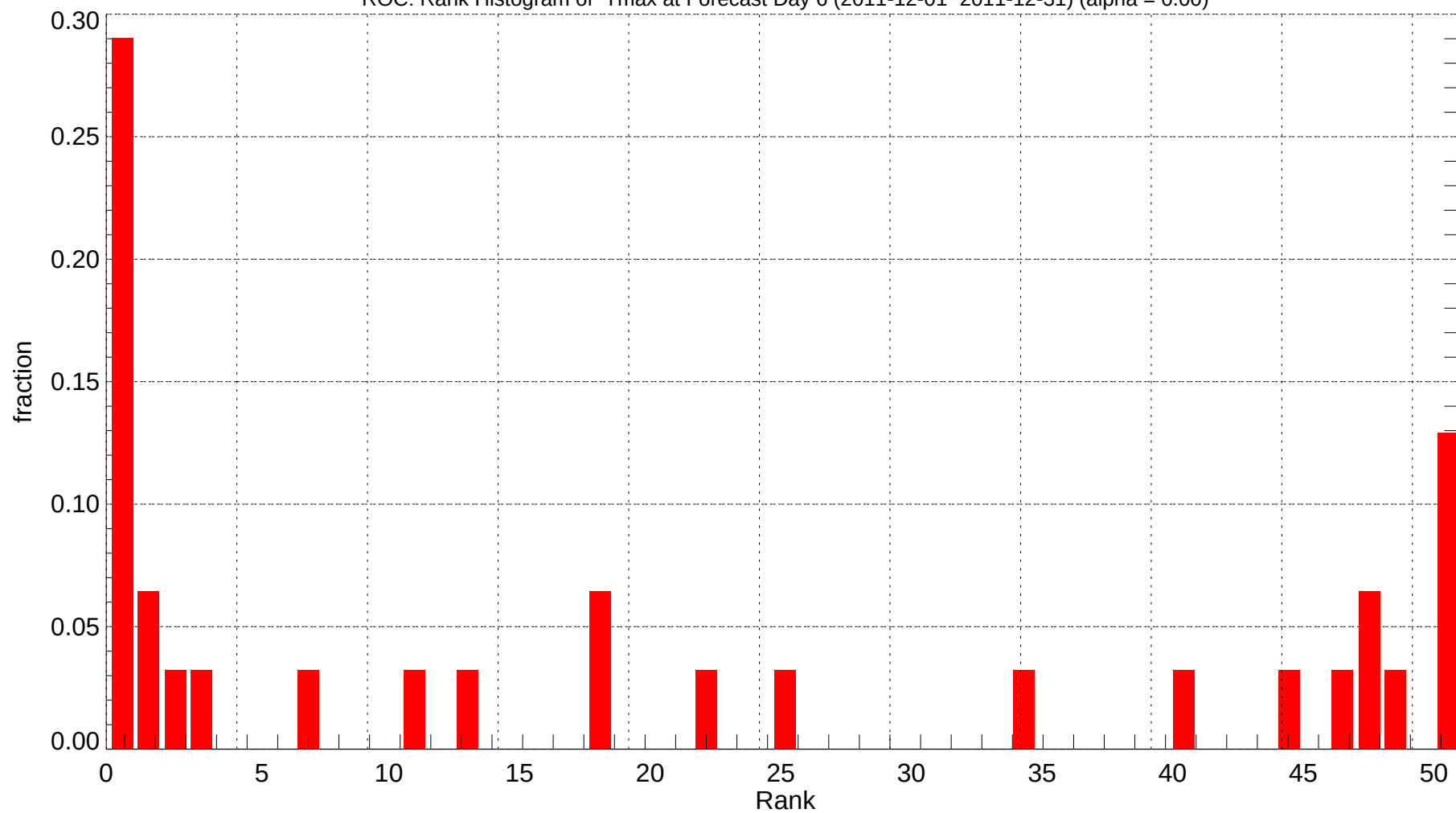
ROC: Rank Histogram of Tmax at Forecast Day 6 (2011-12-01~2011-12-31) (alpha = 0.00)
