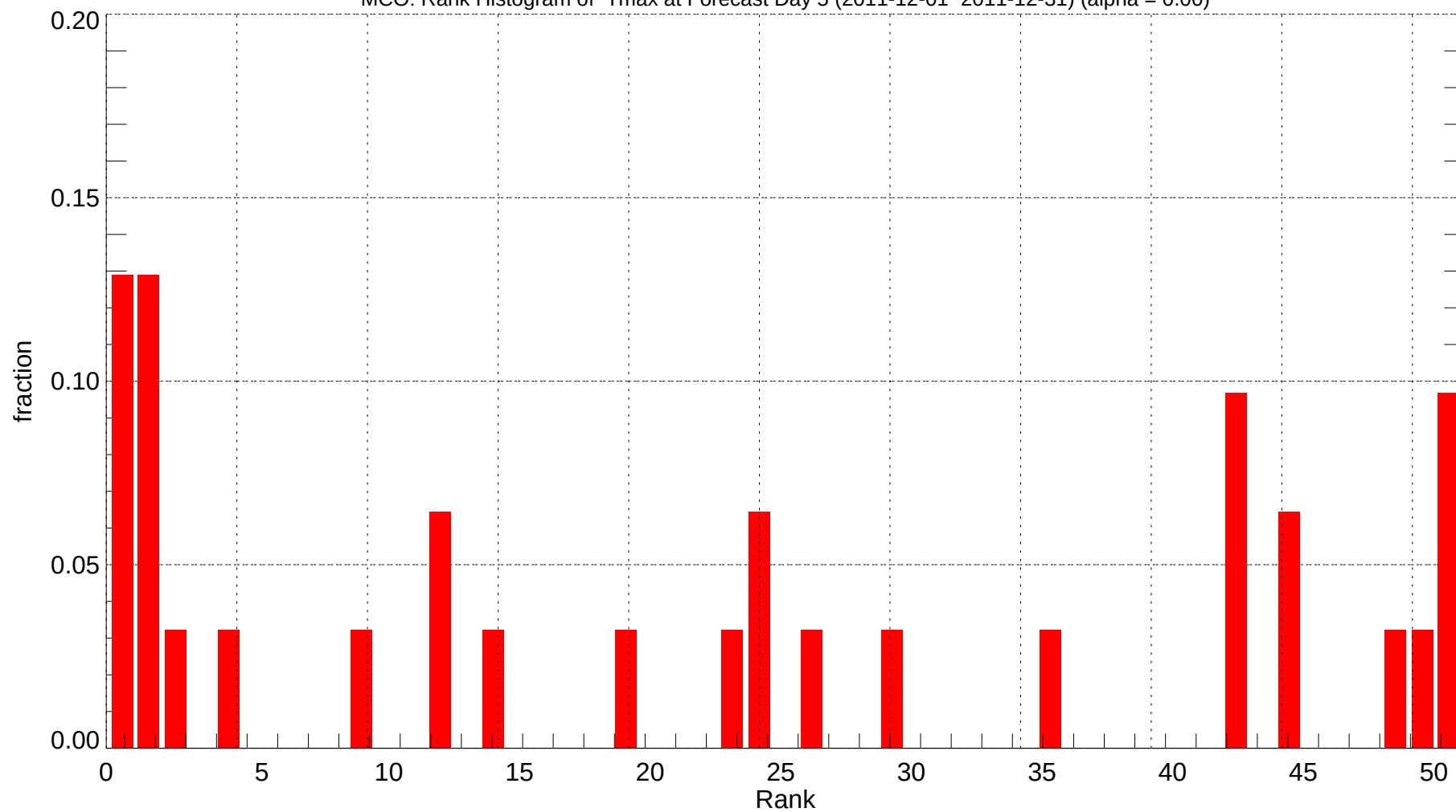
MCO: Rank Histogram of Tmax at Forecast Day 5 (2011-12-01~2011-12-31) (alpha = 0.00)
