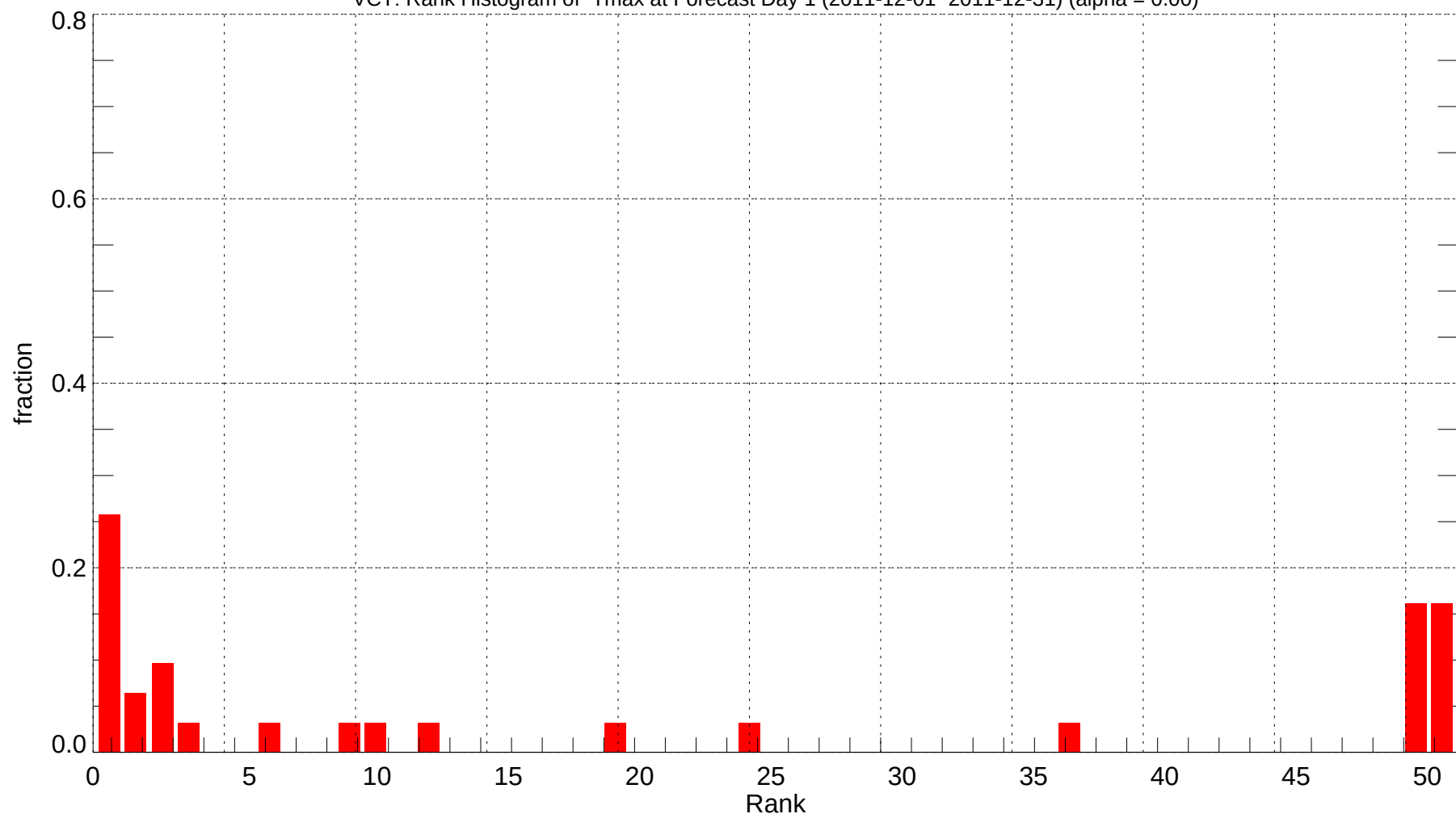
VCT: Rank Histogram of Tmax at Forecast Day 1 (2011-12-01~2011-12-31) (alpha = 0.00)
