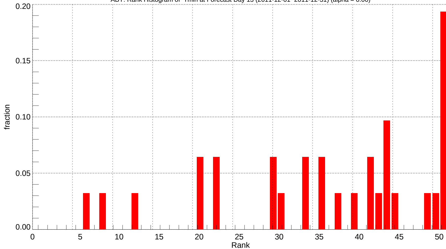
ABY: Rank Histogram of Tmin at Forecast Day 13 (2011-12-01~2011-12-31) (alpha = 0.00)
