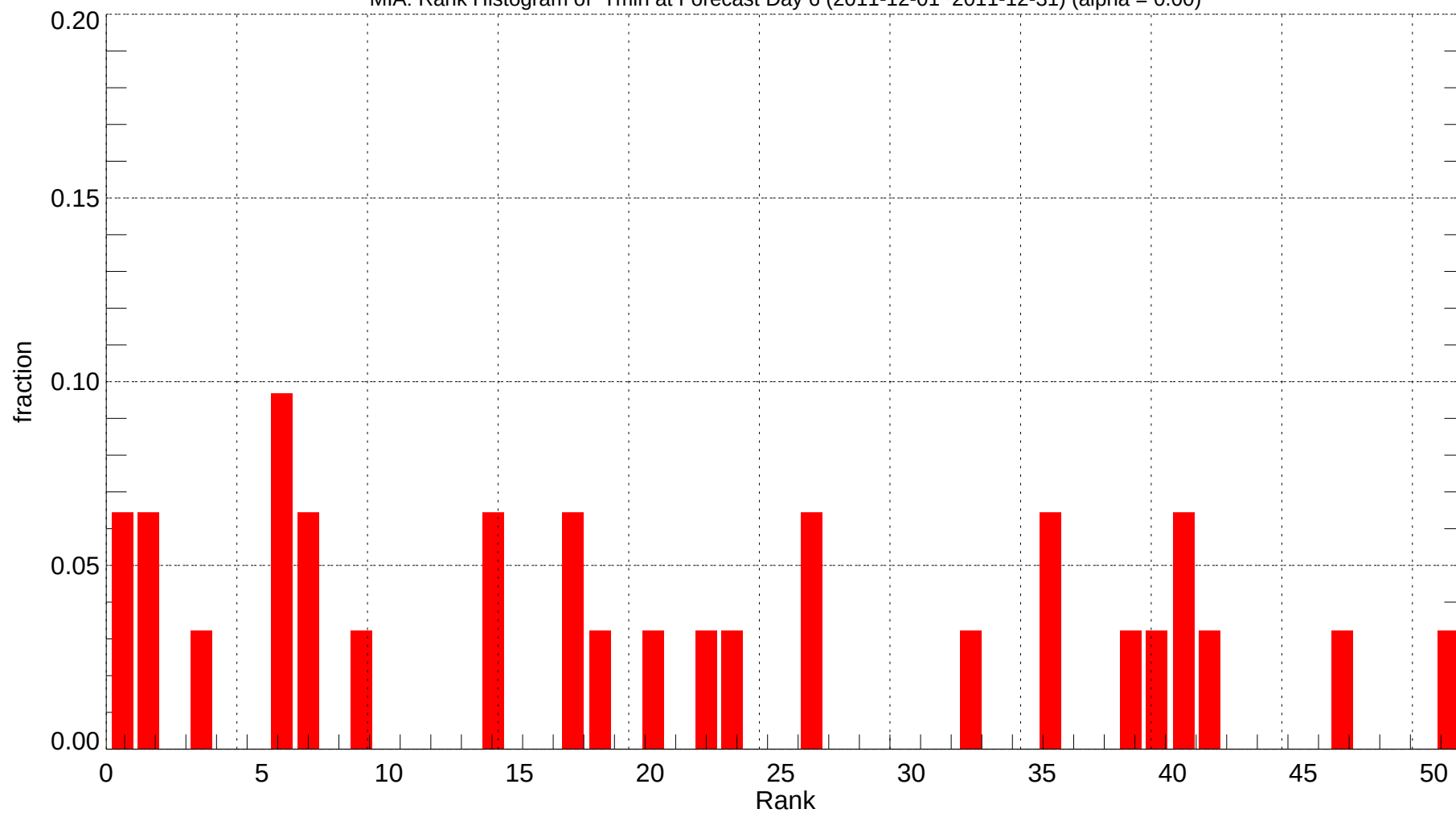
MIA: Rank Histogram of Tmin at Forecast Day 6 (2011-12-01~2011-12-31) (alpha = 0.00)
