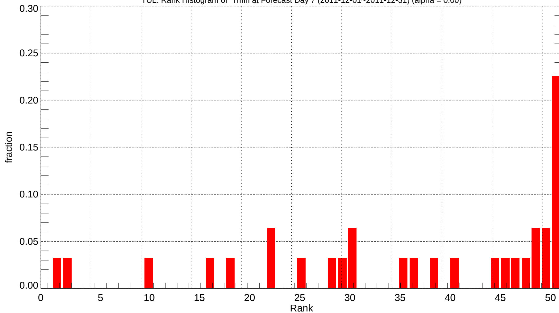
TUL: Rank Histogram of Tmin at Forecast Day 7 (2011-12-01~2011-12-31) (alpha = 0.00)
