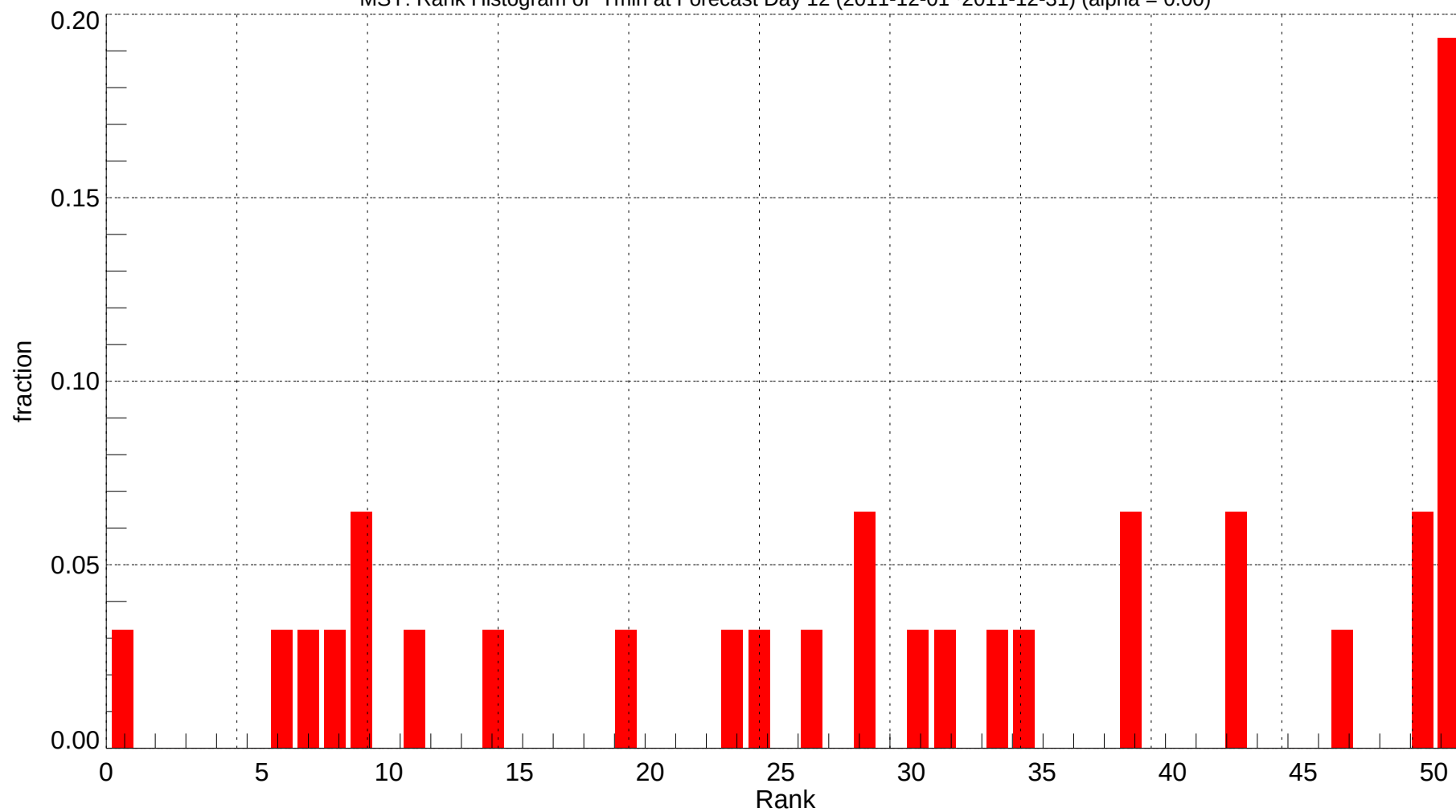
MSY: Rank Histogram of Tmin at Forecast Day 12 (2011-12-01~2011-12-31) (alpha = 0.00)
