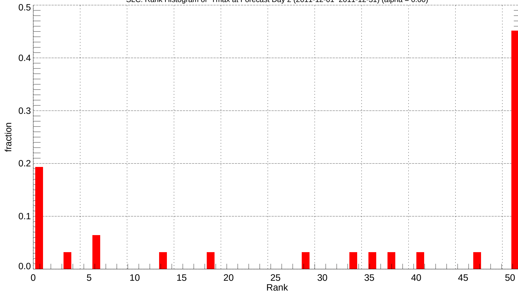
SLC: Rank Histogram of Tmax at Forecast Day 2 (2011-12-01~2011-12-31) (alpha = 0.00)
