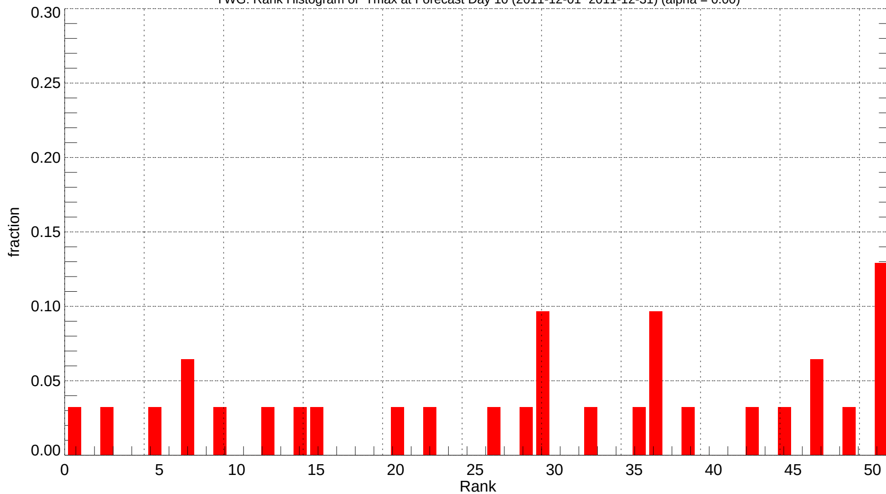
YWG: Rank Histogram of Tmax at Forecast Day 10 (2011-12-01~2011-12-31) (alpha = 0.00)
