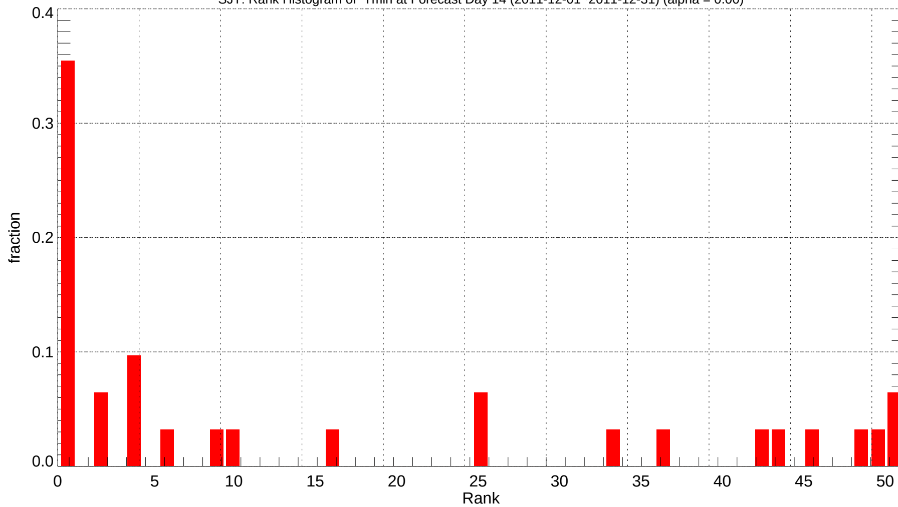
SJT: Rank Histogram of Tmin at Forecast Day 14 (2011-12-01~2011-12-31) (alpha = 0.00)
