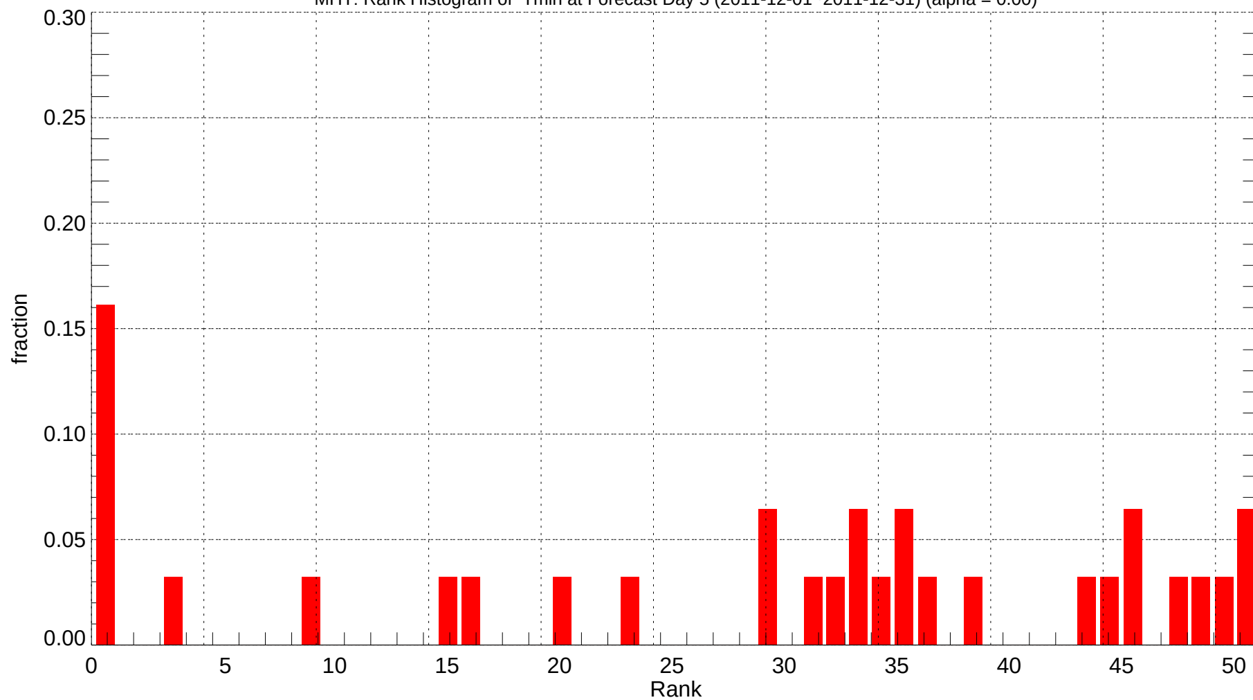
MHT: Rank Histogram of Tmin at Forecast Day 5 (2011-12-01~2011-12-31) (alpha = 0.00)
