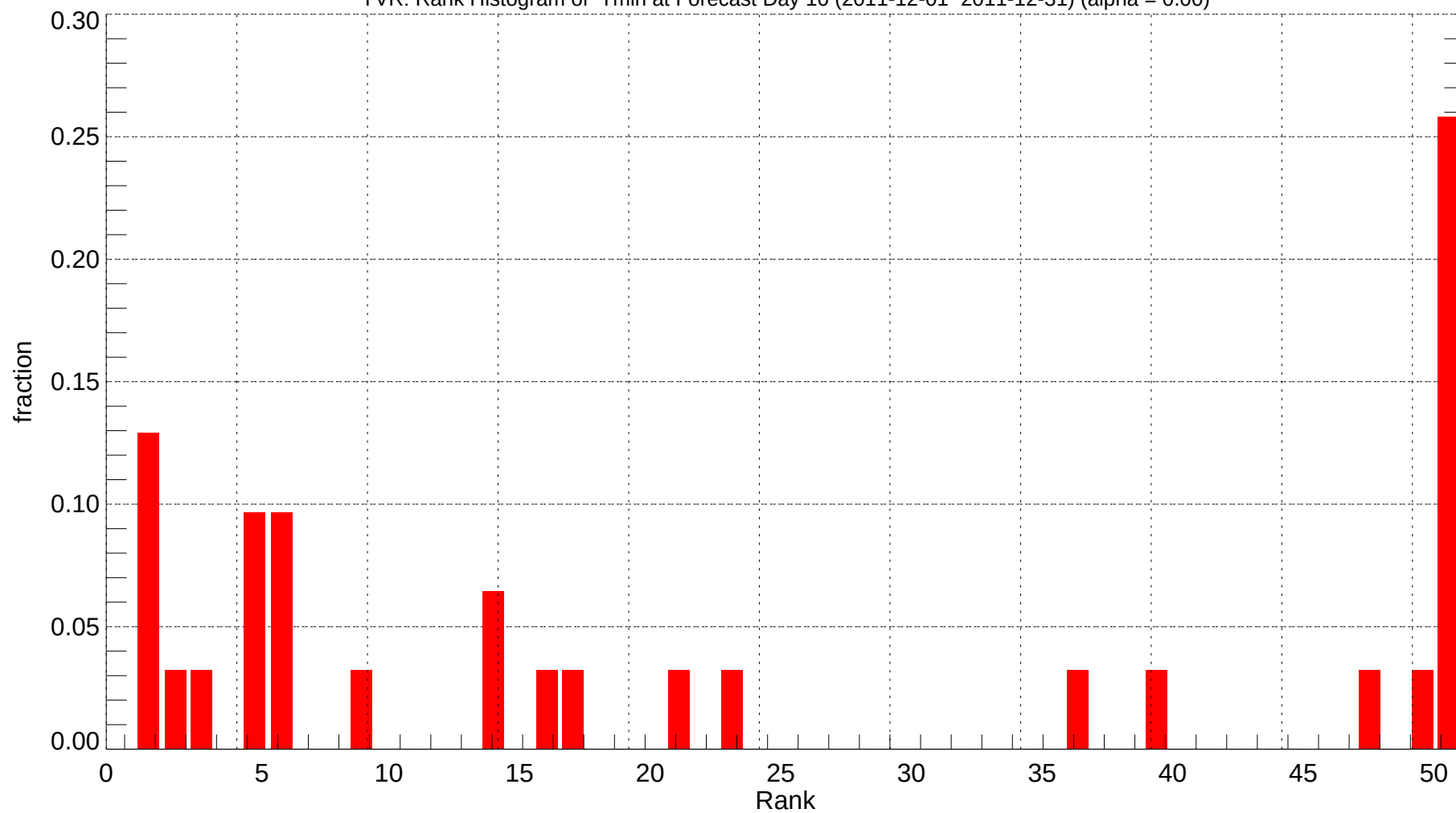
YVR: Rank Histogram of Tmin at Forecast Day 10 (2011-12-01~2011-12-31) (alpha = 0.00)
