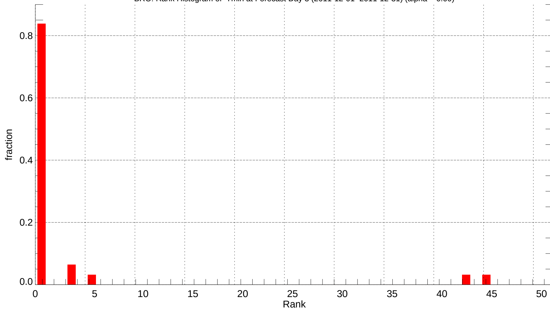
BRO: Rank Histogram of Tmin at Forecast Day 3 (2011-12-01~2011-12-31) (alpha = 0.00)
