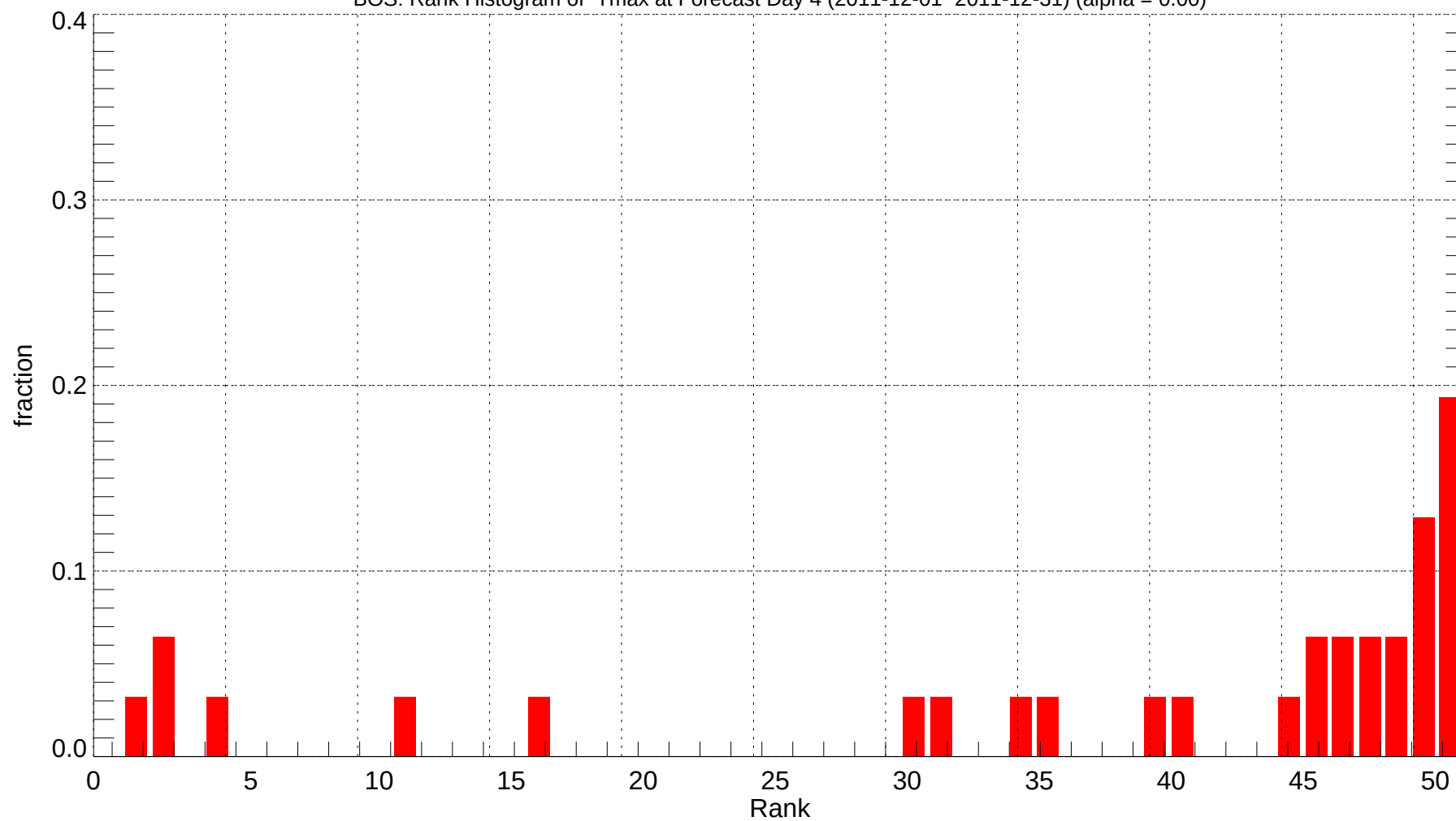
BOS: Rank Histogram of Tmax at Forecast Day 4 (2011-12-01~2011-12-31) (alpha = 0.00)
