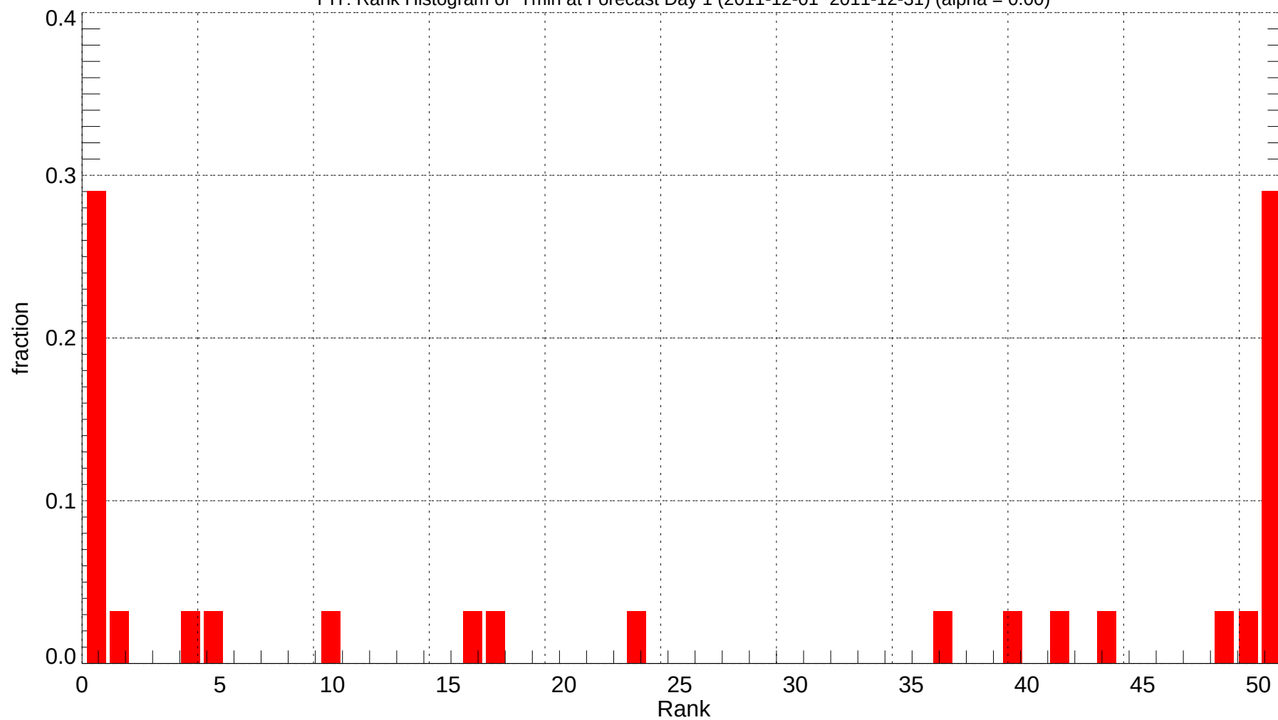
PIT: Rank Histogram of Tmin at Forecast Day 1 (2011-12-01~2011-12-31) (alpha = 0.00)
