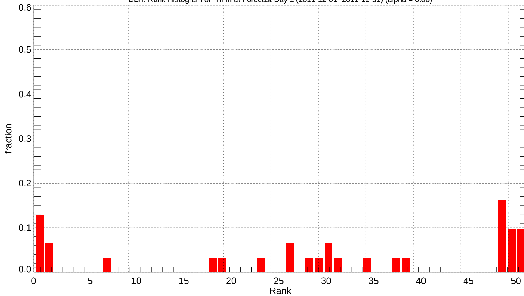
DLH: Rank Histogram of Tmin at Forecast Day 1 (2011-12-01~2011-12-31) (alpha = 0.00)
