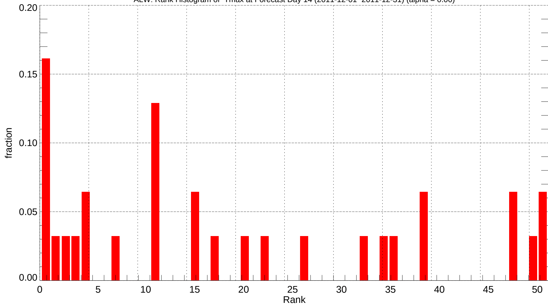
ALW: Rank Histogram of Tmax at Forecast Day 14 (2011-12-01~2011-12-31) (alpha = 0.00)
