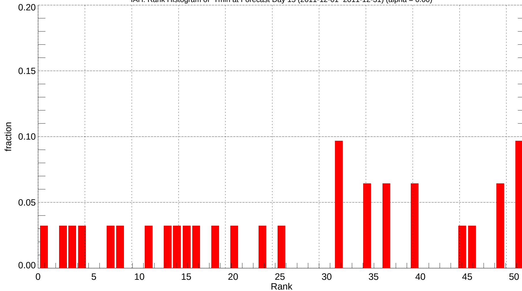
IAH: Rank Histogram of Tmin at Forecast Day 15 (2011-12-01~2011-12-31) (alpha = 0.00)
