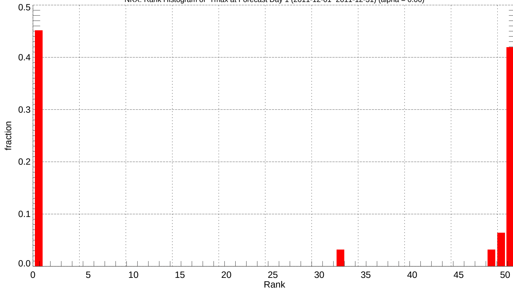
NKX: Rank Histogram of Tmax at Forecast Day 1 (2011-12-01~2011-12-31) (alpha = 0.00)
