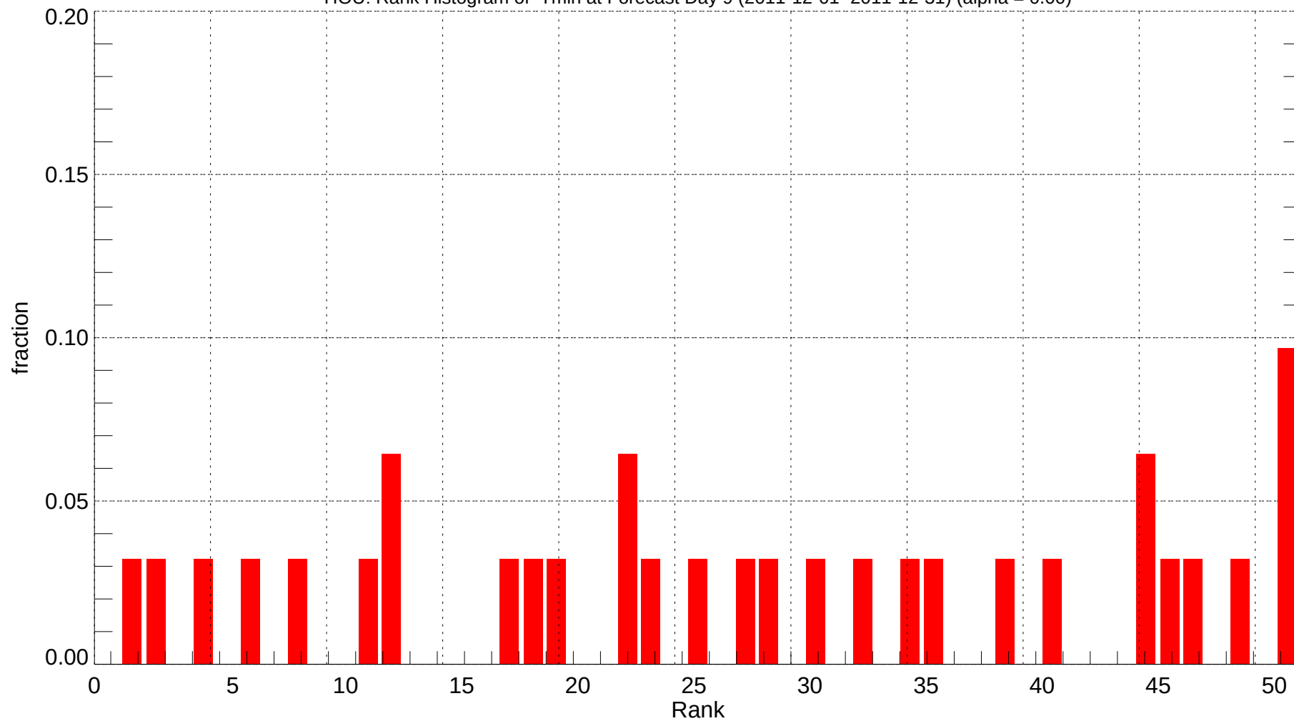
HOU: Rank Histogram of Tmin at Forecast Day 9 (2011-12-01~2011-12-31) (alpha = 0.00)
