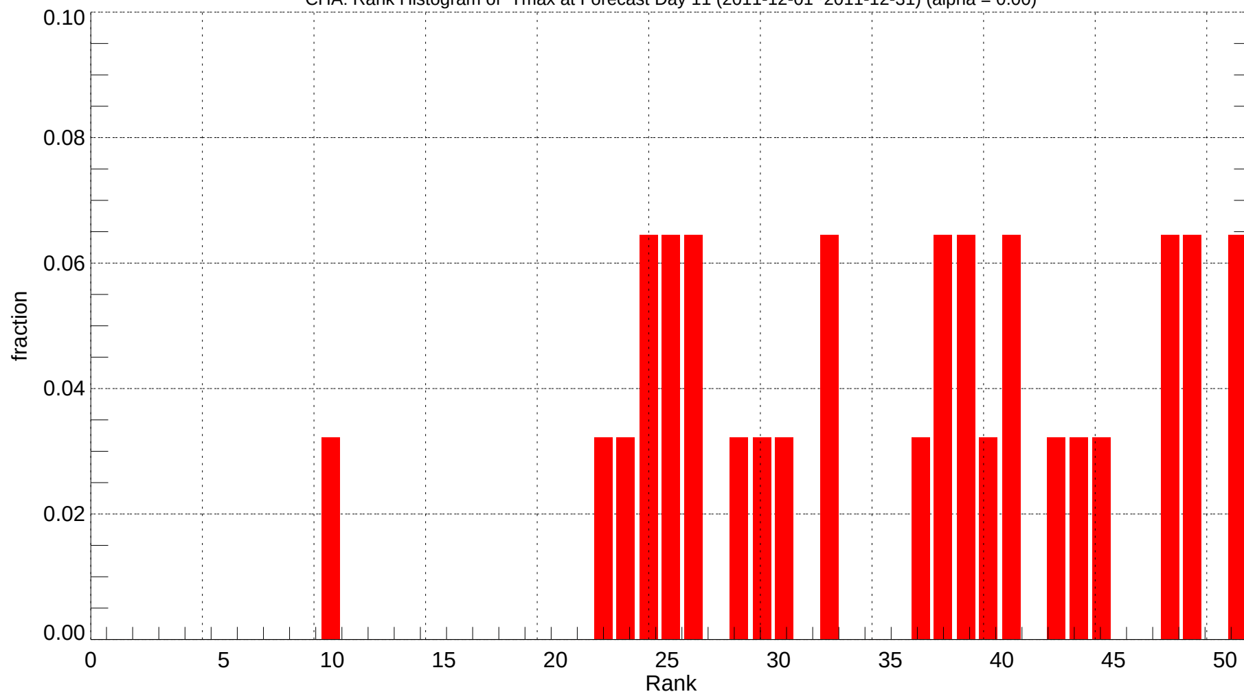
CHA: Rank Histogram of Tmax at Forecast Day 11 (2011-12-01~2011-12-31) (alpha = 0.00)
