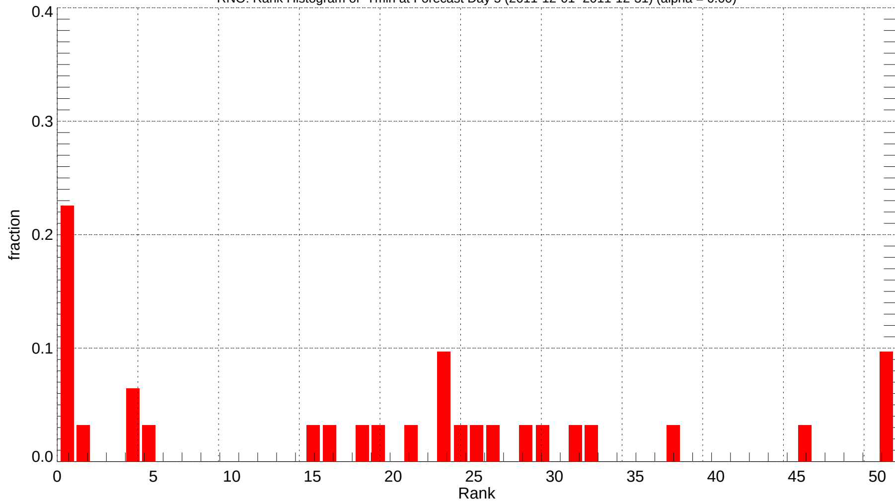
RNO: Rank Histogram of Tmin at Forecast Day 5 (2011-12-01~2011-12-31) (alpha = 0.00)
