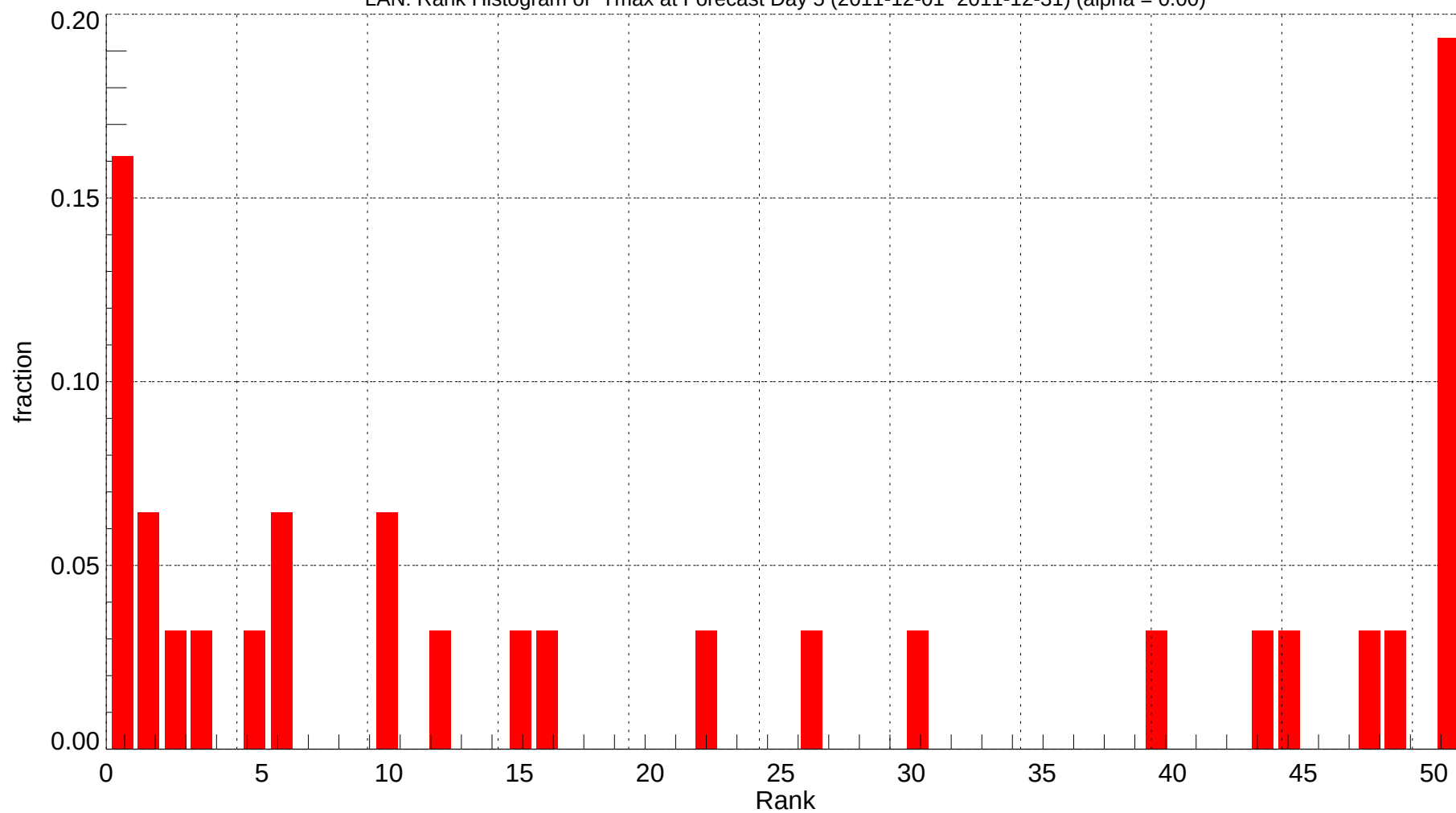
LAN: Rank Histogram of Tmax at Forecast Day 5 (2011-12-01~2011-12-31) (alpha = 0.00)
