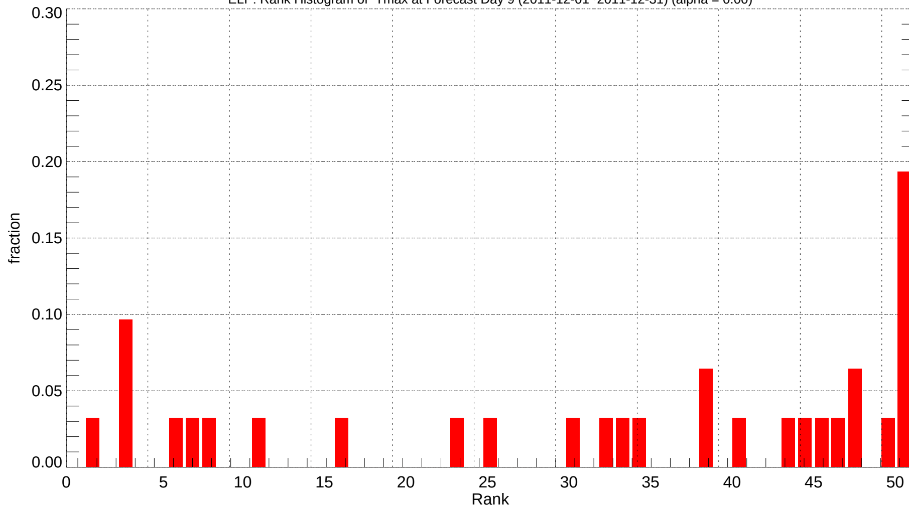
ELP: Rank Histogram of Tmax at Forecast Day 9 (2011-12-01~2011-12-31) (alpha = 0.00)
