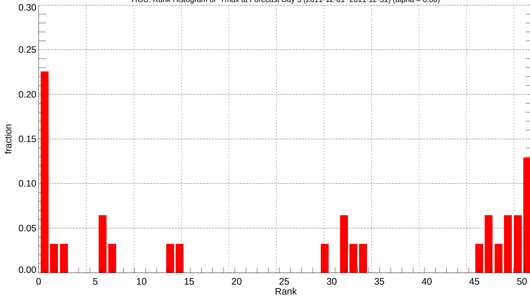
HOU: Rank Histogram of Tmax at Forecast Day 3 (2011-12-01~2011-12-31) (alpha = 0.00)
