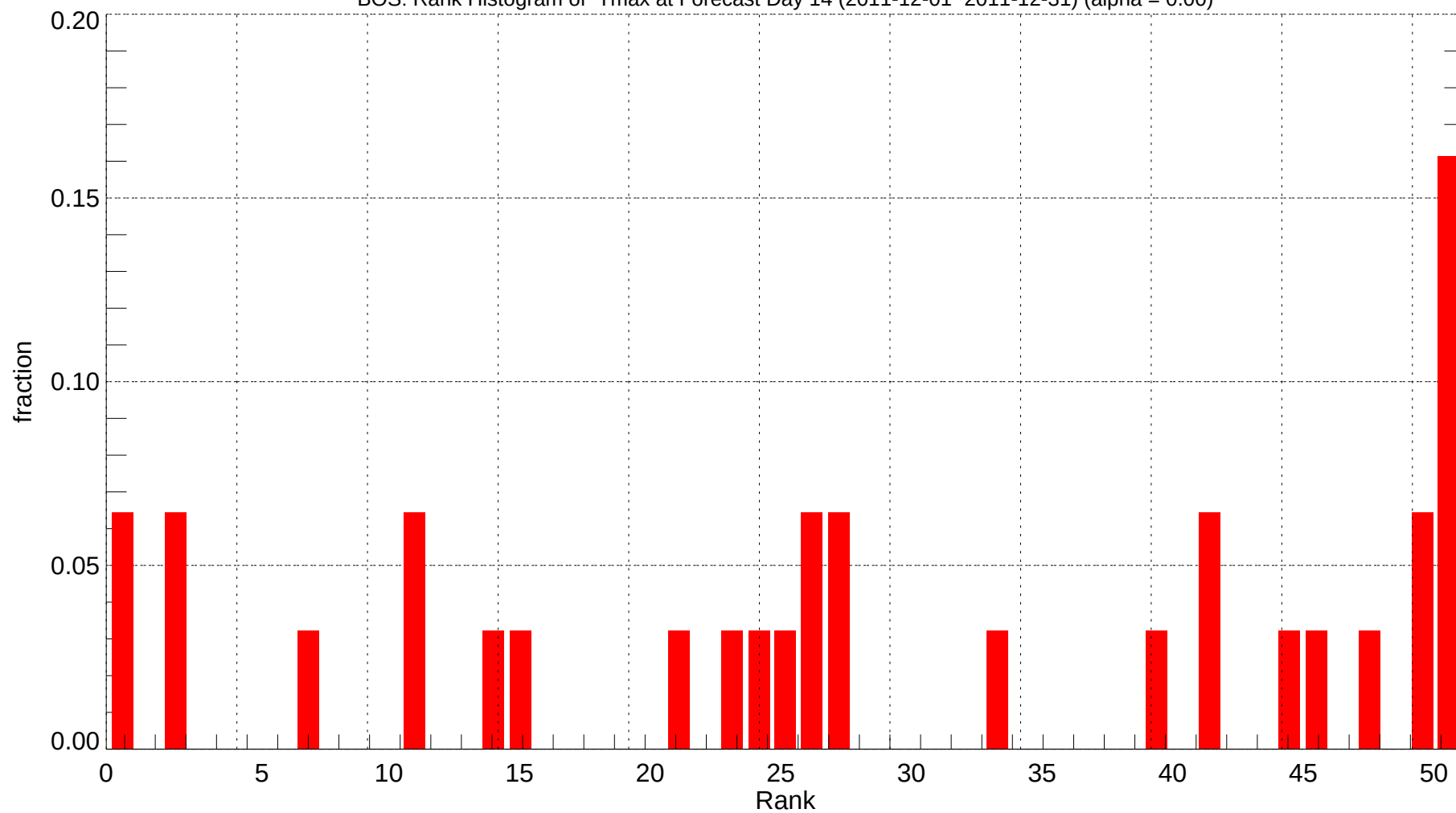
BOS: Rank Histogram of Tmax at Forecast Day 14 (2011-12-01~2011-12-31) (alpha = 0.00)
