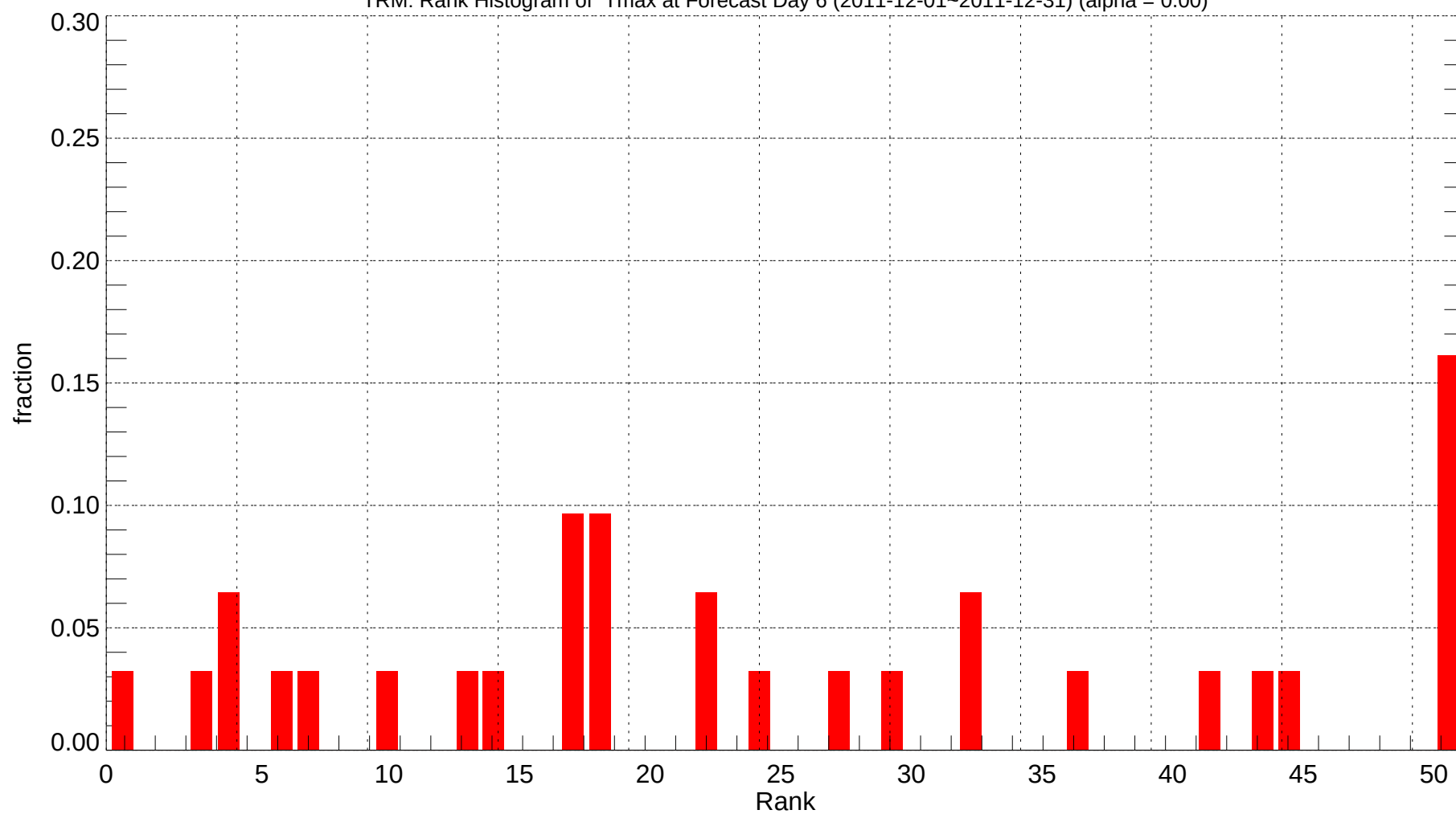
TRM: Rank Histogram of Tmax at Forecast Day 6 (2011-12-01~2011-12-31) (alpha = 0.00)
