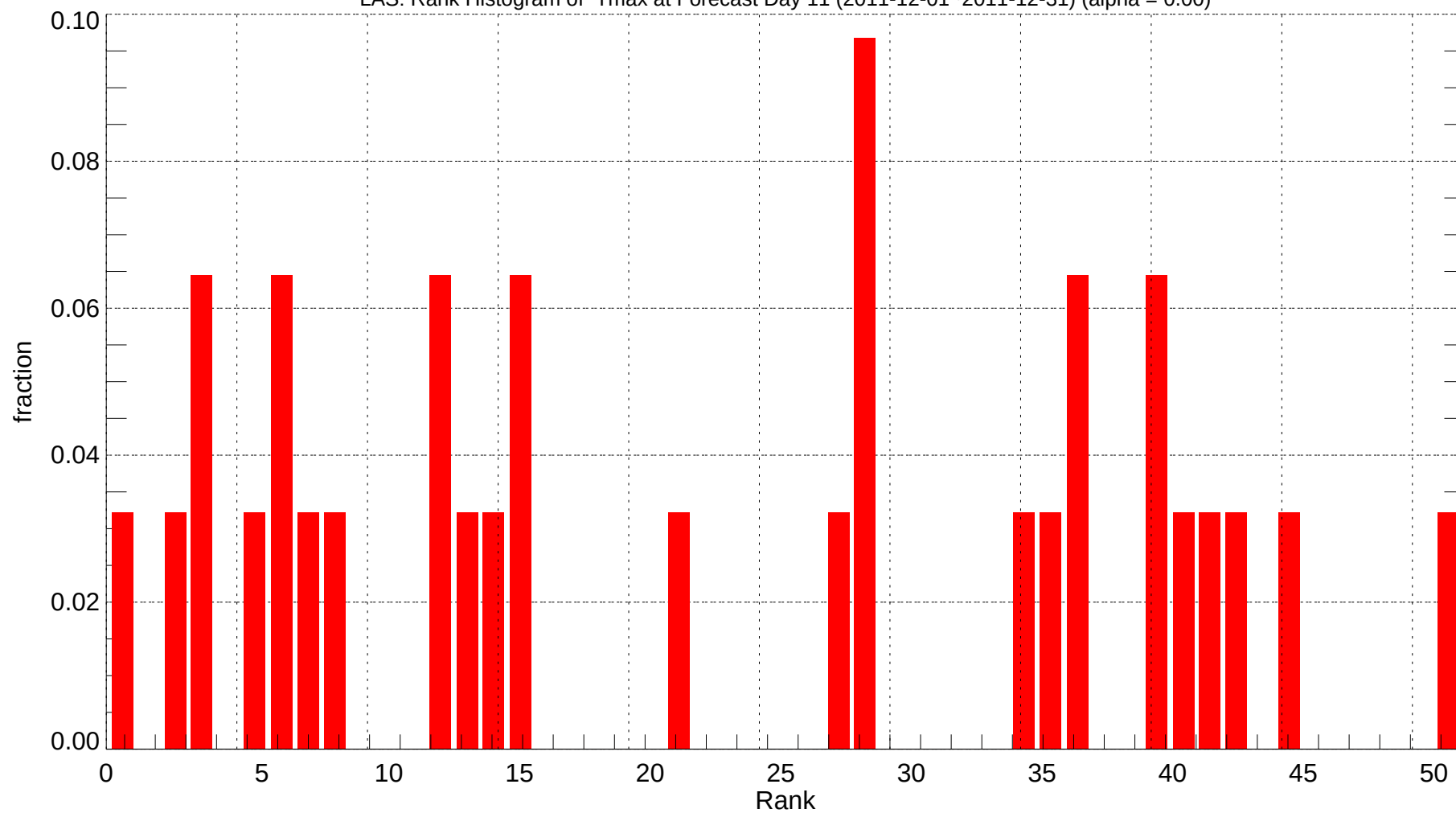
LAS: Rank Histogram of Tmax at Forecast Day 11 (2011-12-01~2011-12-31) (alpha = 0.00)
