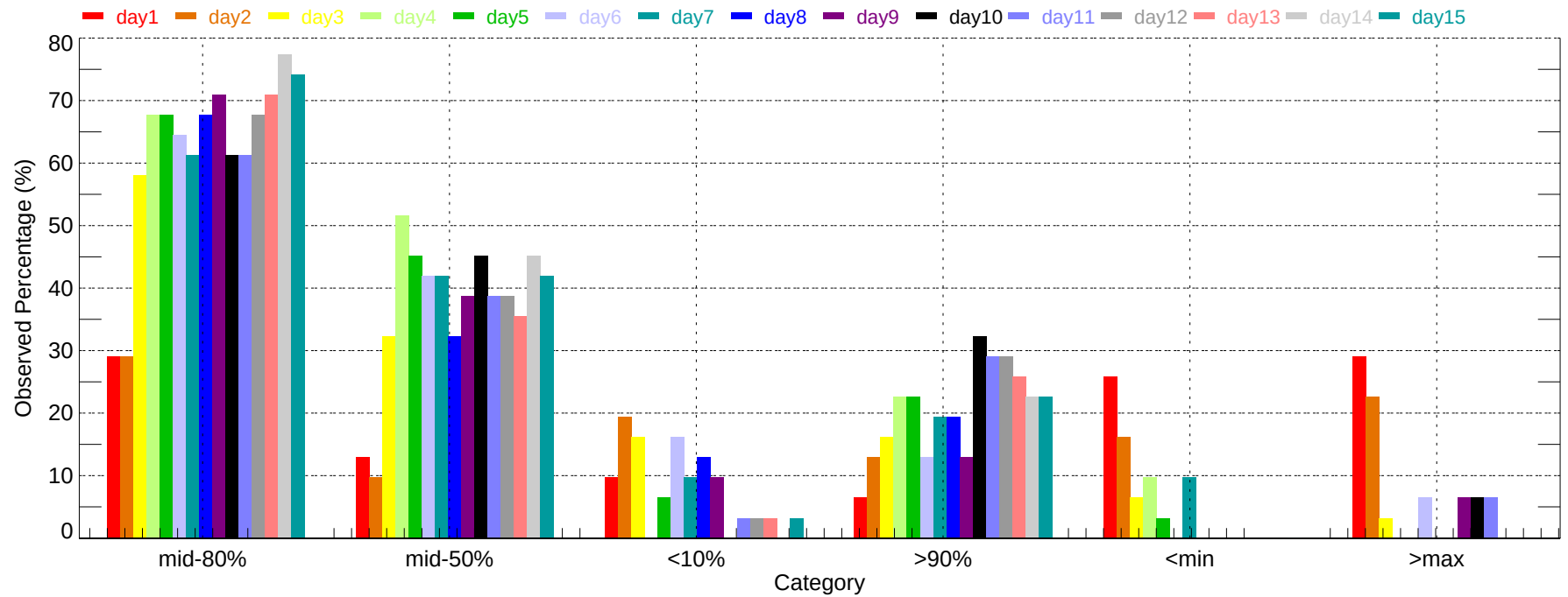
Observed Percentage of Ensembles - ROA: Max Temperature (2011-12-01~2011-12-31)
