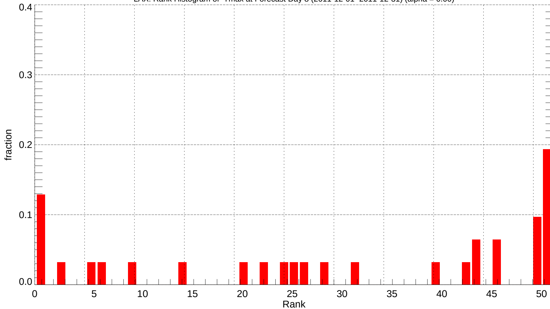
LAX: Rank Histogram of Tmax at Forecast Day 8 (2011-12-01~2011-12-31) (alpha = 0.00)
