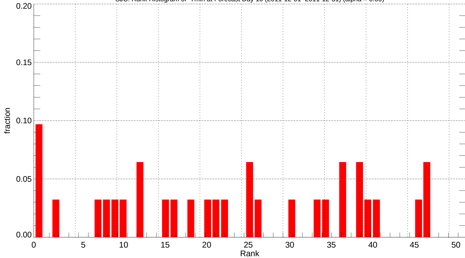
SJC: Rank Histogram of Tmin at Forecast Day 10 (2011-12-01~2011-12-31) (alpha = 0.00)
