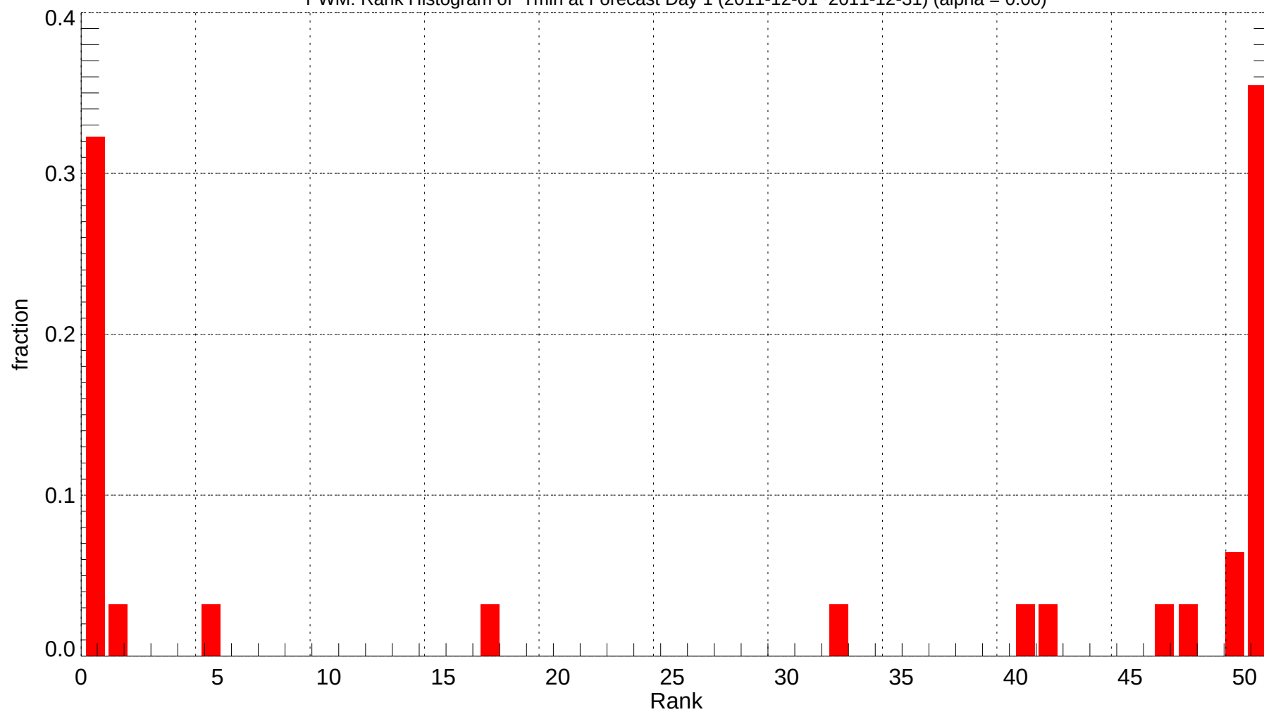
PWM: Rank Histogram of Tmin at Forecast Day 1 (2011-12-01~2011-12-31) (alpha = 0.00)
