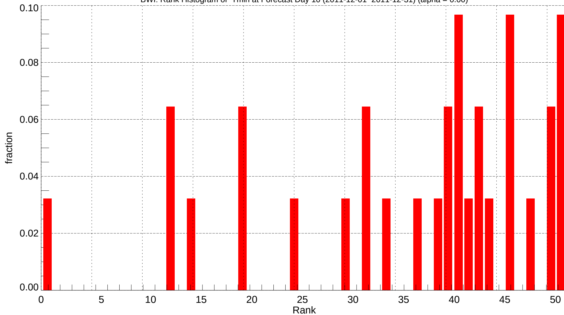
BWl: Rank Histogram of Tmin at Forecast Day 10 (2011-12-01~2011-12-31) (alpha = 0.00)
