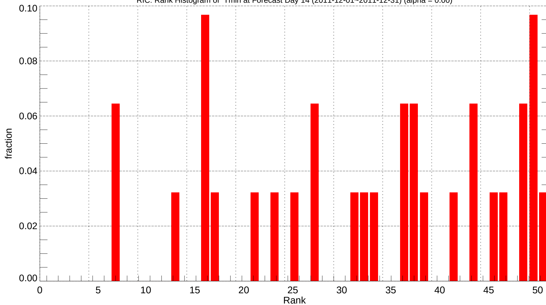
RIC: Rank Histogram of Tmin at Forecast Day 14 (2011-12-01~2011-12-31) (alpha = 0.00)
