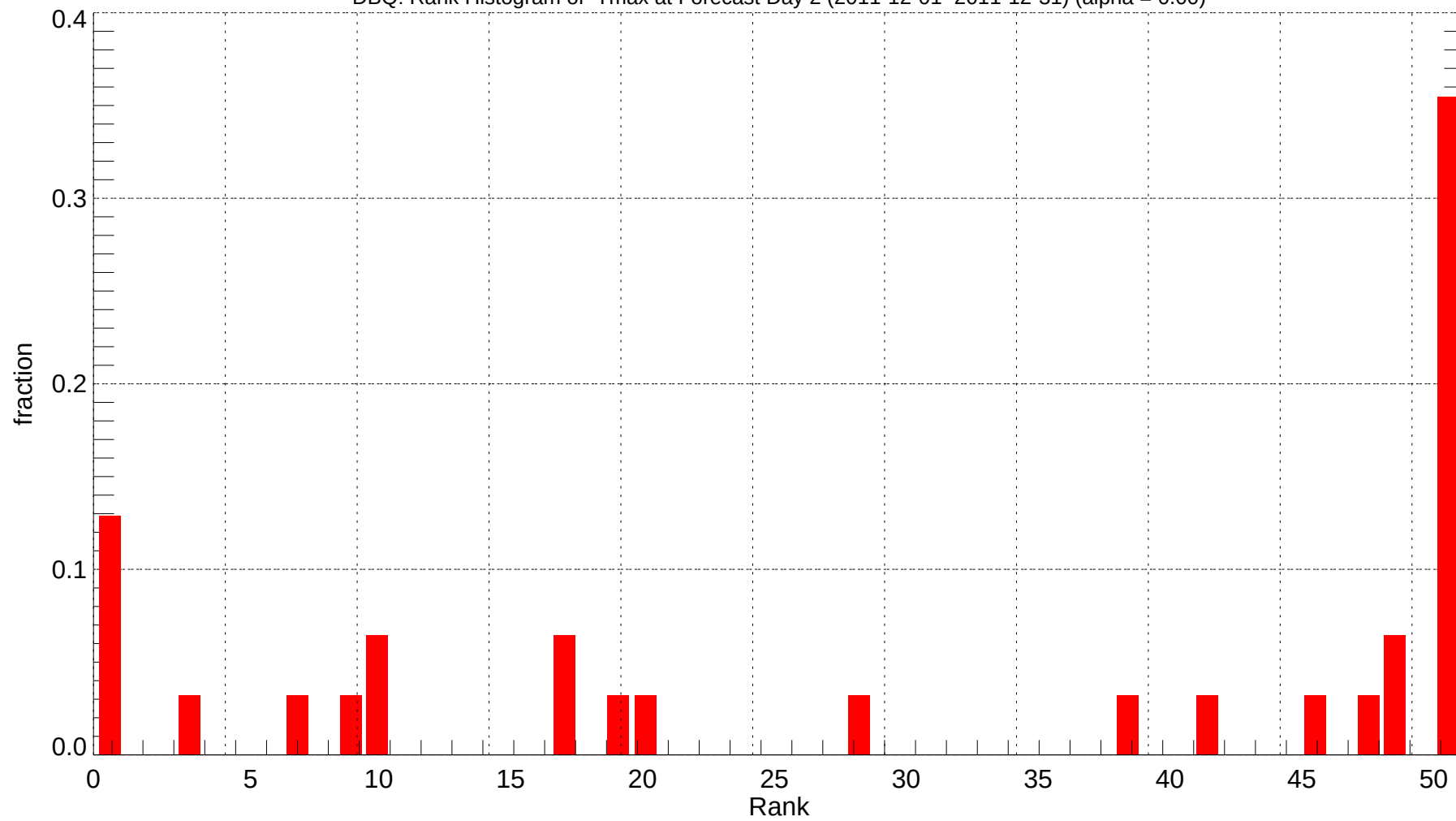
DBQ: Rank Histogram of Tmax at Forecast Day 2 (2011-12-01~2011-12-31) (alpha = 0.00)
