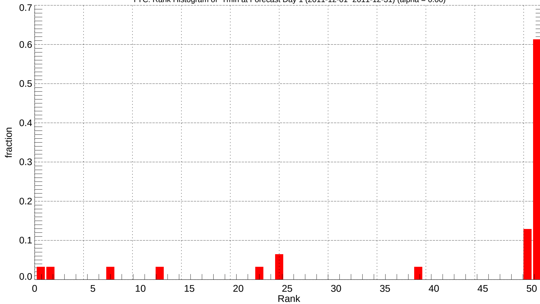
YYC: Rank Histogram of Tmin at Forecast Day 1 (2011-12-01~2011-12-31) (alpha = 0.00)
