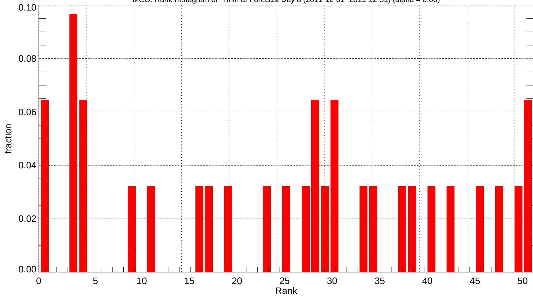
MCO: Rank Histogram of Tmin at Forecast Day 8 (2011-12-01~2011-12-31) (alpha = 0.00)
