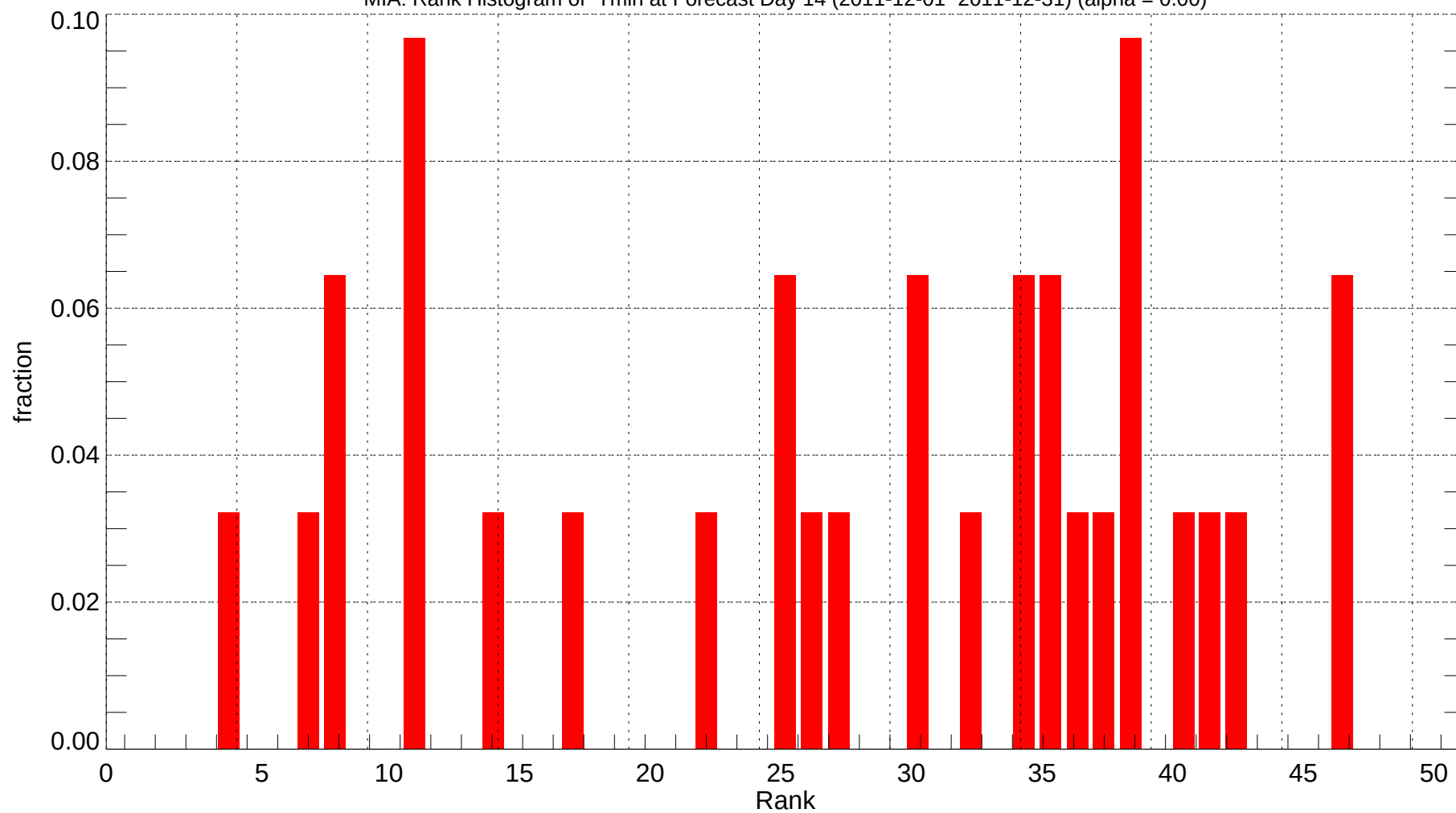
MIA: Rank Histogram of Tmin at Forecast Day 14 (2011-12-01~2011-12-31) (alpha = 0.00)
