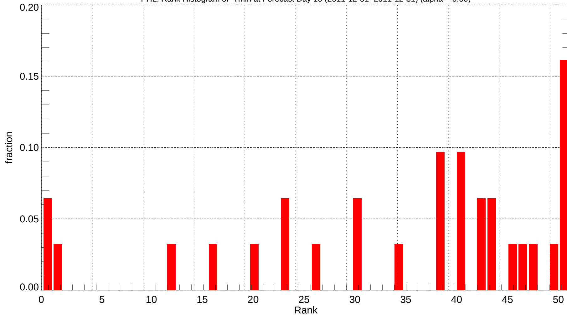
PHL: Rank Histogram of Tmin at Forecast Day 10 (2011-12-01~2011-12-31) (alpha = 0.00)
