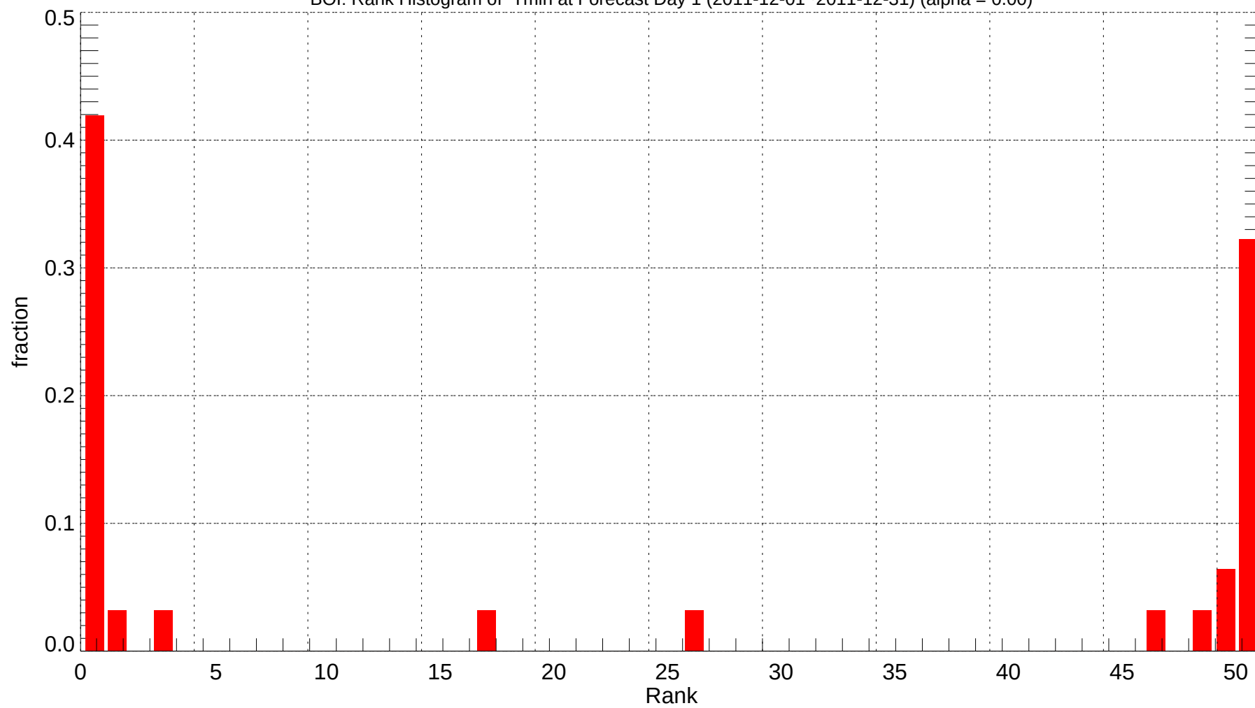
BOI: Rank Histogram of Tmin at Forecast Day 1 (2011-12-01~2011-12-31) (alpha = 0.00)
