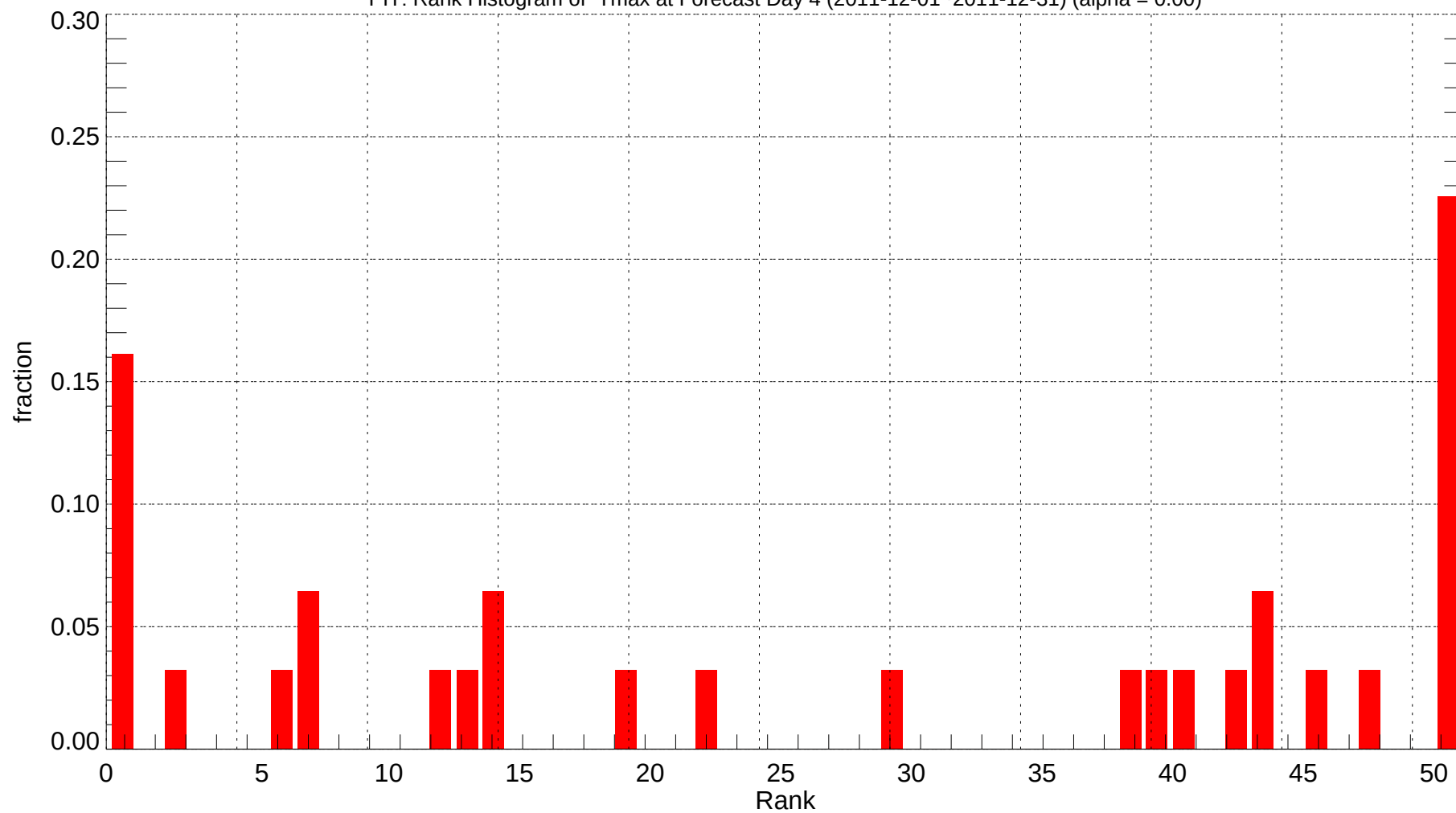
PIT: Rank Histogram of Tmax at Forecast Day 4 (2011-12-01~2011-12-31) (alpha = 0.00)
