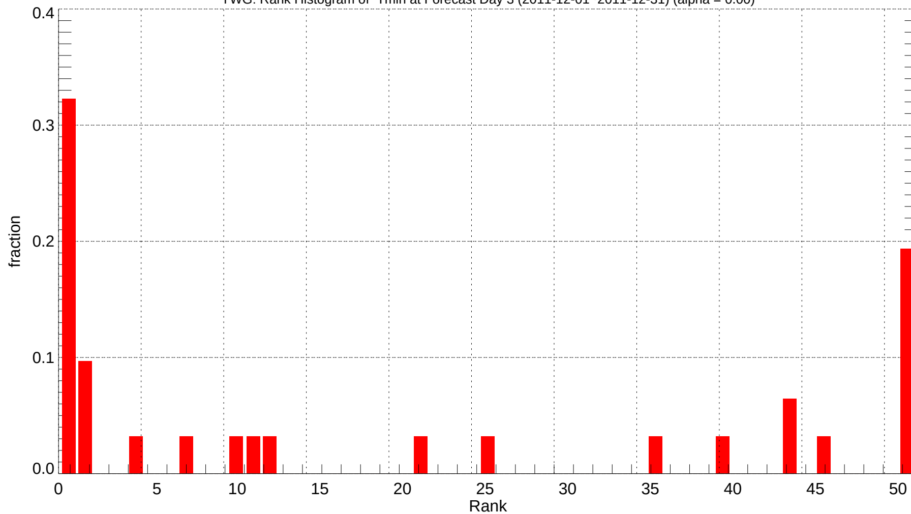
YWG: Rank Histogram of Tmin at Forecast Day 3 (2011-12-01~2011-12-31) (alpha = 0.00)
