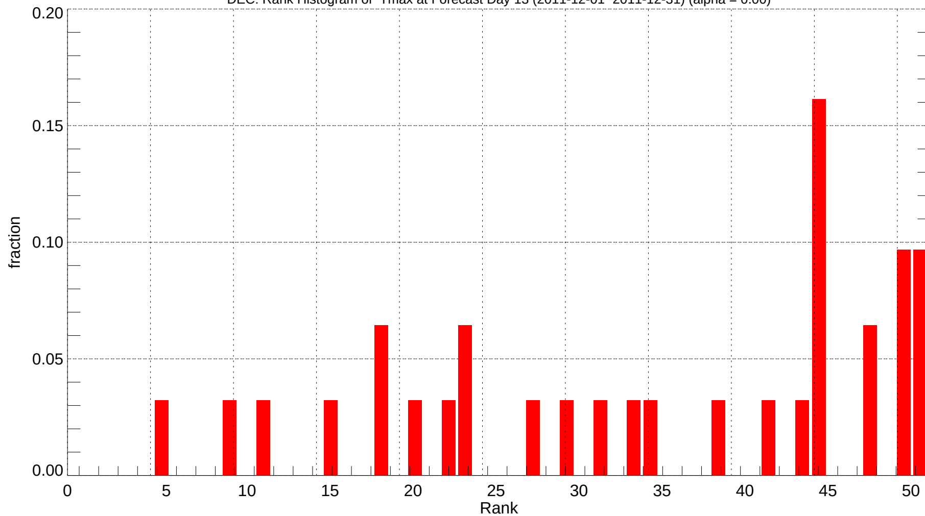
DEC: Rank Histogram of Tmax at Forecast Day 13 (2011-12-01~2011-12-31) (alpha = 0.00)
