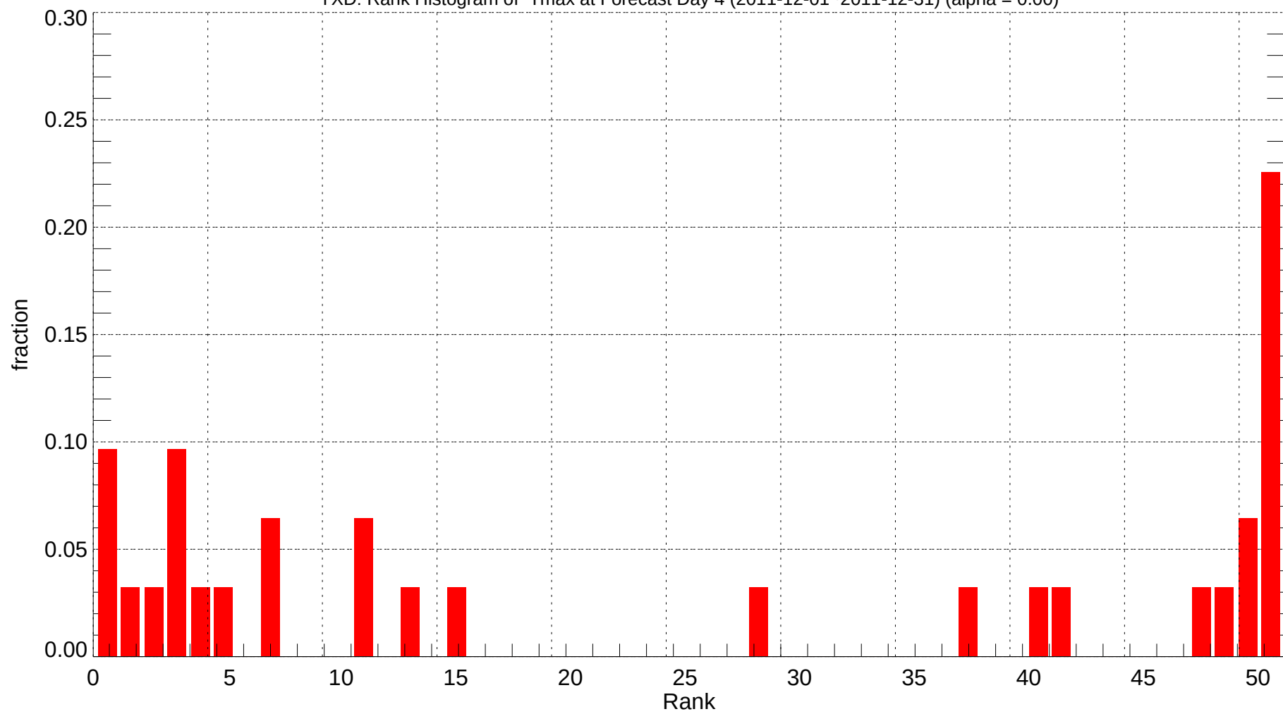
YXD: Rank Histogram of Tmax at Forecast Day 4 (2011-12-01~2011-12-31) (alpha = 0.00)
