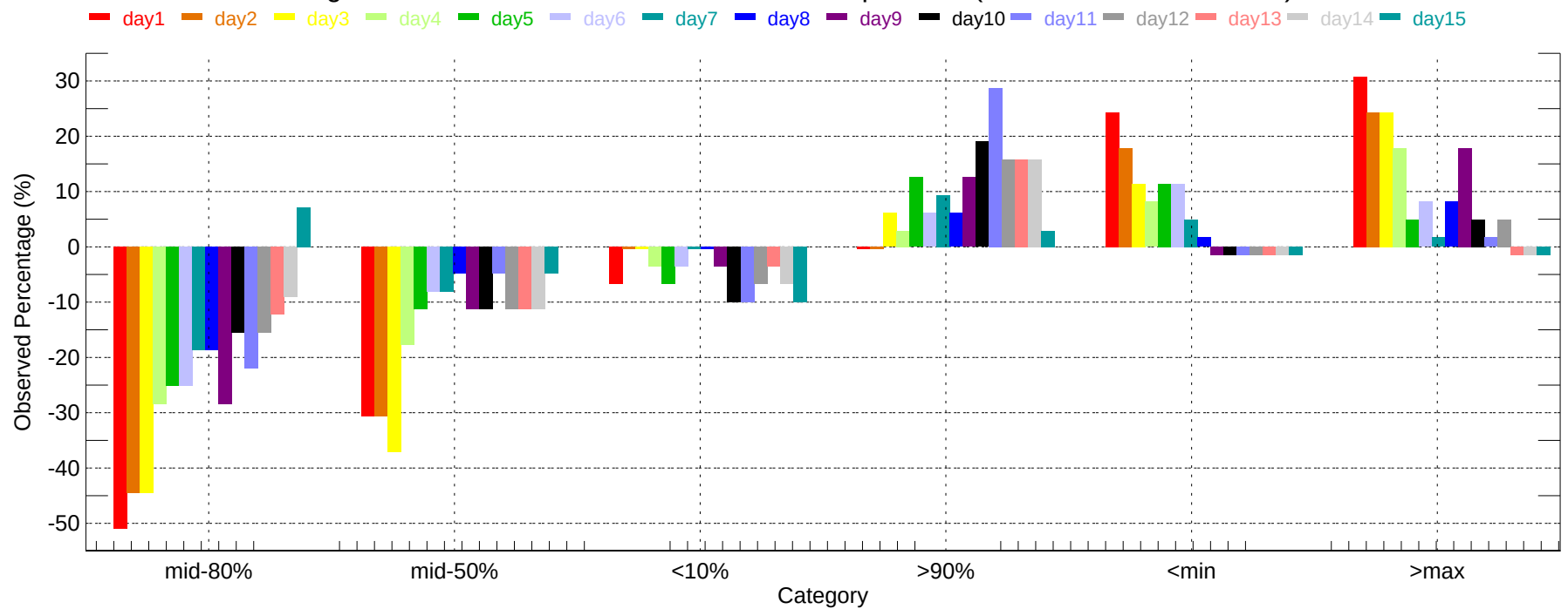
Observed Percentage Deviation of Ensembles - CLE: Min Temperature (2011-12-01~2011-12-31)
