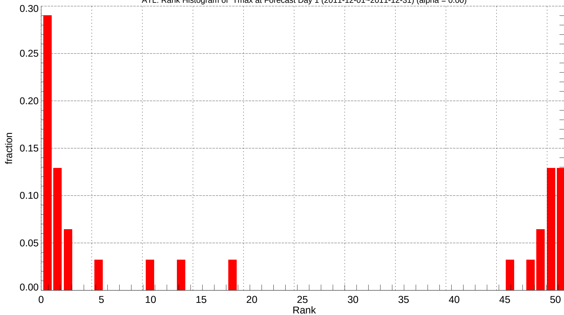
ATL: Rank Histogram of Tmax at Forecast Day 1 (2011-12-01~2011-12-31) (alpha = 0.00)
