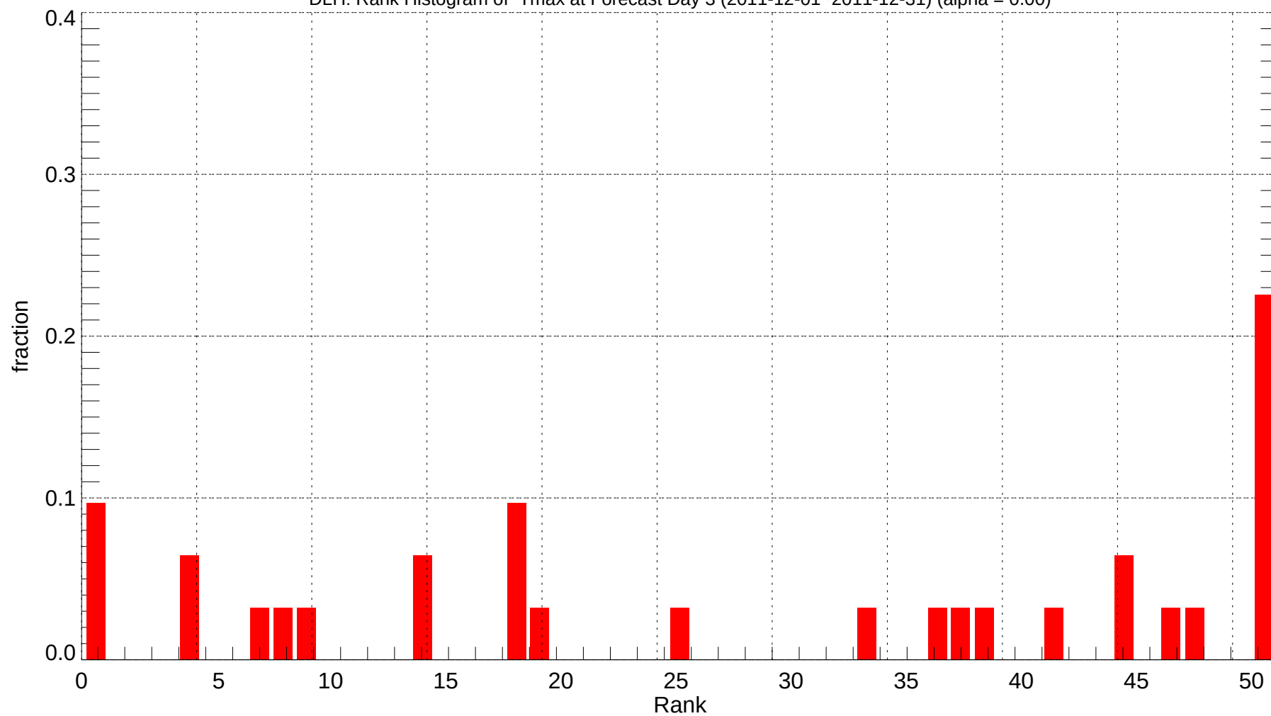
DLH: Rank Histogram of Tmax at Forecast Day 3 (2011-12-01~2011-12-31) (alpha = 0.00)
