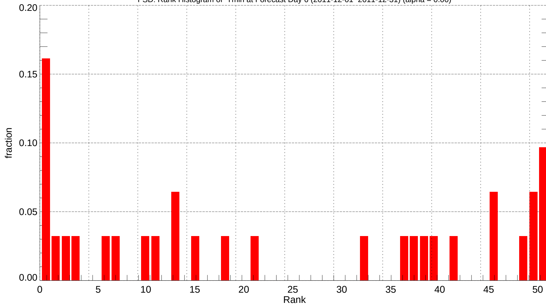
FSD: Rank Histogram of Tmin at Forecast Day 6 (2011-12-01~2011-12-31) (alpha = 0.00)
