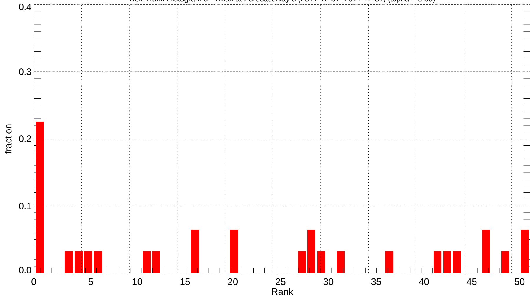
BOI: Rank Histogram of Tmax at Forecast Day 5 (2011-12-01~2011-12-31) (alpha = 0.00)
