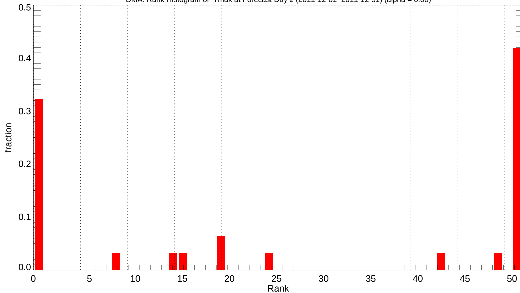
OMA: Rank Histogram of Tmax at Forecast Day 2 (2011-12-01~2011-12-31) (alpha = 0.00)
