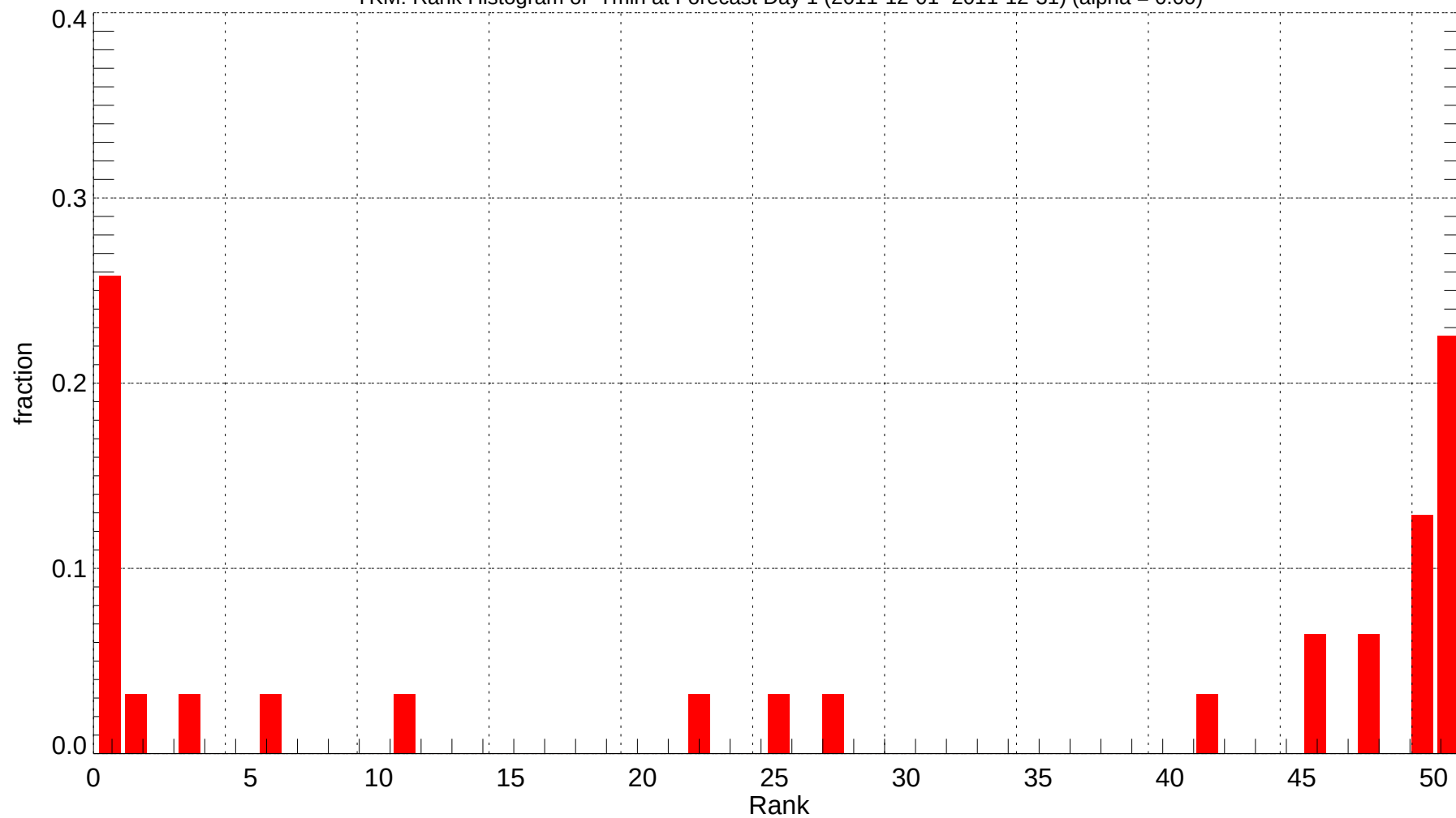
YKM: Rank Histogram of Tmin at Forecast Day 1 (2011-12-01~2011-12-31) (alpha = 0.00)
