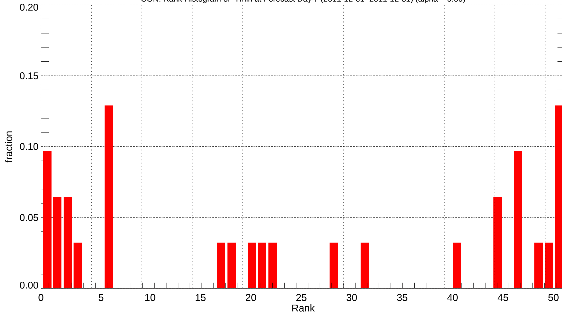
CON: Rank Histogram of Tmin at Forecast Day 7 (2011-12-01~2011-12-31) (alpha = 0.00)
