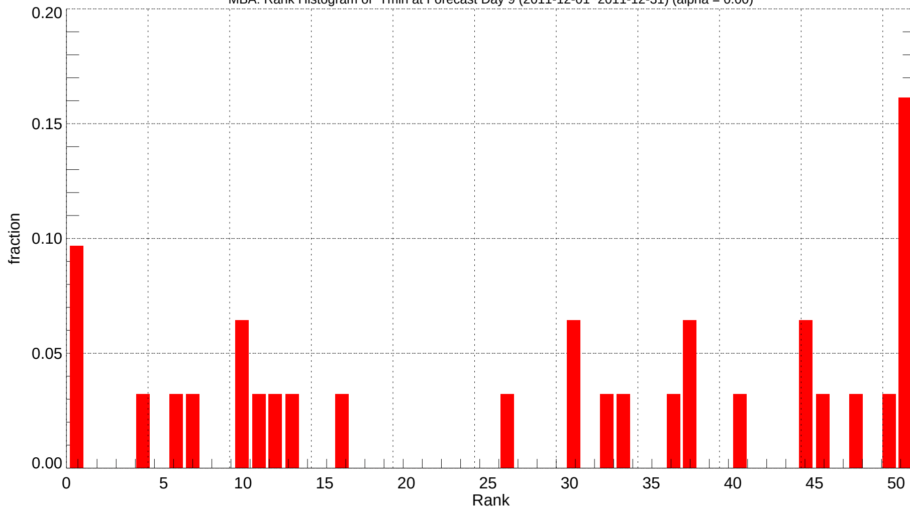
MBA: Rank Histogram of Tmin at Forecast Day 9 (2011-12-01~2011-12-31) (alpha = 0.00)
