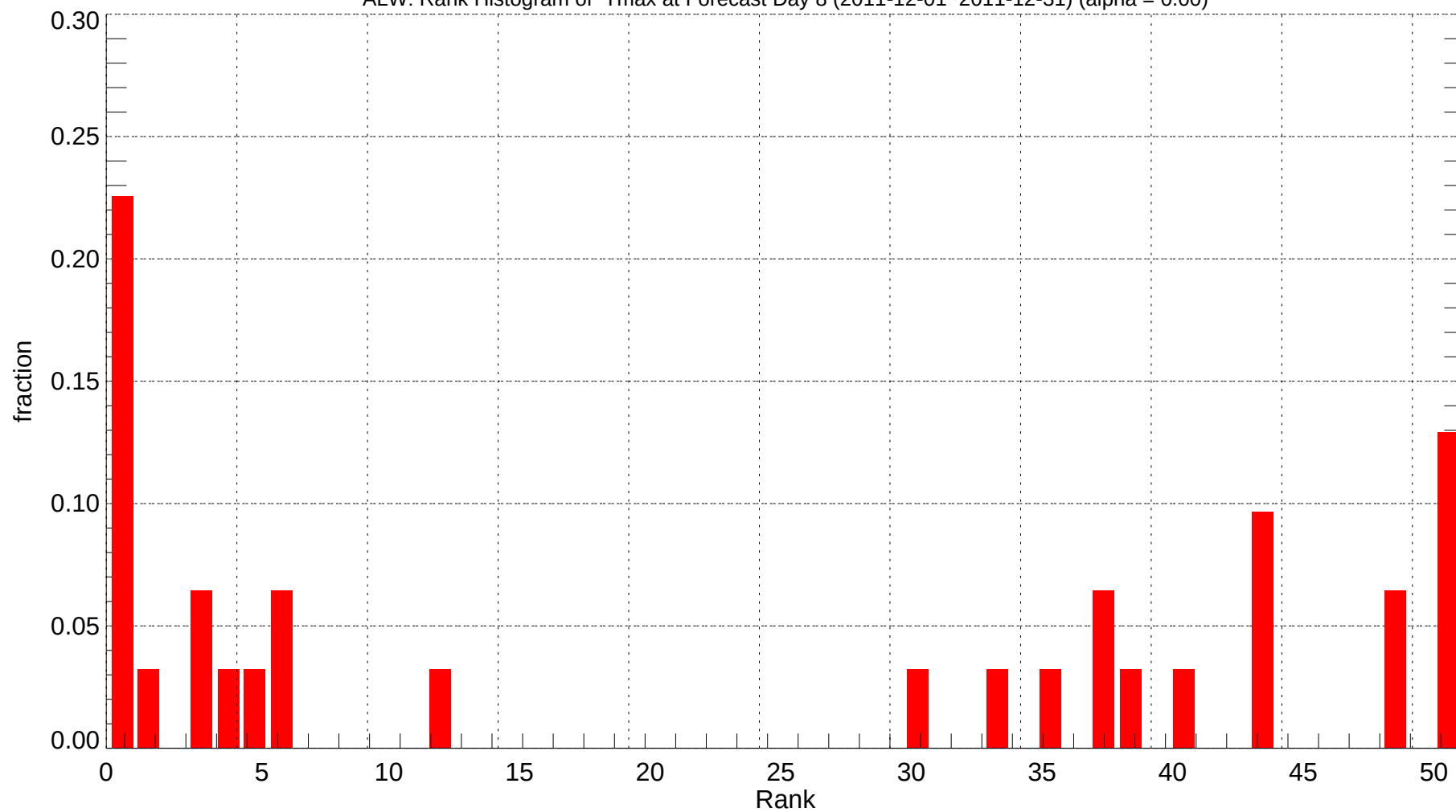
ALW: Rank Histogram of Tmax at Forecast Day 8 (2011-12-01~2011-12-31) (alpha = 0.00)
