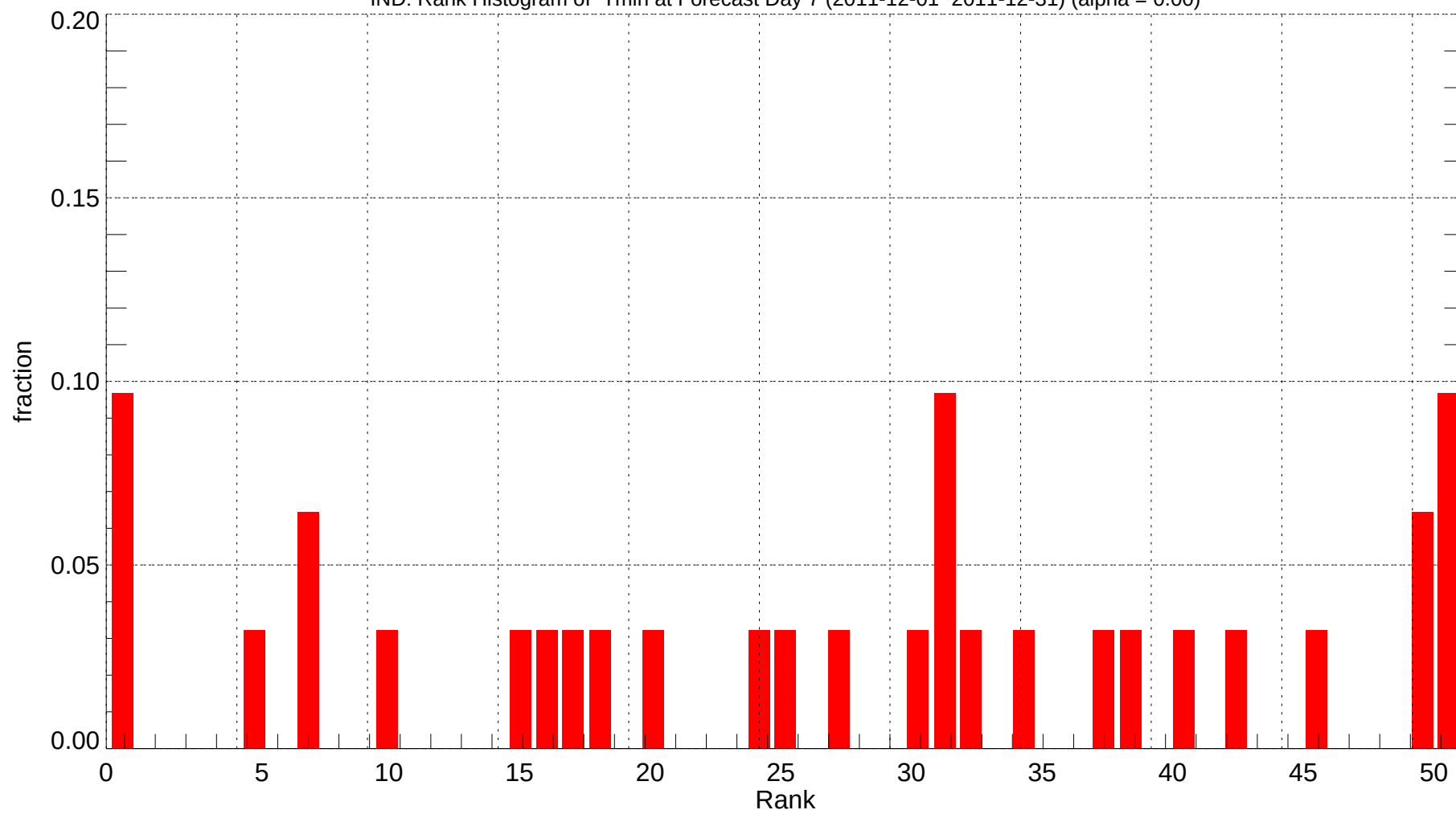
IND: Rank Histogram of Tmin at Forecast Day 7 (2011-12-01~2011-12-31) (alpha = 0.00)
