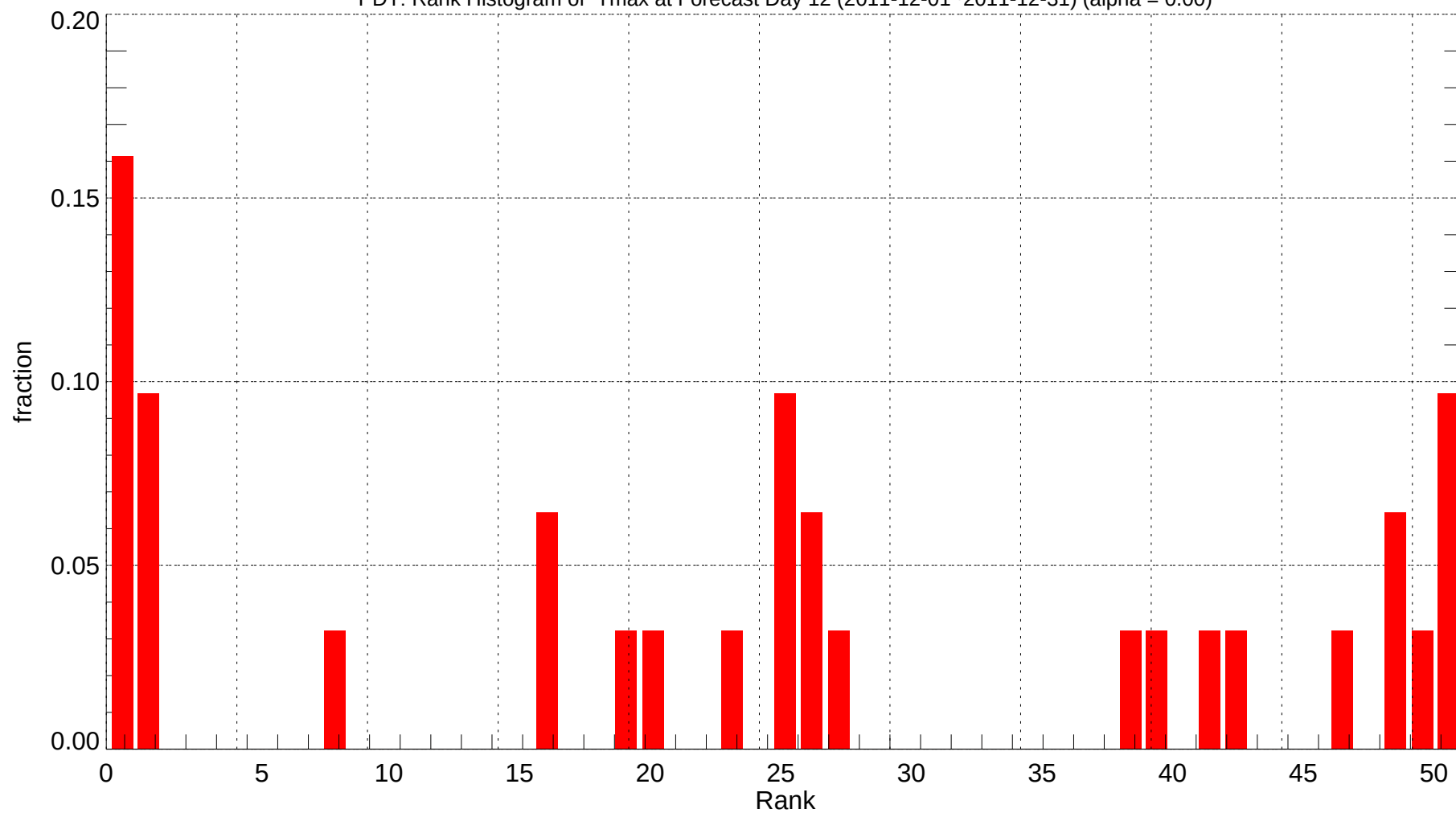
PDT: Rank Histogram of Tmax at Forecast Day 12 (2011-12-01~2011-12-31) (alpha = 0.00)
