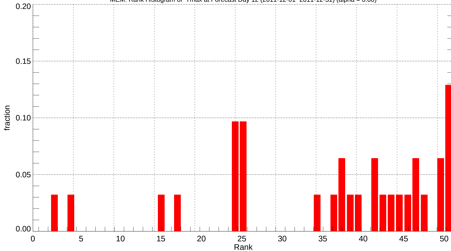
MEM: Rank Histogram of Tmax at Forecast Day 12 (2011-12-01~2011-12-31) (alpha = 0.00)
