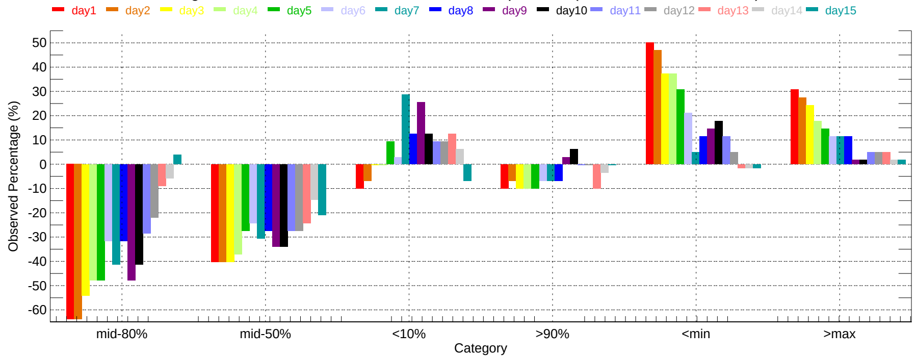
Observed Percentage Deviation of Ensembles - RNO: Min Temperature (2011-12-01~2011-12-31)
