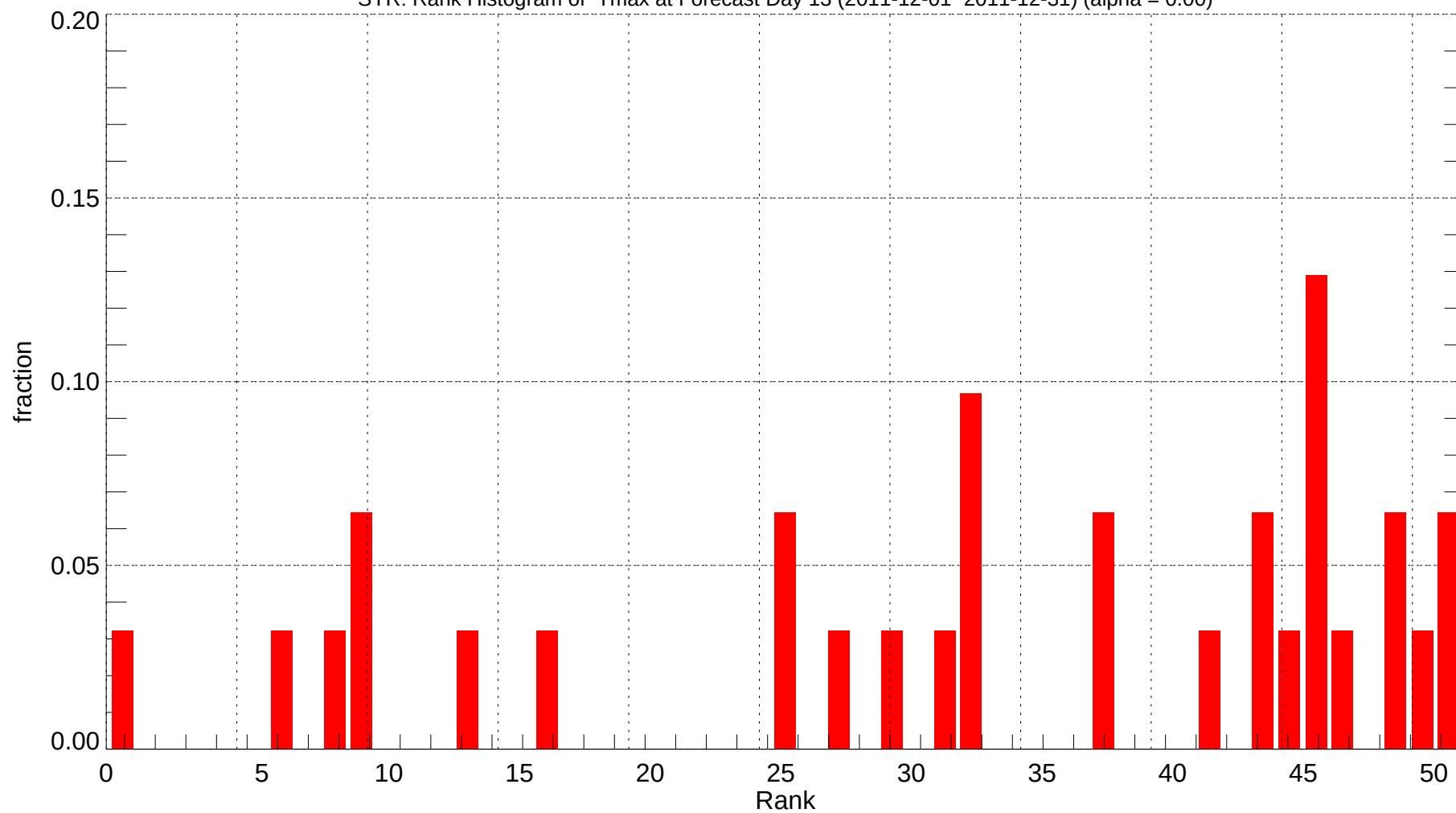
SYR: Rank Histogram of Tmax at Forecast Day 13 (2011-12-01~2011-12-31) (alpha = 0.00)
