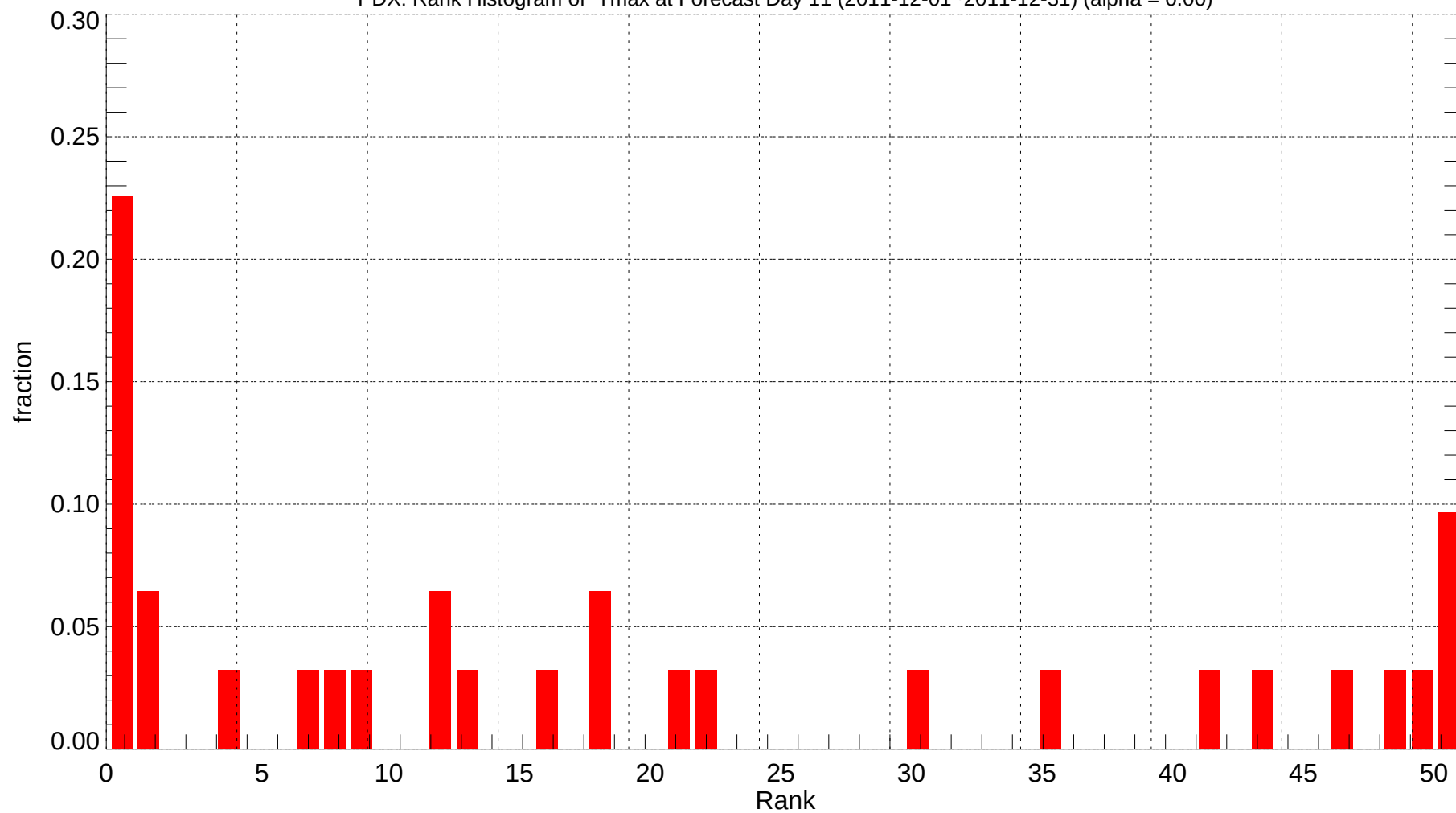
PDX: Rank Histogram of Tmax at Forecast Day 11 (2011-12-01~2011-12-31) (alpha = 0.00)
