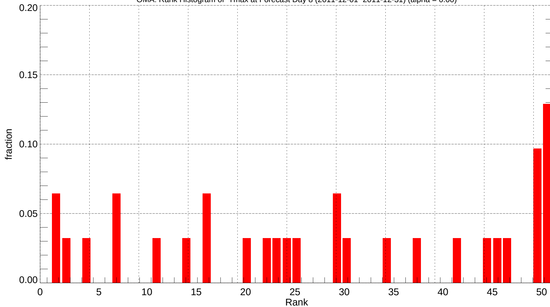
OMA: Rank Histogram of Tmax at Forecast Day 8 (2011-12-01~2011-12-31) (alpha = 0.00)
