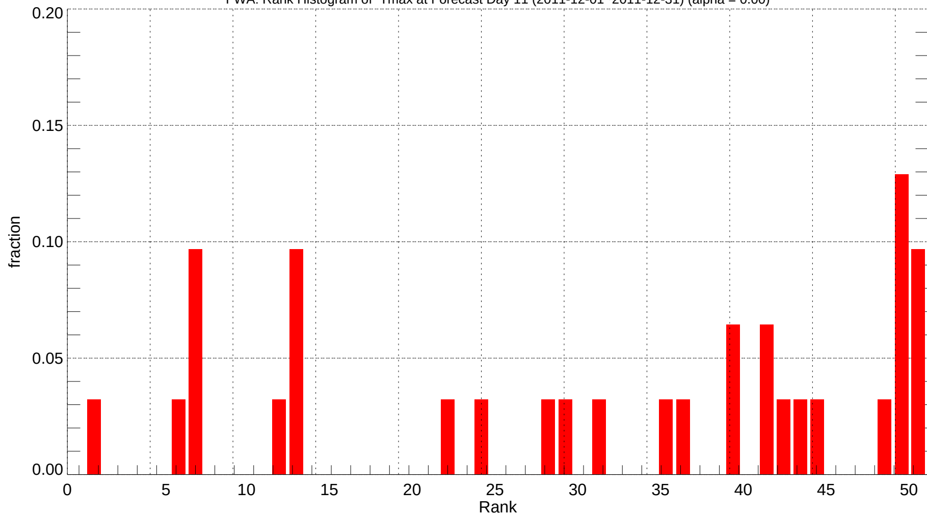
FWA: Rank Histogram of Tmax at Forecast Day 11 (2011-12-01~2011-12-31) (alpha = 0.00)
