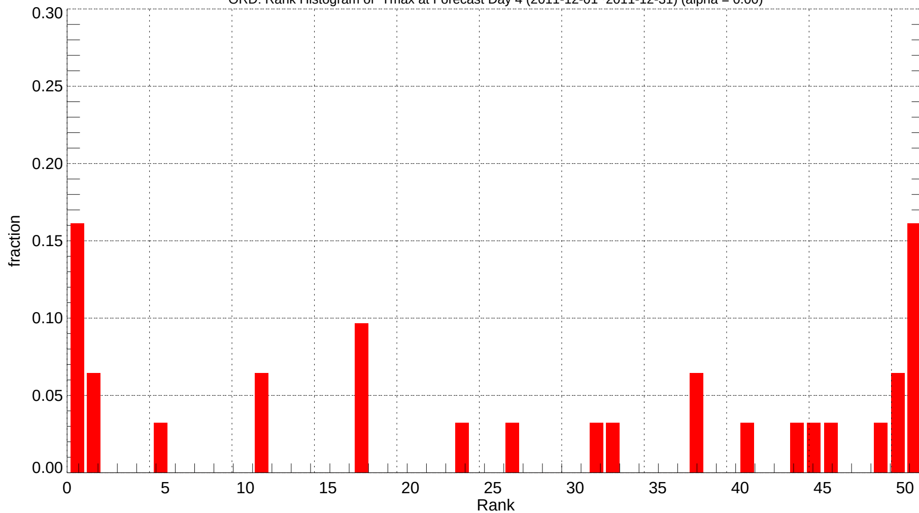
ORD: Rank Histogram of Tmax at Forecast Day 4 (2011-12-01~2011-12-31) (alpha = 0.00)
