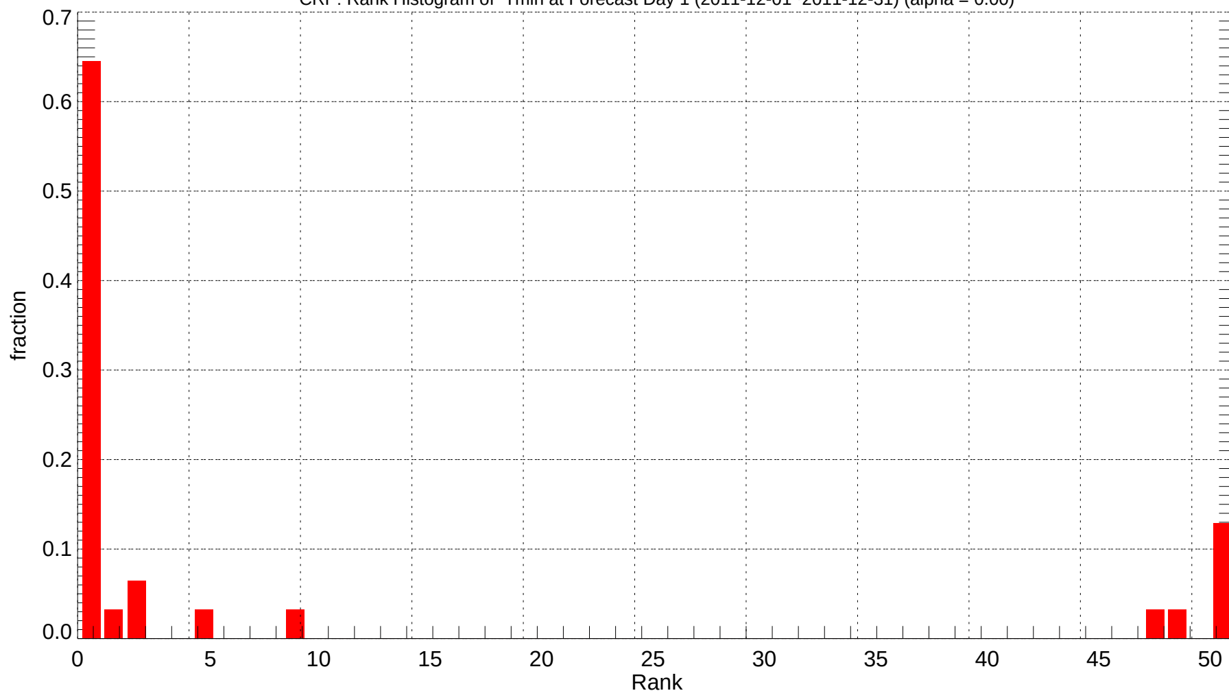
CRP: Rank Histogram of Tmin at Forecast Day 1 (2011-12-01~2011-12-31) (alpha = 0.00)
