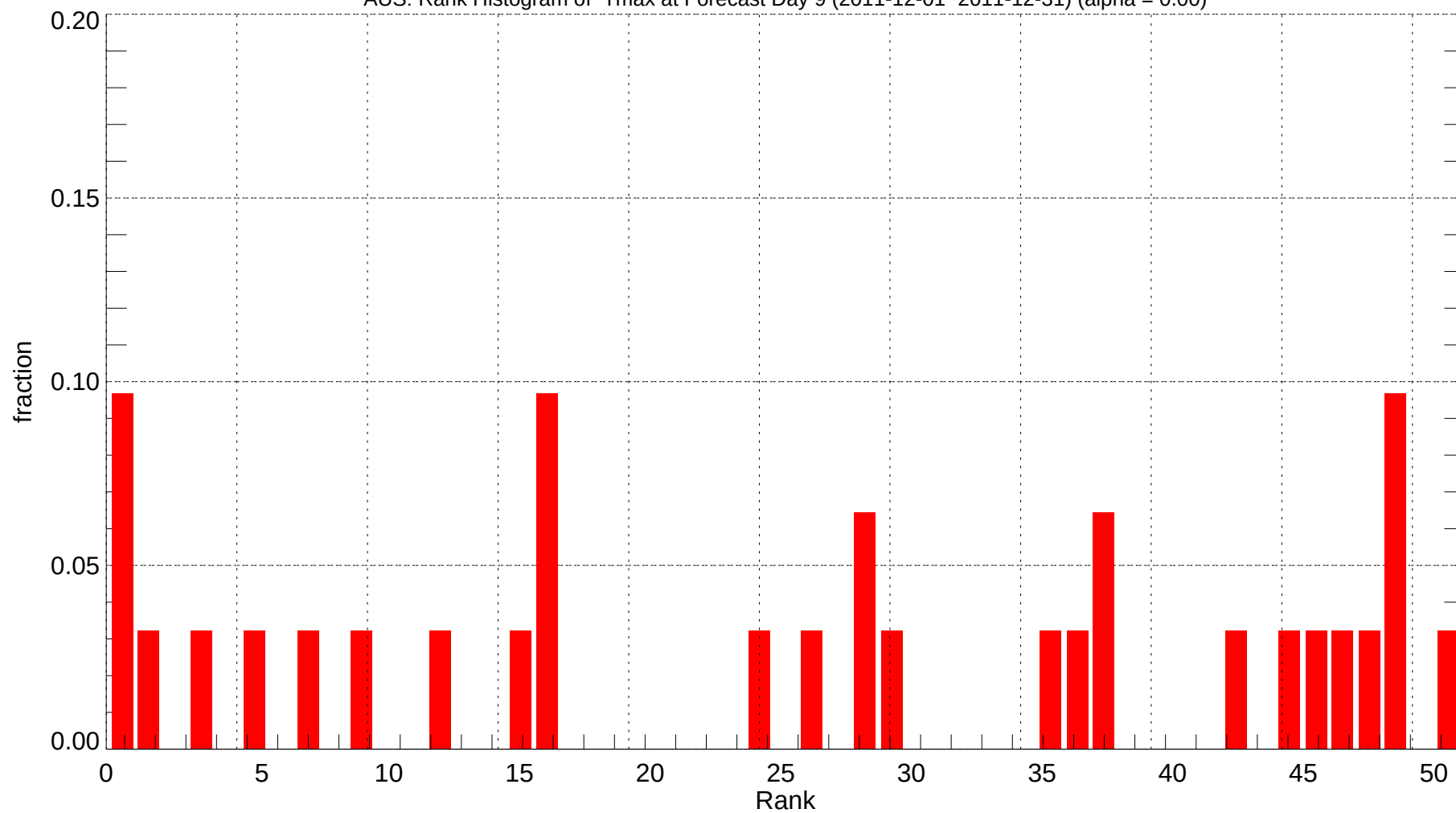
AUS: Rank Histogram of Tmax at Forecast Day 9 (2011-12-01~2011-12-31) (alpha = 0.00)
