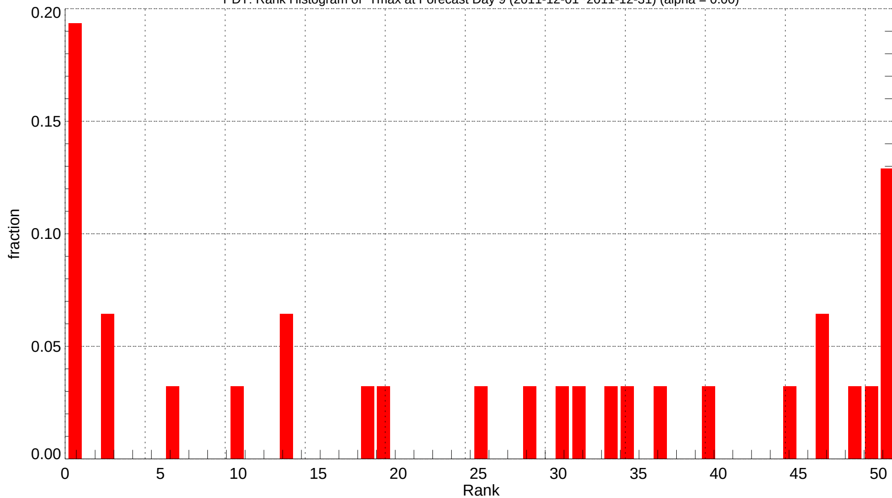
PDT: Rank Histogram of Tmax at Forecast Day 9 (2011-12-01~2011-12-31) (alpha = 0.00)
