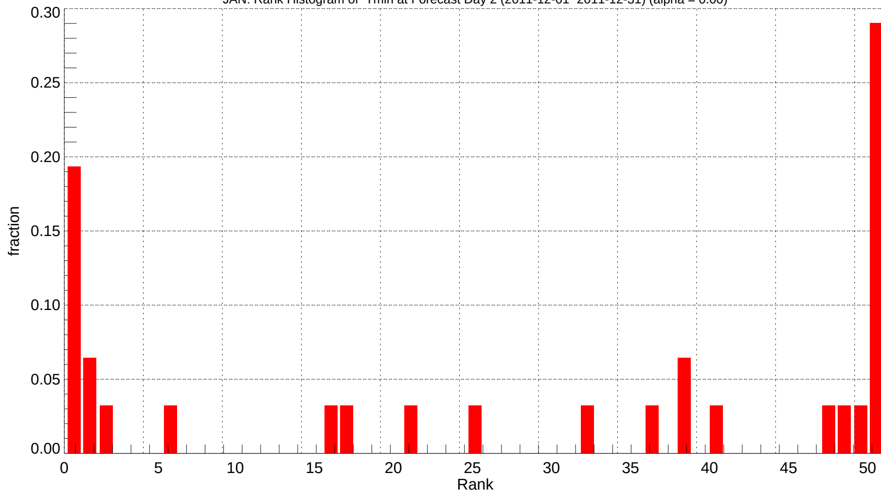
JAN: Rank Histogram of Tmin at Forecast Day 2 (2011-12-01~2011-12-31) (alpha = 0.00)
