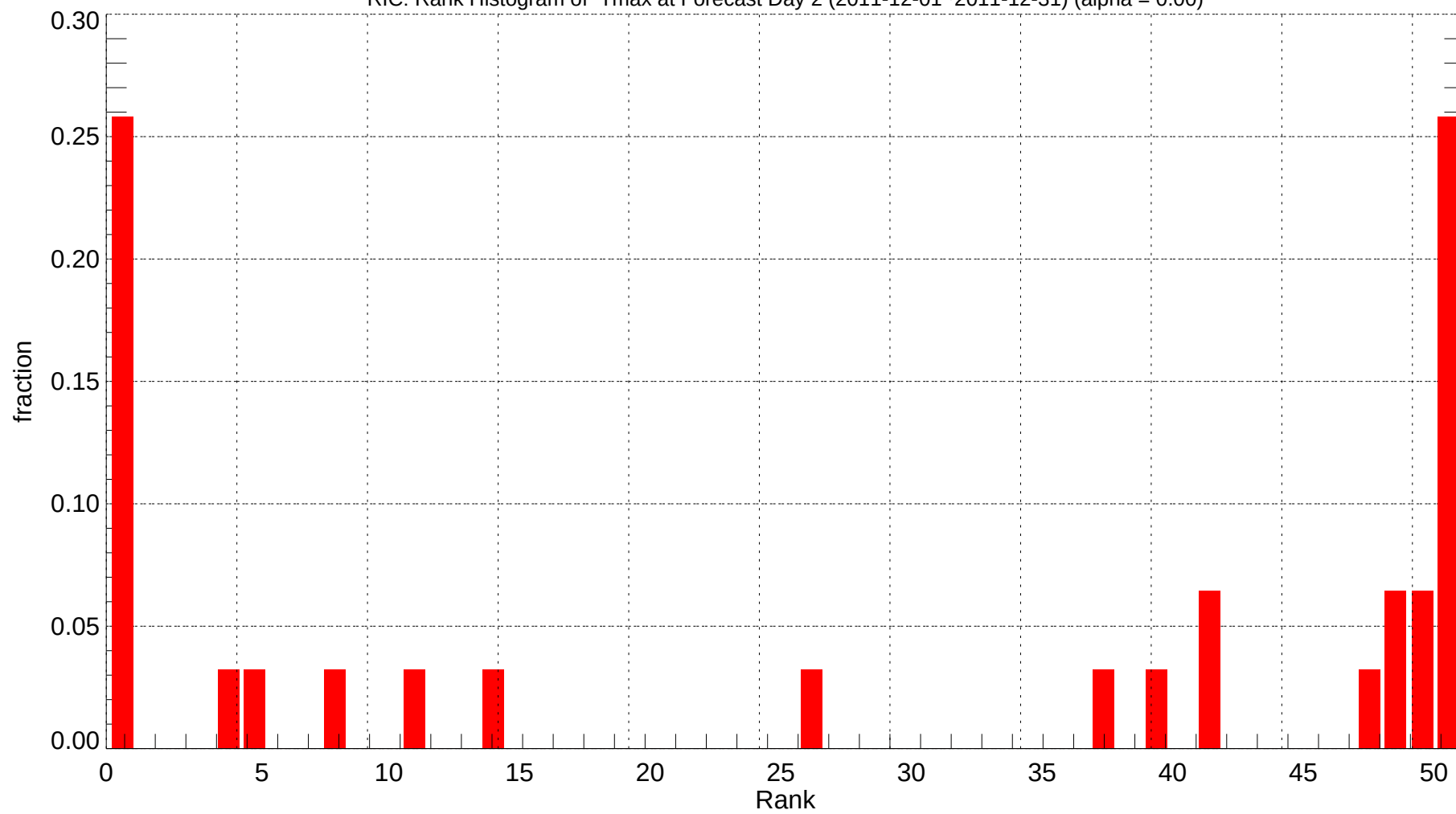
RIC: Rank Histogram of Tmax at Forecast Day 2 (2011-12-01~2011-12-31) (alpha = 0.00)
