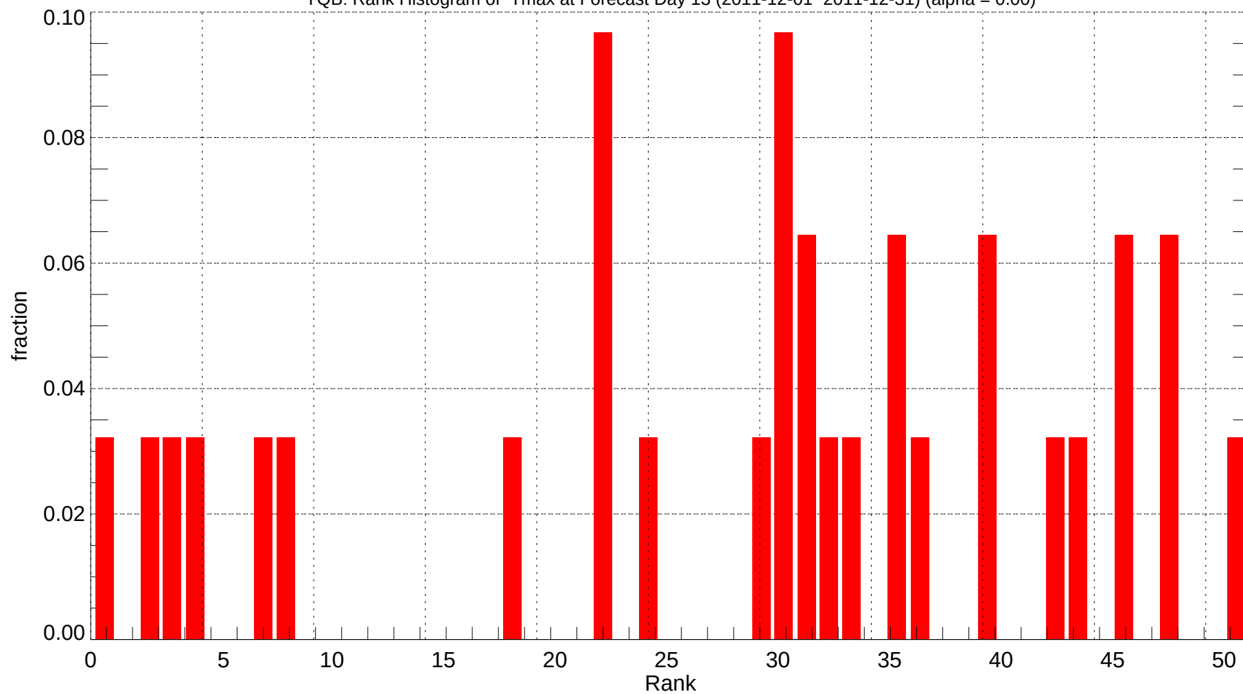
YQB: Rank Histogram of Tmax at Forecast Day 13 (2011-12-01~2011-12-31) (alpha = 0.00)
