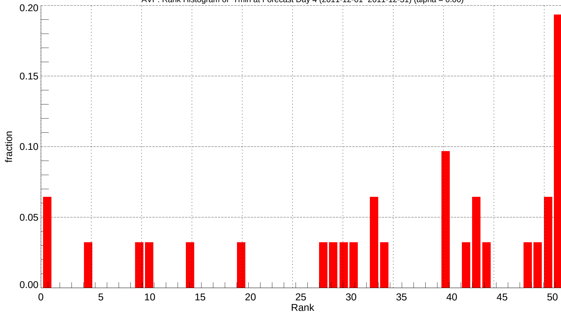
AVP: Rank Histogram of Tmin at Forecast Day 4 (2011-12-01~2011-12-31) (alpha = 0.00)
