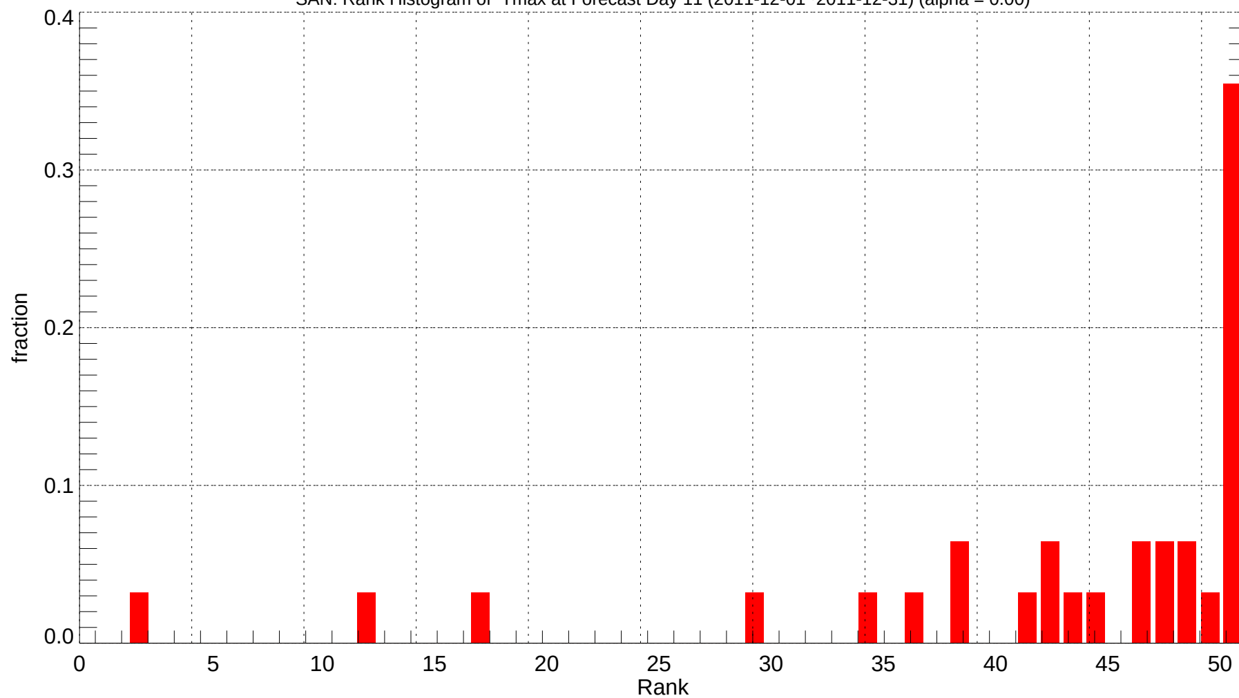
SAN: Rank Histogram of Tmax at Forecast Day 11 (2011-12-01~2011-12-31) (alpha = 0.00)
