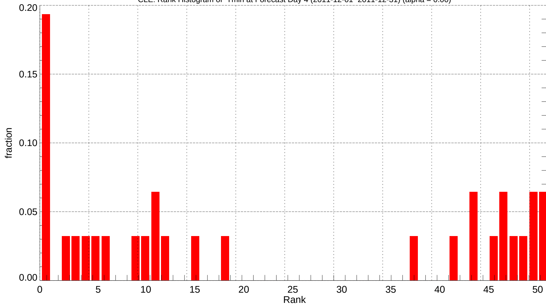
CLE: Rank Histogram of Tmin at Forecast Day 4 (2011-12-01~2011-12-31) (alpha = 0.00)
