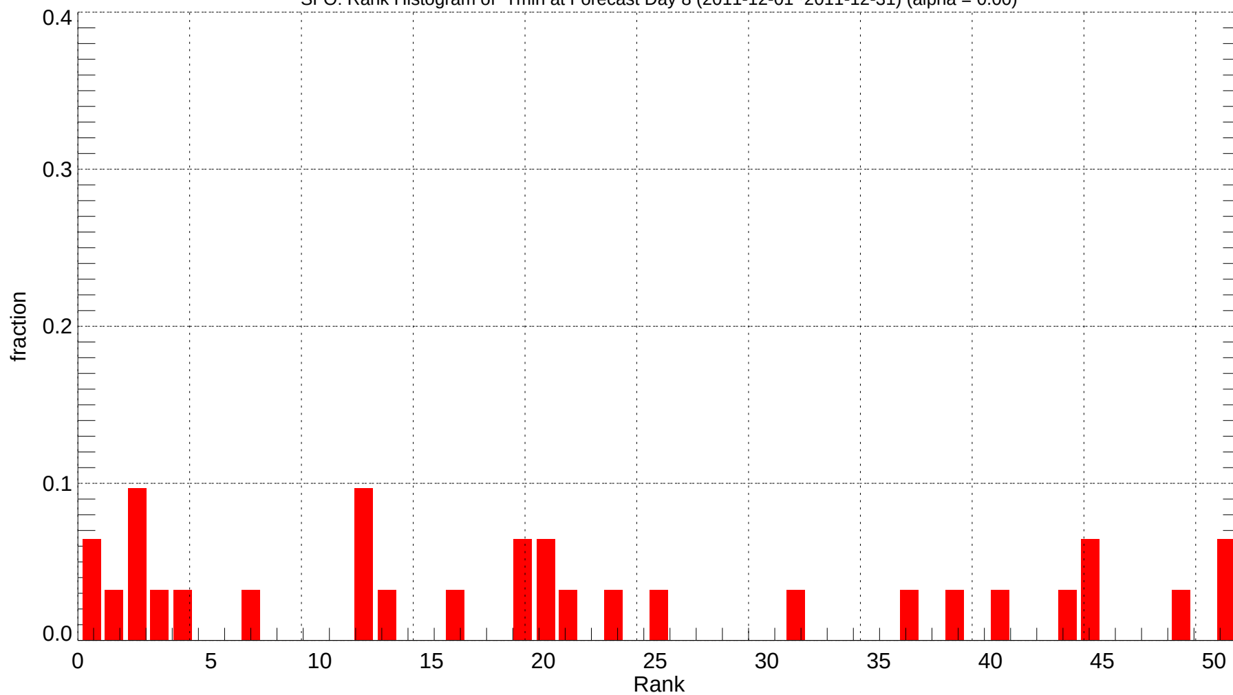
SFO: Rank Histogram of Tmin at Forecast Day 8 (2011-12-01~2011-12-31) (alpha = 0.00)
