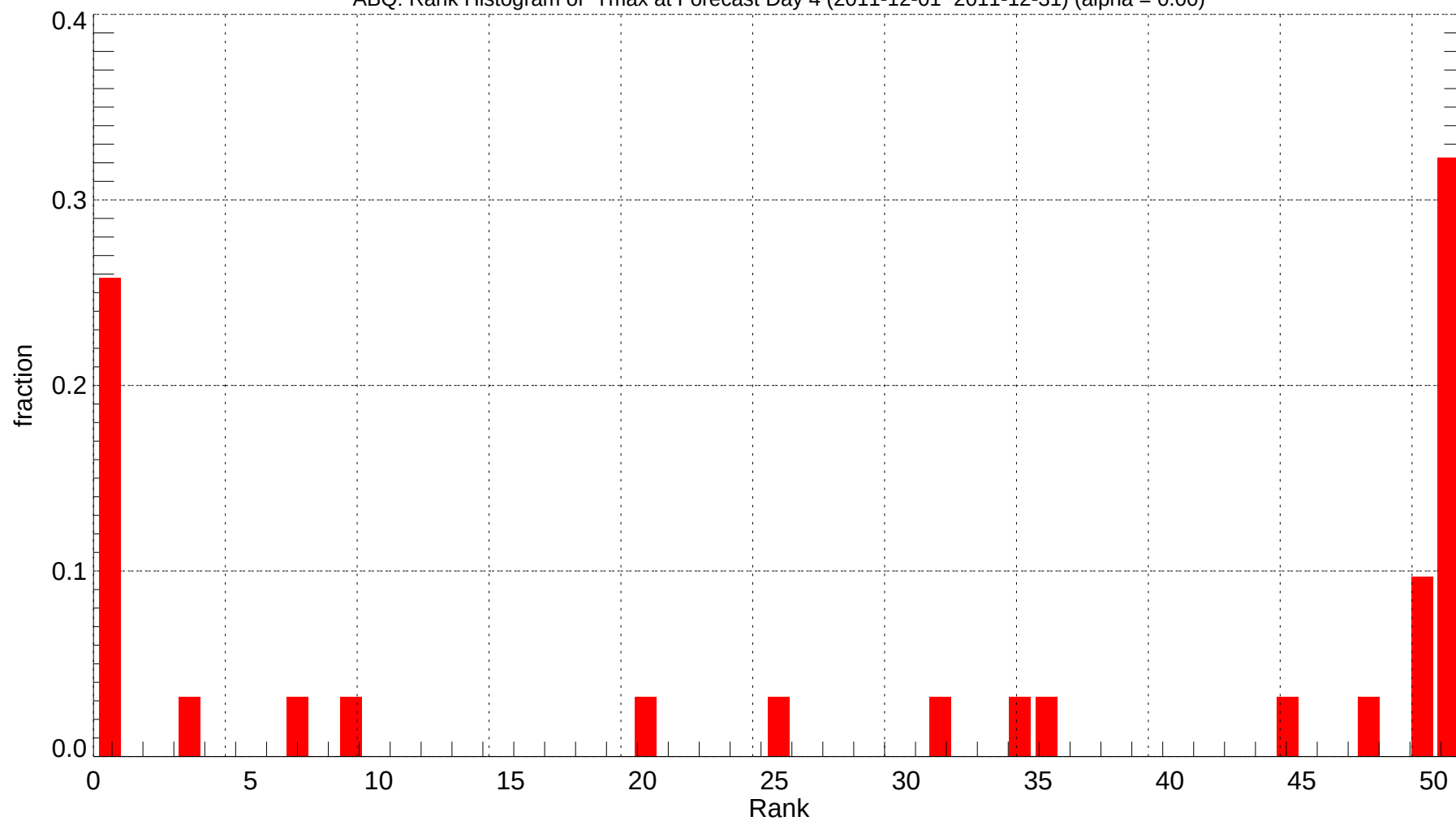
ABQ: Rank Histogram of Tmax at Forecast Day 4 (2011-12-01~2011-12-31) (alpha = 0.00)
