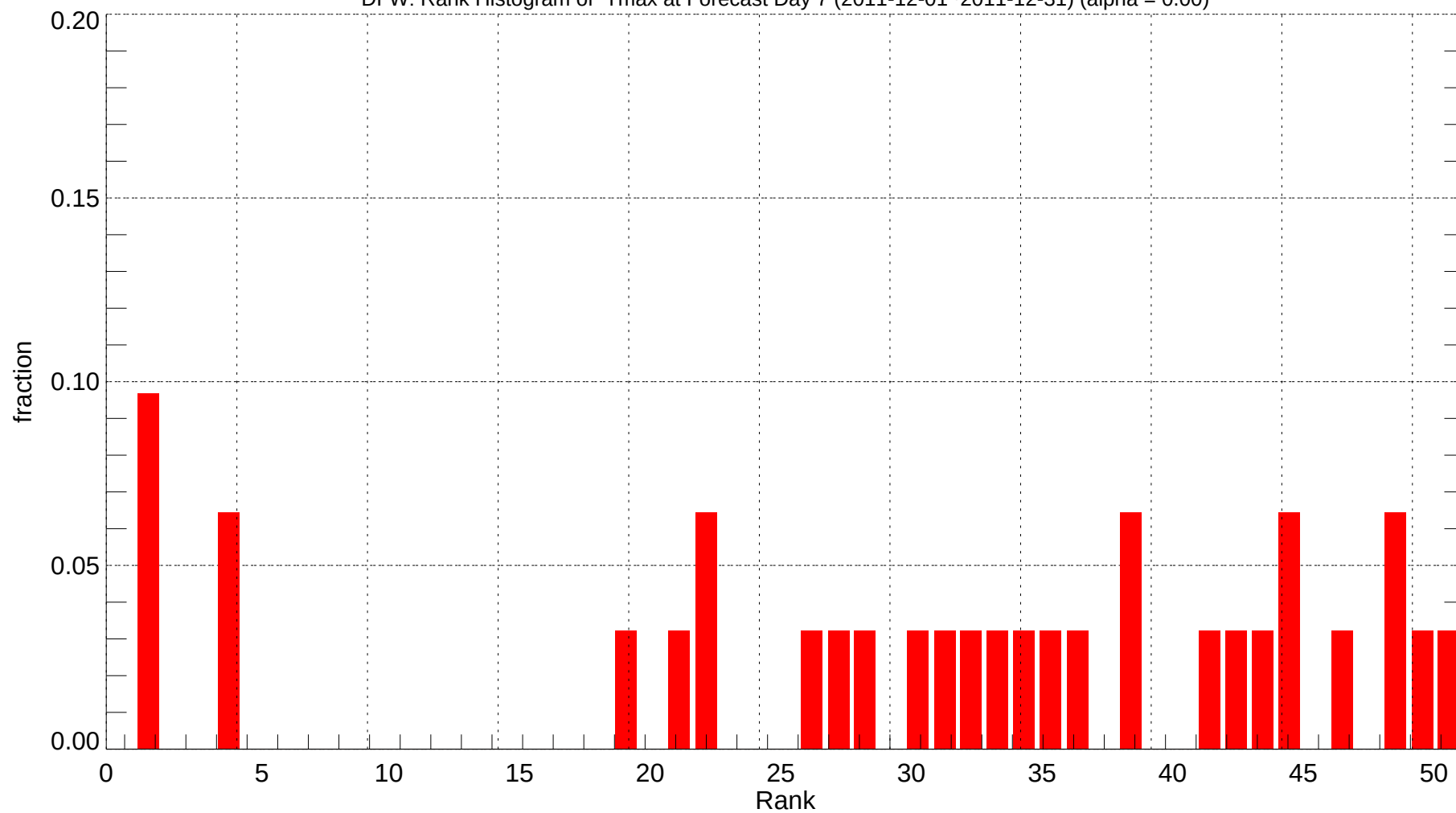
DFW: Rank Histogram of Tmax at Forecast Day 7 (2011-12-01~2011-12-31) (alpha = 0.00)
