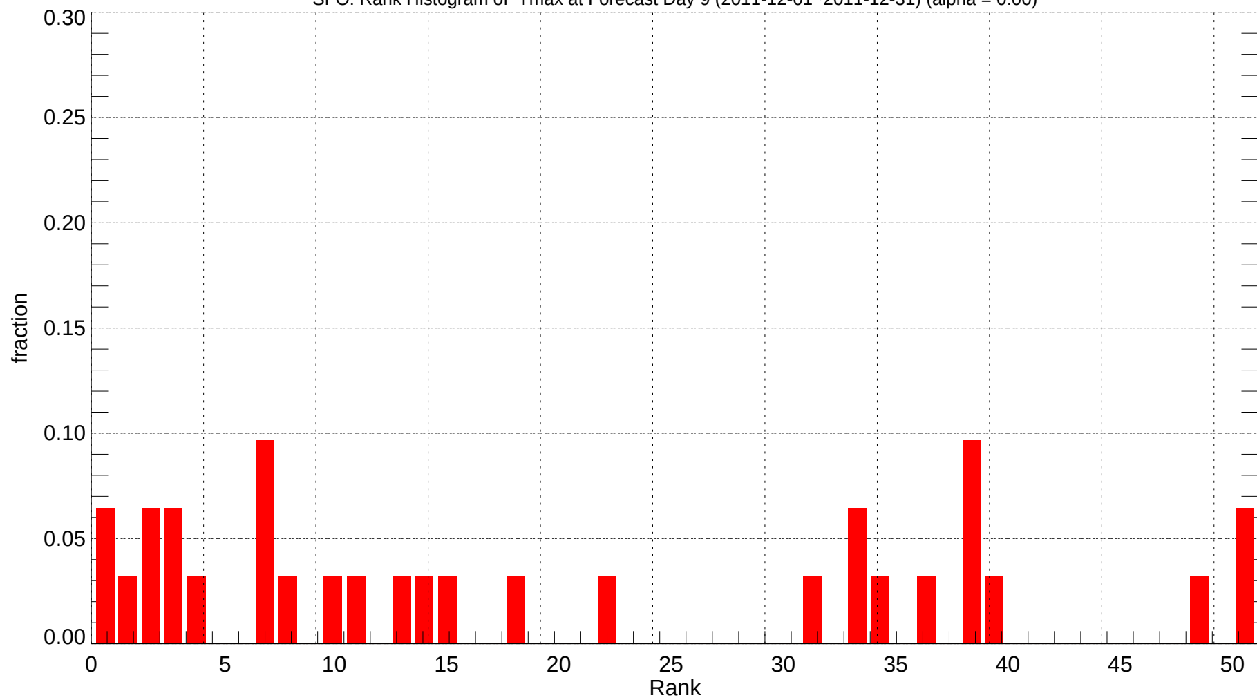
SFO: Rank Histogram of Tmax at Forecast Day 9 (2011-12-01~2011-12-31) (alpha = 0.00)
