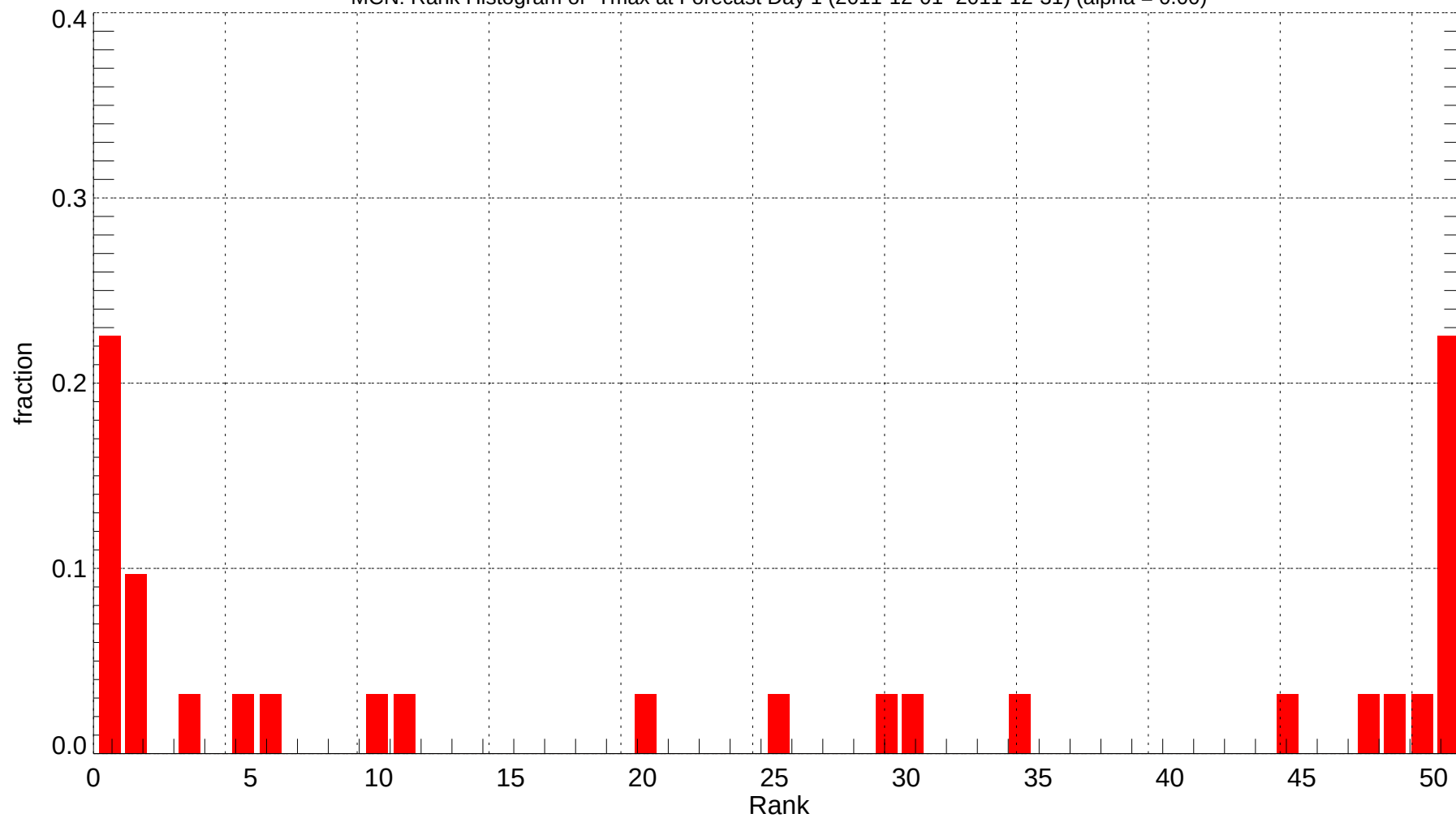
MCN: Rank Histogram of Tmax at Forecast Day 1 (2011-12-01~2011-12-31) (alpha = 0.00)
