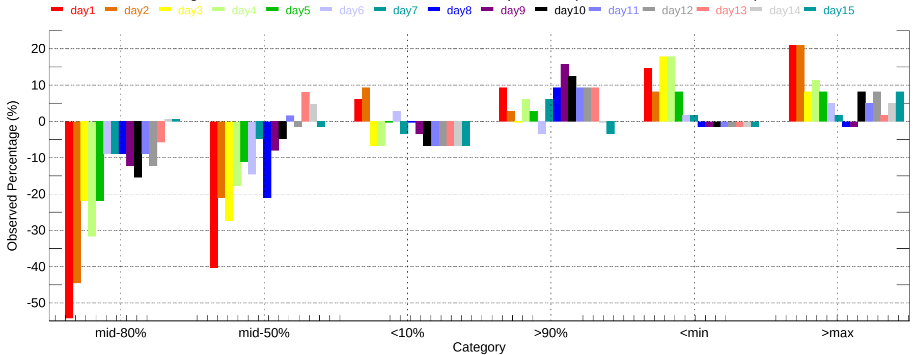
Observed Percentage Deviation of Ensembles - SAV: Max Temperature (2011-12-01~2011-12-31)
