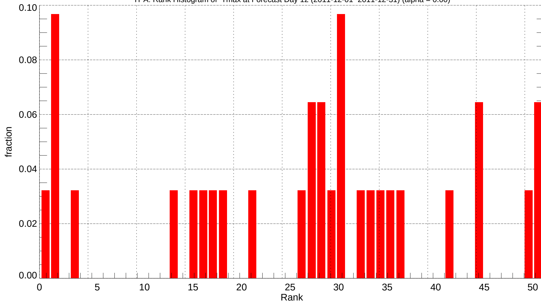
TPA: Rank Histogram of Tmax at Forecast Day 12 (2011-12-01~2011-12-31) (alpha = 0.00)
