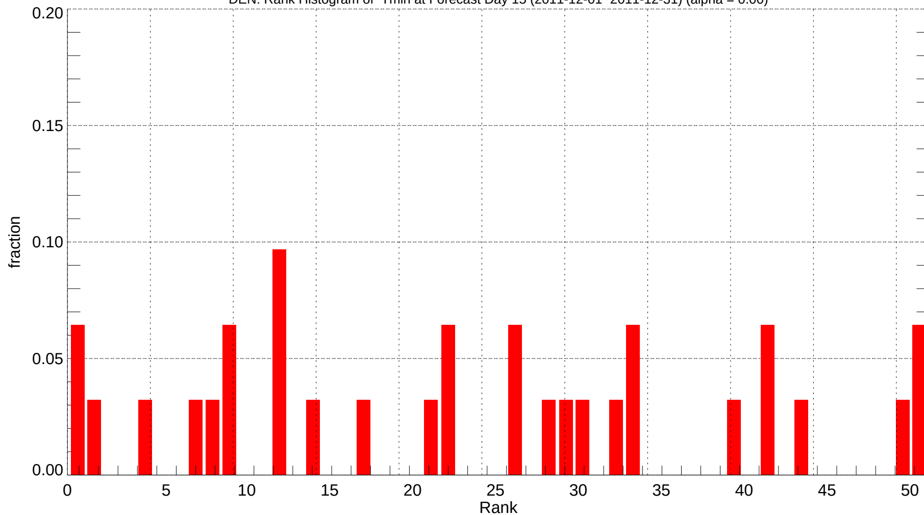
DEN: Rank Histogram of Tmin at Forecast Day 15 (2011-12-01~2011-12-31) (alpha = 0.00)
