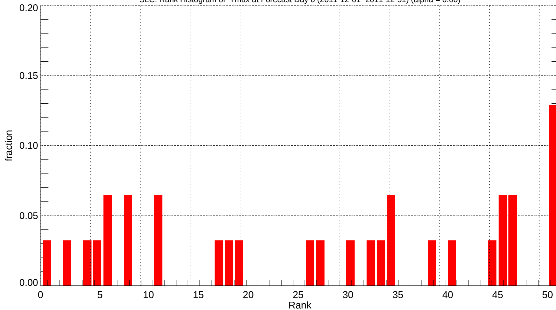
SLC: Rank Histogram of Tmax at Forecast Day 6 (2011-12-01~2011-12-31) (alpha = 0.00)
