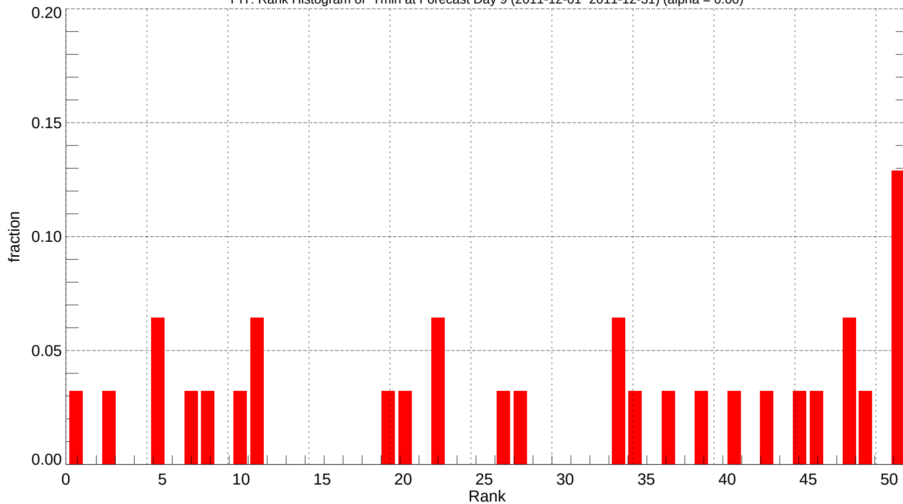
PIT: Rank Histogram of Tmin at Forecast Day 9 (2011-12-01~2011-12-31) (alpha = 0.00)
