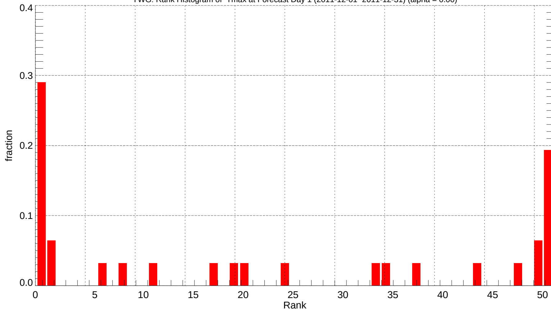
YWG: Rank Histogram of Tmax at Forecast Day 1 (2011-12-01~2011-12-31) (alpha = 0.00)
