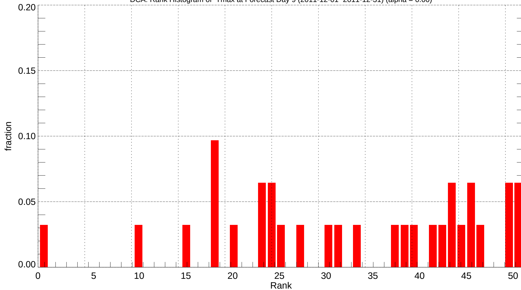
DCA: Rank Histogram of Tmax at Forecast Day 9 (2011-12-01~2011-12-31) (alpha = 0.00)
