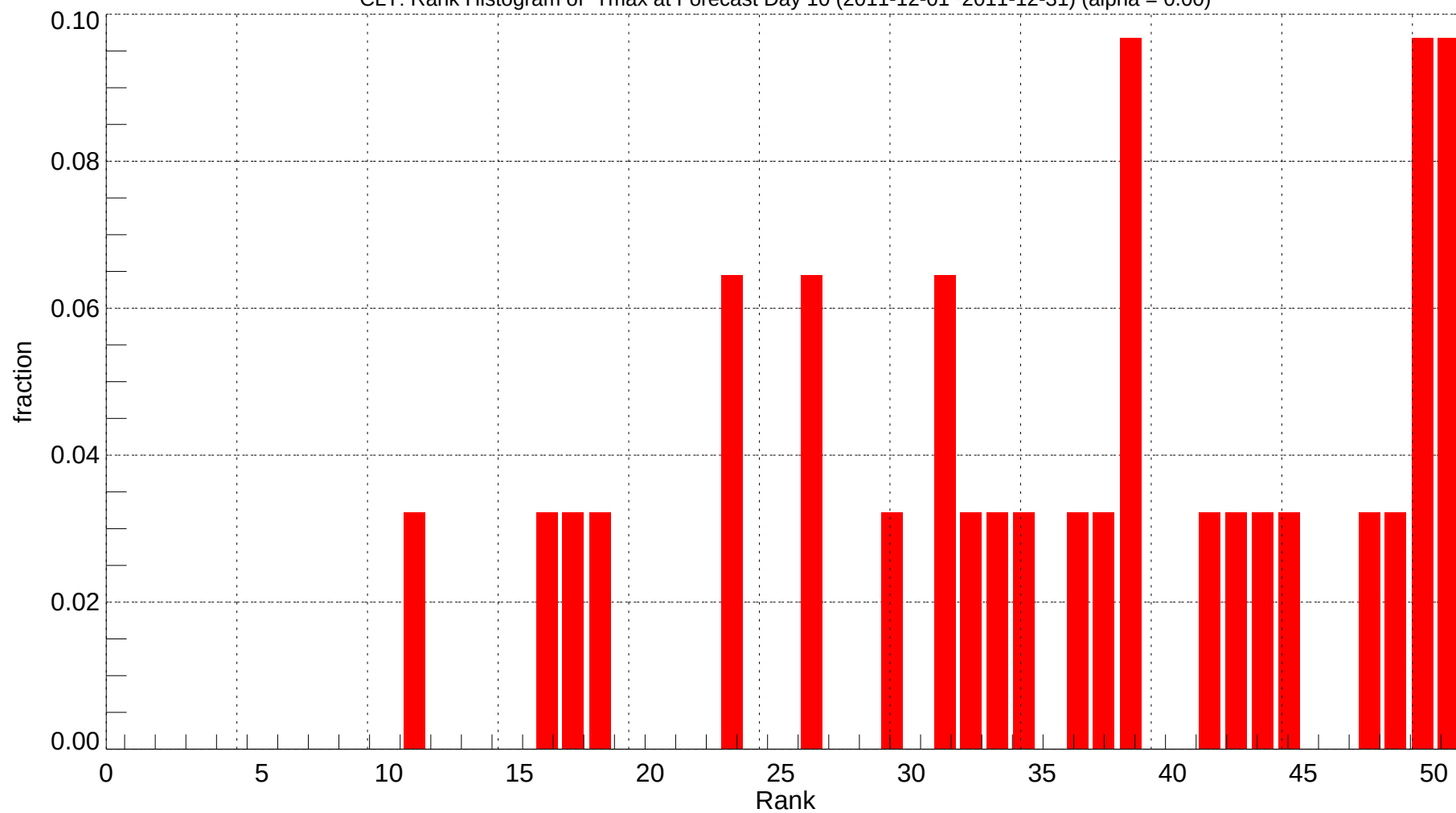
CLT: Rank Histogram of Tmax at Forecast Day 10 (2011-12-01~2011-12-31) (alpha = 0.00)
