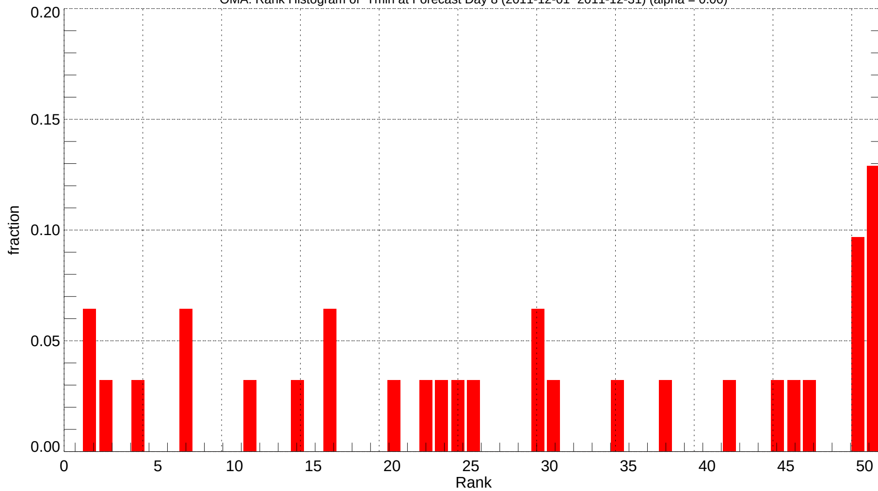
OMA: Rank Histogram of Tmin at Forecast Day 8 (2011-12-01~2011-12-31) (alpha = 0.00)
