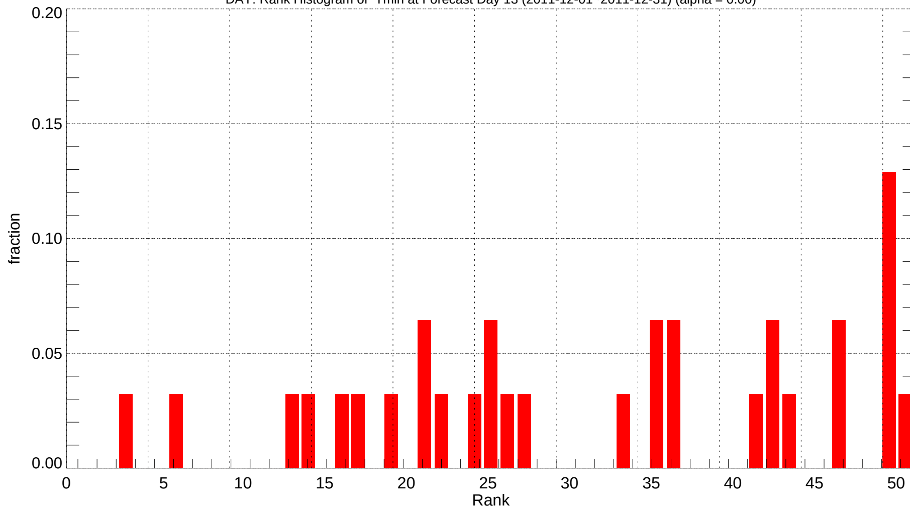
DAY: Rank Histogram of Tmin at Forecast Day 13 (2011-12-01~2011-12-31) (alpha = 0.00)
