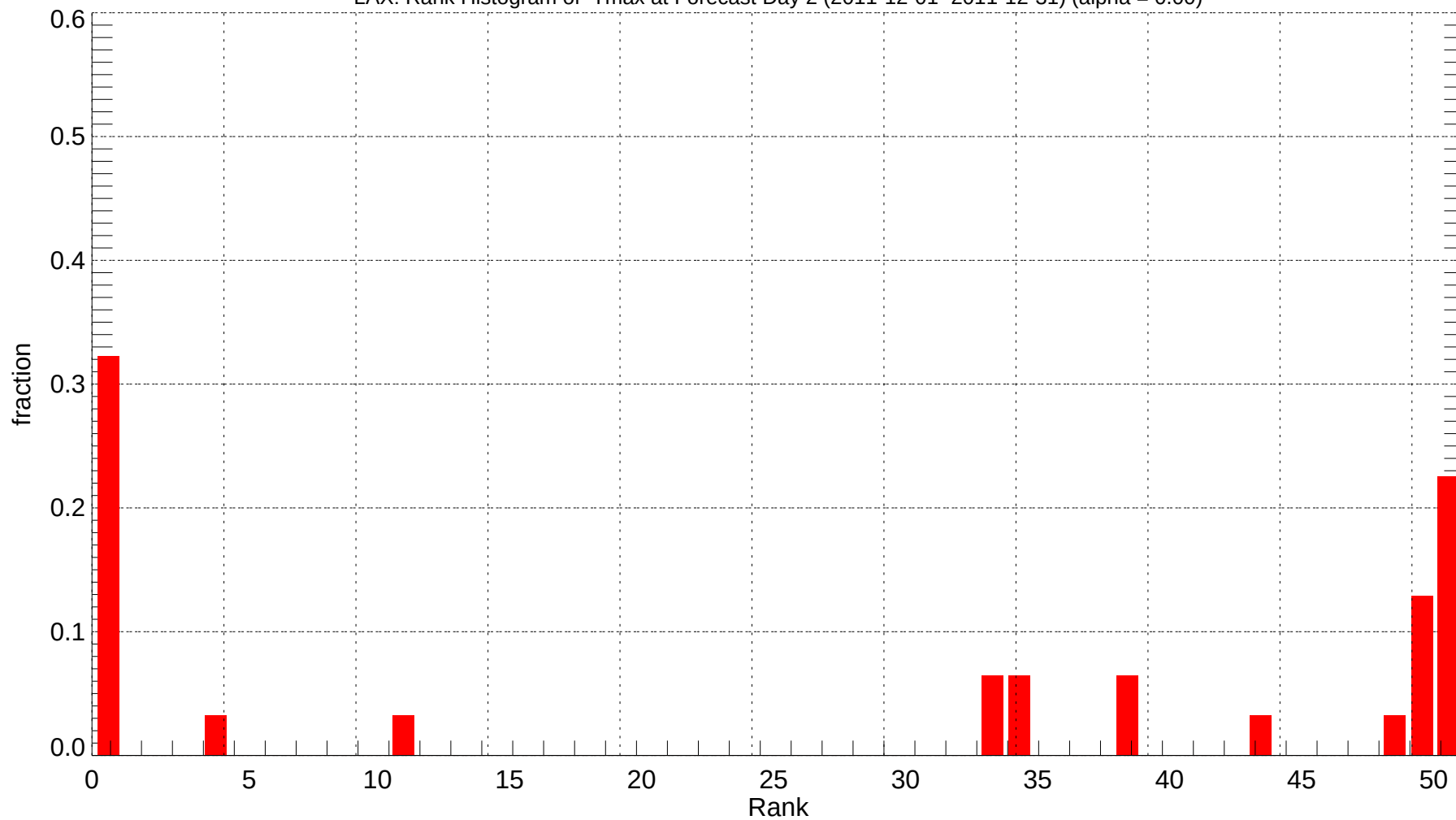
LAX: Rank Histogram of Tmax at Forecast Day 2 (2011-12-01~2011-12-31) (alpha = 0.00)
