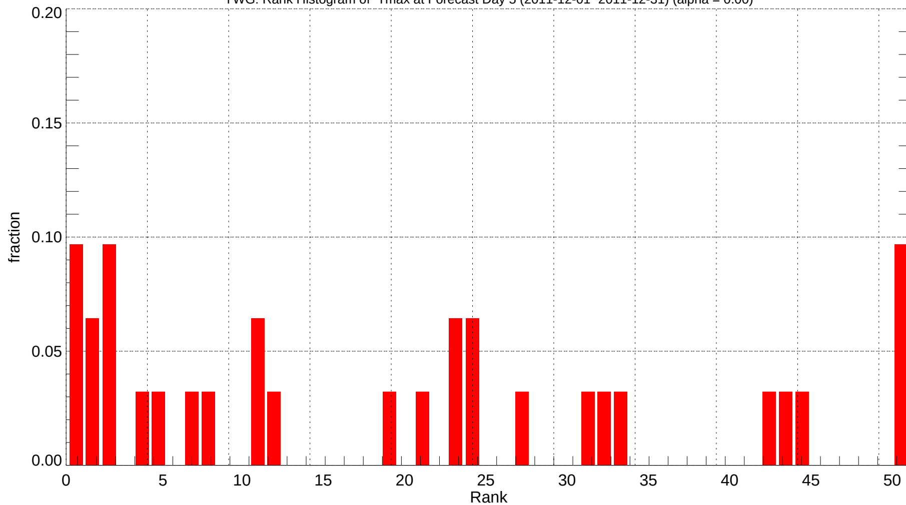
YWG: Rank Histogram of Tmax at Forecast Day 5 (2011-12-01~2011-12-31) (alpha = 0.00)
