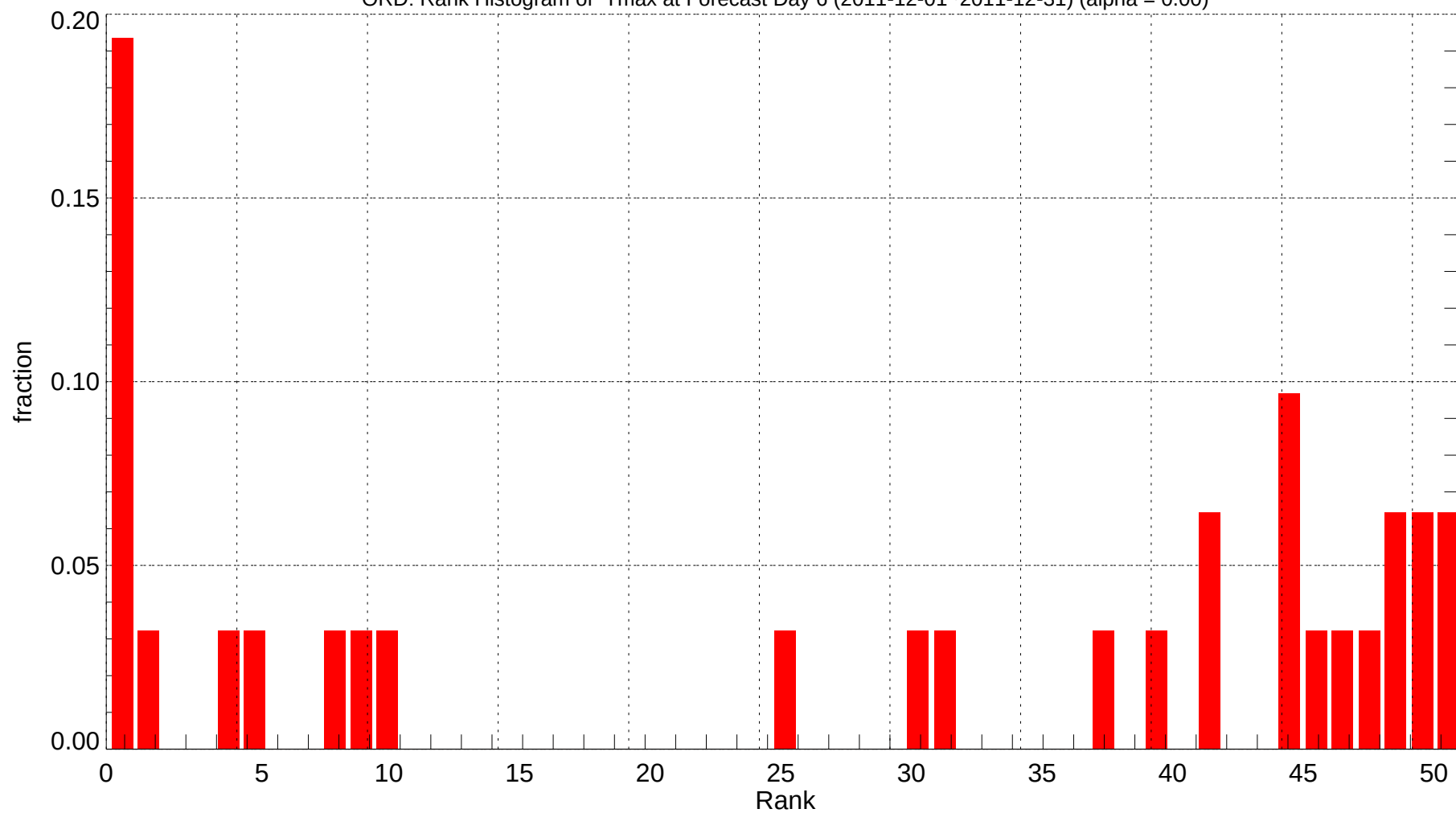
ORD: Rank Histogram of Tmax at Forecast Day 6 (2011-12-01~2011-12-31) (alpha = 0.00)
