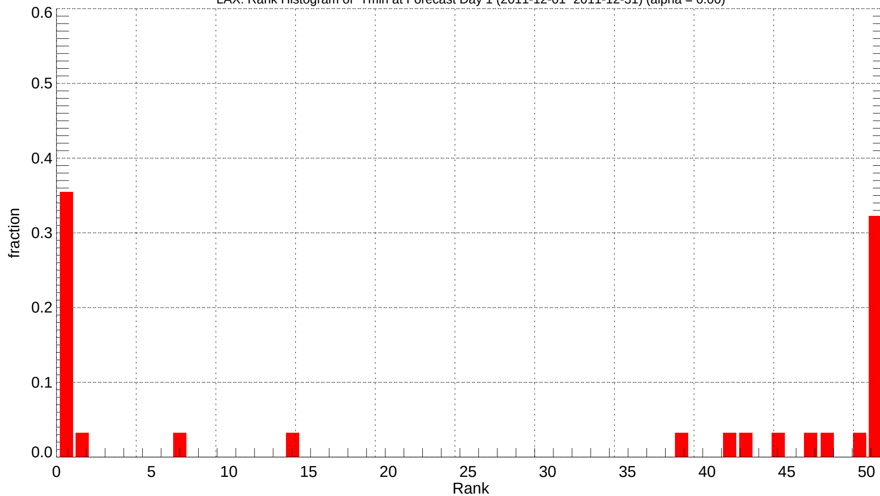
LAX: Rank Histogram of Tmin at Forecast Day 1 (2011-12-01~2011-12-31) (alpha = 0.00)
