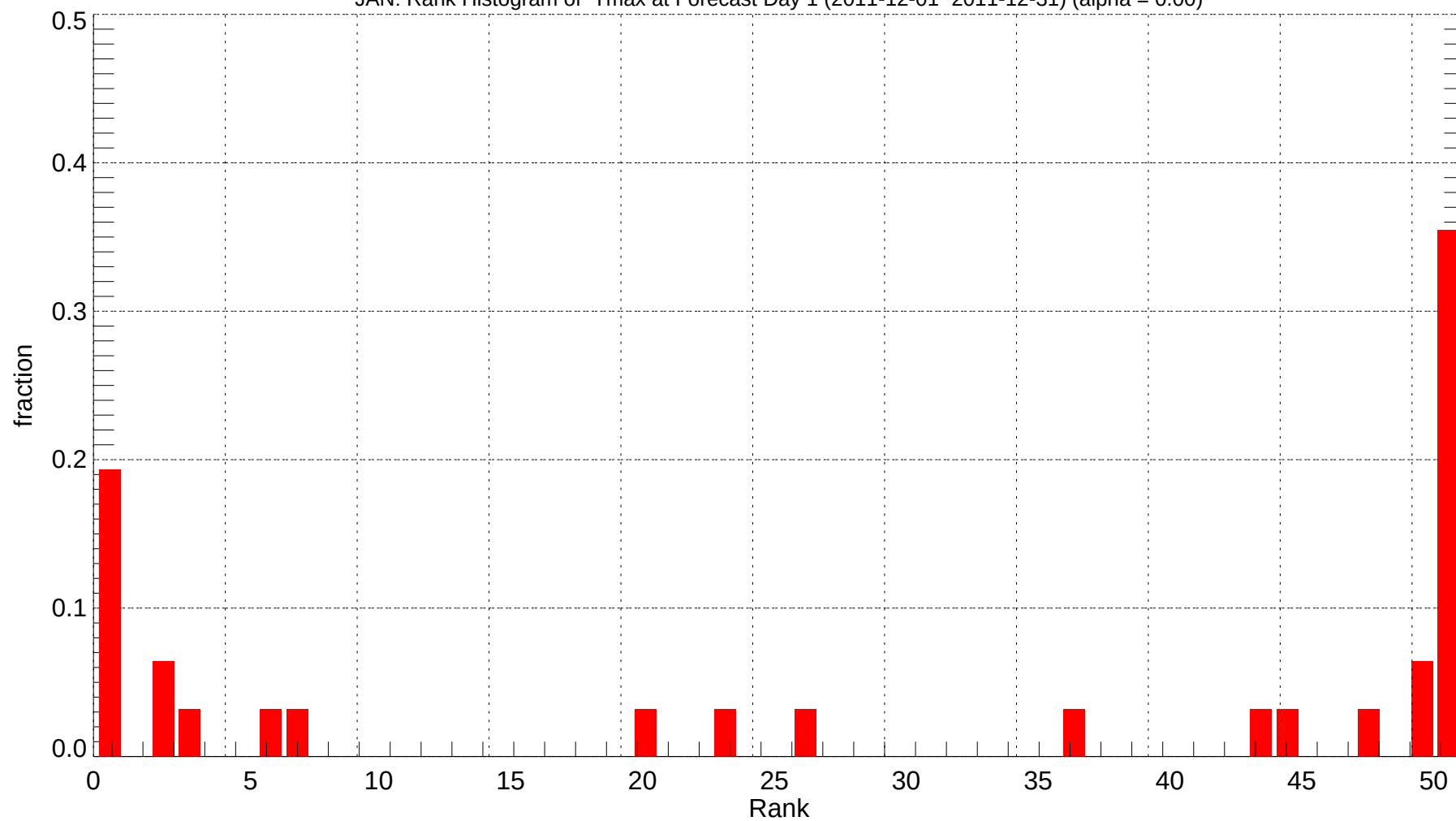
JAN: Rank Histogram of Tmax at Forecast Day 1 (2011-12-01~2011-12-31) (alpha = 0.00)
