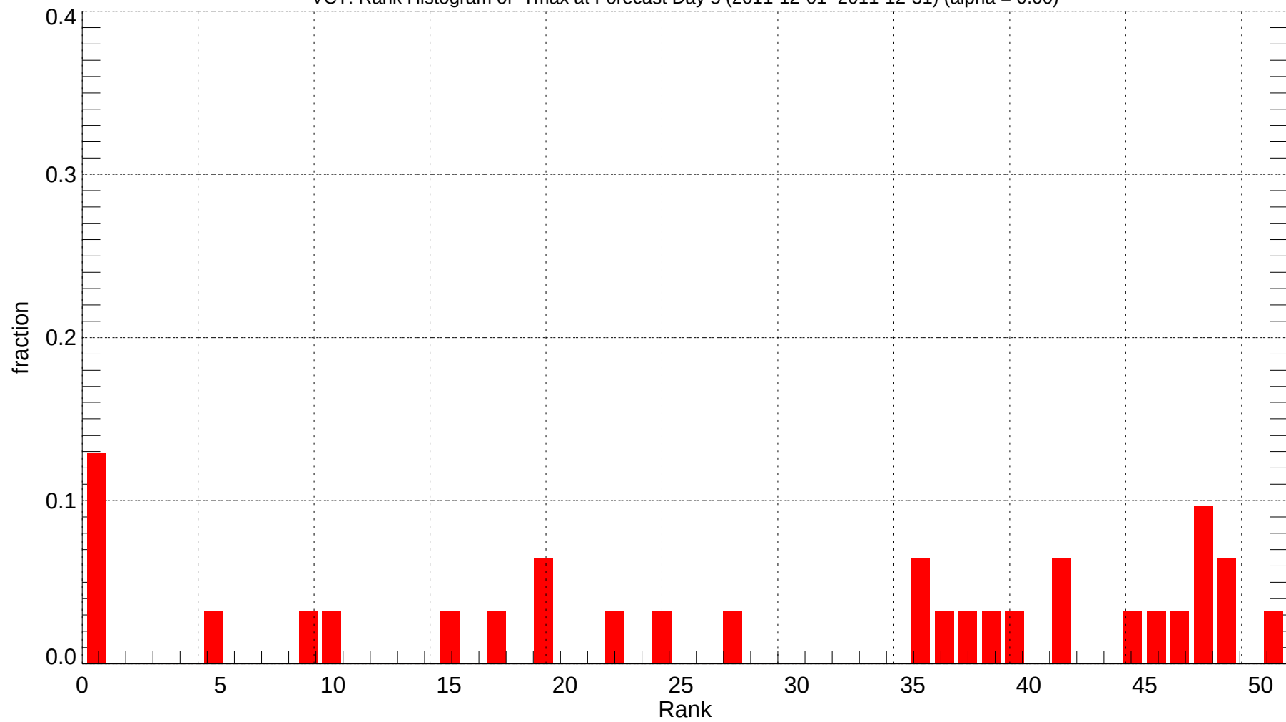
VCT: Rank Histogram of Tmax at Forecast Day 5 (2011-12-01~2011-12-31) (alpha = 0.00)
