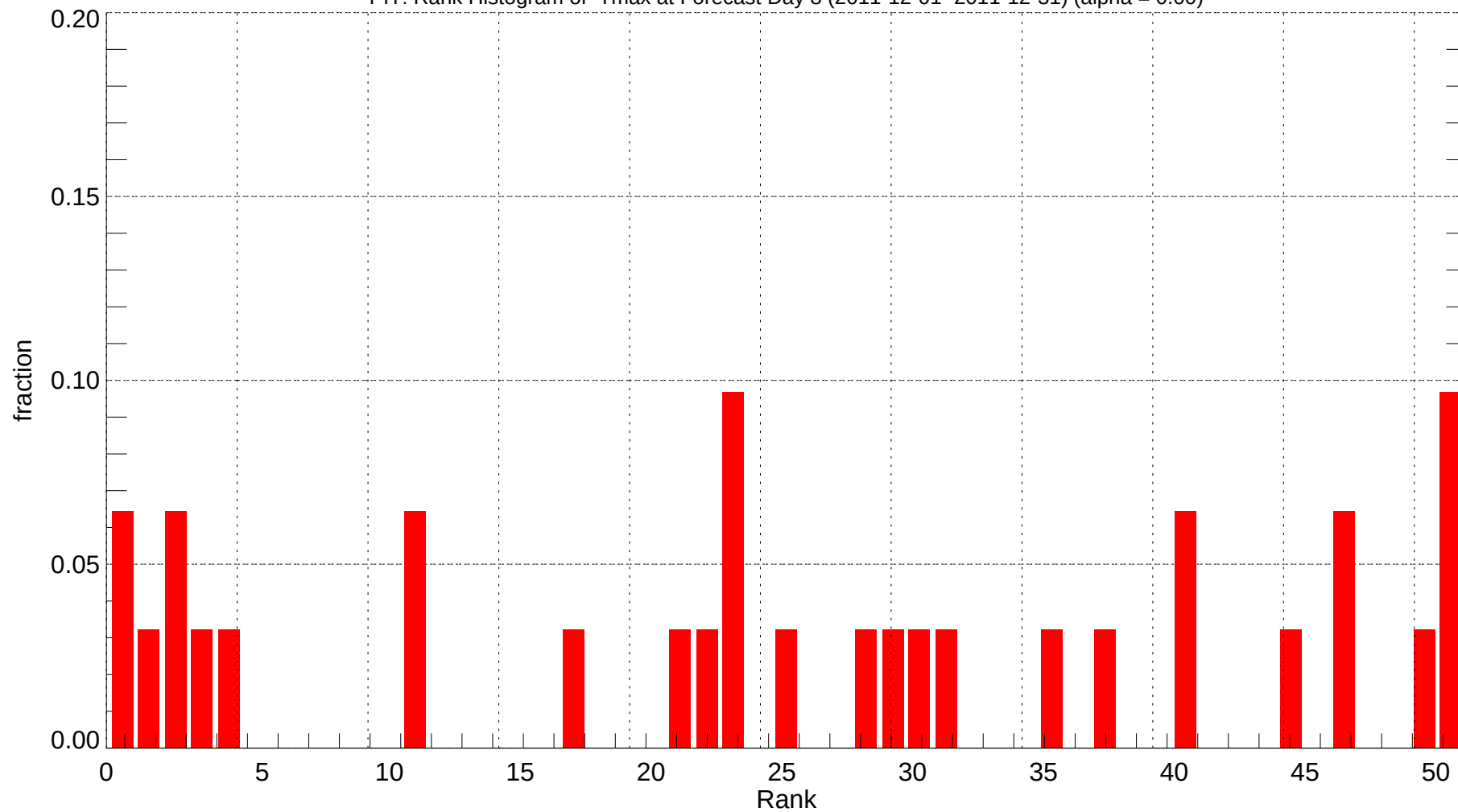
PIT: Rank Histogram of Tmax at Forecast Day 8 (2011-12-01~2011-12-31) (alpha = 0.00)
