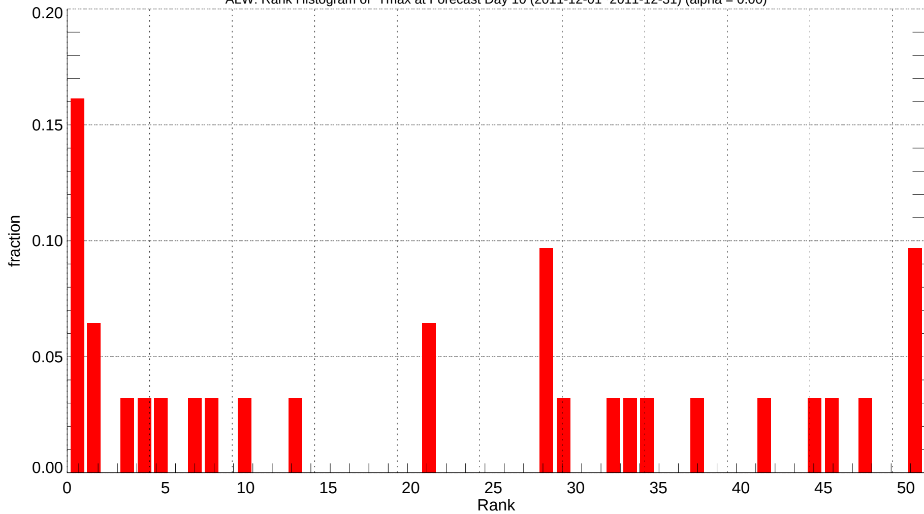
ALW: Rank Histogram of Tmax at Forecast Day 10 (2011-12-01~2011-12-31) (alpha = 0.00)
