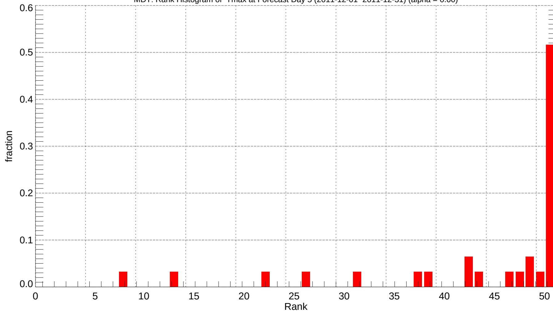
MDT: Rank Histogram of Tmax at Forecast Day 5 (2011-12-01~2011-12-31) (alpha = 0.00)
