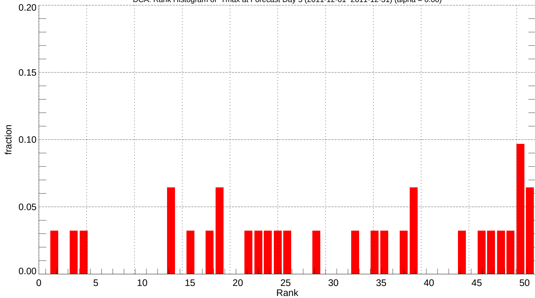
DCA: Rank Histogram of Tmax at Forecast Day 5 (2011-12-01~2011-12-31) (alpha = 0.00)
