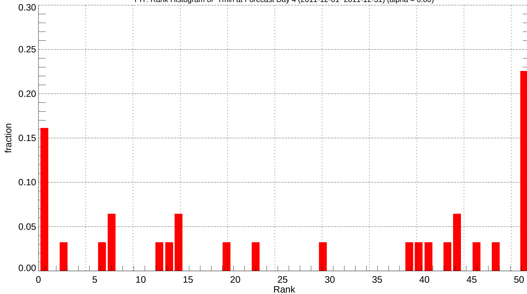
PIT: Rank Histogram of Tmin at Forecast Day 4 (2011-12-01~2011-12-31) (alpha = 0.00)
