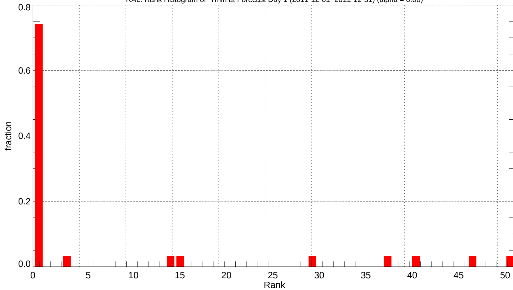
RAL: Rank Histogram of Tmin at Forecast Day 1 (2011-12-01~2011-12-31) (alpha = 0.00)
