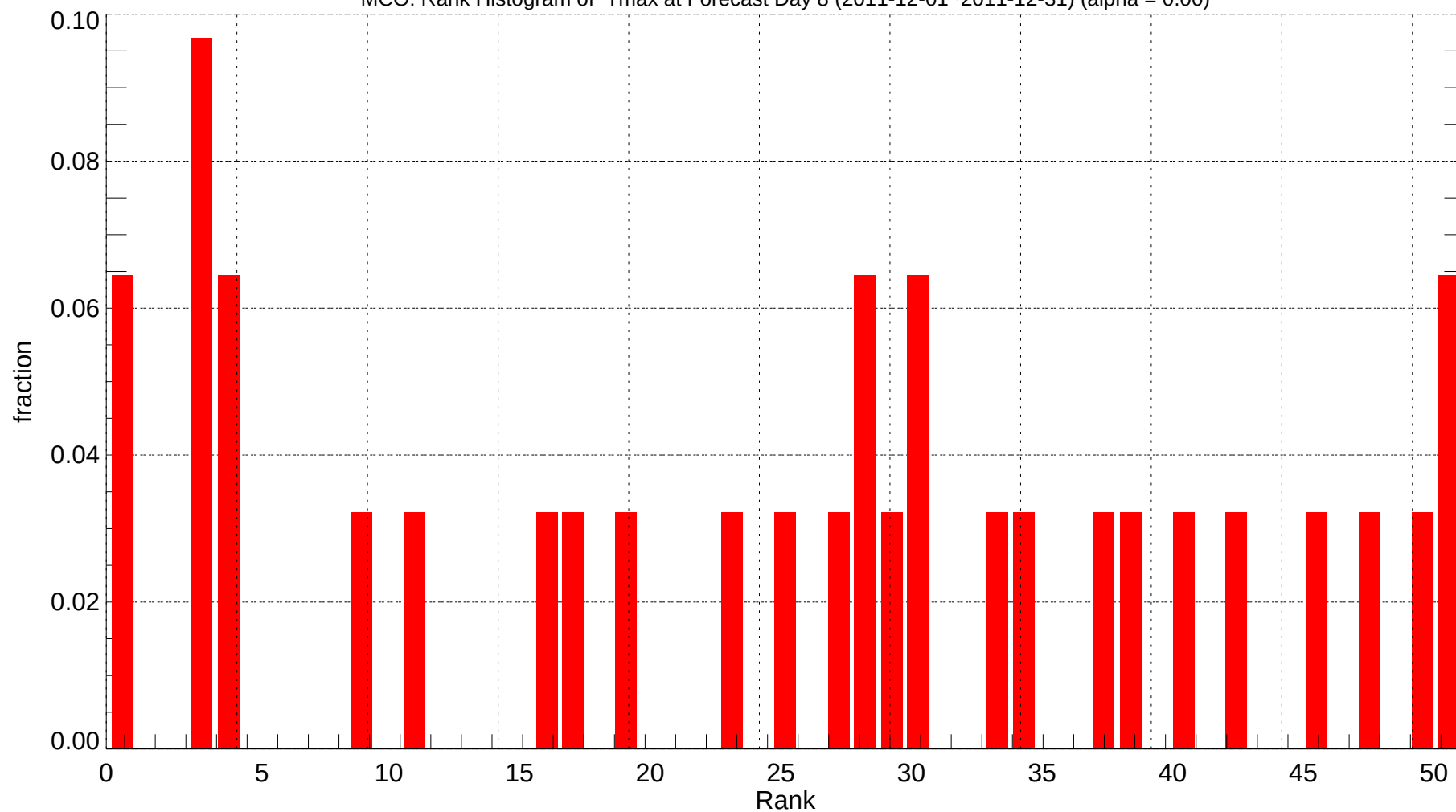
MCO: Rank Histogram of Tmax at Forecast Day 8 (2011-12-01~2011-12-31) (alpha = 0.00)
