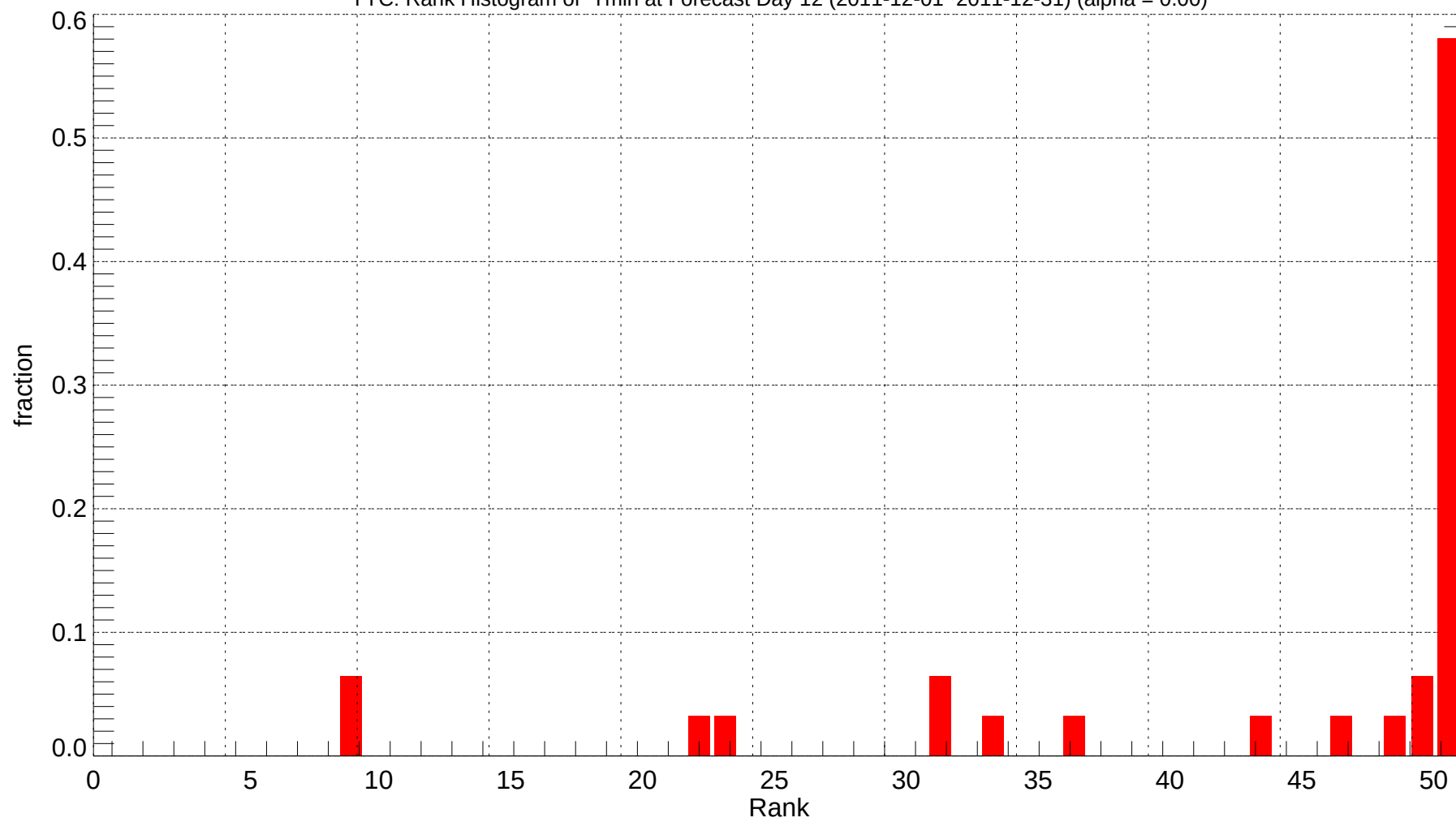
YYC: Rank Histogram of Tmin at Forecast Day 12 (2011-12-01~2011-12-31) (alpha = 0.00)
