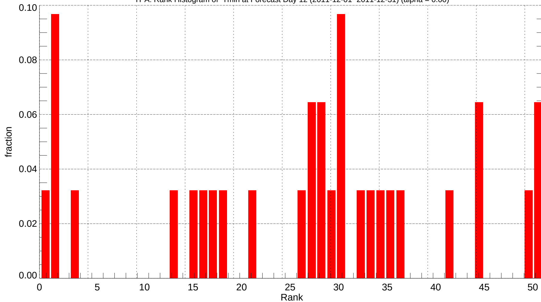
TPA: Rank Histogram of Tmin at Forecast Day 12 (2011-12-01~2011-12-31) (alpha = 0.00)
