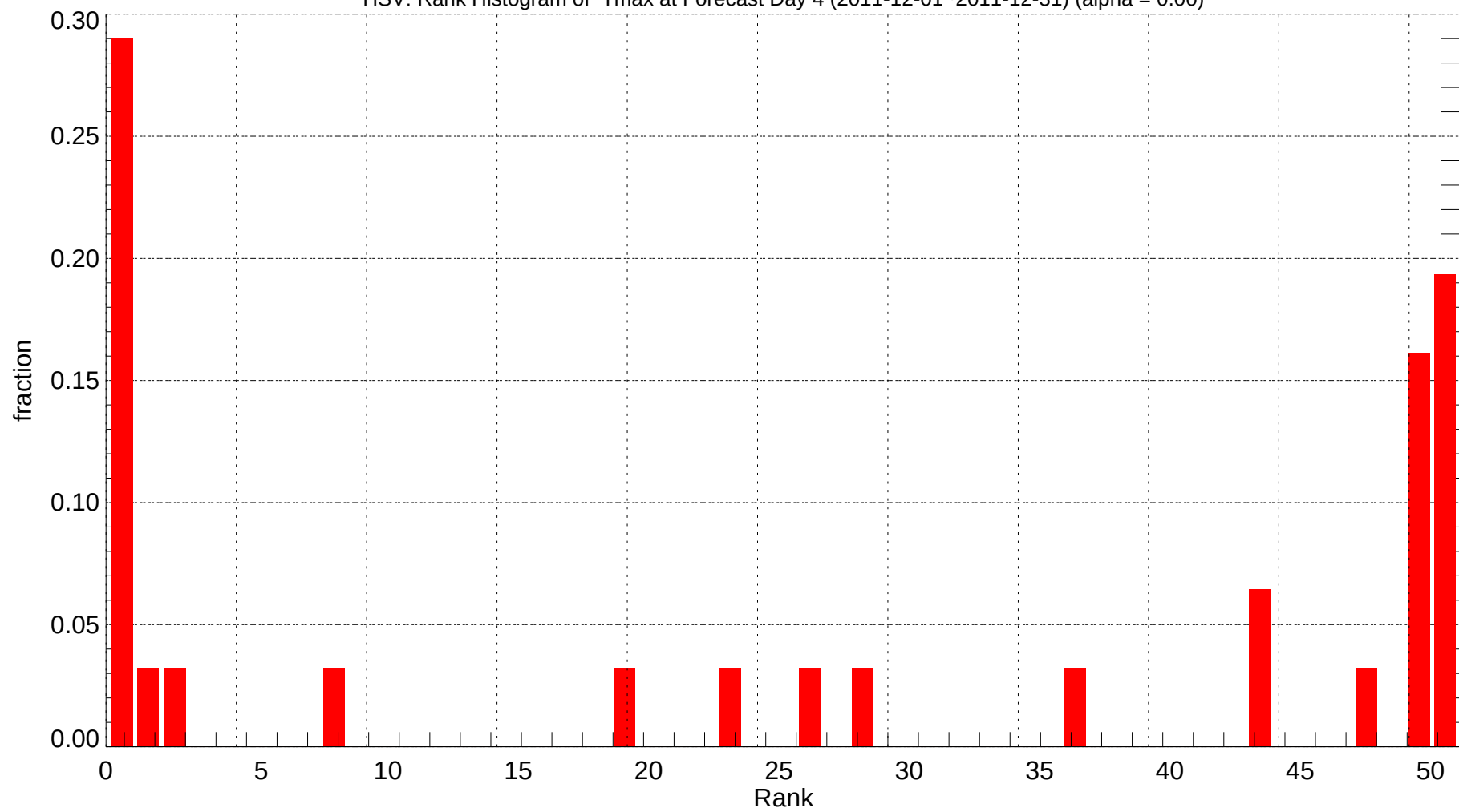
HSV: Rank Histogram of Tmax at Forecast Day 4 (2011-12-01~2011-12-31) (alpha = 0.00)
