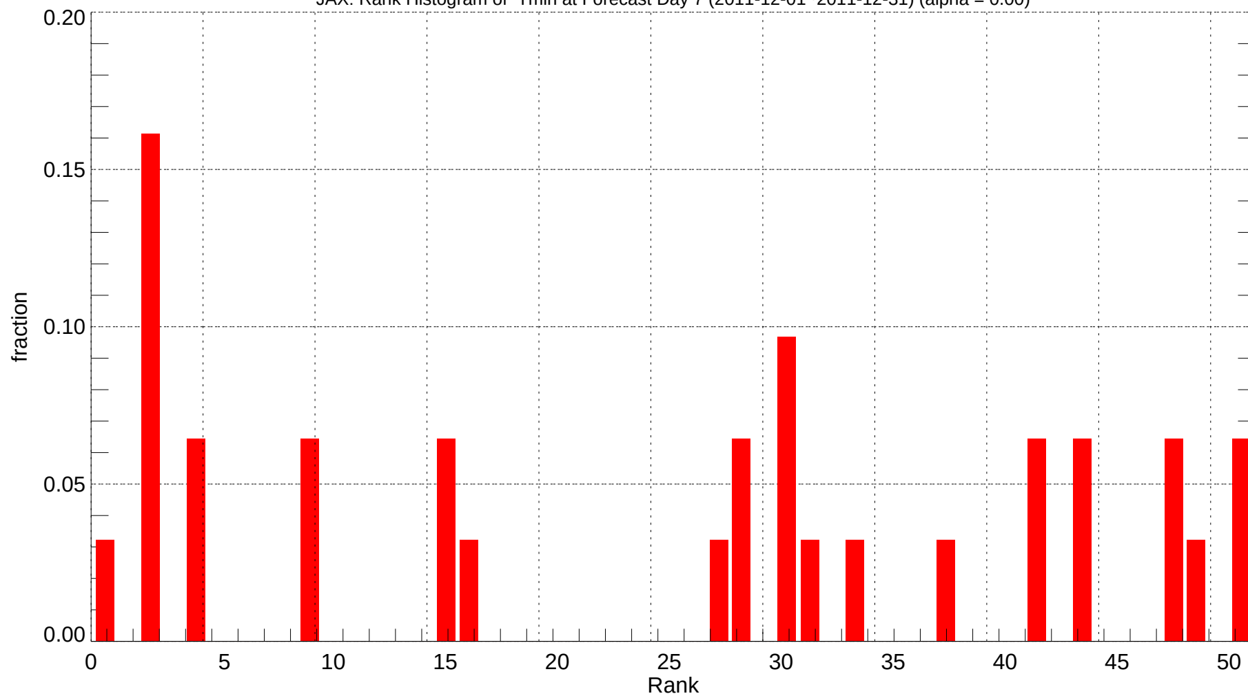
JAX: Rank Histogram of Tmin at Forecast Day 7 (2011-12-01~2011-12-31) (alpha = 0.00)
