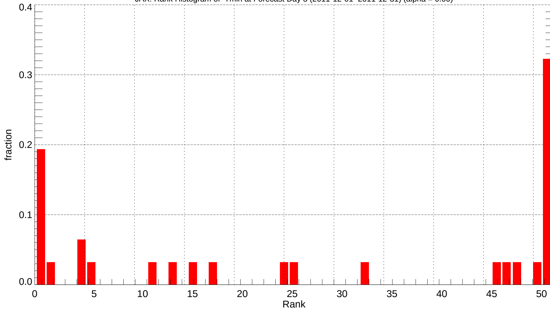
JAX: Rank Histogram of Tmin at Forecast Day 3 (2011-12-01~2011-12-31) (alpha = 0.00)
