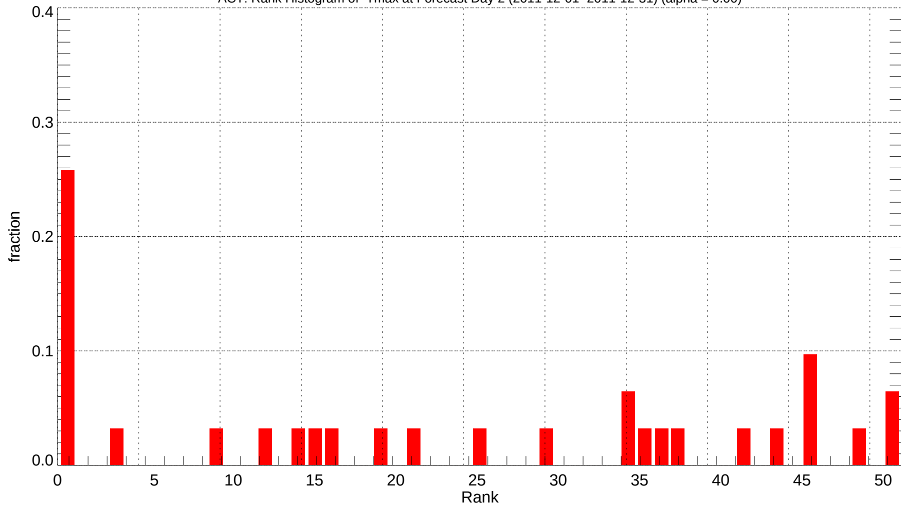
ACT: Rank Histogram of Tmax at Forecast Day 2 (2011-12-01~2011-12-31) (alpha = 0.00)
