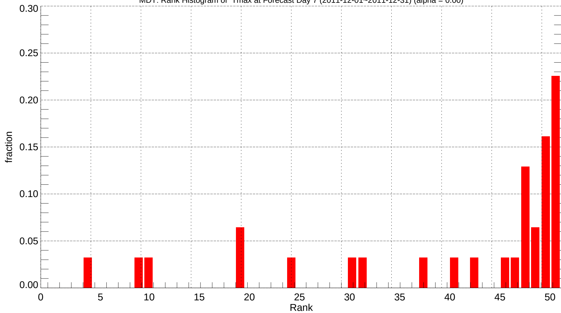
MDT: Rank Histogram of Tmax at Forecast Day 7 (2011-12-01~2011-12-31) (alpha = 0.00)
