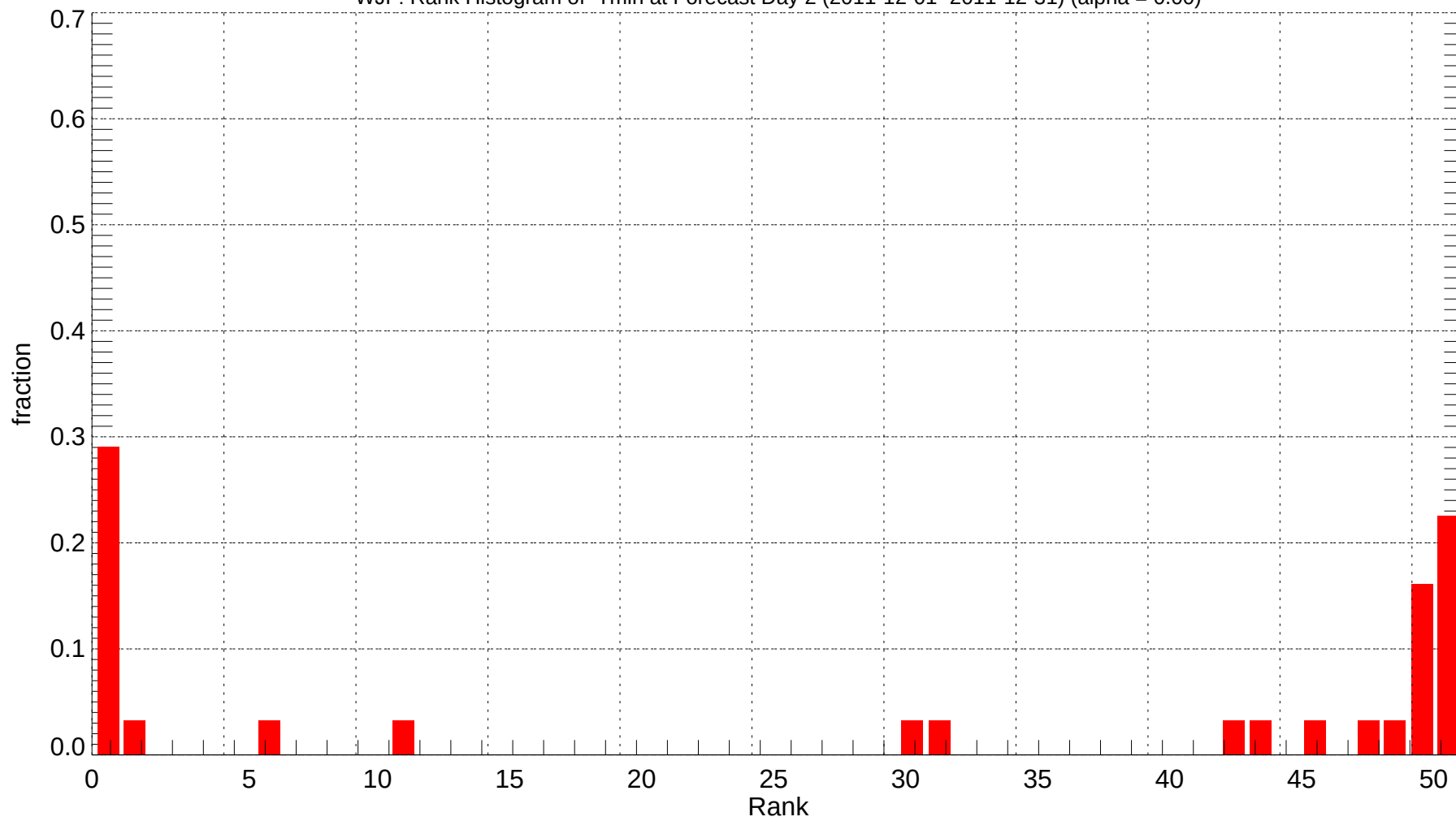
WJF: Rank Histogram of Tmin at Forecast Day 2 (2011-12-01~2011-12-31) (alpha = 0.00)
