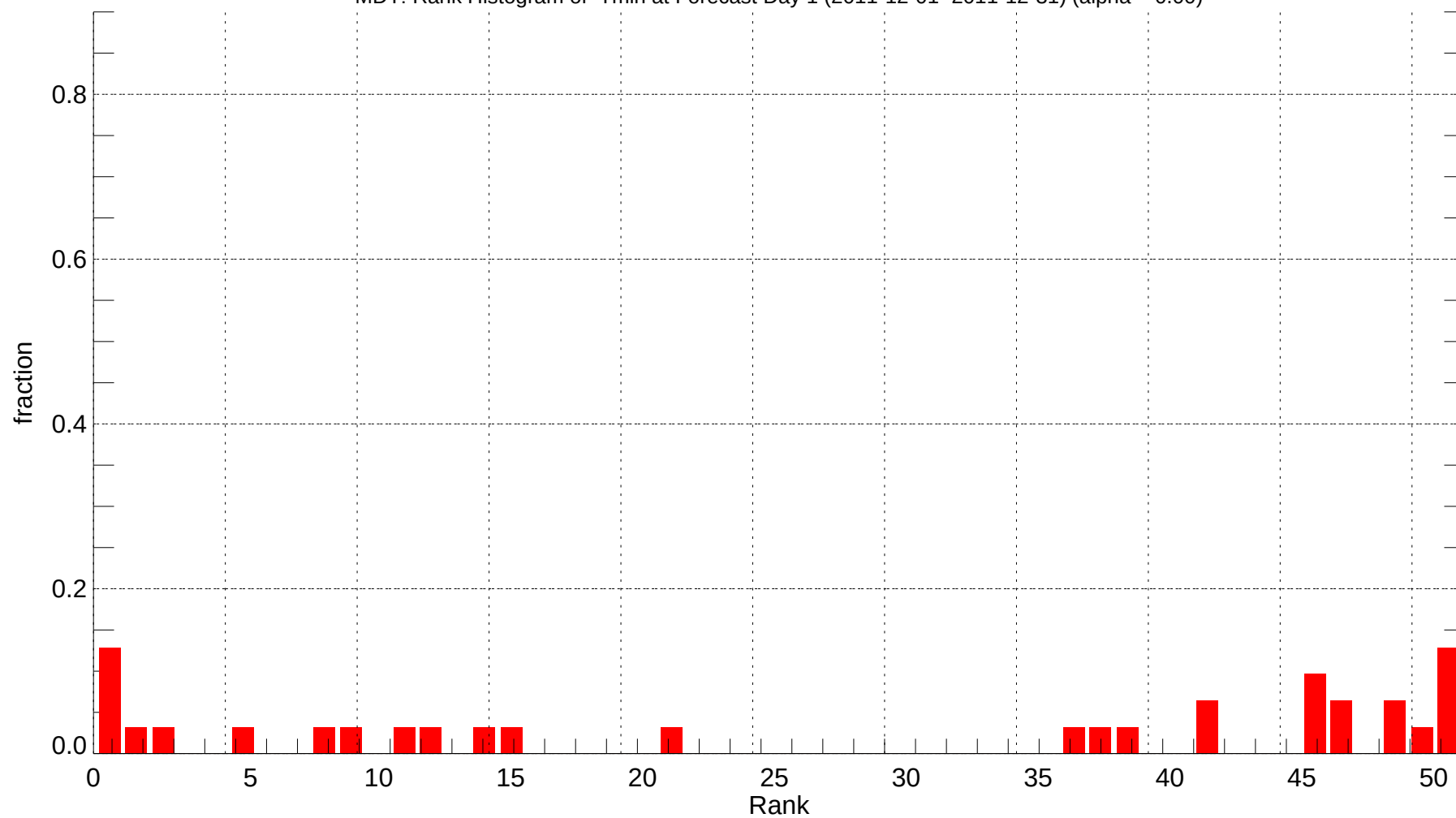
MDT: Rank Histogram of Tmin at Forecast Day 1 (2011-12-01~2011-12-31) (alpha = 0.00)
