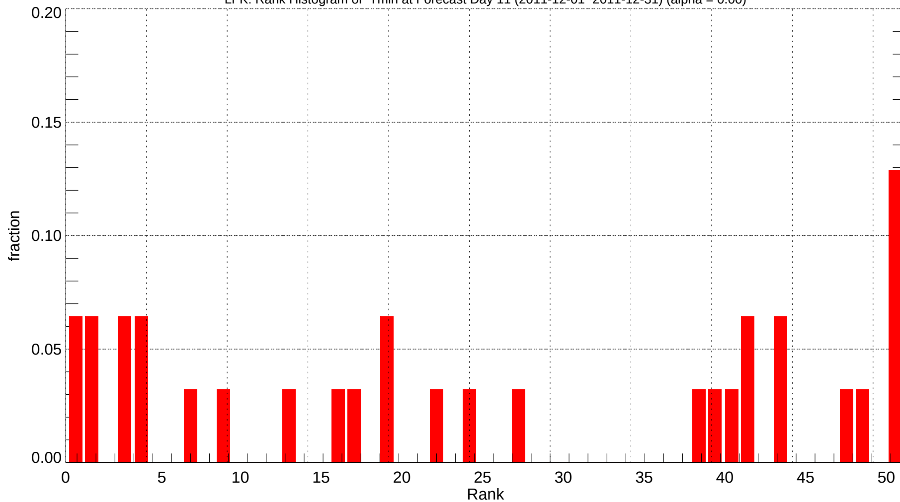
LFK: Rank Histogram of Tmin at Forecast Day 11 (2011-12-01~2011-12-31) (alpha = 0.00)
