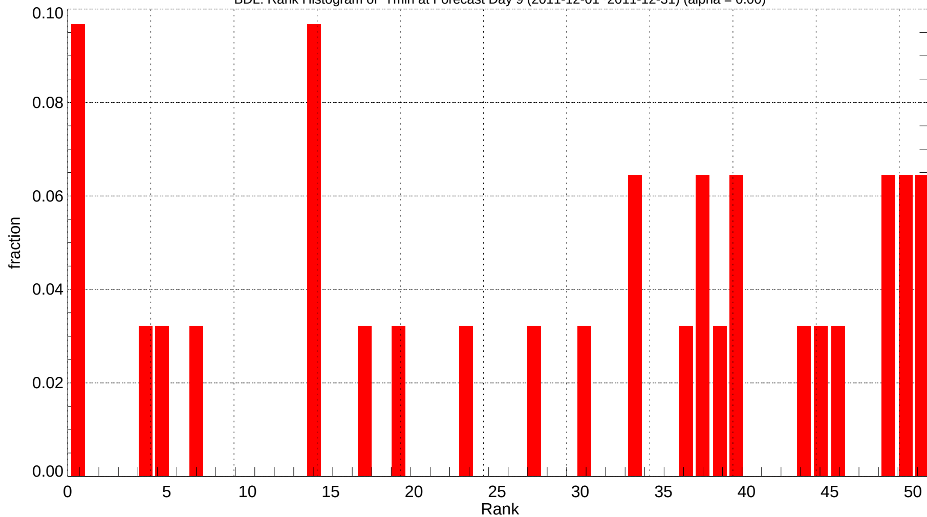
BDL: Rank Histogram of Tmin at Forecast Day 9 (2011-12-01~2011-12-31) (alpha = 0.00)
