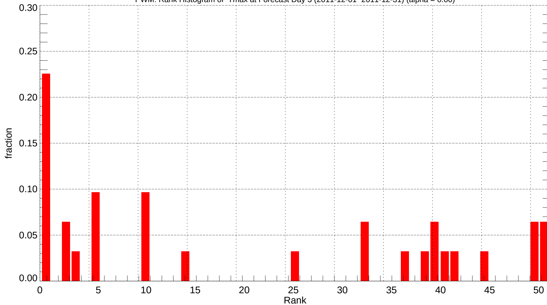
PWM: Rank Histogram of Tmax at Forecast Day 3 (2011-12-01~2011-12-31) (alpha = 0.00)
