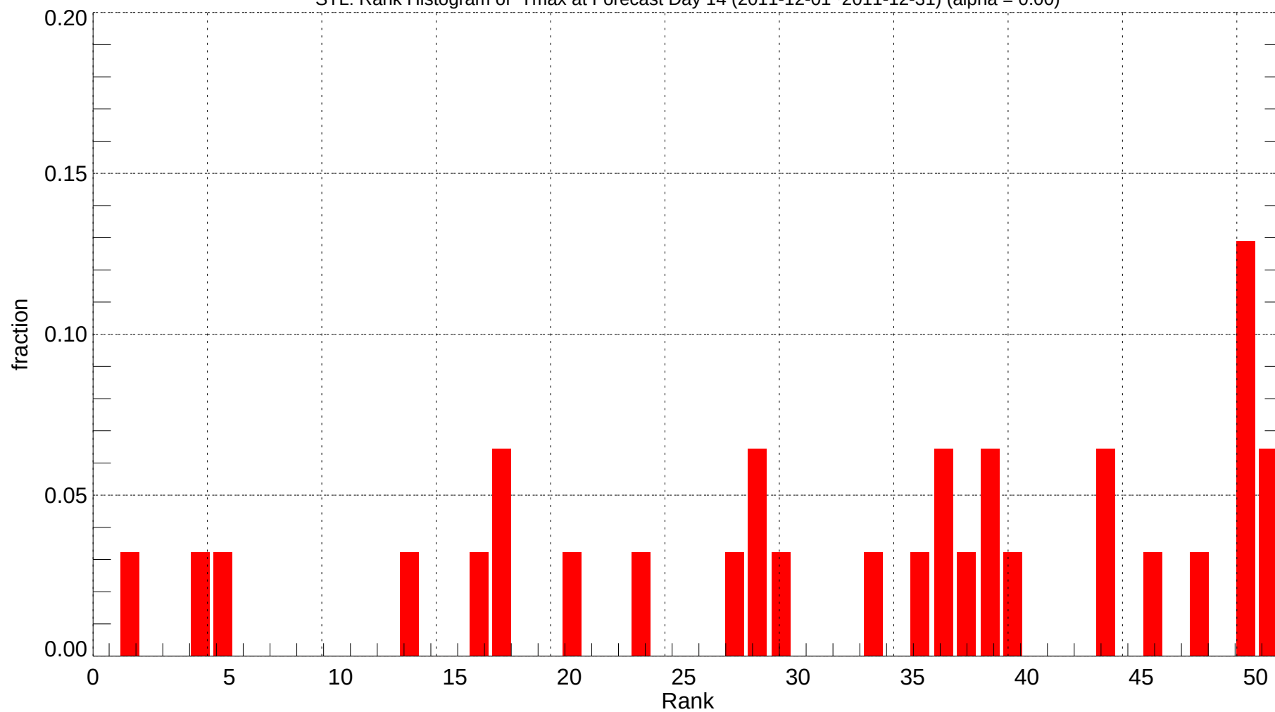
STL: Rank Histogram of Tmax at Forecast Day 14 (2011-12-01~2011-12-31) (alpha = 0.00)
