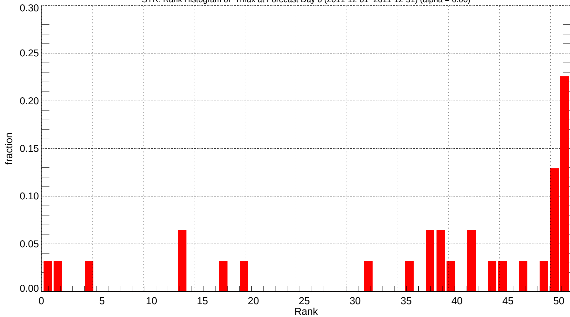
SYR: Rank Histogram of Tmax at Forecast Day 6 (2011-12-01~2011-12-31) (alpha = 0.00)
