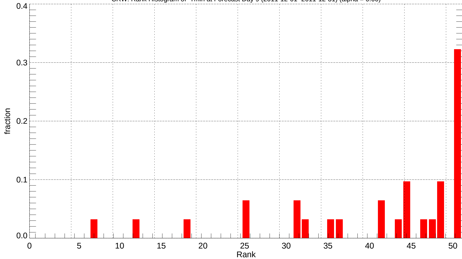
CRW: Rank Histogram of Tmin at Forecast Day 9 (2011-12-01~2011-12-31) (alpha = 0.00)
