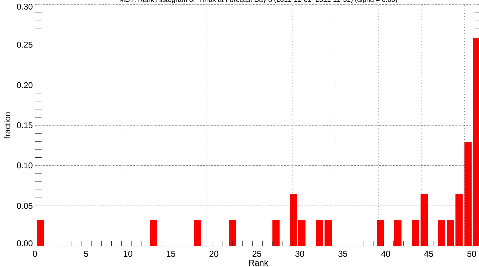
MDT: Rank Histogram of Tmax at Forecast Day 8 (2011-12-01~2011-12-31) (alpha = 0.00)
