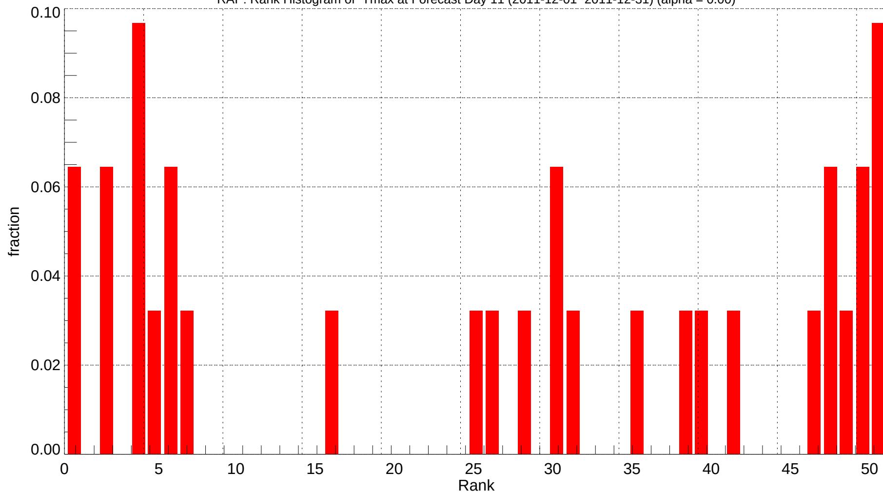
RAP: Rank Histogram of Tmax at Forecast Day 11 (2011-12-01~2011-12-31) (alpha = 0.00)
