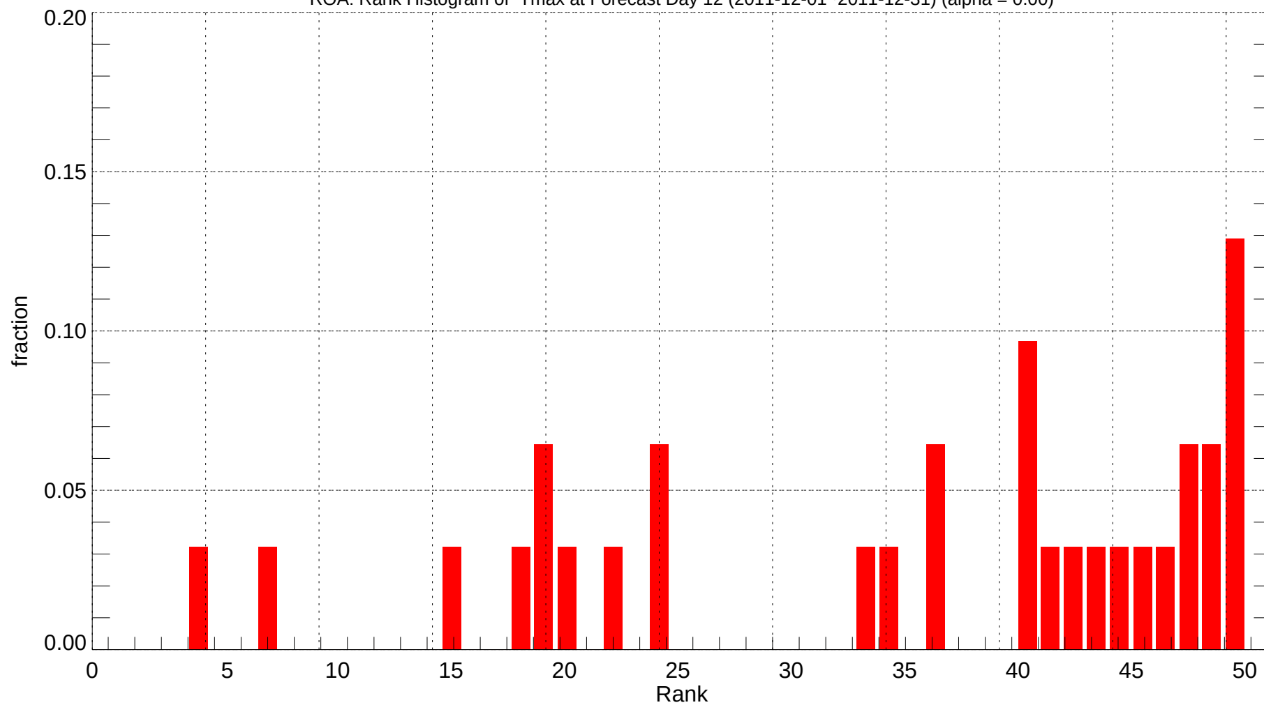
ROA: Rank Histogram of Tmax at Forecast Day 12 (2011-12-01~2011-12-31) (alpha = 0.00)
