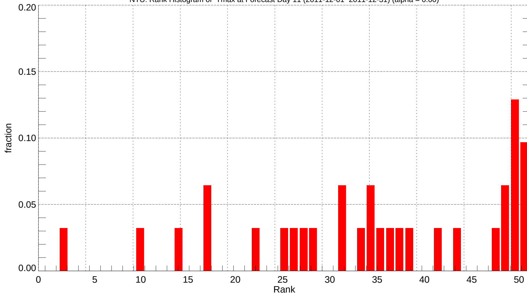
NTU: Rank Histogram of Tmax at Forecast Day 11 (2011-12-01~2011-12-31) (alpha = 0.00)
