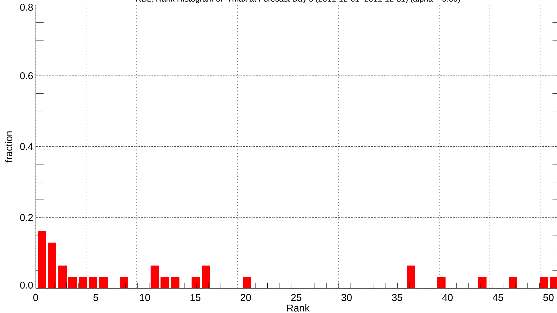
RBL: Rank Histogram of Tmax at Forecast Day 6 (2011-12-01~2011-12-31) (alpha = 0.00)
