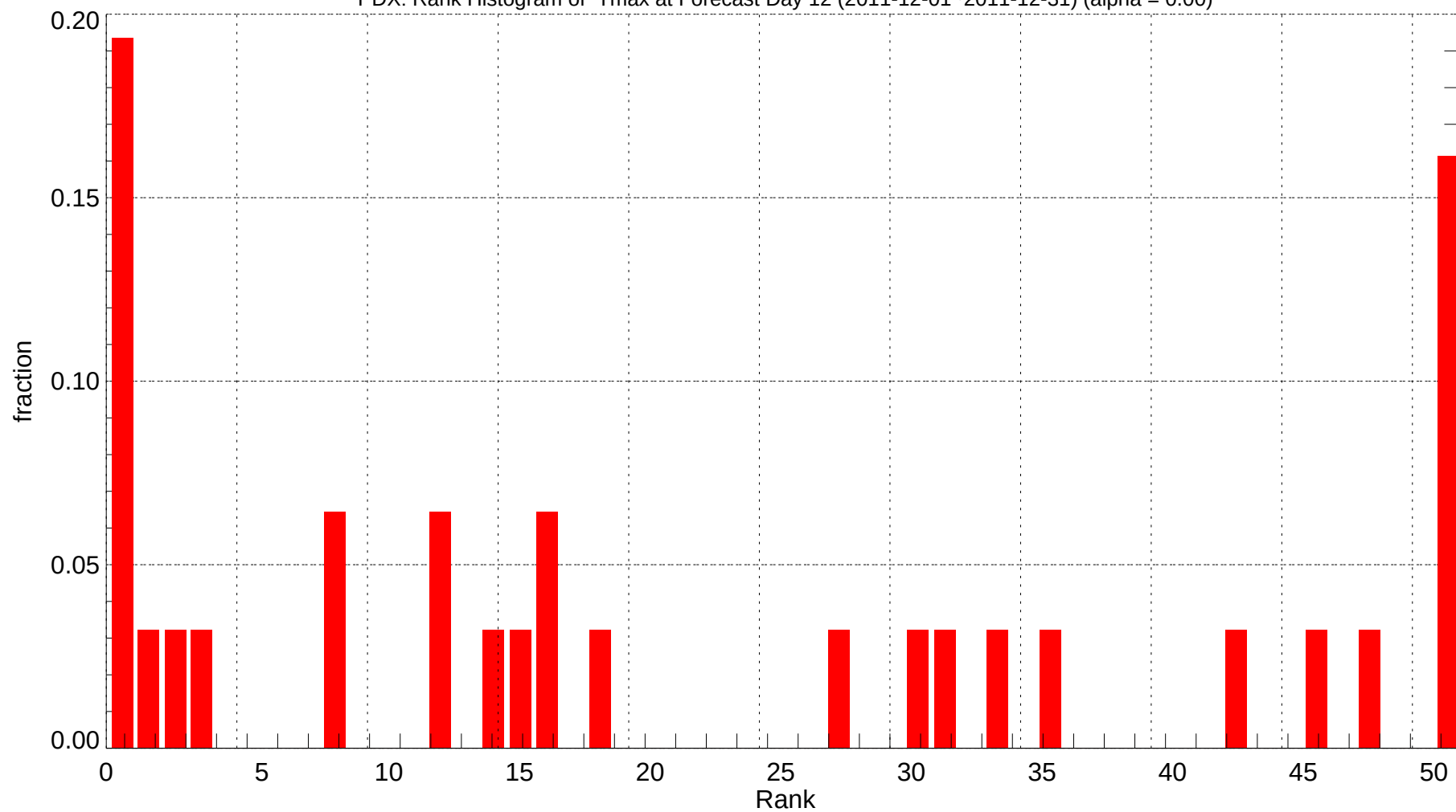
PDX: Rank Histogram of Tmax at Forecast Day 12 (2011-12-01~2011-12-31) (alpha = 0.00)
