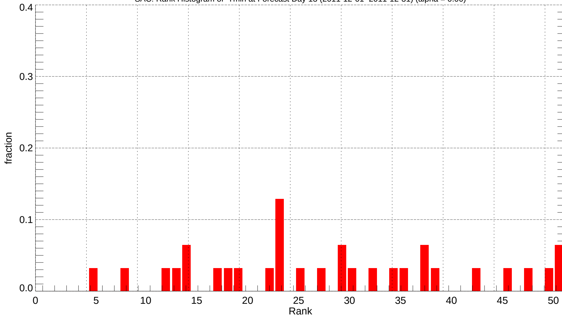
SAC: Rank Histogram of Tmin at Forecast Day 13 (2011-12-01~2011-12-31) (alpha = 0.00)
