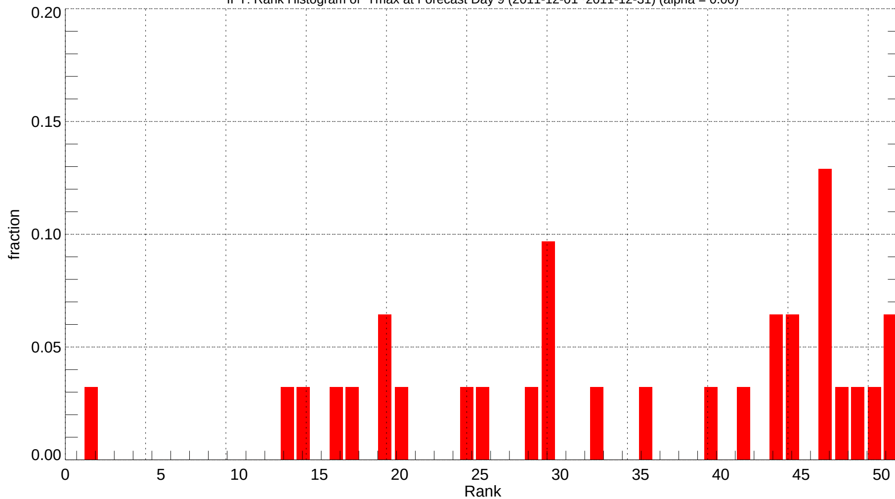
IPT: Rank Histogram of Tmax at Forecast Day 9 (2011-12-01~2011-12-31) (alpha = 0.00)
