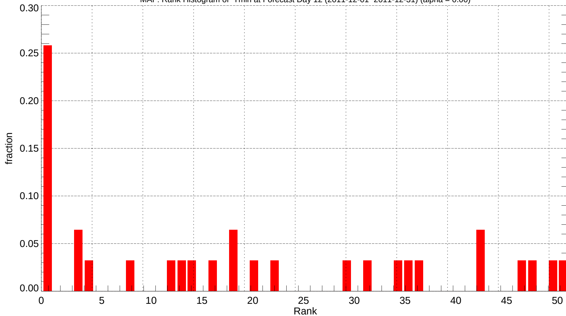
MAF: Rank Histogram of Tmin at Forecast Day 12 (2011-12-01~2011-12-31) (alpha = 0.00)
