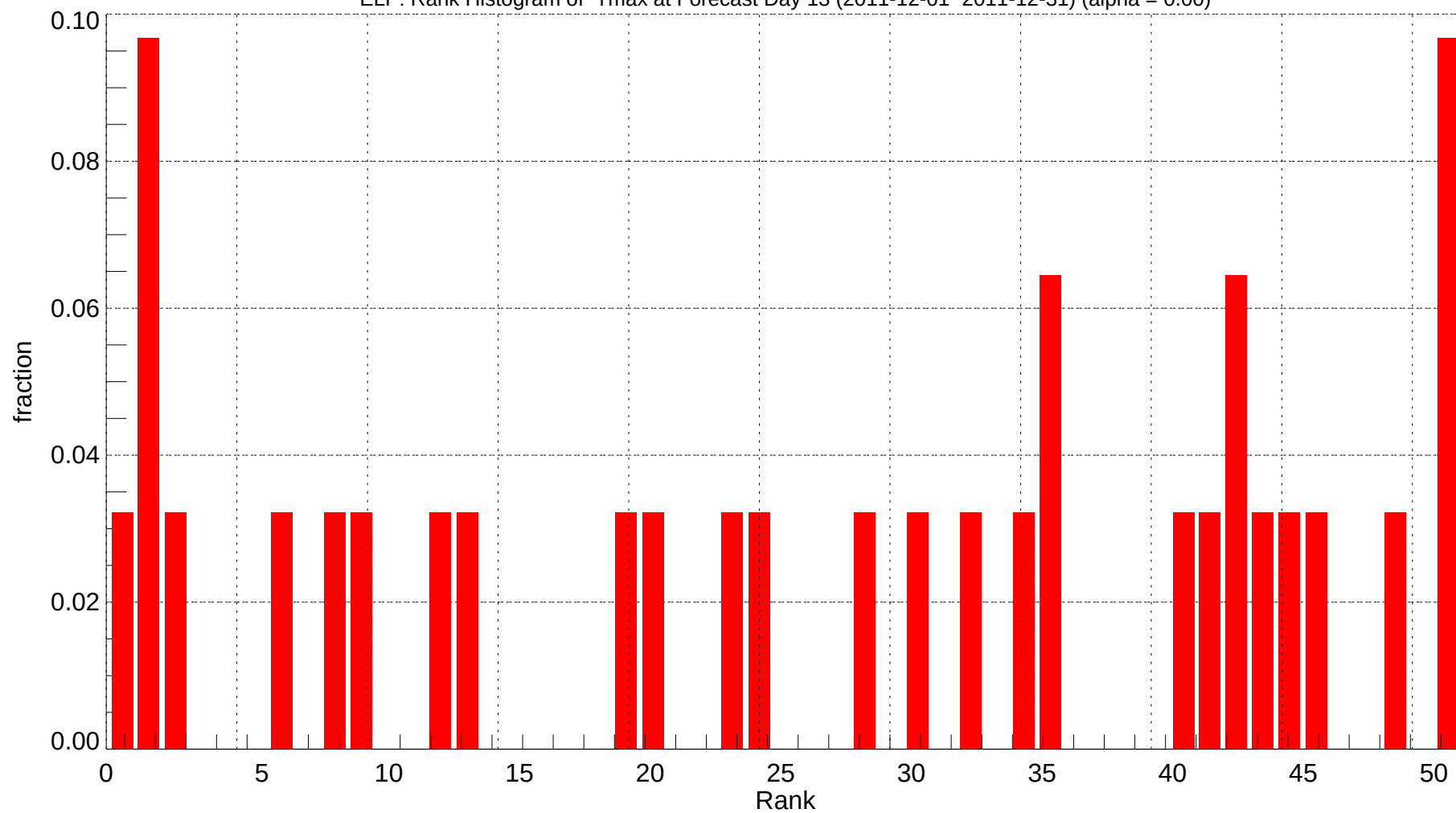
ELP: Rank Histogram of Tmax at Forecast Day 13 (2011-12-01~2011-12-31) (alpha = 0.00)
