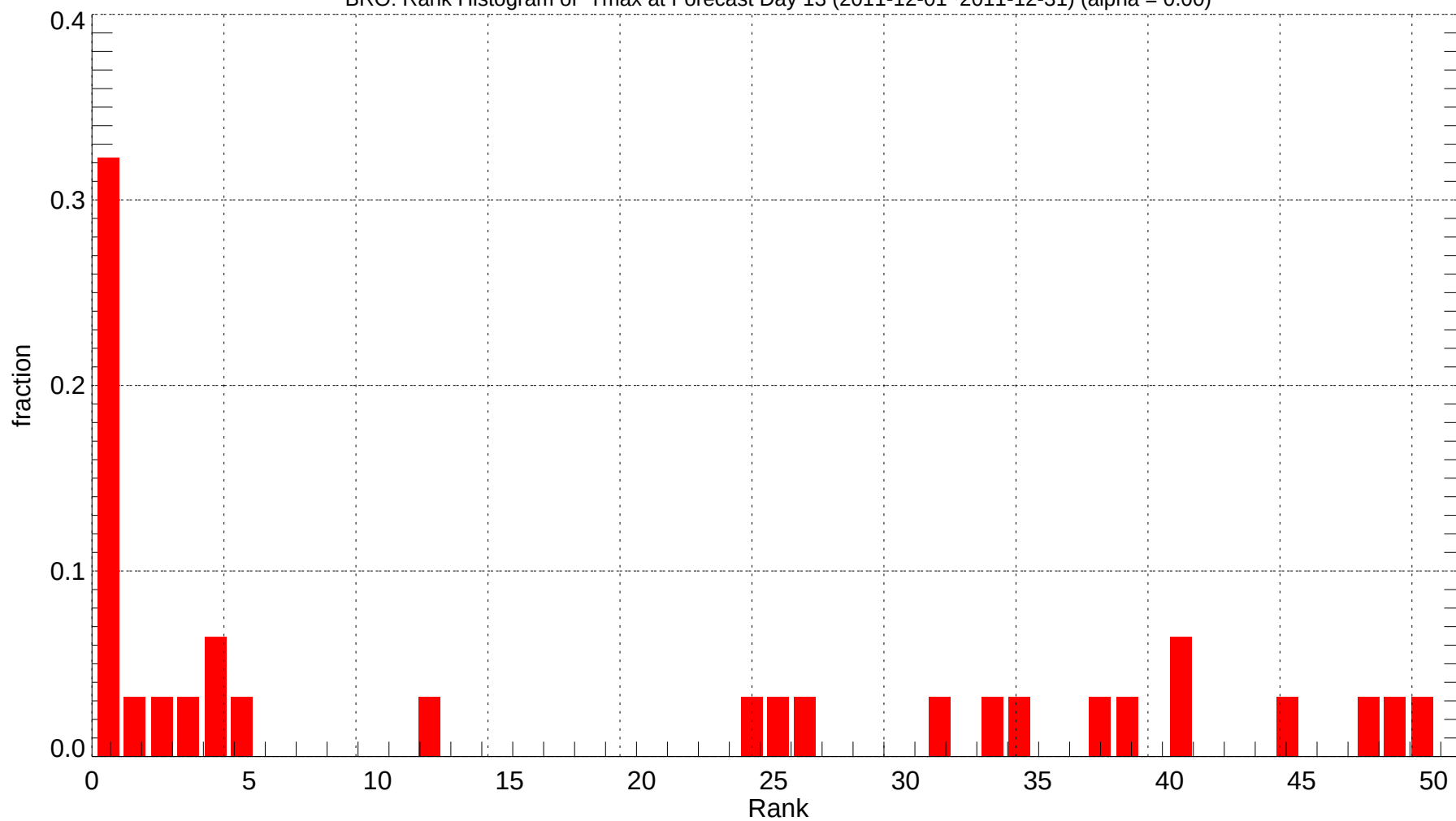
BRO: Rank Histogram of Tmax at Forecast Day 13 (2011-12-01~2011-12-31) (alpha = 0.00)
