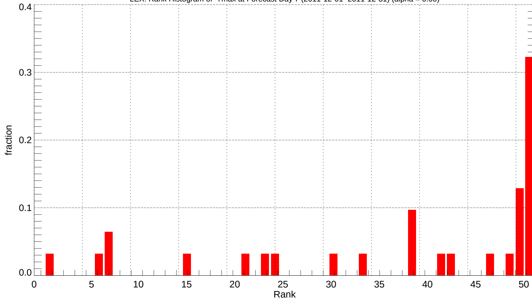
LEX: Rank Histogram of Tmax at Forecast Day 7 (2011-12-01~2011-12-31) (alpha = 0.00)
