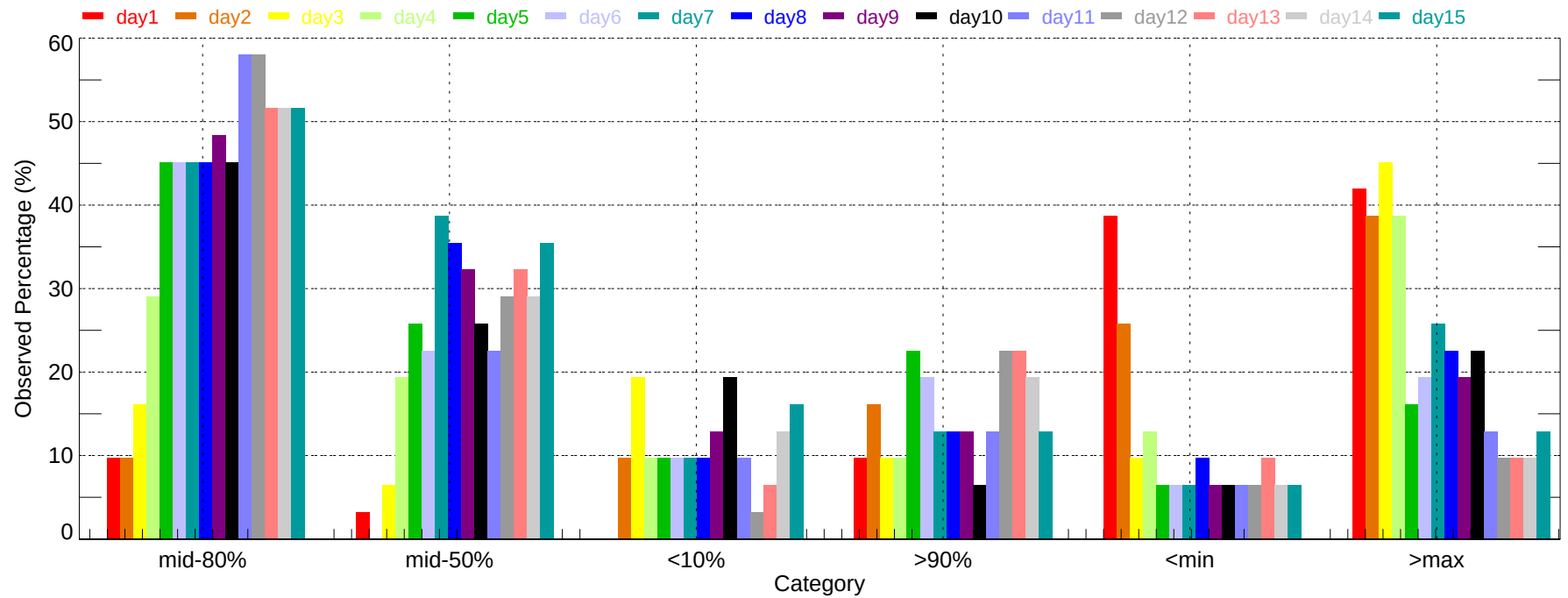
Observed Percentage of Ensembles - PIR: Max Temperature (2011-12-01~2011-12-31)
