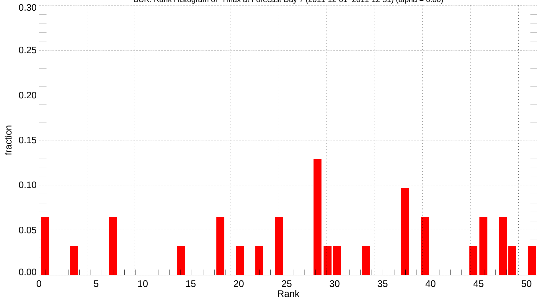
BUR: Rank Histogram of Tmax at Forecast Day 7 (2011-12-01~2011-12-31) (alpha = 0.00)
