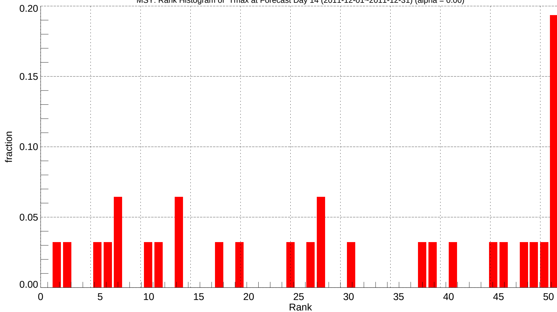
MSY: Rank Histogram of Tmax at Forecast Day 14 (2011-12-01~2011-12-31) (alpha = 0.00)
