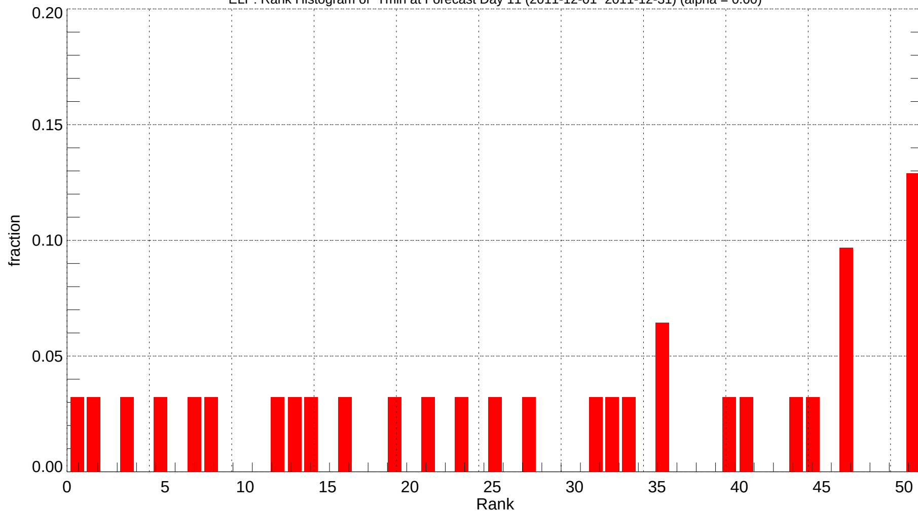
ELP: Rank Histogram of Tmin at Forecast Day 11 (2011-12-01~2011-12-31) (alpha = 0.00)
