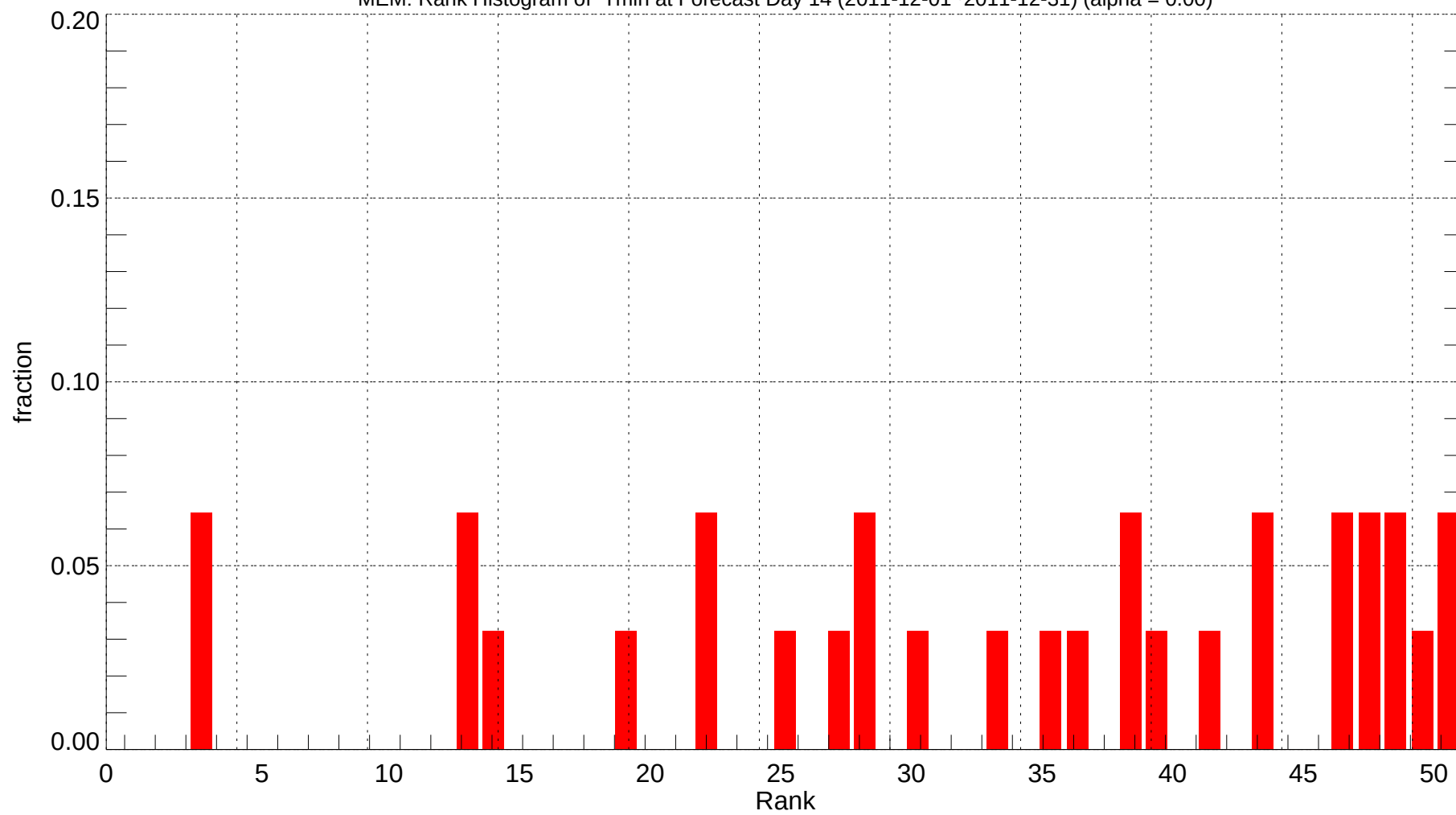
MEM: Rank Histogram of Tmin at Forecast Day 14 (2011-12-01~2011-12-31) (alpha = 0.00)
