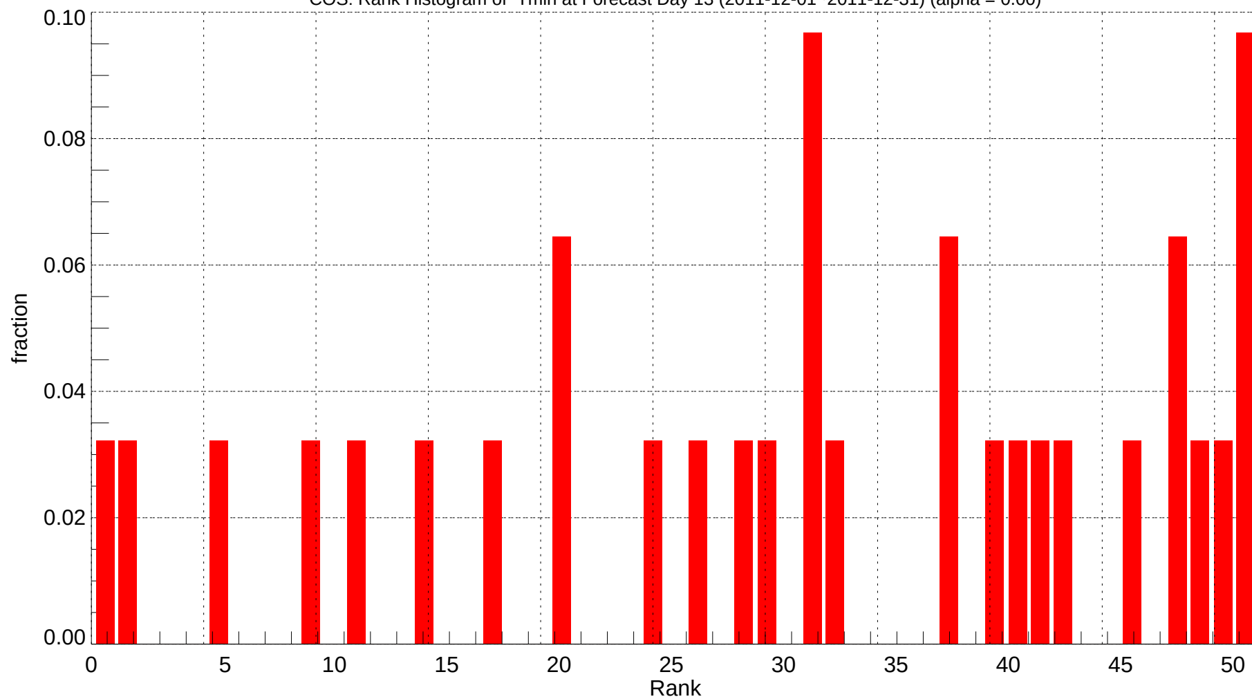
COS: Rank Histogram of Tmin at Forecast Day 13 (2011-12-01~2011-12-31) (alpha = 0.00)
