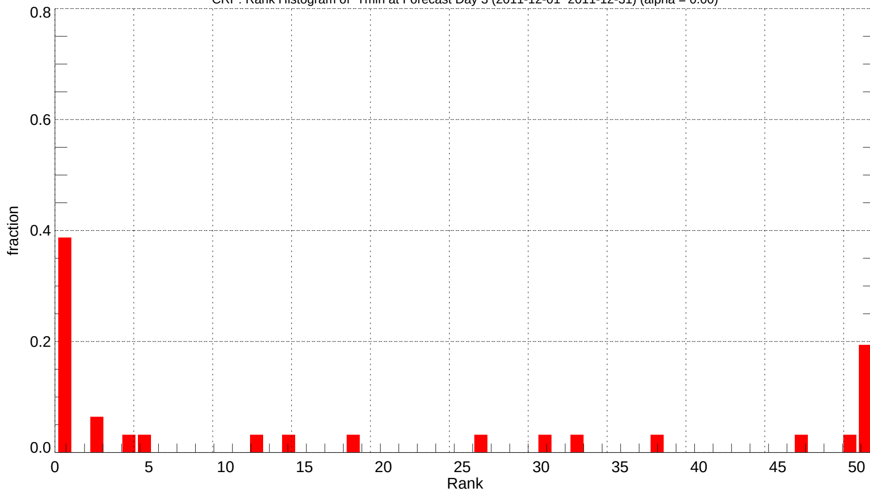
CRP: Rank Histogram of Tmin at Forecast Day 3 (2011-12-01~2011-12-31) (alpha = 0.00)
