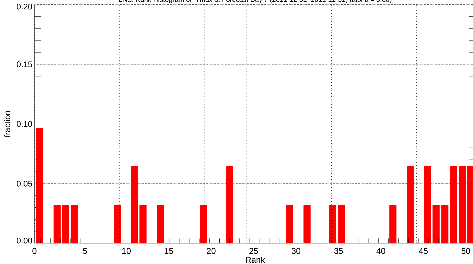
LNS: Rank Histogram of Tmax at Forecast Day 7 (2011-12-01~2011-12-31) (alpha = 0.00)
