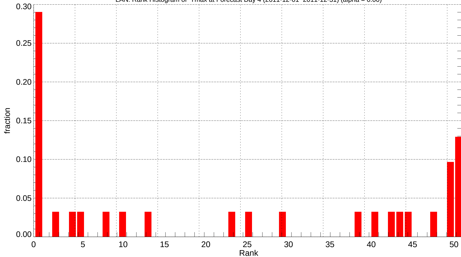
LAN: Rank Histogram of Tmax at Forecast Day 4 (2011-12-01~2011-12-31) (alpha = 0.00)
