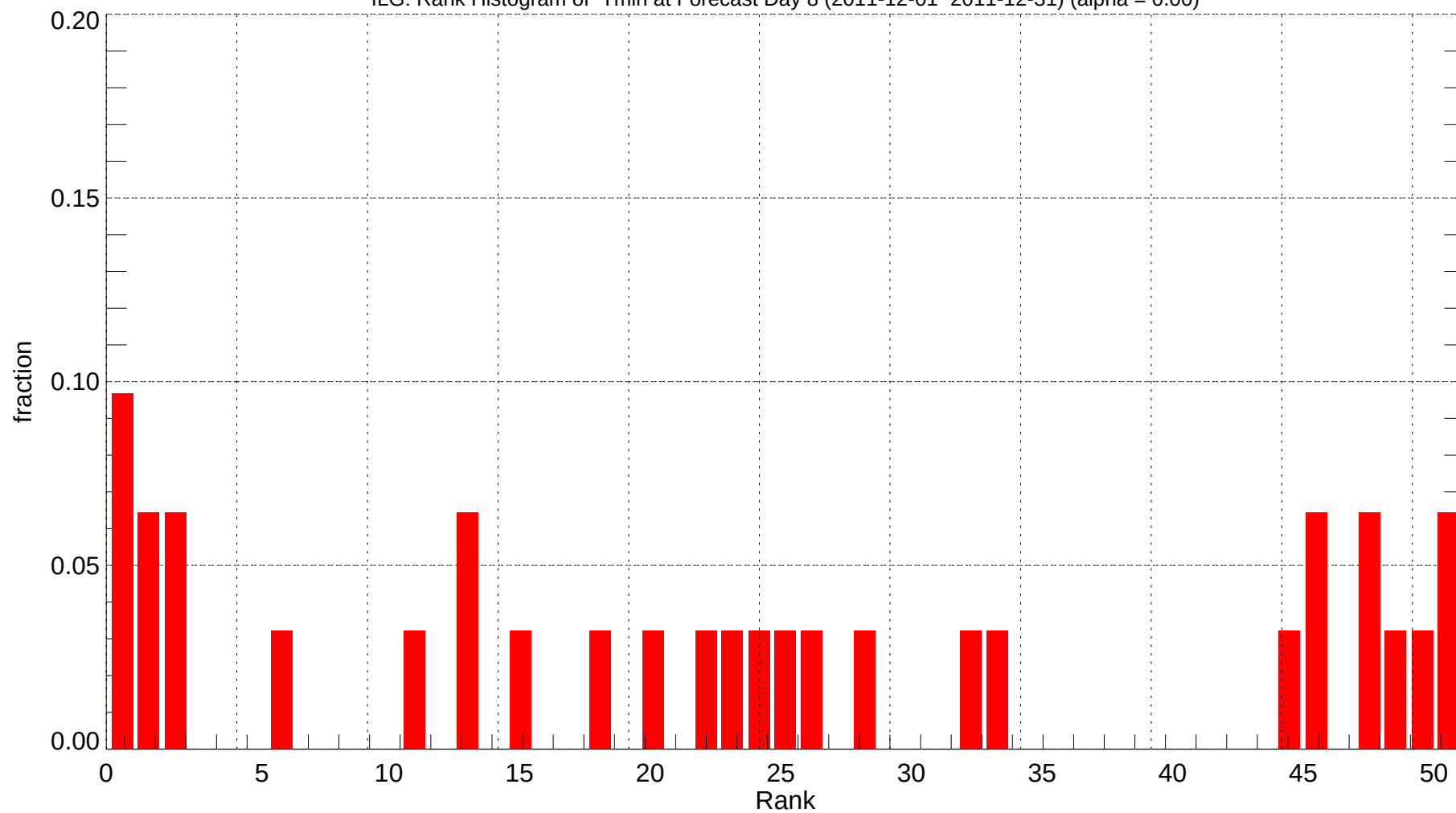
ILG: Rank Histogram of Tmin at Forecast Day 8 (2011-12-01~2011-12-31) (alpha = 0.00)
