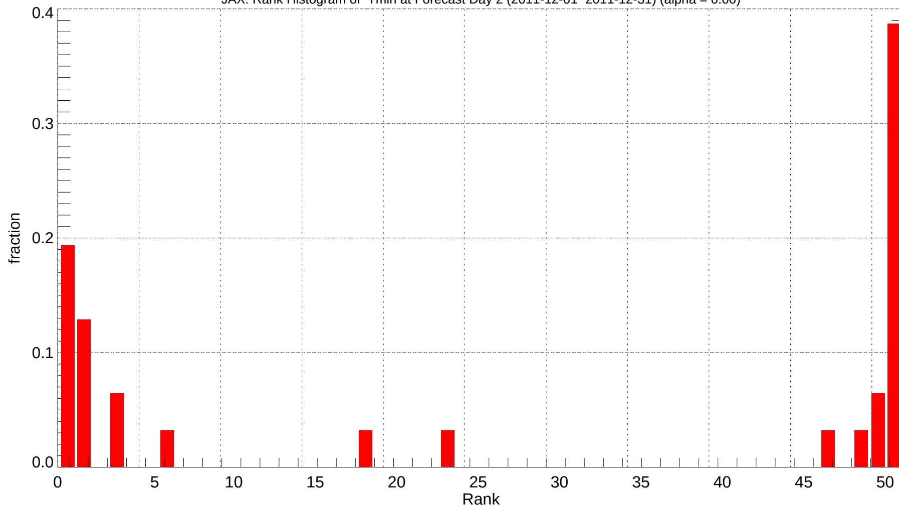
JAX: Rank Histogram of Tmin at Forecast Day 2 (2011-12-01~2011-12-31) (alpha = 0.00)
