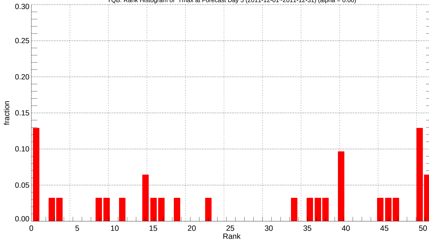
YQB: Rank Histogram of Tmax at Forecast Day 5 (2011-12-01~2011-12-31) (alpha = 0.00)
