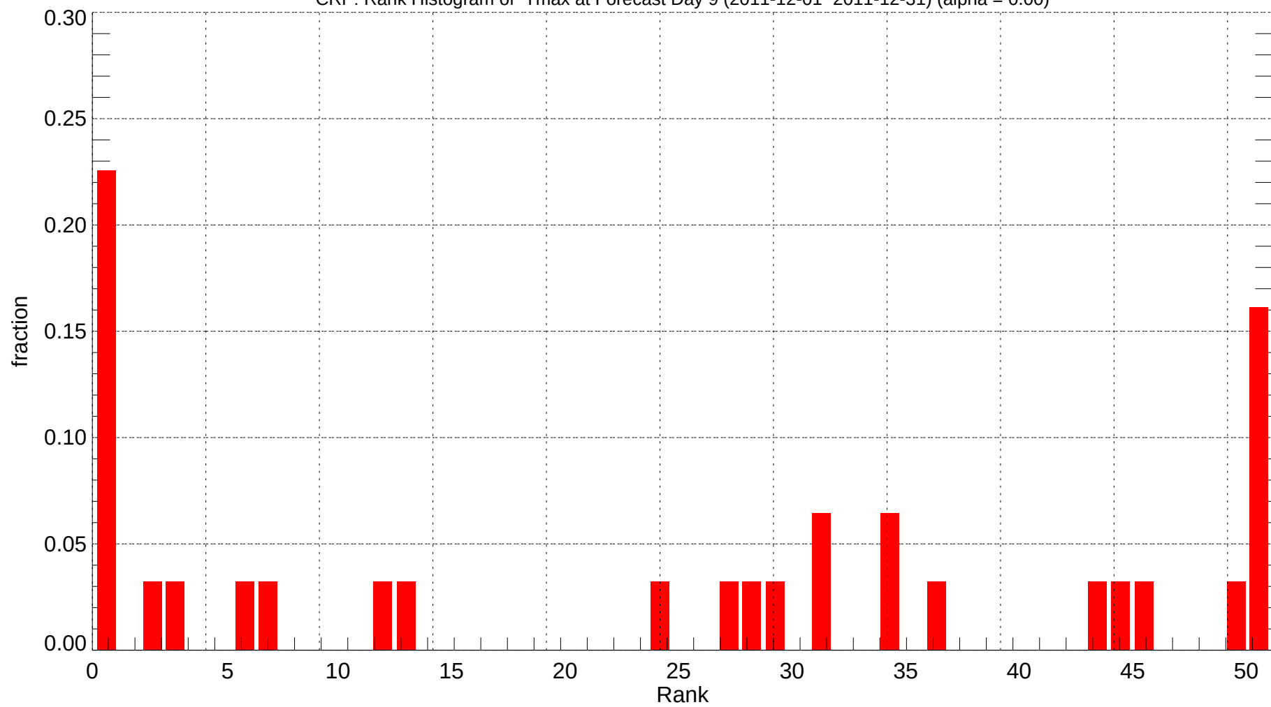
CRP: Rank Histogram of Tmax at Forecast Day 9 (2011-12-01~2011-12-31) (alpha = 0.00)
