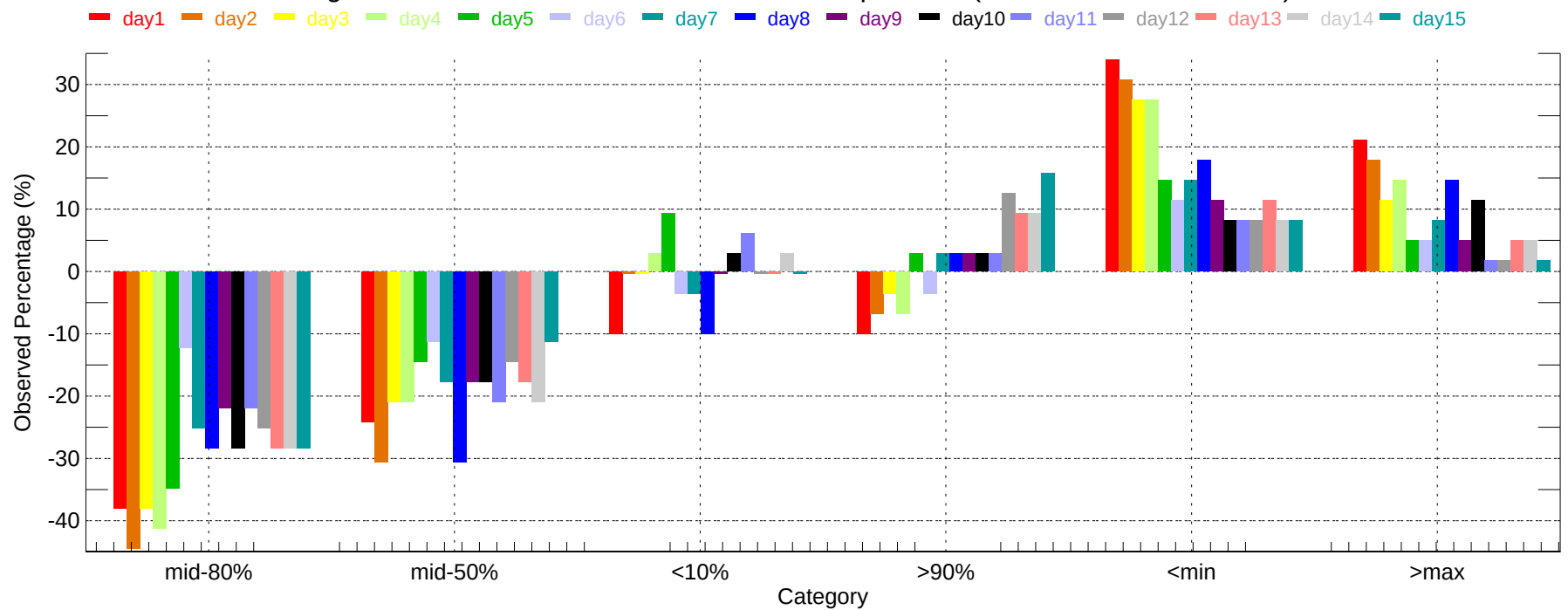
Observed Percentage Deviation of Ensembles - BIS: Max Temperature (2011-12-01~2011-12-31)
