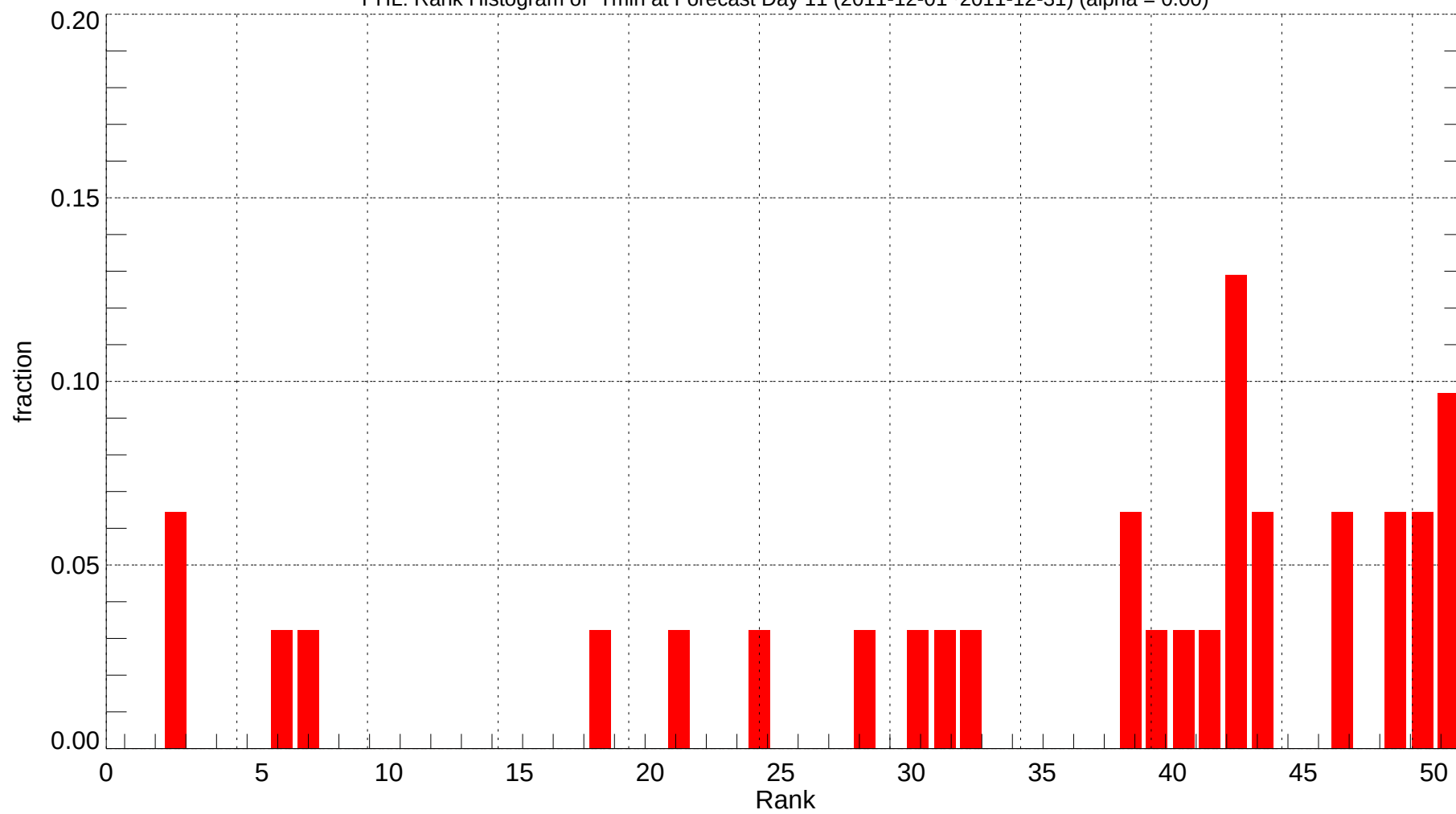
PHL: Rank Histogram of Tmin at Forecast Day 11 (2011-12-01~2011-12-31) (alpha = 0.00)
