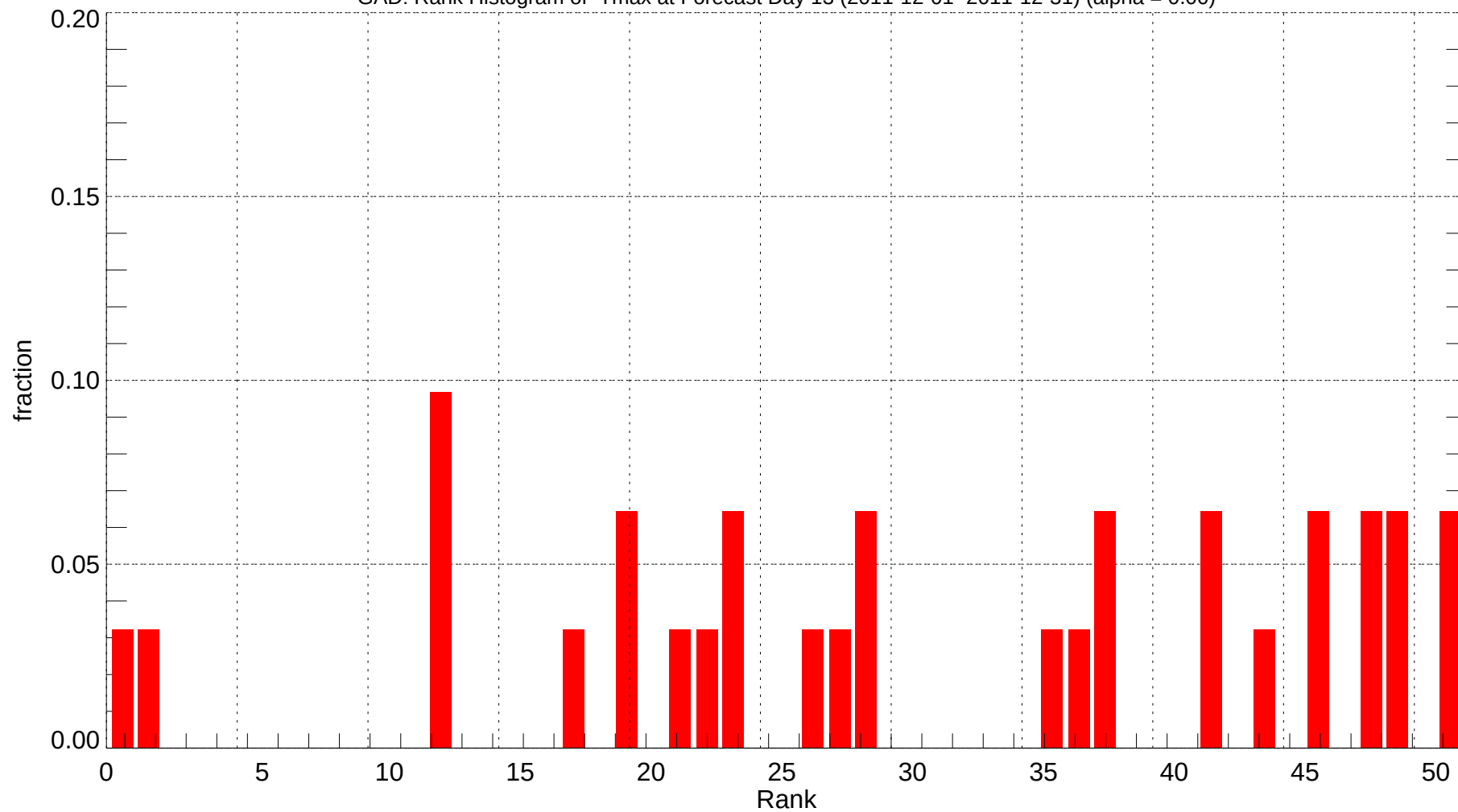
GAD: Rank Histogram of Tmax at Forecast Day 13 (2011-12-01~2011-12-31) (alpha = 0.00)
