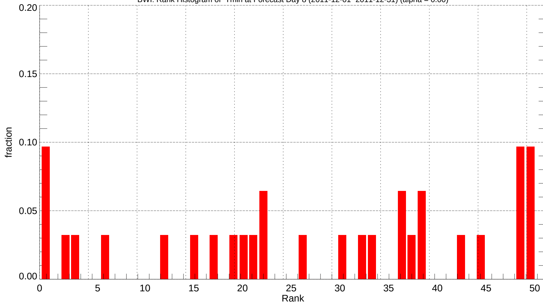
BWI: Rank Histogram of Tmin at Forecast Day 8 (2011-12-01~2011-12-31) (alpha = 0.00)
