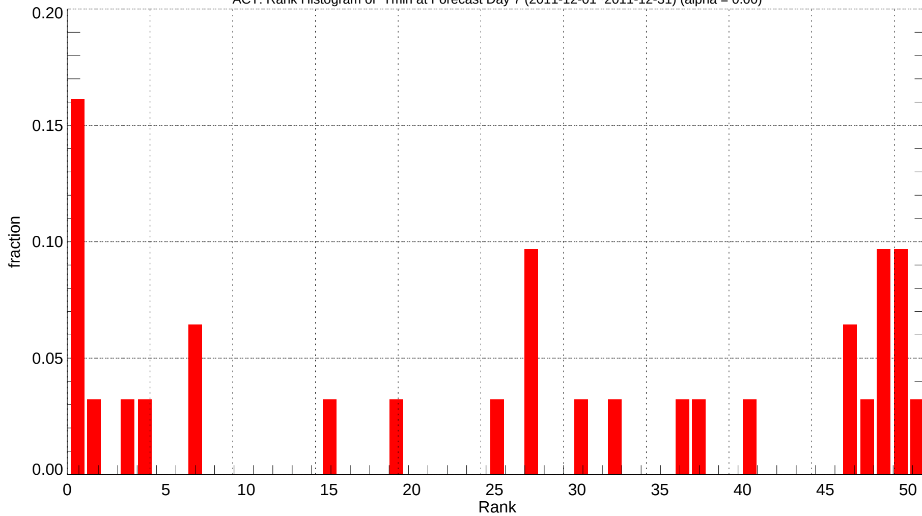
ACT: Rank Histogram of Tmin at Forecast Day 7 (2011-12-01~2011-12-31) (alpha = 0.00)
