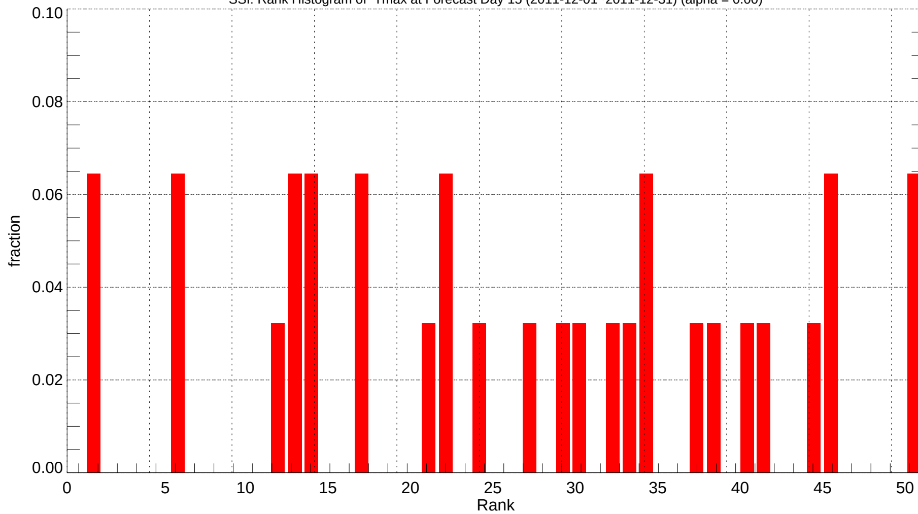
SSI: Rank Histogram of Tmax at Forecast Day 15 (2011-12-01~2011-12-31) (alpha = 0.00)
