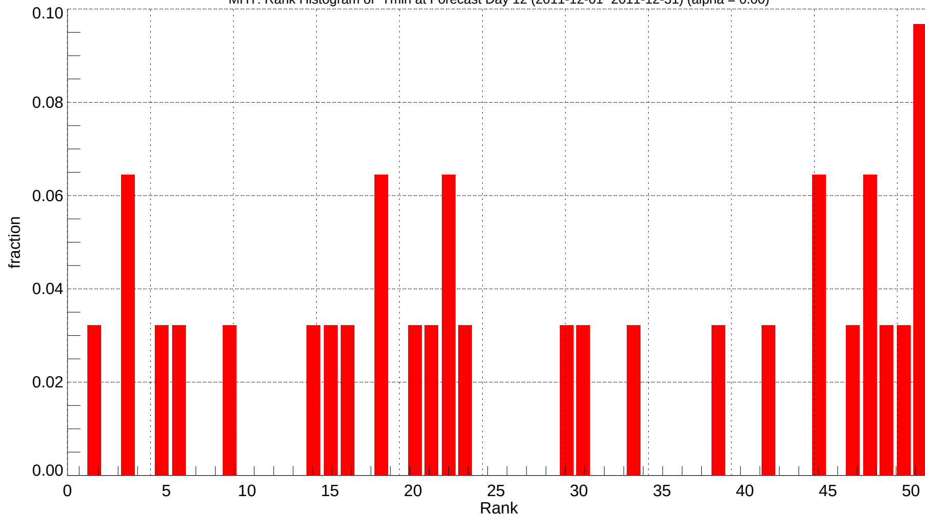
MHT: Rank Histogram of Tmin at Forecast Day 12 (2011-12-01~2011-12-31) (alpha = 0.00)
