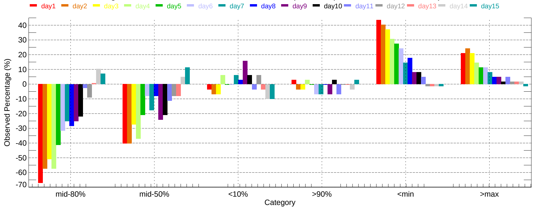
Observed Percentage Deviation of Ensembles - LGB: Min Temperature (2011-12-01~2011-12-31)
