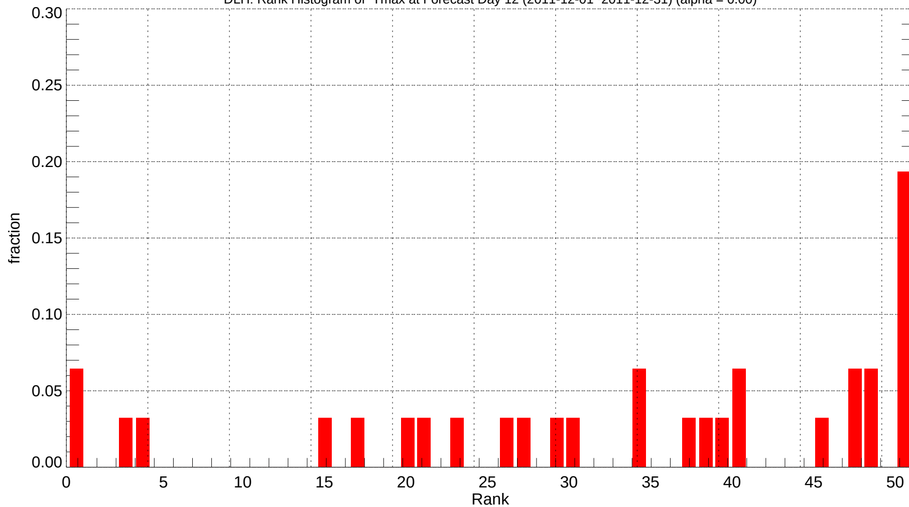
DLH: Rank Histogram of Tmax at Forecast Day 12 (2011-12-01~2011-12-31) (alpha = 0.00)
