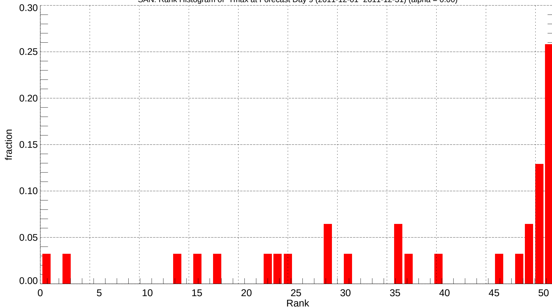
SAN: Rank Histogram of Tmax at Forecast Day 9 (2011-12-01~2011-12-31) (alpha = 0.00)
