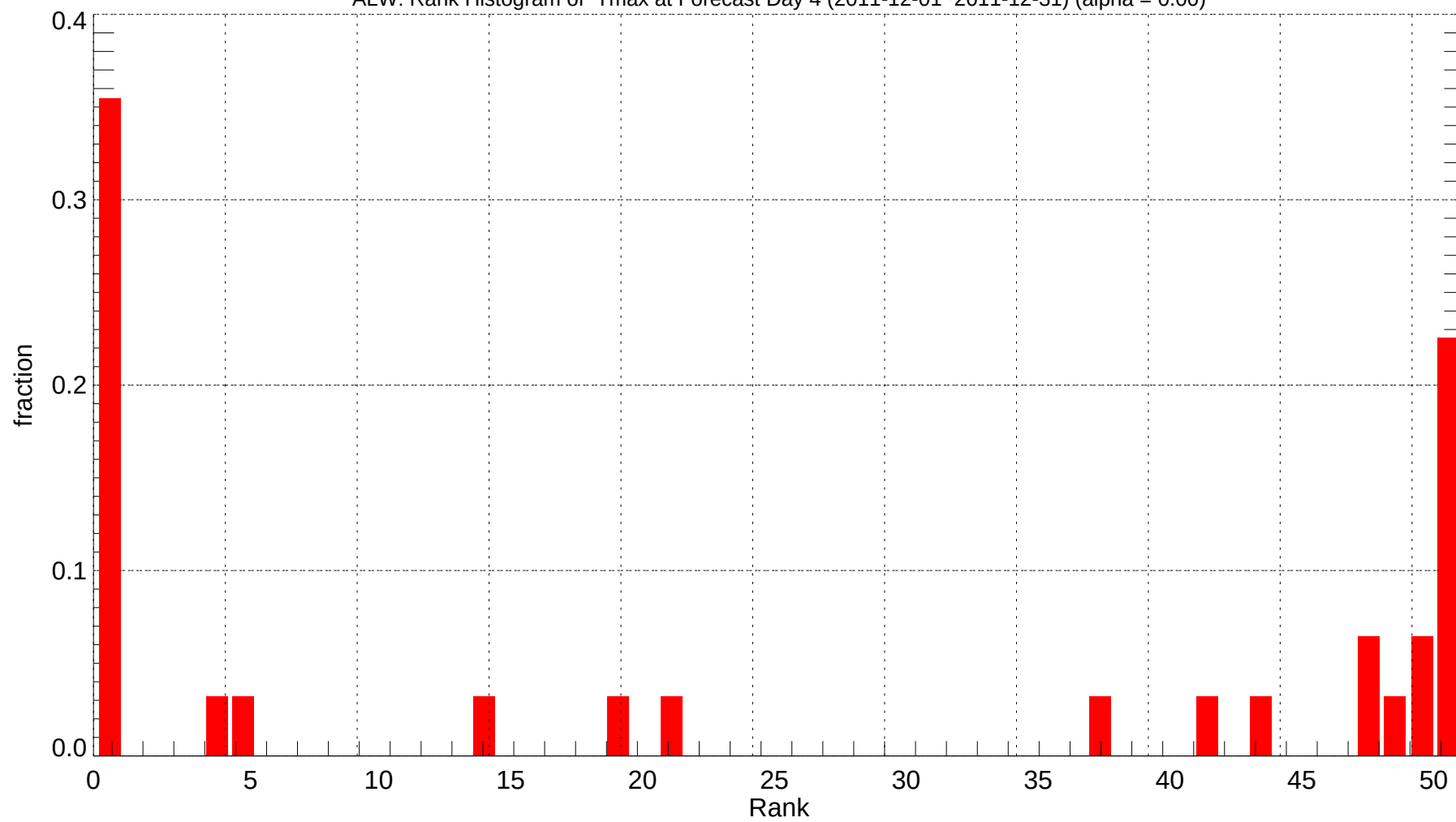
ALW: Rank Histogram of Tmax at Forecast Day 4 (2011-12-01~2011-12-31) (alpha = 0.00)
