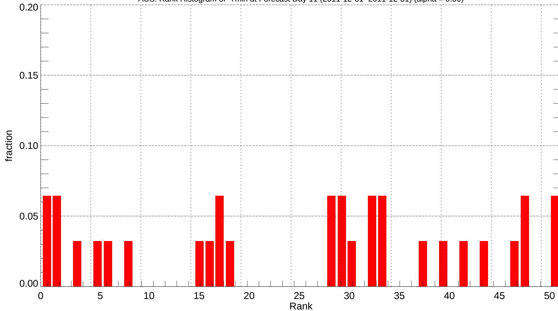
AUS: Rank Histogram of Tmin at Forecast Day 11 (2011-12-01~2011-12-31) (alpha = 0.00)
