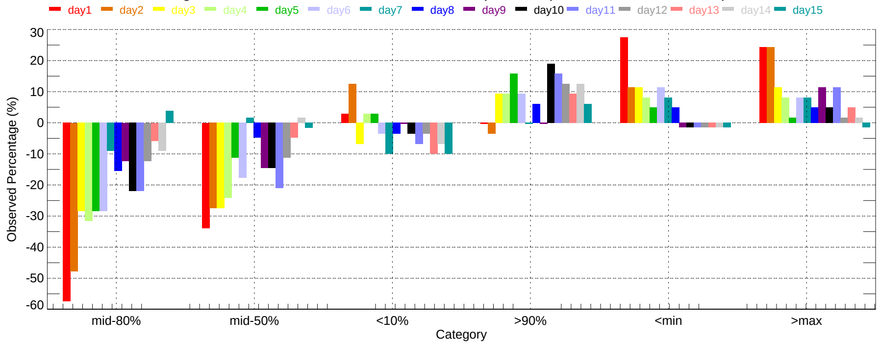
Observed Percentage Deviation of Ensembles - IND: Max Temperature (2011-12-01~2011-12-31)
