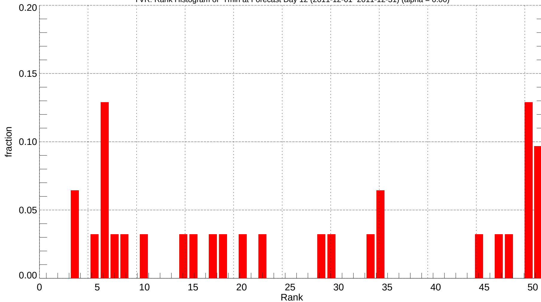
YVR: Rank Histogram of Tmin at Forecast Day 12 (2011-12-01~2011-12-31) (alpha = 0.00)
