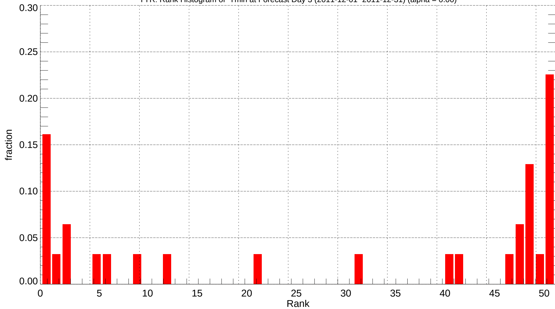
TYR: Rank Histogram of Tmin at Forecast Day 3 (2011-12-01~2011-12-31) (alpha = 0.00)
