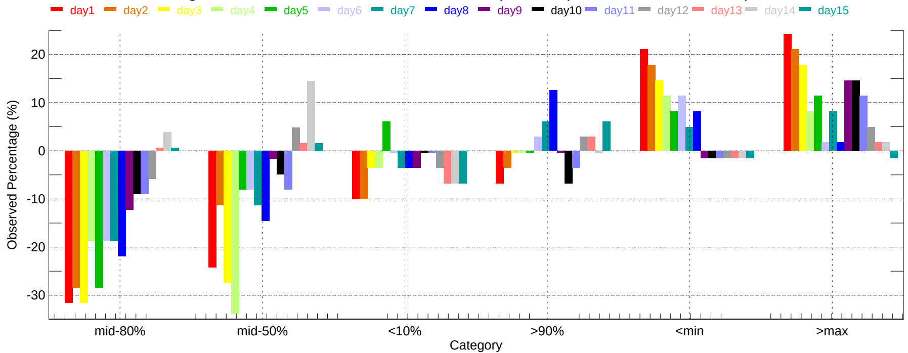
Observed Percentage Deviation of Ensembles - LGA: Min Temperature (2011-12-01~2011-12-31)
