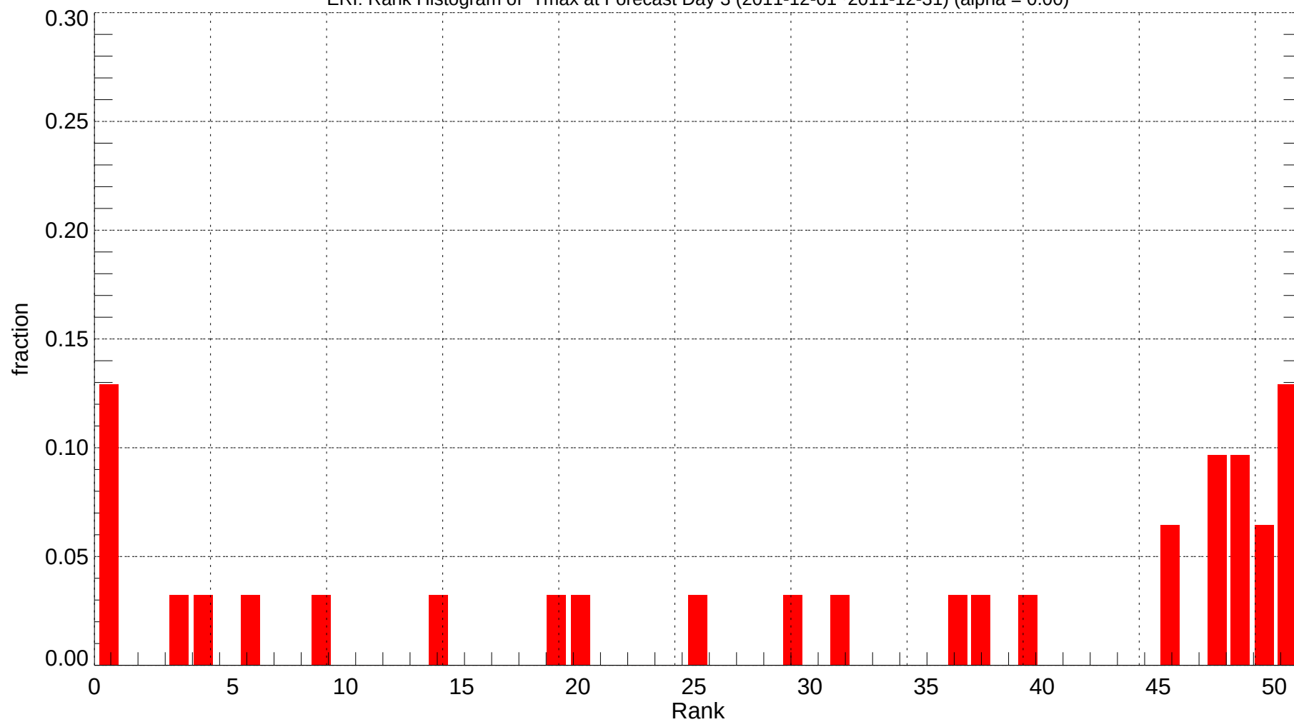
ERI: Rank Histogram of Tmax at Forecast Day 3 (2011-12-01~2011-12-31) (alpha = 0.00)
