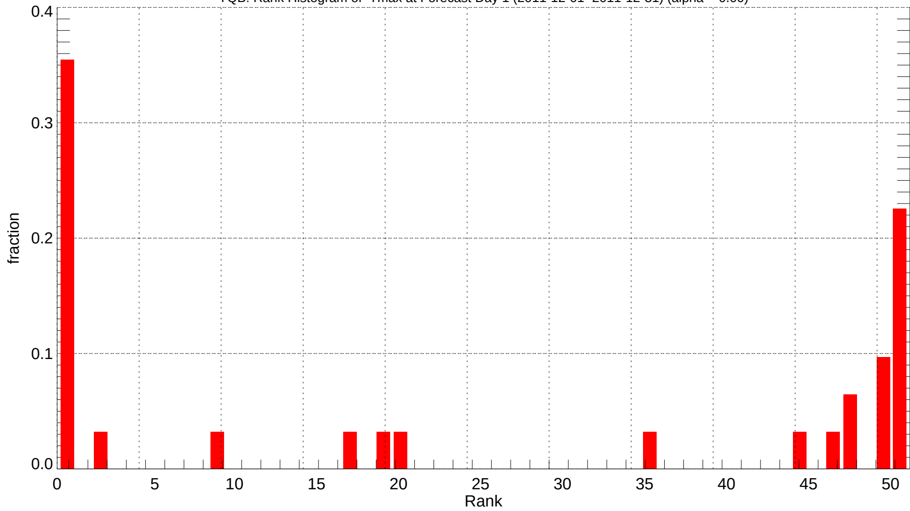
YQB: Rank Histogram of Tmax at Forecast Day 1 (2011-12-01~2011-12-31) (alpha = 0.00)
