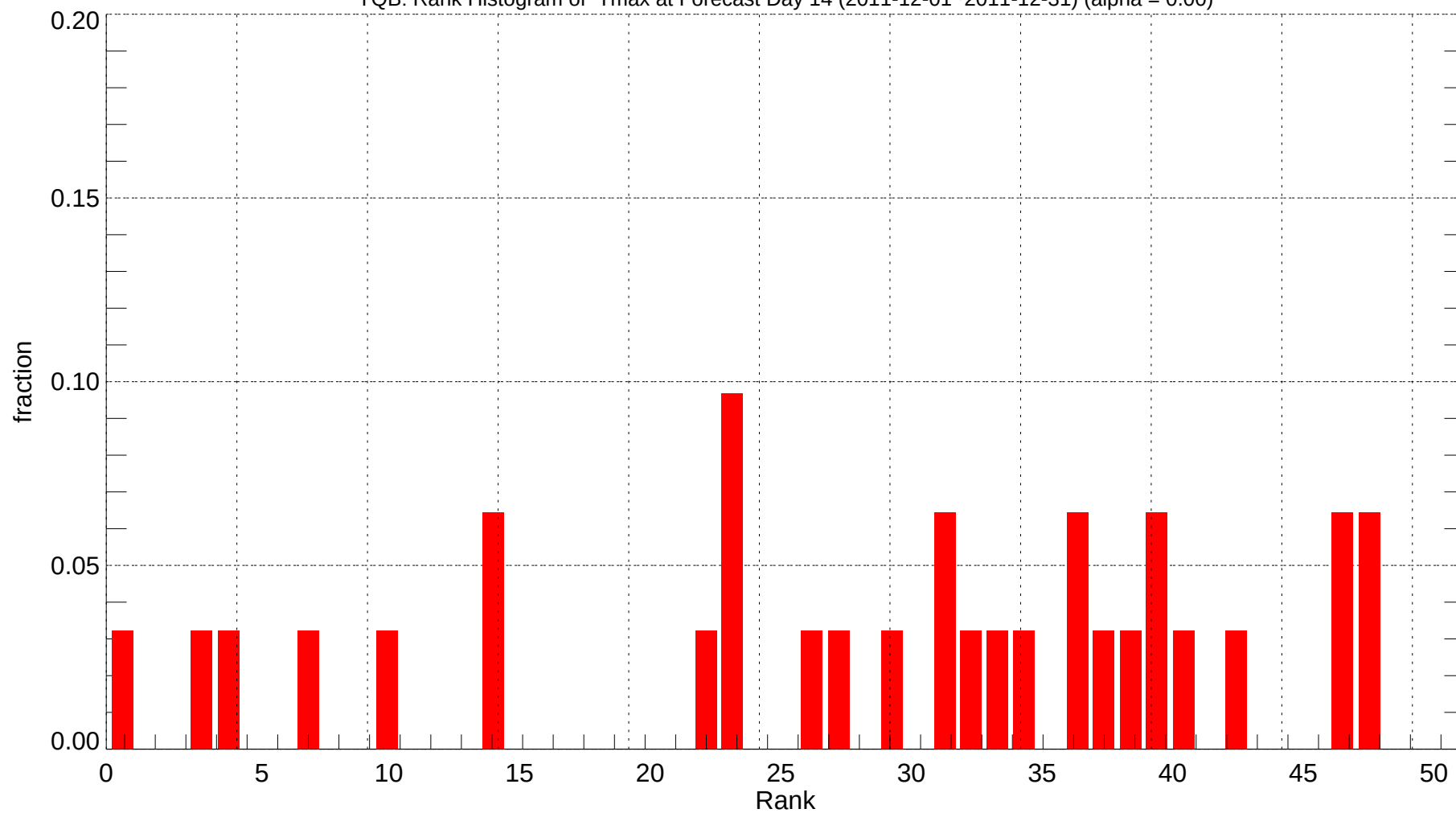
YQB: Rank Histogram of Tmax at Forecast Day 14 (2011-12-01~2011-12-31) (alpha = 0.00)
