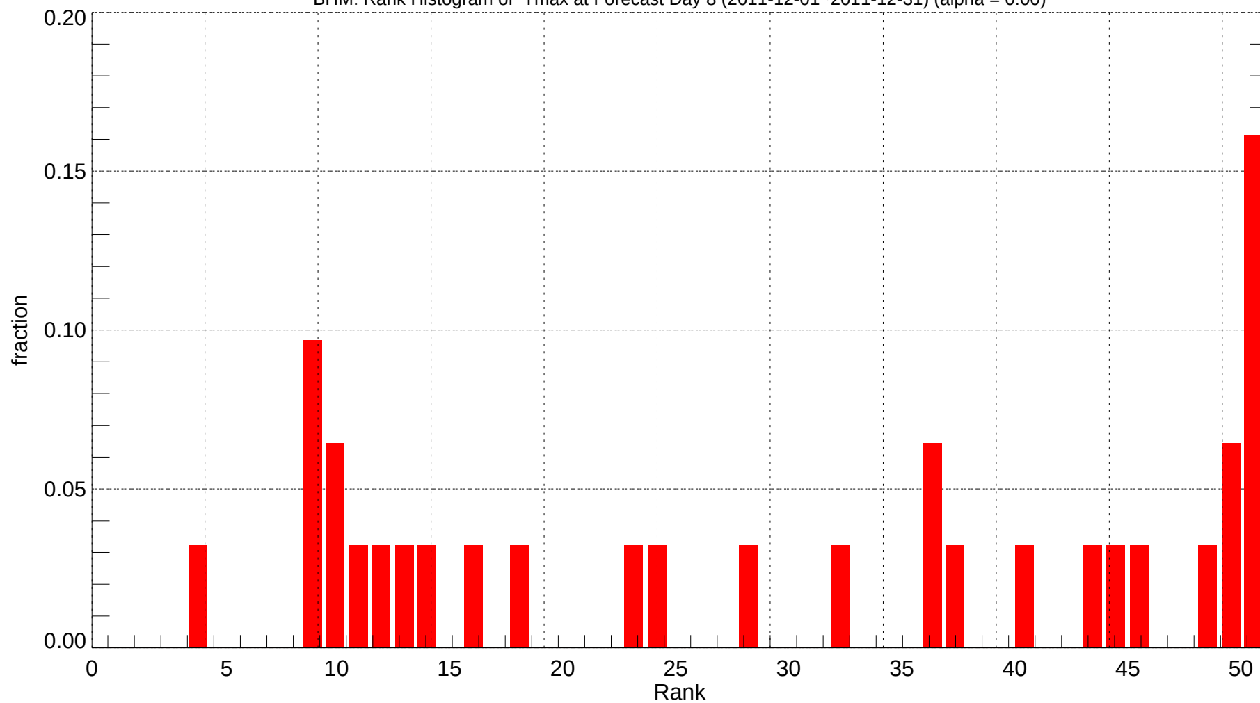
BHM: Rank Histogram of Tmax at Forecast Day 8 (2011-12-01~2011-12-31) (alpha = 0.00)
