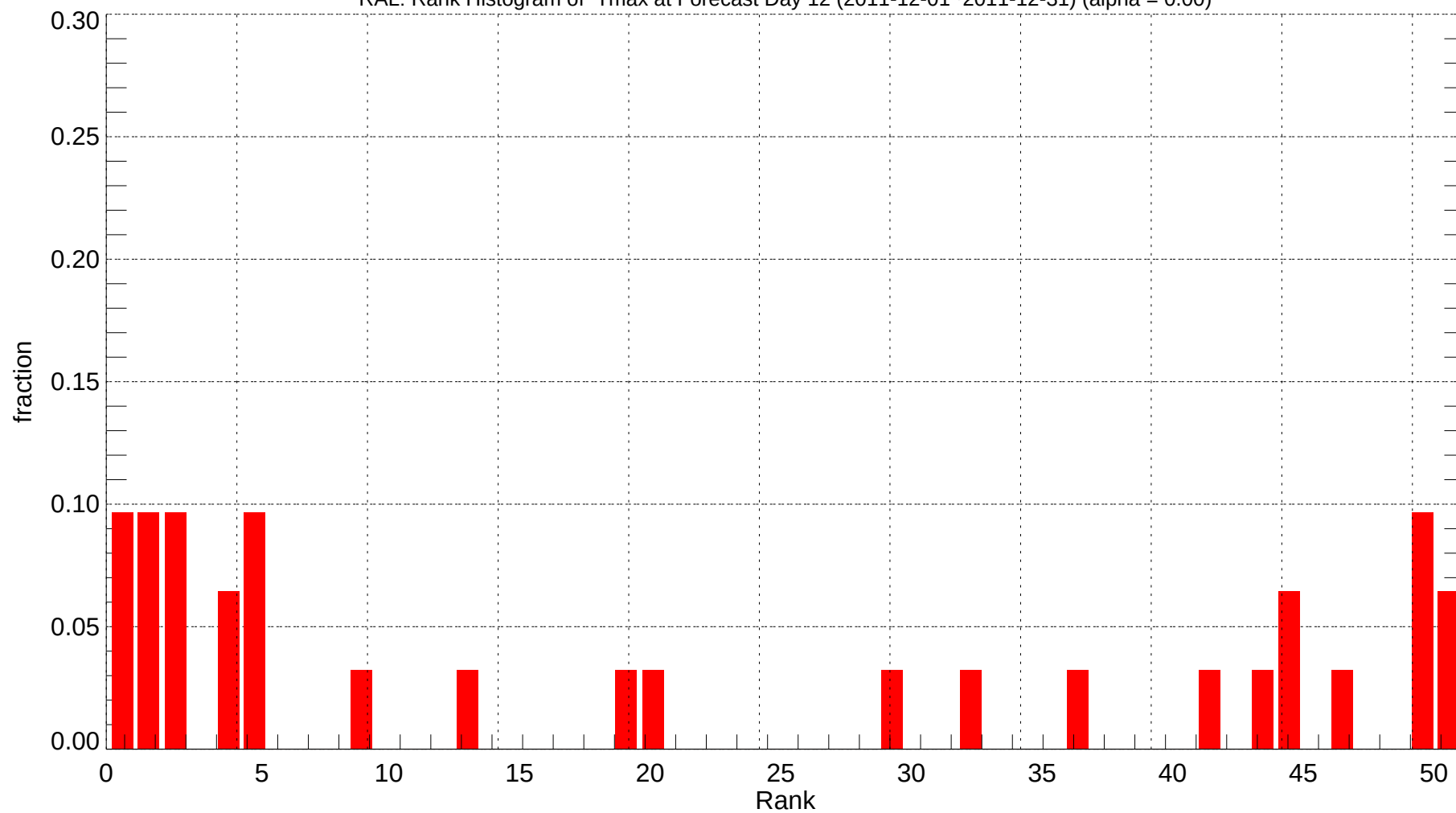
RAL: Rank Histogram of Tmax at Forecast Day 12 (2011-12-01~2011-12-31) (alpha = 0.00)
