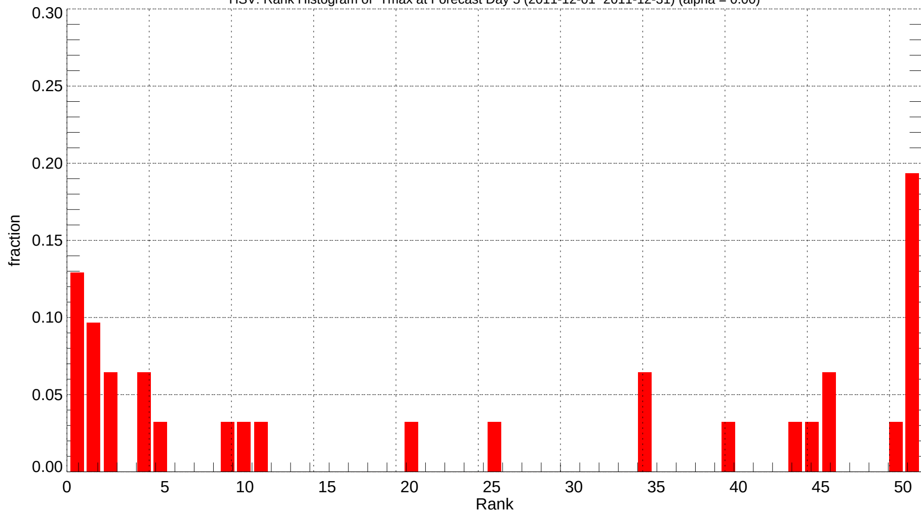
HSV: Rank Histogram of Tmax at Forecast Day 5 (2011-12-01~2011-12-31) (alpha = 0.00)
