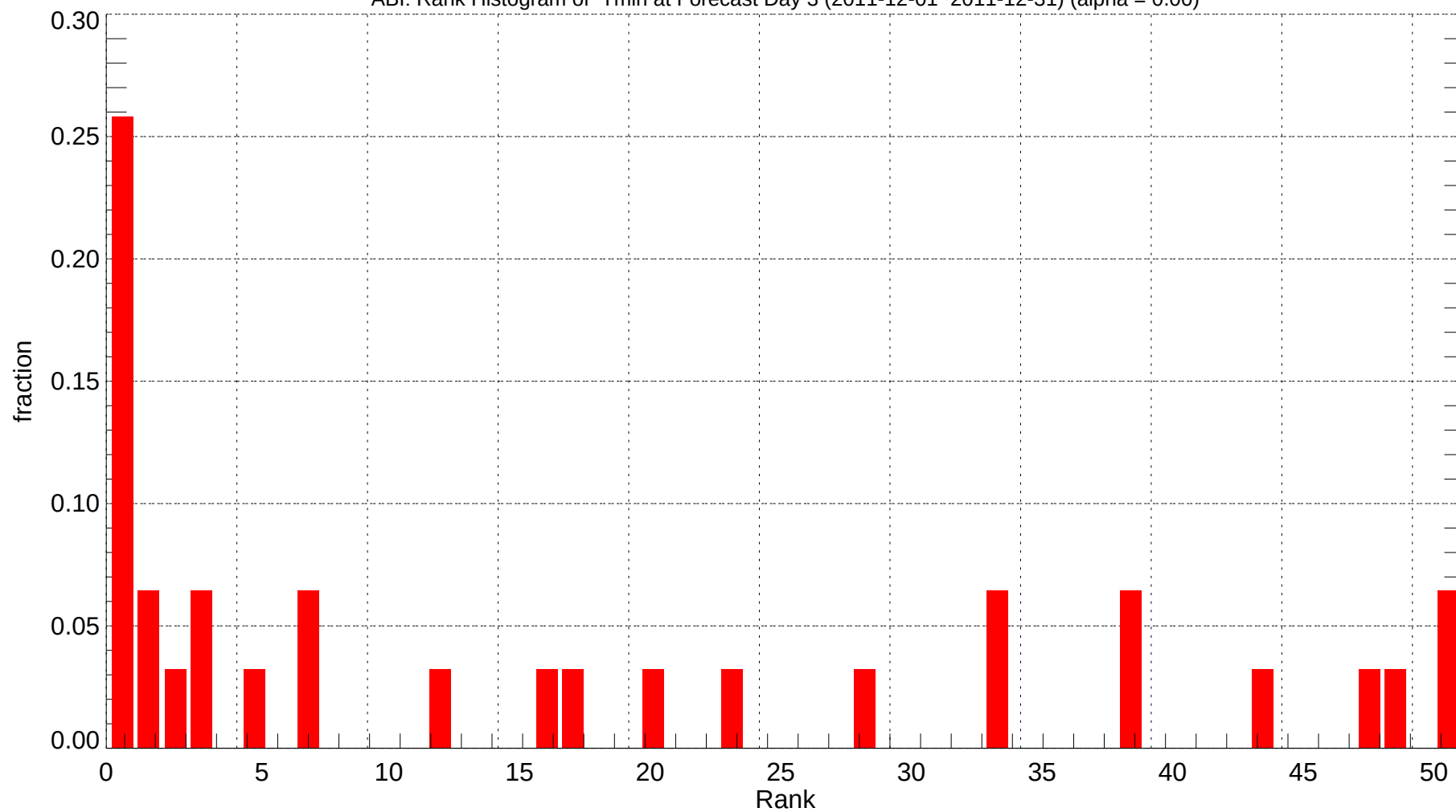
ABI: Rank Histogram of Tmin at Forecast Day 3 (2011-12-01~2011-12-31) (alpha = 0.00)
