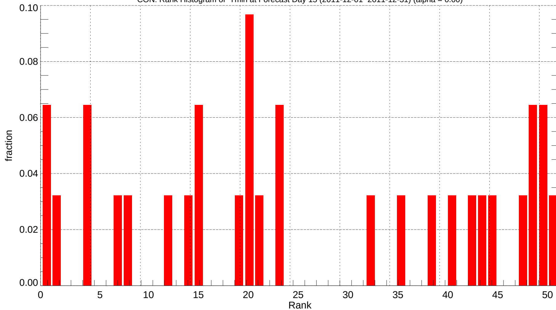
CON: Rank Histogram of Tmin at Forecast Day 15 (2011-12-01~2011-12-31) (alpha = 0.00)
