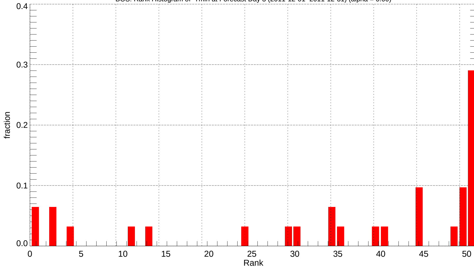
BOS: Rank Histogram of Tmin at Forecast Day 3 (2011-12-01~2011-12-31) (alpha = 0.00)
