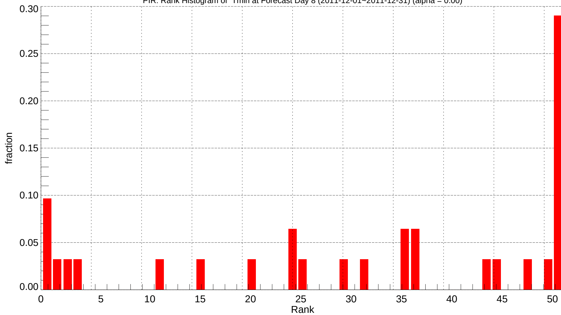
PIR: Rank Histogram of Tmin at Forecast Day 8 (2011-12-01~2011-12-31) (alpha = 0.00)
