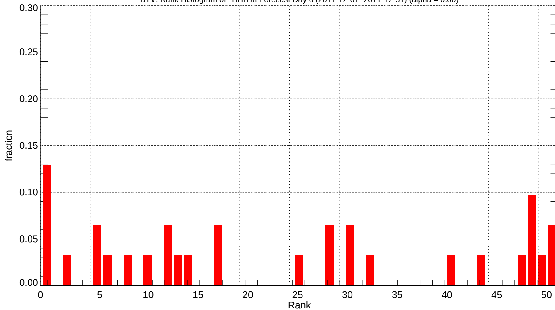
BTV: Rank Histogram of Tmin at Forecast Day 6 (2011-12-01~2011-12-31) (alpha = 0.00)
