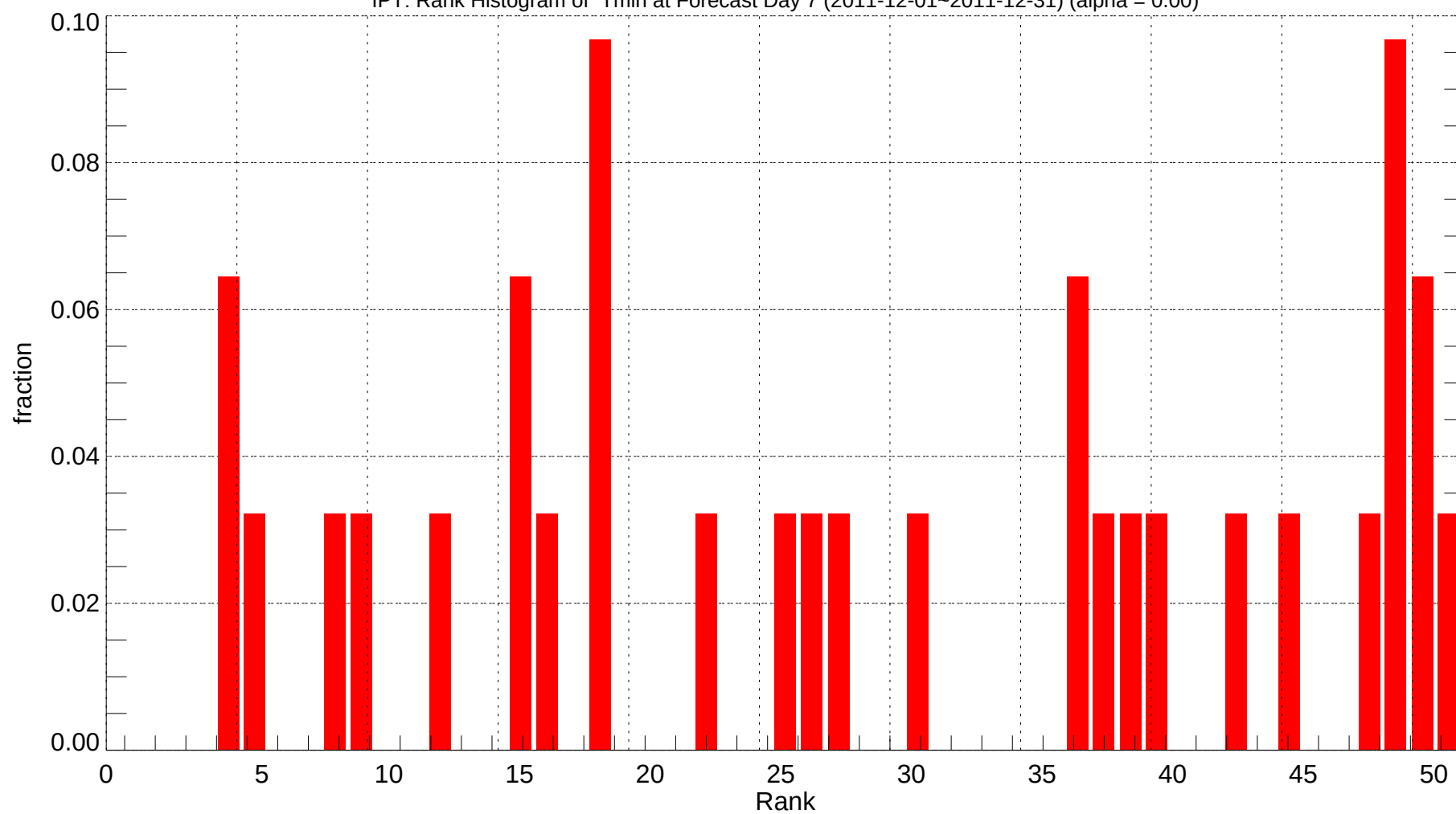
IPT: Rank Histogram of Tmin at Forecast Day 7 (2011-12-01~2011-12-31) (alpha = 0.00)
