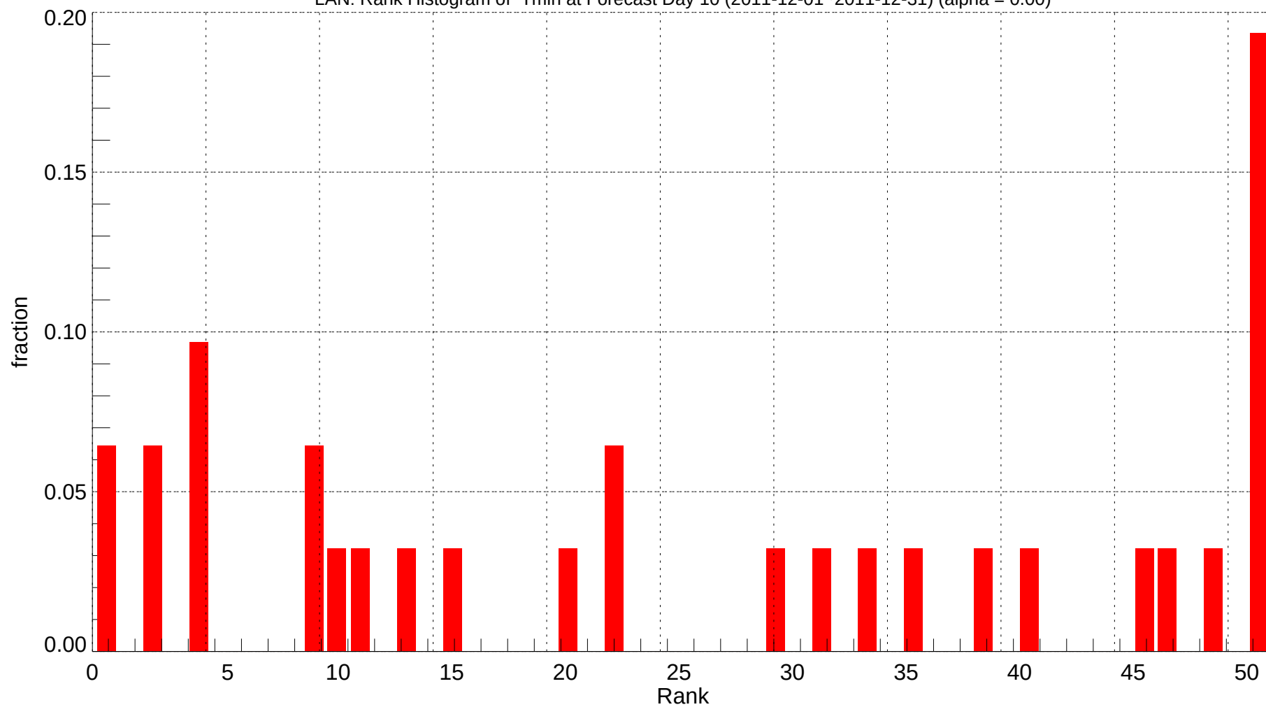
LAN: Rank Histogram of Tmin at Forecast Day 10 (2011-12-01~2011-12-31) (alpha = 0.00)
