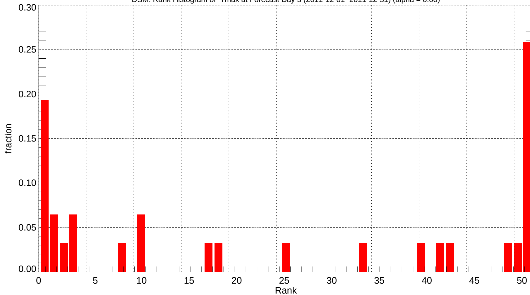
DSM: Rank Histogram of Tmax at Forecast Day 3 (2011-12-01~2011-12-31) (alpha = 0.00)
