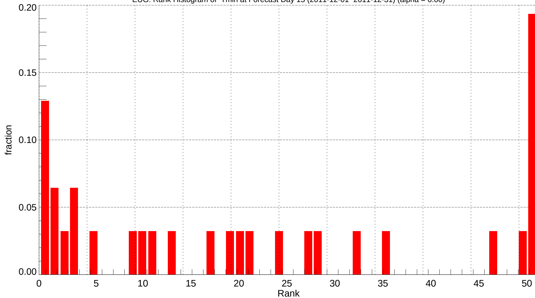
EUG: Rank Histogram of Tmin at Forecast Day 15 (2011-12-01~2011-12-31) (alpha = 0.00)
