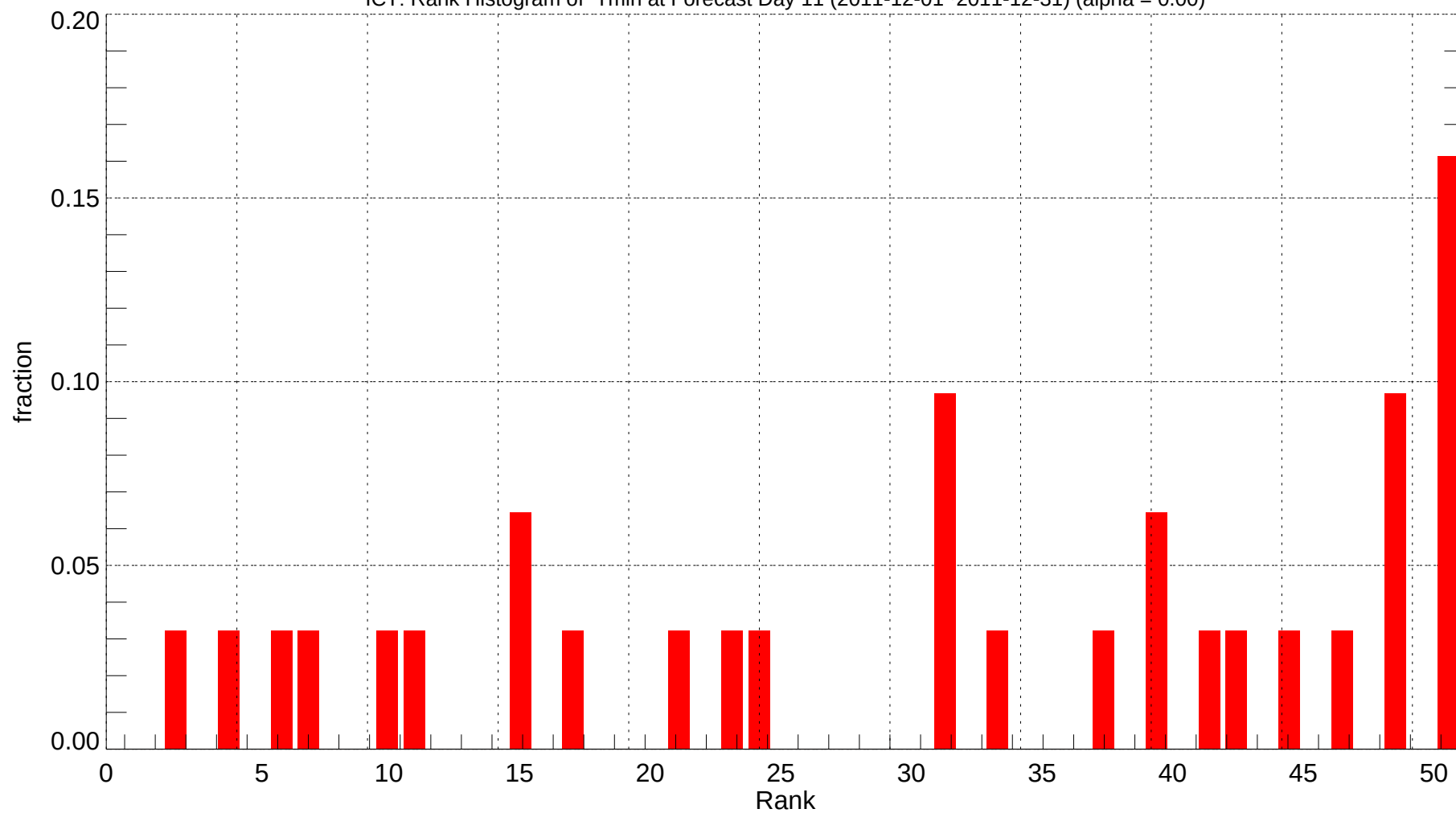
ICT: Rank Histogram of Tmin at Forecast Day 11 (2011-12-01~2011-12-31) (alpha = 0.00)
