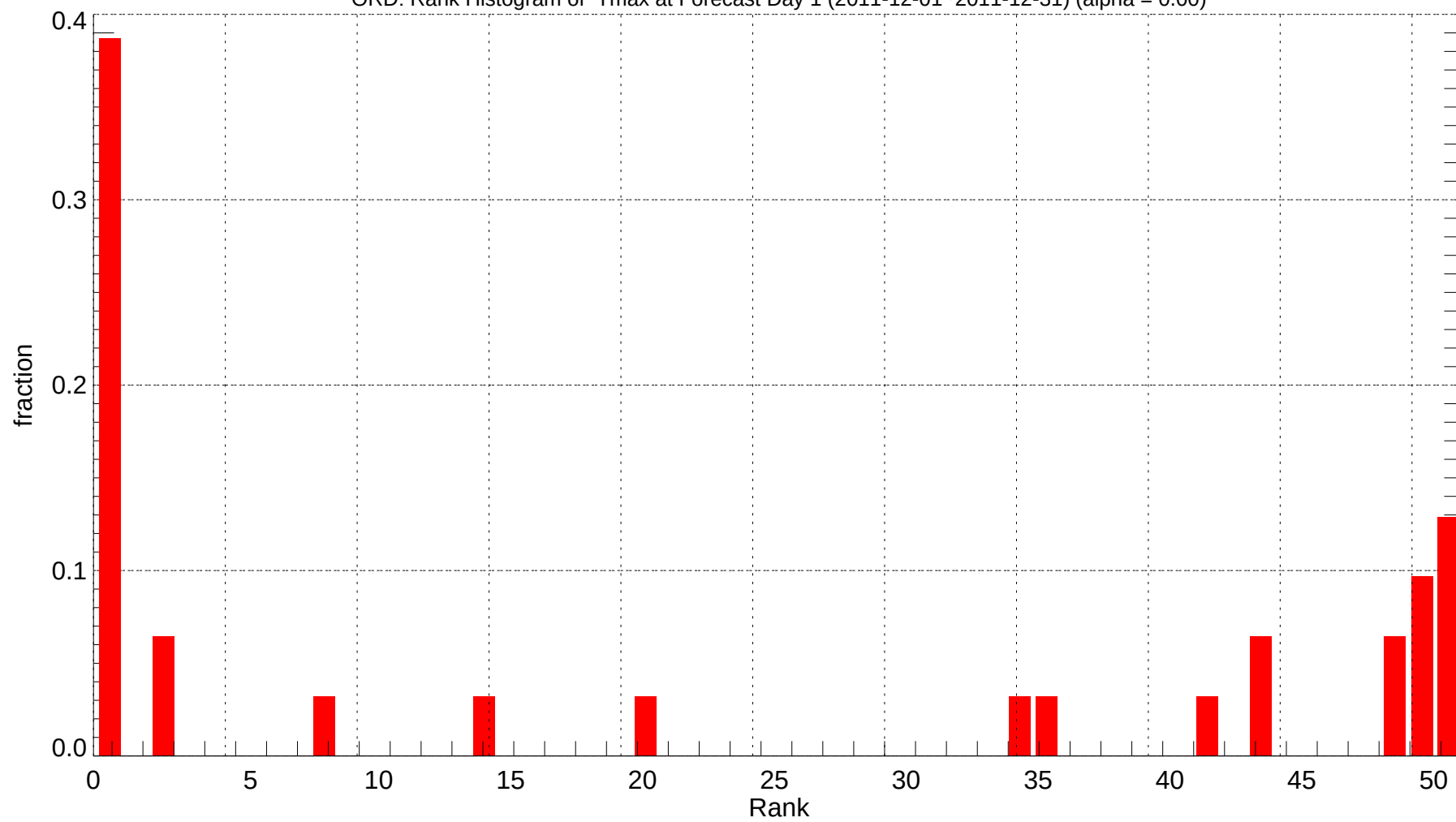
ORD: Rank Histogram of Tmax at Forecast Day 1 (2011-12-01~2011-12-31) (alpha = 0.00)
