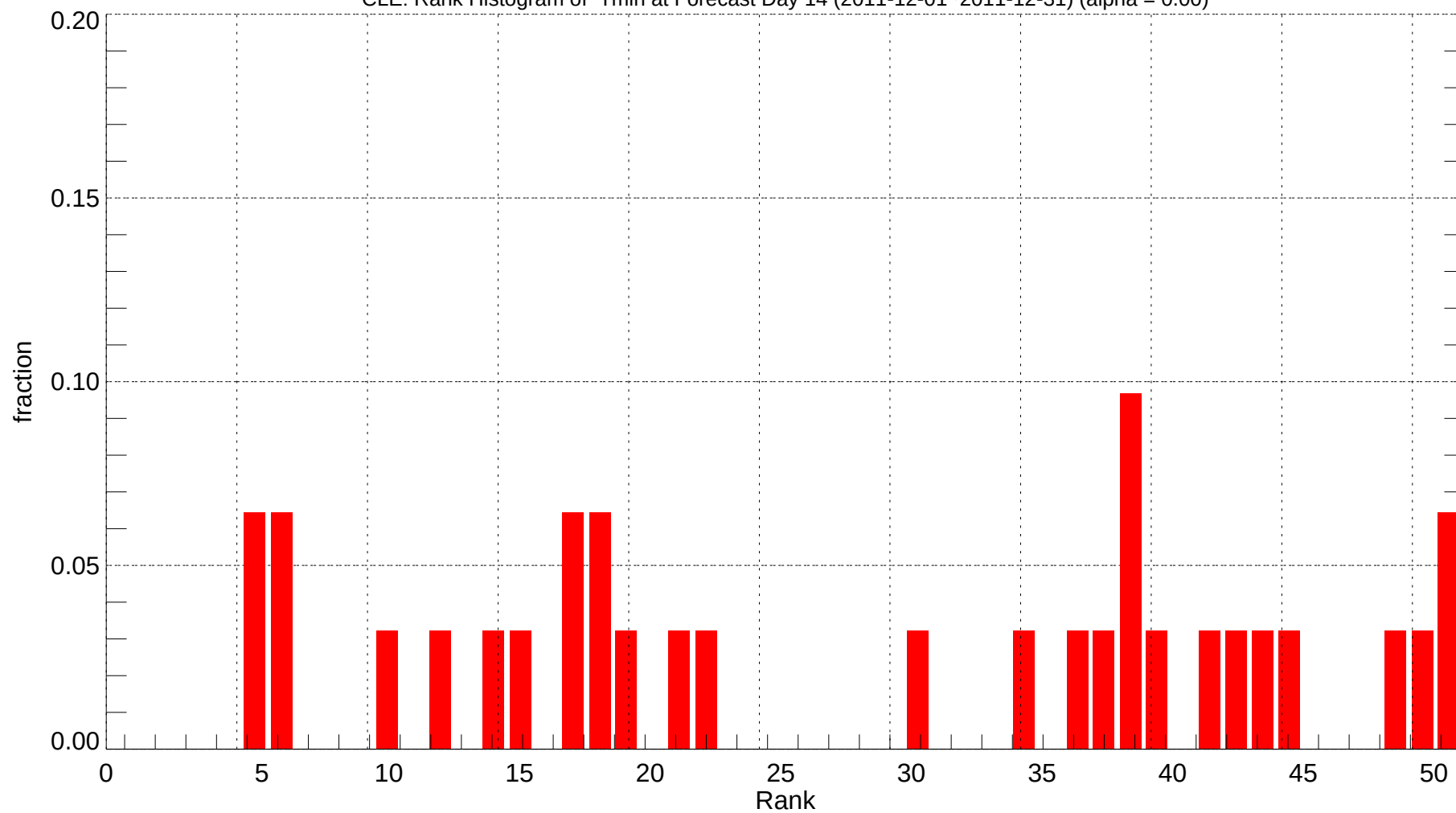
CLE: Rank Histogram of Tmin at Forecast Day 14 (2011-12-01~2011-12-31) (alpha = 0.00)
