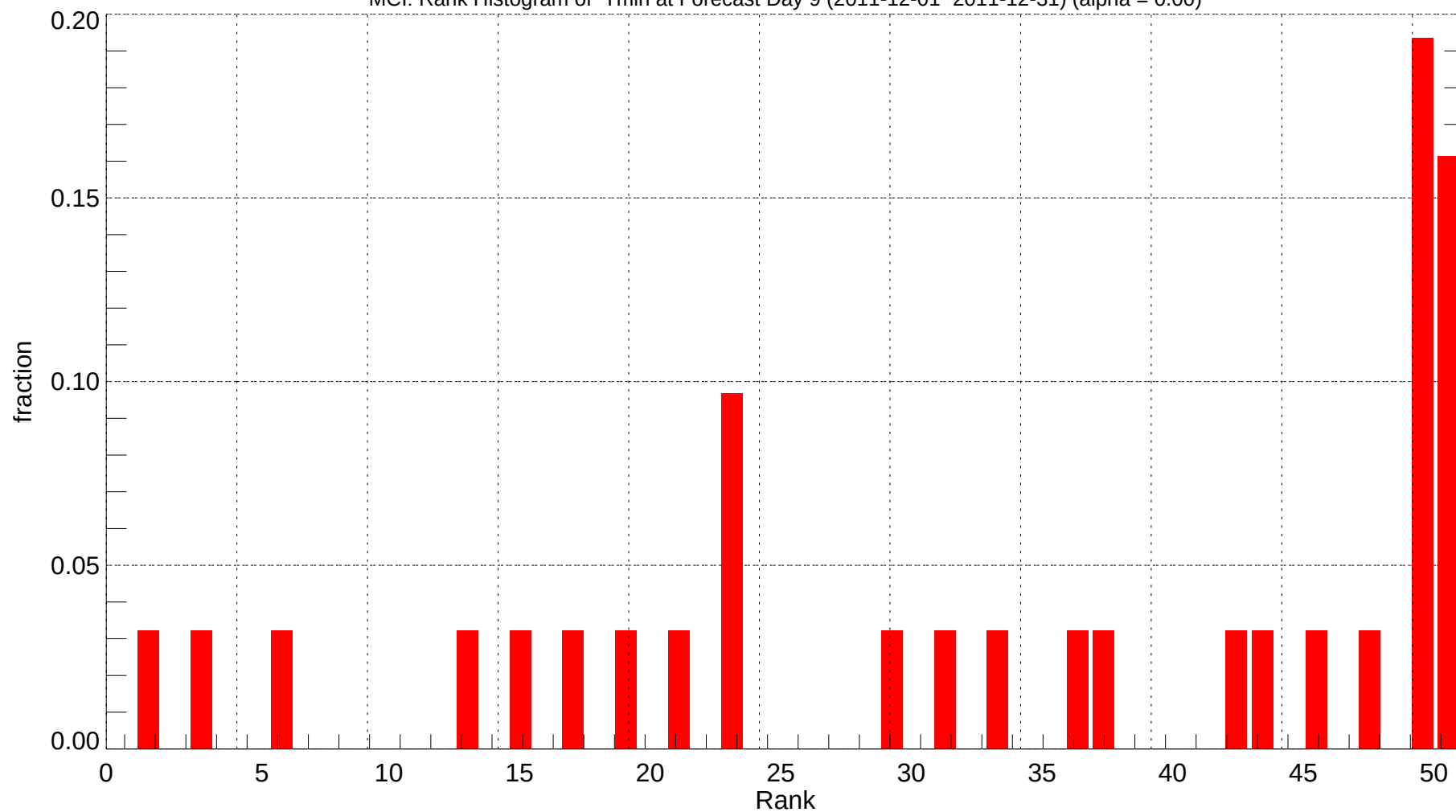
MCI: Rank Histogram of Tmin at Forecast Day 9 (2011-12-01~2011-12-31) (alpha = 0.00)
