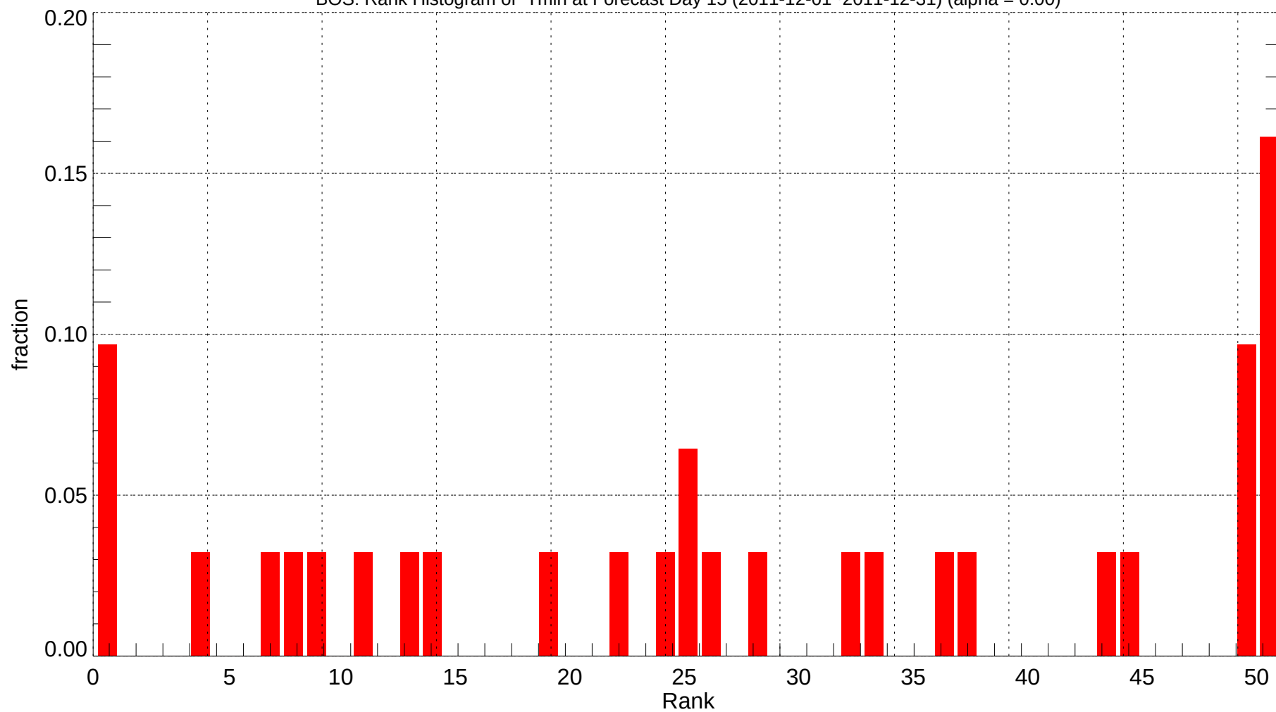
BOS: Rank Histogram of Tmin at Forecast Day 15 (2011-12-01~2011-12-31) (alpha = 0.00)
