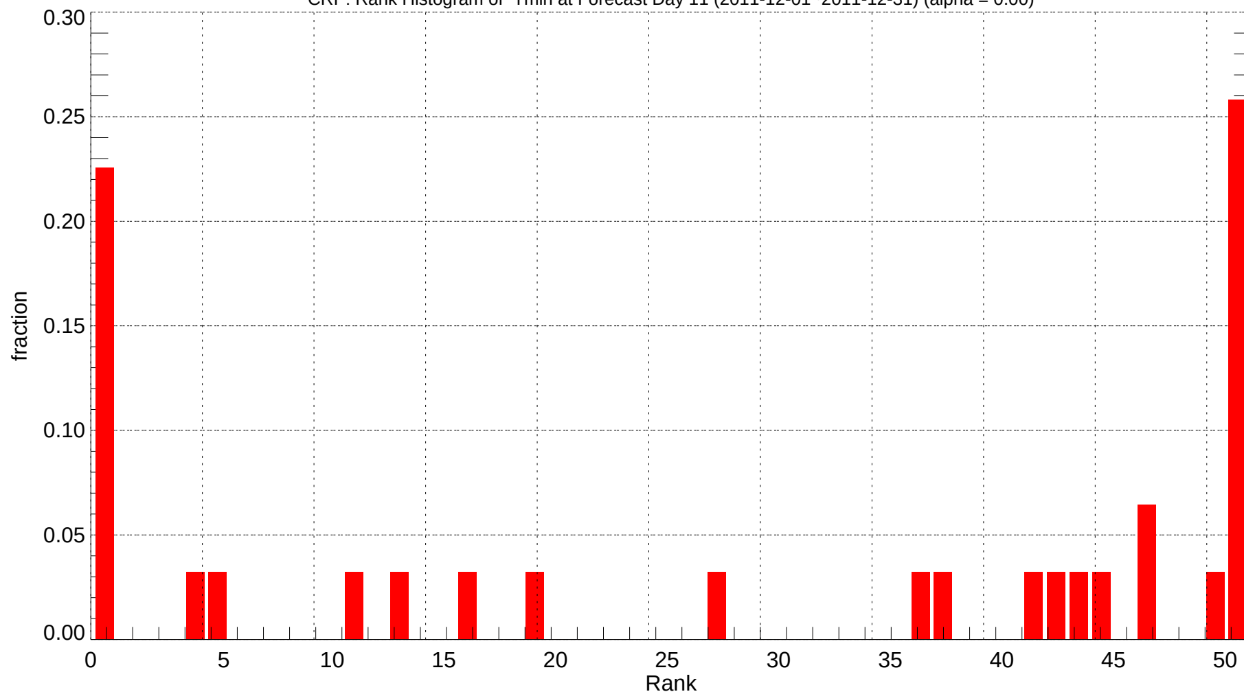
CRP: Rank Histogram of Tmin at Forecast Day 11 (2011-12-01~2011-12-31) (alpha = 0.00)
