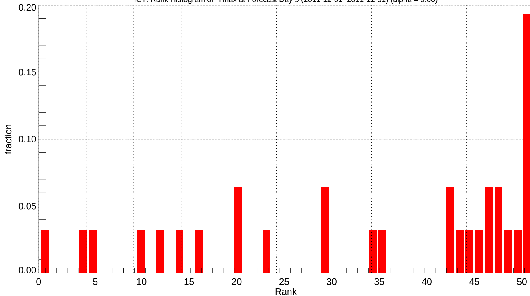
ICT: Rank Histogram of Tmax at Forecast Day 9 (2011-12-01~2011-12-31) (alpha = 0.00)
