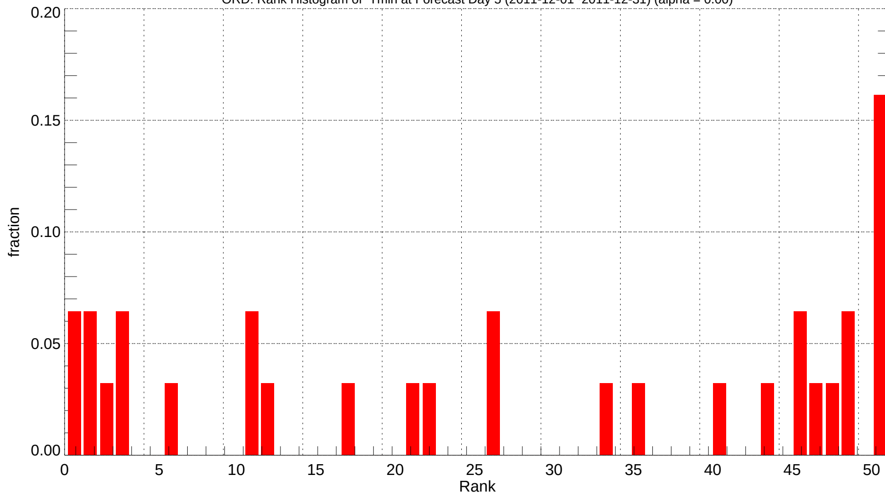
ORD: Rank Histogram of Tmin at Forecast Day 5 (2011-12-01~2011-12-31) (alpha = 0.00)
