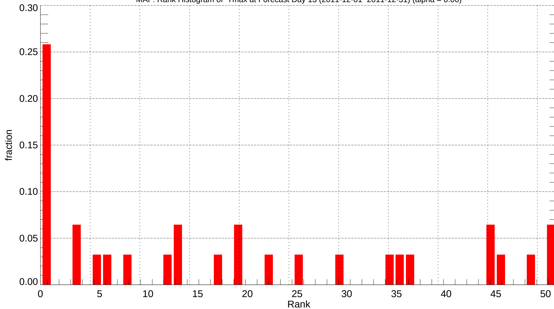
MAF: Rank Histogram of Tmax at Forecast Day 13 (2011-12-01~2011-12-31) (alpha = 0.00)
