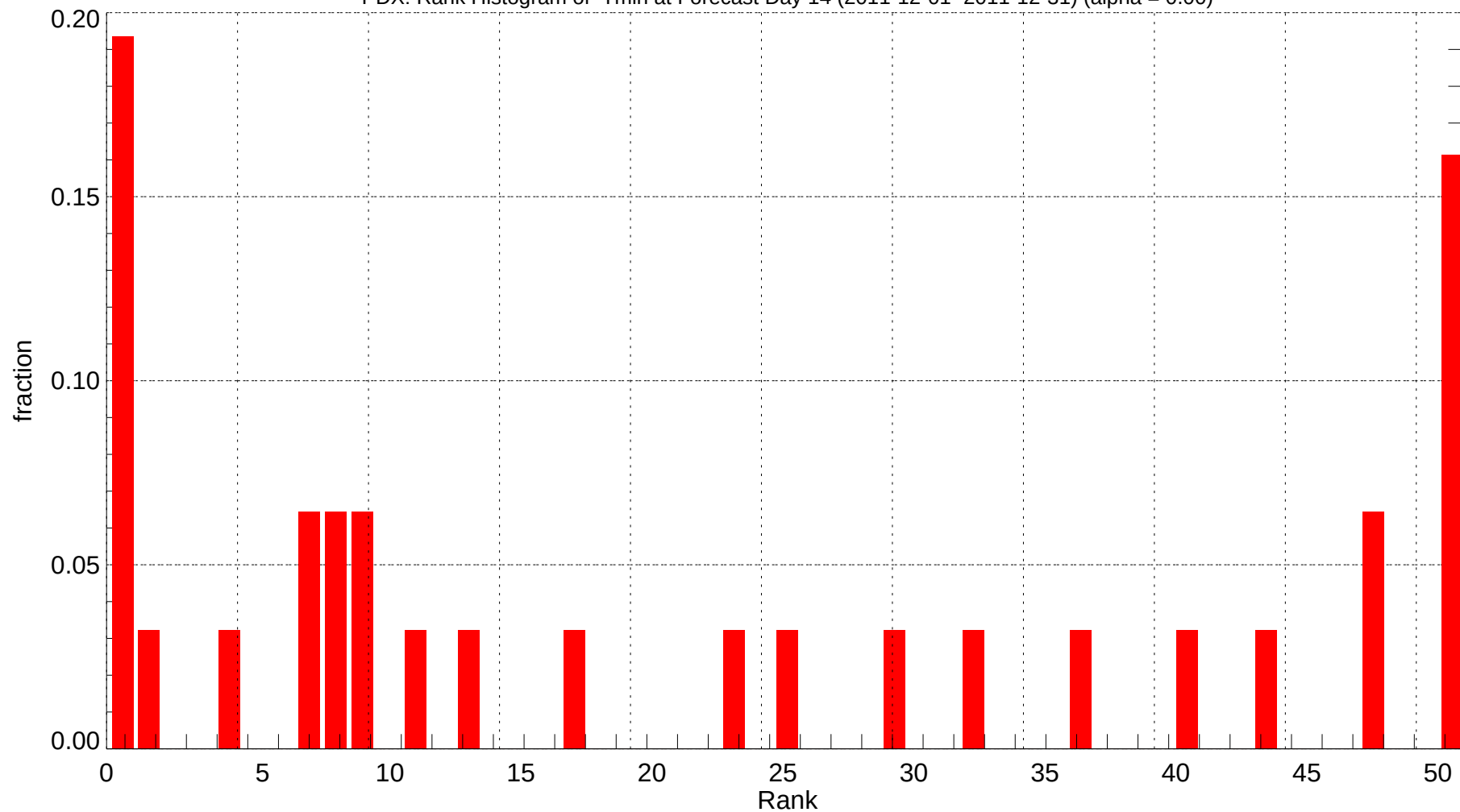
PDX: Rank Histogram of Tmin at Forecast Day 14 (2011-12-01~2011-12-31) (alpha = 0.00)
