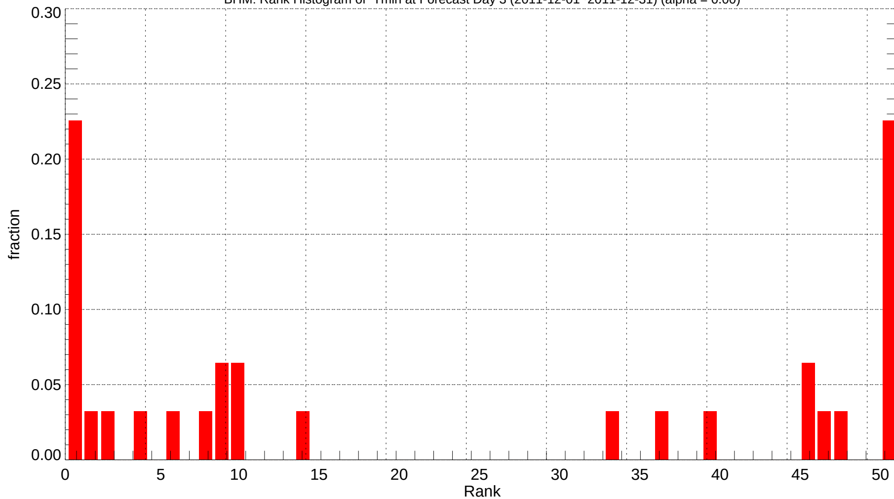
BHM: Rank Histogram of Tmin at Forecast Day 3 (2011-12-01~2011-12-31) (alpha = 0.00)
