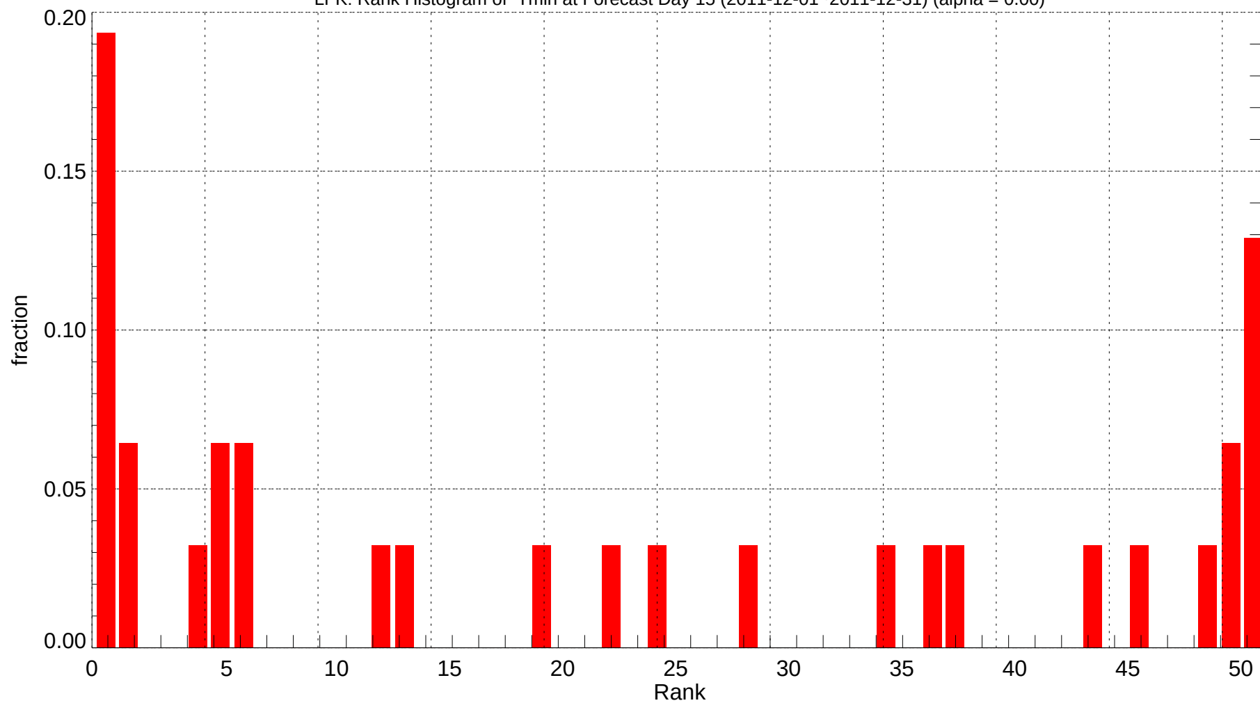
LFK: Rank Histogram of Tmin at Forecast Day 15 (2011-12-01~2011-12-31) (alpha = 0.00)
