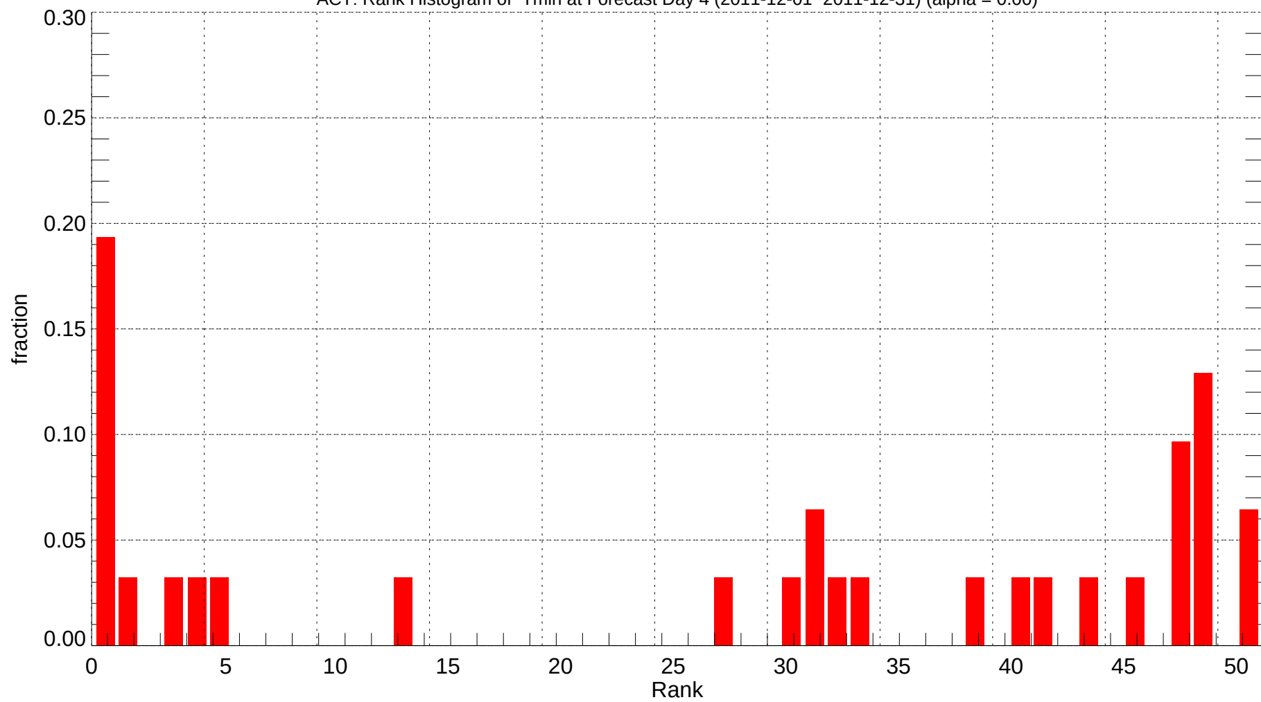
ACT: Rank Histogram of Tmin at Forecast Day 4 (2011-12-01~2011-12-31) (alpha = 0.00)
