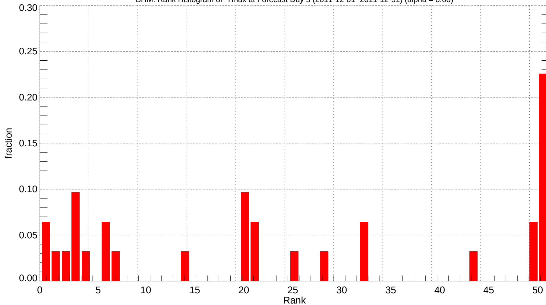
BHM: Rank Histogram of Tmax at Forecast Day 5 (2011-12-01~2011-12-31) (alpha = 0.00)
