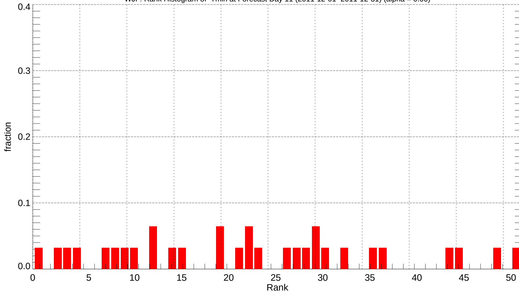
WJF: Rank Histogram of Tmin at Forecast Day 11 (2011-12-01~2011-12-31) (alpha = 0.00)
