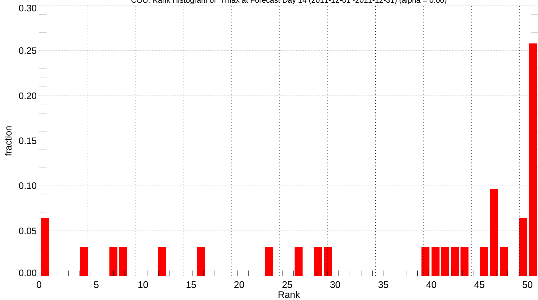
COU: Rank Histogram of Tmax at Forecast Day 14 (2011-12-01~2011-12-31) (alpha = 0.00)
