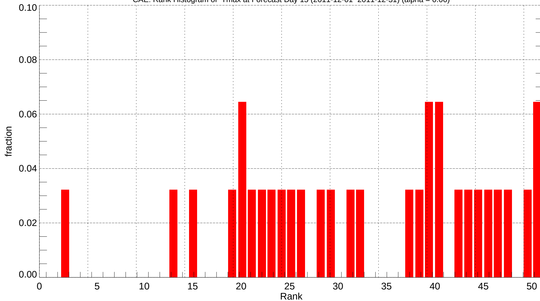
CAE: Rank Histogram of Tmax at Forecast Day 15 (2011-12-01~2011-12-31) (alpha = 0.00)
