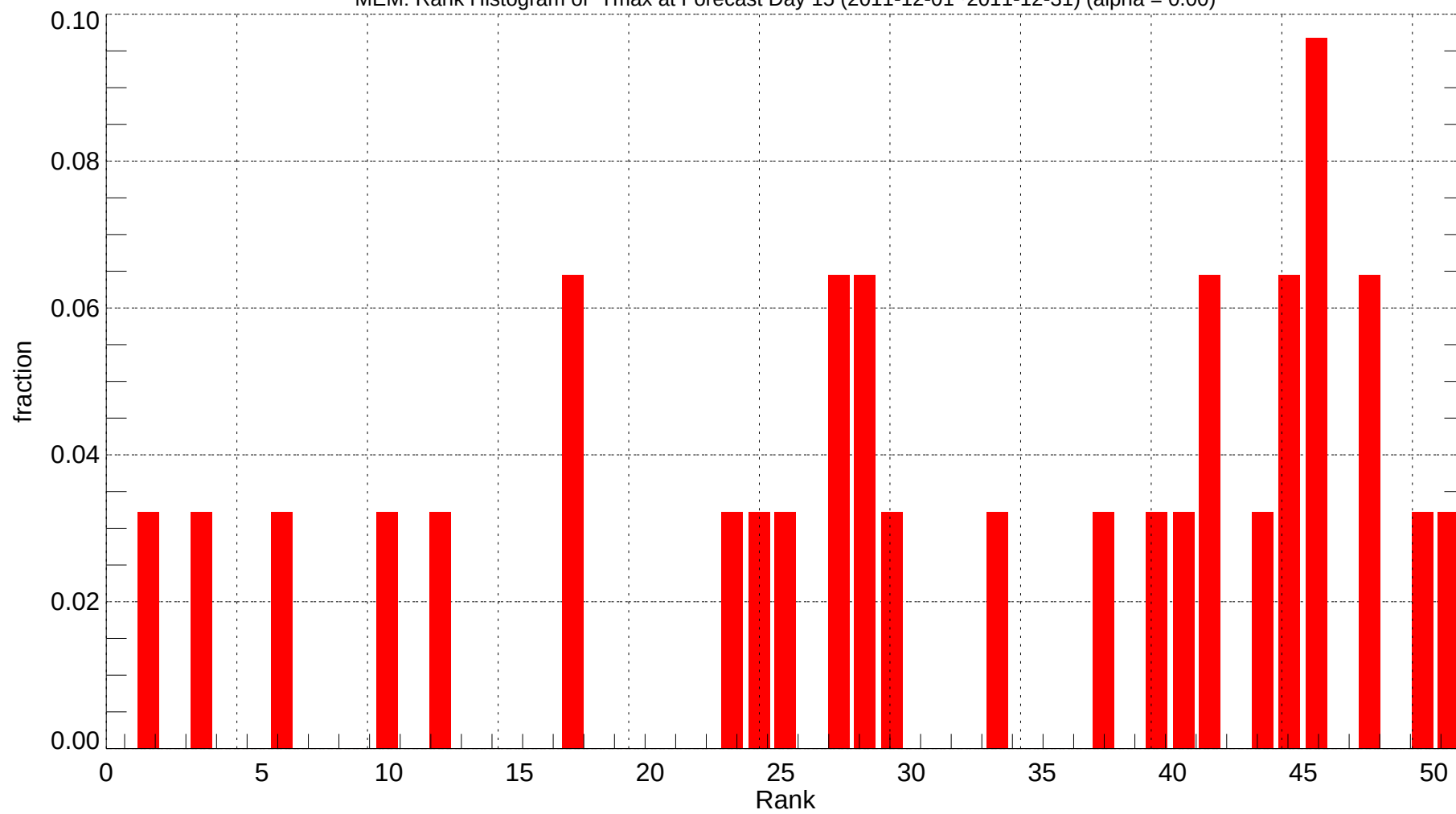
MEM: Rank Histogram of Tmax at Forecast Day 15 (2011-12-01~2011-12-31) (alpha = 0.00)
