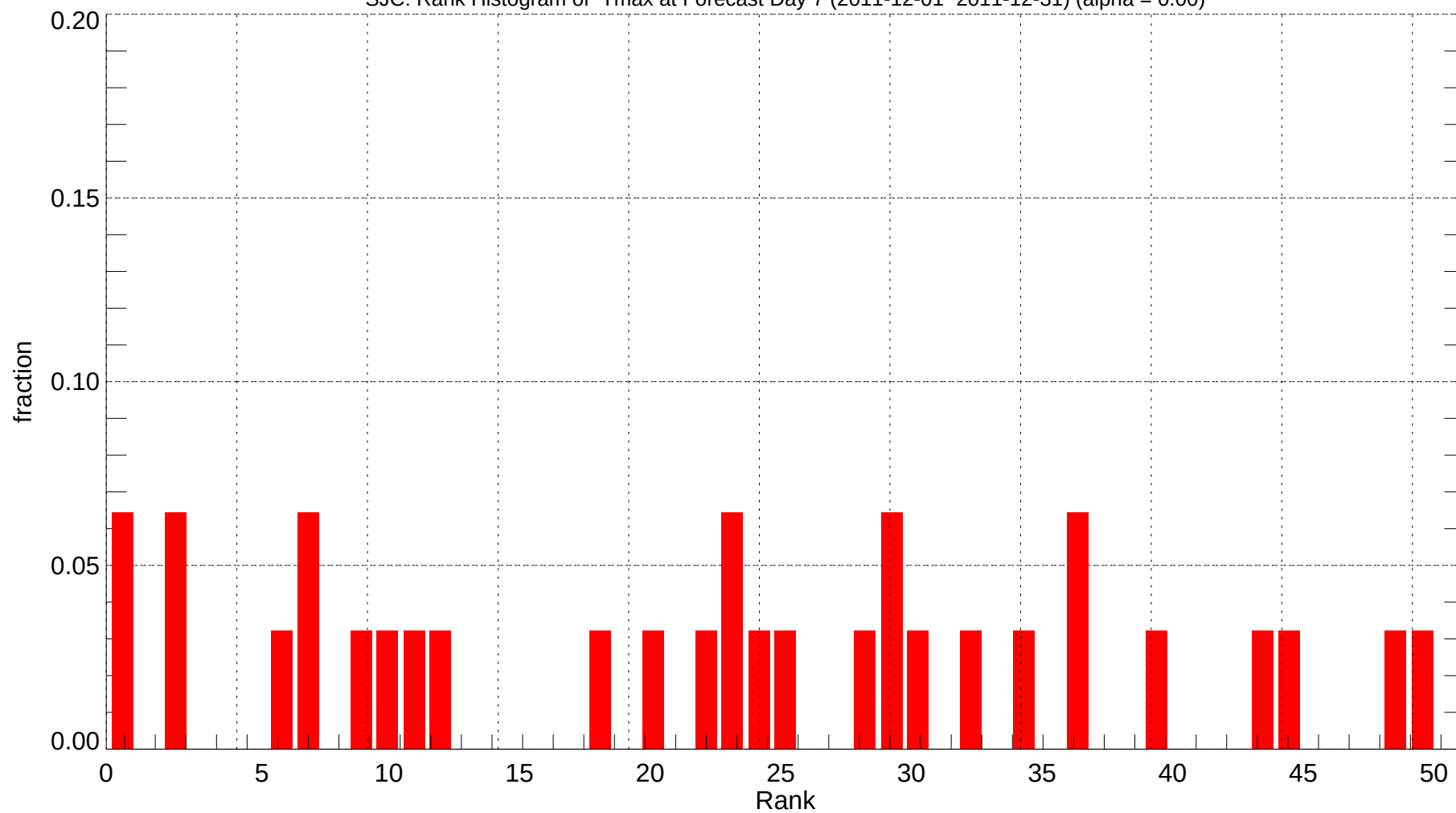
SJC: Rank Histogram of Tmax at Forecast Day 7 (2011-12-01~2011-12-31) (alpha = 0.00)
