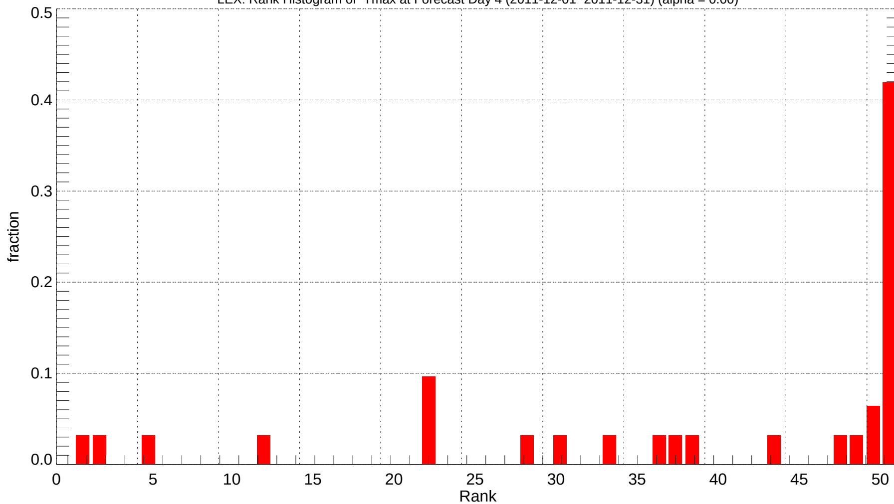
LEX: Rank Histogram of Tmax at Forecast Day 4 (2011-12-01~2011-12-31) (alpha = 0.00)
