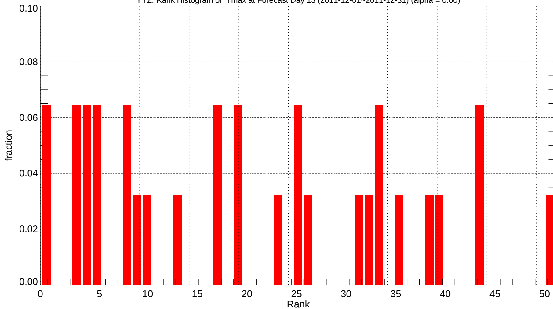
YYZ: Rank Histogram of Tmax at Forecast Day 13 (2011-12-01~2011-12-31) (alpha = 0.00)
