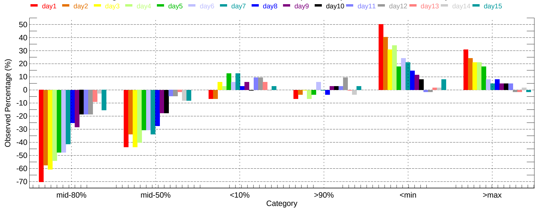
Observed Percentage Deviation of Ensembles - ROC: Max Temperature (2011-12-01~2011-12-31)
