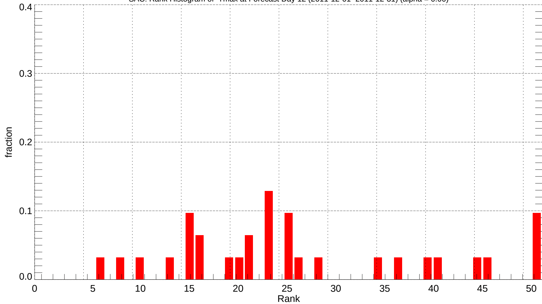
SAC: Rank Histogram of Tmax at Forecast Day 12 (2011-12-01~2011-12-31) (alpha = 0.00)
