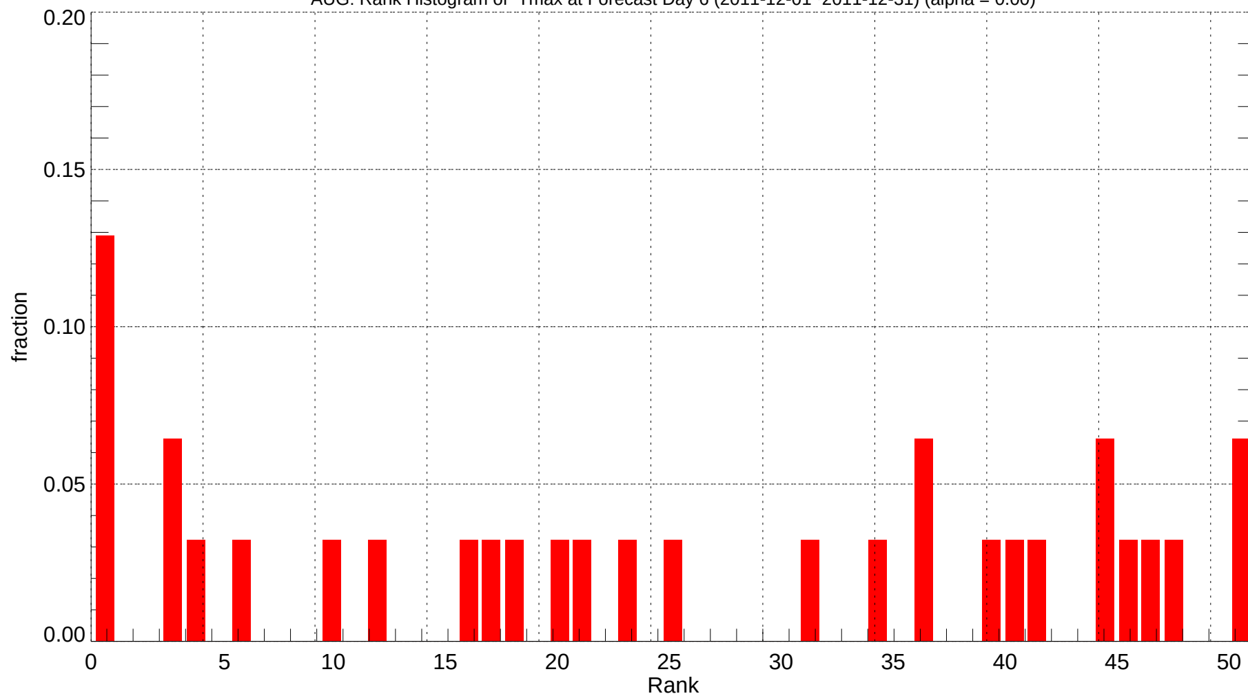
AUG: Rank Histogram of Tmax at Forecast Day 6 (2011-12-01~2011-12-31) (alpha = 0.00)
