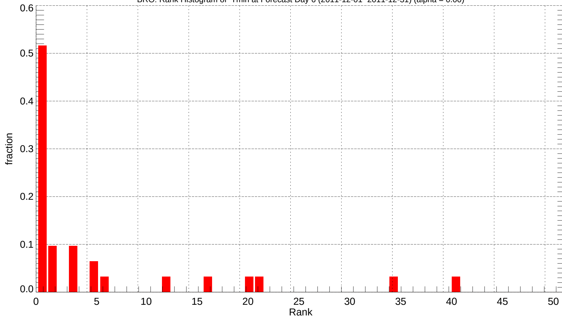
BRO: Rank Histogram of Tmin at Forecast Day 6 (2011-12-01~2011-12-31) (alpha = 0.00)
