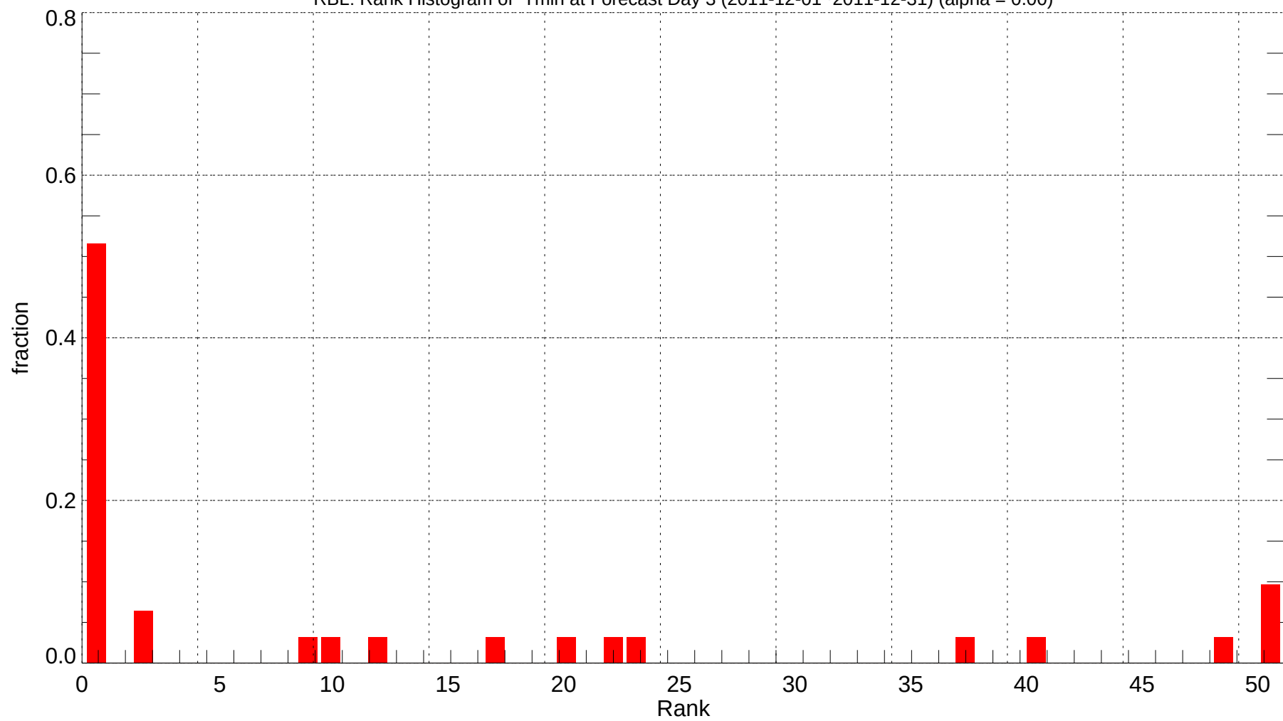
RBL: Rank Histogram of Tmin at Forecast Day 3 (2011-12-01~2011-12-31) (alpha = 0.00)
