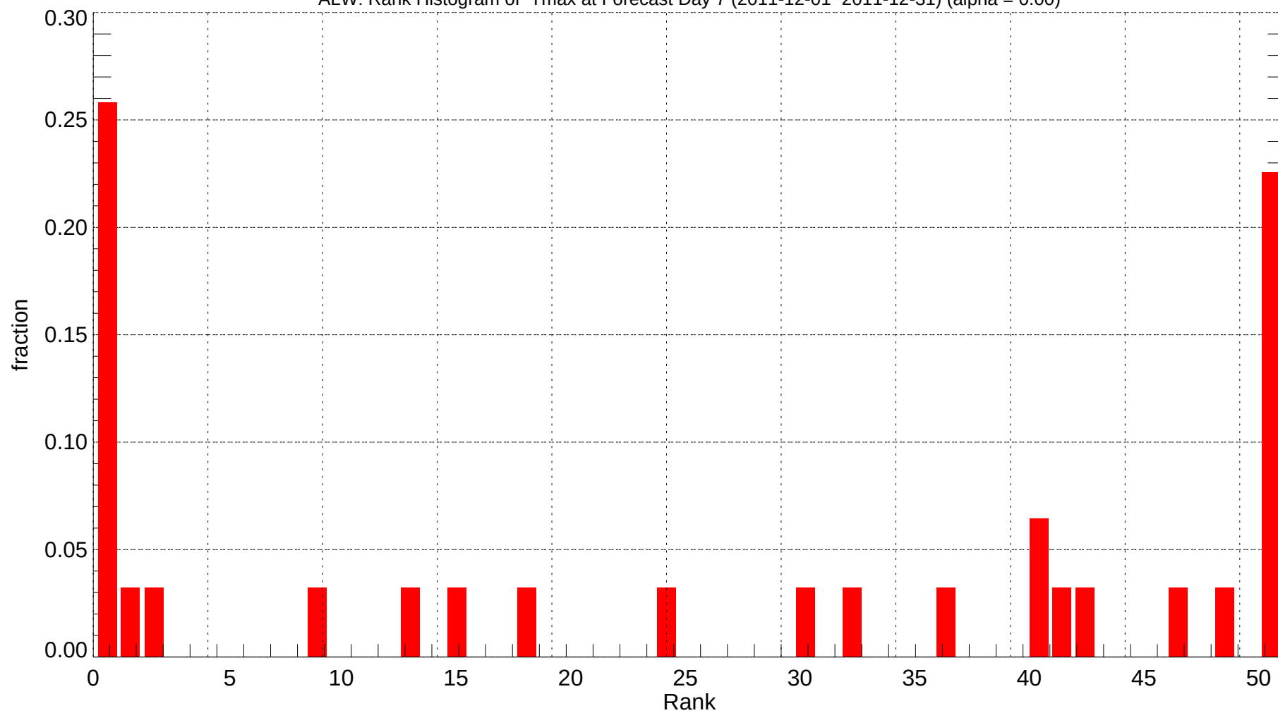
ALW: Rank Histogram of Tmax at Forecast Day 7 (2011-12-01~2011-12-31) (alpha = 0.00)
