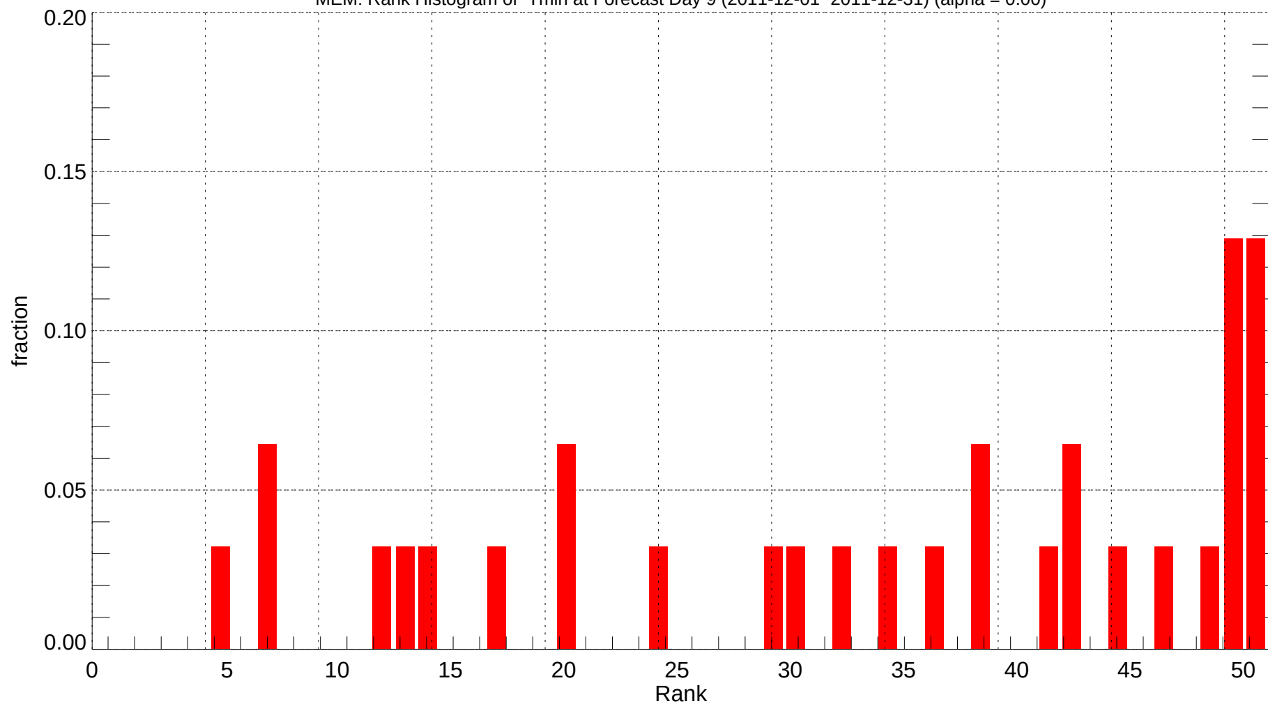
MEM: Rank Histogram of Tmin at Forecast Day 9 (2011-12-01~2011-12-31) (alpha = 0.00)
