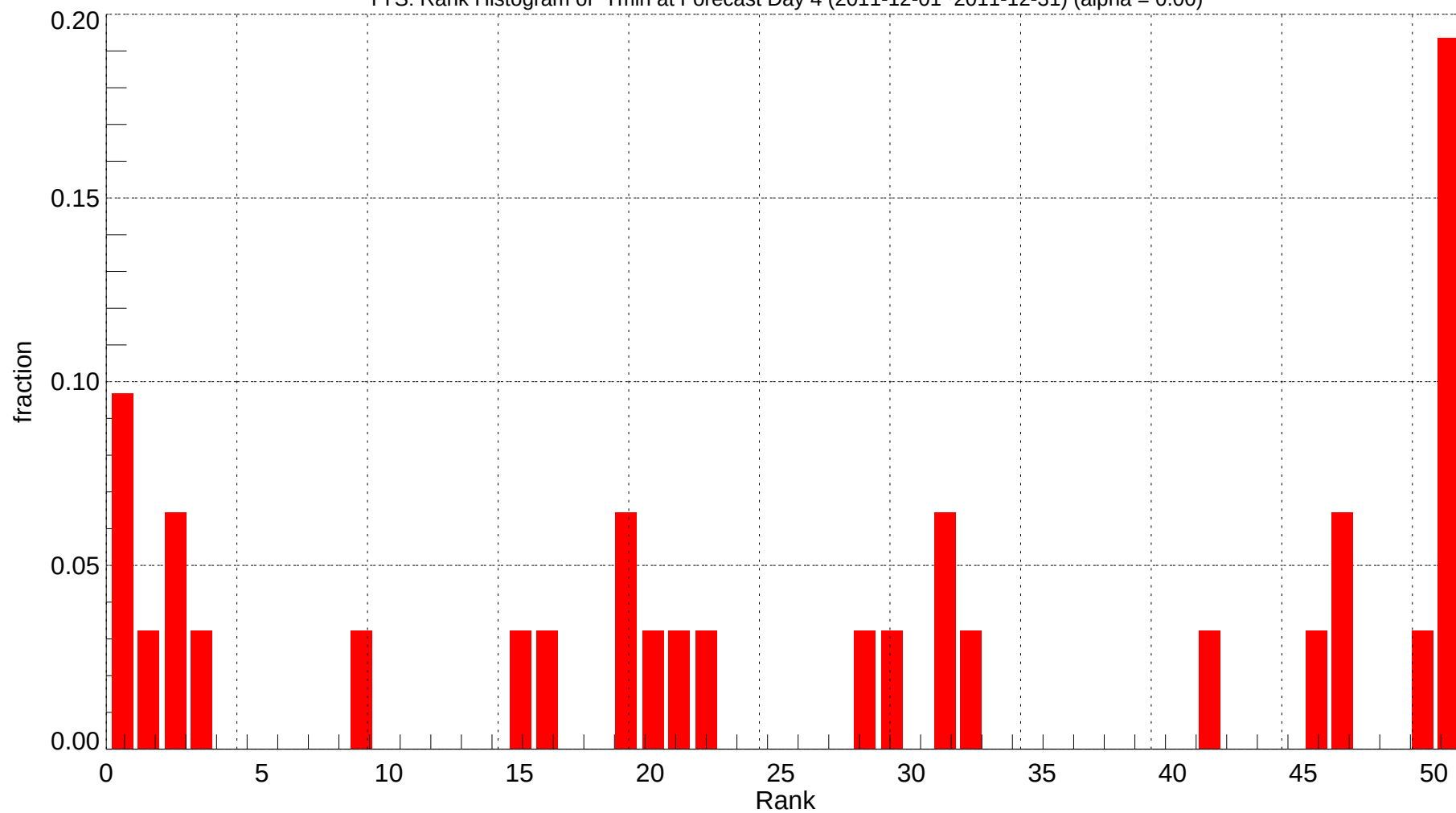
TYS: Rank Histogram of Tmin at Forecast Day 4 (2011-12-01~2011-12-31) (alpha = 0.00)
