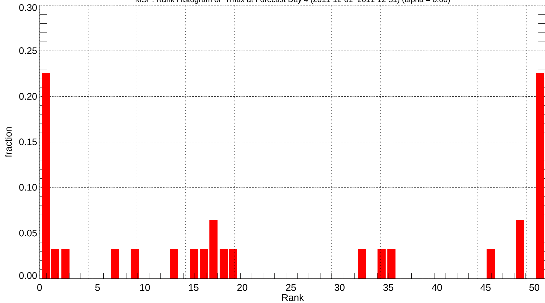
MSP: Rank Histogram of Tmax at Forecast Day 4 (2011-12-01~2011-12-31) (alpha = 0.00)
