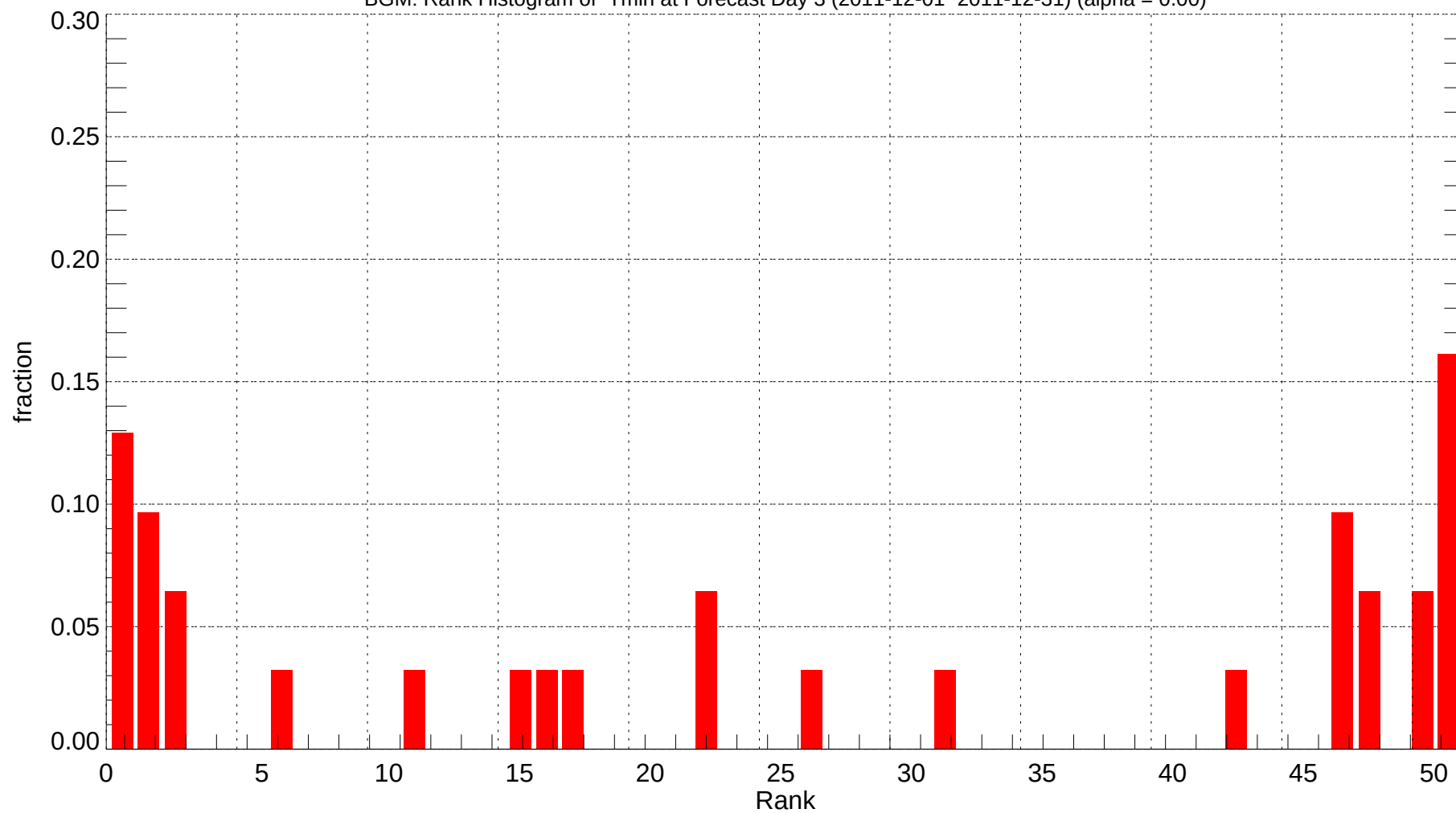
BGM: Rank Histogram of Tmin at Forecast Day 3 (2011-12-01~2011-12-31) (alpha = 0.00)
