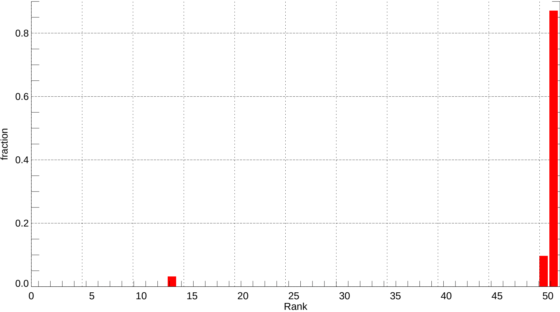
GTF: Rank Histogram of Tmin at Forecast Day 2 (2011-12-01~2011-12-31) (alpha = 0.00)
