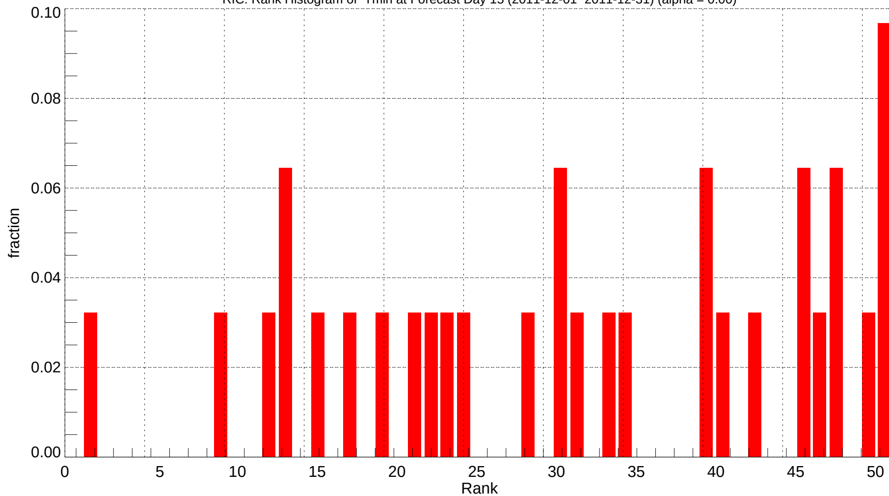
RIC: Rank Histogram of Tmin at Forecast Day 15 (2011-12-01~2011-12-31) (alpha = 0.00)
