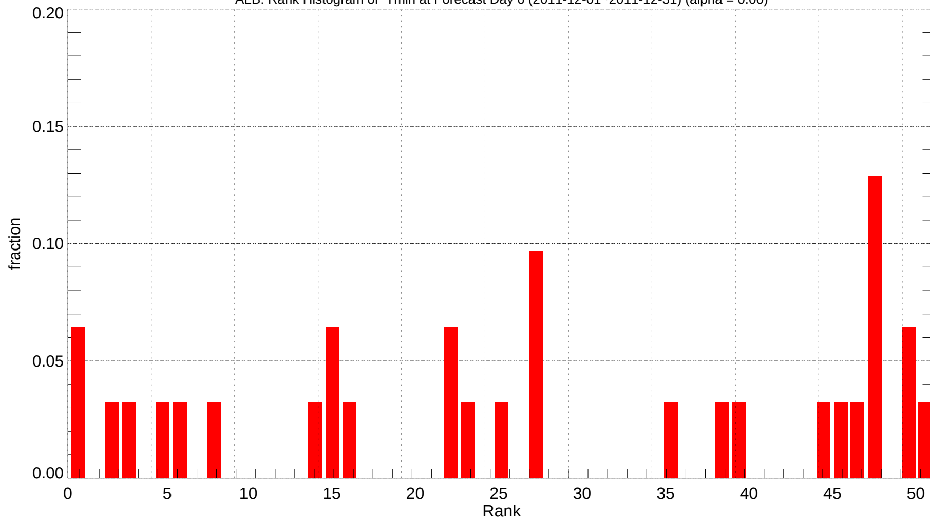
ALB: Rank Histogram of Tmin at Forecast Day 6 (2011-12-01~2011-12-31) (alpha = 0.00)
