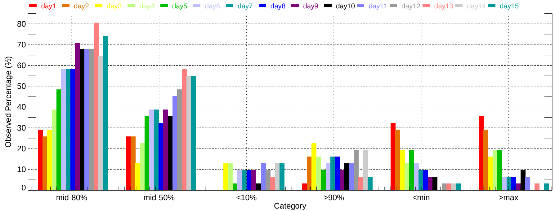
Observed Percentage of Ensembles - YUL: Max Temperature (2011-12-01~2011-12-31)
