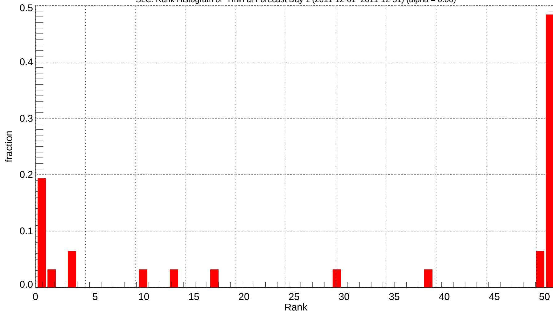
SLC: Rank Histogram of Tmin at Forecast Day 1 (2011-12-01~2011-12-31) (alpha = 0.00)
