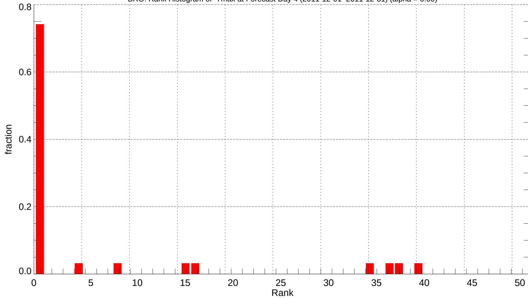
BRO: Rank Histogram of Tmax at Forecast Day 4 (2011-12-01~2011-12-31) (alpha = 0.00)
