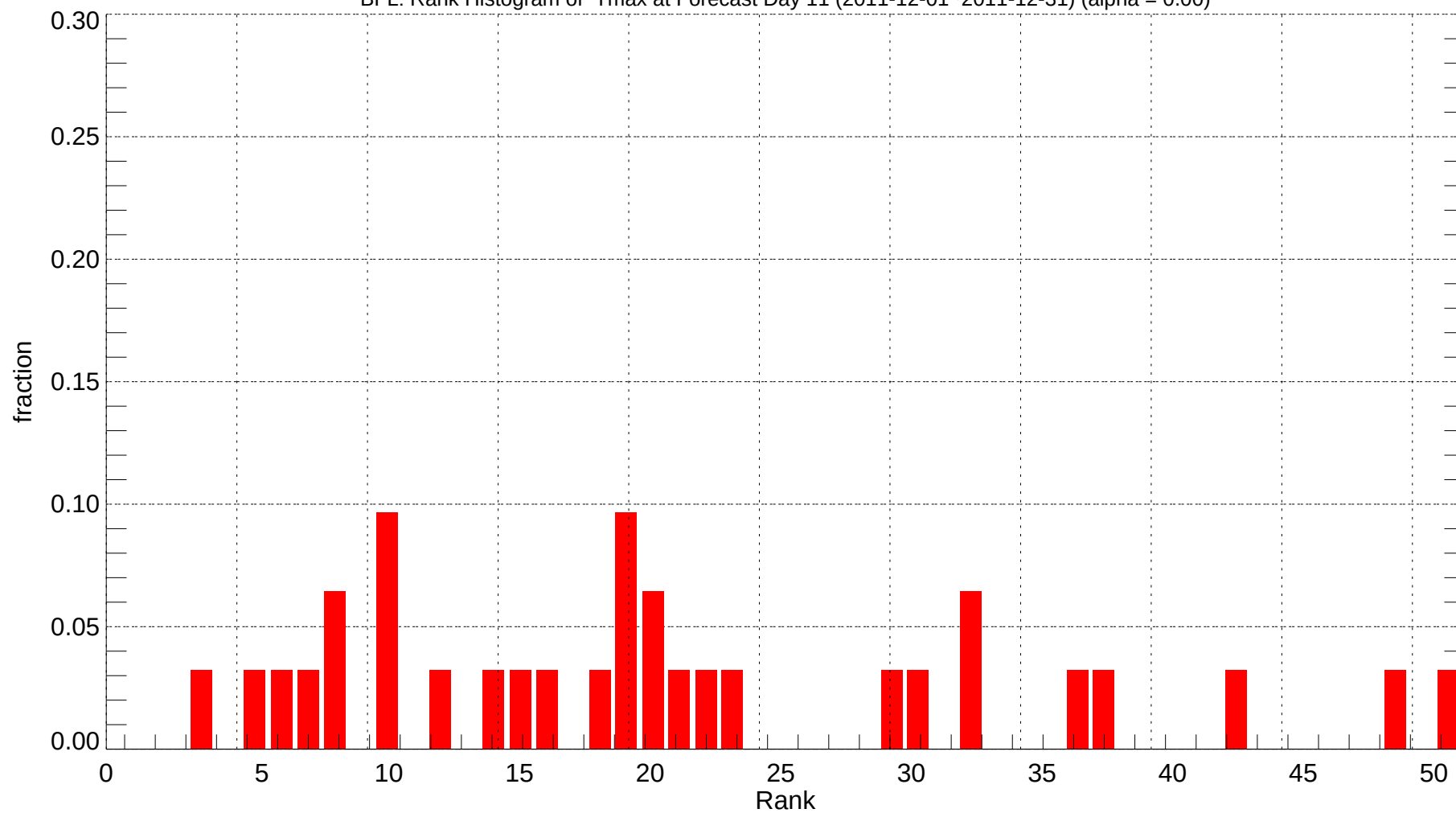
BFL: Rank Histogram of Tmax at Forecast Day 11 (2011-12-01~2011-12-31) (alpha = 0.00)
