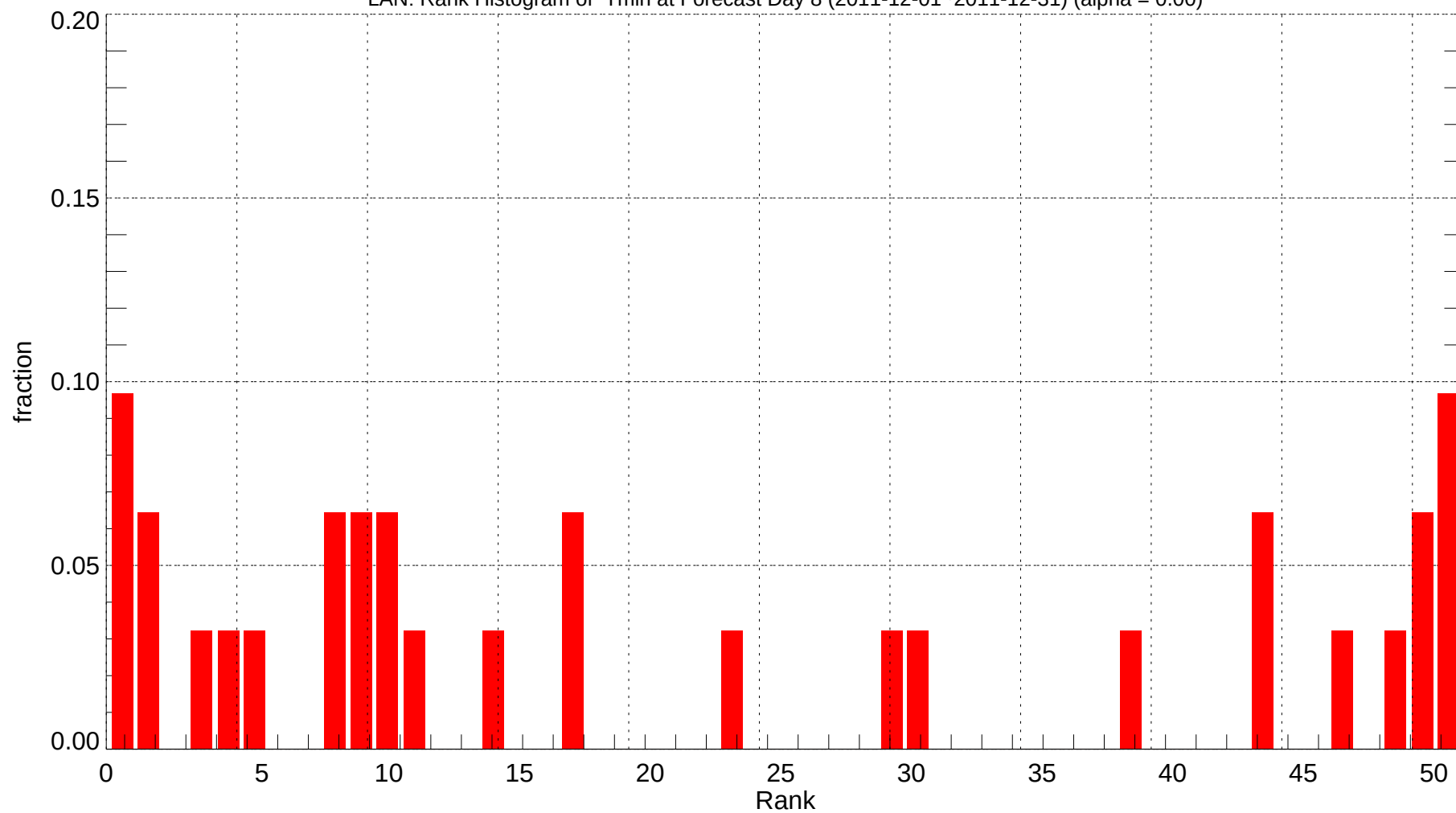
LAN: Rank Histogram of Tmin at Forecast Day 8 (2011-12-01~2011-12-31) (alpha = 0.00)
