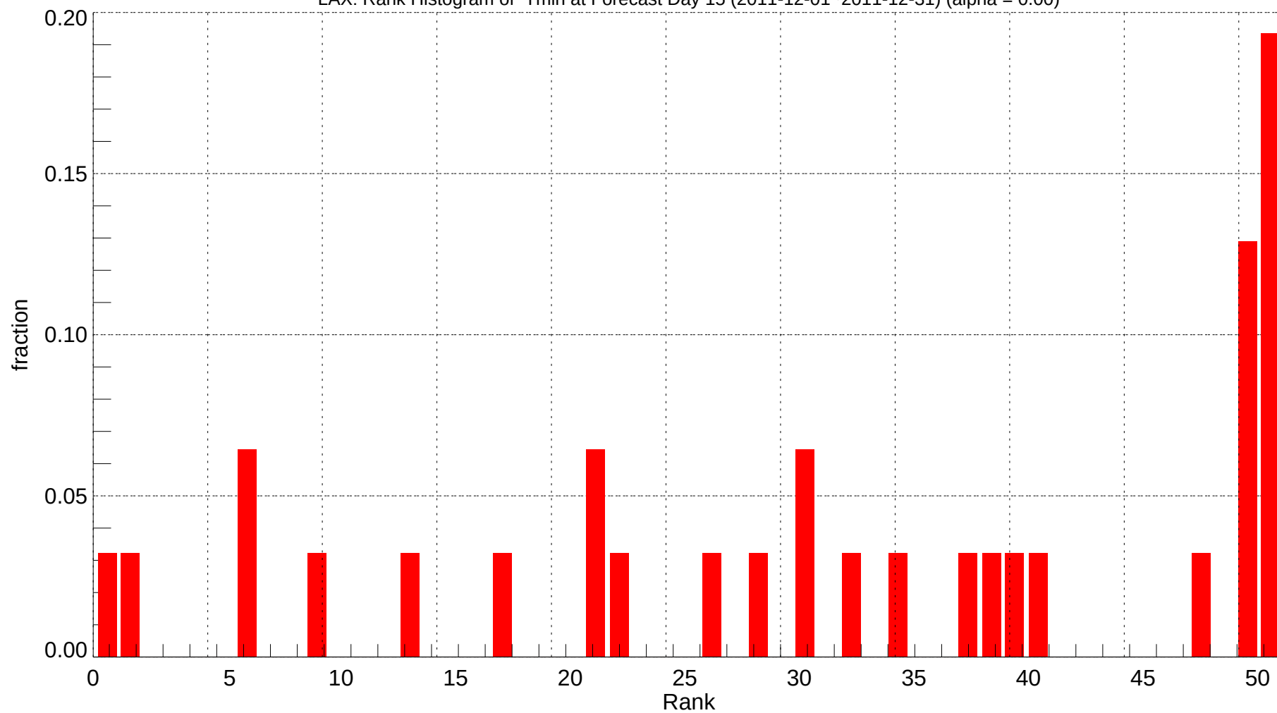
LAX: Rank Histogram of Tmin at Forecast Day 15 (2011-12-01~2011-12-31) (alpha = 0.00)
