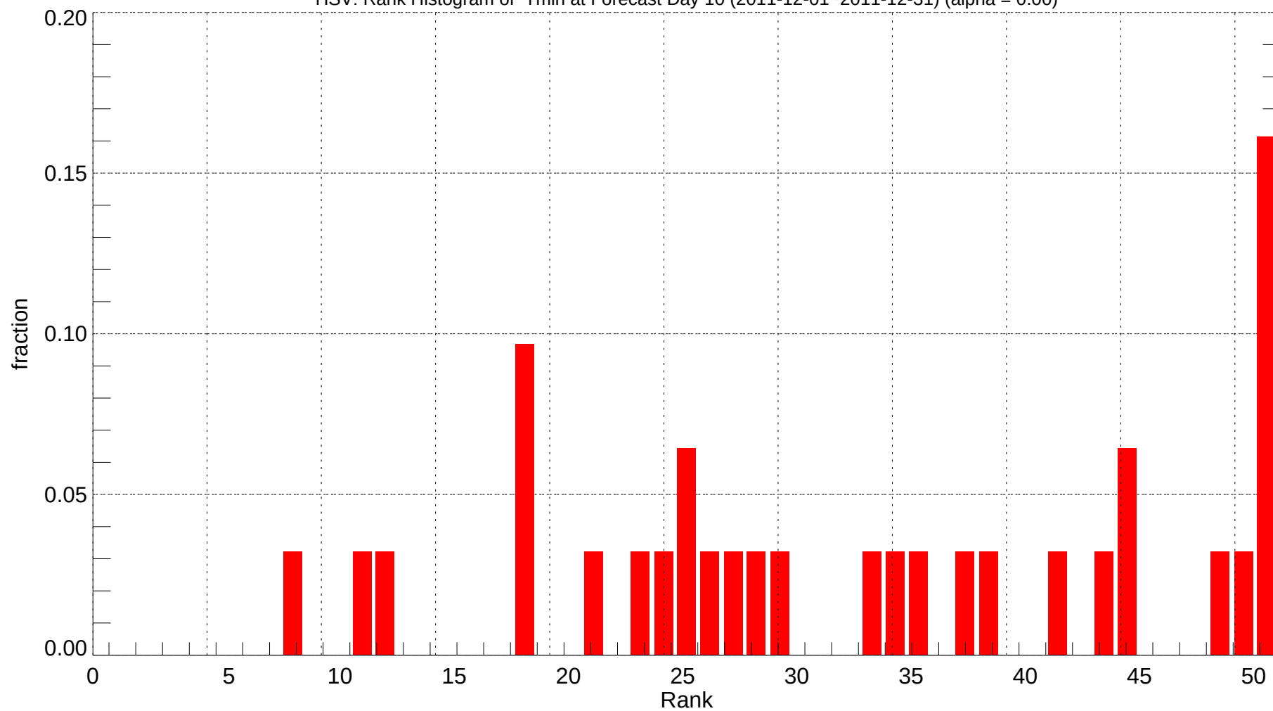
HSV: Rank Histogram of Tmin at Forecast Day 10 (2011-12-01~2011-12-31) (alpha = 0.00)
