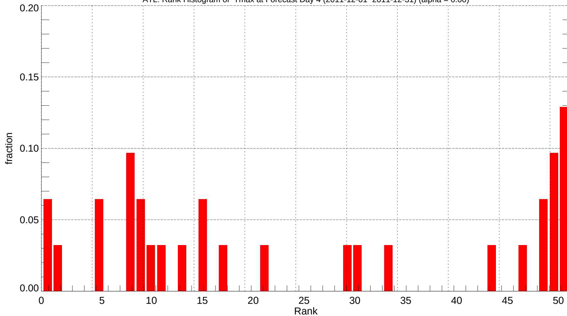
ATL: Rank Histogram of Tmax at Forecast Day 4 (2011-12-01~2011-12-31) (alpha = 0.00)
