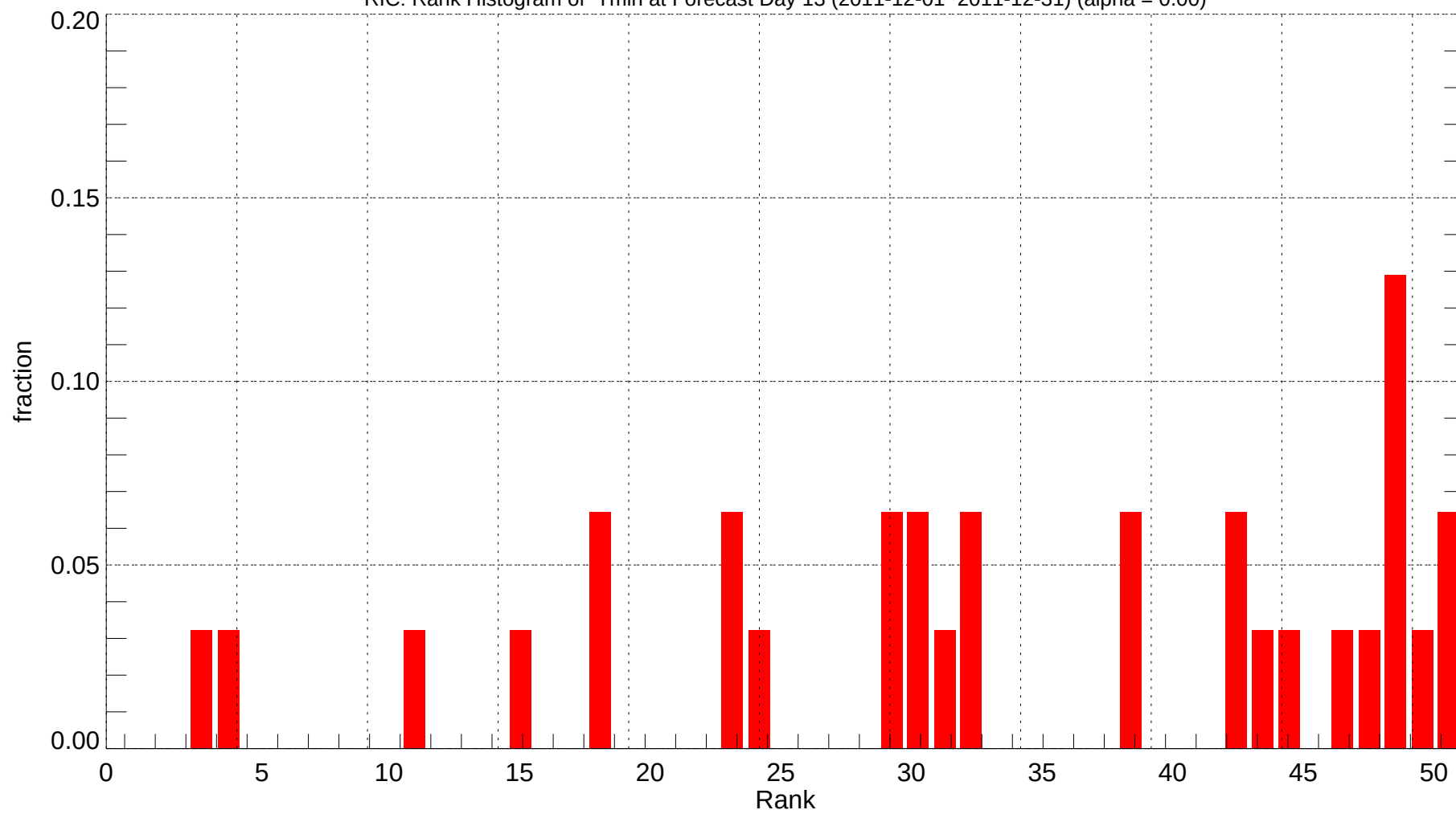
RIC: Rank Histogram of Tmin at Forecast Day 13 (2011-12-01~2011-12-31) (alpha = 0.00)
