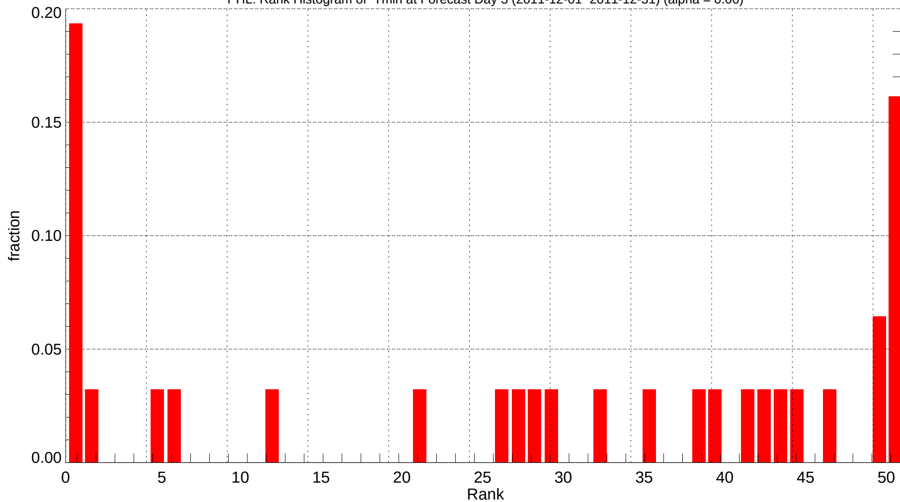
PHL: Rank Histogram of Tmin at Forecast Day 3 (2011-12-01~2011-12-31) (alpha = 0.00)
