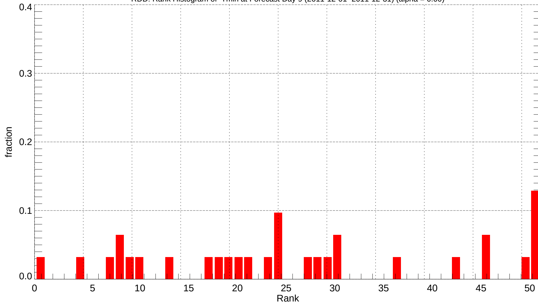
RDD: Rank Histogram of Tmin at Forecast Day 9 (2011-12-01~2011-12-31) (alpha = 0.00)
