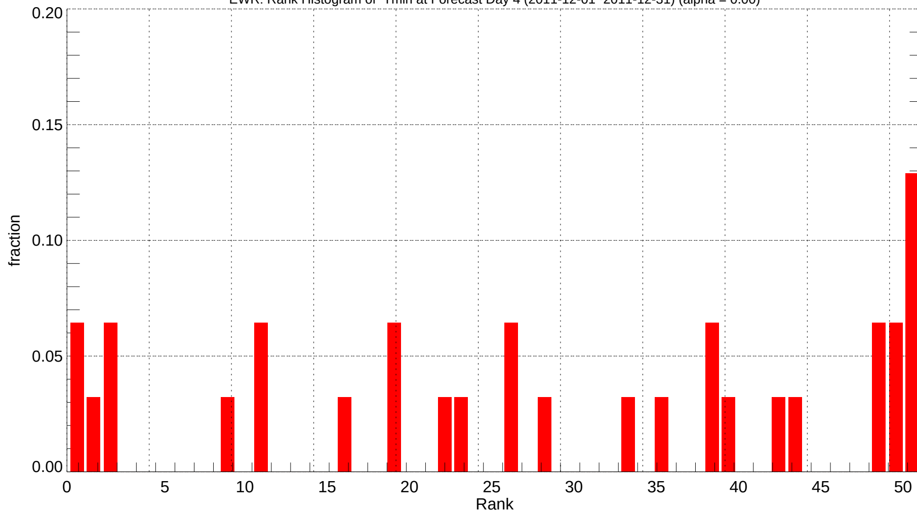
EWR: Rank Histogram of Tmin at Forecast Day 4 (2011-12-01~2011-12-31) (alpha = 0.00)
