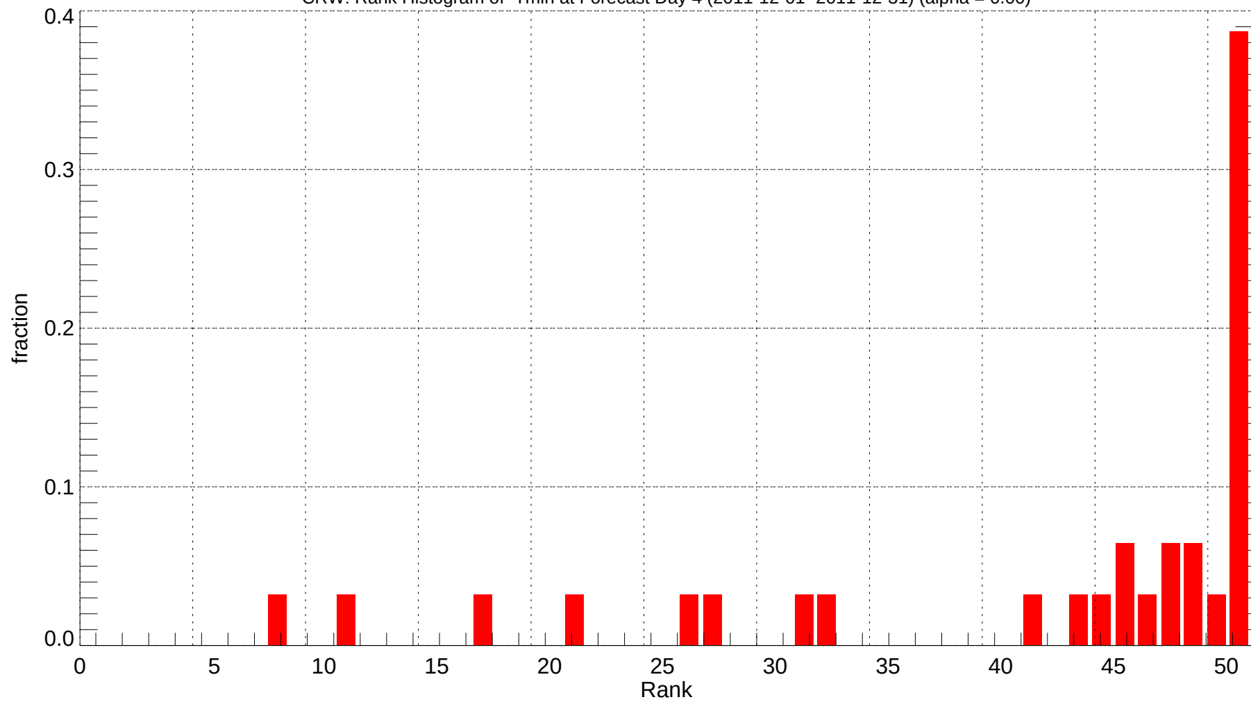
CRW: Rank Histogram of Tmin at Forecast Day 4 (2011-12-01~2011-12-31) (alpha = 0.00)
