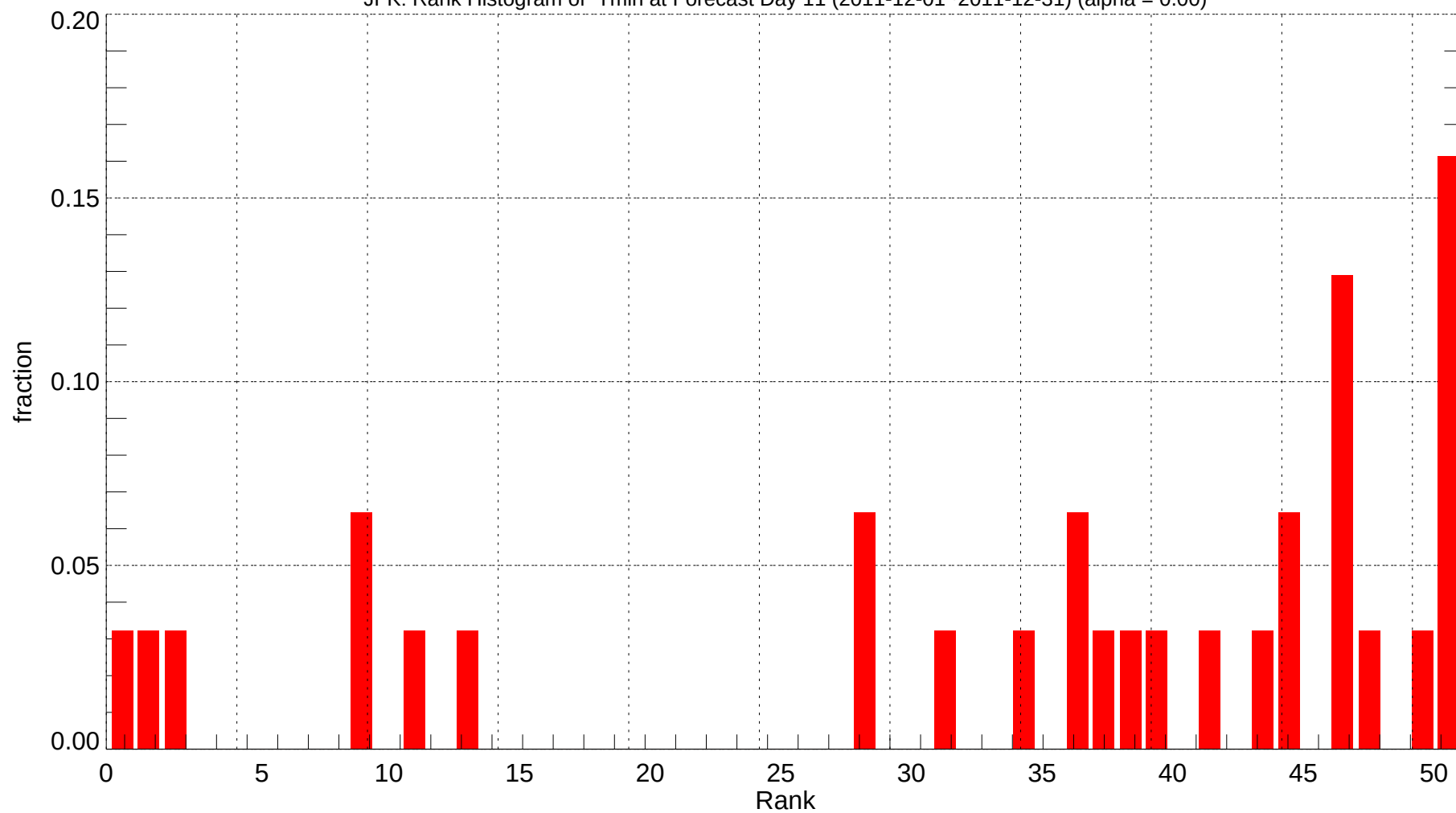
JFK: Rank Histogram of Tmin at Forecast Day 11 (2011-12-01~2011-12-31) (alpha = 0.00)
