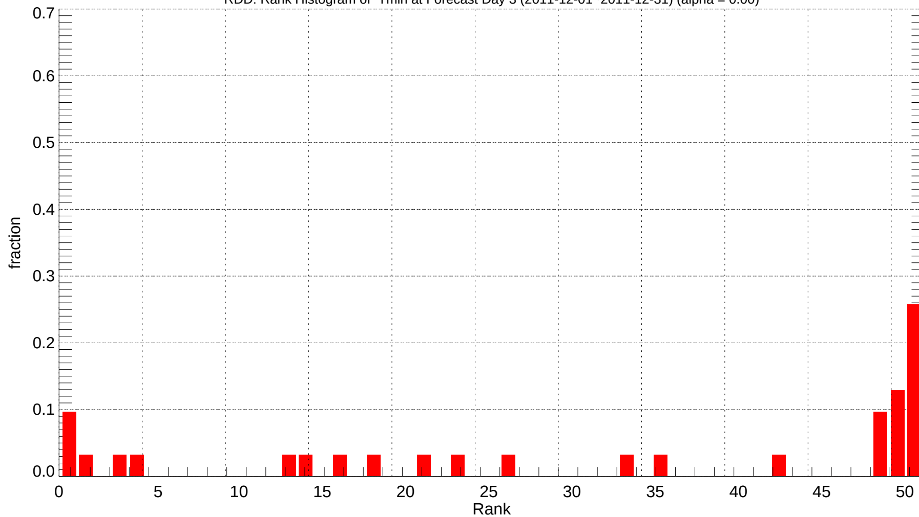
RDD: Rank Histogram of Tmin at Forecast Day 3 (2011-12-01~2011-12-31) (alpha = 0.00)
