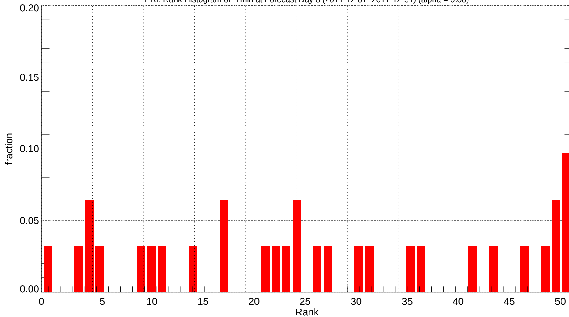
ERI: Rank Histogram of Tmin at Forecast Day 8 (2011-12-01~2011-12-31) (alpha = 0.00)
