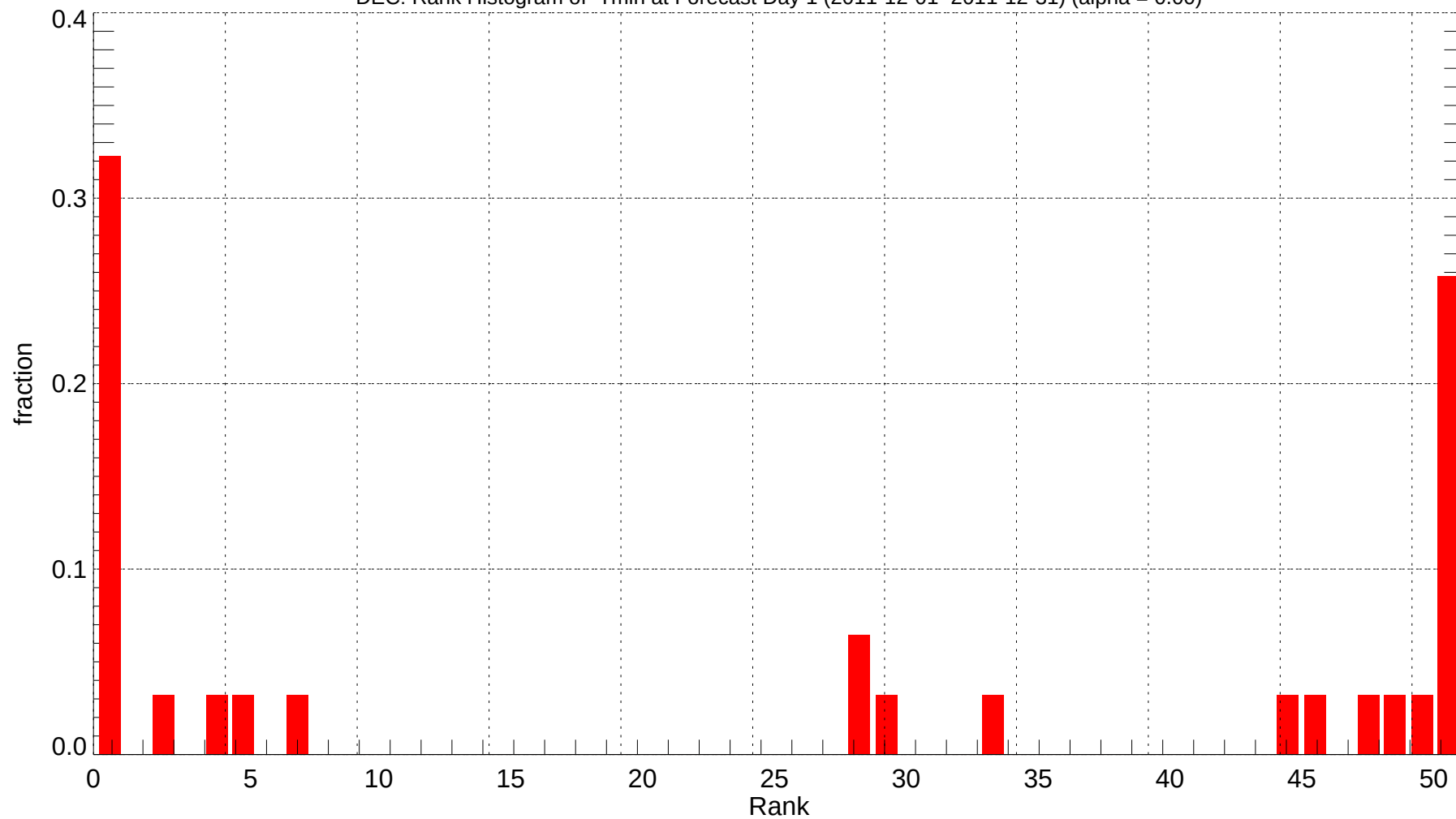
DEC: Rank Histogram of Tmin at Forecast Day 1 (2011-12-01~2011-12-31) (alpha = 0.00)
