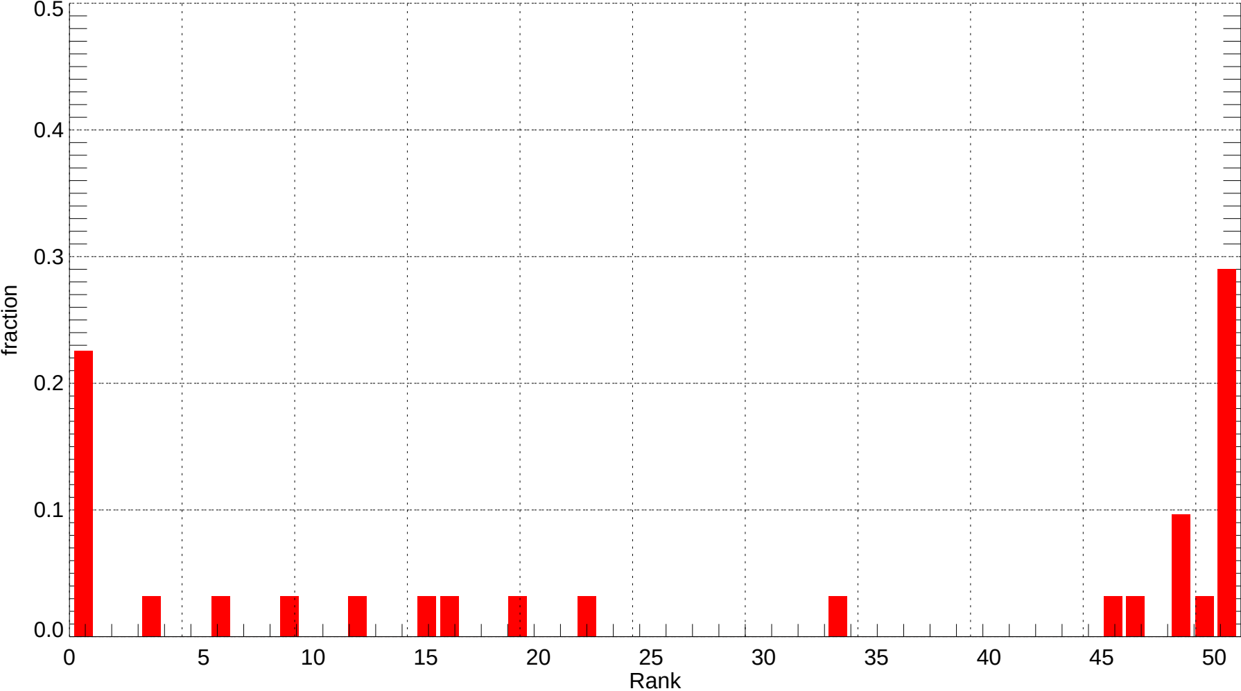
LAX: Rank Histogram of Tmin at Forecast Day 4 (2011-12-01~2011-12-31) (alpha = 0.00)
