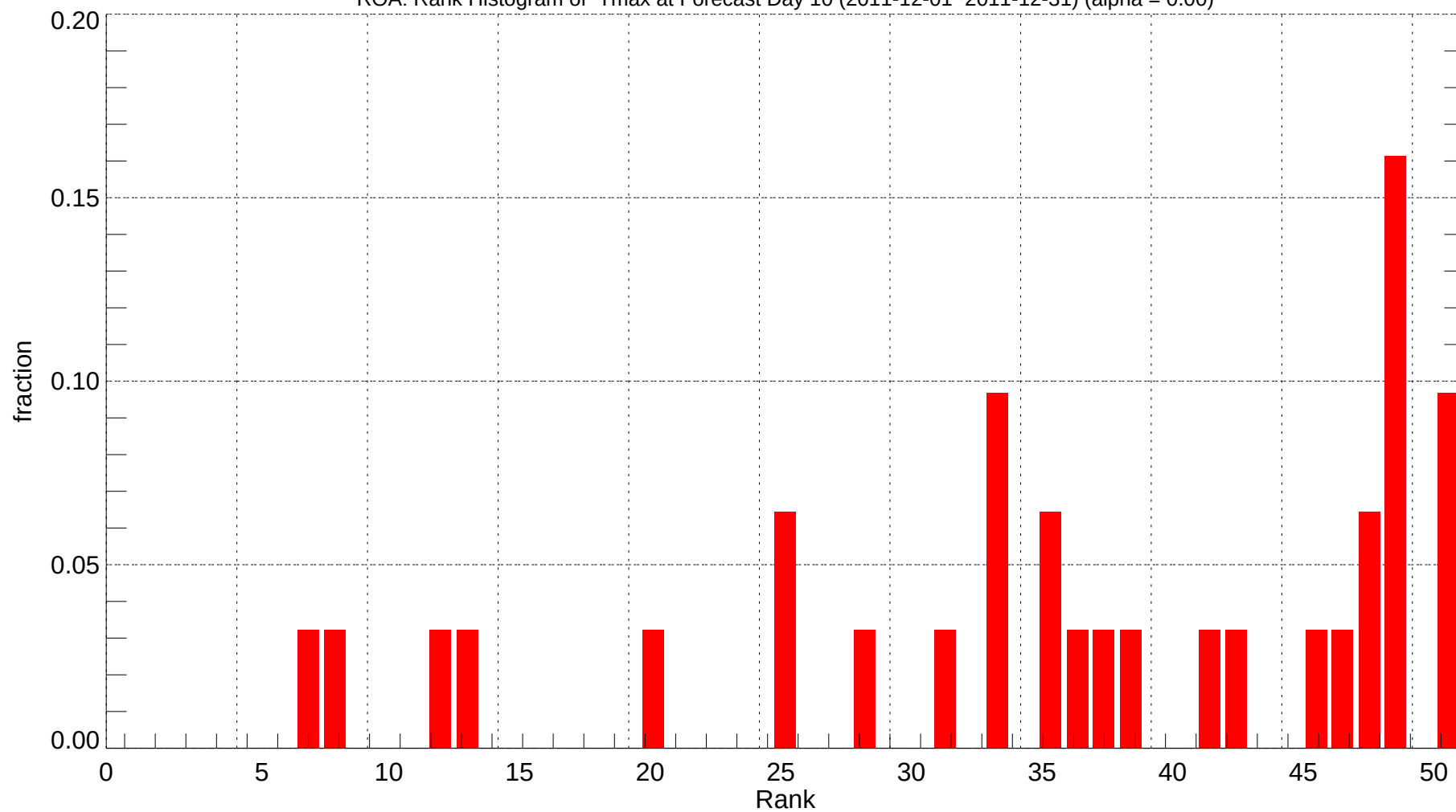
ROA: Rank Histogram of Tmax at Forecast Day 10 (2011-12-01~2011-12-31) (alpha = 0.00)
