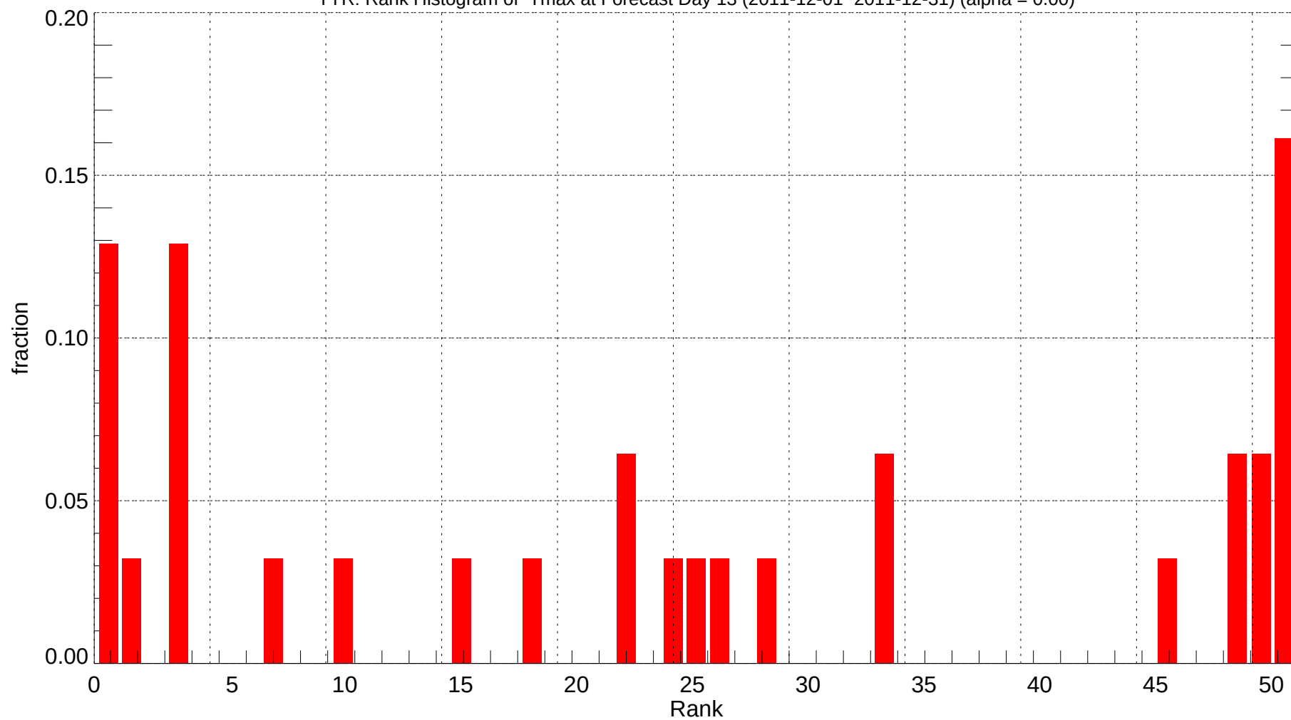
TYR: Rank Histogram of Tmax at Forecast Day 13 (2011-12-01~2011-12-31) (alpha = 0.00)
