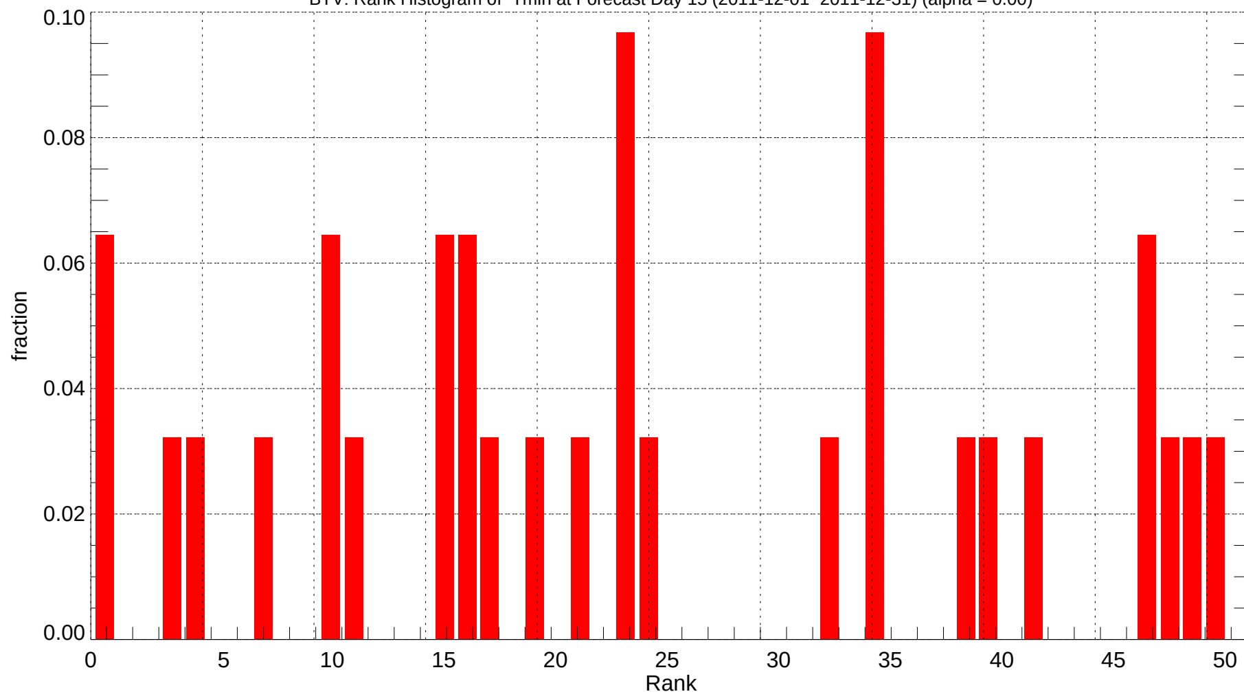
BTV: Rank Histogram of Tmin at Forecast Day 15 (2011-12-01~2011-12-31) (alpha = 0.00)
