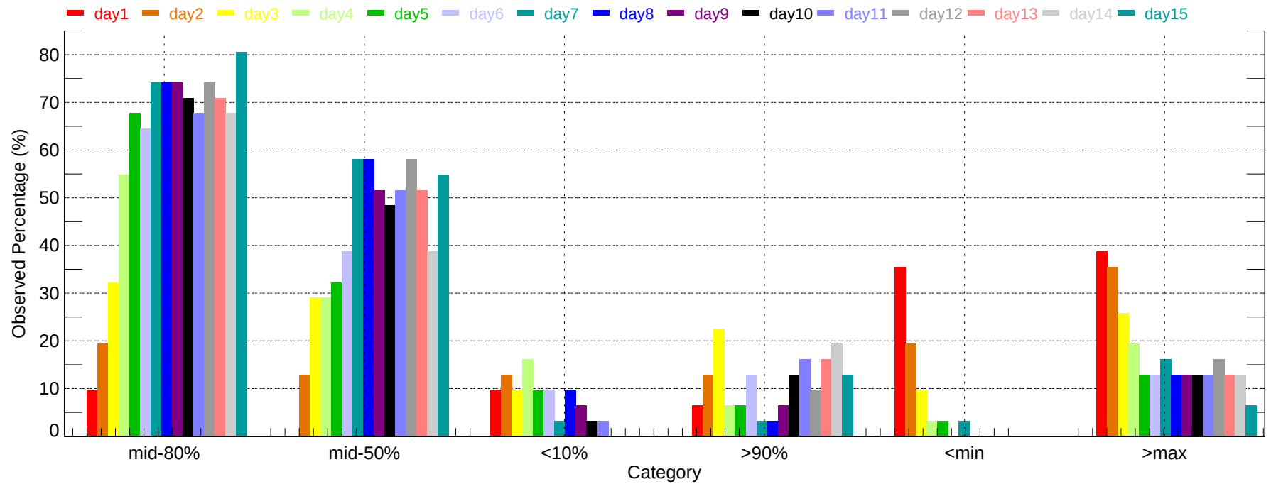
Observed Percentage of Ensembles - RDD: Max Temperature (2011-12-01~2011-12-31)
