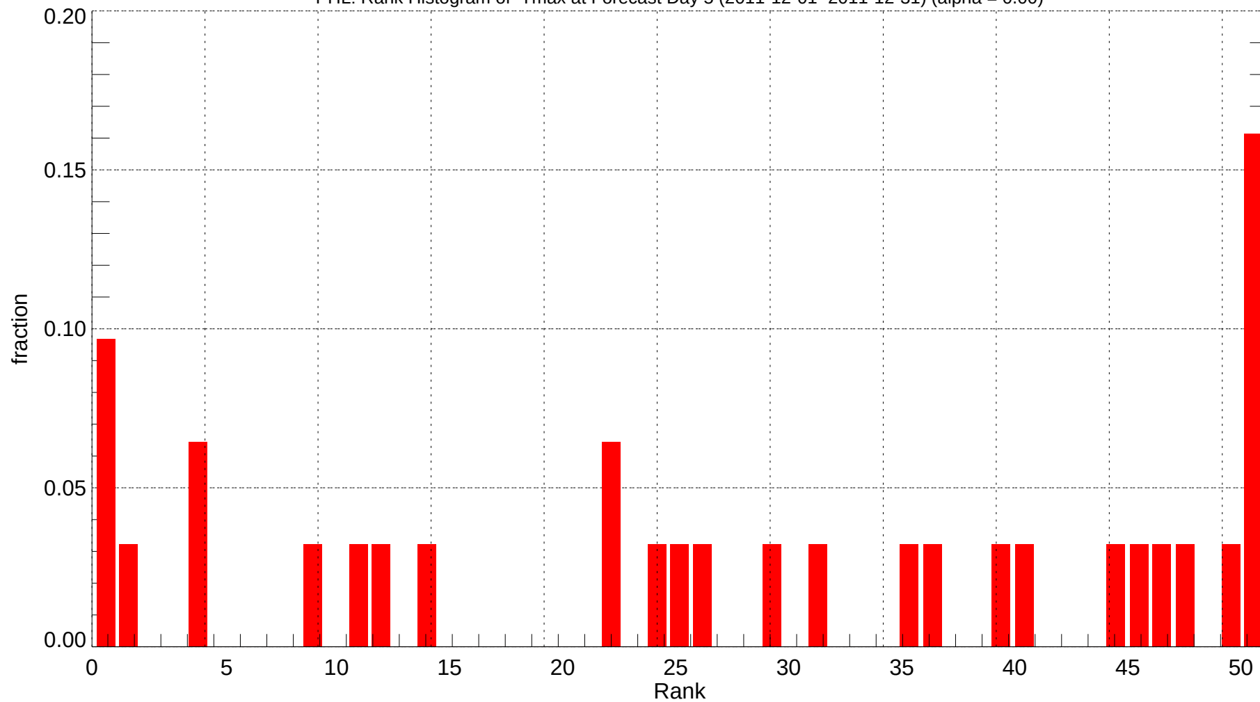
PHL: Rank Histogram of Tmax at Forecast Day 5 (2011-12-01~2011-12-31) (alpha = 0.00)
