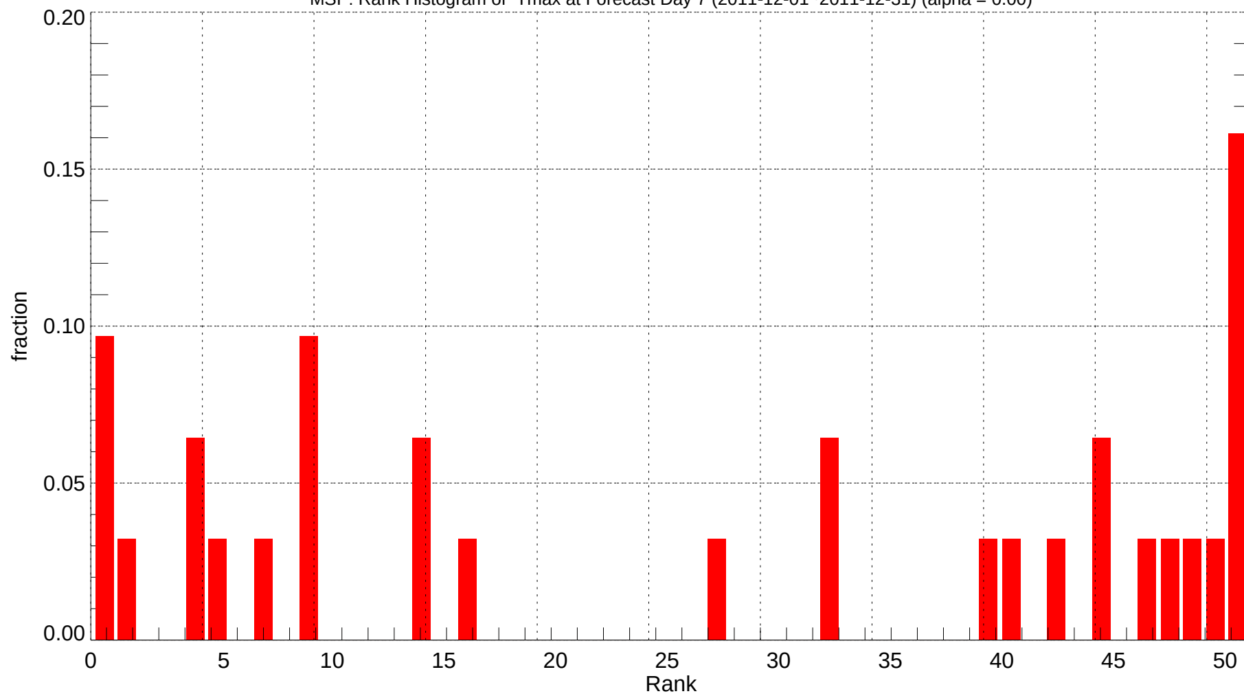
MSP: Rank Histogram of Tmax at Forecast Day 7 (2011-12-01~2011-12-31) (alpha = 0.00)
