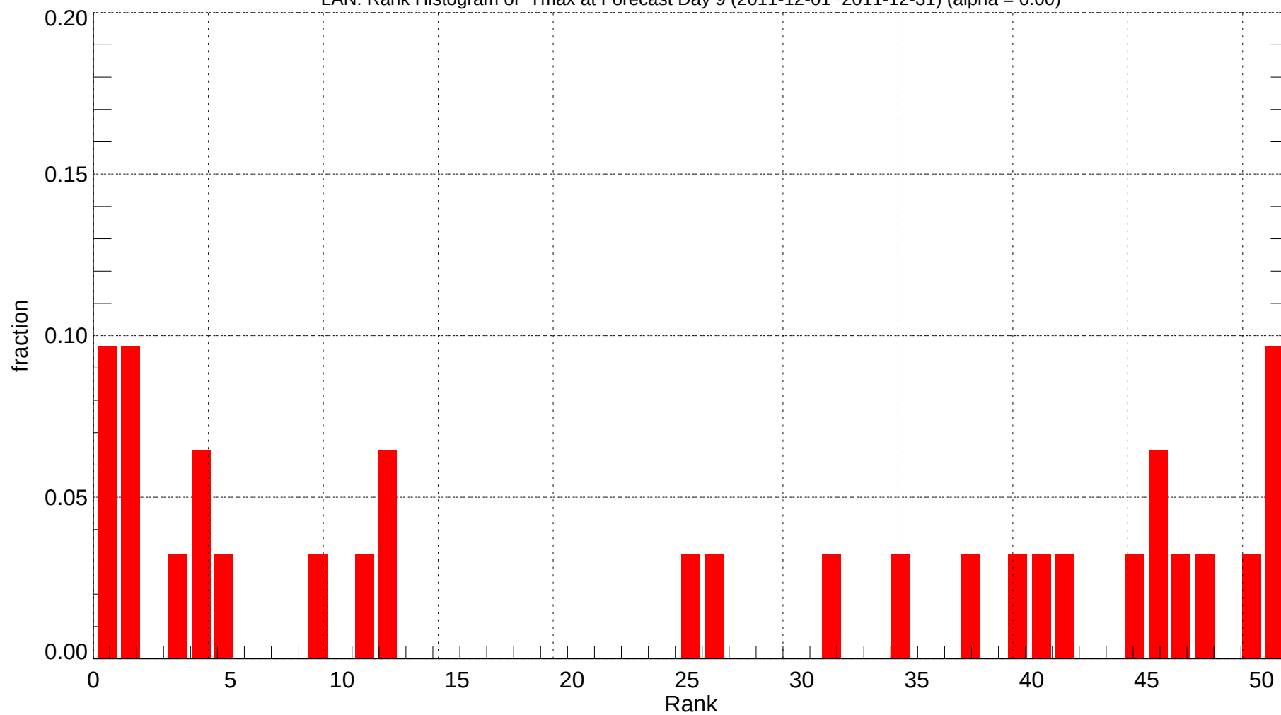
LAN: Rank Histogram of Tmax at Forecast Day 9 (2011-12-01~2011-12-31) (alpha = 0.00)
