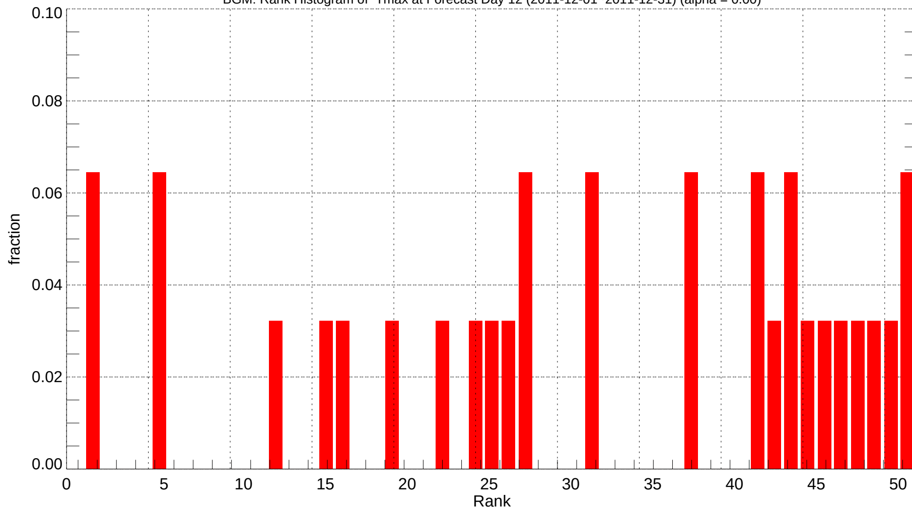
BGM: Rank Histogram of Tmax at Forecast Day 12 (2011-12-01~2011-12-31) (alpha = 0.00)
