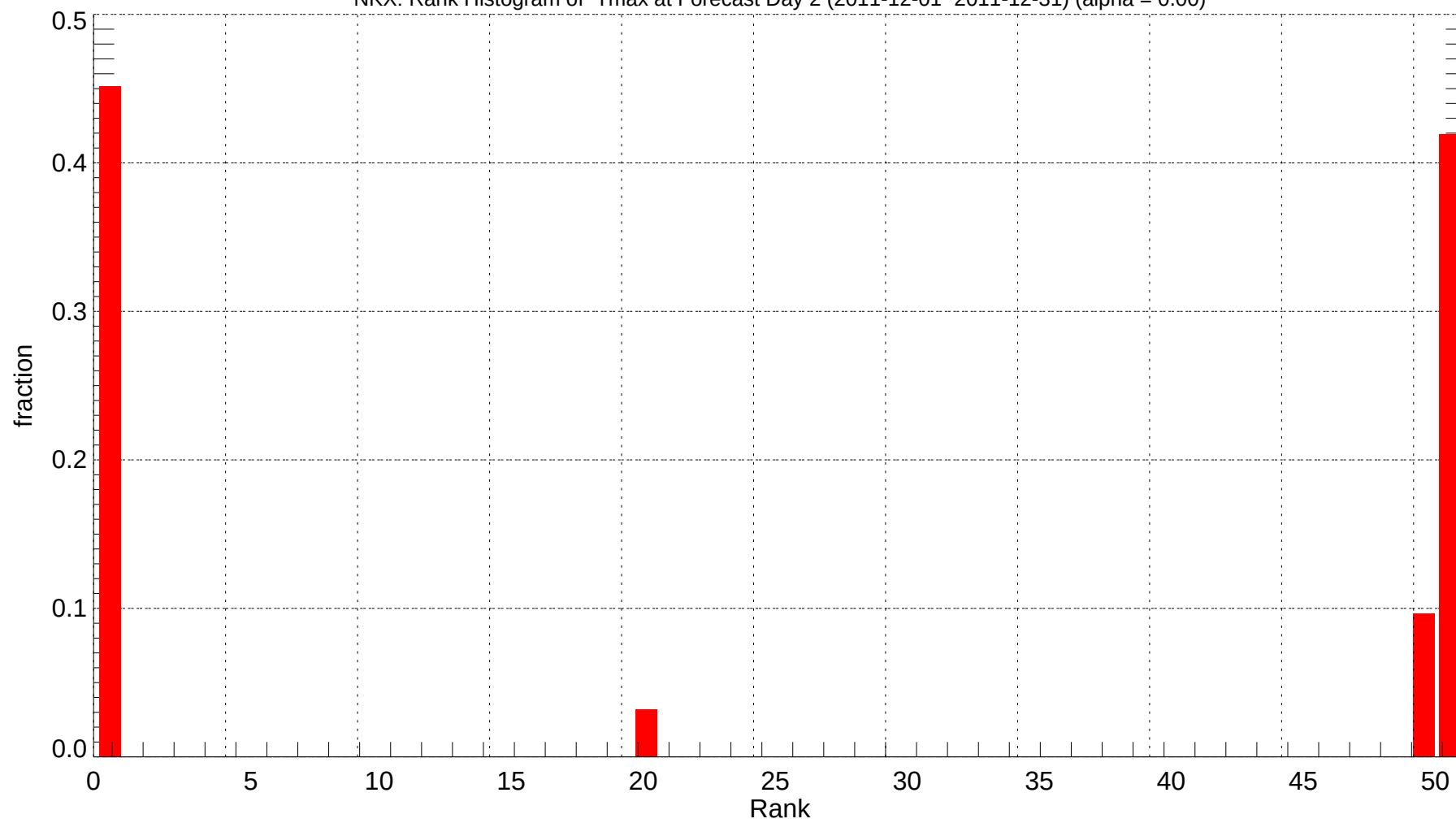
NKX: Rank Histogram of Tmax at Forecast Day 2 (2011-12-01~2011-12-31) (alpha = 0.00)
