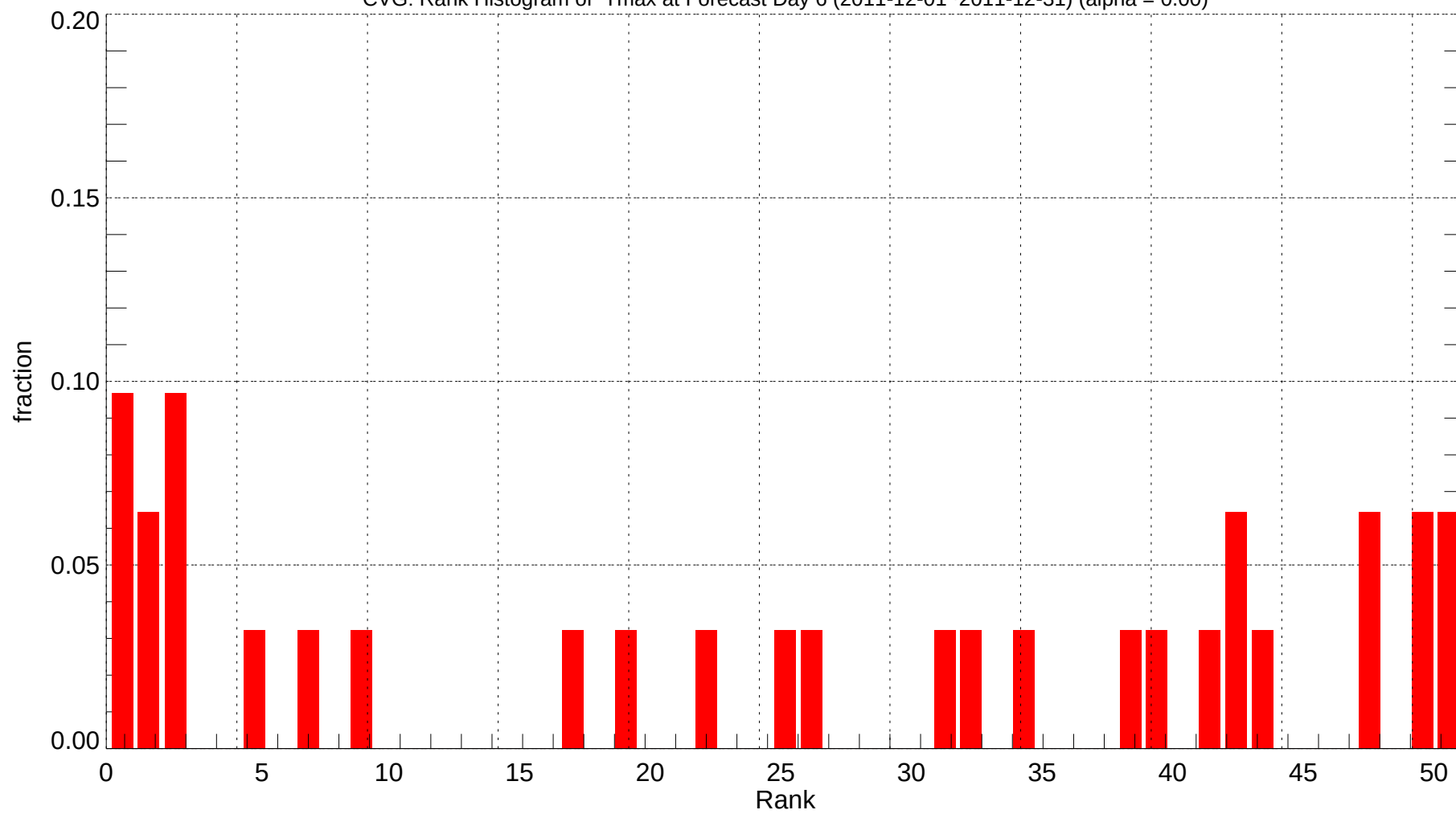
CVG: Rank Histogram of Tmax at Forecast Day 6 (2011-12-01~2011-12-31) (alpha = 0.00)
