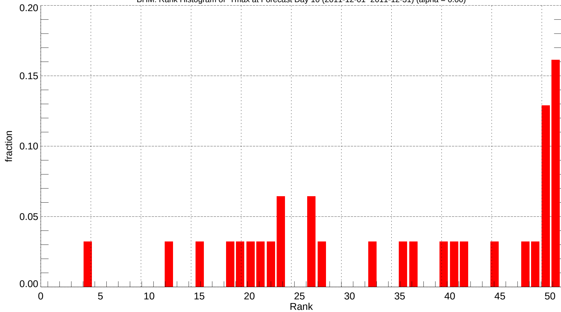
BHM: Rank Histogram of Tmax at Forecast Day 10 (2011-12-01~2011-12-31) (alpha = 0.00)
