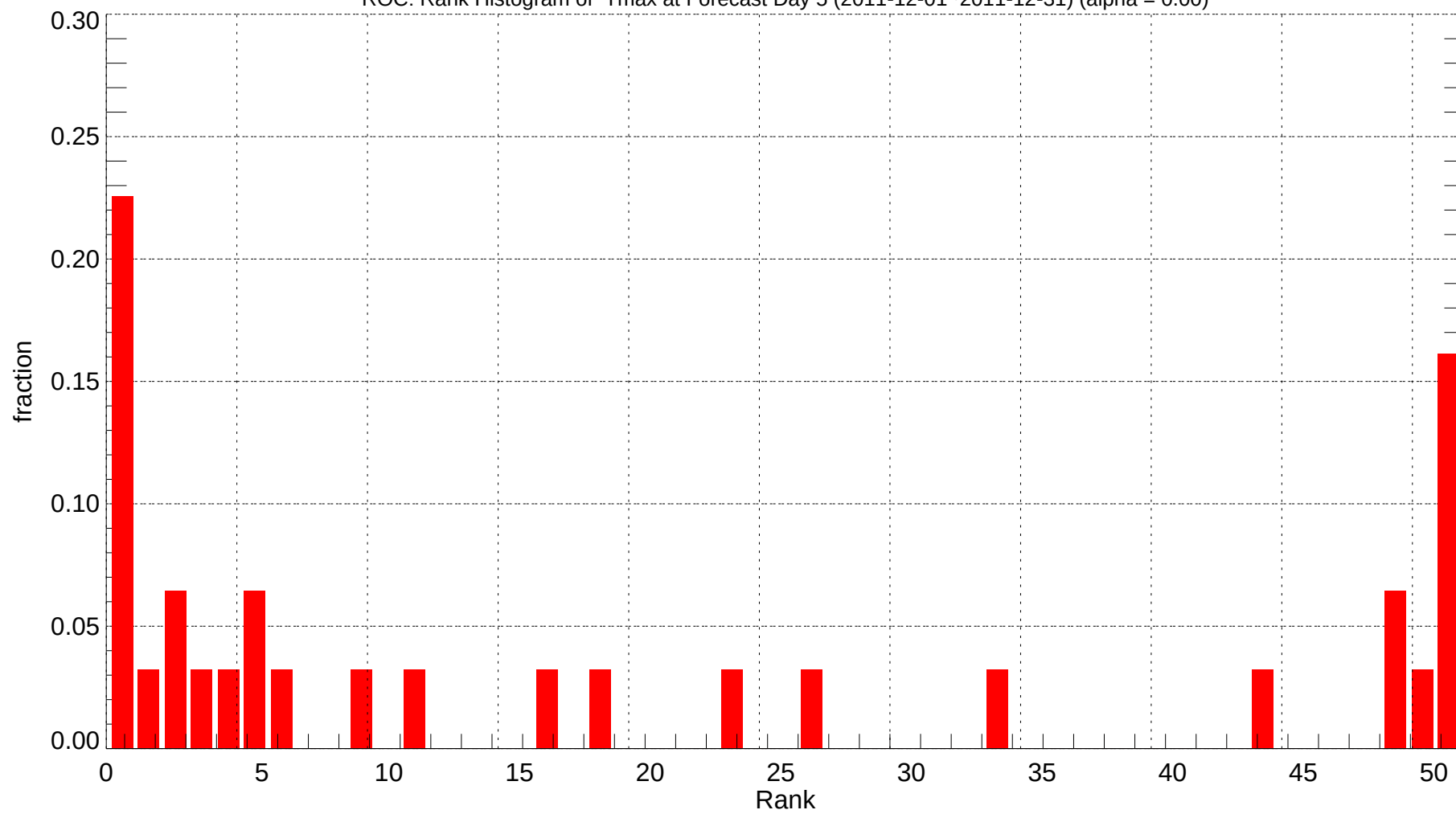
ROC: Rank Histogram of Tmax at Forecast Day 5 (2011-12-01~2011-12-31) (alpha = 0.00)
