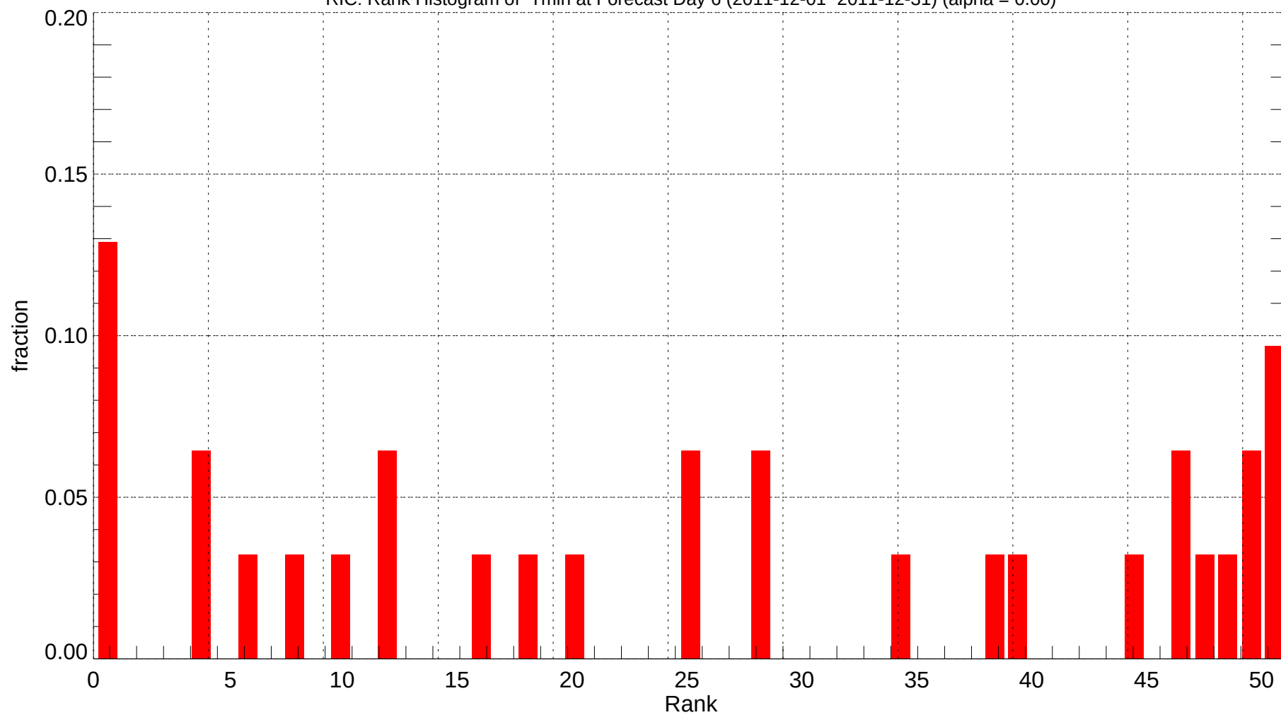
RIC: Rank Histogram of Tmin at Forecast Day 6 (2011-12-01~2011-12-31) (alpha = 0.00)
