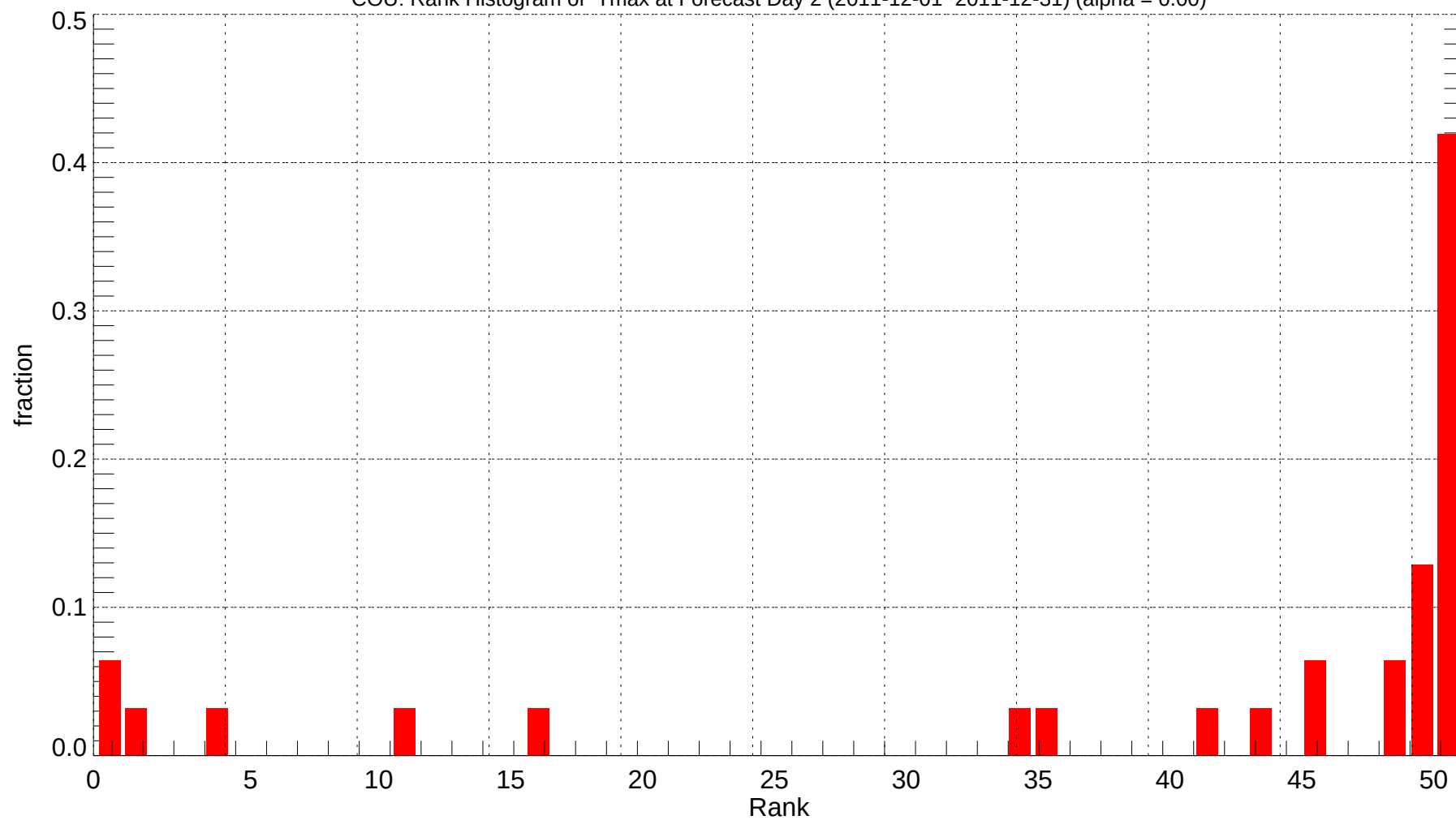
COU: Rank Histogram of Tmax at Forecast Day 2 (2011-12-01~2011-12-31) (alpha = 0.00)
