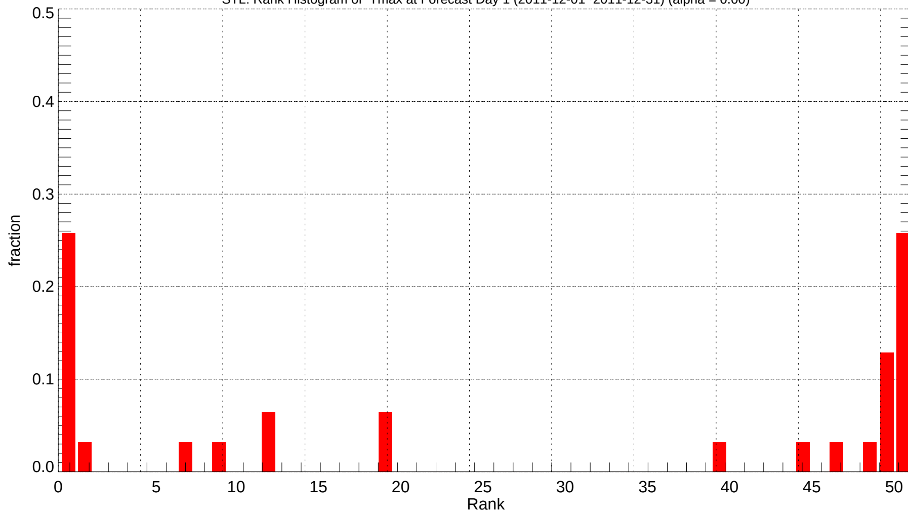
STL: Rank Histogram of Tmax at Forecast Day 1 (2011-12-01~2011-12-31) (alpha = 0.00)
