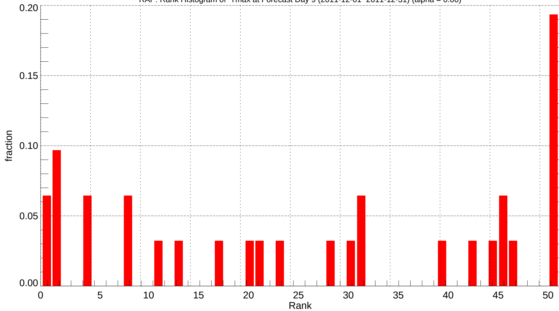
RAP: Rank Histogram of Tmax at Forecast Day 9 (2011-12-01~2011-12-31) (alpha = 0.00)
