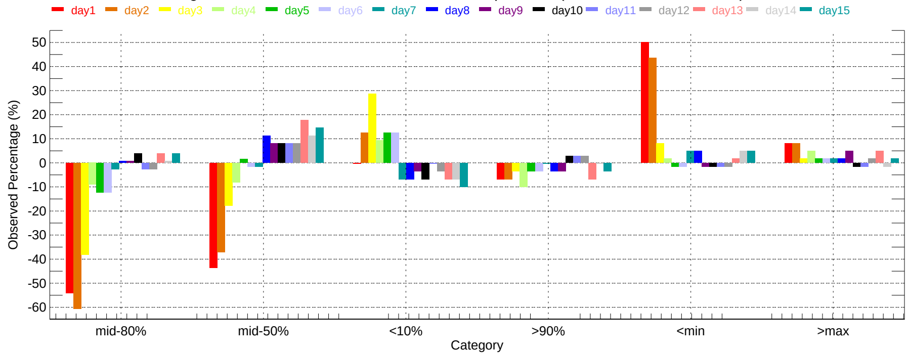
Observed Percentage Deviation of Ensembles - ABI: Min Temperature (2011-12-01~2011-12-31)
