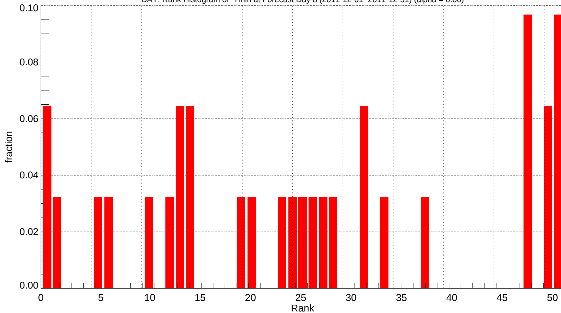
DAY: Rank Histogram of Tmin at Forecast Day 8 (2011-12-01~2011-12-31) (alpha = 0.00)
