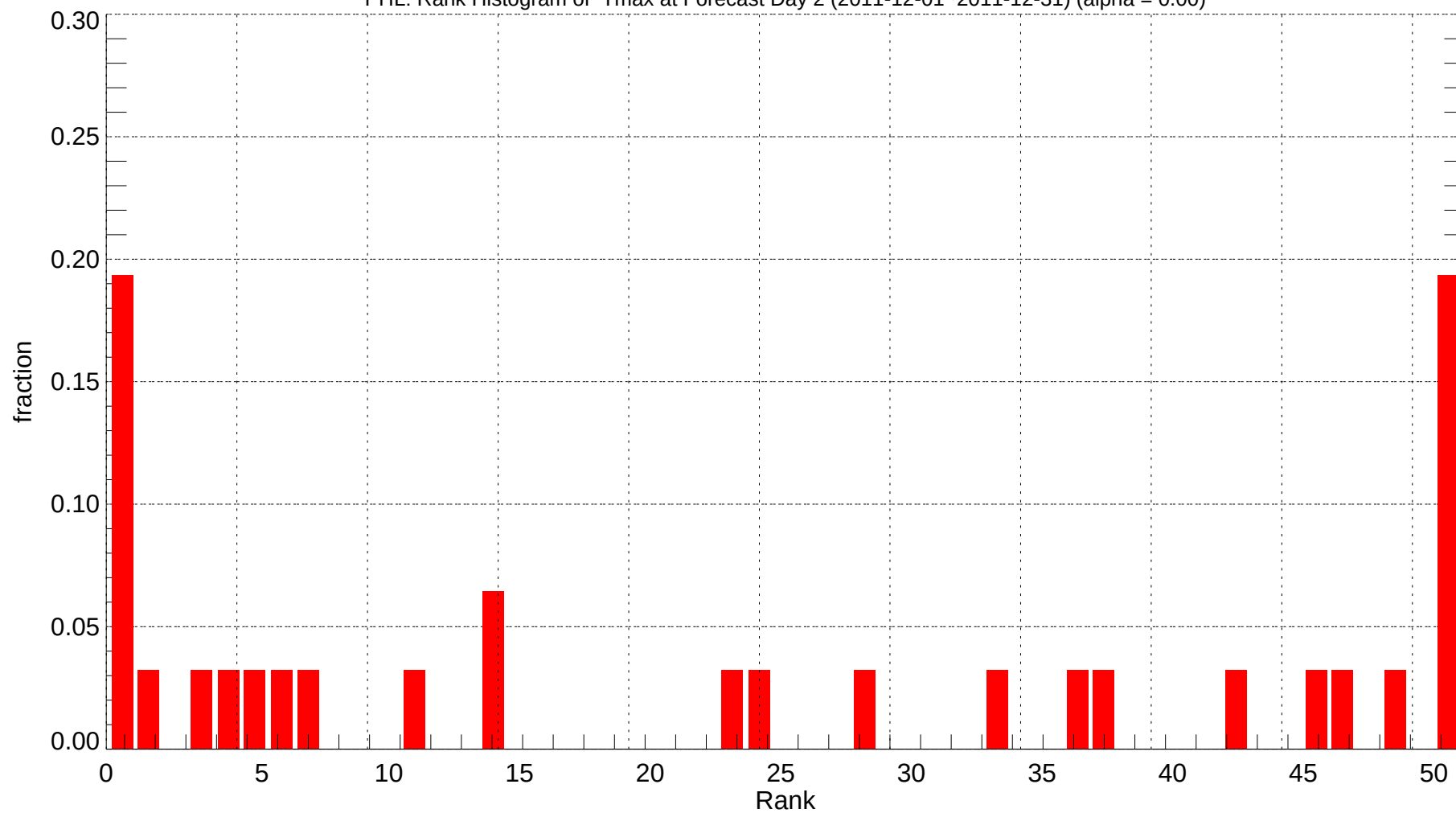
PHL: Rank Histogram of Tmax at Forecast Day 2 (2011-12-01~2011-12-31) (alpha = 0.00)
