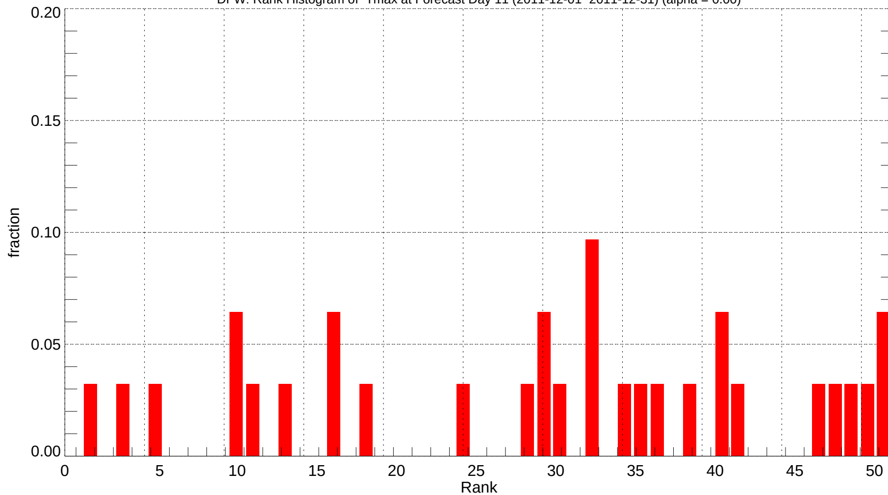
DFW: Rank Histogram of Tmax at Forecast Day 11 (2011-12-01~2011-12-31) (alpha = 0.00)
