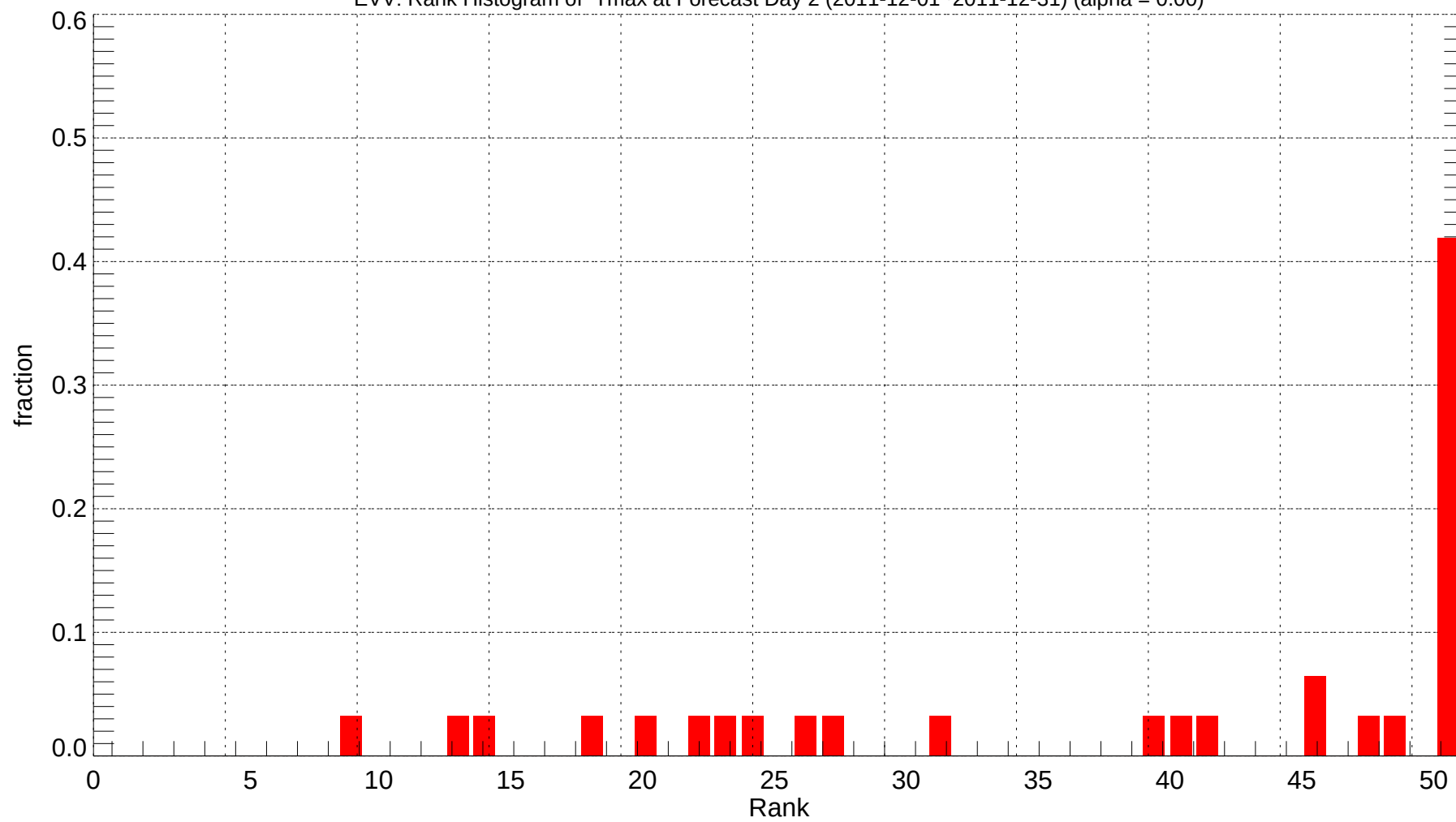
EVV: Rank Histogram of Tmax at Forecast Day 2 (2011-12-01~2011-12-31) (alpha = 0.00)
