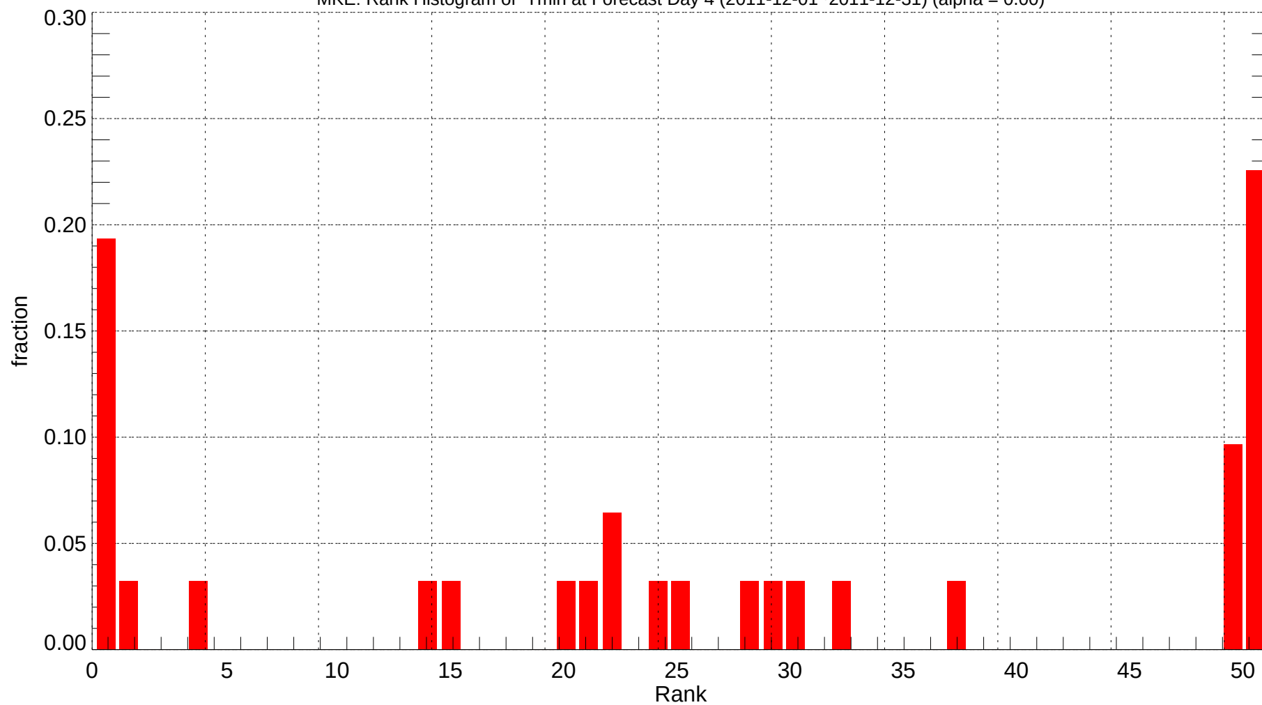
MKE: Rank Histogram of Tmin at Forecast Day 4 (2011-12-01~2011-12-31) (alpha = 0.00)
