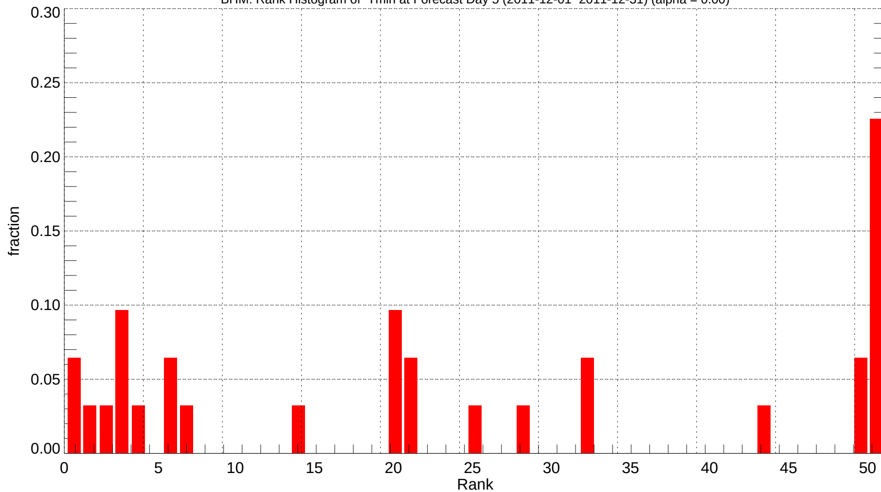
BHM: Rank Histogram of Tmin at Forecast Day 5 (2011-12-01~2011-12-31) (alpha = 0.00)
