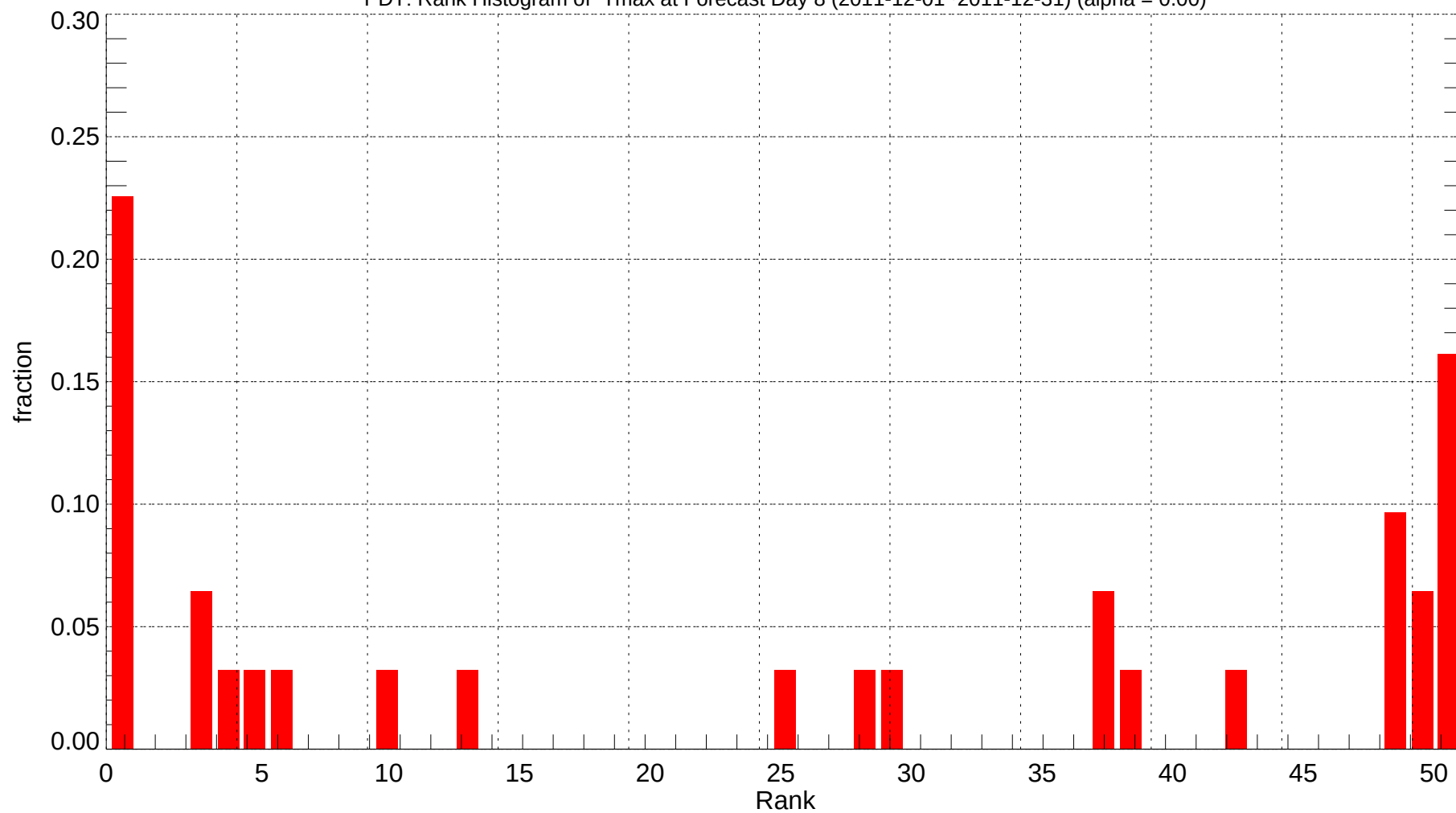
PDT: Rank Histogram of Tmax at Forecast Day 8 (2011-12-01~2011-12-31) (alpha = 0.00)
