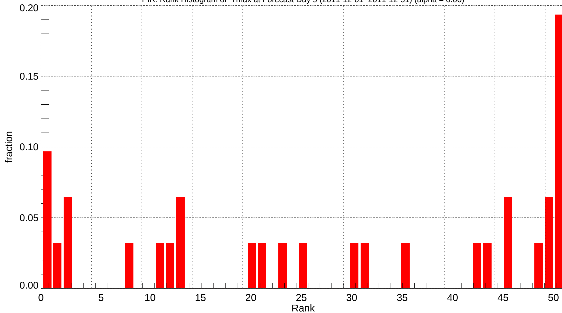
PIR: Rank Histogram of Tmax at Forecast Day 9 (2011-12-01~2011-12-31) (alpha = 0.00)
