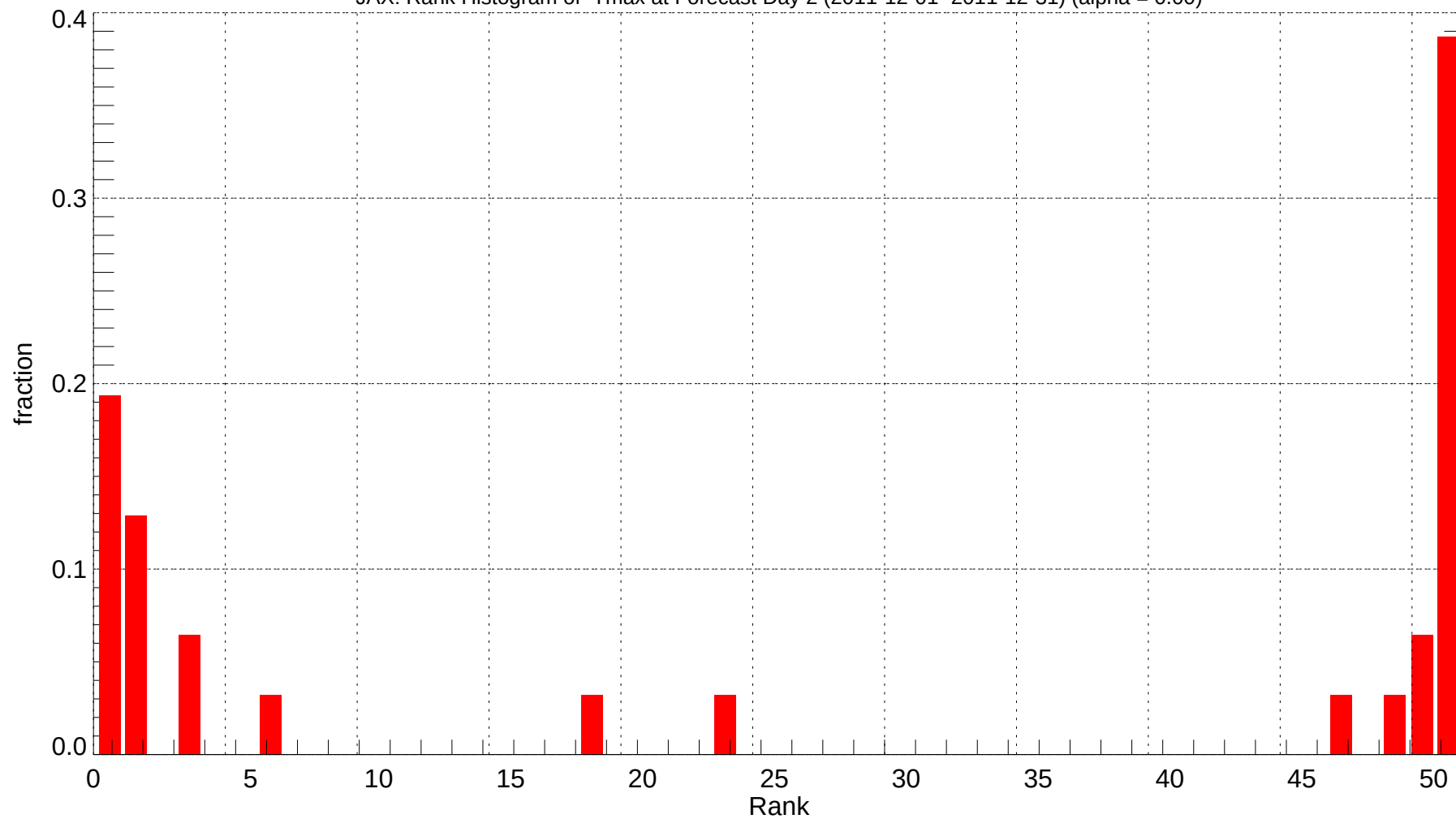
JAX: Rank Histogram of Tmax at Forecast Day 2 (2011-12-01~2011-12-31) (alpha = 0.00)
