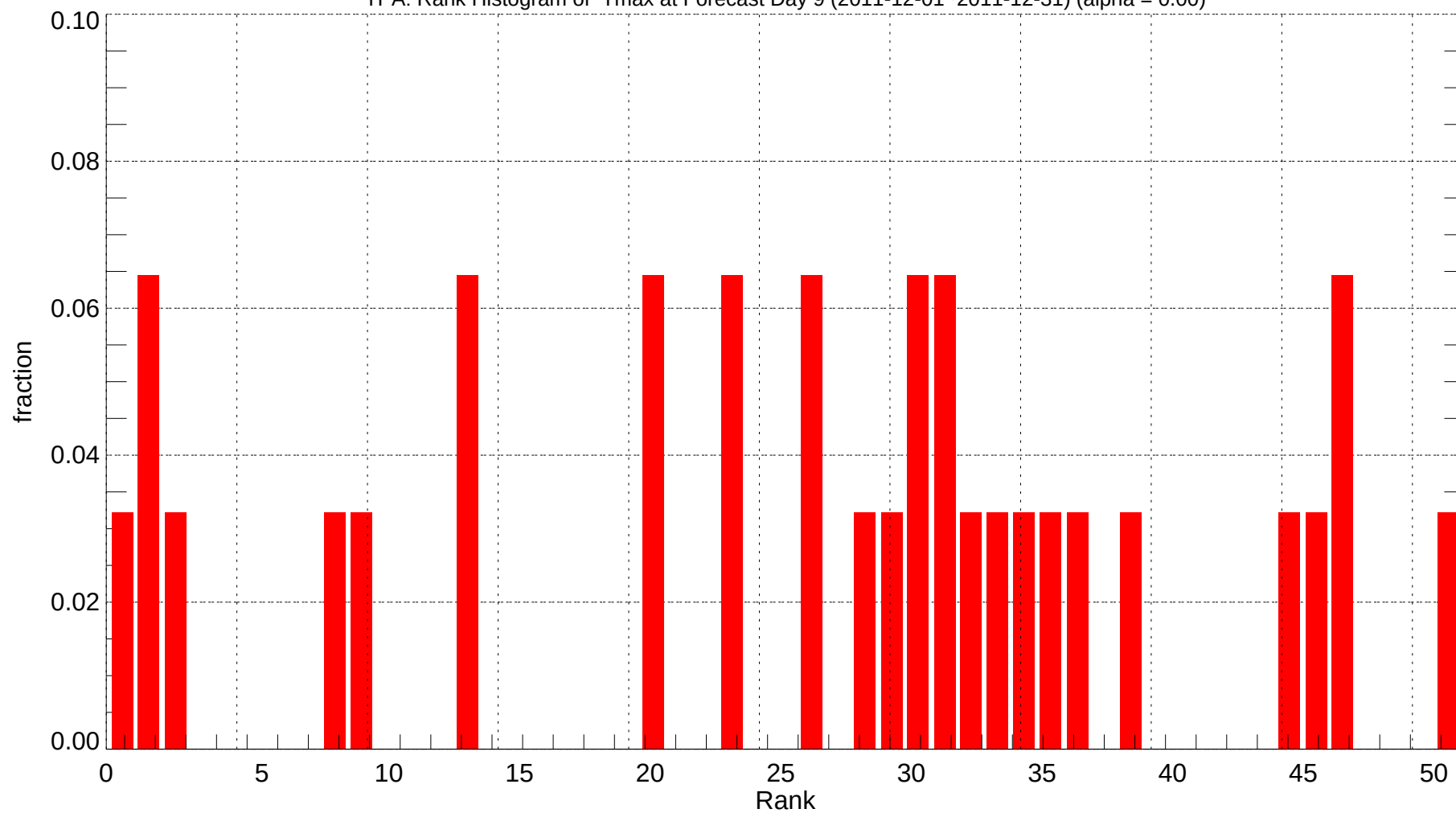
TPA: Rank Histogram of Tmax at Forecast Day 9 (2011-12-01~2011-12-31) (alpha = 0.00)
