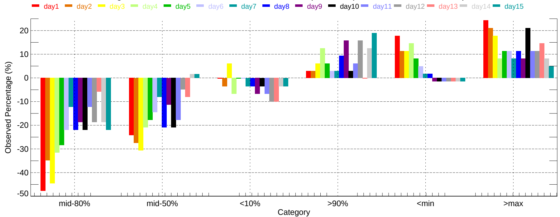
Observed Percentage Deviation of Ensembles - ABY: Max Temperature (2011-12-01~2011-12-31)
