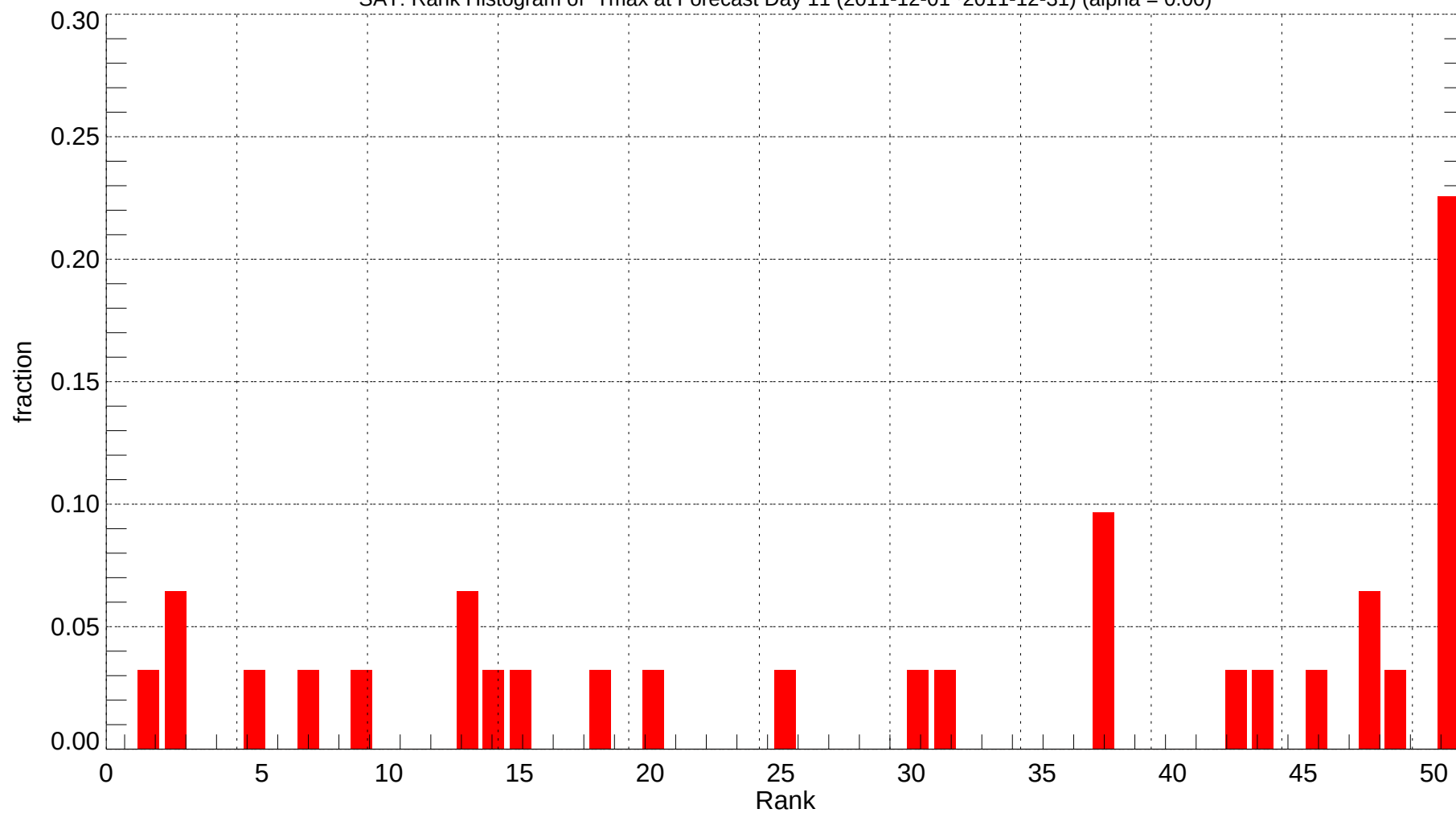
SAT: Rank Histogram of Tmax at Forecast Day 11 (2011-12-01~2011-12-31) (alpha = 0.00)
