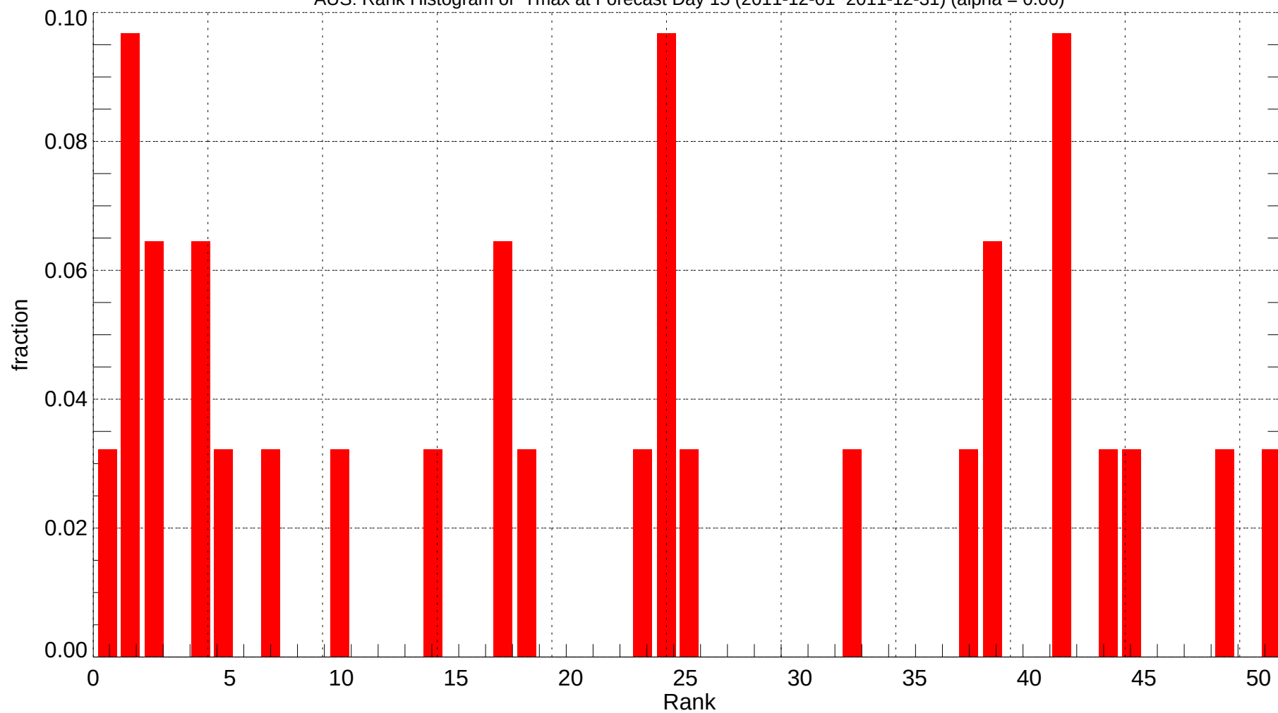
AUS: Rank Histogram of Tmax at Forecast Day 15 (2011-12-01~2011-12-31) (alpha = 0.00)
