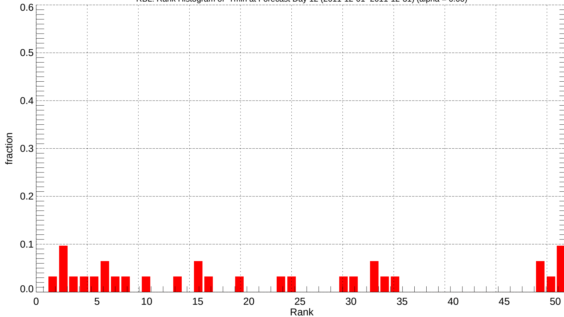
RBL: Rank Histogram of Tmin at Forecast Day 12 (2011-12-01~2011-12-31) (alpha = 0.00)
