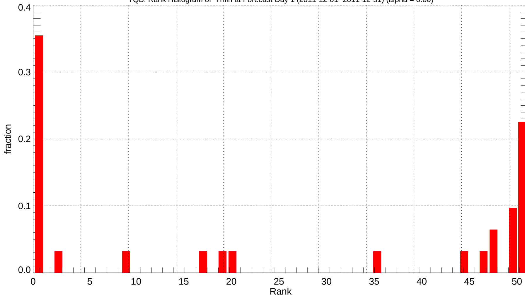
YQB: Rank Histogram of Tmin at Forecast Day 1 (2011-12-01~2011-12-31) (alpha = 0.00)
