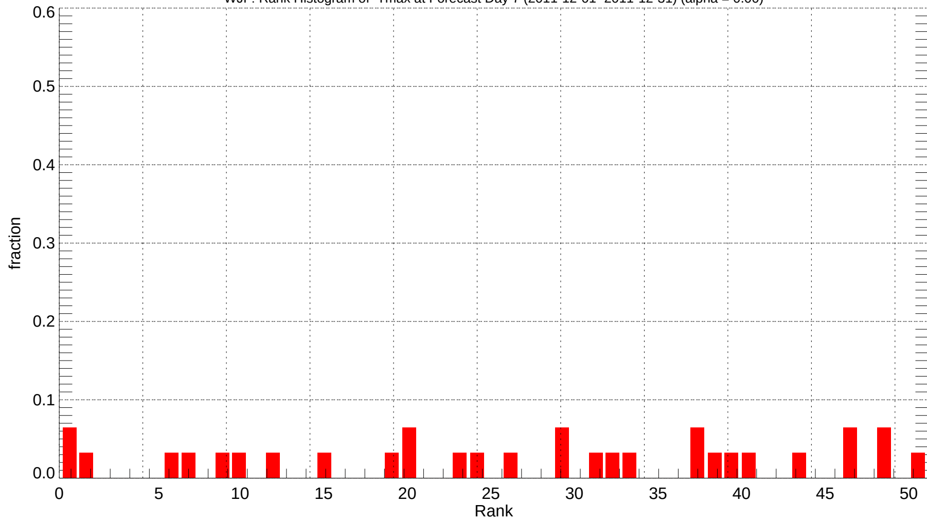
WJF: Rank Histogram of Tmax at Forecast Day 7 (2011-12-01~2011-12-31) (alpha = 0.00)
