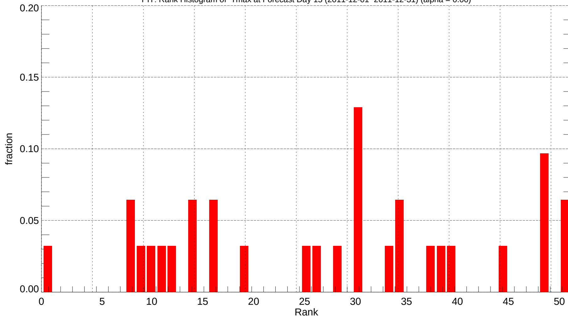
PIT: Rank Histogram of Tmax at Forecast Day 15 (2011-12-01~2011-12-31) (alpha = 0.00)
