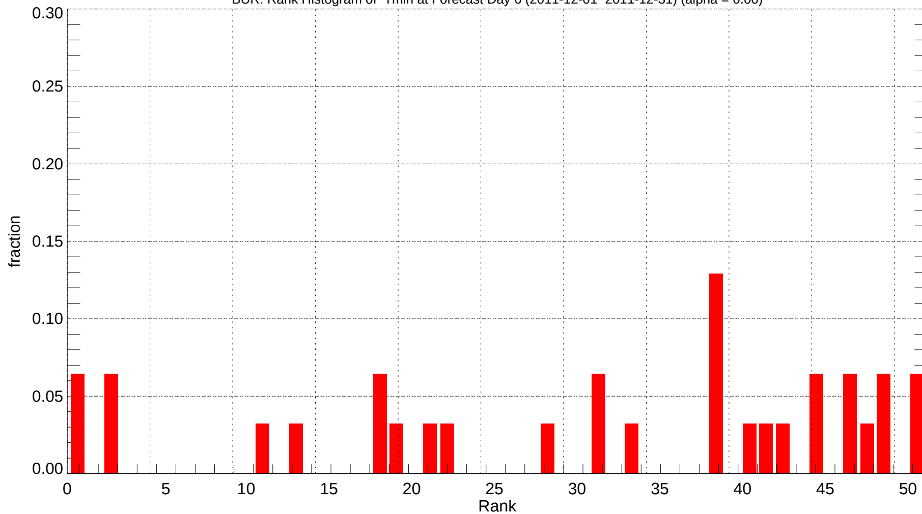
BUR: Rank Histogram of Tmin at Forecast Day 6 (2011-12-01~2011-12-31) (alpha = 0.00)
