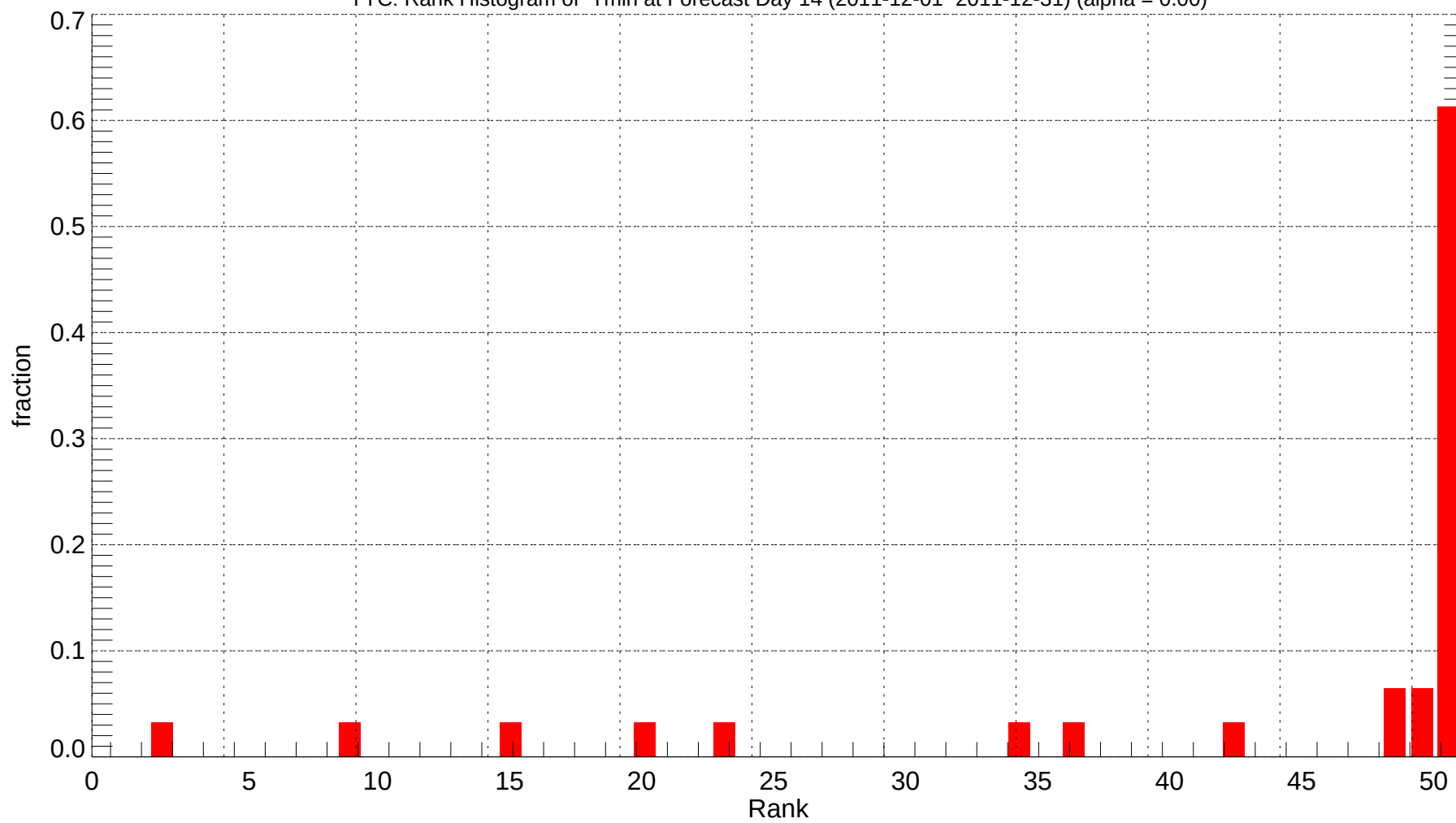
YYC: Rank Histogram of Tmin at Forecast Day 14 (2011-12-01~2011-12-31) (alpha = 0.00)
