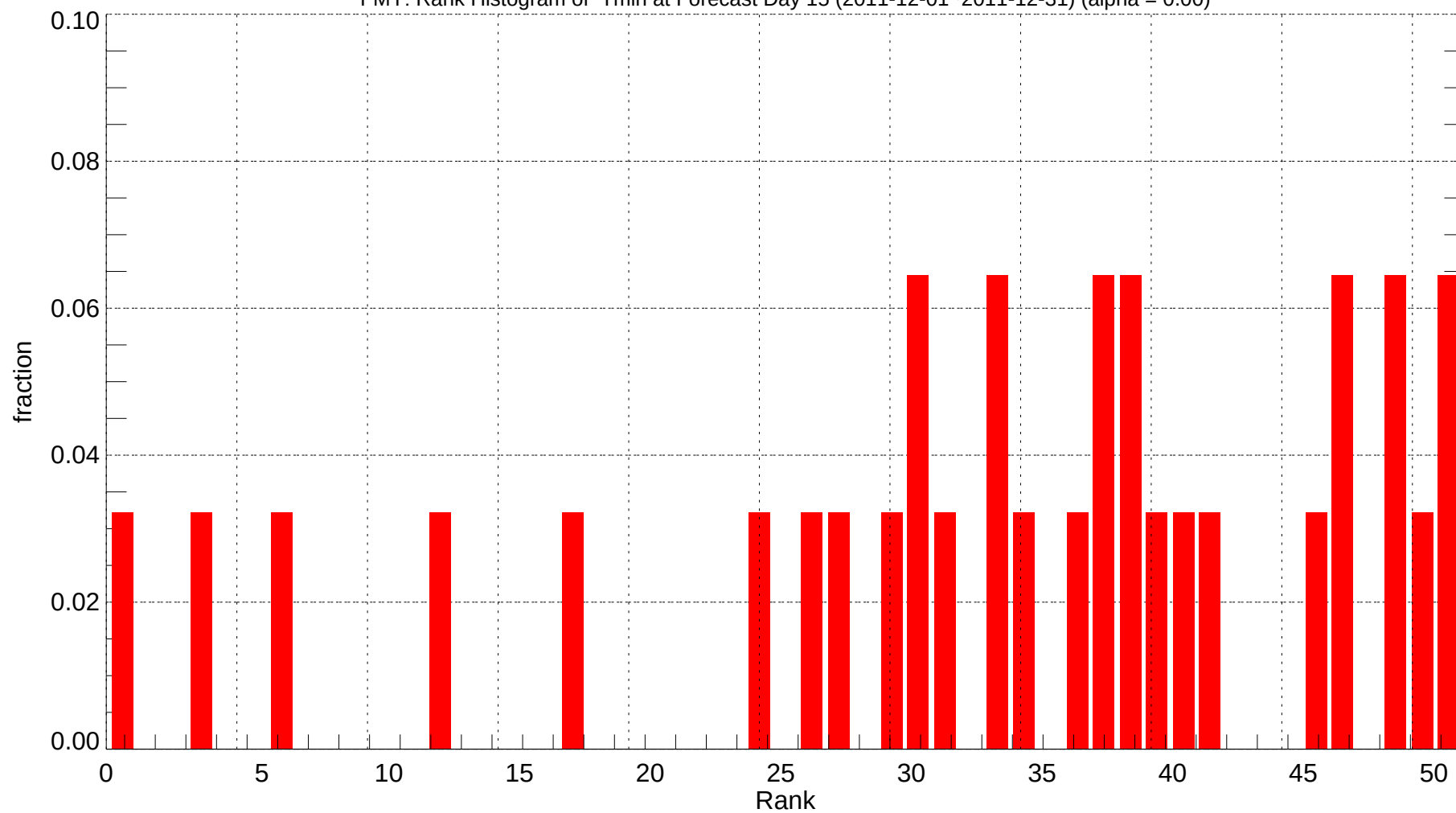
FMY: Rank Histogram of Tmin at Forecast Day 15 (2011-12-01~2011-12-31) (alpha = 0.00)
