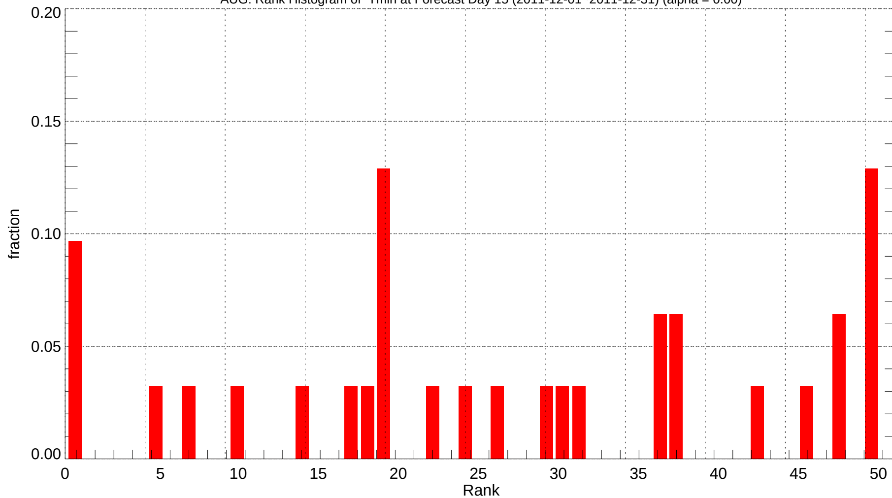
AUG: Rank Histogram of Tmin at Forecast Day 15 (2011-12-01~2011-12-31) (alpha = 0.00)
