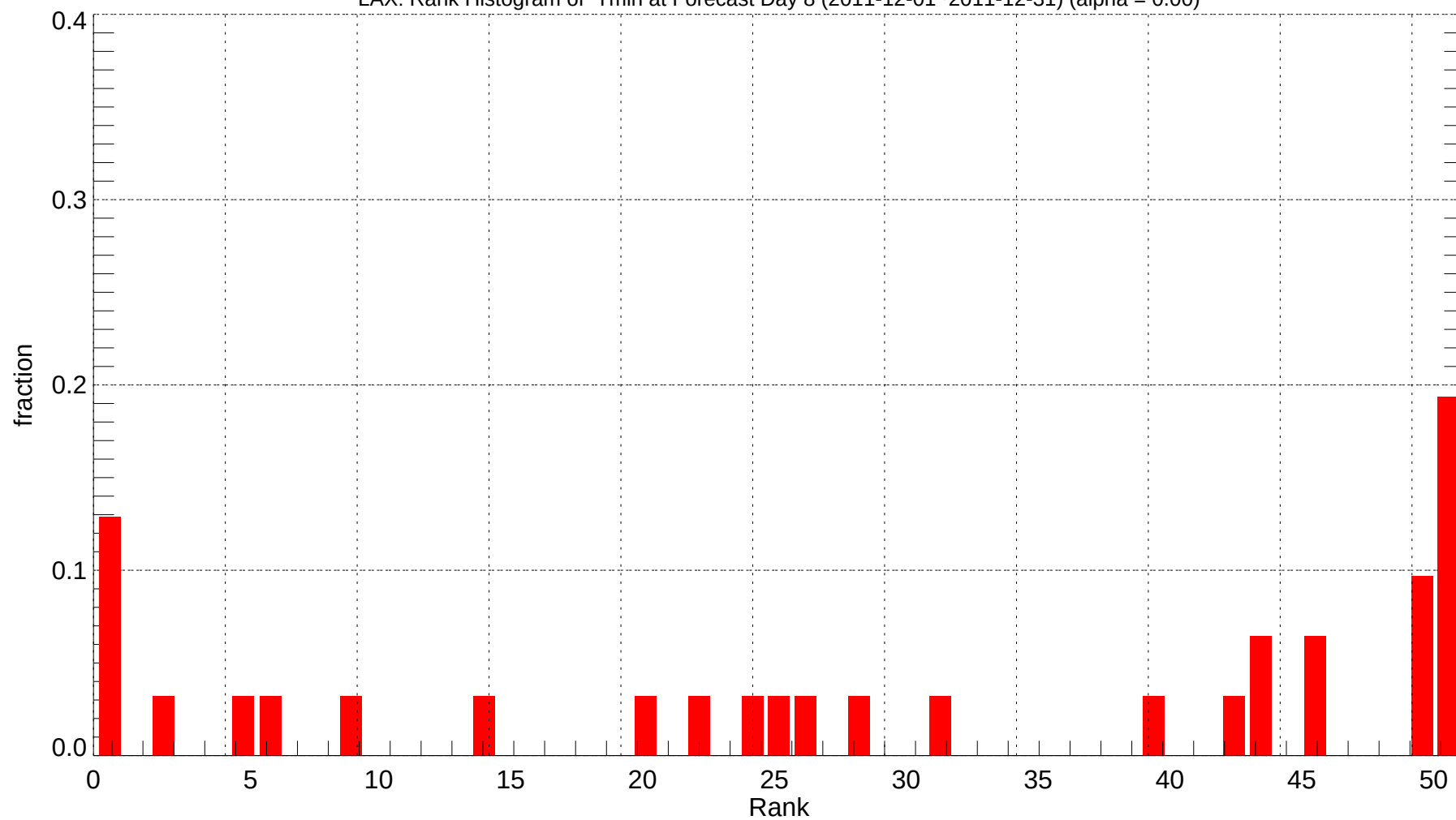
LAX: Rank Histogram of Tmin at Forecast Day 8 (2011-12-01~2011-12-31) (alpha = 0.00)
