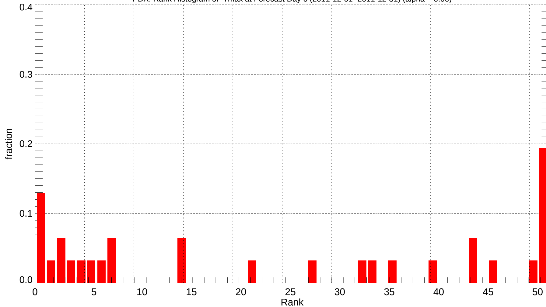
PDX: Rank Histogram of Tmax at Forecast Day 6 (2011-12-01~2011-12-31) (alpha = 0.00)
