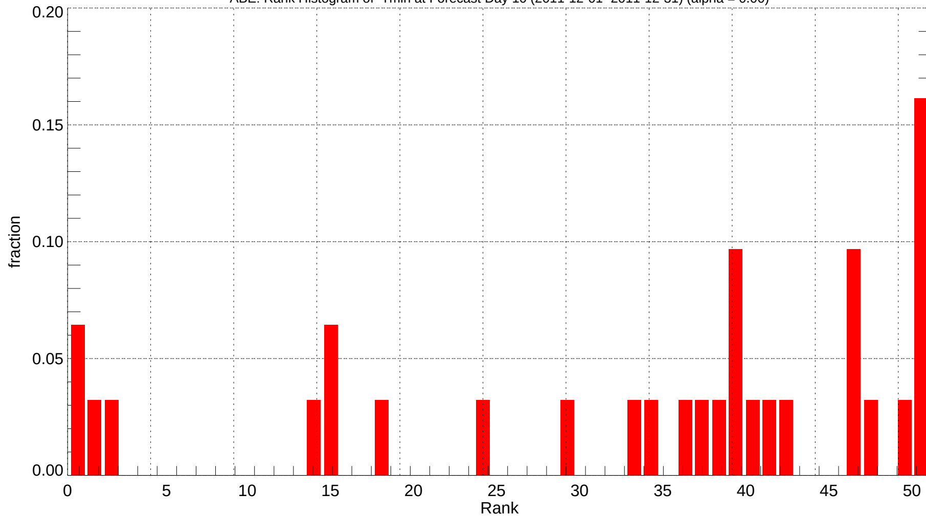
ABE: Rank Histogram of Tmin at Forecast Day 10 (2011-12-01~2011-12-31) (alpha = 0.00)
