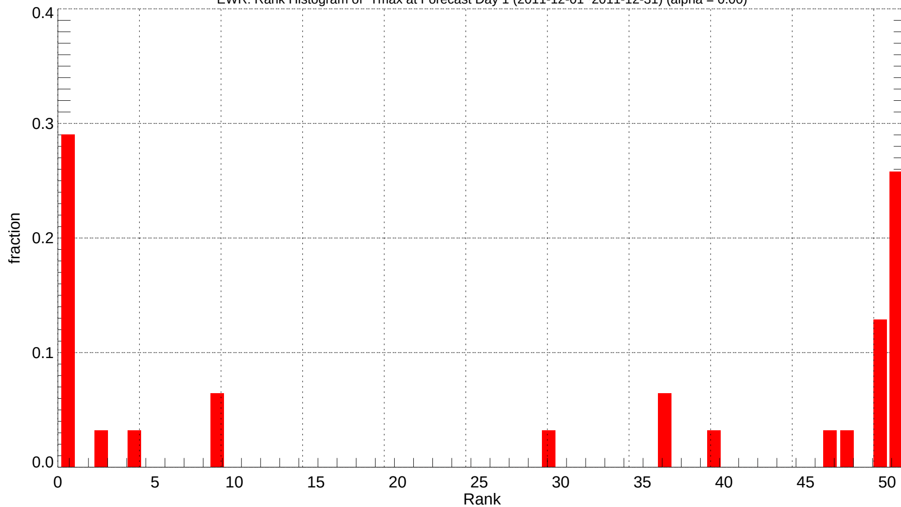
EWR: Rank Histogram of Tmax at Forecast Day 1 (2011-12-01~2011-12-31) (alpha = 0.00)
