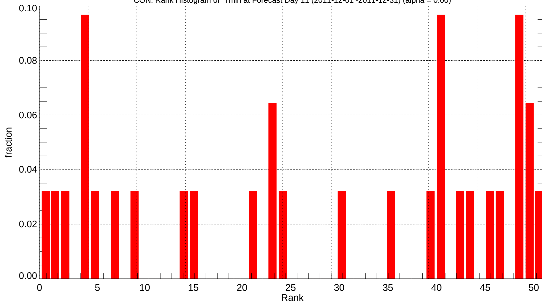
CON: Rank Histogram of Tmin at Forecast Day 11 (2011-12-01~2011-12-31) (alpha = 0.00)
