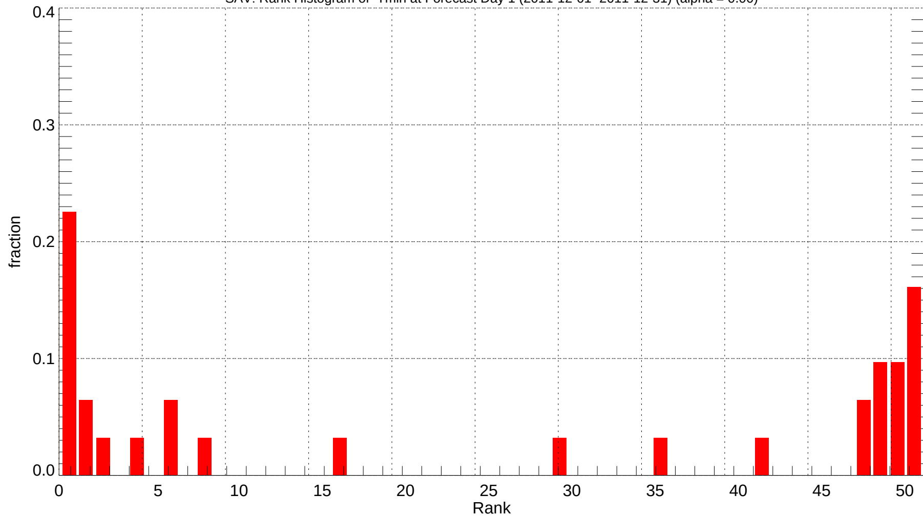
SAV: Rank Histogram of Tmin at Forecast Day 1 (2011-12-01~2011-12-31) (alpha = 0.00)
