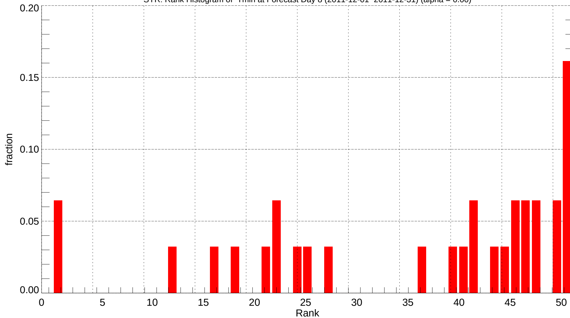
SYR: Rank Histogram of Tmin at Forecast Day 8 (2011-12-01~2011-12-31) (alpha = 0.00)
