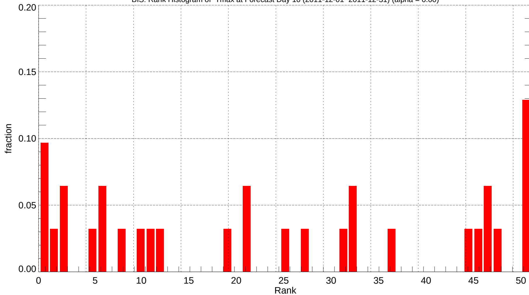
BIS: Rank Histogram of Tmax at Forecast Day 10 (2011-12-01~2011-12-31) (alpha = 0.00)
