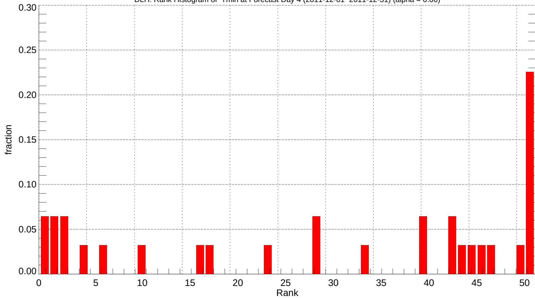
DLH: Rank Histogram of Tmin at Forecast Day 4 (2011-12-01~2011-12-31) (alpha = 0.00)
