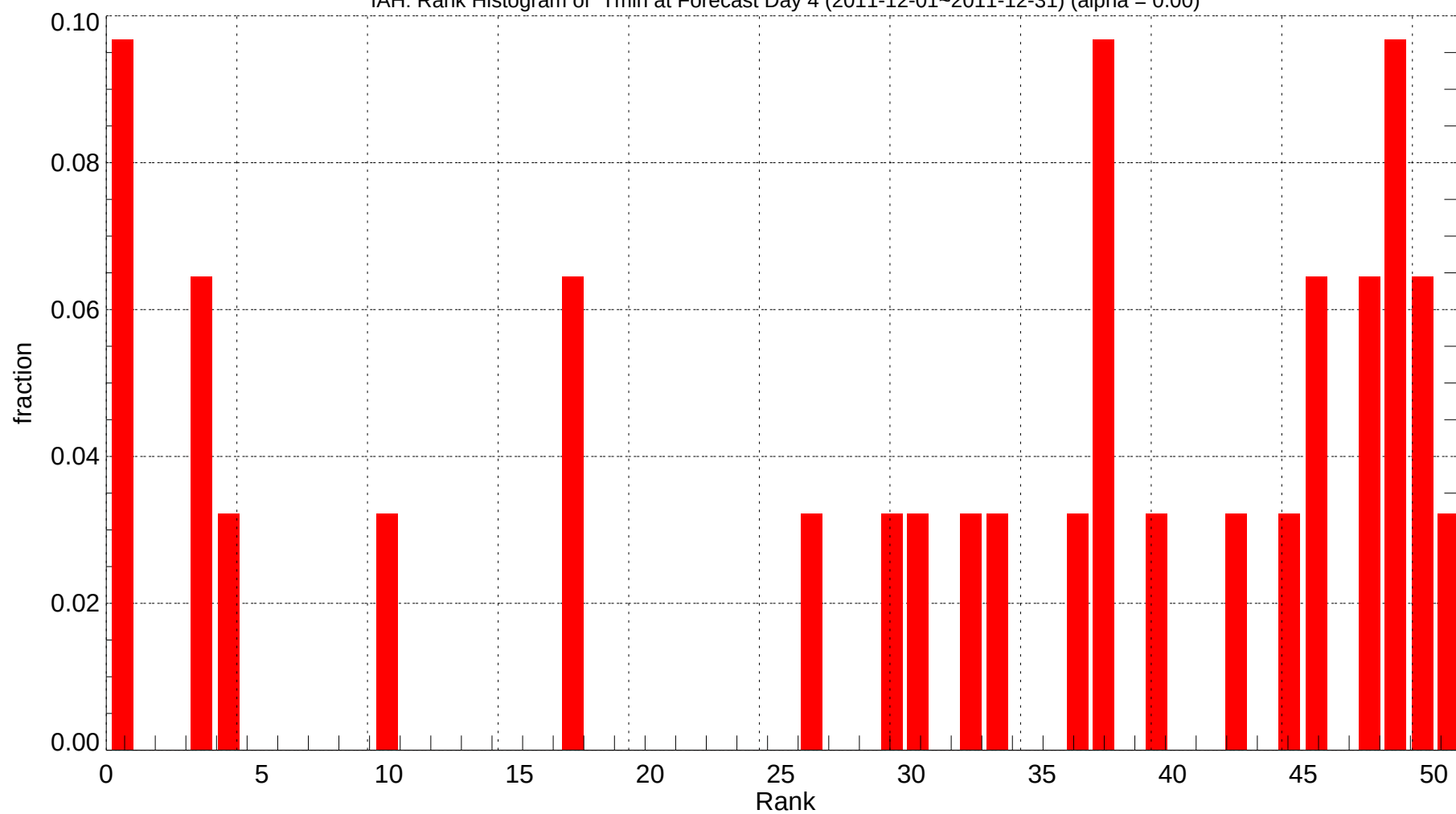
IAH: Rank Histogram of Tmin at Forecast Day 4 (2011-12-01~2011-12-31) (alpha = 0.00)
