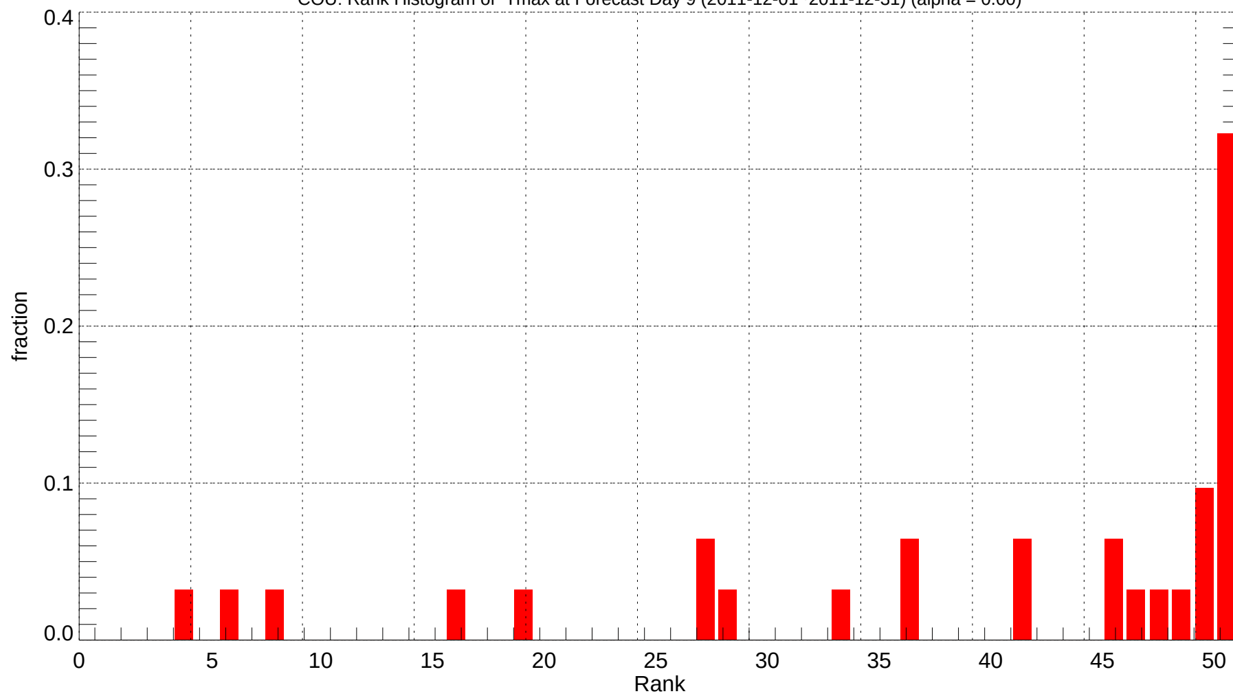
COU: Rank Histogram of Tmax at Forecast Day 9 (2011-12-01~2011-12-31) (alpha = 0.00)
