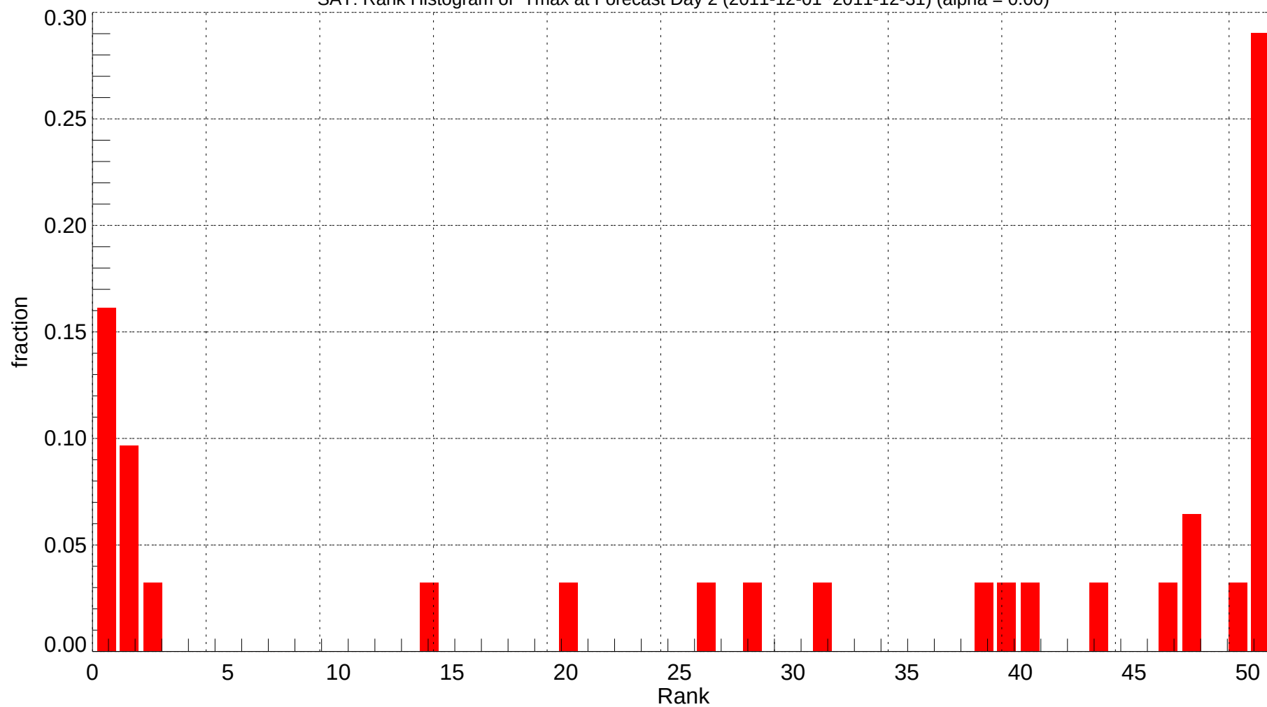
SAT: Rank Histogram of Tmax at Forecast Day 2 (2011-12-01~2011-12-31) (alpha = 0.00)
