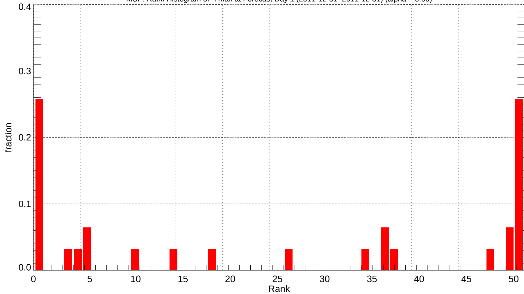
MSP: Rank Histogram of Tmax at Forecast Day 1 (2011-12-01~2011-12-31) (alpha = 0.00)
