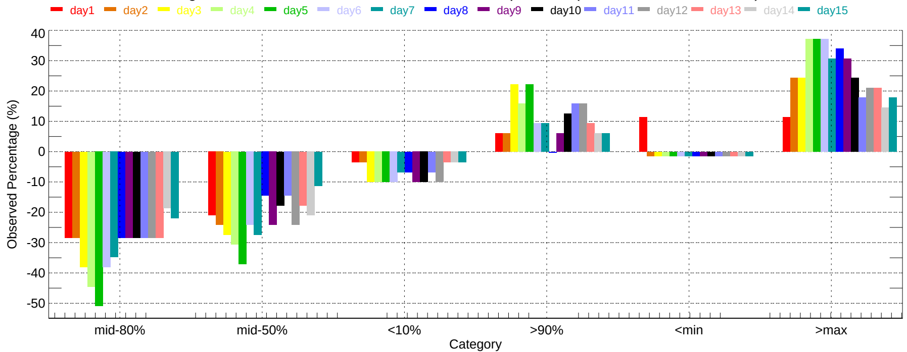
Observed Percentage Deviation of Ensembles - CRW: Max Temperature (2011-12-01~2011-12-31)
