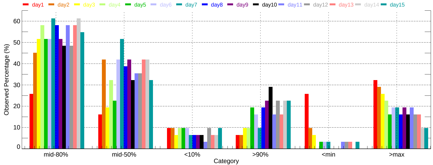
Observed Percentage of Ensembles - MCI: Max Temperature (2011-12-01~2011-12-31)
