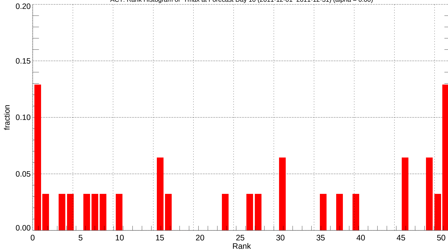
ACT: Rank Histogram of Tmax at Forecast Day 10 (2011-12-01~2011-12-31) (alpha = 0.00)
