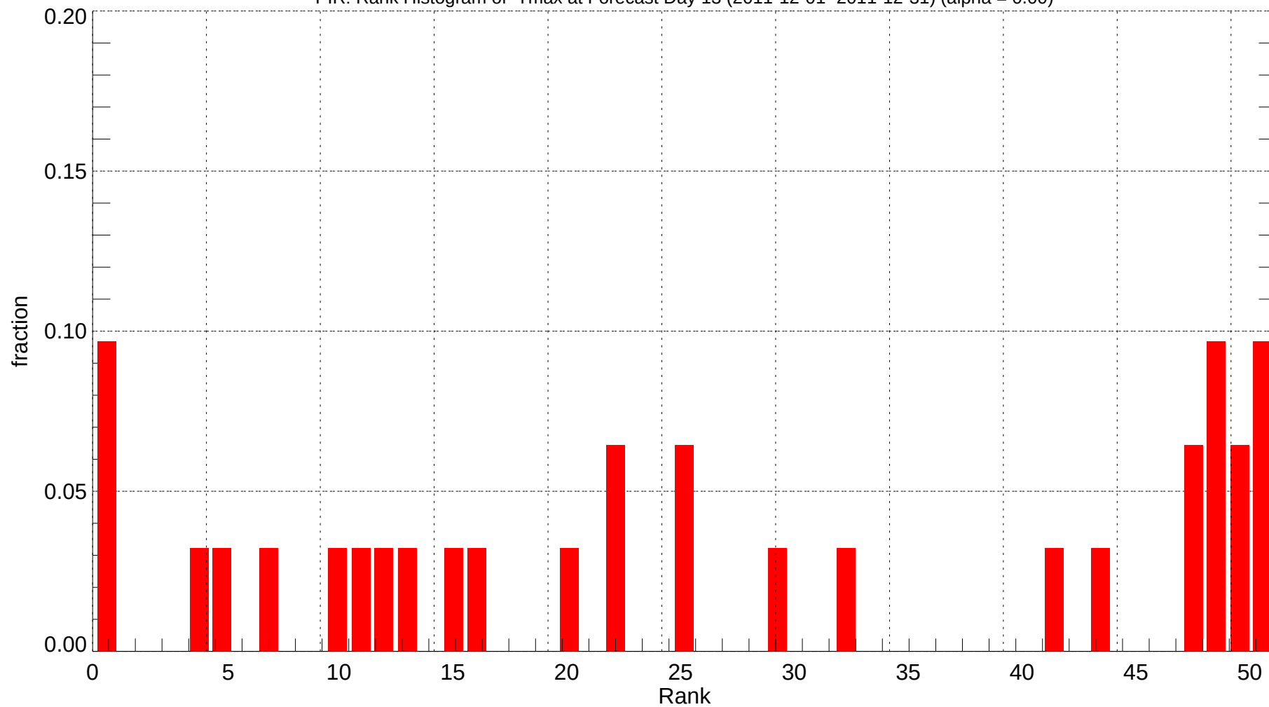
PIR: Rank Histogram of Tmax at Forecast Day 13 (2011-12-01~2011-12-31) (alpha = 0.00)
