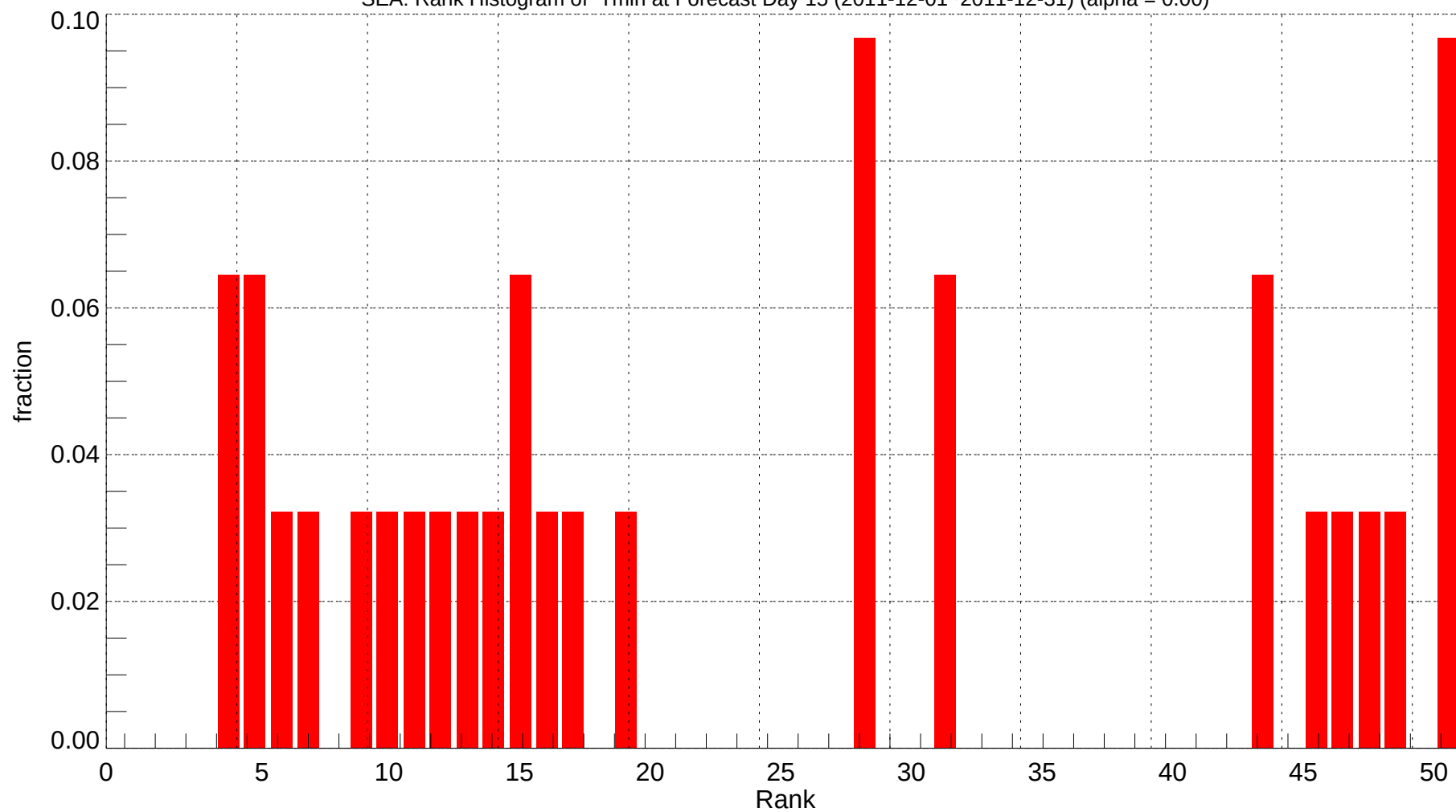
SEA: Rank Histogram of Tmin at Forecast Day 15 (2011-12-01~2011-12-31) (alpha = 0.00)
