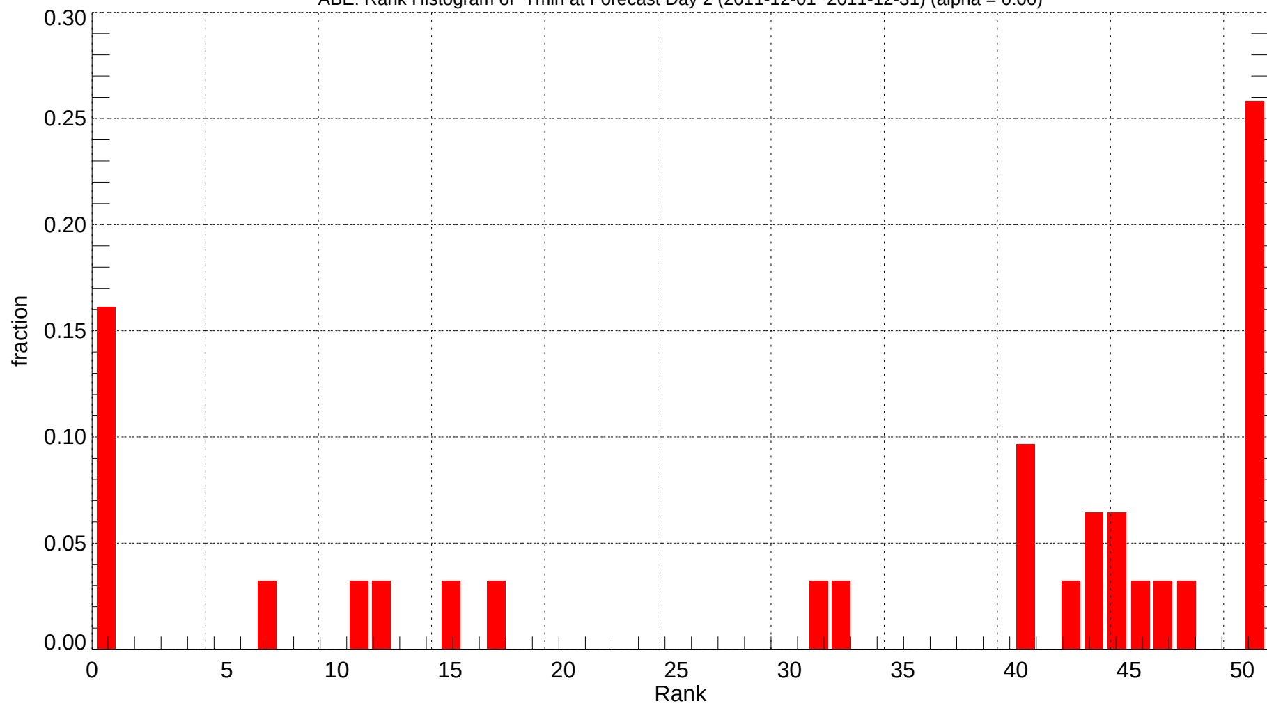
ABE: Rank Histogram of Tmin at Forecast Day 2 (2011-12-01~2011-12-31) (alpha = 0.00)
