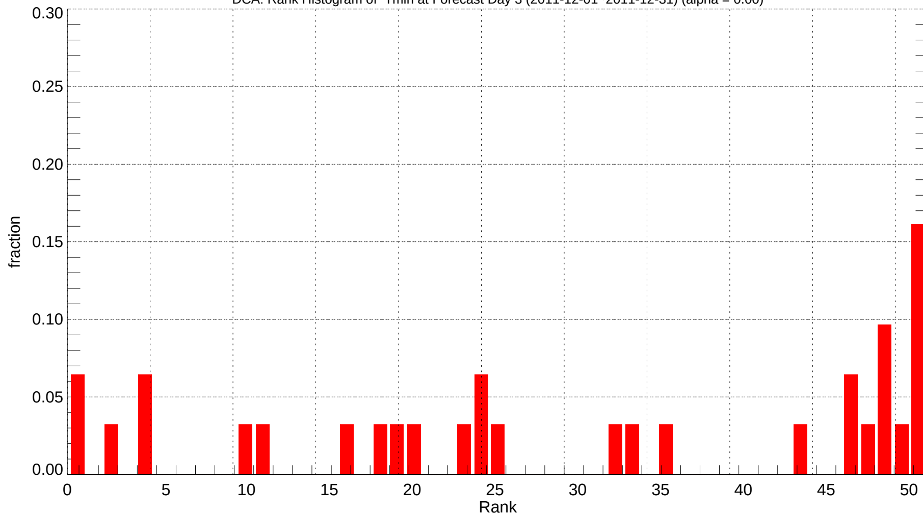
DCA: Rank Histogram of Tmin at Forecast Day 3 (2011-12-01~2011-12-31) (alpha = 0.00)
