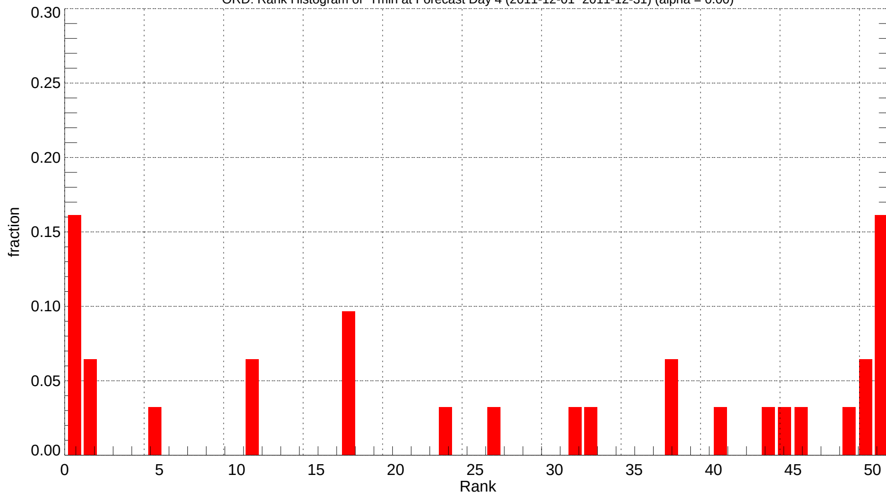
ORD: Rank Histogram of Tmin at Forecast Day 4 (2011-12-01~2011-12-31) (alpha = 0.00)
