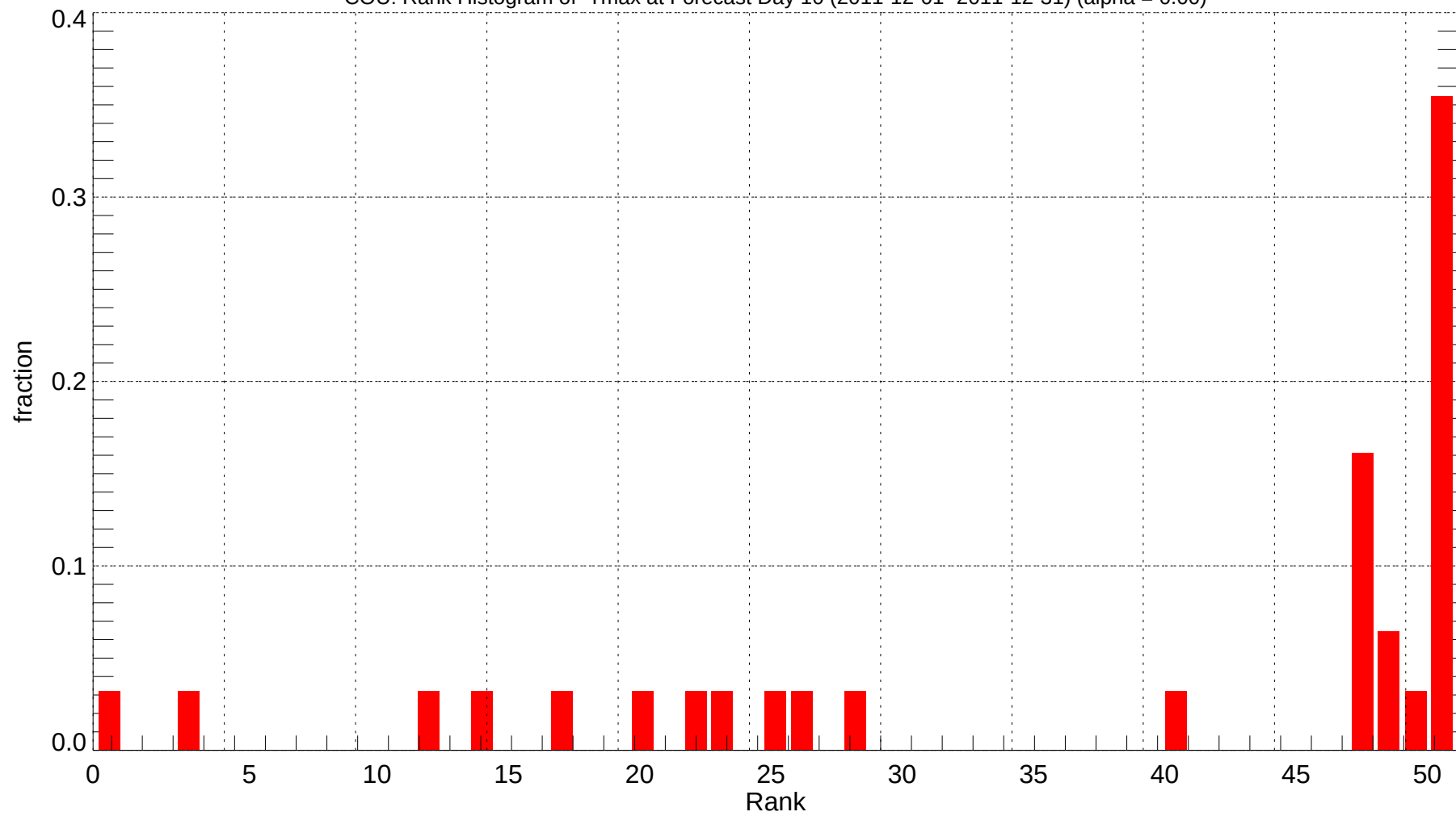
COU: Rank Histogram of Tmax at Forecast Day 10 (2011-12-01~2011-12-31) (alpha = 0.00)
