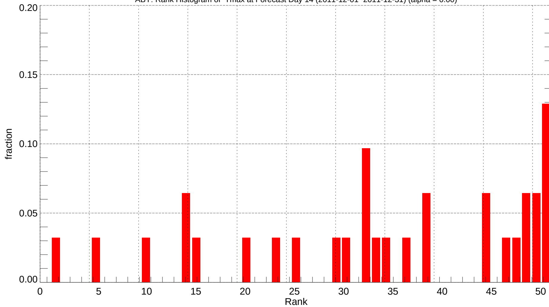
ABY: Rank Histogram of Tmax at Forecast Day 14 (2011-12-01~2011-12-31) (alpha = 0.00)
