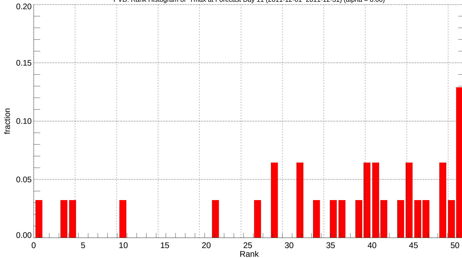
PVD: Rank Histogram of Tmax at Forecast Day 11 (2011-12-01~2011-12-31) (alpha = 0.00)
