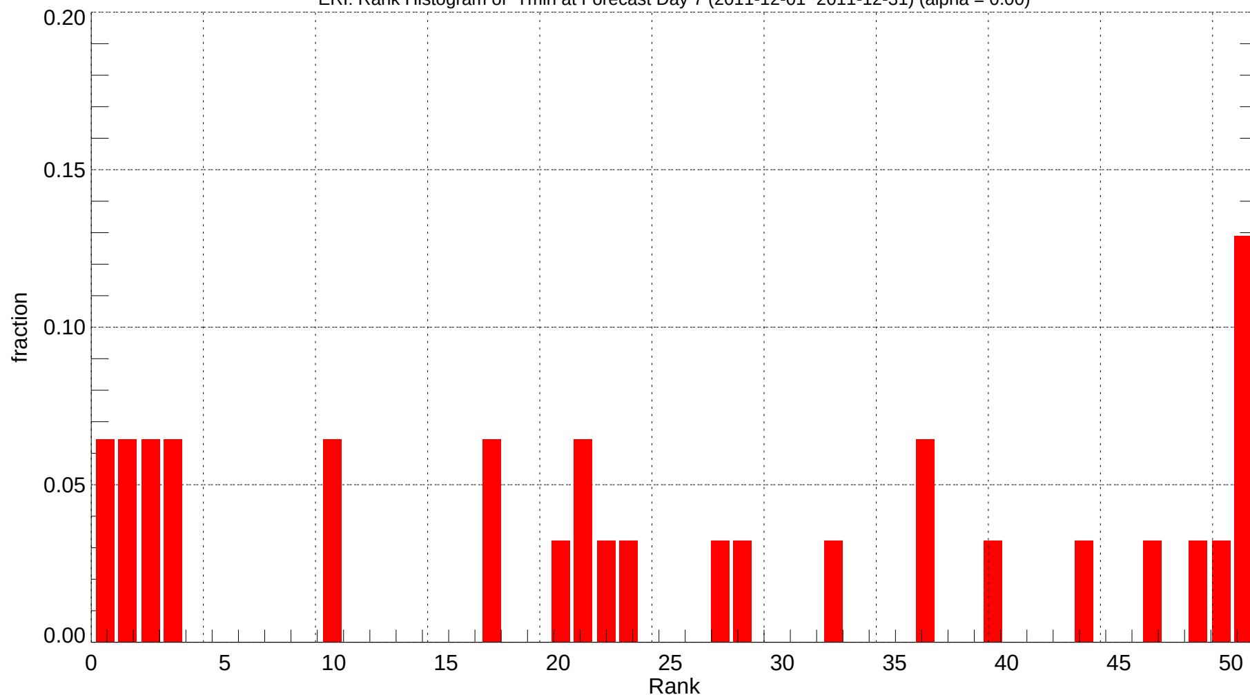
ERI: Rank Histogram of Tmin at Forecast Day 7 (2011-12-01~2011-12-31) (alpha = 0.00)
