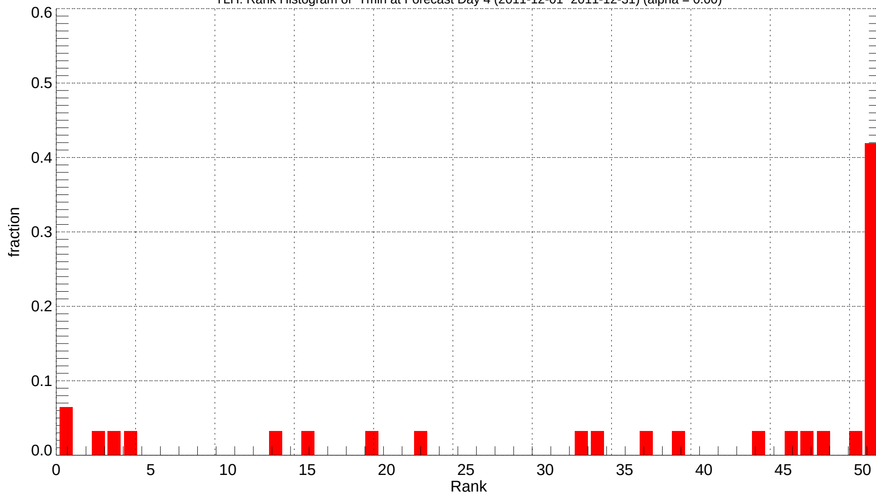
TLH: Rank Histogram of Tmin at Forecast Day 4 (2011-12-01~2011-12-31) (alpha = 0.00)
