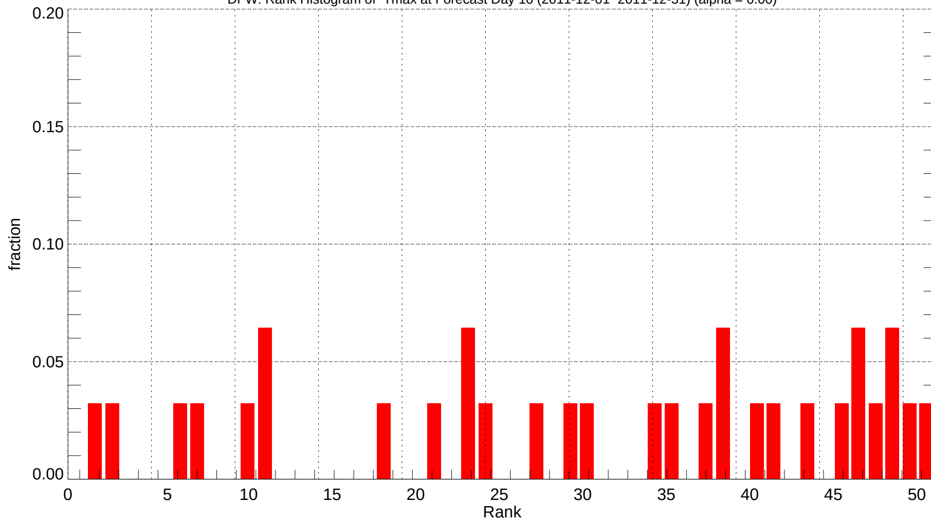
DFW: Rank Histogram of Tmax at Forecast Day 10 (2011-12-01~2011-12-31) (alpha = 0.00)
