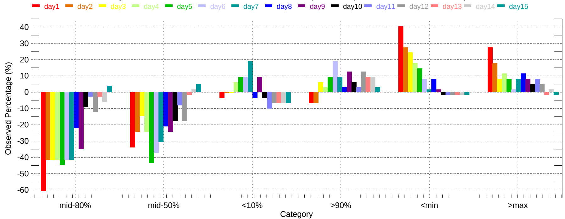
Observed Percentage Deviation of Ensembles - HSV: Min Temperature (2011-12-01~2011-12-31)
