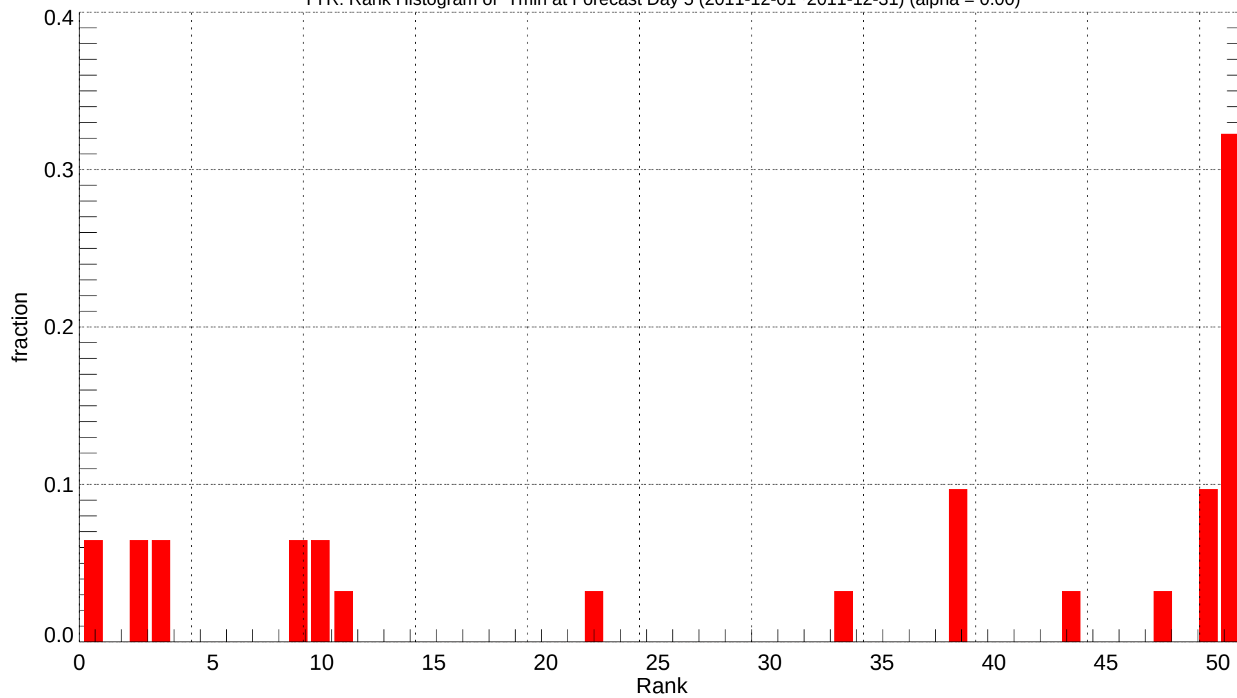
TYR: Rank Histogram of Tmin at Forecast Day 5 (2011-12-01~2011-12-31) (alpha = 0.00)
