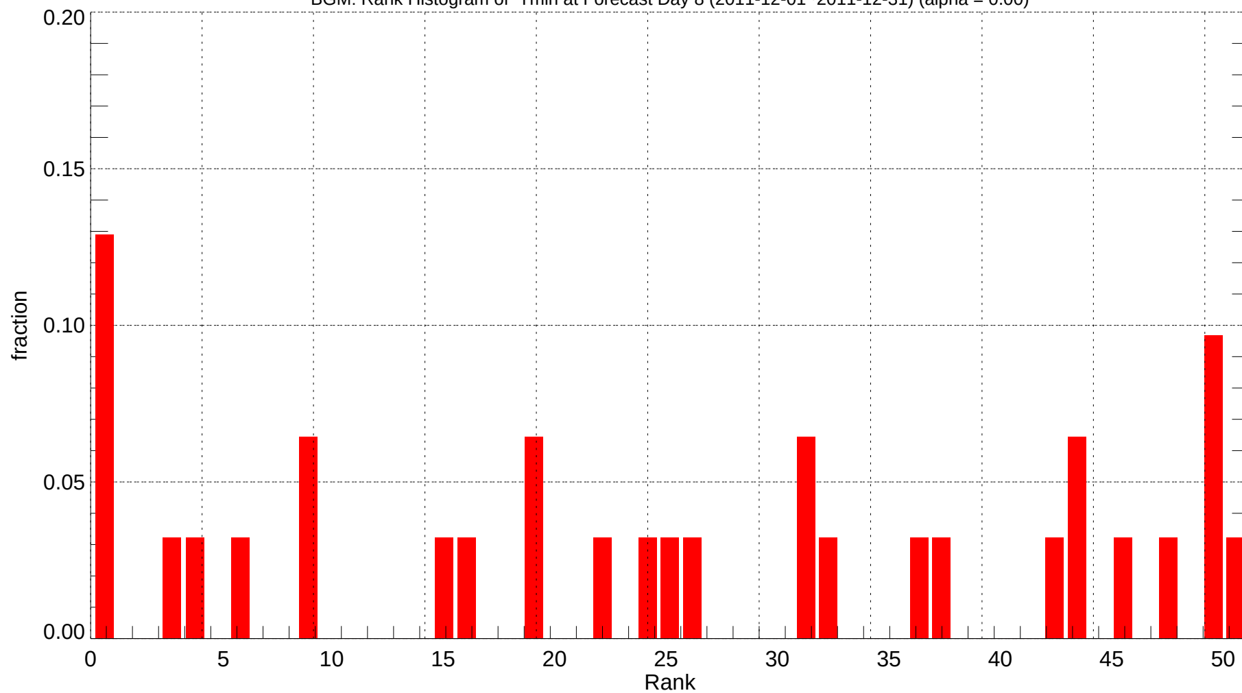
BGM: Rank Histogram of Tmin at Forecast Day 8 (2011-12-01~2011-12-31) (alpha = 0.00)
