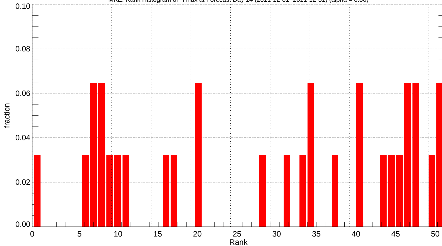
MKE: Rank Histogram of Tmax at Forecast Day 14 (2011-12-01~2011-12-31) (alpha = 0.00)
