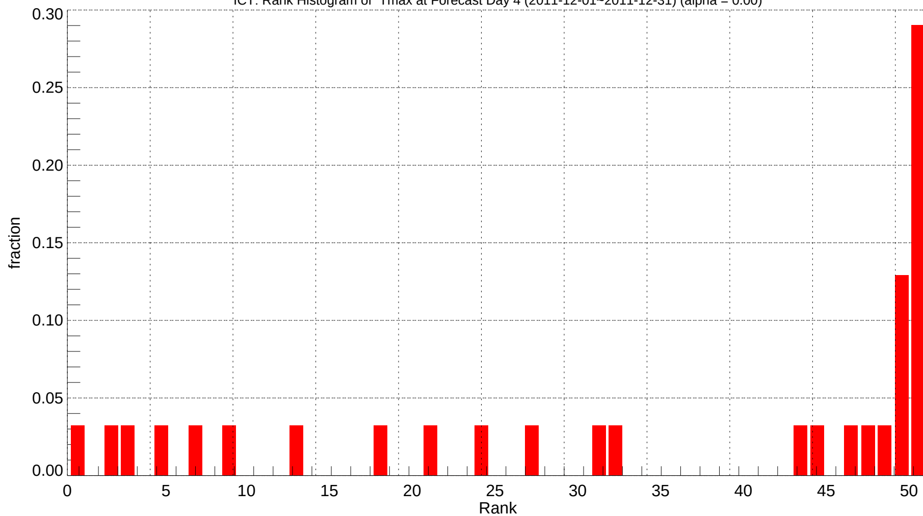
ICT: Rank Histogram of Tmax at Forecast Day 4 (2011-12-01~2011-12-31) (alpha = 0.00)
