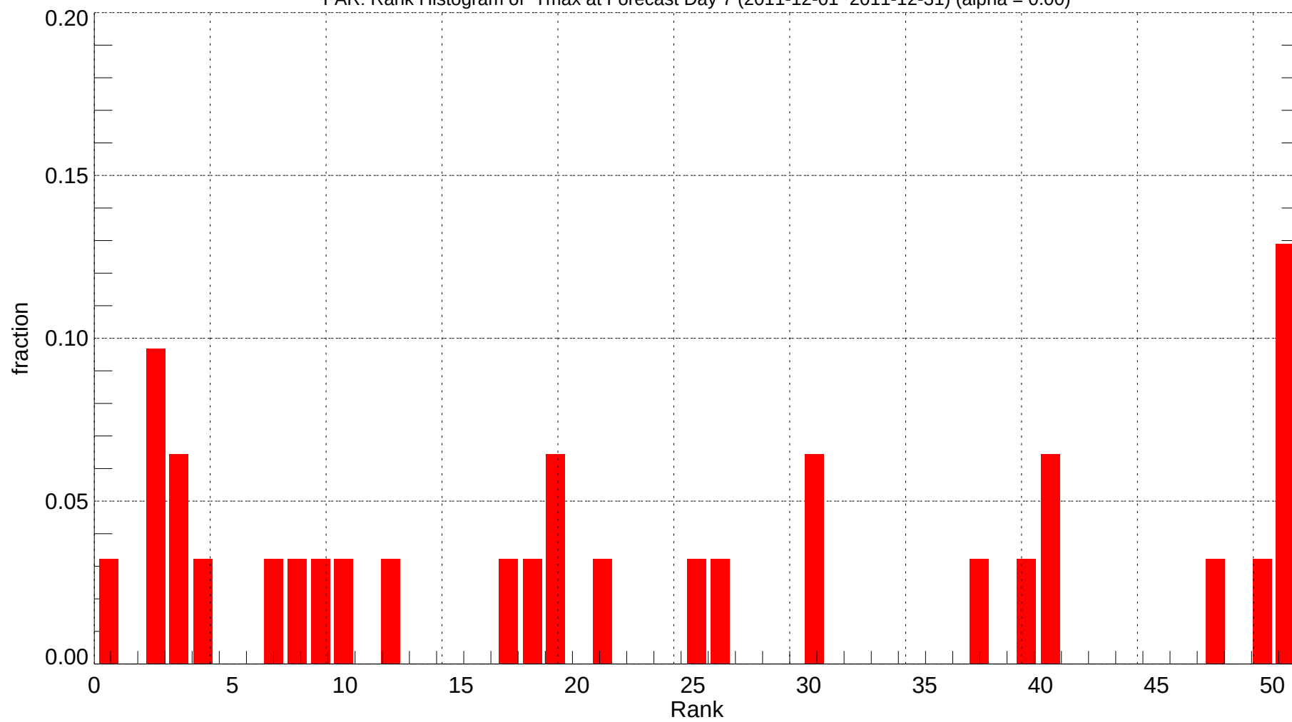
FAR: Rank Histogram of Tmax at Forecast Day 7 (2011-12-01~2011-12-31) (alpha = 0.00)
