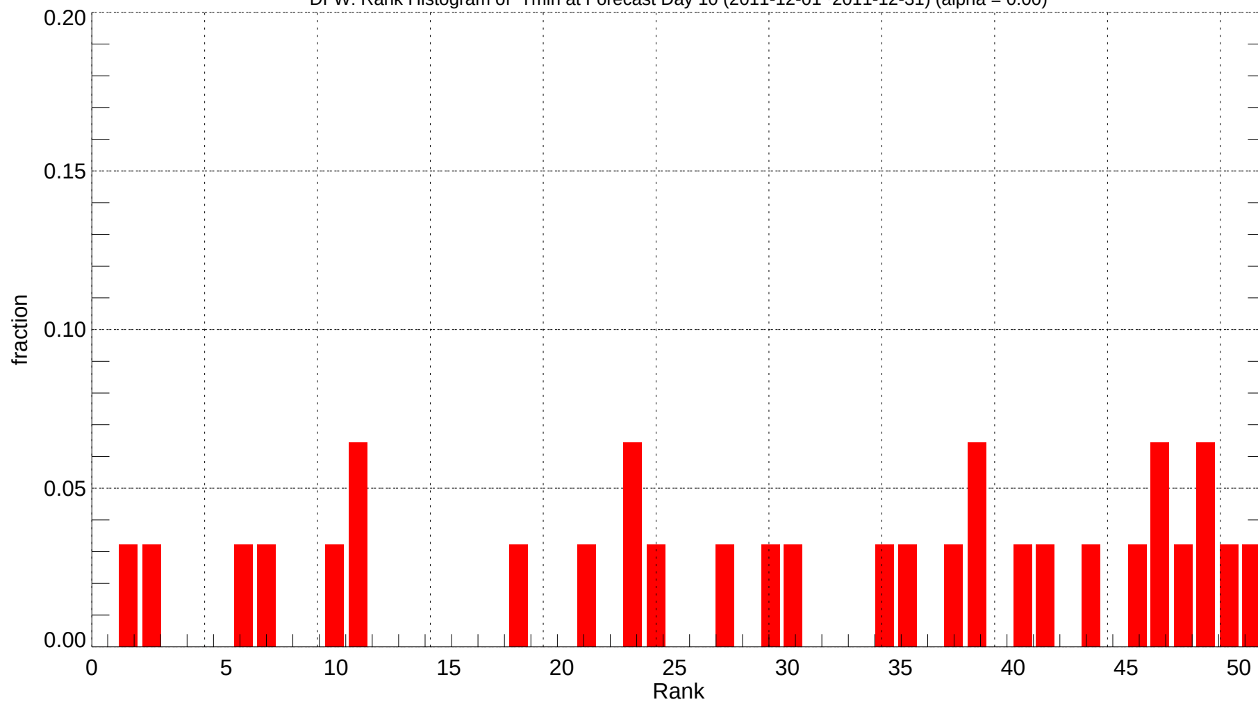
DFW: Rank Histogram of Tmin at Forecast Day 10 (2011-12-01~2011-12-31) (alpha = 0.00)
