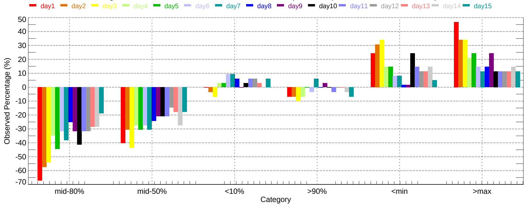
Observed Percentage Deviation of Ensembles - PDX: Max Temperature (2011-12-01~2011-12-31)
