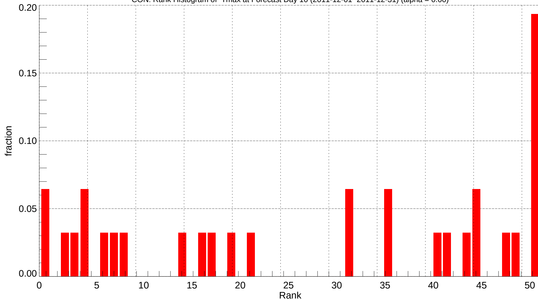
CON: Rank Histogram of Tmax at Forecast Day 10 (2011-12-01~2011-12-31) (alpha = 0.00)
