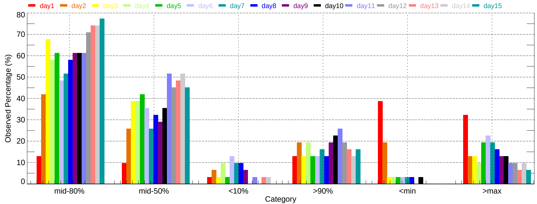
Observed Percentage of Ensembles - JAN: Min Temperature (2011-12-01~2011-12-31)
