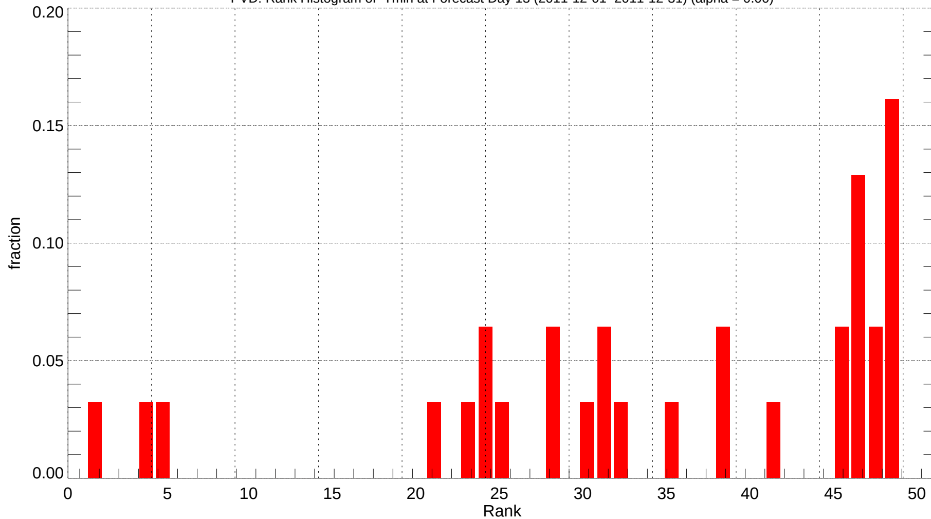
PVD: Rank Histogram of Tmin at Forecast Day 13 (2011-12-01~2011-12-31) (alpha = 0.00)
