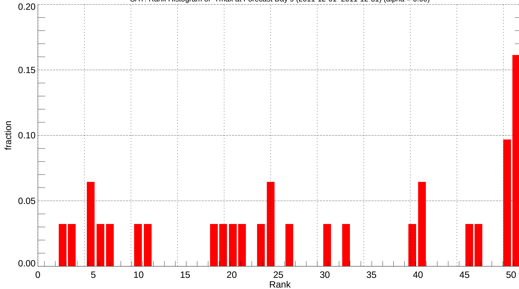
SAT: Rank Histogram of Tmax at Forecast Day 9 (2011-12-01~2011-12-31) (alpha = 0.00)
