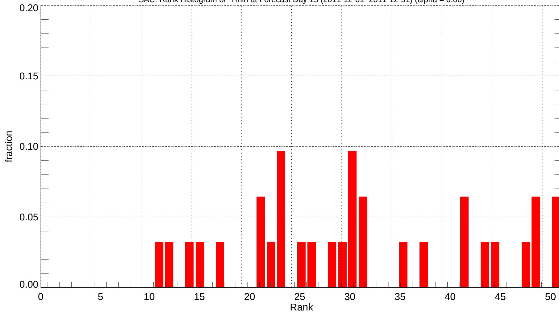
SAC: Rank Histogram of Tmin at Forecast Day 15 (2011-12-01~2011-12-31) (alpha = 0.00)
