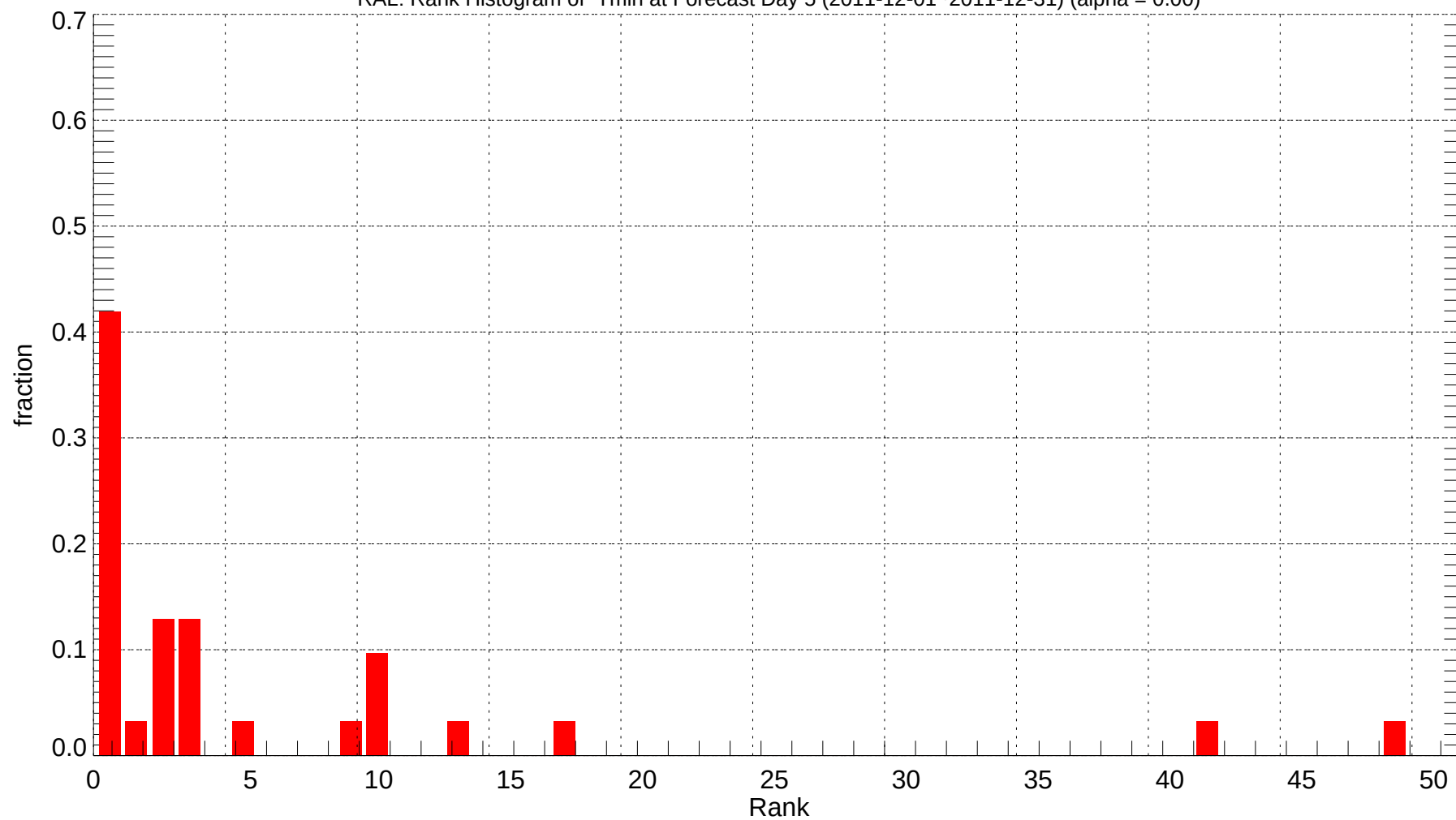
RAL: Rank Histogram of Tmin at Forecast Day 5 (2011-12-01~2011-12-31) (alpha = 0.00)
