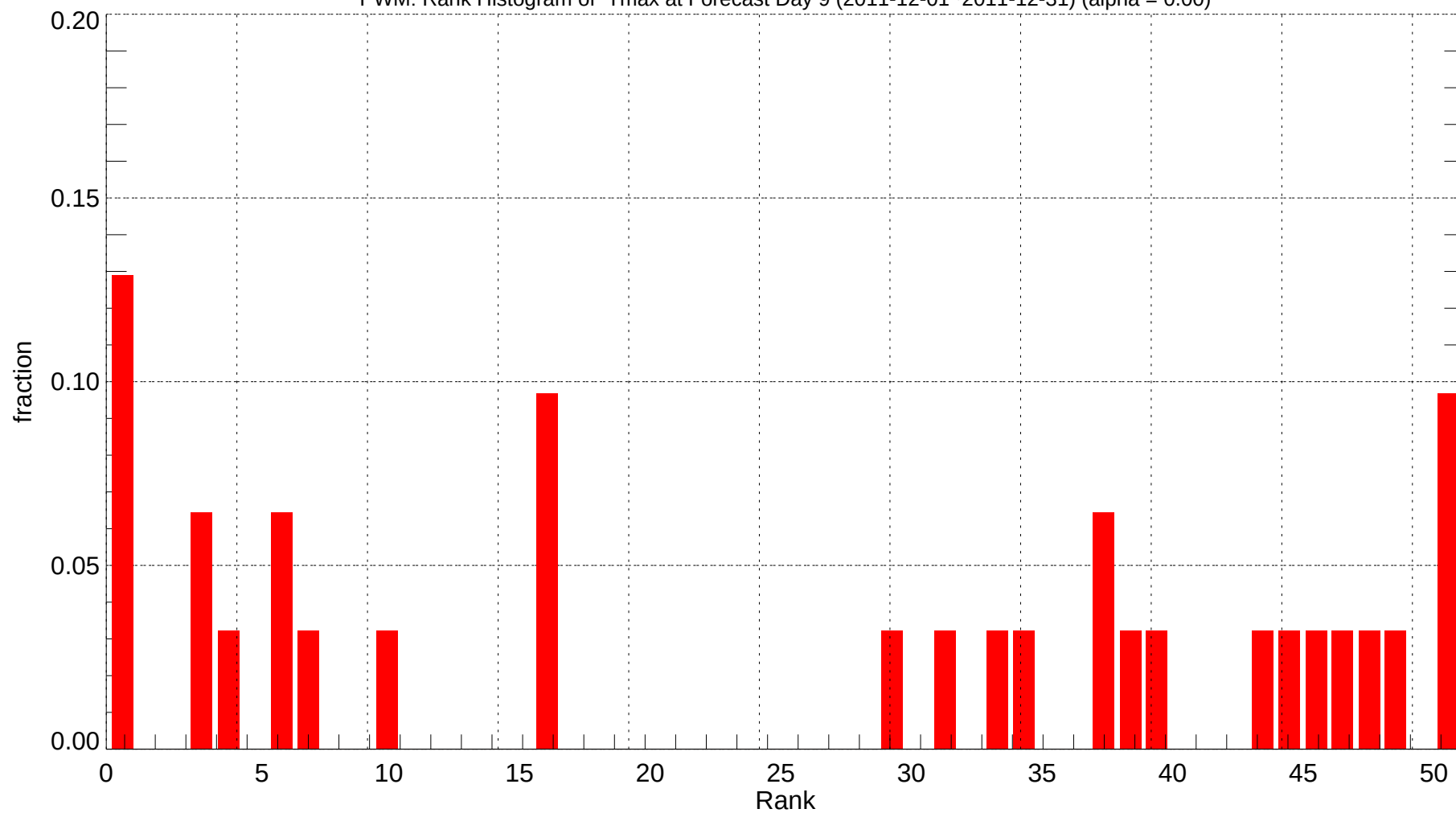
PWM: Rank Histogram of Tmax at Forecast Day 9 (2011-12-01~2011-12-31) (alpha = 0.00)
