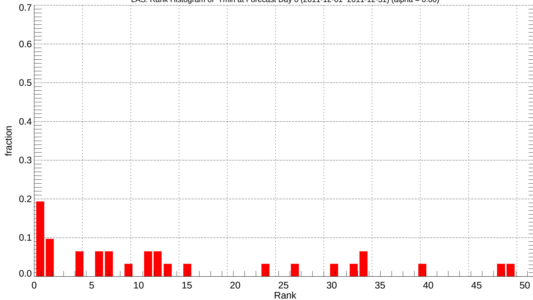
LAS: Rank Histogram of Tmin at Forecast Day 6 (2011-12-01~2011-12-31) (alpha = 0.00)
