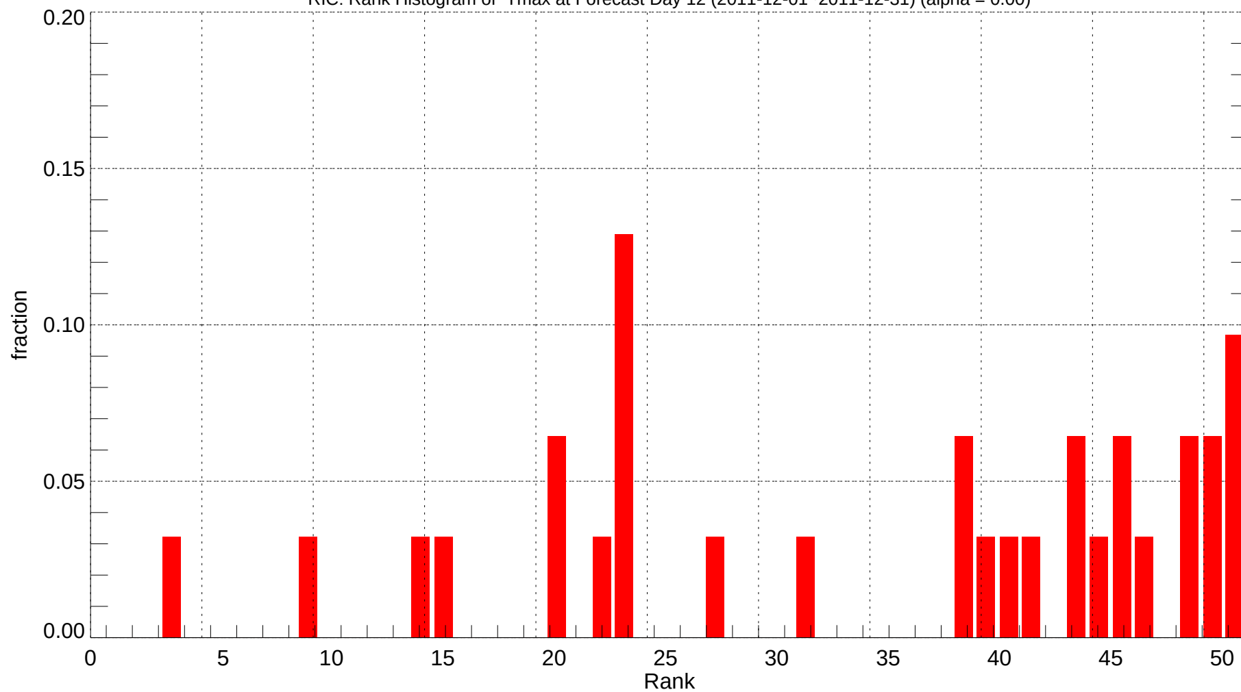
RIC: Rank Histogram of Tmax at Forecast Day 12 (2011-12-01~2011-12-31) (alpha = 0.00)
