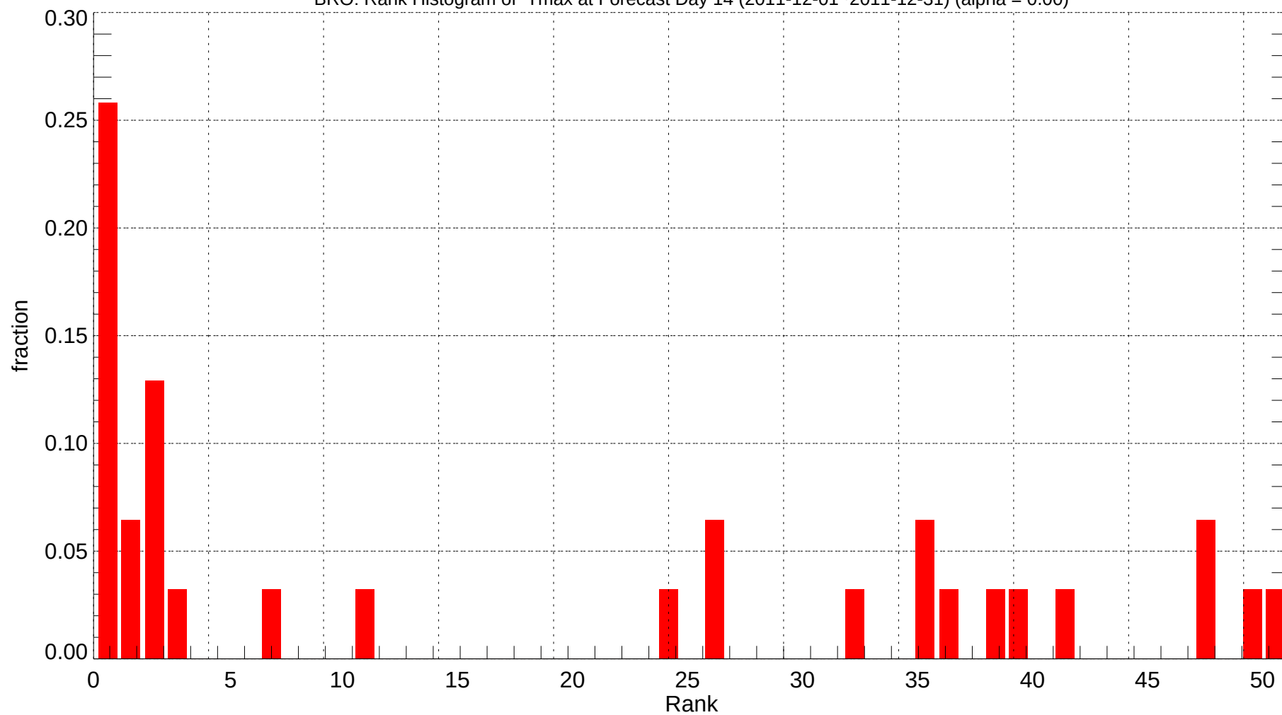
BRO: Rank Histogram of Tmax at Forecast Day 14 (2011-12-01~2011-12-31) (alpha = 0.00)
