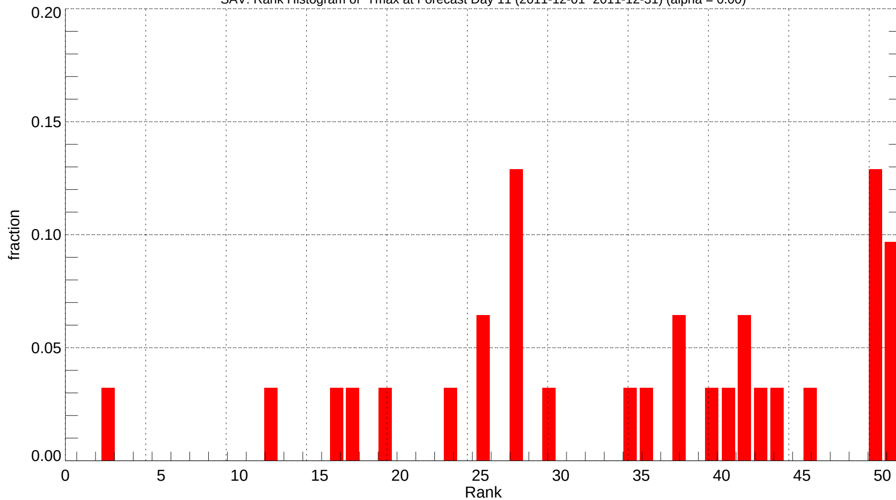
SAV: Rank Histogram of Tmax at Forecast Day 11 (2011-12-01~2011-12-31) (alpha = 0.00)
