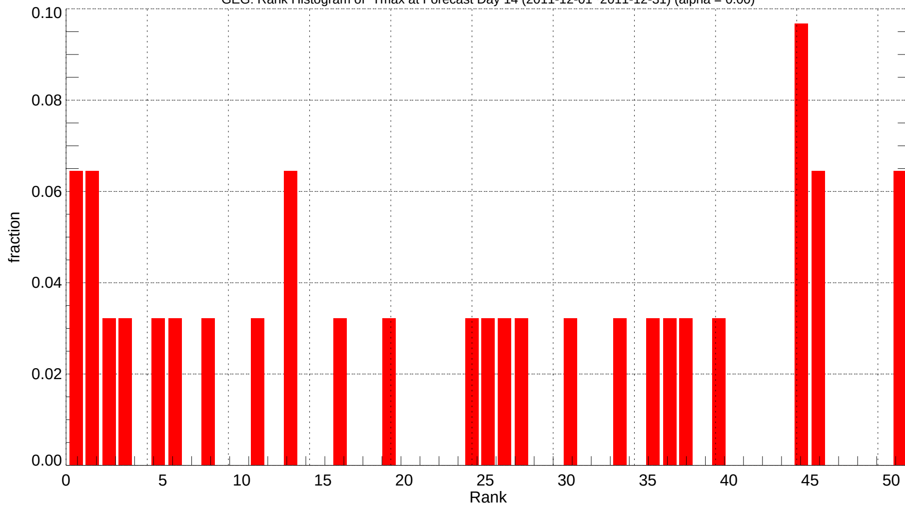
GEG: Rank Histogram of Tmax at Forecast Day 14 (2011-12-01~2011-12-31) (alpha = 0.00)
