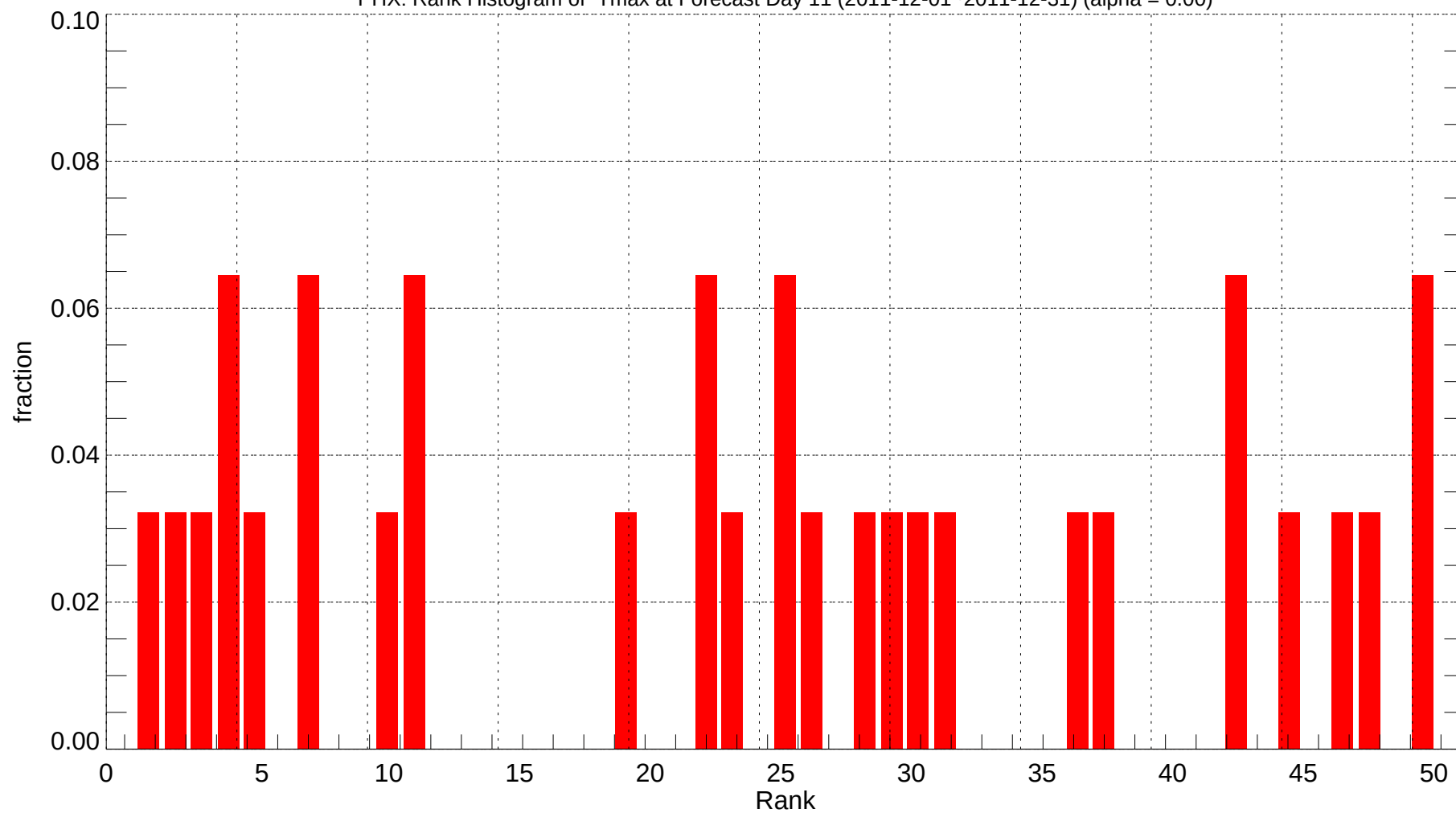
PHX: Rank Histogram of Tmax at Forecast Day 11 (2011-12-01~2011-12-31) (alpha = 0.00)
