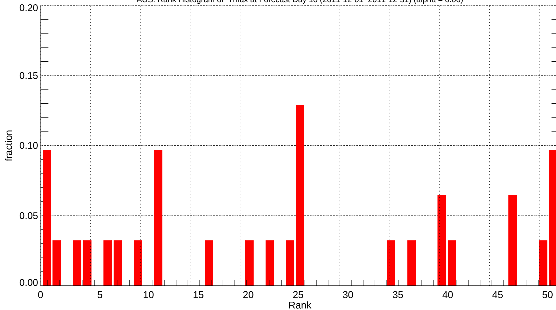
AUS: Rank Histogram of Tmax at Forecast Day 10 (2011-12-01~2011-12-31) (alpha = 0.00)
