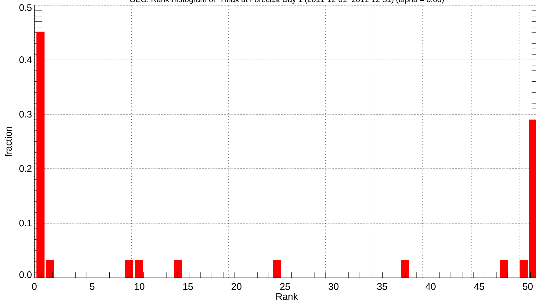
GEG: Rank Histogram of Tmax at Forecast Day 1 (2011-12-01~2011-12-31) (alpha = 0.00)
