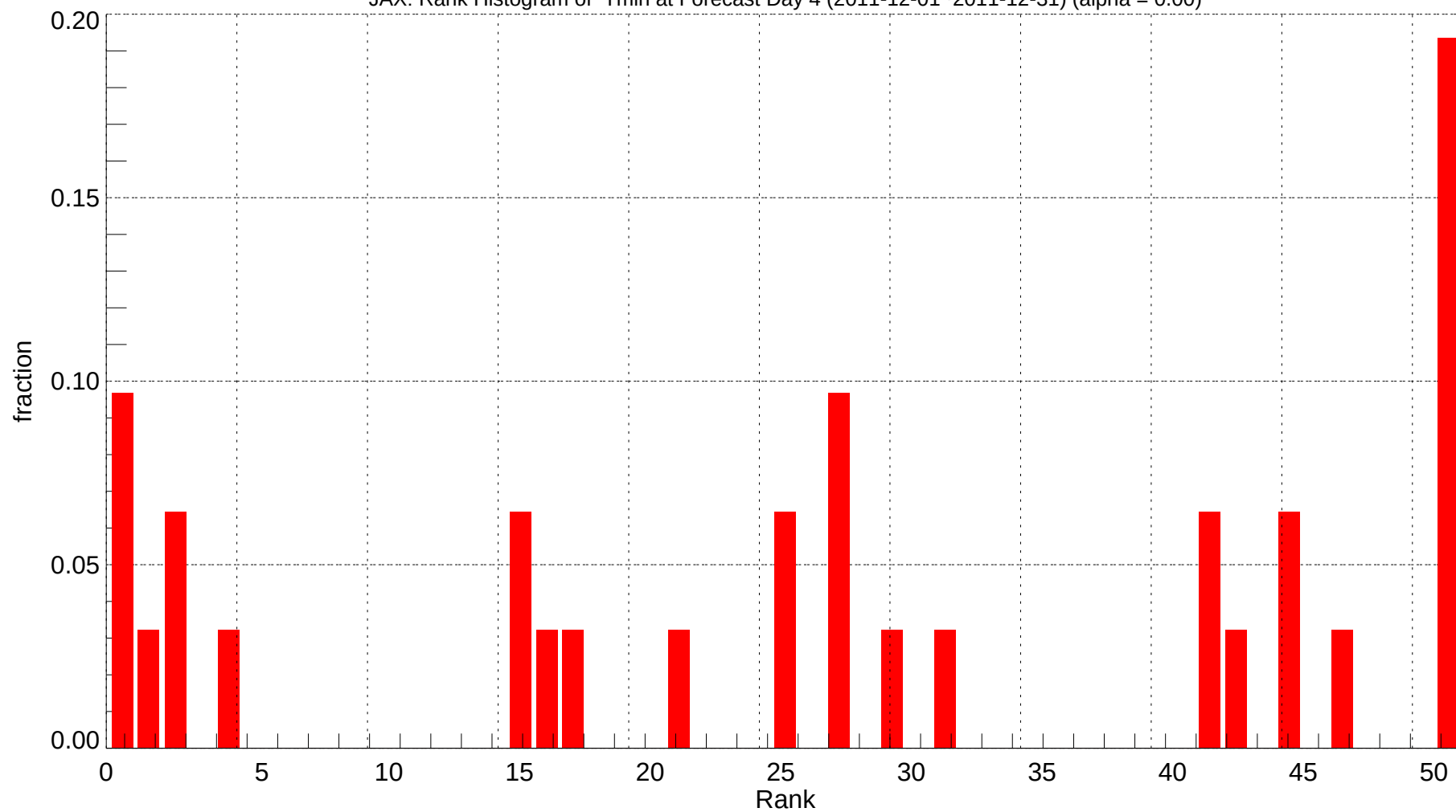
JAX: Rank Histogram of Tmin at Forecast Day 4 (2011-12-01~2011-12-31) (alpha = 0.00)
