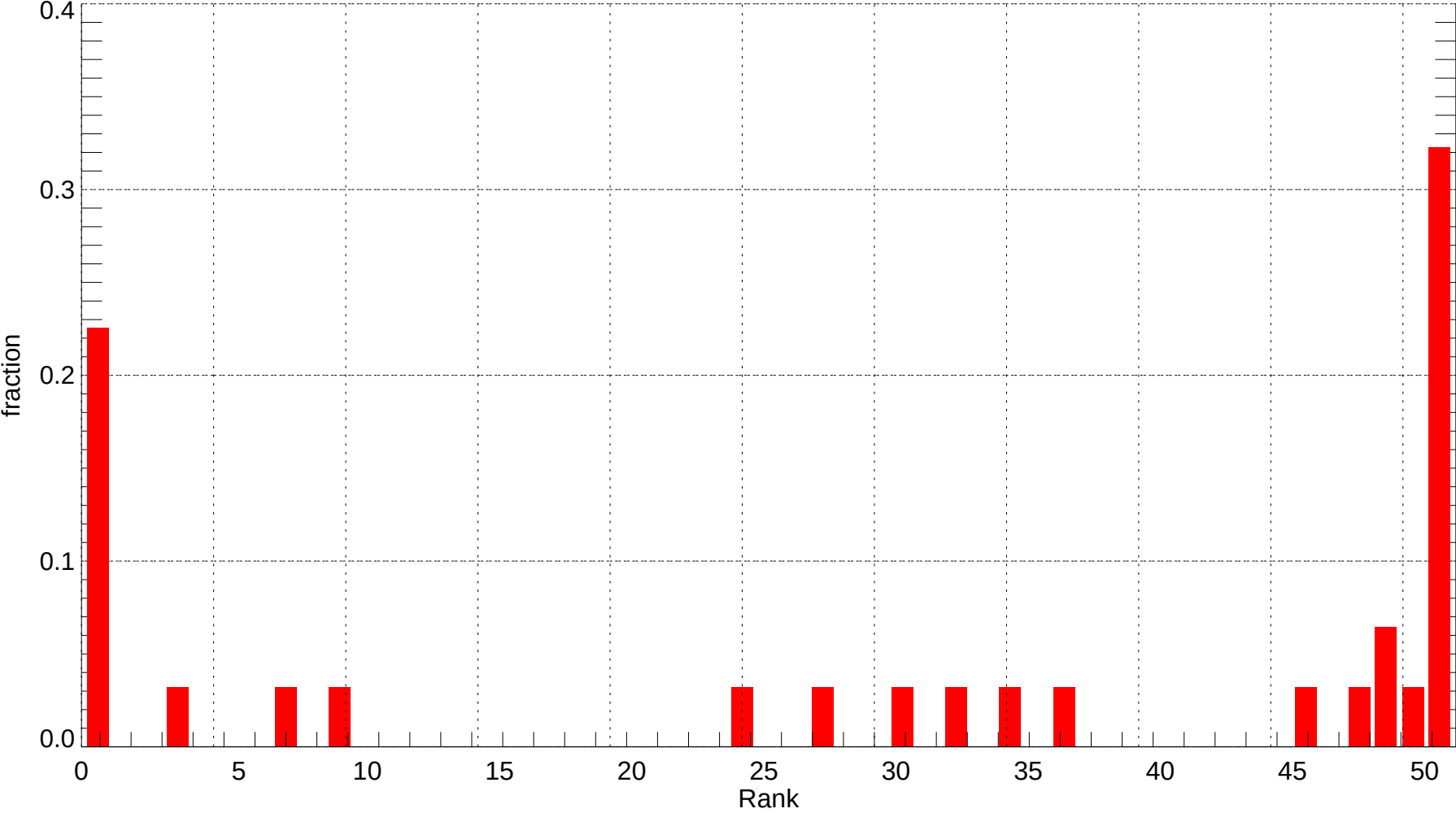
ERI: Rank Histogram of Tmax at Forecast Day 1 (2011-12-01~2011-12-31) (alpha = 0.00)
