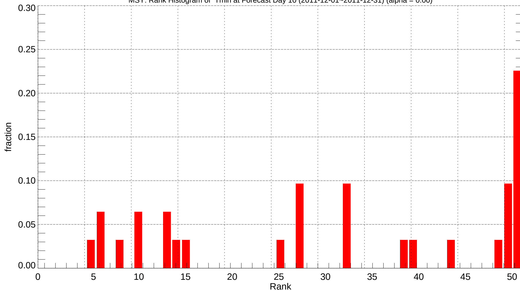
MSY: Rank Histogram of Tmin at Forecast Day 10 (2011-12-01~2011-12-31) (alpha = 0.00)
