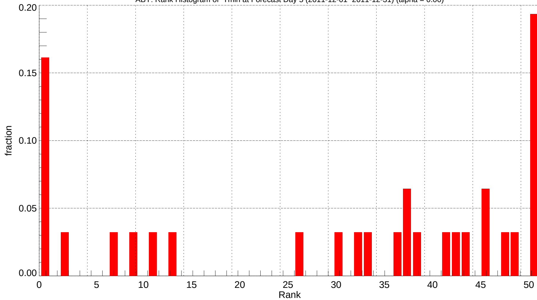
ABY: Rank Histogram of Tmin at Forecast Day 5 (2011-12-01~2011-12-31) (alpha = 0.00)
