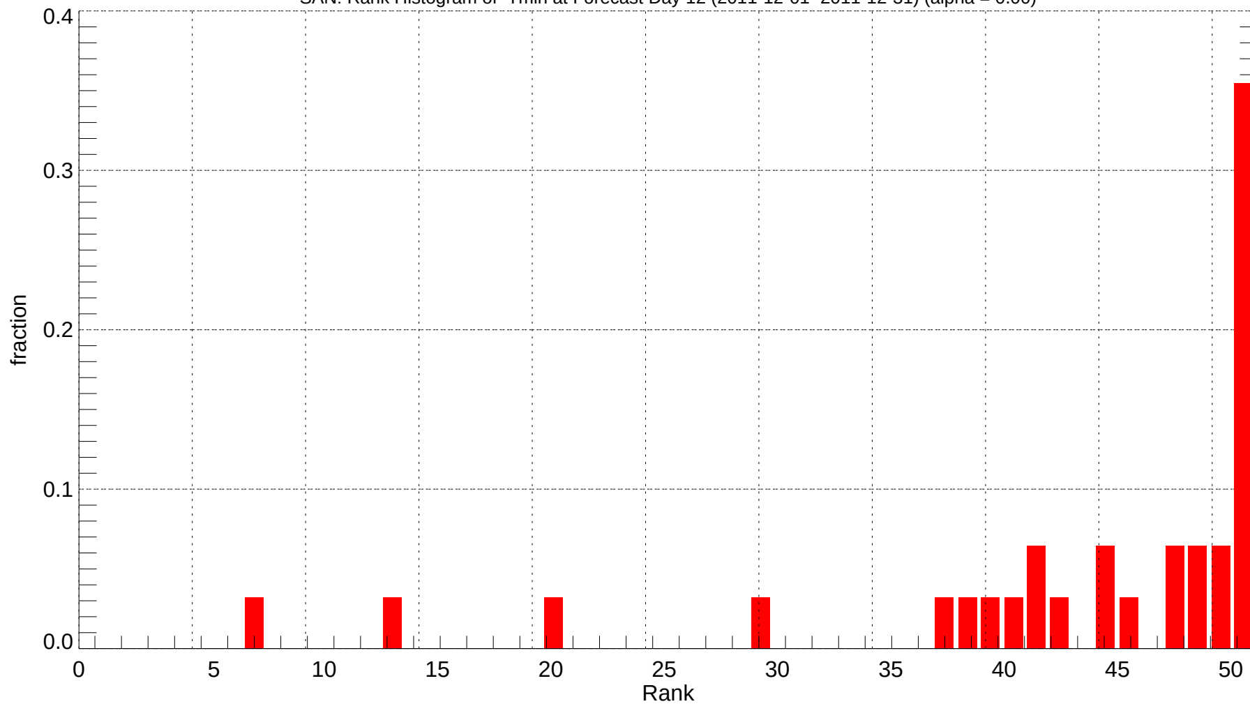
SAN: Rank Histogram of Tmin at Forecast Day 12 (2011-12-01~2011-12-31) (alpha = 0.00)
