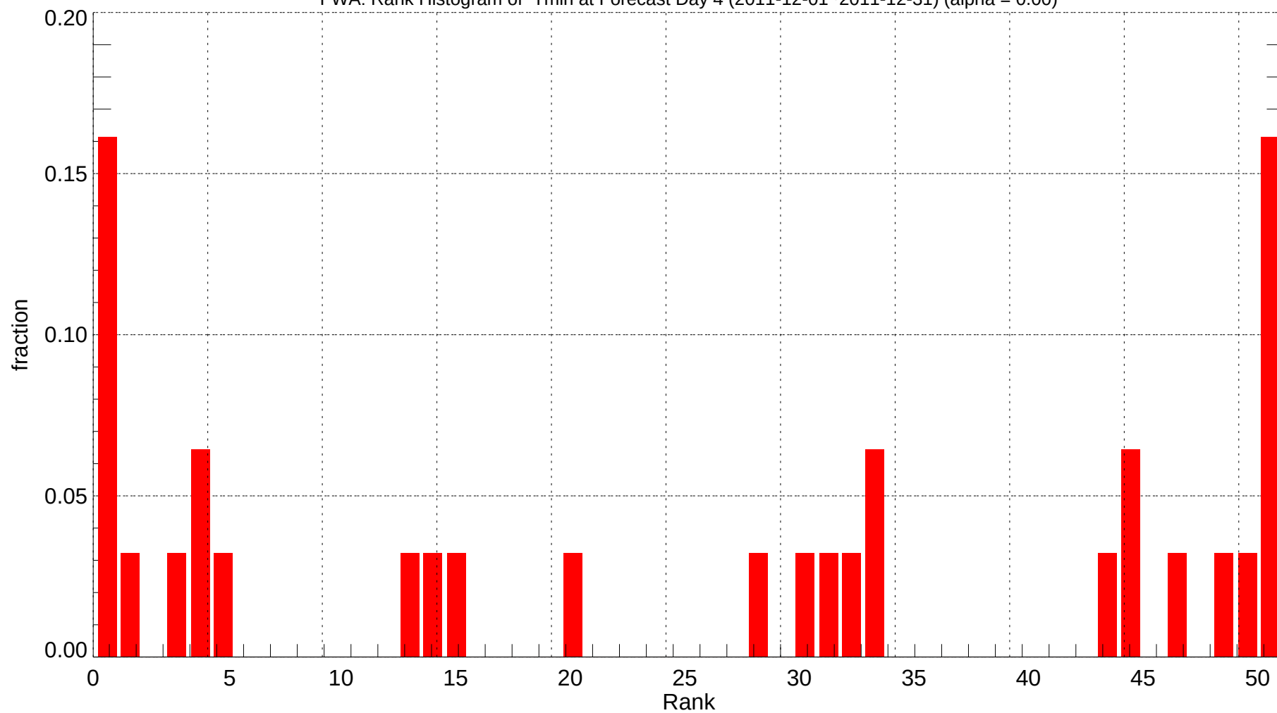
FWA: Rank Histogram of Tmin at Forecast Day 4 (2011-12-01~2011-12-31) (alpha = 0.00)
