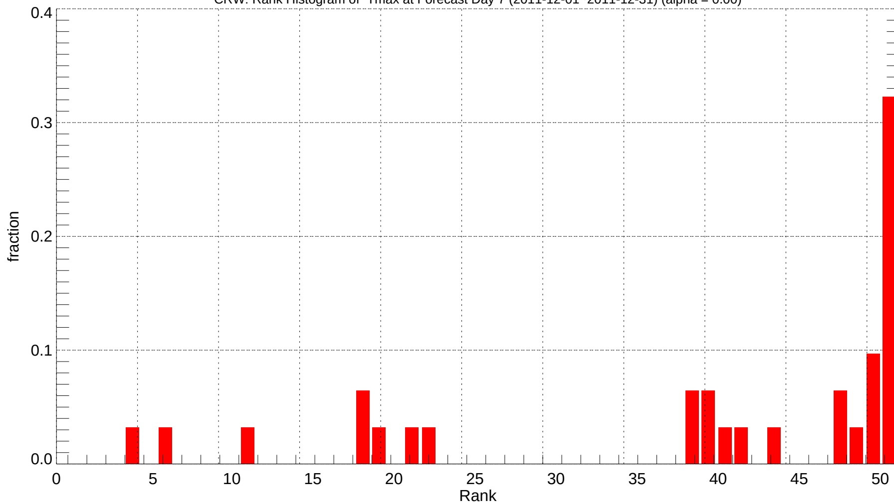
CRW: Rank Histogram of Tmax at Forecast Day 7 (2011-12-01~2011-12-31) (alpha = 0.00)
