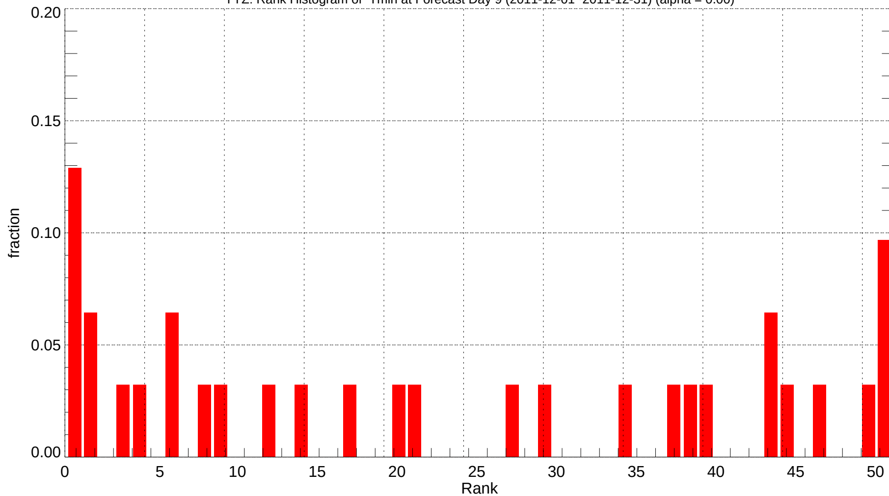
YYZ: Rank Histogram of Tmin at Forecast Day 9 (2011-12-01~2011-12-31) (alpha = 0.00)
