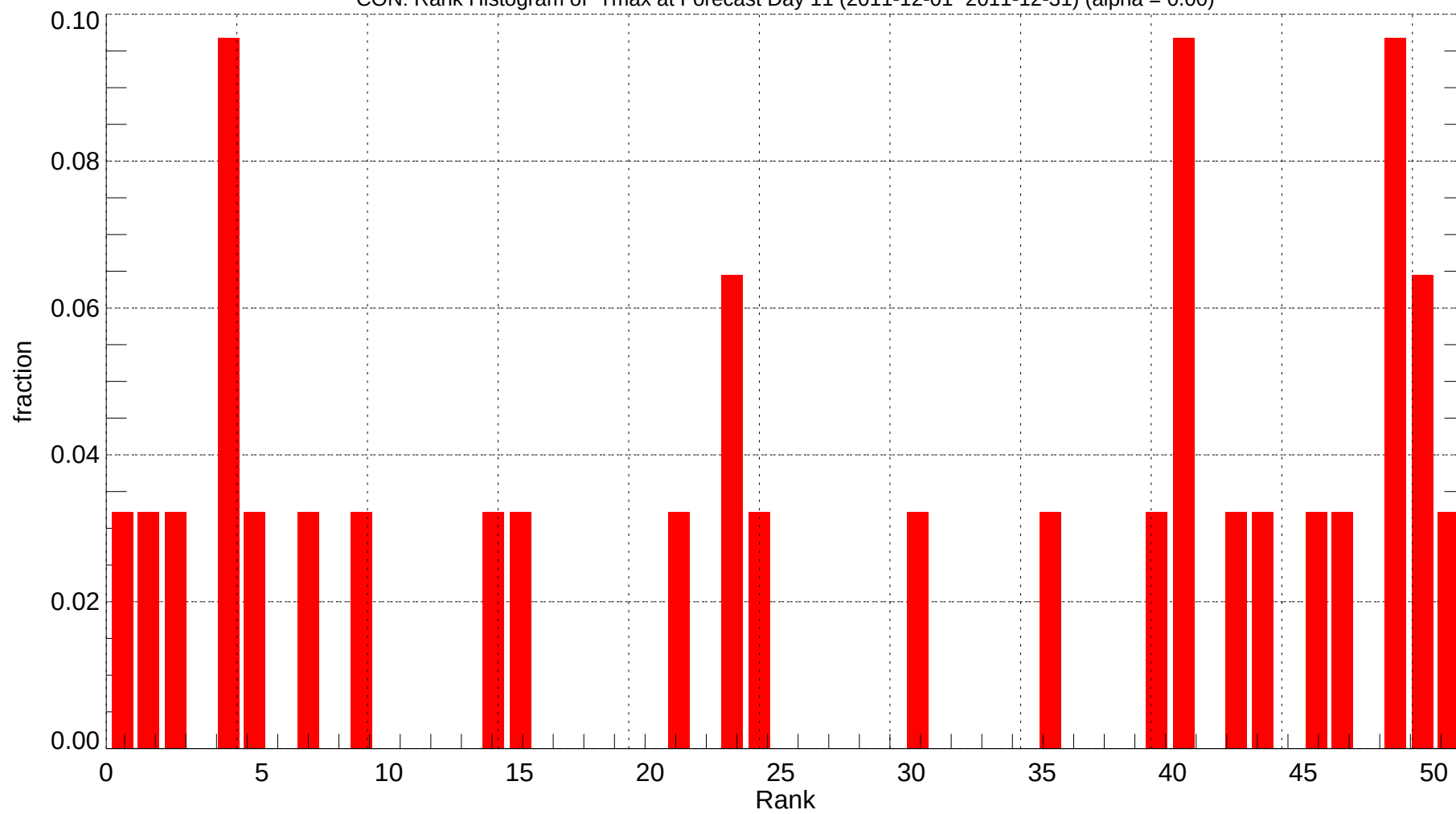
CON: Rank Histogram of Tmax at Forecast Day 11 (2011-12-01~2011-12-31) (alpha = 0.00)
