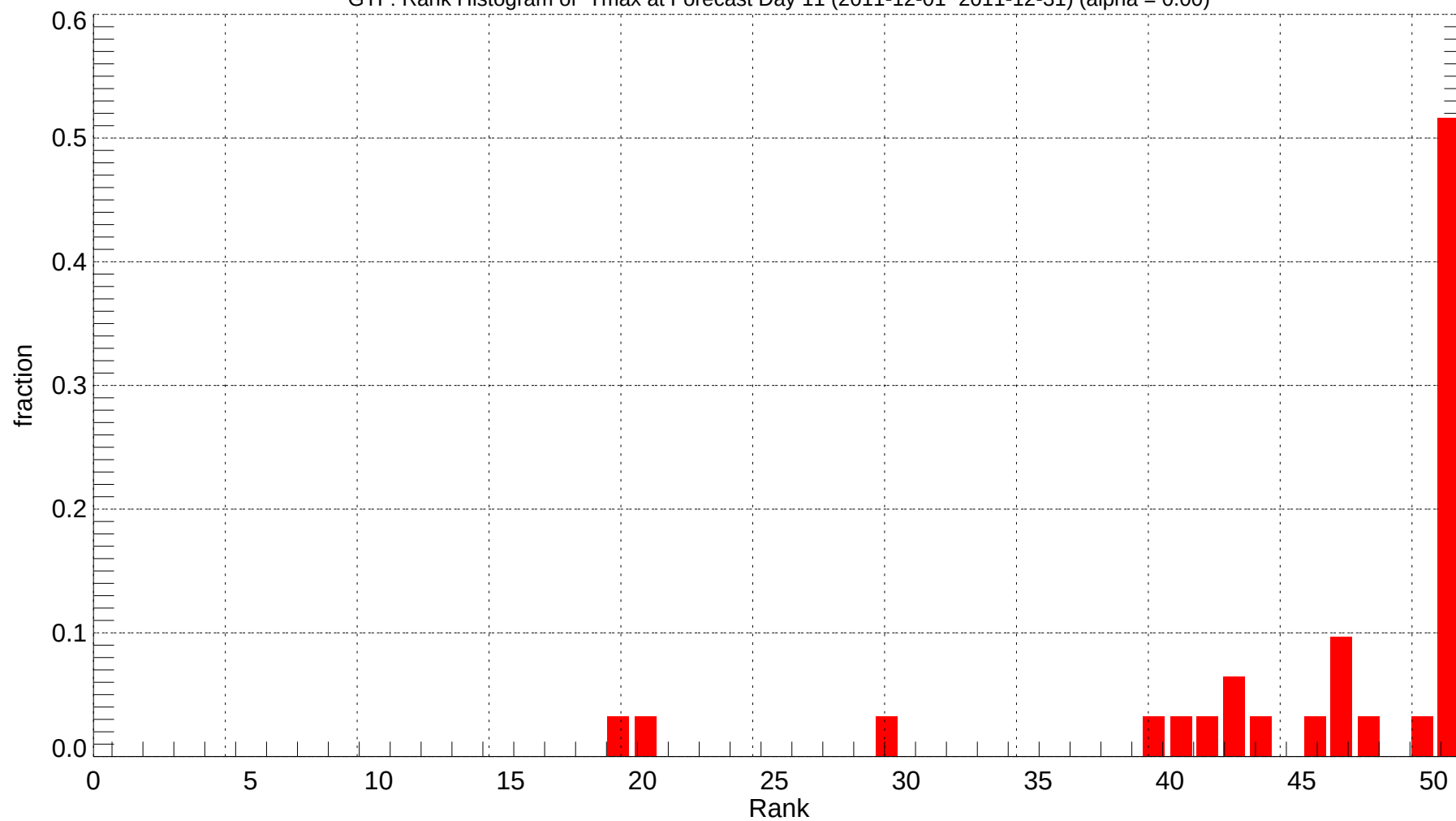
GTF: Rank Histogram of Tmax at Forecast Day 11 (2011-12-01~2011-12-31) (alpha = 0.00)
