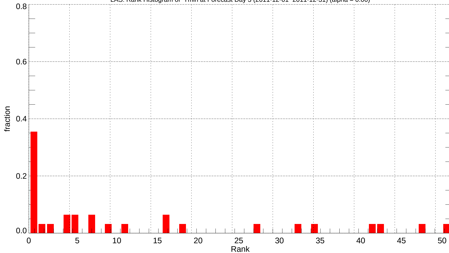
LAS: Rank Histogram of Tmin at Forecast Day 3 (2011-12-01~2011-12-31) (alpha = 0.00)
