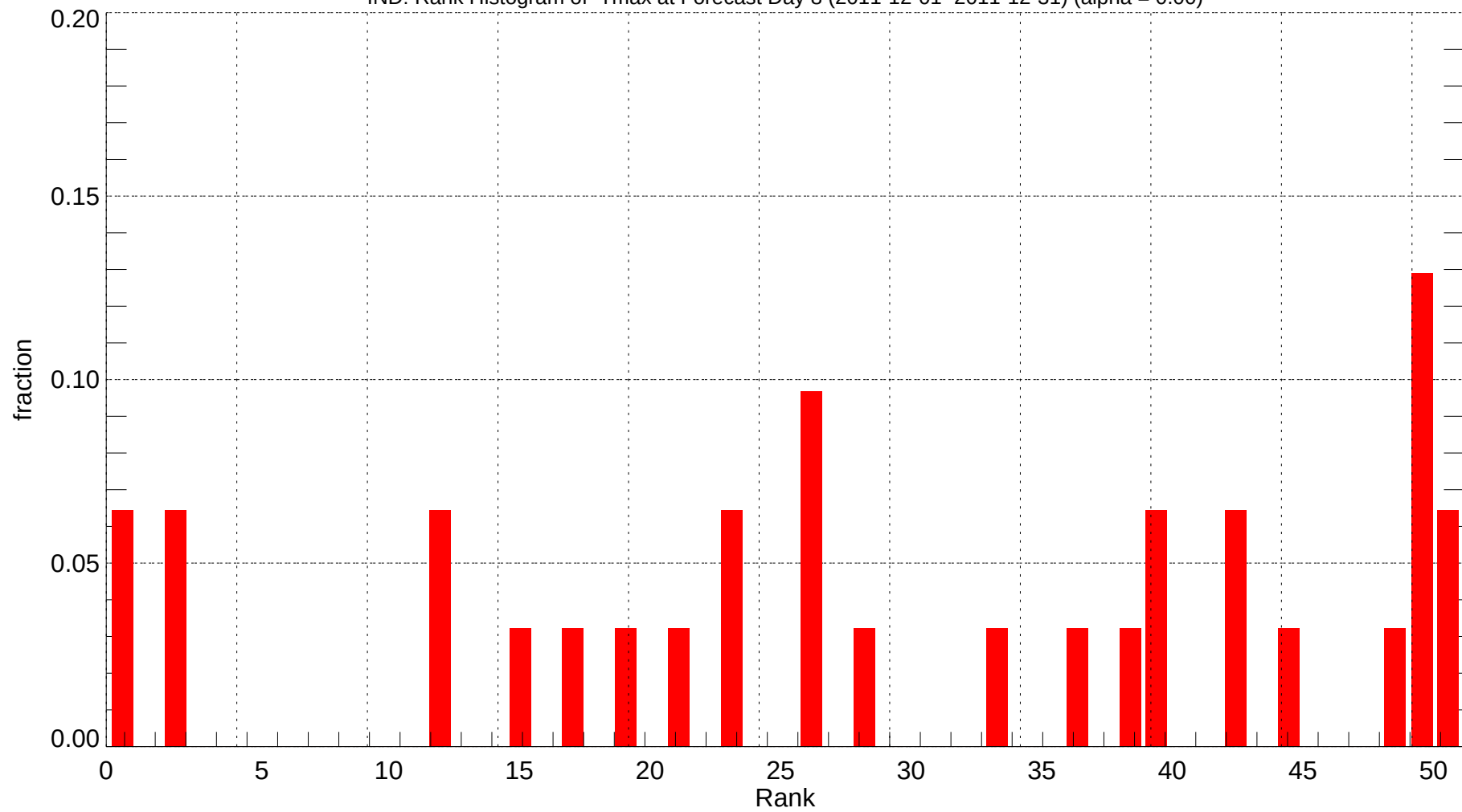
IND: Rank Histogram of Tmax at Forecast Day 8 (2011-12-01~2011-12-31) (alpha = 0.00)
