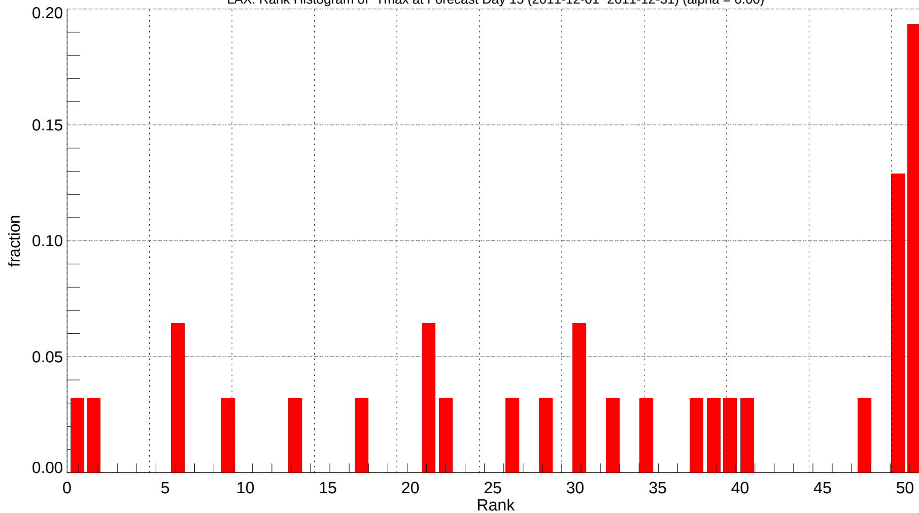
LAX: Rank Histogram of Tmax at Forecast Day 15 (2011-12-01~2011-12-31) (alpha = 0.00)
