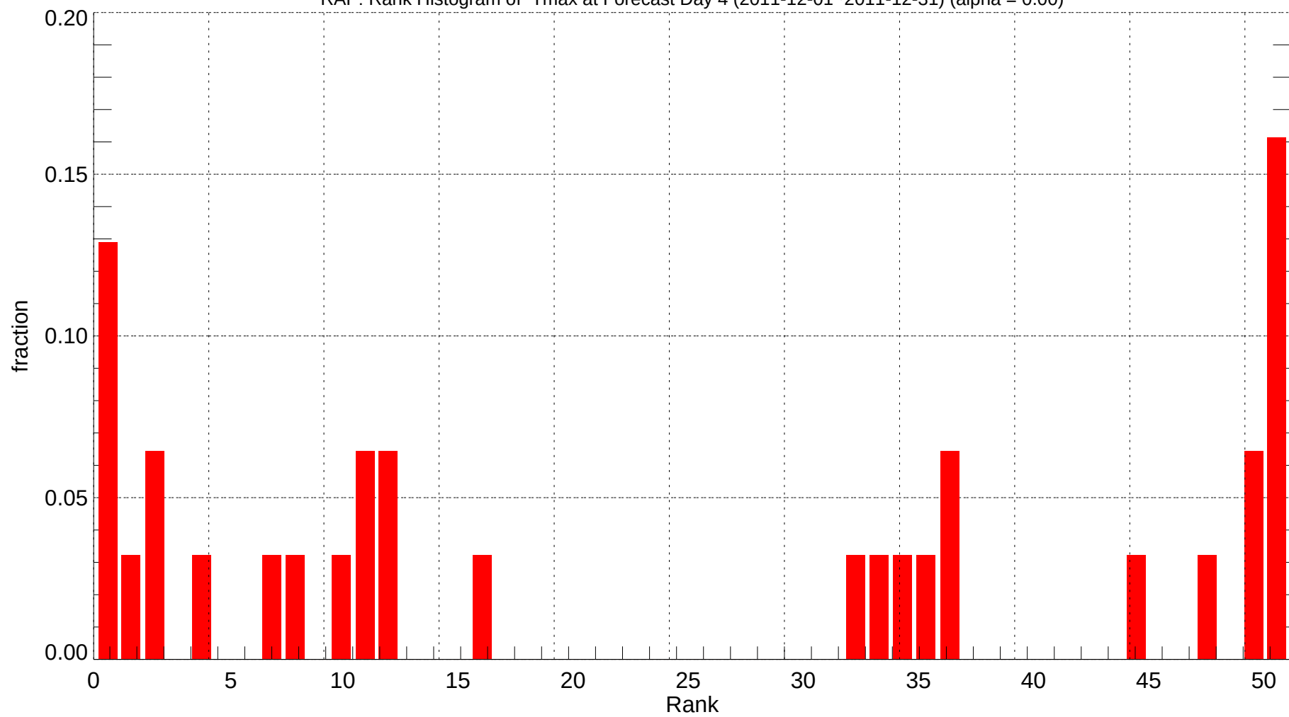
RAP: Rank Histogram of Tmax at Forecast Day 4 (2011-12-01~2011-12-31) (alpha = 0.00)
