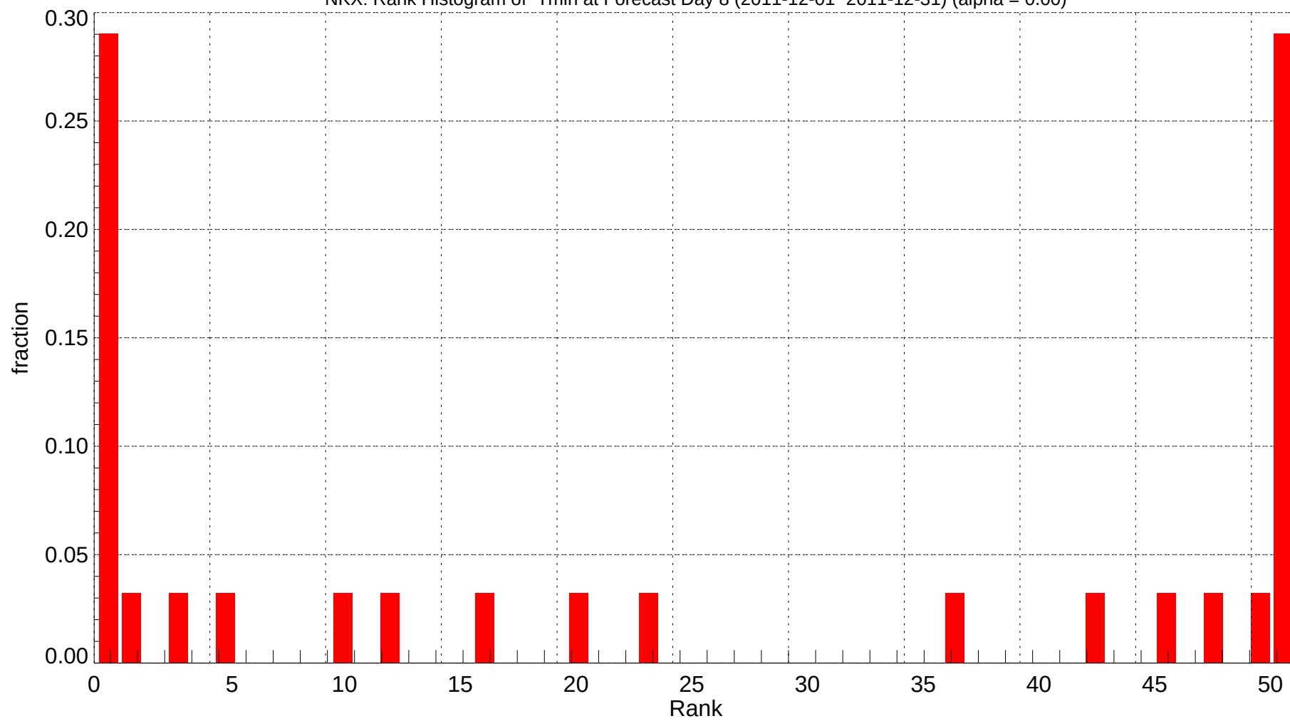
NKX: Rank Histogram of Tmin at Forecast Day 8 (2011-12-01~2011-12-31) (alpha = 0.00)
