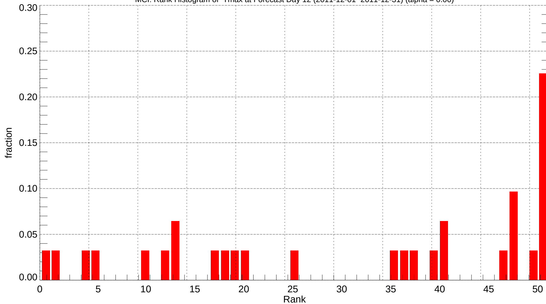
MCI: Rank Histogram of Tmax at Forecast Day 12 (2011-12-01~2011-12-31) (alpha = 0.00)
