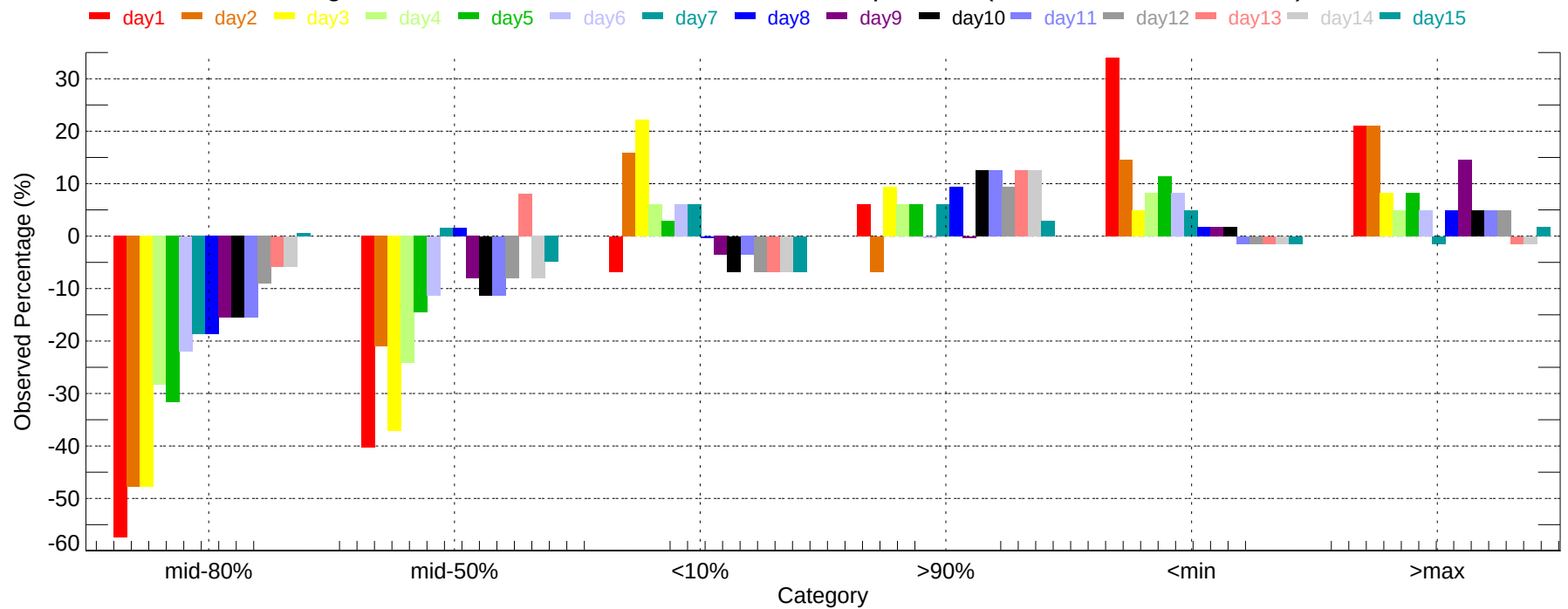
Observed Percentage Deviation of Ensembles - DAY: Max Temperature (2011-12-01~2011-12-31)
