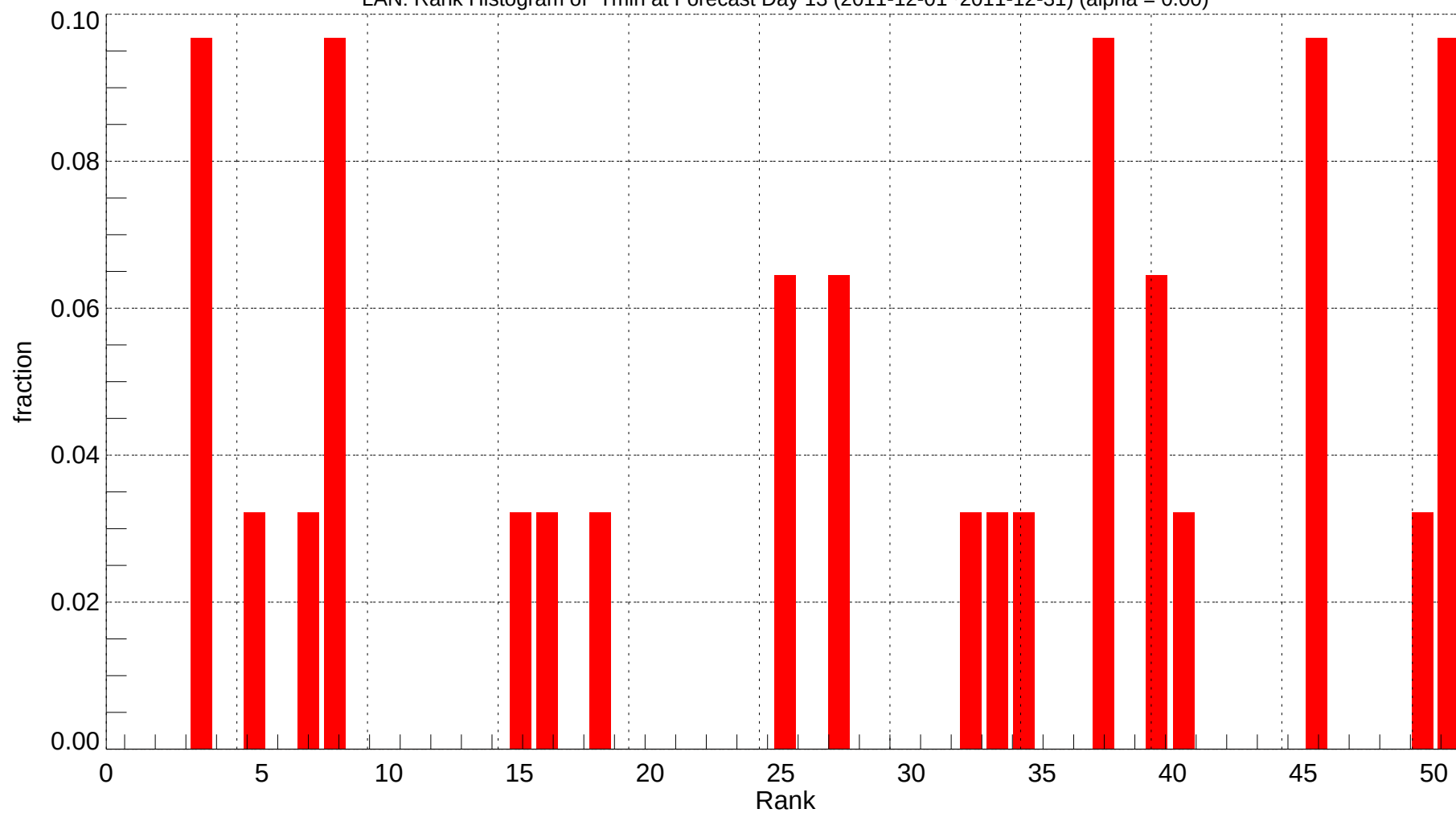
LAN: Rank Histogram of Tmin at Forecast Day 13 (2011-12-01~2011-12-31) (alpha = 0.00)
