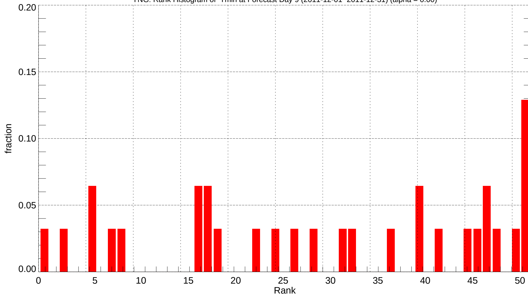
YNG: Rank Histogram of Tmin at Forecast Day 9 (2011-12-01~2011-12-31) (alpha = 0.00)
