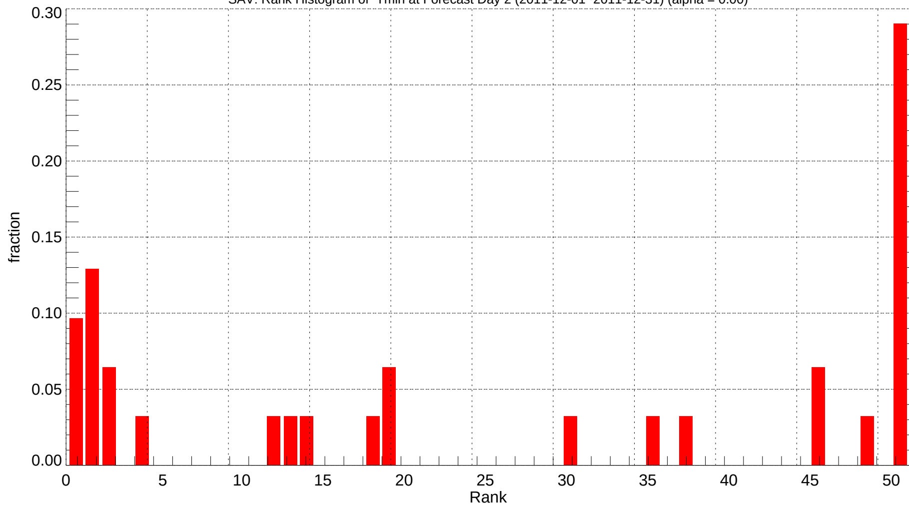
SAV: Rank Histogram of Tmin at Forecast Day 2 (2011-12-01~2011-12-31) (alpha = 0.00)
