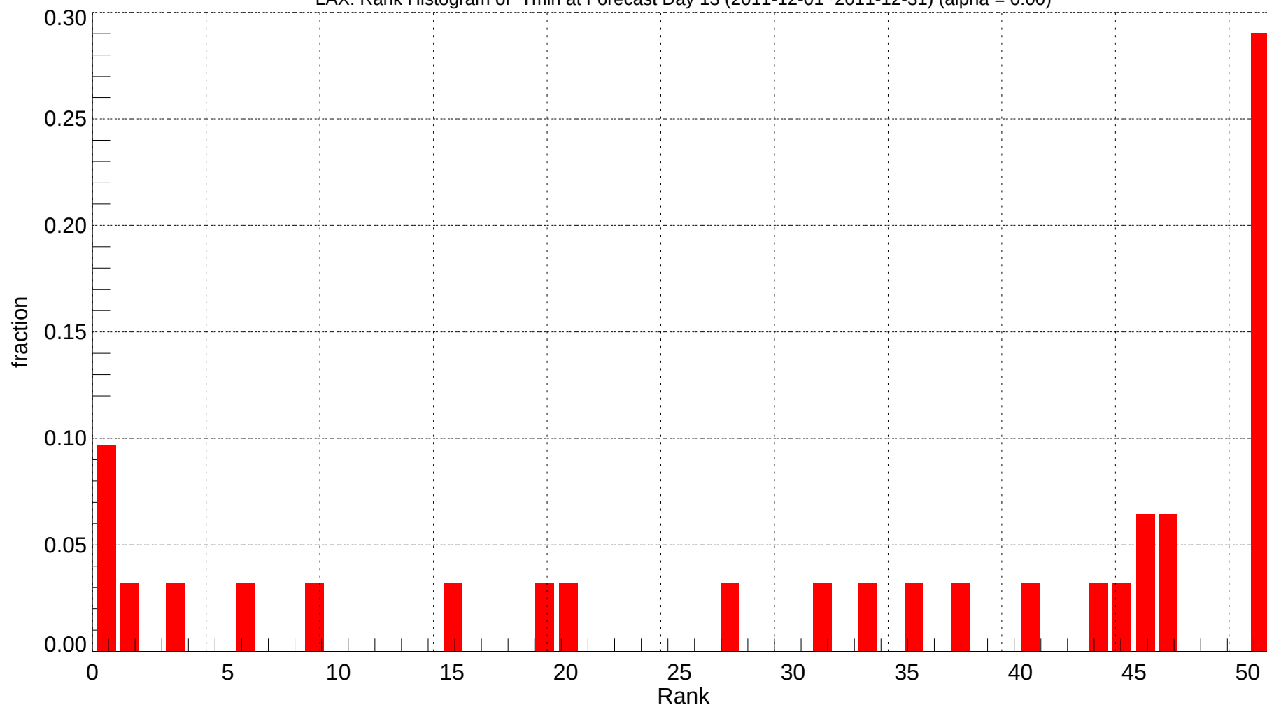
LAX: Rank Histogram of Tmin at Forecast Day 13 (2011-12-01~2011-12-31) (alpha = 0.00)
