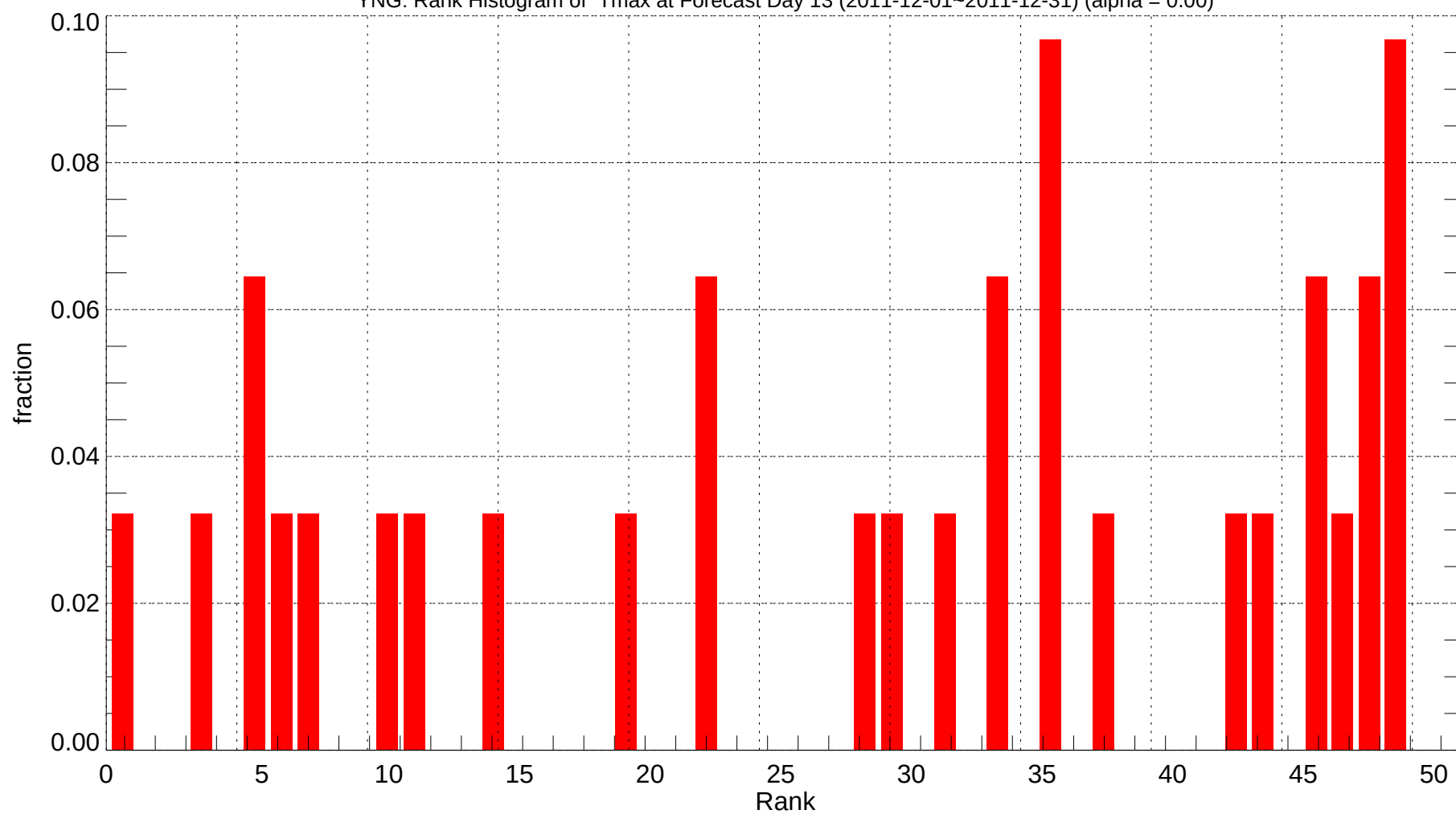
YNG: Rank Histogram of Tmax at Forecast Day 13 (2011-12-01~2011-12-31) (alpha = 0.00)
