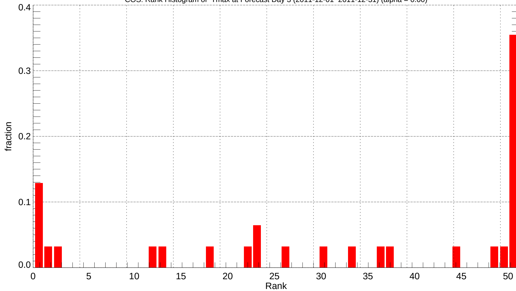
COS: Rank Histogram of Tmax at Forecast Day 3 (2011-12-01~2011-12-31) (alpha = 0.00)
