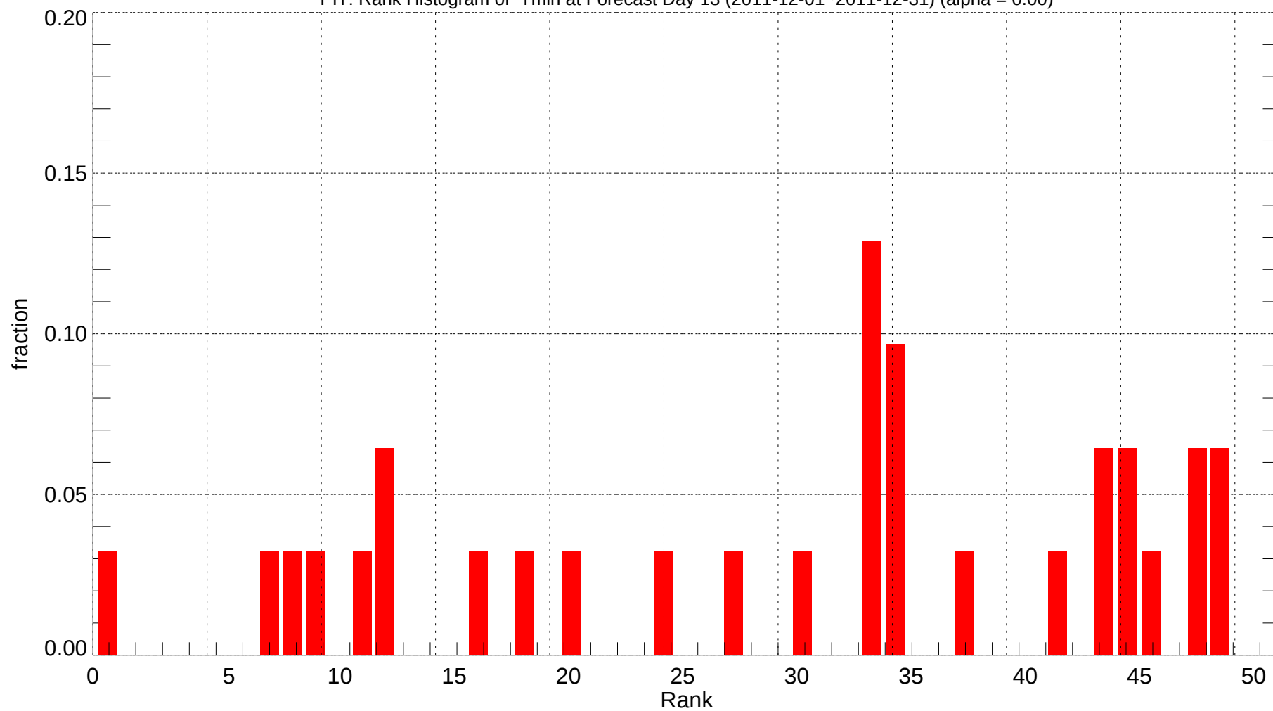
PIT: Rank Histogram of Tmin at Forecast Day 13 (2011-12-01~2011-12-31) (alpha = 0.00)
