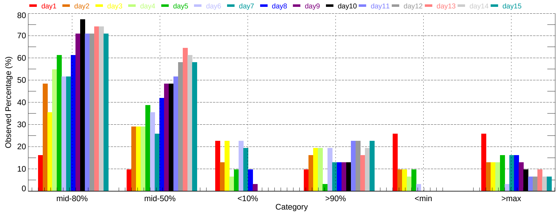
Observed Percentage of Ensembles - ATL: Max Temperature (2011-12-01~2011-12-31)
