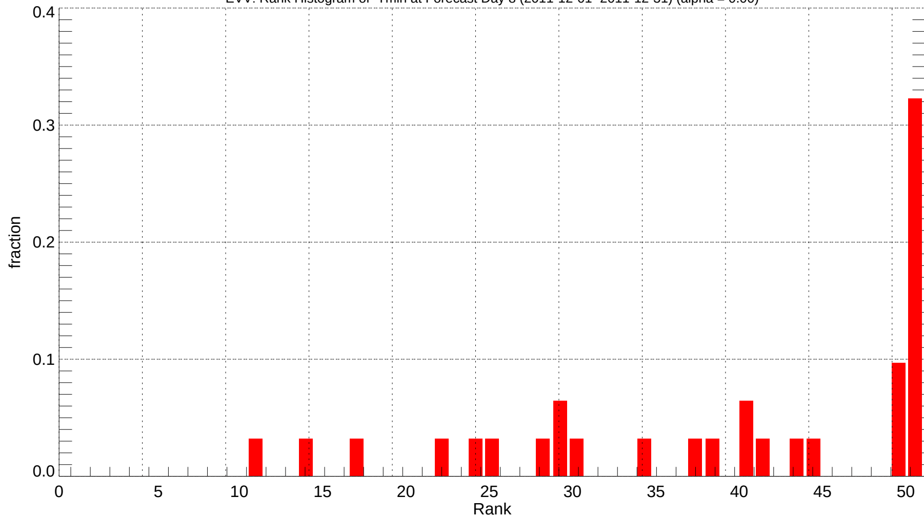
EVV: Rank Histogram of Tmin at Forecast Day 8 (2011-12-01~2011-12-31) (alpha = 0.00)
