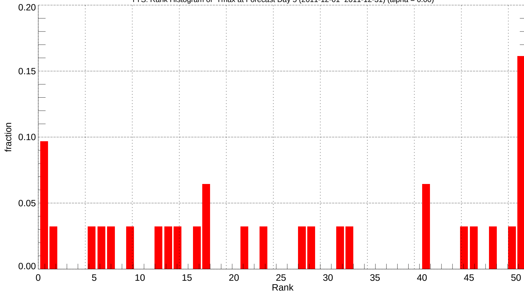
TYS: Rank Histogram of Tmax at Forecast Day 5 (2011-12-01~2011-12-31) (alpha = 0.00)
