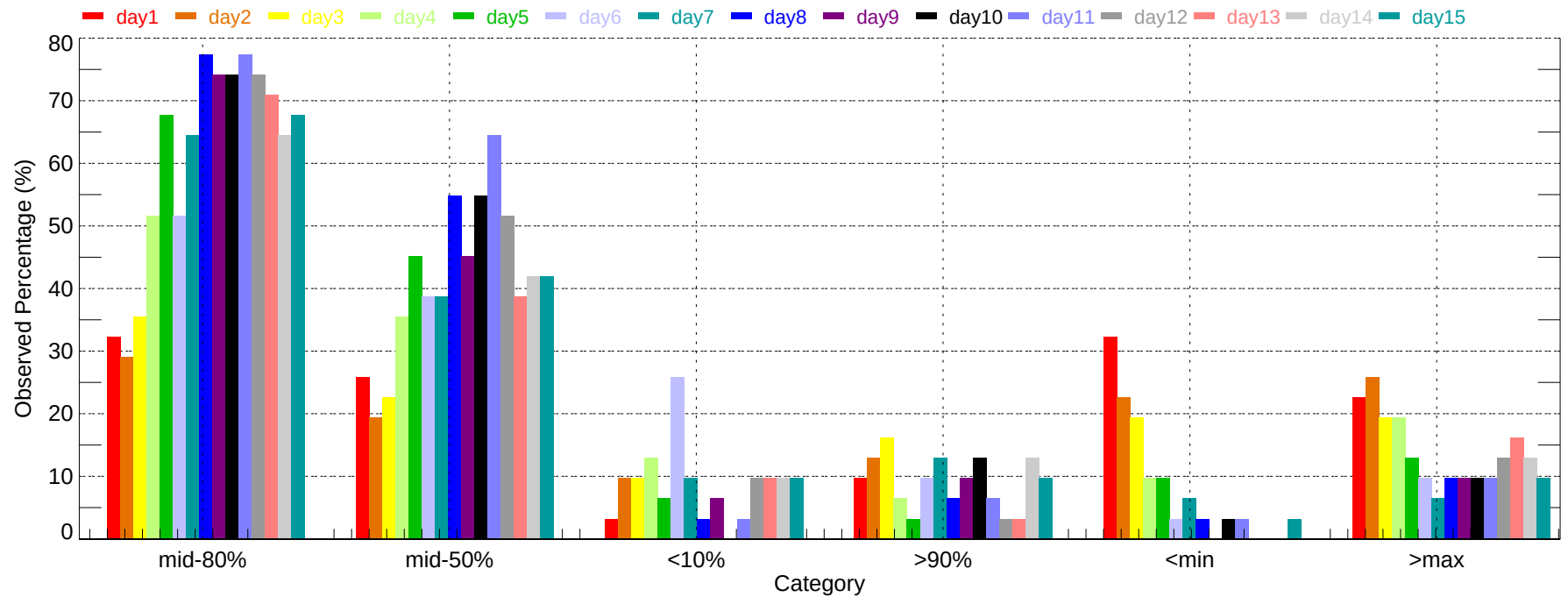
Observed Percentage of Ensembles - HOU: Max Temperature (2011-12-01~2011-12-31)
