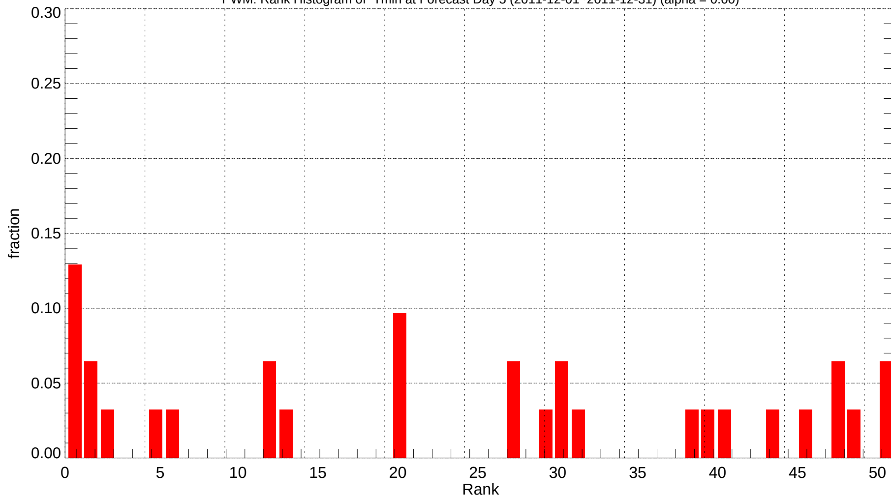
PWM: Rank Histogram of Tmin at Forecast Day 5 (2011-12-01~2011-12-31) (alpha = 0.00)
