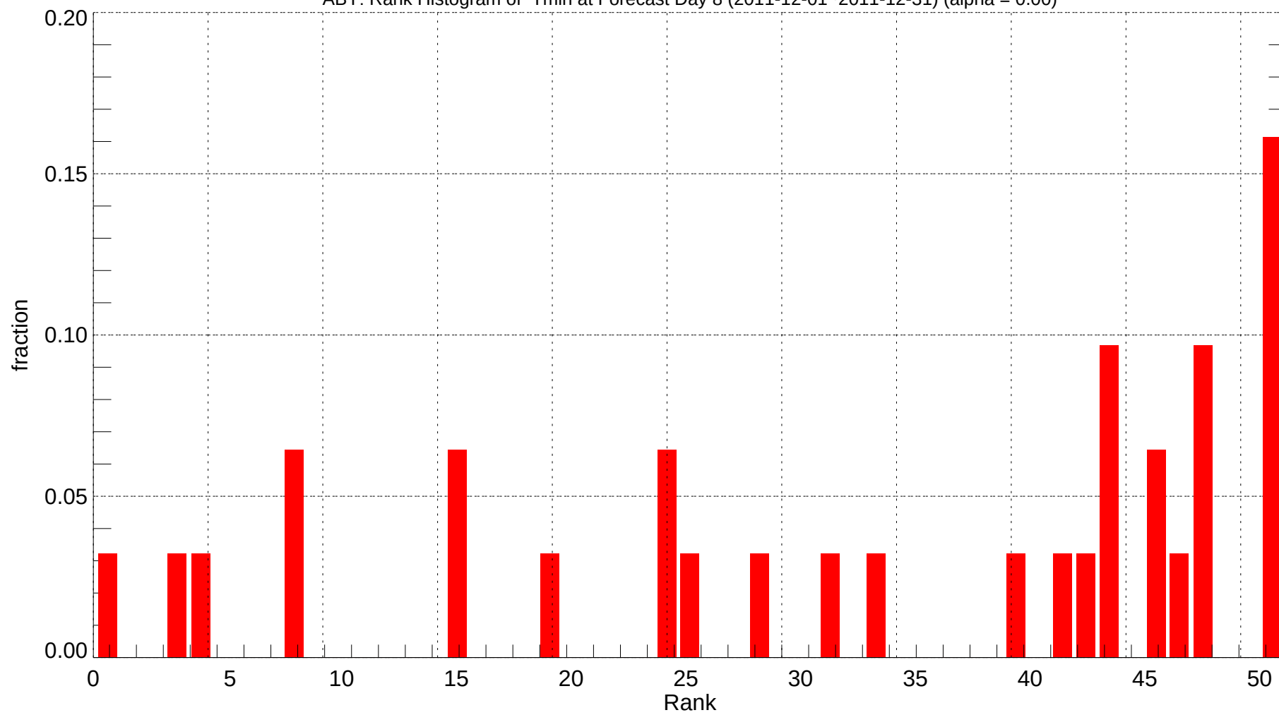
ABY: Rank Histogram of Tmin at Forecast Day 8 (2011-12-01~2011-12-31) (alpha = 0.00)
