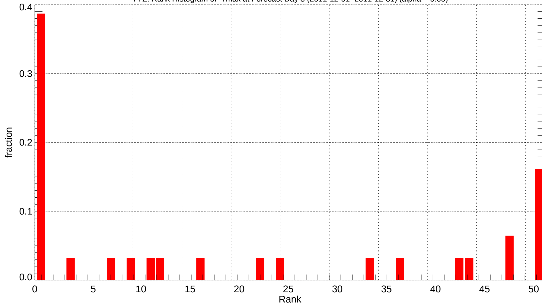
YYZ: Rank Histogram of Tmax at Forecast Day 3 (2011-12-01~2011-12-31) (alpha = 0.00)
