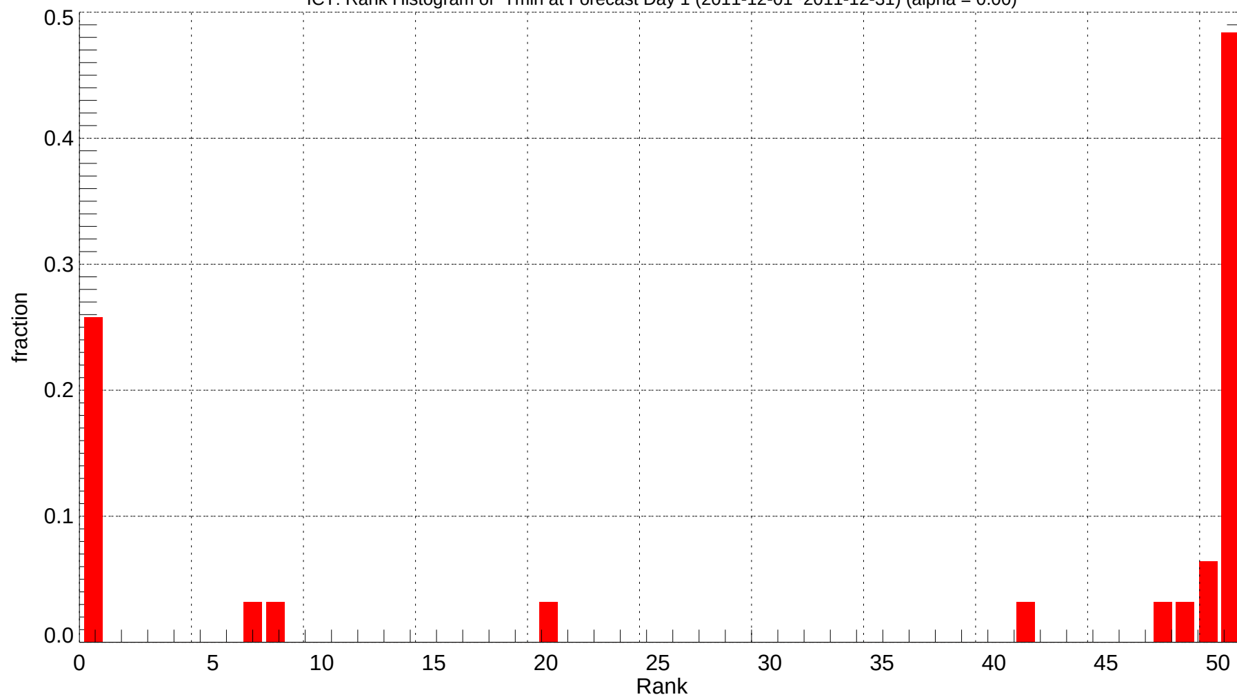
ICT: Rank Histogram of Tmin at Forecast Day 1 (2011-12-01~2011-12-31) (alpha = 0.00)
