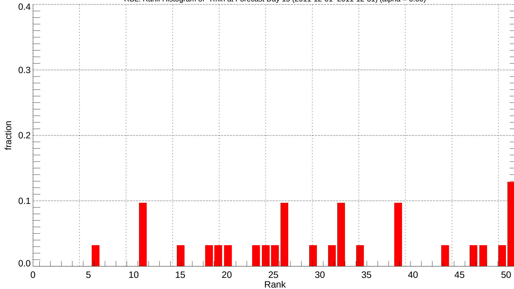
RBL: Rank Histogram of Tmin at Forecast Day 15 (2011-12-01~2011-12-31) (alpha = 0.00)
