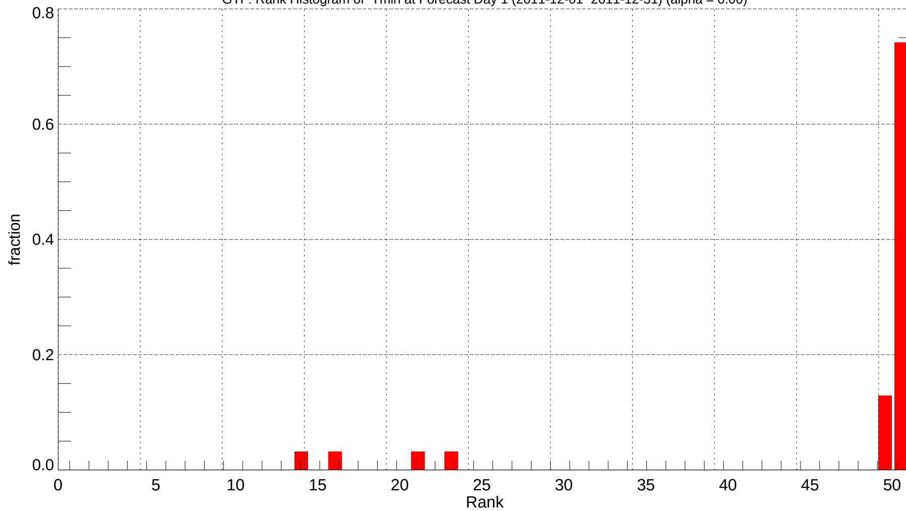
GTF: Rank Histogram of Tmin at Forecast Day 1 (2011-12-01~2011-12-31) (alpha = 0.00)
