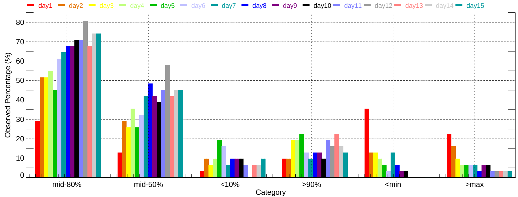
Observed Percentage of Ensembles - LNS: Min Temperature (2011-12-01~2011-12-31)
