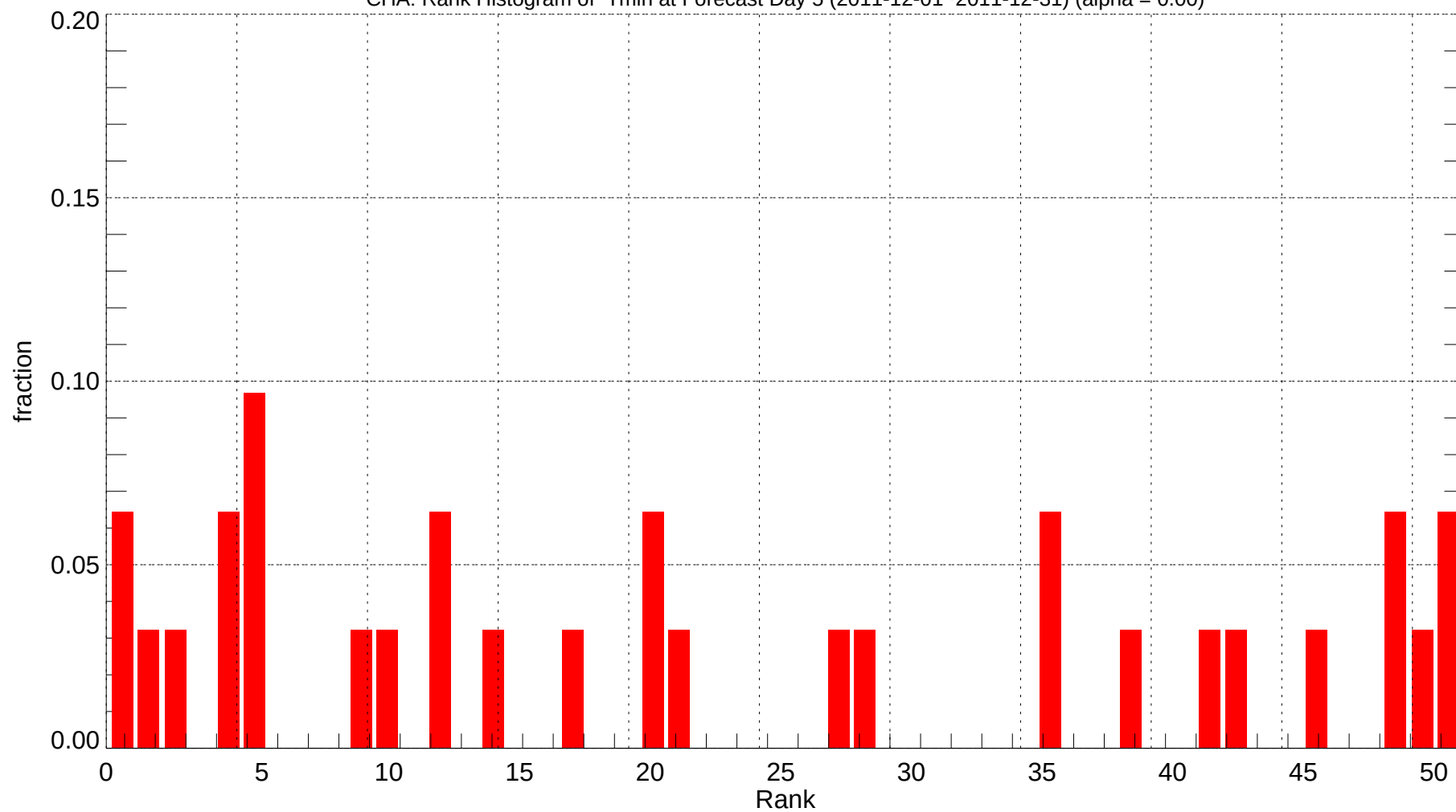
CHA: Rank Histogram of Tmin at Forecast Day 5 (2011-12-01~2011-12-31) (alpha = 0.00)
