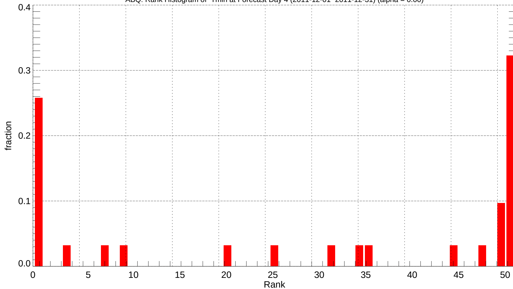
ABQ: Rank Histogram of Tmin at Forecast Day 4 (2011-12-01~2011-12-31) (alpha = 0.00)
