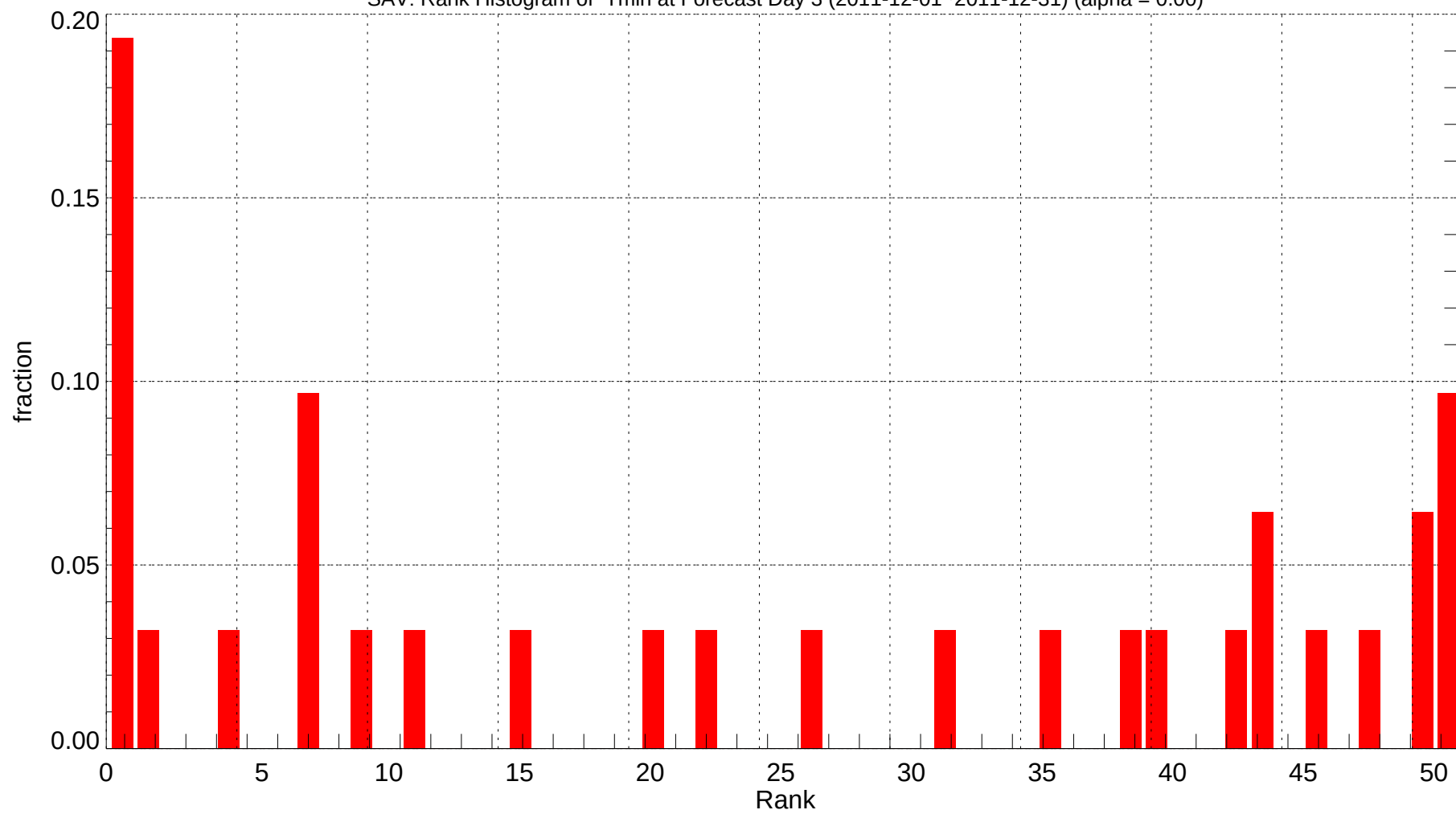
SAV: Rank Histogram of Tmin at Forecast Day 3 (2011-12-01~2011-12-31) (alpha = 0.00)
