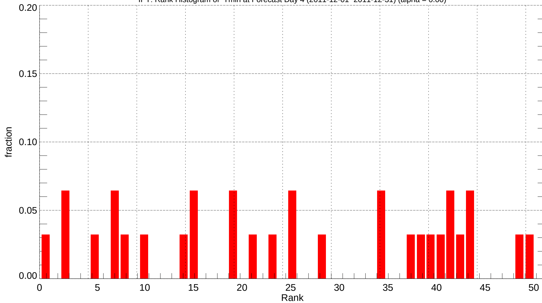
IPT: Rank Histogram of Tmin at Forecast Day 4 (2011-12-01~2011-12-31) (alpha = 0.00)
