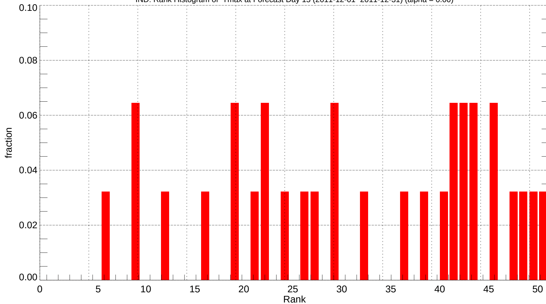
IND: Rank Histogram of Tmax at Forecast Day 15 (2011-12-01~2011-12-31) (alpha = 0.00)
