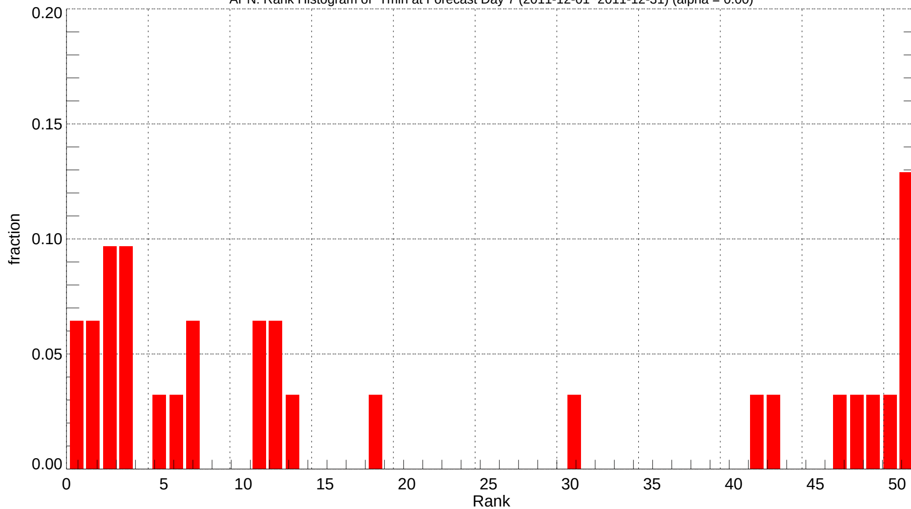
APN: Rank Histogram of Tmin at Forecast Day 7 (2011-12-01~2011-12-31) (alpha = 0.00)
