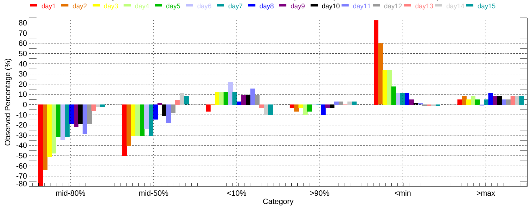
Observed Percentage Deviation of Ensembles - RBL: Max Temperature (2011-12-01~2011-12-31)
