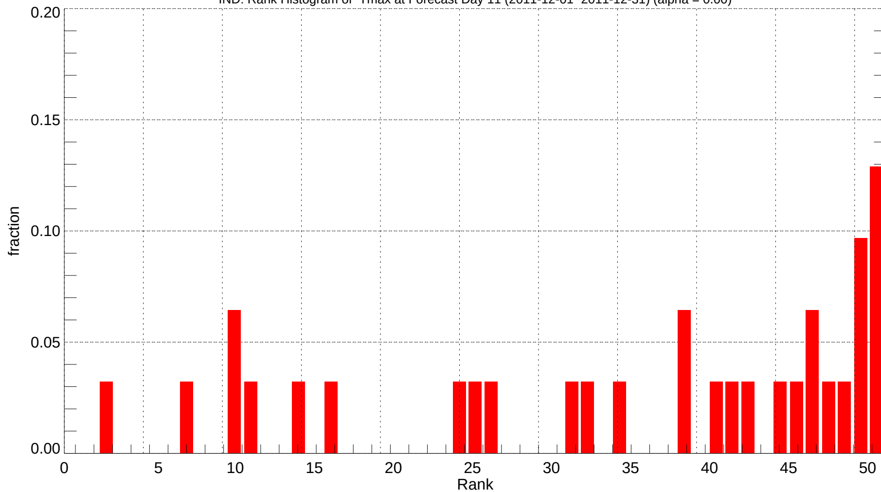
IND: Rank Histogram of Tmax at Forecast Day 11 (2011-12-01~2011-12-31) (alpha = 0.00)
