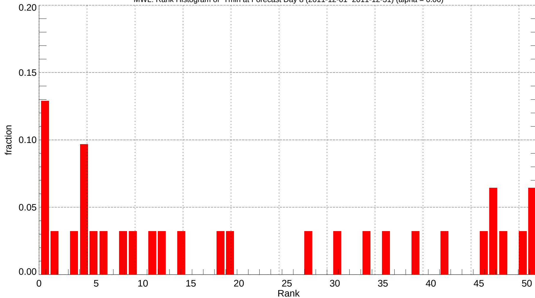
MWL: Rank Histogram of Tmin at Forecast Day 8 (2011-12-01~2011-12-31) (alpha = 0.00)
