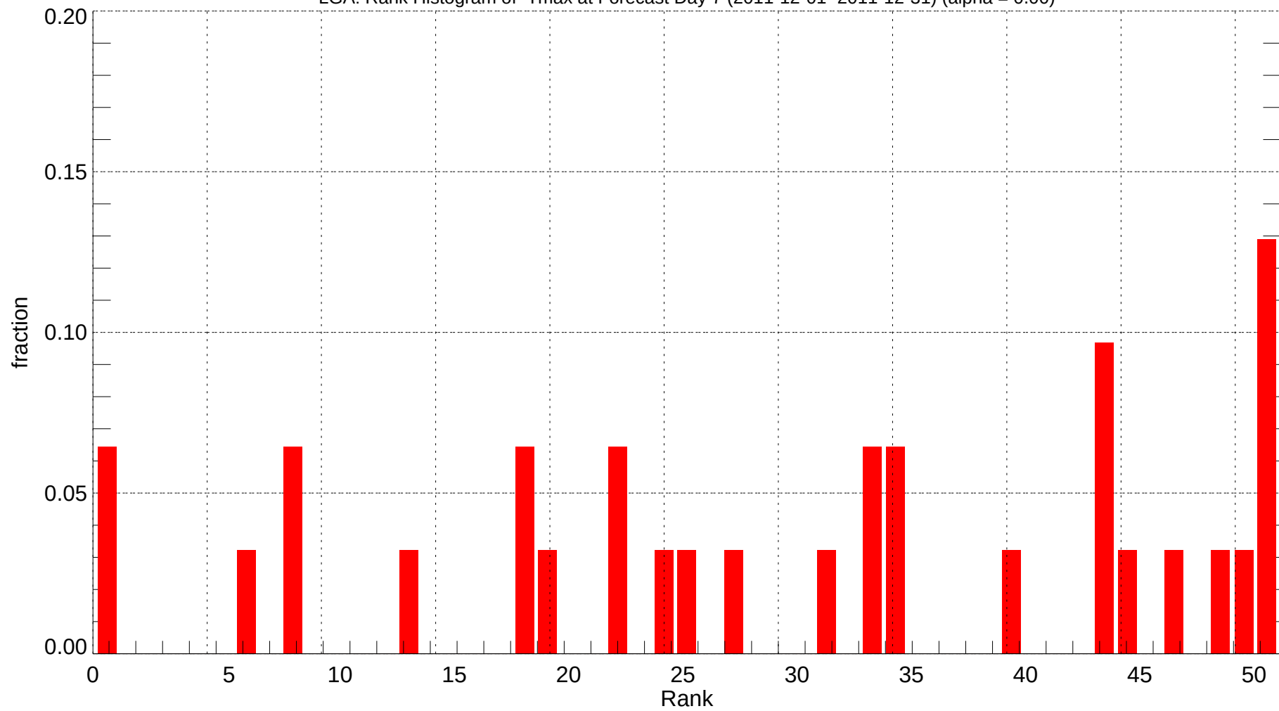
LGA: Rank Histogram of Tmax at Forecast Day 7 (2011-12-01~2011-12-31) (alpha = 0.00)
