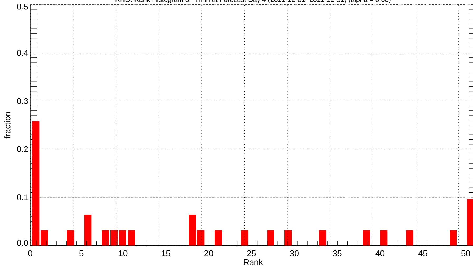
RNO: Rank Histogram of Tmin at Forecast Day 4 (2011-12-01~2011-12-31) (alpha = 0.00)
