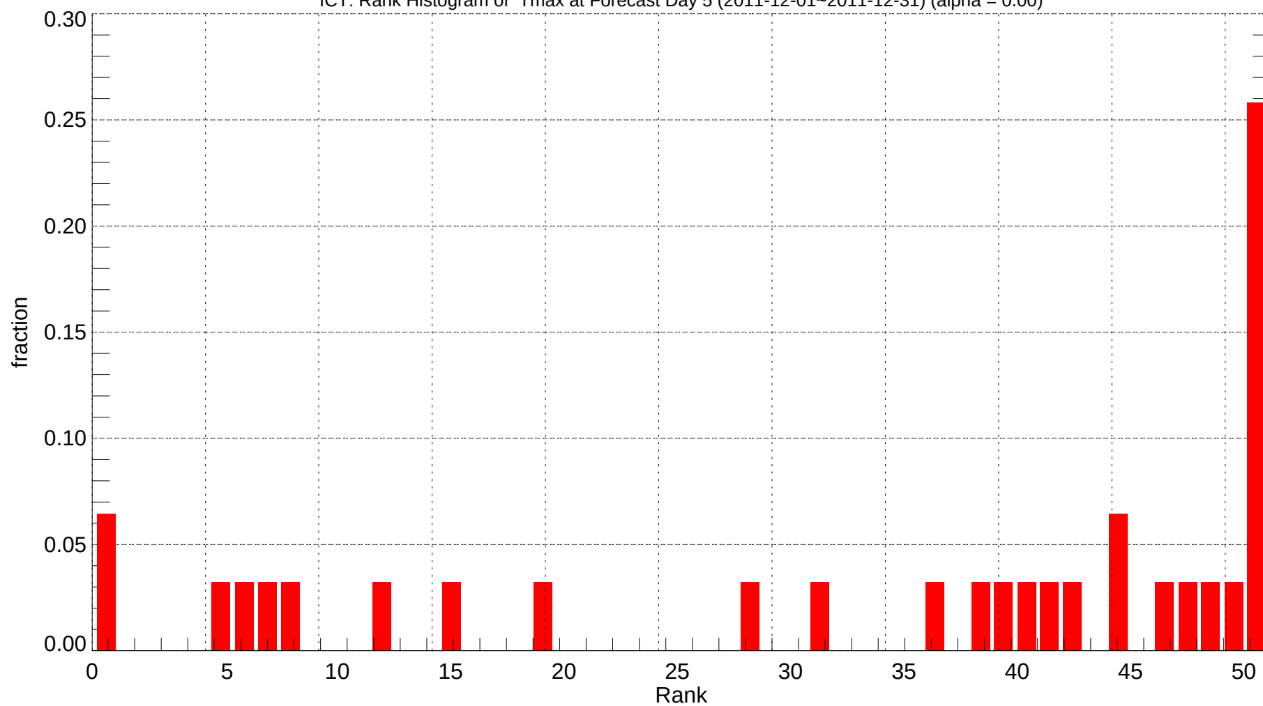
ICT: Rank Histogram of Tmax at Forecast Day 5 (2011-12-01~2011-12-31) (alpha = 0.00)
