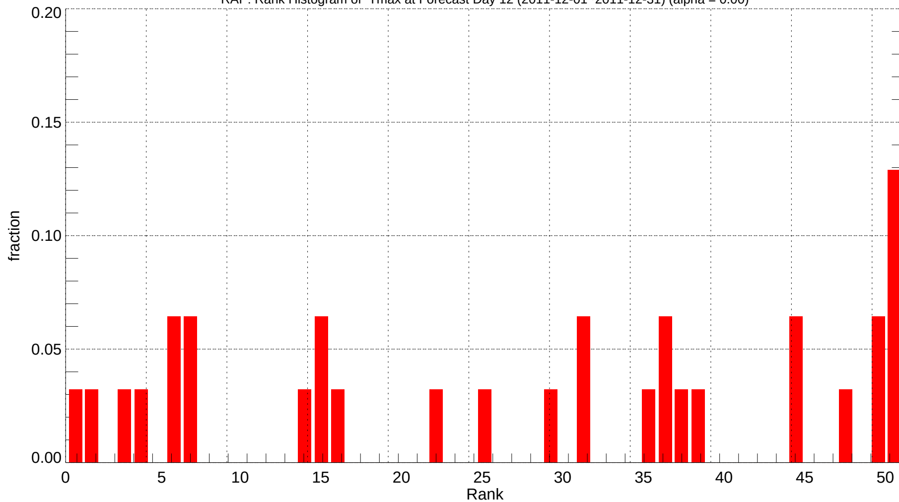
RAP: Rank Histogram of Tmax at Forecast Day 12 (2011-12-01~2011-12-31) (alpha = 0.00)
