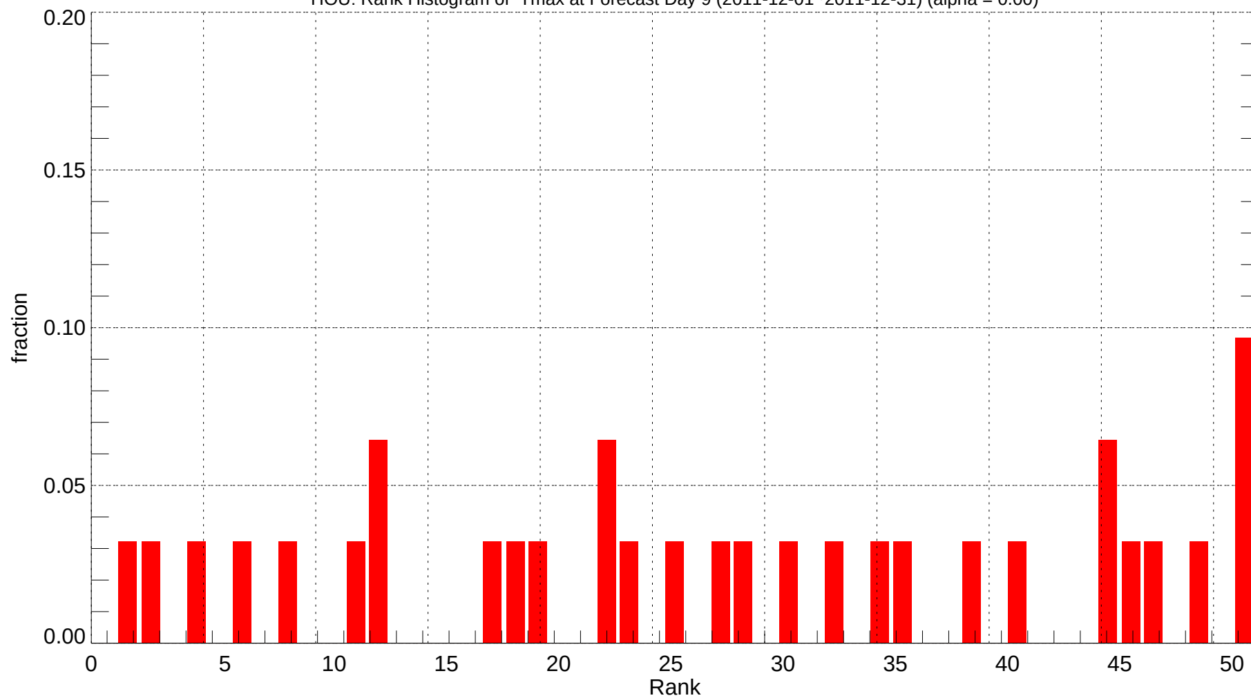
HOU: Rank Histogram of Tmax at Forecast Day 9 (2011-12-01~2011-12-31) (alpha = 0.00)
