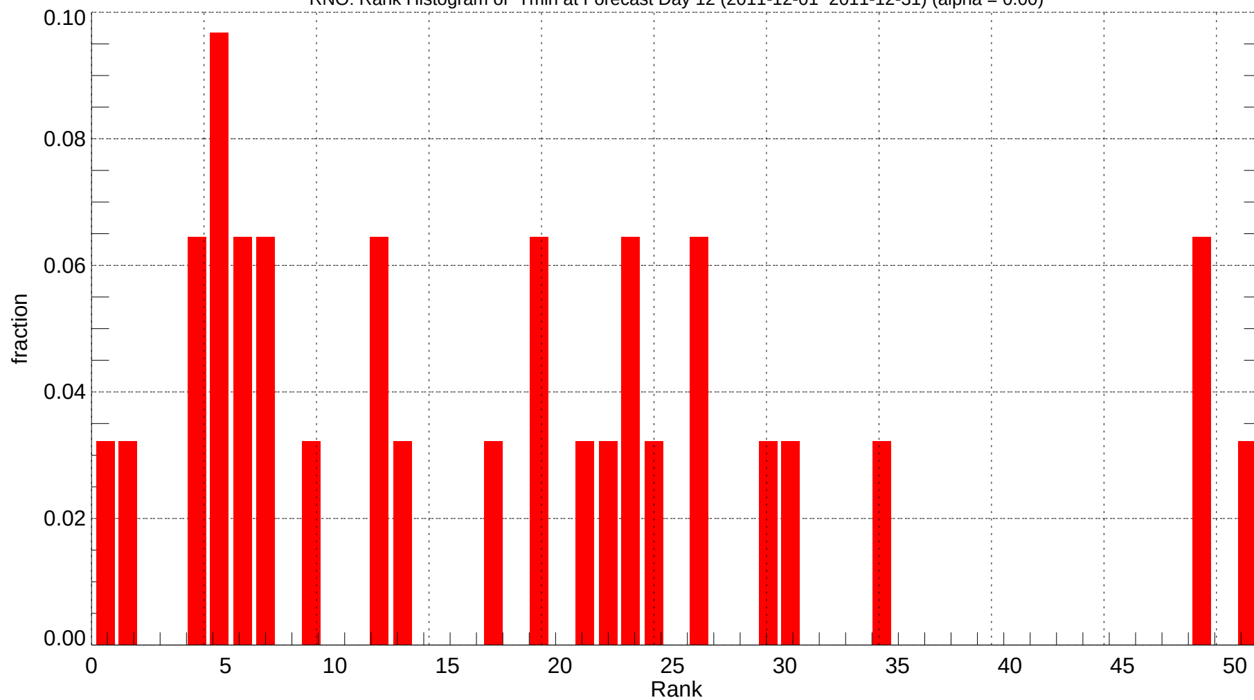
RNO: Rank Histogram of Tmin at Forecast Day 12 (2011-12-01~2011-12-31) (alpha = 0.00)
