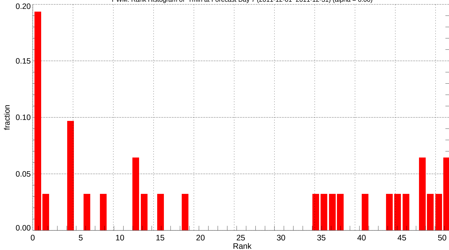
PWM: Rank Histogram of Tmin at Forecast Day 7 (2011-12-01~2011-12-31) (alpha = 0.00)
