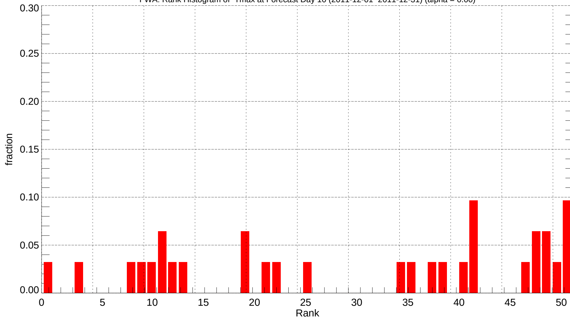
FWA: Rank Histogram of Tmax at Forecast Day 10 (2011-12-01~2011-12-31) (alpha = 0.00)
