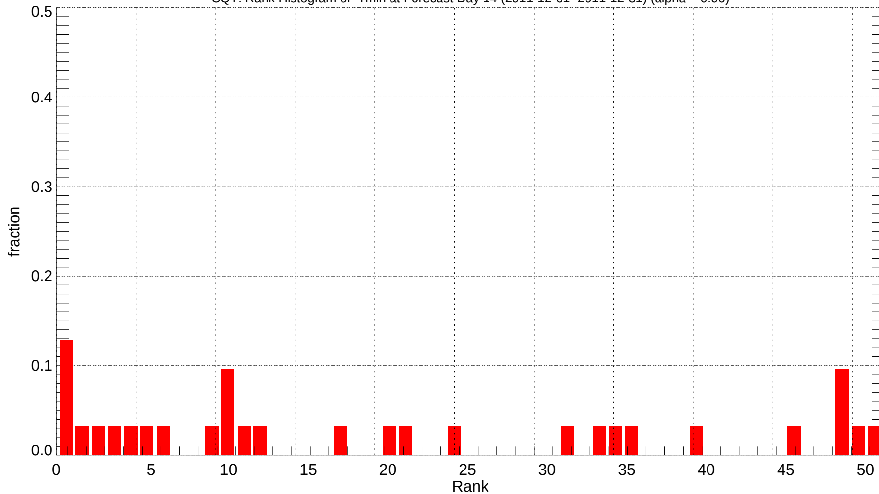
CQT: Rank Histogram of Tmin at Forecast Day 14 (2011-12-01~2011-12-31) (alpha = 0.00)
