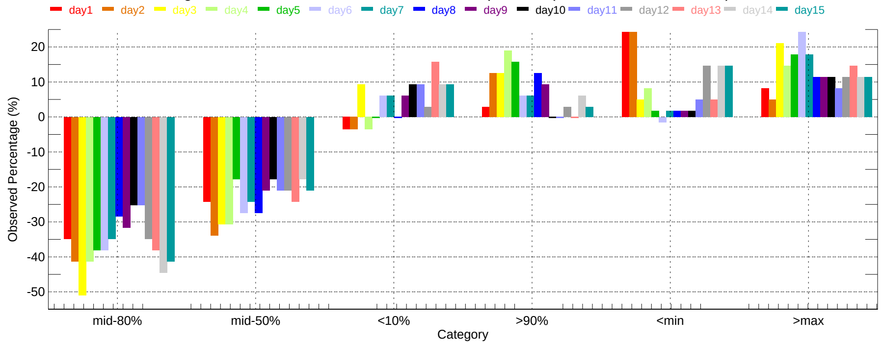
Observed Percentage Deviation of Ensembles - LFK: Max Temperature (2011-12-01~2011-12-31)
