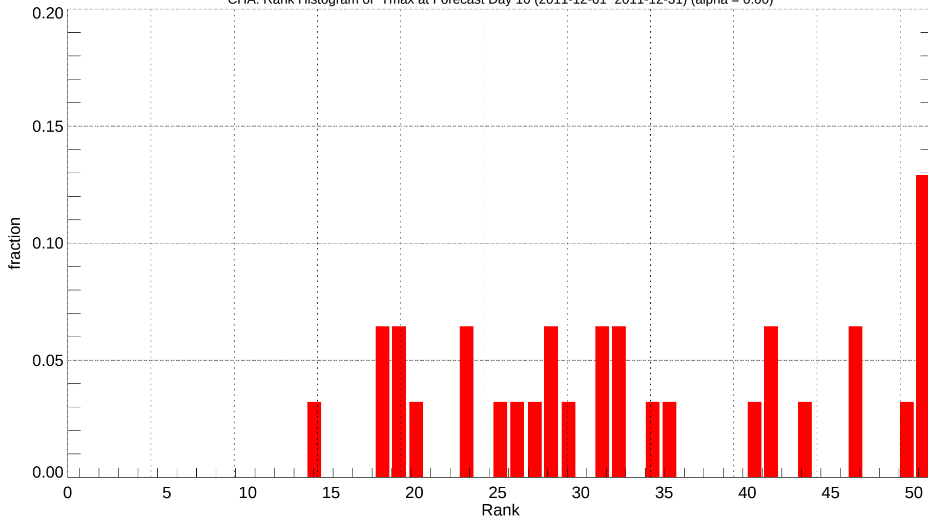
CHA: Rank Histogram of Tmax at Forecast Day 10 (2011-12-01~2011-12-31) (alpha = 0.00)
