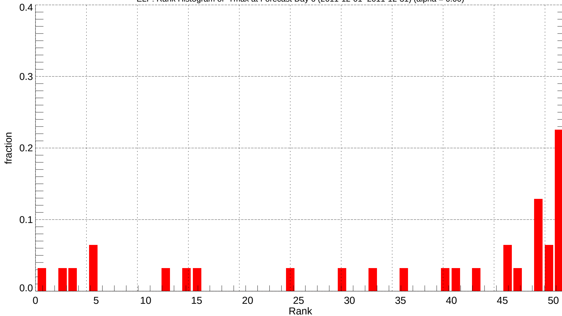
ELP: Rank Histogram of Tmax at Forecast Day 6 (2011-12-01~2011-12-31) (alpha = 0.00)
