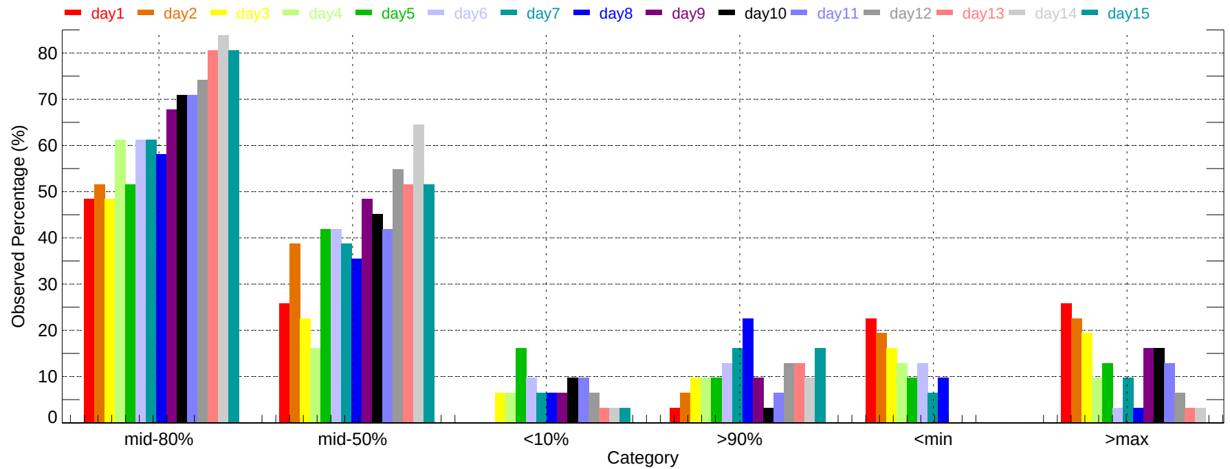
Observed Percentage of Ensembles - LGA: Min Temperature (2011-12-01~2011-12-31)
