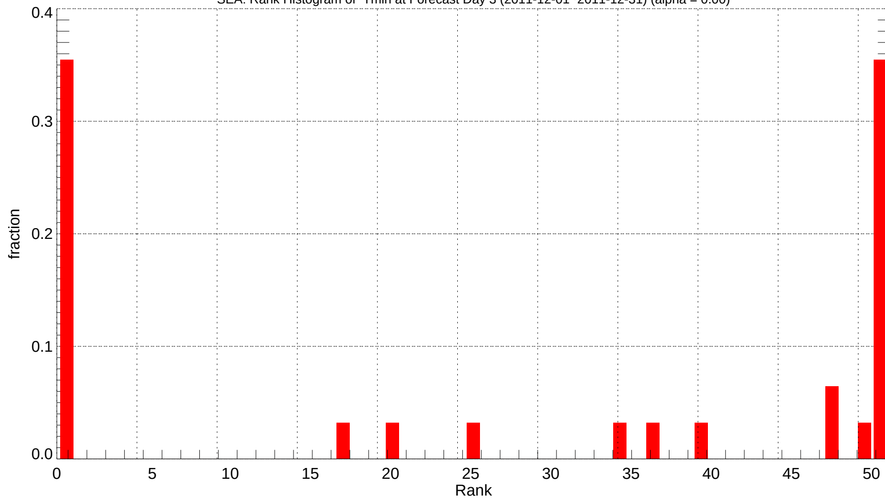
SEA: Rank Histogram of Tmin at Forecast Day 3 (2011-12-01~2011-12-31) (alpha = 0.00)
