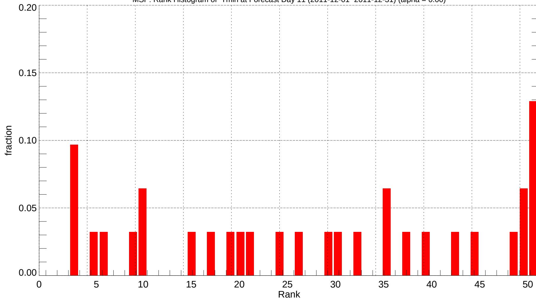
MSP: Rank Histogram of Tmin at Forecast Day 11 (2011-12-01~2011-12-31) (alpha = 0.00)
