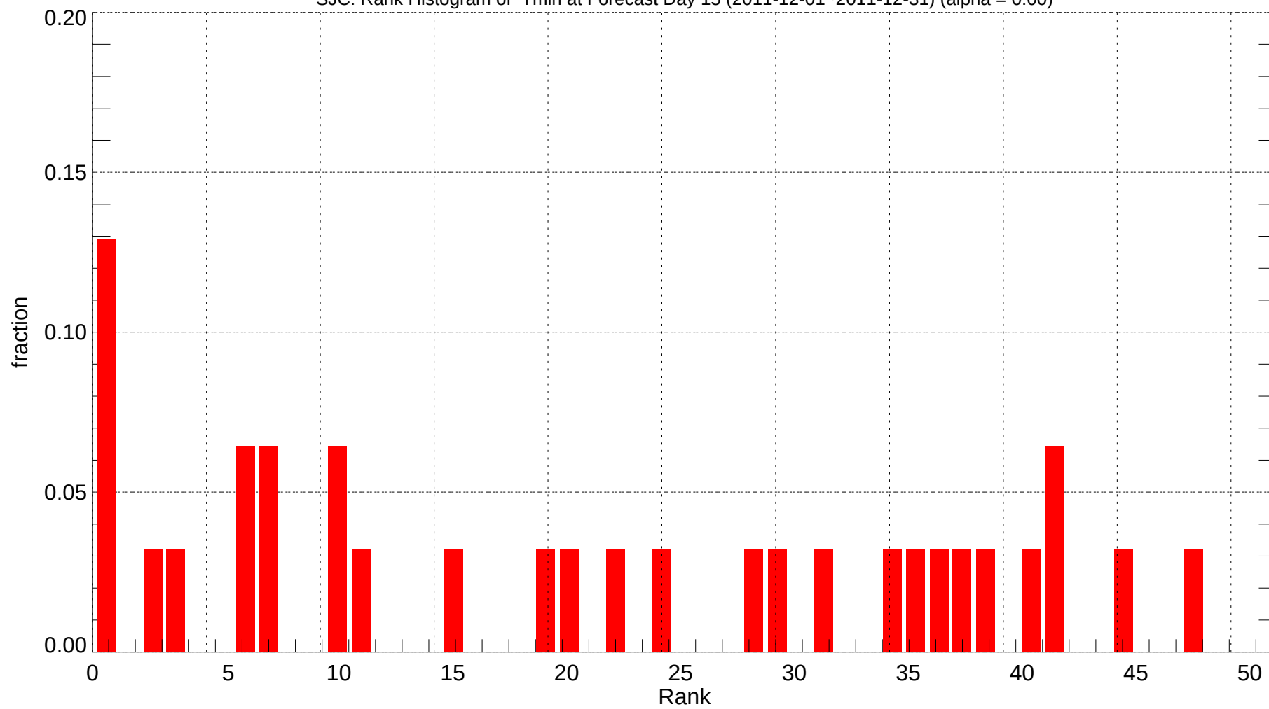
SJC: Rank Histogram of Tmin at Forecast Day 15 (2011-12-01~2011-12-31) (alpha = 0.00)
