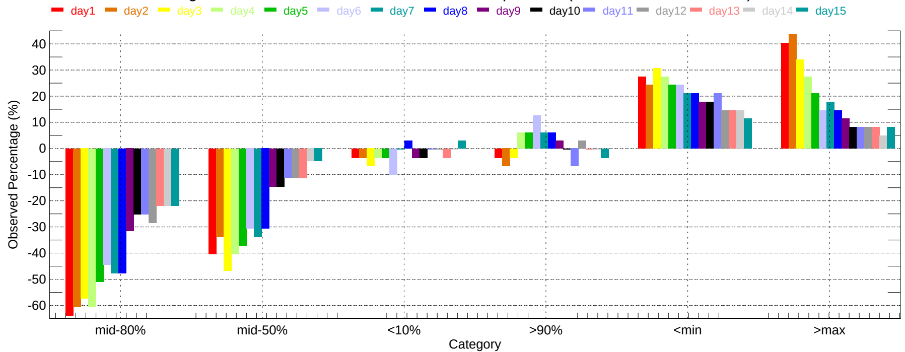
Observed Percentage Deviation of Ensembles - PDT: Max Temperature (2011-12-01~2011-12-31)
