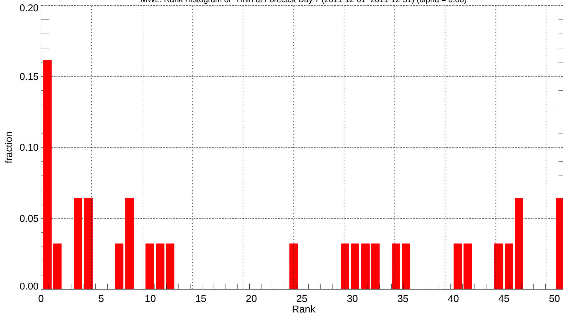
MWL: Rank Histogram of Tmin at Forecast Day 7 (2011-12-01~2011-12-31) (alpha = 0.00)
