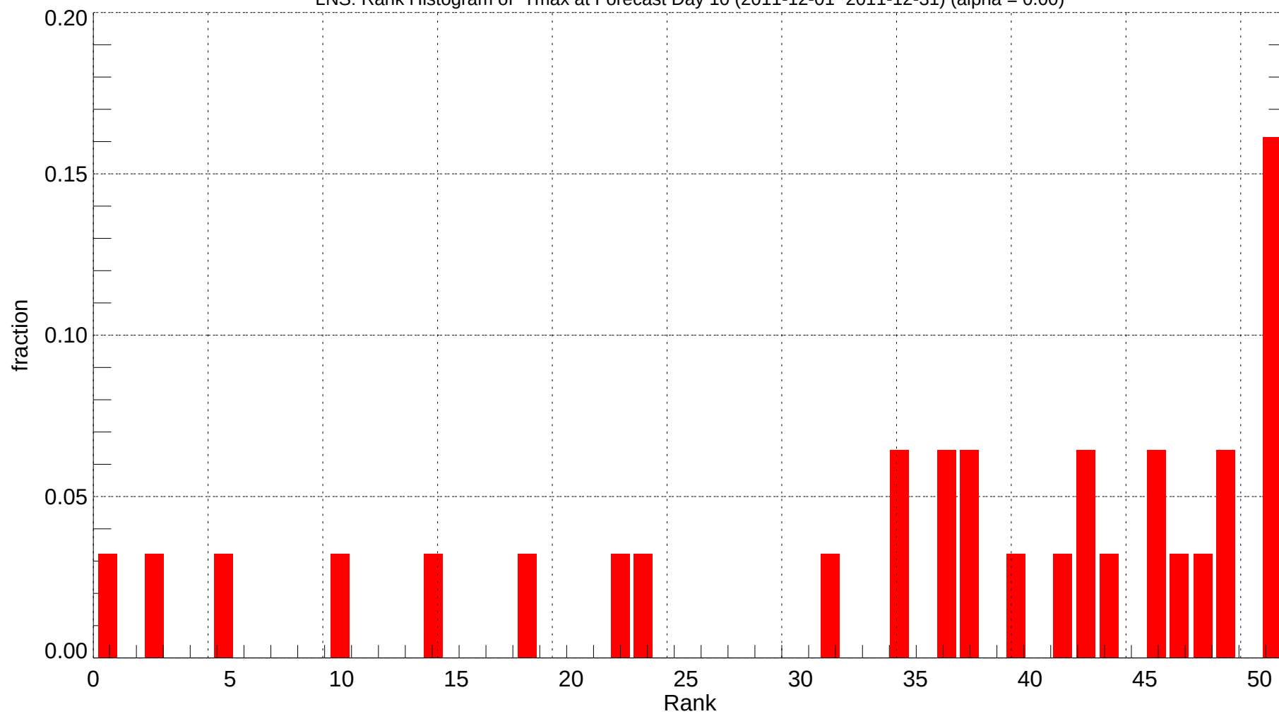
LNS: Rank Histogram of Tmax at Forecast Day 10 (2011-12-01~2011-12-31) (alpha = 0.00)
