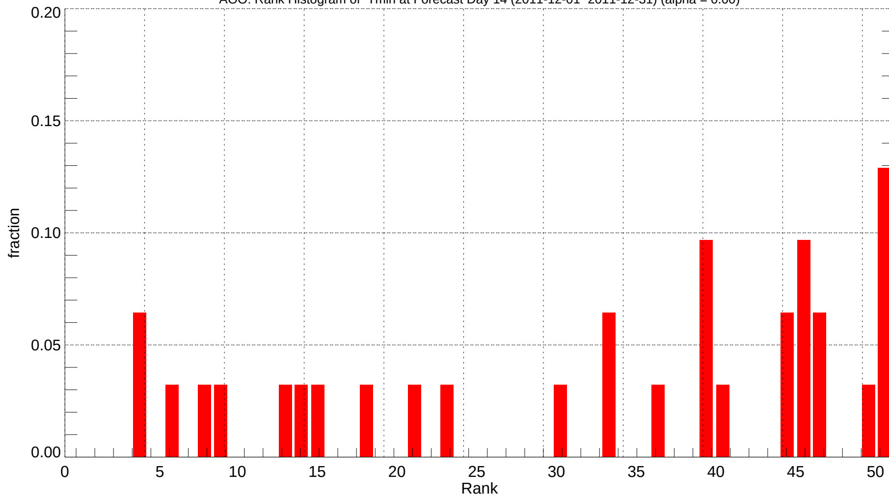
AOO: Rank Histogram of Tmin at Forecast Day 14 (2011-12-01~2011-12-31) (alpha = 0.00)
