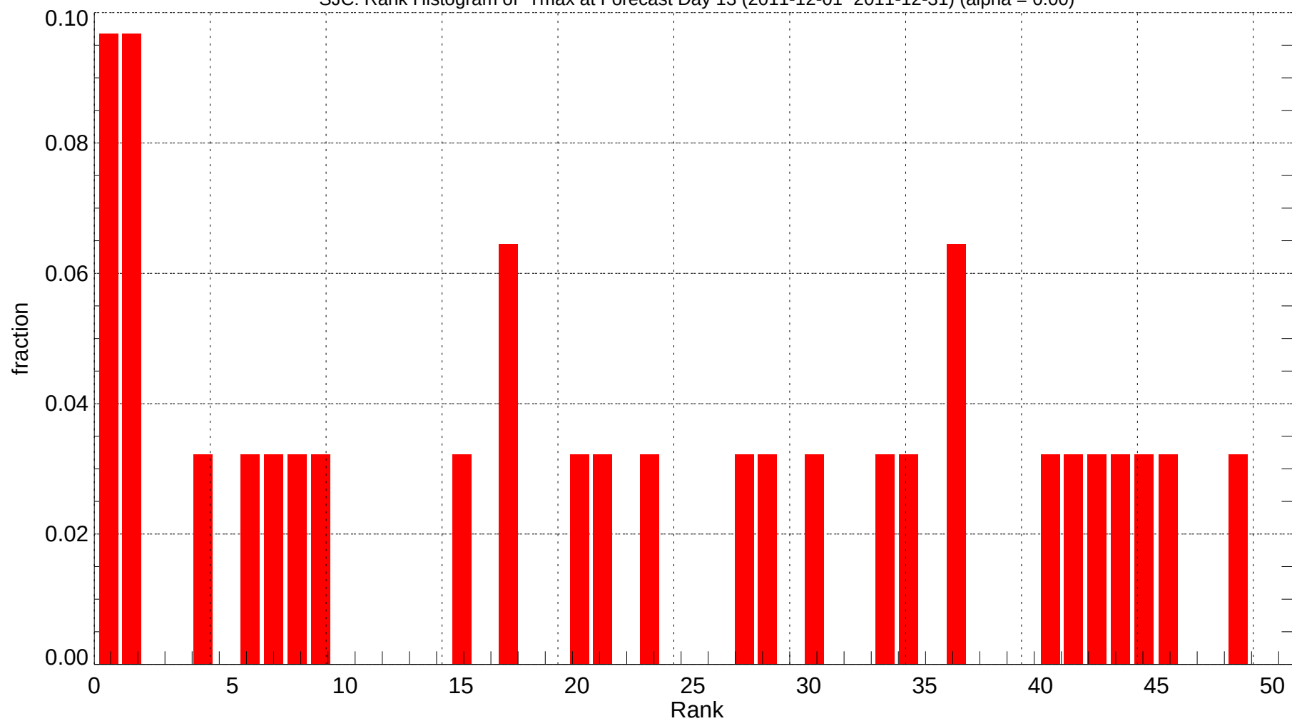
SJC: Rank Histogram of Tmax at Forecast Day 13 (2011-12-01~2011-12-31) (alpha = 0.00)
