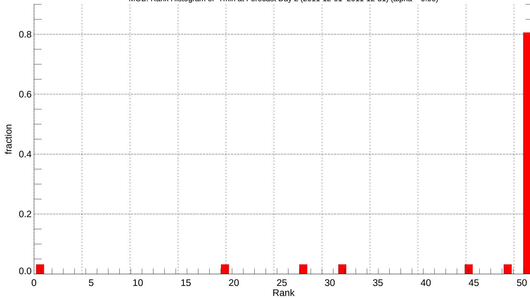
MOB: Rank Histogram of Tmin at Forecast Day 2 (2011-12-01~2011-12-31) (alpha = 0.00)
