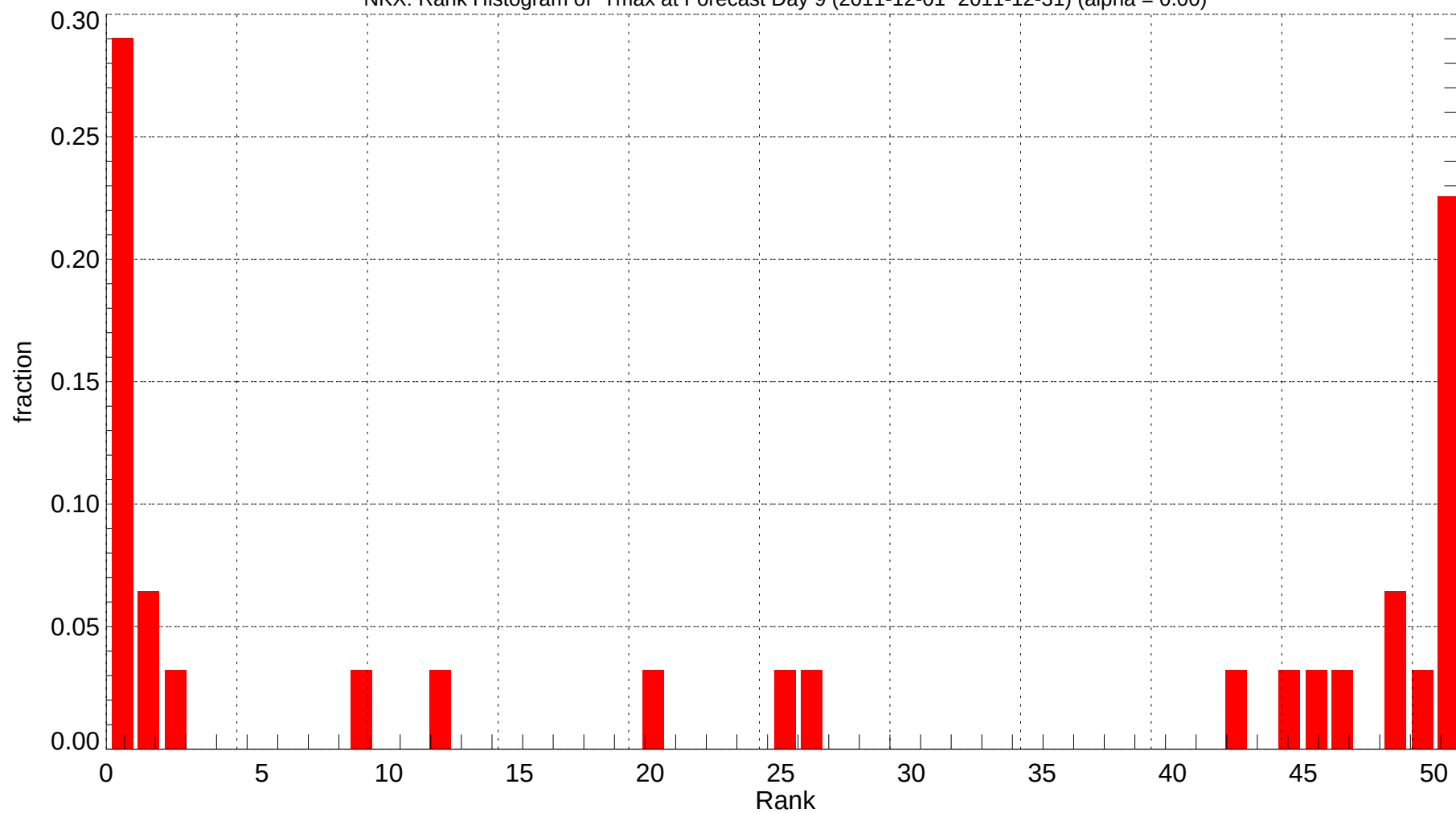
NKX: Rank Histogram of Tmax at Forecast Day 9 (2011-12-01~2011-12-31) (alpha = 0.00)
