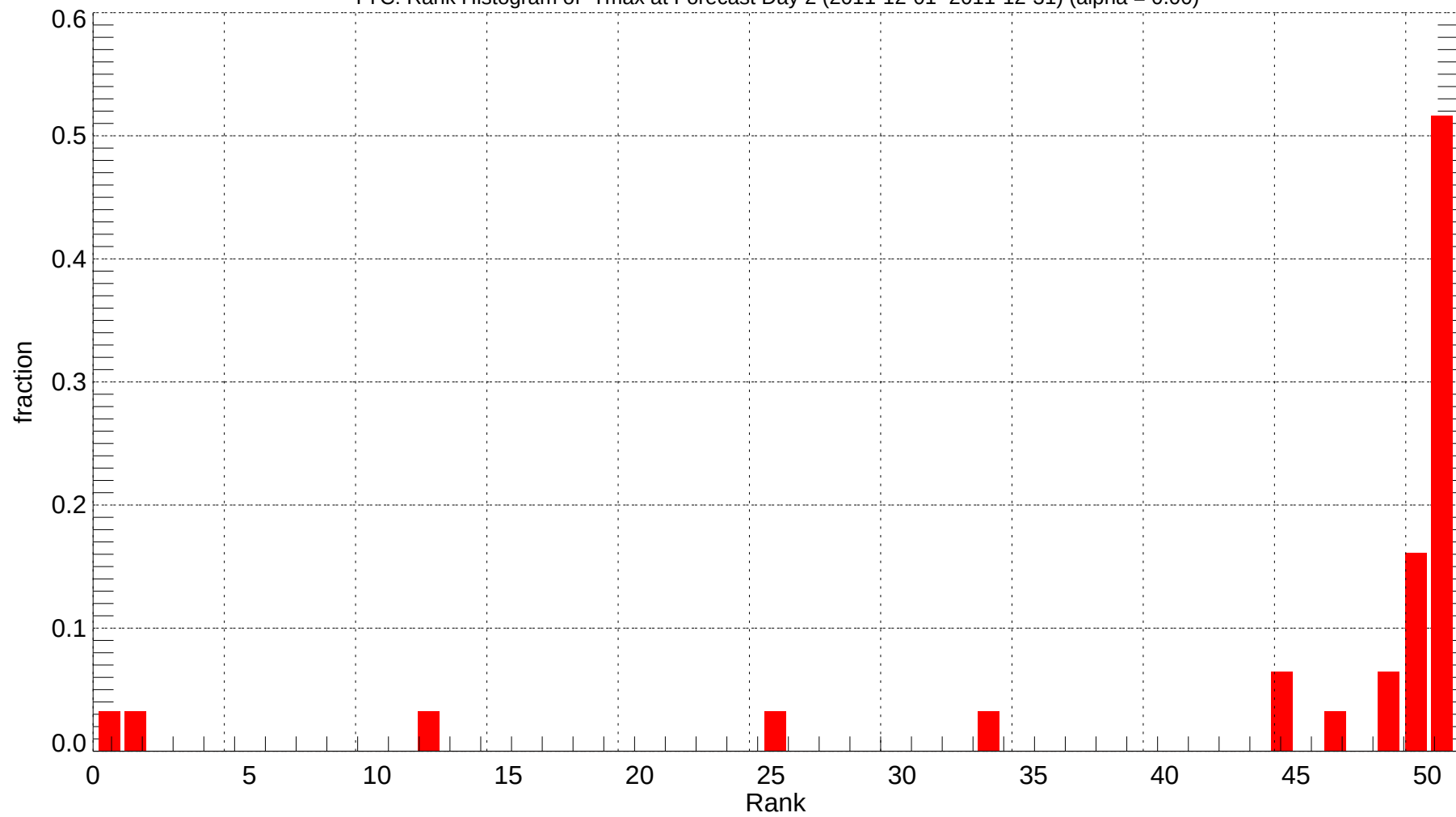
YYC: Rank Histogram of Tmax at Forecast Day 2 (2011-12-01~2011-12-31) (alpha = 0.00)
