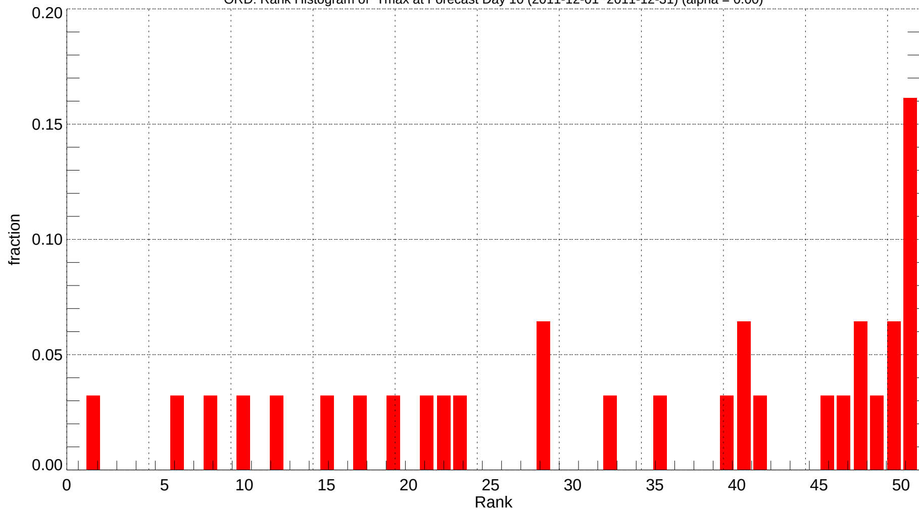
ORD: Rank Histogram of Tmax at Forecast Day 10 (2011-12-01~2011-12-31) (alpha = 0.00)
