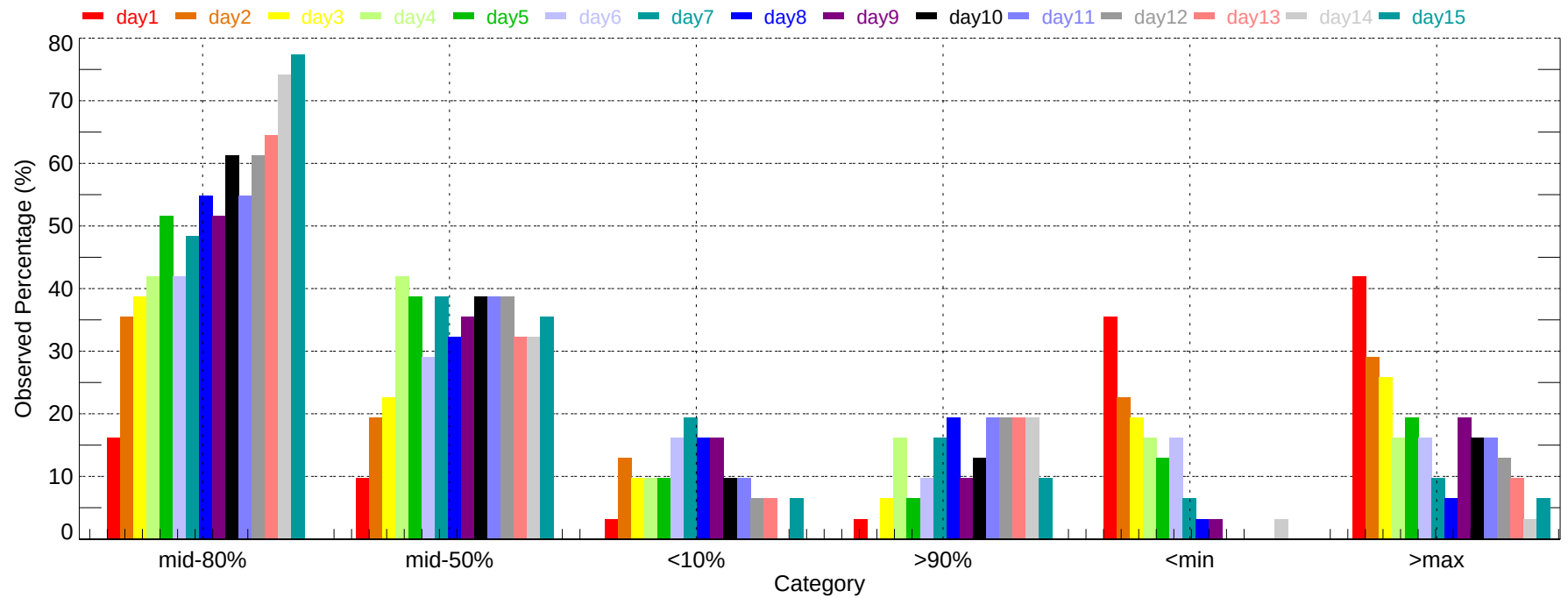
Observed Percentage of Ensembles - MKE: Max Temperature (2011-12-01~2011-12-31)
