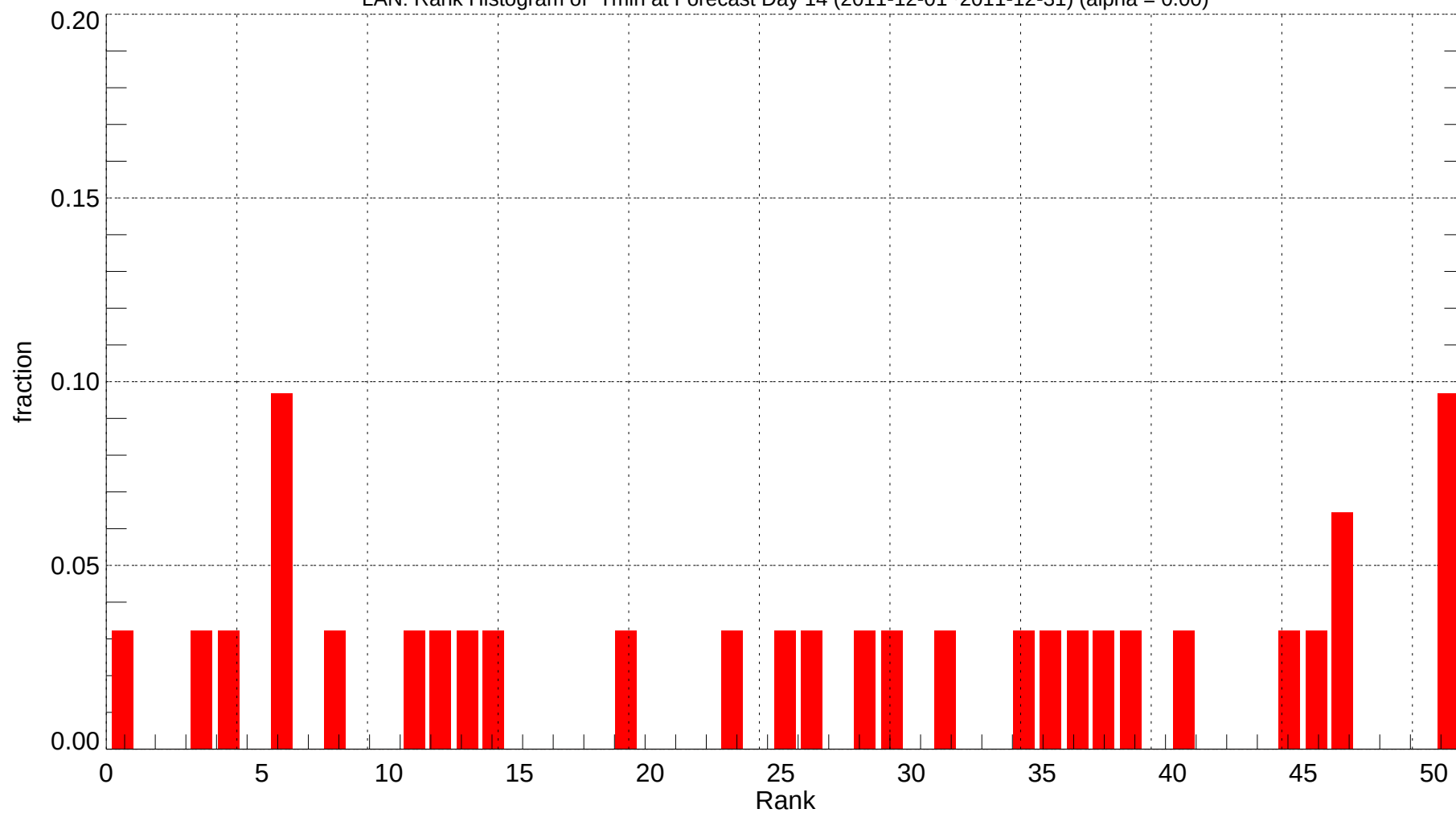
LAN: Rank Histogram of Tmin at Forecast Day 14 (2011-12-01~2011-12-31) (alpha = 0.00)
