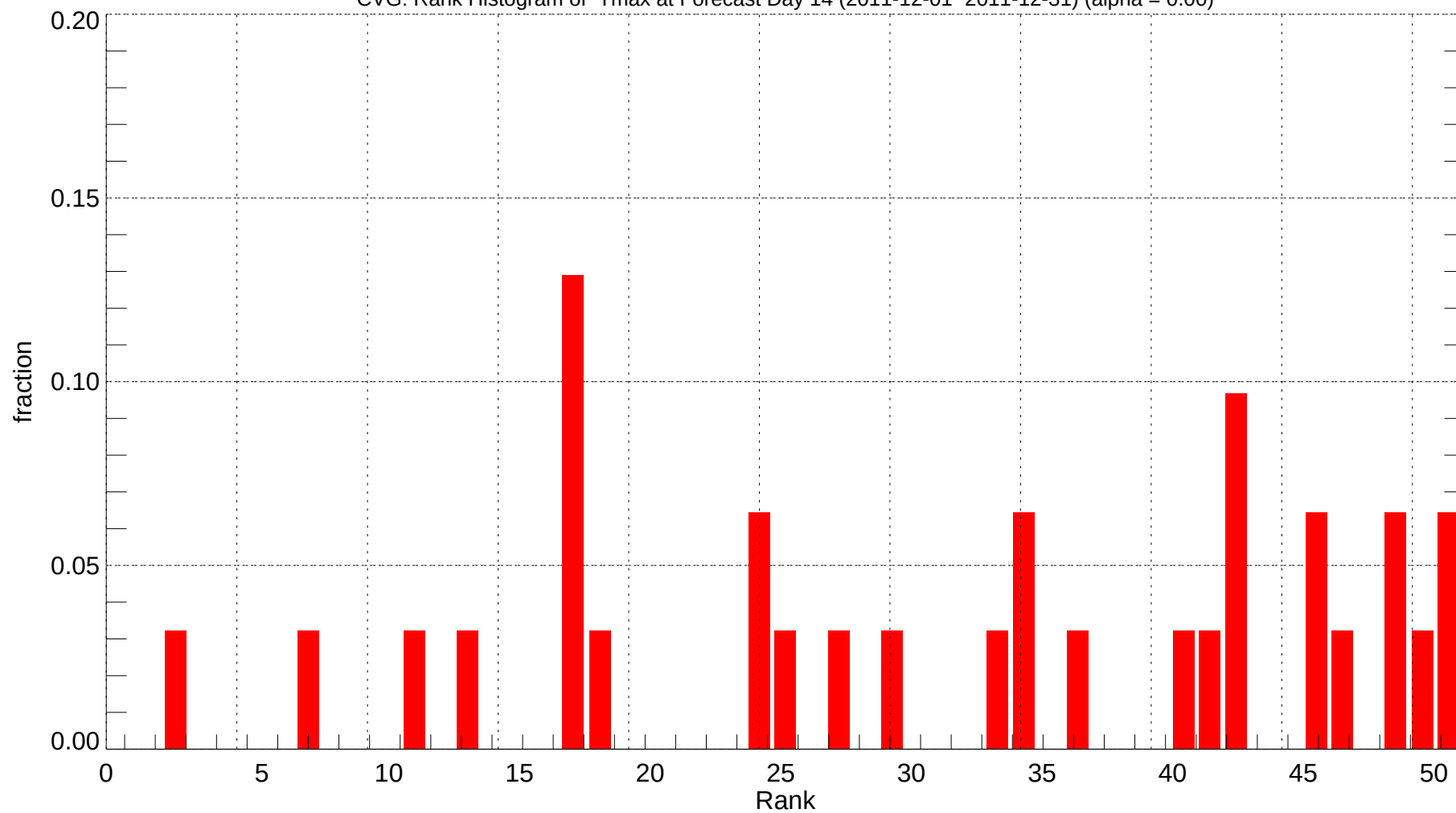
CVG: Rank Histogram of Tmax at Forecast Day 14 (2011-12-01~2011-12-31) (alpha = 0.00)
