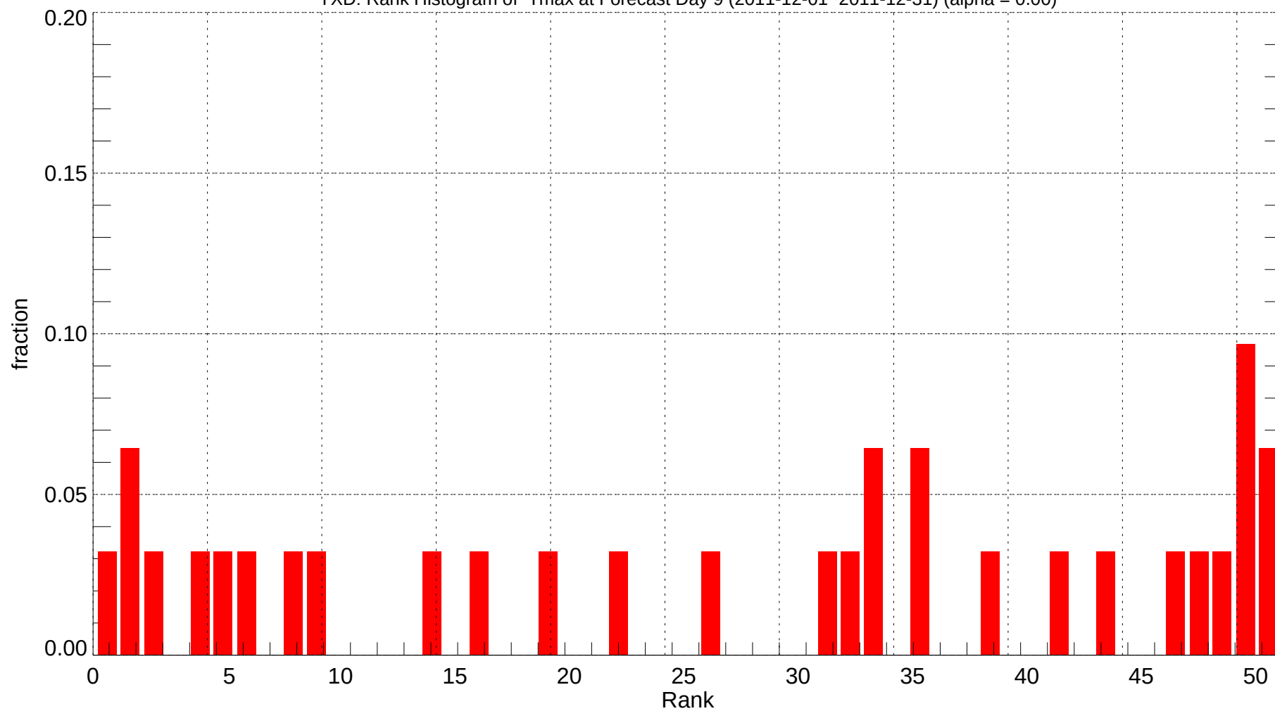
YXD: Rank Histogram of Tmax at Forecast Day 9 (2011-12-01~2011-12-31) (alpha = 0.00)
