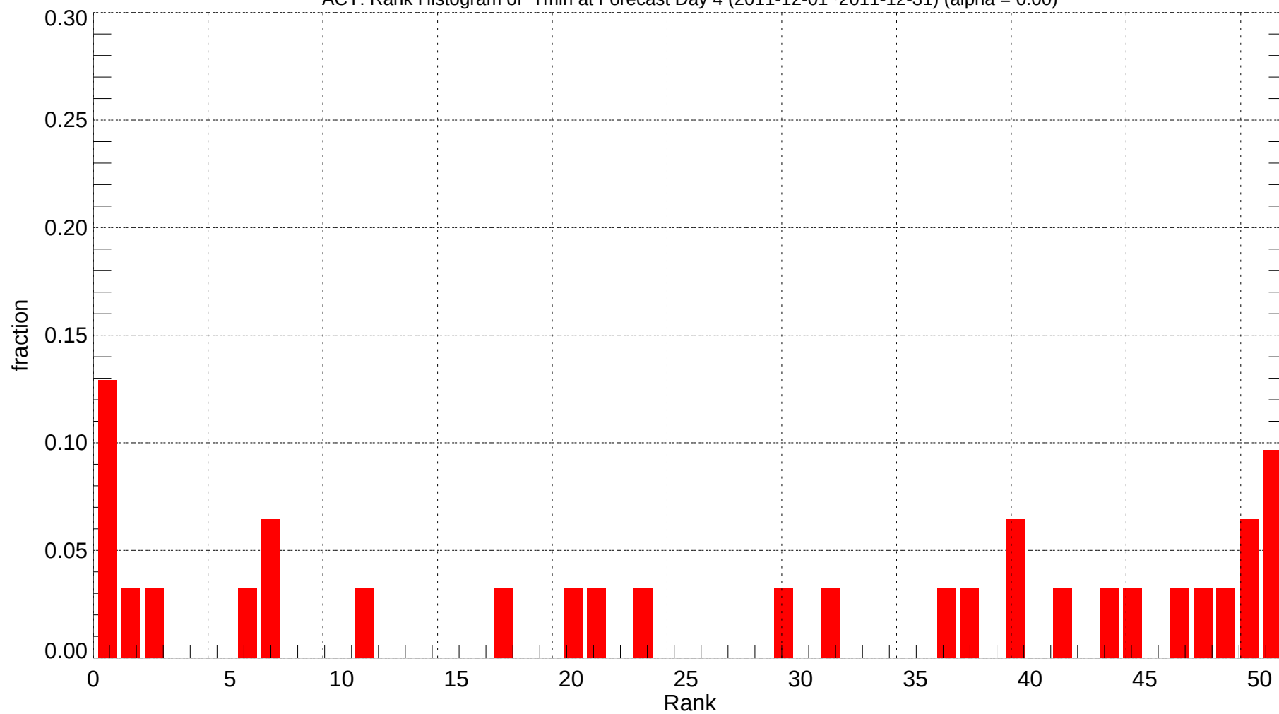
ACY: Rank Histogram of Tmin at Forecast Day 4 (2011-12-01~2011-12-31) (alpha = 0.00)
