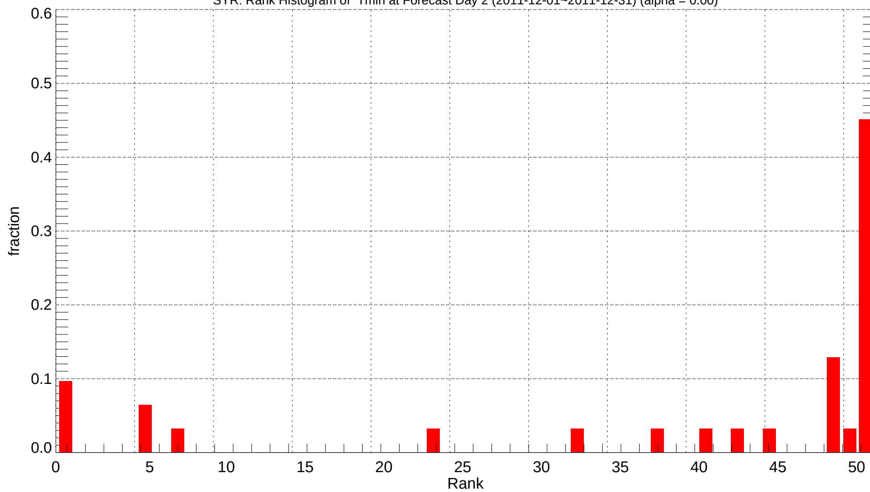
SYR: Rank Histogram of Tmin at Forecast Day 2 (2011-12-01~2011-12-31) (alpha = 0.00)
