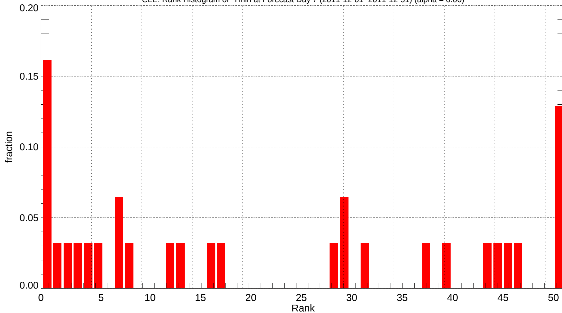
CLE: Rank Histogram of Tmin at Forecast Day 7 (2011-12-01~2011-12-31) (alpha = 0.00)
