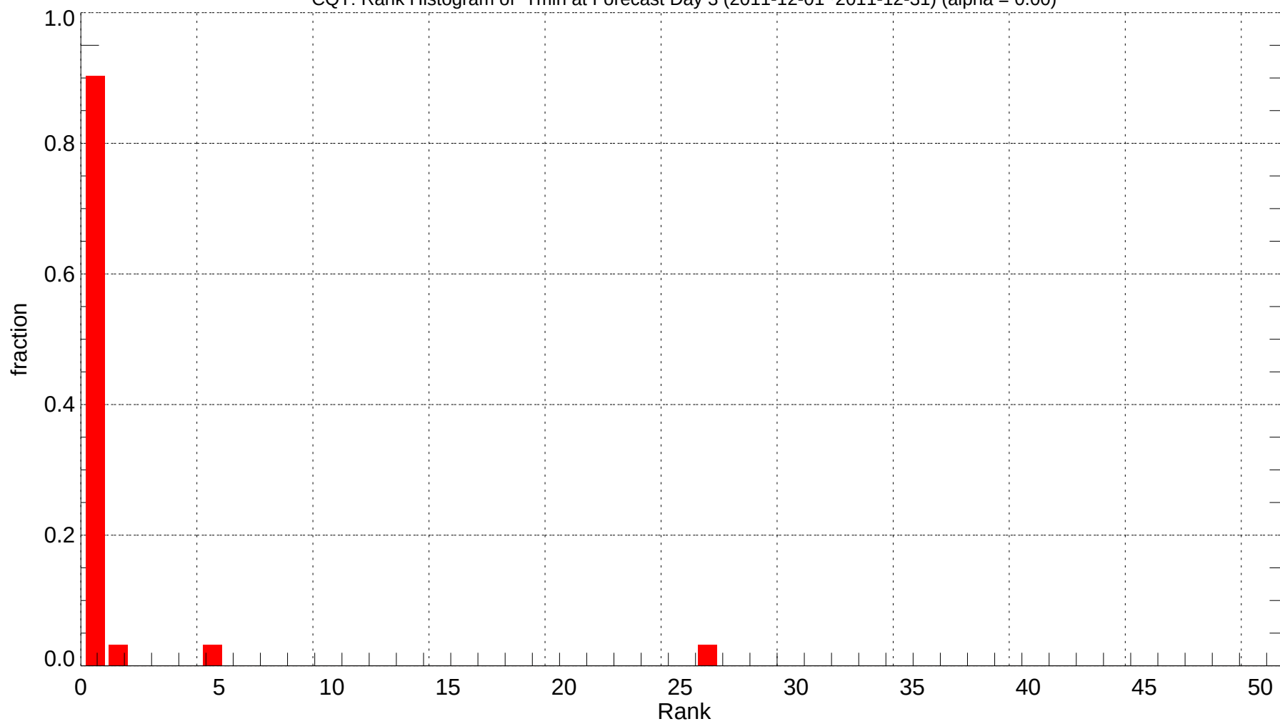
CQT: Rank Histogram of Tmin at Forecast Day 3 (2011-12-01~2011-12-31) (alpha = 0.00)
