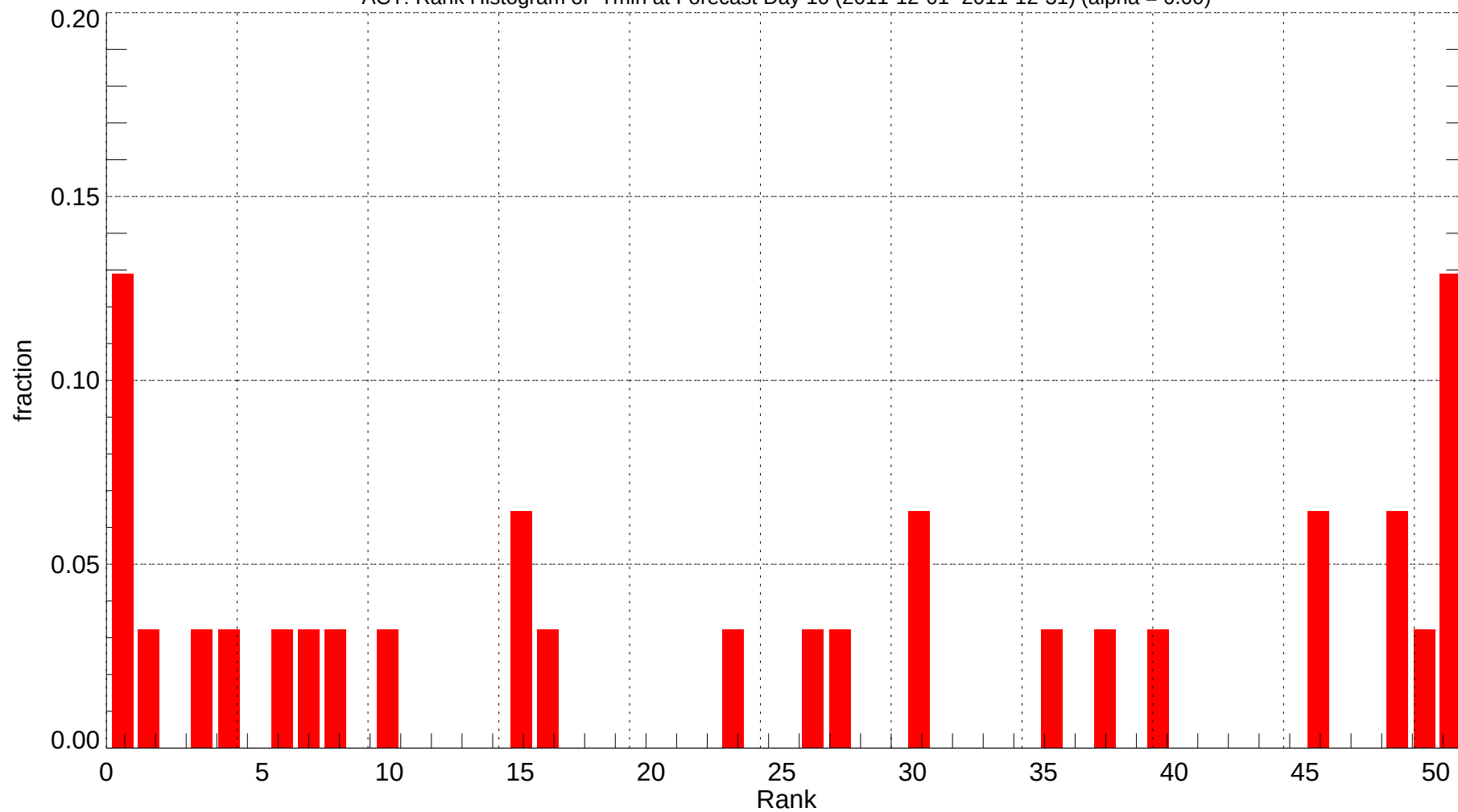
ACT: Rank Histogram of Tmin at Forecast Day 10 (2011-12-01~2011-12-31) (alpha = 0.00)
