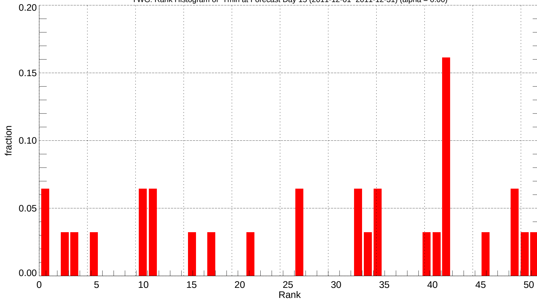
YWG: Rank Histogram of Tmin at Forecast Day 15 (2011-12-01~2011-12-31) (alpha = 0.00)
