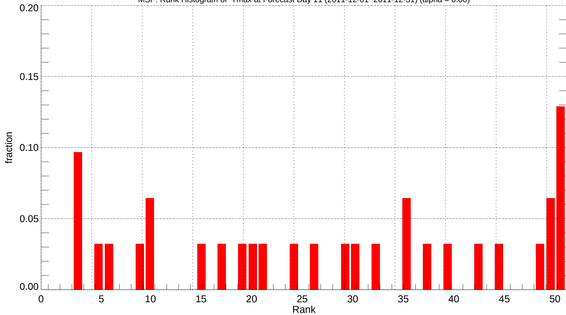
MSP: Rank Histogram of Tmax at Forecast Day 11 (2011-12-01~2011-12-31) (alpha = 0.00)
