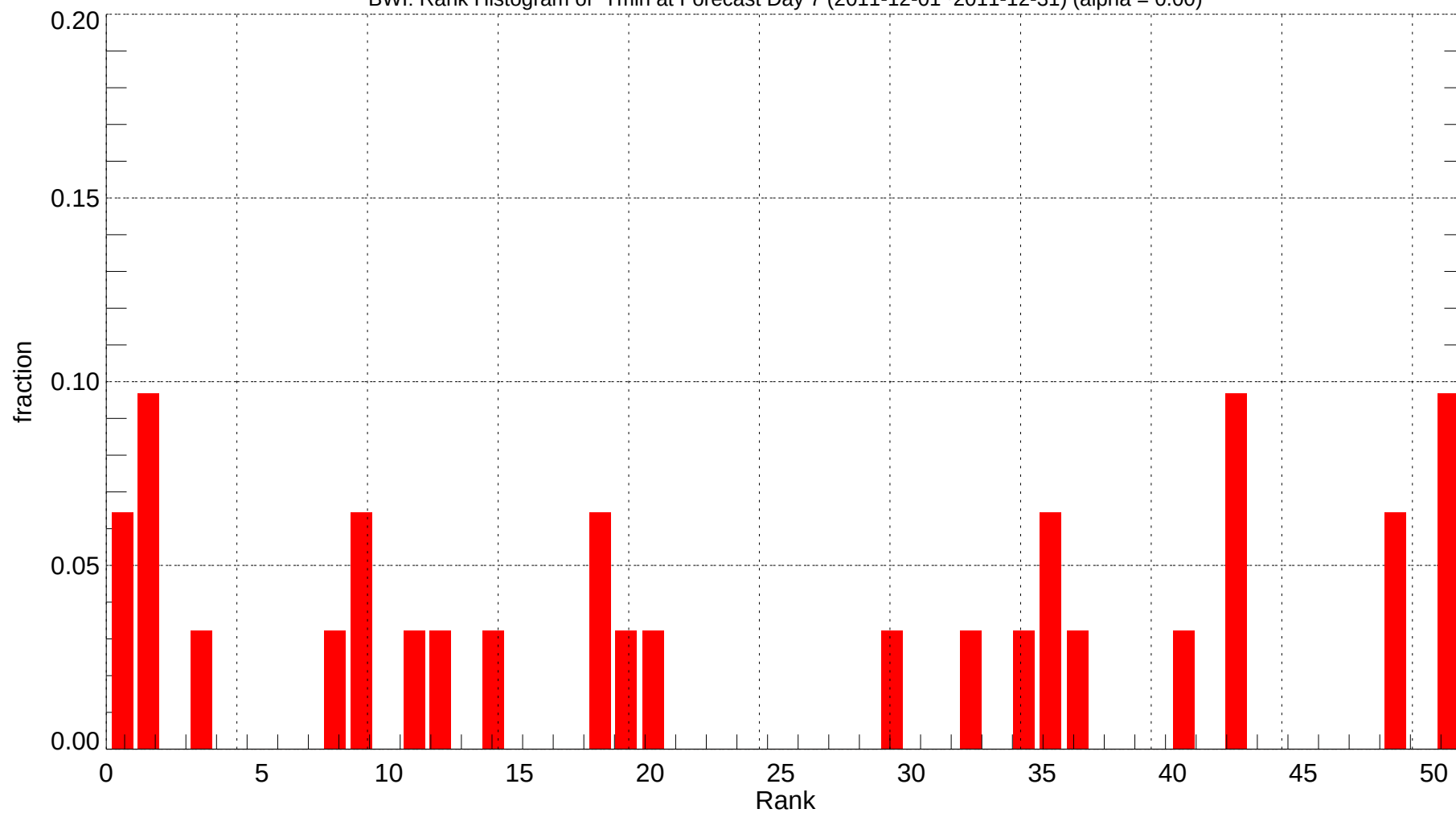
BWI: Rank Histogram of Tmin at Forecast Day 7 (2011-12-01~2011-12-31) (alpha = 0.00)
