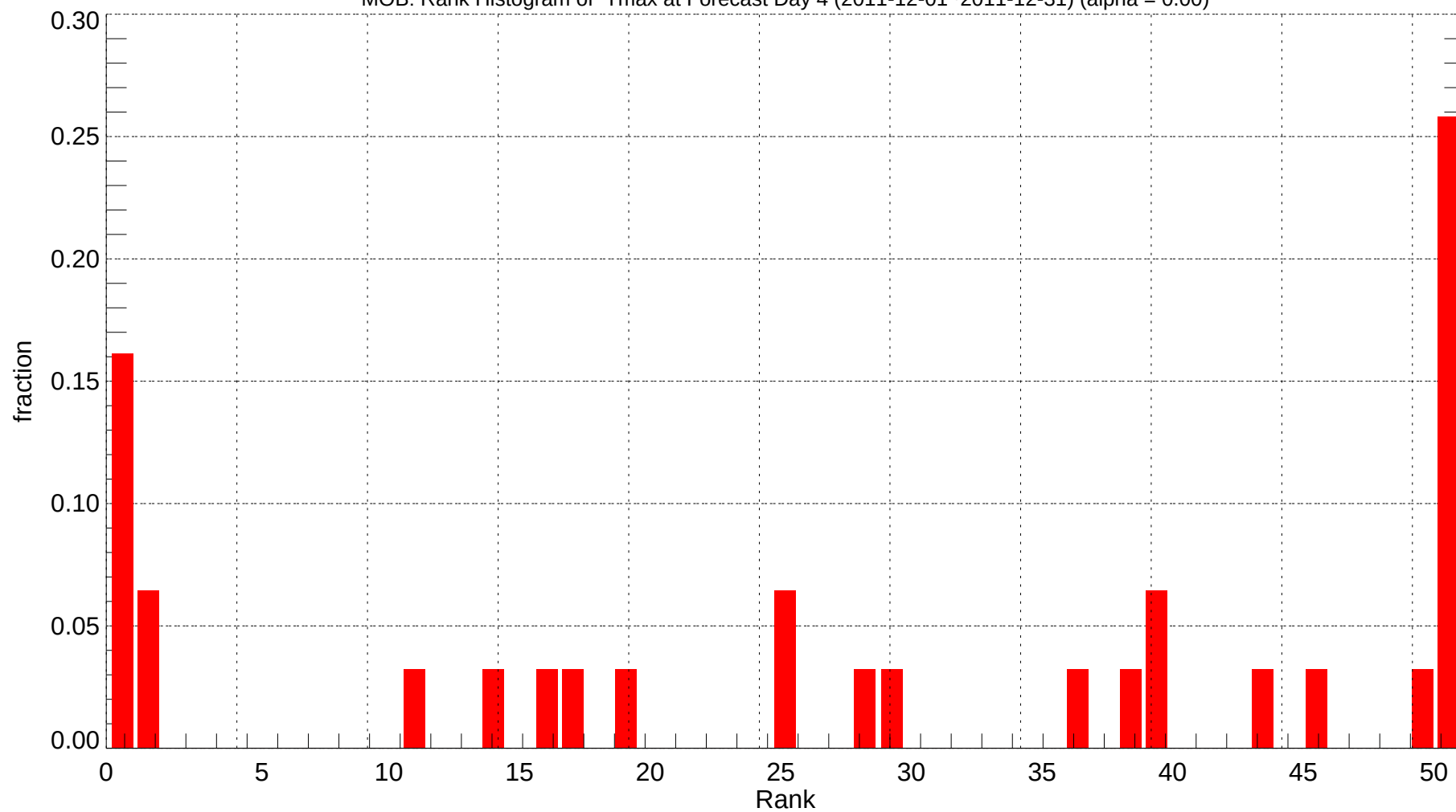
MOB: Rank Histogram of Tmax at Forecast Day 4 (2011-12-01~2011-12-31) (alpha = 0.00)
