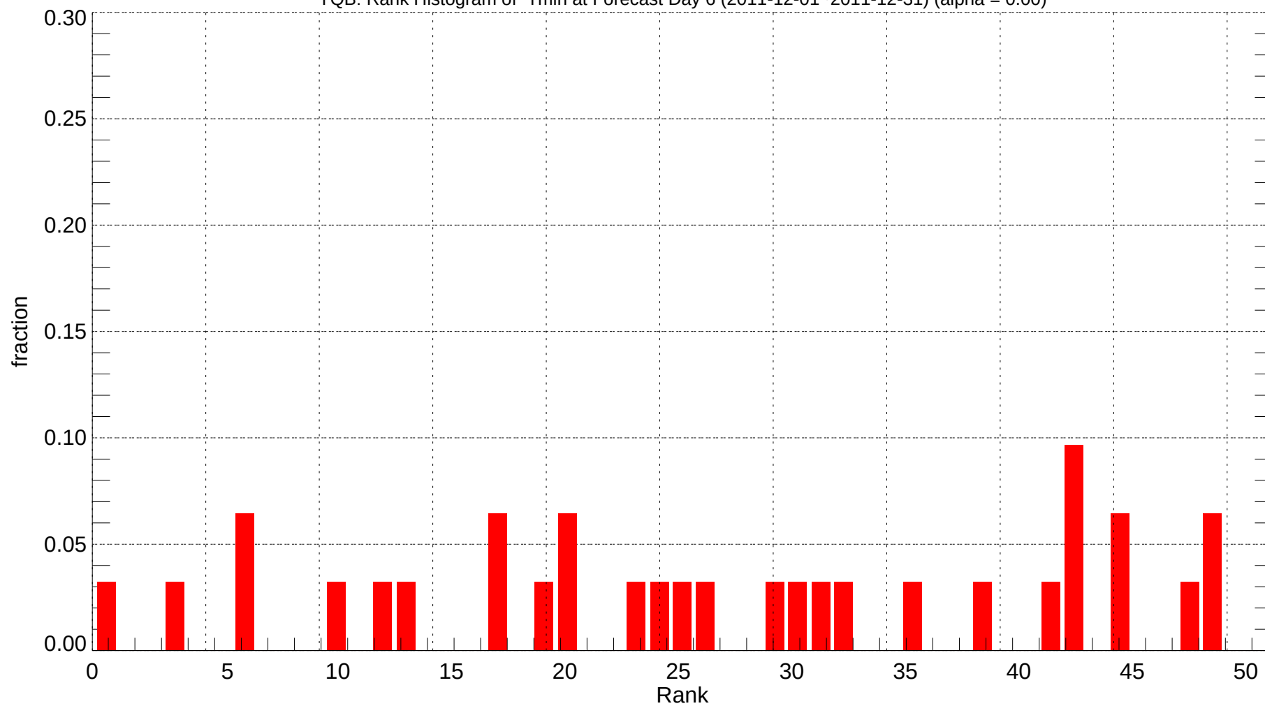
YQB: Rank Histogram of Tmin at Forecast Day 6 (2011-12-01~2011-12-31) (alpha = 0.00)
