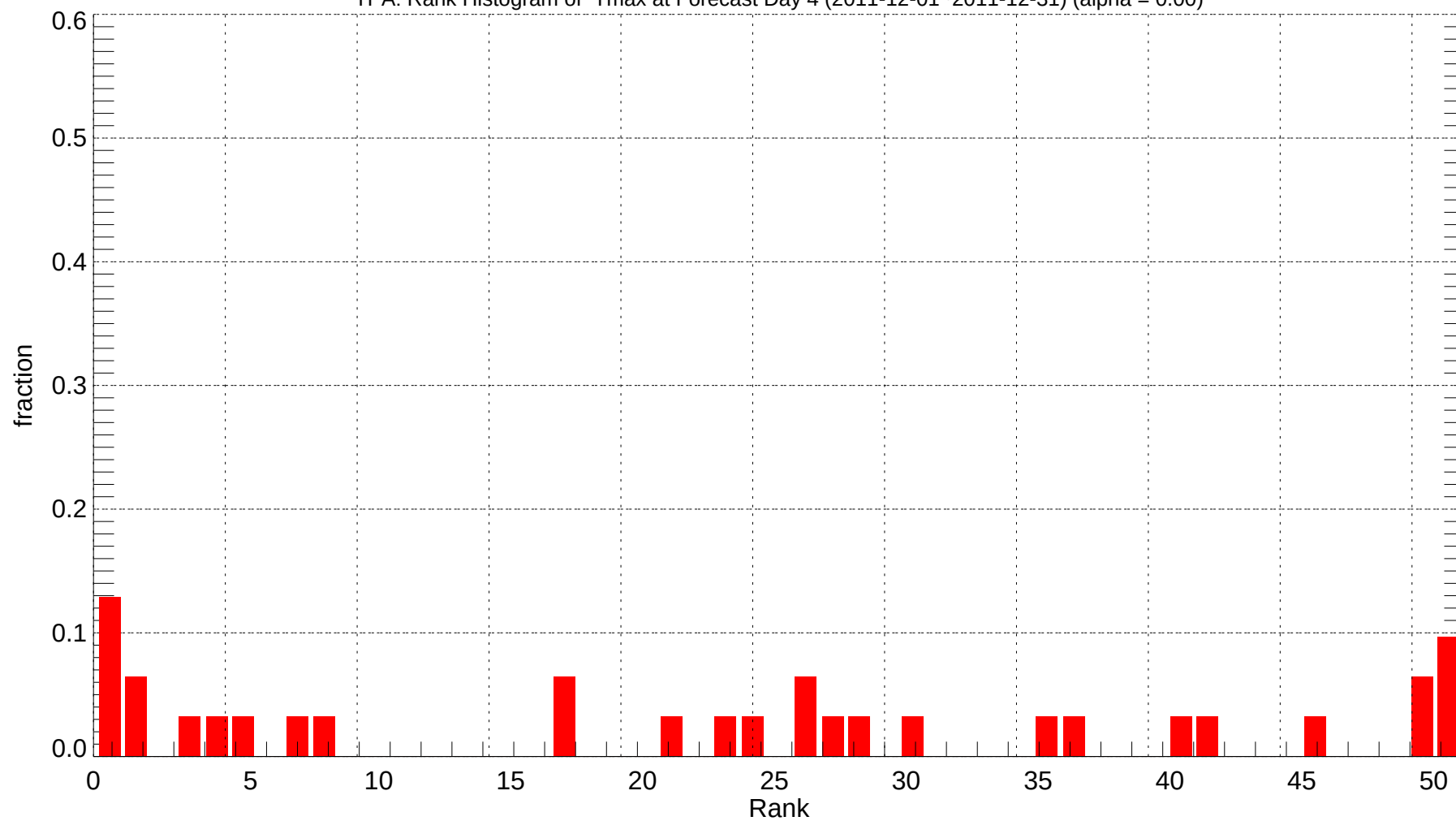
TPA: Rank Histogram of Tmax at Forecast Day 4 (2011-12-01~2011-12-31) (alpha = 0.00)
