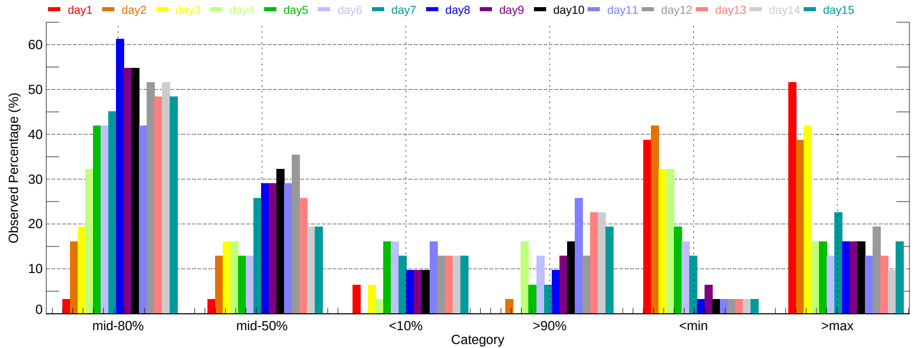
Observed Percentage of Ensembles - FSD: Min Temperature (2011-12-01~2011-12-31)
