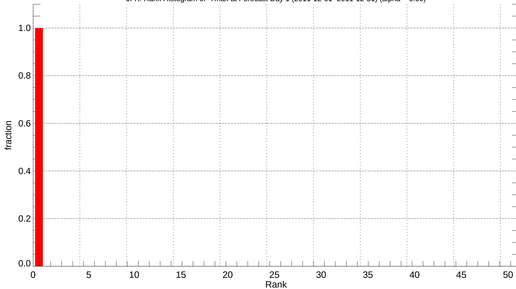
JFK: Rank Histogram of Tmax at Forecast Day 1 (2011-12-01~2011-12-31) (alpha = 0.00)
