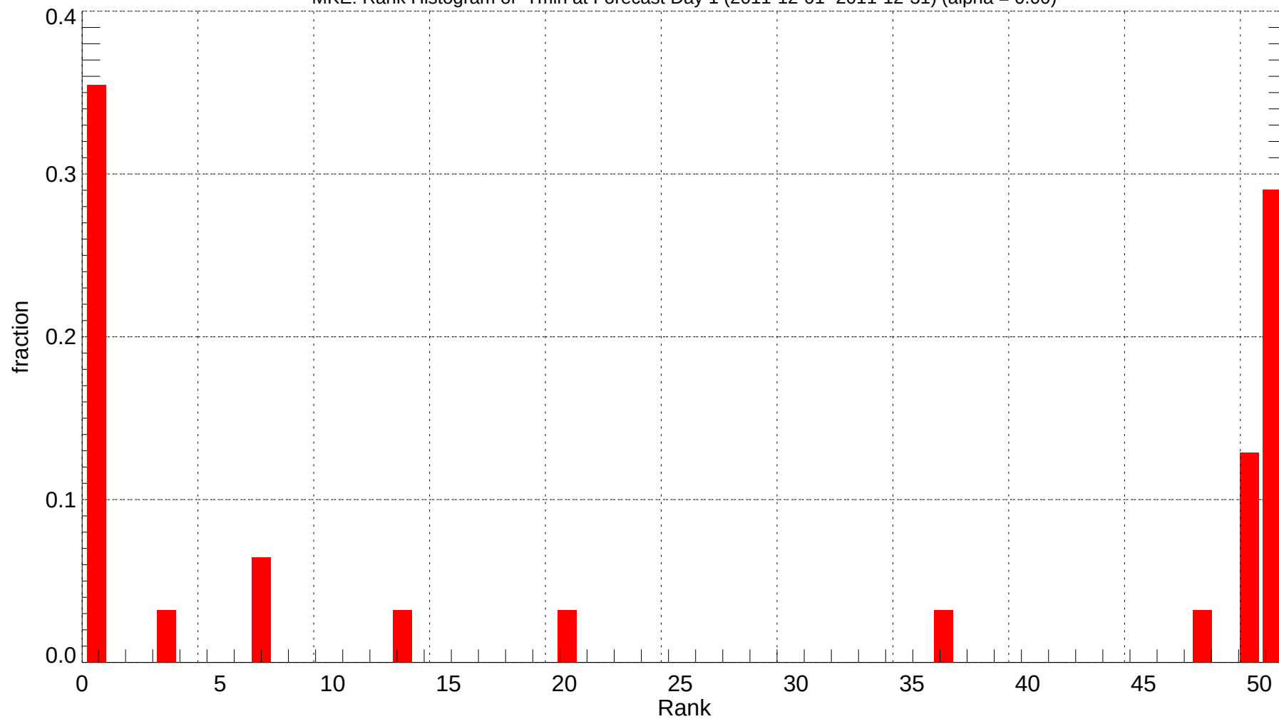
MKE: Rank Histogram of Tmin at Forecast Day 1 (2011-12-01~2011-12-31) (alpha = 0.00)
