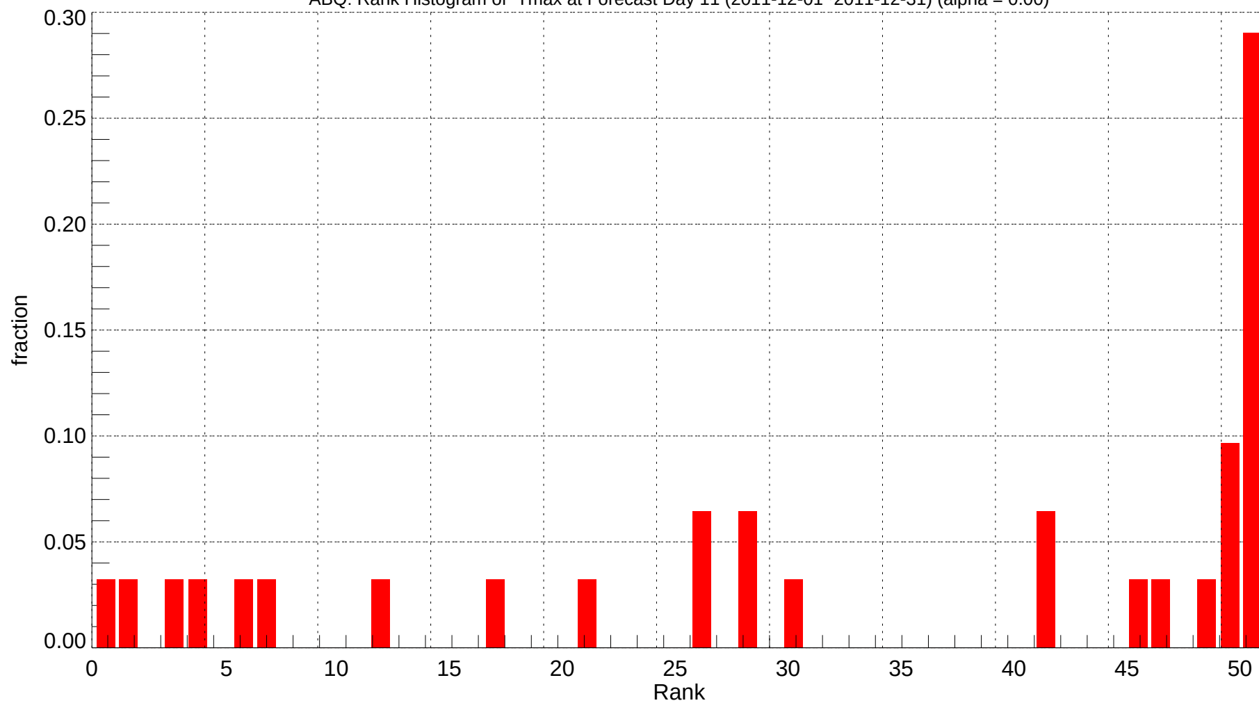
ABQ: Rank Histogram of Tmax at Forecast Day 11 (2011-12-01~2011-12-31) (alpha = 0.00)
