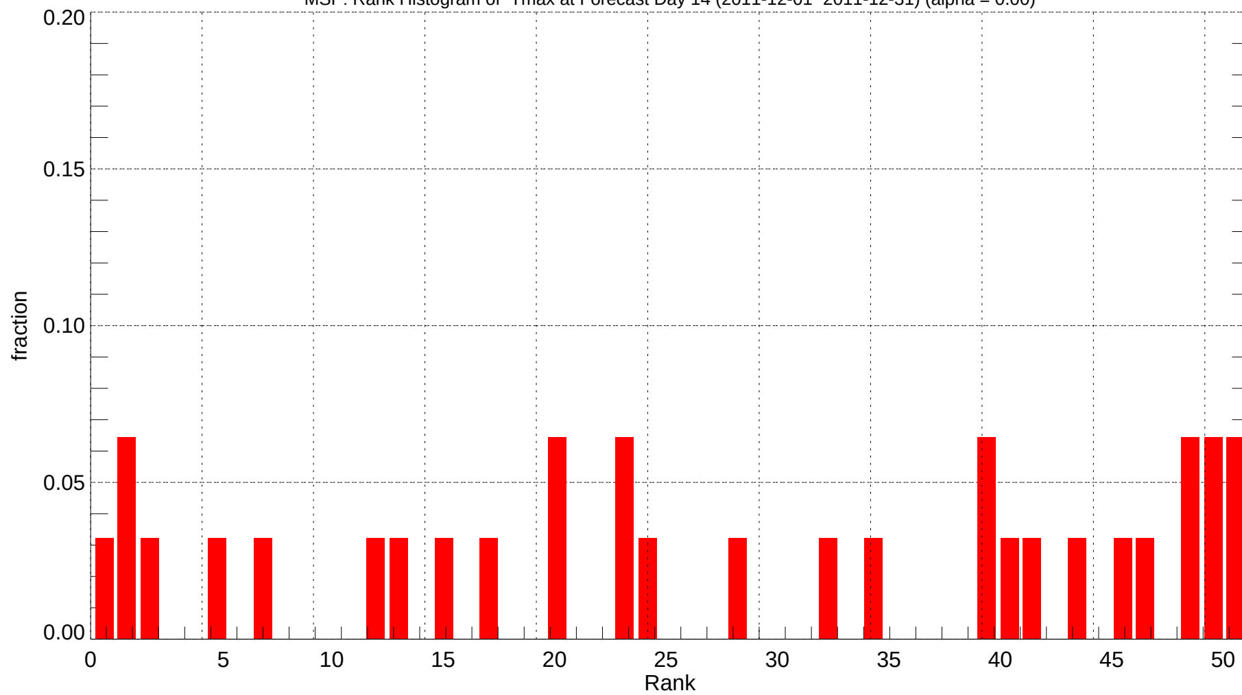
MSP: Rank Histogram of Tmax at Forecast Day 14 (2011-12-01~2011-12-31) (alpha = 0.00)
