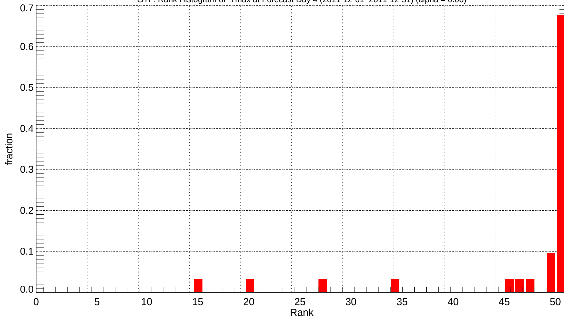
GTF: Rank Histogram of Tmax at Forecast Day 4 (2011-12-01~2011-12-31) (alpha = 0.00)
