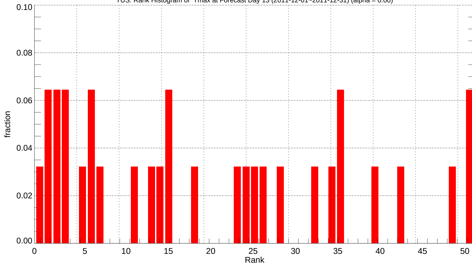
TUS: Rank Histogram of Tmax at Forecast Day 13 (2011-12-01~2011-12-31) (alpha = 0.00)
