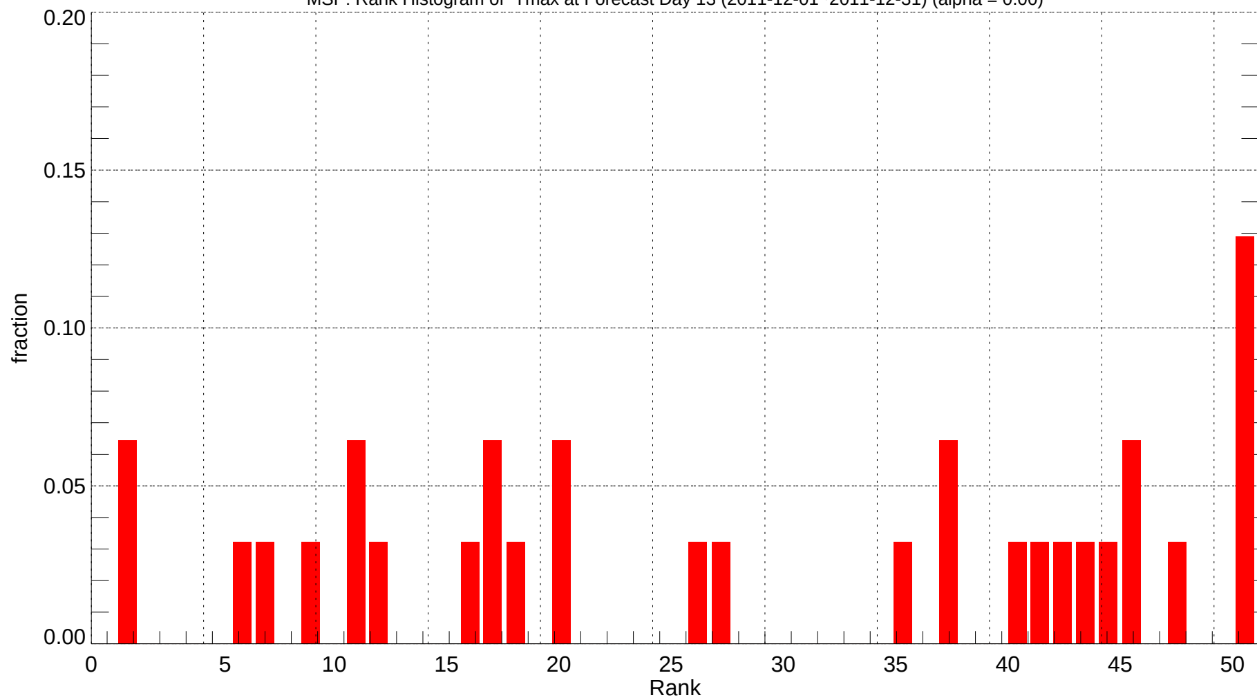
MSP: Rank Histogram of Tmax at Forecast Day 13 (2011-12-01~2011-12-31) (alpha = 0.00)
