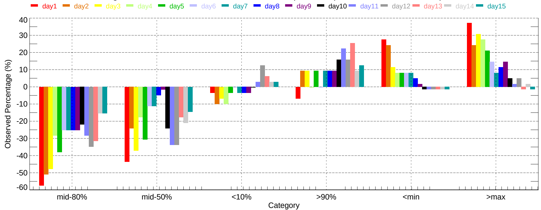
Observed Percentage Deviation of Ensembles - PIT: Min Temperature (2011-12-01~2011-12-31)
