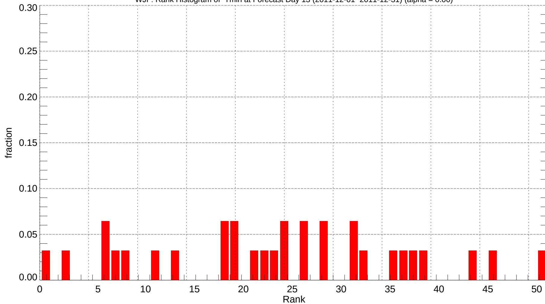
WJF: Rank Histogram of Tmin at Forecast Day 13 (2011-12-01~2011-12-31) (alpha = 0.00)
