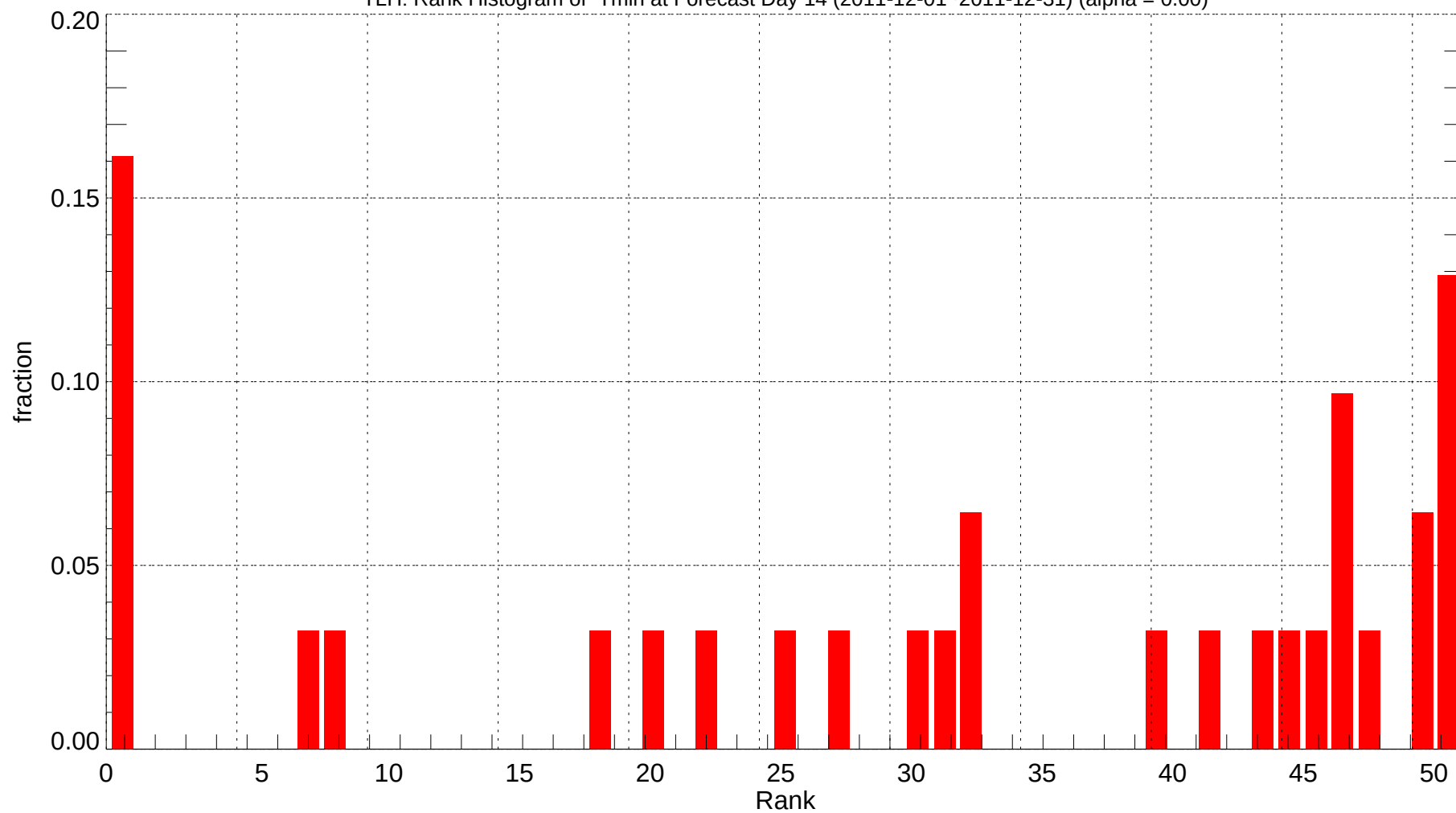
TLH: Rank Histogram of Tmin at Forecast Day 14 (2011-12-01~2011-12-31) (alpha = 0.00)
