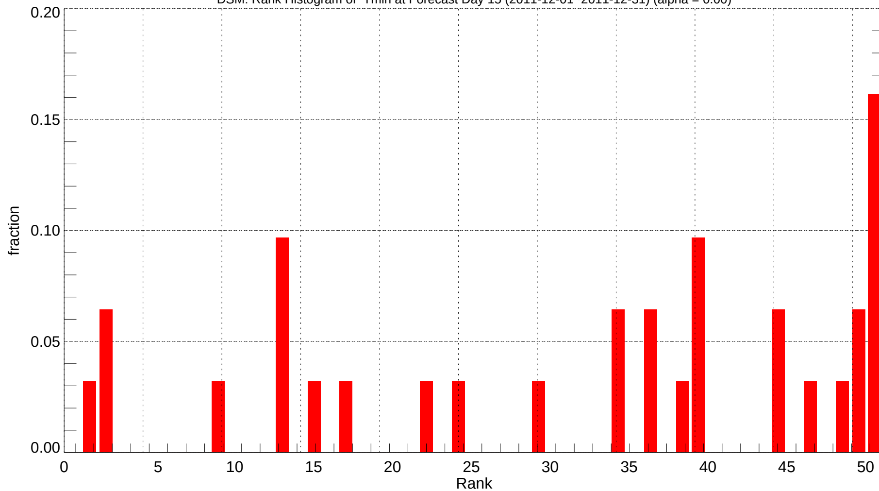
DSM: Rank Histogram of Tmin at Forecast Day 15 (2011-12-01~2011-12-31) (alpha = 0.00)
