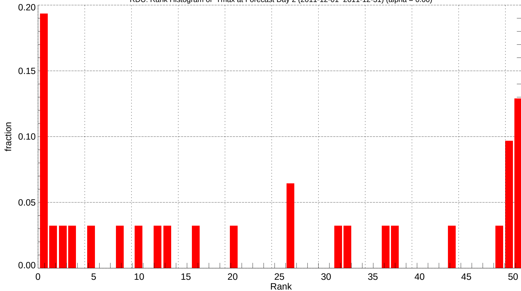
RDU: Rank Histogram of Tmax at Forecast Day 2 (2011-12-01~2011-12-31) (alpha = 0.00)
