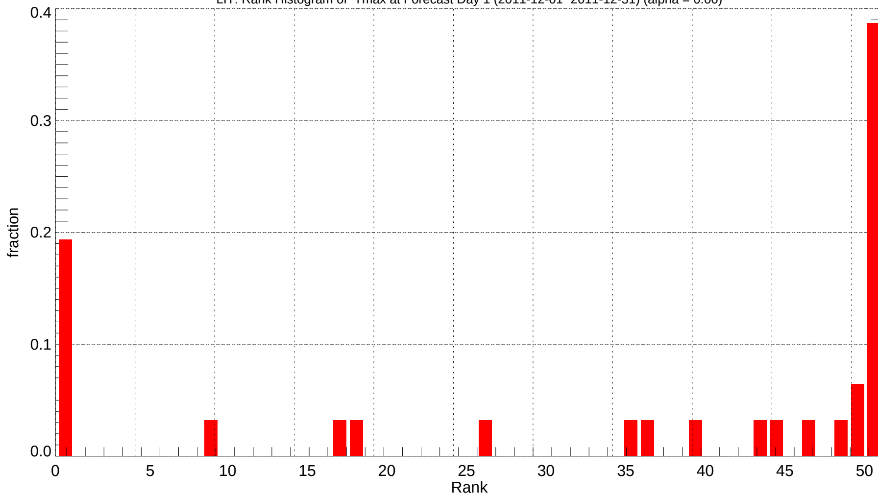
LIT: Rank Histogram of Tmax at Forecast Day 1 (2011-12-01~2011-12-31) (alpha = 0.00)
