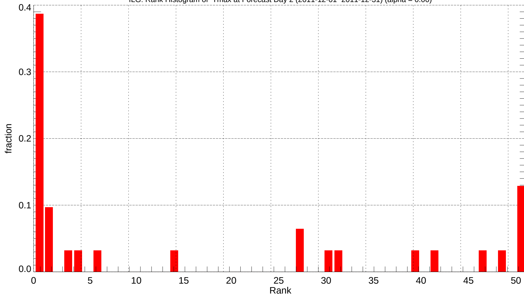
ILG: Rank Histogram of Tmax at Forecast Day 2 (2011-12-01~2011-12-31) (alpha = 0.00)
