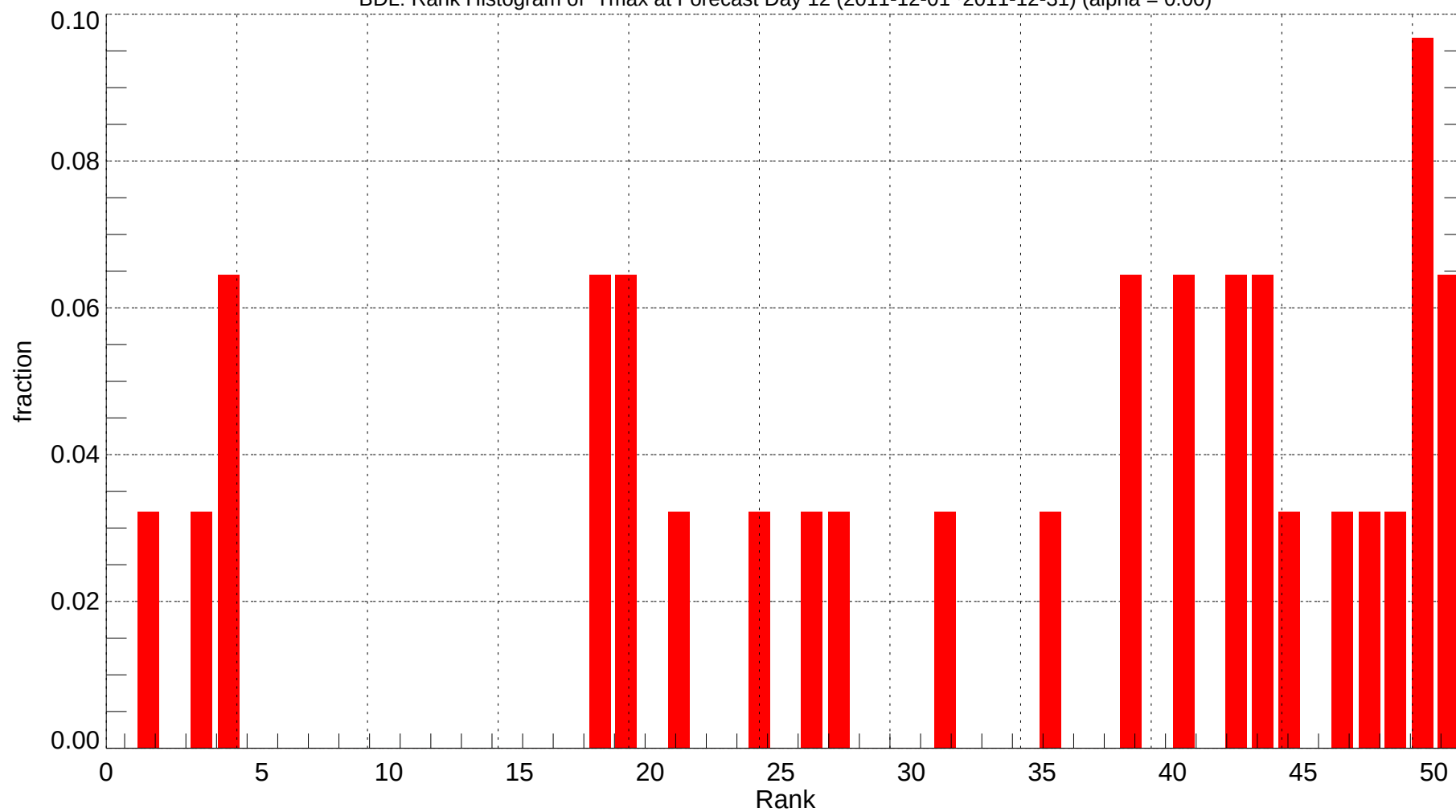
BDL: Rank Histogram of Tmax at Forecast Day 12 (2011-12-01~2011-12-31) (alpha = 0.00)
