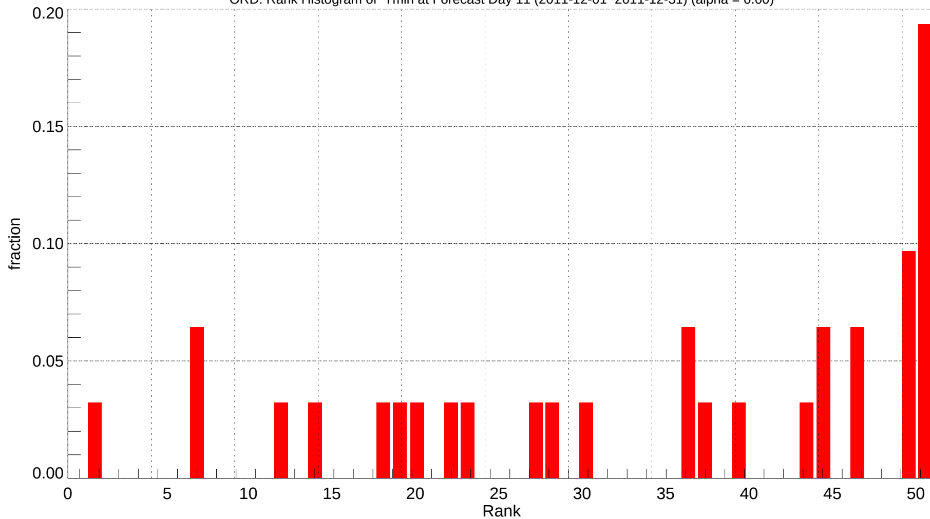
ORD: Rank Histogram of Tmin at Forecast Day 11 (2011-12-01~2011-12-31) (alpha = 0.00)
