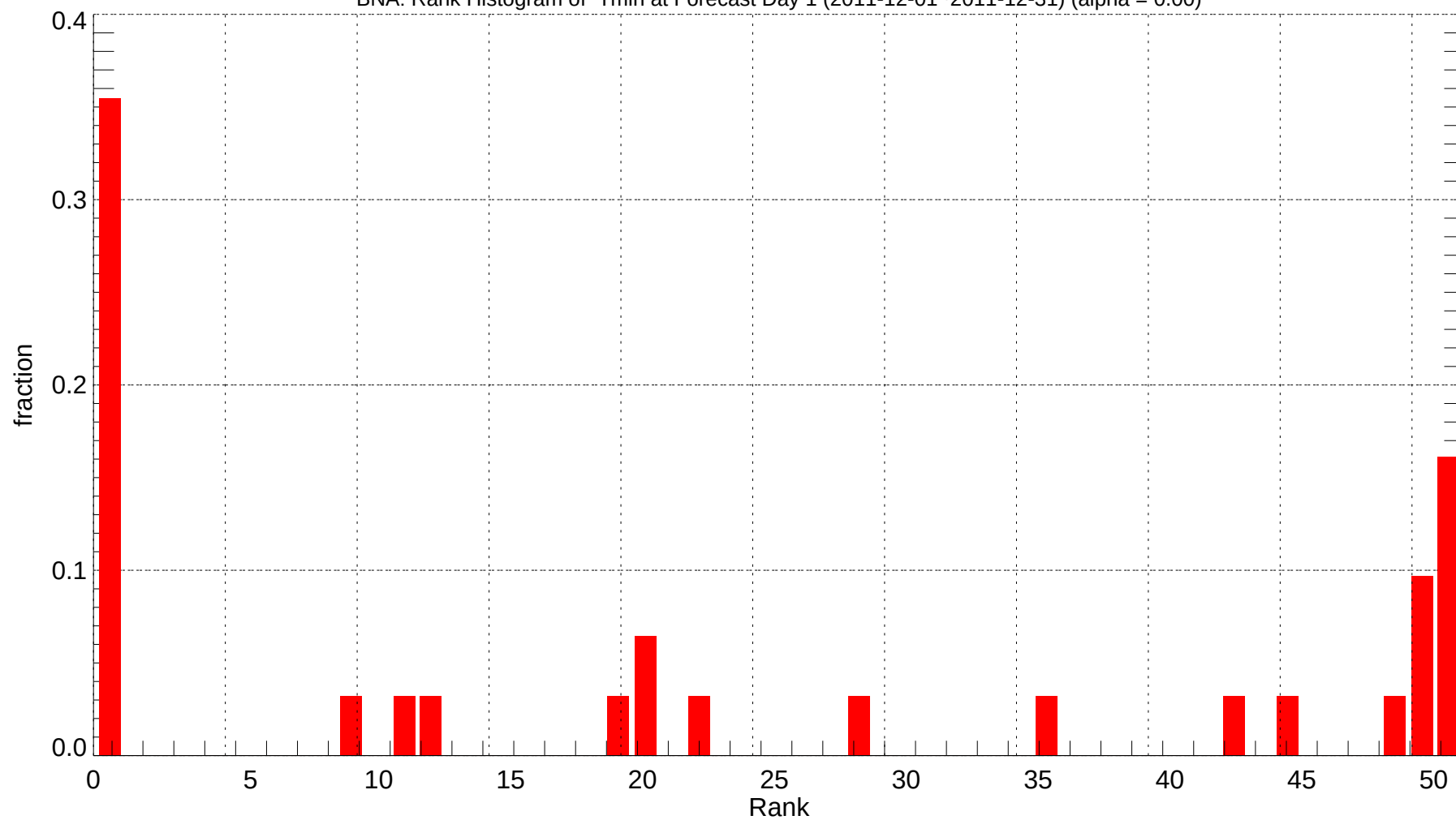
BNA: Rank Histogram of Tmin at Forecast Day 1 (2011-12-01~2011-12-31) (alpha = 0.00)
