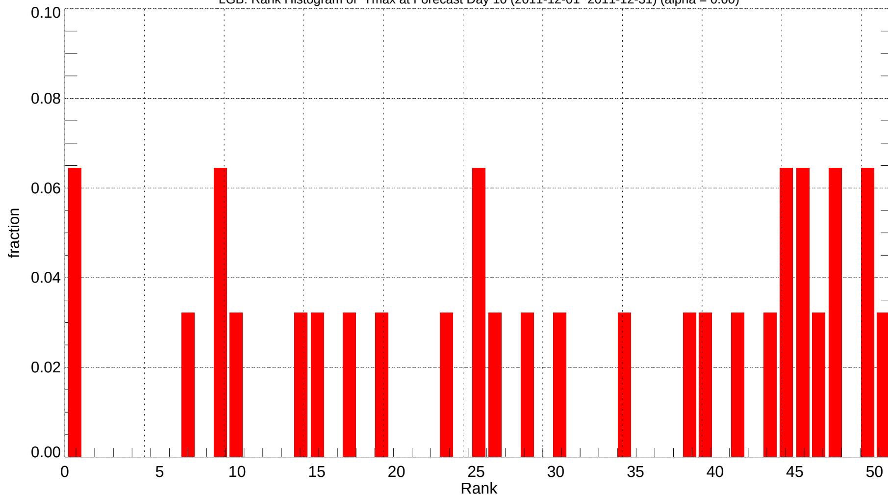
LGB: Rank Histogram of Tmax at Forecast Day 10 (2011-12-01~2011-12-31) (alpha = 0.00)
