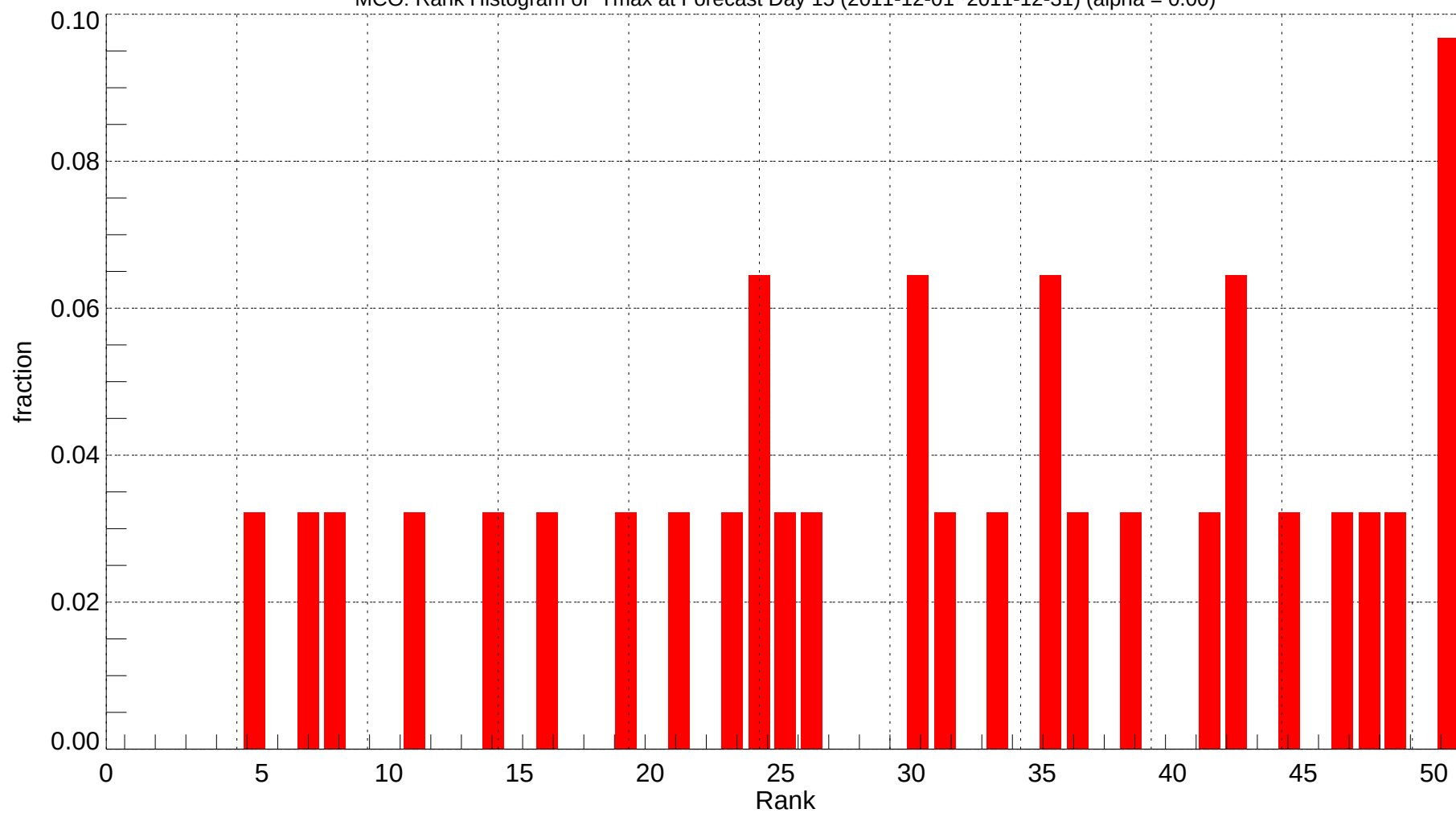
MCO: Rank Histogram of Tmax at Forecast Day 15 (2011-12-01~2011-12-31) (alpha = 0.00)
