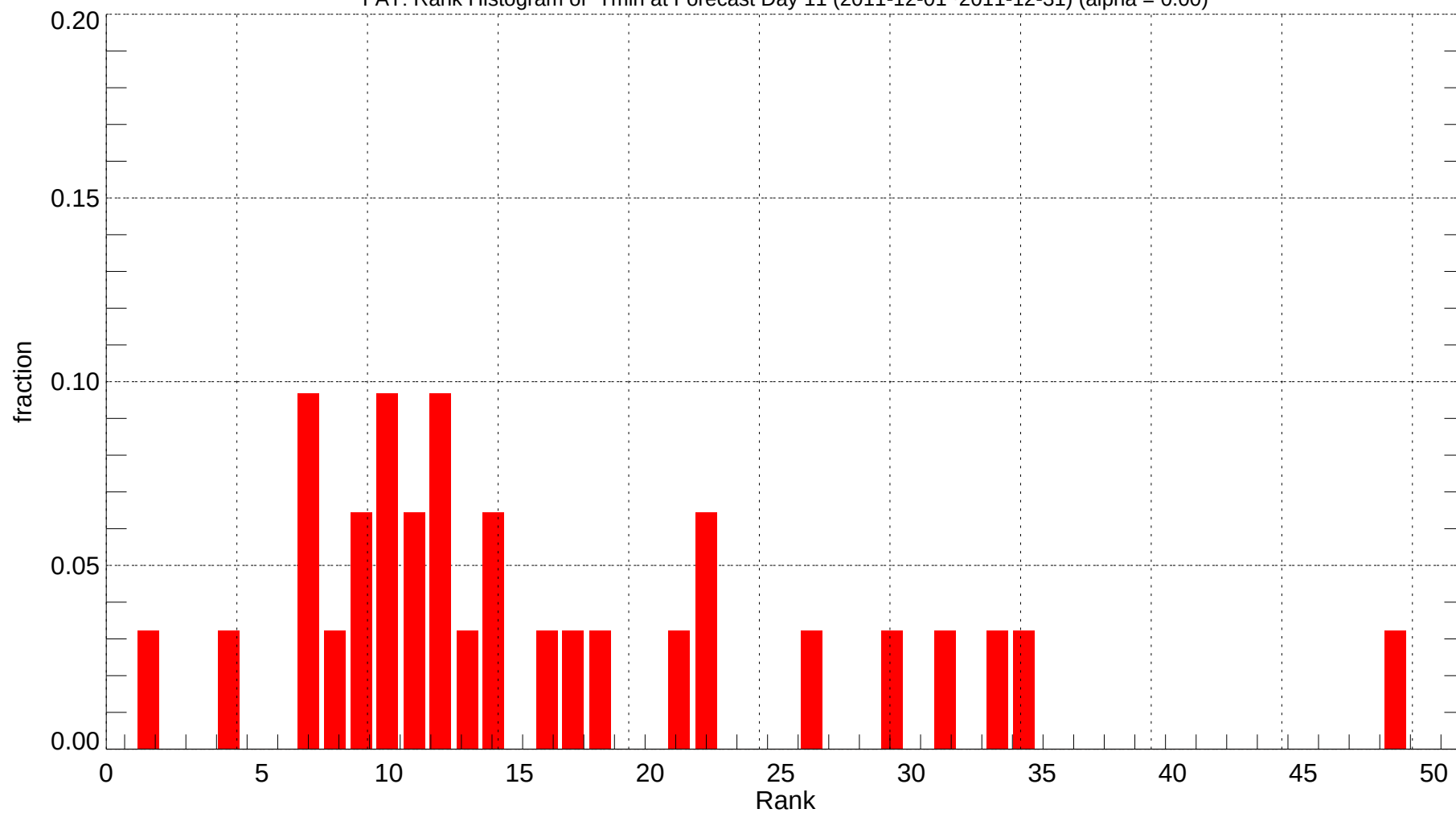
FAT: Rank Histogram of Tmin at Forecast Day 11 (2011-12-01~2011-12-31) (alpha = 0.00)
