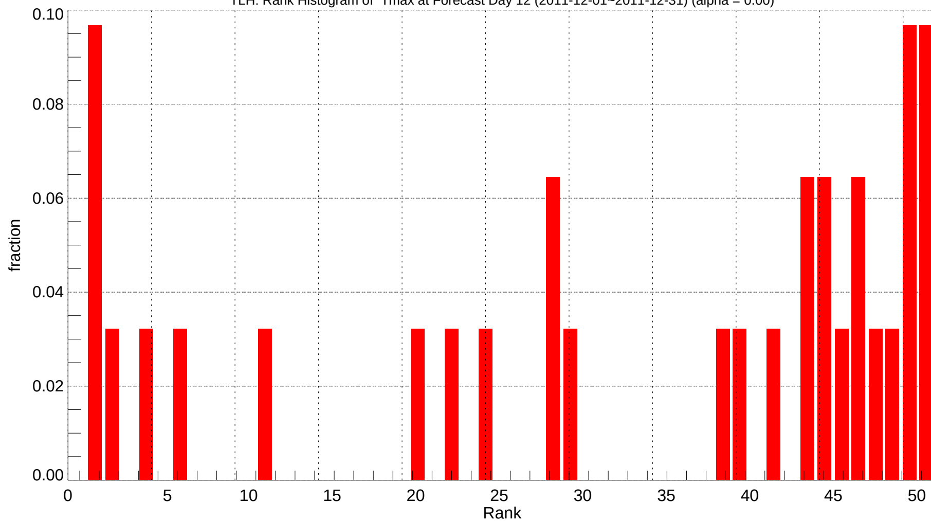
TLH: Rank Histogram of Tmax at Forecast Day 12 (2011-12-01~2011-12-31) (alpha = 0.00)
