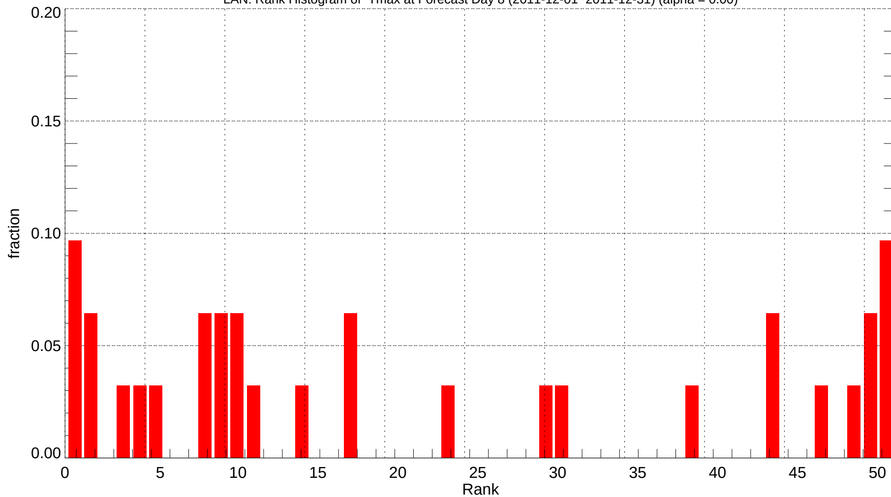
LAN: Rank Histogram of Tmax at Forecast Day 8 (2011-12-01~2011-12-31) (alpha = 0.00)
