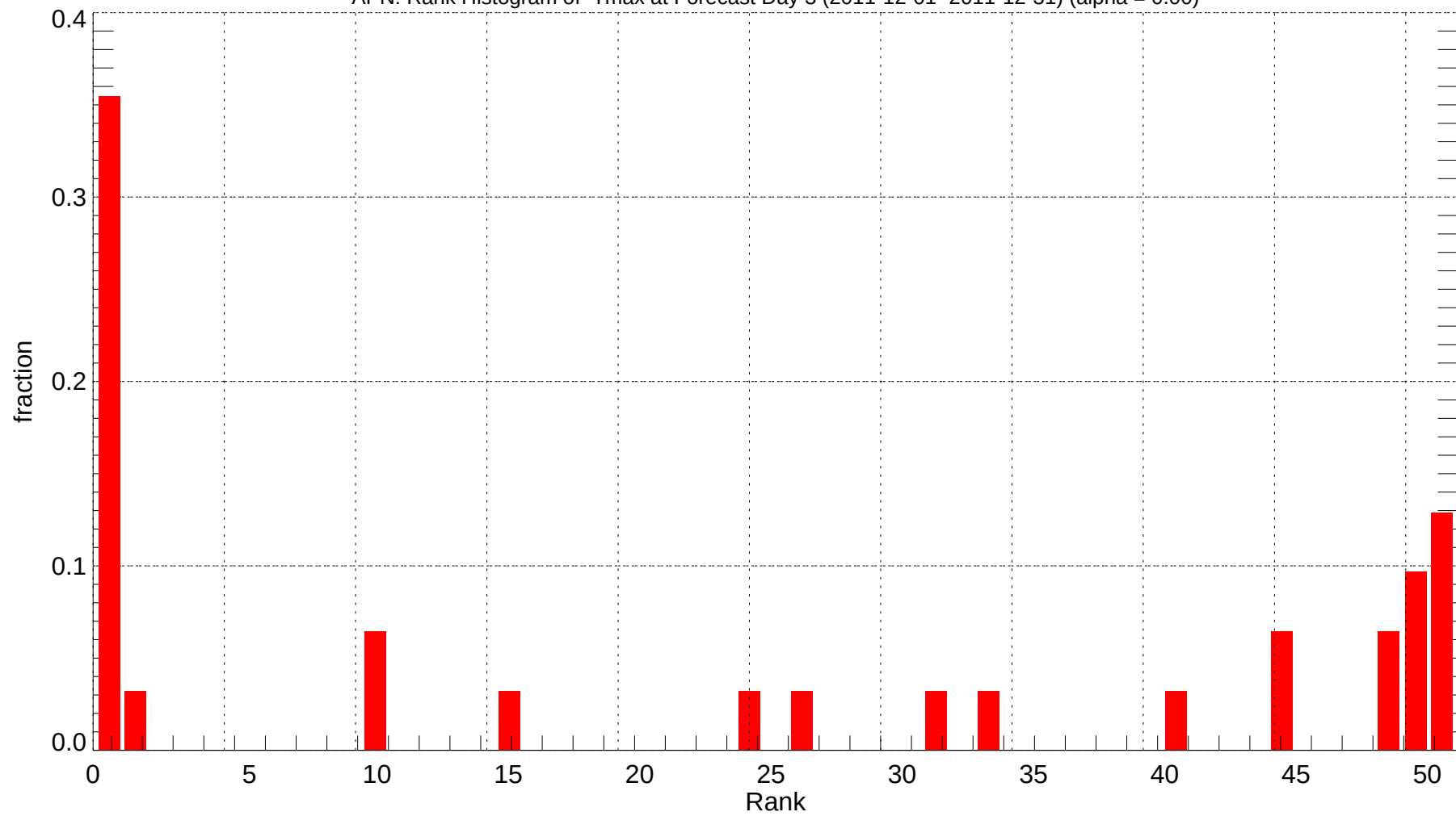
APN: Rank Histogram of Tmax at Forecast Day 3 (2011-12-01~2011-12-31) (alpha = 0.00)
