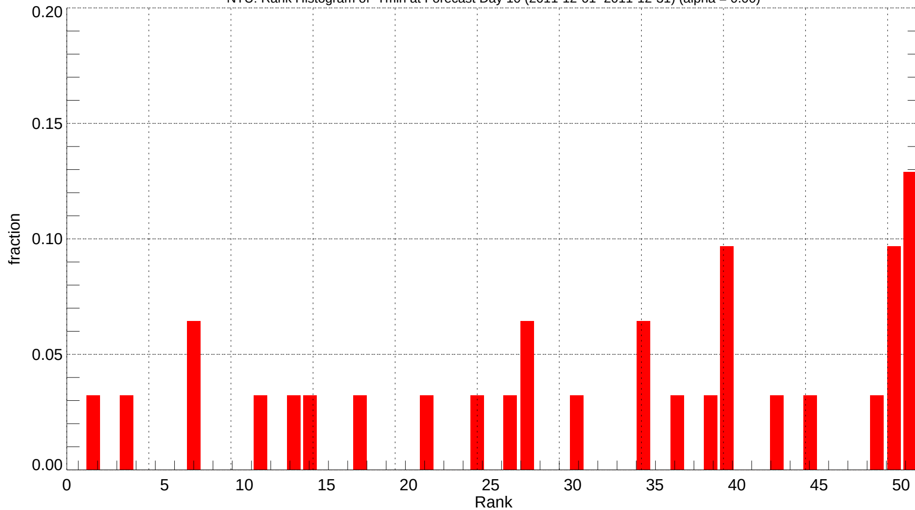
NTU: Rank Histogram of Tmin at Forecast Day 10 (2011-12-01~2011-12-31) (alpha = 0.00)
