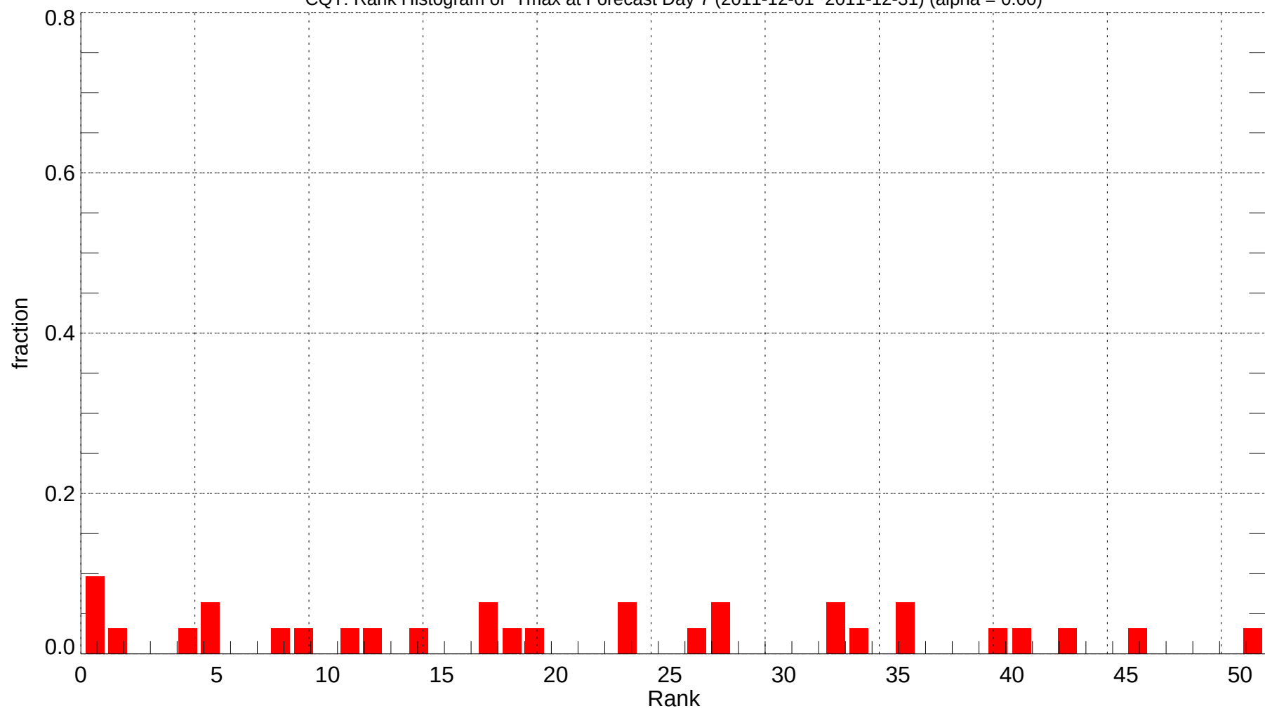
CQT: Rank Histogram of Tmax at Forecast Day 7 (2011-12-01~2011-12-31) (alpha = 0.00)
