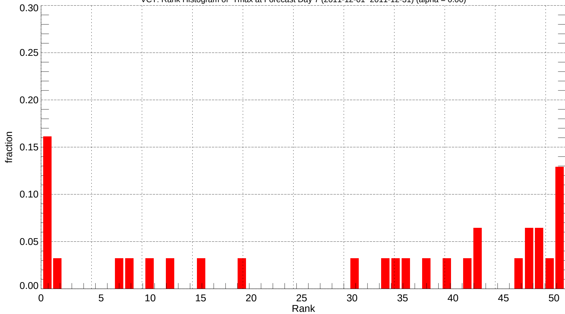
VCT: Rank Histogram of Tmax at Forecast Day 7 (2011-12-01~2011-12-31) (alpha = 0.00)
