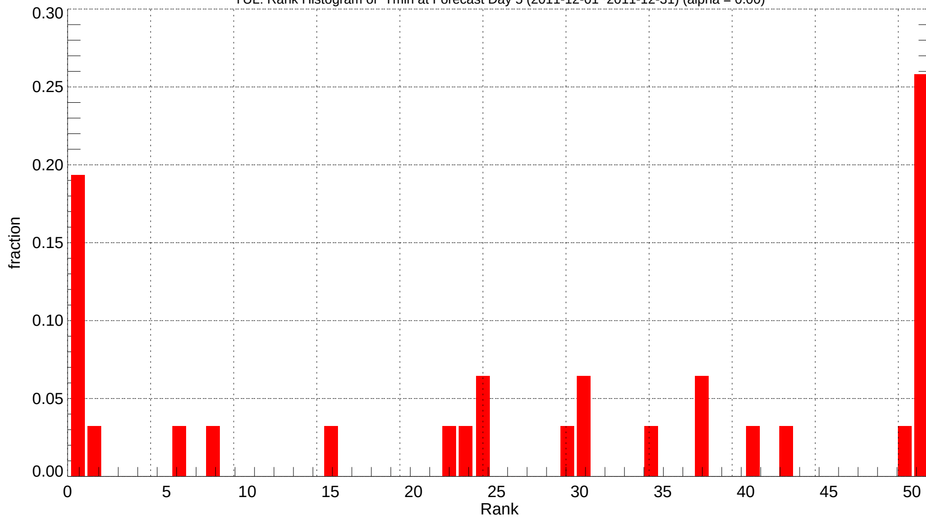
YUL: Rank Histogram of Tmin at Forecast Day 5 (2011-12-01~2011-12-31) (alpha = 0.00)
