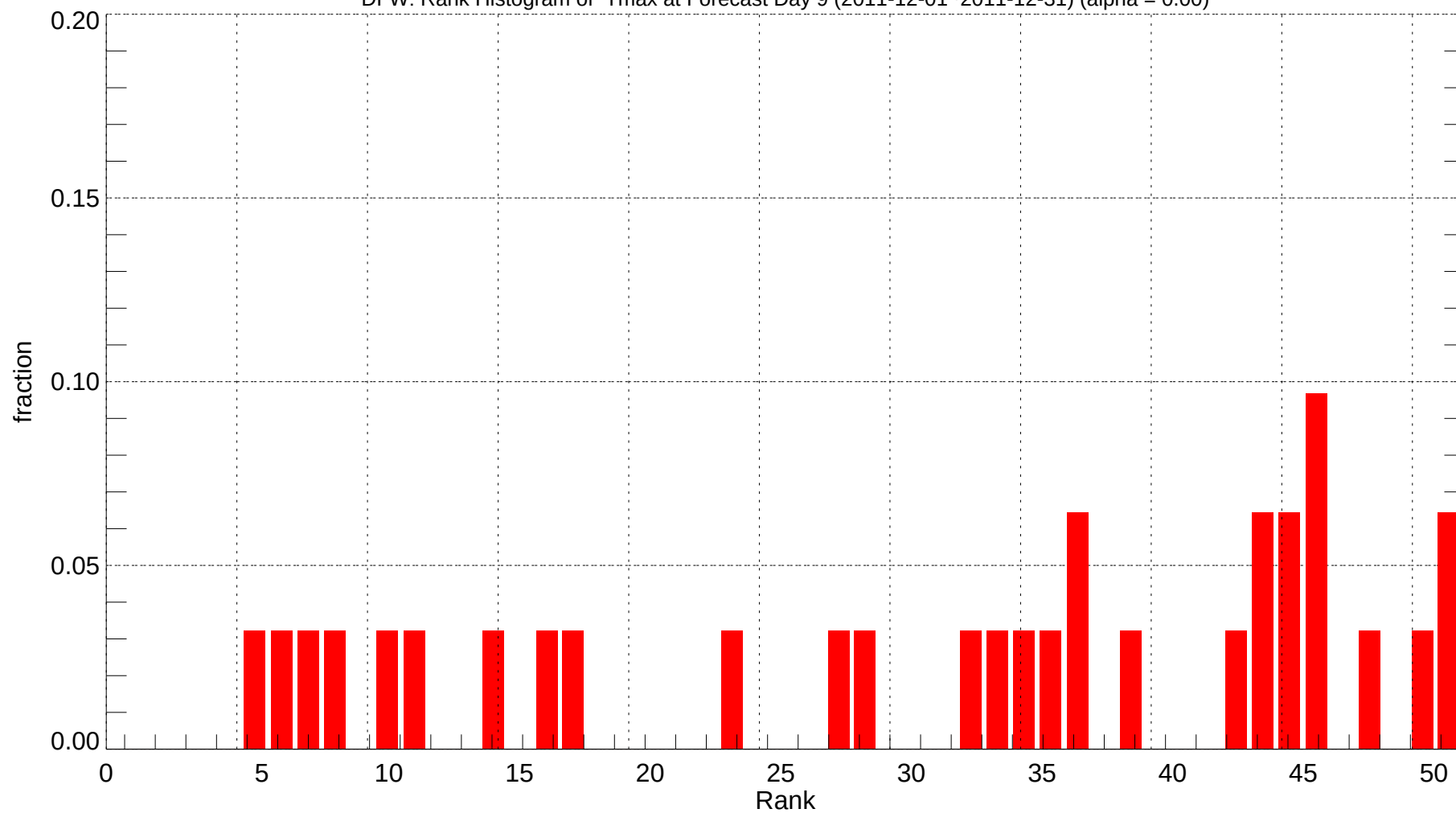
DFW: Rank Histogram of Tmax at Forecast Day 9 (2011-12-01~2011-12-31) (alpha = 0.00)
