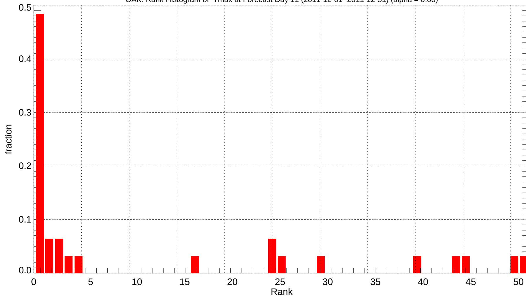
OAK: Rank Histogram of Tmax at Forecast Day 11 (2011-12-01~2011-12-31) (alpha = 0.00)
