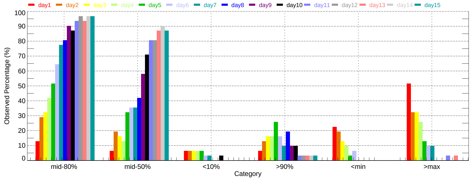
Observed Percentage of Ensembles - SLC: Min Temperature (2011-12-01~2011-12-31)
