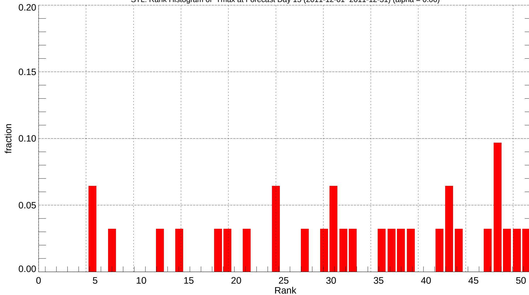
STL: Rank Histogram of Tmax at Forecast Day 15 (2011-12-01~2011-12-31) (alpha = 0.00)
