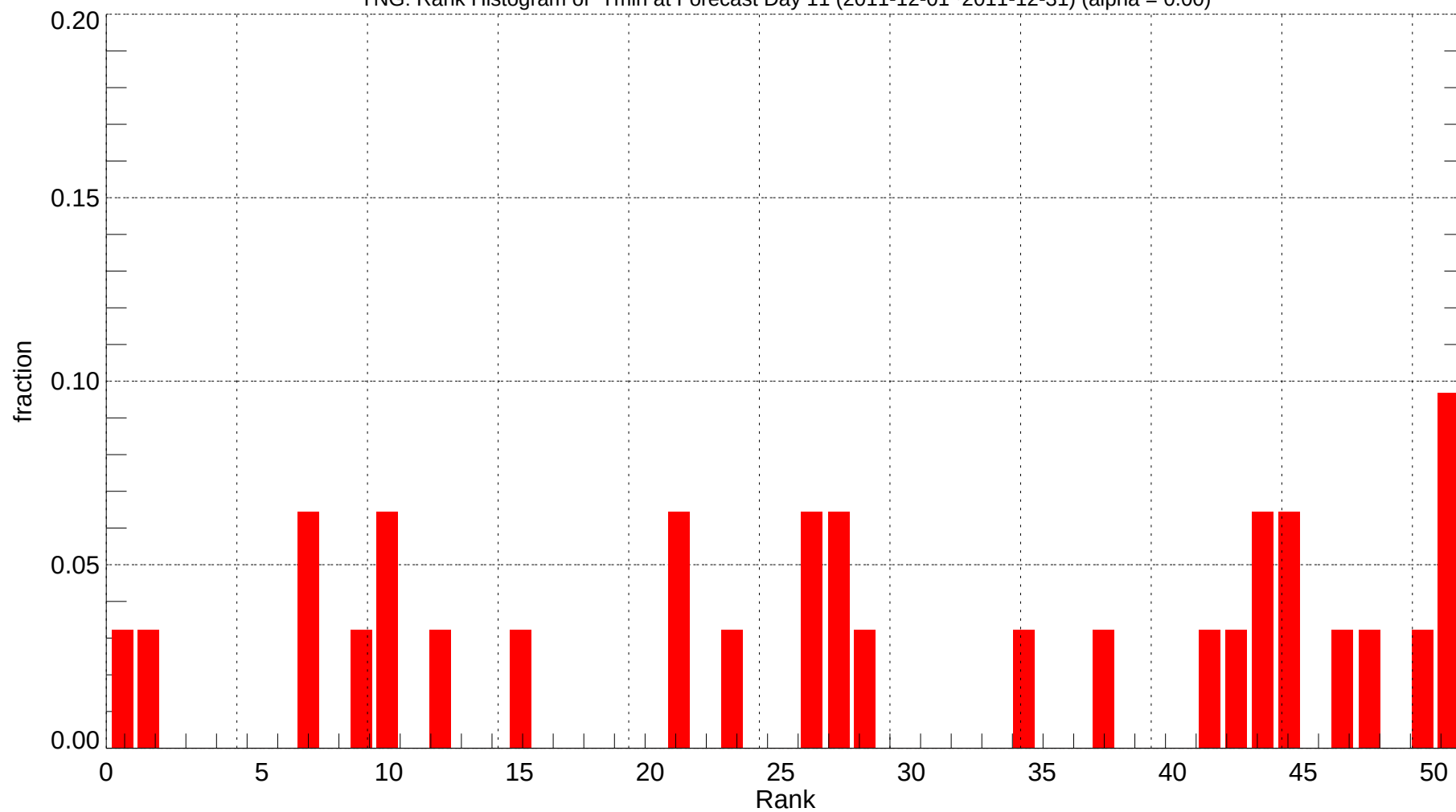
YNG: Rank Histogram of Tmin at Forecast Day 11 (2011-12-01~2011-12-31) (alpha = 0.00)
