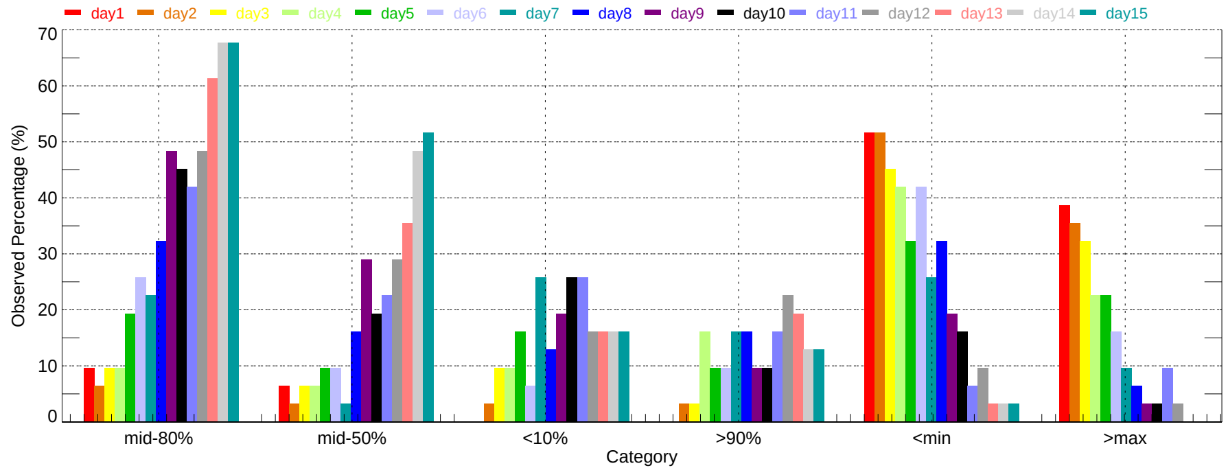
Observed Percentage of Ensembles - LAX: Min Temperature (2011-12-01~2011-12-31)
