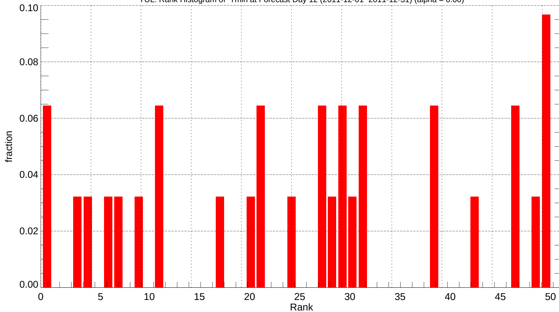
YUL: Rank Histogram of Tmin at Forecast Day 12 (2011-12-01~2011-12-31) (alpha = 0.00)
