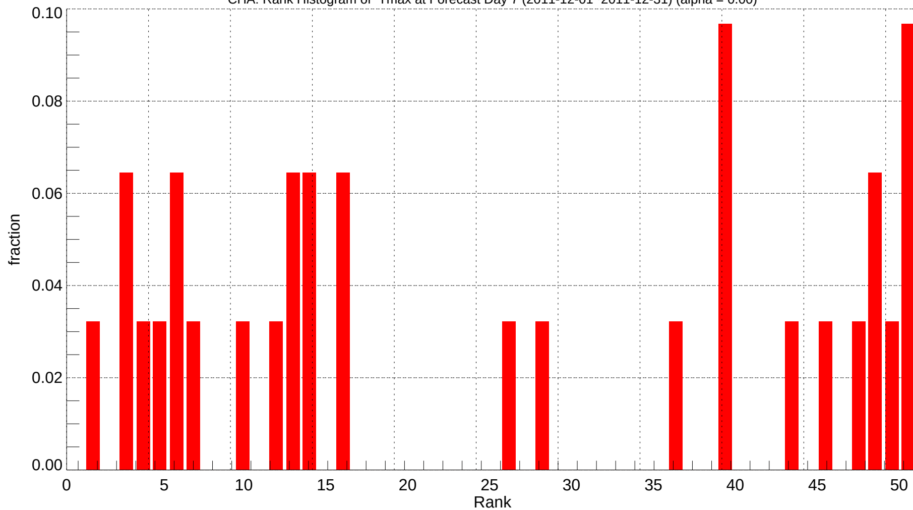
CHA: Rank Histogram of Tmax at Forecast Day 7 (2011-12-01~2011-12-31) (alpha = 0.00)
