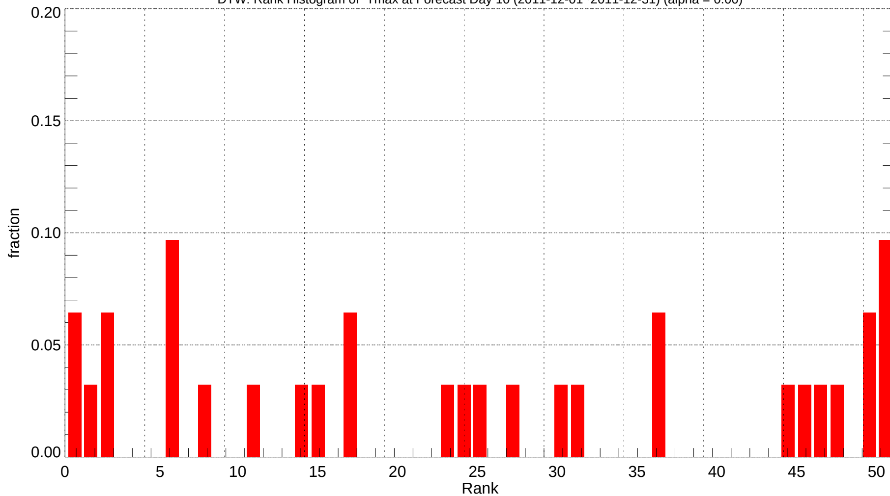
DTW: Rank Histogram of Tmax at Forecast Day 10 (2011-12-01~2011-12-31) (alpha = 0.00)
