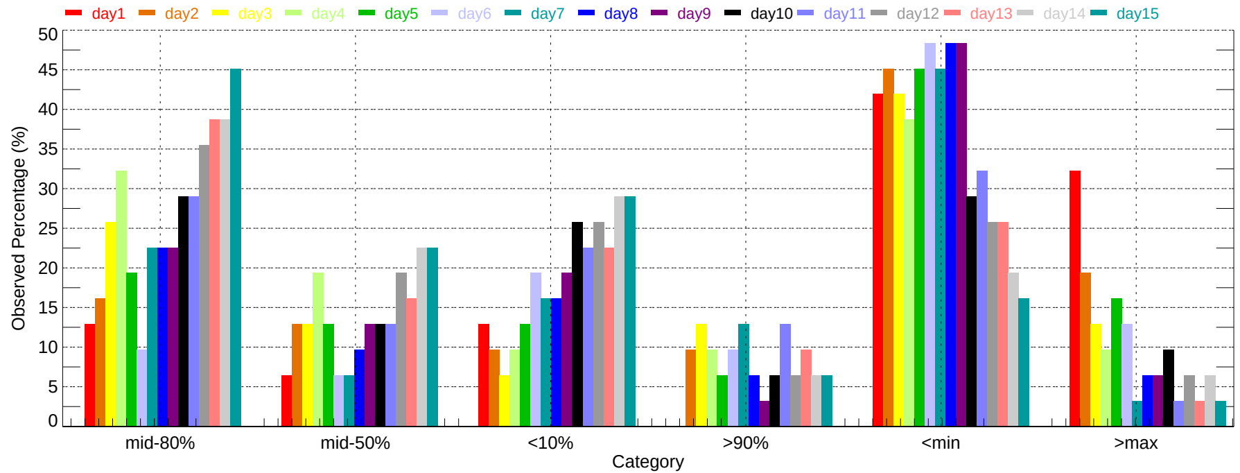
Observed Percentage of Ensembles - OAK: Min Temperature (2011-12-01~2011-12-31)
