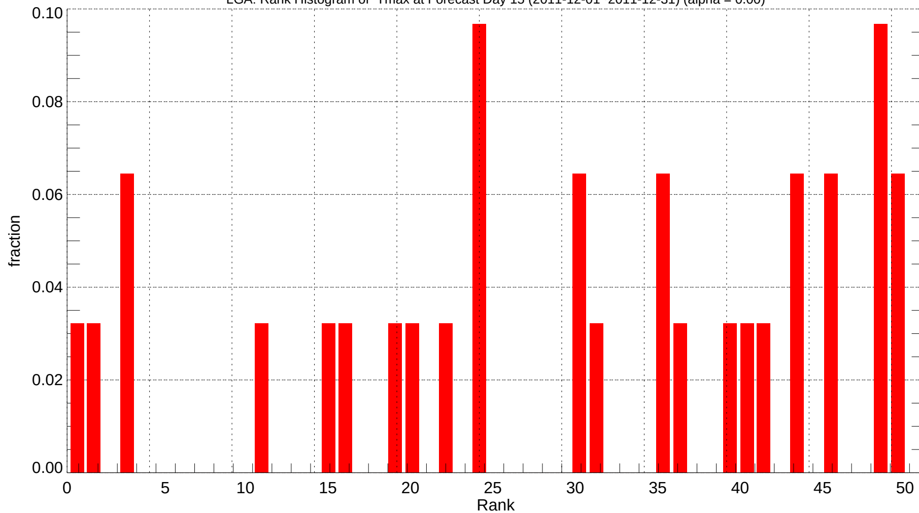
LGA: Rank Histogram of Tmax at Forecast Day 15 (2011-12-01~2011-12-31) (alpha = 0.00)
