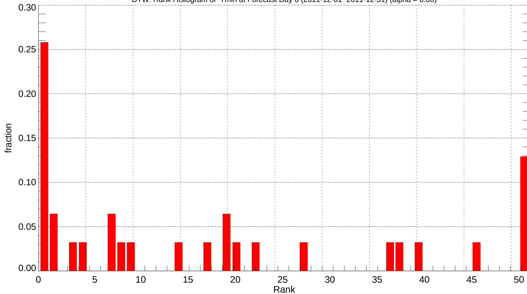
DTW: Rank Histogram of Tmin at Forecast Day 6 (2011-12-01~2011-12-31) (alpha = 0.00)
