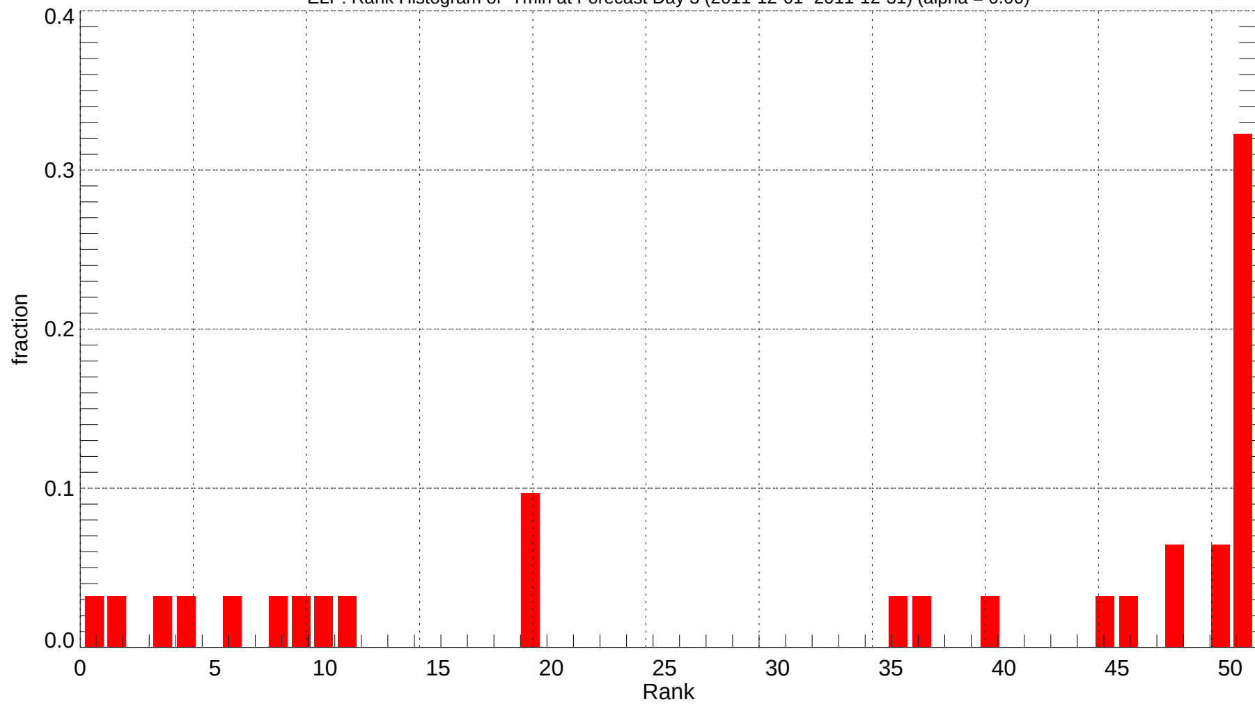
ELP: Rank Histogram of Tmin at Forecast Day 3 (2011-12-01~2011-12-31) (alpha = 0.00)
