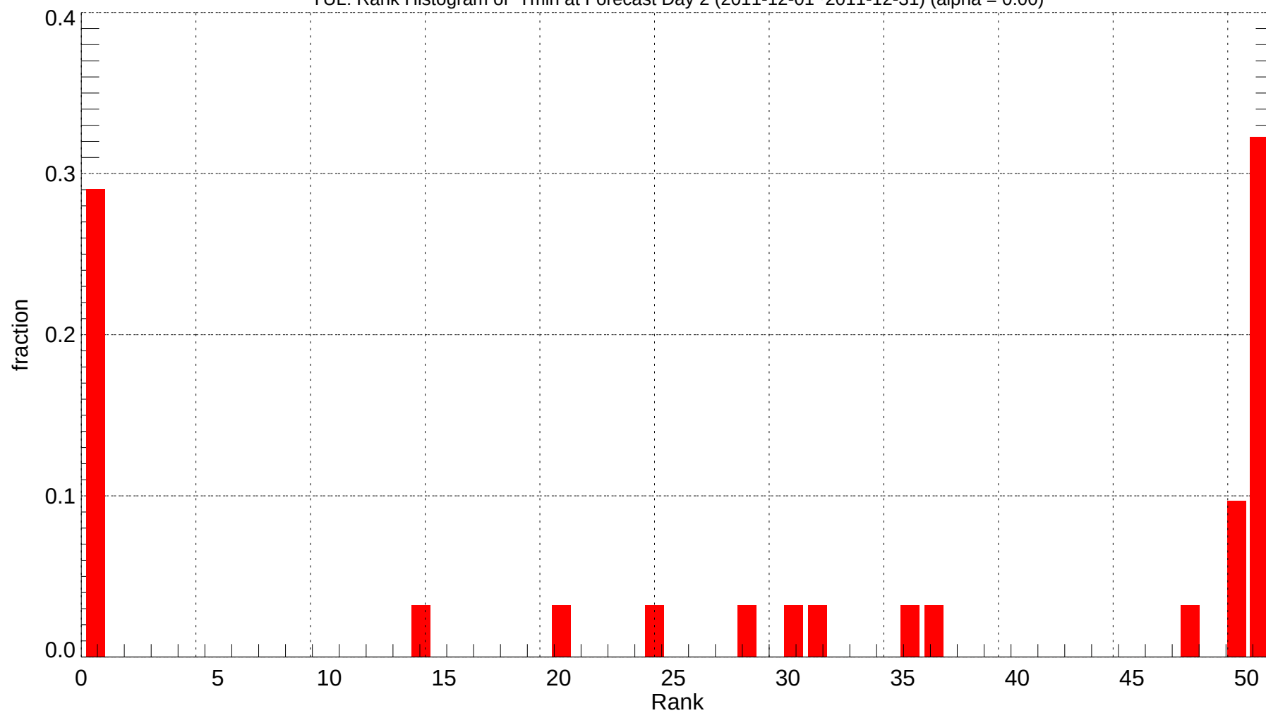
YUL: Rank Histogram of Tmin at Forecast Day 2 (2011-12-01~2011-12-31) (alpha = 0.00)
