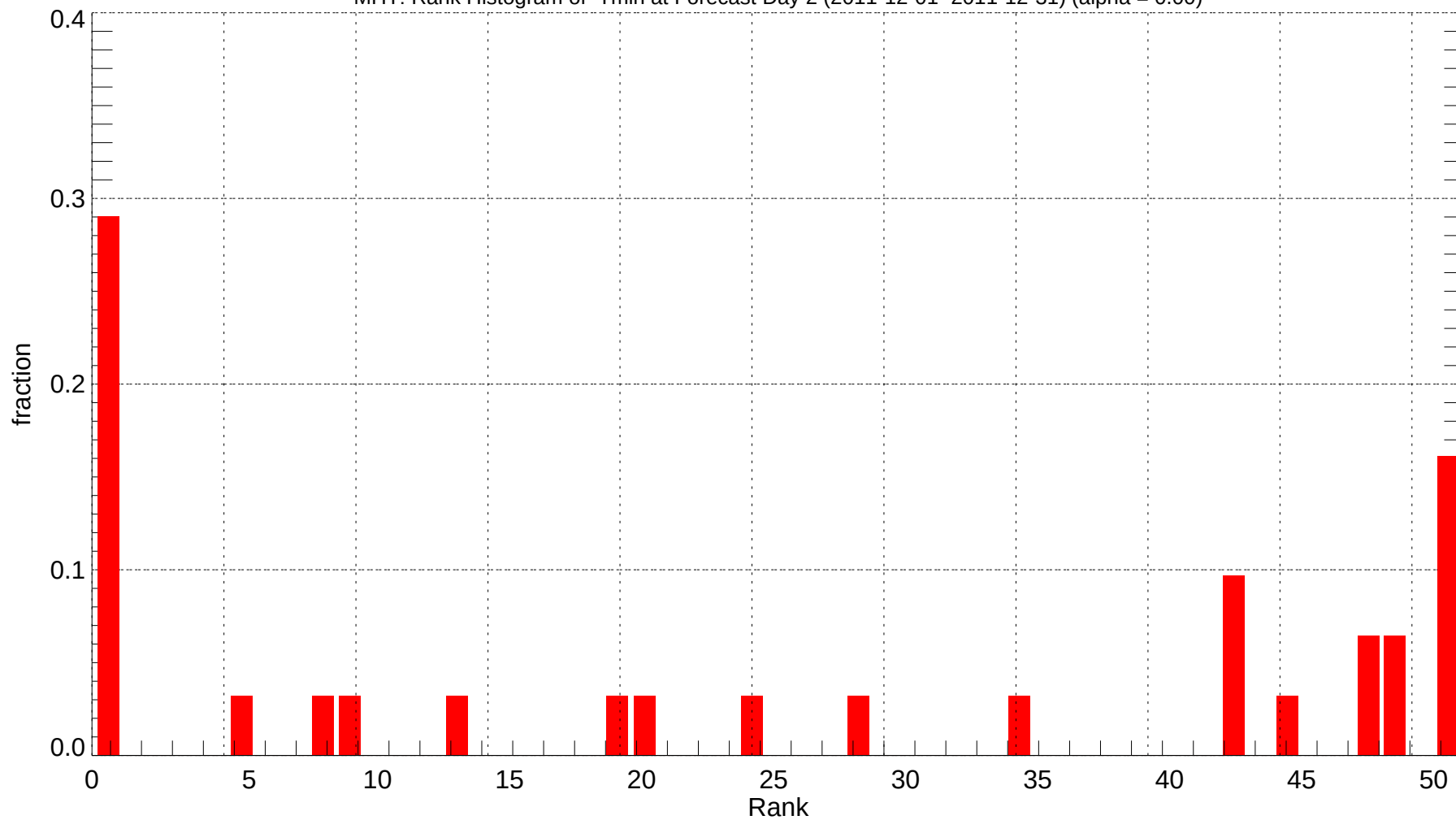
MHT: Rank Histogram of Tmin at Forecast Day 2 (2011-12-01~2011-12-31) (alpha = 0.00)
