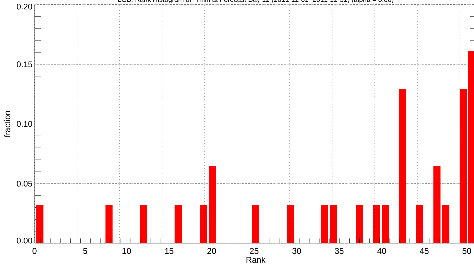
LGB: Rank Histogram of Tmin at Forecast Day 12 (2011-12-01~2011-12-31) (alpha = 0.00)
