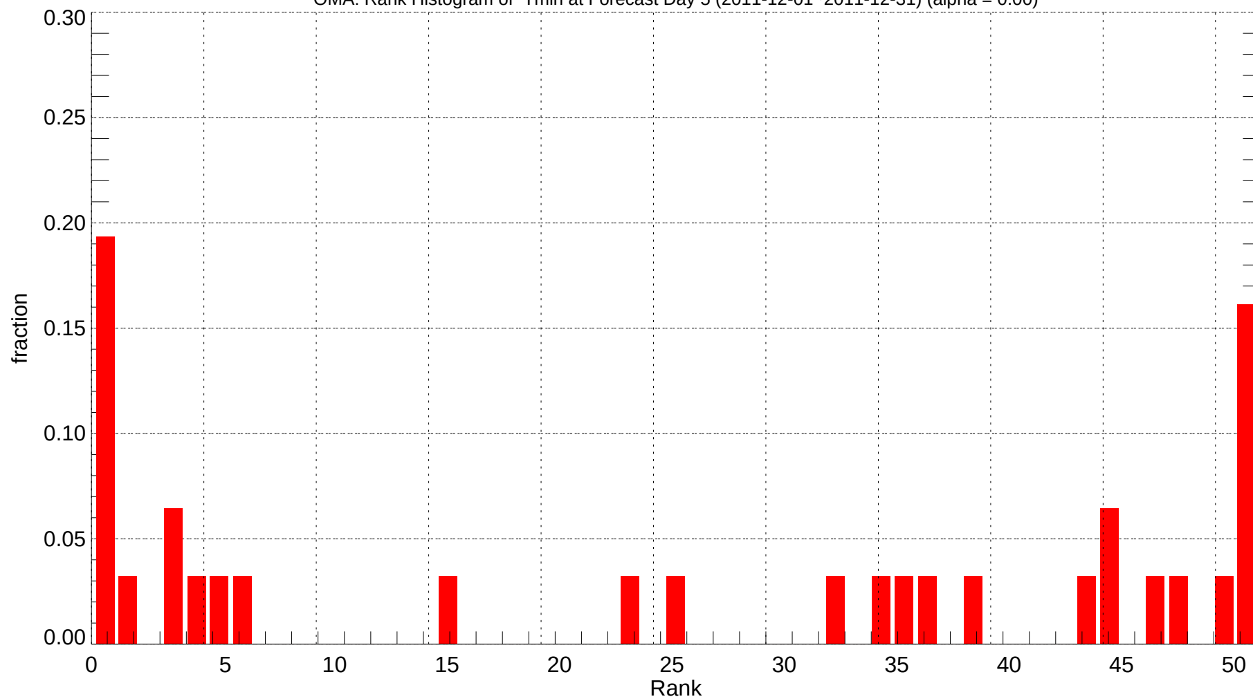
OMA: Rank Histogram of Tmin at Forecast Day 5 (2011-12-01~2011-12-31) (alpha = 0.00)
