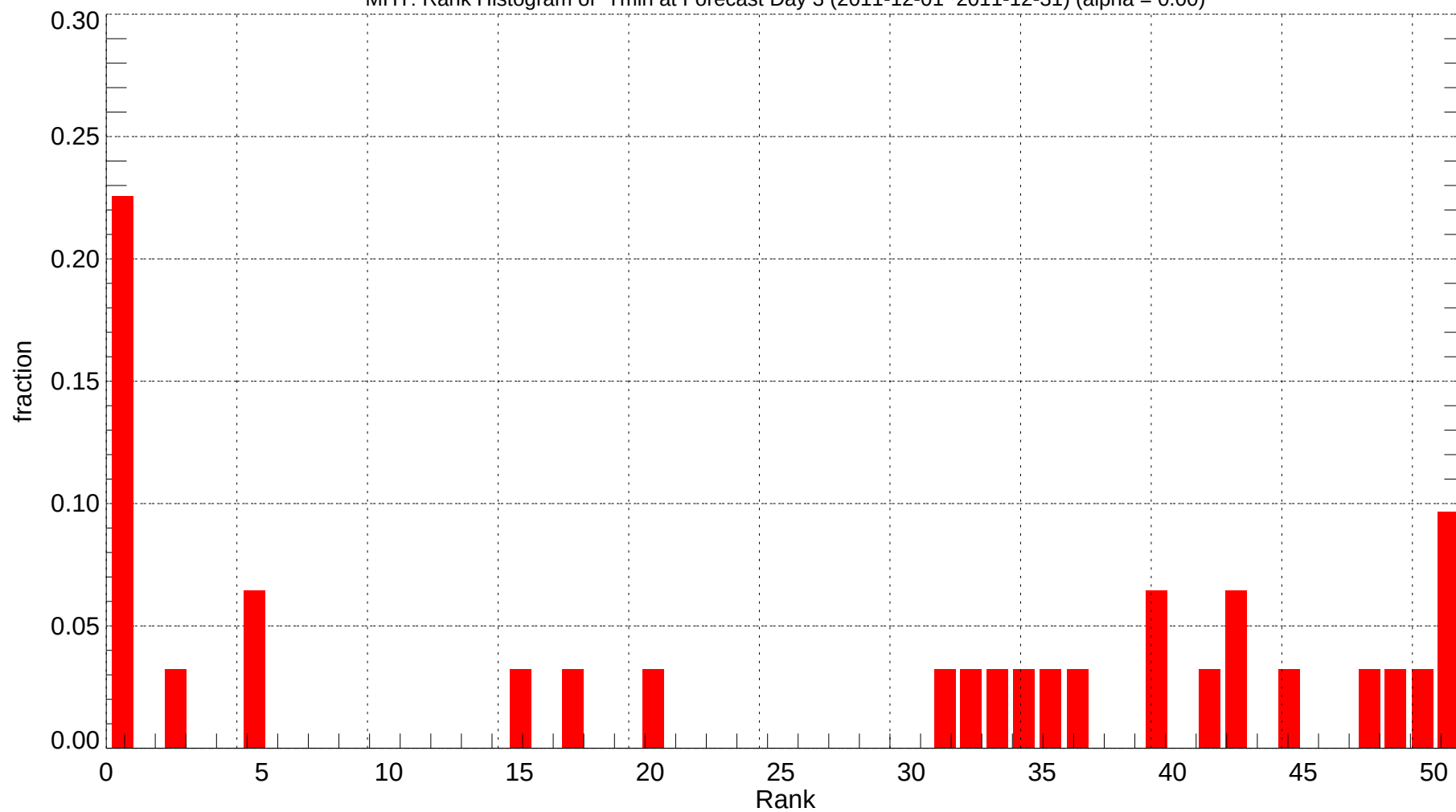
MHT: Rank Histogram of Tmin at Forecast Day 3 (2011-12-01~2011-12-31) (alpha = 0.00)
