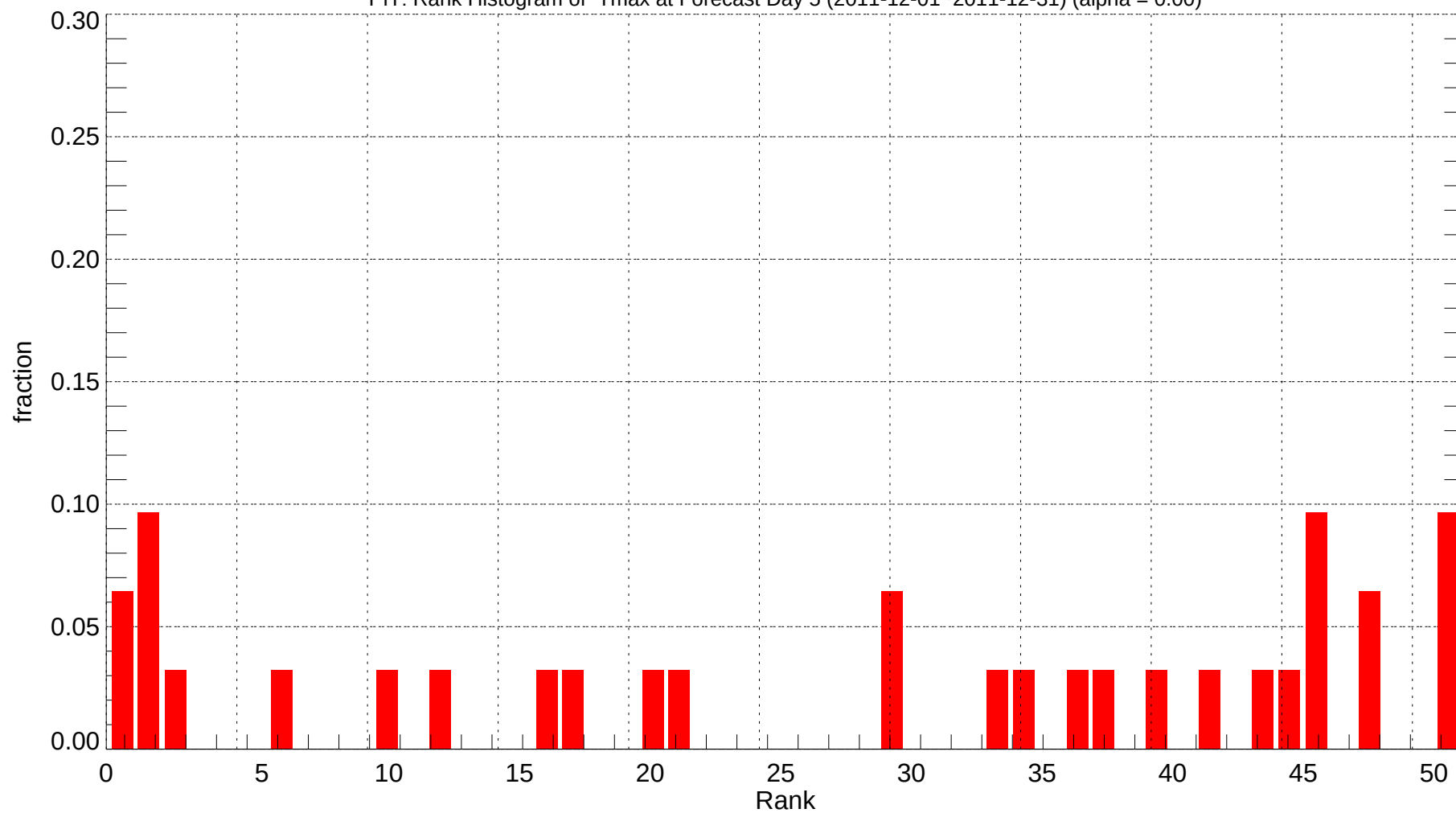
PIT: Rank Histogram of Tmax at Forecast Day 5 (2011-12-01~2011-12-31) (alpha = 0.00)
