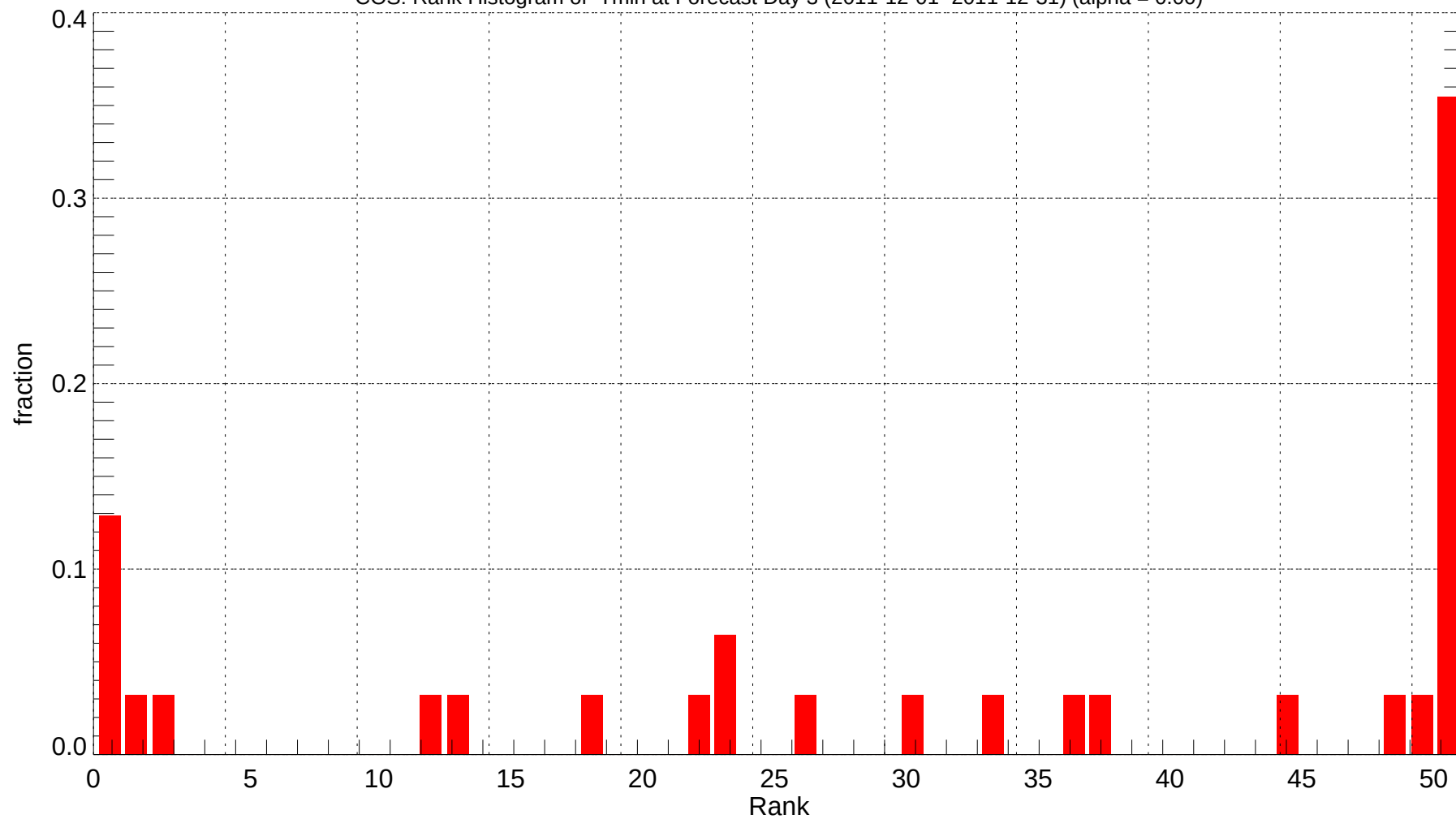
COS: Rank Histogram of Tmin at Forecast Day 3 (2011-12-01~2011-12-31) (alpha = 0.00)
