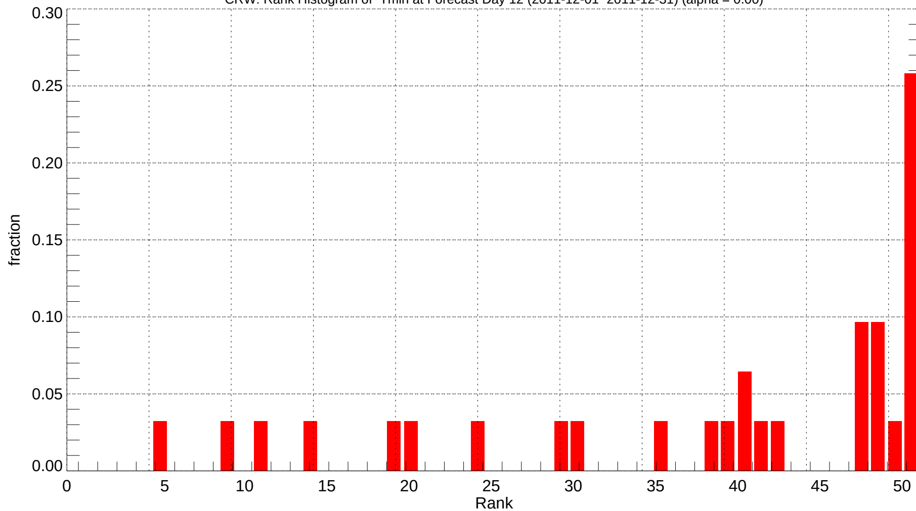
CRW: Rank Histogram of Tmin at Forecast Day 12 (2011-12-01~2011-12-31) (alpha = 0.00)
