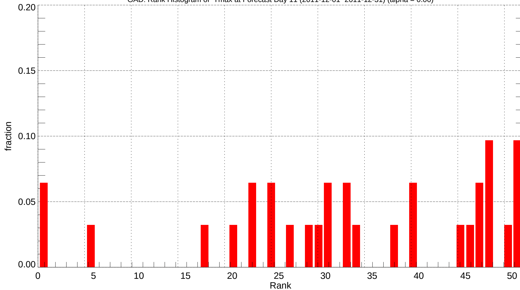
GAD: Rank Histogram of Tmax at Forecast Day 11 (2011-12-01~2011-12-31) (alpha = 0.00)
