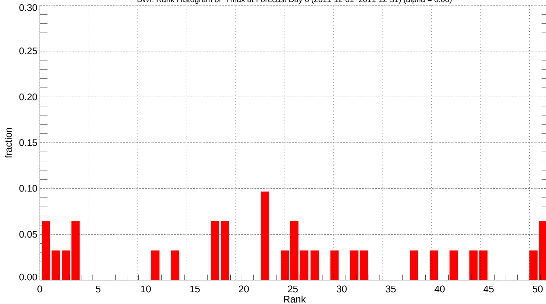
BWI: Rank Histogram of Tmax at Forecast Day 6 (2011-12-01~2011-12-31) (alpha = 0.00)
