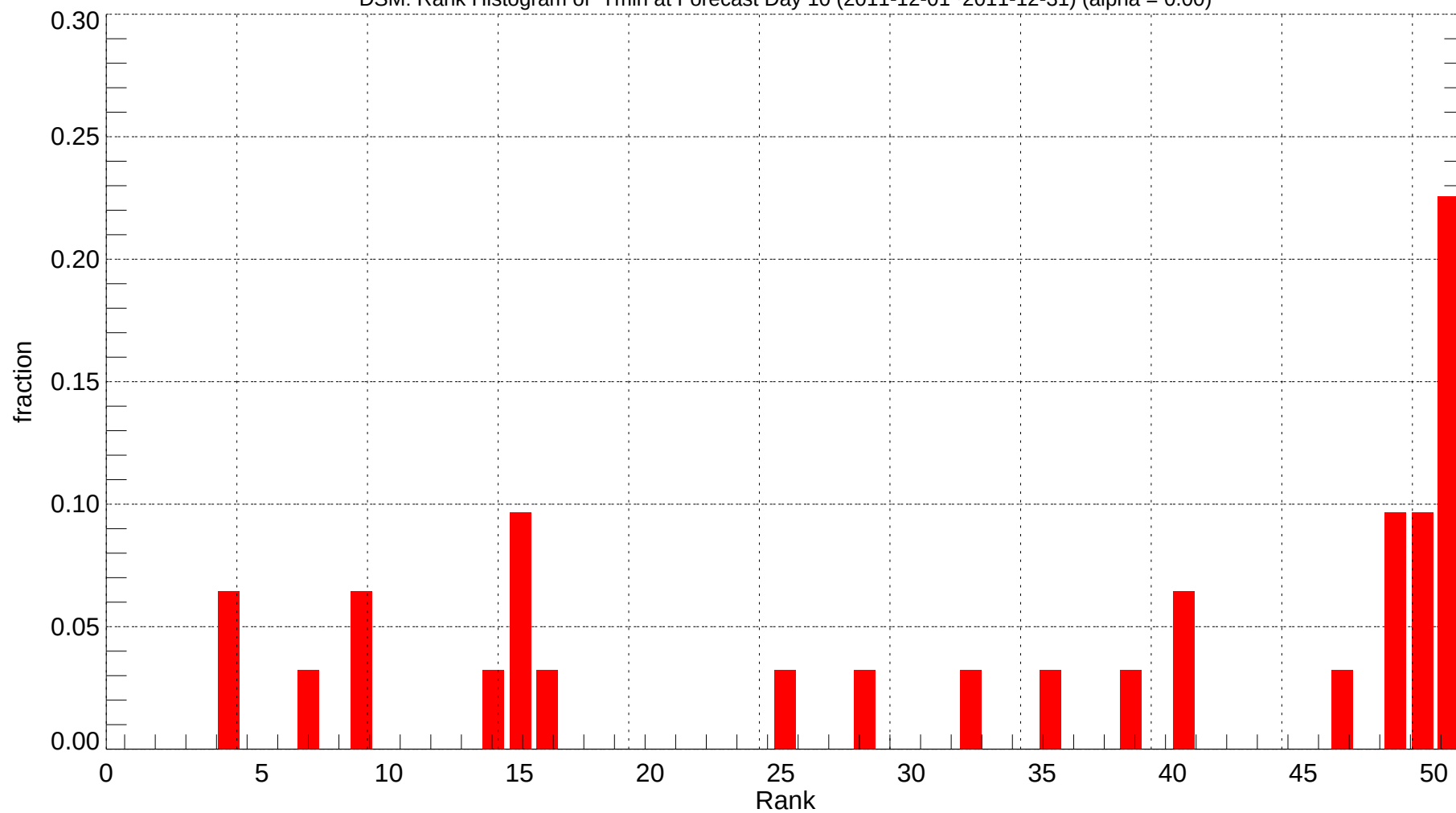
DSM: Rank Histogram of Tmin at Forecast Day 10 (2011-12-01~2011-12-31) (alpha = 0.00)
