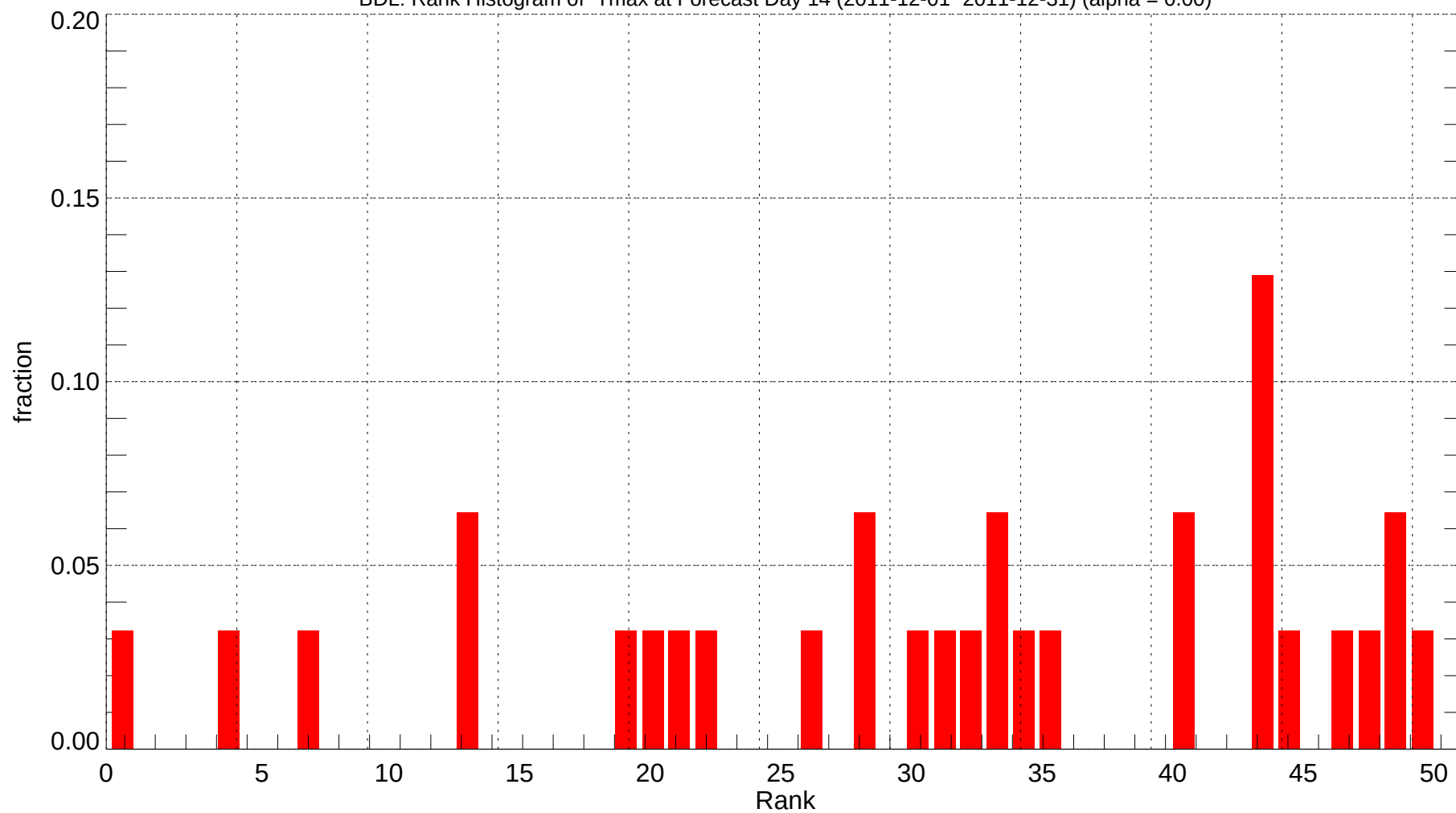
BDL: Rank Histogram of Tmax at Forecast Day 14 (2011-12-01~2011-12-31) (alpha = 0.00)
