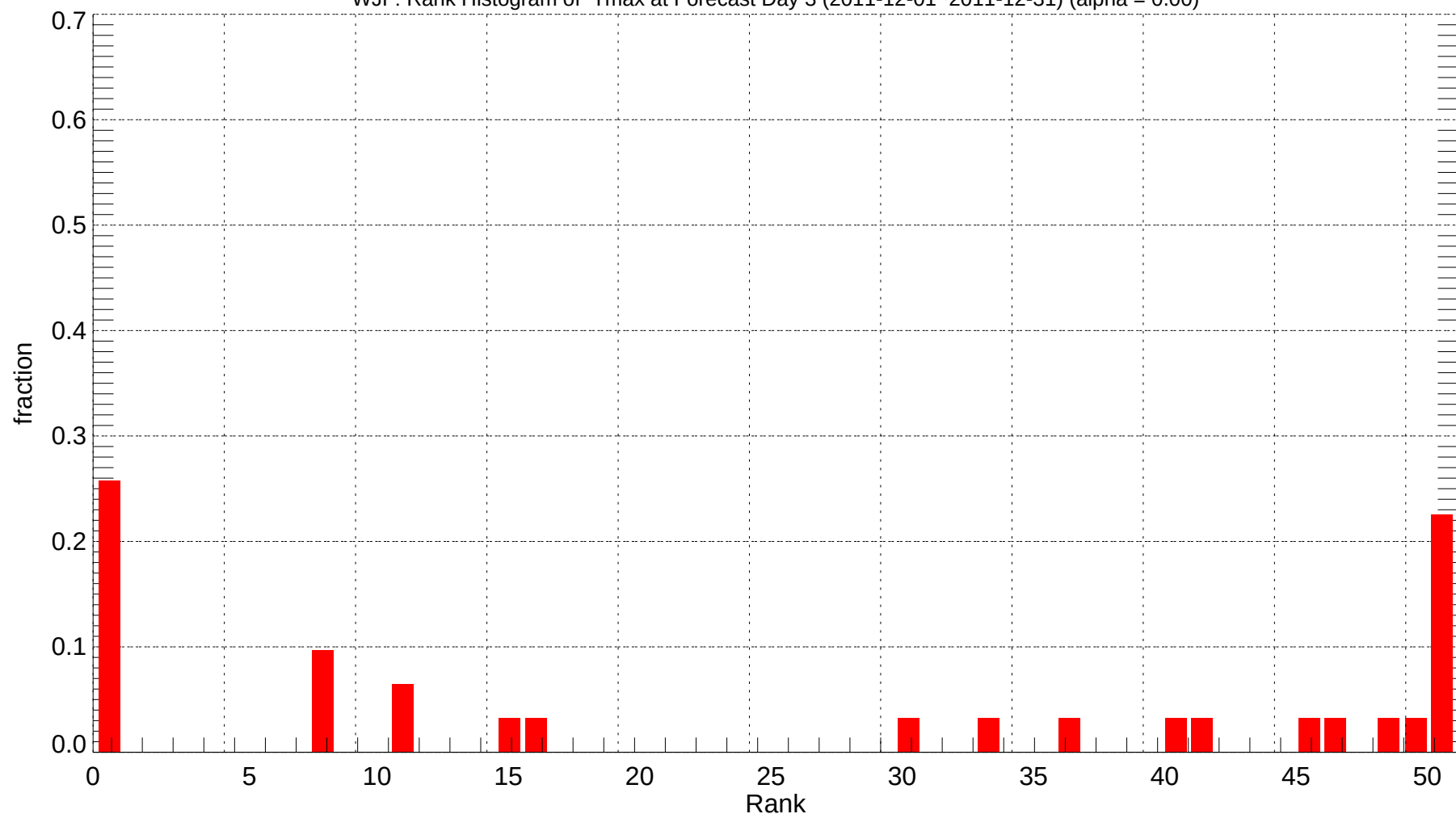
WJF: Rank Histogram of Tmax at Forecast Day 3 (2011-12-01~2011-12-31) (alpha = 0.00)
