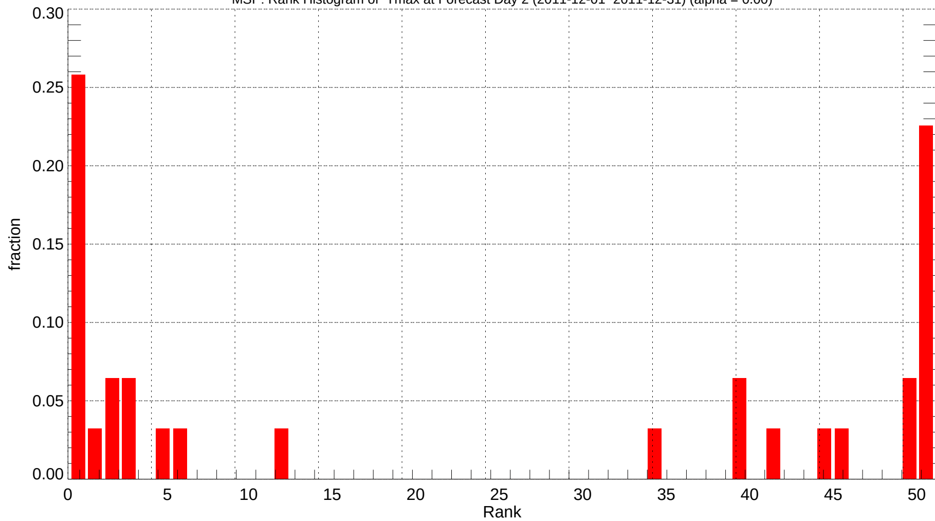
MSP: Rank Histogram of Tmax at Forecast Day 2 (2011-12-01~2011-12-31) (alpha = 0.00)
