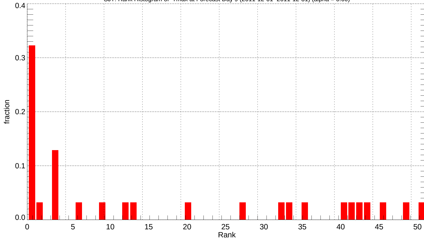
SJT: Rank Histogram of Tmax at Forecast Day 9 (2011-12-01~2011-12-31) (alpha = 0.00)
