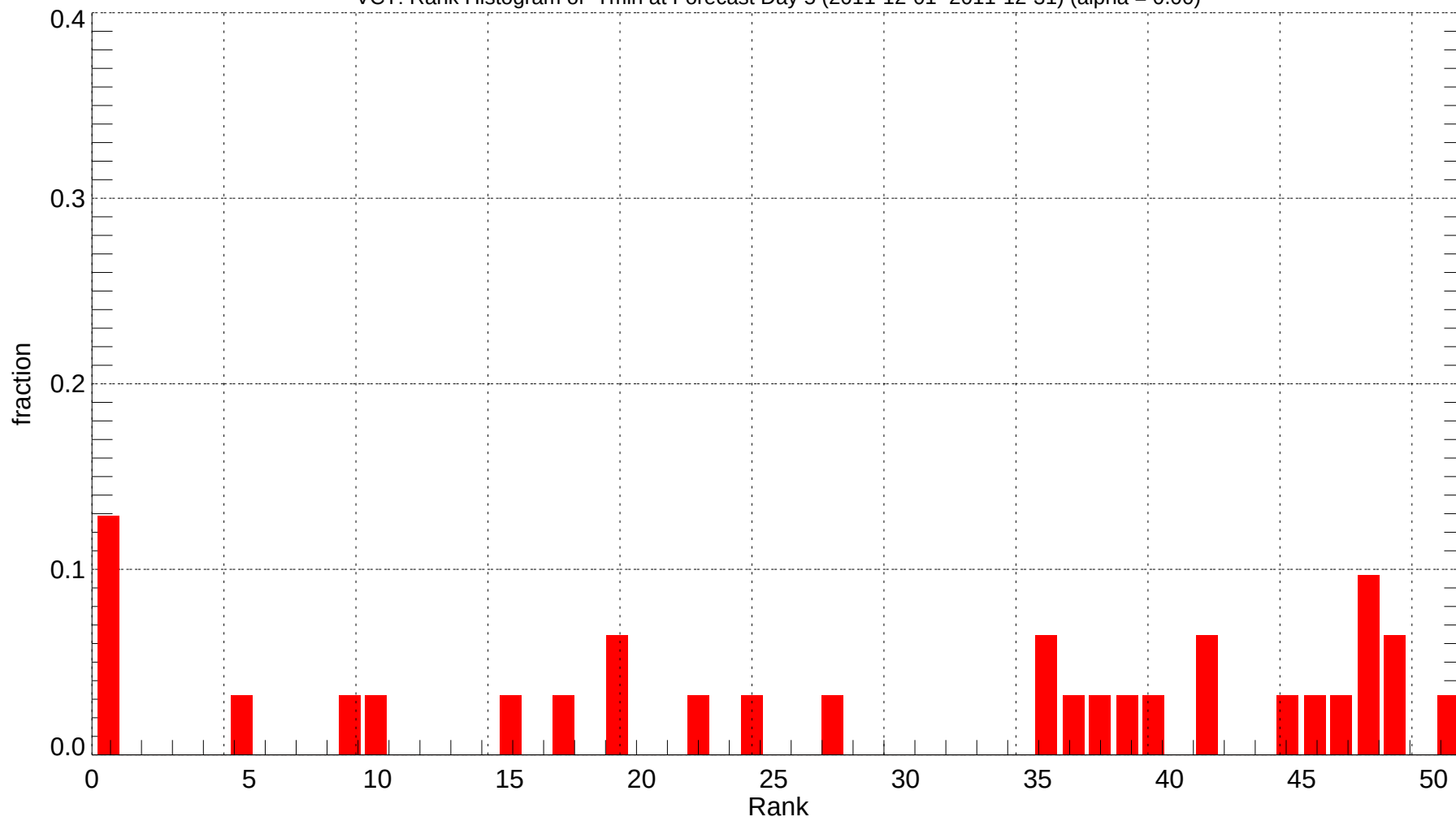
VCT: Rank Histogram of Tmin at Forecast Day 5 (2011-12-01~2011-12-31) (alpha = 0.00)
