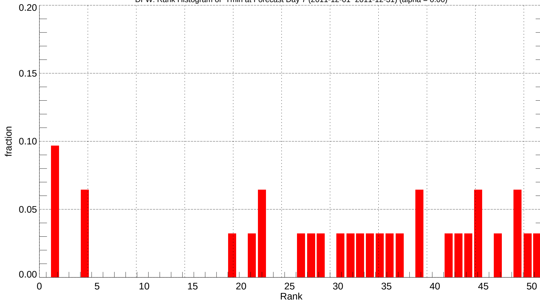
DFW: Rank Histogram of Tmin at Forecast Day 7 (2011-12-01~2011-12-31) (alpha = 0.00)
