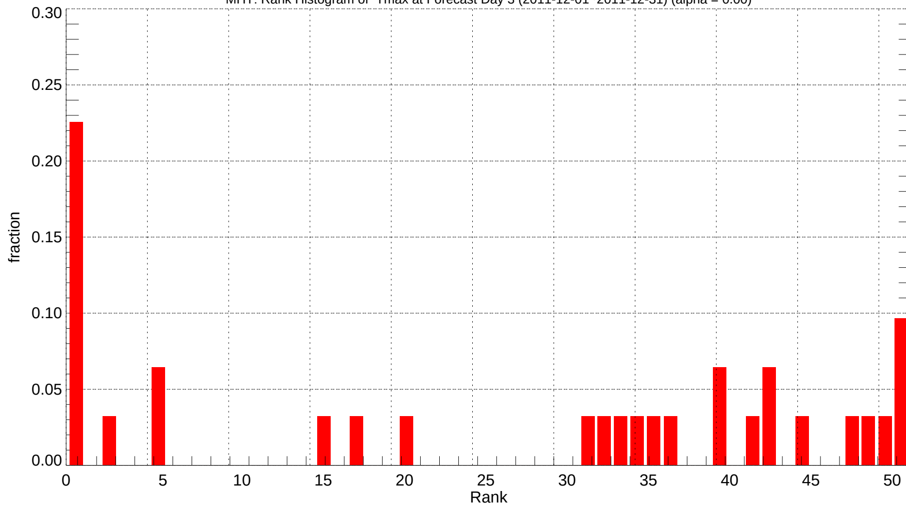
MHT: Rank Histogram of Tmax at Forecast Day 3 (2011-12-01~2011-12-31) (alpha = 0.00)
