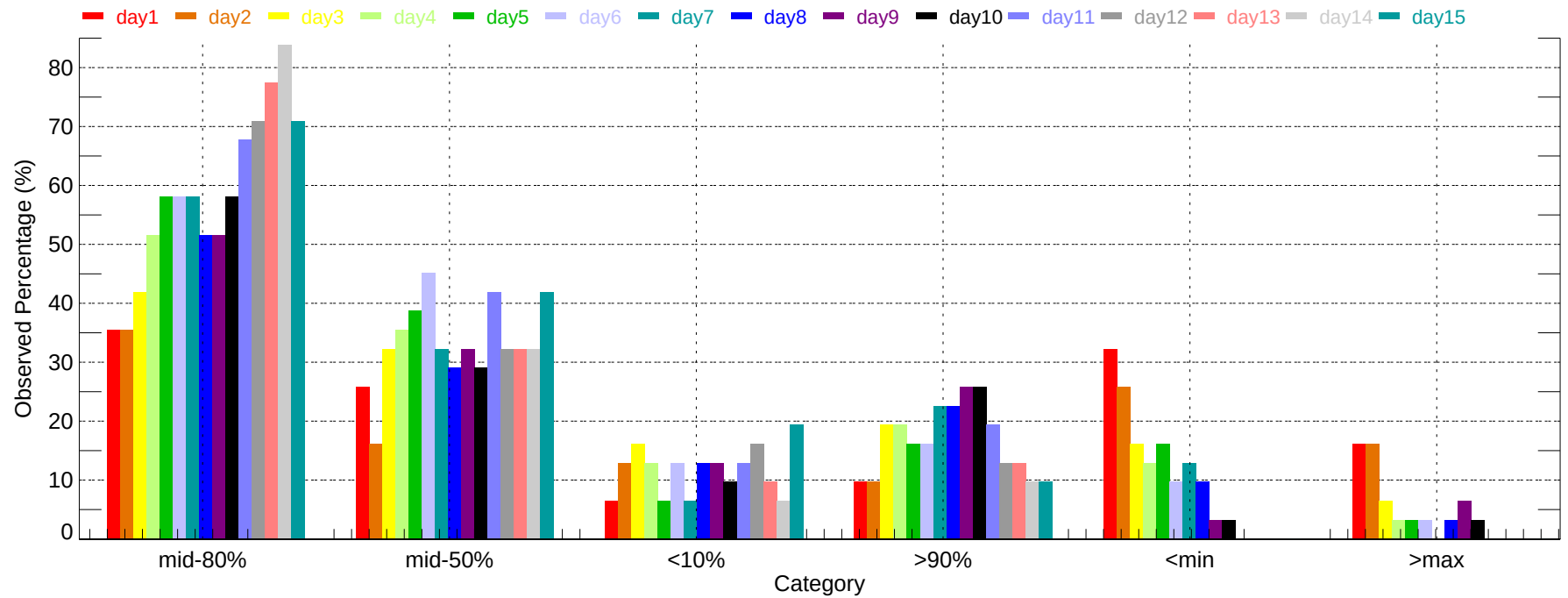
Observed Percentage of Ensembles - BUF: Min Temperature (2011-12-01~2011-12-31)
