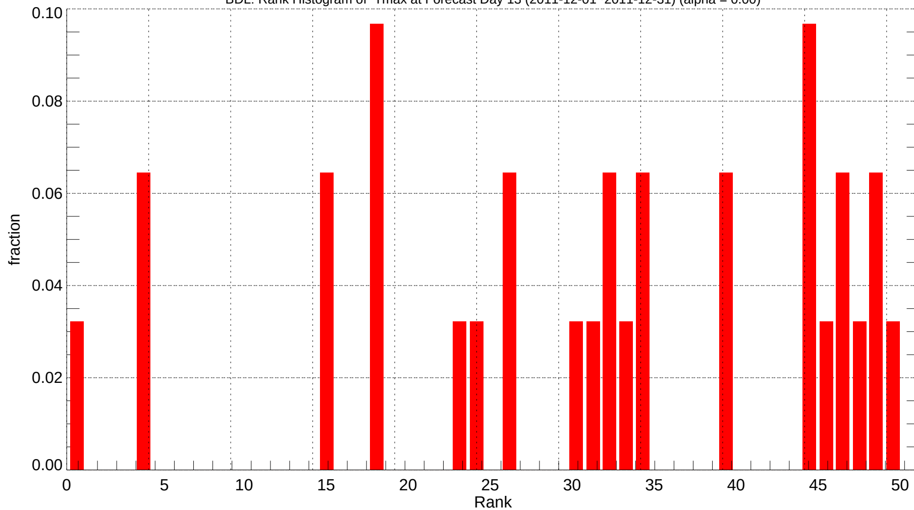
BDL: Rank Histogram of Tmax at Forecast Day 13 (2011-12-01~2011-12-31) (alpha = 0.00)
