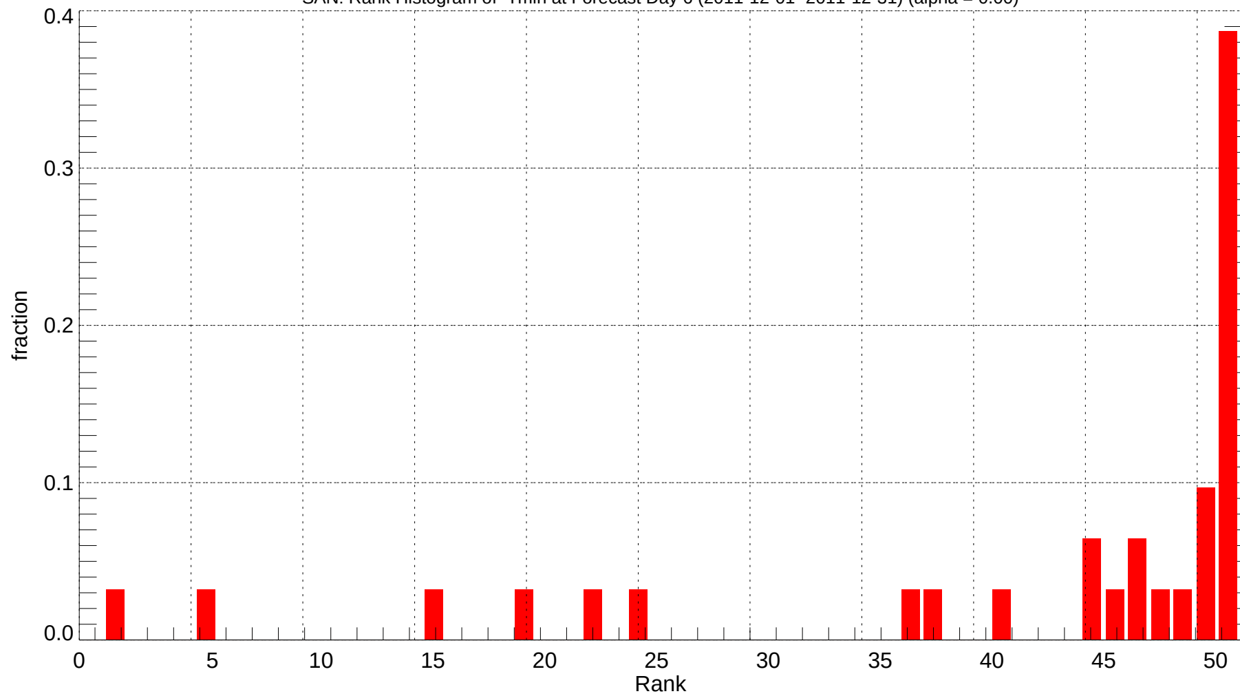
SAN: Rank Histogram of Tmin at Forecast Day 6 (2011-12-01~2011-12-31) (alpha = 0.00)
