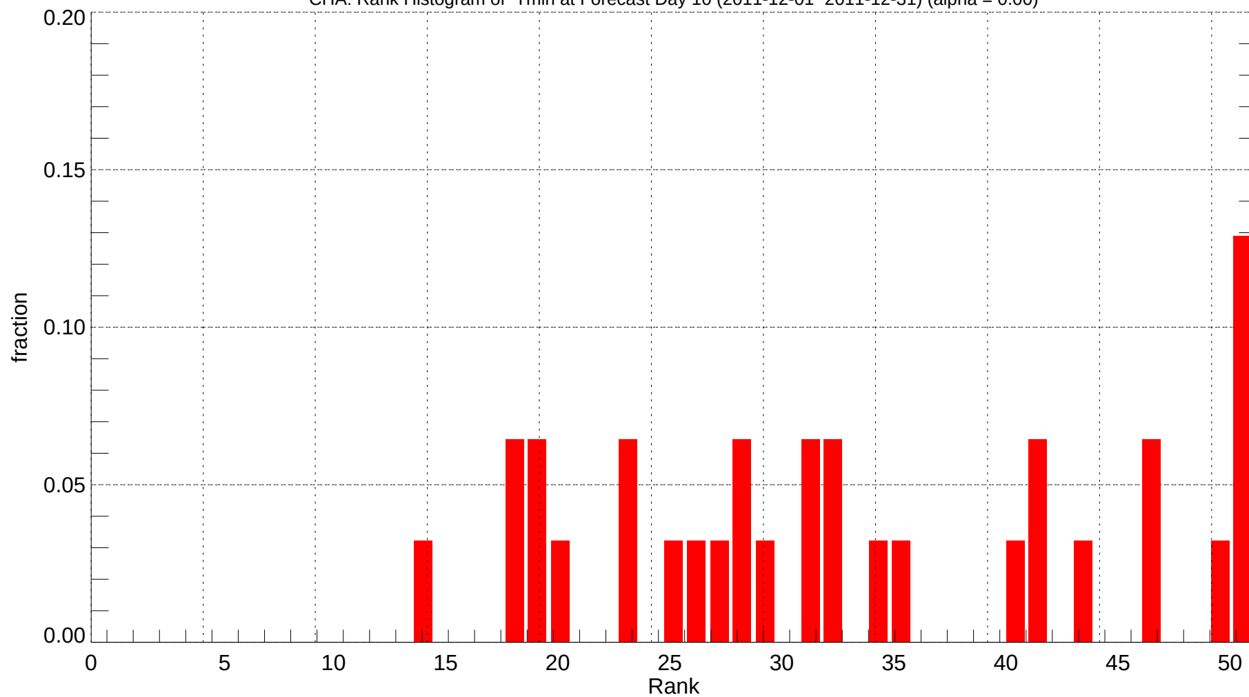
CHA: Rank Histogram of Tmin at Forecast Day 10 (2011-12-01~2011-12-31) (alpha = 0.00)
