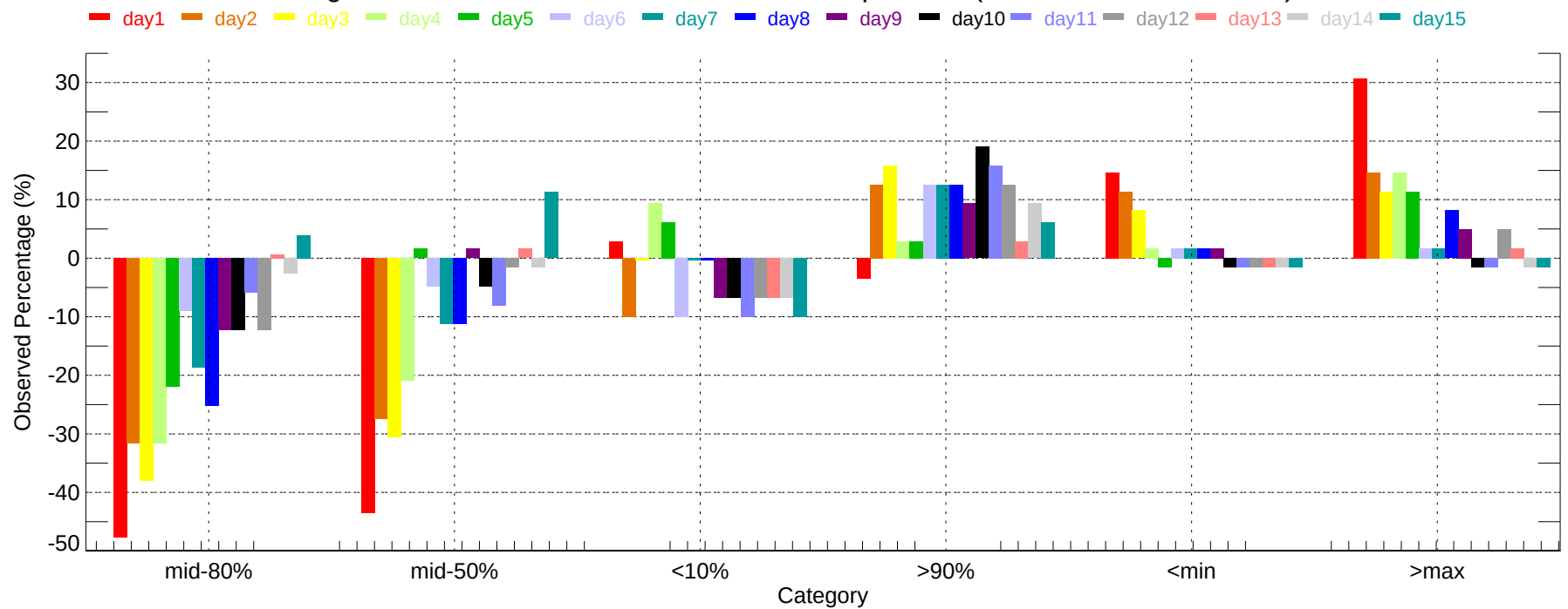
Observed Percentage Deviation of Ensembles - TYS: Min Temperature (2011-12-01~2011-12-31)
