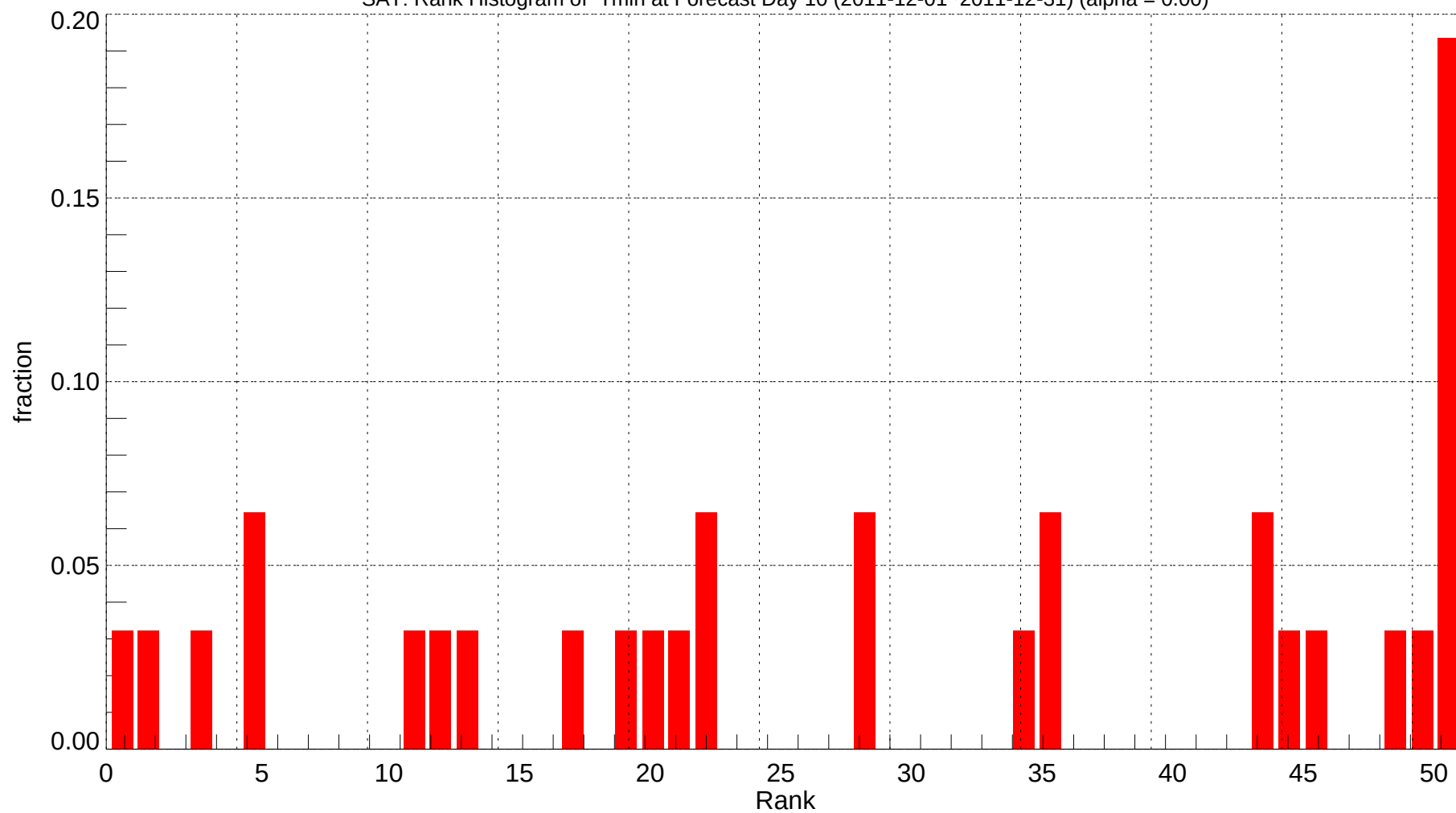
SAT: Rank Histogram of Tmin at Forecast Day 10 (2011-12-01~2011-12-31) (alpha = 0.00)
