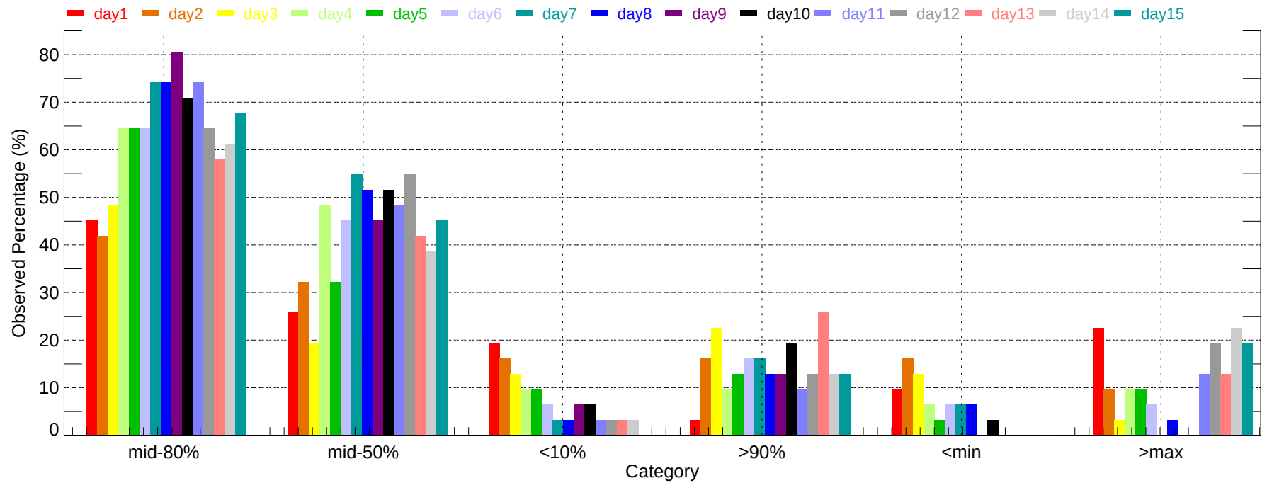
Observed Percentage of Ensembles - BUR: Max Temperature (2011-12-01~2011-12-31)
