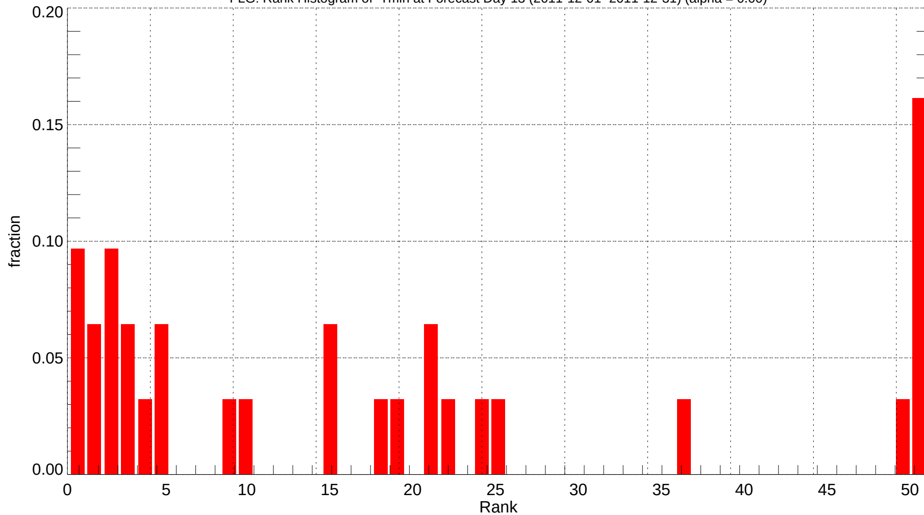
FLG: Rank Histogram of Tmin at Forecast Day 13 (2011-12-01~2011-12-31) (alpha = 0.00)
