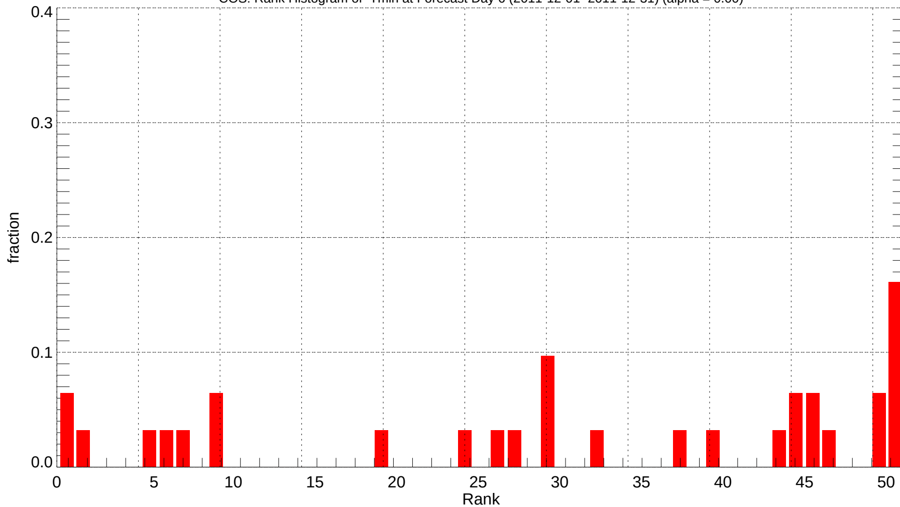
COS: Rank Histogram of Tmin at Forecast Day 6 (2011-12-01~2011-12-31) (alpha = 0.00)
