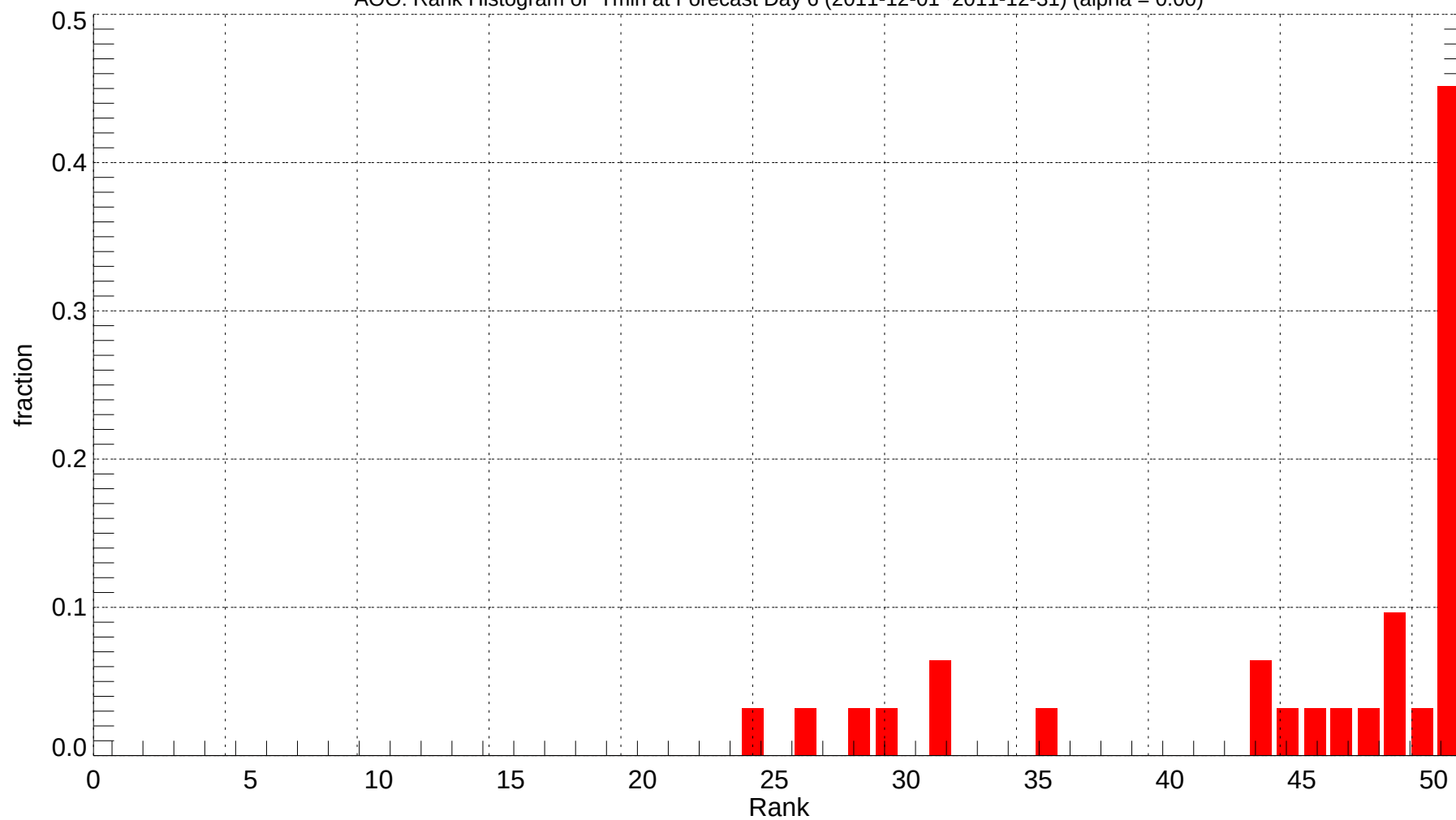
AOO: Rank Histogram of Tmin at Forecast Day 6 (2011-12-01~2011-12-31) (alpha = 0.00)
