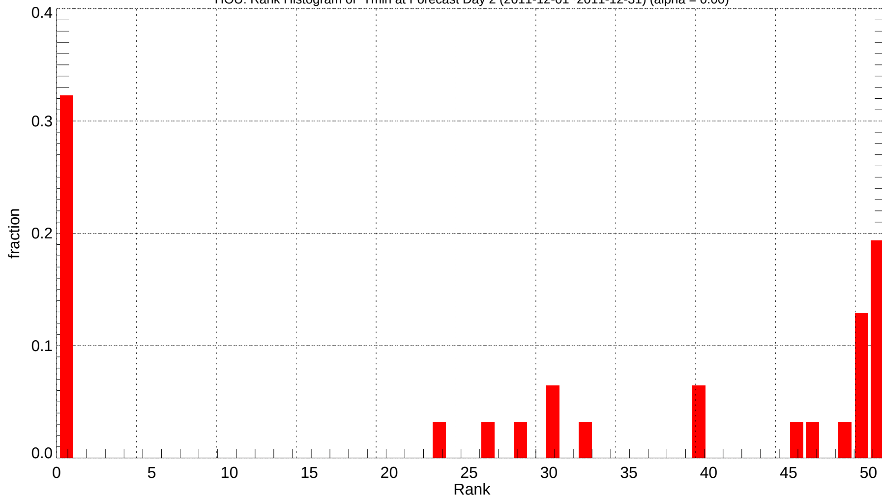
HOU: Rank Histogram of Tmin at Forecast Day 2 (2011-12-01~2011-12-31) (alpha = 0.00)
