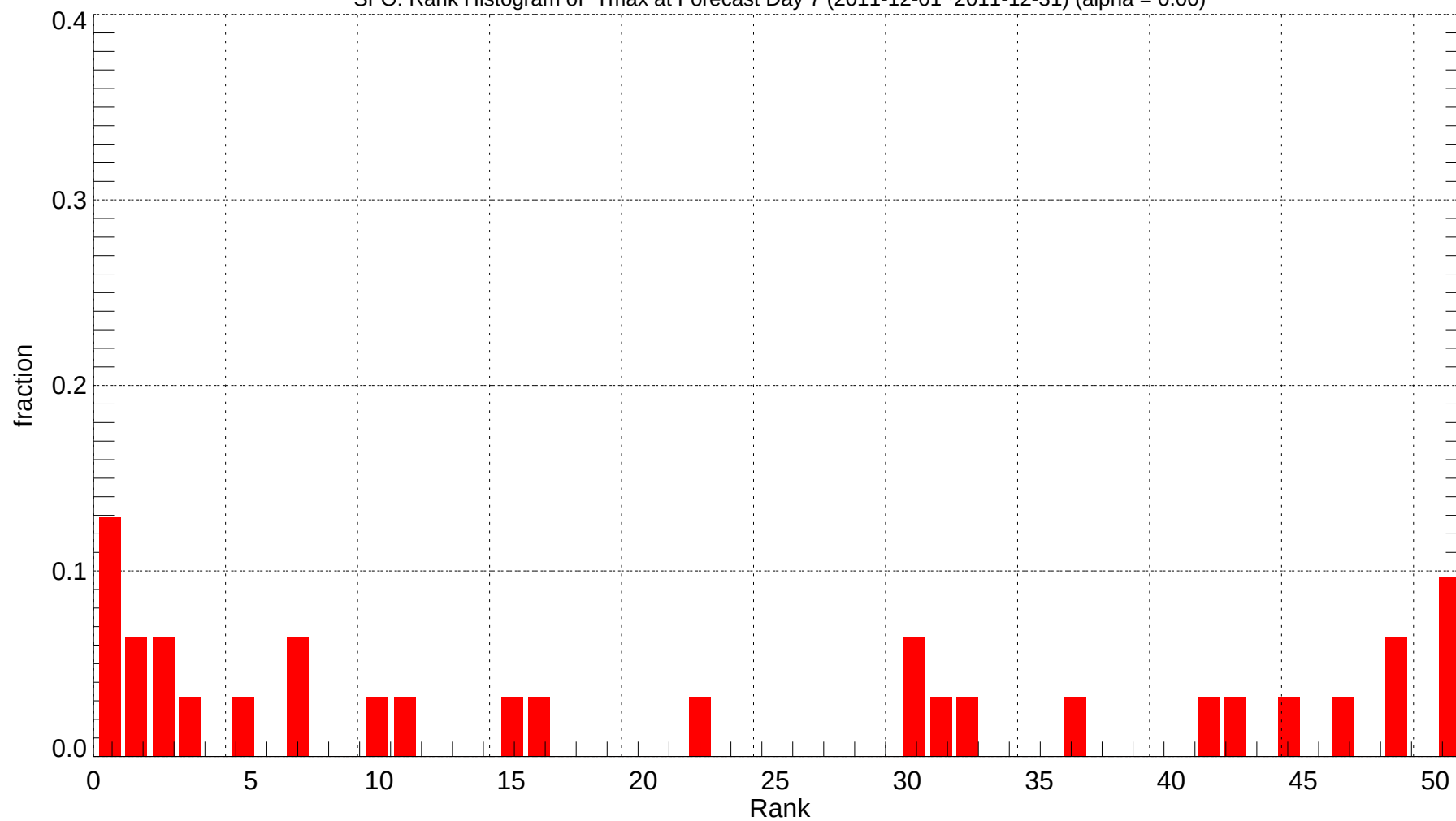
SFO: Rank Histogram of Tmax at Forecast Day 7 (2011-12-01~2011-12-31) (alpha = 0.00)
