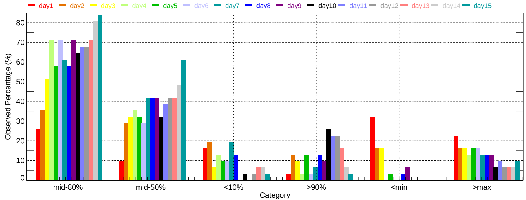
Observed Percentage of Ensembles - MCN: Min Temperature (2011-12-01~2011-12-31)
