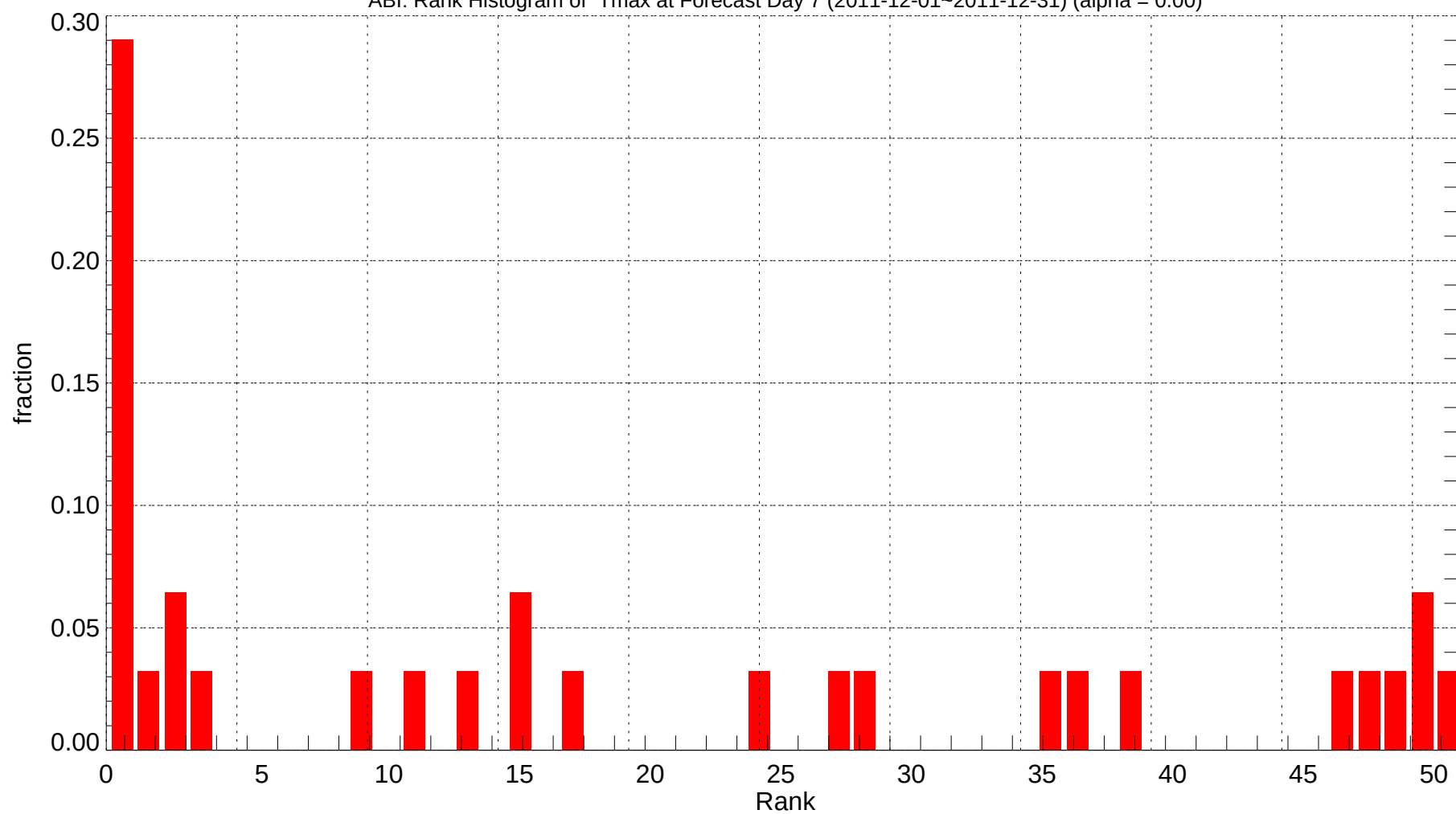
ABI: Rank Histogram of Tmax at Forecast Day 7 (2011-12-01~2011-12-31) (alpha = 0.00)
