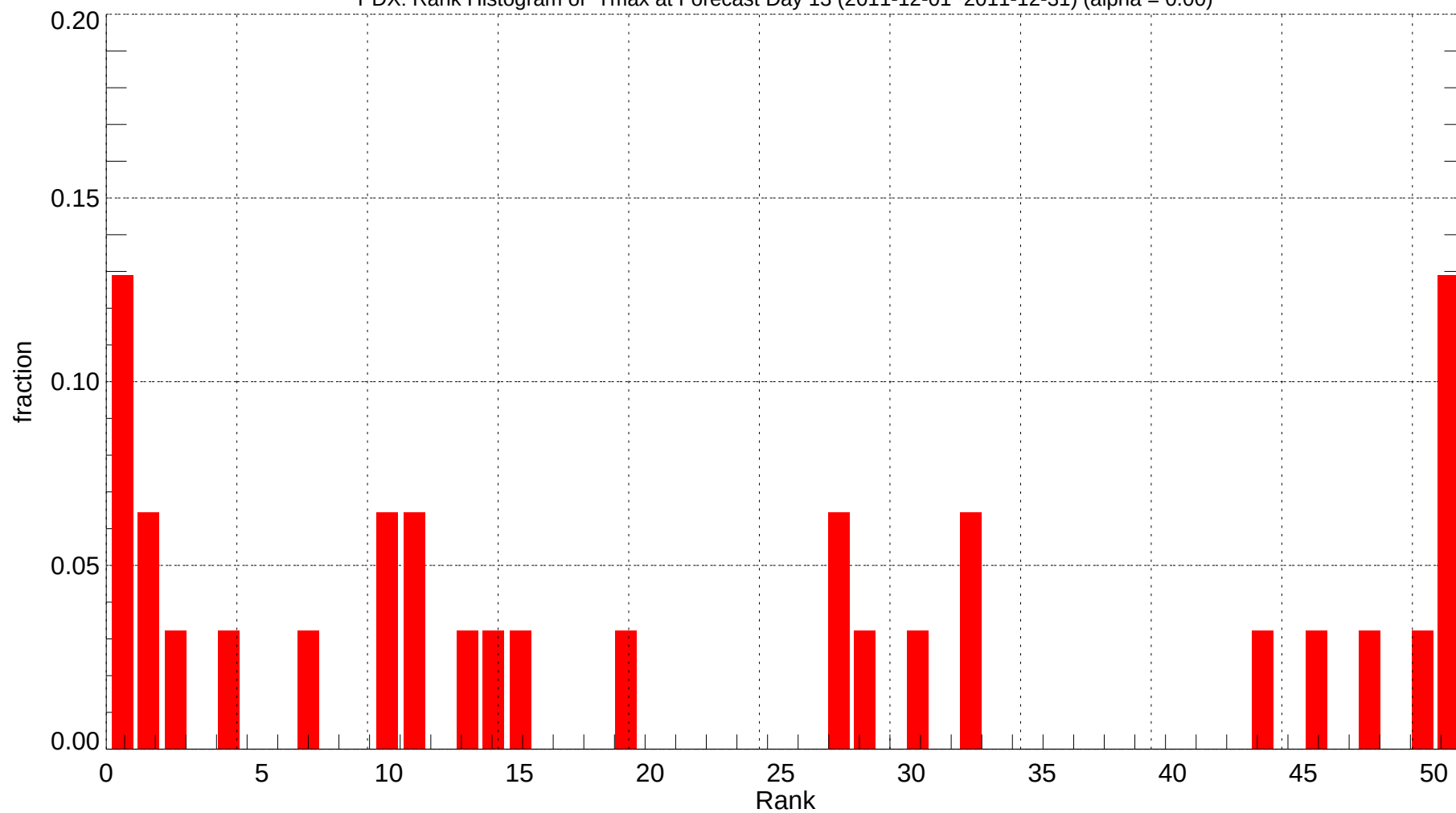
PDX: Rank Histogram of Tmax at Forecast Day 13 (2011-12-01~2011-12-31) (alpha = 0.00)
