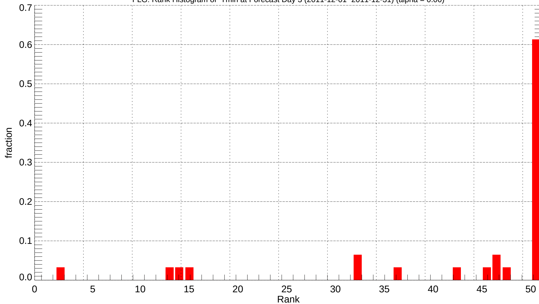
FLG: Rank Histogram of Tmin at Forecast Day 3 (2011-12-01~2011-12-31) (alpha = 0.00)
