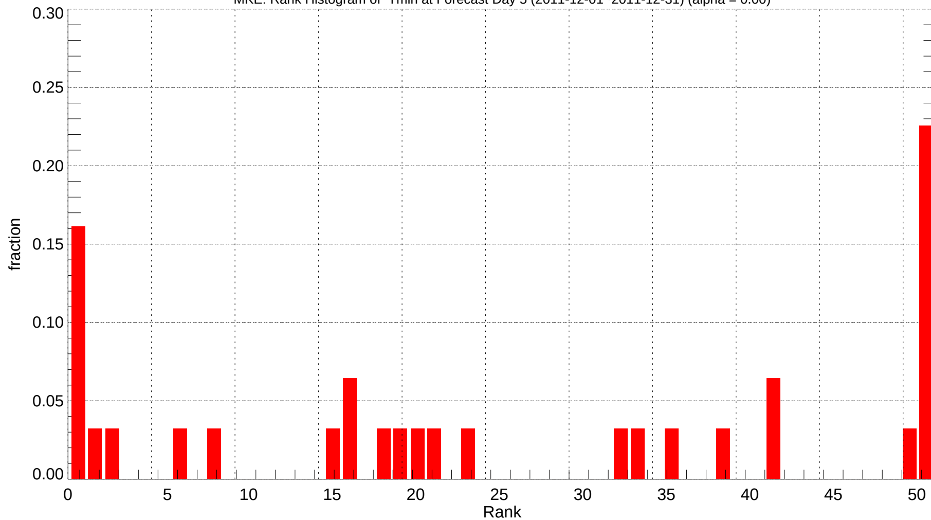
MKE: Rank Histogram of Tmin at Forecast Day 5 (2011-12-01~2011-12-31) (alpha = 0.00)
