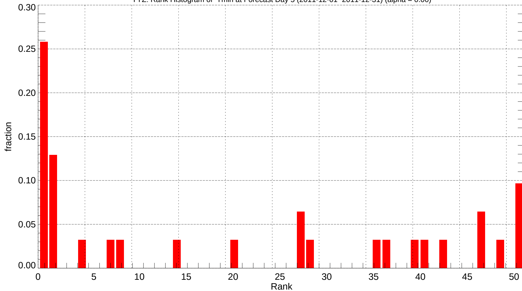
YYZ: Rank Histogram of Tmin at Forecast Day 5 (2011-12-01~2011-12-31) (alpha = 0.00)
