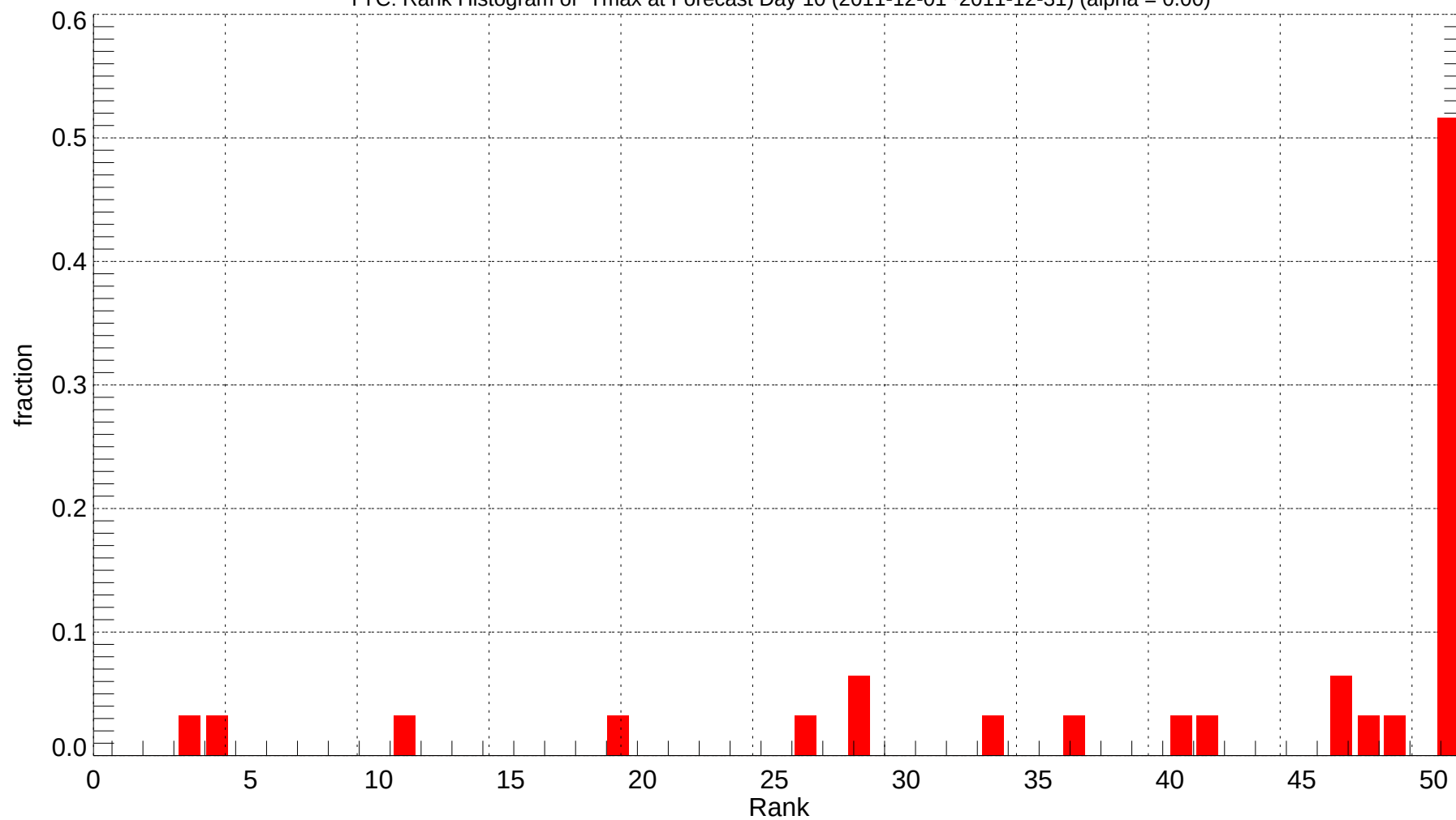
YYC: Rank Histogram of Tmax at Forecast Day 10 (2011-12-01~2011-12-31) (alpha = 0.00)
