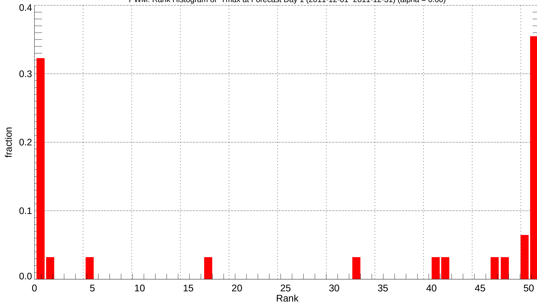
PWM: Rank Histogram of Tmax at Forecast Day 1 (2011-12-01~2011-12-31) (alpha = 0.00)
