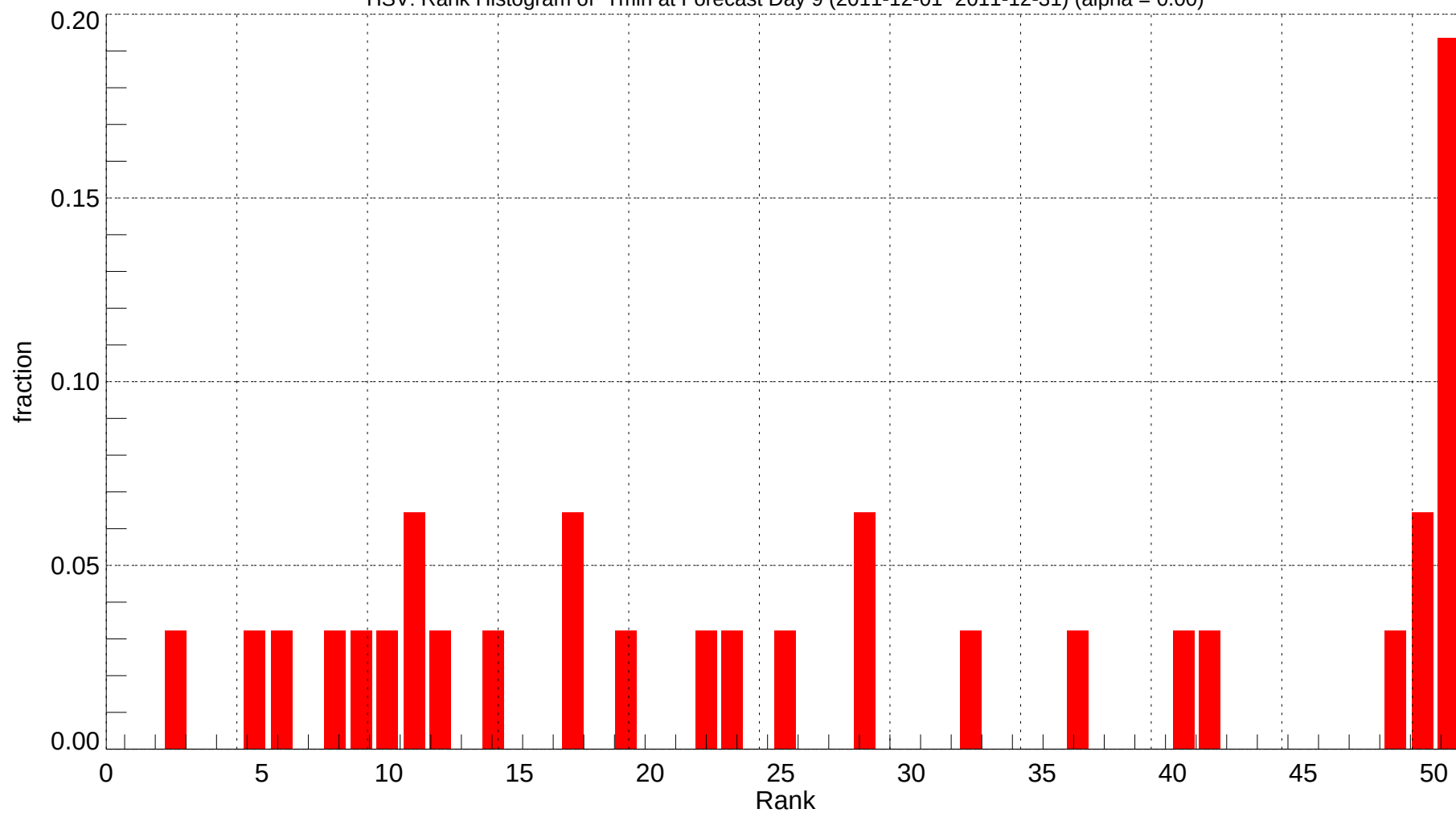
HSV: Rank Histogram of Tmin at Forecast Day 9 (2011-12-01~2011-12-31) (alpha = 0.00)
