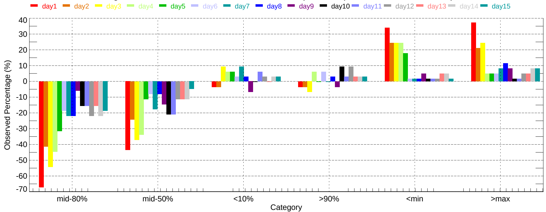
Observed Percentage Deviation of Ensembles - FAR: Max Temperature (2011-12-01~2011-12-31)
