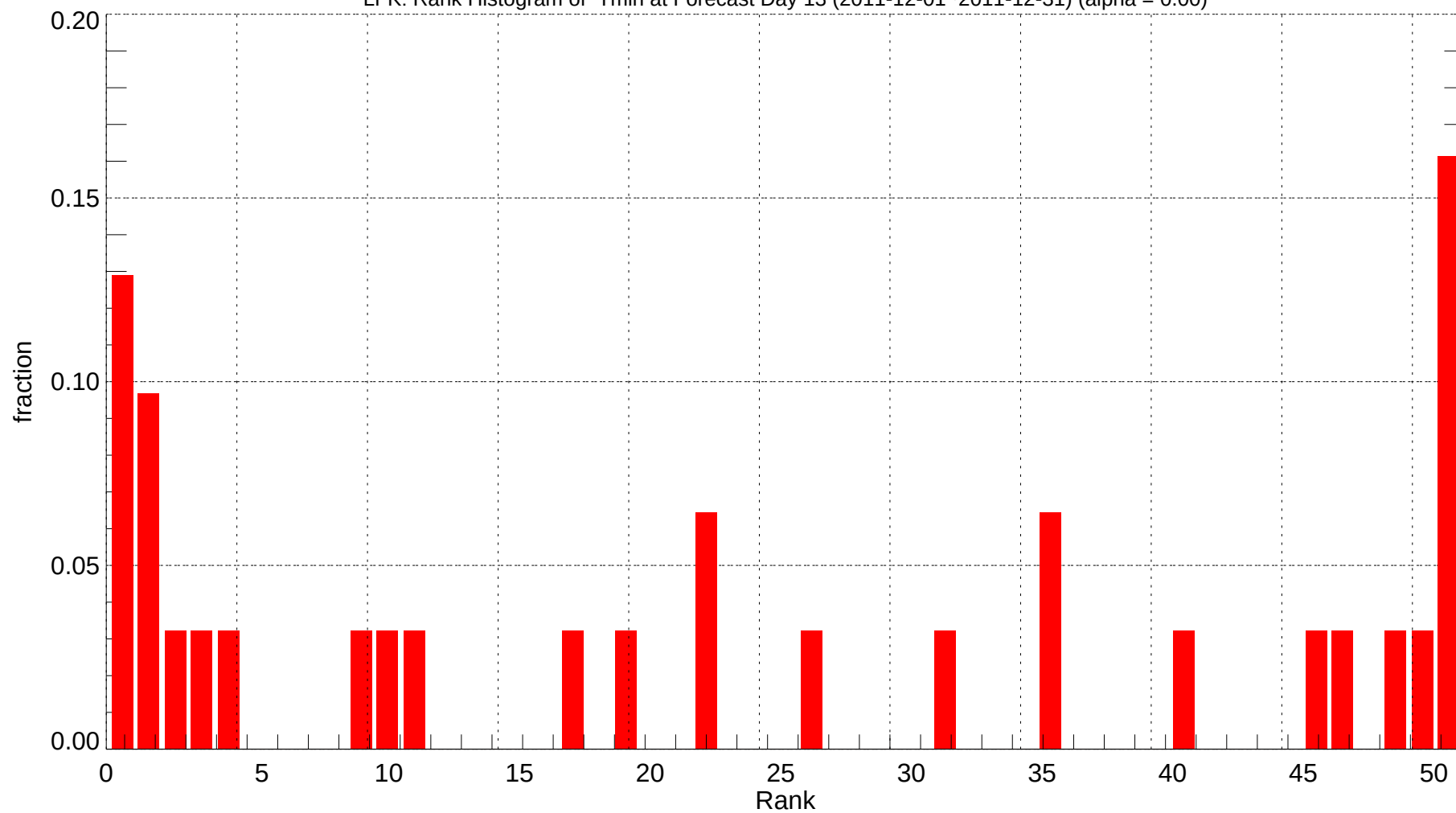
LFK: Rank Histogram of Tmin at Forecast Day 13 (2011-12-01~2011-12-31) (alpha = 0.00)
