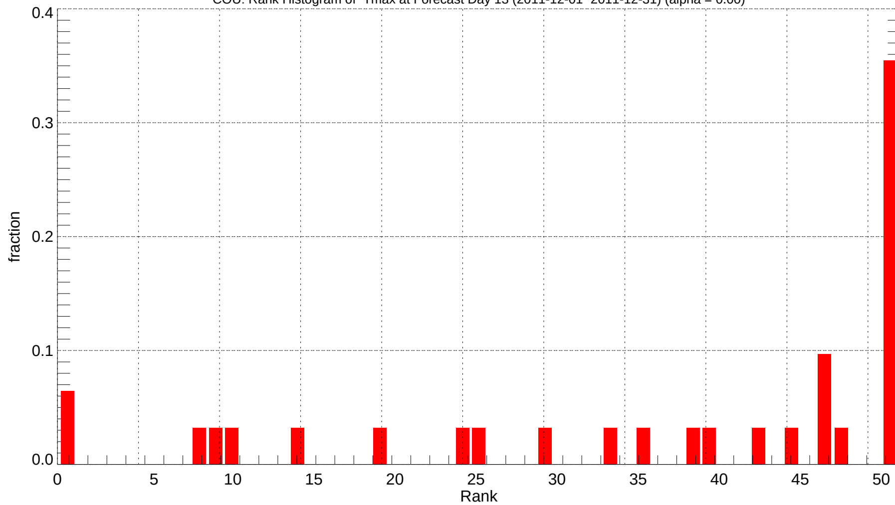
COU: Rank Histogram of Tmax at Forecast Day 13 (2011-12-01~2011-12-31) (alpha = 0.00)
