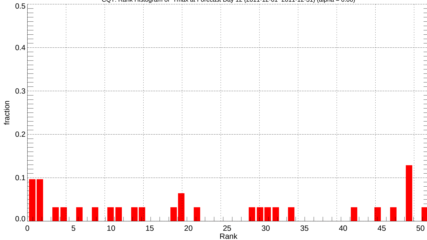
CQT: Rank Histogram of Tmax at Forecast Day 12 (2011-12-01~2011-12-31) (alpha = 0.00)
