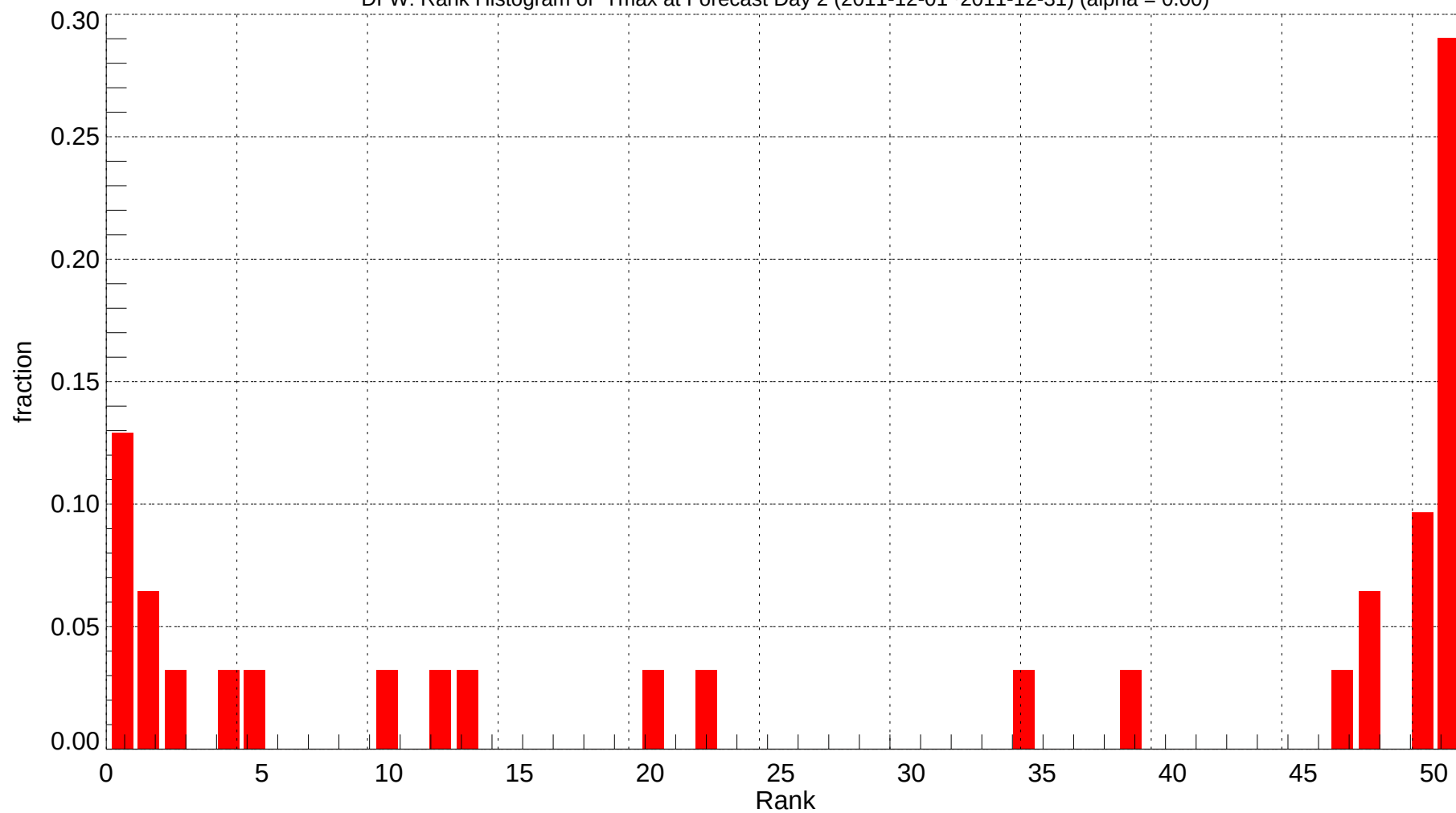
DFW: Rank Histogram of Tmax at Forecast Day 2 (2011-12-01~2011-12-31) (alpha = 0.00)
