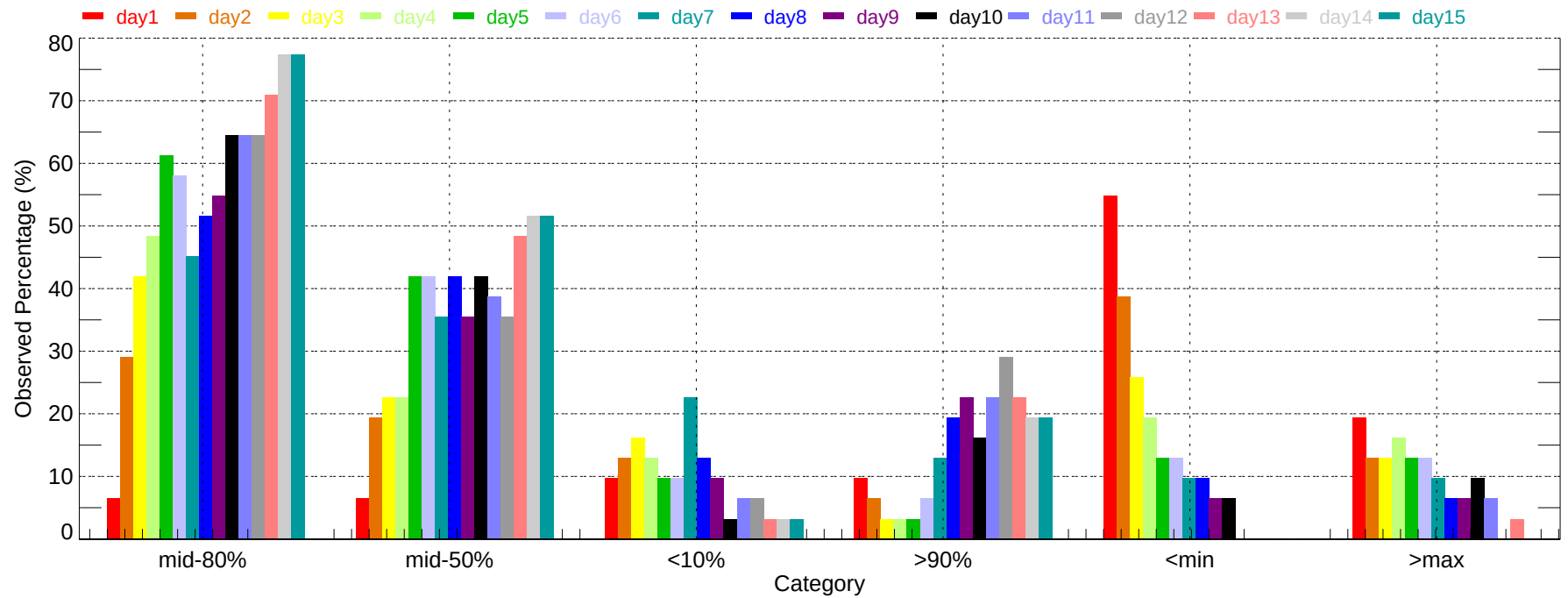
Observed Percentage of Ensembles - ILG: Max Temperature (2011-12-01~2011-12-31)
