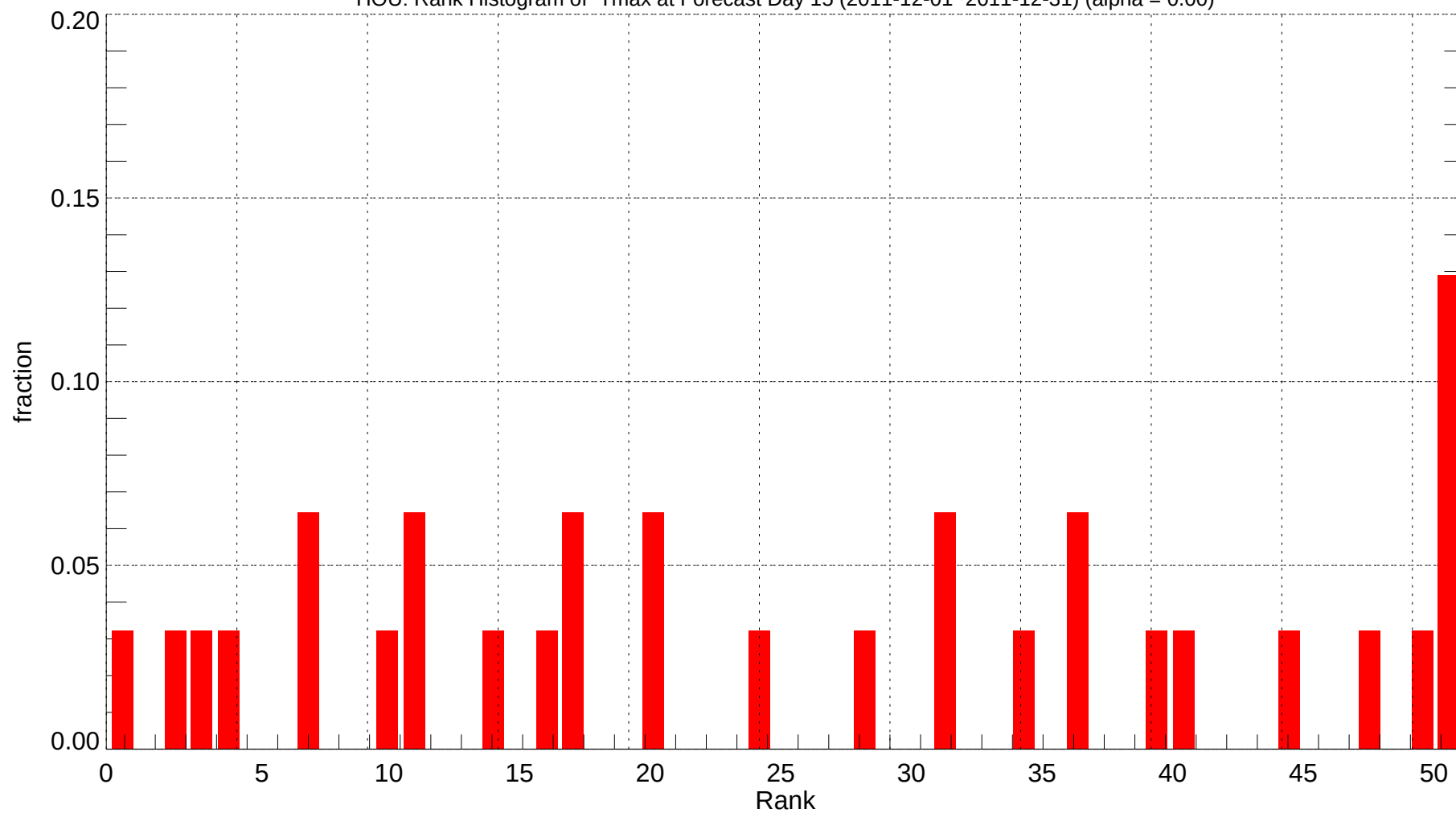
HOU: Rank Histogram of Tmax at Forecast Day 15 (2011-12-01~2011-12-31) (alpha = 0.00)
