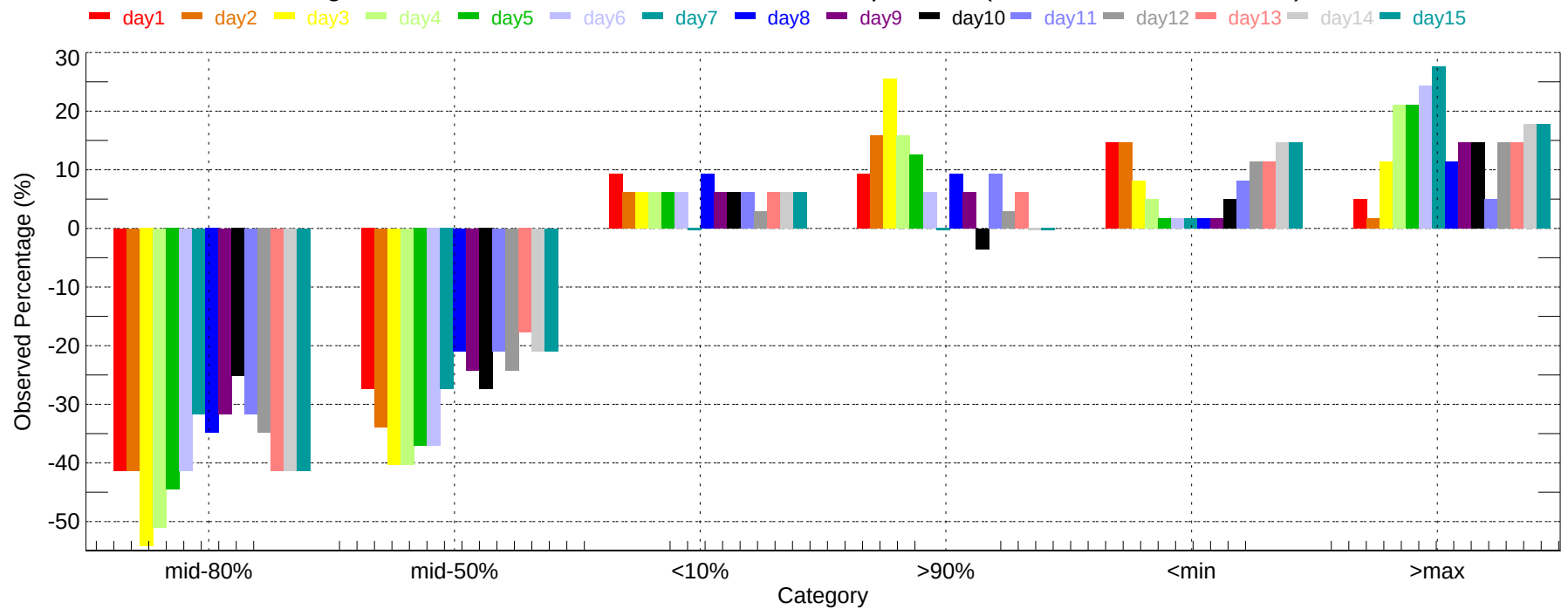
Observed Percentage Deviation of Ensembles - TYR: Max Temperature (2011-12-01~2011-12-31)
