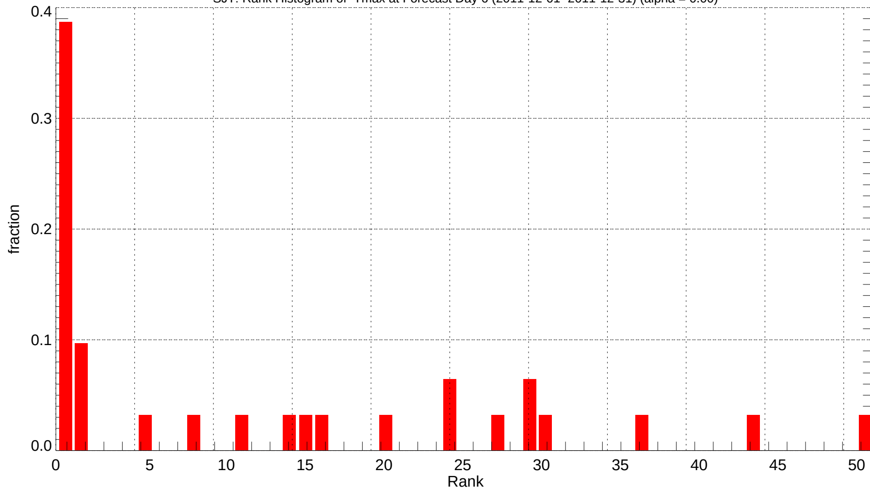
SJT: Rank Histogram of Tmax at Forecast Day 6 (2011-12-01~2011-12-31) (alpha = 0.00)
