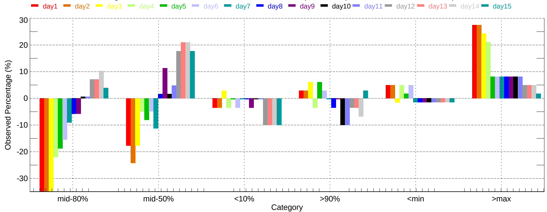
Observed Percentage Deviation of Ensembles - SAC: Max Temperature (2011-12-01~2011-12-31)
