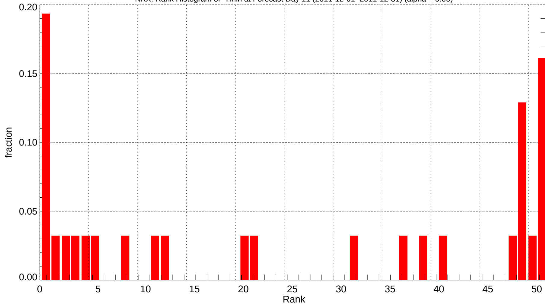
NKX: Rank Histogram of Tmin at Forecast Day 11 (2011-12-01~2011-12-31) (alpha = 0.00)
