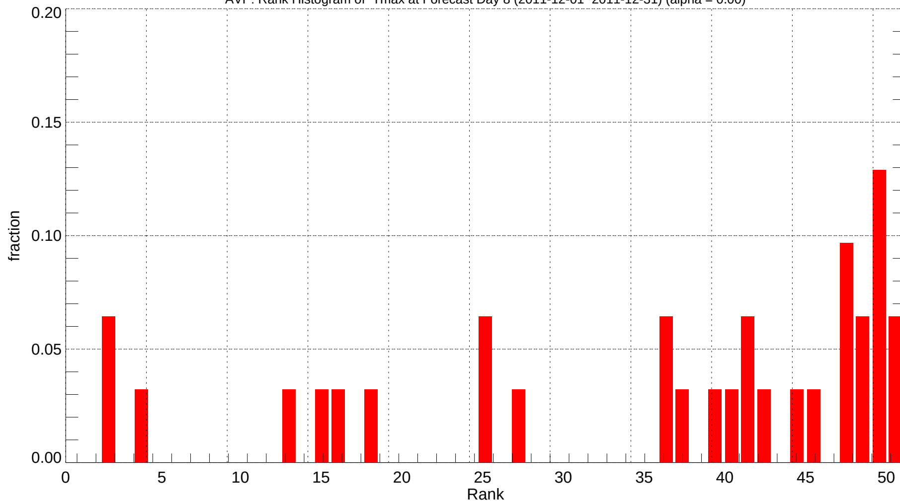
AVP: Rank Histogram of Tmax at Forecast Day 8 (2011-12-01~2011-12-31) (alpha = 0.00)
