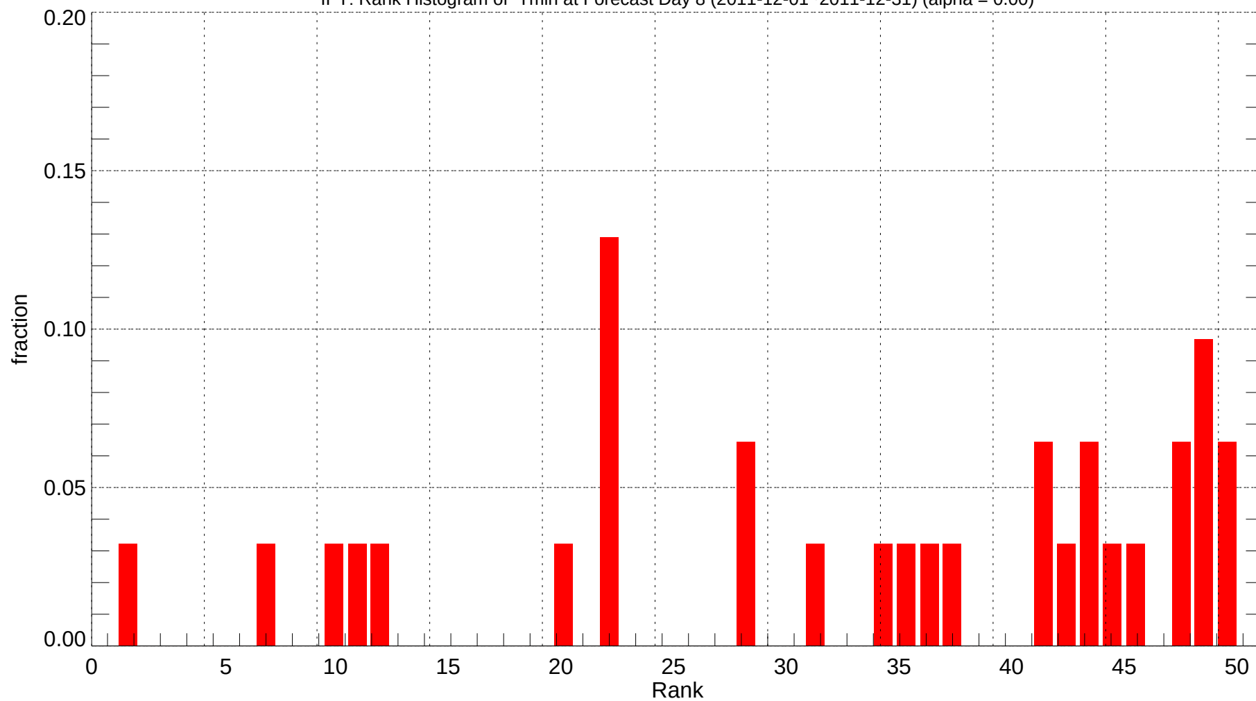
IPT: Rank Histogram of Tmin at Forecast Day 8 (2011-12-01~2011-12-31) (alpha = 0.00)
