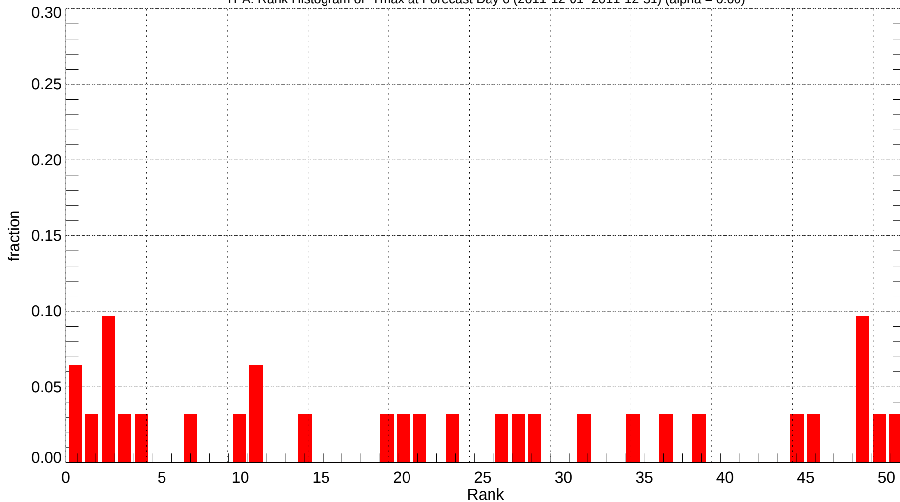
TPA: Rank Histogram of Tmax at Forecast Day 6 (2011-12-01~2011-12-31) (alpha = 0.00)
