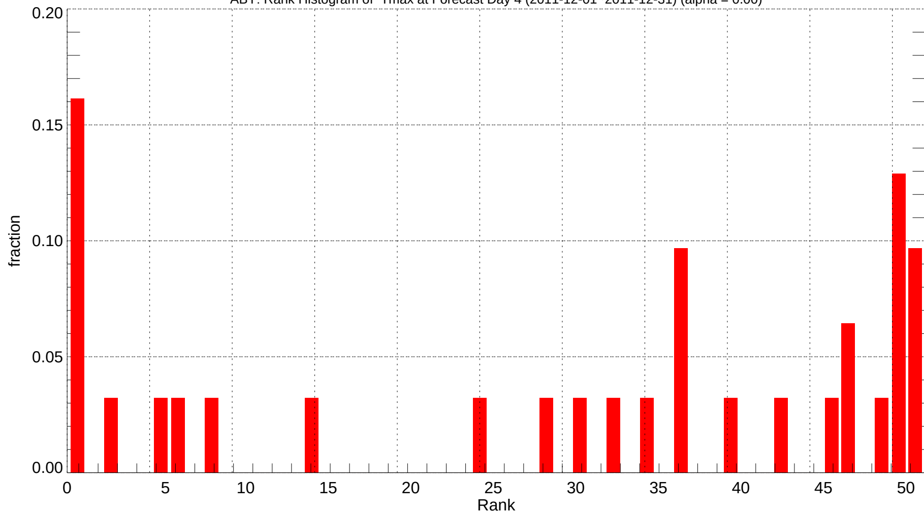
ABY: Rank Histogram of Tmax at Forecast Day 4 (2011-12-01~2011-12-31) (alpha = 0.00)
