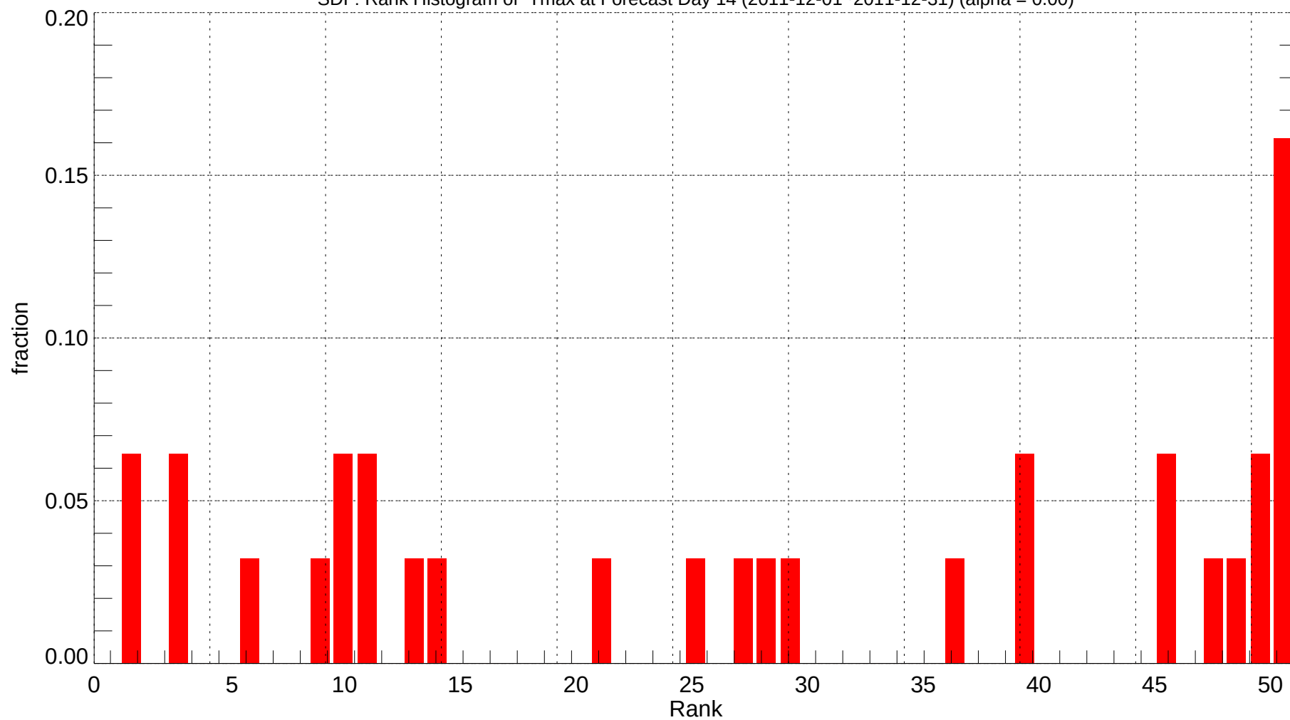
SDF: Rank Histogram of Tmax at Forecast Day 14 (2011-12-01~2011-12-31) (alpha = 0.00)
