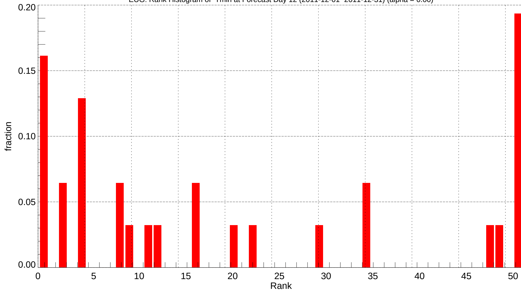
EUG: Rank Histogram of Tmin at Forecast Day 12 (2011-12-01~2011-12-31) (alpha = 0.00)
