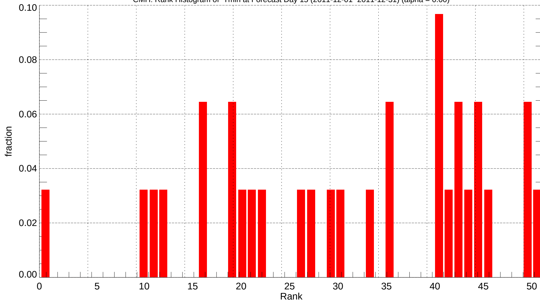
CMH: Rank Histogram of Tmin at Forecast Day 15 (2011-12-01~2011-12-31) (alpha = 0.00)
