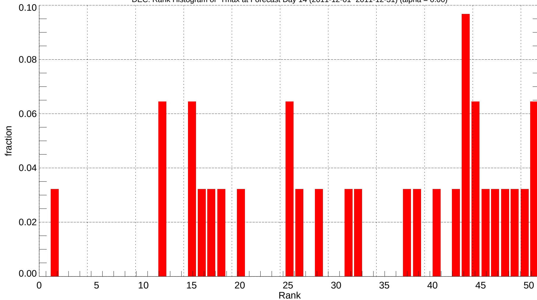
DEC: Rank Histogram of Tmax at Forecast Day 14 (2011-12-01~2011-12-31) (alpha = 0.00)
