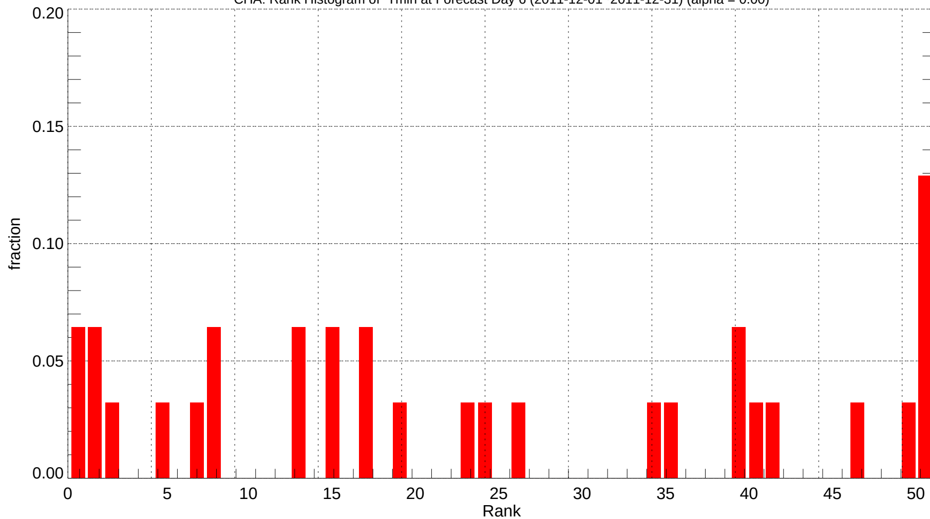
CHA: Rank Histogram of Tmin at Forecast Day 6 (2011-12-01~2011-12-31) (alpha = 0.00)
