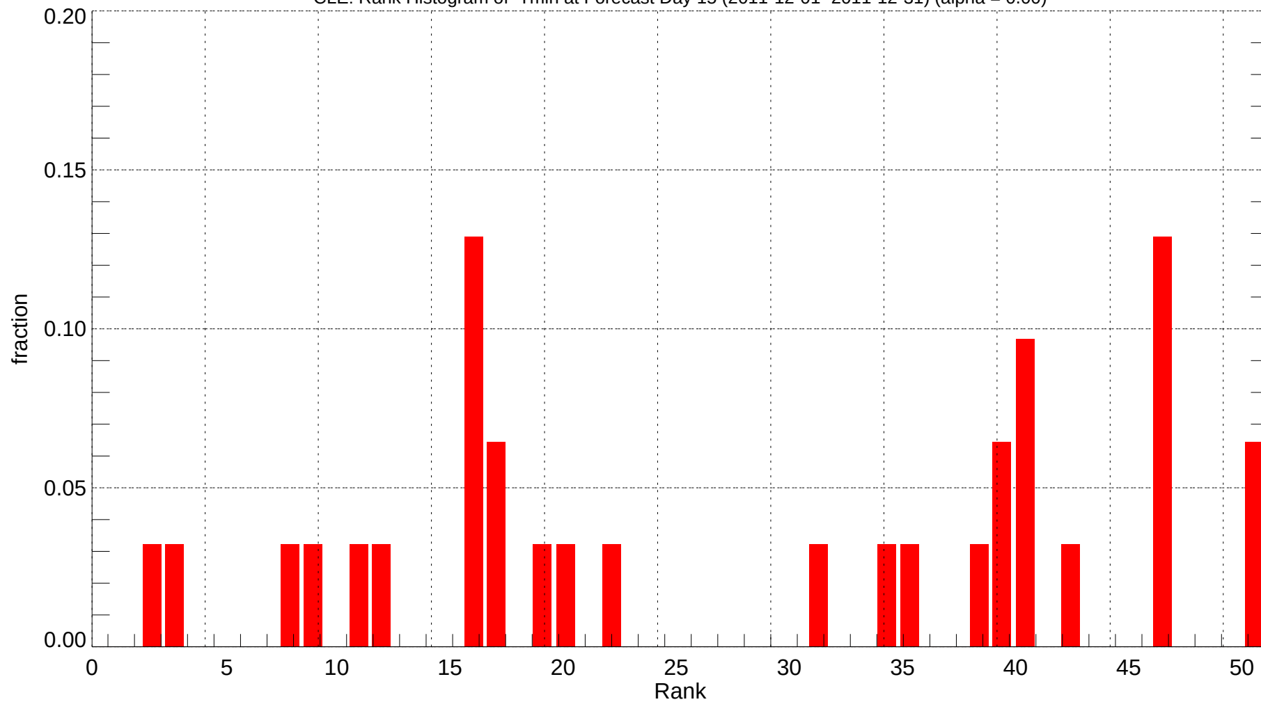
CLE: Rank Histogram of Tmin at Forecast Day 15 (2011-12-01~2011-12-31) (alpha = 0.00)
