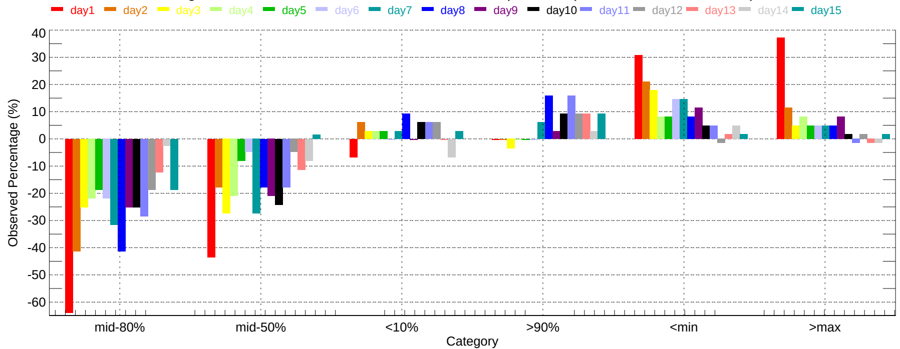
Observed Percentage Deviation of Ensembles - PWM: Max Temperature (2011-12-01~2011-12-31)
