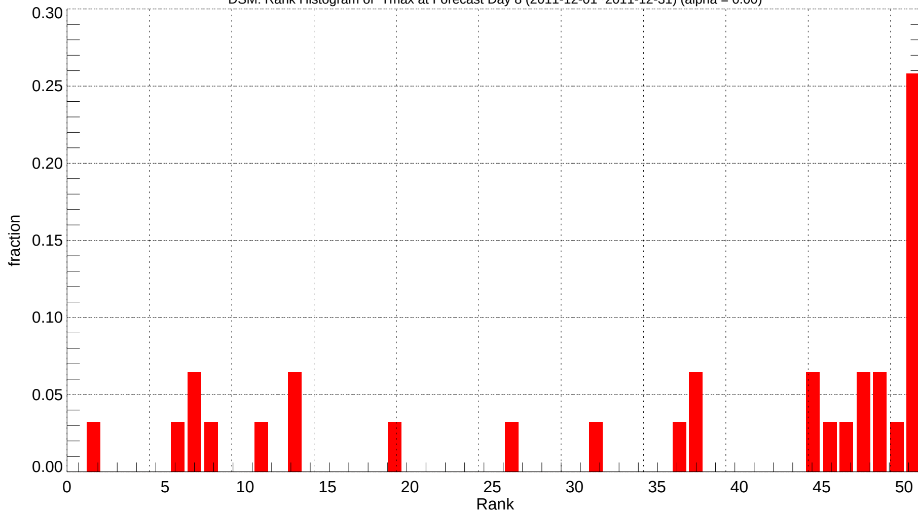
DSM: Rank Histogram of Tmax at Forecast Day 8 (2011-12-01~2011-12-31) (alpha = 0.00)
