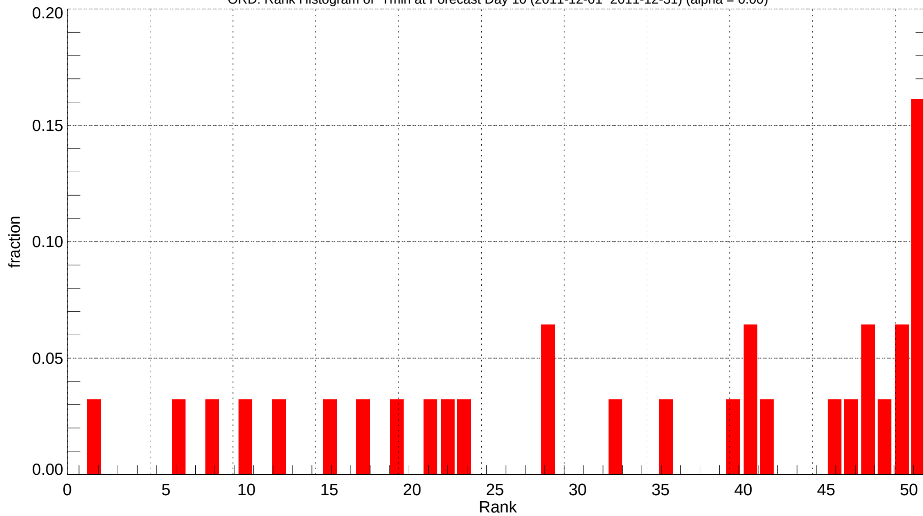
ORD: Rank Histogram of Tmin at Forecast Day 10 (2011-12-01~2011-12-31) (alpha = 0.00)
