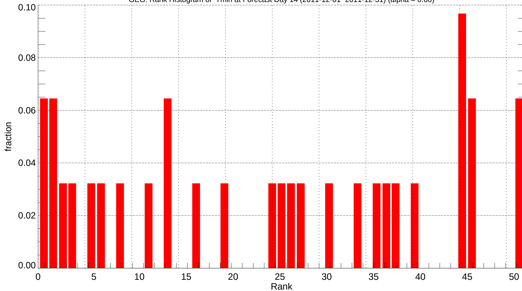
GEG: Rank Histogram of Tmin at Forecast Day 14 (2011-12-01~2011-12-31) (alpha = 0.00)
