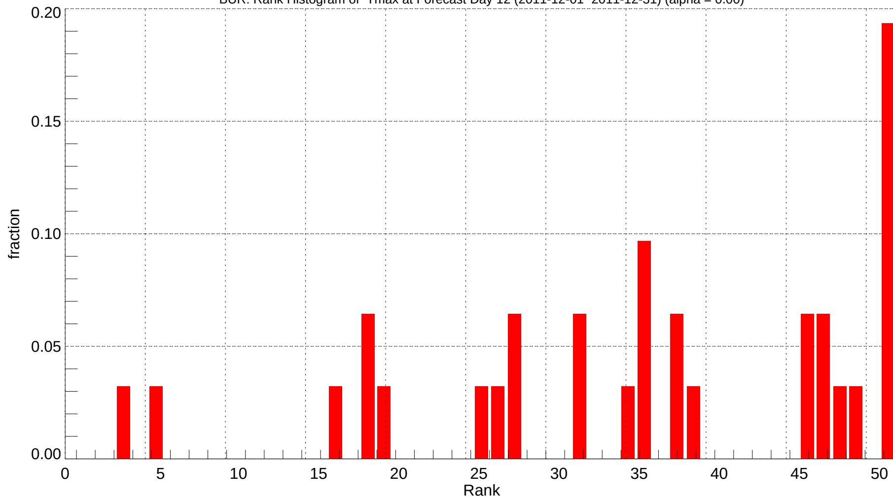
BUR: Rank Histogram of Tmax at Forecast Day 12 (2011-12-01~2011-12-31) (alpha = 0.00)
