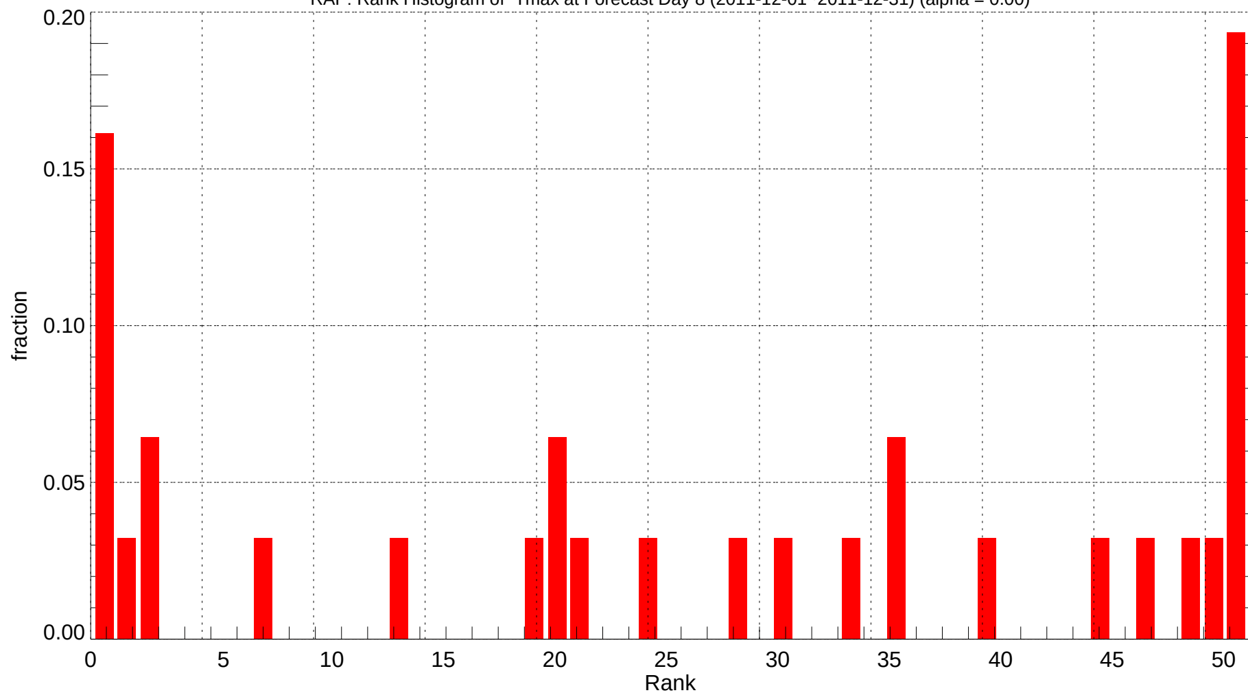
RAP: Rank Histogram of Tmax at Forecast Day 8 (2011-12-01~2011-12-31) (alpha = 0.00)
