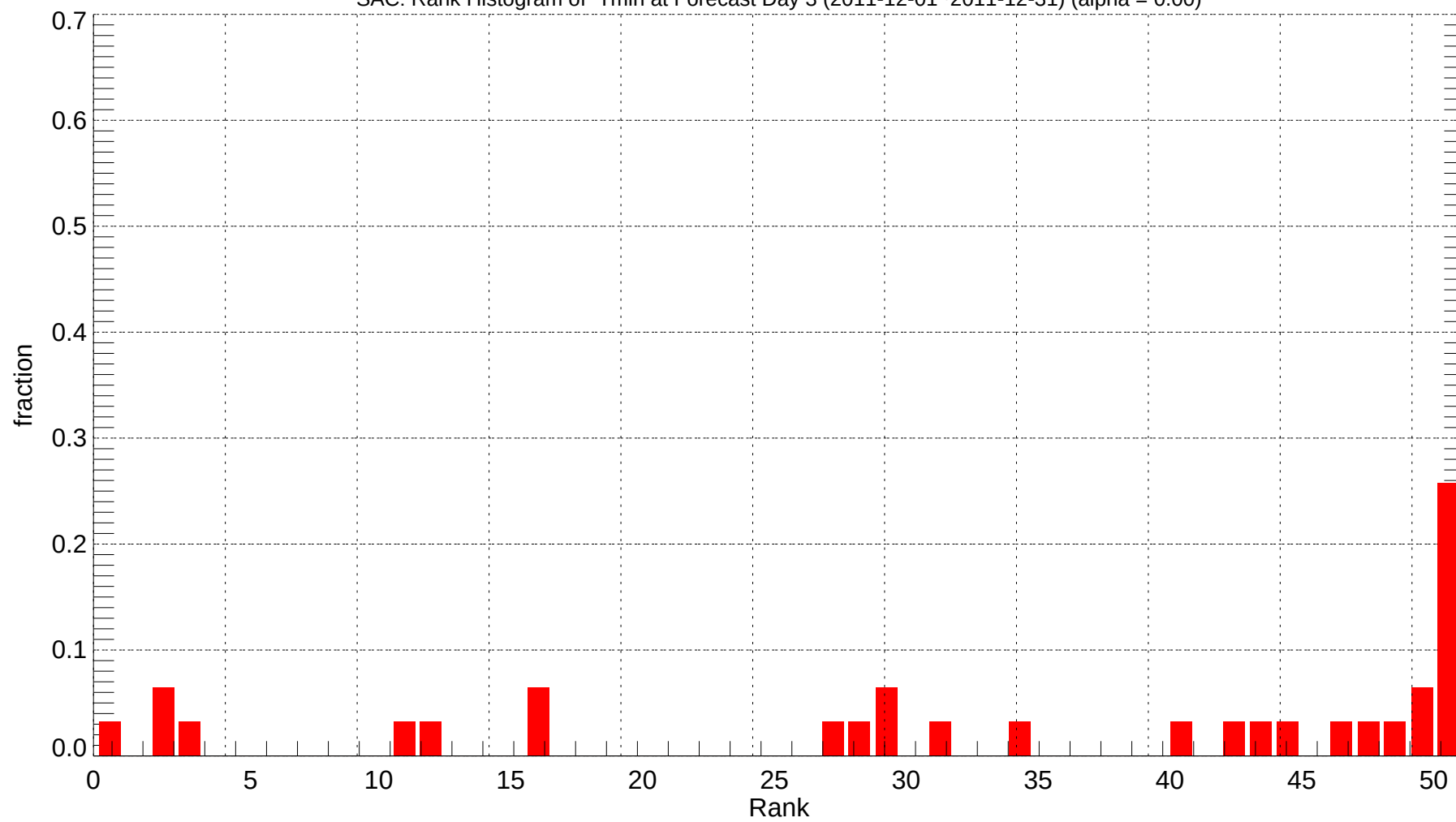
SAC: Rank Histogram of Tmin at Forecast Day 3 (2011-12-01~2011-12-31) (alpha = 0.00)
