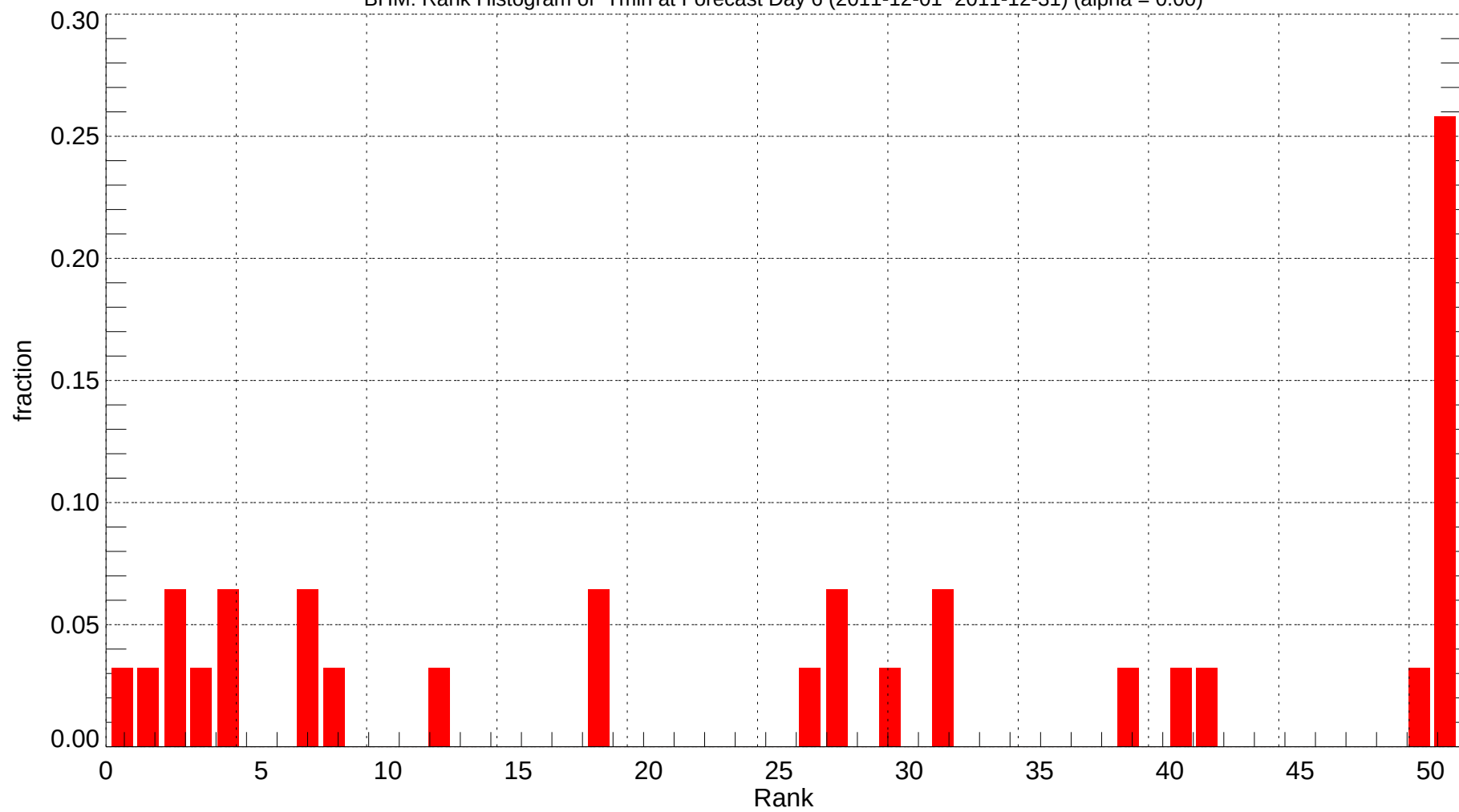
BHM: Rank Histogram of Tmin at Forecast Day 6 (2011-12-01~2011-12-31) (alpha = 0.00)
