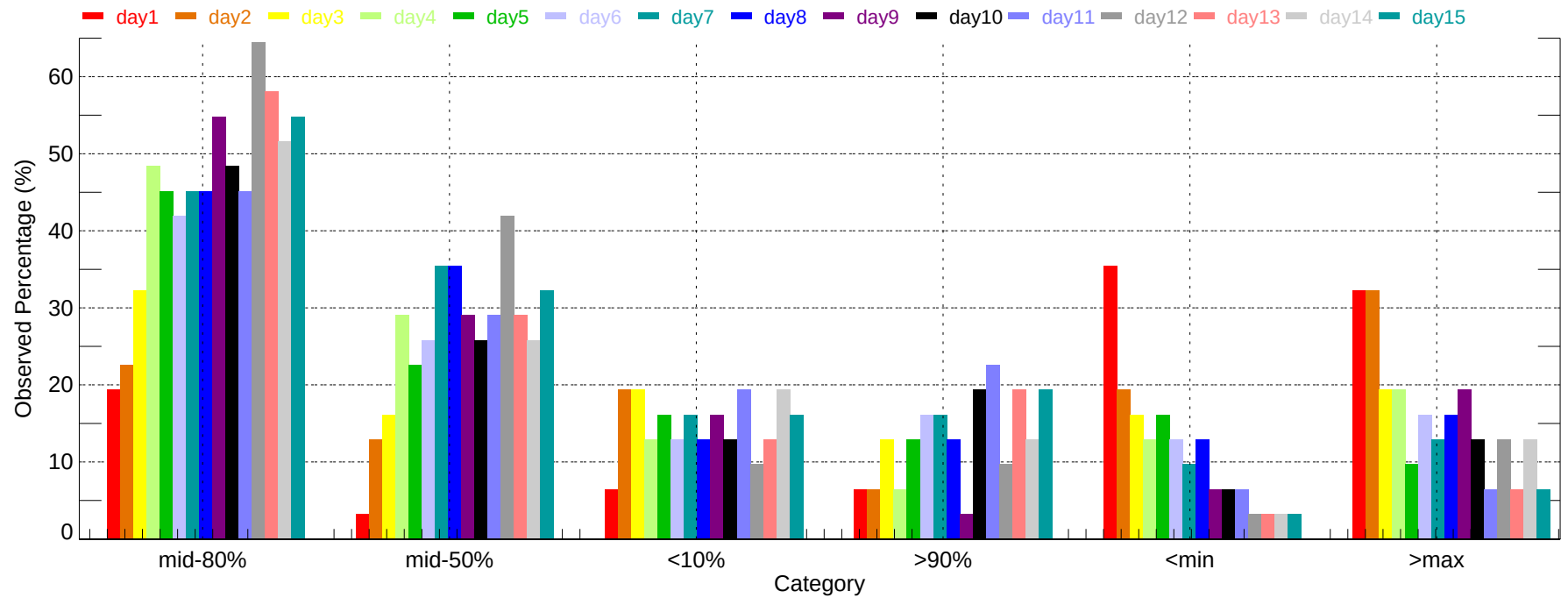
Observed Percentage of Ensembles - RAP: Max Temperature (2011-12-01~2011-12-31)
