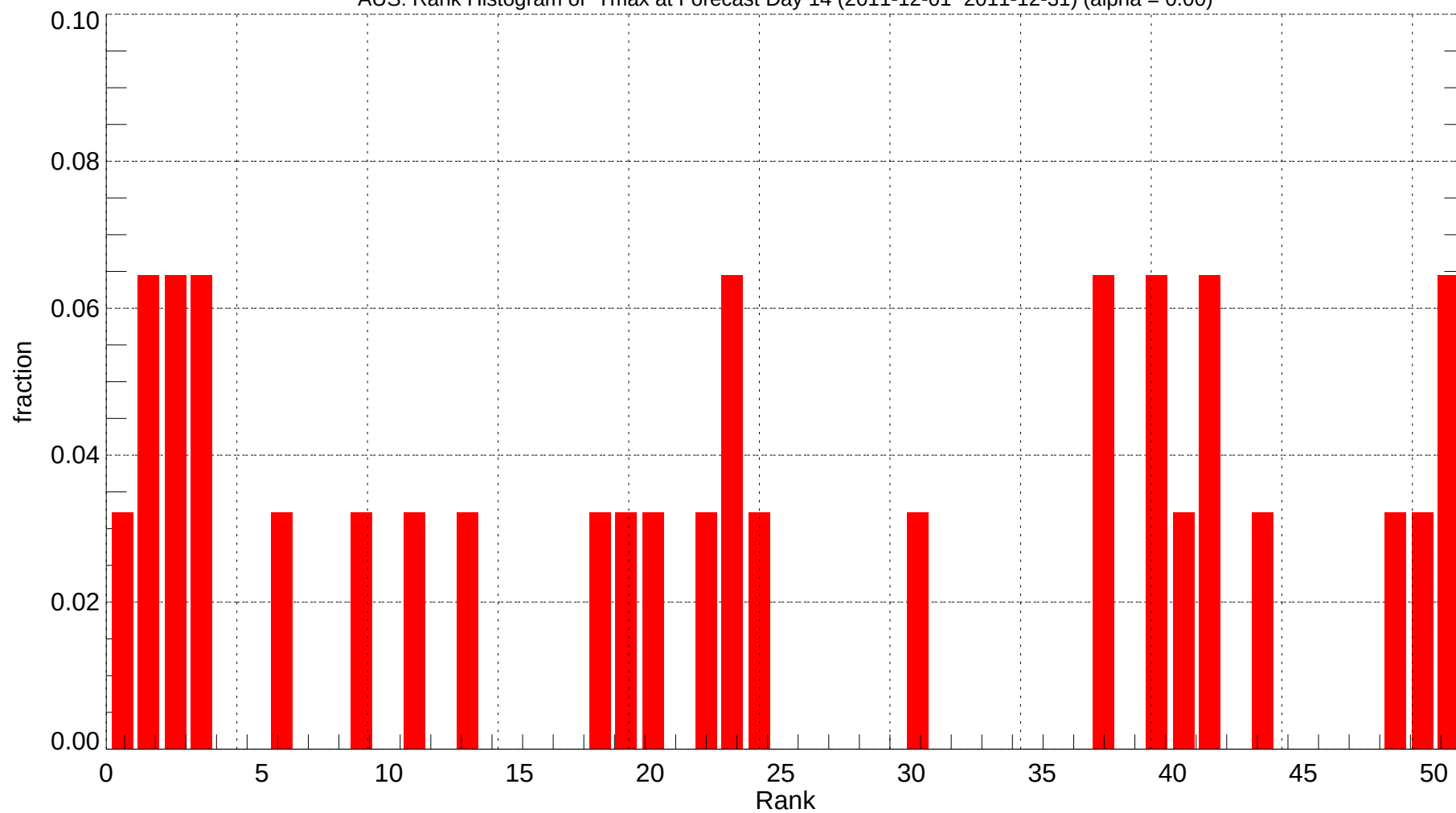
AUS: Rank Histogram of Tmax at Forecast Day 14 (2011-12-01~2011-12-31) (alpha = 0.00)
