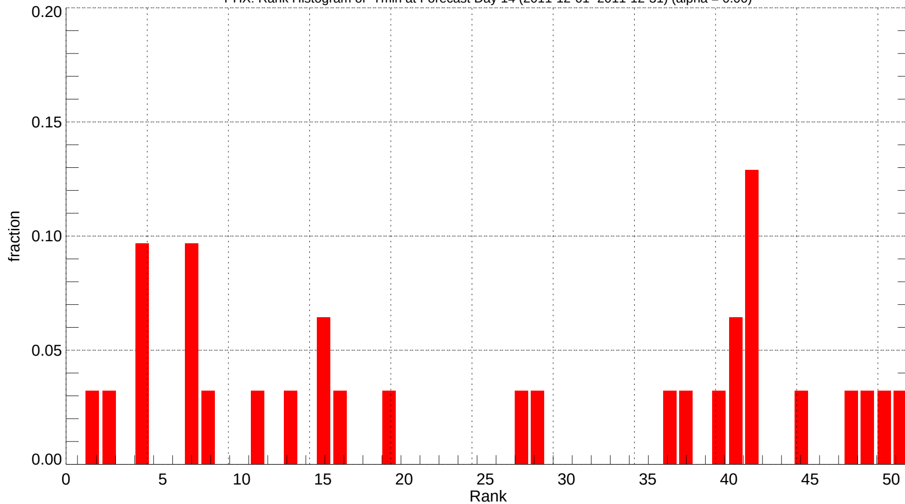
PHX: Rank Histogram of Tmin at Forecast Day 14 (2011-12-01~2011-12-31) (alpha = 0.00)
