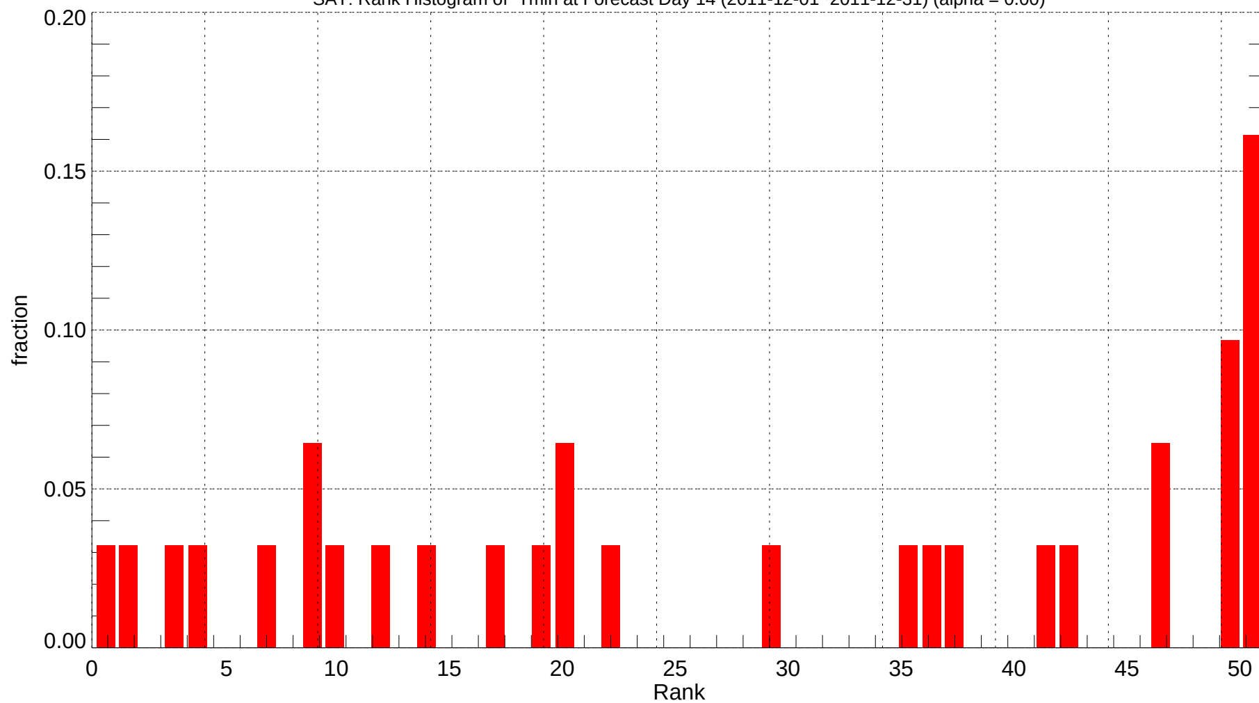
SAT: Rank Histogram of Tmin at Forecast Day 14 (2011-12-01~2011-12-31) (alpha = 0.00)
