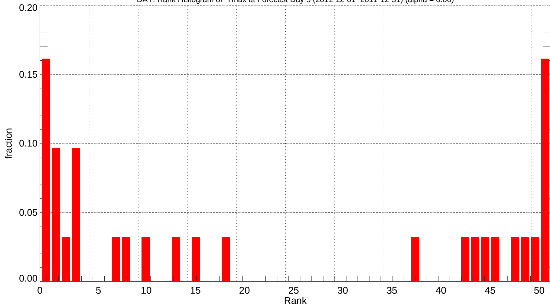
DAY: Rank Histogram of Tmax at Forecast Day 3 (2011-12-01~2011-12-31) (alpha = 0.00)
