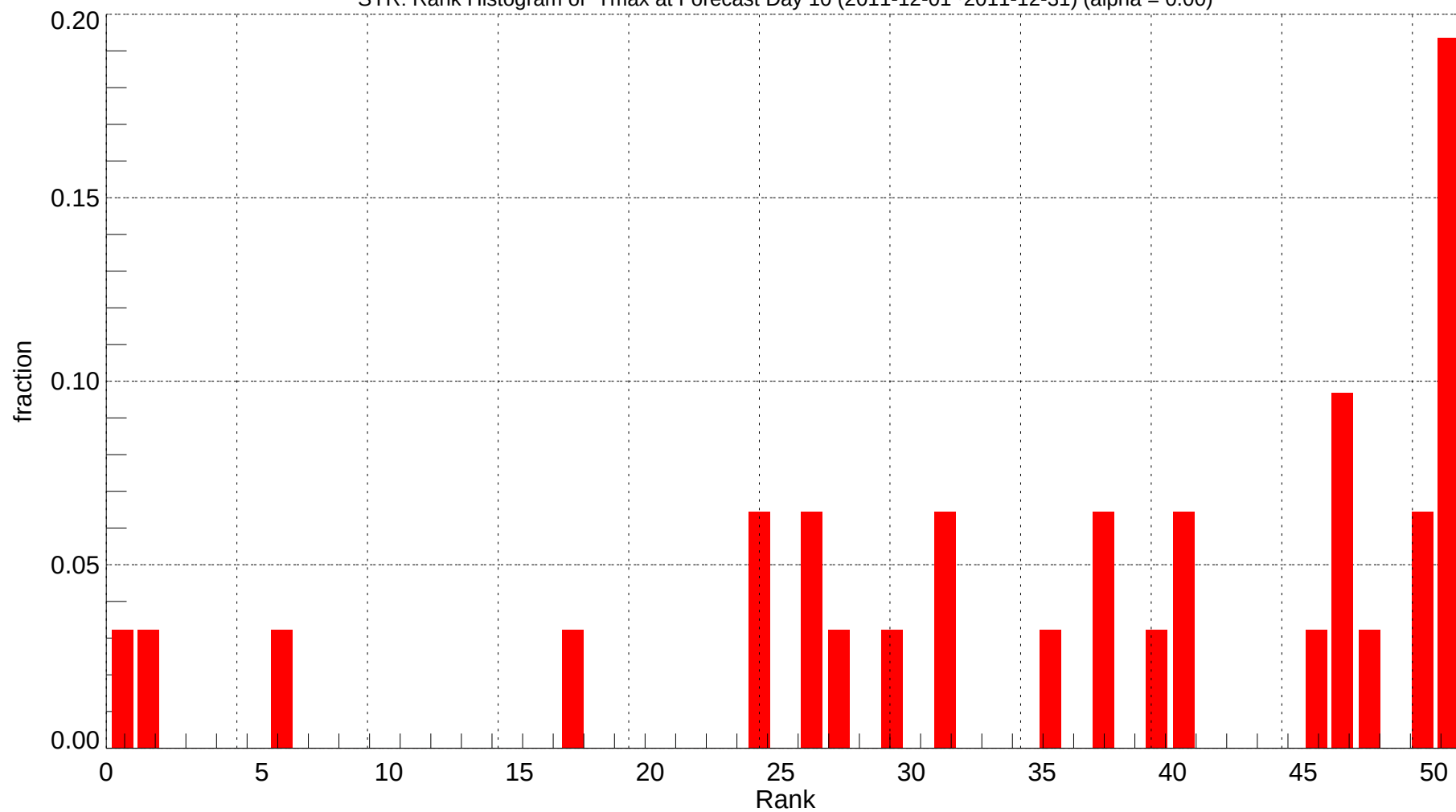
SYR: Rank Histogram of Tmax at Forecast Day 10 (2011-12-01~2011-12-31) (alpha = 0.00)
