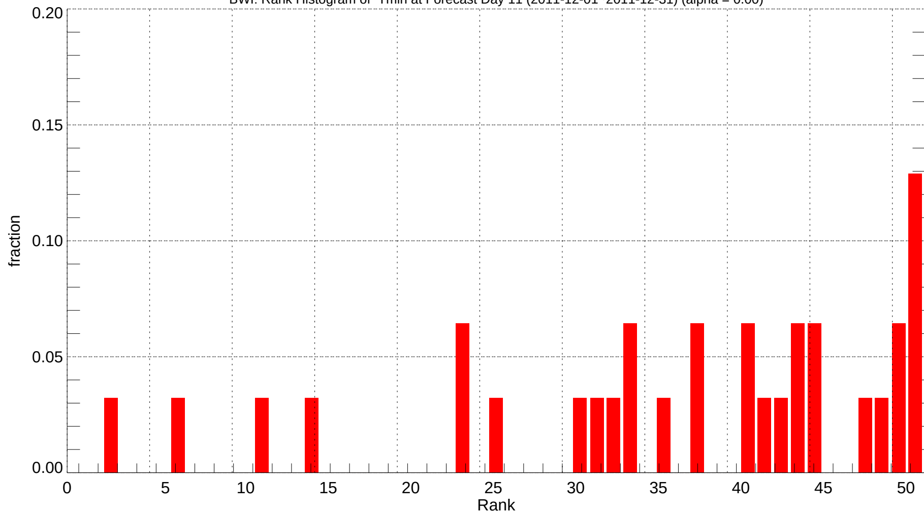
BWl: Rank Histogram of Tmin at Forecast Day 11 (2011-12-01~2011-12-31) (alpha = 0.00)
