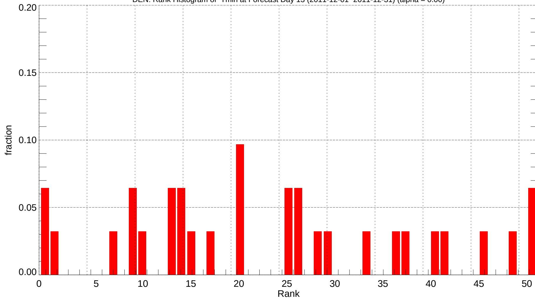
DEN: Rank Histogram of Tmin at Forecast Day 13 (2011-12-01~2011-12-31) (alpha = 0.00)
