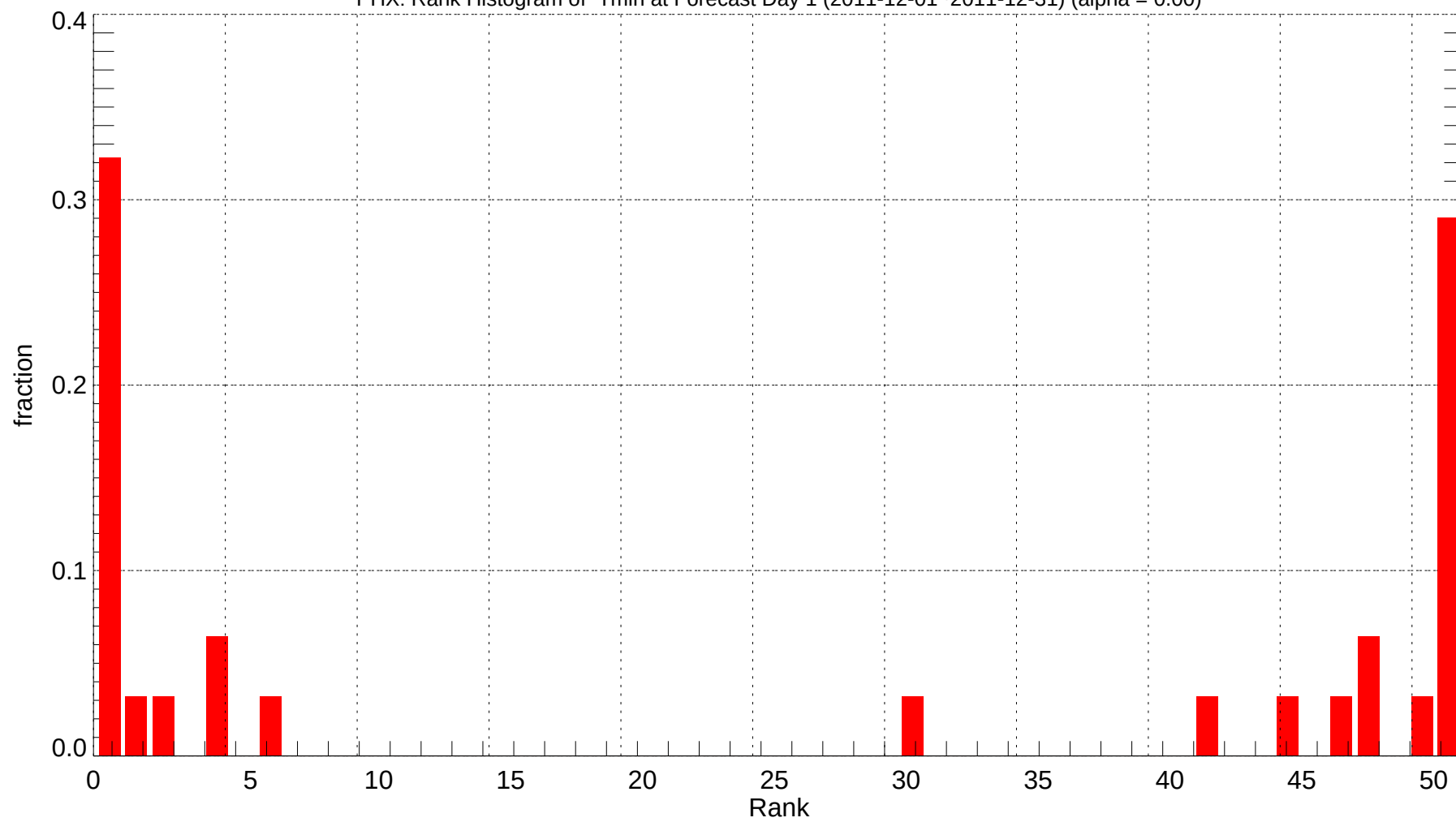
PHX: Rank Histogram of Tmin at Forecast Day 1 (2011-12-01~2011-12-31) (alpha = 0.00)
