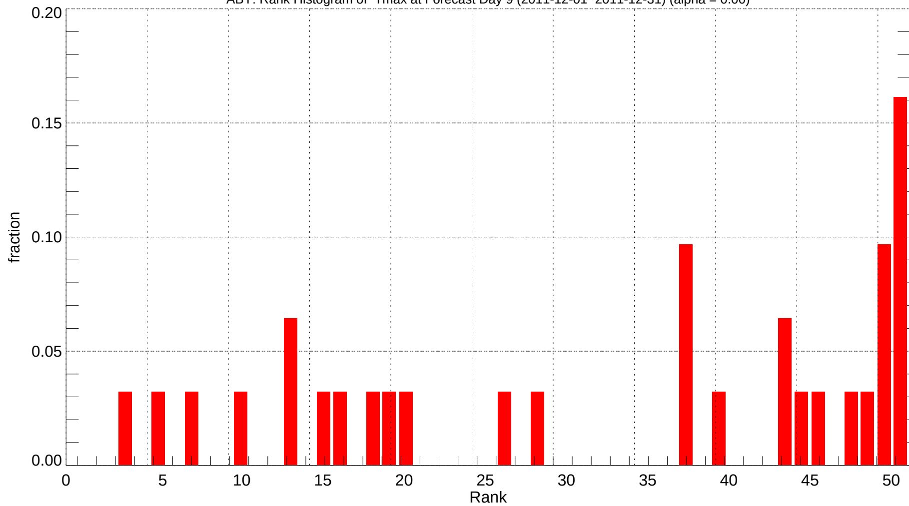
ABY: Rank Histogram of Tmax at Forecast Day 9 (2011-12-01~2011-12-31) (alpha = 0.00)
