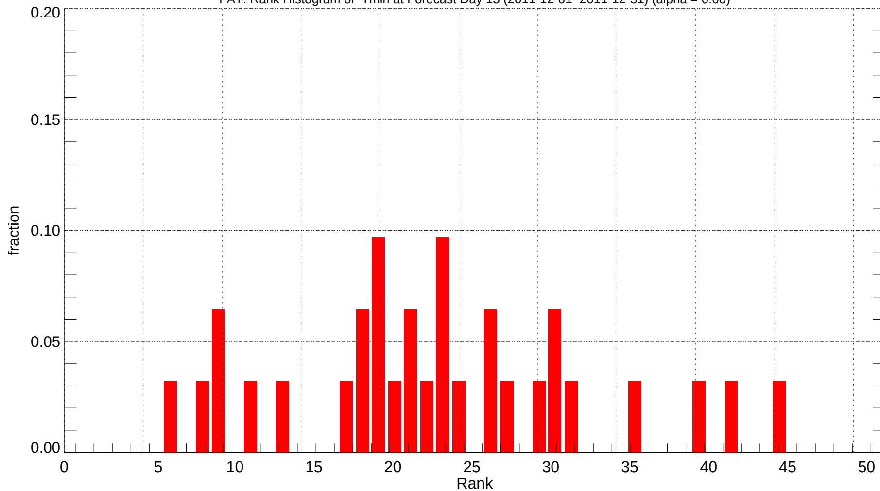
FAT: Rank Histogram of Tmin at Forecast Day 15 (2011-12-01~2011-12-31) (alpha = 0.00)
