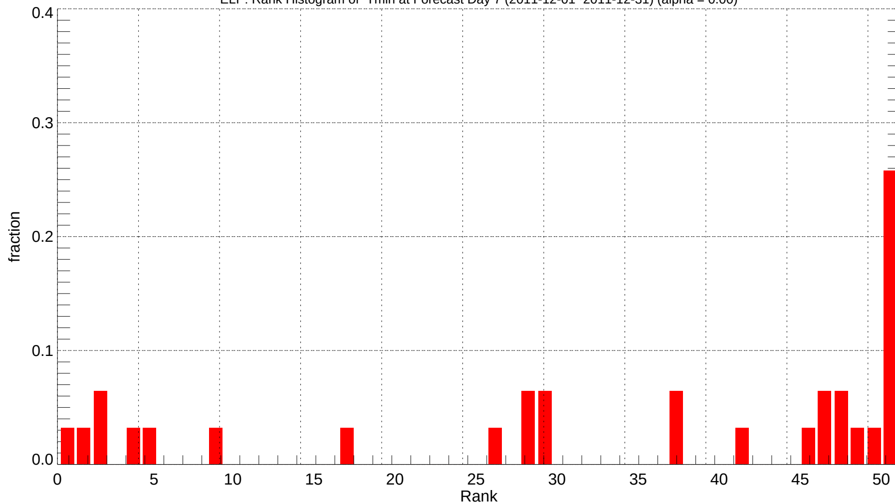
ELP: Rank Histogram of Tmin at Forecast Day 7 (2011-12-01~2011-12-31) (alpha = 0.00)
