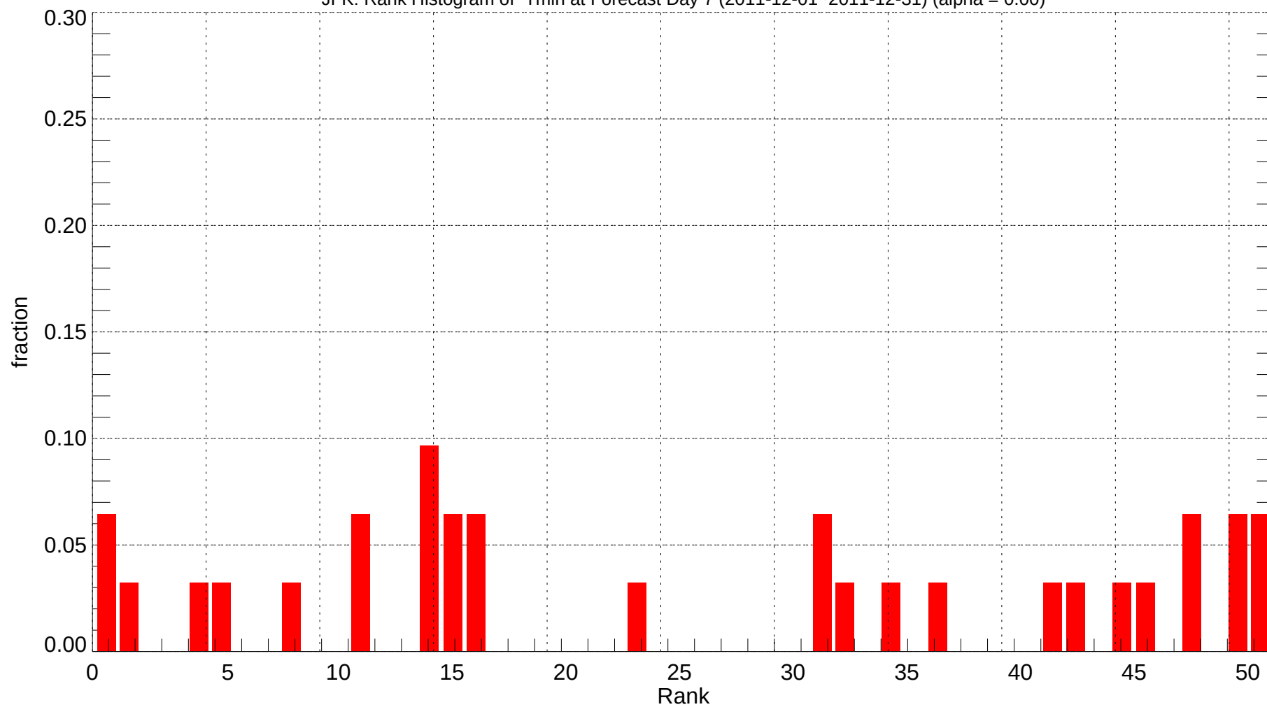
JFK: Rank Histogram of Tmin at Forecast Day 7 (2011-12-01~2011-12-31) (alpha = 0.00)
