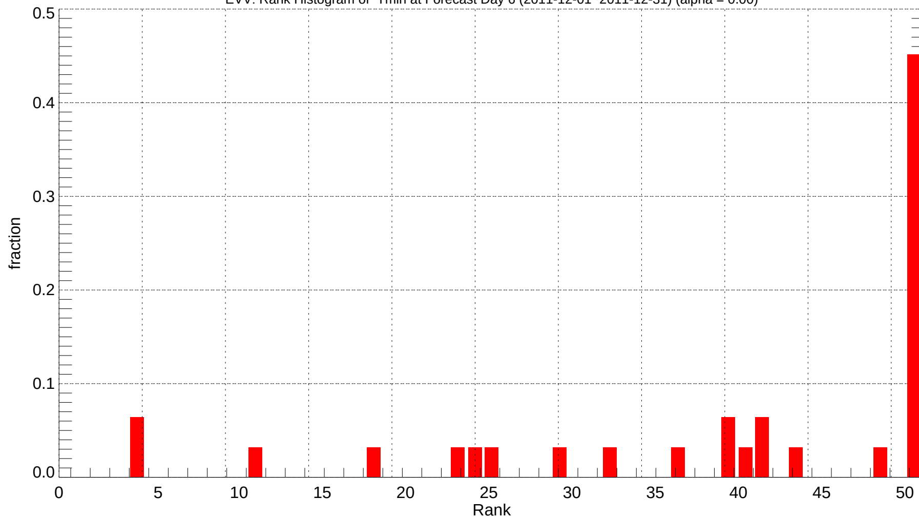
EVV: Rank Histogram of Tmin at Forecast Day 6 (2011-12-01~2011-12-31) (alpha = 0.00)
