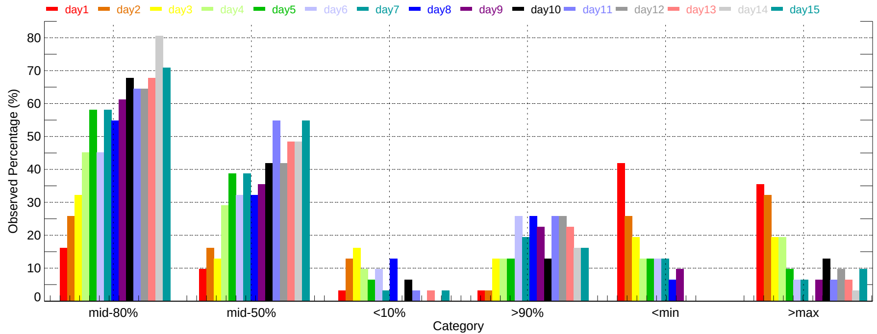
Observed Percentage of Ensembles - NTU: Max Temperature (2011-12-01~2011-12-31)
