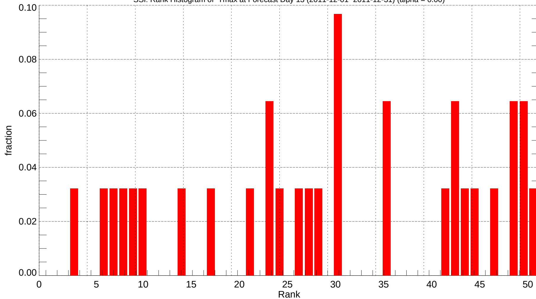
SSI: Rank Histogram of Tmax at Forecast Day 13 (2011-12-01~2011-12-31) (alpha = 0.00)
