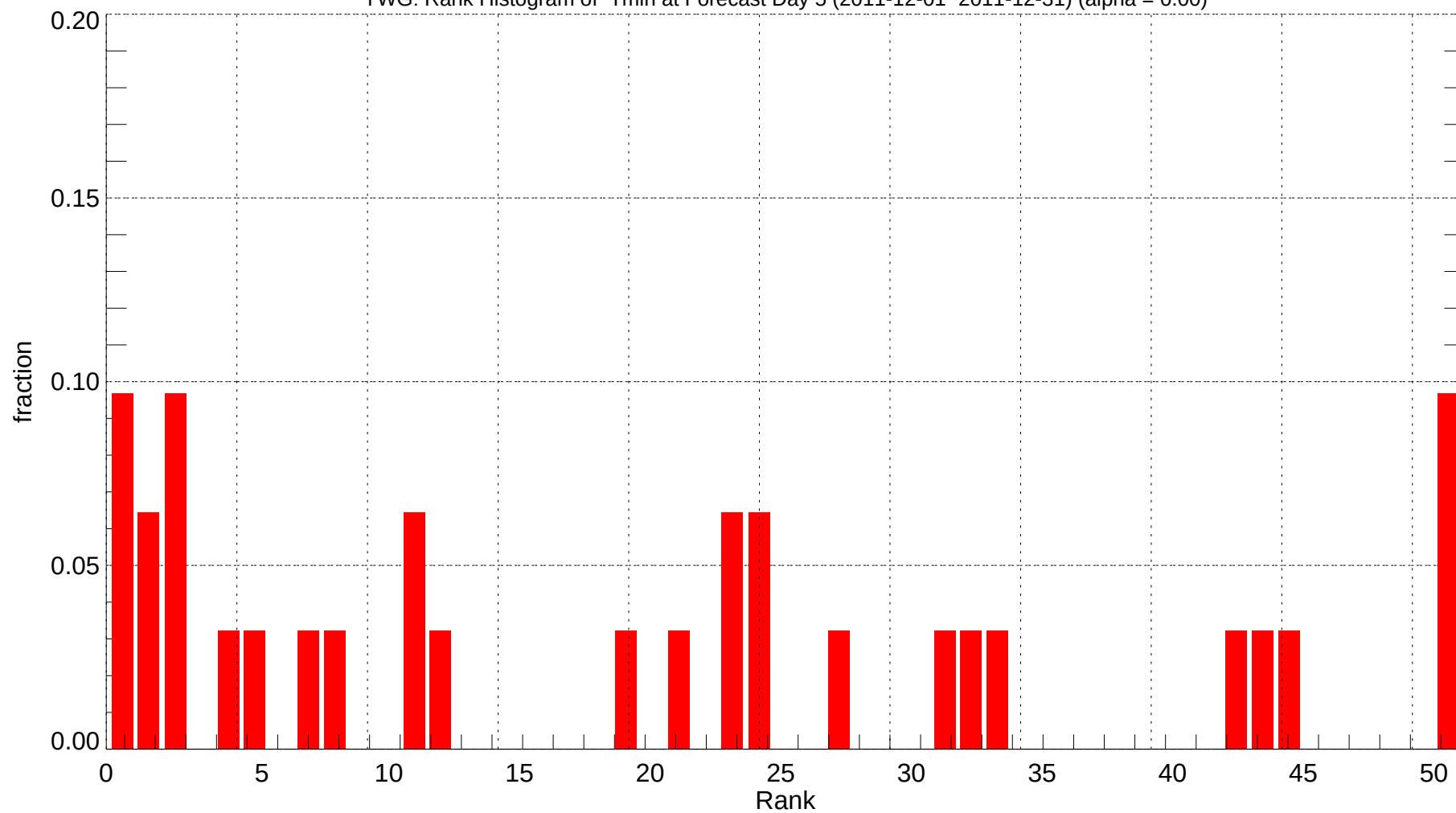
YWG: Rank Histogram of Tmin at Forecast Day 5 (2011-12-01~2011-12-31) (alpha = 0.00)
