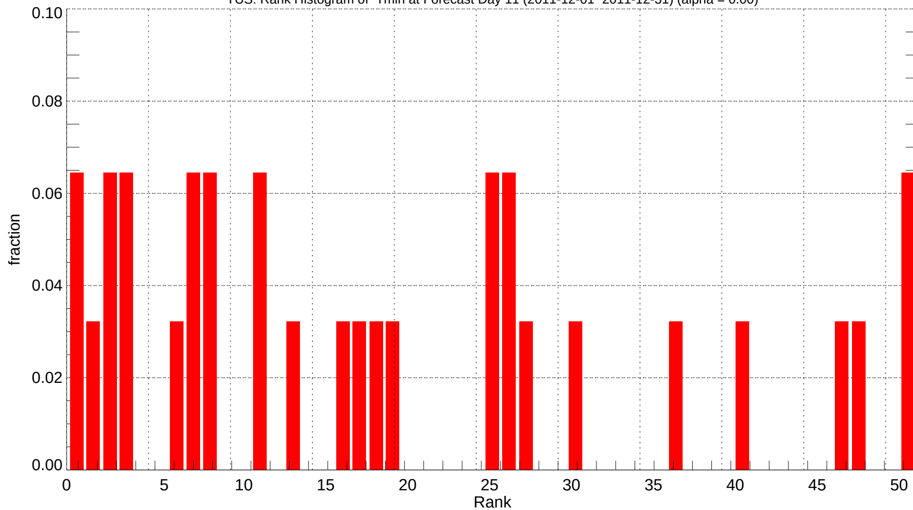
TUS: Rank Histogram of Tmin at Forecast Day 11 (2011-12-01~2011-12-31) (alpha = 0.00)
