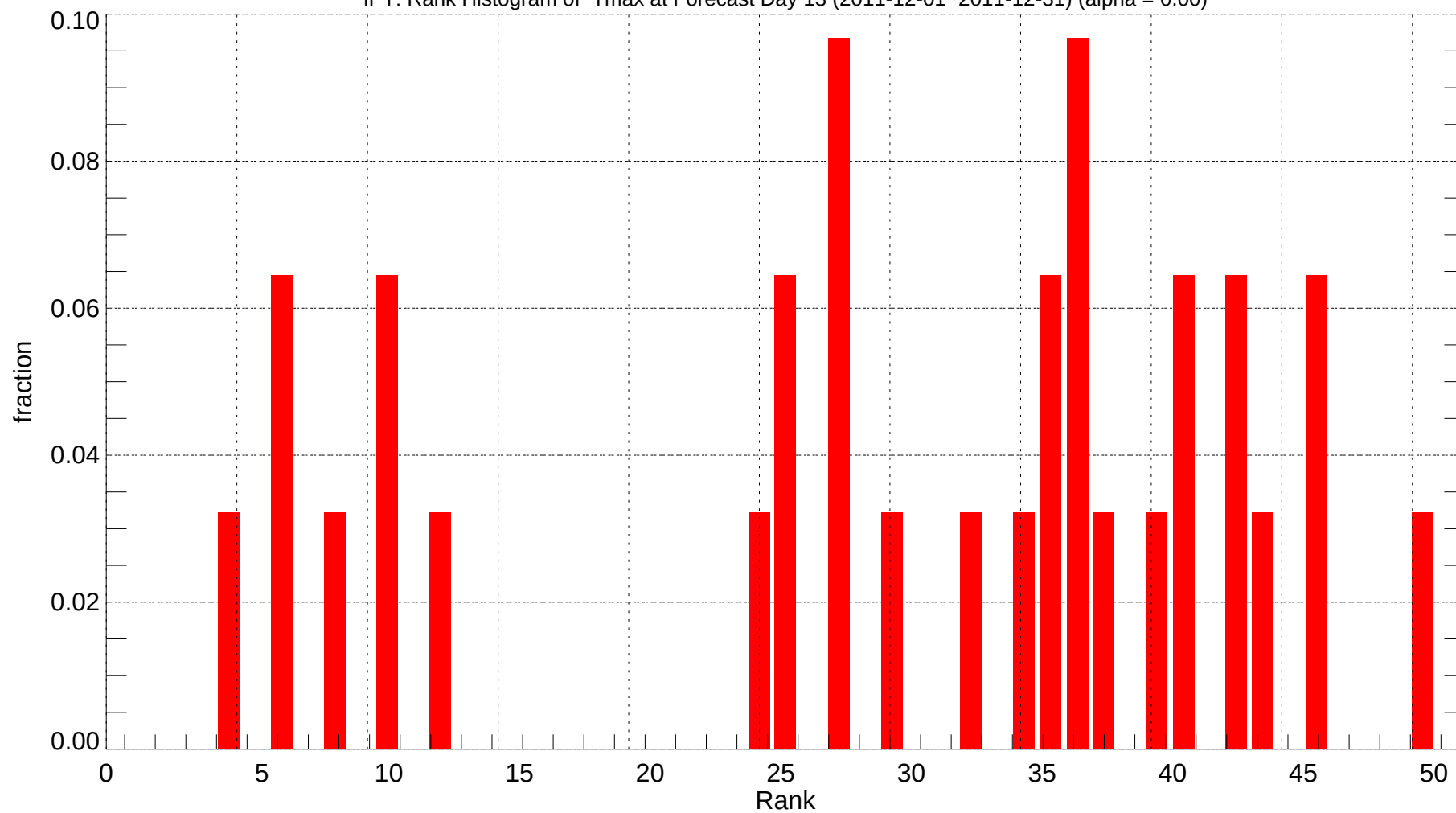
IPT: Rank Histogram of Tmax at Forecast Day 13 (2011-12-01~2011-12-31) (alpha = 0.00)
