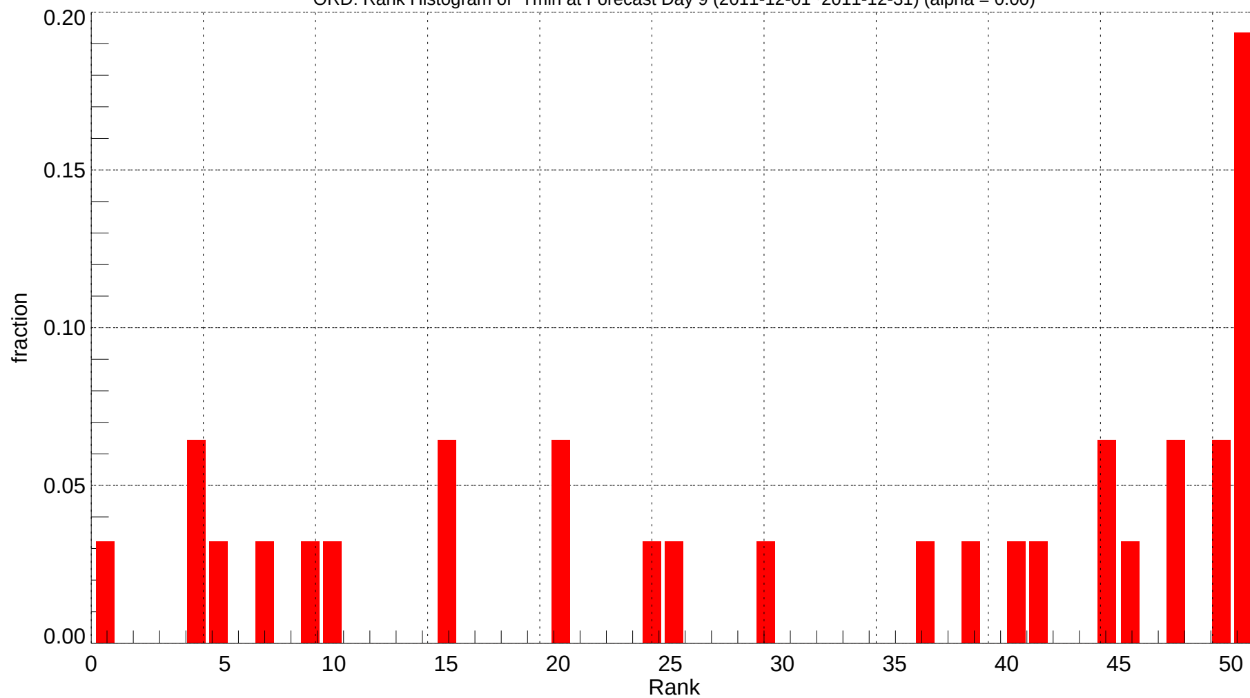
ORD: Rank Histogram of Tmin at Forecast Day 9 (2011-12-01~2011-12-31) (alpha = 0.00)
