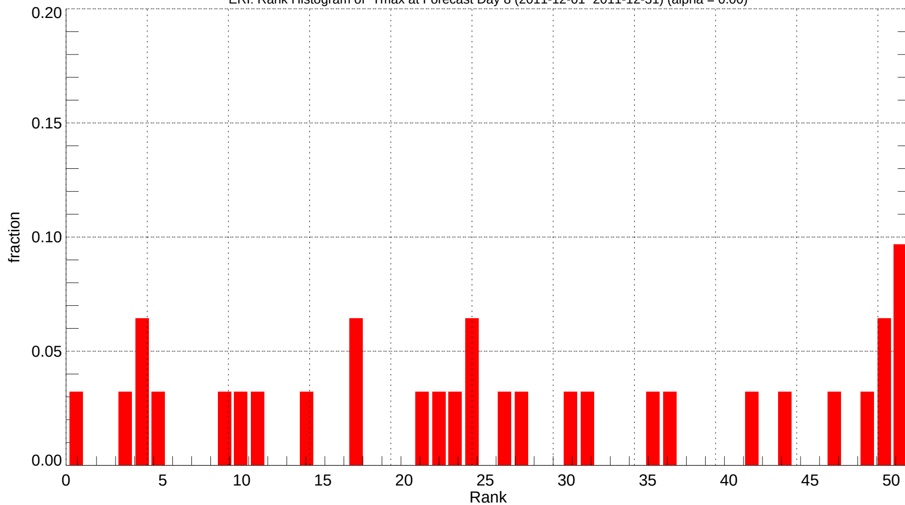
ERI: Rank Histogram of Tmax at Forecast Day 8 (2011-12-01~2011-12-31) (alpha = 0.00)
