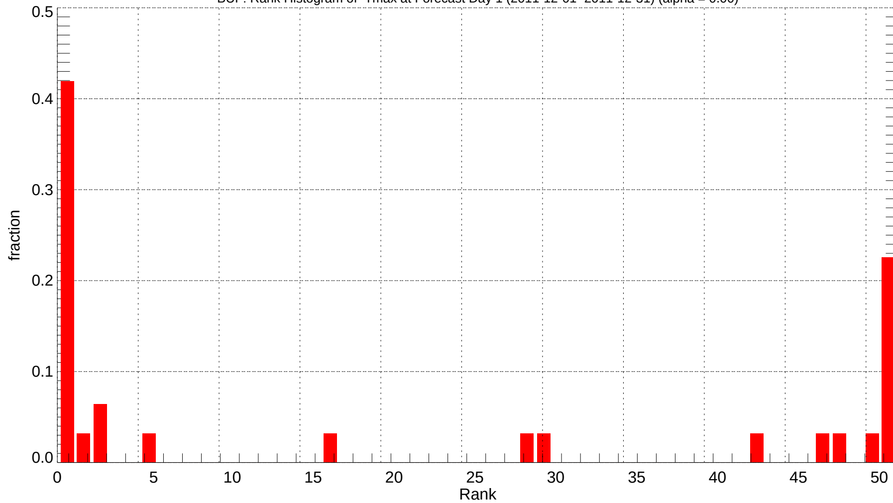
BUF: Rank Histogram of Tmax at Forecast Day 1 (2011-12-01~2011-12-31) (alpha = 0.00)
