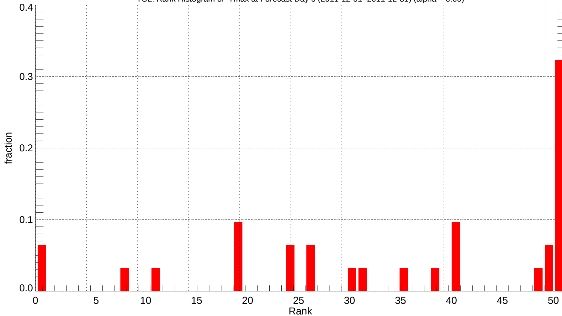
TUL: Rank Histogram of Tmax at Forecast Day 6 (2011-12-01~2011-12-31) (alpha = 0.00)
