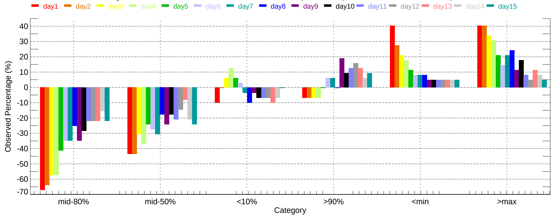
Observed Percentage Deviation of Ensembles - PIR: Min Temperature (2011-12-01~2011-12-31)
