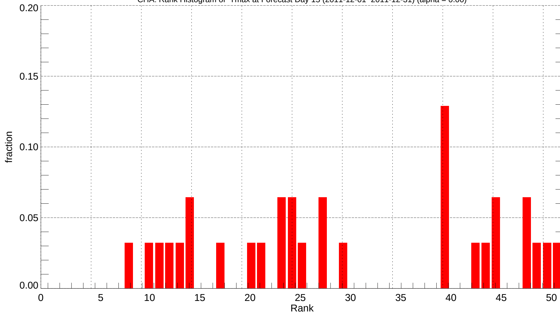
CHA: Rank Histogram of Tmax at Forecast Day 15 (2011-12-01~2011-12-31) (alpha = 0.00)
