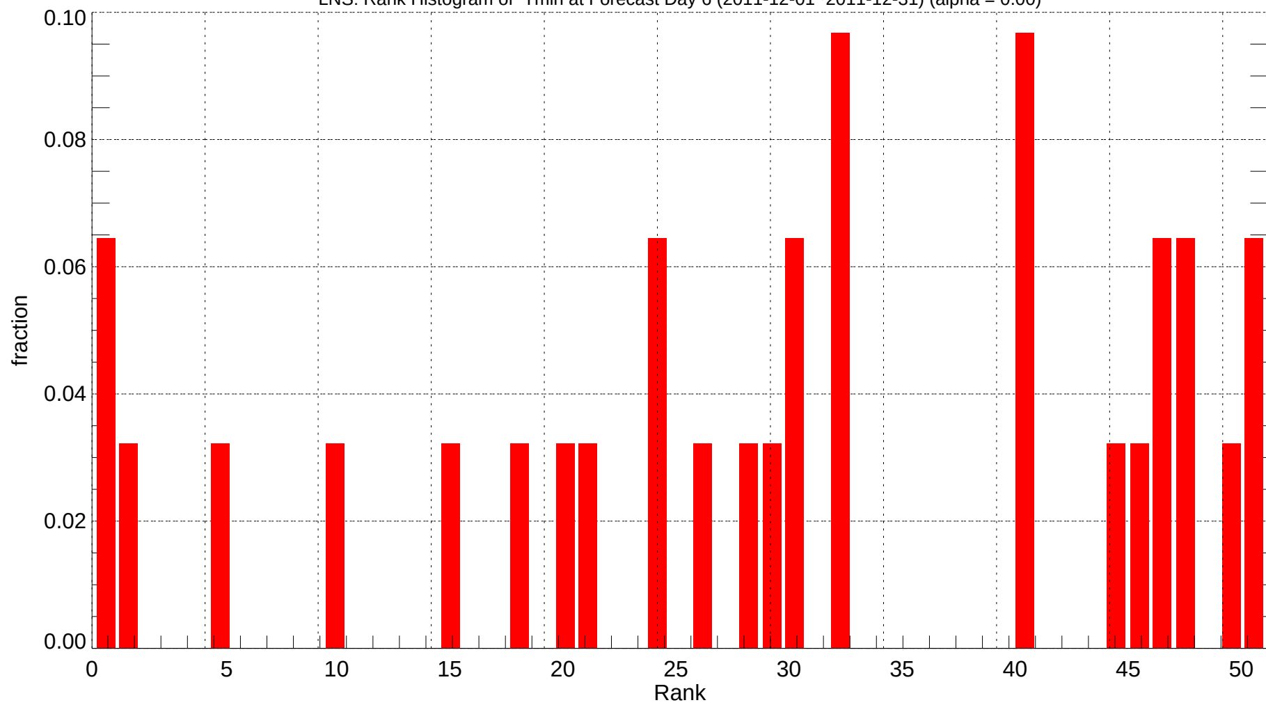
LNS: Rank Histogram of Tmin at Forecast Day 6 (2011-12-01~2011-12-31) (alpha = 0.00)
