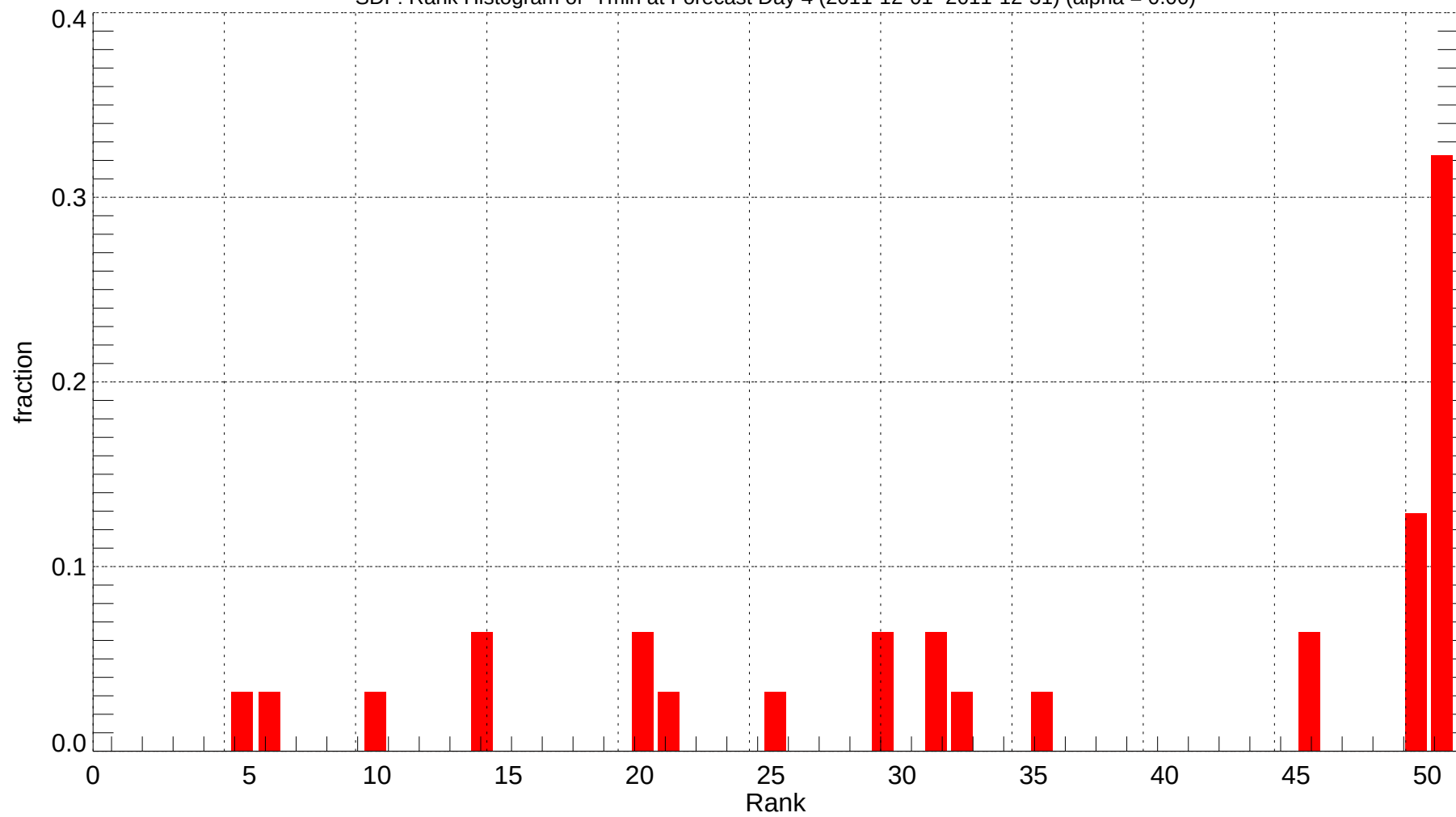
SDF: Rank Histogram of Tmin at Forecast Day 4 (2011-12-01~2011-12-31) (alpha = 0.00)
