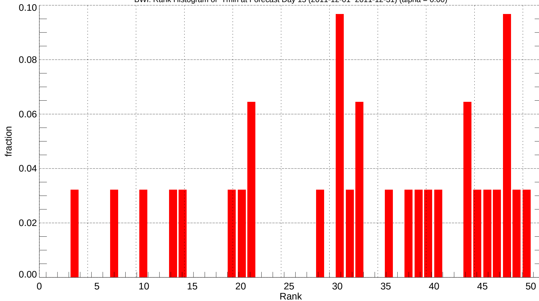
BWl: Rank Histogram of Tmin at Forecast Day 15 (2011-12-01~2011-12-31) (alpha = 0.00)
