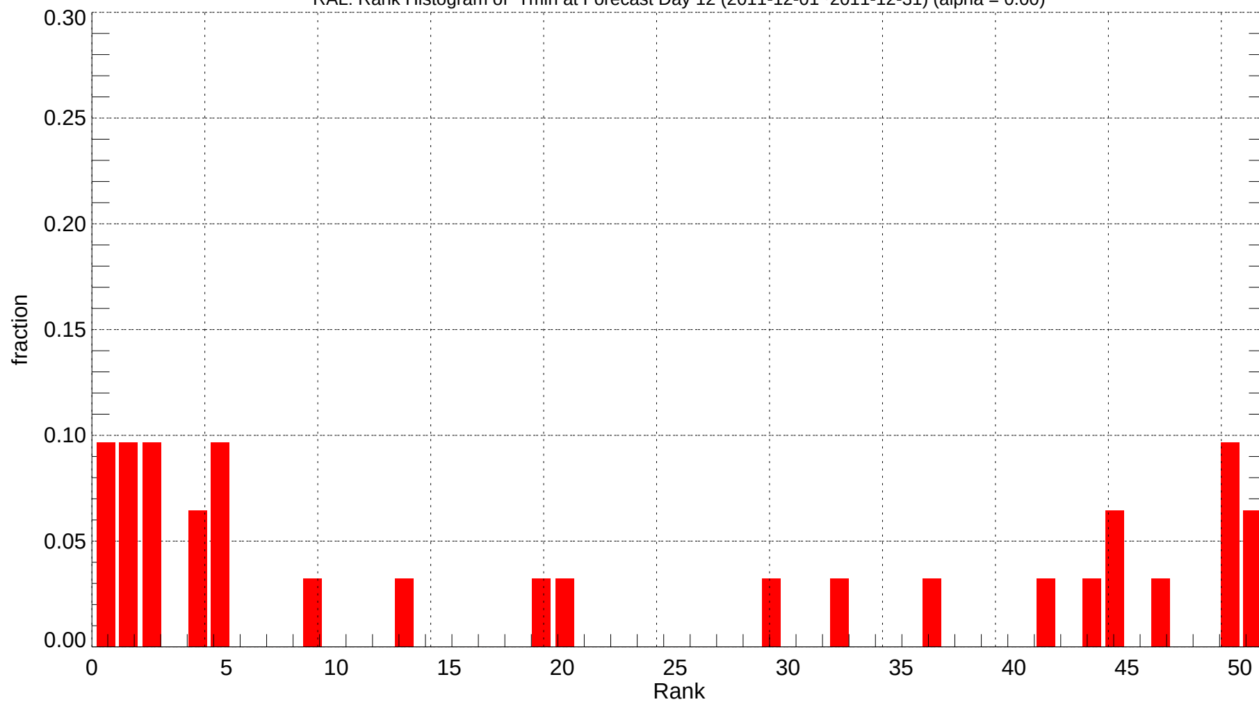
RAL: Rank Histogram of Tmin at Forecast Day 12 (2011-12-01~2011-12-31) (alpha = 0.00)
