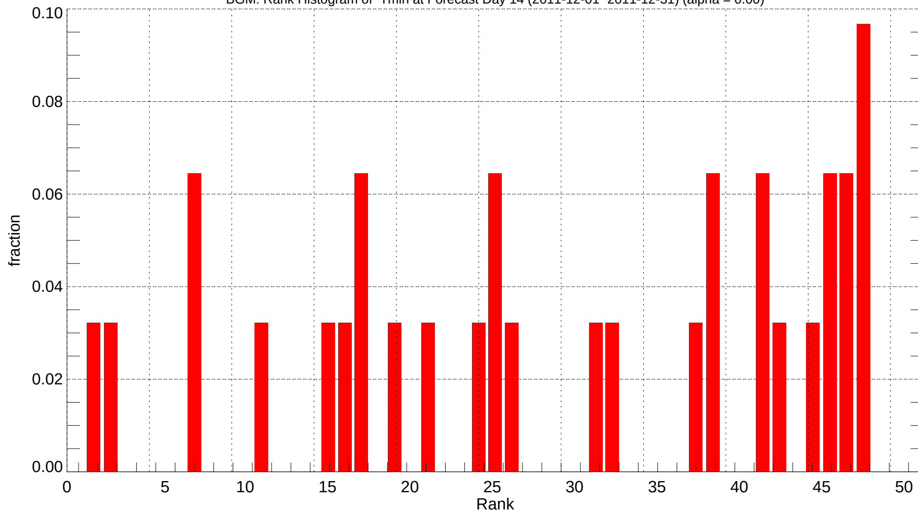
BGM: Rank Histogram of Tmin at Forecast Day 14 (2011-12-01~2011-12-31) (alpha = 0.00)
