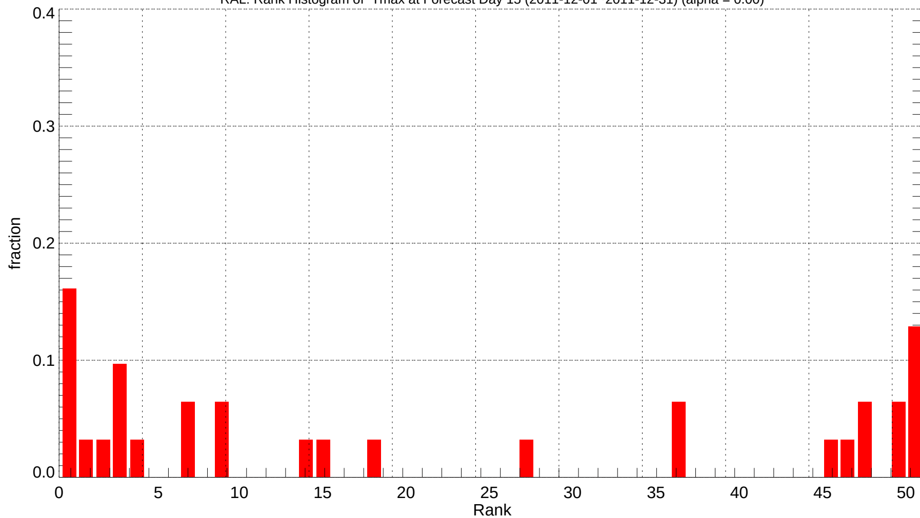
RAL: Rank Histogram of Tmax at Forecast Day 15 (2011-12-01~2011-12-31) (alpha = 0.00)
