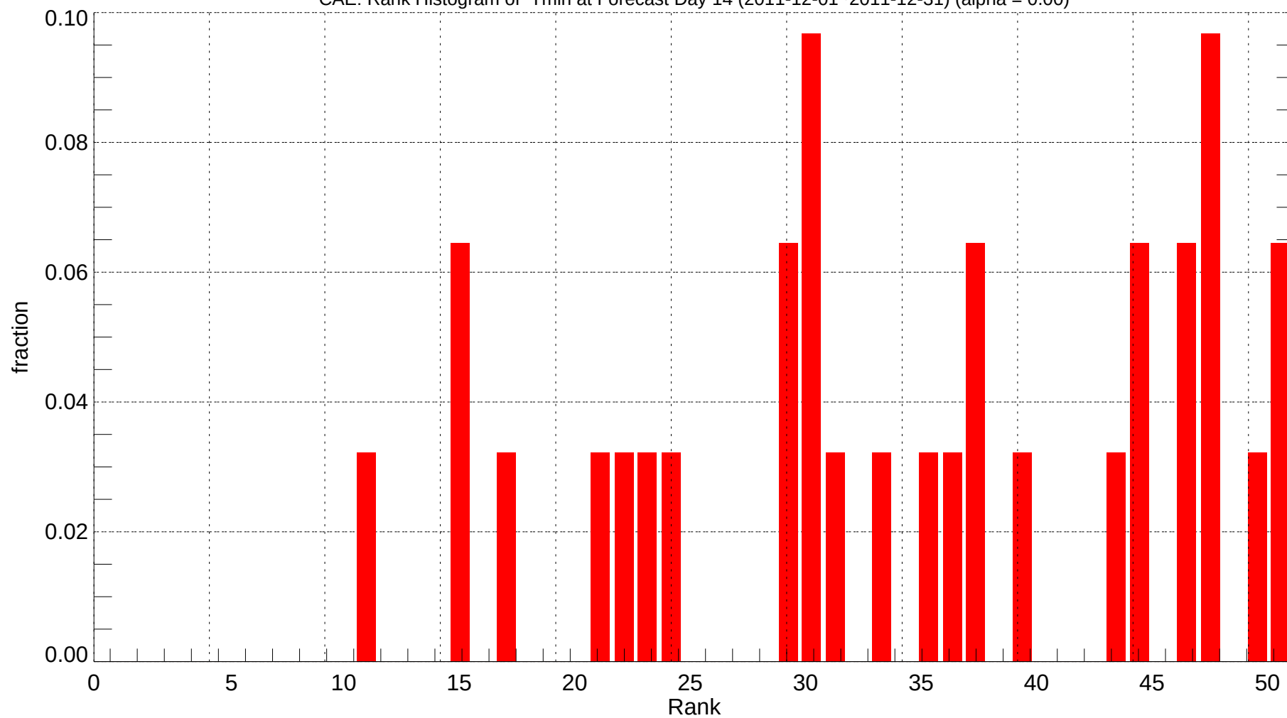
CAE: Rank Histogram of Tmin at Forecast Day 14 (2011-12-01~2011-12-31) (alpha = 0.00)
