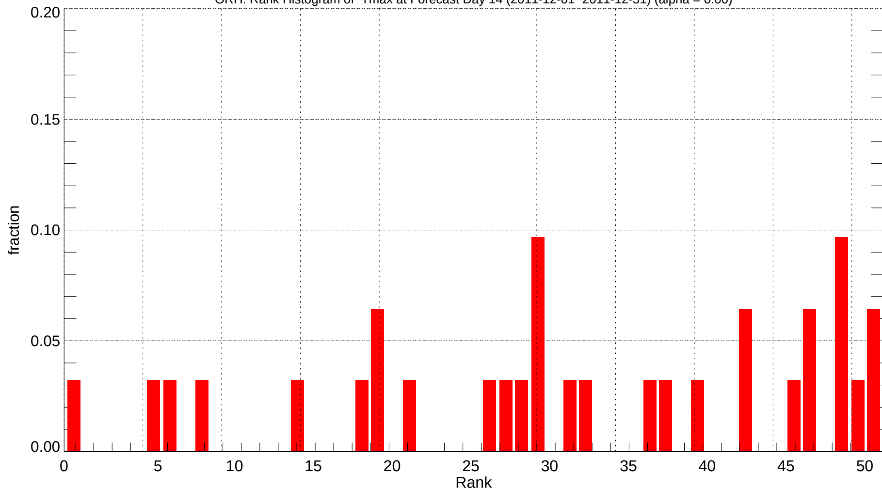
ORH: Rank Histogram of Tmax at Forecast Day 14 (2011-12-01~2011-12-31) (alpha = 0.00)
