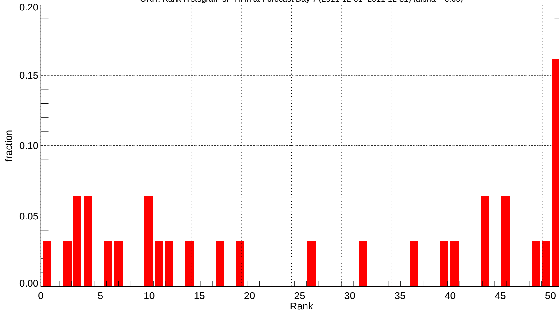
ORH: Rank Histogram of Tmin at Forecast Day 7 (2011-12-01~2011-12-31) (alpha = 0.00)
