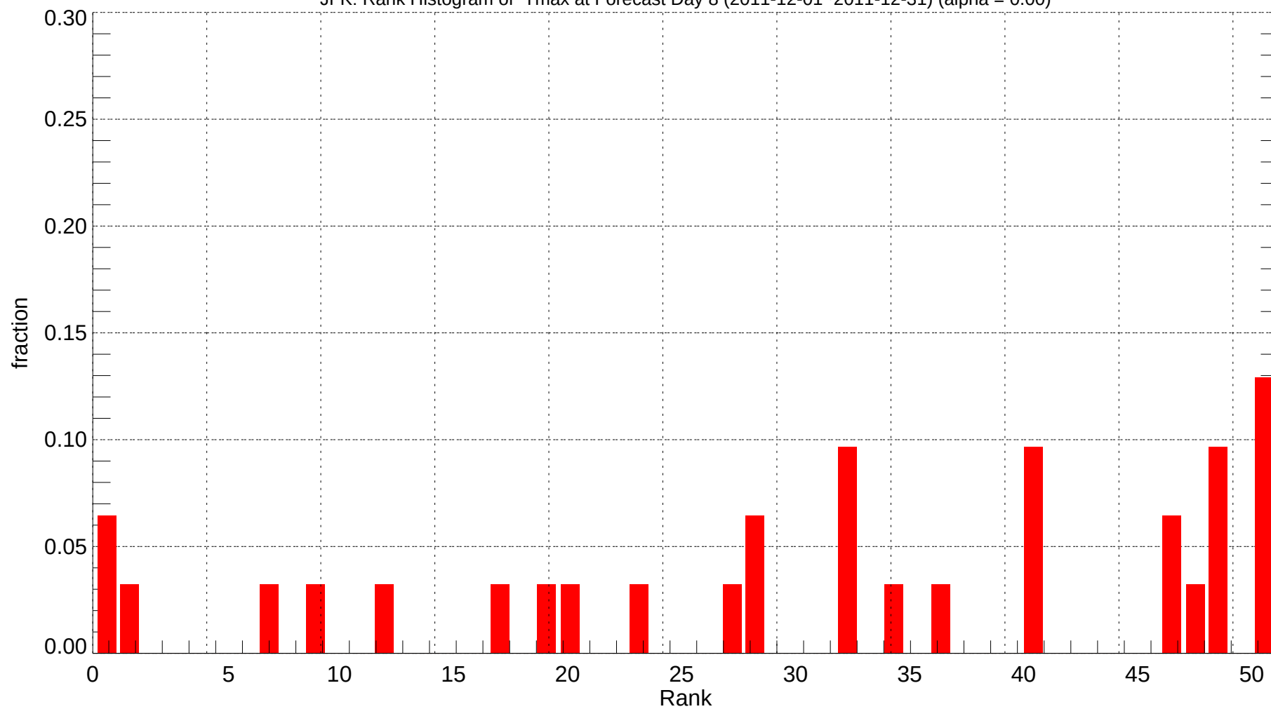
JFK: Rank Histogram of Tmax at Forecast Day 8 (2011-12-01~2011-12-31) (alpha = 0.00)
