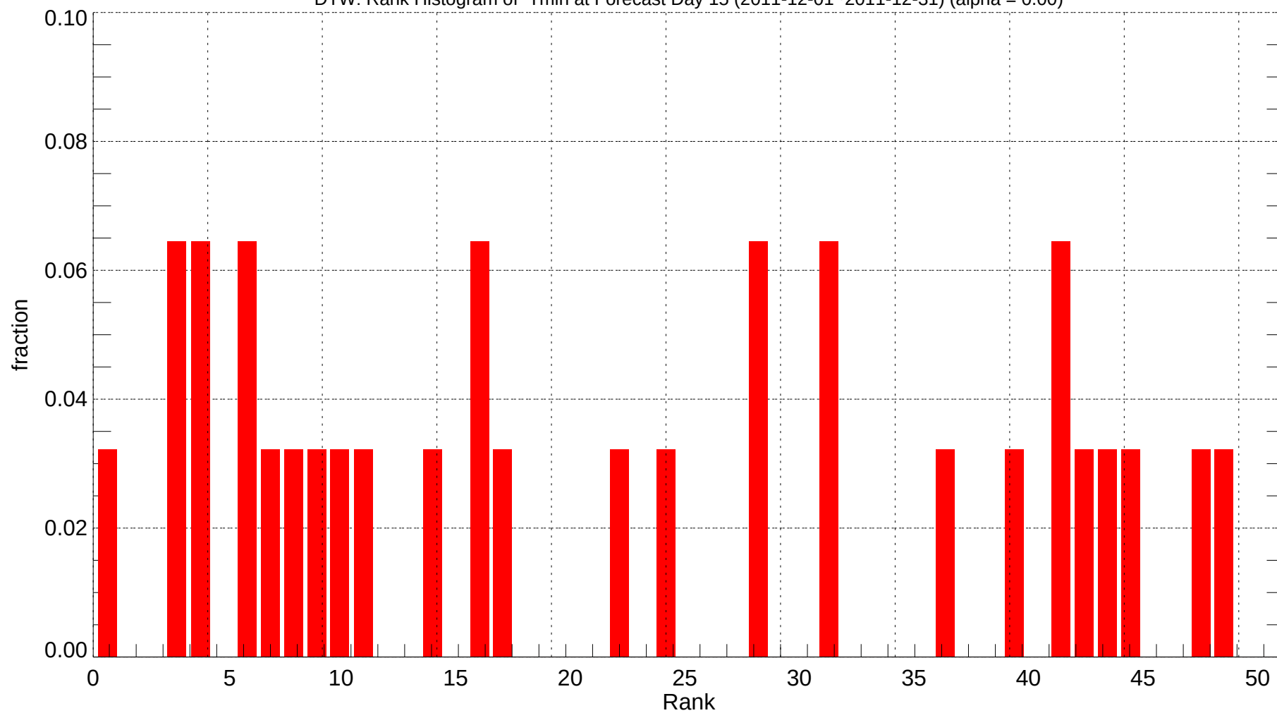
DTW: Rank Histogram of Tmin at Forecast Day 15 (2011-12-01~2011-12-31) (alpha = 0.00)
