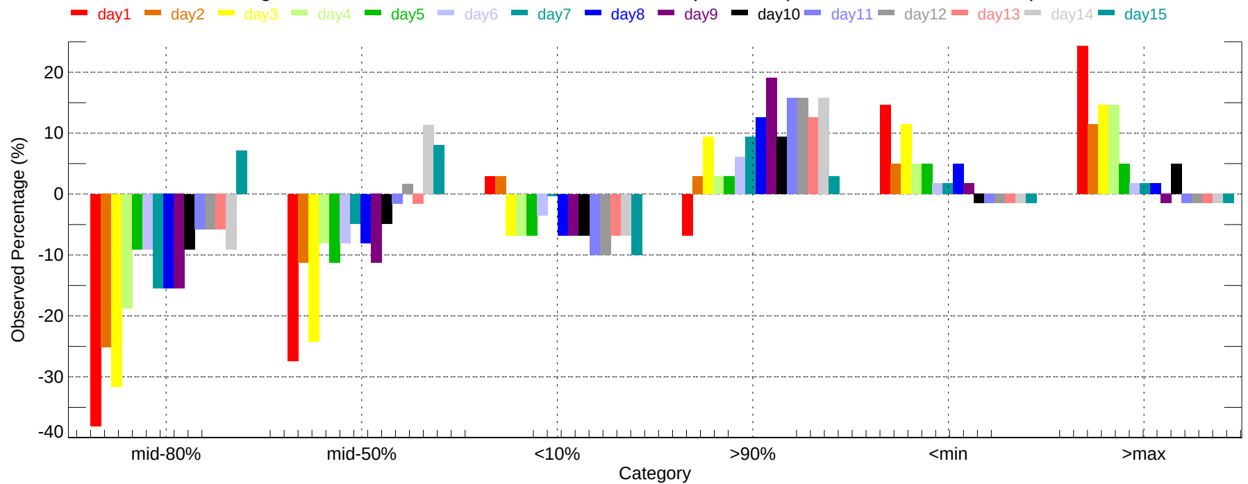
Observed Percentage Deviation of Ensembles - DTW: Min Temperature (2011-12-01~2011-12-31)
