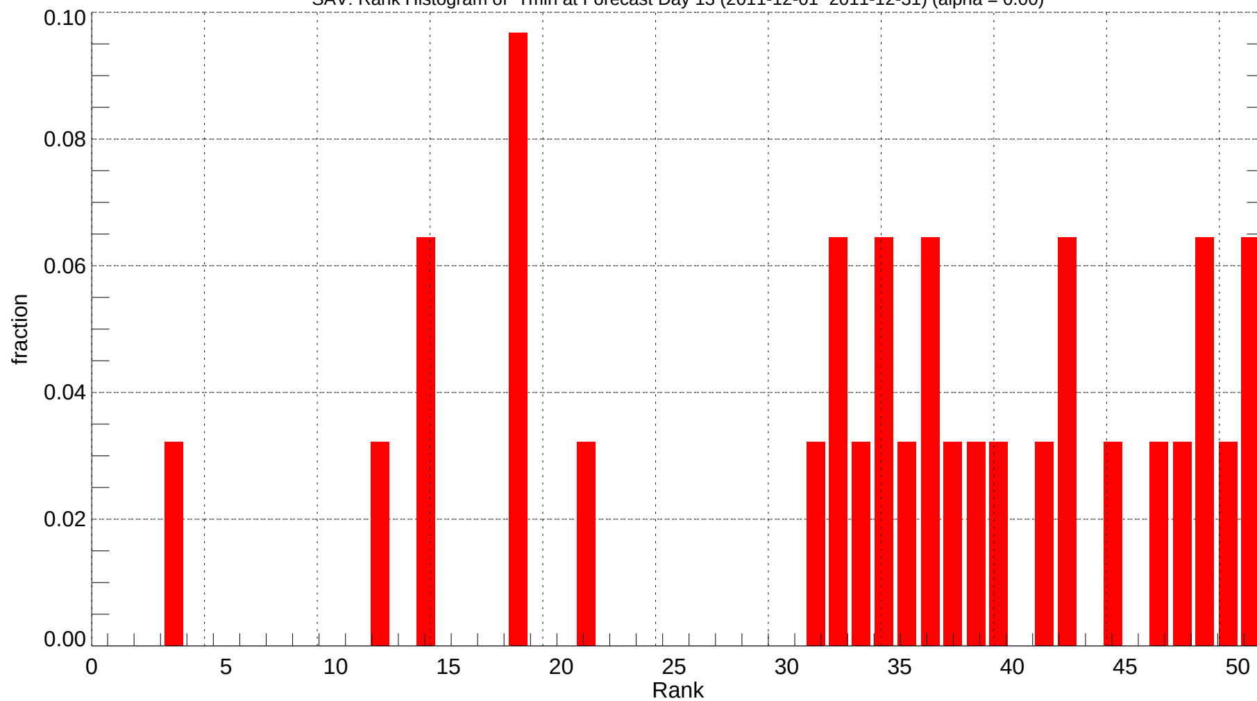
SAV: Rank Histogram of Tmin at Forecast Day 13 (2011-12-01~2011-12-31) (alpha = 0.00)
