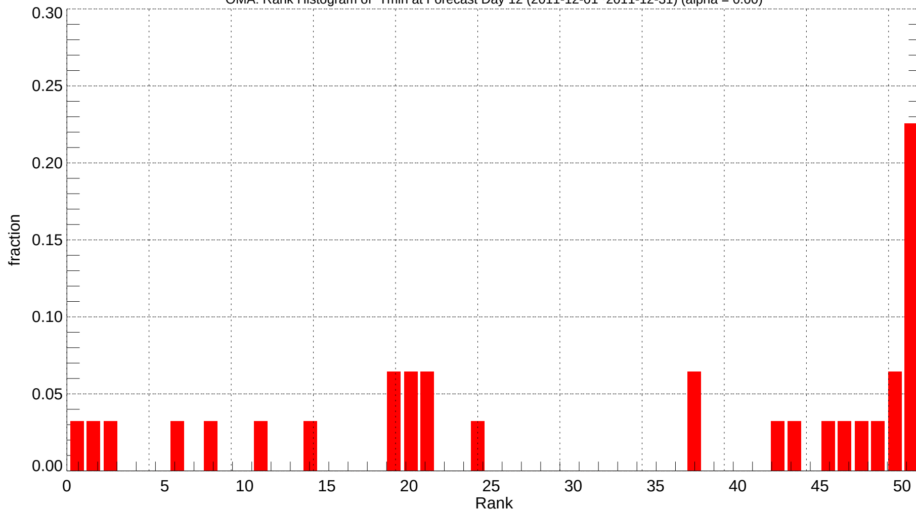
OMA: Rank Histogram of Tmin at Forecast Day 12 (2011-12-01~2011-12-31) (alpha = 0.00)
