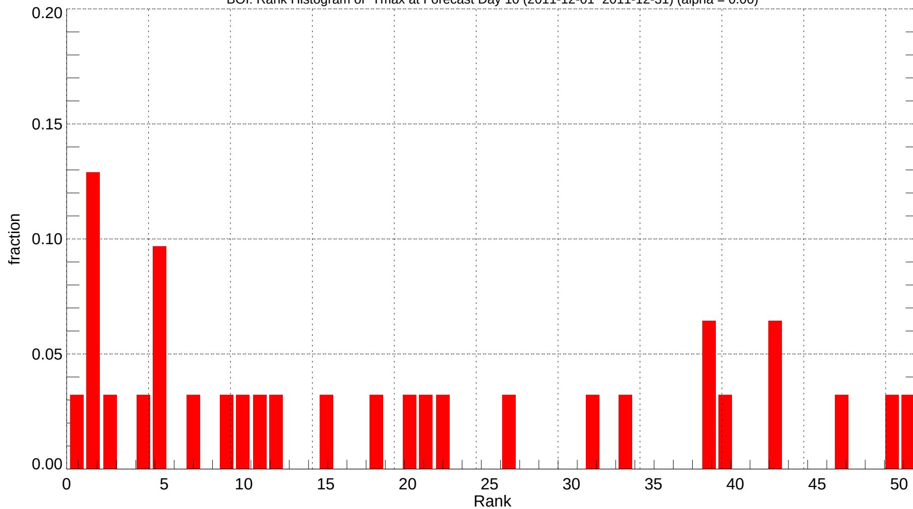
BOI: Rank Histogram of Tmax at Forecast Day 10 (2011-12-01~2011-12-31) (alpha = 0.00)
