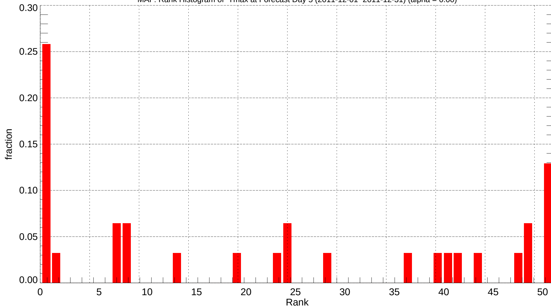
MAF: Rank Histogram of Tmax at Forecast Day 5 (2011-12-01~2011-12-31) (alpha = 0.00)
