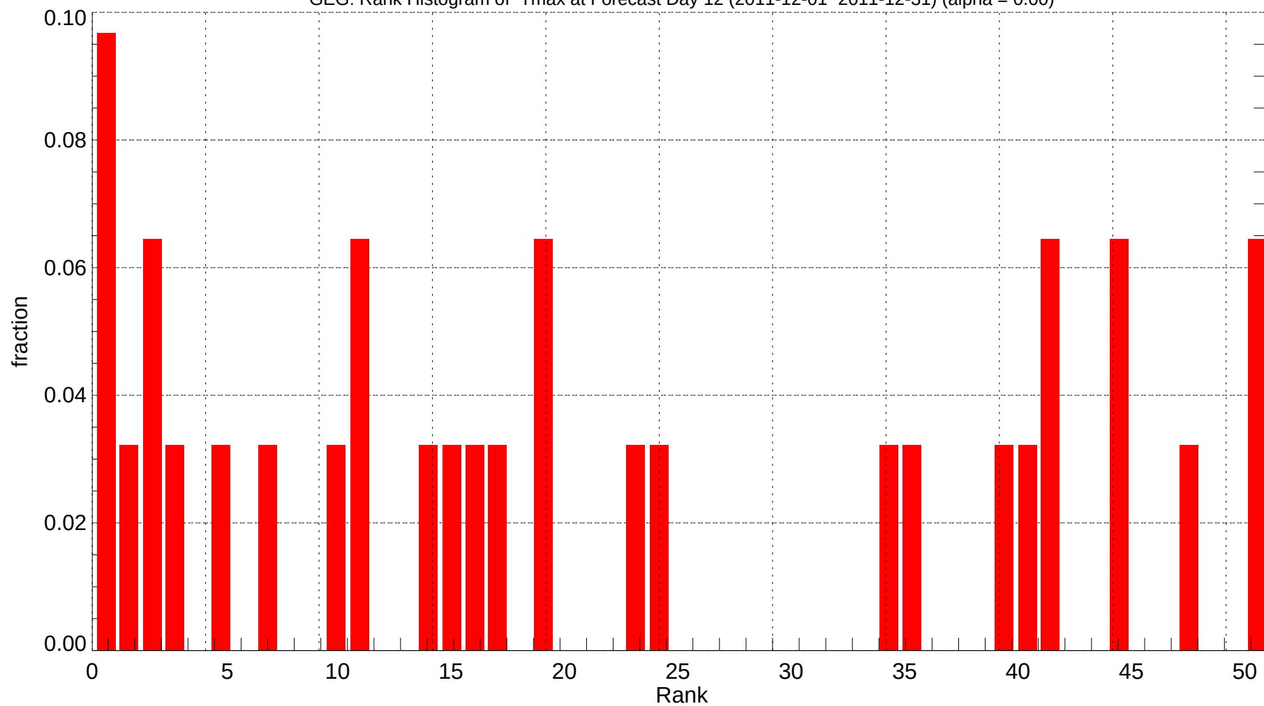
GEG: Rank Histogram of Tmax at Forecast Day 12 (2011-12-01~2011-12-31) (alpha = 0.00)
