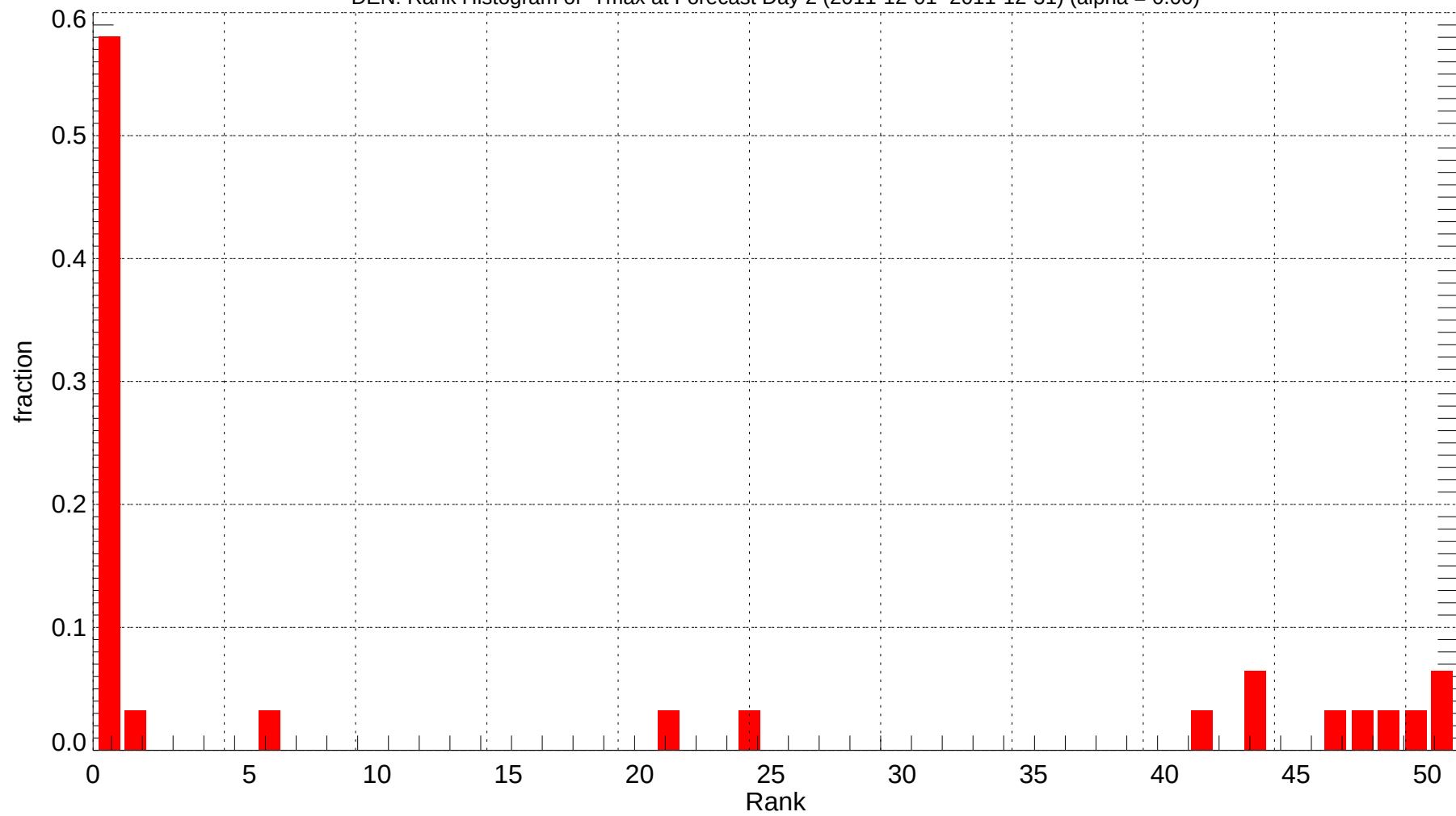
DEN: Rank Histogram of Tmax at Forecast Day 2 (2011-12-01~2011-12-31) (alpha = 0.00)
