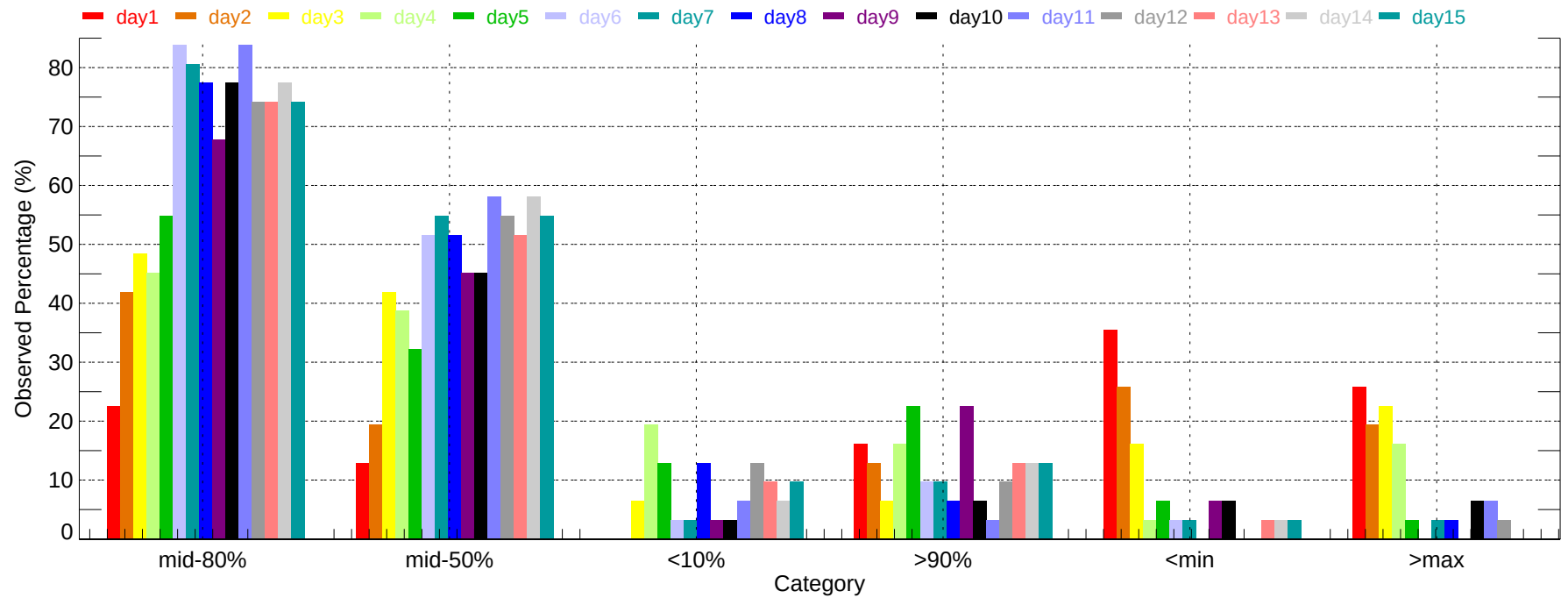
Observed Percentage of Ensembles - YQB: Max Temperature (2011-12-01~2011-12-31)
