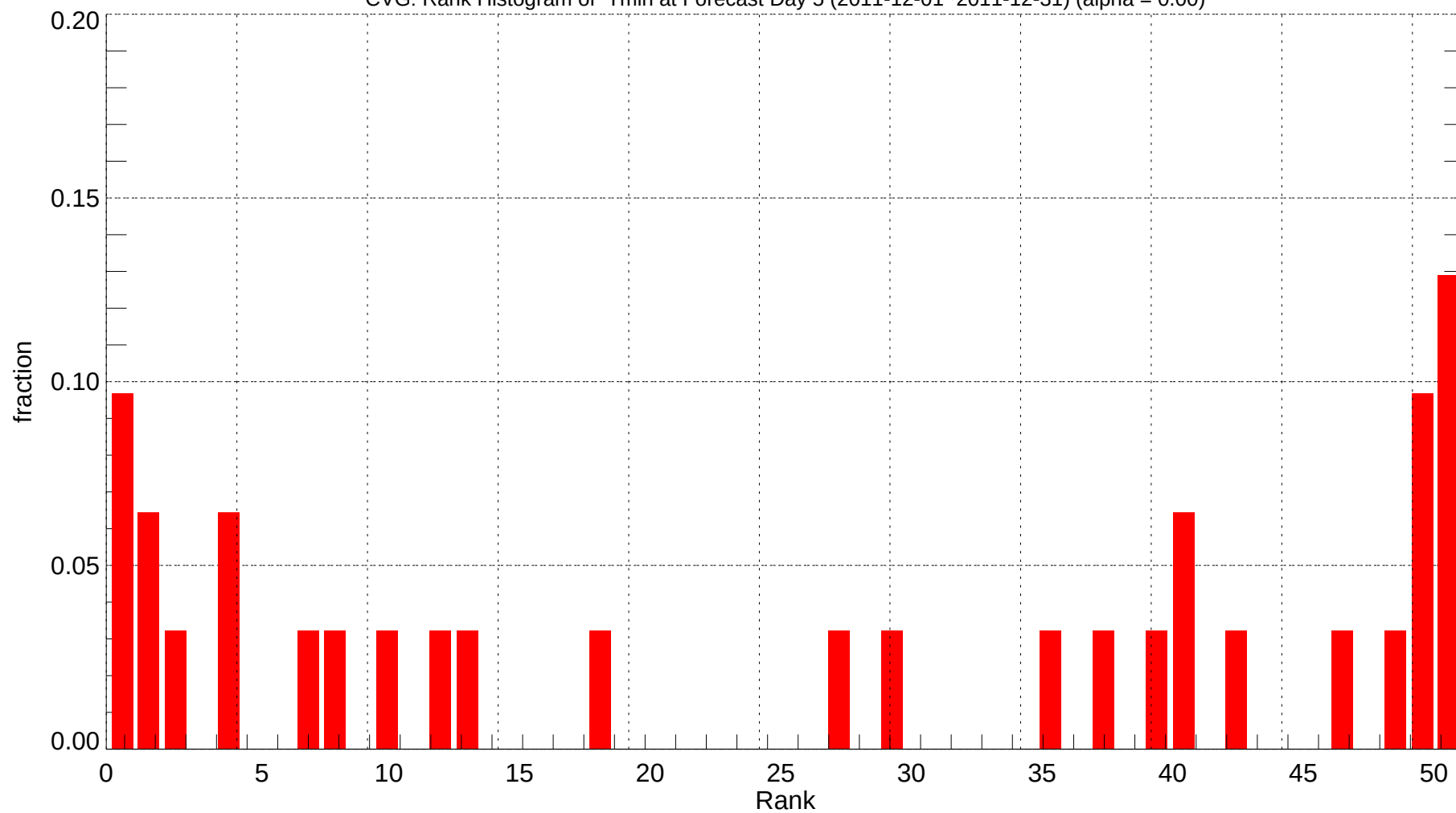
CVG: Rank Histogram of Tmin at Forecast Day 5 (2011-12-01~2011-12-31) (alpha = 0.00)
