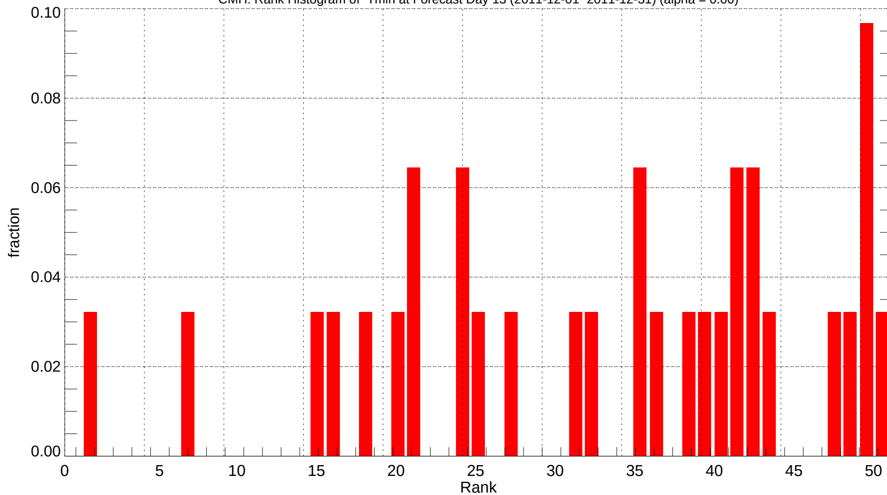
CMH: Rank Histogram of Tmin at Forecast Day 13 (2011-12-01~2011-12-31) (alpha = 0.00)
