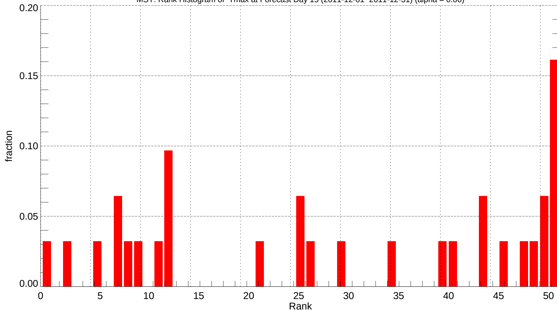
MSY: Rank Histogram of Tmax at Forecast Day 15 (2011-12-01~2011-12-31) (alpha = 0.00)
