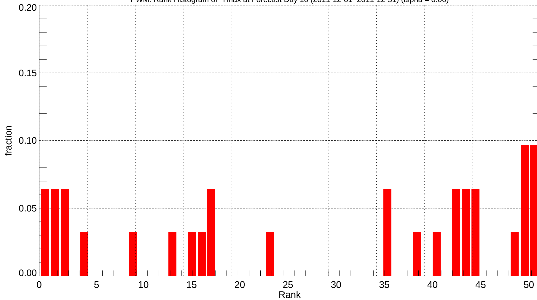
PWM: Rank Histogram of Tmax at Forecast Day 10 (2011-12-01~2011-12-31) (alpha = 0.00)
