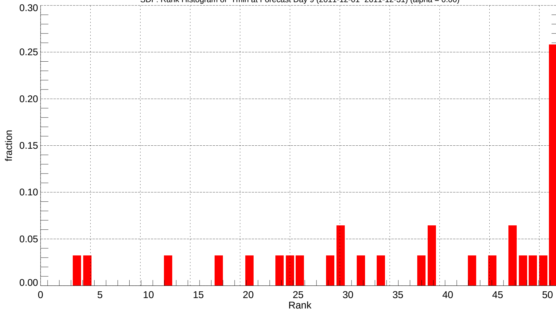
SDF: Rank Histogram of Tmin at Forecast Day 9 (2011-12-01~2011-12-31) (alpha = 0.00)
