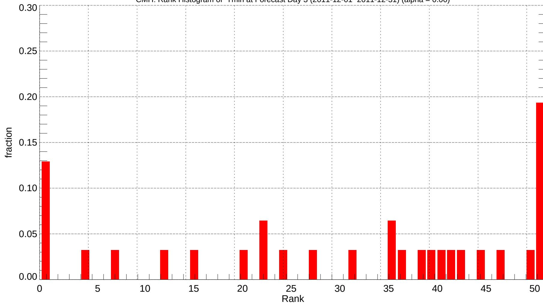
CMH: Rank Histogram of Tmin at Forecast Day 3 (2011-12-01~2011-12-31) (alpha = 0.00)
