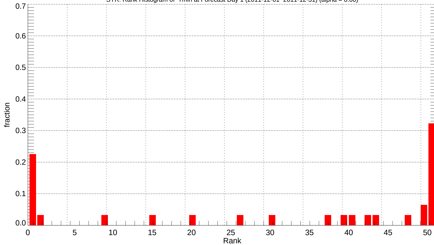
SYR: Rank Histogram of Tmin at Forecast Day 1 (2011-12-01~2011-12-31) (alpha = 0.00)
