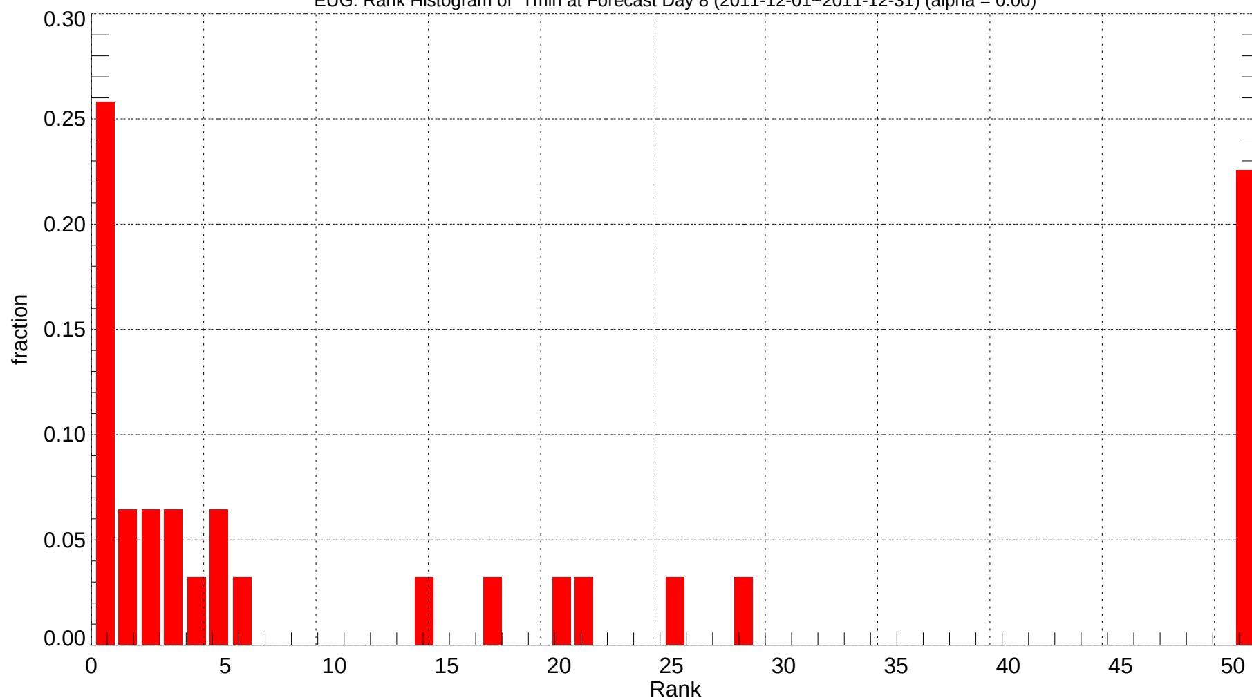
EUG: Rank Histogram of Tmin at Forecast Day 8 (2011-12-01~2011-12-31) (alpha = 0.00)
