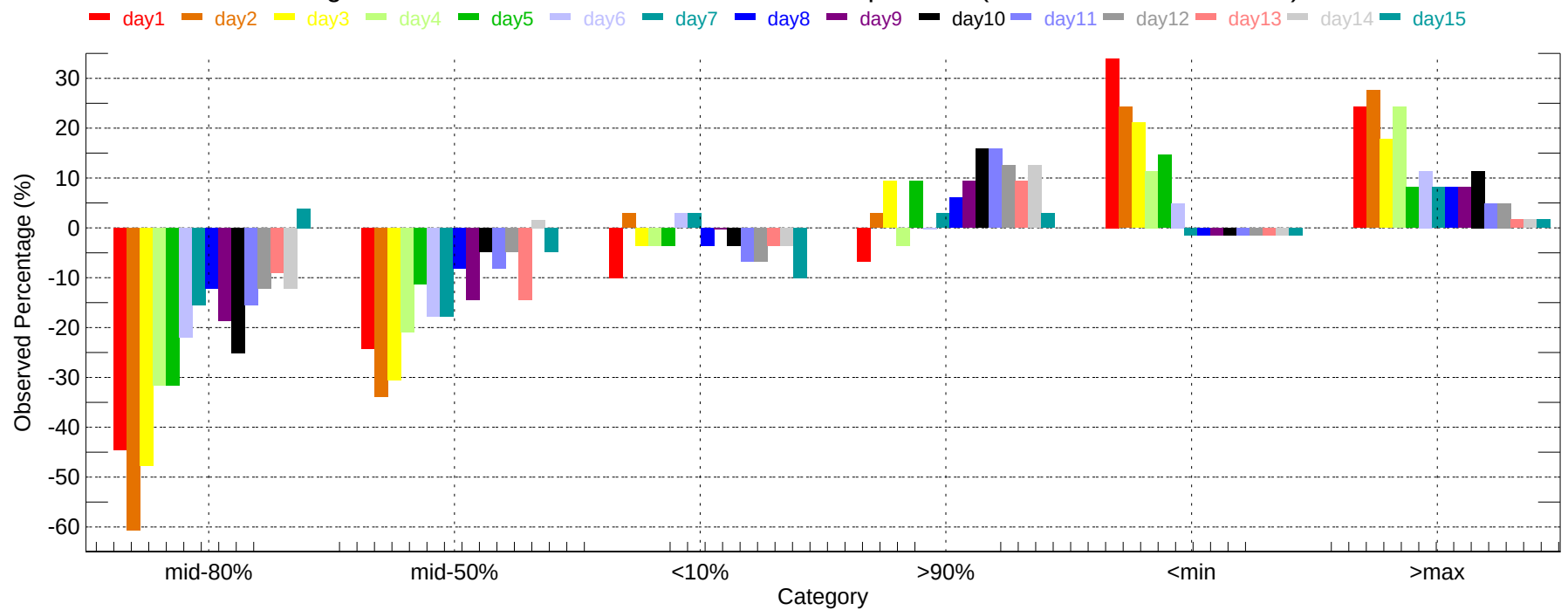
Observed Percentage Deviation of Ensembles - CVG: Min Temperature (2011-12-01~2011-12-31)
