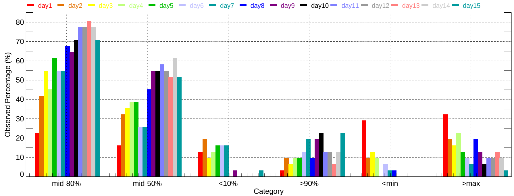
Observed Percentage of Ensembles - TYS: Max Temperature (2011-12-01~2011-12-31)
