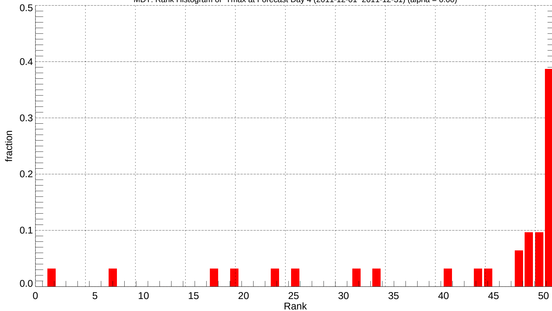
MDT: Rank Histogram of Tmax at Forecast Day 4 (2011-12-01~2011-12-31) (alpha = 0.00)
