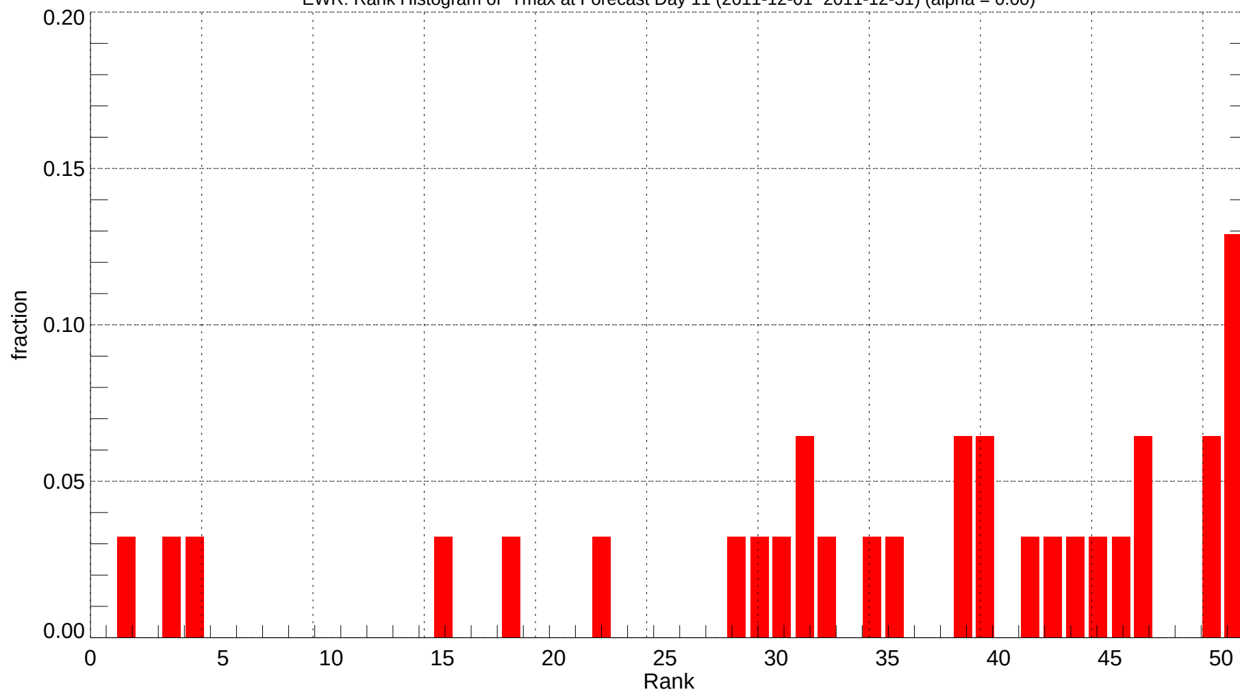
EWR: Rank Histogram of Tmax at Forecast Day 11 (2011-12-01~2011-12-31) (alpha = 0.00)
