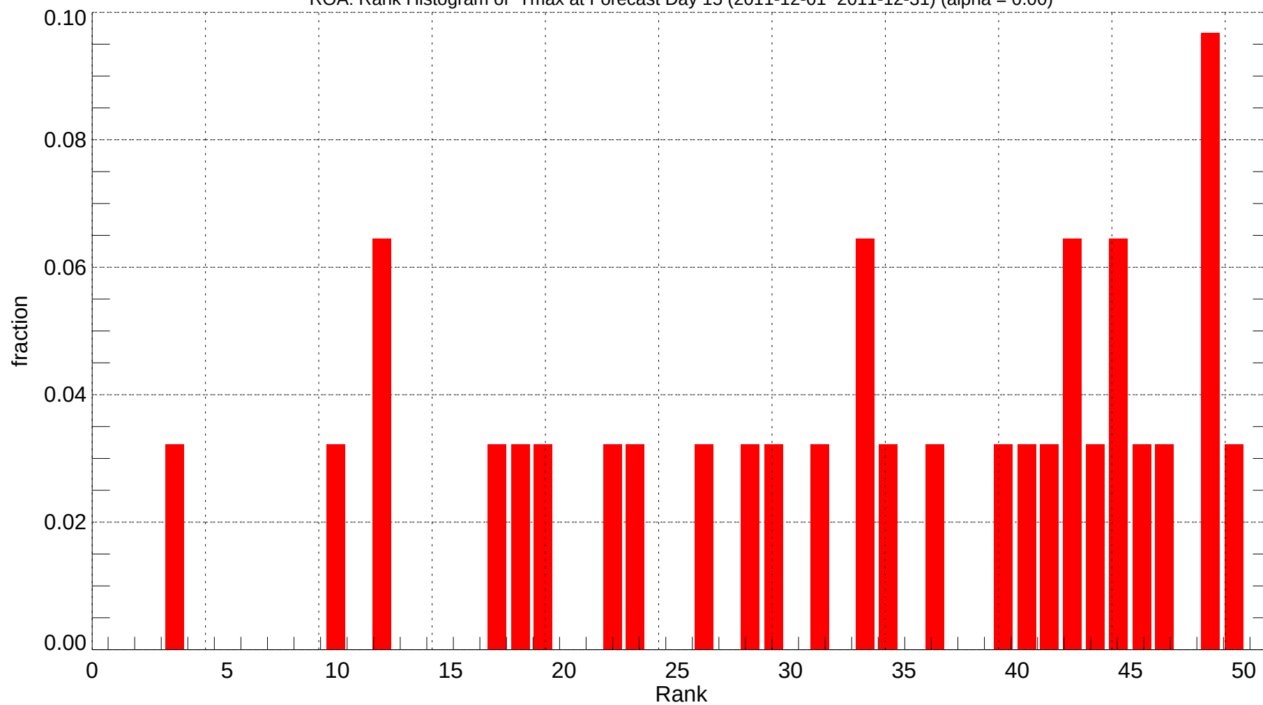
ROA: Rank Histogram of Tmax at Forecast Day 15 (2011-12-01~2011-12-31) (alpha = 0.00)
