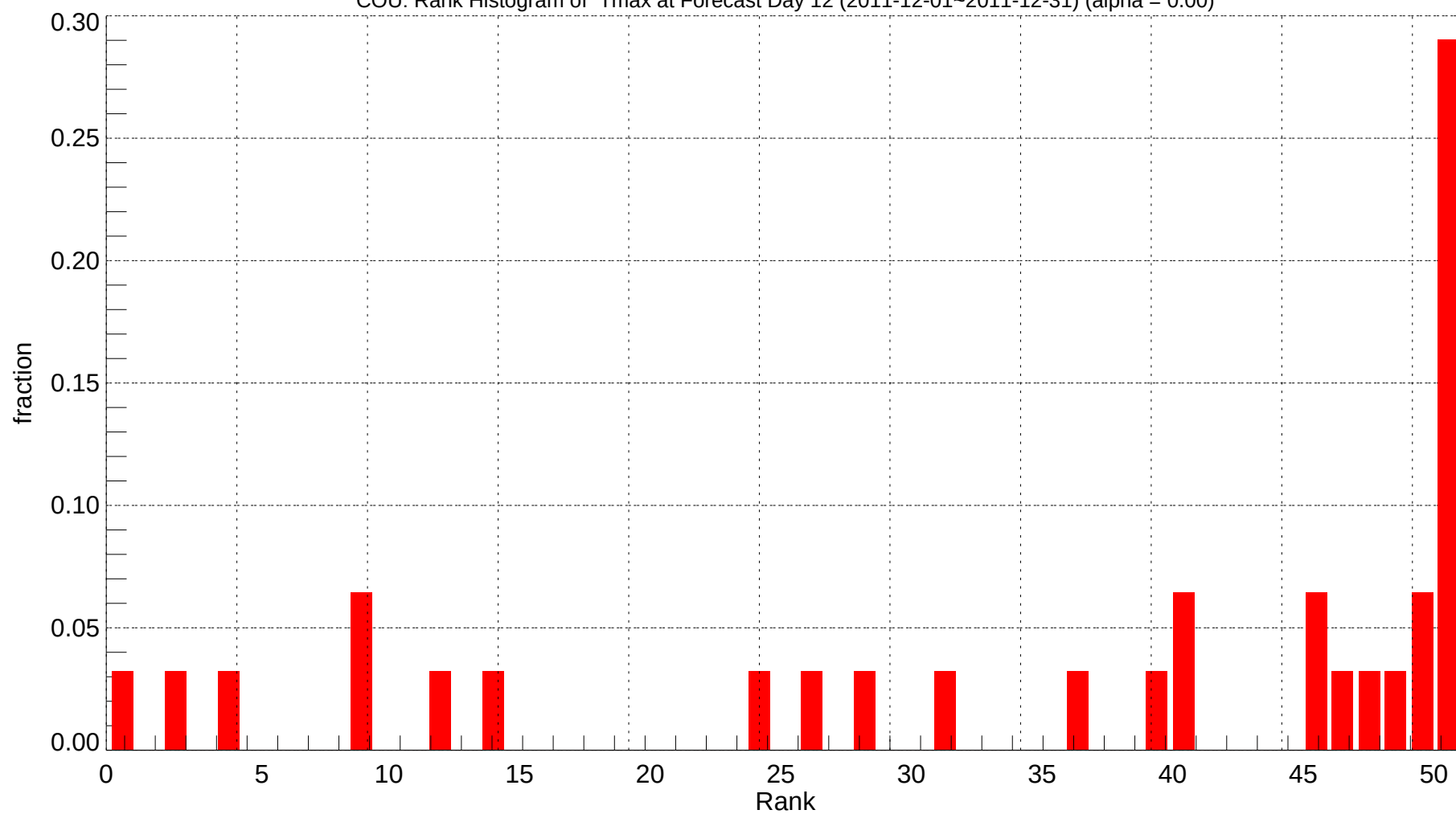
COU: Rank Histogram of Tmax at Forecast Day 12 (2011-12-01~2011-12-31) (alpha = 0.00)
