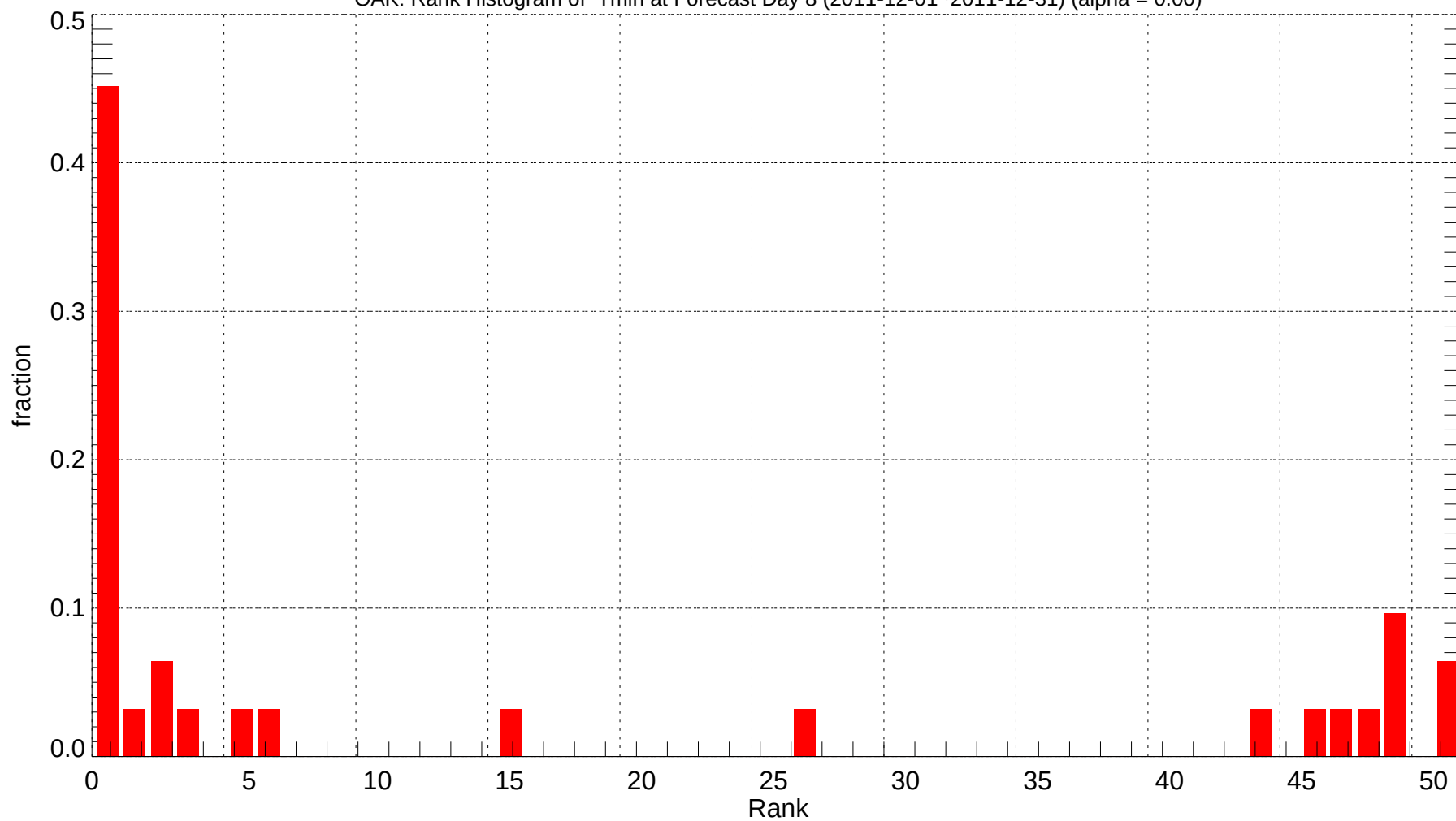
OAK: Rank Histogram of Tmin at Forecast Day 8 (2011-12-01~2011-12-31) (alpha = 0.00)
