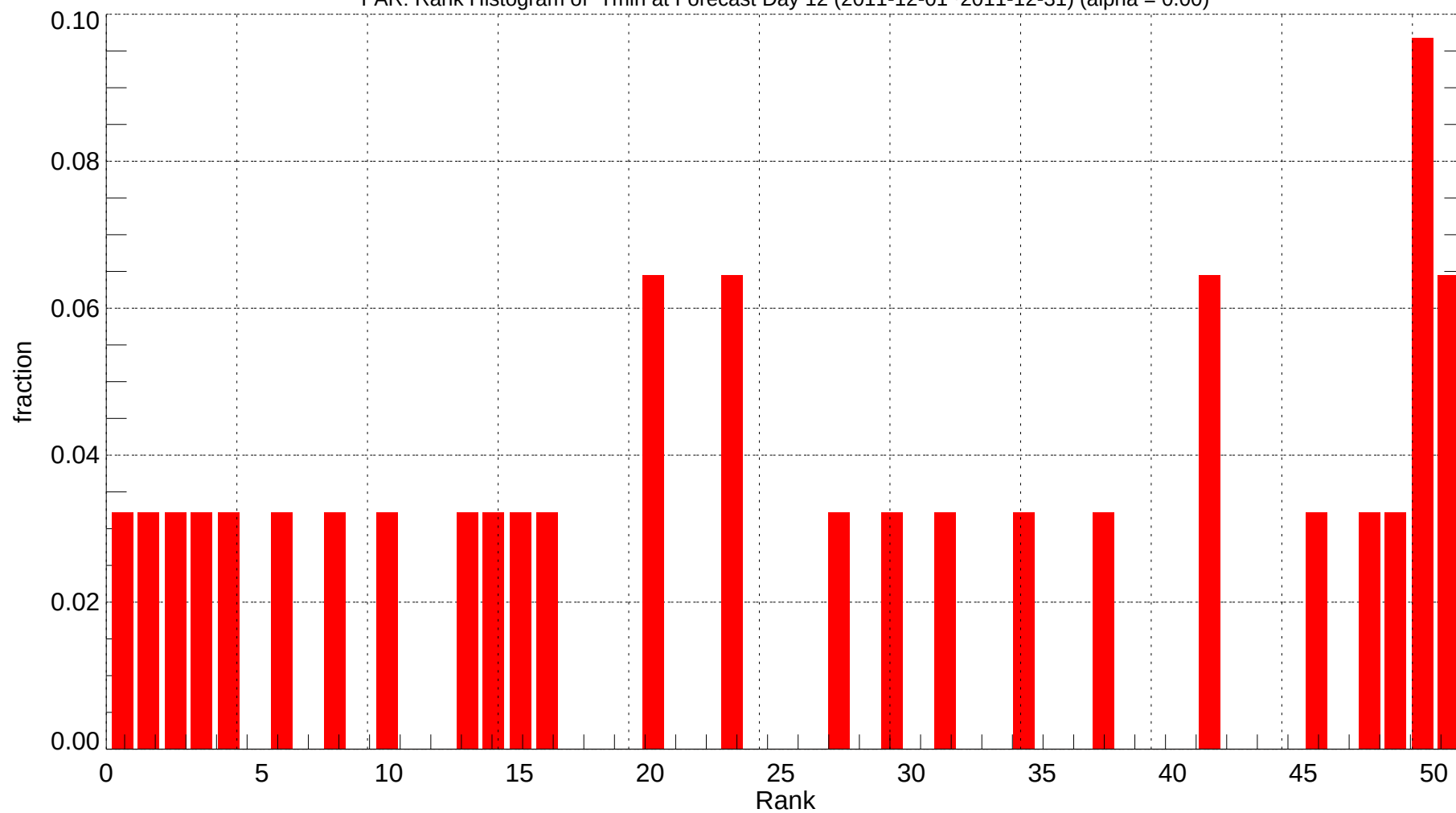
FAR: Rank Histogram of Tmin at Forecast Day 12 (2011-12-01~2011-12-31) (alpha = 0.00)
