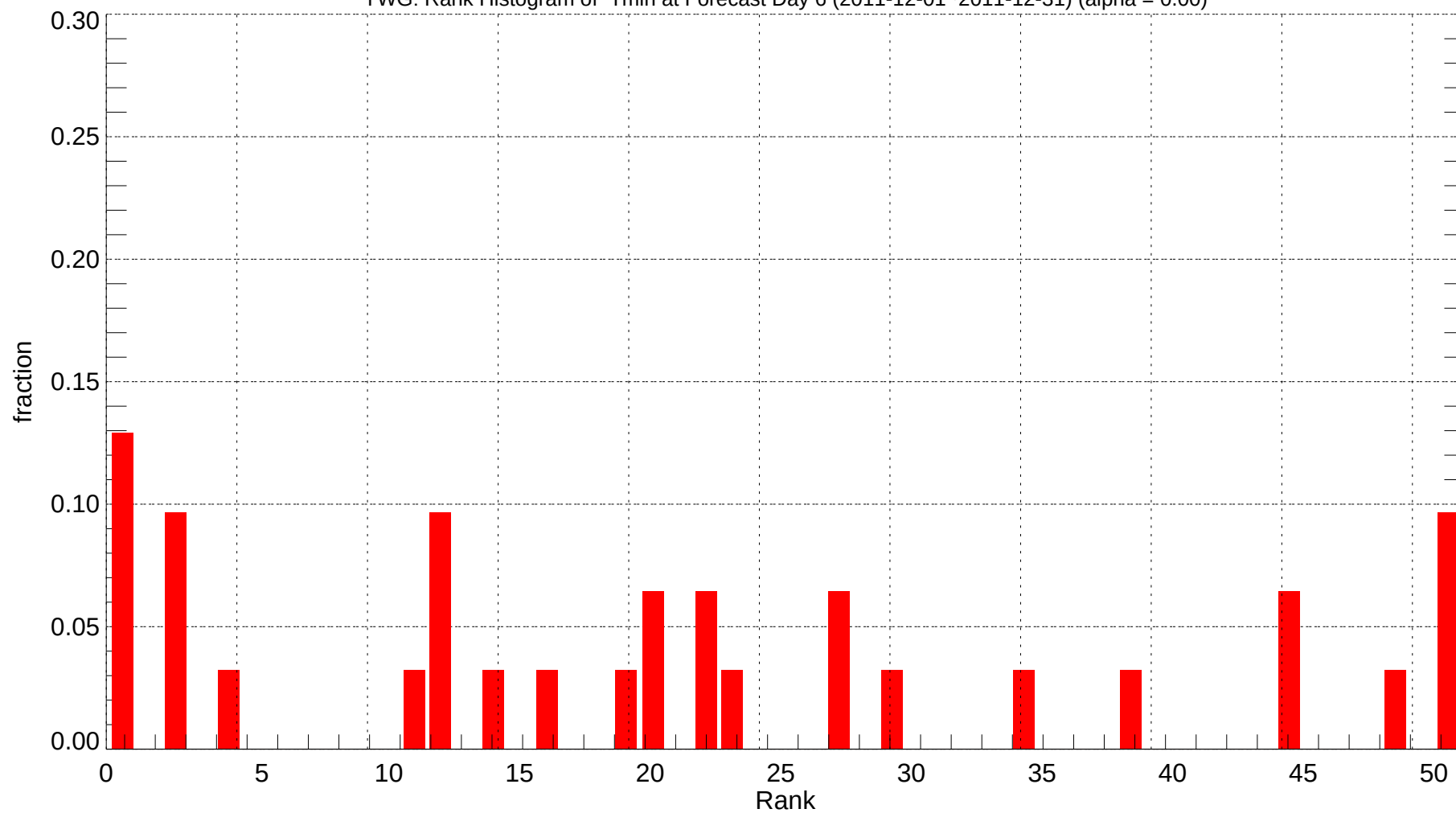
YWG: Rank Histogram of Tmin at Forecast Day 6 (2011-12-01~2011-12-31) (alpha = 0.00)
