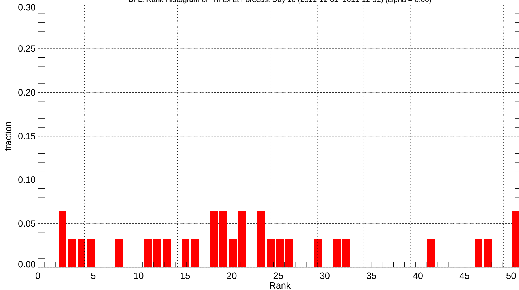
BFL: Rank Histogram of Tmax at Forecast Day 10 (2011-12-01~2011-12-31) (alpha = 0.00)
