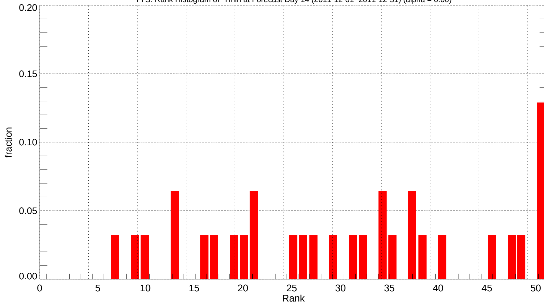
TYS: Rank Histogram of Tmin at Forecast Day 14 (2011-12-01~2011-12-31) (alpha = 0.00)
