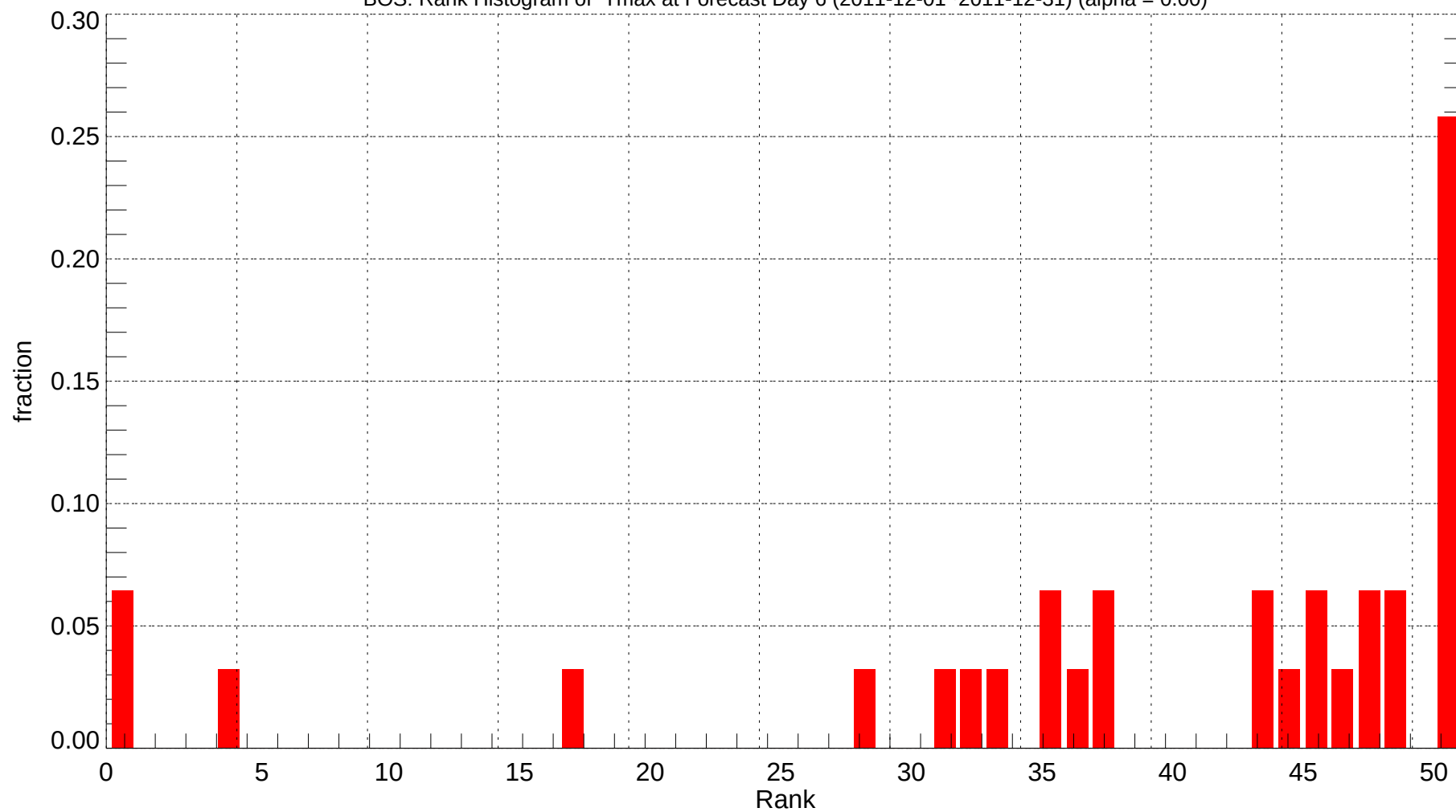
BOS: Rank Histogram of Tmax at Forecast Day 6 (2011-12-01~2011-12-31) (alpha = 0.00)
