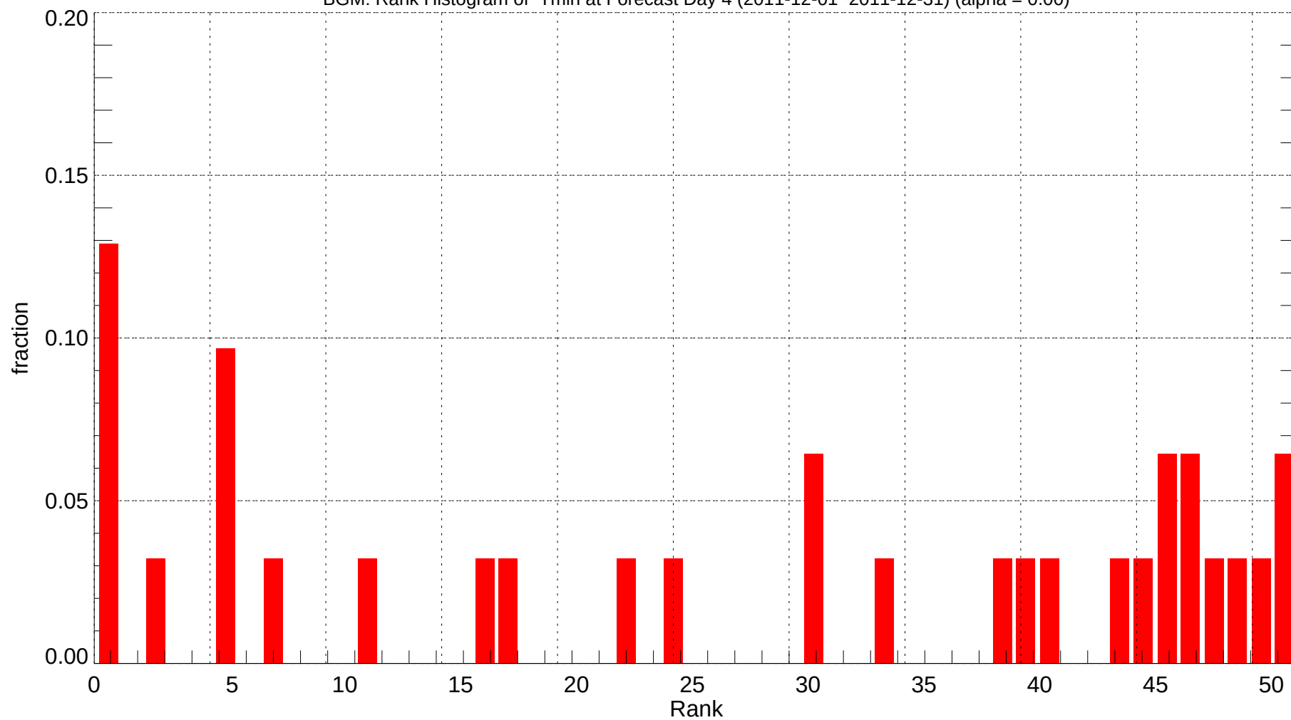
BGM: Rank Histogram of Tmin at Forecast Day 4 (2011-12-01~2011-12-31) (alpha = 0.00)
