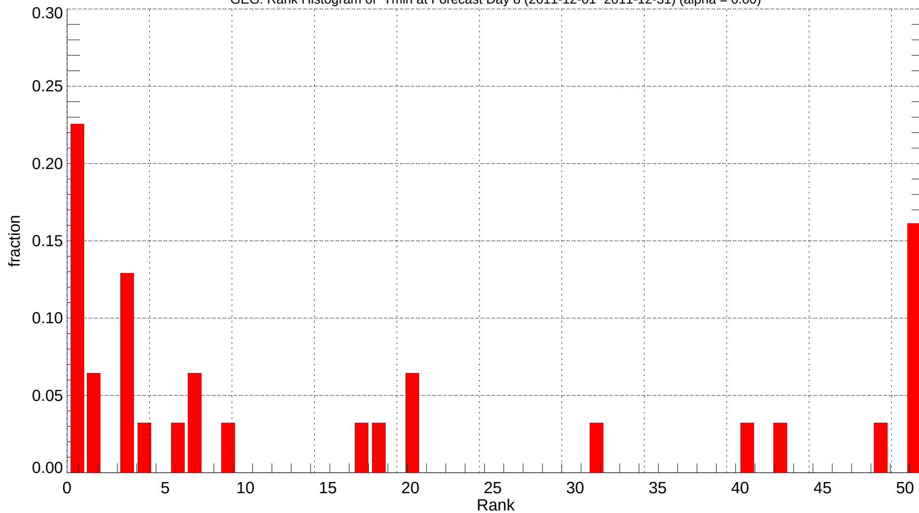
GEG: Rank Histogram of Tmin at Forecast Day 8 (2011-12-01~2011-12-31) (alpha = 0.00)
