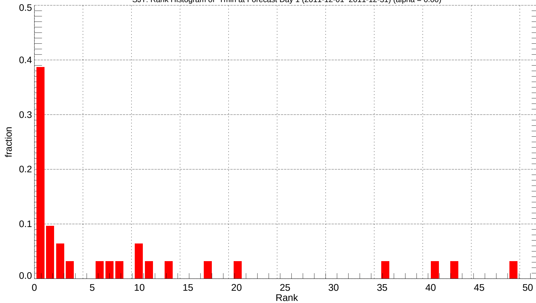
SJT: Rank Histogram of Tmin at Forecast Day 1 (2011-12-01~2011-12-31) (alpha = 0.00)
