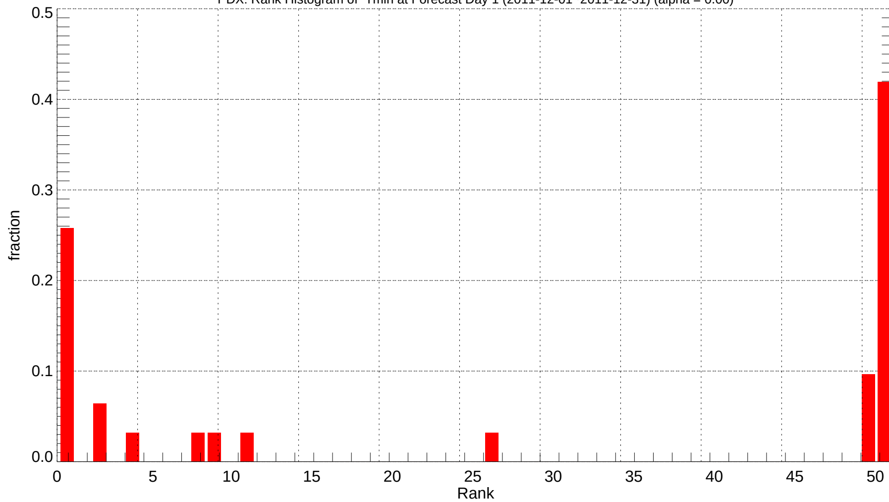
PDX: Rank Histogram of Tmin at Forecast Day 1 (2011-12-01~2011-12-31) (alpha = 0.00)
