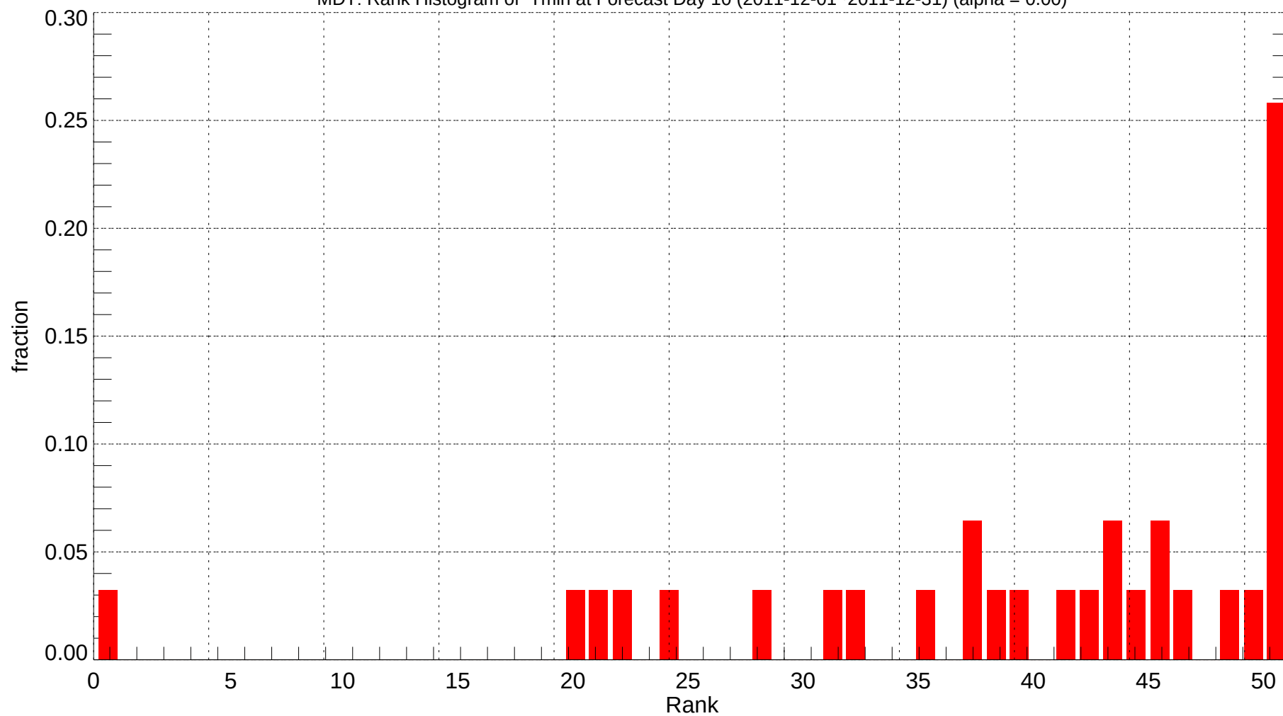
MDT: Rank Histogram of Tmin at Forecast Day 10 (2011-12-01~2011-12-31) (alpha = 0.00)
