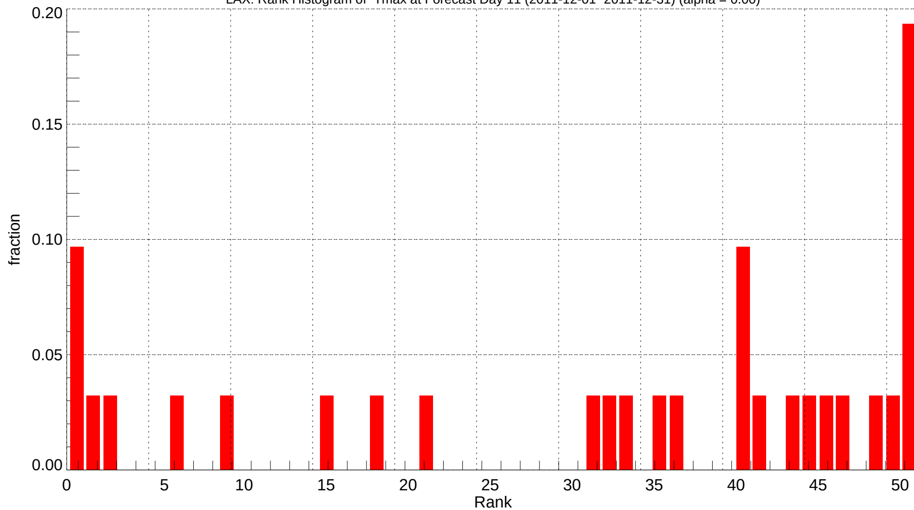
LAX: Rank Histogram of Tmax at Forecast Day 11 (2011-12-01~2011-12-31) (alpha = 0.00)
