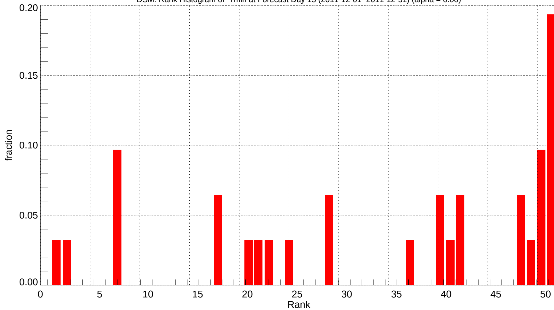
DSM: Rank Histogram of Tmin at Forecast Day 13 (2011-12-01~2011-12-31) (alpha = 0.00)
