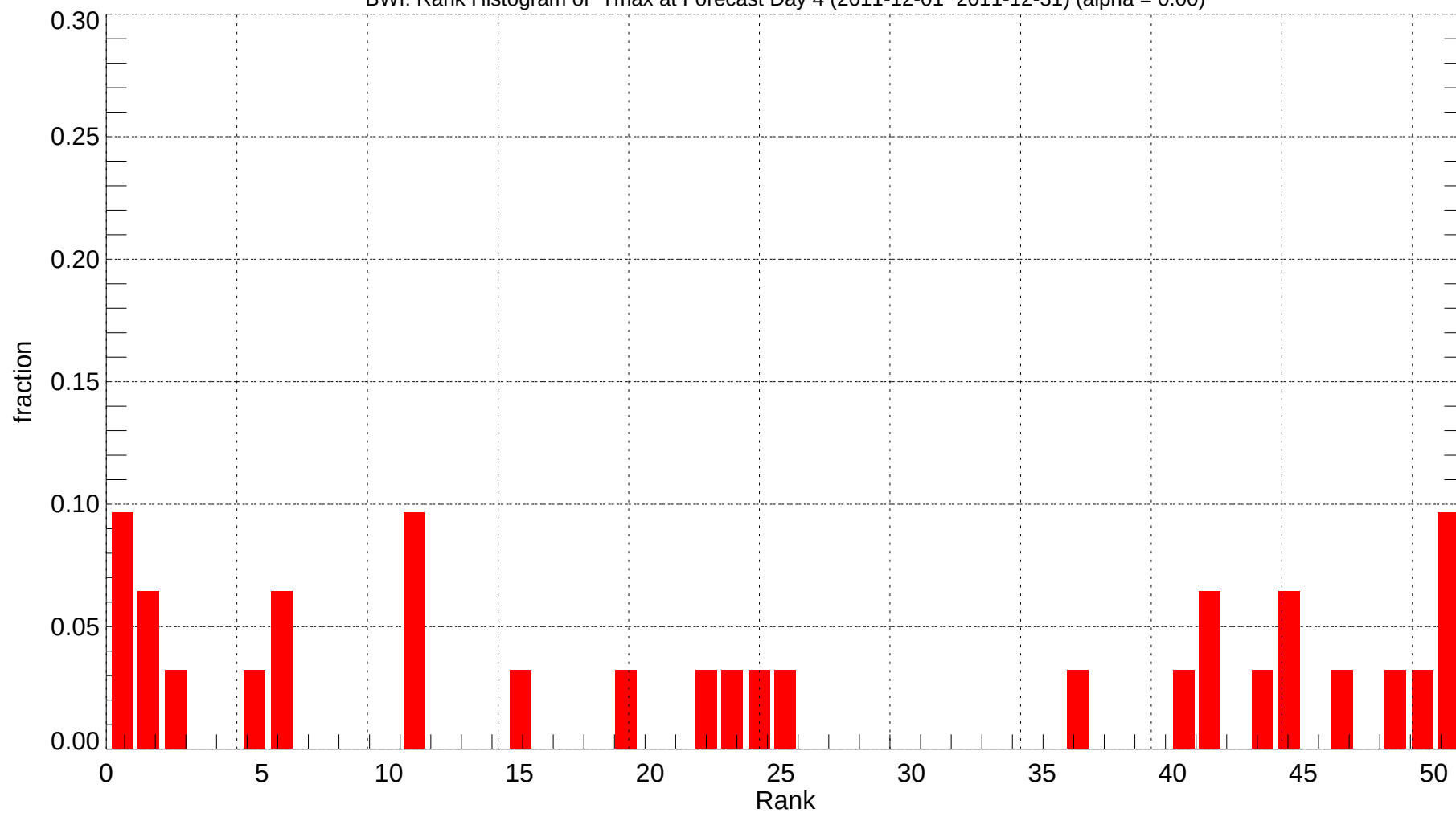
BWI: Rank Histogram of Tmax at Forecast Day 4 (2011-12-01~2011-12-31) (alpha = 0.00)
