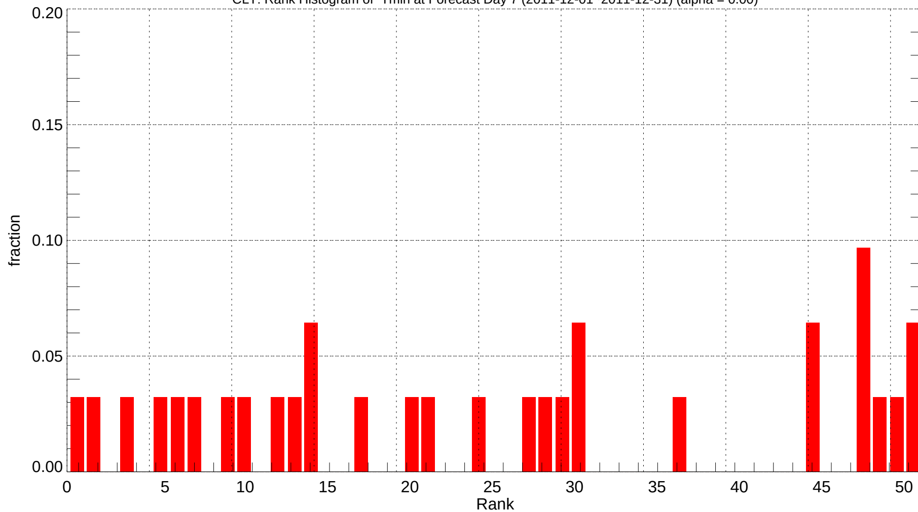
CLT: Rank Histogram of Tmin at Forecast Day 7 (2011-12-01~2011-12-31) (alpha = 0.00)
