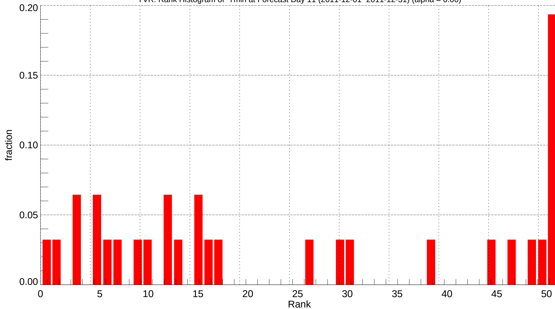
YVR: Rank Histogram of Tmin at Forecast Day 11 (2011-12-01~2011-12-31) (alpha = 0.00)
