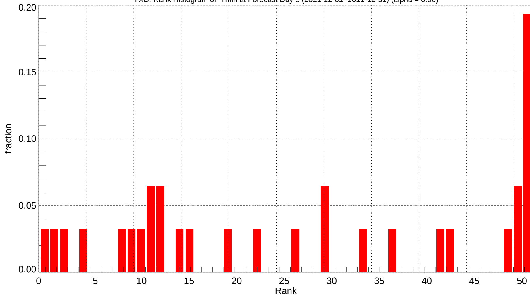
YXD: Rank Histogram of Tmin at Forecast Day 5 (2011-12-01~2011-12-31) (alpha = 0.00)
