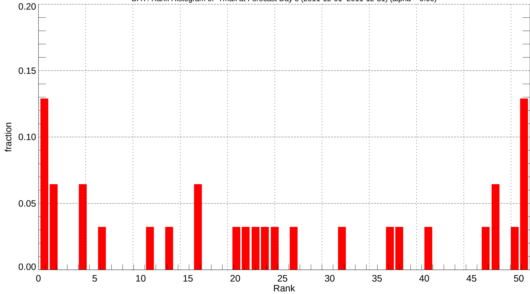
DAY: Rank Histogram of Tmax at Forecast Day 5 (2011-12-01~2011-12-31) (alpha = 0.00)
