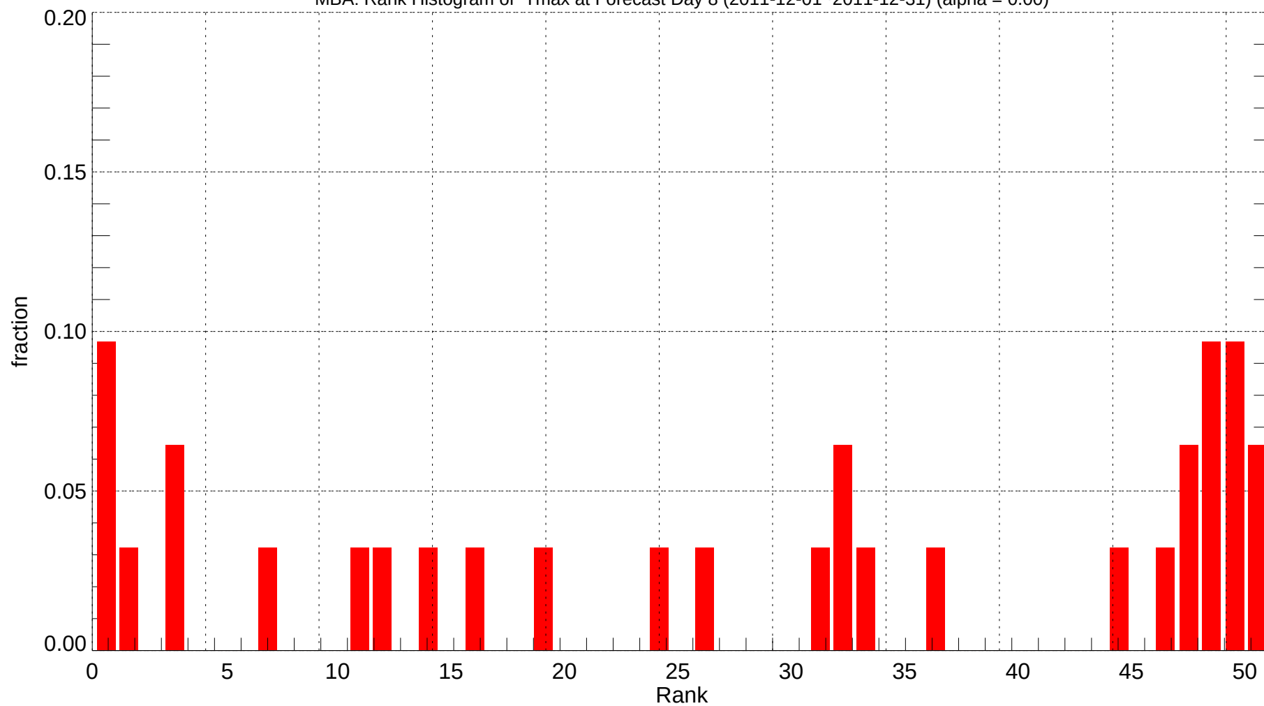
MBA: Rank Histogram of Tmax at Forecast Day 8 (2011-12-01~2011-12-31) (alpha = 0.00)
