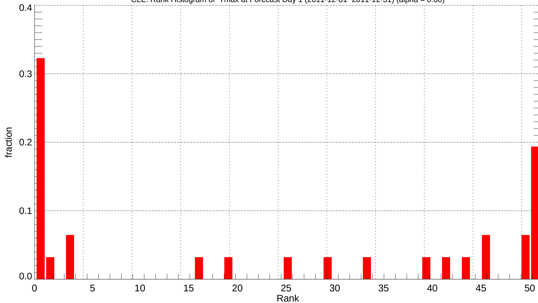
CLE: Rank Histogram of Tmax at Forecast Day 1 (2011-12-01~2011-12-31) (alpha = 0.00)
