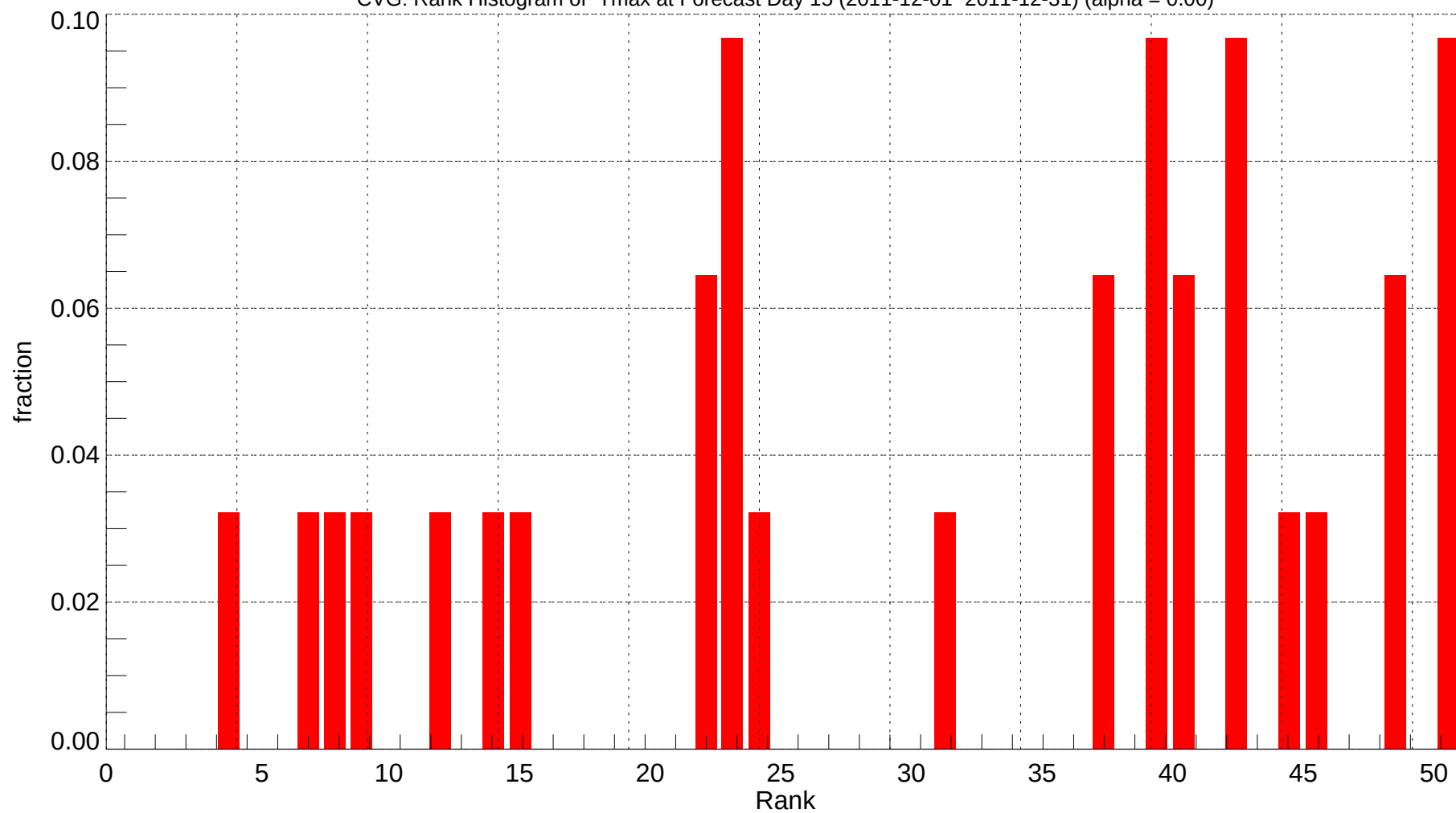
CVG: Rank Histogram of Tmax at Forecast Day 15 (2011-12-01~2011-12-31) (alpha = 0.00)
