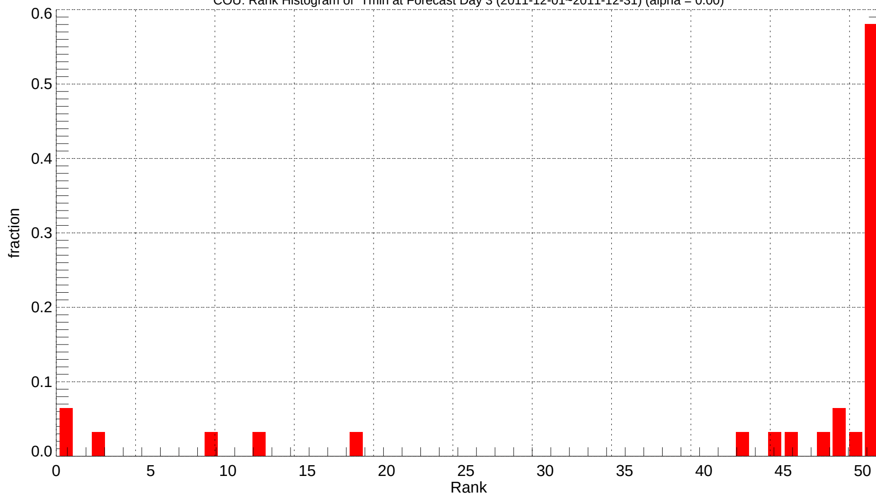
COU: Rank Histogram of Tmin at Forecast Day 3 (2011-12-01~2011-12-31) (alpha = 0.00)
