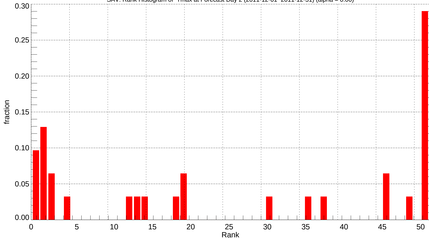
SAV: Rank Histogram of Tmax at Forecast Day 2 (2011-12-01~2011-12-31) (alpha = 0.00)
