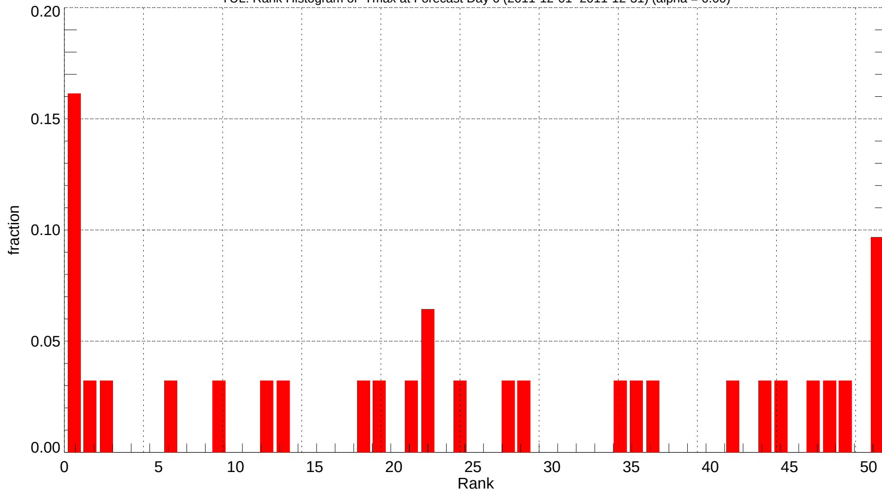
YUL: Rank Histogram of Tmax at Forecast Day 6 (2011-12-01~2011-12-31) (alpha = 0.00)
