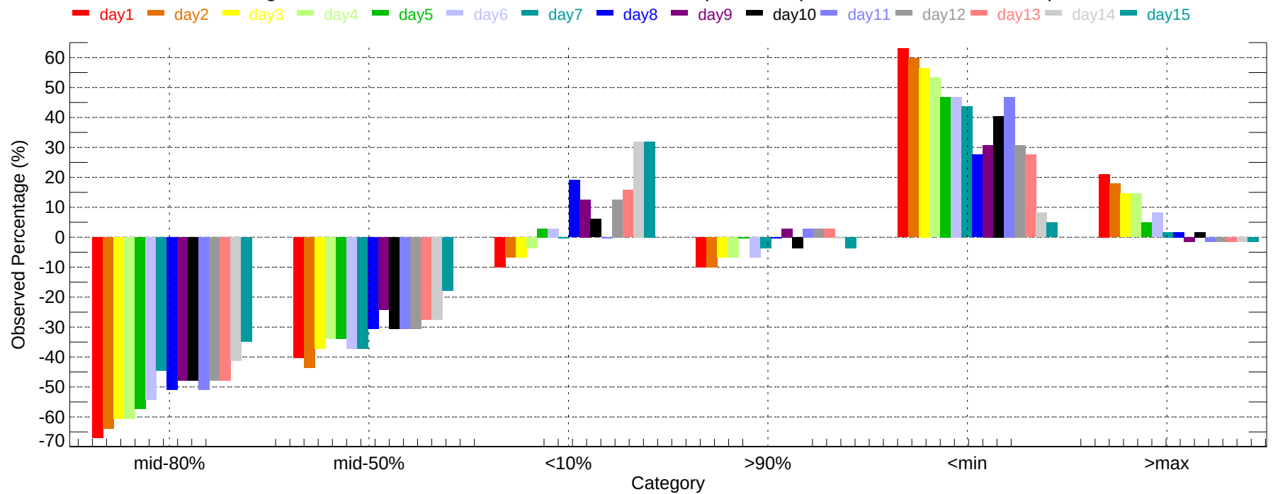
Observed Percentage Deviation of Ensembles - RDD: Min Temperature (2011-12-01~2011-12-31)
