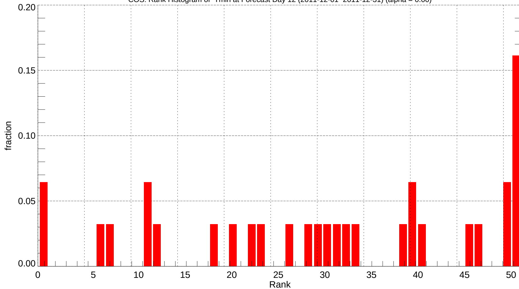
COS: Rank Histogram of Tmin at Forecast Day 12 (2011-12-01~2011-12-31) (alpha = 0.00)
