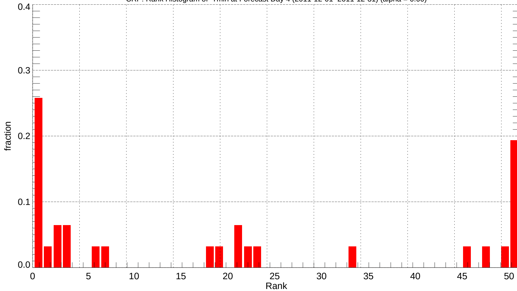
CRP: Rank Histogram of Tmin at Forecast Day 4 (2011-12-01~2011-12-31) (alpha = 0.00)
