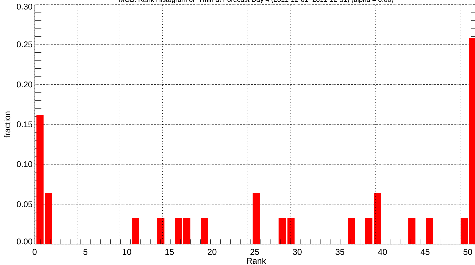
MOB: Rank Histogram of Tmin at Forecast Day 4 (2011-12-01~2011-12-31) (alpha = 0.00)
