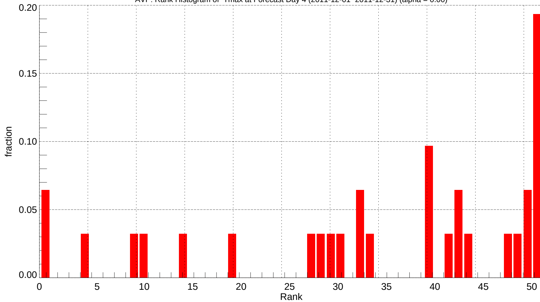
AVP: Rank Histogram of Tmax at Forecast Day 4 (2011-12-01~2011-12-31) (alpha = 0.00)
