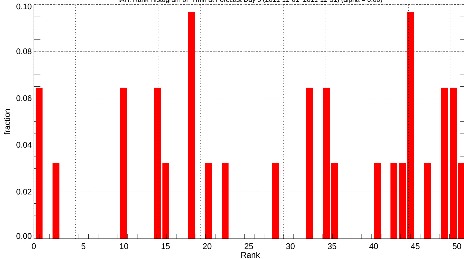
IAH: Rank Histogram of Tmin at Forecast Day 5 (2011-12-01~2011-12-31) (alpha = 0.00)
