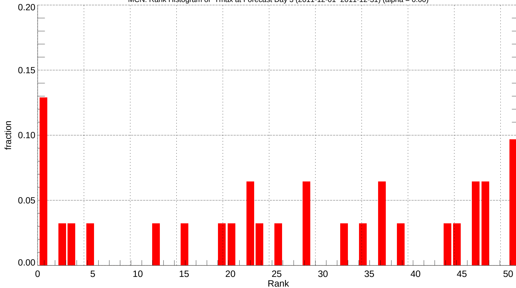
MCN: Rank Histogram of Tmax at Forecast Day 3 (2011-12-01~2011-12-31) (alpha = 0.00)
