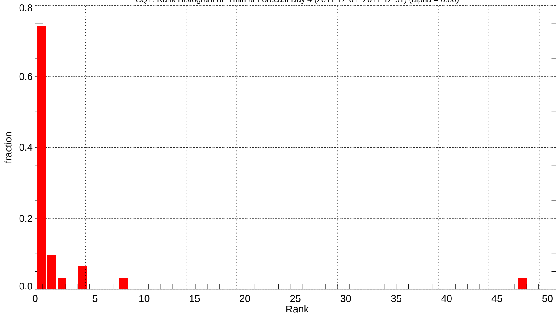
CQT: Rank Histogram of Tmin at Forecast Day 4 (2011-12-01~2011-12-31) (alpha = 0.00)
