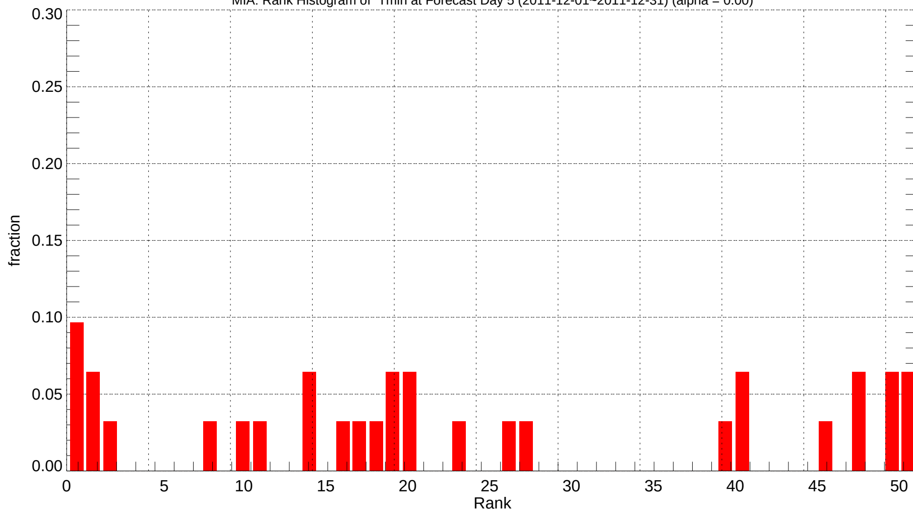
MIA: Rank Histogram of Tmin at Forecast Day 5 (2011-12-01~2011-12-31) (alpha = 0.00)
