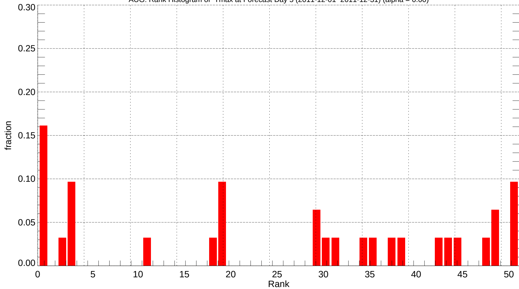
AUG: Rank Histogram of Tmax at Forecast Day 5 (2011-12-01~2011-12-31) (alpha = 0.00)
