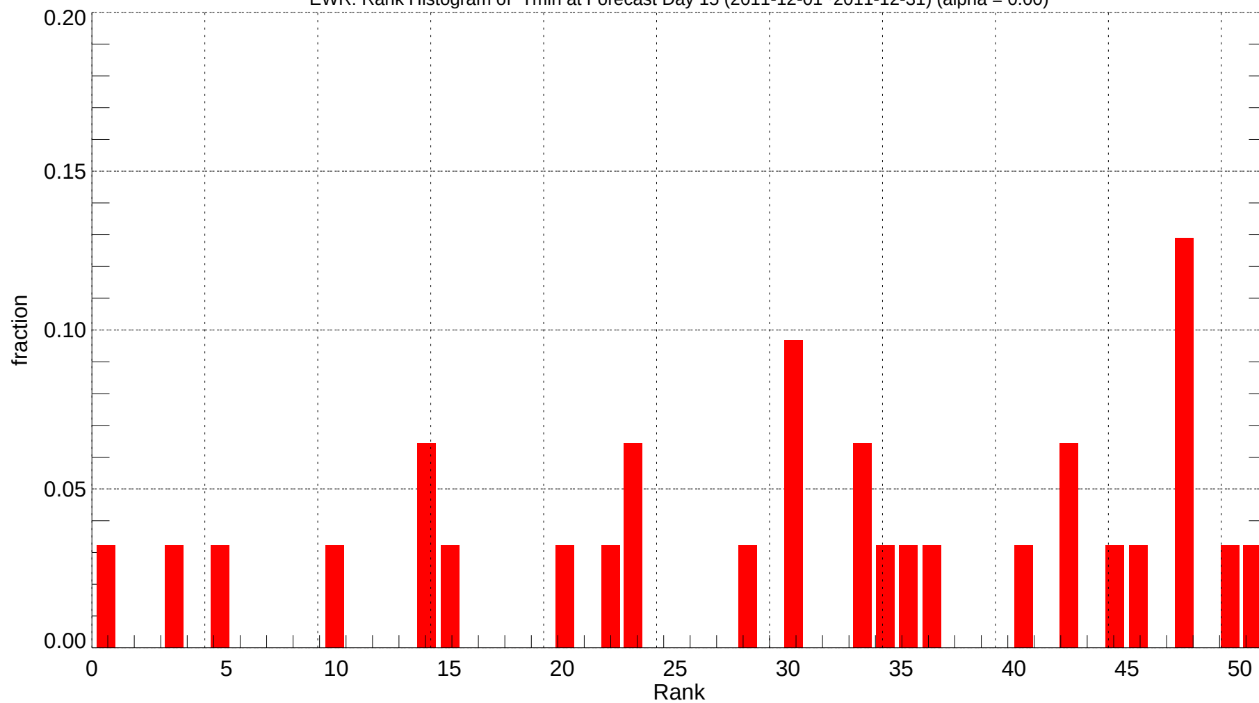
EWR: Rank Histogram of Tmin at Forecast Day 15 (2011-12-01~2011-12-31) (alpha = 0.00)
