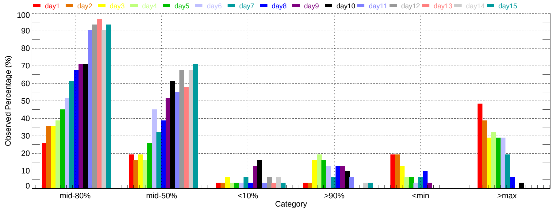
Observed Percentage of Ensembles - BFL: Max Temperature (2011-12-01~2011-12-31)
