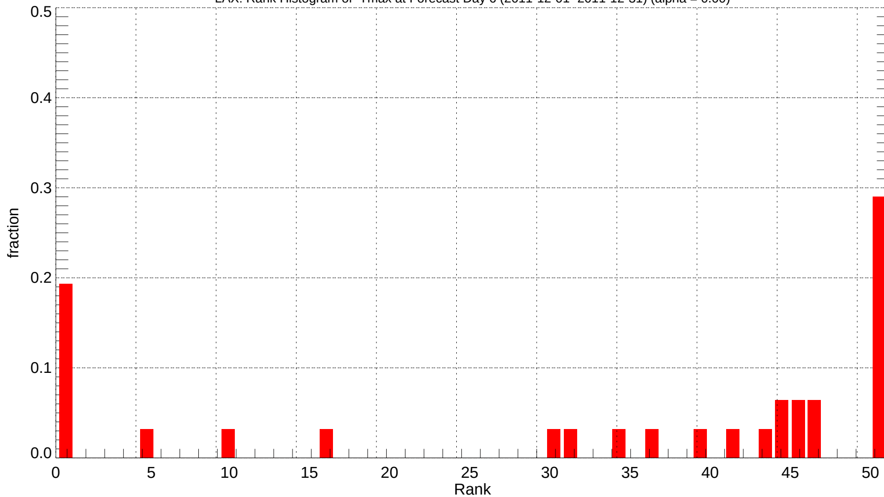
LAX: Rank Histogram of Tmax at Forecast Day 6 (2011-12-01~2011-12-31) (alpha = 0.00)
