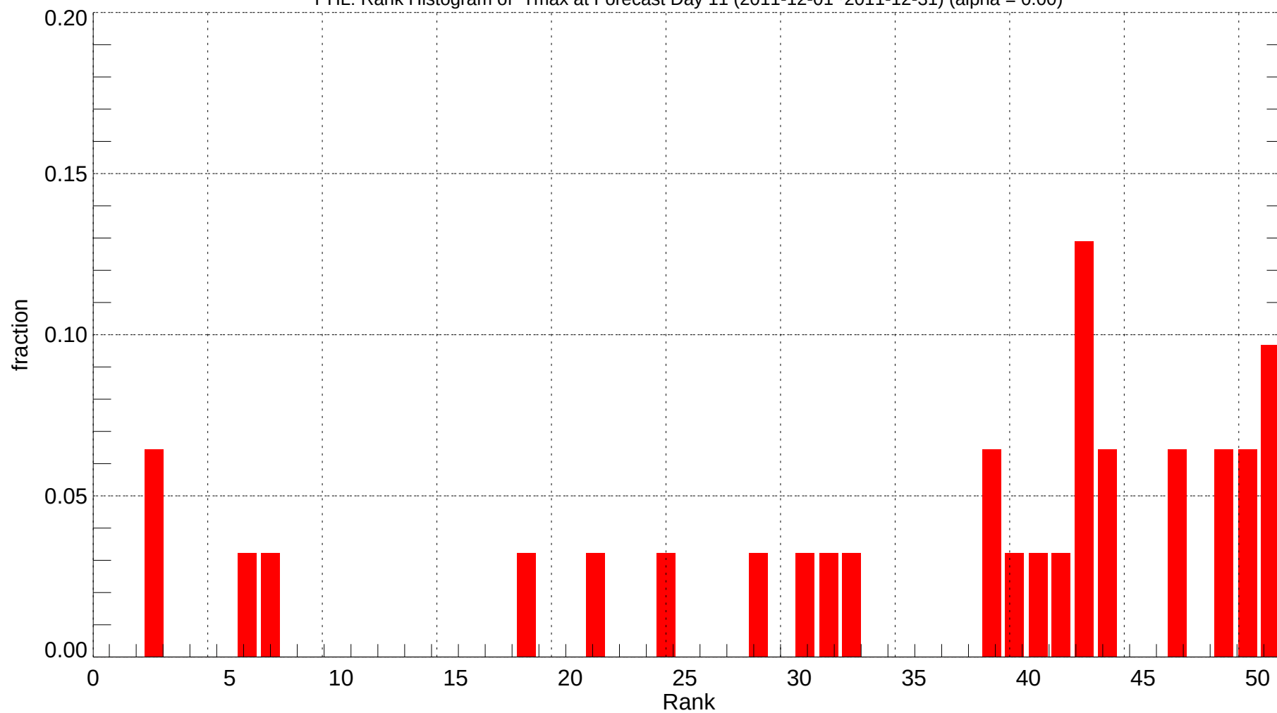
PHL: Rank Histogram of Tmax at Forecast Day 11 (2011-12-01~2011-12-31) (alpha = 0.00)
