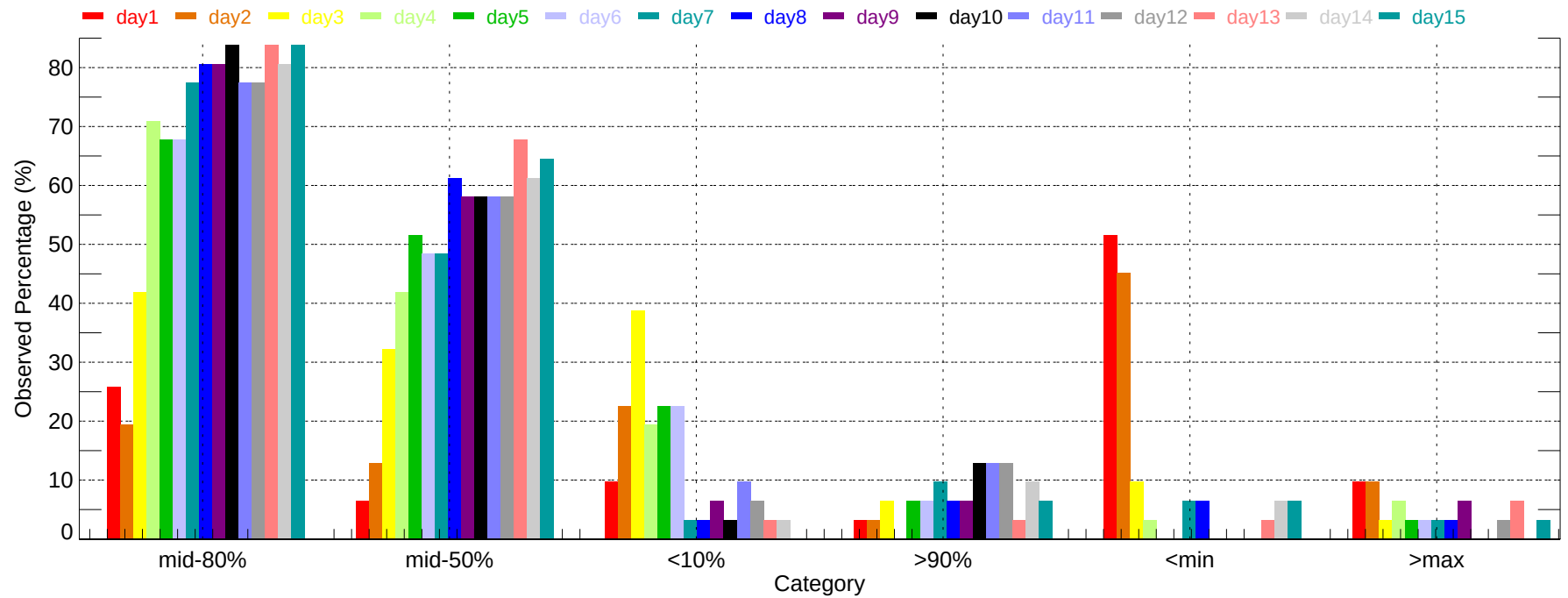
Observed Percentage of Ensembles - ABI: Min Temperature (2011-12-01~2011-12-31)
