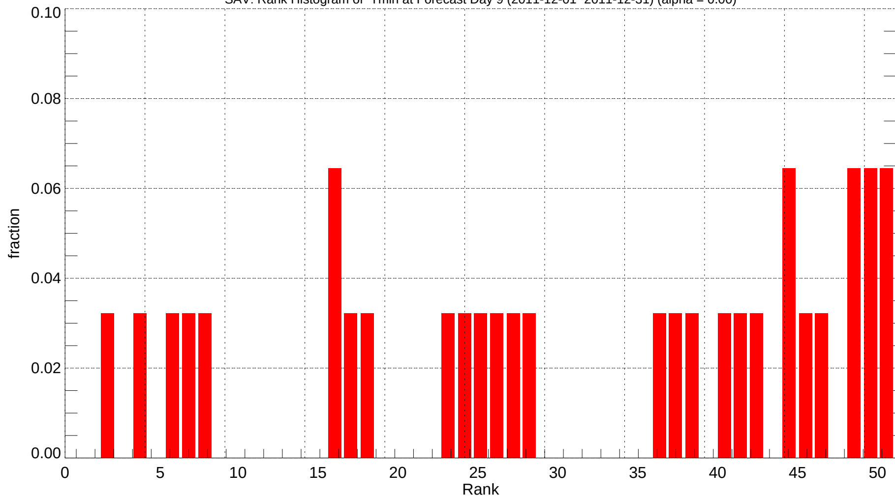
SAV: Rank Histogram of Tmin at Forecast Day 9 (2011-12-01~2011-12-31) (alpha = 0.00)
