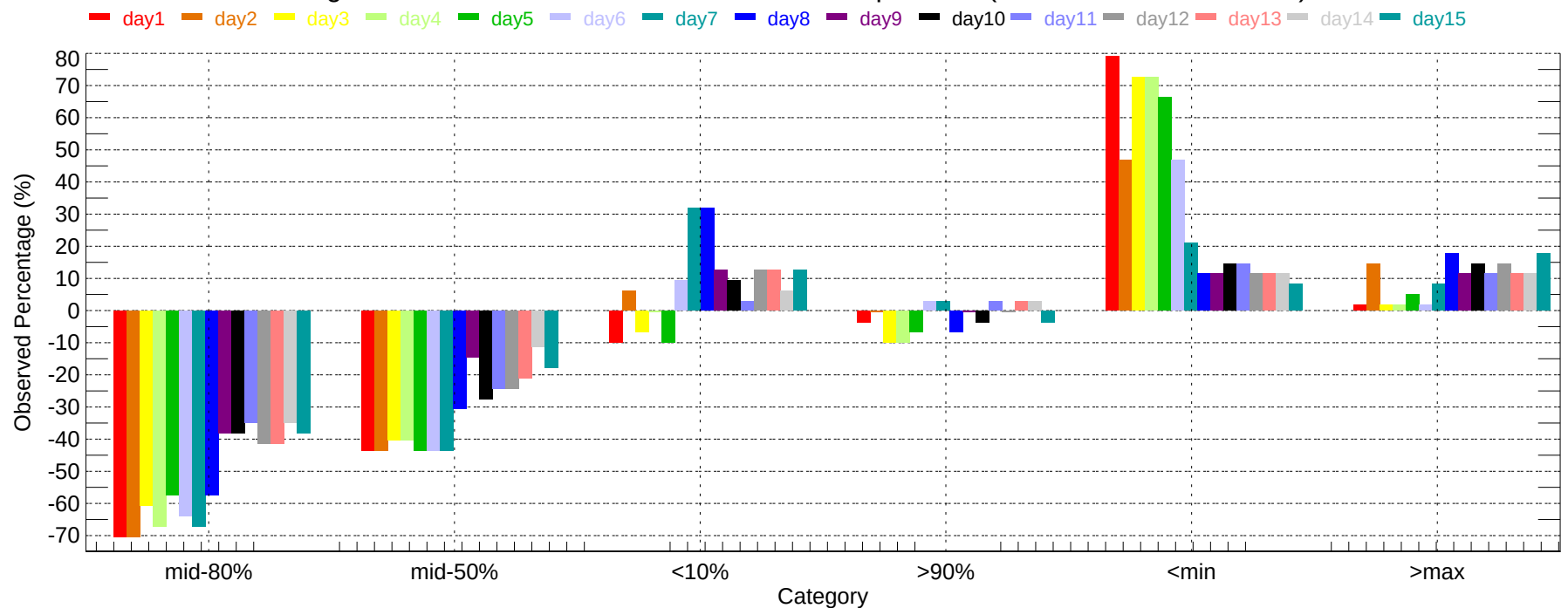
Observed Percentage Deviation of Ensembles - EUG: Max Temperature (2011-12-01~2011-12-31)
