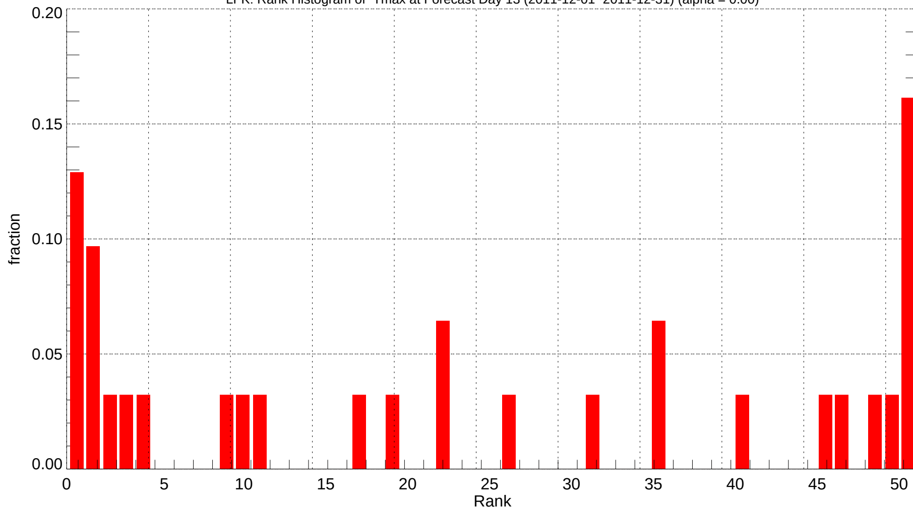
LFK: Rank Histogram of Tmax at Forecast Day 13 (2011-12-01~2011-12-31) (alpha = 0.00)
