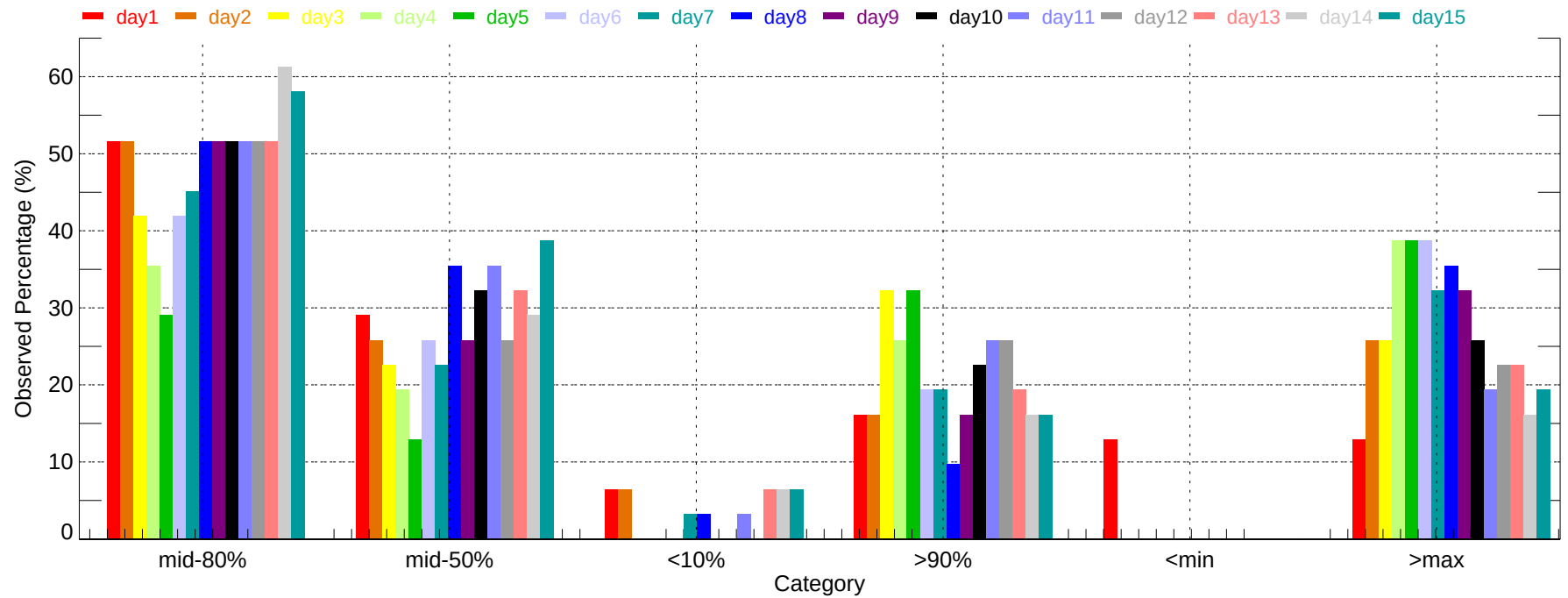
Observed Percentage of Ensembles - CRW: Max Temperature (2011-12-01~2011-12-31)
