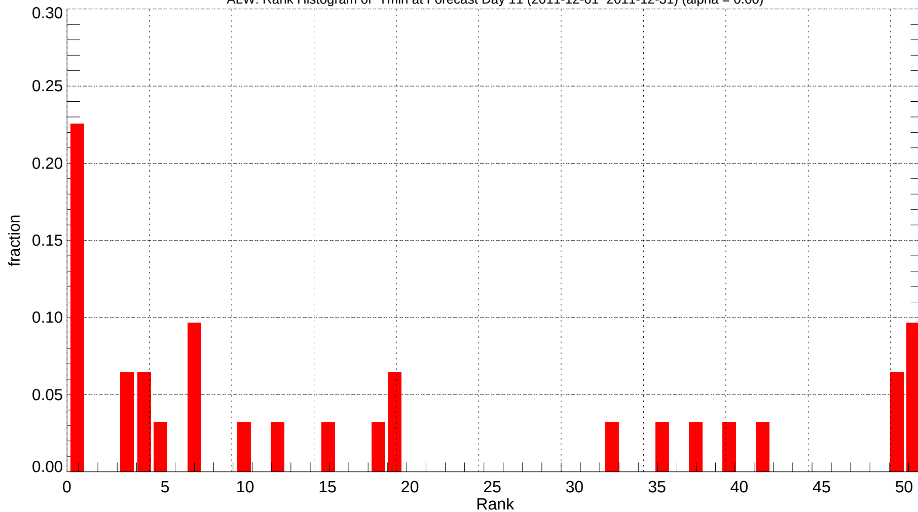
ALW: Rank Histogram of Tmin at Forecast Day 11 (2011-12-01~2011-12-31) (alpha = 0.00)
