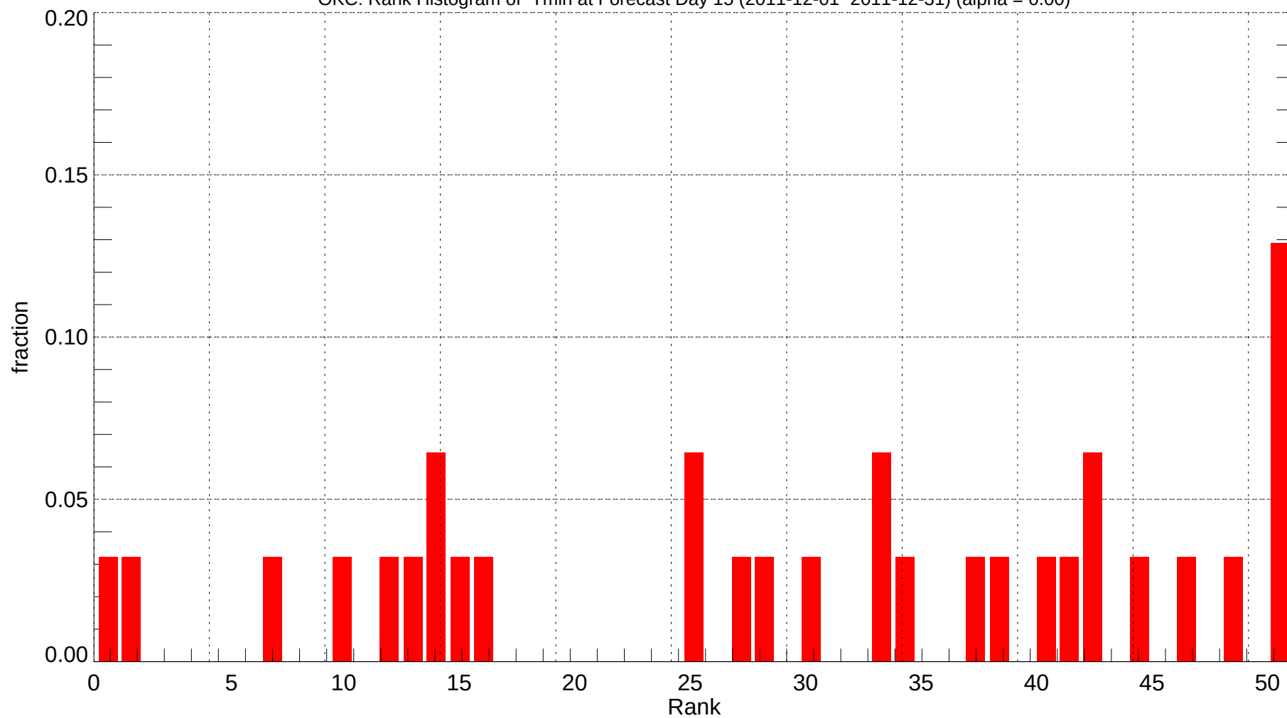
OKC: Rank Histogram of Tmin at Forecast Day 15 (2011-12-01~2011-12-31) (alpha = 0.00)
