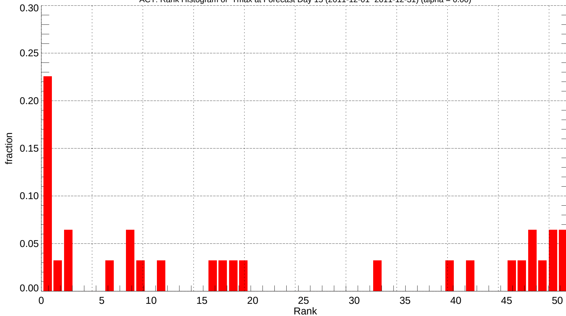
ACT: Rank Histogram of Tmax at Forecast Day 15 (2011-12-01~2011-12-31) (alpha = 0.00)
