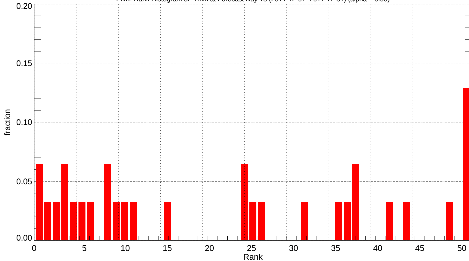
PDX: Rank Histogram of Tmin at Forecast Day 15 (2011-12-01~2011-12-31) (alpha = 0.00)
