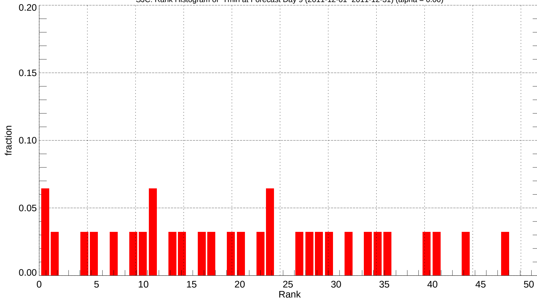
SJC: Rank Histogram of Tmin at Forecast Day 9 (2011-12-01~2011-12-31) (alpha = 0.00)
