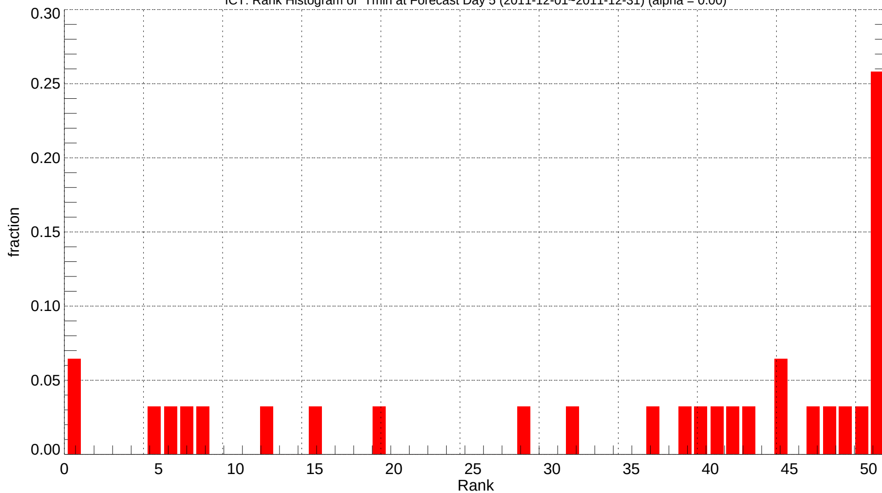
ICT: Rank Histogram of Tmin at Forecast Day 5 (2011-12-01~2011-12-31) (alpha = 0.00)
