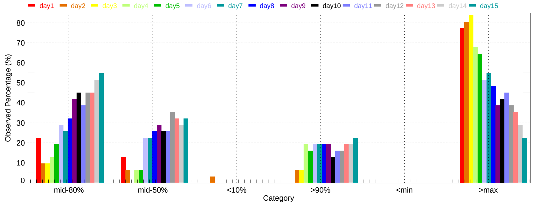
Observed Percentage of Ensembles - GTF: Min Temperature (2011-12-01~2011-12-31)
