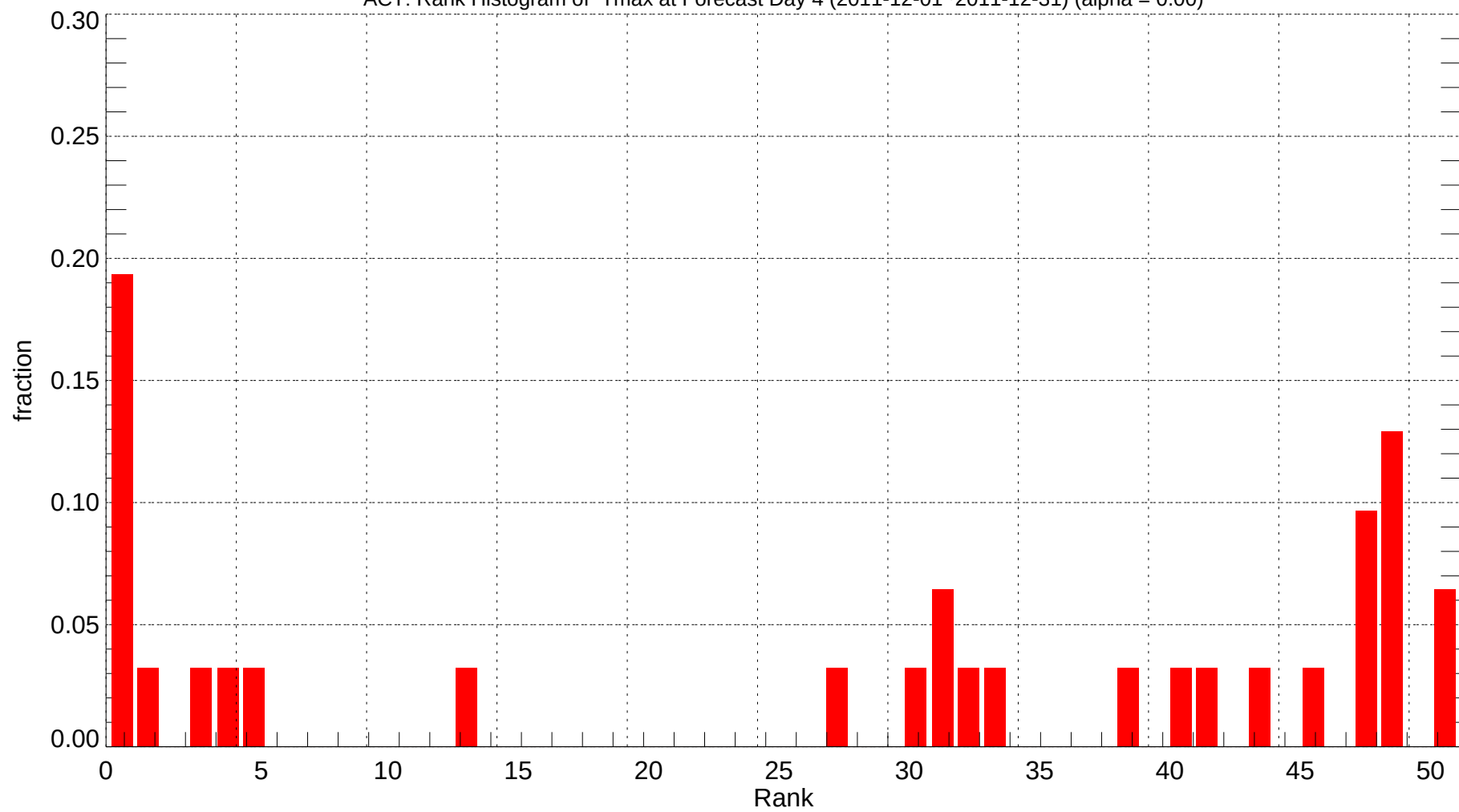
ACT: Rank Histogram of Tmax at Forecast Day 4 (2011-12-01~2011-12-31) (alpha = 0.00)
