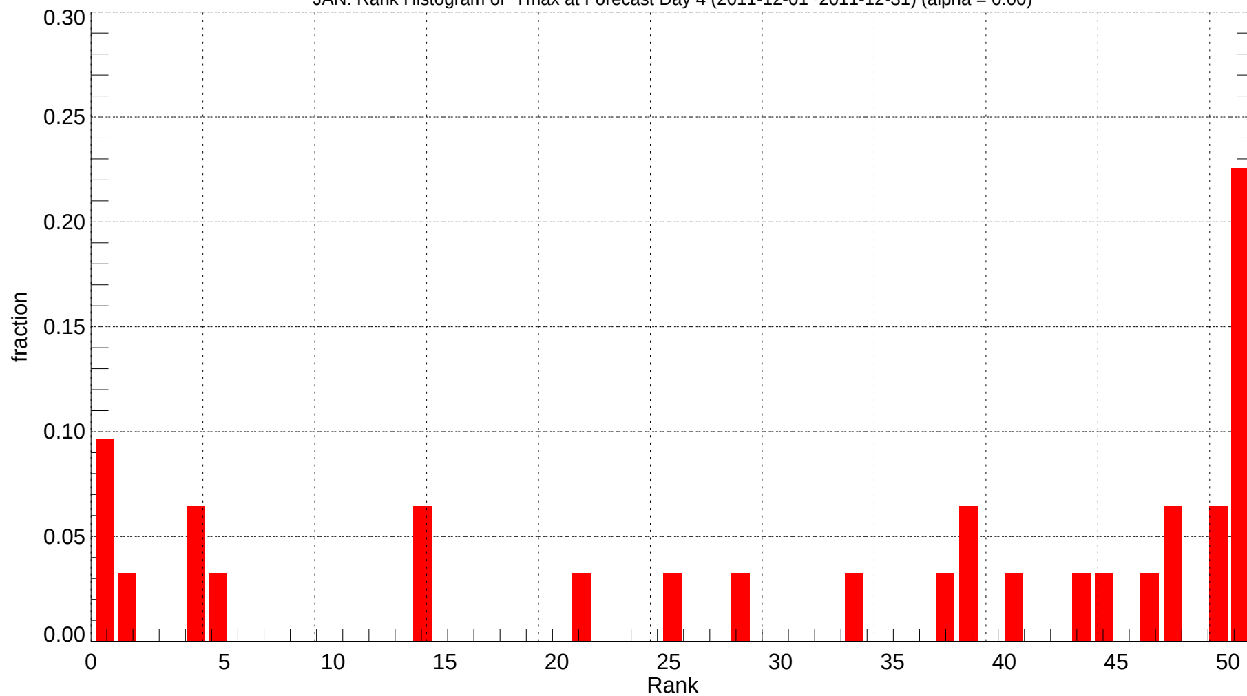
JAN: Rank Histogram of Tmax at Forecast Day 4 (2011-12-01~2011-12-31) (alpha = 0.00)
