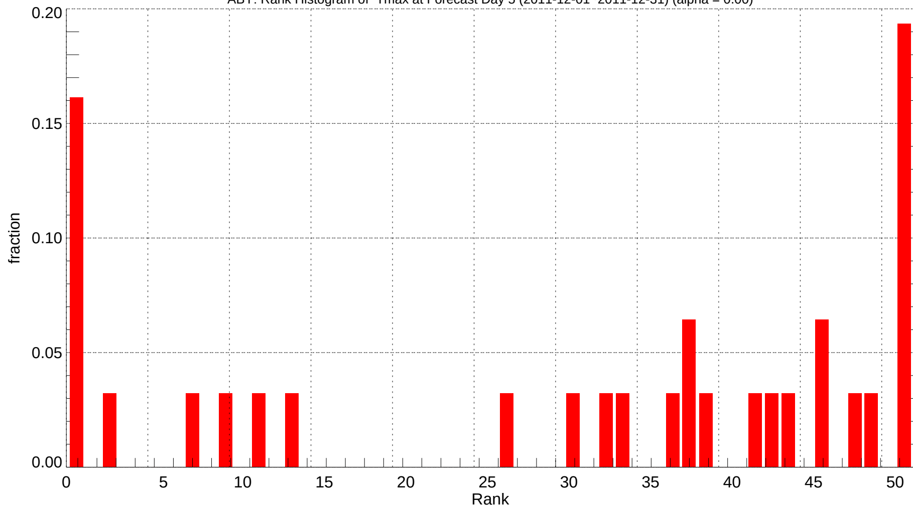
ABY: Rank Histogram of Tmax at Forecast Day 5 (2011-12-01~2011-12-31) (alpha = 0.00)
