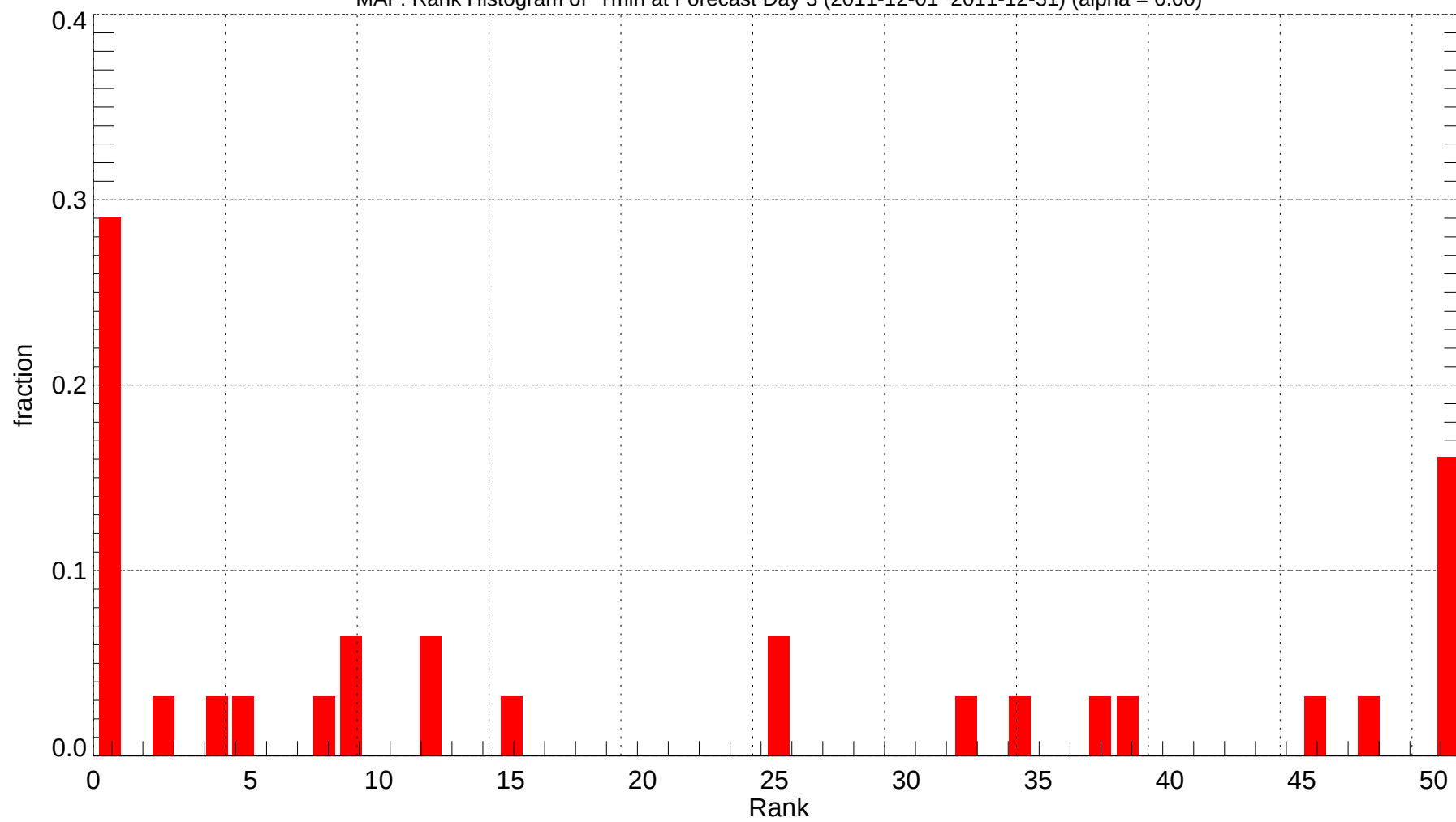
MAF: Rank Histogram of Tmin at Forecast Day 3 (2011-12-01~2011-12-31) (alpha = 0.00)
