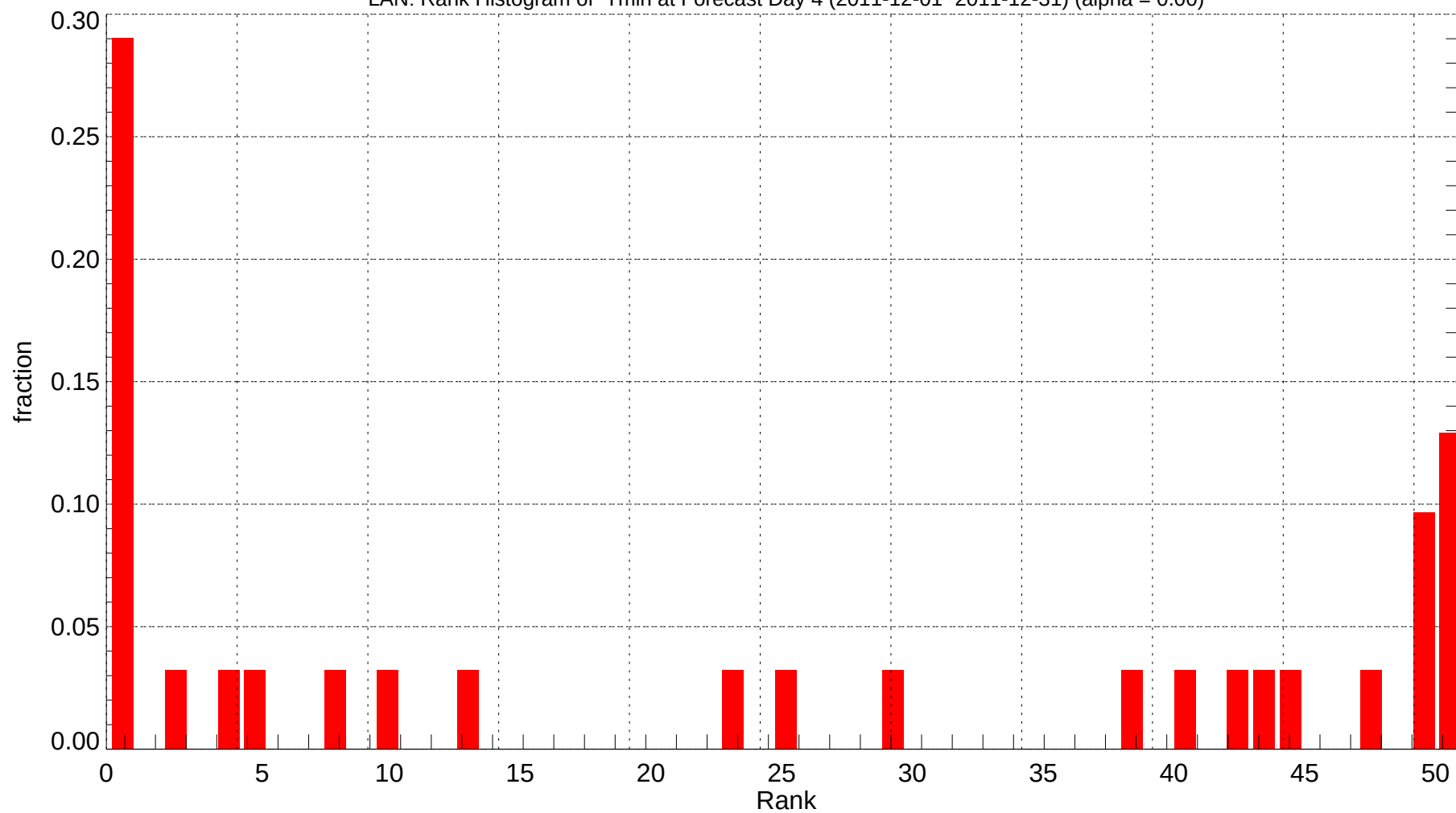
LAN: Rank Histogram of Tmin at Forecast Day 4 (2011-12-01~2011-12-31) (alpha = 0.00)
