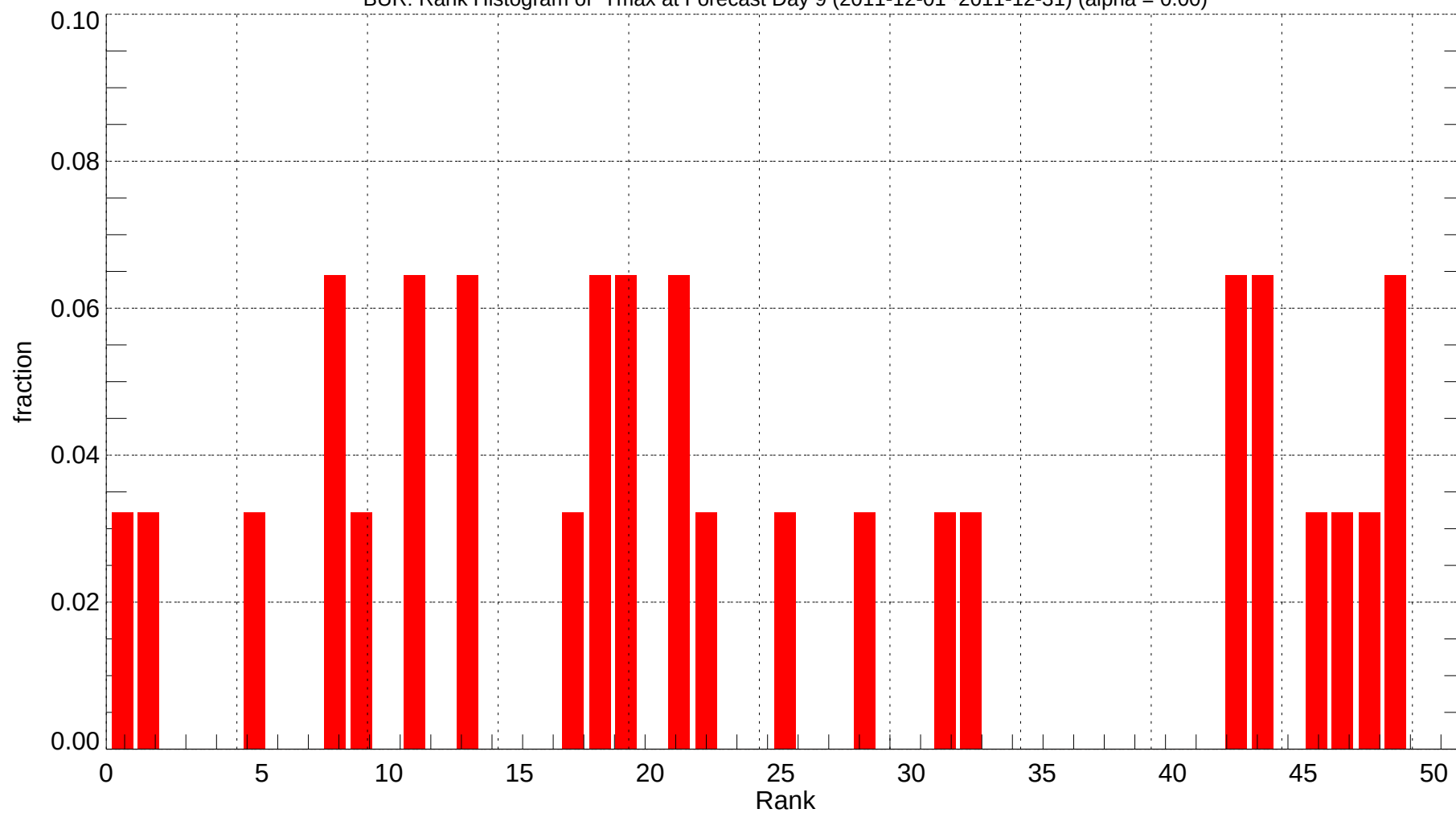
BUR: Rank Histogram of Tmax at Forecast Day 9 (2011-12-01~2011-12-31) (alpha = 0.00)
