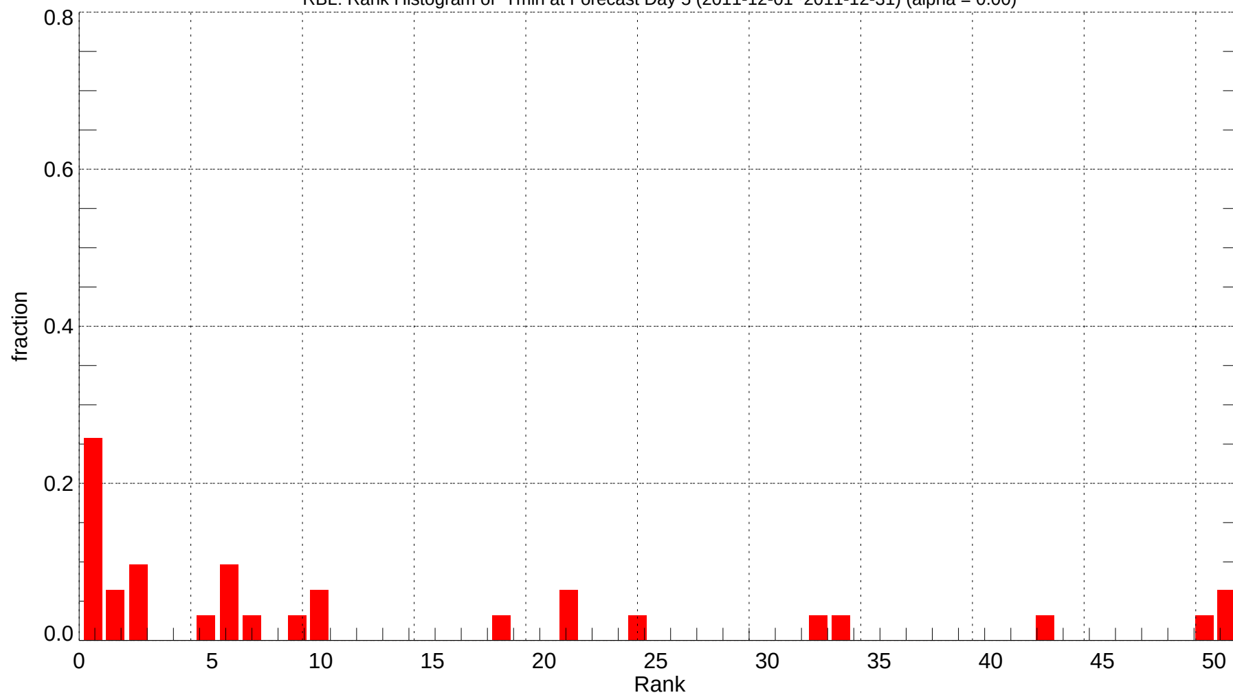
RBL: Rank Histogram of Tmin at Forecast Day 5 (2011-12-01~2011-12-31) (alpha = 0.00)
