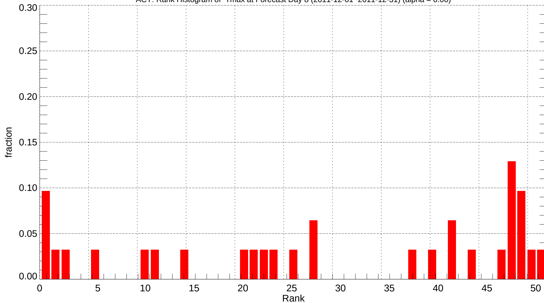
ACY: Rank Histogram of Tmax at Forecast Day 8 (2011-12-01~2011-12-31) (alpha = 0.00)
