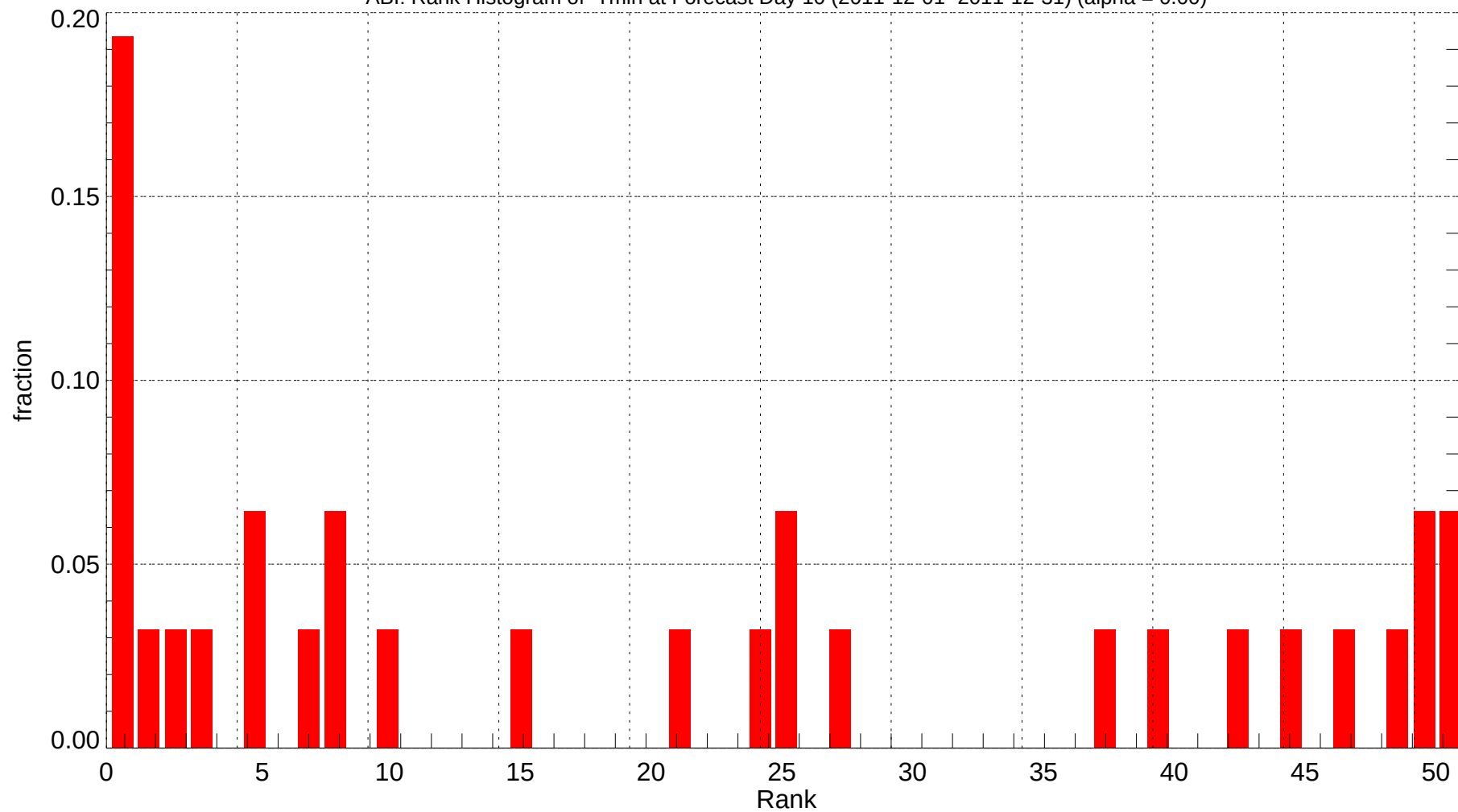
ABI: Rank Histogram of Tmin at Forecast Day 10 (2011-12-01~2011-12-31) (alpha = 0.00)
