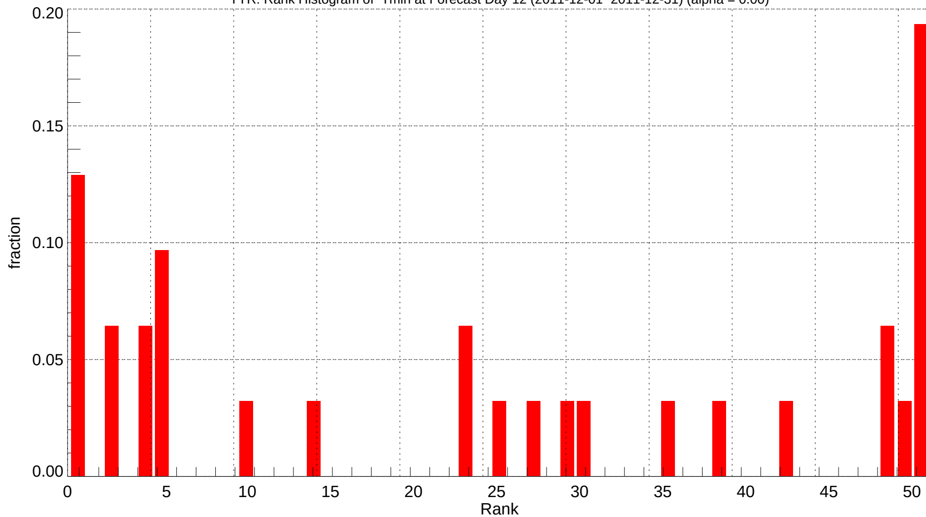
TYR: Rank Histogram of Tmin at Forecast Day 12 (2011-12-01~2011-12-31) (alpha = 0.00)
