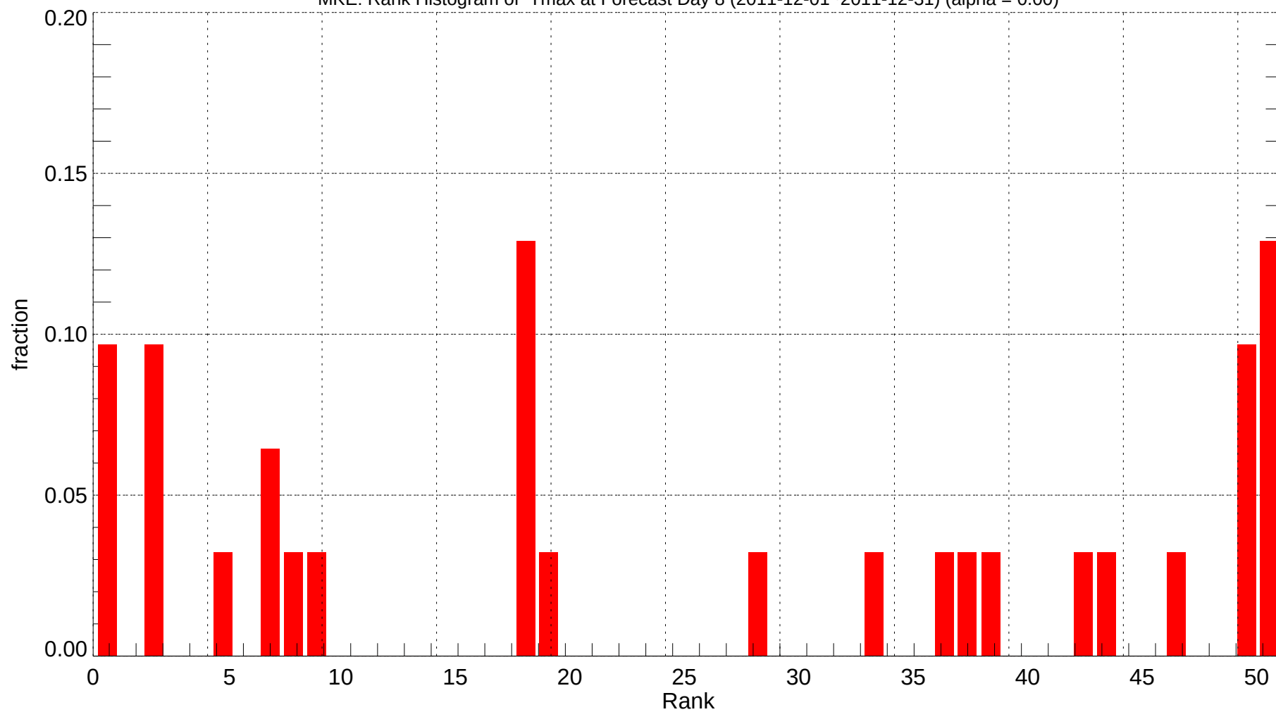
MKE: Rank Histogram of Tmax at Forecast Day 8 (2011-12-01~2011-12-31) (alpha = 0.00)
