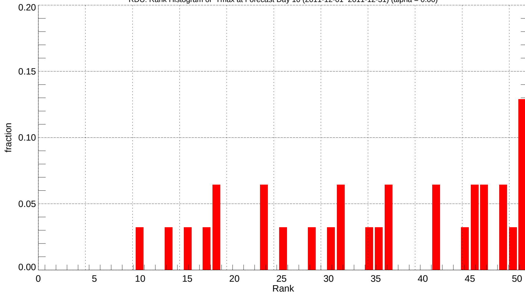
RDU: Rank Histogram of Tmax at Forecast Day 10 (2011-12-01~2011-12-31) (alpha = 0.00)
