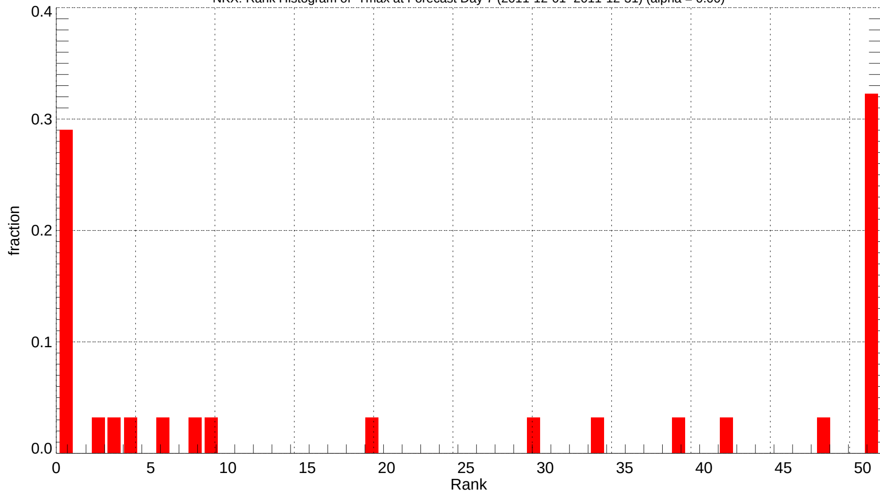
NKX: Rank Histogram of Tmax at Forecast Day 7 (2011-12-01~2011-12-31) (alpha = 0.00)
