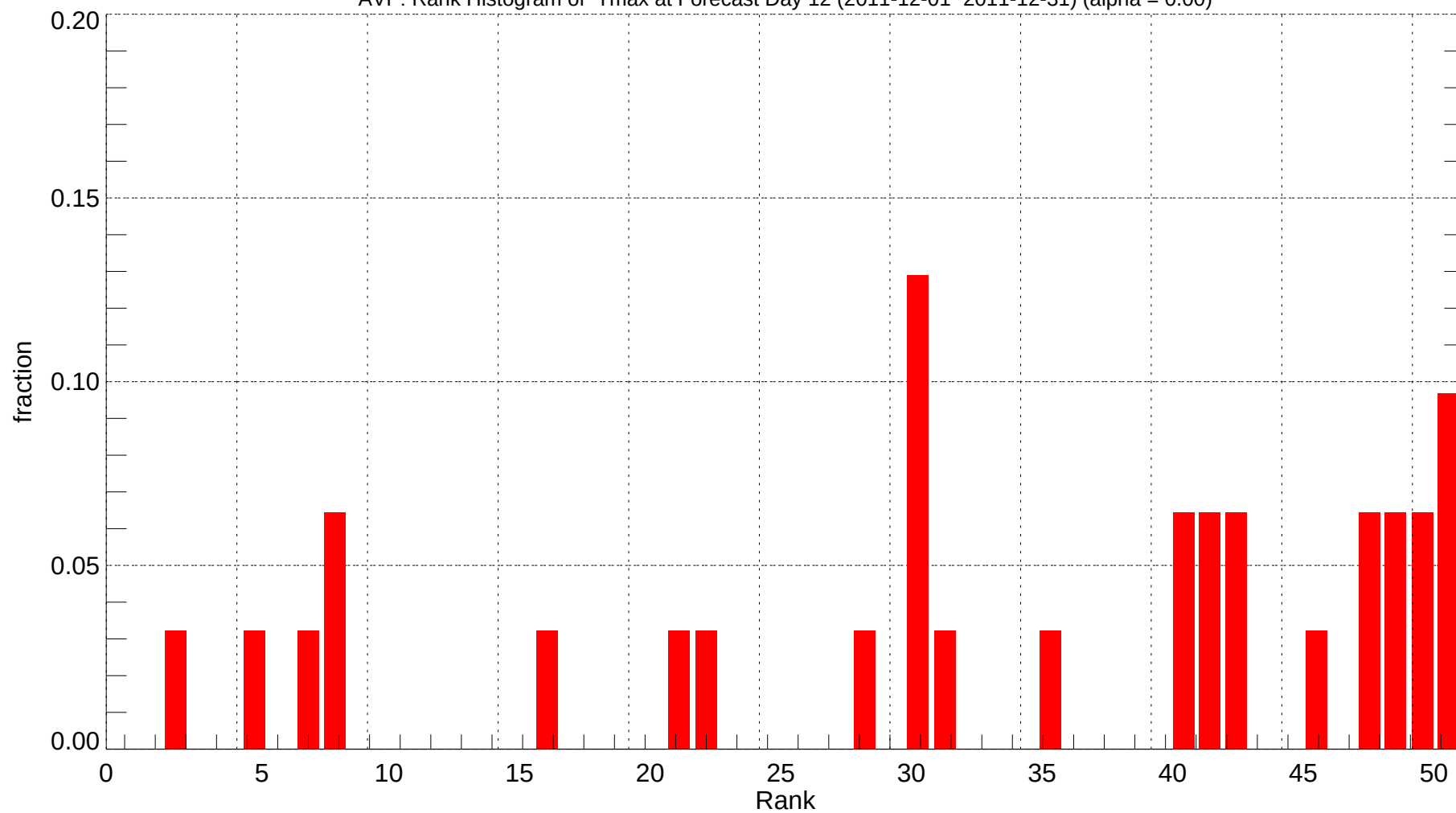
AVP: Rank Histogram of Tmax at Forecast Day 12 (2011-12-01~2011-12-31) (alpha = 0.00)
