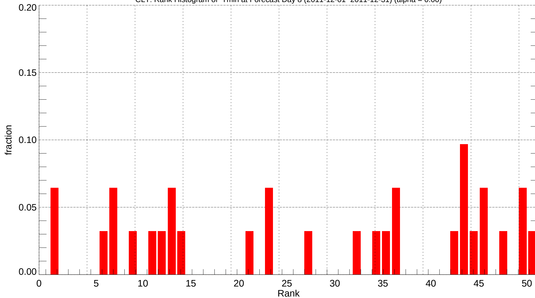
CLT: Rank Histogram of Tmin at Forecast Day 8 (2011-12-01~2011-12-31) (alpha = 0.00)
