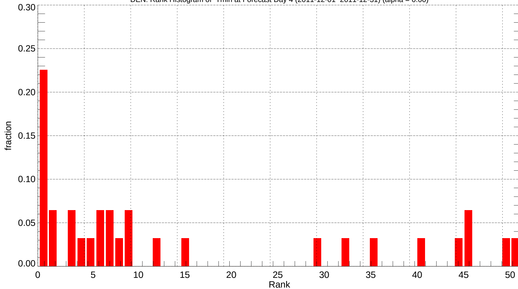
DEN: Rank Histogram of Tmin at Forecast Day 4 (2011-12-01~2011-12-31) (alpha = 0.00)
