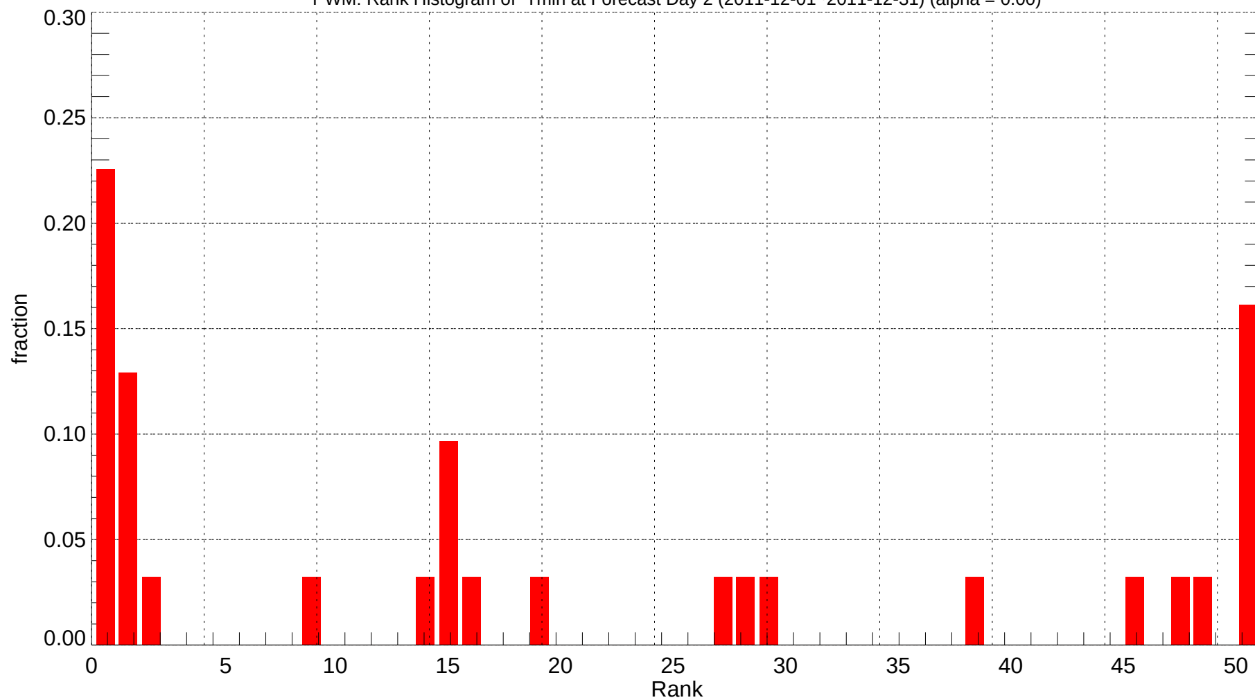
PWM: Rank Histogram of Tmin at Forecast Day 2 (2011-12-01~2011-12-31) (alpha = 0.00)
