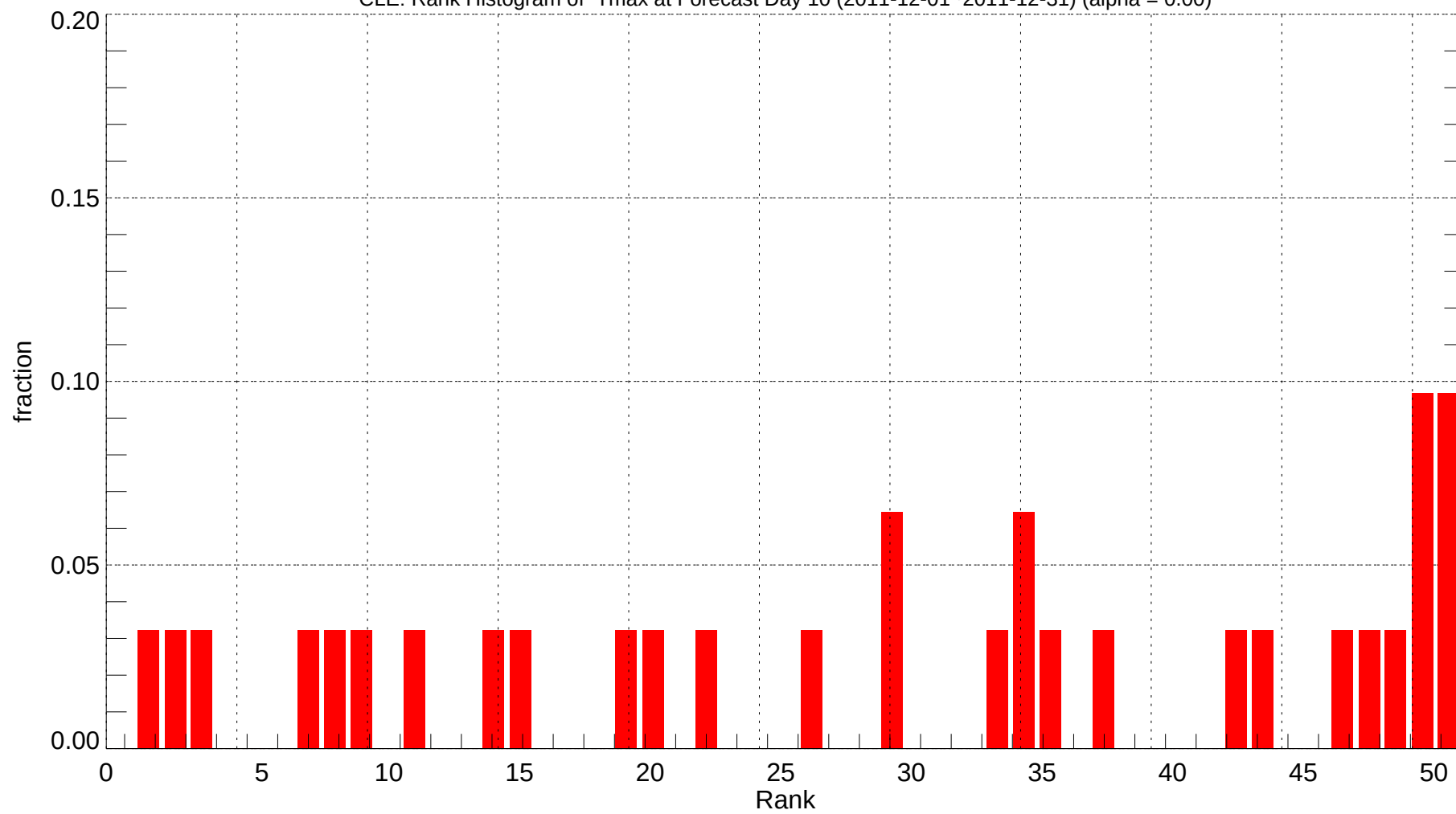
CLE: Rank Histogram of Tmax at Forecast Day 10 (2011-12-01~2011-12-31) (alpha = 0.00)
