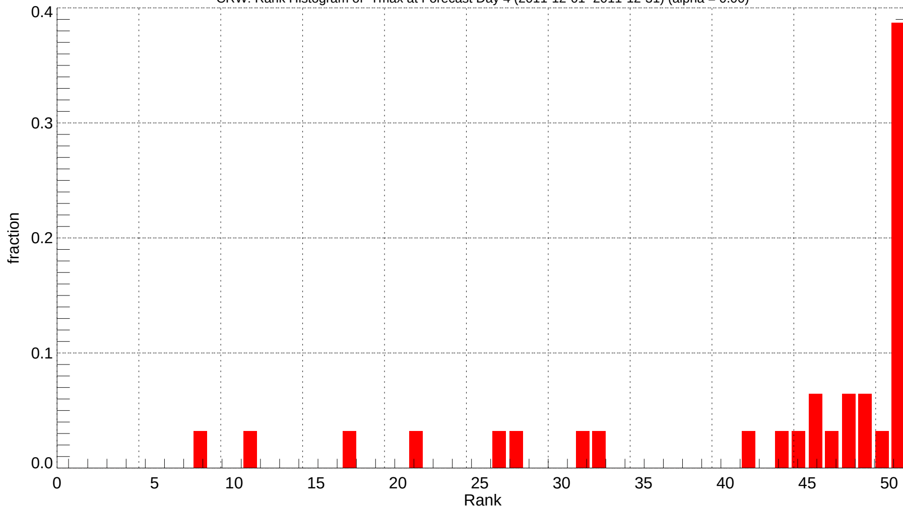
CRW: Rank Histogram of Tmax at Forecast Day 4 (2011-12-01~2011-12-31) (alpha = 0.00)
