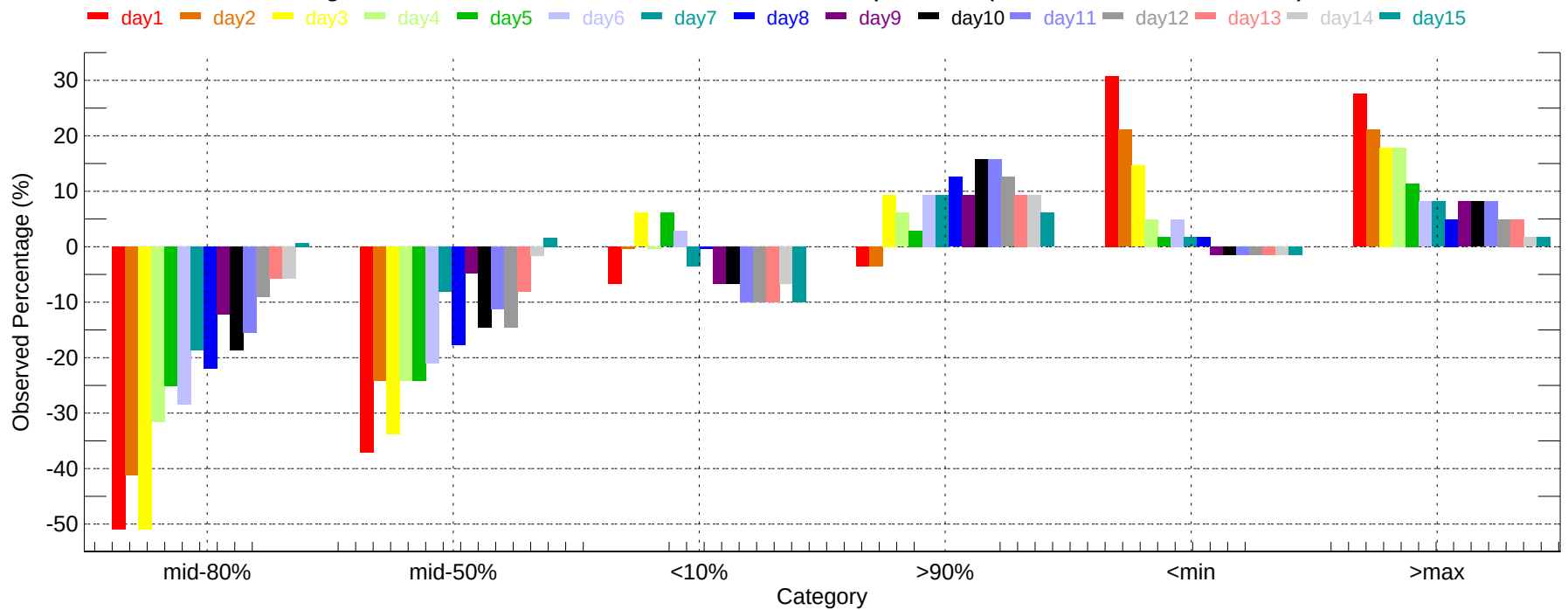
Observed Percentage Deviation of Ensembles - DEC: Max Temperature (2011-12-01~2011-12-31)
