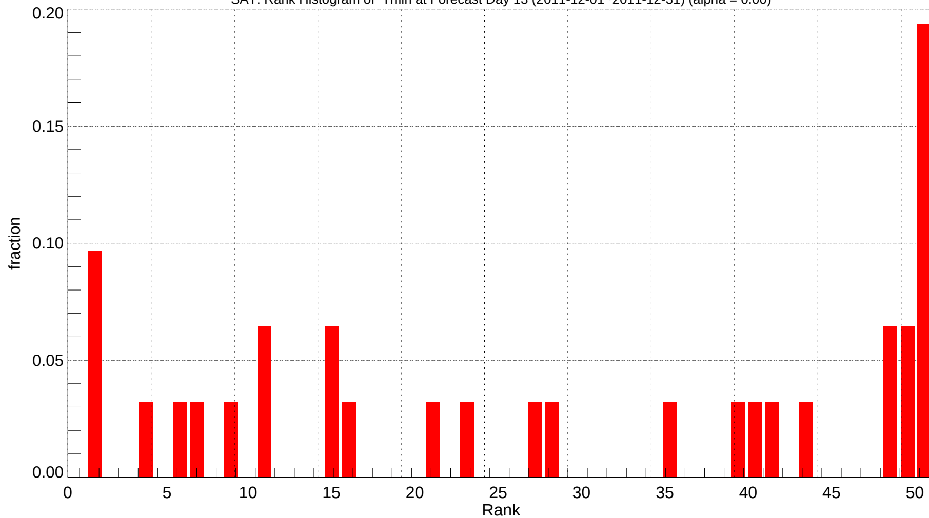
SAT: Rank Histogram of Tmin at Forecast Day 13 (2011-12-01~2011-12-31) (alpha = 0.00)
