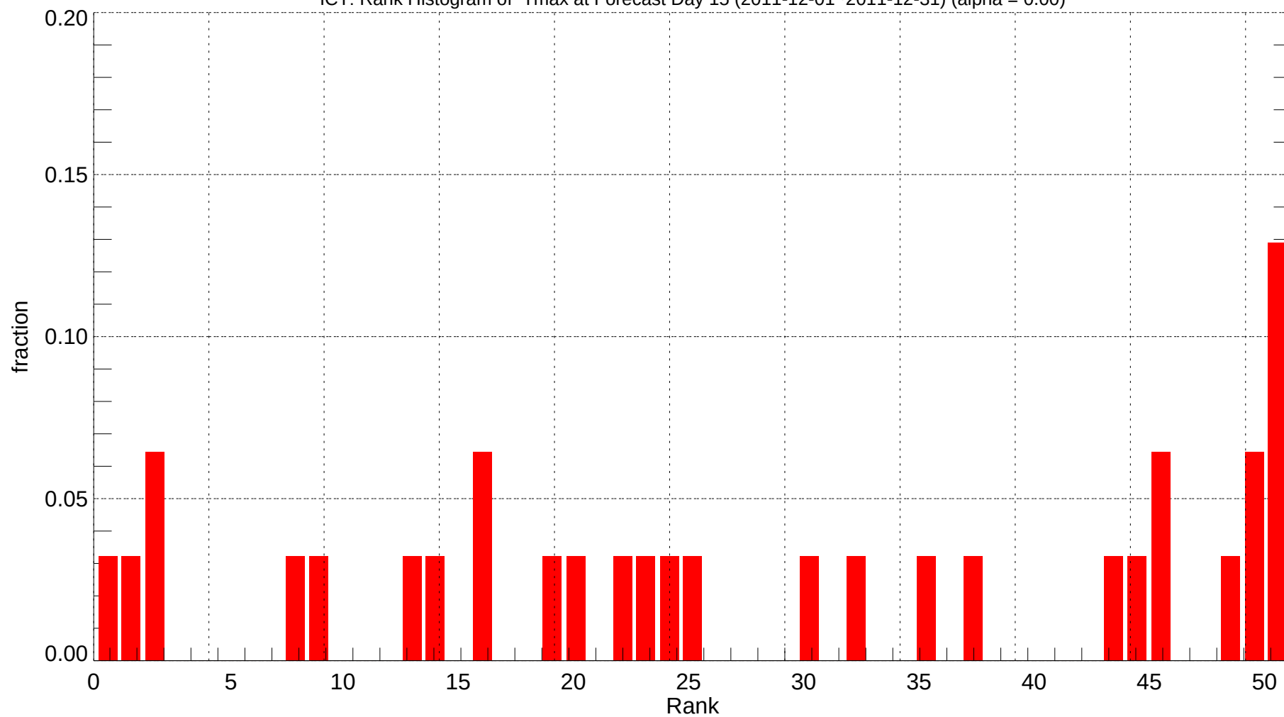
ICT: Rank Histogram of Tmax at Forecast Day 15 (2011-12-01~2011-12-31) (alpha = 0.00)
