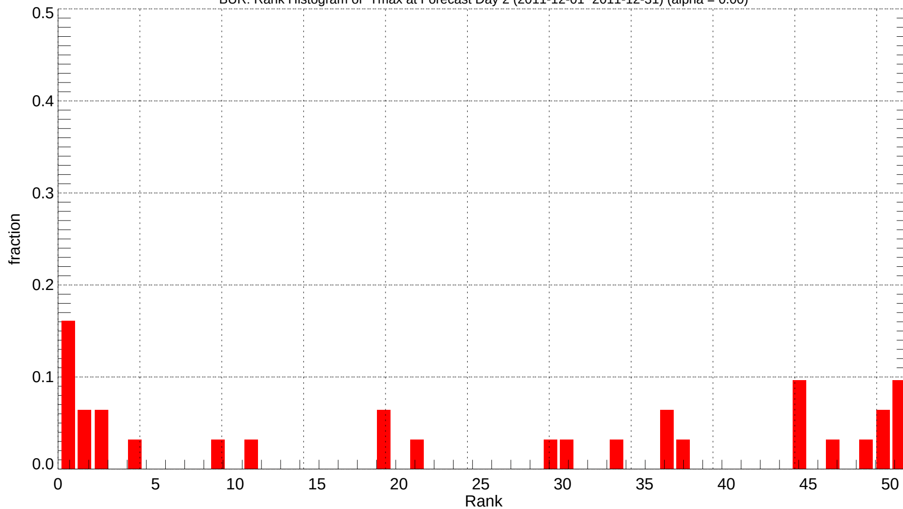
BUR: Rank Histogram of Tmax at Forecast Day 2 (2011-12-01~2011-12-31) (alpha = 0.00)
