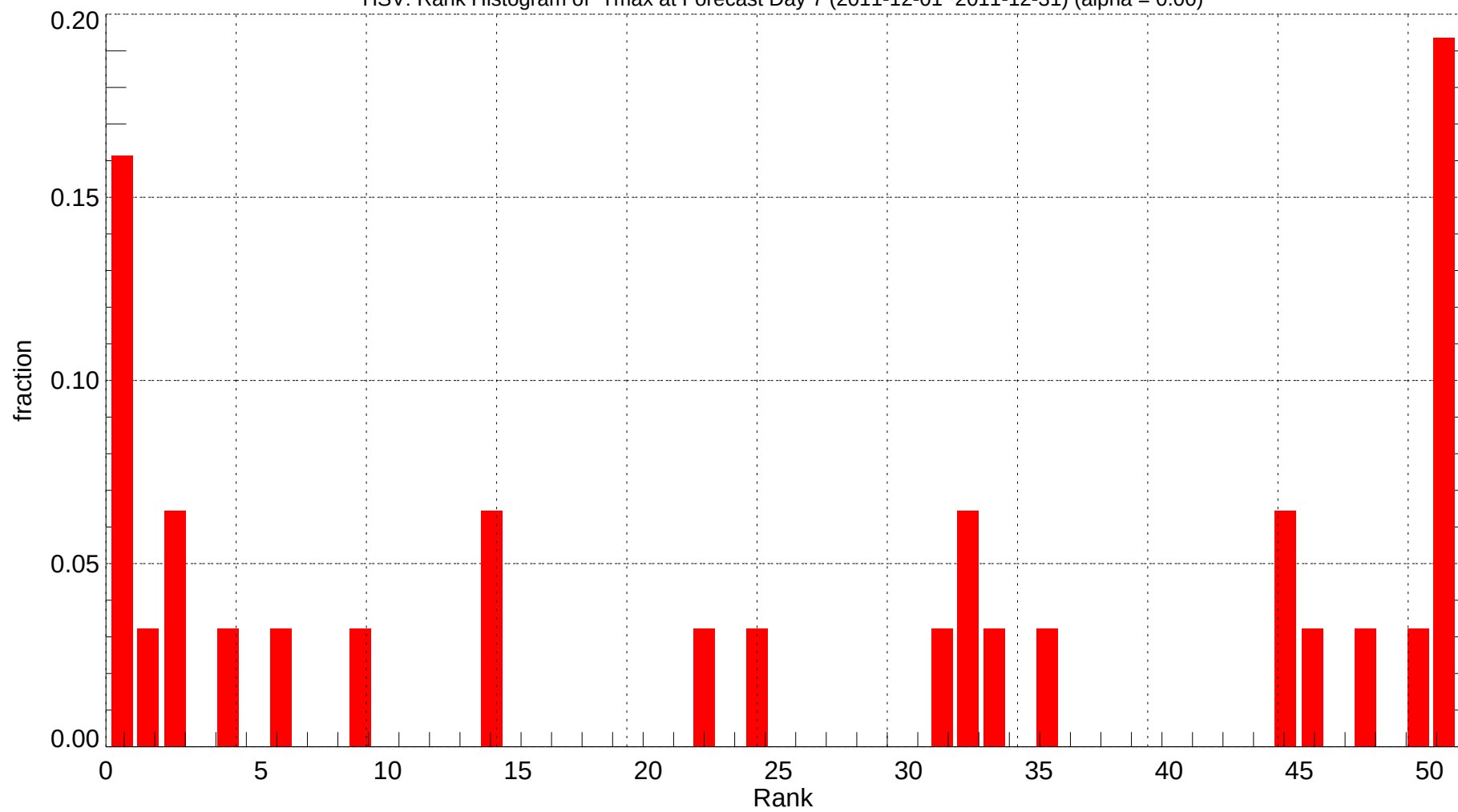
HSV: Rank Histogram of Tmax at Forecast Day 7 (2011-12-01~2011-12-31) (alpha = 0.00)
