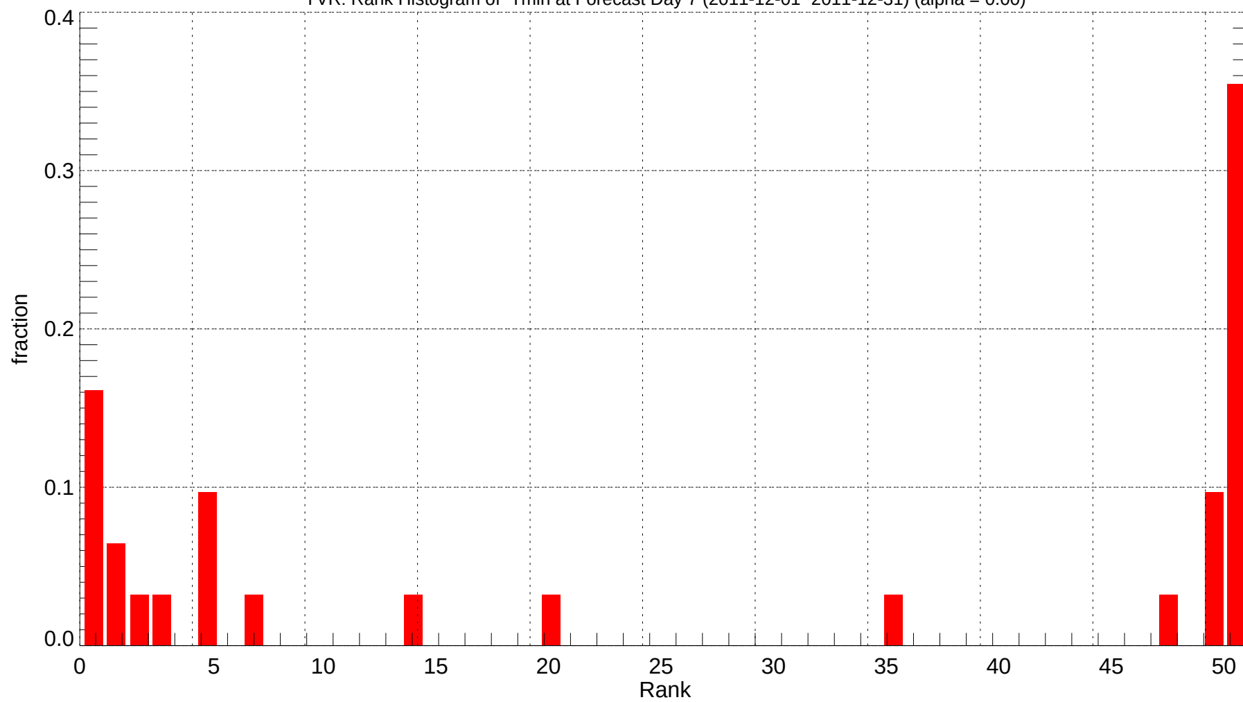
YVR: Rank Histogram of Tmin at Forecast Day 7 (2011-12-01~2011-12-31) (alpha = 0.00)
