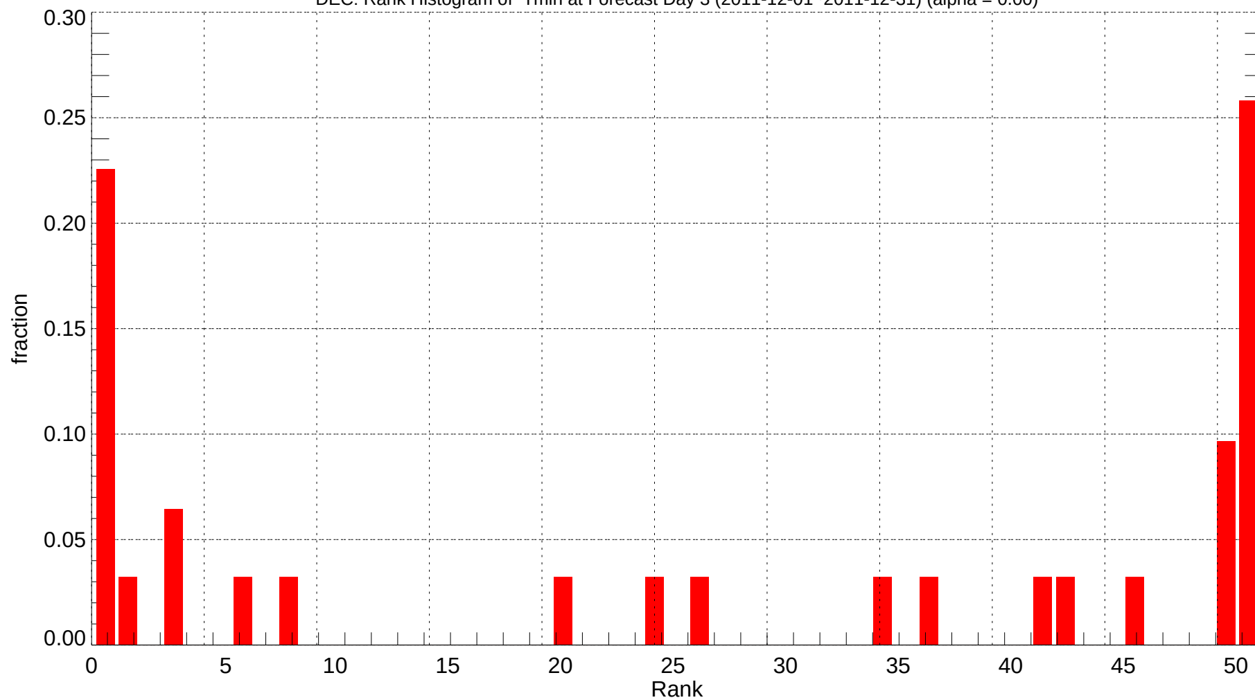
DEC: Rank Histogram of Tmin at Forecast Day 3 (2011-12-01~2011-12-31) (alpha = 0.00)
