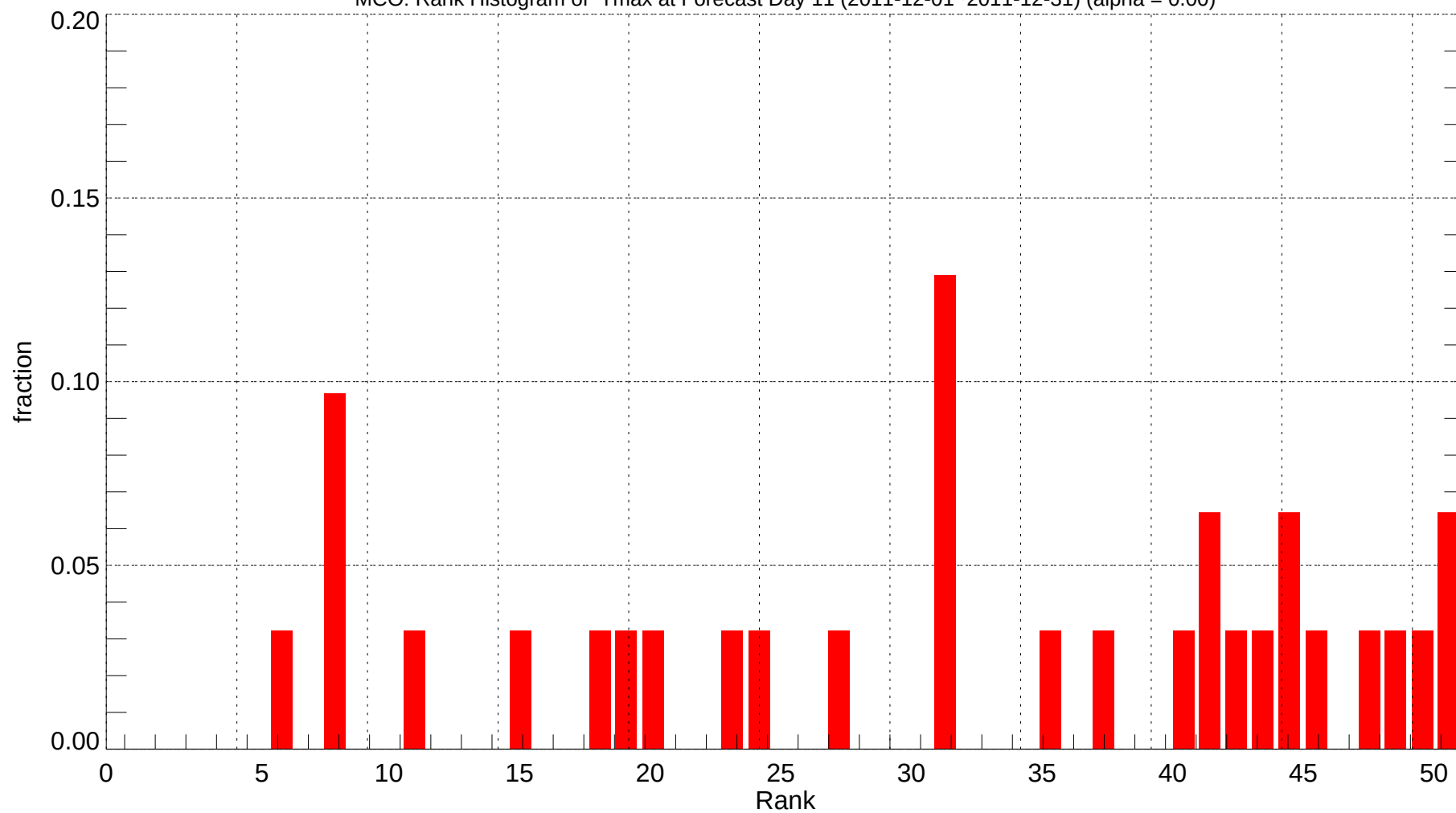
MCO: Rank Histogram of Tmax at Forecast Day 11 (2011-12-01~2011-12-31) (alpha = 0.00)
