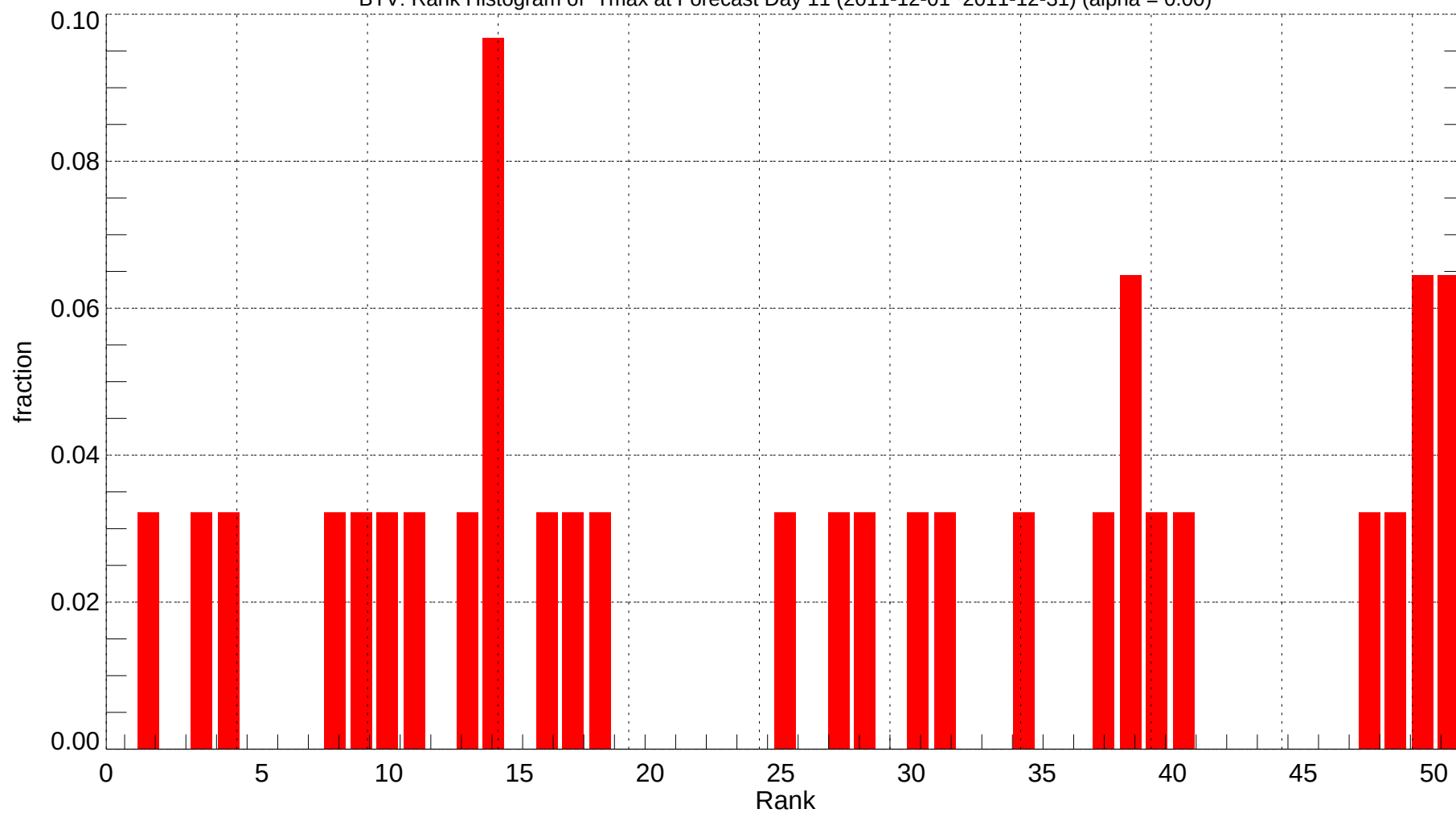
BTV: Rank Histogram of Tmax at Forecast Day 11 (2011-12-01~2011-12-31) (alpha = 0.00)
