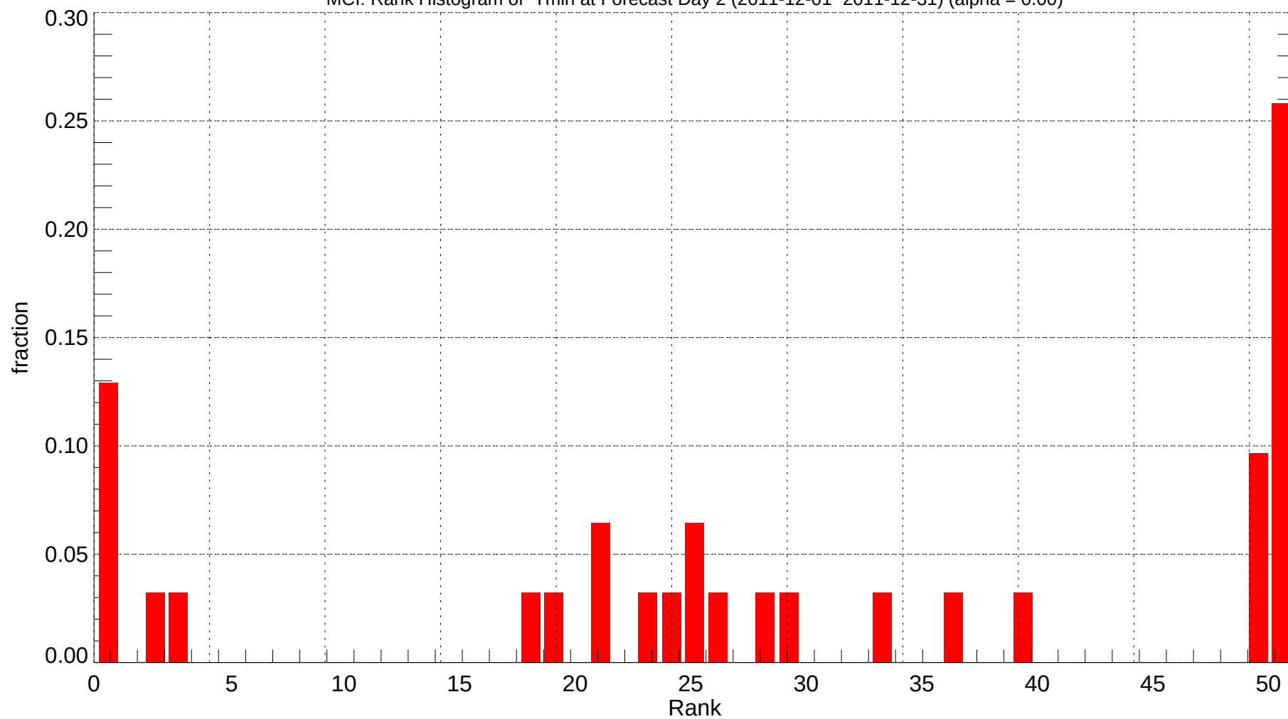
MCI: Rank Histogram of Tmin at Forecast Day 2 (2011-12-01~2011-12-31) (alpha = 0.00)
