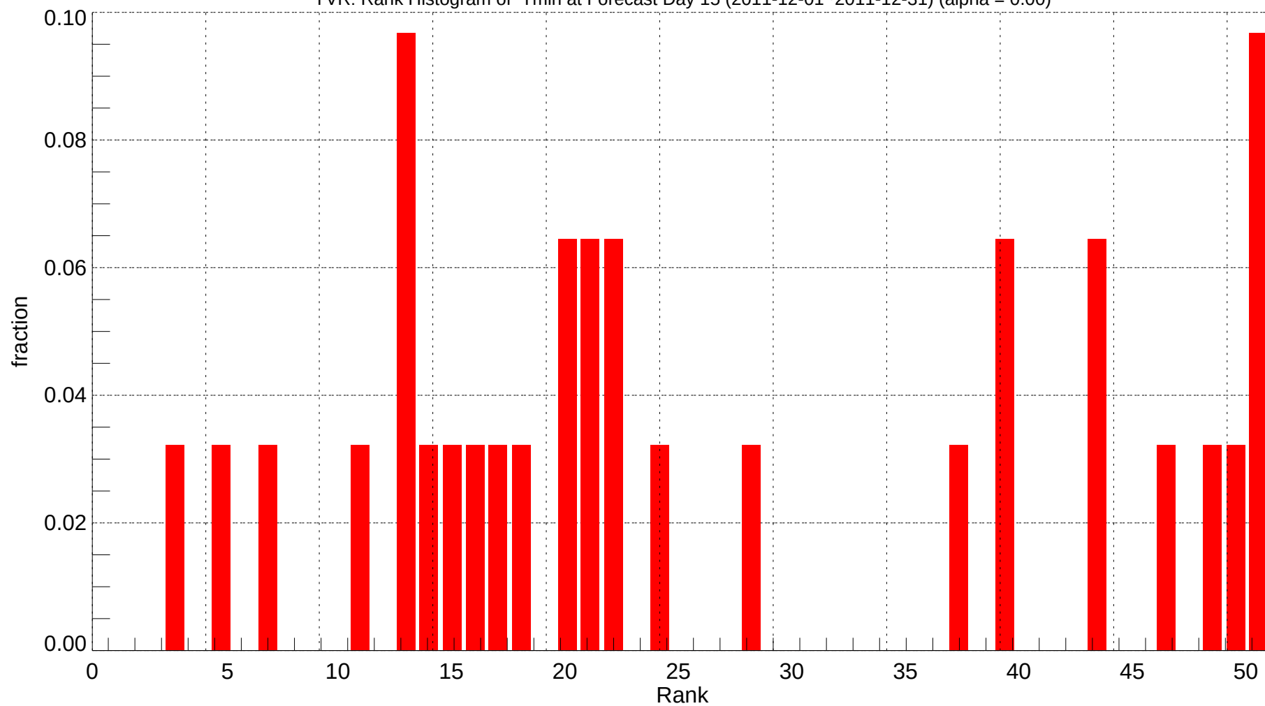
YVR: Rank Histogram of Tmin at Forecast Day 15 (2011-12-01~2011-12-31) (alpha = 0.00)
