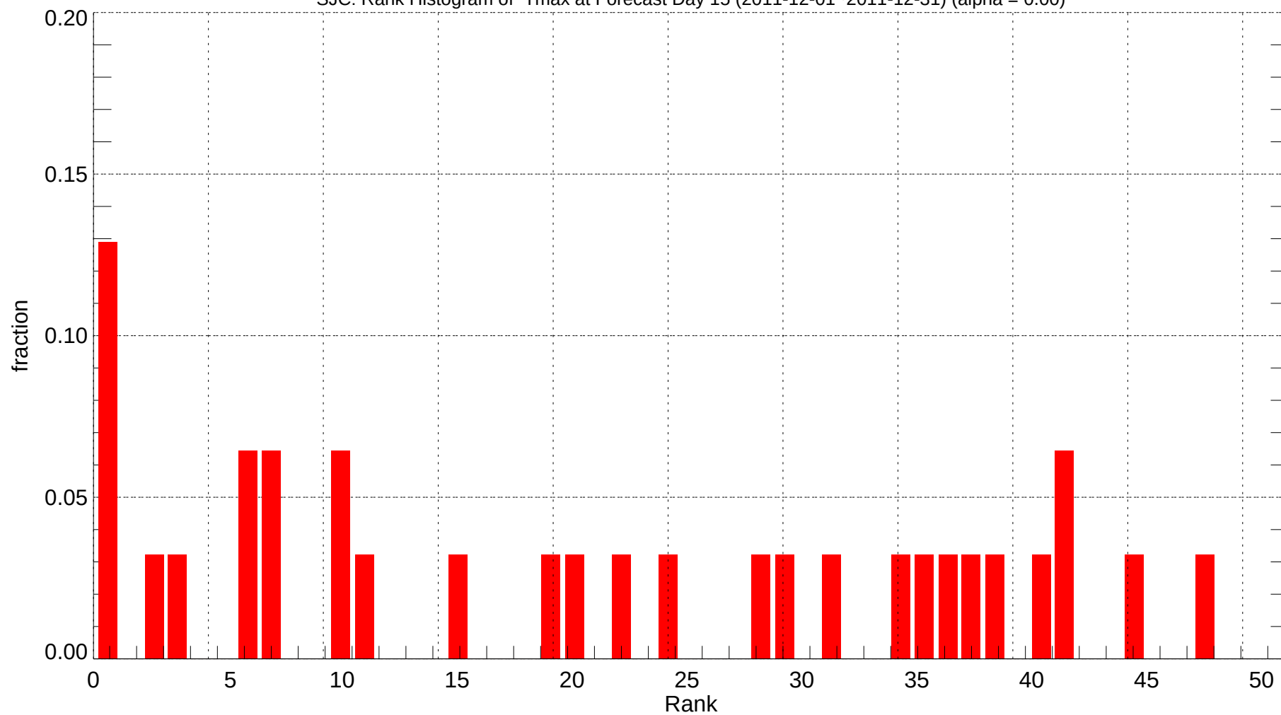
SJC: Rank Histogram of Tmax at Forecast Day 15 (2011-12-01~2011-12-31) (alpha = 0.00)
