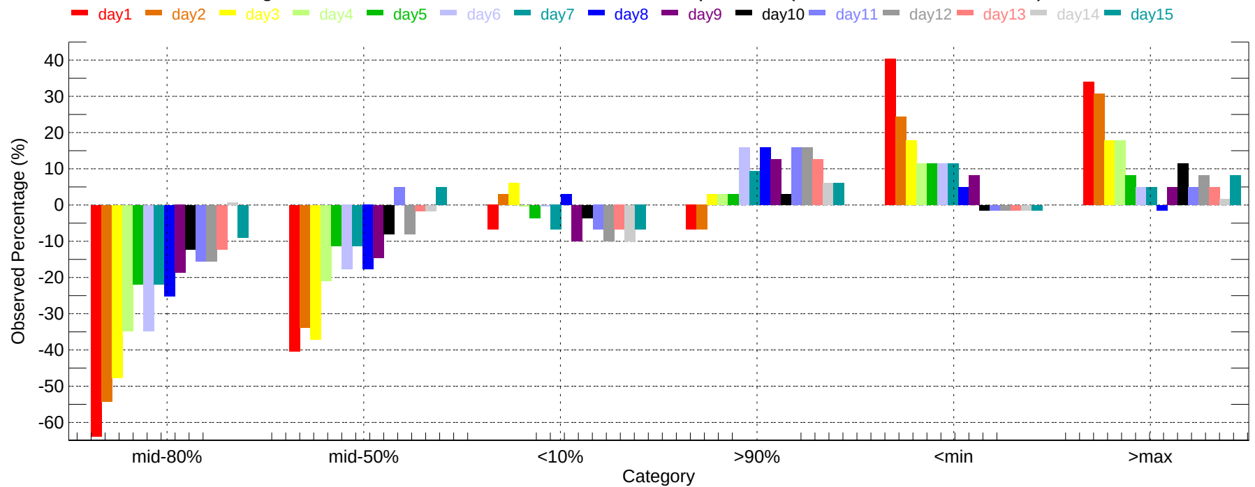
Observed Percentage Deviation of Ensembles - NTU: Max Temperature (2011-12-01~2011-12-31)
