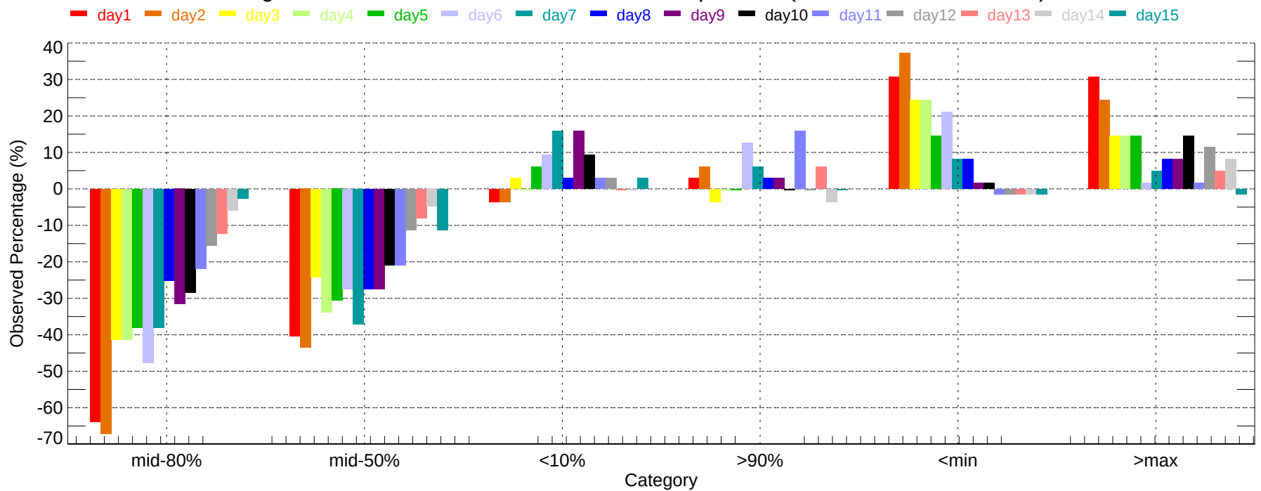
Observed Percentage Deviation of Ensembles - LAN: Max Temperature (2011-12-01~2011-12-31)
