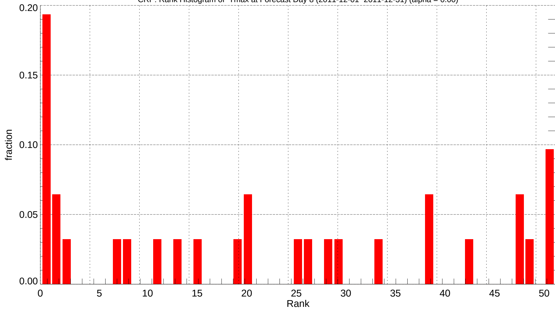
CRP: Rank Histogram of Tmax at Forecast Day 8 (2011-12-01~2011-12-31) (alpha = 0.00)
