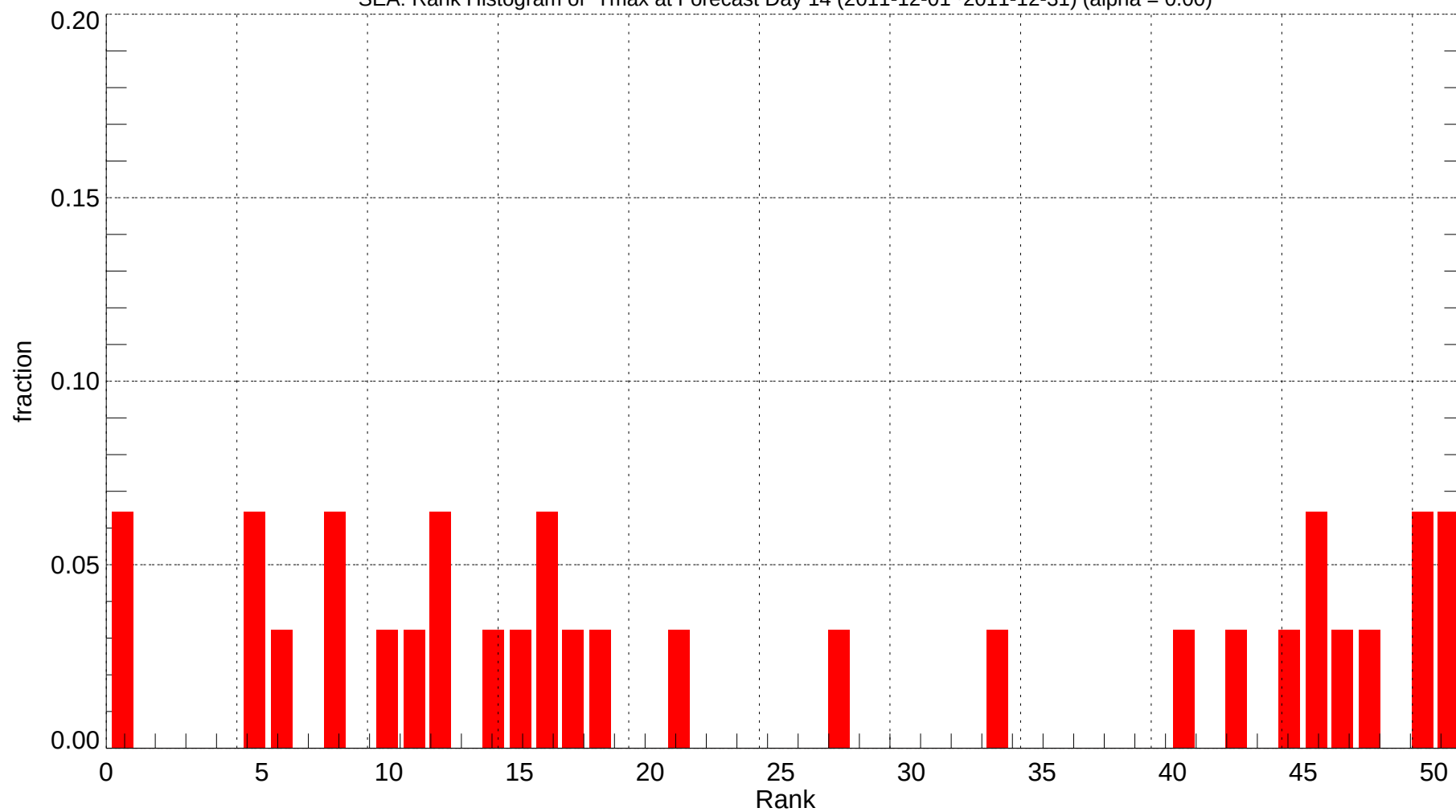
SEA: Rank Histogram of Tmax at Forecast Day 14 (2011-12-01~2011-12-31) (alpha = 0.00)
