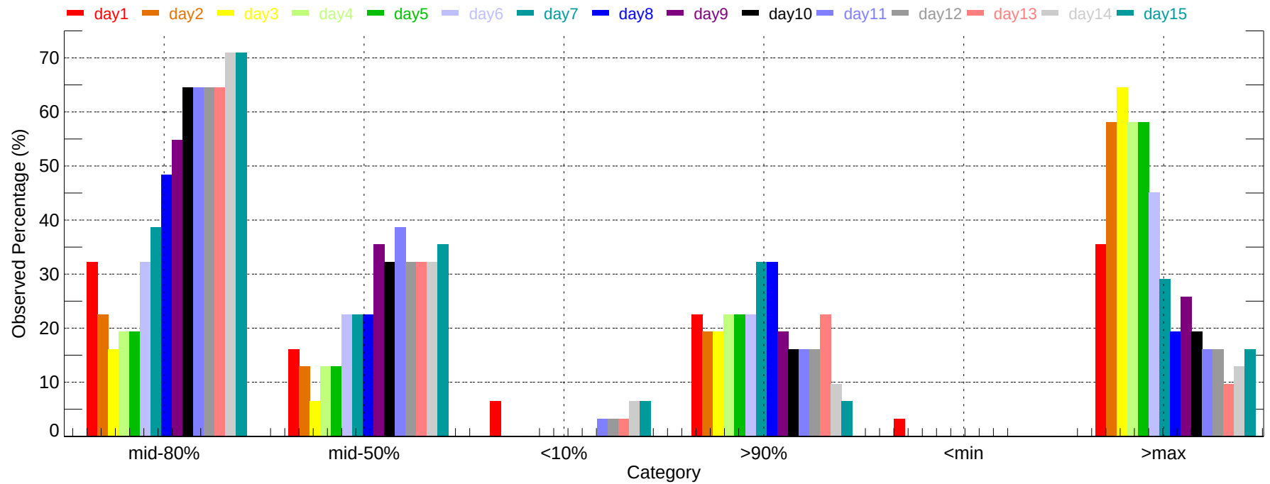
Observed Percentage of Ensembles - AOO: Max Temperature (2011-12-01~2011-12-31)
