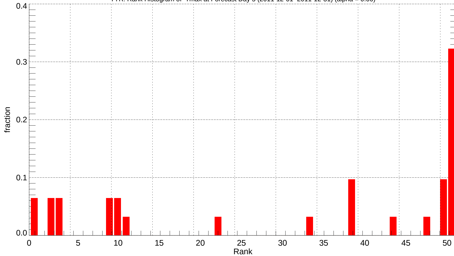
TYR: Rank Histogram of Tmax at Forecast Day 5 (2011-12-01~2011-12-31) (alpha = 0.00)
