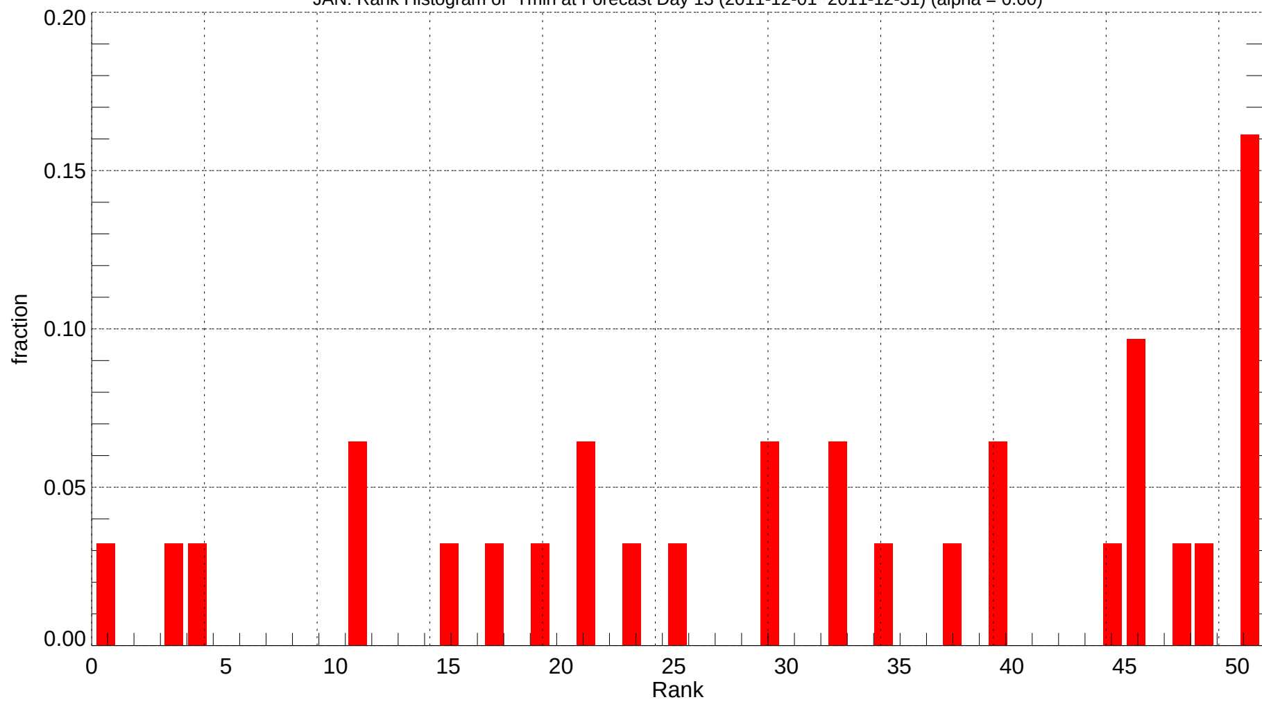
JAN: Rank Histogram of Tmin at Forecast Day 13 (2011-12-01~2011-12-31) (alpha = 0.00)
