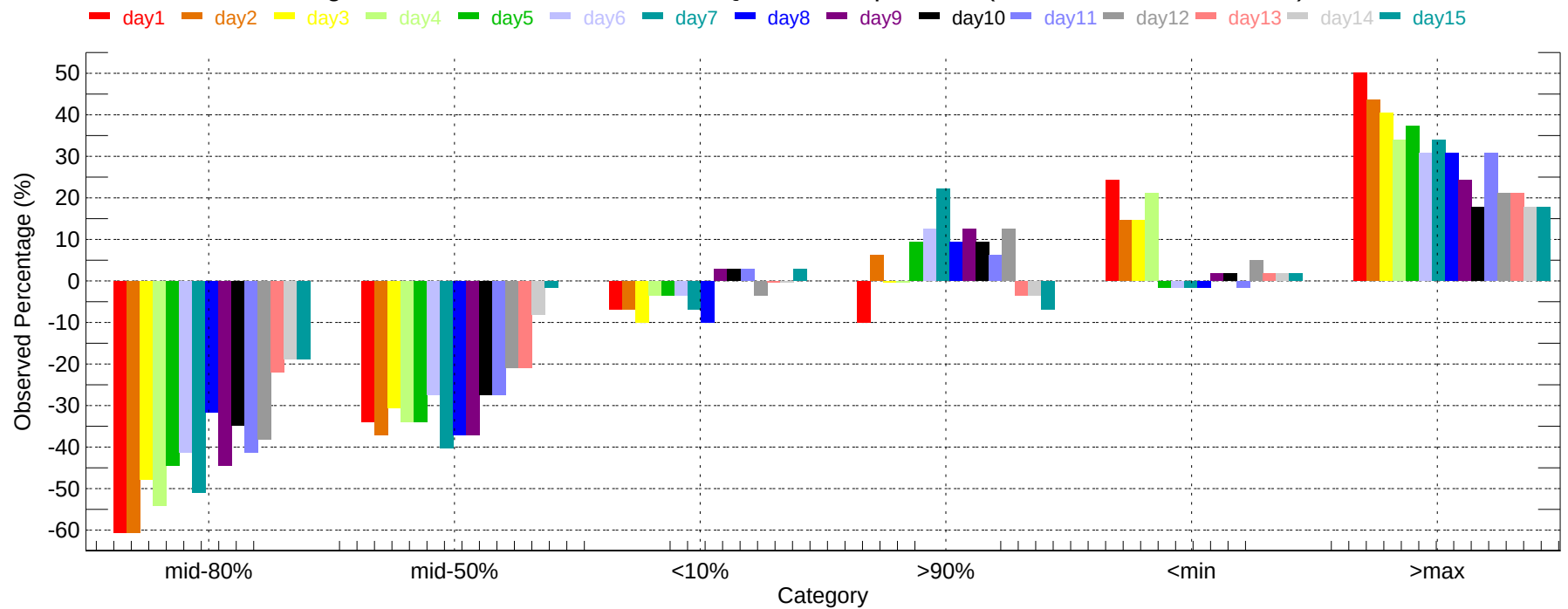
Observed Percentage Deviation of Ensembles - ABQ: Max Temperature (2011-12-01~2011-12-31)
