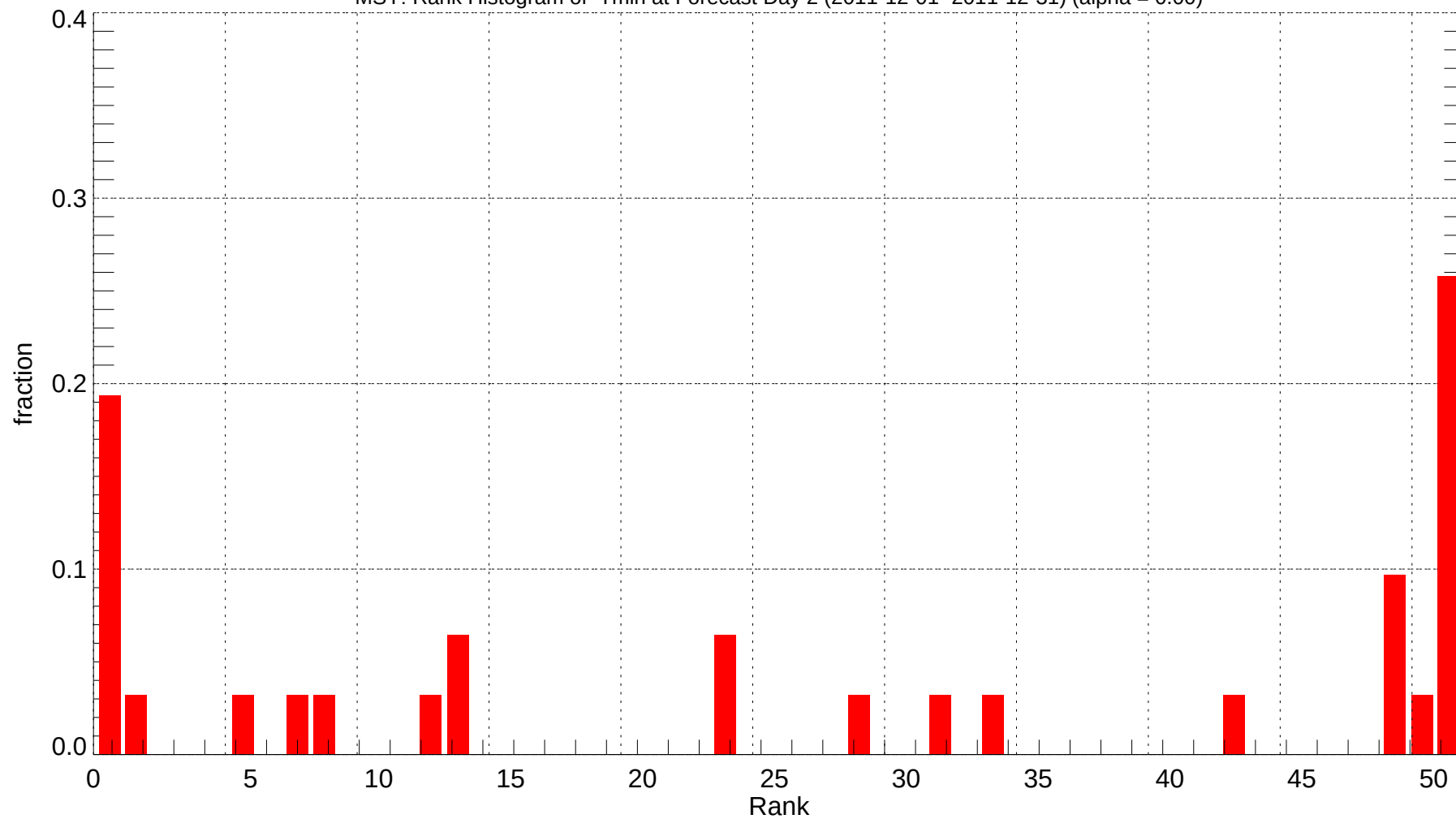
MSY: Rank Histogram of Tmin at Forecast Day 2 (2011-12-01~2011-12-31) (alpha = 0.00)
