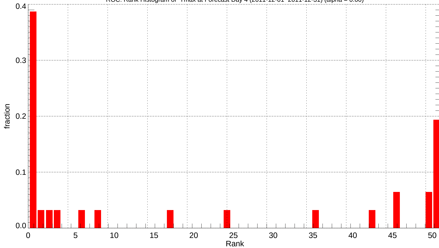
ROC: Rank Histogram of Tmax at Forecast Day 4 (2011-12-01~2011-12-31) (alpha = 0.00)
