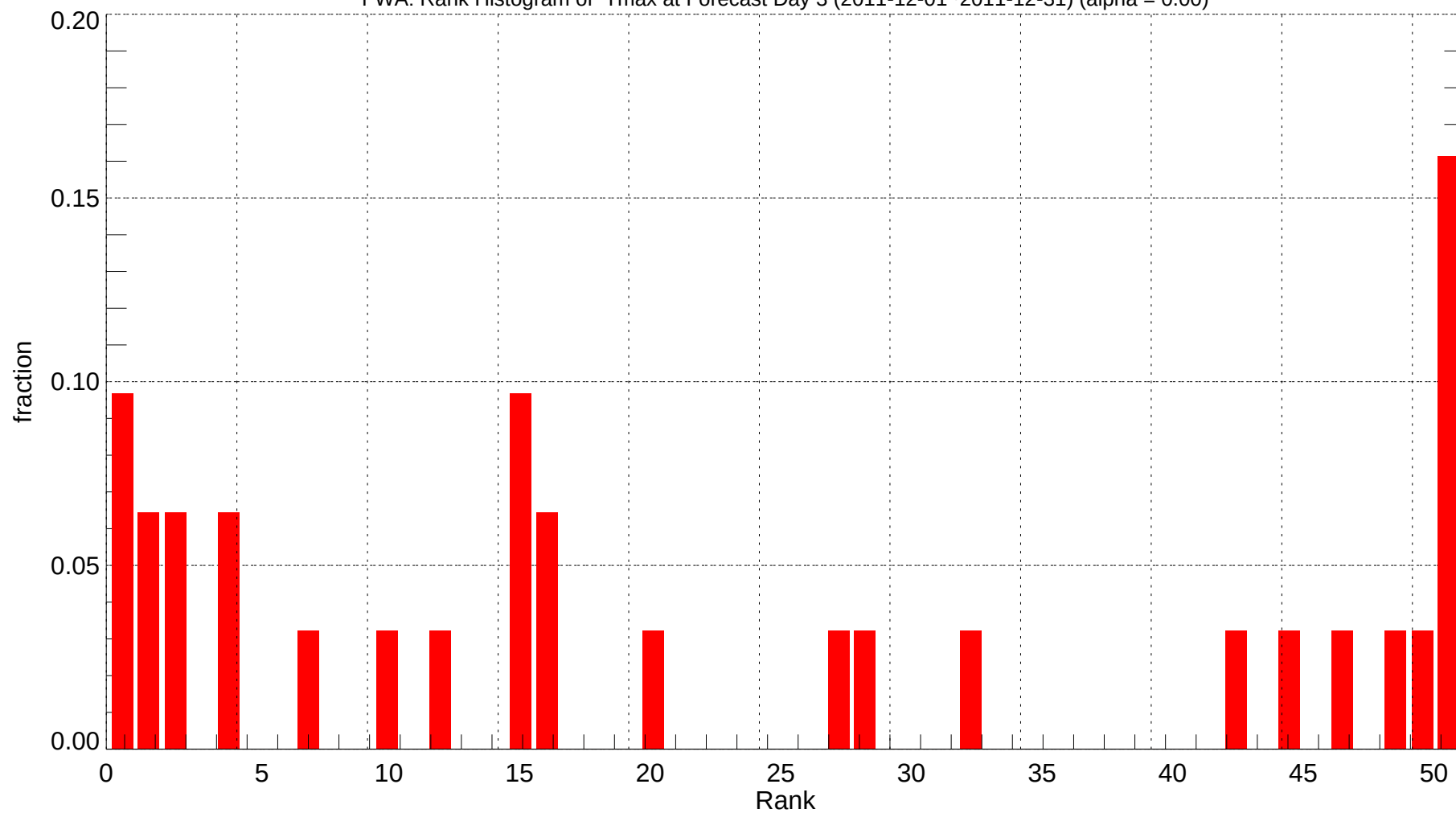
FWA: Rank Histogram of Tmax at Forecast Day 3 (2011-12-01~2011-12-31) (alpha = 0.00)
