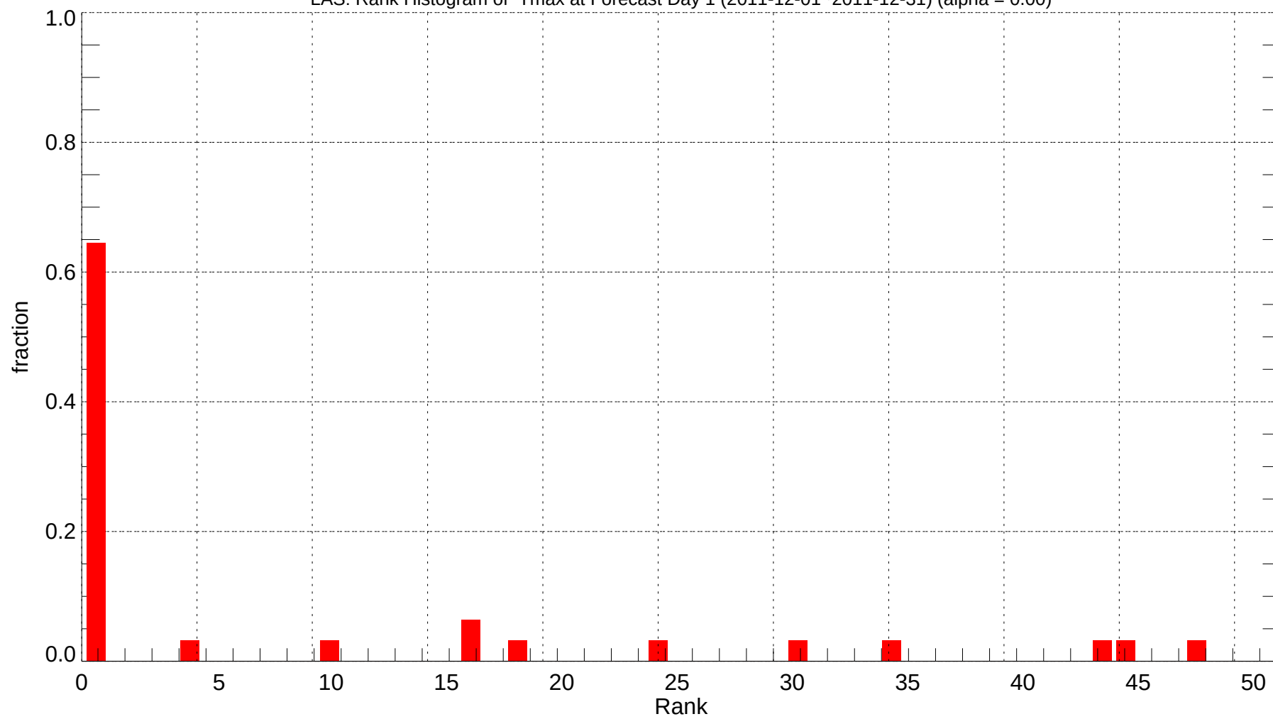
LAS: Rank Histogram of Tmax at Forecast Day 1 (2011-12-01~2011-12-31) (alpha = 0.00)
