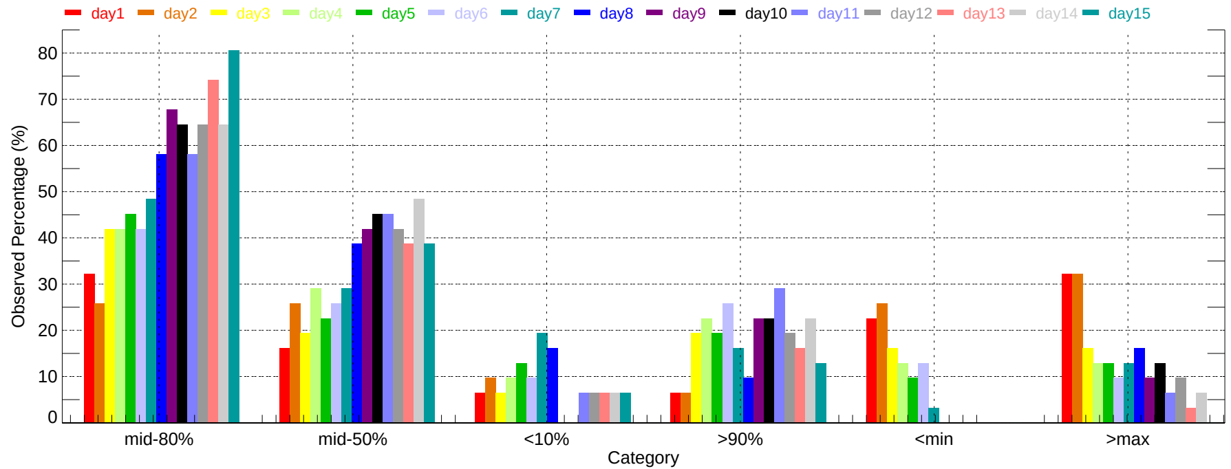
Observed Percentage of Ensembles - MEM: Max Temperature (2011-12-01~2011-12-31)
