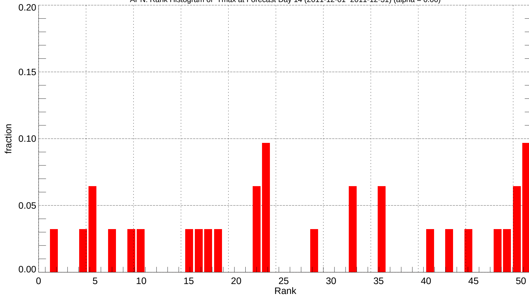
APN: Rank Histogram of Tmax at Forecast Day 14 (2011-12-01~2011-12-31) (alpha = 0.00)
