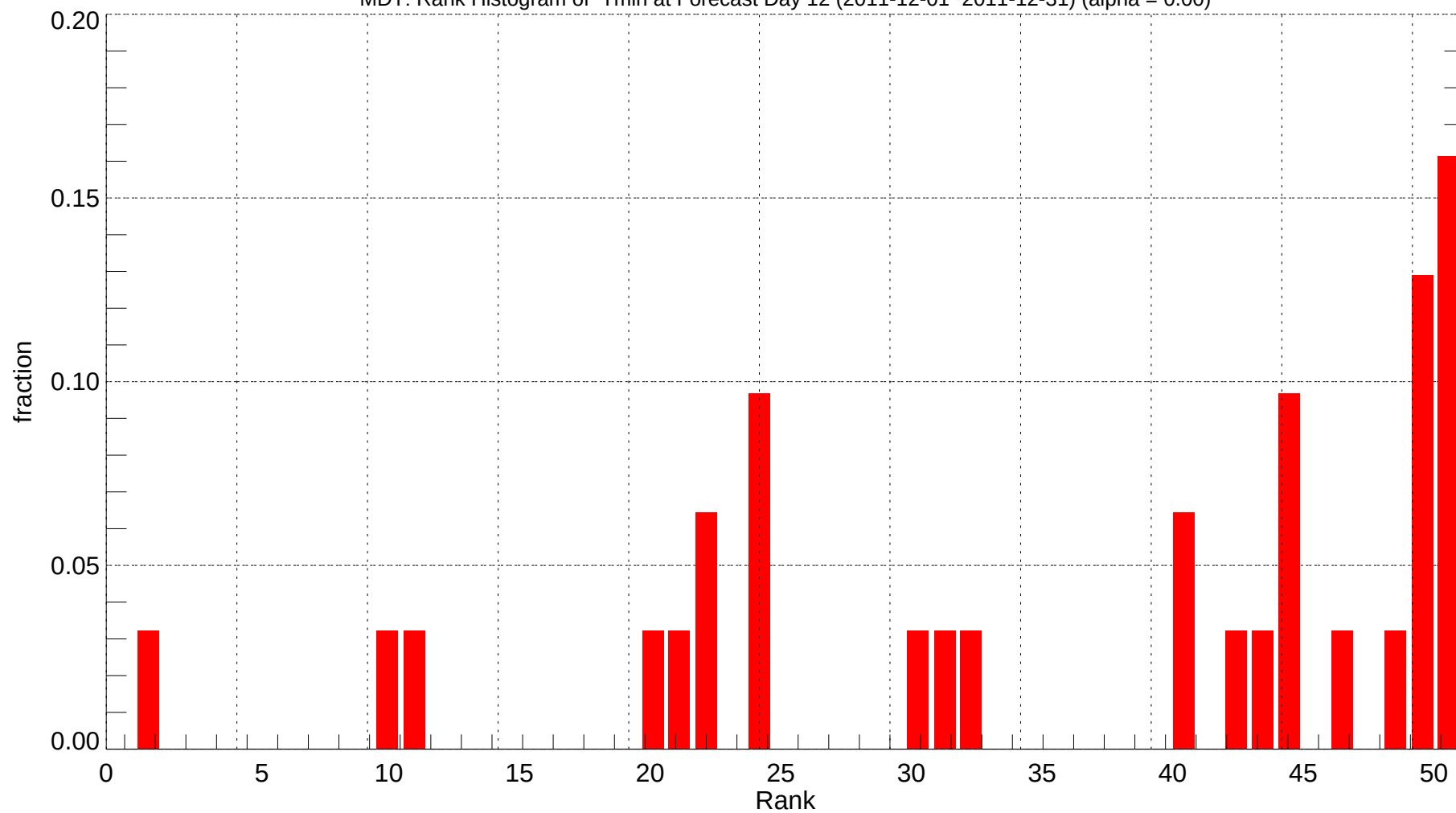
MDT: Rank Histogram of Tmin at Forecast Day 12 (2011-12-01~2011-12-31) (alpha = 0.00)
