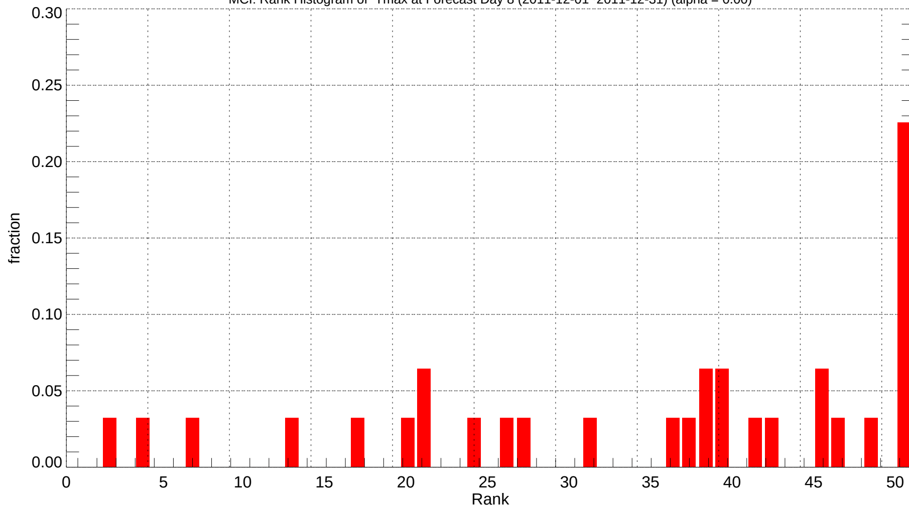
MCI: Rank Histogram of Tmax at Forecast Day 8 (2011-12-01~2011-12-31) (alpha = 0.00)
