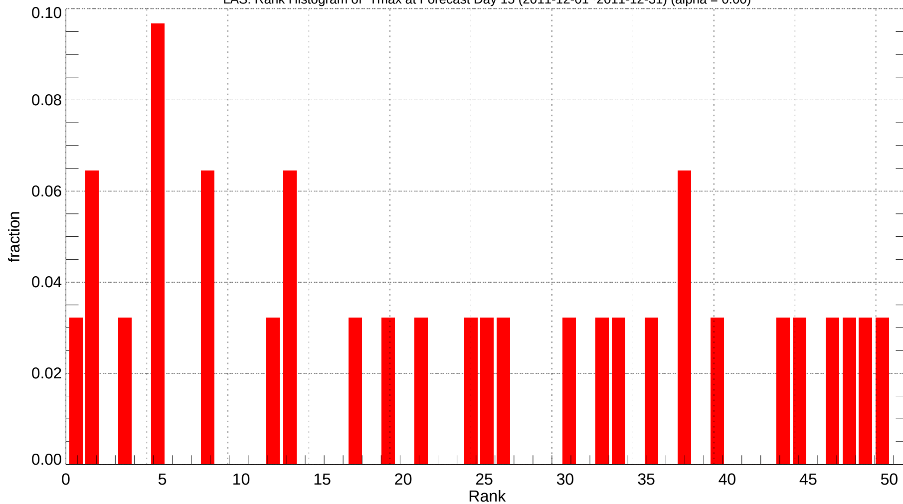
LAS: Rank Histogram of Tmax at Forecast Day 15 (2011-12-01~2011-12-31) (alpha = 0.00)
