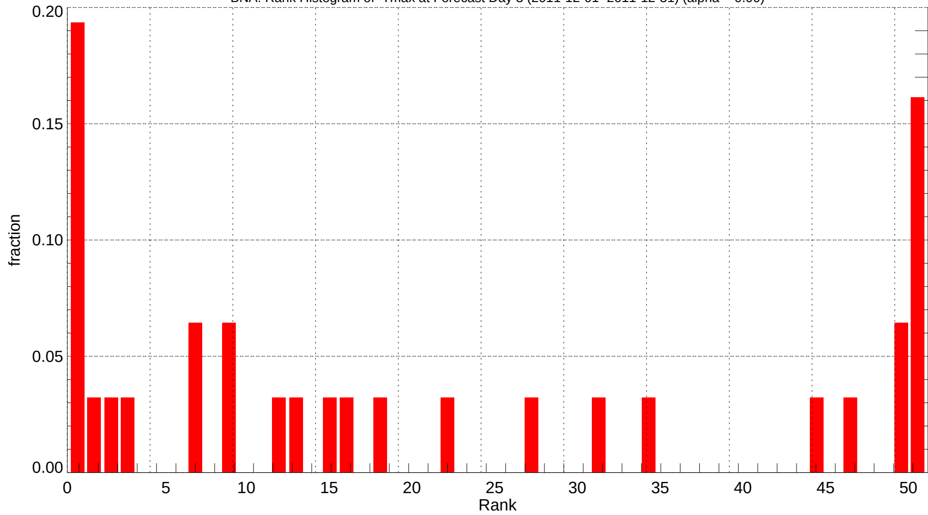
BNA: Rank Histogram of Tmax at Forecast Day 3 (2011-12-01~2011-12-31) (alpha = 0.00)
