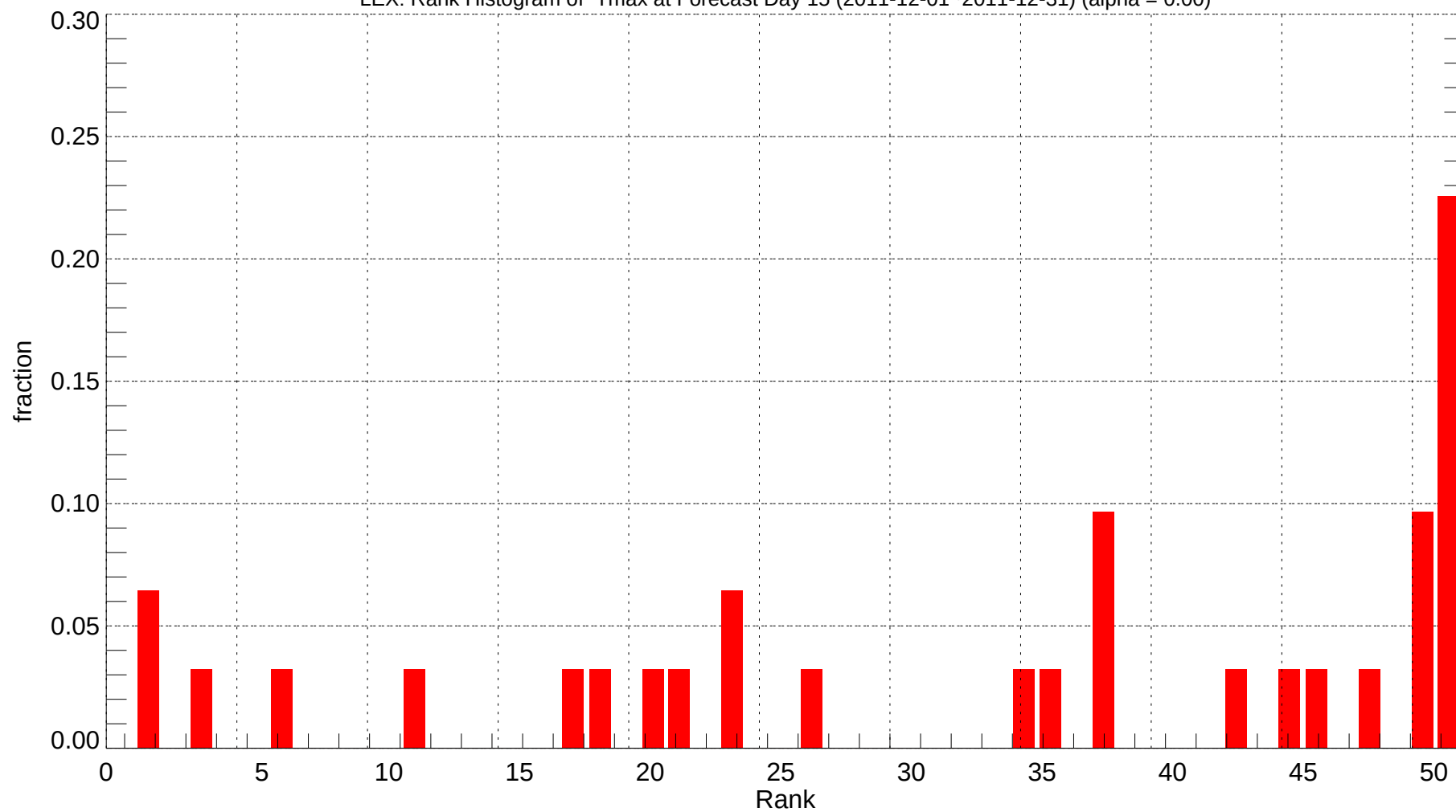
LEX: Rank Histogram of Tmax at Forecast Day 15 (2011-12-01~2011-12-31) (alpha = 0.00)
