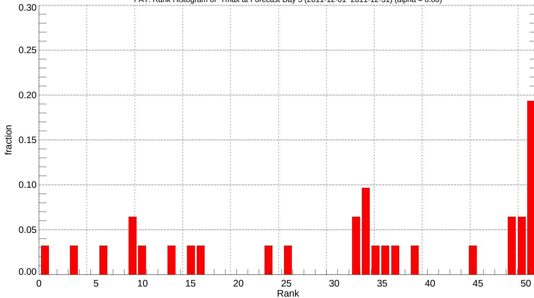
FAT: Rank Histogram of Tmax at Forecast Day 5 (2011-12-01~2011-12-31) (alpha = 0.00)
