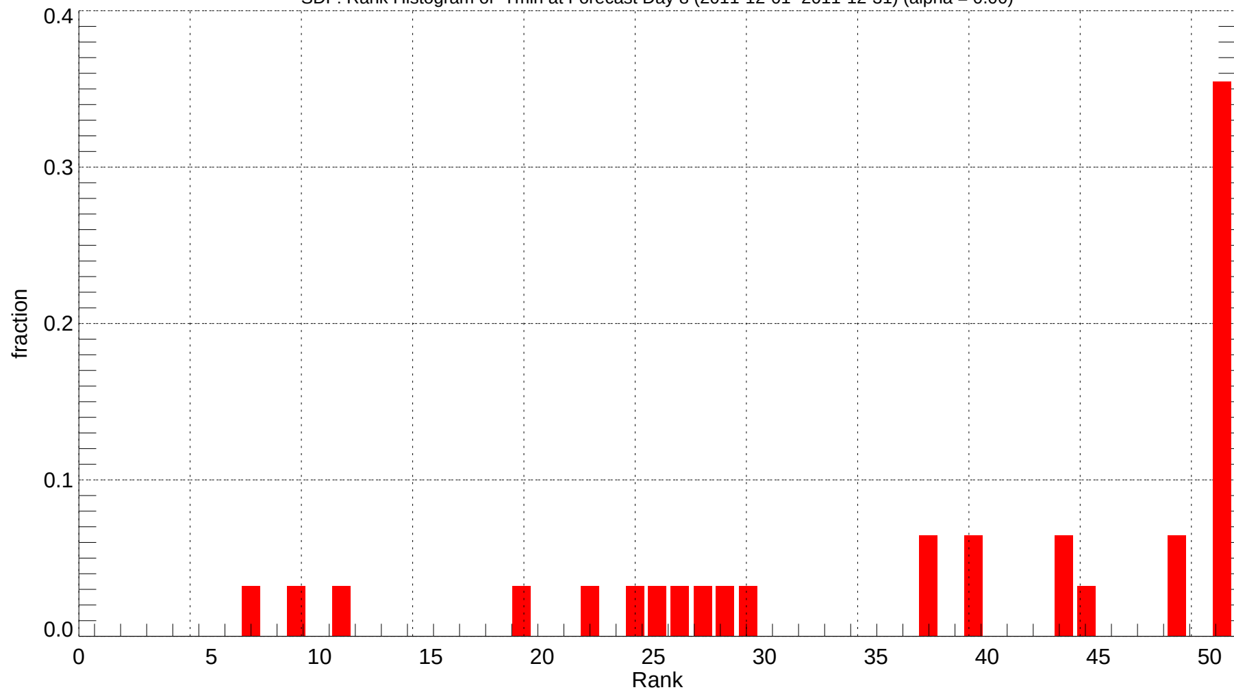
SDF: Rank Histogram of Tmin at Forecast Day 8 (2011-12-01~2011-12-31) (alpha = 0.00)
