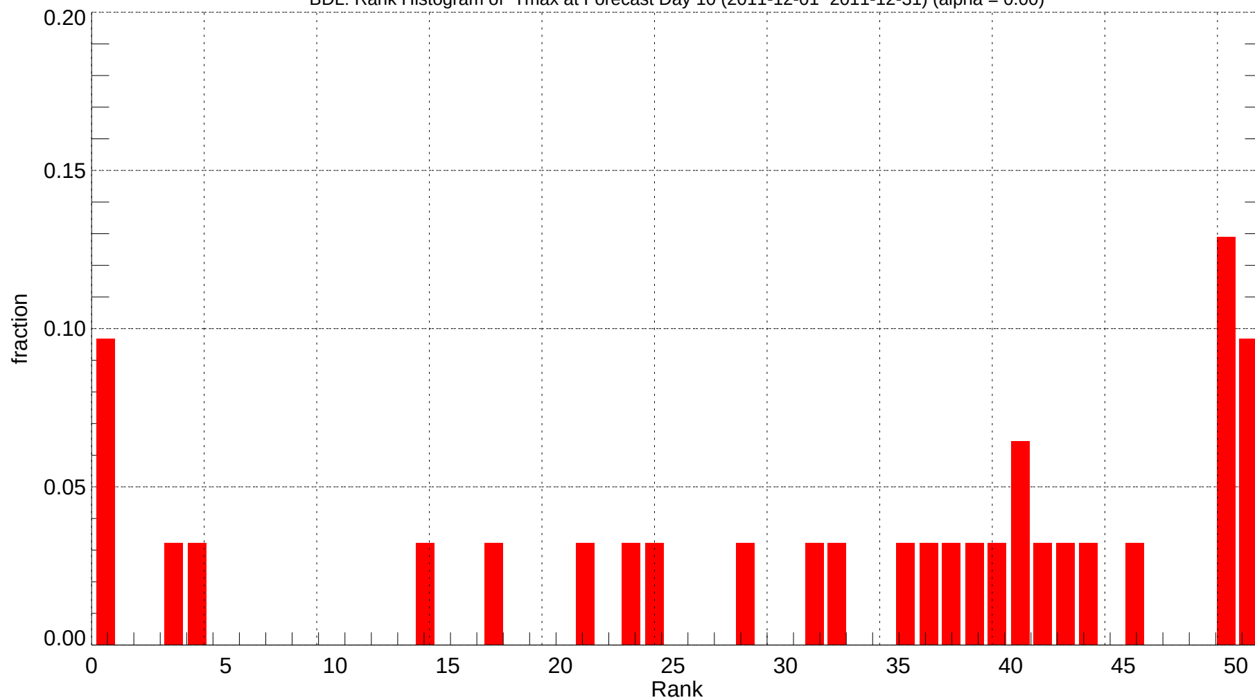
BDL: Rank Histogram of Tmax at Forecast Day 10 (2011-12-01~2011-12-31) (alpha = 0.00)
