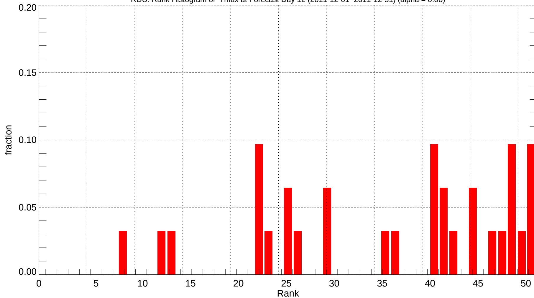
RDU: Rank Histogram of Tmax at Forecast Day 12 (2011-12-01~2011-12-31) (alpha = 0.00)
