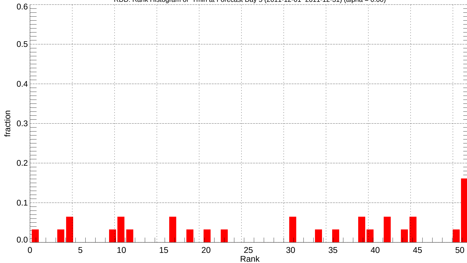
RDD: Rank Histogram of Tmin at Forecast Day 5 (2011-12-01~2011-12-31) (alpha = 0.00)
