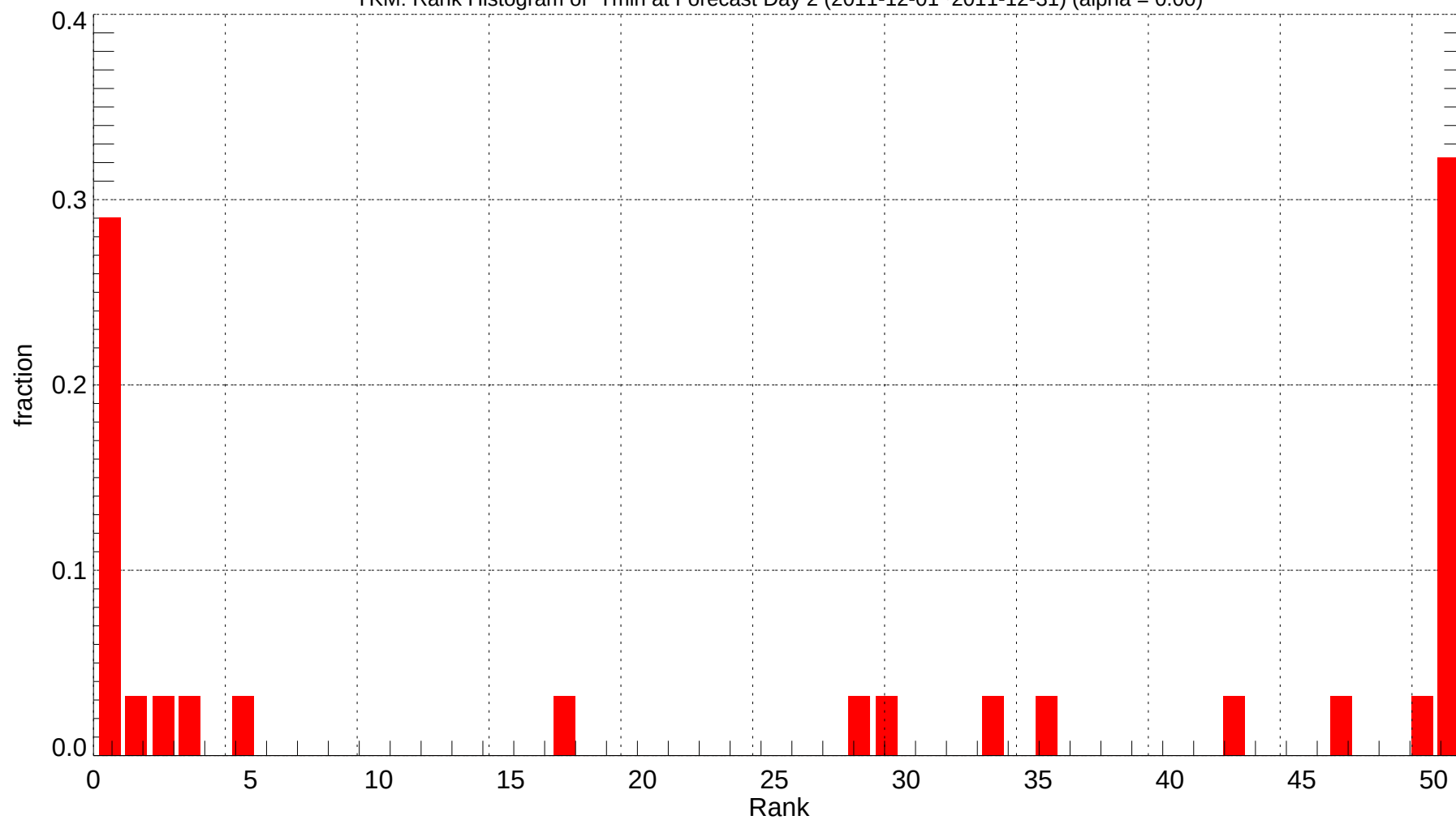
YKM: Rank Histogram of Tmin at Forecast Day 2 (2011-12-01~2011-12-31) (alpha = 0.00)
