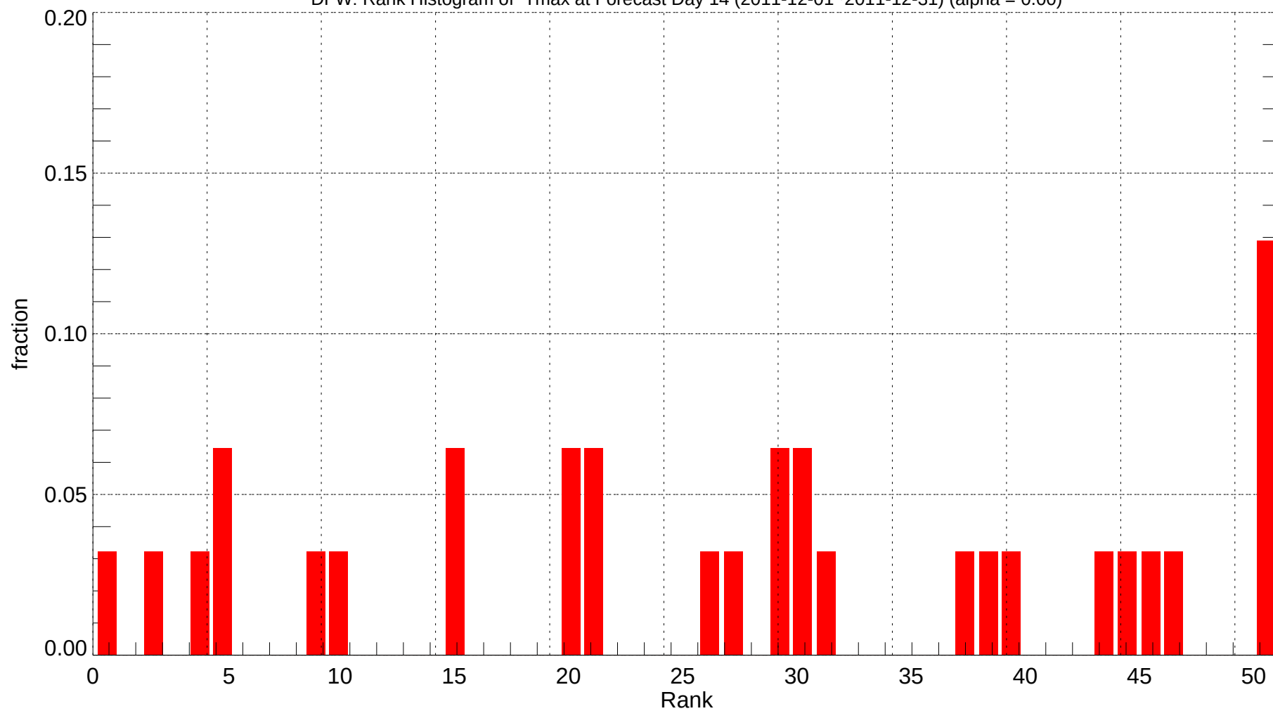
DFW: Rank Histogram of Tmax at Forecast Day 14 (2011-12-01~2011-12-31) (alpha = 0.00)
