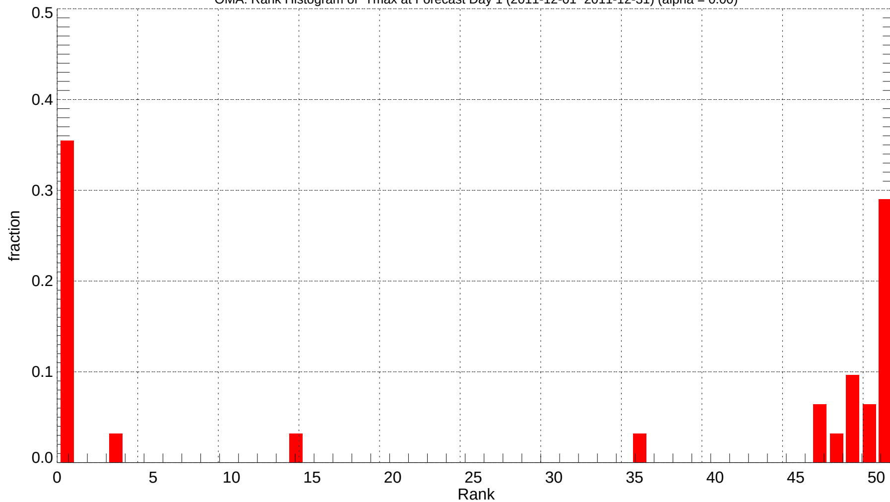
OMA: Rank Histogram of Tmax at Forecast Day 1 (2011-12-01~2011-12-31) (alpha = 0.00)
