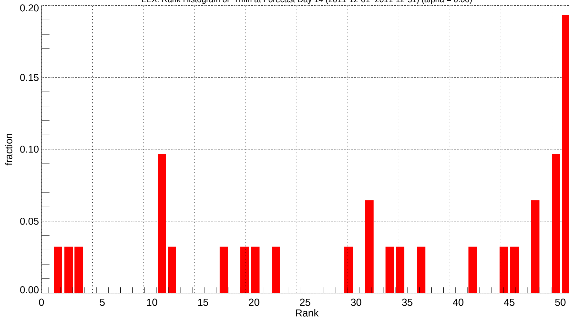
LEX: Rank Histogram of Tmin at Forecast Day 14 (2011-12-01~2011-12-31) (alpha = 0.00)
