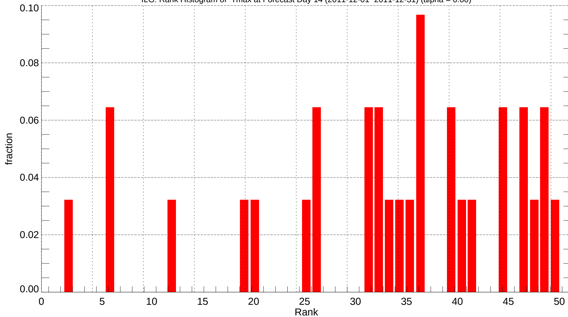
ILG: Rank Histogram of Tmax at Forecast Day 14 (2011-12-01~2011-12-31) (alpha = 0.00)
