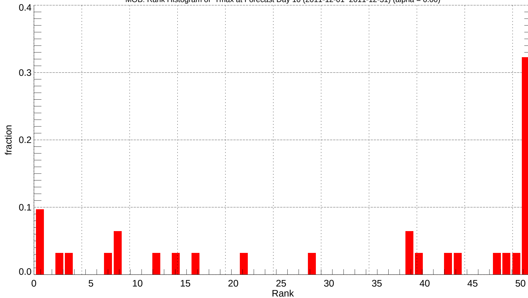
MOB: Rank Histogram of Tmax at Forecast Day 10 (2011-12-01~2011-12-31) (alpha = 0.00)
