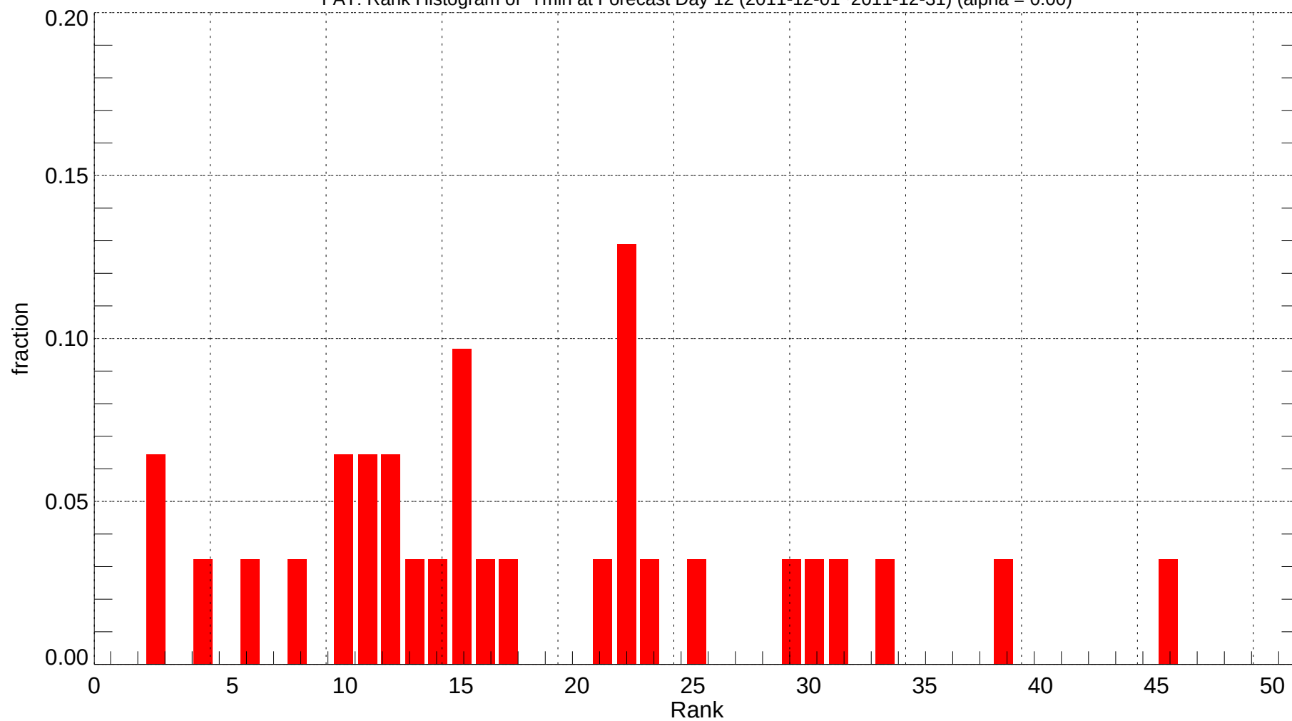
FAT: Rank Histogram of Tmin at Forecast Day 12 (2011-12-01~2011-12-31) (alpha = 0.00)
