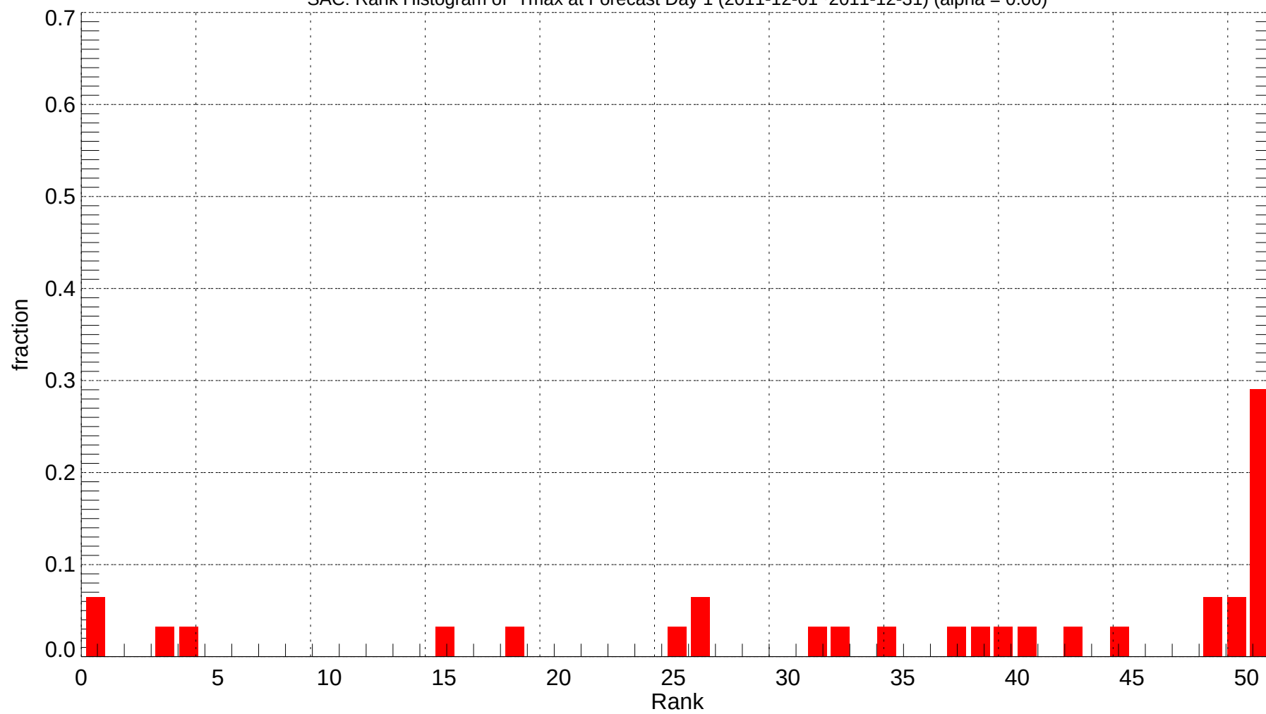
SAC: Rank Histogram of Tmax at Forecast Day 1 (2011-12-01~2011-12-31) (alpha = 0.00)
