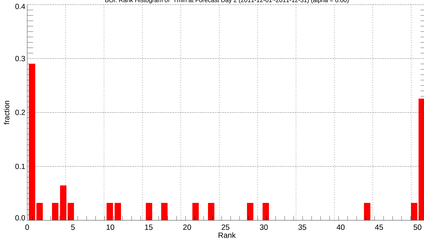
BOI: Rank Histogram of Tmin at Forecast Day 2 (2011-12-01~2011-12-31) (alpha = 0.00)
