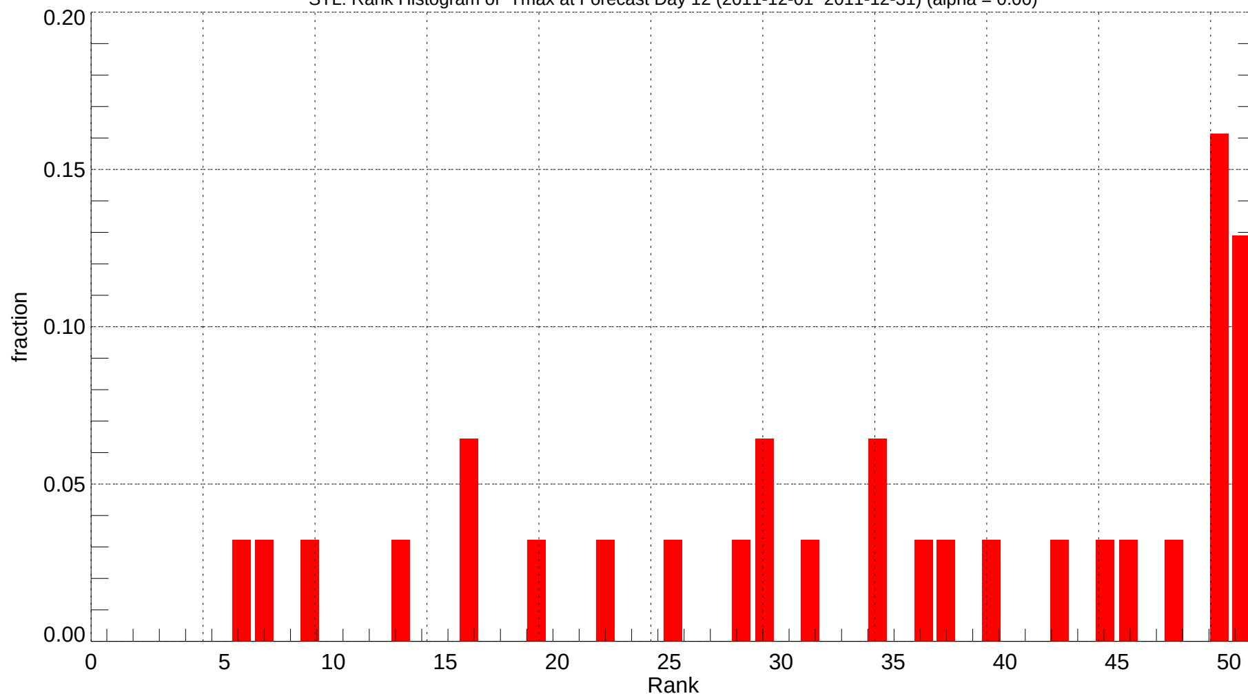
STL: Rank Histogram of Tmax at Forecast Day 12 (2011-12-01~2011-12-31) (alpha = 0.00)
