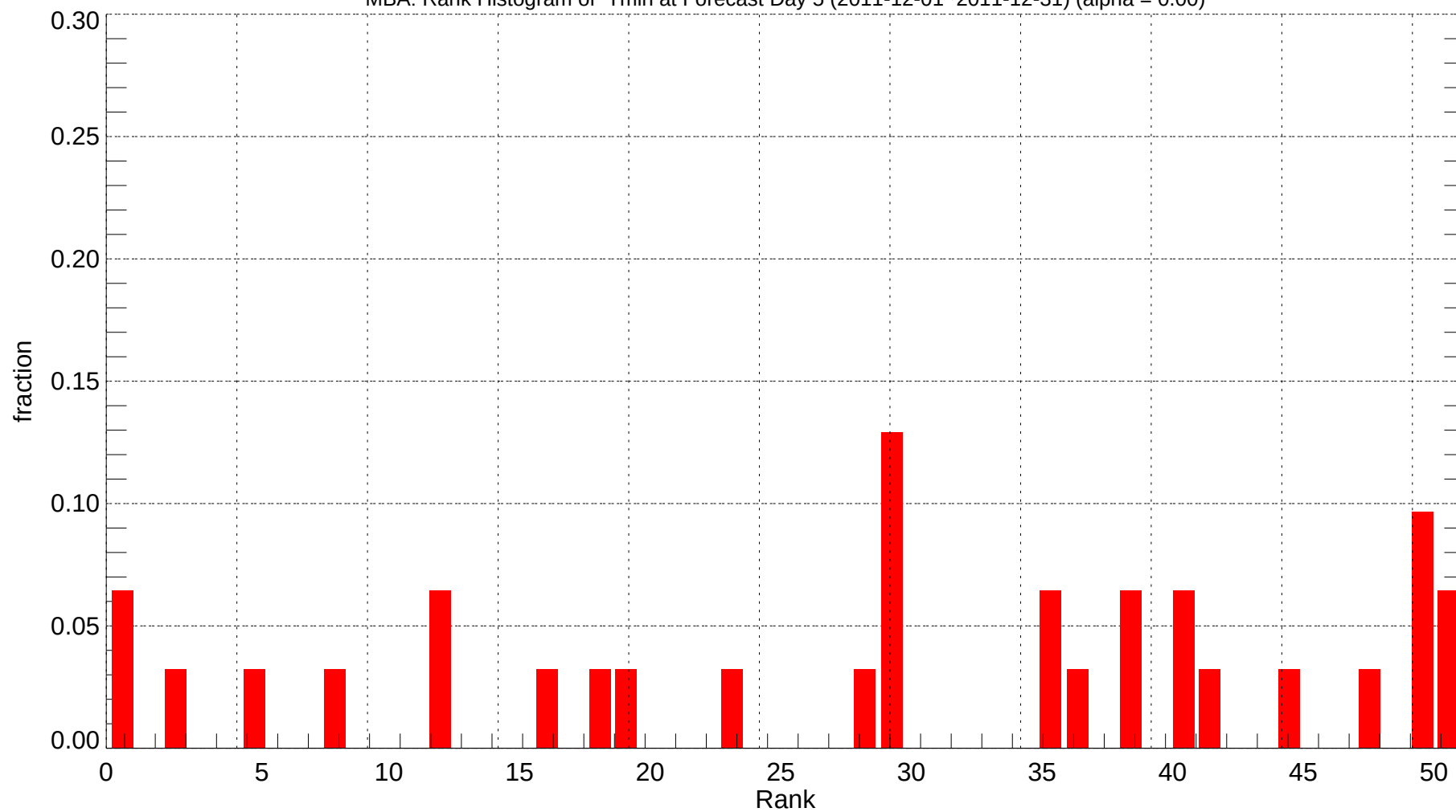
MBA: Rank Histogram of Tmin at Forecast Day 5 (2011-12-01~2011-12-31) (alpha = 0.00)
