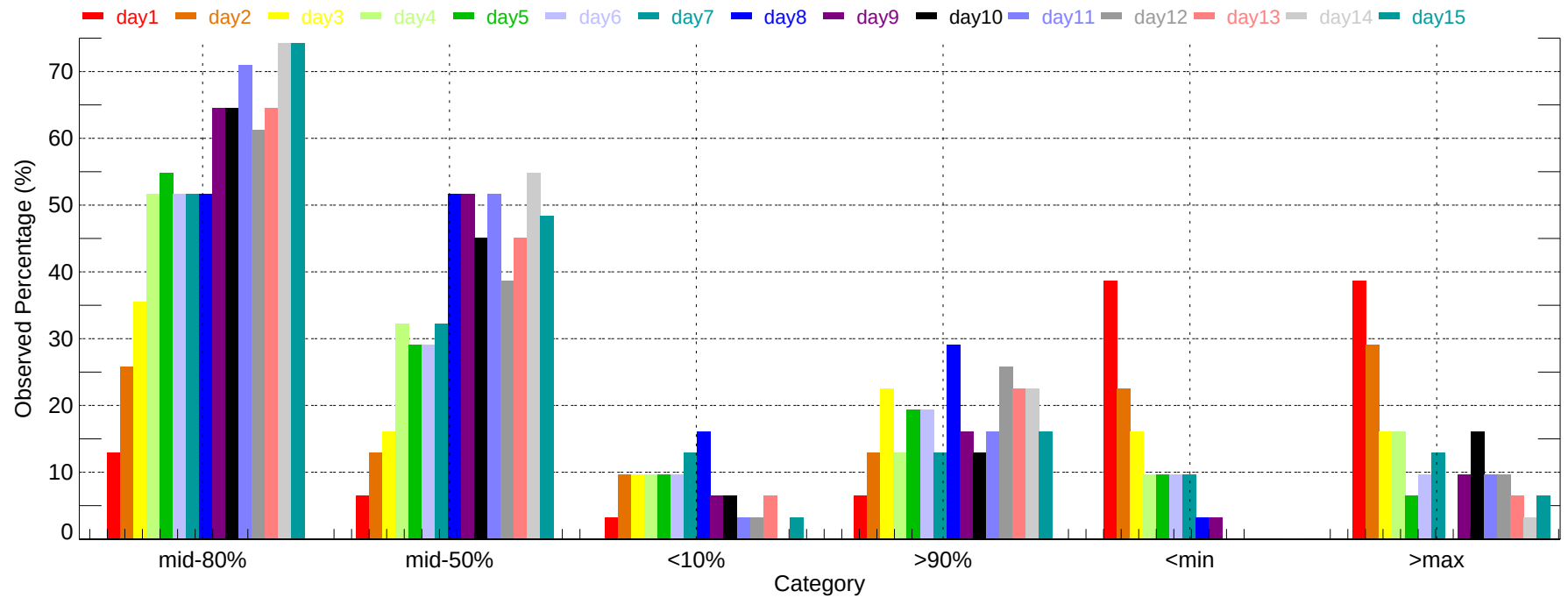
Observed Percentage of Ensembles - RIC: Max Temperature (2011-12-01~2011-12-31)
