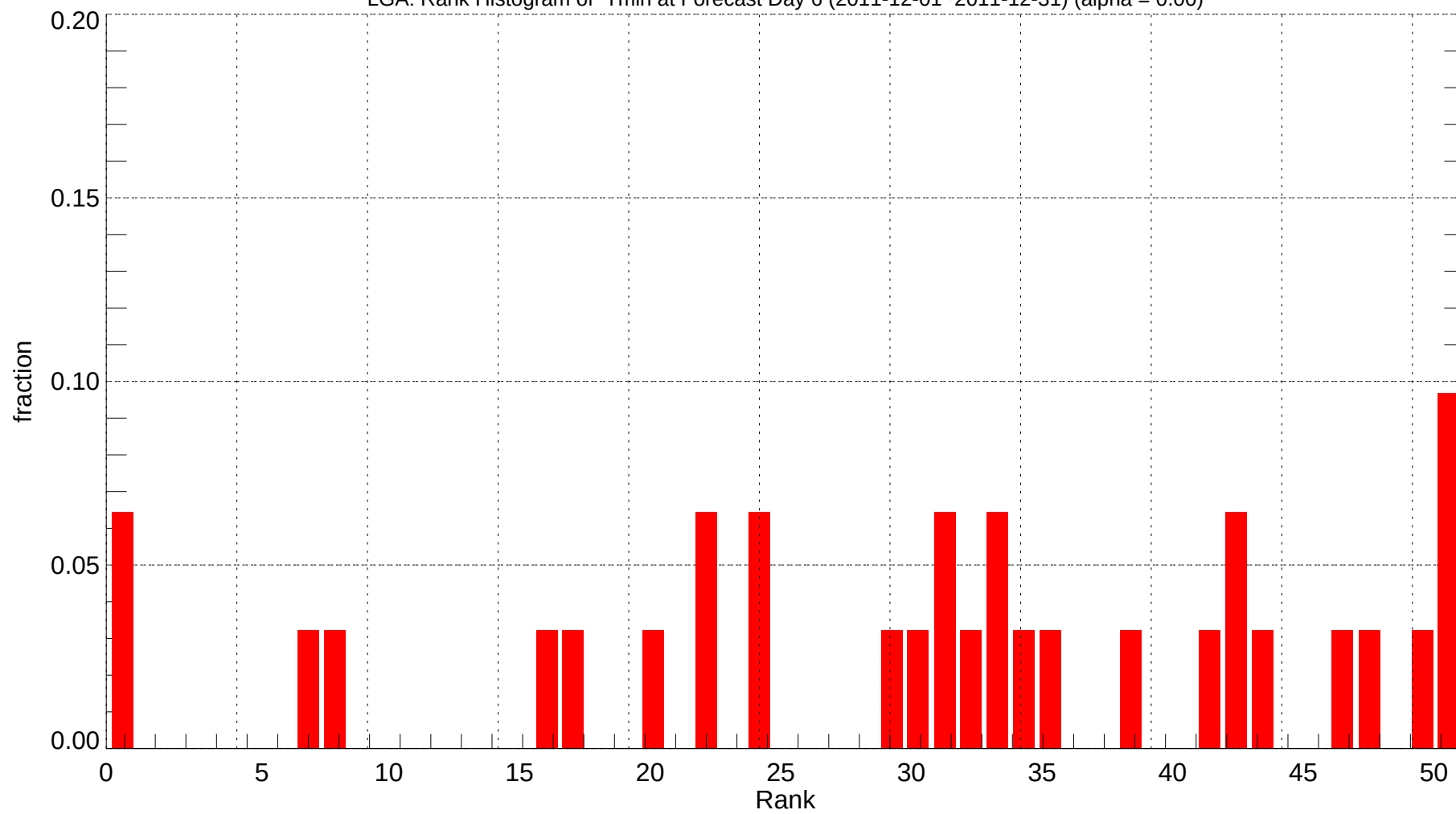
LGA: Rank Histogram of Tmin at Forecast Day 6 (2011-12-01~2011-12-31) (alpha = 0.00)
