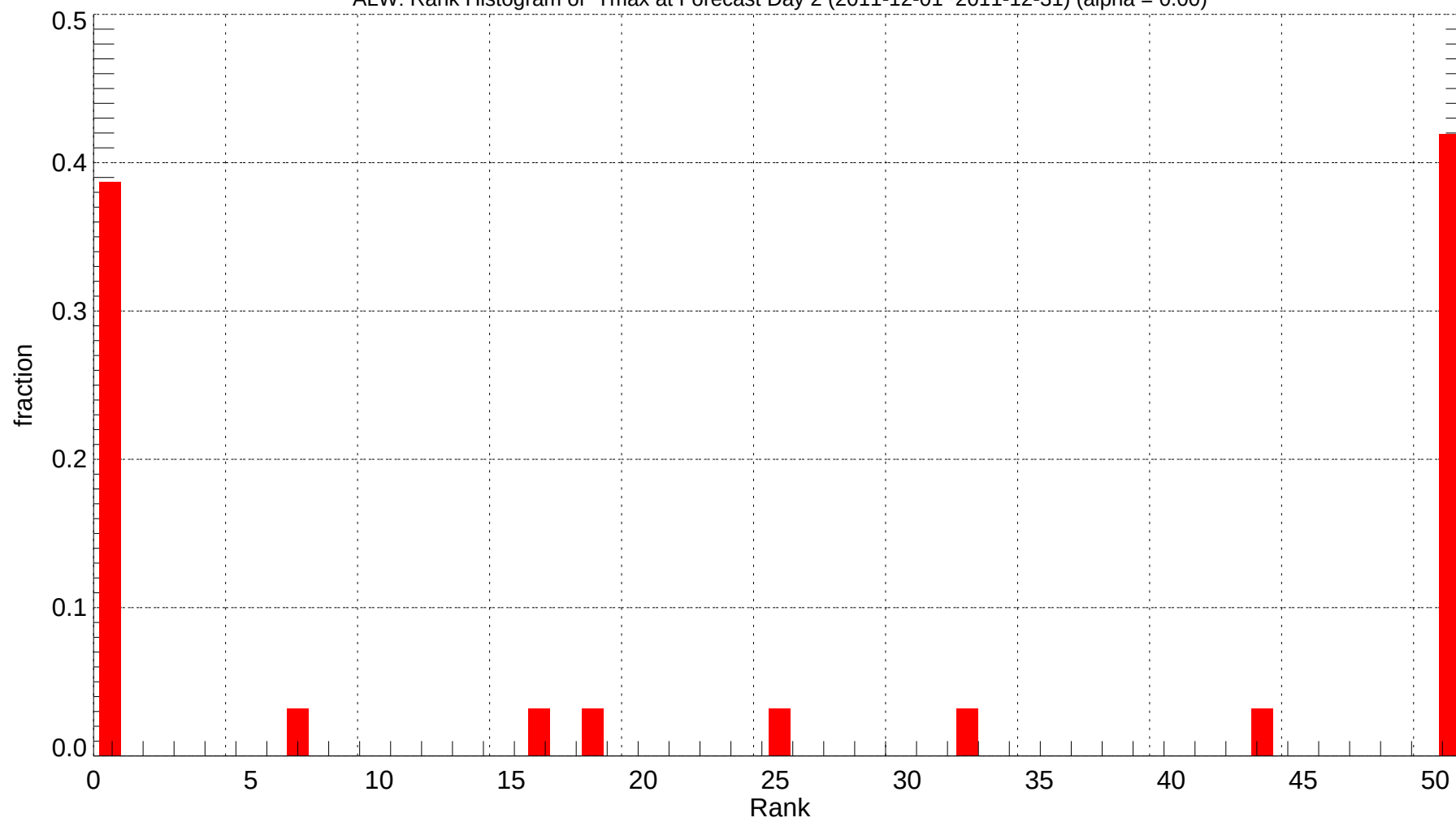
ALW: Rank Histogram of Tmax at Forecast Day 2 (2011-12-01~2011-12-31) (alpha = 0.00)
