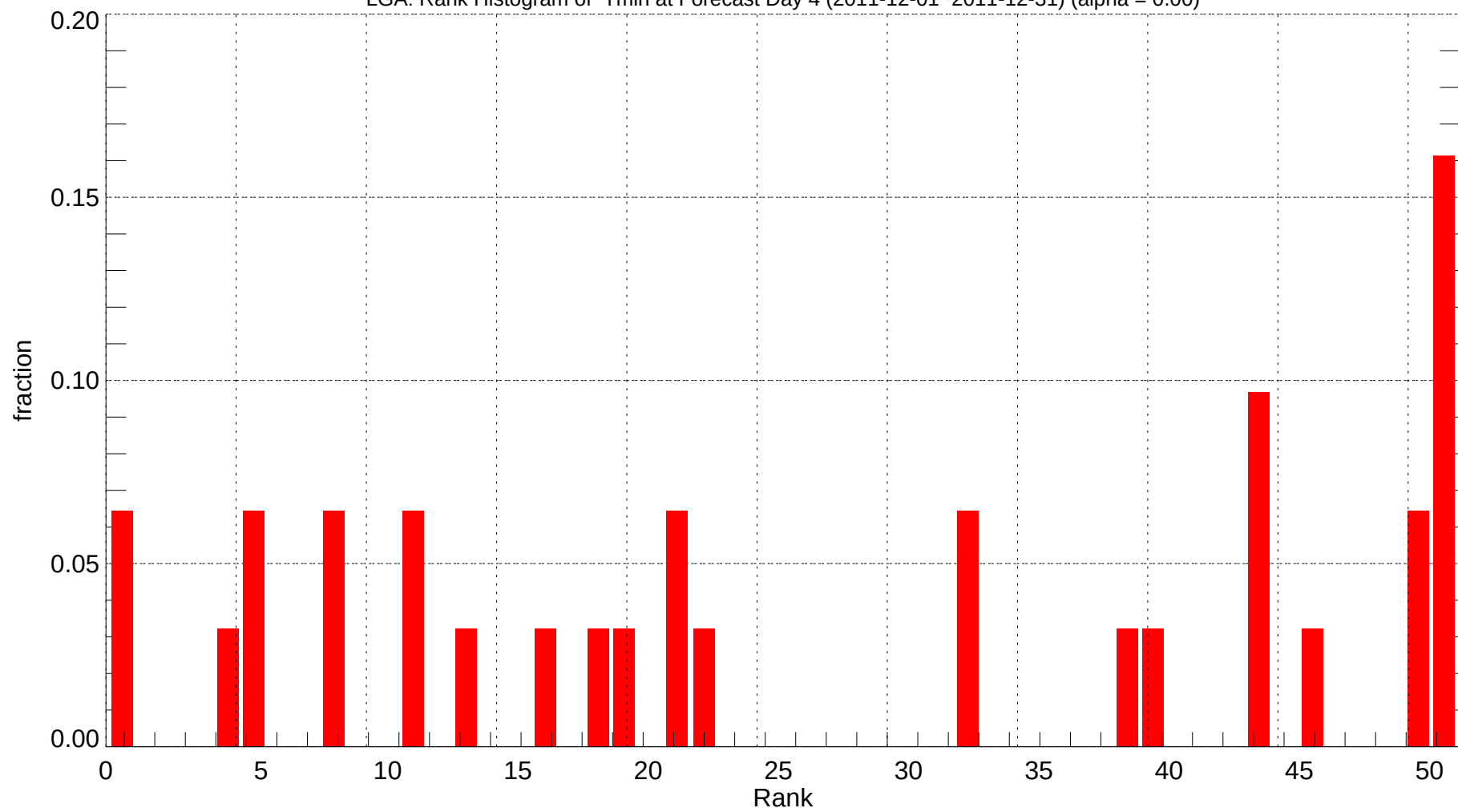
LGA: Rank Histogram of Tmin at Forecast Day 4 (2011-12-01~2011-12-31) (alpha = 0.00)
