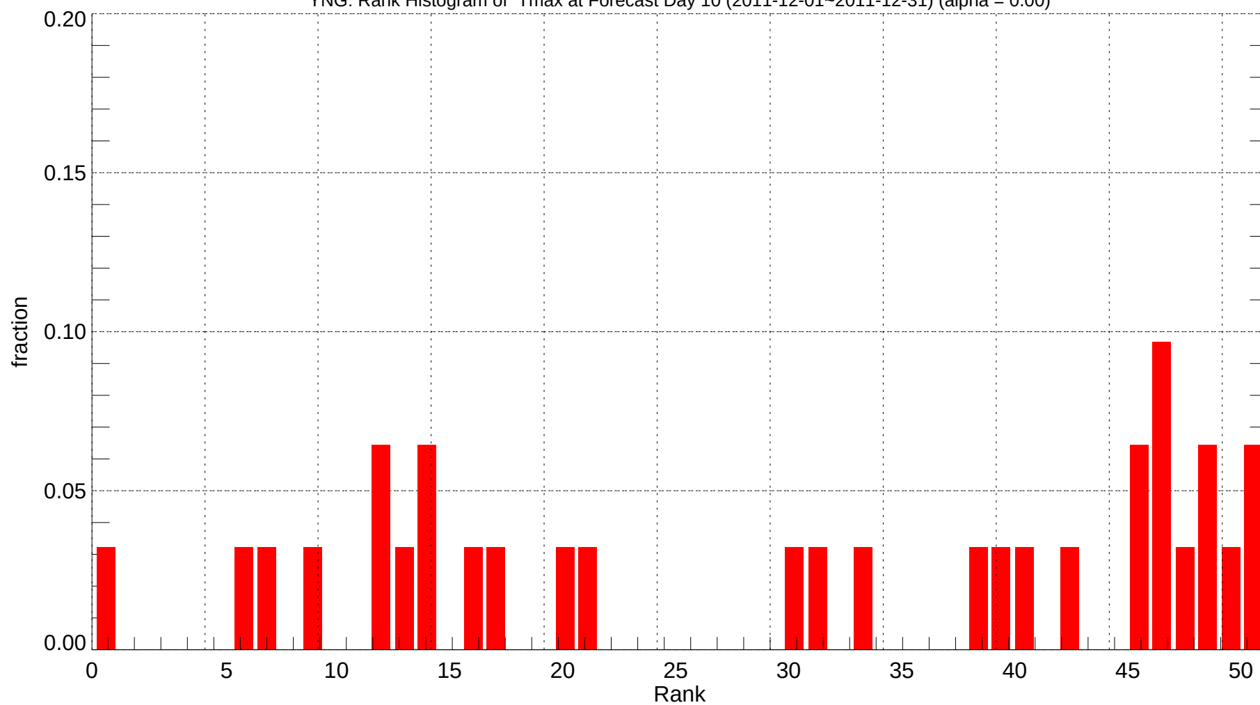
YNG: Rank Histogram of Tmax at Forecast Day 10 (2011-12-01~2011-12-31) (alpha = 0.00)
