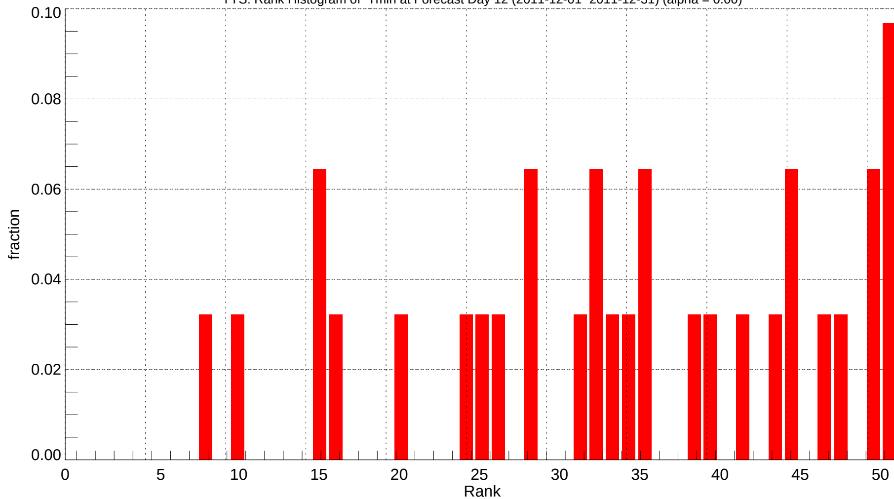
TYS: Rank Histogram of Tmin at Forecast Day 12 (2011-12-01~2011-12-31) (alpha = 0.00)
