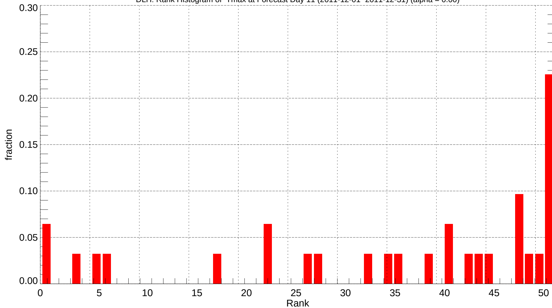
DLH: Rank Histogram of Tmax at Forecast Day 11 (2011-12-01~2011-12-31) (alpha = 0.00)
