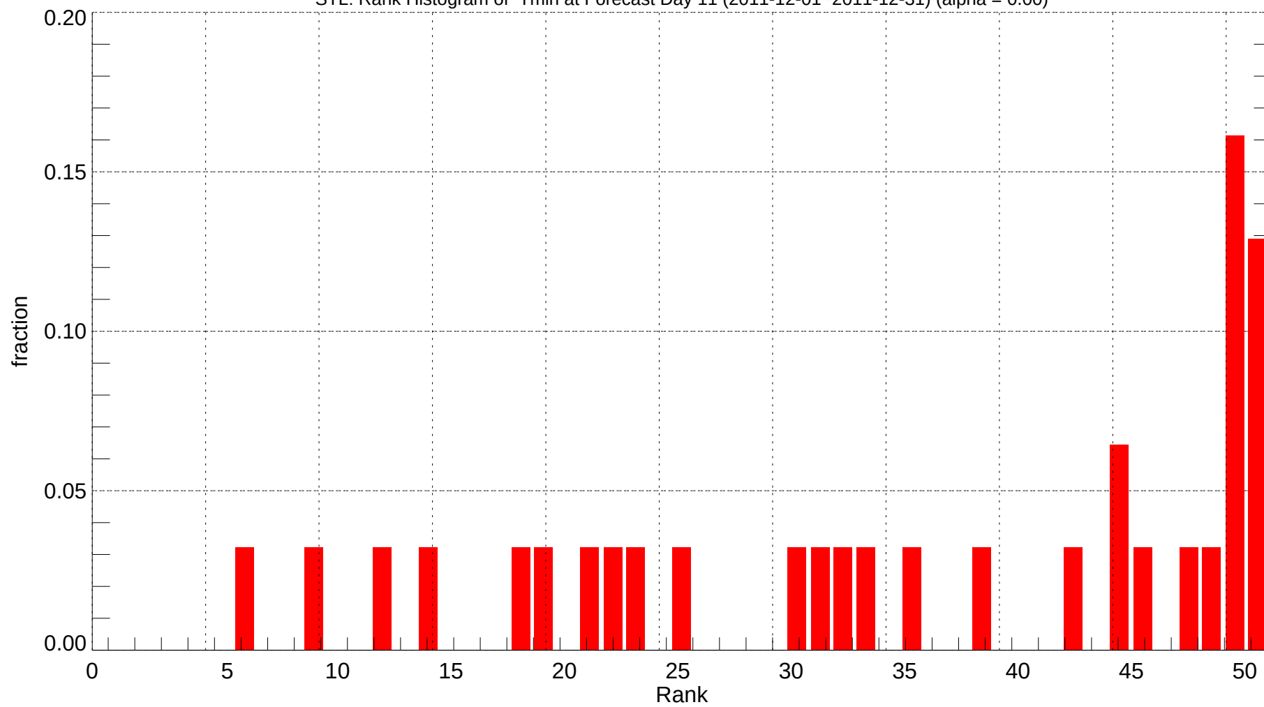
STL: Rank Histogram of Tmin at Forecast Day 11 (2011-12-01~2011-12-31) (alpha = 0.00)
