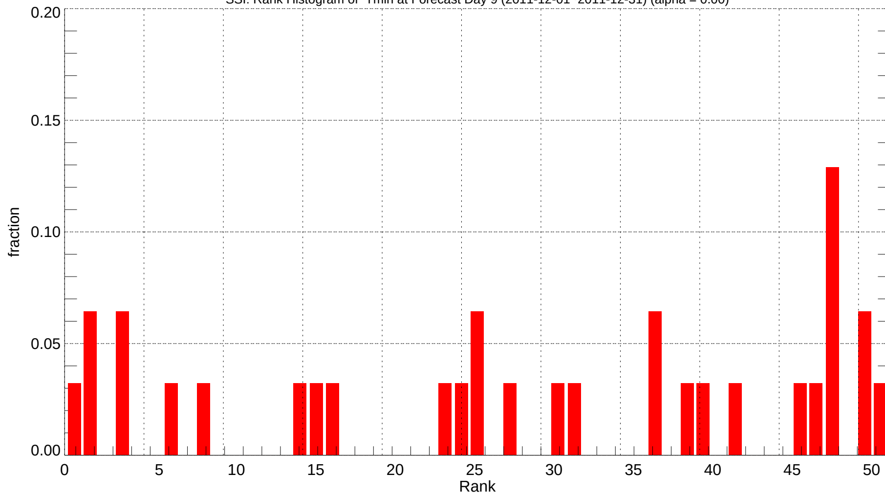
SSI: Rank Histogram of Tmin at Forecast Day 9 (2011-12-01~2011-12-31) (alpha = 0.00)
