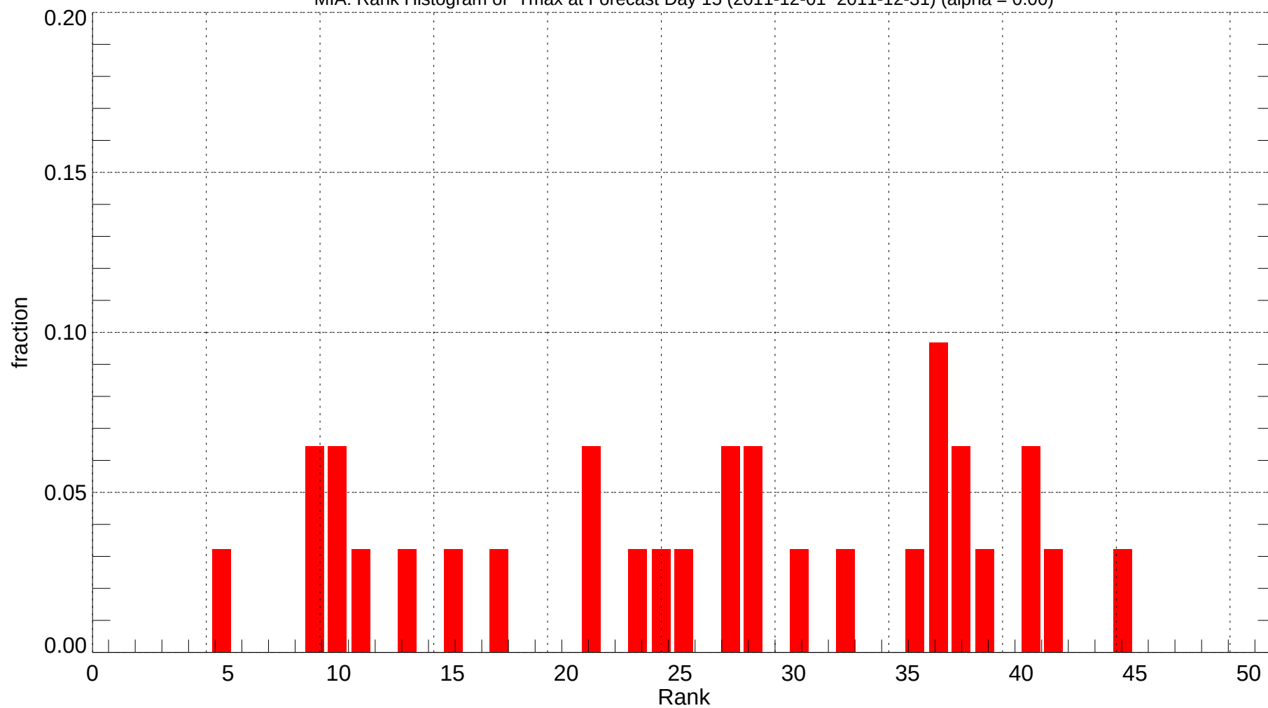
MIA: Rank Histogram of Tmax at Forecast Day 15 (2011-12-01~2011-12-31) (alpha = 0.00)
