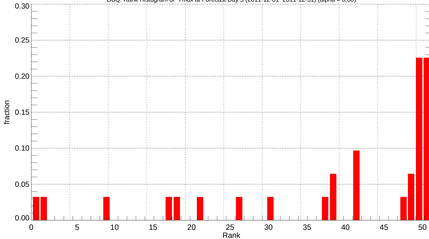
DBQ: Rank Histogram of Tmax at Forecast Day 5 (2011-12-01~2011-12-31) (alpha = 0.00)
