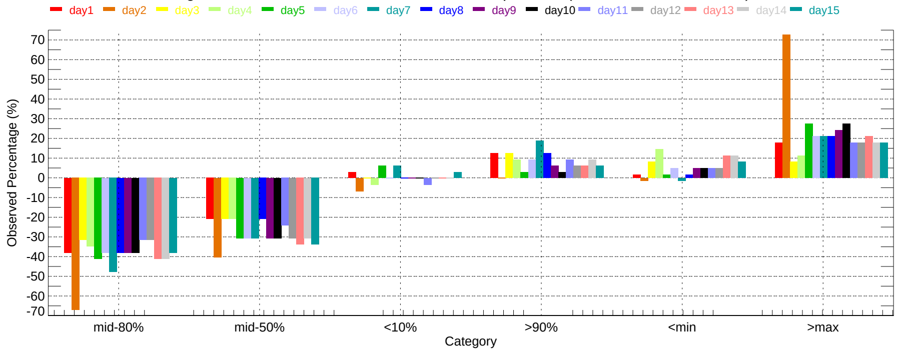
Observed Percentage Deviation of Ensembles - MOB: Max Temperature (2011-12-01~2011-12-31)
