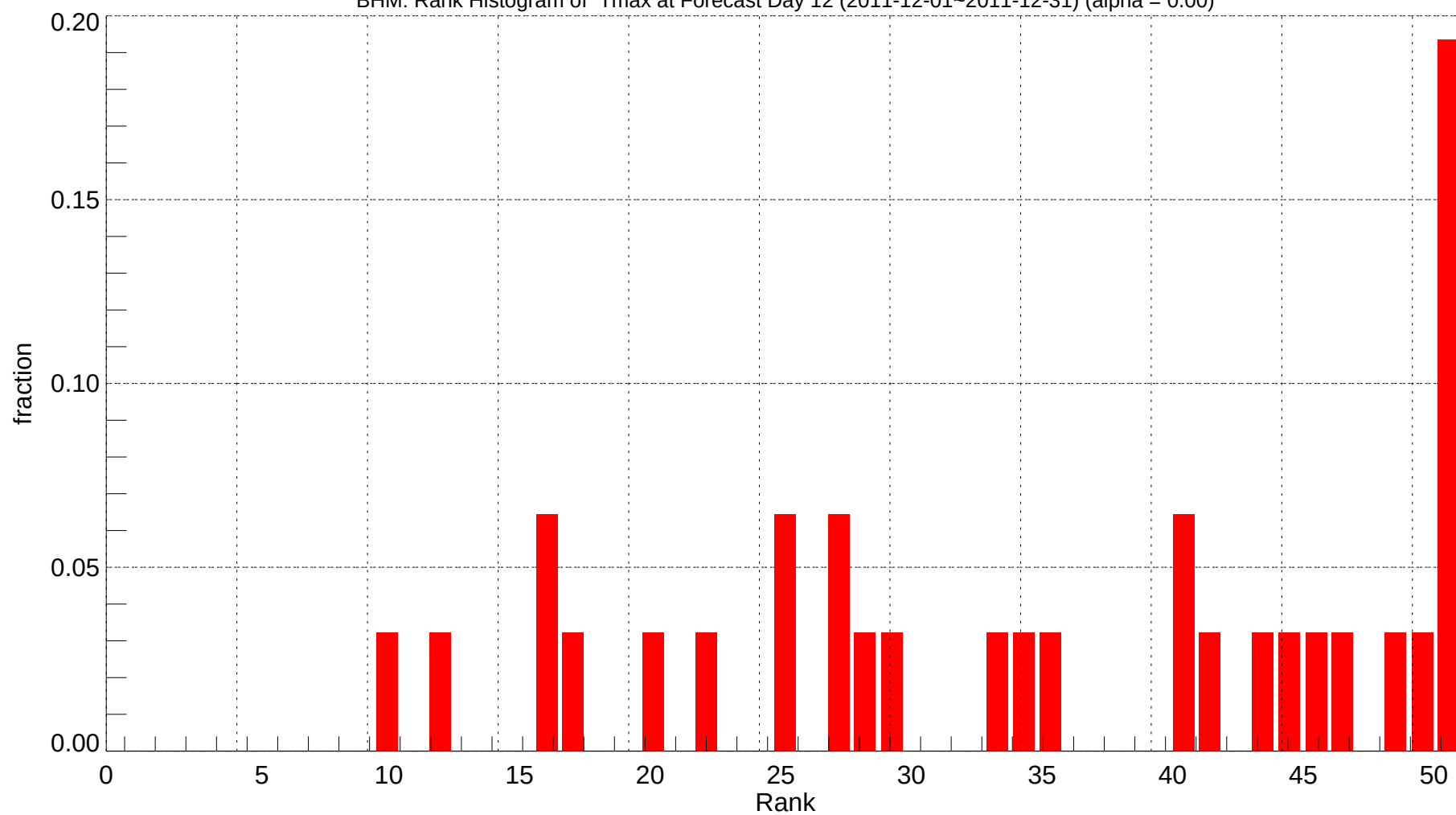
BHM: Rank Histogram of Tmax at Forecast Day 12 (2011-12-01~2011-12-31) (alpha = 0.00)
