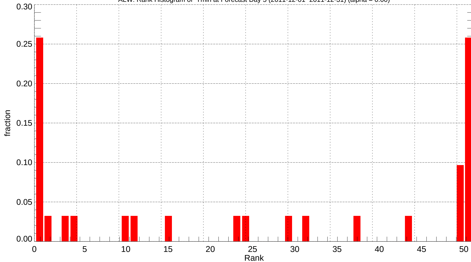
ALW: Rank Histogram of Tmin at Forecast Day 5 (2011-12-01~2011-12-31) (alpha = 0.00)
