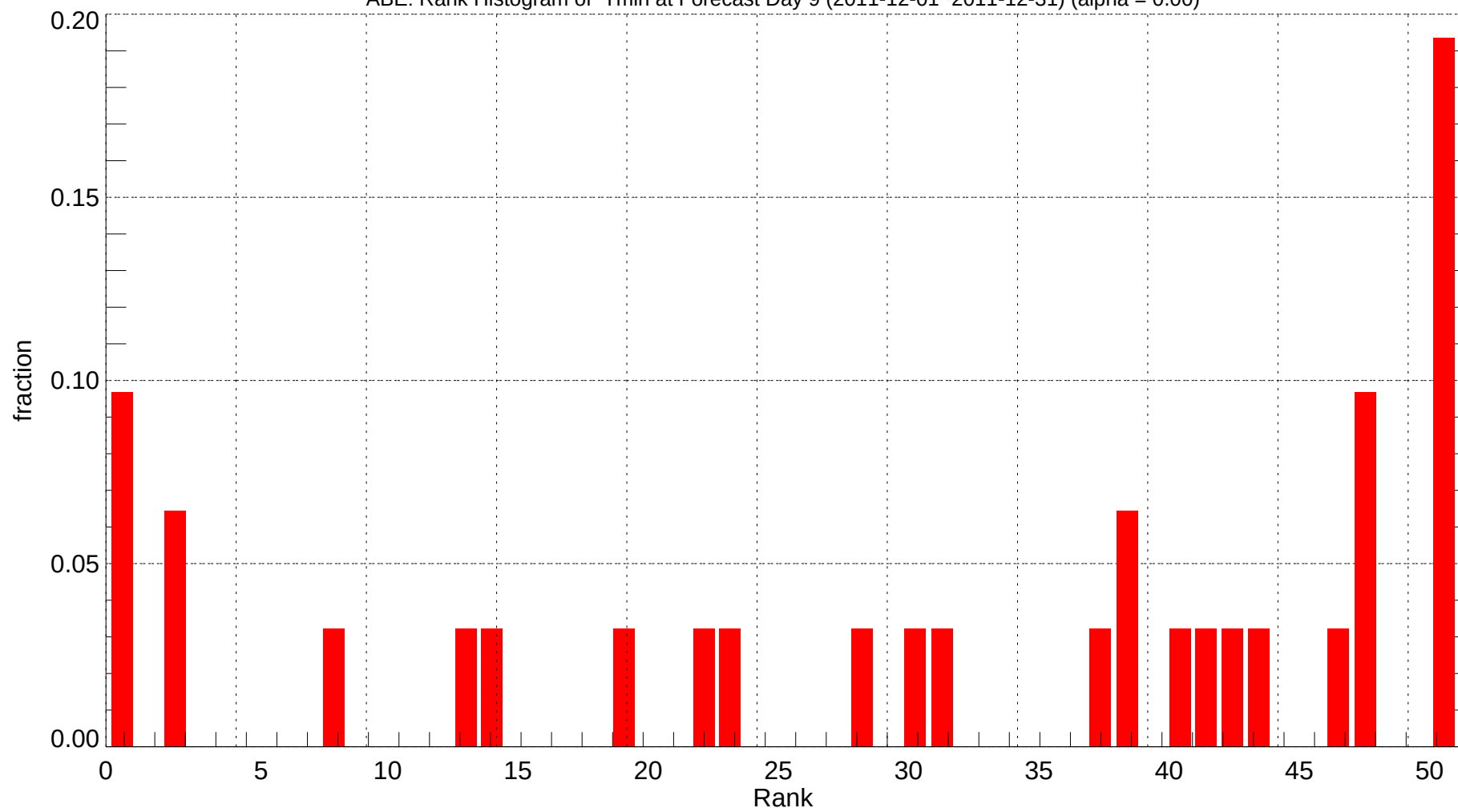
ABE: Rank Histogram of Tmin at Forecast Day 9 (2011-12-01~2011-12-31) (alpha = 0.00)
