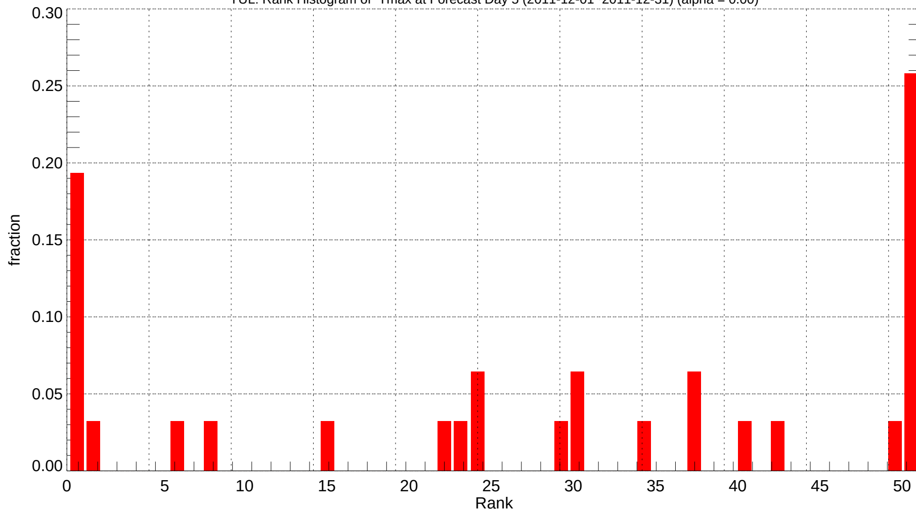
YUL: Rank Histogram of Tmax at Forecast Day 5 (2011-12-01~2011-12-31) (alpha = 0.00)
