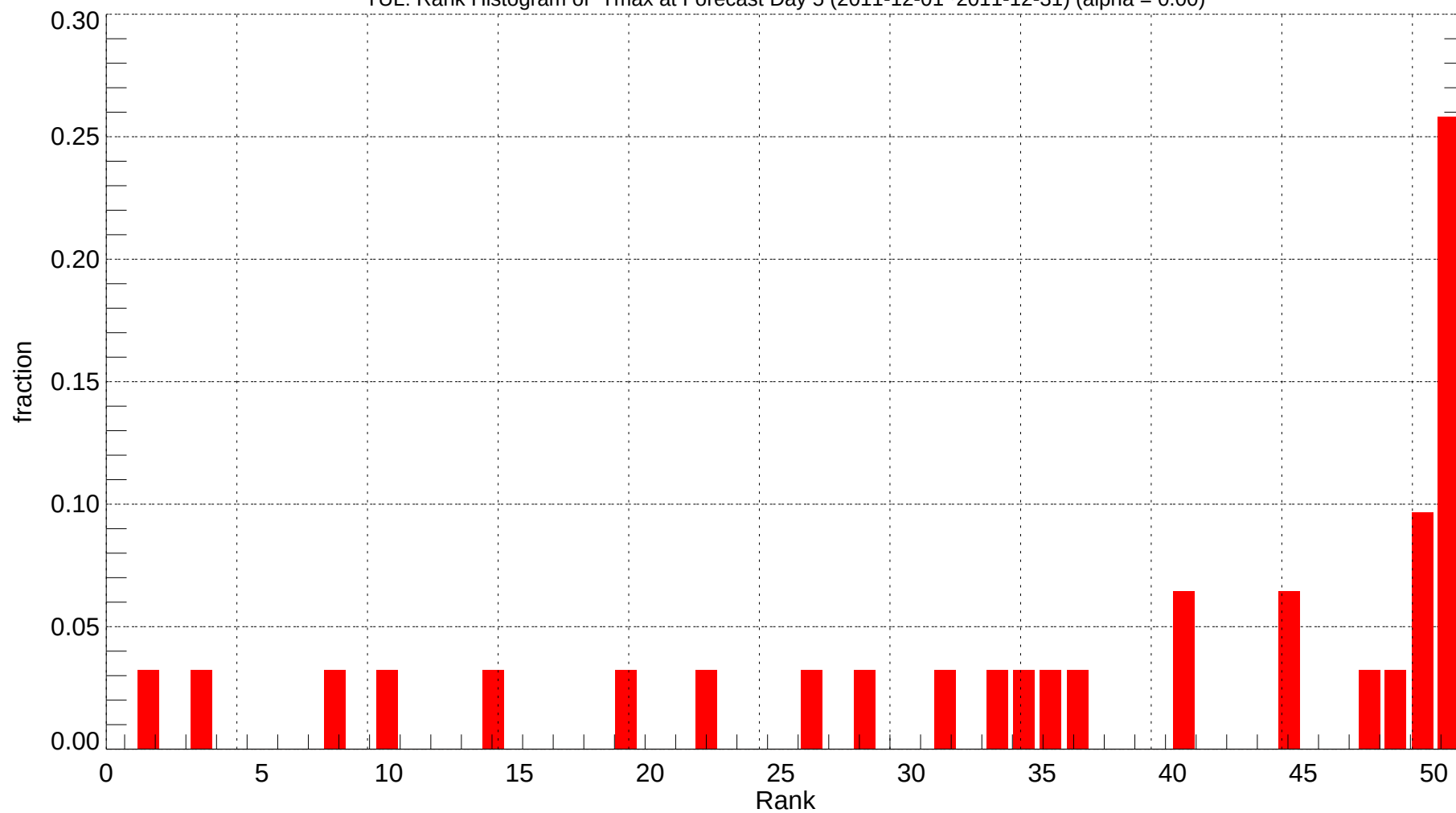
TUL: Rank Histogram of Tmax at Forecast Day 5 (2011-12-01~2011-12-31) (alpha = 0.00)
