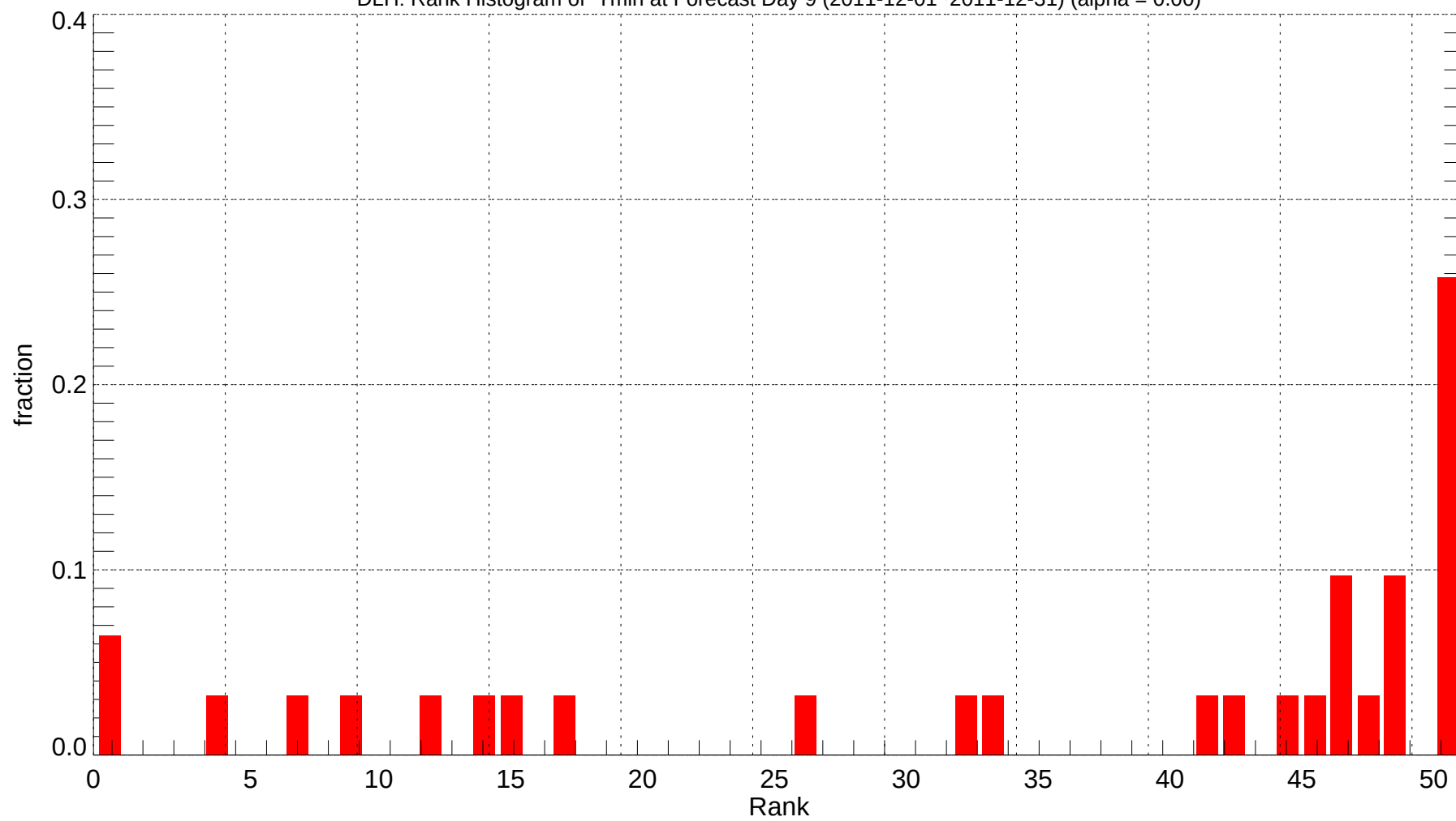
DLH: Rank Histogram of Tmin at Forecast Day 9 (2011-12-01~2011-12-31) (alpha = 0.00)
