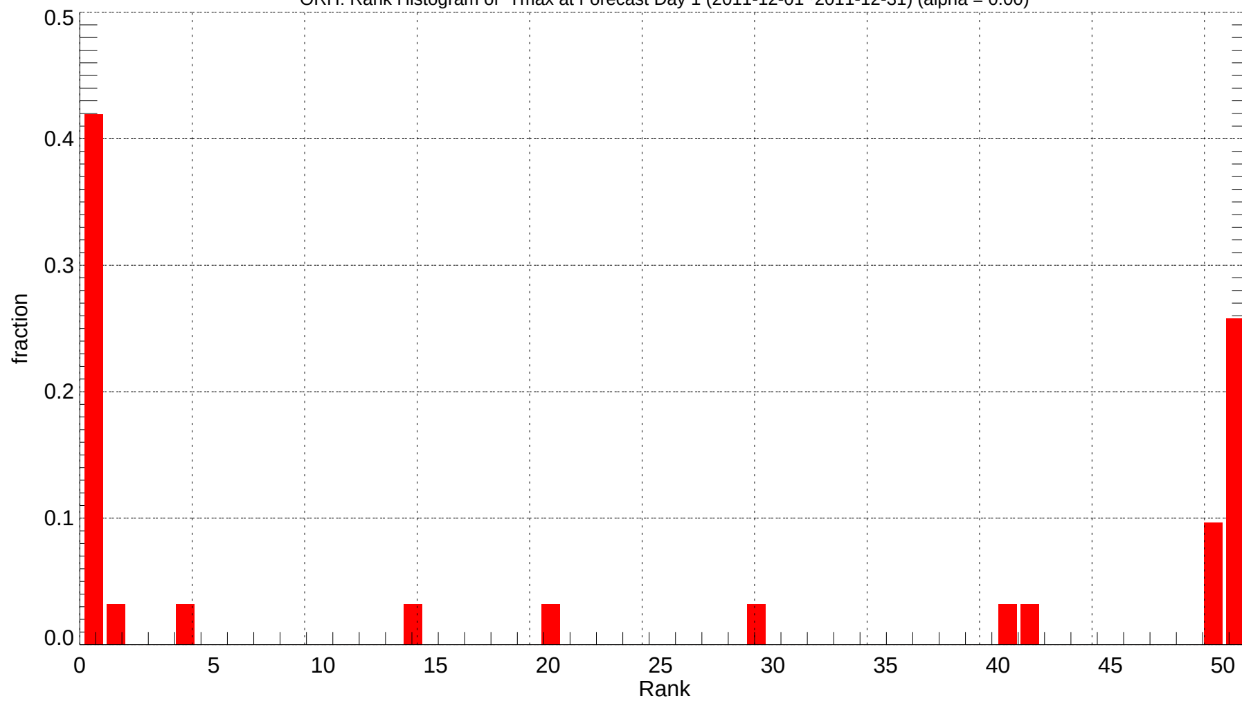
ORH: Rank Histogram of Tmax at Forecast Day 1 (2011-12-01~2011-12-31) (alpha = 0.00)
