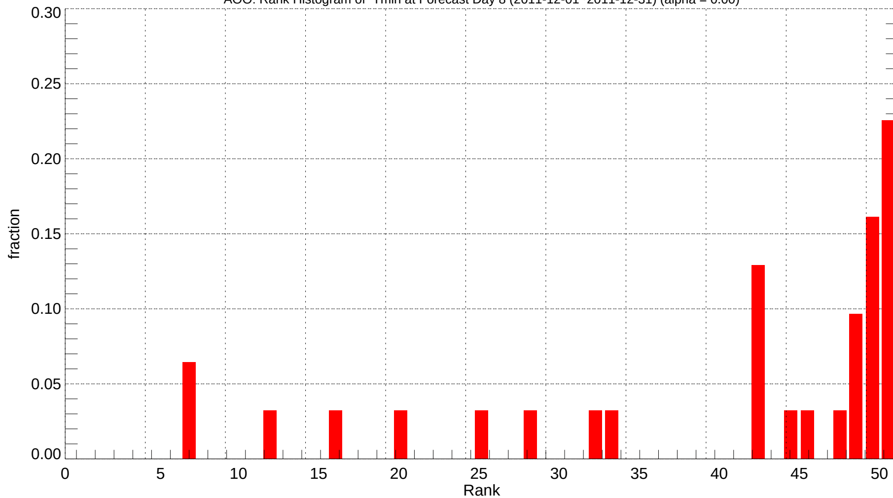
AOO: Rank Histogram of Tmin at Forecast Day 8 (2011-12-01~2011-12-31) (alpha = 0.00)
