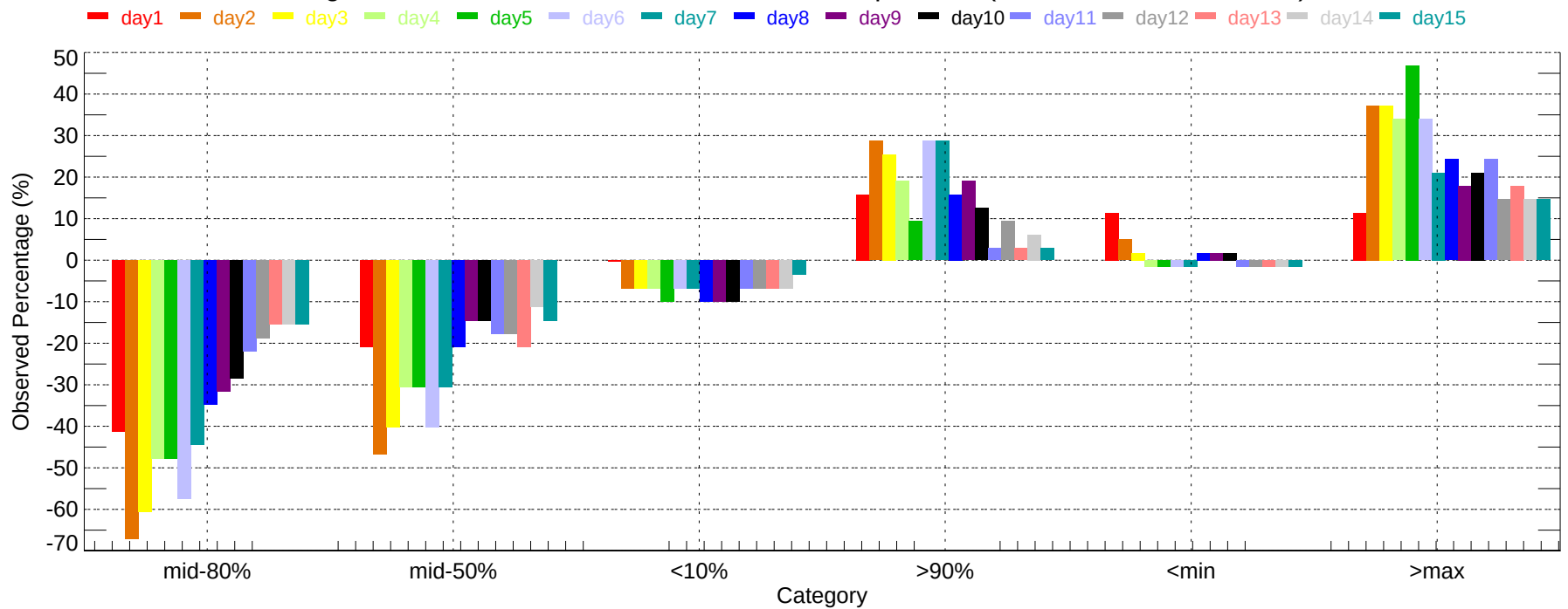
Observed Percentage Deviation of Ensembles - MDT: Max Temperature (2011-12-01~2011-12-31)
