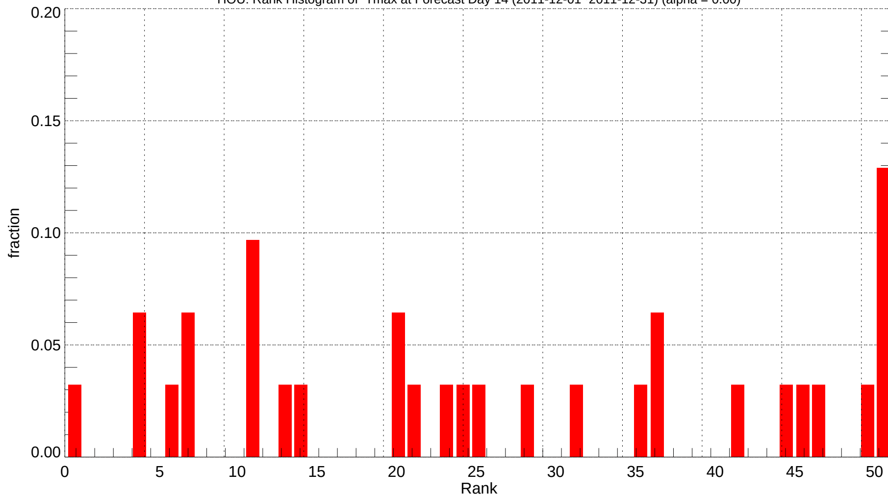
HOU: Rank Histogram of Tmax at Forecast Day 14 (2011-12-01~2011-12-31) (alpha = 0.00)
