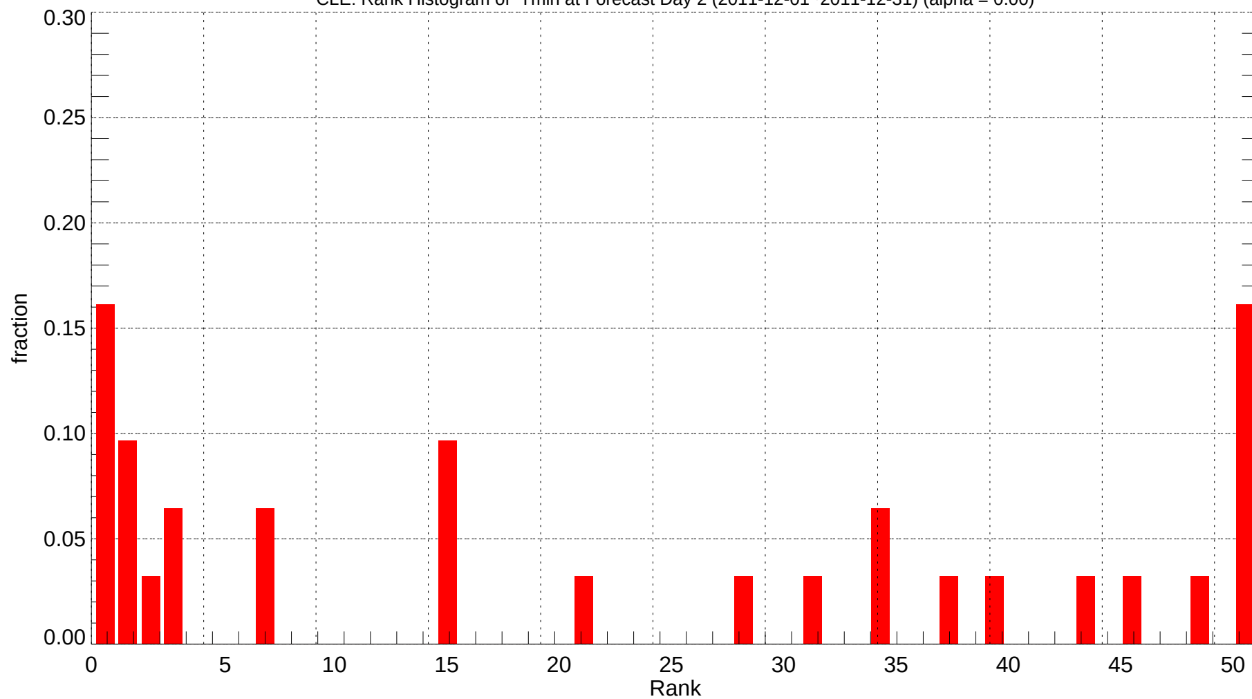
CLE: Rank Histogram of Tmin at Forecast Day 2 (2011-12-01~2011-12-31) (alpha = 0.00)
