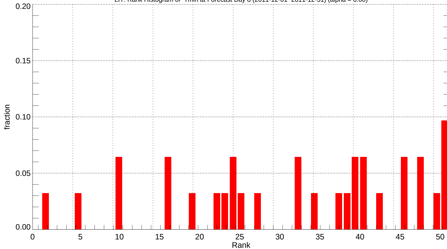
LIT: Rank Histogram of Tmin at Forecast Day 8 (2011-12-01~2011-12-31) (alpha = 0.00)
