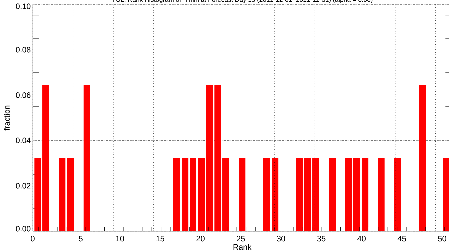
YUL: Rank Histogram of Tmin at Forecast Day 15 (2011-12-01~2011-12-31) (alpha = 0.00)
