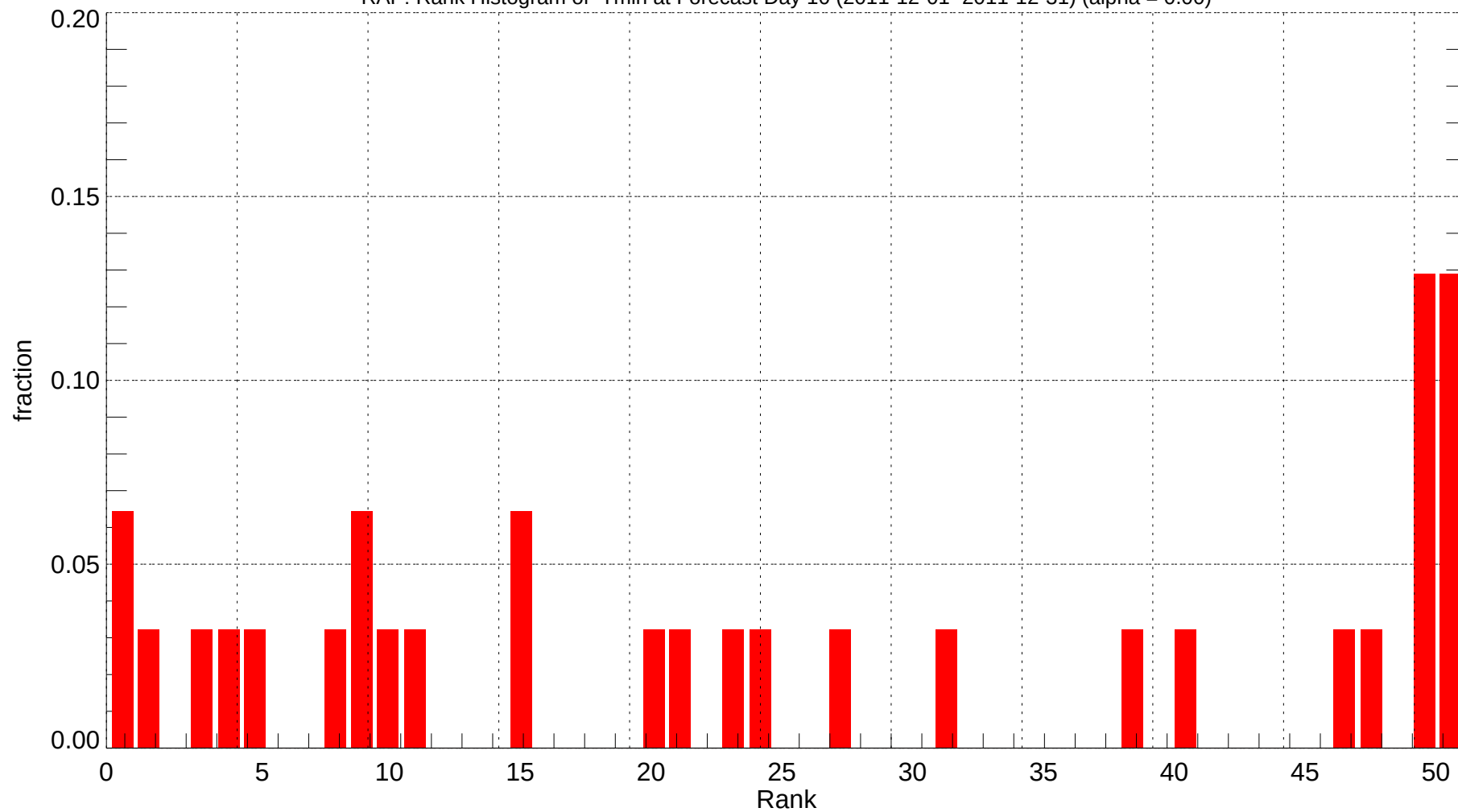
RAP: Rank Histogram of Tmin at Forecast Day 10 (2011-12-01~2011-12-31) (alpha = 0.00)
