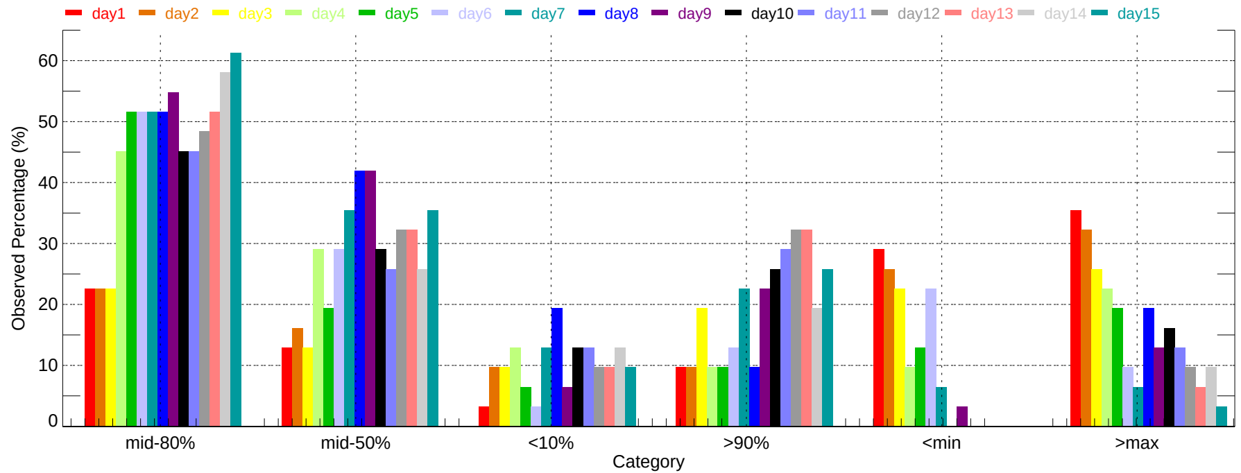
Observed Percentage of Ensembles - YWG: Min Temperature (2011-12-01~2011-12-31)
