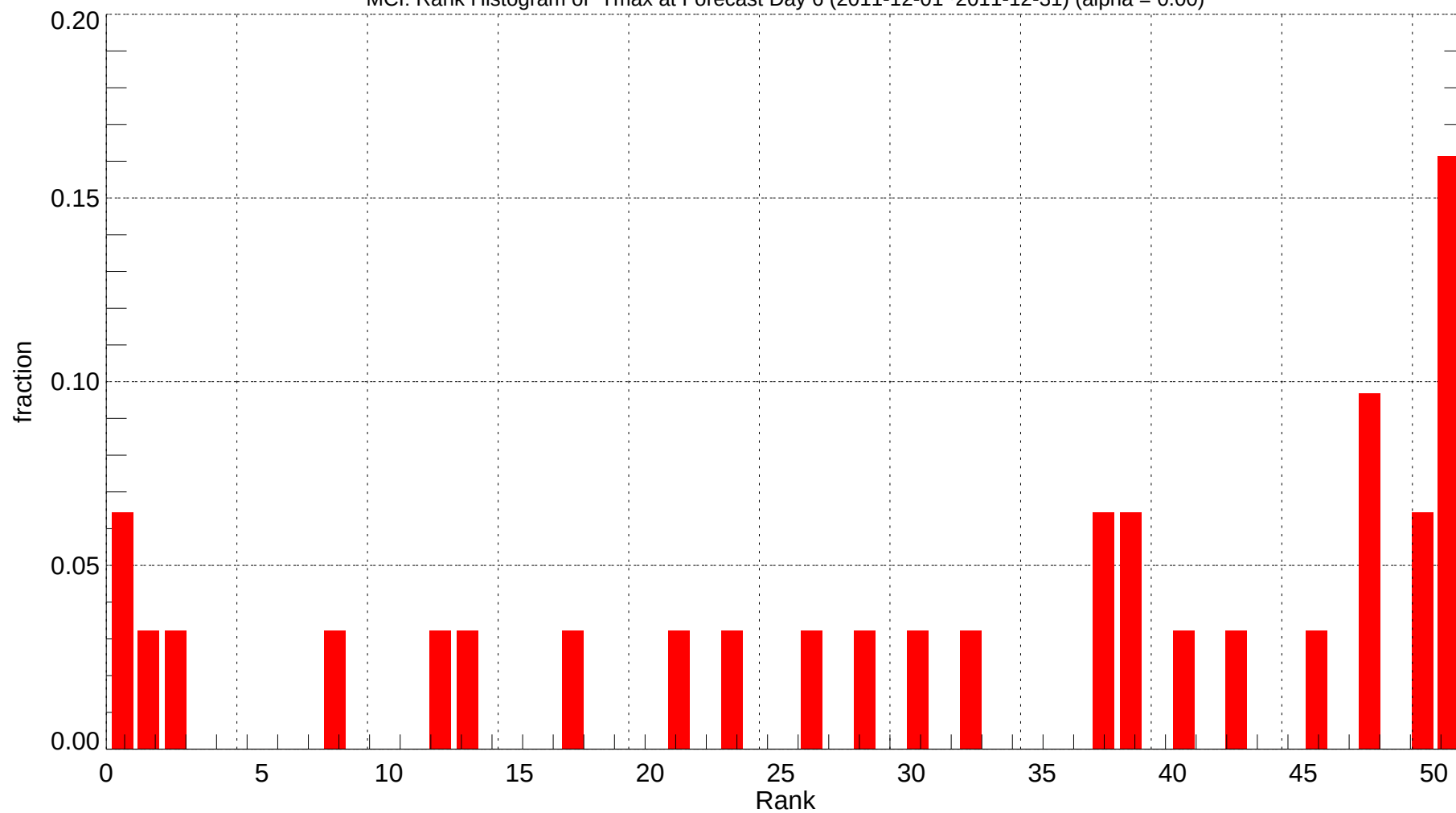
MCI: Rank Histogram of Tmax at Forecast Day 6 (2011-12-01~2011-12-31) (alpha = 0.00)
