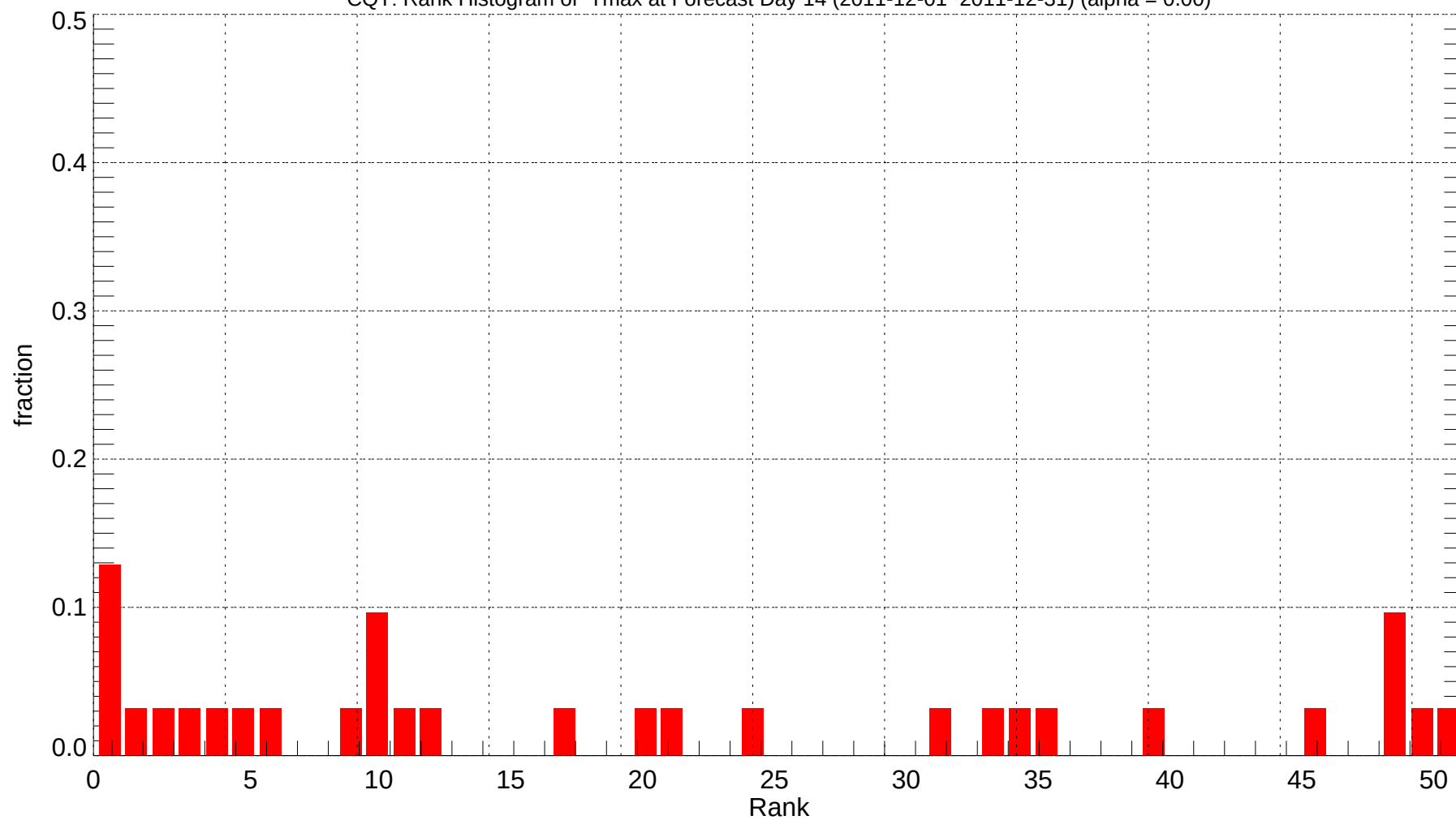
CQT: Rank Histogram of Tmax at Forecast Day 14 (2011-12-01~2011-12-31) (alpha = 0.00)
