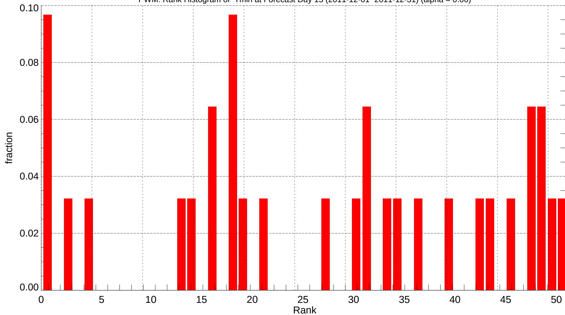
PWM: Rank Histogram of Tmin at Forecast Day 15 (2011-12-01~2011-12-31) (alpha = 0.00)
