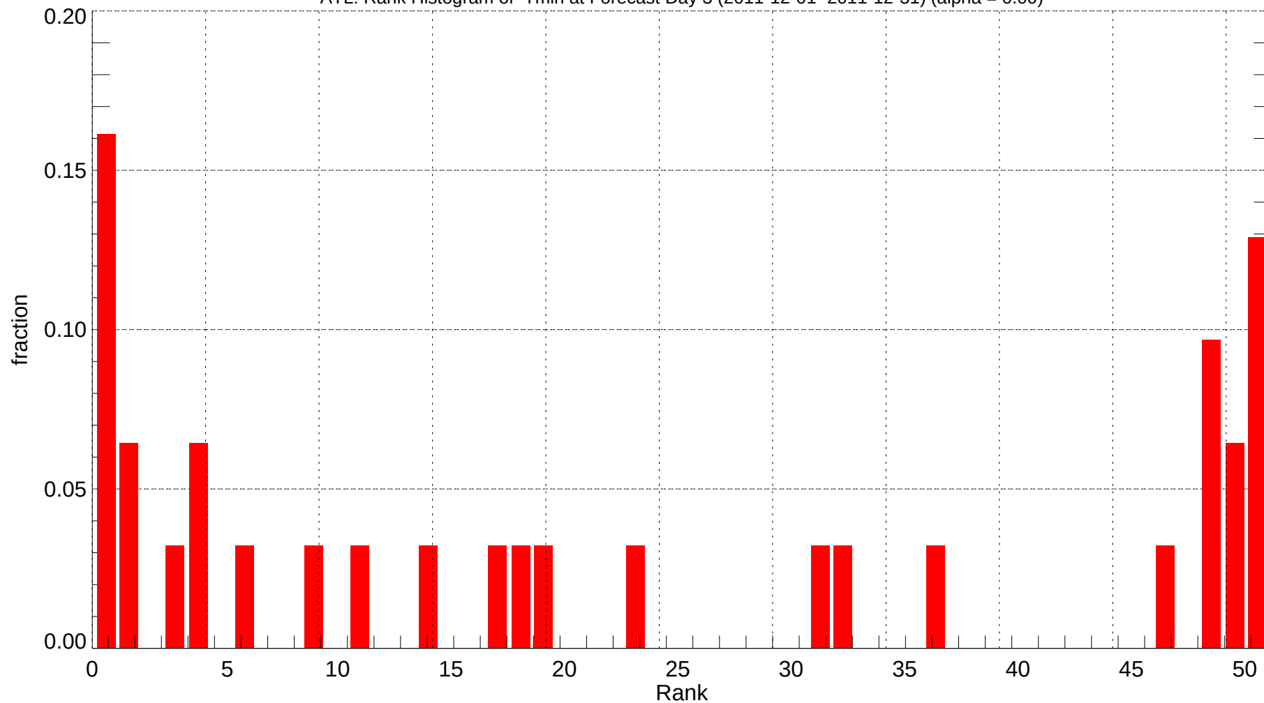
ATL: Rank Histogram of Tmin at Forecast Day 3 (2011-12-01~2011-12-31) (alpha = 0.00)
