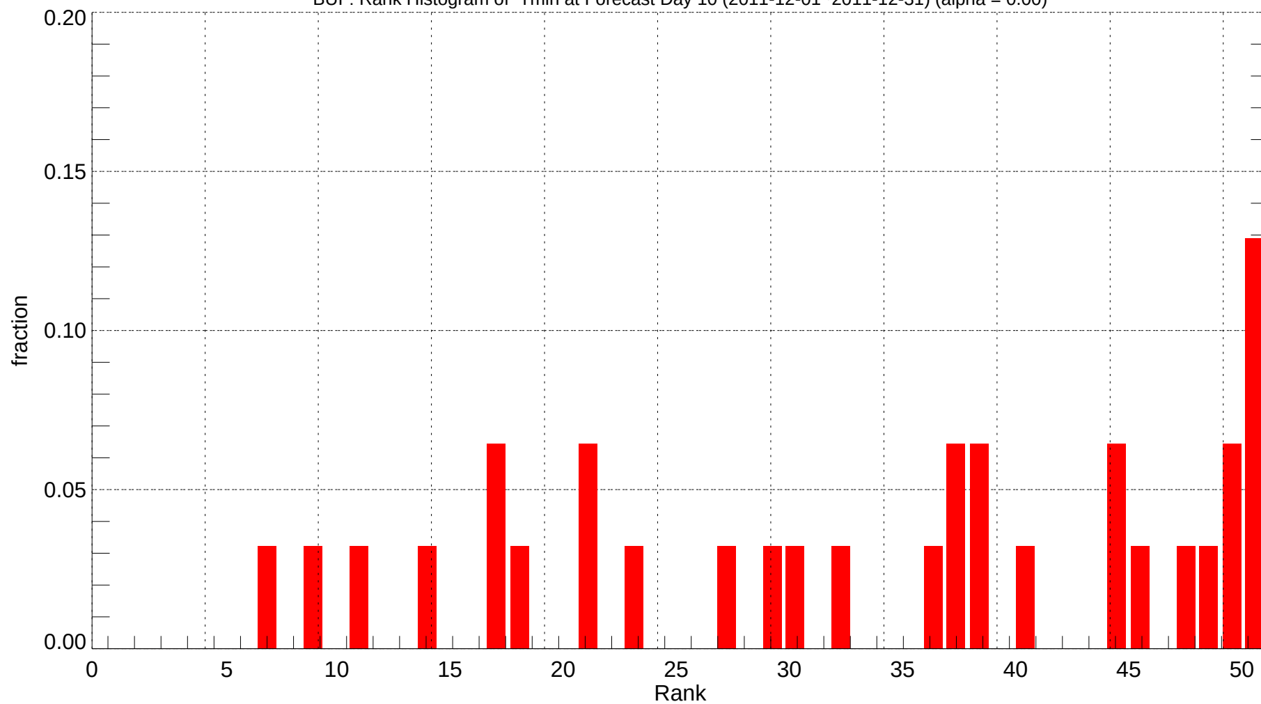
BUF: Rank Histogram of Tmin at Forecast Day 10 (2011-12-01~2011-12-31) (alpha = 0.00)
