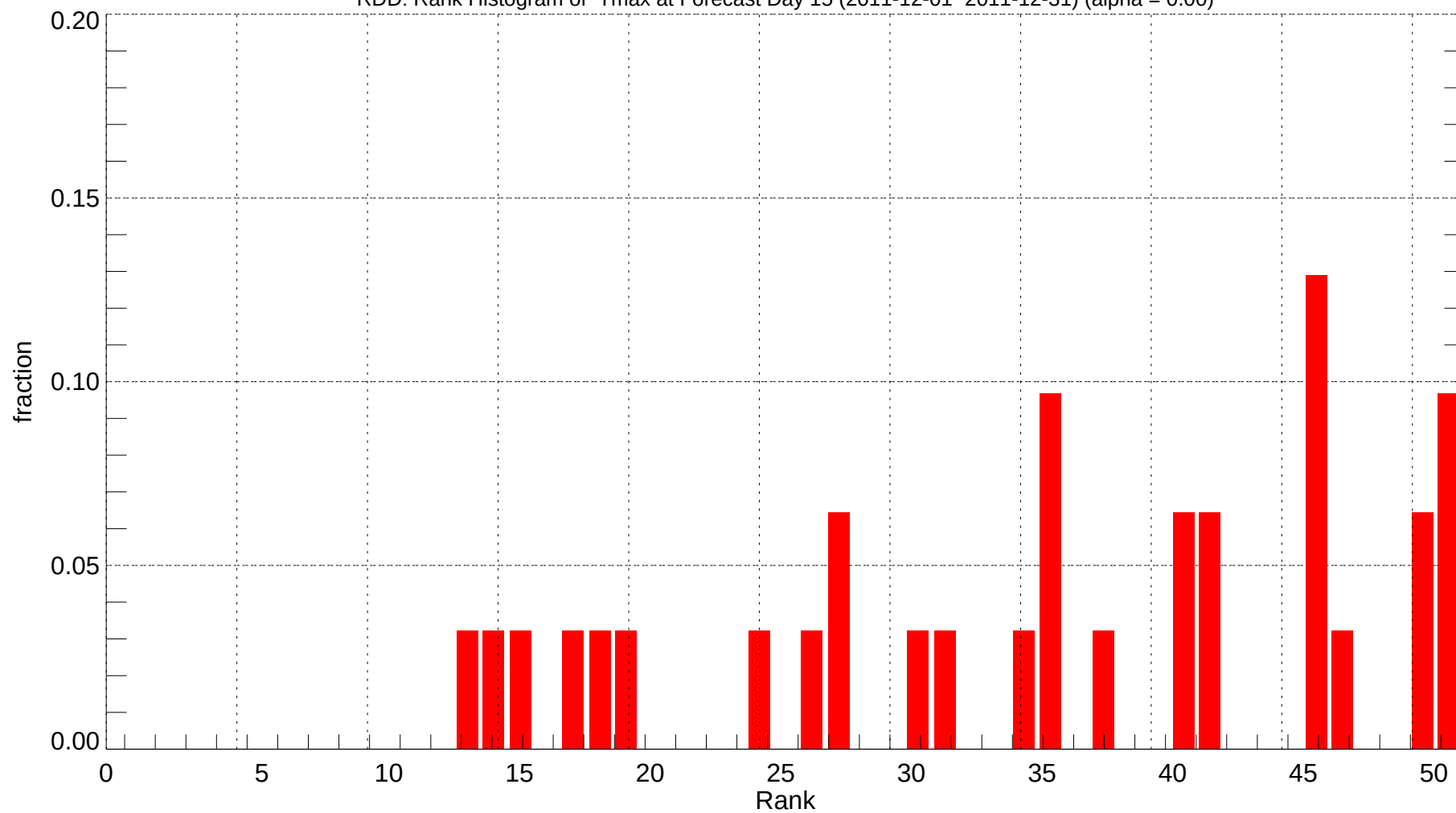
RDD: Rank Histogram of Tmax at Forecast Day 15 (2011-12-01~2011-12-31) (alpha = 0.00)
