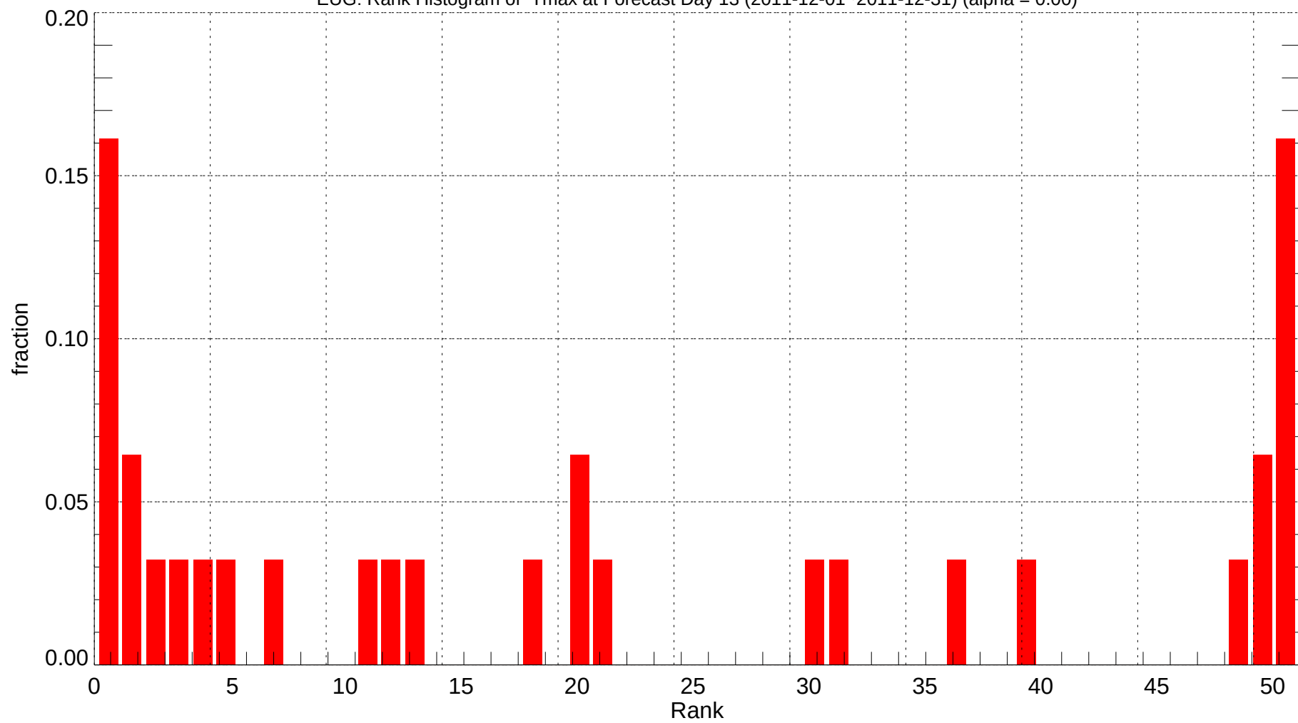
EUG: Rank Histogram of Tmax at Forecast Day 13 (2011-12-01~2011-12-31) (alpha = 0.00)
