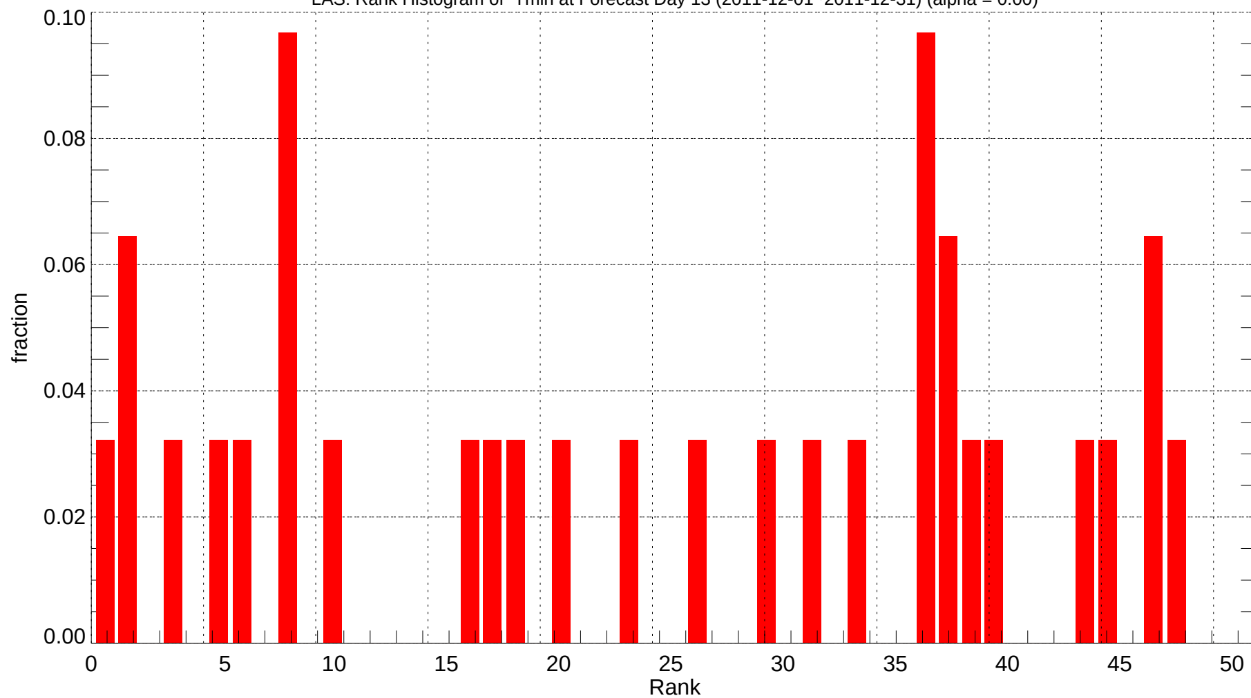
LAS: Rank Histogram of Tmin at Forecast Day 13 (2011-12-01~2011-12-31) (alpha = 0.00)
