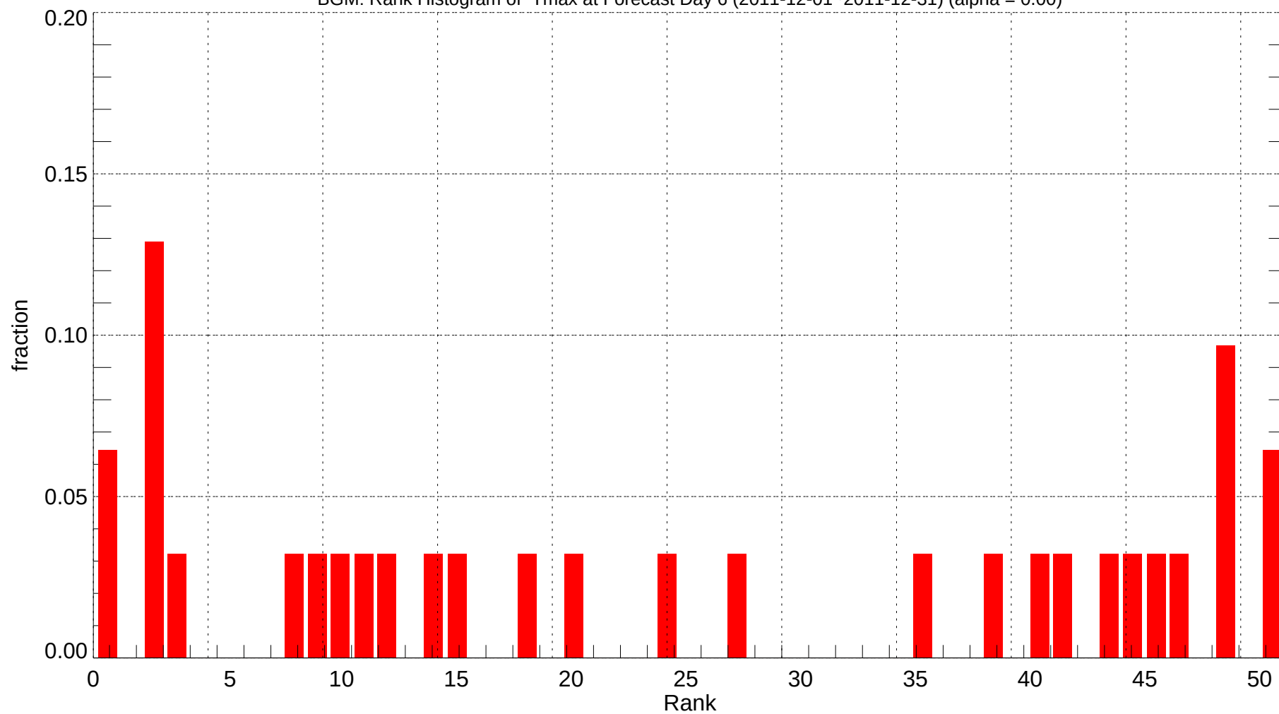
BGM: Rank Histogram of Tmax at Forecast Day 6 (2011-12-01~2011-12-31) (alpha = 0.00)
