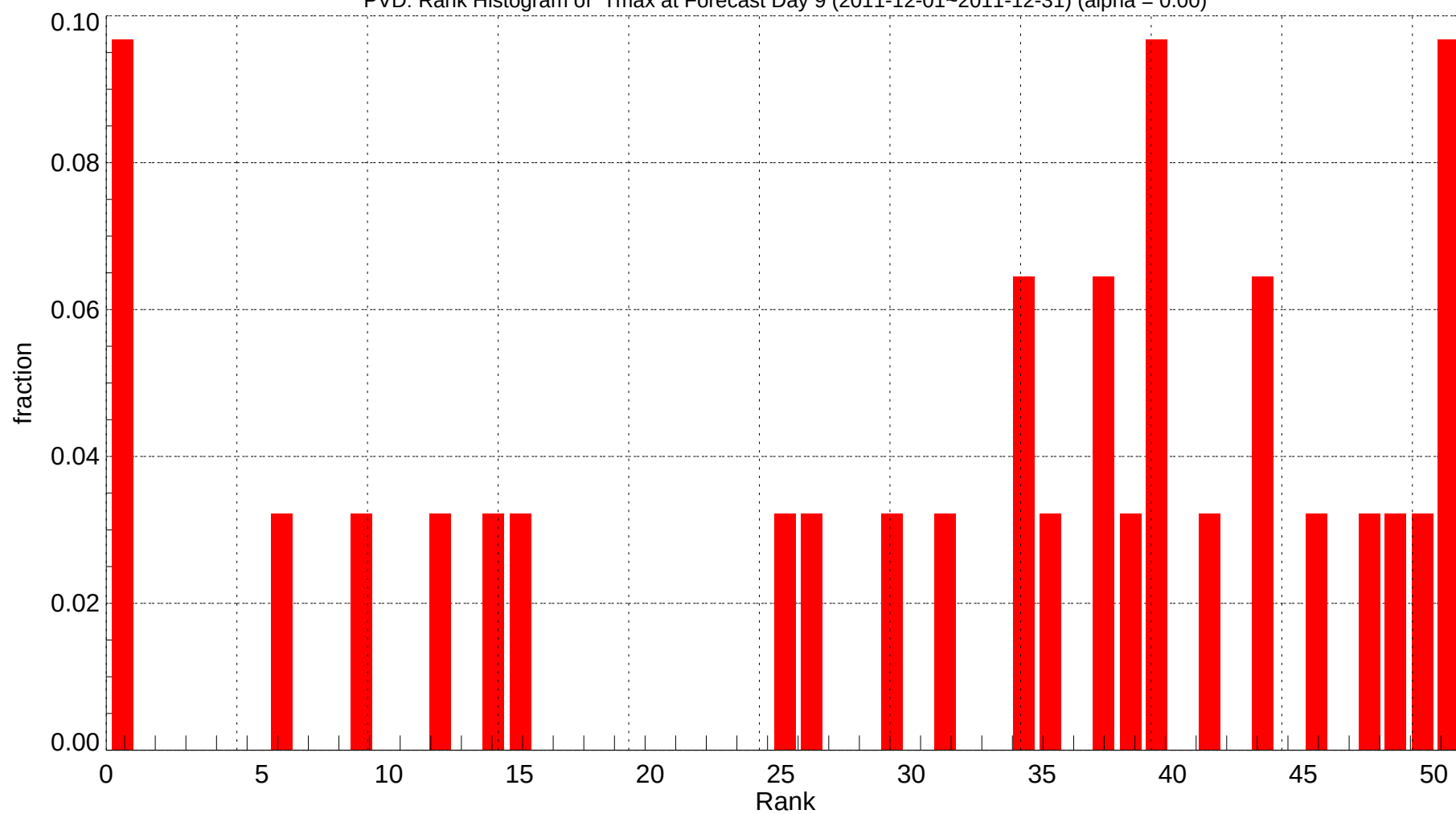
PVD: Rank Histogram of Tmax at Forecast Day 9 (2011-12-01~2011-12-31) (alpha = 0.00)
