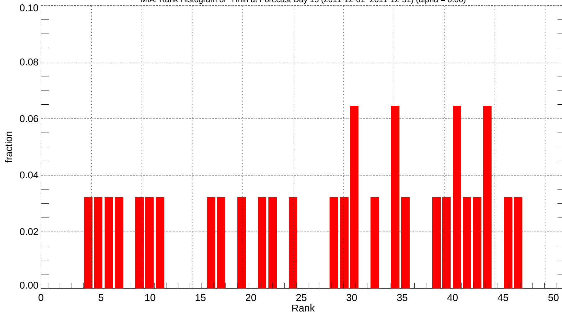
MIA: Rank Histogram of Tmin at Forecast Day 13 (2011-12-01~2011-12-31) (alpha = 0.00)
