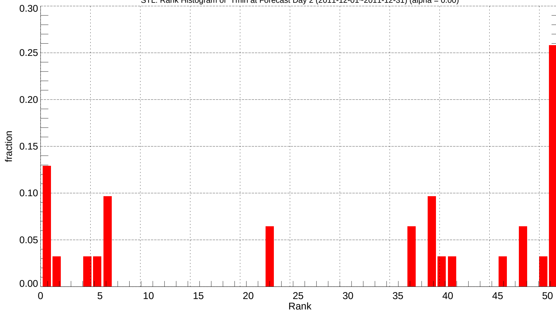
STL: Rank Histogram of Tmin at Forecast Day 2 (2011-12-01~2011-12-31) (alpha = 0.00)
