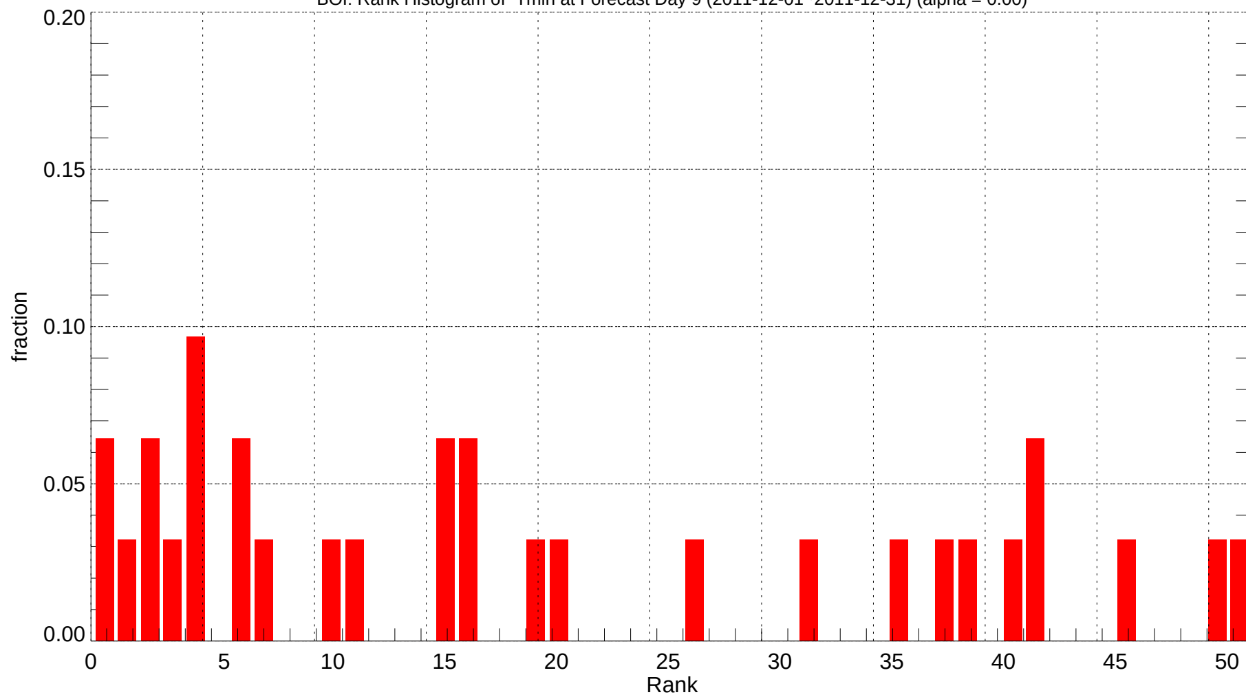
BOI: Rank Histogram of Tmin at Forecast Day 9 (2011-12-01~2011-12-31) (alpha = 0.00)
