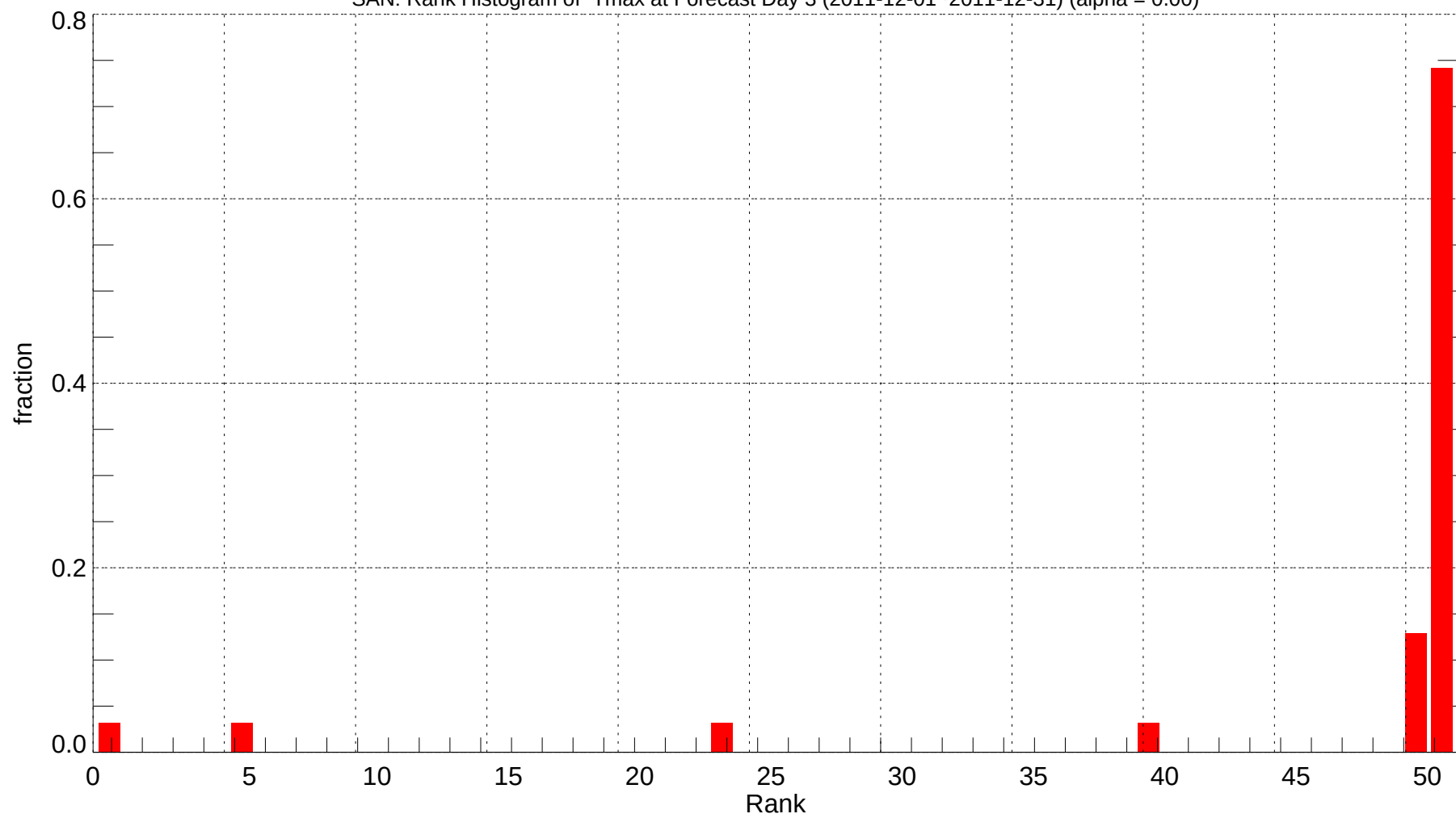
SAN: Rank Histogram of Tmax at Forecast Day 3 (2011-12-01~2011-12-31) (alpha = 0.00)
