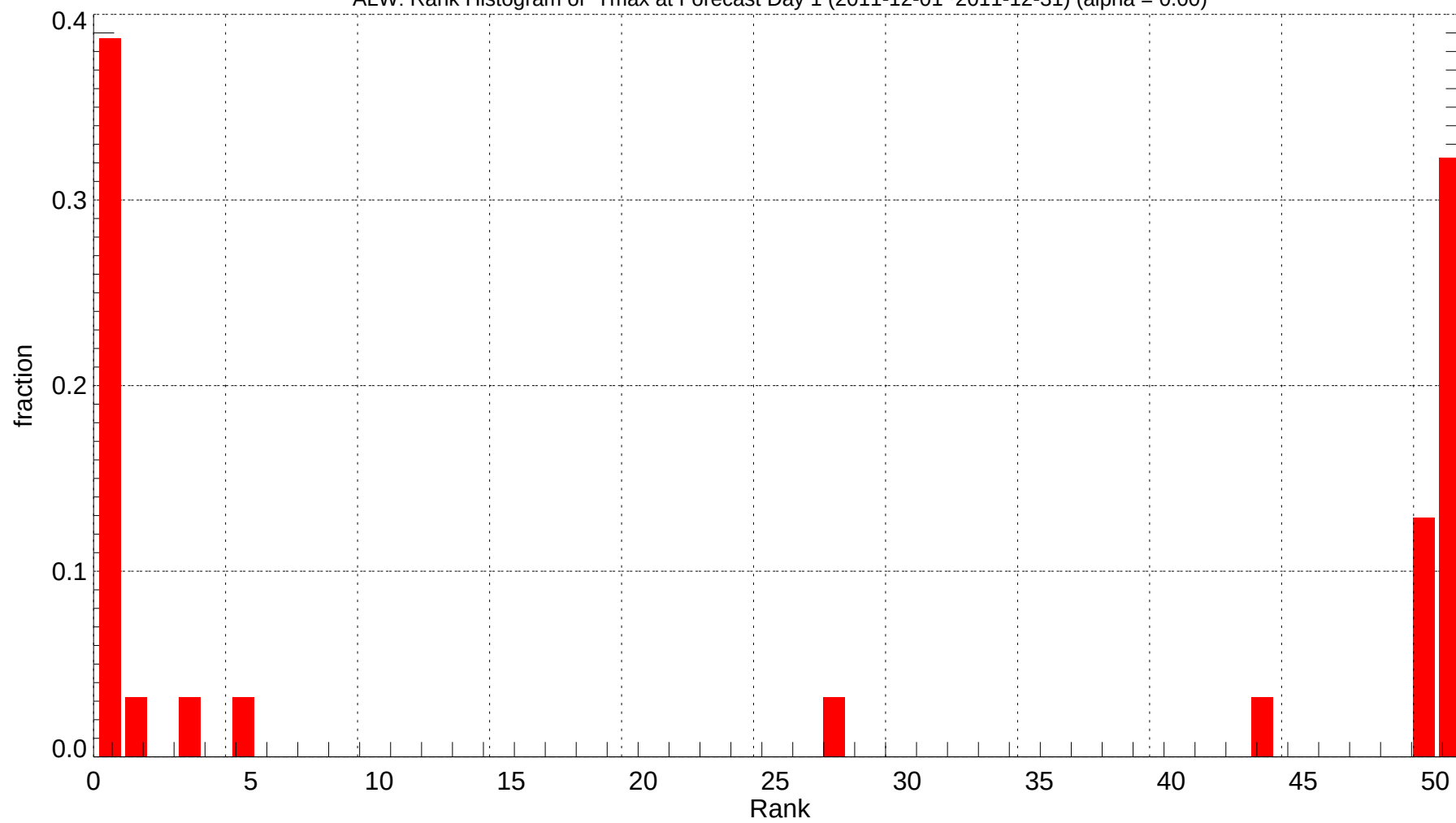
ALW: Rank Histogram of Tmax at Forecast Day 1 (2011-12-01~2011-12-31) (alpha = 0.00)
