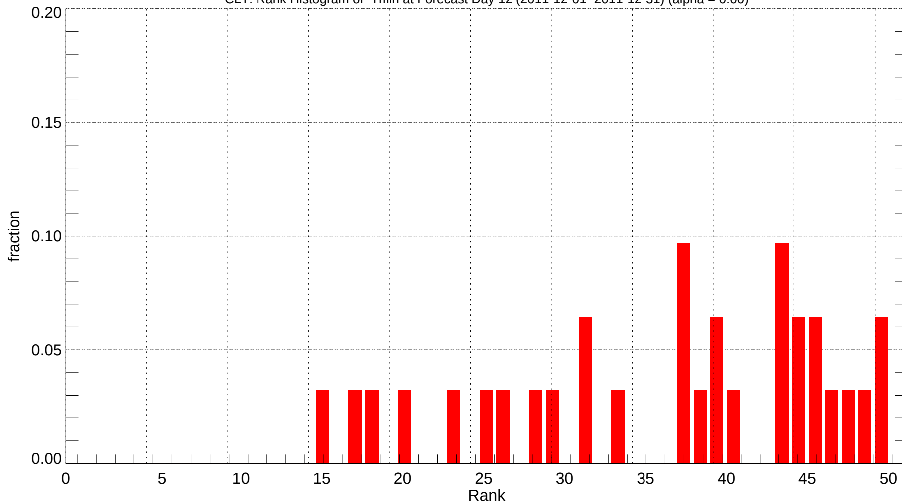
CLT: Rank Histogram of Tmin at Forecast Day 12 (2011-12-01~2011-12-31) (alpha = 0.00)
