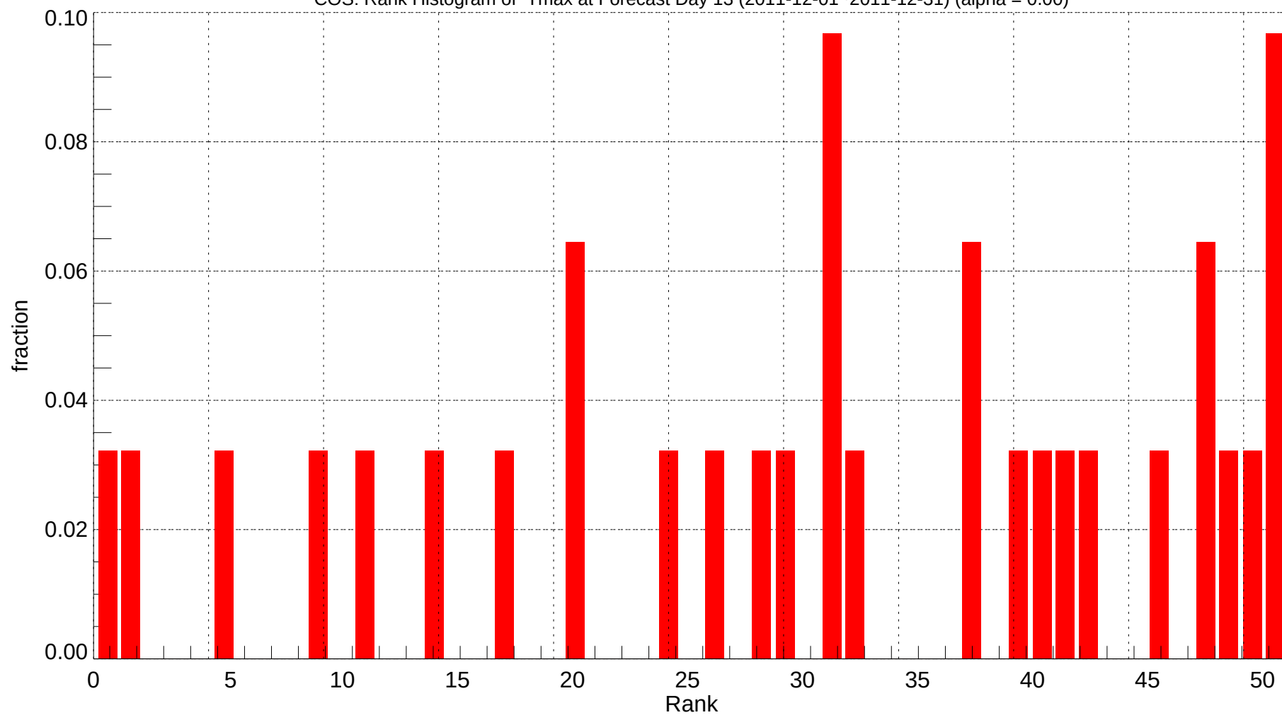
COS: Rank Histogram of Tmax at Forecast Day 13 (2011-12-01~2011-12-31) (alpha = 0.00)
