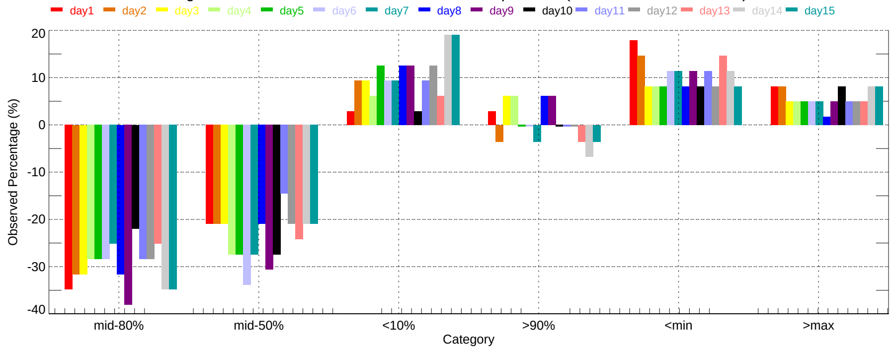
Observed Percentage Deviation of Ensembles - MWL: Max Temperature (2011-12-01~2011-12-31)
