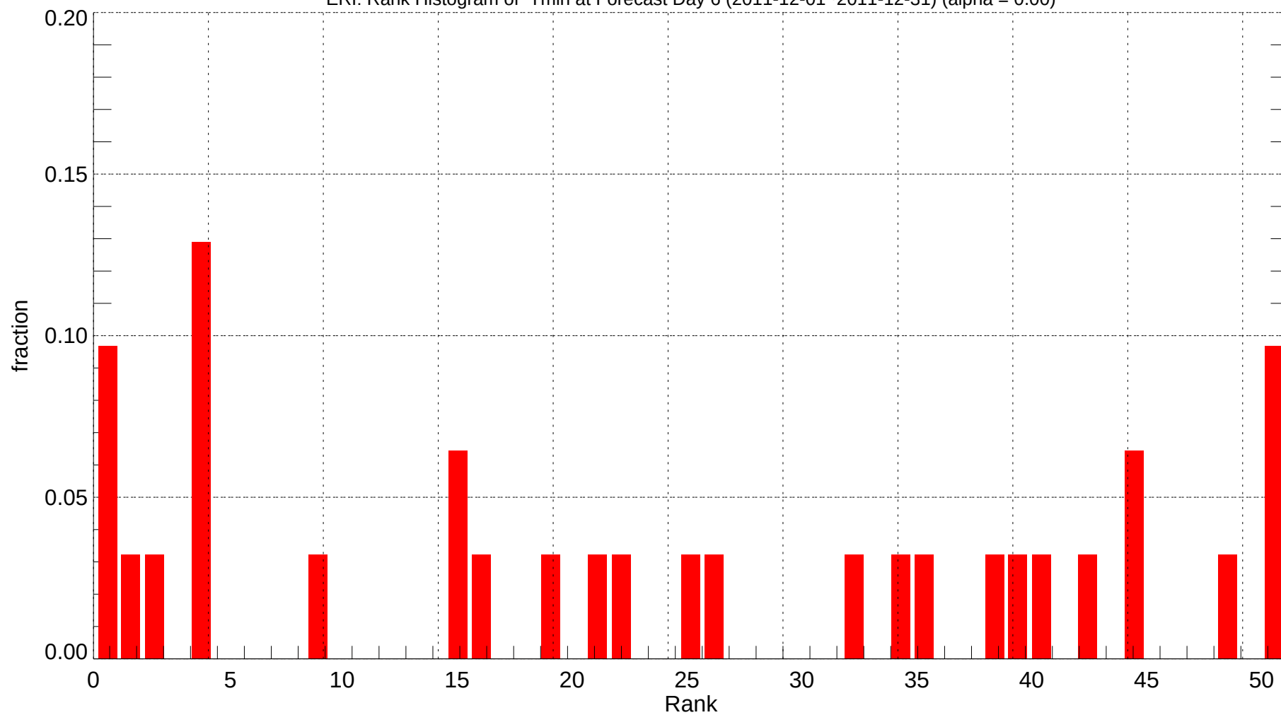
ERI: Rank Histogram of Tmin at Forecast Day 6 (2011-12-01~2011-12-31) (alpha = 0.00)
