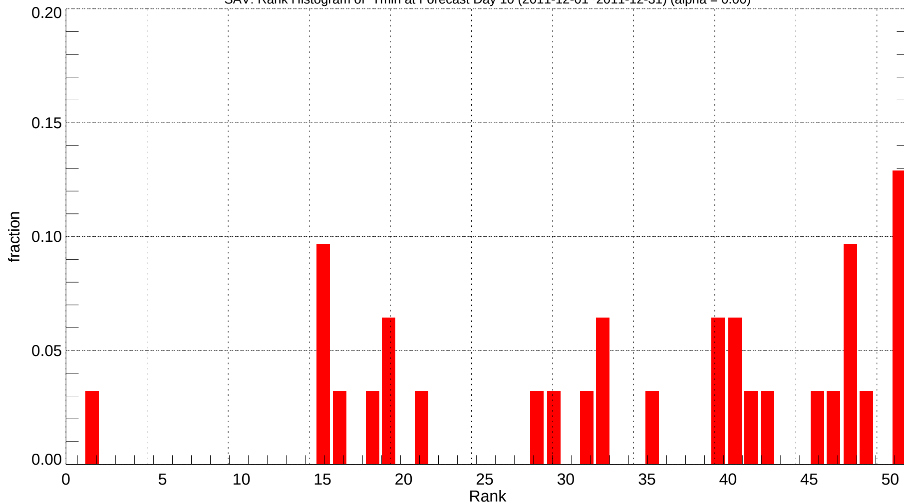
SAV: Rank Histogram of Tmin at Forecast Day 10 (2011-12-01~2011-12-31) (alpha = 0.00)
