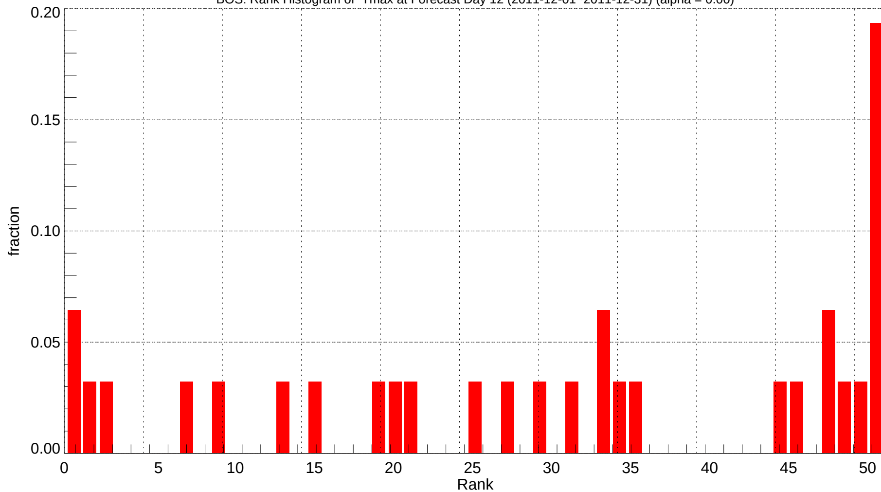
BOS: Rank Histogram of Tmax at Forecast Day 12 (2011-12-01~2011-12-31) (alpha = 0.00)
