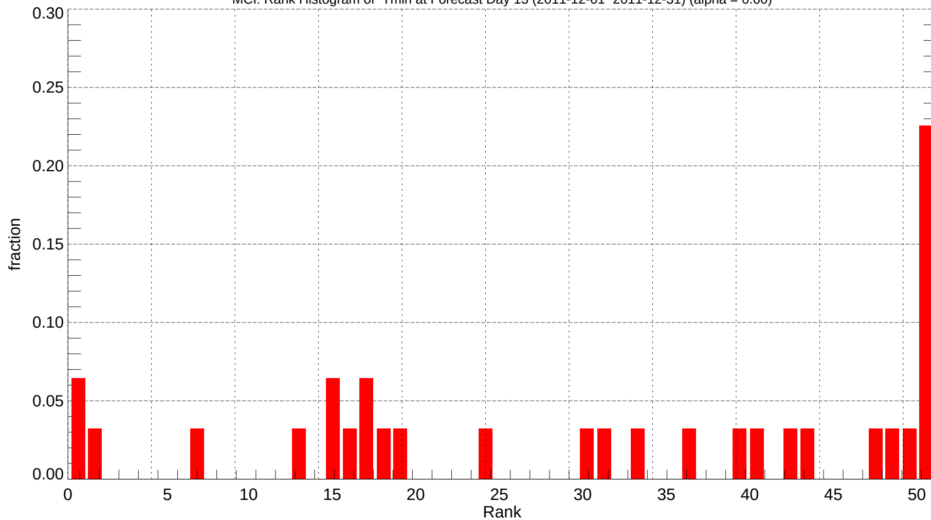
MCI: Rank Histogram of Tmin at Forecast Day 13 (2011-12-01~2011-12-31) (alpha = 0.00)
