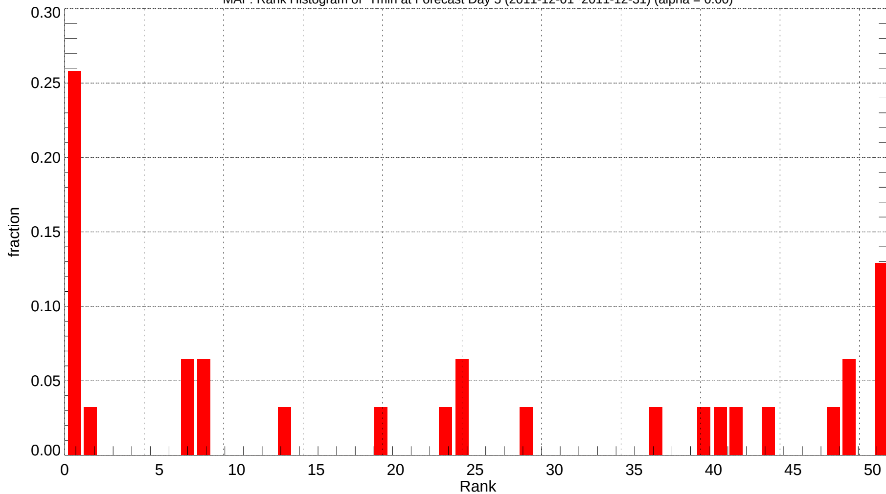
MAF: Rank Histogram of Tmin at Forecast Day 5 (2011-12-01~2011-12-31) (alpha = 0.00)
