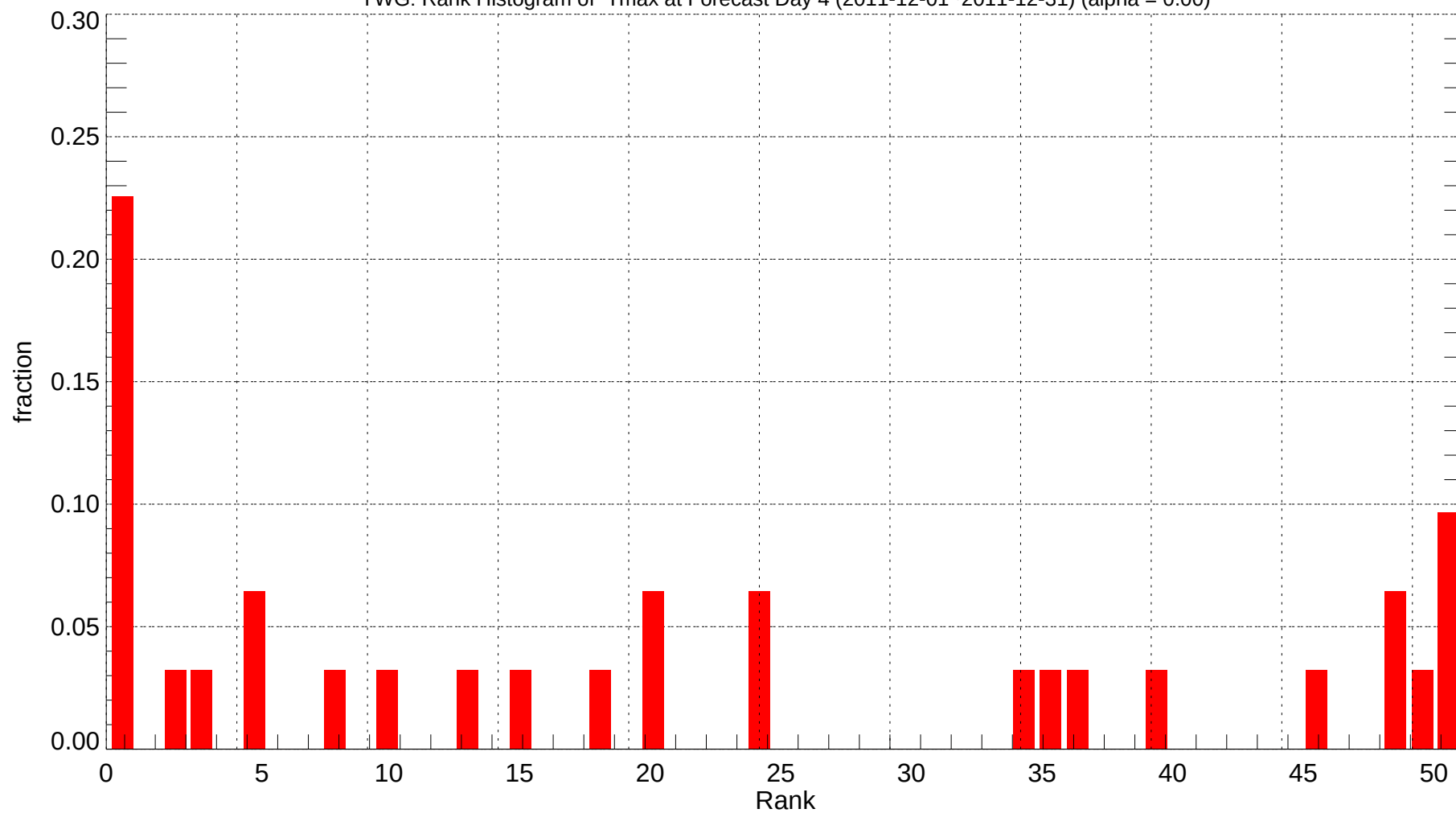
YWG: Rank Histogram of Tmax at Forecast Day 4 (2011-12-01~2011-12-31) (alpha = 0.00)
