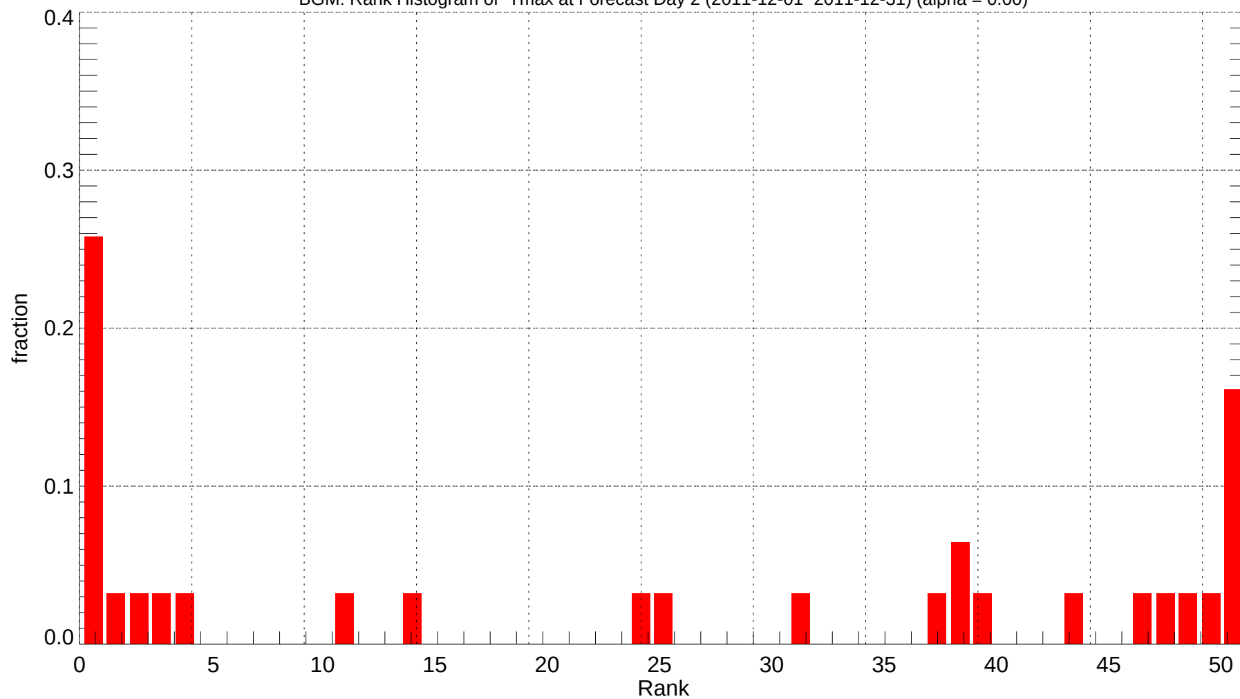
BGM: Rank Histogram of Tmax at Forecast Day 2 (2011-12-01~2011-12-31) (alpha = 0.00)
