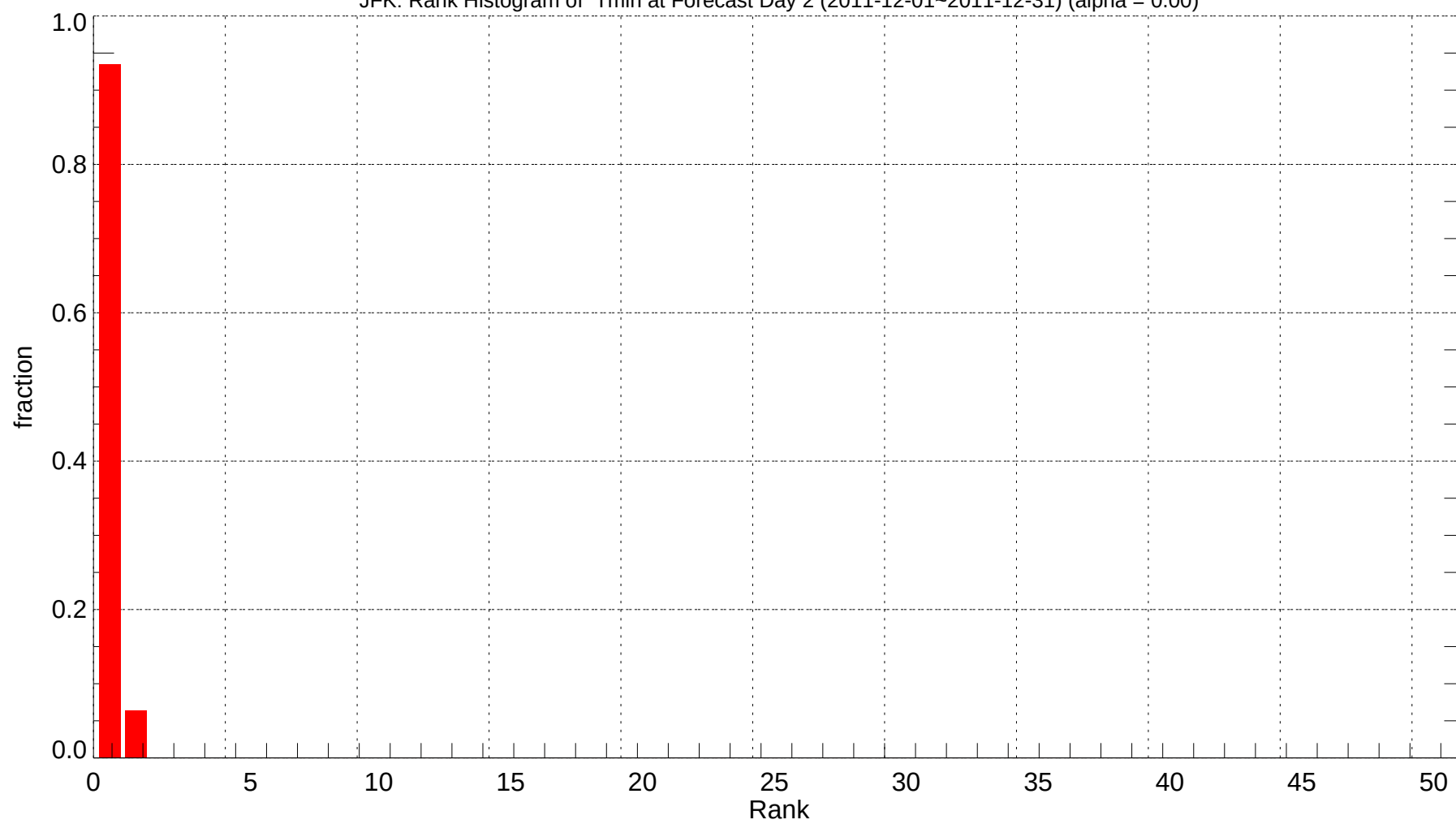
JFK: Rank Histogram of Tmin at Forecast Day 2 (2011-12-01~2011-12-31) (alpha = 0.00)
