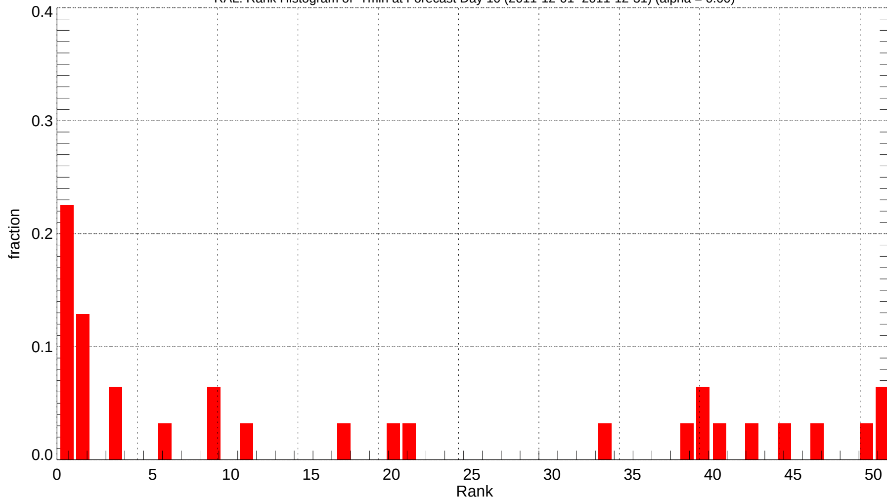
RAL: Rank Histogram of Tmin at Forecast Day 10 (2011-12-01~2011-12-31) (alpha = 0.00)
