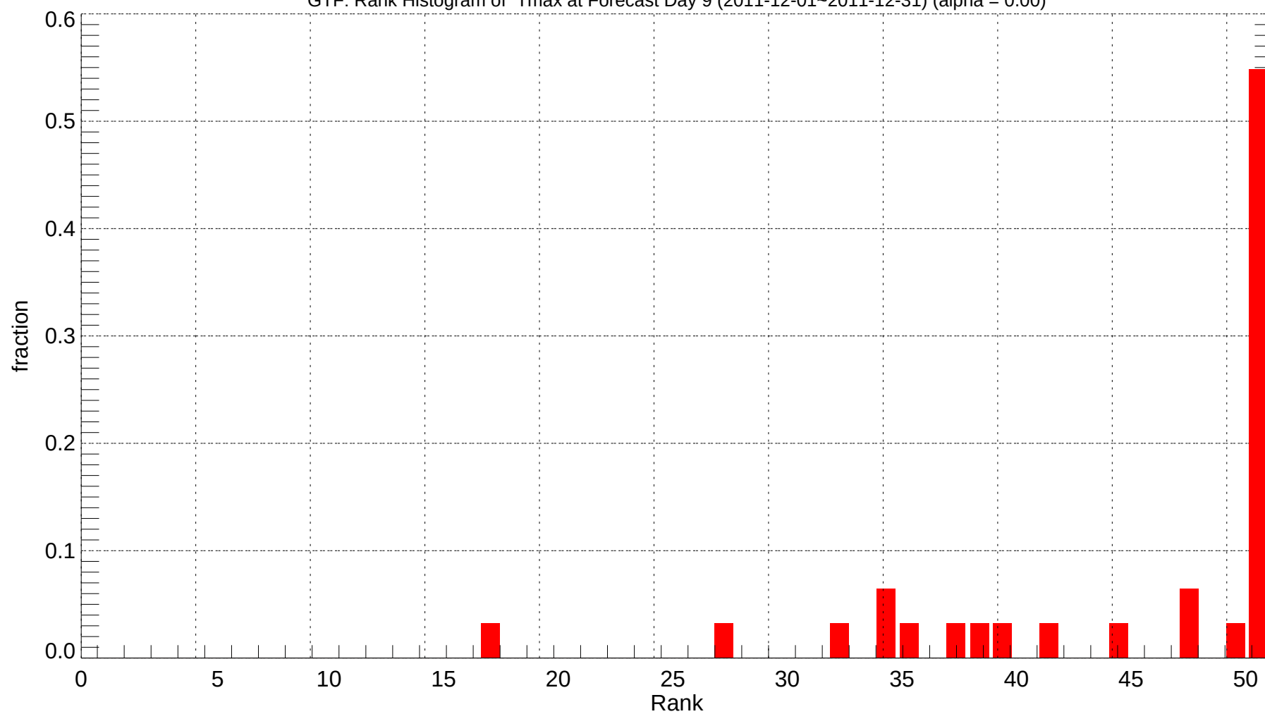
GTF: Rank Histogram of Tmax at Forecast Day 9 (2011-12-01~2011-12-31) (alpha = 0.00)
