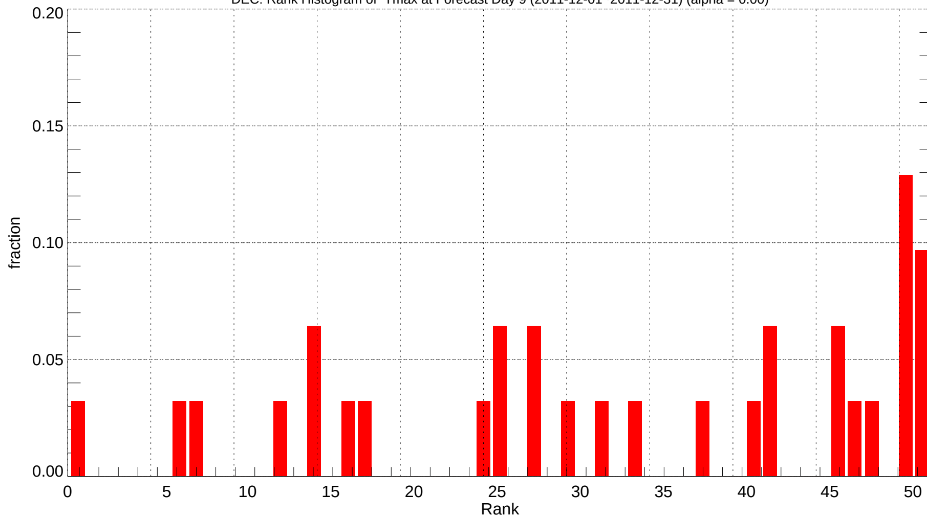
DEC: Rank Histogram of Tmax at Forecast Day 9 (2011-12-01~2011-12-31) (alpha = 0.00)
