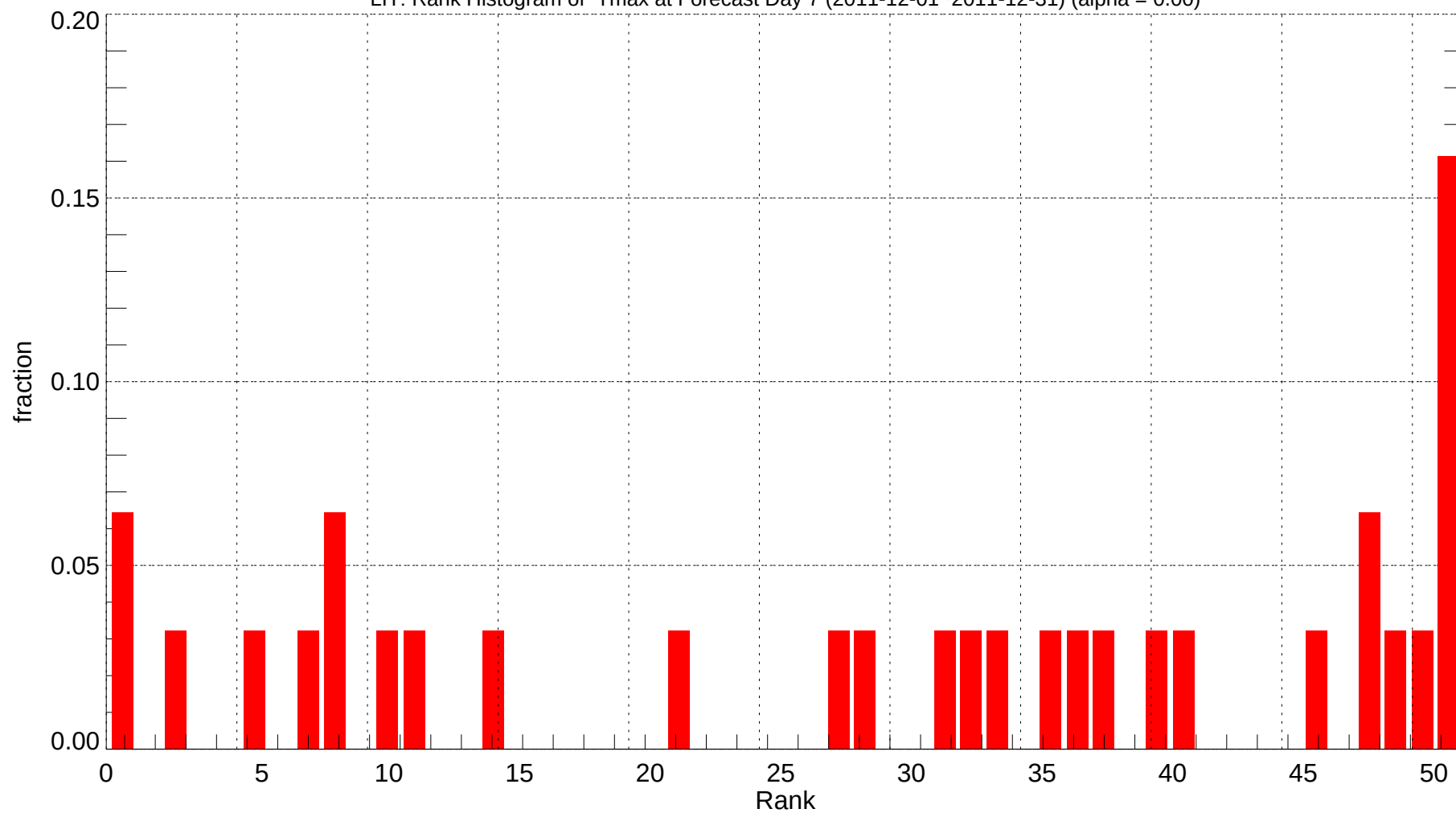
LIT: Rank Histogram of Tmax at Forecast Day 7 (2011-12-01~2011-12-31) (alpha = 0.00)
