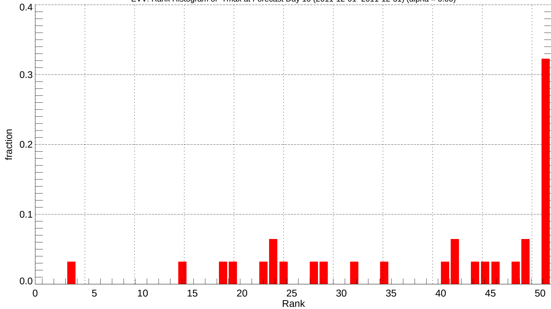
EVV: Rank Histogram of Tmax at Forecast Day 10 (2011-12-01~2011-12-31) (alpha = 0.00)
