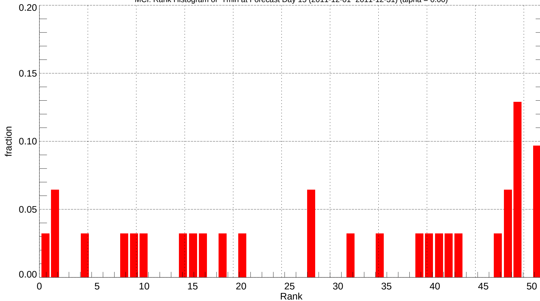
MCI: Rank Histogram of Tmin at Forecast Day 15 (2011-12-01~2011-12-31) (alpha = 0.00)
