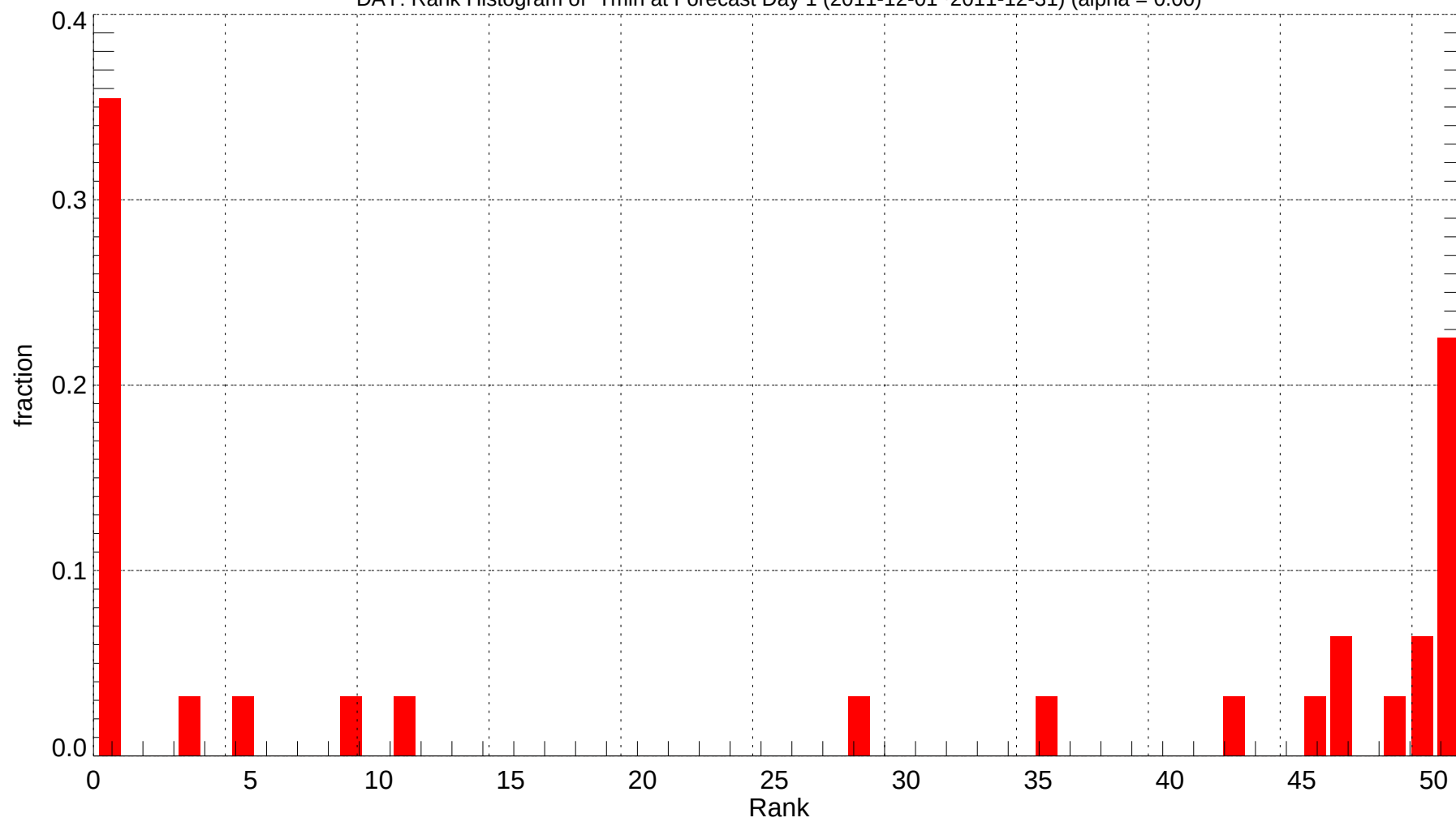
DAY: Rank Histogram of Tmin at Forecast Day 1 (2011-12-01~2011-12-31) (alpha = 0.00)
