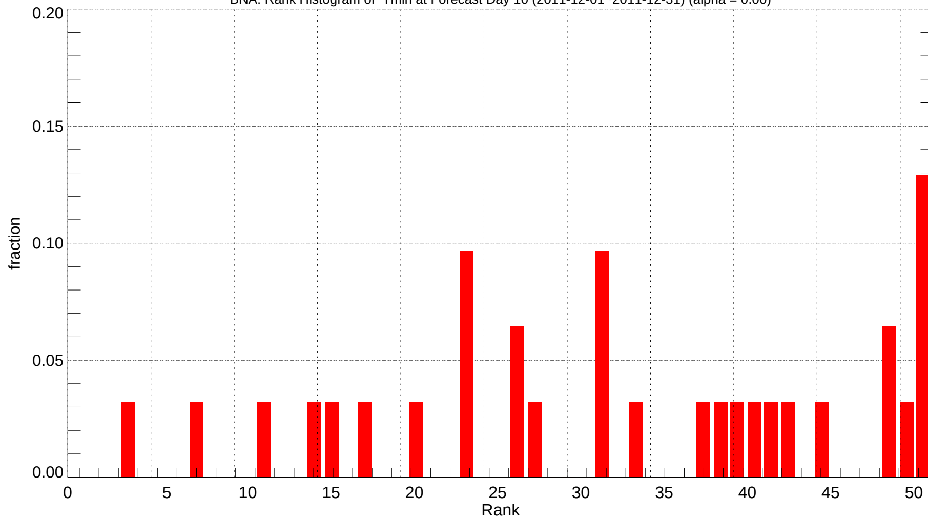
BNA: Rank Histogram of Tmin at Forecast Day 10 (2011-12-01~2011-12-31) (alpha = 0.00)
