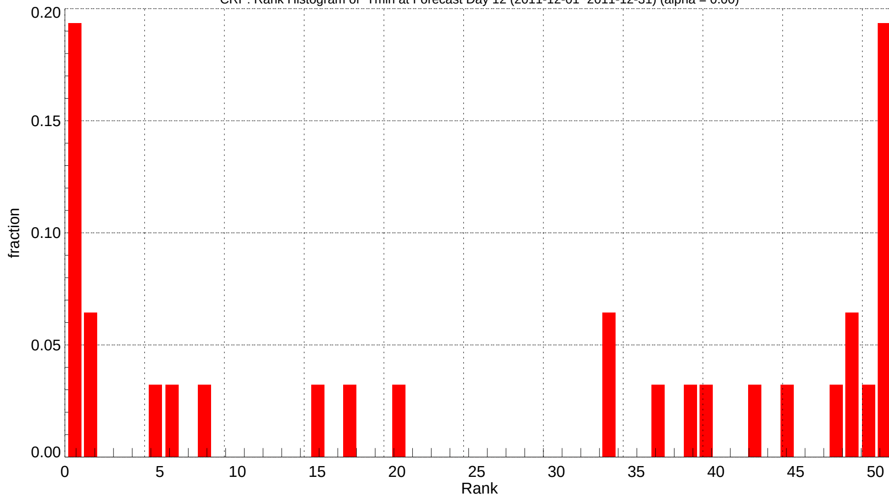
CRP: Rank Histogram of Tmin at Forecast Day 12 (2011-12-01~2011-12-31) (alpha = 0.00)
