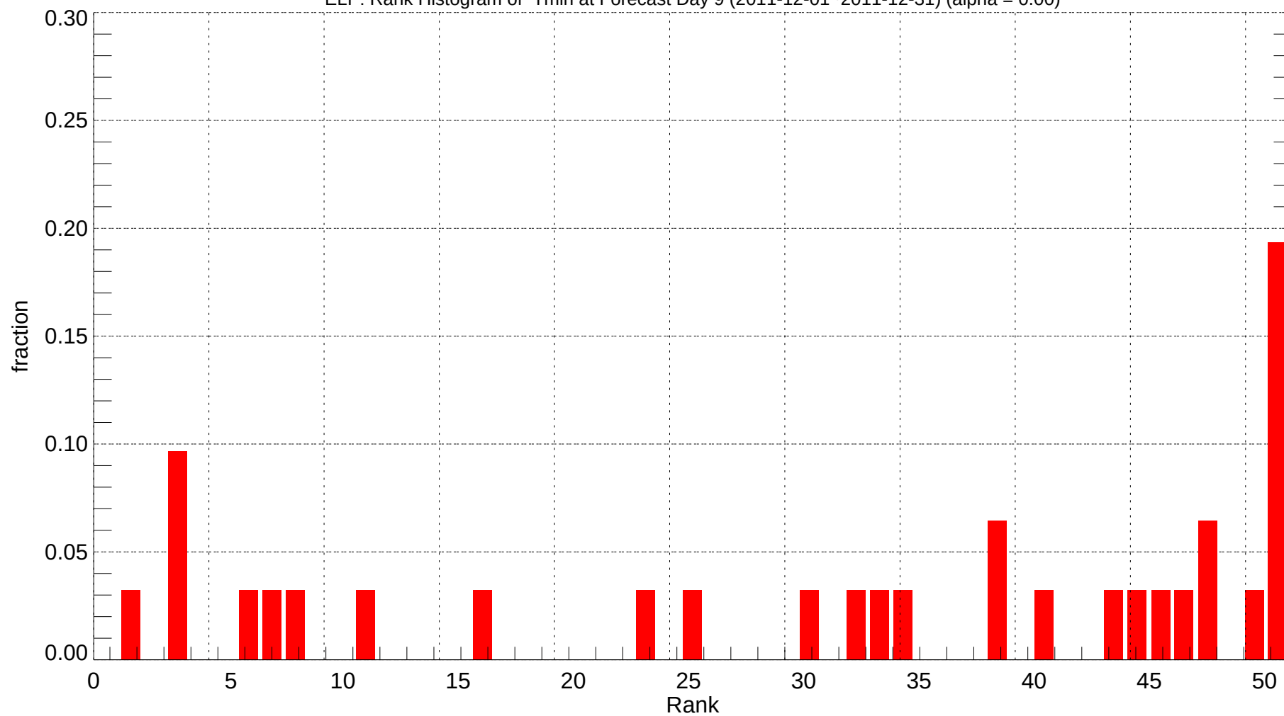
ELP: Rank Histogram of Tmin at Forecast Day 9 (2011-12-01~2011-12-31) (alpha = 0.00)
