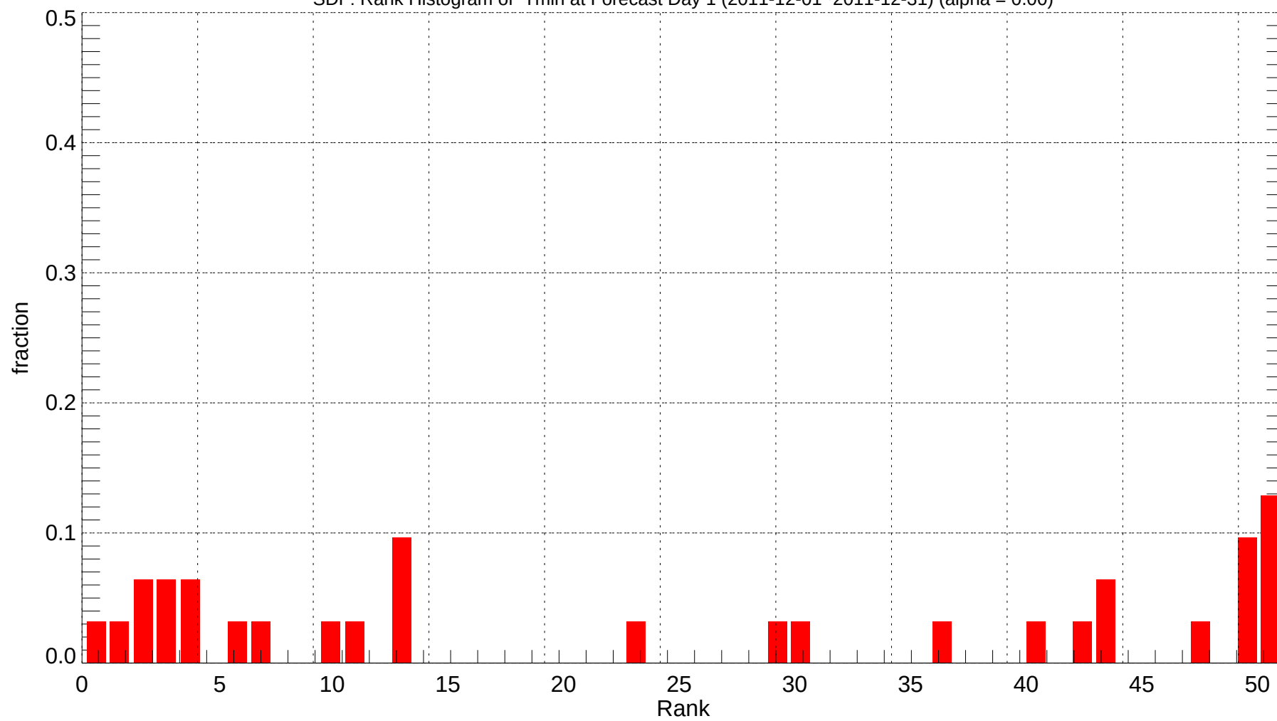
SDF: Rank Histogram of Tmin at Forecast Day 1 (2011-12-01~2011-12-31) (alpha = 0.00)
