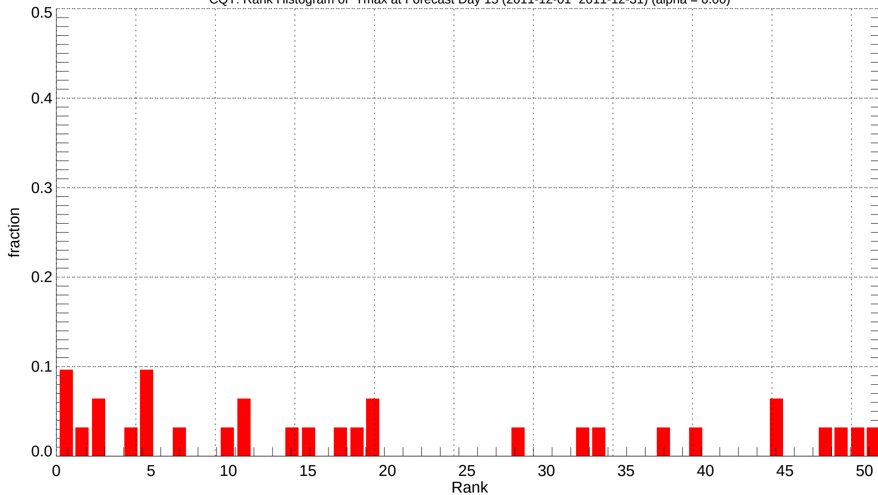
CQT: Rank Histogram of Tmax at Forecast Day 15 (2011-12-01~2011-12-31) (alpha = 0.00)
