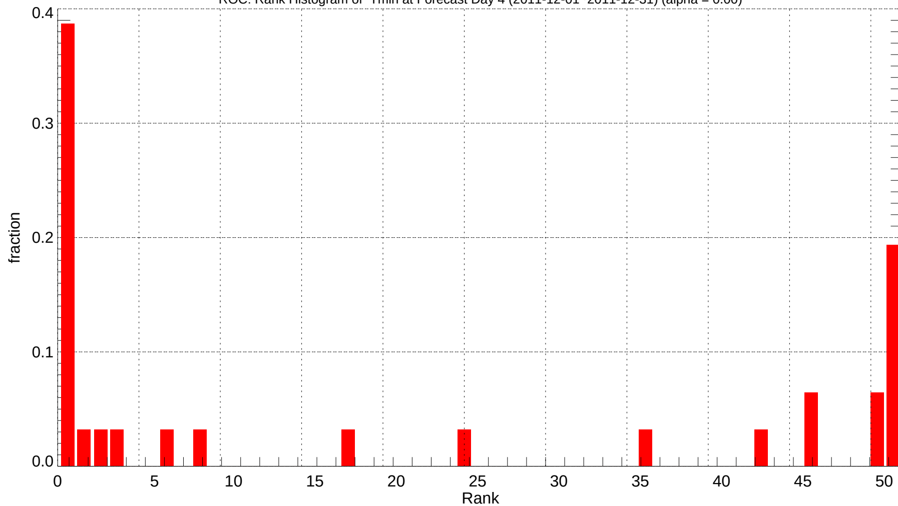
ROC: Rank Histogram of Tmin at Forecast Day 4 (2011-12-01~2011-12-31) (alpha = 0.00)
