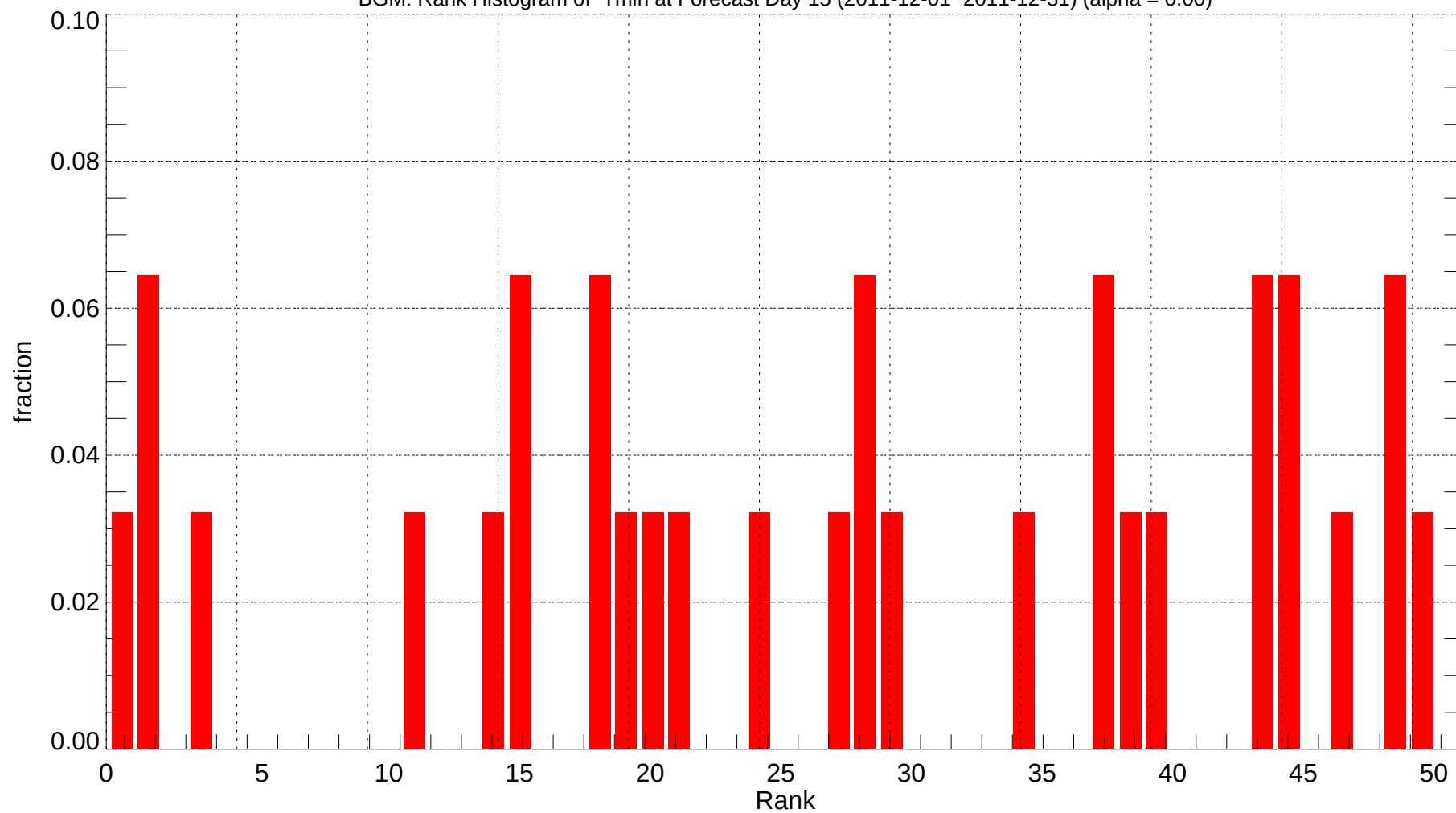
BGM: Rank Histogram of Tmin at Forecast Day 15 (2011-12-01~2011-12-31) (alpha = 0.00)
