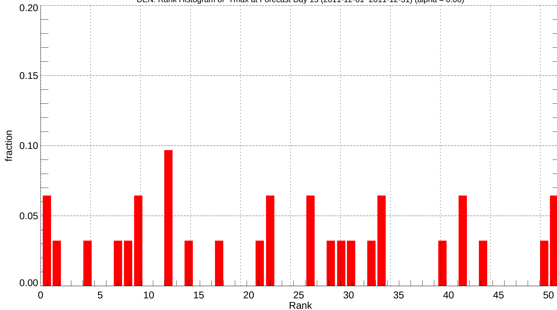
DEN: Rank Histogram of Tmax at Forecast Day 15 (2011-12-01~2011-12-31) (alpha = 0.00)
