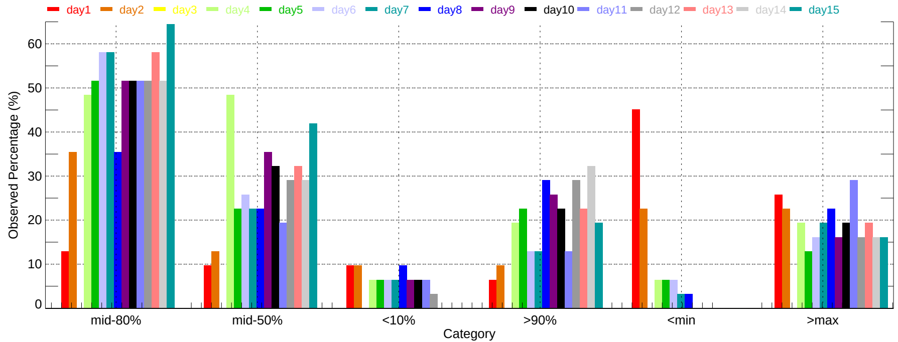
Observed Percentage of Ensembles - YYC: Min Temperature (2011-12-01~2011-12-31)
