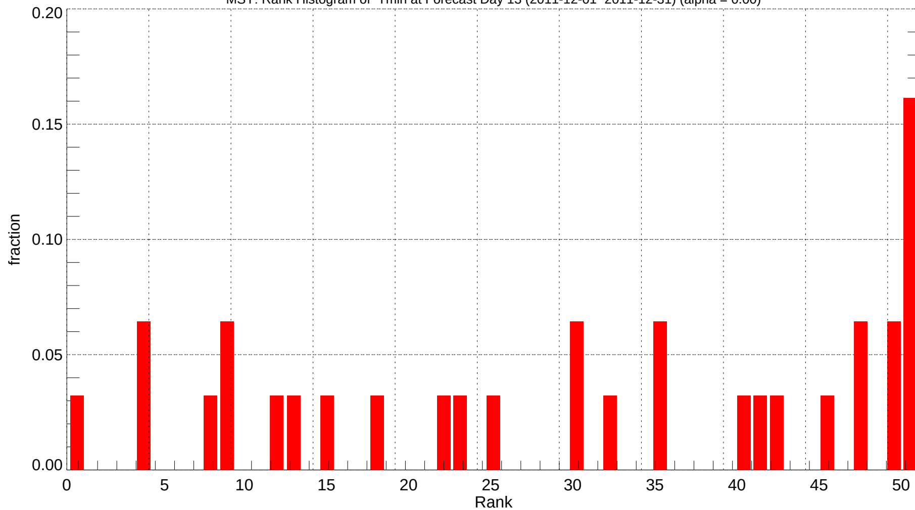
MSY: Rank Histogram of Tmin at Forecast Day 13 (2011-12-01~2011-12-31) (alpha = 0.00)
