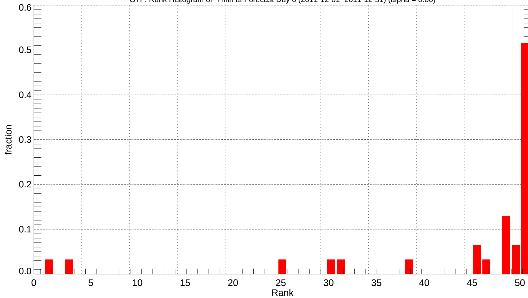
GTF: Rank Histogram of Tmin at Forecast Day 6 (2011-12-01~2011-12-31) (alpha = 0.00)
