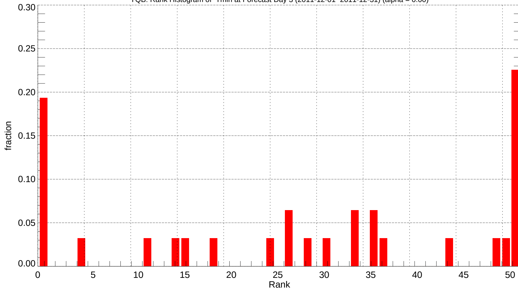
YQB: Rank Histogram of Tmin at Forecast Day 3 (2011-12-01~2011-12-31) (alpha = 0.00)
