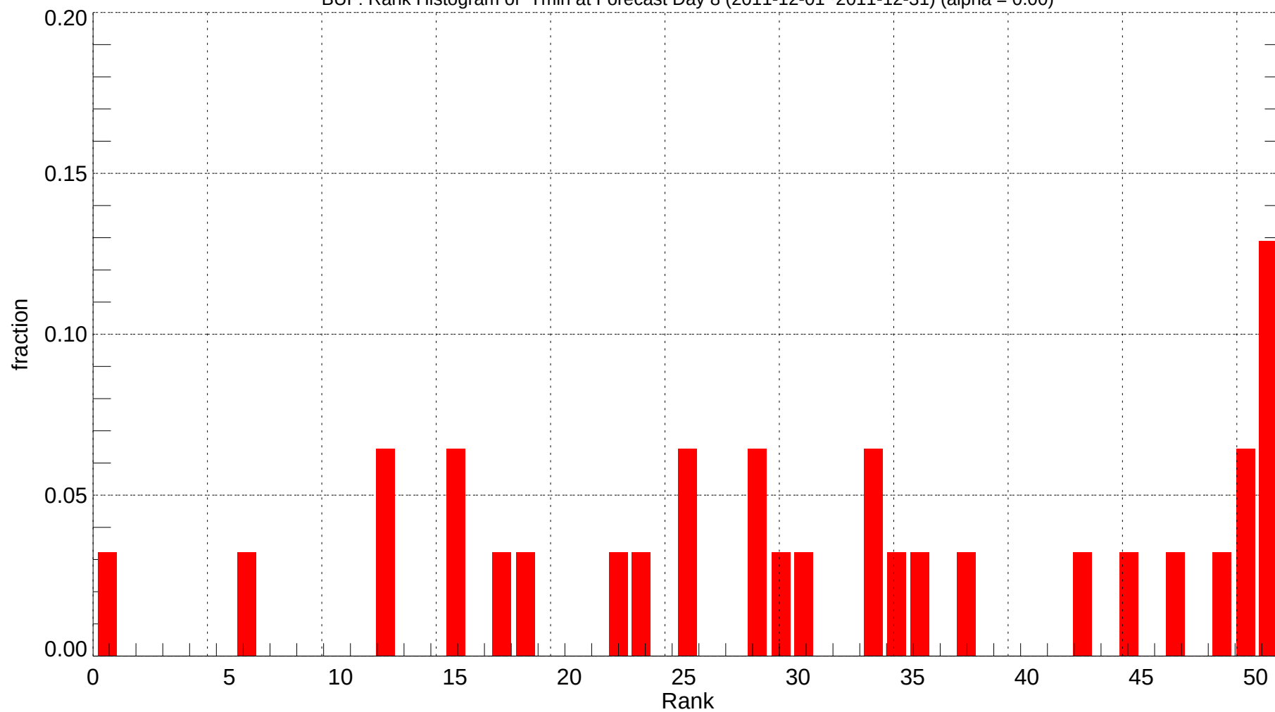
BUF: Rank Histogram of Tmin at Forecast Day 8 (2011-12-01~2011-12-31) (alpha = 0.00)
