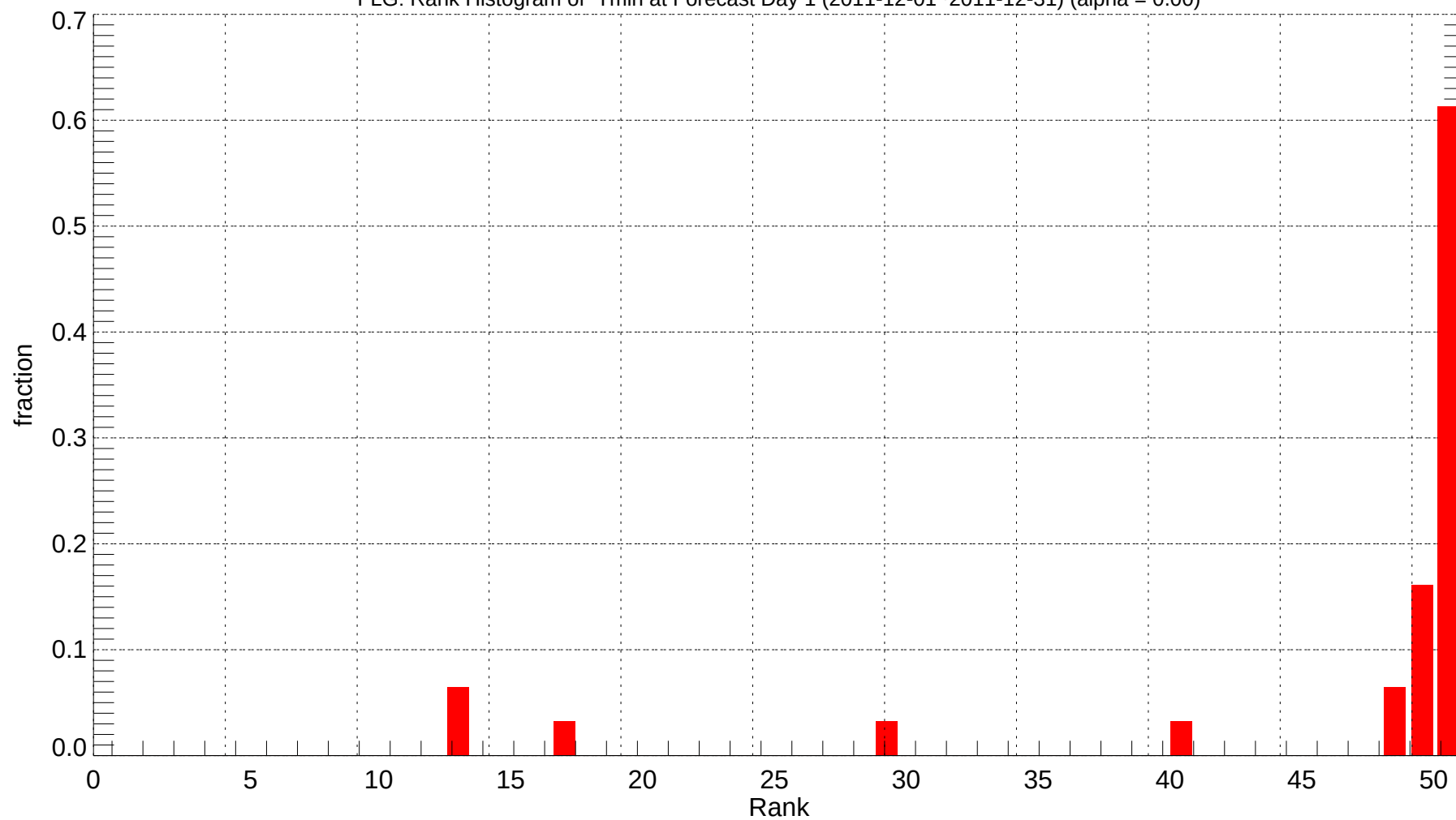
FLG: Rank Histogram of Tmin at Forecast Day 1 (2011-12-01~2011-12-31) (alpha = 0.00)
