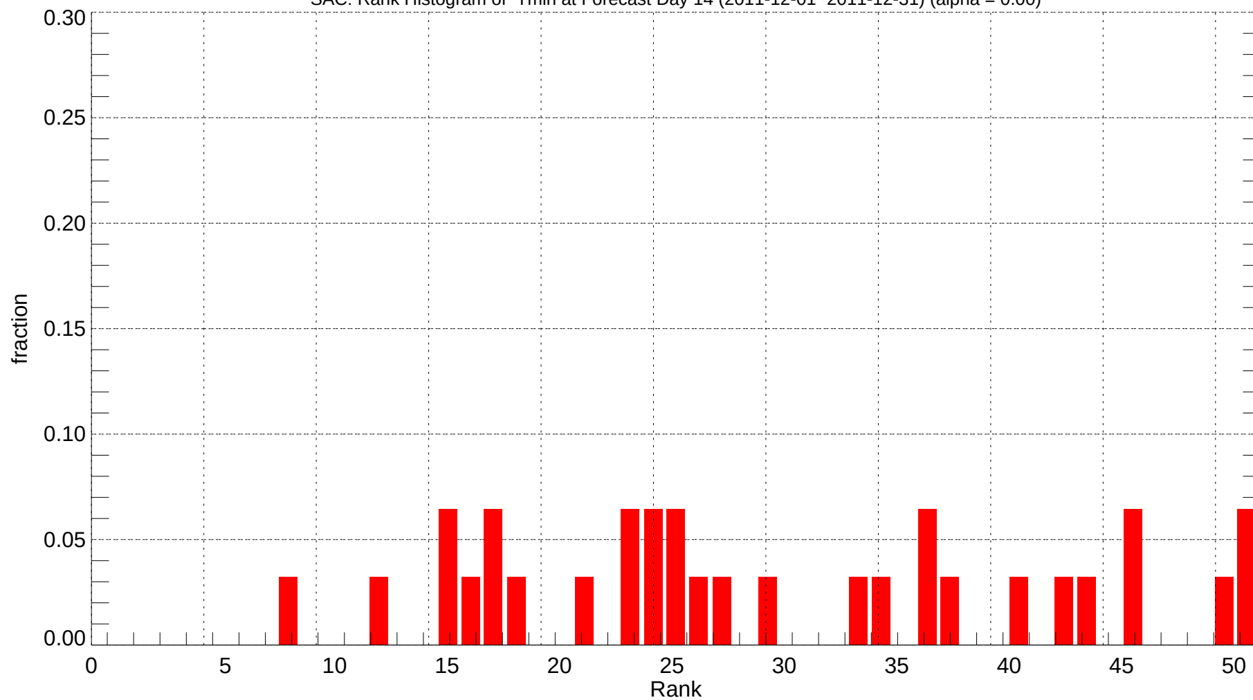
SAC: Rank Histogram of Tmin at Forecast Day 14 (2011-12-01~2011-12-31) (alpha = 0.00)
