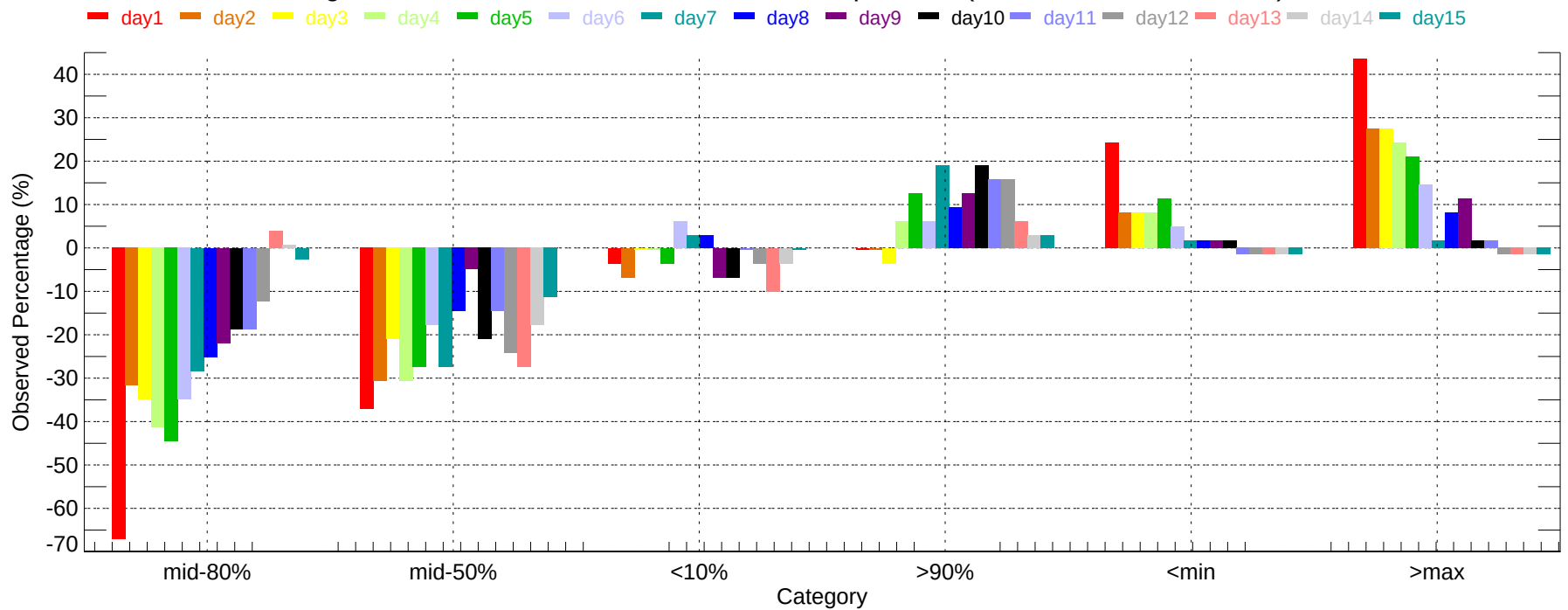
Observed Percentage Deviation of Ensembles - ERI: Min Temperature (2011-12-01~2011-12-31)
