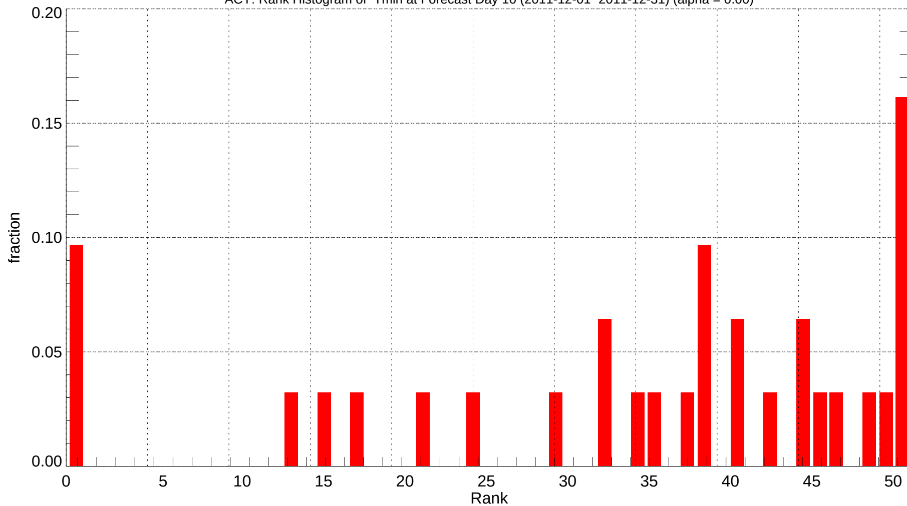
ACY: Rank Histogram of Tmin at Forecast Day 10 (2011-12-01~2011-12-31) (alpha = 0.00)
