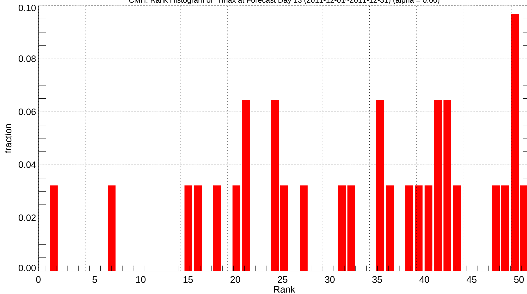
CMH: Rank Histogram of Tmax at Forecast Day 13 (2011-12-01~2011-12-31) (alpha = 0.00)
