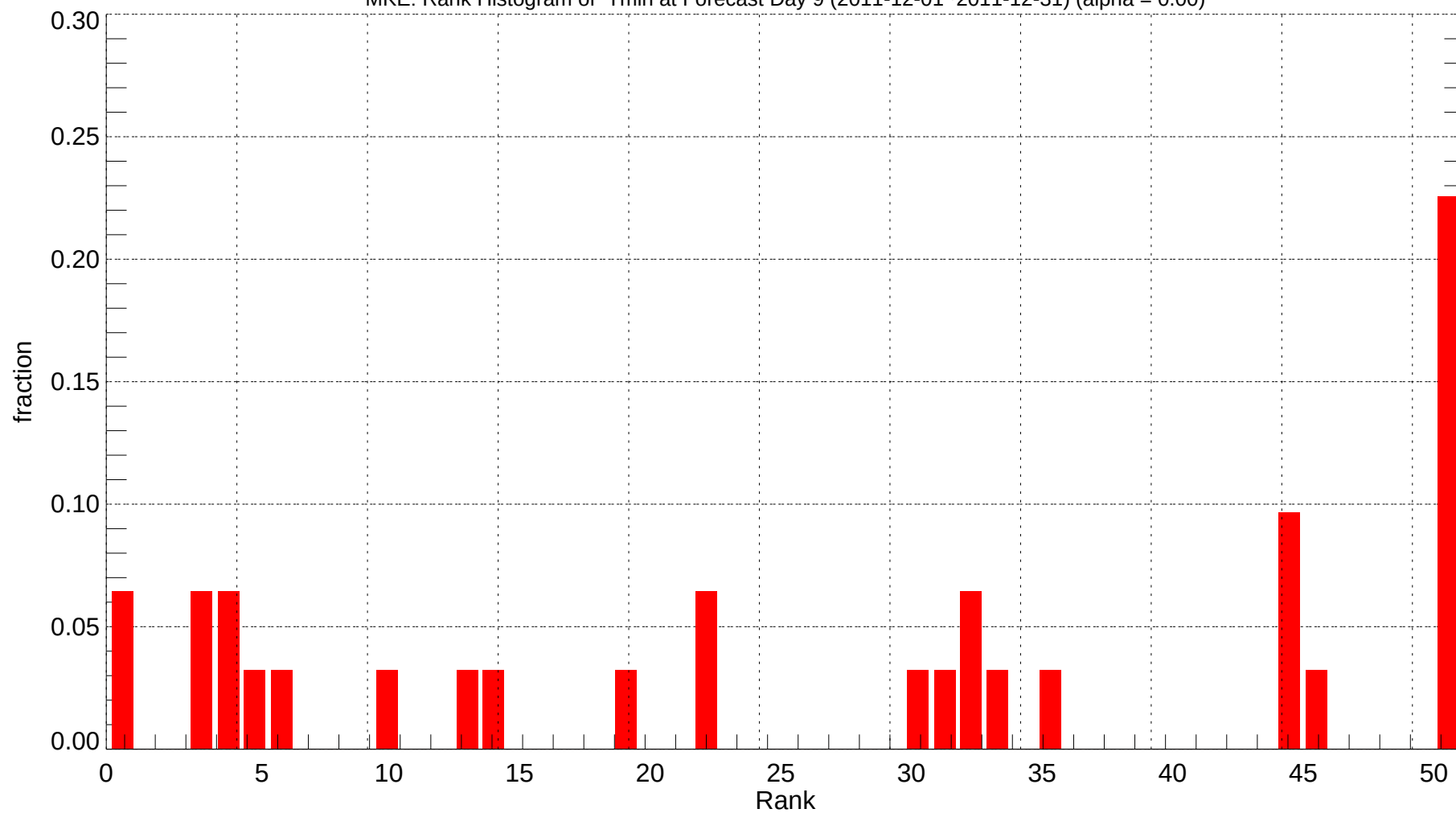
MKE: Rank Histogram of Tmin at Forecast Day 9 (2011-12-01~2011-12-31) (alpha = 0.00)
