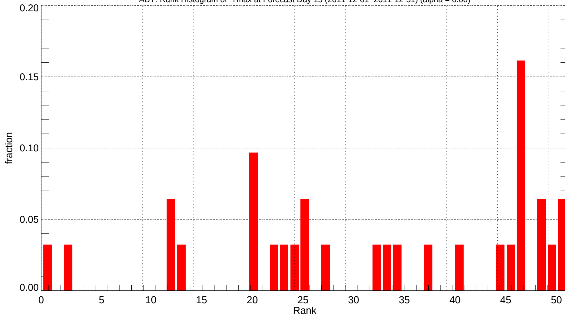
ABY: Rank Histogram of Tmax at Forecast Day 15 (2011-12-01~2011-12-31) (alpha = 0.00)
