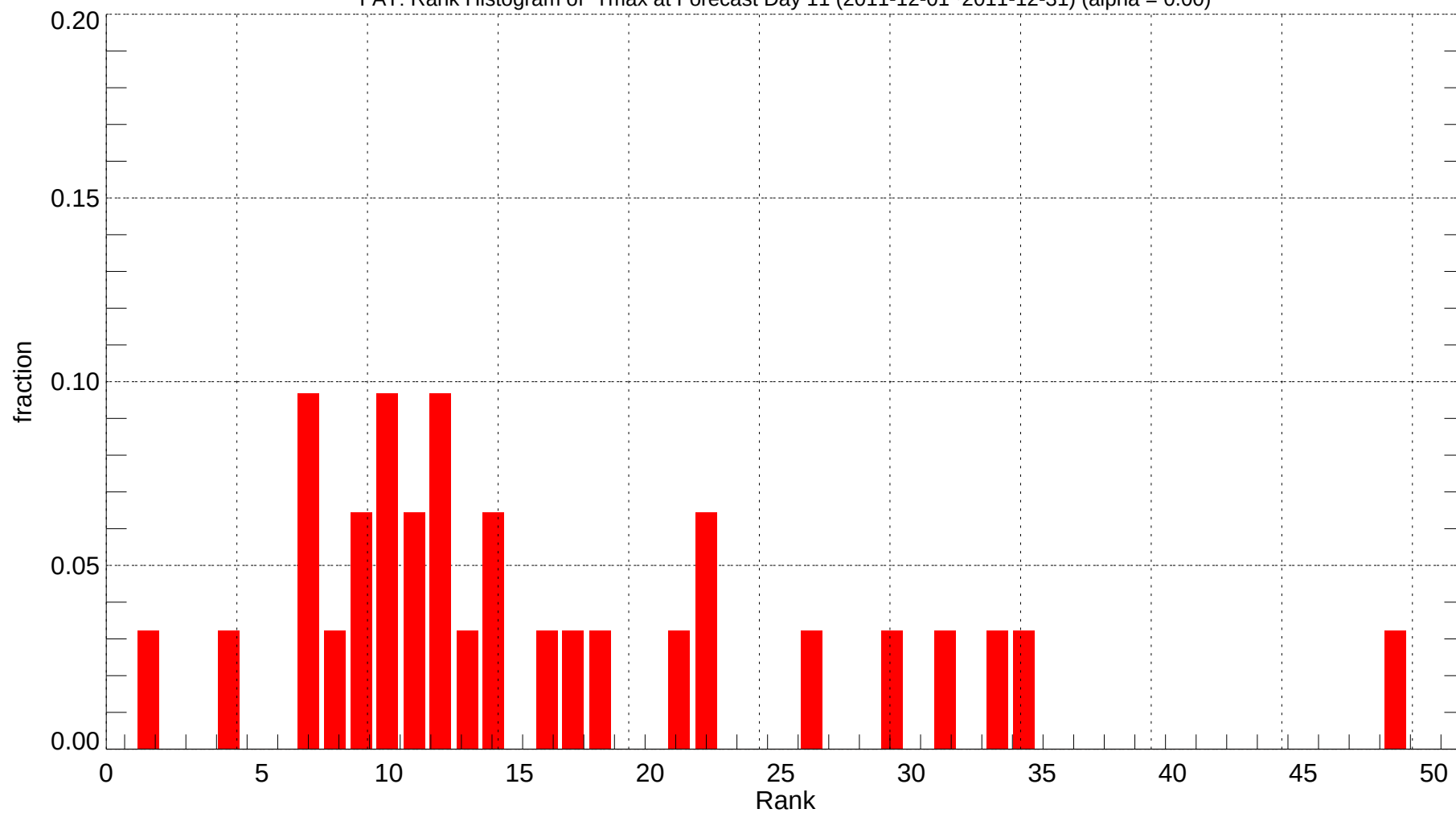
FAT: Rank Histogram of Tmax at Forecast Day 11 (2011-12-01~2011-12-31) (alpha = 0.00)
