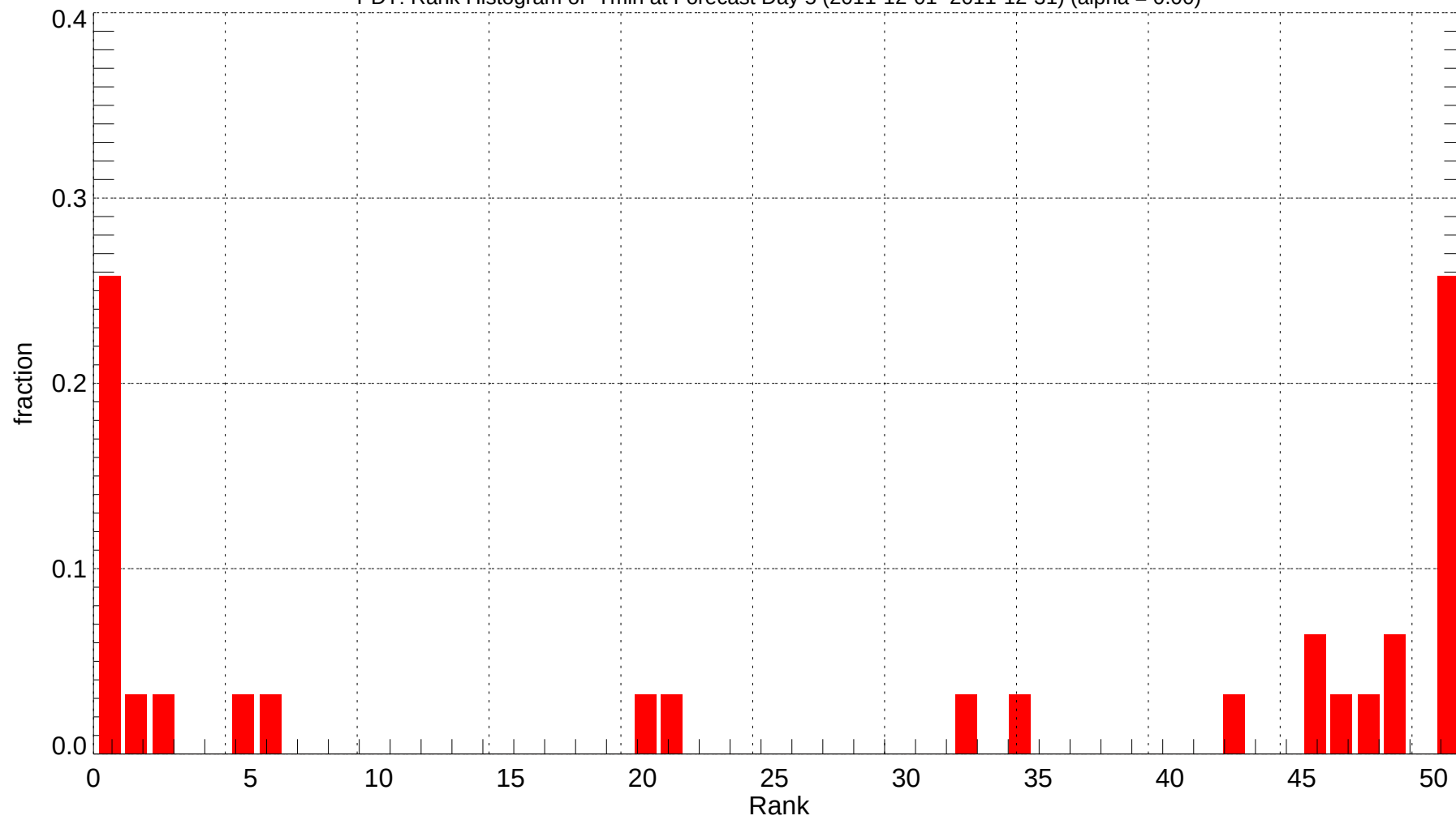
PDT: Rank Histogram of Tmin at Forecast Day 5 (2011-12-01~2011-12-31) (alpha = 0.00)
