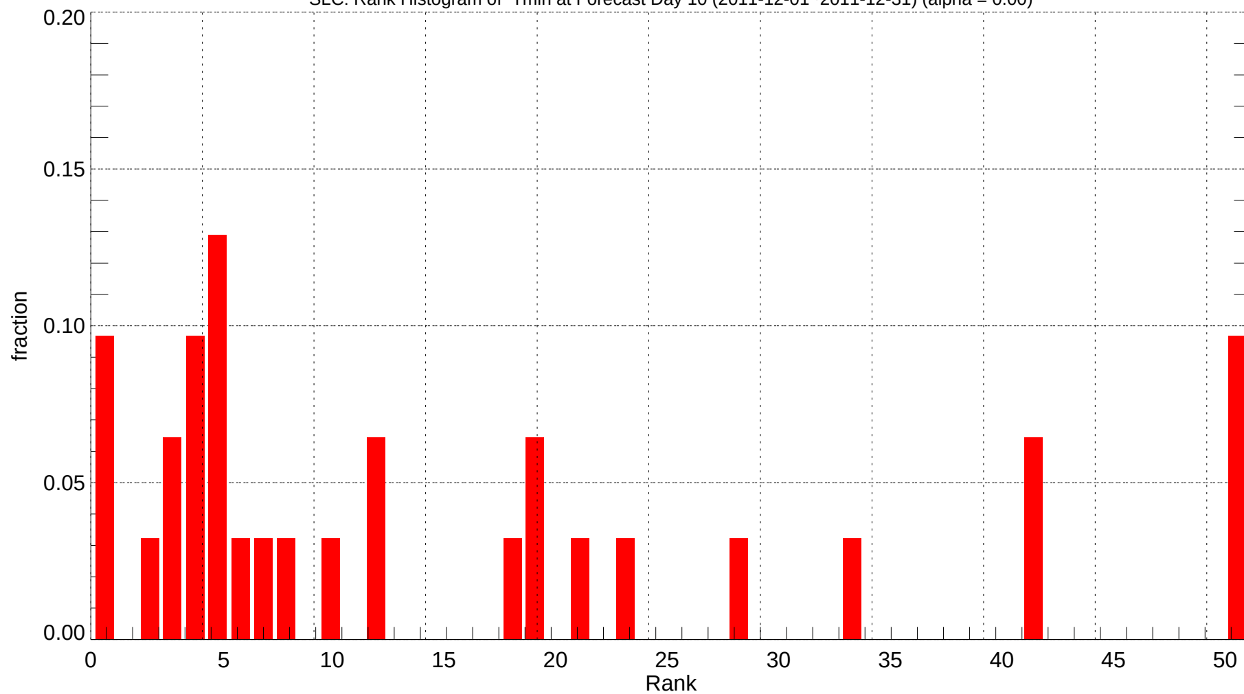
SLC: Rank Histogram of Tmin at Forecast Day 10 (2011-12-01~2011-12-31) (alpha = 0.00)
