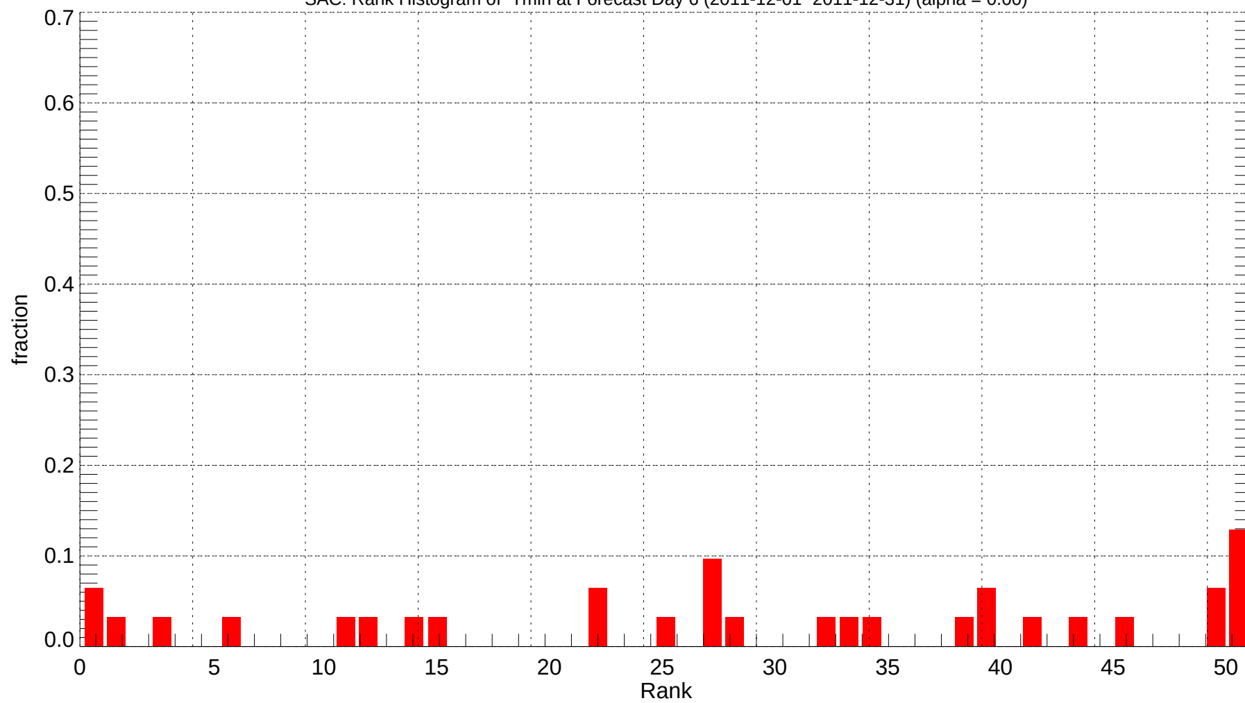
SAC: Rank Histogram of Tmin at Forecast Day 6 (2011-12-01~2011-12-31) (alpha = 0.00)
