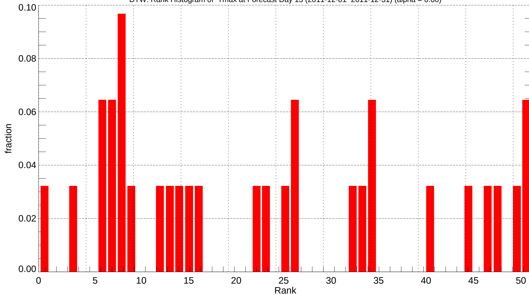
DTW: Rank Histogram of Tmax at Forecast Day 13 (2011-12-01~2011-12-31) (alpha = 0.00)
