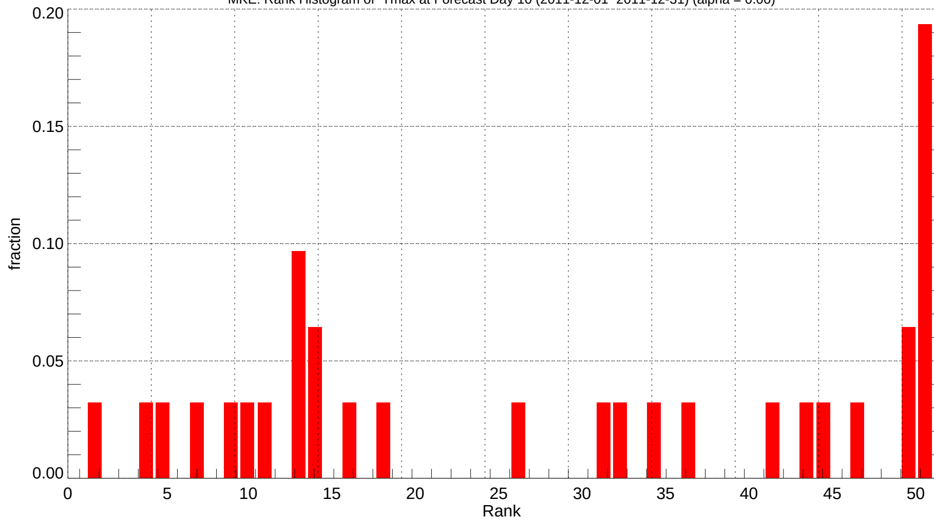
MKE: Rank Histogram of Tmax at Forecast Day 10 (2011-12-01~2011-12-31) (alpha = 0.00)
