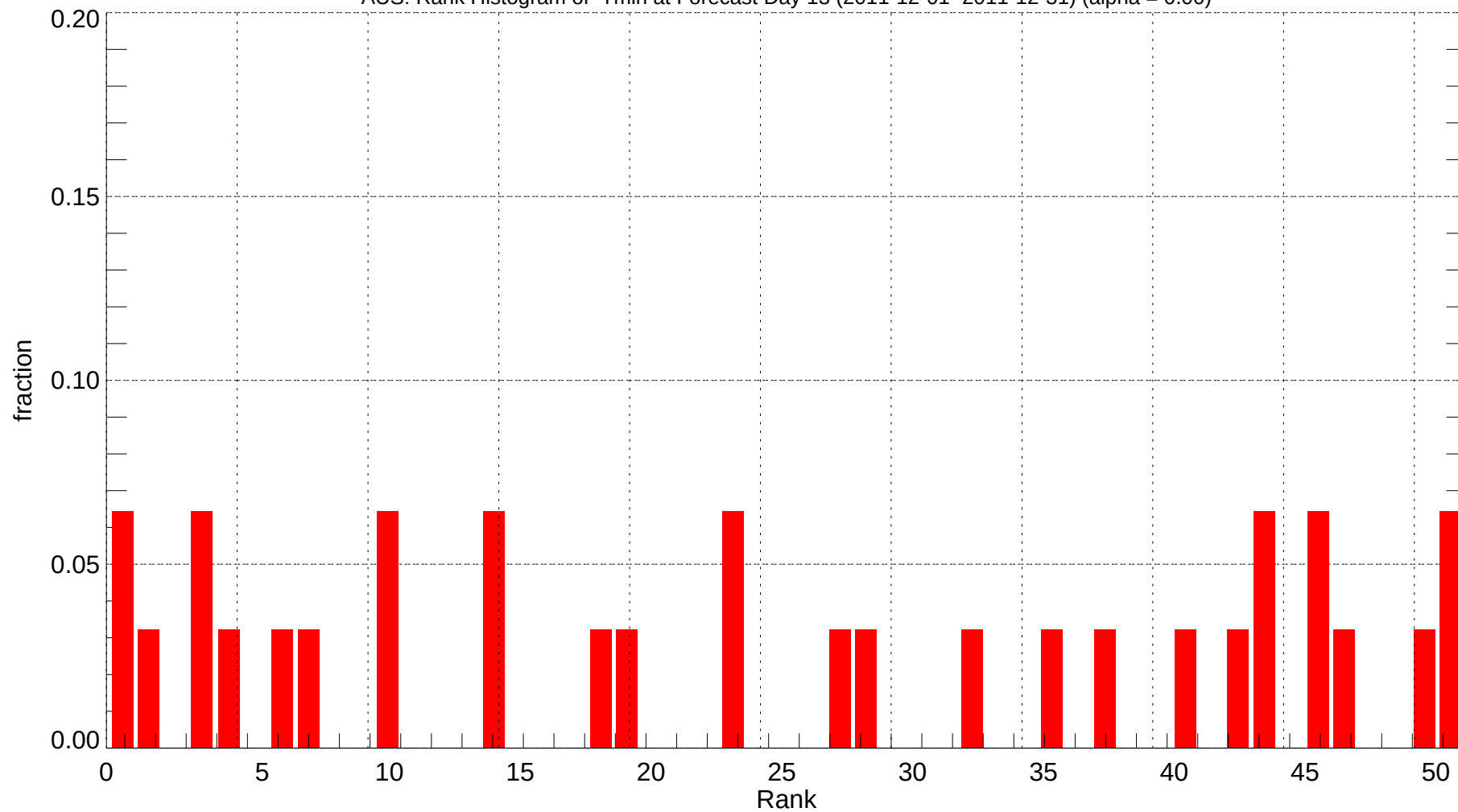
AUS: Rank Histogram of Tmin at Forecast Day 13 (2011-12-01~2011-12-31) (alpha = 0.00)
