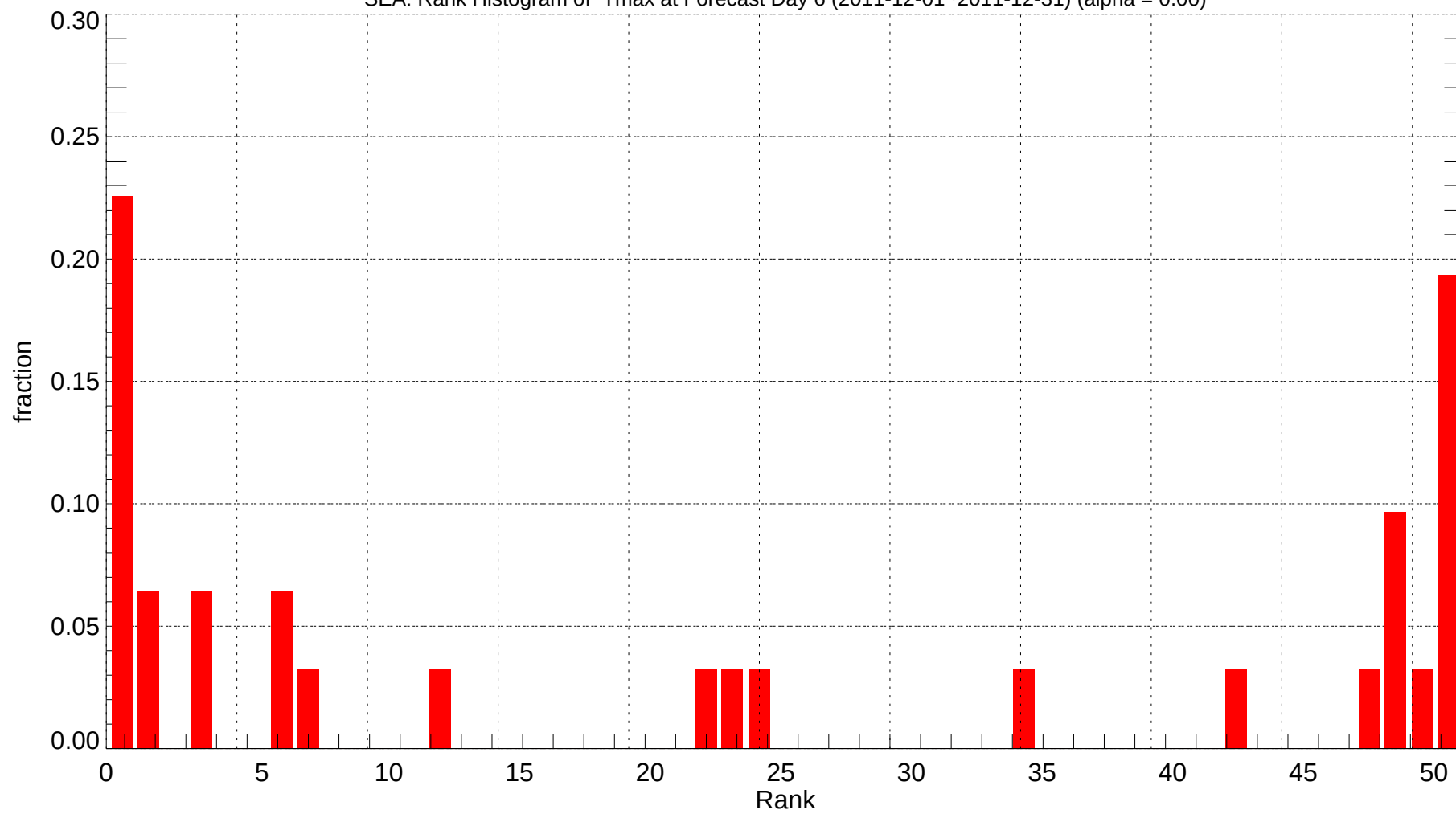
SEA: Rank Histogram of Tmax at Forecast Day 6 (2011-12-01~2011-12-31) (alpha = 0.00)
