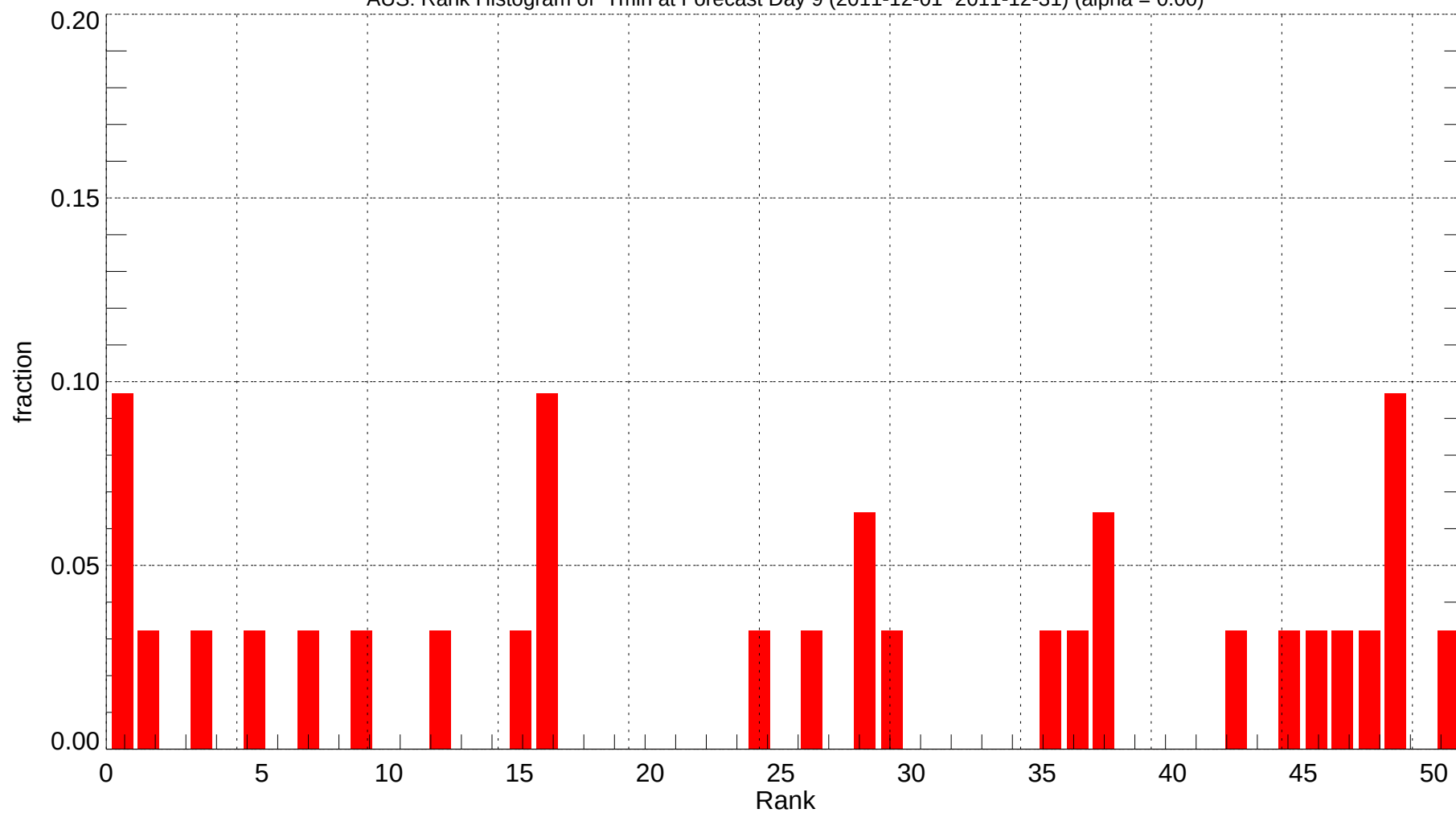
AUS: Rank Histogram of Tmin at Forecast Day 9 (2011-12-01~2011-12-31) (alpha = 0.00)
