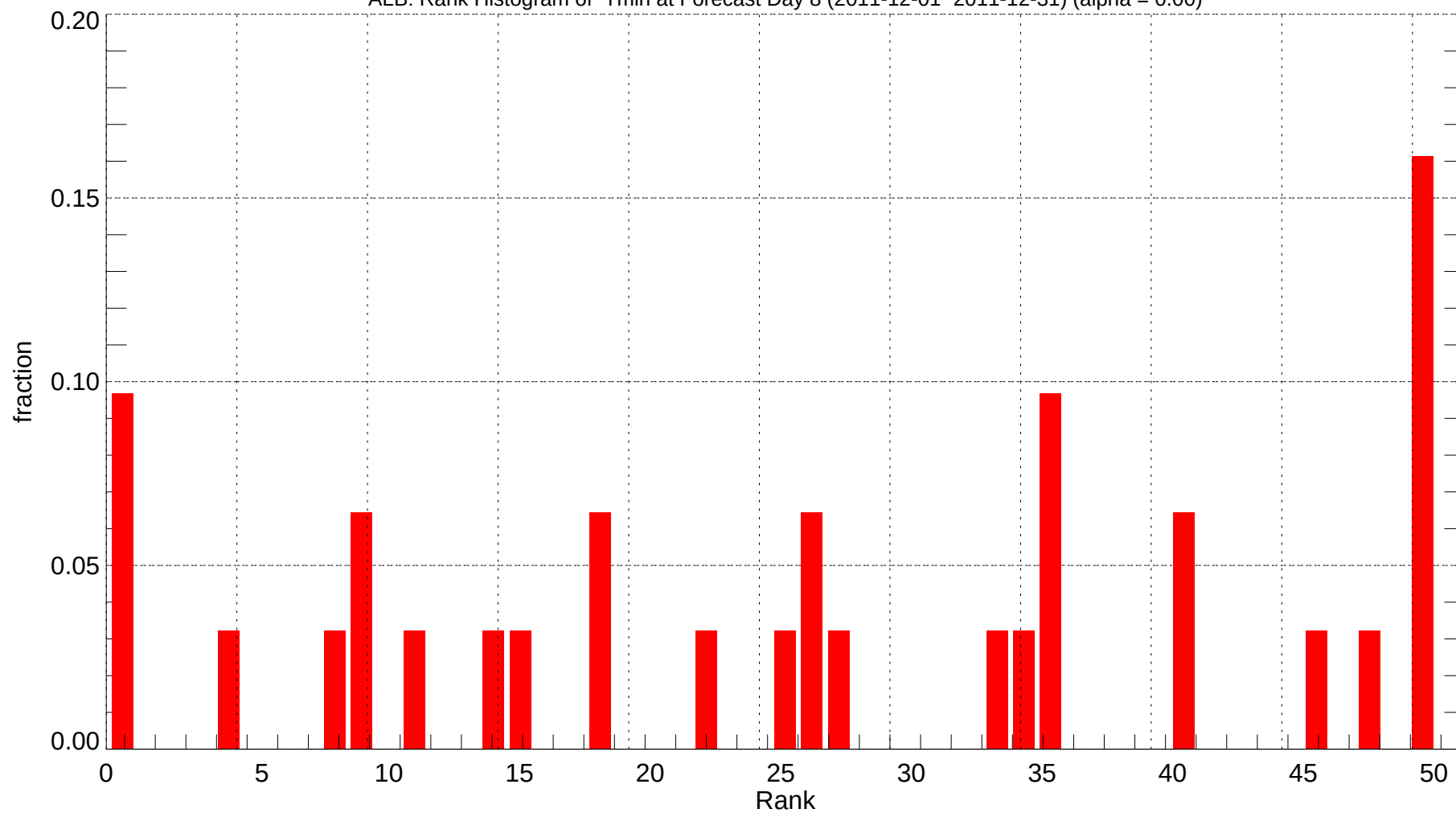
ALB: Rank Histogram of Tmin at Forecast Day 8 (2011-12-01~2011-12-31) (alpha = 0.00)
