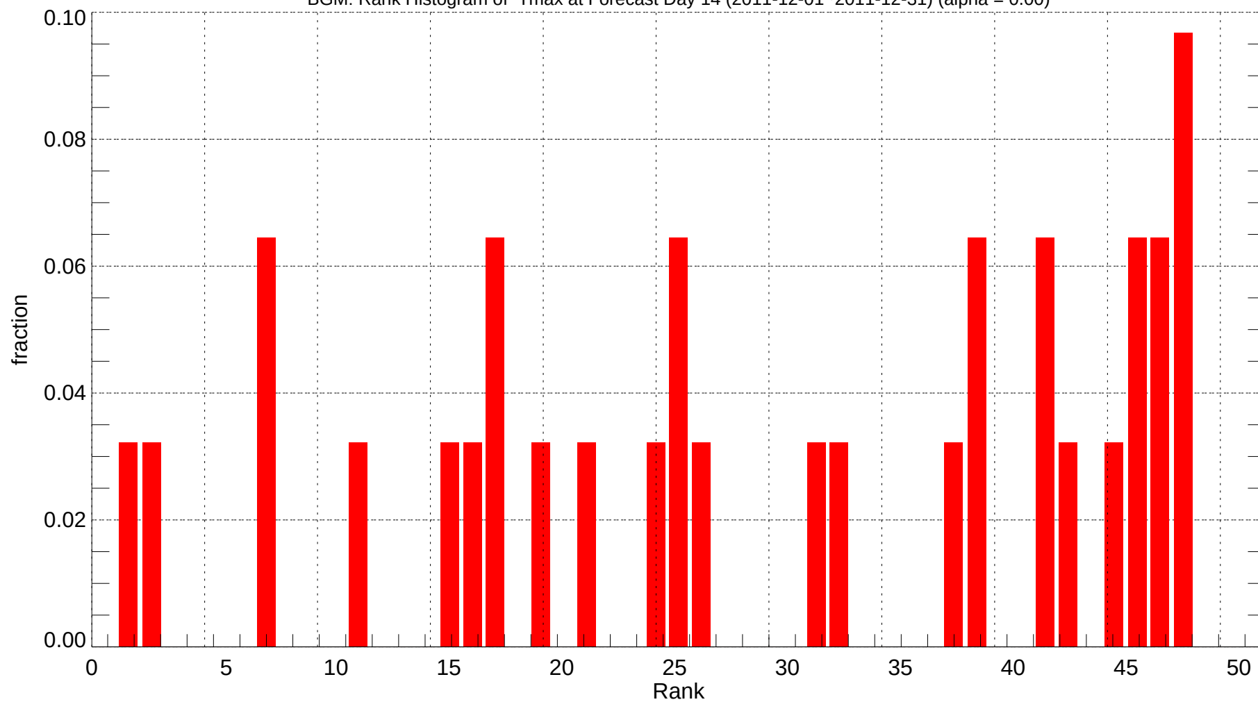
BGM: Rank Histogram of Tmax at Forecast Day 14 (2011-12-01~2011-12-31) (alpha = 0.00)
