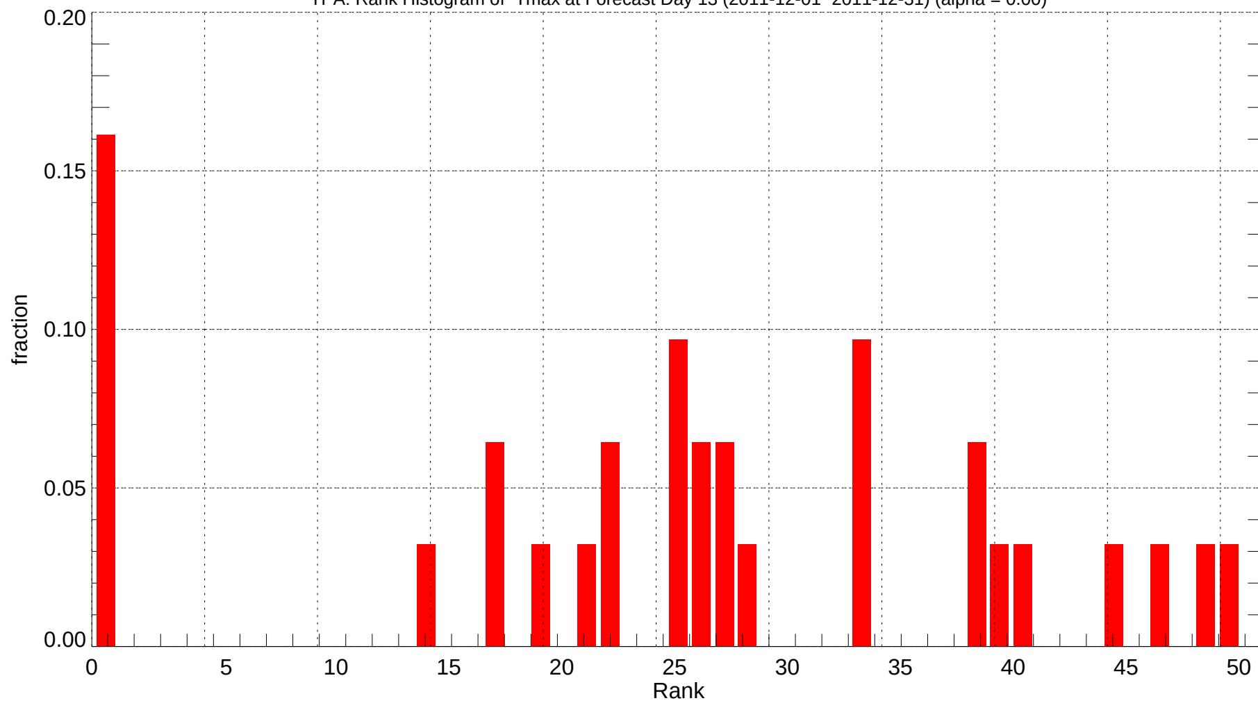
TPA: Rank Histogram of Tmax at Forecast Day 13 (2011-12-01~2011-12-31) (alpha = 0.00)
