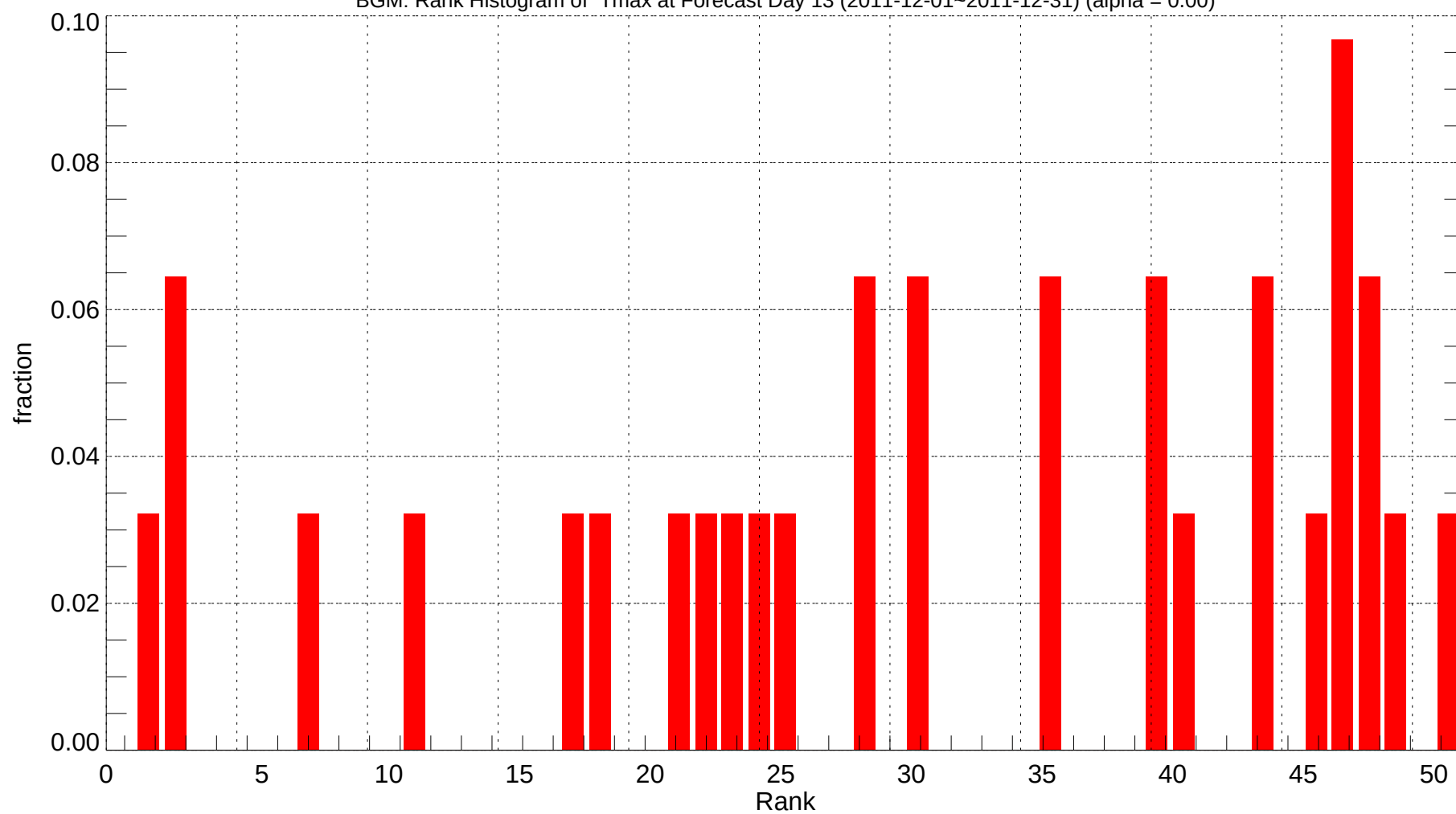
BGM: Rank Histogram of Tmax at Forecast Day 13 (2011-12-01~2011-12-31) (alpha = 0.00)
