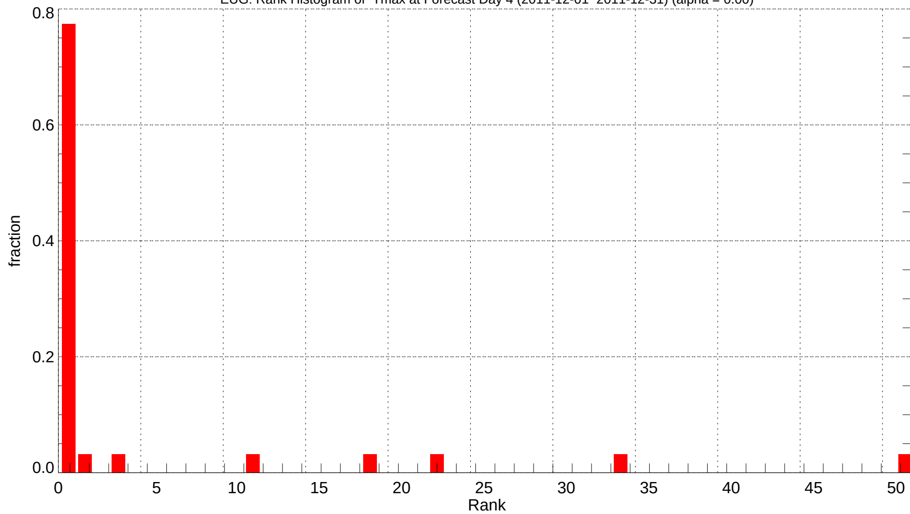
EUG: Rank Histogram of Tmax at Forecast Day 4 (2011-12-01~2011-12-31) (alpha = 0.00)
