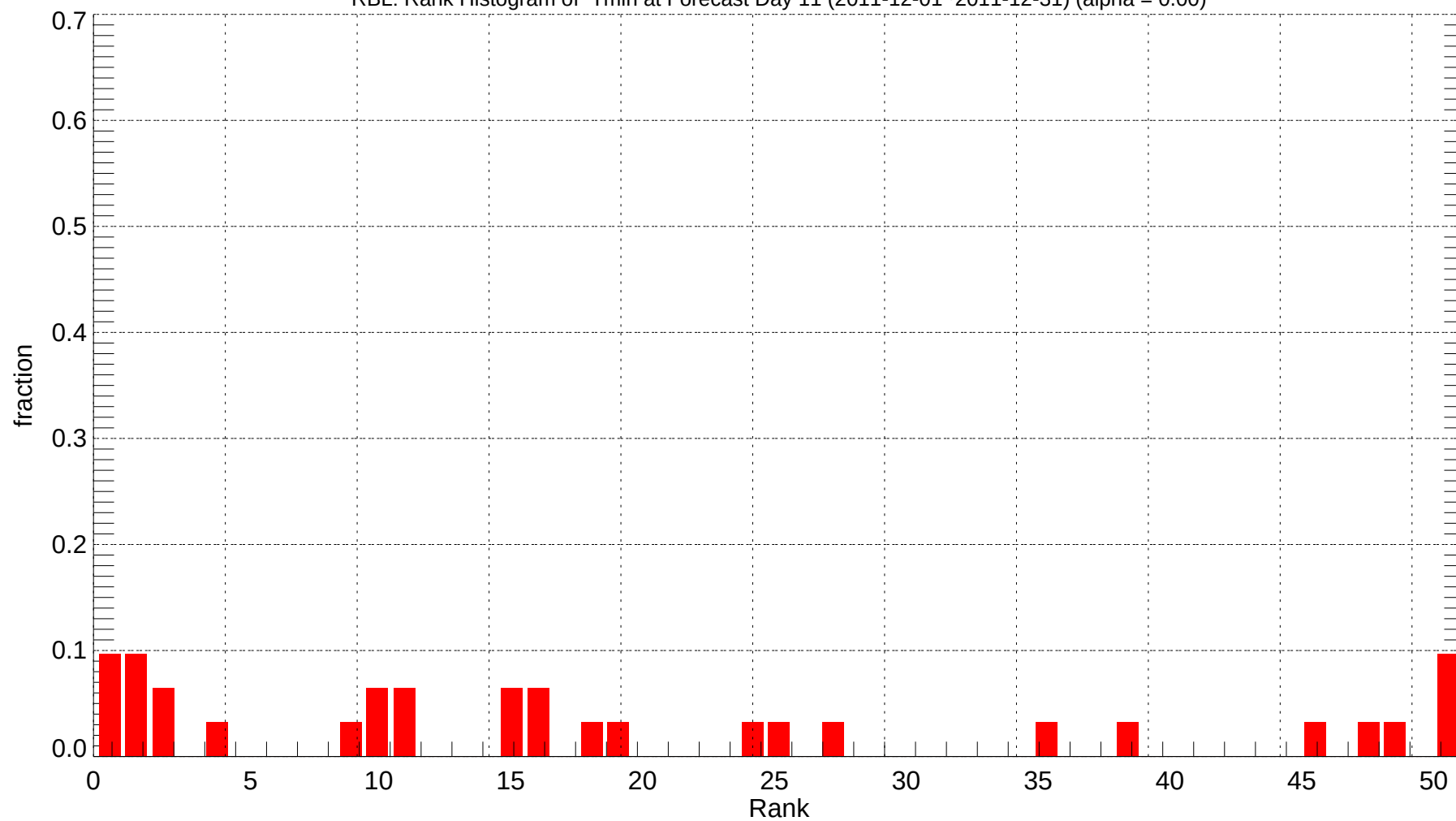
RBL: Rank Histogram of Tmin at Forecast Day 11 (2011-12-01~2011-12-31) (alpha = 0.00)
