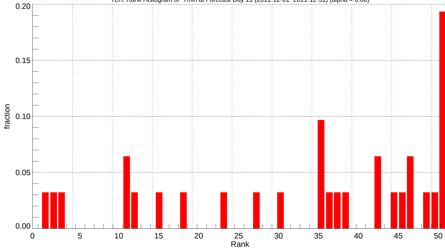
TLH: Rank Histogram of Tmin at Forecast Day 11 (2011-12-01~2011-12-31) (alpha = 0.00)
