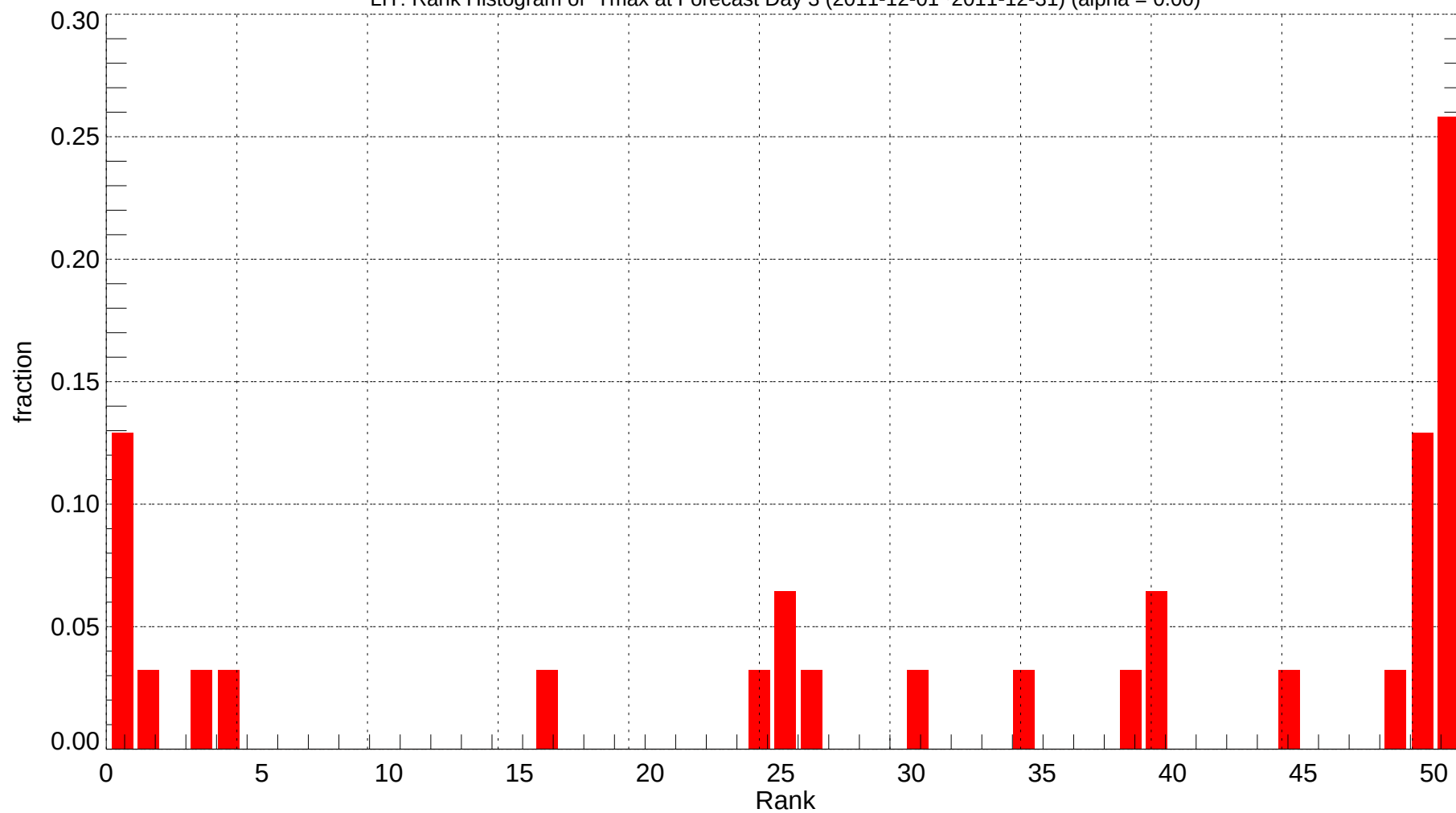
LIT: Rank Histogram of Tmax at Forecast Day 3 (2011-12-01~2011-12-31) (alpha = 0.00)
