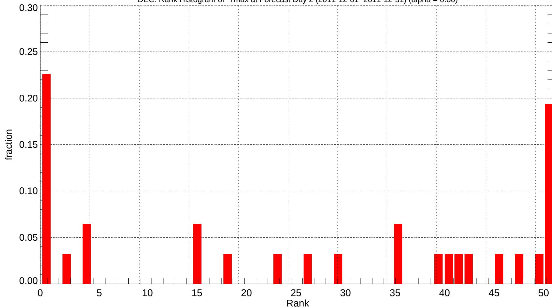
DEC: Rank Histogram of Tmax at Forecast Day 2 (2011-12-01~2011-12-31) (alpha = 0.00)
