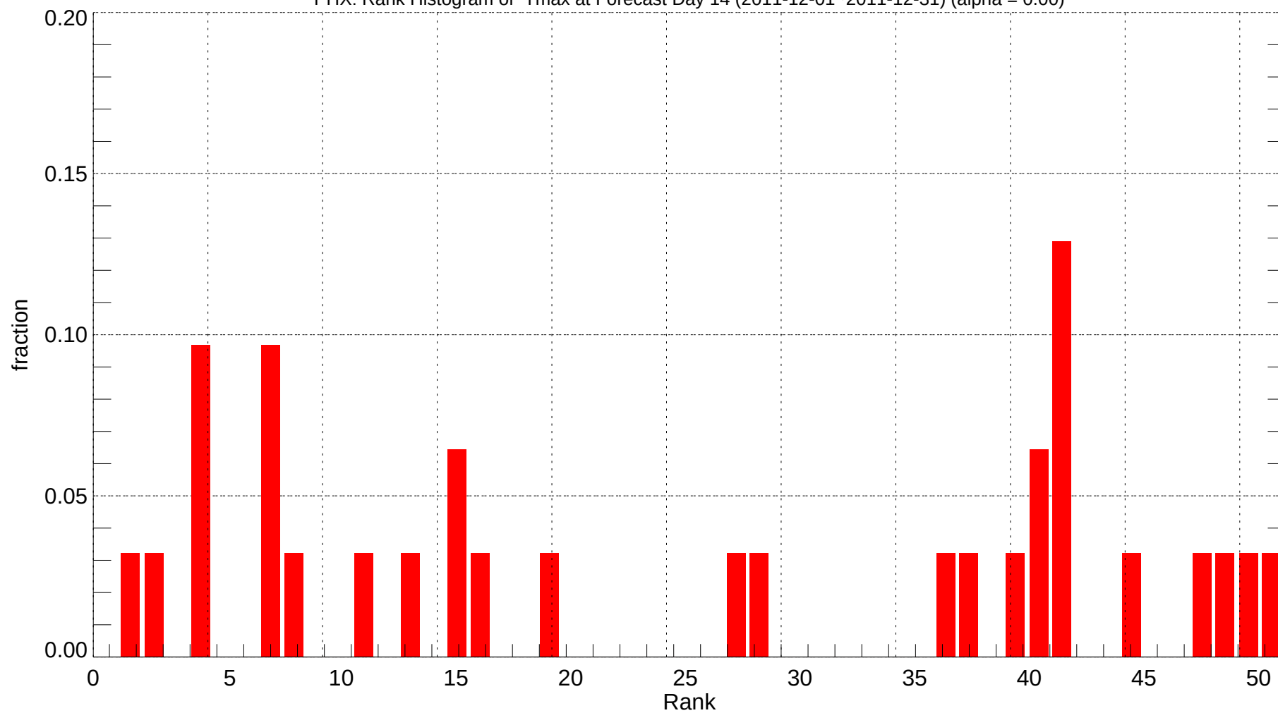
PHX: Rank Histogram of Tmax at Forecast Day 14 (2011-12-01~2011-12-31) (alpha = 0.00)
