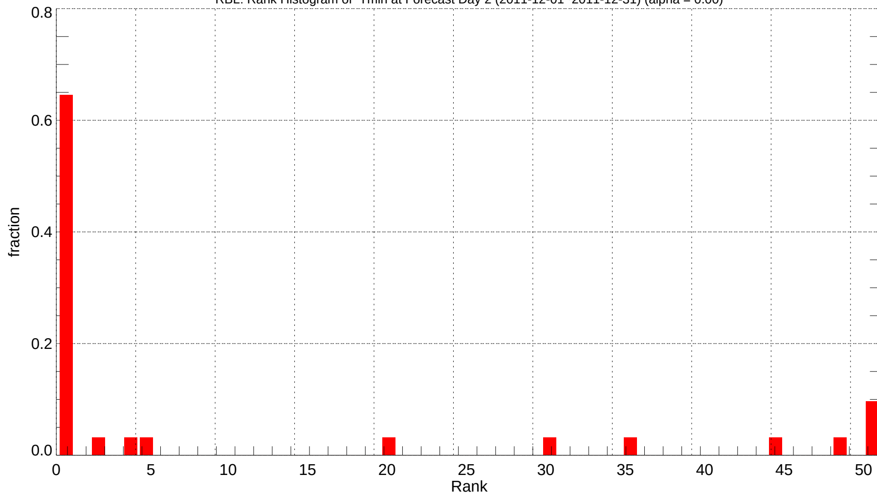
RBL: Rank Histogram of Tmin at Forecast Day 2 (2011-12-01~2011-12-31) (alpha = 0.00)
