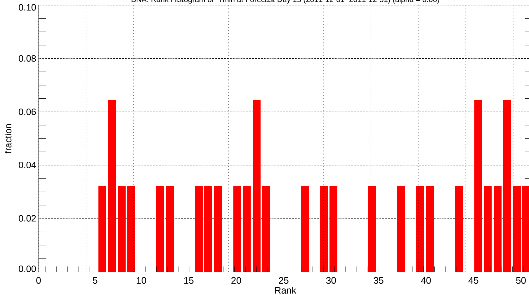
BNA: Rank Histogram of Tmin at Forecast Day 15 (2011-12-01~2011-12-31) (alpha = 0.00)
