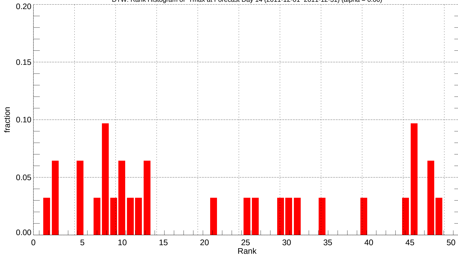
DTW: Rank Histogram of Tmax at Forecast Day 14 (2011-12-01~2011-12-31) (alpha = 0.00)
