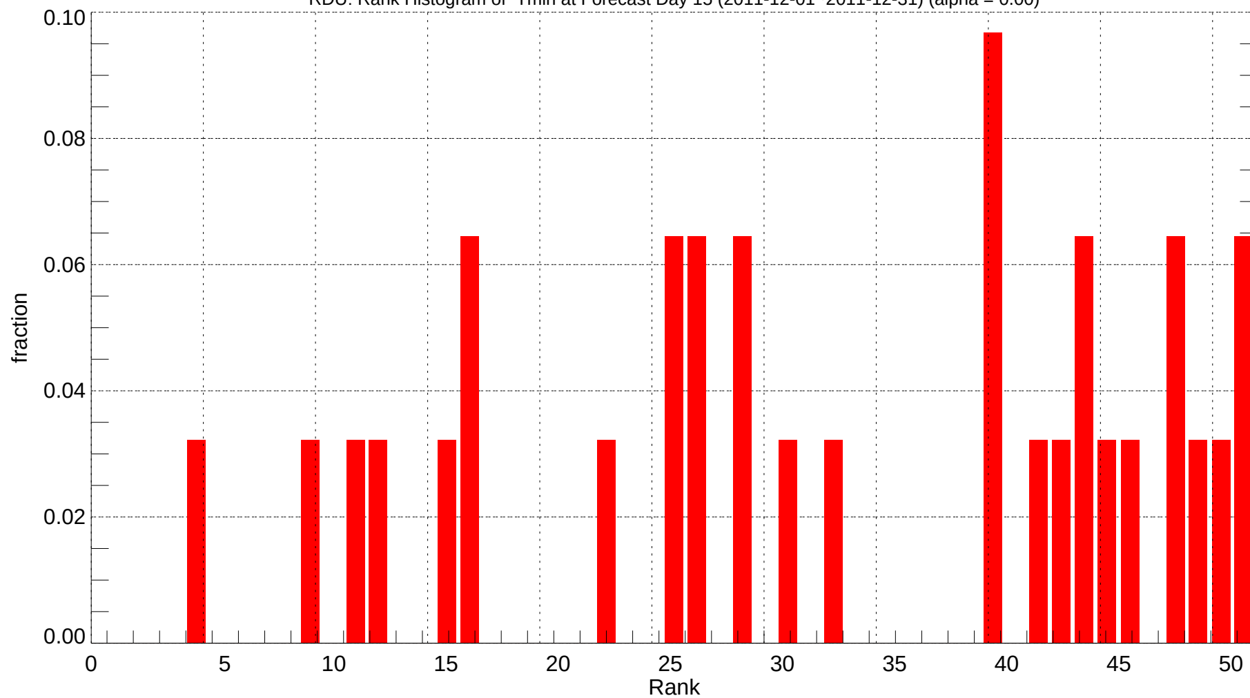
RDU: Rank Histogram of Tmin at Forecast Day 15 (2011-12-01~2011-12-31) (alpha = 0.00)
