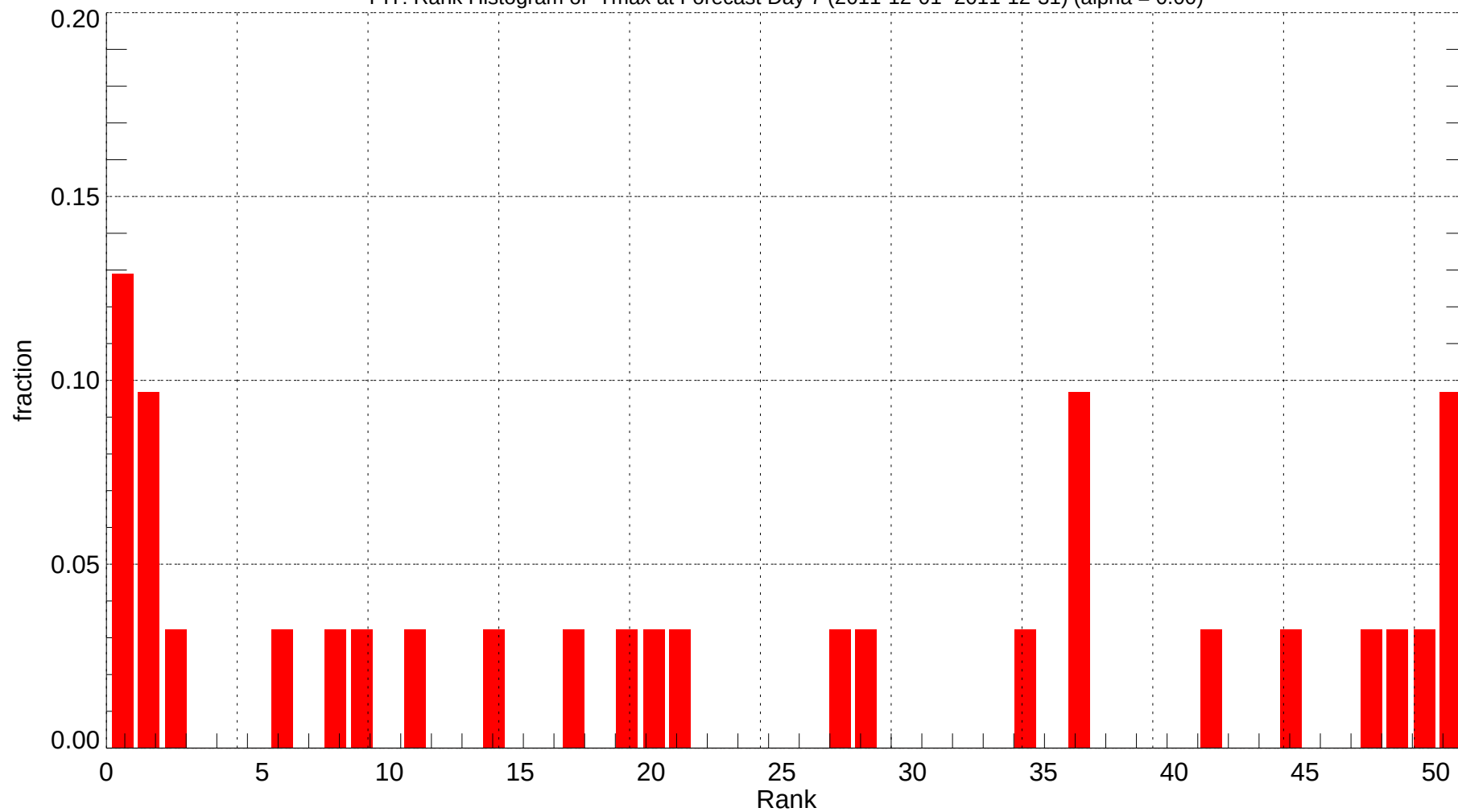
PIT: Rank Histogram of Tmax at Forecast Day 7 (2011-12-01~2011-12-31) (alpha = 0.00)
