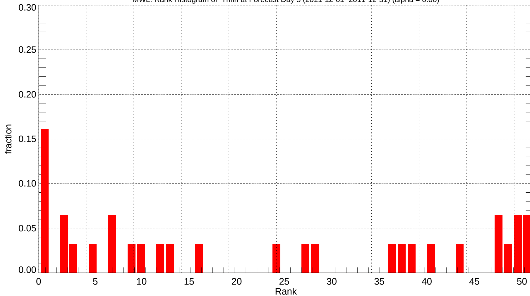
MWL: Rank Histogram of Tmin at Forecast Day 3 (2011-12-01~2011-12-31) (alpha = 0.00)
