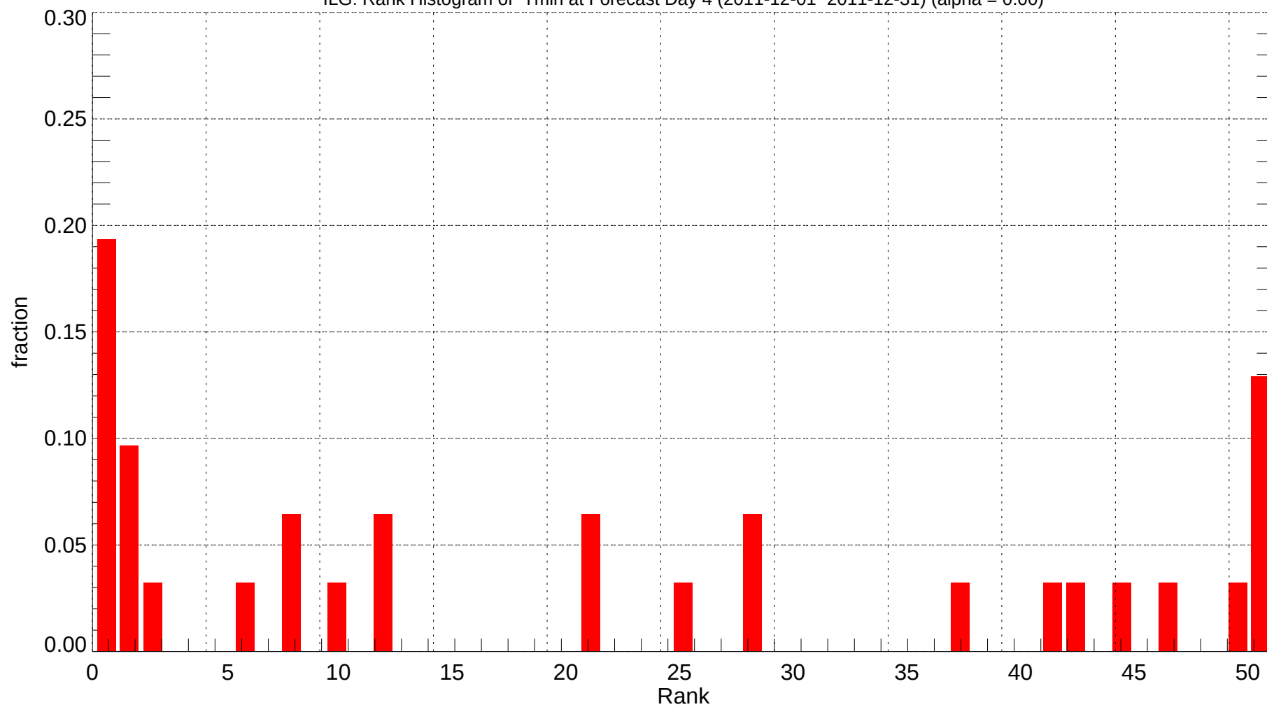
ILG: Rank Histogram of Tmin at Forecast Day 4 (2011-12-01~2011-12-31) (alpha = 0.00)
