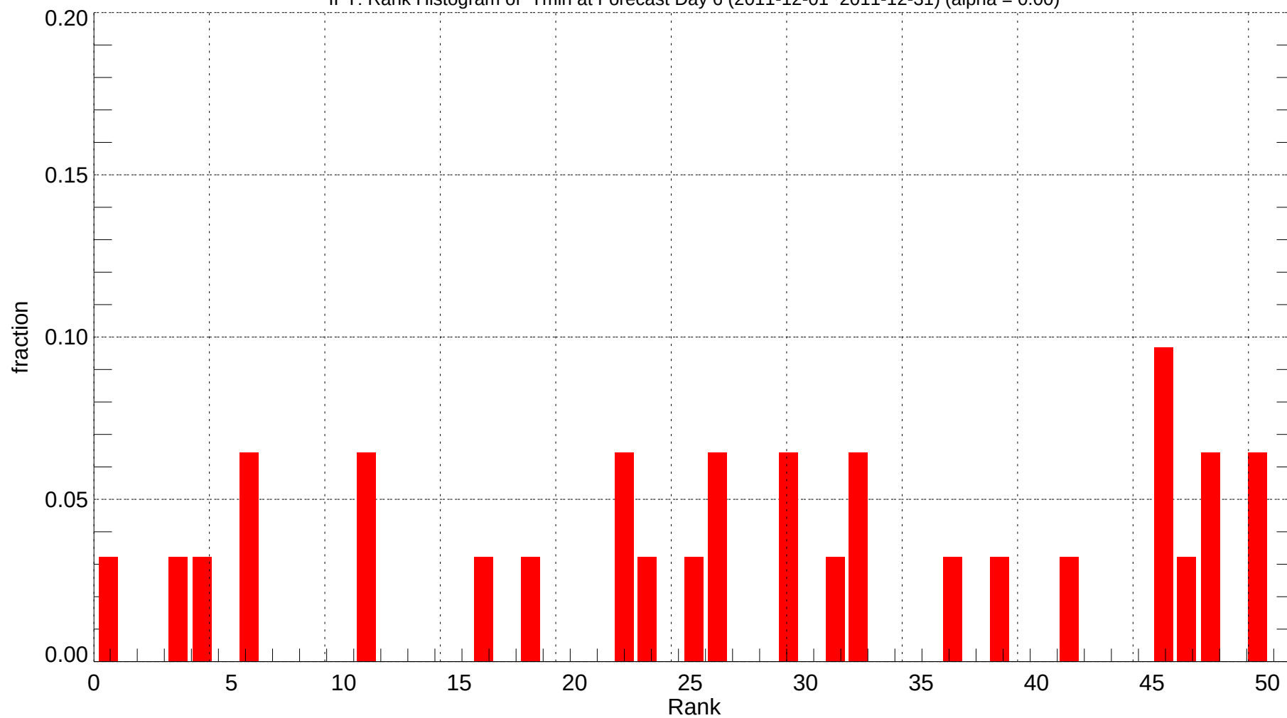
IPT: Rank Histogram of Tmin at Forecast Day 6 (2011-12-01~2011-12-31) (alpha = 0.00)
