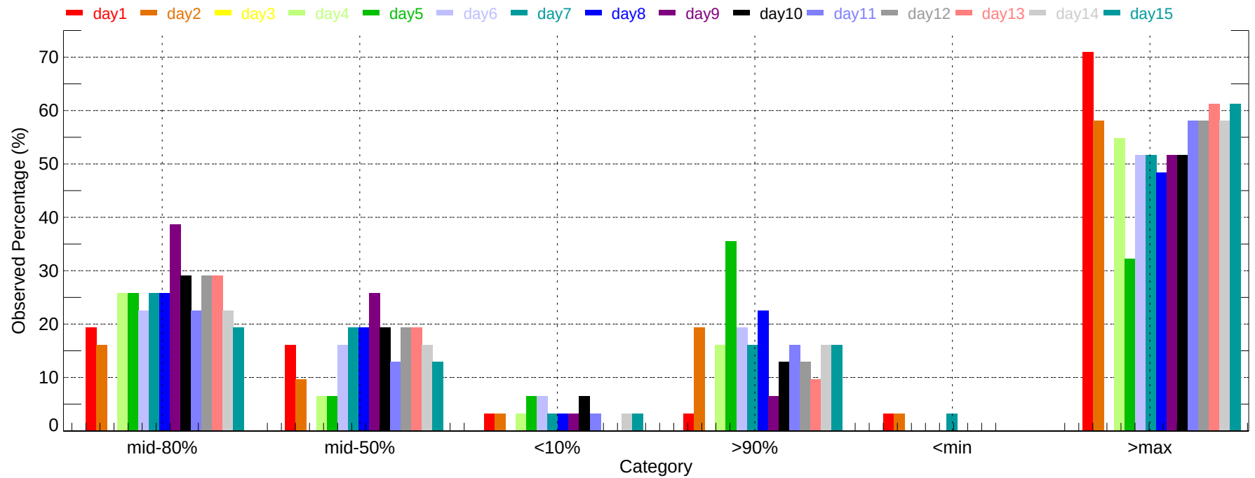
Observed Percentage of Ensembles - YYC: Max Temperature (2011-12-01~2011-12-31)
