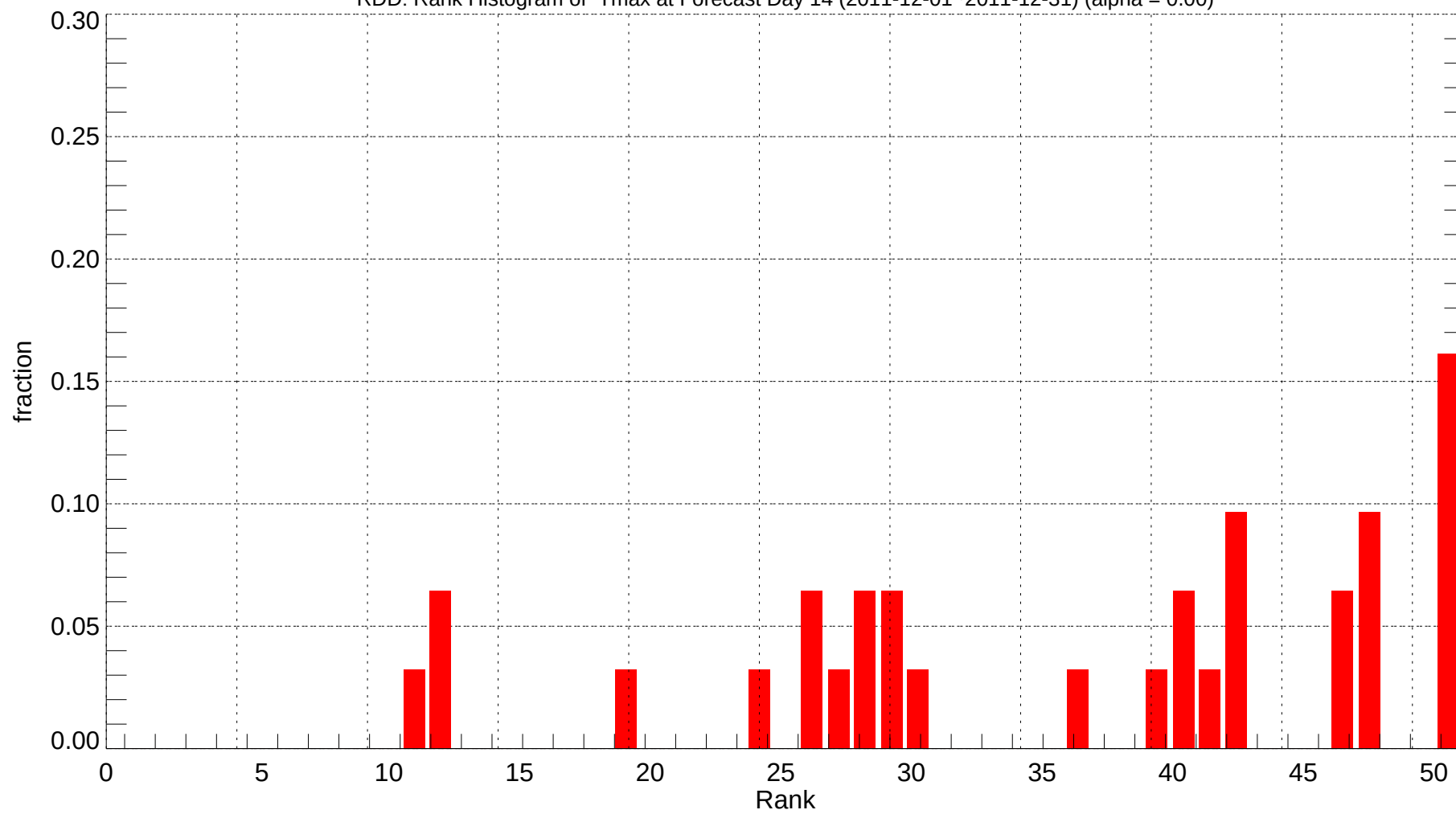
RDD: Rank Histogram of Tmax at Forecast Day 14 (2011-12-01~2011-12-31) (alpha = 0.00)
