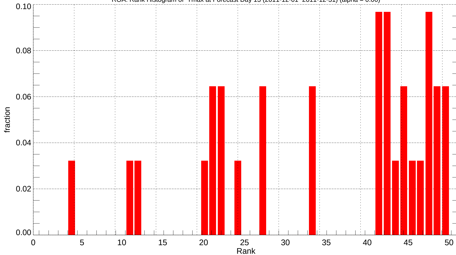
ROA: Rank Histogram of Tmax at Forecast Day 13 (2011-12-01~2011-12-31) (alpha = 0.00)
