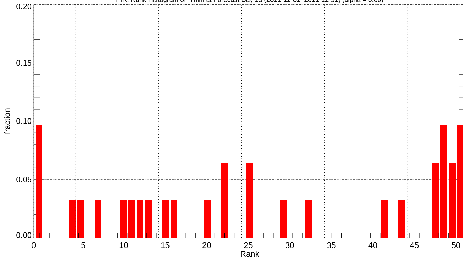
PIR: Rank Histogram of Tmin at Forecast Day 13 (2011-12-01~2011-12-31) (alpha = 0.00)
