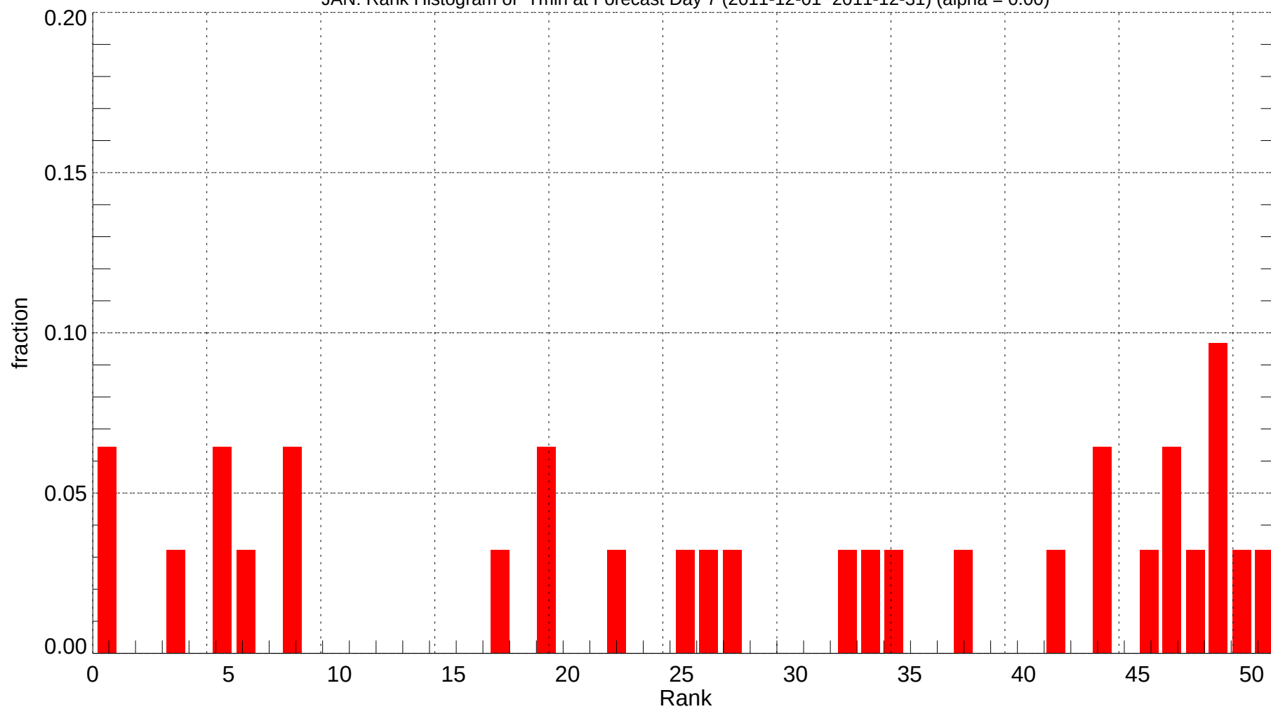
JAN: Rank Histogram of Tmin at Forecast Day 7 (2011-12-01~2011-12-31) (alpha = 0.00)
