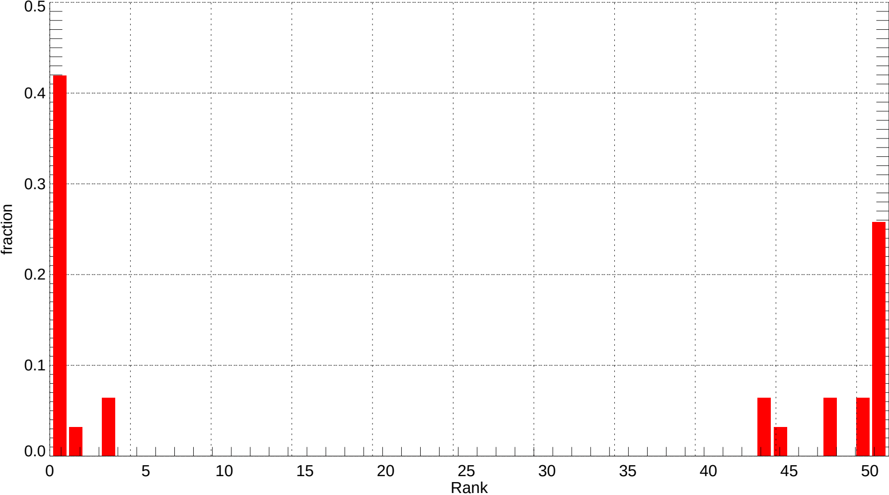
SJC: Rank Histogram of Tmin at Forecast Day 1 (2011-12-01~2011-12-31) (alpha = 0.00)
