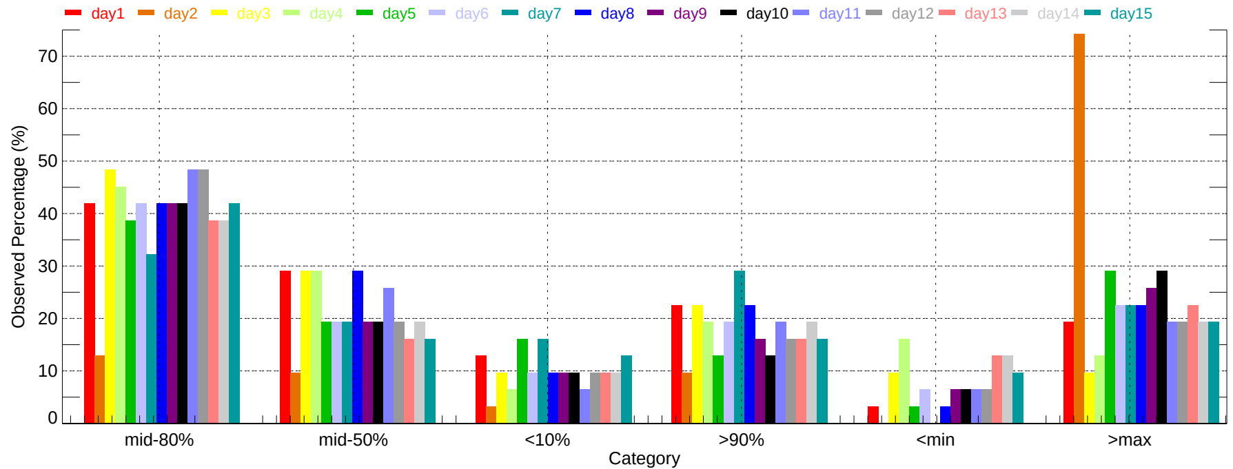
Observed Percentage of Ensembles - MOB: Max Temperature (2011-12-01~2011-12-31)
