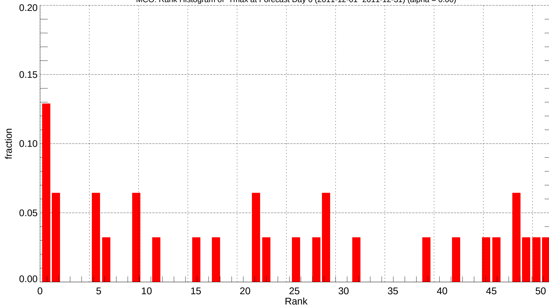
MCO: Rank Histogram of Tmax at Forecast Day 6 (2011-12-01~2011-12-31) (alpha = 0.00)
