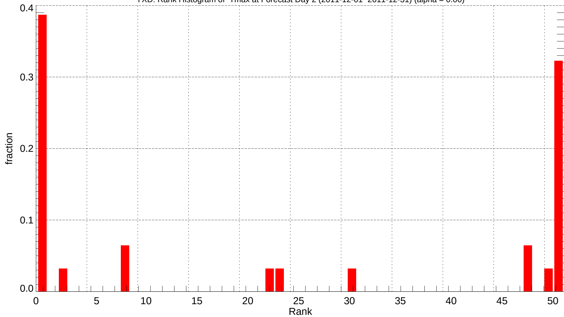
YXD: Rank Histogram of Tmax at Forecast Day 2 (2011-12-01~2011-12-31) (alpha = 0.00)
