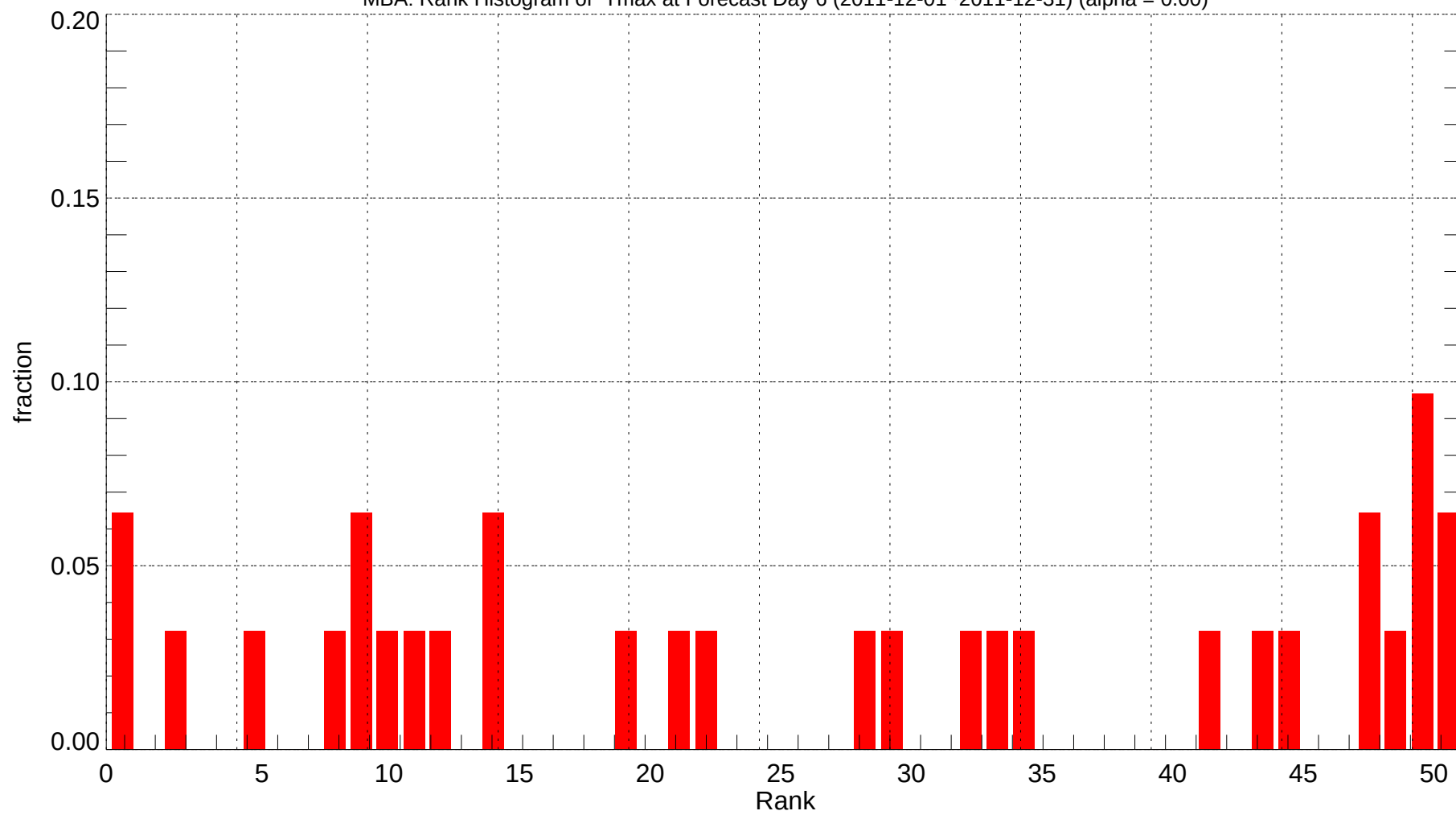
MBA: Rank Histogram of Tmax at Forecast Day 6 (2011-12-01~2011-12-31) (alpha = 0.00)
