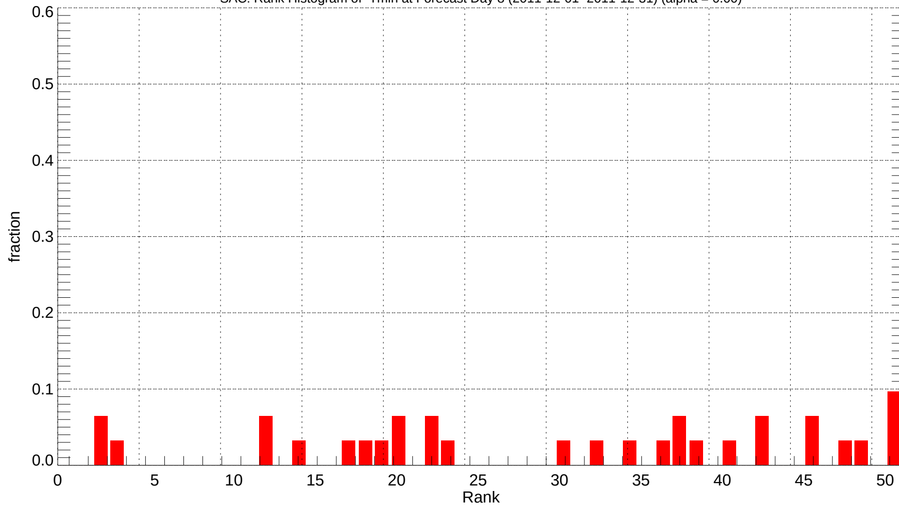
SAC: Rank Histogram of Tmin at Forecast Day 8 (2011-12-01~2011-12-31) (alpha = 0.00)
