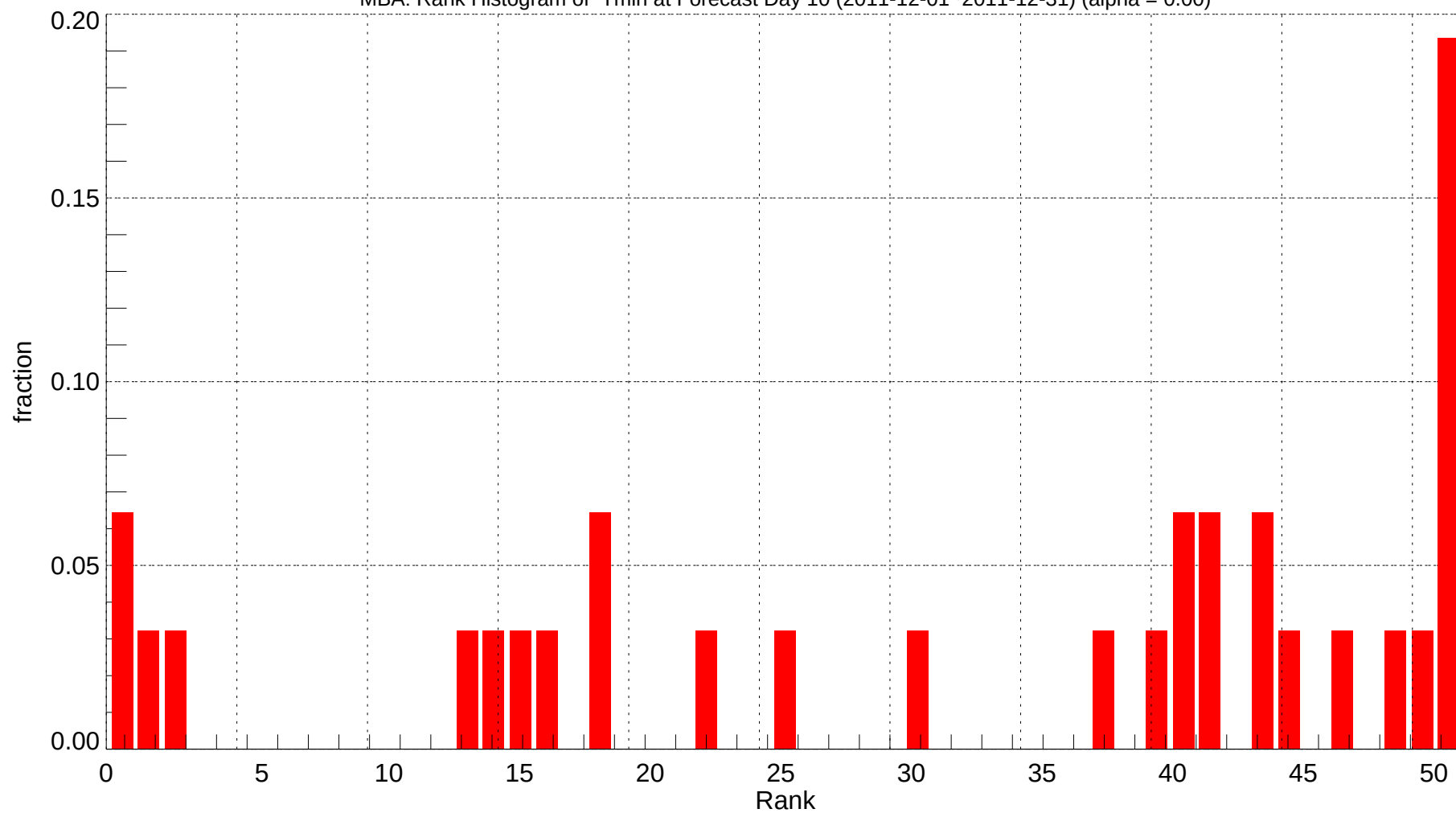
MBA: Rank Histogram of Tmin at Forecast Day 10 (2011-12-01~2011-12-31) (alpha = 0.00)
