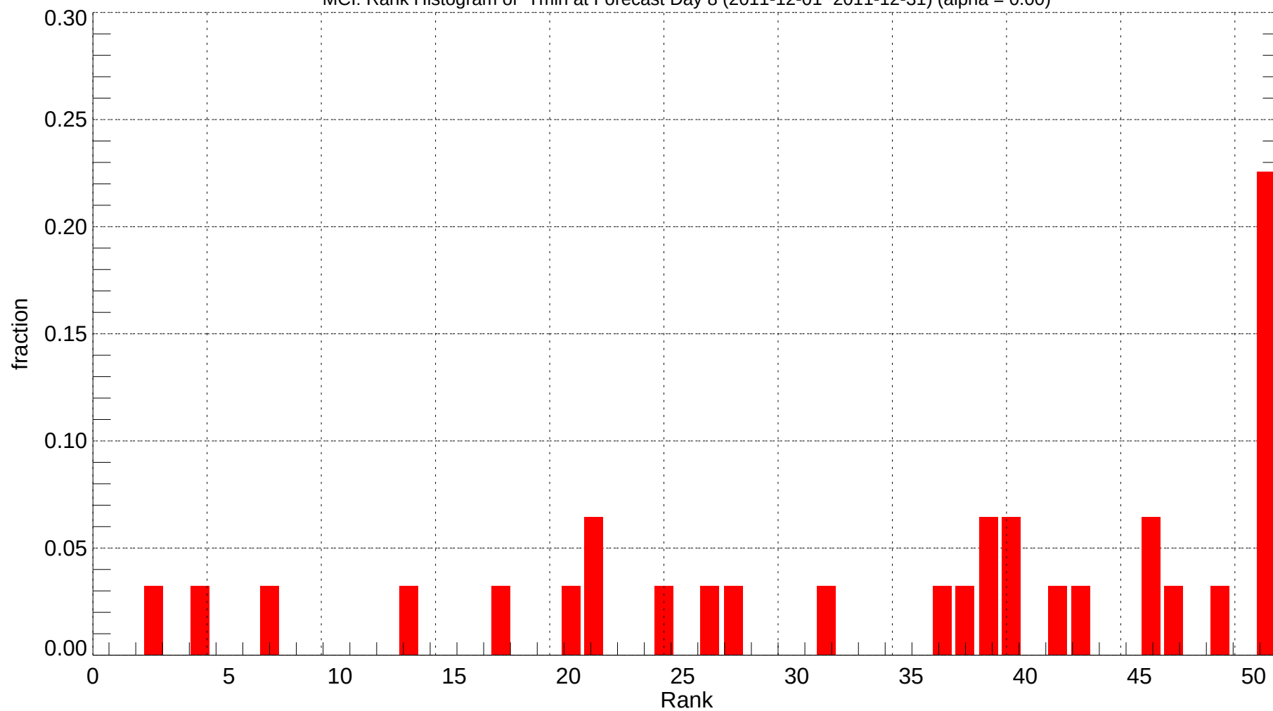
MCI: Rank Histogram of Tmin at Forecast Day 8 (2011-12-01~2011-12-31) (alpha = 0.00)
