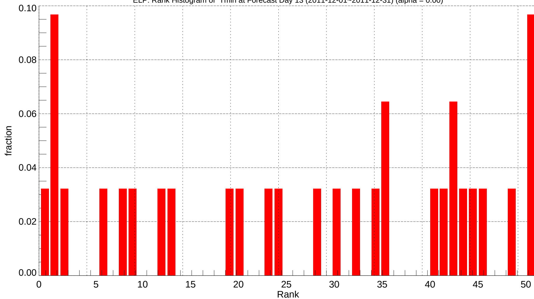
ELP: Rank Histogram of Tmin at Forecast Day 13 (2011-12-01~2011-12-31) (alpha = 0.00)
