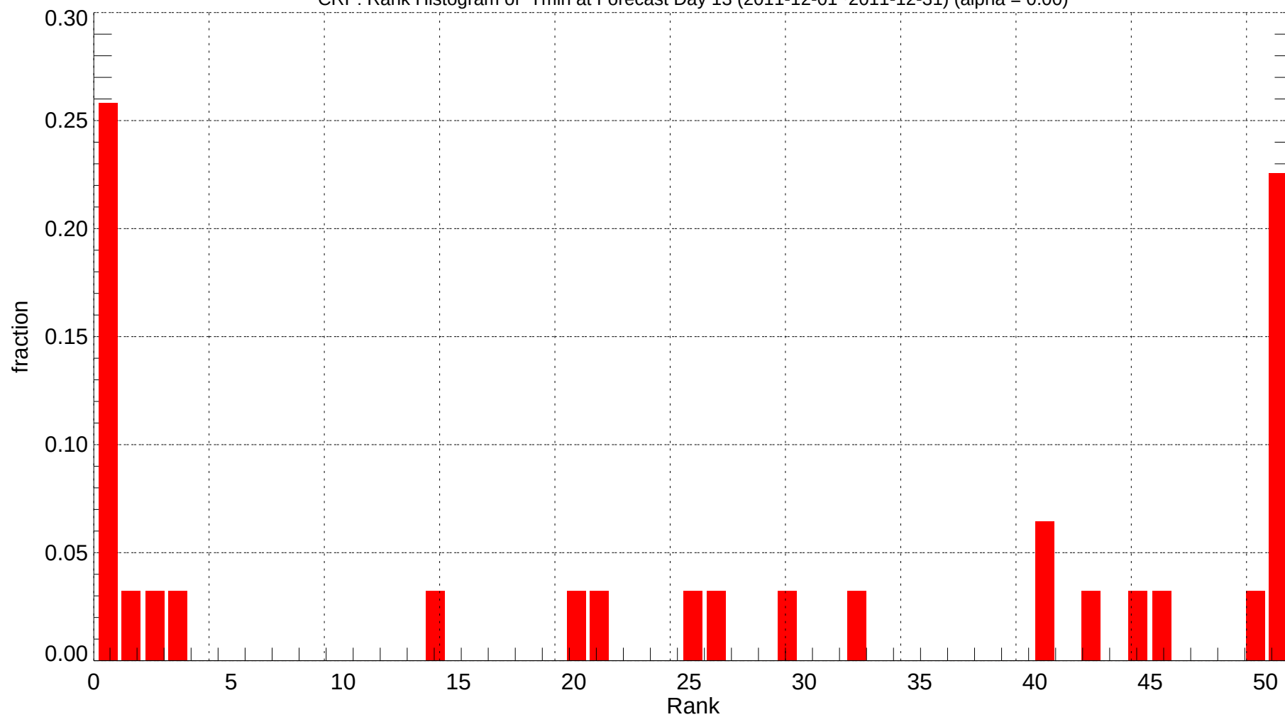
CRP: Rank Histogram of Tmin at Forecast Day 13 (2011-12-01~2011-12-31) (alpha = 0.00)
