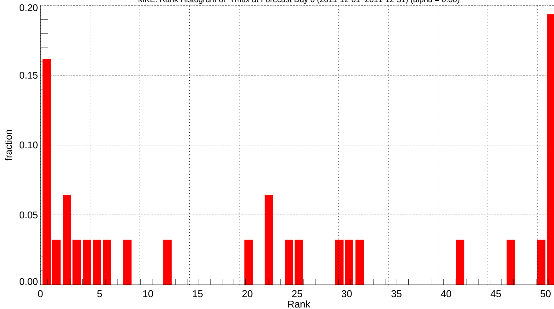
MKE: Rank Histogram of Tmax at Forecast Day 6 (2011-12-01~2011-12-31) (alpha = 0.00)
