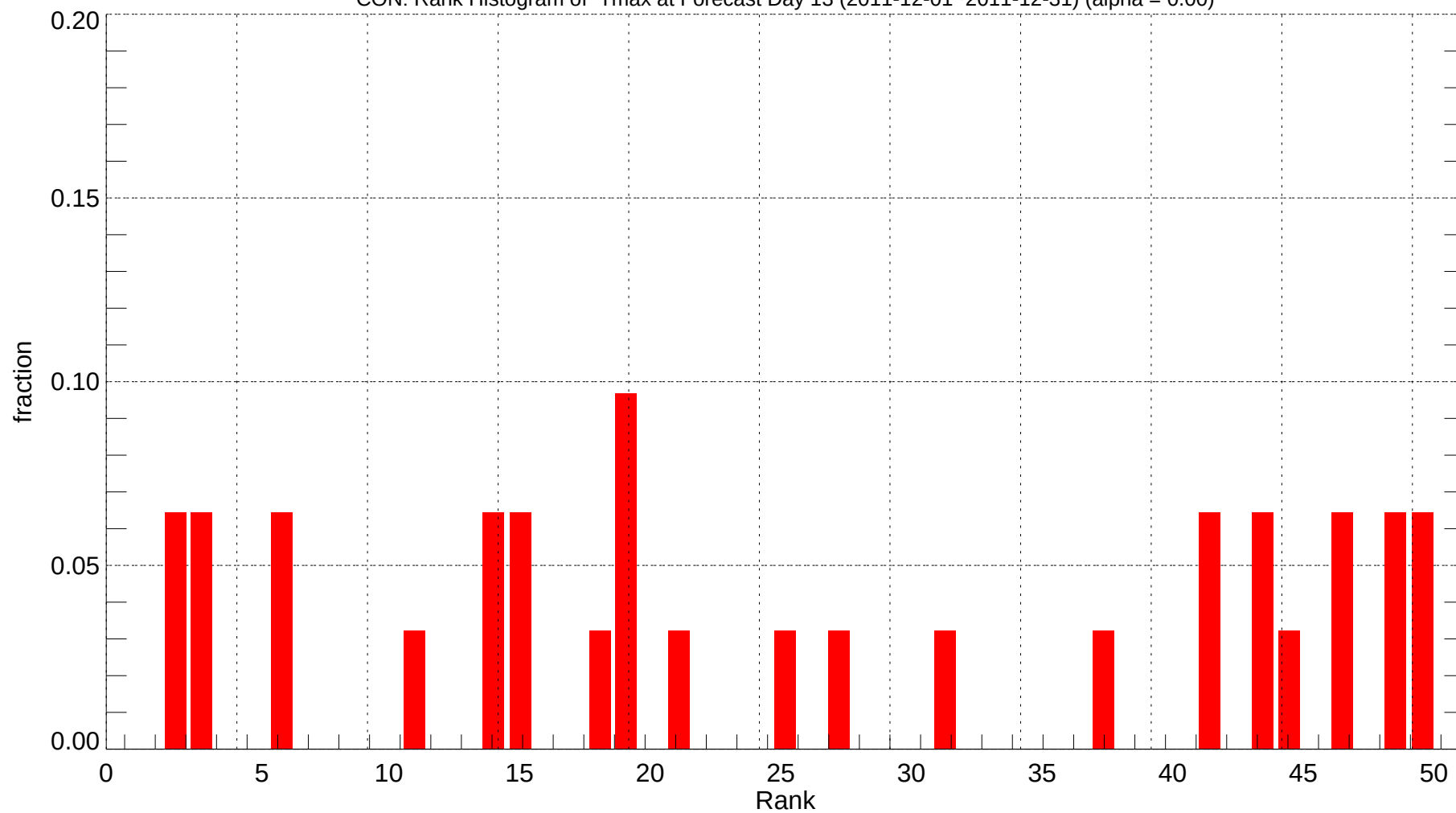
CON: Rank Histogram of Tmax at Forecast Day 13 (2011-12-01~2011-12-31) (alpha = 0.00)
