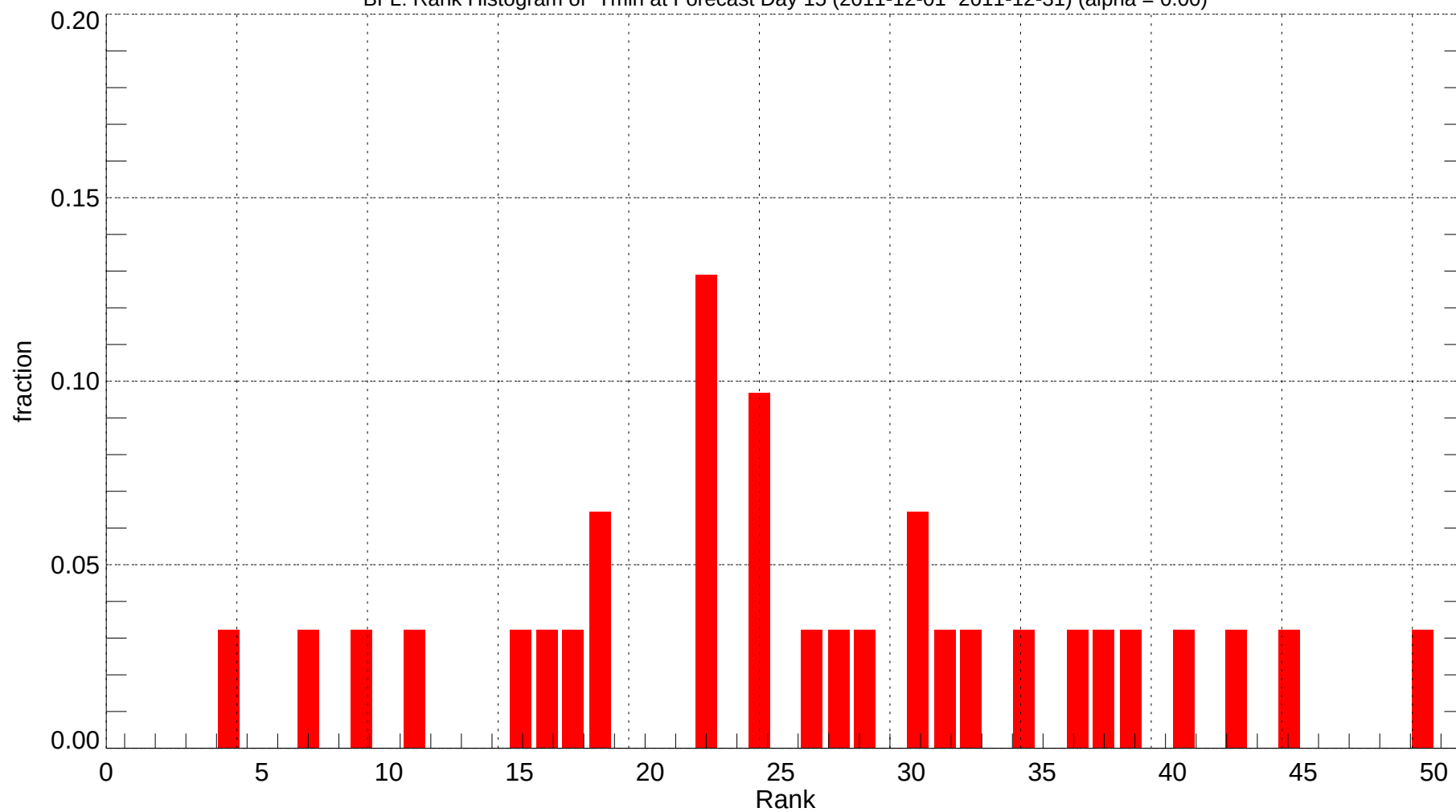
BFL: Rank Histogram of Tmin at Forecast Day 15 (2011-12-01~2011-12-31) (alpha = 0.00)
