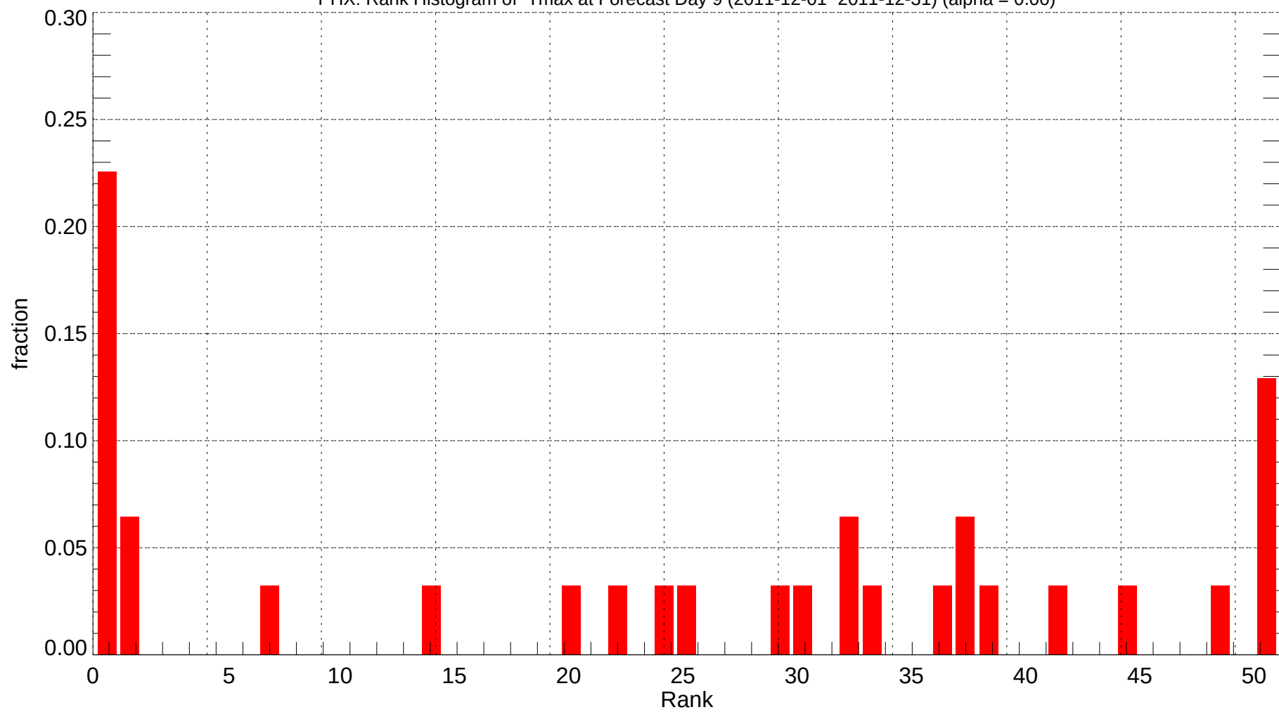
PHX: Rank Histogram of Tmax at Forecast Day 9 (2011-12-01~2011-12-31) (alpha = 0.00)
