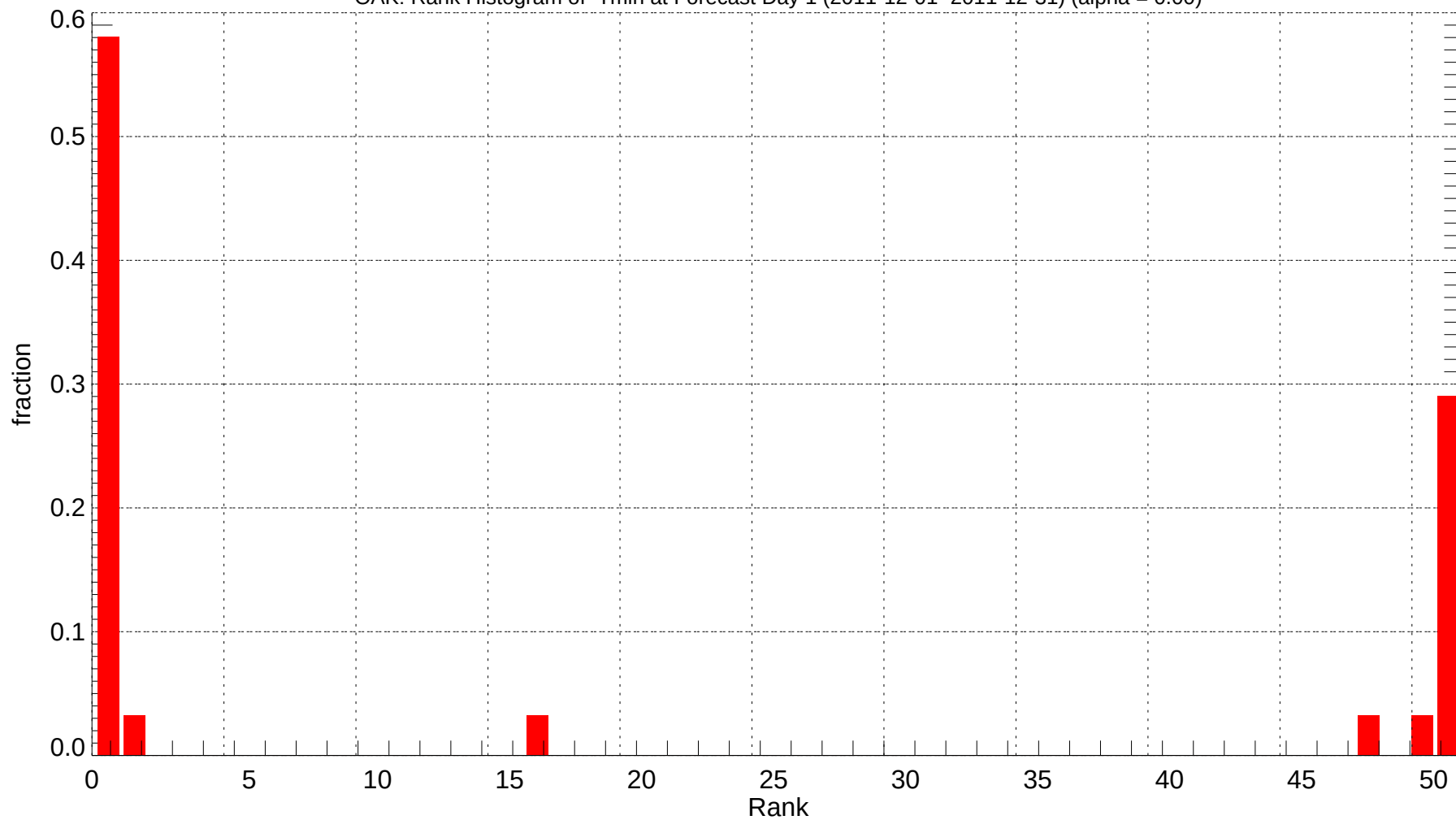
OAK: Rank Histogram of Tmin at Forecast Day 1 (2011-12-01~2011-12-31) (alpha = 0.00)
