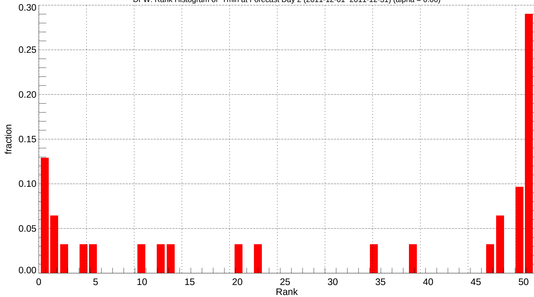
DFW: Rank Histogram of Tmin at Forecast Day 2 (2011-12-01~2011-12-31) (alpha = 0.00)
