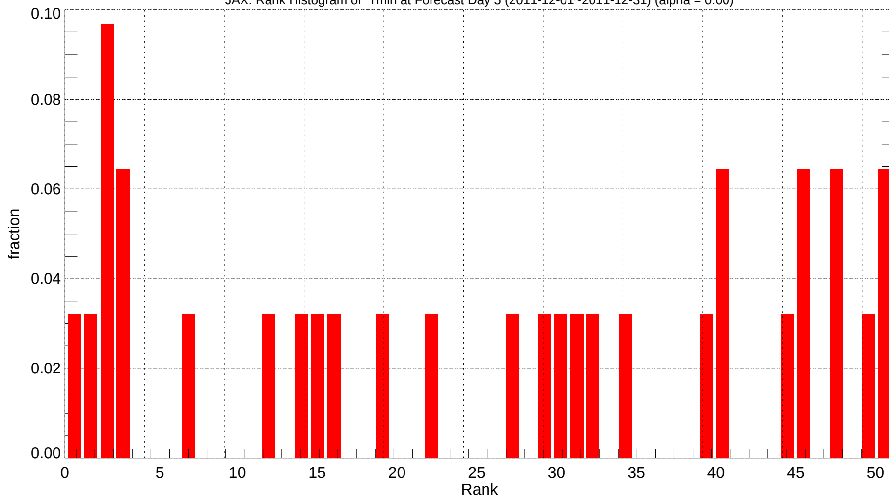
JAX: Rank Histogram of Tmin at Forecast Day 5 (2011-12-01~2011-12-31) (alpha = 0.00)
