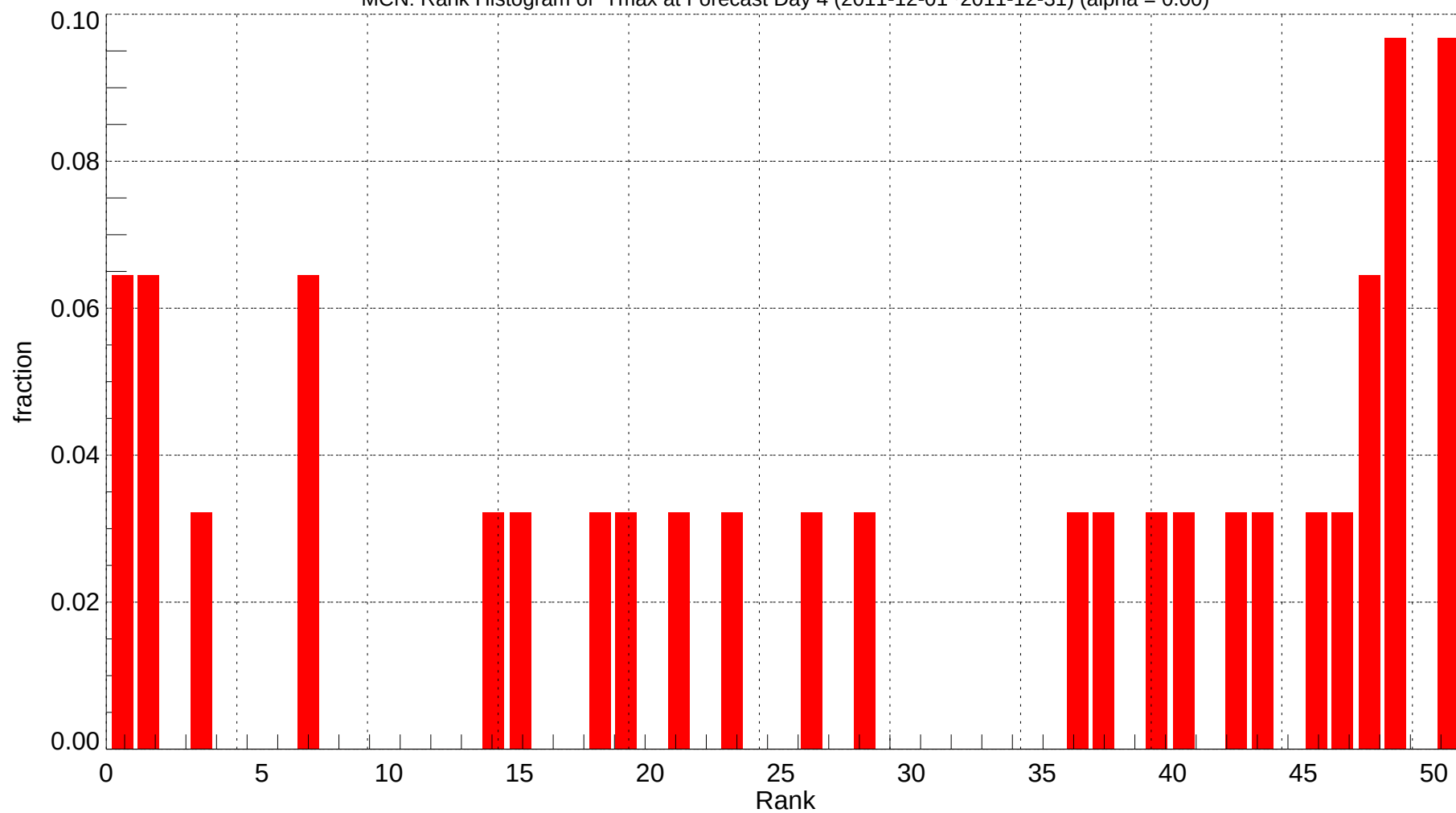
MCN: Rank Histogram of Tmax at Forecast Day 4 (2011-12-01~2011-12-31) (alpha = 0.00)
