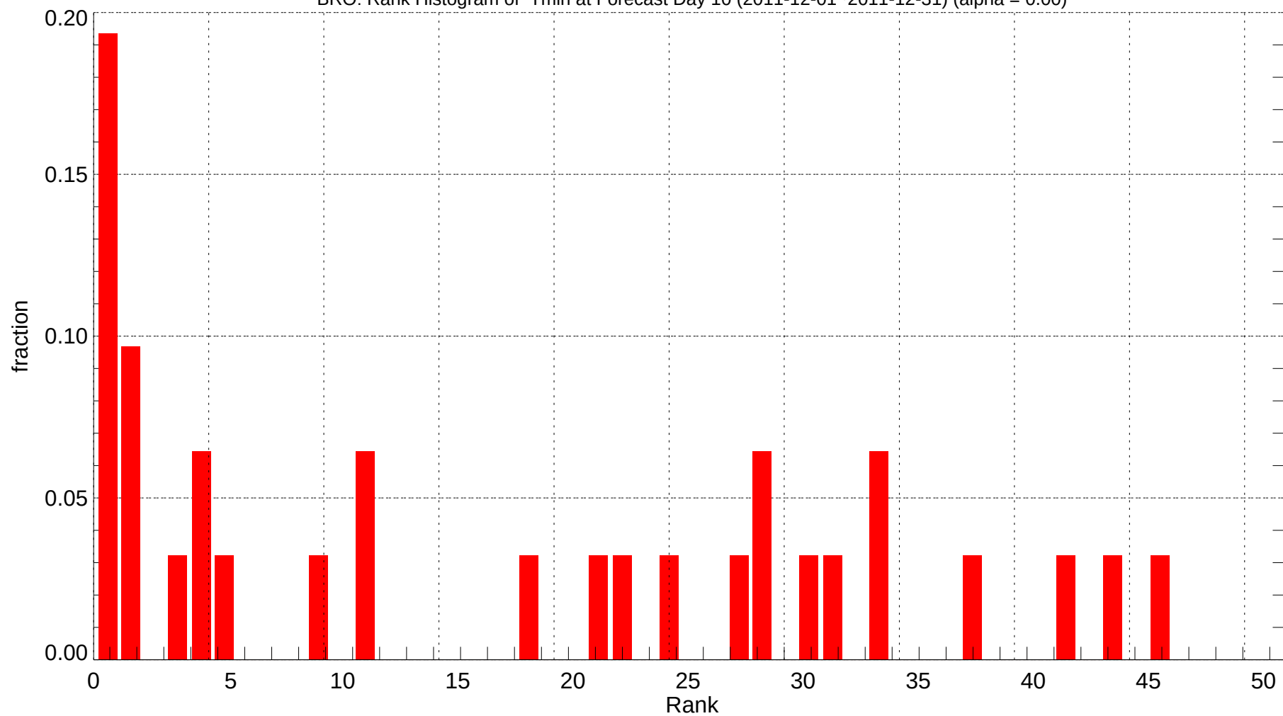
BRO: Rank Histogram of Tmin at Forecast Day 10 (2011-12-01~2011-12-31) (alpha = 0.00)
