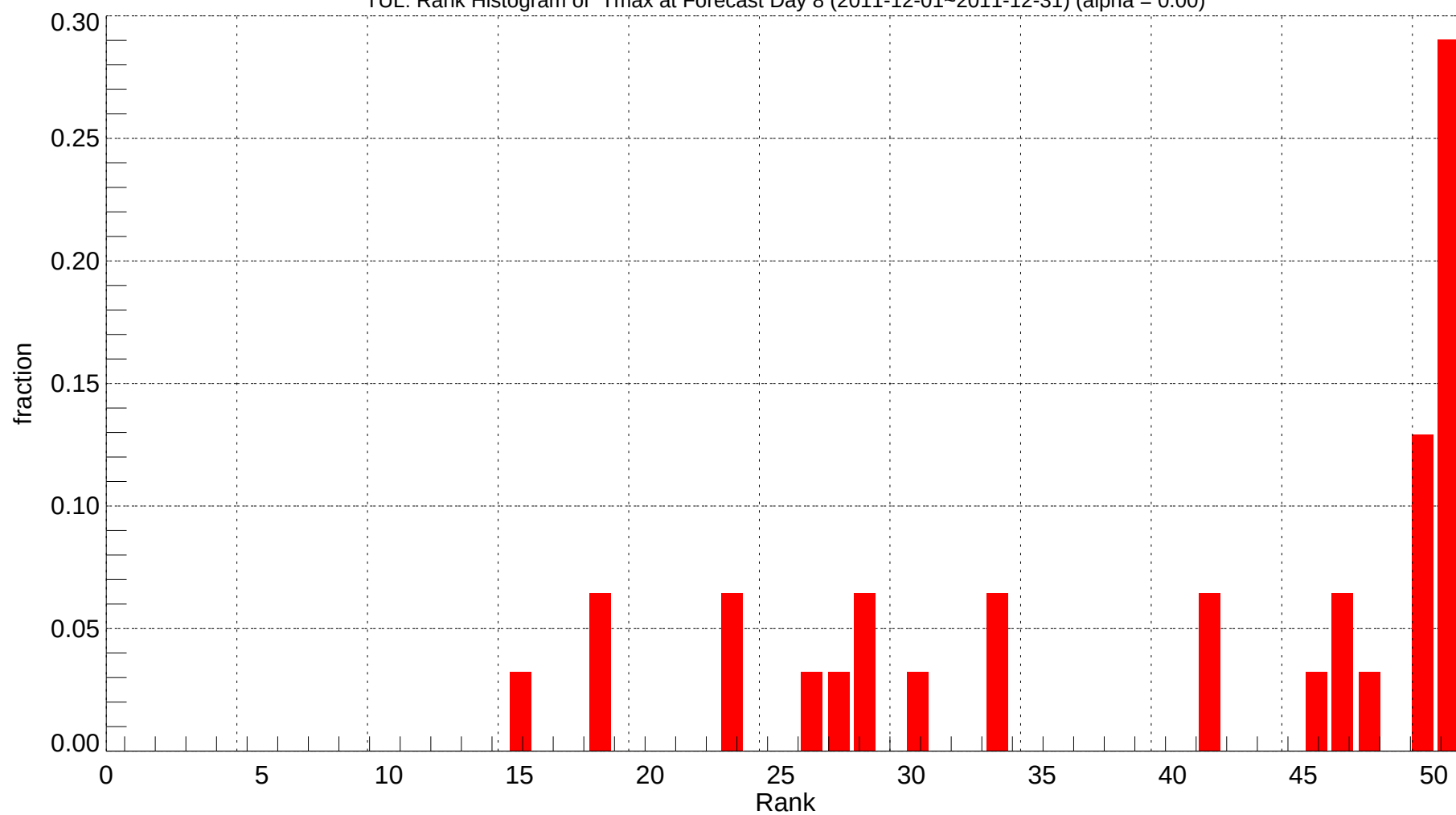
TUL: Rank Histogram of Tmax at Forecast Day 8 (2011-12-01~2011-12-31) (alpha = 0.00)
