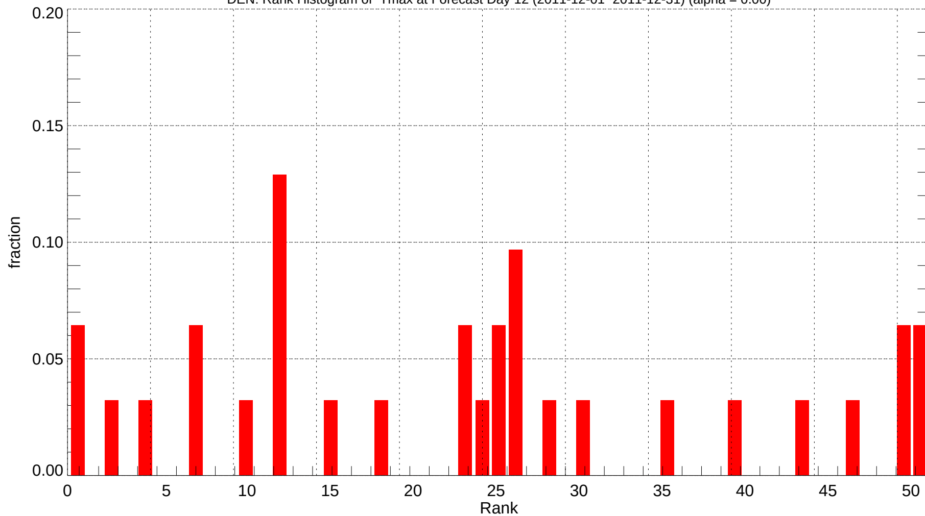
DEN: Rank Histogram of Tmax at Forecast Day 12 (2011-12-01~2011-12-31) (alpha = 0.00)
