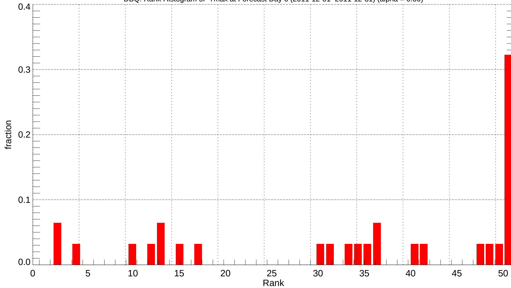
DBQ: Rank Histogram of Tmax at Forecast Day 6 (2011-12-01~2011-12-31) (alpha = 0.00)
