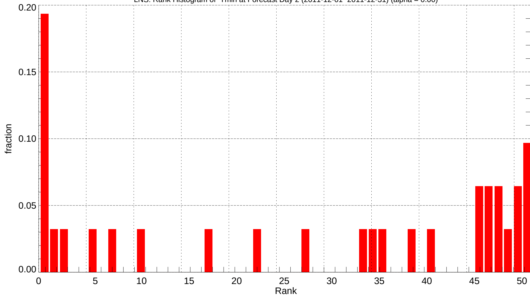
LNS: Rank Histogram of Tmin at Forecast Day 2 (2011-12-01~2011-12-31) (alpha = 0.00)
