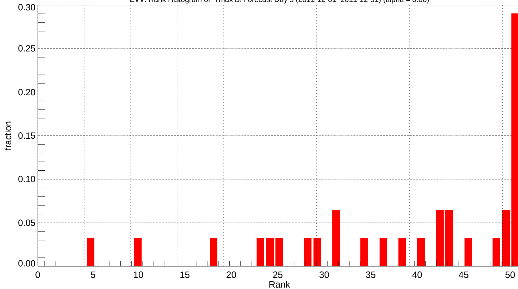
EVV: Rank Histogram of Tmax at Forecast Day 9 (2011-12-01~2011-12-31) (alpha = 0.00)
