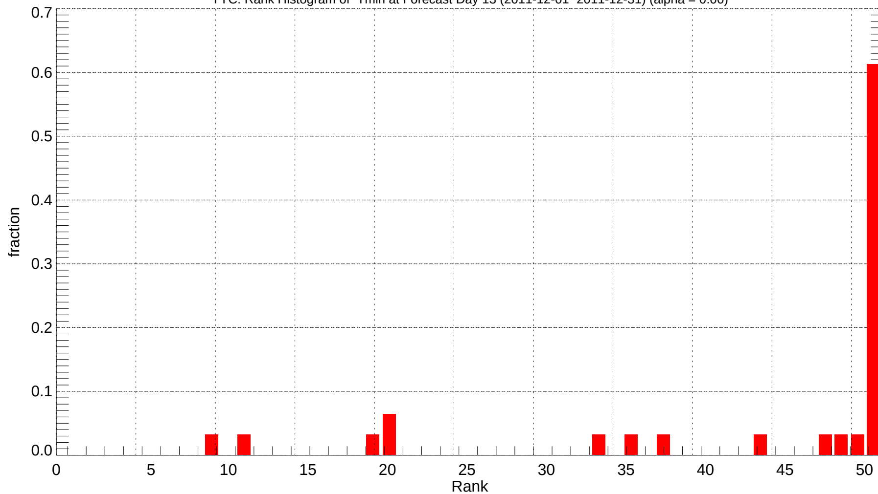
YYC: Rank Histogram of Tmin at Forecast Day 13 (2011-12-01~2011-12-31) (alpha = 0.00)
