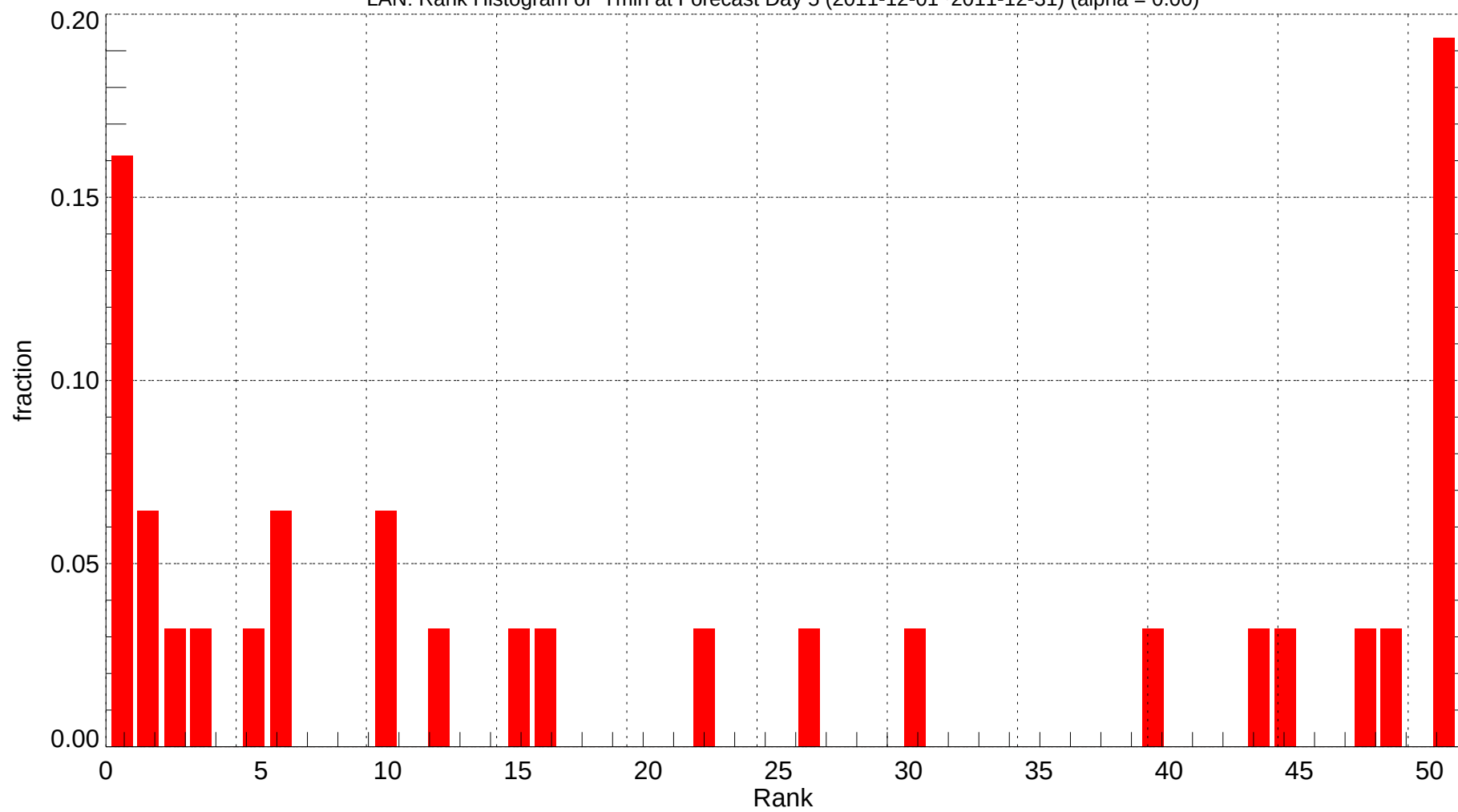
LAN: Rank Histogram of Tmin at Forecast Day 5 (2011-12-01~2011-12-31) (alpha = 0.00)
