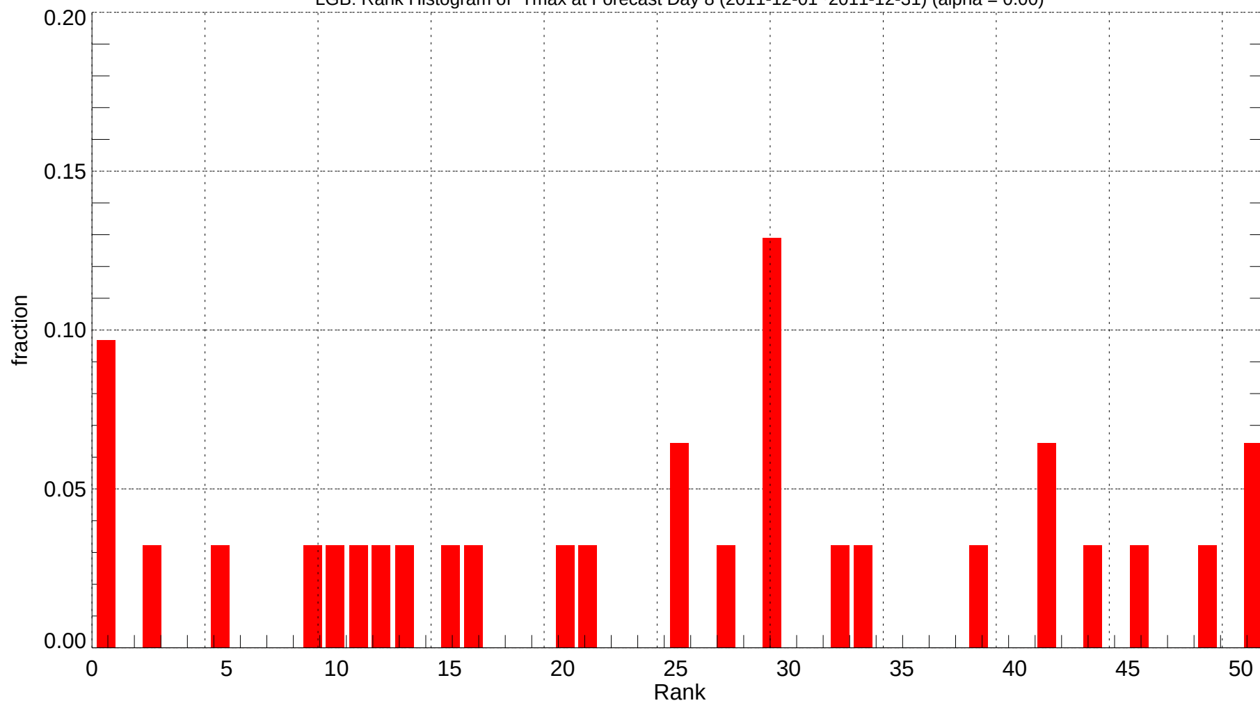
LGB: Rank Histogram of Tmax at Forecast Day 8 (2011-12-01~2011-12-31) (alpha = 0.00)
