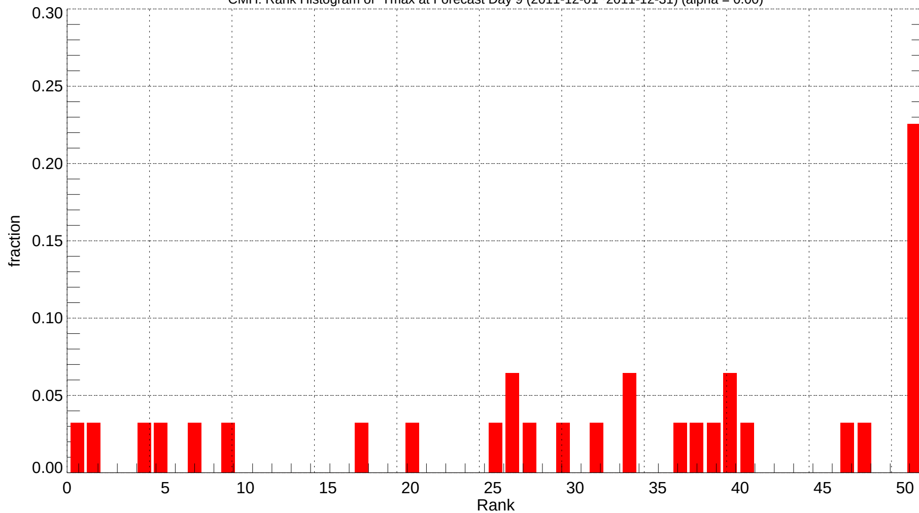
CMH: Rank Histogram of Tmax at Forecast Day 9 (2011-12-01~2011-12-31) (alpha = 0.00)
