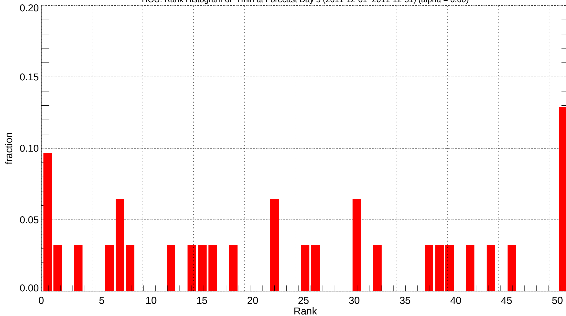
HOU: Rank Histogram of Tmin at Forecast Day 5 (2011-12-01~2011-12-31) (alpha = 0.00)
