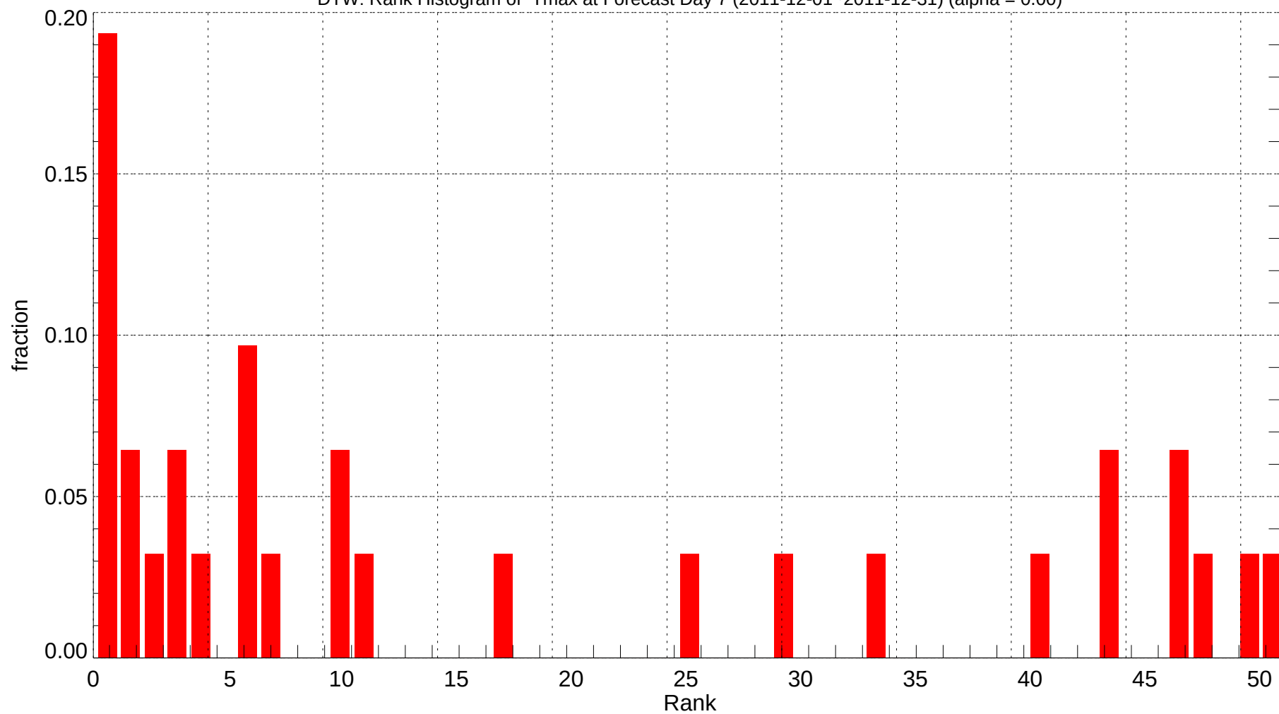
DTW: Rank Histogram of Tmax at Forecast Day 7 (2011-12-01~2011-12-31) (alpha = 0.00)
