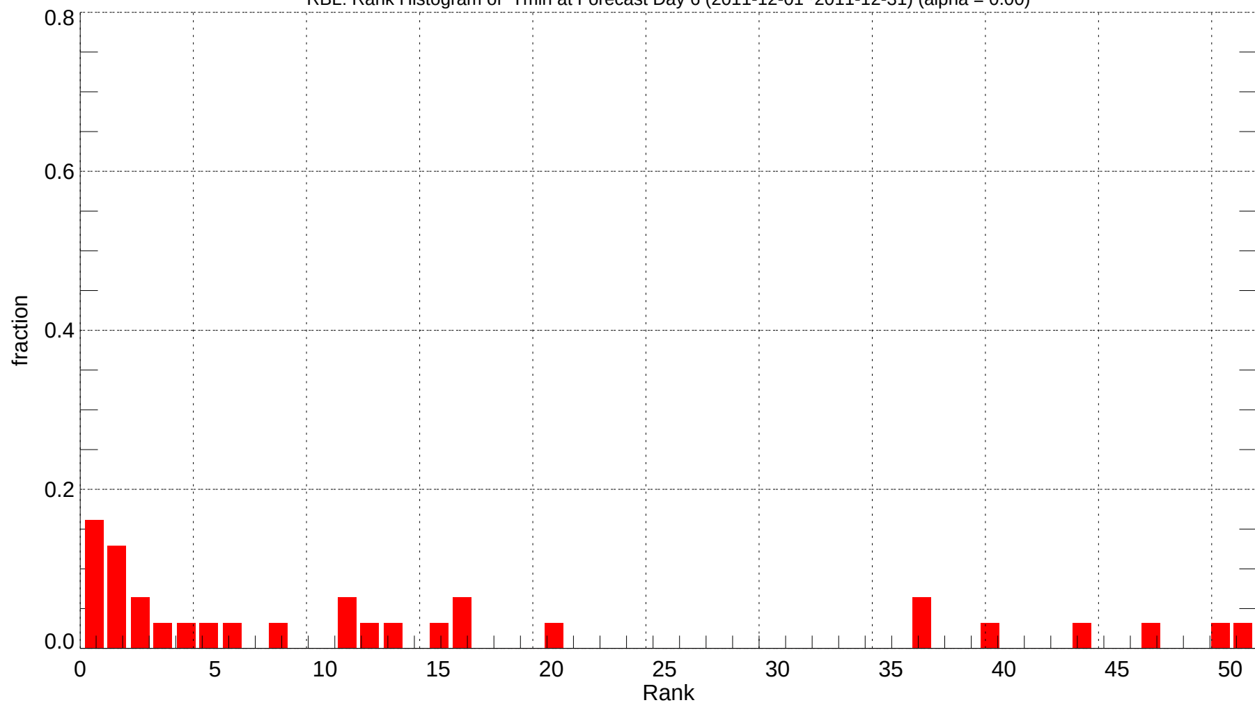
RBL: Rank Histogram of Tmin at Forecast Day 6 (2011-12-01~2011-12-31) (alpha = 0.00)
