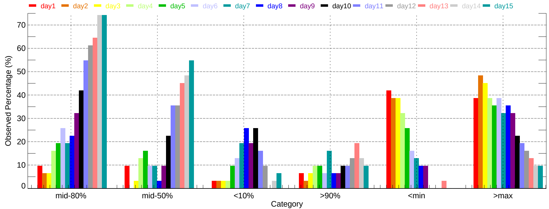
Observed Percentage of Ensembles - YVR: Max Temperature (2011-12-01~2011-12-31)
