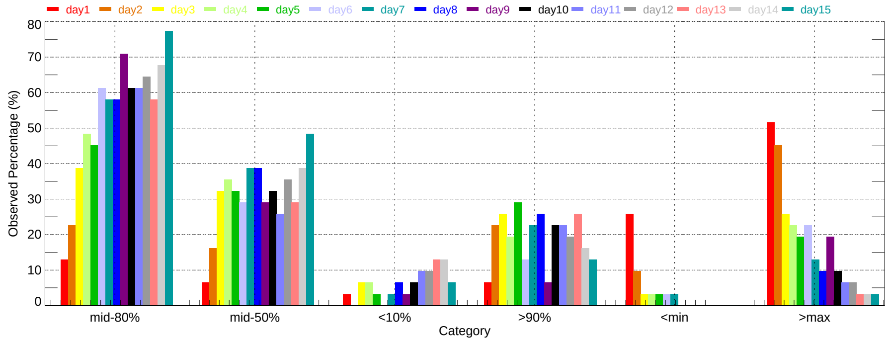
Observed Percentage of Ensembles - SDF: Min Temperature (2011-12-01~2011-12-31)
