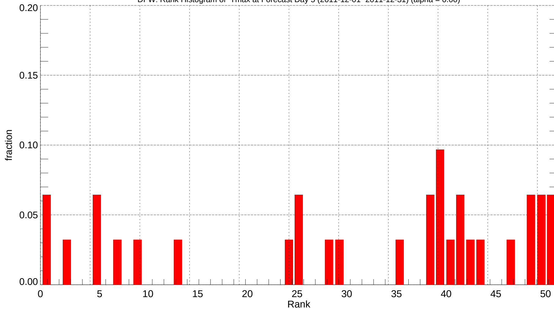
DFW: Rank Histogram of Tmax at Forecast Day 5 (2011-12-01~2011-12-31) (alpha = 0.00)
