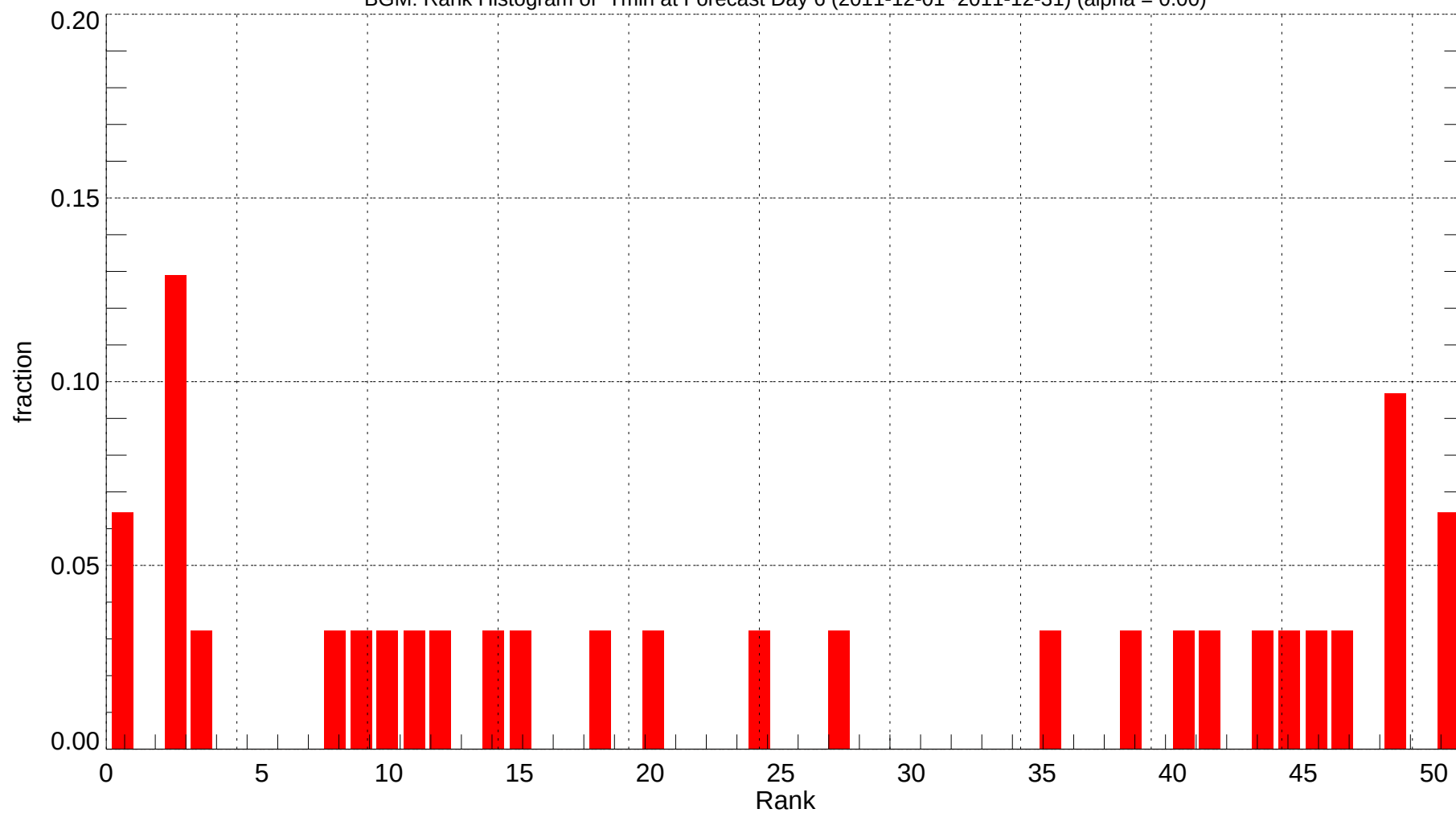
BGM: Rank Histogram of Tmin at Forecast Day 6 (2011-12-01~2011-12-31) (alpha = 0.00)
