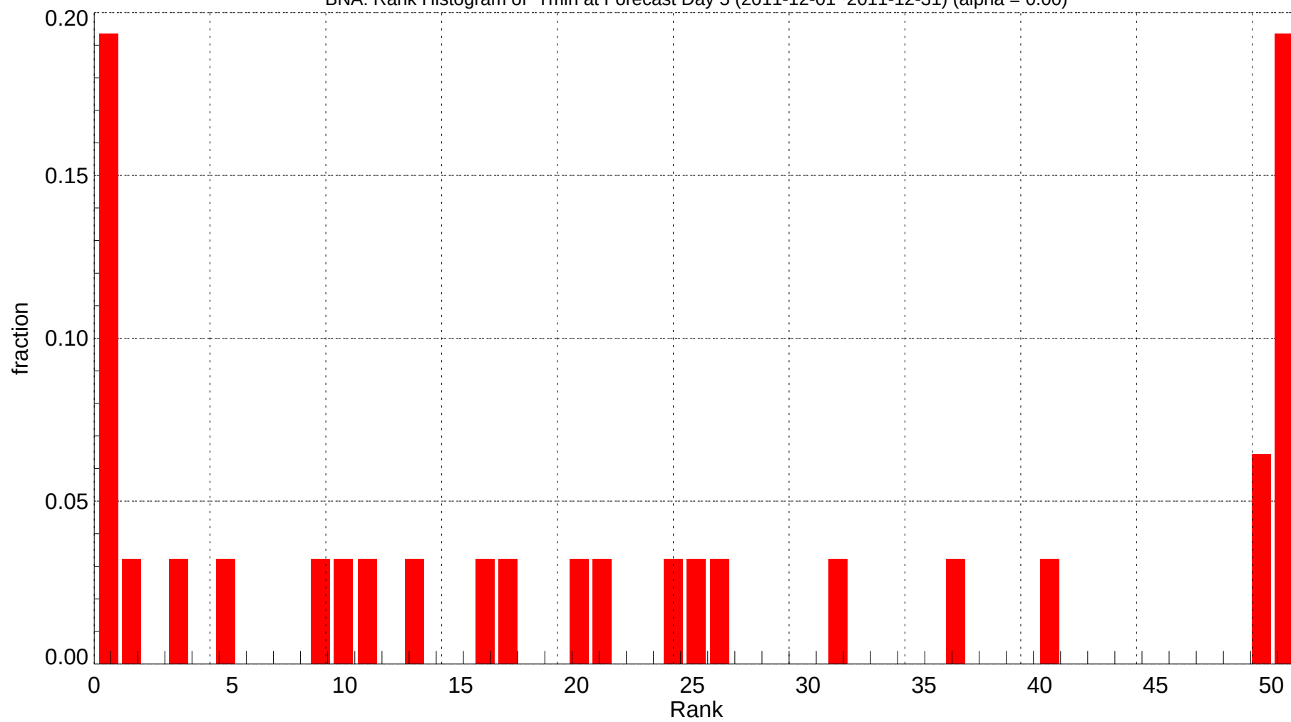
BNA: Rank Histogram of Tmin at Forecast Day 5 (2011-12-01~2011-12-31) (alpha = 0.00)
