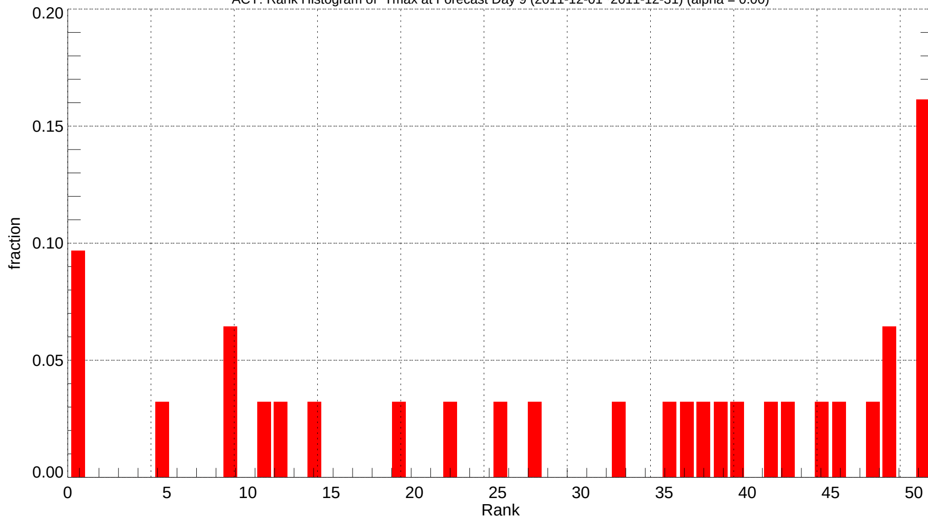
ACY: Rank Histogram of Tmax at Forecast Day 9 (2011-12-01~2011-12-31) (alpha = 0.00)
