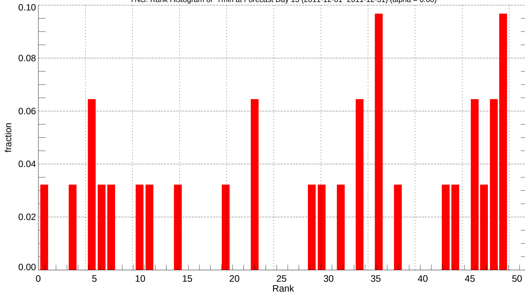
YNG: Rank Histogram of Tmin at Forecast Day 13 (2011-12-01~2011-12-31) (alpha = 0.00)
