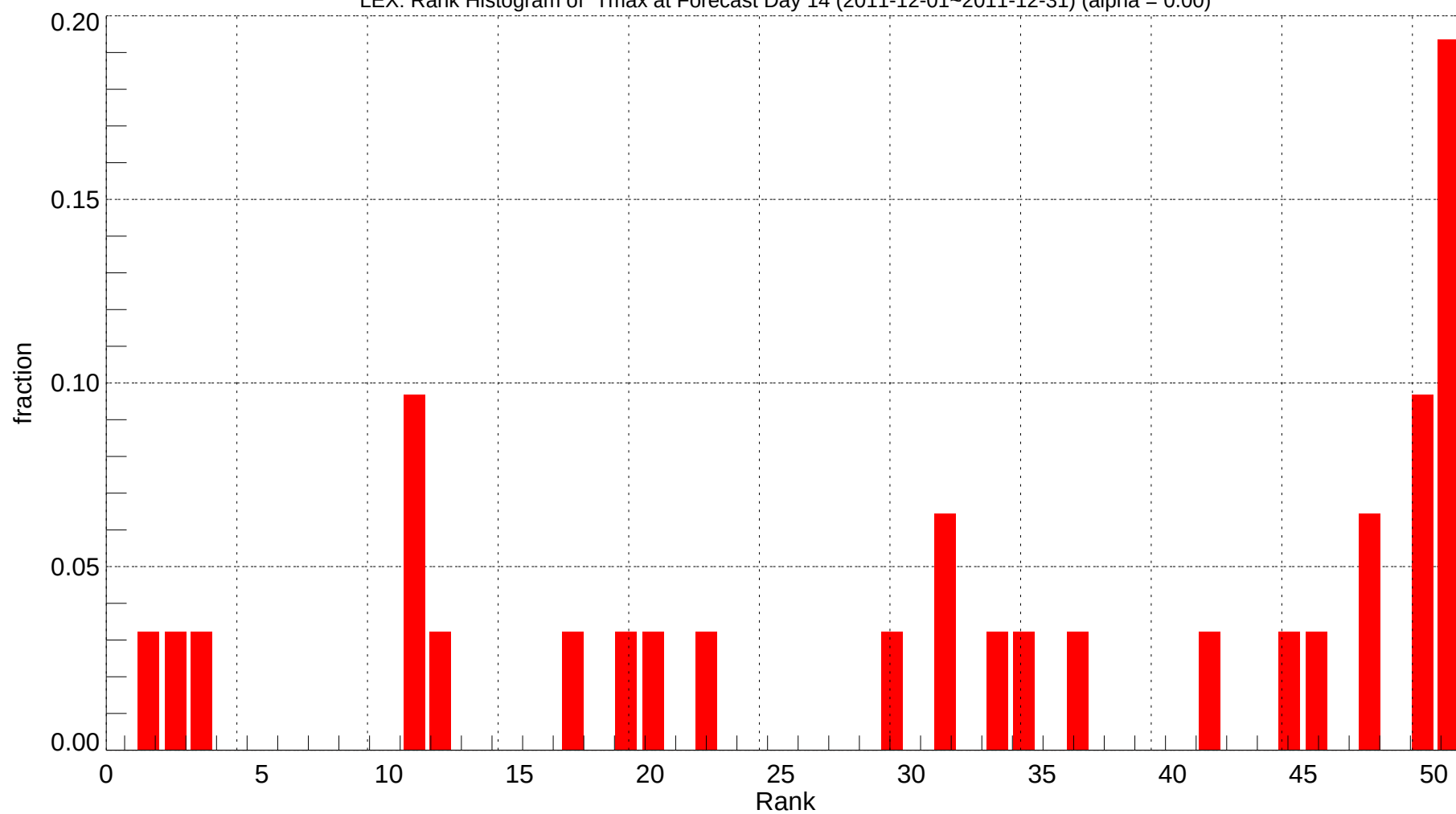
LEX: Rank Histogram of Tmax at Forecast Day 14 (2011-12-01~2011-12-31) (alpha = 0.00)
