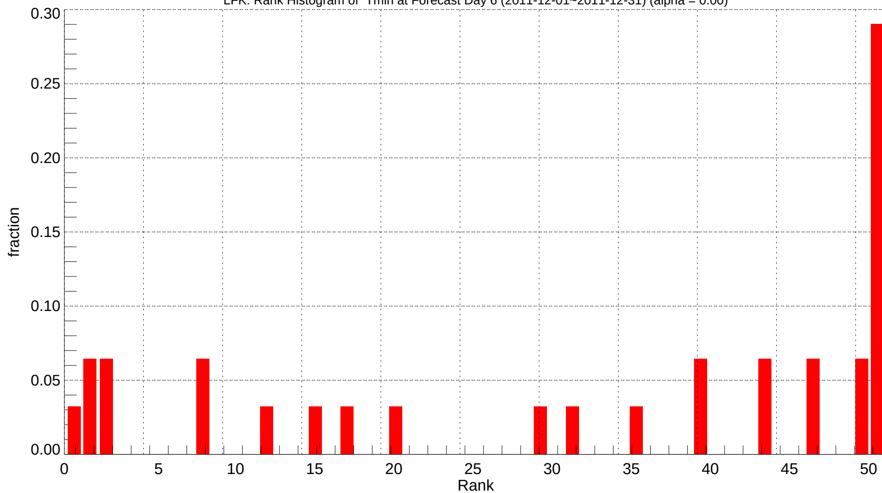
LFK: Rank Histogram of Tmin at Forecast Day 6 (2011-12-01~2011-12-31) (alpha = 0.00)
