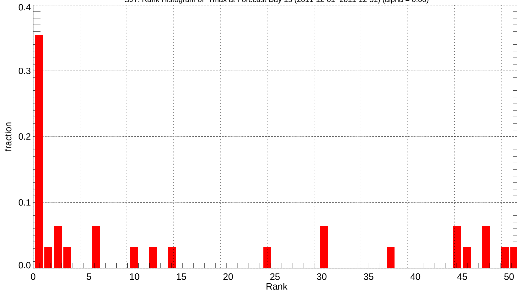
SJT: Rank Histogram of Tmax at Forecast Day 15 (2011-12-01~2011-12-31) (alpha = 0.00)
