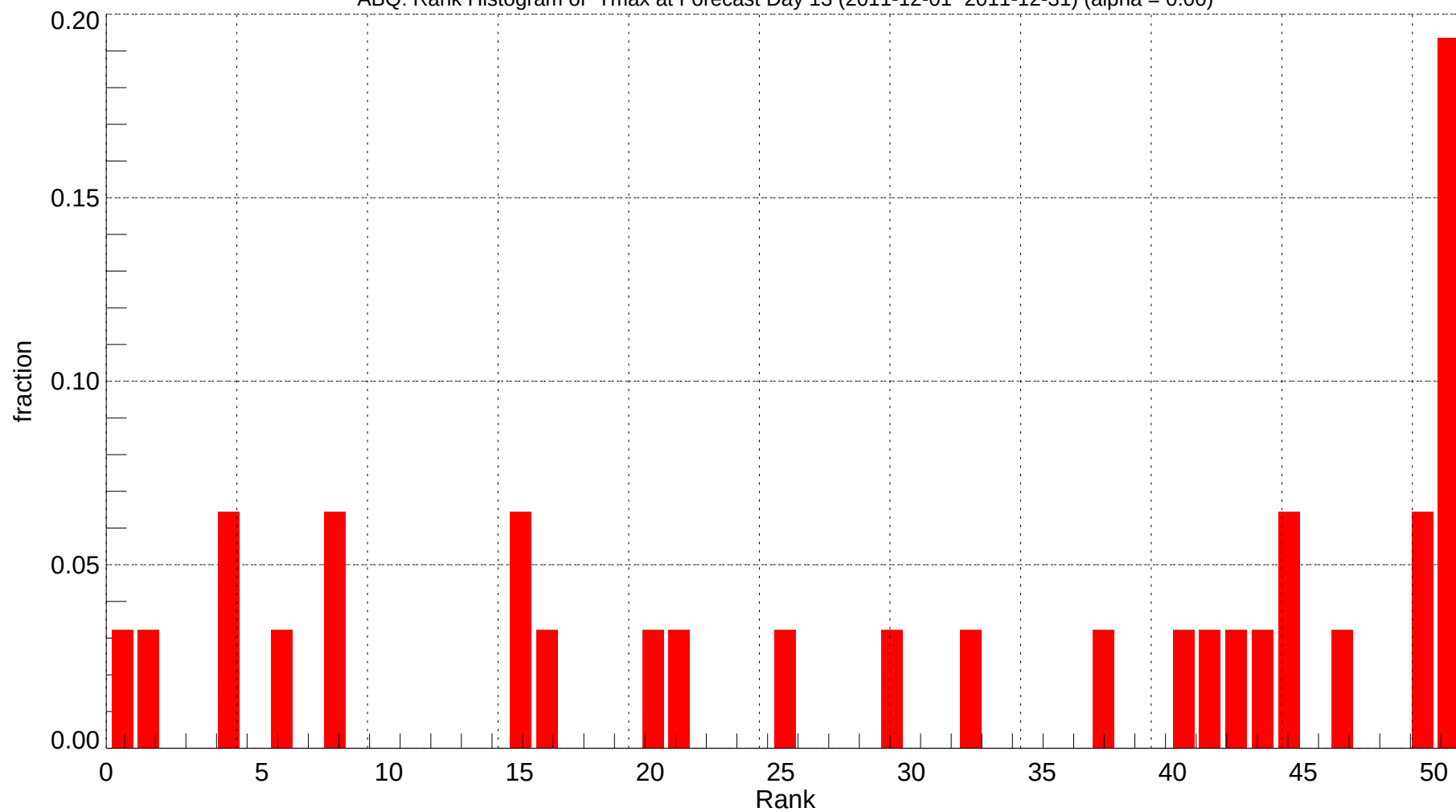
ABQ: Rank Histogram of Tmax at Forecast Day 13 (2011-12-01~2011-12-31) (alpha = 0.00)
