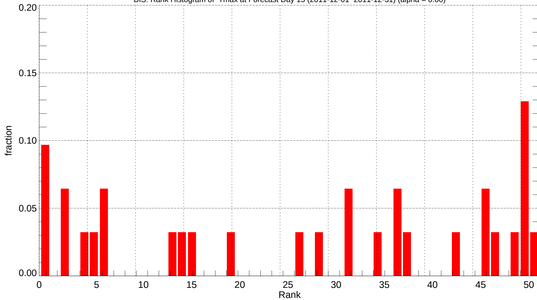
BIS: Rank Histogram of Tmax at Forecast Day 15 (2011-12-01~2011-12-31) (alpha = 0.00)
