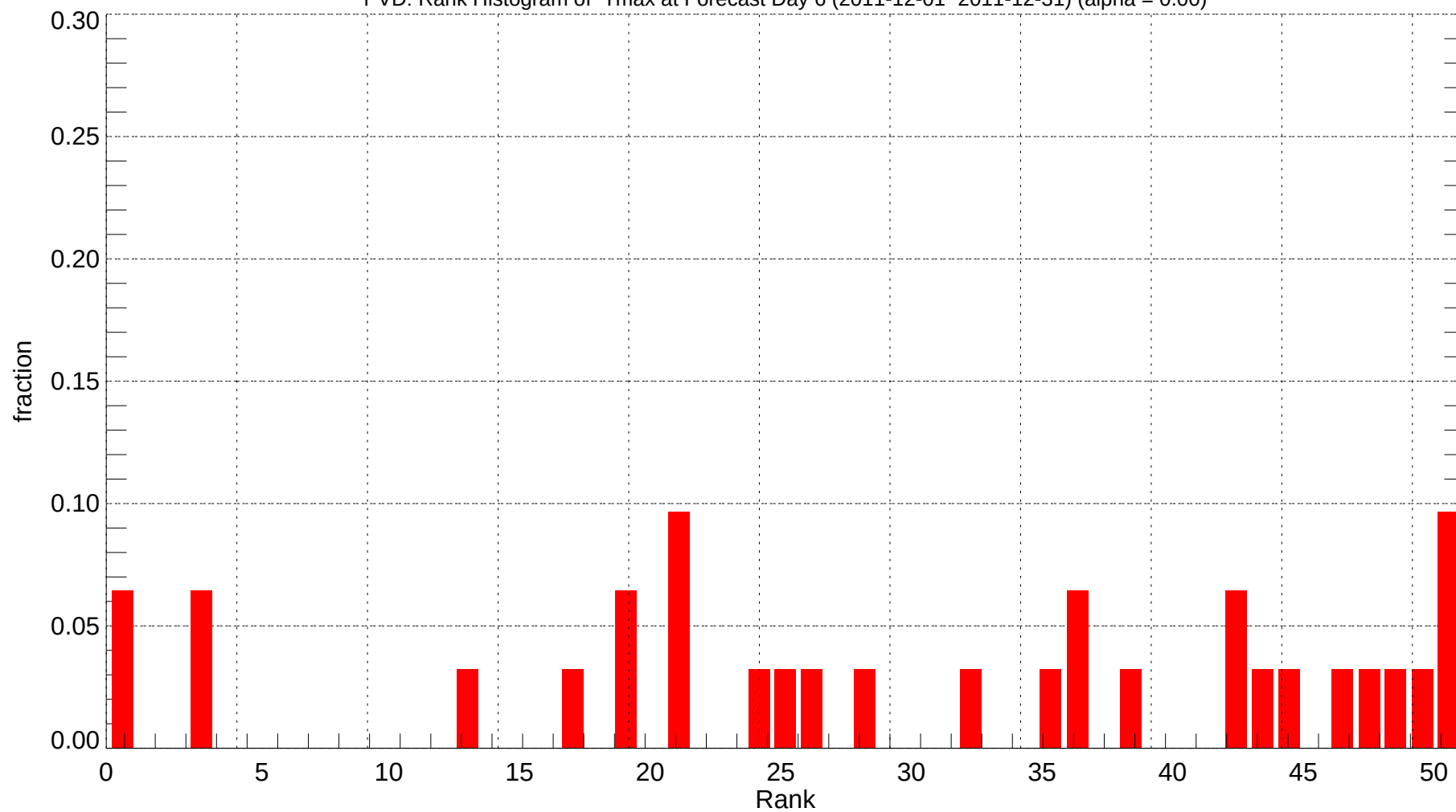
PVD: Rank Histogram of Tmax at Forecast Day 6 (2011-12-01~2011-12-31) (alpha = 0.00)
