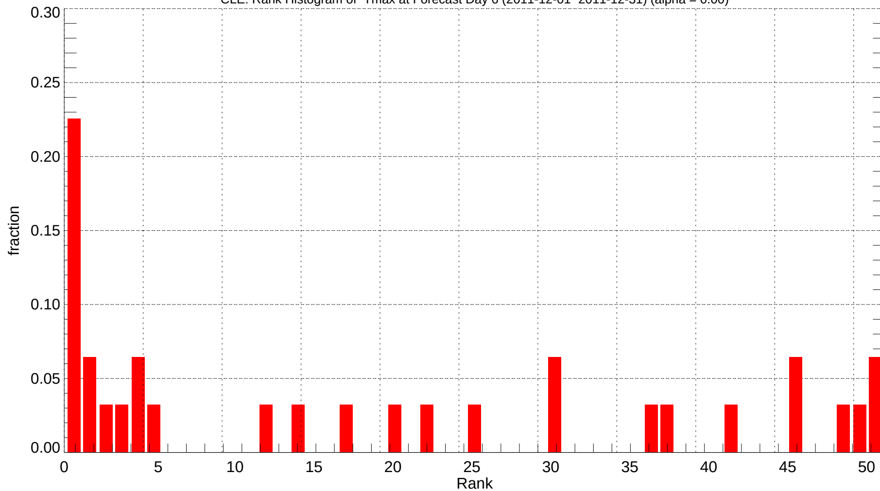
CLE: Rank Histogram of Tmax at Forecast Day 6 (2011-12-01~2011-12-31) (alpha = 0.00)
