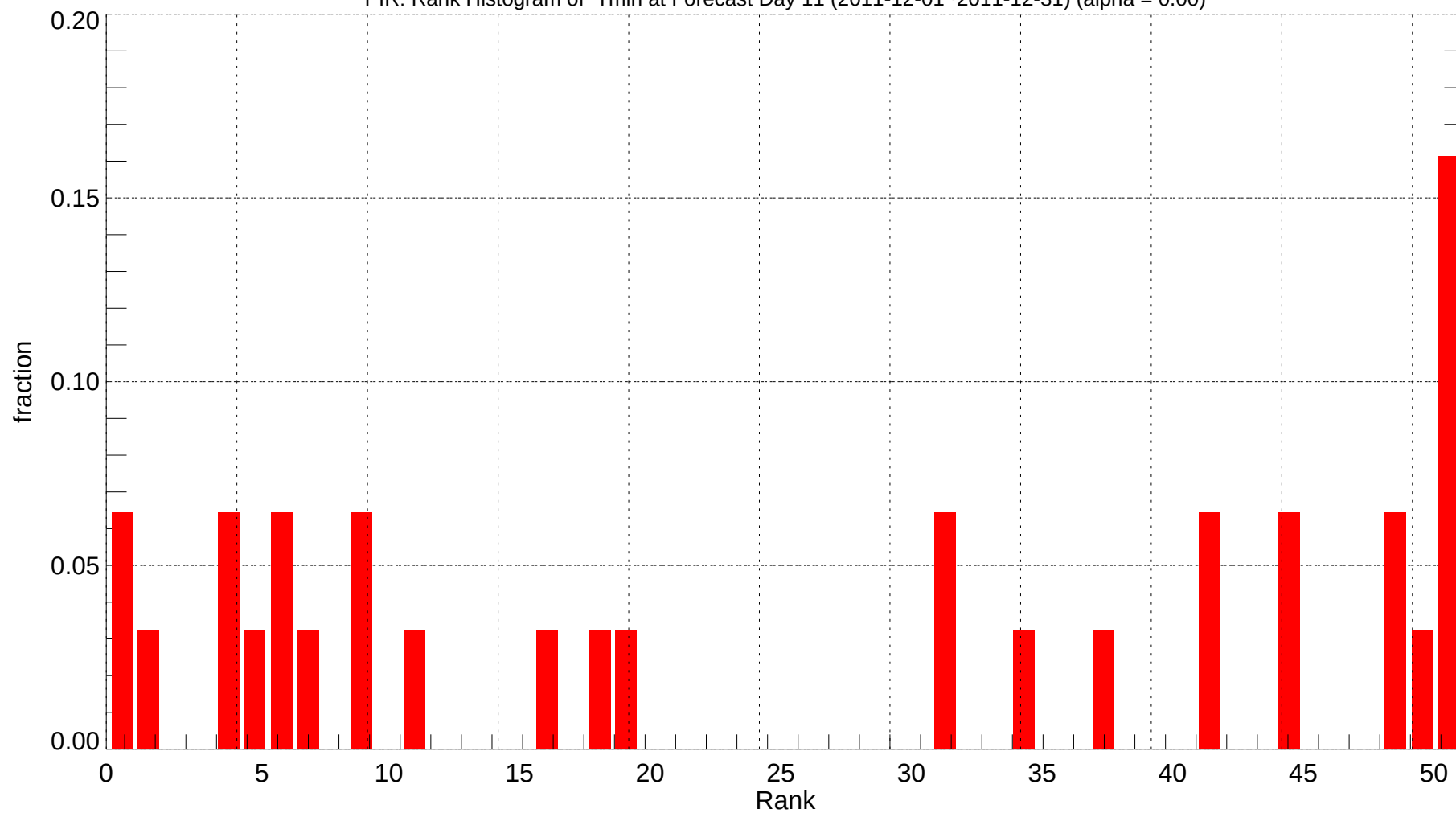
PIR: Rank Histogram of Tmin at Forecast Day 11 (2011-12-01~2011-12-31) (alpha = 0.00)
