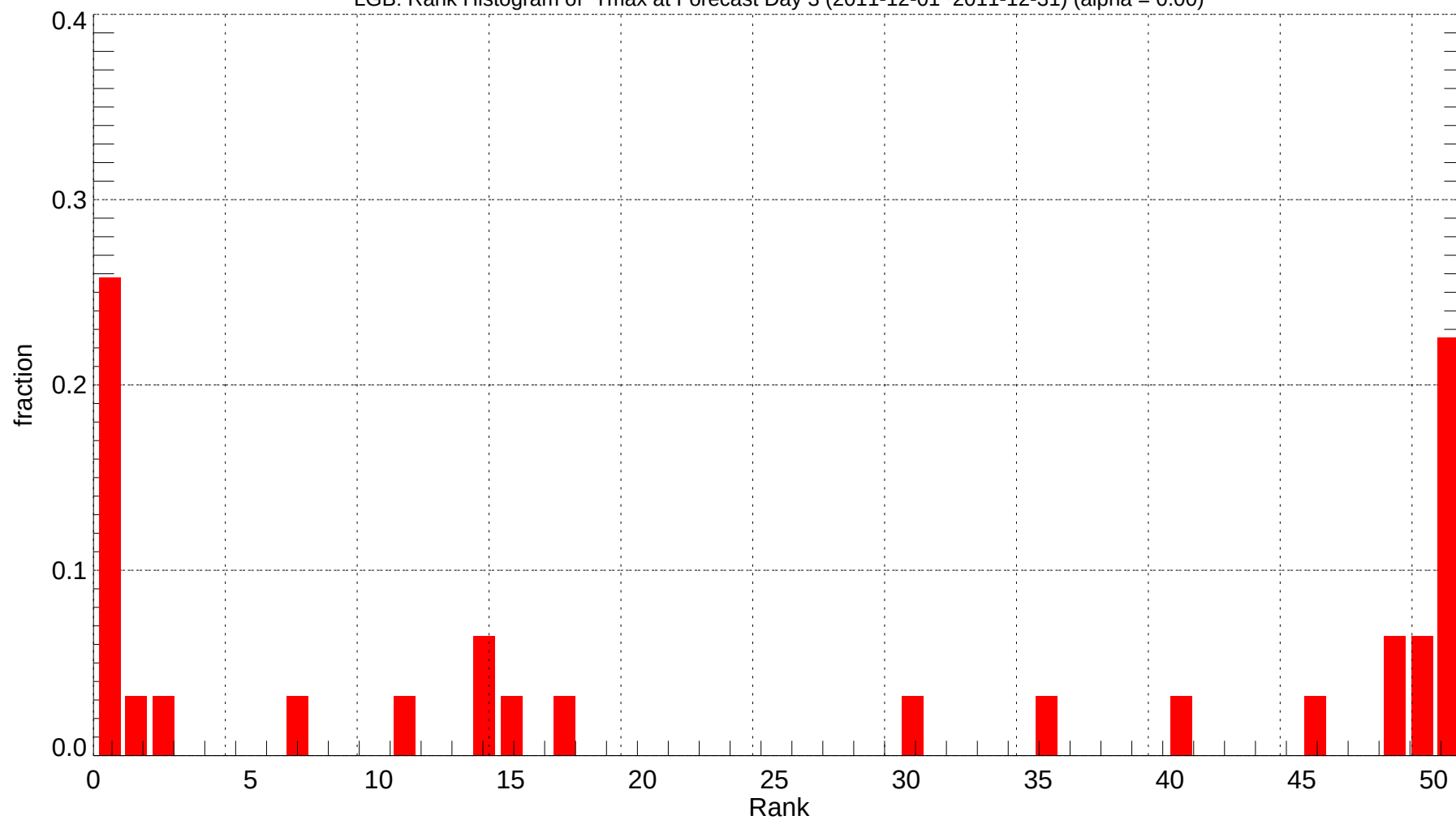
LGB: Rank Histogram of Tmax at Forecast Day 3 (2011-12-01~2011-12-31) (alpha = 0.00)
