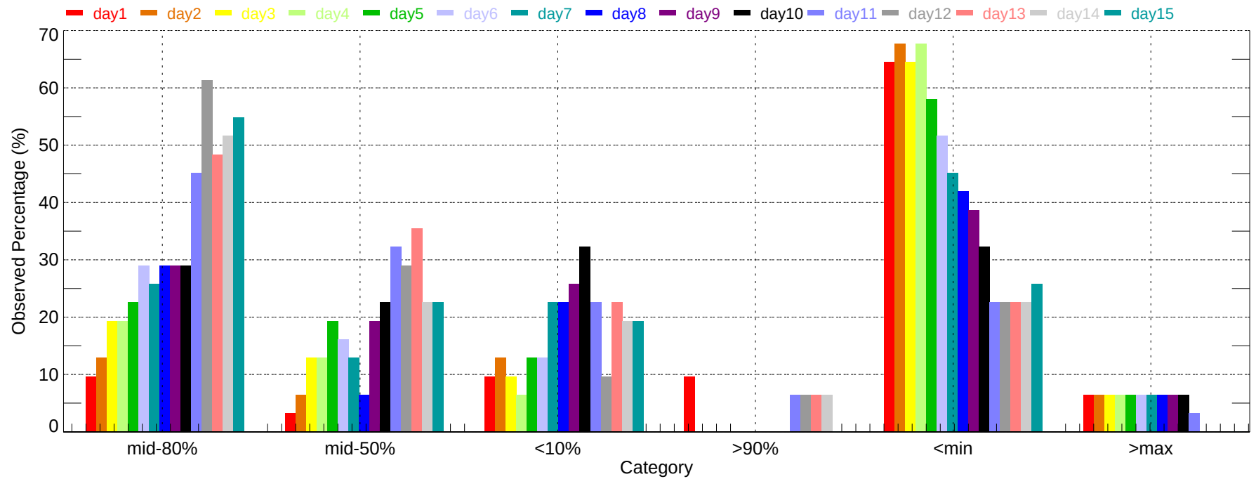
Observed Percentage of Ensembles - RAL: Min Temperature (2011-12-01~2011-12-31)
