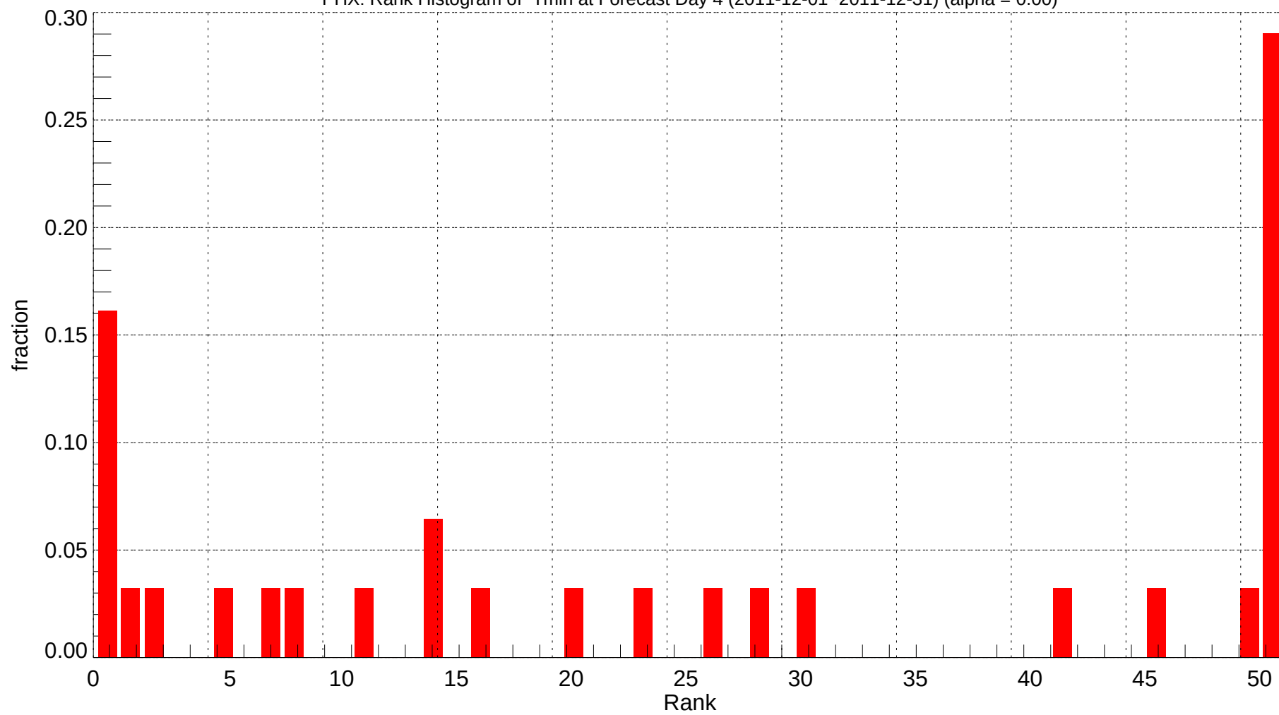
PHX: Rank Histogram of Tmin at Forecast Day 4 (2011-12-01~2011-12-31) (alpha = 0.00)
