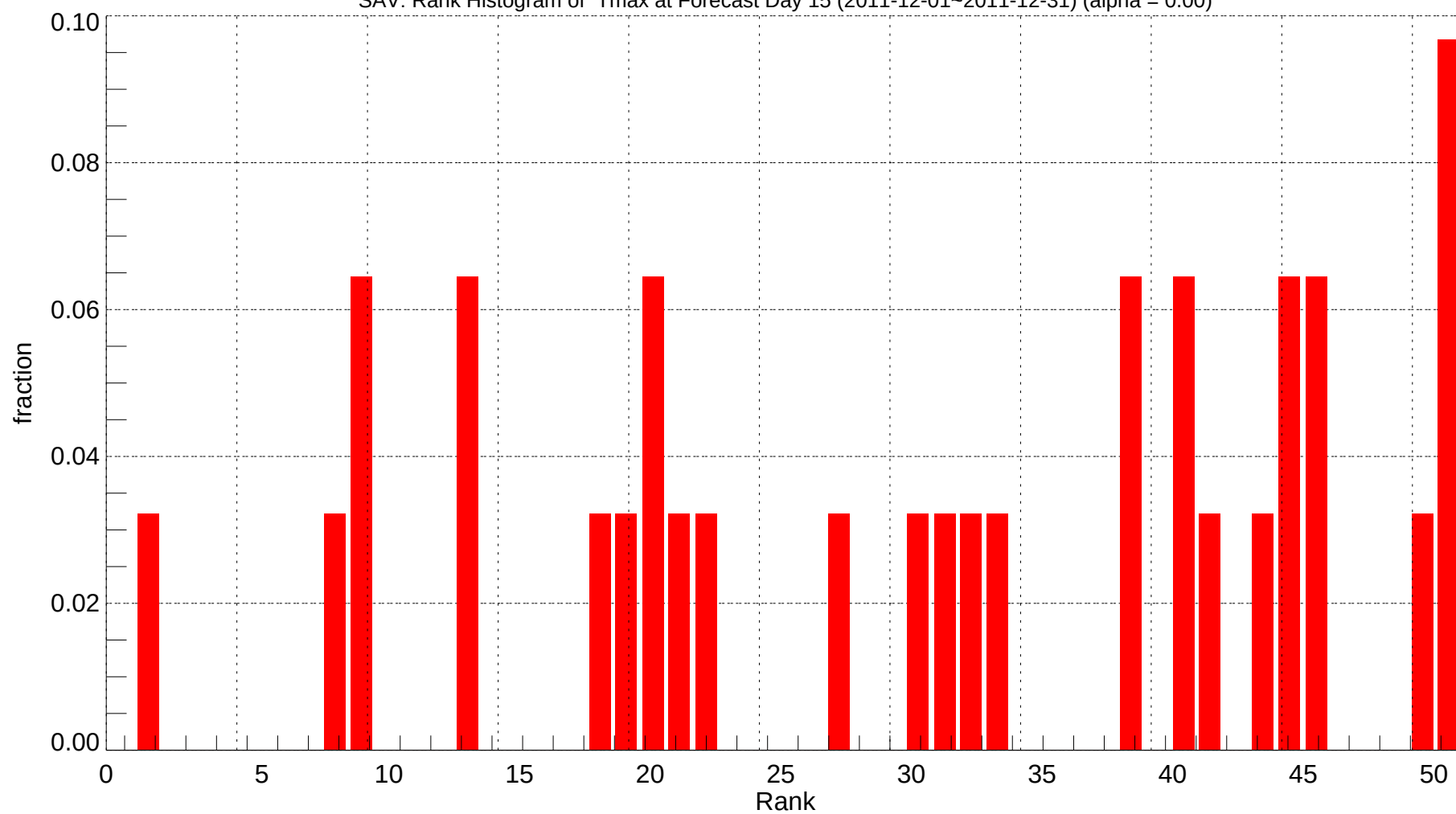
SAV: Rank Histogram of Tmax at Forecast Day 15 (2011-12-01~2011-12-31) (alpha = 0.00)
