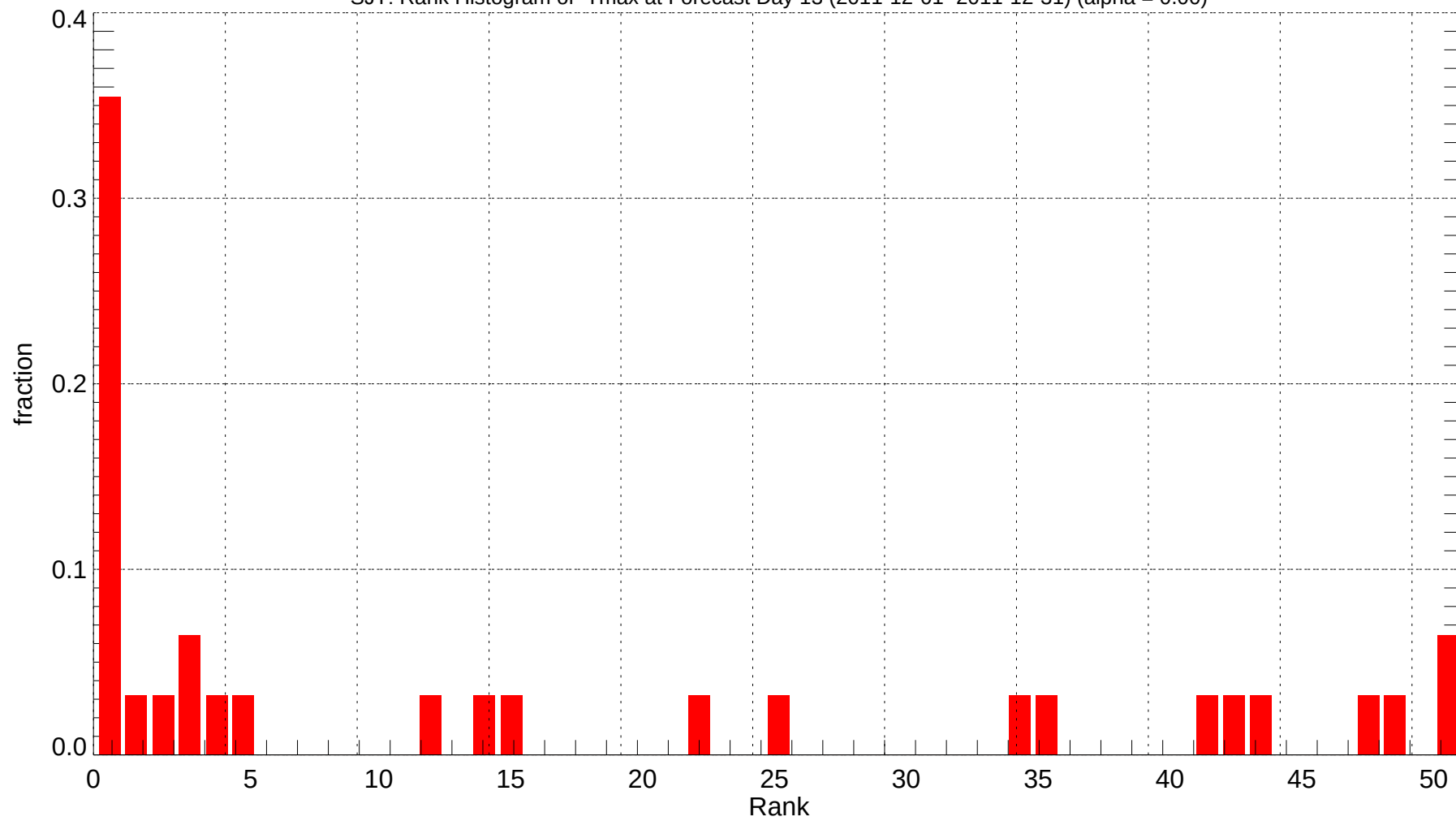
SJT: Rank Histogram of Tmax at Forecast Day 13 (2011-12-01~2011-12-31) (alpha = 0.00)
