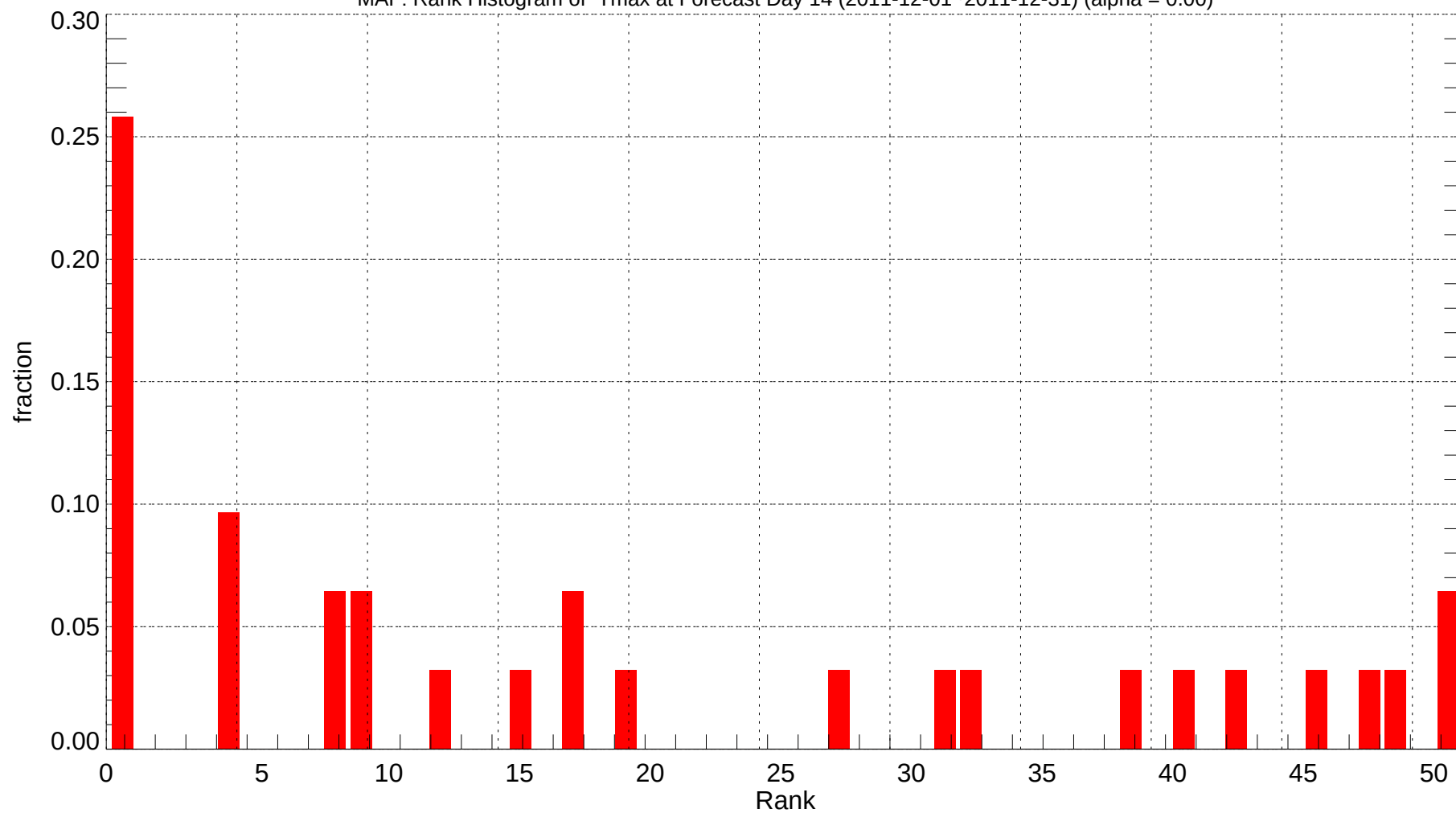
MAF: Rank Histogram of Tmax at Forecast Day 14 (2011-12-01~2011-12-31) (alpha = 0.00)
