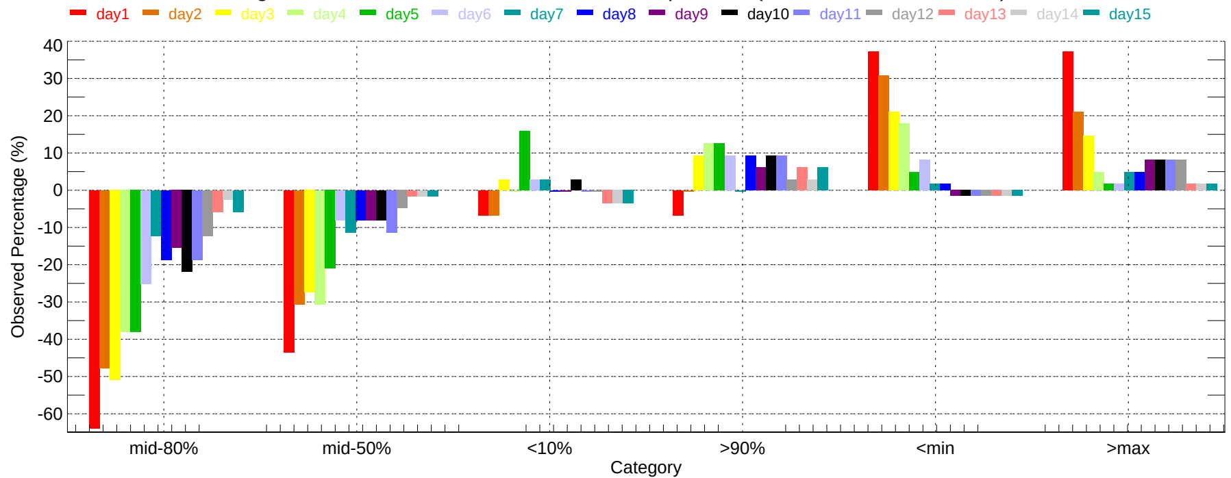
Observed Percentage Deviation of Ensembles - IPT: Min Temperature (2011-12-01~2011-12-31)
