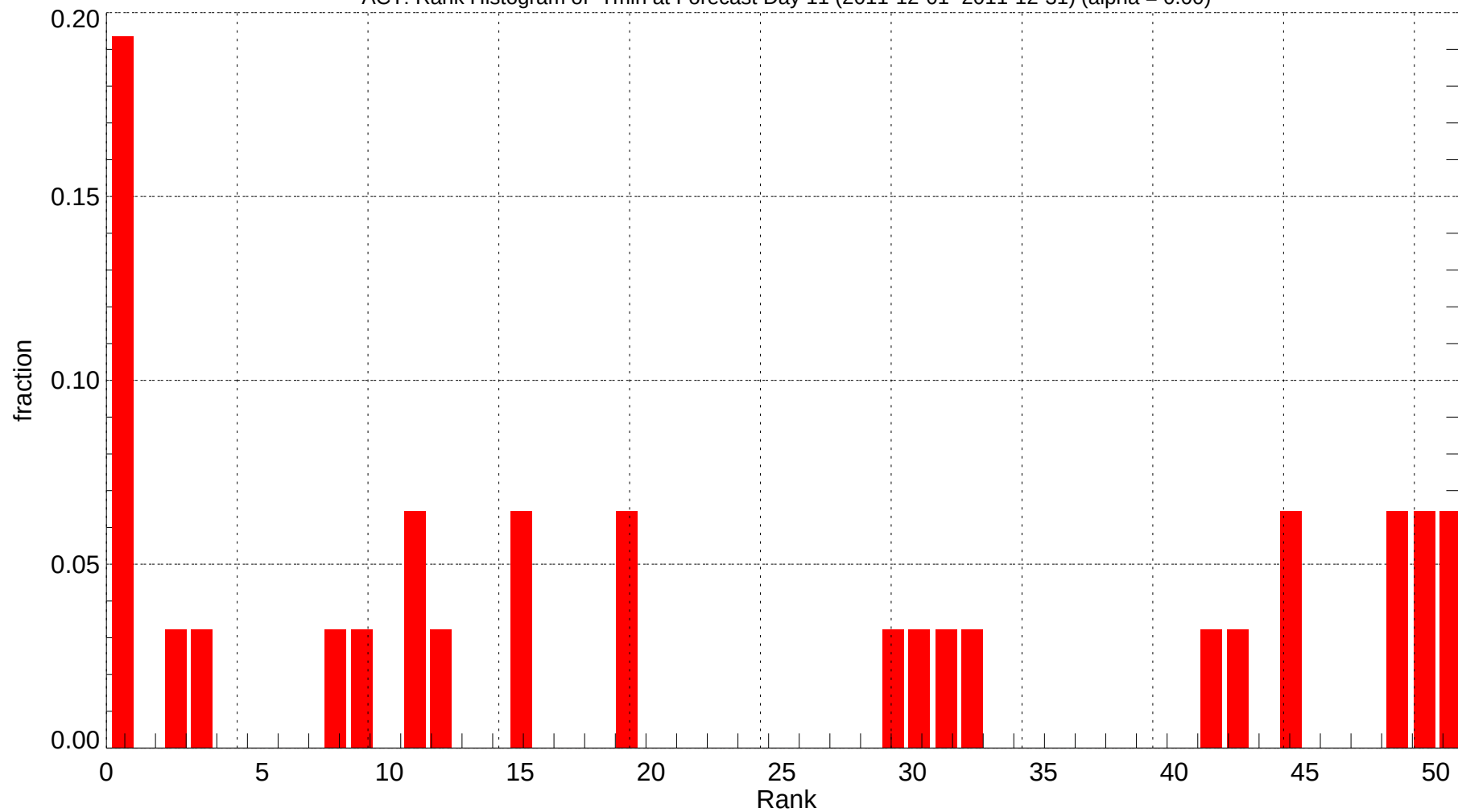
ACT: Rank Histogram of Tmin at Forecast Day 11 (2011-12-01~2011-12-31) (alpha = 0.00)
