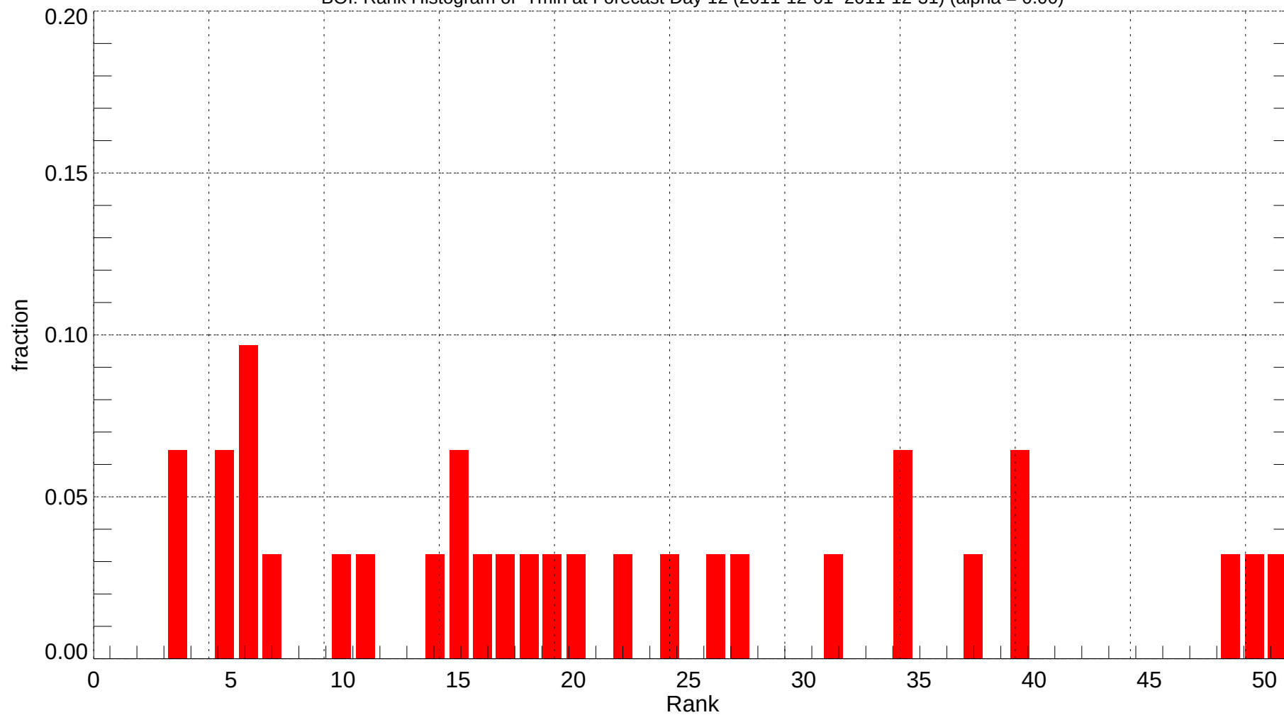
BOI: Rank Histogram of Tmin at Forecast Day 12 (2011-12-01~2011-12-31) (alpha = 0.00)
