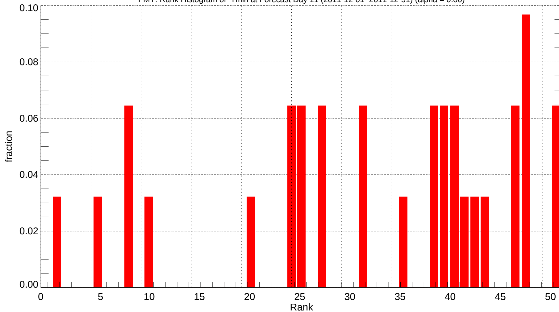
FMY: Rank Histogram of Tmin at Forecast Day 11 (2011-12-01~2011-12-31) (alpha = 0.00)
