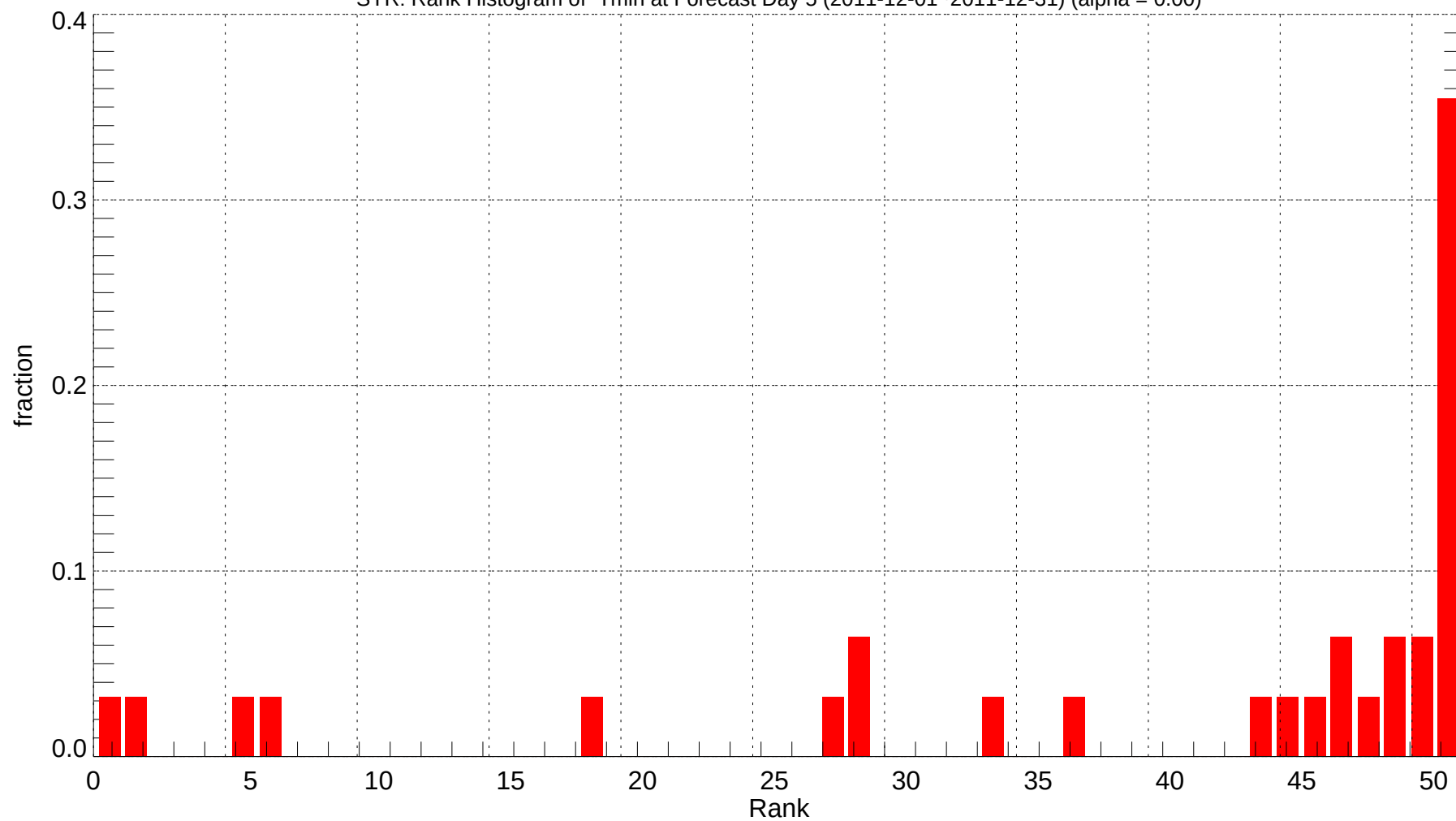
SYR: Rank Histogram of Tmin at Forecast Day 5 (2011-12-01~2011-12-31) (alpha = 0.00)
