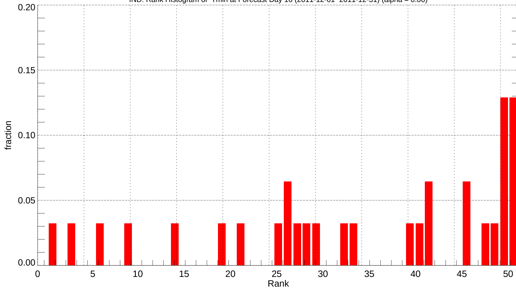
IND: Rank Histogram of Tmin at Forecast Day 10 (2011-12-01~2011-12-31) (alpha = 0.00)
