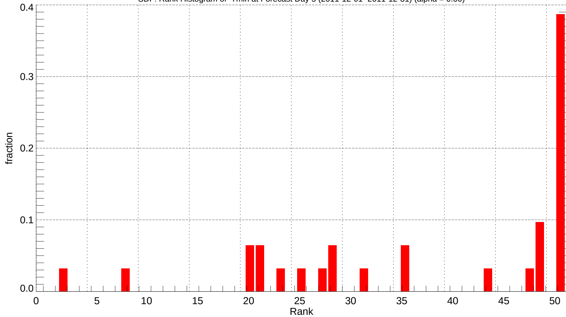
SDF: Rank Histogram of Tmin at Forecast Day 5 (2011-12-01~2011-12-31) (alpha = 0.00)
