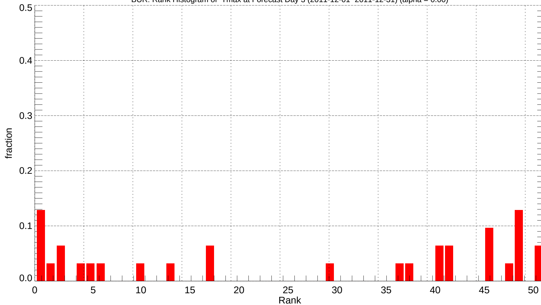
BUR: Rank Histogram of Tmax at Forecast Day 3 (2011-12-01~2011-12-31) (alpha = 0.00)
