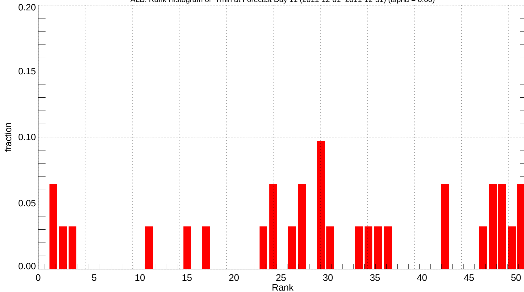
ALB: Rank Histogram of Tmin at Forecast Day 11 (2011-12-01~2011-12-31) (alpha = 0.00)
