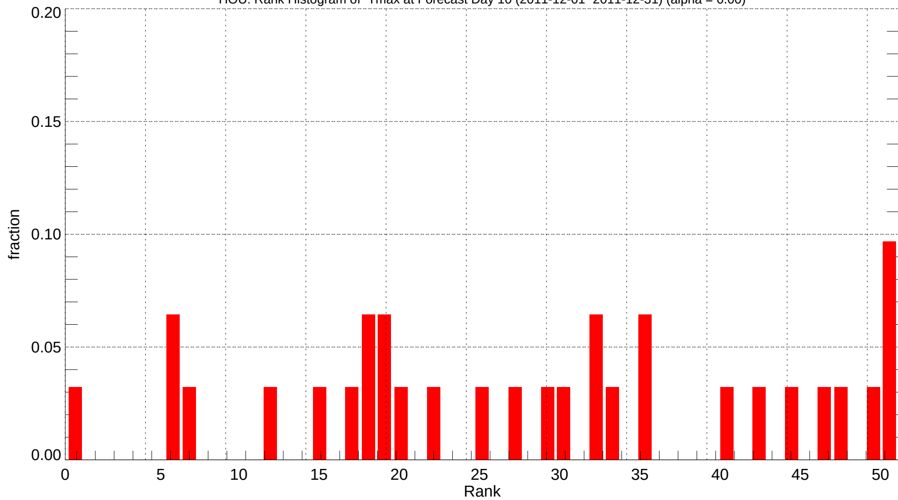
HOU: Rank Histogram of Tmax at Forecast Day 10 (2011-12-01~2011-12-31) (alpha = 0.00)
