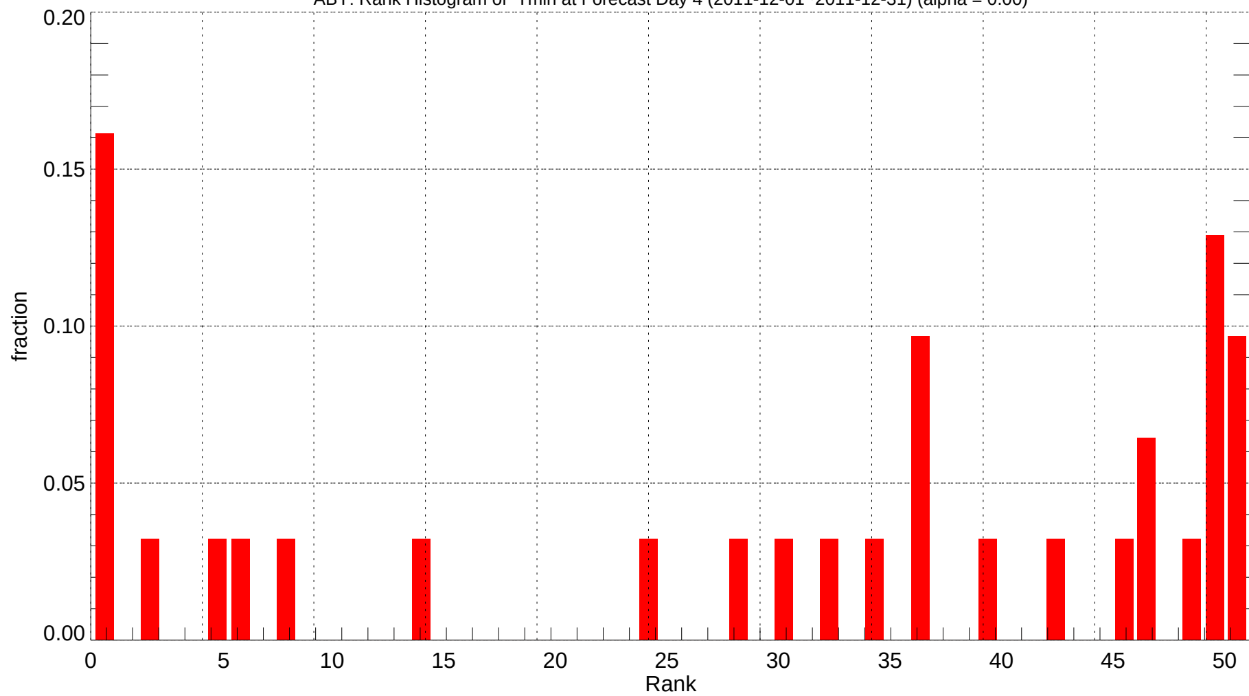
ABY: Rank Histogram of Tmin at Forecast Day 4 (2011-12-01~2011-12-31) (alpha = 0.00)
