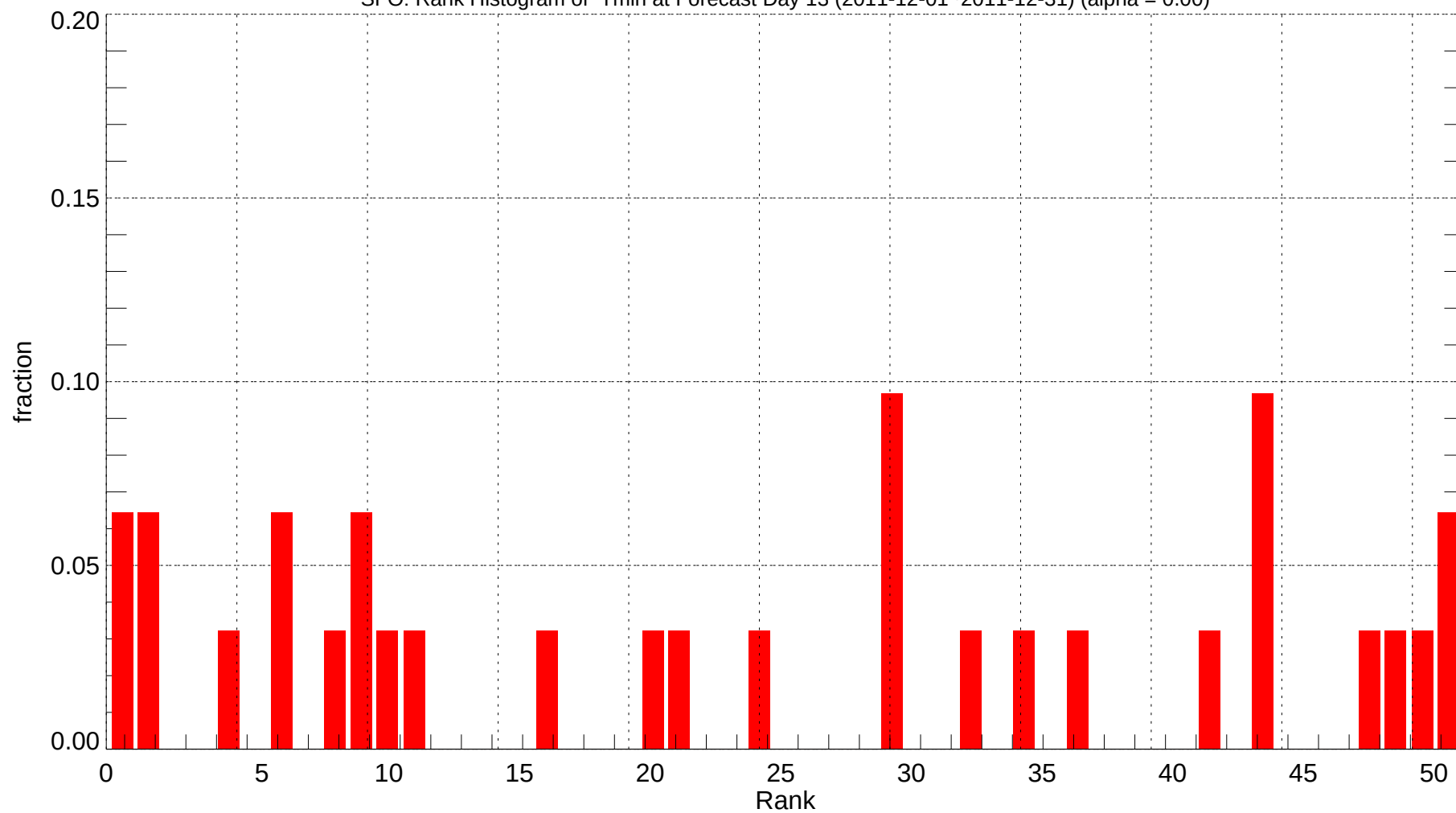
SFO: Rank Histogram of Tmin at Forecast Day 13 (2011-12-01~2011-12-31) (alpha = 0.00)
