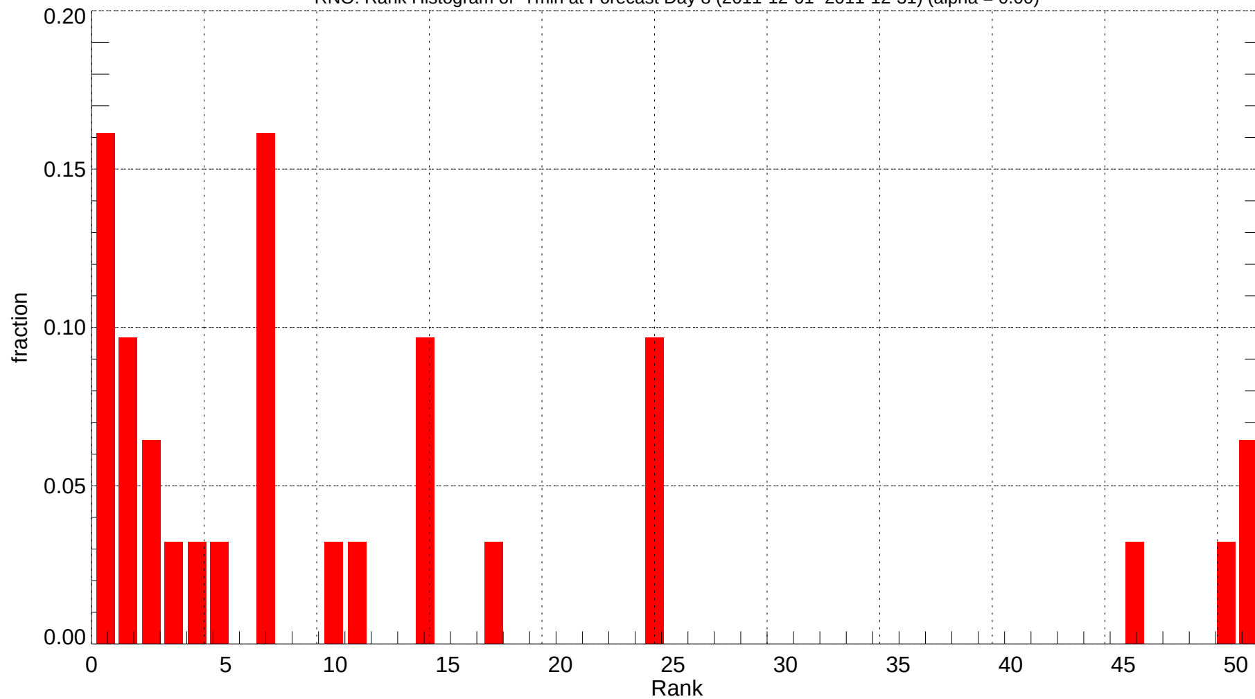
RNO: Rank Histogram of Tmin at Forecast Day 8 (2011-12-01~2011-12-31) (alpha = 0.00)
