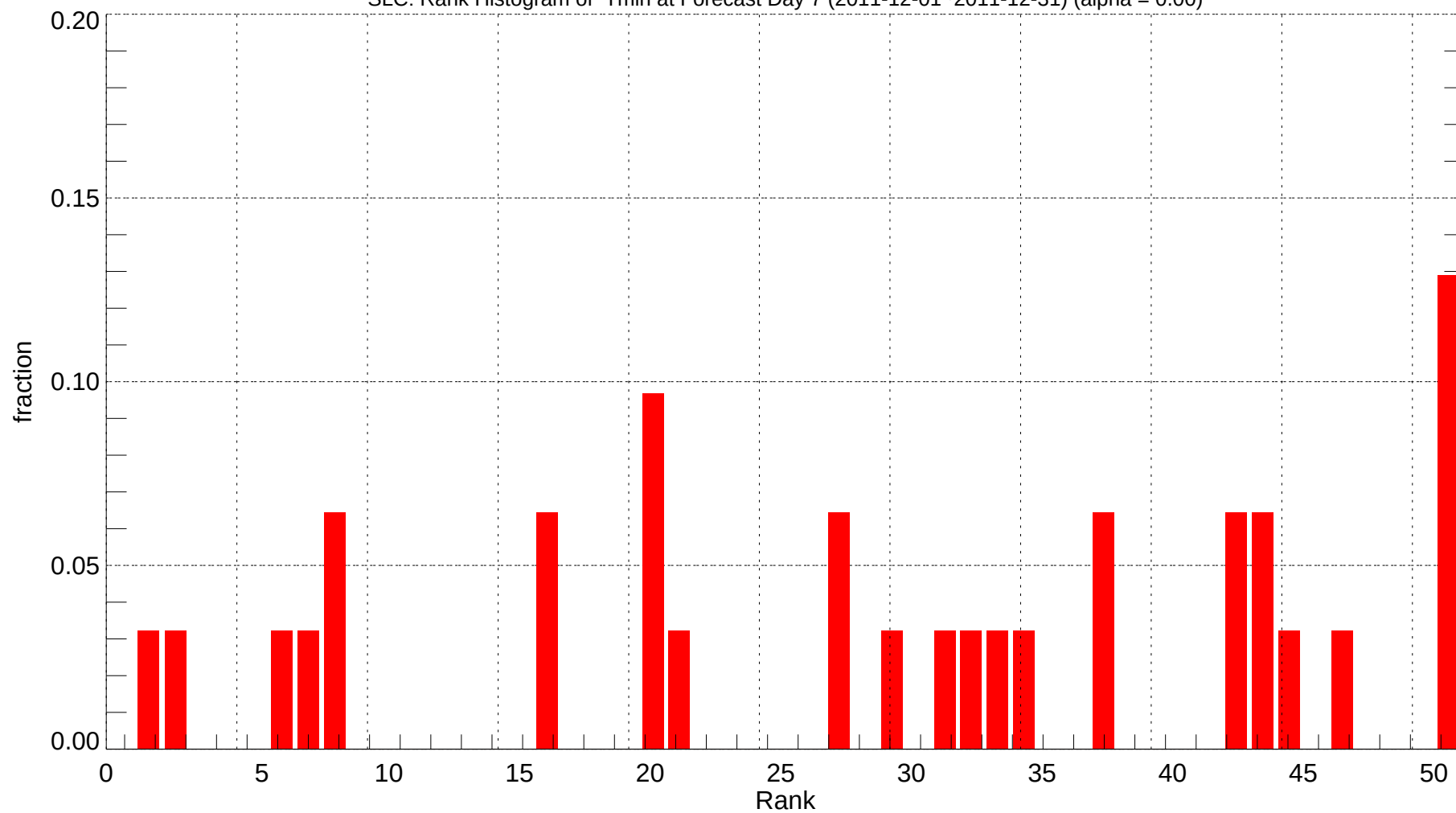
SLC: Rank Histogram of Tmin at Forecast Day 7 (2011-12-01~2011-12-31) (alpha = 0.00)
