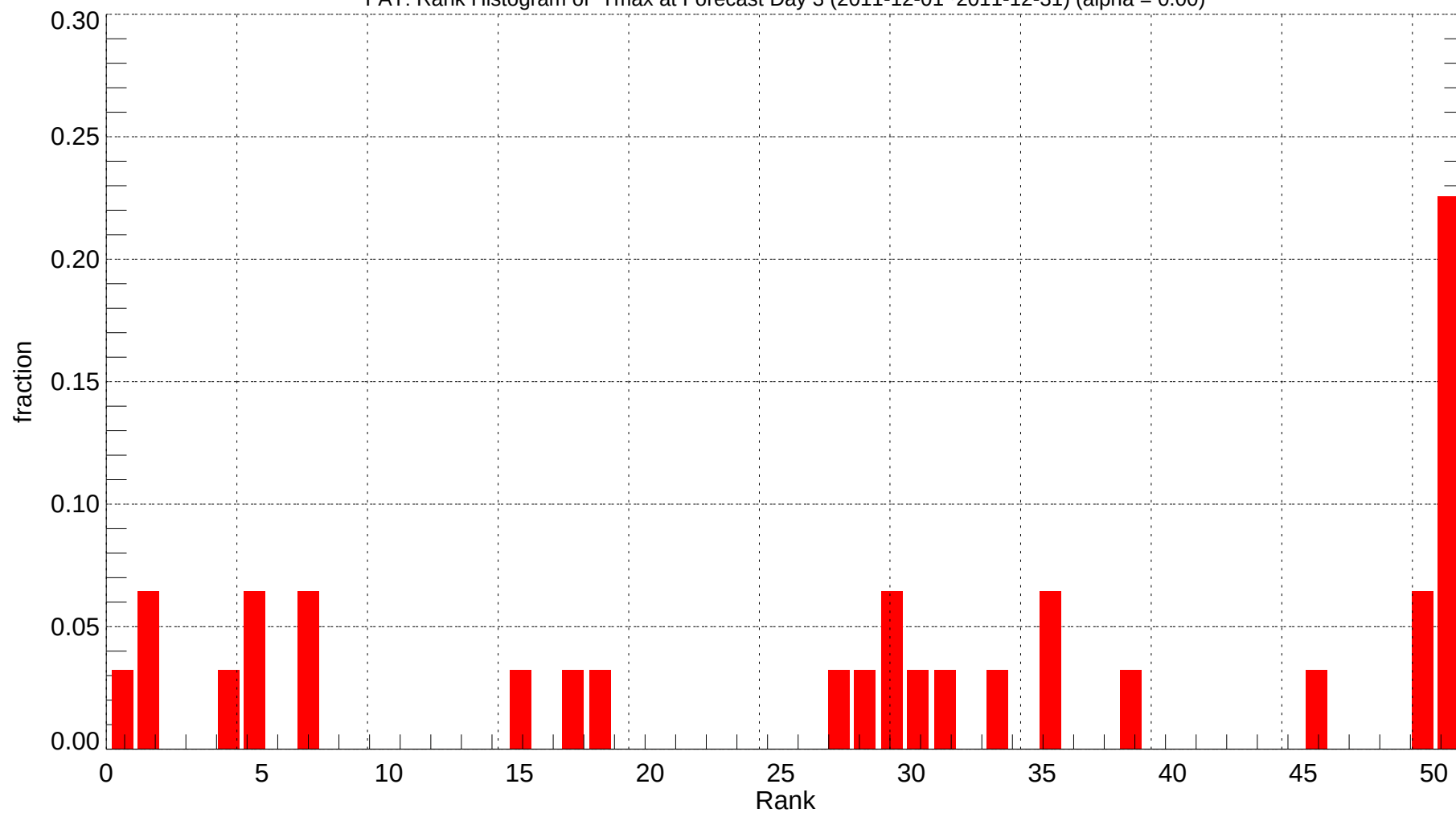
FAT: Rank Histogram of Tmax at Forecast Day 3 (2011-12-01~2011-12-31) (alpha = 0.00)
