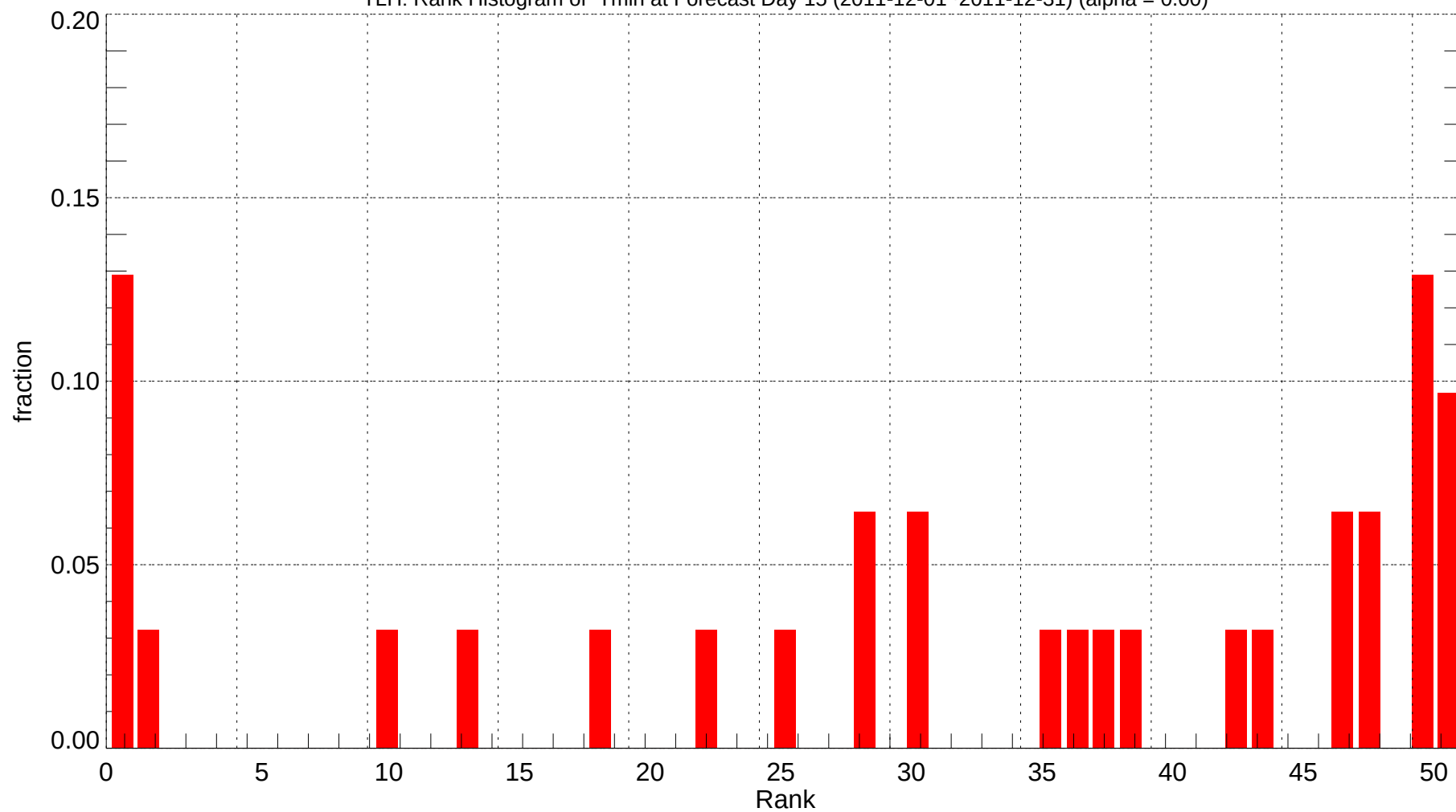
TLH: Rank Histogram of Tmin at Forecast Day 15 (2011-12-01~2011-12-31) (alpha = 0.00)
