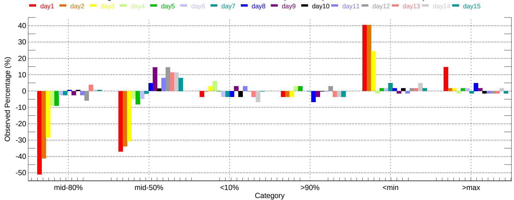
Observed Percentage Deviation of Ensembles - MAF: Min Temperature (2011-12-01~2011-12-31)
