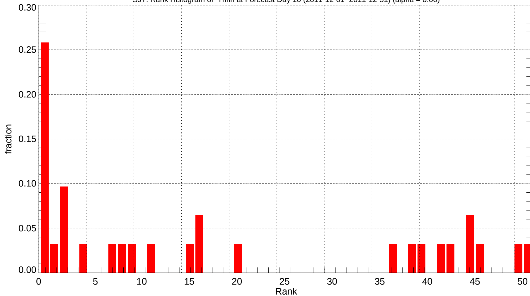
SJT: Rank Histogram of Tmin at Forecast Day 10 (2011-12-01~2011-12-31) (alpha = 0.00)
