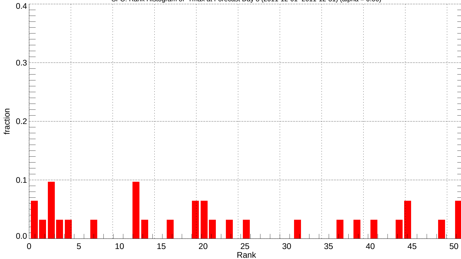
SFO: Rank Histogram of Tmax at Forecast Day 8 (2011-12-01~2011-12-31) (alpha = 0.00)
