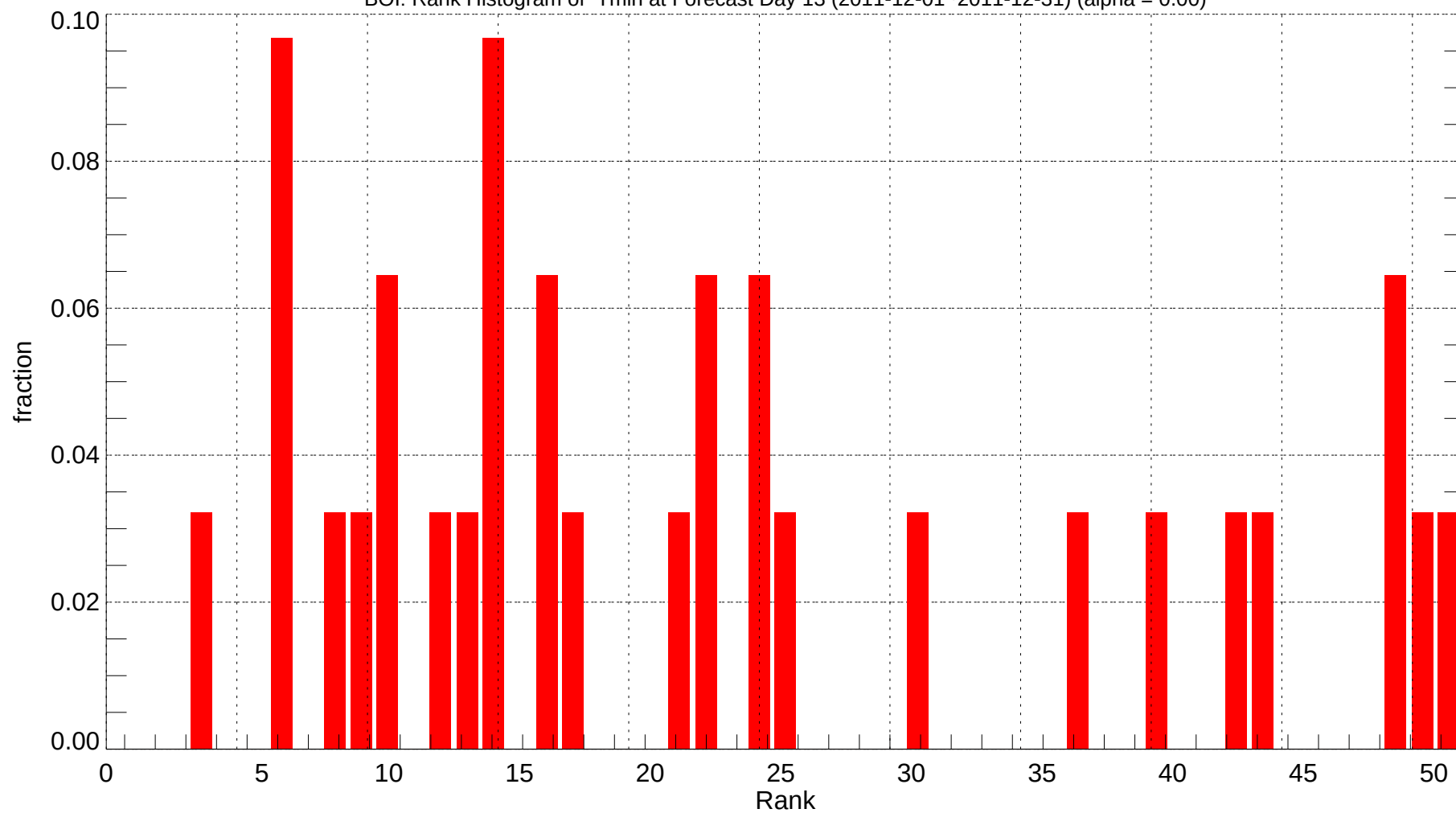
BOI: Rank Histogram of Tmin at Forecast Day 13 (2011-12-01~2011-12-31) (alpha = 0.00)
