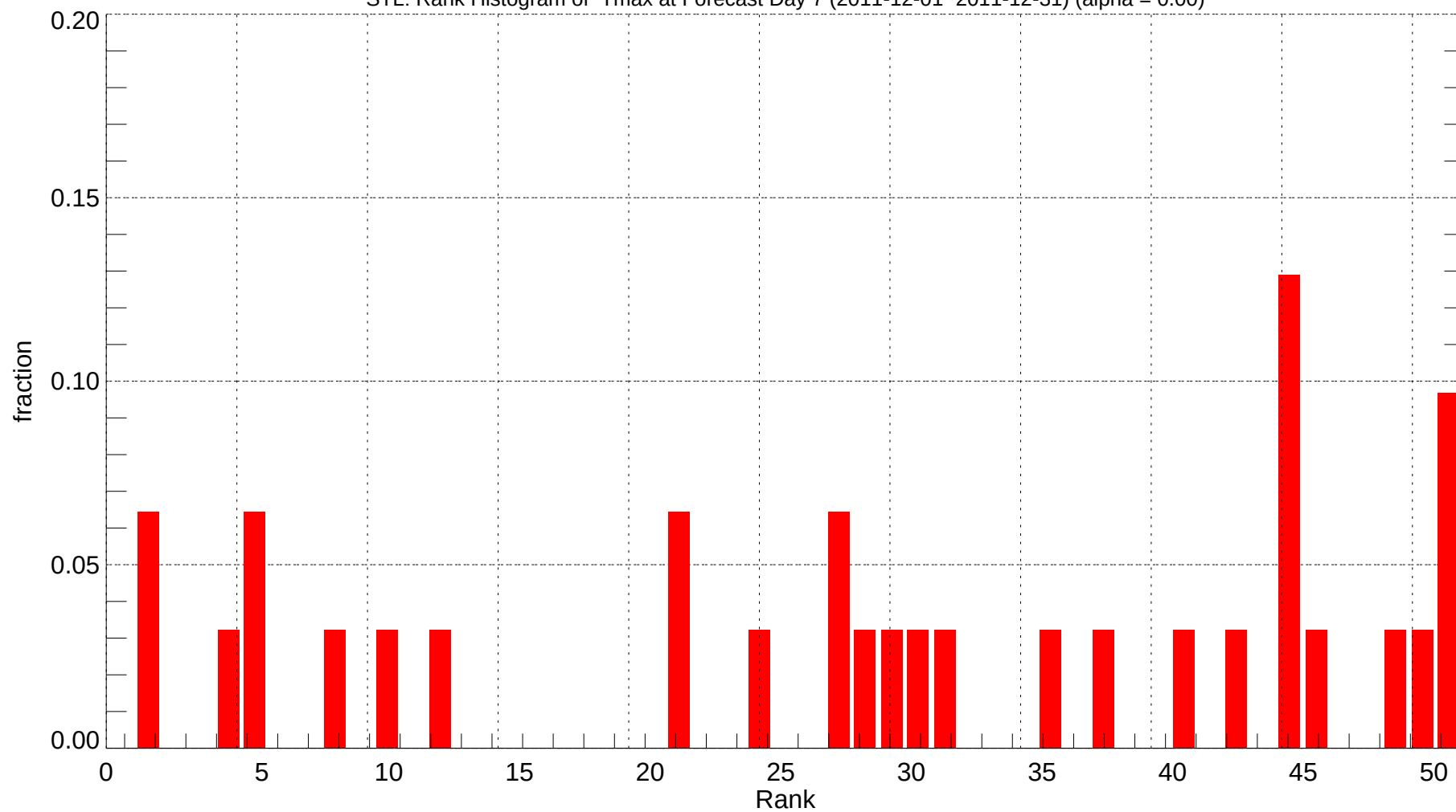
STL: Rank Histogram of Tmax at Forecast Day 7 (2011-12-01~2011-12-31) (alpha = 0.00)
