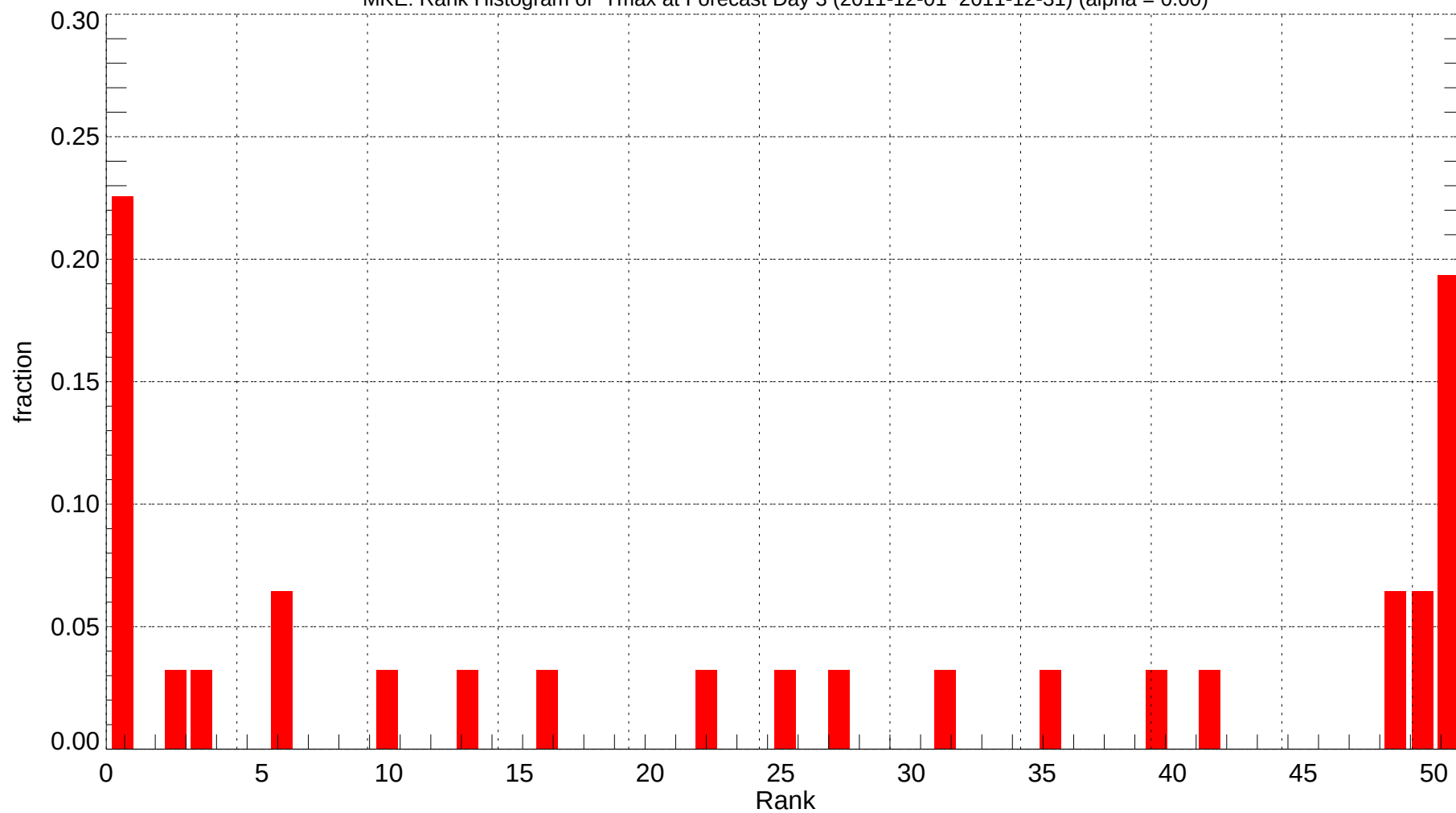
MKE: Rank Histogram of Tmax at Forecast Day 3 (2011-12-01~2011-12-31) (alpha = 0.00)
