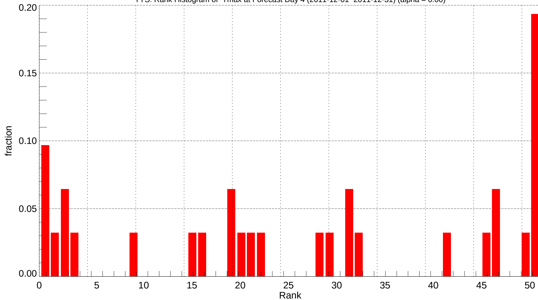
TYS: Rank Histogram of Tmax at Forecast Day 4 (2011-12-01~2011-12-31) (alpha = 0.00)
