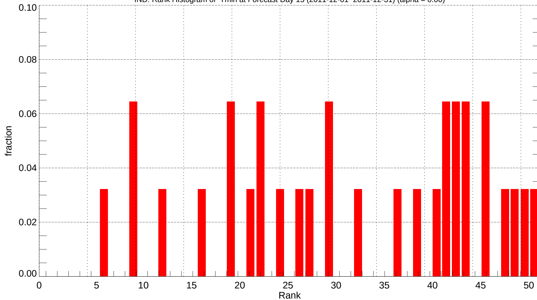
IND: Rank Histogram of Tmin at Forecast Day 15 (2011-12-01~2011-12-31) (alpha = 0.00)
