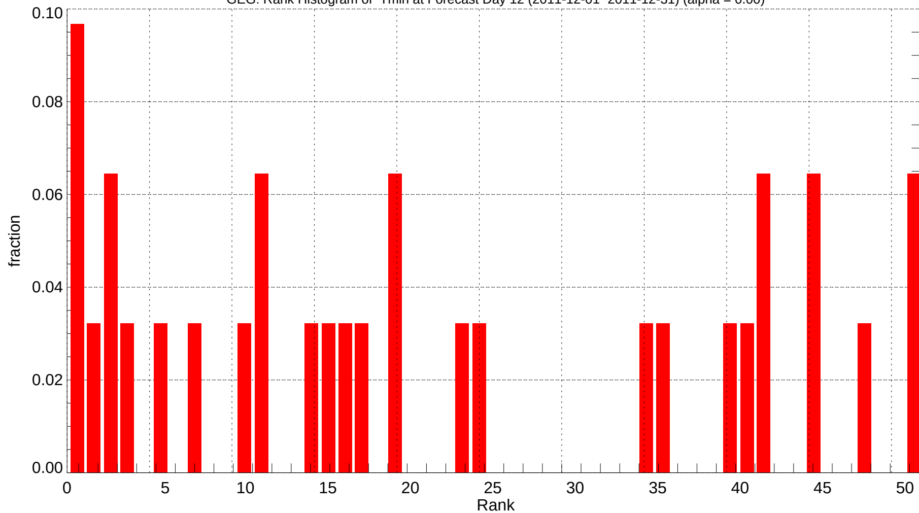
GEG: Rank Histogram of Tmin at Forecast Day 12 (2011-12-01~2011-12-31) (alpha = 0.00)
