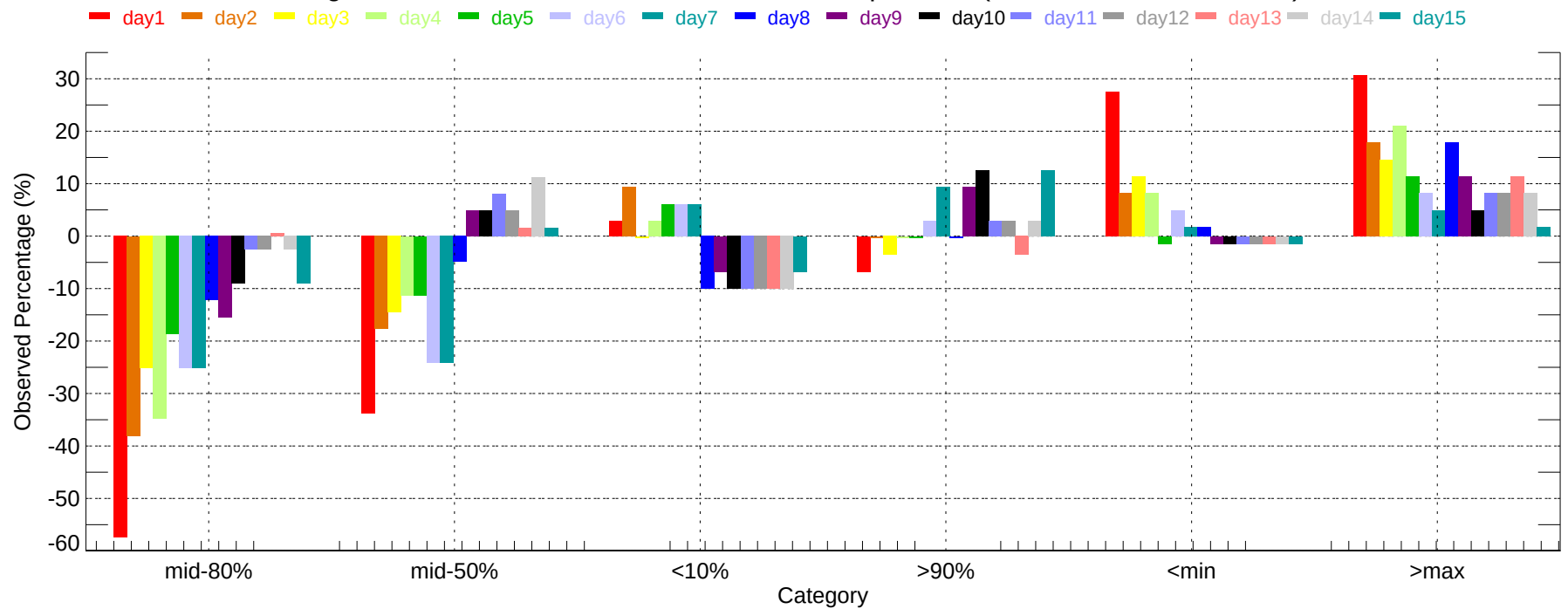
Observed Percentage Deviation of Ensembles - TYS: Max Temperature (2011-12-01~2011-12-31)
