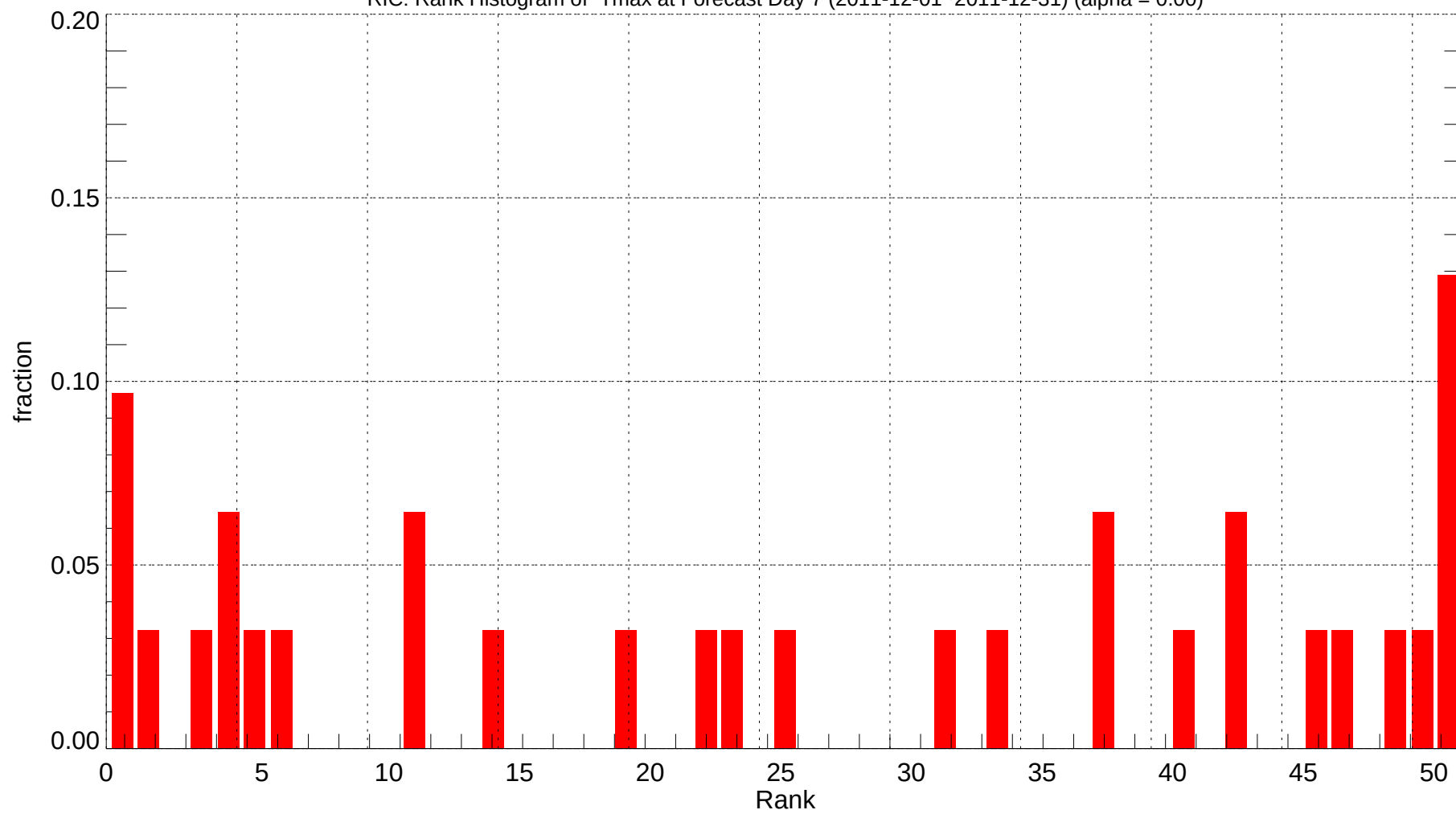
RIC: Rank Histogram of Tmax at Forecast Day 7 (2011-12-01~2011-12-31) (alpha = 0.00)
