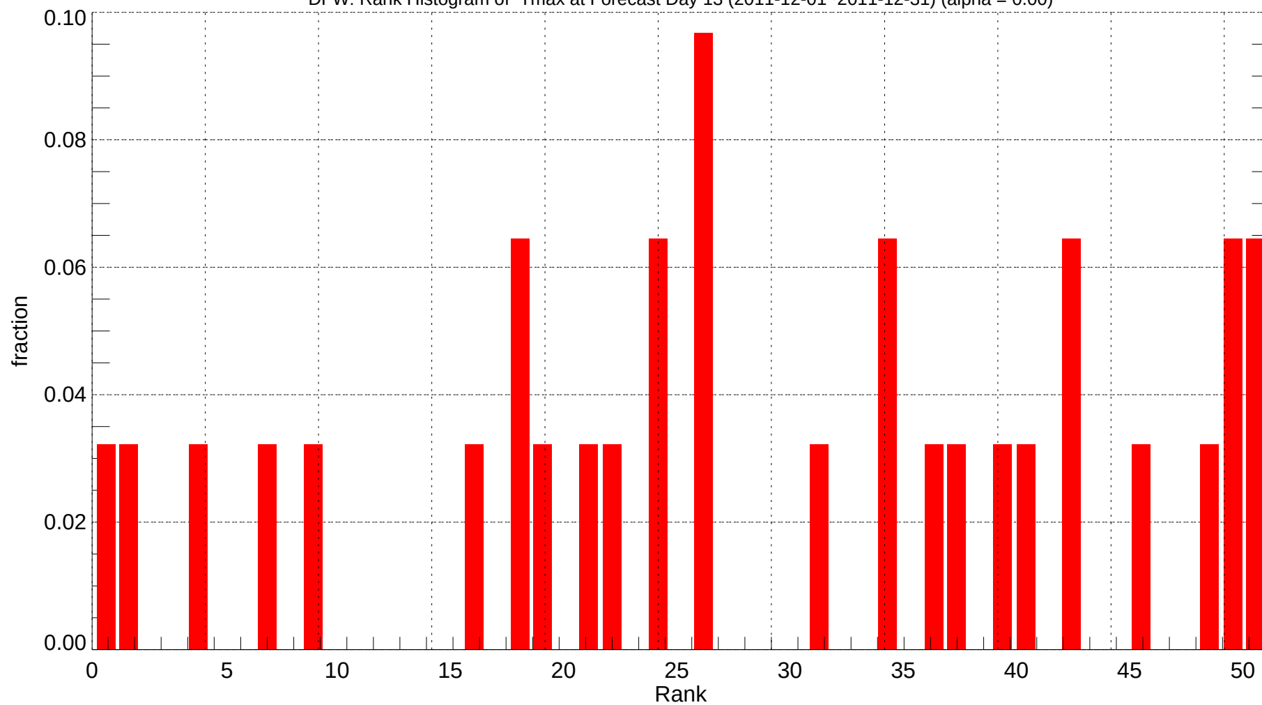
DFW: Rank Histogram of Tmax at Forecast Day 13 (2011-12-01~2011-12-31) (alpha = 0.00)
