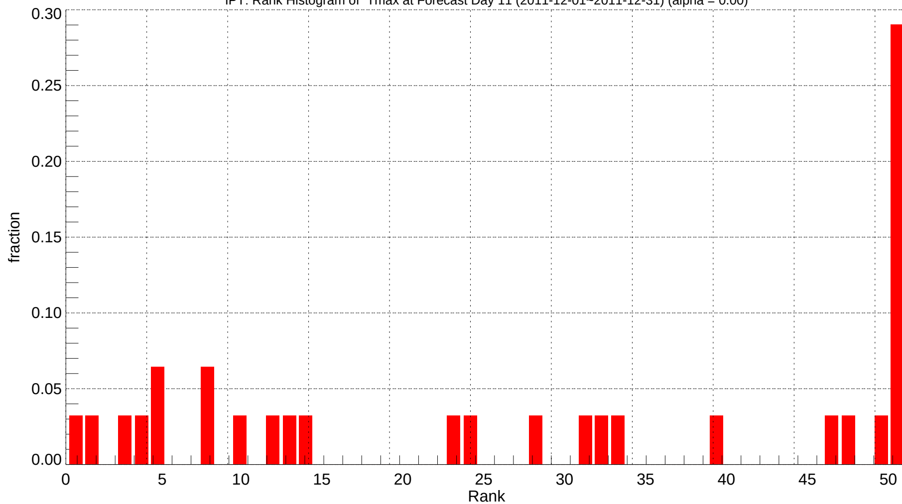
IPT: Rank Histogram of Tmax at Forecast Day 11 (2011-12-01~2011-12-31) (alpha = 0.00)
