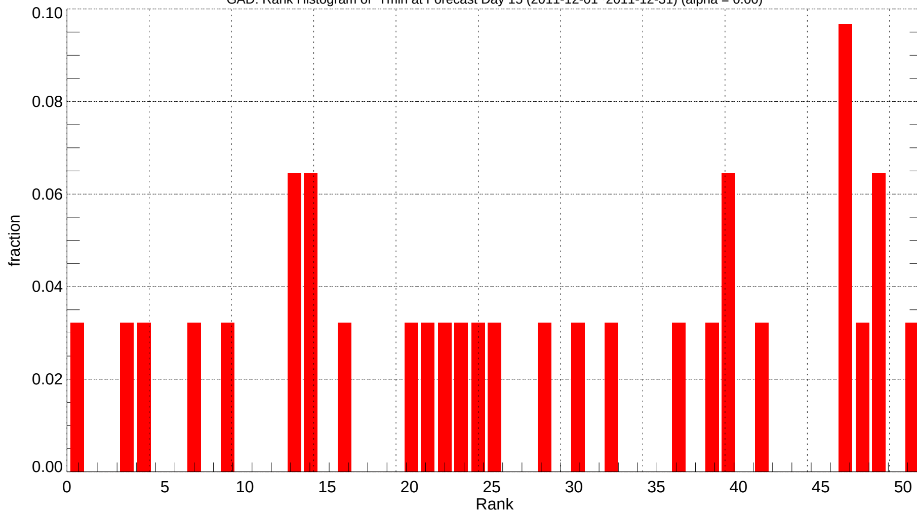
GAD: Rank Histogram of Tmin at Forecast Day 15 (2011-12-01~2011-12-31) (alpha = 0.00)
