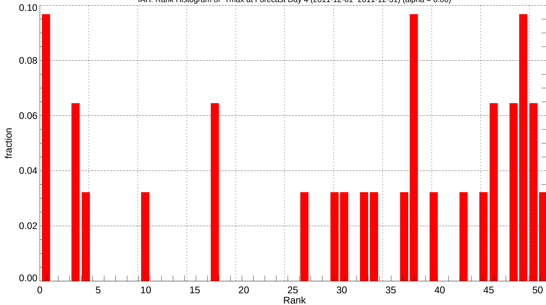
IAH: Rank Histogram of Tmax at Forecast Day 4 (2011-12-01~2011-12-31) (alpha = 0.00)
