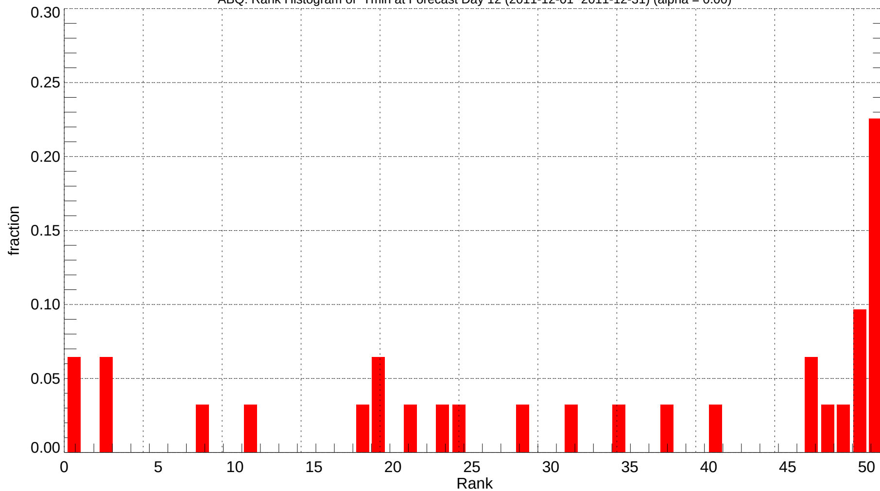
ABQ: Rank Histogram of Tmin at Forecast Day 12 (2011-12-01~2011-12-31) (alpha = 0.00)
