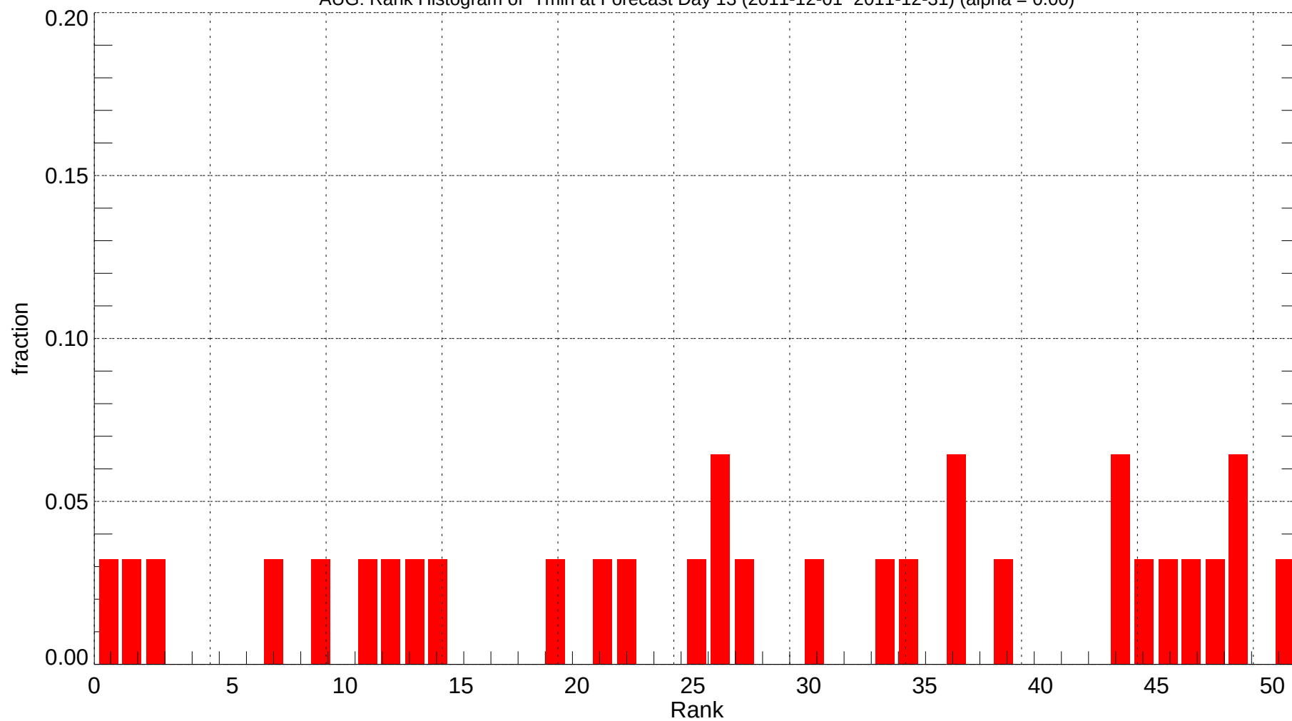
AUG: Rank Histogram of Tmin at Forecast Day 13 (2011-12-01~2011-12-31) (alpha = 0.00)
