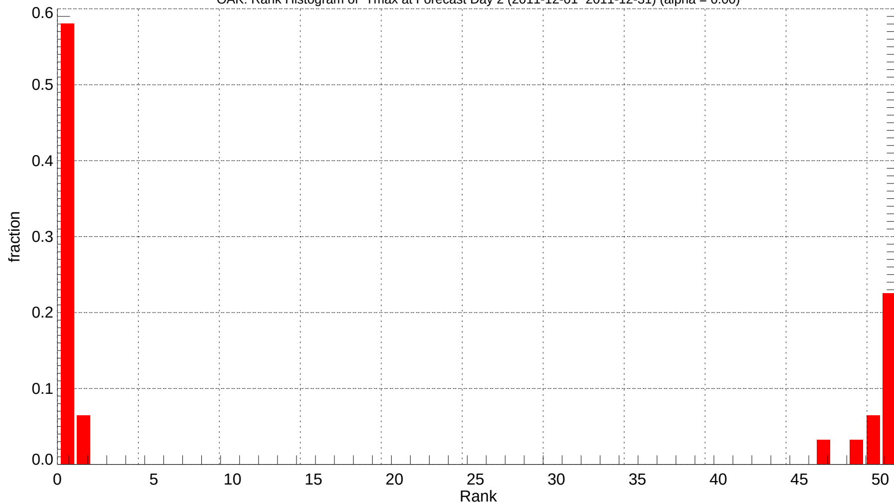
OAK: Rank Histogram of Tmax at Forecast Day 2 (2011-12-01~2011-12-31) (alpha = 0.00)
