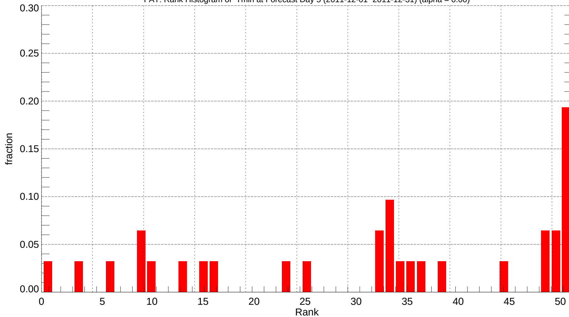
FAT: Rank Histogram of Tmin at Forecast Day 5 (2011-12-01~2011-12-31) (alpha = 0.00)
