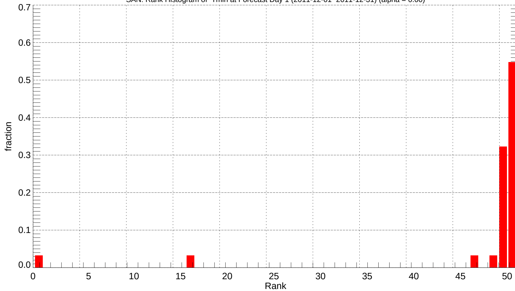
SAN: Rank Histogram of Tmin at Forecast Day 1 (2011-12-01~2011-12-31) (alpha = 0.00)
