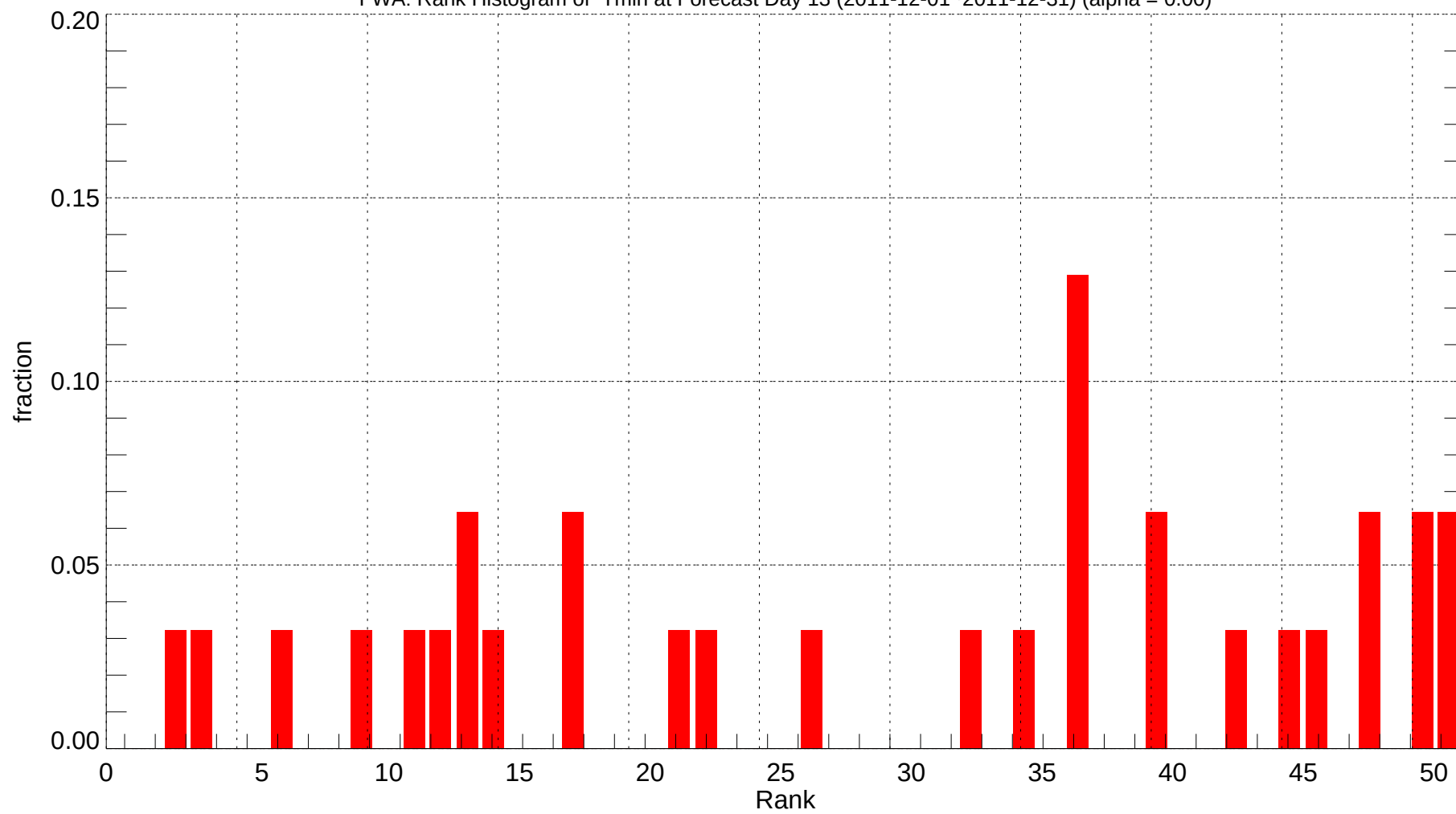
FWA: Rank Histogram of Tmin at Forecast Day 13 (2011-12-01~2011-12-31) (alpha = 0.00)
