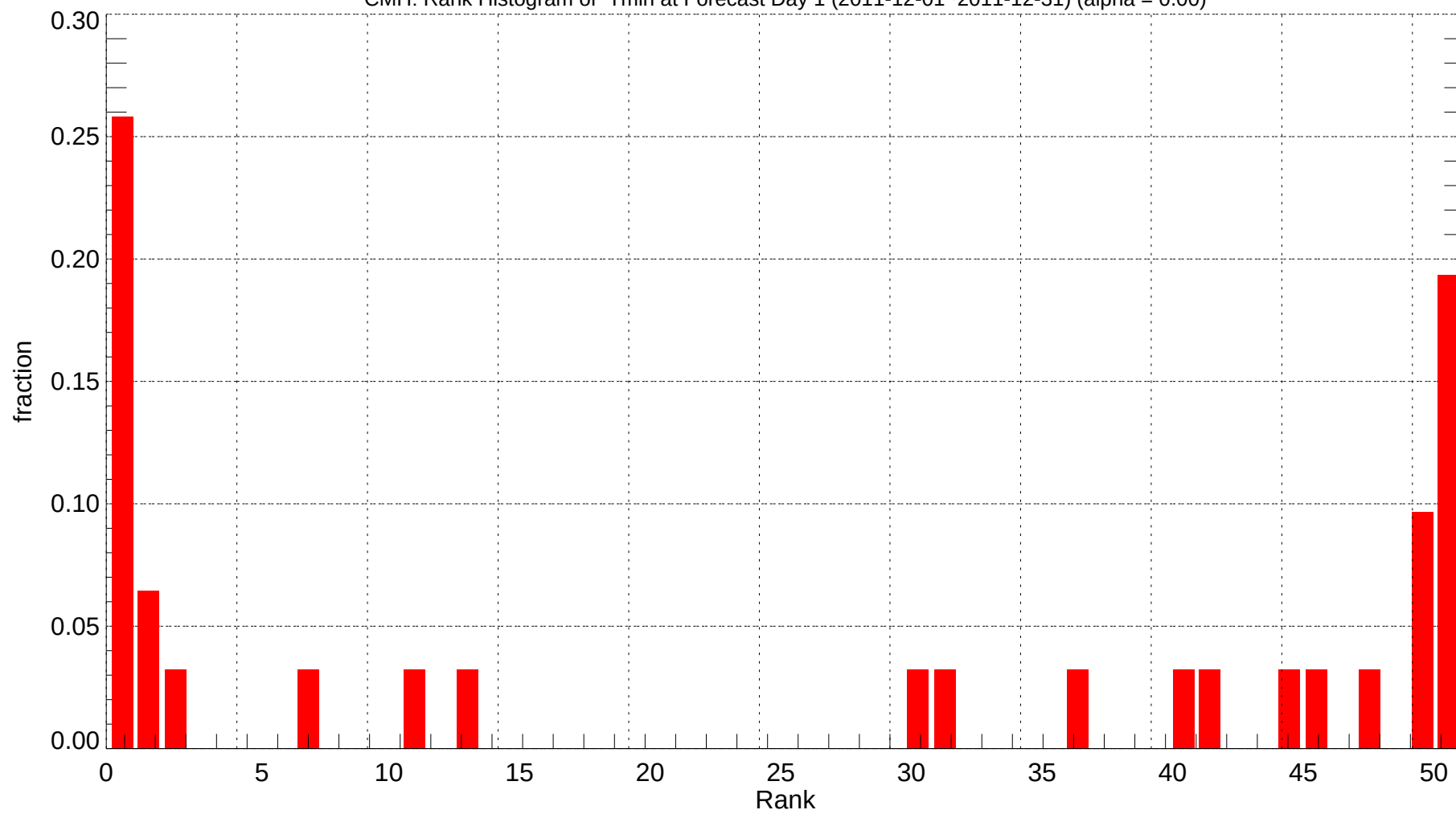
CMH: Rank Histogram of Tmin at Forecast Day 1 (2011-12-01~2011-12-31) (alpha = 0.00)
