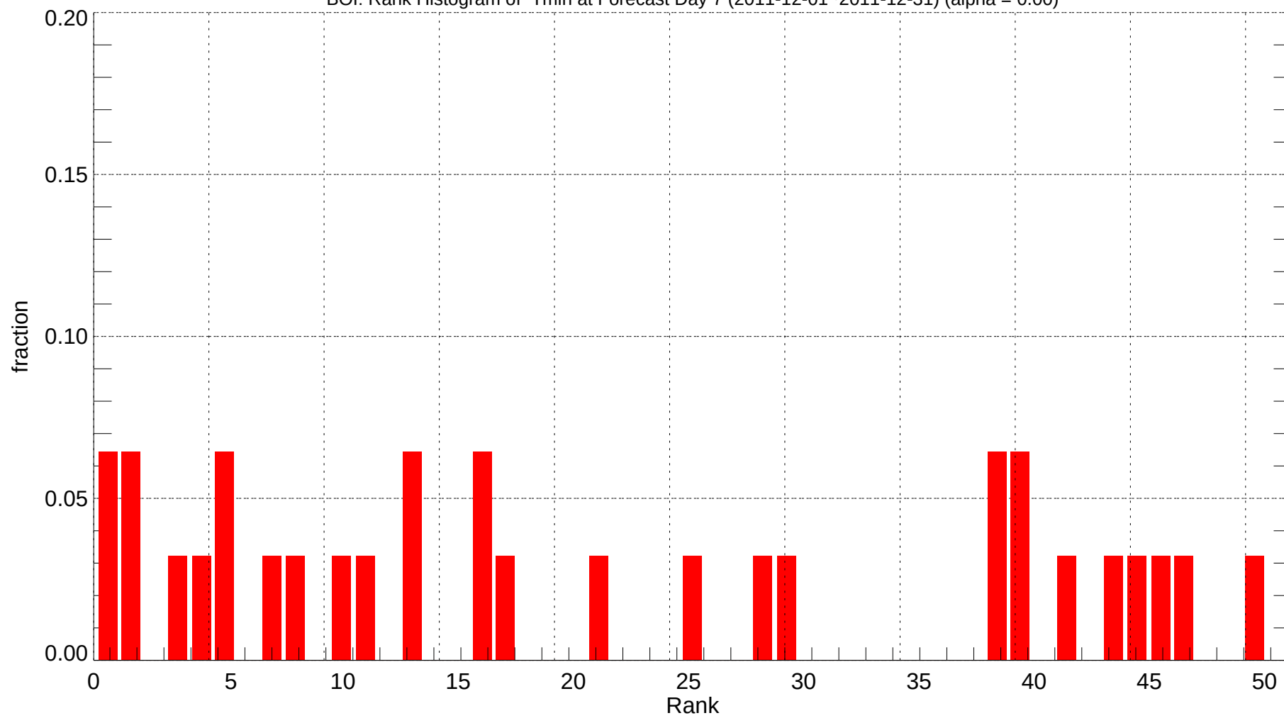
BOI: Rank Histogram of Tmin at Forecast Day 7 (2011-12-01~2011-12-31) (alpha = 0.00)
