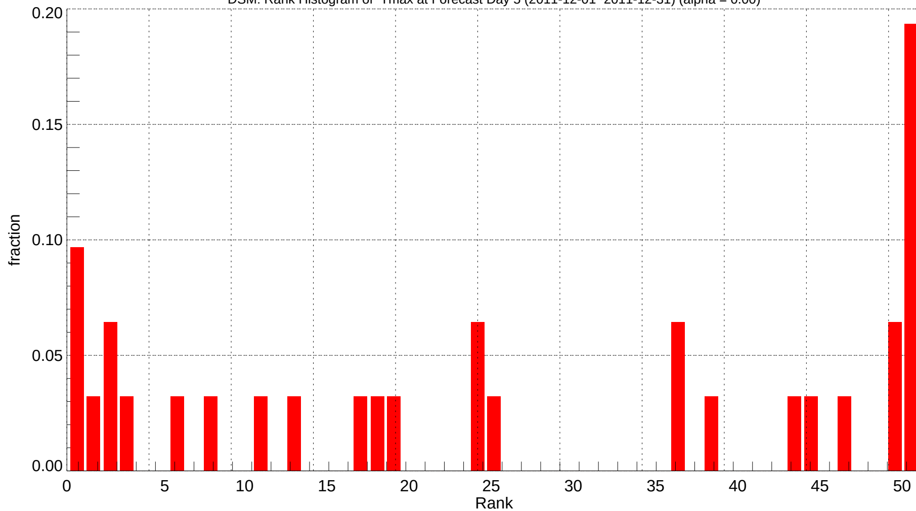
DSM: Rank Histogram of Tmax at Forecast Day 5 (2011-12-01~2011-12-31) (alpha = 0.00)
