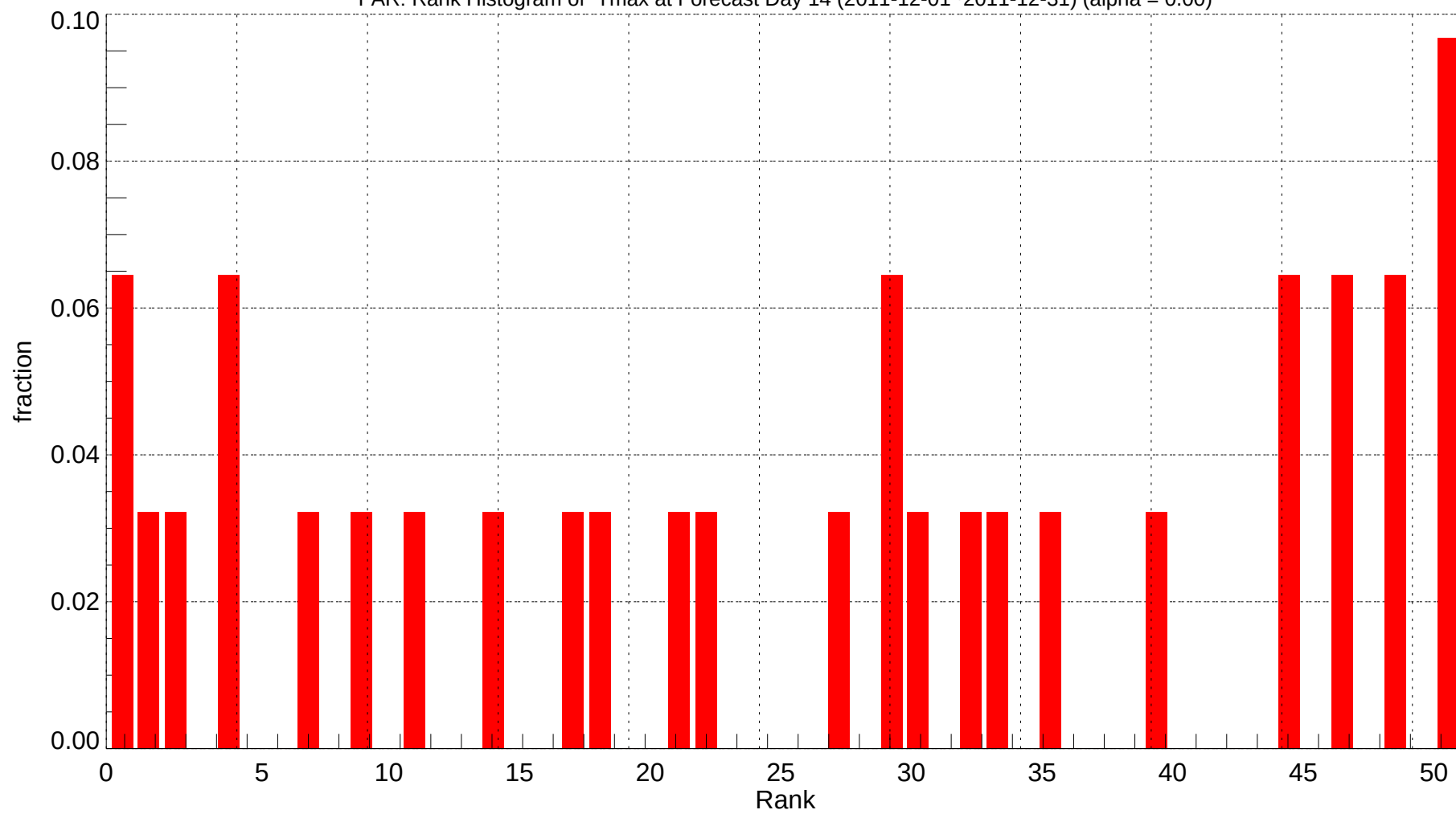
FAR: Rank Histogram of Tmax at Forecast Day 14 (2011-12-01~2011-12-31) (alpha = 0.00)
