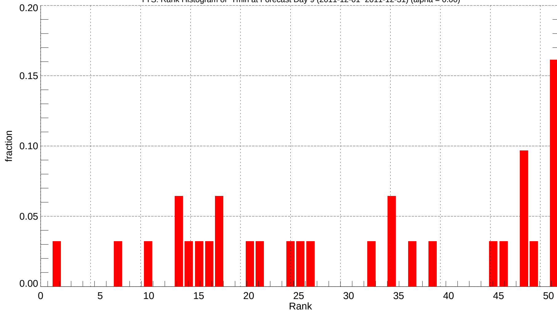
TYS: Rank Histogram of Tmin at Forecast Day 9 (2011-12-01~2011-12-31) (alpha = 0.00)
