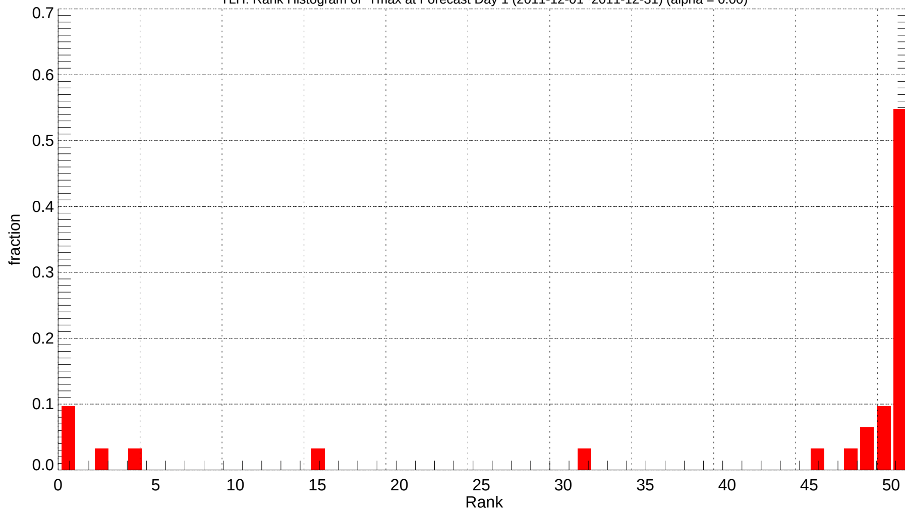
TLH: Rank Histogram of Tmax at Forecast Day 1 (2011-12-01~2011-12-31) (alpha = 0.00)
