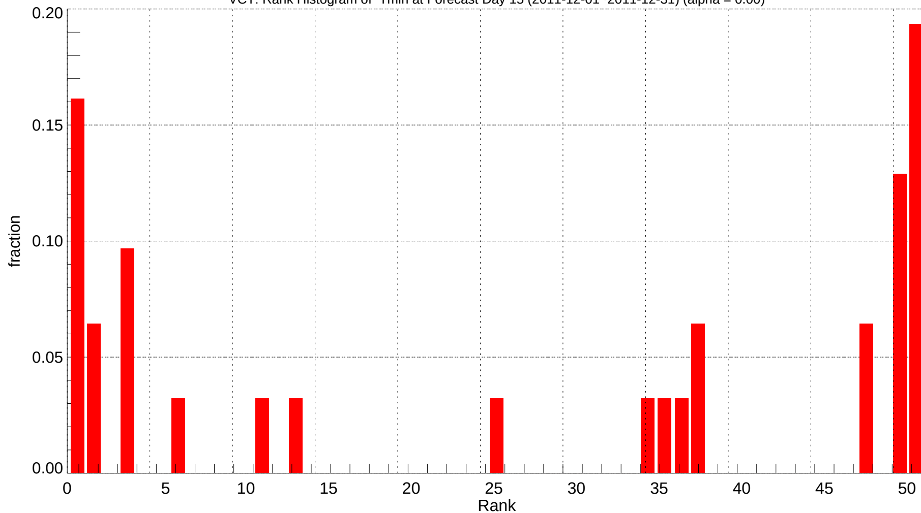
VCT: Rank Histogram of Tmin at Forecast Day 15 (2011-12-01~2011-12-31) (alpha = 0.00)
