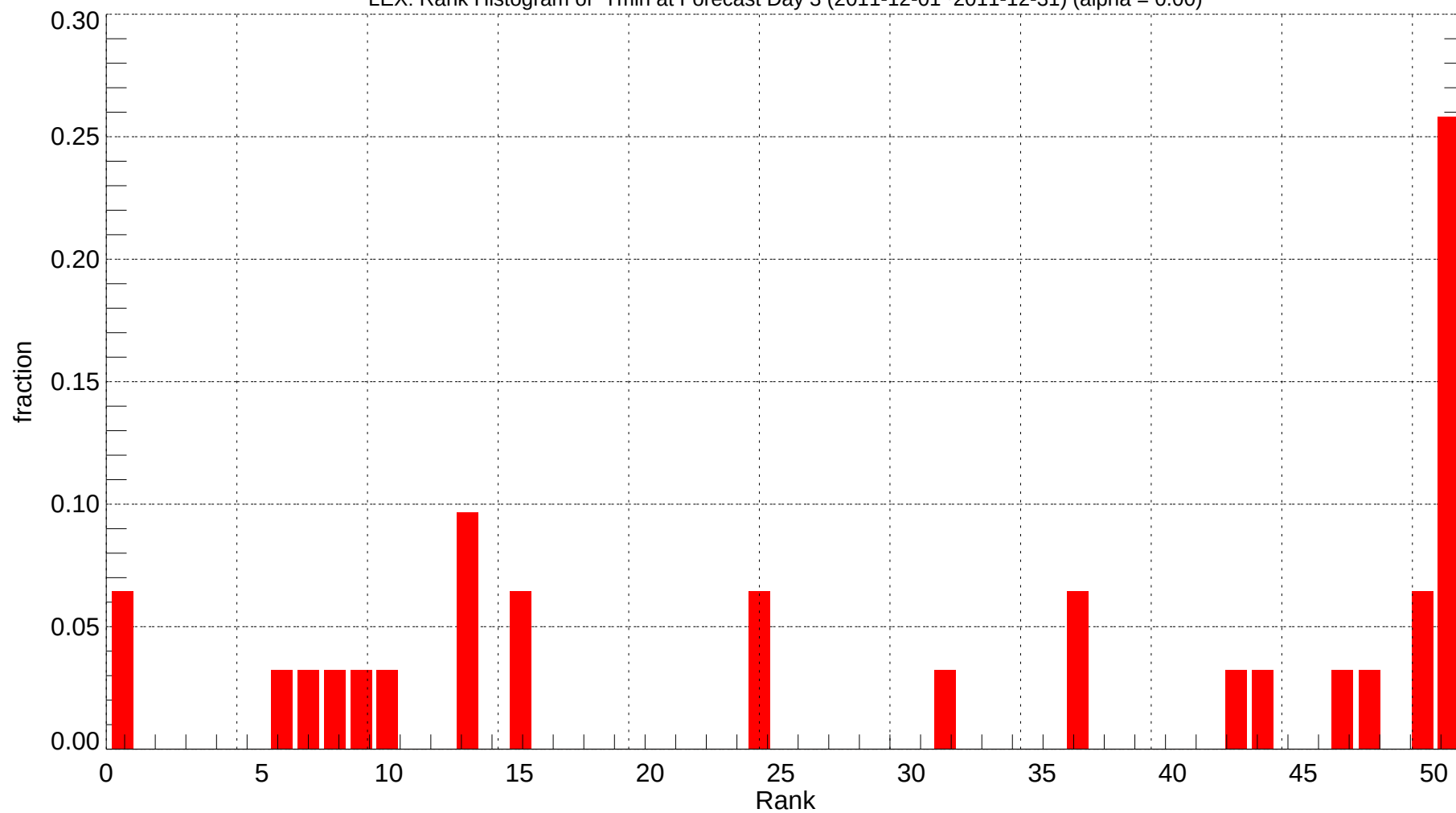
LEX: Rank Histogram of Tmin at Forecast Day 3 (2011-12-01~2011-12-31) (alpha = 0.00)
