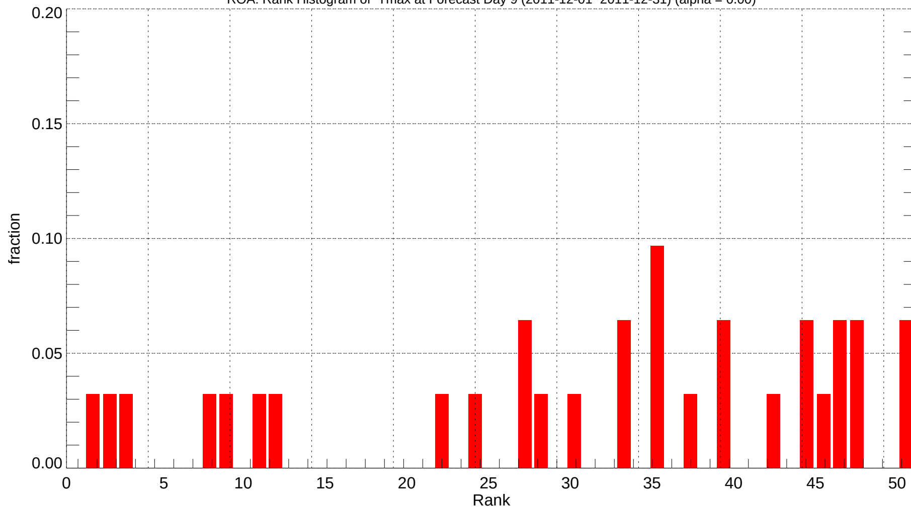
ROA: Rank Histogram of Tmax at Forecast Day 9 (2011-12-01~2011-12-31) (alpha = 0.00)
