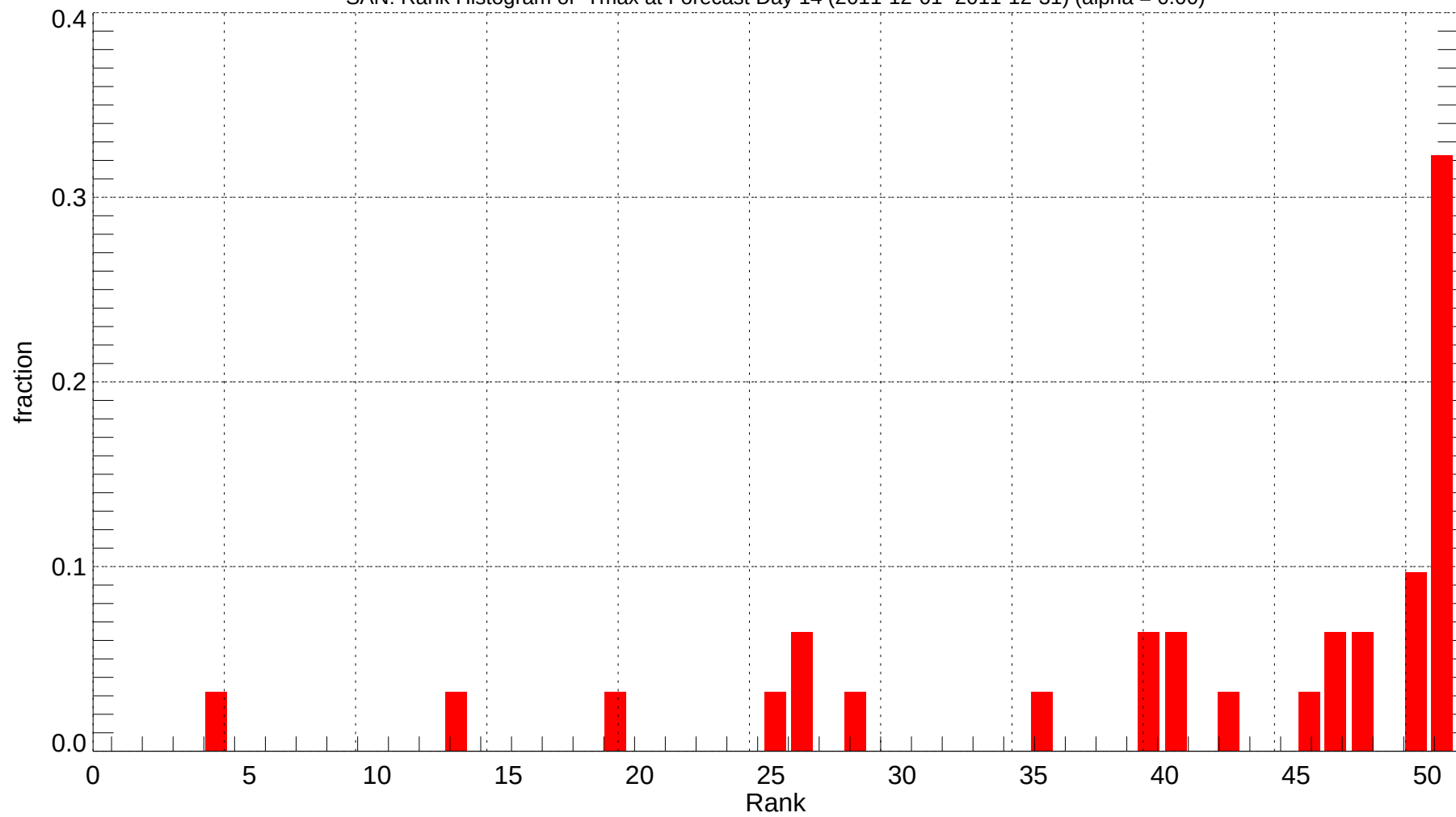
SAN: Rank Histogram of Tmax at Forecast Day 14 (2011-12-01~2011-12-31) (alpha = 0.00)
