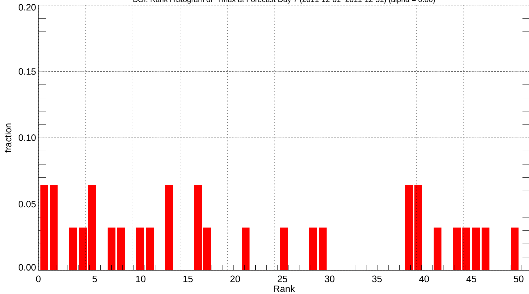
BOI: Rank Histogram of Tmax at Forecast Day 7 (2011-12-01~2011-12-31) (alpha = 0.00)
