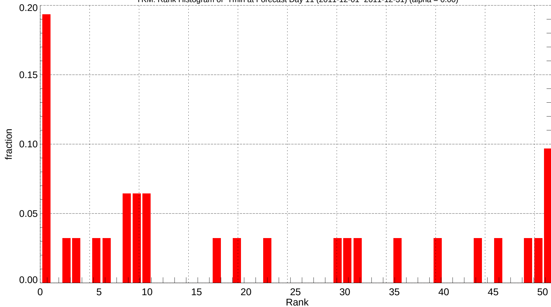
YKM: Rank Histogram of Tmin at Forecast Day 11 (2011-12-01~2011-12-31) (alpha = 0.00)
