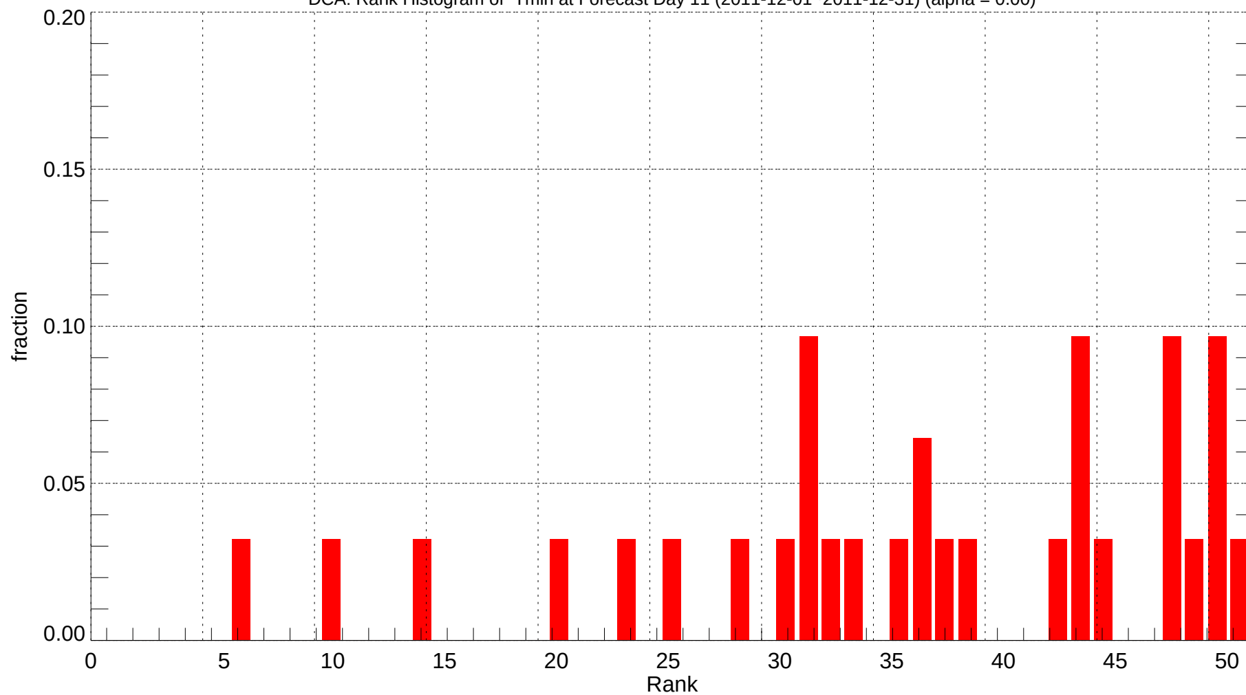
DCA: Rank Histogram of Tmin at Forecast Day 11 (2011-12-01~2011-12-31) (alpha = 0.00)
