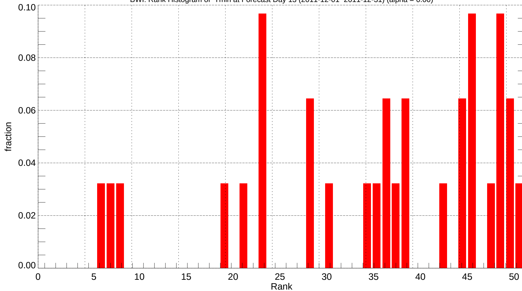
BWl: Rank Histogram of Tmin at Forecast Day 13 (2011-12-01~2011-12-31) (alpha = 0.00)
