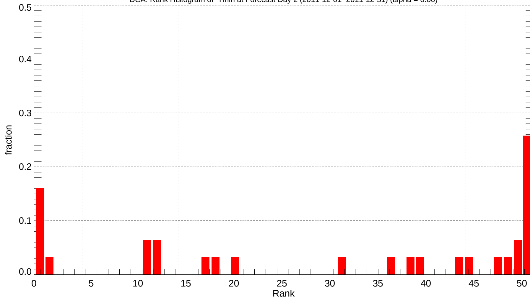
DCA: Rank Histogram of Tmin at Forecast Day 2 (2011-12-01~2011-12-31) (alpha = 0.00)
