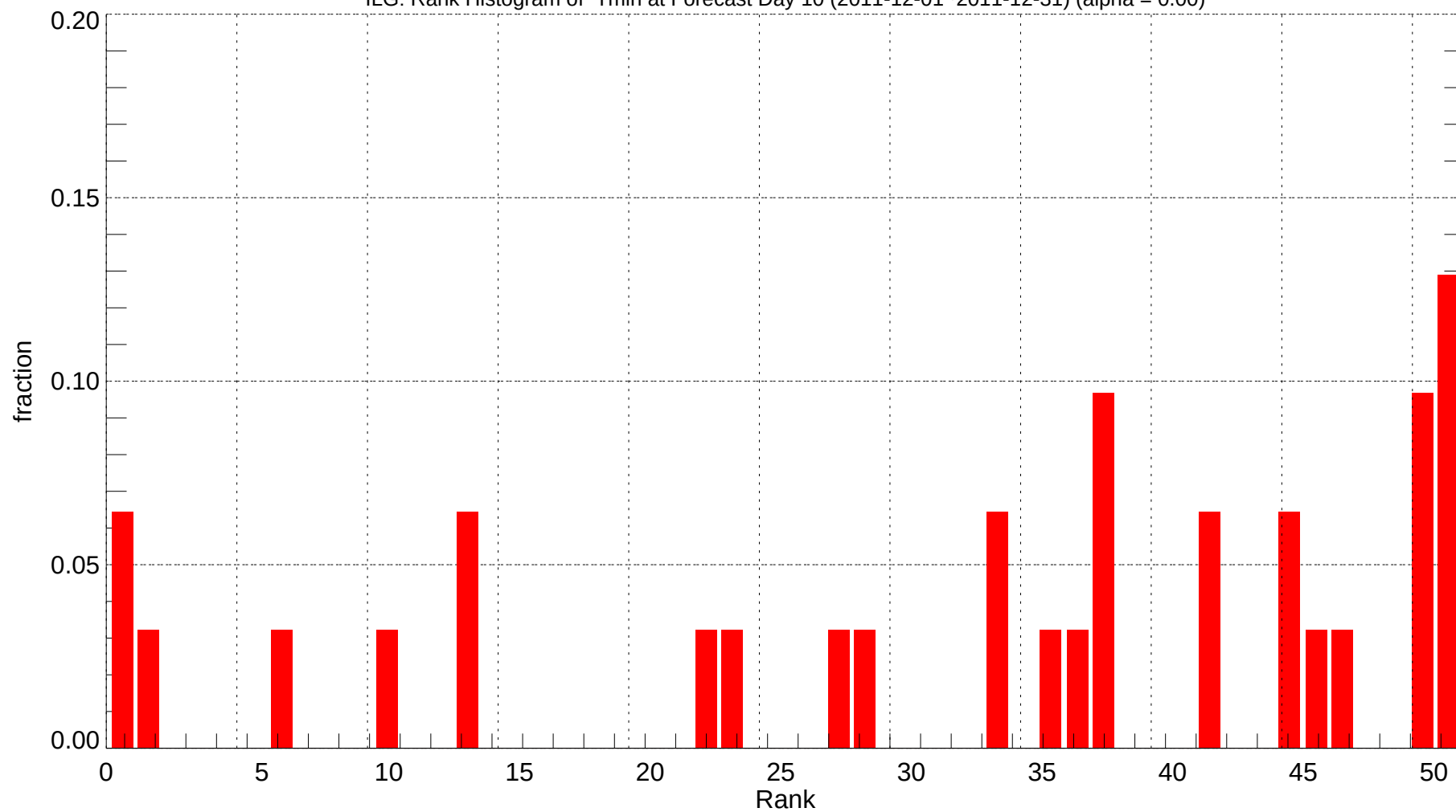
ILG: Rank Histogram of Tmin at Forecast Day 10 (2011-12-01~2011-12-31) (alpha = 0.00)
