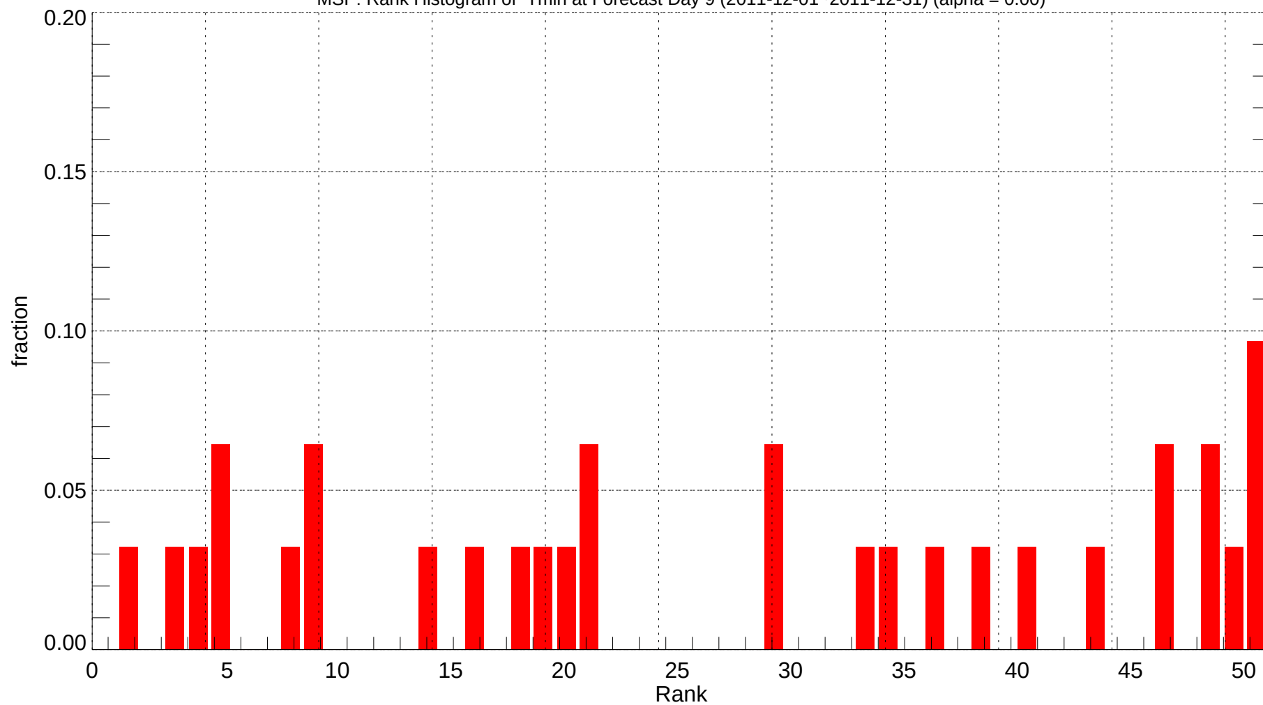
MSP: Rank Histogram of Tmin at Forecast Day 9 (2011-12-01~2011-12-31) (alpha = 0.00)
