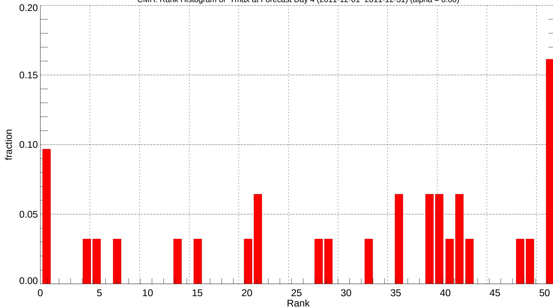
CMH: Rank Histogram of Tmax at Forecast Day 4 (2011-12-01~2011-12-31) (alpha = 0.00)
