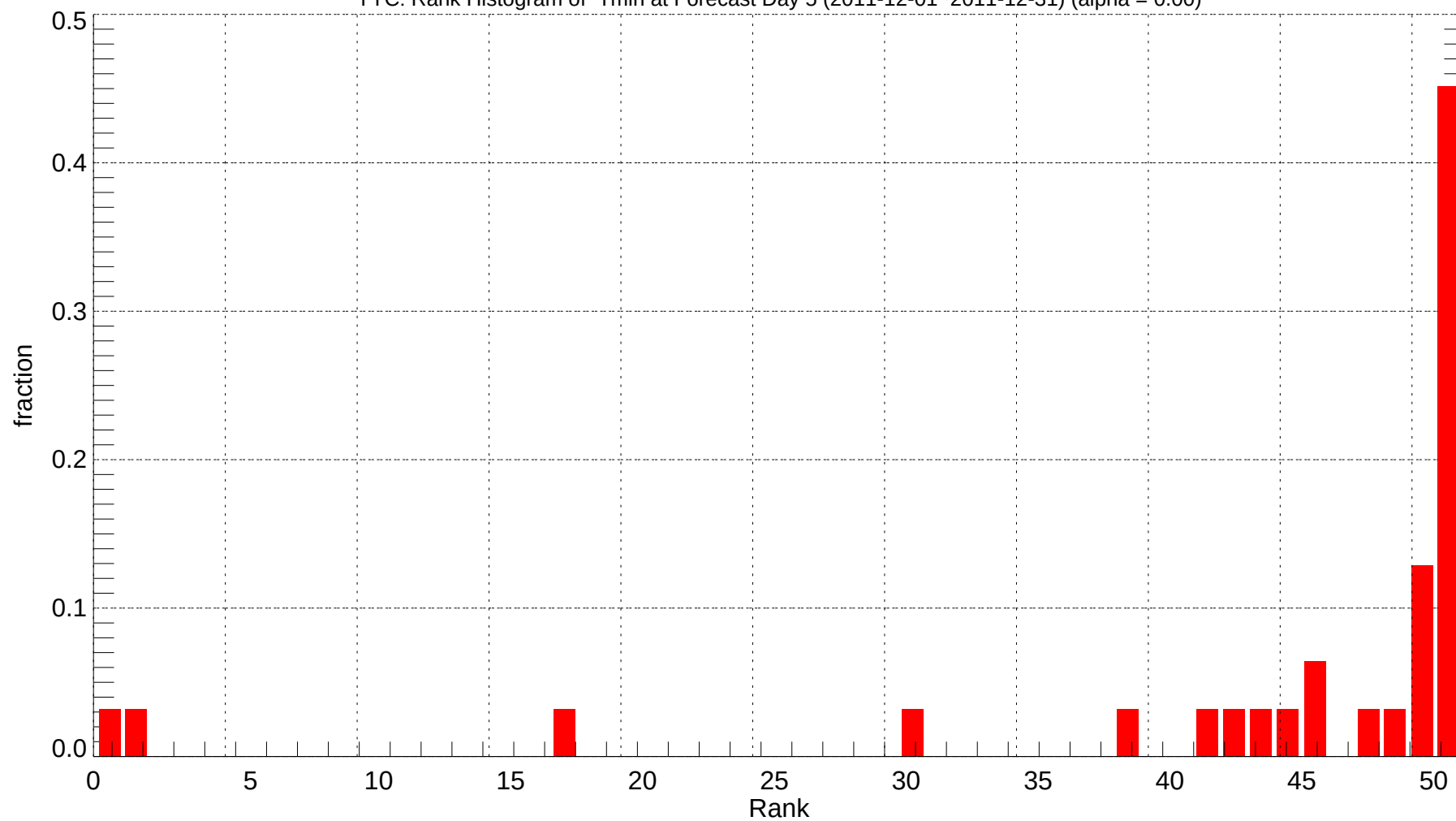
YYC: Rank Histogram of Tmin at Forecast Day 5 (2011-12-01~2011-12-31) (alpha = 0.00)
