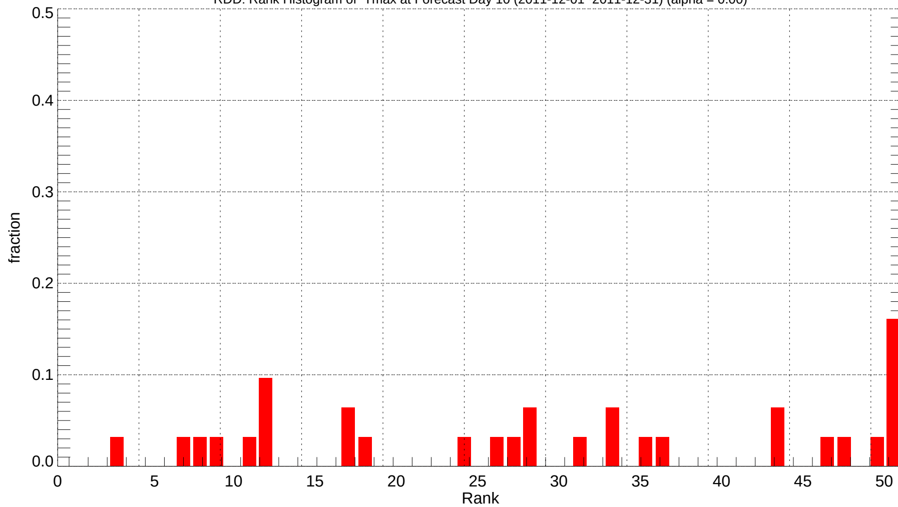
RDD: Rank Histogram of Tmax at Forecast Day 10 (2011-12-01~2011-12-31) (alpha = 0.00)
