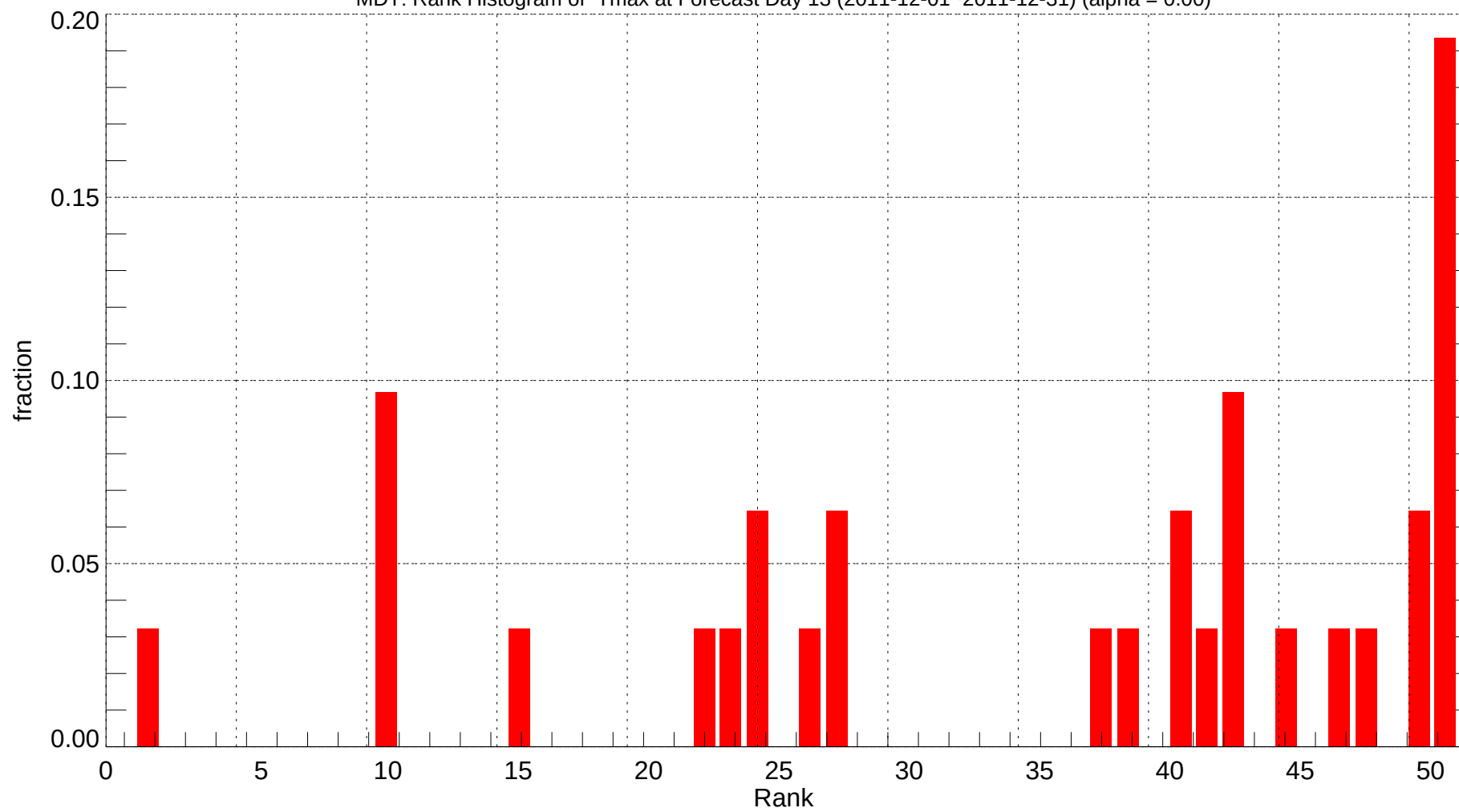
MDT: Rank Histogram of Tmax at Forecast Day 13 (2011-12-01~2011-12-31) (alpha = 0.00)
