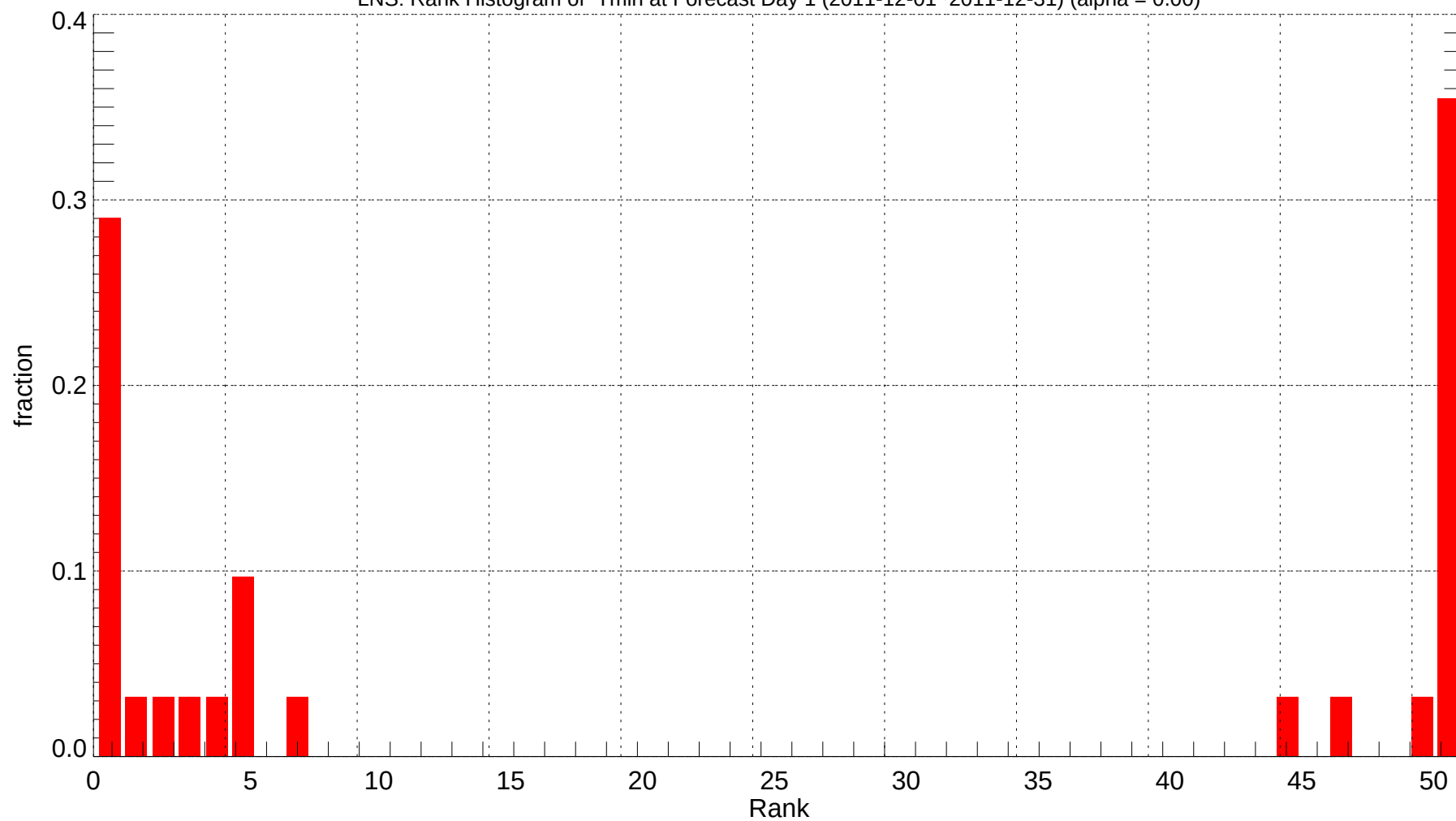
LNS: Rank Histogram of Tmin at Forecast Day 1 (2011-12-01~2011-12-31) (alpha = 0.00)
