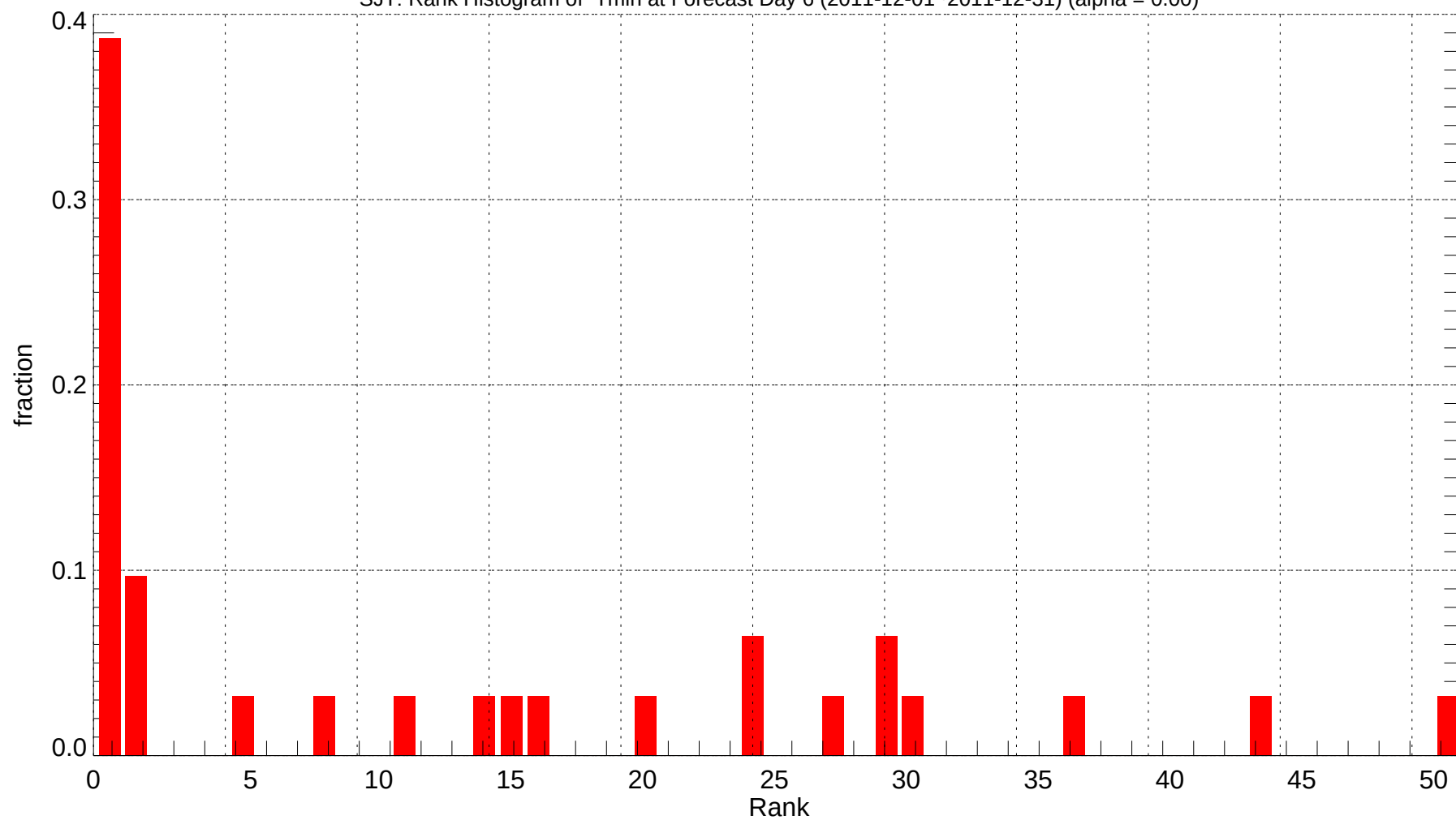
SJT: Rank Histogram of Tmin at Forecast Day 6 (2011-12-01~2011-12-31) (alpha = 0.00)
