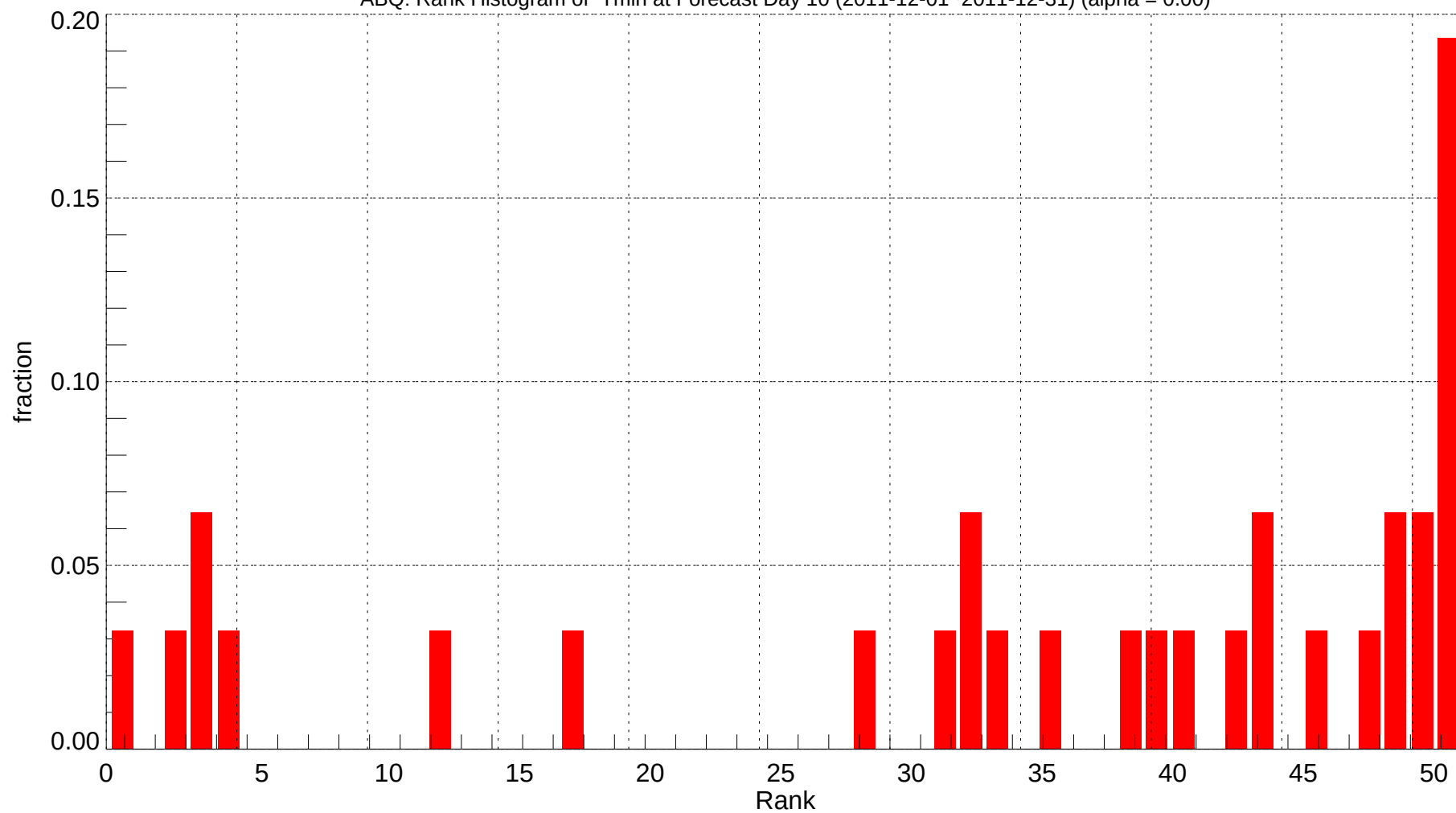
ABQ: Rank Histogram of Tmin at Forecast Day 10 (2011-12-01~2011-12-31) (alpha = 0.00)
