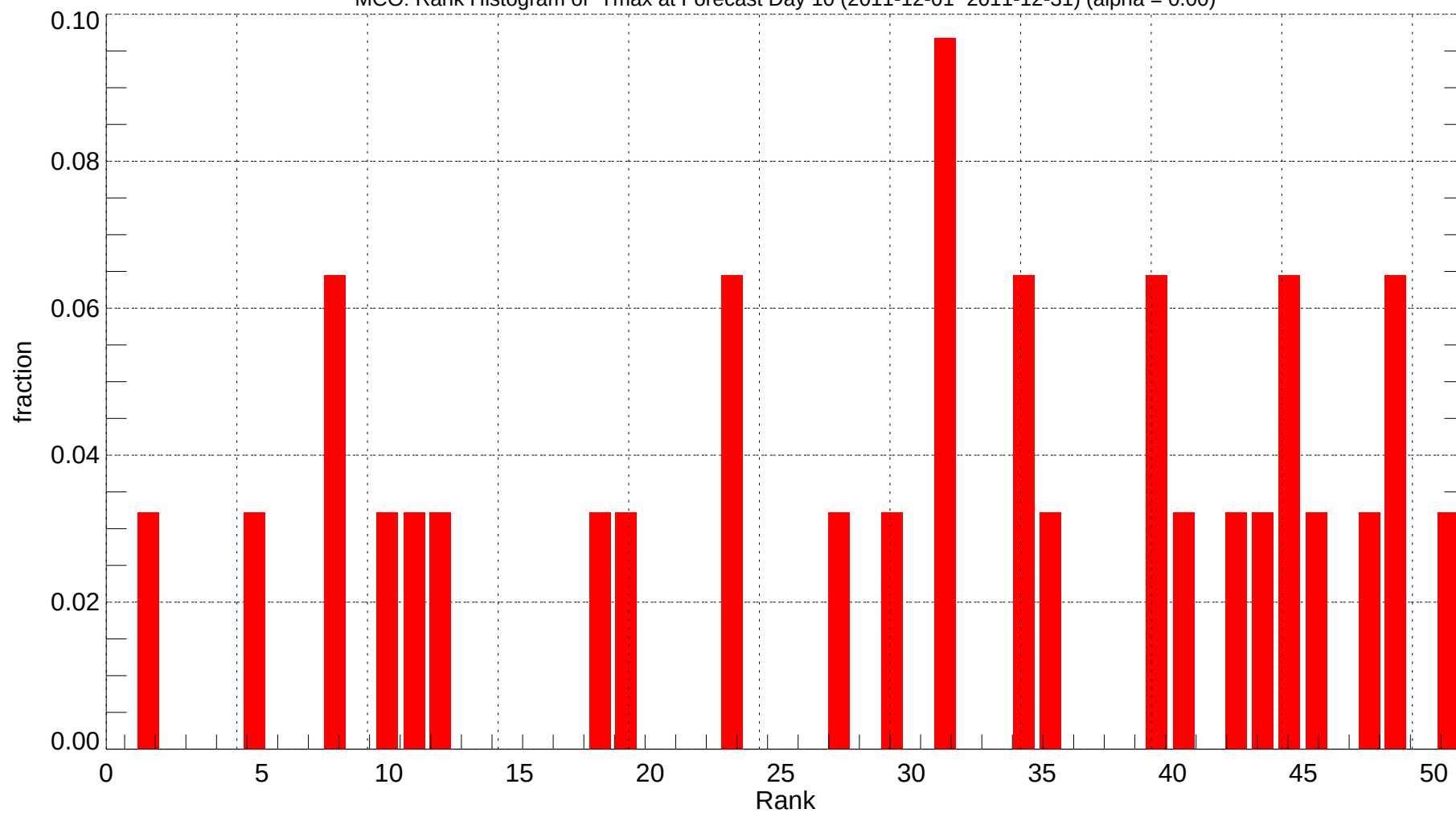
MCO: Rank Histogram of Tmax at Forecast Day 10 (2011-12-01~2011-12-31) (alpha = 0.00)
