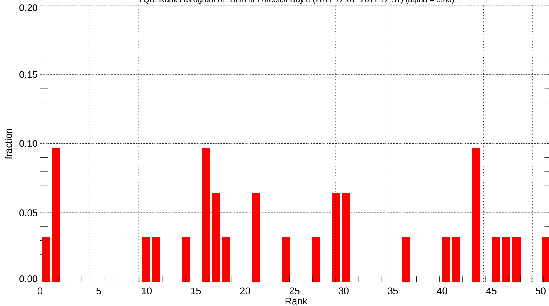
YQB: Rank Histogram of Tmin at Forecast Day 8 (2011-12-01~2011-12-31) (alpha = 0.00)
