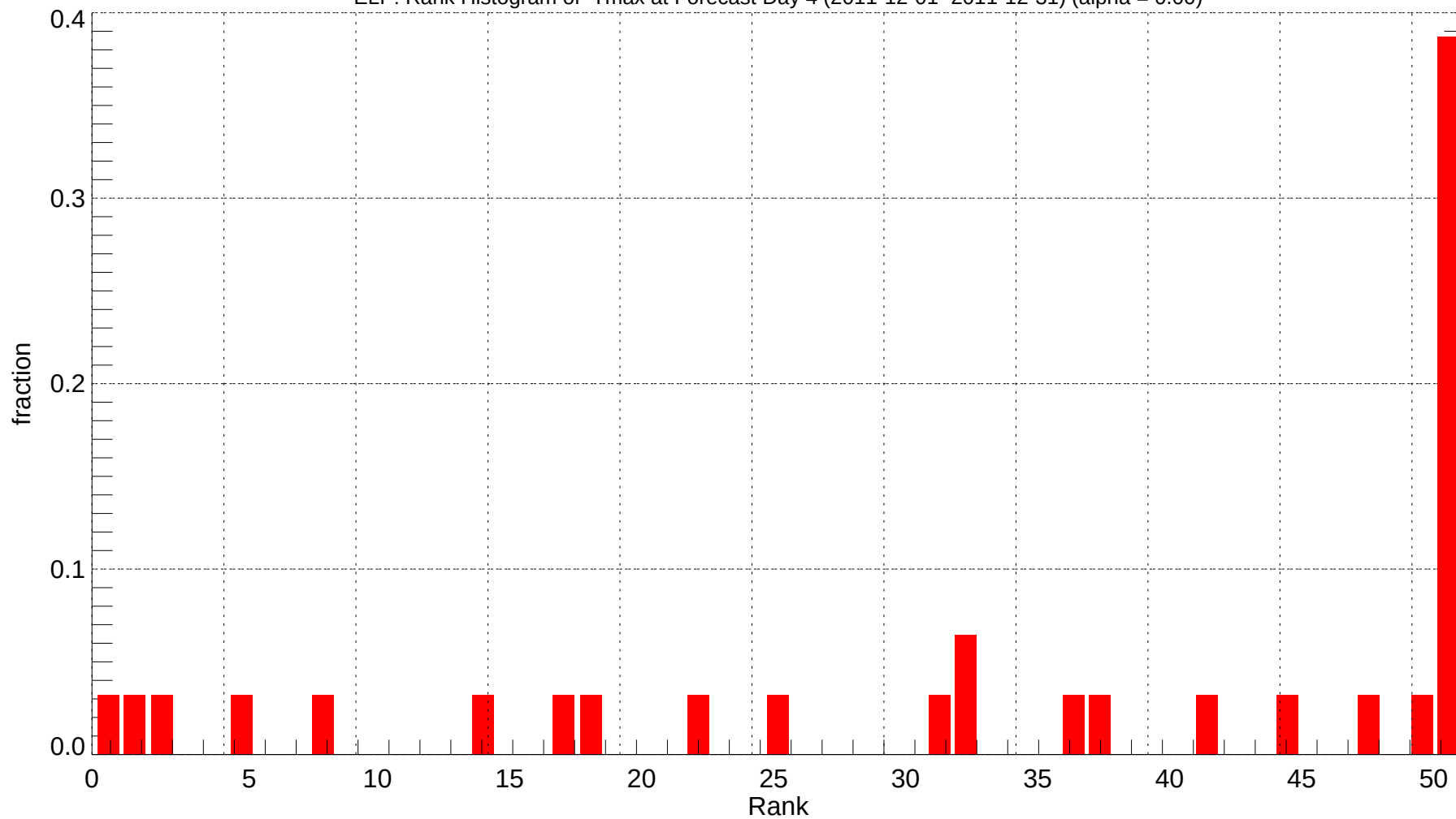
ELP: Rank Histogram of Tmax at Forecast Day 4 (2011-12-01~2011-12-31) (alpha = 0.00)
