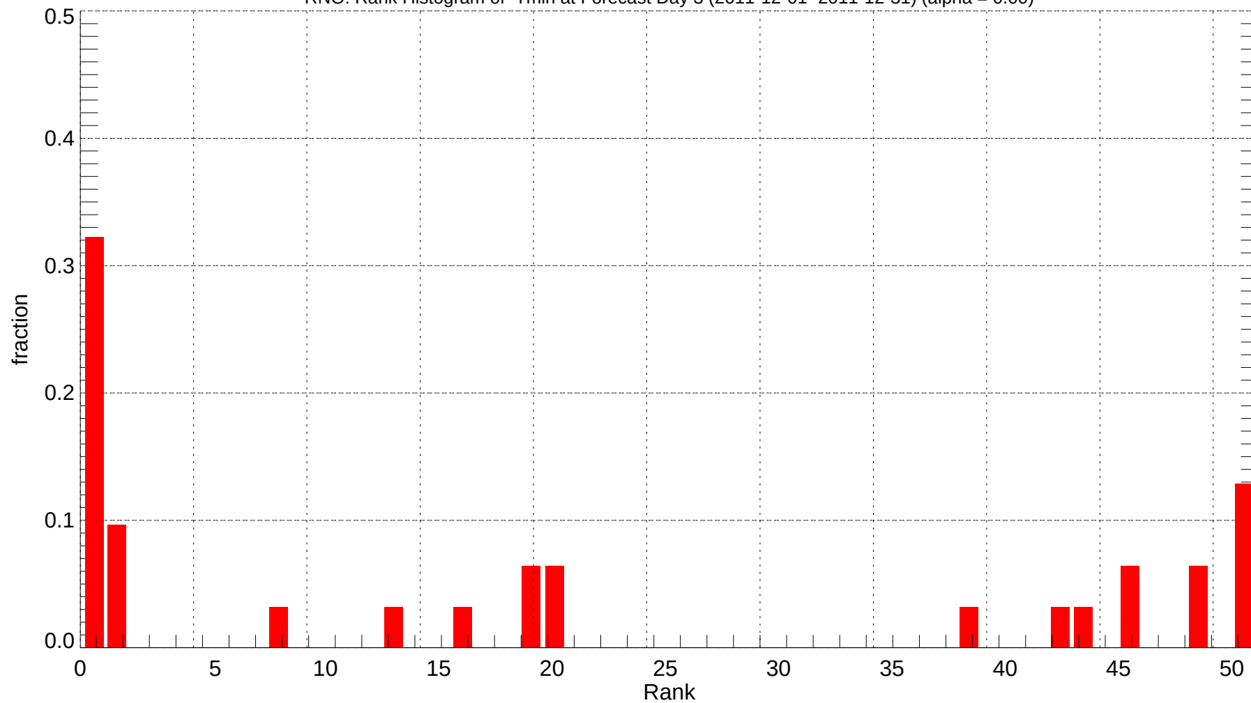
RNO: Rank Histogram of Tmin at Forecast Day 3 (2011-12-01~2011-12-31) (alpha = 0.00)
