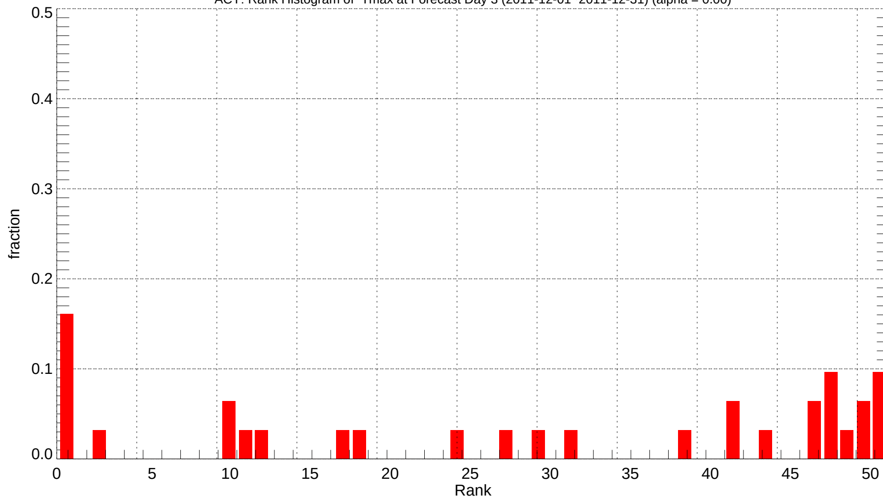
ACY: Rank Histogram of Tmax at Forecast Day 3 (2011-12-01~2011-12-31) (alpha = 0.00)
