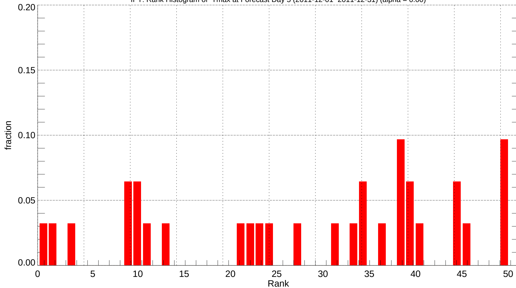
IPT: Rank Histogram of Tmax at Forecast Day 5 (2011-12-01~2011-12-31) (alpha = 0.00)
