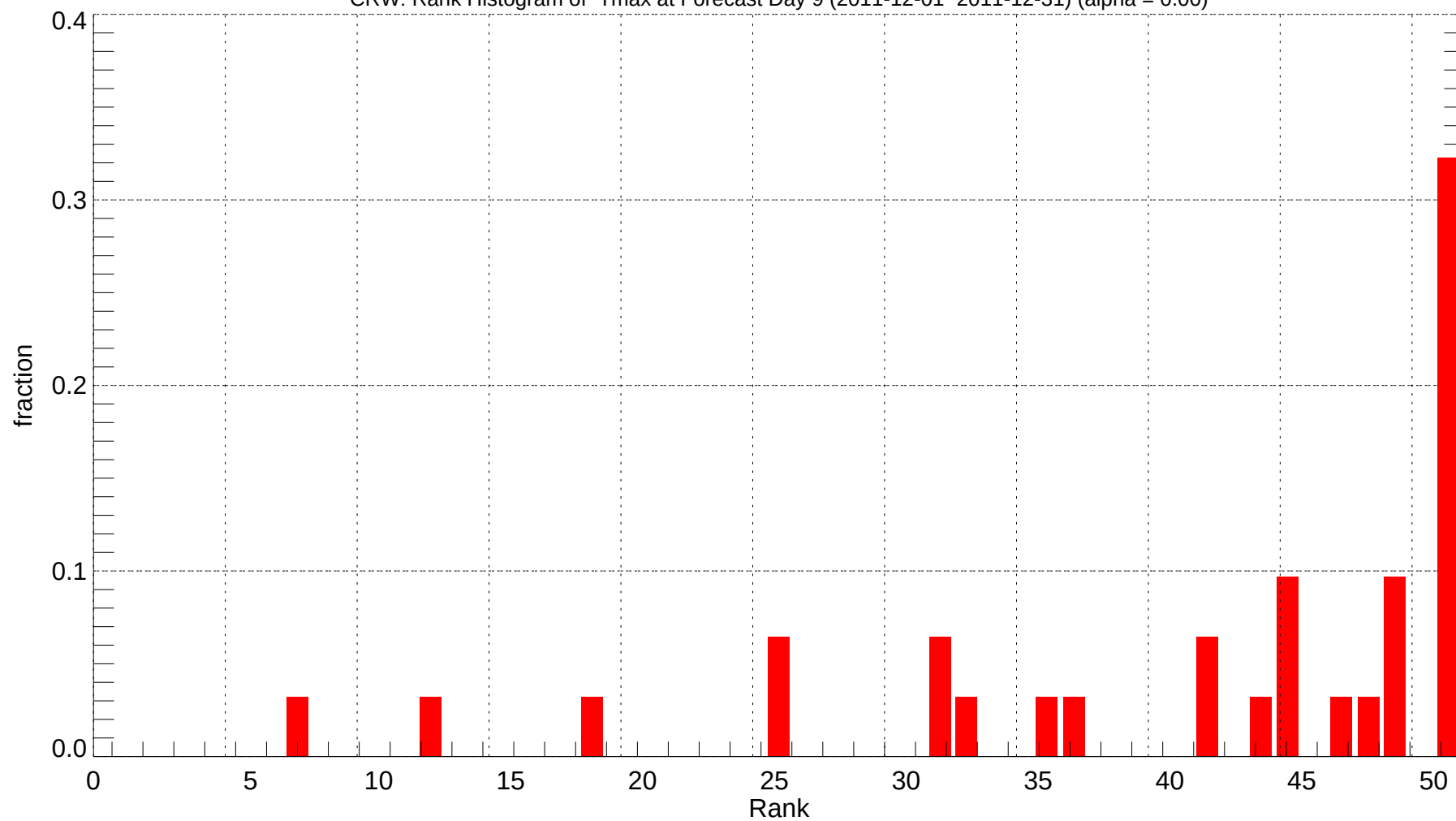
CRW: Rank Histogram of Tmax at Forecast Day 9 (2011-12-01~2011-12-31) (alpha = 0.00)
