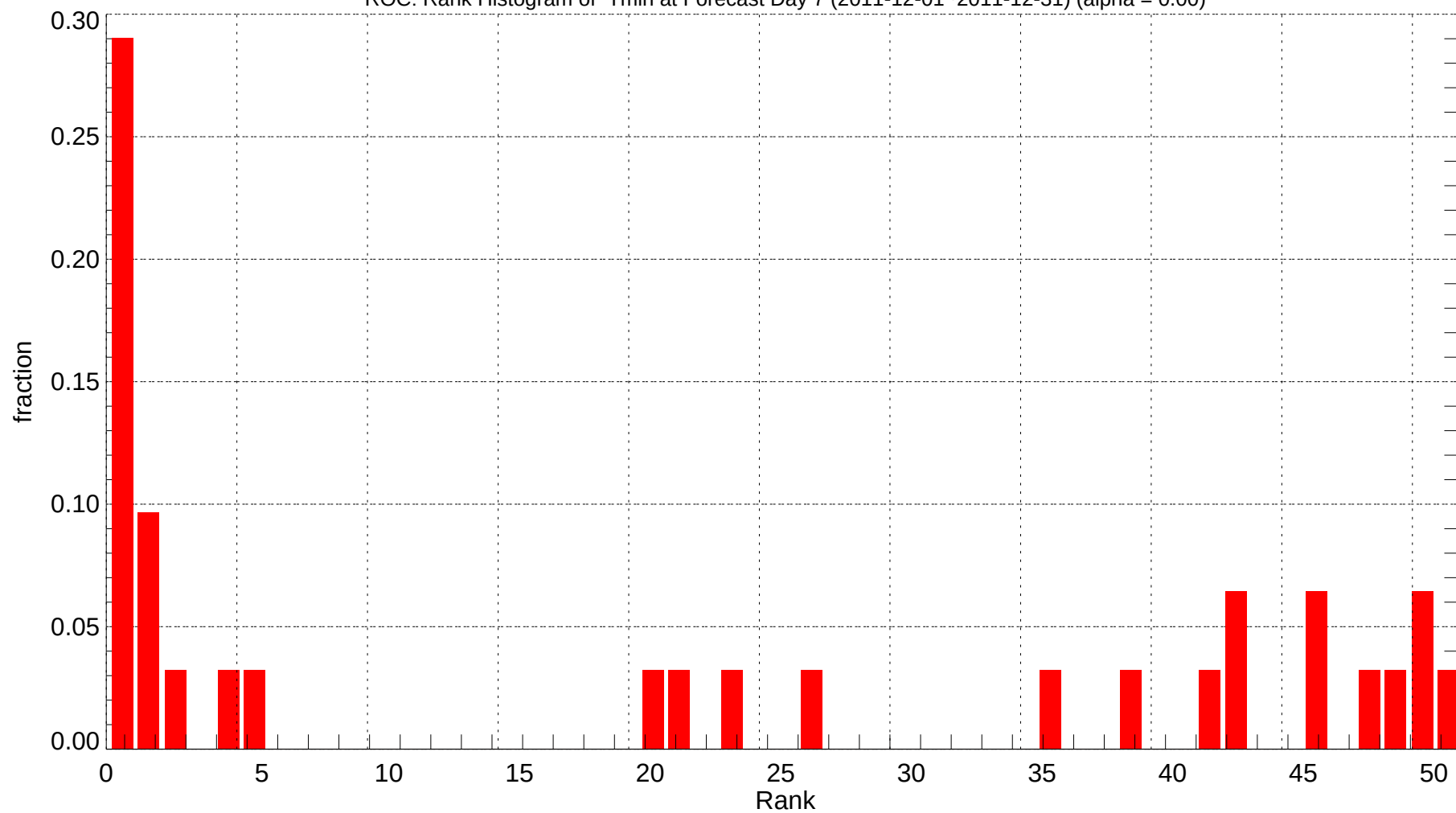
ROC: Rank Histogram of Tmin at Forecast Day 7 (2011-12-01~2011-12-31) (alpha = 0.00)
