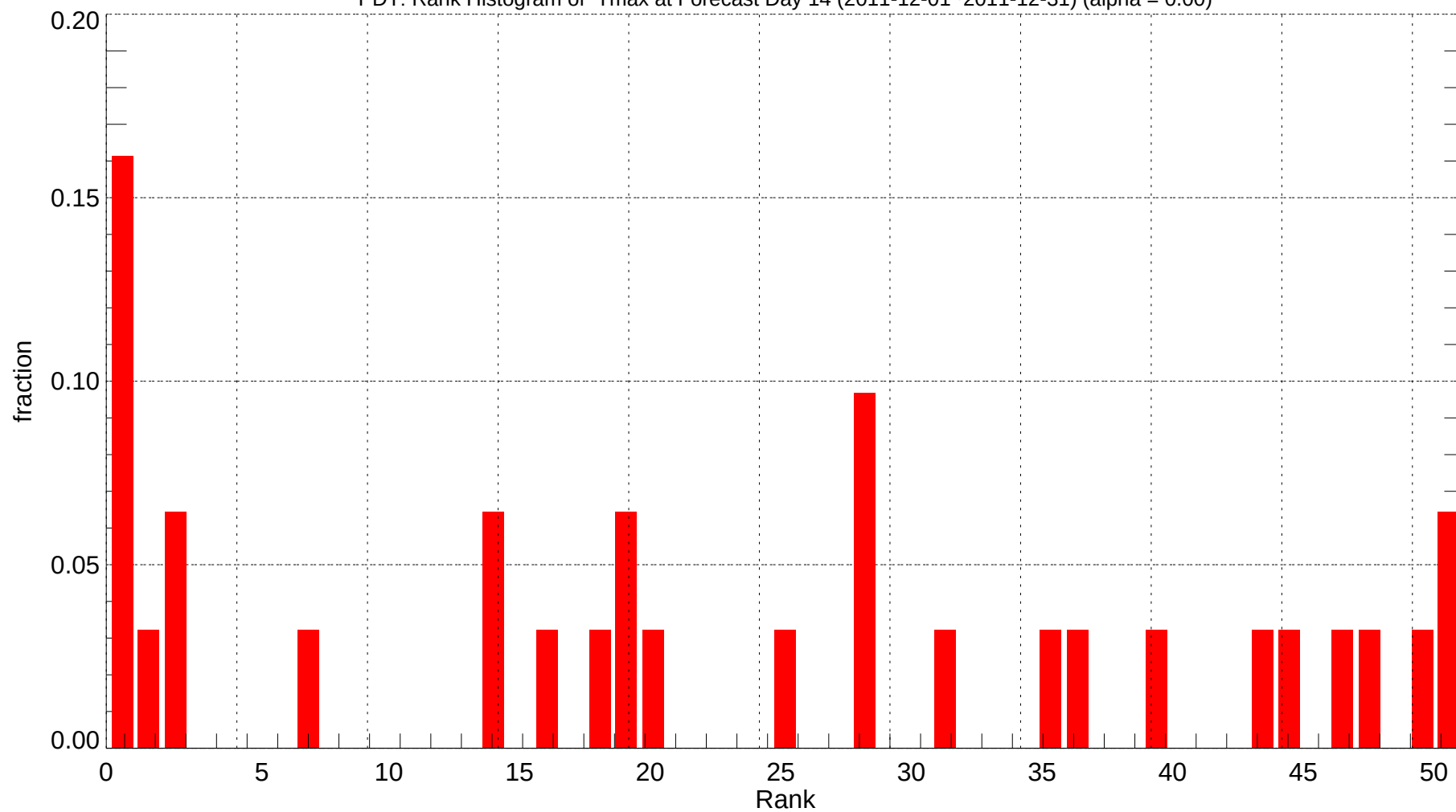
PDT: Rank Histogram of Tmax at Forecast Day 14 (2011-12-01~2011-12-31) (alpha = 0.00)
