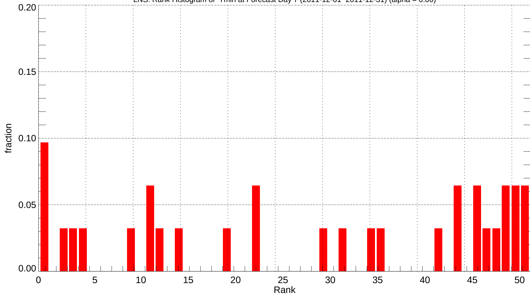
LNS: Rank Histogram of Tmin at Forecast Day 7 (2011-12-01~2011-12-31) (alpha = 0.00)
