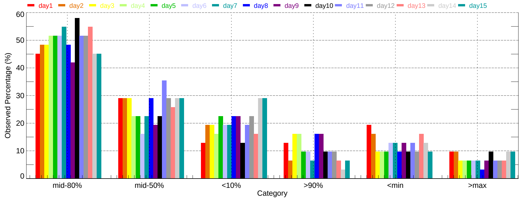
Observed Percentage of Ensembles - MWL: Max Temperature (2011-12-01~2011-12-31)
