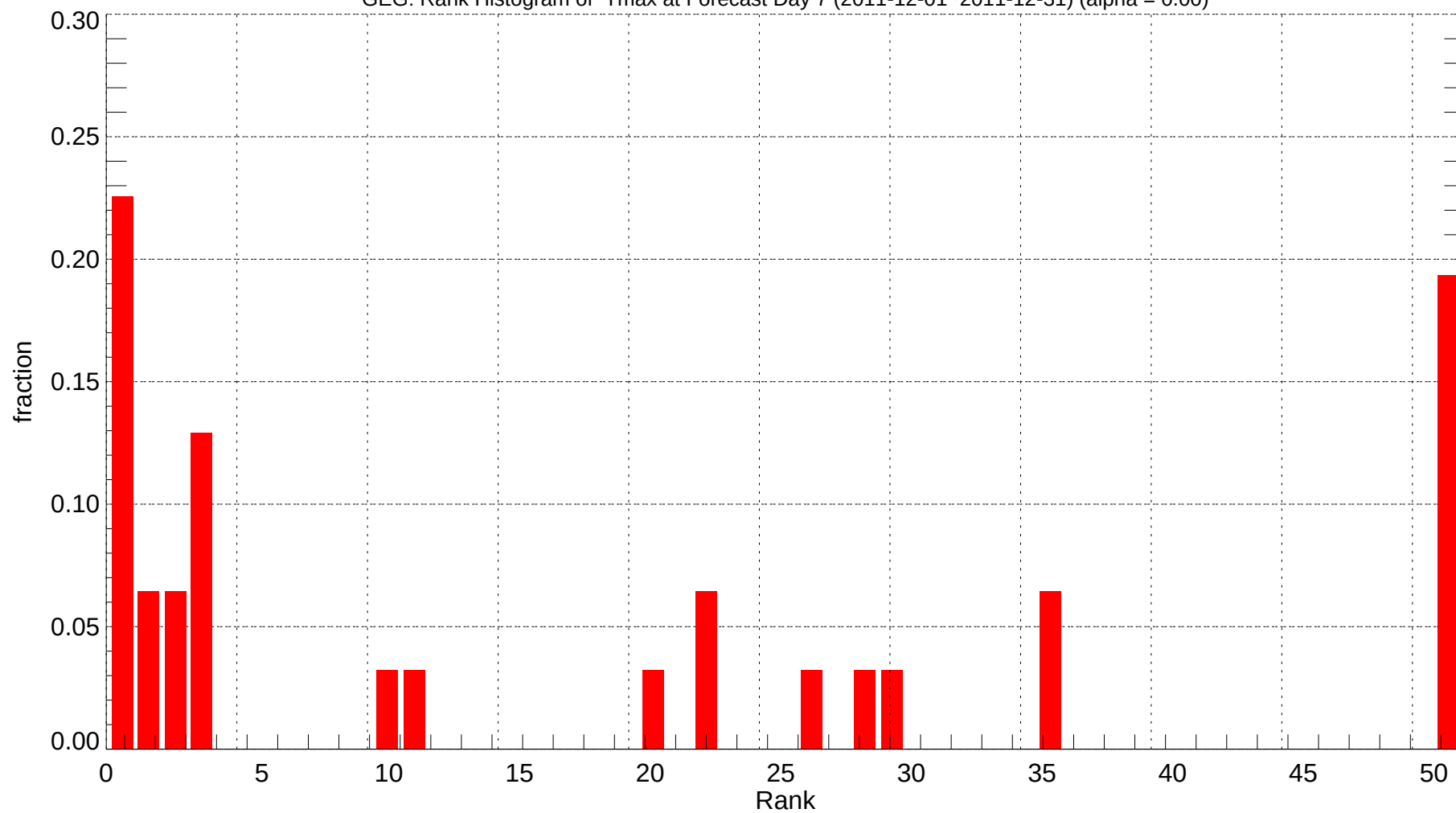
GEG: Rank Histogram of Tmax at Forecast Day 7 (2011-12-01~2011-12-31) (alpha = 0.00)
