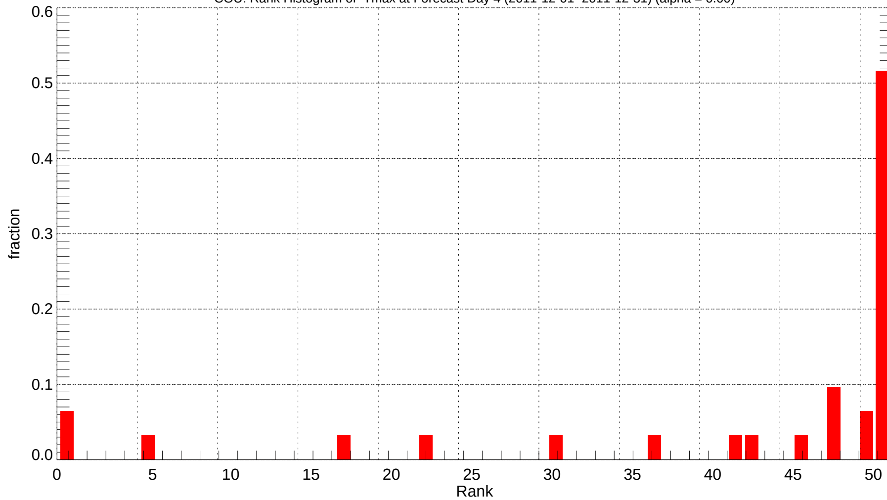
COU: Rank Histogram of Tmax at Forecast Day 4 (2011-12-01~2011-12-31) (alpha = 0.00)
