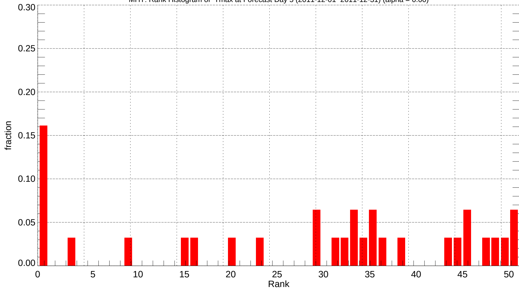
MHT: Rank Histogram of Tmax at Forecast Day 5 (2011-12-01~2011-12-31) (alpha = 0.00)
