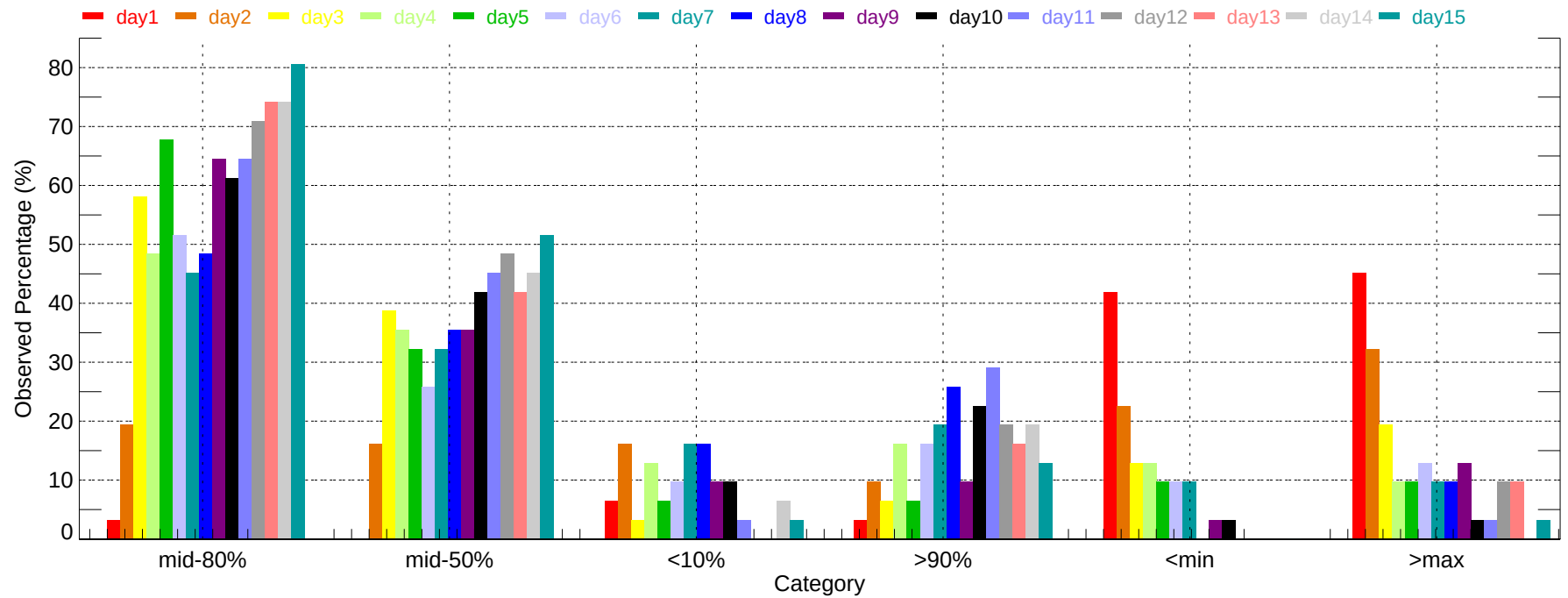
Observed Percentage of Ensembles - ROA: Min Temperature (2011-12-01~2011-12-31)
