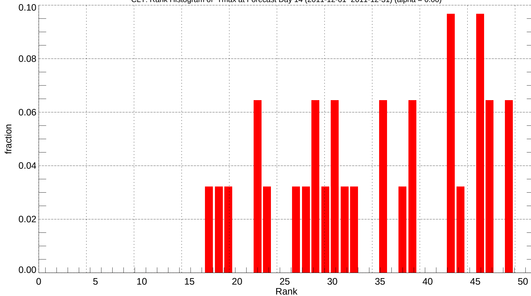
CLT: Rank Histogram of Tmax at Forecast Day 14 (2011-12-01~2011-12-31) (alpha = 0.00)
