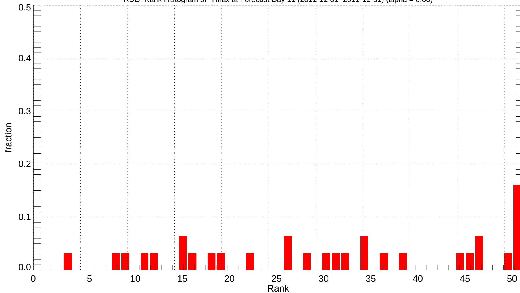
RDD: Rank Histogram of Tmax at Forecast Day 11 (2011-12-01~2011-12-31) (alpha = 0.00)
