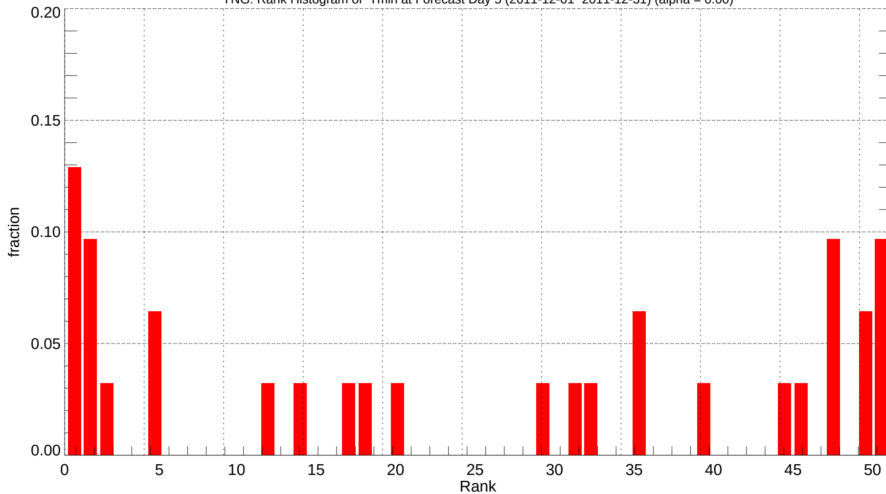
YNG: Rank Histogram of Tmin at Forecast Day 5 (2011-12-01~2011-12-31) (alpha = 0.00)
