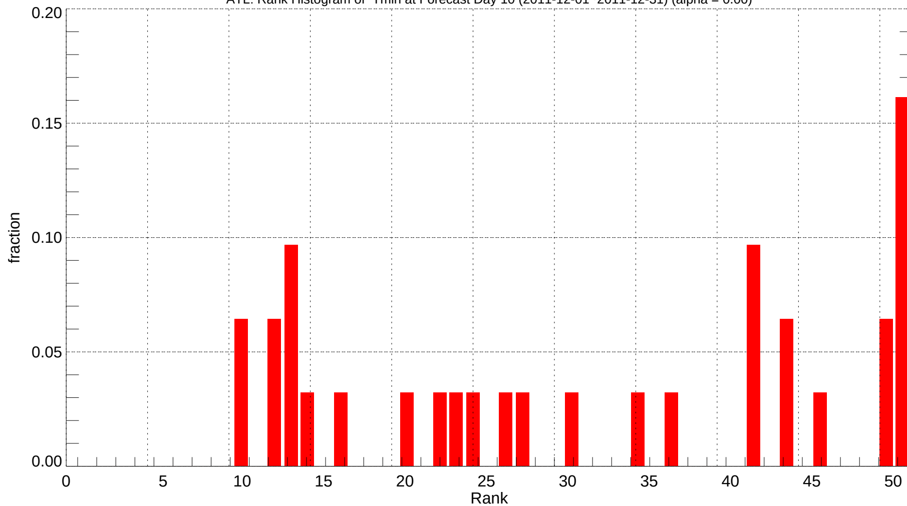
ATL: Rank Histogram of Tmin at Forecast Day 10 (2011-12-01~2011-12-31) (alpha = 0.00)
