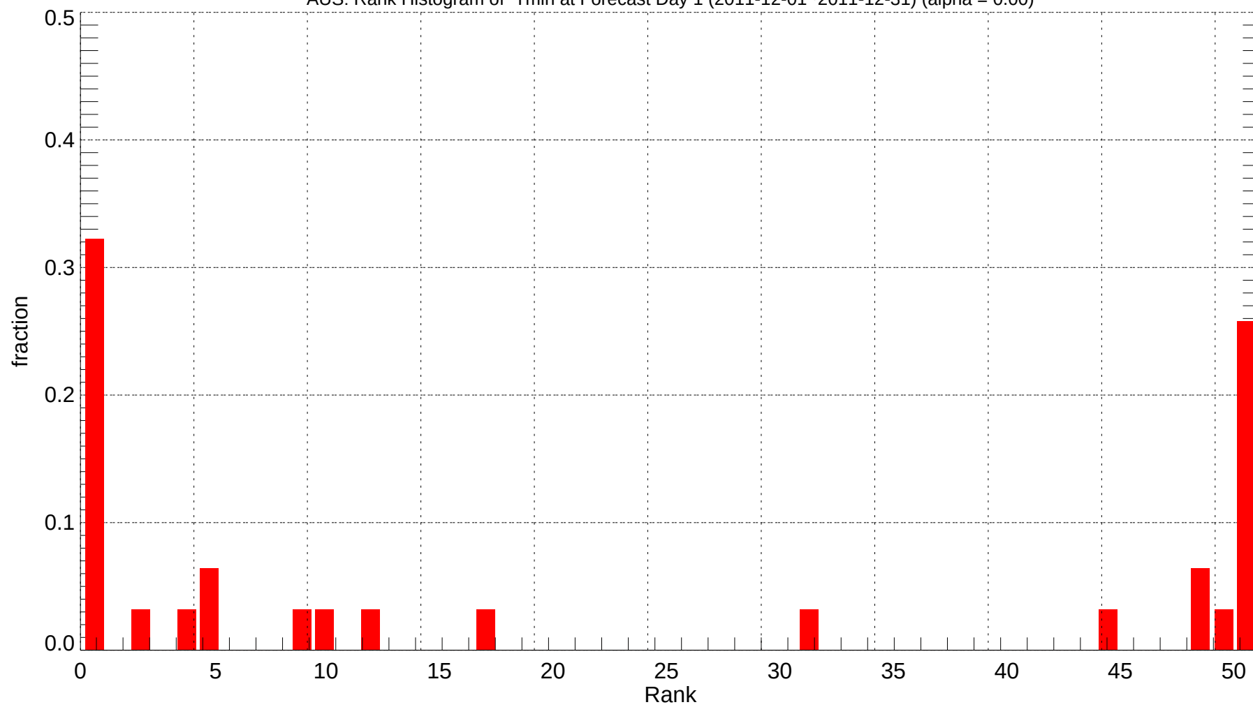
AUS: Rank Histogram of Tmin at Forecast Day 1 (2011-12-01~2011-12-31) (alpha = 0.00)
