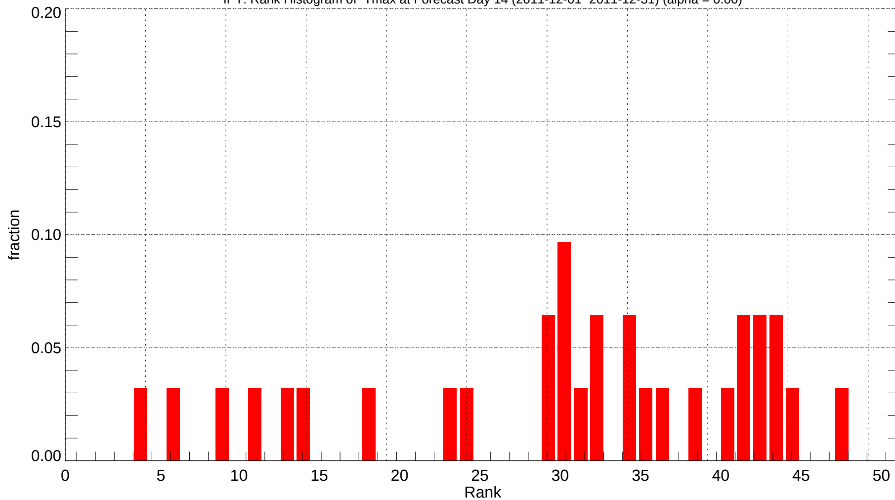
IPT: Rank Histogram of Tmax at Forecast Day 14 (2011-12-01~2011-12-31) (alpha = 0.00)
