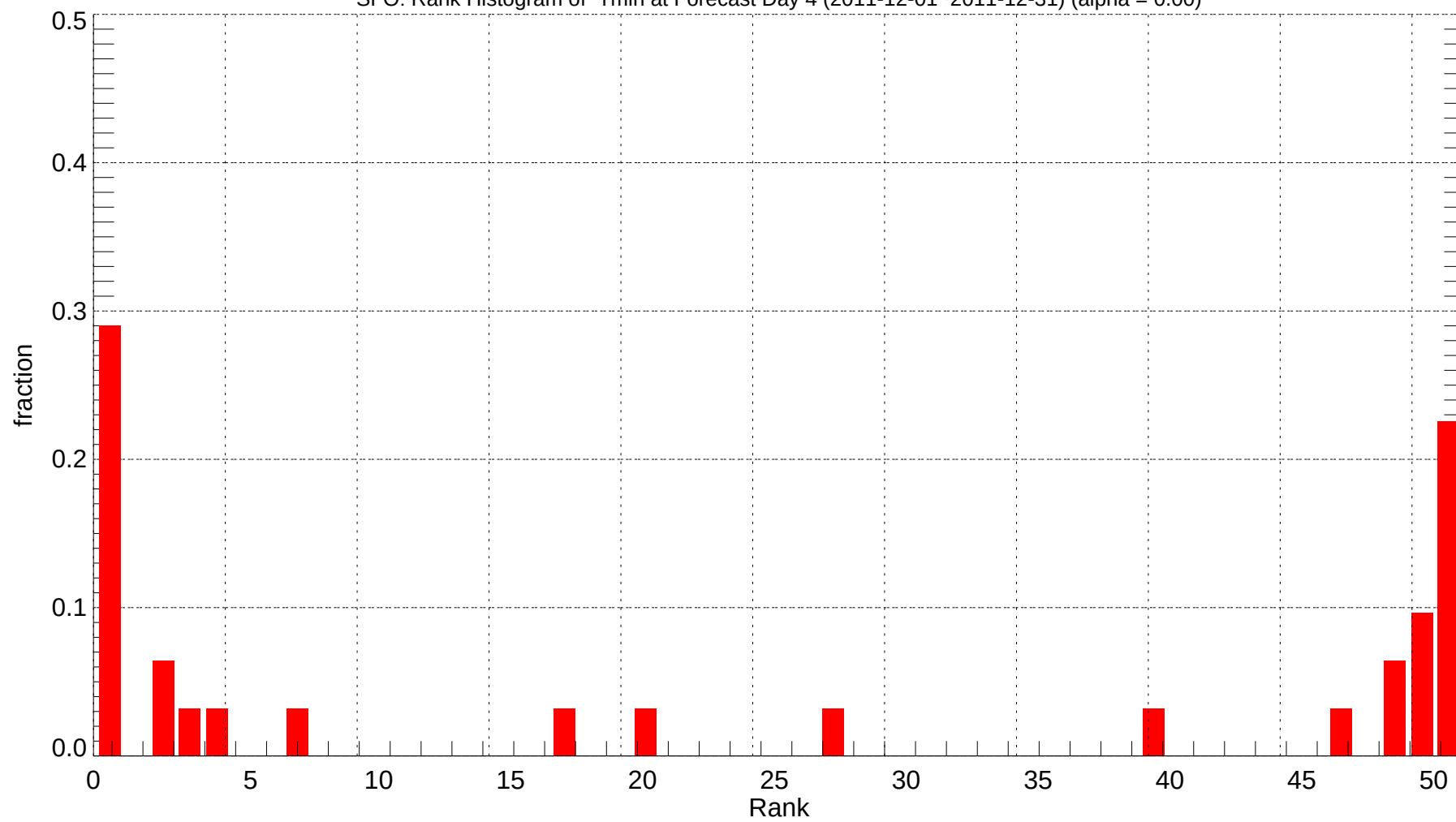
SFO: Rank Histogram of Tmin at Forecast Day 4 (2011-12-01~2011-12-31) (alpha = 0.00)
