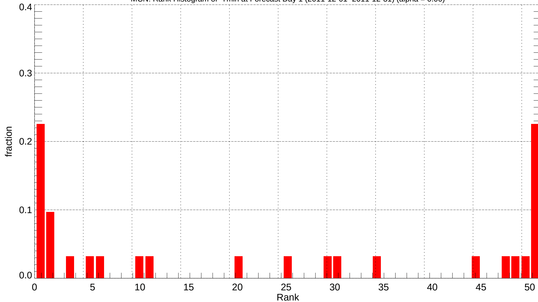
MCN: Rank Histogram of Tmin at Forecast Day 1 (2011-12-01~2011-12-31) (alpha = 0.00)
