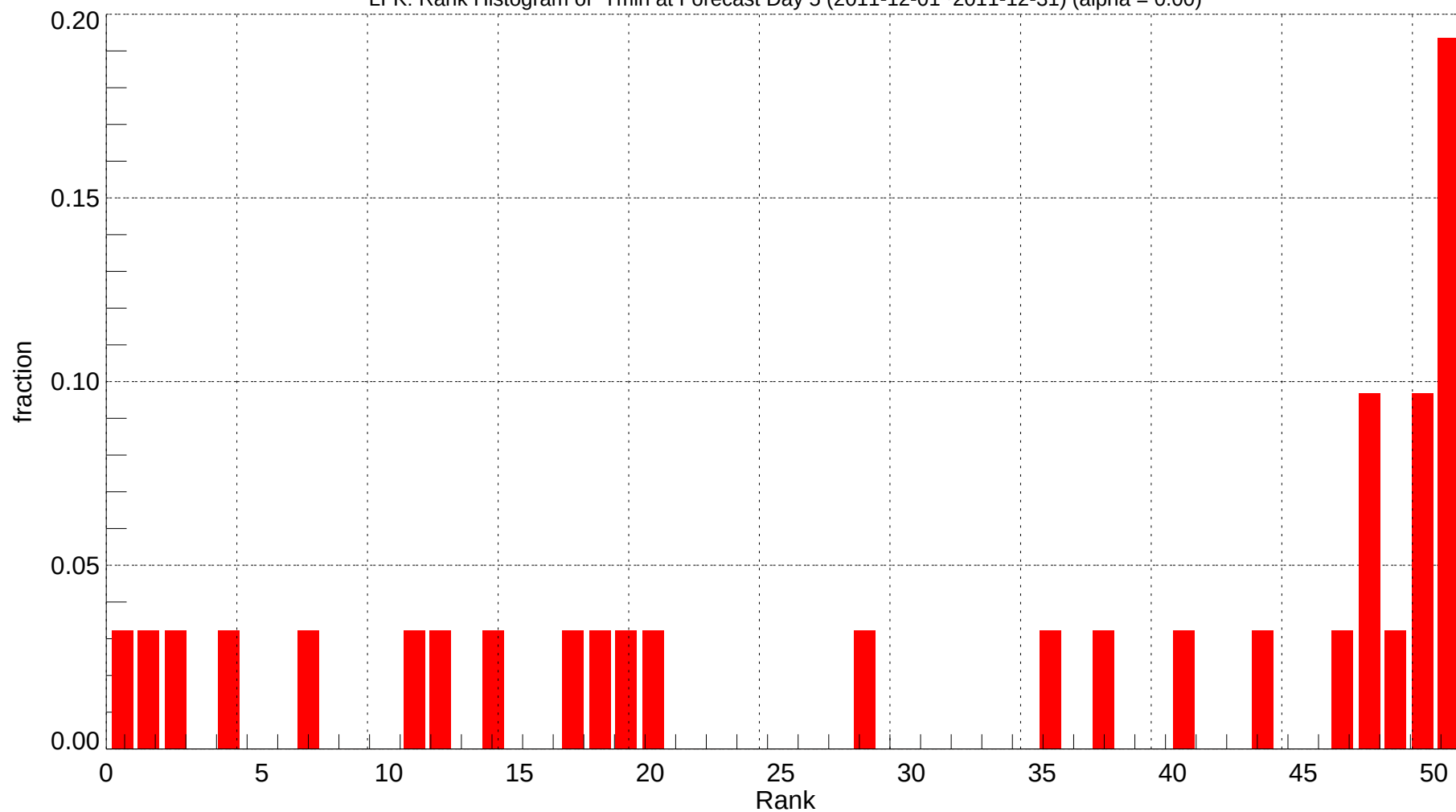
LFK: Rank Histogram of Tmin at Forecast Day 5 (2011-12-01~2011-12-31) (alpha = 0.00)
