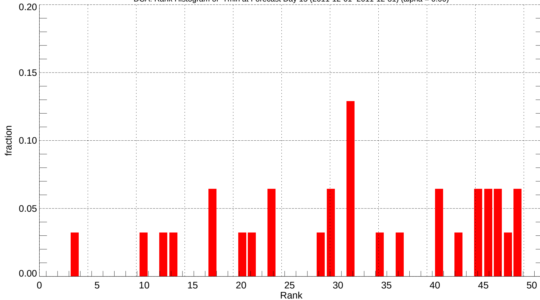
DCA: Rank Histogram of Tmin at Forecast Day 15 (2011-12-01~2011-12-31) (alpha = 0.00)
