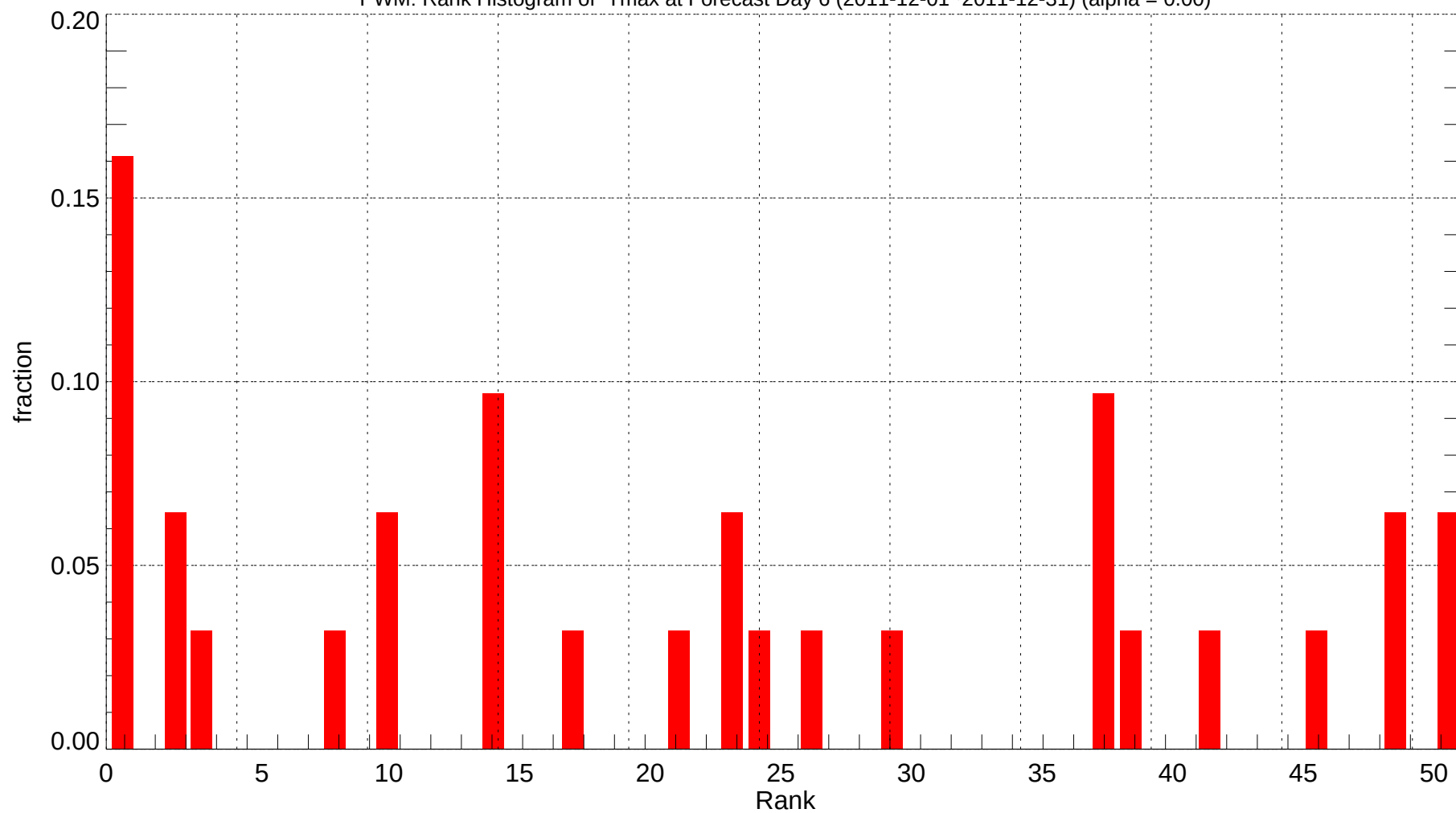
PWM: Rank Histogram of Tmax at Forecast Day 6 (2011-12-01~2011-12-31) (alpha = 0.00)
