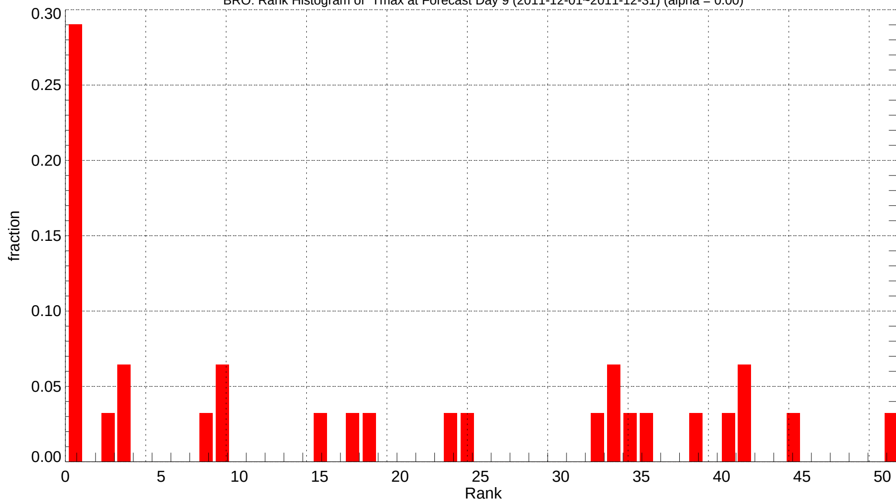
BRO: Rank Histogram of Tmax at Forecast Day 9 (2011-12-01~2011-12-31) (alpha = 0.00)
