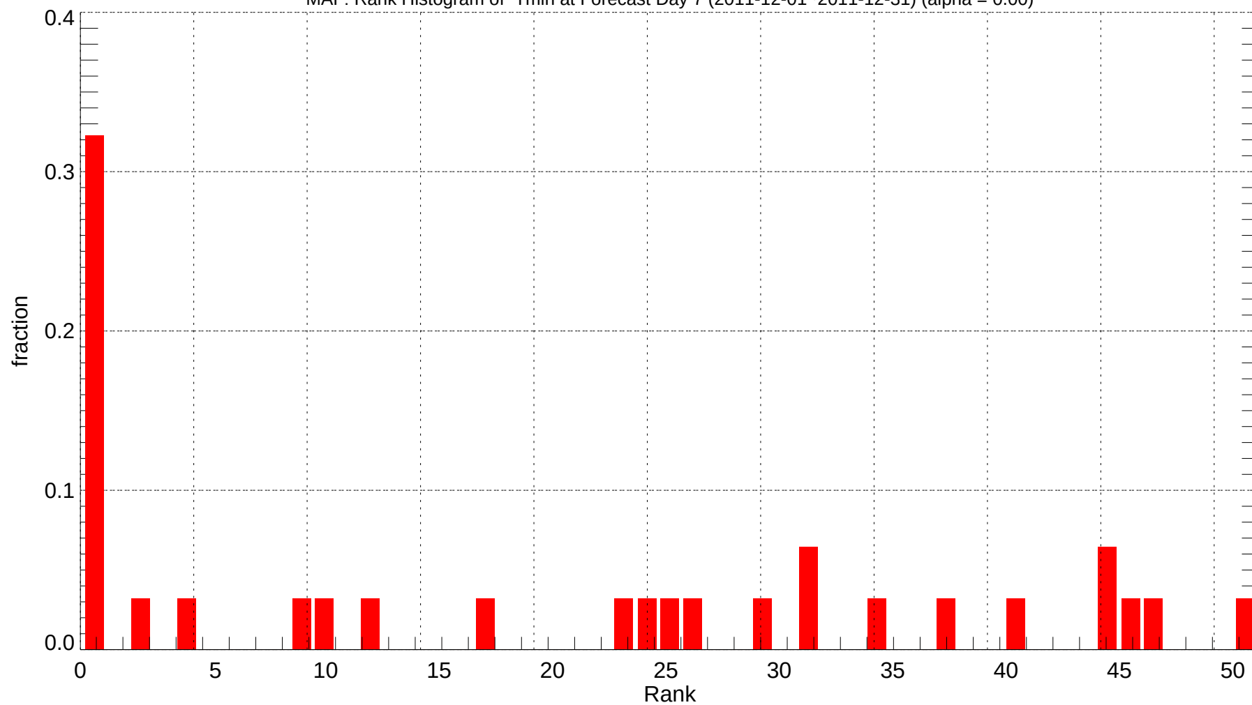
MAF: Rank Histogram of Tmin at Forecast Day 7 (2011-12-01~2011-12-31) (alpha = 0.00)
