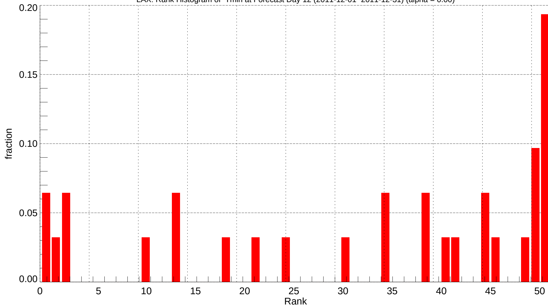
LAX: Rank Histogram of Tmin at Forecast Day 12 (2011-12-01~2011-12-31) (alpha = 0.00)
