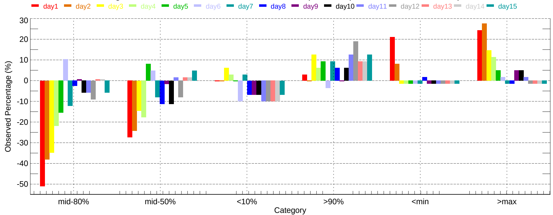
Observed Percentage Deviation of Ensembles - DCA: Max Temperature (2011-12-01~2011-12-31)
