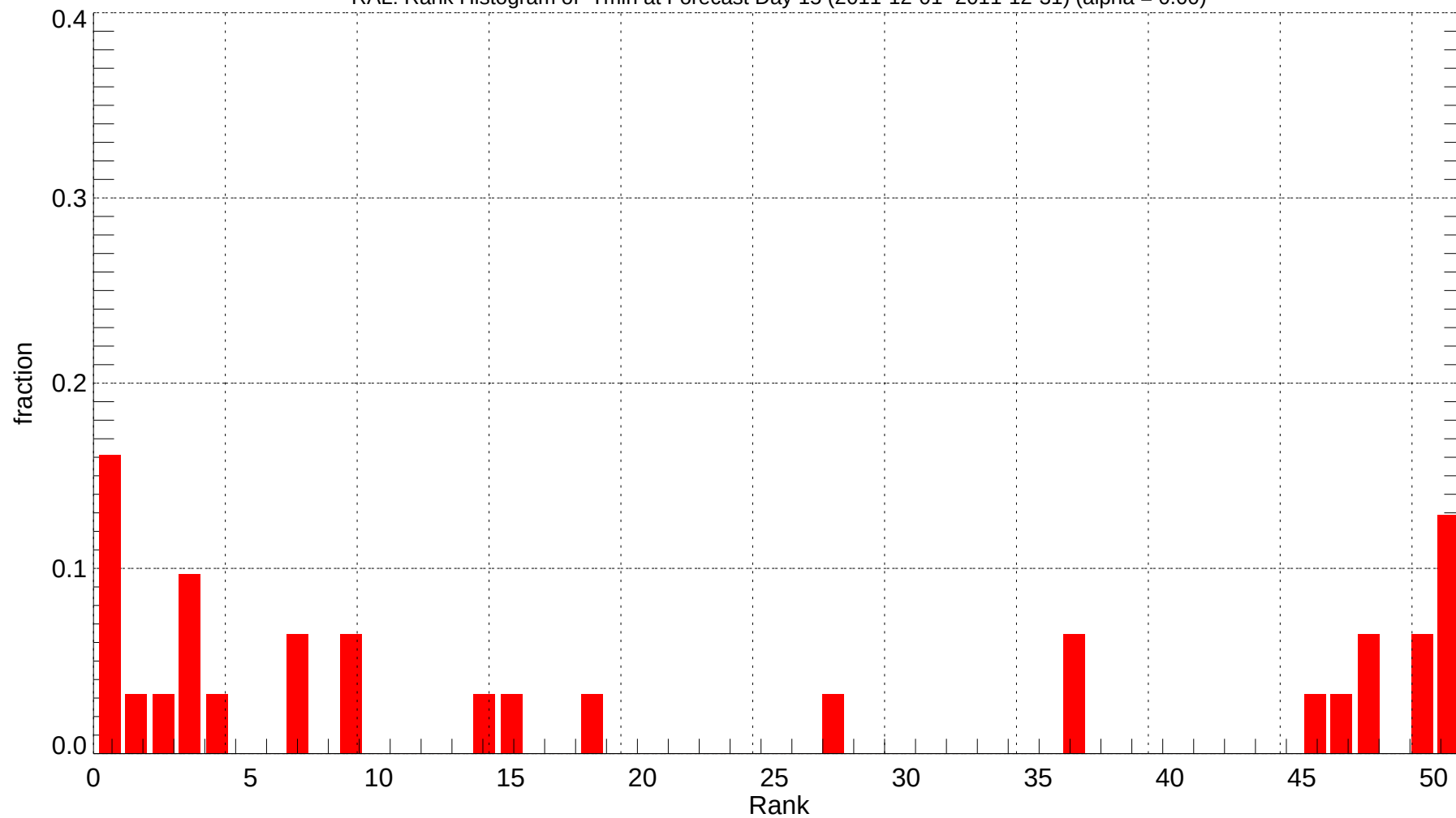
RAL: Rank Histogram of Tmin at Forecast Day 15 (2011-12-01~2011-12-31) (alpha = 0.00)
