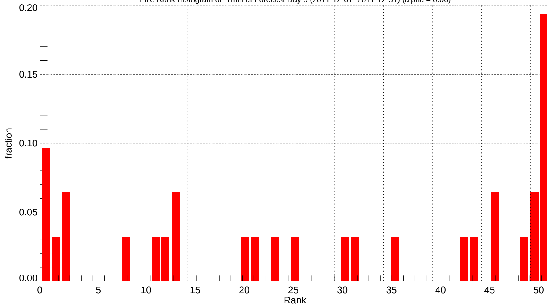
PIR: Rank Histogram of Tmin at Forecast Day 9 (2011-12-01~2011-12-31) (alpha = 0.00)
