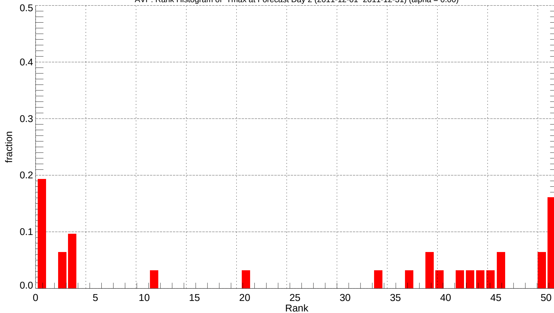
AVP: Rank Histogram of Tmax at Forecast Day 2 (2011-12-01~2011-12-31) (alpha = 0.00)
