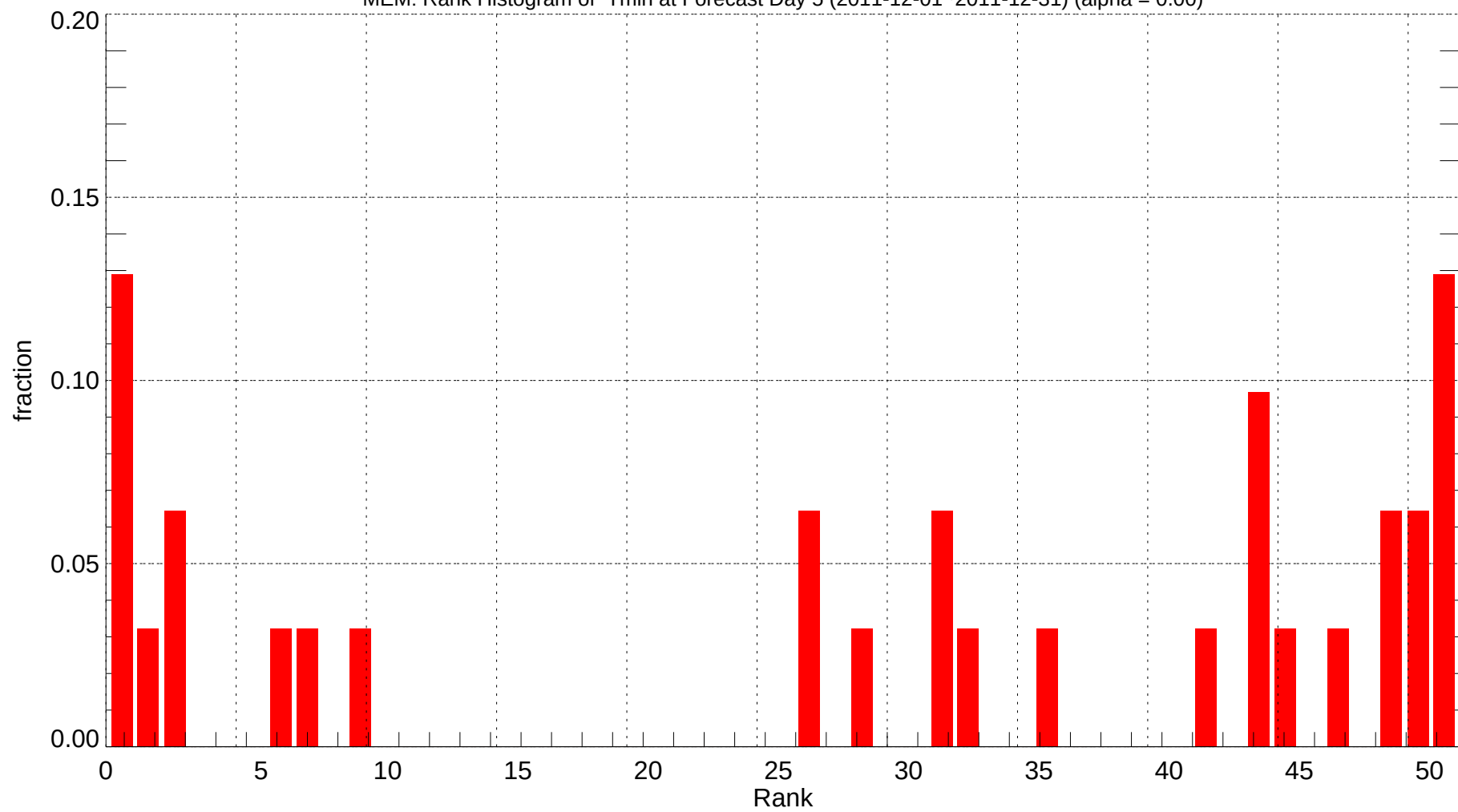
MEM: Rank Histogram of Tmin at Forecast Day 5 (2011-12-01~2011-12-31) (alpha = 0.00)
