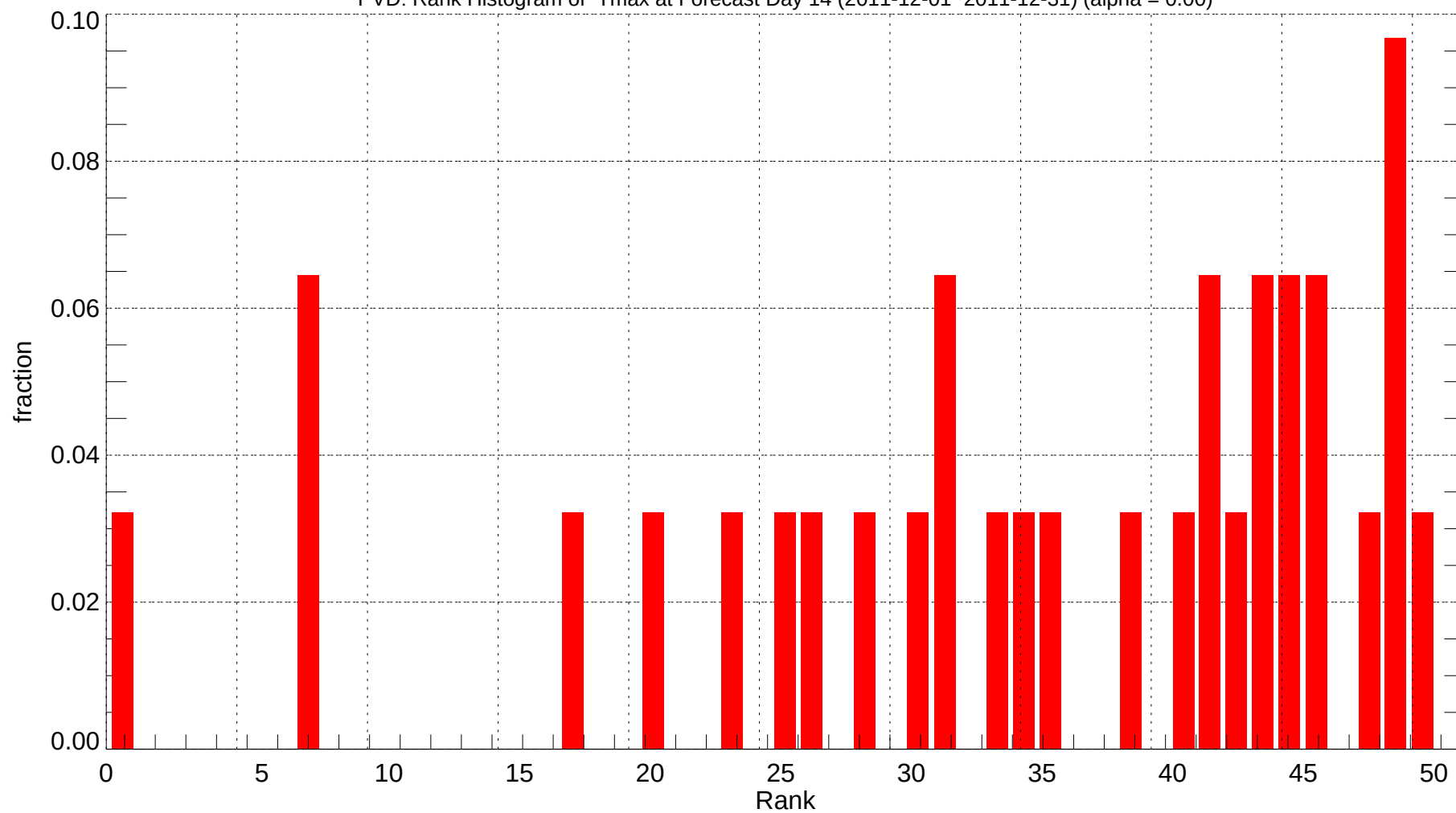
PVD: Rank Histogram of Tmax at Forecast Day 14 (2011-12-01~2011-12-31) (alpha = 0.00)
