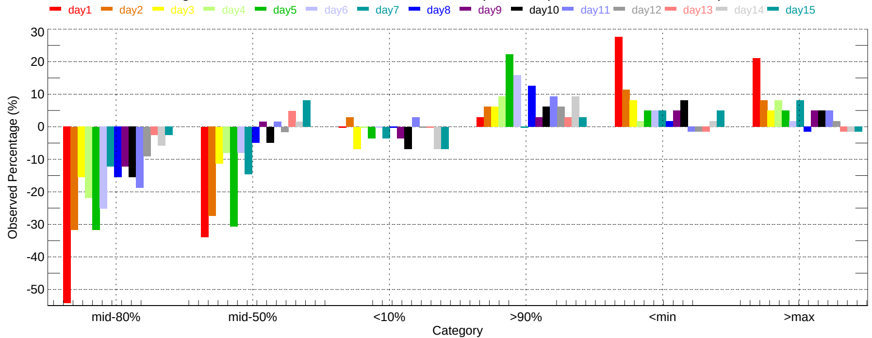
Observed Percentage Deviation of Ensembles - ALB: Max Temperature (2011-12-01~2011-12-31)
