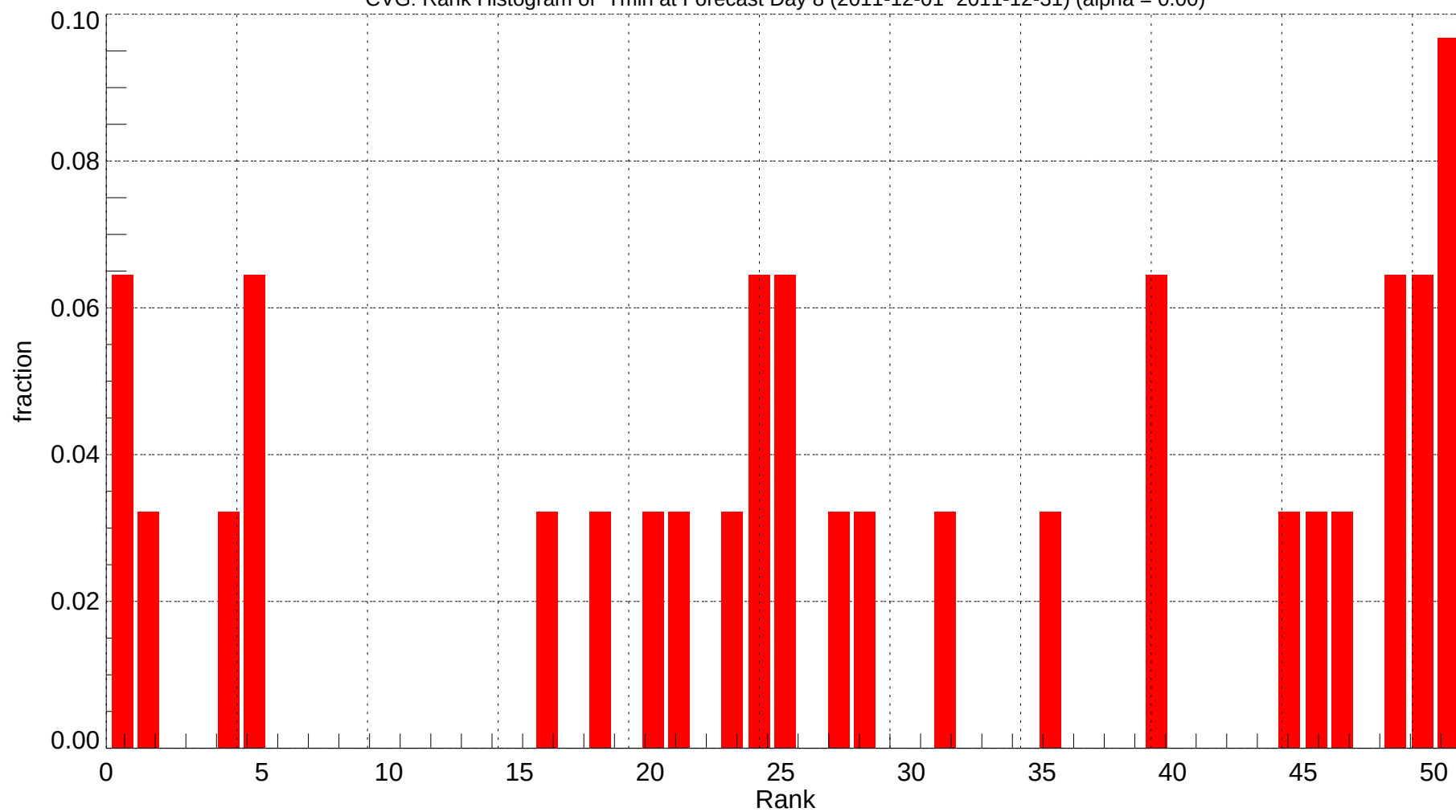
CVG: Rank Histogram of Tmin at Forecast Day 8 (2011-12-01~2011-12-31) (alpha = 0.00)
