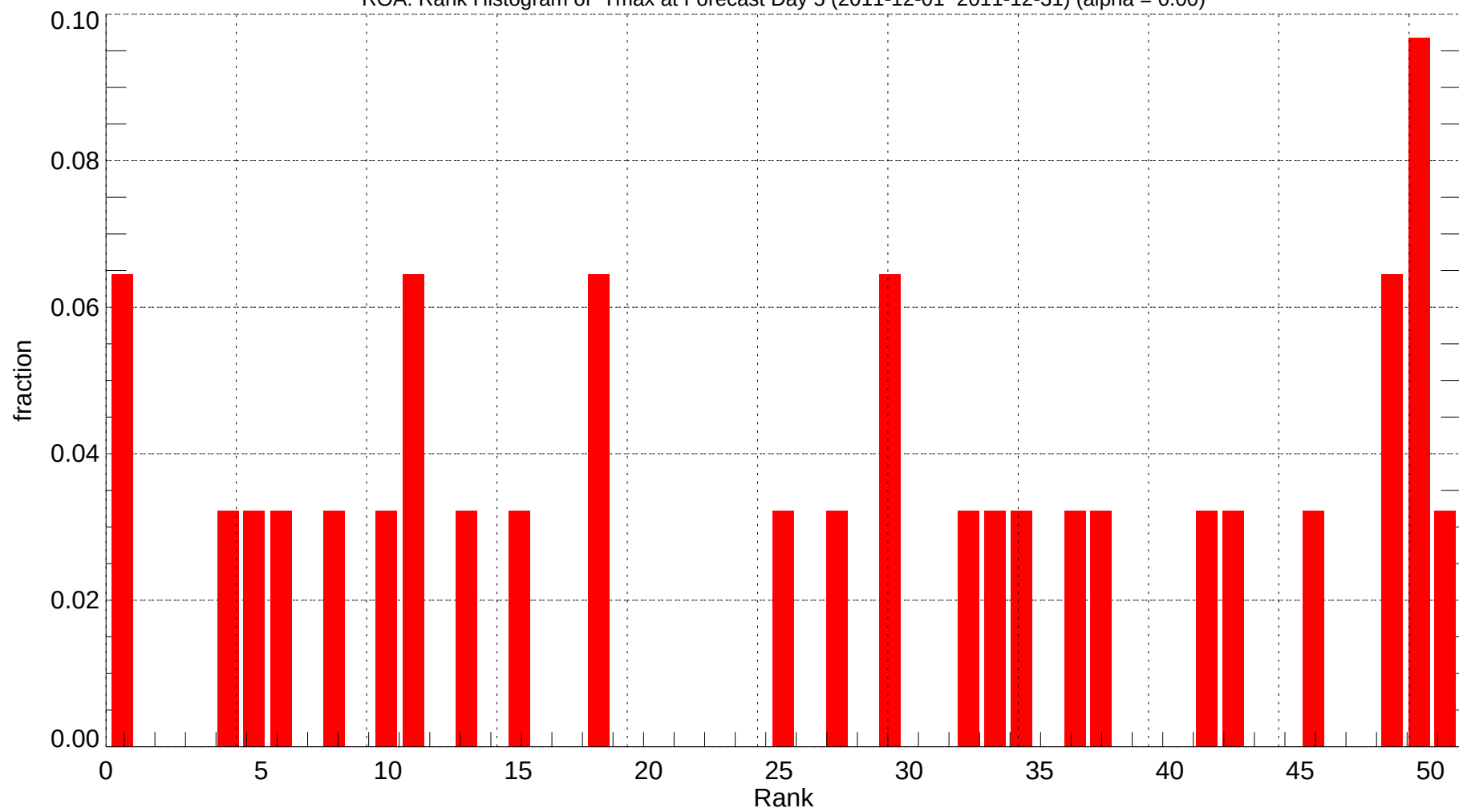
ROA: Rank Histogram of Tmax at Forecast Day 5 (2011-12-01~2011-12-31) (alpha = 0.00)
