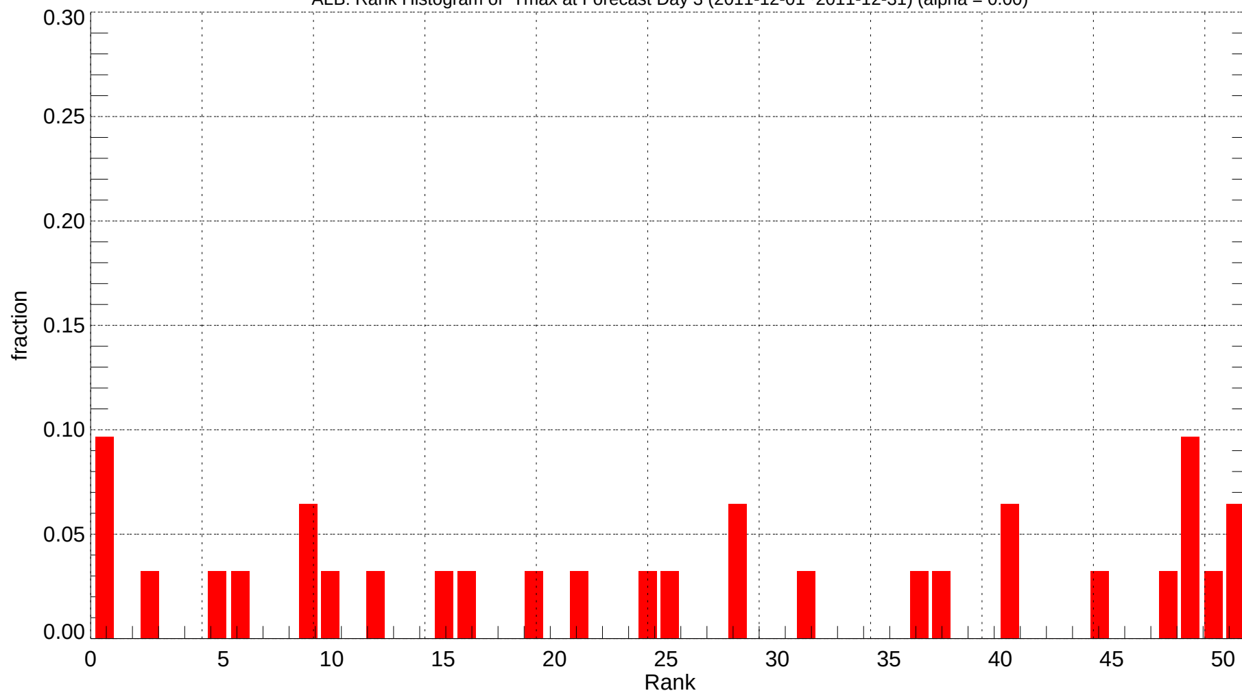
ALB: Rank Histogram of Tmax at Forecast Day 3 (2011-12-01~2011-12-31) (alpha = 0.00)
