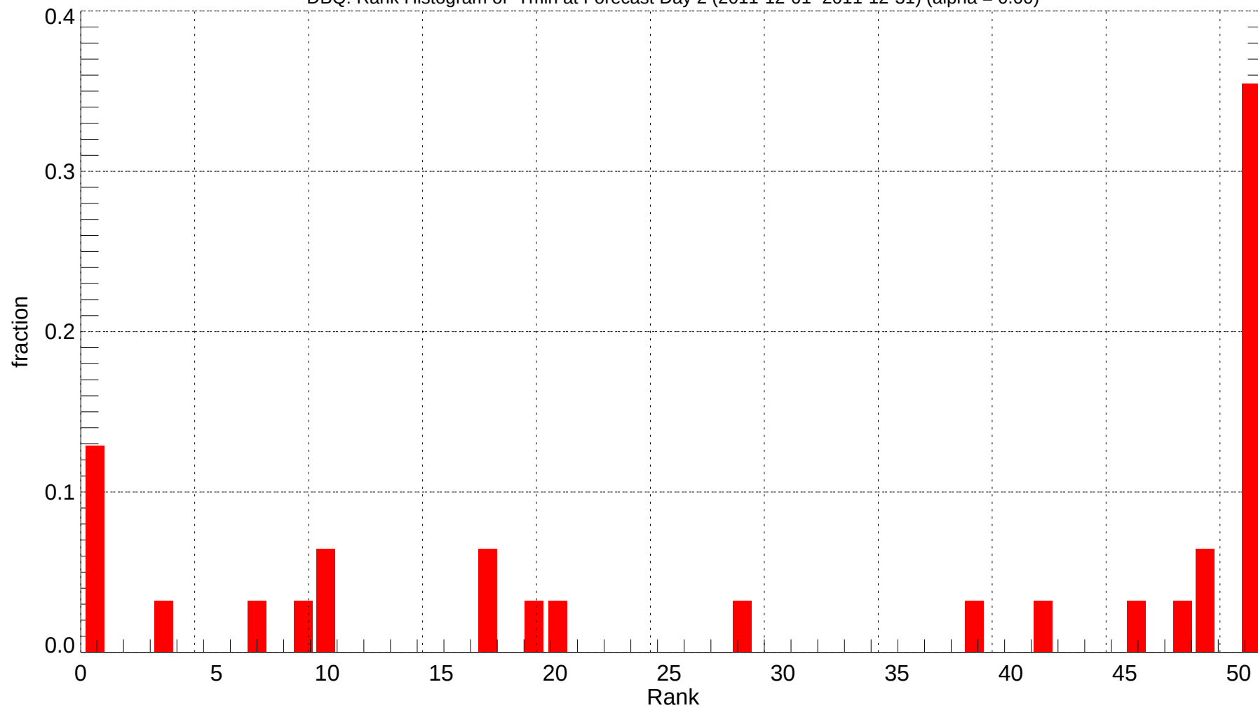
DBQ: Rank Histogram of Tmin at Forecast Day 2 (2011-12-01~2011-12-31) (alpha = 0.00)
