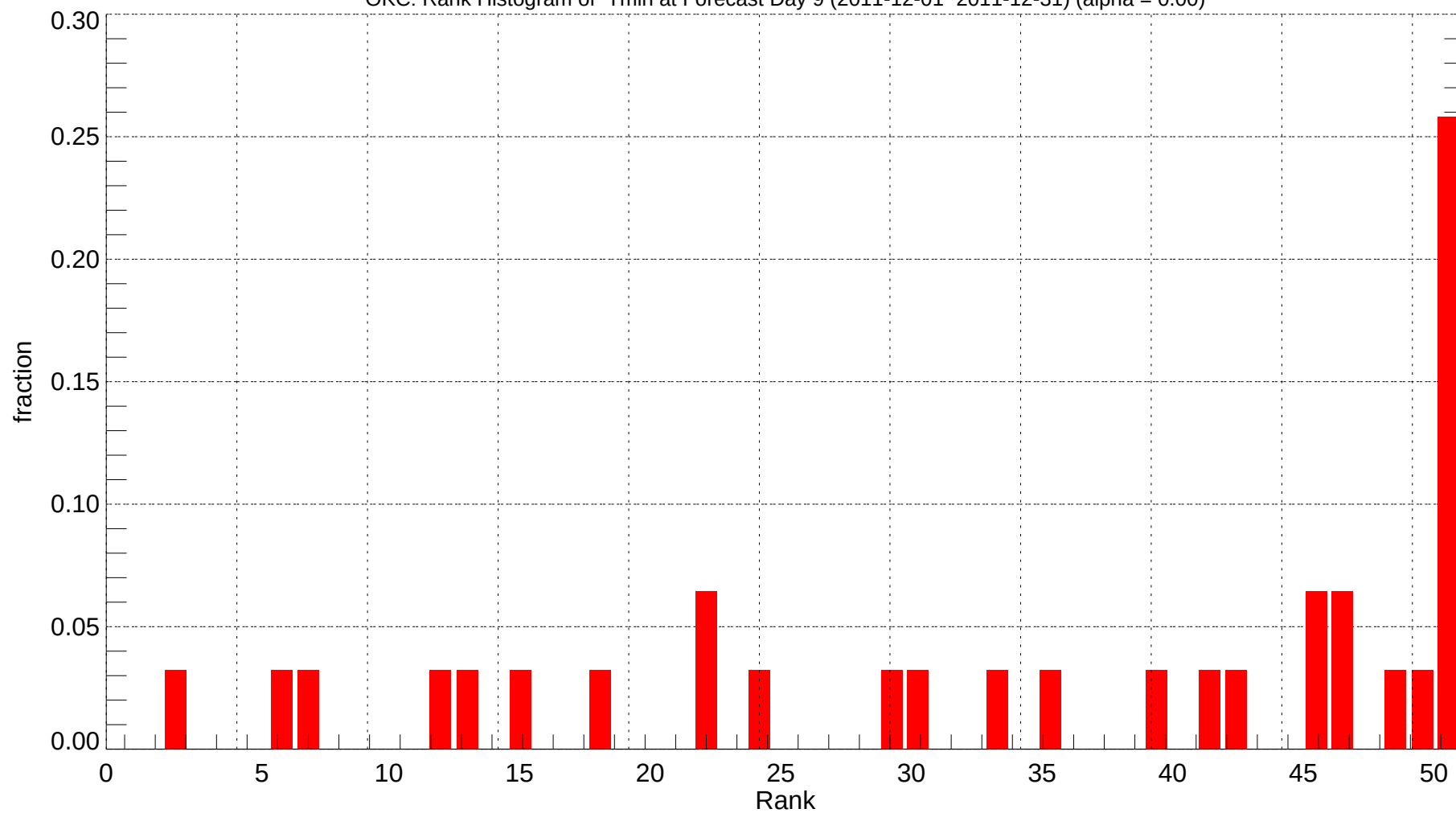
OKC: Rank Histogram of Tmin at Forecast Day 9 (2011-12-01~2011-12-31) (alpha = 0.00)
