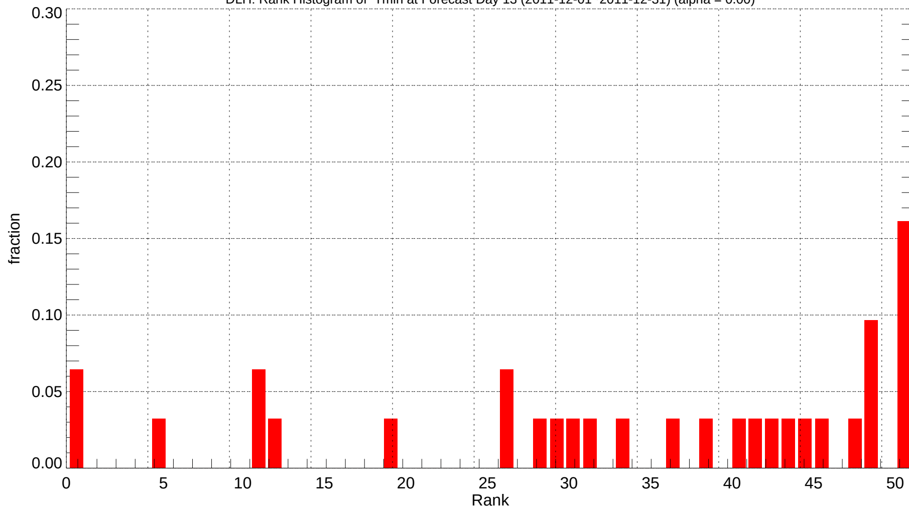
DLH: Rank Histogram of Tmin at Forecast Day 13 (2011-12-01~2011-12-31) (alpha = 0.00)
