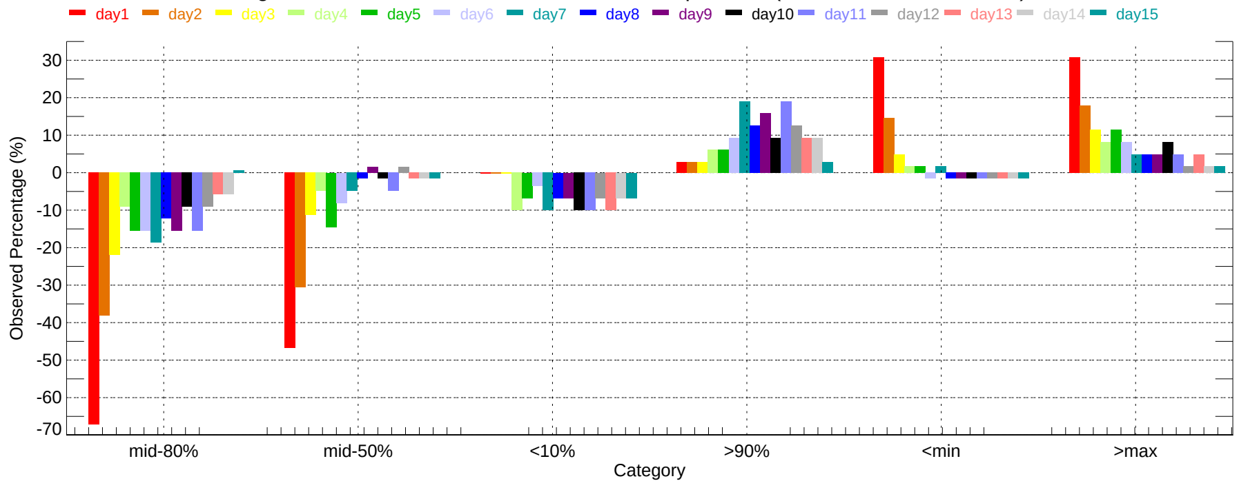
Observed Percentage Deviation of Ensembles - OKC: Min Temperature (2011-12-01~2011-12-31)
