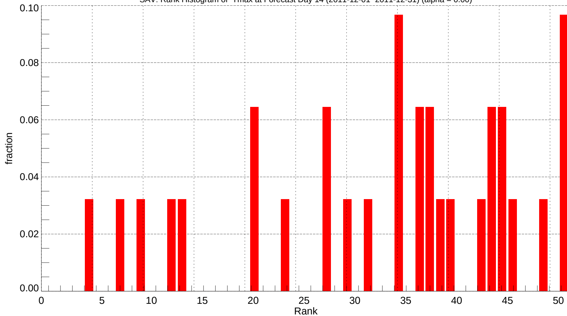
SAV: Rank Histogram of Tmax at Forecast Day 14 (2011-12-01~2011-12-31) (alpha = 0.00)
