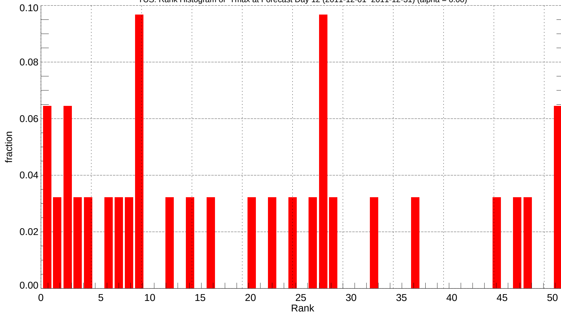
TUS: Rank Histogram of Tmax at Forecast Day 12 (2011-12-01~2011-12-31) (alpha = 0.00)
