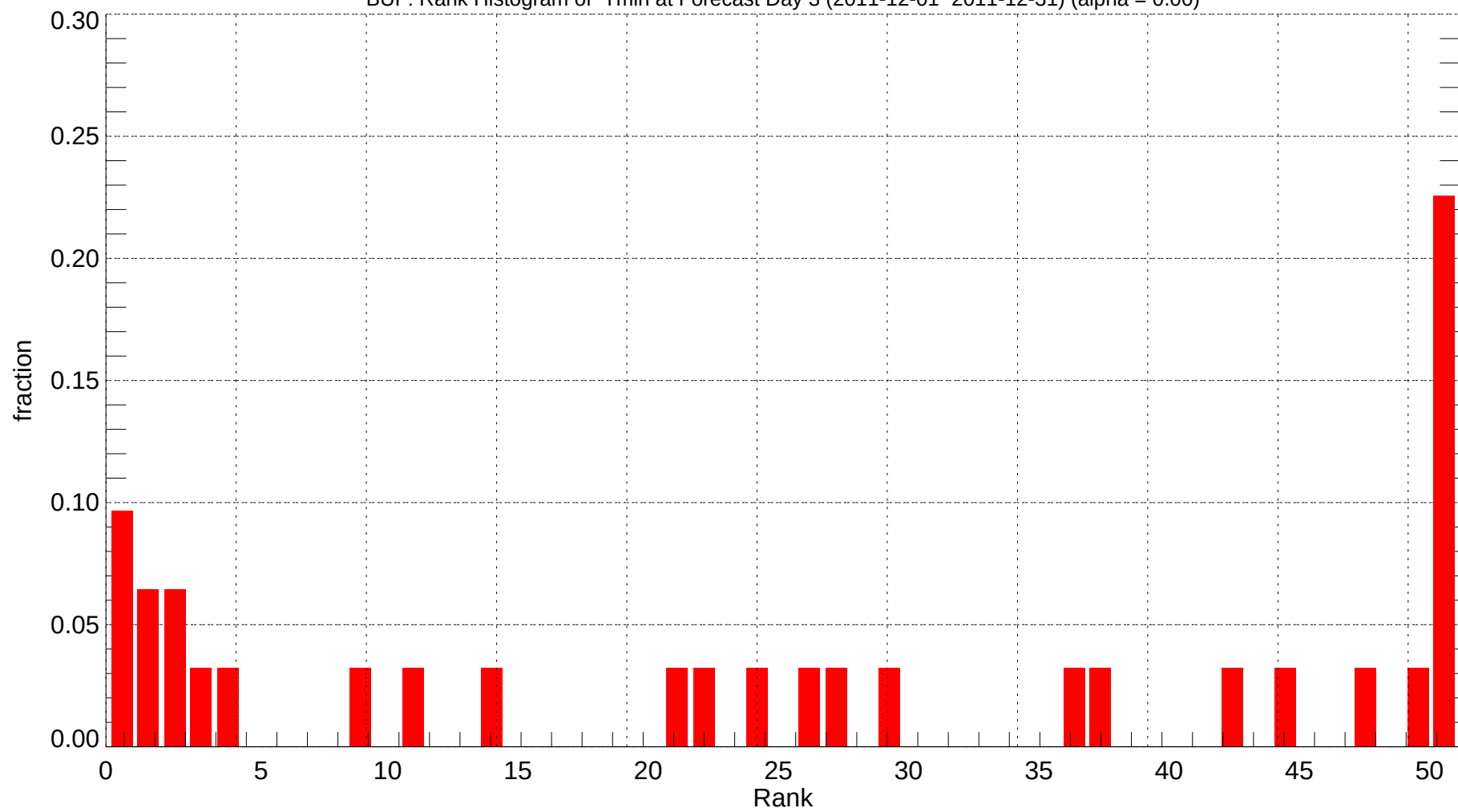
BUF: Rank Histogram of Tmin at Forecast Day 3 (2011-12-01~2011-12-31) (alpha = 0.00)
