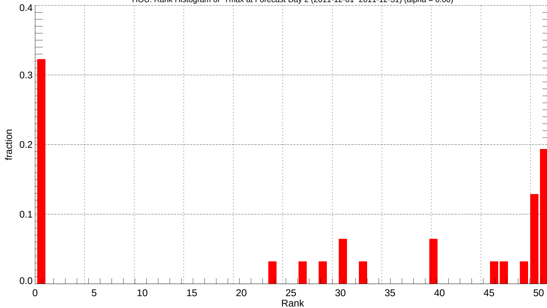
HOU: Rank Histogram of Tmax at Forecast Day 2 (2011-12-01~2011-12-31) (alpha = 0.00)
