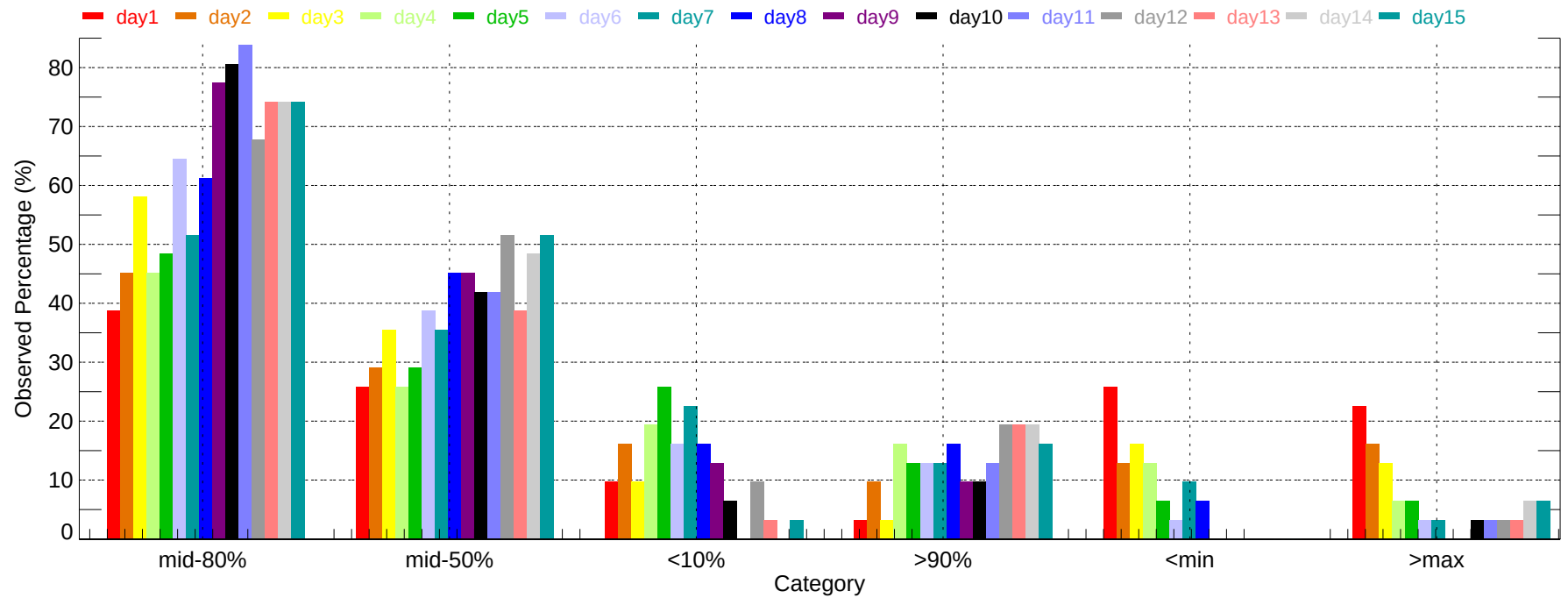
Observed Percentage of Ensembles - MCO: Max Temperature (2011-12-01~2011-12-31)
