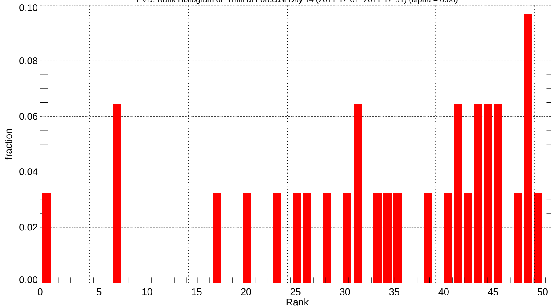
PVD: Rank Histogram of Tmin at Forecast Day 14 (2011-12-01~2011-12-31) (alpha = 0.00)
