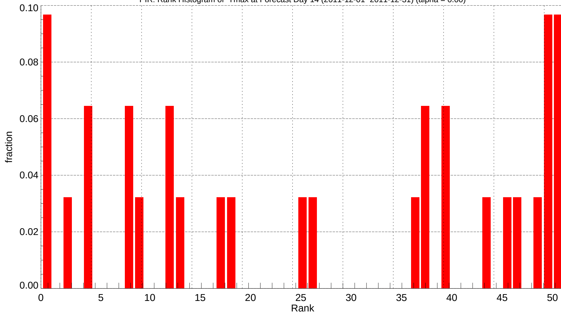
PIR: Rank Histogram of Tmax at Forecast Day 14 (2011-12-01~2011-12-31) (alpha = 0.00)
