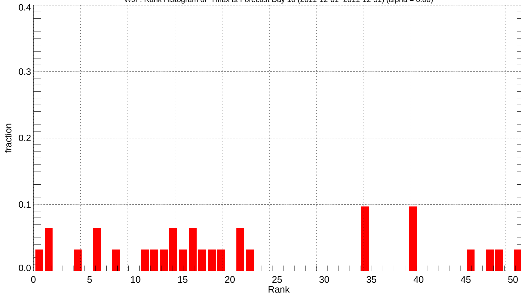
WJF: Rank Histogram of Tmax at Forecast Day 10 (2011-12-01~2011-12-31) (alpha = 0.00)
