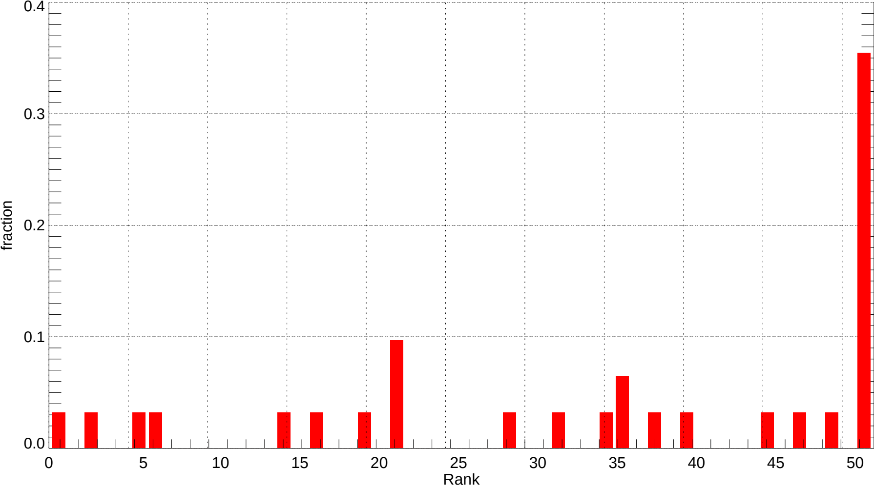
TUL: Rank Histogram of Tmin at Forecast Day 3 (2011-12-01~2011-12-31) (alpha = 0.00)
