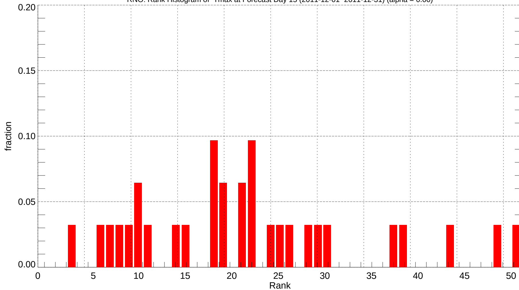
RNO: Rank Histogram of Tmax at Forecast Day 15 (2011-12-01~2011-12-31) (alpha = 0.00)
