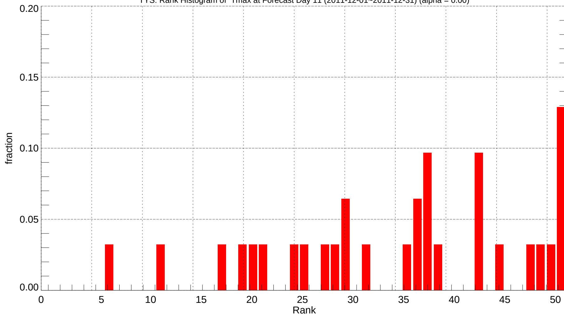
TYS: Rank Histogram of Tmax at Forecast Day 11 (2011-12-01~2011-12-31) (alpha = 0.00)
