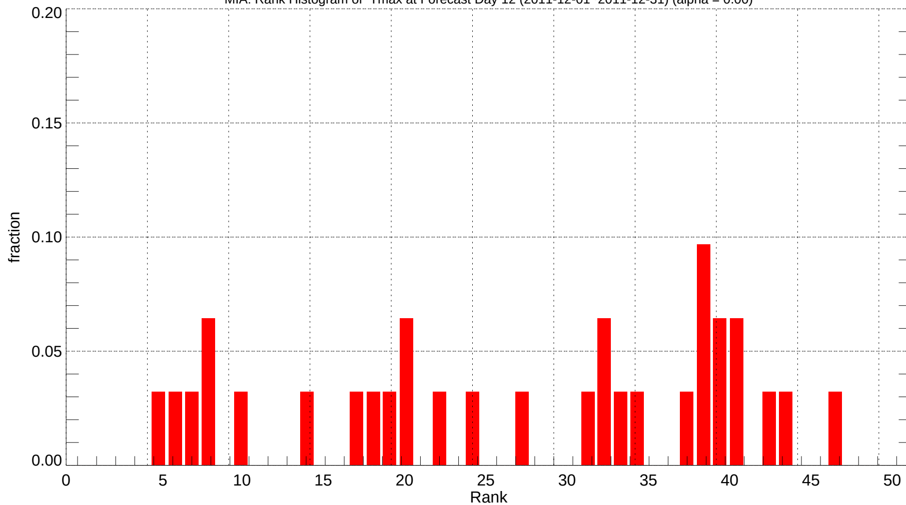
MIA: Rank Histogram of Tmax at Forecast Day 12 (2011-12-01~2011-12-31) (alpha = 0.00)
