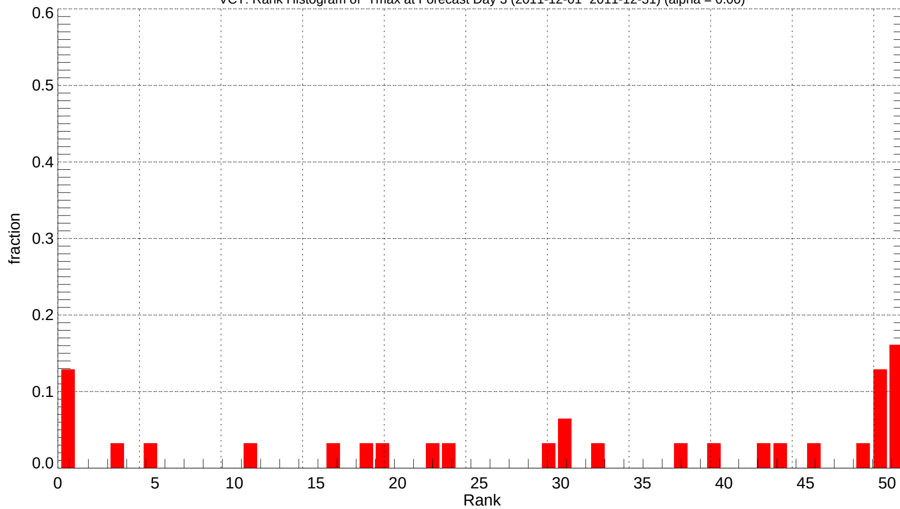
VCT: Rank Histogram of Tmax at Forecast Day 3 (2011-12-01~2011-12-31) (alpha = 0.00)
