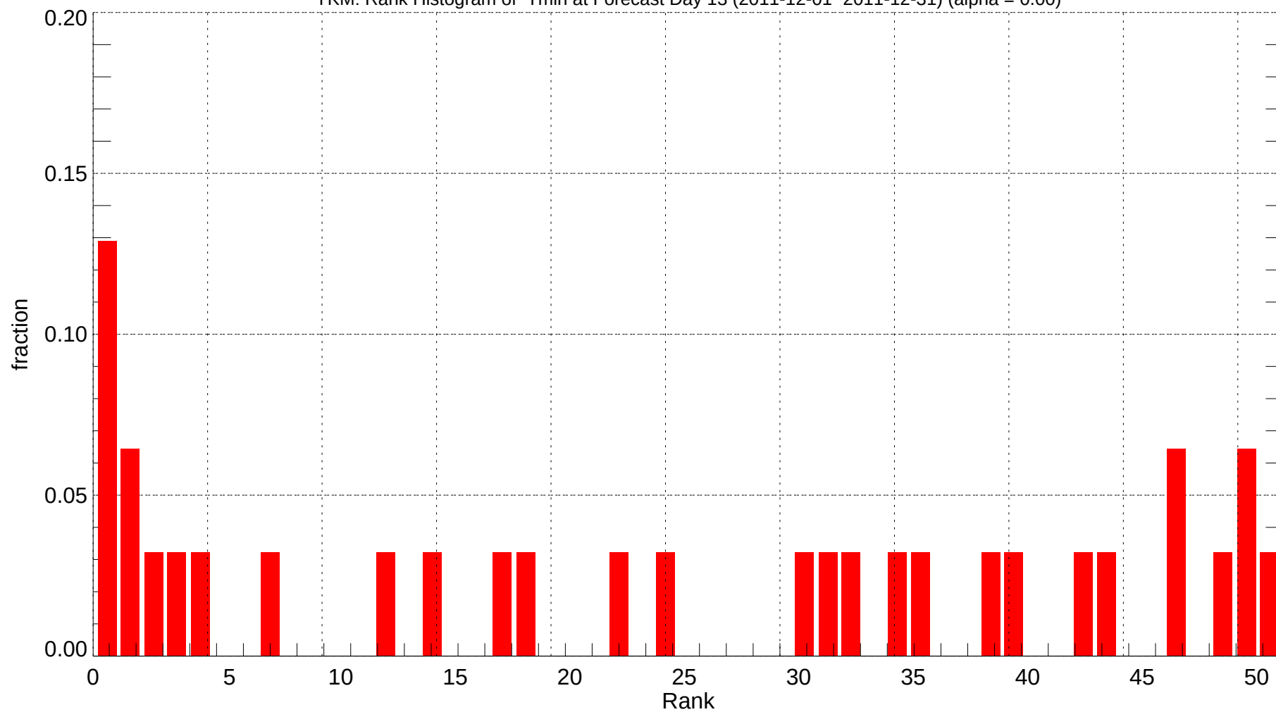
YKM: Rank Histogram of Tmin at Forecast Day 13 (2011-12-01~2011-12-31) (alpha = 0.00)
