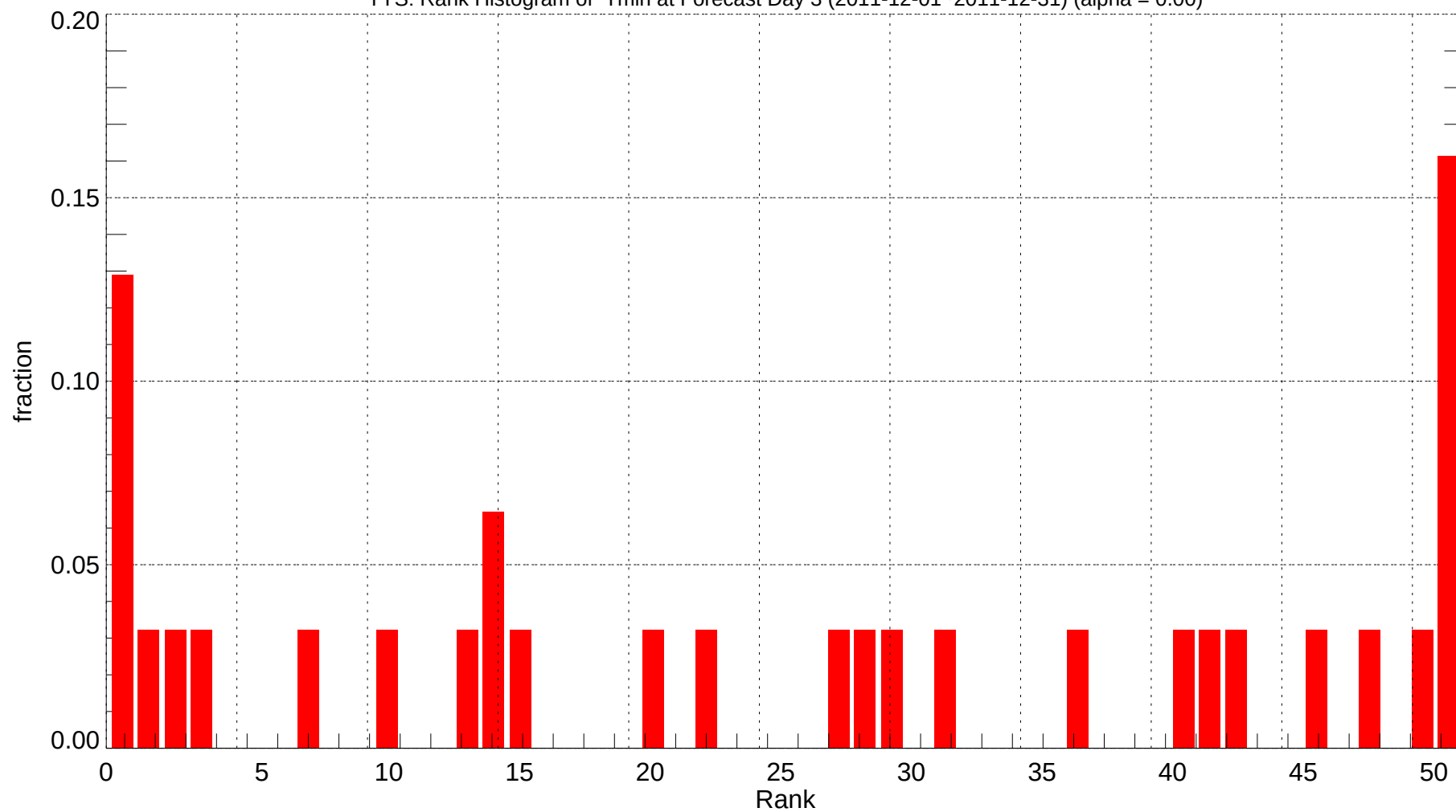
TYS: Rank Histogram of Tmin at Forecast Day 3 (2011-12-01~2011-12-31) (alpha = 0.00)
