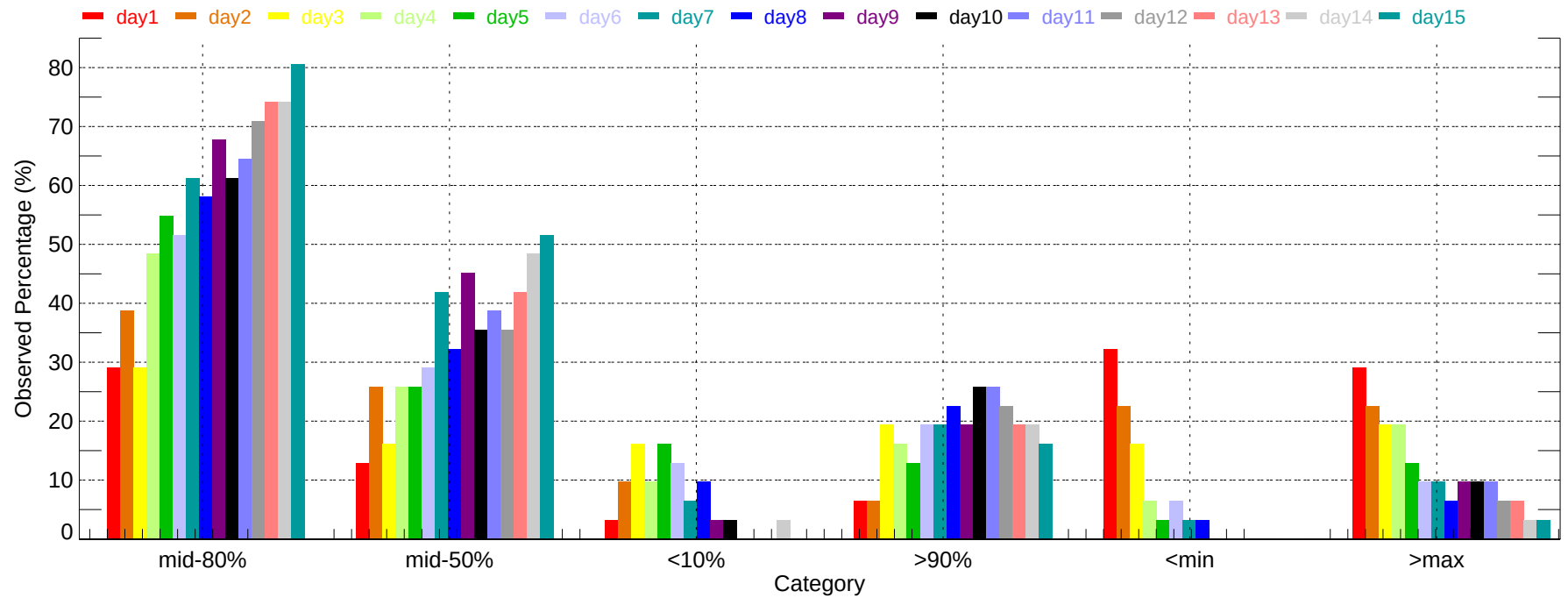
Observed Percentage of Ensembles - DEC: Max Temperature (2011-12-01~2011-12-31)
