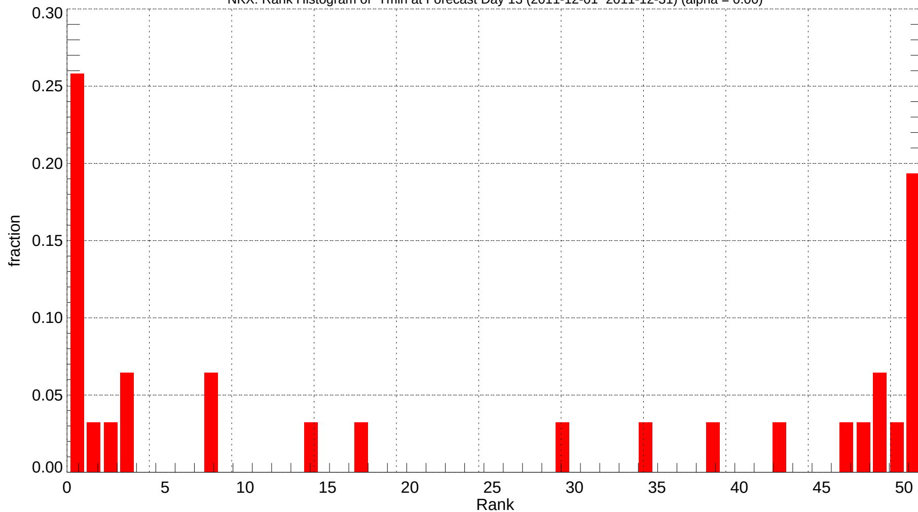
NKX: Rank Histogram of Tmin at Forecast Day 13 (2011-12-01~2011-12-31) (alpha = 0.00)
