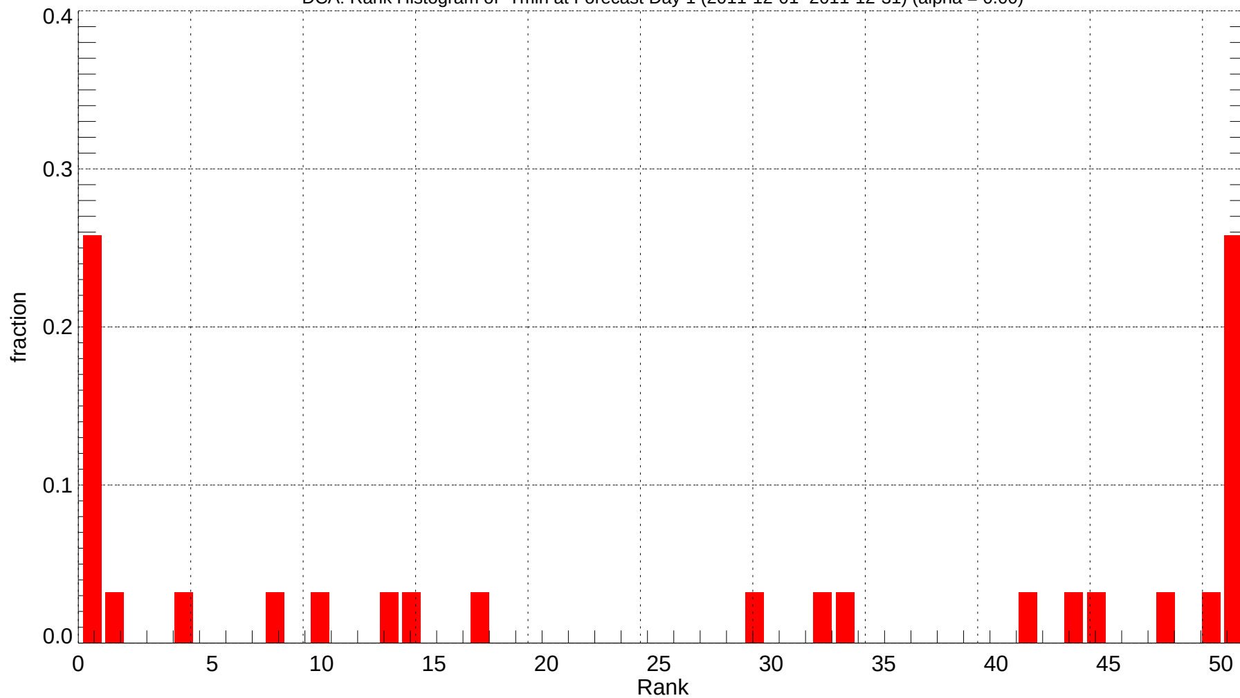
DCA: Rank Histogram of Tmin at Forecast Day 1 (2011-12-01~2011-12-31) (alpha = 0.00)
