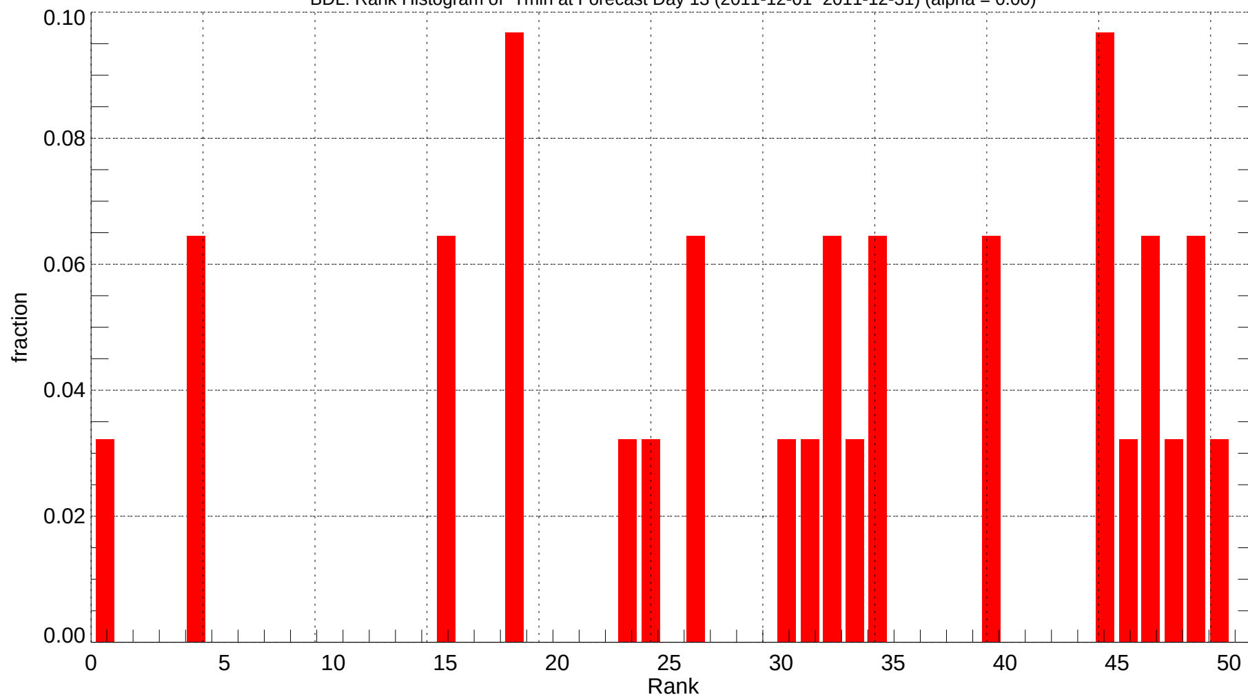
BDL: Rank Histogram of Tmin at Forecast Day 13 (2011-12-01~2011-12-31) (alpha = 0.00)
