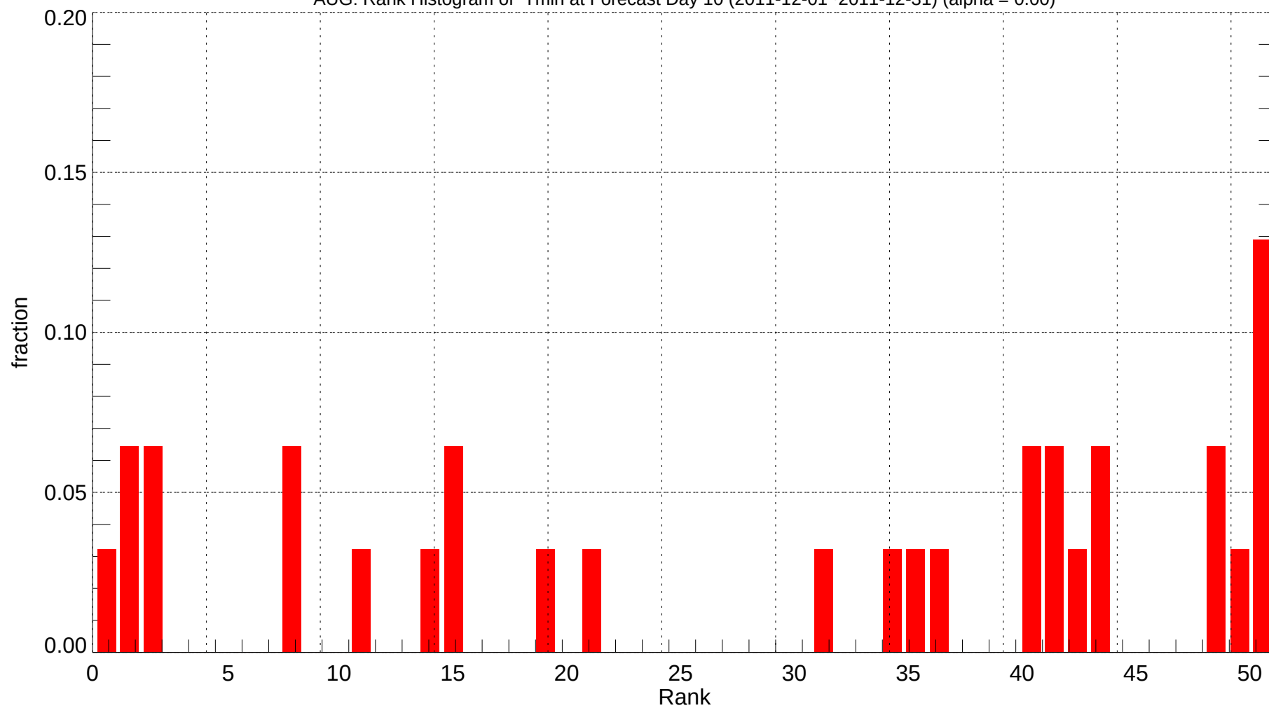
AUG: Rank Histogram of Tmin at Forecast Day 10 (2011-12-01~2011-12-31) (alpha = 0.00)
