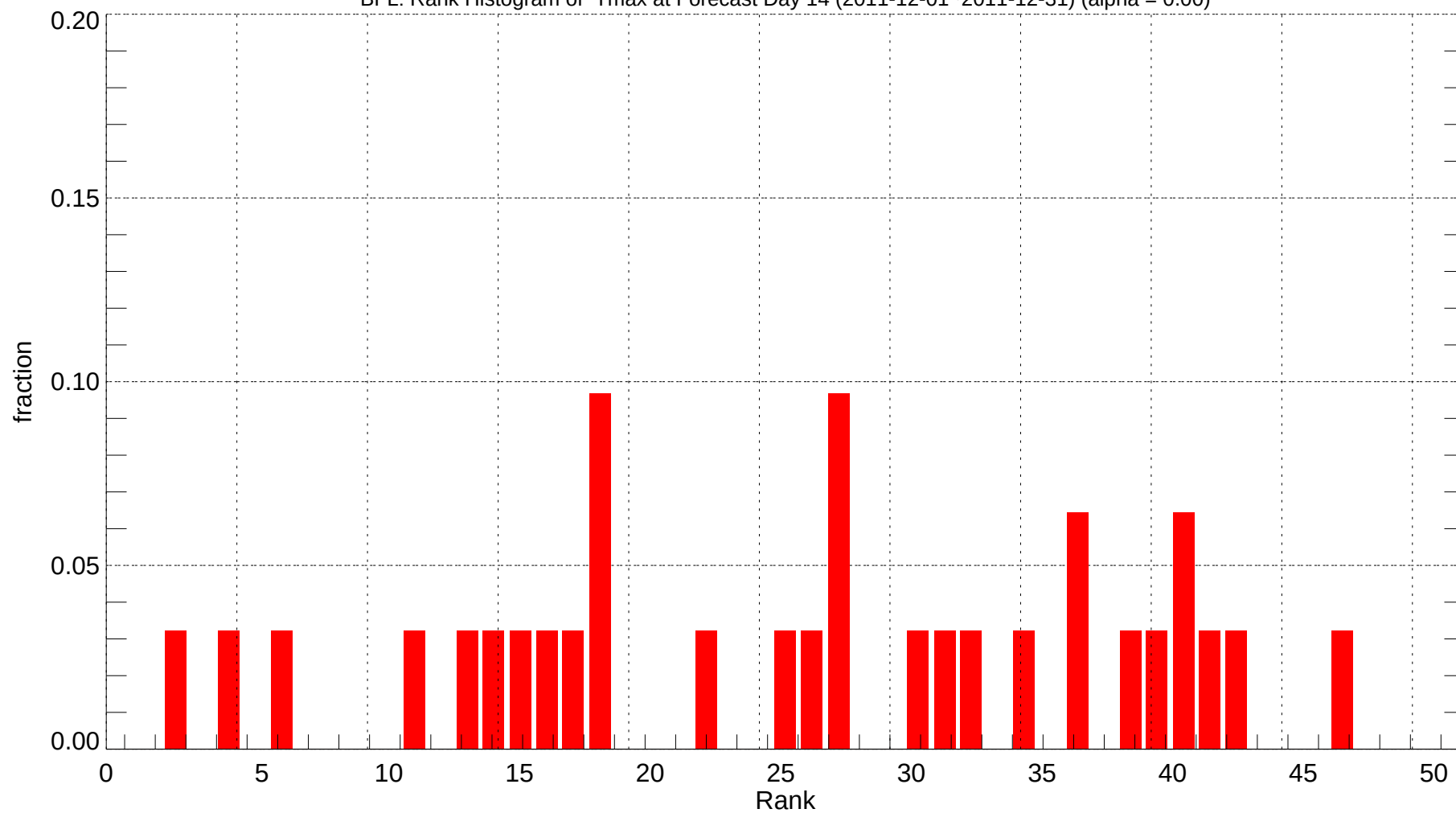
BFL: Rank Histogram of Tmax at Forecast Day 14 (2011-12-01~2011-12-31) (alpha = 0.00)
