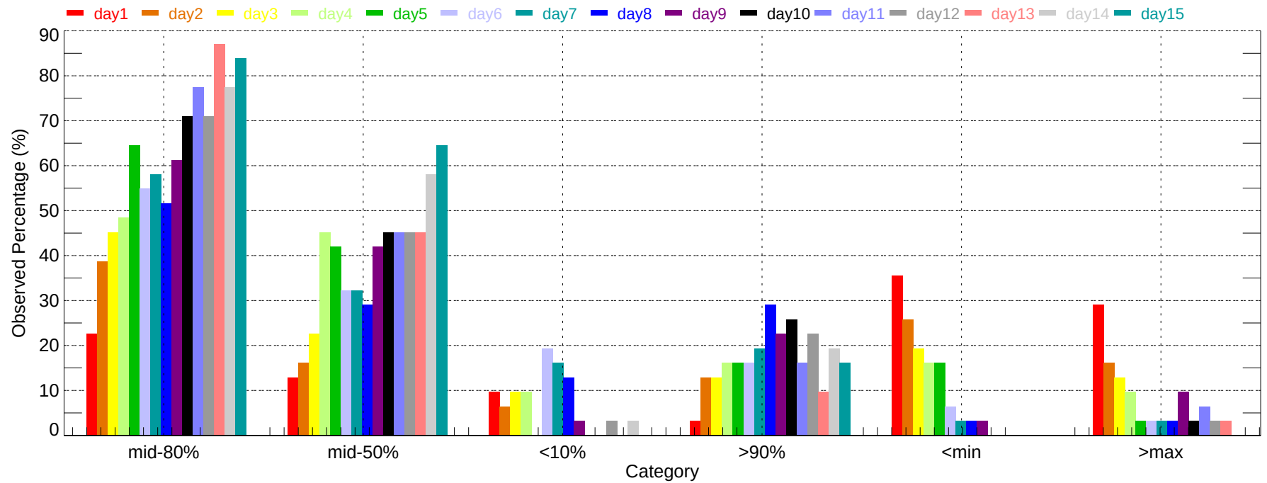
Observed Percentage of Ensembles - CHA: Min Temperature (2011-12-01~2011-12-31)
