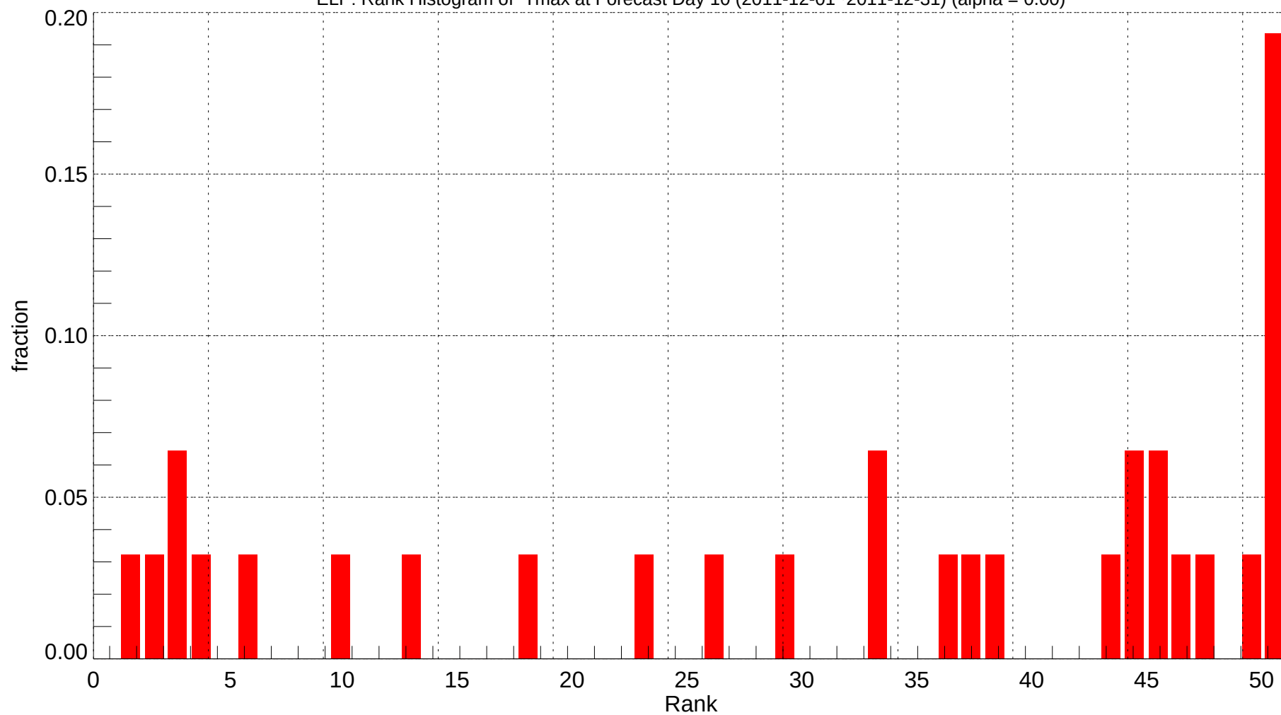
ELP: Rank Histogram of Tmax at Forecast Day 10 (2011-12-01~2011-12-31) (alpha = 0.00)
