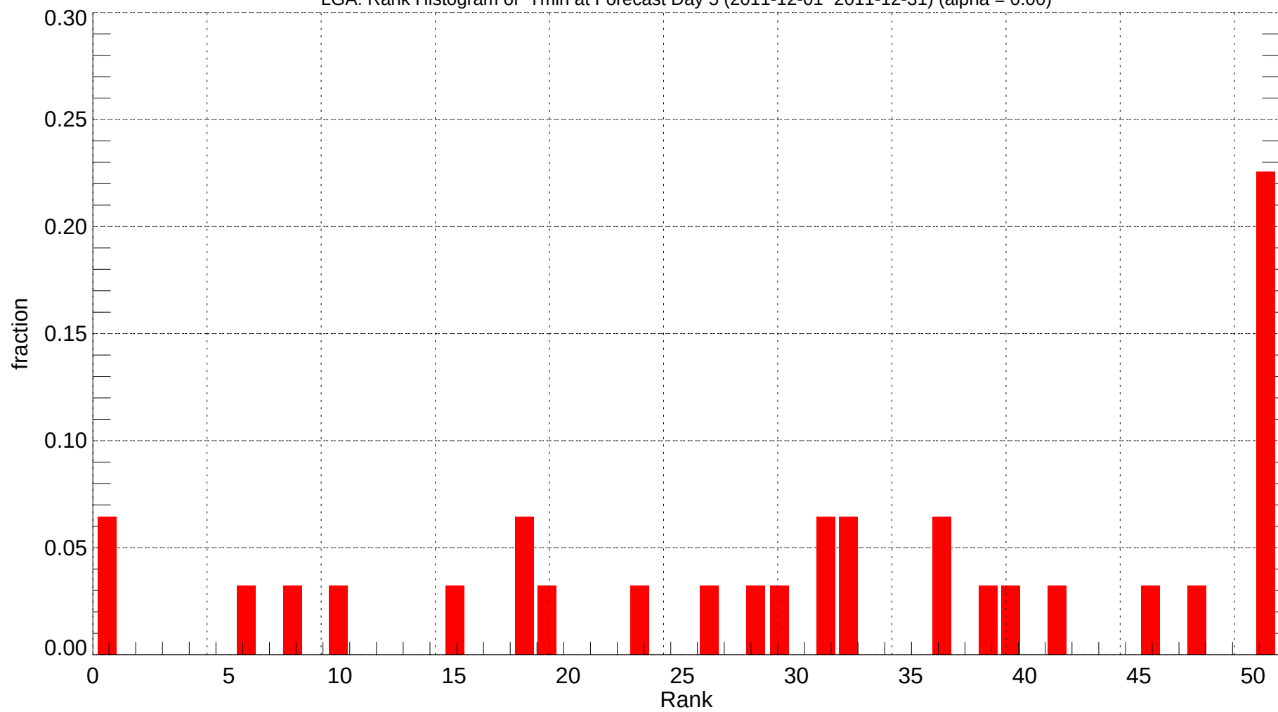
LGA: Rank Histogram of Tmin at Forecast Day 5 (2011-12-01~2011-12-31) (alpha = 0.00)
