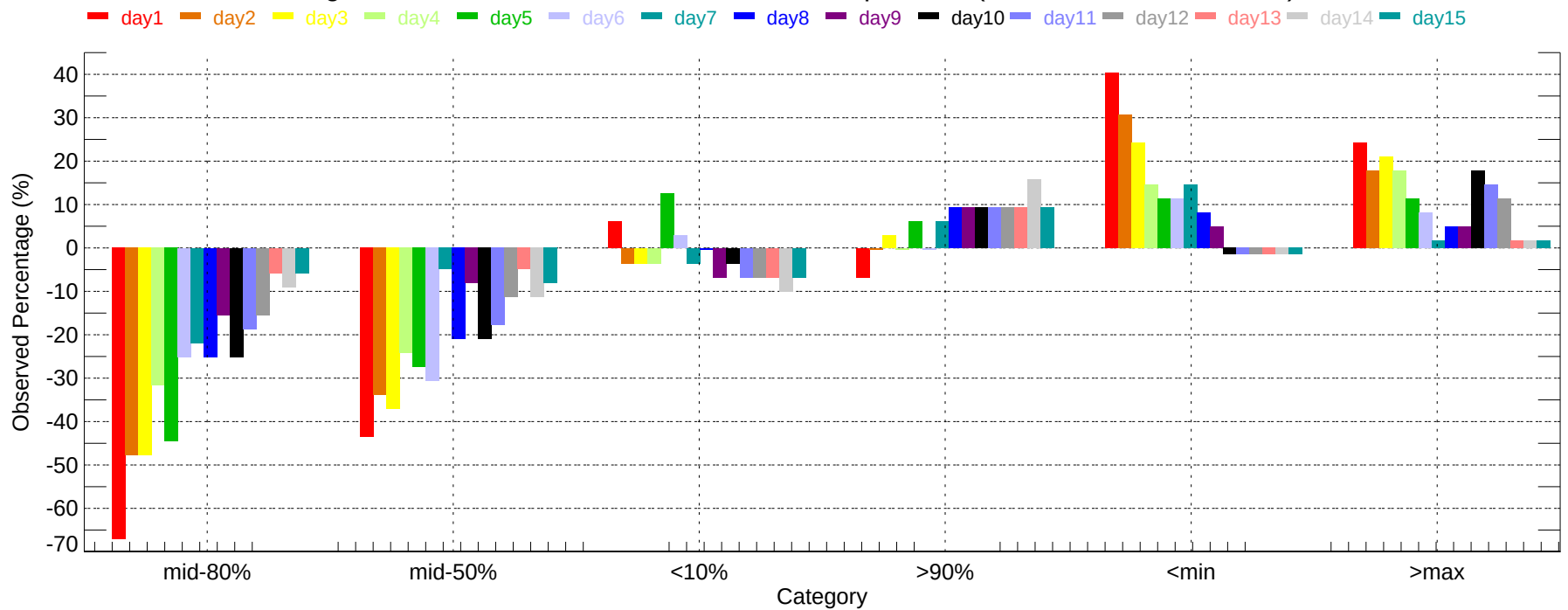
Observed Percentage Deviation of Ensembles - APN: Min Temperature (2011-12-01~2011-12-31)
