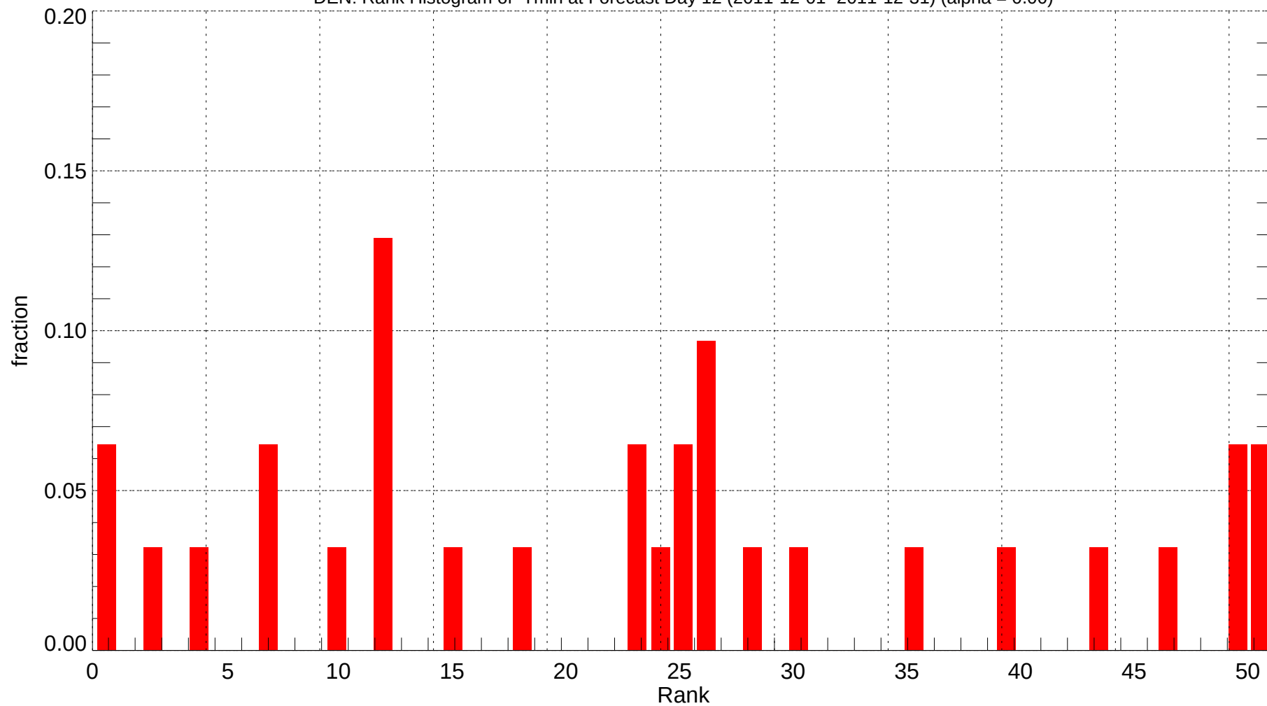
DEN: Rank Histogram of Tmin at Forecast Day 12 (2011-12-01~2011-12-31) (alpha = 0.00)
