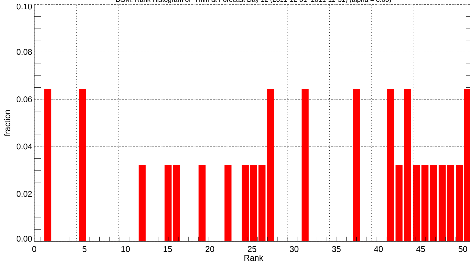
BGM: Rank Histogram of Tmin at Forecast Day 12 (2011-12-01~2011-12-31) (alpha = 0.00)
