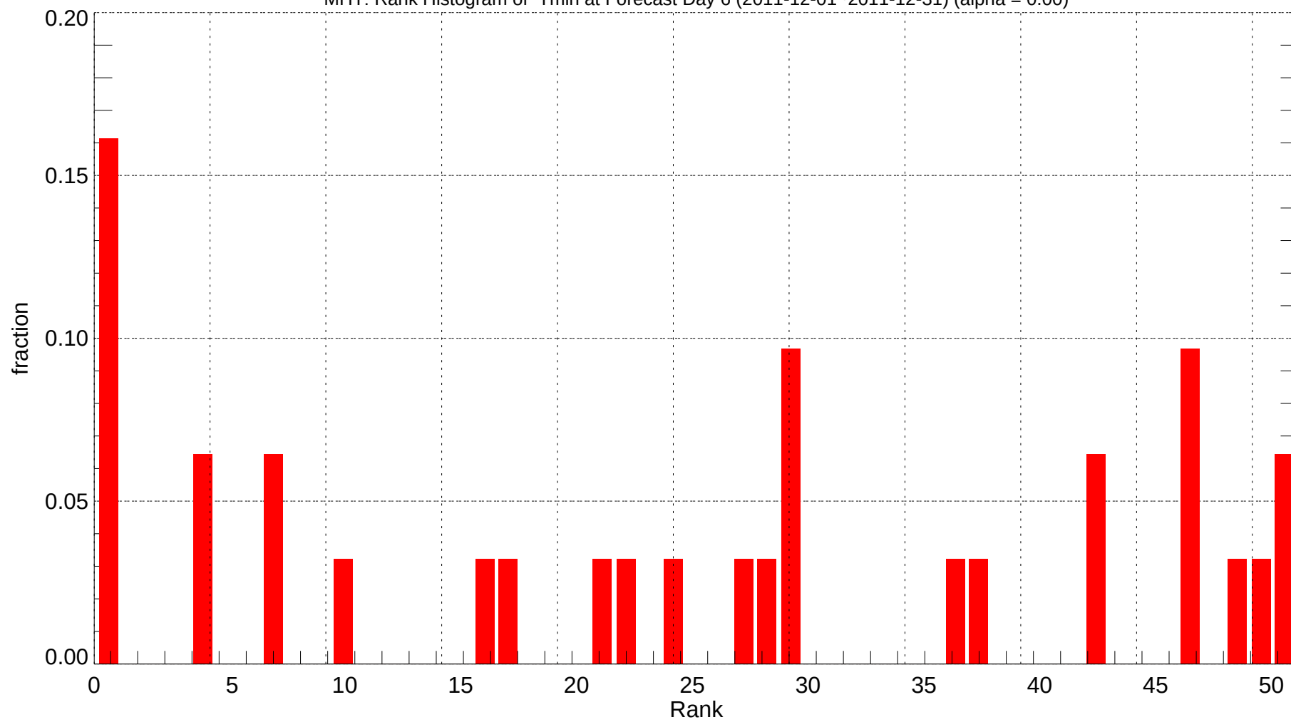
MHT: Rank Histogram of Tmin at Forecast Day 6 (2011-12-01~2011-12-31) (alpha = 0.00)
