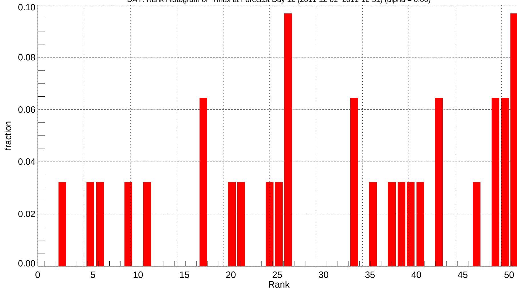
DAY: Rank Histogram of Tmax at Forecast Day 12 (2011-12-01~2011-12-31) (alpha = 0.00)
