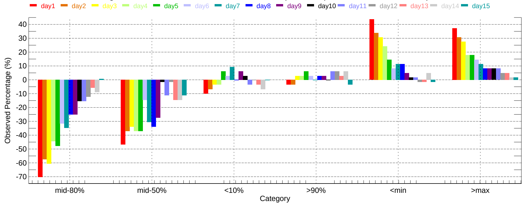
Observed Percentage Deviation of Ensembles - ILG: Min Temperature (2011-12-01~2011-12-31)
