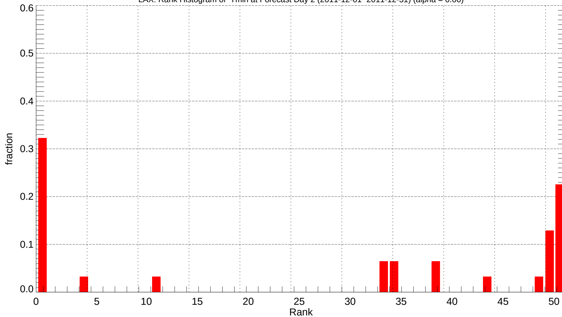
LAX: Rank Histogram of Tmin at Forecast Day 2 (2011-12-01~2011-12-31) (alpha = 0.00)
