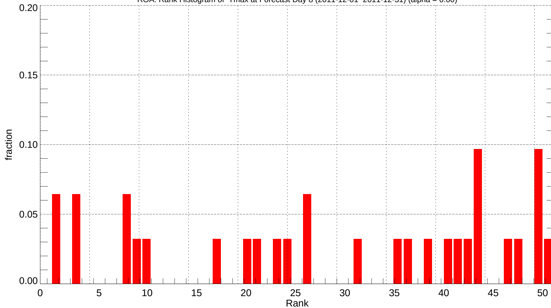
ROA: Rank Histogram of Tmax at Forecast Day 8 (2011-12-01~2011-12-31) (alpha = 0.00)
