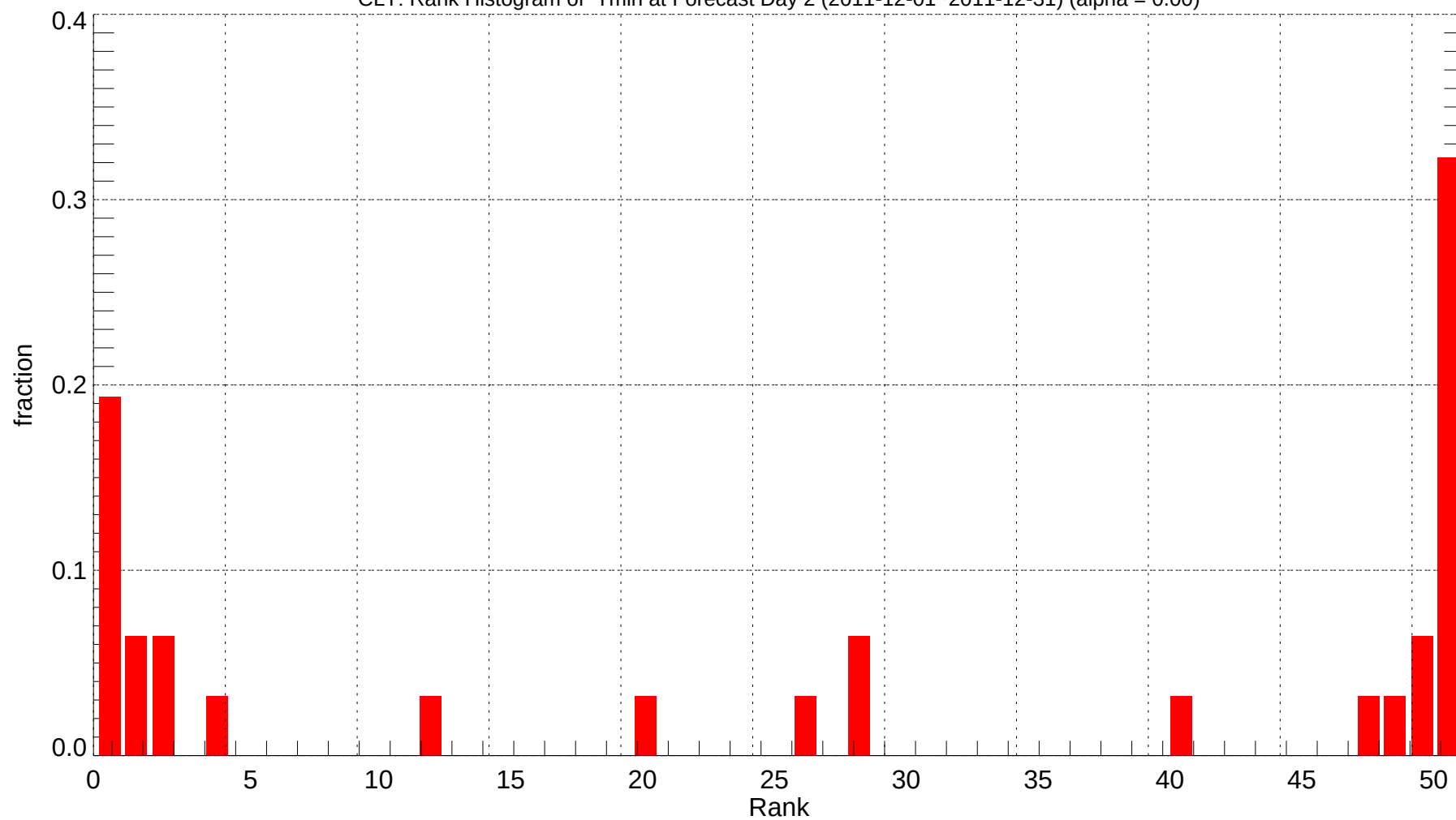
CLT: Rank Histogram of Tmin at Forecast Day 2 (2011-12-01~2011-12-31) (alpha = 0.00)
