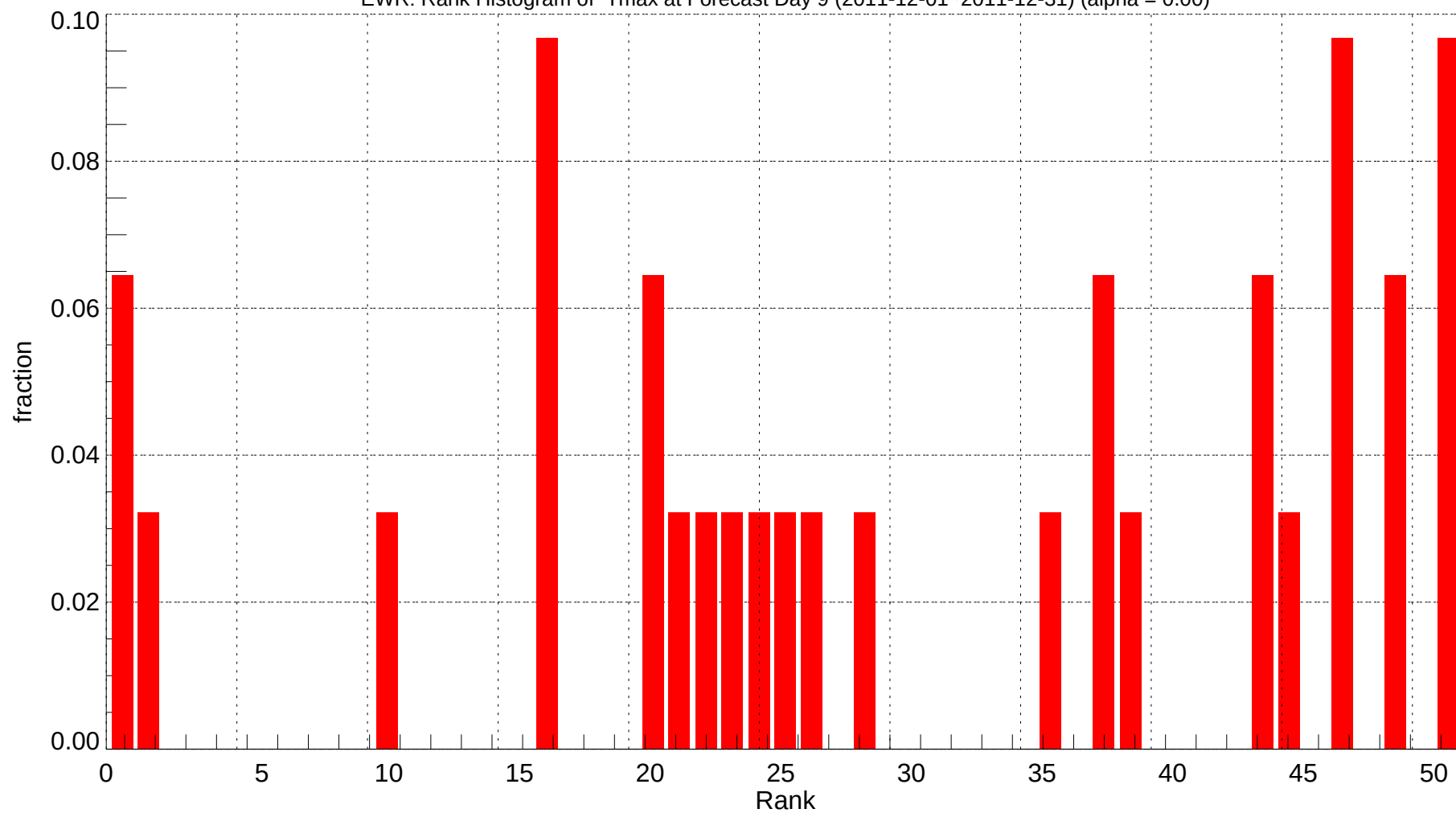
EWR: Rank Histogram of Tmax at Forecast Day 9 (2011-12-01~2011-12-31) (alpha = 0.00)
