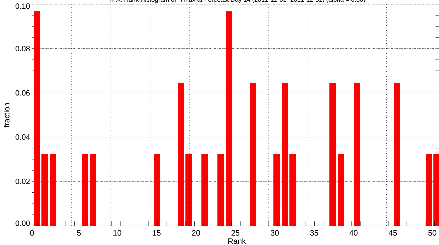
TPA: Rank Histogram of Tmax at Forecast Day 14 (2011-12-01~2011-12-31) (alpha = 0.00)
