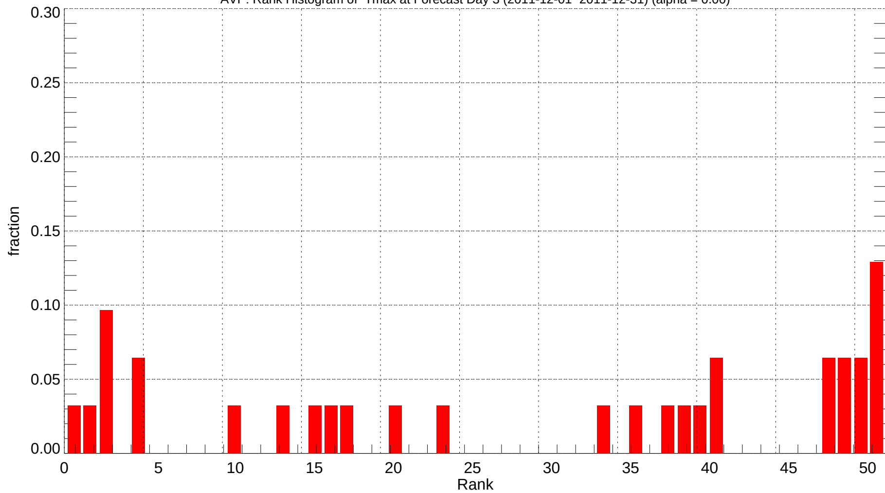
AVP: Rank Histogram of Tmax at Forecast Day 3 (2011-12-01~2011-12-31) (alpha = 0.00)
