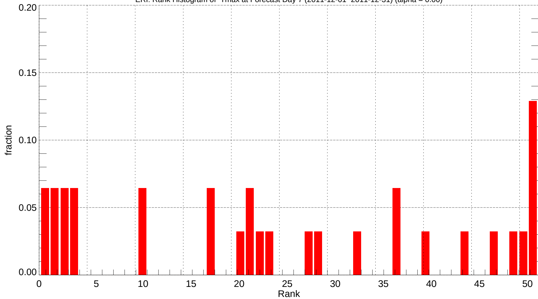
ERI: Rank Histogram of Tmax at Forecast Day 7 (2011-12-01~2011-12-31) (alpha = 0.00)
