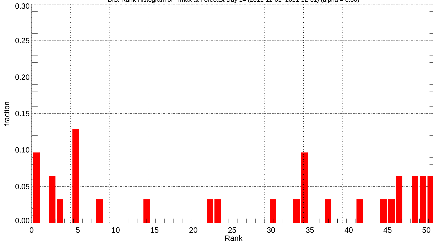
BIS: Rank Histogram of Tmax at Forecast Day 14 (2011-12-01~2011-12-31) (alpha = 0.00)
