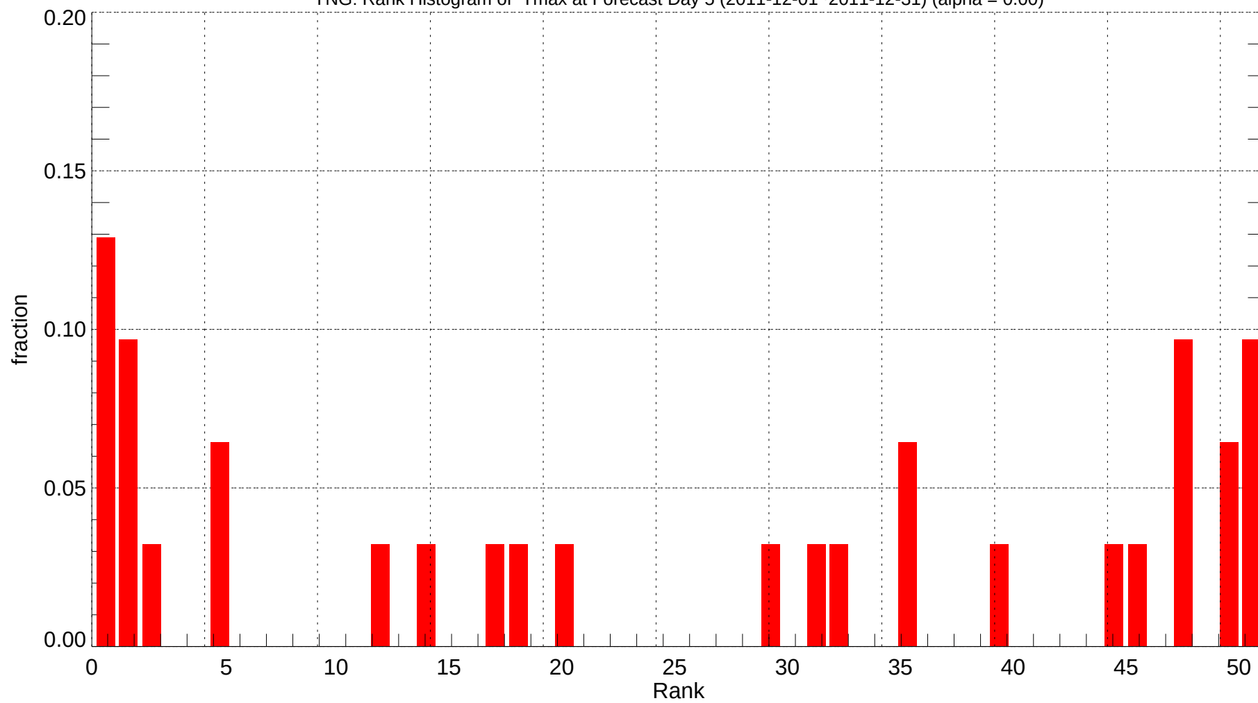
YNG: Rank Histogram of Tmax at Forecast Day 5 (2011-12-01~2011-12-31) (alpha = 0.00)
