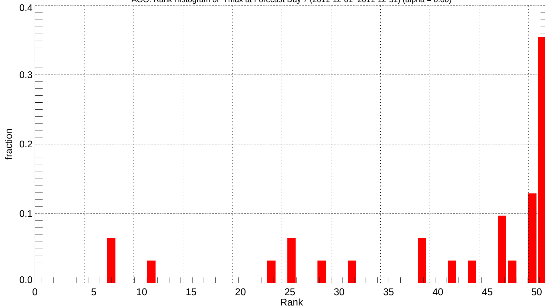
AOO: Rank Histogram of Tmax at Forecast Day 7 (2011-12-01~2011-12-31) (alpha = 0.00)
