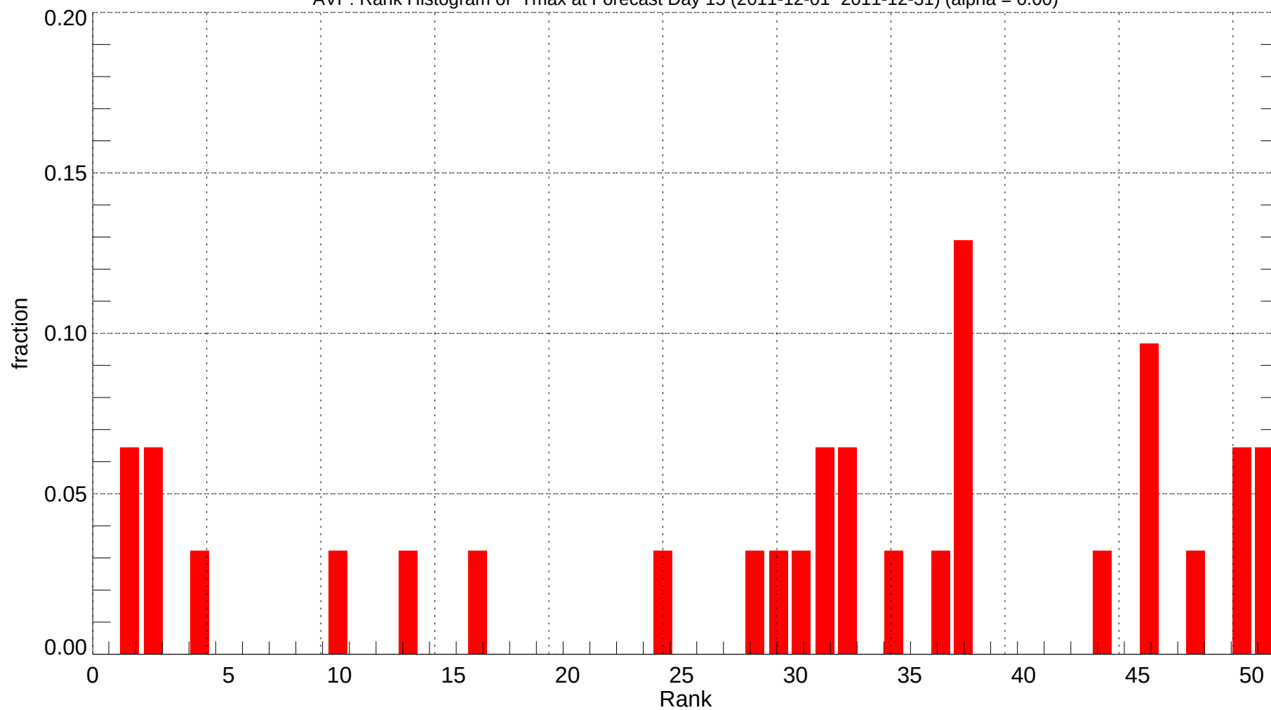
AVP: Rank Histogram of Tmax at Forecast Day 15 (2011-12-01~2011-12-31) (alpha = 0.00)
