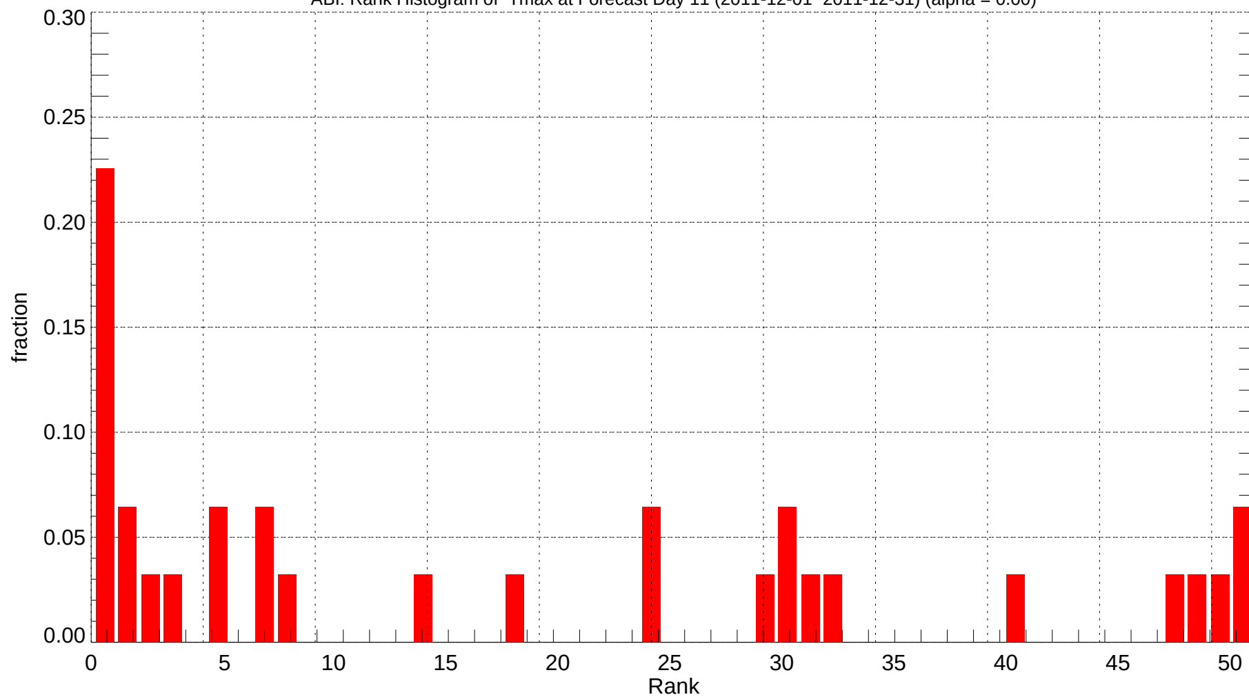
ABI: Rank Histogram of Tmax at Forecast Day 11 (2011-12-01~2011-12-31) (alpha = 0.00)
