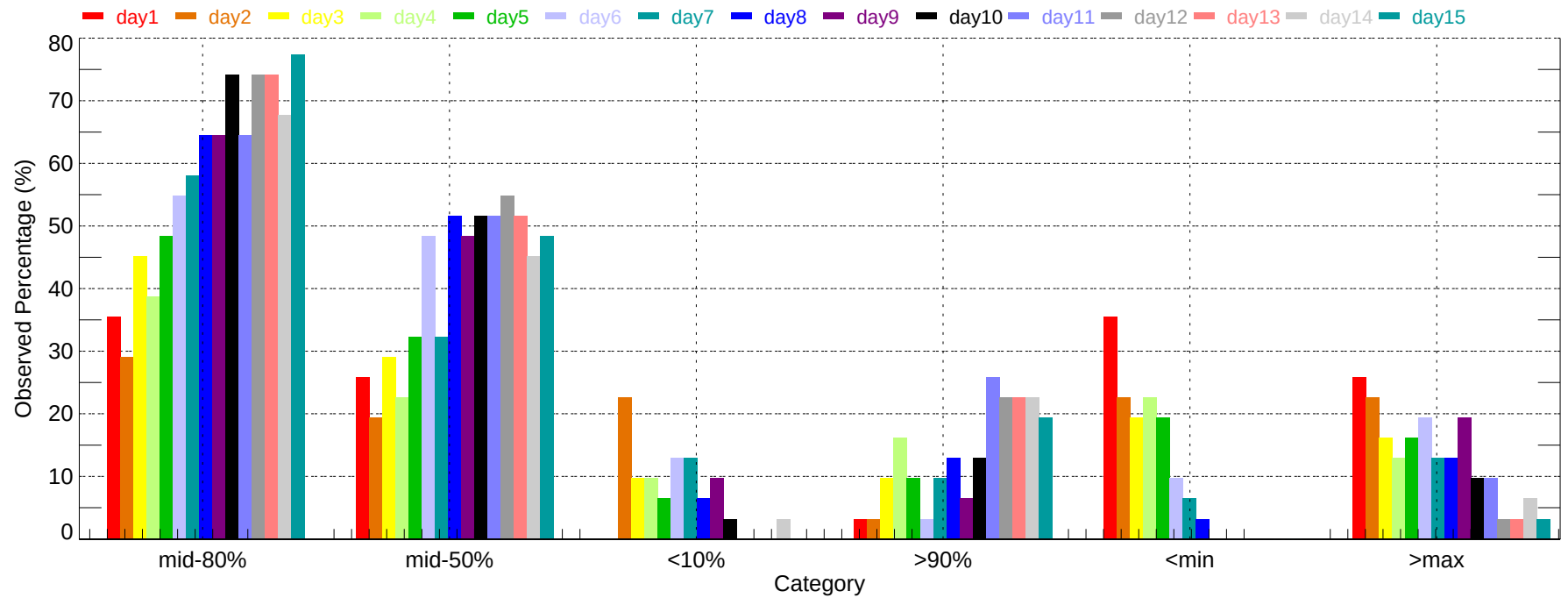
Observed Percentage of Ensembles - BNA: Max Temperature (2011-12-01~2011-12-31)
