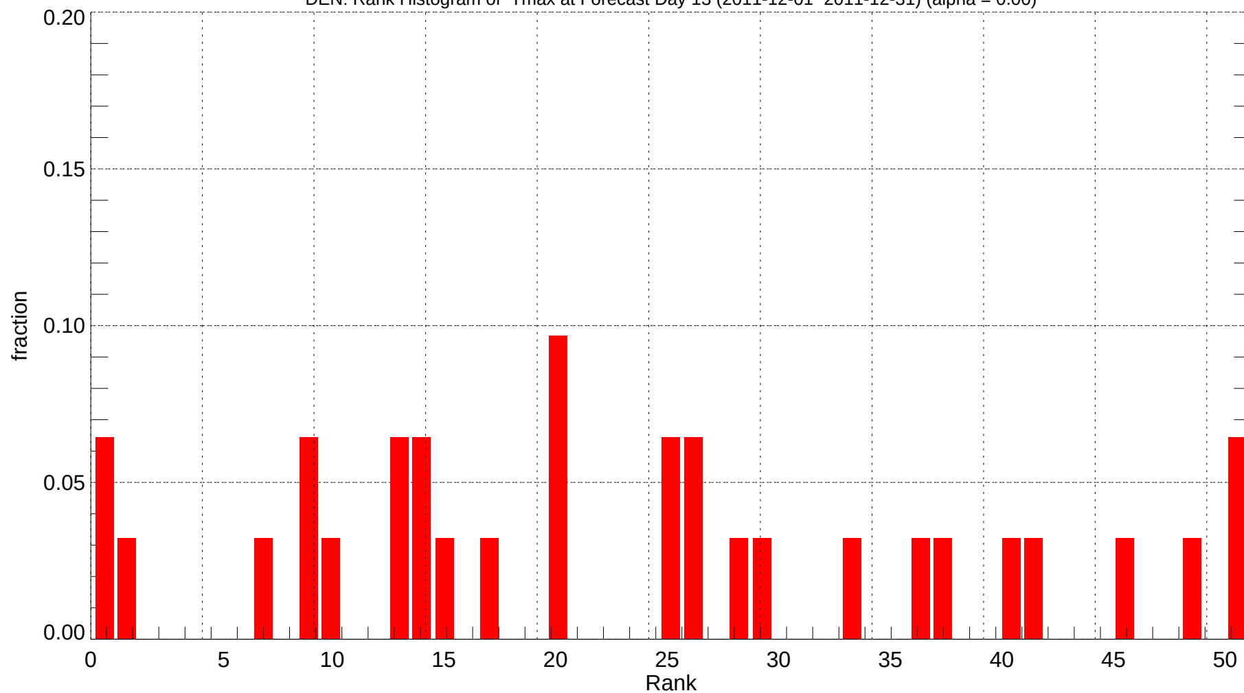
DEN: Rank Histogram of Tmax at Forecast Day 13 (2011-12-01~2011-12-31) (alpha = 0.00)
