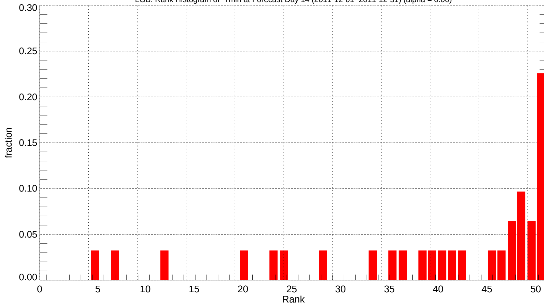
LGB: Rank Histogram of Tmin at Forecast Day 14 (2011-12-01~2011-12-31) (alpha = 0.00)
