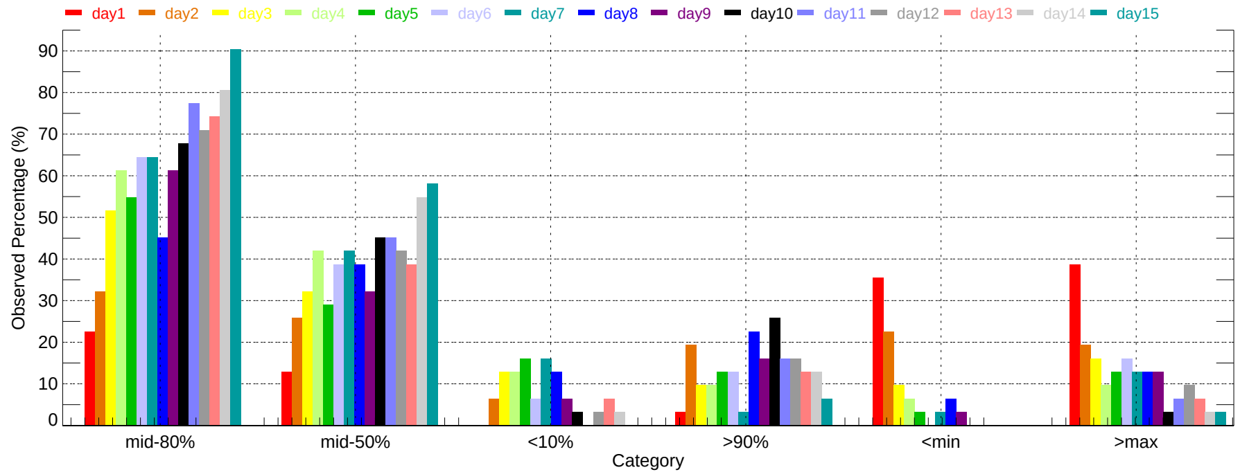
Observed Percentage of Ensembles - CAE: Min Temperature (2011-12-01~2011-12-31)
