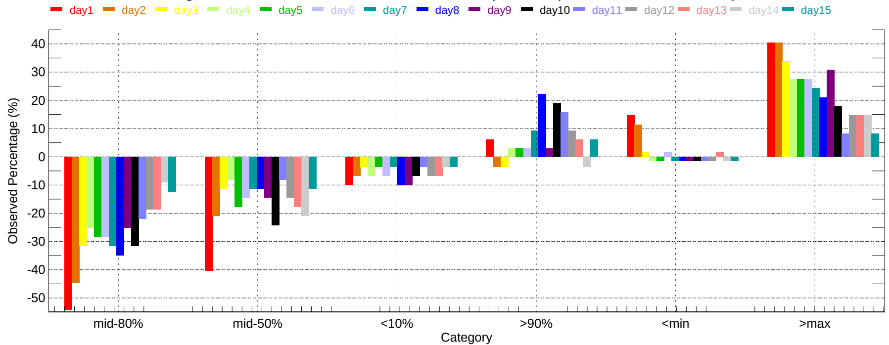
Observed Percentage Deviation of Ensembles - TUL: Max Temperature (2011-12-01~2011-12-31)
