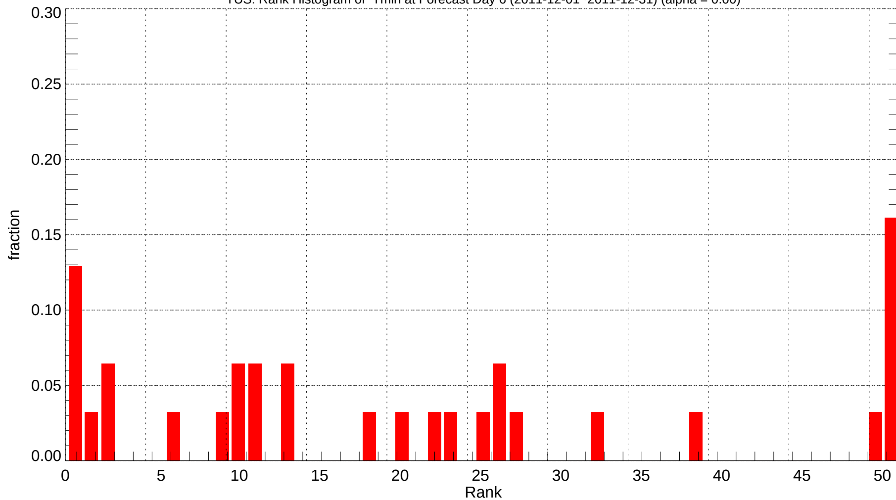
TUS: Rank Histogram of Tmin at Forecast Day 6 (2011-12-01~2011-12-31) (alpha = 0.00)
