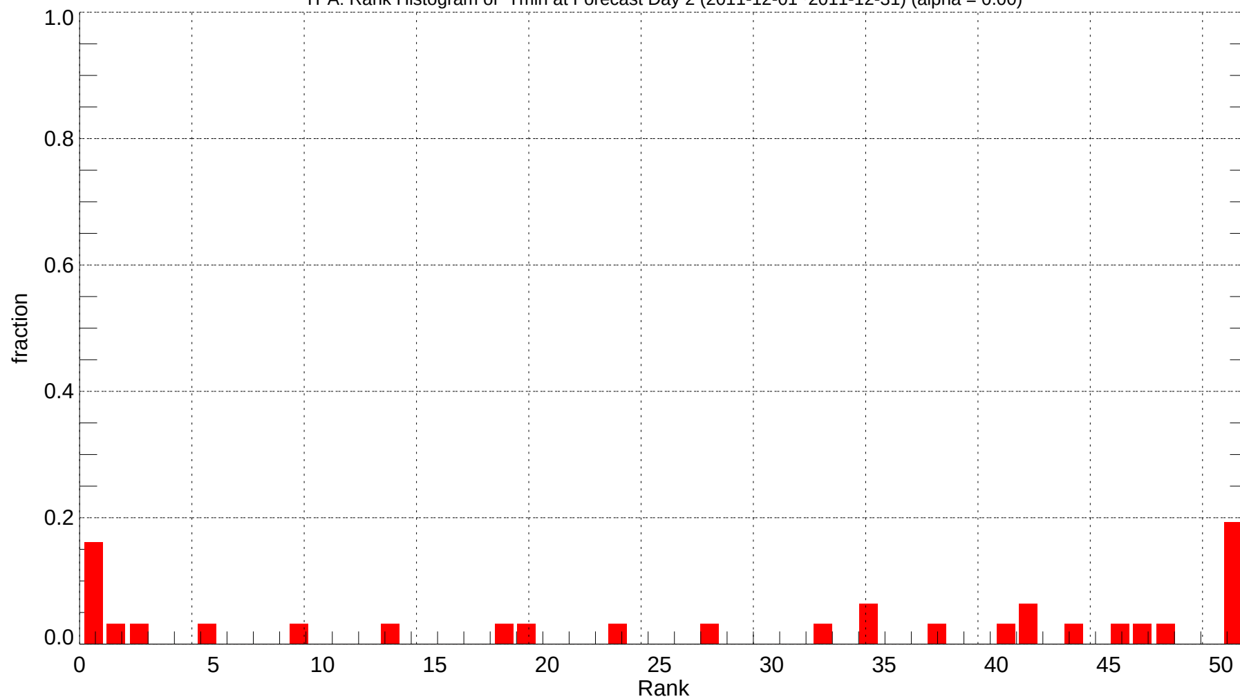
TPA: Rank Histogram of Tmin at Forecast Day 2 (2011-12-01~2011-12-31) (alpha = 0.00)
