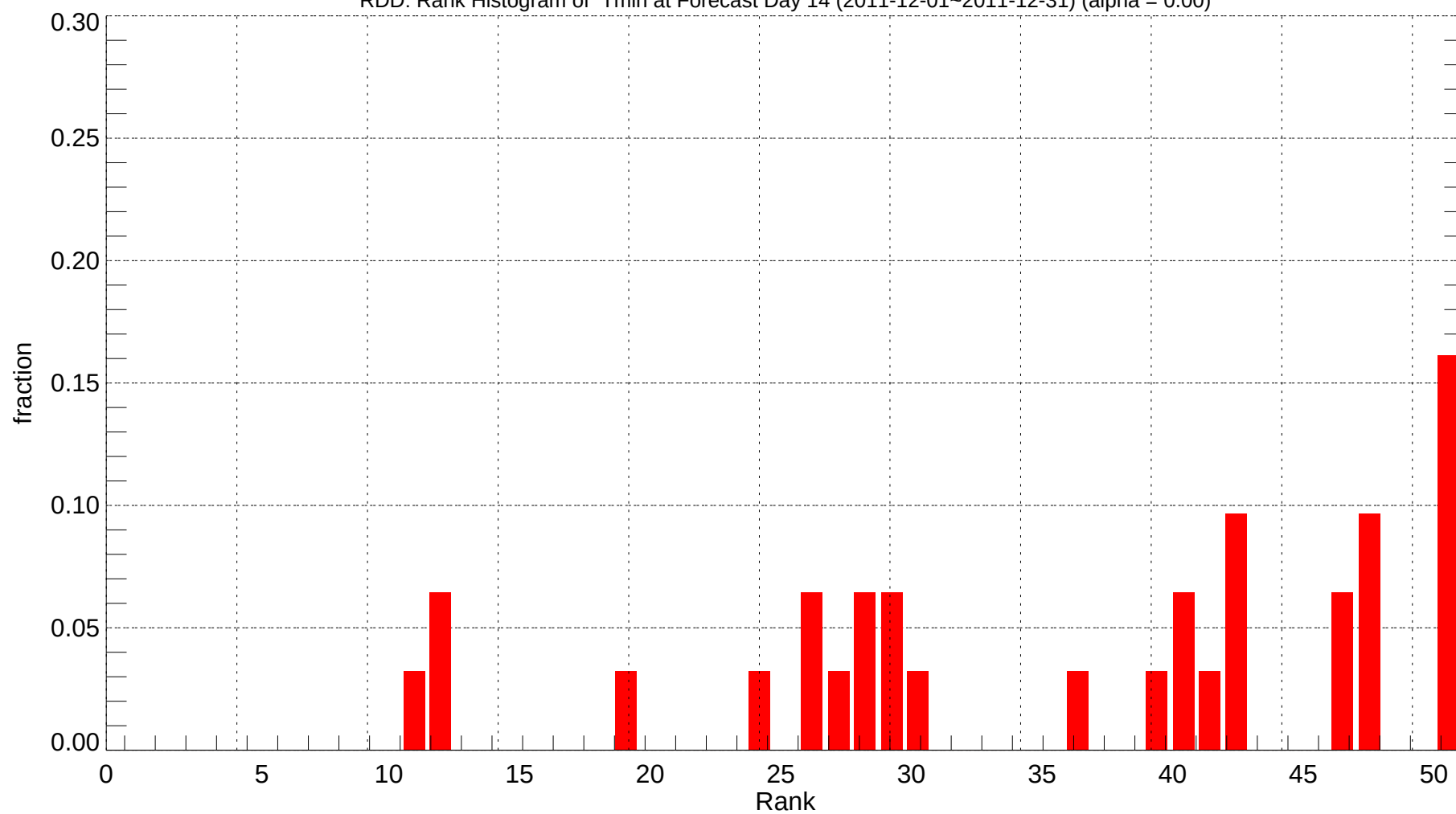
RDD: Rank Histogram of Tmin at Forecast Day 14 (2011-12-01~2011-12-31) (alpha = 0.00)
