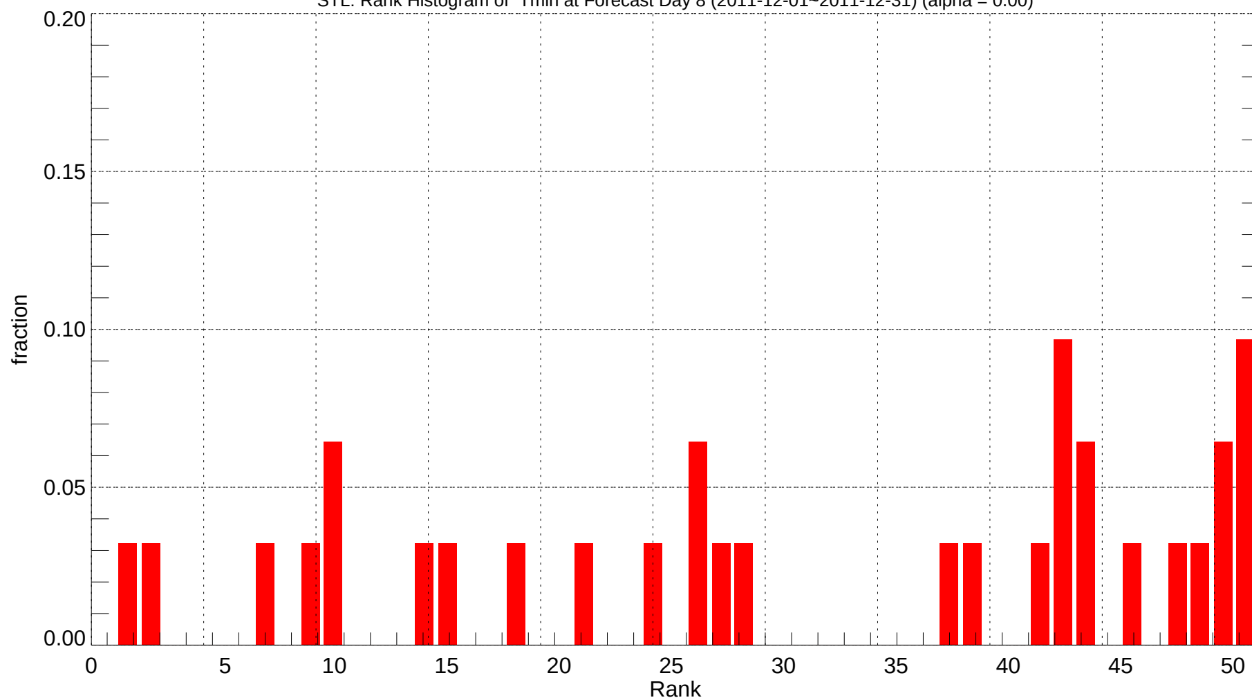
STL: Rank Histogram of Tmin at Forecast Day 8 (2011-12-01~2011-12-31) (alpha = 0.00)
