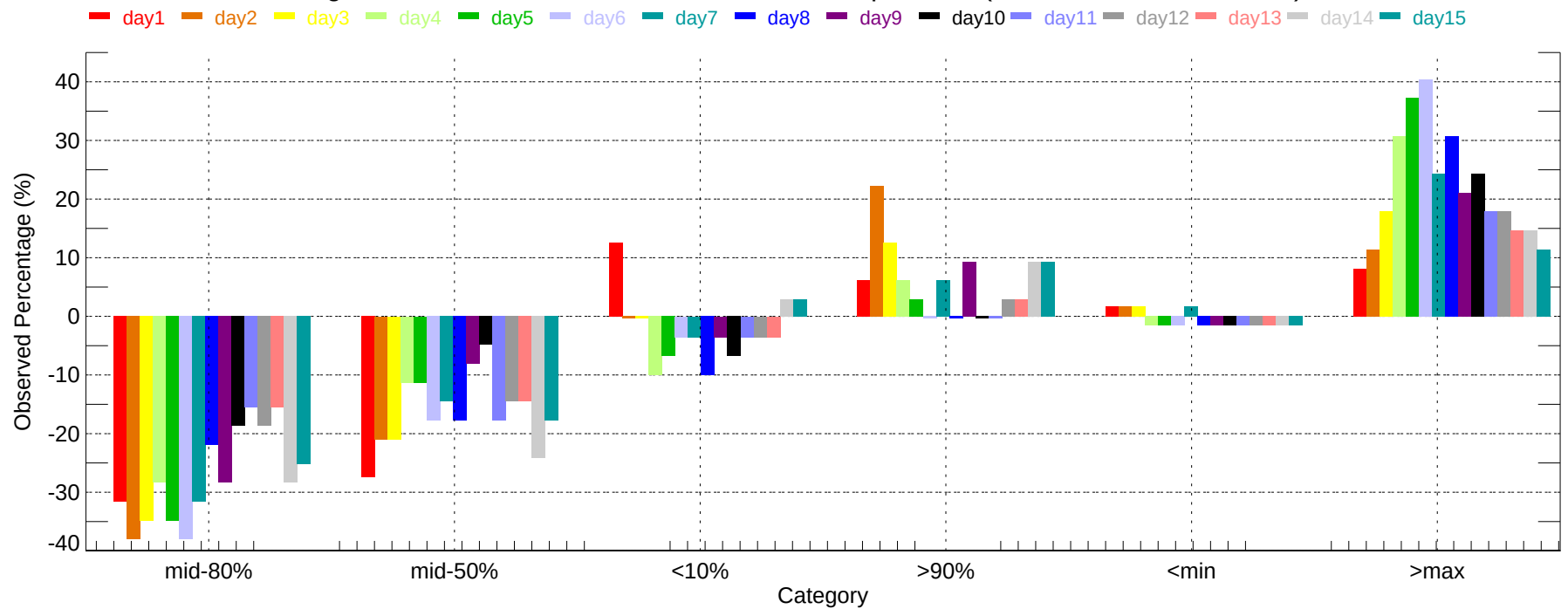
Observed Percentage Deviation of Ensembles - SDF: Max Temperature (2011-12-01~2011-12-31)
