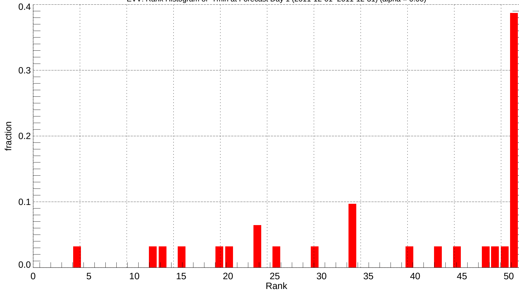
EVV: Rank Histogram of Tmin at Forecast Day 1 (2011-12-01~2011-12-31) (alpha = 0.00)
