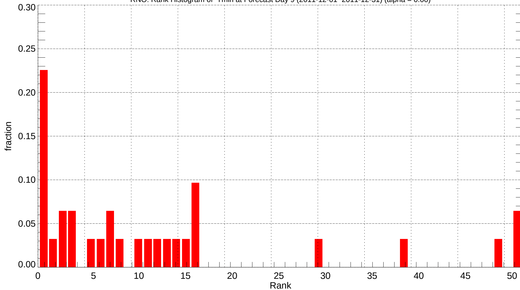
RNO: Rank Histogram of Tmin at Forecast Day 9 (2011-12-01~2011-12-31) (alpha = 0.00)
