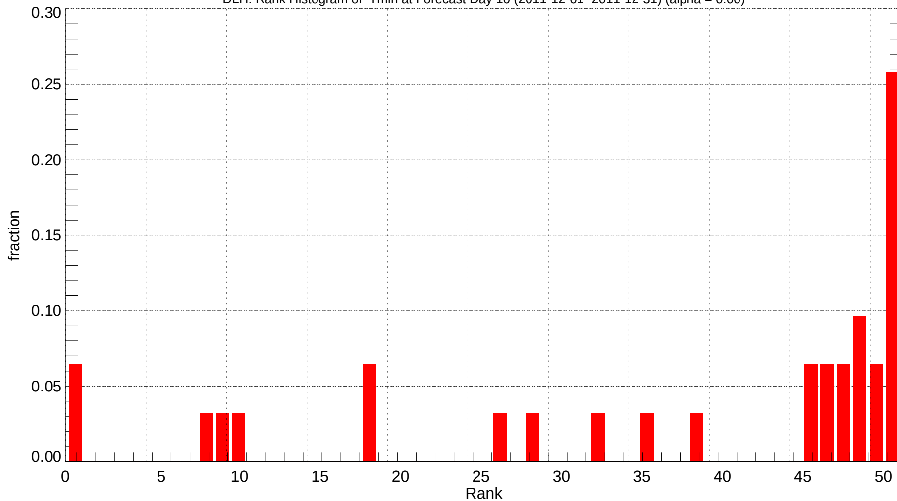
DLH: Rank Histogram of Tmin at Forecast Day 10 (2011-12-01~2011-12-31) (alpha = 0.00)
