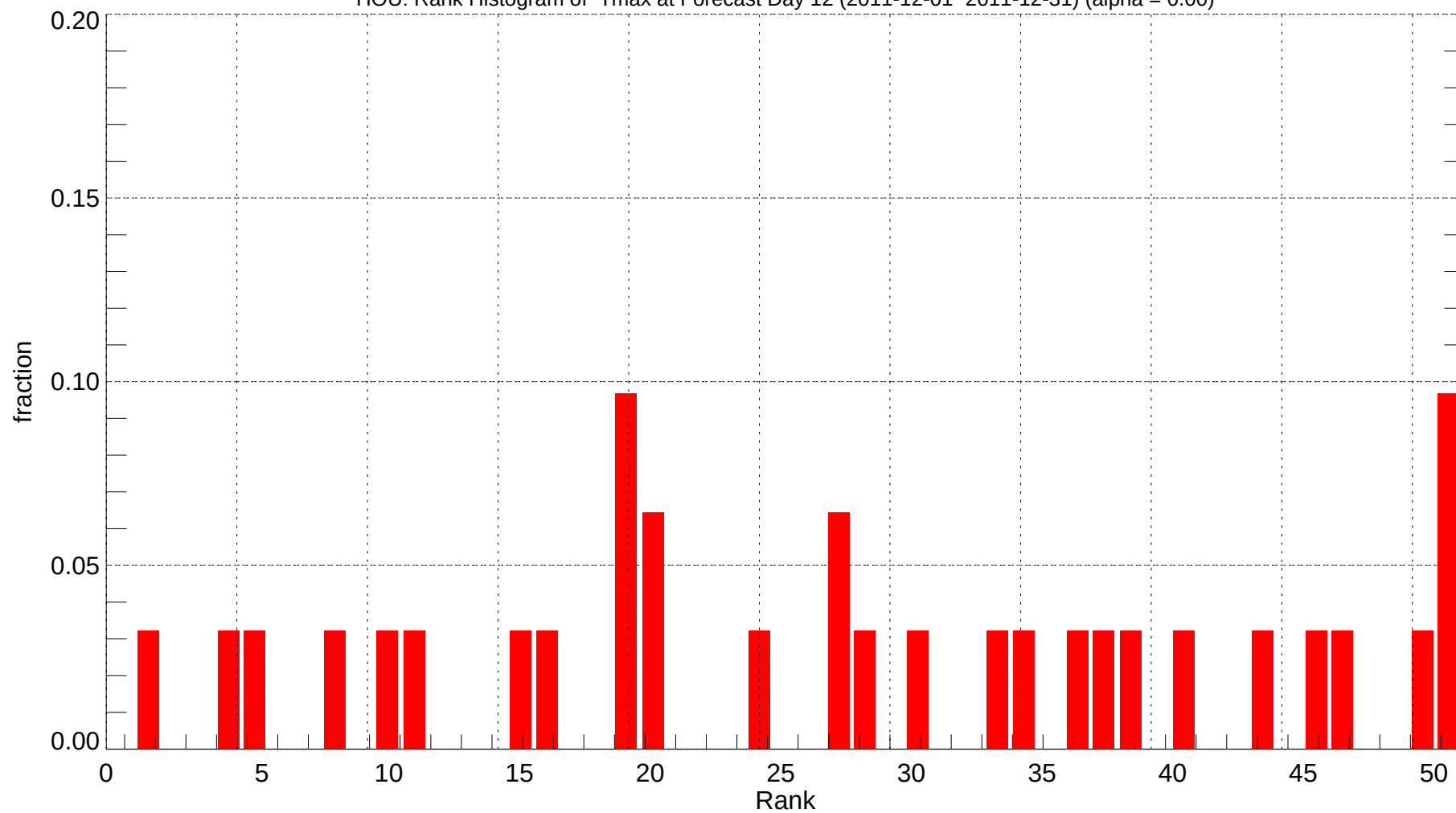
HOU: Rank Histogram of Tmax at Forecast Day 12 (2011-12-01~2011-12-31) (alpha = 0.00)
