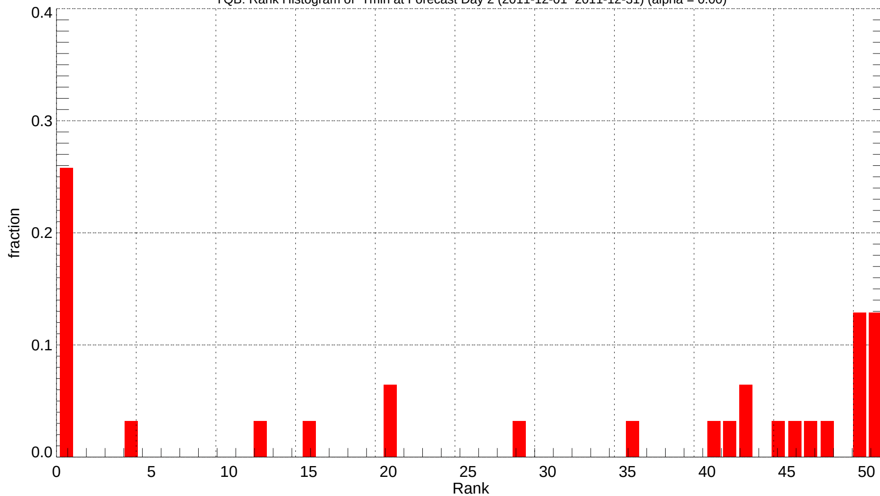
YQB: Rank Histogram of Tmin at Forecast Day 2 (2011-12-01~2011-12-31) (alpha = 0.00)
