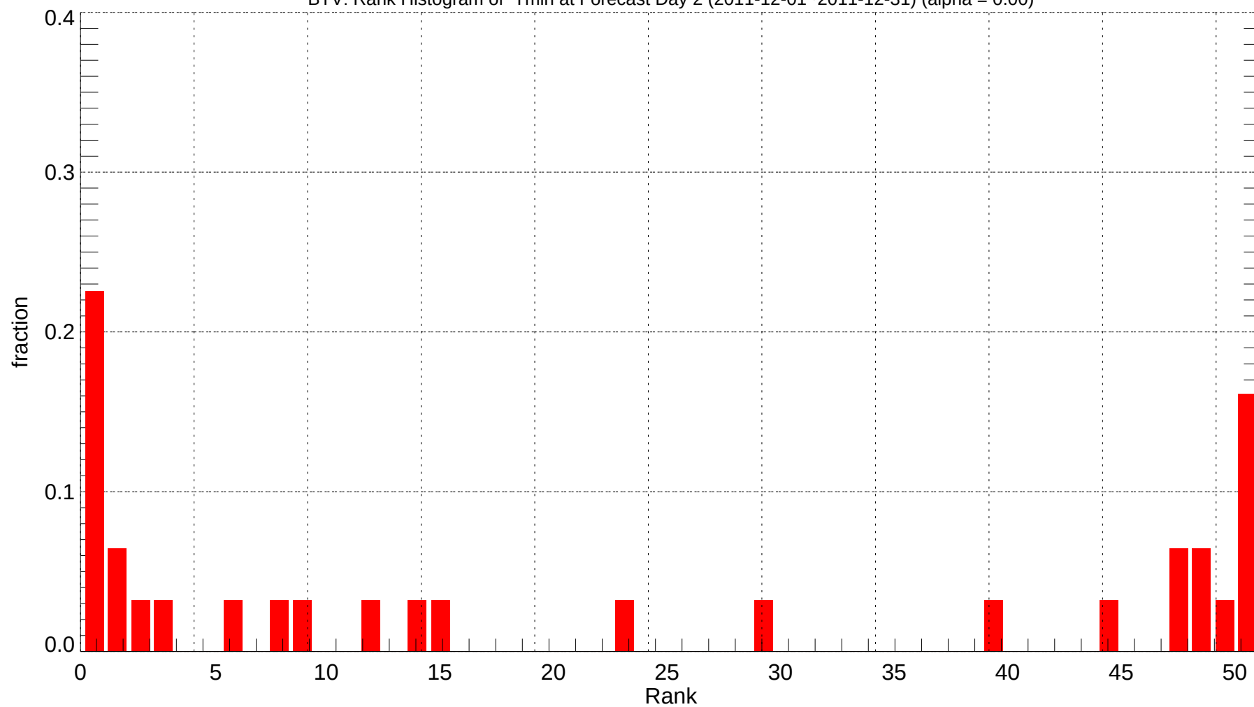
BTV: Rank Histogram of Tmin at Forecast Day 2 (2011-12-01~2011-12-31) (alpha = 0.00)
