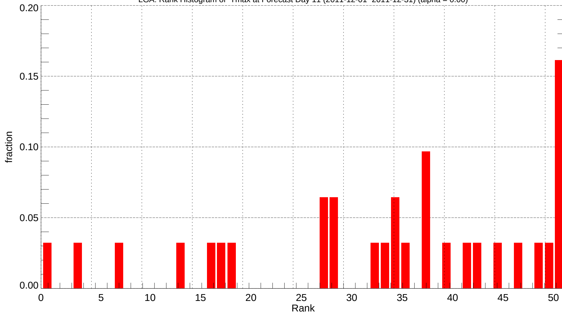
LGA: Rank Histogram of Tmax at Forecast Day 11 (2011-12-01~2011-12-31) (alpha = 0.00)
