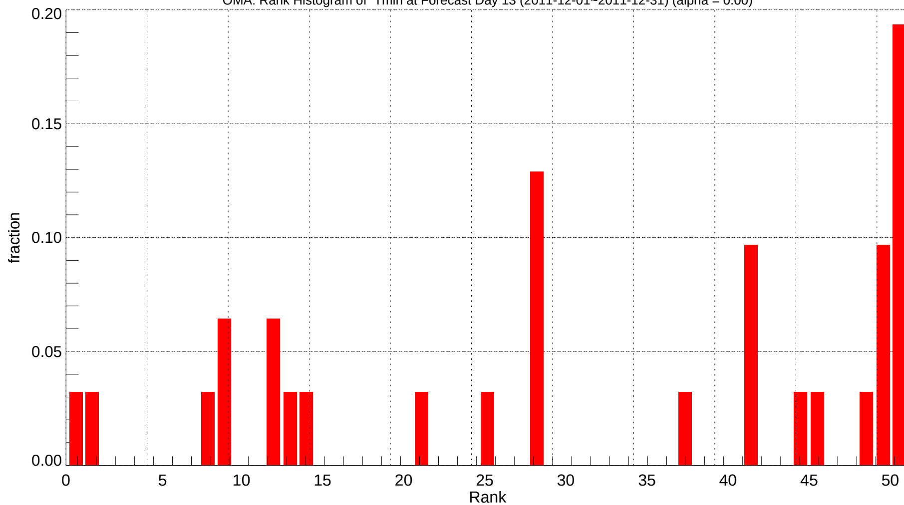
OMA: Rank Histogram of Tmin at Forecast Day 13 (2011-12-01~2011-12-31) (alpha = 0.00)
