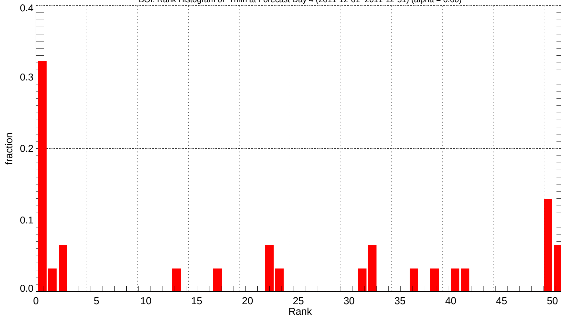
BOI: Rank Histogram of Tmin at Forecast Day 4 (2011-12-01~2011-12-31) (alpha = 0.00)
