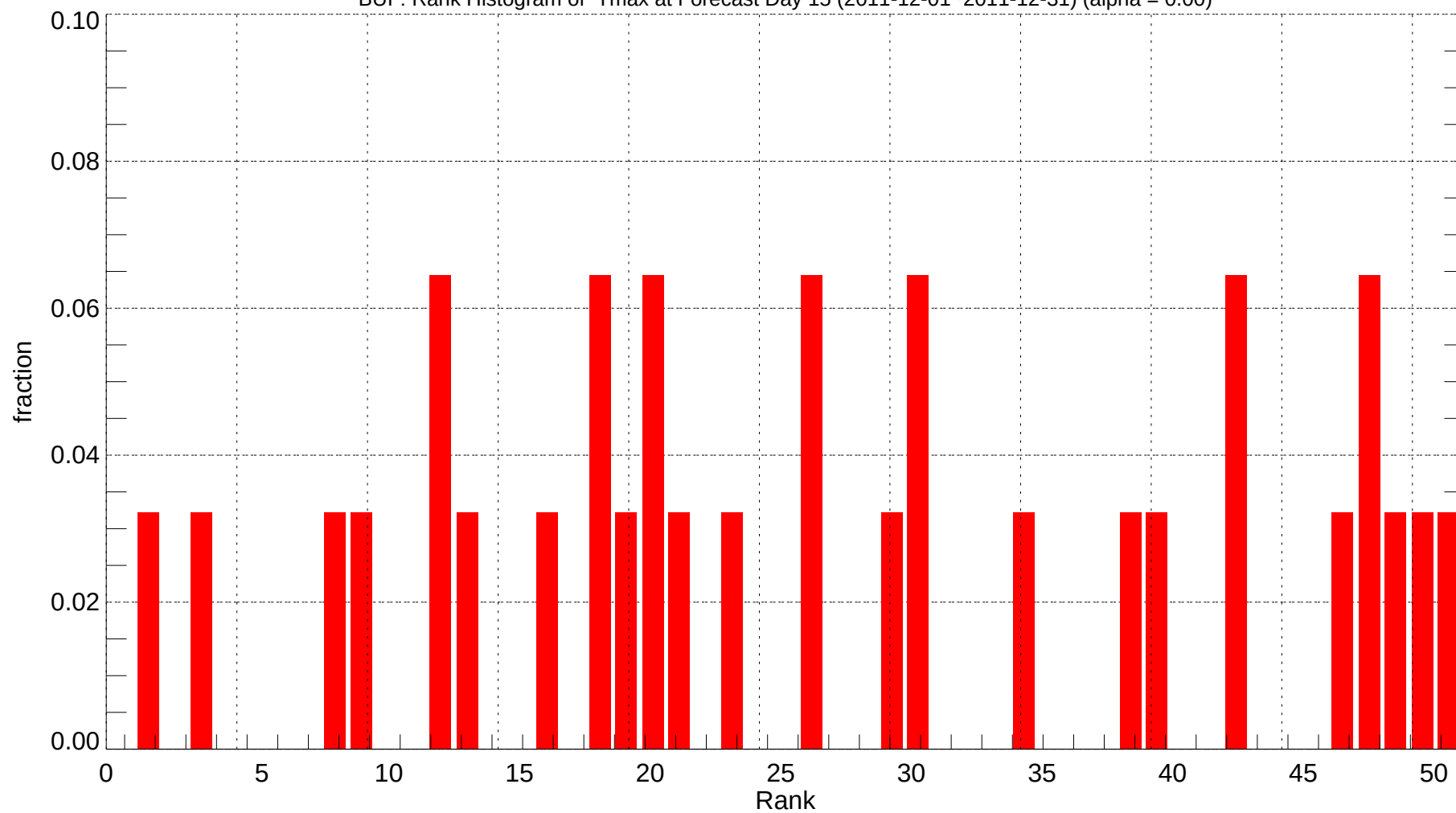
BUF: Rank Histogram of Tmax at Forecast Day 15 (2011-12-01~2011-12-31) (alpha = 0.00)
