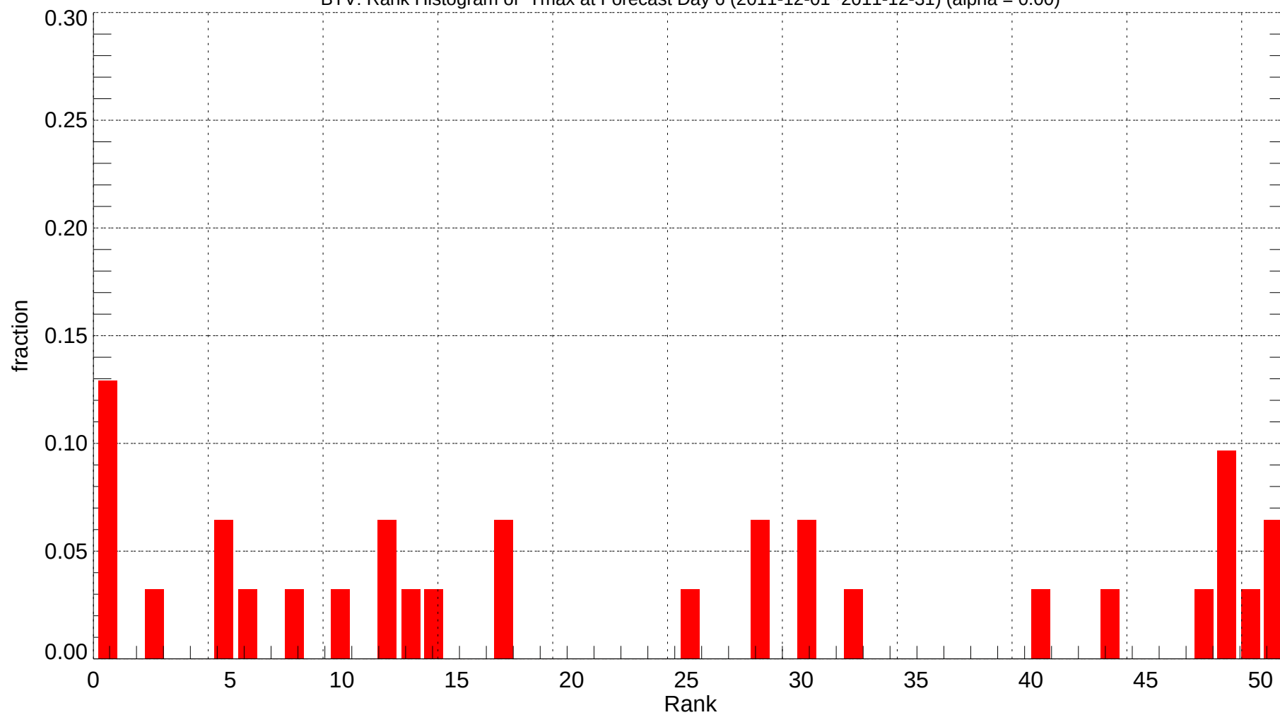
BTV: Rank Histogram of Tmax at Forecast Day 6 (2011-12-01~2011-12-31) (alpha = 0.00)
