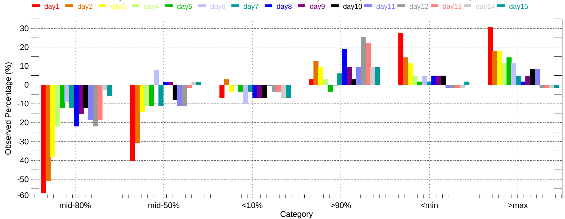
Observed Percentage Deviation of Ensembles - EWR: Max Temperature (2011-12-01~2011-12-31)
