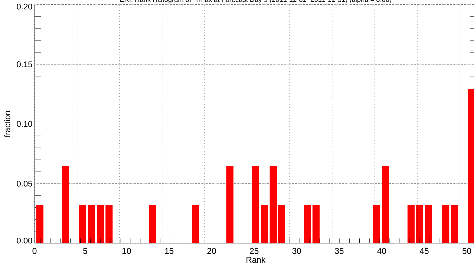
ERI: Rank Histogram of Tmax at Forecast Day 9 (2011-12-01~2011-12-31) (alpha = 0.00)
