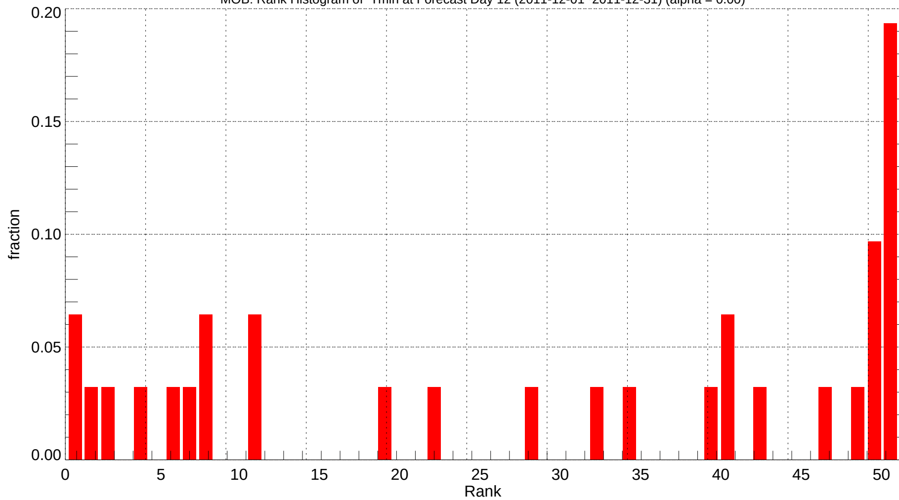
MOB: Rank Histogram of Tmin at Forecast Day 12 (2011-12-01~2011-12-31) (alpha = 0.00)
