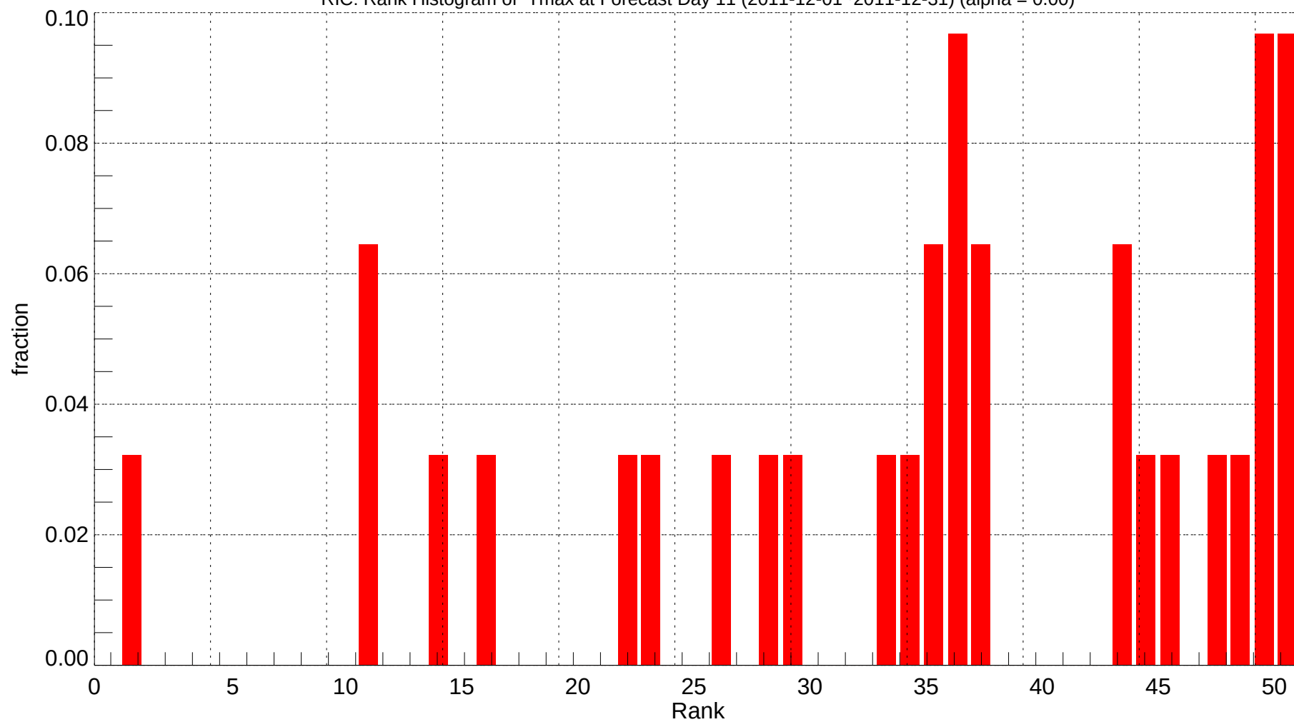
RIC: Rank Histogram of Tmax at Forecast Day 11 (2011-12-01~2011-12-31) (alpha = 0.00)
