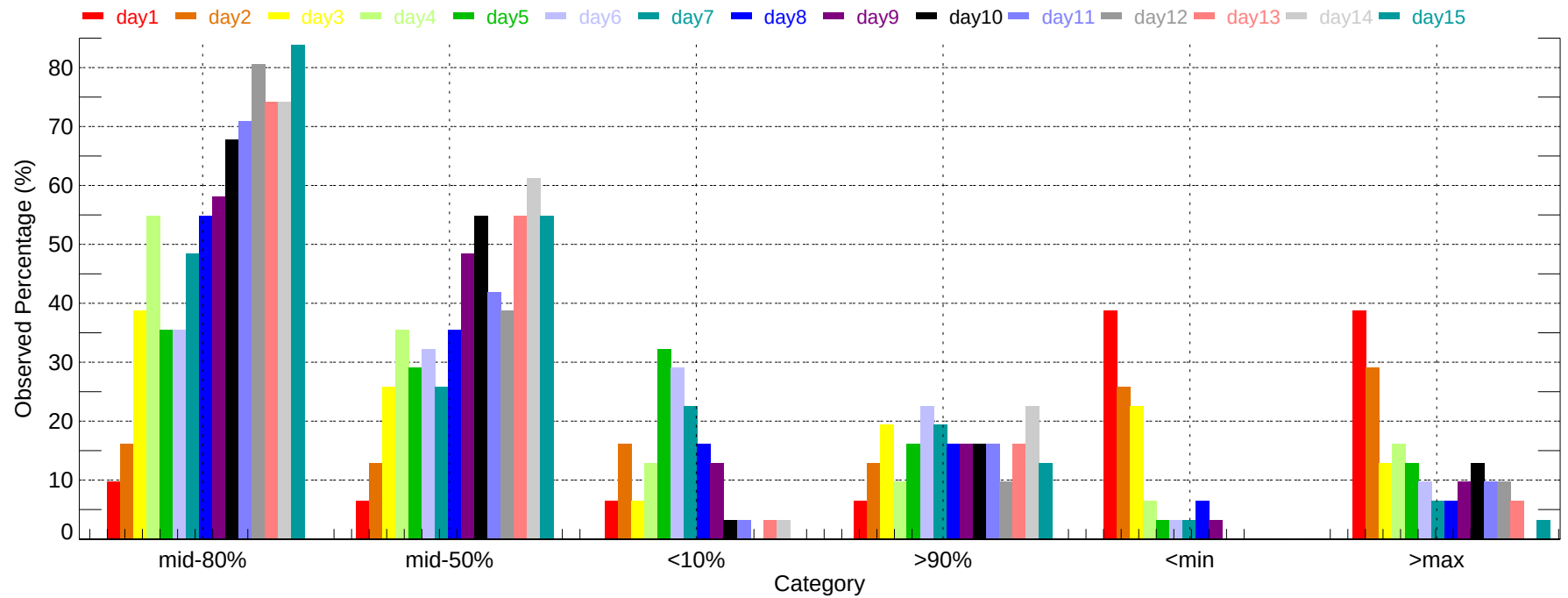
Observed Percentage of Ensembles - MKE: Min Temperature (2011-12-01~2011-12-31)
