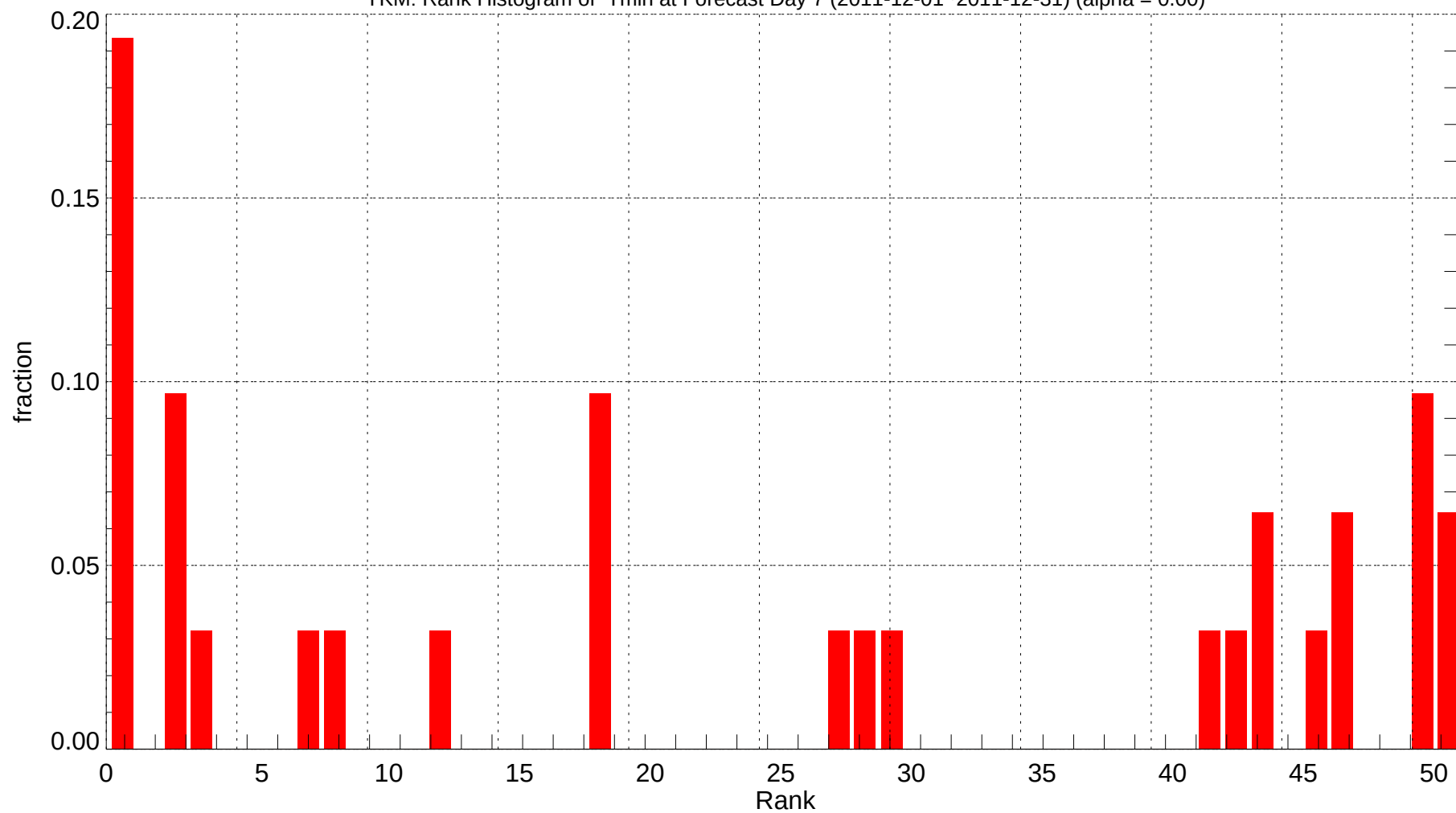
YKM: Rank Histogram of Tmin at Forecast Day 7 (2011-12-01~2011-12-31) (alpha = 0.00)
