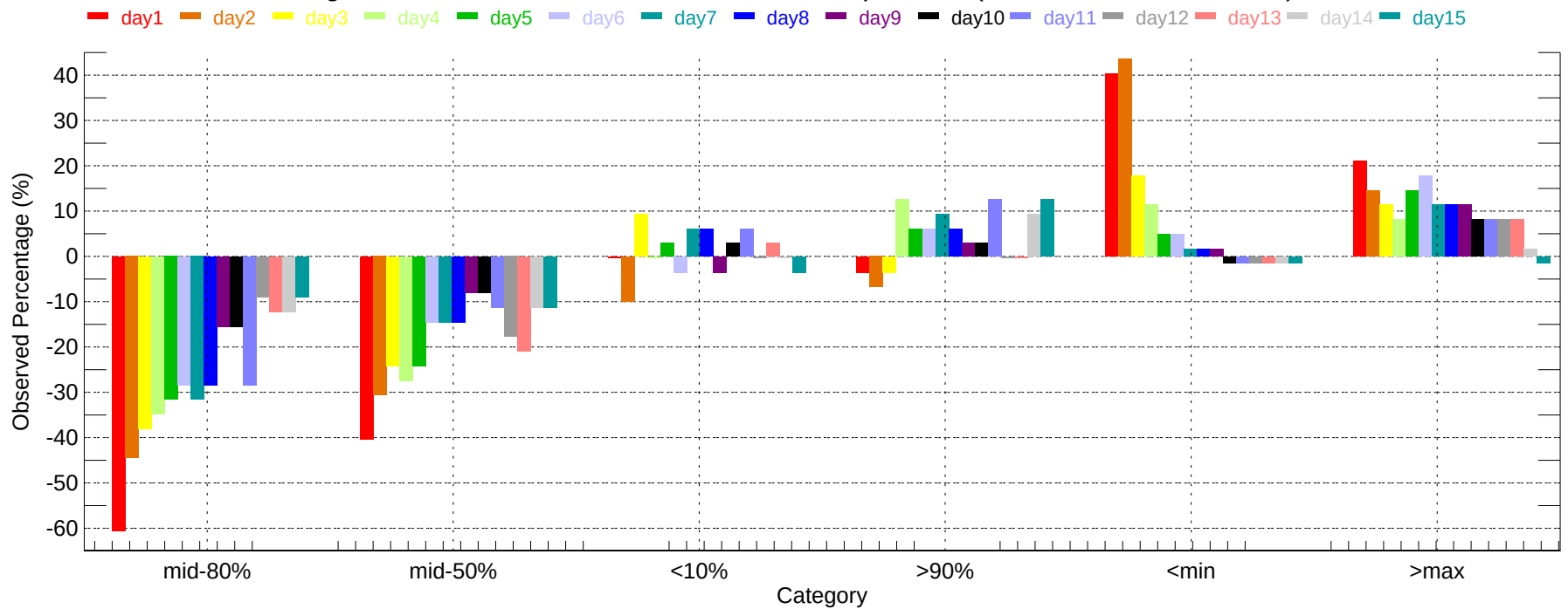
Observed Percentage Deviation of Ensembles - AVP: Min Temperature (2011-12-01~2011-12-31)
