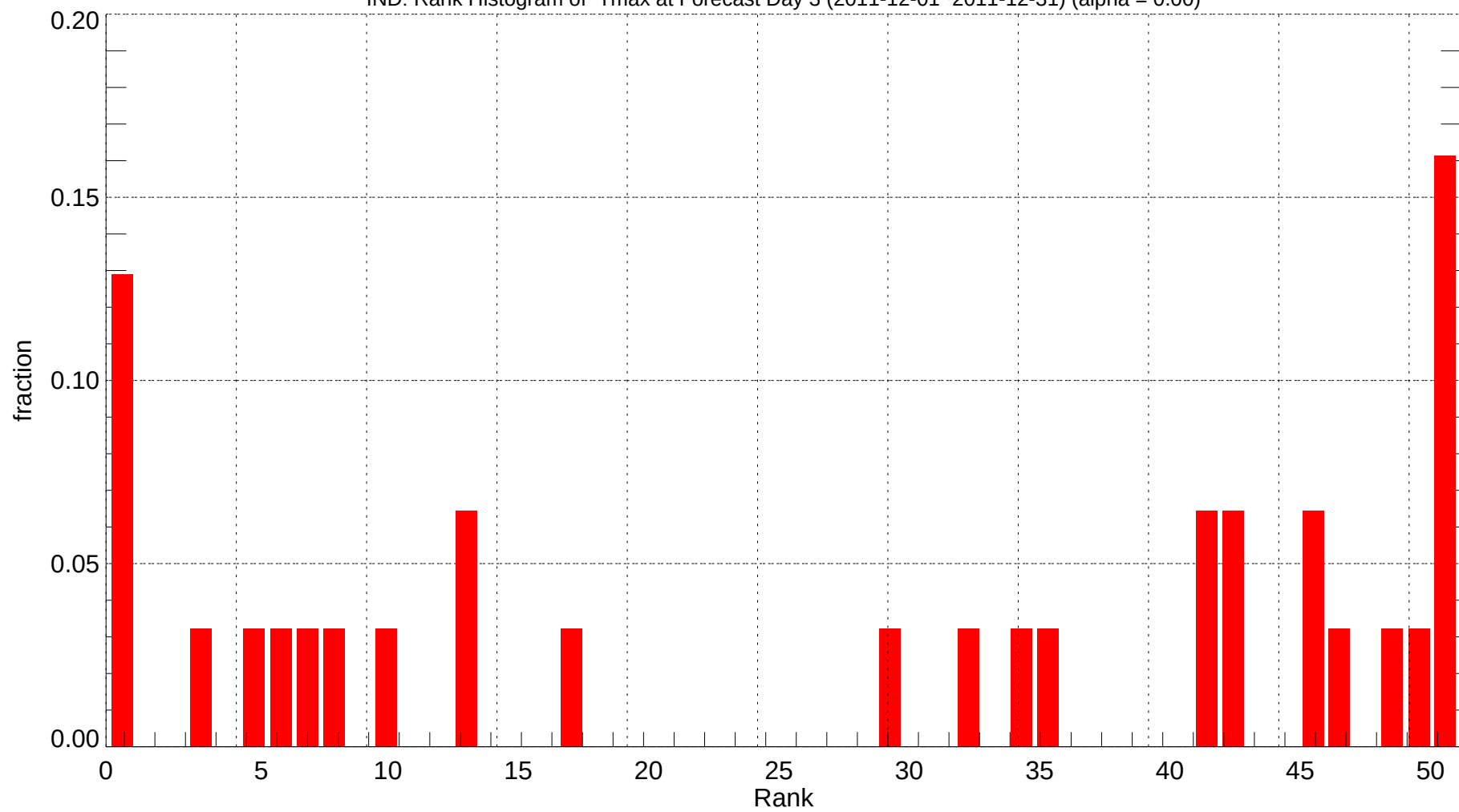
IND: Rank Histogram of Tmax at Forecast Day 3 (2011-12-01~2011-12-31) (alpha = 0.00)
