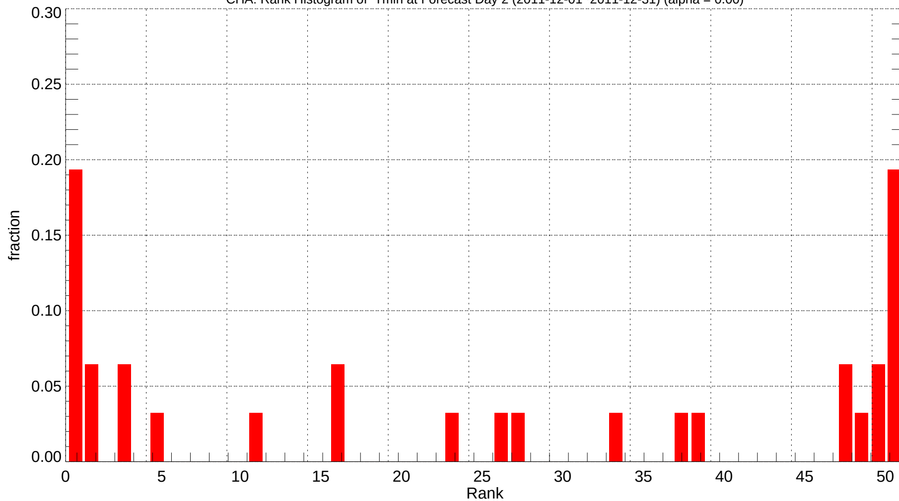
CHA: Rank Histogram of Tmin at Forecast Day 2 (2011-12-01~2011-12-31) (alpha = 0.00)
