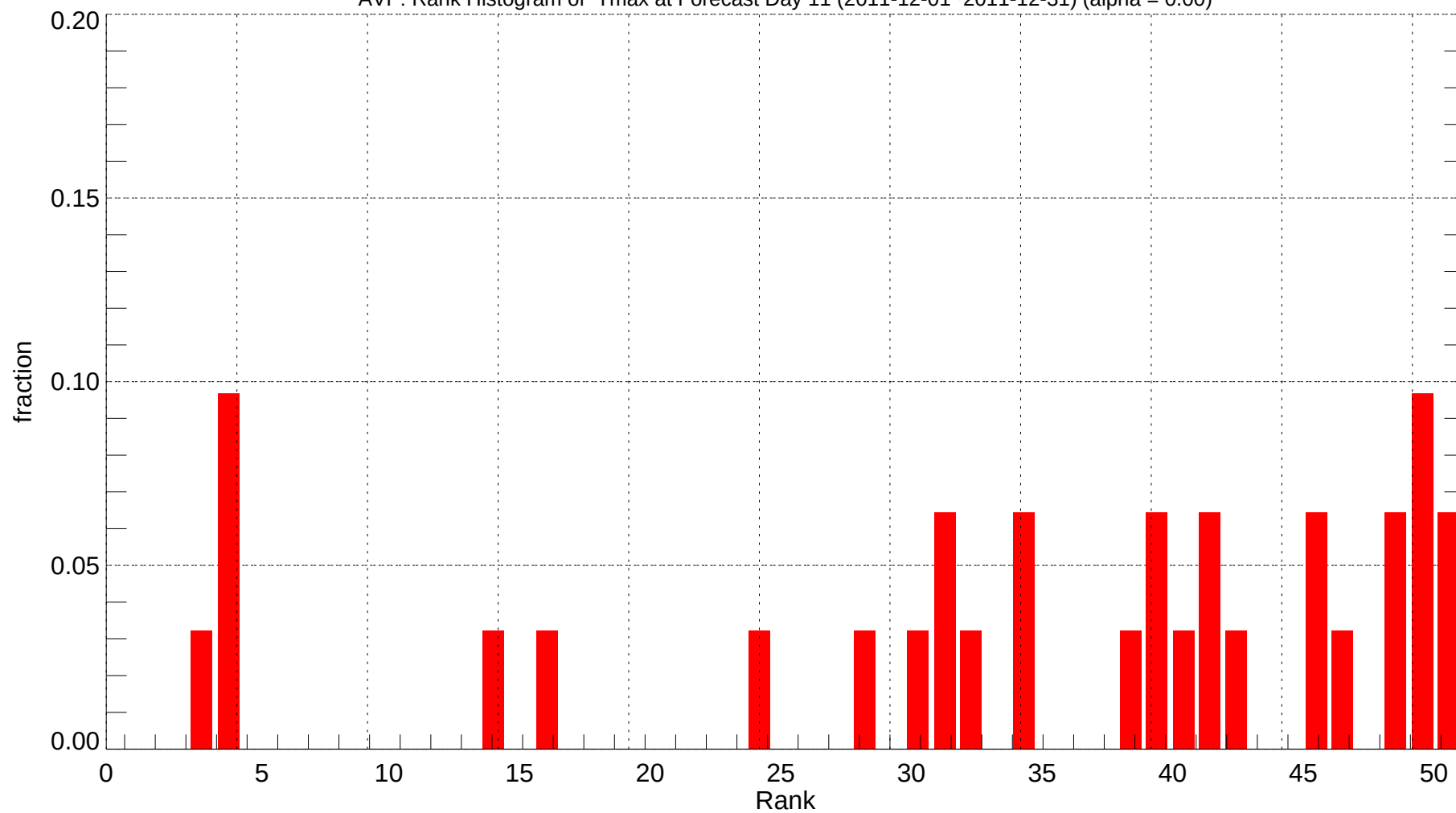
AVP: Rank Histogram of Tmax at Forecast Day 11 (2011-12-01~2011-12-31) (alpha = 0.00)
