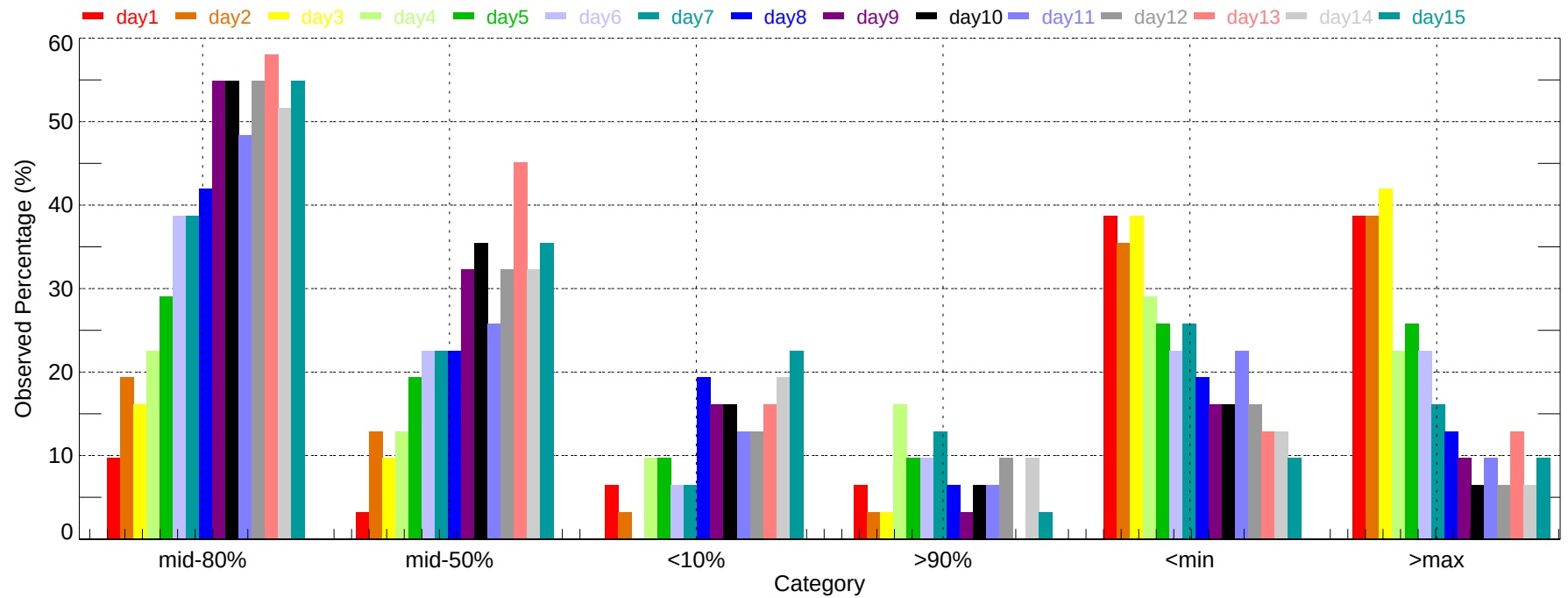
Observed Percentage of Ensembles - ALW: Max Temperature (2011-12-01~2011-12-31)
