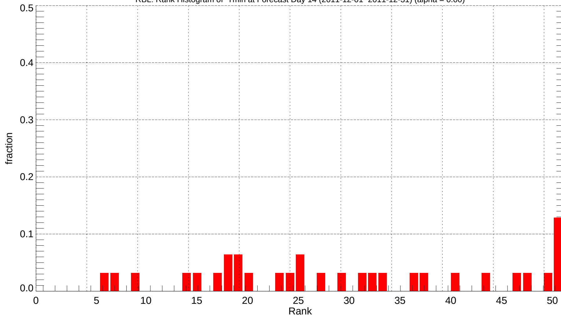
RBL: Rank Histogram of Tmin at Forecast Day 14 (2011-12-01~2011-12-31) (alpha = 0.00)
