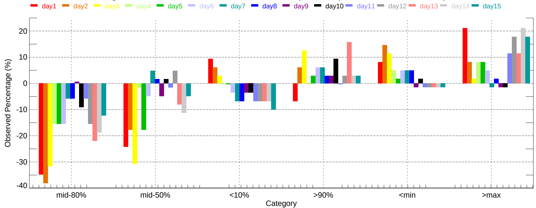
Observed Percentage Deviation of Ensembles - BUR: Max Temperature (2011-12-01~2011-12-31)
