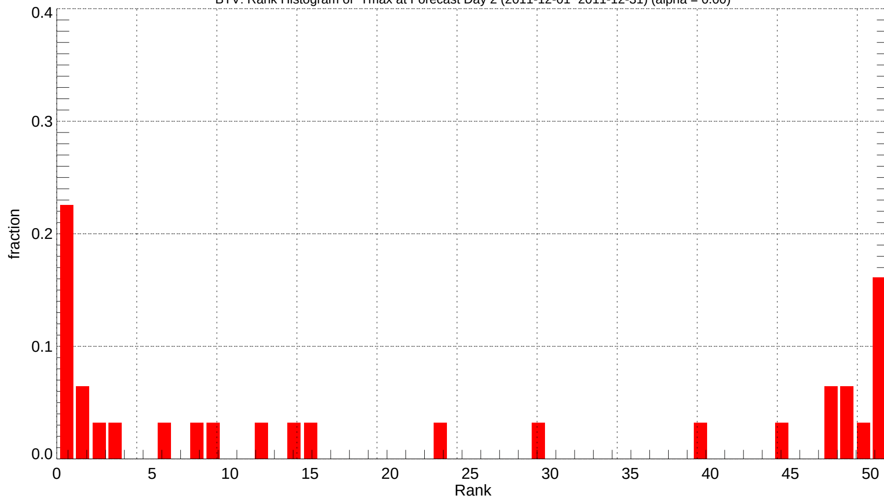
BTV: Rank Histogram of Tmax at Forecast Day 2 (2011-12-01~2011-12-31) (alpha = 0.00)
