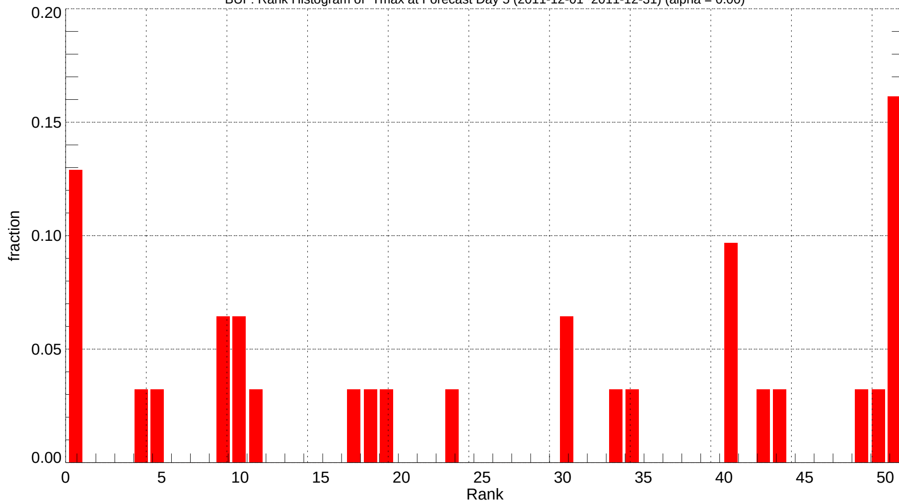
BUF: Rank Histogram of Tmax at Forecast Day 5 (2011-12-01~2011-12-31) (alpha = 0.00)
