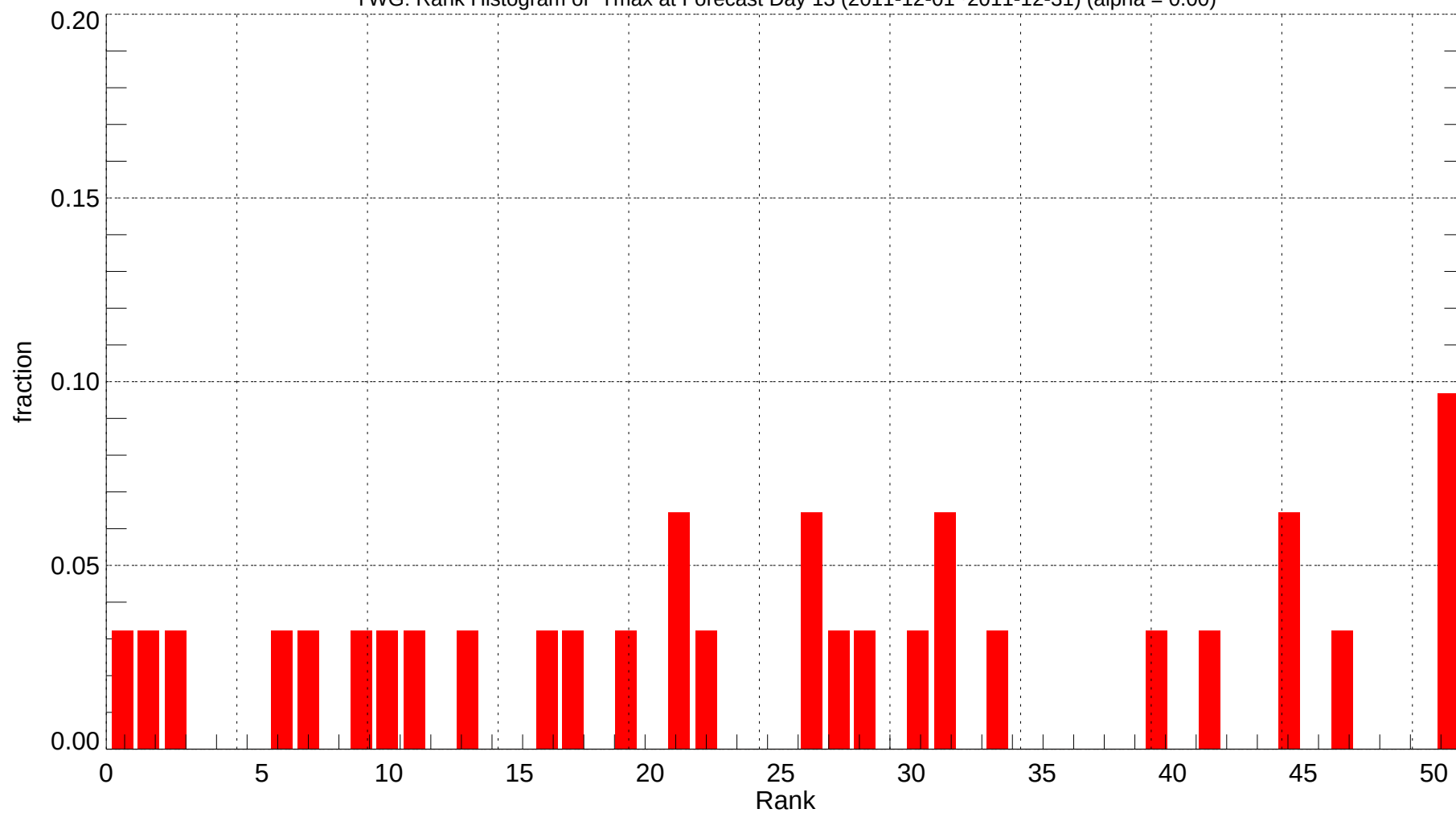
YWG: Rank Histogram of Tmax at Forecast Day 13 (2011-12-01~2011-12-31) (alpha = 0.00)
