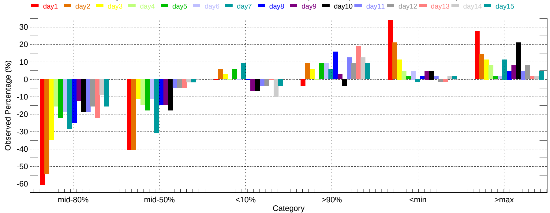
Observed Percentage Deviation of Ensembles - ORH: Max Temperature (2011-12-01~2011-12-31)
