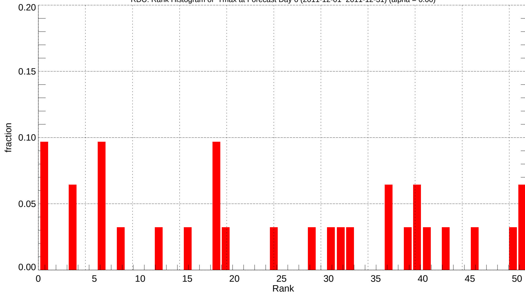
RDU: Rank Histogram of Tmax at Forecast Day 6 (2011-12-01~2011-12-31) (alpha = 0.00)
