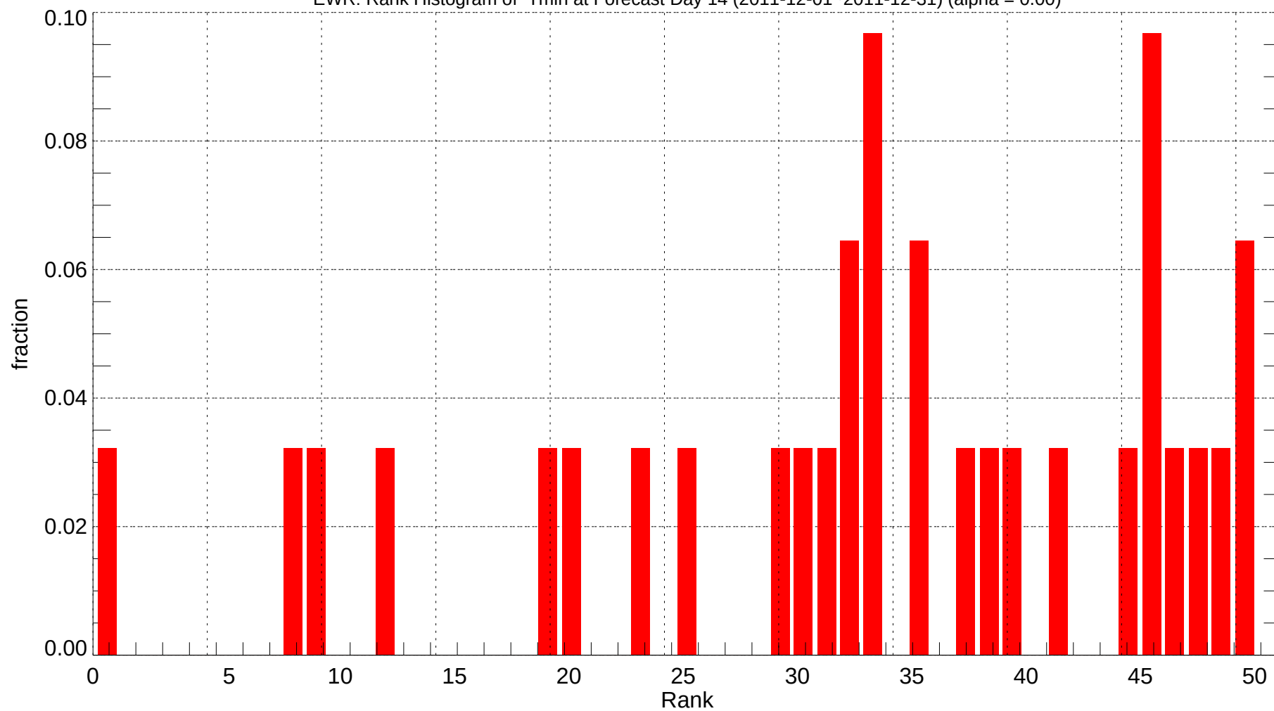
EWR: Rank Histogram of Tmin at Forecast Day 14 (2011-12-01~2011-12-31) (alpha = 0.00)
