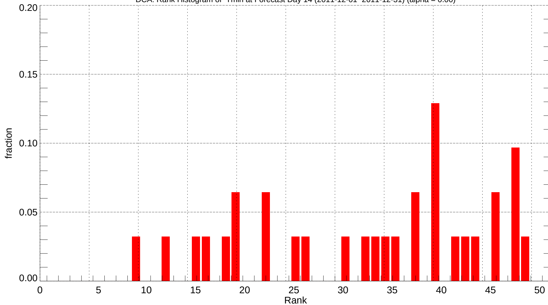
DCA: Rank Histogram of Tmin at Forecast Day 14 (2011-12-01~2011-12-31) (alpha = 0.00)
