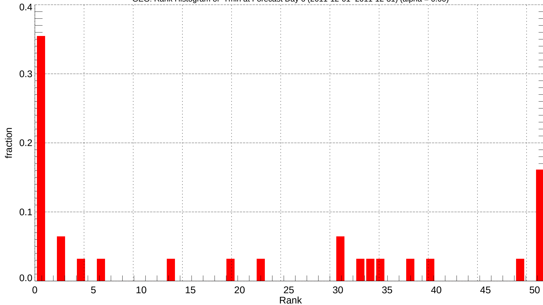
GEG: Rank Histogram of Tmin at Forecast Day 6 (2011-12-01~2011-12-31) (alpha = 0.00)
