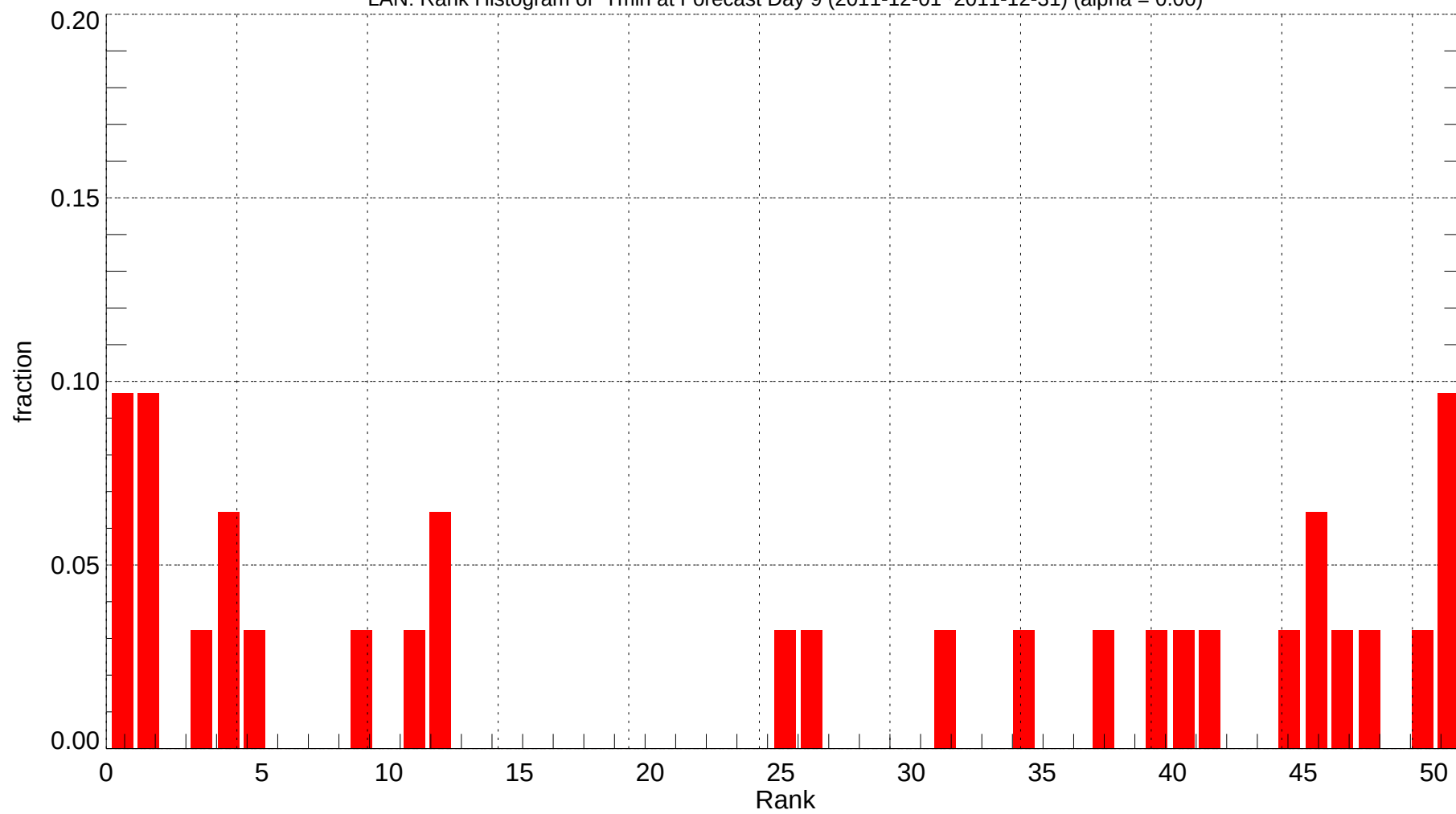
LAN: Rank Histogram of Tmin at Forecast Day 9 (2011-12-01~2011-12-31) (alpha = 0.00)
