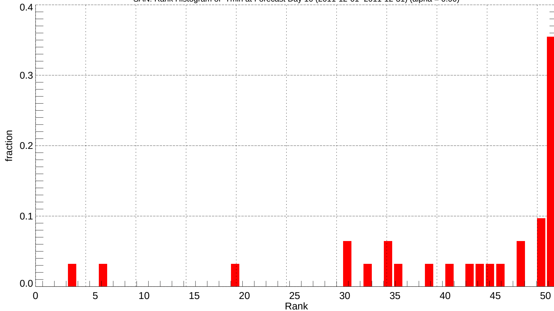
SAN: Rank Histogram of Tmin at Forecast Day 10 (2011-12-01~2011-12-31) (alpha = 0.00)
