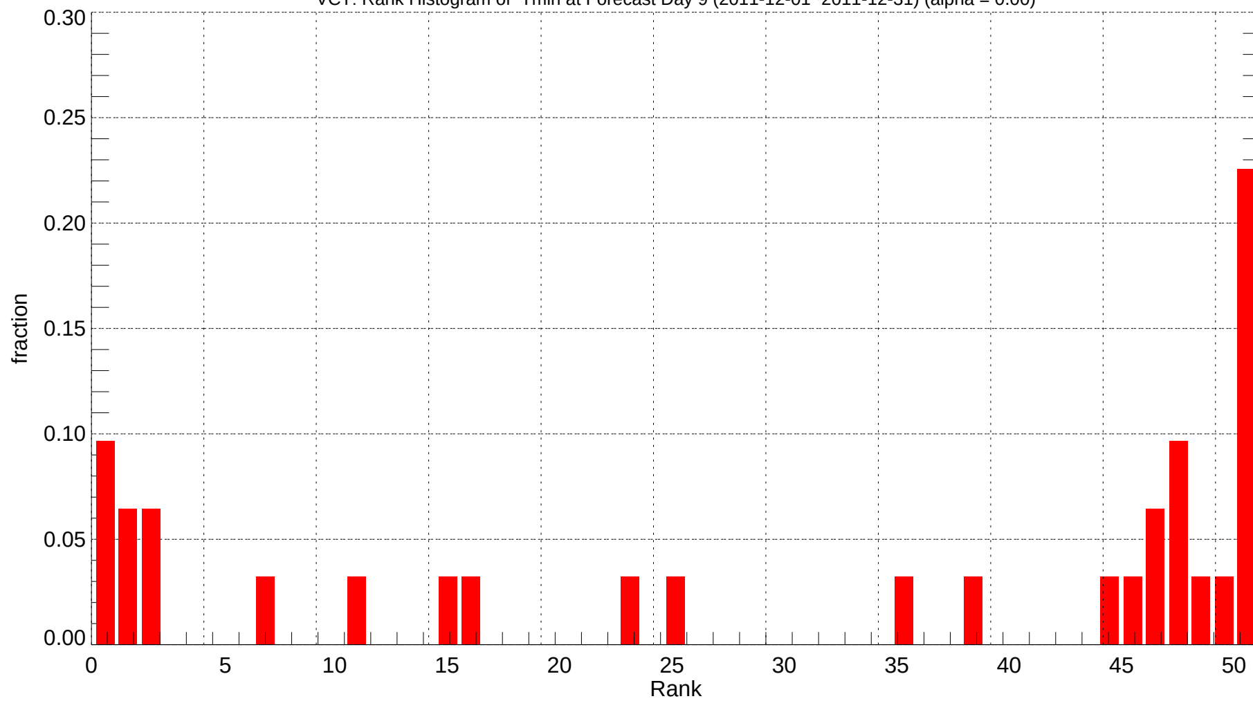
VCT: Rank Histogram of Tmin at Forecast Day 9 (2011-12-01~2011-12-31) (alpha = 0.00)
