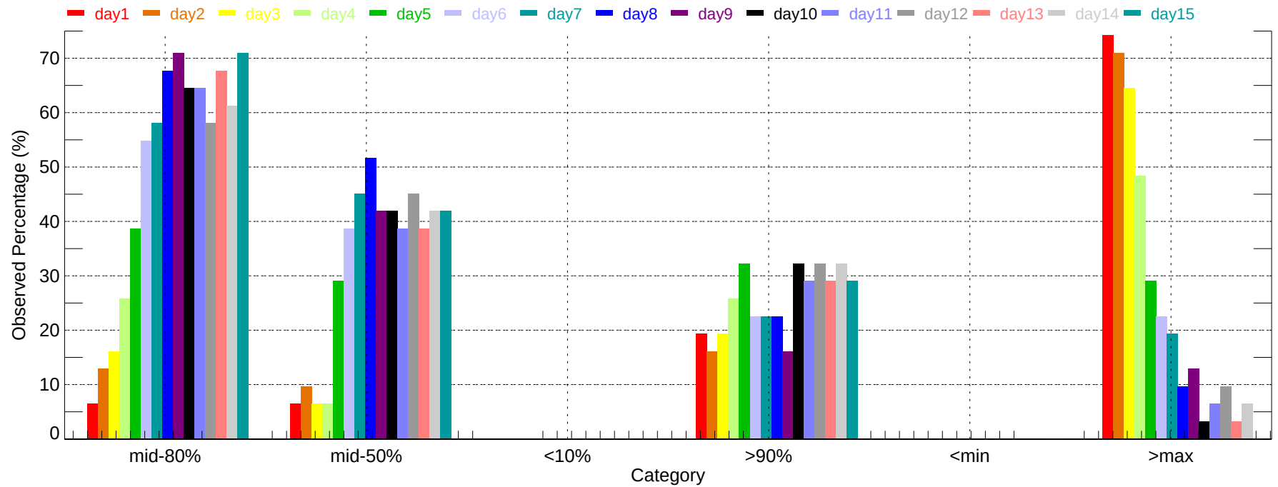
Observed Percentage of Ensembles - SAN: Min Temperature (2011-12-01~2011-12-31)
