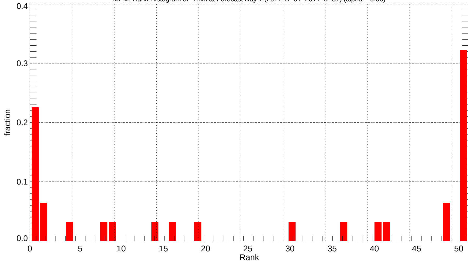
MEM: Rank Histogram of Tmin at Forecast Day 1 (2011-12-01~2011-12-31) (alpha = 0.00)
