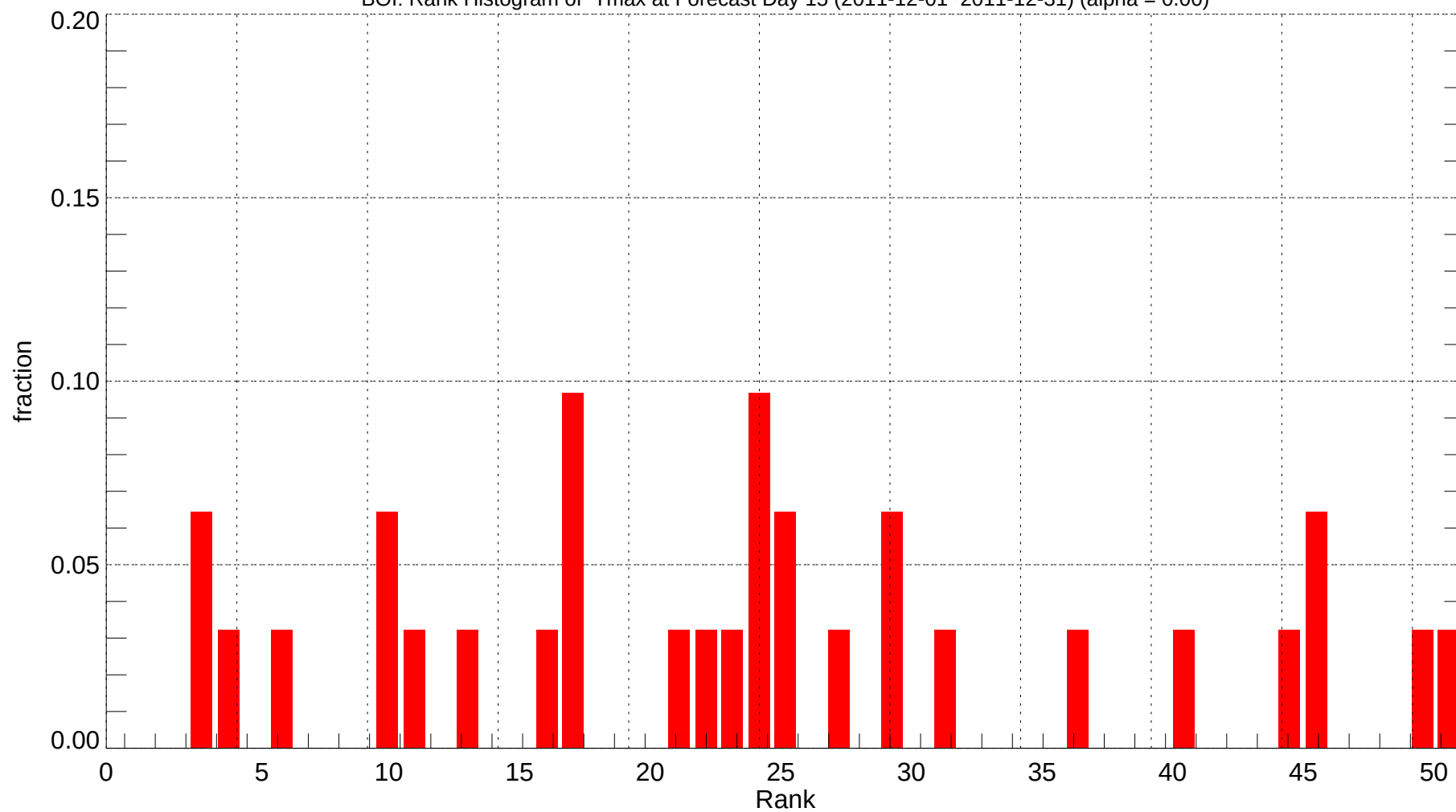
BOI: Rank Histogram of Tmax at Forecast Day 15 (2011-12-01~2011-12-31) (alpha = 0.00)
