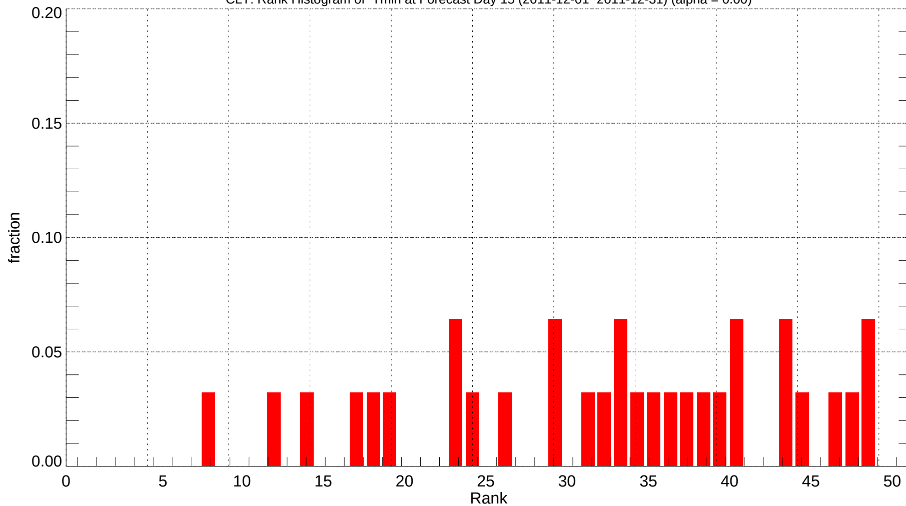
CLT: Rank Histogram of Tmin at Forecast Day 15 (2011-12-01~2011-12-31) (alpha = 0.00)
