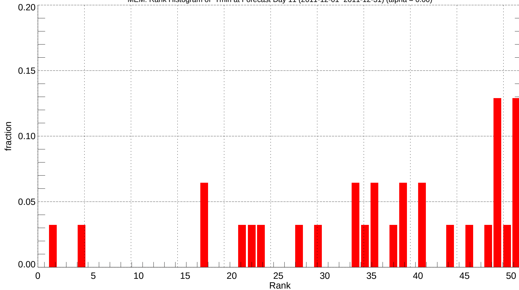
MEM: Rank Histogram of Tmin at Forecast Day 11 (2011-12-01~2011-12-31) (alpha = 0.00)
