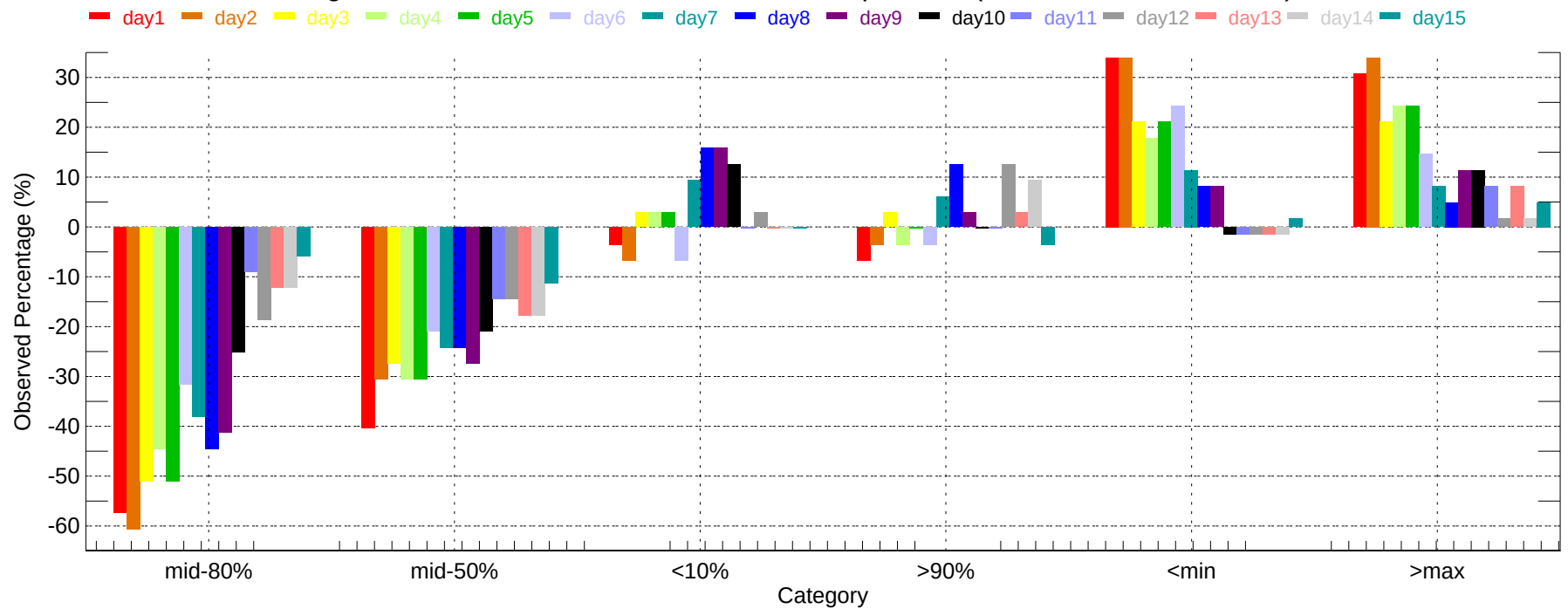
Observed Percentage Deviation of Ensembles - BTV: Min Temperature (2011-12-01~2011-12-31)
