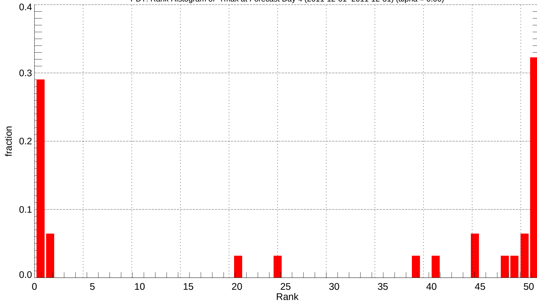
PDT: Rank Histogram of Tmax at Forecast Day 4 (2011-12-01~2011-12-31) (alpha = 0.00)
