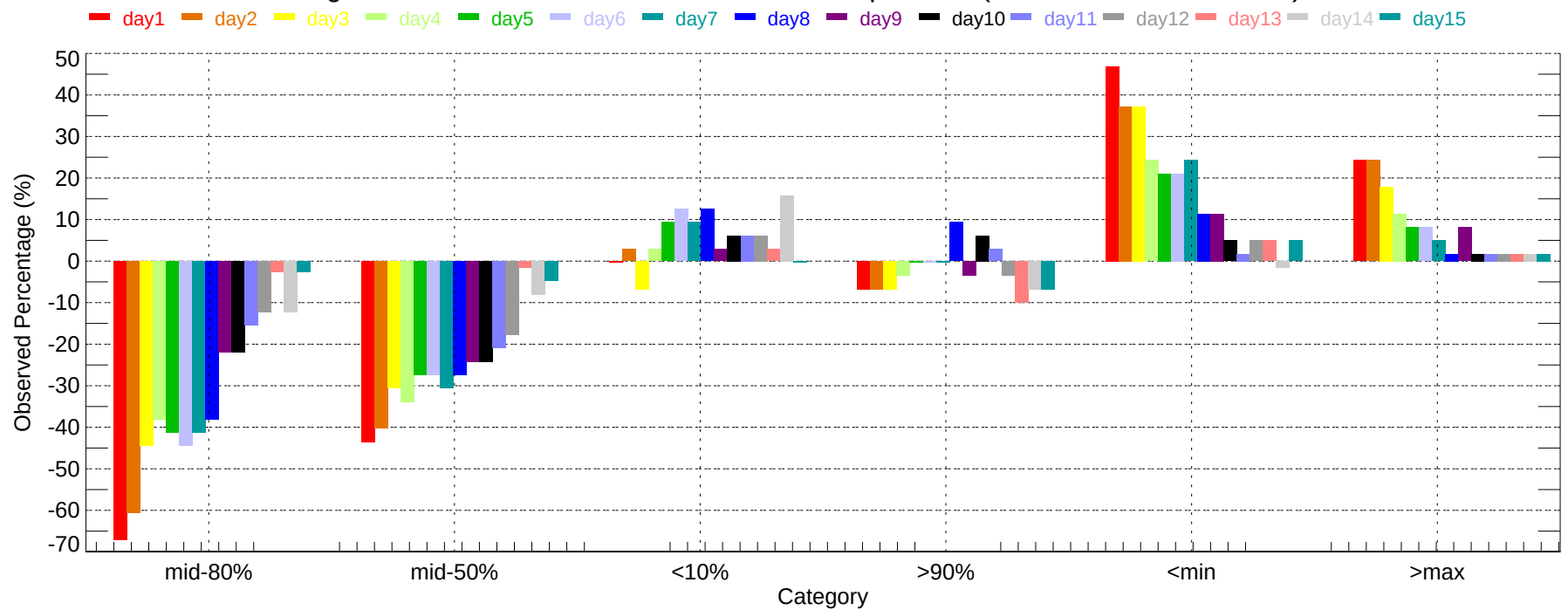
Observed Percentage Deviation of Ensembles - YYZ: Max Temperature (2011-12-01~2011-12-31)
