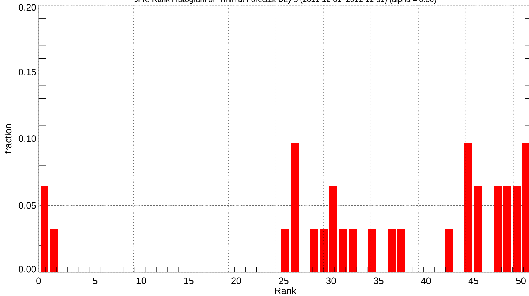
JFK: Rank Histogram of Tmin at Forecast Day 9 (2011-12-01~2011-12-31) (alpha = 0.00)
