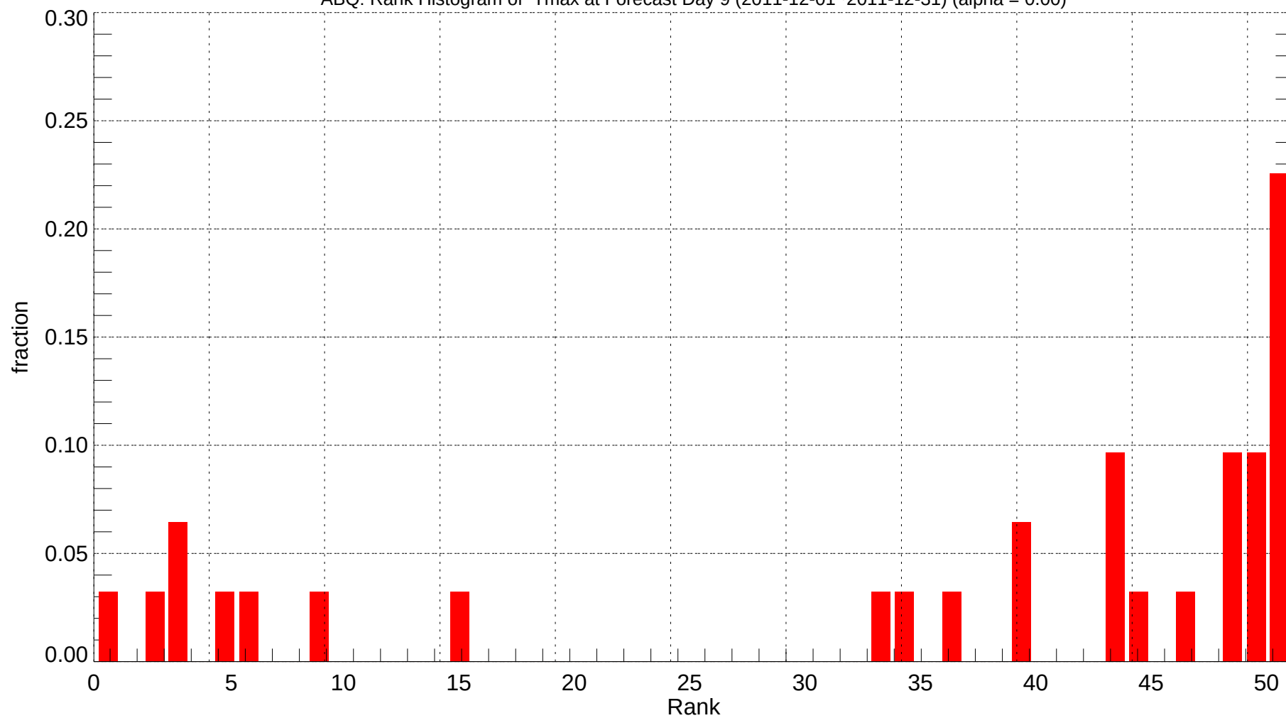
ABQ: Rank Histogram of Tmax at Forecast Day 9 (2011-12-01~2011-12-31) (alpha = 0.00)
