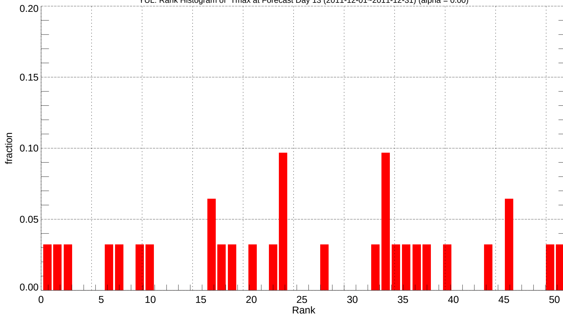
YUL: Rank Histogram of Tmax at Forecast Day 13 (2011-12-01~2011-12-31) (alpha = 0.00)
