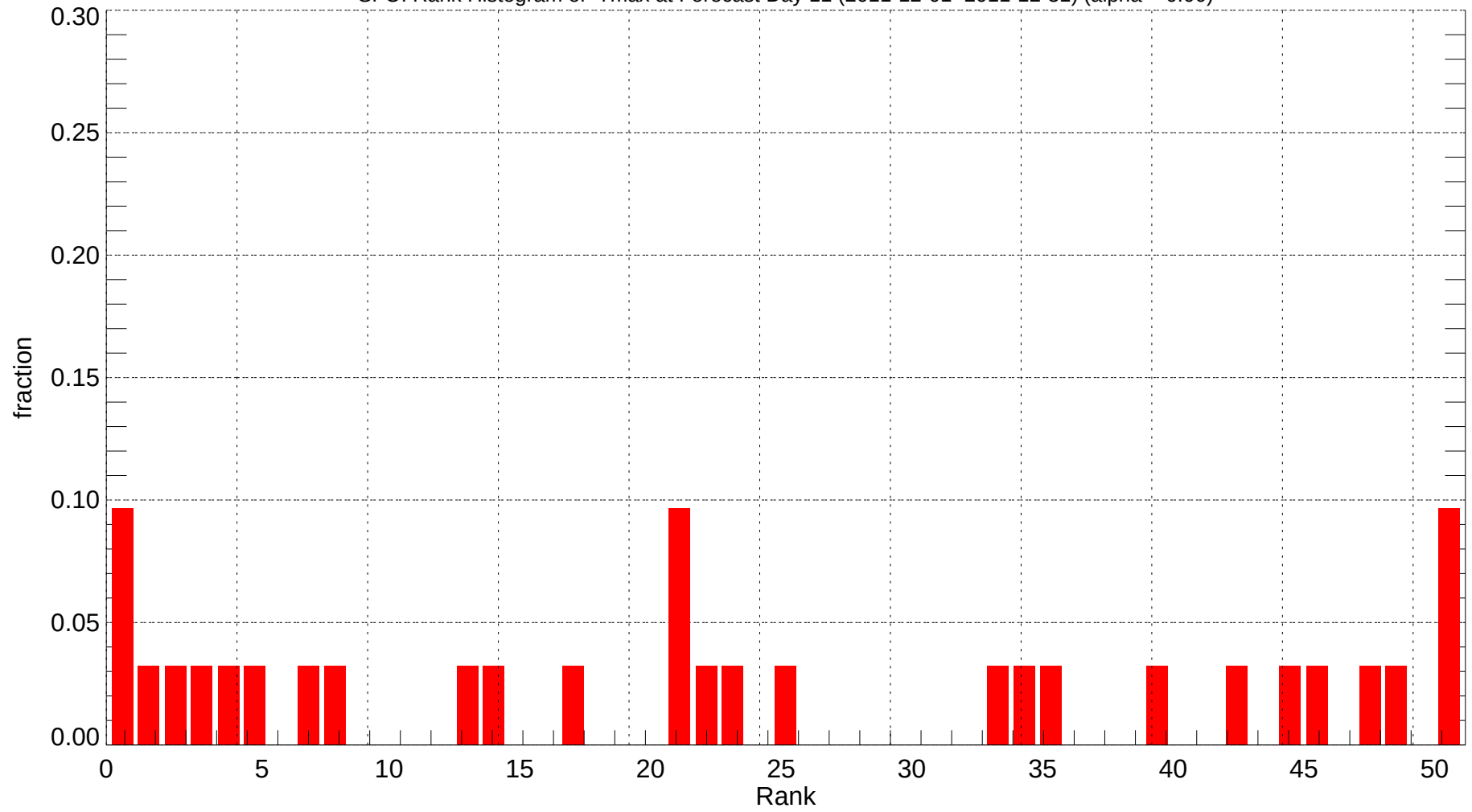
SFO: Rank Histogram of Tmax at Forecast Day 11 (2011-12-01~2011-12-31) (alpha = 0.00)
