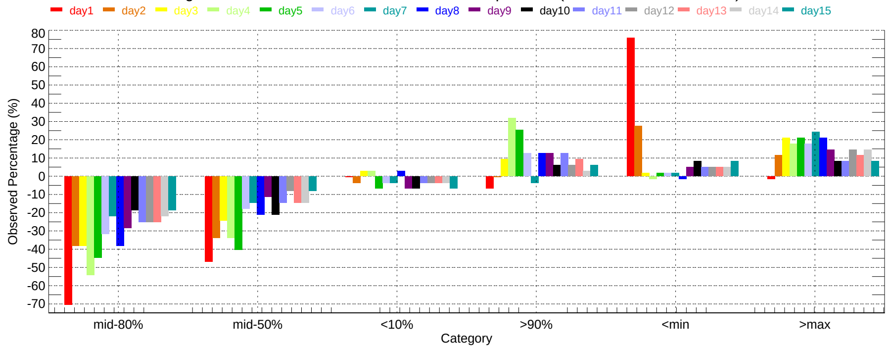
Observed Percentage Deviation of Ensembles - BOS: Max Temperature (2011-12-01~2011-12-31)
