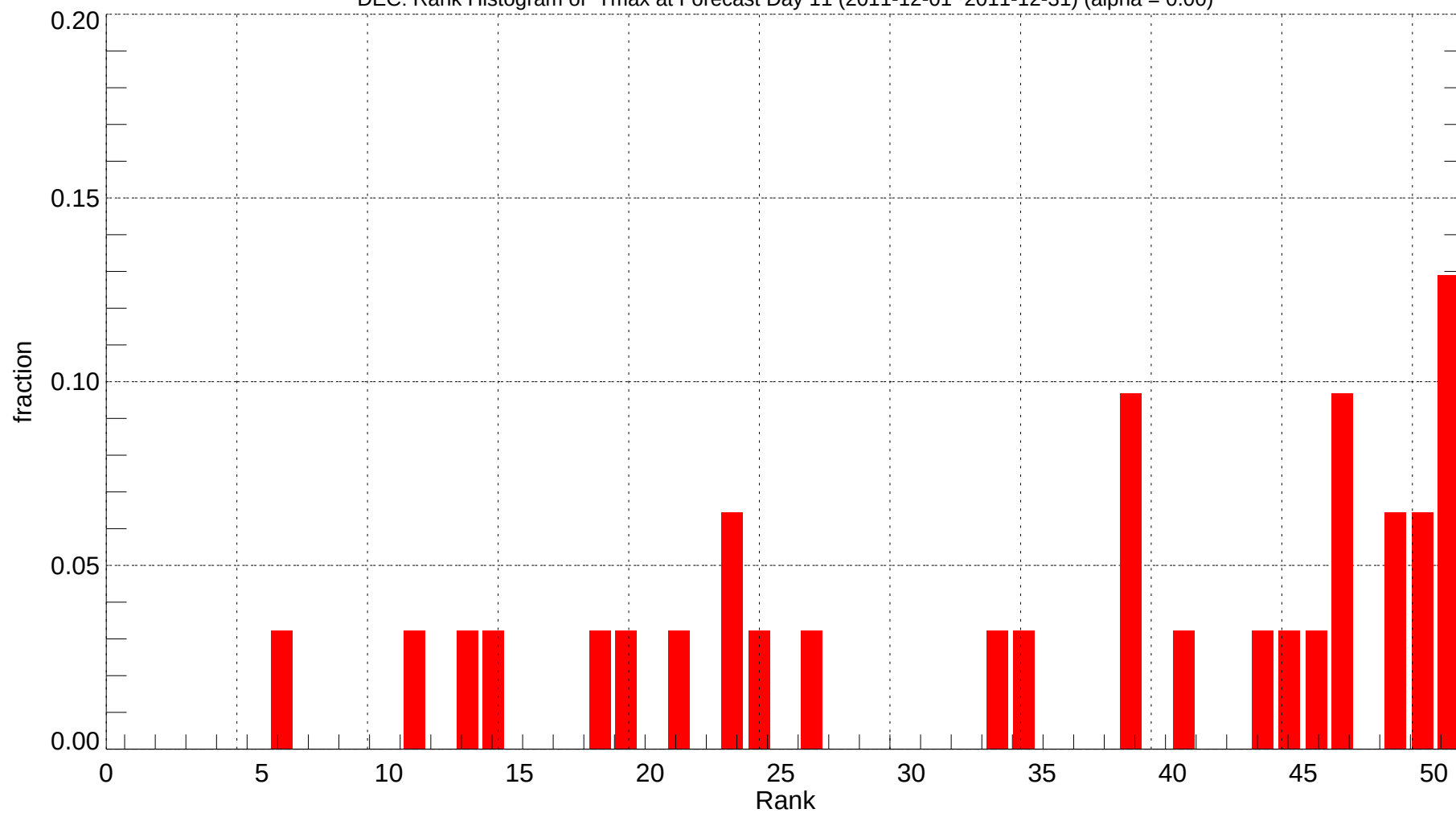
DEC: Rank Histogram of Tmax at Forecast Day 11 (2011-12-01~2011-12-31) (alpha = 0.00)
