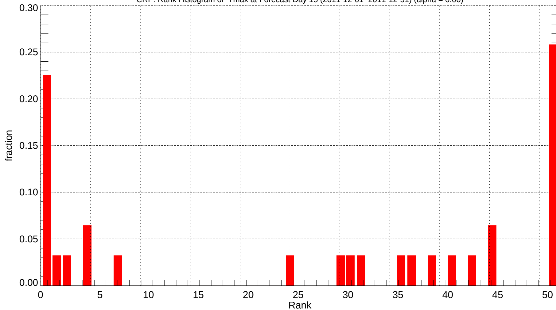
CRP: Rank Histogram of Tmax at Forecast Day 15 (2011-12-01~2011-12-31) (alpha = 0.00)
