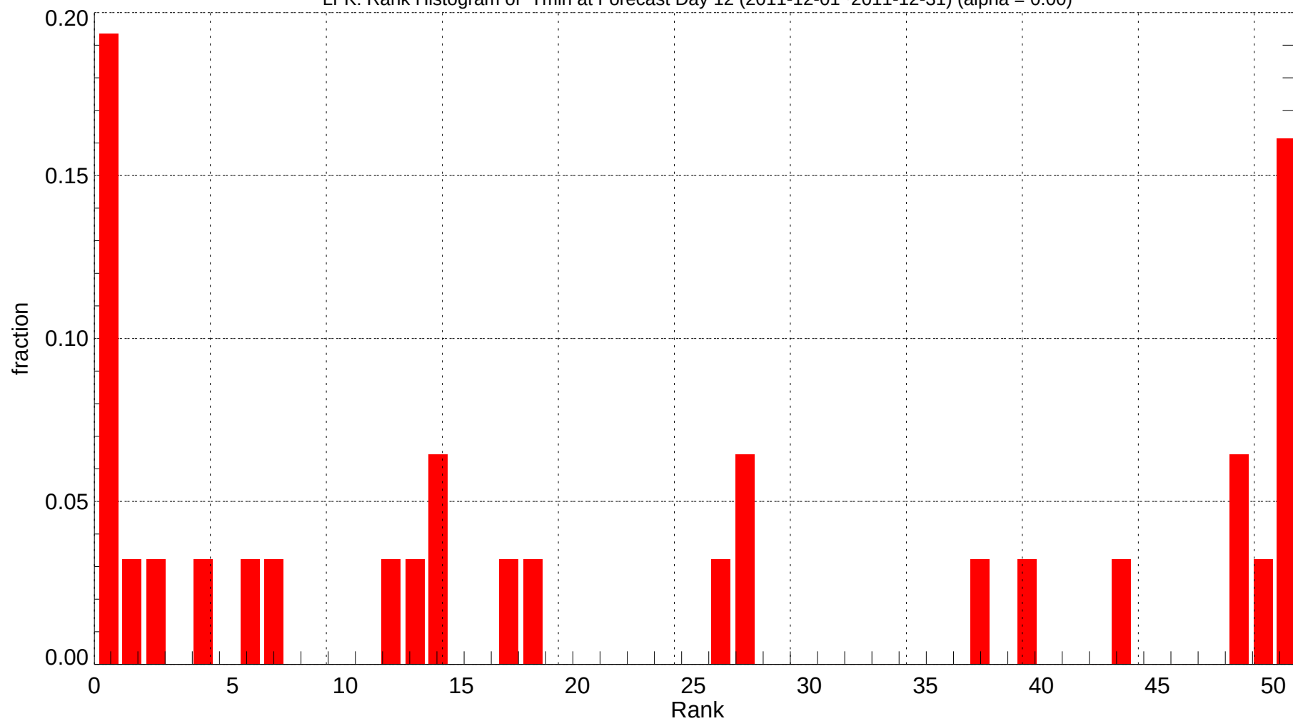
LFK: Rank Histogram of Tmin at Forecast Day 12 (2011-12-01~2011-12-31) (alpha = 0.00)
