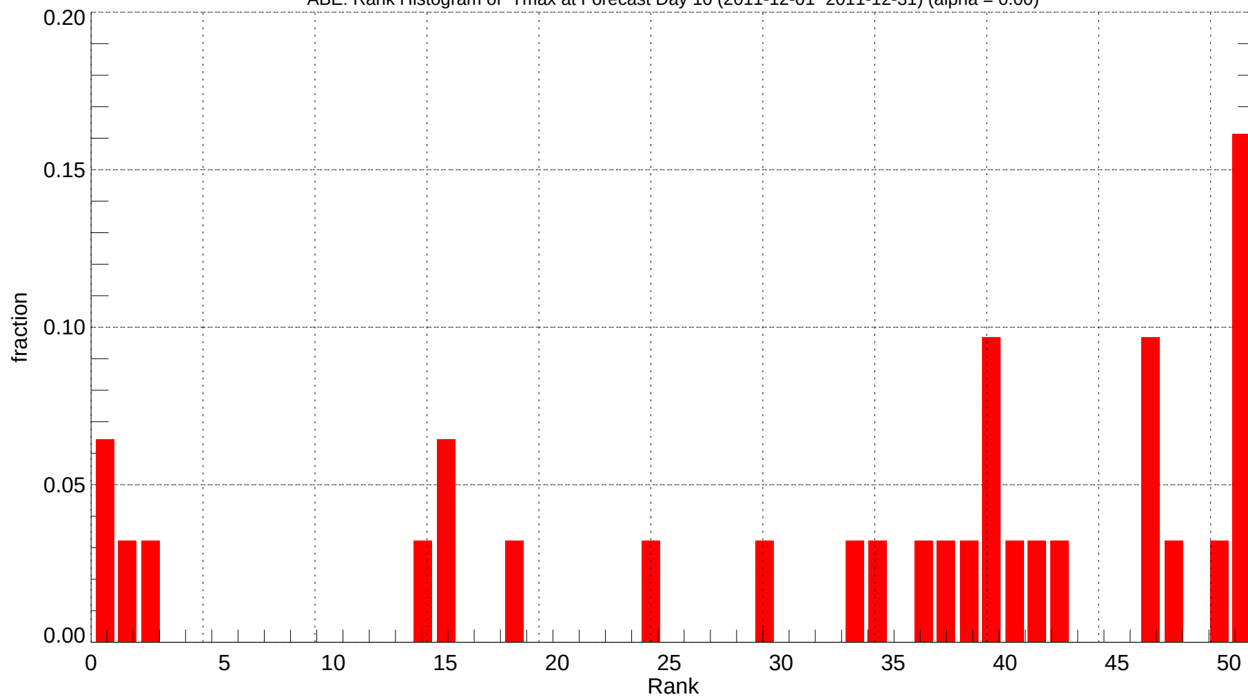
ABE: Rank Histogram of Tmax at Forecast Day 10 (2011-12-01~2011-12-31) (alpha = 0.00)
