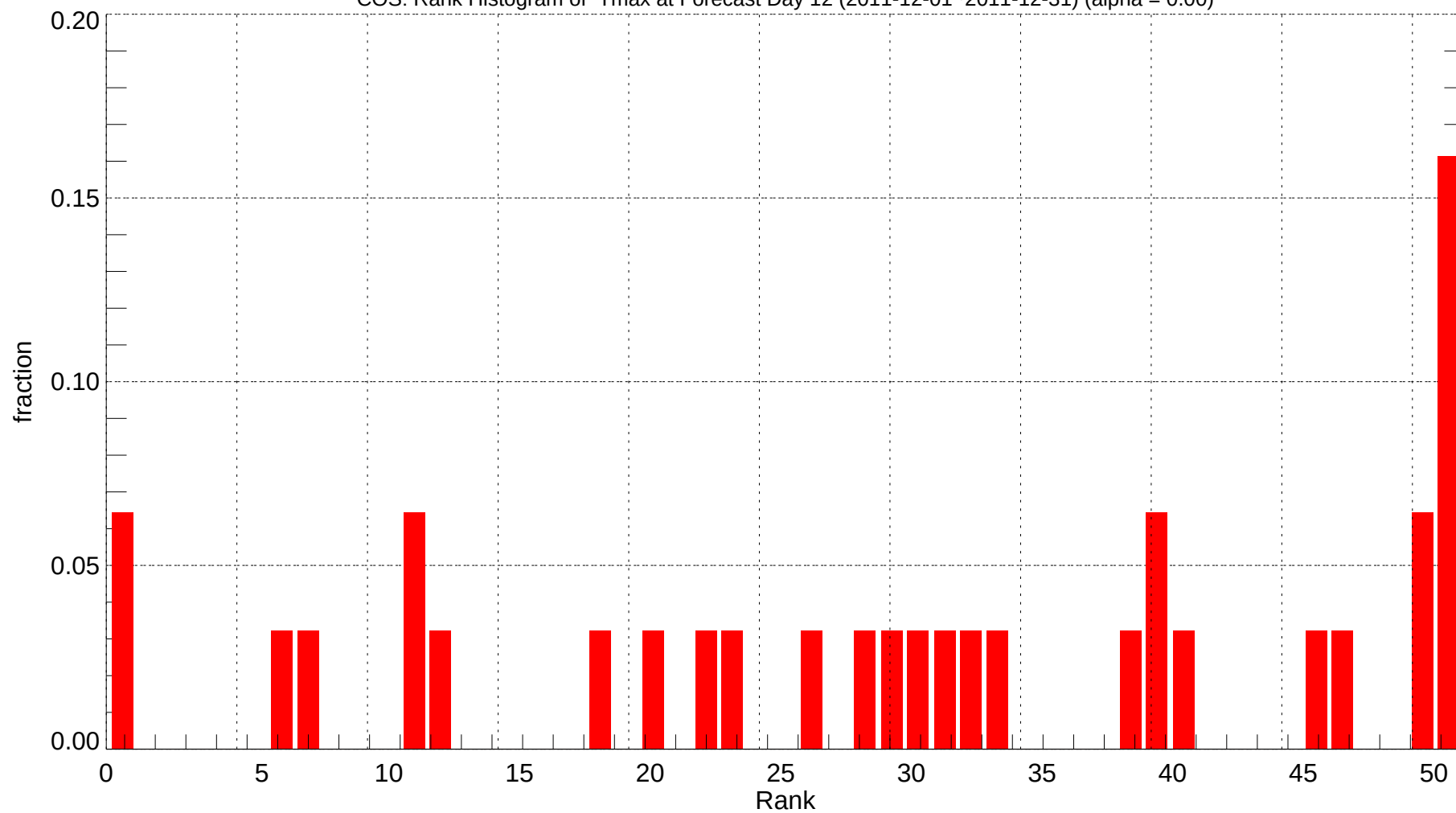
COS: Rank Histogram of Tmax at Forecast Day 12 (2011-12-01~2011-12-31) (alpha = 0.00)
