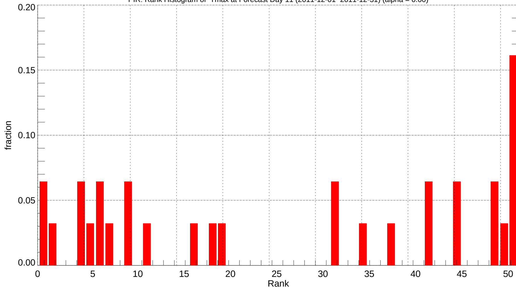
PIR: Rank Histogram of Tmax at Forecast Day 11 (2011-12-01~2011-12-31) (alpha = 0.00)
