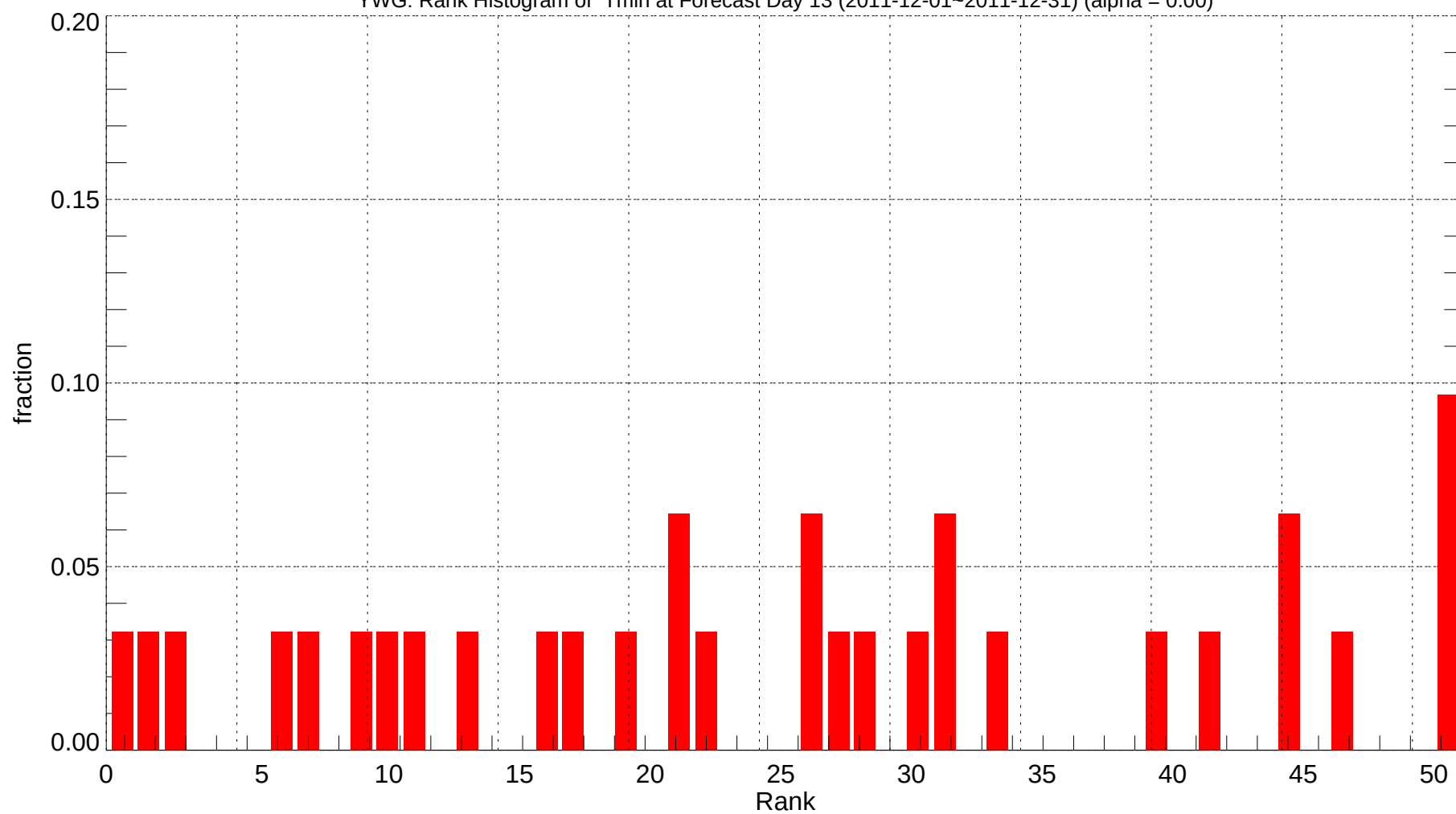
YWG: Rank Histogram of Tmin at Forecast Day 13 (2011-12-01~2011-12-31) (alpha = 0.00)
