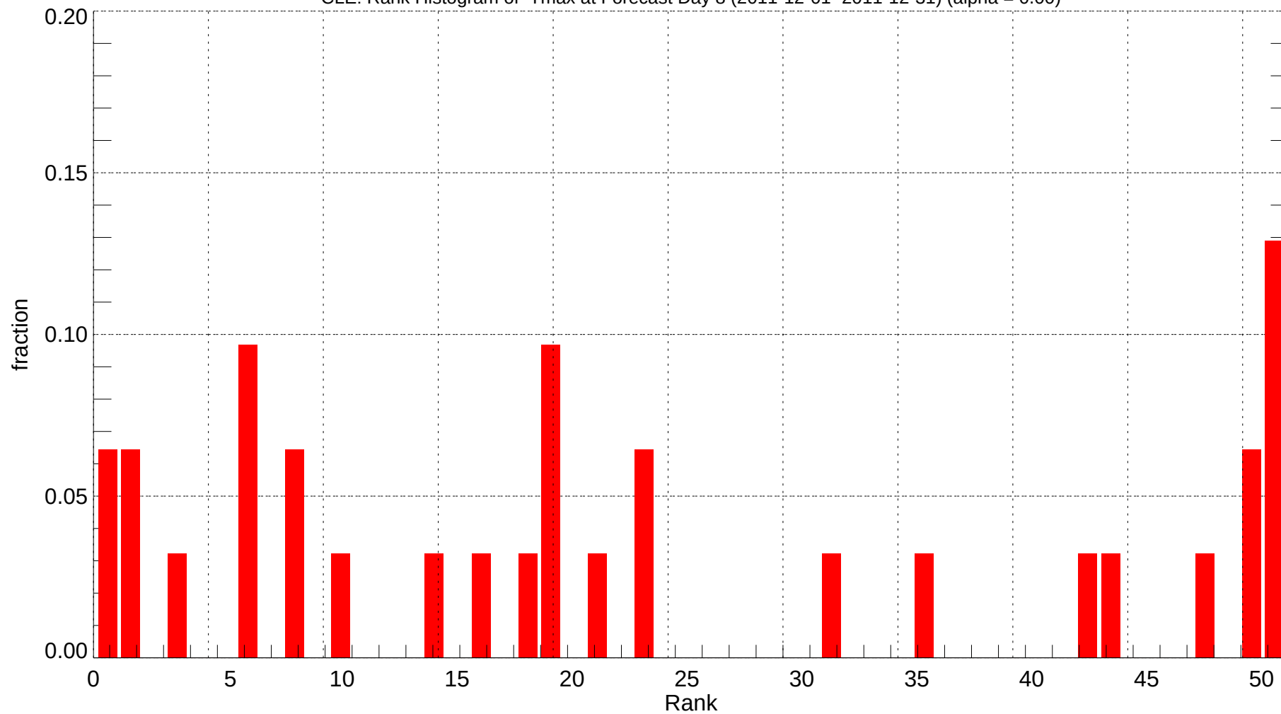
CLE: Rank Histogram of Tmax at Forecast Day 8 (2011-12-01~2011-12-31) (alpha = 0.00)
