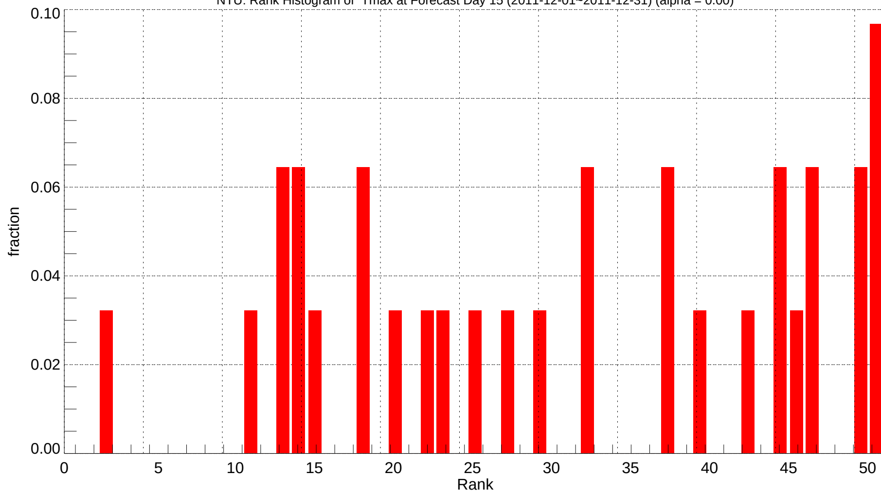
NTU: Rank Histogram of Tmax at Forecast Day 15 (2011-12-01~2011-12-31) (alpha = 0.00)
