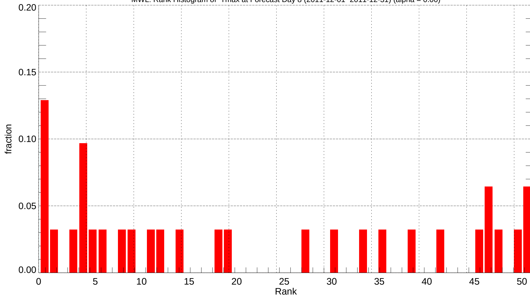
MWL: Rank Histogram of Tmax at Forecast Day 8 (2011-12-01~2011-12-31) (alpha = 0.00)
