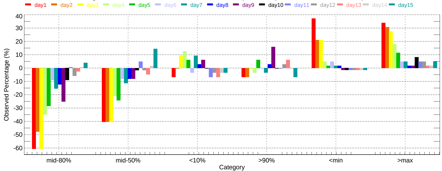
Observed Percentage Deviation of Ensembles - SSI: Max Temperature (2011-12-01~2011-12-31)
