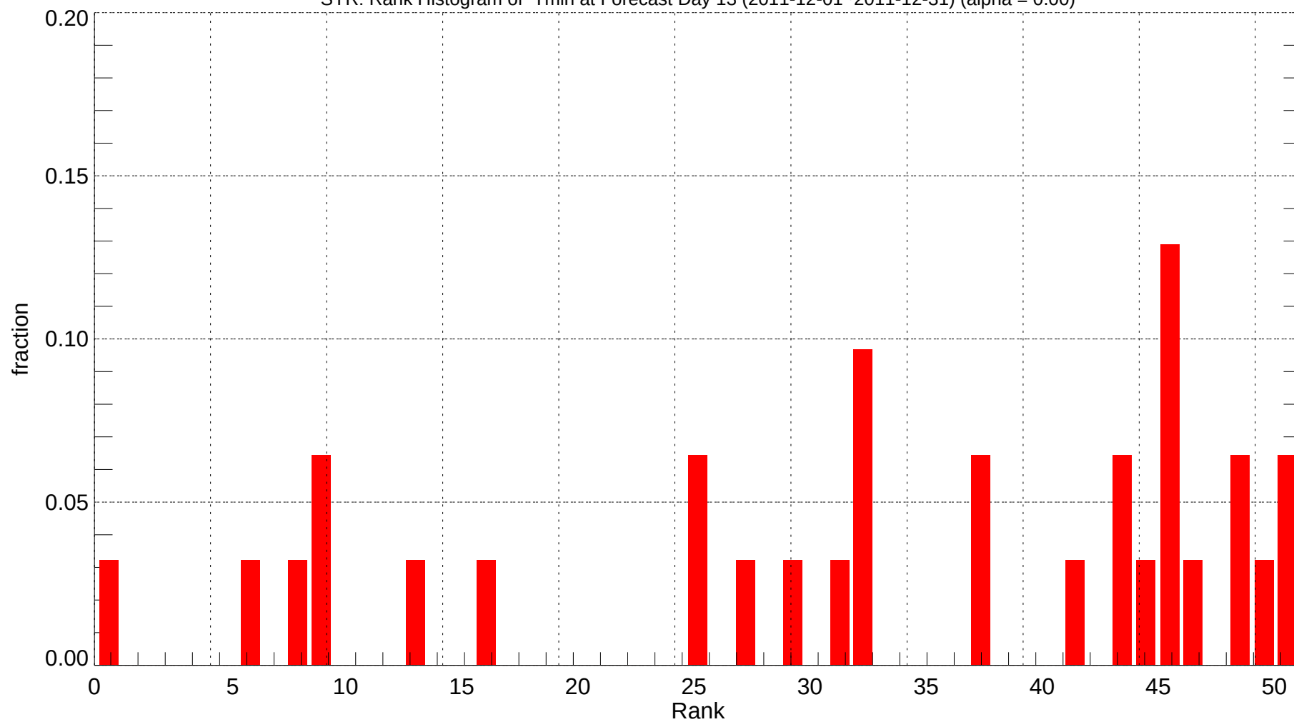
SYR: Rank Histogram of Tmin at Forecast Day 13 (2011-12-01~2011-12-31) (alpha = 0.00)
