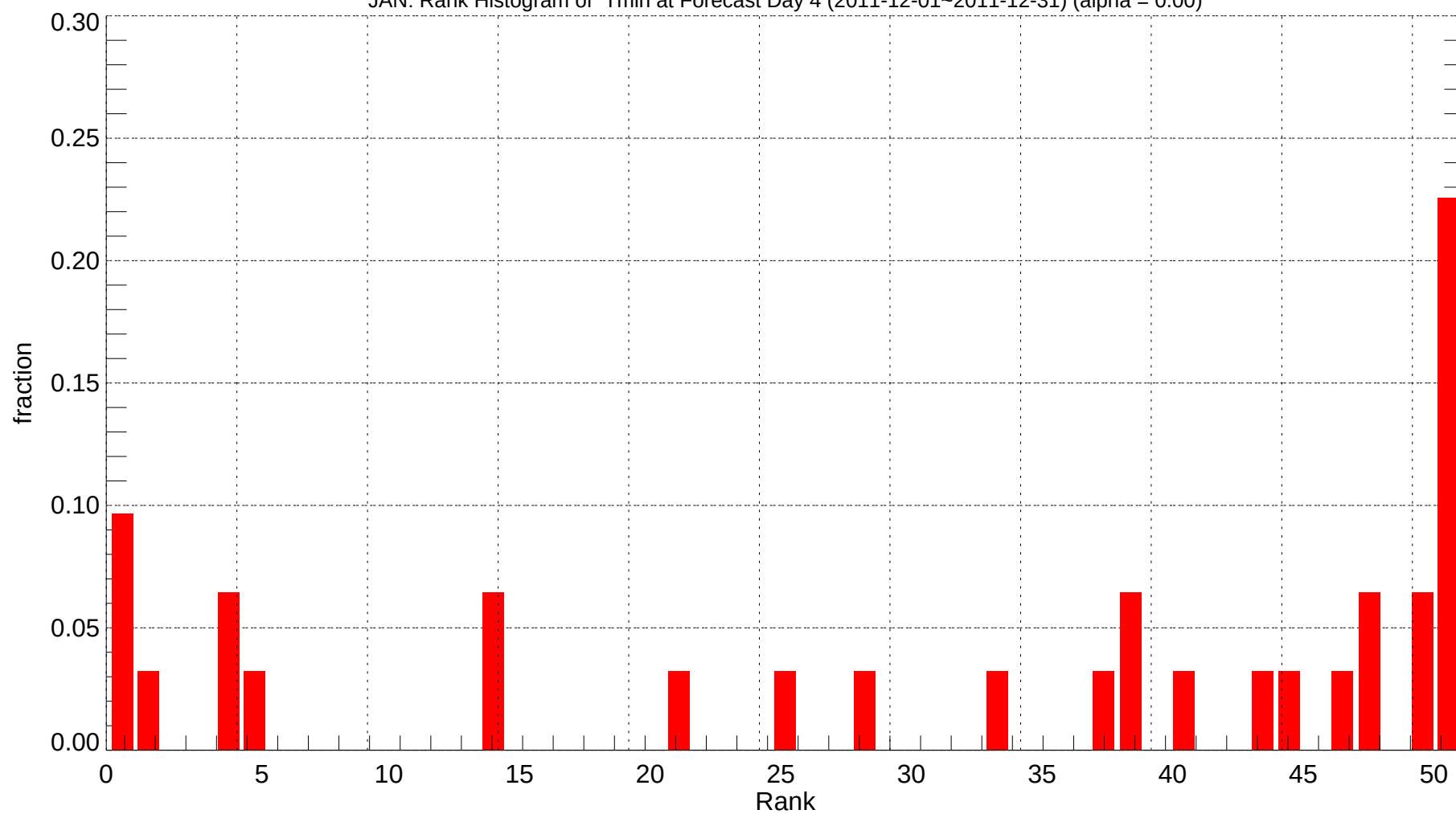
JAN: Rank Histogram of Tmin at Forecast Day 4 (2011-12-01~2011-12-31) (alpha = 0.00)
