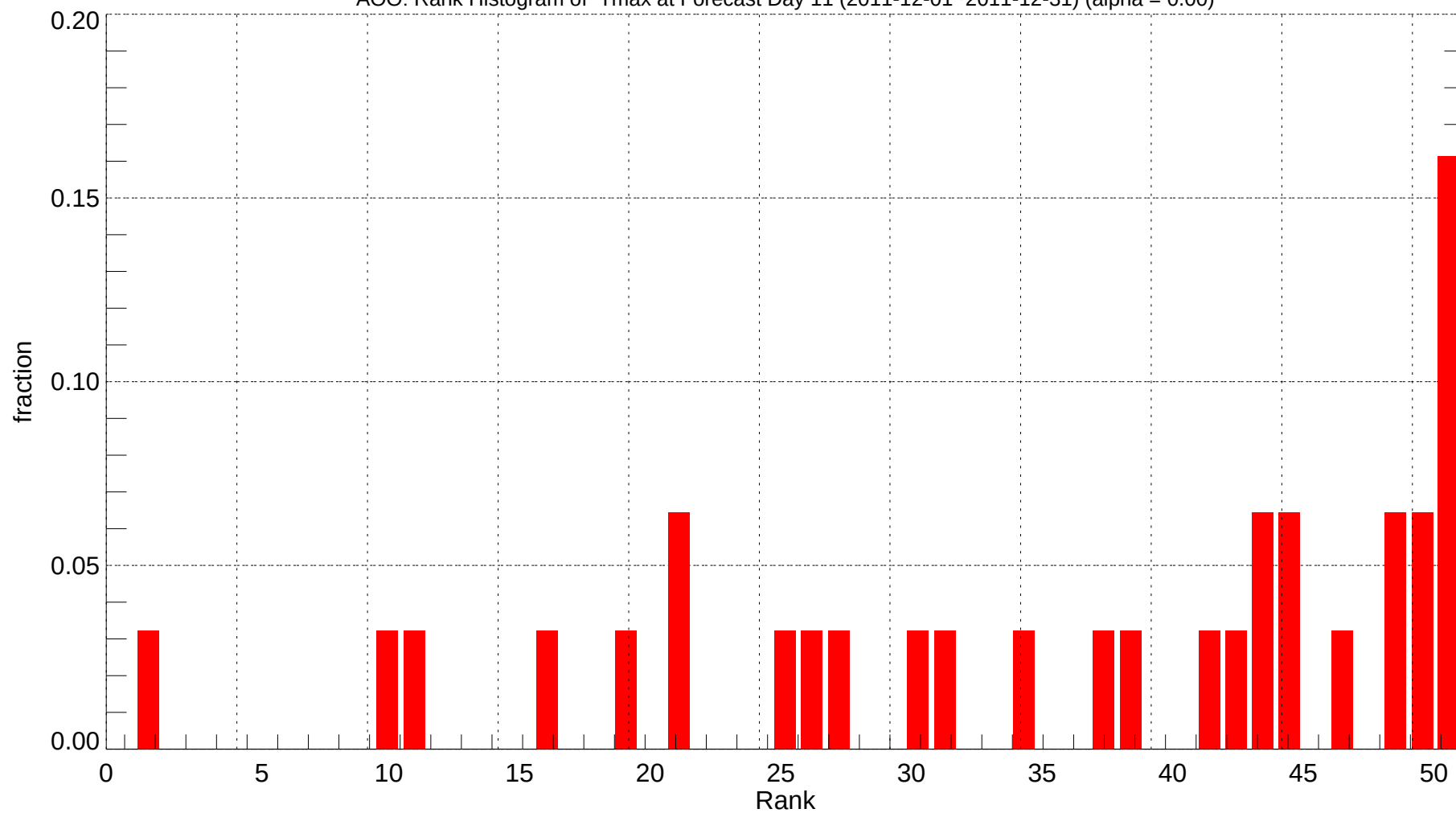
AOO: Rank Histogram of Tmax at Forecast Day 11 (2011-12-01~2011-12-31) (alpha = 0.00)
