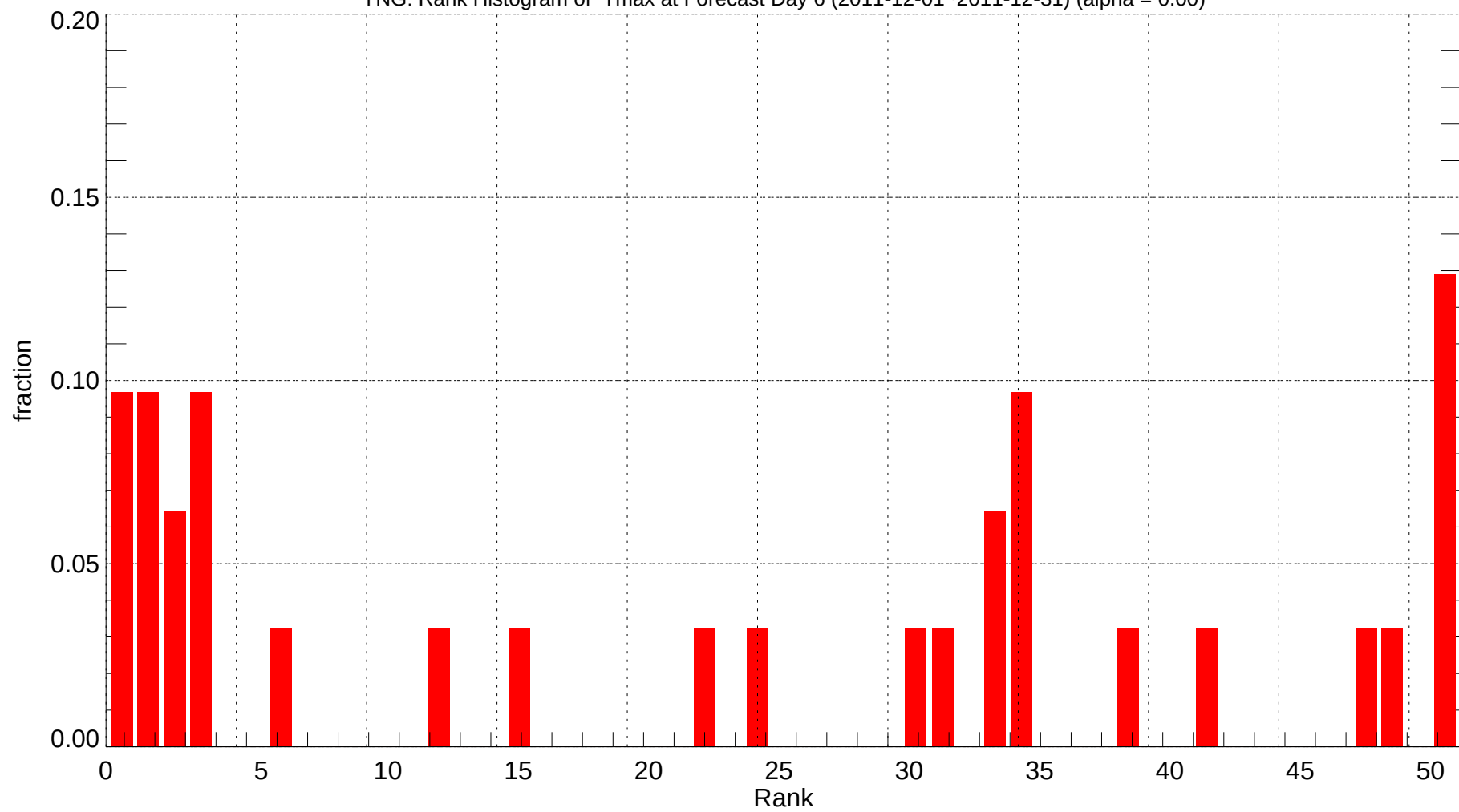
YNG: Rank Histogram of Tmax at Forecast Day 6 (2011-12-01~2011-12-31) (alpha = 0.00)
