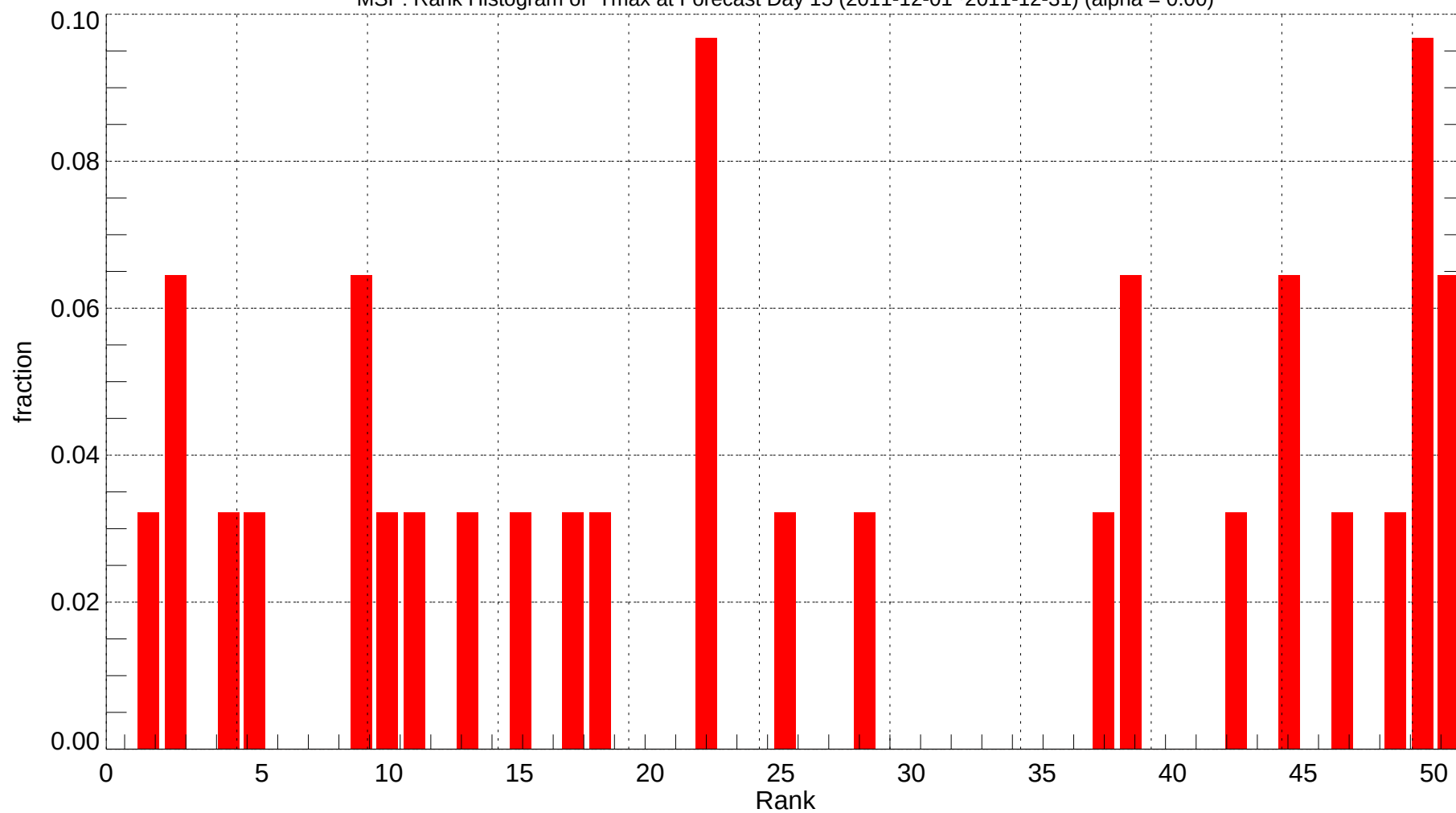
MSP: Rank Histogram of Tmax at Forecast Day 15 (2011-12-01~2011-12-31) (alpha = 0.00)
