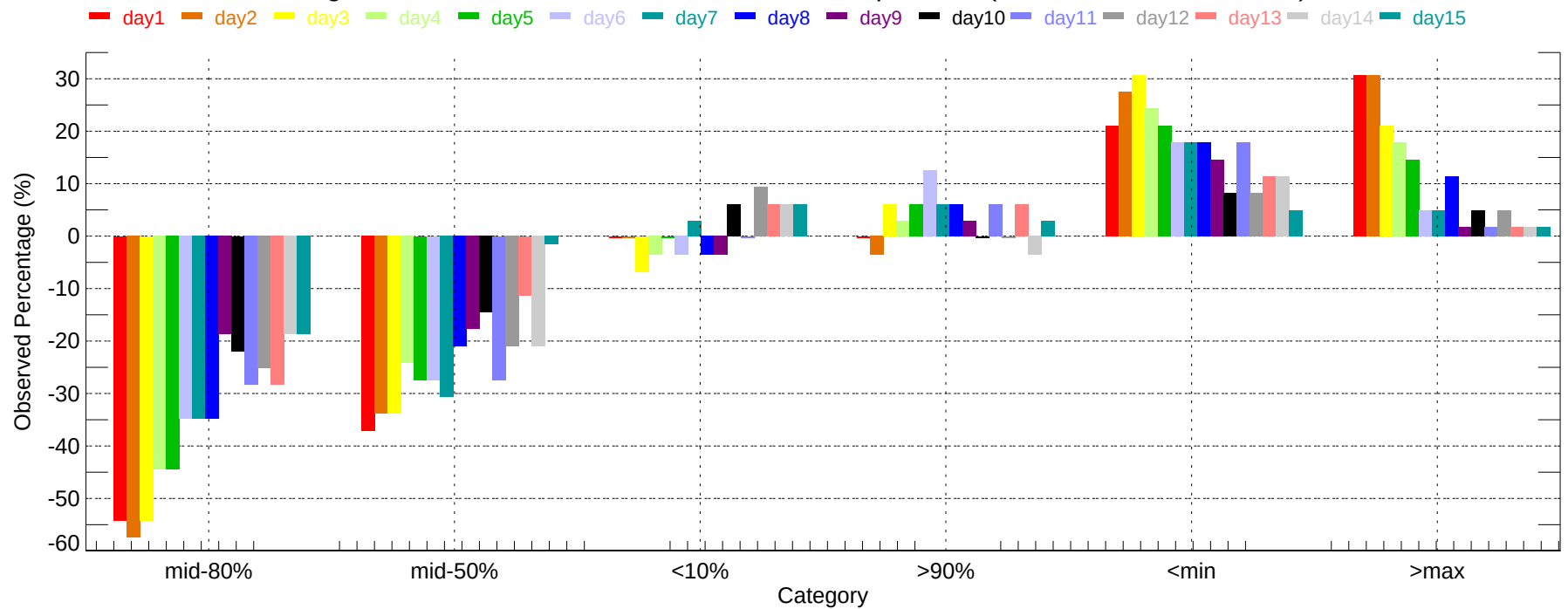
Observed Percentage Deviation of Ensembles - YKM: Max Temperature (2011-12-01~2011-12-31)
