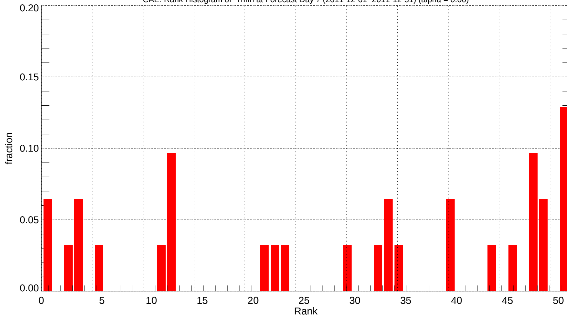
CAE: Rank Histogram of Tmin at Forecast Day 7 (2011-12-01~2011-12-31) (alpha = 0.00)
