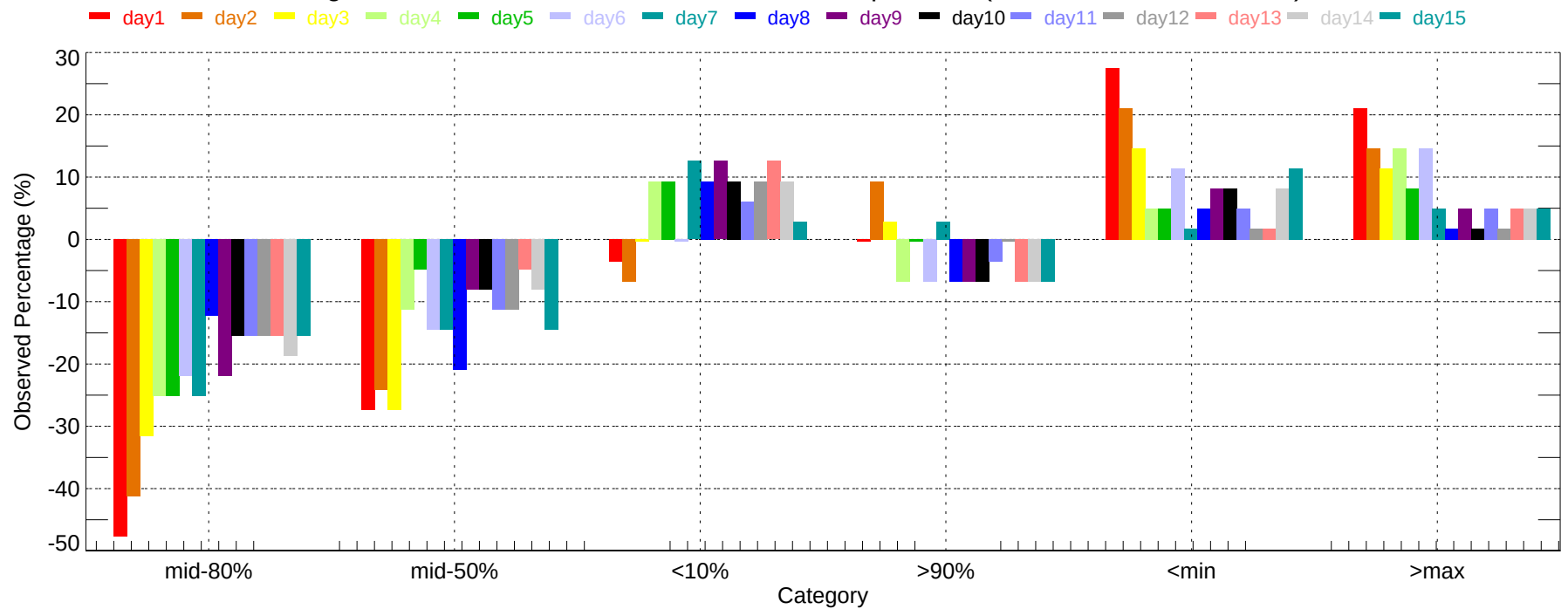
Observed Percentage Deviation of Ensembles - TUS: Max Temperature (2011-12-01~2011-12-31)
