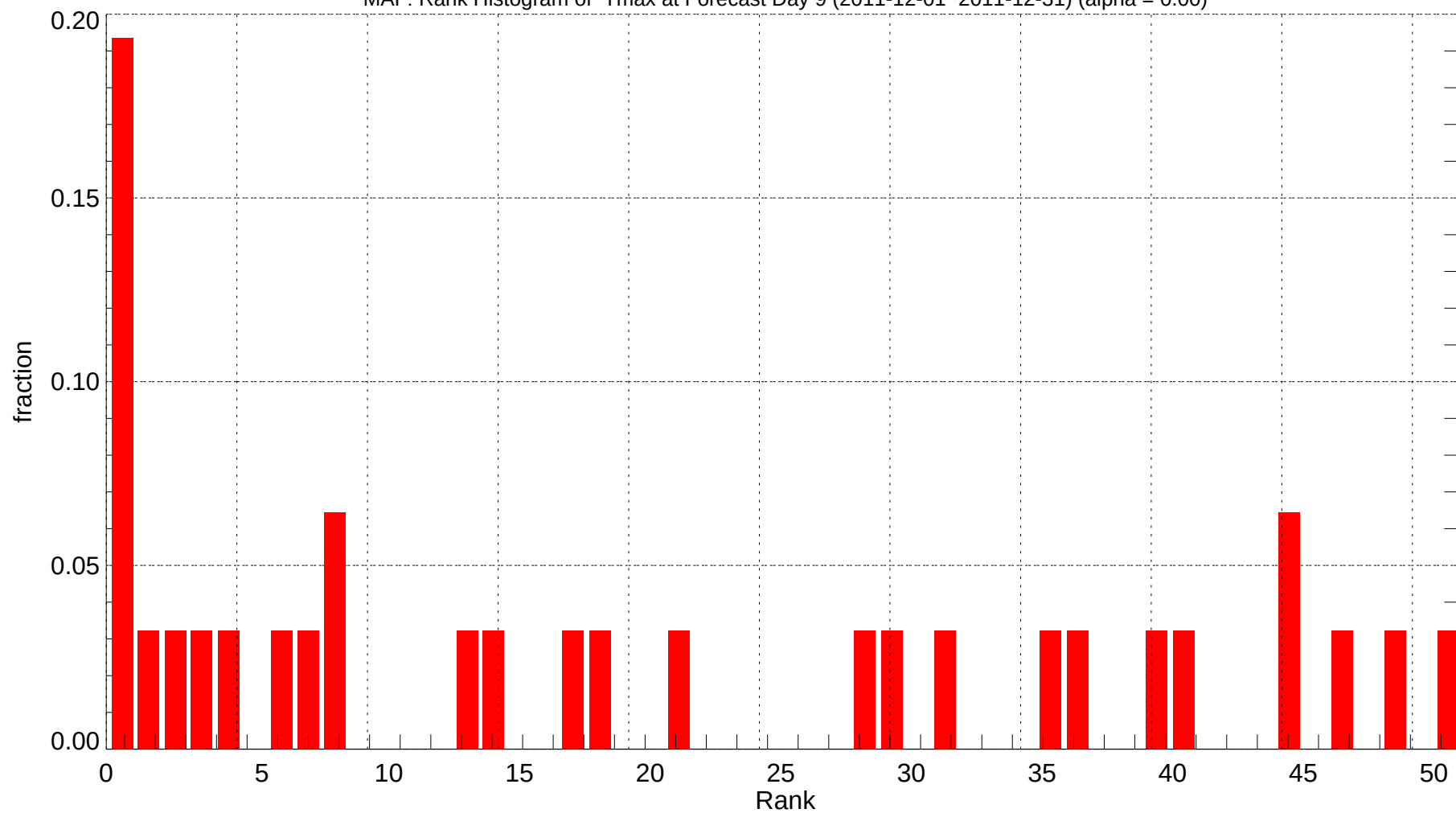
MAF: Rank Histogram of Tmax at Forecast Day 9 (2011-12-01~2011-12-31) (alpha = 0.00)
