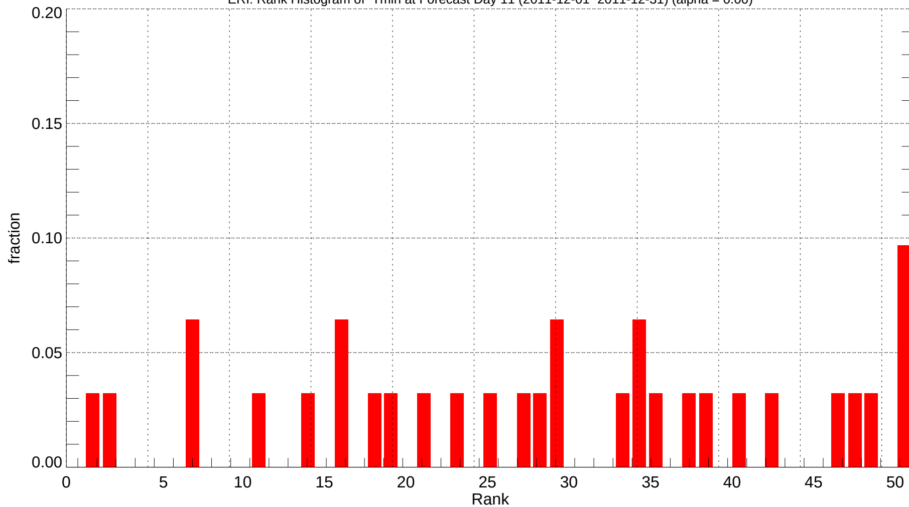
ERI: Rank Histogram of Tmin at Forecast Day 11 (2011-12-01~2011-12-31) (alpha = 0.00)
