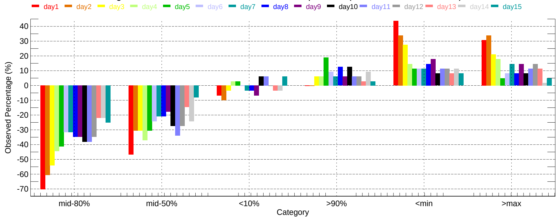
Observed Percentage Deviation of Ensembles - DEN: Min Temperature (2011-12-01~2011-12-31)
