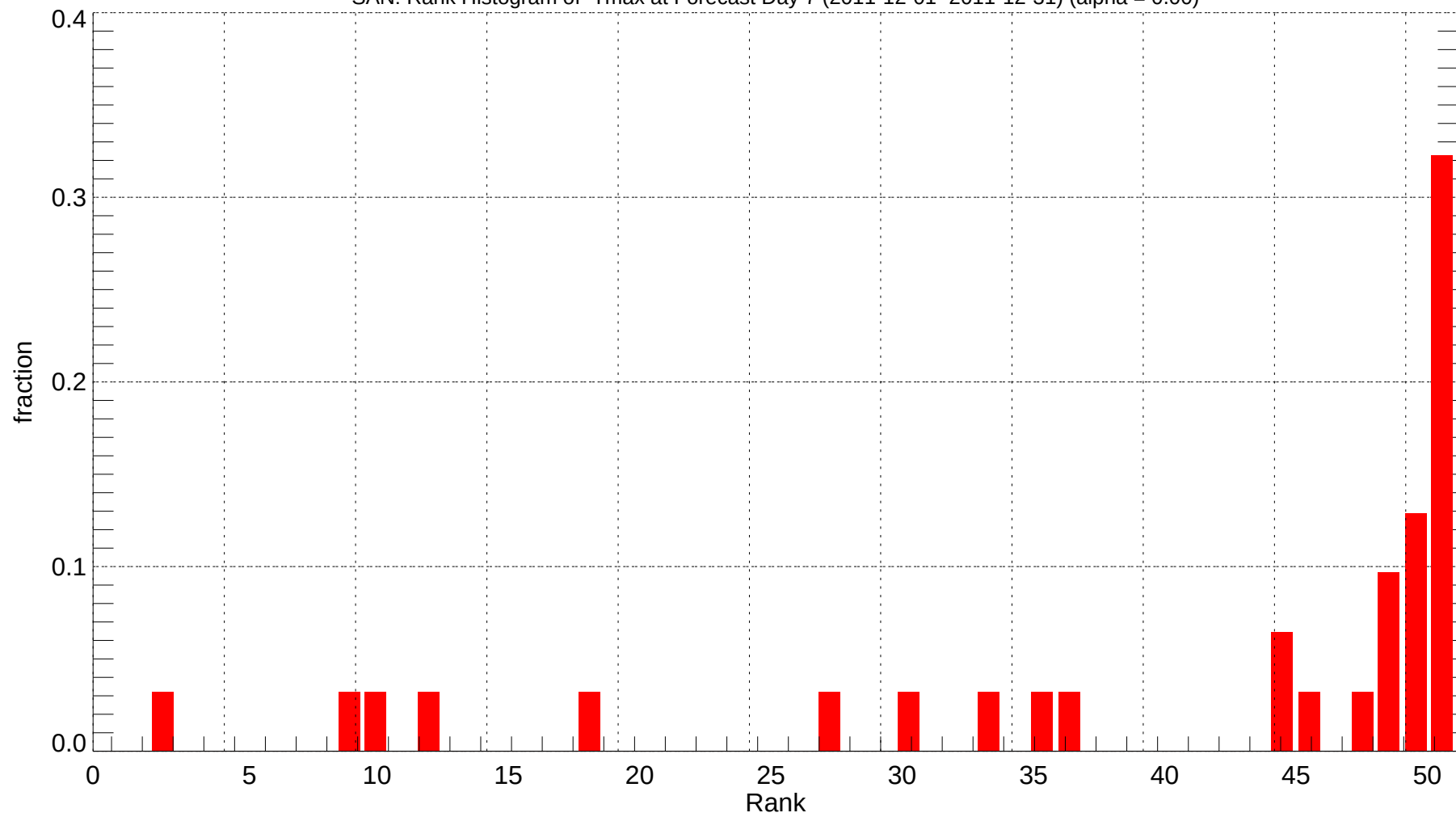
SAN: Rank Histogram of Tmax at Forecast Day 7 (2011-12-01~2011-12-31) (alpha = 0.00)
