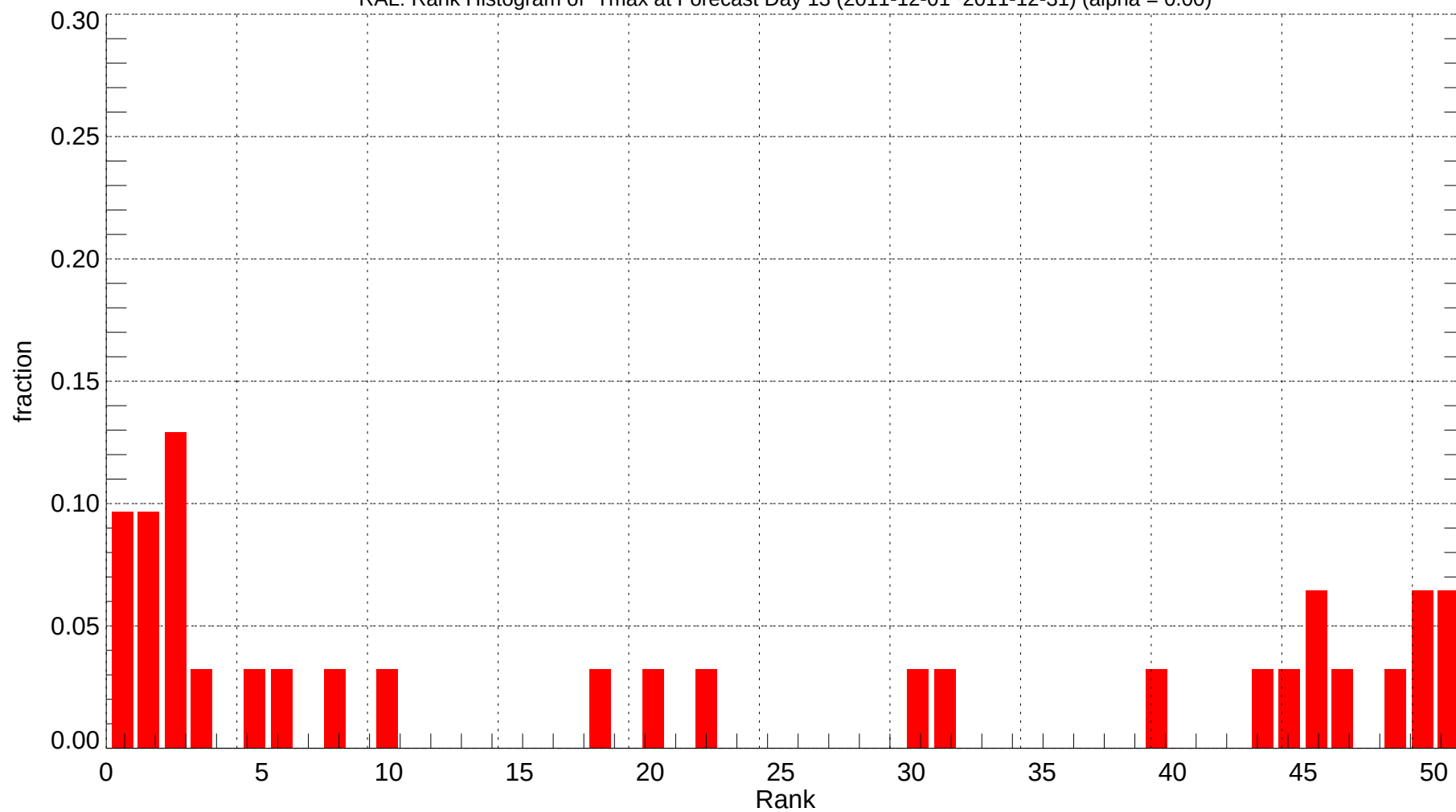
RAL: Rank Histogram of Tmax at Forecast Day 13 (2011-12-01~2011-12-31) (alpha = 0.00)
