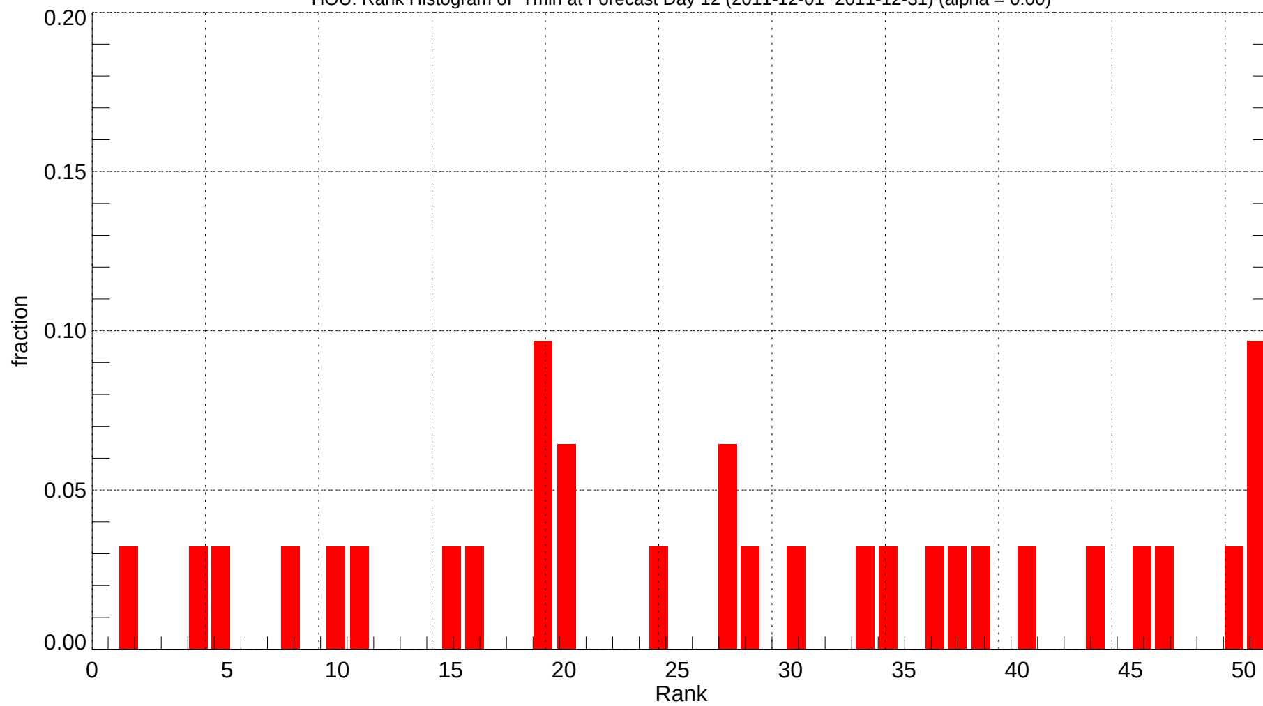
HOU: Rank Histogram of Tmin at Forecast Day 12 (2011-12-01~2011-12-31) (alpha = 0.00)
