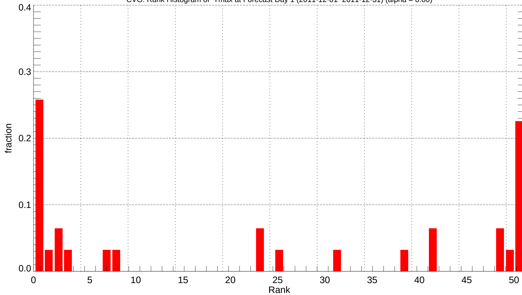
CVG: Rank Histogram of Tmax at Forecast Day 1 (2011-12-01~2011-12-31) (alpha = 0.00)
