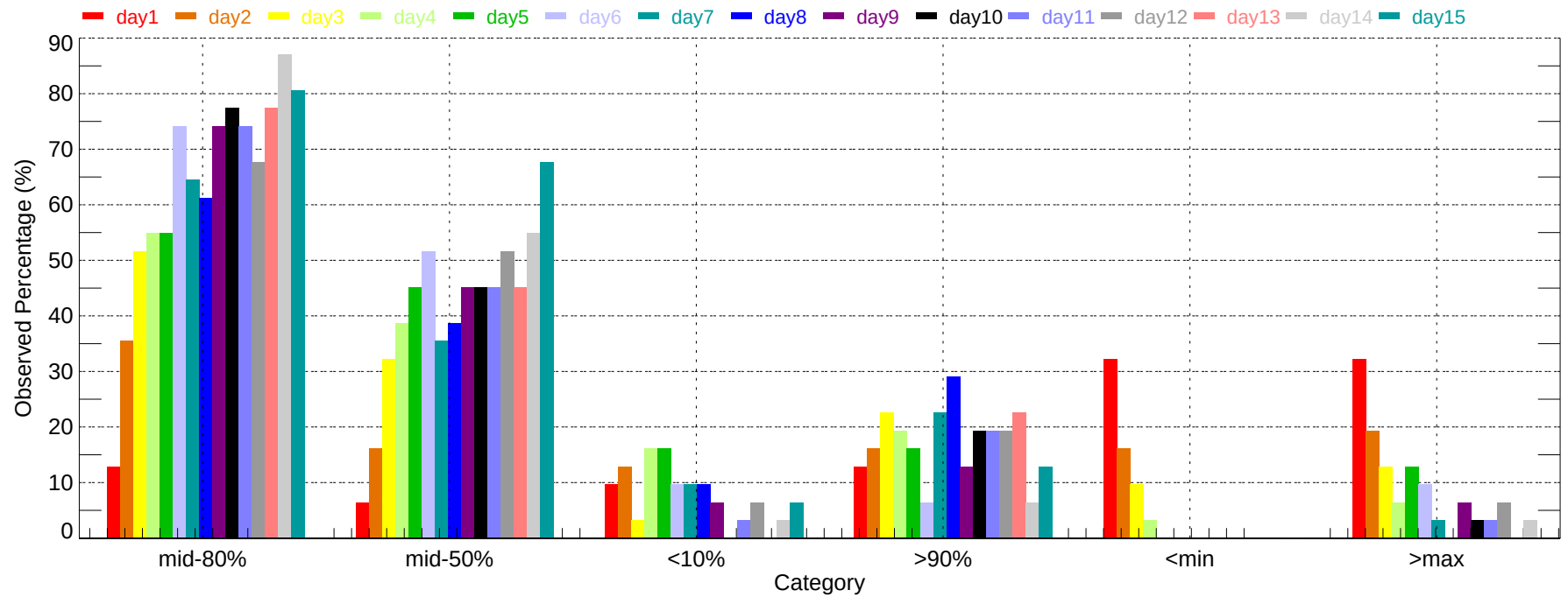
Observed Percentage of Ensembles - SAV: Min Temperature (2011-12-01~2011-12-31)
