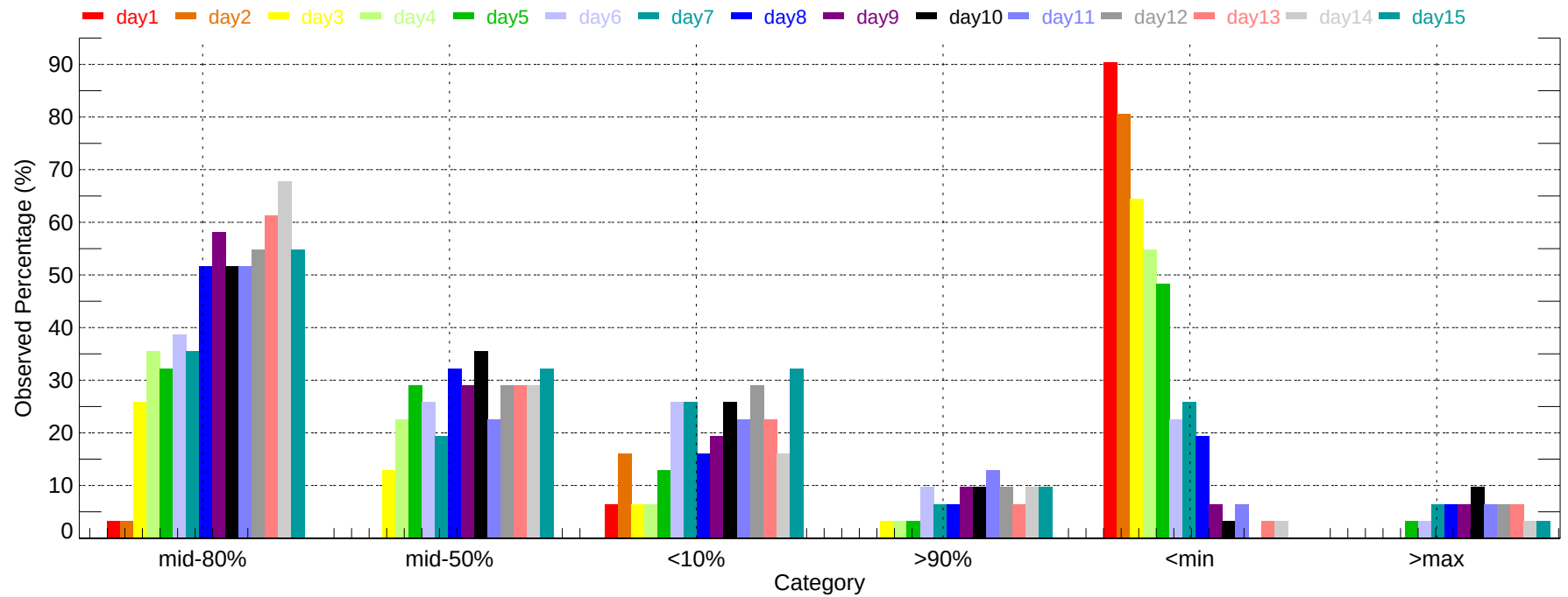
Observed Percentage of Ensembles - JFK: Min Temperature (2011-12-01~2011-12-31)
