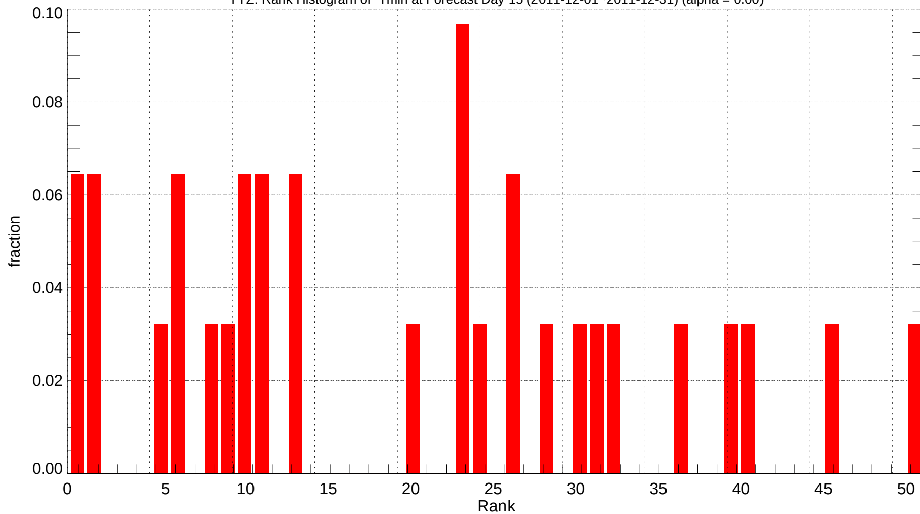
YYZ: Rank Histogram of Tmin at Forecast Day 15 (2011-12-01~2011-12-31) (alpha = 0.00)
