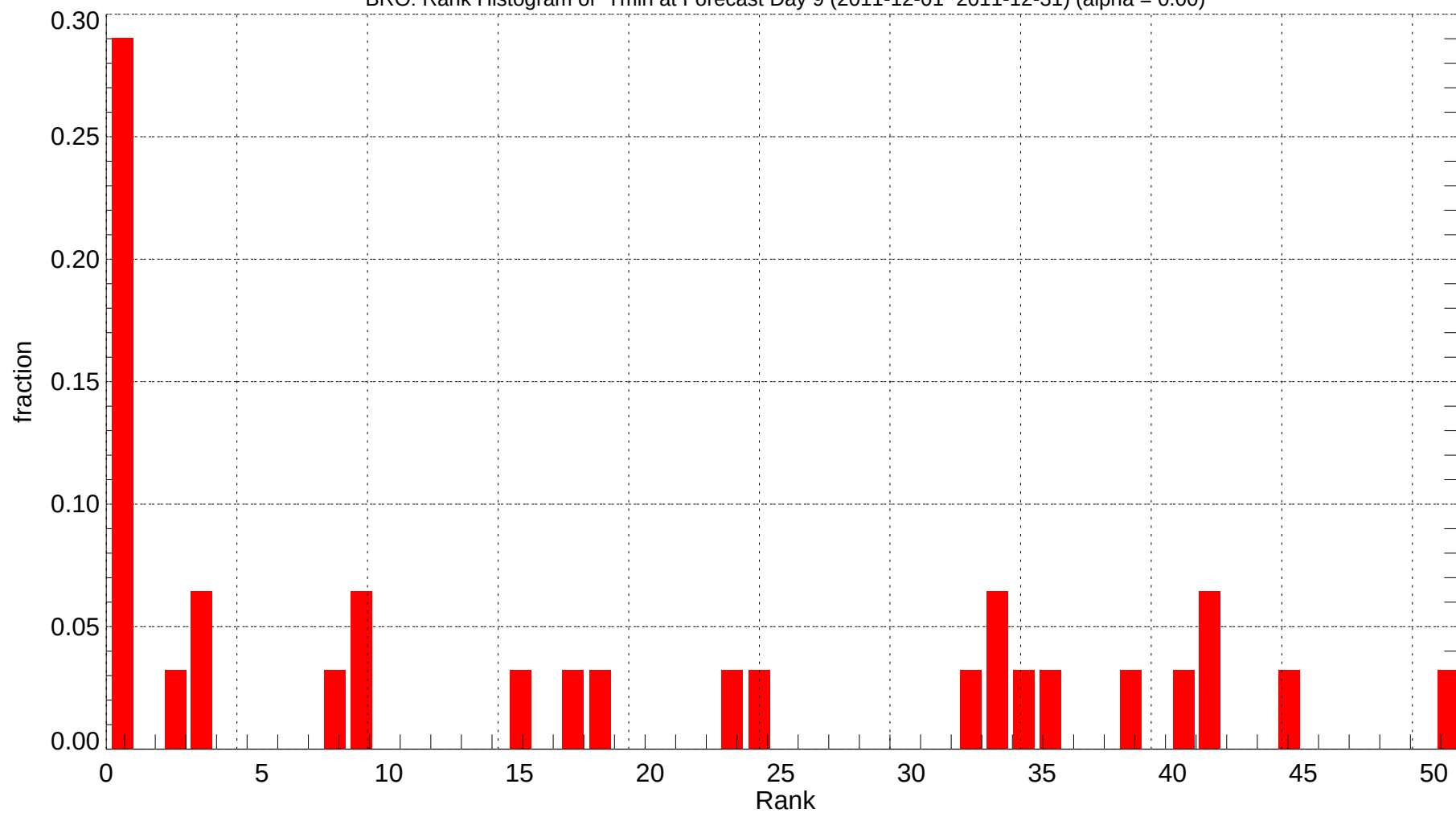
BRO: Rank Histogram of Tmin at Forecast Day 9 (2011-12-01~2011-12-31) (alpha = 0.00)
