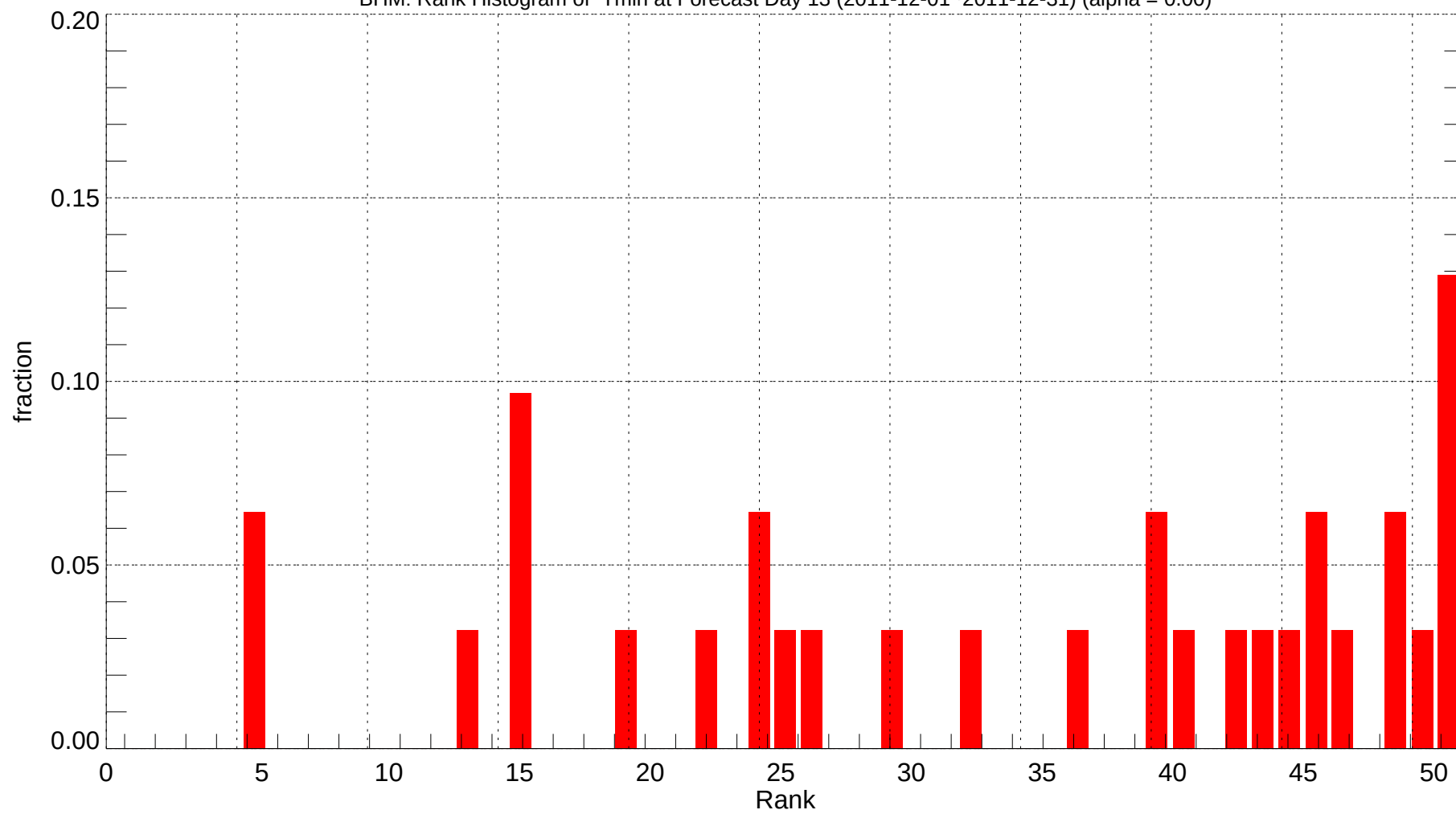
BHM: Rank Histogram of Tmin at Forecast Day 13 (2011-12-01~2011-12-31) (alpha = 0.00)
