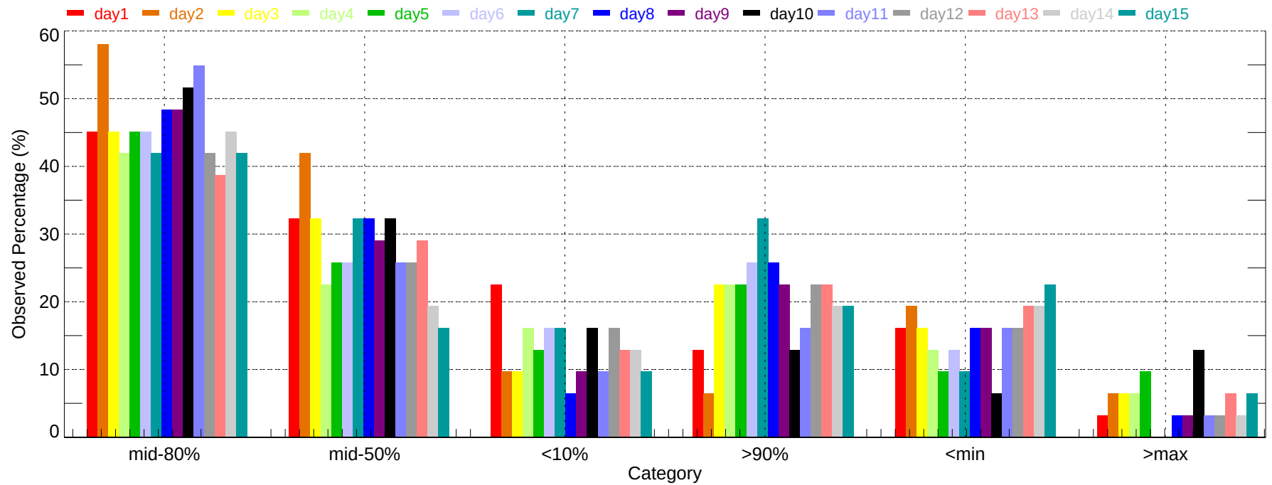
Observed Percentage of Ensembles - ACT: Max Temperature (2011-12-01~2011-12-31)
