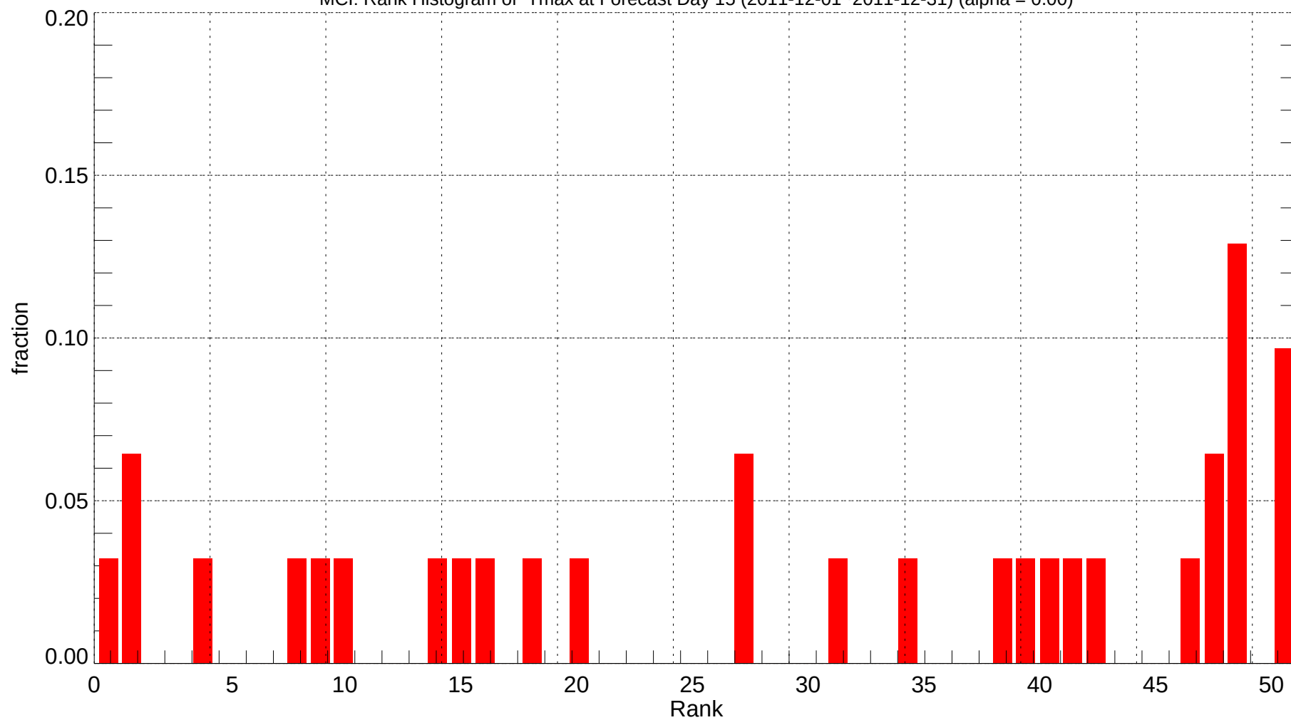
MCI: Rank Histogram of Tmax at Forecast Day 15 (2011-12-01~2011-12-31) (alpha = 0.00)
