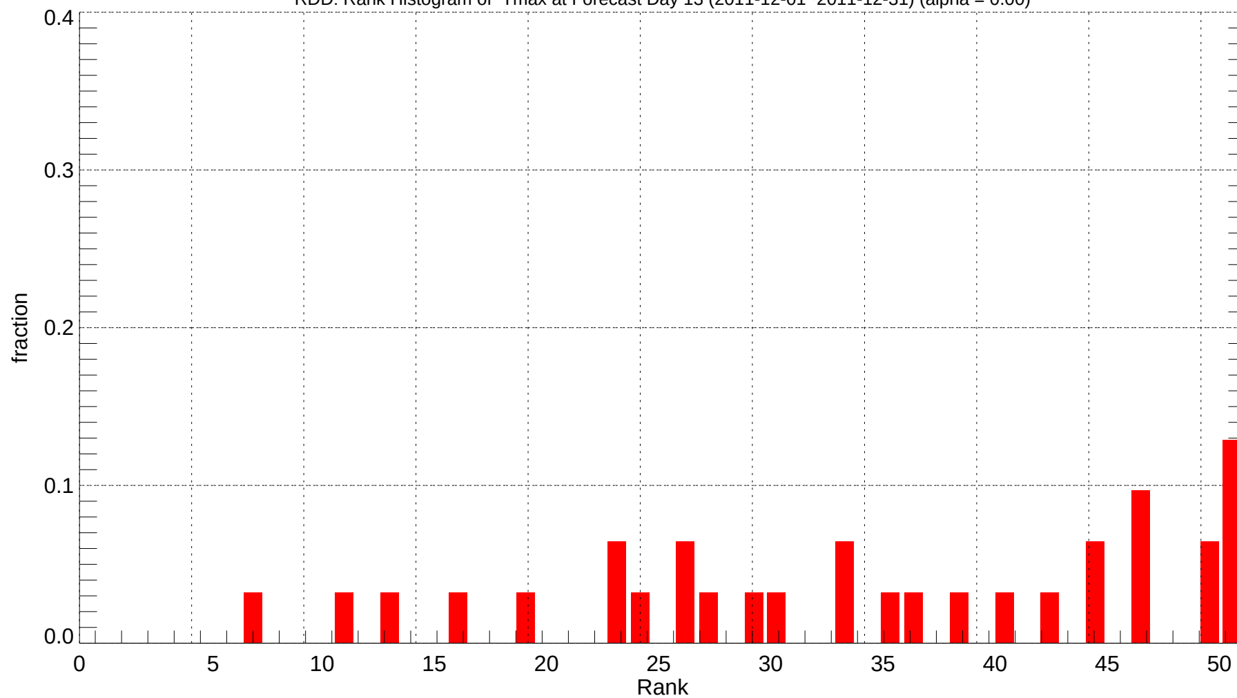
RDD: Rank Histogram of Tmax at Forecast Day 13 (2011-12-01~2011-12-31) (alpha = 0.00)
