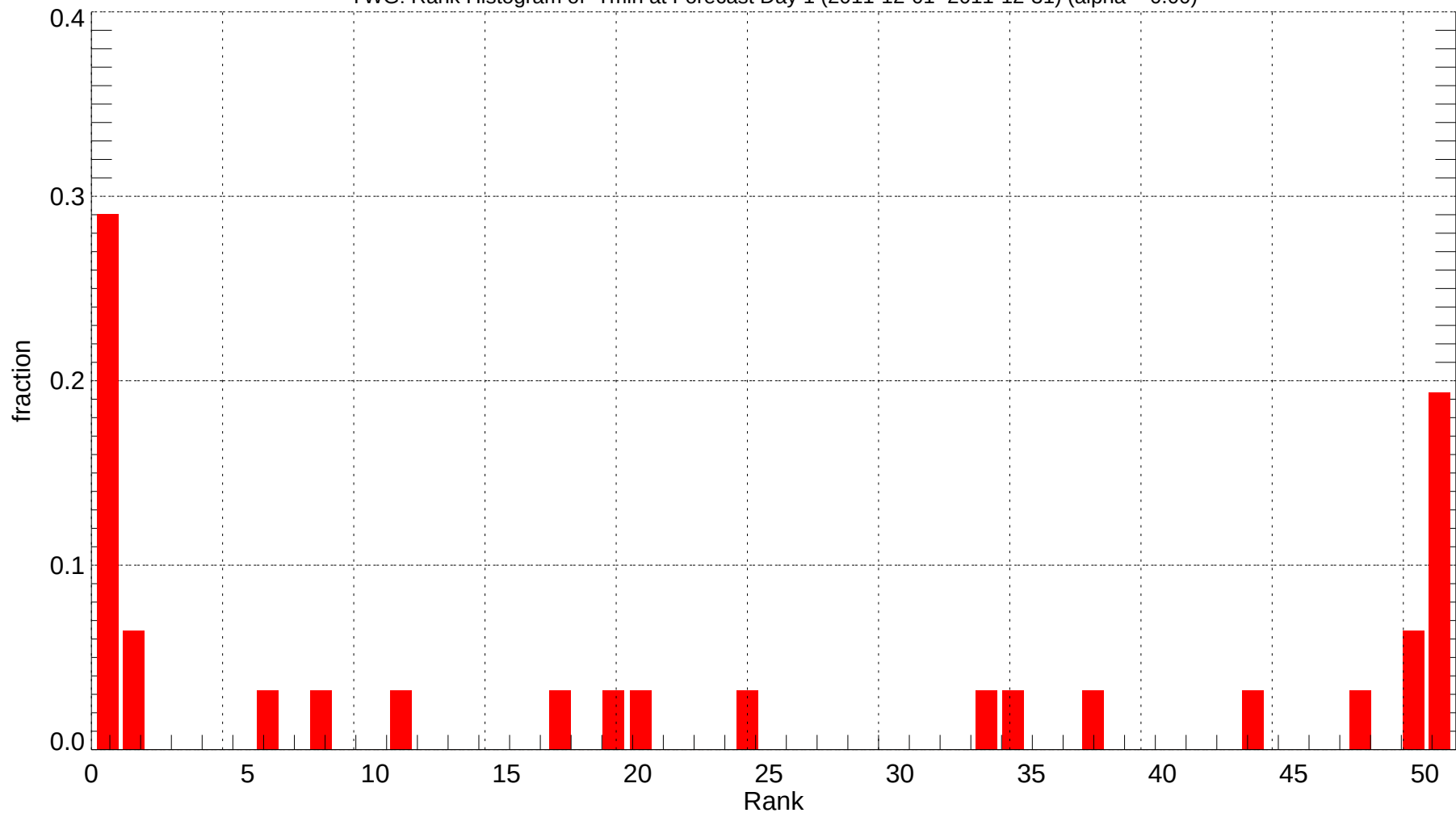
YWG: Rank Histogram of Tmin at Forecast Day 1 (2011-12-01~2011-12-31) (alpha = 0.00)
