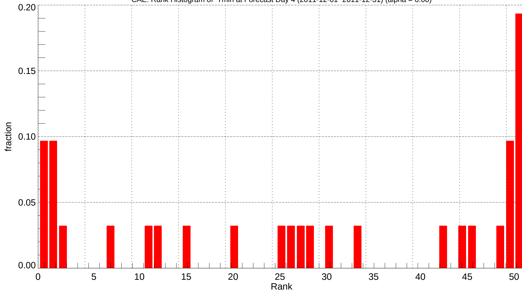
CAE: Rank Histogram of Tmin at Forecast Day 4 (2011-12-01~2011-12-31) (alpha = 0.00)
