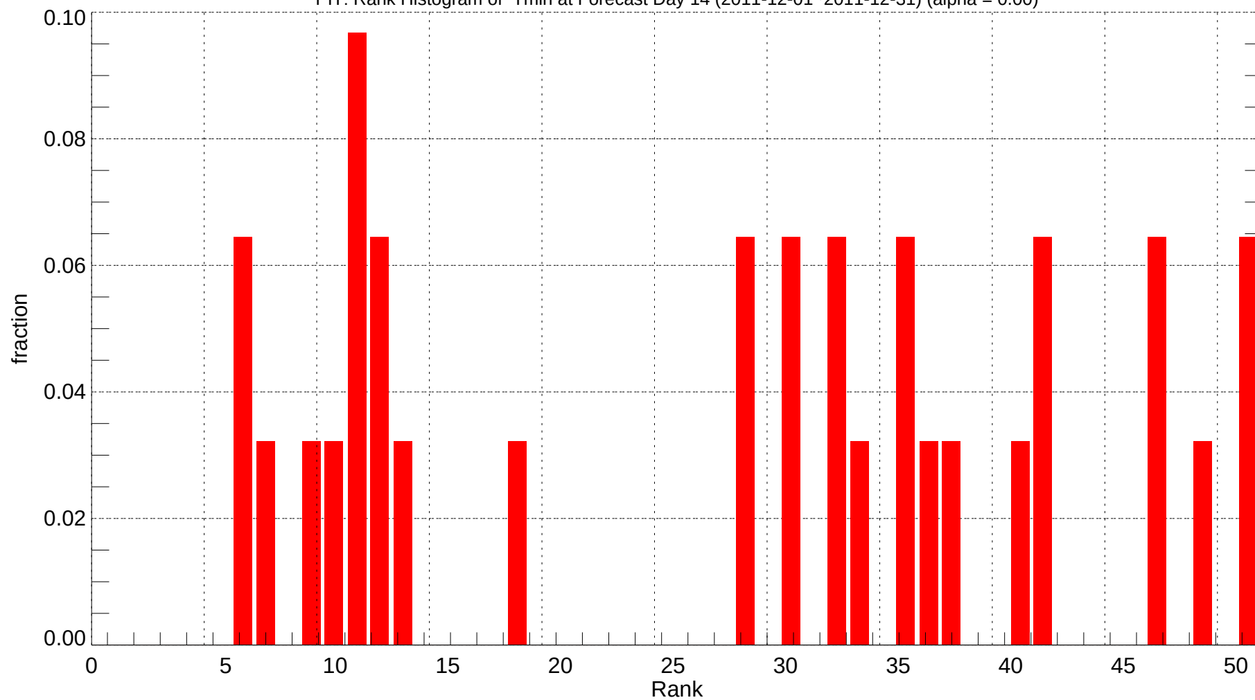
PIT: Rank Histogram of Tmin at Forecast Day 14 (2011-12-01~2011-12-31) (alpha = 0.00)
