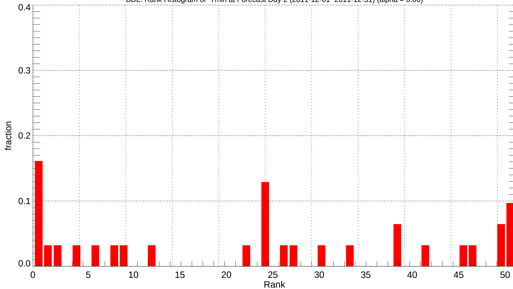
BDL: Rank Histogram of Tmin at Forecast Day 2 (2011-12-01~2011-12-31) (alpha = 0.00)
