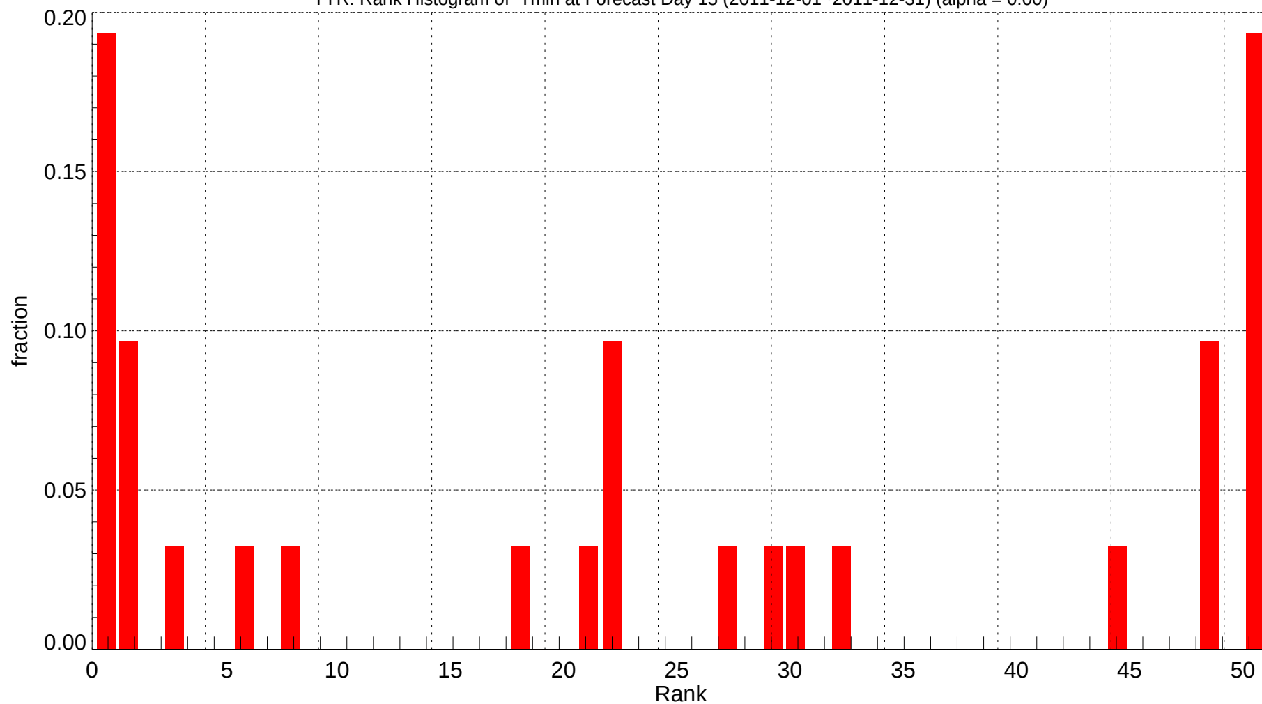
TYR: Rank Histogram of Tmin at Forecast Day 15 (2011-12-01~2011-12-31) (alpha = 0.00)
