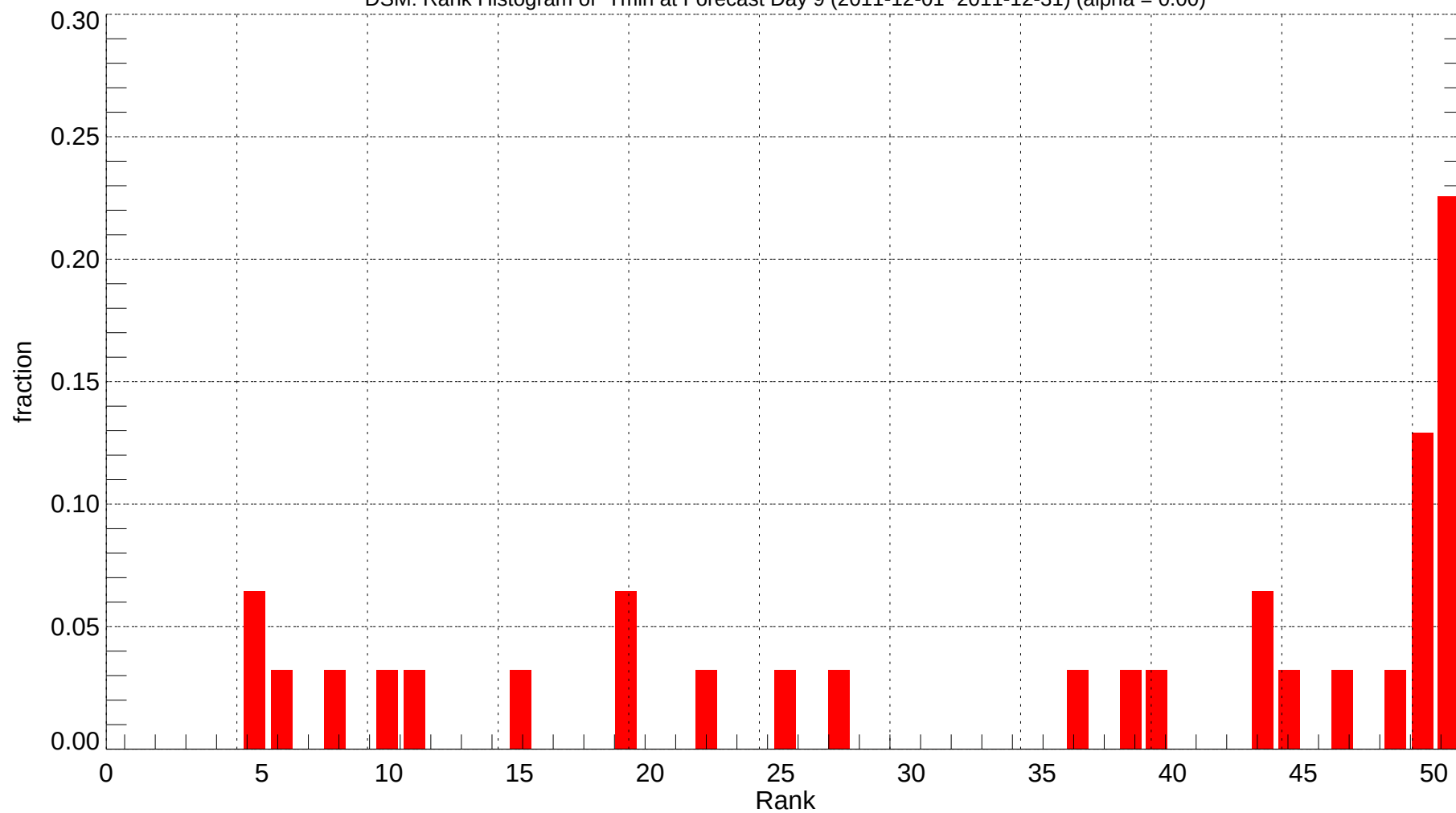
DSM: Rank Histogram of Tmin at Forecast Day 9 (2011-12-01~2011-12-31) (alpha = 0.00)
