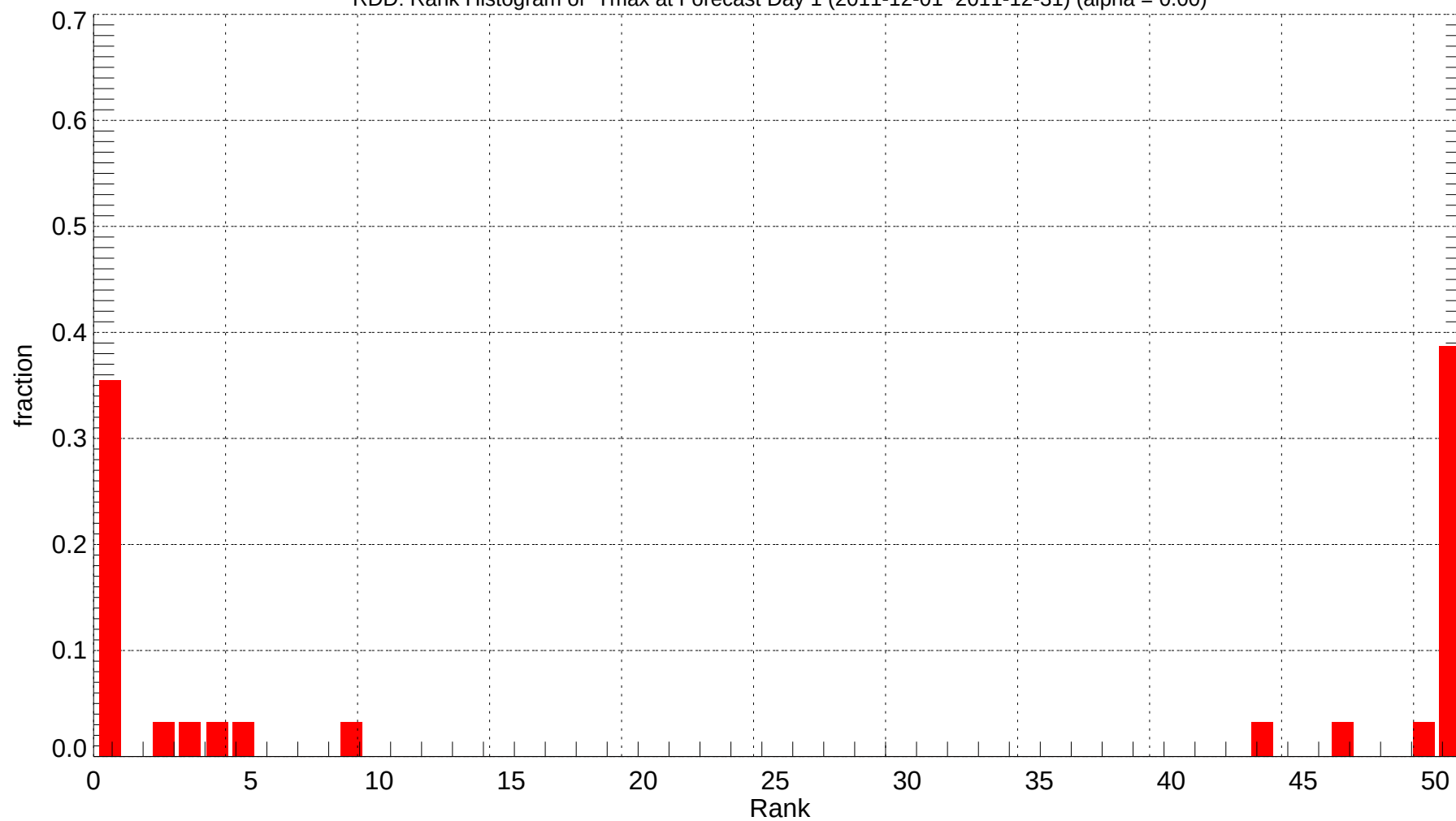
RDD: Rank Histogram of Tmax at Forecast Day 1 (2011-12-01~2011-12-31) (alpha = 0.00)
