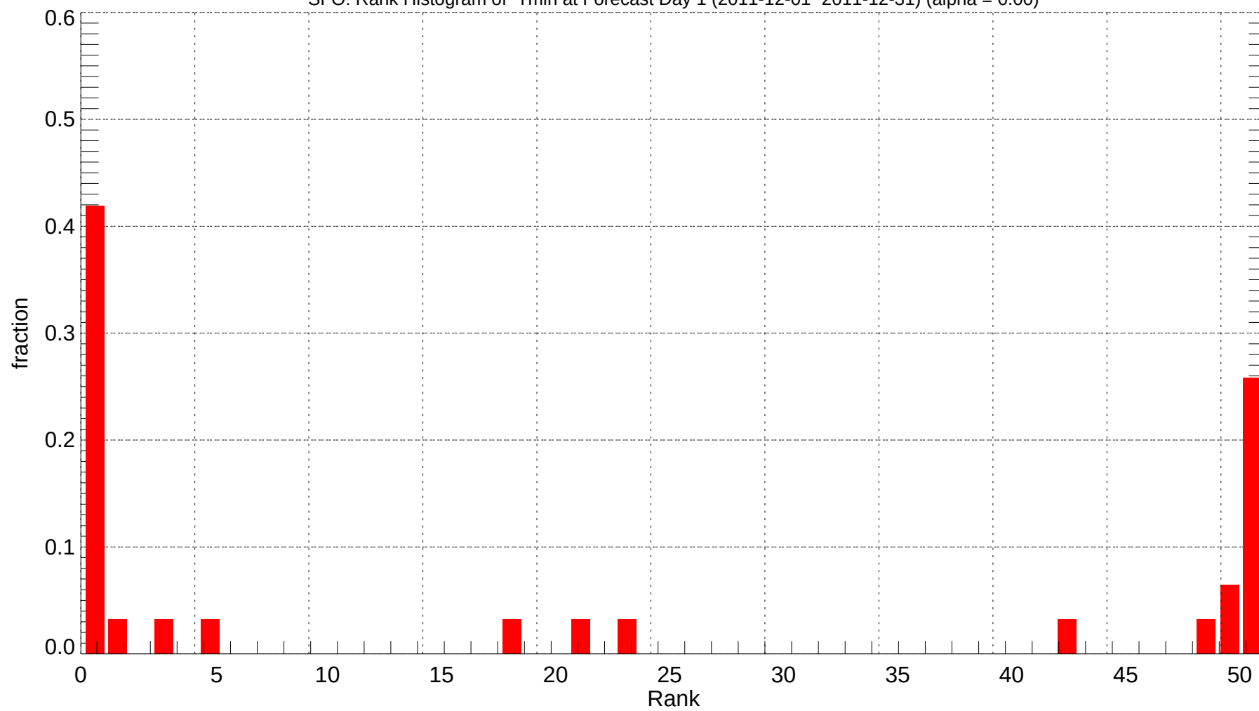
SFO: Rank Histogram of Tmin at Forecast Day 1 (2011-12-01~2011-12-31) (alpha = 0.00)
