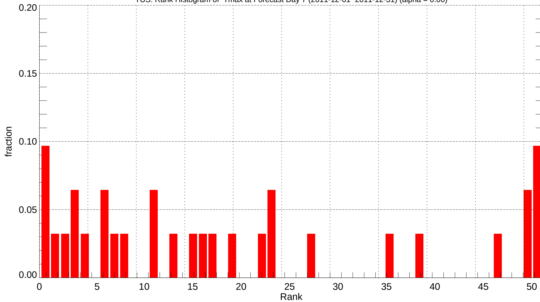
TUS: Rank Histogram of Tmax at Forecast Day 7 (2011-12-01~2011-12-31) (alpha = 0.00)
