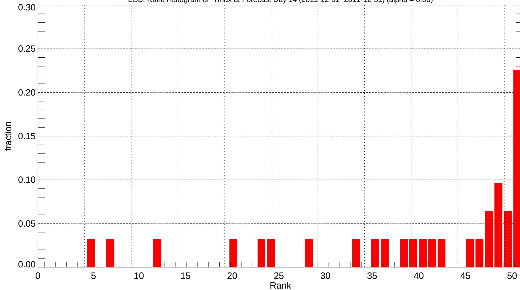
LGB: Rank Histogram of Tmax at Forecast Day 14 (2011-12-01~2011-12-31) (alpha = 0.00)
