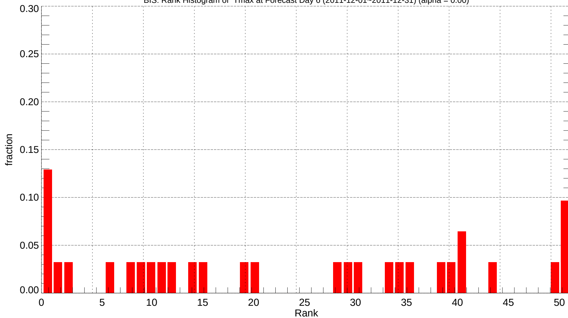
BIS: Rank Histogram of Tmax at Forecast Day 6 (2011-12-01~2011-12-31) (alpha = 0.00)
