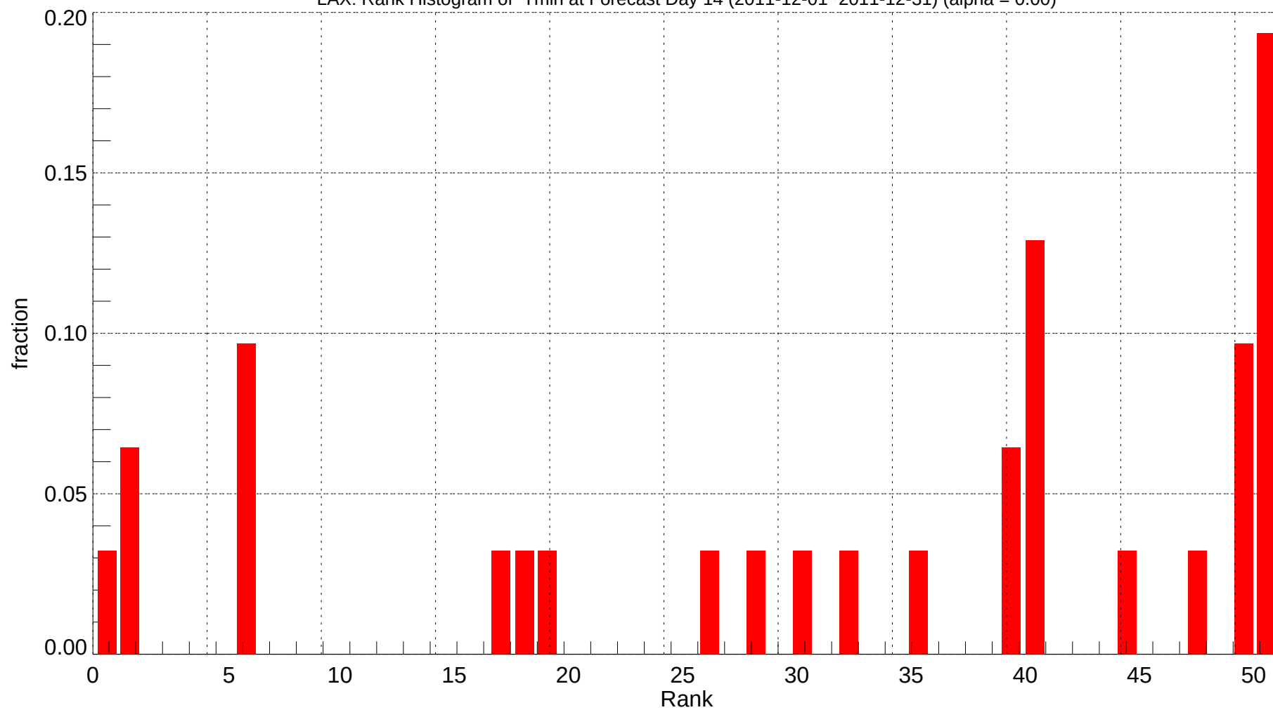
LAX: Rank Histogram of Tmin at Forecast Day 14 (2011-12-01~2011-12-31) (alpha = 0.00)
