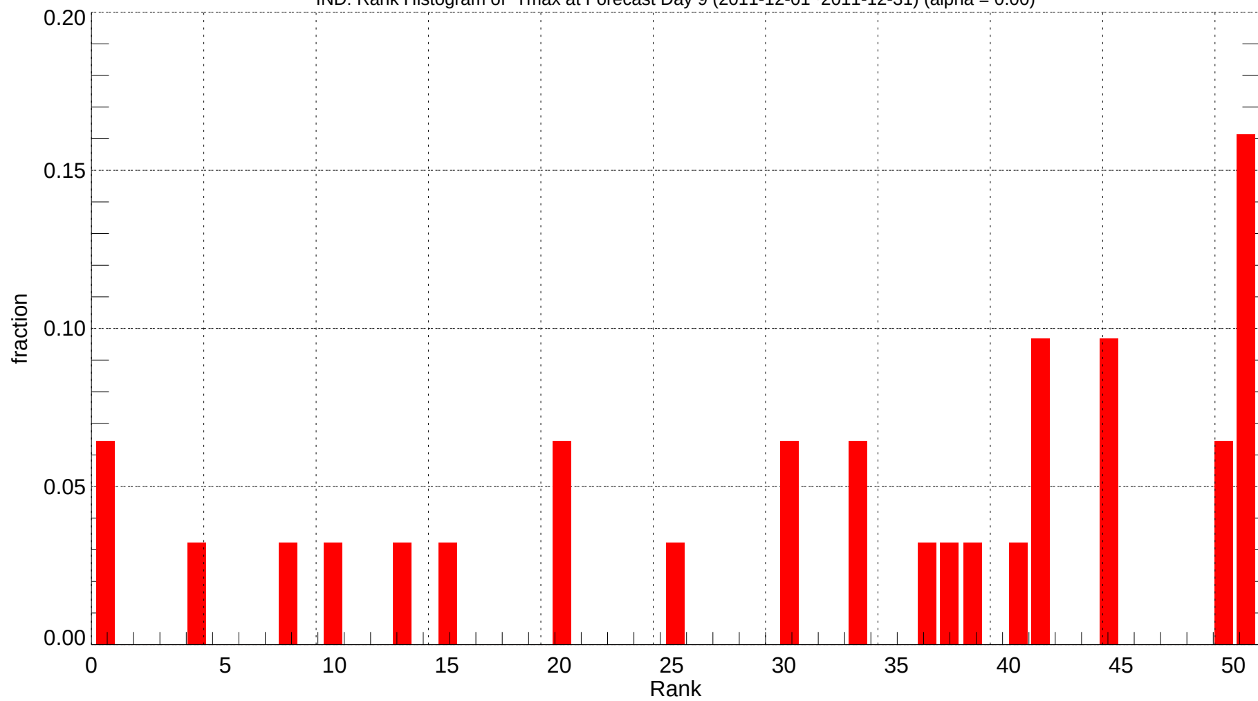
IND: Rank Histogram of Tmax at Forecast Day 9 (2011-12-01~2011-12-31) (alpha = 0.00)
