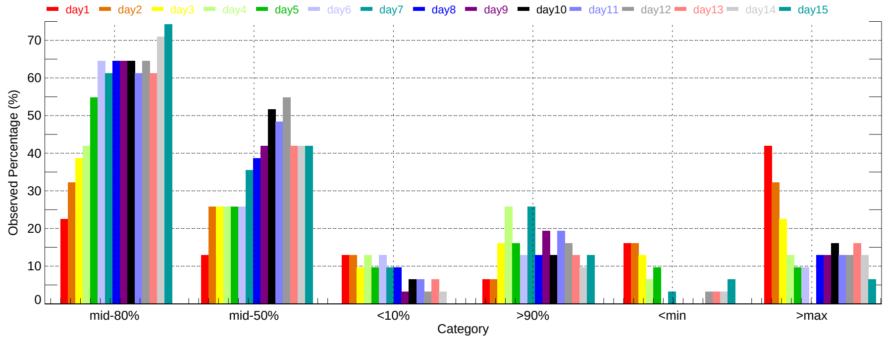
Observed Percentage of Ensembles - JAN: Max Temperature (2011-12-01~2011-12-31)
