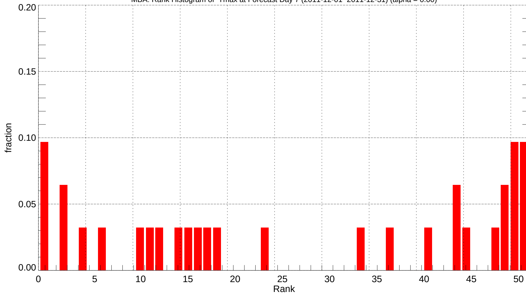
MBA: Rank Histogram of Tmax at Forecast Day 7 (2011-12-01~2011-12-31) (alpha = 0.00)
