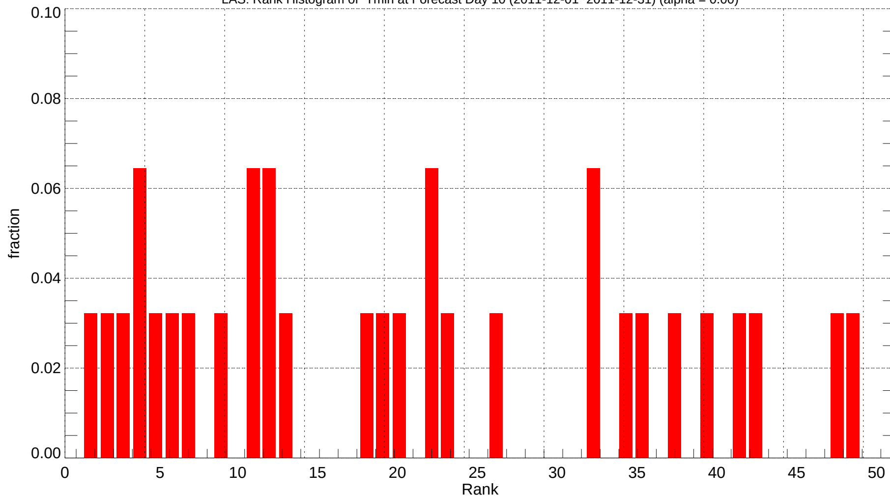
LAS: Rank Histogram of Tmin at Forecast Day 10 (2011-12-01~2011-12-31) (alpha = 0.00)
