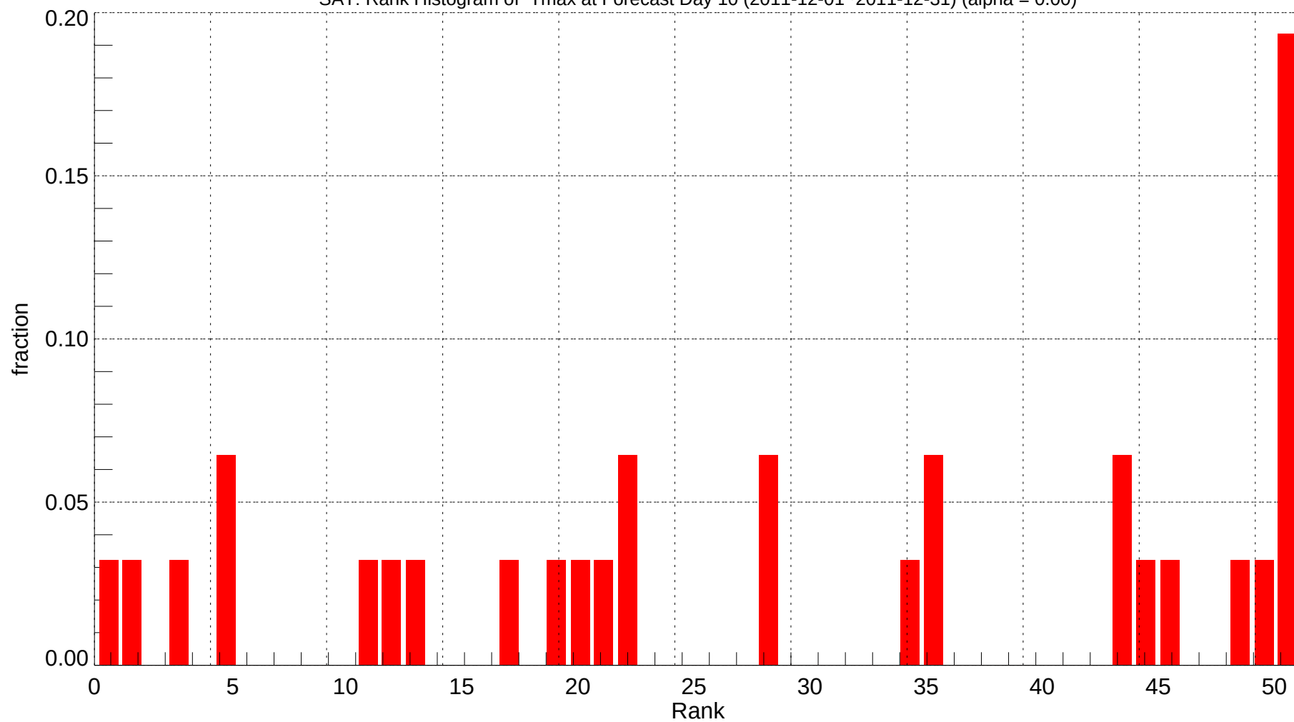
SAT: Rank Histogram of Tmax at Forecast Day 10 (2011-12-01~2011-12-31) (alpha = 0.00)
