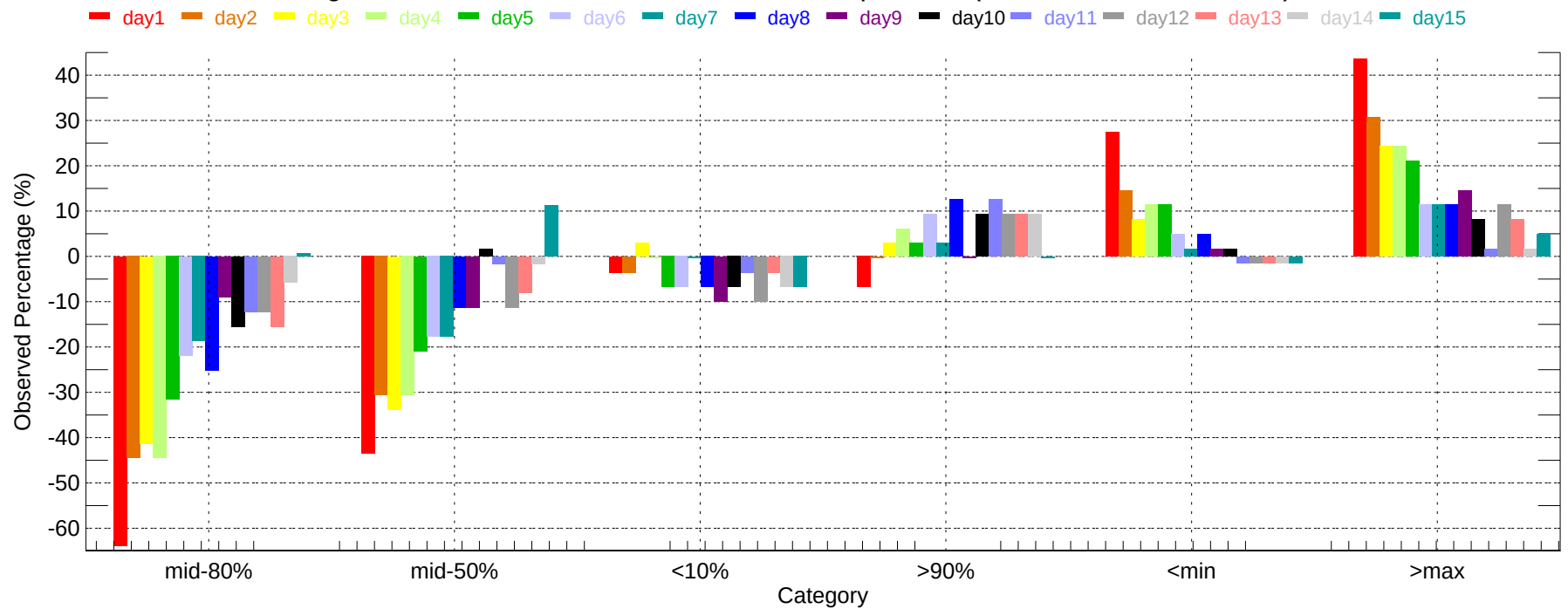
Observed Percentage Deviation of Ensembles - CLT: Min Temperature (2011-12-01~2011-12-31)
