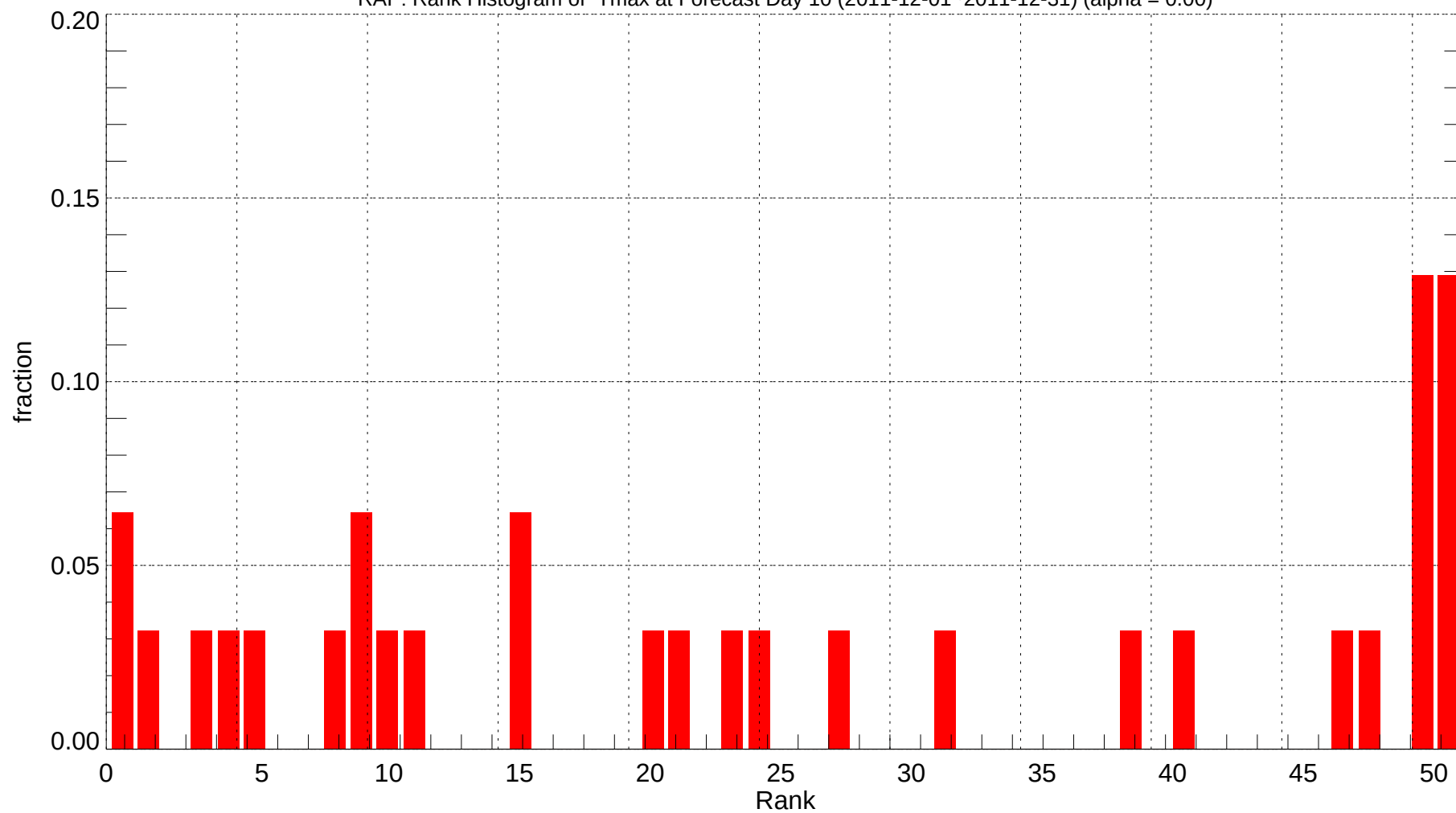
RAP: Rank Histogram of Tmax at Forecast Day 10 (2011-12-01~2011-12-31) (alpha = 0.00)
