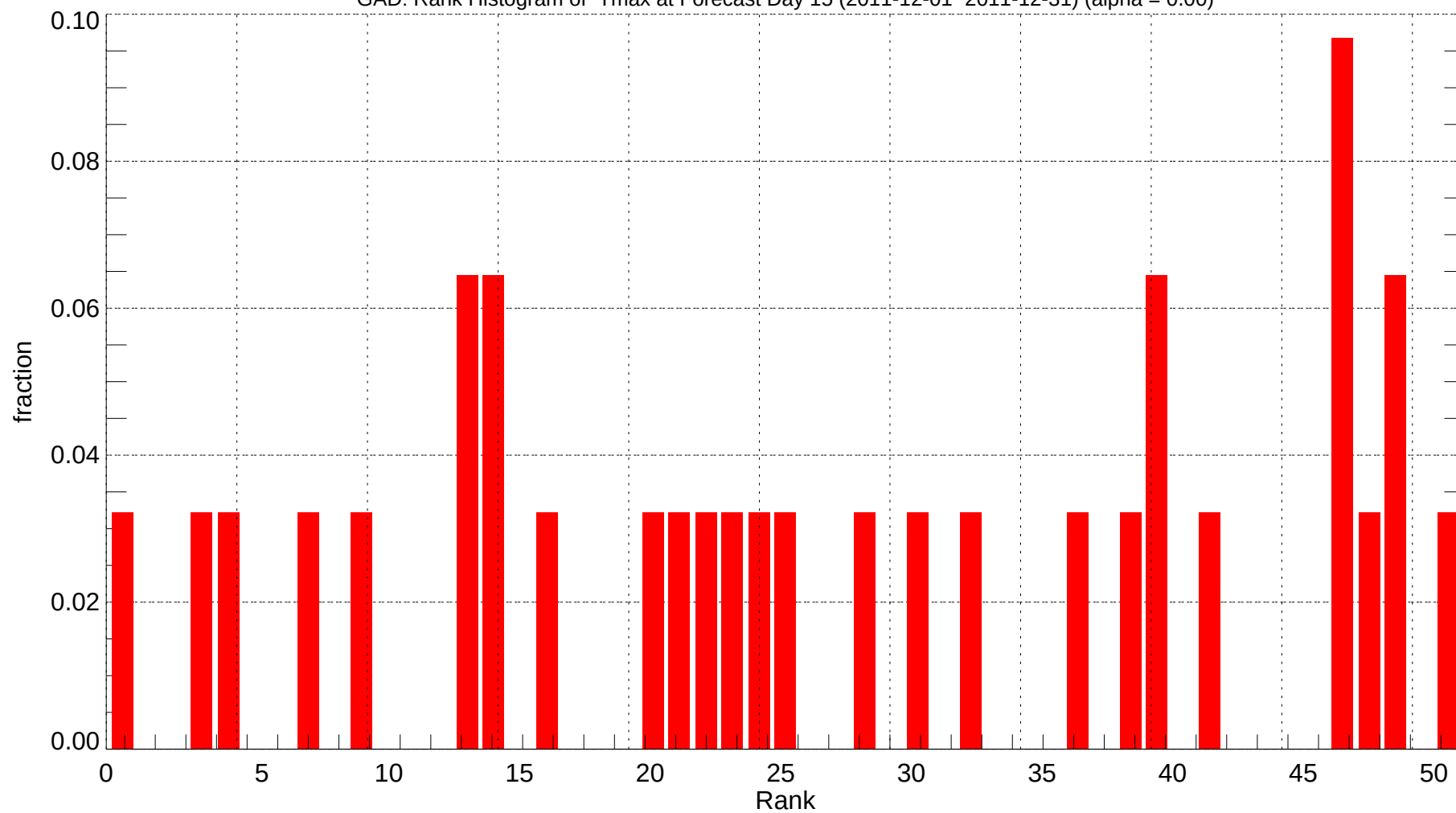
GAD: Rank Histogram of Tmax at Forecast Day 15 (2011-12-01~2011-12-31) (alpha = 0.00)
