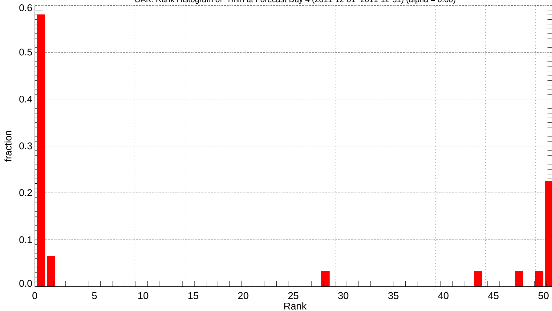
OAK: Rank Histogram of Tmin at Forecast Day 4 (2011-12-01~2011-12-31) (alpha = 0.00)
