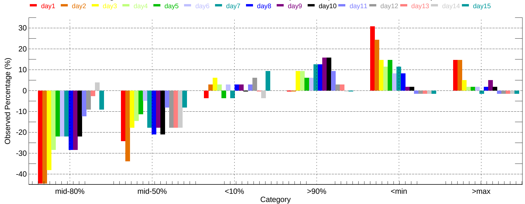
Observed Percentage Deviation of Ensembles - BUF: Min Temperature (2011-12-01~2011-12-31)
