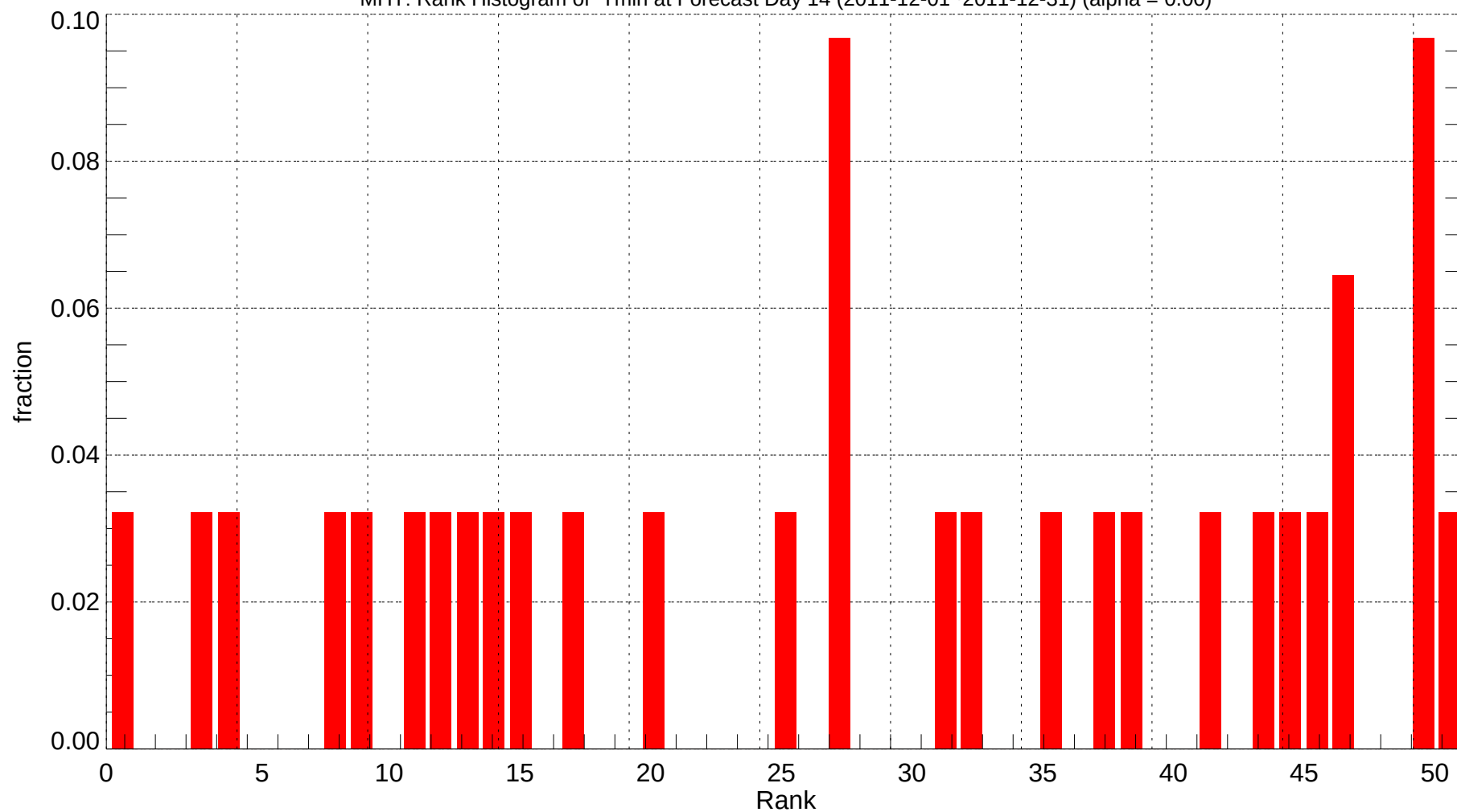
MHT: Rank Histogram of Tmin at Forecast Day 14 (2011-12-01~2011-12-31) (alpha = 0.00)
