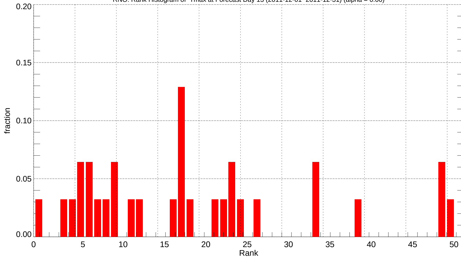
RNO: Rank Histogram of Tmax at Forecast Day 13 (2011-12-01~2011-12-31) (alpha = 0.00)
