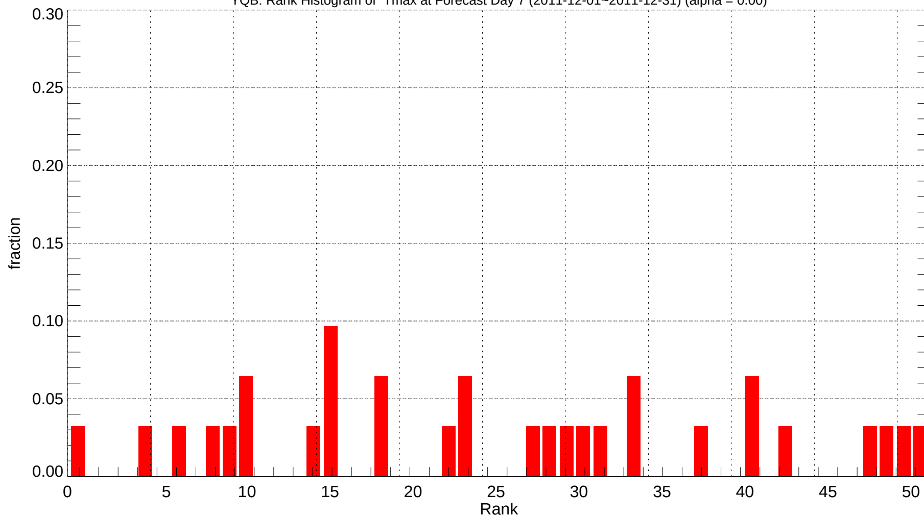
YQB: Rank Histogram of Tmax at Forecast Day 7 (2011-12-01~2011-12-31) (alpha = 0.00)
