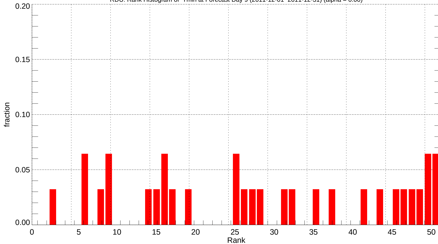
RDU: Rank Histogram of Tmin at Forecast Day 9 (2011-12-01~2011-12-31) (alpha = 0.00)
