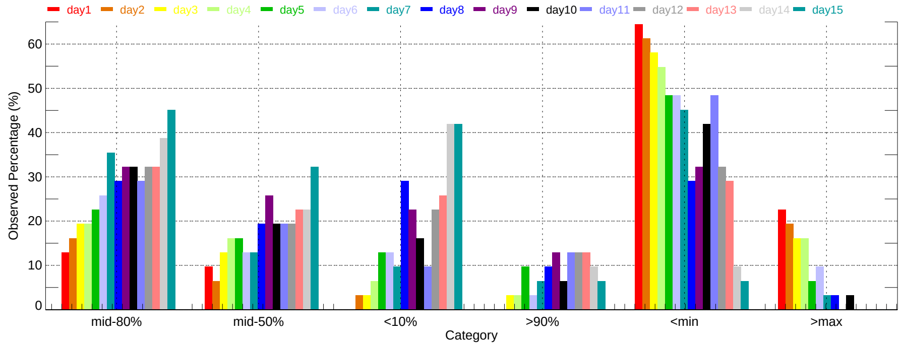
Observed Percentage of Ensembles - RDD: Min Temperature (2011-12-01~2011-12-31)
