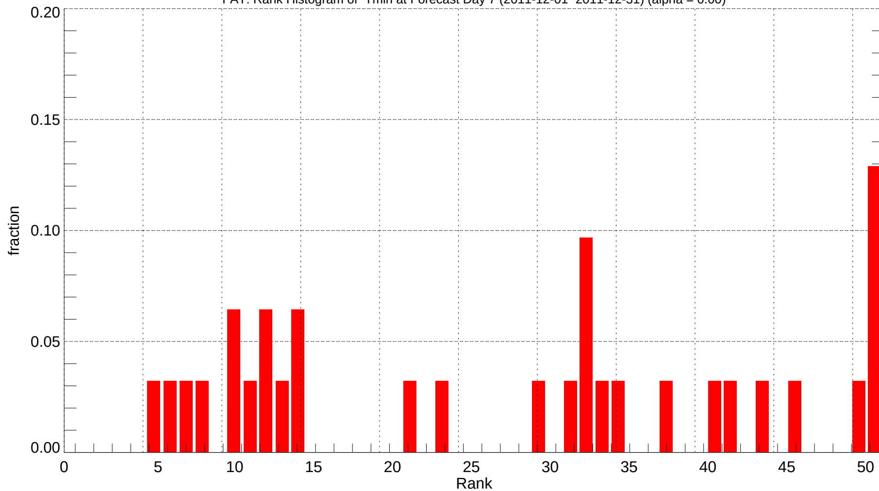
FAT: Rank Histogram of Tmin at Forecast Day 7 (2011-12-01~2011-12-31) (alpha = 0.00)
