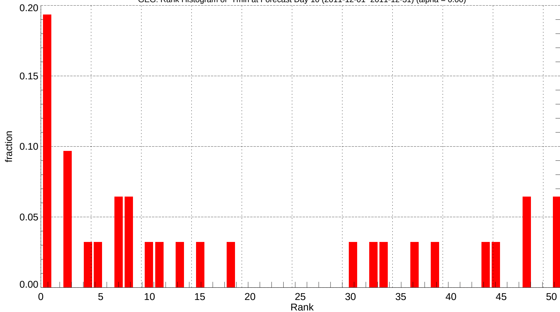
GEG: Rank Histogram of Tmin at Forecast Day 10 (2011-12-01~2011-12-31) (alpha = 0.00)
