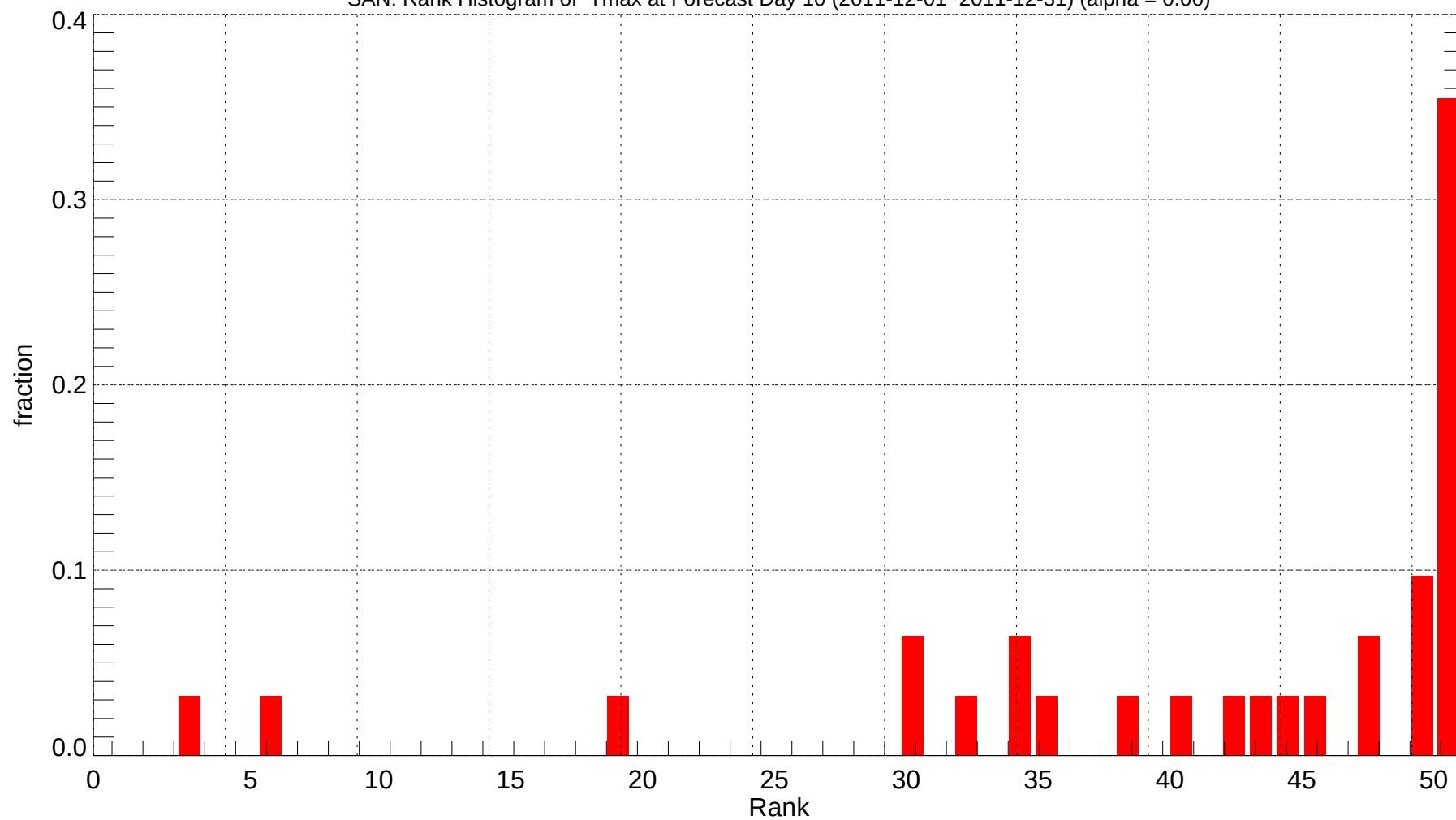
SAN: Rank Histogram of Tmax at Forecast Day 10 (2011-12-01~2011-12-31) (alpha = 0.00)
