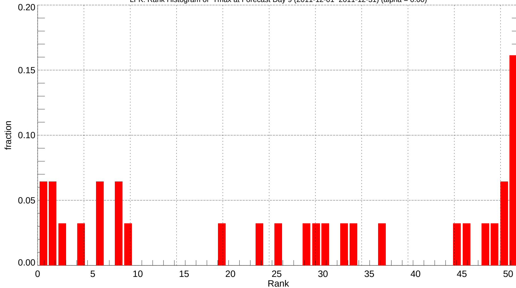
LFK: Rank Histogram of Tmax at Forecast Day 9 (2011-12-01~2011-12-31) (alpha = 0.00)
