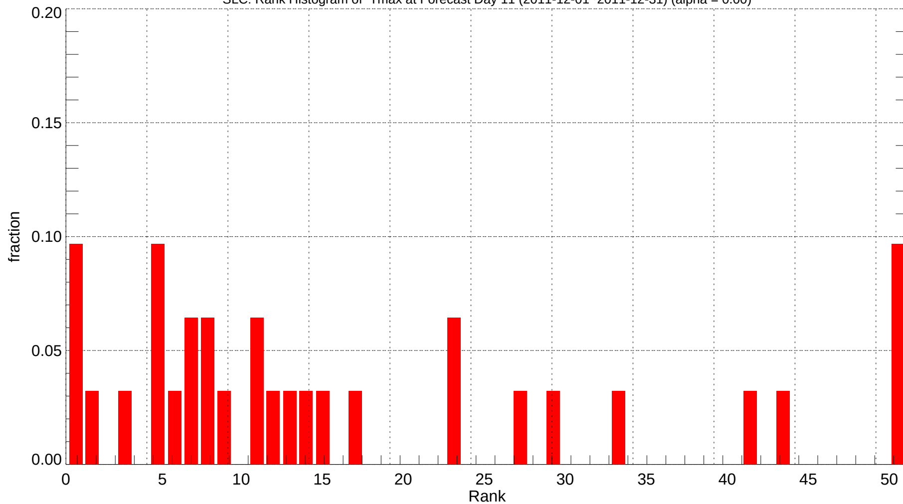
SLC: Rank Histogram of Tmax at Forecast Day 11 (2011-12-01~2011-12-31) (alpha = 0.00)
