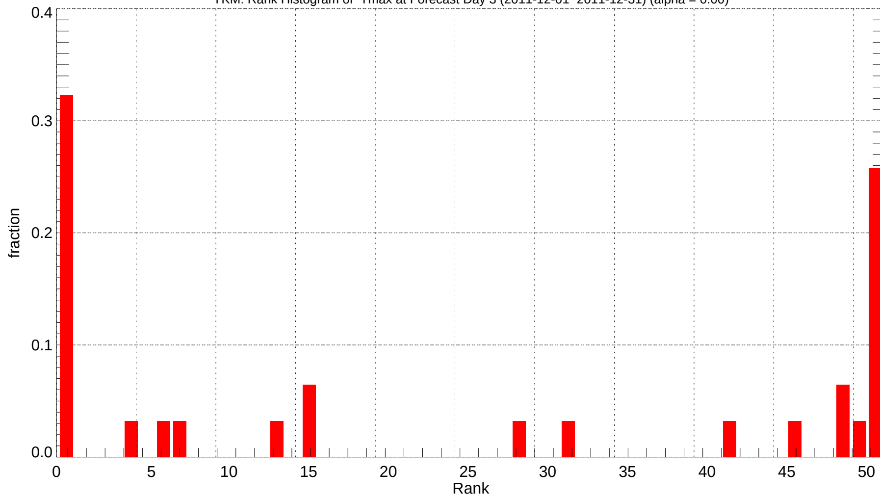
YKM: Rank Histogram of Tmax at Forecast Day 3 (2011-12-01~2011-12-31) (alpha = 0.00)
