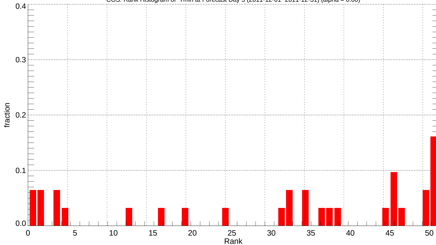
COS: Rank Histogram of Tmin at Forecast Day 5 (2011-12-01~2011-12-31) (alpha = 0.00)
