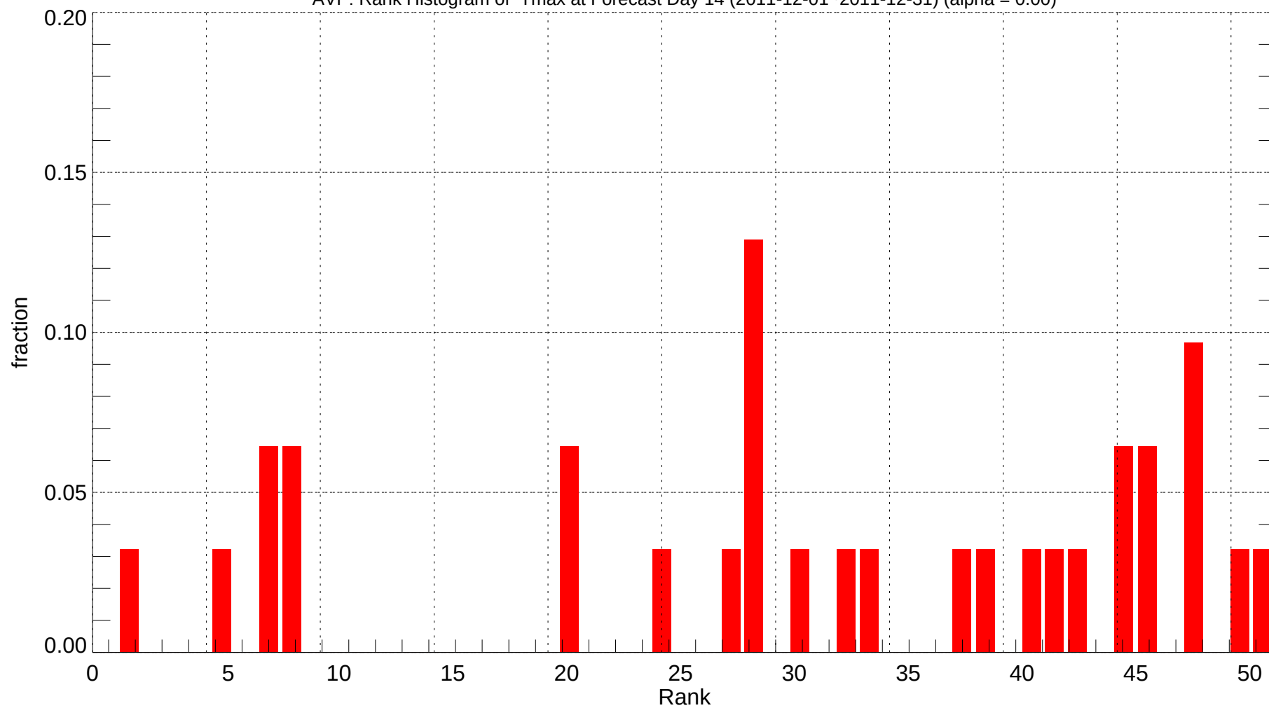
AVP: Rank Histogram of Tmax at Forecast Day 14 (2011-12-01~2011-12-31) (alpha = 0.00)
