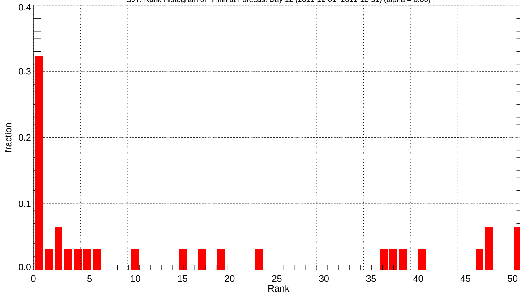
SJT: Rank Histogram of Tmin at Forecast Day 12 (2011-12-01~2011-12-31) (alpha = 0.00)
