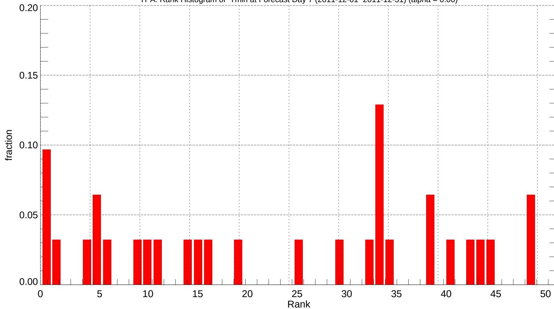
TPA: Rank Histogram of Tmin at Forecast Day 7 (2011-12-01~2011-12-31) (alpha = 0.00)
