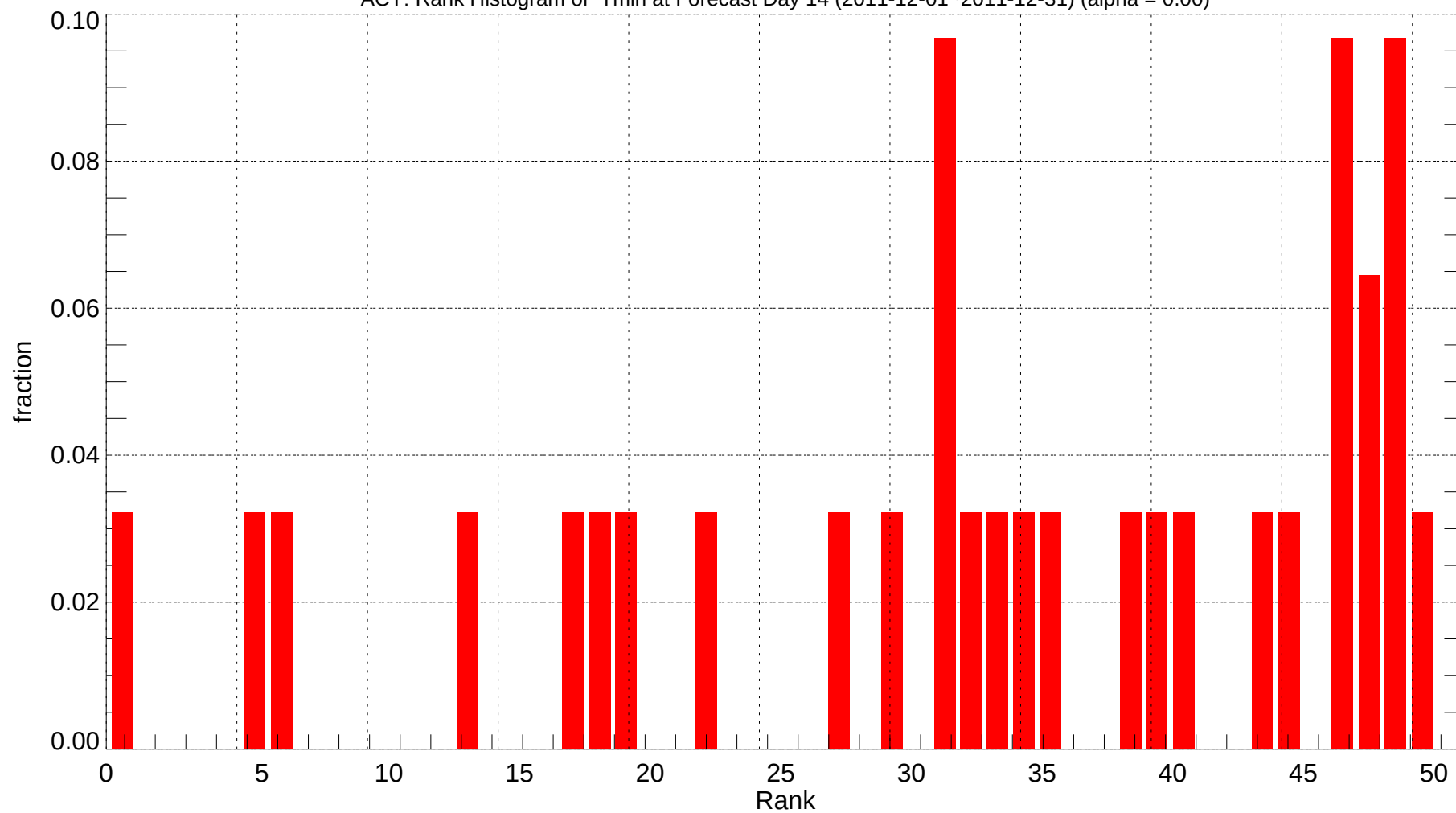
ACY: Rank Histogram of Tmin at Forecast Day 14 (2011-12-01~2011-12-31) (alpha = 0.00)
