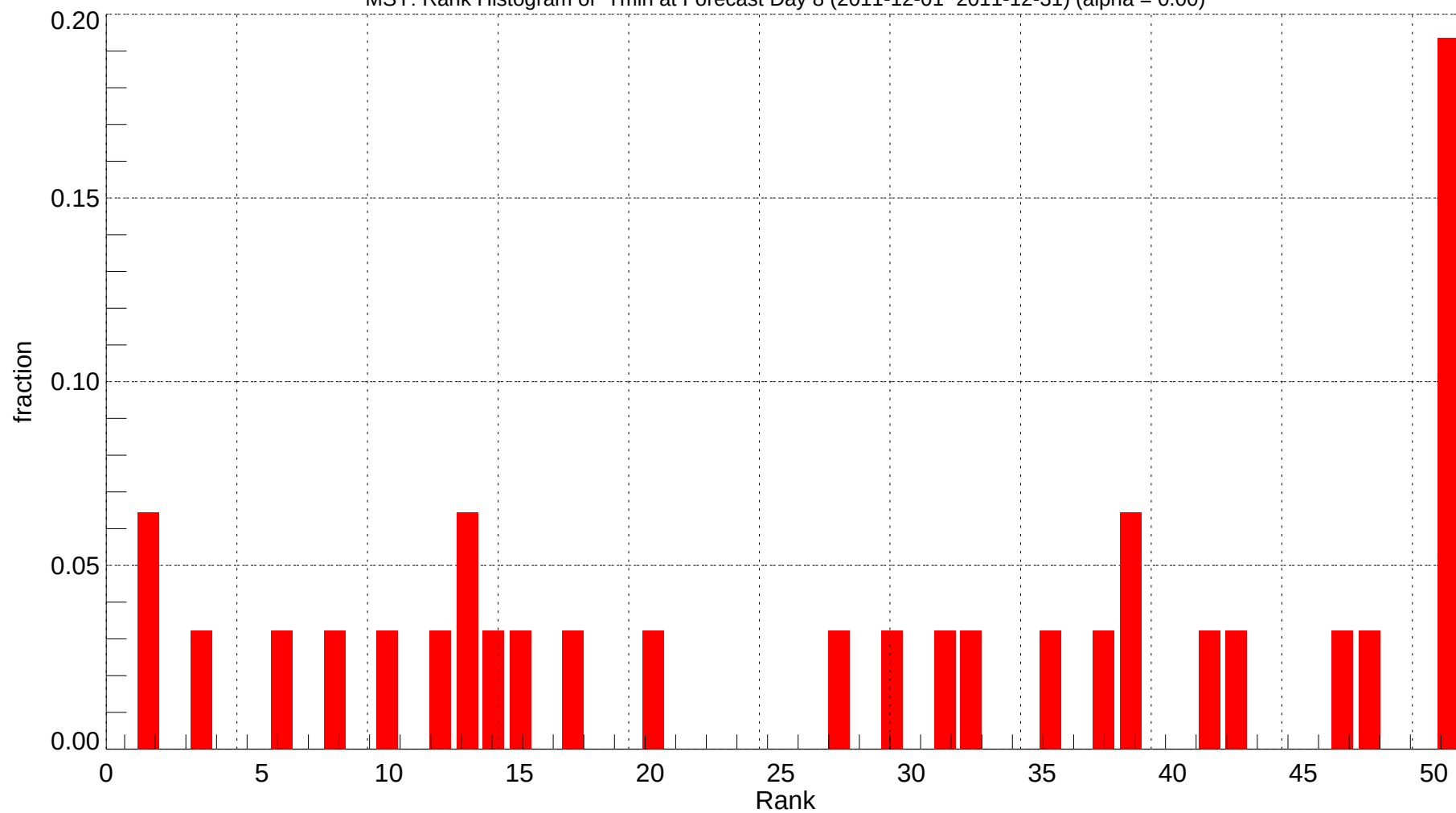
MSY: Rank Histogram of Tmin at Forecast Day 8 (2011-12-01~2011-12-31) (alpha = 0.00)
