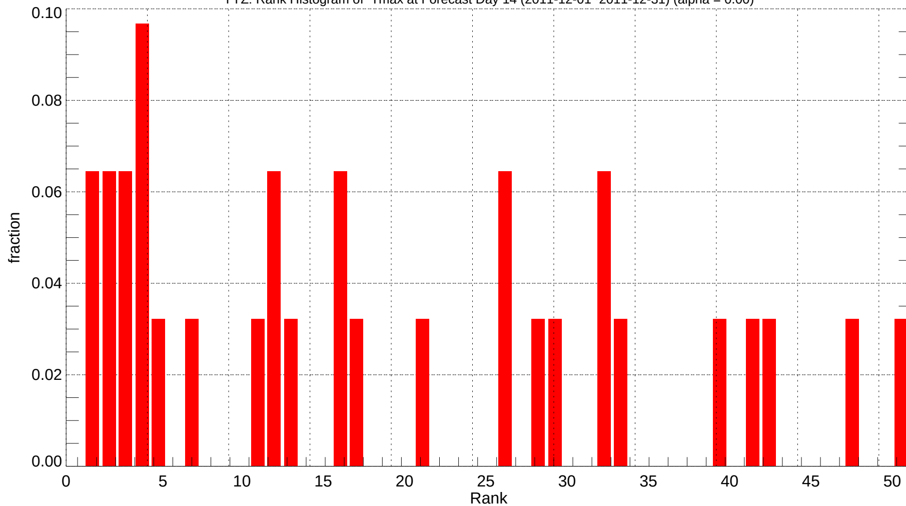
YYZ: Rank Histogram of Tmax at Forecast Day 14 (2011-12-01~2011-12-31) (alpha = 0.00)
