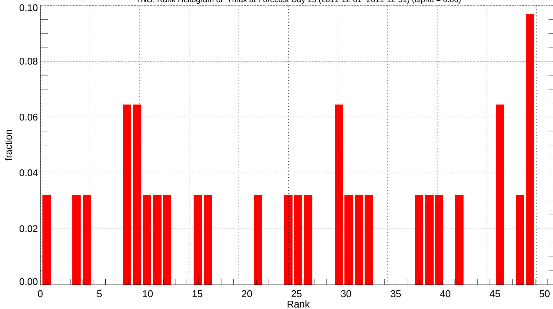
YNG: Rank Histogram of Tmax at Forecast Day 15 (2011-12-01~2011-12-31) (alpha = 0.00)
