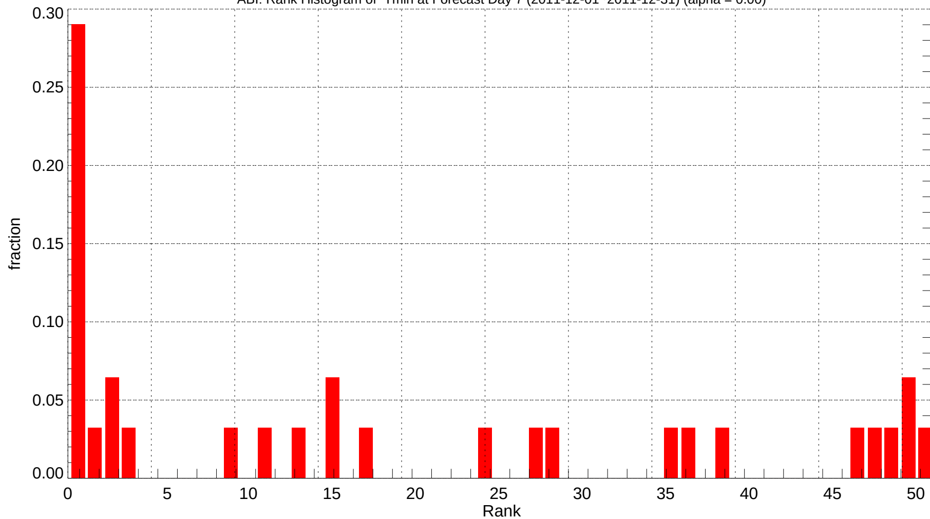
ABI: Rank Histogram of Tmin at Forecast Day 7 (2011-12-01~2011-12-31) (alpha = 0.00)
