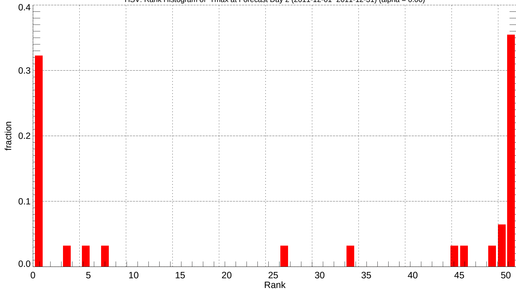
HSV: Rank Histogram of Tmax at Forecast Day 2 (2011-12-01~2011-12-31) (alpha = 0.00)
