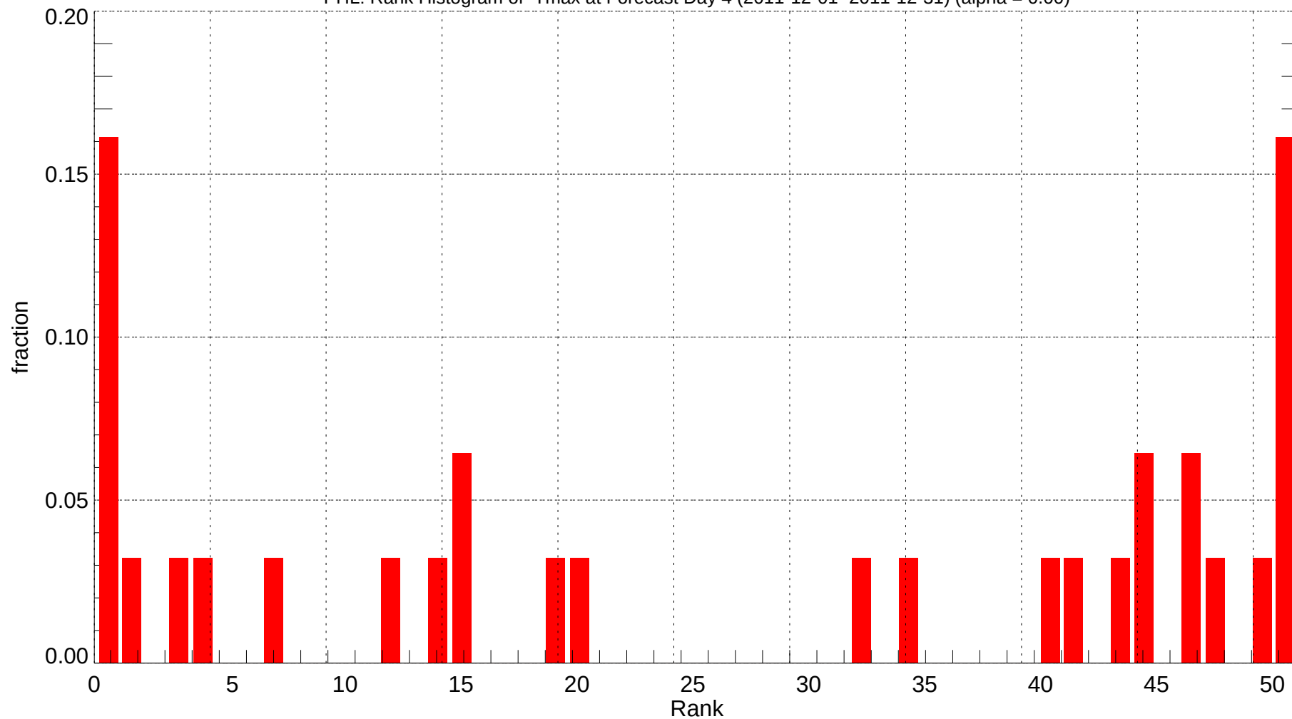
PHL: Rank Histogram of Tmax at Forecast Day 4 (2011-12-01~2011-12-31) (alpha = 0.00)
