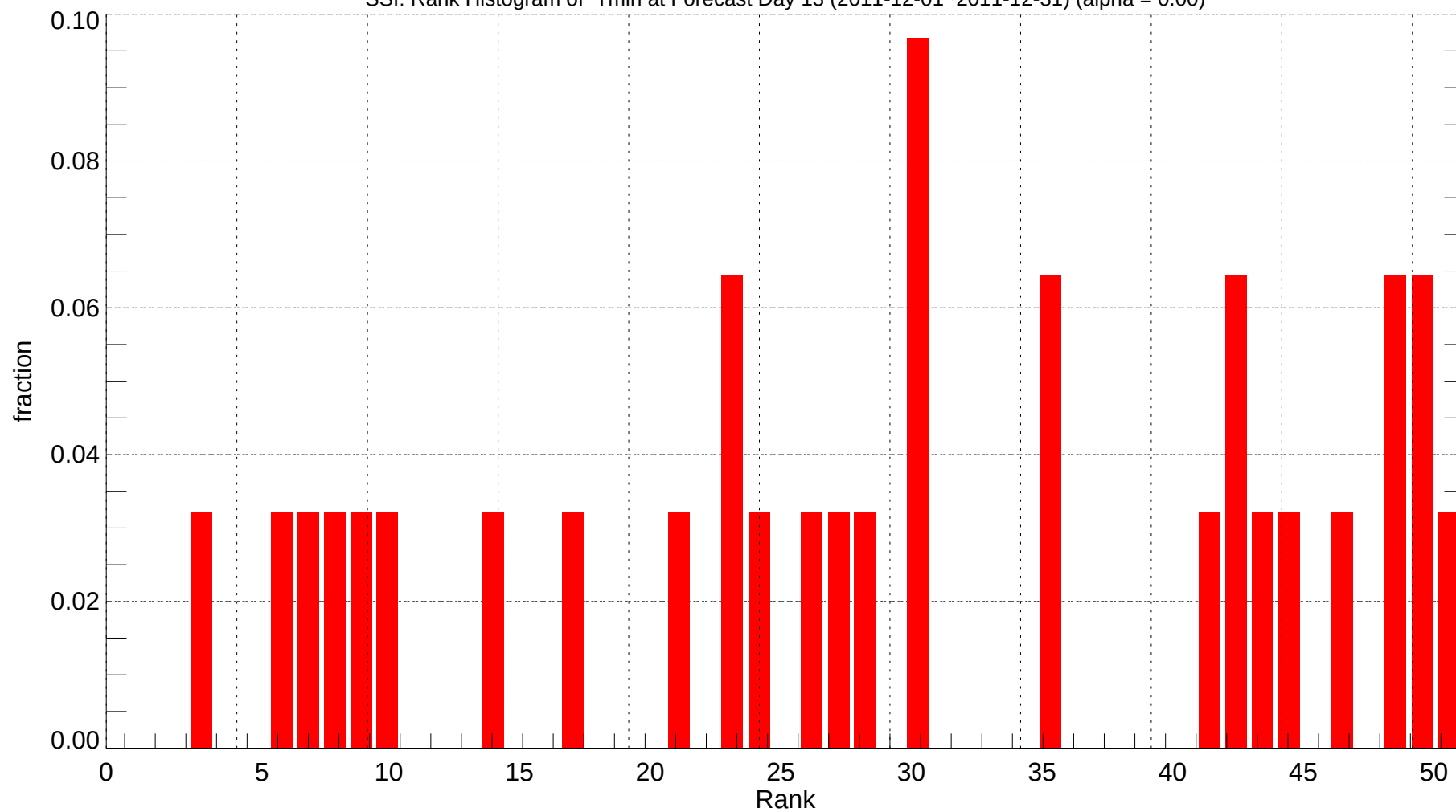
SSI: Rank Histogram of Tmin at Forecast Day 13 (2011-12-01~2011-12-31) (alpha = 0.00)
