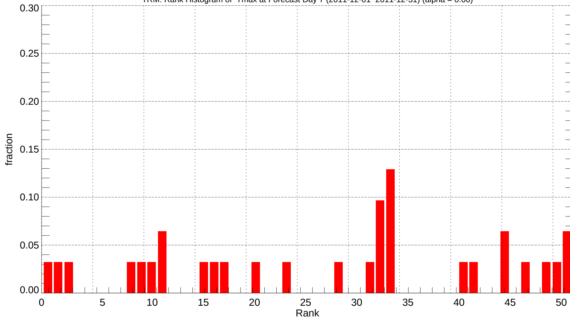
TRM: Rank Histogram of Tmax at Forecast Day 7 (2011-12-01~2011-12-31) (alpha = 0.00)
