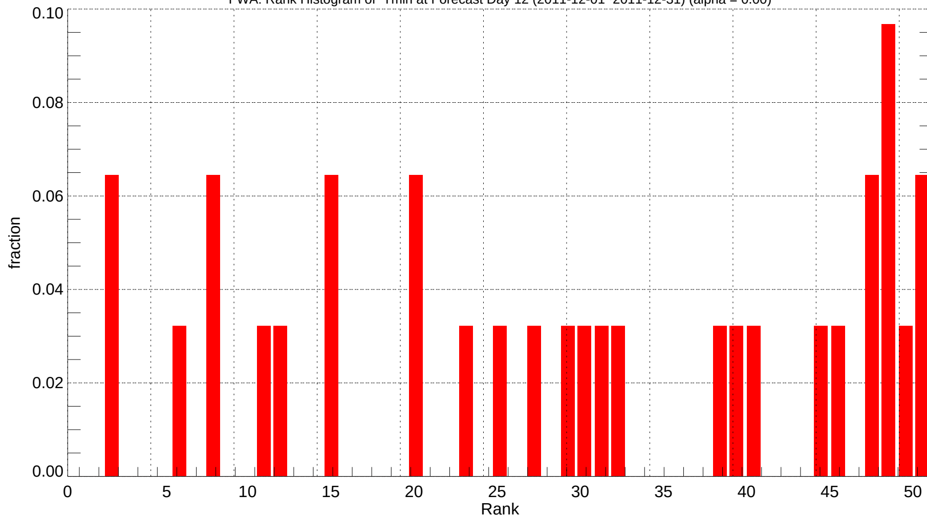
FWA: Rank Histogram of Tmin at Forecast Day 12 (2011-12-01~2011-12-31) (alpha = 0.00)
