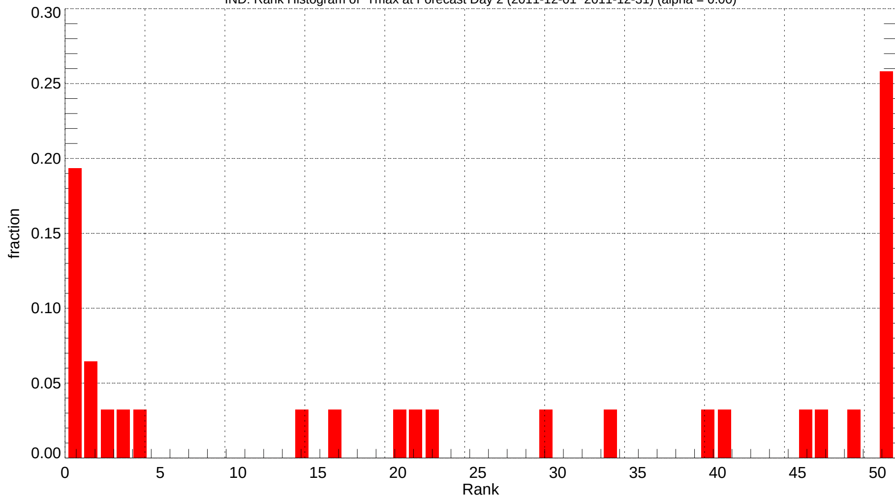
IND: Rank Histogram of Tmax at Forecast Day 2 (2011-12-01~2011-12-31) (alpha = 0.00)
