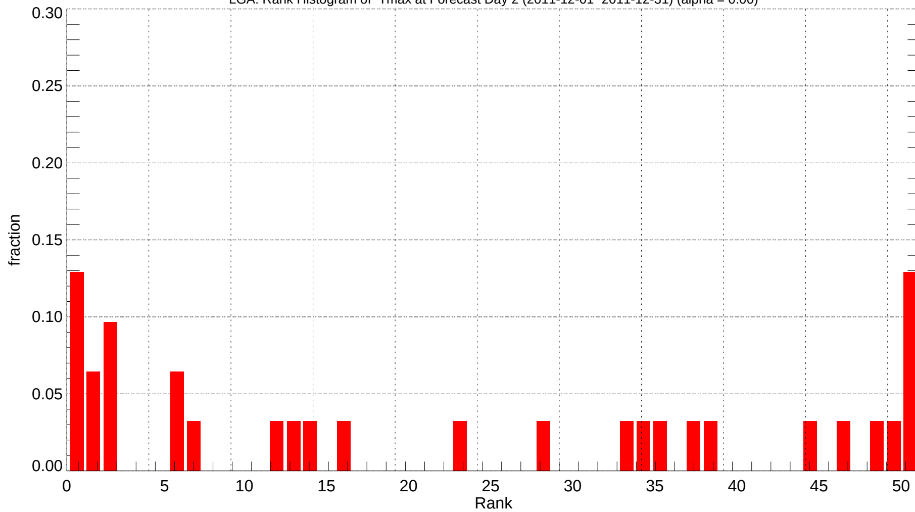
LGA: Rank Histogram of Tmax at Forecast Day 2 (2011-12-01~2011-12-31) (alpha = 0.00)
