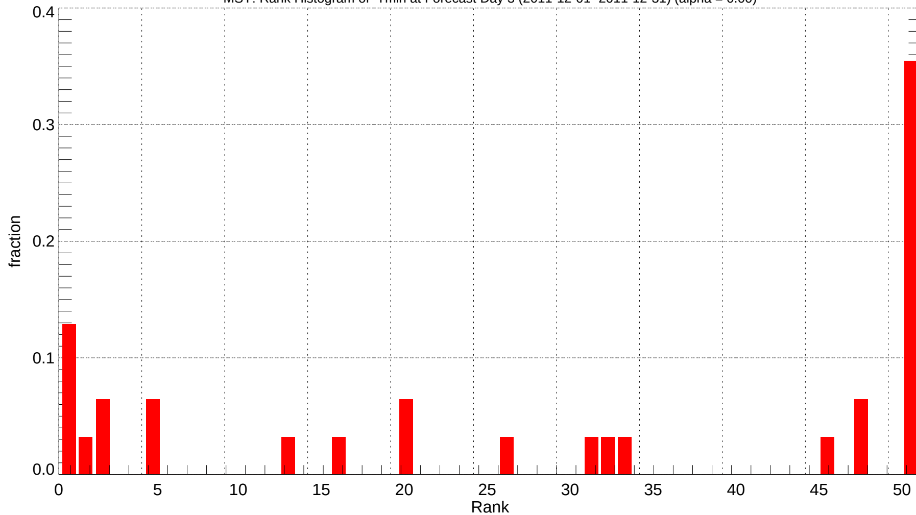
MSY: Rank Histogram of Tmin at Forecast Day 3 (2011-12-01~2011-12-31) (alpha = 0.00)
