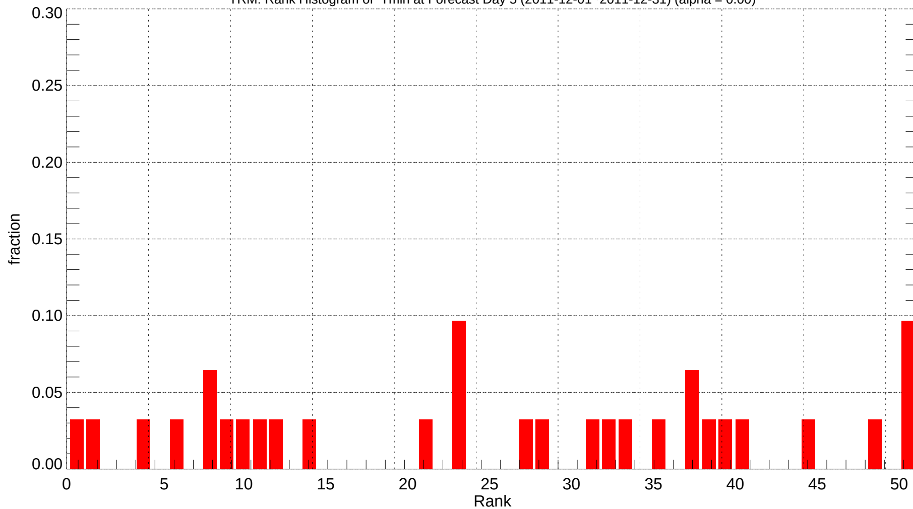
TRM: Rank Histogram of Tmin at Forecast Day 5 (2011-12-01~2011-12-31) (alpha = 0.00)
