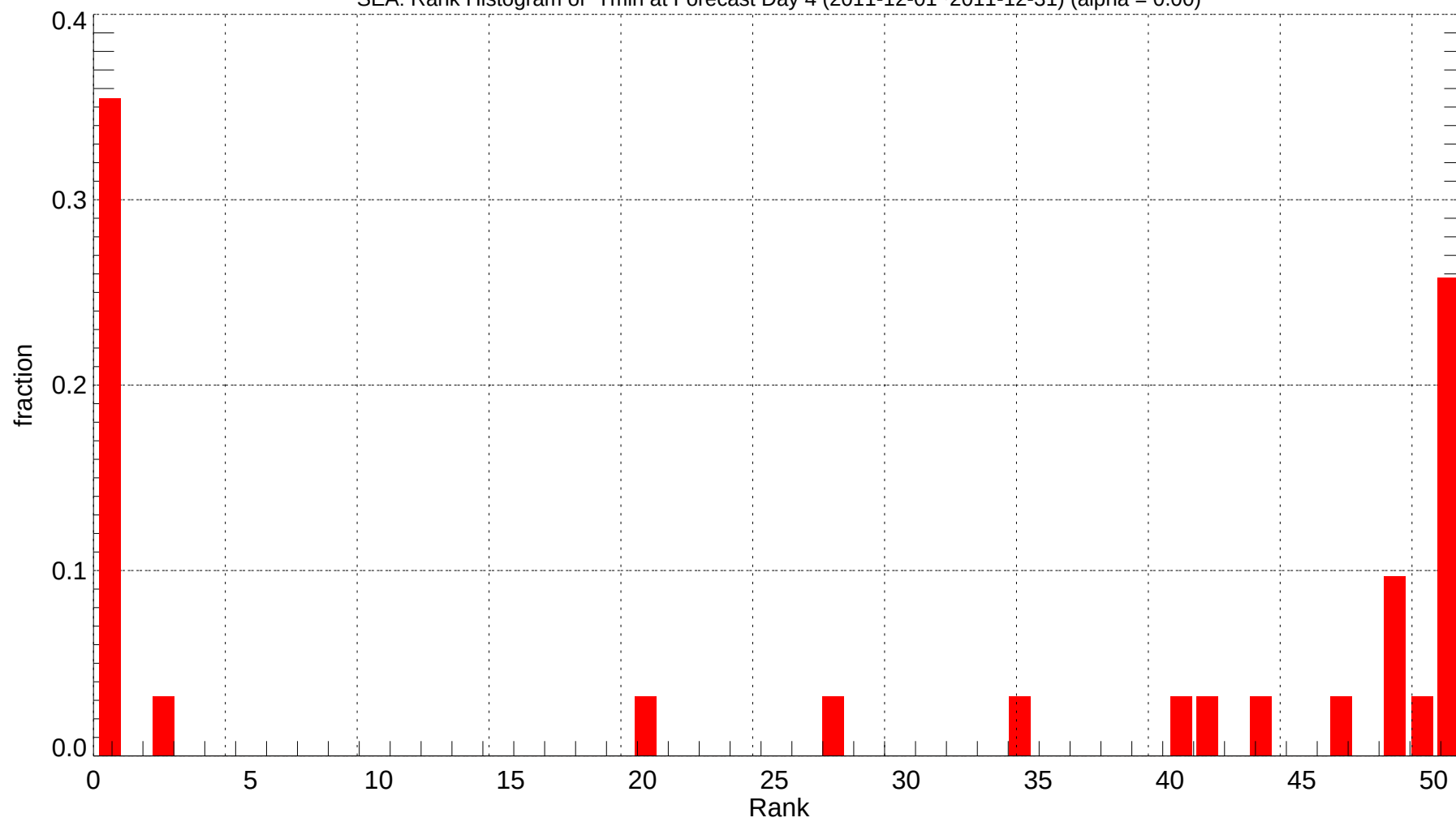
SEA: Rank Histogram of Tmin at Forecast Day 4 (2011-12-01~2011-12-31) (alpha = 0.00)
