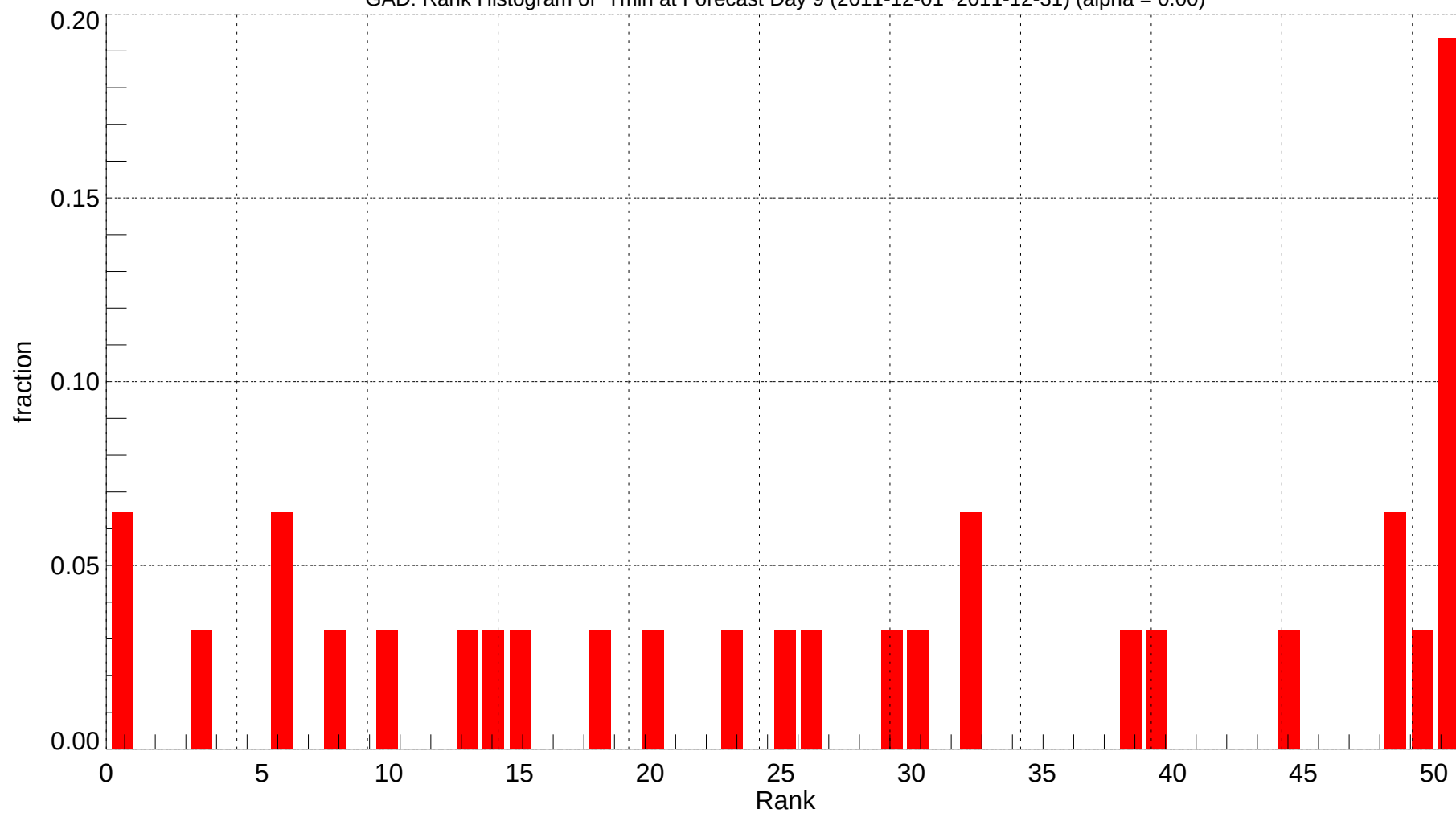
GAD: Rank Histogram of Tmin at Forecast Day 9 (2011-12-01~2011-12-31) (alpha = 0.00)
