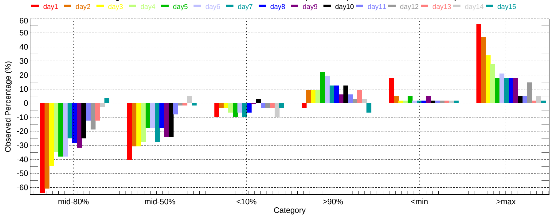
Observed Percentage Deviation of Ensembles - COS: Min Temperature (2011-12-01~2011-12-31)
