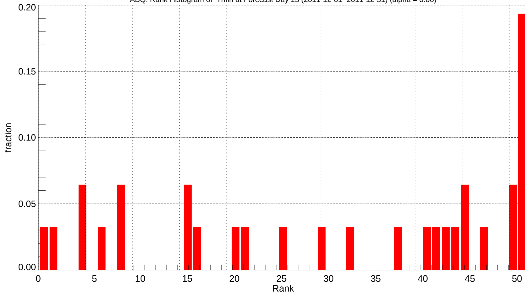
ABQ: Rank Histogram of Tmin at Forecast Day 13 (2011-12-01~2011-12-31) (alpha = 0.00)
