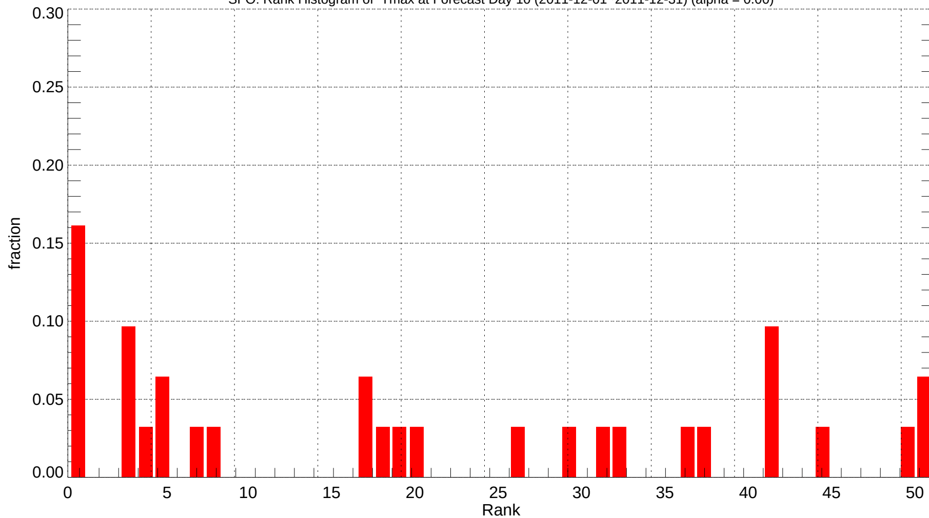
SFO: Rank Histogram of Tmax at Forecast Day 10 (2011-12-01~2011-12-31) (alpha = 0.00)
