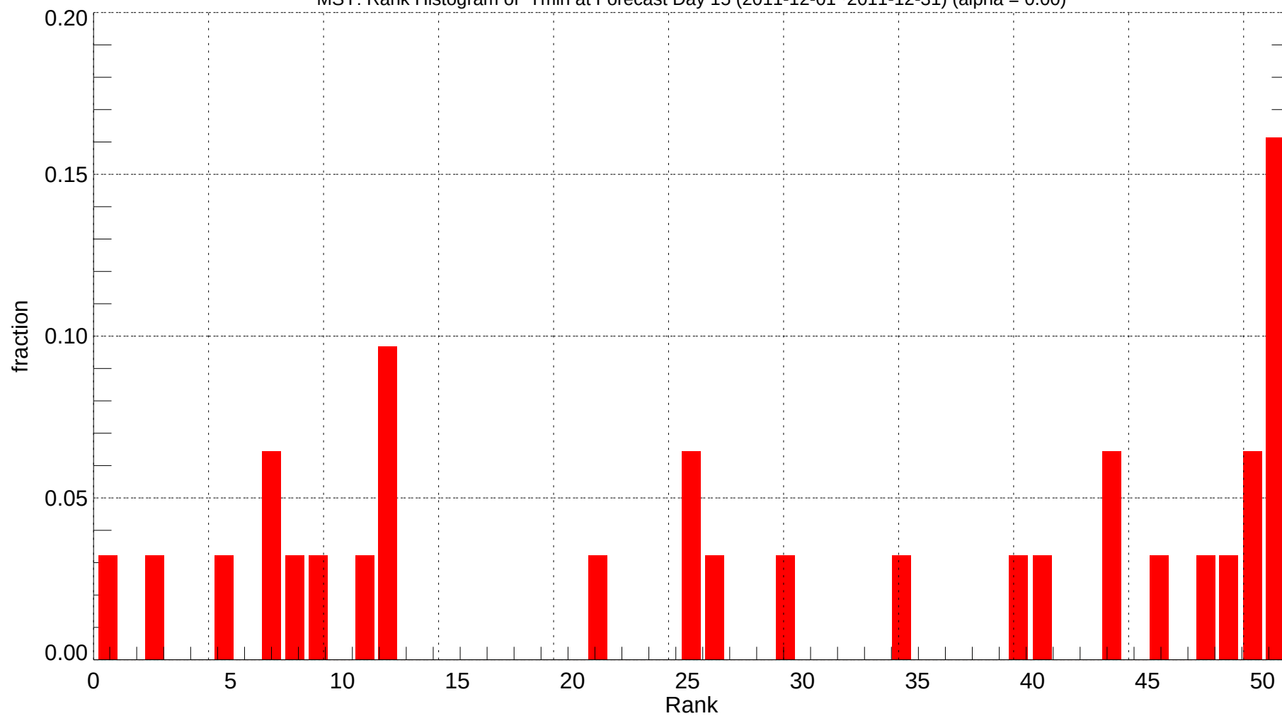
MSY: Rank Histogram of Tmin at Forecast Day 15 (2011-12-01~2011-12-31) (alpha = 0.00)
