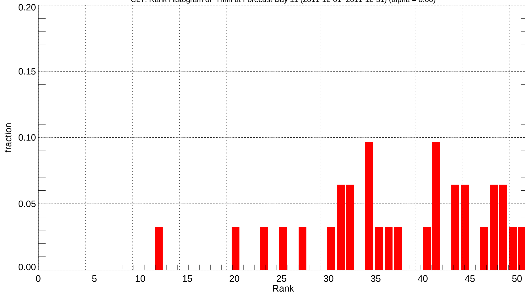
CLT: Rank Histogram of Tmin at Forecast Day 11 (2011-12-01~2011-12-31) (alpha = 0.00)
