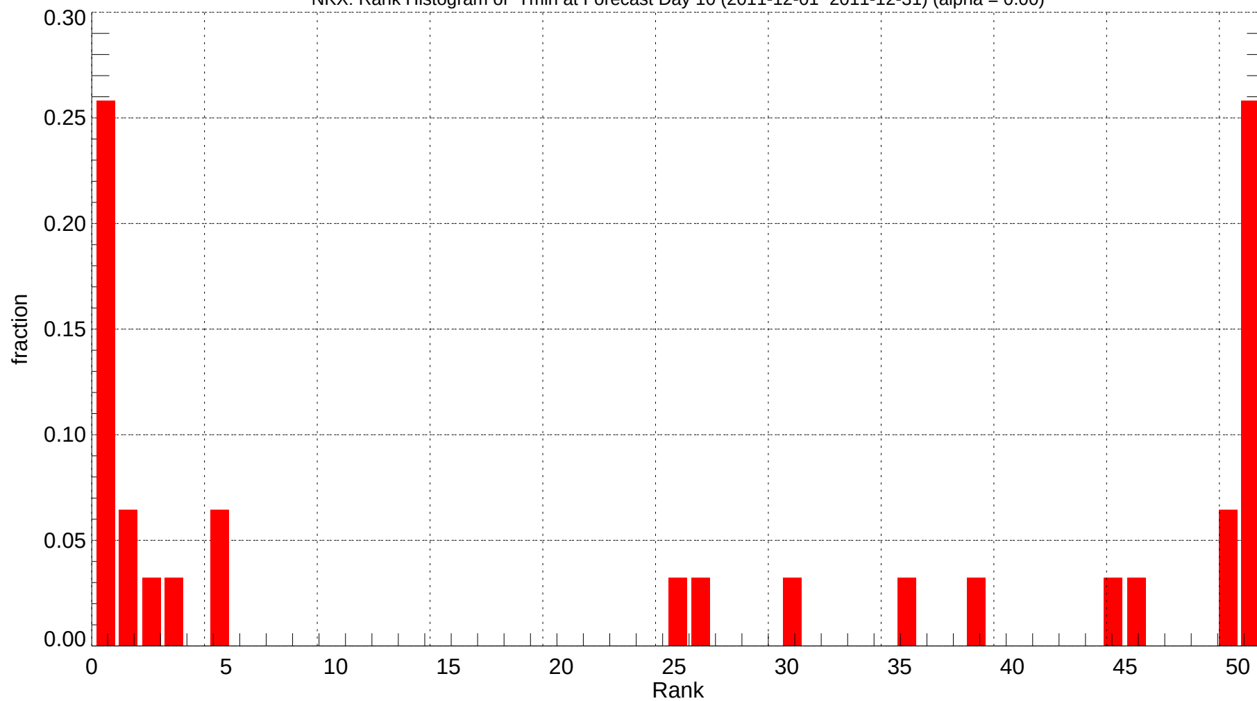
NKX: Rank Histogram of Tmin at Forecast Day 10 (2011-12-01~2011-12-31) (alpha = 0.00)
