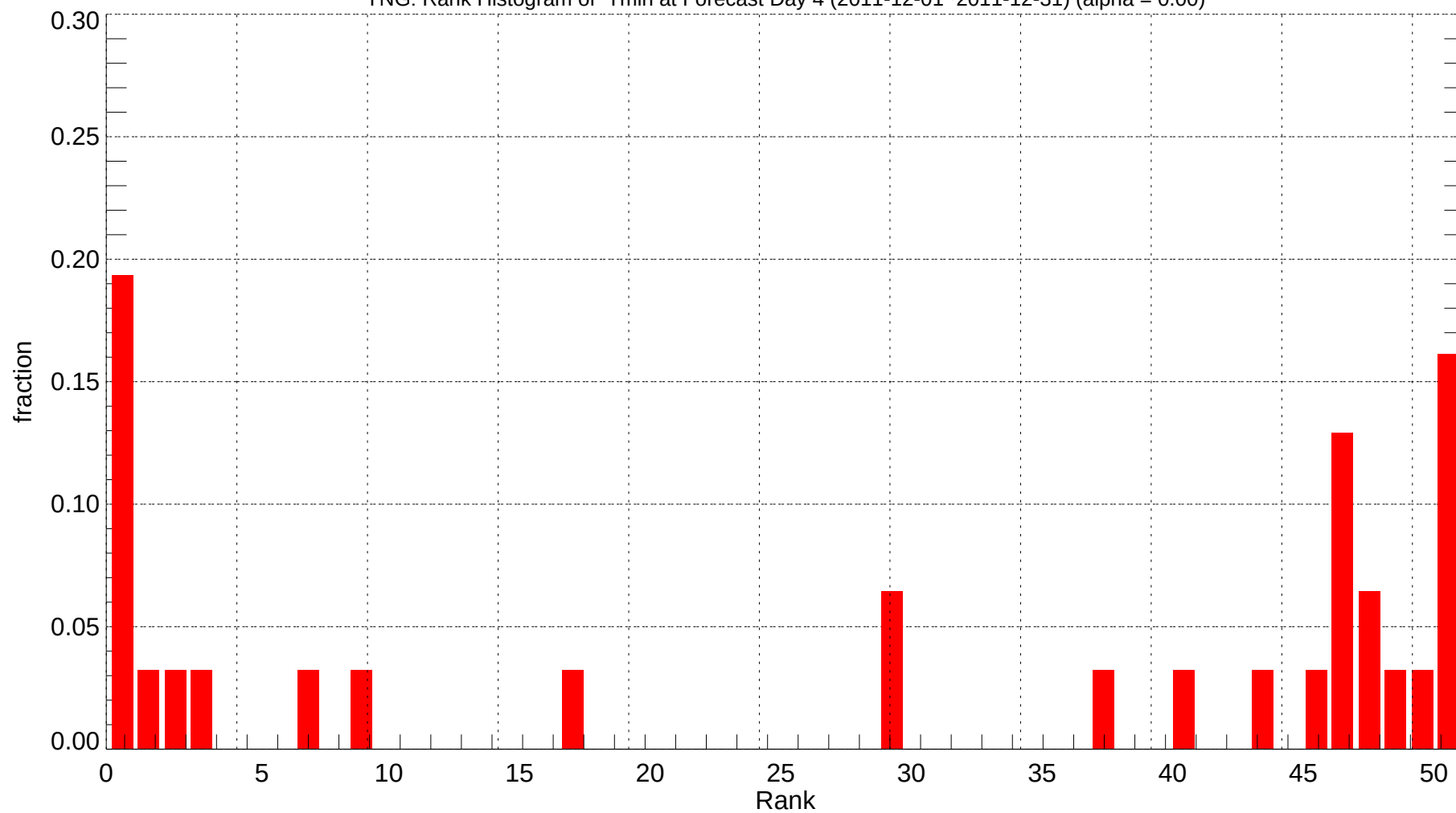
YNG: Rank Histogram of Tmin at Forecast Day 4 (2011-12-01~2011-12-31) (alpha = 0.00)
