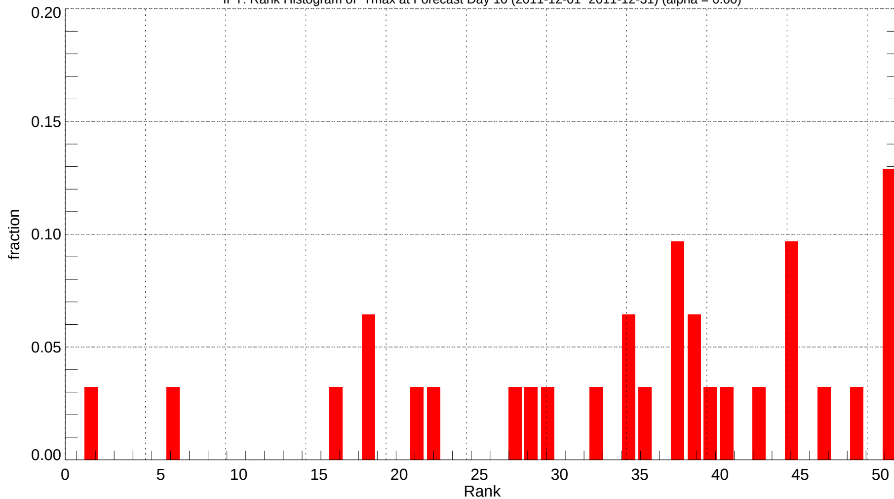
IPT: Rank Histogram of Tmax at Forecast Day 10 (2011-12-01~2011-12-31) (alpha = 0.00)
