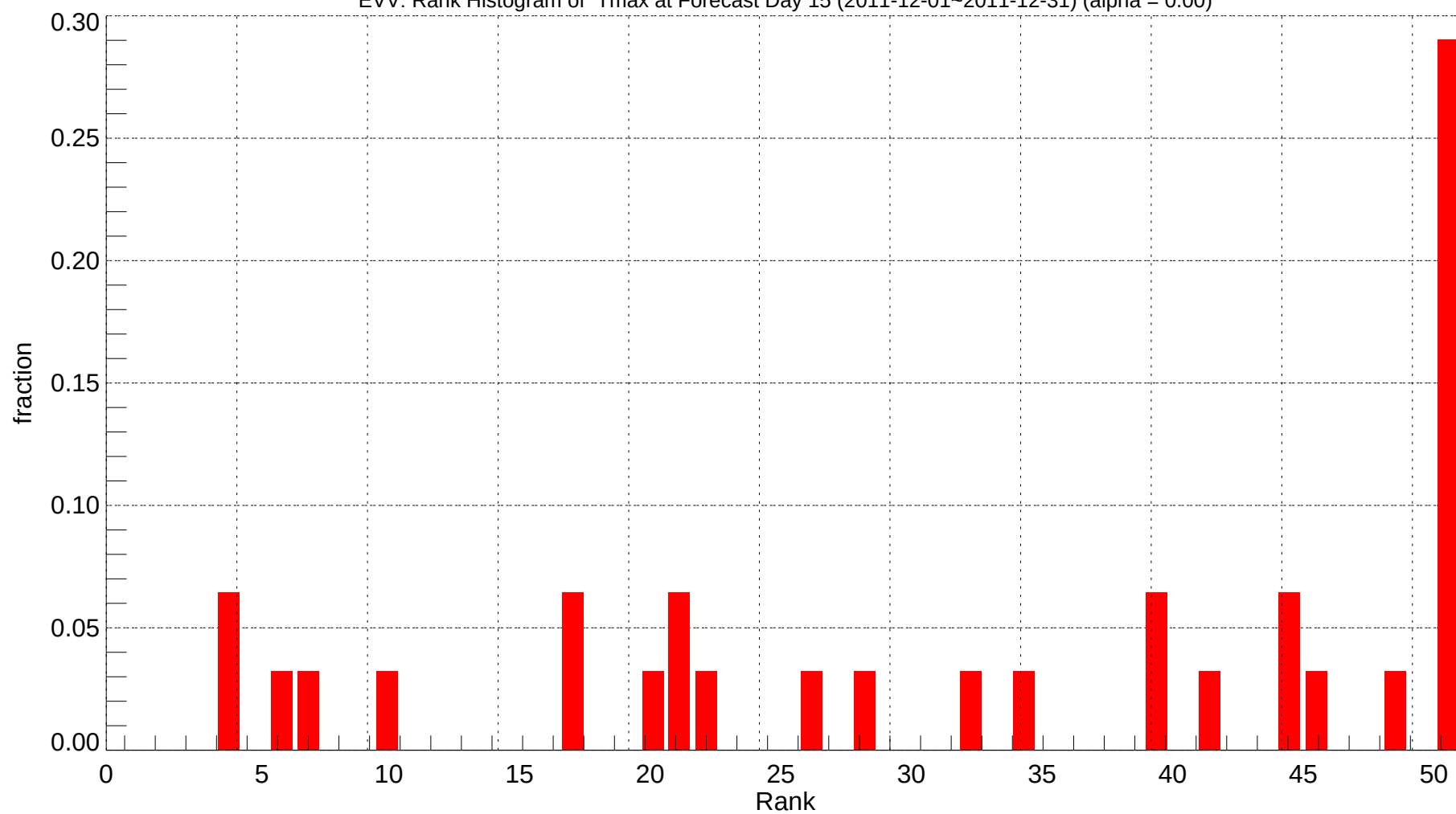
EVV: Rank Histogram of Tmax at Forecast Day 15 (2011-12-01~2011-12-31) (alpha = 0.00)
