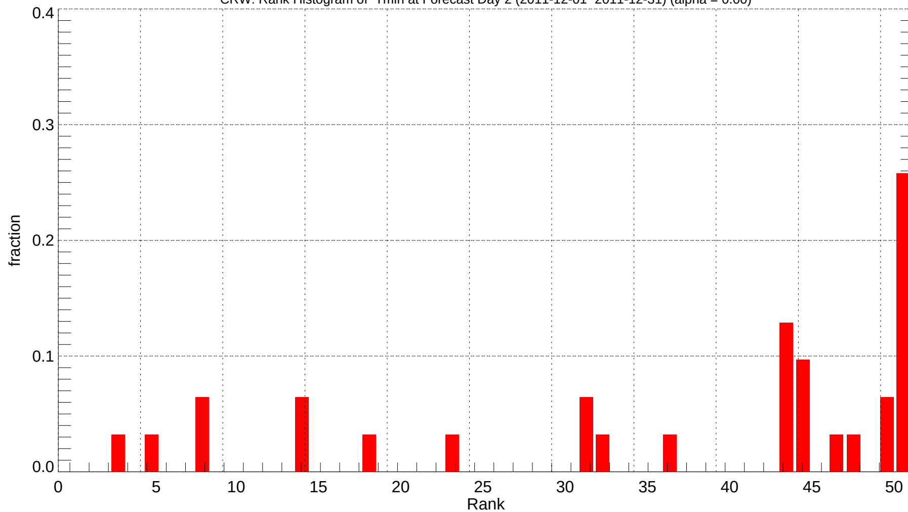
CRW: Rank Histogram of Tmin at Forecast Day 2 (2011-12-01~2011-12-31) (alpha = 0.00)
