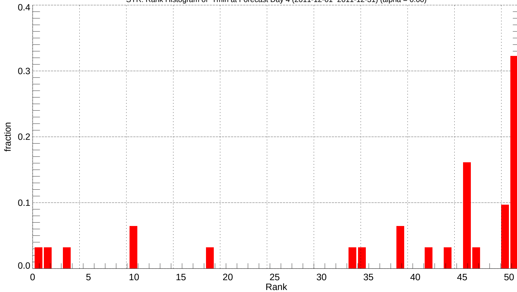
SYR: Rank Histogram of Tmin at Forecast Day 4 (2011-12-01~2011-12-31) (alpha = 0.00)
