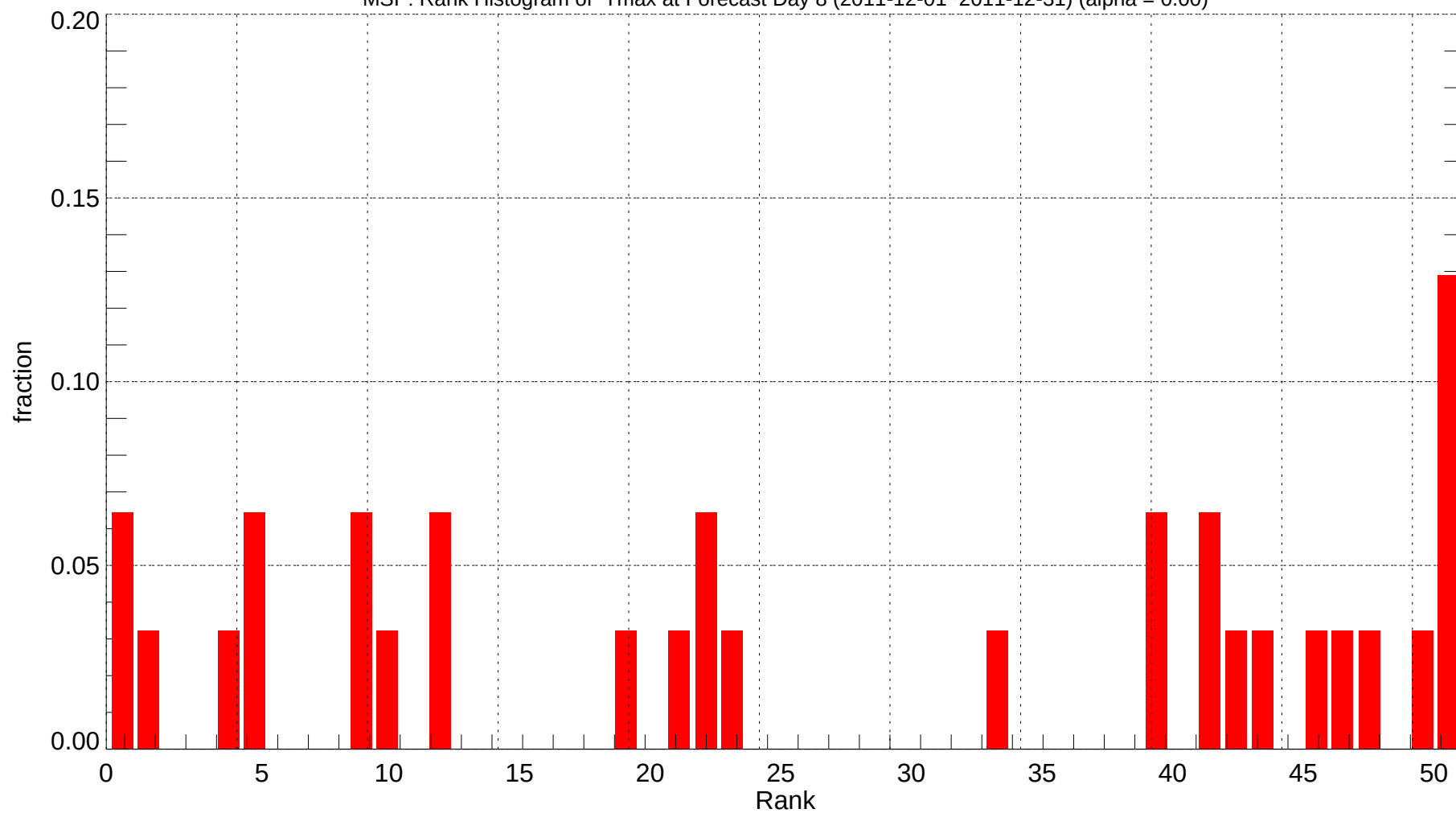
MSP: Rank Histogram of Tmax at Forecast Day 8 (2011-12-01~2011-12-31) (alpha = 0.00)
