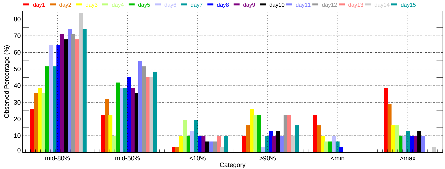
Observed Percentage of Ensembles - ERI: Max Temperature (2011-12-01~2011-12-31)
