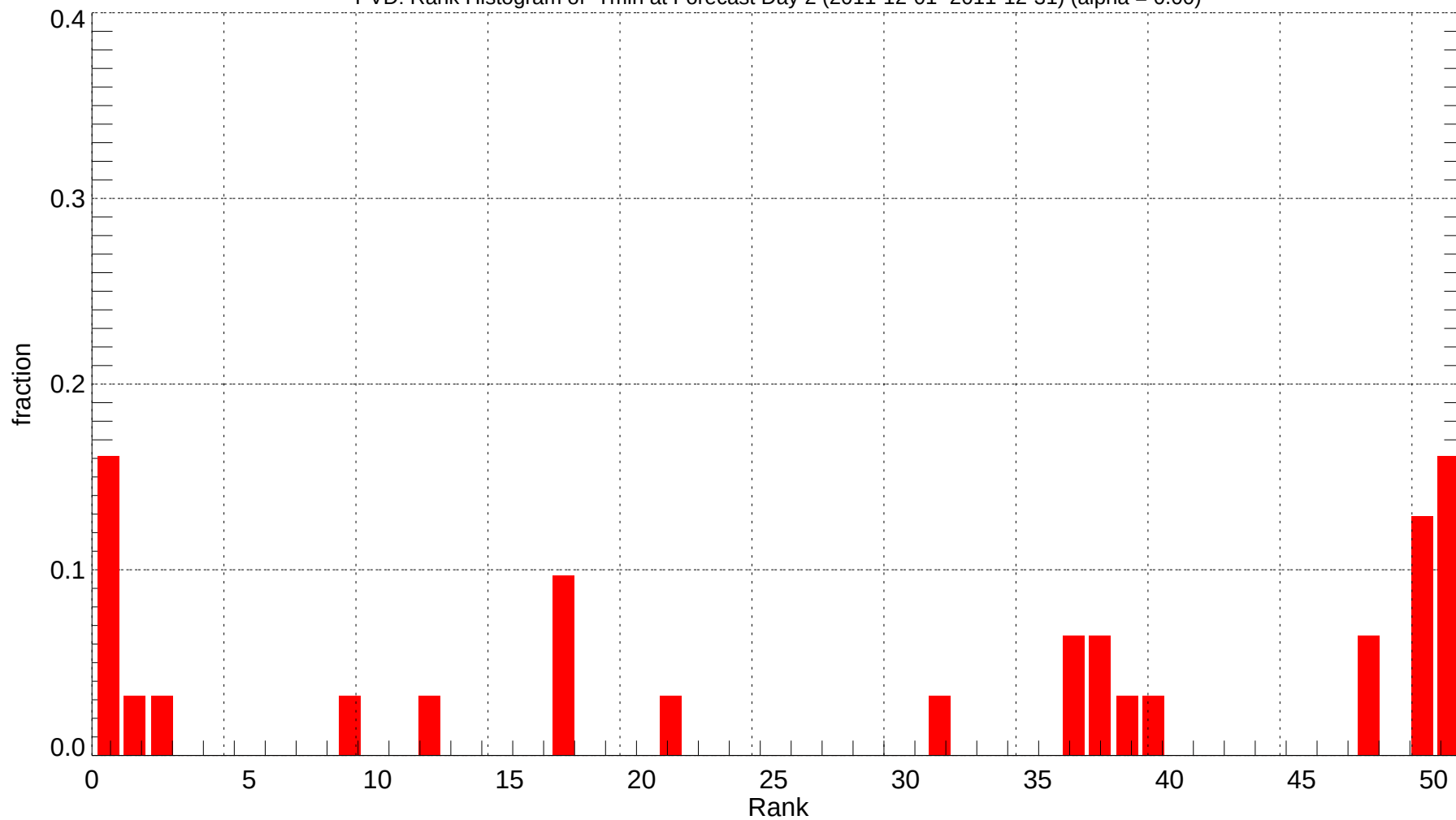
PVD: Rank Histogram of Tmin at Forecast Day 2 (2011-12-01~2011-12-31) (alpha = 0.00)
