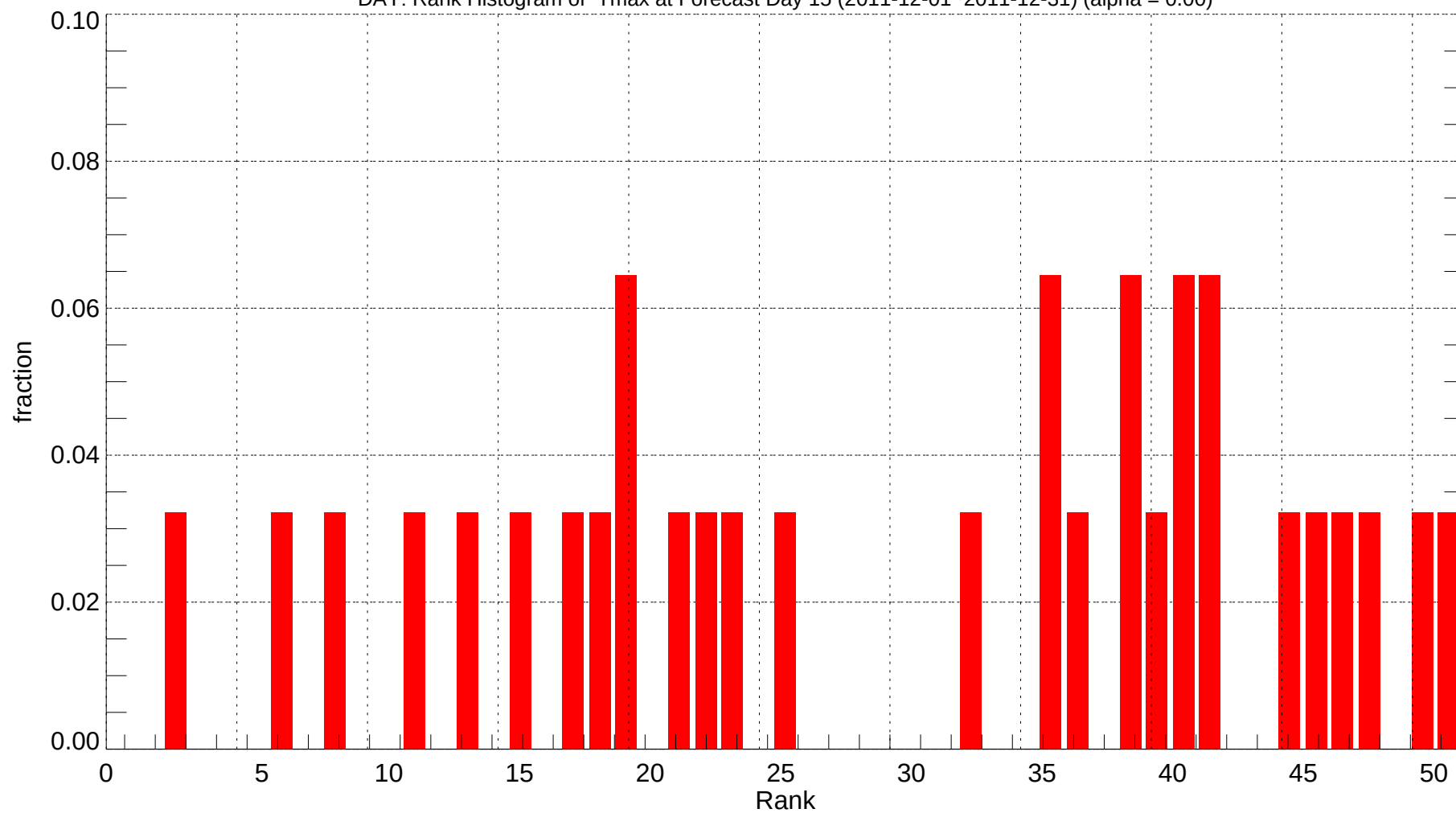
DAY: Rank Histogram of Tmax at Forecast Day 15 (2011-12-01~2011-12-31) (alpha = 0.00)
