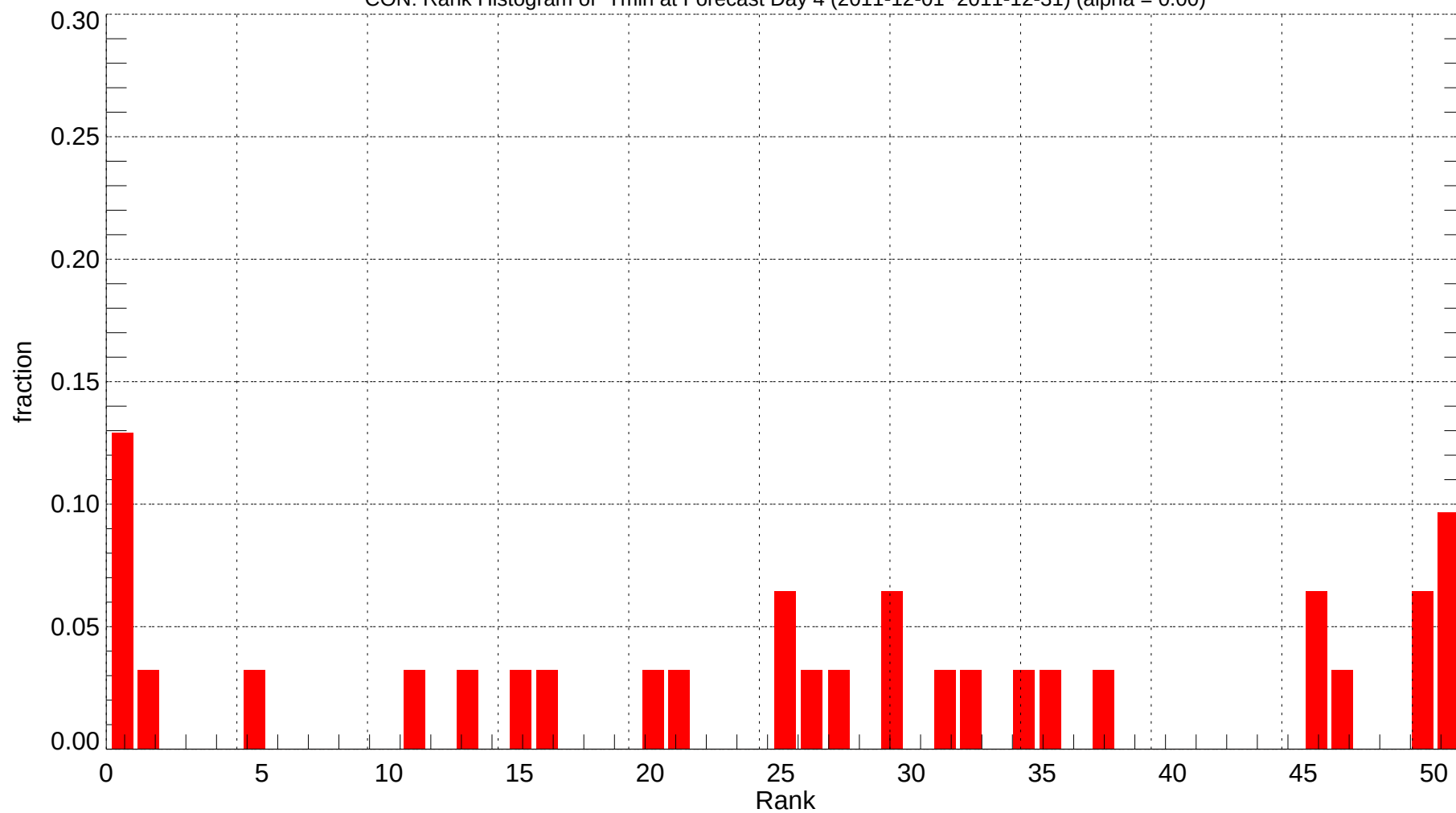
CON: Rank Histogram of Tmin at Forecast Day 4 (2011-12-01~2011-12-31) (alpha = 0.00)
