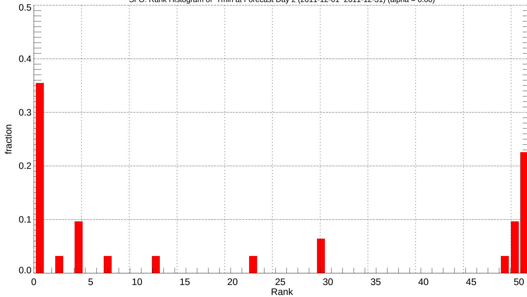
SFO: Rank Histogram of Tmin at Forecast Day 2 (2011-12-01~2011-12-31) (alpha = 0.00)
