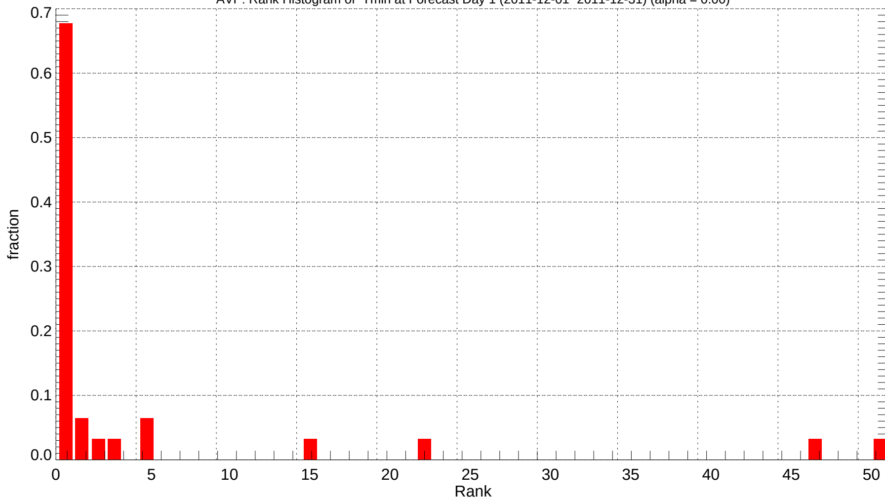
AVP: Rank Histogram of Tmin at Forecast Day 1 (2011-12-01~2011-12-31) (alpha = 0.00)
