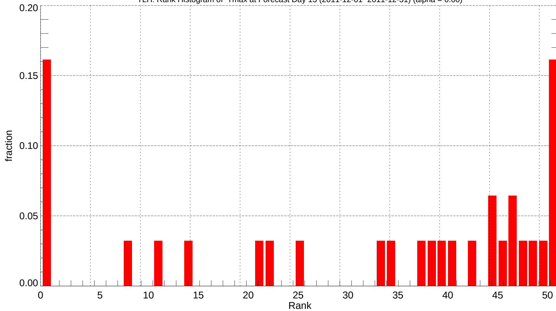
TLH: Rank Histogram of Tmax at Forecast Day 13 (2011-12-01~2011-12-31) (alpha = 0.00)
