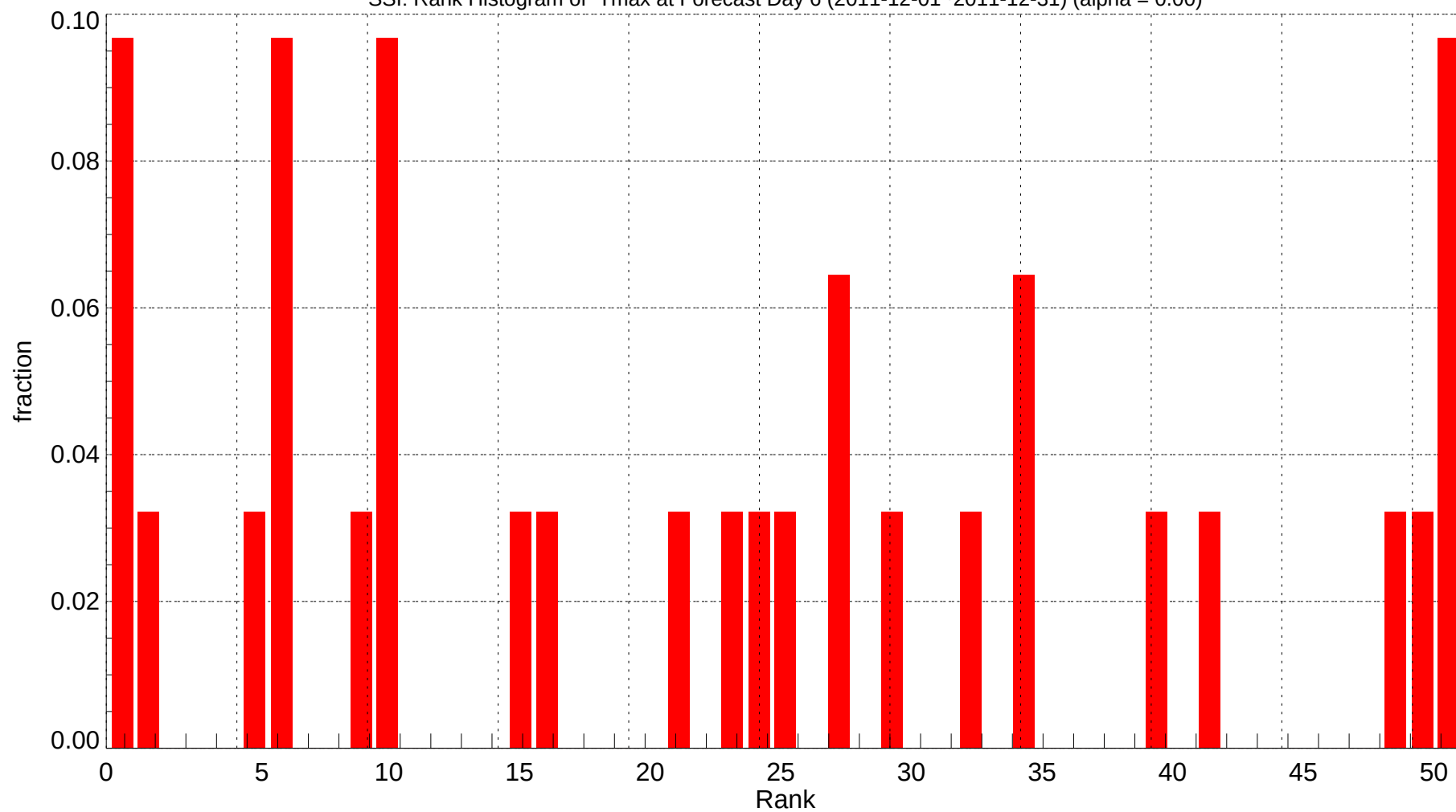
SSI: Rank Histogram of Tmax at Forecast Day 6 (2011-12-01~2011-12-31) (alpha = 0.00)
