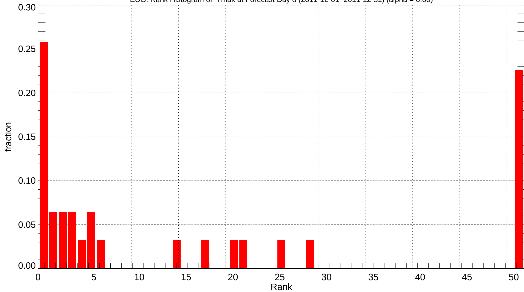
EUG: Rank Histogram of Tmax at Forecast Day 8 (2011-12-01~2011-12-31) (alpha = 0.00)
