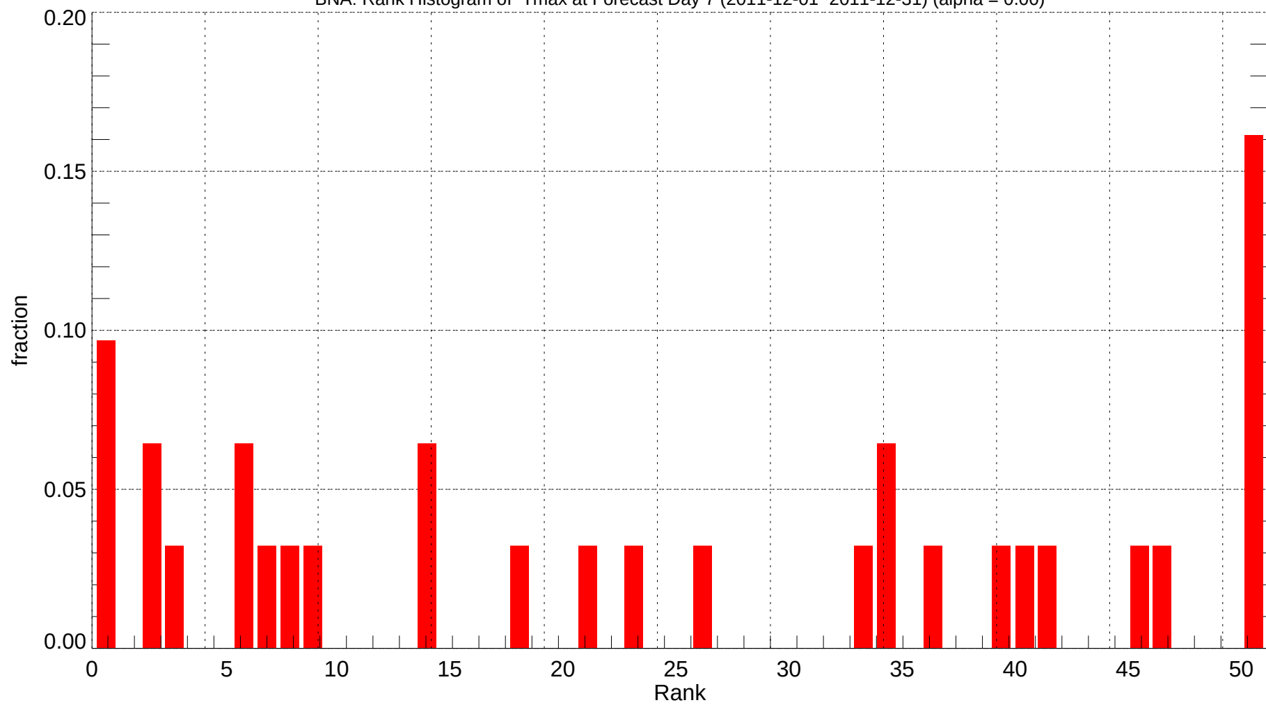
BNA: Rank Histogram of Tmax at Forecast Day 7 (2011-12-01~2011-12-31) (alpha = 0.00)
