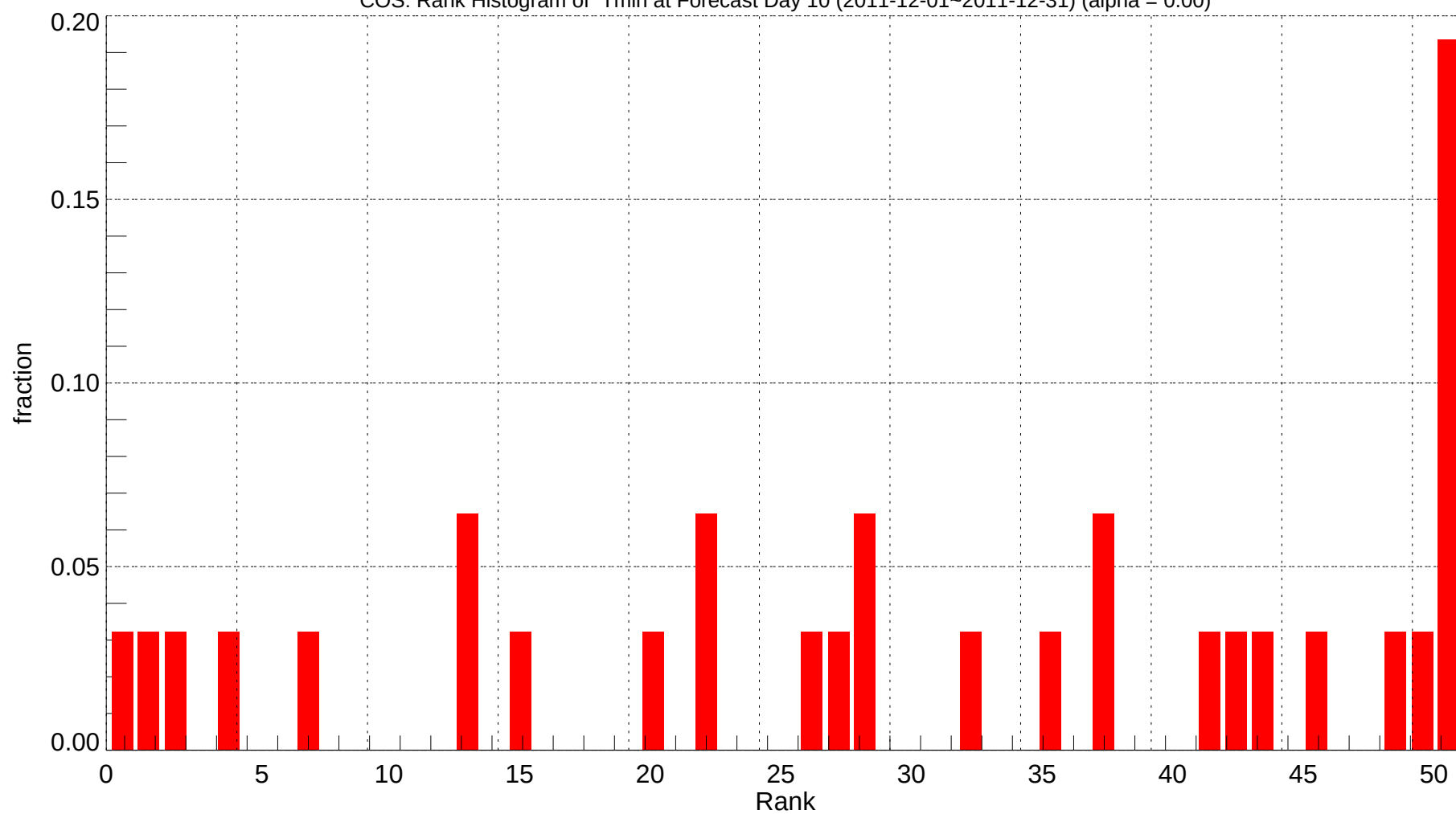
COS: Rank Histogram of Tmin at Forecast Day 10 (2011-12-01~2011-12-31) (alpha = 0.00)
