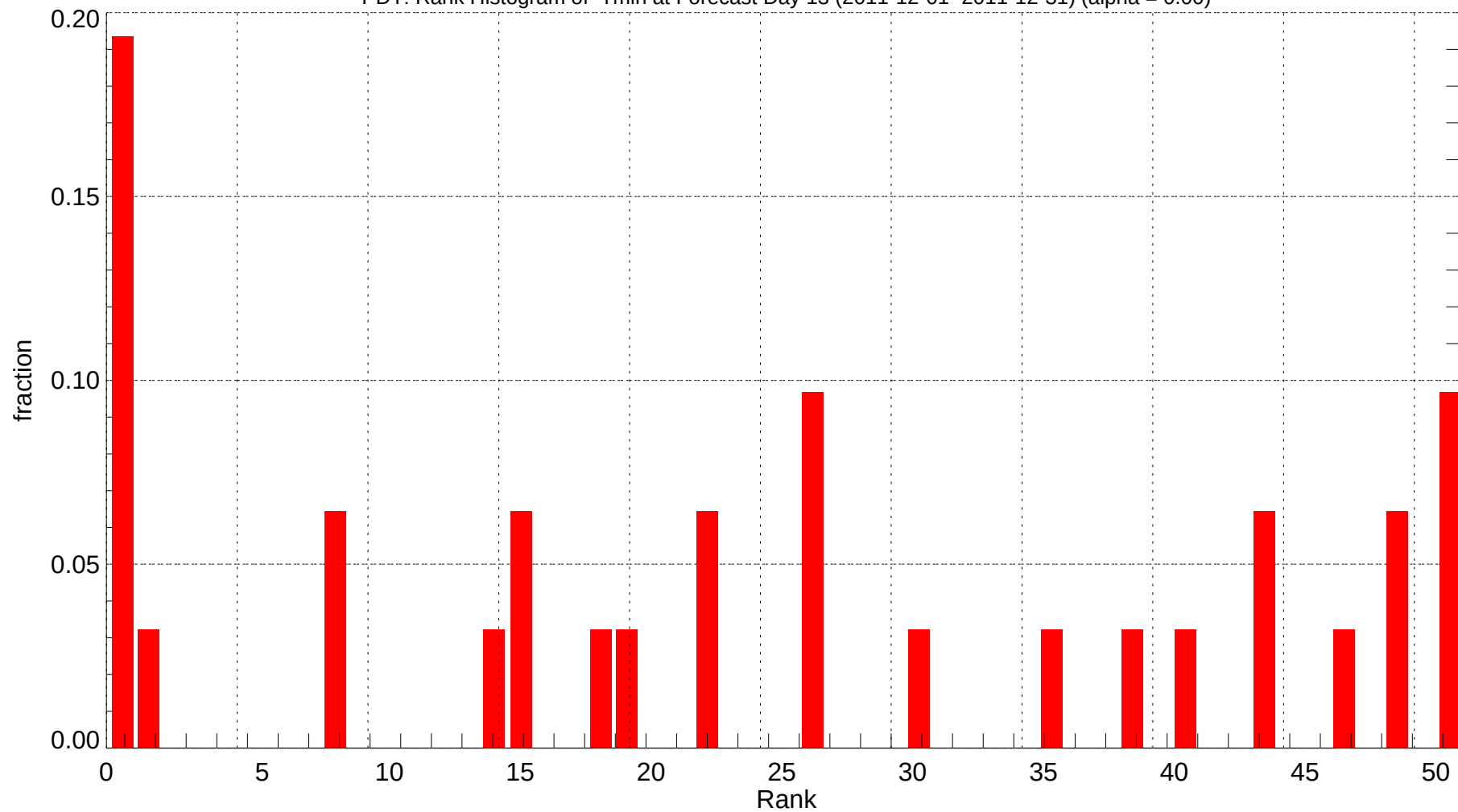
PDT: Rank Histogram of Tmin at Forecast Day 13 (2011-12-01~2011-12-31) (alpha = 0.00)
