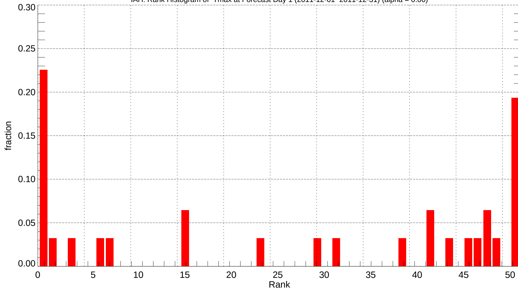
IAH: Rank Histogram of Tmax at Forecast Day 1 (2011-12-01~2011-12-31) (alpha = 0.00)
