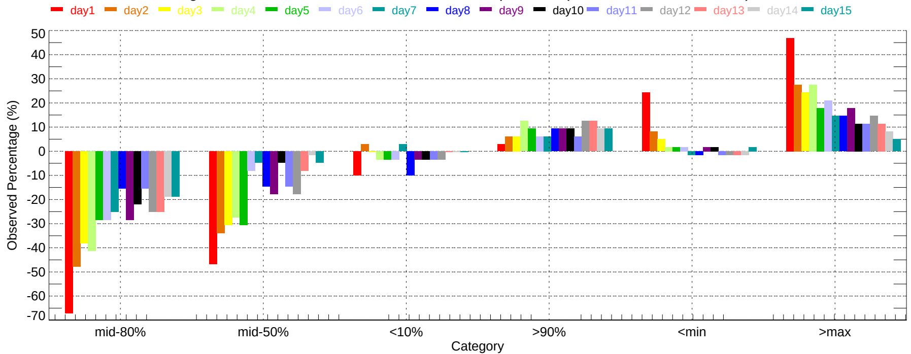
Observed Percentage Deviation of Ensembles - ICT: Max Temperature (2011-12-01~2011-12-31)
