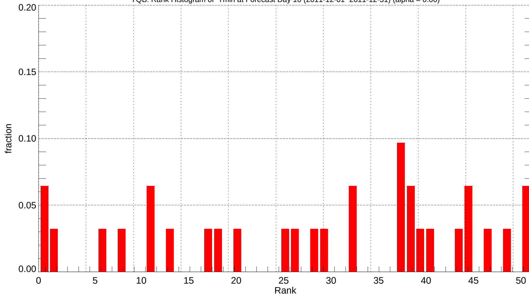
YQB: Rank Histogram of Tmin at Forecast Day 10 (2011-12-01~2011-12-31) (alpha = 0.00)
