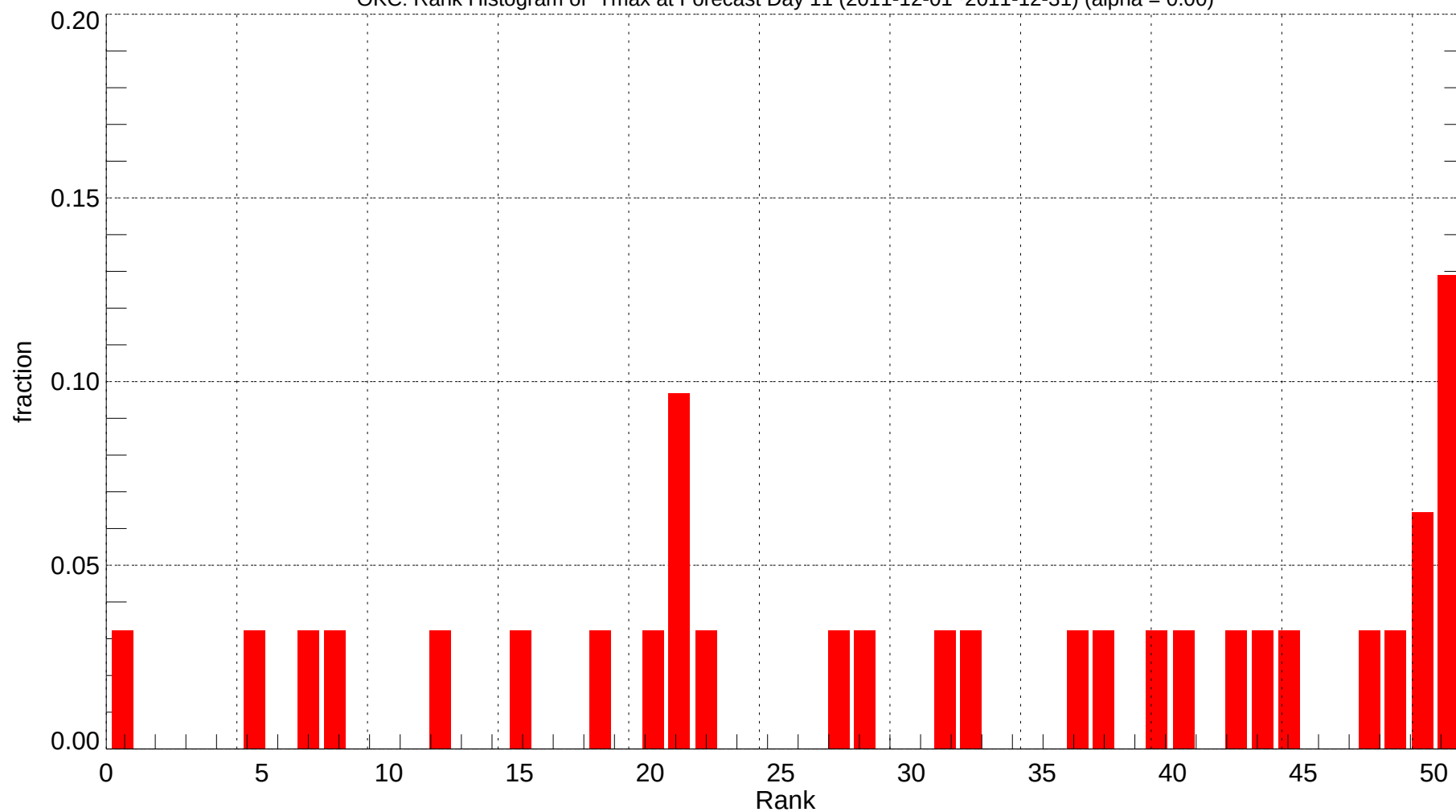
OKC: Rank Histogram of Tmax at Forecast Day 11 (2011-12-01~2011-12-31) (alpha = 0.00)
