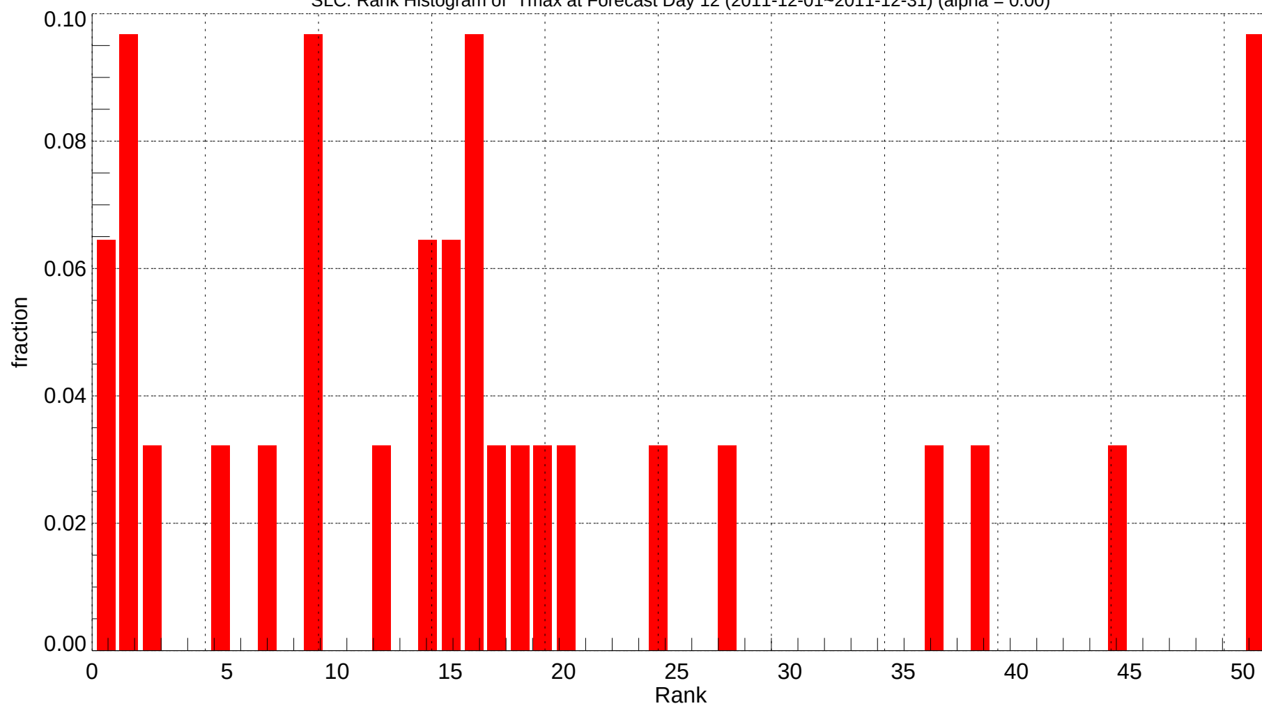
SLC: Rank Histogram of Tmax at Forecast Day 12 (2011-12-01~2011-12-31) (alpha = 0.00)
