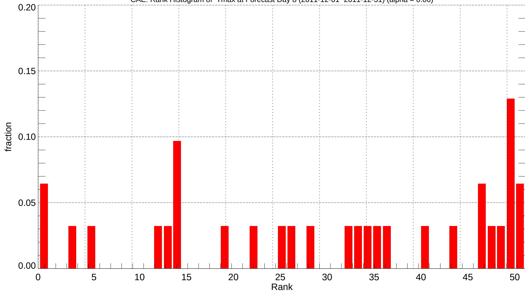
CAE: Rank Histogram of Tmax at Forecast Day 8 (2011-12-01~2011-12-31) (alpha = 0.00)
