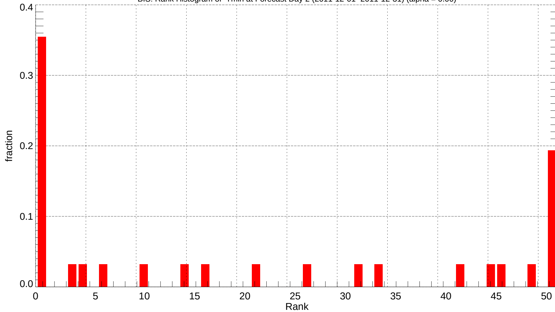
BIS: Rank Histogram of Tmin at Forecast Day 2 (2011-12-01~2011-12-31) (alpha = 0.00)
