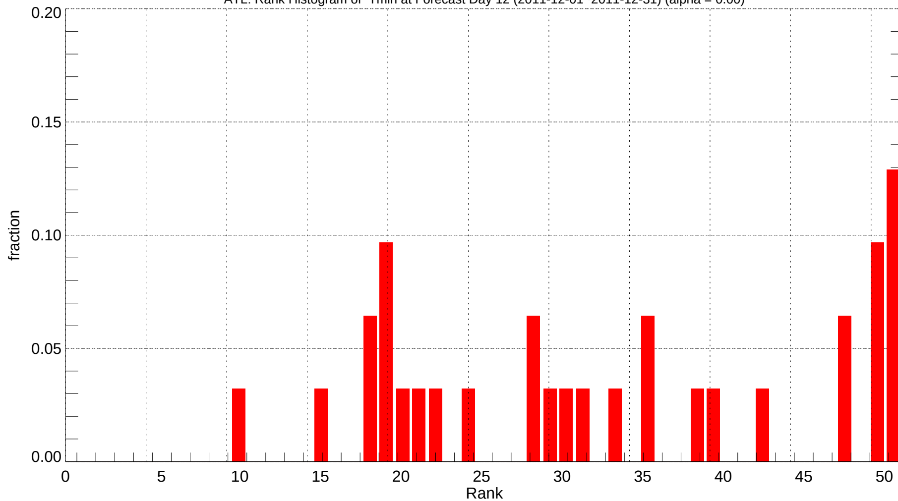
ATL: Rank Histogram of Tmin at Forecast Day 12 (2011-12-01~2011-12-31) (alpha = 0.00)
