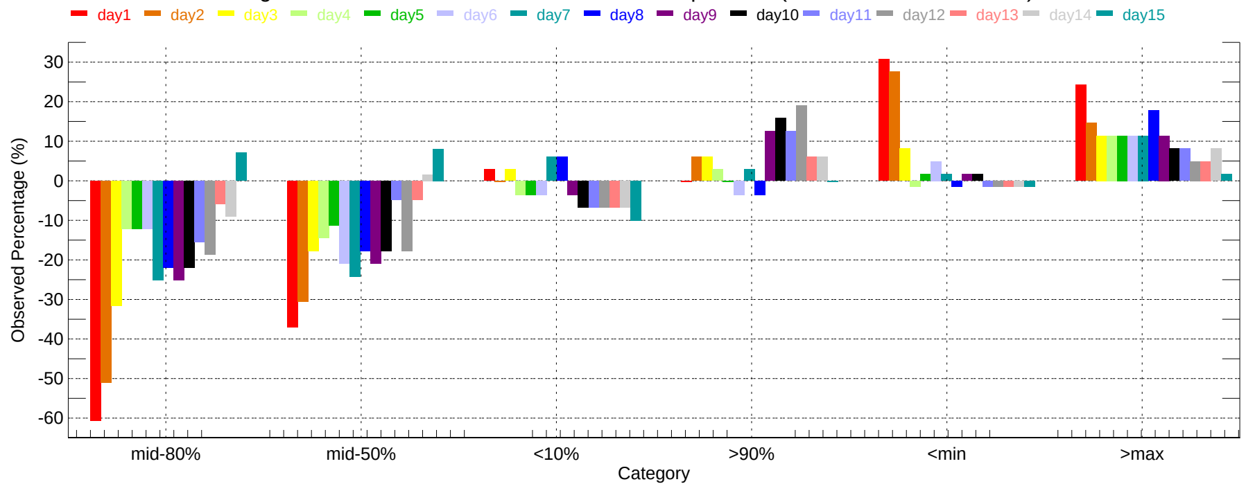
Observed Percentage Deviation of Ensembles - BHM: Min Temperature (2011-12-01~2011-12-31)
