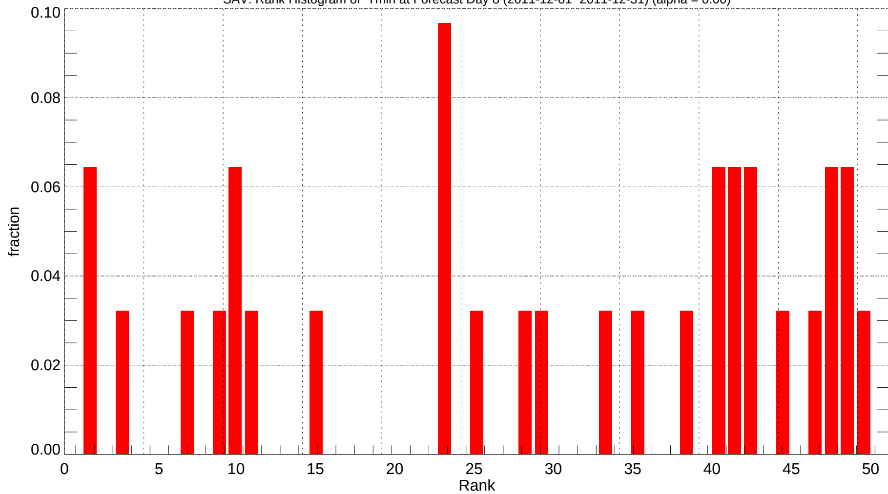
SAV: Rank Histogram of Tmin at Forecast Day 8 (2011-12-01~2011-12-31) (alpha = 0.00)
