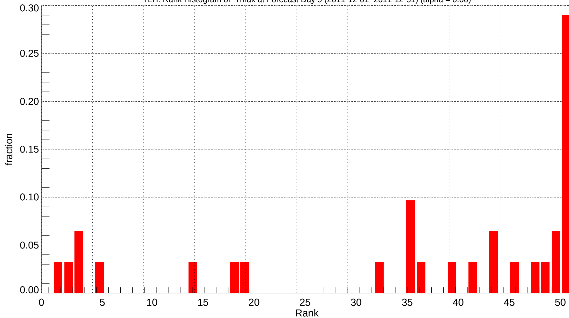
TLH: Rank Histogram of Tmax at Forecast Day 9 (2011-12-01~2011-12-31) (alpha = 0.00)
