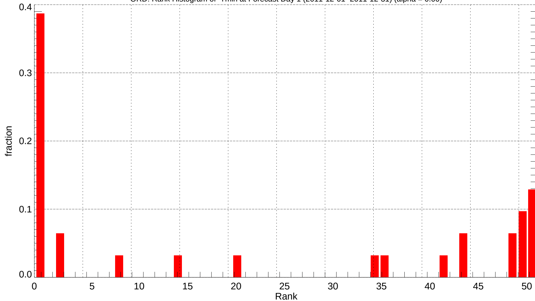
ORD: Rank Histogram of Tmin at Forecast Day 1 (2011-12-01~2011-12-31) (alpha = 0.00)
