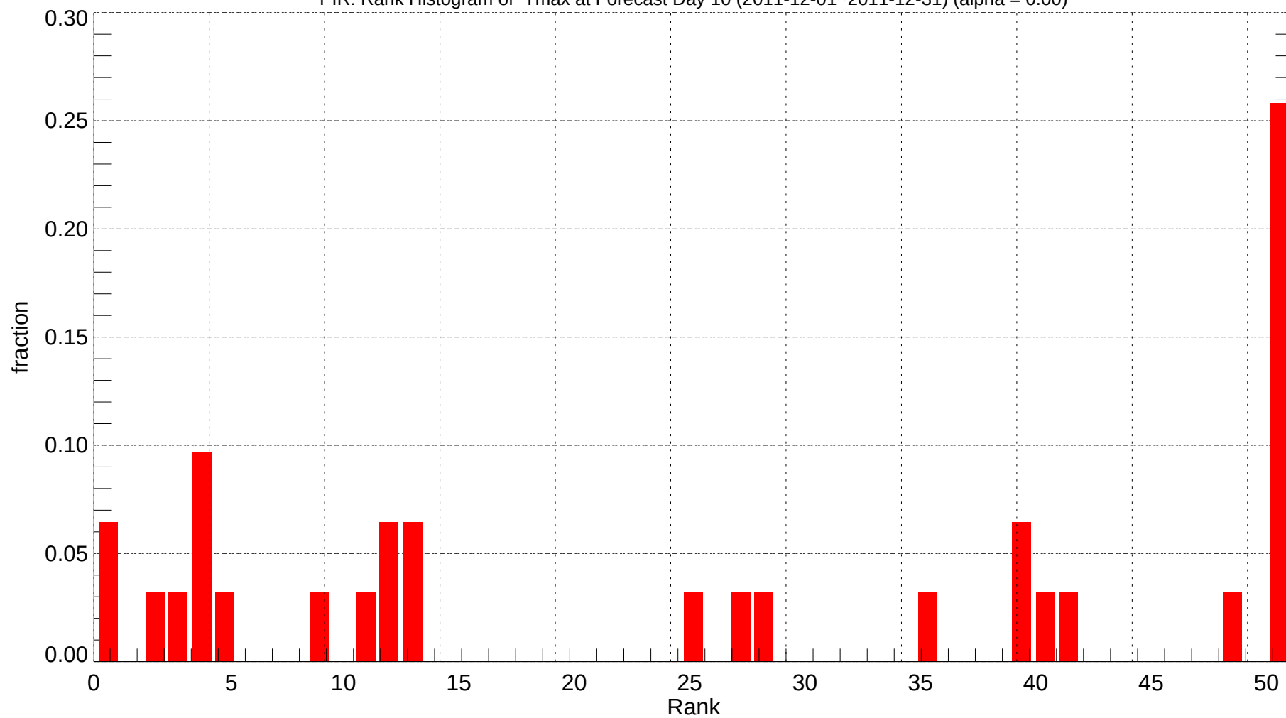
PIR: Rank Histogram of Tmax at Forecast Day 10 (2011-12-01~2011-12-31) (alpha = 0.00)
