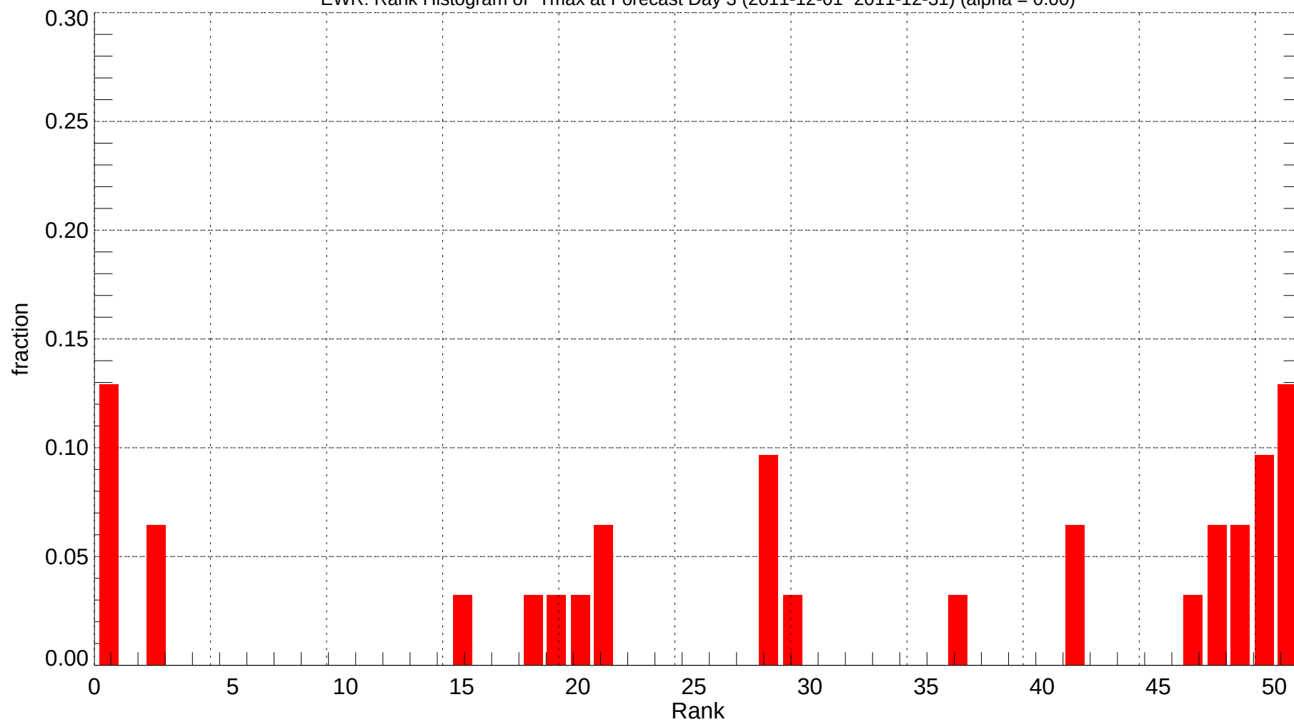
EWR: Rank Histogram of Tmax at Forecast Day 3 (2011-12-01~2011-12-31) (alpha = 0.00)
