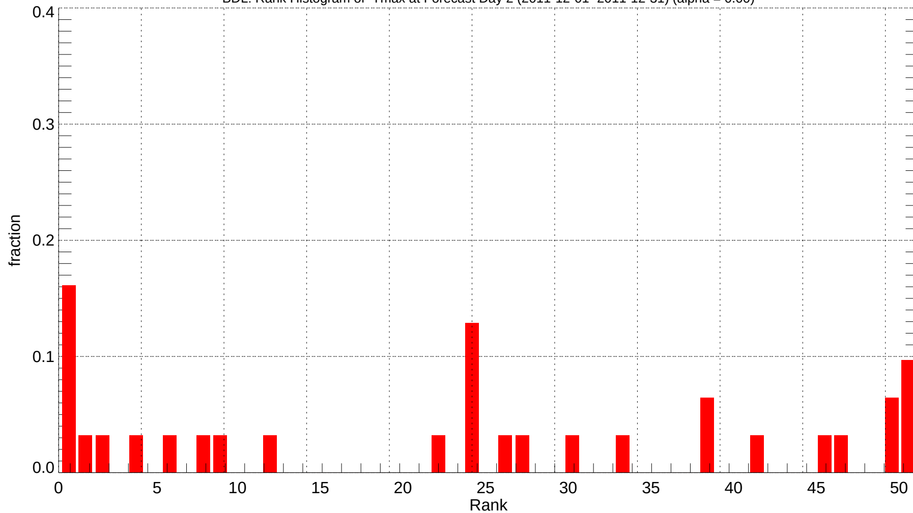
BDL: Rank Histogram of Tmax at Forecast Day 2 (2011-12-01~2011-12-31) (alpha = 0.00)
