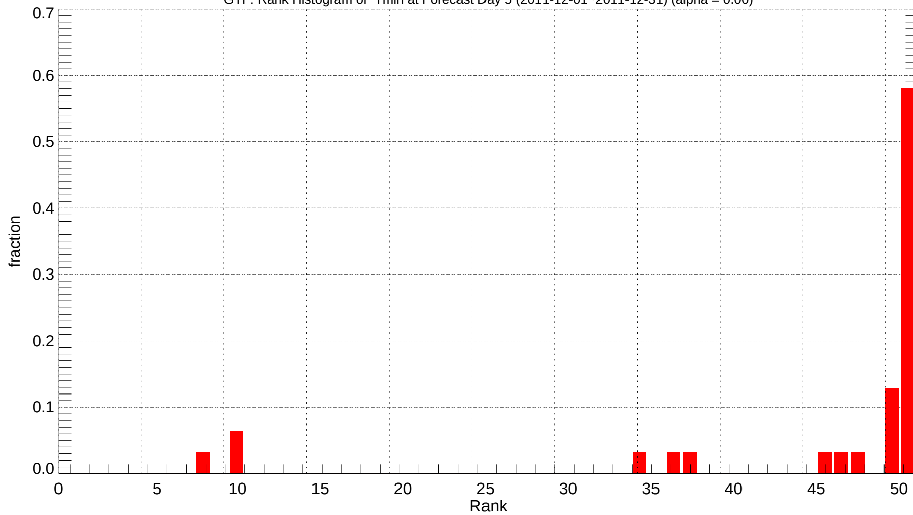
GTF: Rank Histogram of Tmin at Forecast Day 5 (2011-12-01~2011-12-31) (alpha = 0.00)
