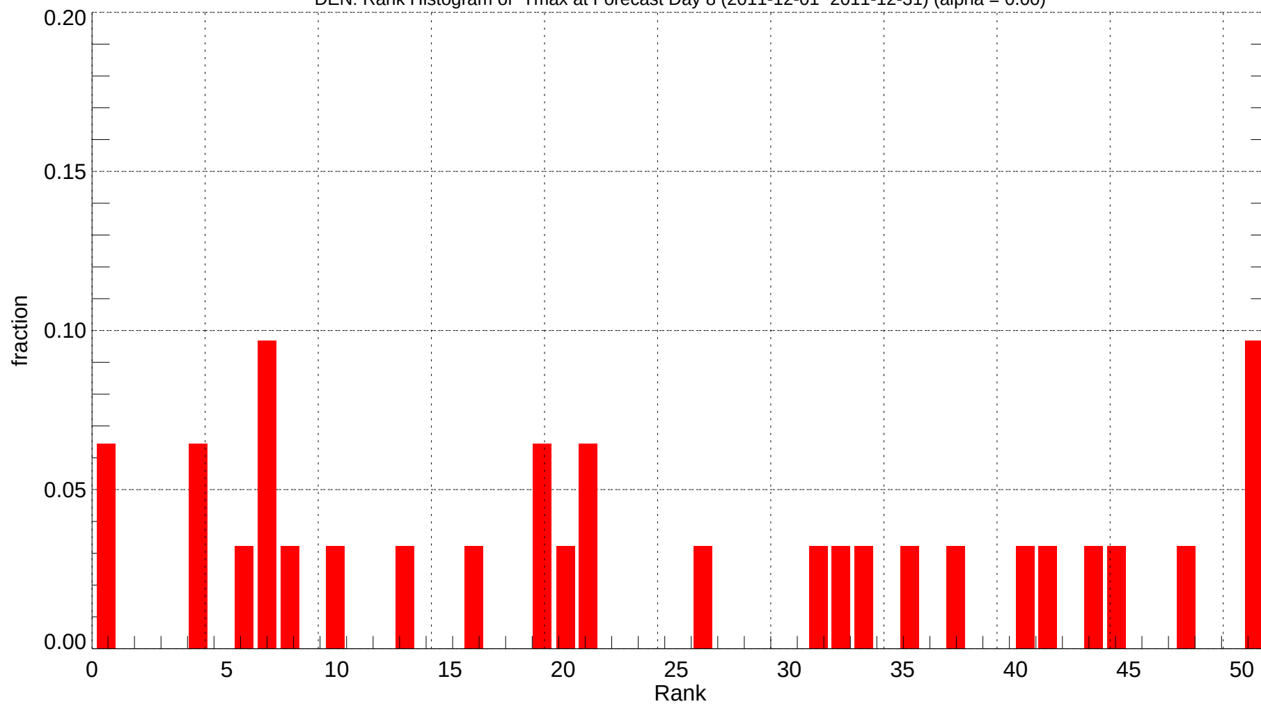
DEN: Rank Histogram of Tmax at Forecast Day 8 (2011-12-01~2011-12-31) (alpha = 0.00)
