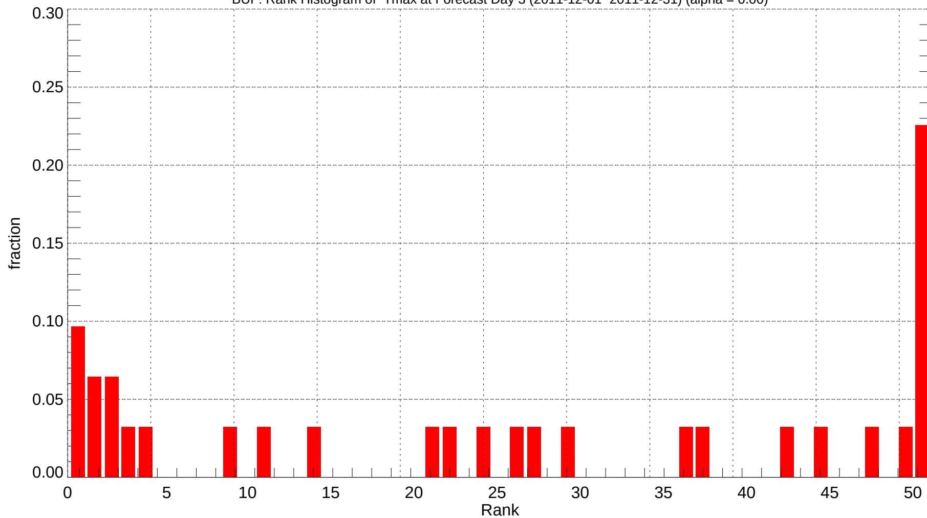
BUF: Rank Histogram of Tmax at Forecast Day 3 (2011-12-01~2011-12-31) (alpha = 0.00)
