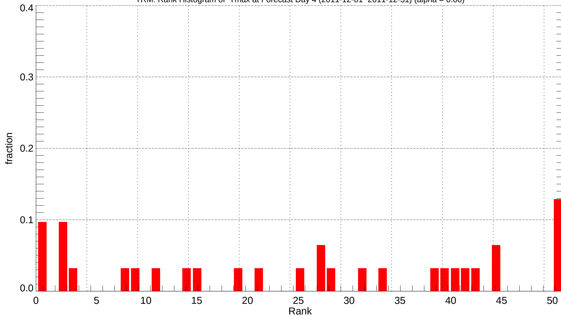
TRM: Rank Histogram of Tmax at Forecast Day 4 (2011-12-01~2011-12-31) (alpha = 0.00)
