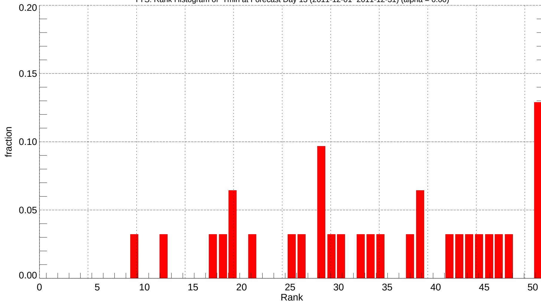
TYS: Rank Histogram of Tmin at Forecast Day 13 (2011-12-01~2011-12-31) (alpha = 0.00)
