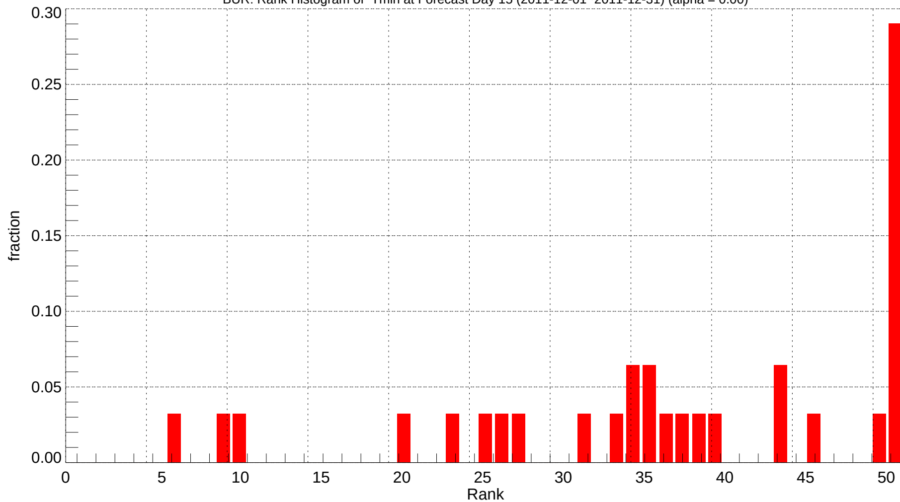
BUR: Rank Histogram of Tmin at Forecast Day 15 (2011-12-01~2011-12-31) (alpha = 0.00)
