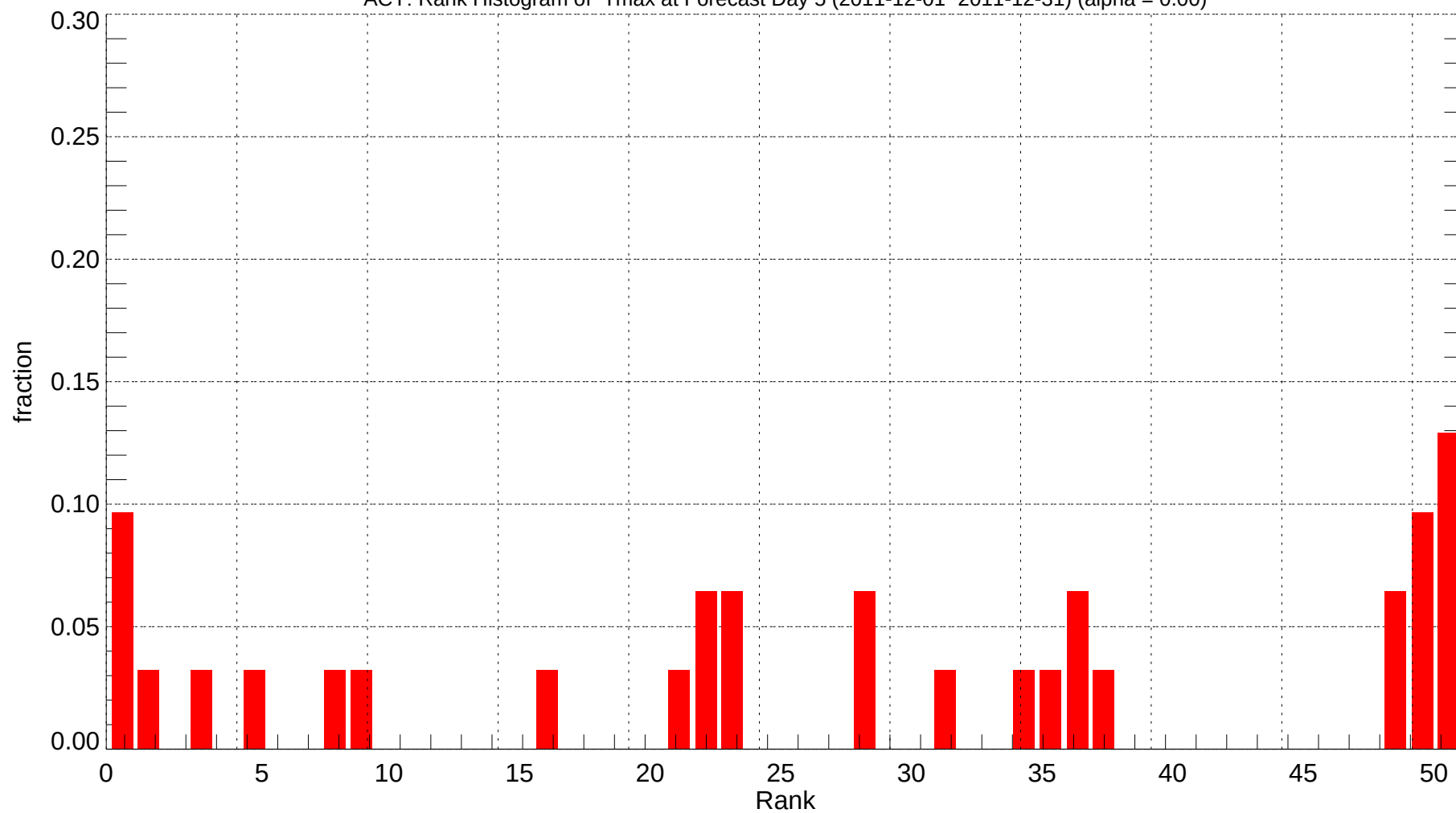
ACY: Rank Histogram of Tmax at Forecast Day 5 (2011-12-01~2011-12-31) (alpha = 0.00)
