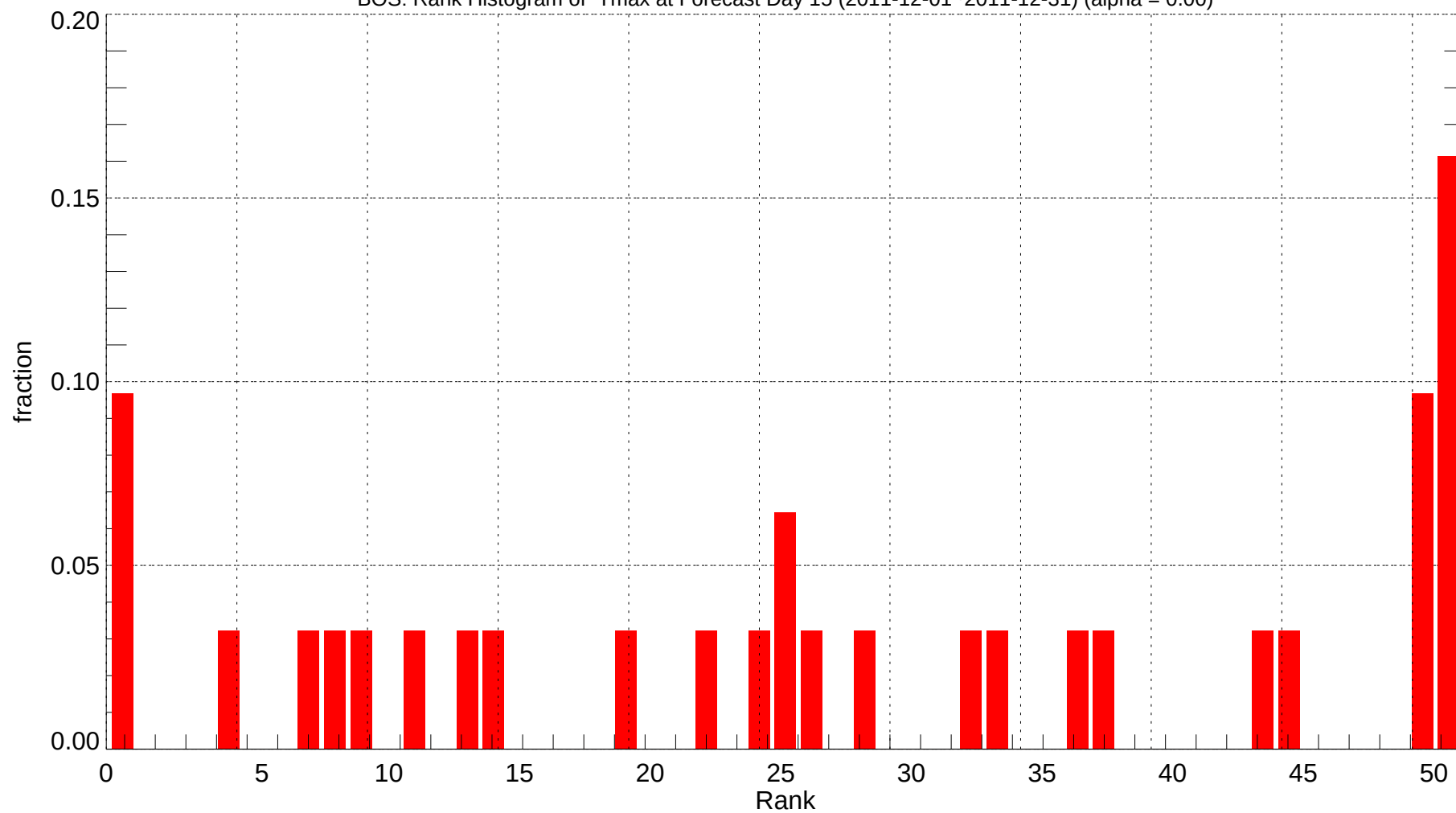
BOS: Rank Histogram of Tmax at Forecast Day 15 (2011-12-01~2011-12-31) (alpha = 0.00)
