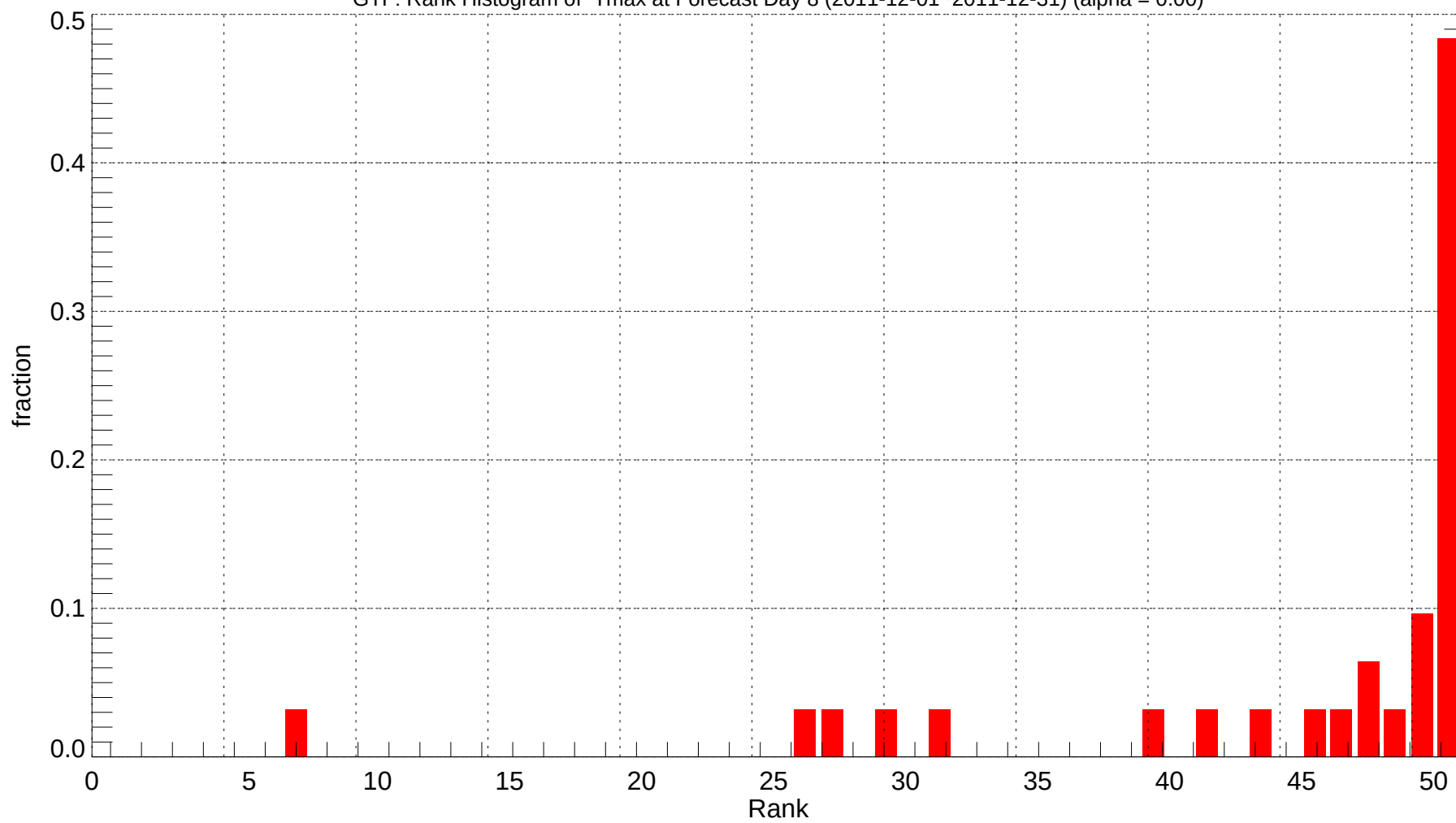
GTF: Rank Histogram of Tmax at Forecast Day 8 (2011-12-01~2011-12-31) (alpha = 0.00)
