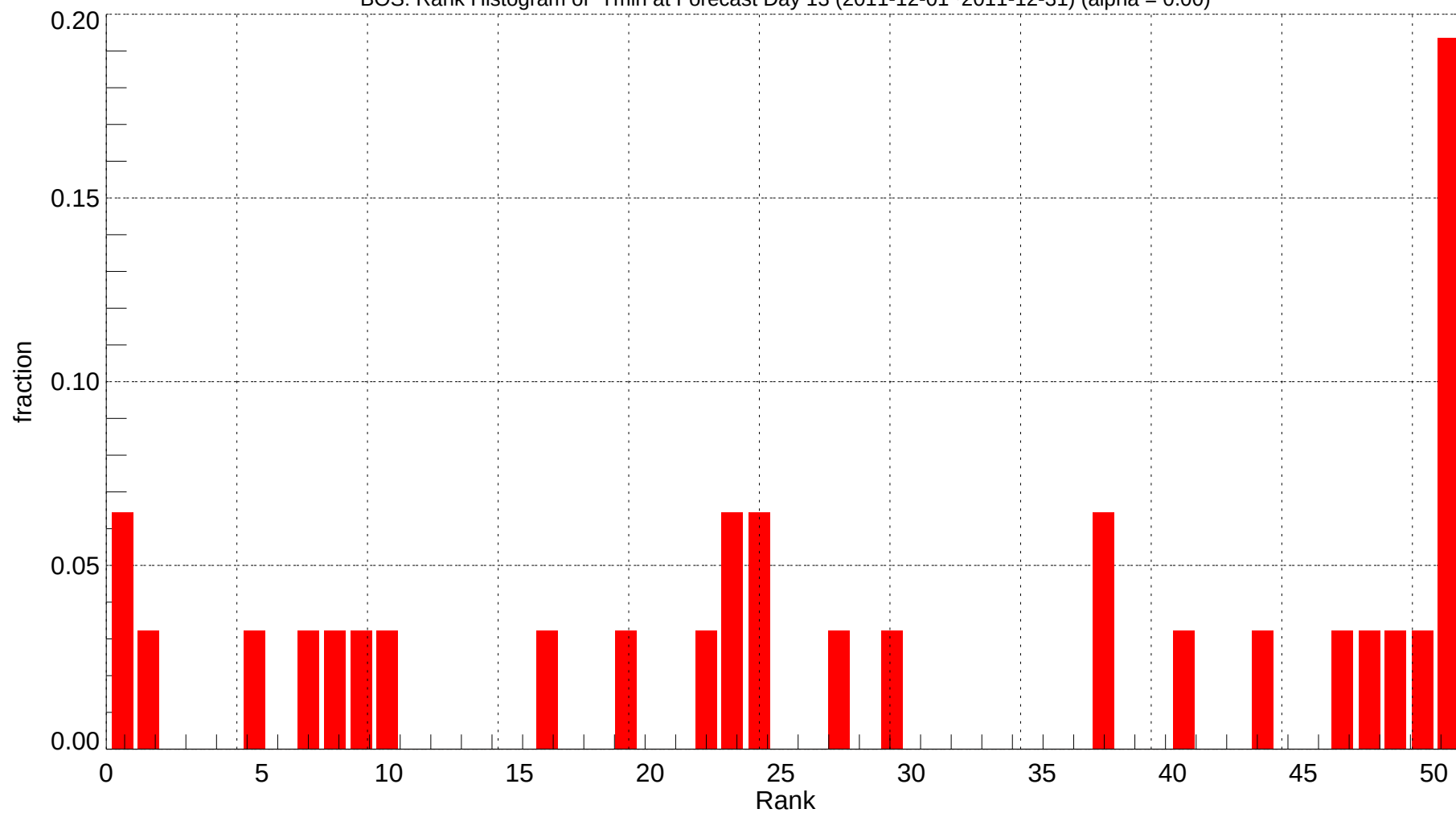
BOS: Rank Histogram of Tmin at Forecast Day 13 (2011-12-01~2011-12-31) (alpha = 0.00)
