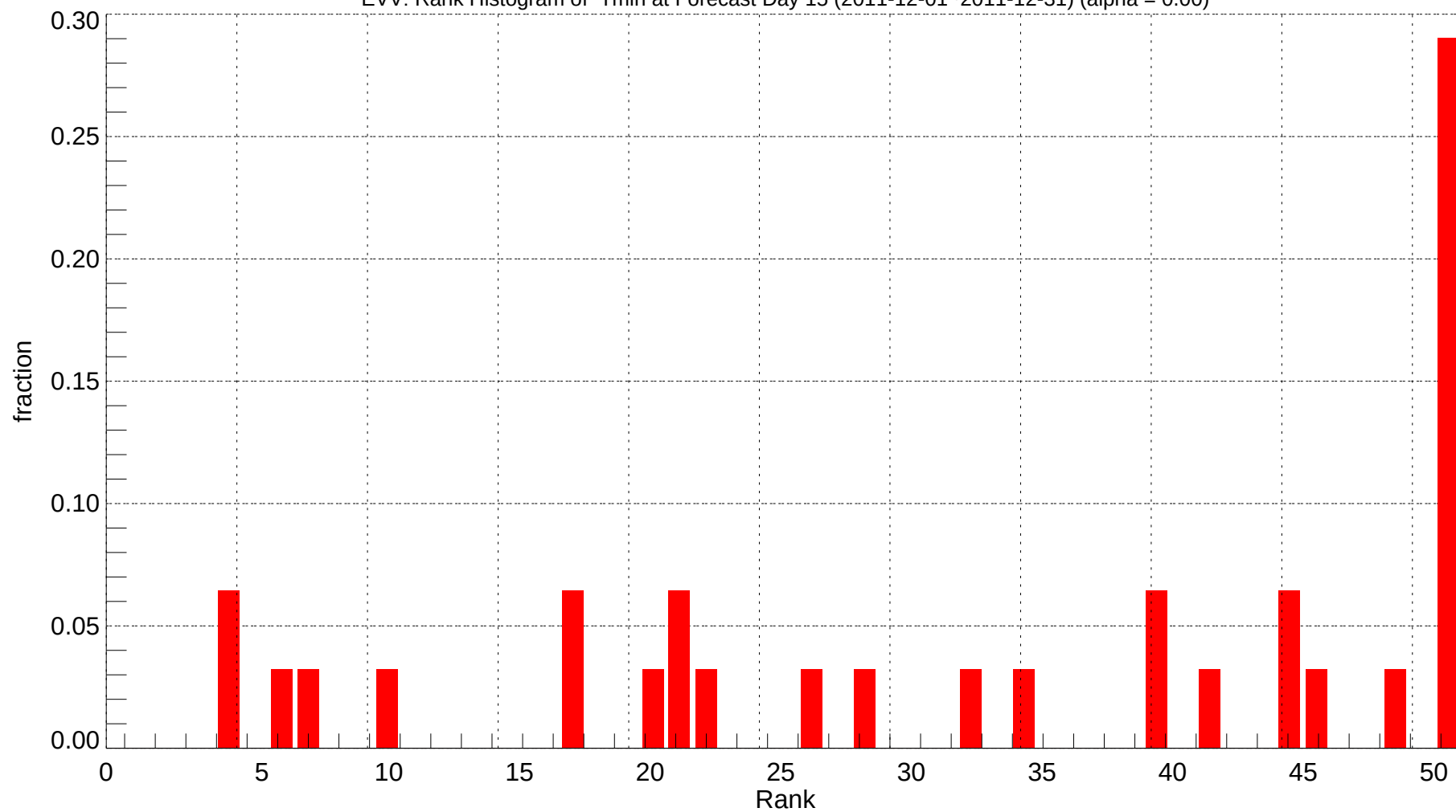
EVV: Rank Histogram of Tmin at Forecast Day 15 (2011-12-01~2011-12-31) (alpha = 0.00)
