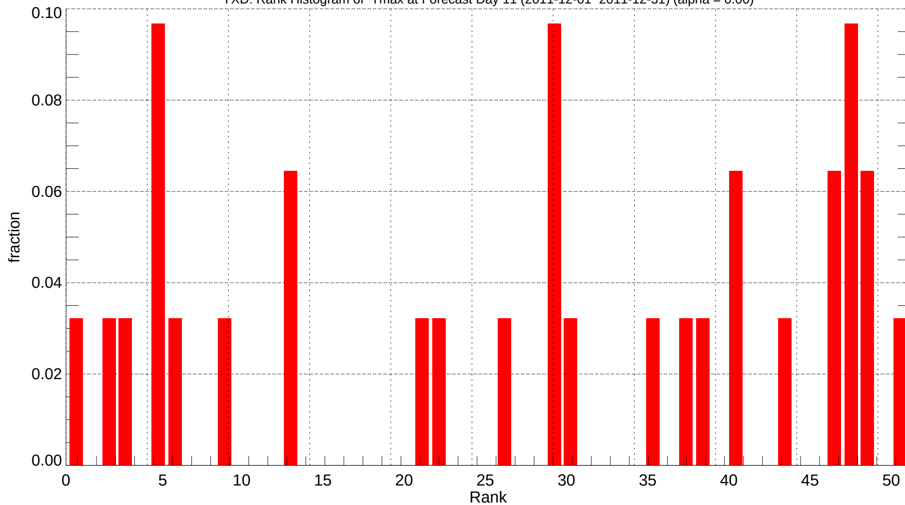
YXD: Rank Histogram of Tmax at Forecast Day 11 (2011-12-01~2011-12-31) (alpha = 0.00)
