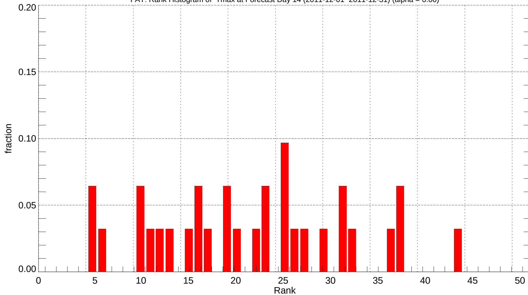
FAT: Rank Histogram of Tmax at Forecast Day 14 (2011-12-01~2011-12-31) (alpha = 0.00)
