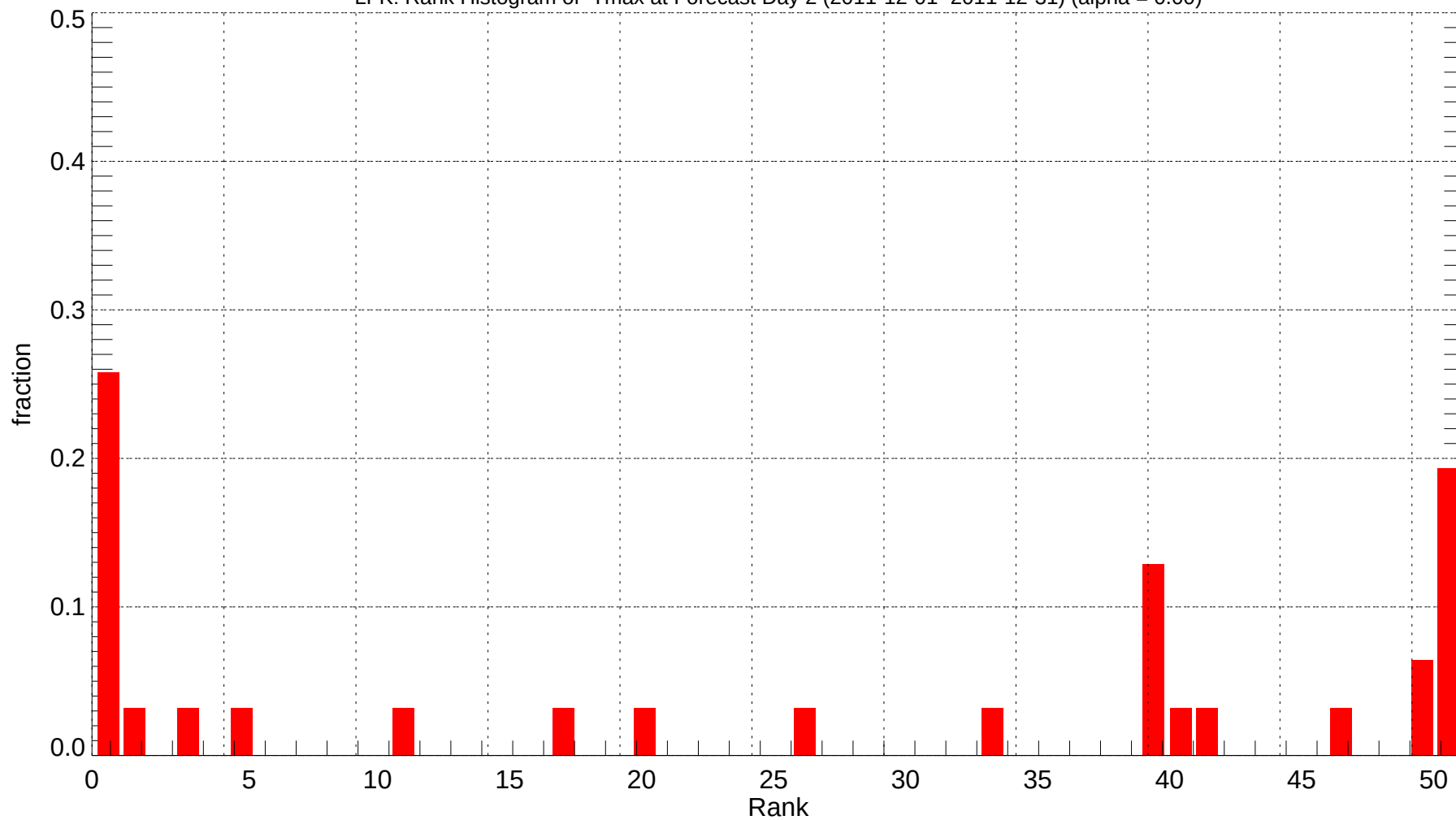
LFK: Rank Histogram of Tmax at Forecast Day 2 (2011-12-01~2011-12-31) (alpha = 0.00)
