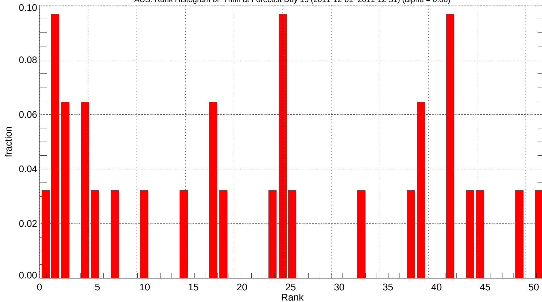
AUS: Rank Histogram of Tmin at Forecast Day 15 (2011-12-01~2011-12-31) (alpha = 0.00)
