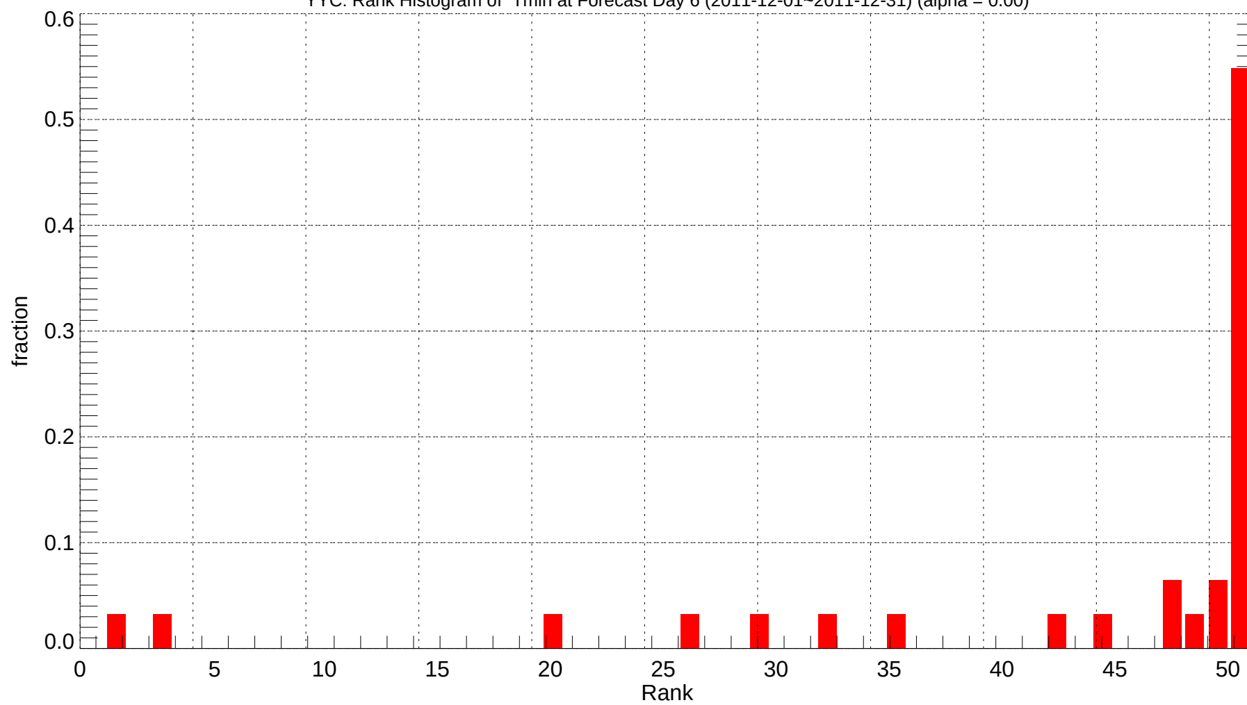
YYC: Rank Histogram of Tmin at Forecast Day 6 (2011-12-01~2011-12-31) (alpha = 0.00)
