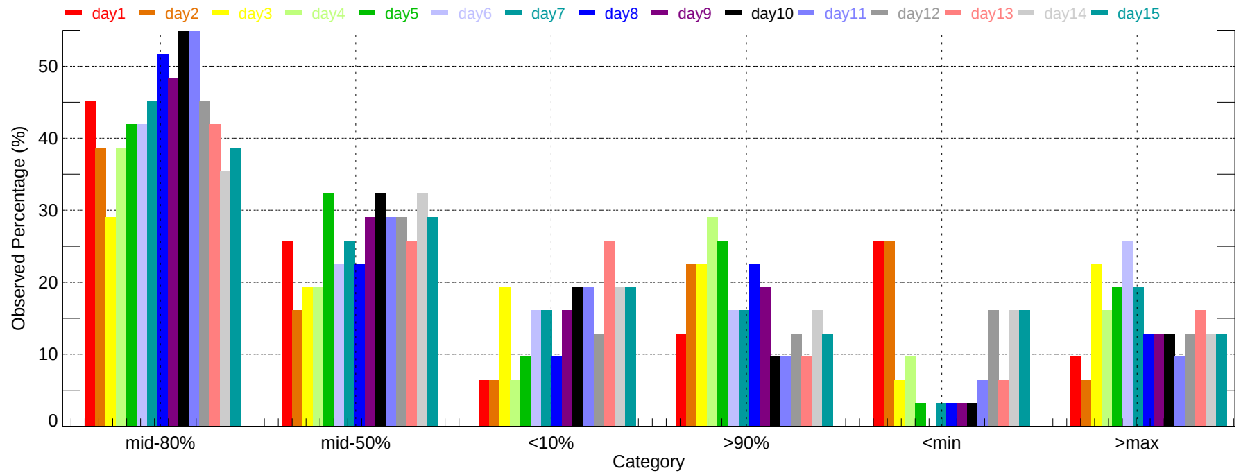
Observed Percentage of Ensembles - LFK: Max Temperature (2011-12-01~2011-12-31)
