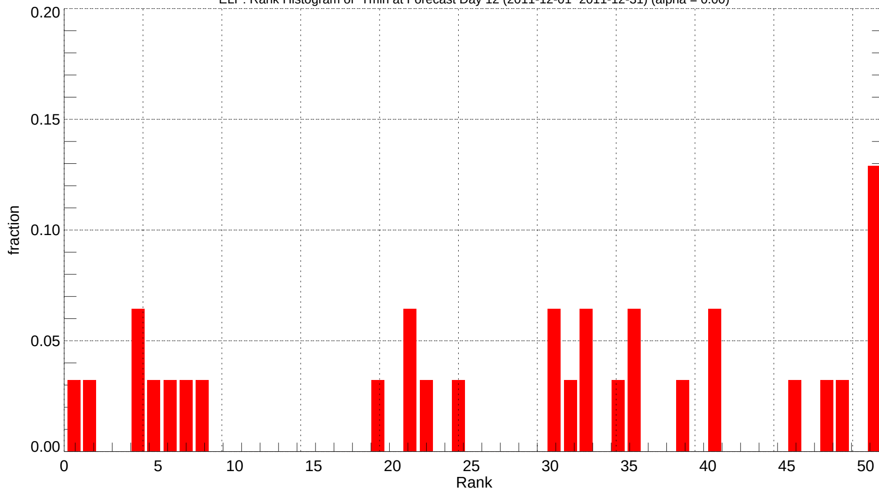
ELP: Rank Histogram of Tmin at Forecast Day 12 (2011-12-01~2011-12-31) (alpha = 0.00)
