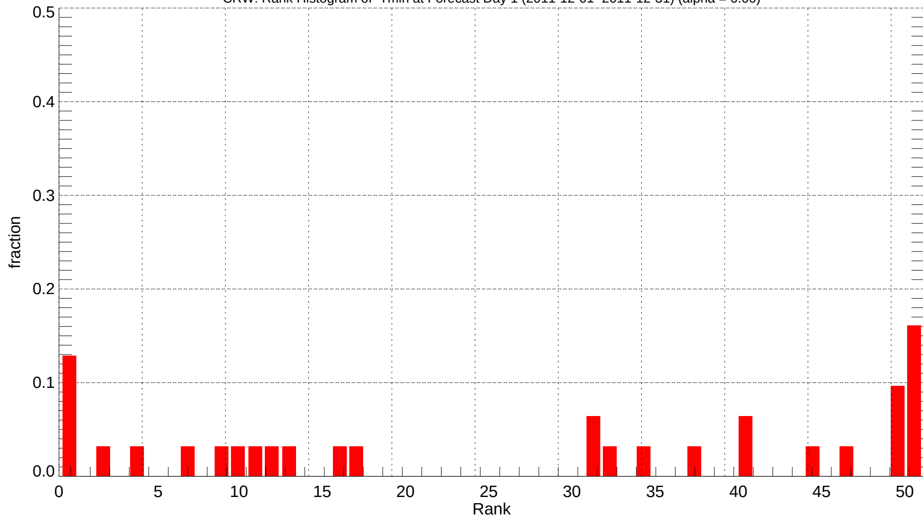
CRW: Rank Histogram of Tmin at Forecast Day 1 (2011-12-01~2011-12-31) (alpha = 0.00)
