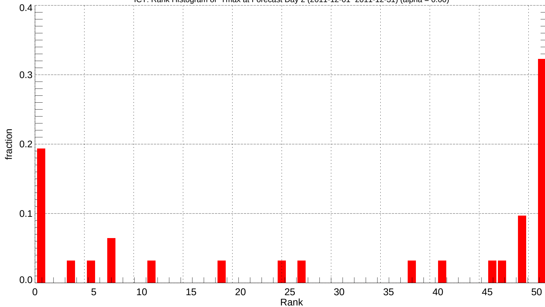
ICT: Rank Histogram of Tmax at Forecast Day 2 (2011-12-01~2011-12-31) (alpha = 0.00)
