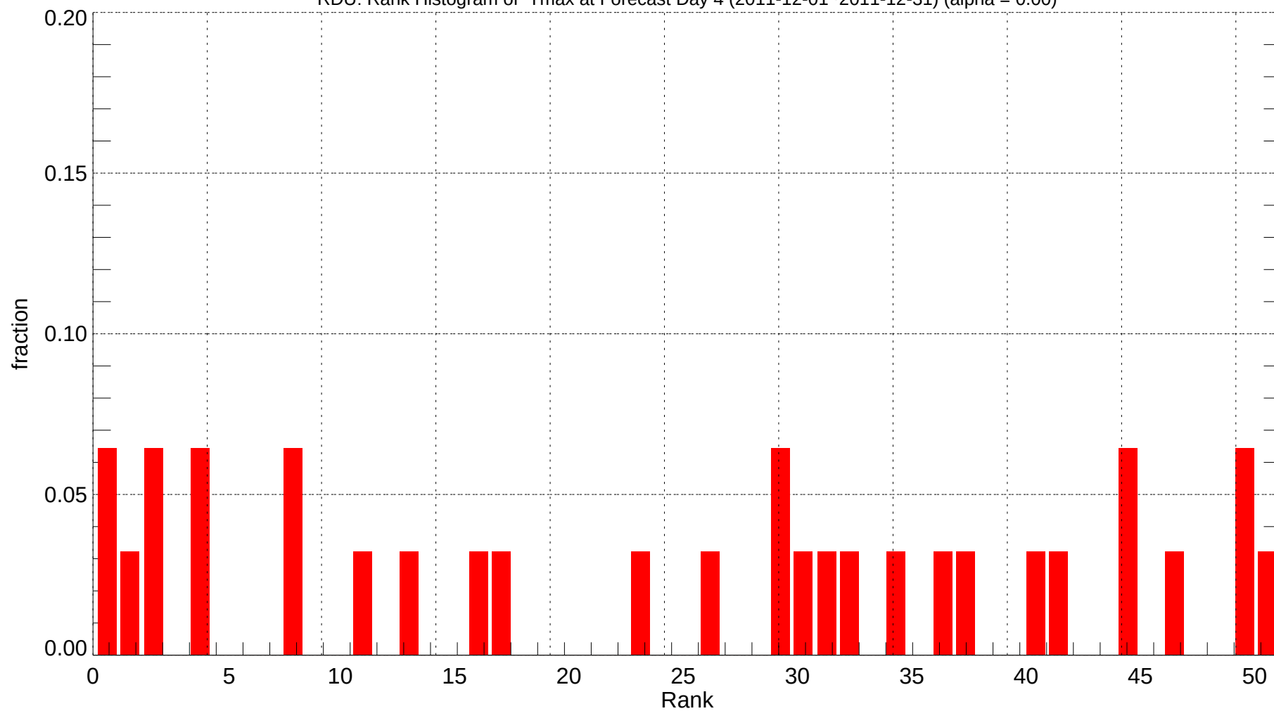
RDU: Rank Histogram of Tmax at Forecast Day 4 (2011-12-01~2011-12-31) (alpha = 0.00)
