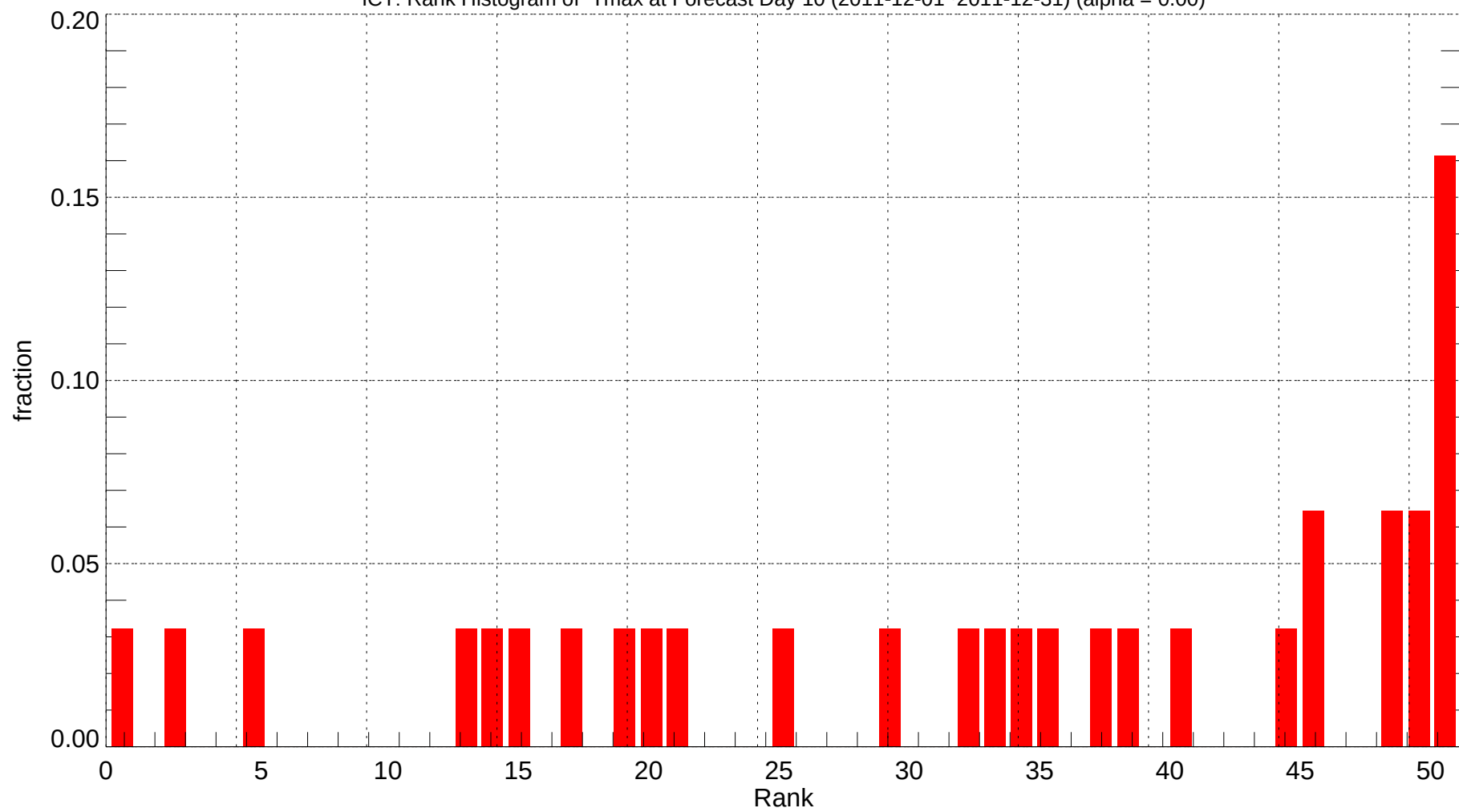
ICT: Rank Histogram of Tmax at Forecast Day 10 (2011-12-01~2011-12-31) (alpha = 0.00)
