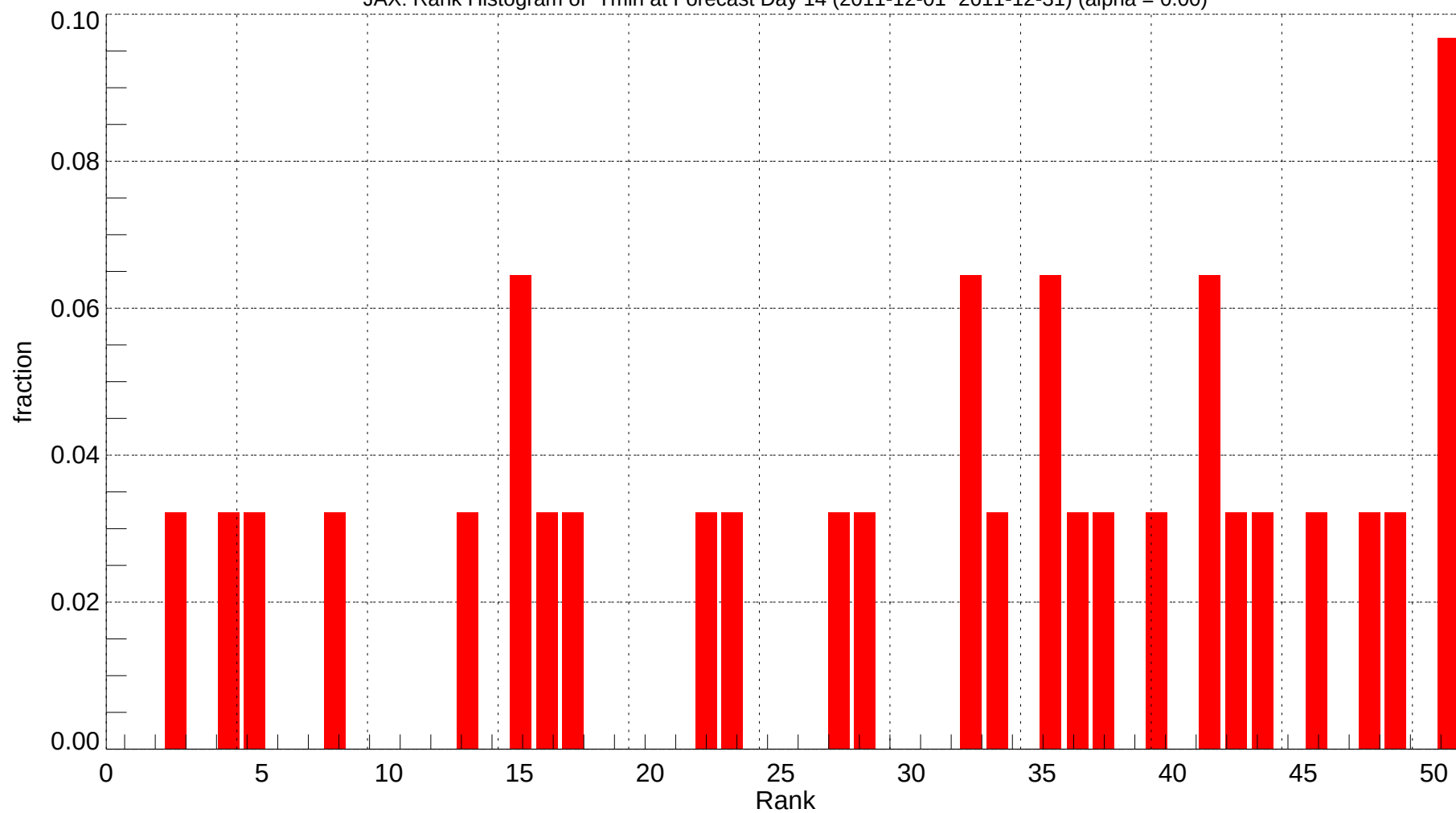
JAX: Rank Histogram of Tmin at Forecast Day 14 (2011-12-01~2011-12-31) (alpha = 0.00)
