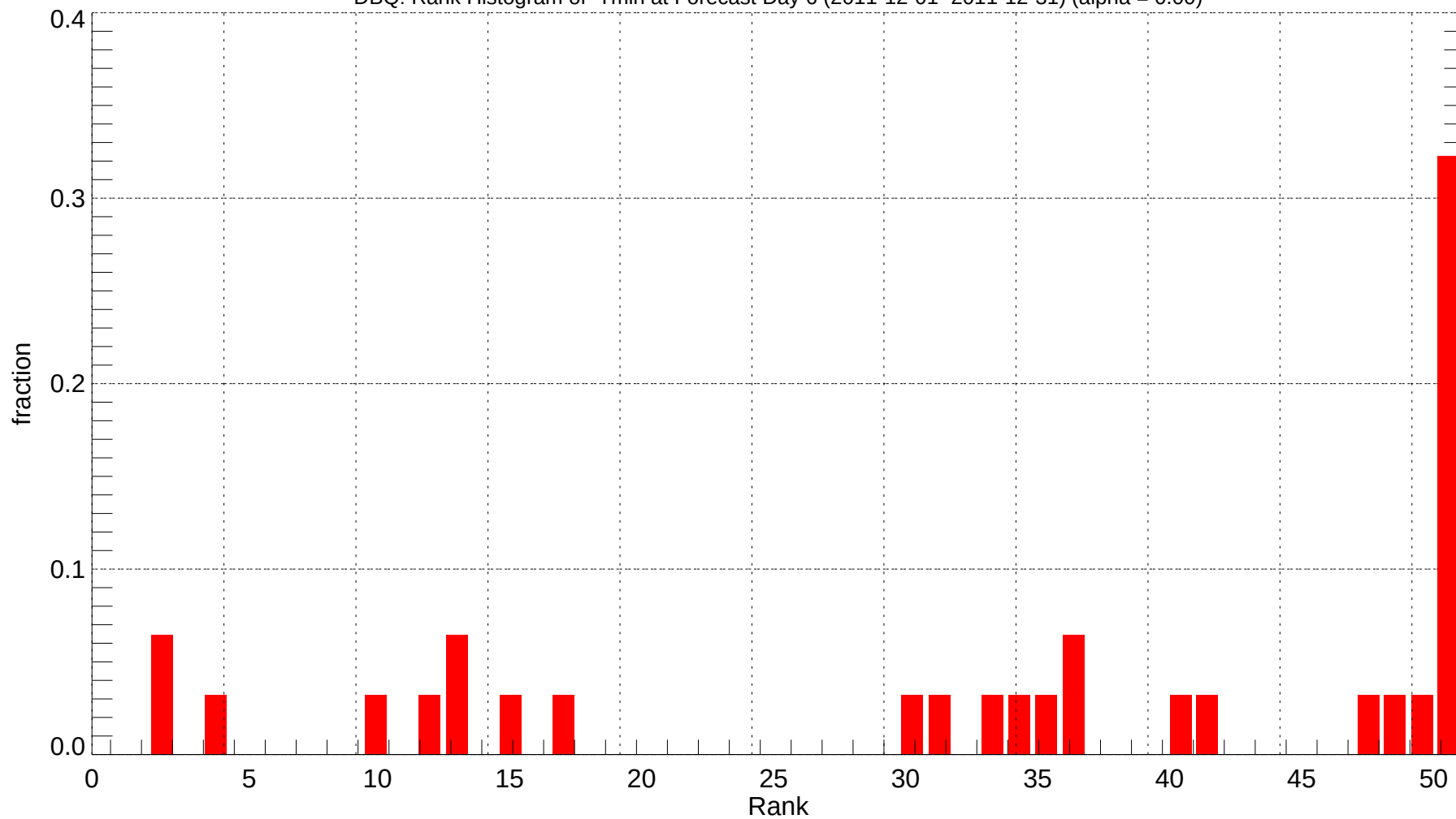
DBQ: Rank Histogram of Tmin at Forecast Day 6 (2011-12-01~2011-12-31) (alpha = 0.00)
