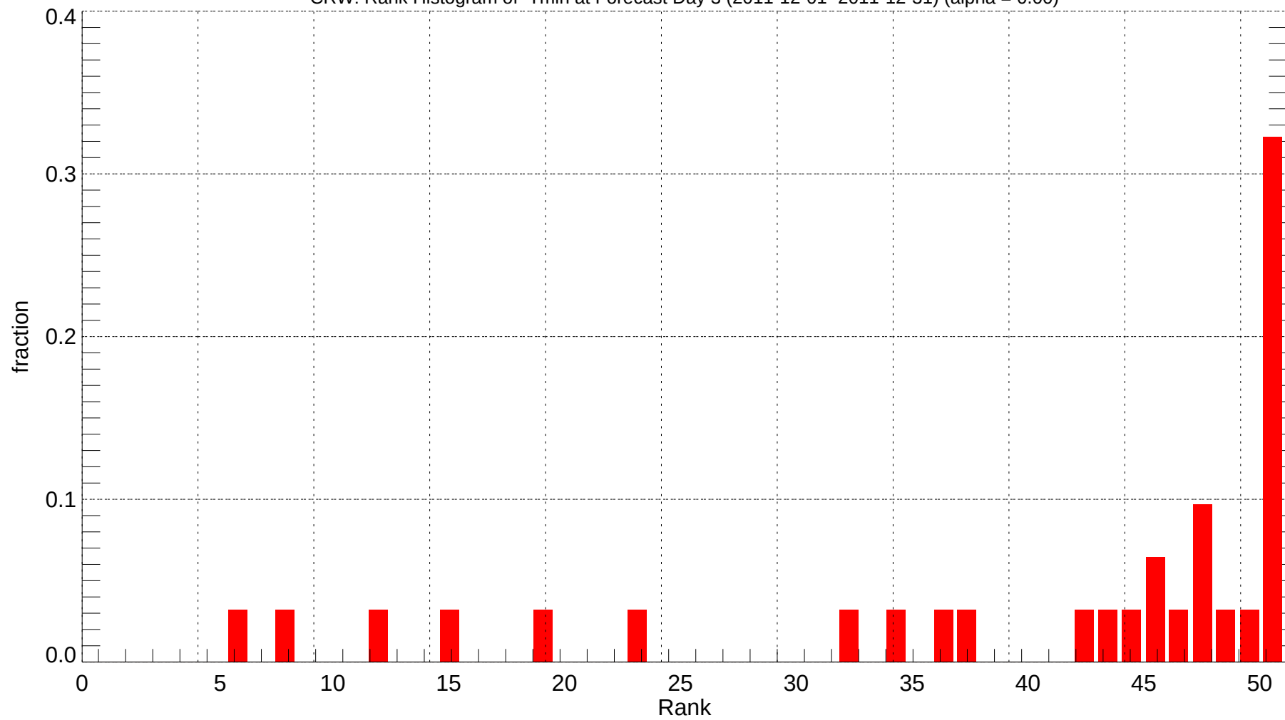
CRW: Rank Histogram of Tmin at Forecast Day 3 (2011-12-01~2011-12-31) (alpha = 0.00)
