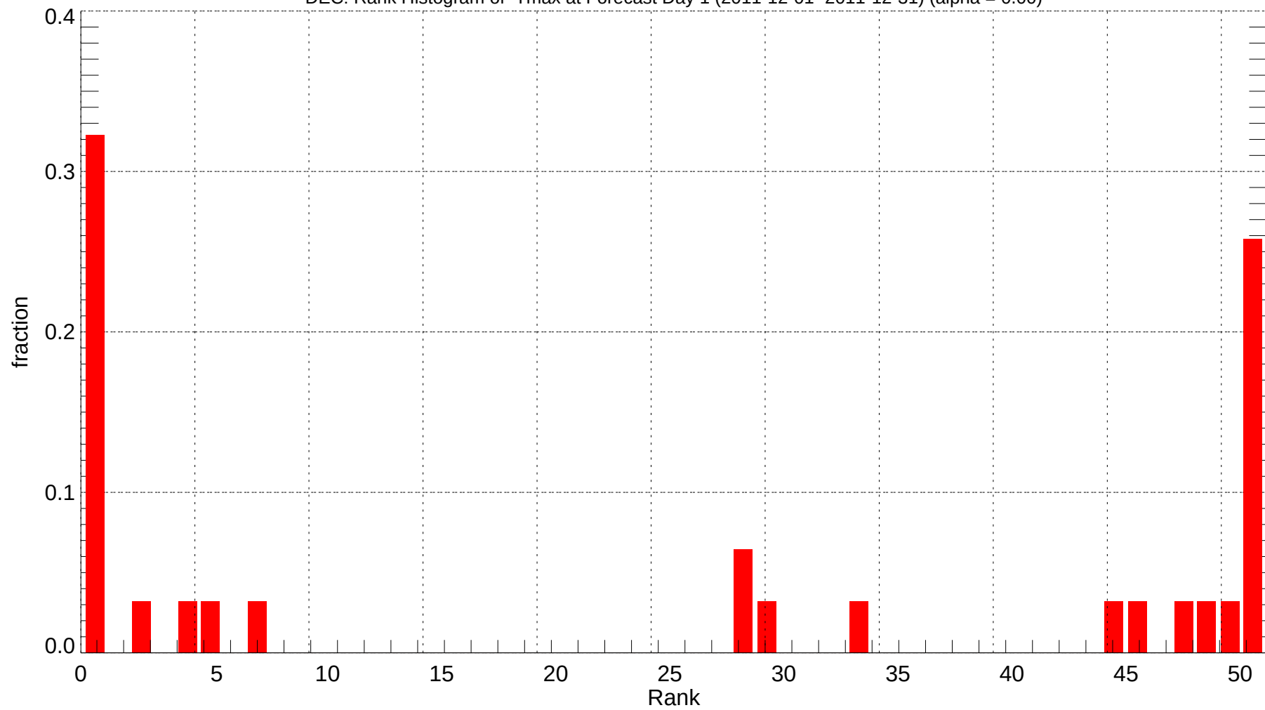
DEC: Rank Histogram of Tmax at Forecast Day 1 (2011-12-01~2011-12-31) (alpha = 0.00)
