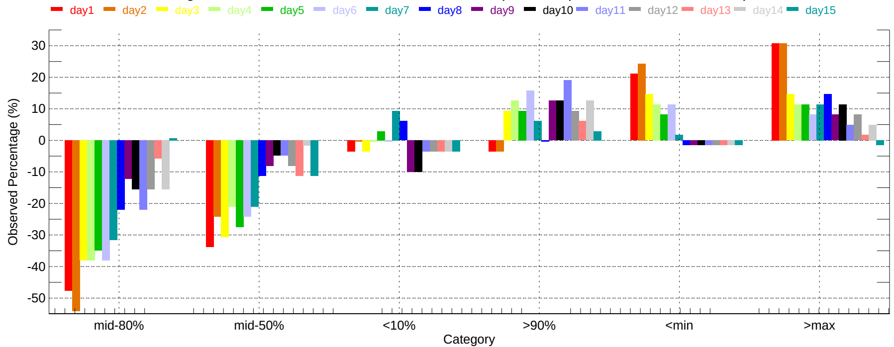
Observed Percentage Deviation of Ensembles - MEM: Max Temperature (2011-12-01~2011-12-31)
