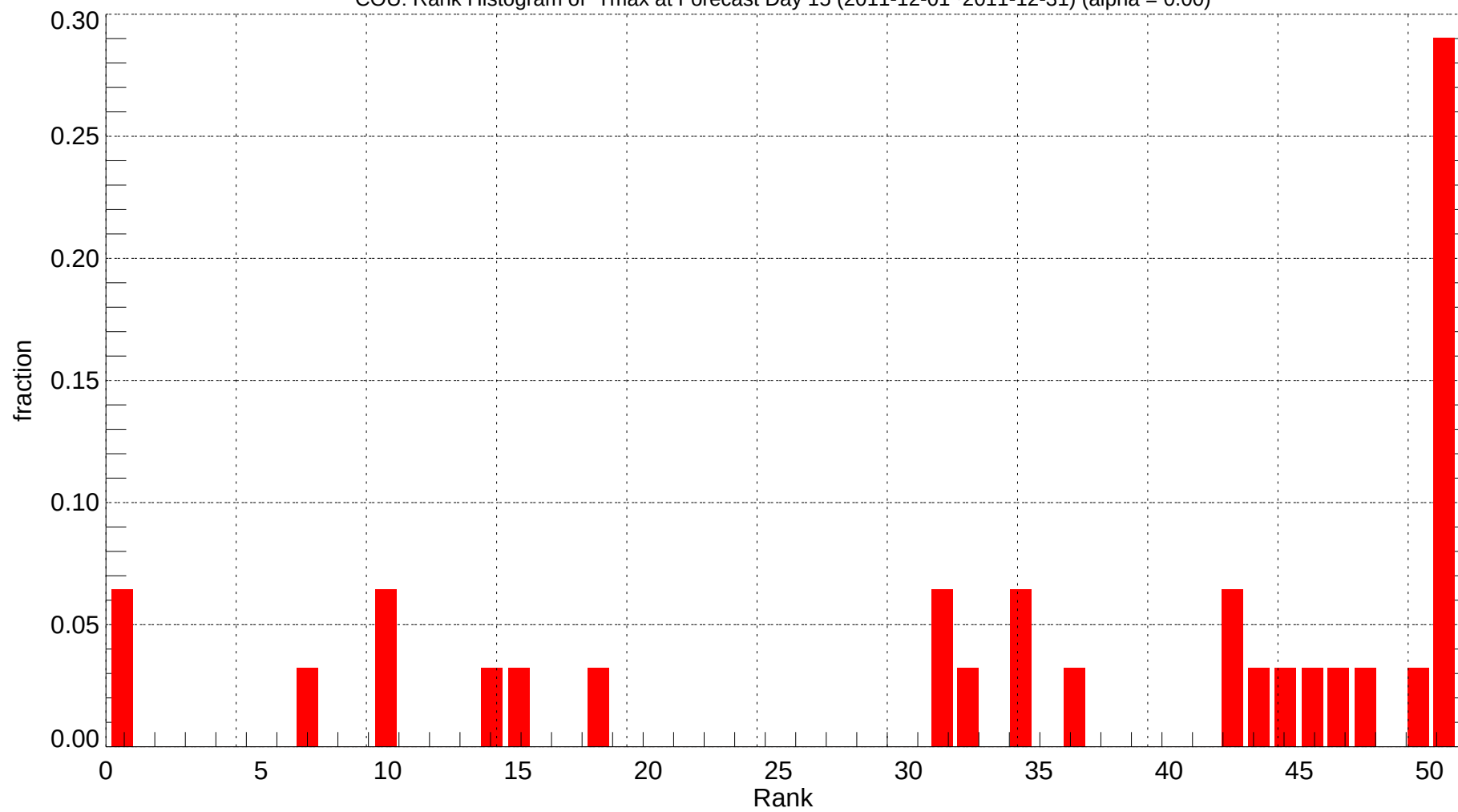
COU: Rank Histogram of Tmax at Forecast Day 15 (2011-12-01~2011-12-31) (alpha = 0.00)
