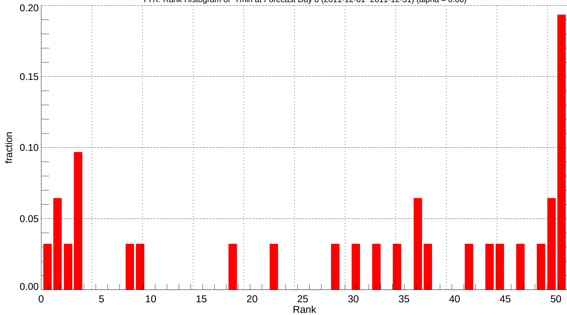
TYR: Rank Histogram of Tmin at Forecast Day 8 (2011-12-01~2011-12-31) (alpha = 0.00)
