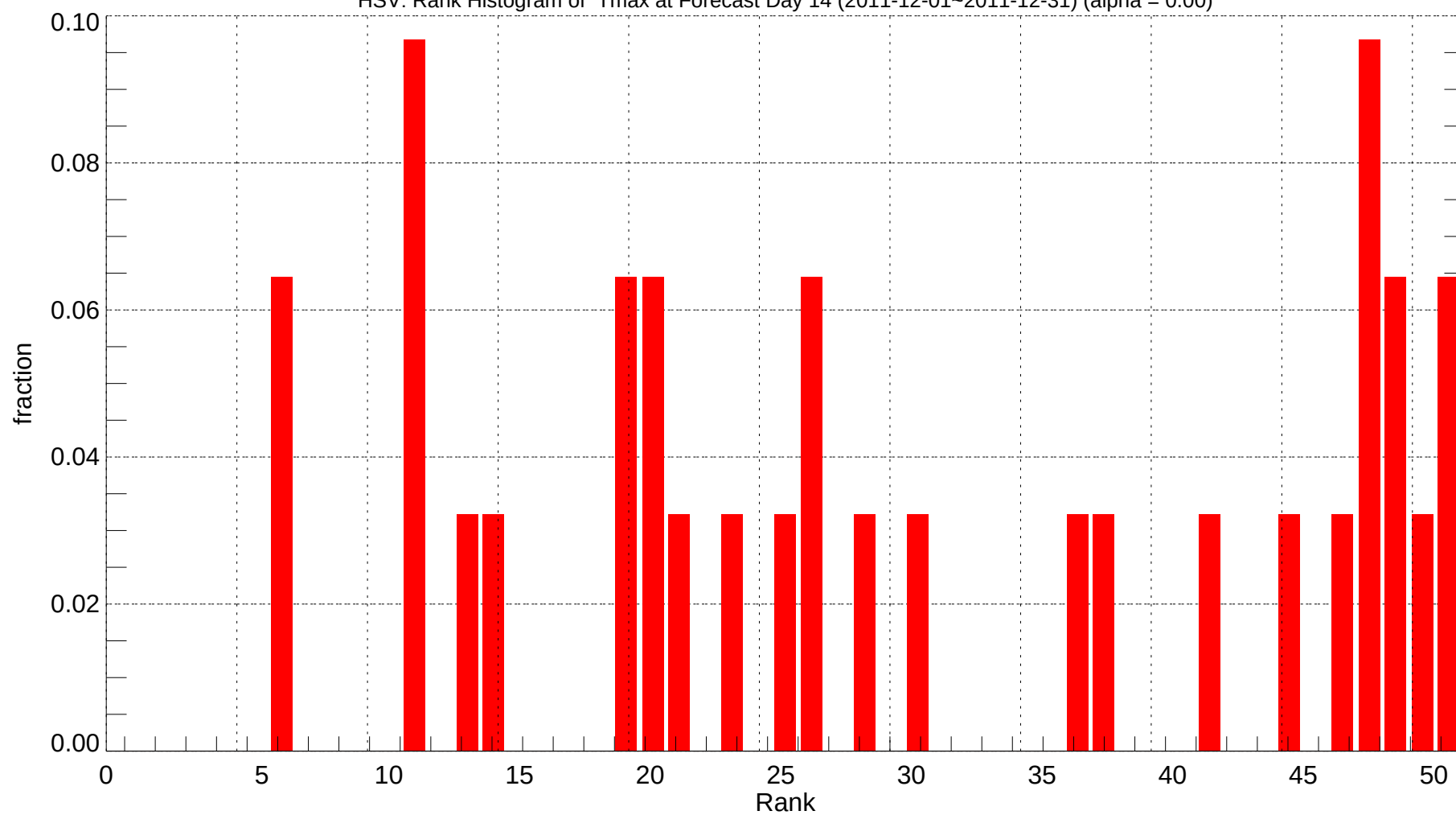
HSV: Rank Histogram of Tmax at Forecast Day 14 (2011-12-01~2011-12-31) (alpha = 0.00)
