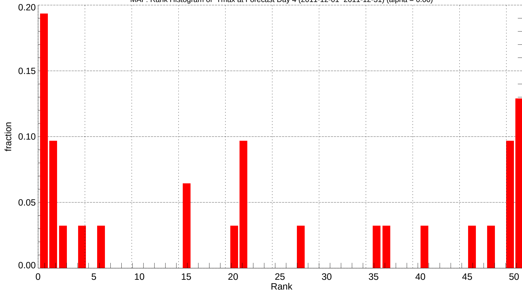
MAF: Rank Histogram of Tmax at Forecast Day 4 (2011-12-01~2011-12-31) (alpha = 0.00)
