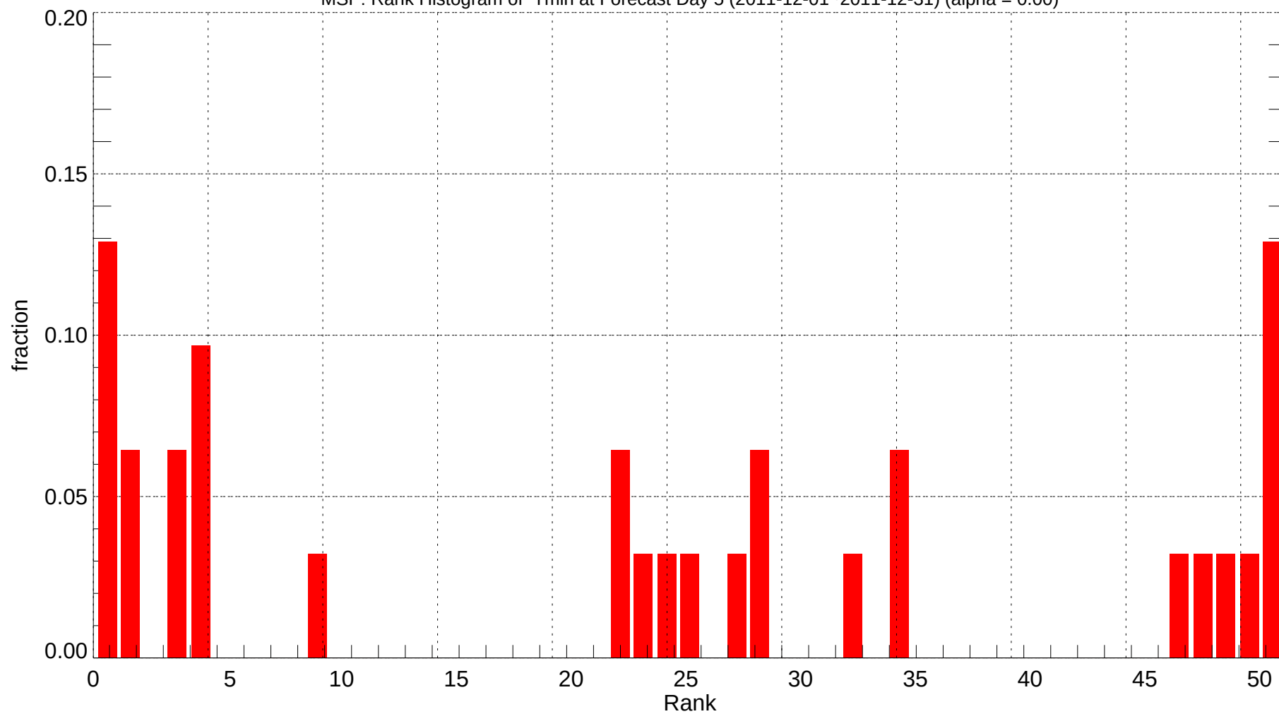
MSP: Rank Histogram of Tmin at Forecast Day 5 (2011-12-01~2011-12-31) (alpha = 0.00)
