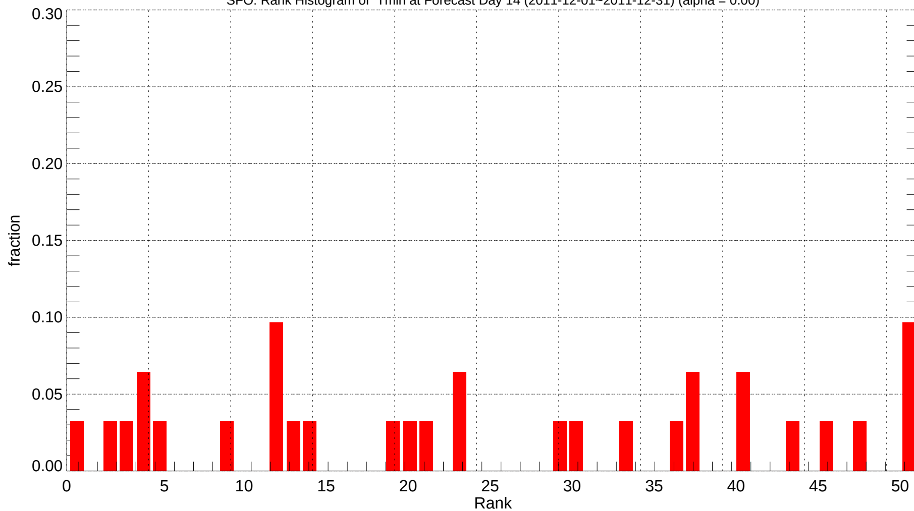
SFO: Rank Histogram of Tmin at Forecast Day 14 (2011-12-01~2011-12-31) (alpha = 0.00)
