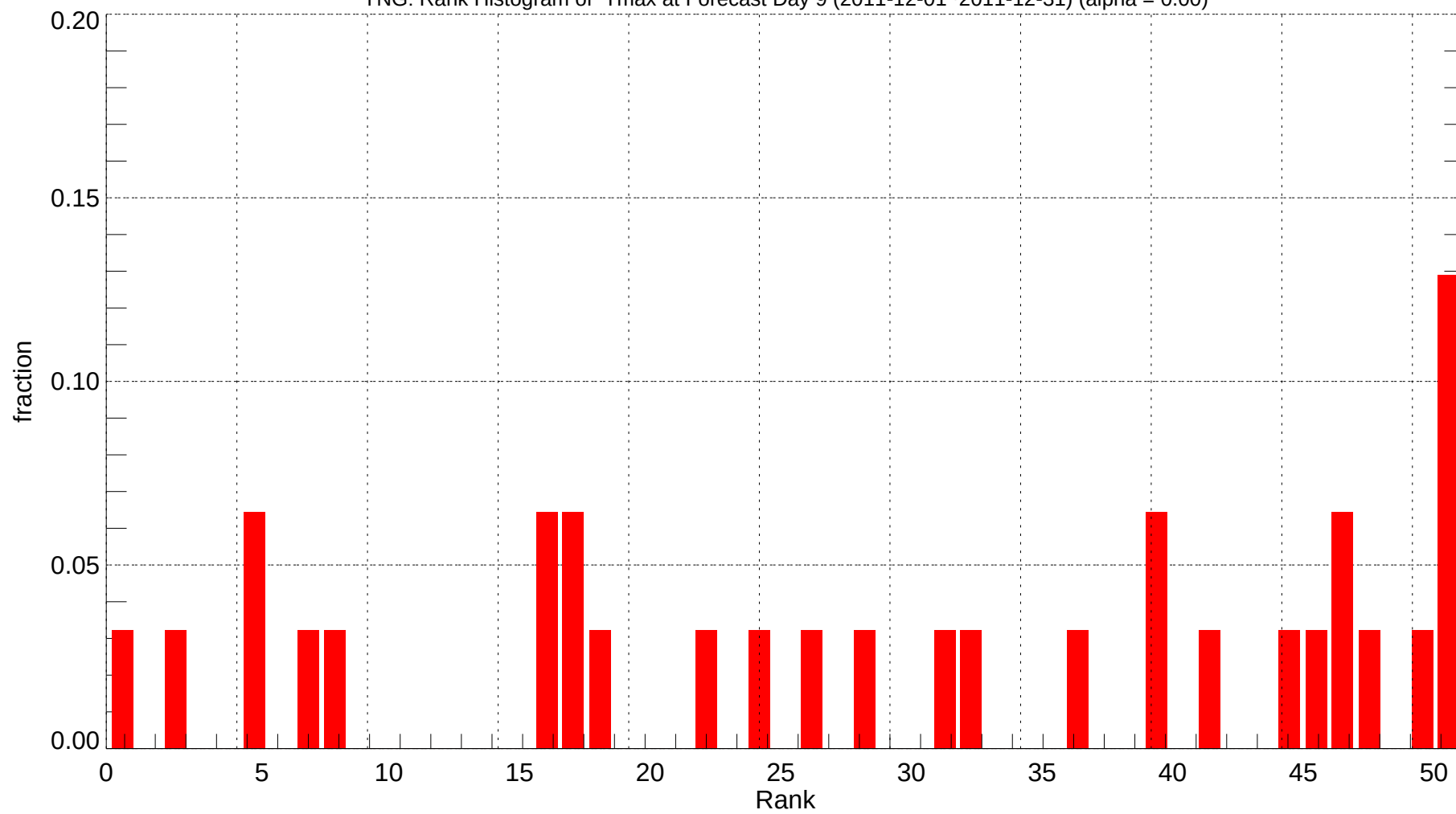
YNG: Rank Histogram of Tmax at Forecast Day 9 (2011-12-01~2011-12-31) (alpha = 0.00)
