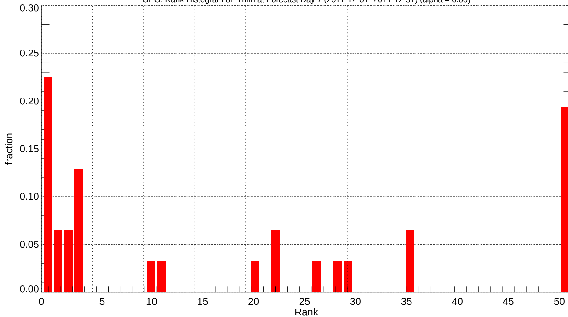
GEG: Rank Histogram of Tmin at Forecast Day 7 (2011-12-01~2011-12-31) (alpha = 0.00)
