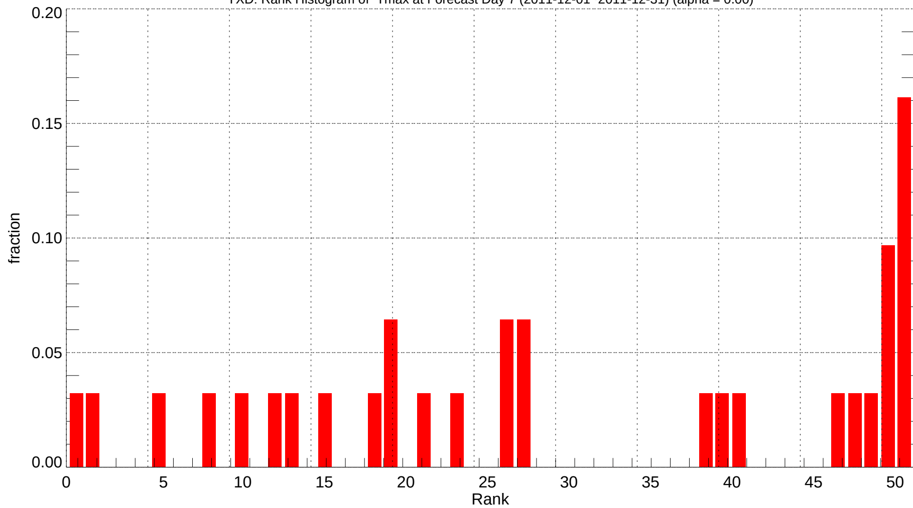
YXD: Rank Histogram of Tmax at Forecast Day 7 (2011-12-01~2011-12-31) (alpha = 0.00)
