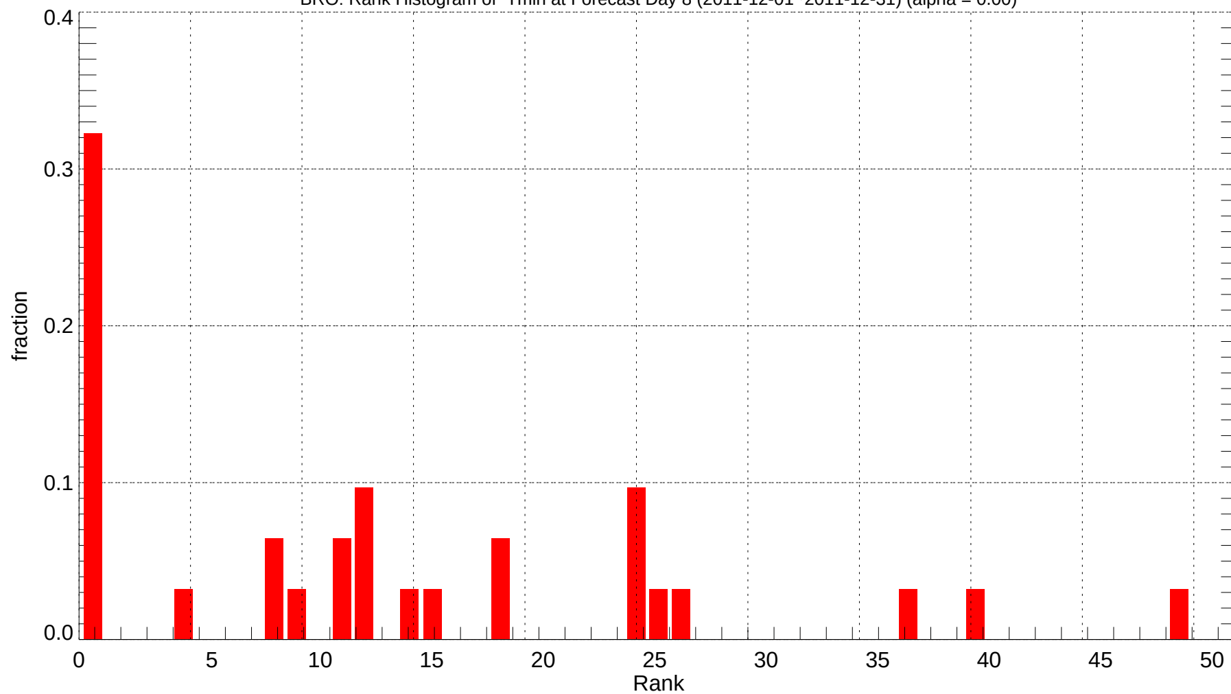
BRO: Rank Histogram of Tmin at Forecast Day 8 (2011-12-01~2011-12-31) (alpha = 0.00)
