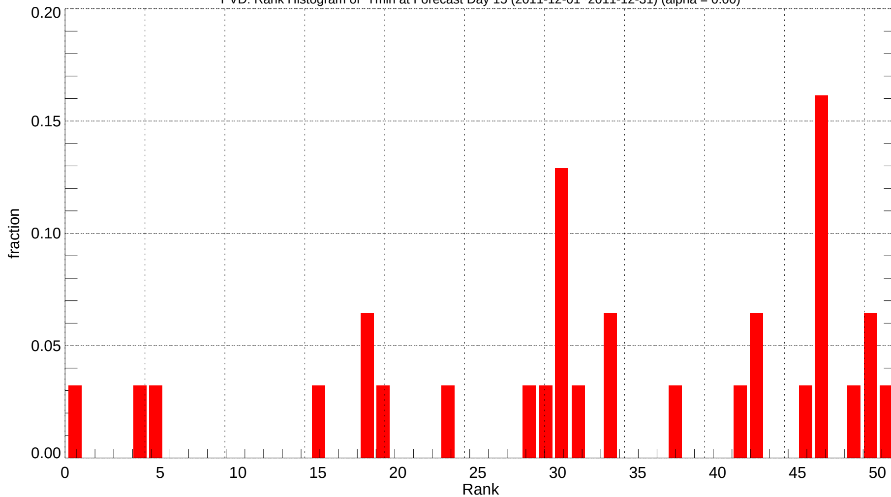
PVD: Rank Histogram of Tmin at Forecast Day 15 (2011-12-01~2011-12-31) (alpha = 0.00)
