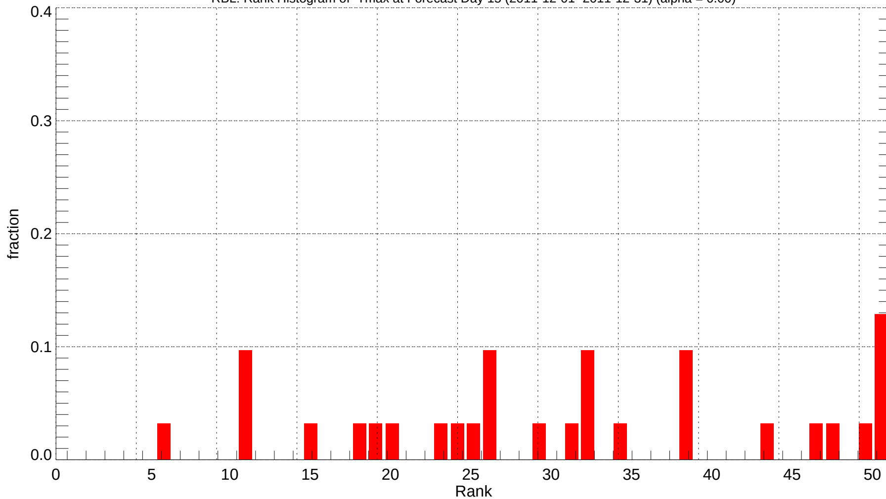
RBL: Rank Histogram of Tmax at Forecast Day 15 (2011-12-01~2011-12-31) (alpha = 0.00)
