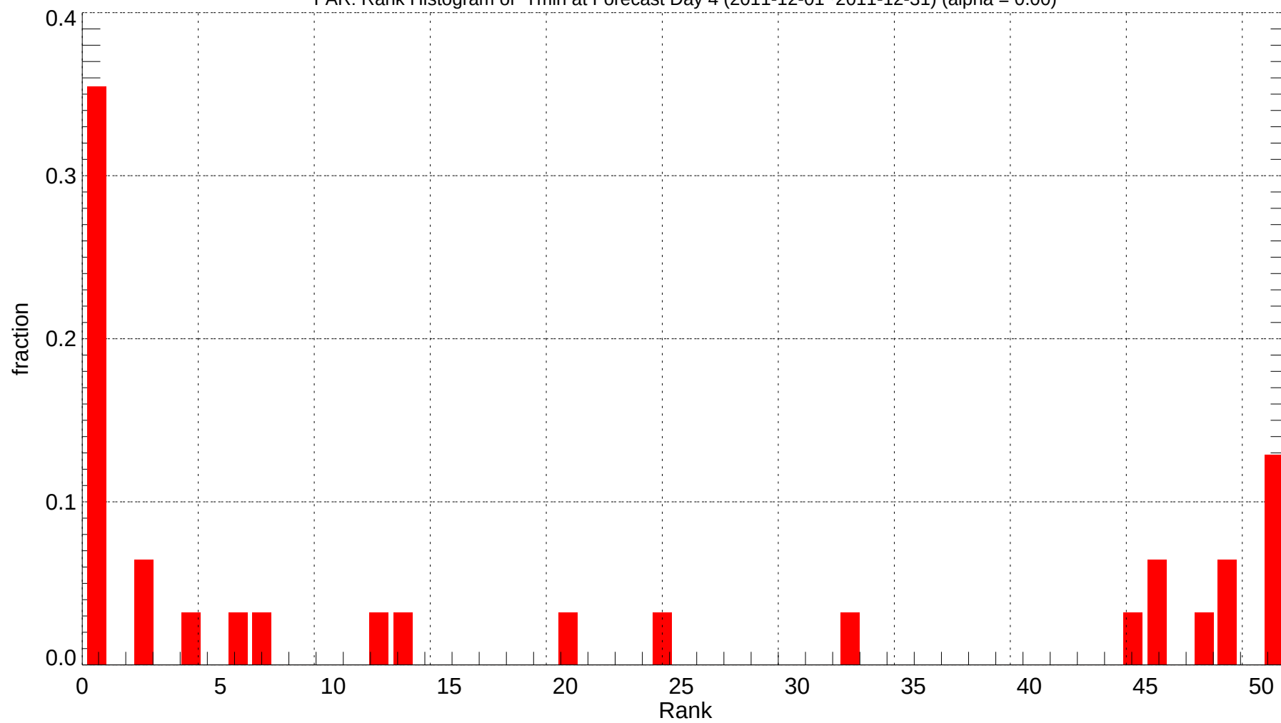
FAR: Rank Histogram of Tmin at Forecast Day 4 (2011-12-01~2011-12-31) (alpha = 0.00)
