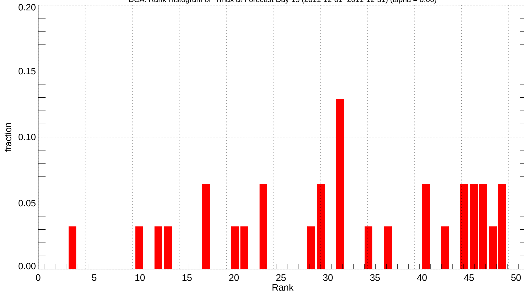
DCA: Rank Histogram of Tmax at Forecast Day 15 (2011-12-01~2011-12-31) (alpha = 0.00)
