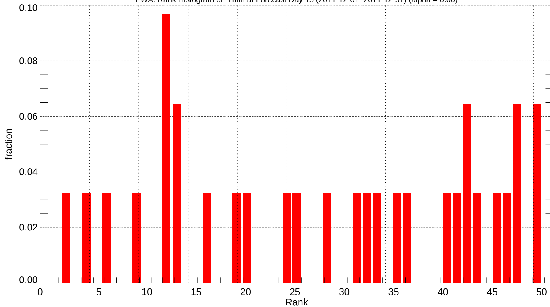
FWA: Rank Histogram of Tmin at Forecast Day 15 (2011-12-01~2011-12-31) (alpha = 0.00)
