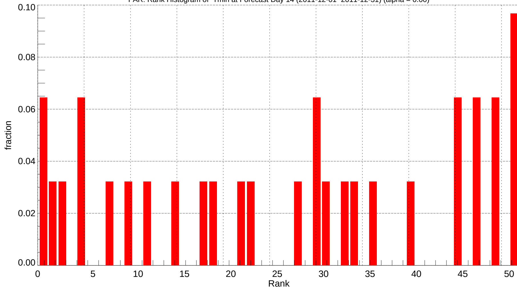
FAR: Rank Histogram of Tmin at Forecast Day 14 (2011-12-01~2011-12-31) (alpha = 0.00)
