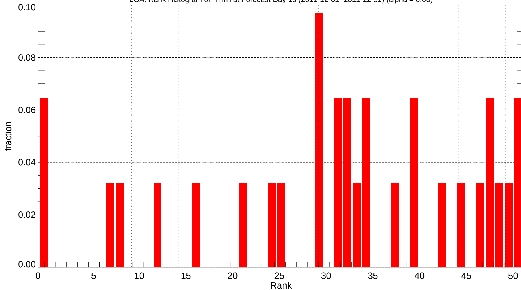
LGA: Rank Histogram of Tmin at Forecast Day 13 (2011-12-01~2011-12-31) (alpha = 0.00)
