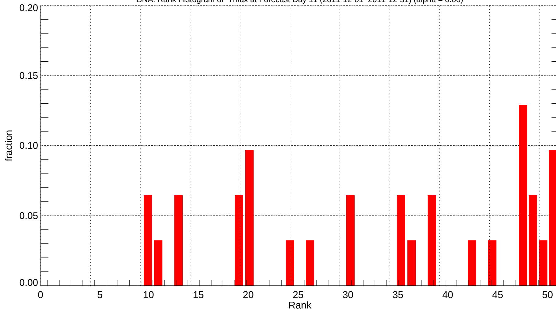
BNA: Rank Histogram of Tmax at Forecast Day 11 (2011-12-01~2011-12-31) (alpha = 0.00)
