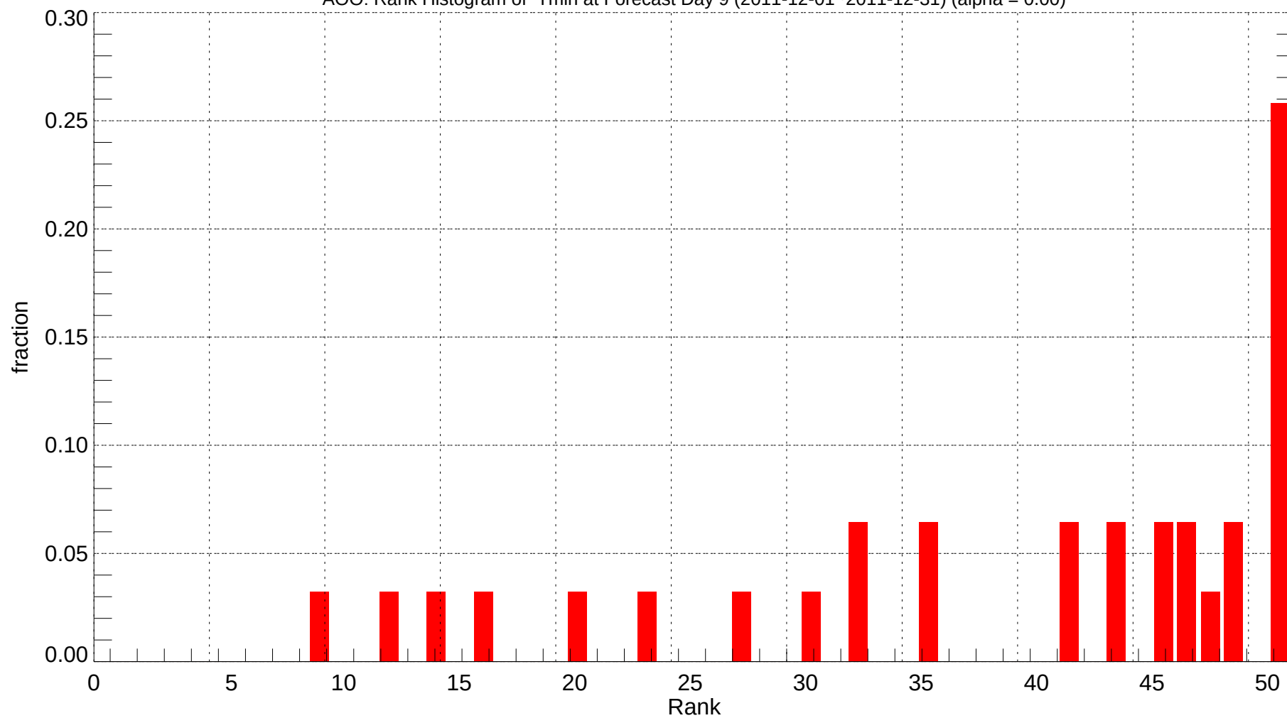
AOO: Rank Histogram of Tmin at Forecast Day 9 (2011-12-01~2011-12-31) (alpha = 0.00)
