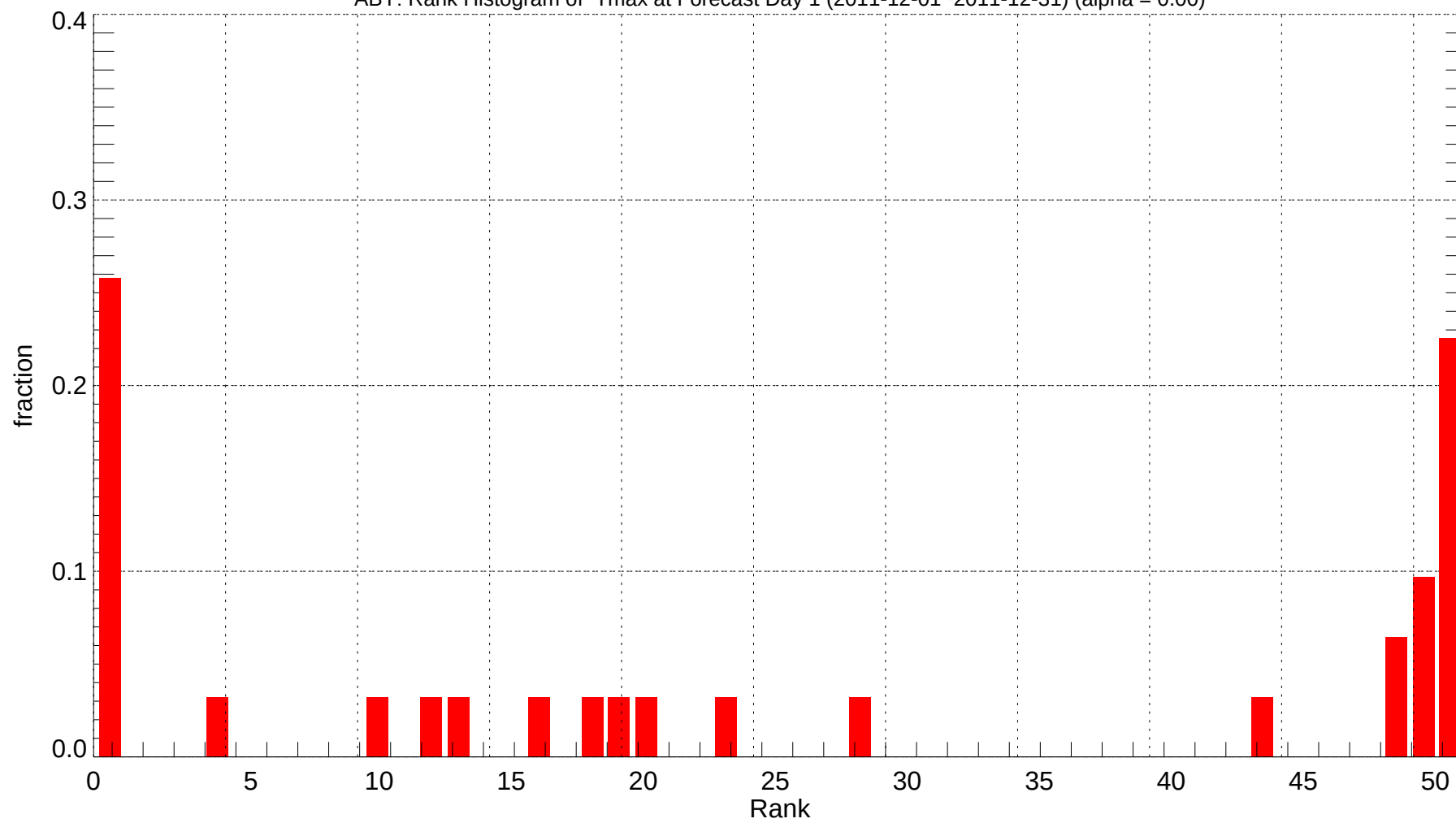
ABY: Rank Histogram of Tmax at Forecast Day 1 (2011-12-01~2011-12-31) (alpha = 0.00)
