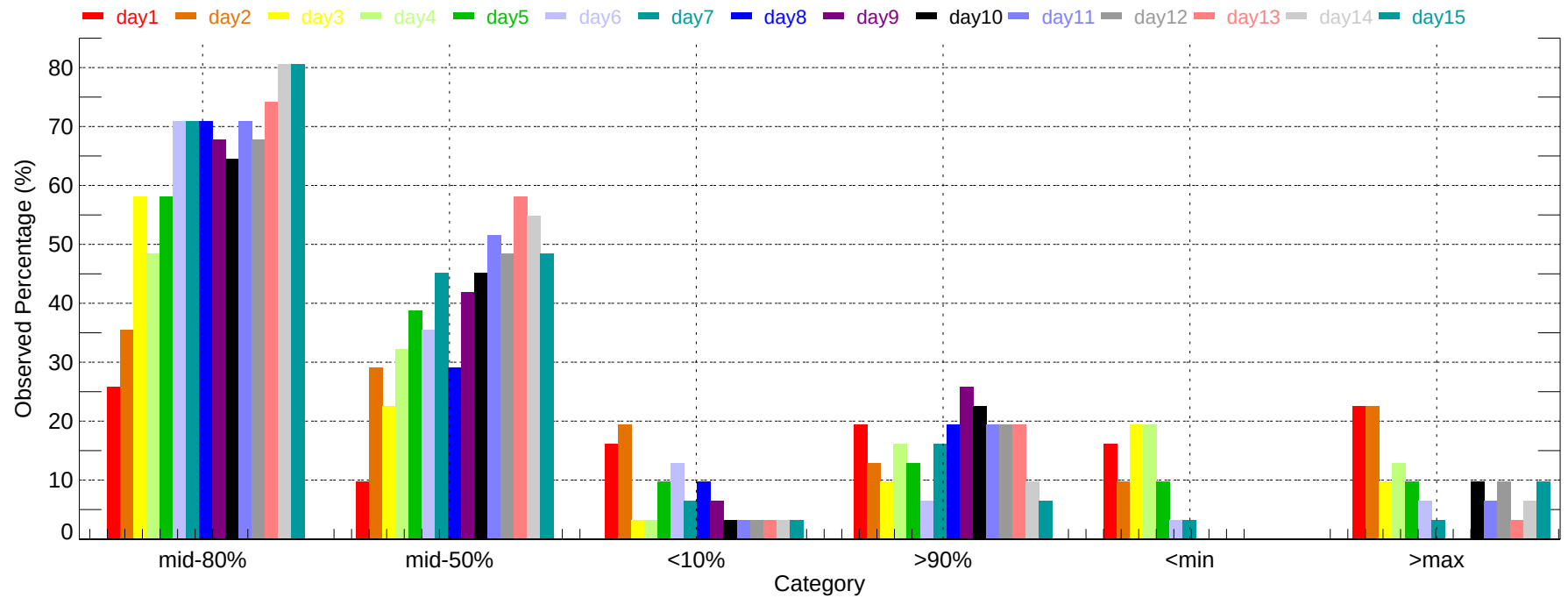
Observed Percentage of Ensembles - SAV: Max Temperature (2011-12-01~2011-12-31)
