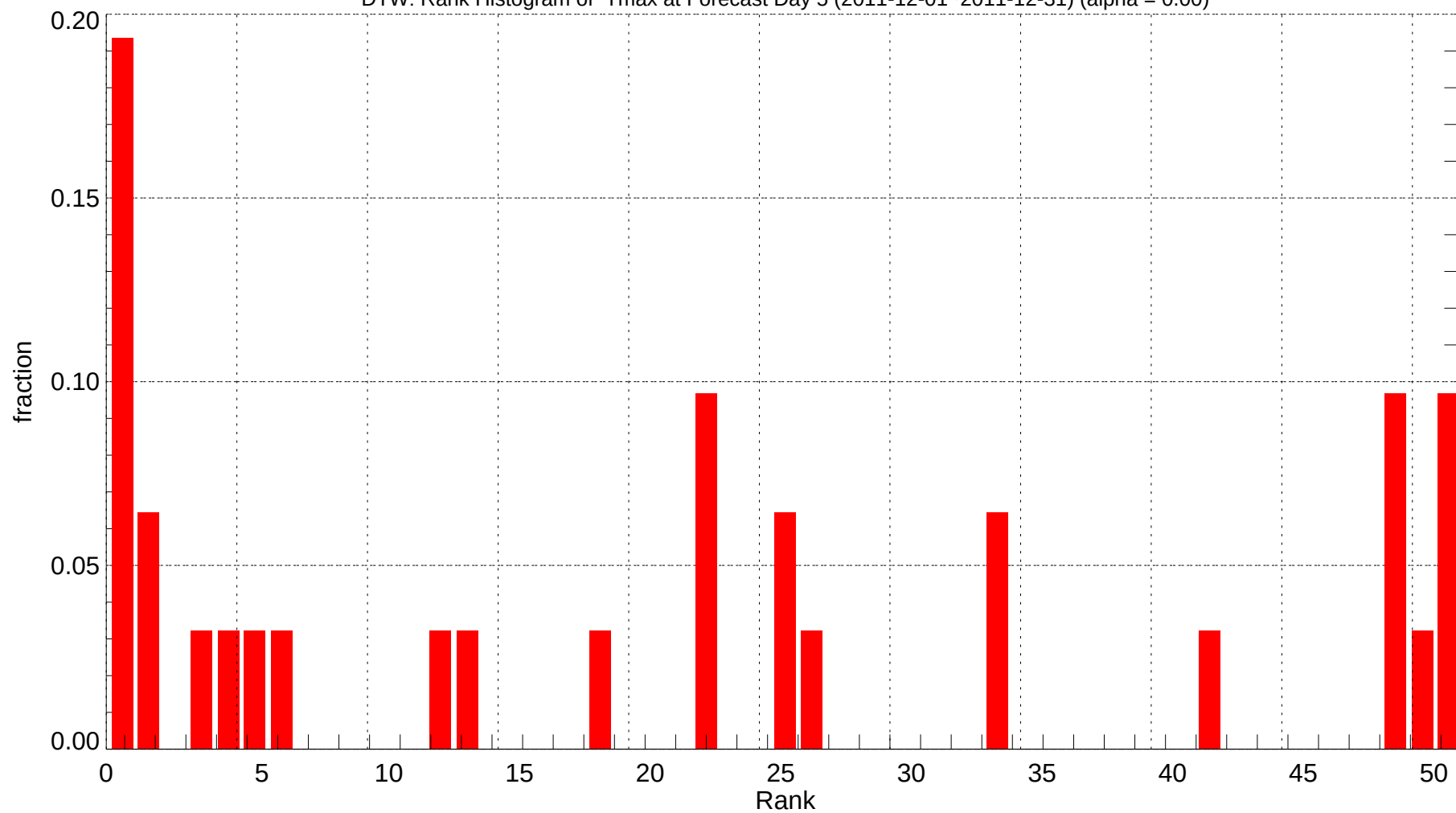
DTW: Rank Histogram of Tmax at Forecast Day 5 (2011-12-01~2011-12-31) (alpha = 0.00)
