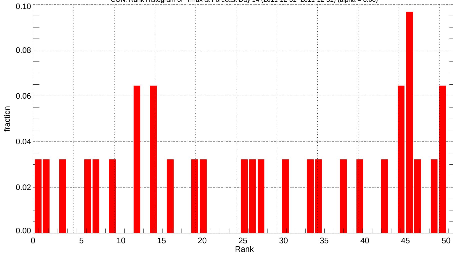
CON: Rank Histogram of Tmax at Forecast Day 14 (2011-12-01~2011-12-31) (alpha = 0.00)
