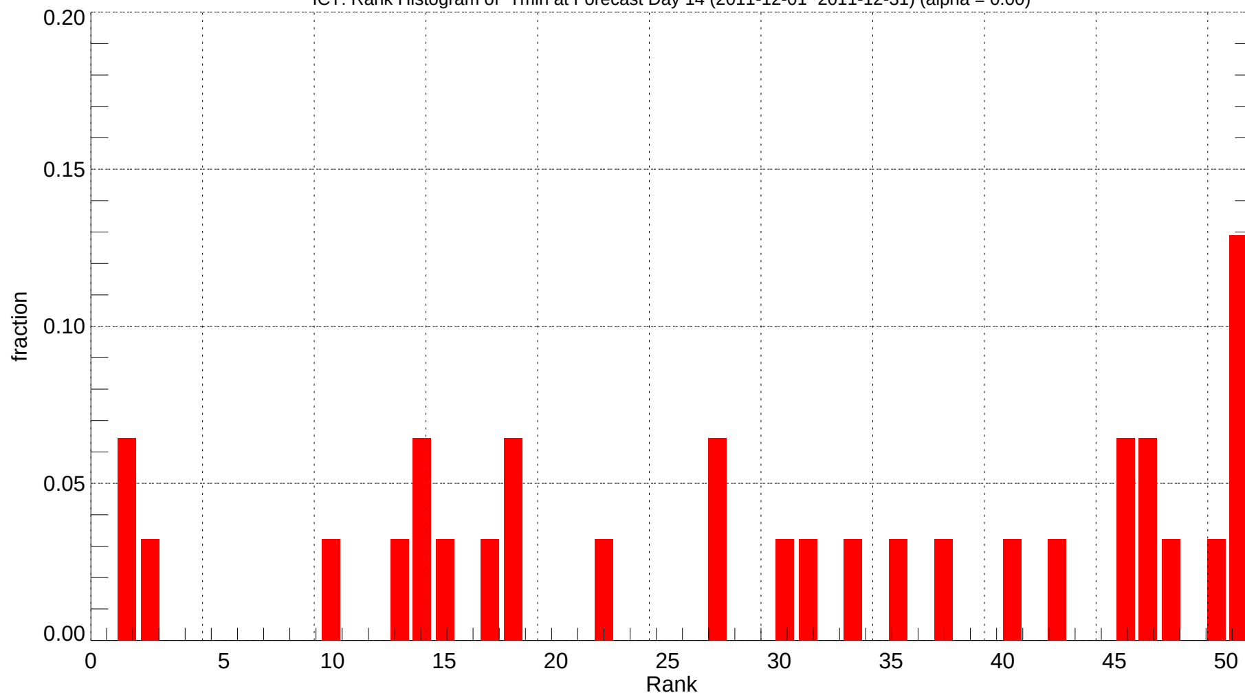
ICT: Rank Histogram of Tmin at Forecast Day 14 (2011-12-01~2011-12-31) (alpha = 0.00)
