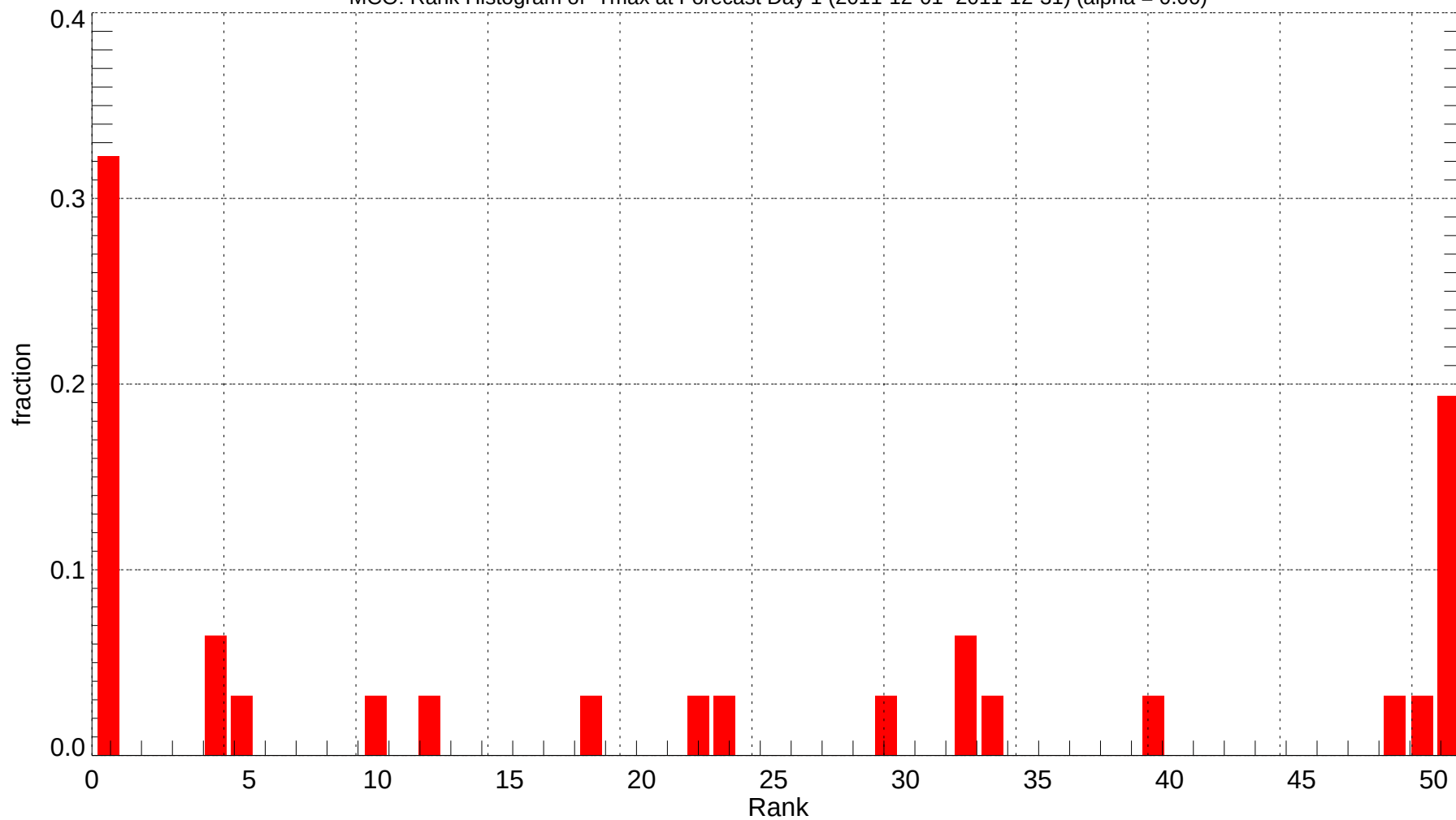
MCO: Rank Histogram of Tmax at Forecast Day 1 (2011-12-01~2011-12-31) (alpha = 0.00)
