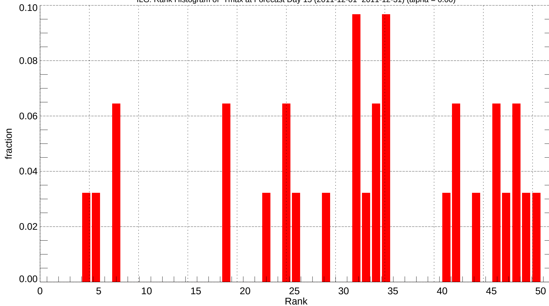
ILG: Rank Histogram of Tmax at Forecast Day 15 (2011-12-01~2011-12-31) (alpha = 0.00)
