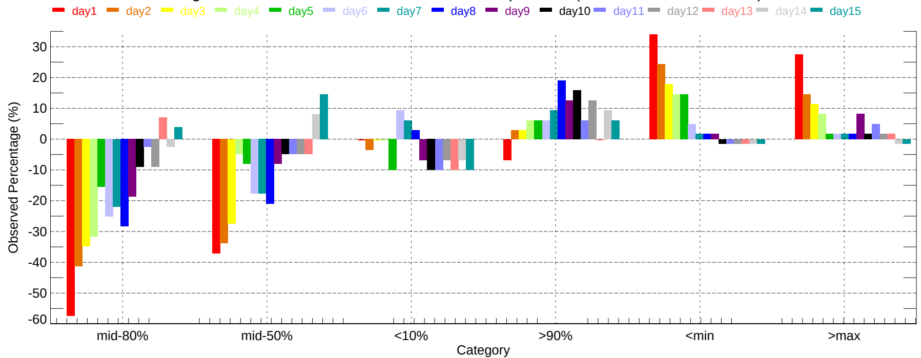
Observed Percentage Deviation of Ensembles - CHA: Min Temperature (2011-12-01~2011-12-31)
