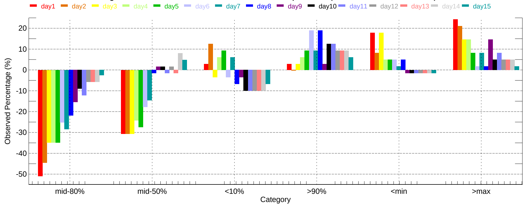
Observed Percentage Deviation of Ensembles - CAE: Max Temperature (2011-12-01~2011-12-31)
