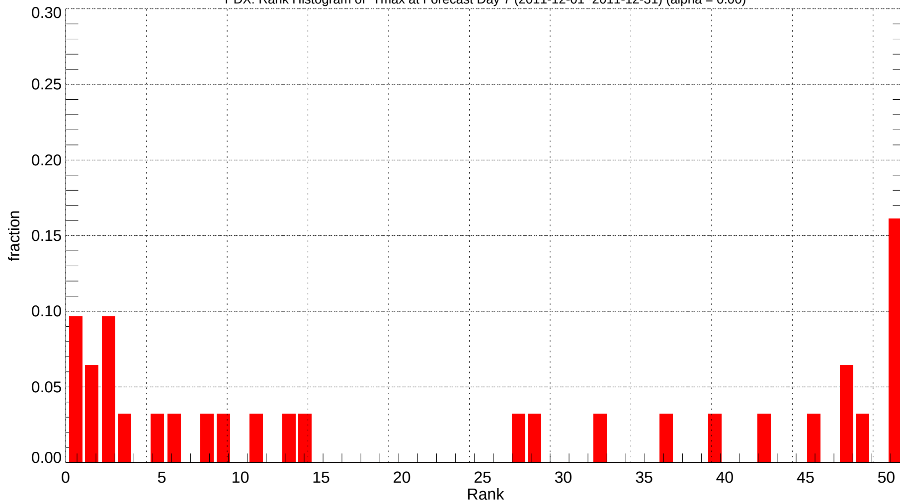
PDX: Rank Histogram of Tmax at Forecast Day 7 (2011-12-01~2011-12-31) (alpha = 0.00)
