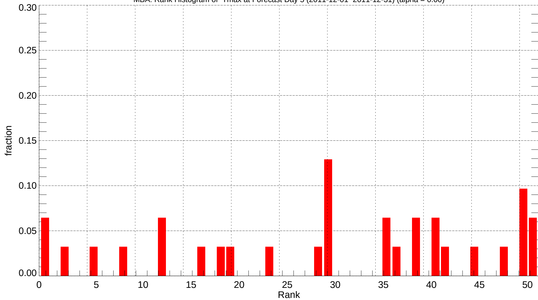
MBA: Rank Histogram of Tmax at Forecast Day 5 (2011-12-01~2011-12-31) (alpha = 0.00)
