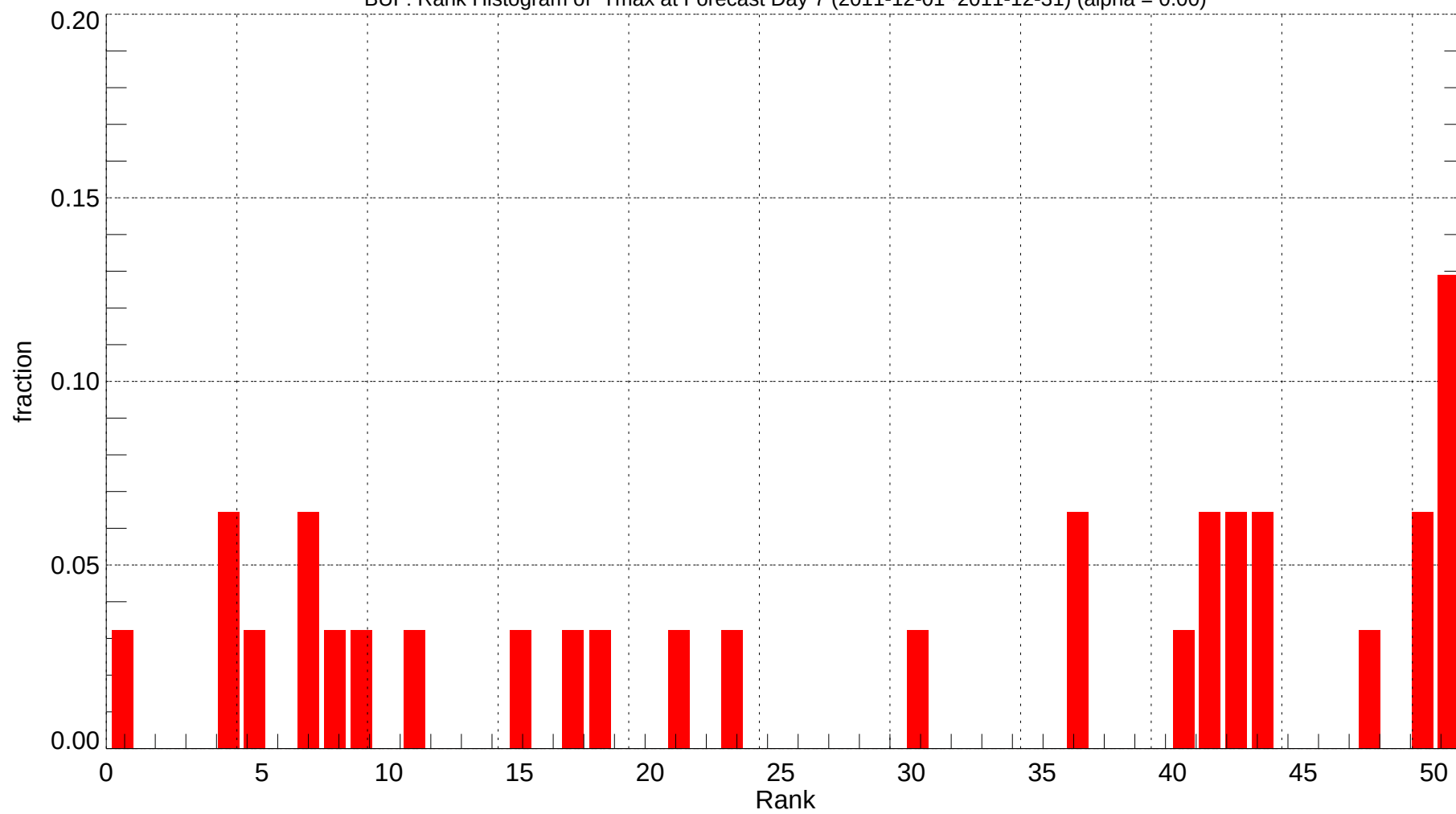
BUF: Rank Histogram of Tmax at Forecast Day 7 (2011-12-01~2011-12-31) (alpha = 0.00)
