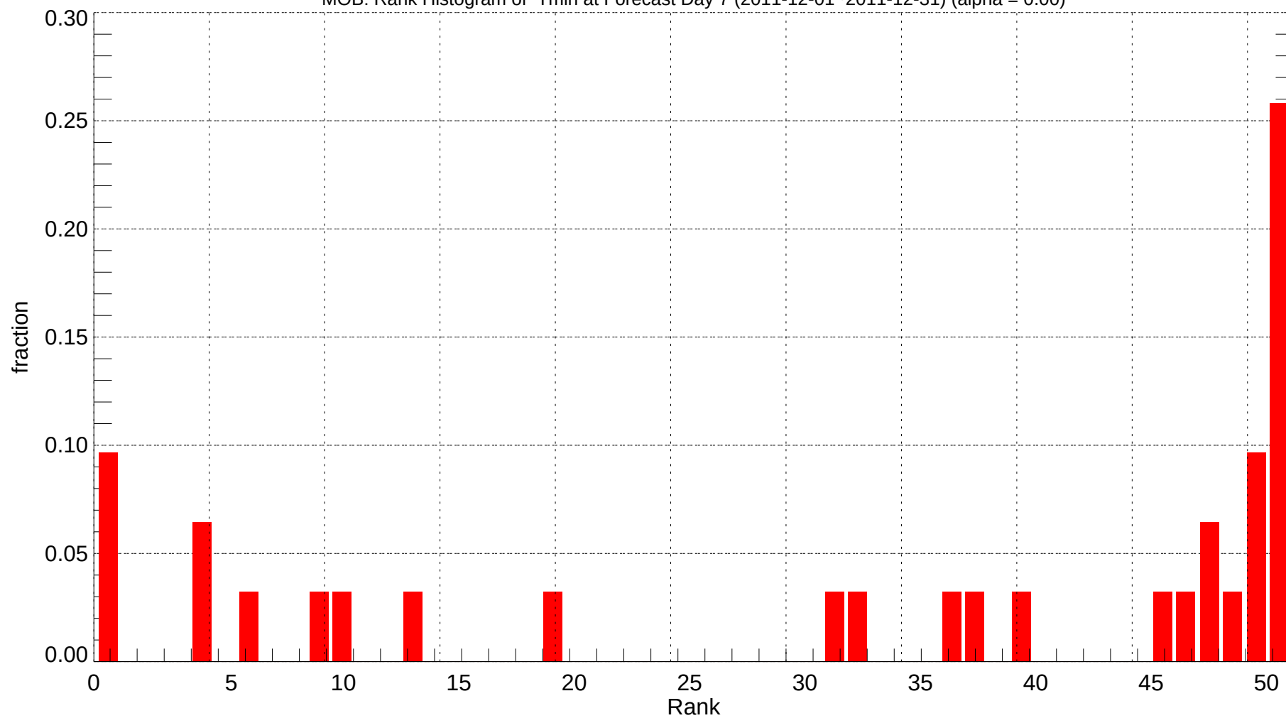
MOB: Rank Histogram of Tmin at Forecast Day 7 (2011-12-01~2011-12-31) (alpha = 0.00)
