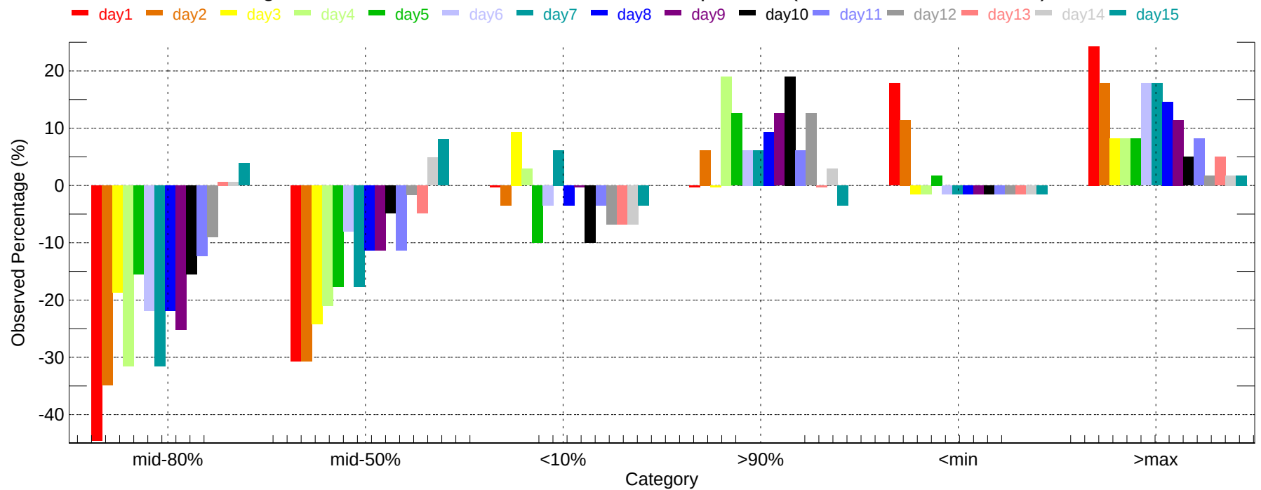
Observed Percentage Deviation of Ensembles - DFW: Min Temperature (2011-12-01~2011-12-31)
