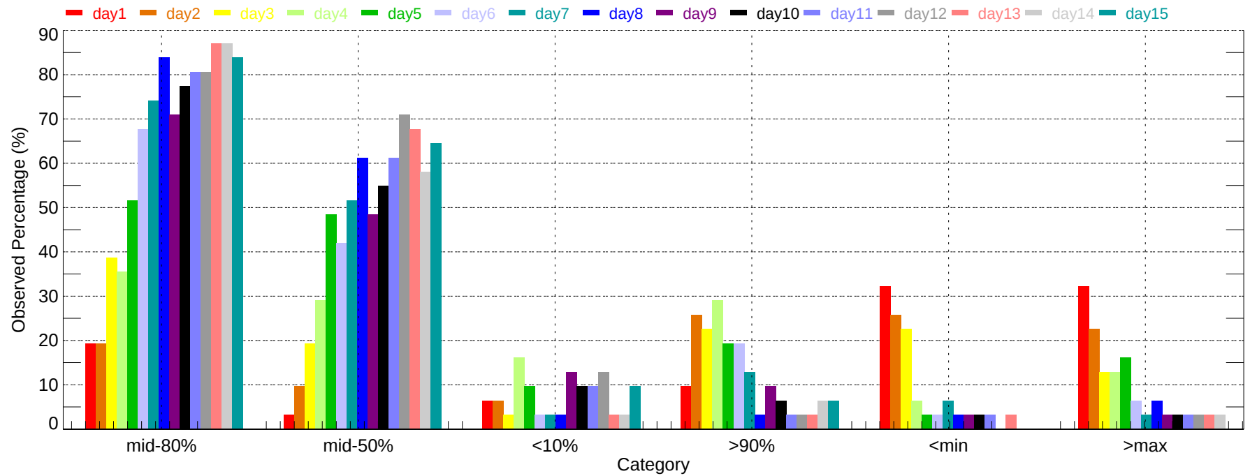
Observed Percentage of Ensembles - WJF: Max Temperature (2011-12-01~2011-12-31)
