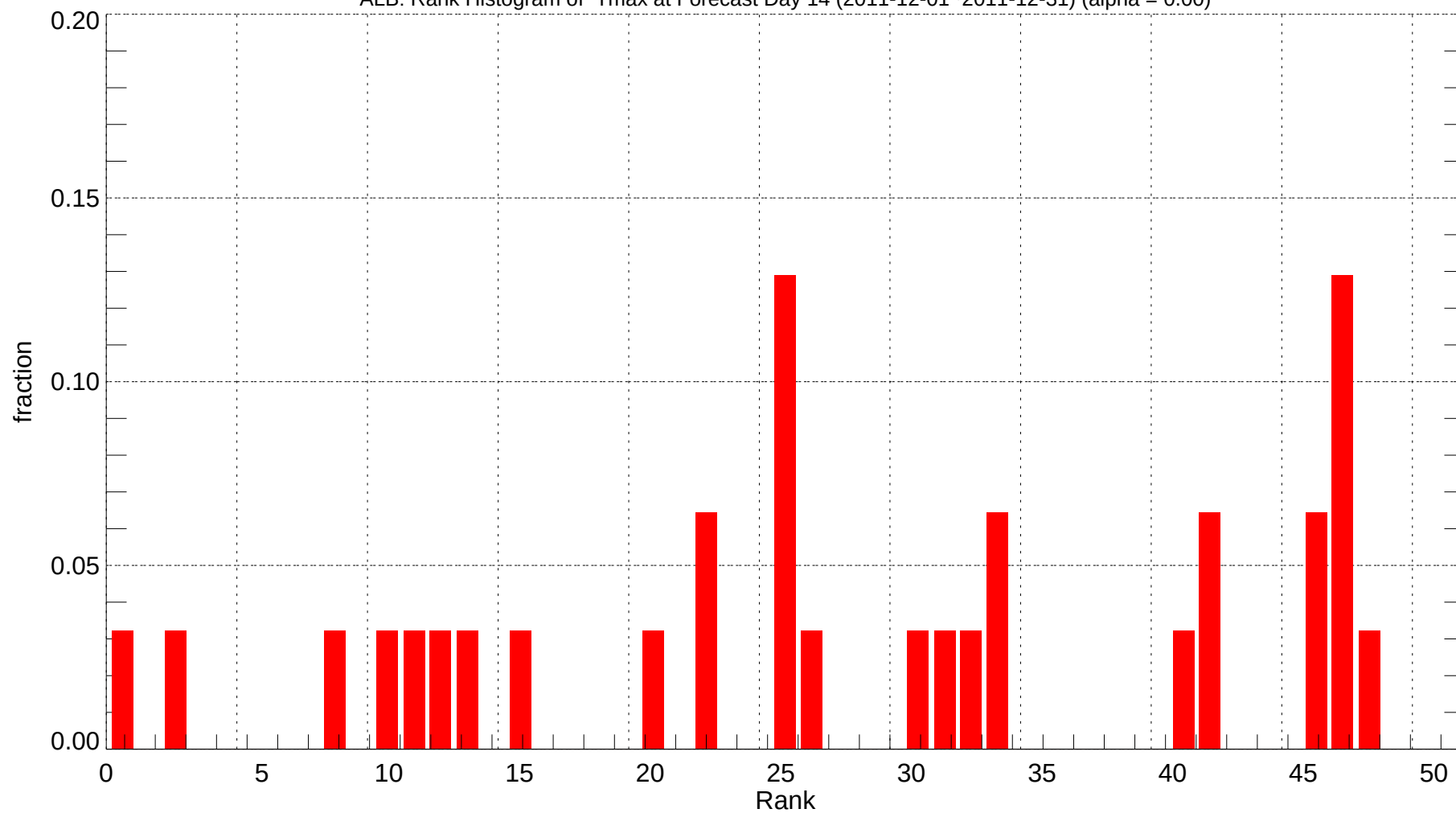
ALB: Rank Histogram of Tmax at Forecast Day 14 (2011-12-01~2011-12-31) (alpha = 0.00)
