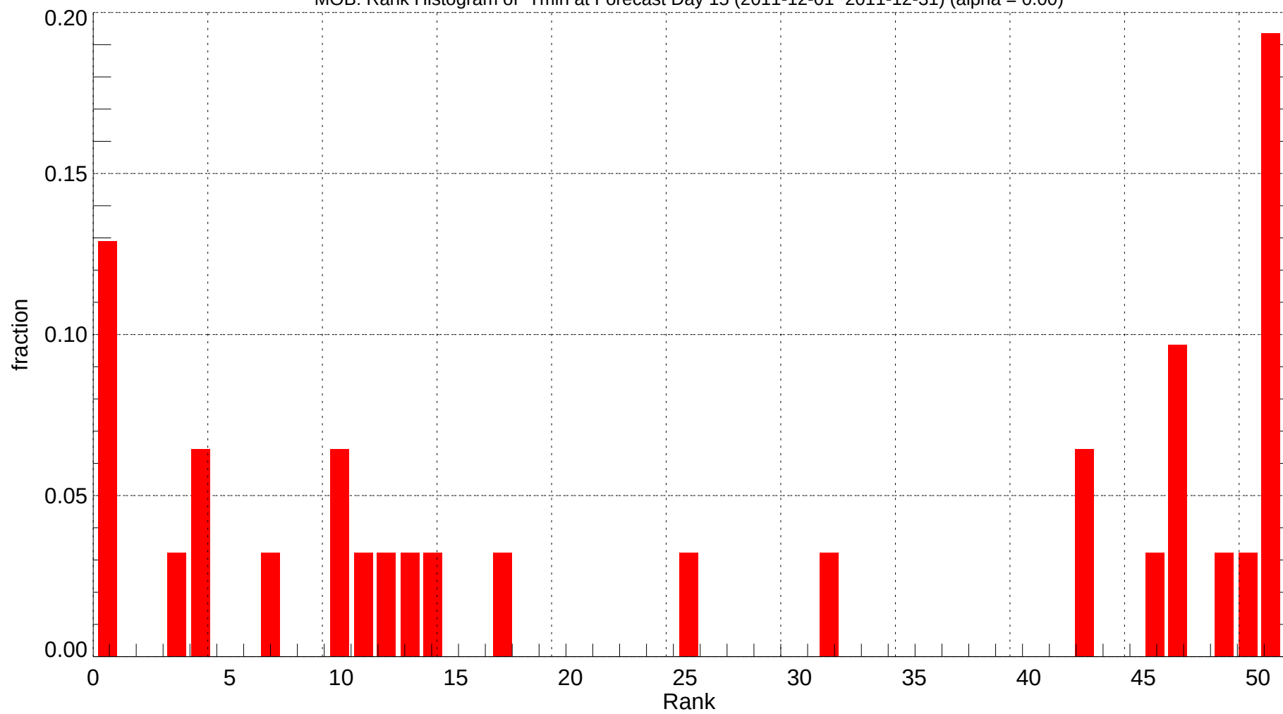
MOB: Rank Histogram of Tmin at Forecast Day 15 (2011-12-01~2011-12-31) (alpha = 0.00)
