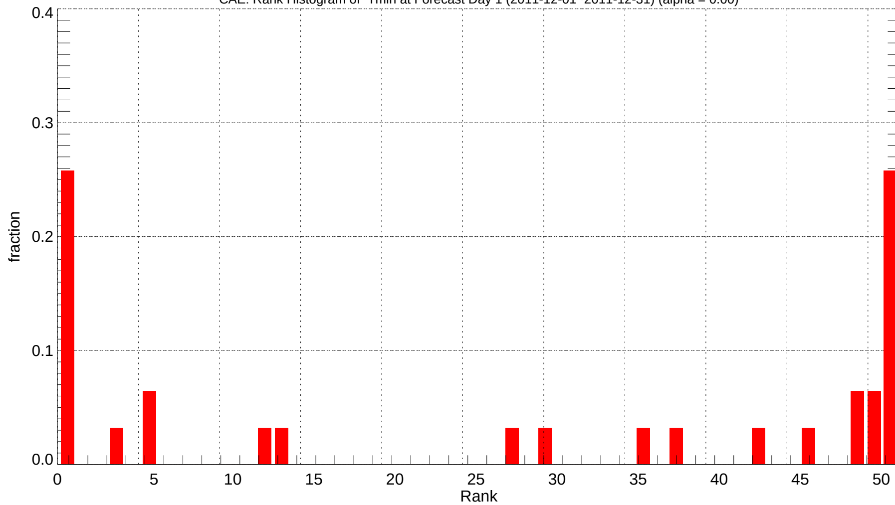
CAE: Rank Histogram of Tmin at Forecast Day 1 (2011-12-01~2011-12-31) (alpha = 0.00)
