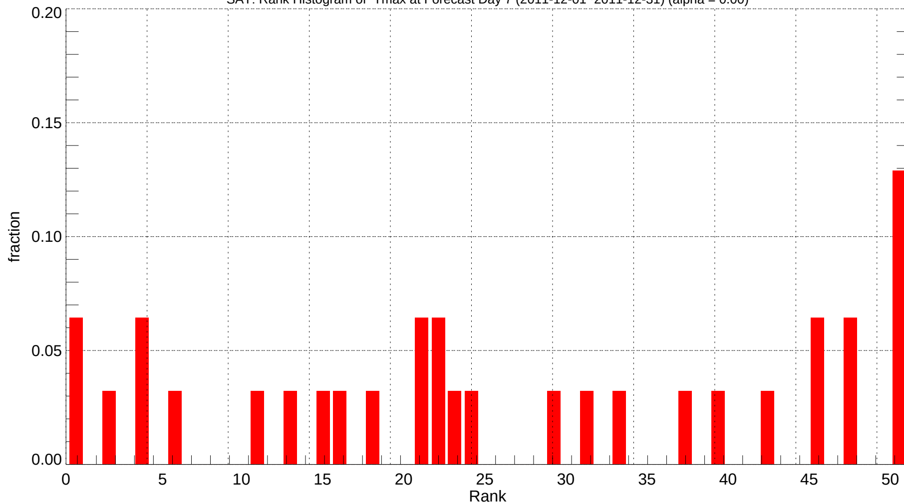
SAT: Rank Histogram of Tmax at Forecast Day 7 (2011-12-01~2011-12-31) (alpha = 0.00)
