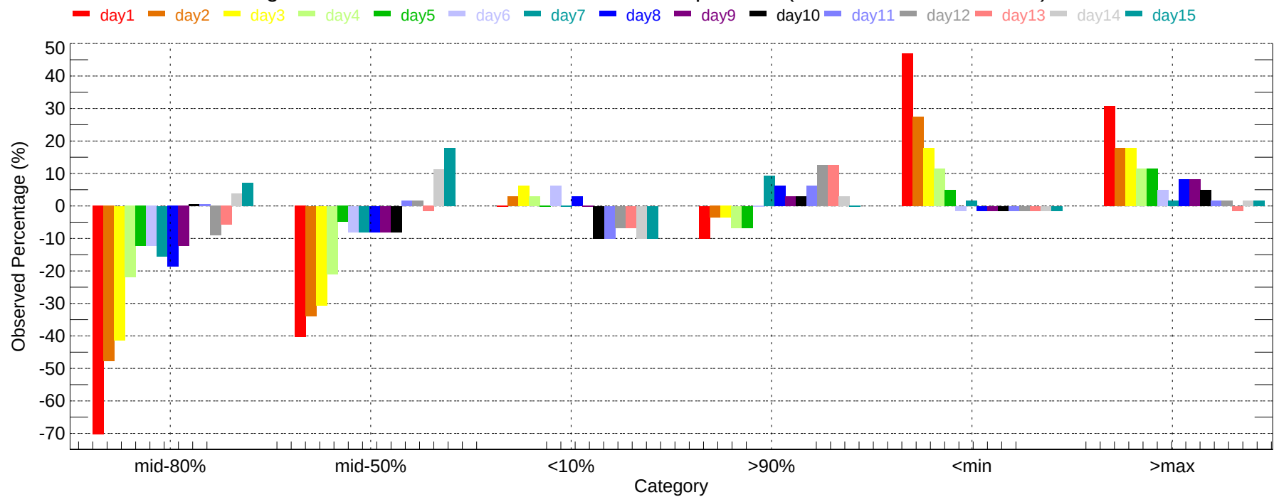
Observed Percentage Deviation of Ensembles - SSI: Min Temperature (2011-12-01~2011-12-31)
