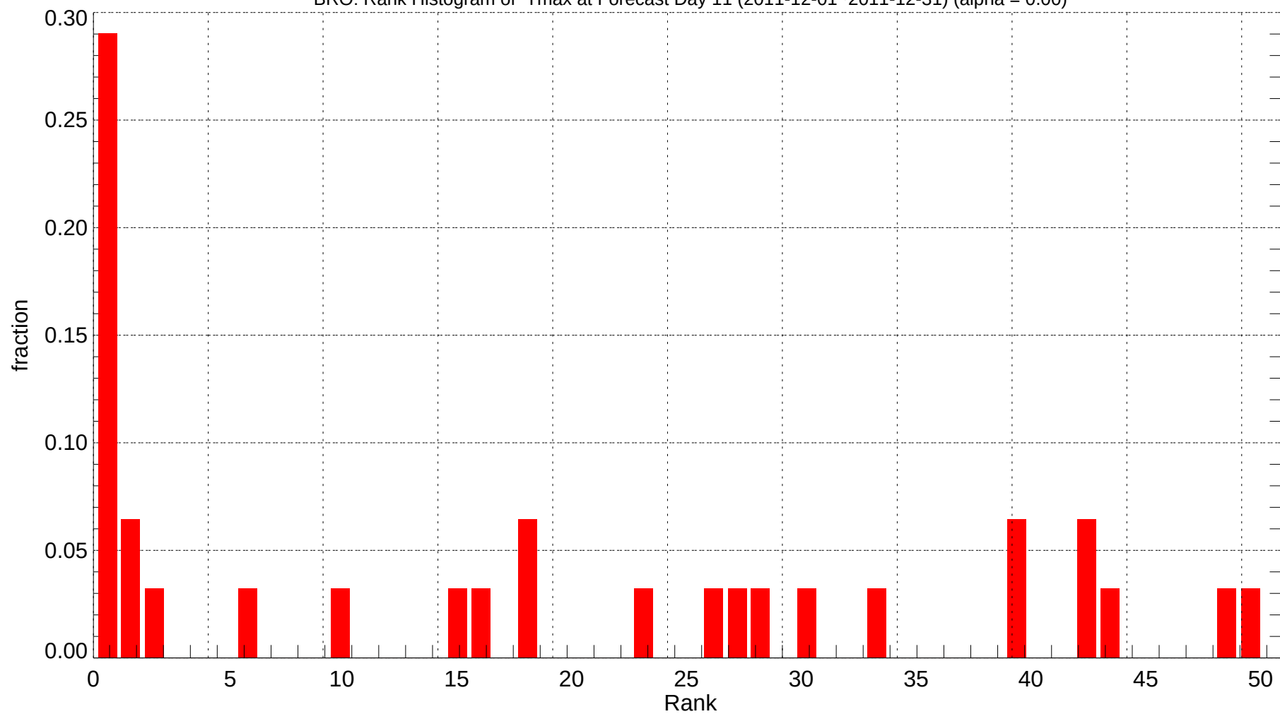
BRO: Rank Histogram of Tmax at Forecast Day 11 (2011-12-01~2011-12-31) (alpha = 0.00)
