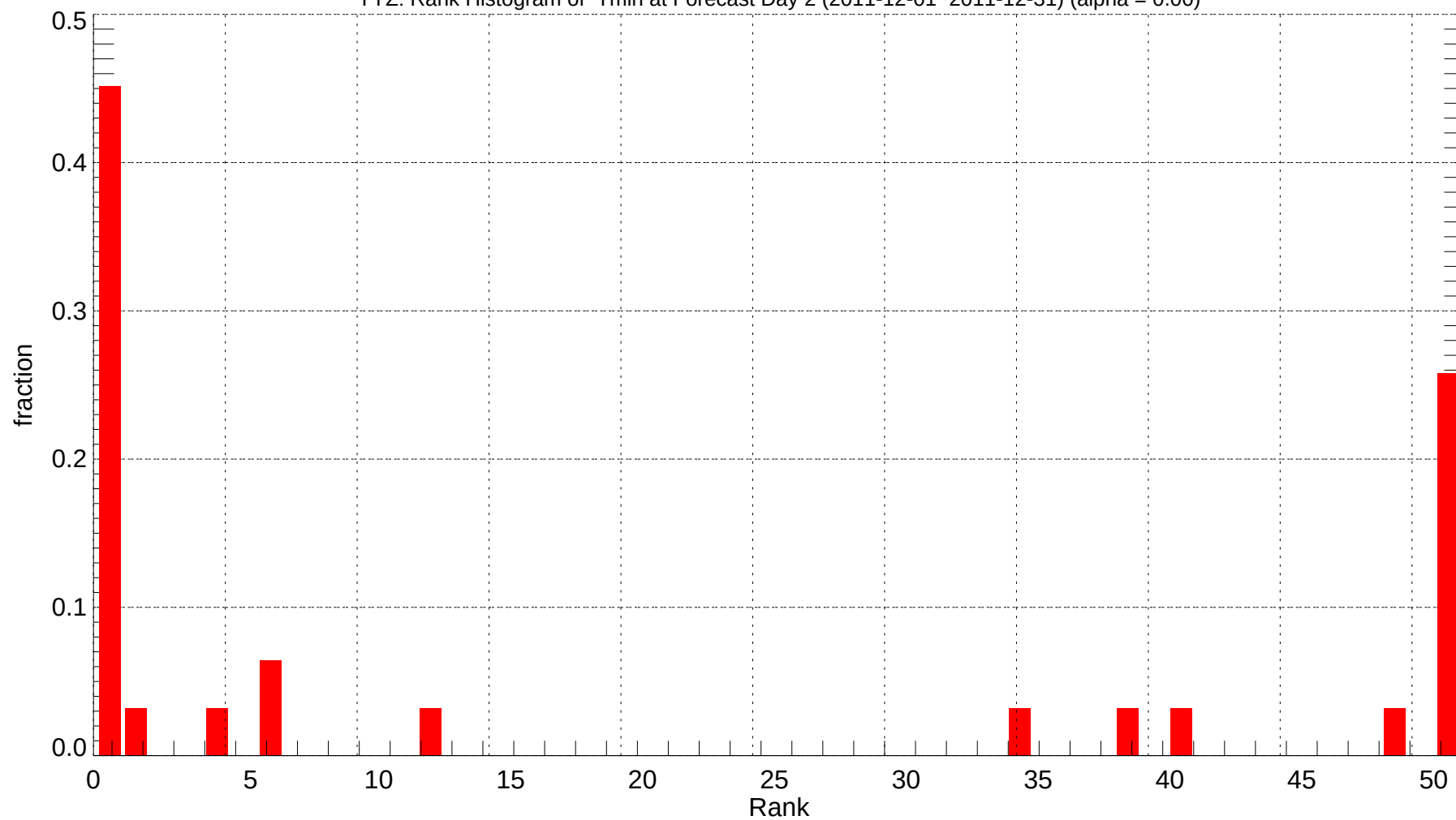
YYZ: Rank Histogram of Tmin at Forecast Day 2 (2011-12-01~2011-12-31) (alpha = 0.00)
