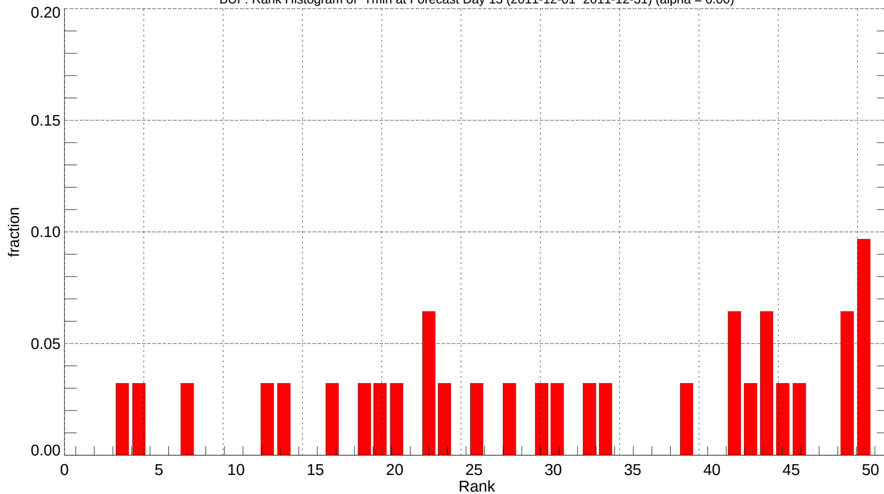
BUF: Rank Histogram of Tmin at Forecast Day 13 (2011-12-01~2011-12-31) (alpha = 0.00)
