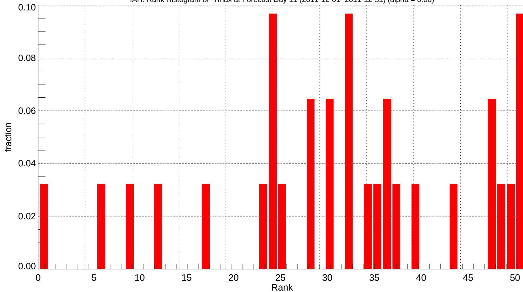
IAH: Rank Histogram of Tmax at Forecast Day 11 (2011-12-01~2011-12-31) (alpha = 0.00)
