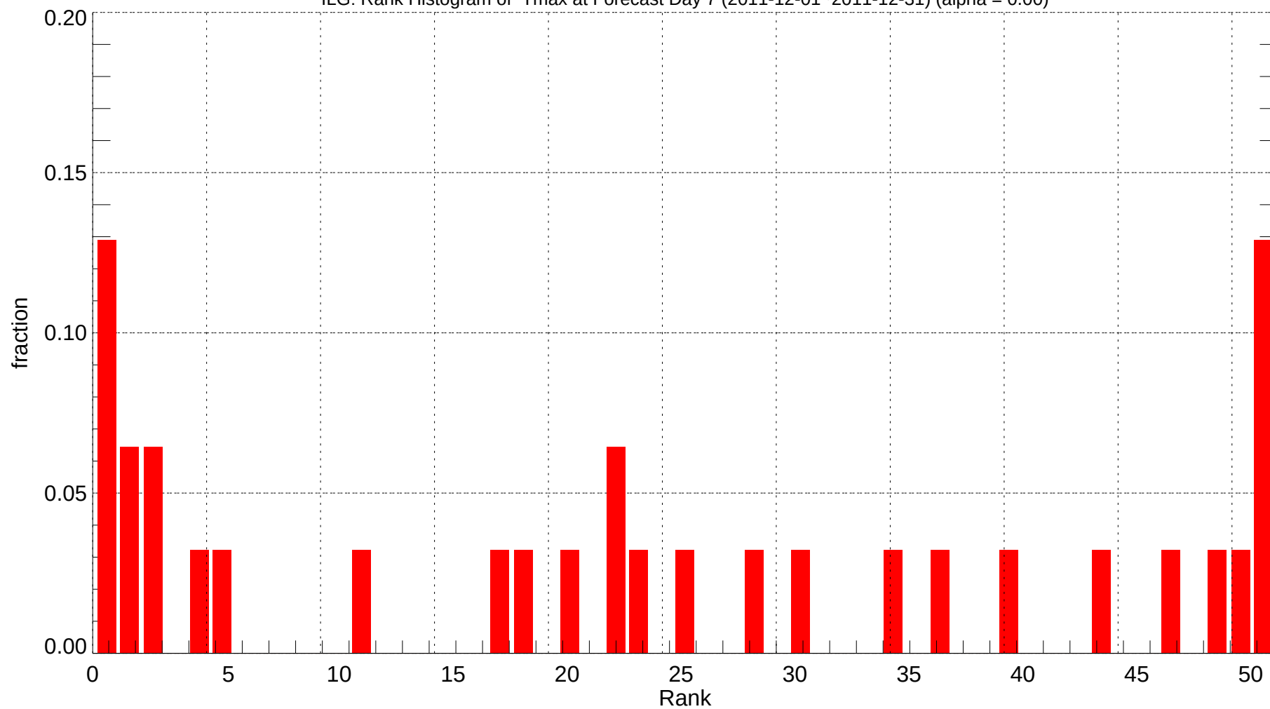
ILG: Rank Histogram of Tmax at Forecast Day 7 (2011-12-01~2011-12-31) (alpha = 0.00)
