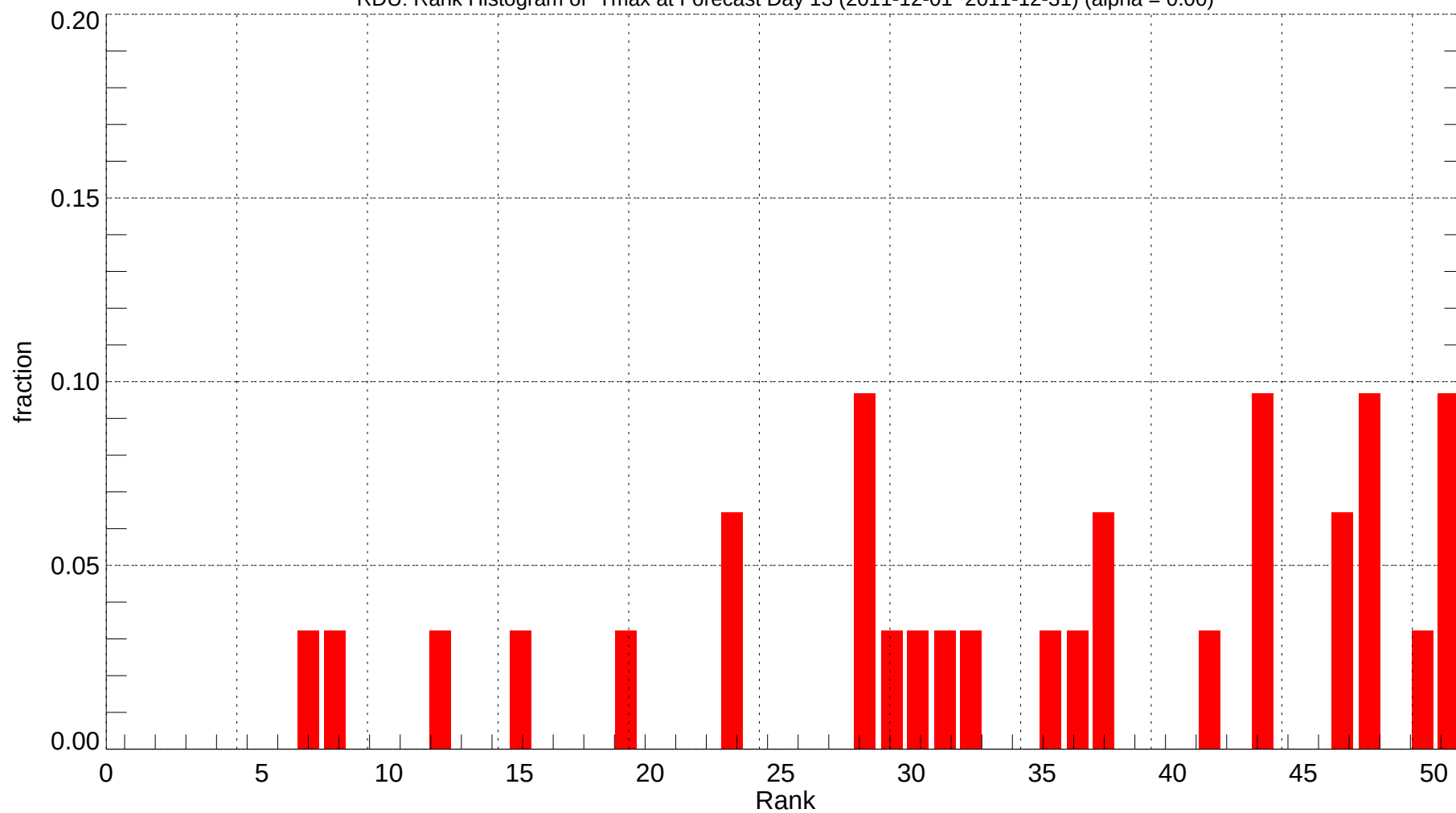
RDU: Rank Histogram of Tmax at Forecast Day 13 (2011-12-01~2011-12-31) (alpha = 0.00)
