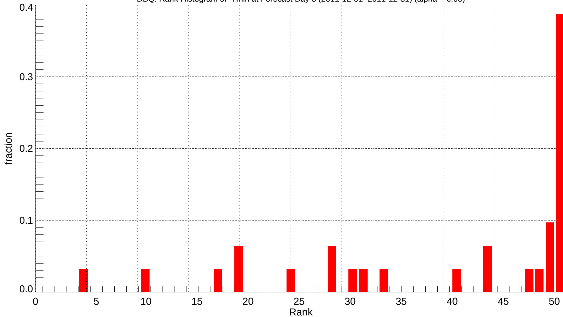
DBQ: Rank Histogram of Tmin at Forecast Day 8 (2011-12-01~2011-12-31) (alpha = 0.00)
