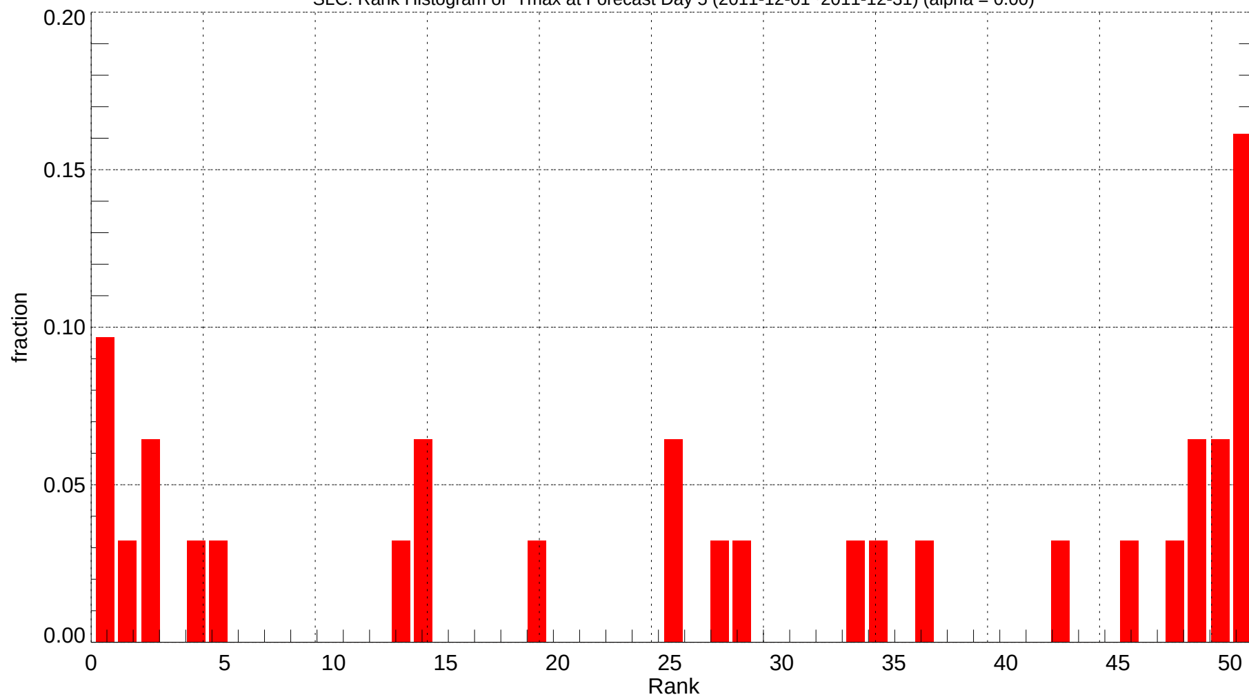
SLC: Rank Histogram of Tmax at Forecast Day 5 (2011-12-01~2011-12-31) (alpha = 0.00)
