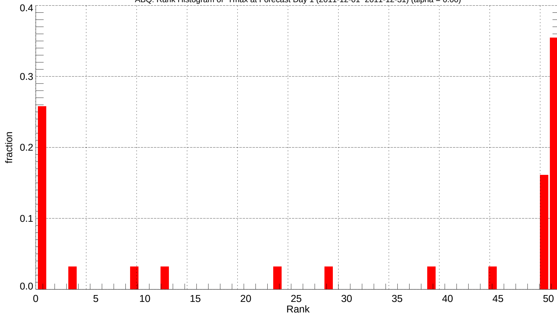
ABQ: Rank Histogram of Tmax at Forecast Day 1 (2011-12-01~2011-12-31) (alpha = 0.00)
