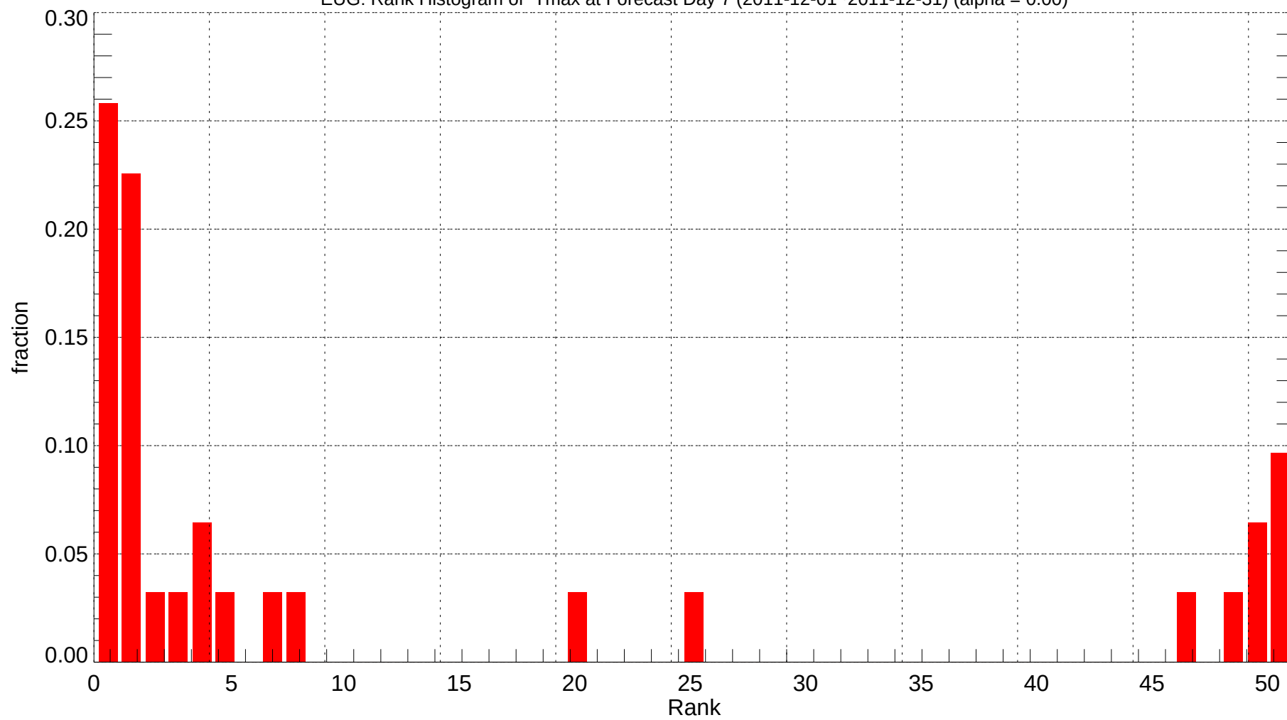
EUG: Rank Histogram of Tmax at Forecast Day 7 (2011-12-01~2011-12-31) (alpha = 0.00)
