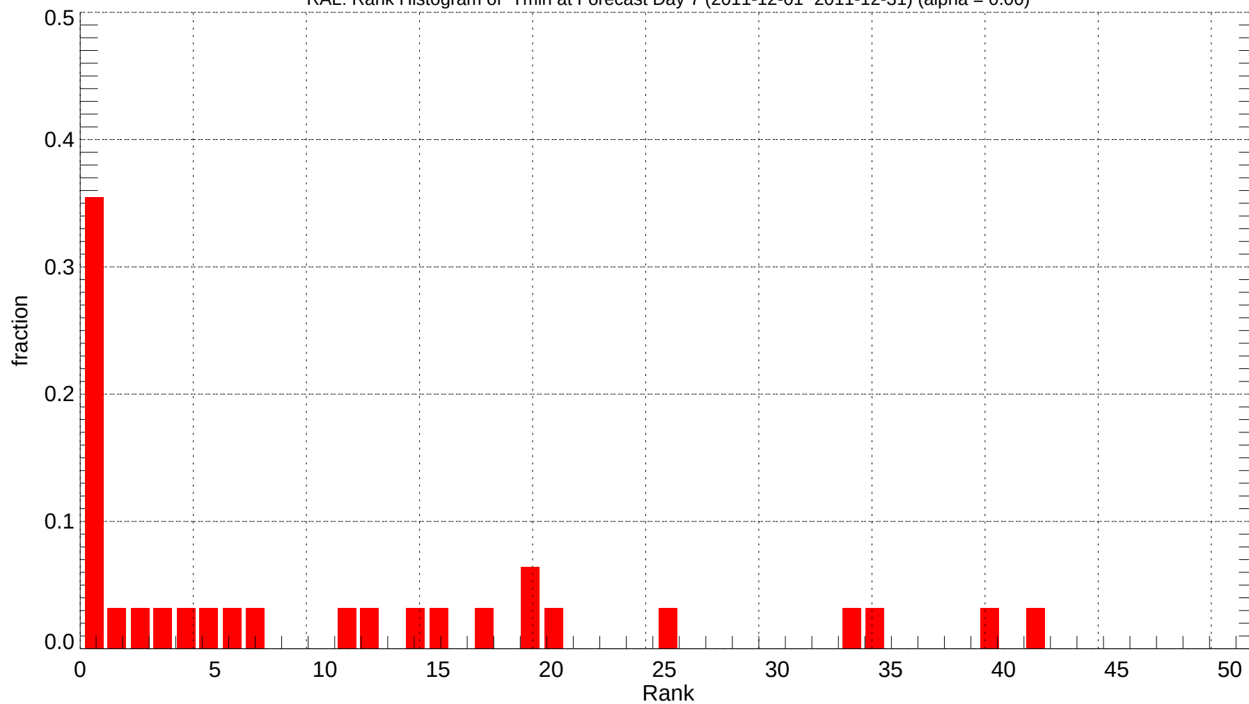
RAL: Rank Histogram of Tmin at Forecast Day 7 (2011-12-01~2011-12-31) (alpha = 0.00)
