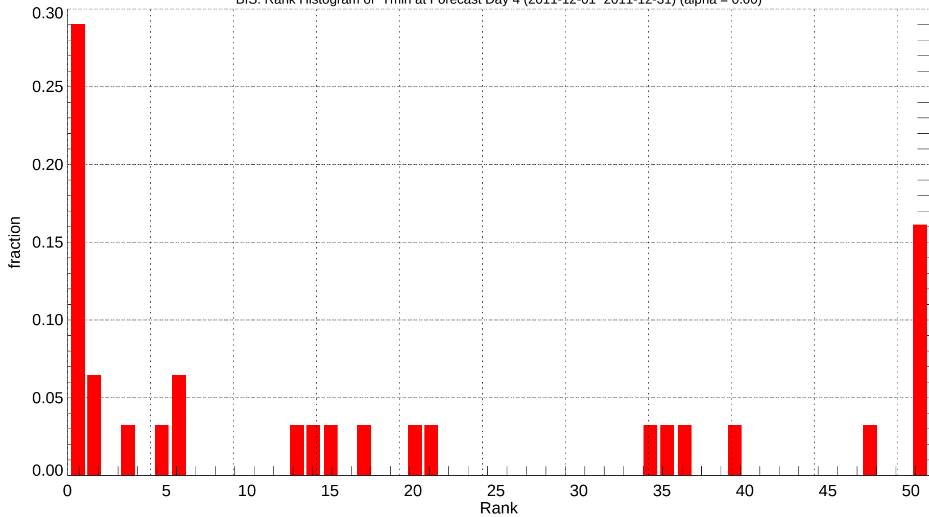
BIS: Rank Histogram of Tmin at Forecast Day 4 (2011-12-01~2011-12-31) (alpha = 0.00)
