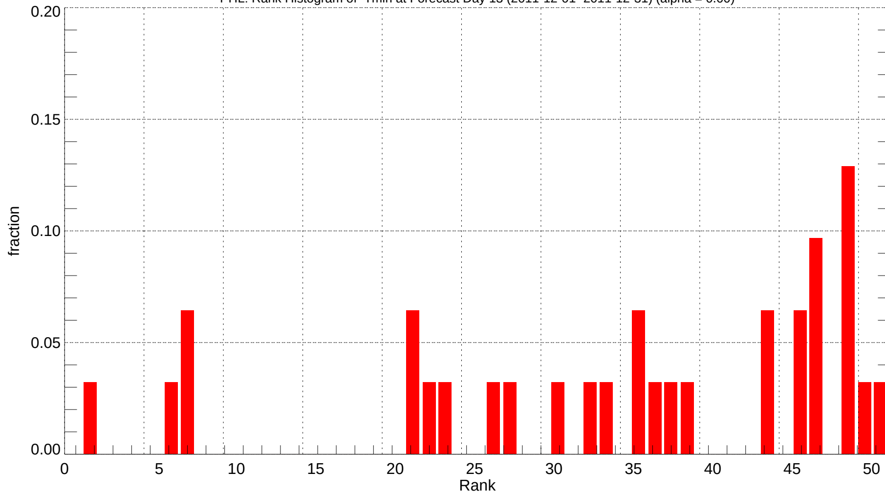
PHL: Rank Histogram of Tmin at Forecast Day 13 (2011-12-01~2011-12-31) (alpha = 0.00)
