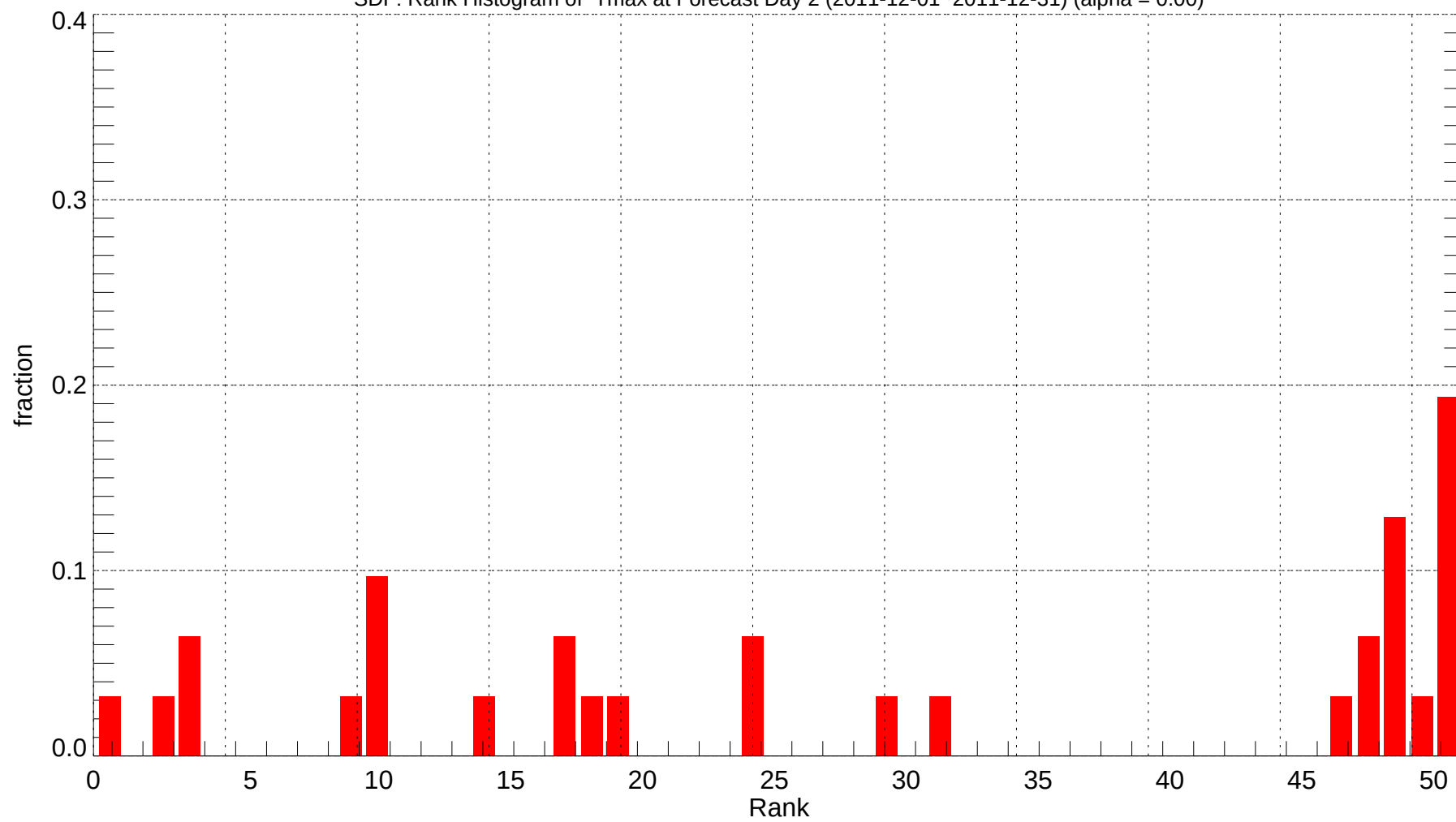
SDF: Rank Histogram of Tmax at Forecast Day 2 (2011-12-01~2011-12-31) (alpha = 0.00)
