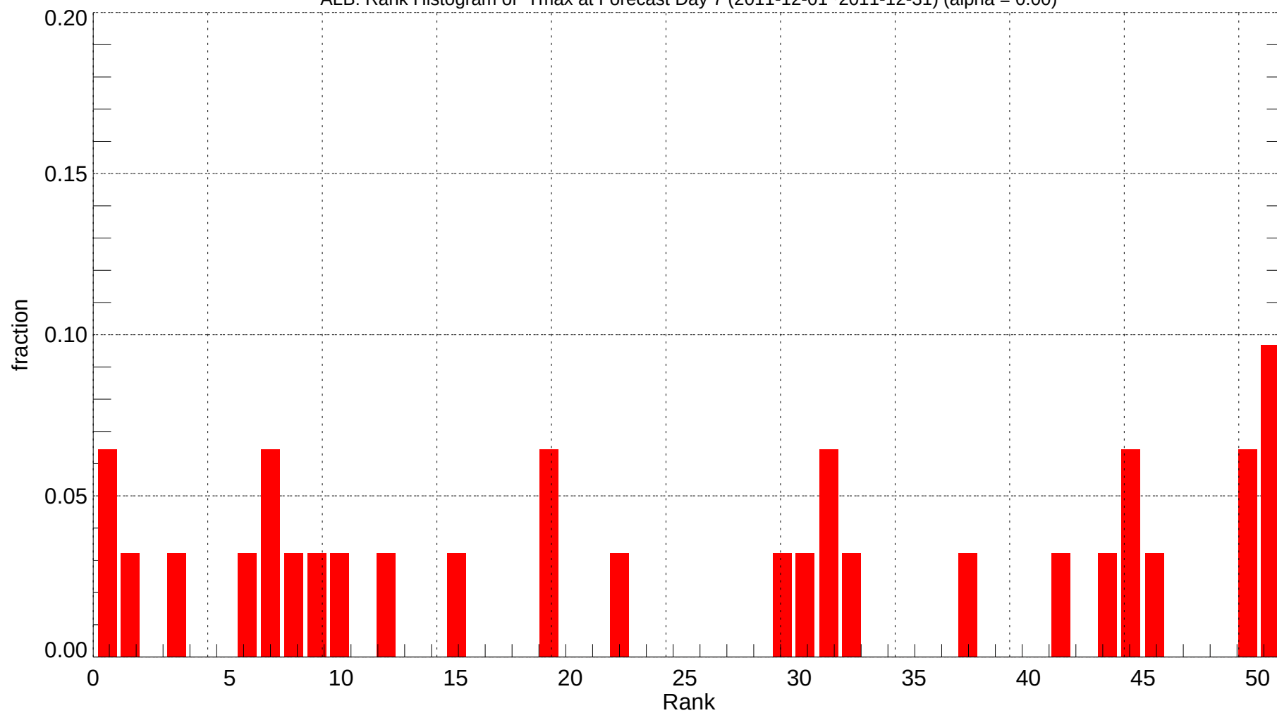
ALB: Rank Histogram of Tmax at Forecast Day 7 (2011-12-01~2011-12-31) (alpha = 0.00)
