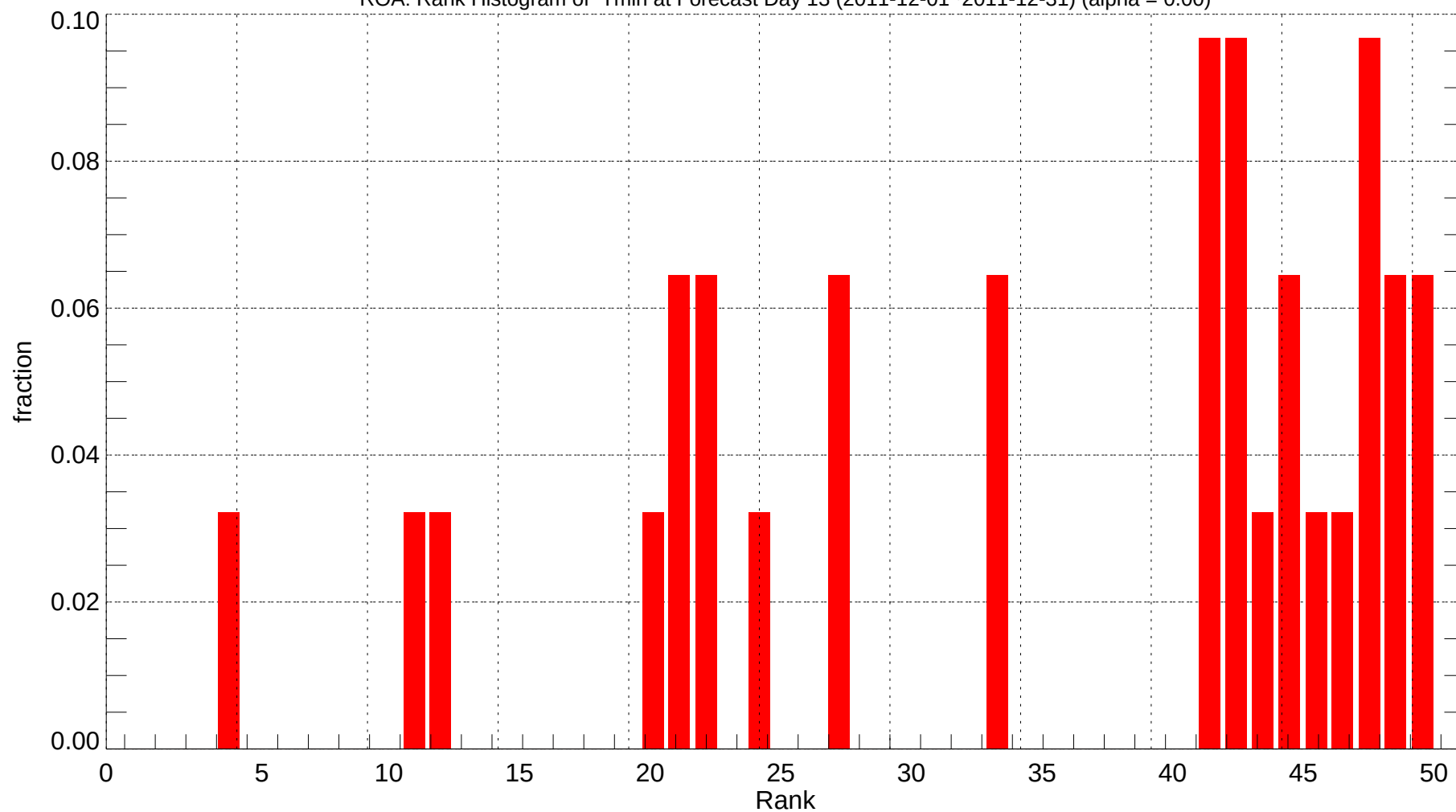
ROA: Rank Histogram of Tmin at Forecast Day 13 (2011-12-01~2011-12-31) (alpha = 0.00)
