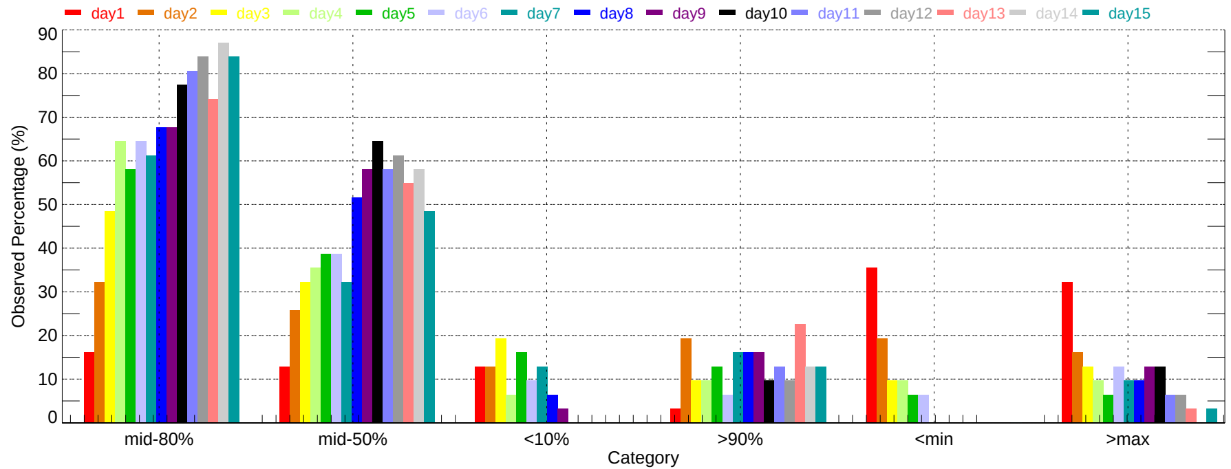
Observed Percentage of Ensembles - CHA: Max Temperature (2011-12-01~2011-12-31)
