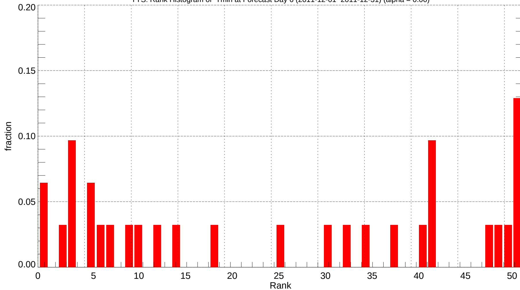
TYS: Rank Histogram of Tmin at Forecast Day 6 (2011-12-01~2011-12-31) (alpha = 0.00)
