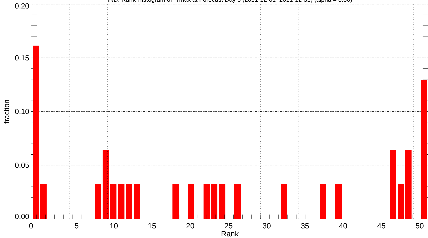
IND: Rank Histogram of Tmax at Forecast Day 6 (2011-12-01~2011-12-31) (alpha = 0.00)
