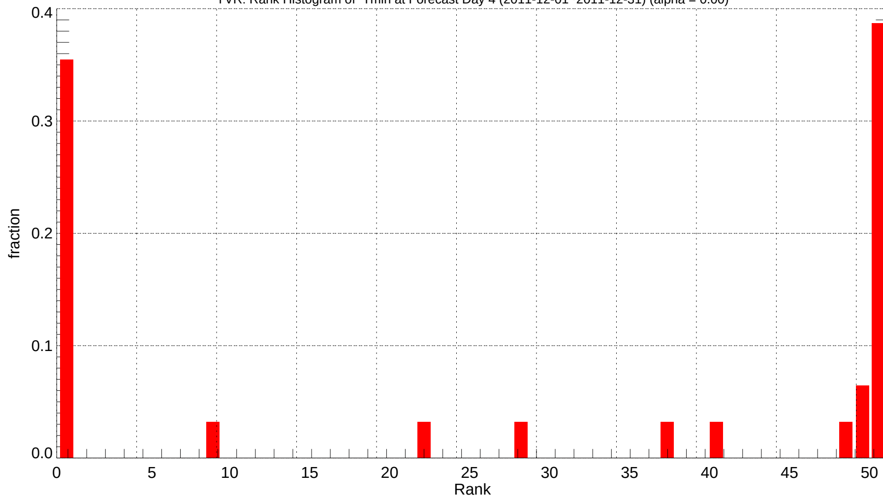
YVR: Rank Histogram of Tmin at Forecast Day 4 (2011-12-01~2011-12-31) (alpha = 0.00)
