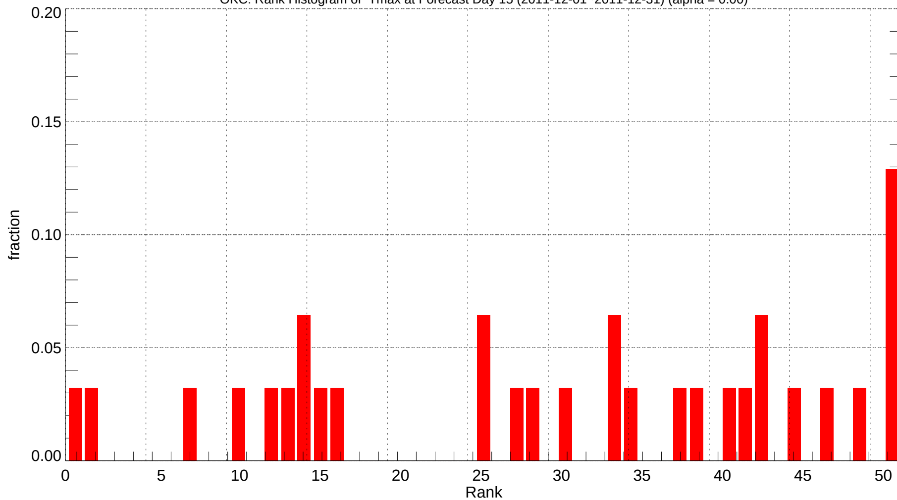
OKC: Rank Histogram of Tmax at Forecast Day 15 (2011-12-01~2011-12-31) (alpha = 0.00)
