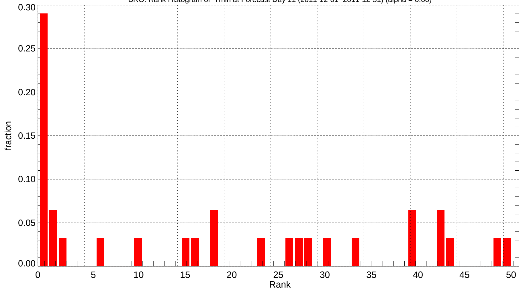
BRO: Rank Histogram of Tmin at Forecast Day 11 (2011-12-01~2011-12-31) (alpha = 0.00)
