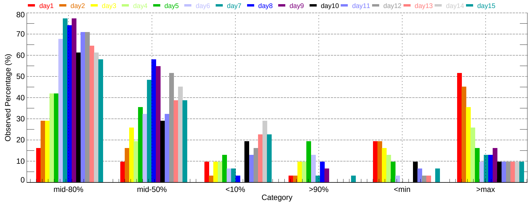
Observed Percentage of Ensembles - SLC: Max Temperature (2011-12-01~2011-12-31)
