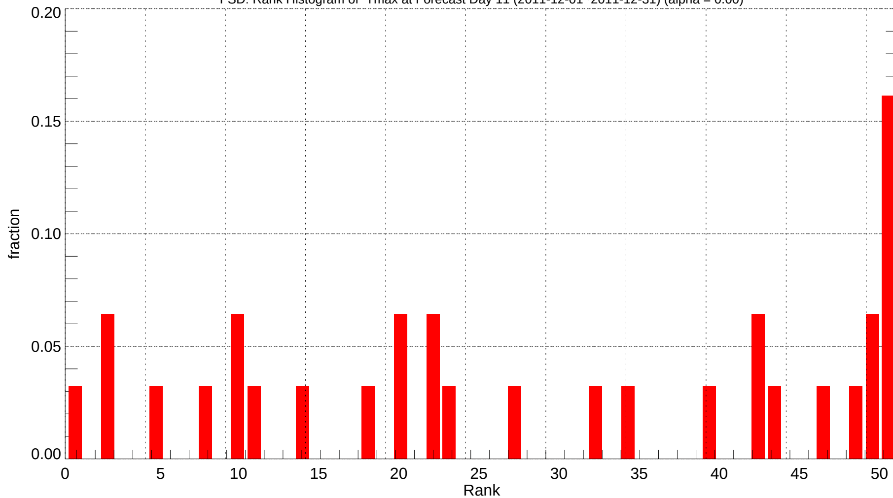
FSD: Rank Histogram of Tmax at Forecast Day 11 (2011-12-01~2011-12-31) (alpha = 0.00)
