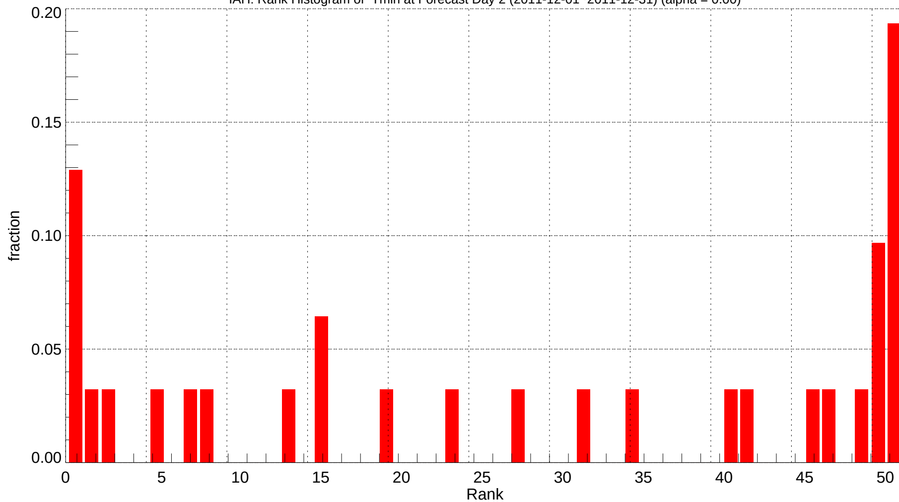
IAH: Rank Histogram of Tmin at Forecast Day 2 (2011-12-01~2011-12-31) (alpha = 0.00)
