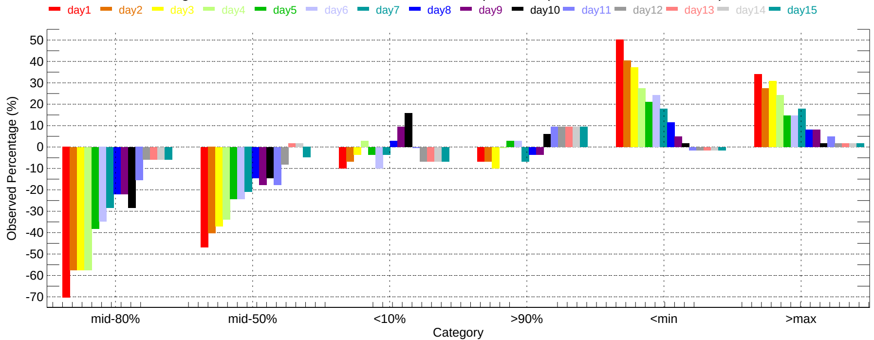
Observed Percentage Deviation of Ensembles - BUR: Min Temperature (2011-12-01~2011-12-31)
