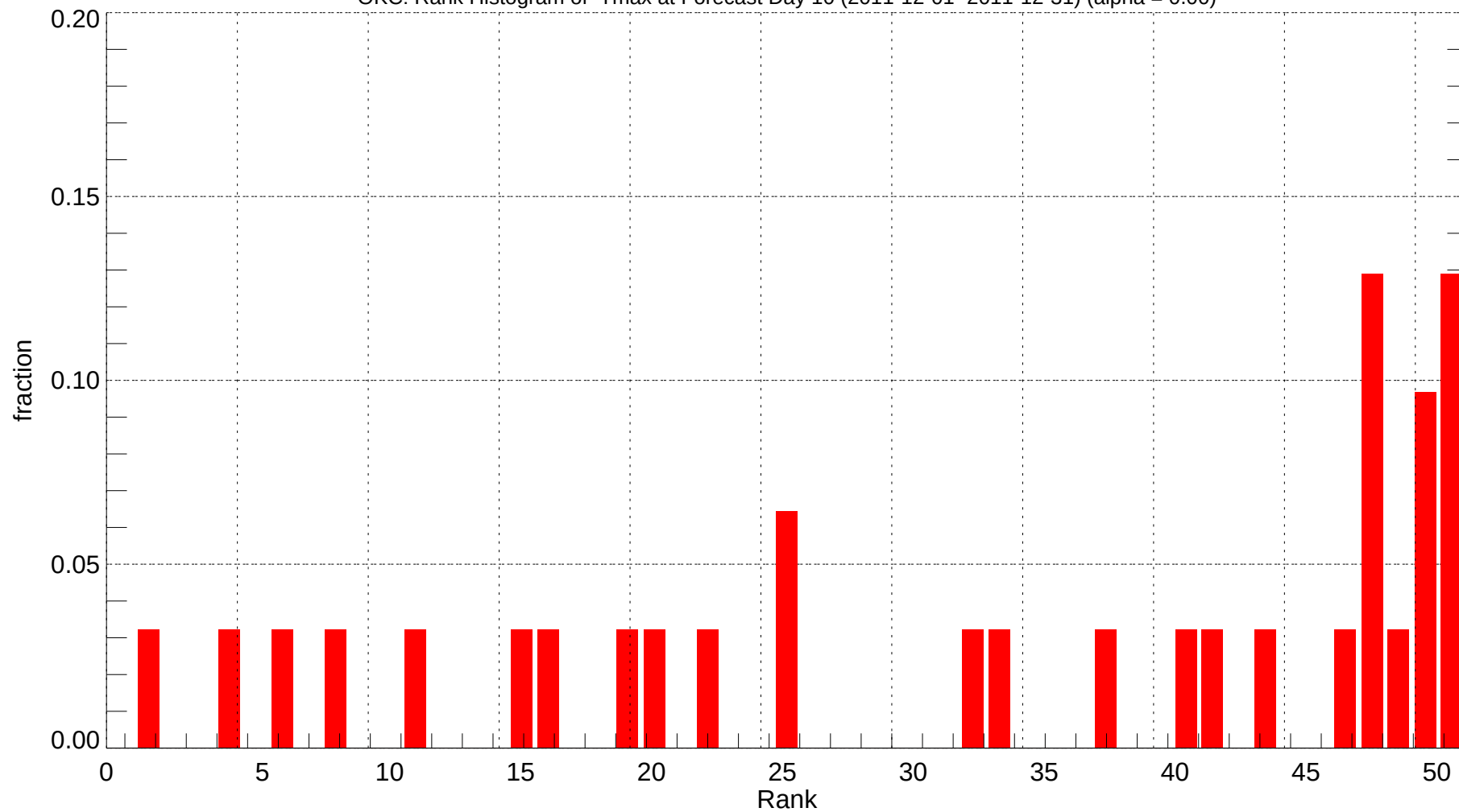
OKC: Rank Histogram of Tmax at Forecast Day 10 (2011-12-01~2011-12-31) (alpha = 0.00)
