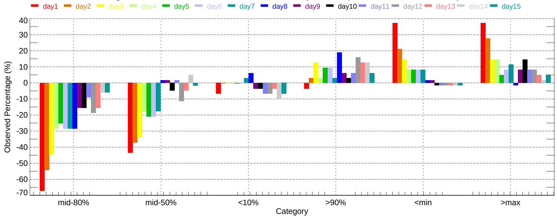
Observed Percentage Deviation of Ensembles - RIC: Max Temperature (2011-12-01~2011-12-31)
