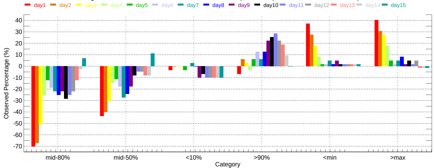
Observed Percentage Deviation of Ensembles - GAD: Min Temperature (2011-12-01~2011-12-31)
