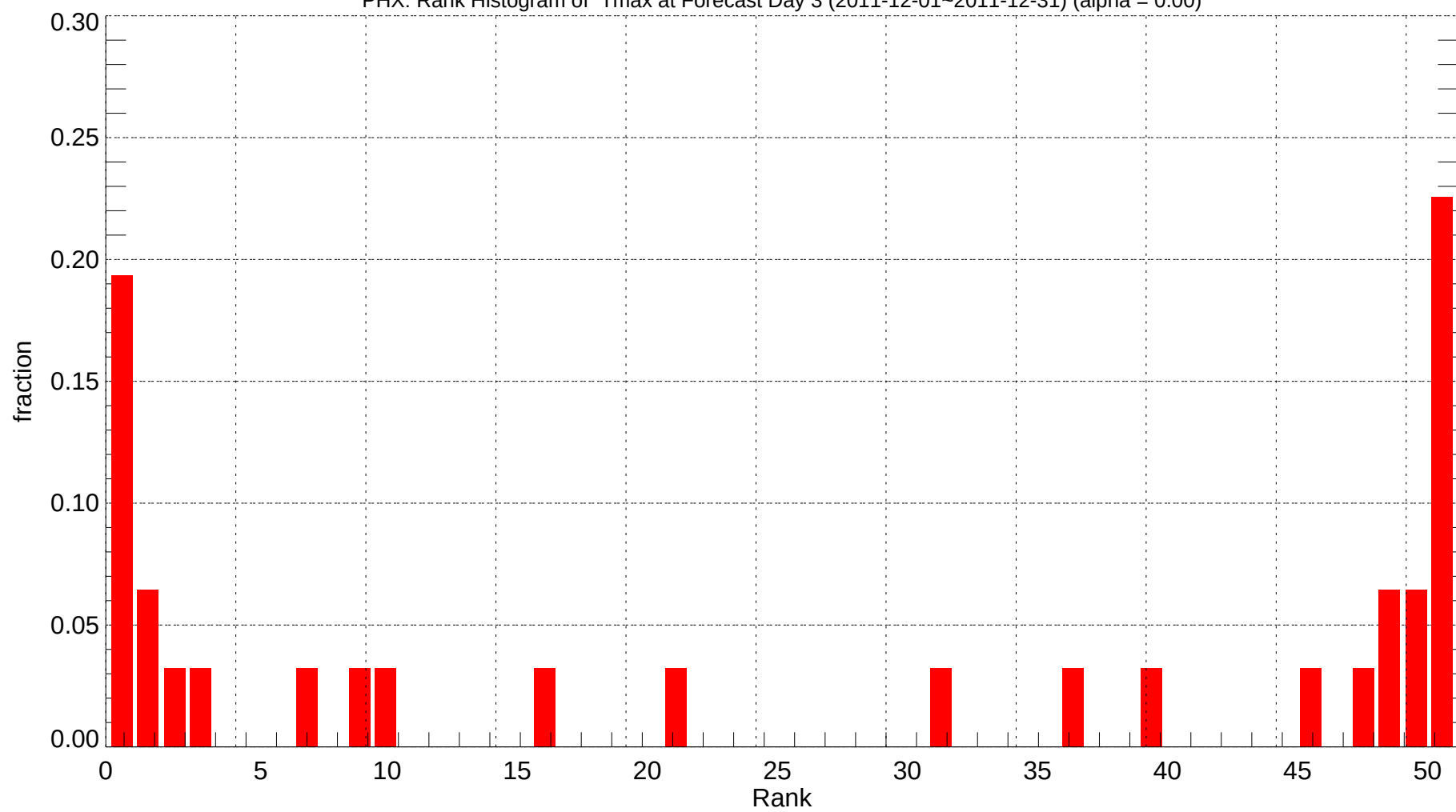
PHX: Rank Histogram of Tmax at Forecast Day 3 (2011-12-01~2011-12-31) (alpha = 0.00)
