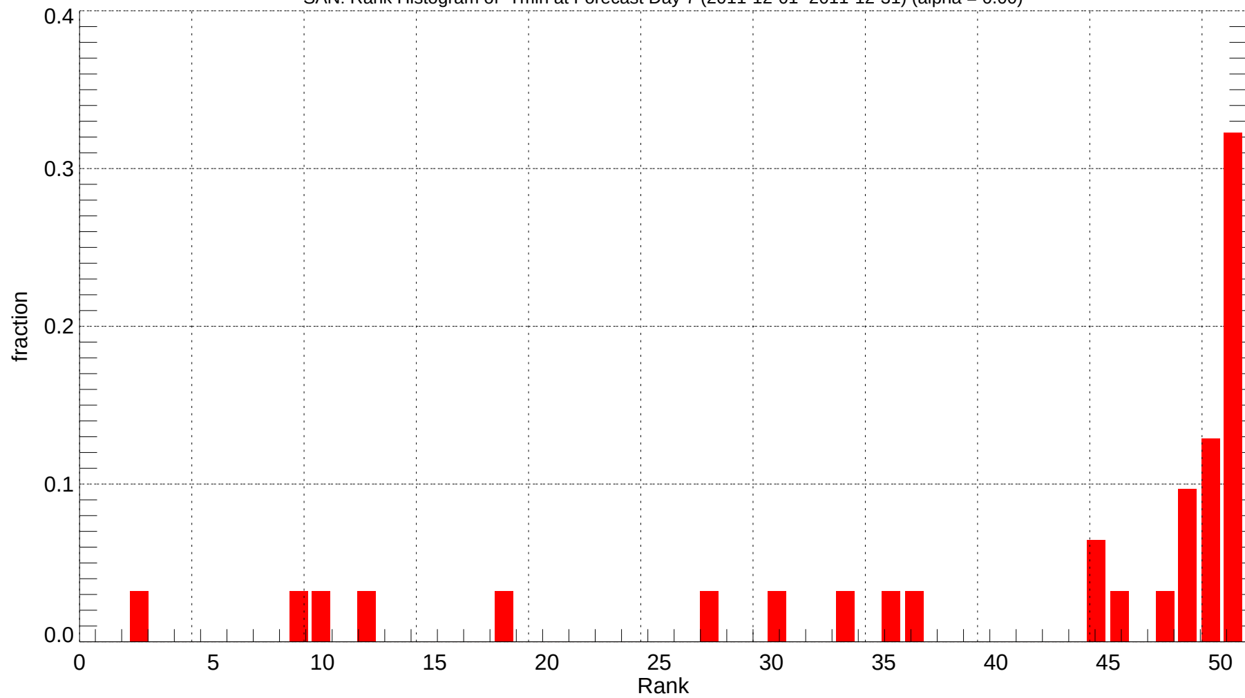
SAN: Rank Histogram of Tmin at Forecast Day 7 (2011-12-01~2011-12-31) (alpha = 0.00)
