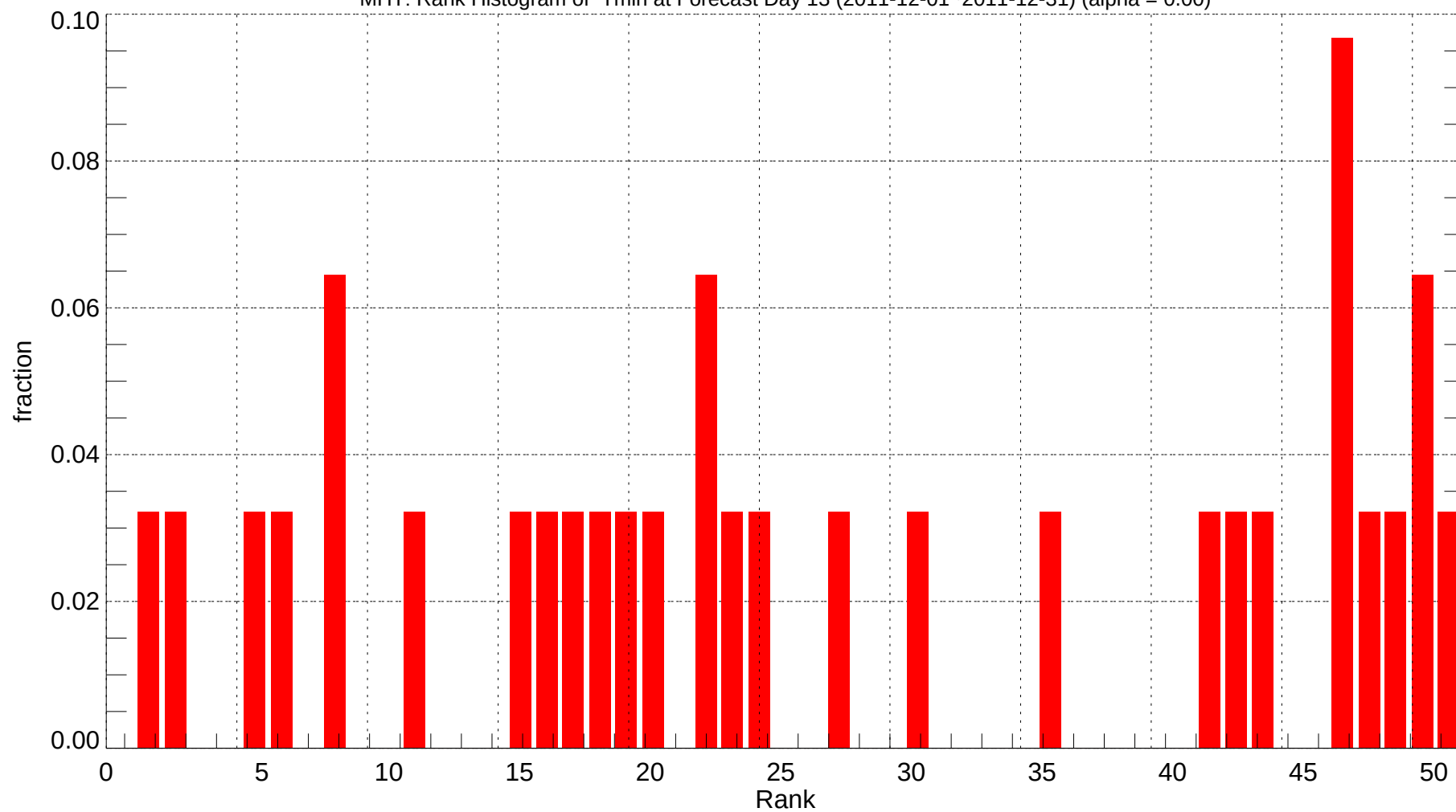
MHT: Rank Histogram of Tmin at Forecast Day 13 (2011-12-01~2011-12-31) (alpha = 0.00)
