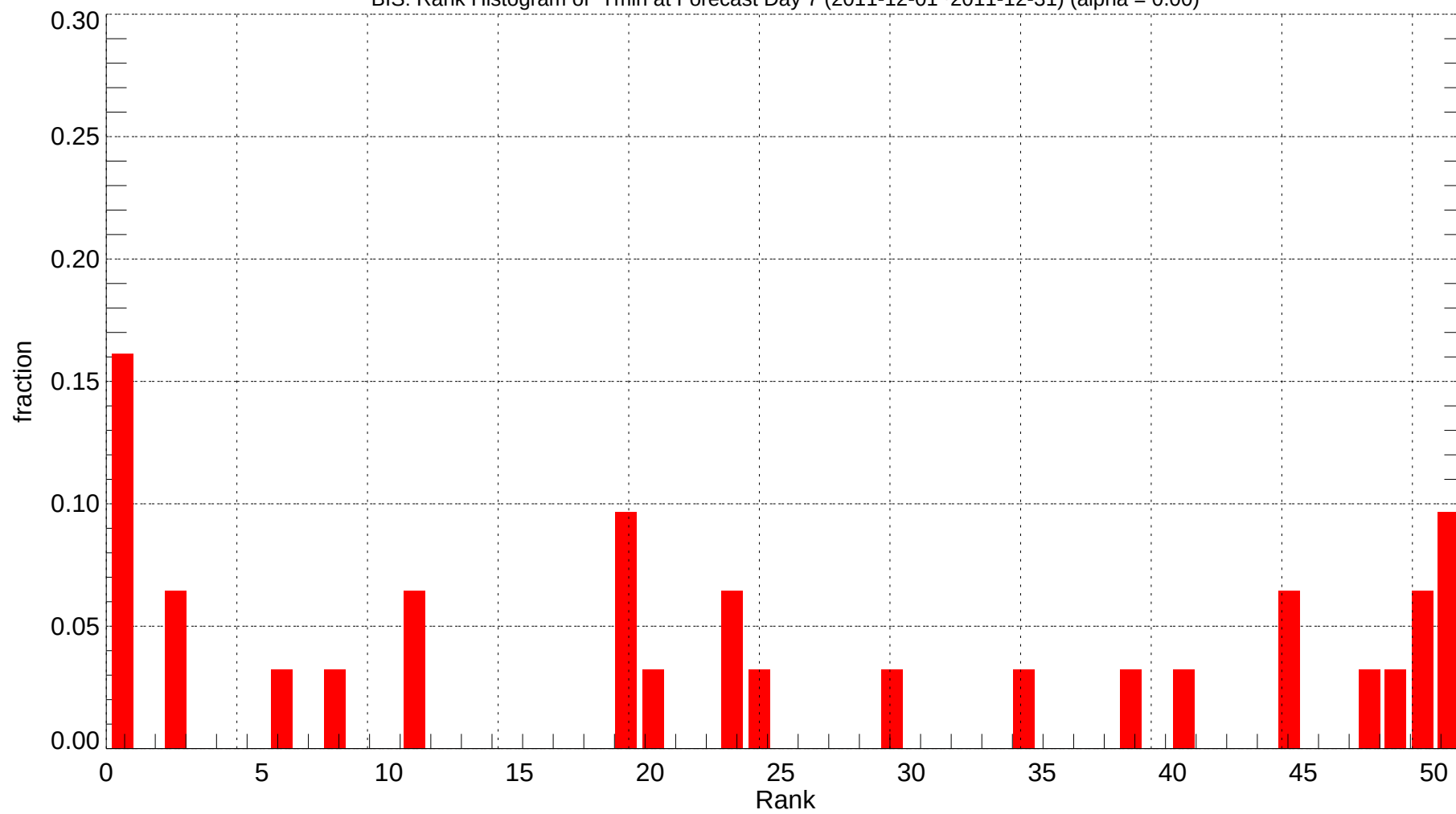
BIS: Rank Histogram of Tmin at Forecast Day 7 (2011-12-01~2011-12-31) (alpha = 0.00)
