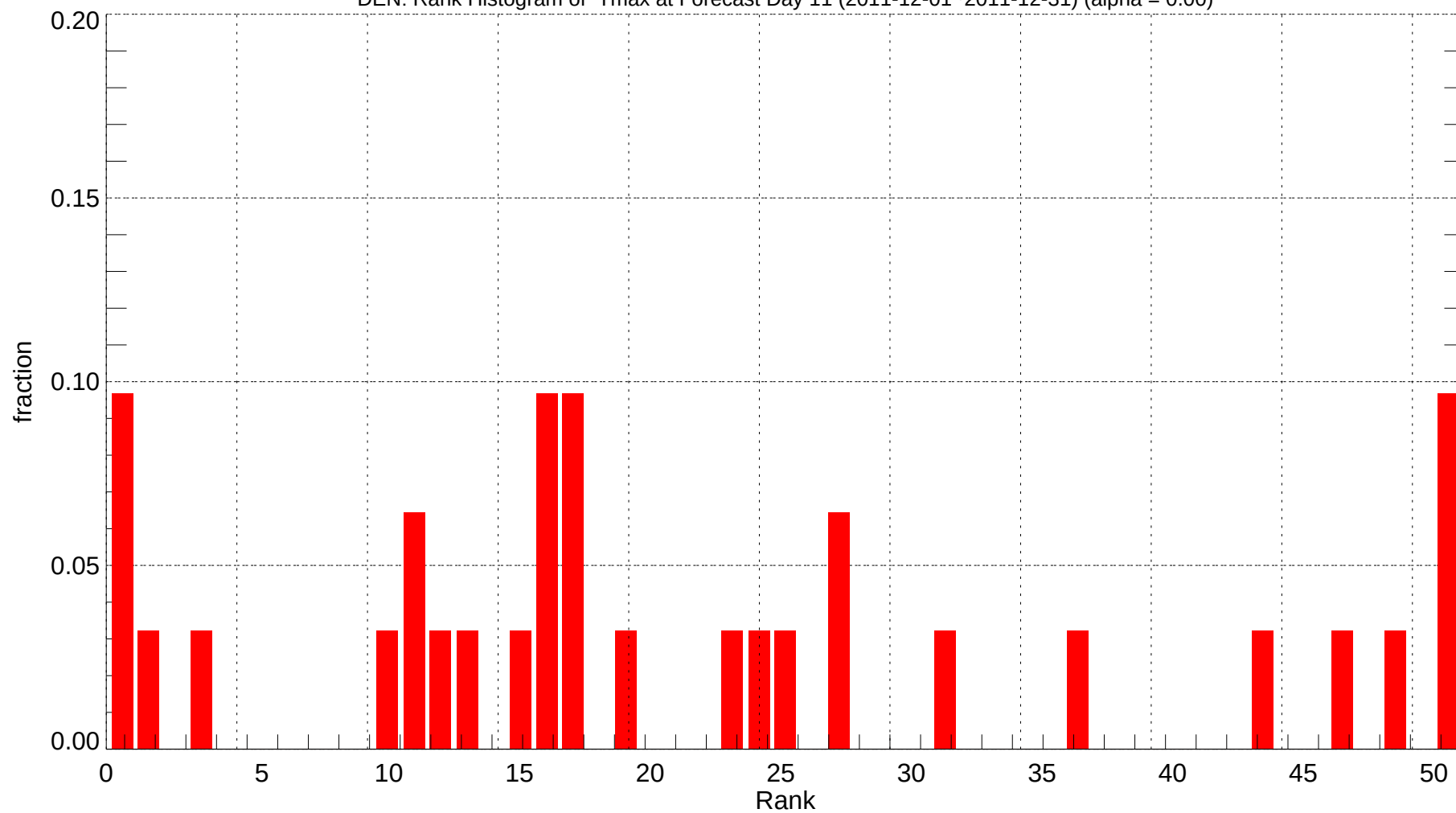
DEN: Rank Histogram of Tmax at Forecast Day 11 (2011-12-01~2011-12-31) (alpha = 0.00)
