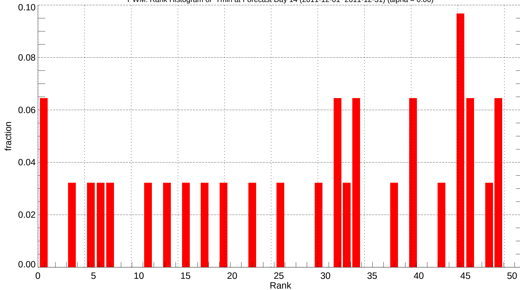
PWM: Rank Histogram of Tmin at Forecast Day 14 (2011-12-01~2011-12-31) (alpha = 0.00)
