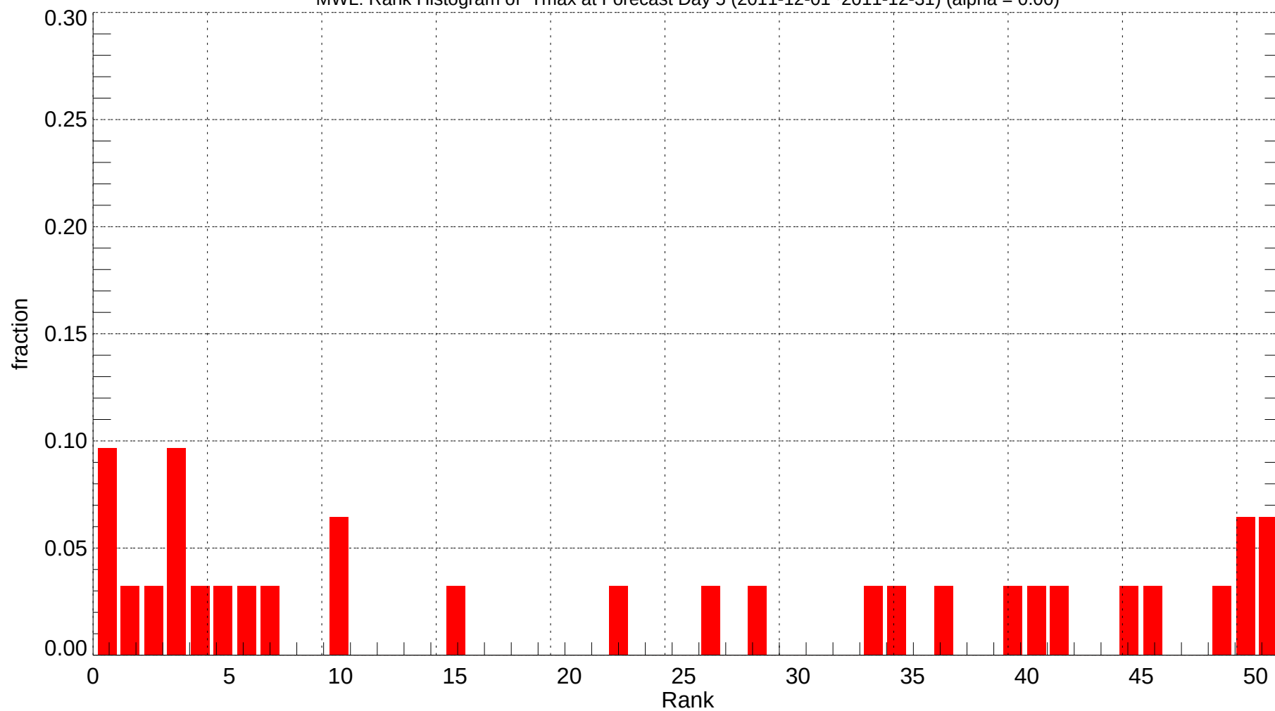
MWL: Rank Histogram of Tmax at Forecast Day 5 (2011-12-01~2011-12-31) (alpha = 0.00)
