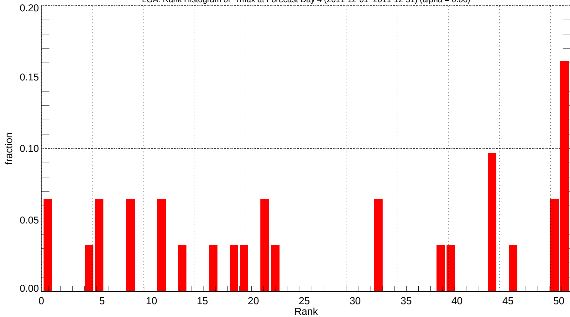
LGA: Rank Histogram of Tmax at Forecast Day 4 (2011-12-01~2011-12-31) (alpha = 0.00)
