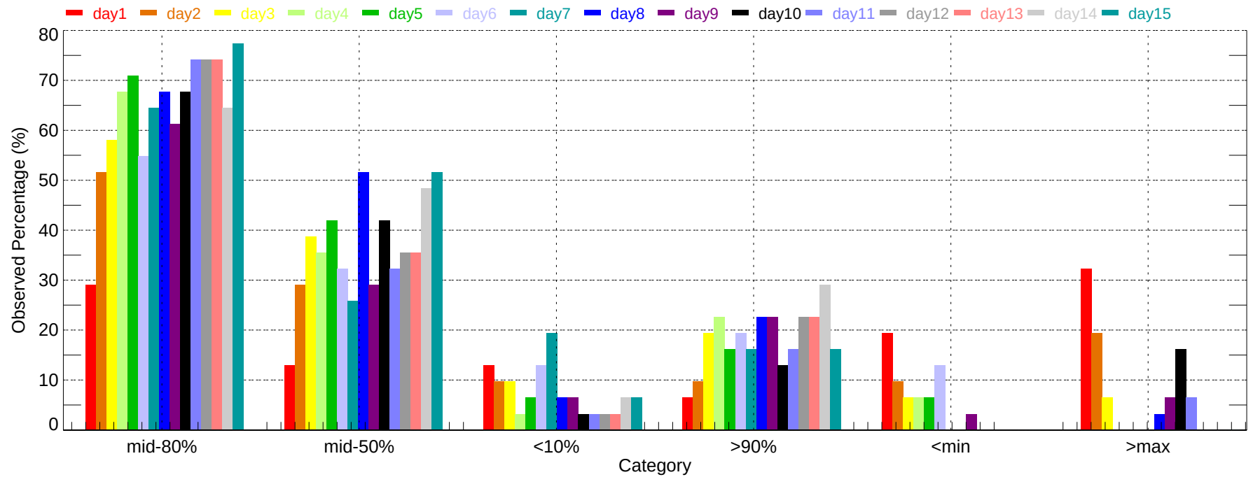
Observed Percentage of Ensembles - IND: Min Temperature (2011-12-01~2011-12-31)
