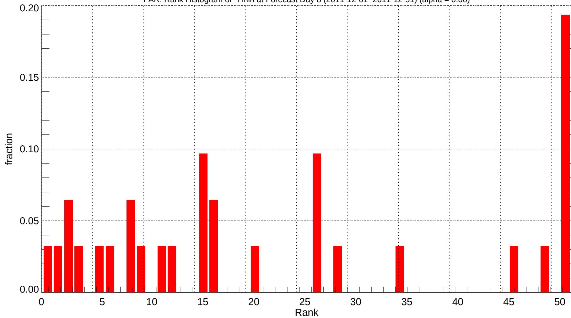
FAR: Rank Histogram of Tmin at Forecast Day 8 (2011-12-01~2011-12-31) (alpha = 0.00)
