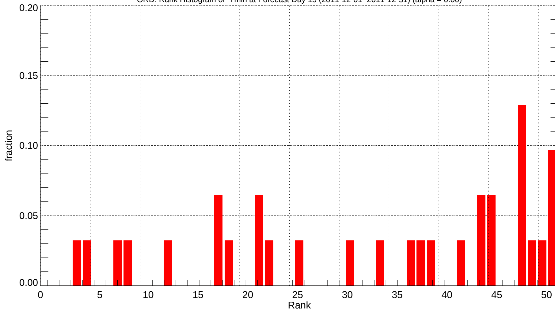
ORD: Rank Histogram of Tmin at Forecast Day 13 (2011-12-01~2011-12-31) (alpha = 0.00)
