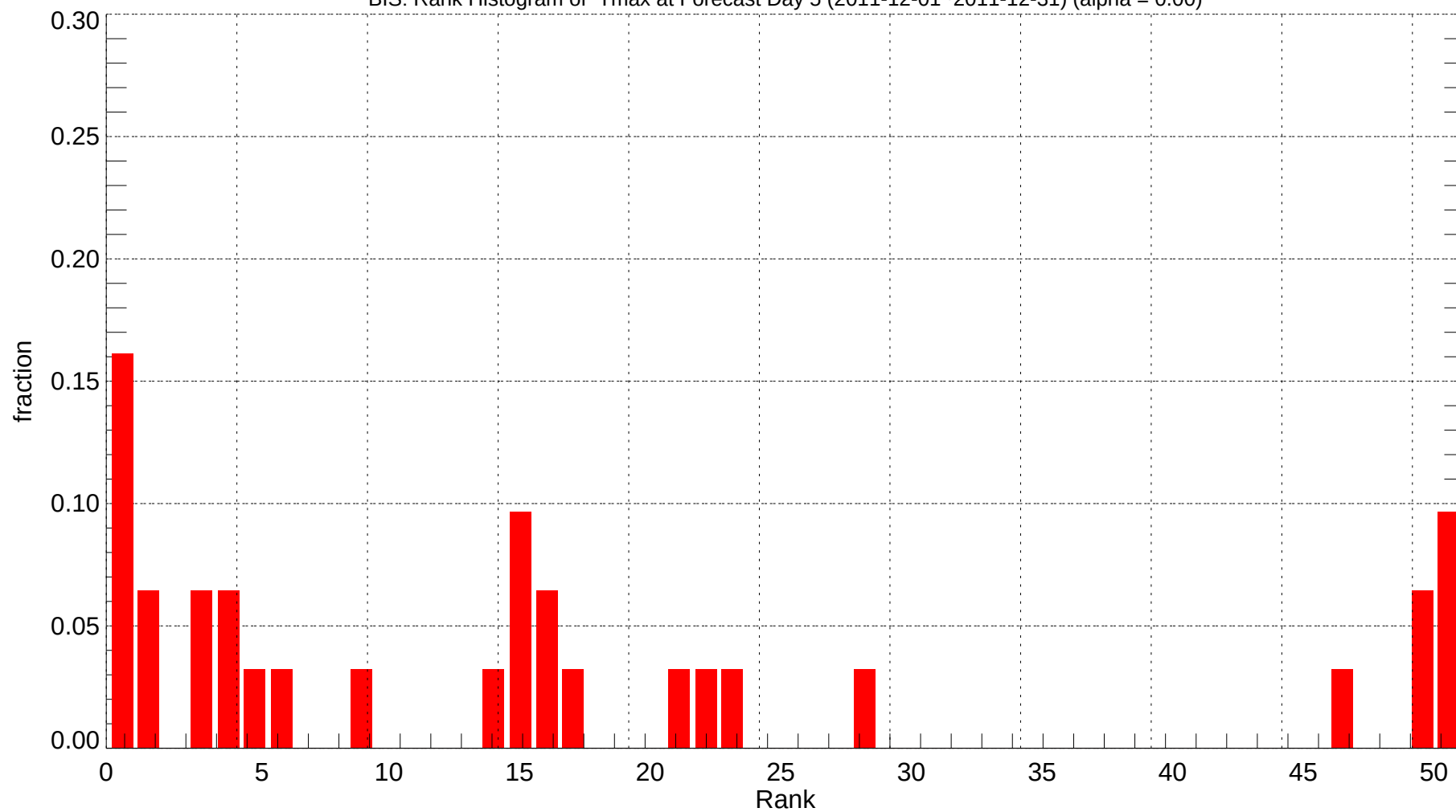
BIS: Rank Histogram of Tmax at Forecast Day 5 (2011-12-01~2011-12-31) (alpha = 0.00)
