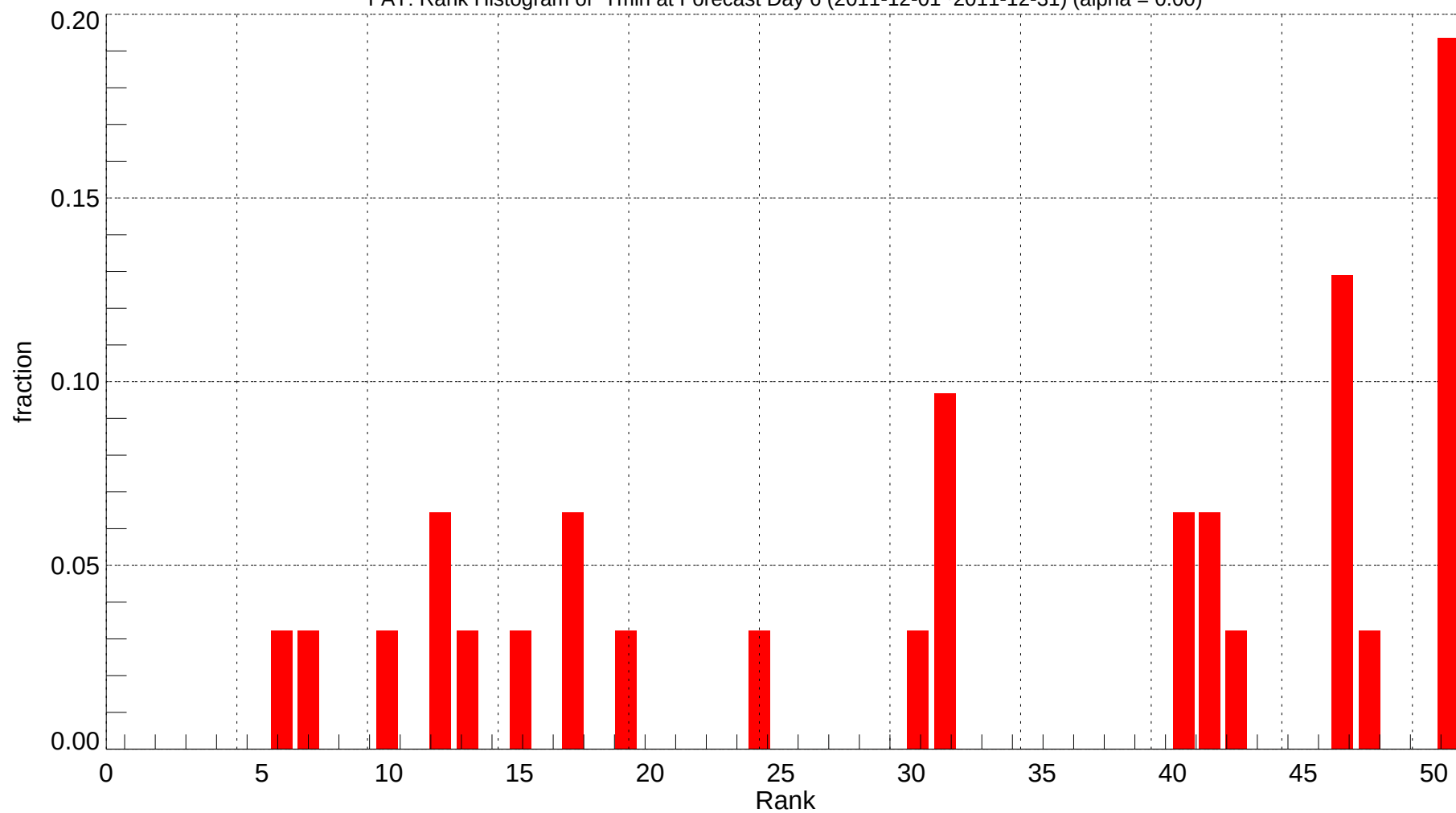
FAT: Rank Histogram of Tmin at Forecast Day 6 (2011-12-01~2011-12-31) (alpha = 0.00)
