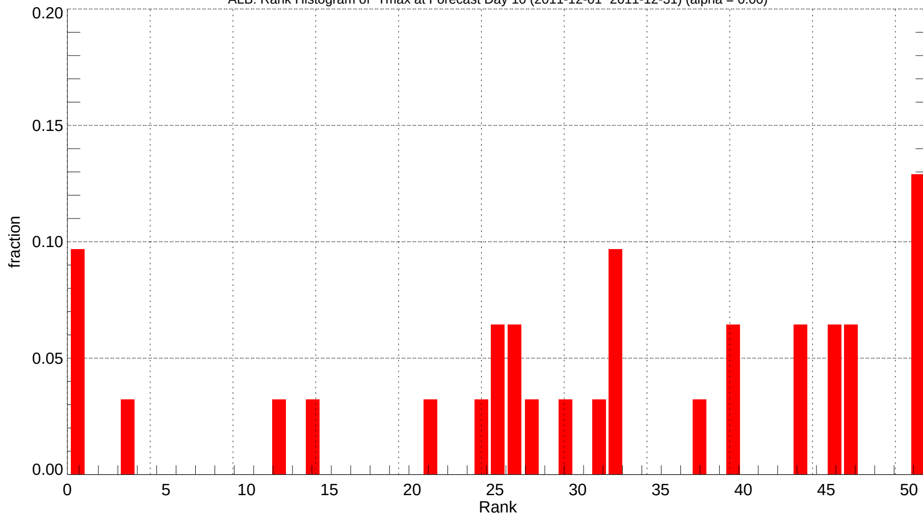
ALB: Rank Histogram of Tmax at Forecast Day 10 (2011-12-01~2011-12-31) (alpha = 0.00)
