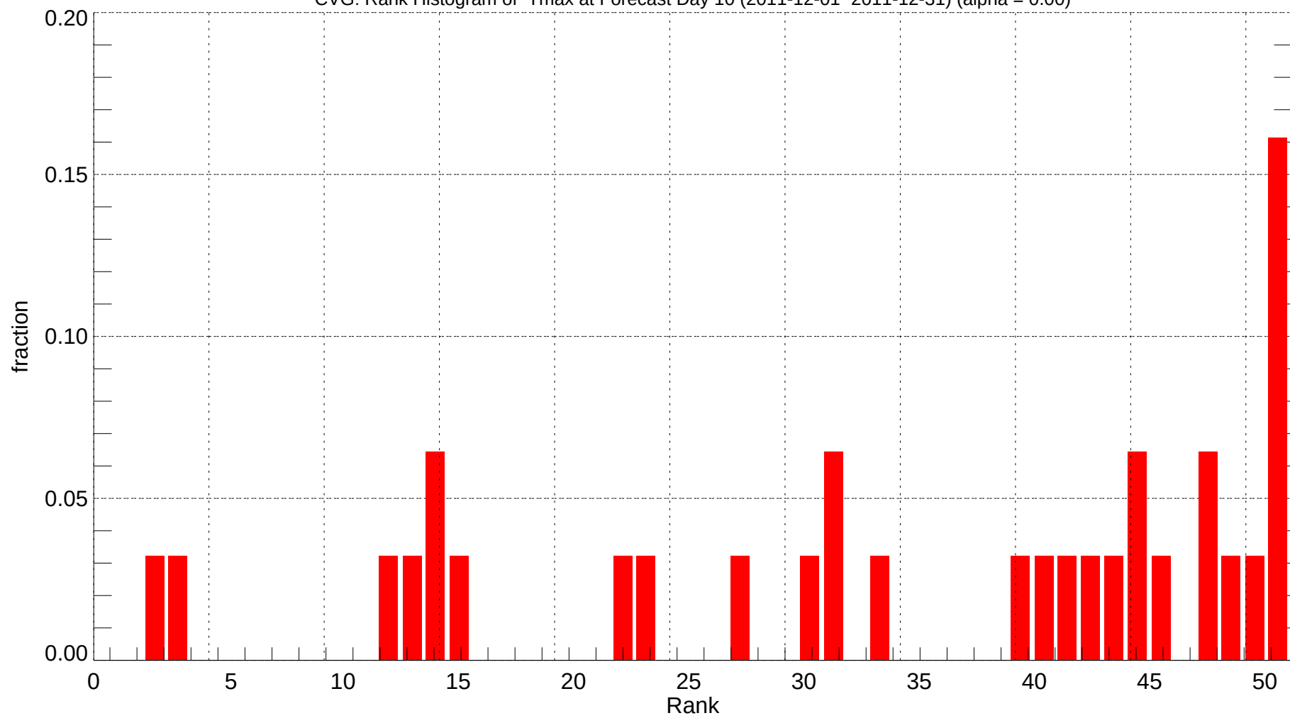
CVG: Rank Histogram of Tmax at Forecast Day 10 (2011-12-01~2011-12-31) (alpha = 0.00)
