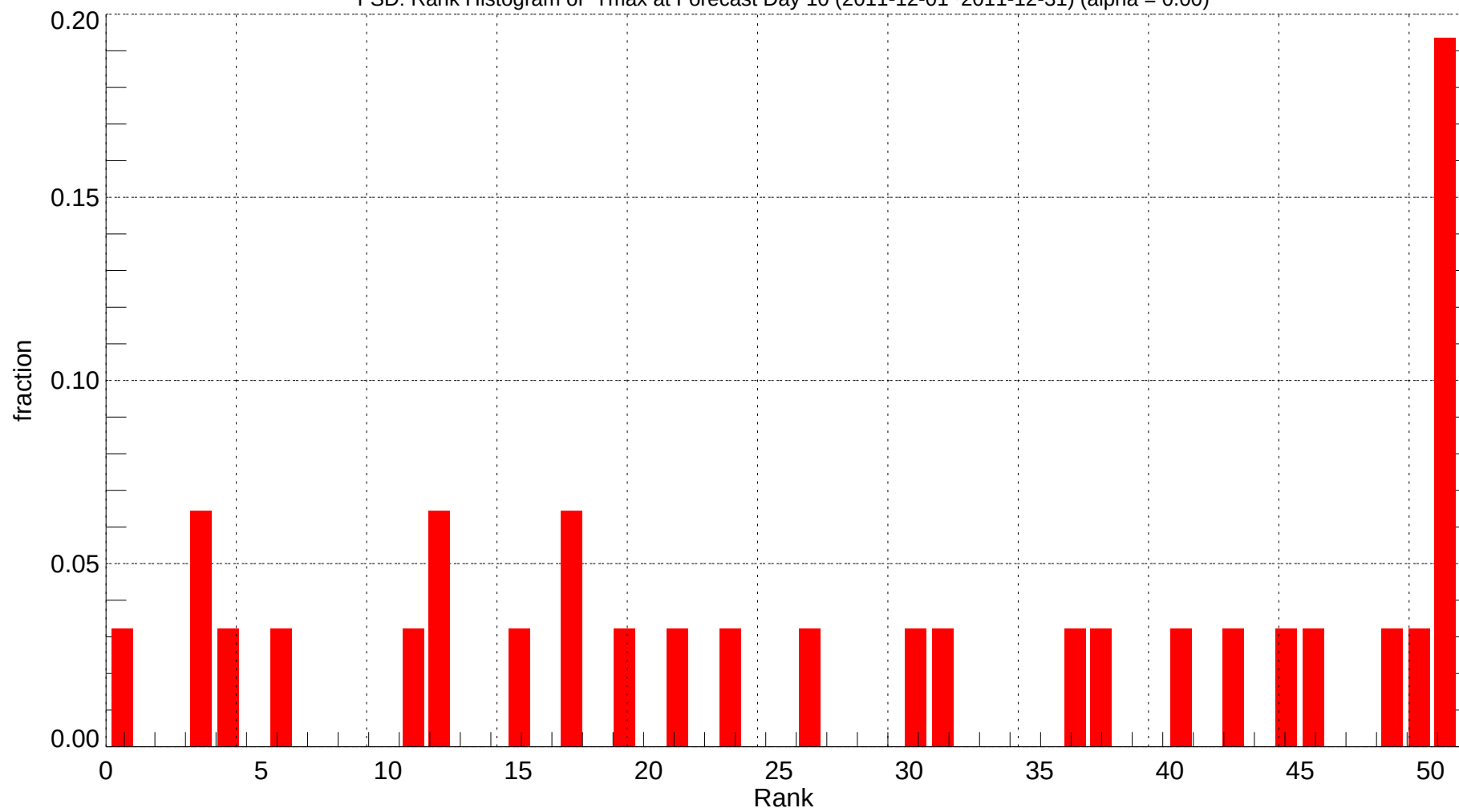
FSD: Rank Histogram of Tmax at Forecast Day 10 (2011-12-01~2011-12-31) (alpha = 0.00)
