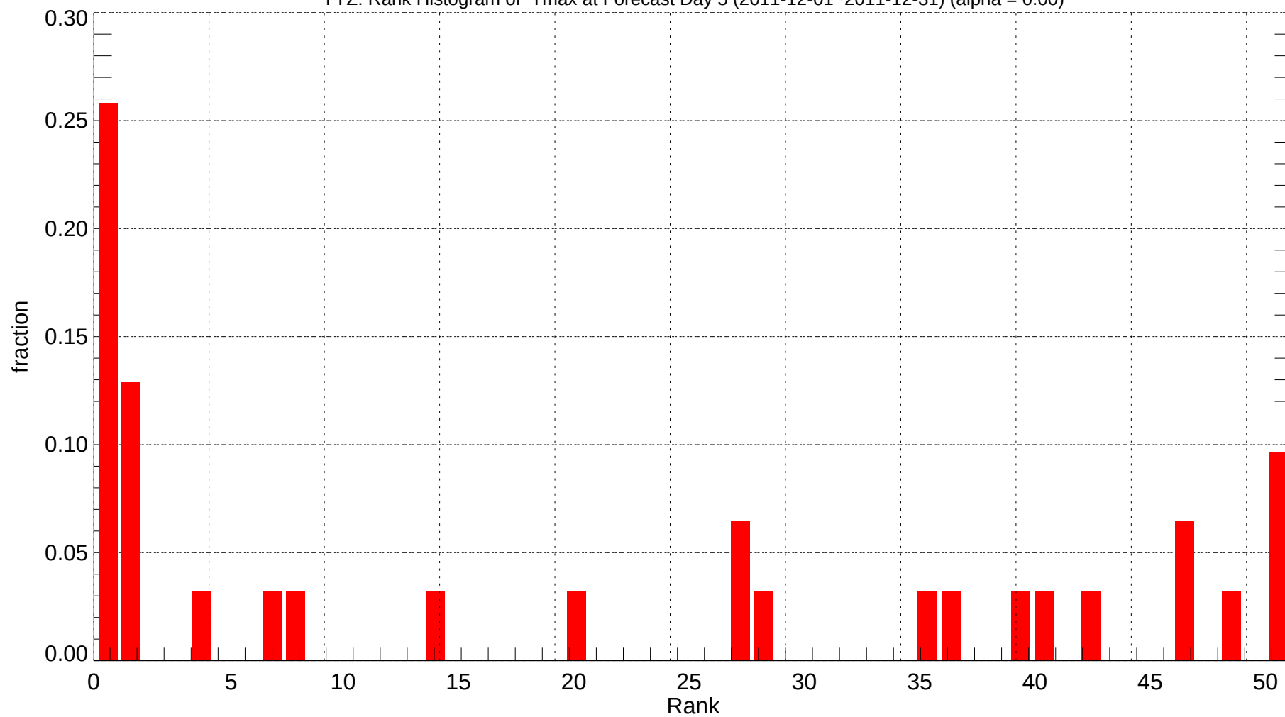
YYZ: Rank Histogram of Tmax at Forecast Day 5 (2011-12-01~2011-12-31) (alpha = 0.00)
