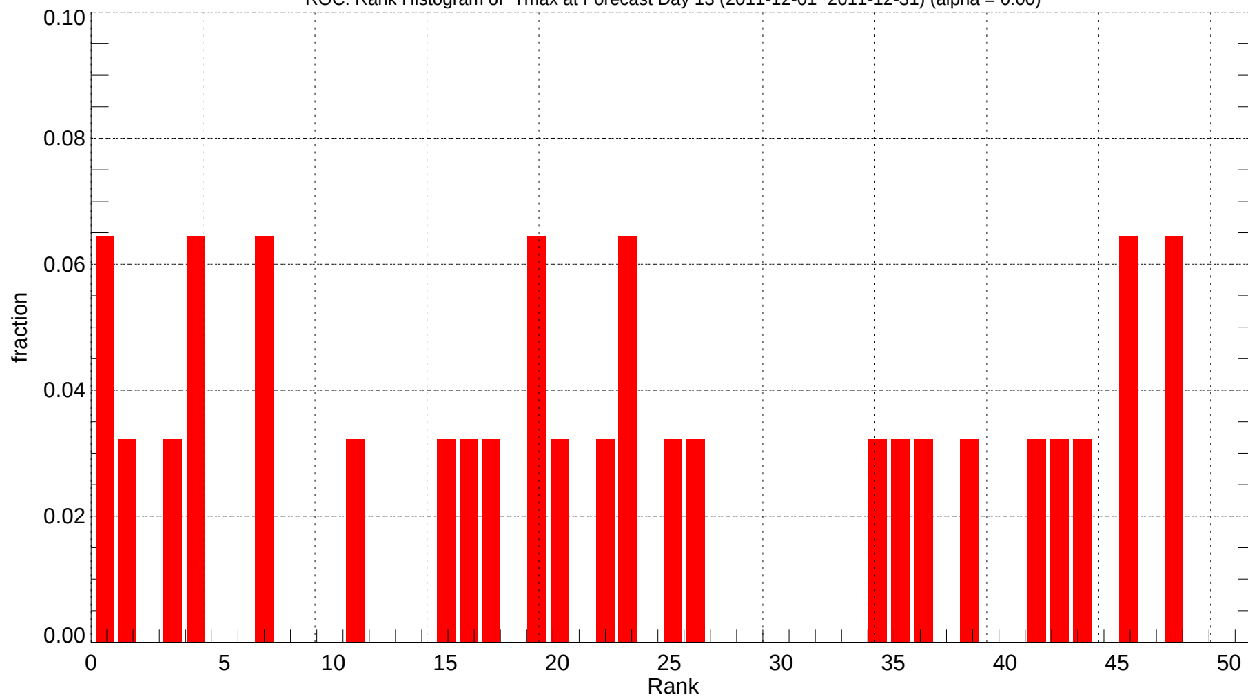
ROC: Rank Histogram of Tmax at Forecast Day 13 (2011-12-01~2011-12-31) (alpha = 0.00)
