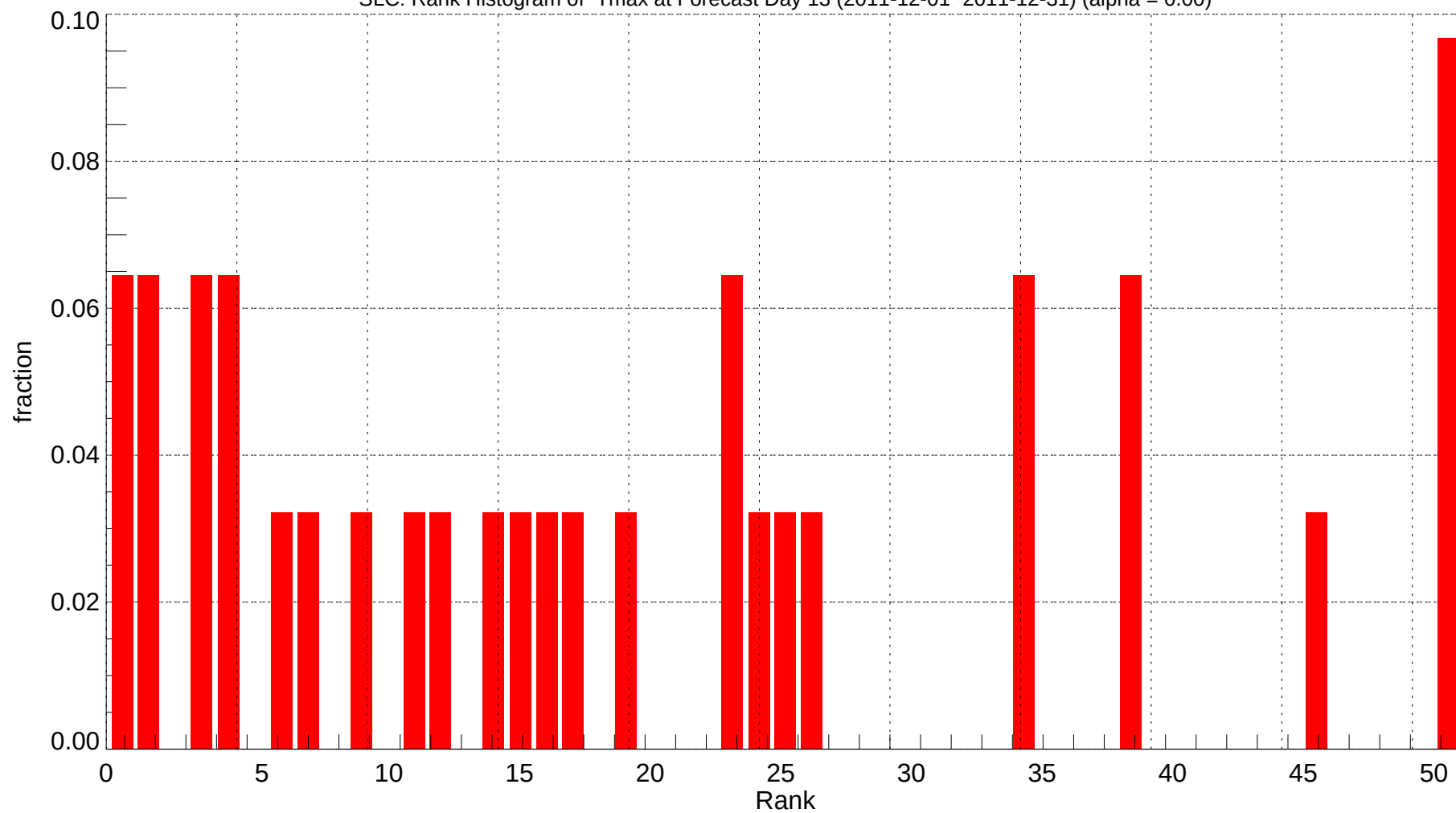
SLC: Rank Histogram of Tmax at Forecast Day 13 (2011-12-01~2011-12-31) (alpha = 0.00)
