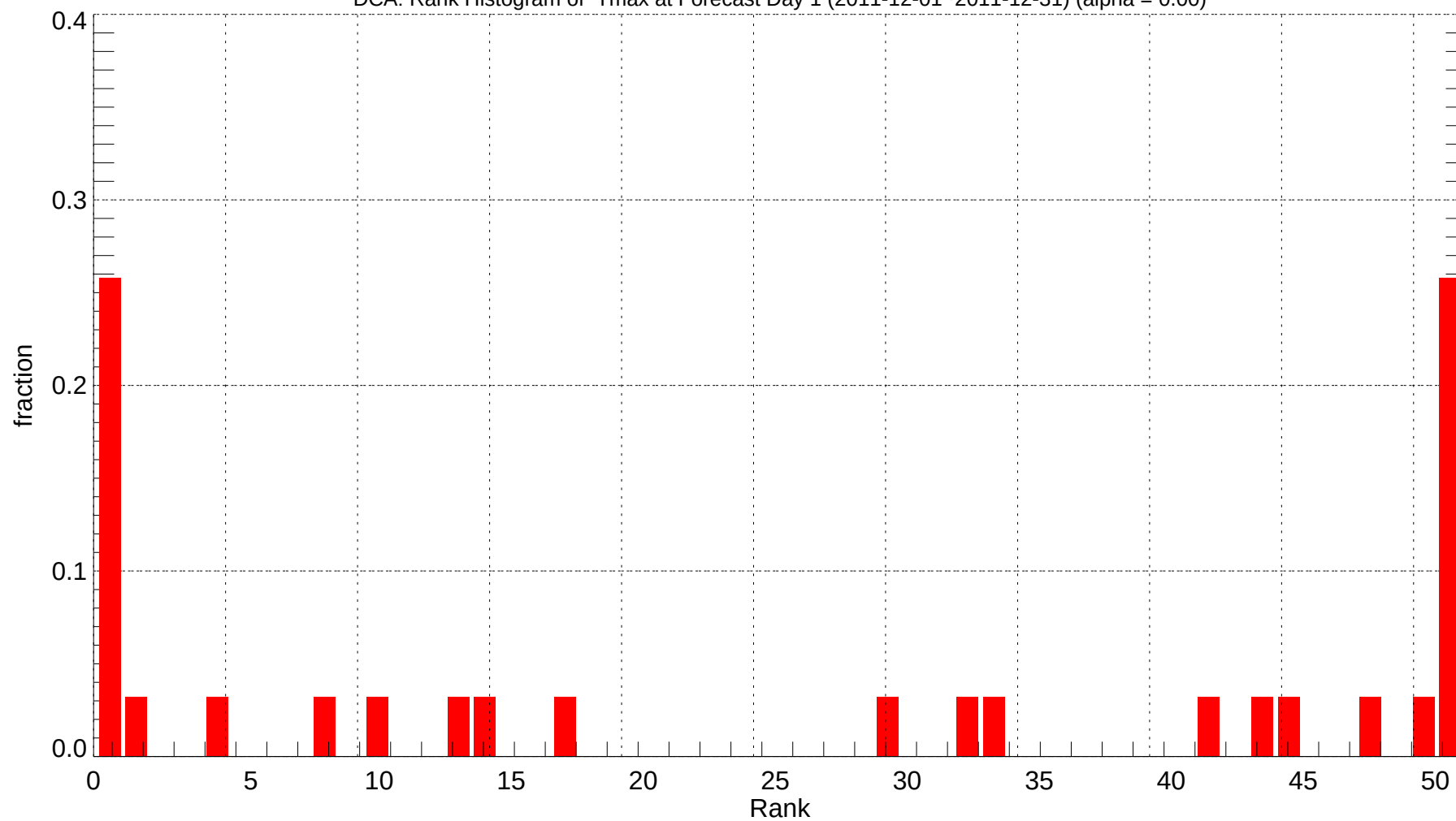
DCA: Rank Histogram of Tmax at Forecast Day 1 (2011-12-01~2011-12-31) (alpha = 0.00)
