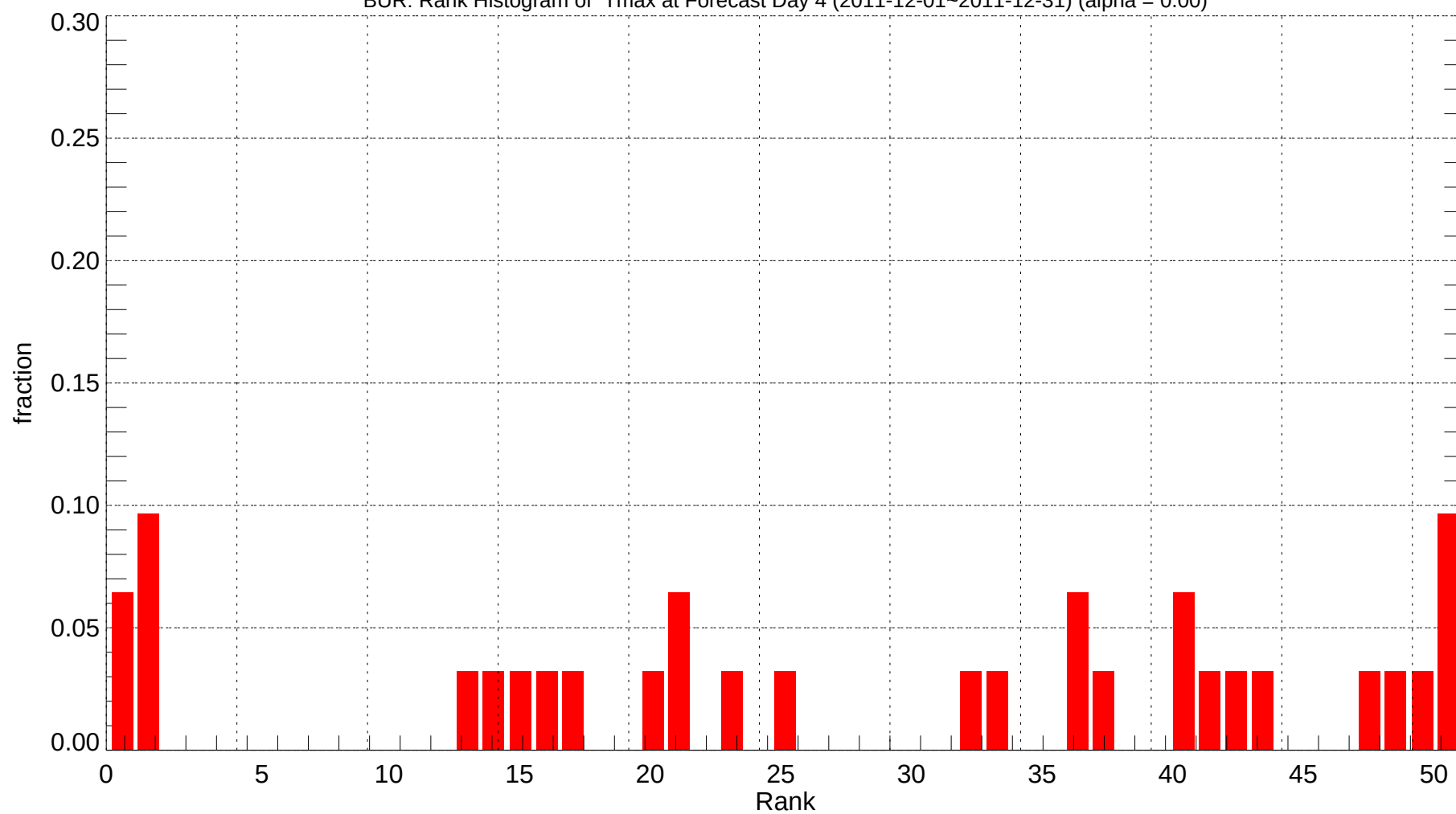
BUR: Rank Histogram of Tmax at Forecast Day 4 (2011-12-01~2011-12-31) (alpha = 0.00)
