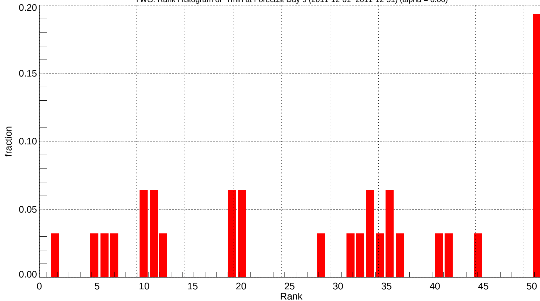
YWG: Rank Histogram of Tmin at Forecast Day 9 (2011-12-01~2011-12-31) (alpha = 0.00)
