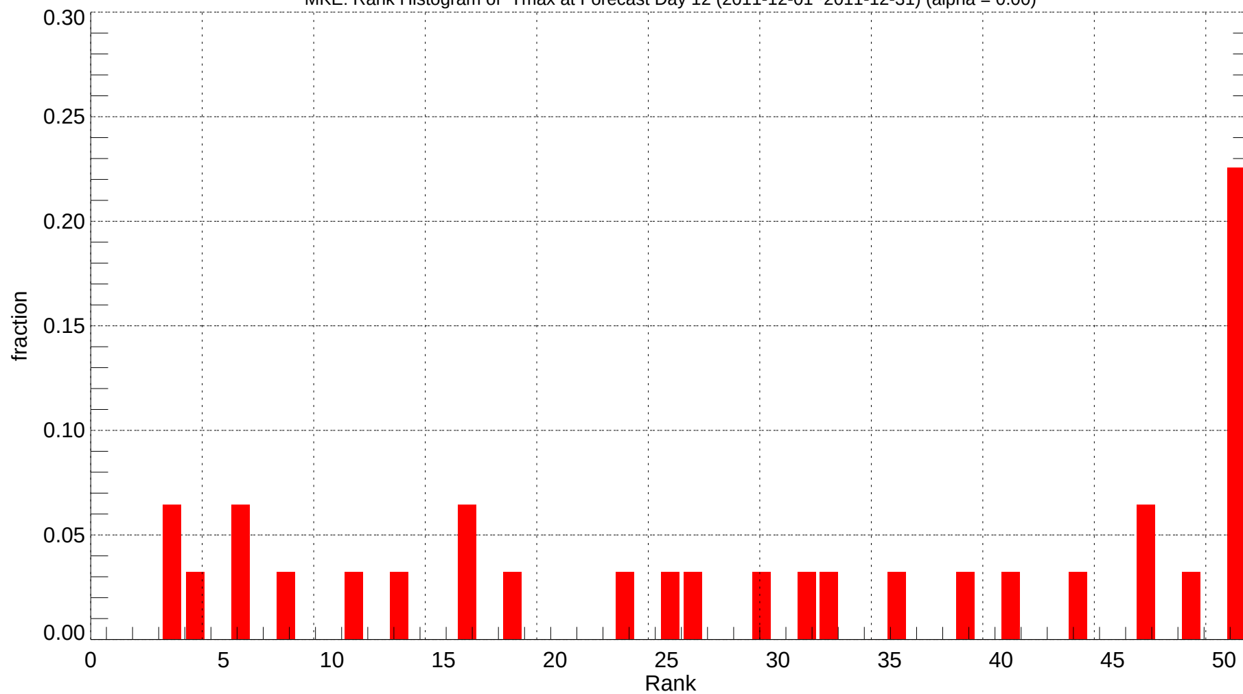
MKE: Rank Histogram of Tmax at Forecast Day 12 (2011-12-01~2011-12-31) (alpha = 0.00)
