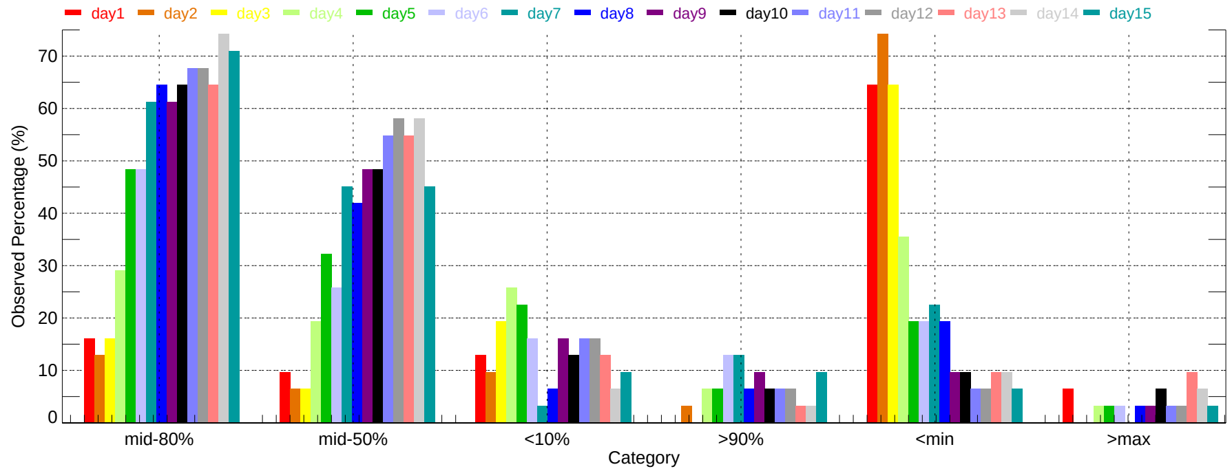
Observed Percentage of Ensembles - CRP: Min Temperature (2011-12-01~2011-12-31)
