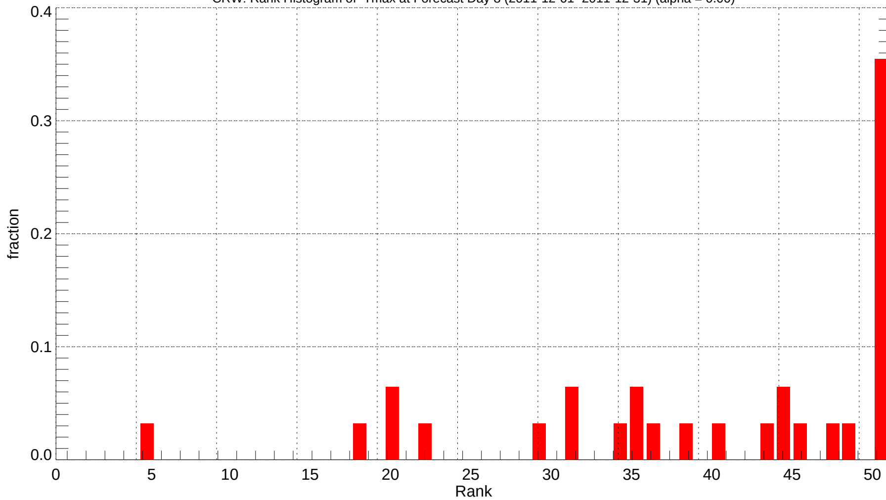
CRW: Rank Histogram of Tmax at Forecast Day 8 (2011-12-01~2011-12-31) (alpha = 0.00)
