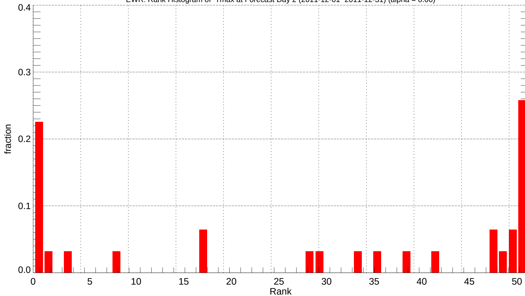
EWR: Rank Histogram of Tmax at Forecast Day 2 (2011-12-01~2011-12-31) (alpha = 0.00)
