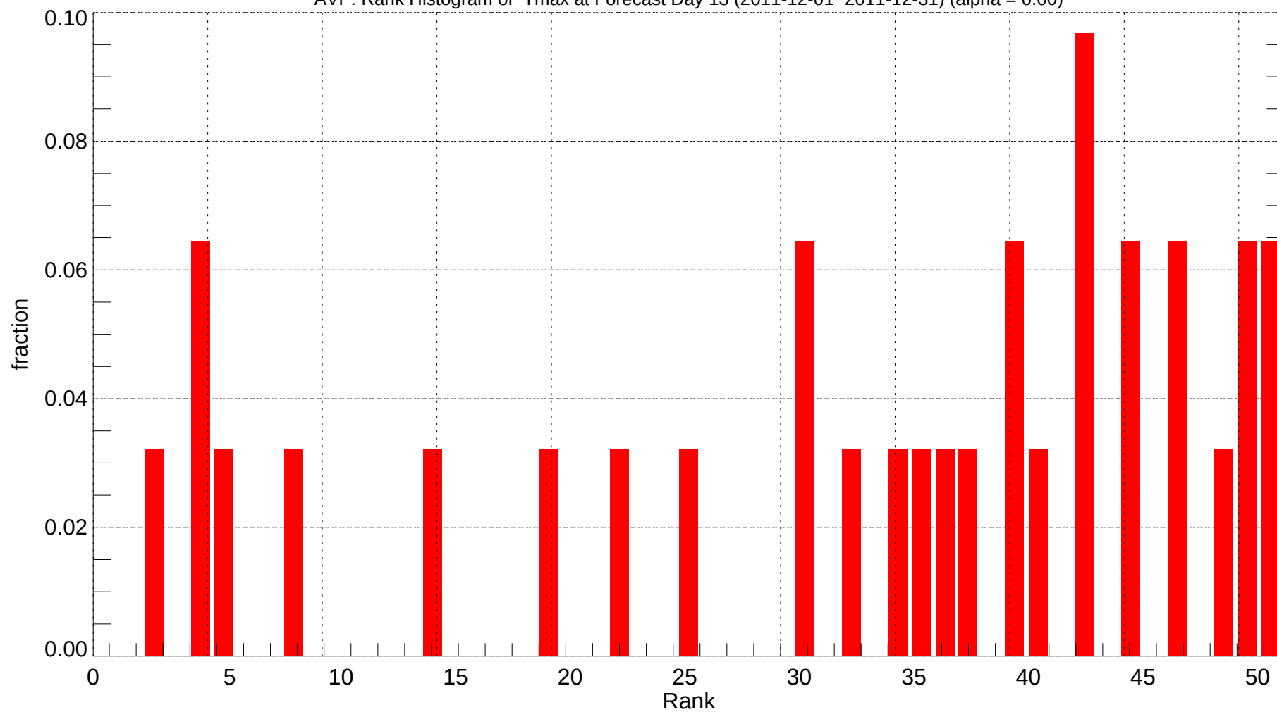
AVP: Rank Histogram of Tmax at Forecast Day 13 (2011-12-01~2011-12-31) (alpha = 0.00)
