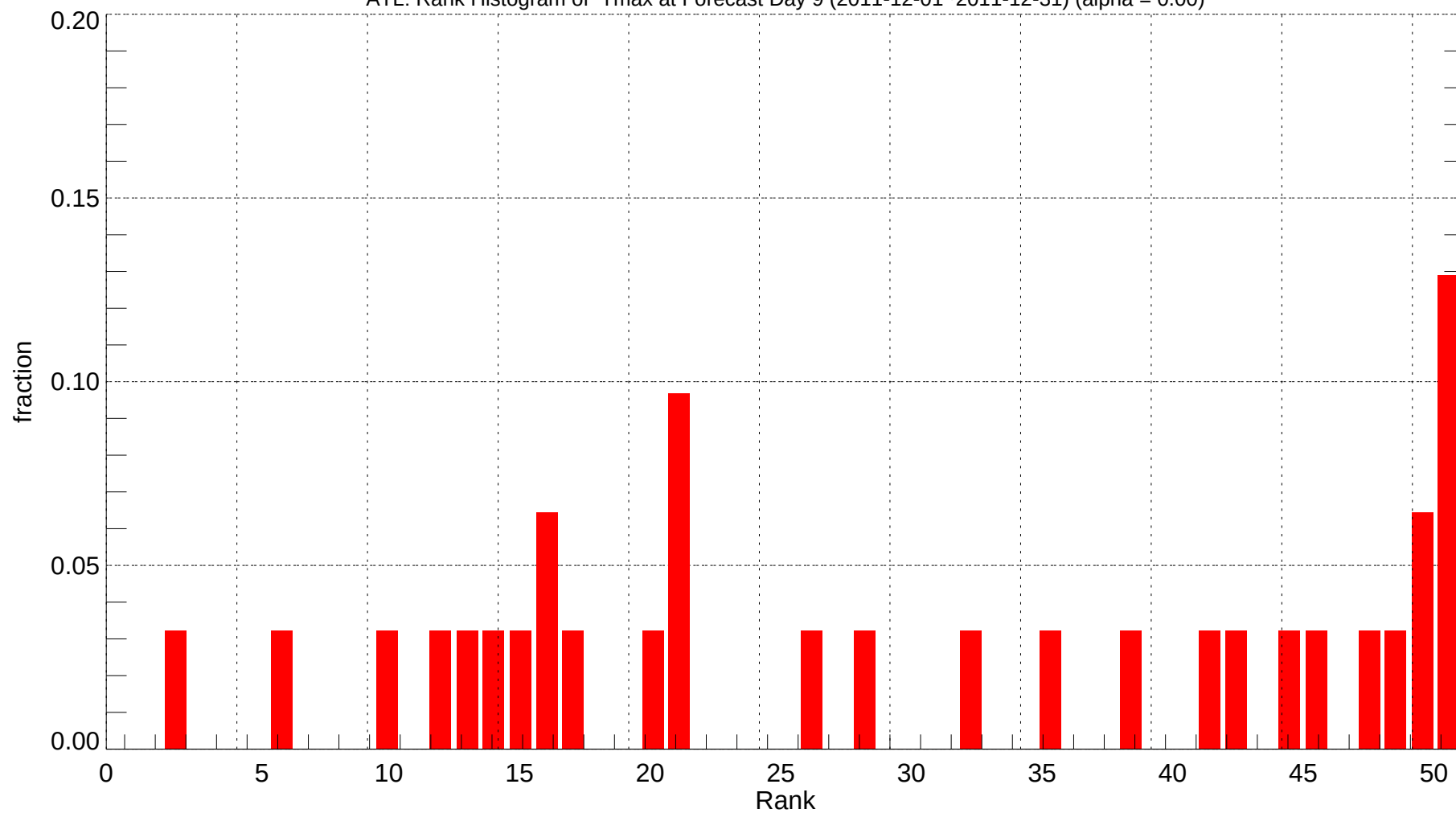
ATL: Rank Histogram of Tmax at Forecast Day 9 (2011-12-01~2011-12-31) (alpha = 0.00)
