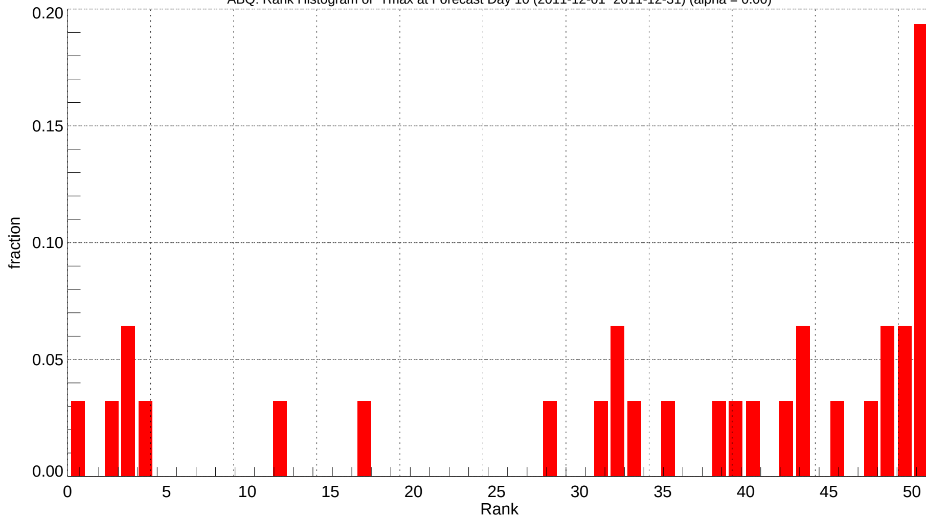
ABQ: Rank Histogram of Tmax at Forecast Day 10 (2011-12-01~2011-12-31) (alpha = 0.00)
