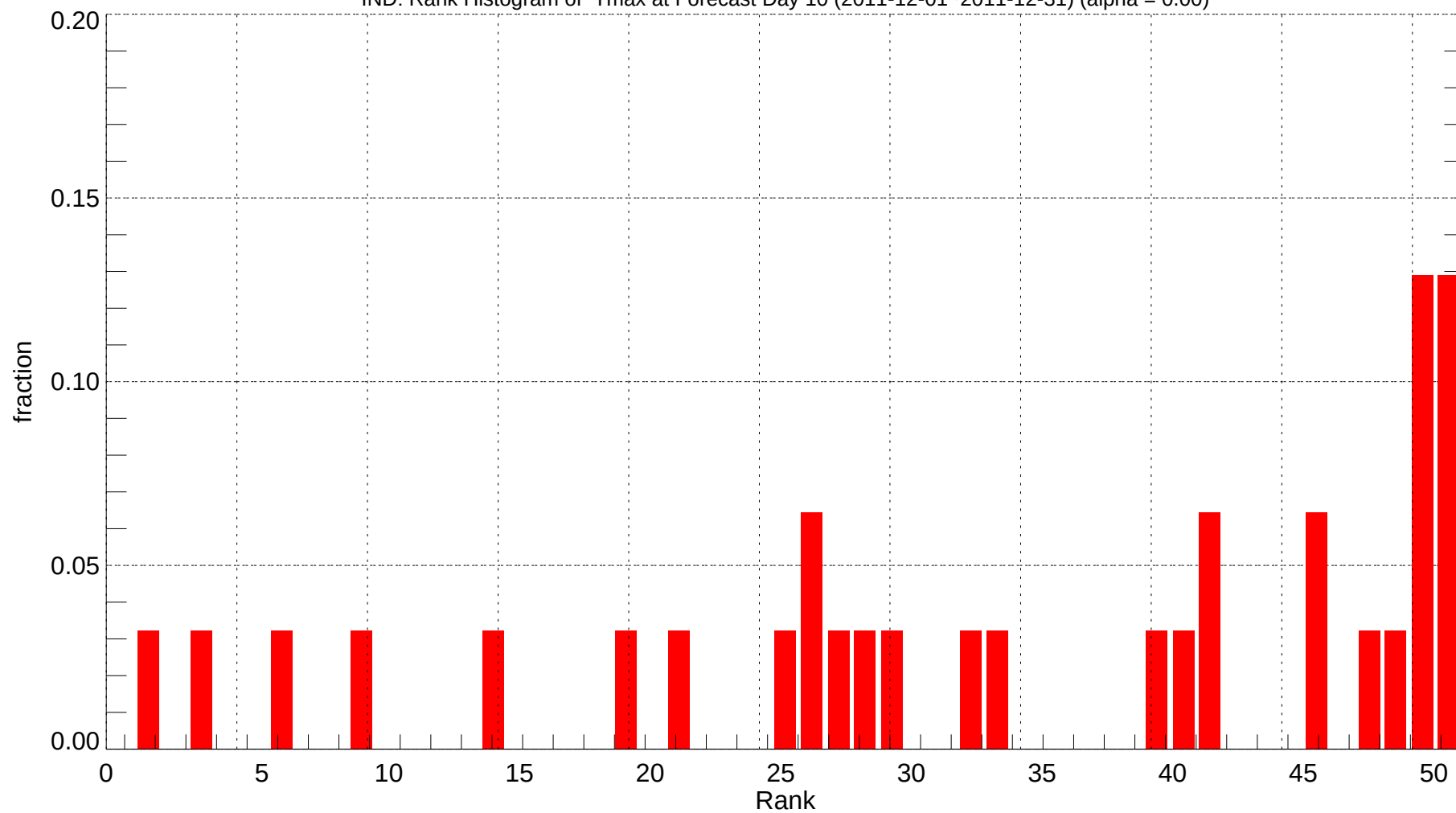
IND: Rank Histogram of Tmax at Forecast Day 10 (2011-12-01~2011-12-31) (alpha = 0.00)
