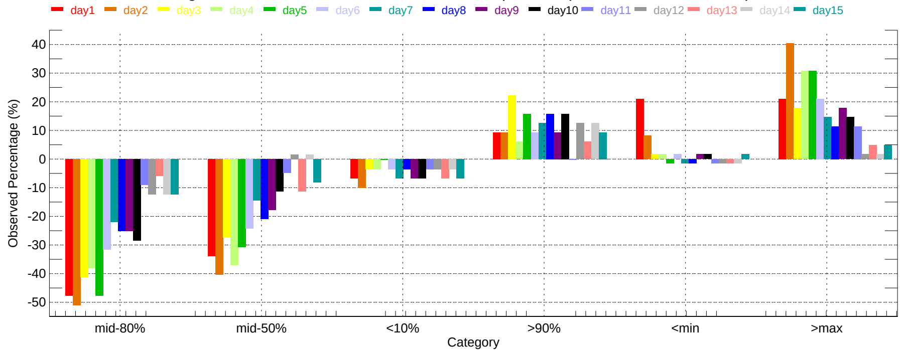
Observed Percentage Deviation of Ensembles - SYR: Max Temperature (2011-12-01~2011-12-31)
