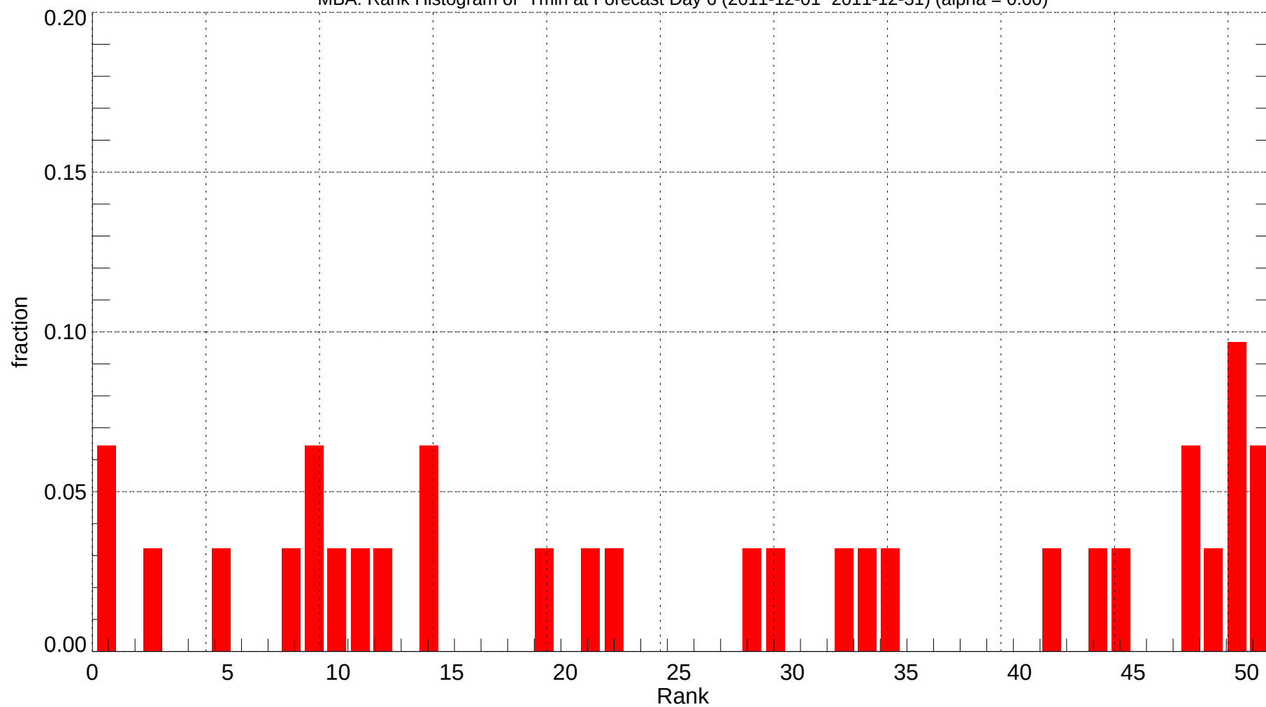
MBA: Rank Histogram of Tmin at Forecast Day 6 (2011-12-01~2011-12-31) (alpha = 0.00)
