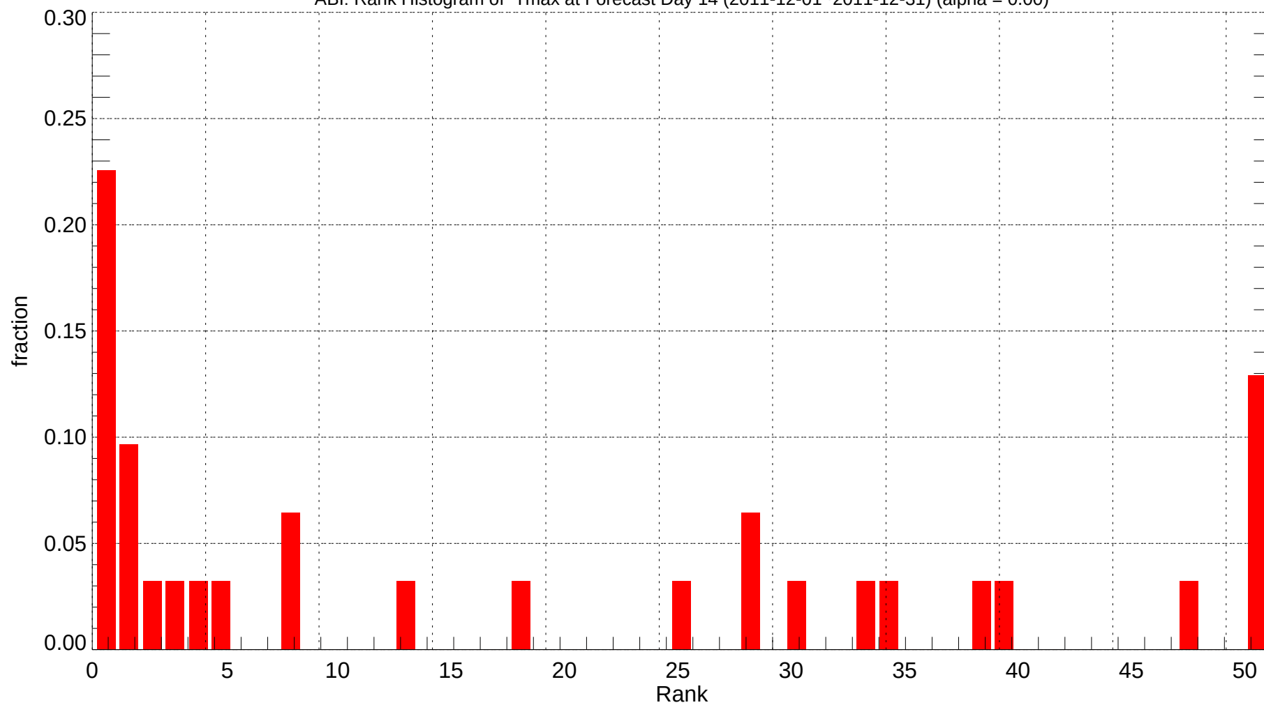
ABI: Rank Histogram of Tmax at Forecast Day 14 (2011-12-01~2011-12-31) (alpha = 0.00)
