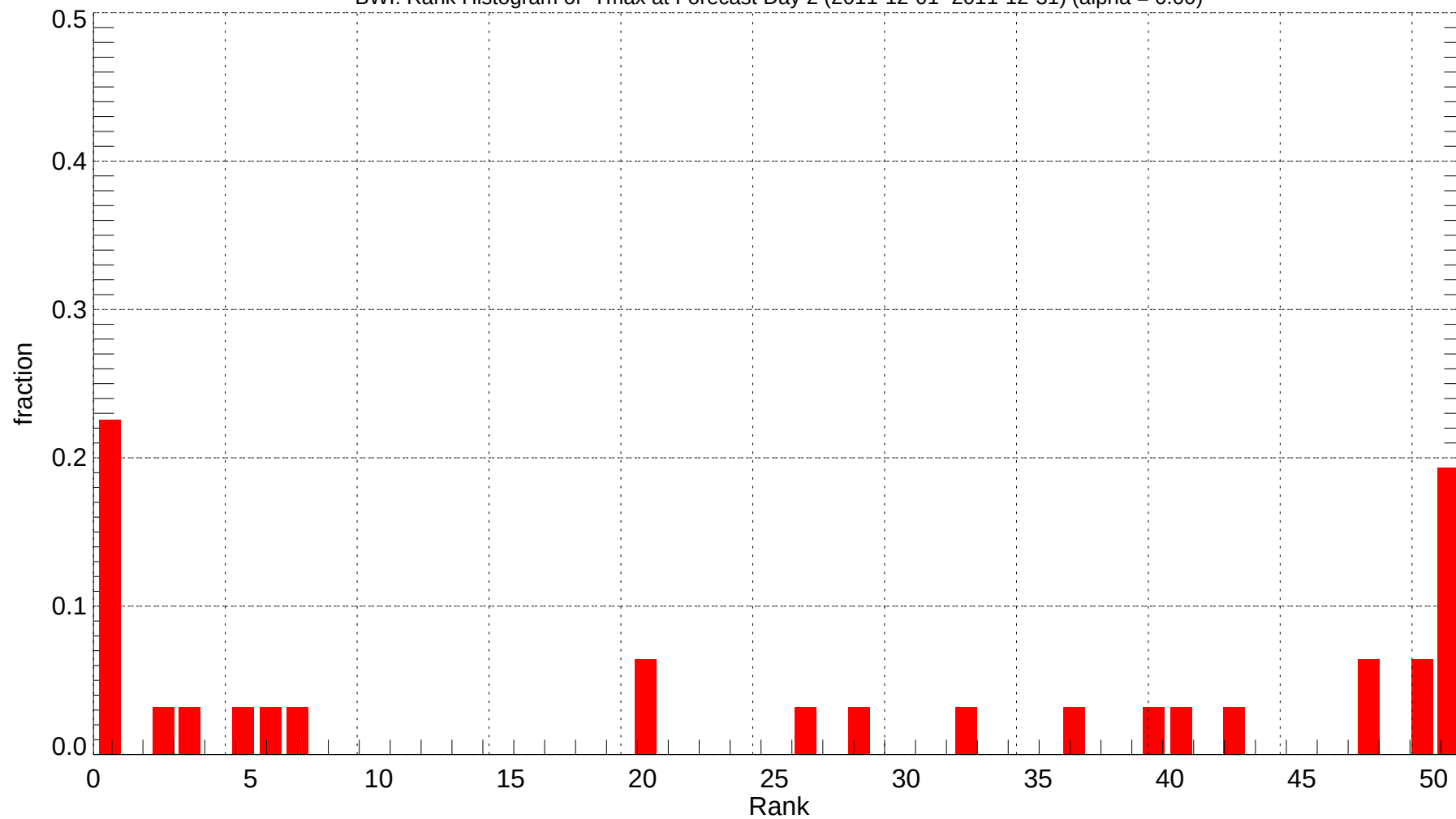
BWI: Rank Histogram of Tmax at Forecast Day 2 (2011-12-01~2011-12-31) (alpha = 0.00)
