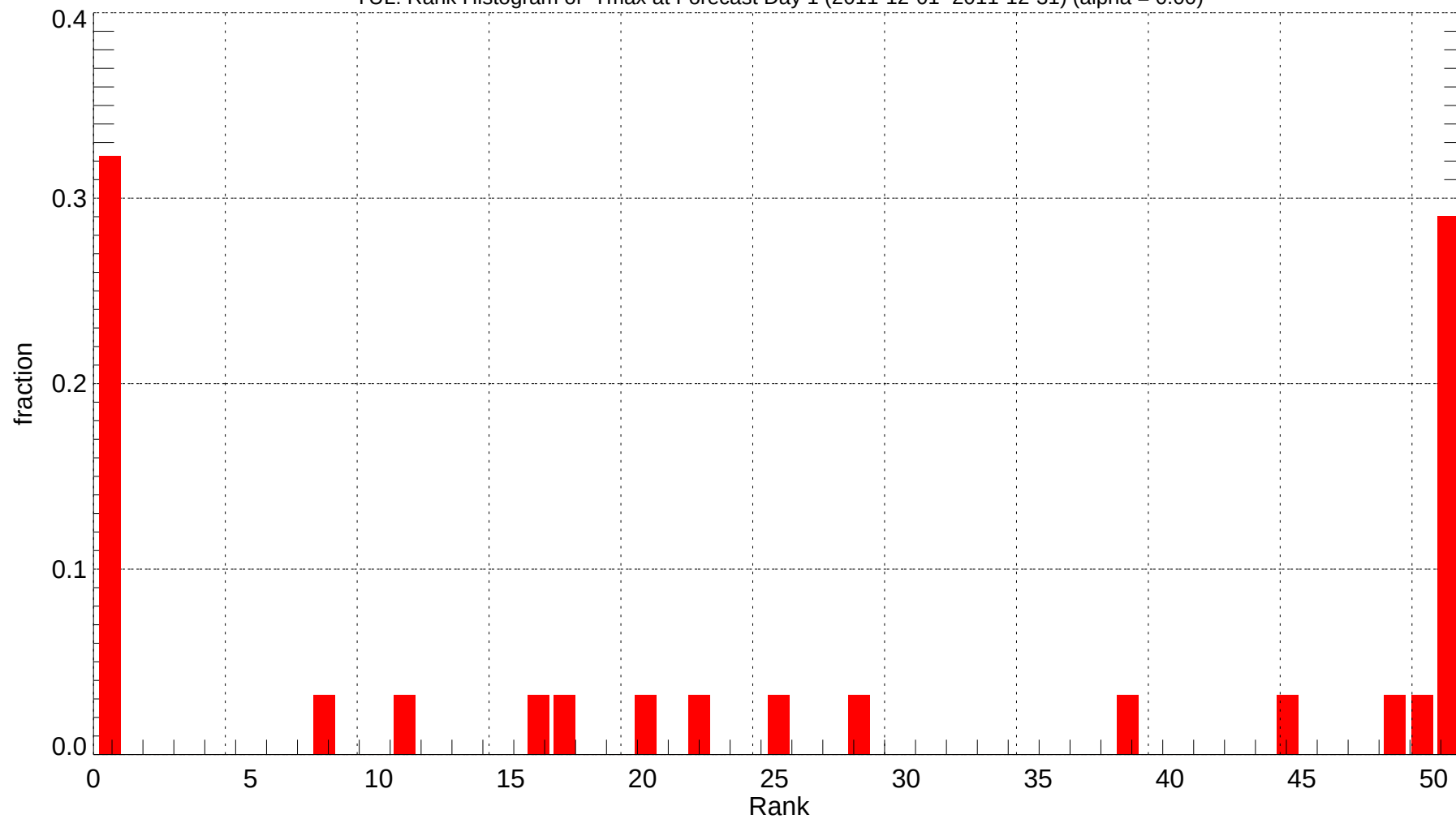
YUL: Rank Histogram of Tmax at Forecast Day 1 (2011-12-01~2011-12-31) (alpha = 0.00)
