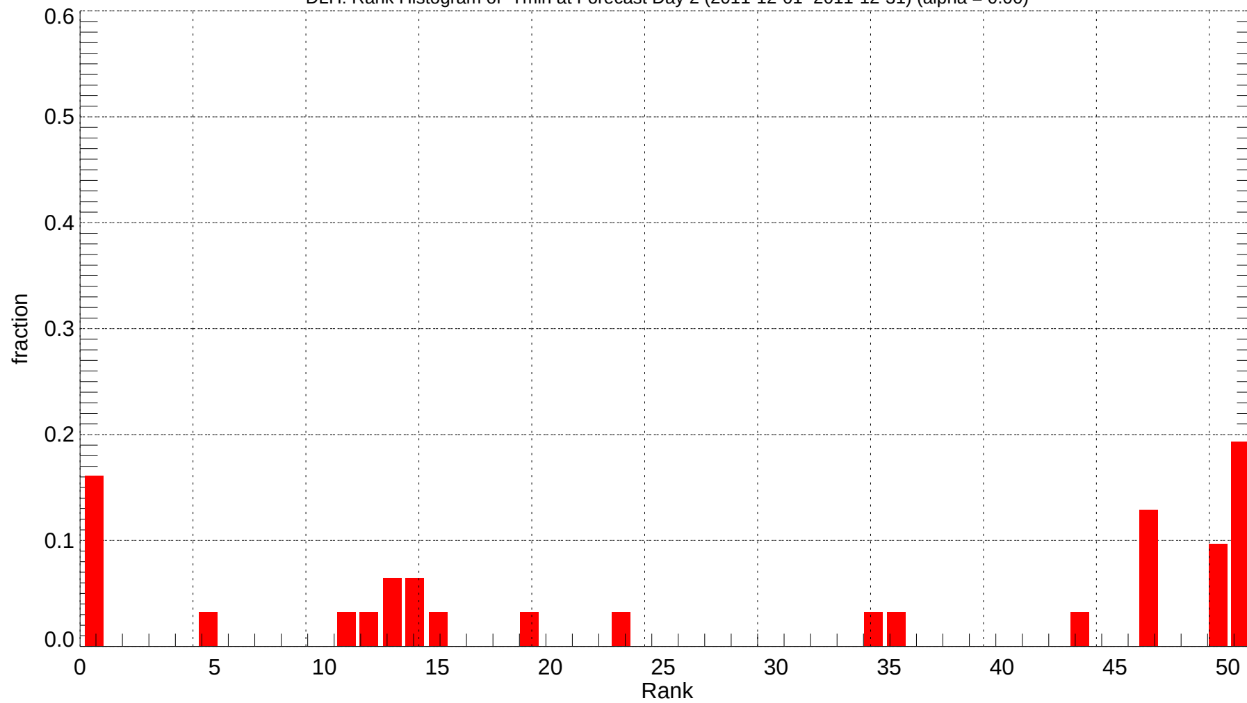
DLH: Rank Histogram of Tmin at Forecast Day 2 (2011-12-01~2011-12-31) (alpha = 0.00)
