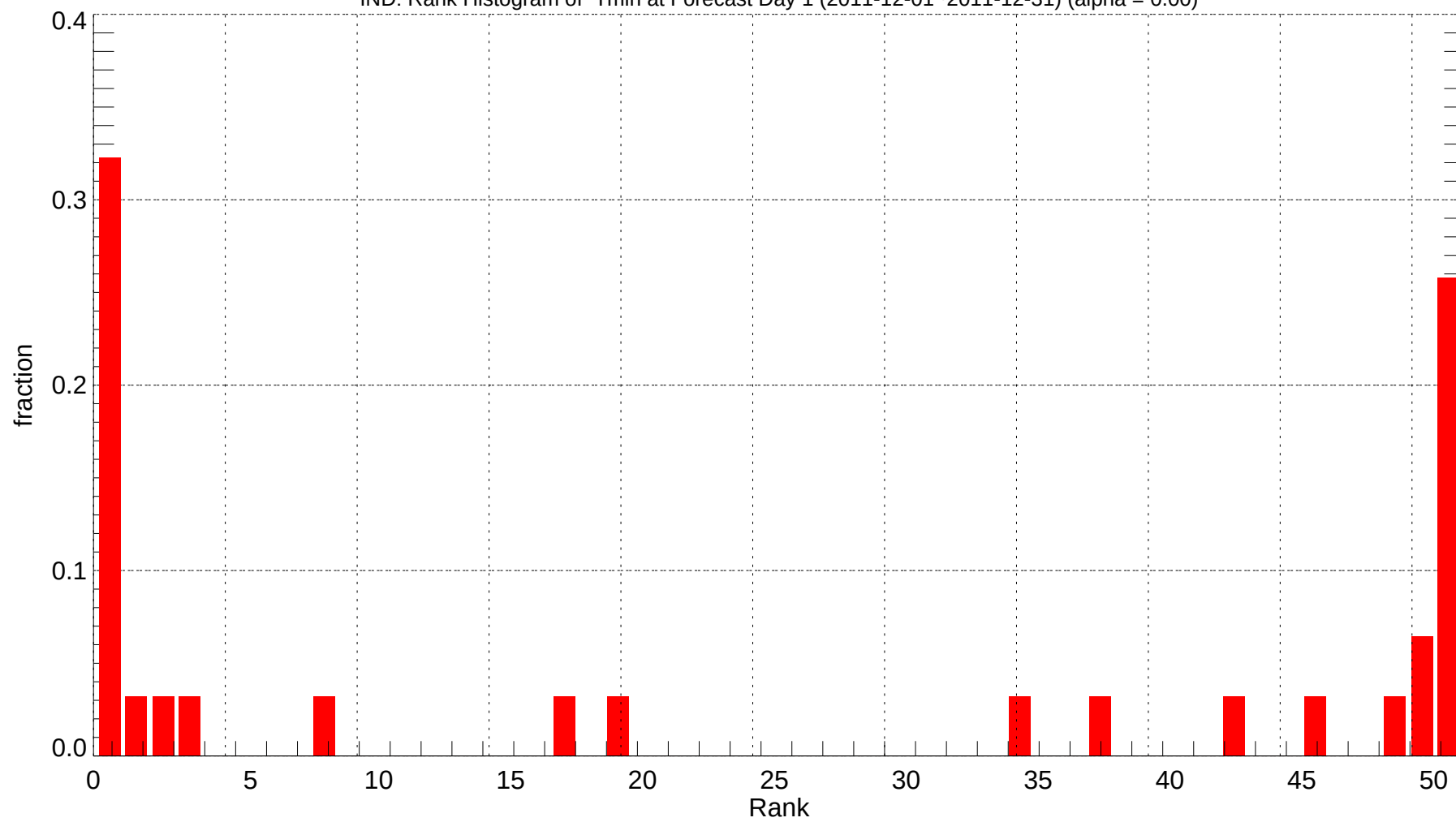
IND: Rank Histogram of Tmin at Forecast Day 1 (2011-12-01~2011-12-31) (alpha = 0.00)
