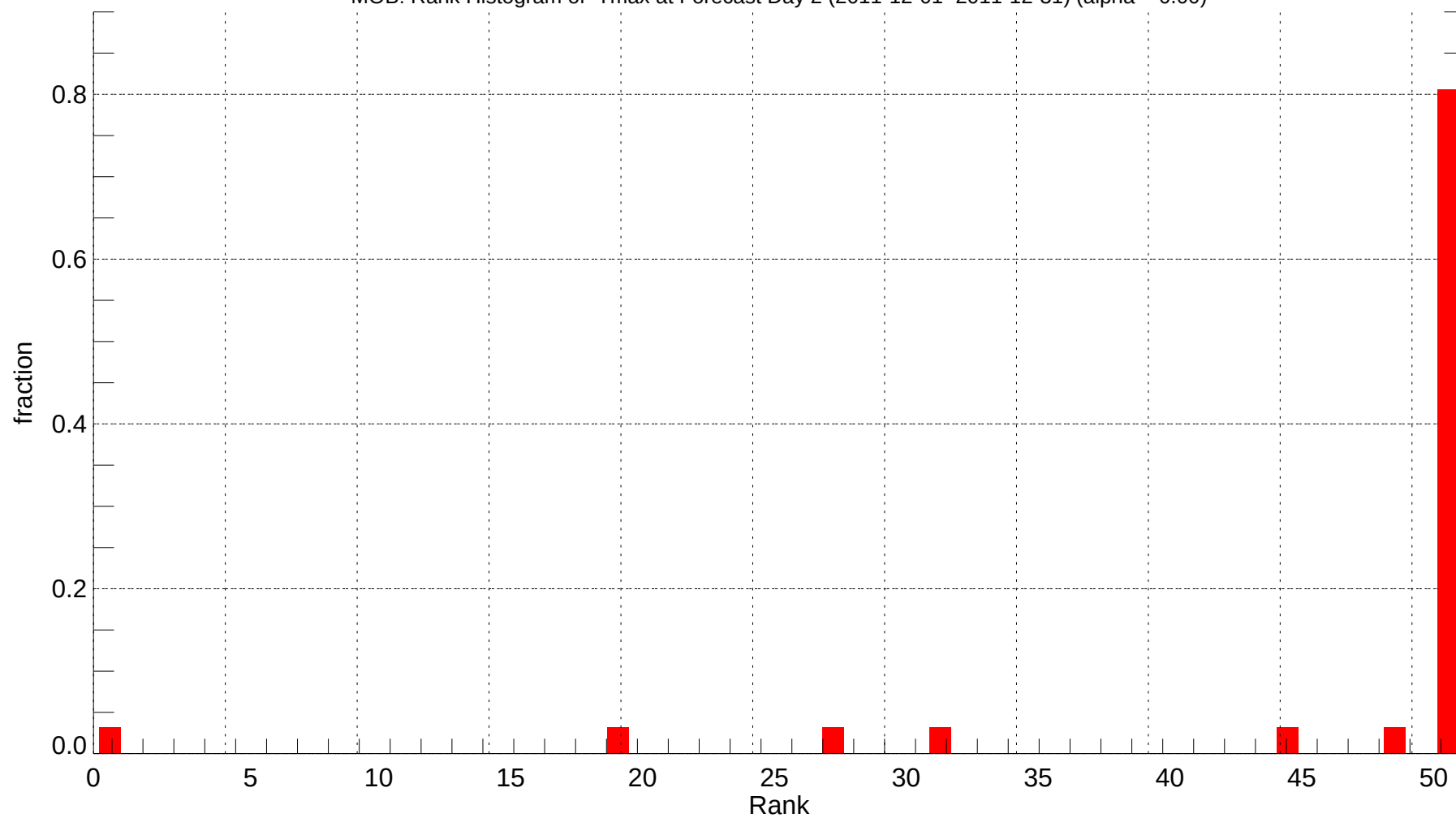
MOB: Rank Histogram of Tmax at Forecast Day 2 (2011-12-01~2011-12-31) (alpha = 0.00)
