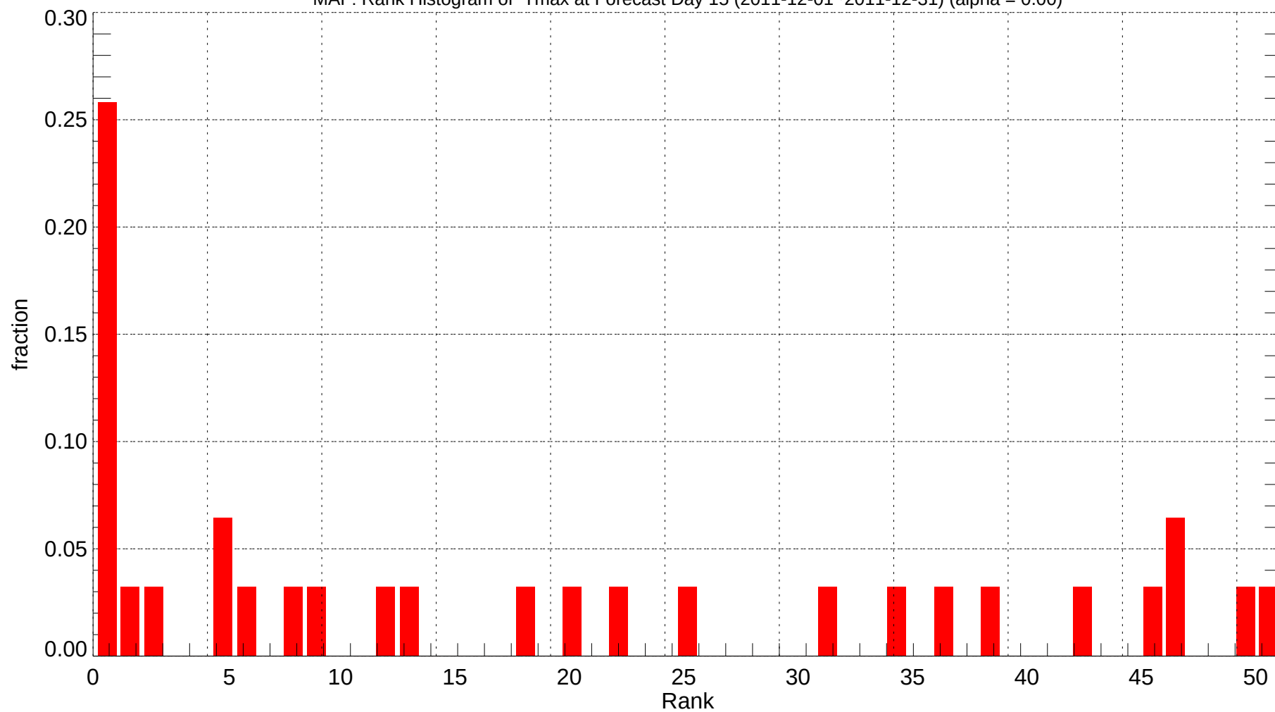
MAF: Rank Histogram of Tmax at Forecast Day 15 (2011-12-01~2011-12-31) (alpha = 0.00)
