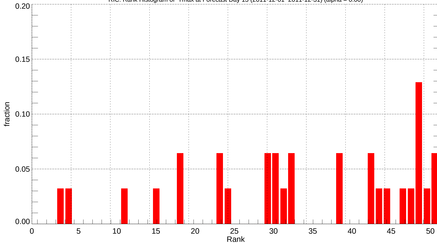
RIC: Rank Histogram of Tmax at Forecast Day 13 (2011-12-01~2011-12-31) (alpha = 0.00)
