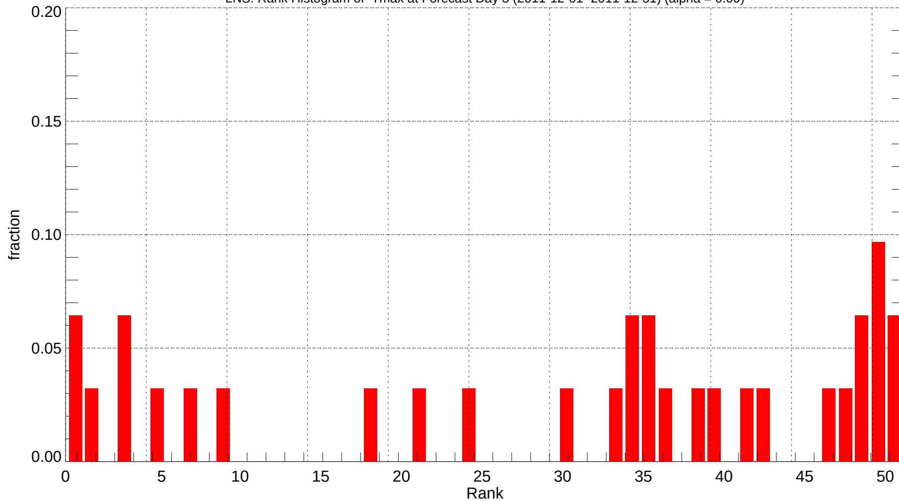
LNS: Rank Histogram of Tmax at Forecast Day 3 (2011-12-01~2011-12-31) (alpha = 0.00)
