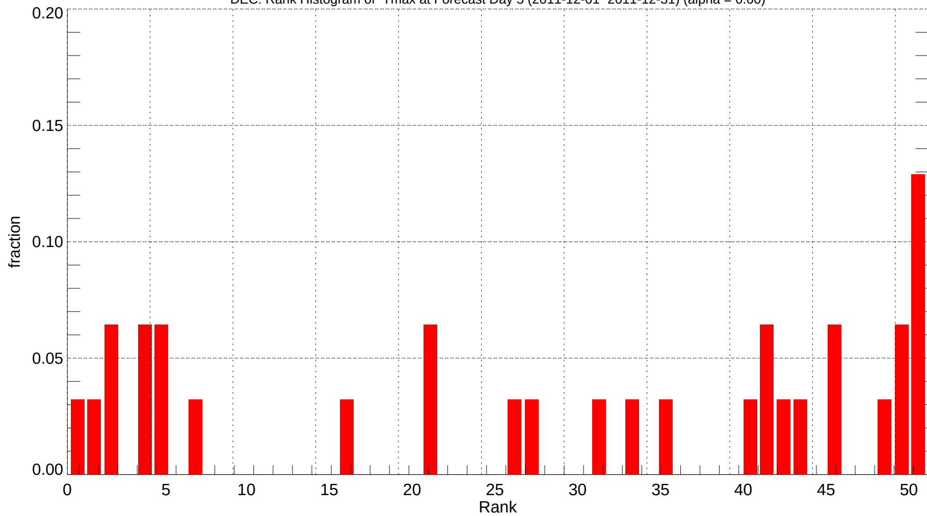
DEC: Rank Histogram of Tmax at Forecast Day 5 (2011-12-01~2011-12-31) (alpha = 0.00)
