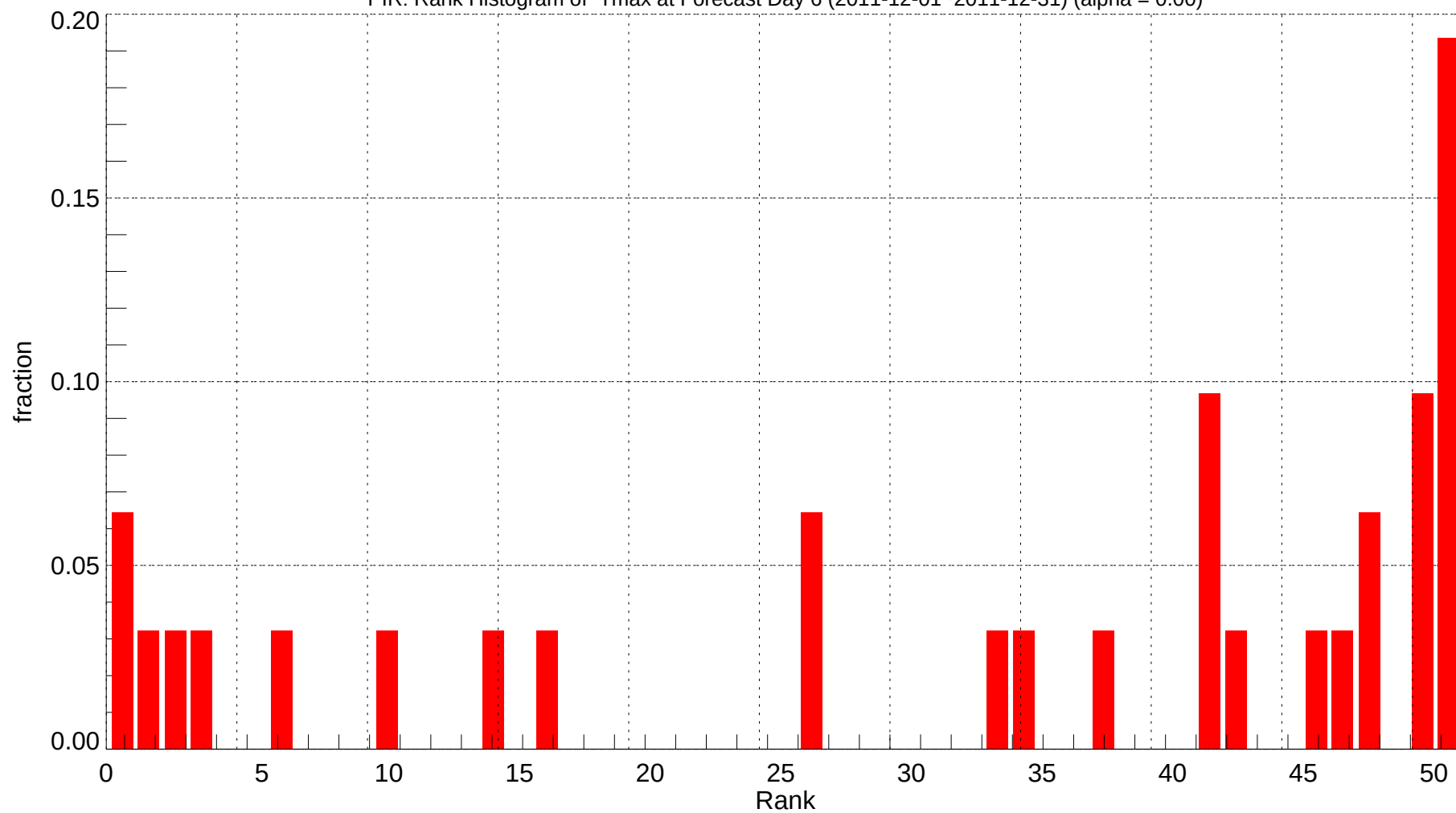
PIR: Rank Histogram of Tmax at Forecast Day 6 (2011-12-01~2011-12-31) (alpha = 0.00)
