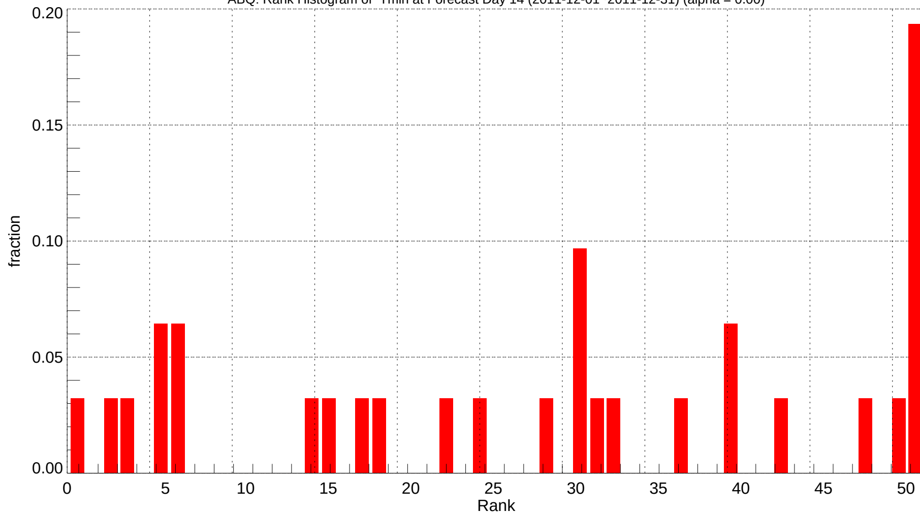
ABQ: Rank Histogram of Tmin at Forecast Day 14 (2011-12-01~2011-12-31) (alpha = 0.00)
