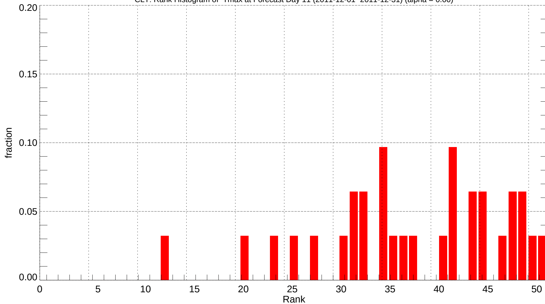
CLT: Rank Histogram of Tmax at Forecast Day 11 (2011-12-01~2011-12-31) (alpha = 0.00)
