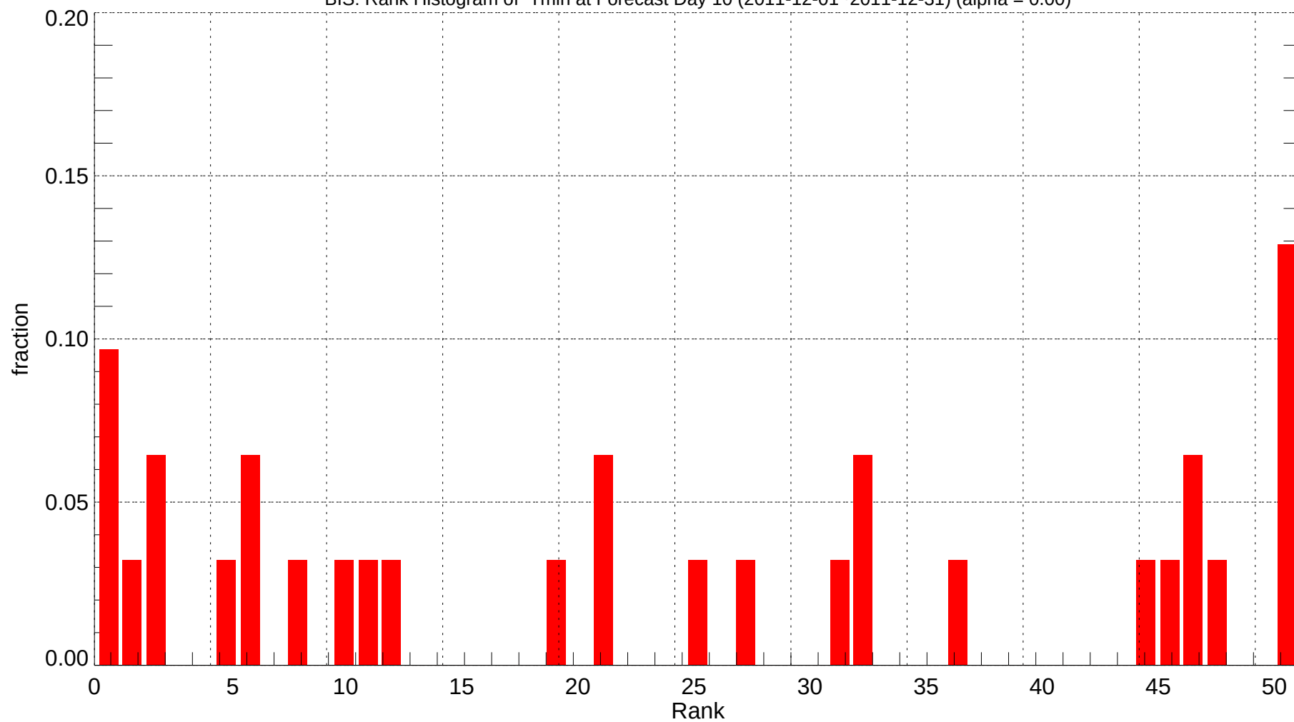
BIS: Rank Histogram of Tmin at Forecast Day 10 (2011-12-01~2011-12-31) (alpha = 0.00)
