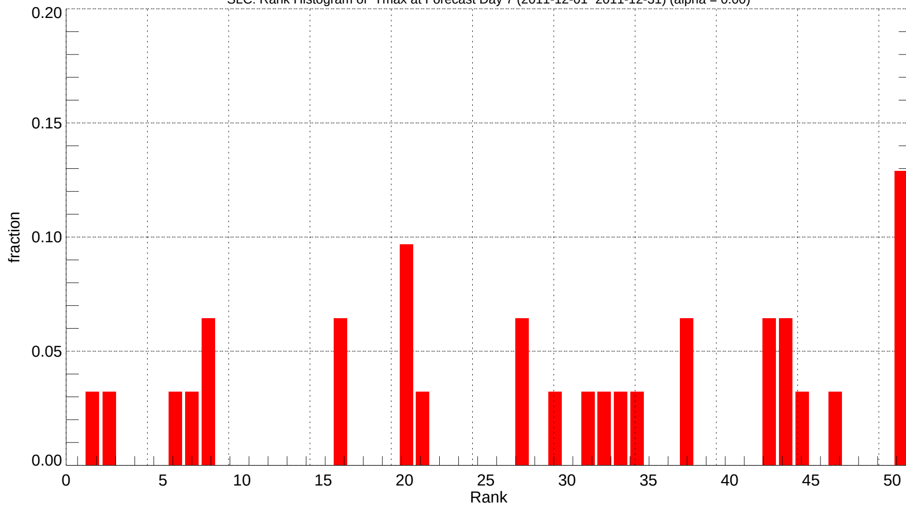
SLC: Rank Histogram of Tmax at Forecast Day 7 (2011-12-01~2011-12-31) (alpha = 0.00)
