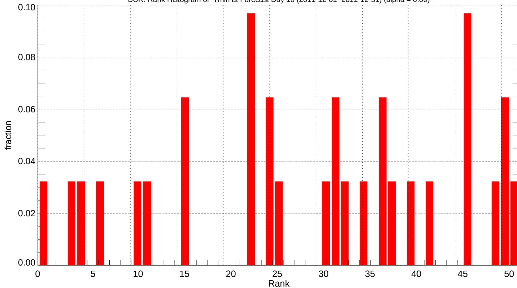
BUR: Rank Histogram of Tmin at Forecast Day 10 (2011-12-01~2011-12-31) (alpha = 0.00)
