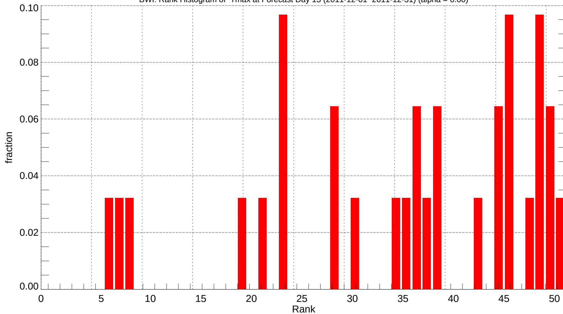
BWI: Rank Histogram of Tmax at Forecast Day 13 (2011-12-01~2011-12-31) (alpha = 0.00)
