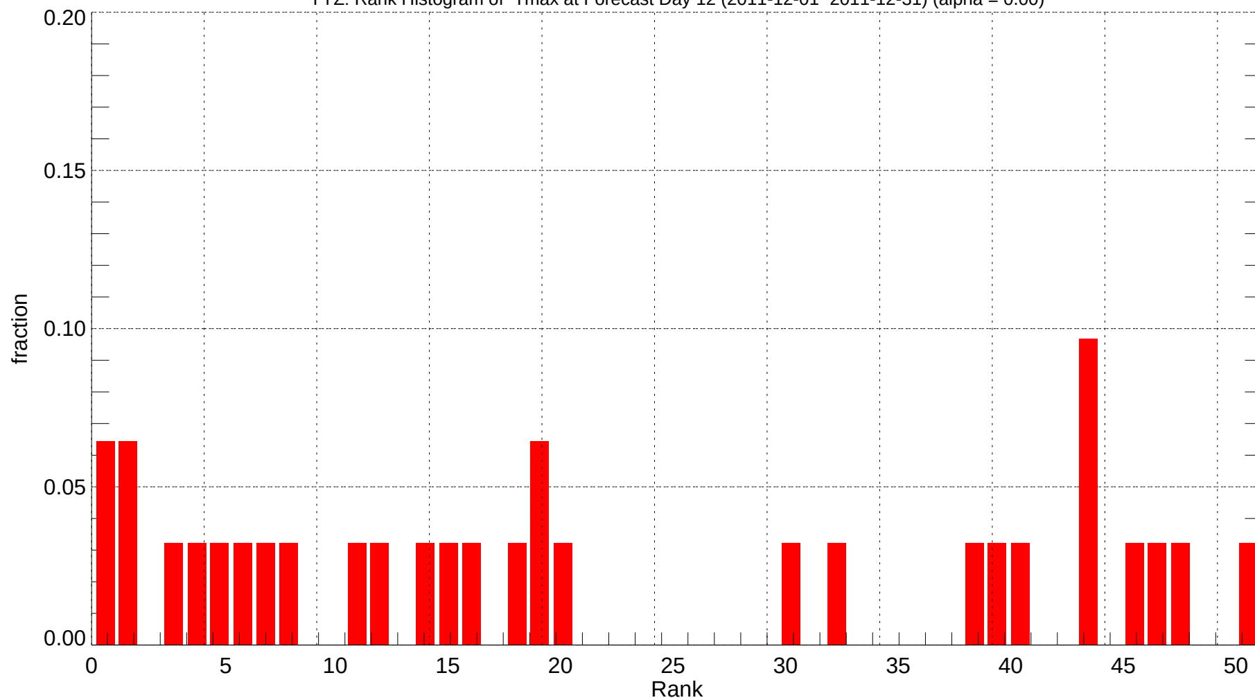
YYZ: Rank Histogram of Tmax at Forecast Day 12 (2011-12-01~2011-12-31) (alpha = 0.00)
