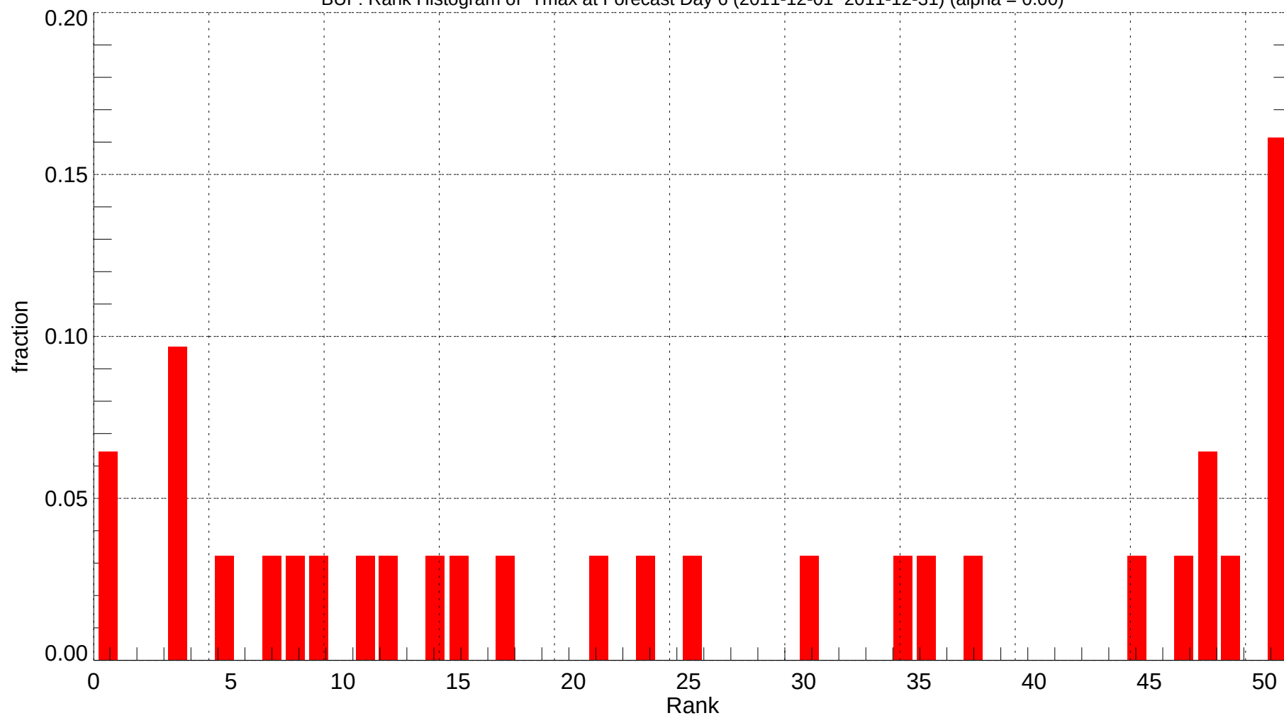
BUF: Rank Histogram of Tmax at Forecast Day 6 (2011-12-01~2011-12-31) (alpha = 0.00)
