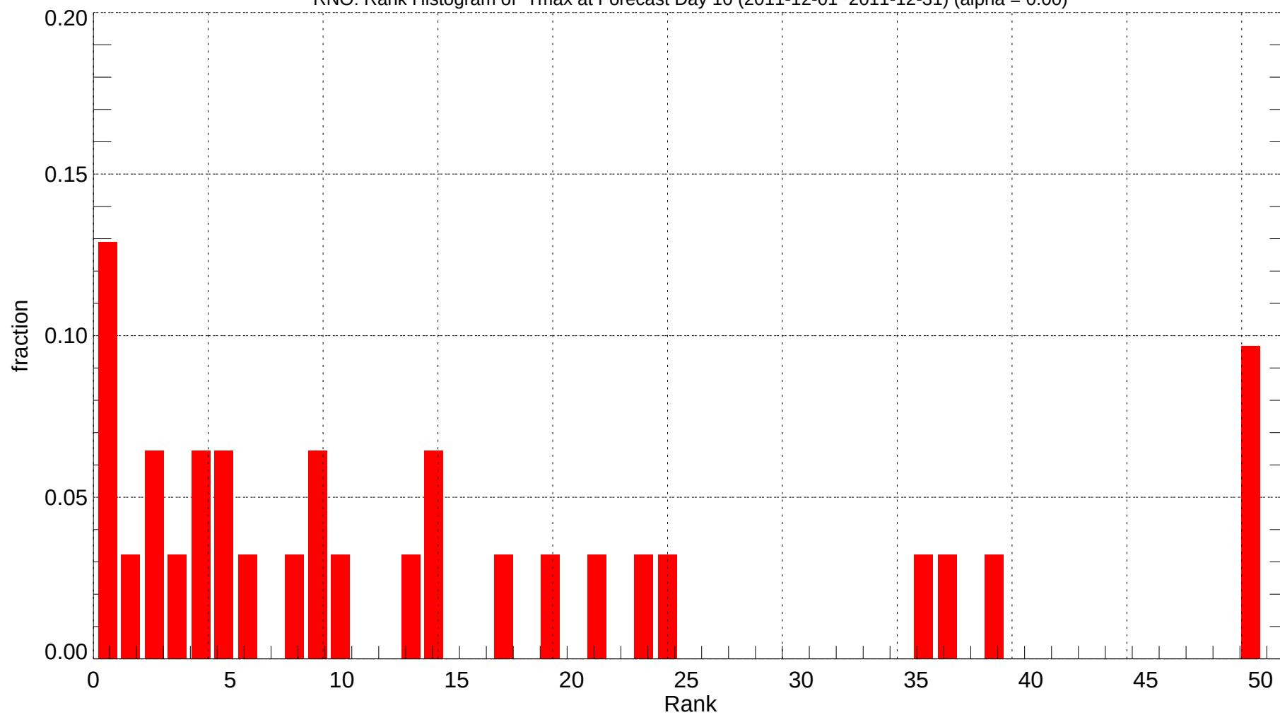
RNO: Rank Histogram of Tmax at Forecast Day 10 (2011-12-01~2011-12-31) (alpha = 0.00)
