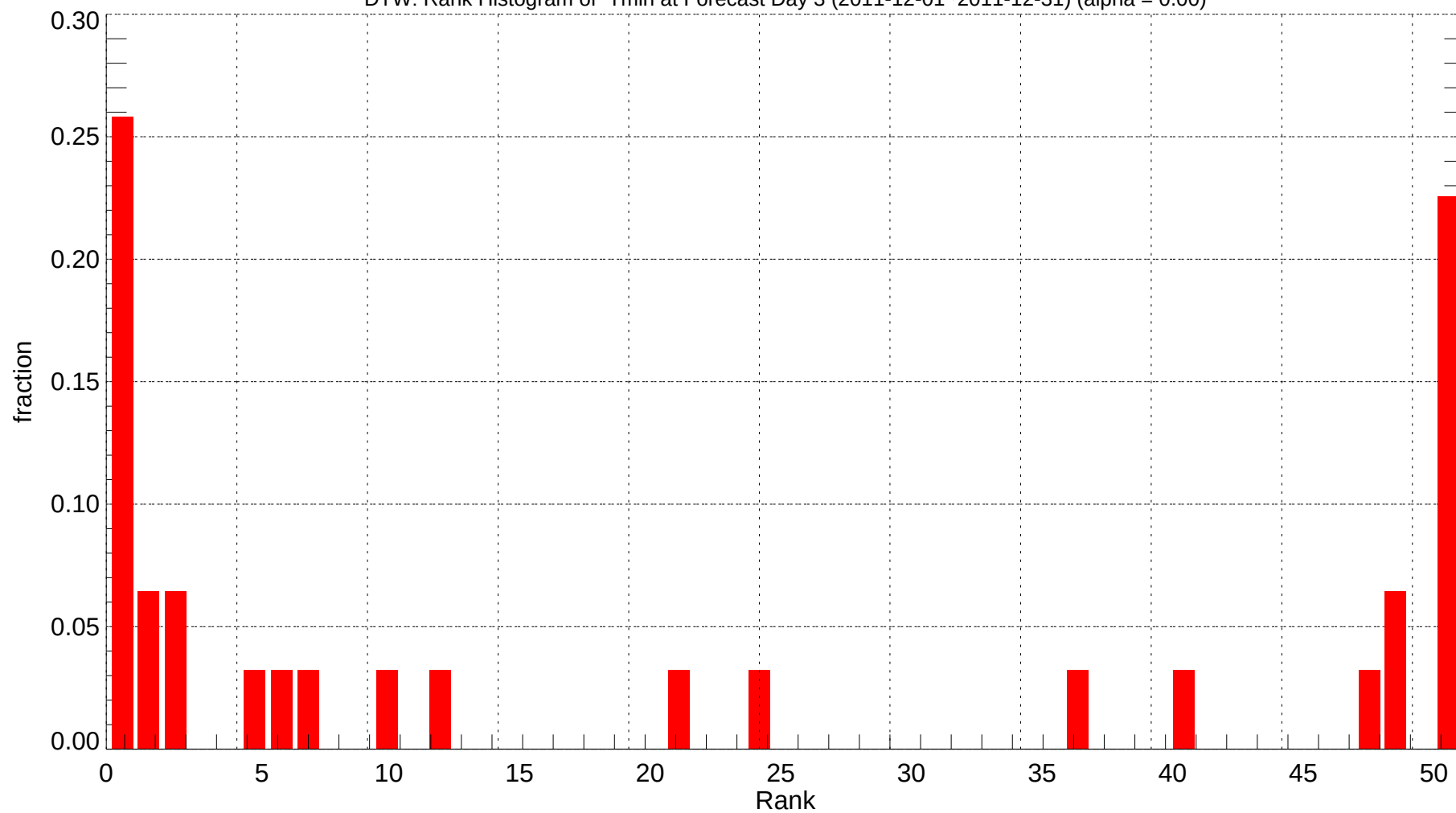
DTW: Rank Histogram of Tmin at Forecast Day 3 (2011-12-01~2011-12-31) (alpha = 0.00)
