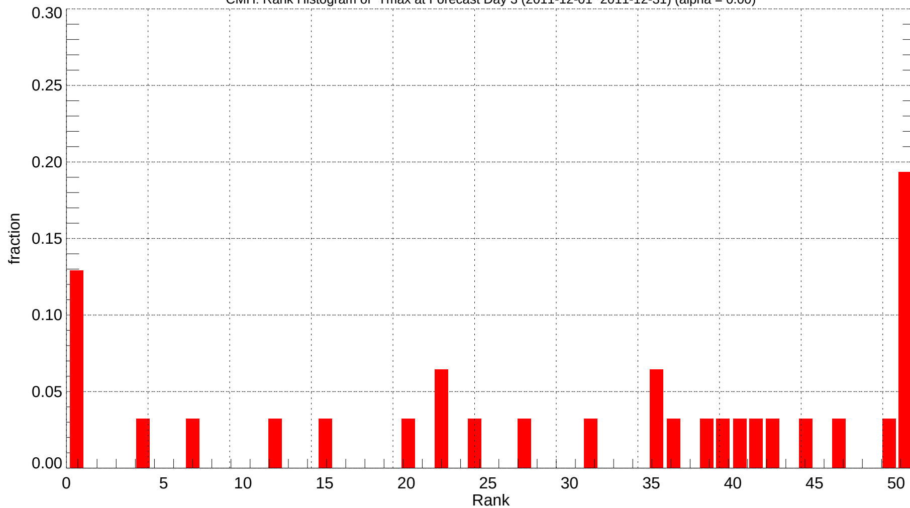
CMH: Rank Histogram of Tmax at Forecast Day 3 (2011-12-01~2011-12-31) (alpha = 0.00)
