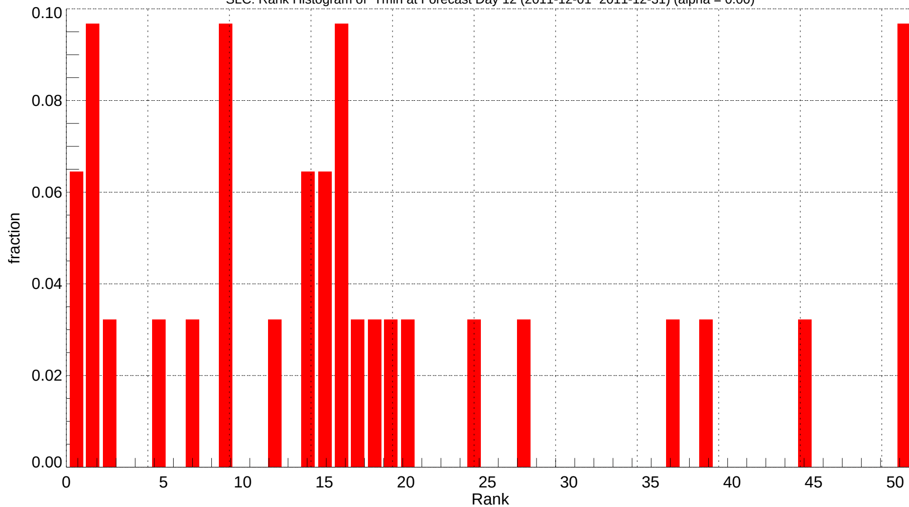
SLC: Rank Histogram of Tmin at Forecast Day 12 (2011-12-01~2011-12-31) (alpha = 0.00)
