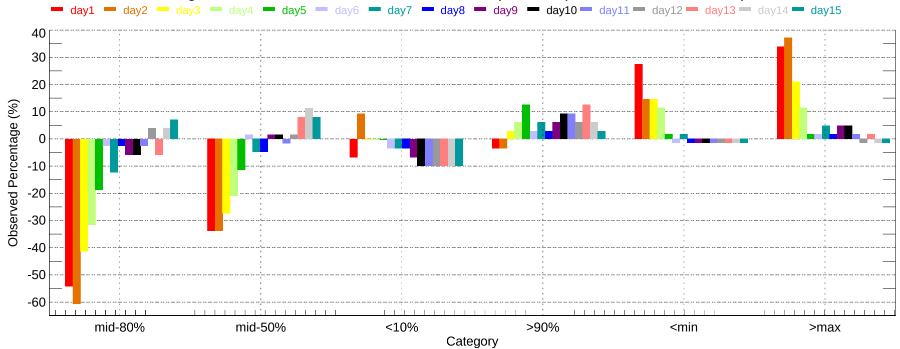
Observed Percentage Deviation of Ensembles - CLT: Max Temperature (2011-12-01~2011-12-31)
