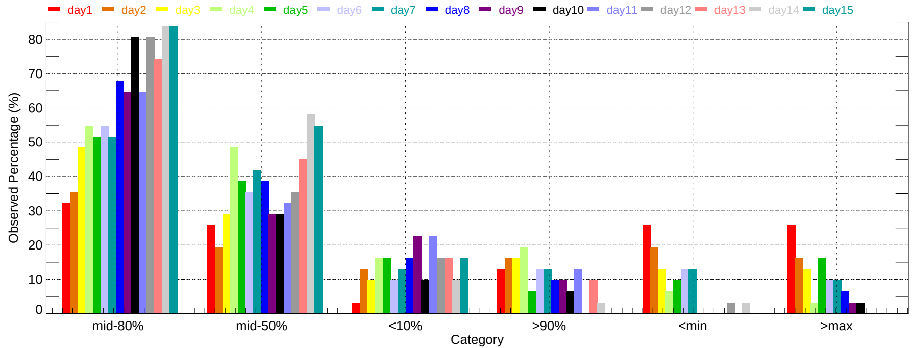
Observed Percentage of Ensembles - PHX: Min Temperature (2011-12-01~2011-12-31)
