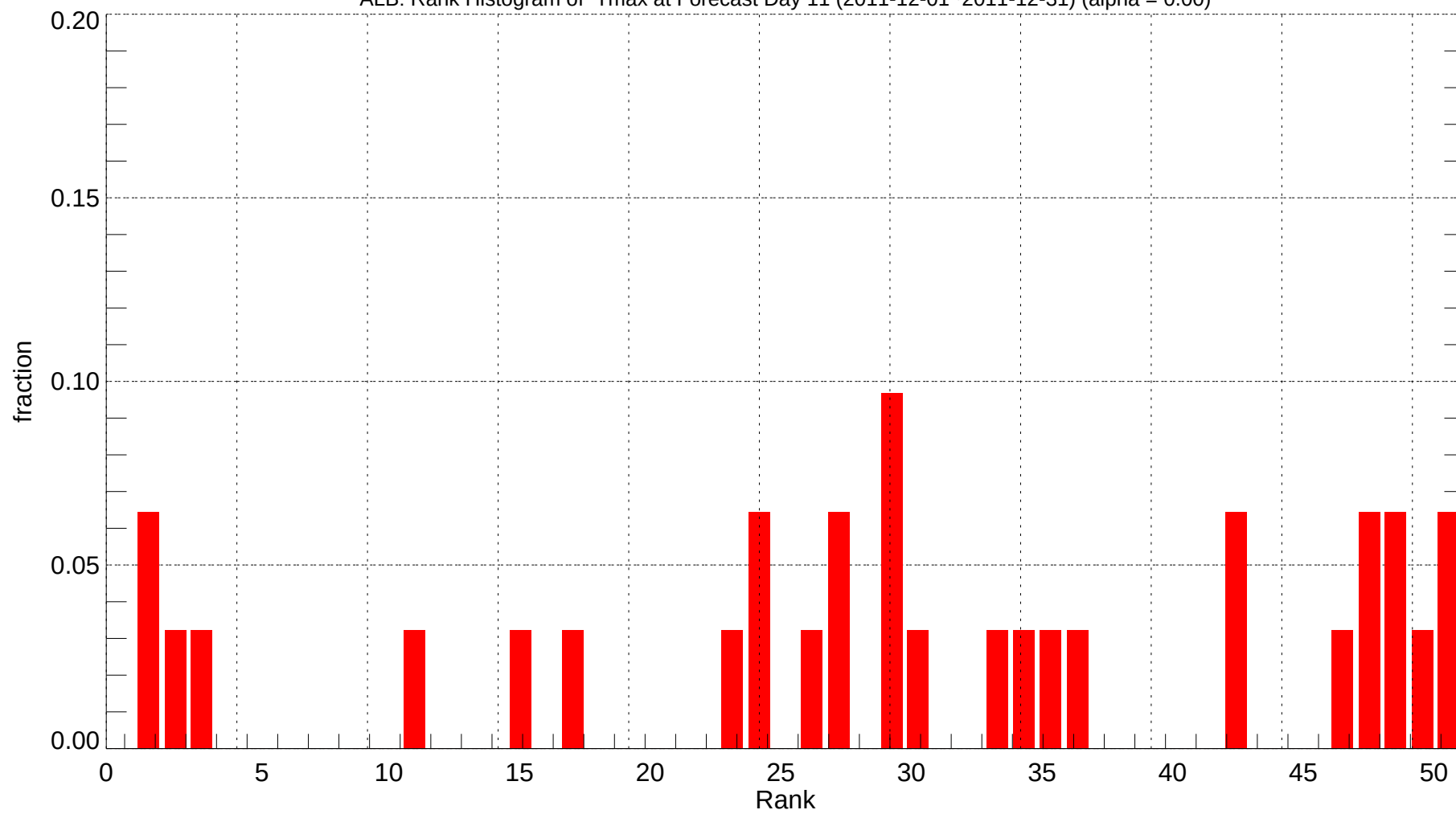
ALB: Rank Histogram of Tmax at Forecast Day 11 (2011-12-01~2011-12-31) (alpha = 0.00)
