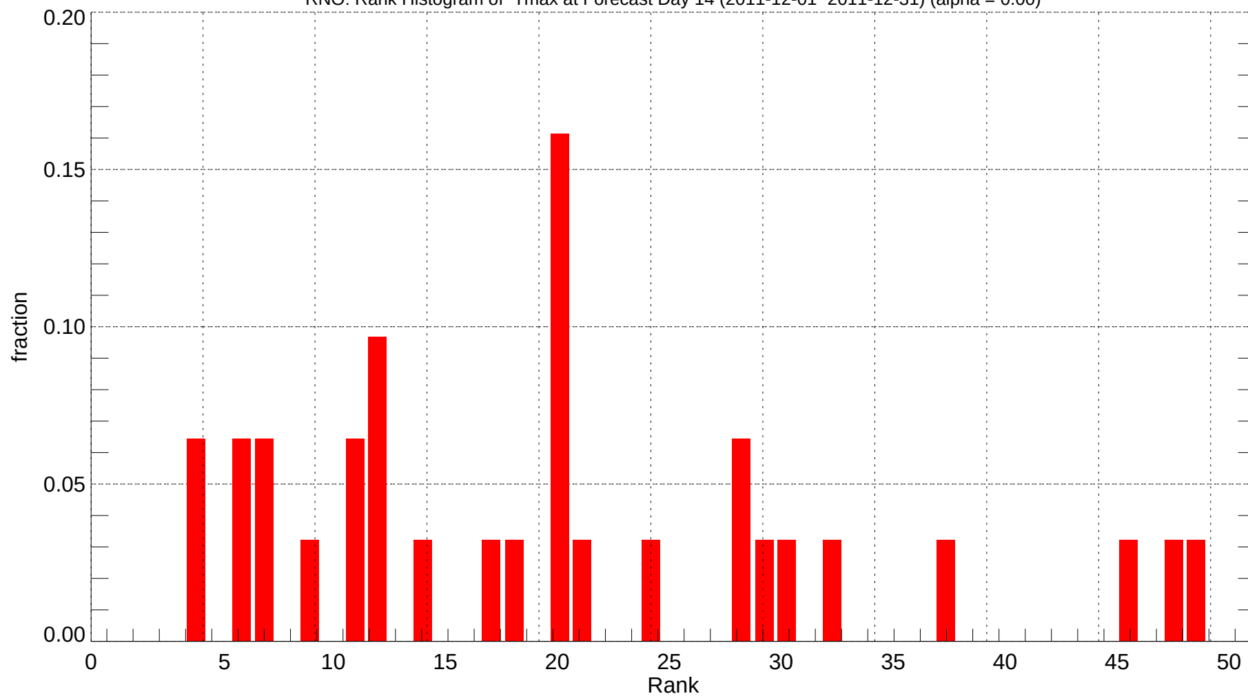
RNO: Rank Histogram of Tmax at Forecast Day 14 (2011-12-01~2011-12-31) (alpha = 0.00)
