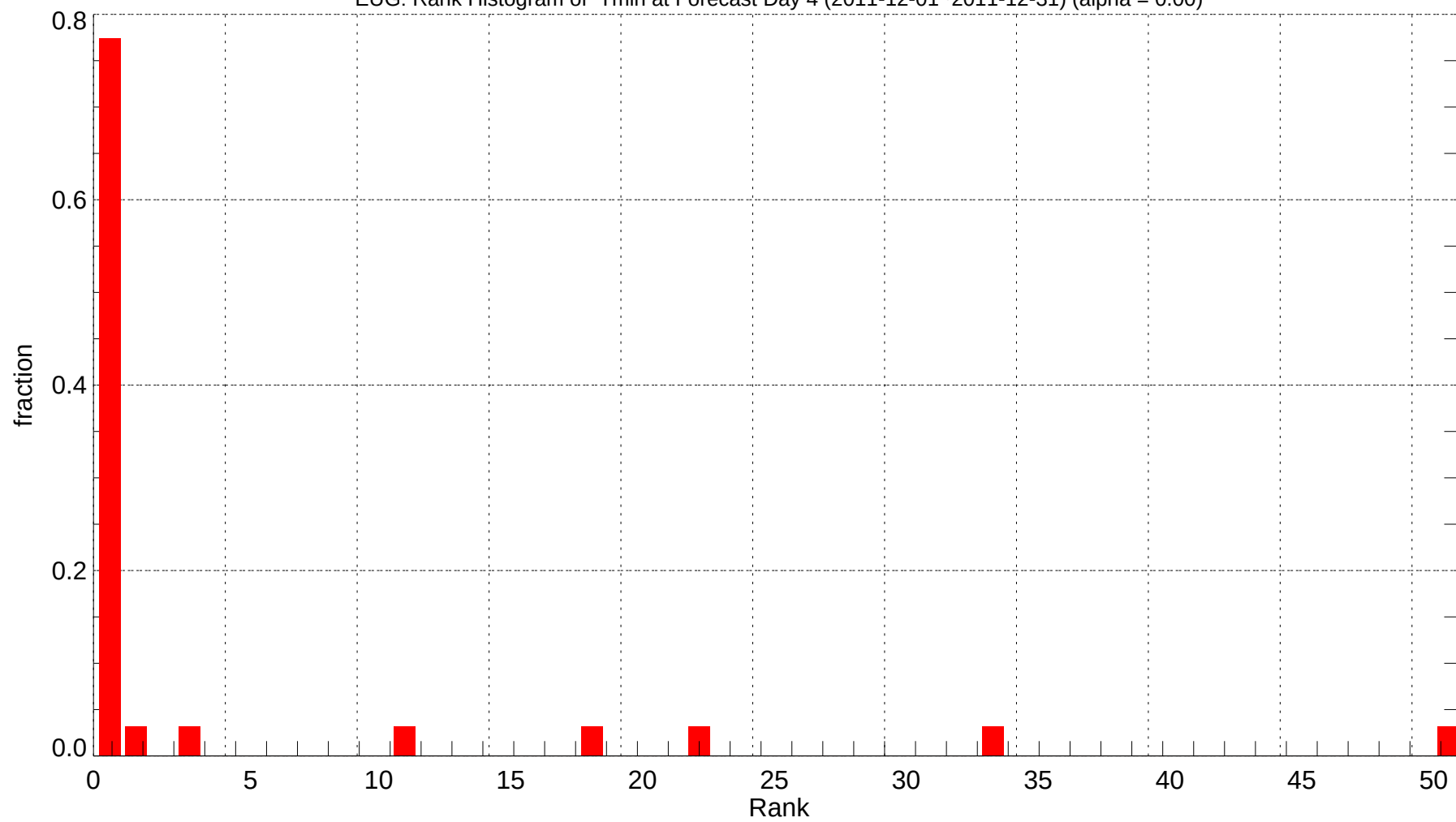
EUG: Rank Histogram of Tmin at Forecast Day 4 (2011-12-01~2011-12-31) (alpha = 0.00)
