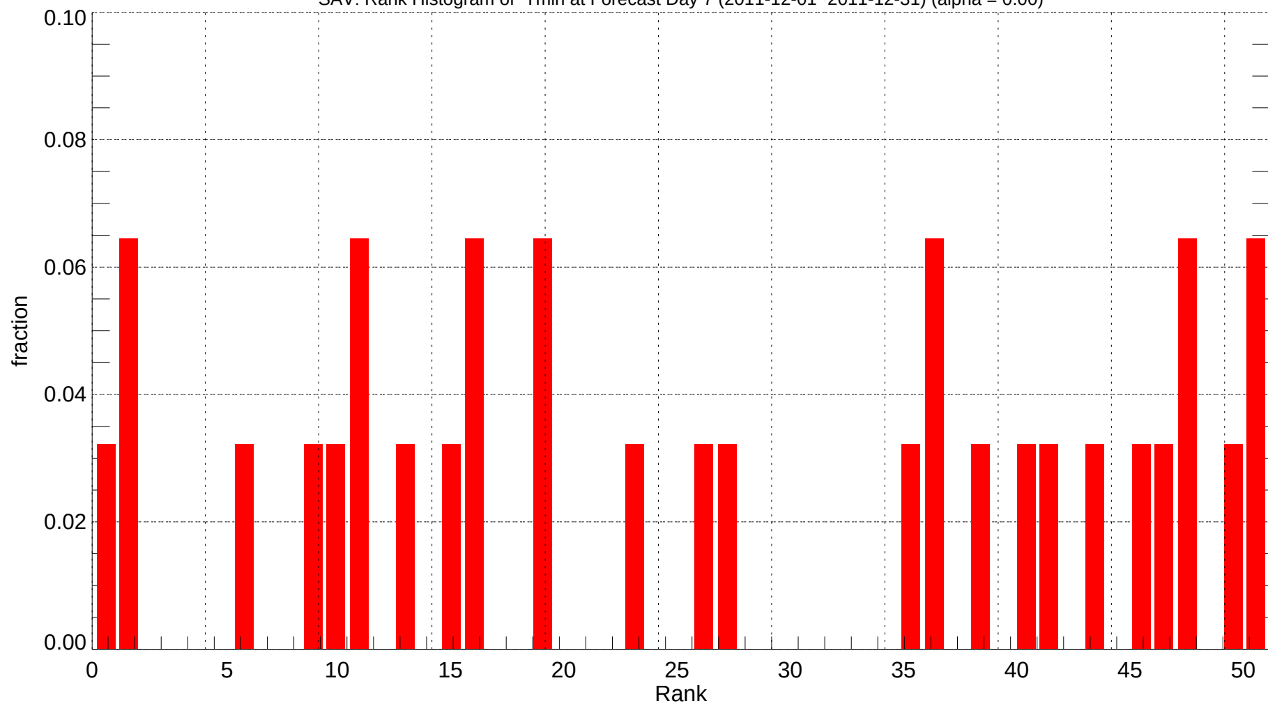
SAV: Rank Histogram of Tmin at Forecast Day 7 (2011-12-01~2011-12-31) (alpha = 0.00)
