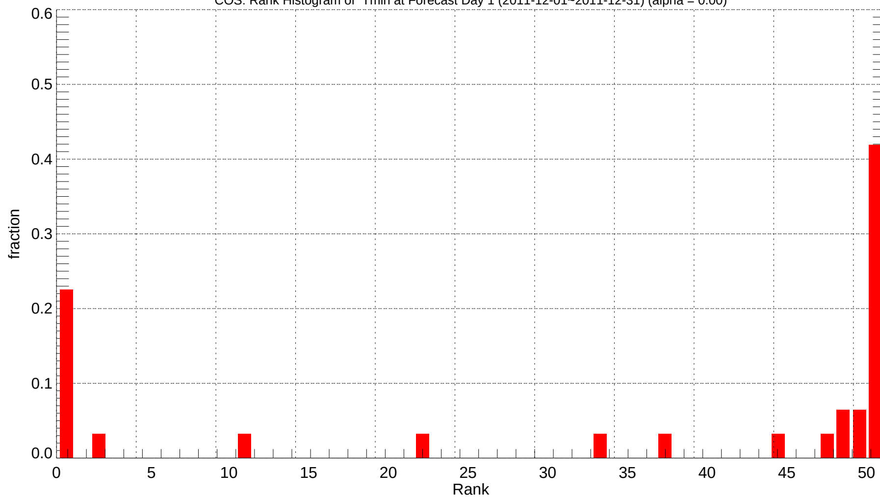
COS: Rank Histogram of Tmin at Forecast Day 1 (2011-12-01~2011-12-31) (alpha = 0.00)
