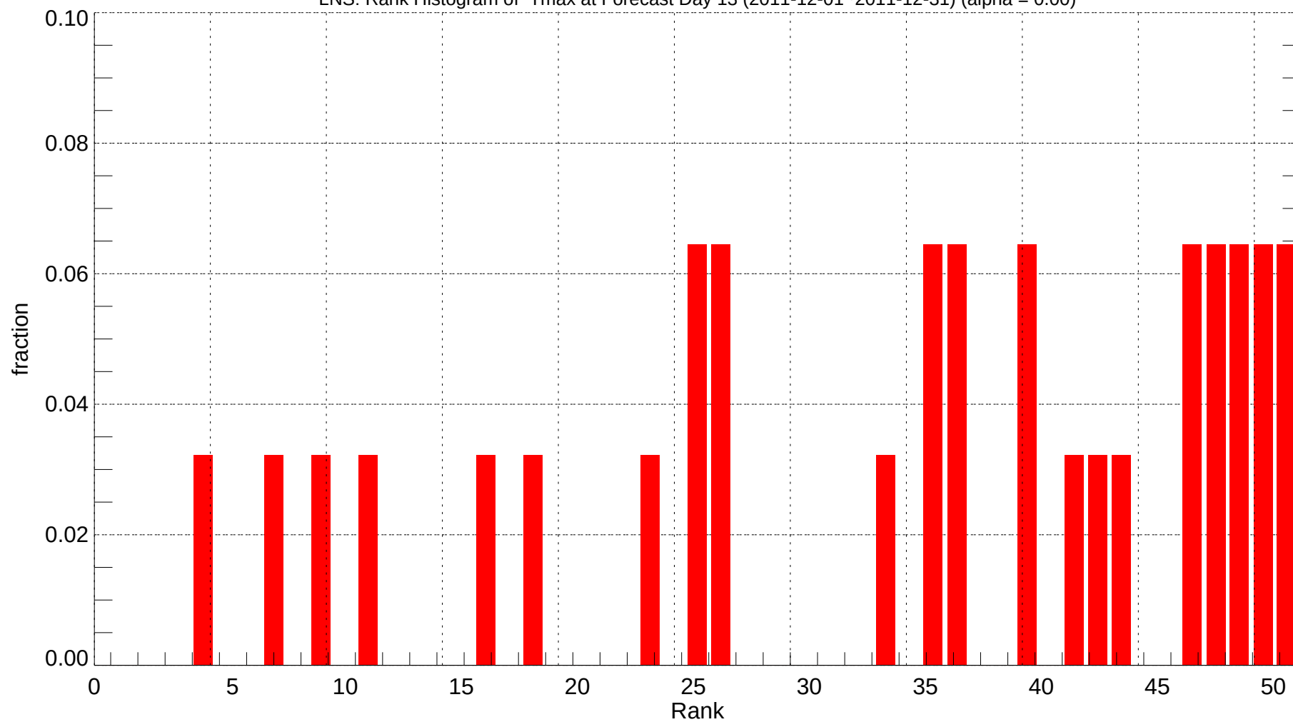
LNS: Rank Histogram of Tmax at Forecast Day 13 (2011-12-01~2011-12-31) (alpha = 0.00)
