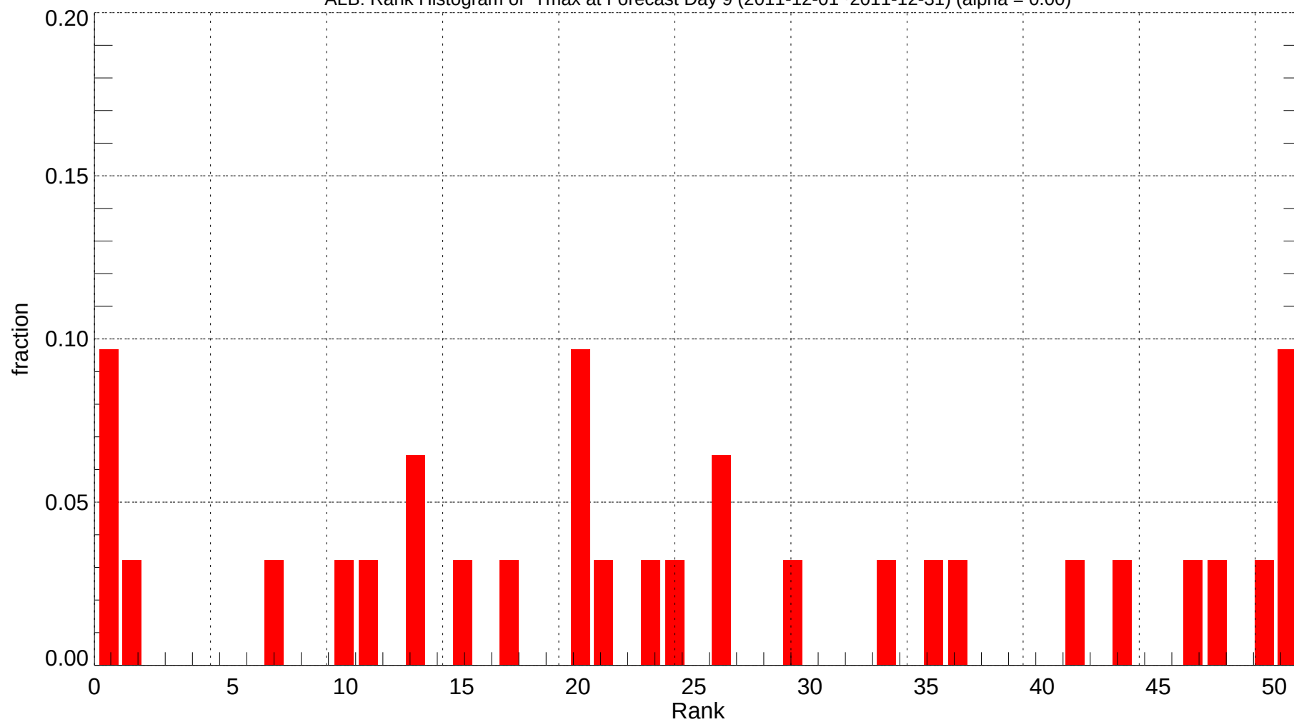
ALB: Rank Histogram of Tmax at Forecast Day 9 (2011-12-01~2011-12-31) (alpha = 0.00)
