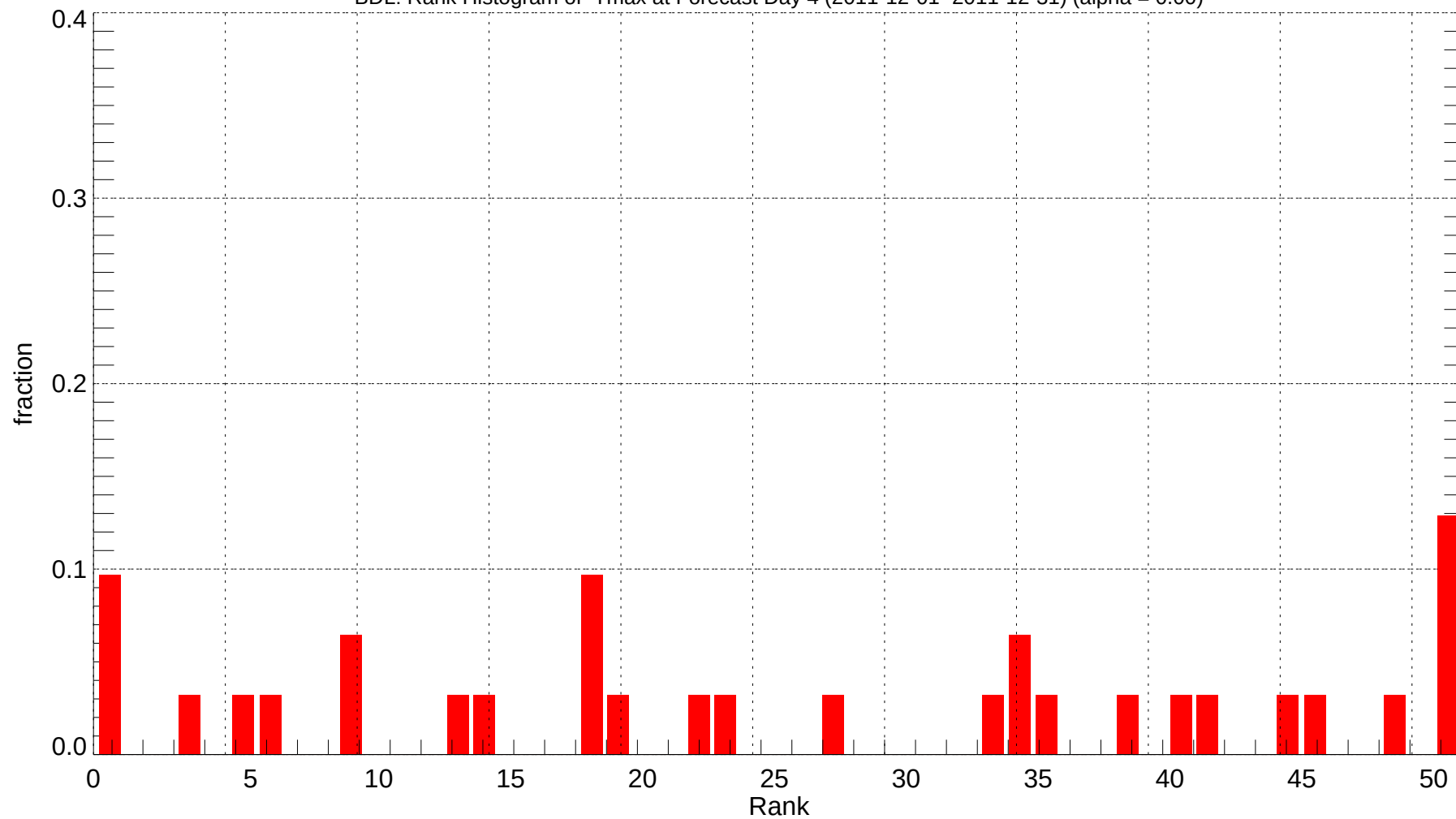
BDL: Rank Histogram of Tmax at Forecast Day 4 (2011-12-01~2011-12-31) (alpha = 0.00)
