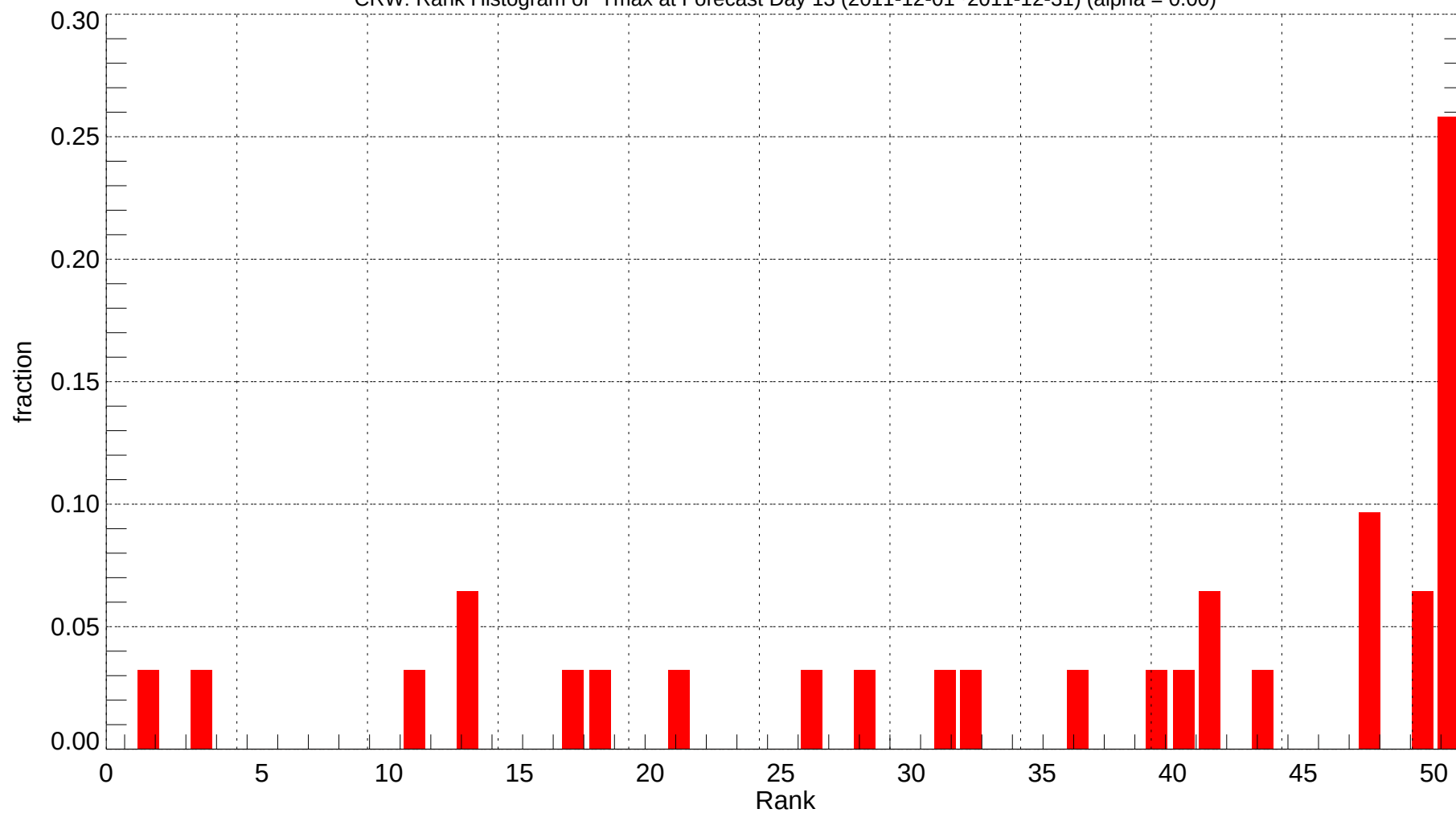
CRW: Rank Histogram of Tmax at Forecast Day 13 (2011-12-01~2011-12-31) (alpha = 0.00)
