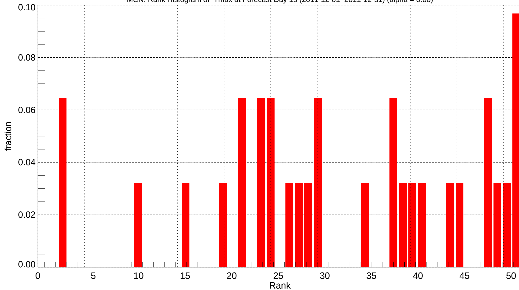
MCN: Rank Histogram of Tmax at Forecast Day 15 (2011-12-01~2011-12-31) (alpha = 0.00)
