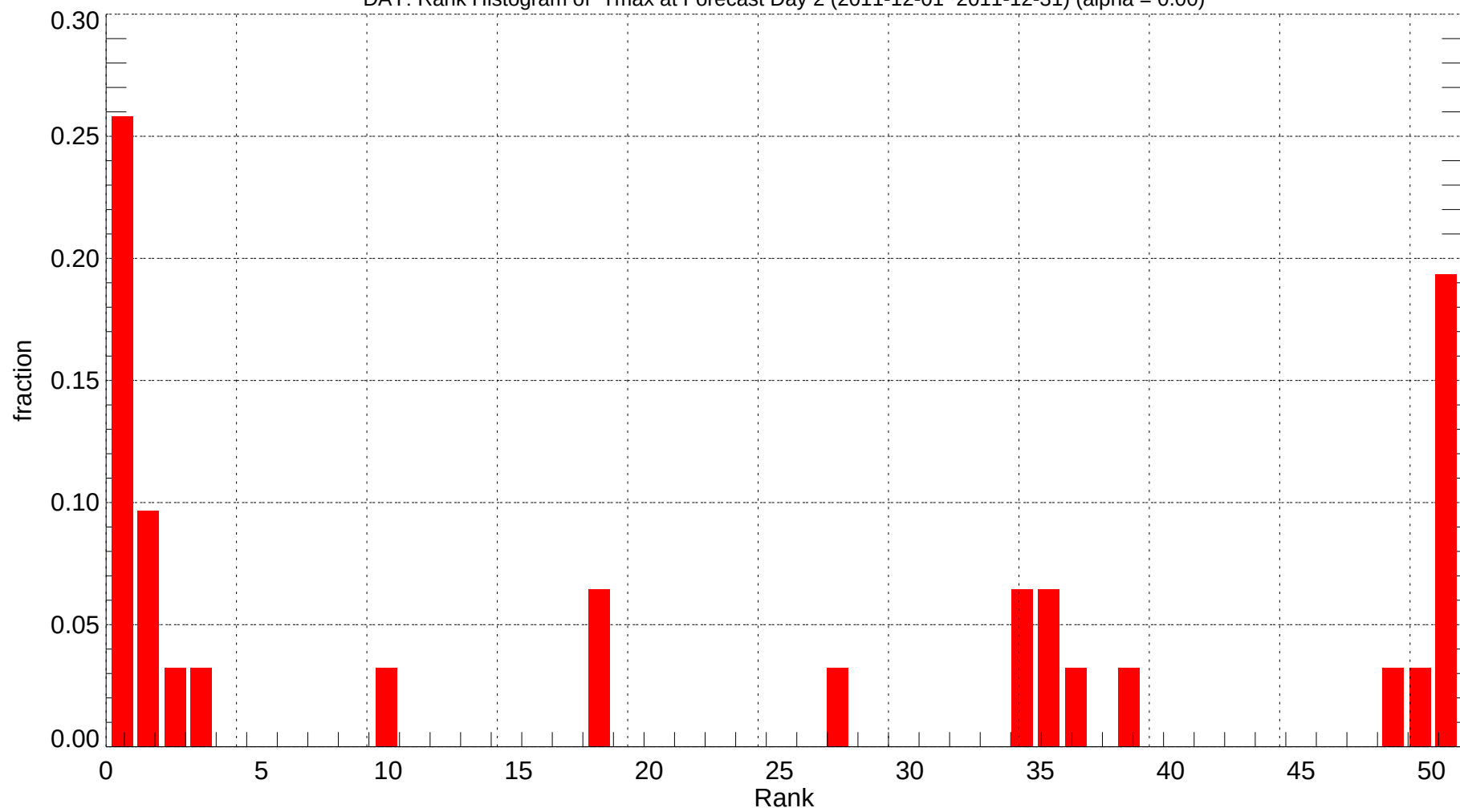
DAY: Rank Histogram of Tmax at Forecast Day 2 (2011-12-01~2011-12-31) (alpha = 0.00)
