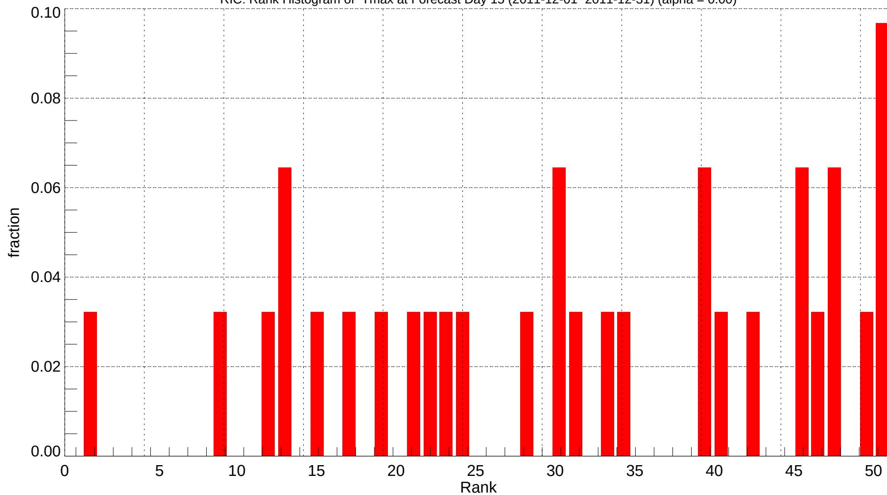
RIC: Rank Histogram of Tmax at Forecast Day 15 (2011-12-01~2011-12-31) (alpha = 0.00)
