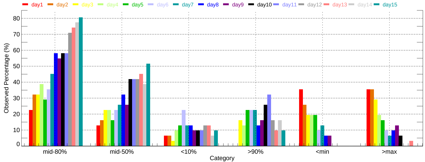
Observed Percentage of Ensembles - YYZ: Min Temperature (2011-12-01~2011-12-31)
