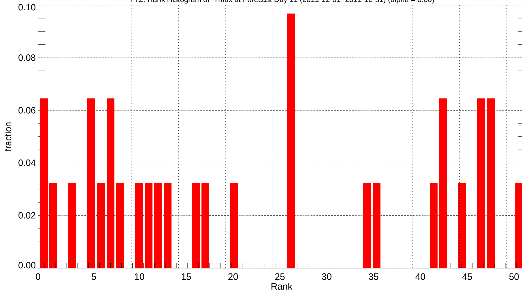
YYZ: Rank Histogram of Tmax at Forecast Day 11 (2011-12-01~2011-12-31) (alpha = 0.00)
