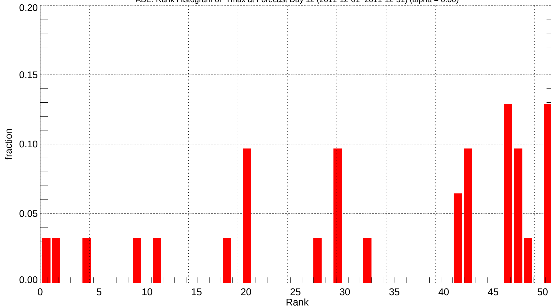
ABE: Rank Histogram of Tmax at Forecast Day 12 (2011-12-01~2011-12-31) (alpha = 0.00)
