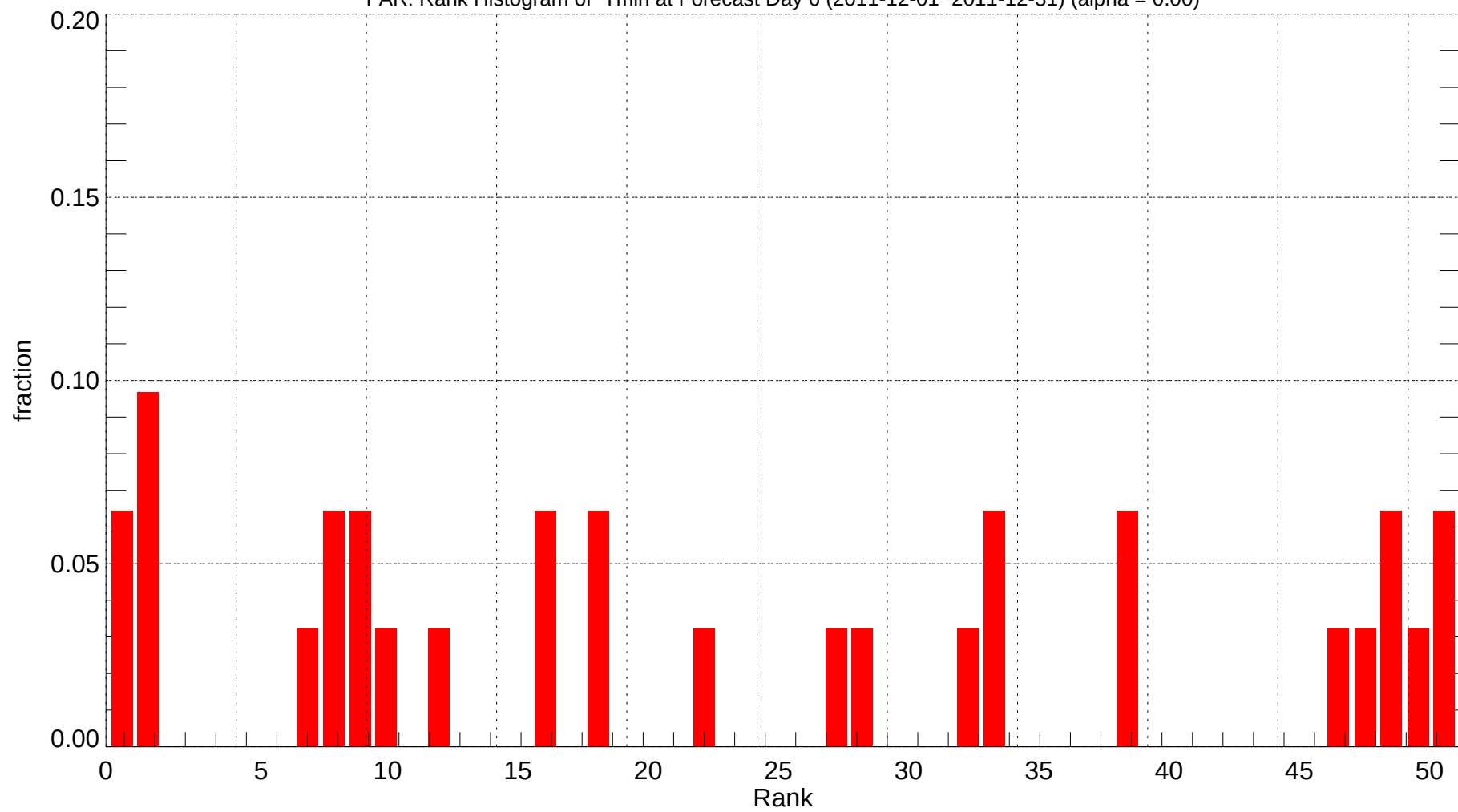
FAR: Rank Histogram of Tmin at Forecast Day 6 (2011-12-01~2011-12-31) (alpha = 0.00)
