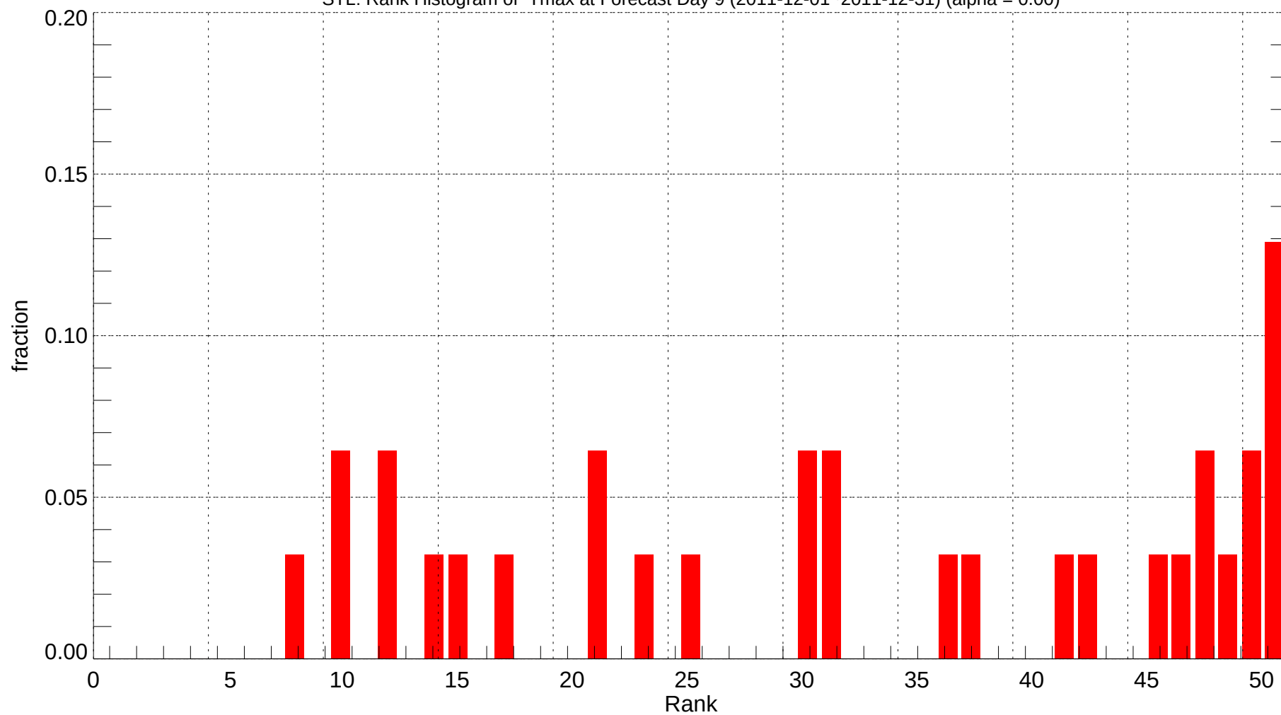
STL: Rank Histogram of Tmax at Forecast Day 9 (2011-12-01~2011-12-31) (alpha = 0.00)
