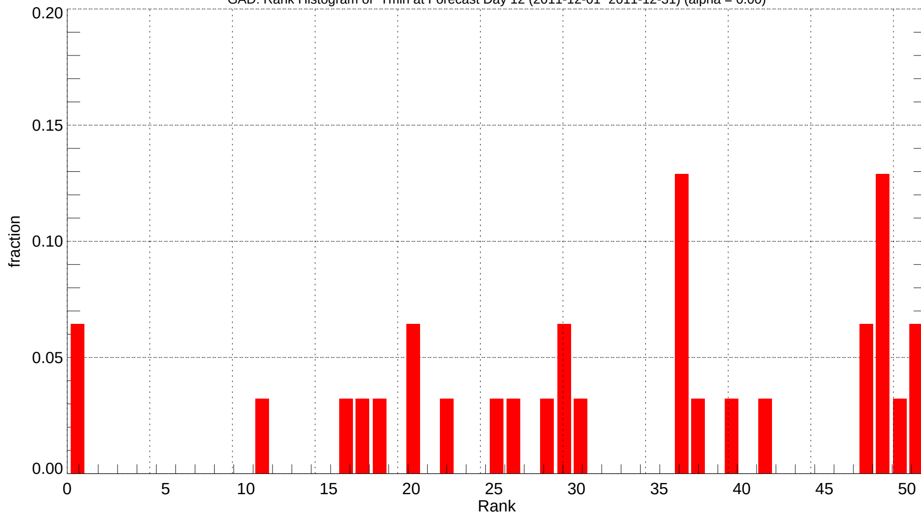
GAD: Rank Histogram of Tmin at Forecast Day 12 (2011-12-01~2011-12-31) (alpha = 0.00)
