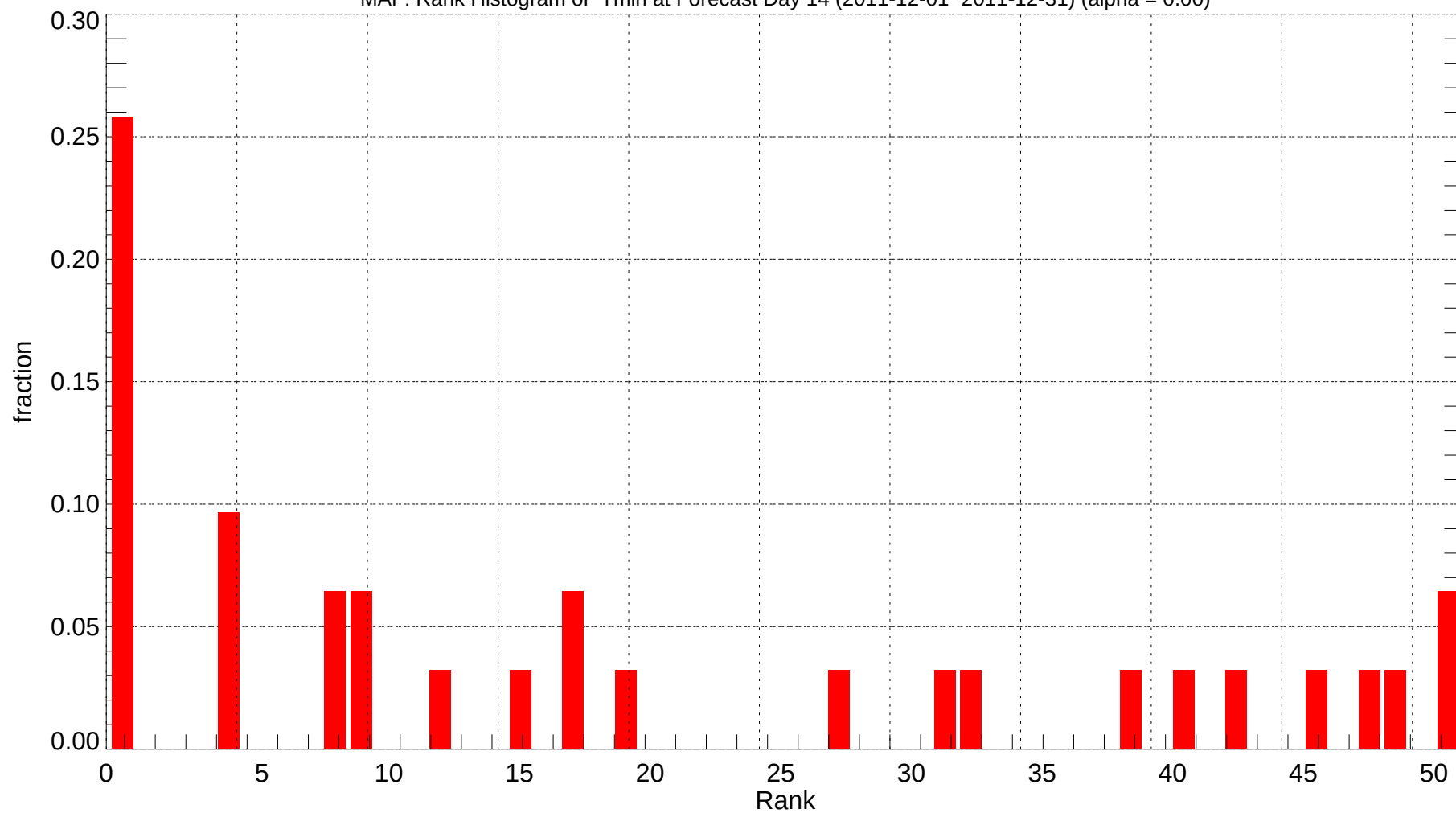
MAF: Rank Histogram of Tmin at Forecast Day 14 (2011-12-01~2011-12-31) (alpha = 0.00)
