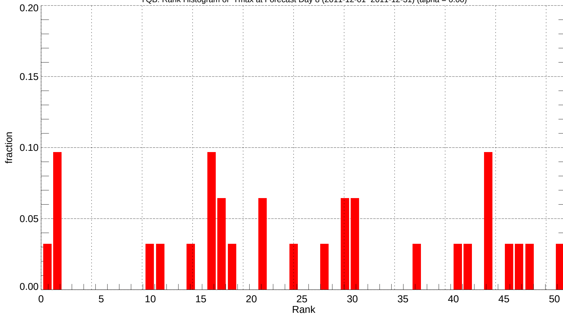
YQB: Rank Histogram of Tmax at Forecast Day 8 (2011-12-01~2011-12-31) (alpha = 0.00)
