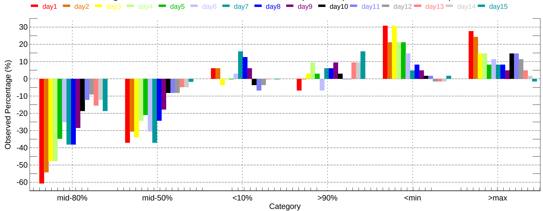
Observed Percentage Deviation of Ensembles - APN: Max Temperature (2011-12-01~2011-12-31)
