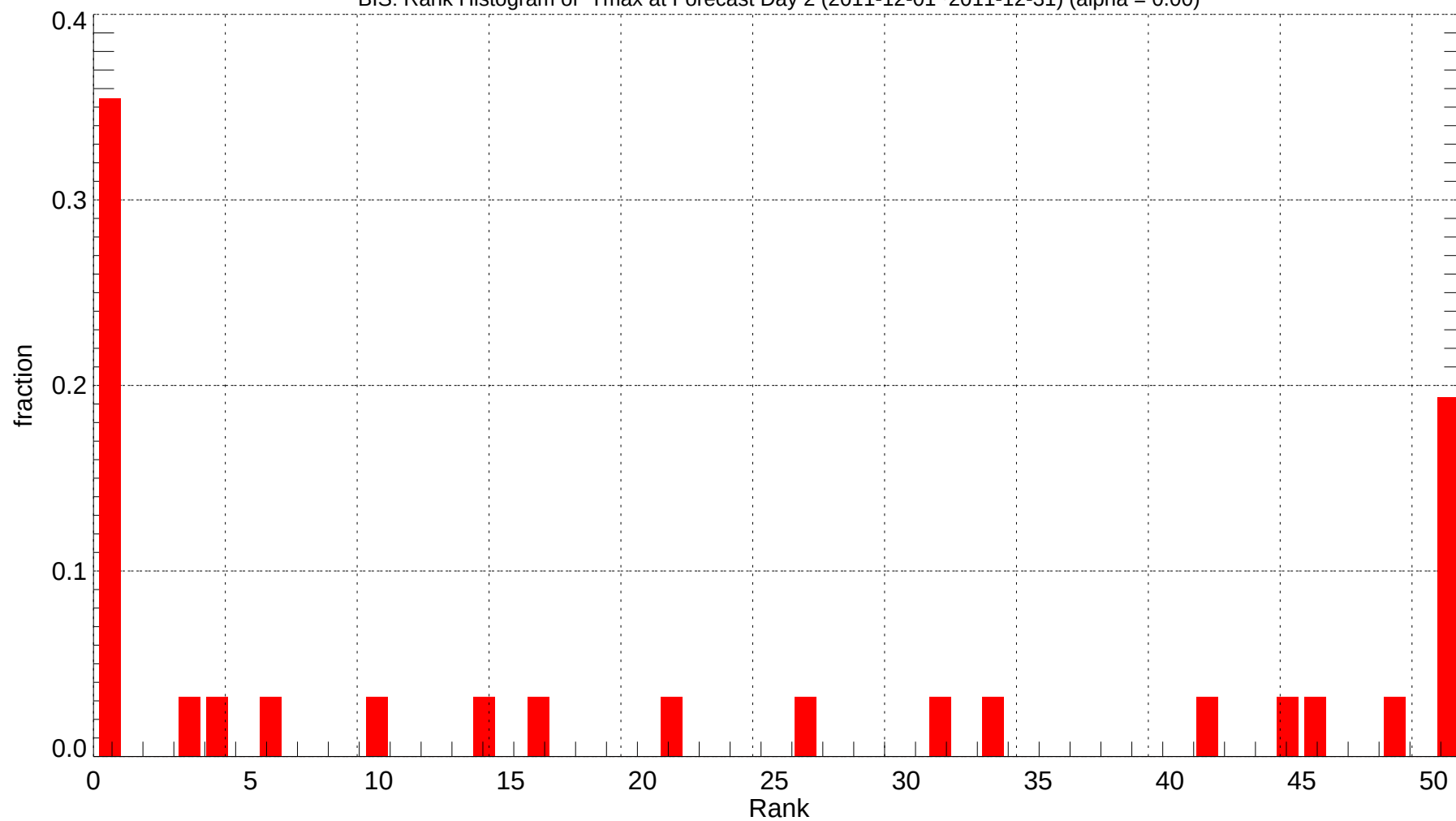
BIS: Rank Histogram of Tmax at Forecast Day 2 (2011-12-01~2011-12-31) (alpha = 0.00)
