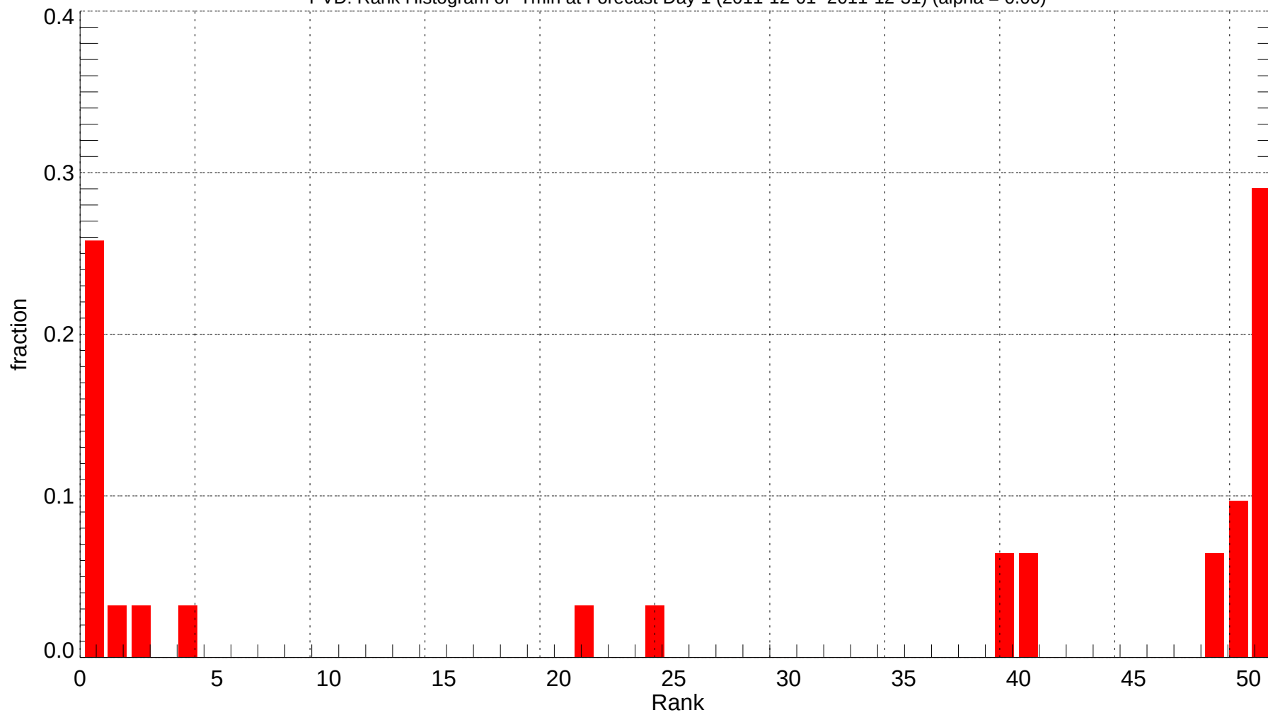
PVD: Rank Histogram of Tmin at Forecast Day 1 (2011-12-01~2011-12-31) (alpha = 0.00)
