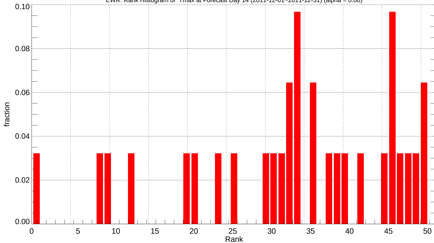
EWR: Rank Histogram of Tmax at Forecast Day 14 (2011-12-01~2011-12-31) (alpha = 0.00)
