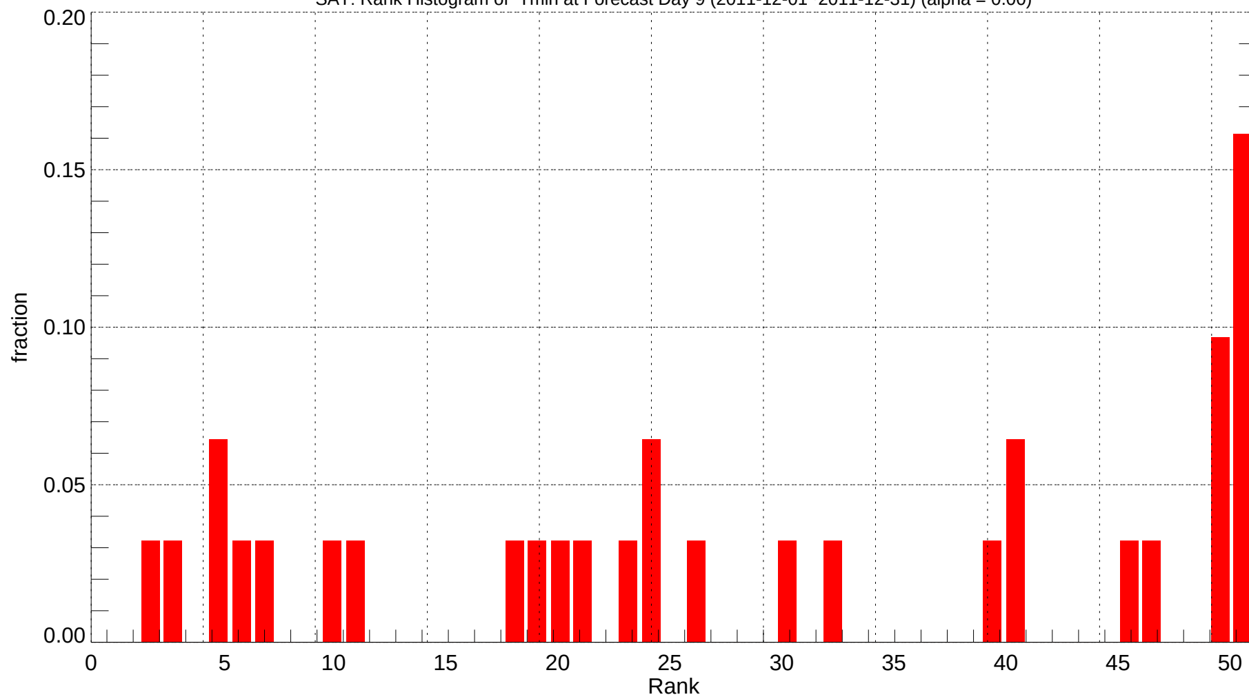
SAT: Rank Histogram of Tmin at Forecast Day 9 (2011-12-01~2011-12-31) (alpha = 0.00)
