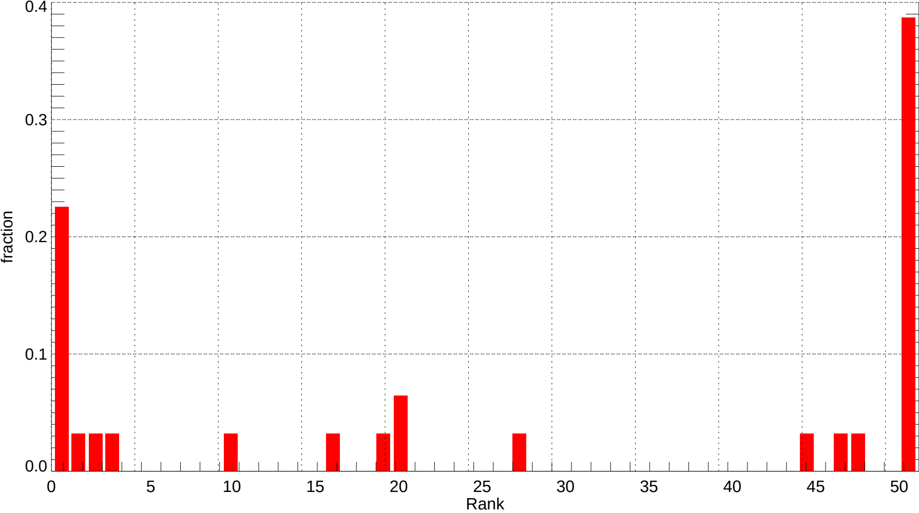
ELP: Rank Histogram of Tmin at Forecast Day 1 (2011-12-01~2011-12-31) (alpha = 0.00)
