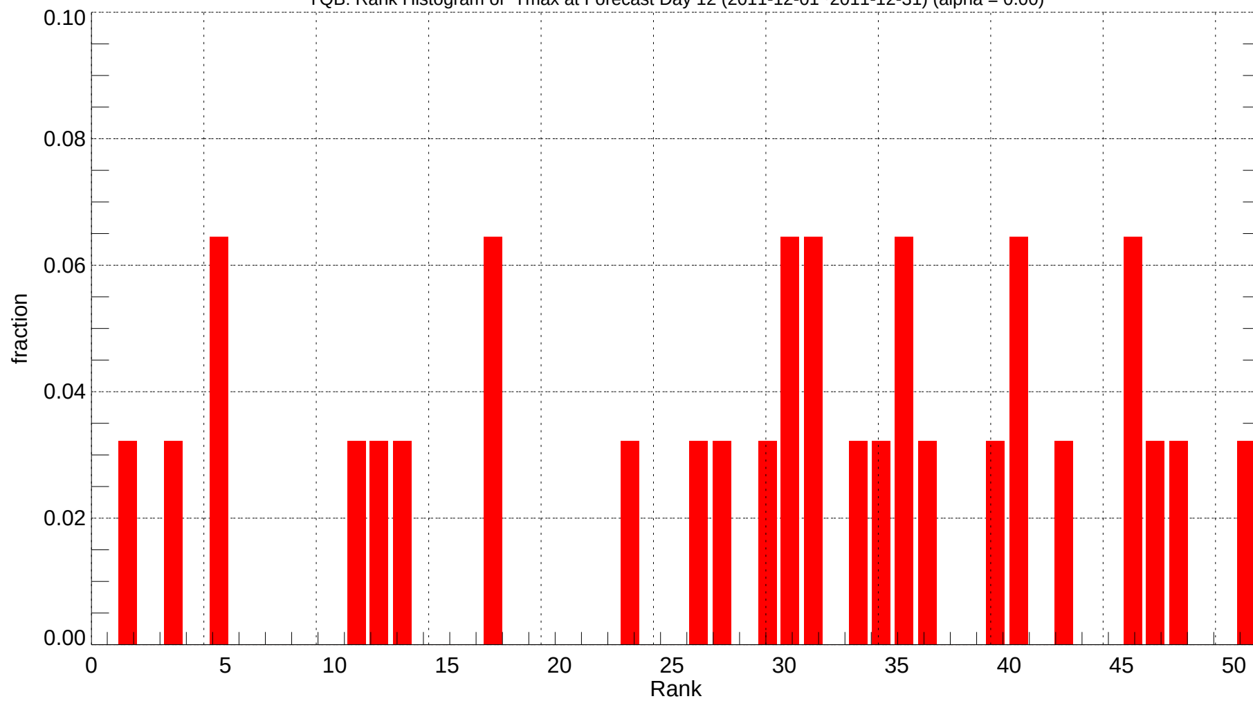
YQB: Rank Histogram of Tmax at Forecast Day 12 (2011-12-01~2011-12-31) (alpha = 0.00)
