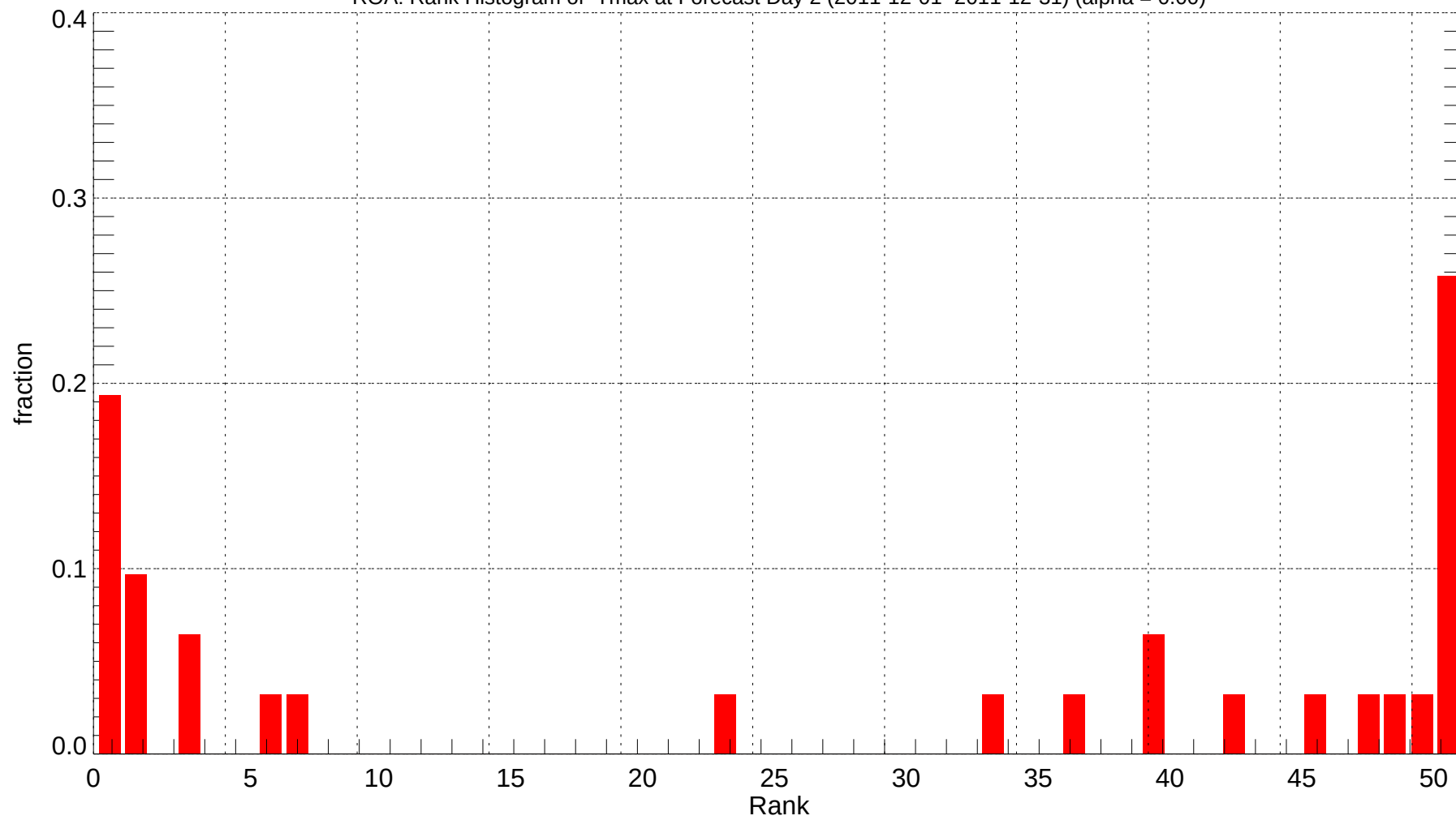
ROA: Rank Histogram of Tmax at Forecast Day 2 (2011-12-01~2011-12-31) (alpha = 0.00)
