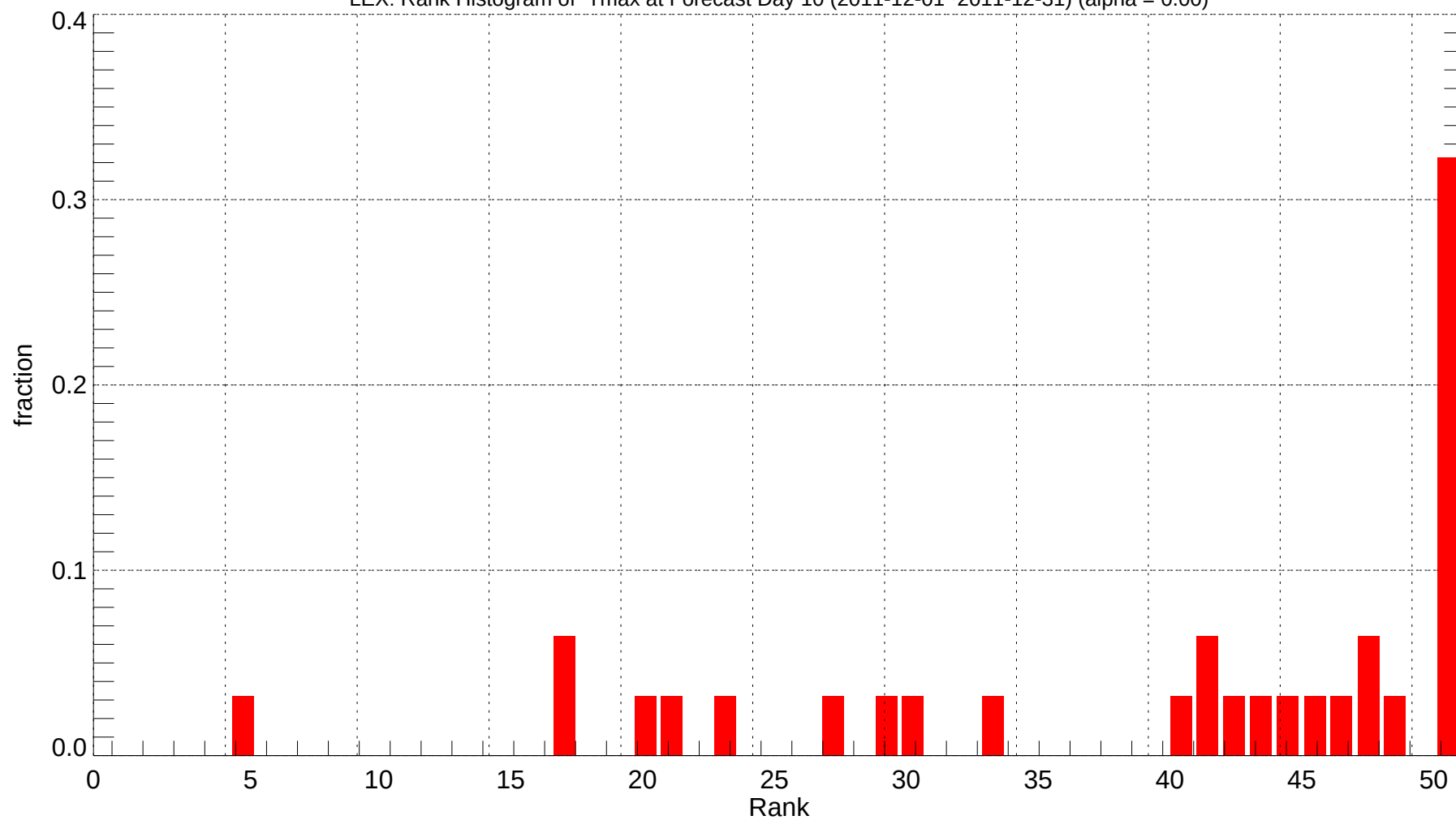
LEX: Rank Histogram of Tmax at Forecast Day 10 (2011-12-01~2011-12-31) (alpha = 0.00)
