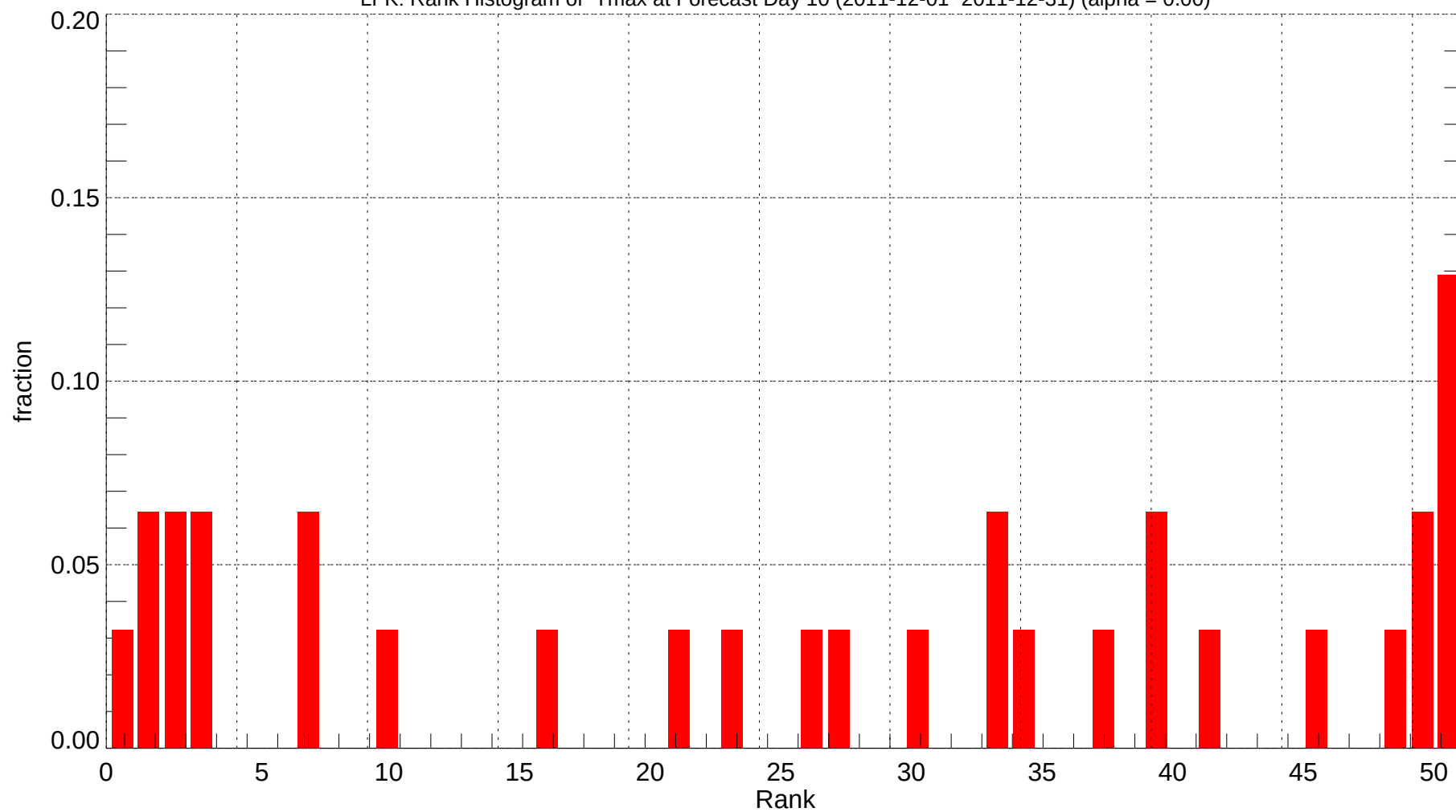
LFK: Rank Histogram of Tmax at Forecast Day 10 (2011-12-01~2011-12-31) (alpha = 0.00)
