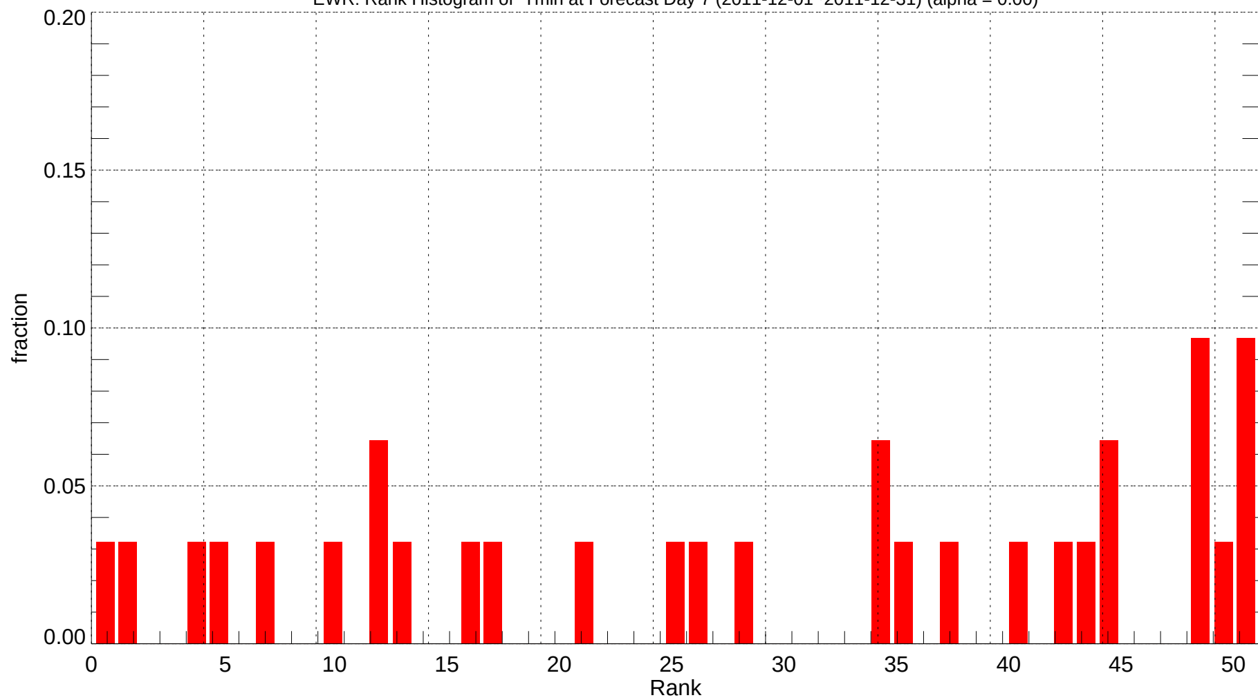
EWR: Rank Histogram of Tmin at Forecast Day 7 (2011-12-01~2011-12-31) (alpha = 0.00)
