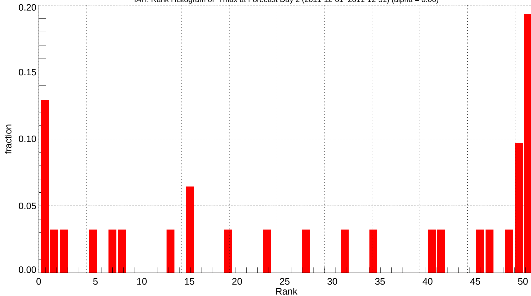
IAH: Rank Histogram of Tmax at Forecast Day 2 (2011-12-01~2011-12-31) (alpha = 0.00)
