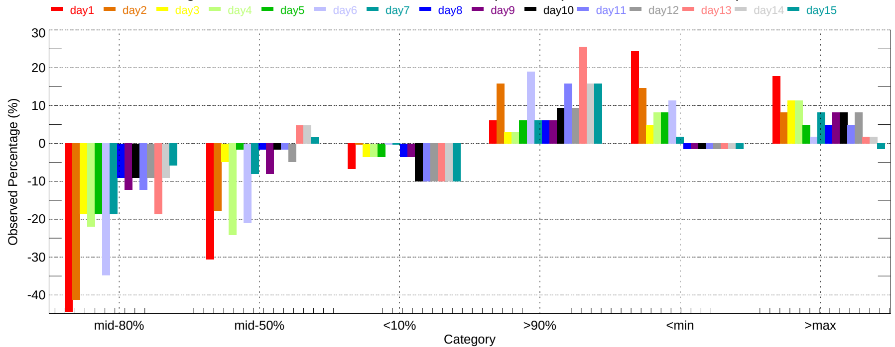
Observed Percentage Deviation of Ensembles - DEC: Min Temperature (2011-12-01~2011-12-31)
