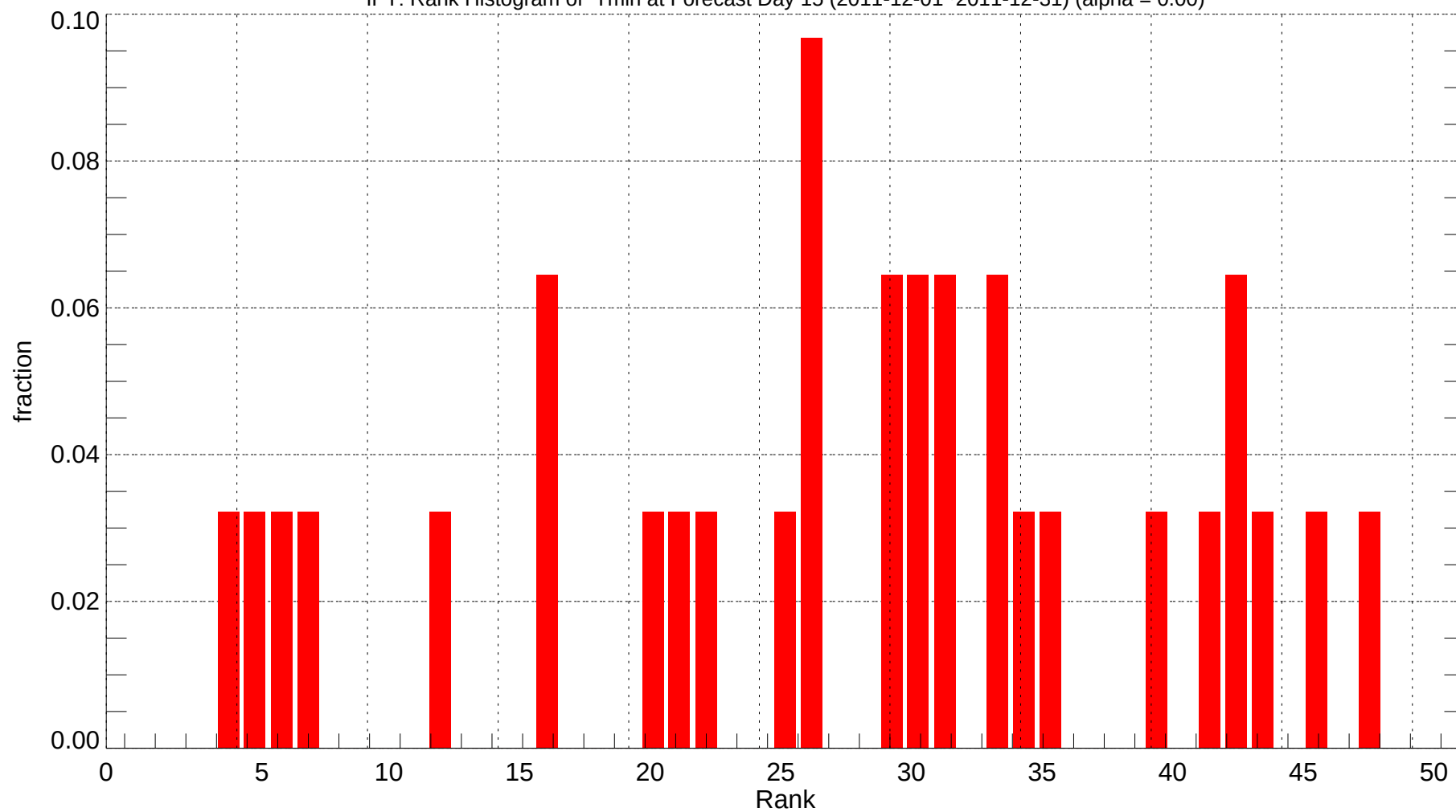
IPT: Rank Histogram of Tmin at Forecast Day 15 (2011-12-01~2011-12-31) (alpha = 0.00)
