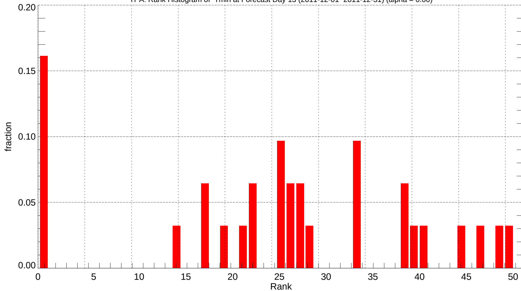
TPA: Rank Histogram of Tmin at Forecast Day 13 (2011-12-01~2011-12-31) (alpha = 0.00)
