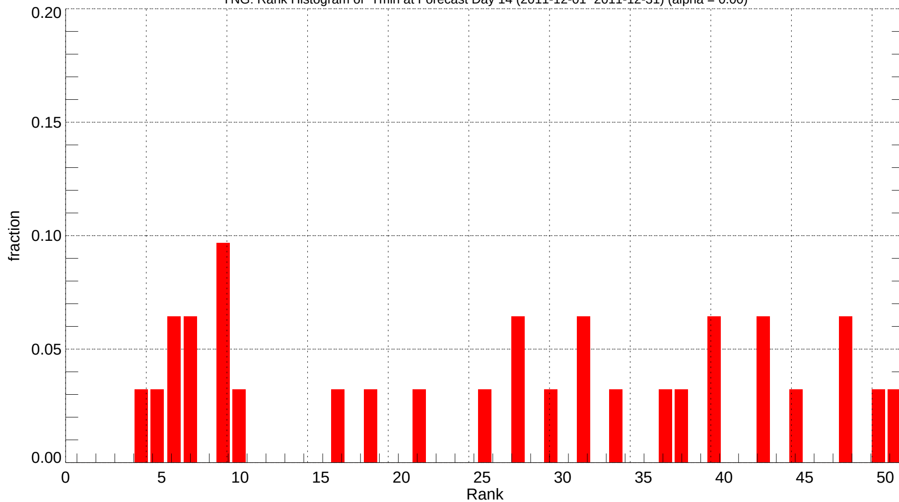
YNG: Rank Histogram of Tmin at Forecast Day 14 (2011-12-01~2011-12-31) (alpha = 0.00)
