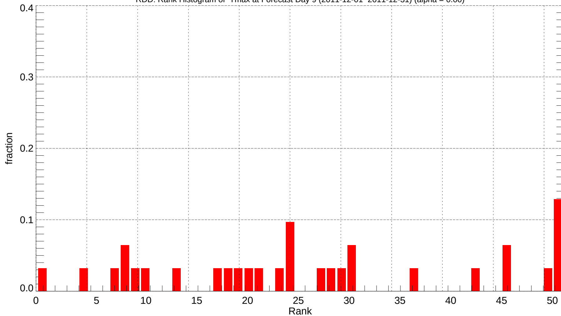
RDD: Rank Histogram of Tmax at Forecast Day 9 (2011-12-01~2011-12-31) (alpha = 0.00)
