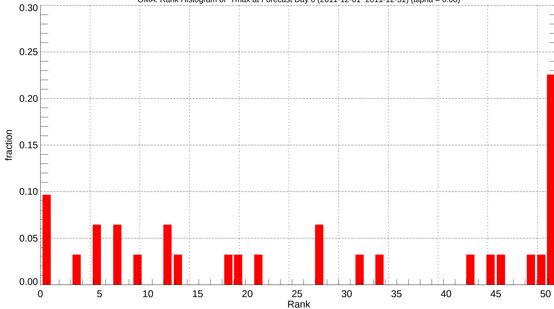
OMA: Rank Histogram of Tmax at Forecast Day 6 (2011-12-01~2011-12-31) (alpha = 0.00)
