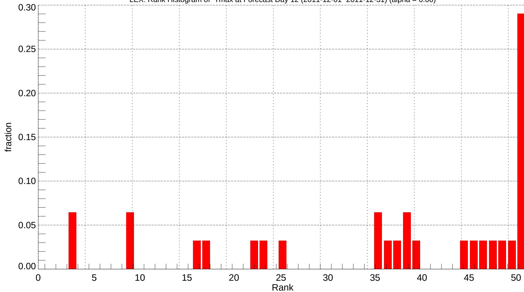
LEX: Rank Histogram of Tmax at Forecast Day 12 (2011-12-01~2011-12-31) (alpha = 0.00)
