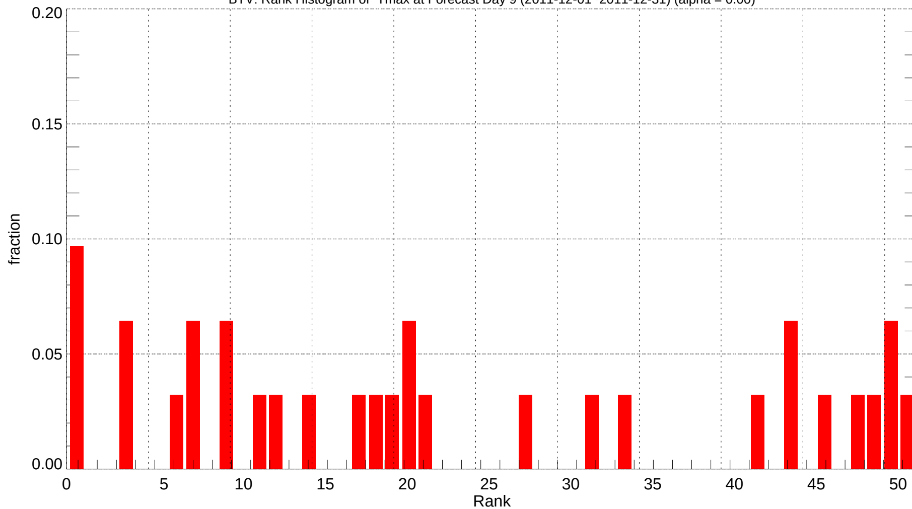
BTV: Rank Histogram of Tmax at Forecast Day 9 (2011-12-01~2011-12-31) (alpha = 0.00)
