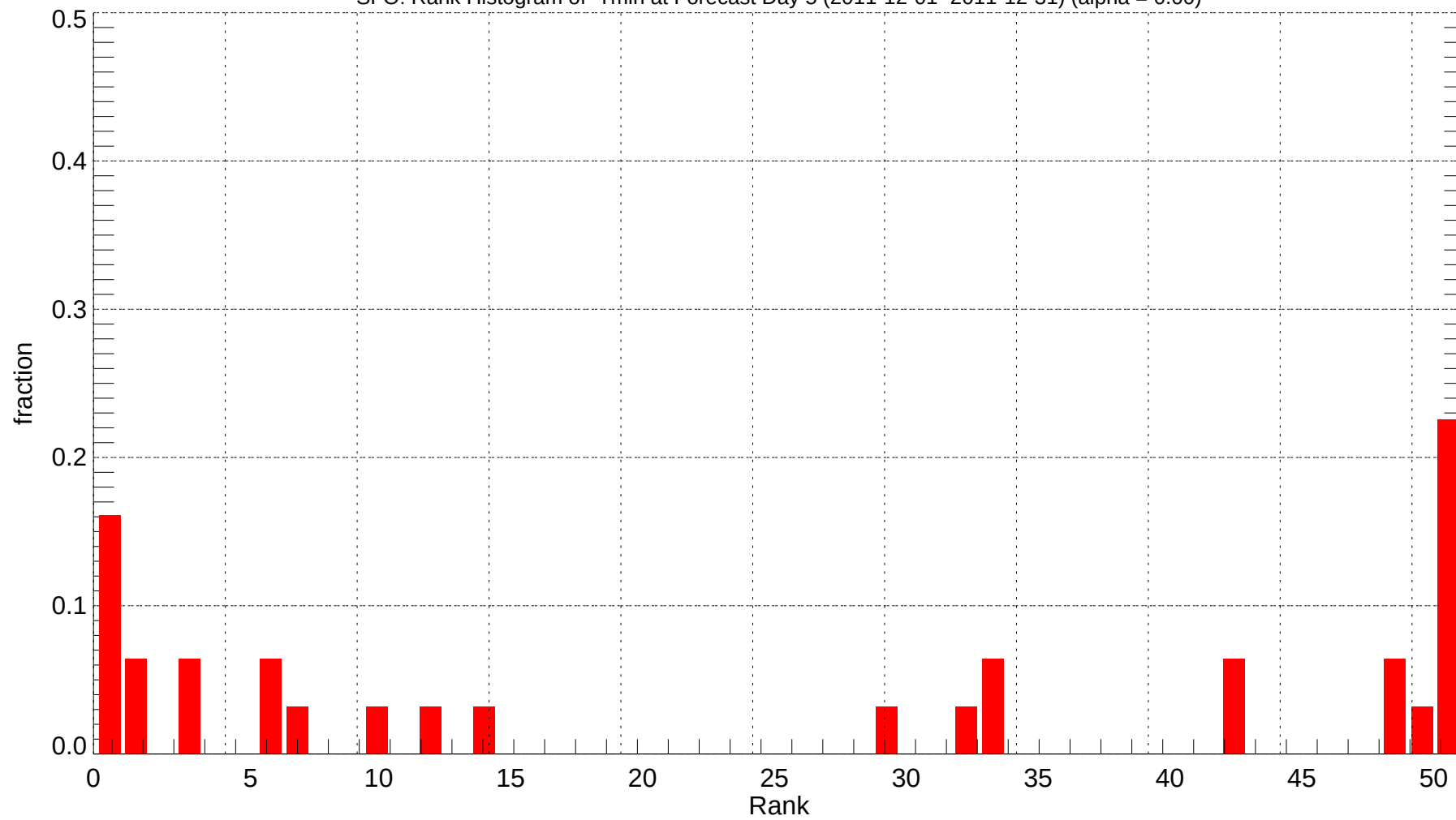
SFO: Rank Histogram of Tmin at Forecast Day 5 (2011-12-01~2011-12-31) (alpha = 0.00)
