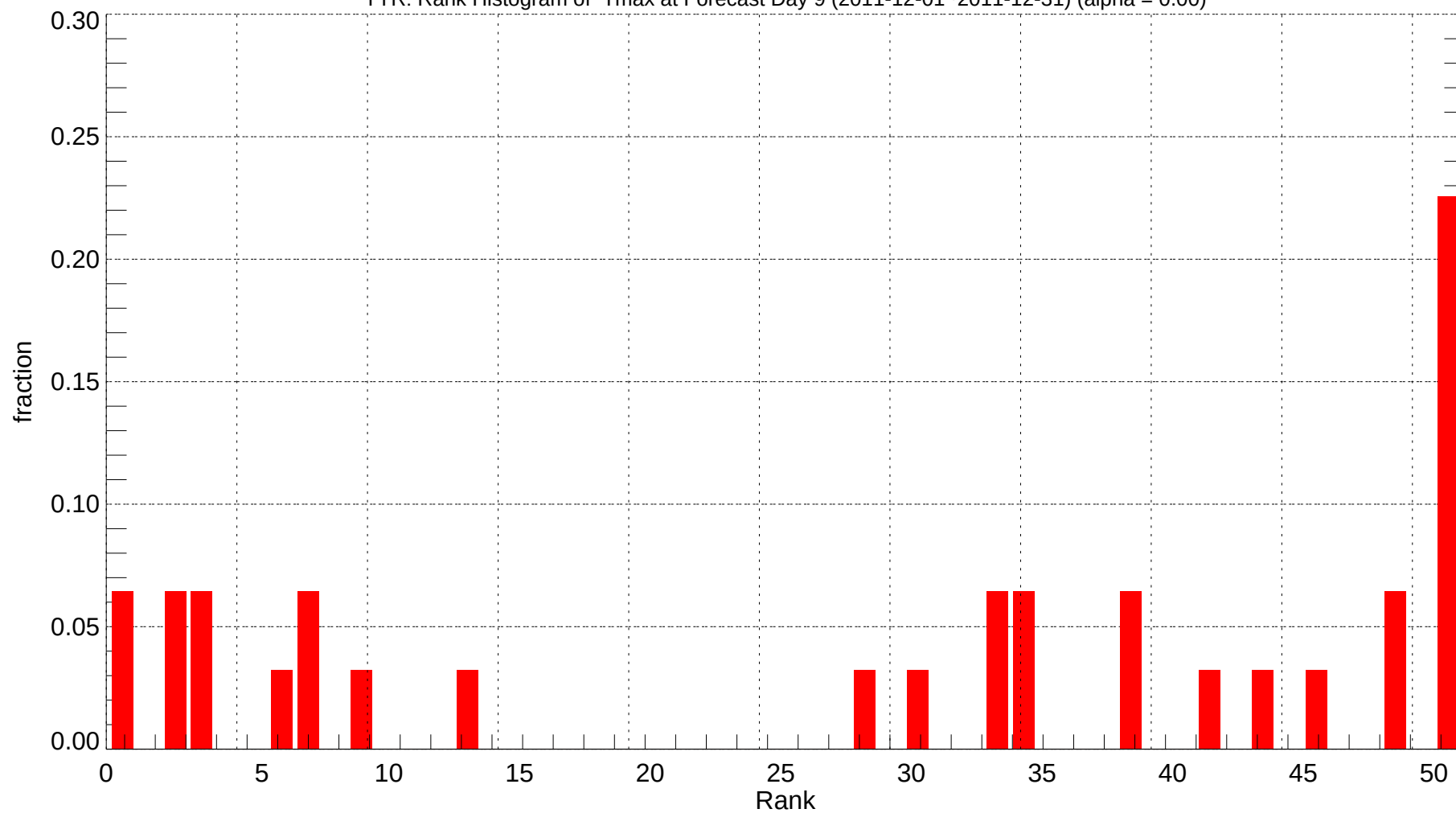
TYR: Rank Histogram of Tmax at Forecast Day 9 (2011-12-01~2011-12-31) (alpha = 0.00)
