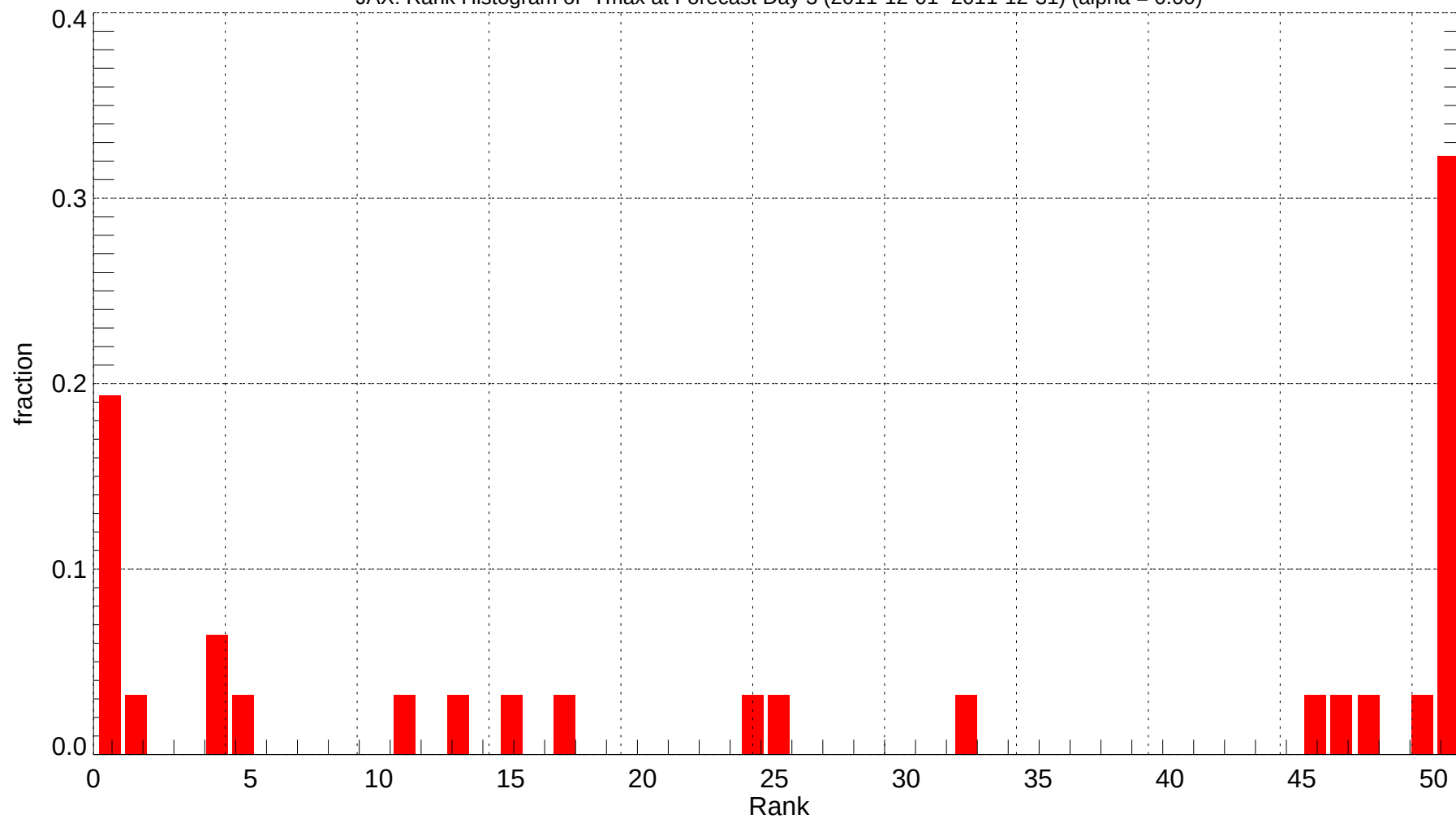
JAX: Rank Histogram of Tmax at Forecast Day 3 (2011-12-01~2011-12-31) (alpha = 0.00)
