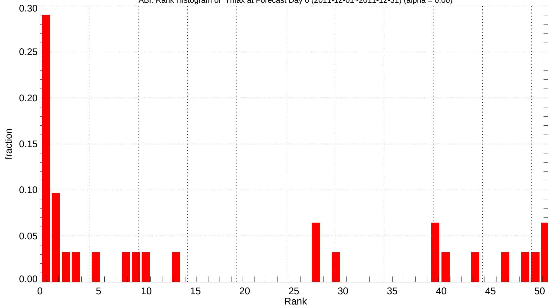
ABI: Rank Histogram of Tmax at Forecast Day 6 (2011-12-01~2011-12-31) (alpha = 0.00)
