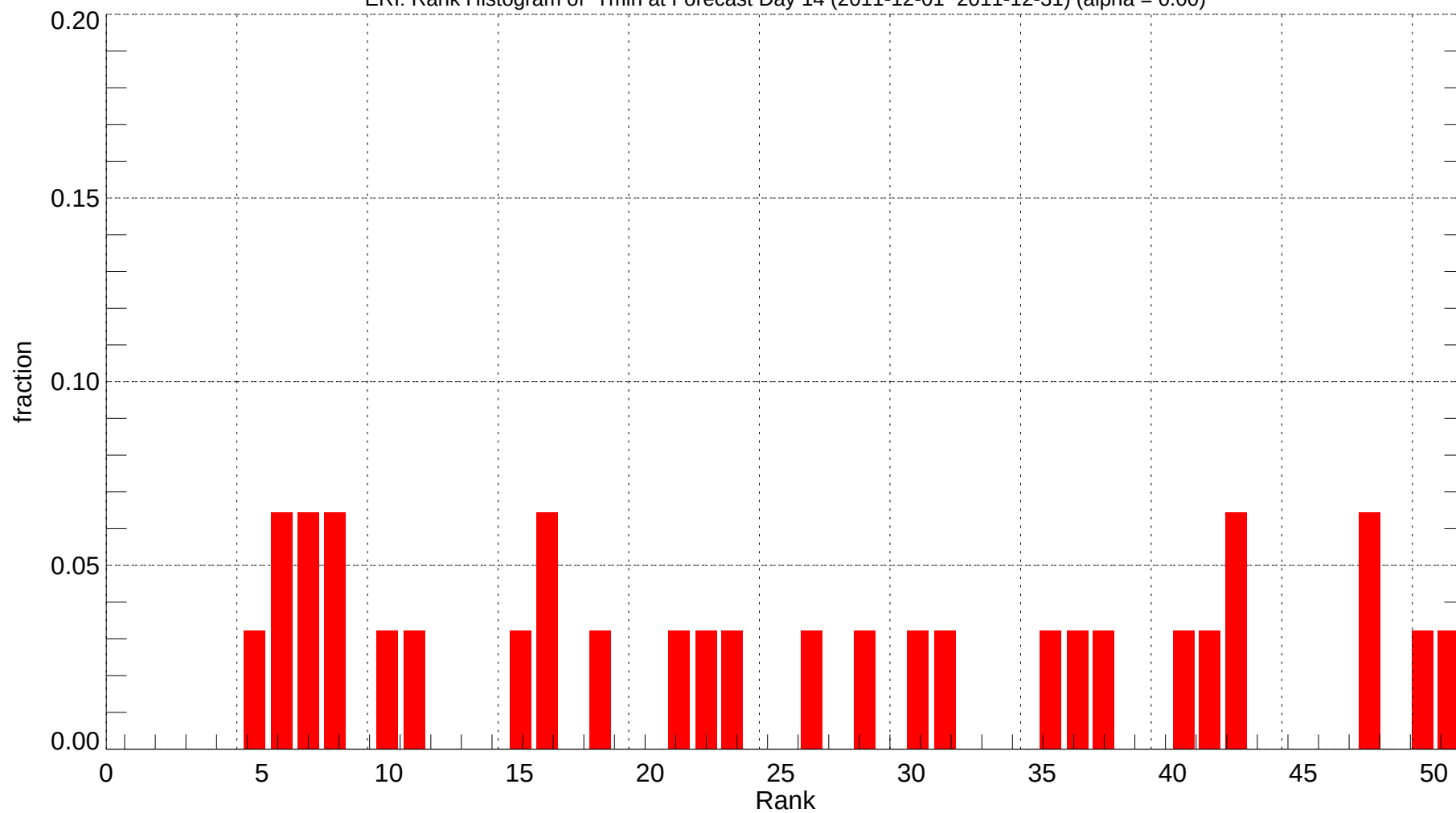
ERI: Rank Histogram of Tmin at Forecast Day 14 (2011-12-01~2011-12-31) (alpha = 0.00)
