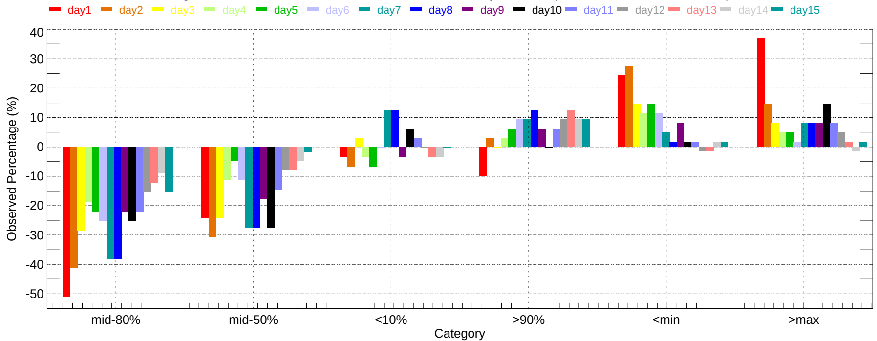
Observed Percentage Deviation of Ensembles - MHT: Max Temperature (2011-12-01~2011-12-31)
