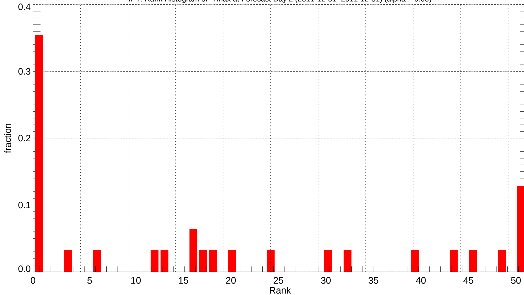
IPT: Rank Histogram of Tmax at Forecast Day 2 (2011-12-01~2011-12-31) (alpha = 0.00)
