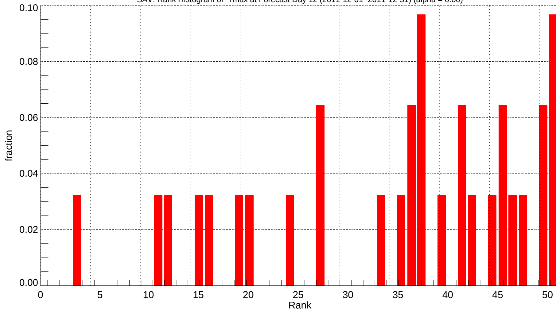
SAV: Rank Histogram of Tmax at Forecast Day 12 (2011-12-01~2011-12-31) (alpha = 0.00)
