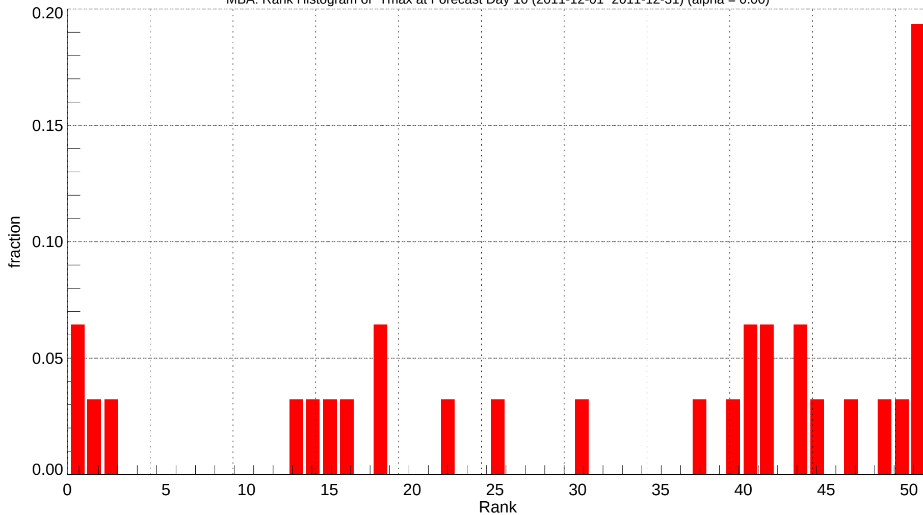
MBA: Rank Histogram of Tmax at Forecast Day 10 (2011-12-01~2011-12-31) (alpha = 0.00)
