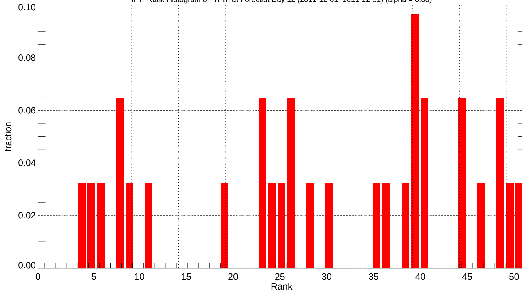
IPT: Rank Histogram of Tmin at Forecast Day 12 (2011-12-01~2011-12-31) (alpha = 0.00)
