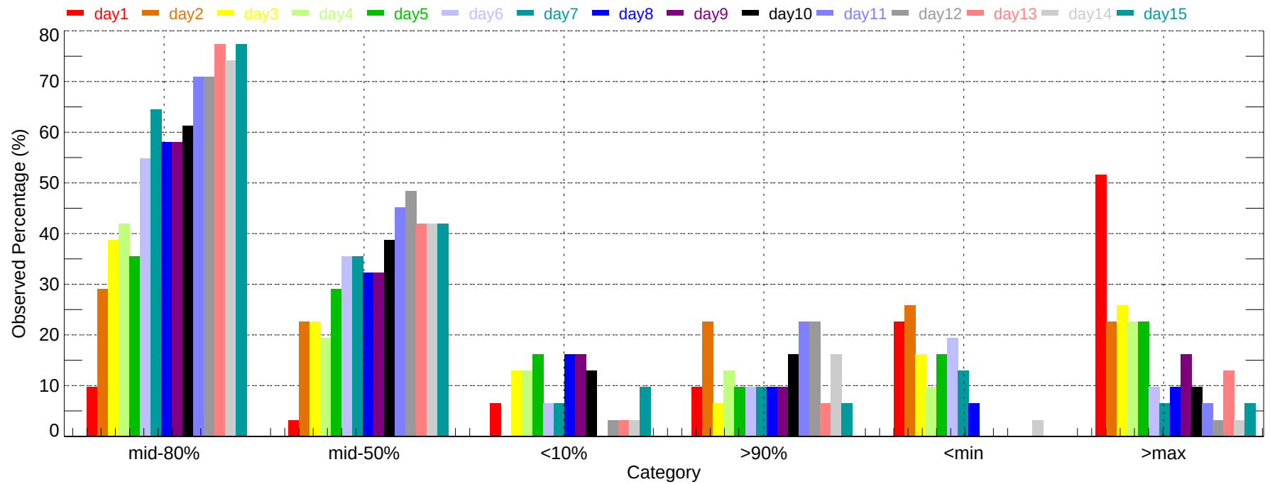
Observed Percentage of Ensembles - ALB: Min Temperature (2011-12-01~2011-12-31)
