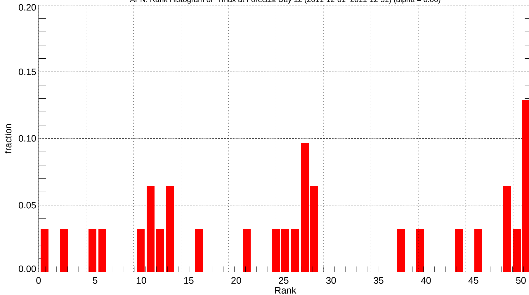
APN: Rank Histogram of Tmax at Forecast Day 12 (2011-12-01~2011-12-31) (alpha = 0.00)
