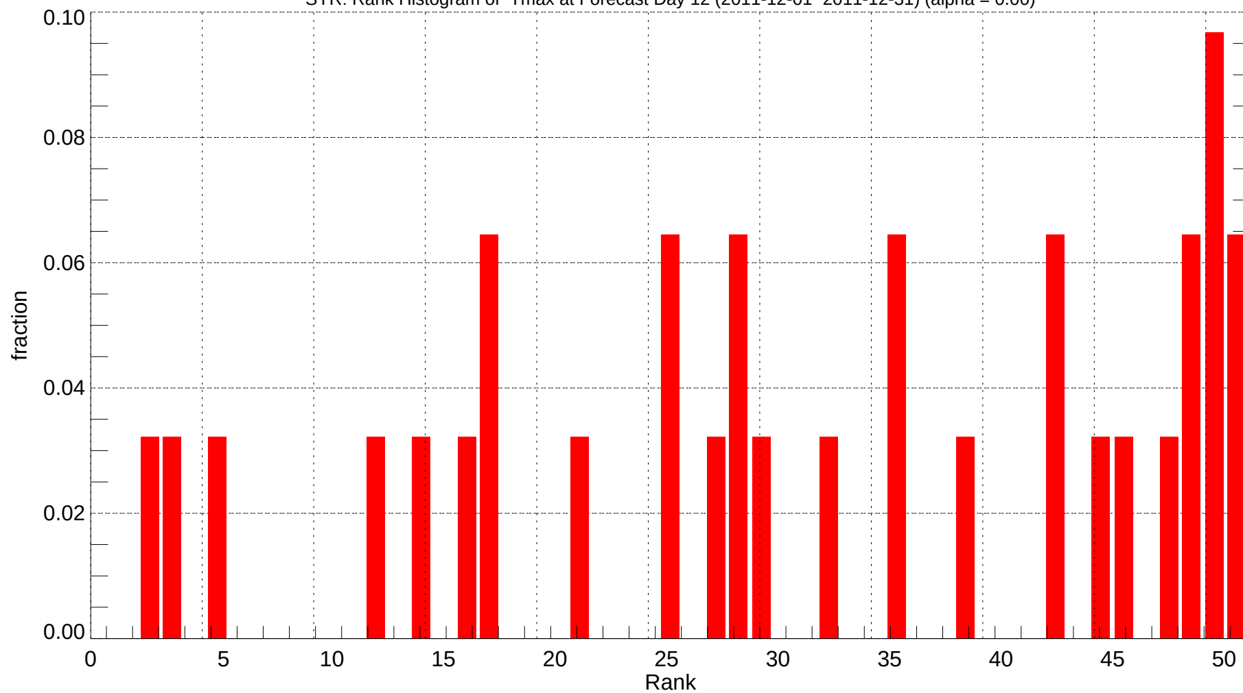
SYR: Rank Histogram of Tmax at Forecast Day 12 (2011-12-01~2011-12-31) (alpha = 0.00)
