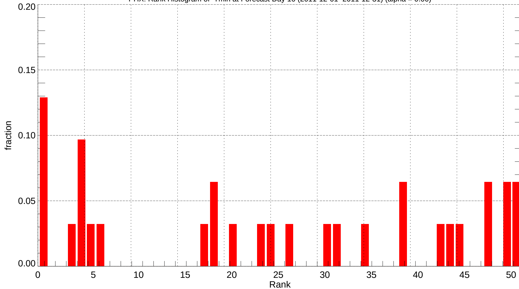
PHX: Rank Histogram of Tmin at Forecast Day 10 (2011-12-01~2011-12-31) (alpha = 0.00)
