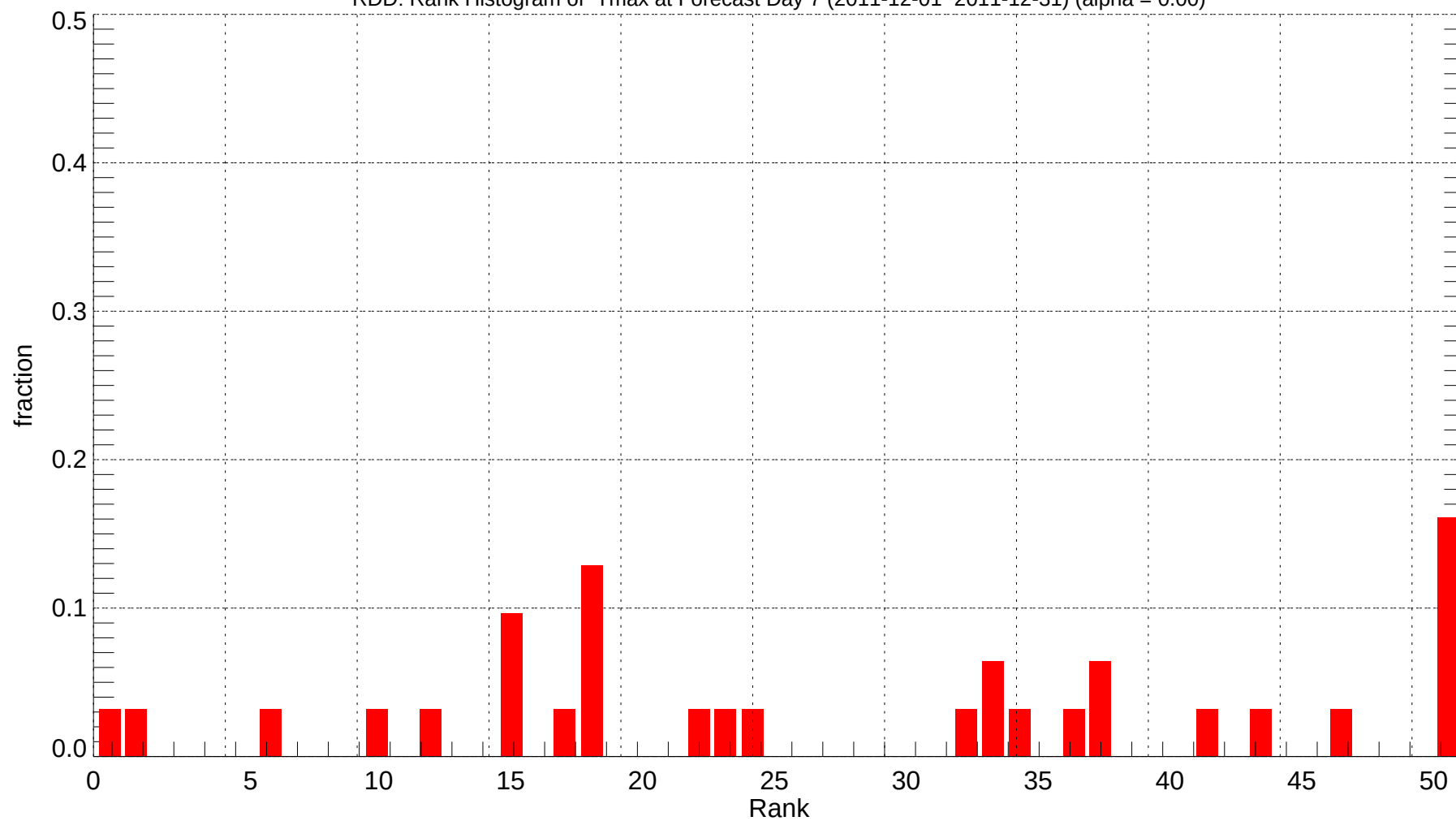
RDD: Rank Histogram of Tmax at Forecast Day 7 (2011-12-01~2011-12-31) (alpha = 0.00)
