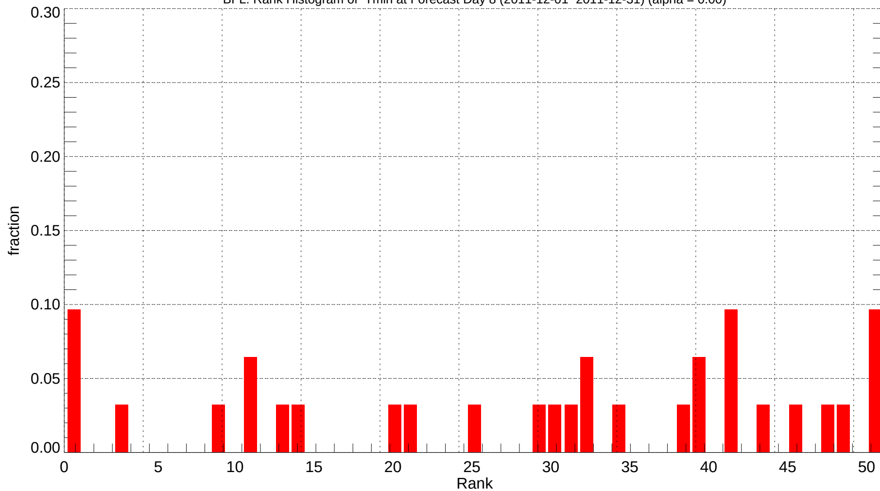
BFL: Rank Histogram of Tmin at Forecast Day 8 (2011-12-01~2011-12-31) (alpha = 0.00)
