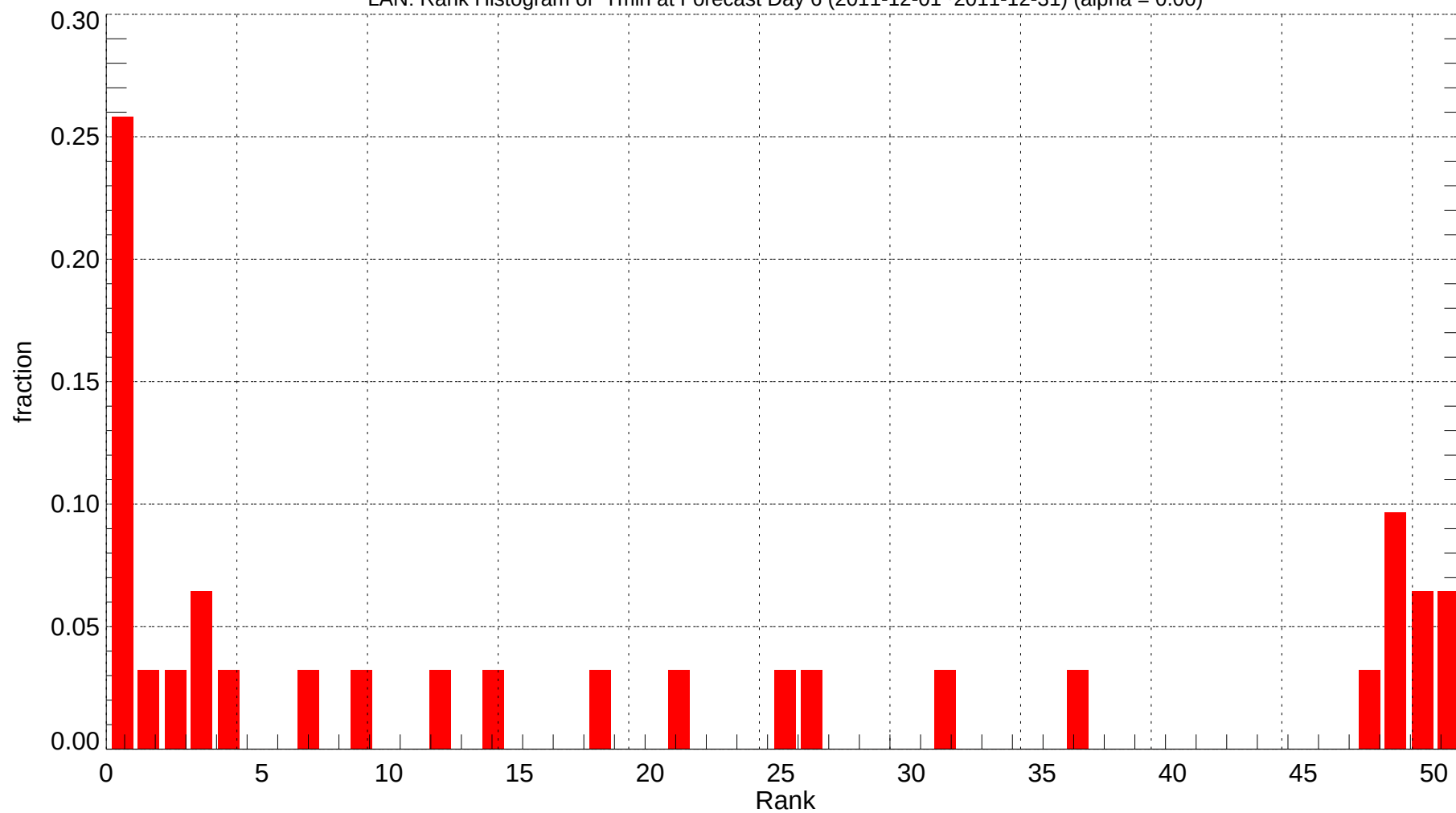
LAN: Rank Histogram of Tmin at Forecast Day 6 (2011-12-01~2011-12-31) (alpha = 0.00)
