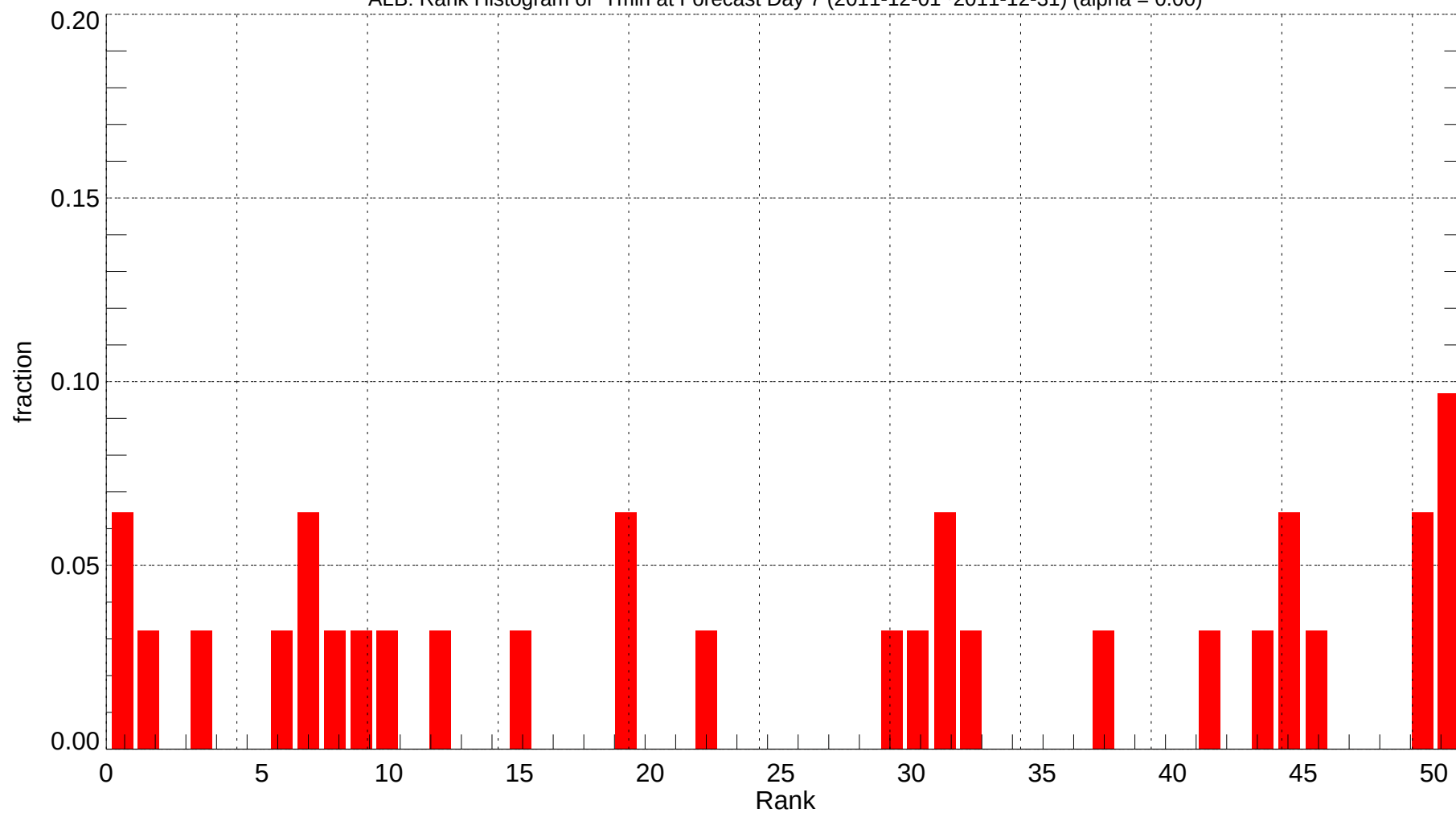
ALB: Rank Histogram of Tmin at Forecast Day 7 (2011-12-01~2011-12-31) (alpha = 0.00)
