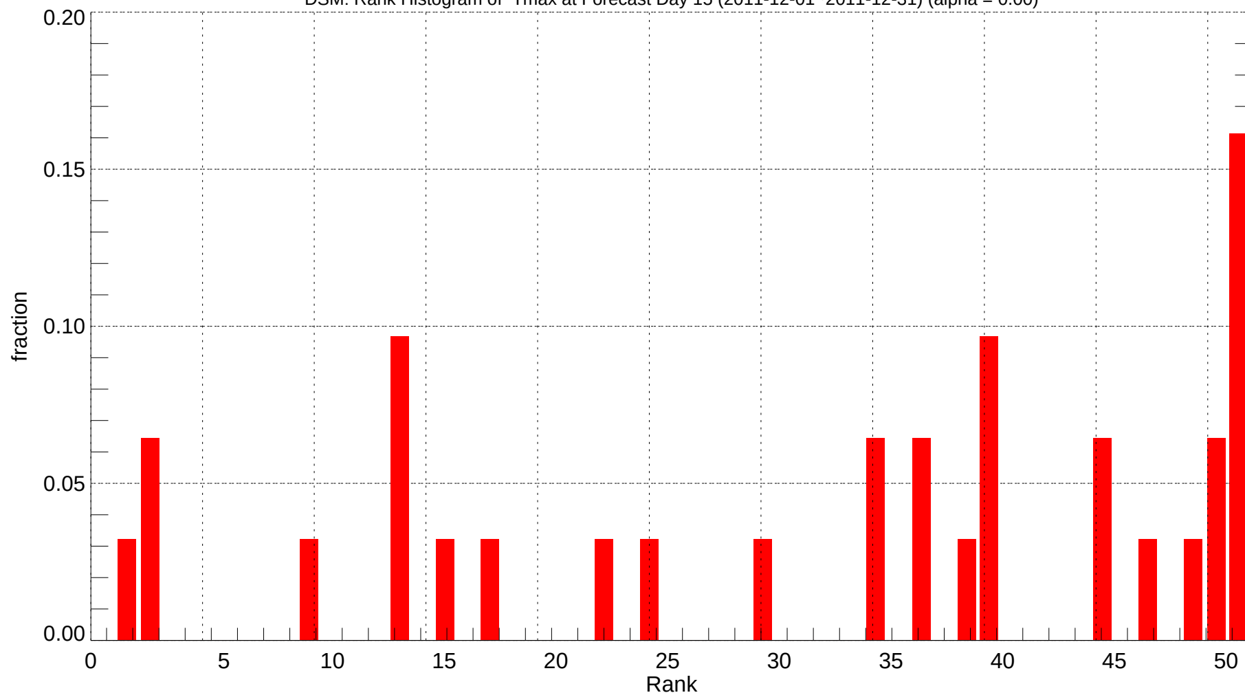
DSM: Rank Histogram of Tmax at Forecast Day 15 (2011-12-01~2011-12-31) (alpha = 0.00)
