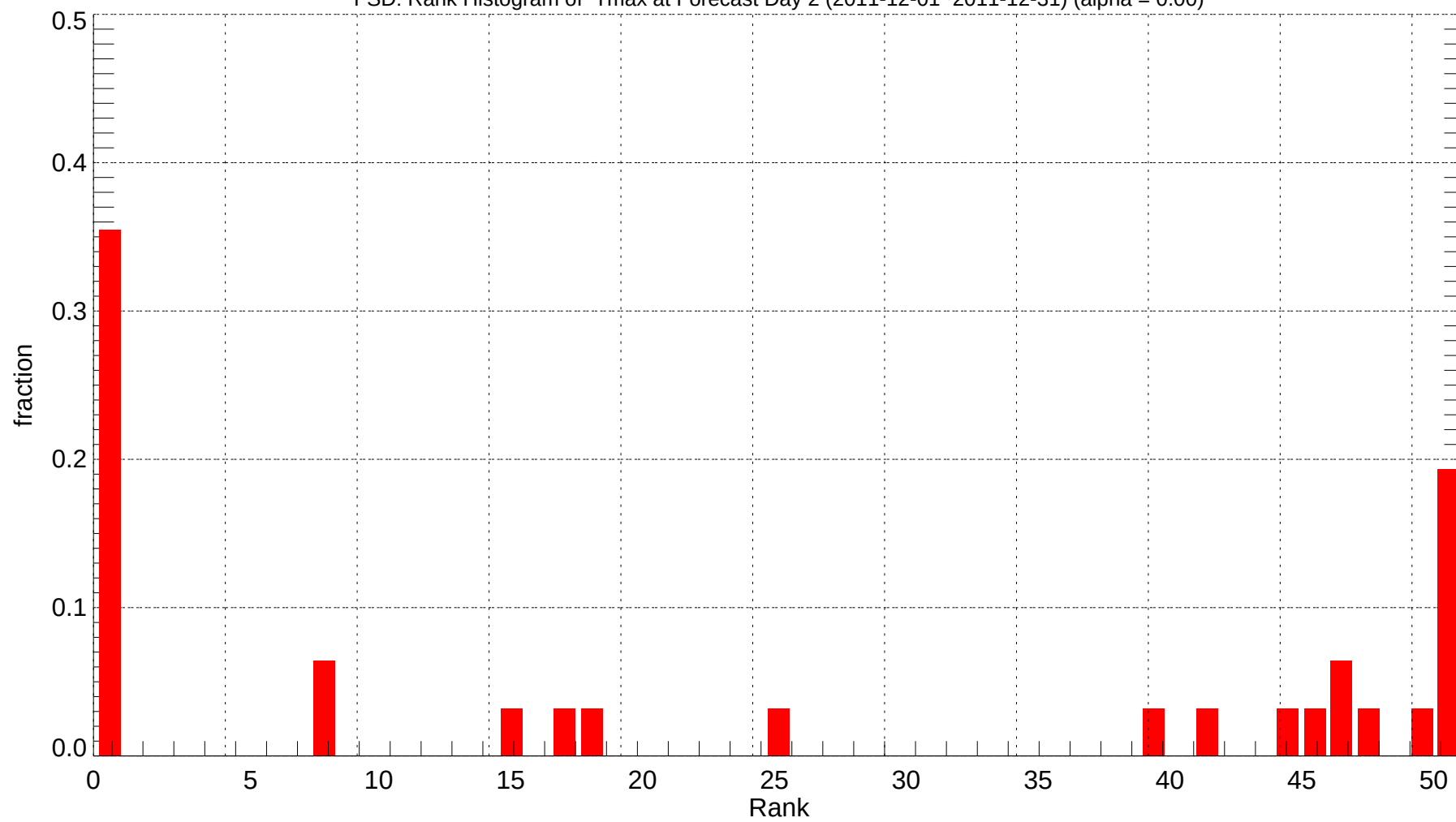
FSD: Rank Histogram of Tmax at Forecast Day 2 (2011-12-01~2011-12-31) (alpha = 0.00)
