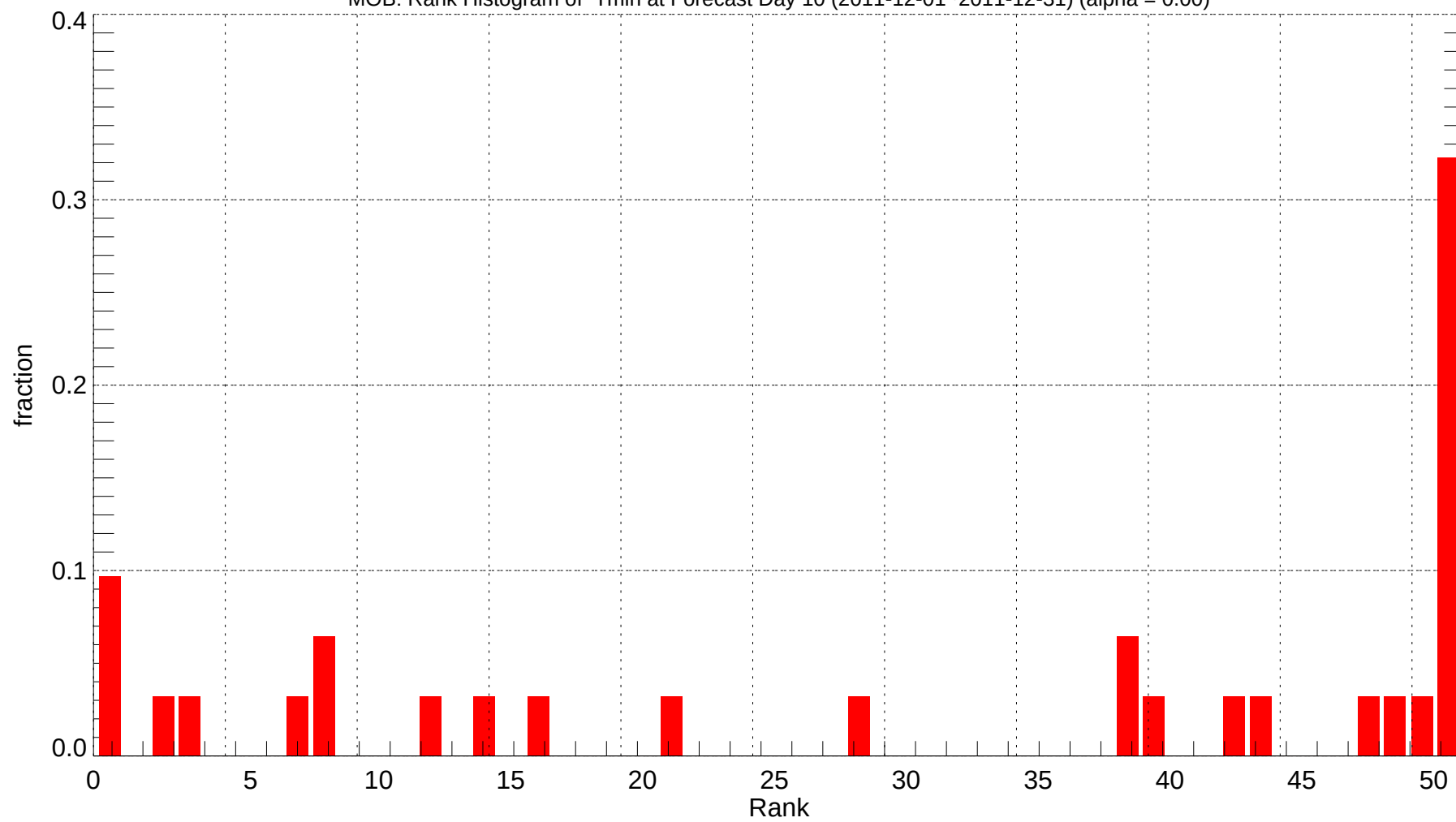
MOB: Rank Histogram of Tmin at Forecast Day 10 (2011-12-01~2011-12-31) (alpha = 0.00)
