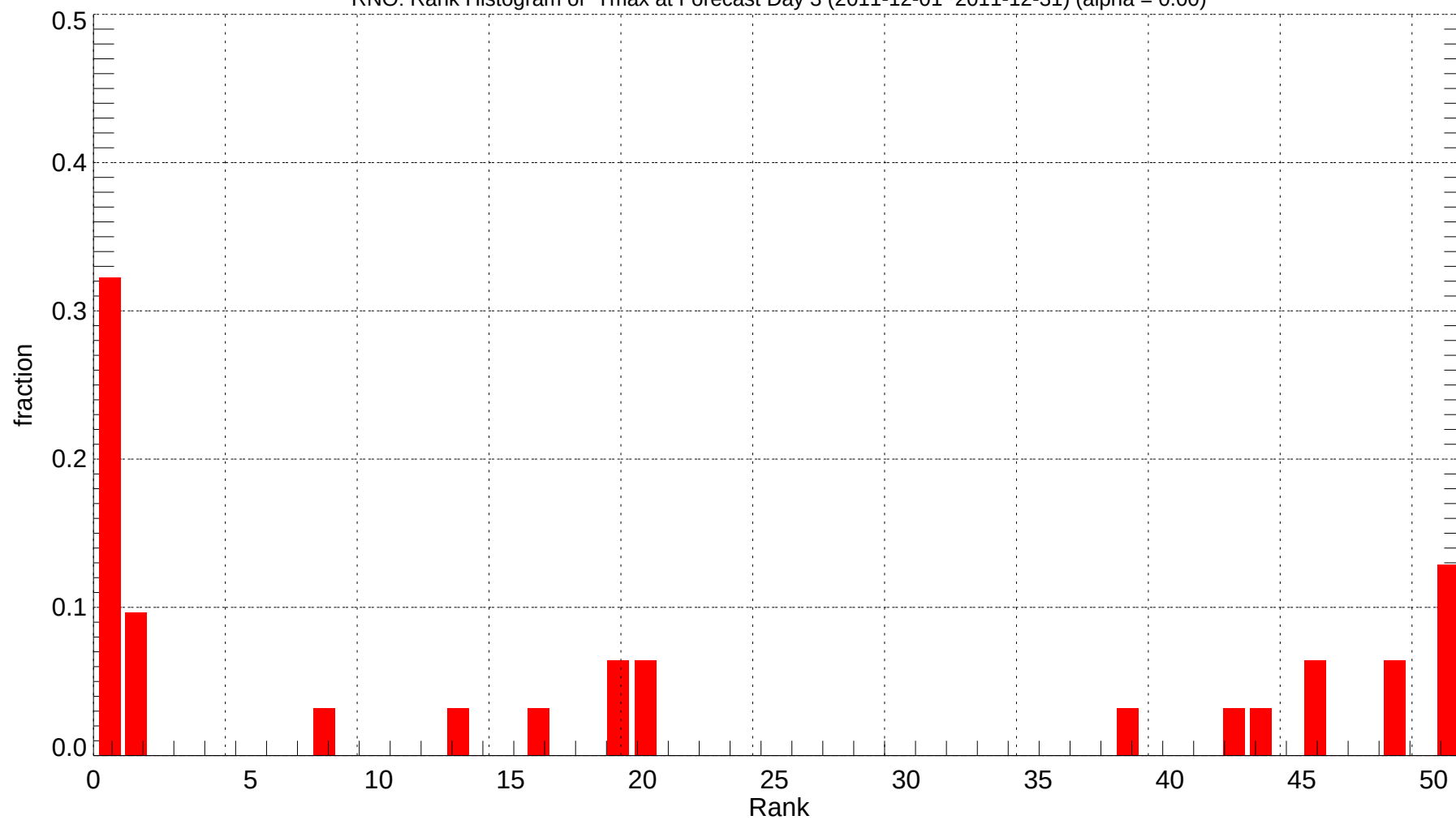
RNO: Rank Histogram of Tmax at Forecast Day 3 (2011-12-01~2011-12-31) (alpha = 0.00)
