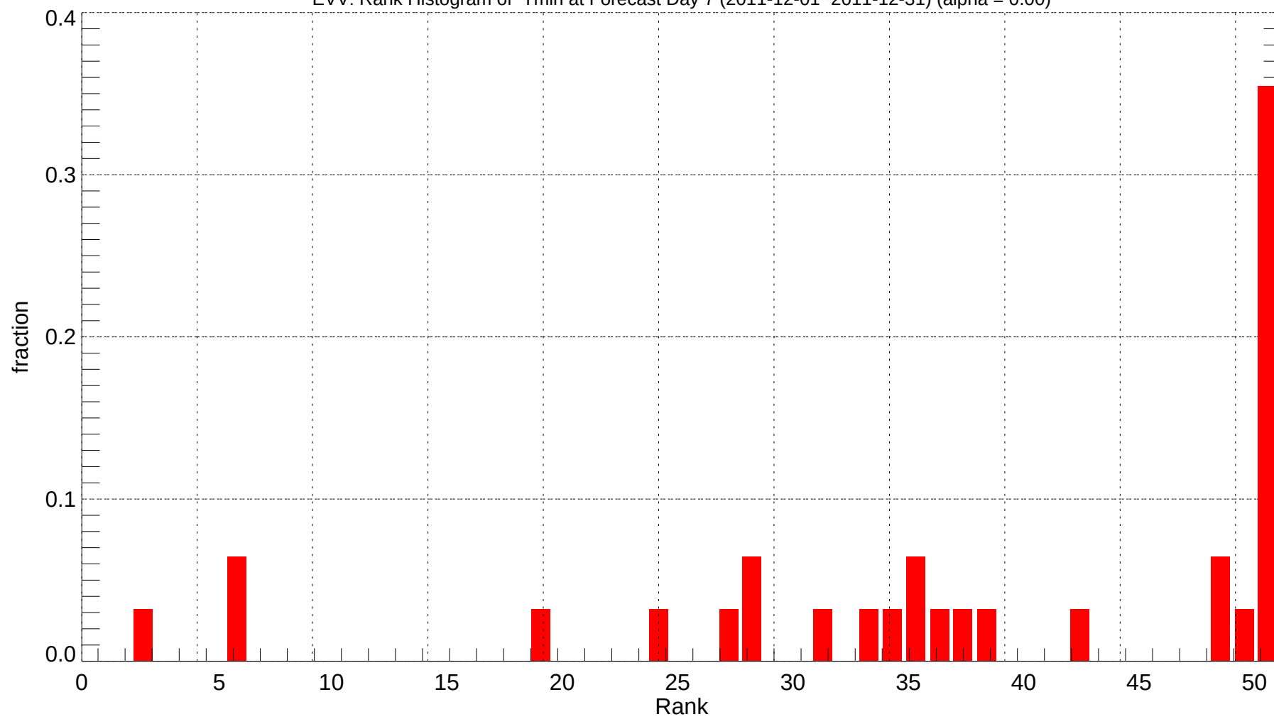
EVV: Rank Histogram of Tmin at Forecast Day 7 (2011-12-01~2011-12-31) (alpha = 0.00)
