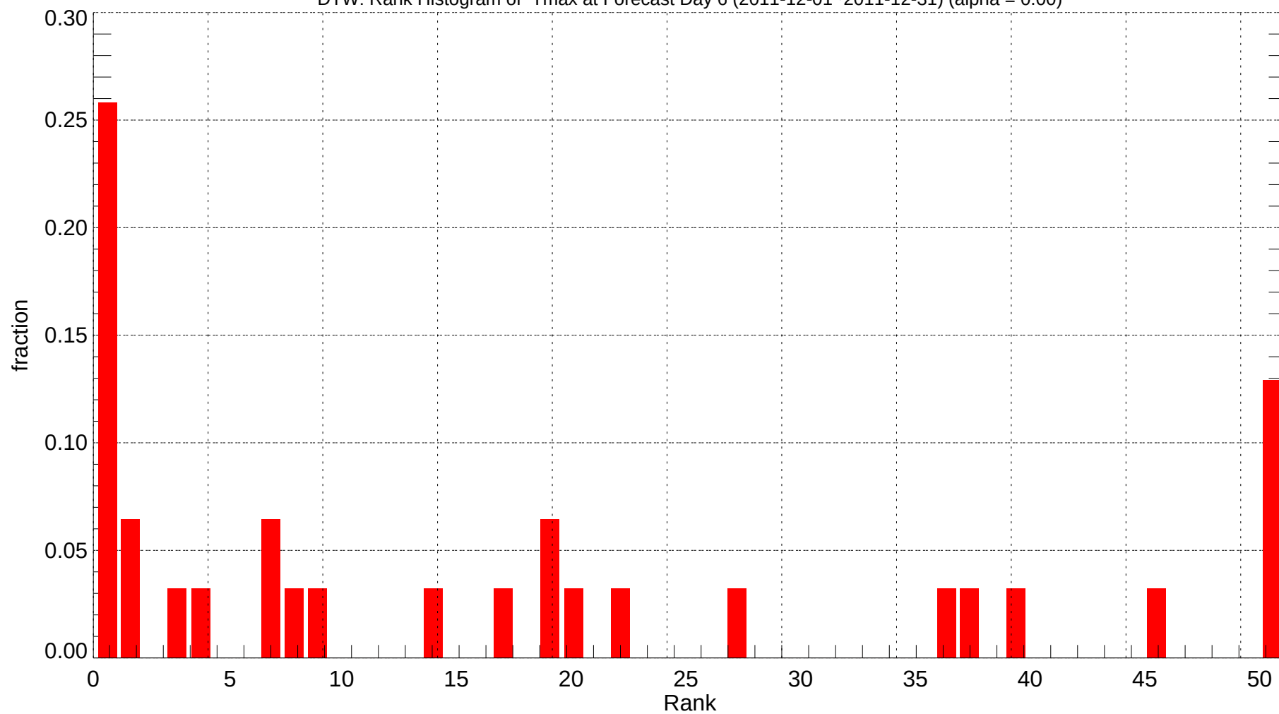
DTW: Rank Histogram of Tmax at Forecast Day 6 (2011-12-01~2011-12-31) (alpha = 0.00)
