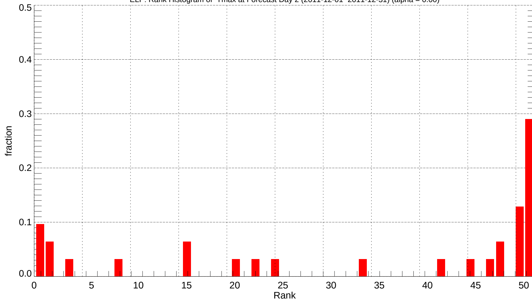
ELP: Rank Histogram of Tmax at Forecast Day 2 (2011-12-01~2011-12-31) (alpha = 0.00)
