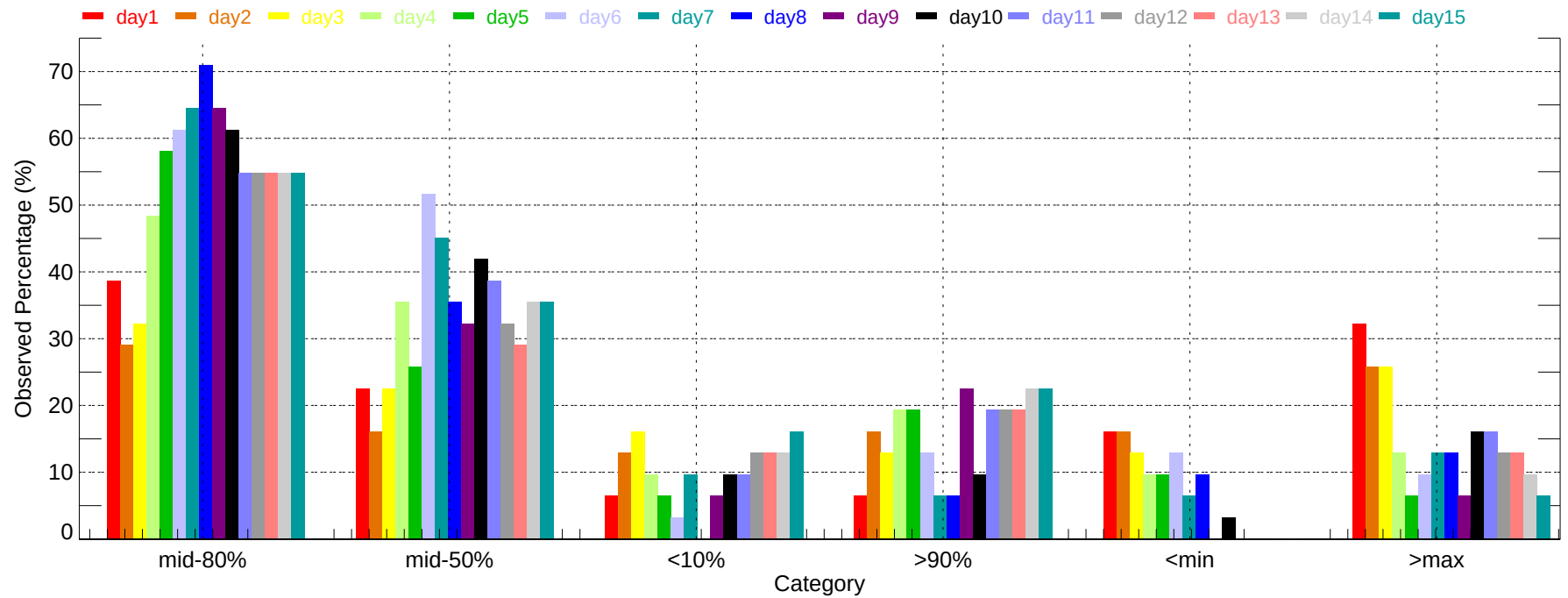
Observed Percentage of Ensembles - SAT: Max Temperature (2011-12-01~2011-12-31)
