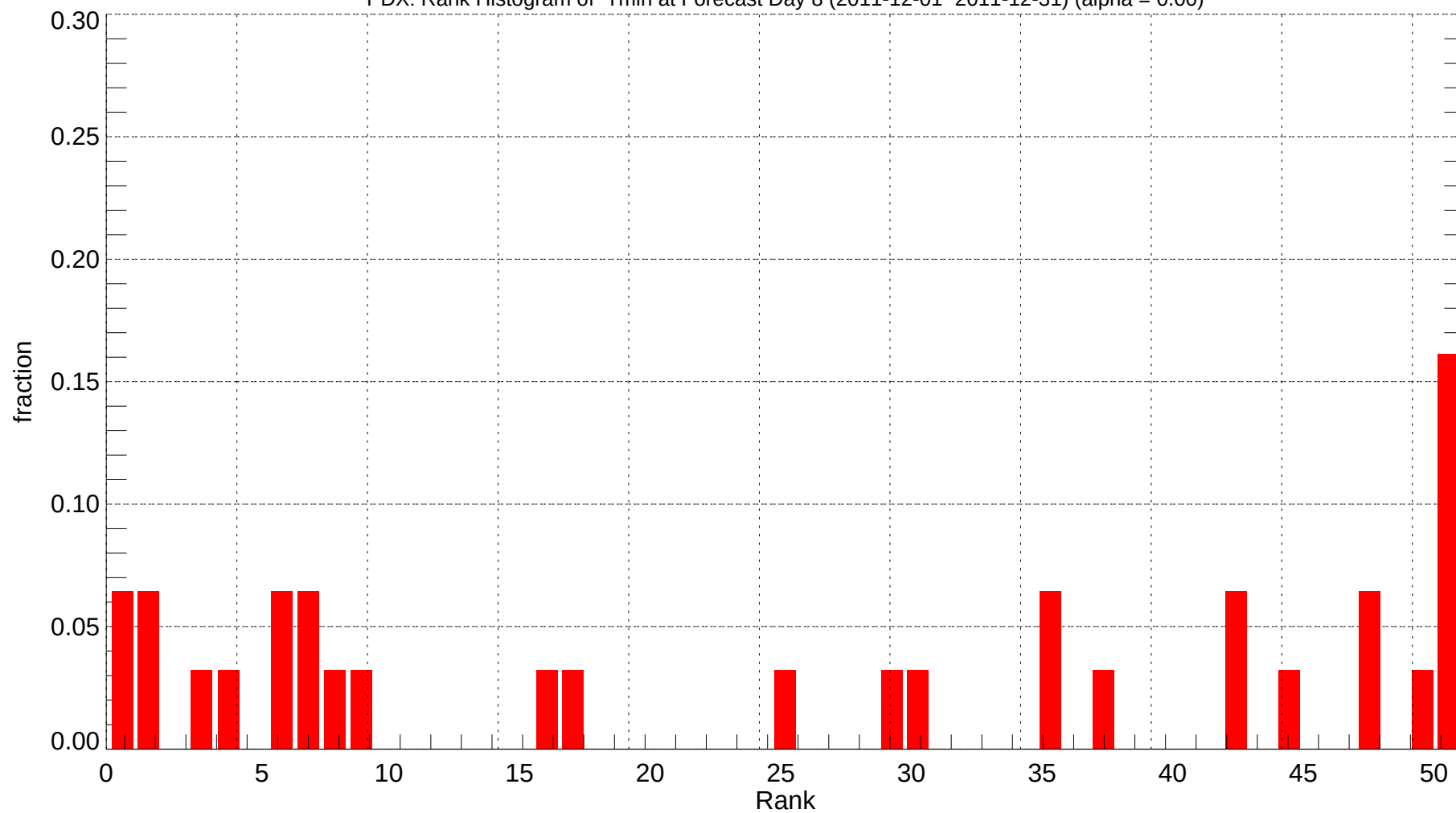
PDX: Rank Histogram of Tmin at Forecast Day 8 (2011-12-01~2011-12-31) (alpha = 0.00)
