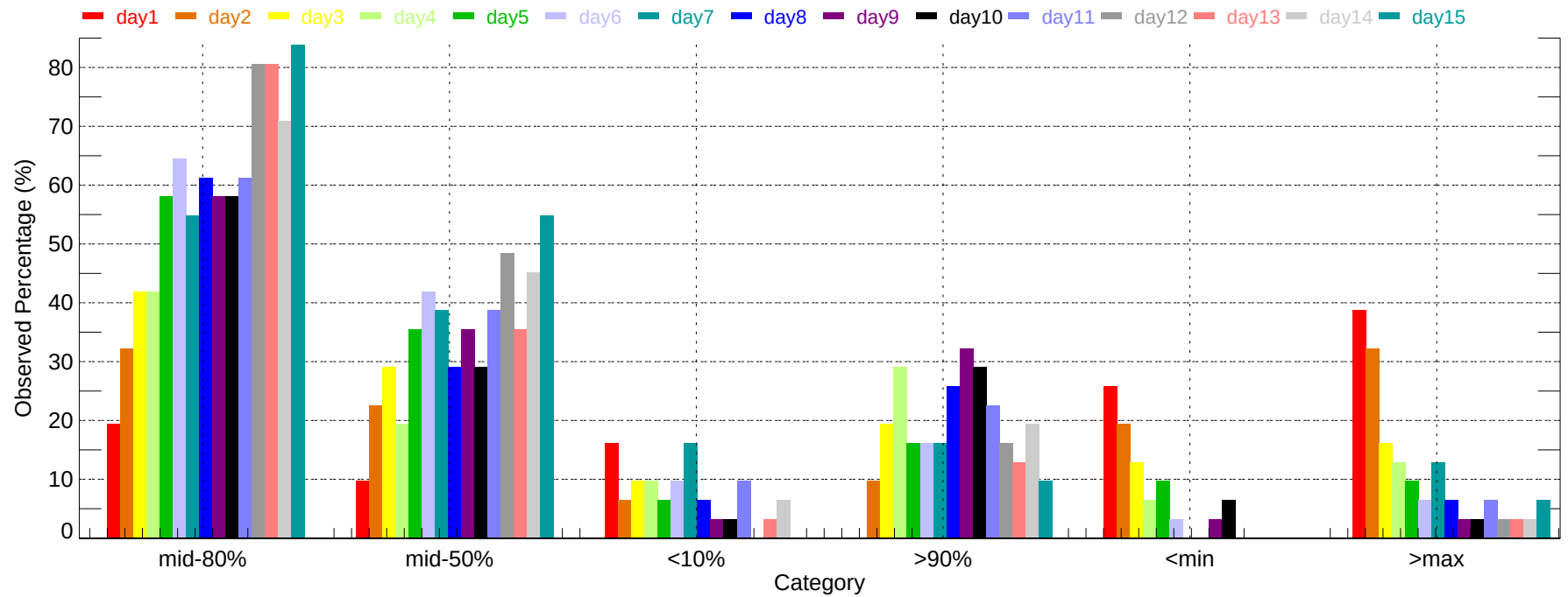
Observed Percentage of Ensembles - MSY: Min Temperature (2011-12-01~2011-12-31)
