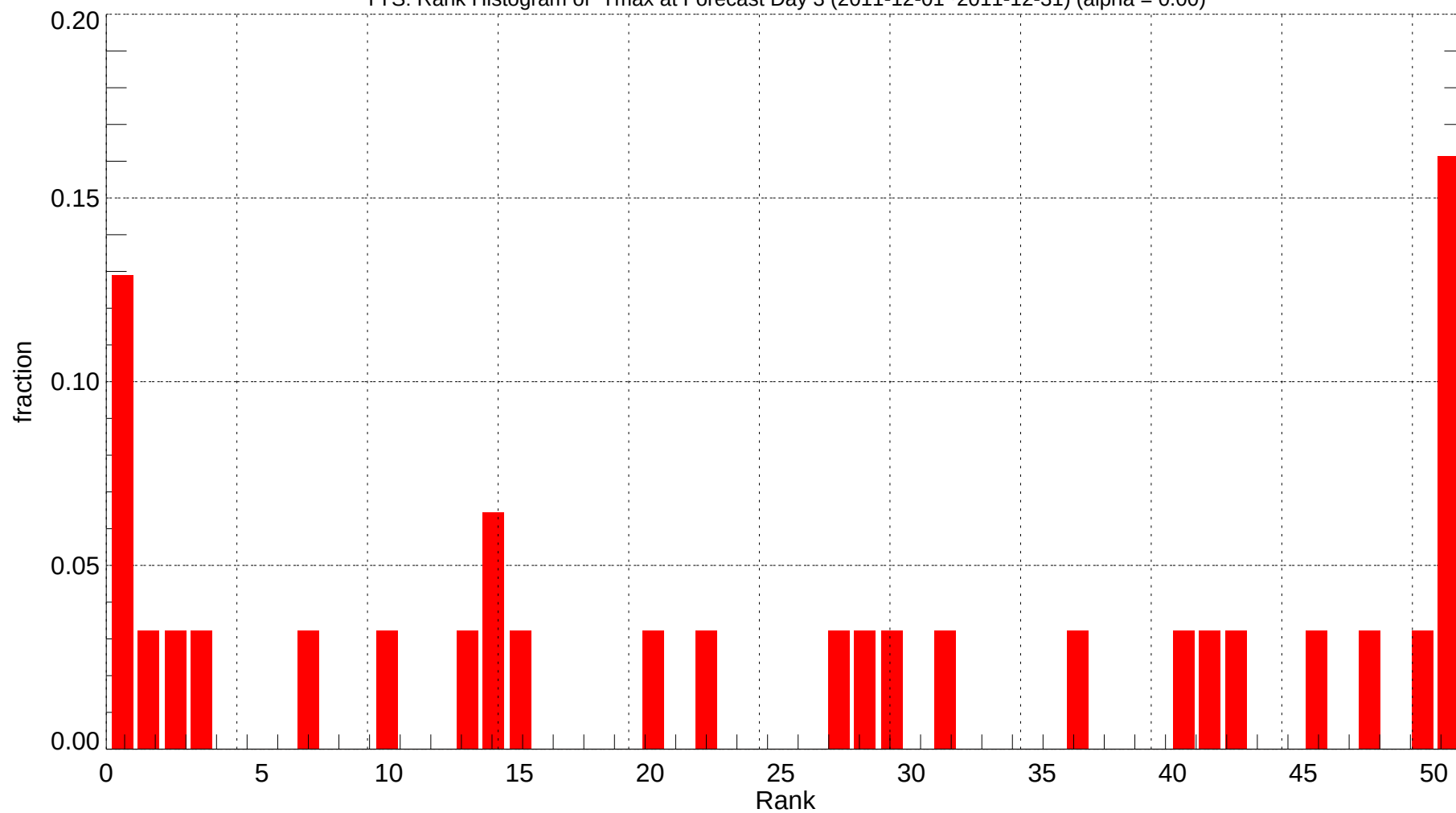
TYS: Rank Histogram of Tmax at Forecast Day 3 (2011-12-01~2011-12-31) (alpha = 0.00)
