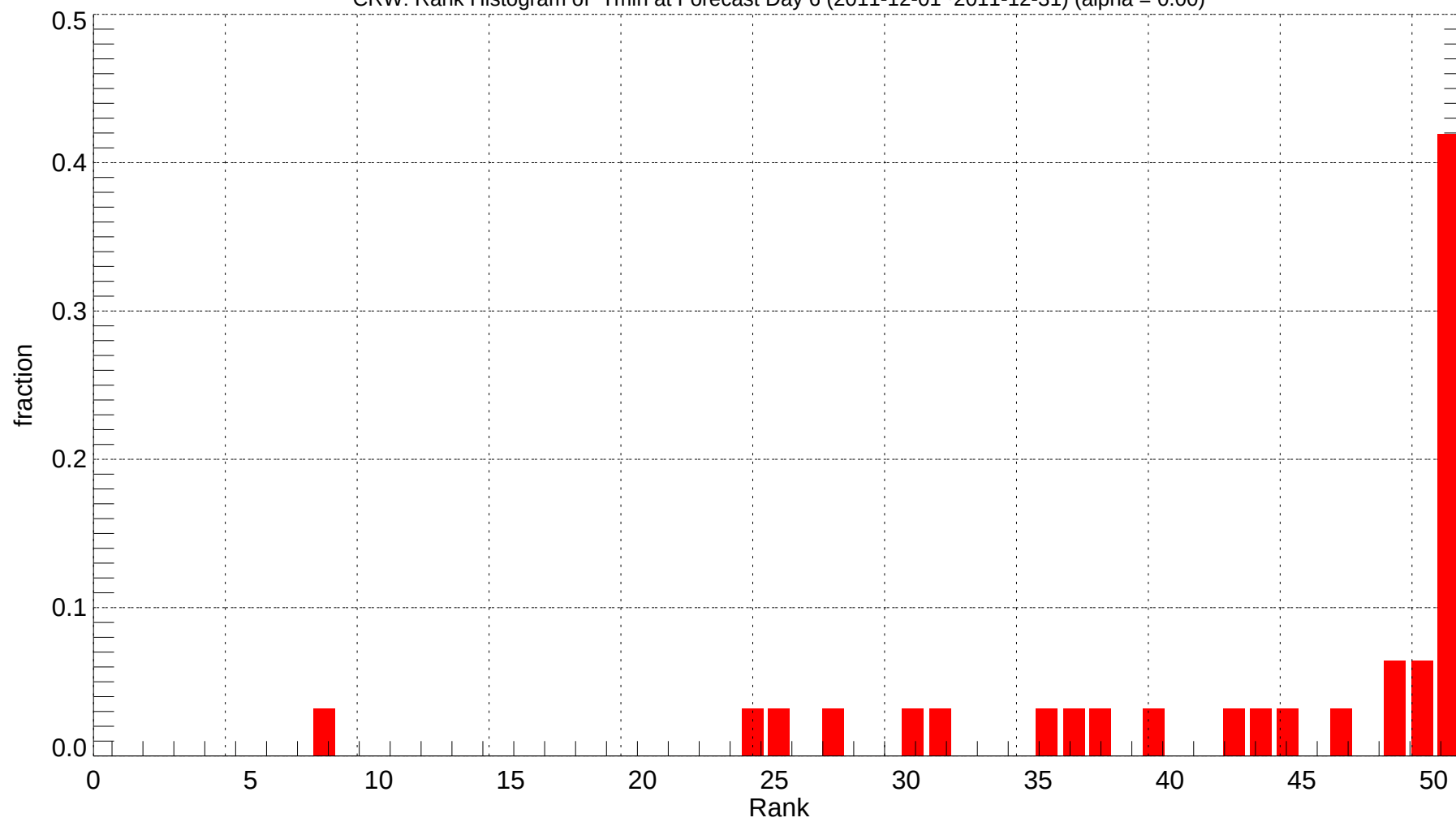
CRW: Rank Histogram of Tmin at Forecast Day 6 (2011-12-01~2011-12-31) (alpha = 0.00)
