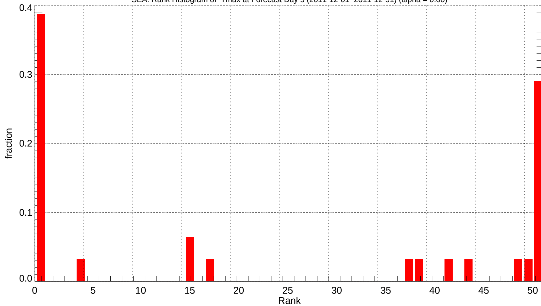
SEA: Rank Histogram of Tmax at Forecast Day 5 (2011-12-01~2011-12-31) (alpha = 0.00)
