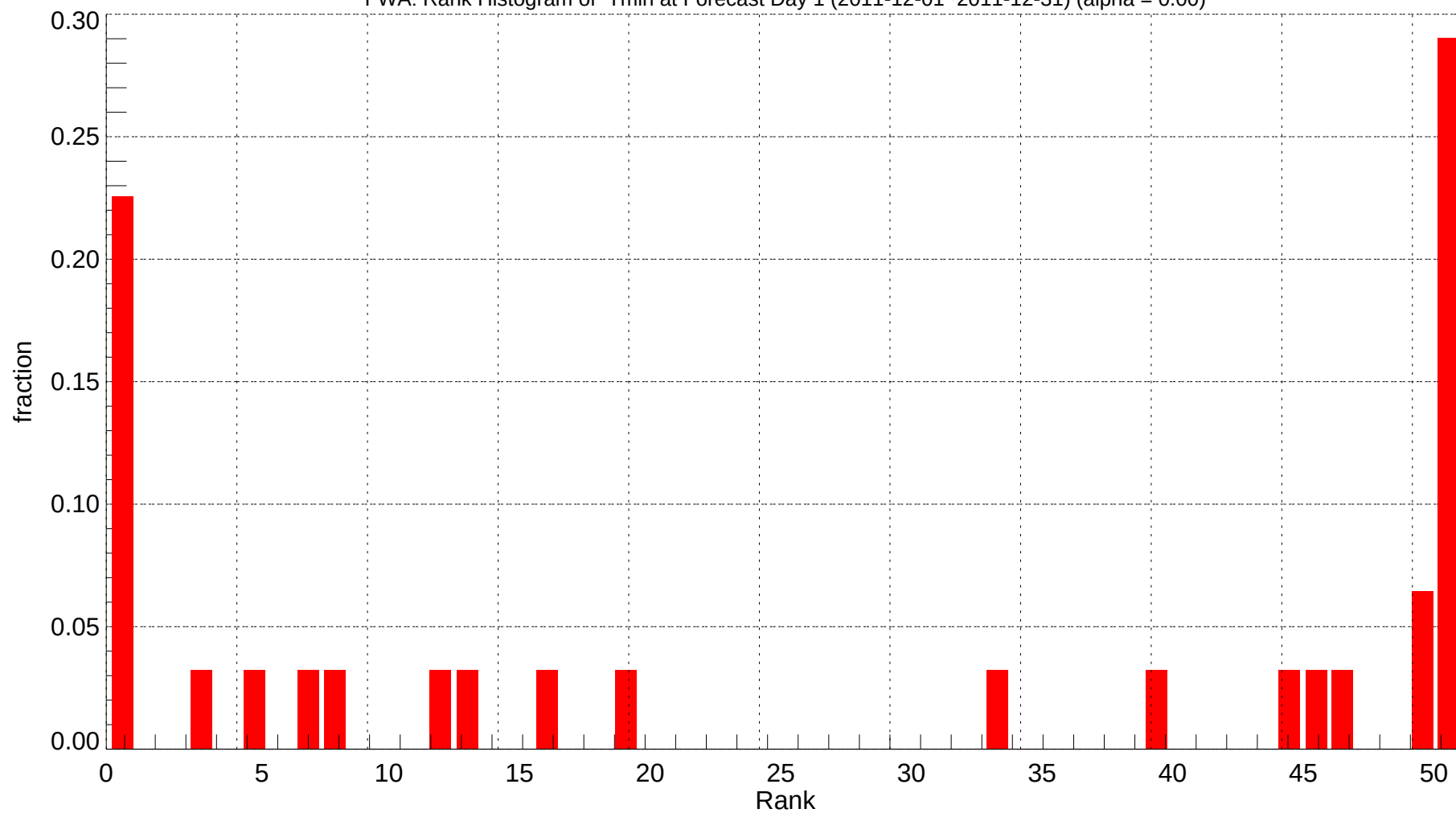
FWA: Rank Histogram of Tmin at Forecast Day 1 (2011-12-01~2011-12-31) (alpha = 0.00)
