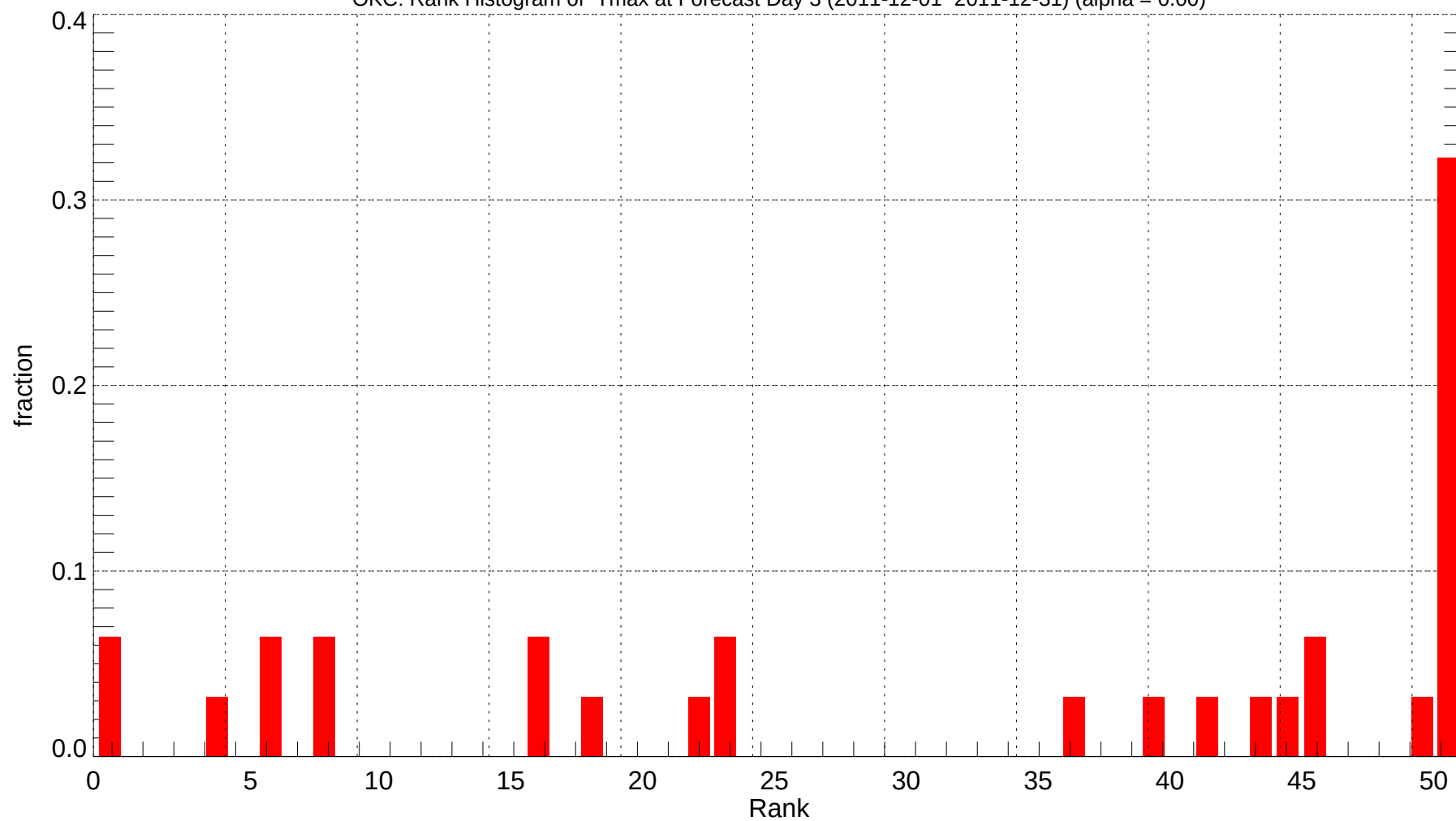
OKC: Rank Histogram of Tmax at Forecast Day 3 (2011-12-01~2011-12-31) (alpha = 0.00)
