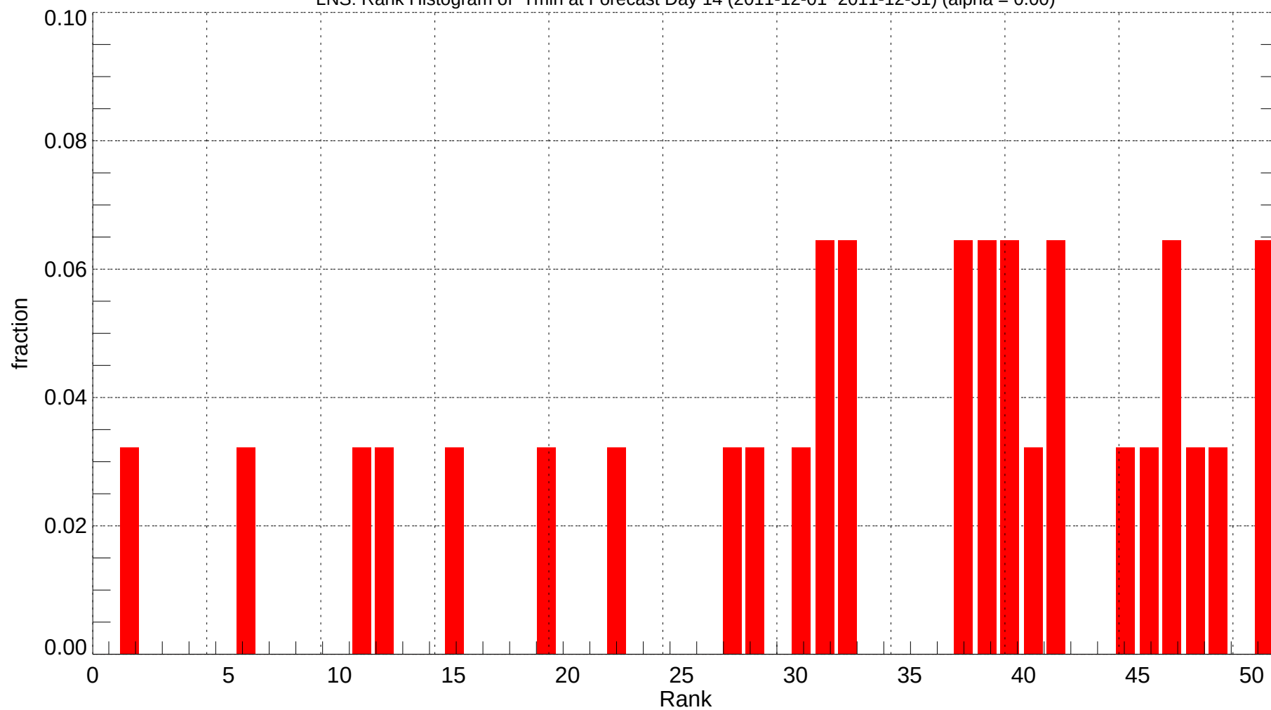
LNS: Rank Histogram of Tmin at Forecast Day 14 (2011-12-01~2011-12-31) (alpha = 0.00)
