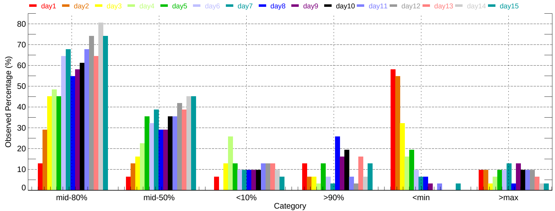
Observed Percentage of Ensembles - SYR: Min Temperature (2011-12-01~2011-12-31)
