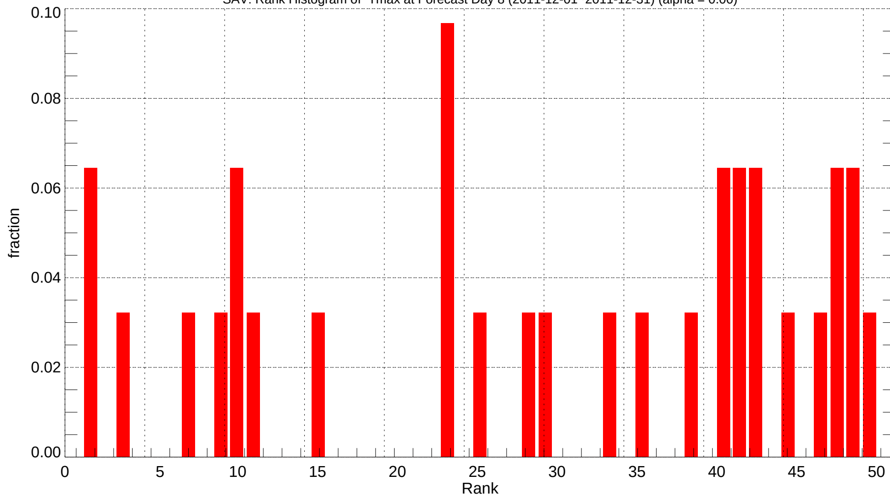
SAV: Rank Histogram of Tmax at Forecast Day 8 (2011-12-01~2011-12-31) (alpha = 0.00)
