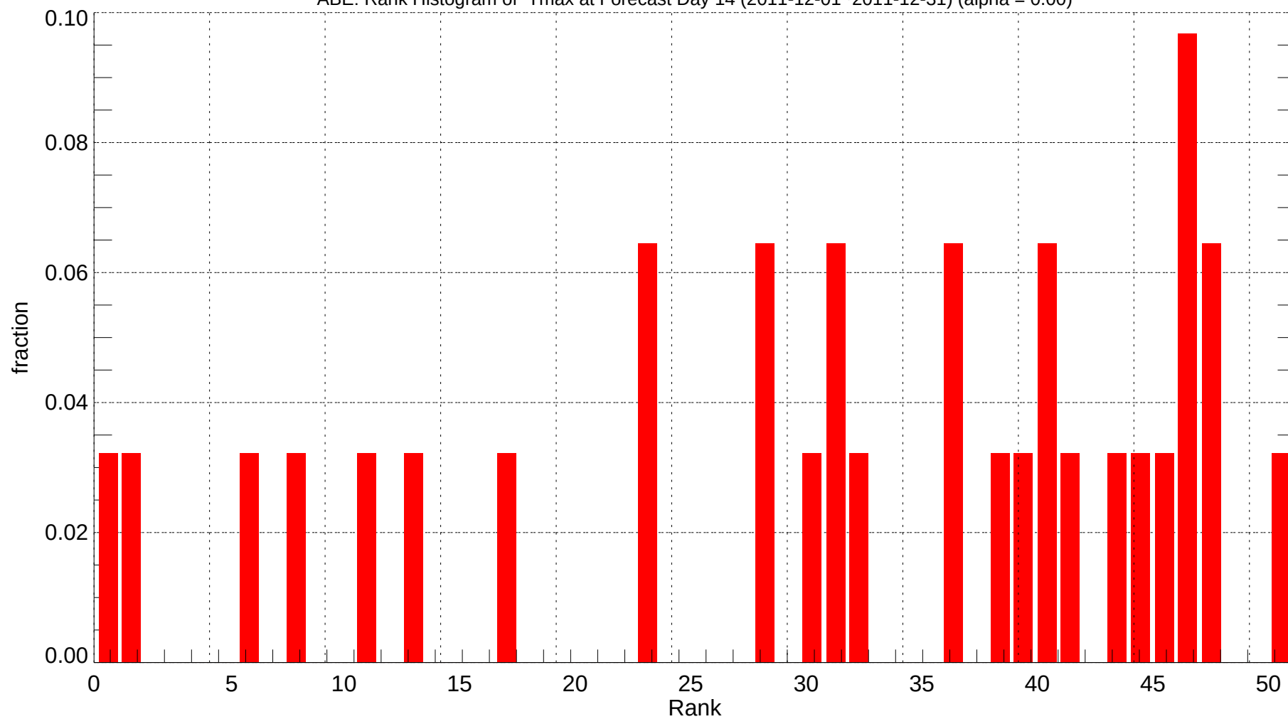
ABE: Rank Histogram of Tmax at Forecast Day 14 (2011-12-01~2011-12-31) (alpha = 0.00)
