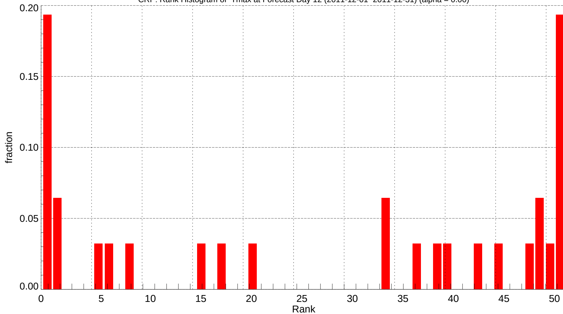
CRP: Rank Histogram of Tmax at Forecast Day 12 (2011-12-01~2011-12-31) (alpha = 0.00)
