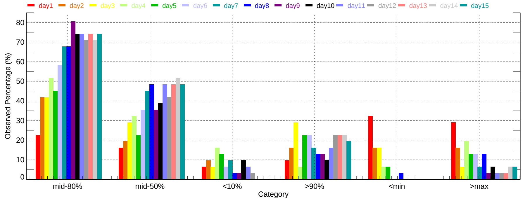
Observed Percentage of Ensembles - YXD: Min Temperature (2011-12-01~2011-12-31)
