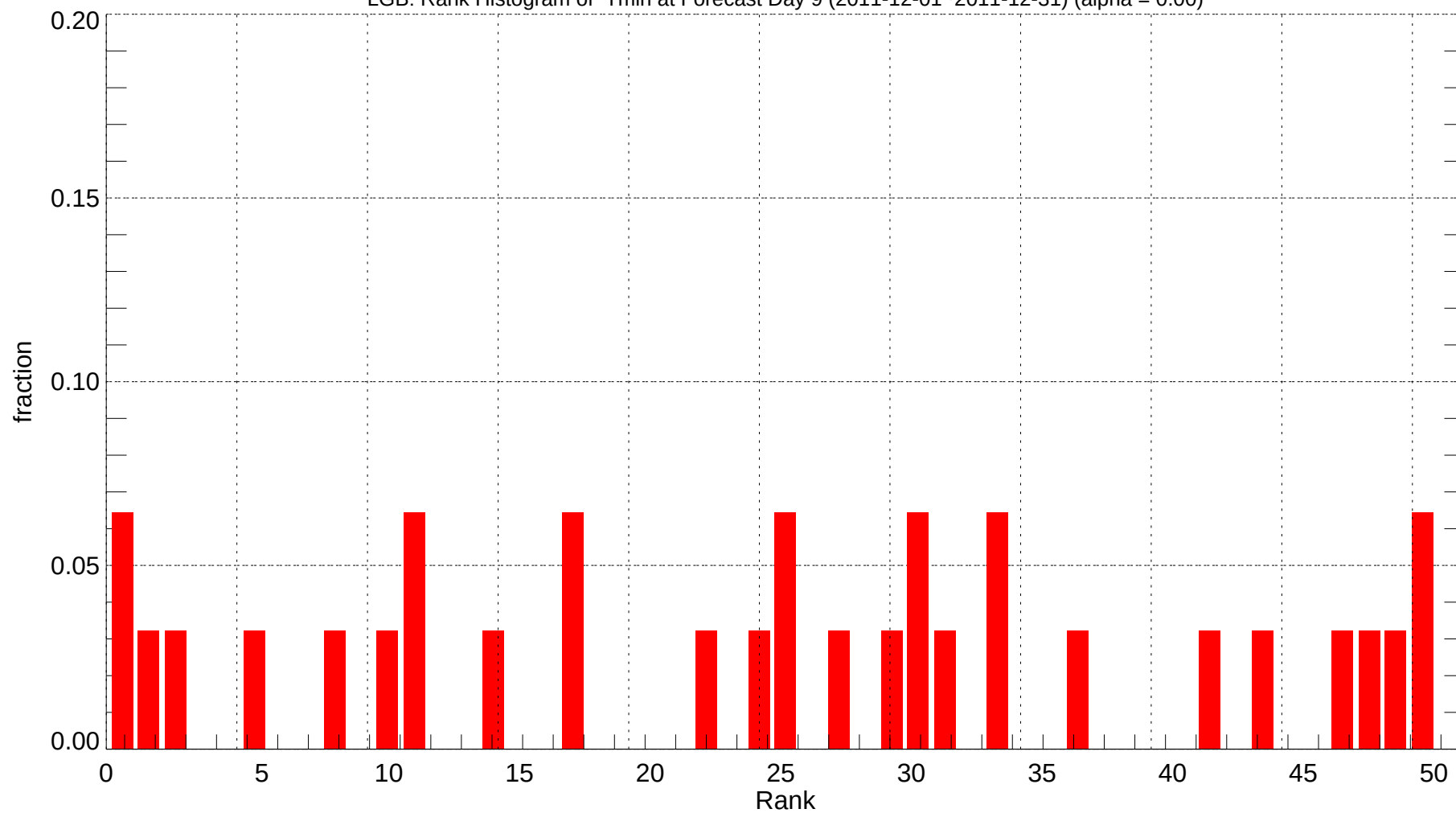
LGB: Rank Histogram of Tmin at Forecast Day 9 (2011-12-01~2011-12-31) (alpha = 0.00)
