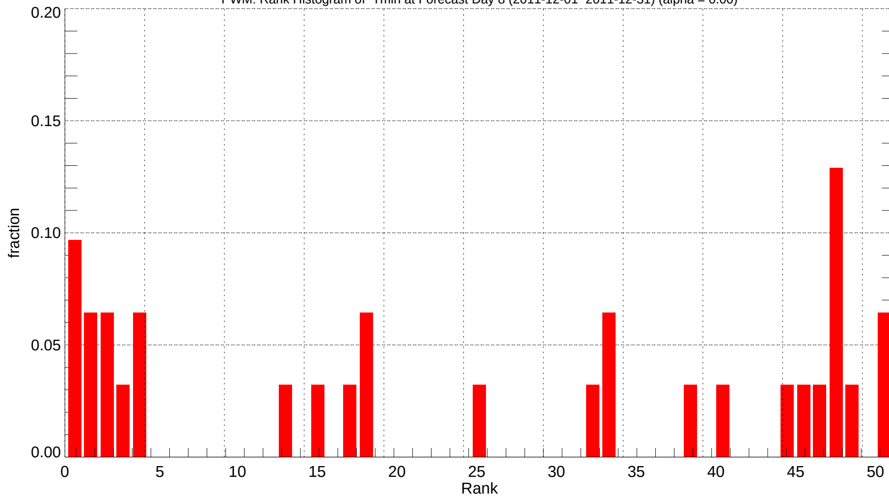
PWM: Rank Histogram of Tmin at Forecast Day 8 (2011-12-01~2011-12-31) (alpha = 0.00)
