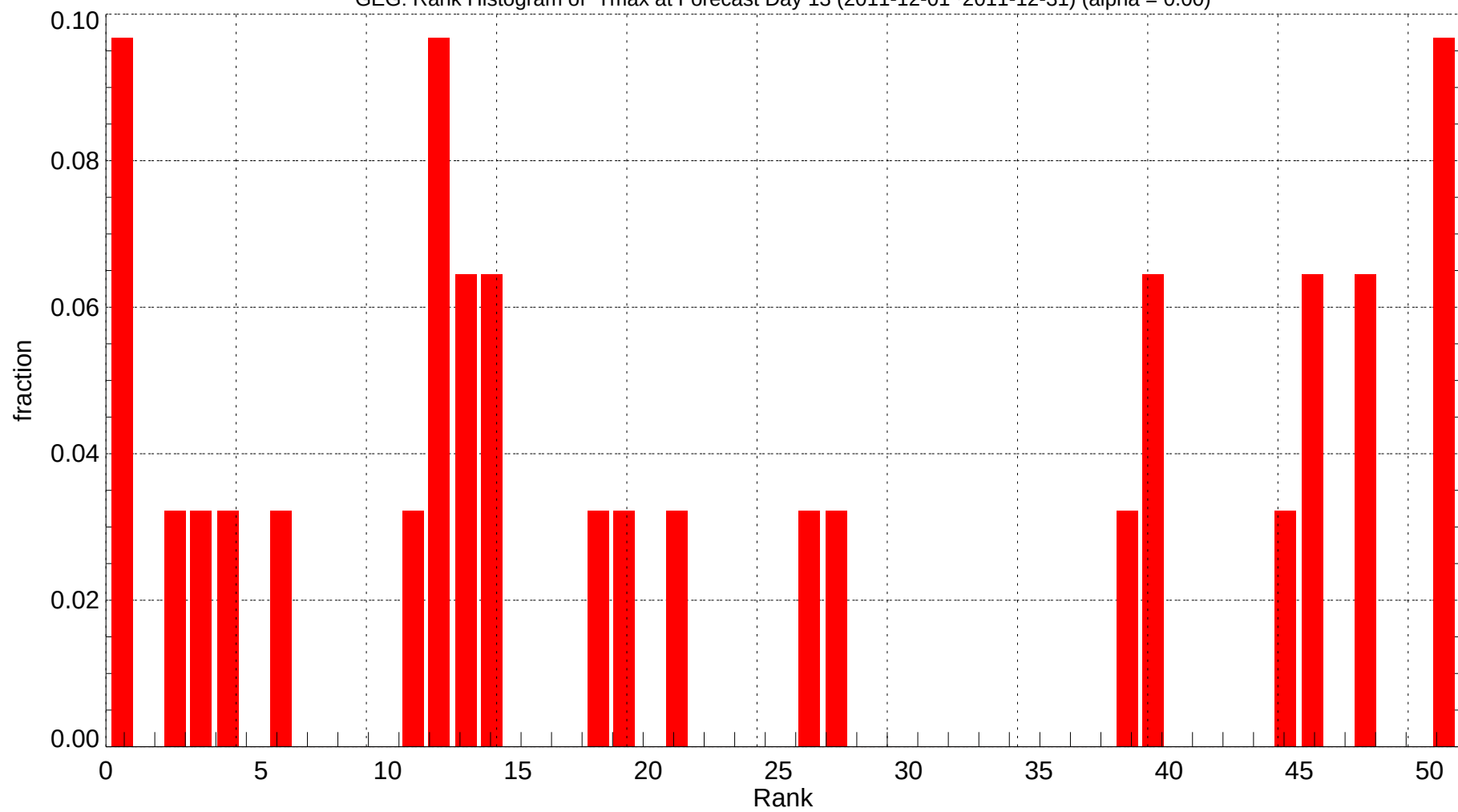
GEG: Rank Histogram of Tmax at Forecast Day 13 (2011-12-01~2011-12-31) (alpha = 0.00)
