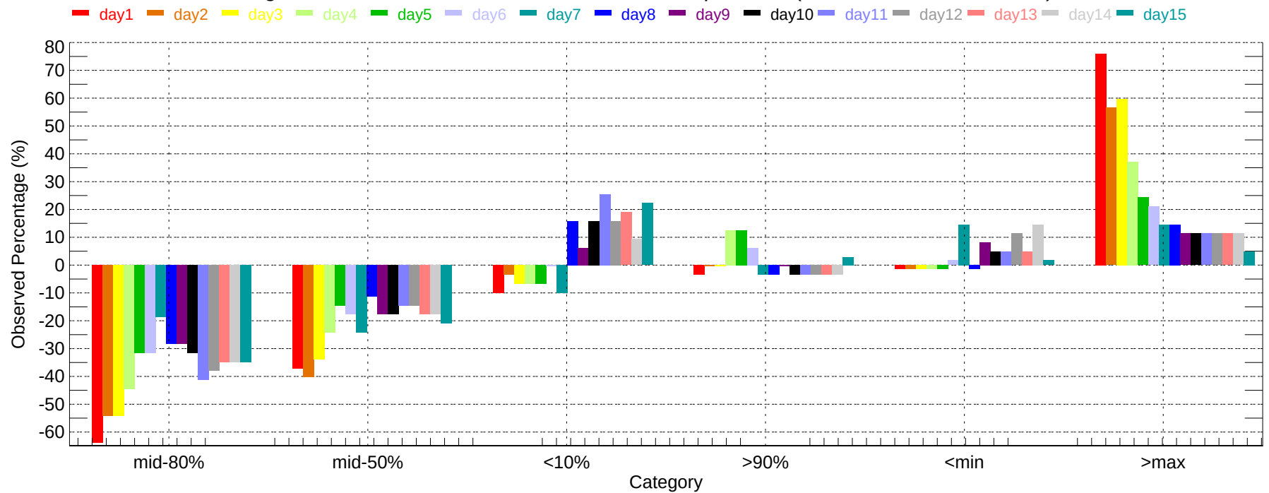
Observed Percentage Deviation of Ensembles - FLG: Max Temperature (2011-12-01~2011-12-31)
