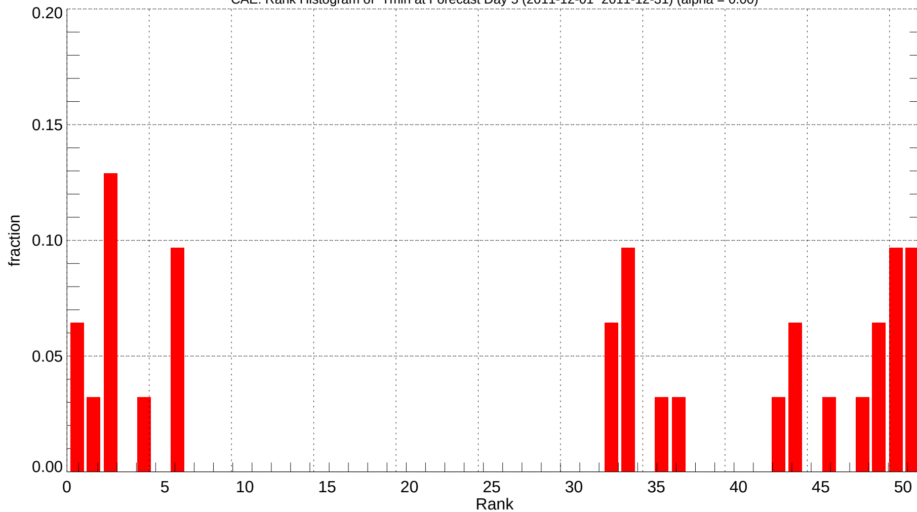
CAE: Rank Histogram of Tmin at Forecast Day 5 (2011-12-01~2011-12-31) (alpha = 0.00)
