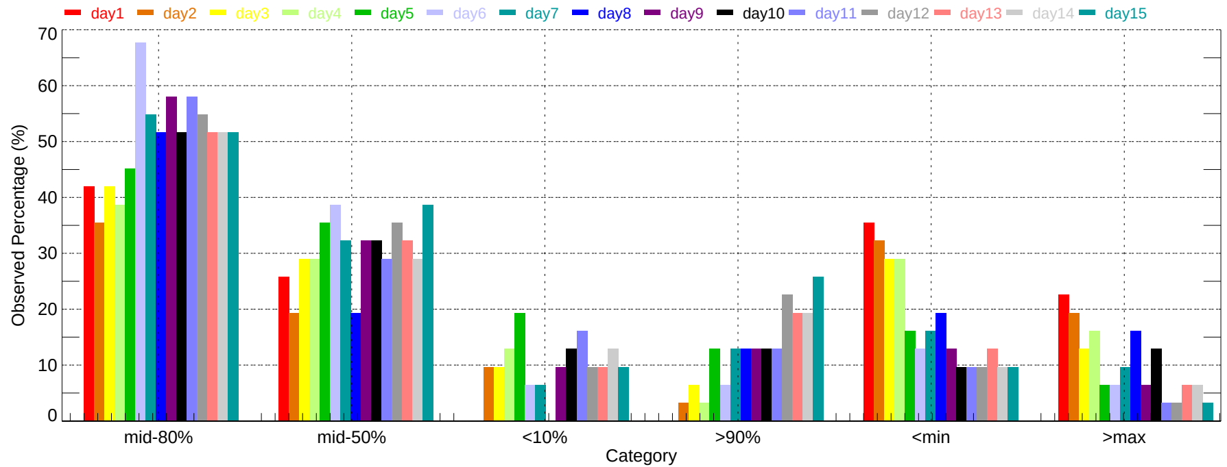
Observed Percentage of Ensembles - BIS: Max Temperature (2011-12-01~2011-12-31)
