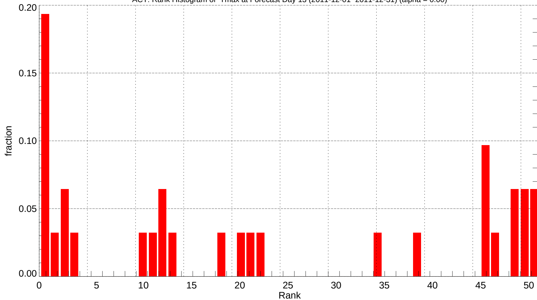
ACT: Rank Histogram of Tmax at Forecast Day 13 (2011-12-01~2011-12-31) (alpha = 0.00)
