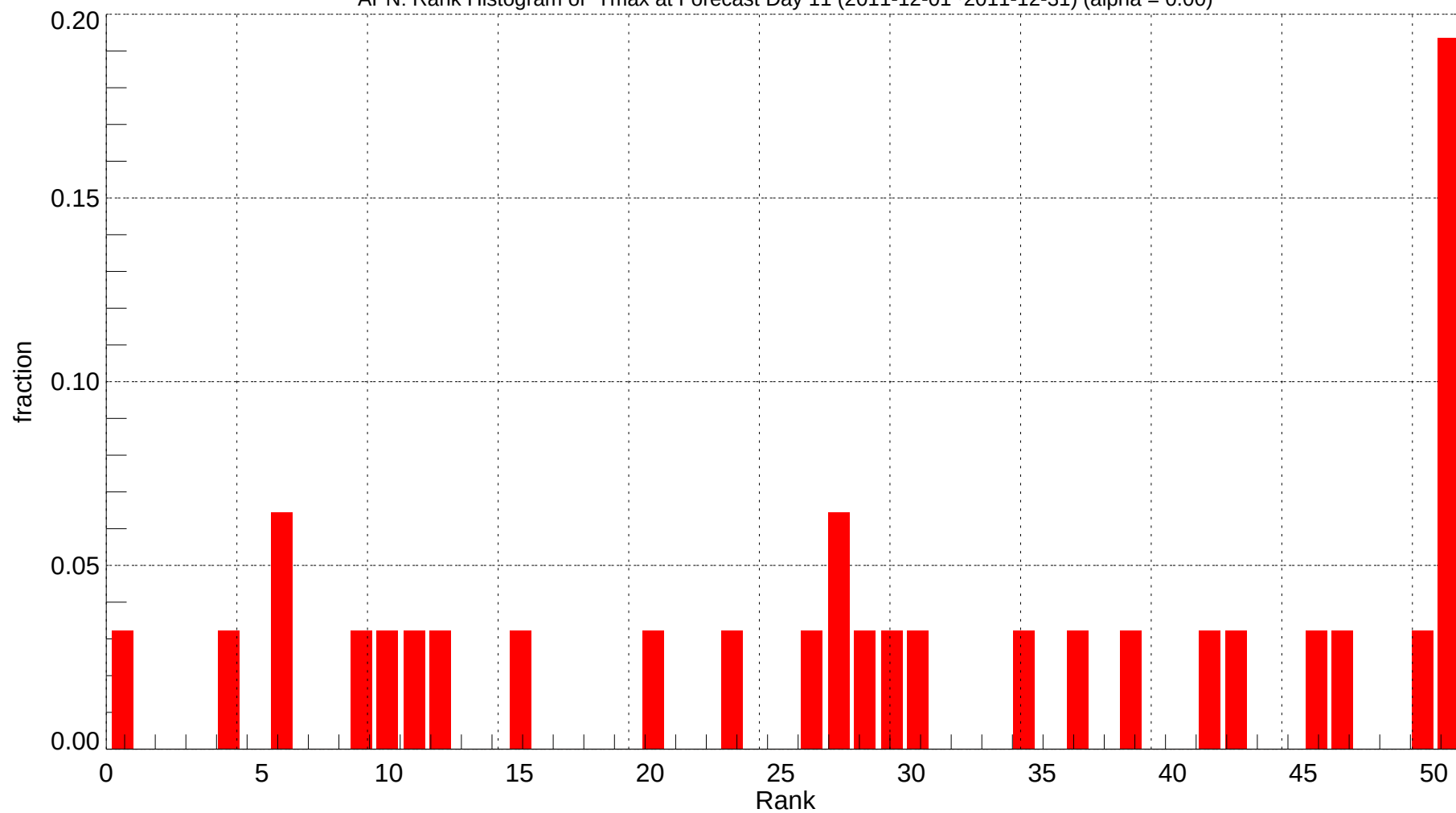
APN: Rank Histogram of Tmax at Forecast Day 11 (2011-12-01~2011-12-31) (alpha = 0.00)
