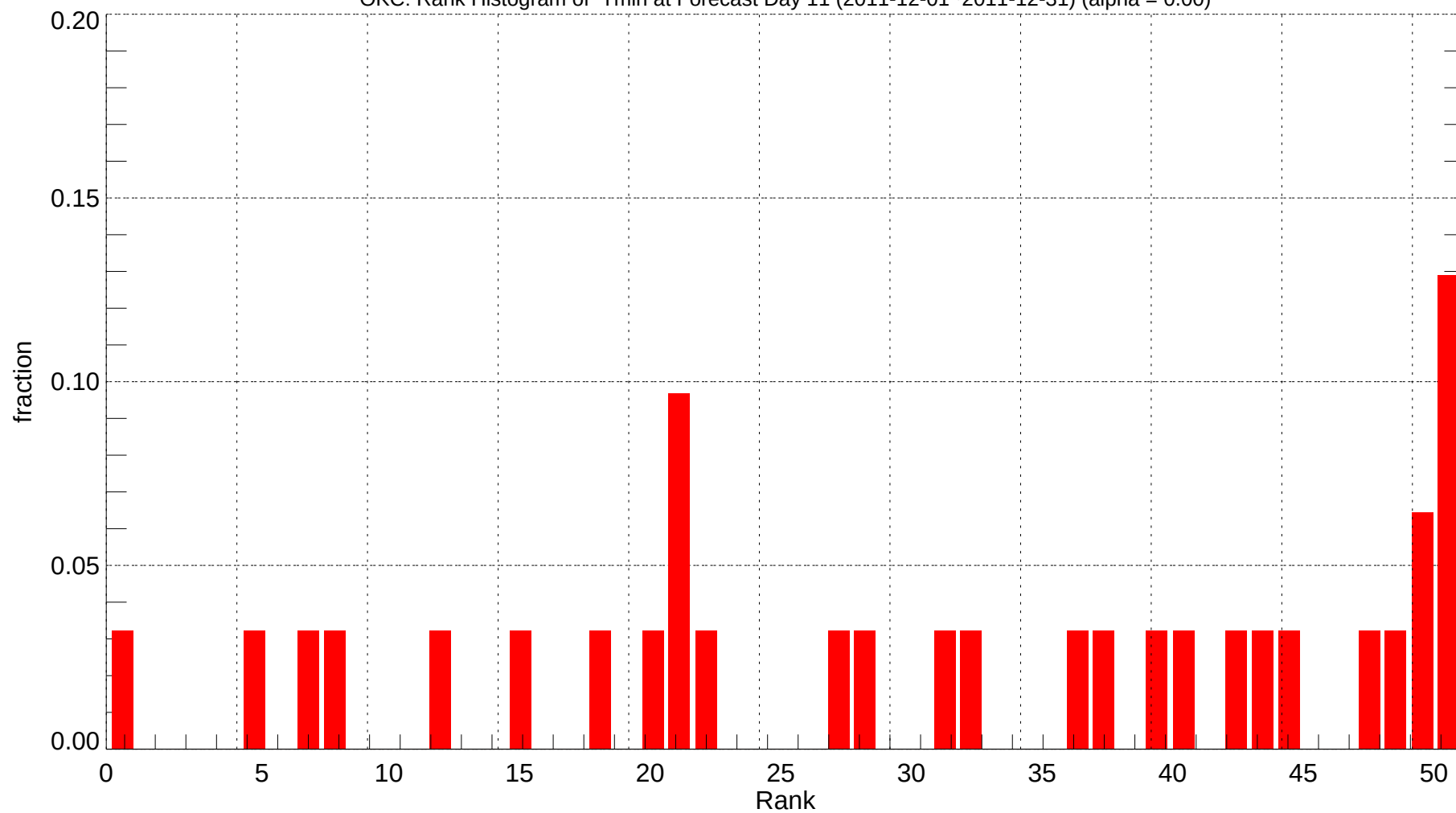
OKC: Rank Histogram of Tmin at Forecast Day 11 (2011-12-01~2011-12-31) (alpha = 0.00)
