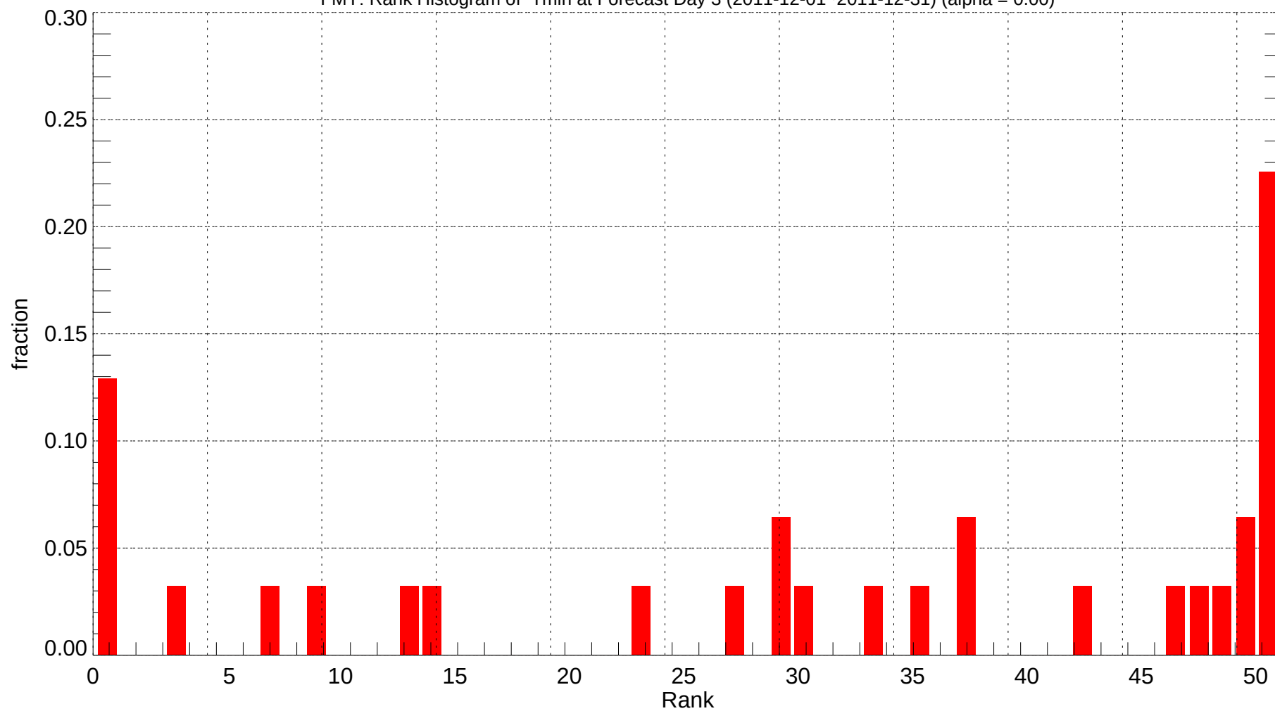
FMY: Rank Histogram of Tmin at Forecast Day 3 (2011-12-01~2011-12-31) (alpha = 0.00)
