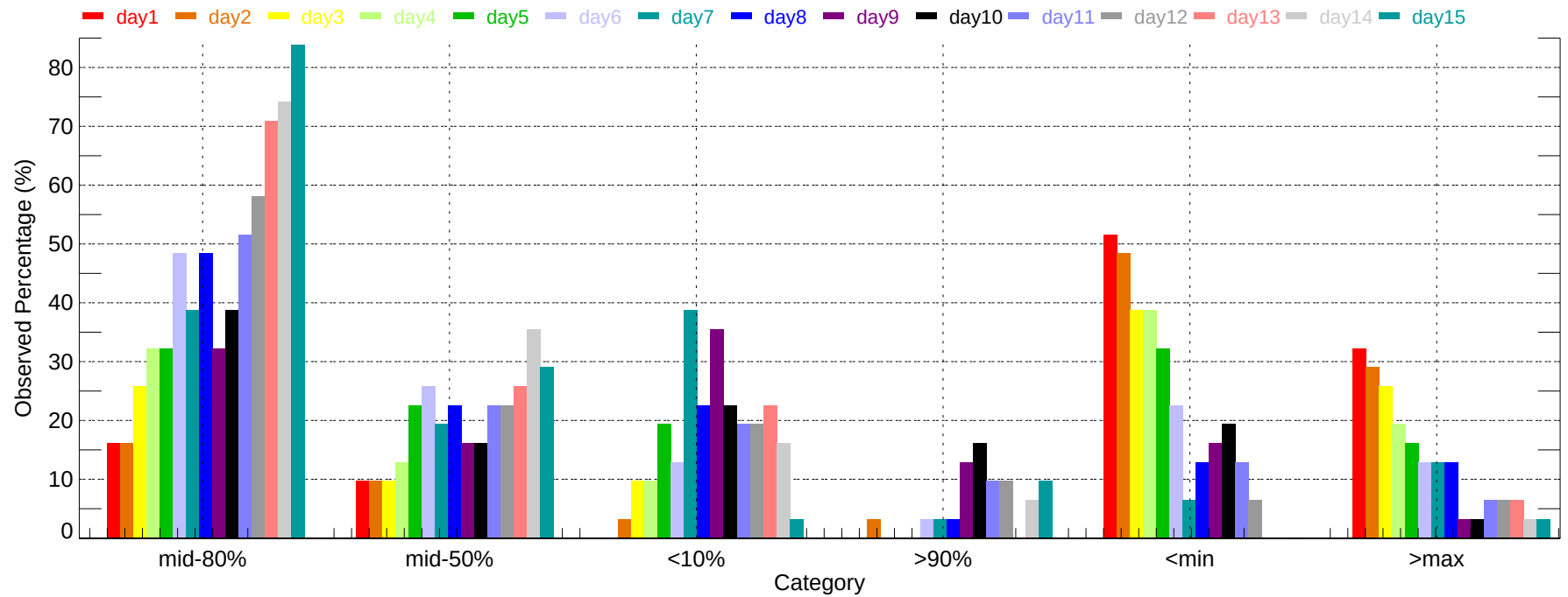
Observed Percentage of Ensembles - RNO: Min Temperature (2011-12-01~2011-12-31)
