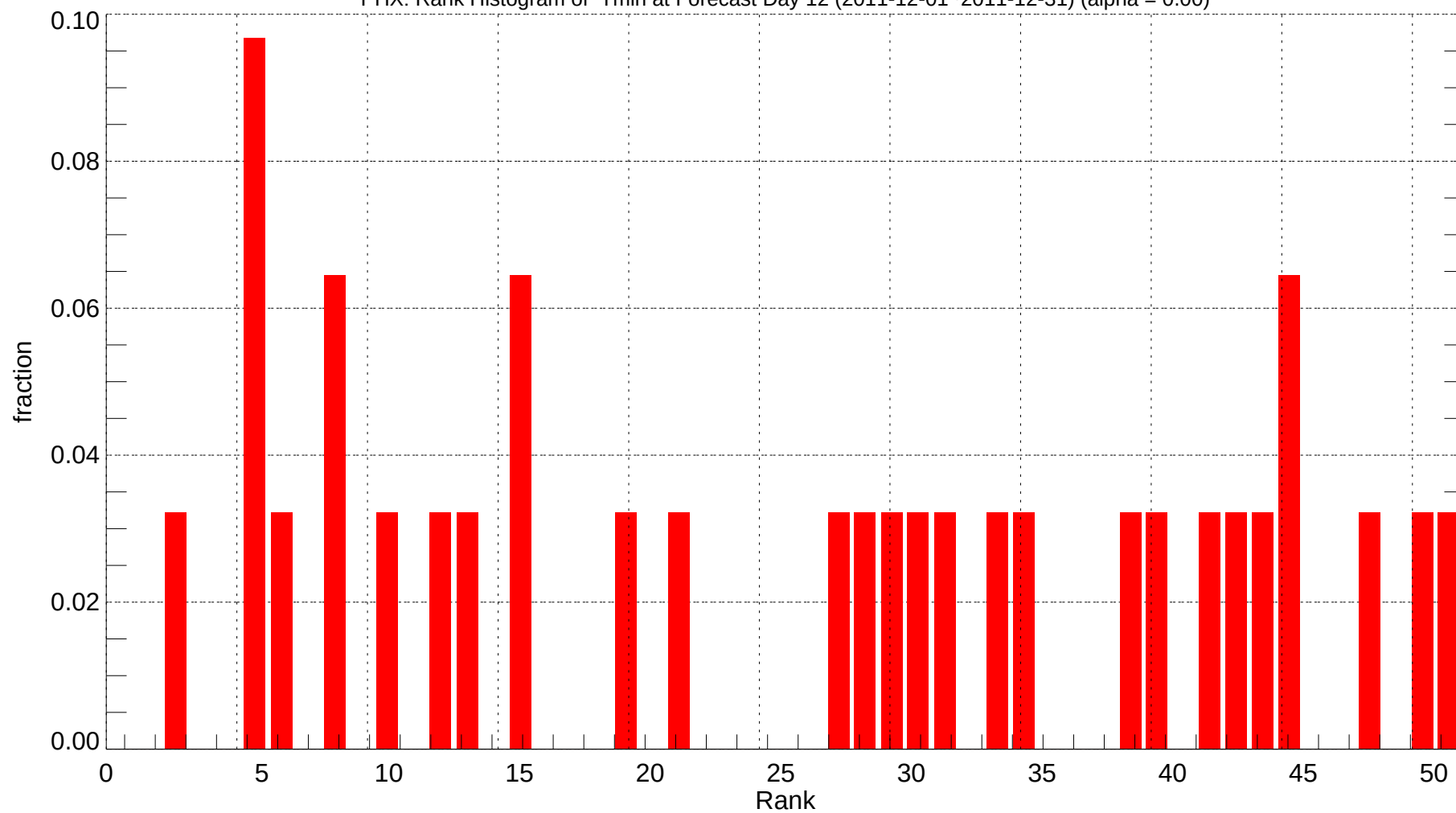
PHX: Rank Histogram of Tmin at Forecast Day 12 (2011-12-01~2011-12-31) (alpha = 0.00)
