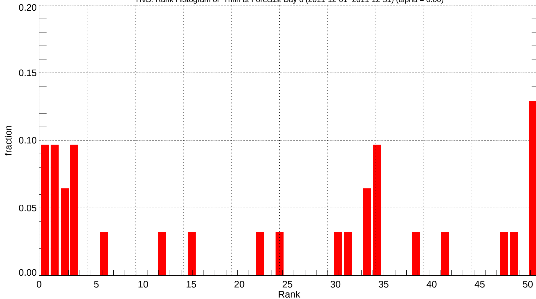
YNG: Rank Histogram of Tmin at Forecast Day 6 (2011-12-01~2011-12-31) (alpha = 0.00)
