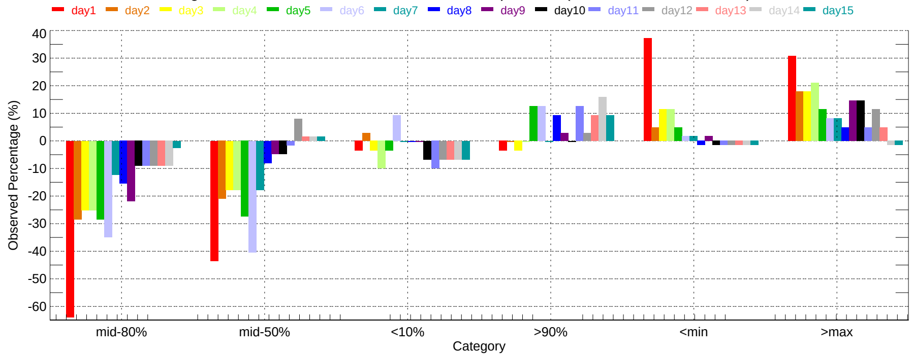
Observed Percentage Deviation of Ensembles - STL: Min Temperature (2011-12-01~2011-12-31)
