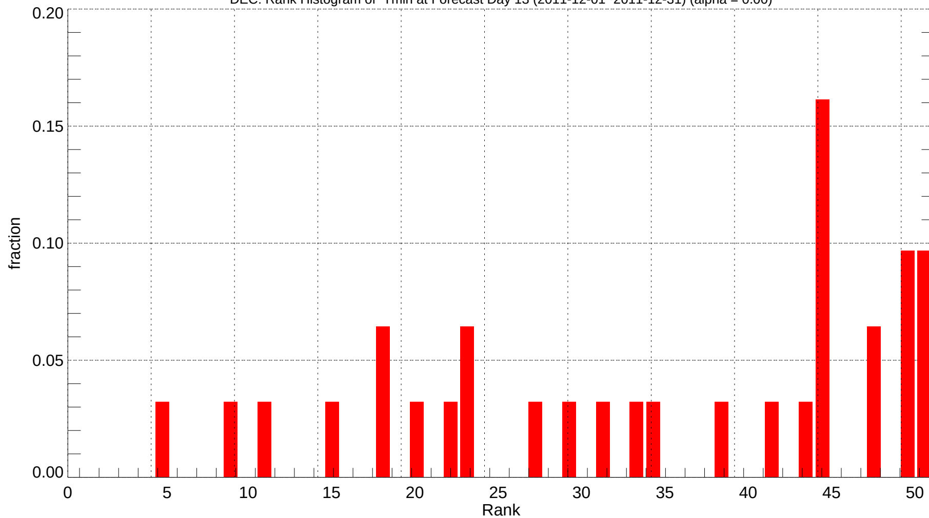
DEC: Rank Histogram of Tmin at Forecast Day 13 (2011-12-01~2011-12-31) (alpha = 0.00)
