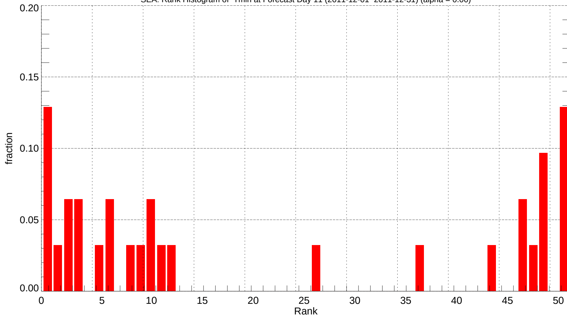
SEA: Rank Histogram of Tmin at Forecast Day 11 (2011-12-01~2011-12-31) (alpha = 0.00)
