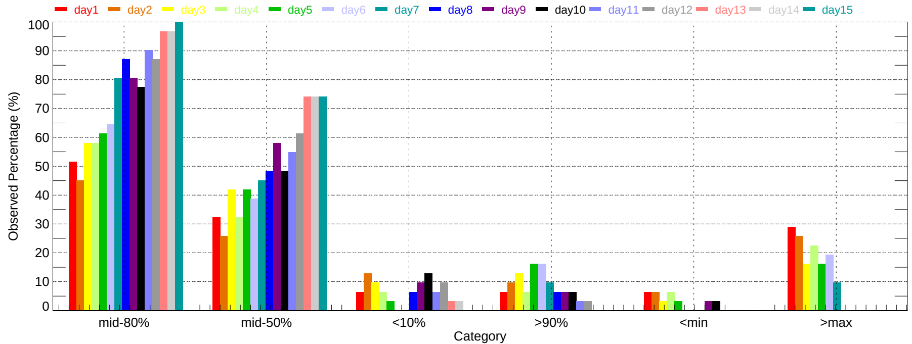
Observed Percentage of Ensembles - FAT: Max Temperature (2011-12-01~2011-12-31)
