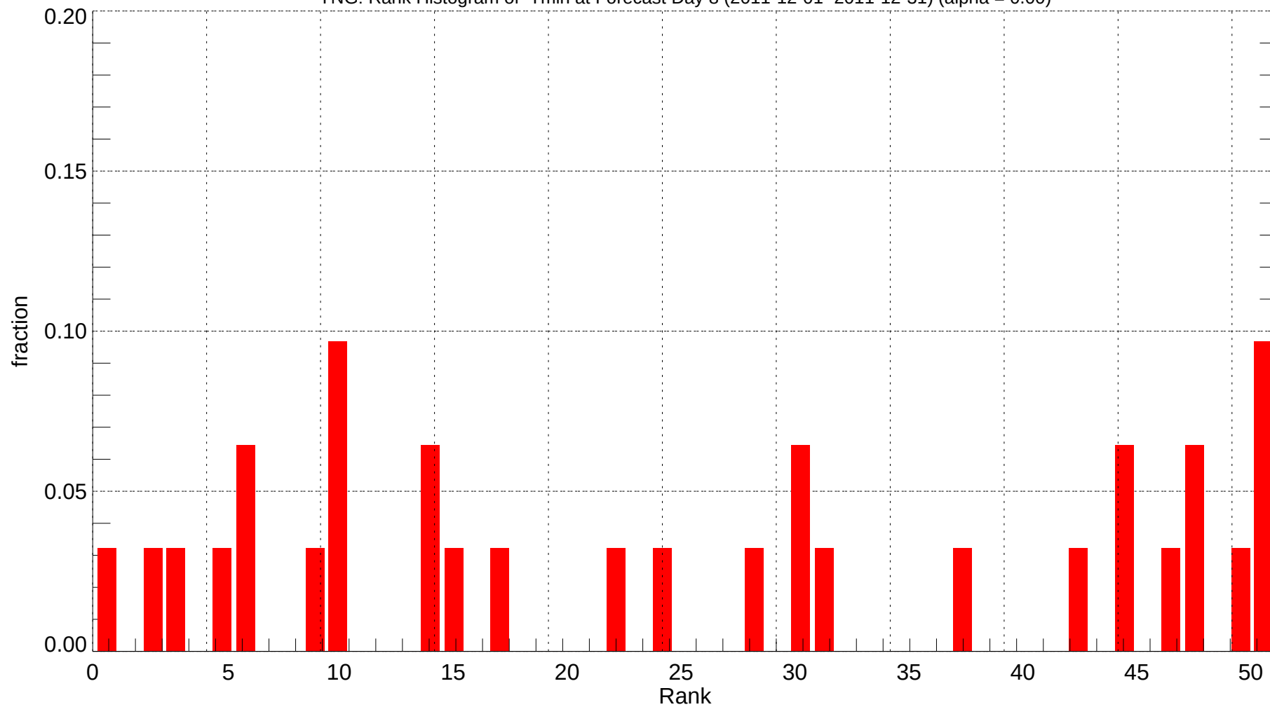
YNG: Rank Histogram of Tmin at Forecast Day 8 (2011-12-01~2011-12-31) (alpha = 0.00)
