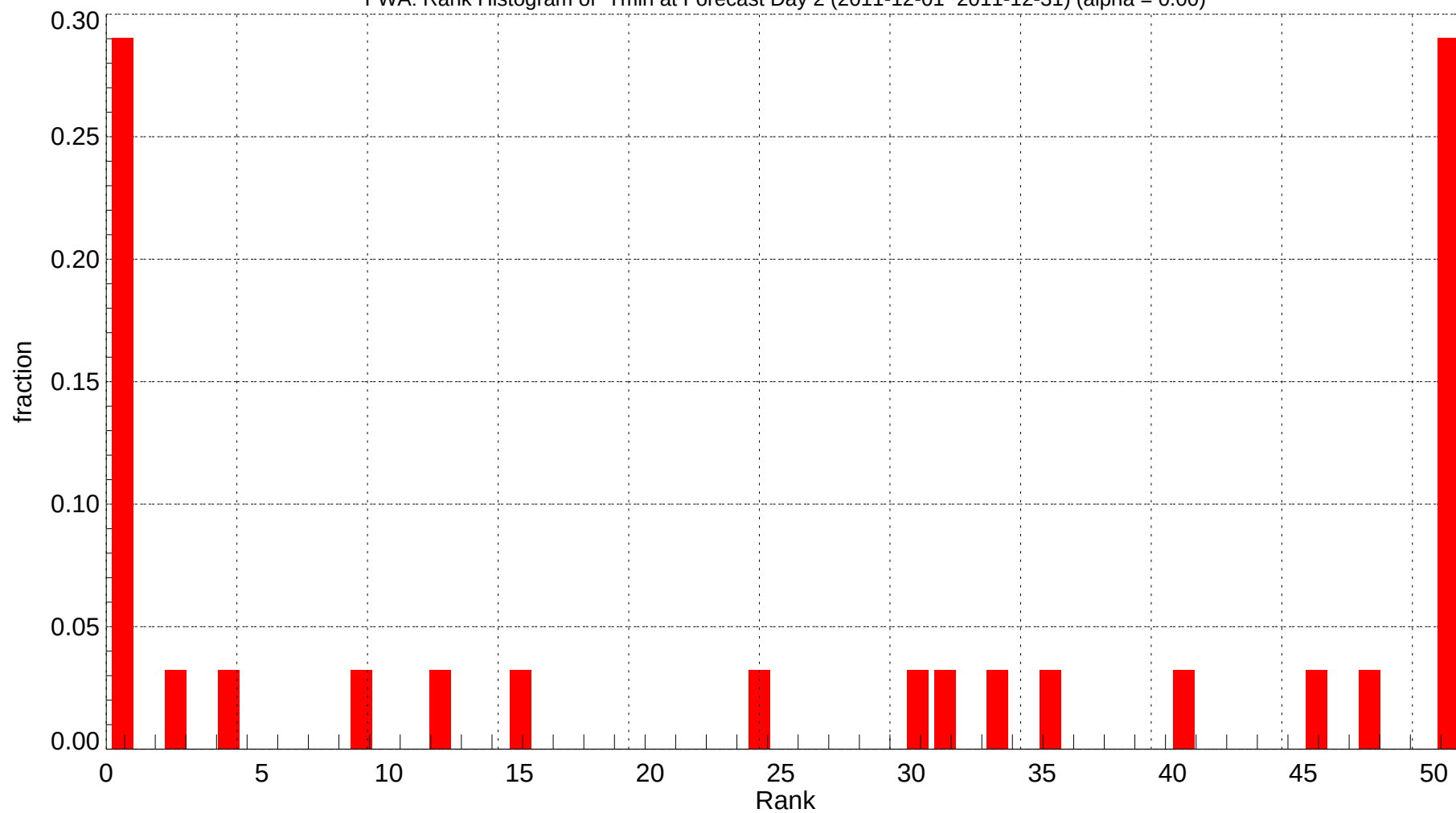
FWA: Rank Histogram of Tmin at Forecast Day 2 (2011-12-01~2011-12-31) (alpha = 0.00)
