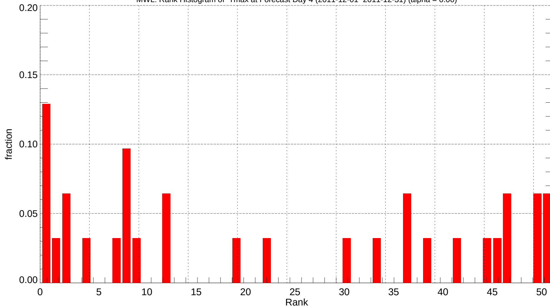
MWL: Rank Histogram of Tmax at Forecast Day 4 (2011-12-01~2011-12-31) (alpha = 0.00)
