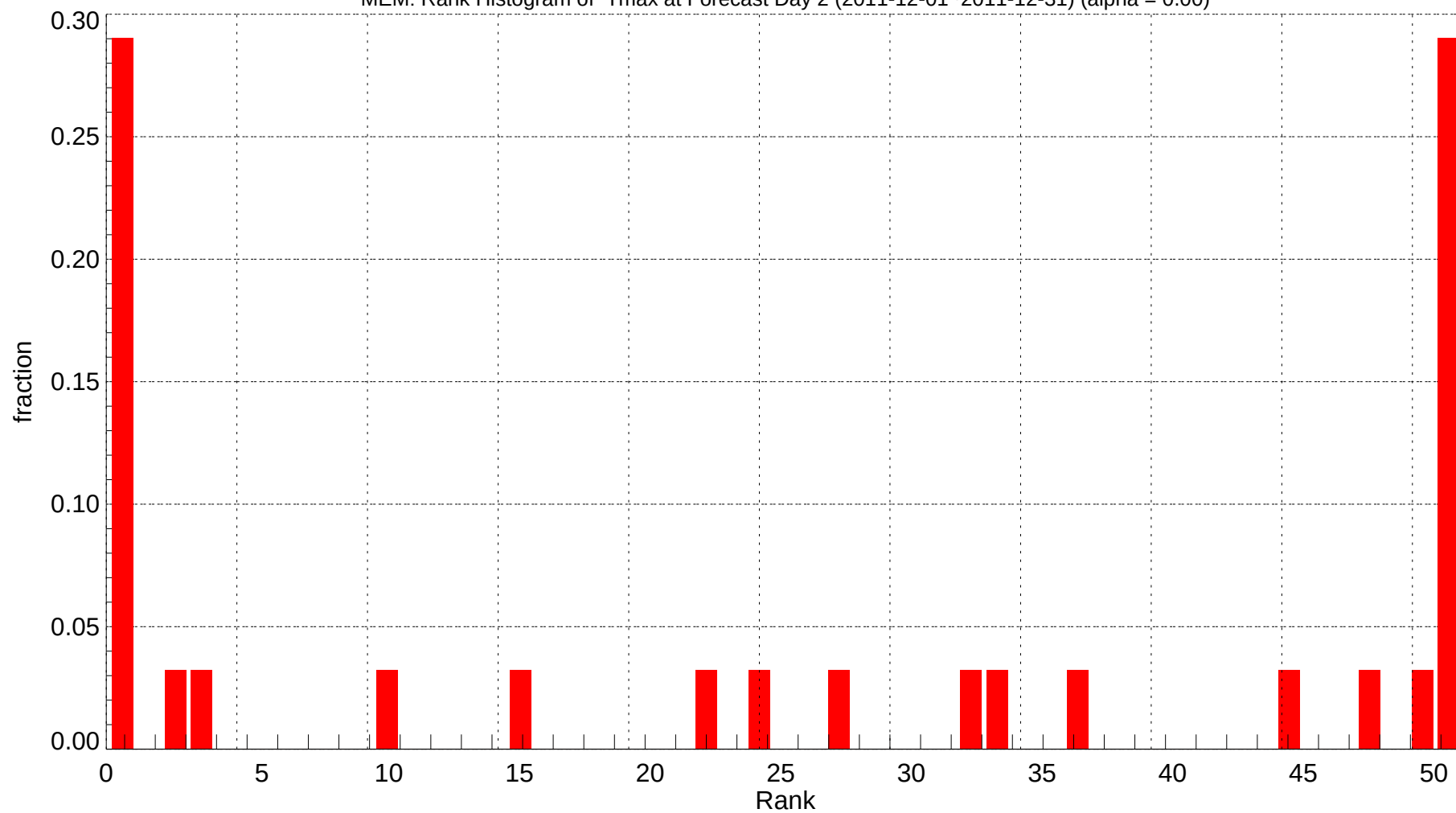
MEM: Rank Histogram of Tmax at Forecast Day 2 (2011-12-01~2011-12-31) (alpha = 0.00)
