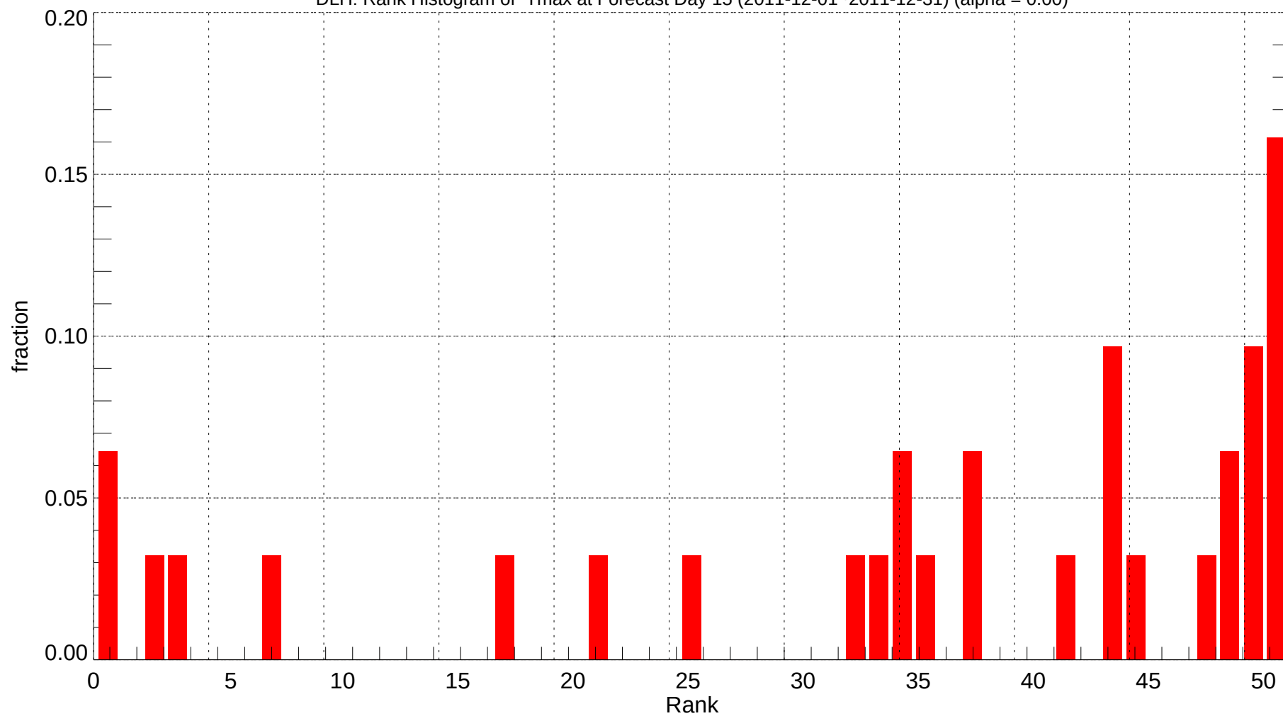
DLH: Rank Histogram of Tmax at Forecast Day 15 (2011-12-01~2011-12-31) (alpha = 0.00)
