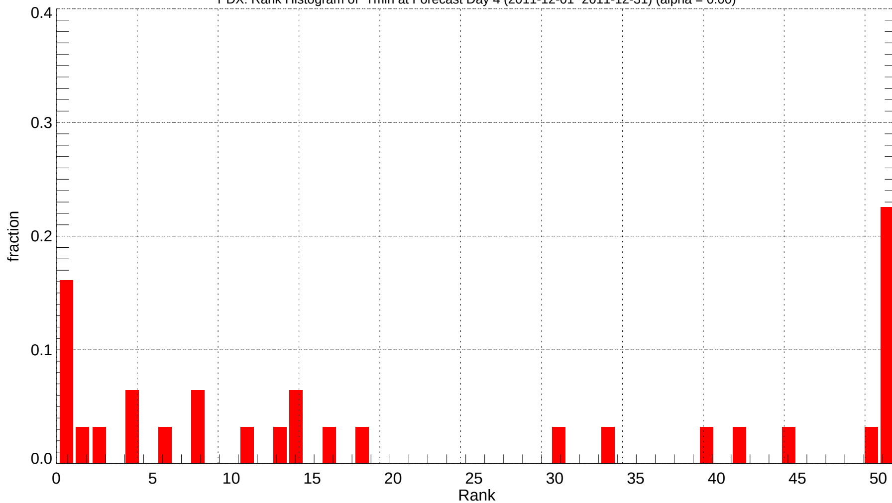
PDX: Rank Histogram of Tmin at Forecast Day 4 (2011-12-01~2011-12-31) (alpha = 0.00)
