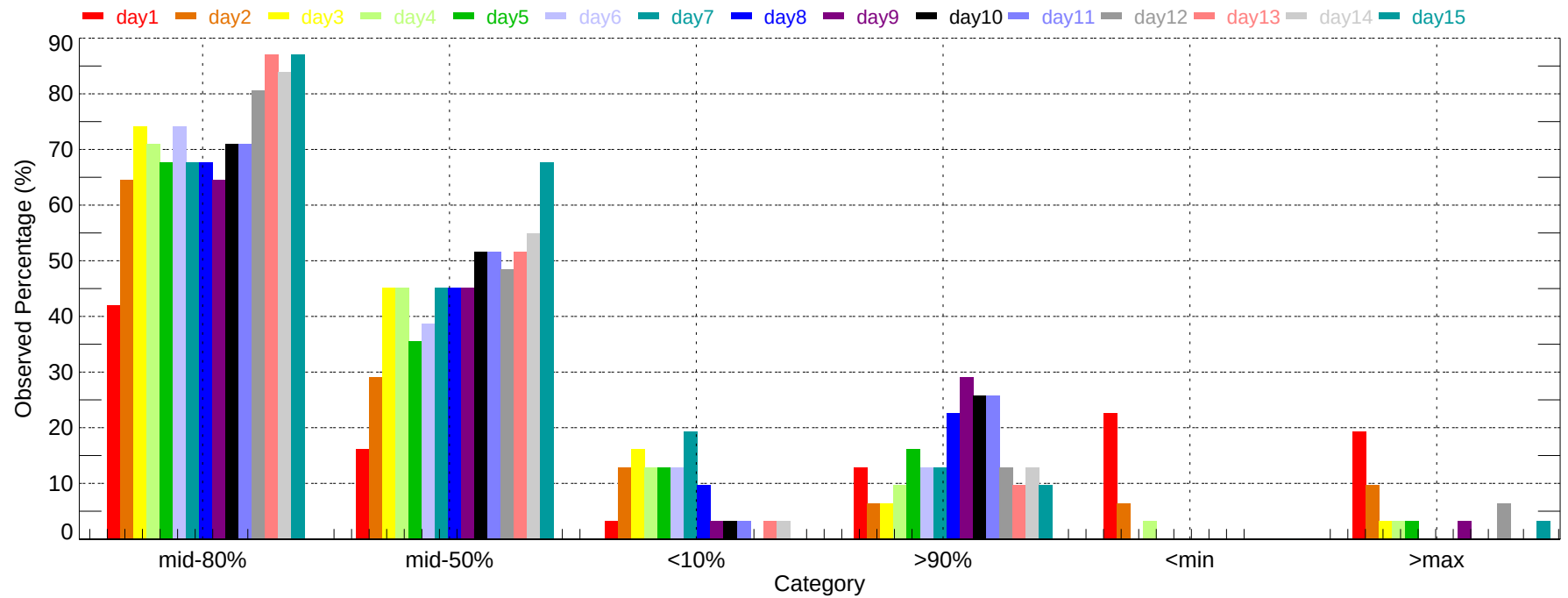
Observed Percentage of Ensembles - ATL: Min Temperature (2011-12-01~2011-12-31)
