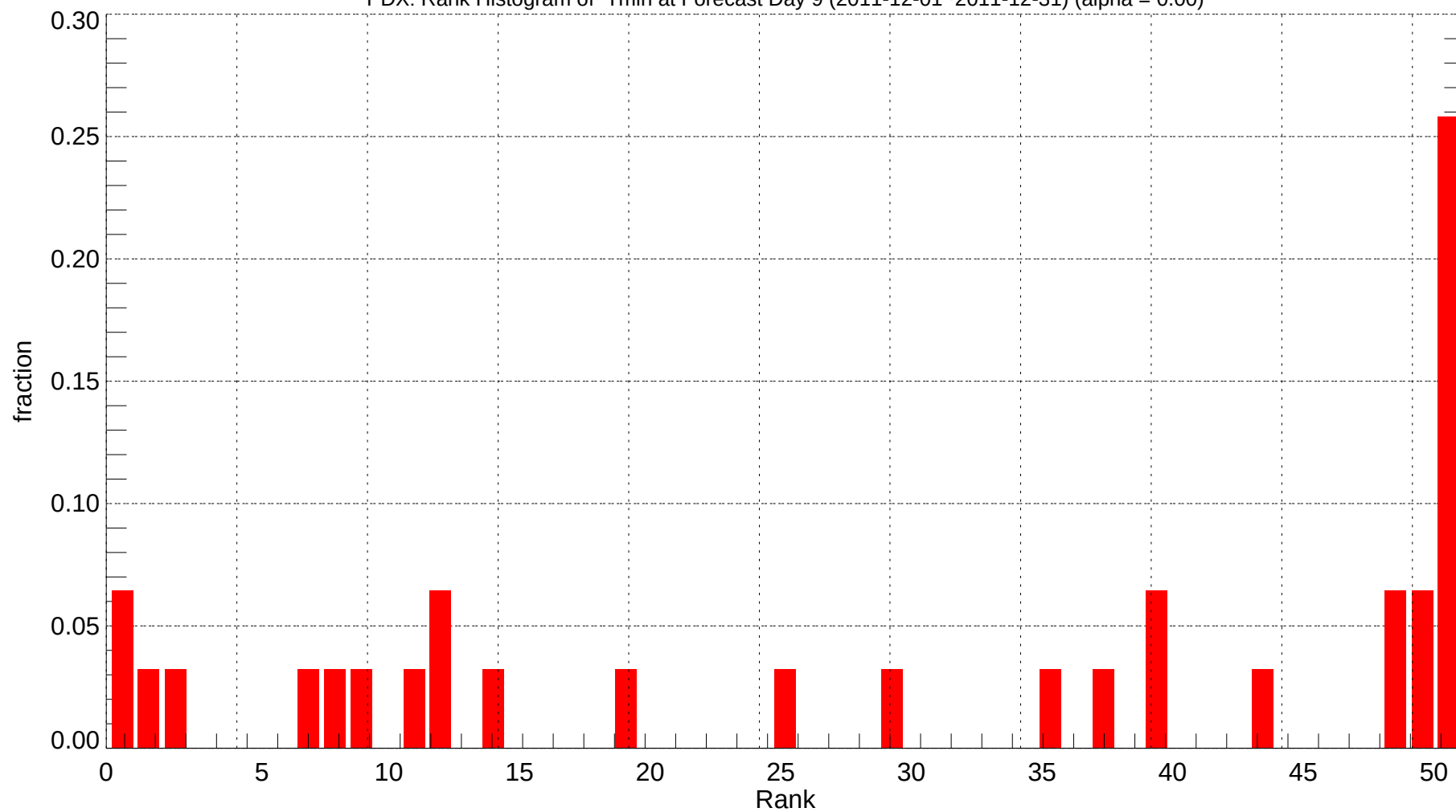
PDX: Rank Histogram of Tmin at Forecast Day 9 (2011-12-01~2011-12-31) (alpha = 0.00)
