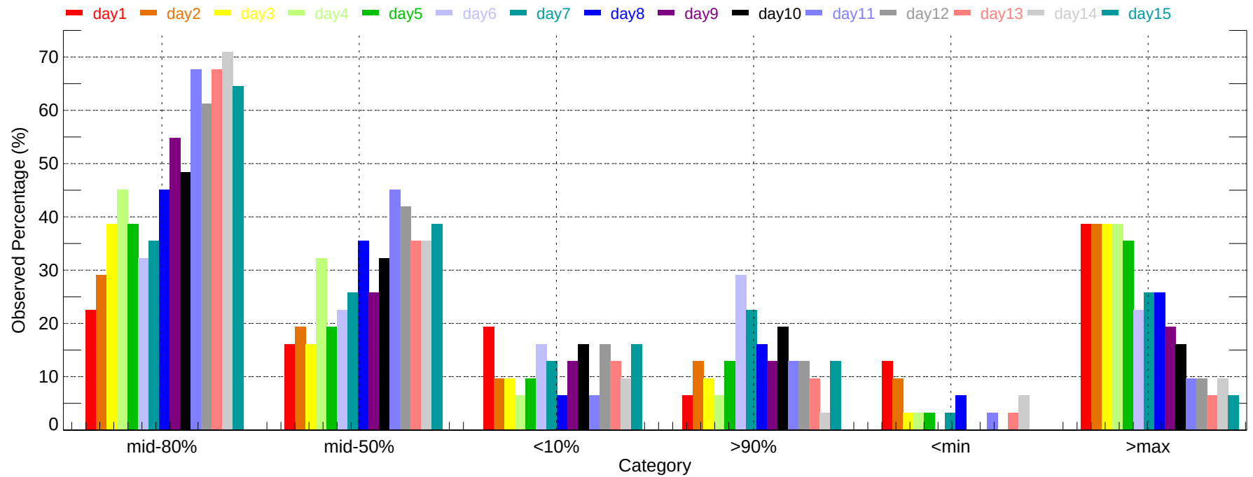
Observed Percentage of Ensembles - ELP: Max Temperature (2011-12-01~2011-12-31)
