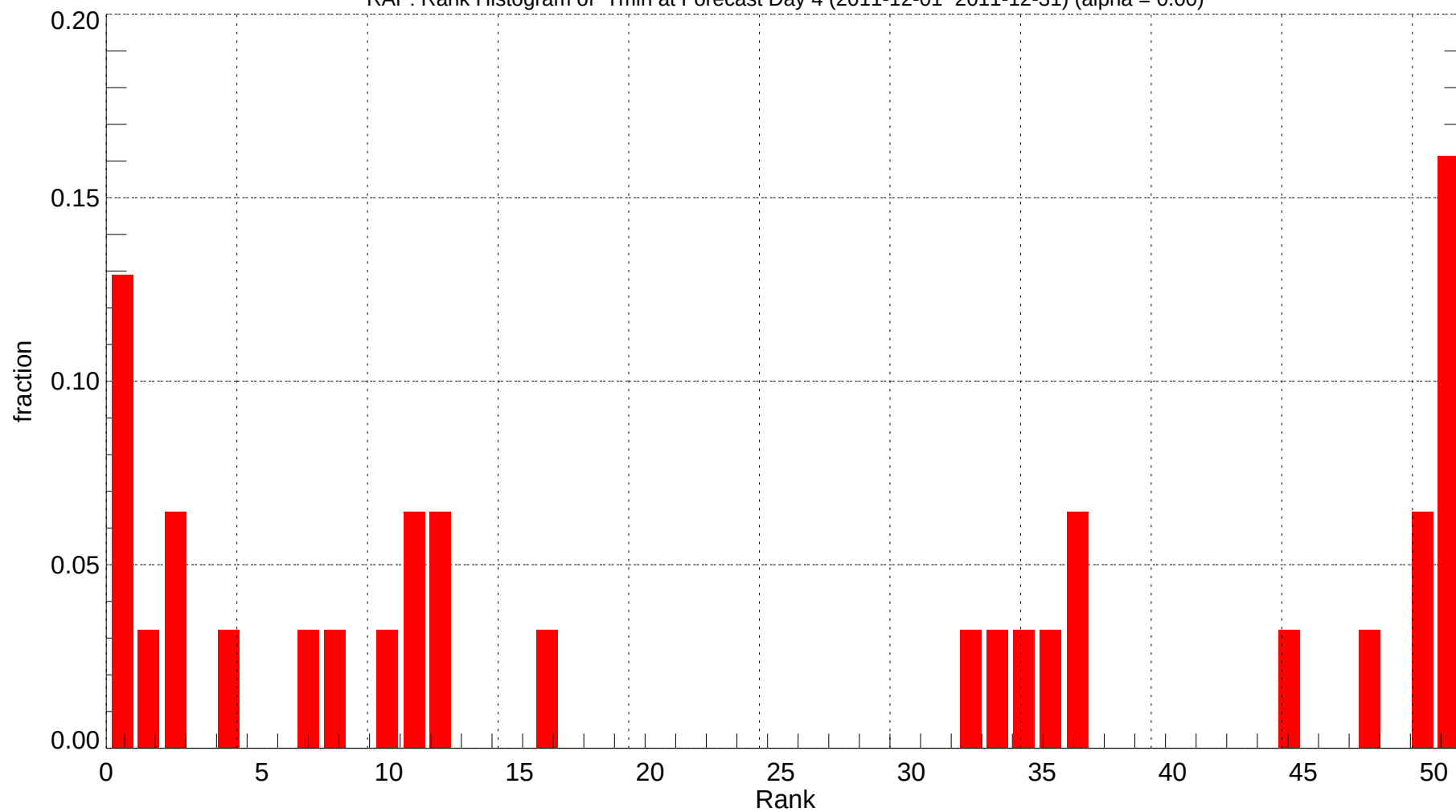
RAP: Rank Histogram of Tmin at Forecast Day 4 (2011-12-01~2011-12-31) (alpha = 0.00)
