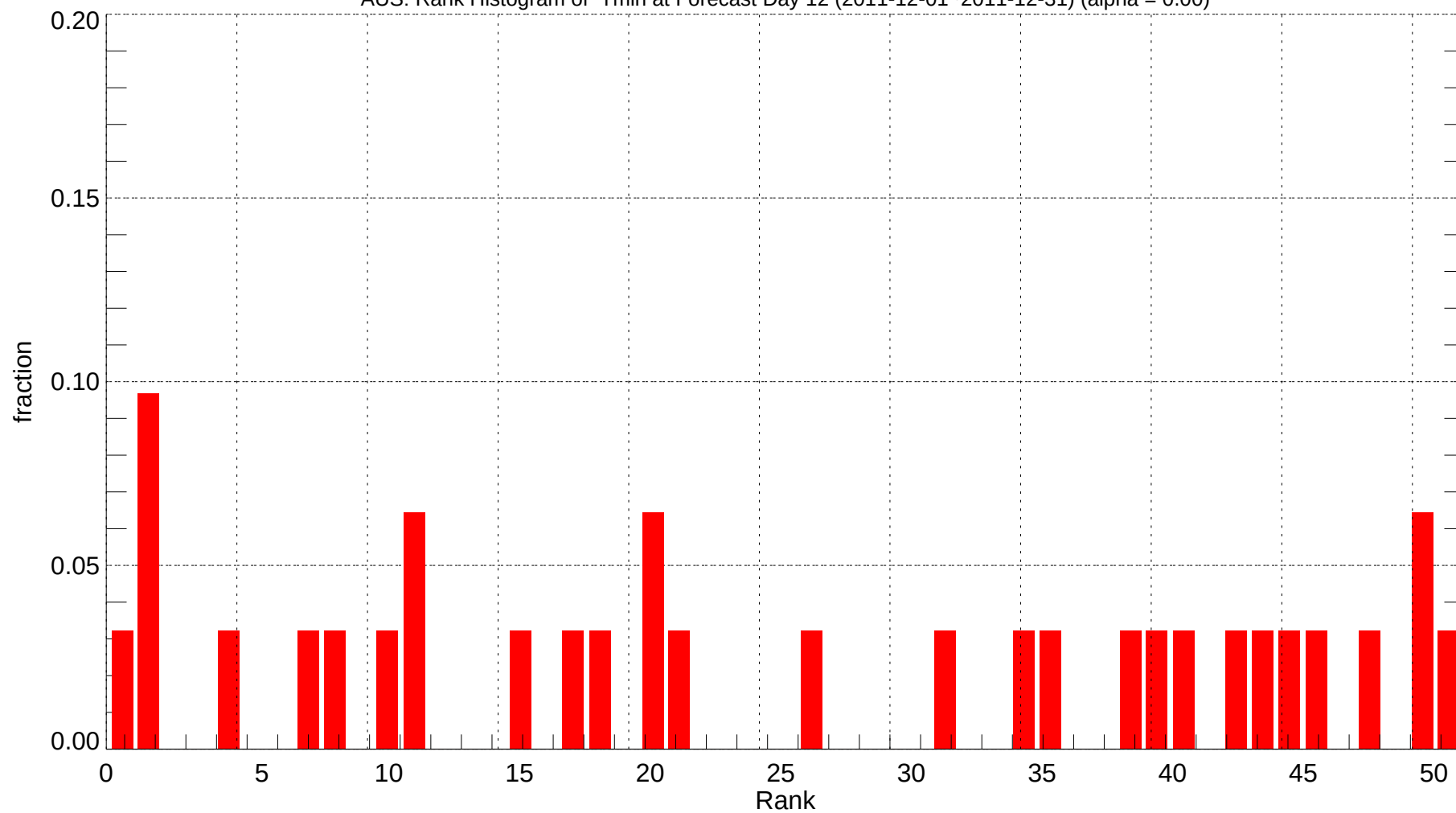
AUS: Rank Histogram of Tmin at Forecast Day 12 (2011-12-01~2011-12-31) (alpha = 0.00)
