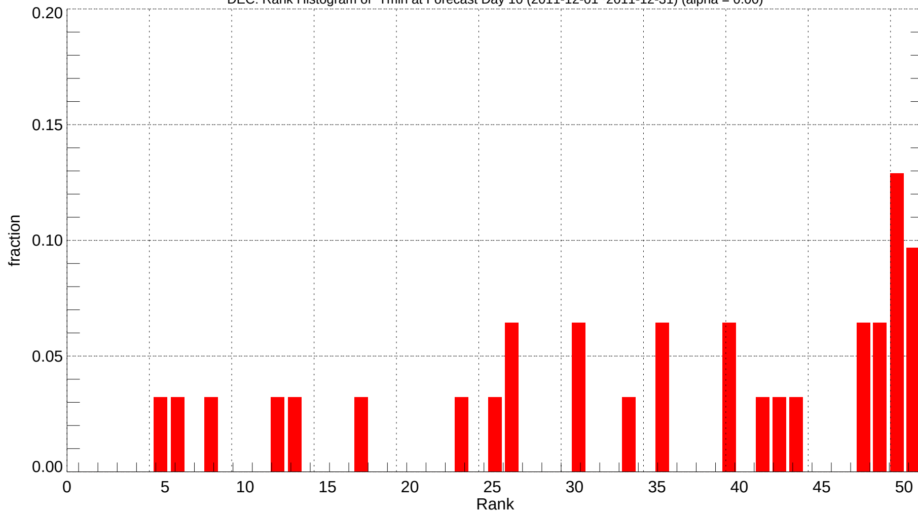
DEC: Rank Histogram of Tmin at Forecast Day 10 (2011-12-01~2011-12-31) (alpha = 0.00)
