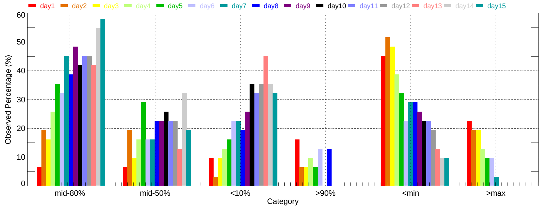
Observed Percentage of Ensembles - BFL: Min Temperature (2011-12-01~2011-12-31)
