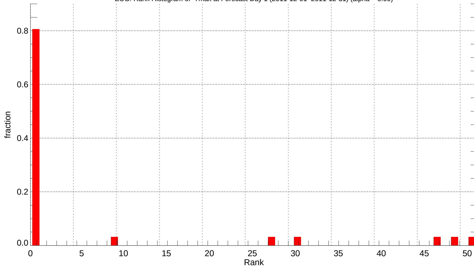
EUG: Rank Histogram of Tmax at Forecast Day 1 (2011-12-01~2011-12-31) (alpha = 0.00)
