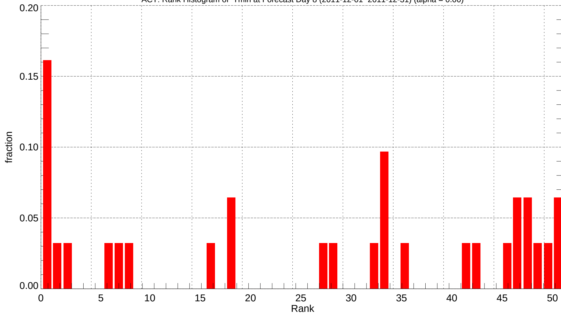
ACT: Rank Histogram of Tmin at Forecast Day 8 (2011-12-01~2011-12-31) (alpha = 0.00)
