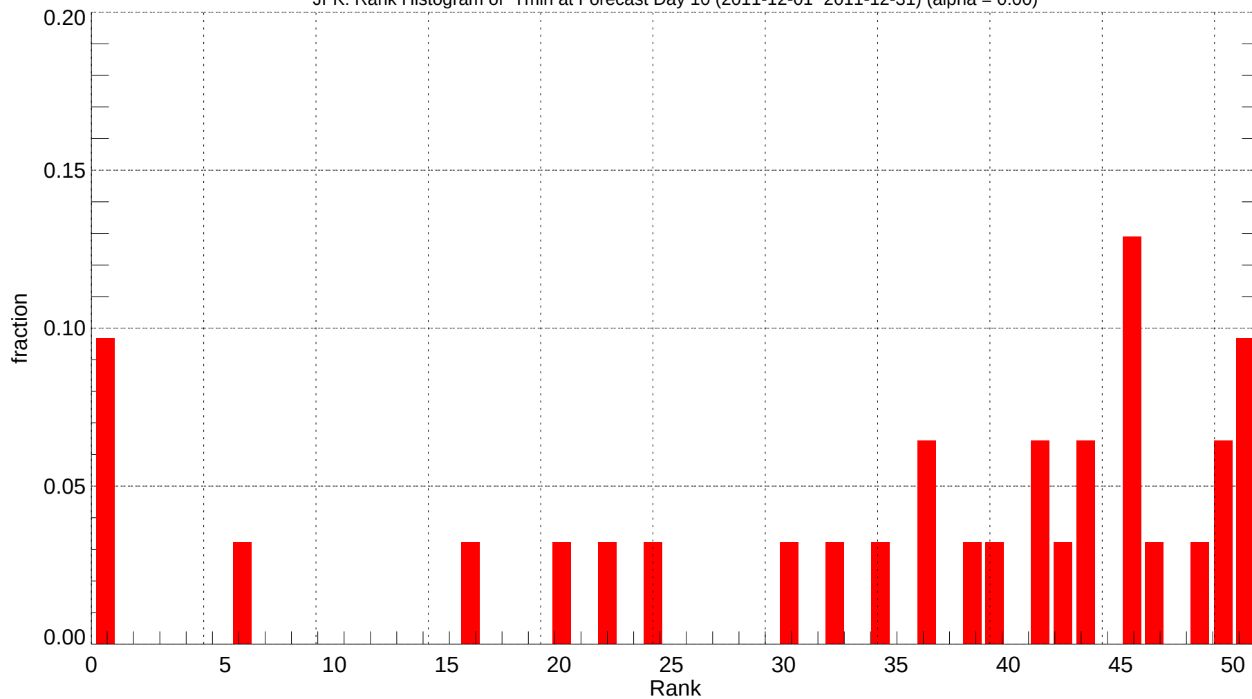
JFK: Rank Histogram of Tmin at Forecast Day 10 (2011-12-01~2011-12-31) (alpha = 0.00)
