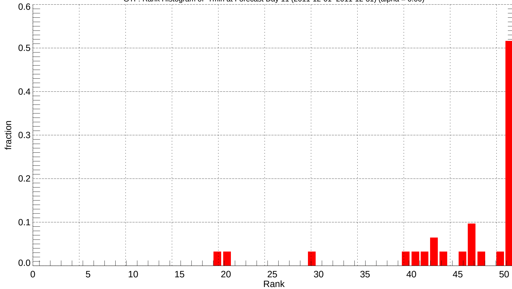
GTF: Rank Histogram of Tmin at Forecast Day 11 (2011-12-01~2011-12-31) (alpha = 0.00)
