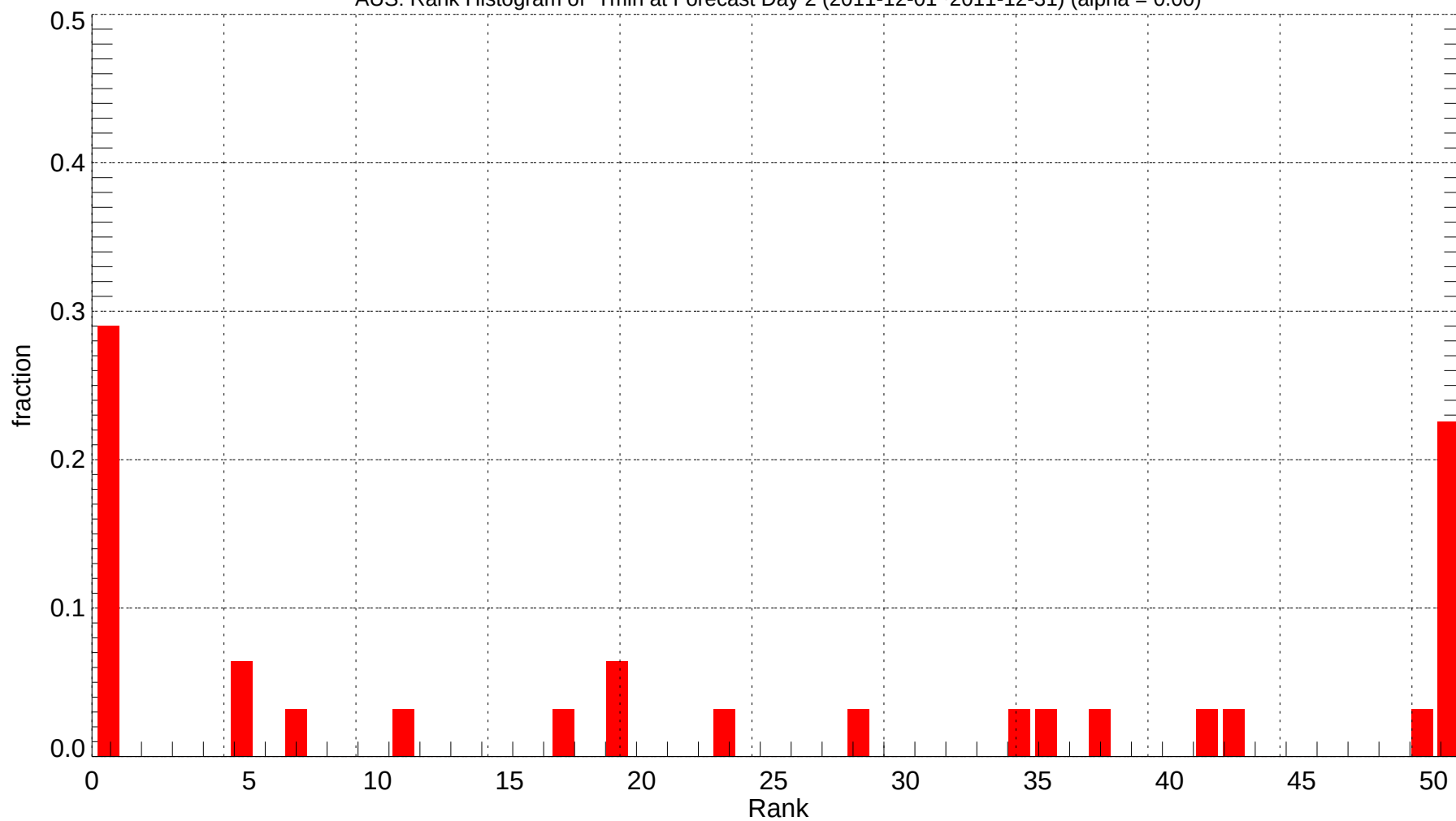
AUS: Rank Histogram of Tmin at Forecast Day 2 (2011-12-01~2011-12-31) (alpha = 0.00)
