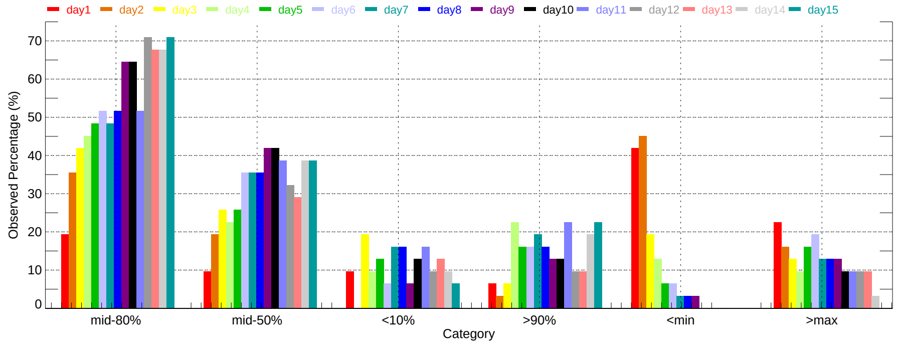
Observed Percentage of Ensembles - AVP: Min Temperature (2011-12-01~2011-12-31)
