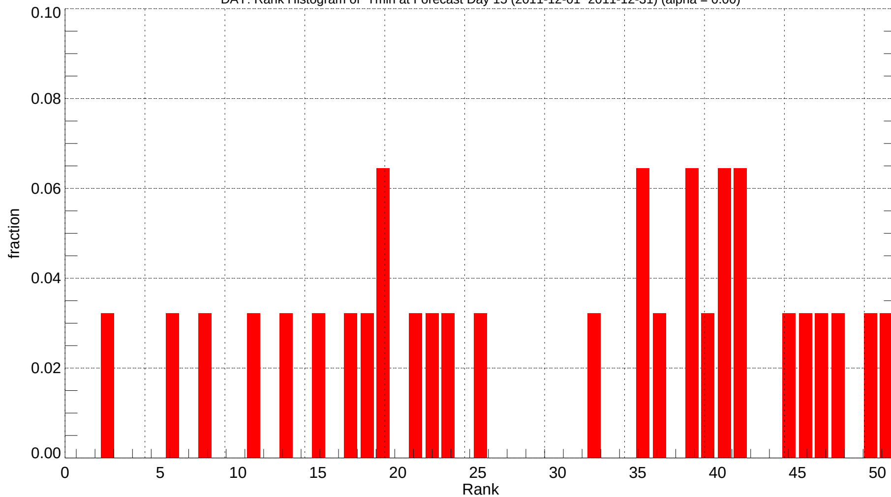
DAY: Rank Histogram of Tmin at Forecast Day 15 (2011-12-01~2011-12-31) (alpha = 0.00)
