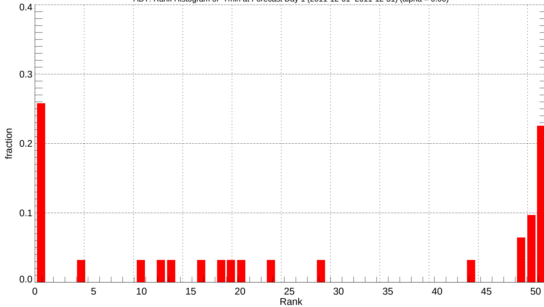
ABY: Rank Histogram of Tmin at Forecast Day 1 (2011-12-01~2011-12-31) (alpha = 0.00)
