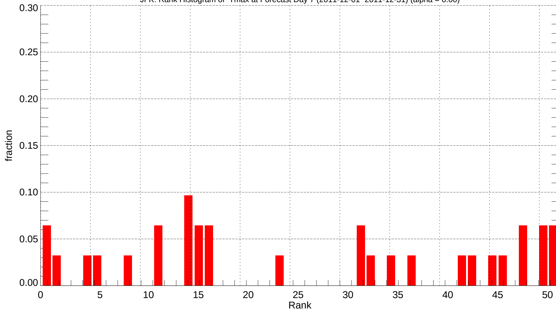
JFK: Rank Histogram of Tmax at Forecast Day 7 (2011-12-01~2011-12-31) (alpha = 0.00)
