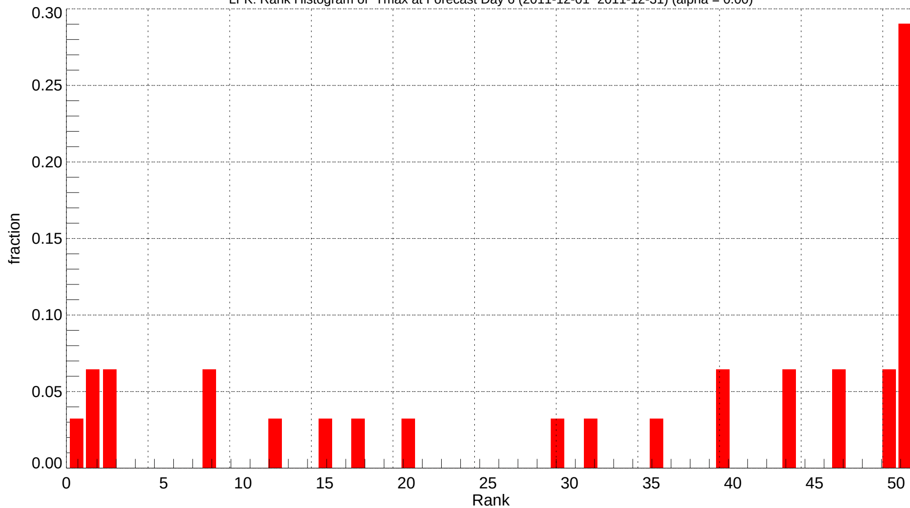
LFK: Rank Histogram of Tmax at Forecast Day 6 (2011-12-01~2011-12-31) (alpha = 0.00)
