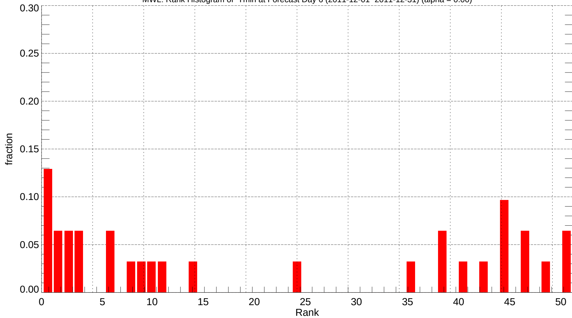
MWL: Rank Histogram of Tmin at Forecast Day 6 (2011-12-01~2011-12-31) (alpha = 0.00)
