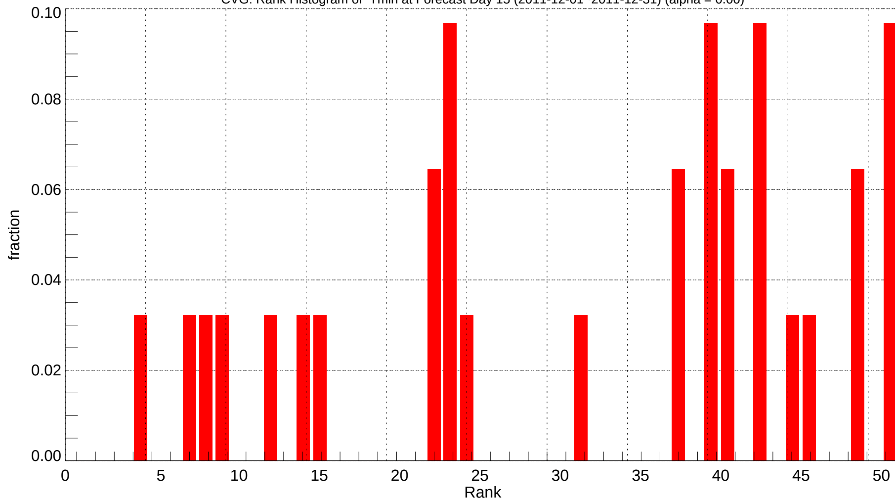
CVG: Rank Histogram of Tmin at Forecast Day 15 (2011-12-01~2011-12-31) (alpha = 0.00)
