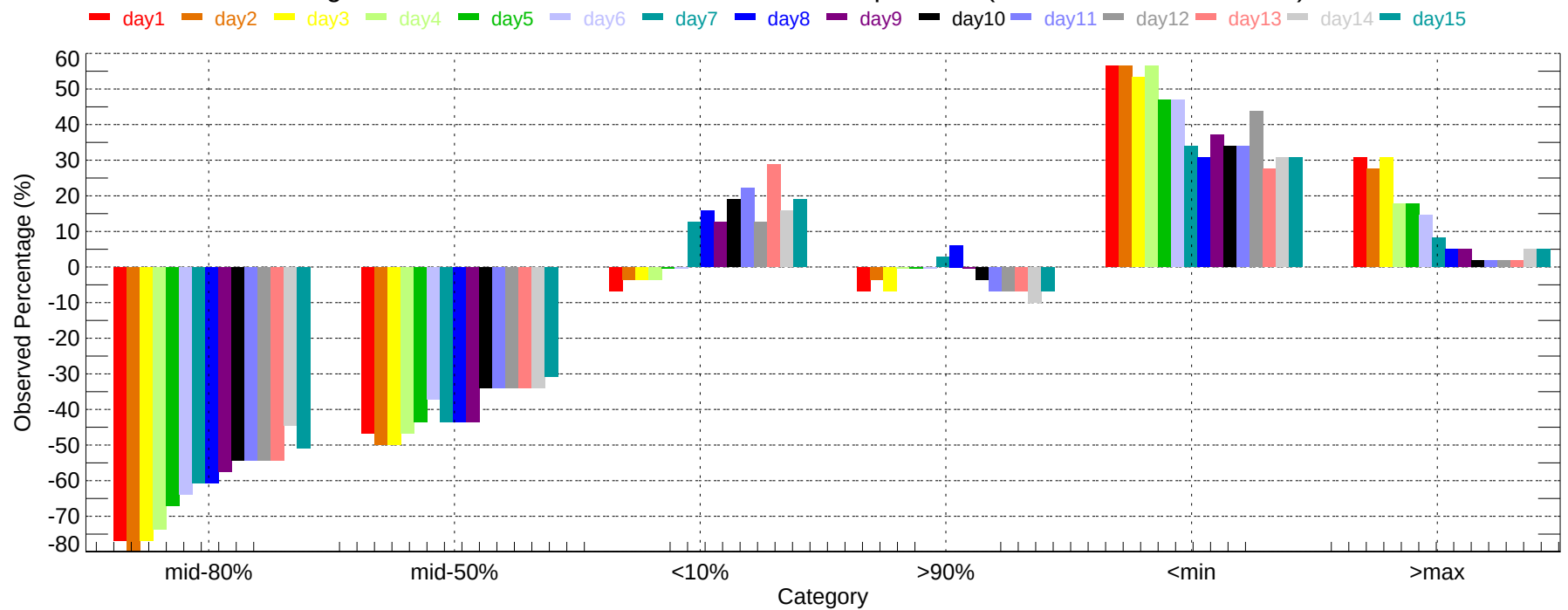
Observed Percentage Deviation of Ensembles - OAK: Max Temperature (2011-12-01~2011-12-31)
