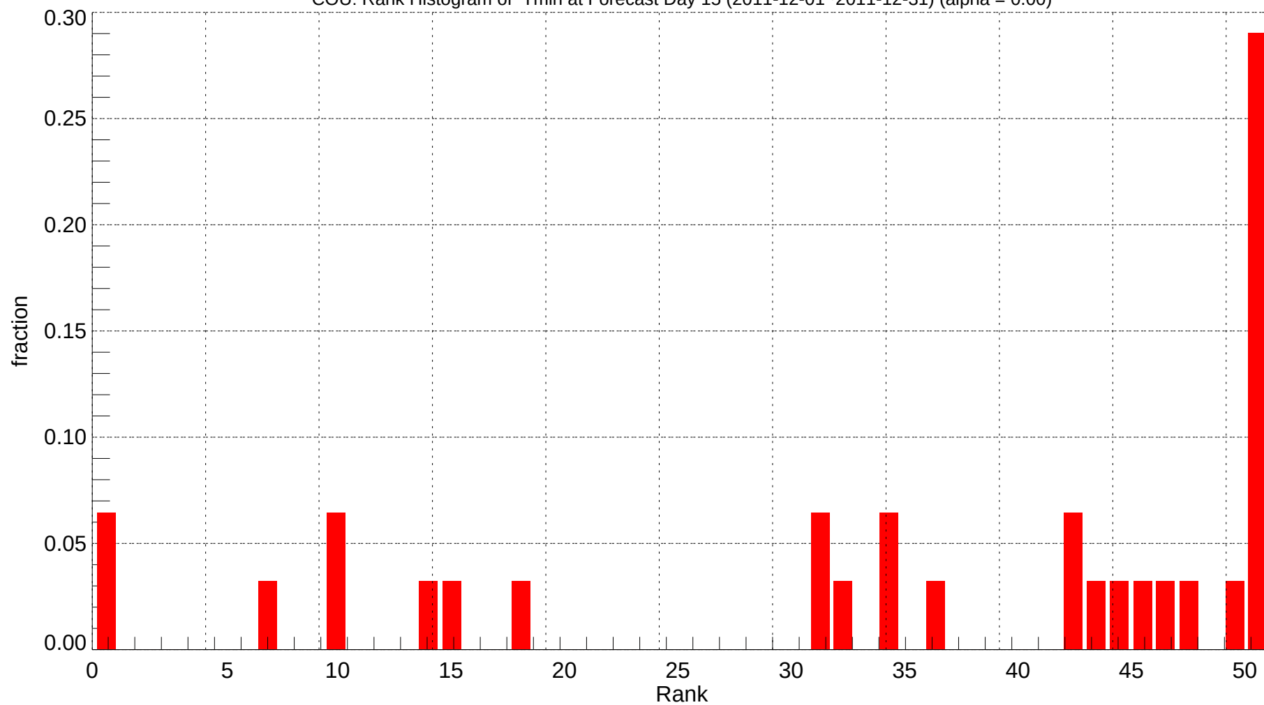
COU: Rank Histogram of Tmin at Forecast Day 15 (2011-12-01~2011-12-31) (alpha = 0.00)
