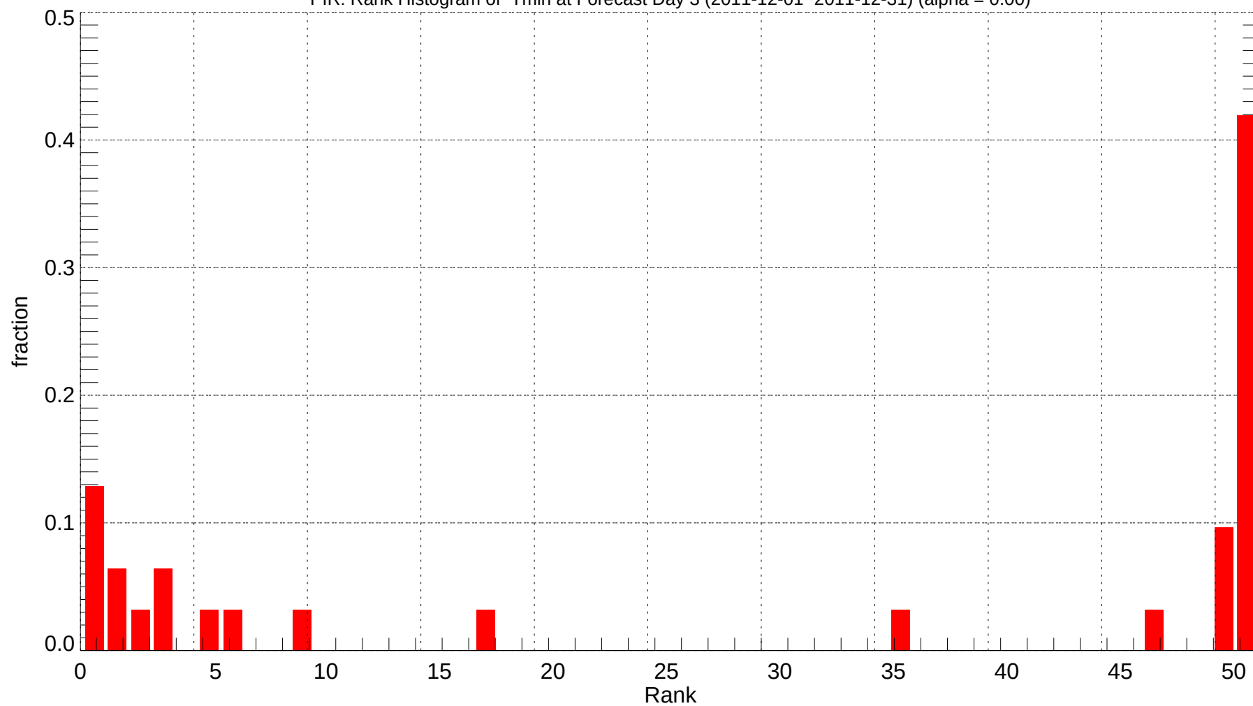
PIR: Rank Histogram of Tmin at Forecast Day 3 (2011-12-01~2011-12-31) (alpha = 0.00)
