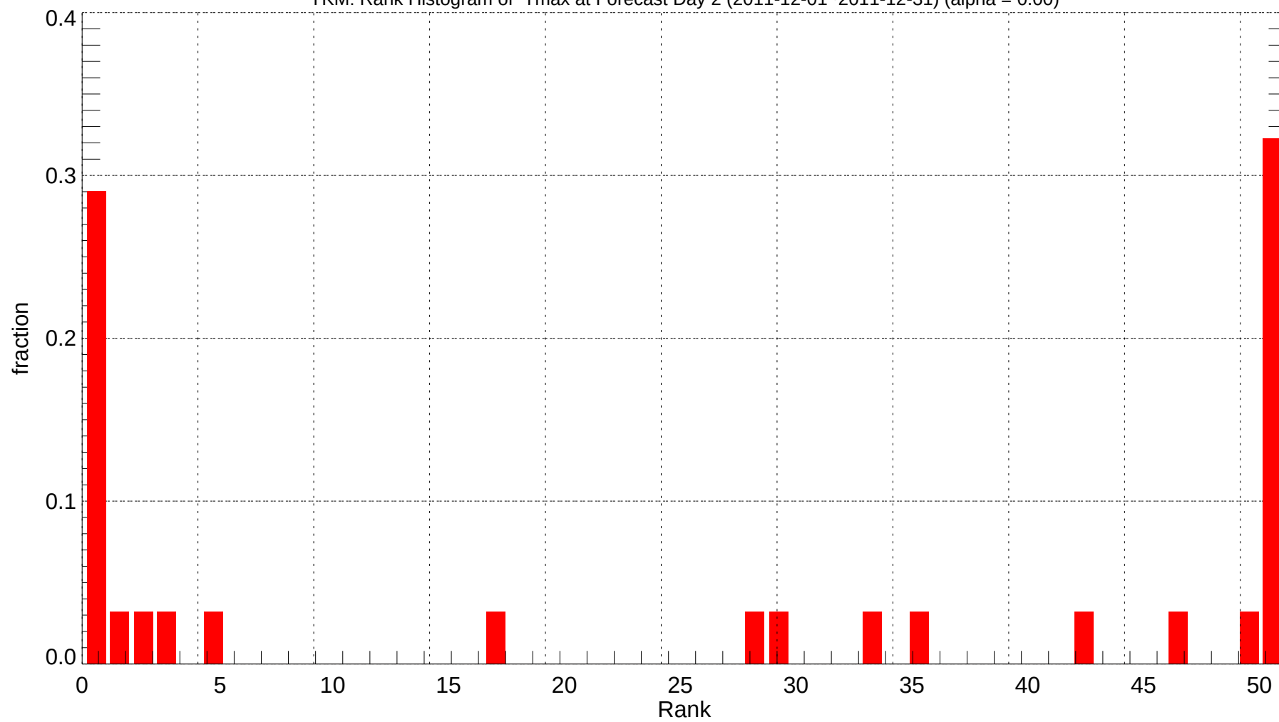
YKM: Rank Histogram of Tmax at Forecast Day 2 (2011-12-01~2011-12-31) (alpha = 0.00)
