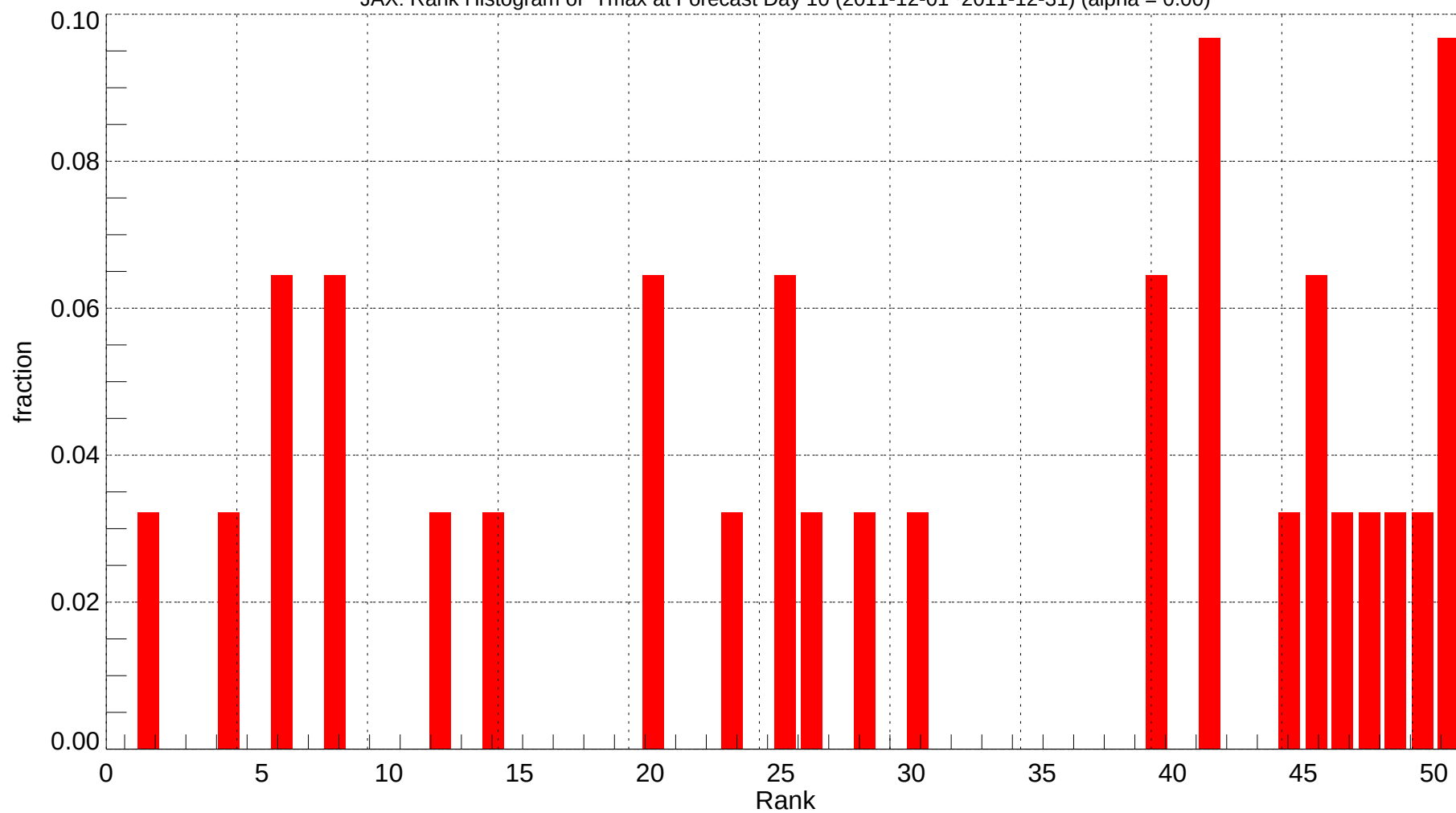
JAX: Rank Histogram of Tmax at Forecast Day 10 (2011-12-01~2011-12-31) (alpha = 0.00)
