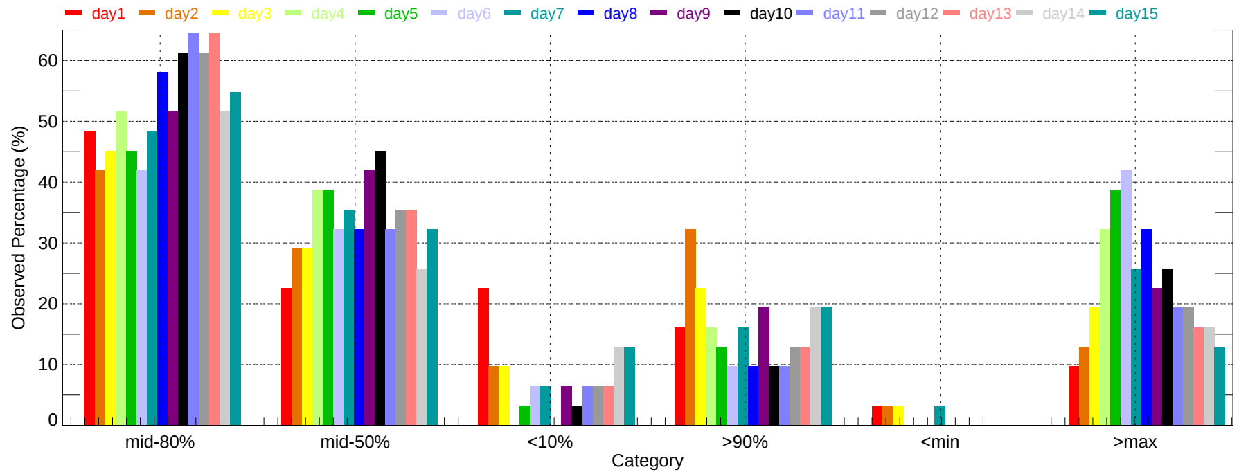
Observed Percentage of Ensembles - SDF: Max Temperature (2011-12-01~2011-12-31)
