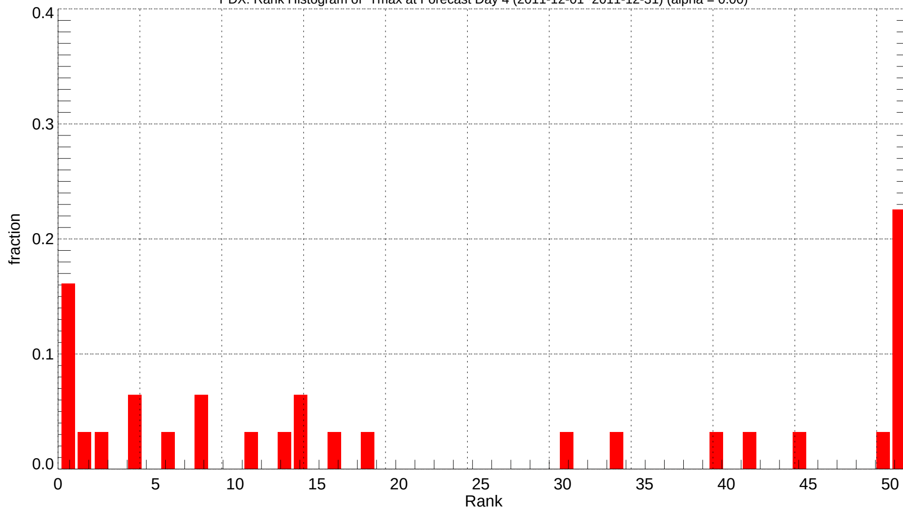
PDX: Rank Histogram of Tmax at Forecast Day 4 (2011-12-01~2011-12-31) (alpha = 0.00)
