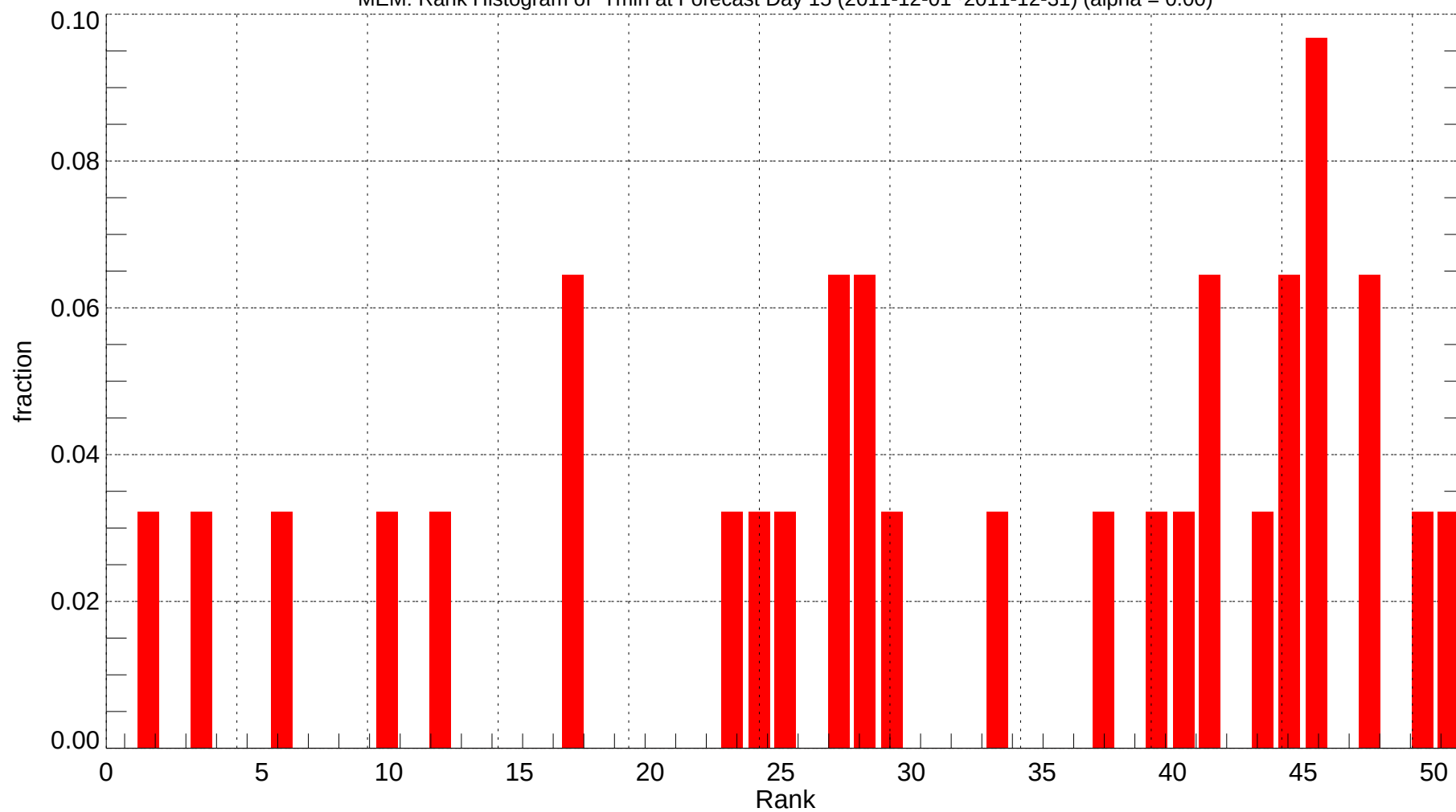
MEM: Rank Histogram of Tmin at Forecast Day 15 (2011-12-01~2011-12-31) (alpha = 0.00)
