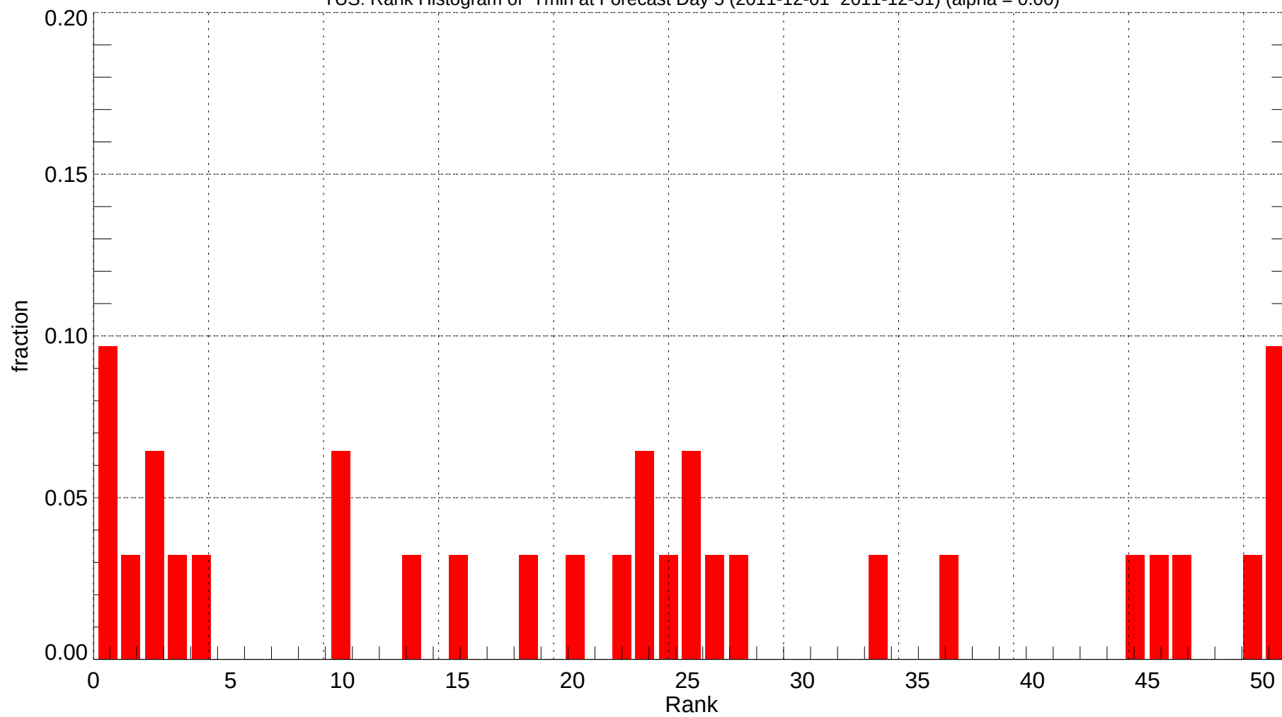
TUS: Rank Histogram of Tmin at Forecast Day 5 (2011-12-01~2011-12-31) (alpha = 0.00)
