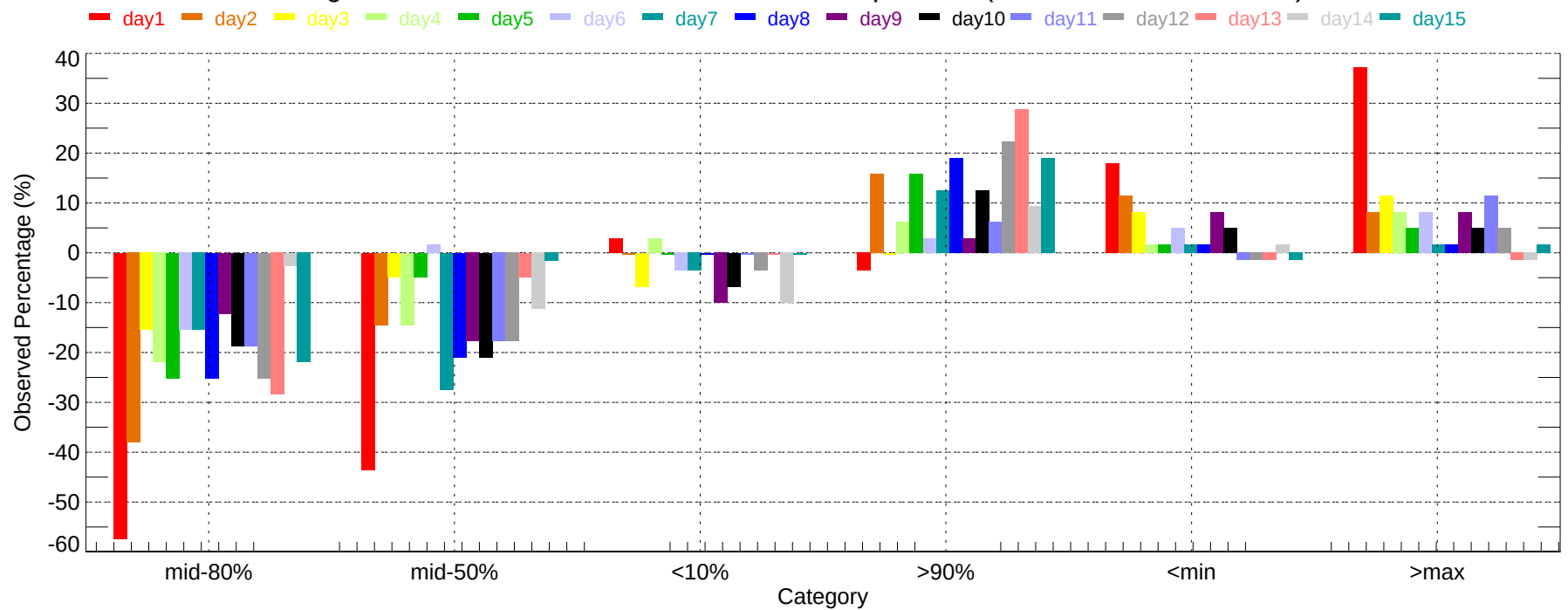
Observed Percentage Deviation of Ensembles - PVD: Max Temperature (2011-12-01~2011-12-31)
