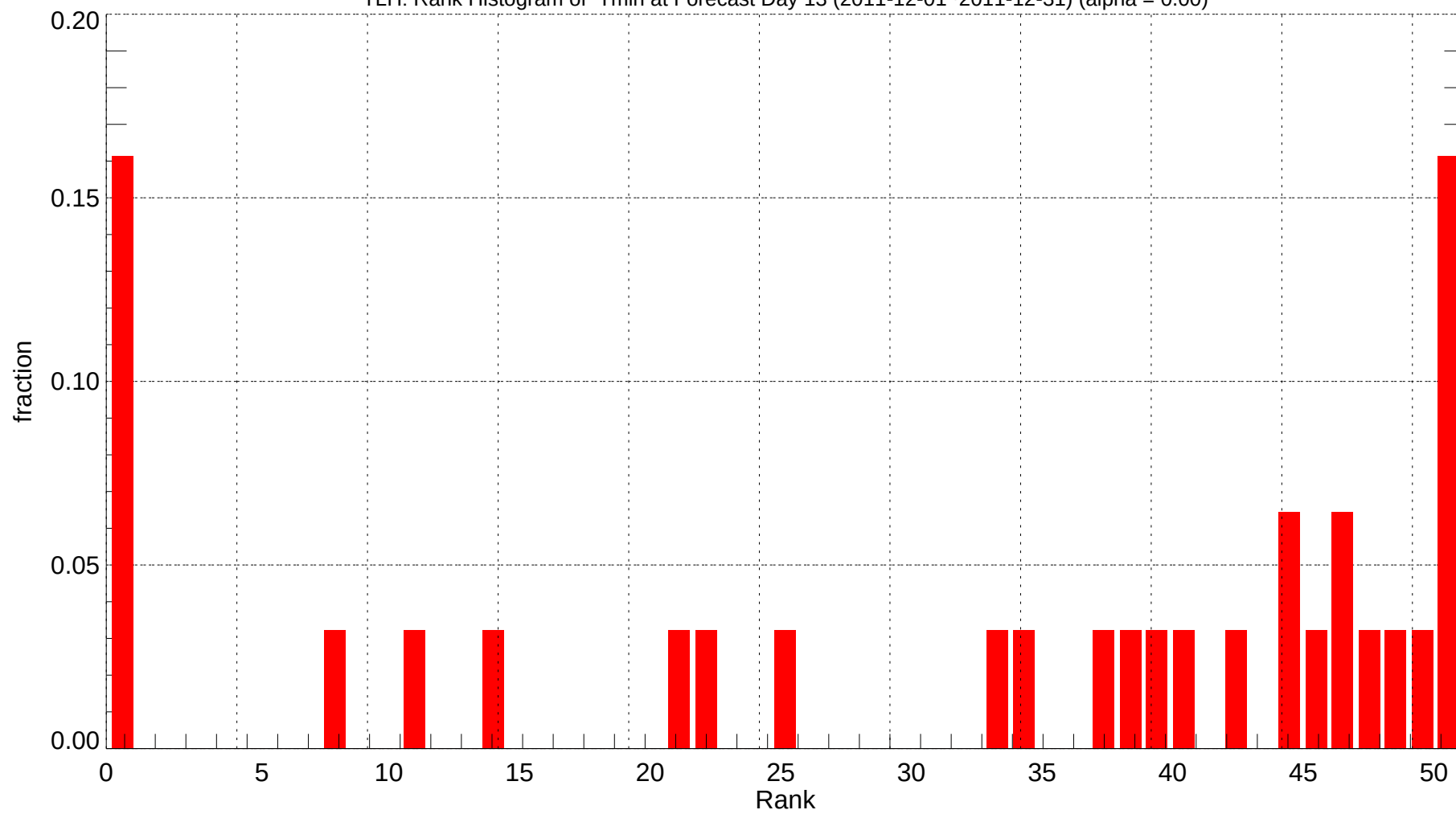
TLH: Rank Histogram of Tmin at Forecast Day 13 (2011-12-01~2011-12-31) (alpha = 0.00)
