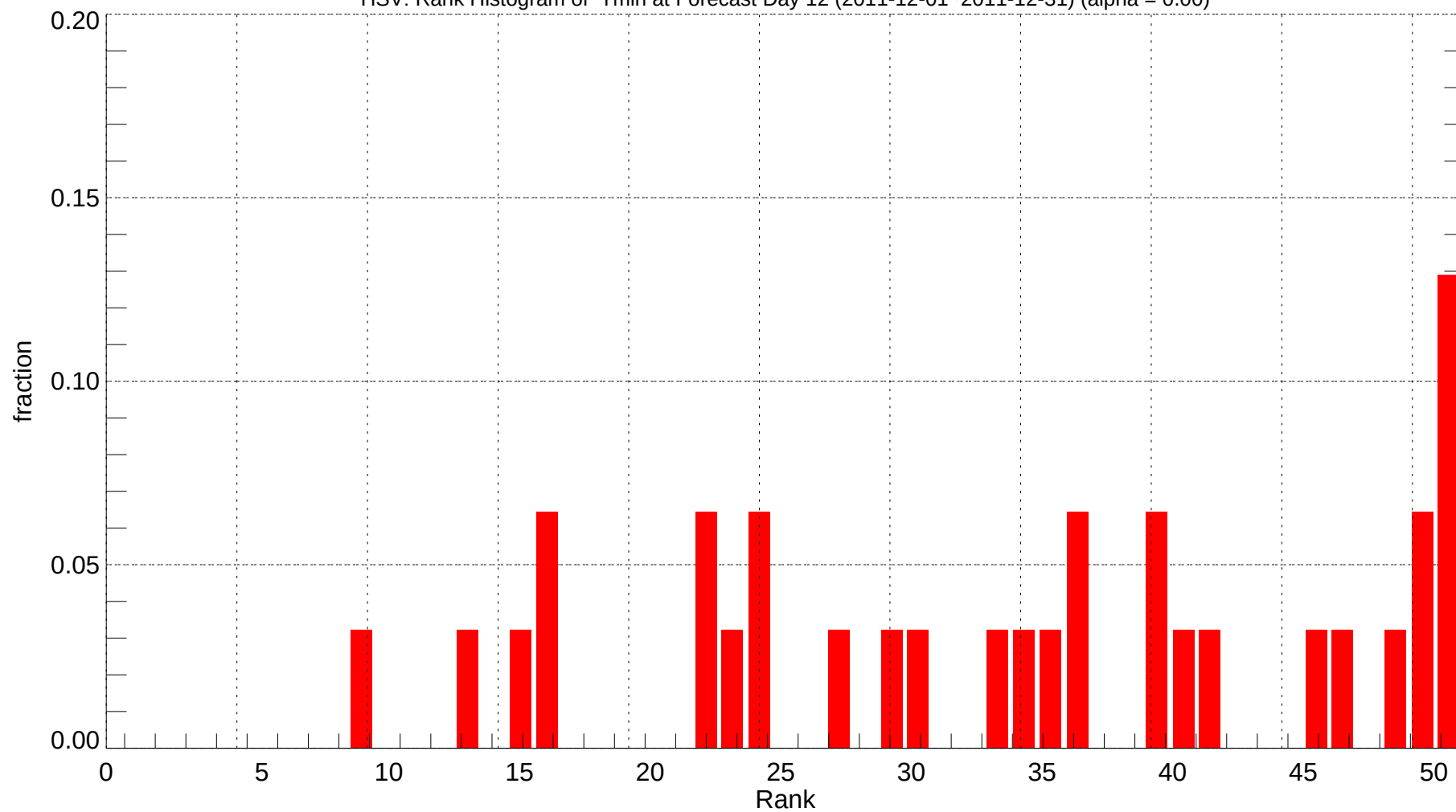
HSV: Rank Histogram of Tmin at Forecast Day 12 (2011-12-01~2011-12-31) (alpha = 0.00)
