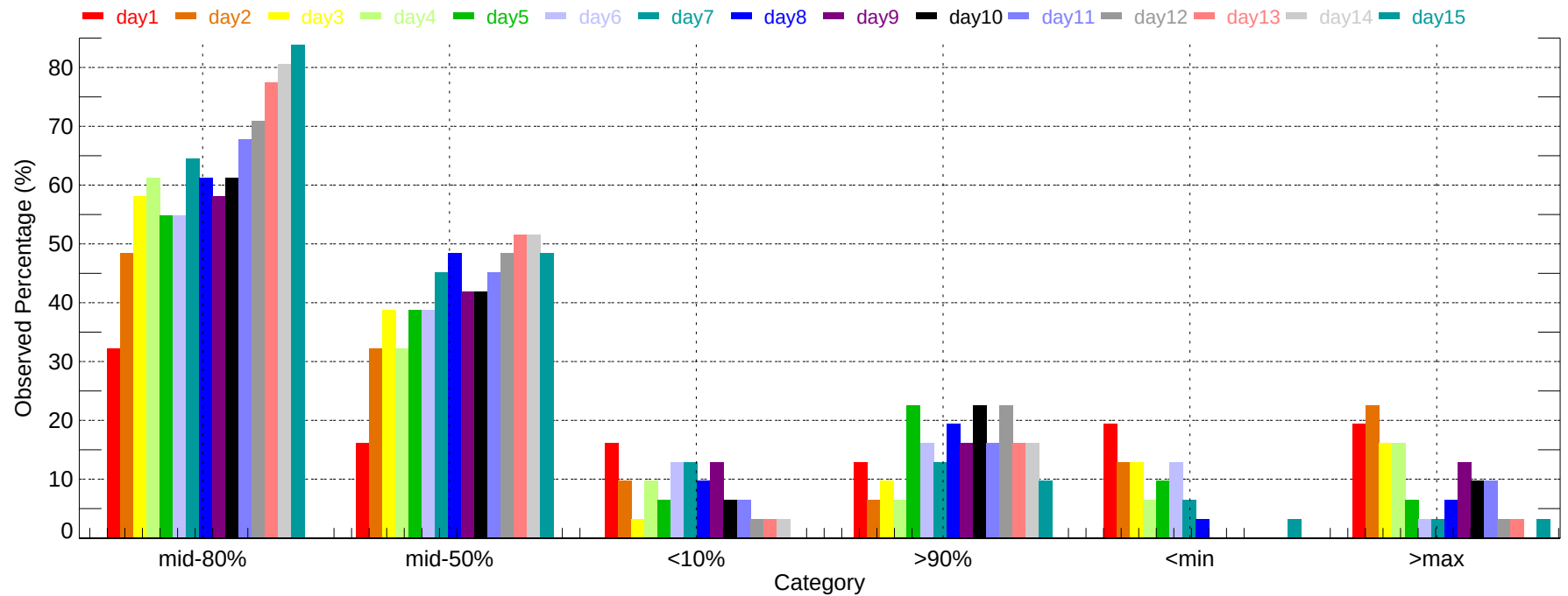
Observed Percentage of Ensembles - CMH: Max Temperature (2011-12-01~2011-12-31)
