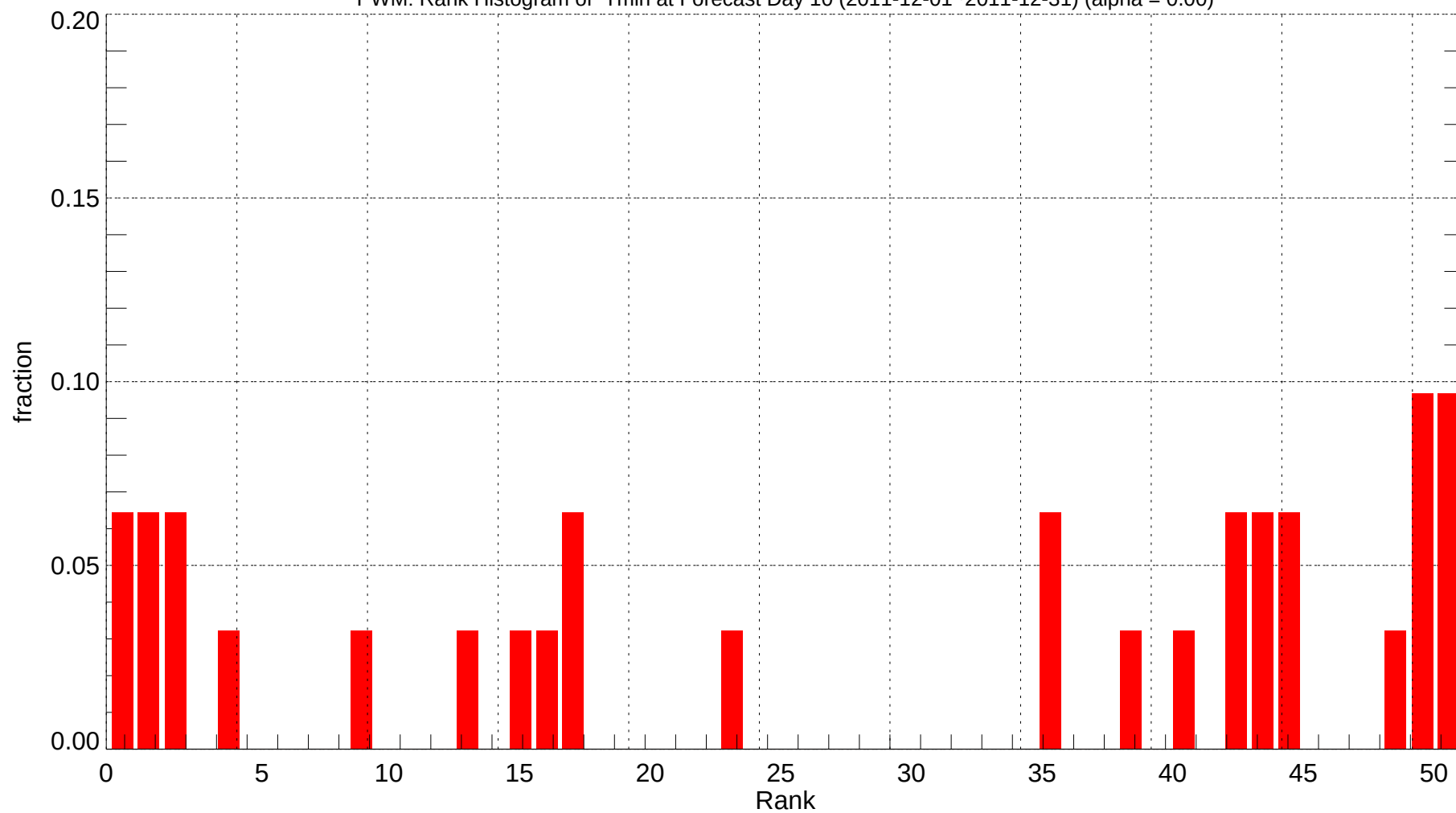
PWM: Rank Histogram of Tmin at Forecast Day 10 (2011-12-01~2011-12-31) (alpha = 0.00)
