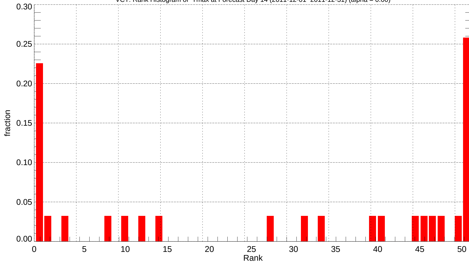
VCT: Rank Histogram of Tmax at Forecast Day 14 (2011-12-01~2011-12-31) (alpha = 0.00)
