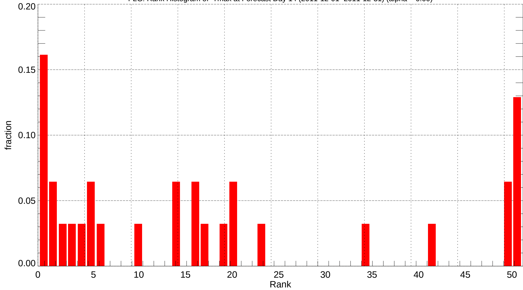
FLG: Rank Histogram of Tmax at Forecast Day 14 (2011-12-01~2011-12-31) (alpha = 0.00)
