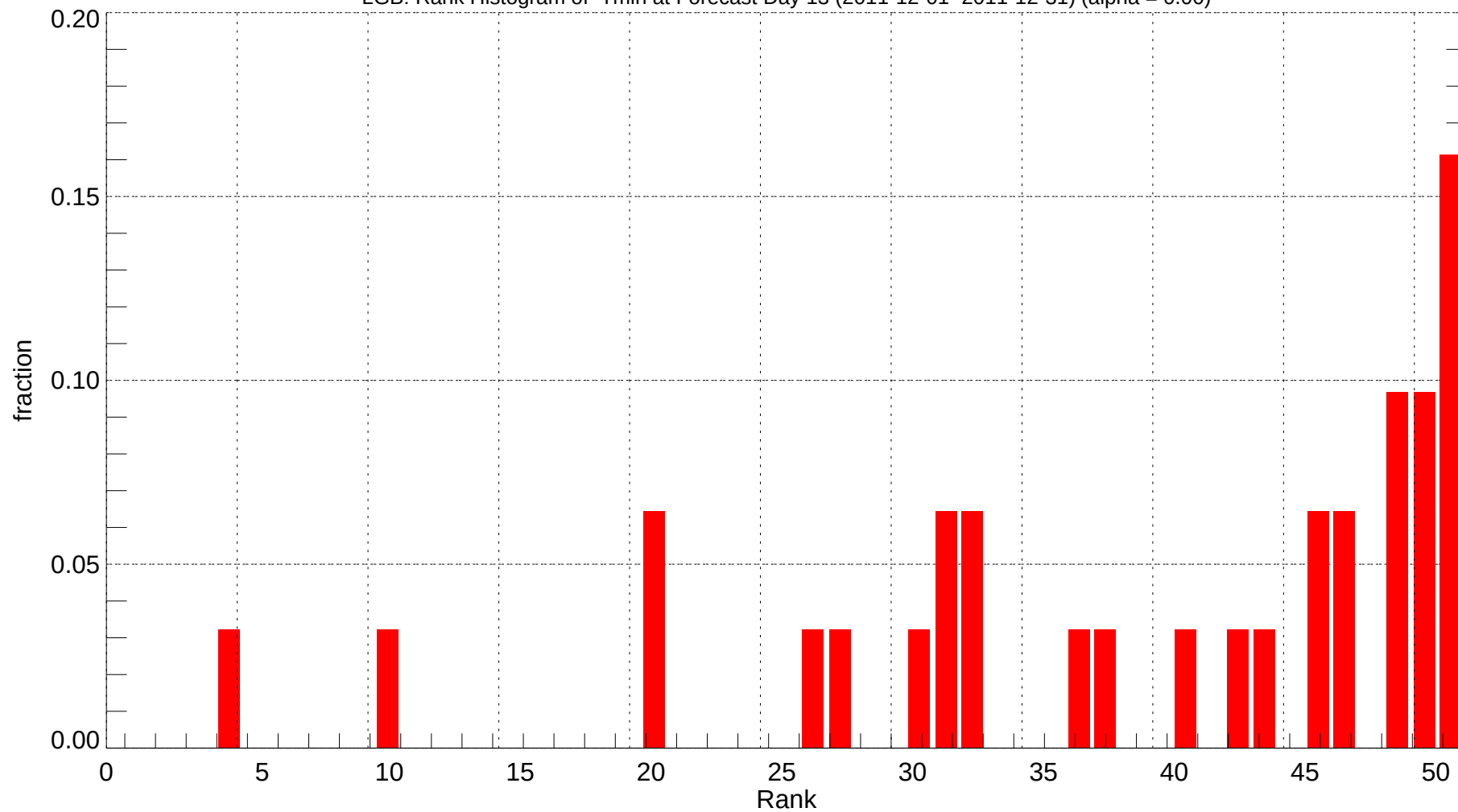
LGB: Rank Histogram of Tmin at Forecast Day 13 (2011-12-01~2011-12-31) (alpha = 0.00)
