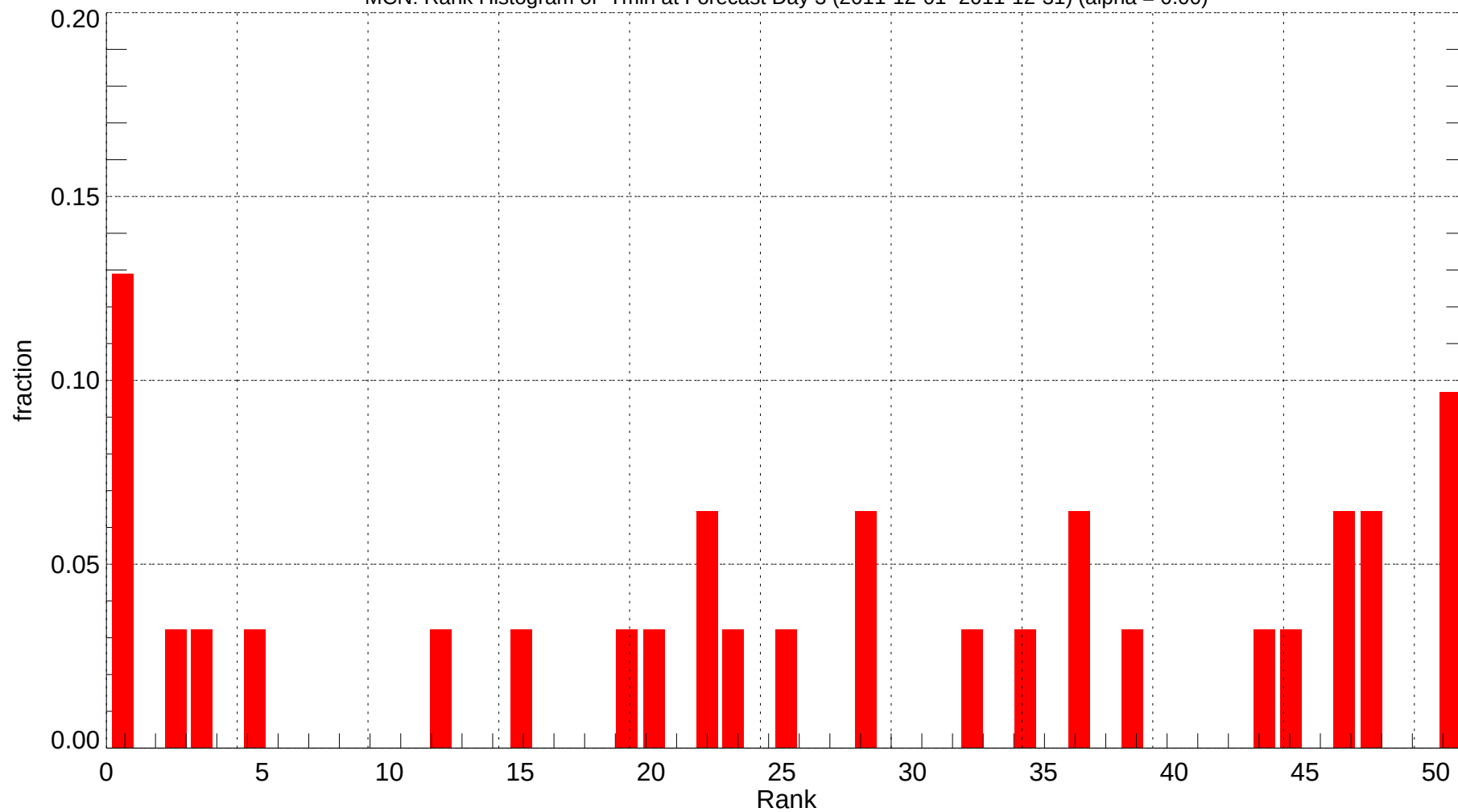
MCN: Rank Histogram of Tmin at Forecast Day 3 (2011-12-01~2011-12-31) (alpha = 0.00)
