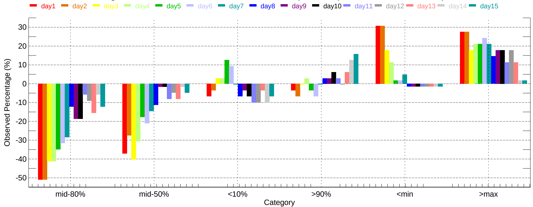
Observed Percentage Deviation of Ensembles - BHM: Max Temperature (2011-12-01~2011-12-31)
