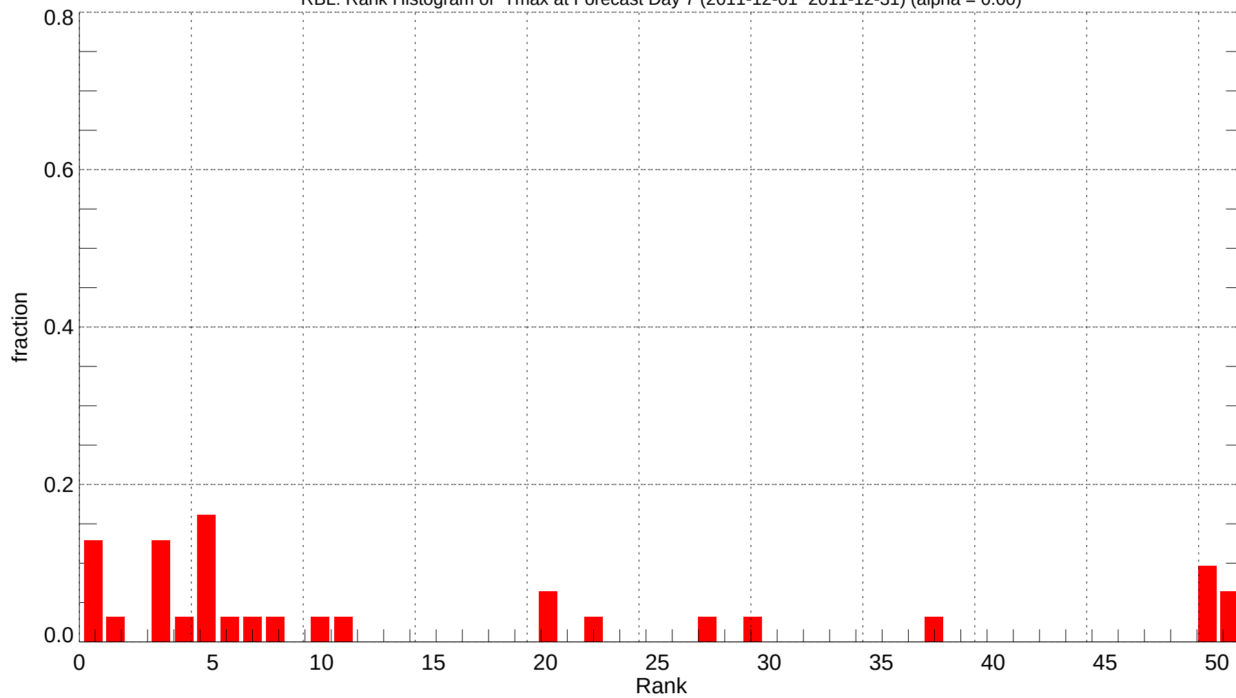
RBL: Rank Histogram of Tmax at Forecast Day 7 (2011-12-01~2011-12-31) (alpha = 0.00)
