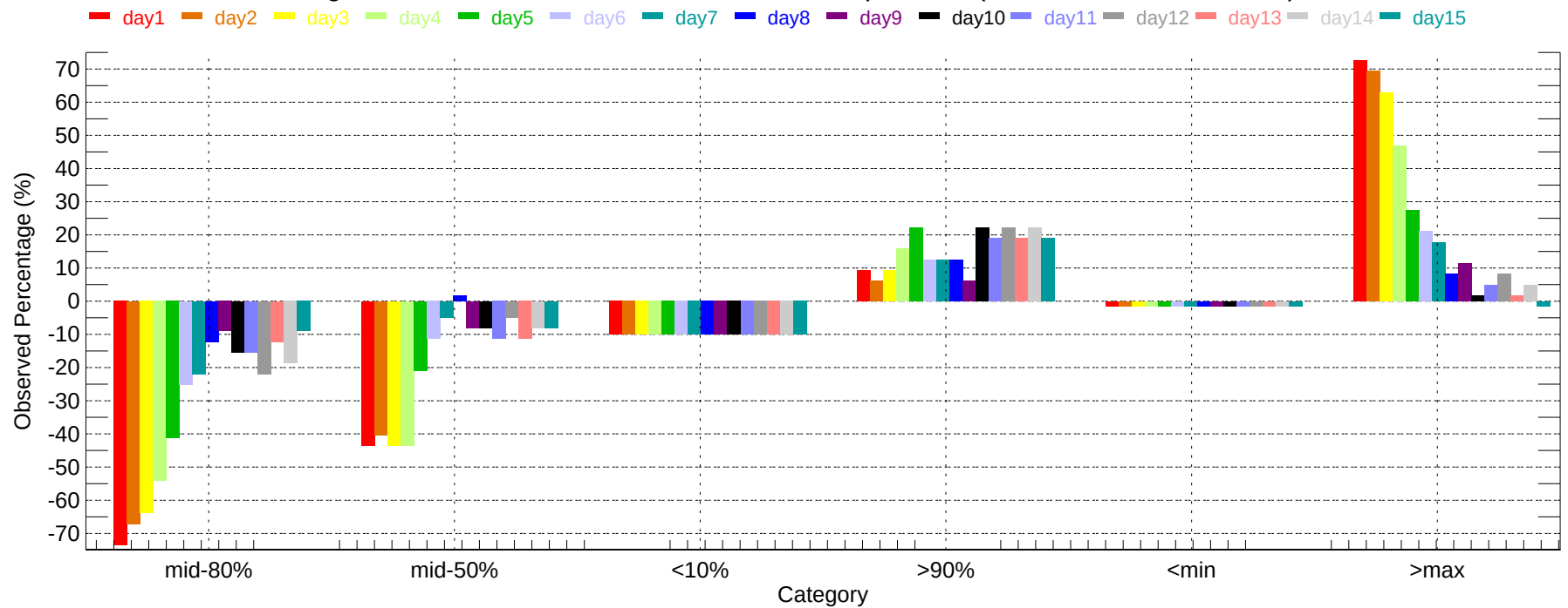
Observed Percentage Deviation of Ensembles - SAN: Min Temperature (2011-12-01~2011-12-31)
