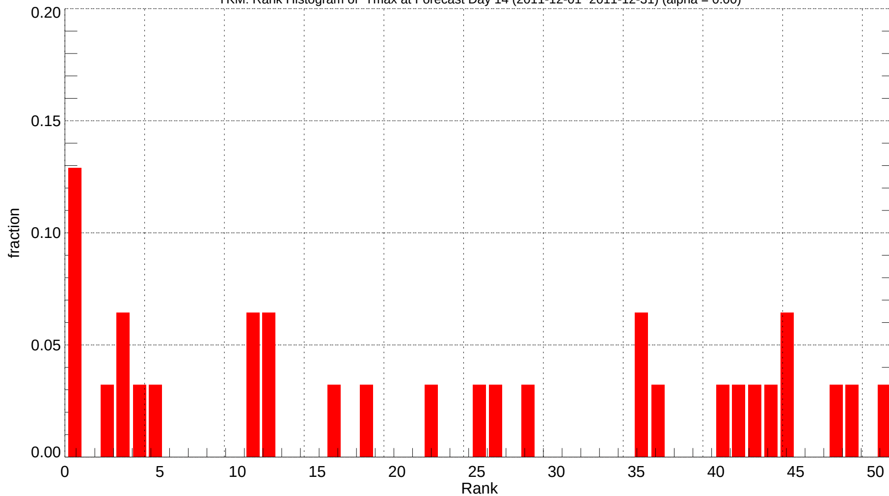
YKM: Rank Histogram of Tmax at Forecast Day 14 (2011-12-01~2011-12-31) (alpha = 0.00)
