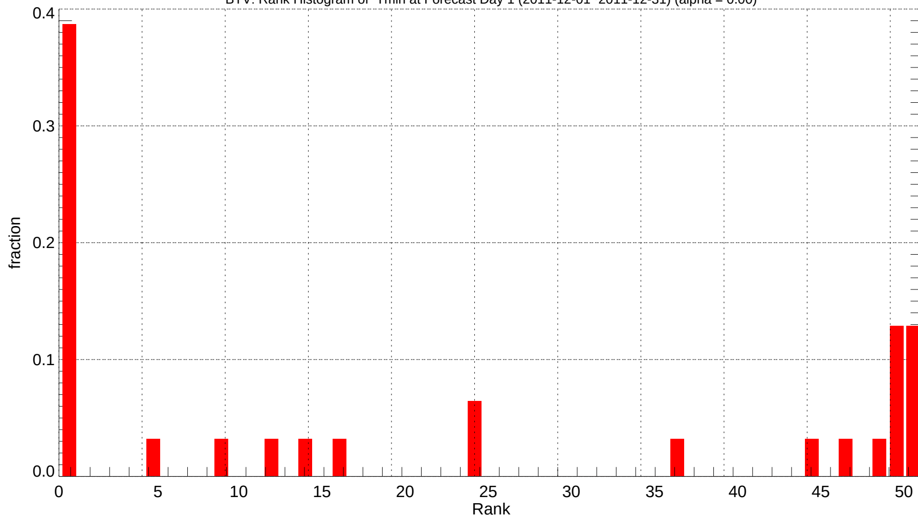
BTV: Rank Histogram of Tmin at Forecast Day 1 (2011-12-01~2011-12-31) (alpha = 0.00)
