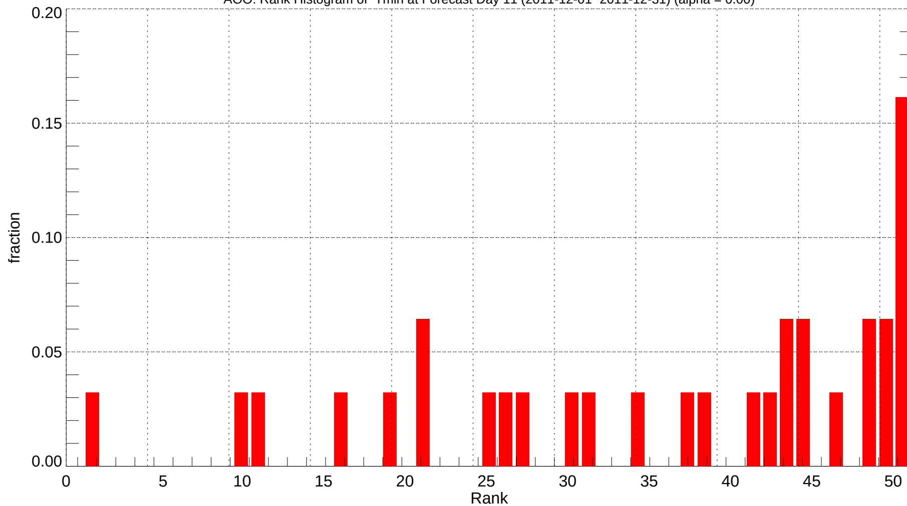
AOO: Rank Histogram of Tmin at Forecast Day 11 (2011-12-01~2011-12-31) (alpha = 0.00)
