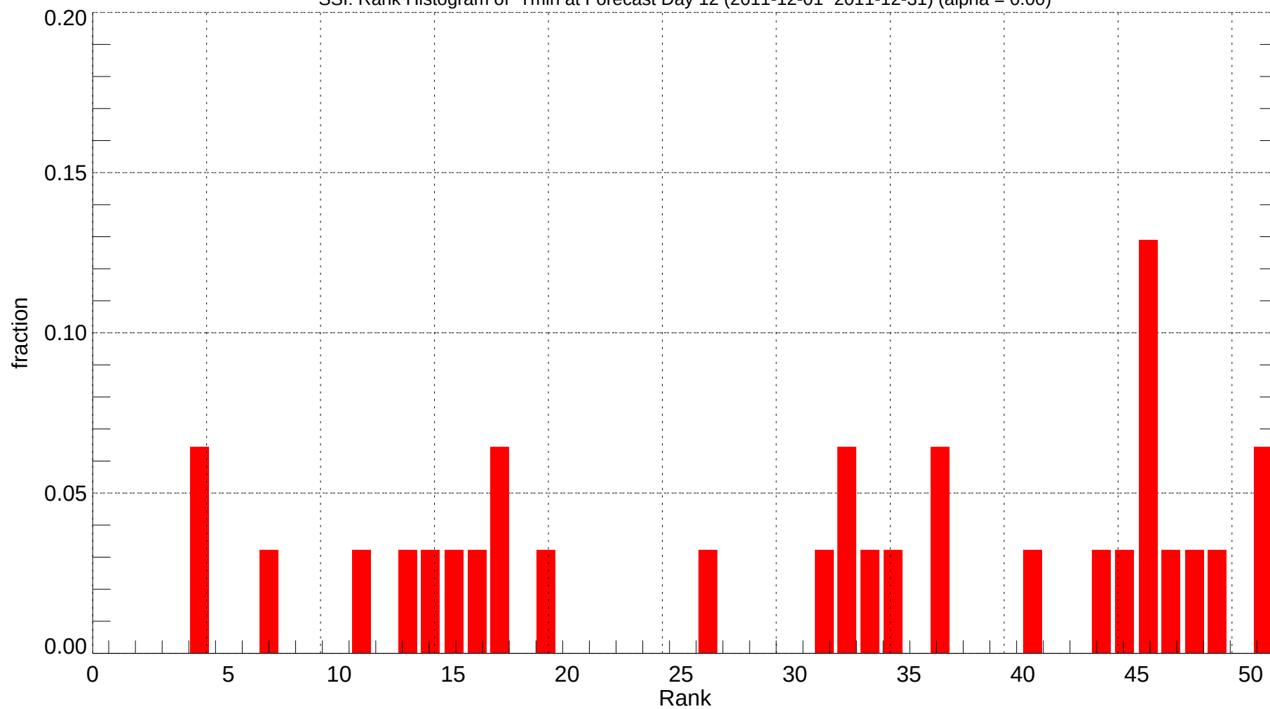
SSI: Rank Histogram of Tmin at Forecast Day 12 (2011-12-01~2011-12-31) (alpha = 0.00)
