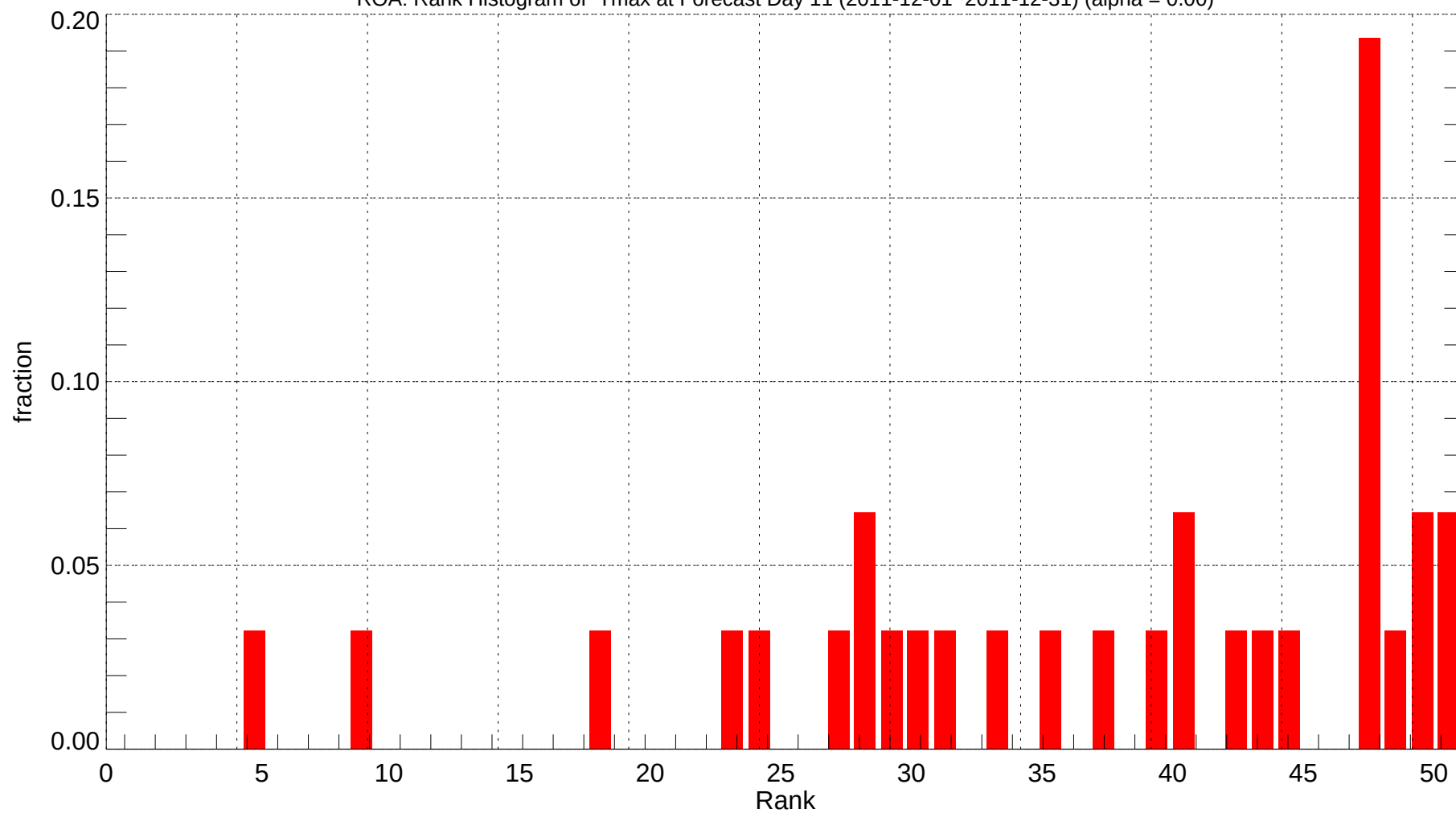
ROA: Rank Histogram of Tmax at Forecast Day 11 (2011-12-01~2011-12-31) (alpha = 0.00)
