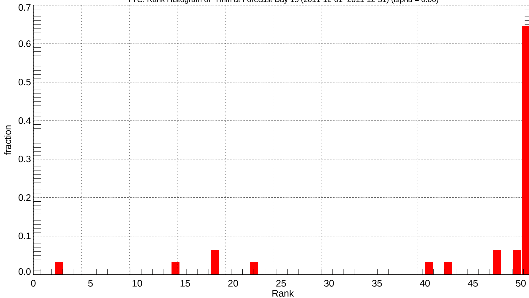
YYC: Rank Histogram of Tmin at Forecast Day 15 (2011-12-01~2011-12-31) (alpha = 0.00)
