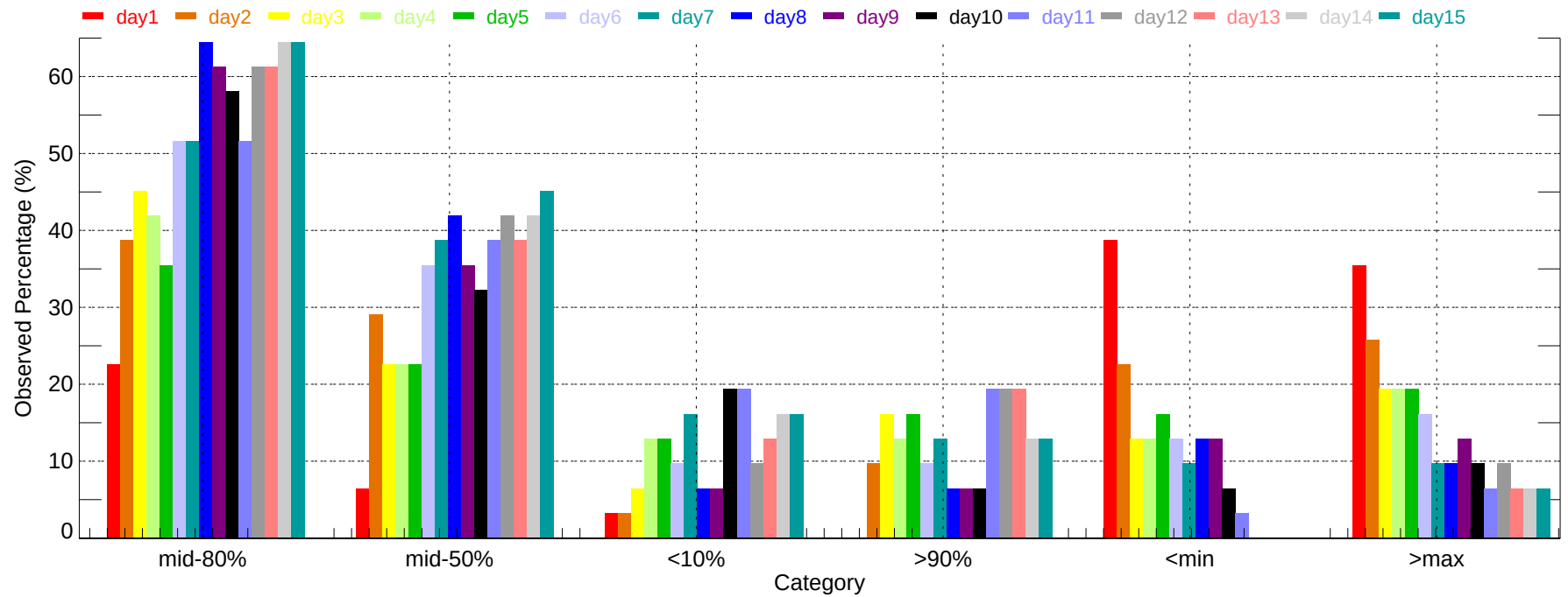
Observed Percentage of Ensembles - ABE: Min Temperature (2011-12-01~2011-12-31)
