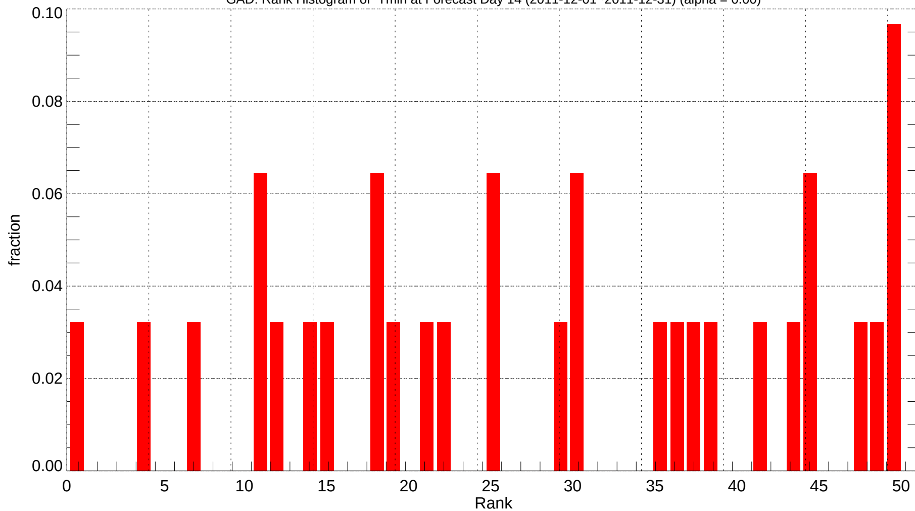
GAD: Rank Histogram of Tmin at Forecast Day 14 (2011-12-01~2011-12-31) (alpha = 0.00)
