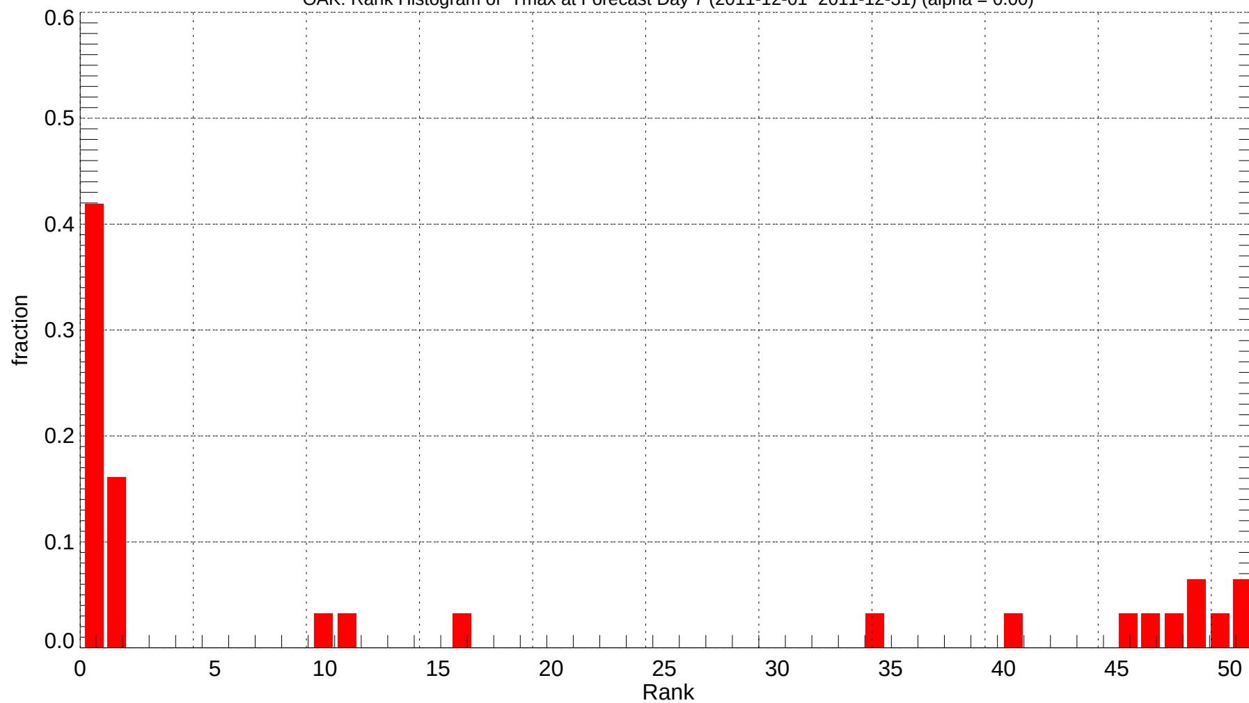
OAK: Rank Histogram of Tmax at Forecast Day 7 (2011-12-01~2011-12-31) (alpha = 0.00)
