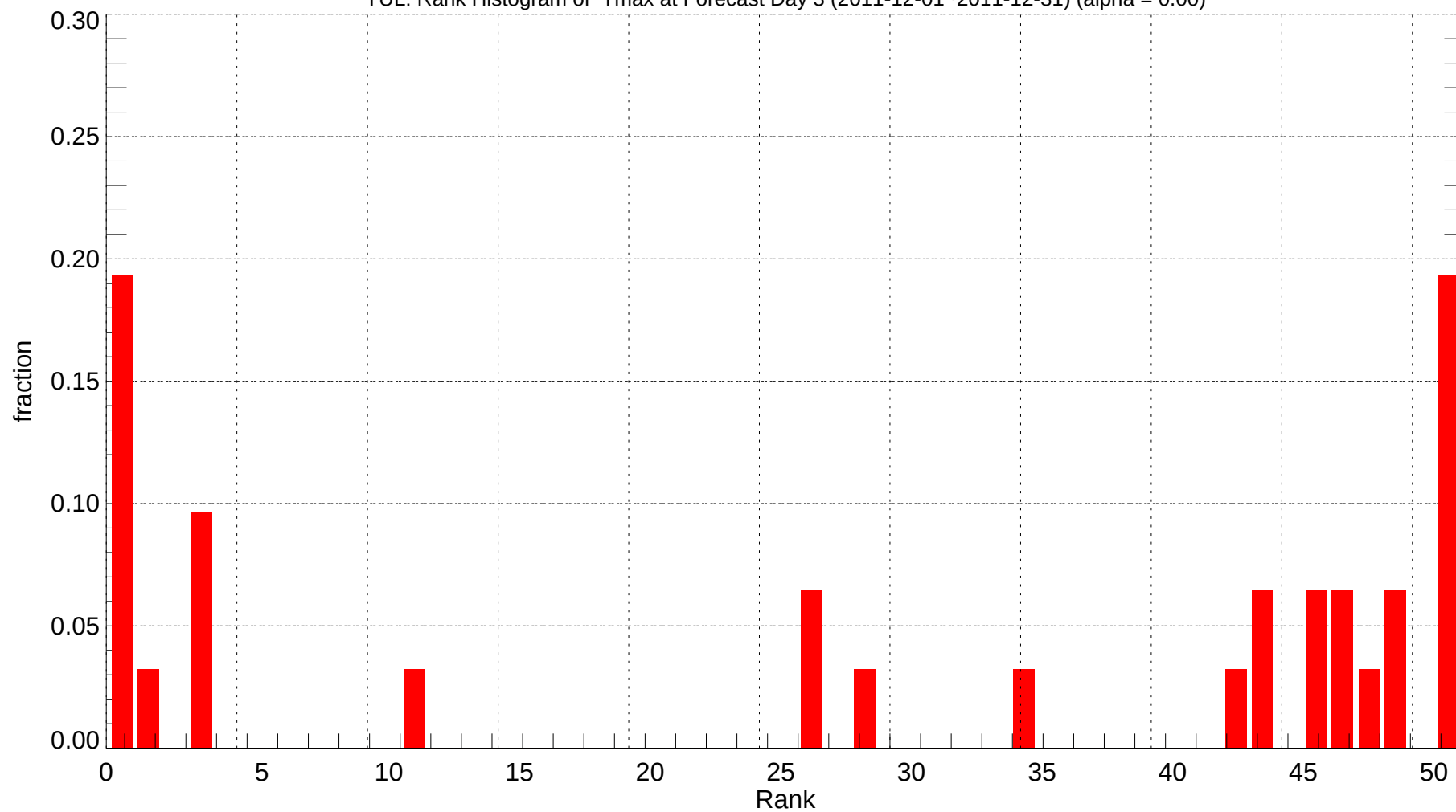
YUL: Rank Histogram of Tmax at Forecast Day 3 (2011-12-01~2011-12-31) (alpha = 0.00)
