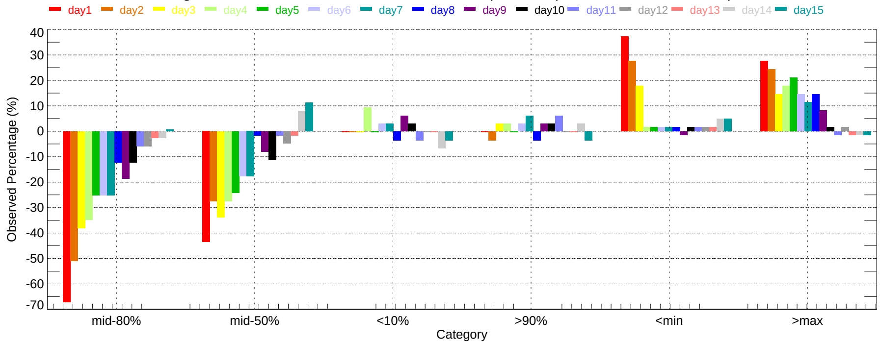
Observed Percentage Deviation of Ensembles - MWL: Min Temperature (2011-12-01~2011-12-31)
