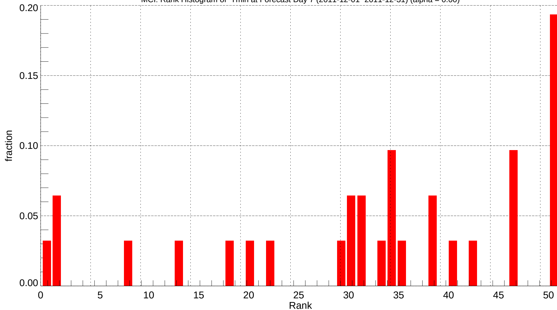
MCI: Rank Histogram of Tmin at Forecast Day 7 (2011-12-01~2011-12-31) (alpha = 0.00)
