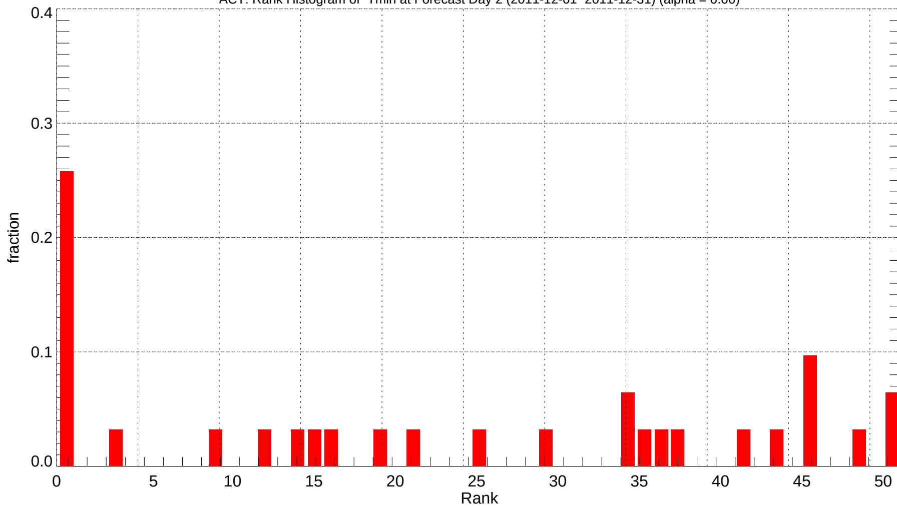
ACT: Rank Histogram of Tmin at Forecast Day 2 (2011-12-01~2011-12-31) (alpha = 0.00)
