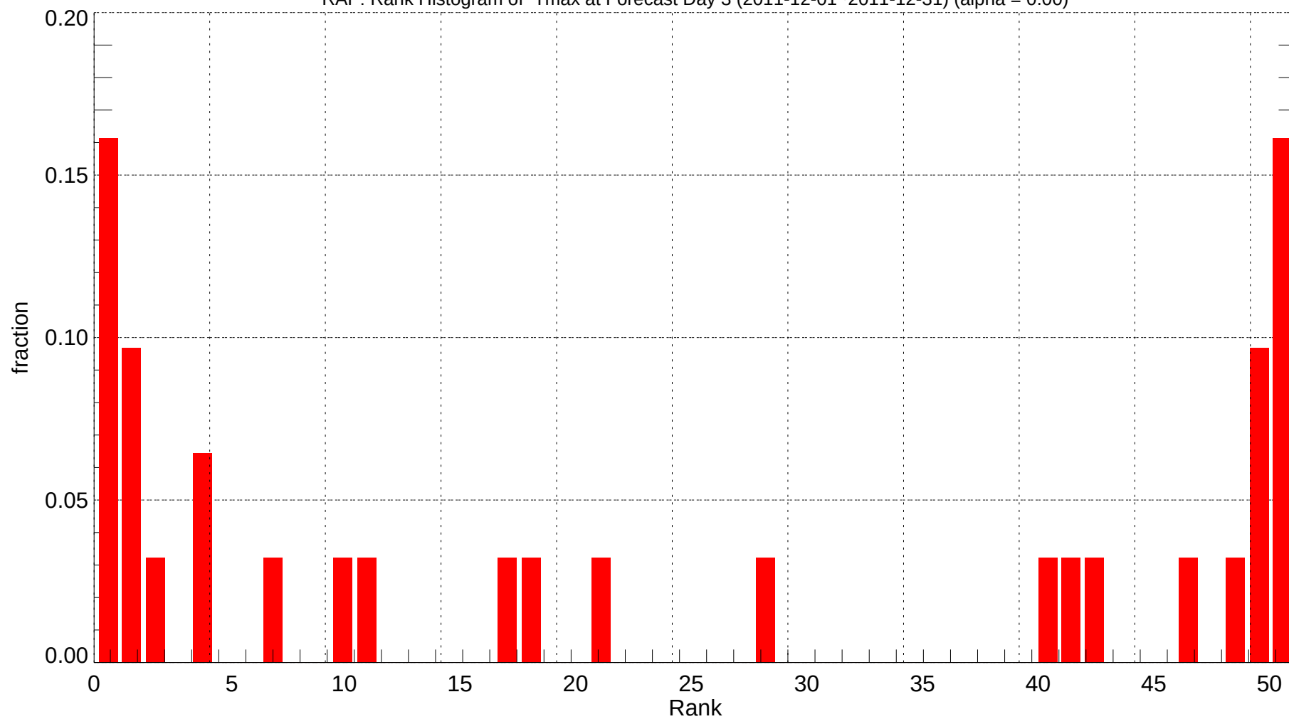
RAP: Rank Histogram of Tmax at Forecast Day 3 (2011-12-01~2011-12-31) (alpha = 0.00)
