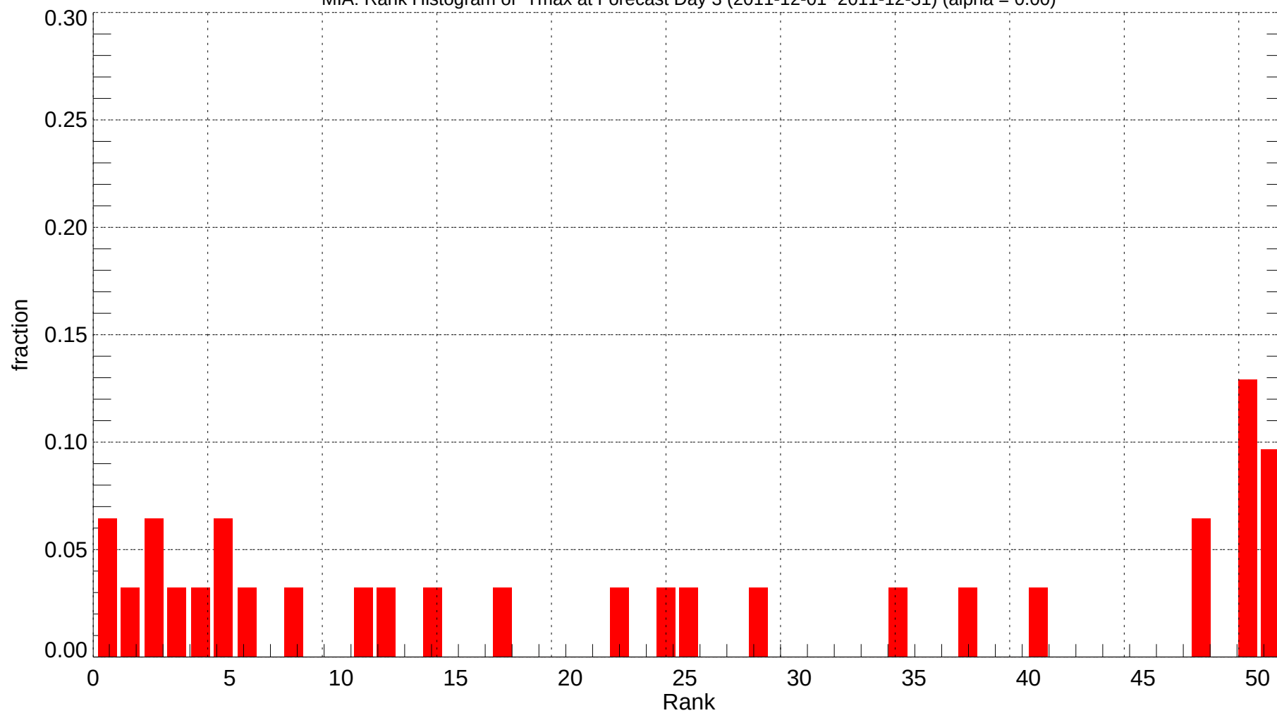
MIA: Rank Histogram of Tmax at Forecast Day 3 (2011-12-01~2011-12-31) (alpha = 0.00)
