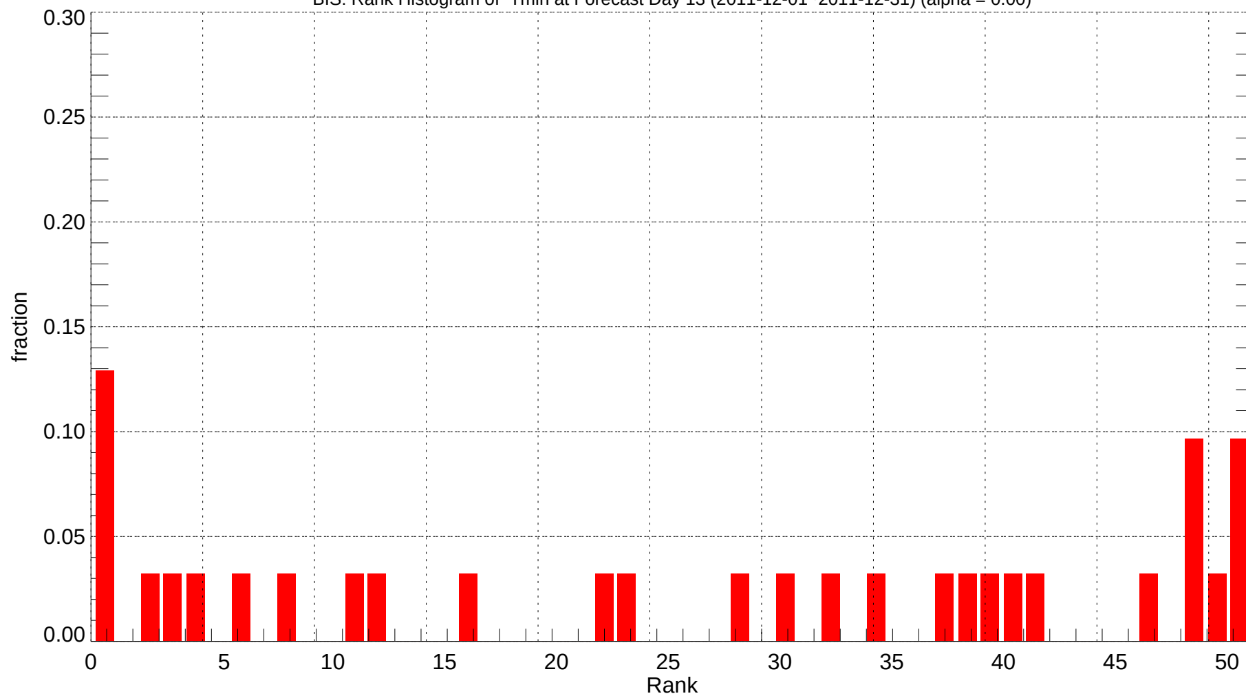
BIS: Rank Histogram of Tmin at Forecast Day 13 (2011-12-01~2011-12-31) (alpha = 0.00)
