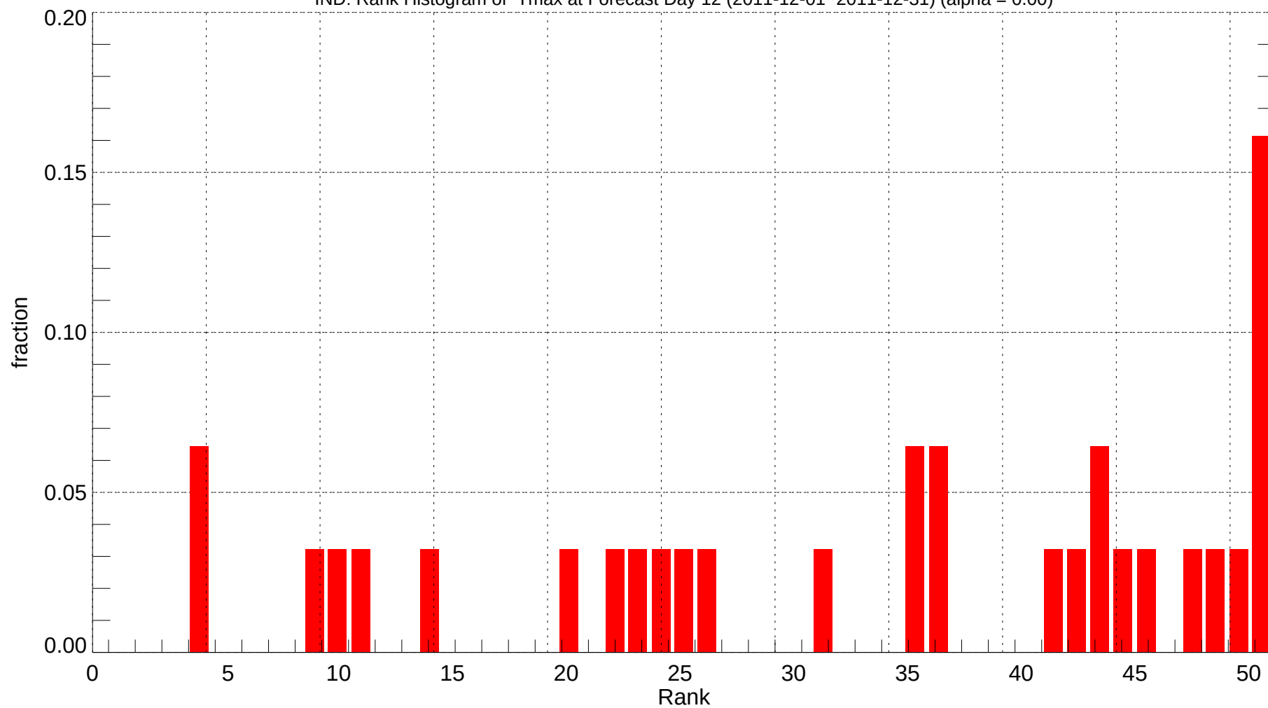
IND: Rank Histogram of Tmax at Forecast Day 12 (2011-12-01~2011-12-31) (alpha = 0.00)
