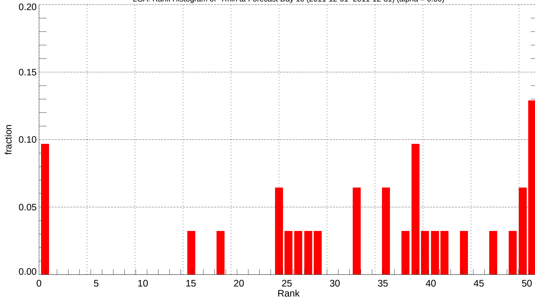
LGA: Rank Histogram of Tmin at Forecast Day 10 (2011-12-01~2011-12-31) (alpha = 0.00)
