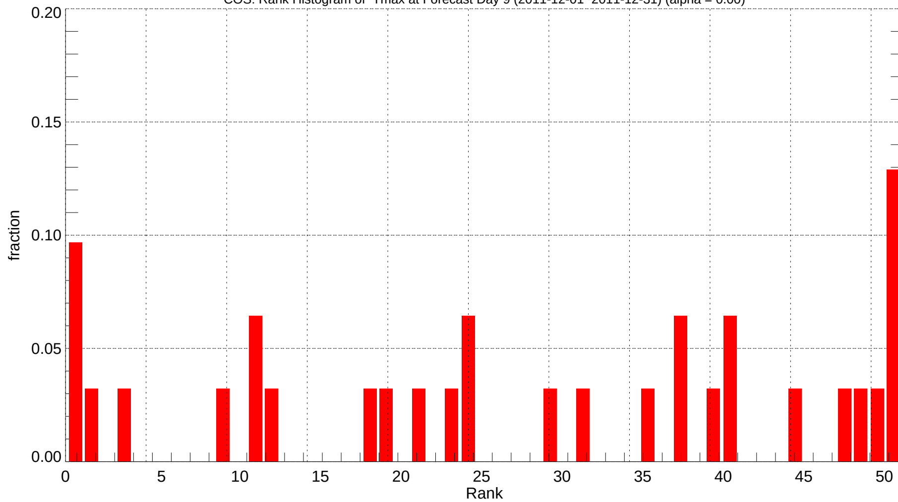
COS: Rank Histogram of Tmax at Forecast Day 9 (2011-12-01~2011-12-31) (alpha = 0.00)
