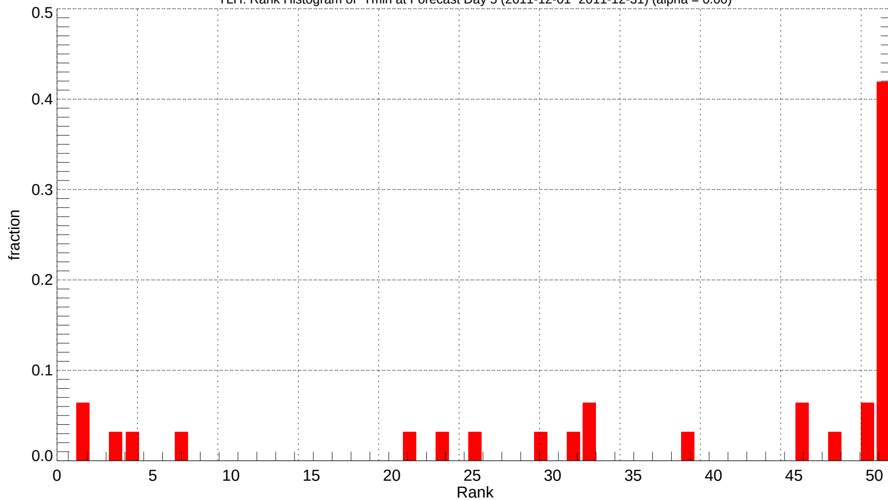
TLH: Rank Histogram of Tmin at Forecast Day 5 (2011-12-01~2011-12-31) (alpha = 0.00)
