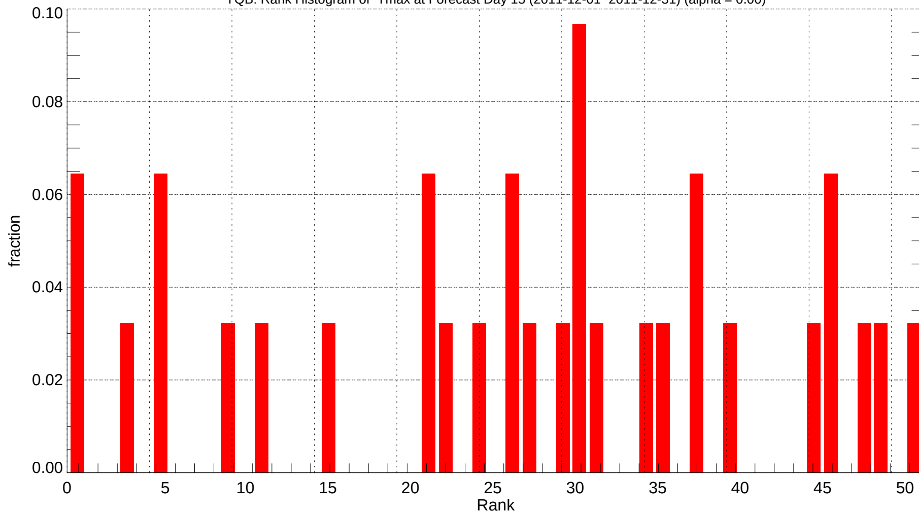
YQB: Rank Histogram of Tmax at Forecast Day 15 (2011-12-01~2011-12-31) (alpha = 0.00)
