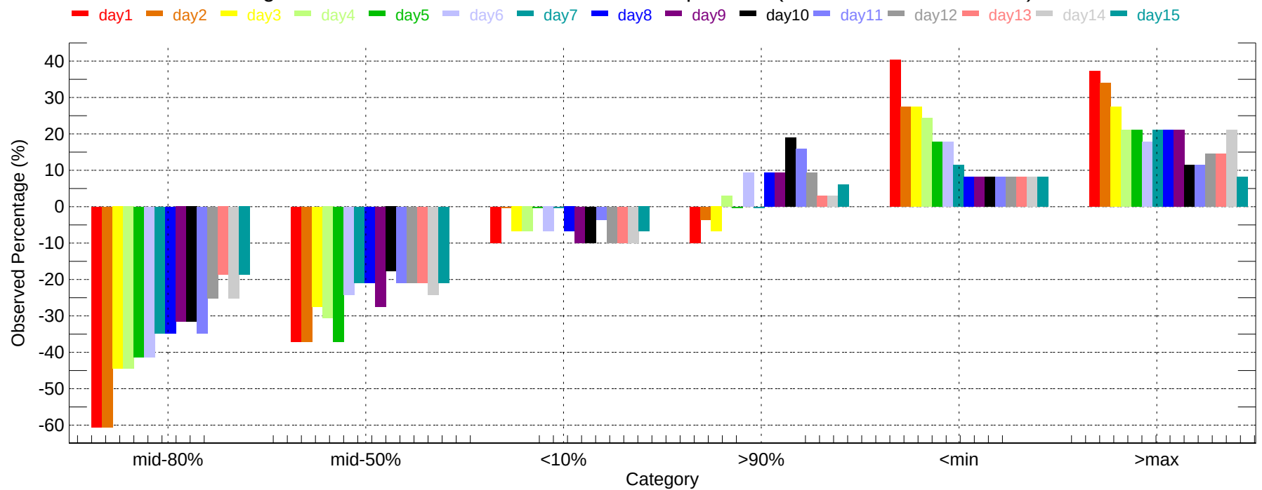
Observed Percentage Deviation of Ensembles - BIS: Min Temperature (2011-12-01~2011-12-31)
