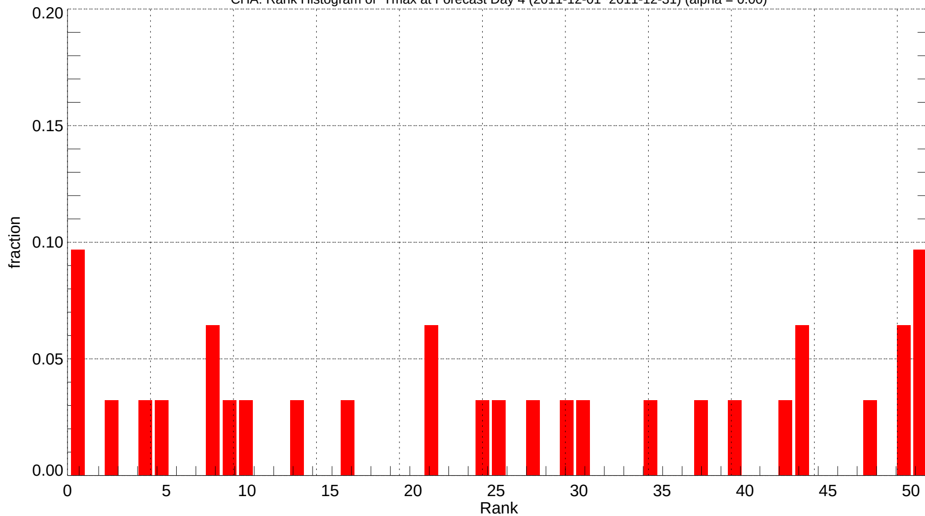
CHA: Rank Histogram of Tmax at Forecast Day 4 (2011-12-01~2011-12-31) (alpha = 0.00)
