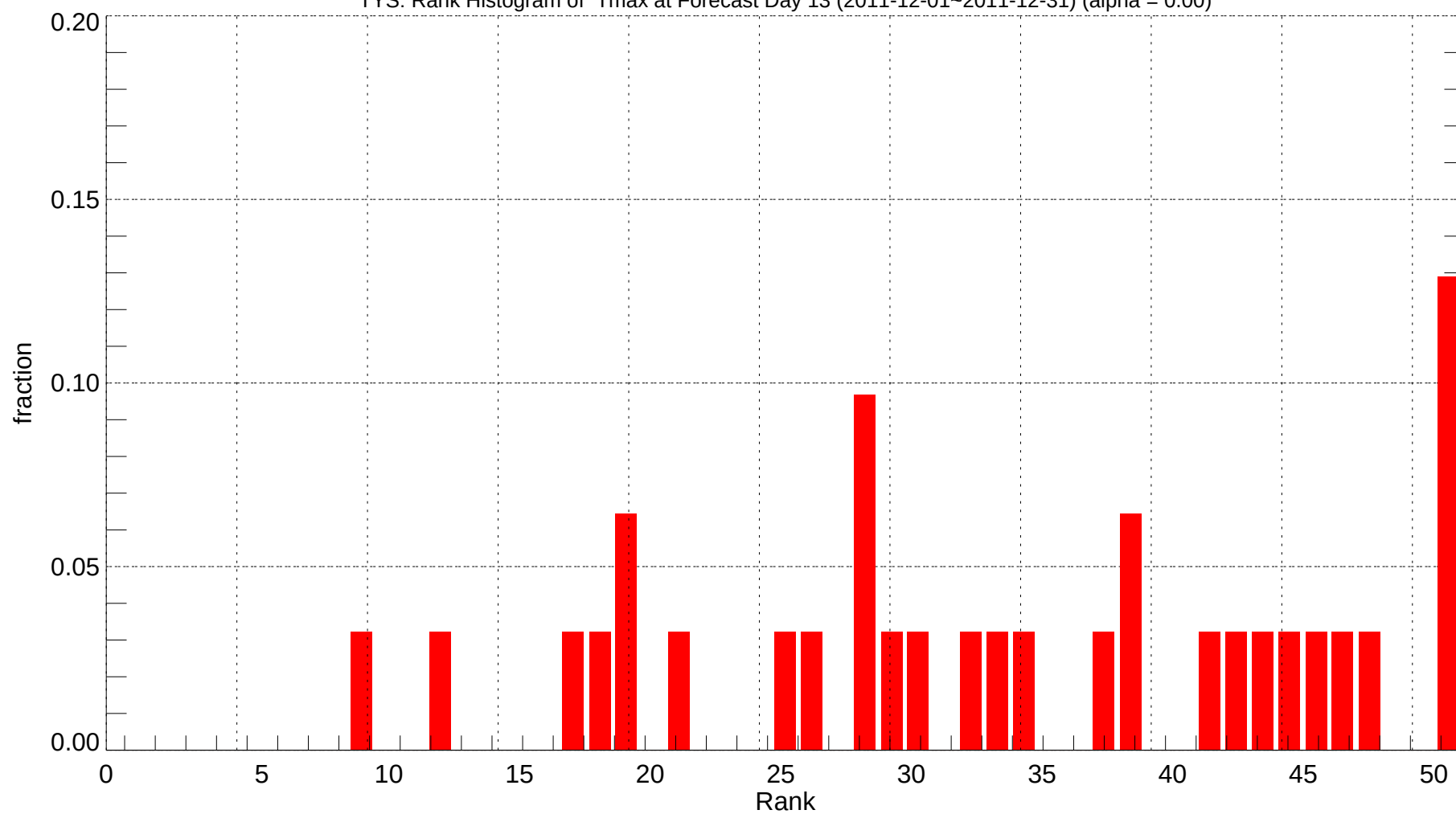
TYS: Rank Histogram of Tmax at Forecast Day 13 (2011-12-01~2011-12-31) (alpha = 0.00)
