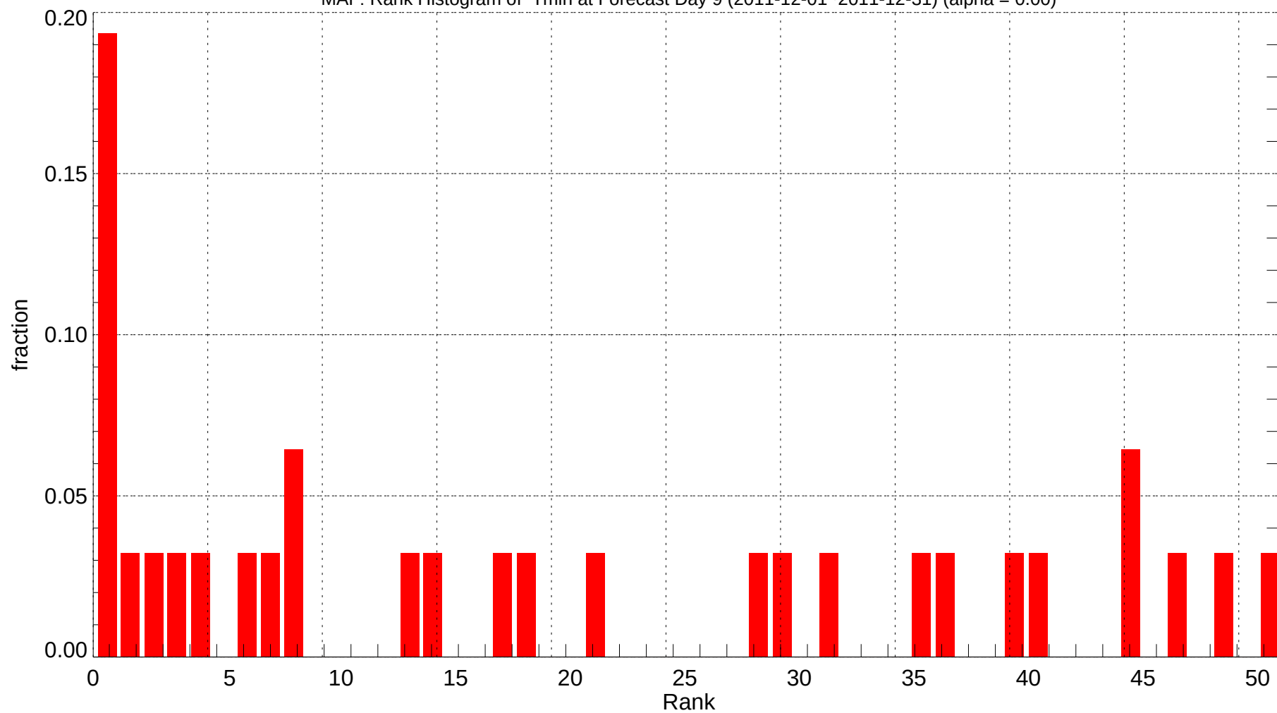
MAF: Rank Histogram of Tmin at Forecast Day 9 (2011-12-01~2011-12-31) (alpha = 0.00)
