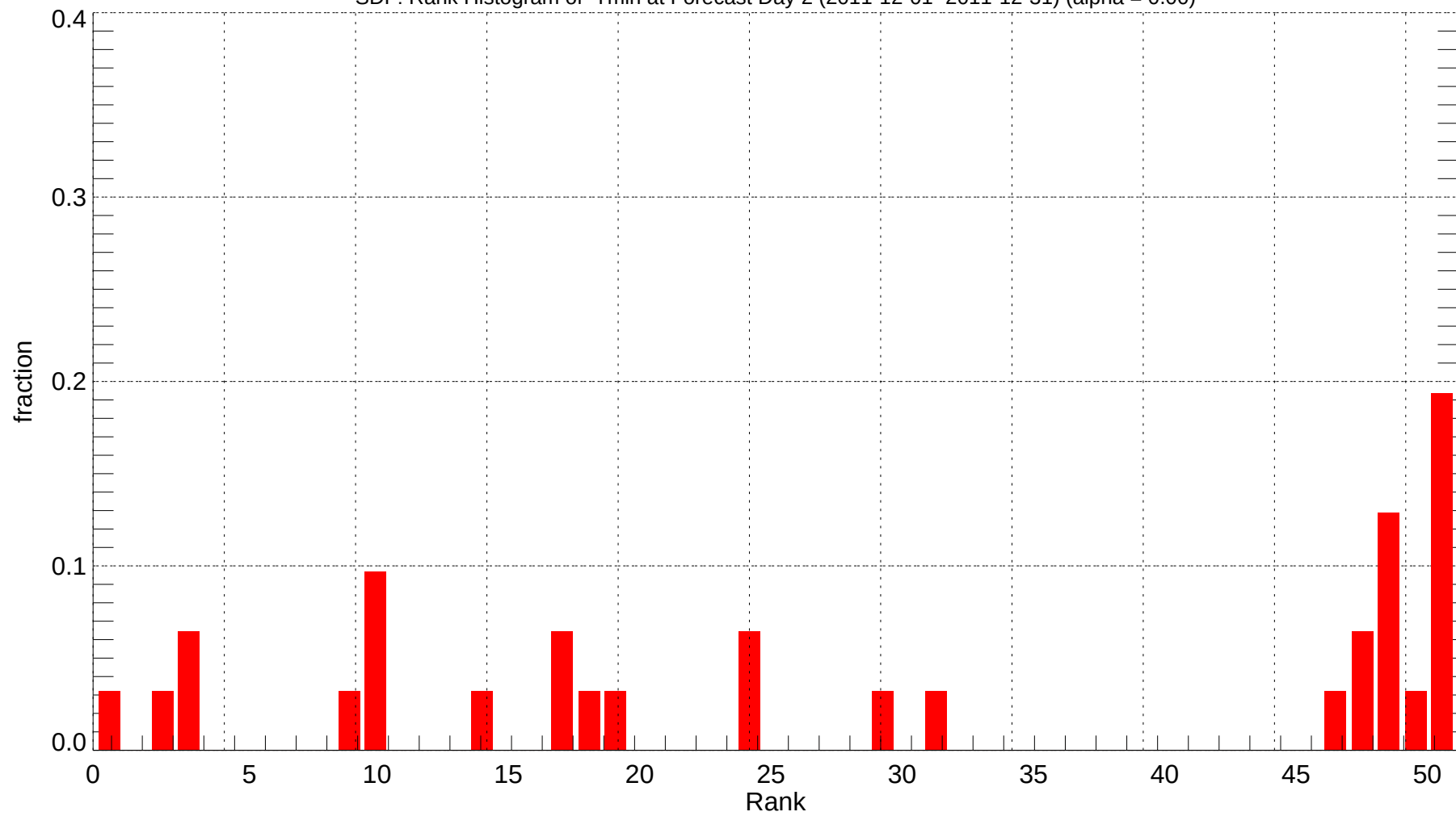
SDF: Rank Histogram of Tmin at Forecast Day 2 (2011-12-01~2011-12-31) (alpha = 0.00)
