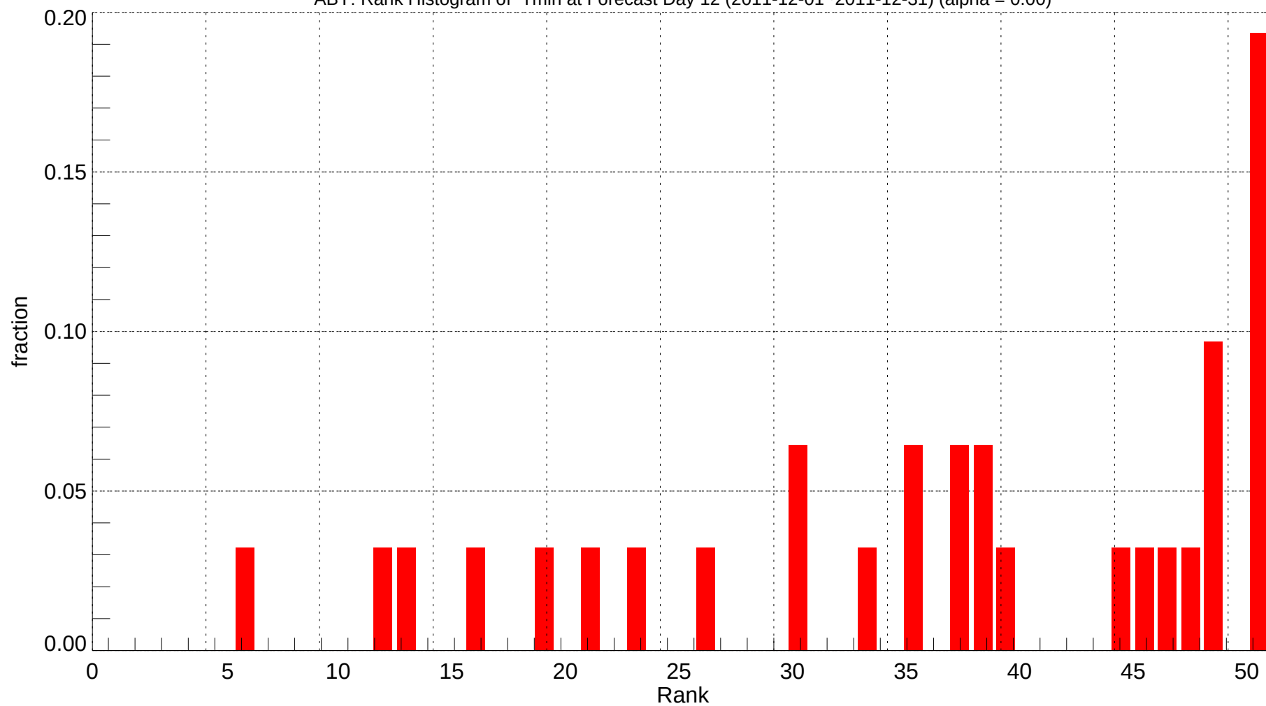
ABY: Rank Histogram of Tmin at Forecast Day 12 (2011-12-01~2011-12-31) (alpha = 0.00)
