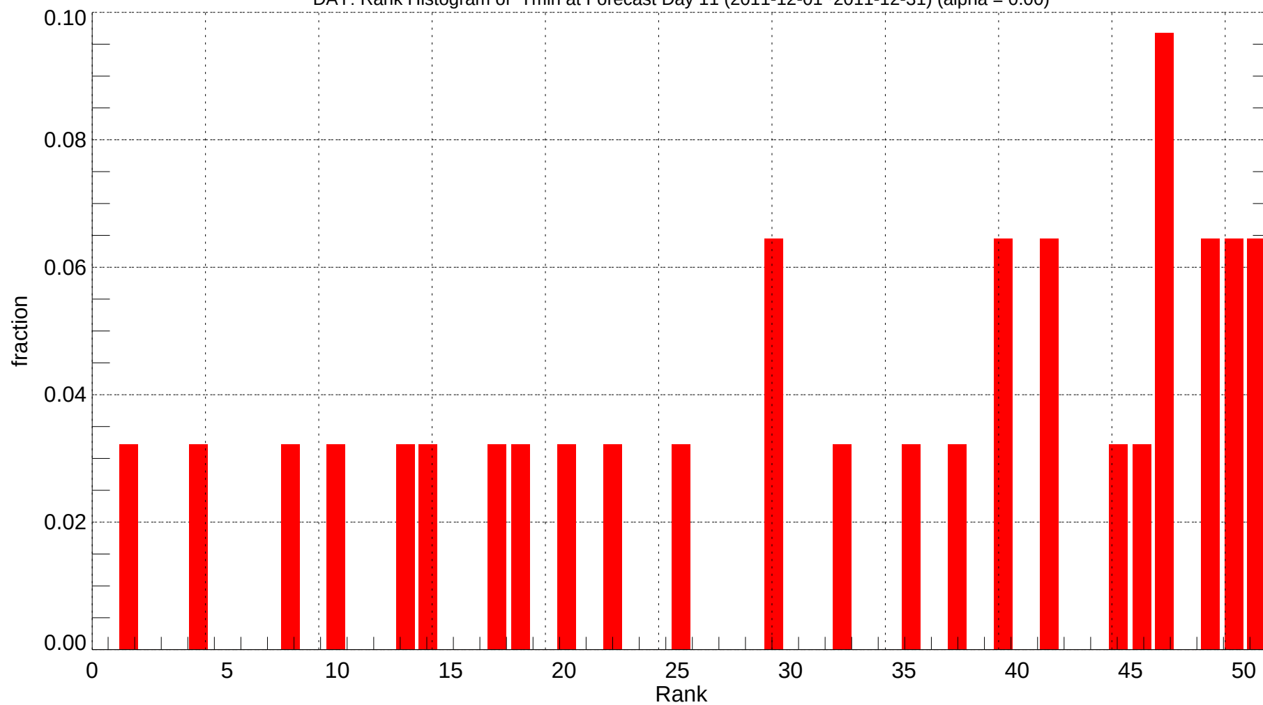
DAY: Rank Histogram of Tmin at Forecast Day 11 (2011-12-01~2011-12-31) (alpha = 0.00)
