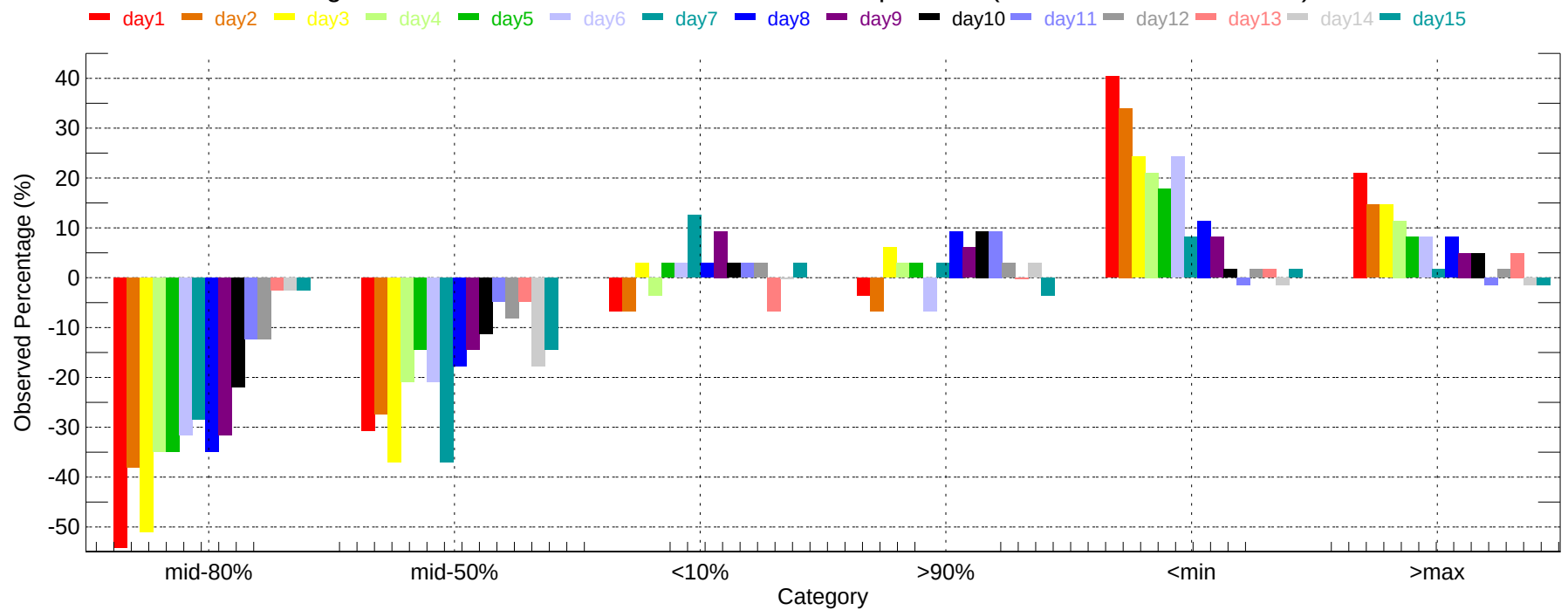
Observed Percentage Deviation of Ensembles - DTW: Max Temperature (2011-12-01~2011-12-31)
