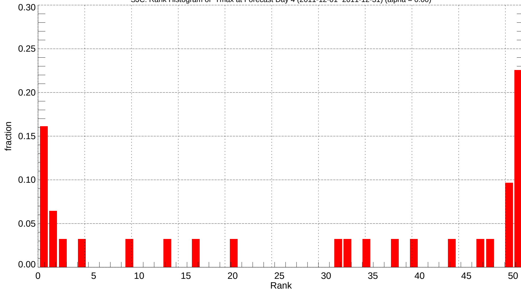
SJC: Rank Histogram of Tmax at Forecast Day 4 (2011-12-01~2011-12-31) (alpha = 0.00)
