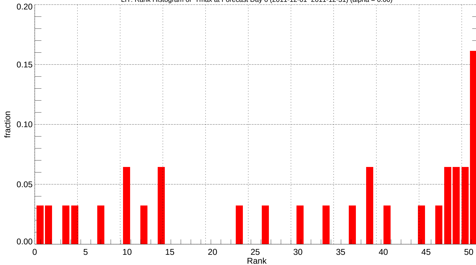
LIT: Rank Histogram of Tmax at Forecast Day 6 (2011-12-01~2011-12-31) (alpha = 0.00)
