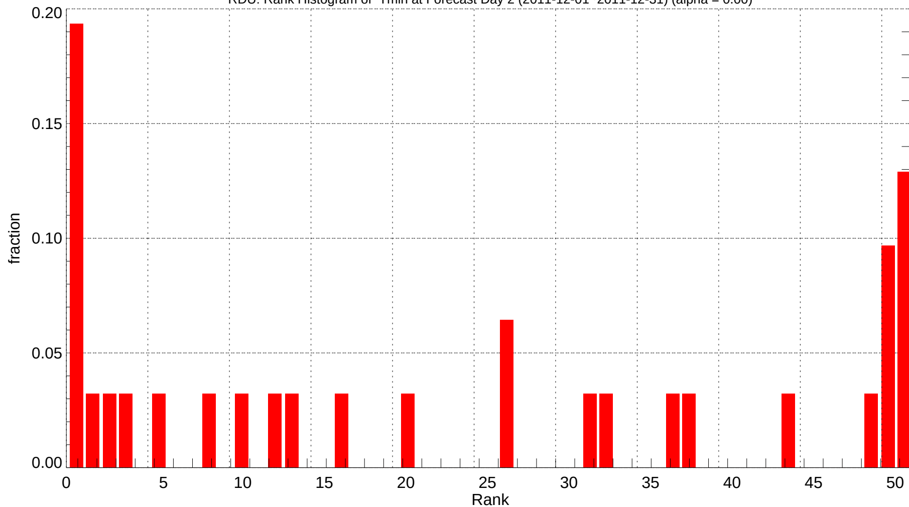
RDU: Rank Histogram of Tmin at Forecast Day 2 (2011-12-01~2011-12-31) (alpha = 0.00)
