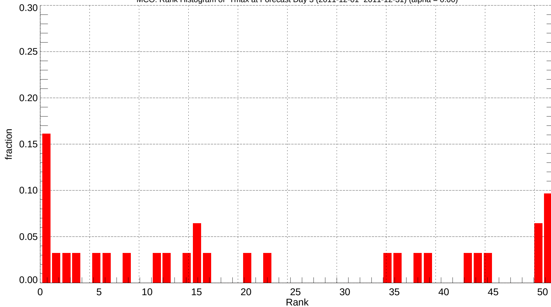
MCO: Rank Histogram of Tmax at Forecast Day 3 (2011-12-01~2011-12-31) (alpha = 0.00)
