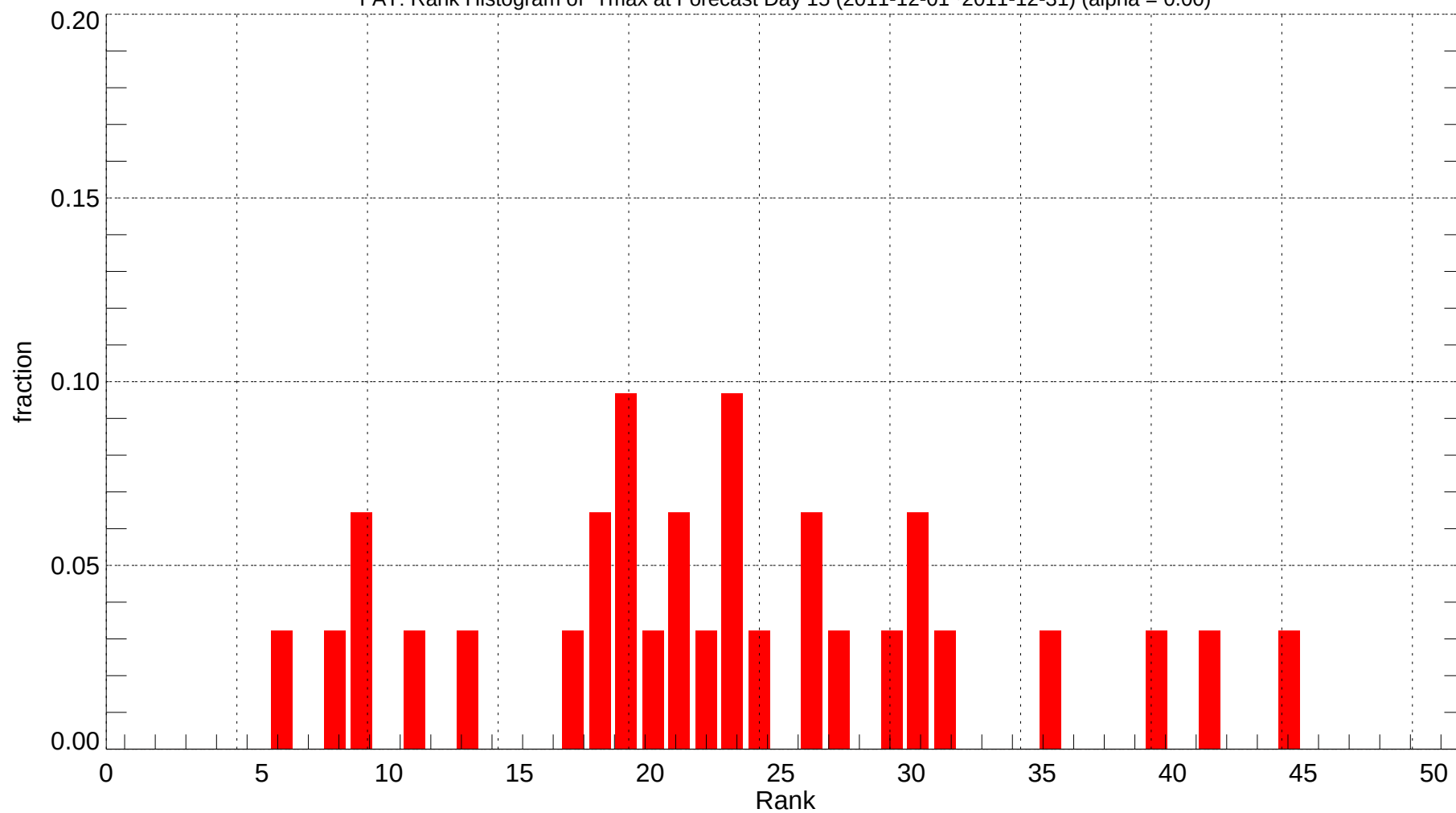
FAT: Rank Histogram of Tmax at Forecast Day 15 (2011-12-01~2011-12-31) (alpha = 0.00)
