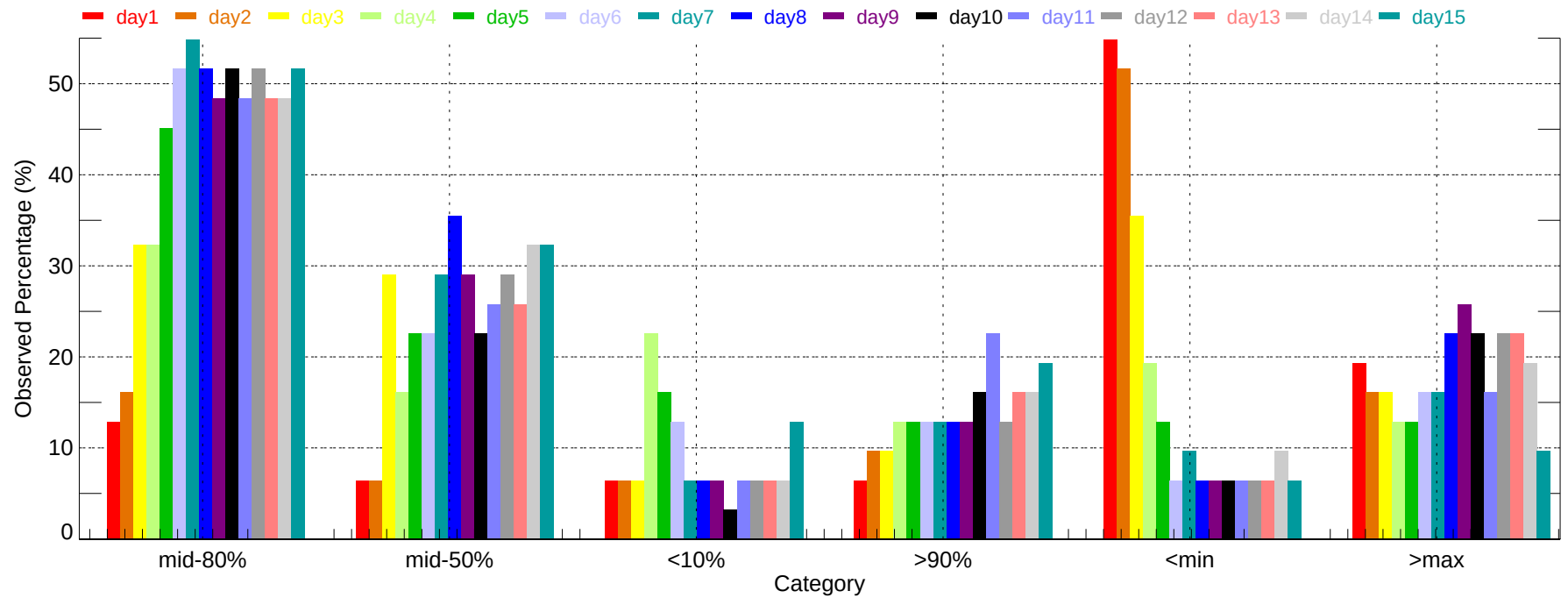
Observed Percentage of Ensembles - DLH: Min Temperature (2011-12-01~2011-12-31)
