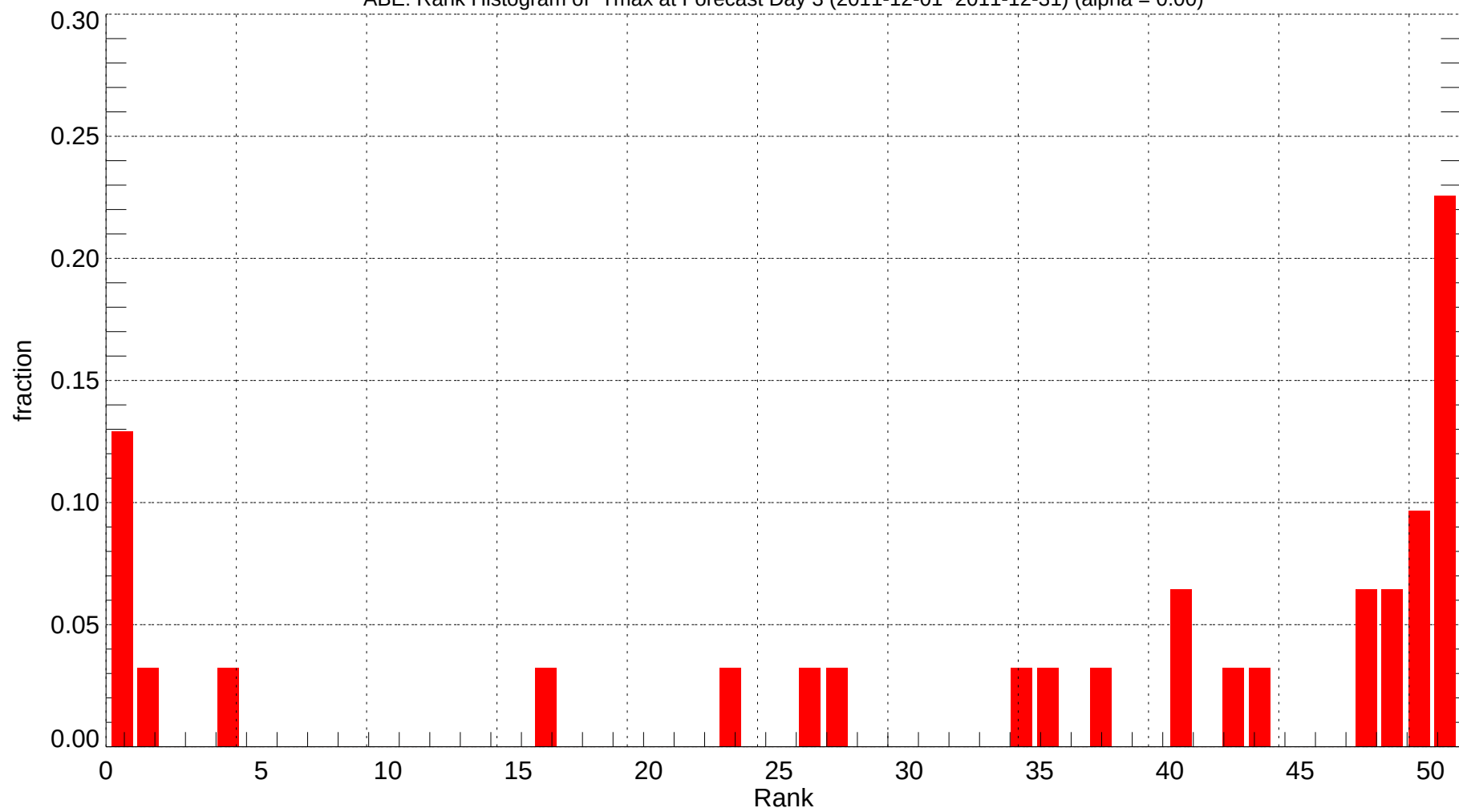
ABE: Rank Histogram of Tmax at Forecast Day 3 (2011-12-01~2011-12-31) (alpha = 0.00)
