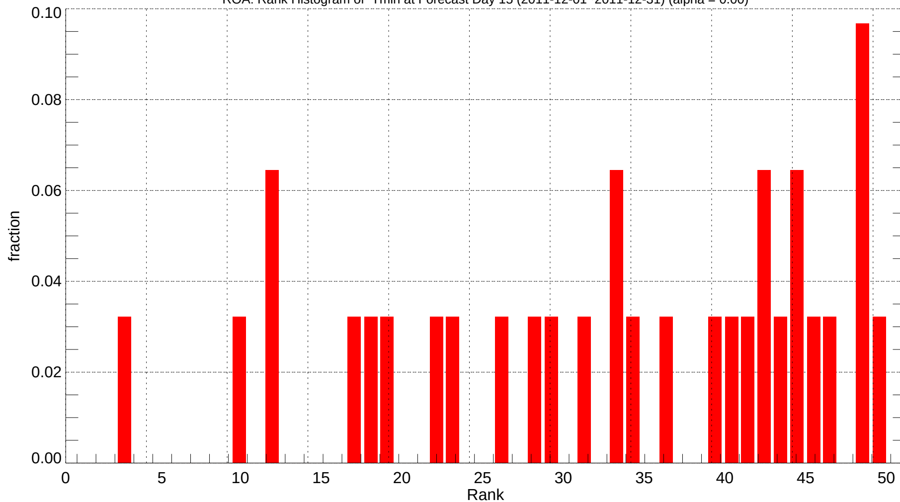
ROA: Rank Histogram of Tmin at Forecast Day 15 (2011-12-01~2011-12-31) (alpha = 0.00)
