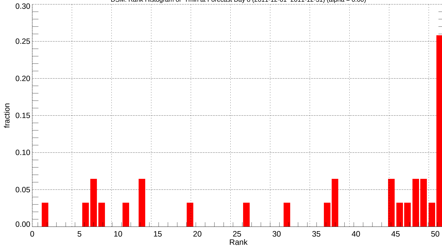
DSM: Rank Histogram of Tmin at Forecast Day 8 (2011-12-01~2011-12-31) (alpha = 0.00)
