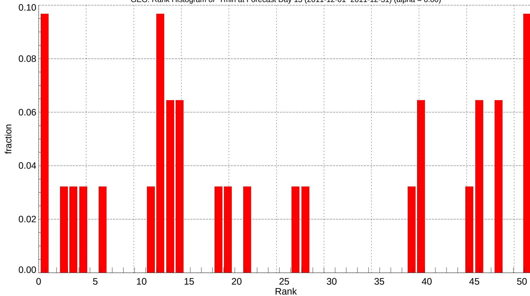
GEG: Rank Histogram of Tmin at Forecast Day 13 (2011-12-01~2011-12-31) (alpha = 0.00)
