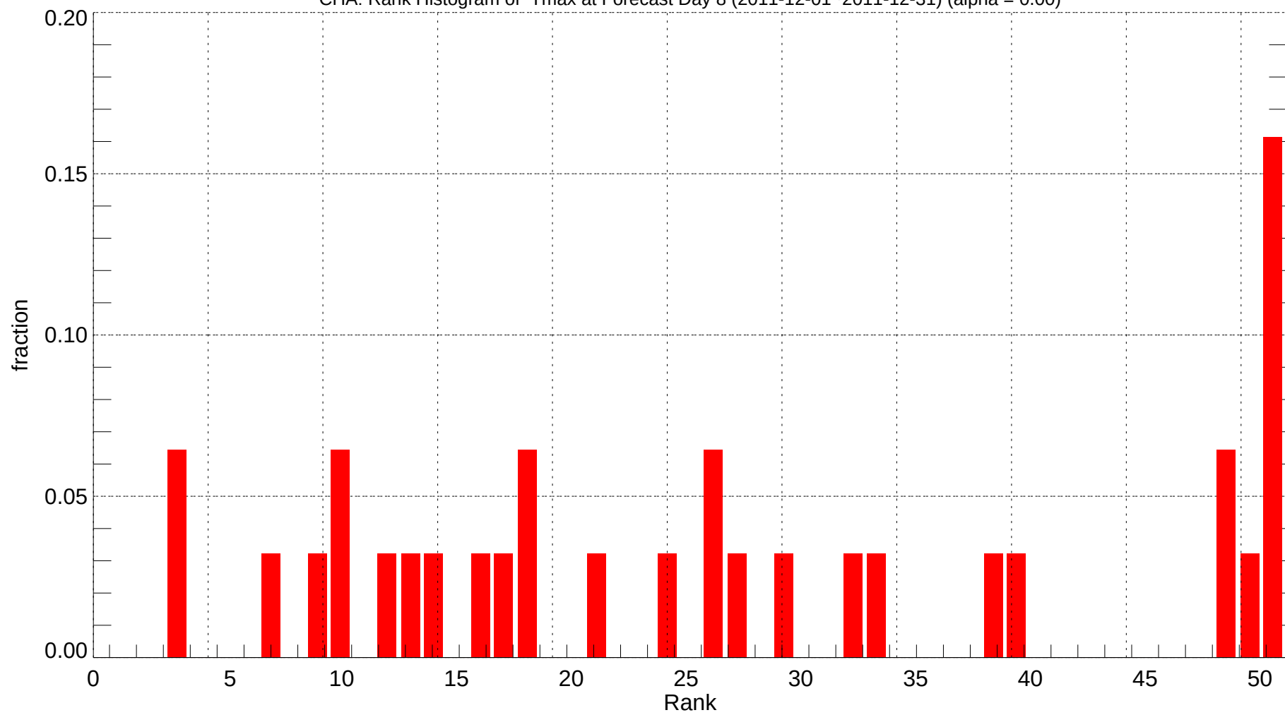
CHA: Rank Histogram of Tmax at Forecast Day 8 (2011-12-01~2011-12-31) (alpha = 0.00)
