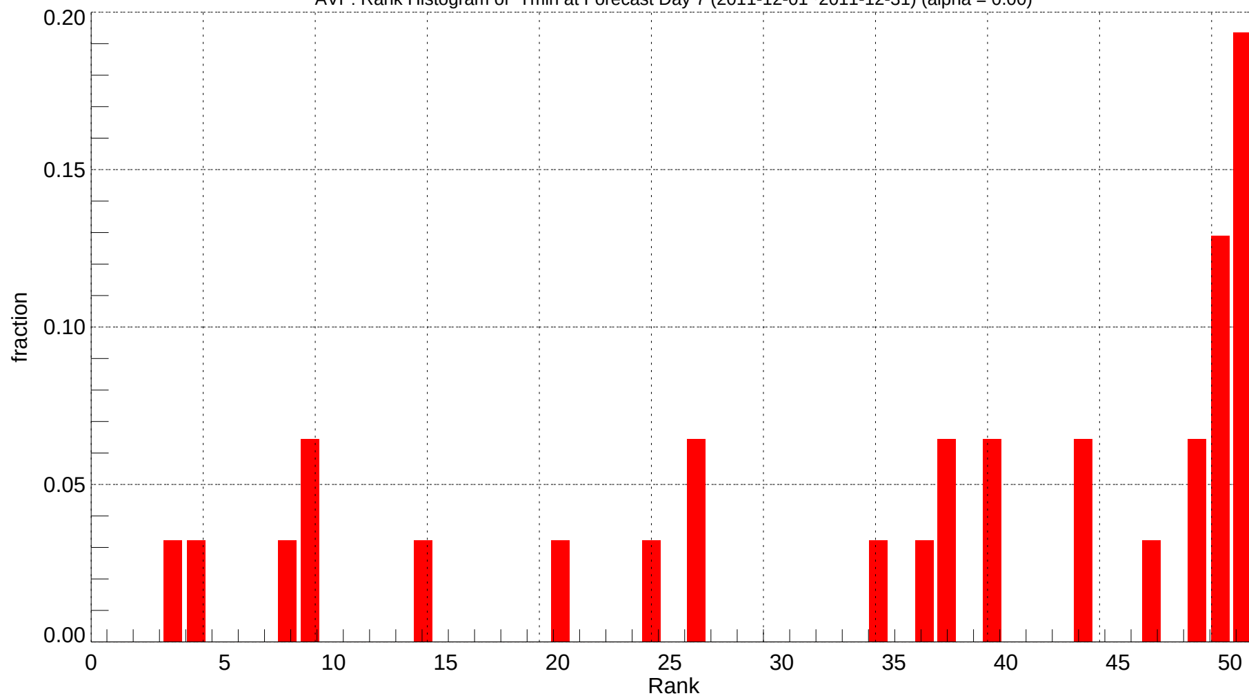
AVP: Rank Histogram of Tmin at Forecast Day 7 (2011-12-01~2011-12-31) (alpha = 0.00)
