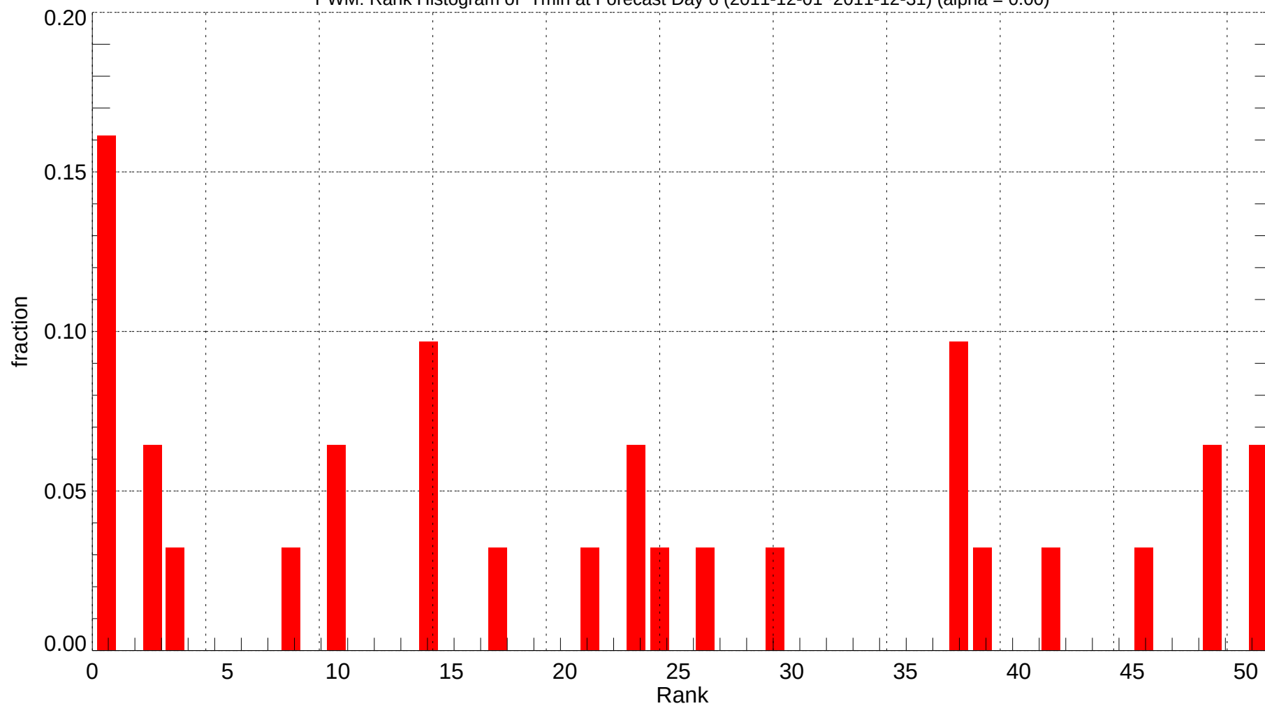
PWM: Rank Histogram of Tmin at Forecast Day 6 (2011-12-01~2011-12-31) (alpha = 0.00)
