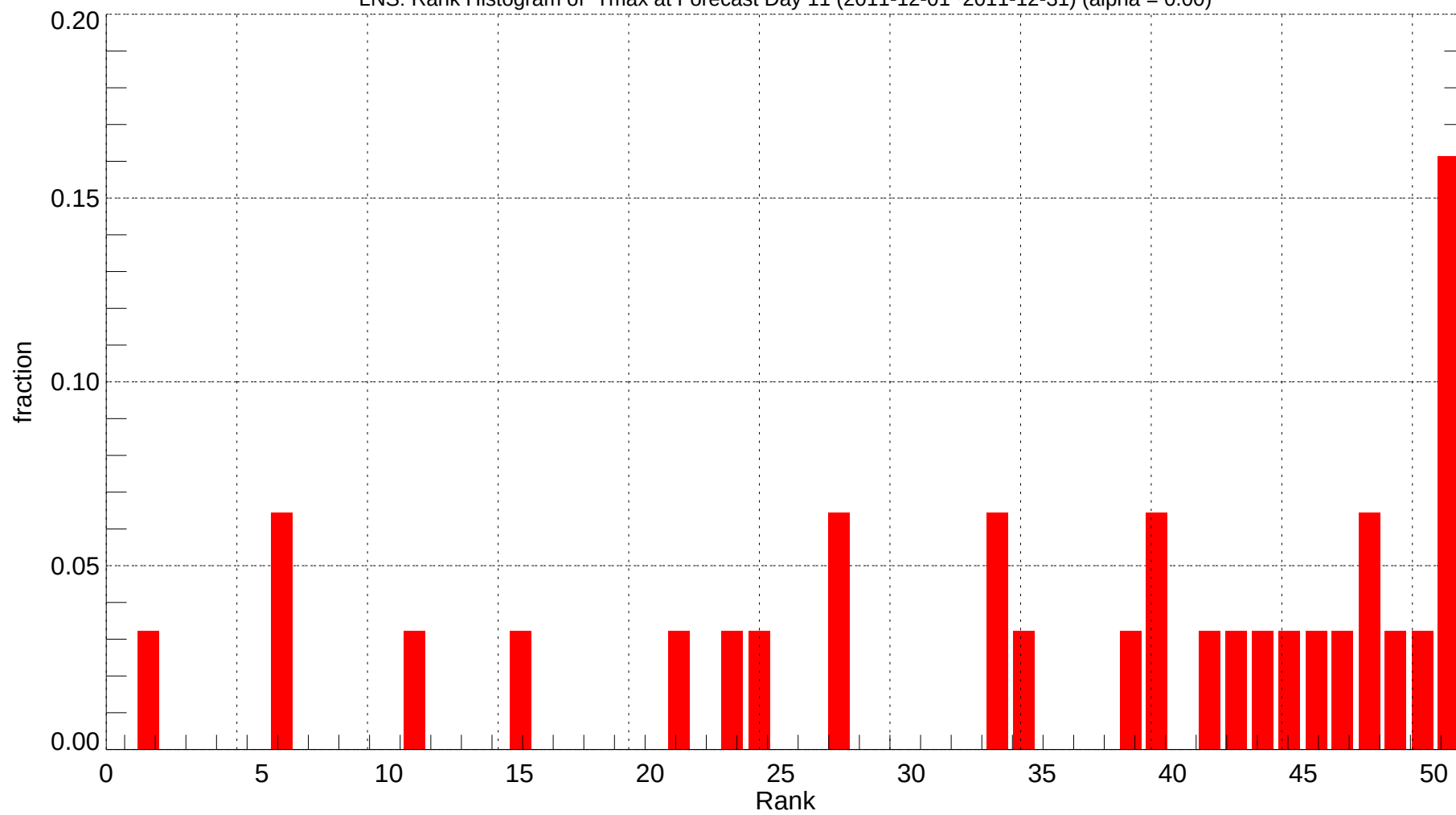
LNS: Rank Histogram of Tmax at Forecast Day 11 (2011-12-01~2011-12-31) (alpha = 0.00)
