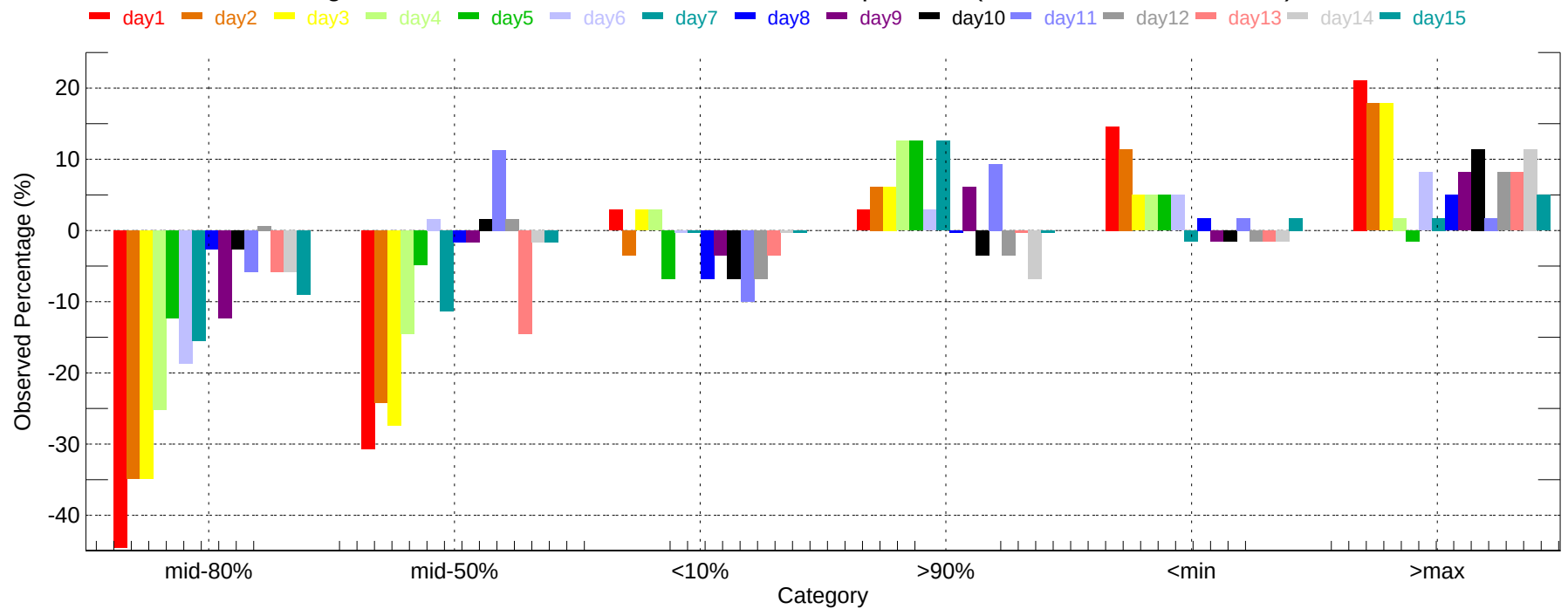
Observed Percentage Deviation of Ensembles - IAH: Max Temperature (2011-12-01~2011-12-31)
