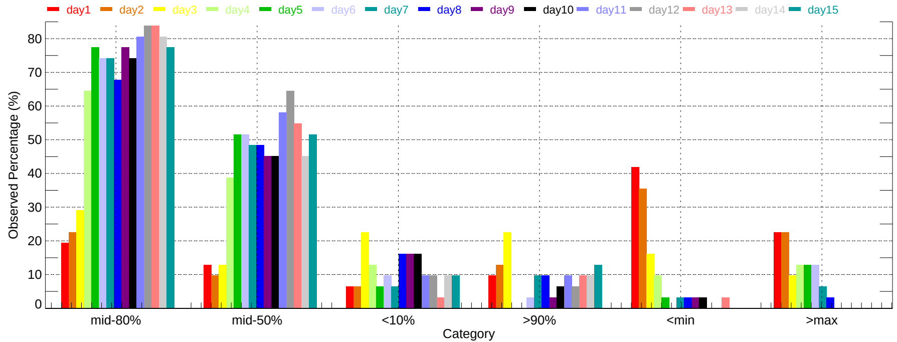
Observed Percentage of Ensembles - TRM: Max Temperature (2011-12-01~2011-12-31)
