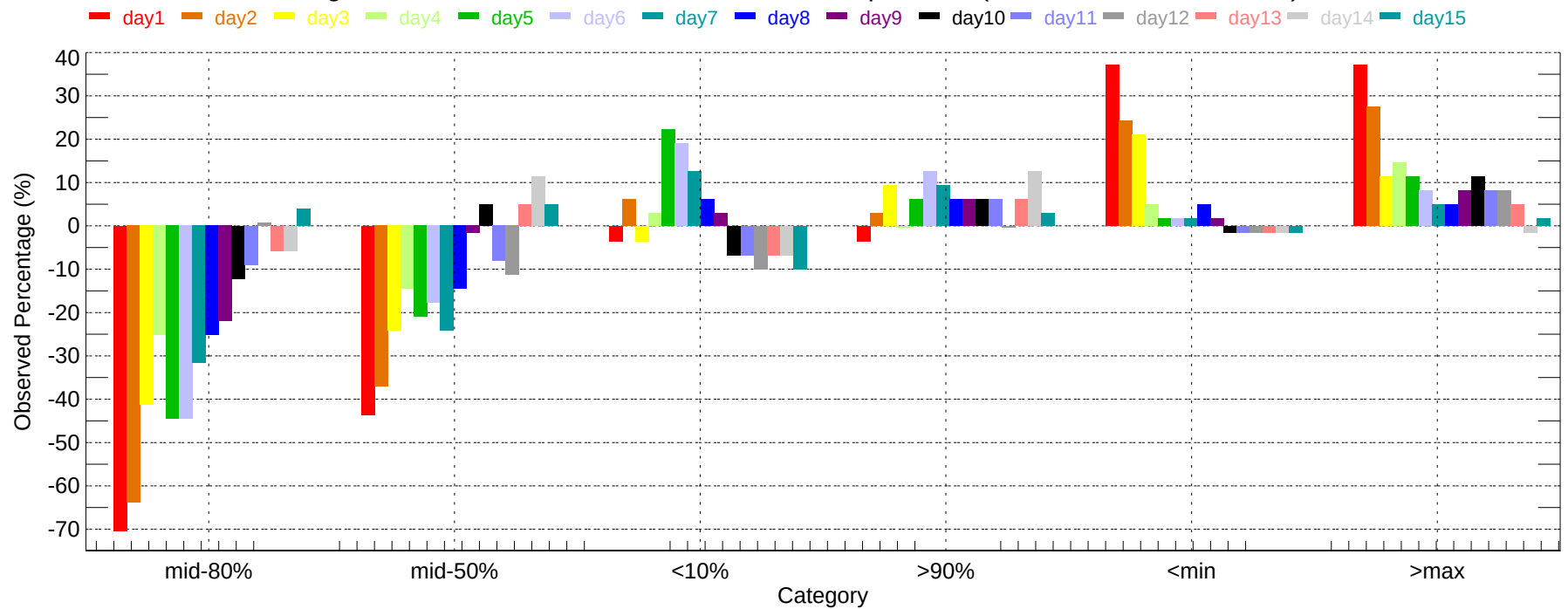
Observed Percentage Deviation of Ensembles - MKE: Min Temperature (2011-12-01~2011-12-31)
