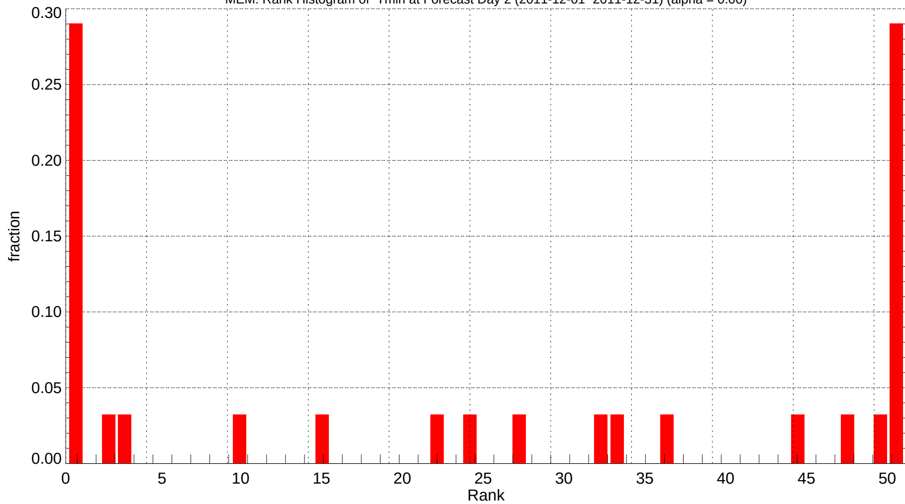
MEM: Rank Histogram of Tmin at Forecast Day 2 (2011-12-01~2011-12-31) (alpha = 0.00)
