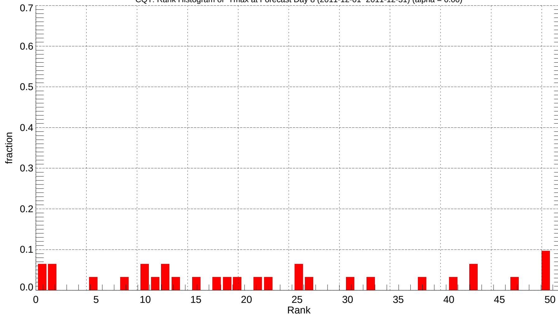
CQT: Rank Histogram of Tmax at Forecast Day 8 (2011-12-01~2011-12-31) (alpha = 0.00)
