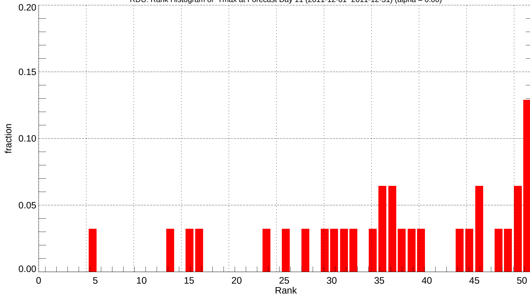
RDU: Rank Histogram of Tmax at Forecast Day 11 (2011-12-01~2011-12-31) (alpha = 0.00)
