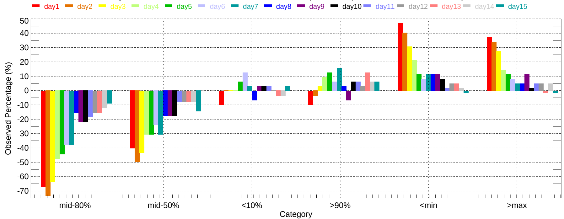
Observed Percentage Deviation of Ensembles - SJC: Min Temperature (2011-12-01~2011-12-31)
