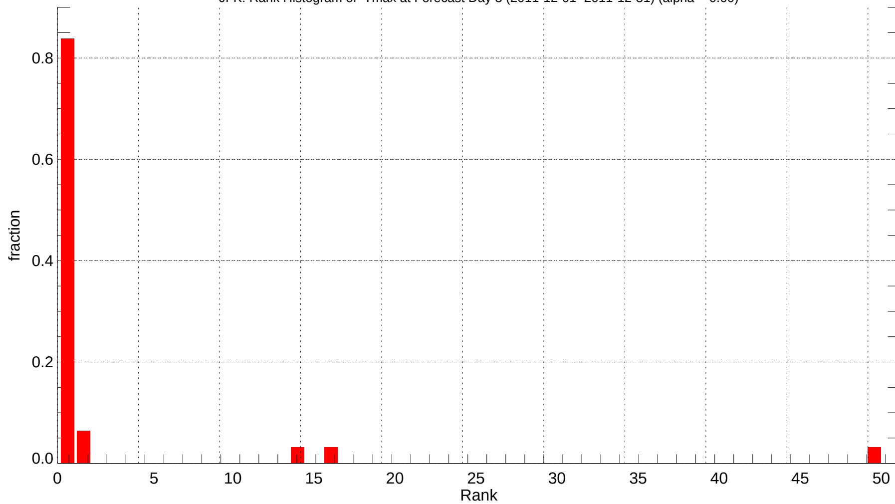
JFK: Rank Histogram of Tmax at Forecast Day 3 (2011-12-01~2011-12-31) (alpha = 0.00)
