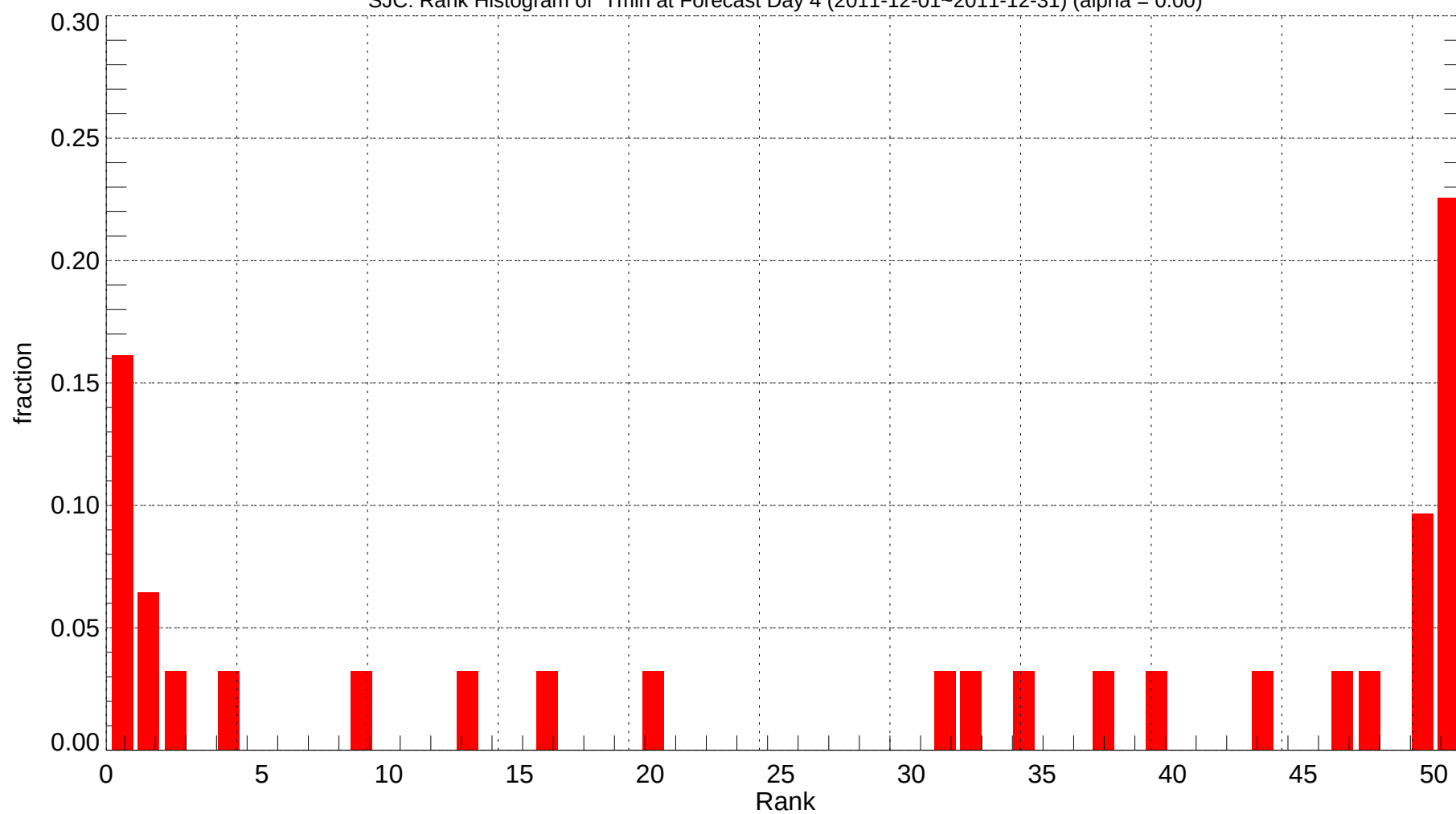
SJC: Rank Histogram of Tmin at Forecast Day 4 (2011-12-01~2011-12-31) (alpha = 0.00)
