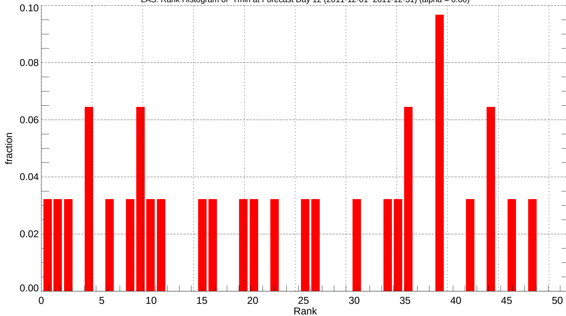
LAS: Rank Histogram of Tmin at Forecast Day 12 (2011-12-01~2011-12-31) (alpha = 0.00)
