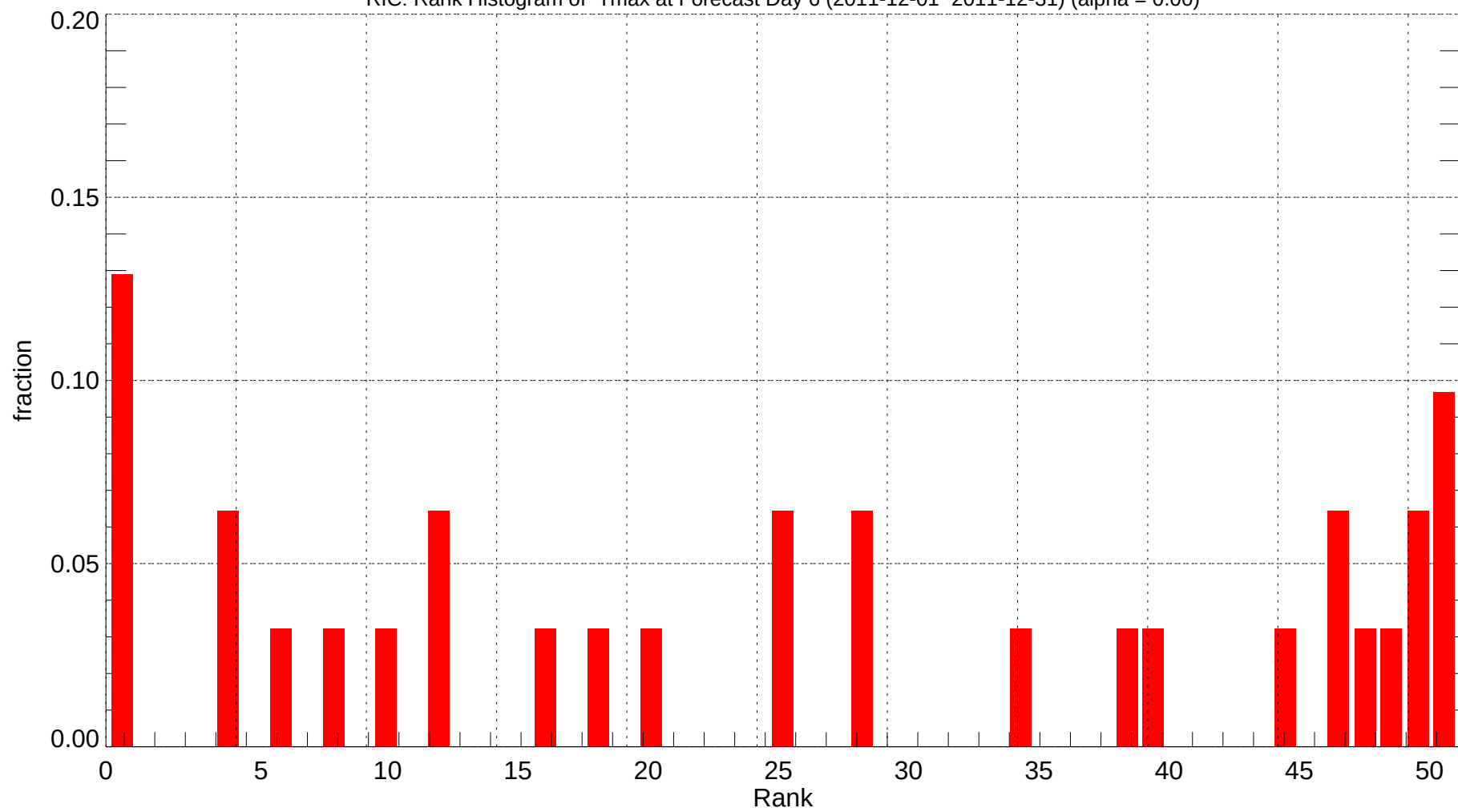
RIC: Rank Histogram of Tmax at Forecast Day 6 (2011-12-01~2011-12-31) (alpha = 0.00)
