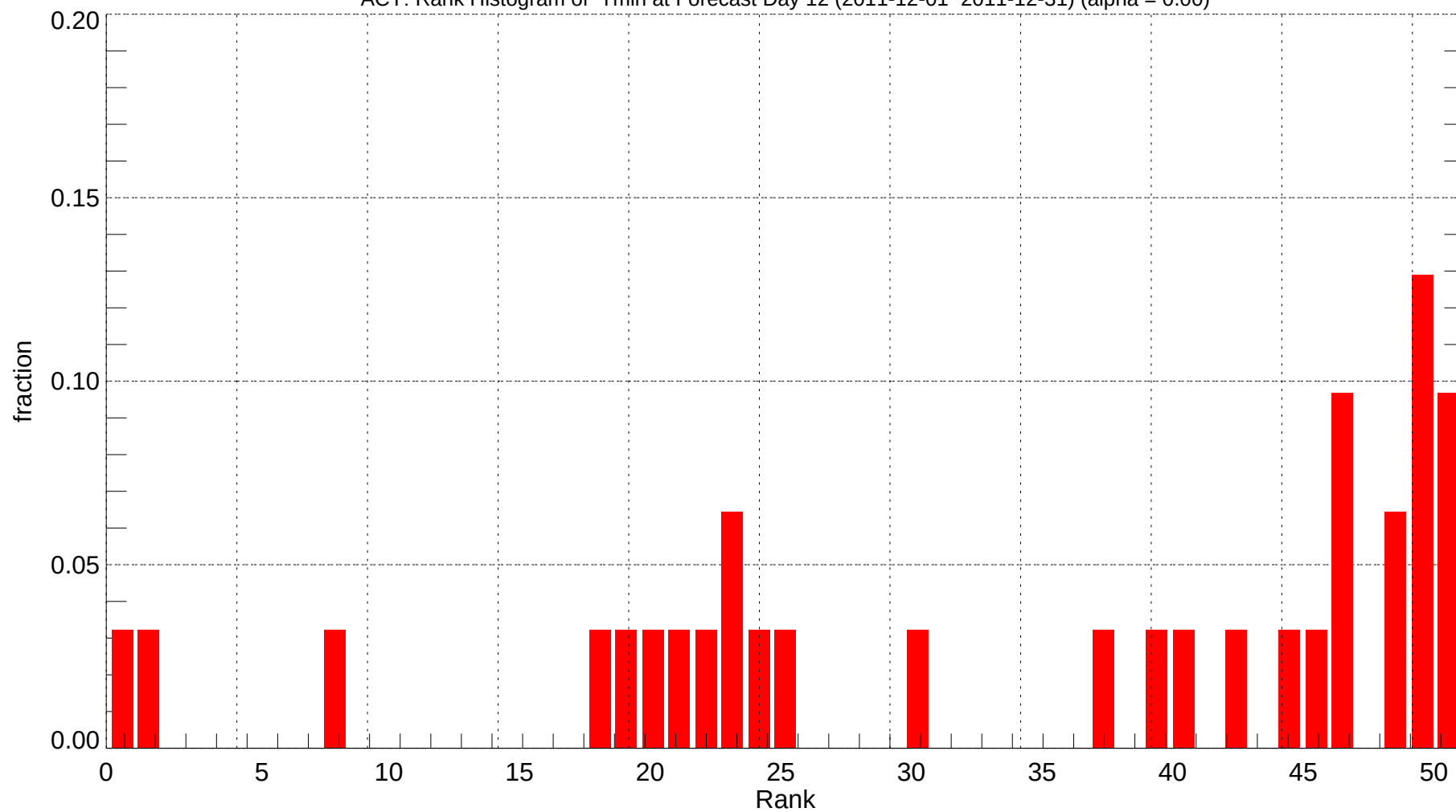
ACY: Rank Histogram of Tmin at Forecast Day 12 (2011-12-01~2011-12-31) (alpha = 0.00)
