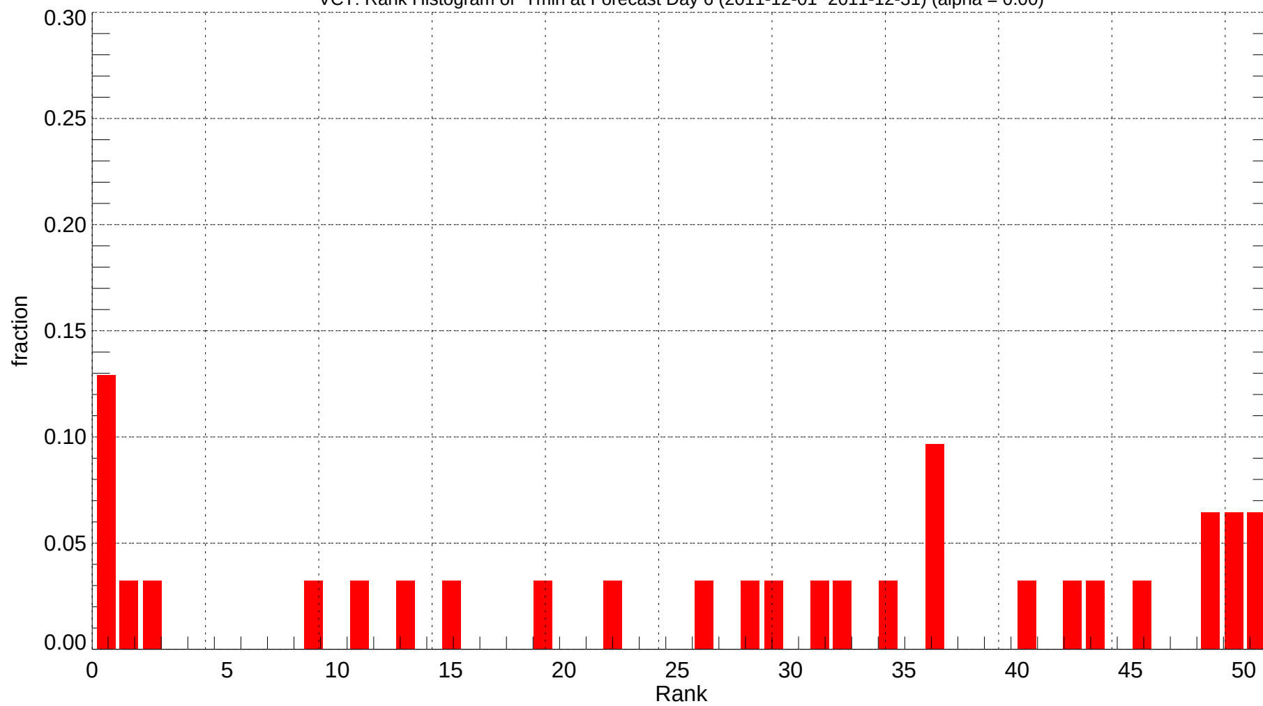
VCT: Rank Histogram of Tmin at Forecast Day 6 (2011-12-01~2011-12-31) (alpha = 0.00)
