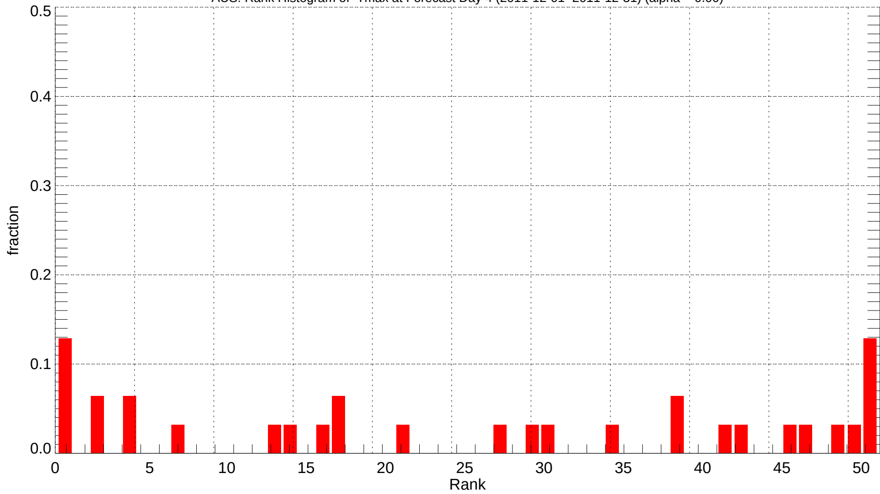
AUS: Rank Histogram of Tmax at Forecast Day 4 (2011-12-01~2011-12-31) (alpha = 0.00)
