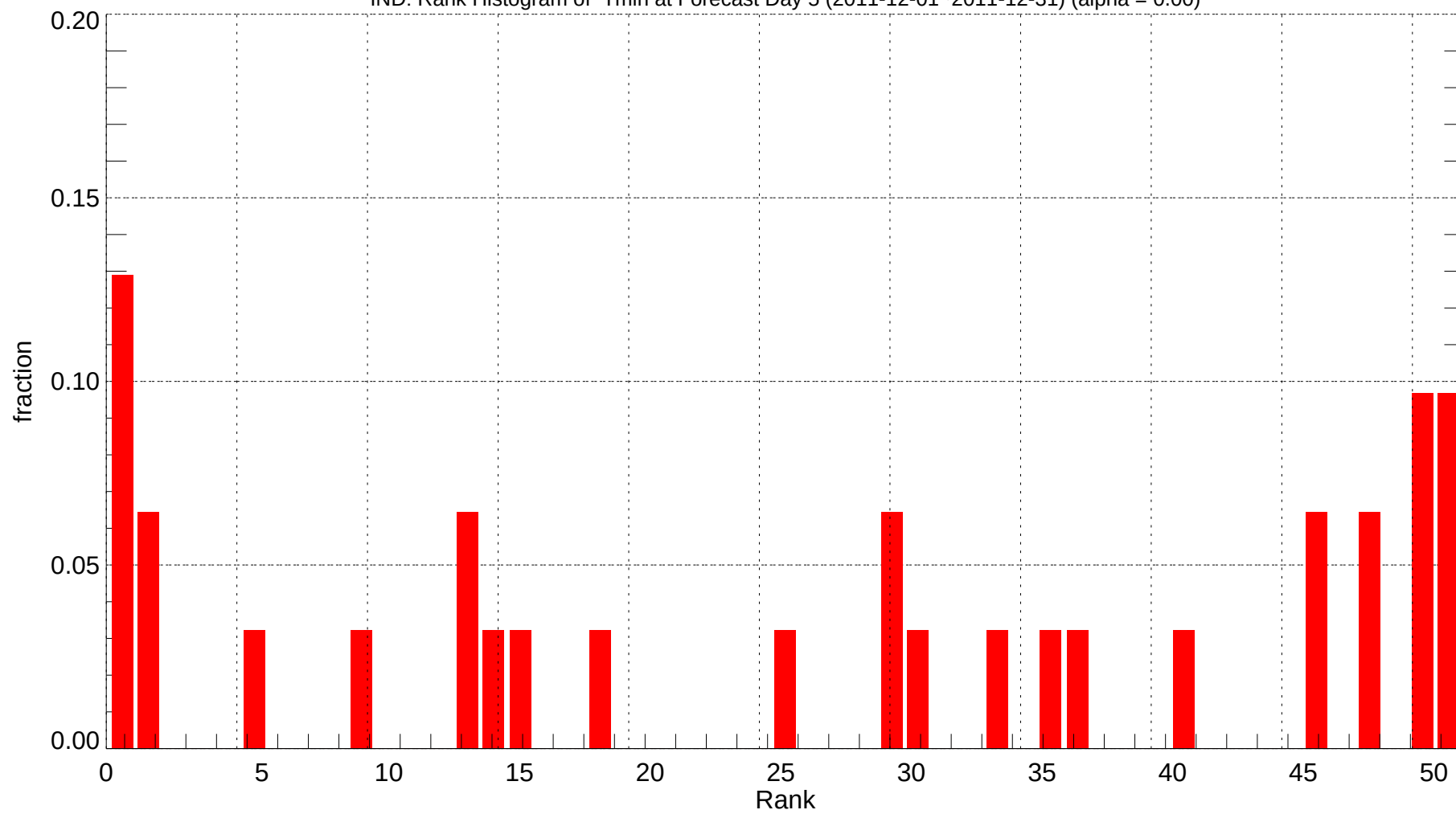
IND: Rank Histogram of Tmin at Forecast Day 5 (2011-12-01~2011-12-31) (alpha = 0.00)
