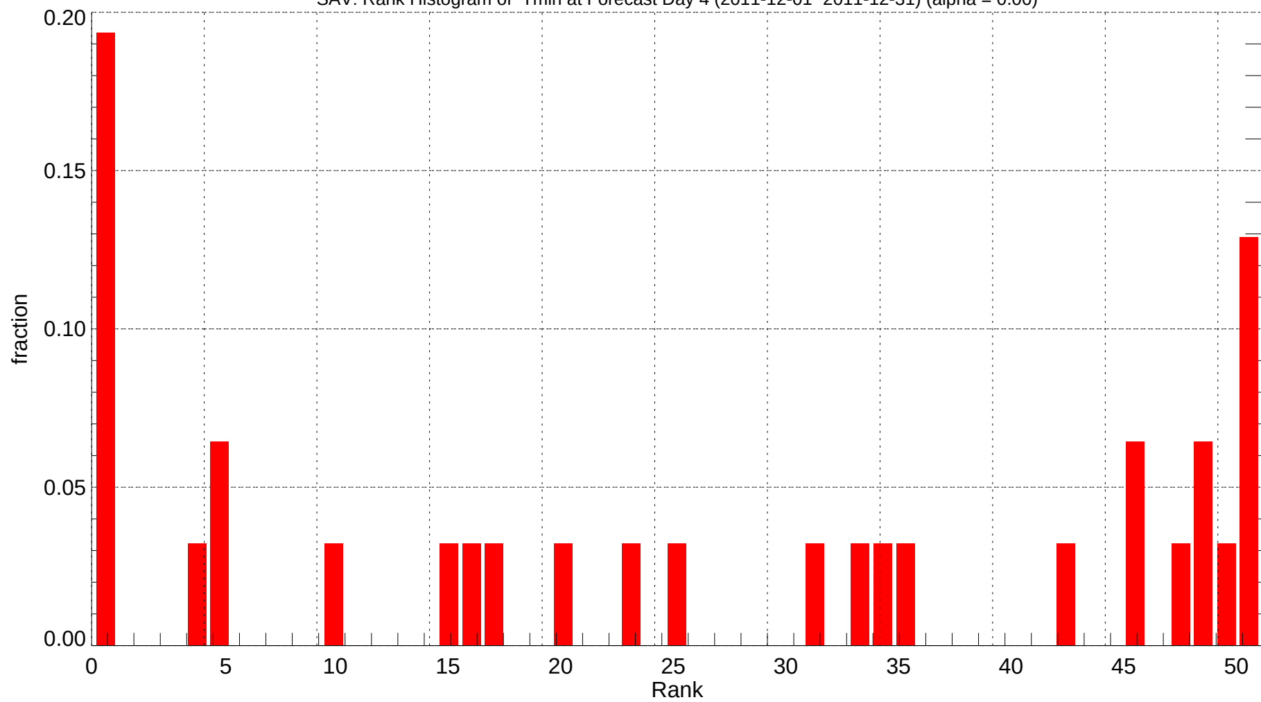
SAV: Rank Histogram of Tmin at Forecast Day 4 (2011-12-01~2011-12-31) (alpha = 0.00)
