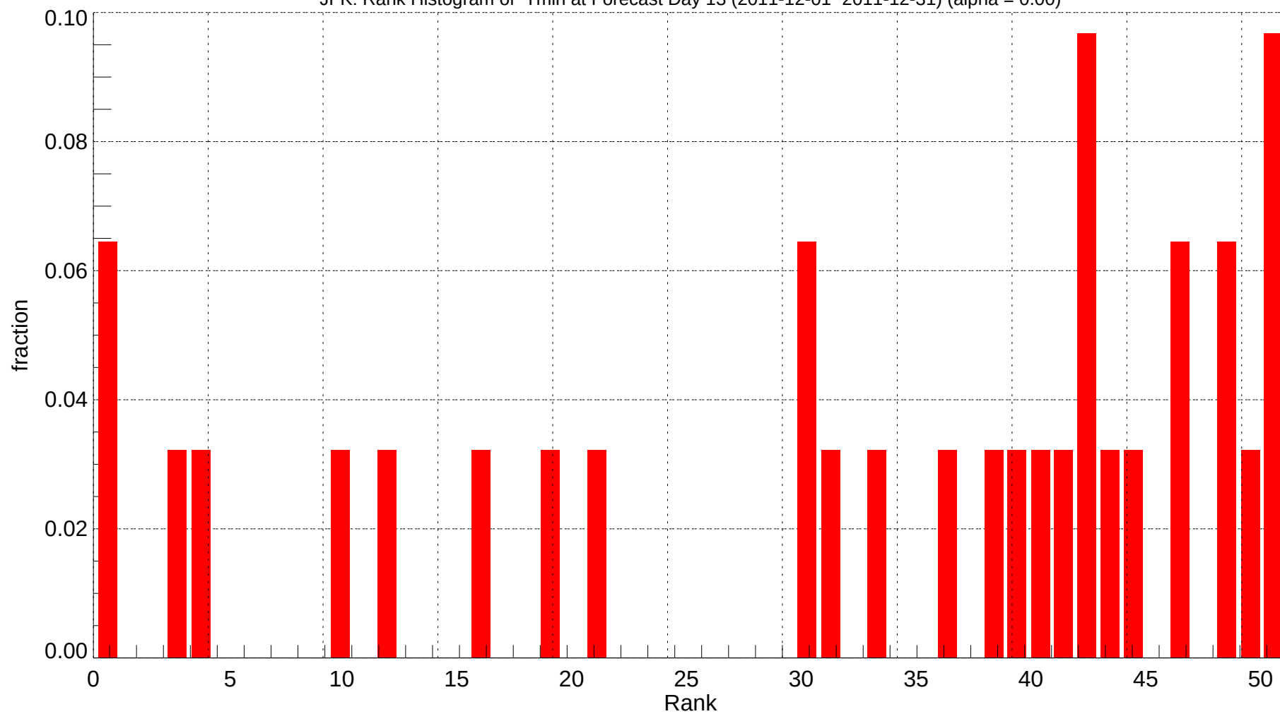
JFK: Rank Histogram of Tmin at Forecast Day 13 (2011-12-01~2011-12-31) (alpha = 0.00)
