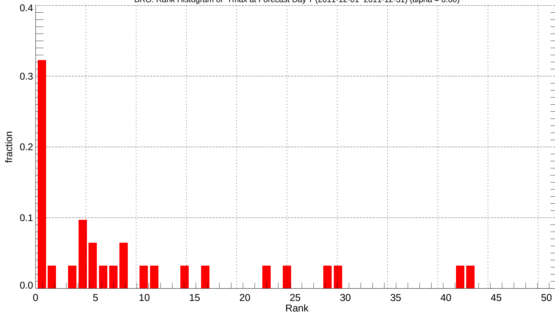
BRO: Rank Histogram of Tmax at Forecast Day 7 (2011-12-01~2011-12-31) (alpha = 0.00)
