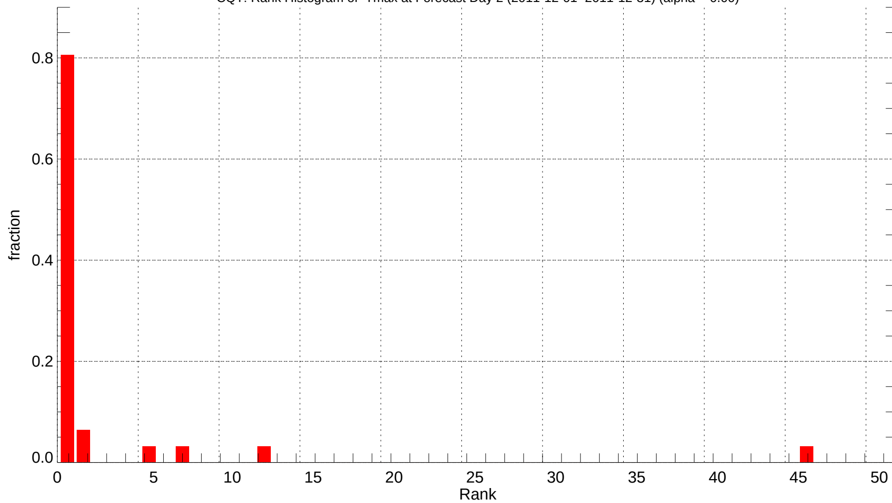
CQT: Rank Histogram of Tmax at Forecast Day 2 (2011-12-01~2011-12-31) (alpha = 0.00)
