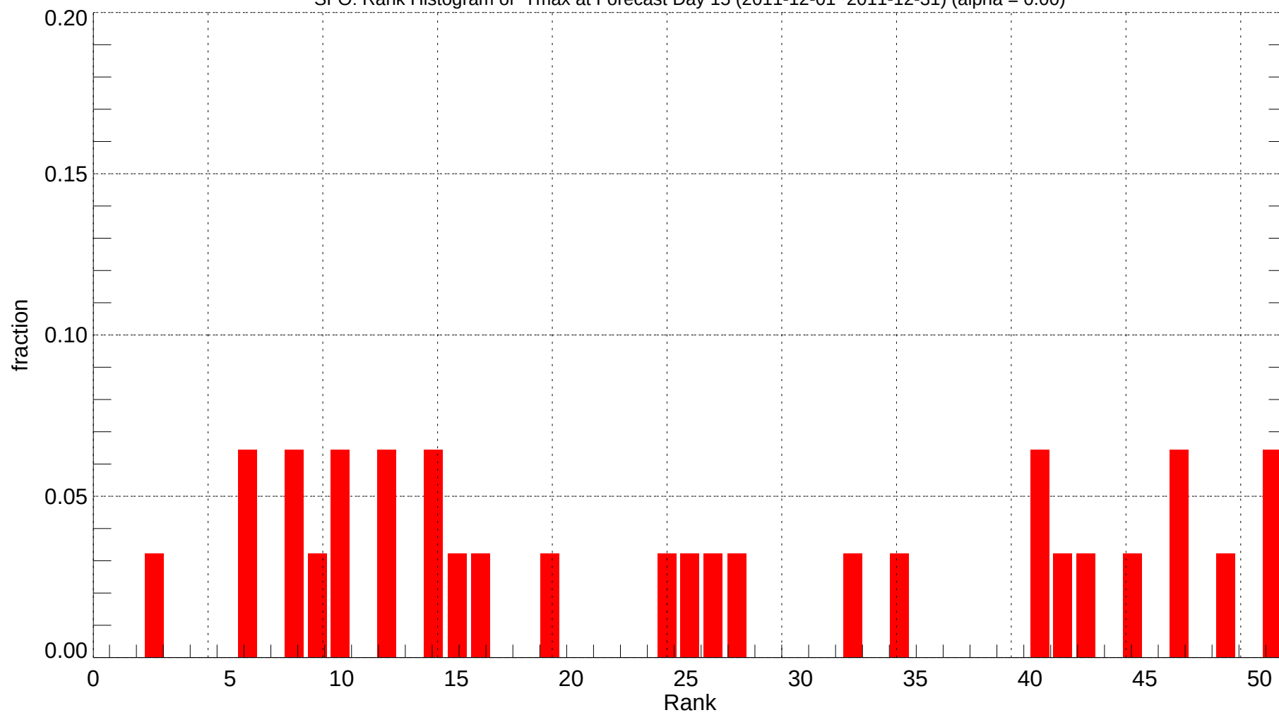
SFO: Rank Histogram of Tmax at Forecast Day 15 (2011-12-01~2011-12-31) (alpha = 0.00)
