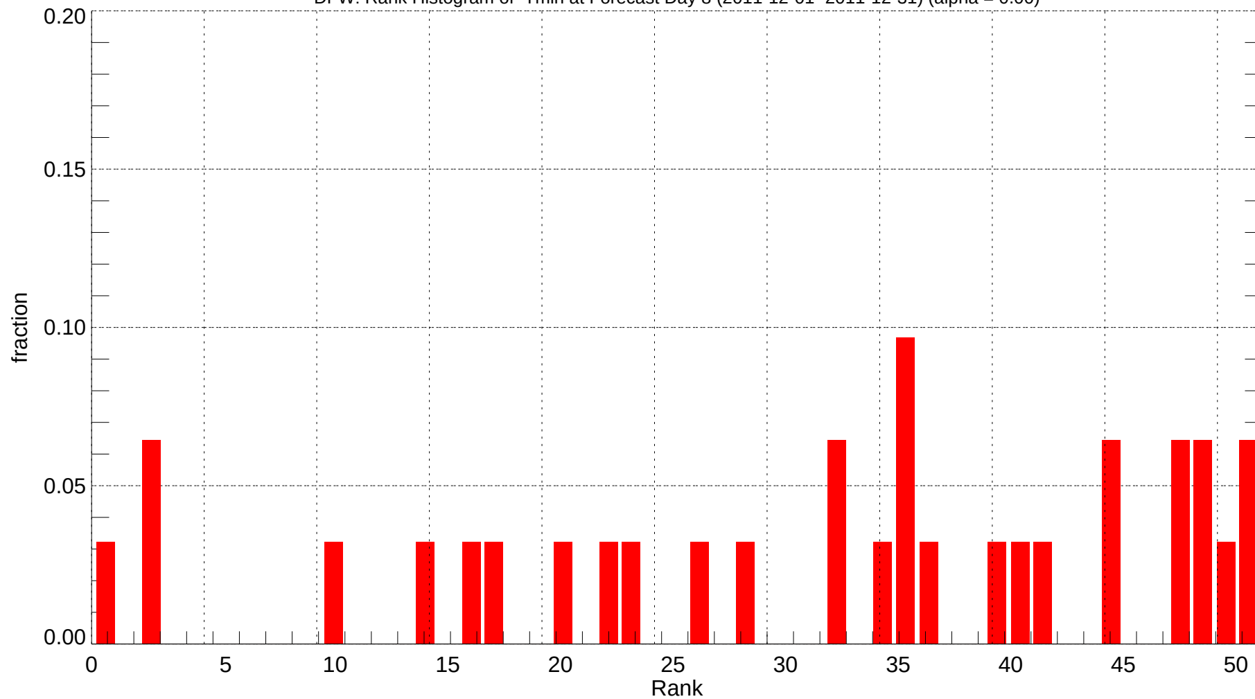
DFW: Rank Histogram of Tmin at Forecast Day 8 (2011-12-01~2011-12-31) (alpha = 0.00)
