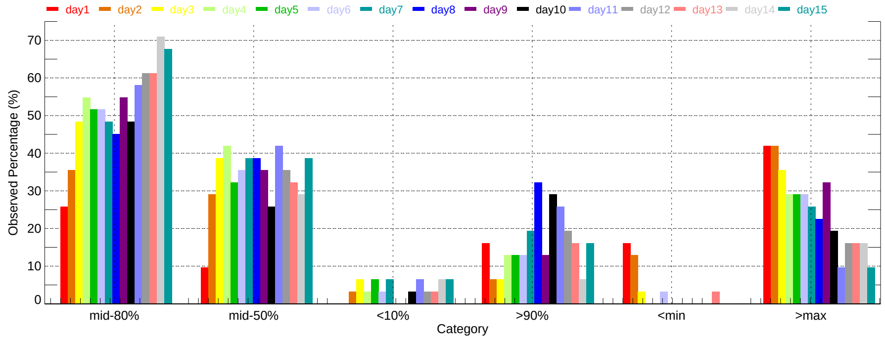
Observed Percentage of Ensembles - TUL: Max Temperature (2011-12-01~2011-12-31)
