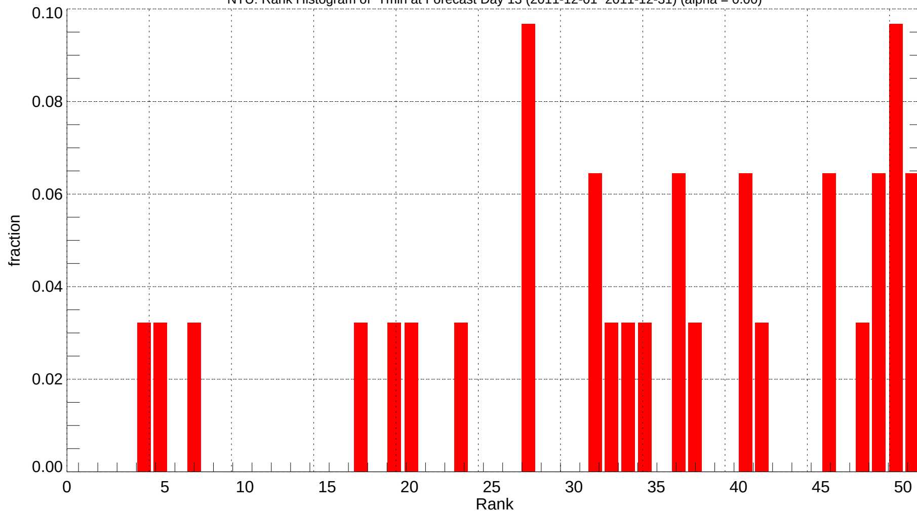
NTU: Rank Histogram of Tmin at Forecast Day 13 (2011-12-01~2011-12-31) (alpha = 0.00)
