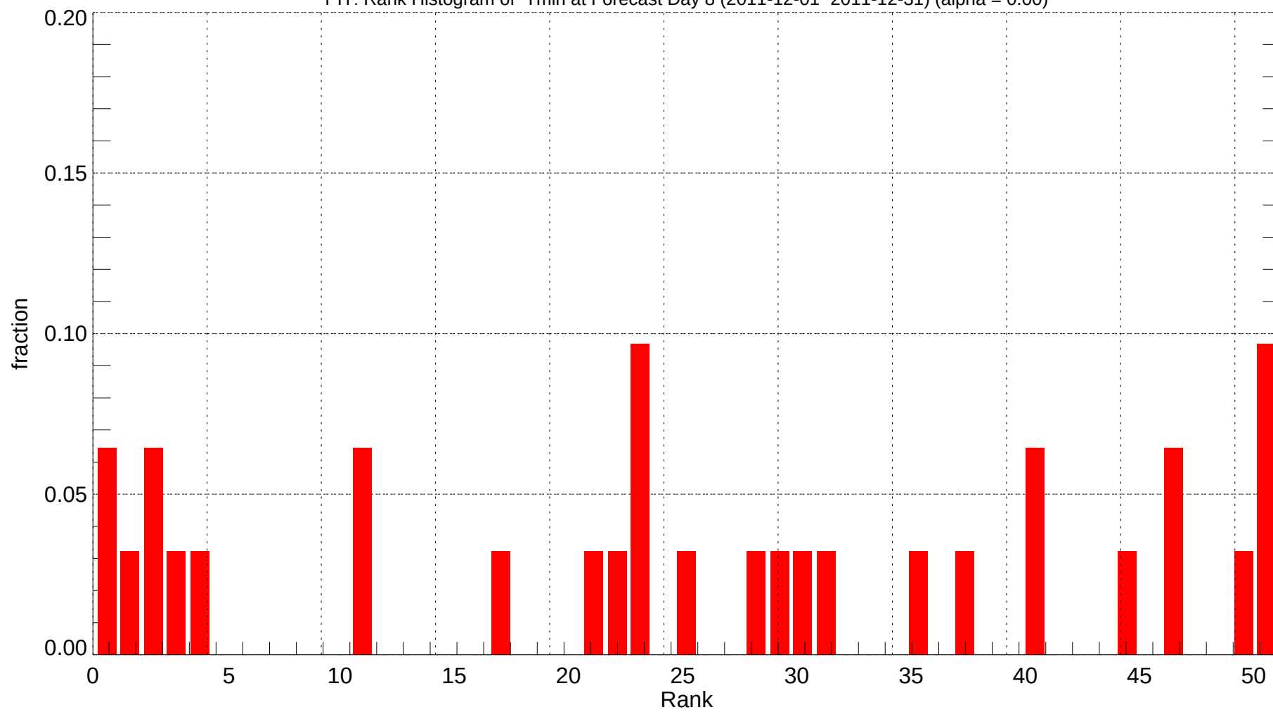
PIT: Rank Histogram of Tmin at Forecast Day 8 (2011-12-01~2011-12-31) (alpha = 0.00)
