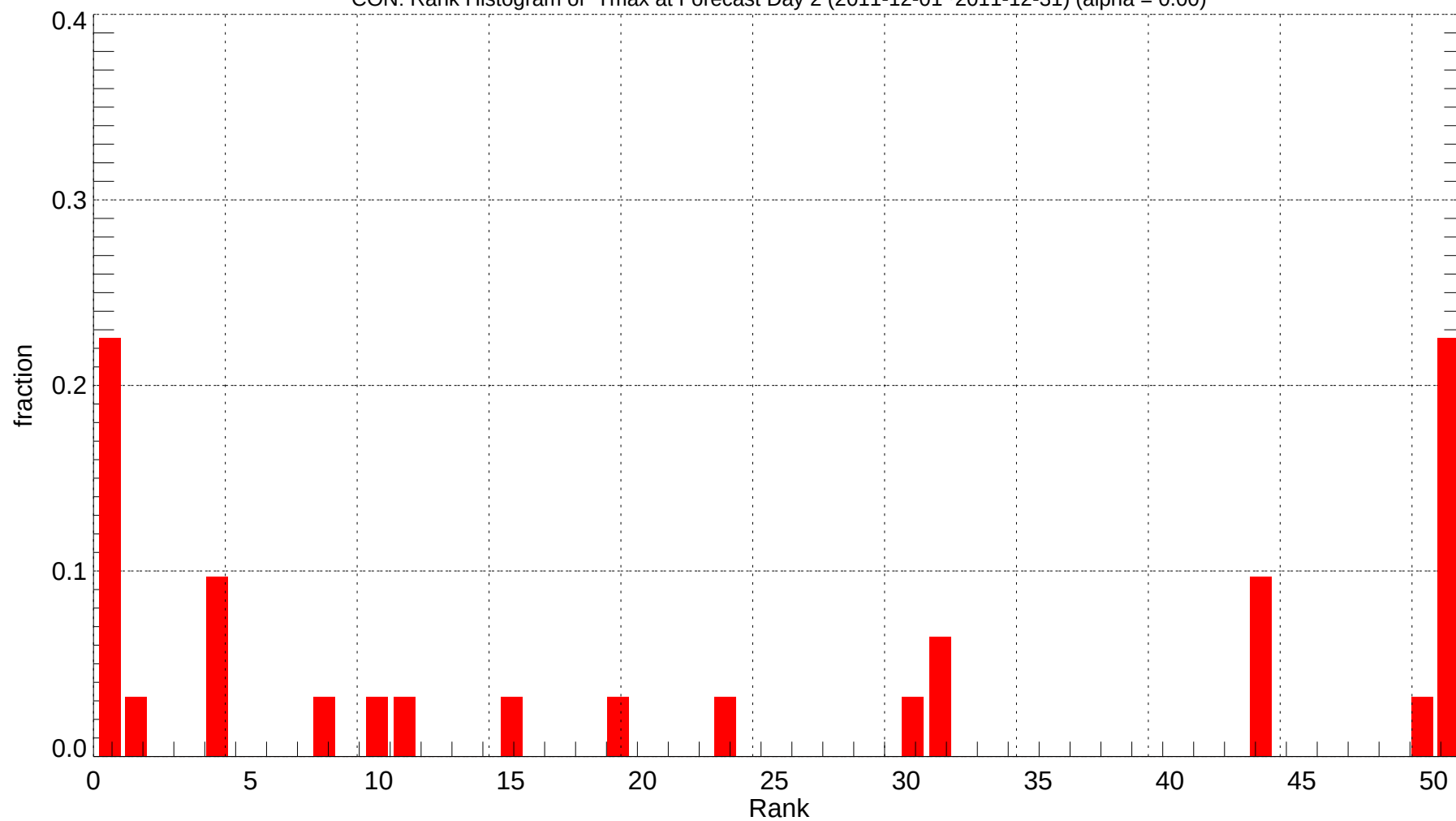
CON: Rank Histogram of Tmax at Forecast Day 2 (2011-12-01~2011-12-31) (alpha = 0.00)
