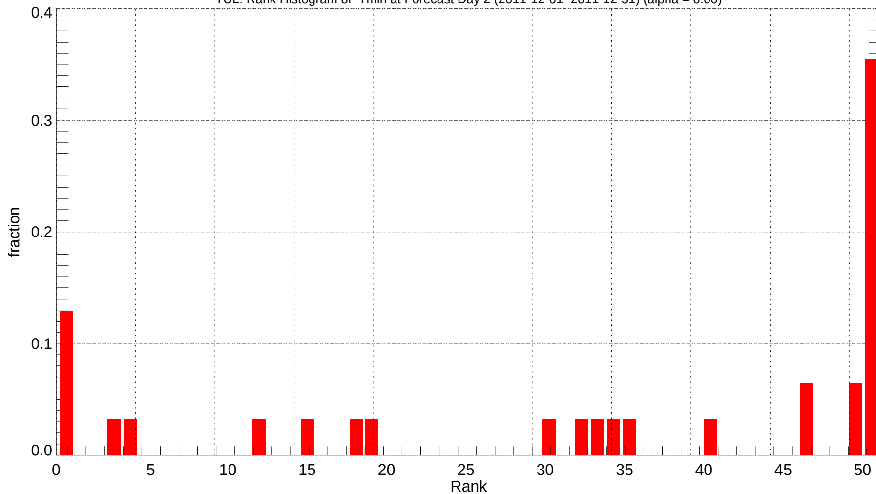
TUL: Rank Histogram of Tmin at Forecast Day 2 (2011-12-01~2011-12-31) (alpha = 0.00)
