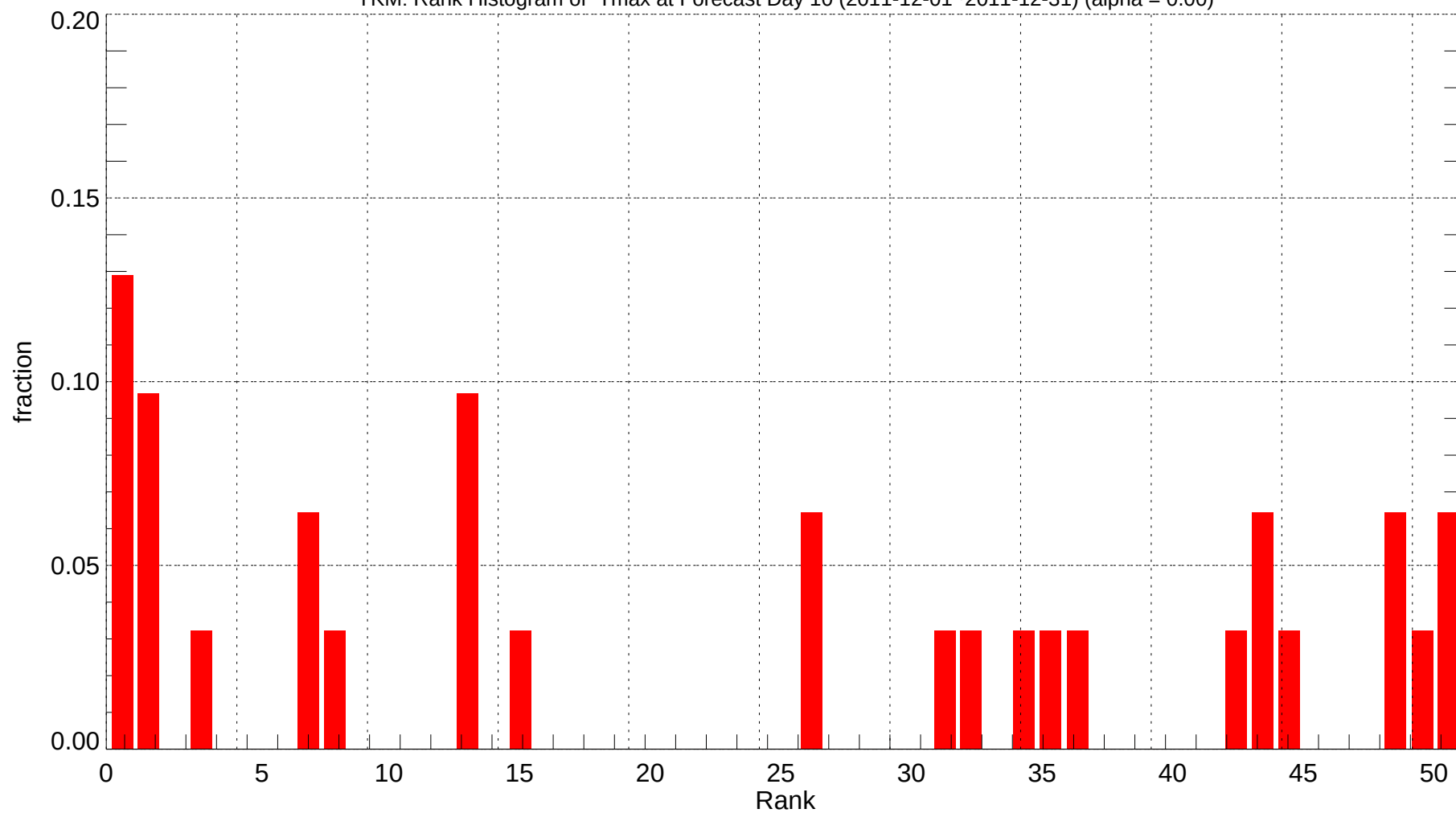
YKM: Rank Histogram of Tmax at Forecast Day 10 (2011-12-01~2011-12-31) (alpha = 0.00)
