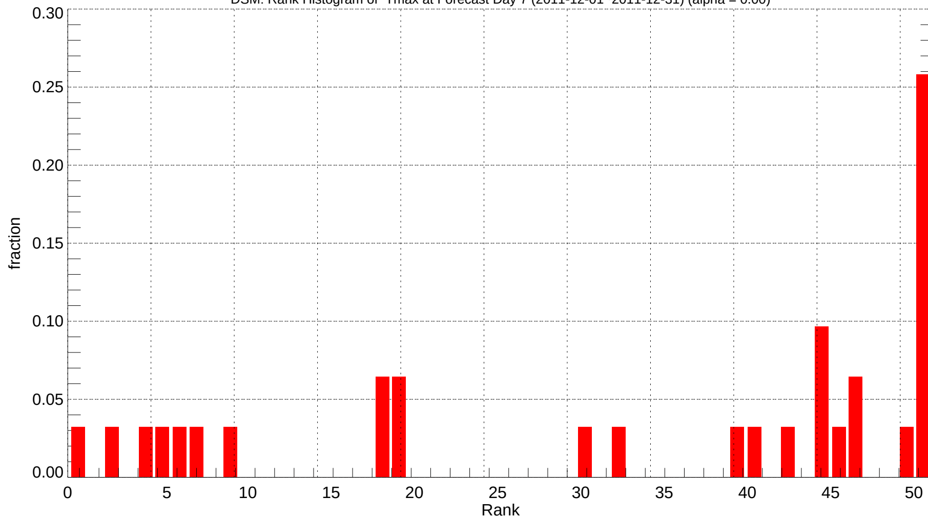
DSM: Rank Histogram of Tmax at Forecast Day 7 (2011-12-01~2011-12-31) (alpha = 0.00)
