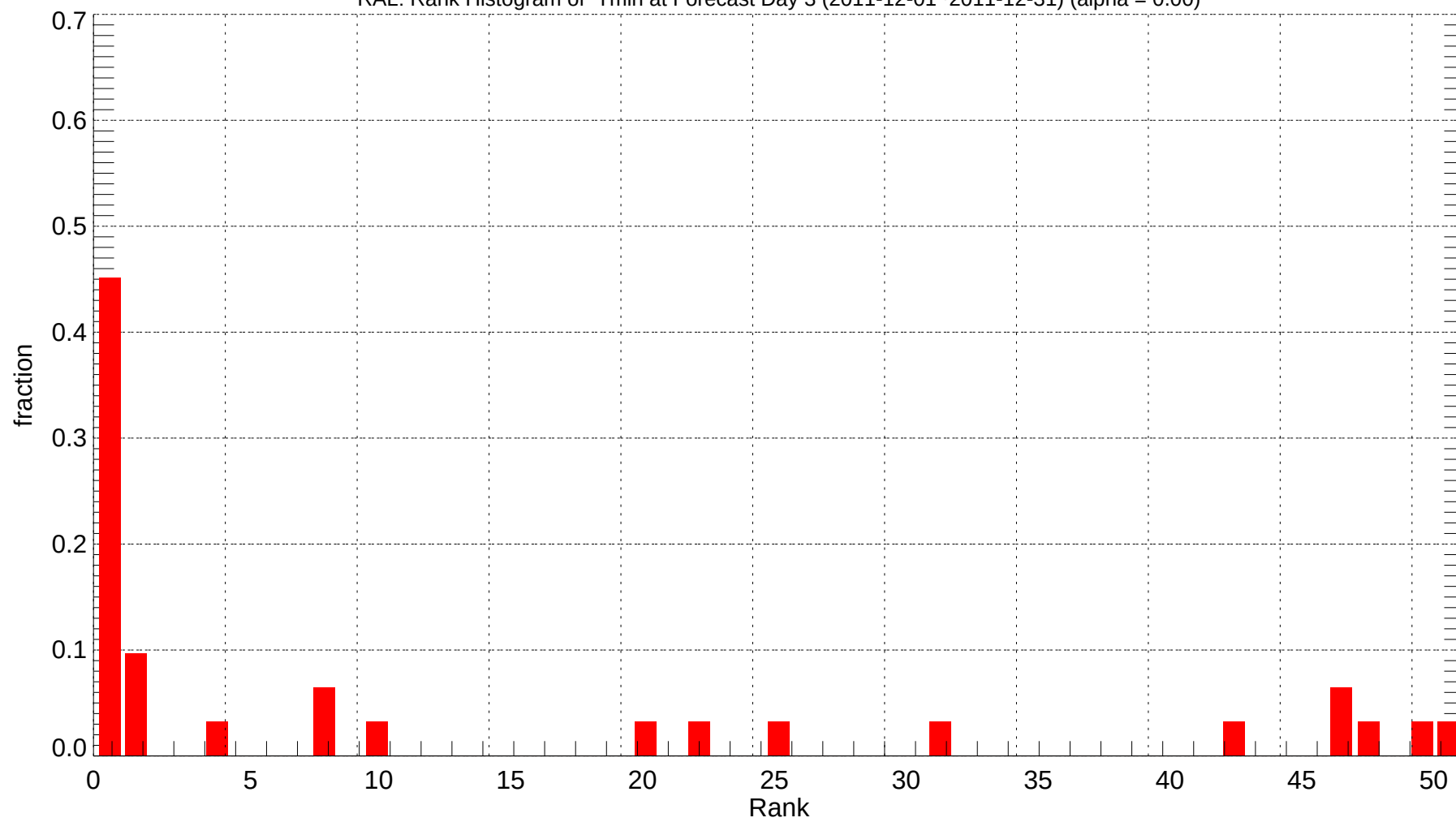
RAL: Rank Histogram of Tmin at Forecast Day 3 (2011-12-01~2011-12-31) (alpha = 0.00)
