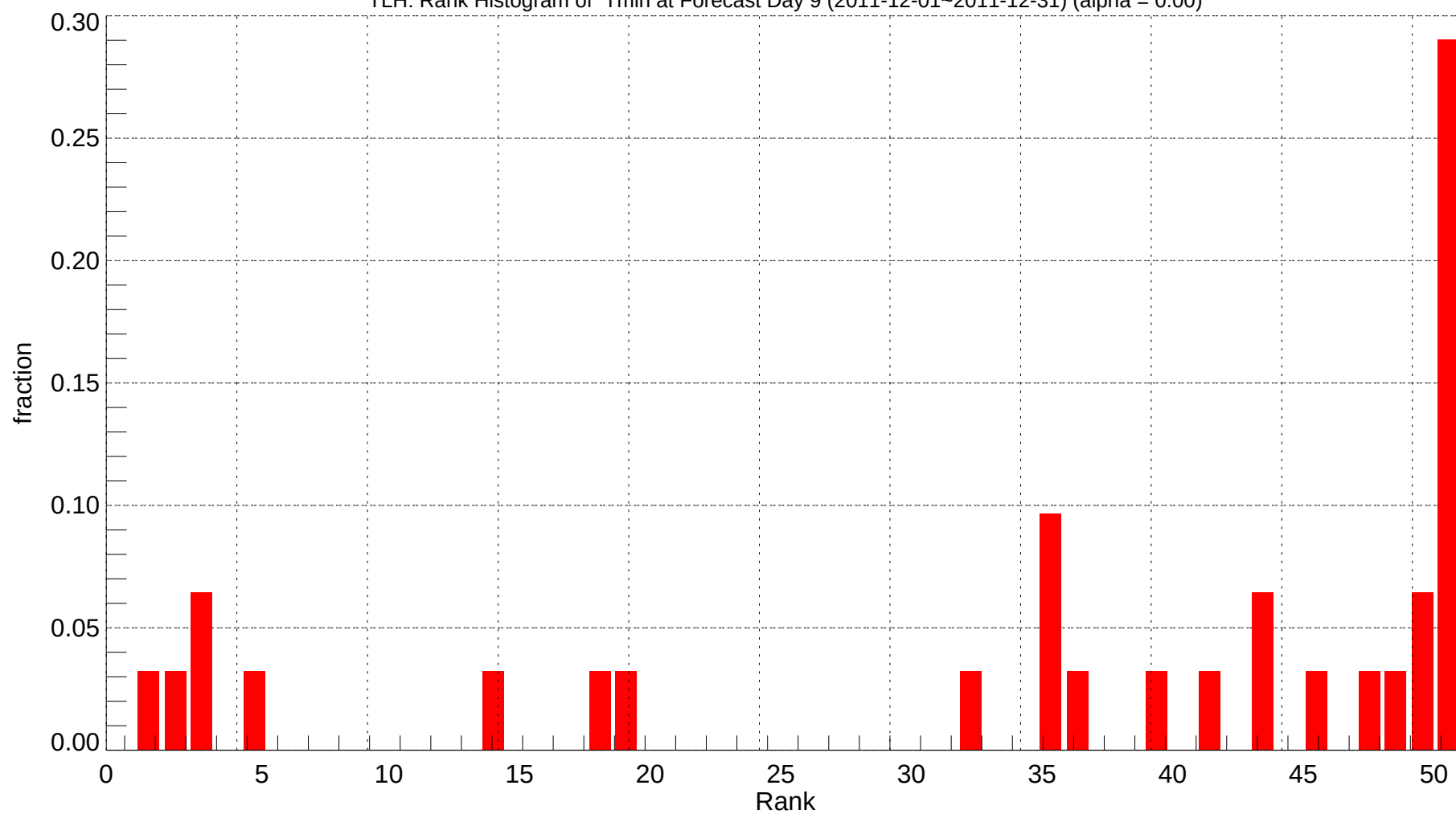
TLH: Rank Histogram of Tmin at Forecast Day 9 (2011-12-01~2011-12-31) (alpha = 0.00)
