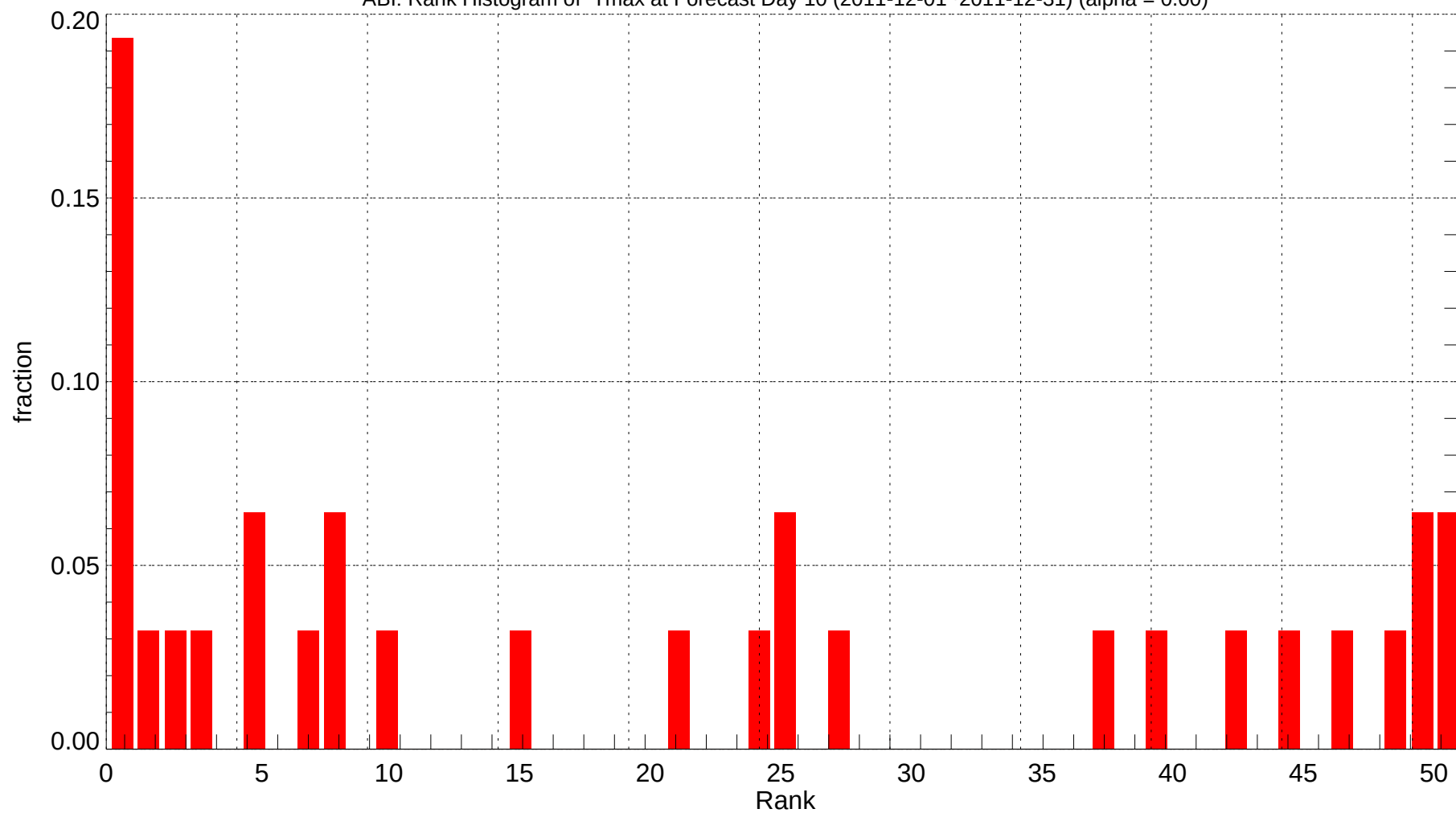
ABI: Rank Histogram of Tmax at Forecast Day 10 (2011-12-01~2011-12-31) (alpha = 0.00)
