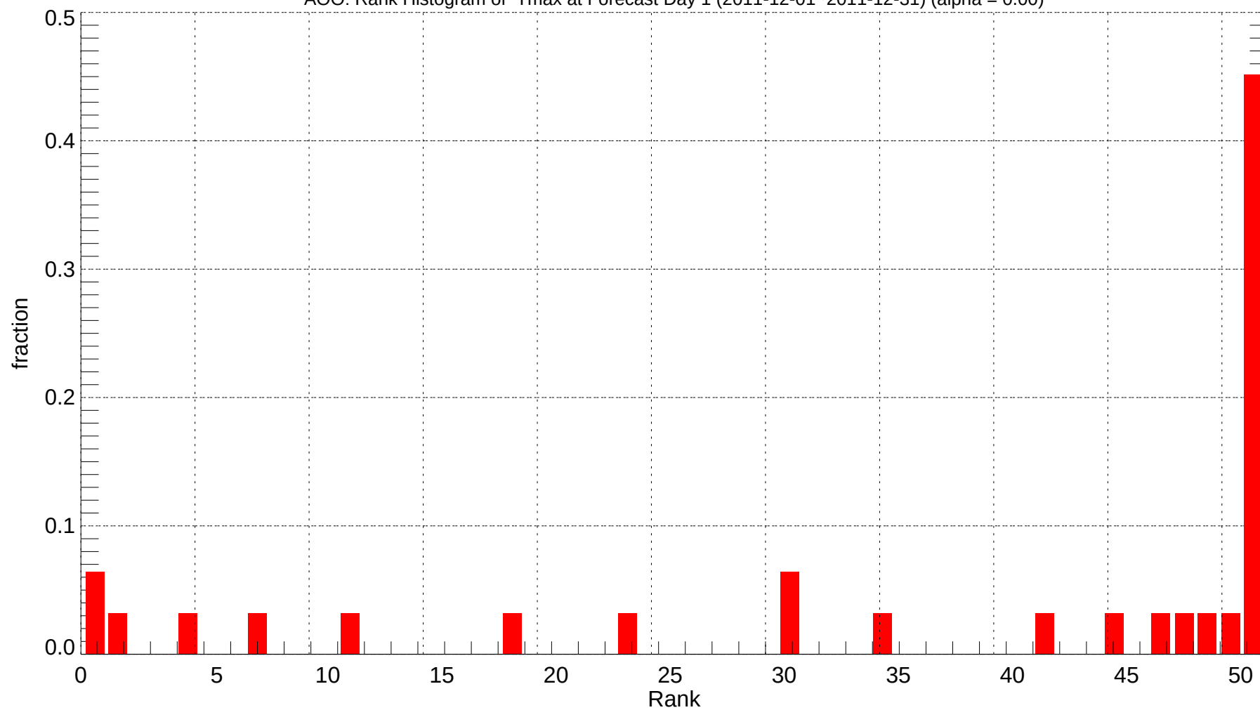
AOO: Rank Histogram of Tmax at Forecast Day 1 (2011-12-01~2011-12-31) (alpha = 0.00)
