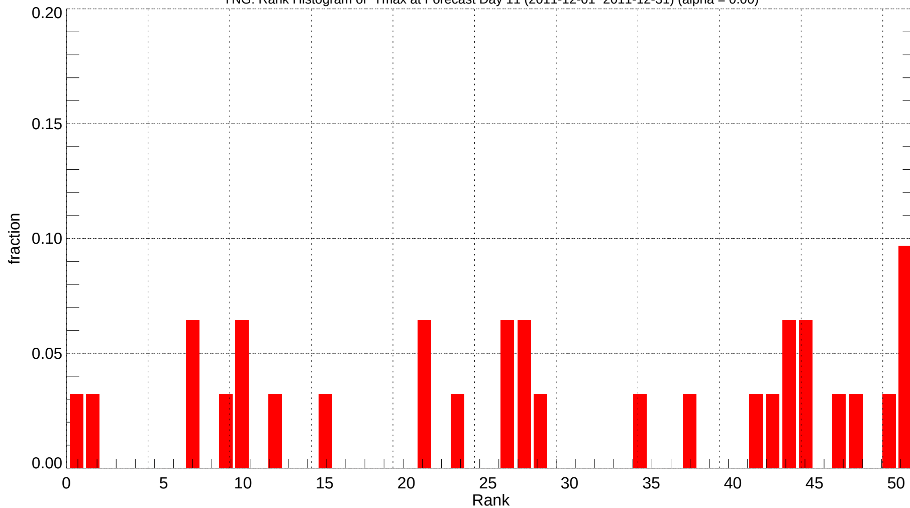
YNG: Rank Histogram of Tmax at Forecast Day 11 (2011-12-01~2011-12-31) (alpha = 0.00)
