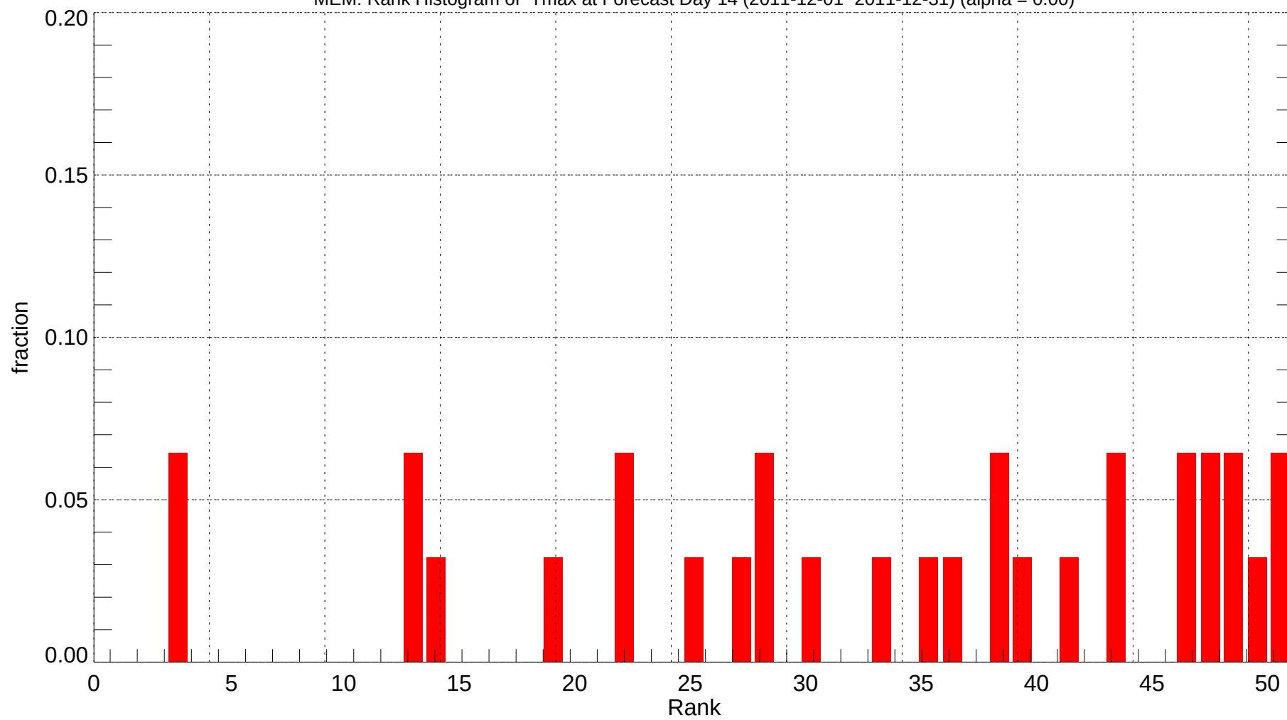
MEM: Rank Histogram of Tmax at Forecast Day 14 (2011-12-01~2011-12-31) (alpha = 0.00)
