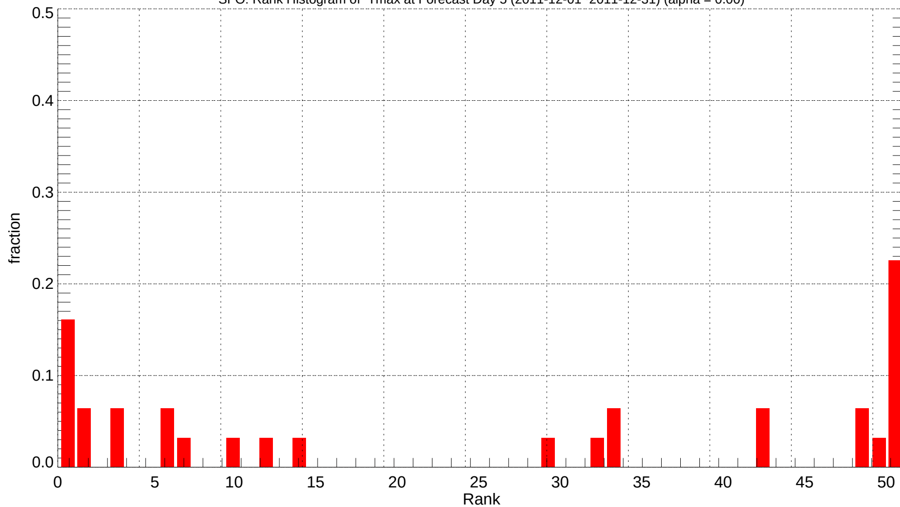
SFO: Rank Histogram of Tmax at Forecast Day 5 (2011-12-01~2011-12-31) (alpha = 0.00)
