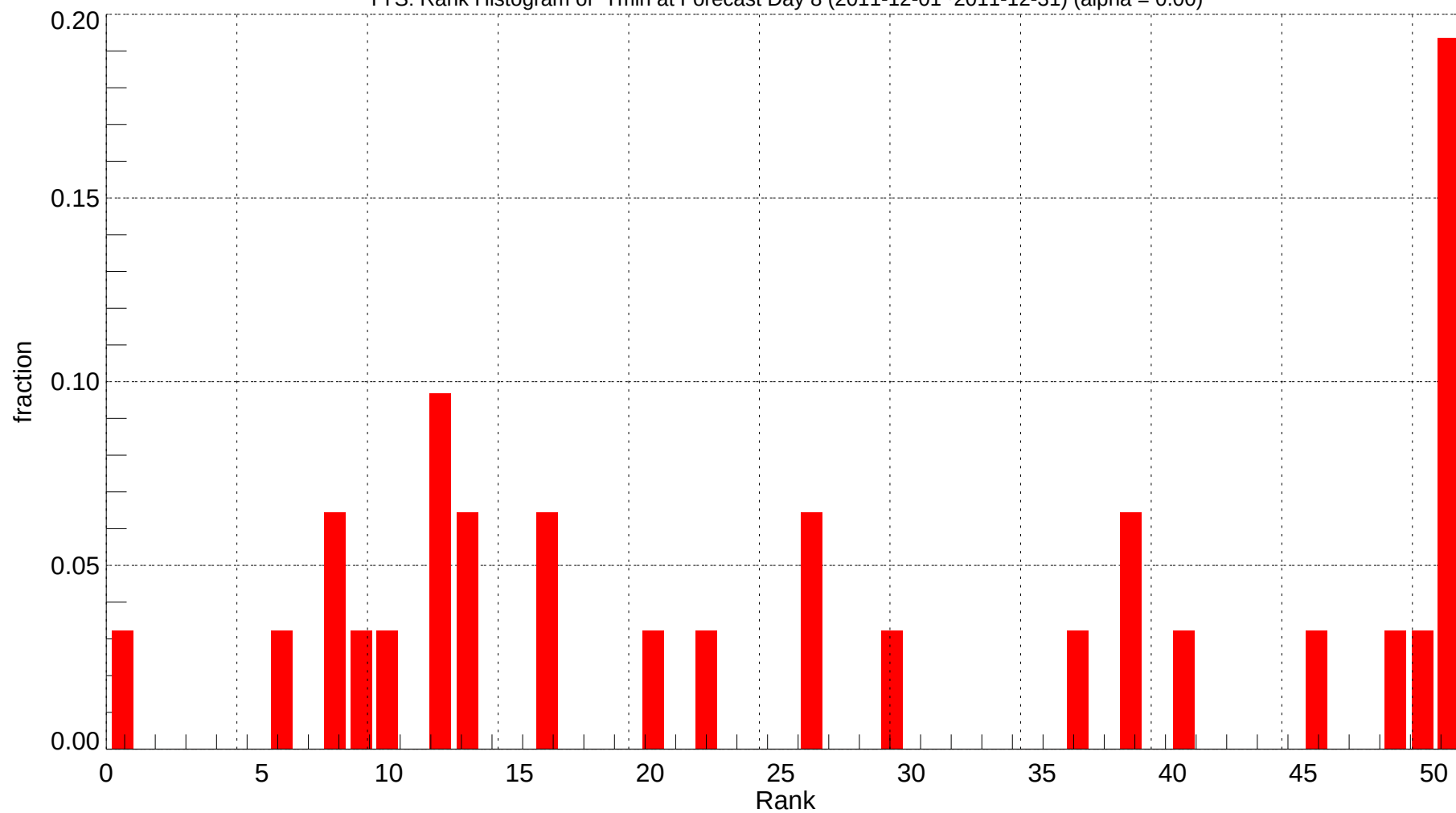
TYS: Rank Histogram of Tmin at Forecast Day 8 (2011-12-01~2011-12-31) (alpha = 0.00)
