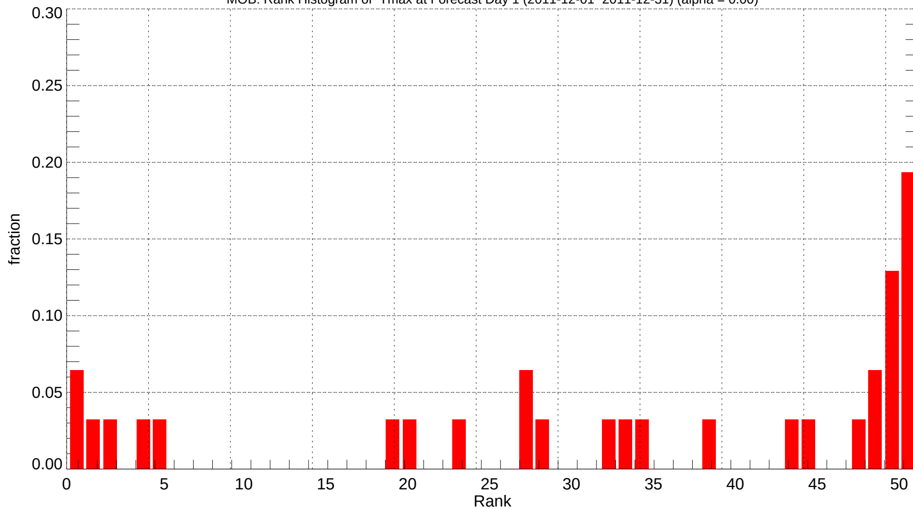
MOB: Rank Histogram of Tmax at Forecast Day 1 (2011-12-01~2011-12-31) (alpha = 0.00)
