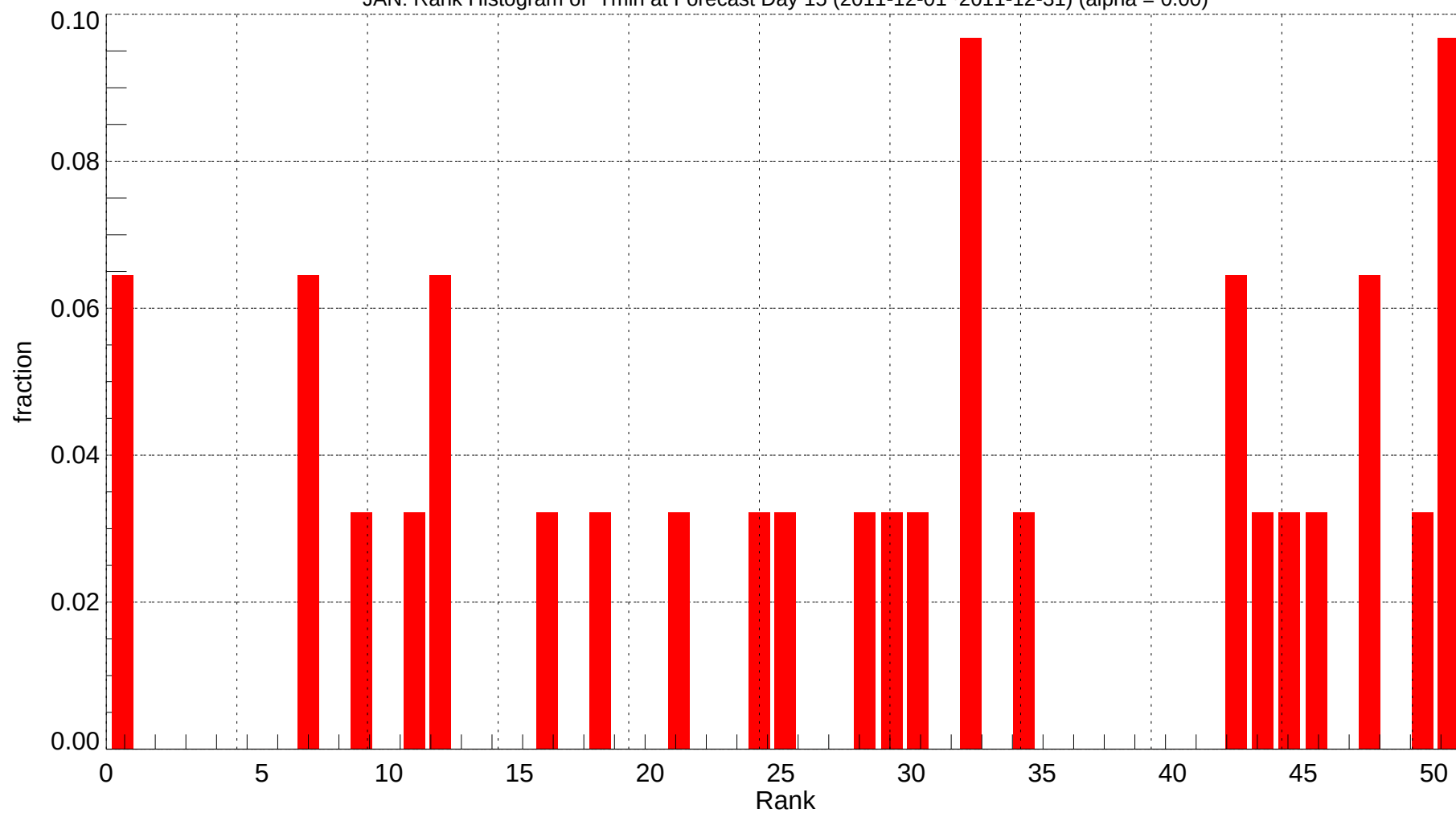
JAN: Rank Histogram of Tmin at Forecast Day 15 (2011-12-01~2011-12-31) (alpha = 0.00)
