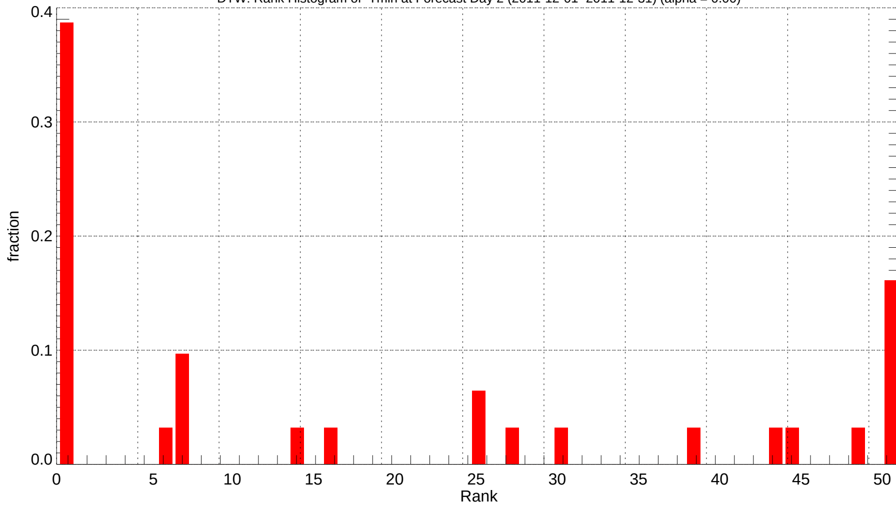
DTW: Rank Histogram of Tmin at Forecast Day 2 (2011-12-01~2011-12-31) (alpha = 0.00)
