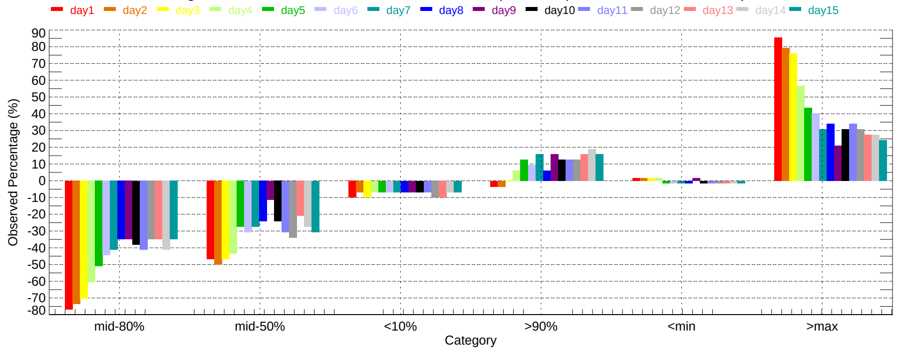
Observed Percentage Deviation of Ensembles - SAN: Max Temperature (2011-12-01~2011-12-31)
