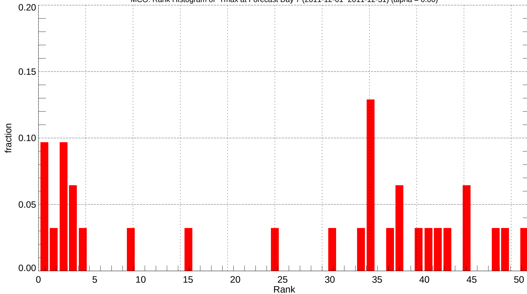
MCO: Rank Histogram of Tmax at Forecast Day 7 (2011-12-01~2011-12-31) (alpha = 0.00)
