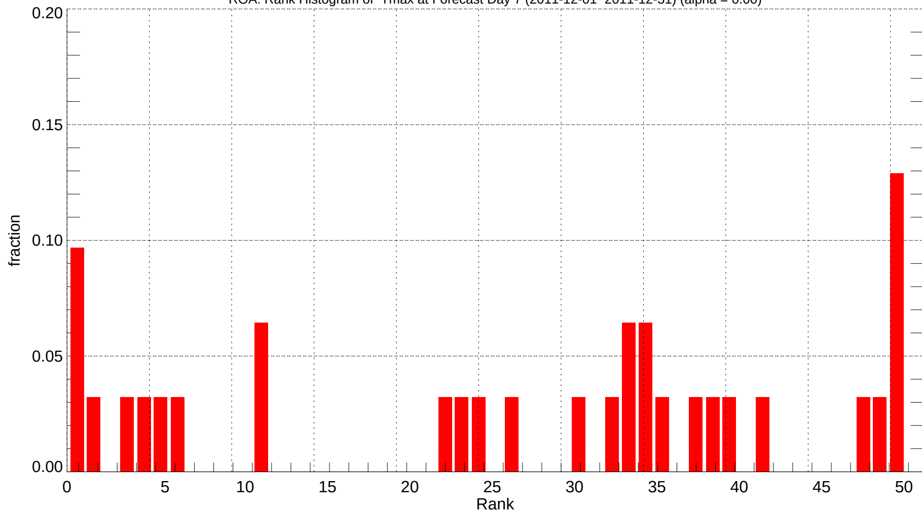
ROA: Rank Histogram of Tmax at Forecast Day 7 (2011-12-01~2011-12-31) (alpha = 0.00)
