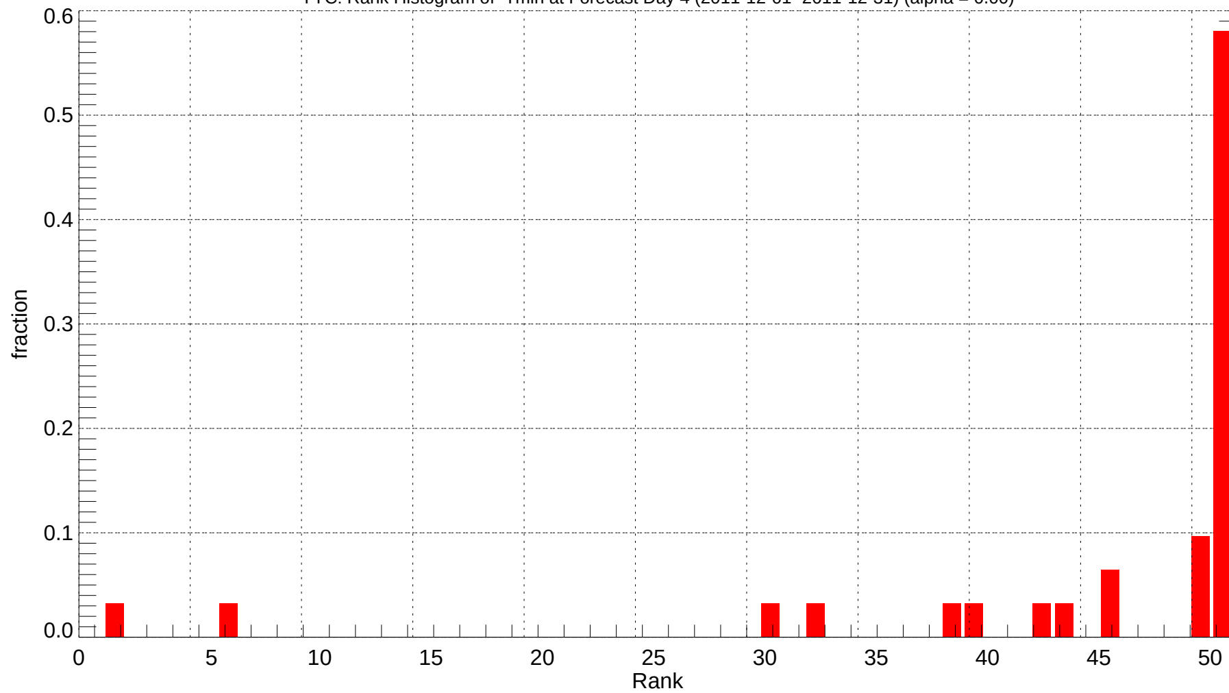
YYC: Rank Histogram of Tmin at Forecast Day 4 (2011-12-01~2011-12-31) (alpha = 0.00)
