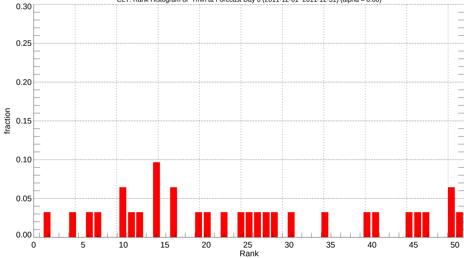
CLT: Rank Histogram of Tmin at Forecast Day 6 (2011-12-01~2011-12-31) (alpha = 0.00)
