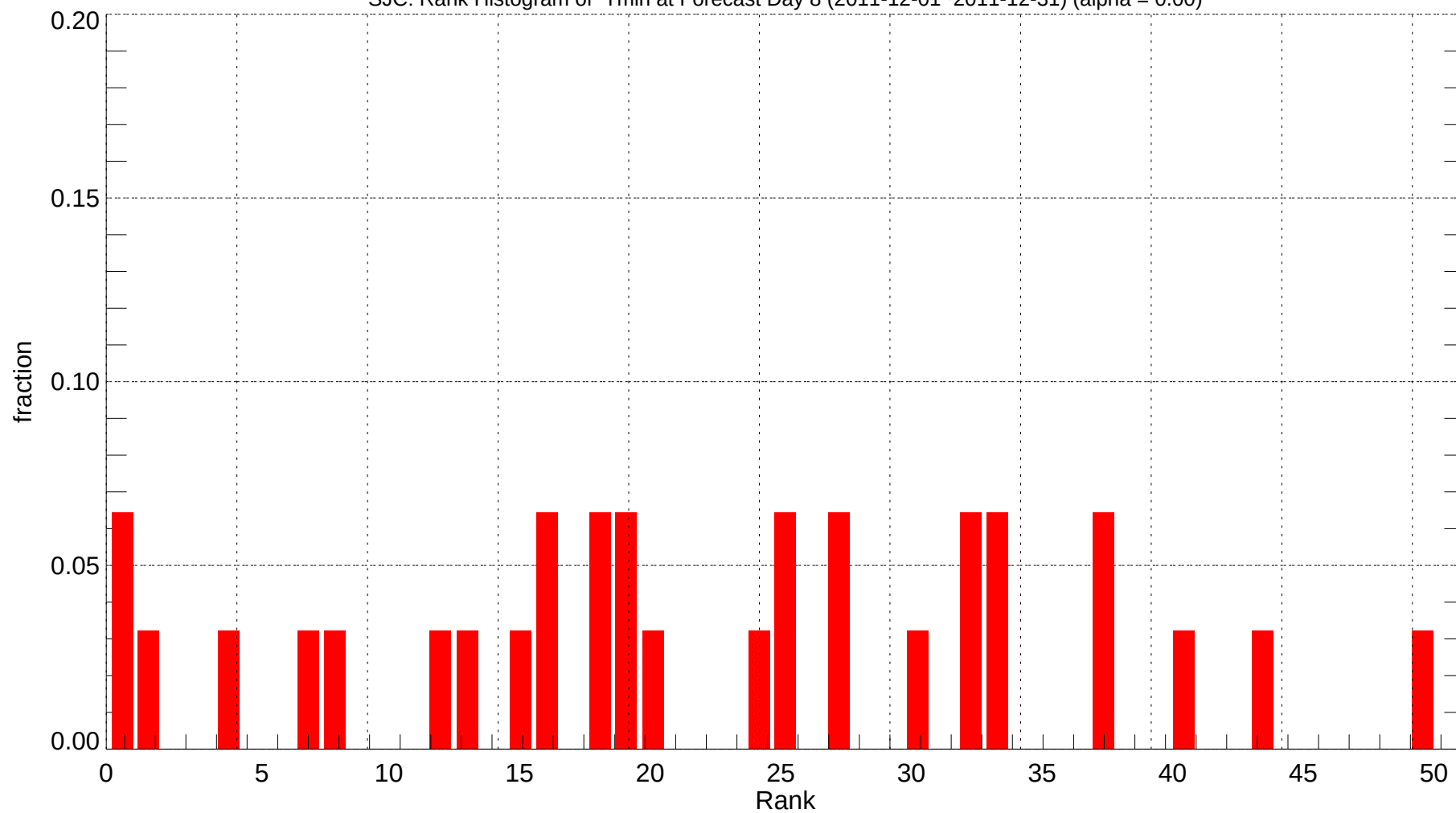
SJC: Rank Histogram of Tmin at Forecast Day 8 (2011-12-01~2011-12-31) (alpha = 0.00)
