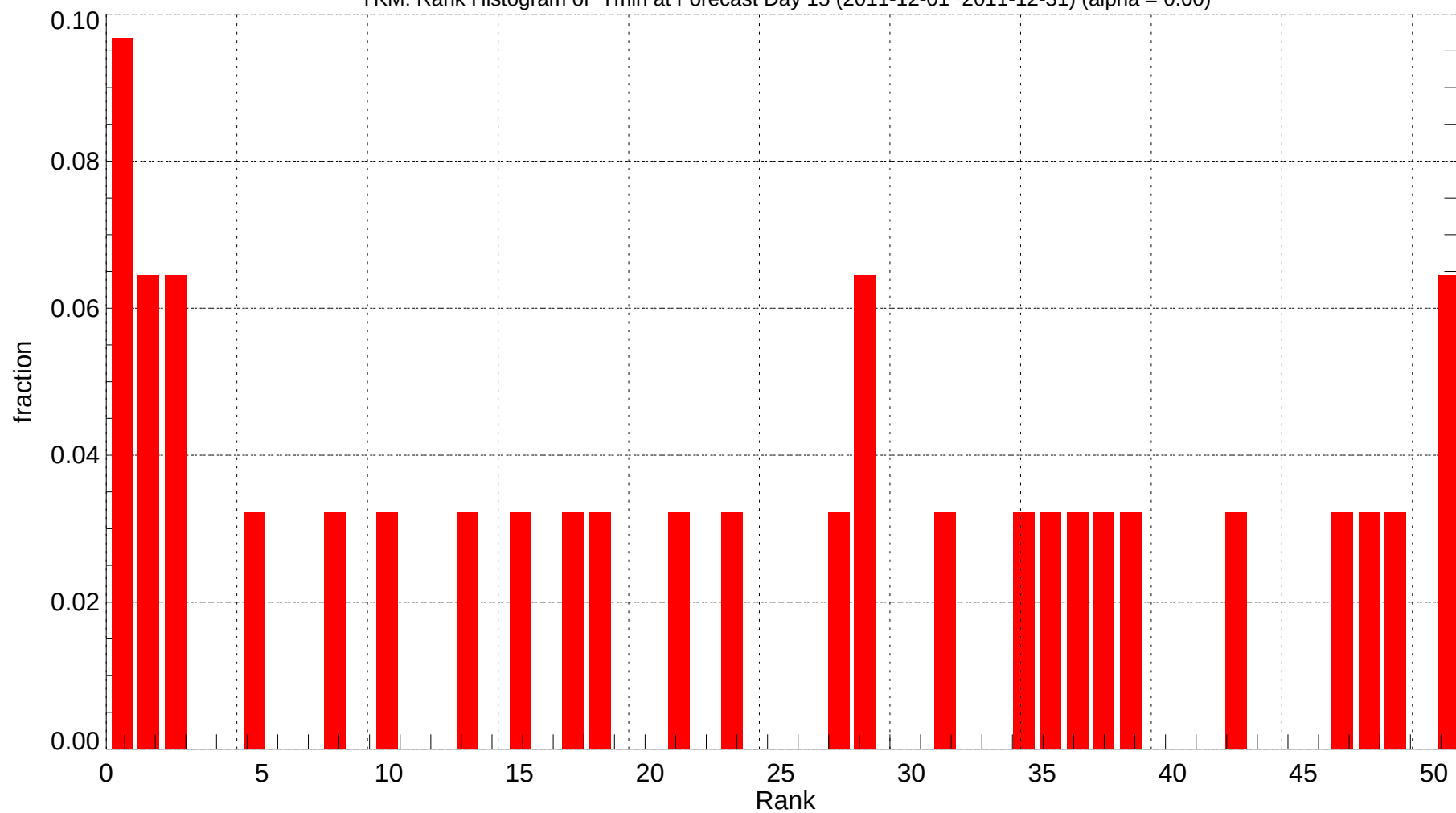
YKM: Rank Histogram of Tmin at Forecast Day 15 (2011-12-01~2011-12-31) (alpha = 0.00)
