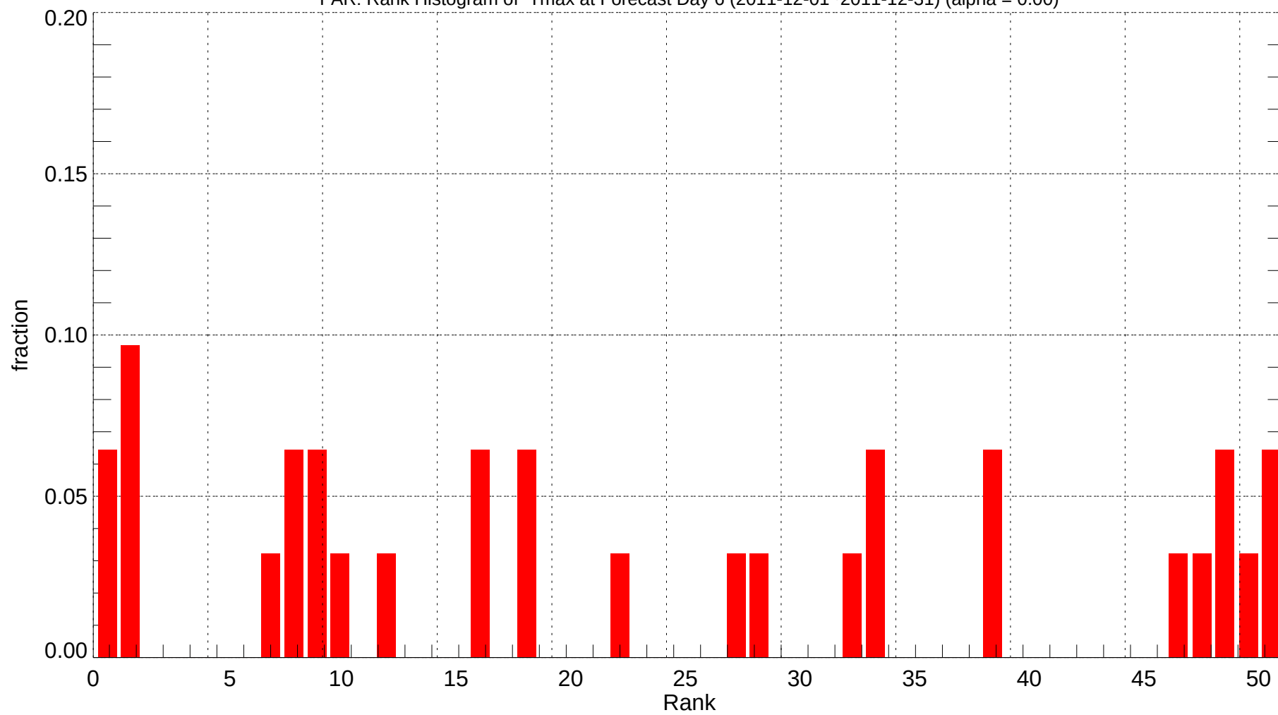
FAR: Rank Histogram of Tmax at Forecast Day 6 (2011-12-01~2011-12-31) (alpha = 0.00)
