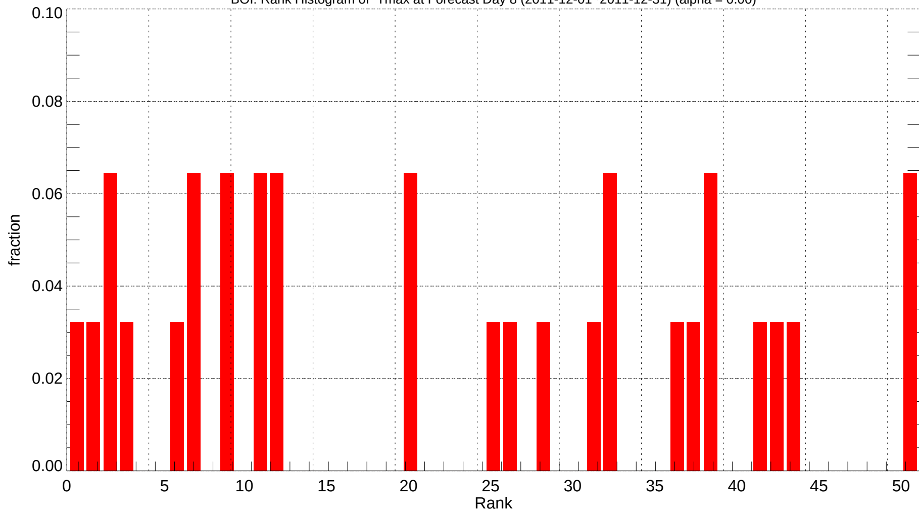
BOI: Rank Histogram of Tmax at Forecast Day 8 (2011-12-01~2011-12-31) (alpha = 0.00)
