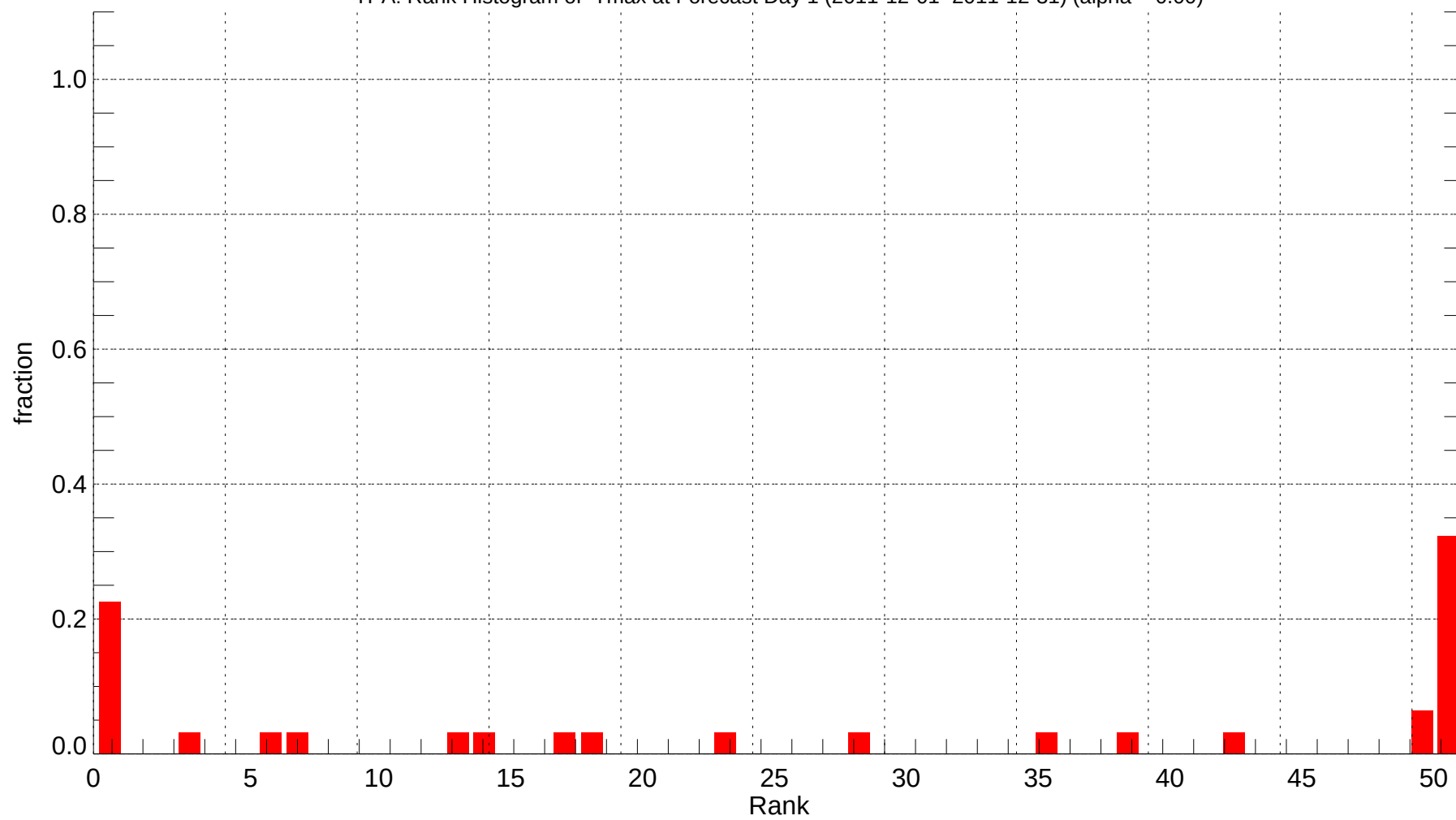
TPA: Rank Histogram of Tmax at Forecast Day 1 (2011-12-01~2011-12-31) (alpha = 0.00)
