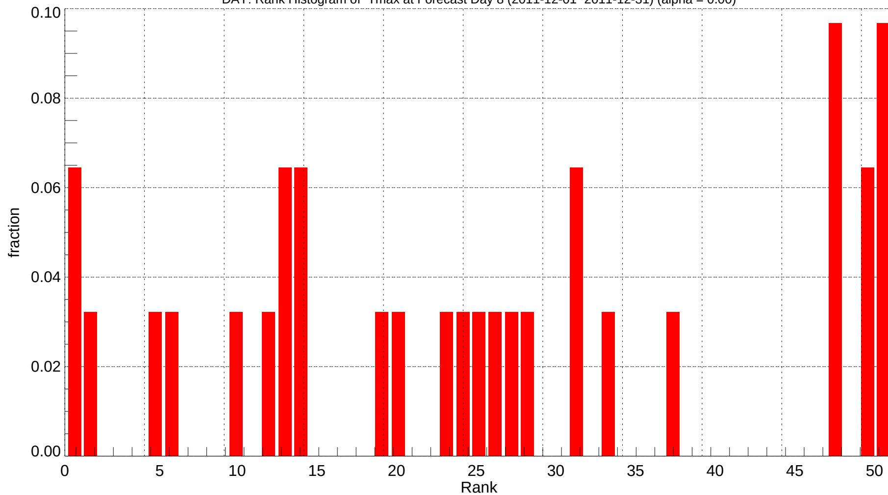
DAY: Rank Histogram of Tmax at Forecast Day 8 (2011-12-01~2011-12-31) (alpha = 0.00)
