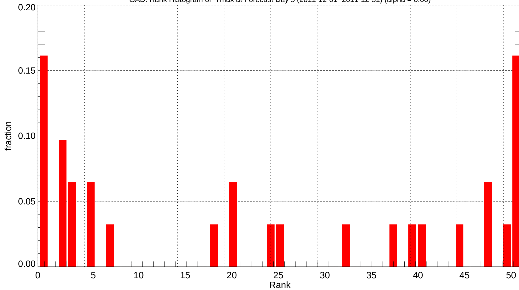
GAD: Rank Histogram of Tmax at Forecast Day 5 (2011-12-01~2011-12-31) (alpha = 0.00)
