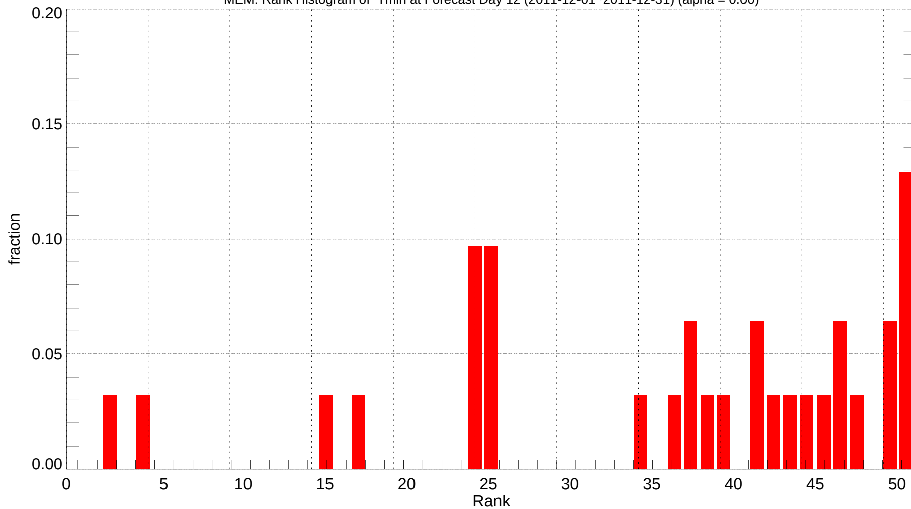
MEM: Rank Histogram of Tmin at Forecast Day 12 (2011-12-01~2011-12-31) (alpha = 0.00)
