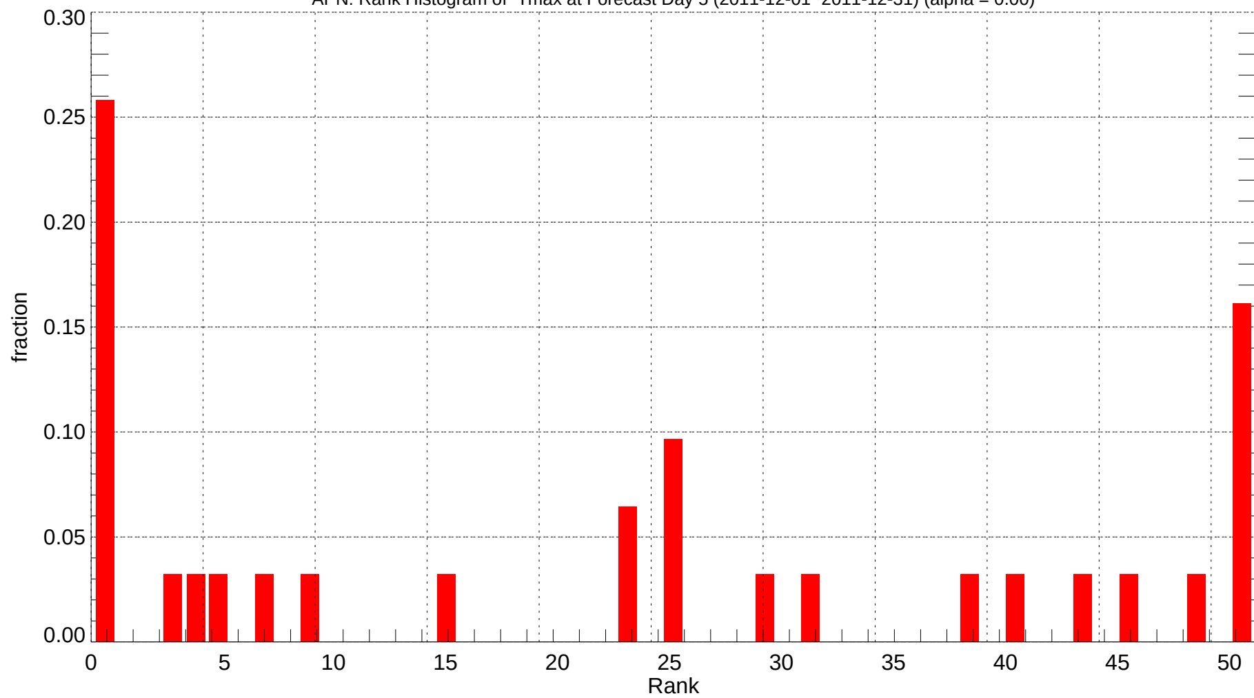
APN: Rank Histogram of Tmax at Forecast Day 5 (2011-12-01~2011-12-31) (alpha = 0.00)
