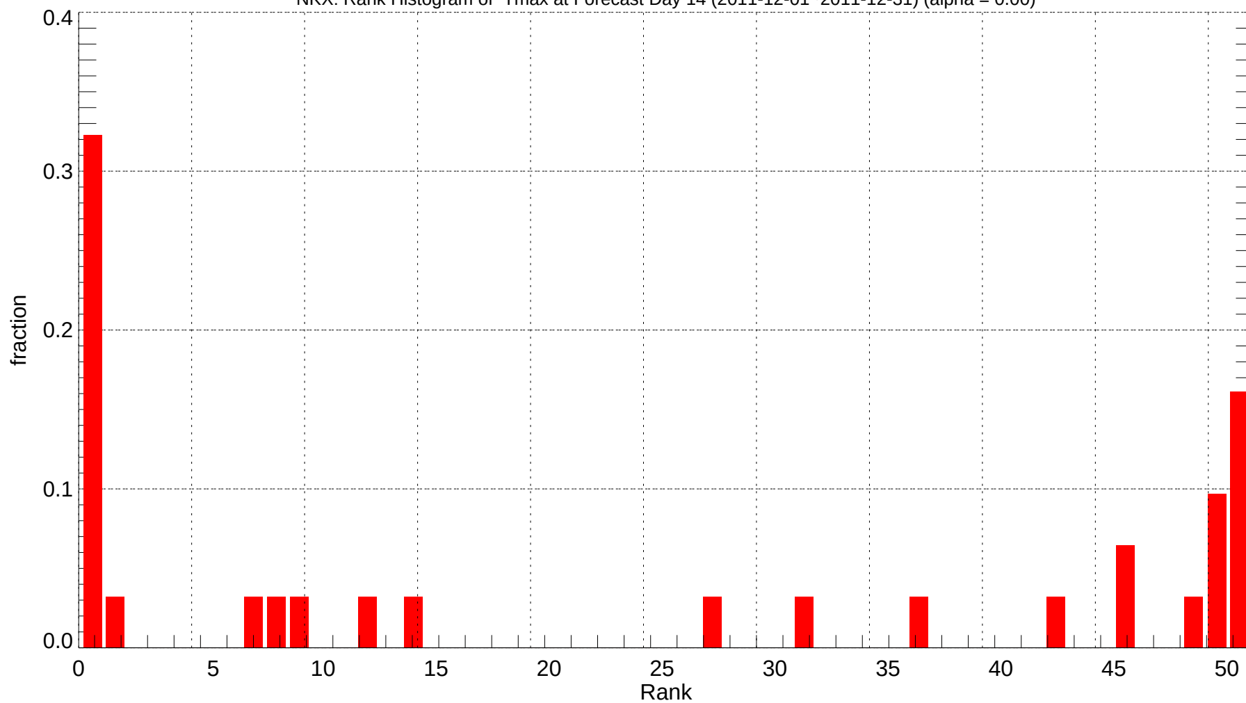
NKX: Rank Histogram of Tmax at Forecast Day 14 (2011-12-01~2011-12-31) (alpha = 0.00)
