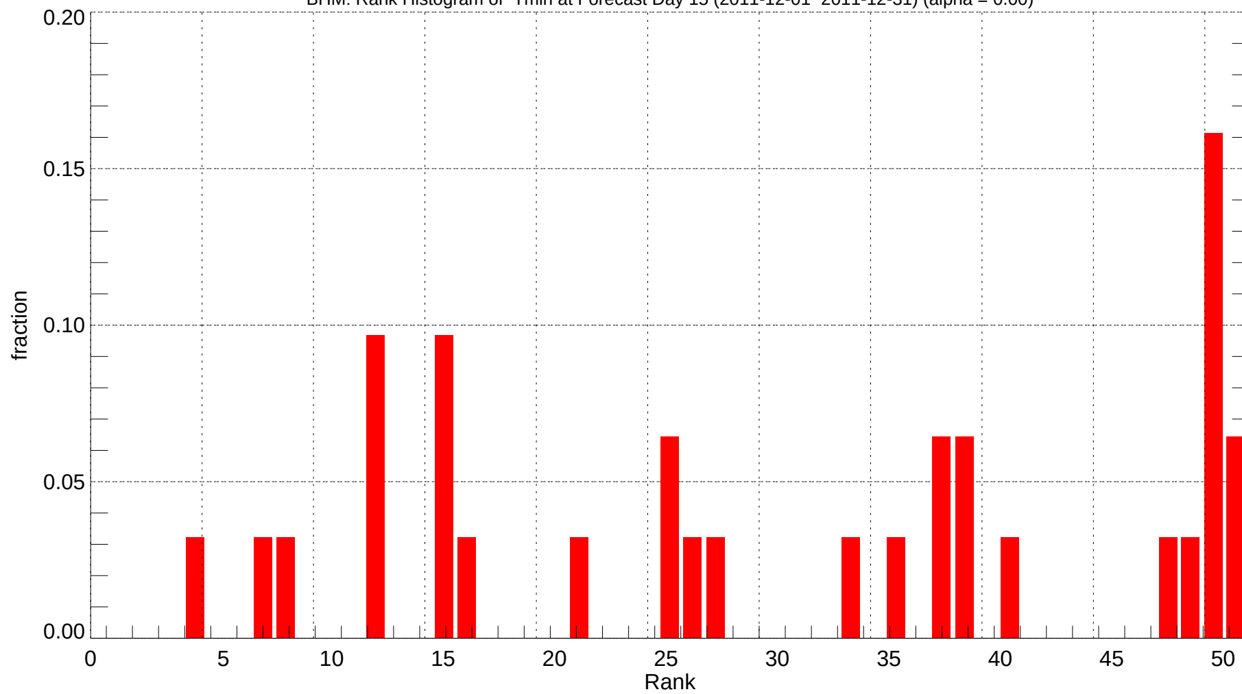
BHM: Rank Histogram of Tmin at Forecast Day 15 (2011-12-01~2011-12-31) (alpha = 0.00)
