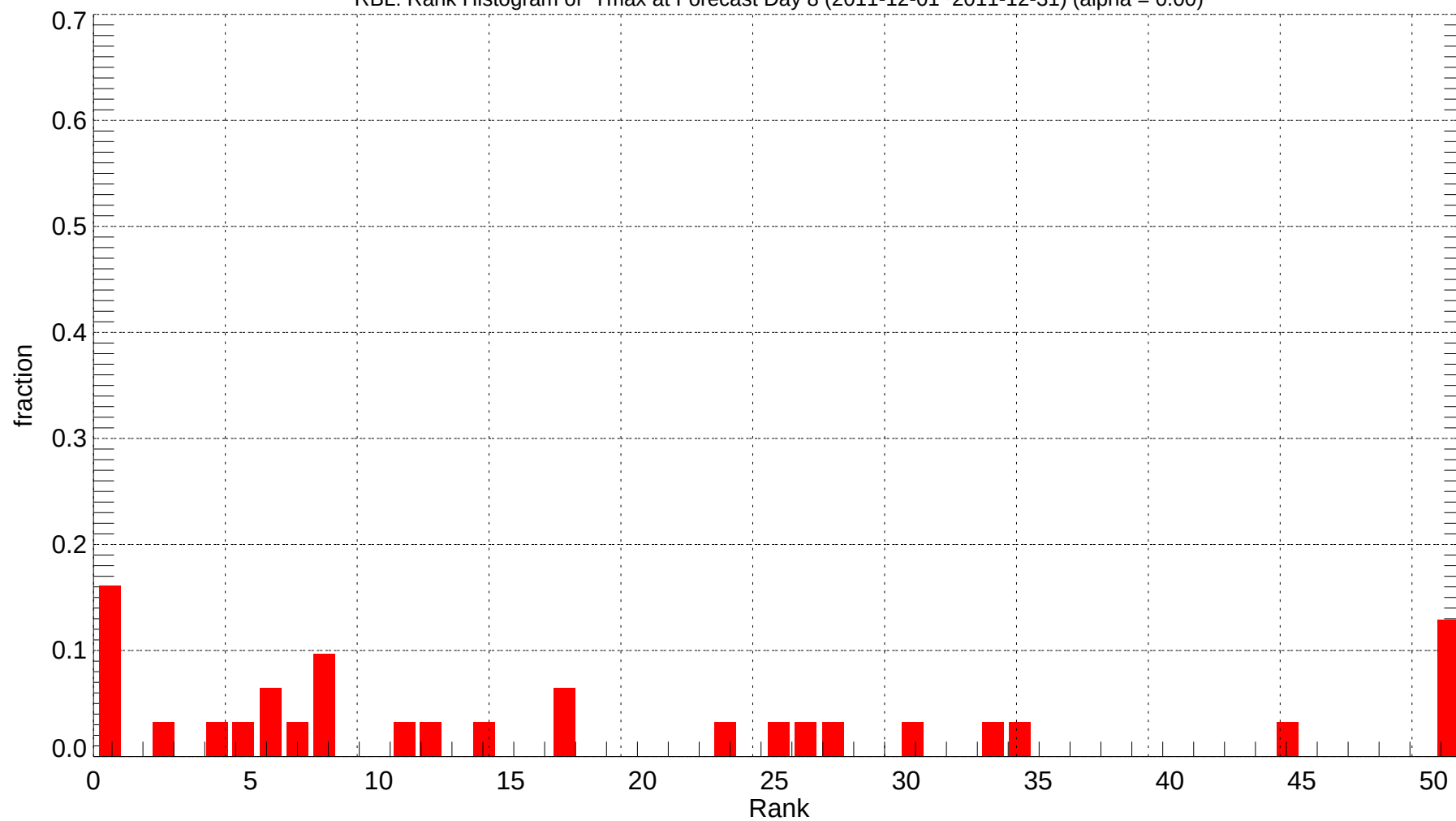
RBL: Rank Histogram of Tmax at Forecast Day 8 (2011-12-01~2011-12-31) (alpha = 0.00)
