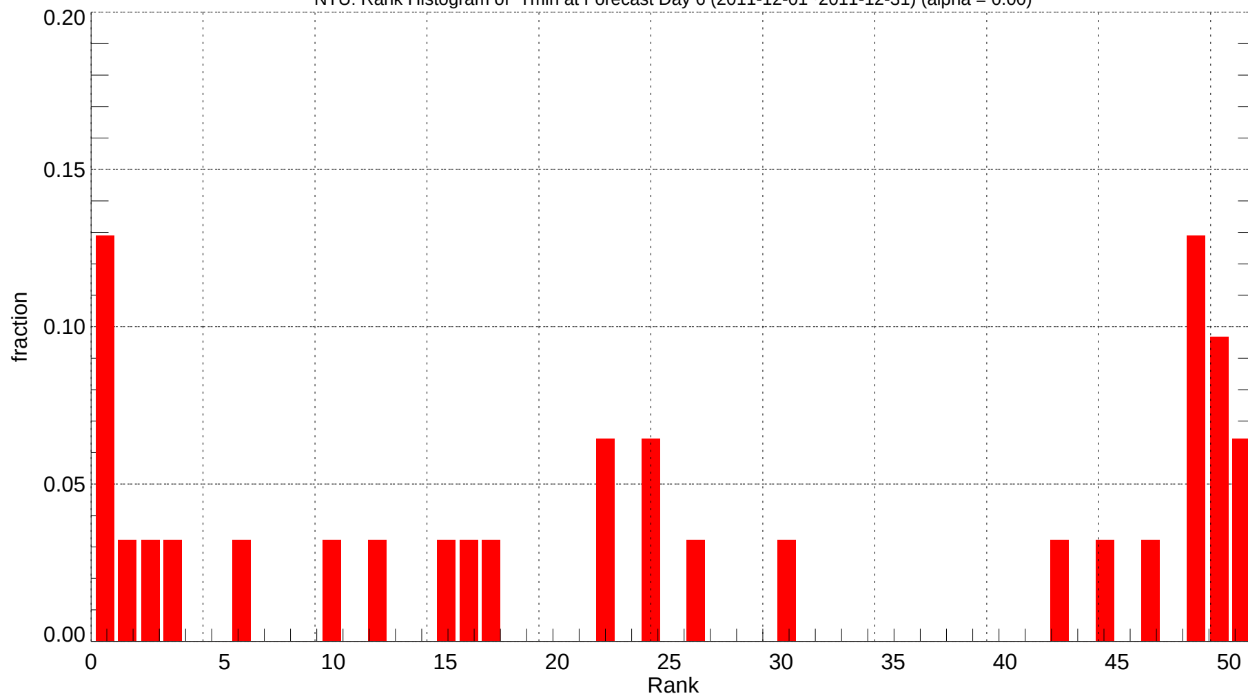
NTU: Rank Histogram of Tmin at Forecast Day 6 (2011-12-01~2011-12-31) (alpha = 0.00)
