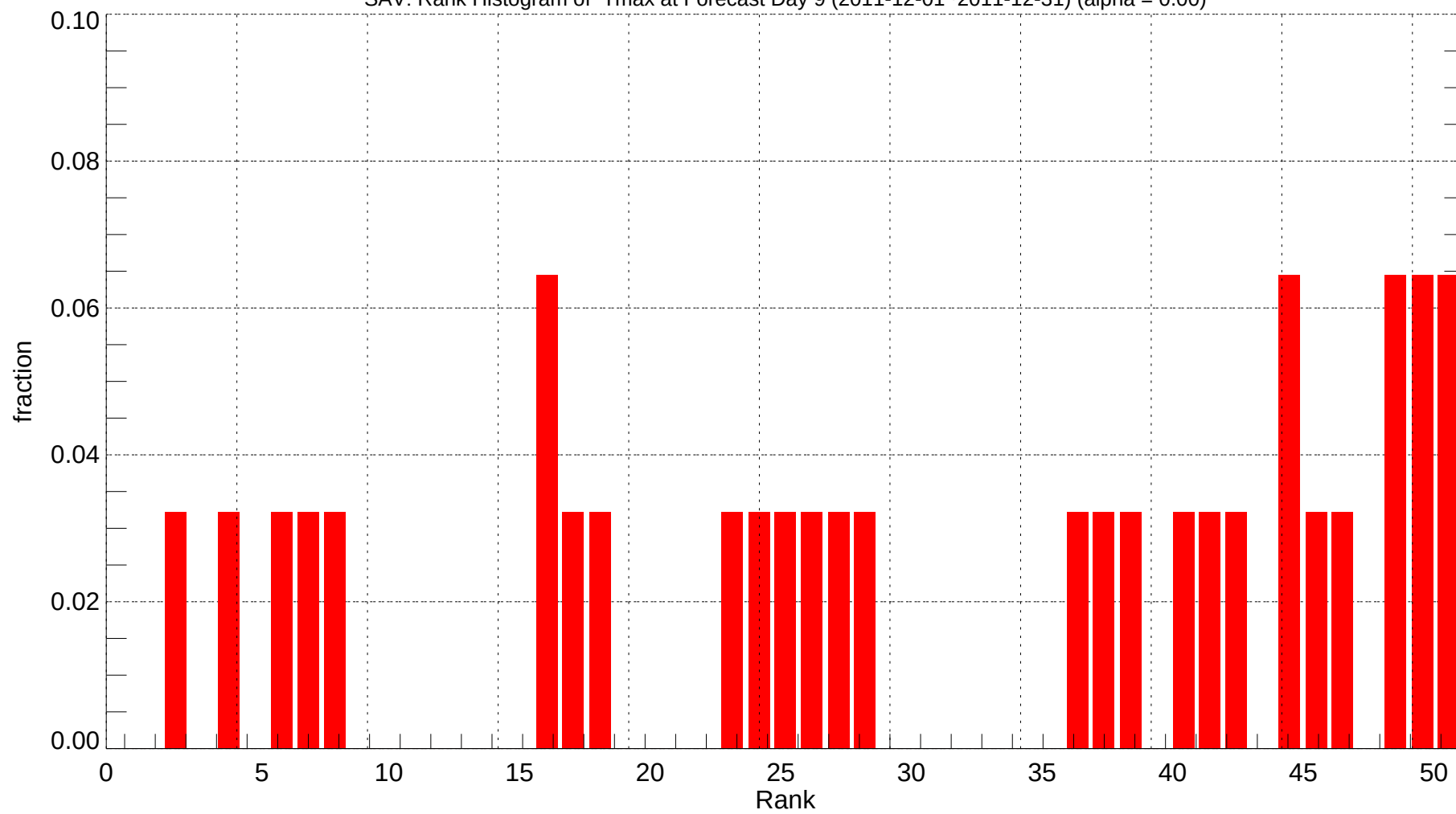
SAV: Rank Histogram of Tmax at Forecast Day 9 (2011-12-01~2011-12-31) (alpha = 0.00)
