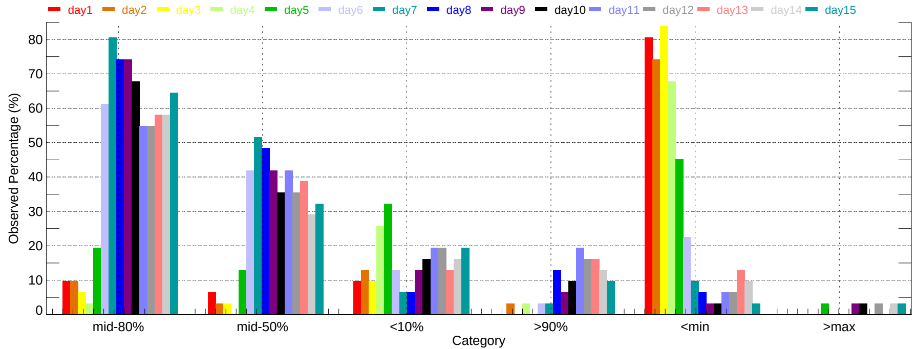
Observed Percentage of Ensembles - CQT: Max Temperature (2011-12-01~2011-12-31)
