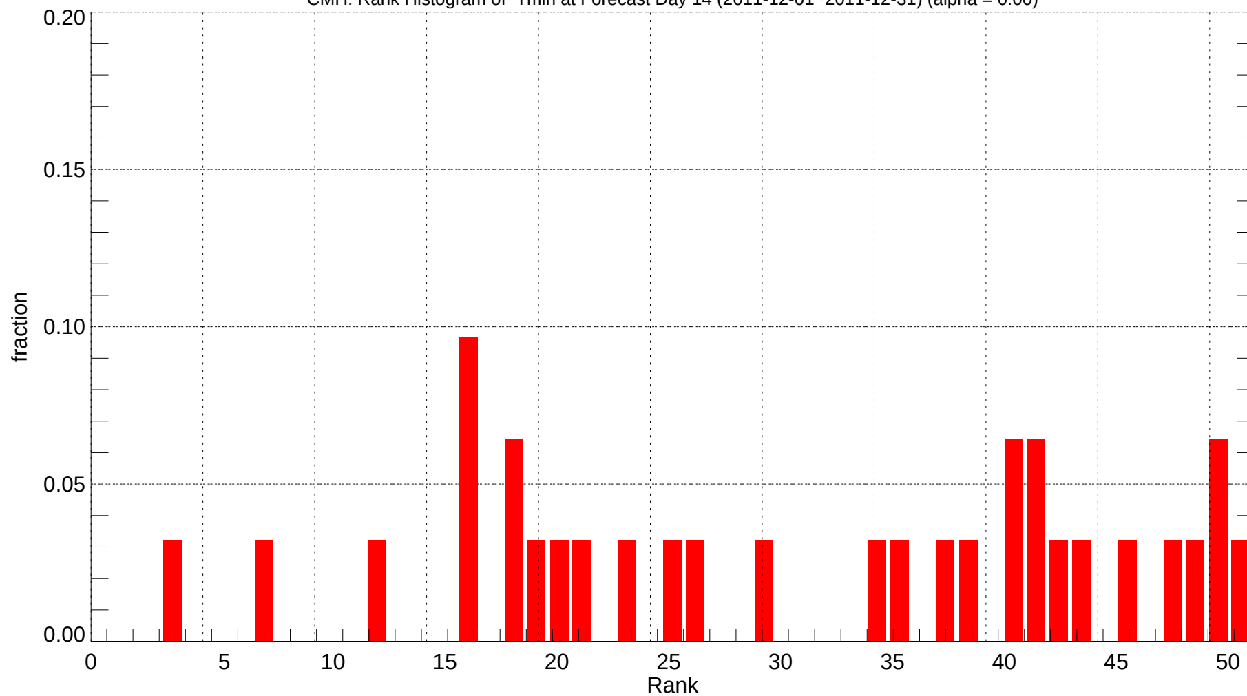
CMH: Rank Histogram of Tmin at Forecast Day 14 (2011-12-01~2011-12-31) (alpha = 0.00)
