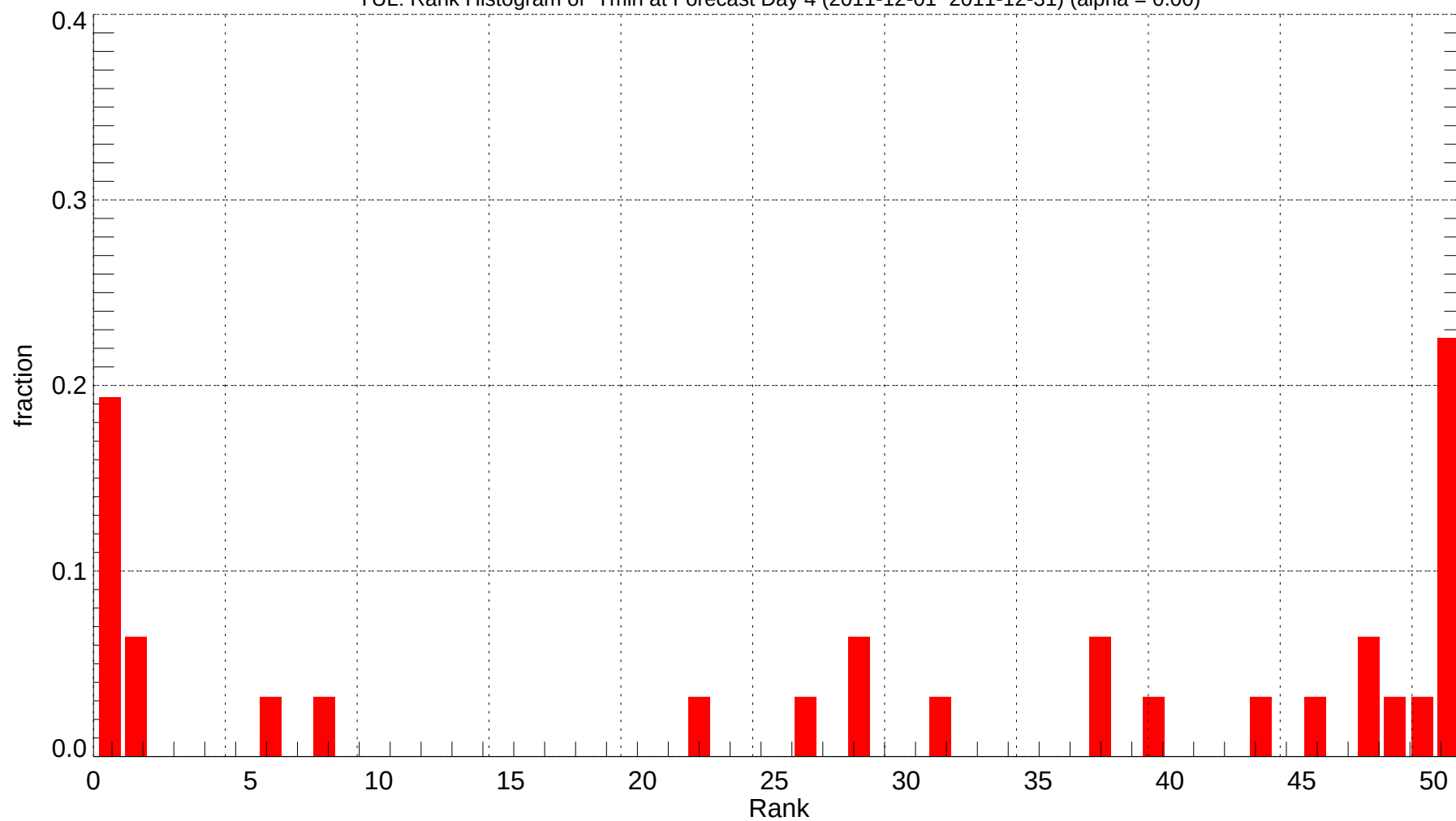
YUL: Rank Histogram of Tmin at Forecast Day 4 (2011-12-01~2011-12-31) (alpha = 0.00)
