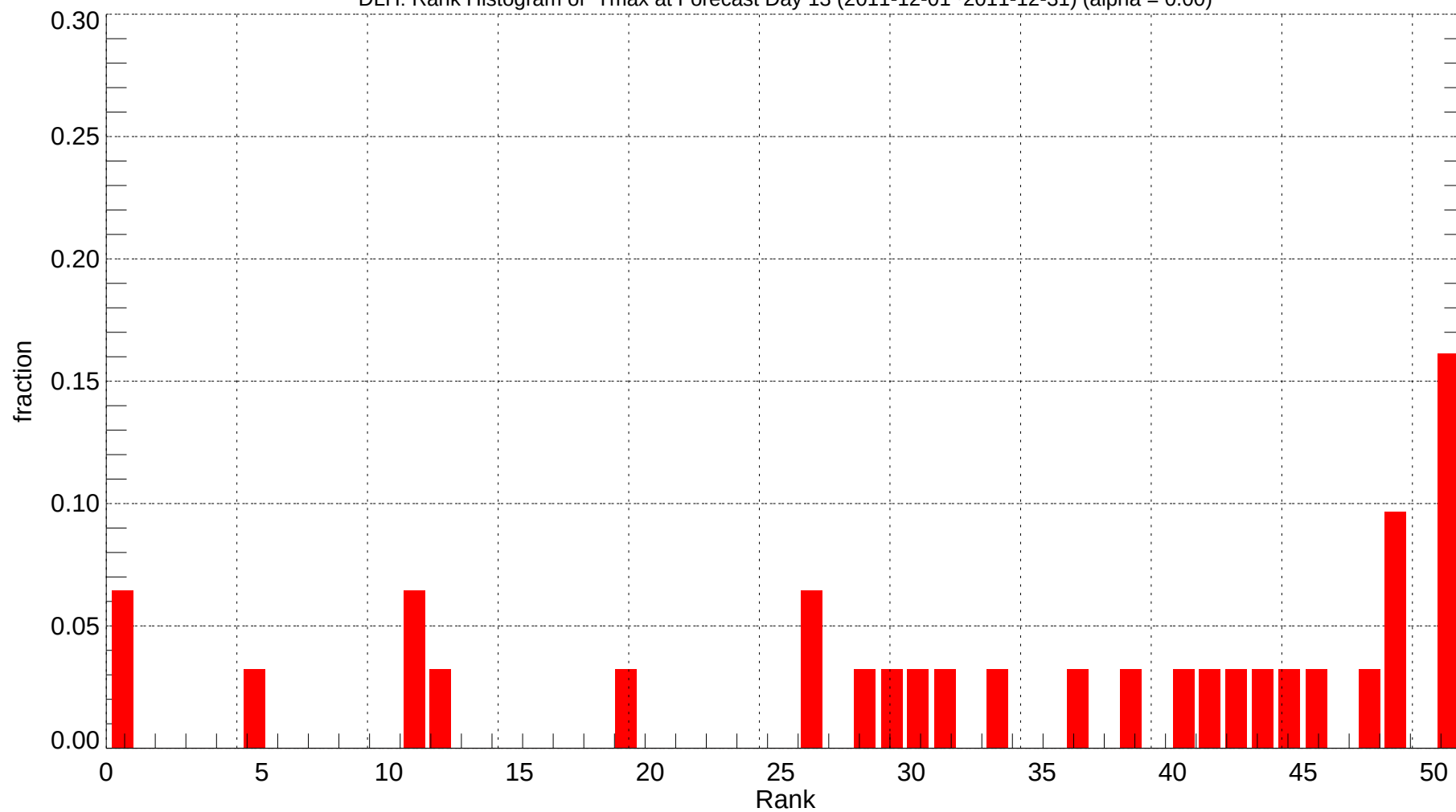
DLH: Rank Histogram of Tmax at Forecast Day 13 (2011-12-01~2011-12-31) (alpha = 0.00)
