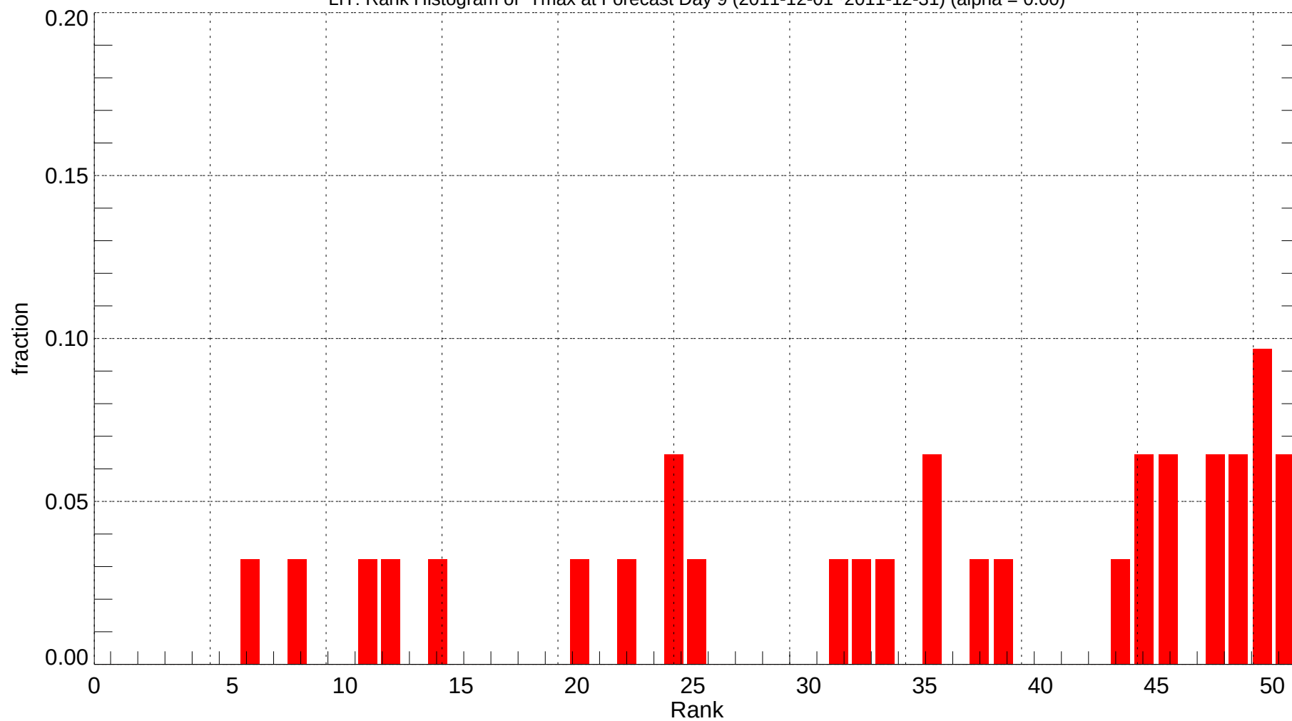
LIT: Rank Histogram of Tmax at Forecast Day 9 (2011-12-01~2011-12-31) (alpha = 0.00)
