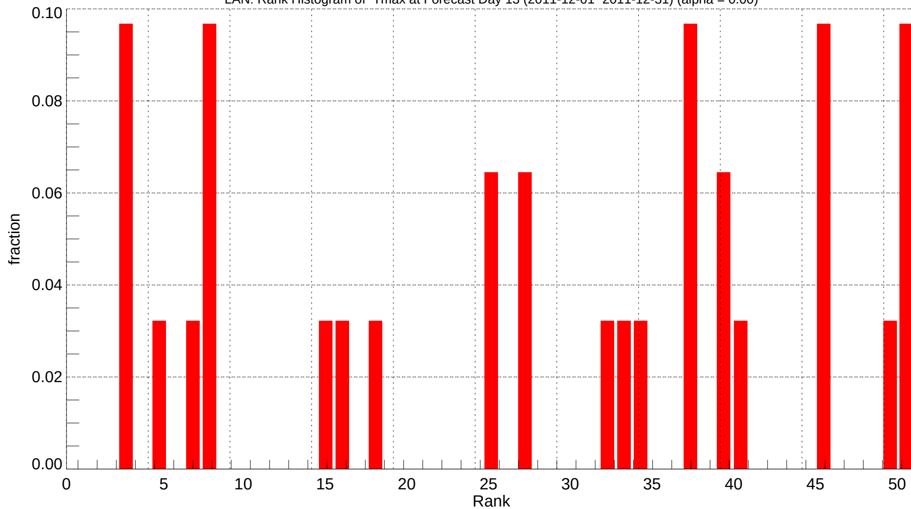
LAN: Rank Histogram of Tmax at Forecast Day 13 (2011-12-01~2011-12-31) (alpha = 0.00)
