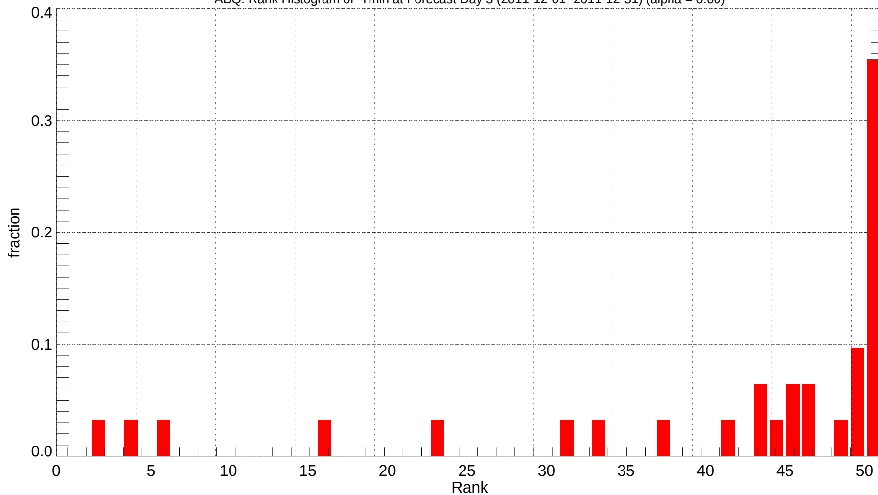
ABQ: Rank Histogram of Tmin at Forecast Day 5 (2011-12-01~2011-12-31) (alpha = 0.00)
