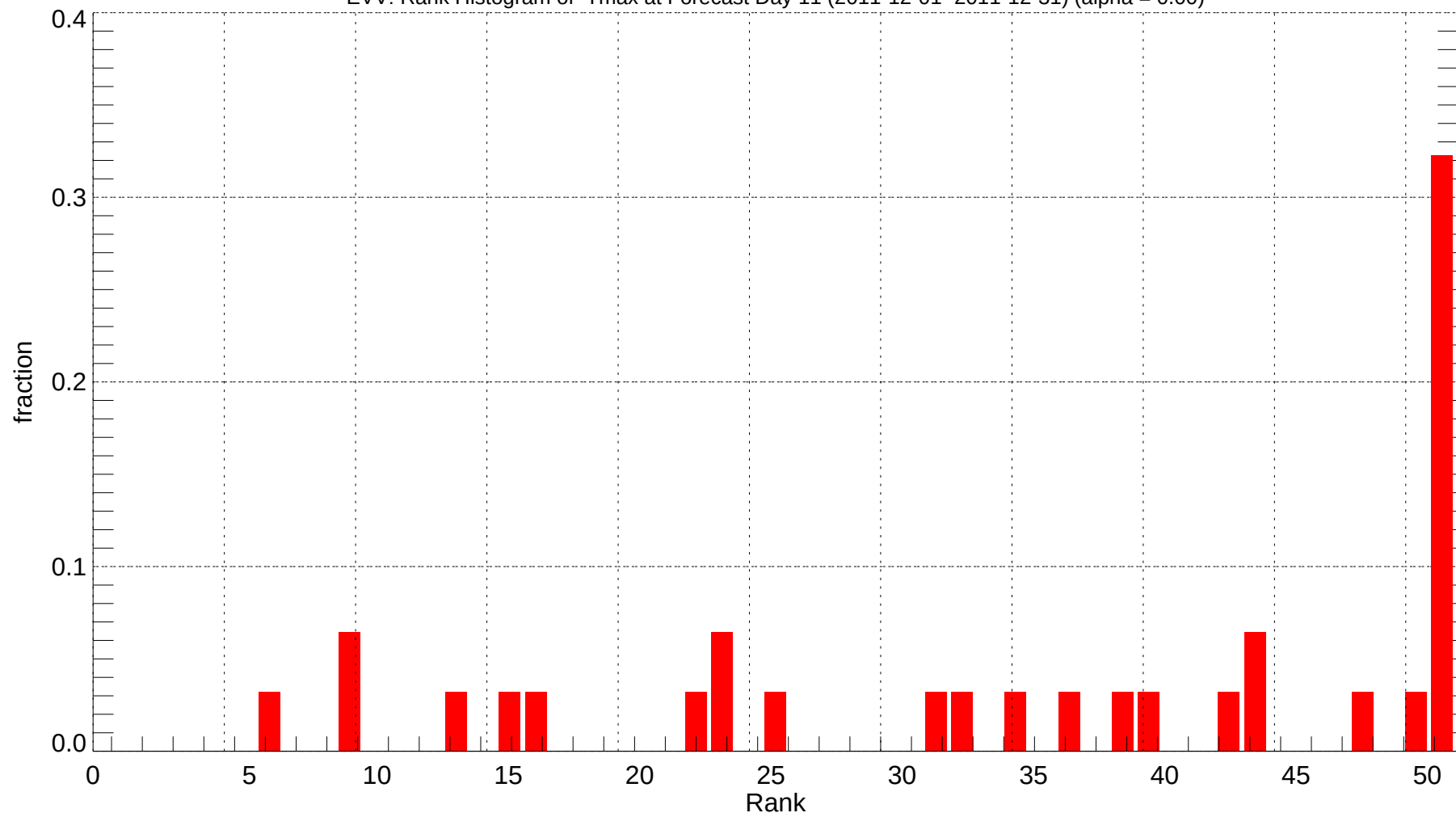
EVV: Rank Histogram of Tmax at Forecast Day 11 (2011-12-01~2011-12-31) (alpha = 0.00)
