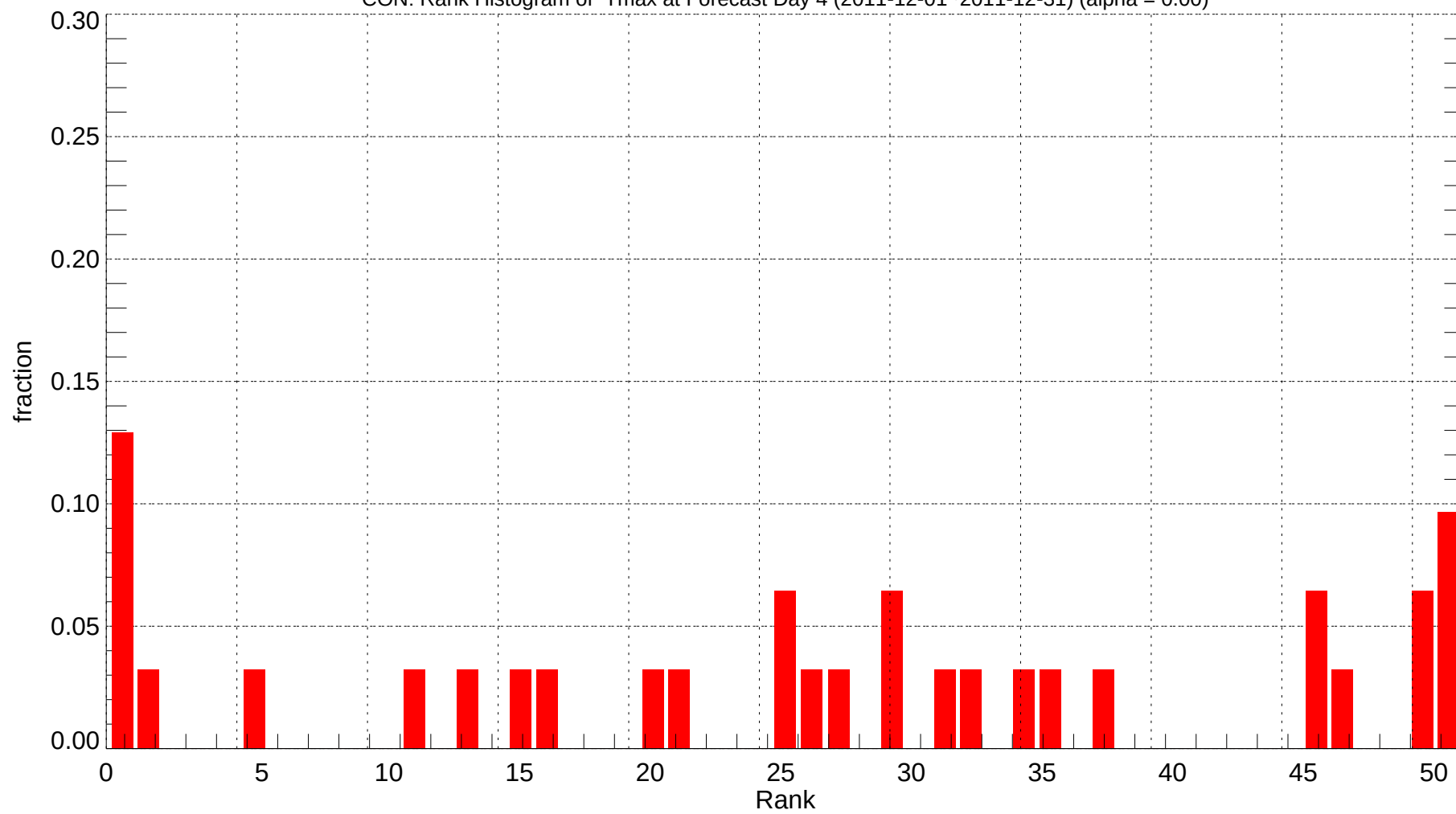
CON: Rank Histogram of Tmax at Forecast Day 4 (2011-12-01~2011-12-31) (alpha = 0.00)
