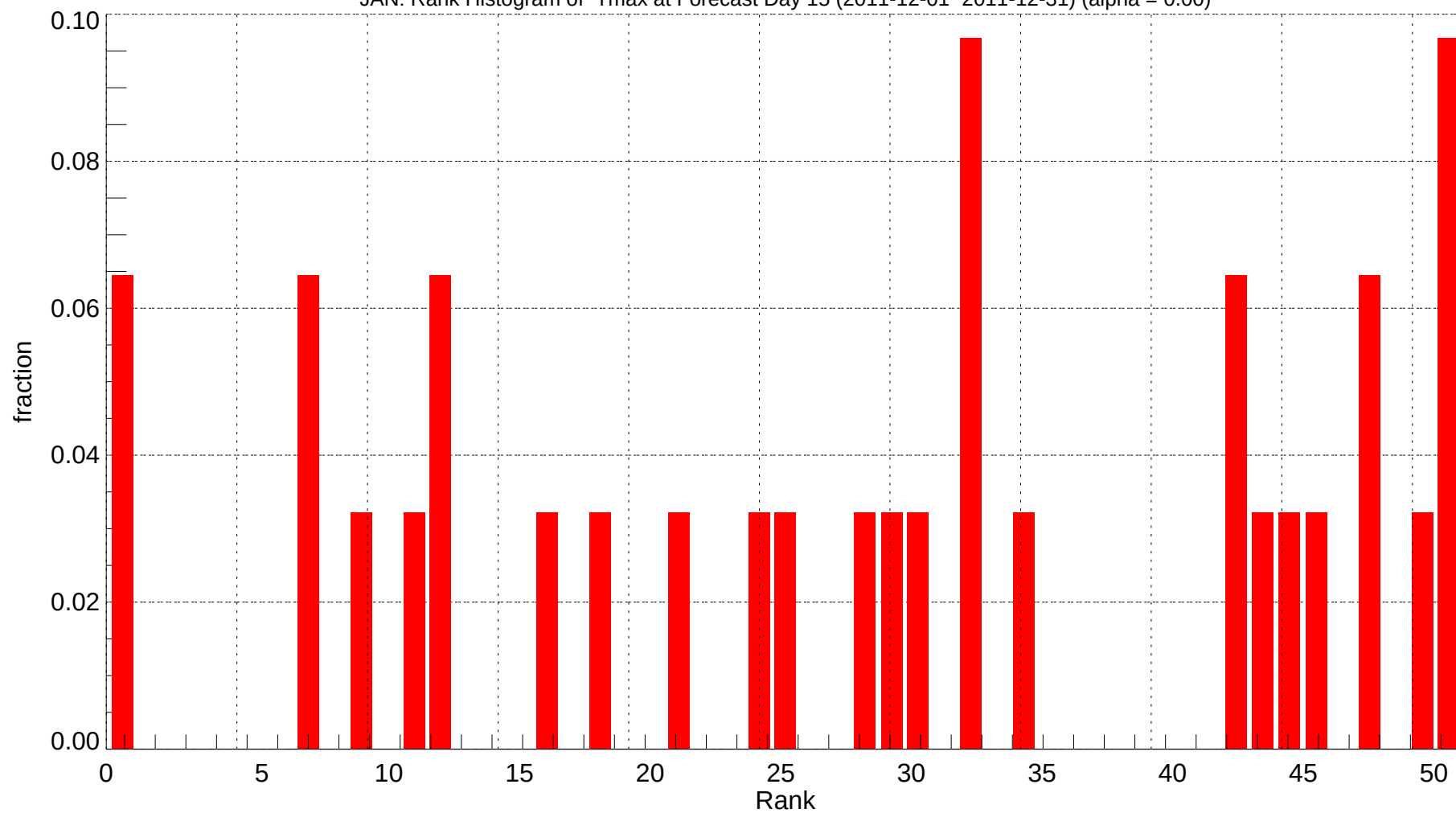
JAN: Rank Histogram of Tmax at Forecast Day 15 (2011-12-01~2011-12-31) (alpha = 0.00)
