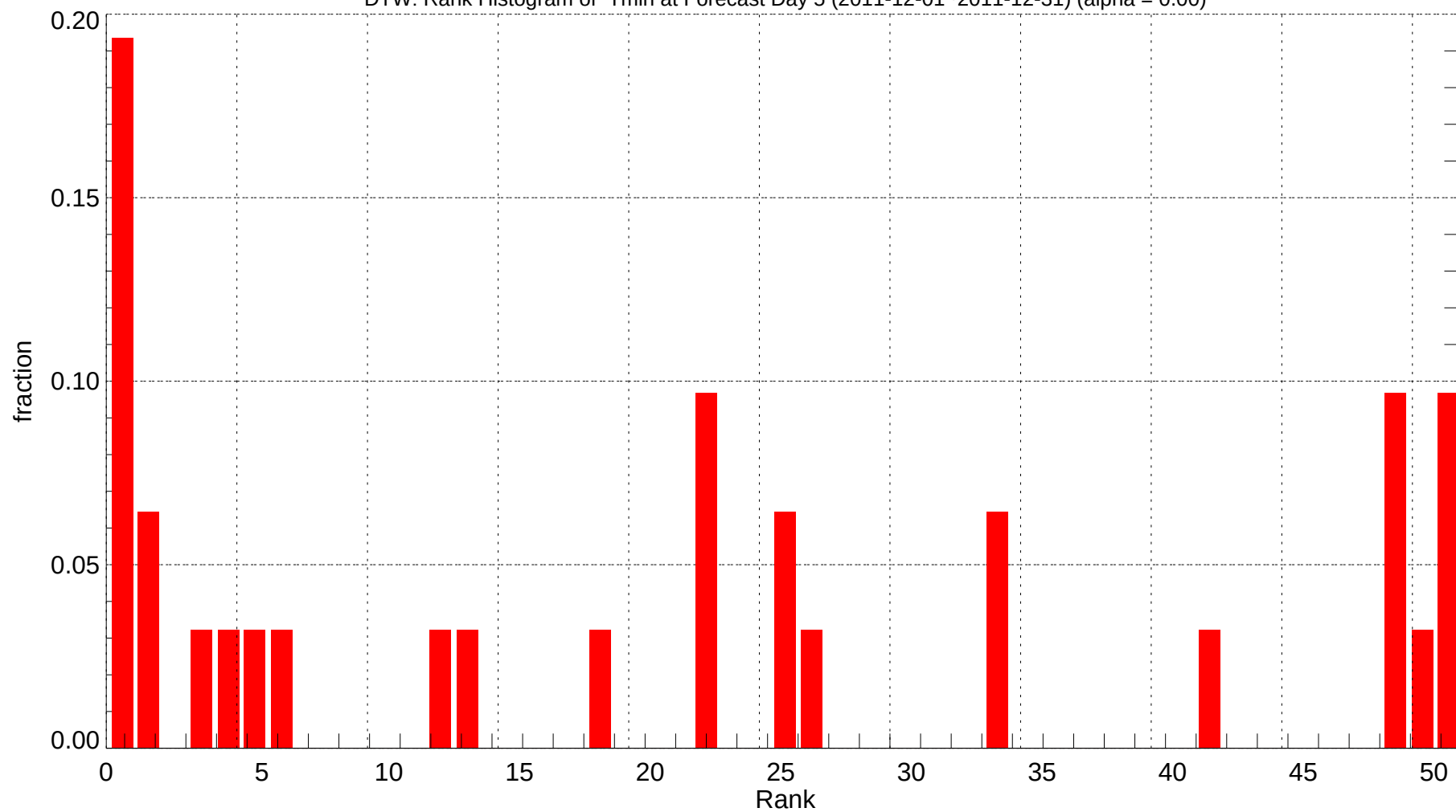
DTW: Rank Histogram of Tmin at Forecast Day 5 (2011-12-01~2011-12-31) (alpha = 0.00)
