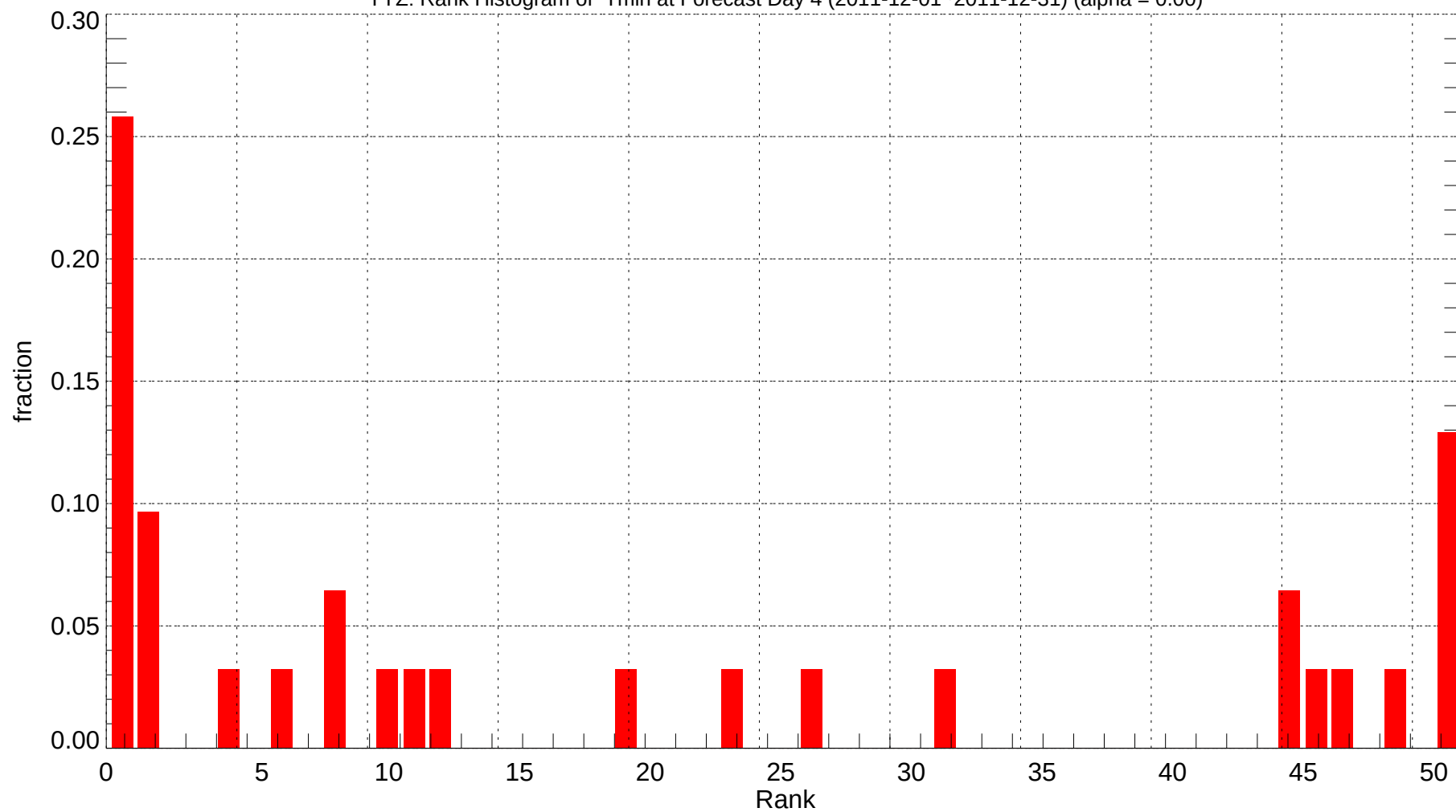
YYZ: Rank Histogram of Tmin at Forecast Day 4 (2011-12-01~2011-12-31) (alpha = 0.00)
