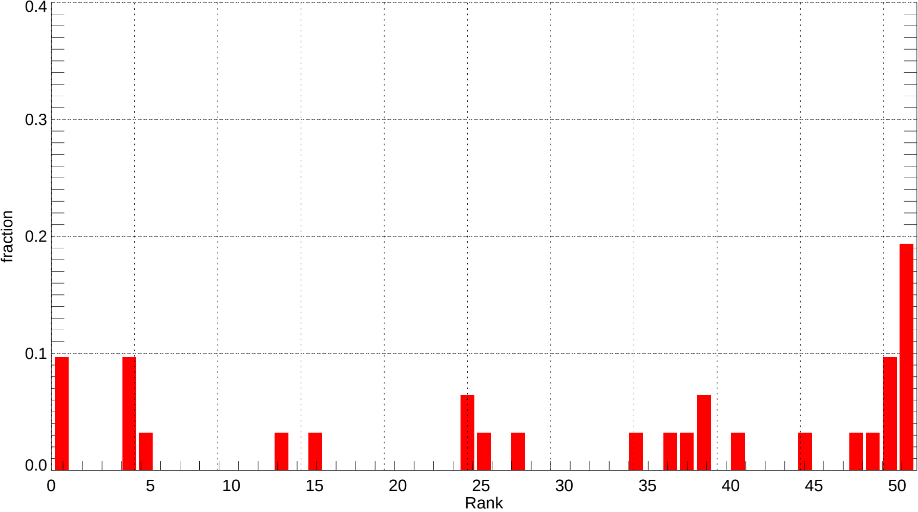
FAT: Rank Histogram of Tmin at Forecast Day 1 (2011-12-01~2011-12-31) (alpha = 0.00)
