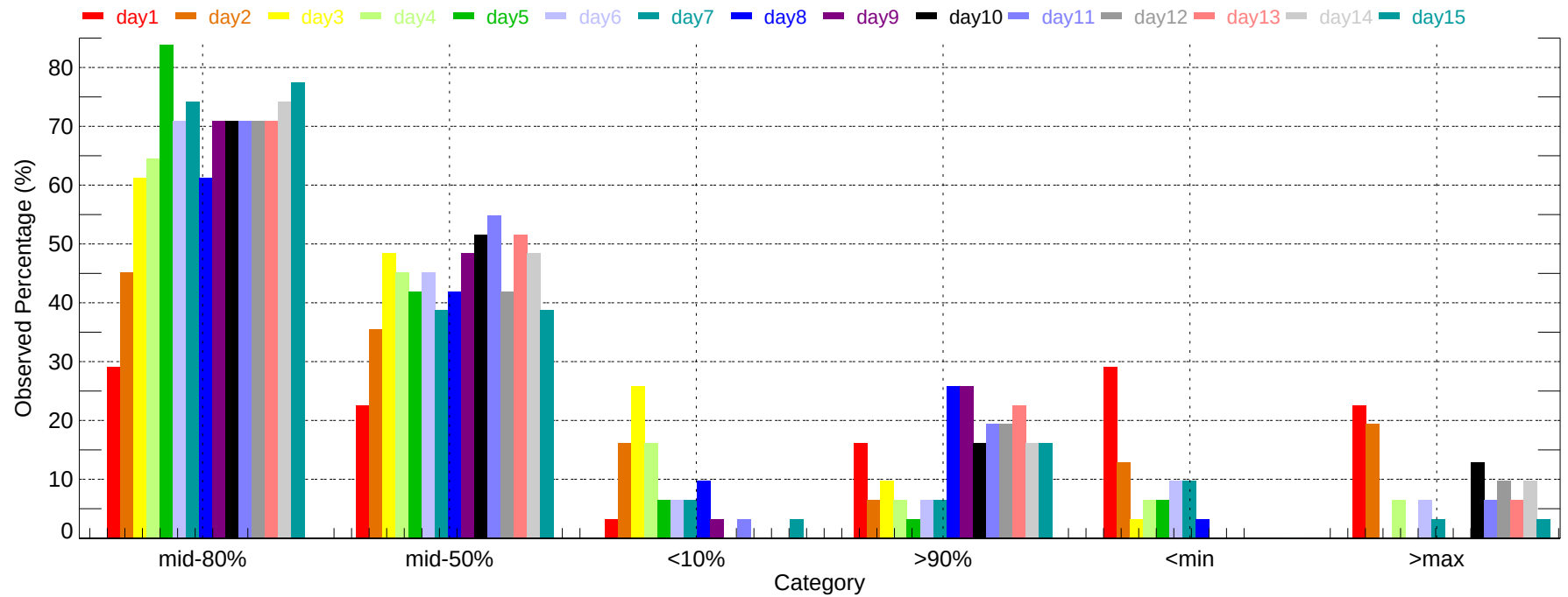
Observed Percentage of Ensembles - RDU: Max Temperature (2011-12-01~2011-12-31)
