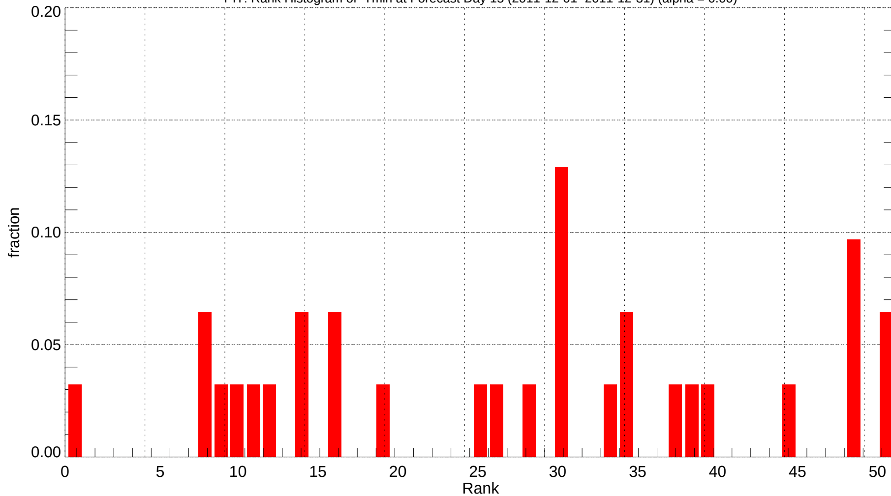
PIT: Rank Histogram of Tmin at Forecast Day 15 (2011-12-01~2011-12-31) (alpha = 0.00)
