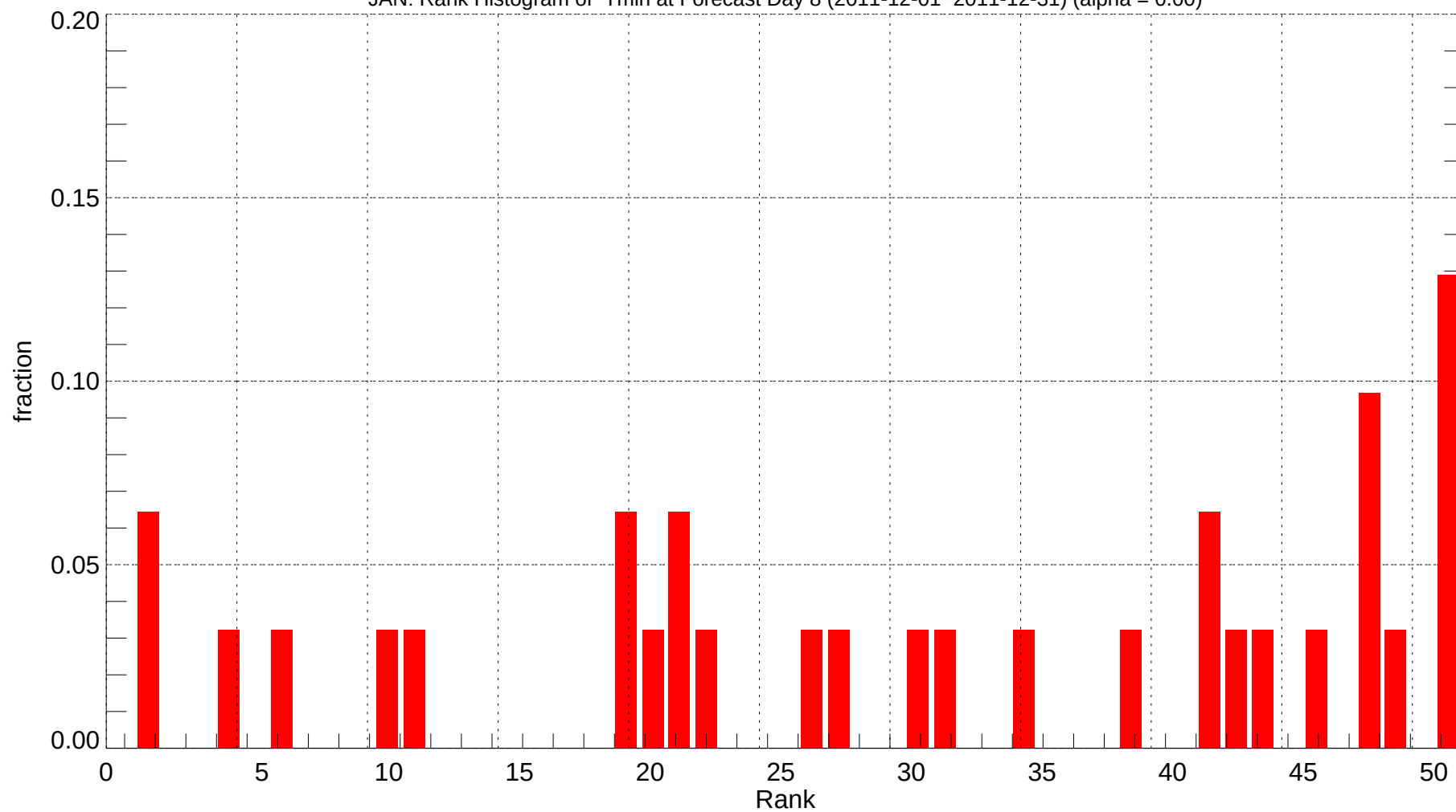
JAN: Rank Histogram of Tmin at Forecast Day 8 (2011-12-01~2011-12-31) (alpha = 0.00)
