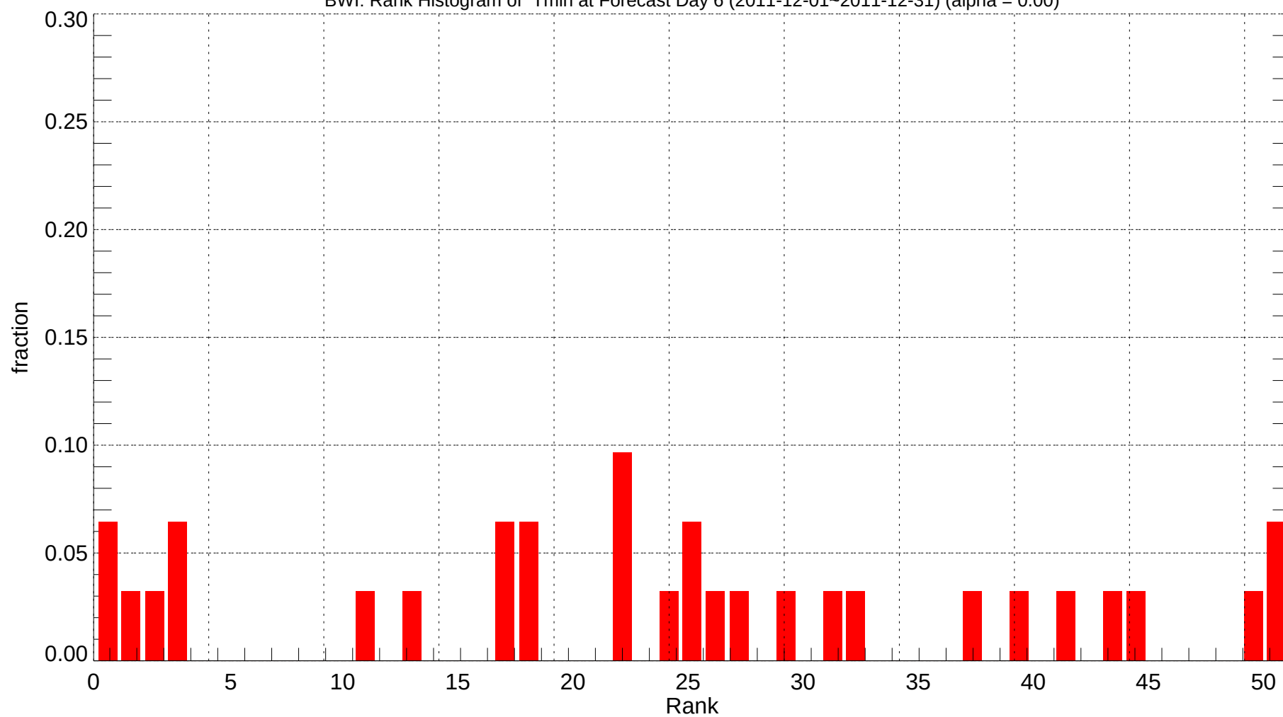
BWI: Rank Histogram of Tmin at Forecast Day 6 (2011-12-01~2011-12-31) (alpha = 0.00)
