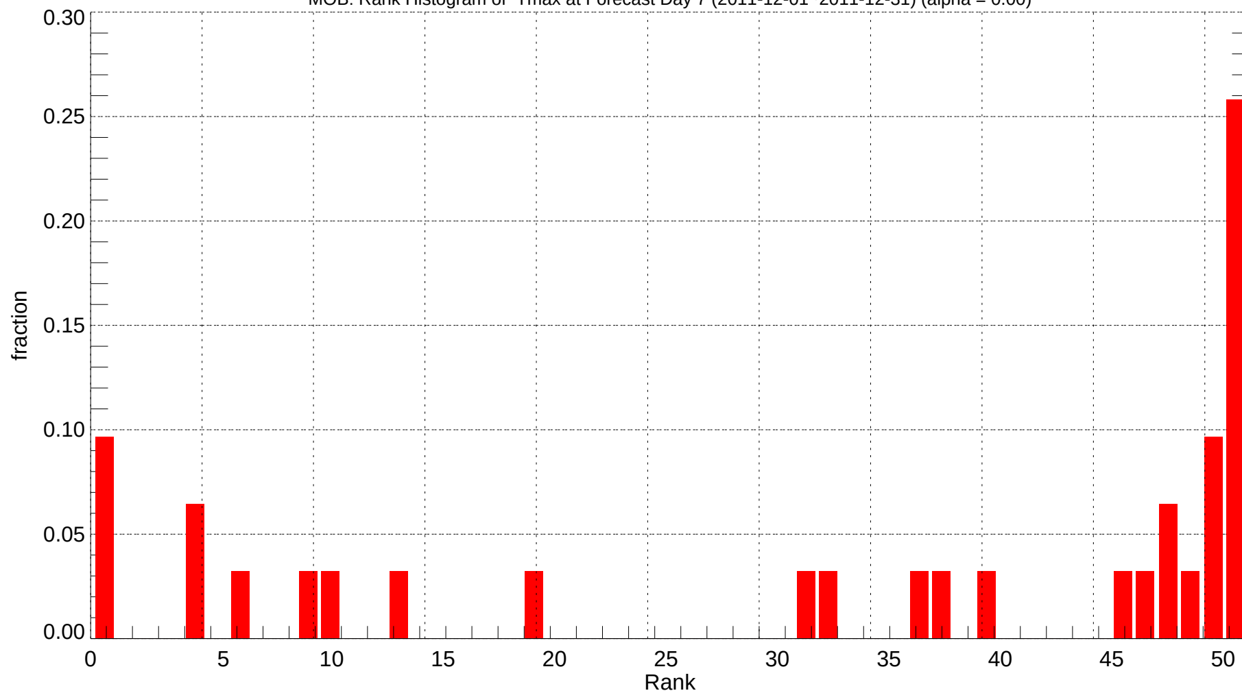
MOB: Rank Histogram of Tmax at Forecast Day 7 (2011-12-01~2011-12-31) (alpha = 0.00)
