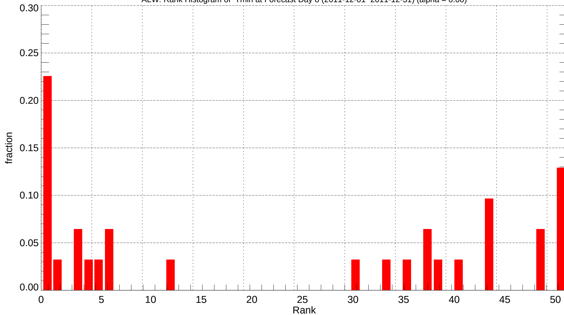
ALW: Rank Histogram of Tmin at Forecast Day 8 (2011-12-01~2011-12-31) (alpha = 0.00)
