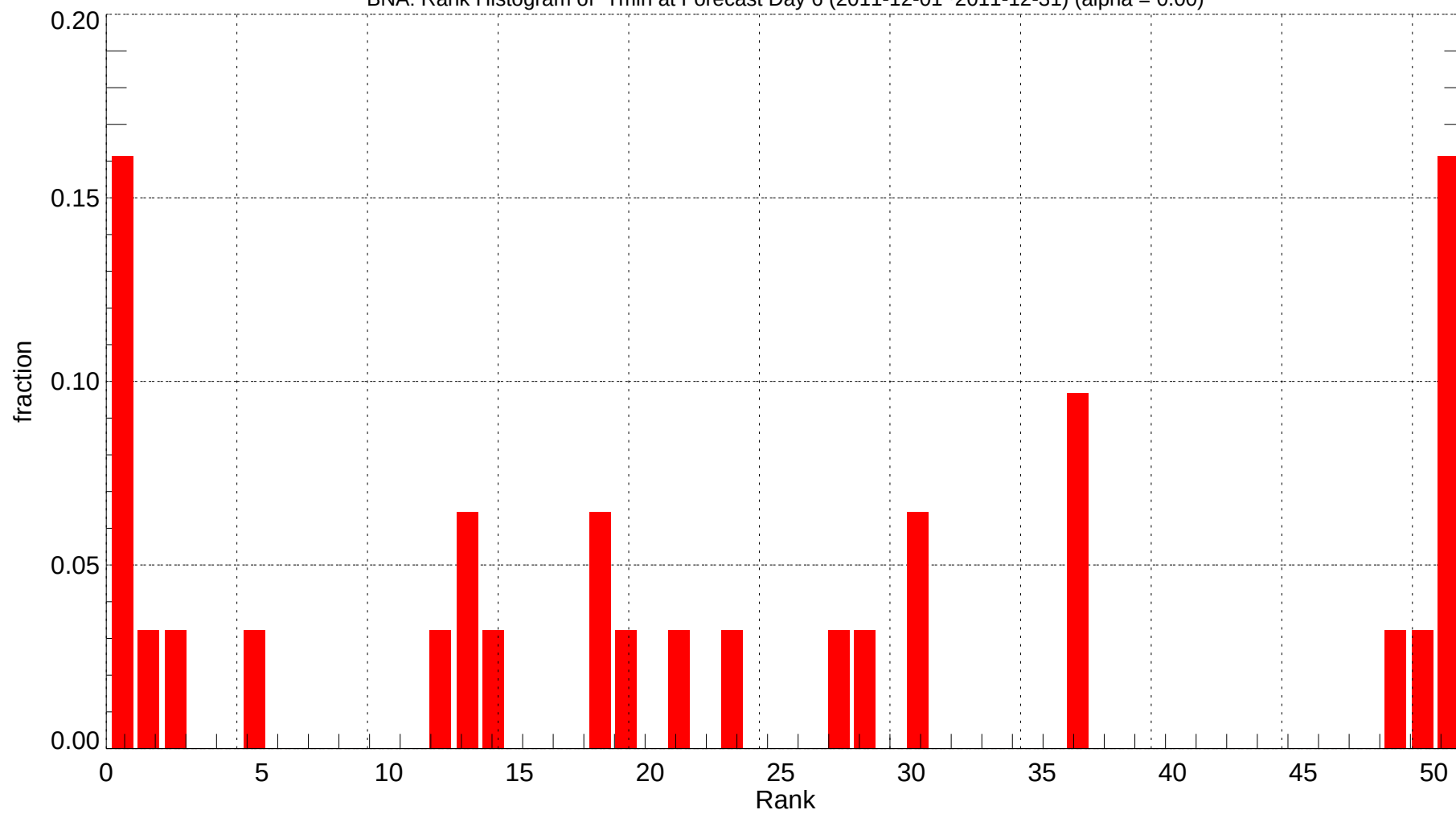
BNA: Rank Histogram of Tmin at Forecast Day 6 (2011-12-01~2011-12-31) (alpha = 0.00)
