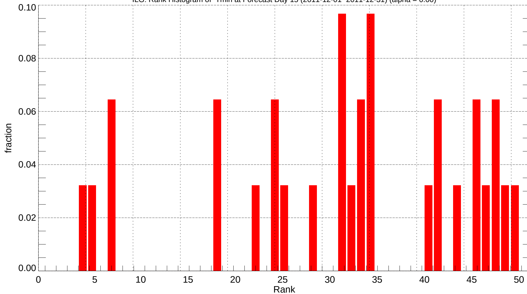
ILG: Rank Histogram of Tmin at Forecast Day 15 (2011-12-01~2011-12-31) (alpha = 0.00)
