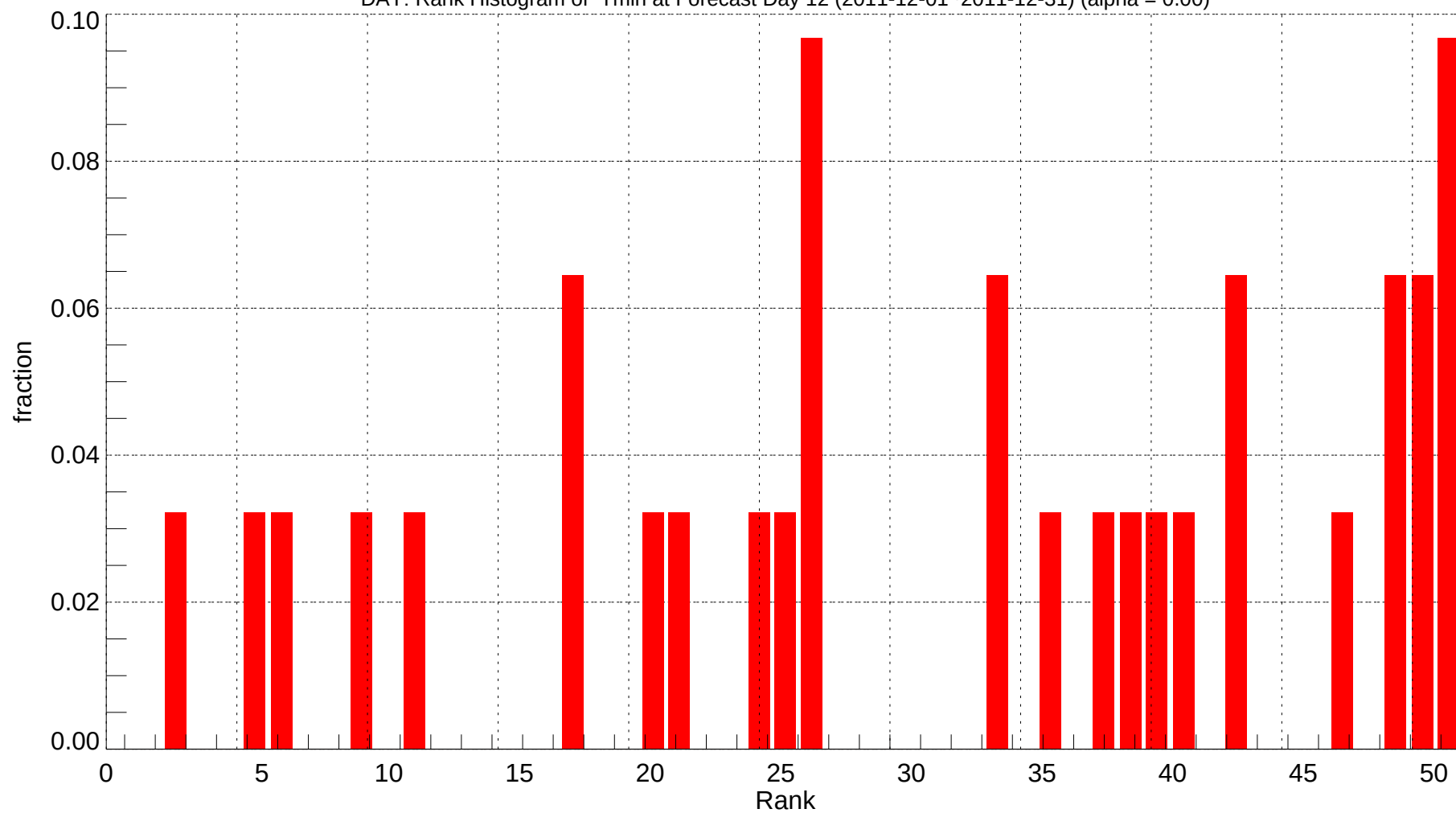
DAY: Rank Histogram of Tmin at Forecast Day 12 (2011-12-01~2011-12-31) (alpha = 0.00)
