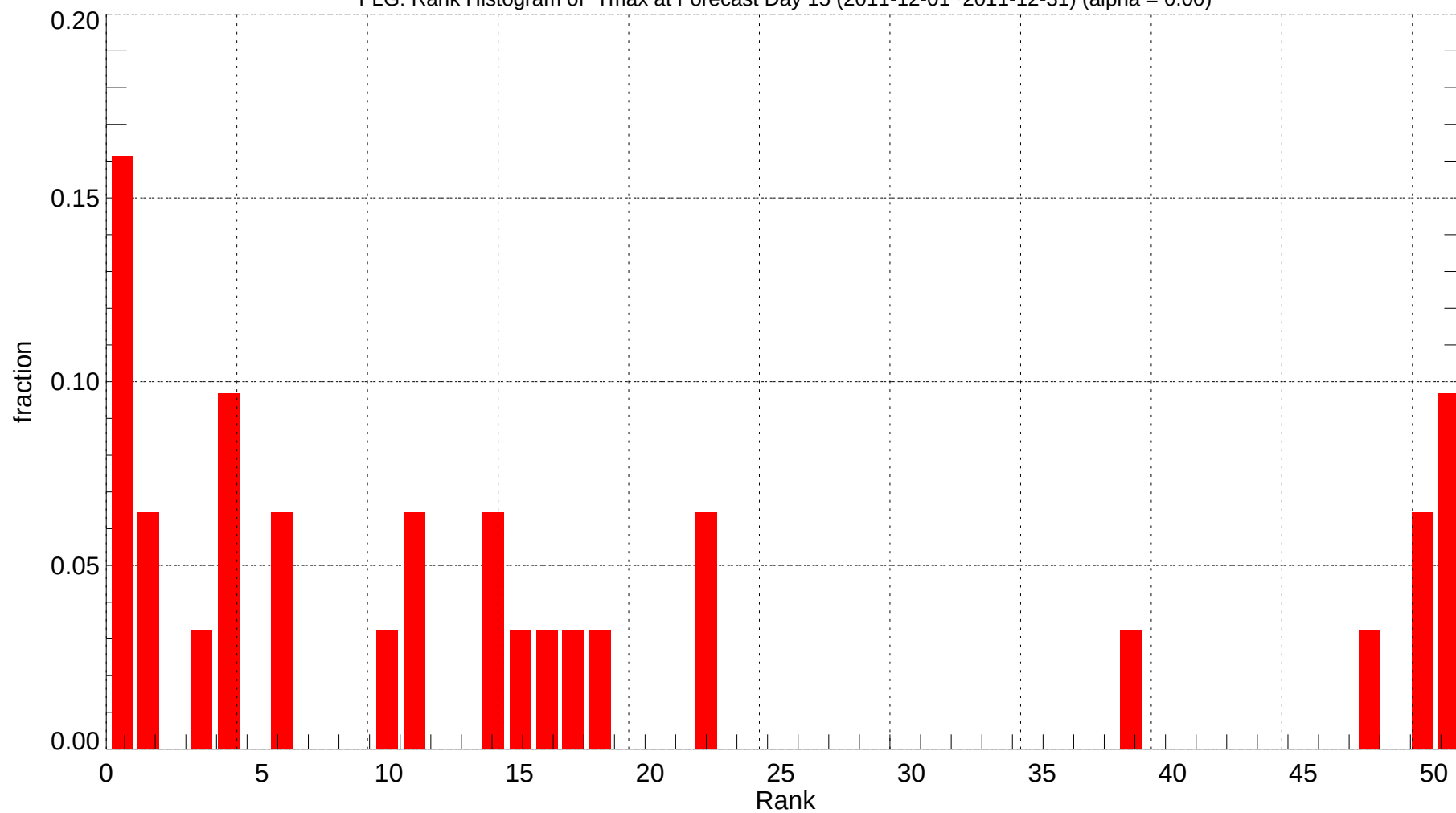
FLG: Rank Histogram of Tmax at Forecast Day 15 (2011-12-01~2011-12-31) (alpha = 0.00)
