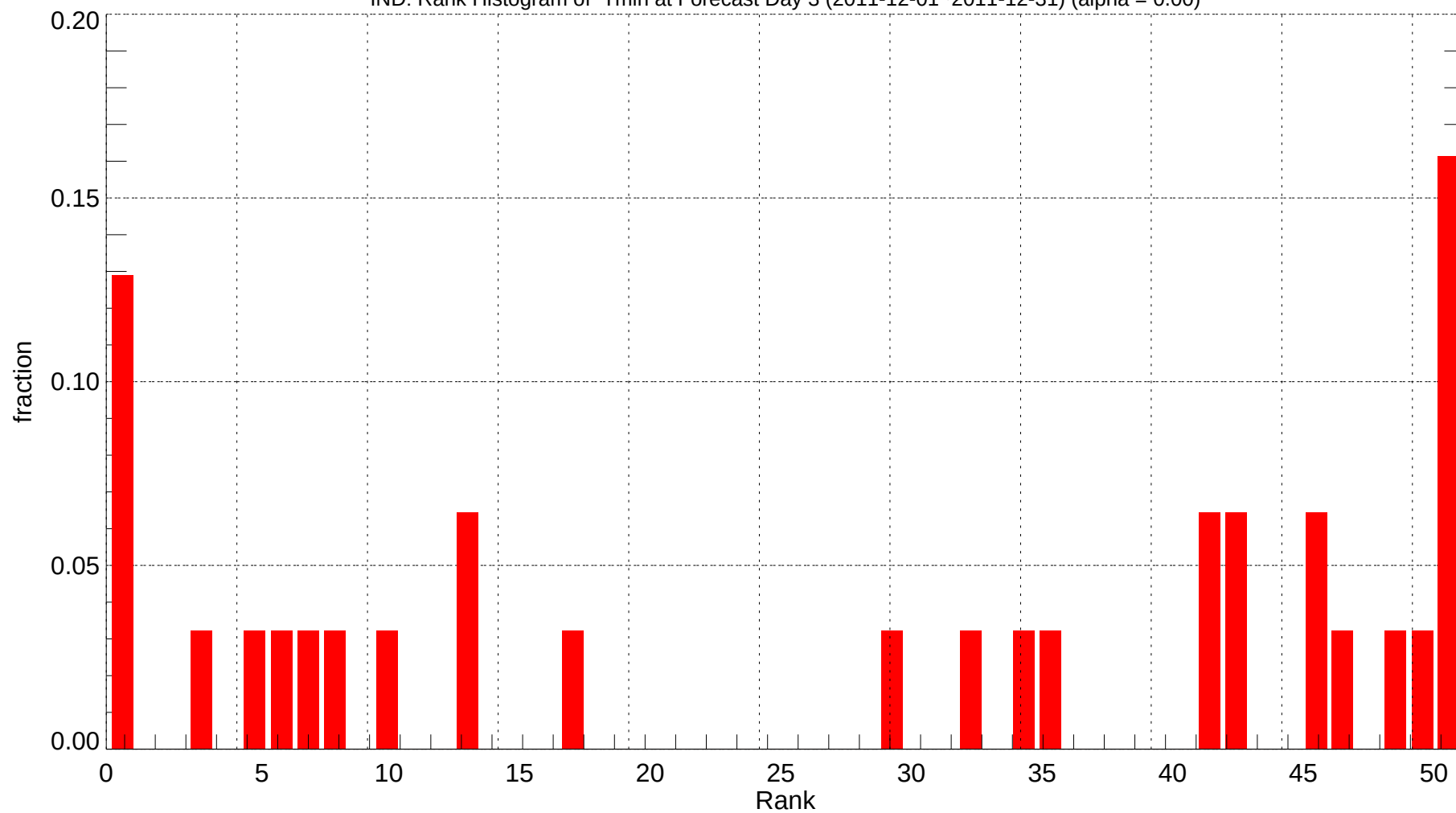
IND: Rank Histogram of Tmin at Forecast Day 3 (2011-12-01~2011-12-31) (alpha = 0.00)
