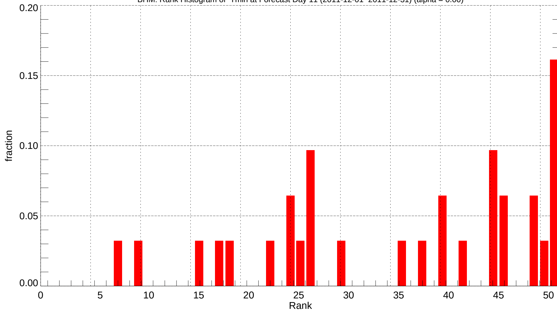
BHM: Rank Histogram of Tmin at Forecast Day 11 (2011-12-01~2011-12-31) (alpha = 0.00)
