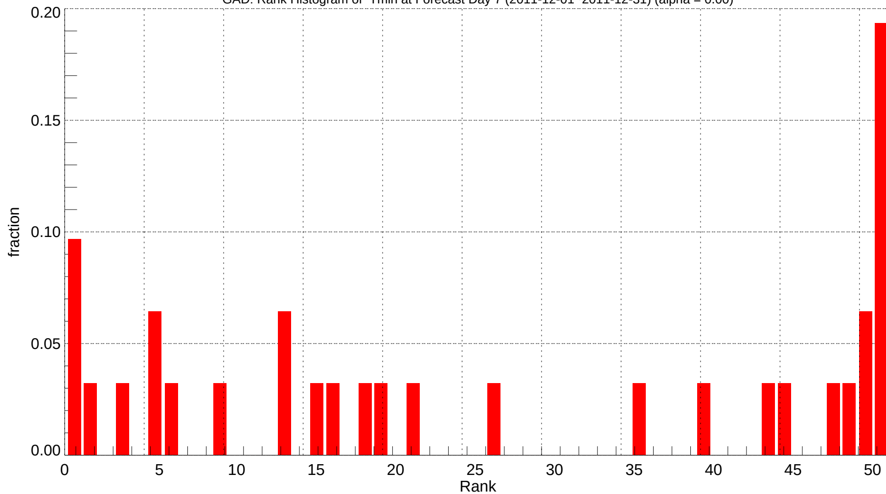
GAD: Rank Histogram of Tmin at Forecast Day 7 (2011-12-01~2011-12-31) (alpha = 0.00)
