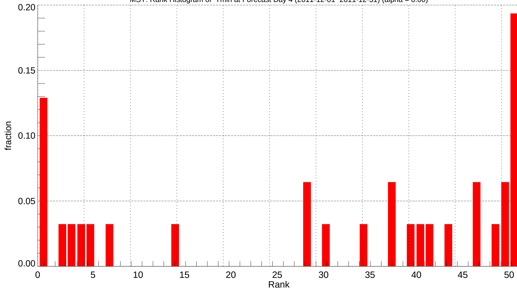
MSY: Rank Histogram of Tmin at Forecast Day 4 (2011-12-01~2011-12-31) (alpha = 0.00)
