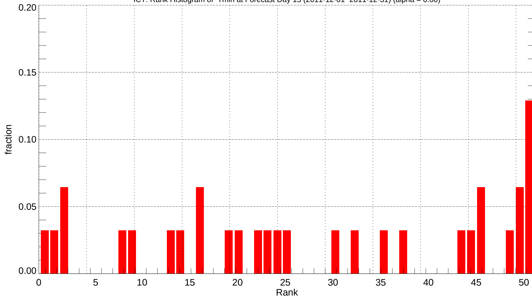
ICT: Rank Histogram of Tmin at Forecast Day 15 (2011-12-01~2011-12-31) (alpha = 0.00)
