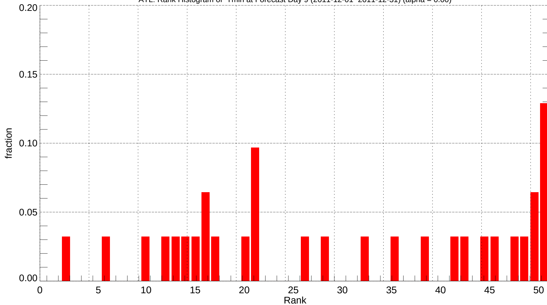
ATL: Rank Histogram of Tmin at Forecast Day 9 (2011-12-01~2011-12-31) (alpha = 0.00)
