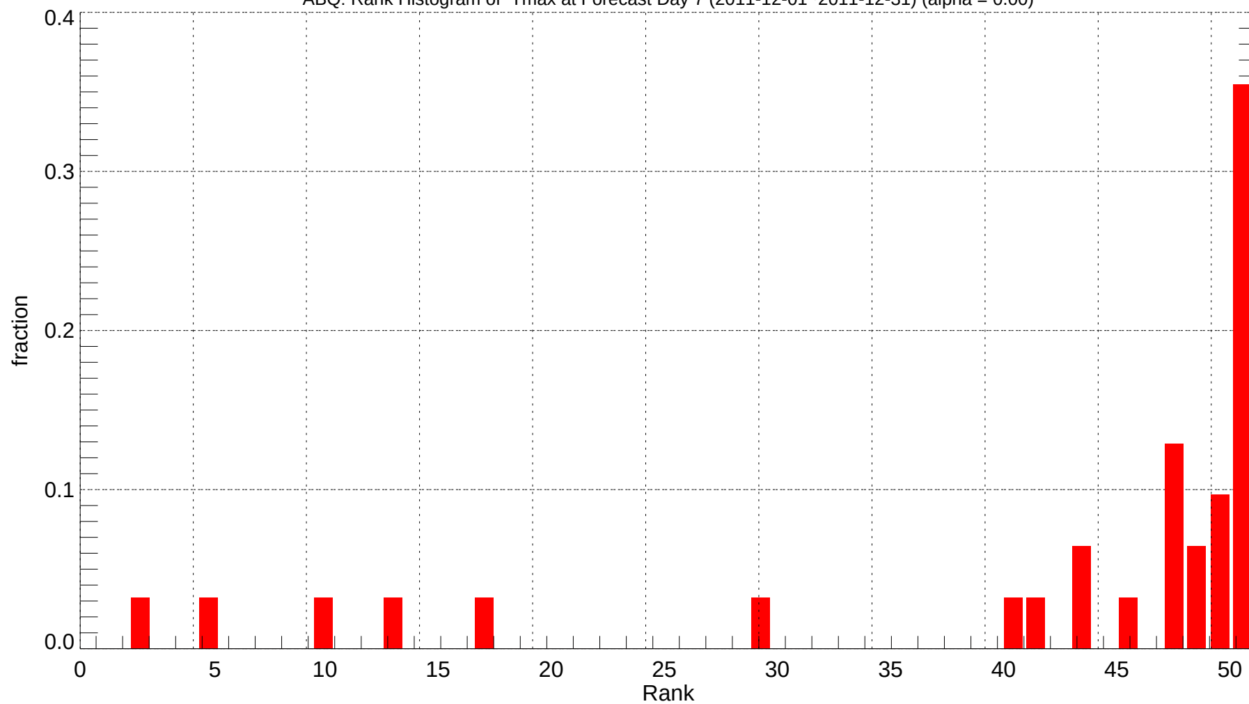
ABQ: Rank Histogram of Tmax at Forecast Day 7 (2011-12-01~2011-12-31) (alpha = 0.00)
