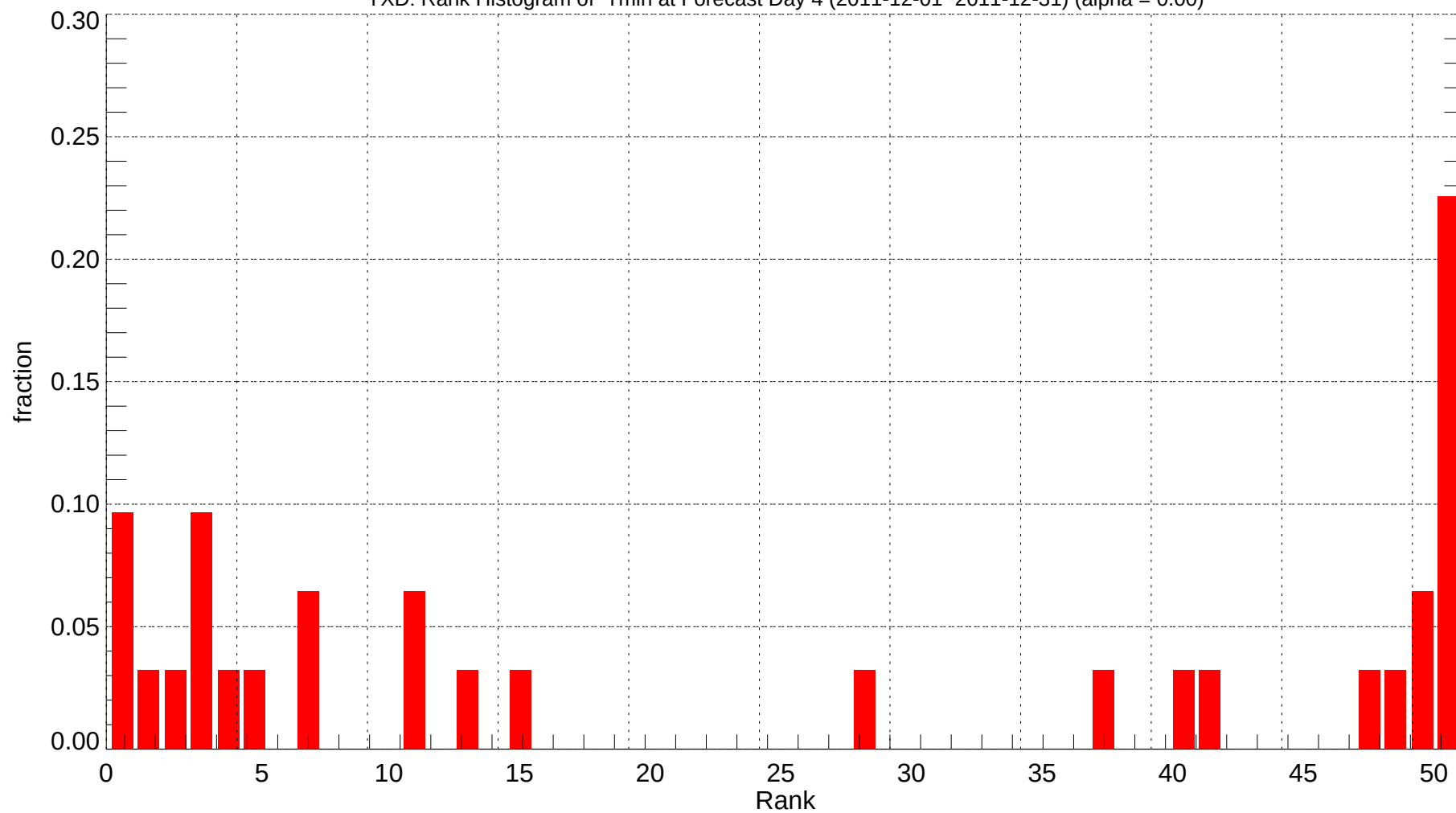
YXD: Rank Histogram of Tmin at Forecast Day 4 (2011-12-01~2011-12-31) (alpha = 0.00)
