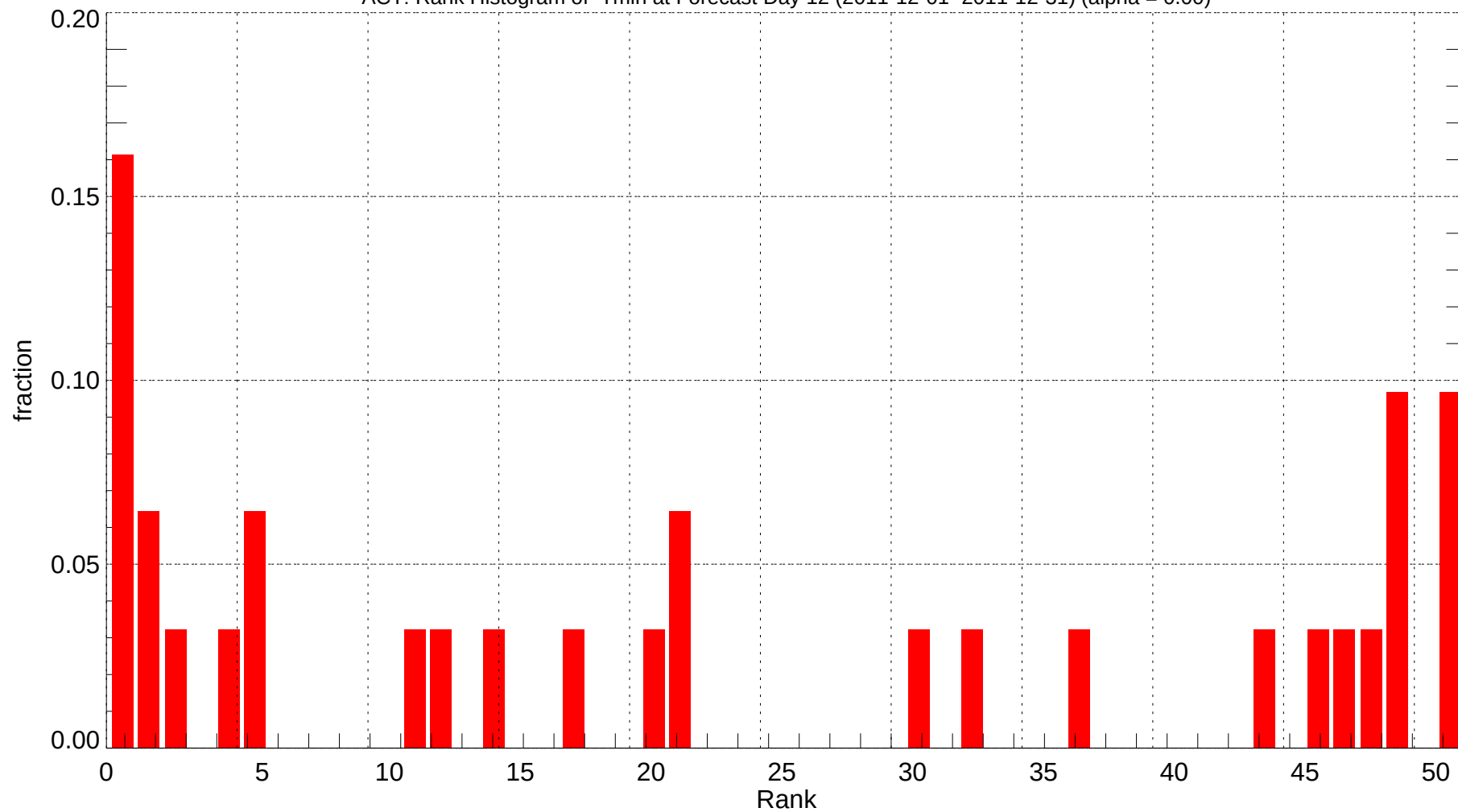
ACT: Rank Histogram of Tmin at Forecast Day 12 (2011-12-01~2011-12-31) (alpha = 0.00)
