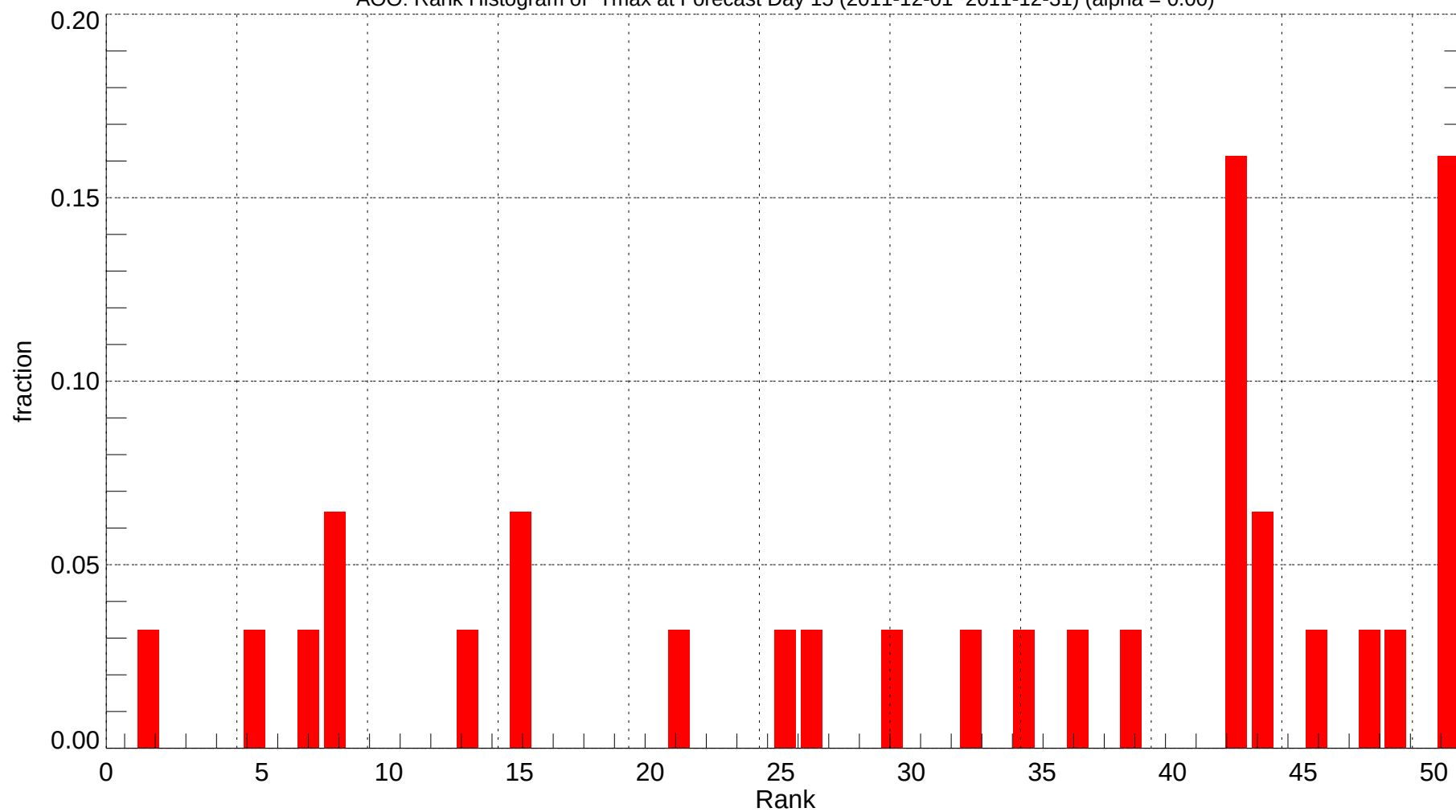
AOO: Rank Histogram of Tmax at Forecast Day 15 (2011-12-01~2011-12-31) (alpha = 0.00)
