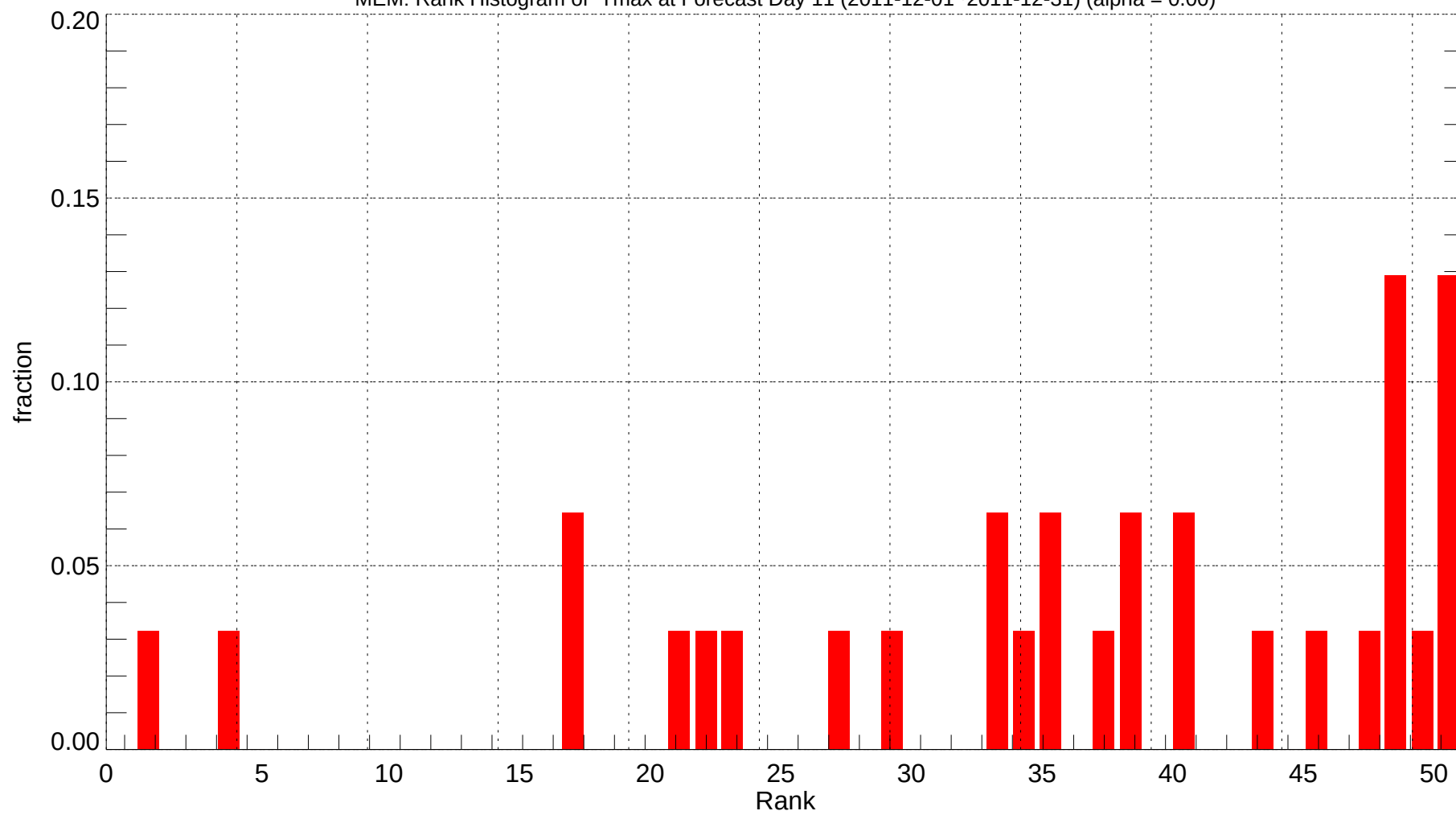
MEM: Rank Histogram of Tmax at Forecast Day 11 (2011-12-01~2011-12-31) (alpha = 0.00)
