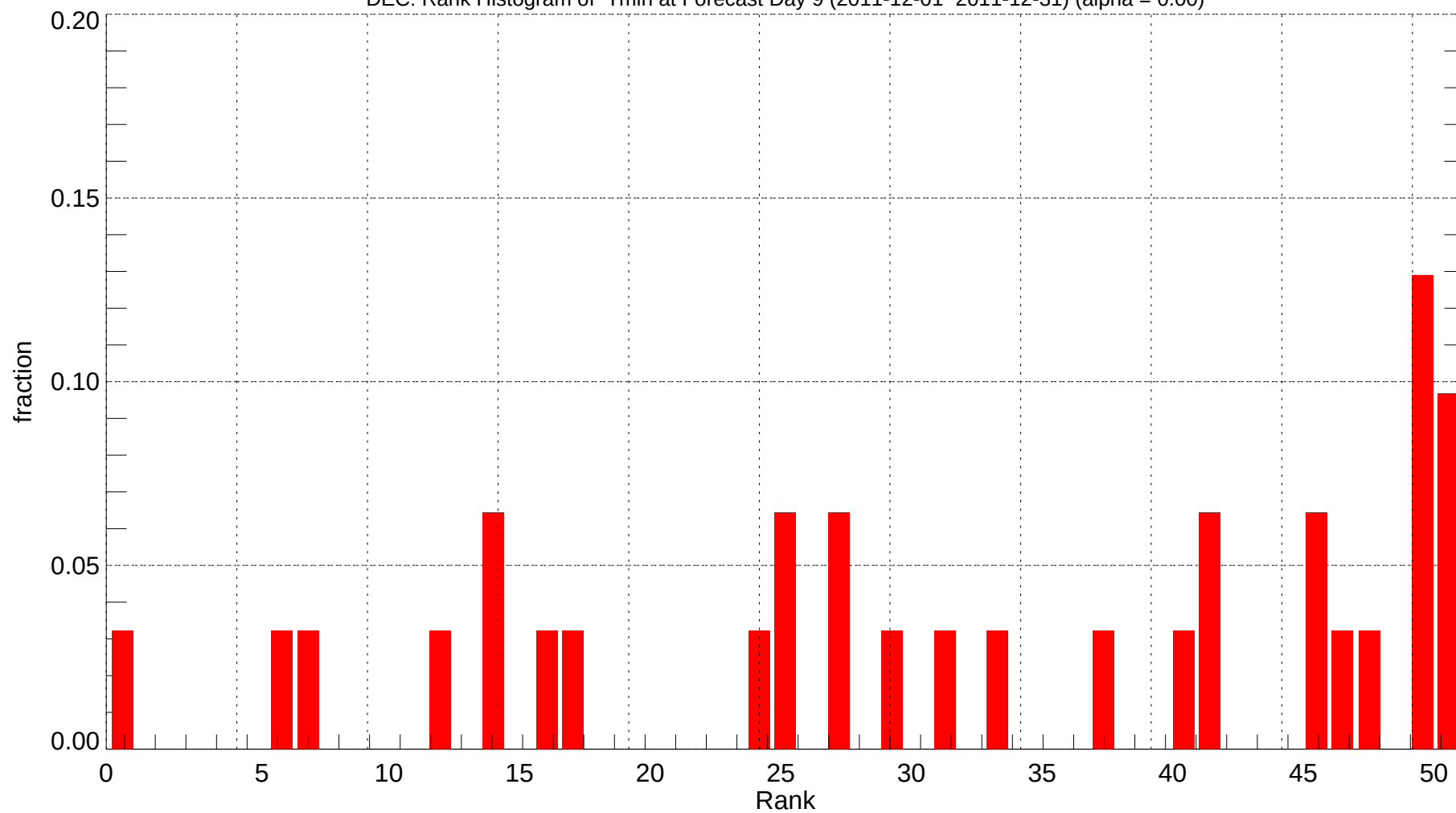
DEC: Rank Histogram of Tmin at Forecast Day 9 (2011-12-01~2011-12-31) (alpha = 0.00)
