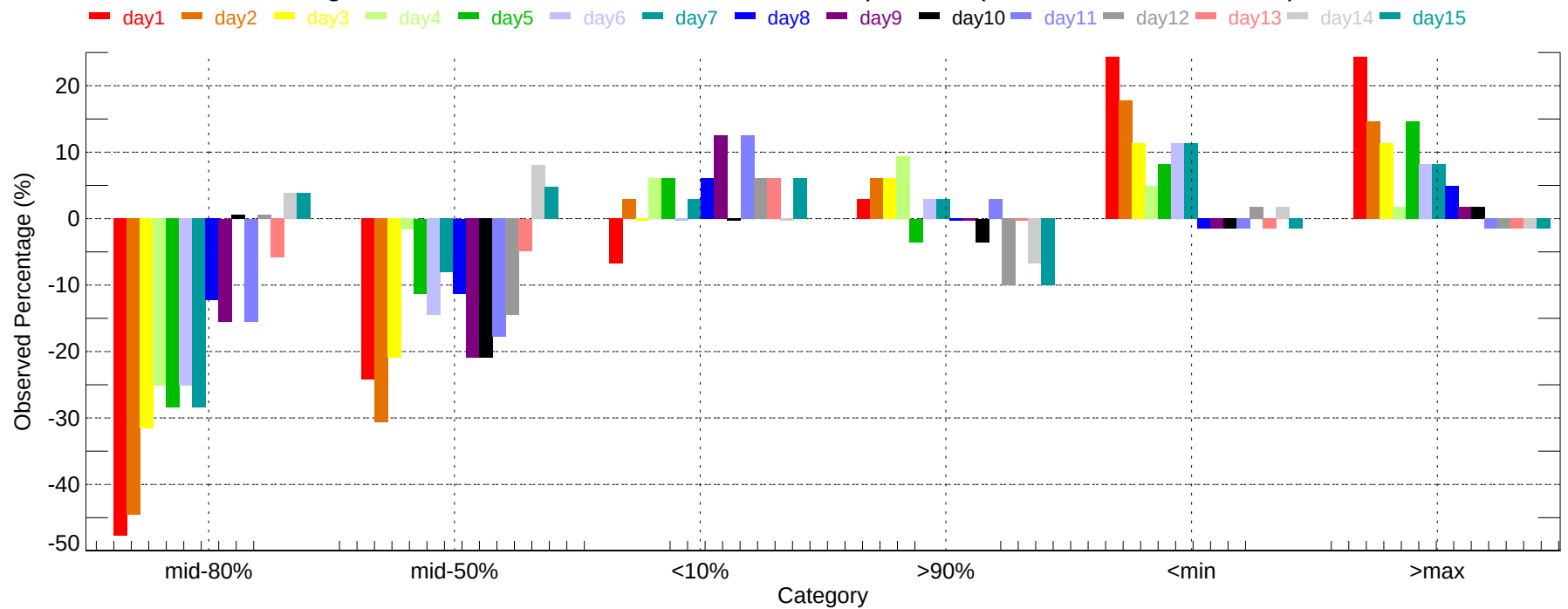
Observed Percentage Deviation of Ensembles - PHX: Min Temperature (2011-12-01~2011-12-31)
