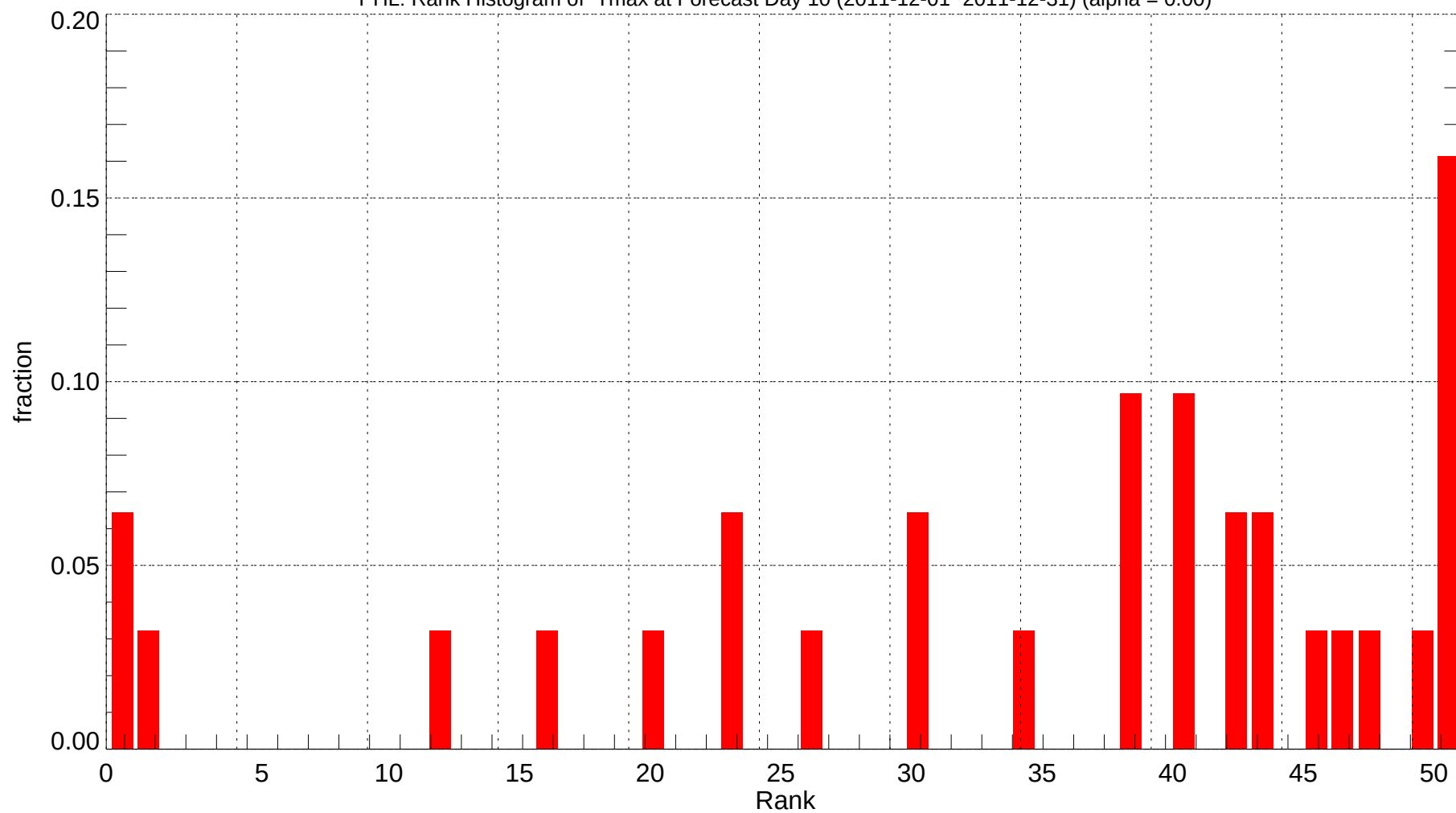
PHL: Rank Histogram of Tmax at Forecast Day 10 (2011-12-01~2011-12-31) (alpha = 0.00)
