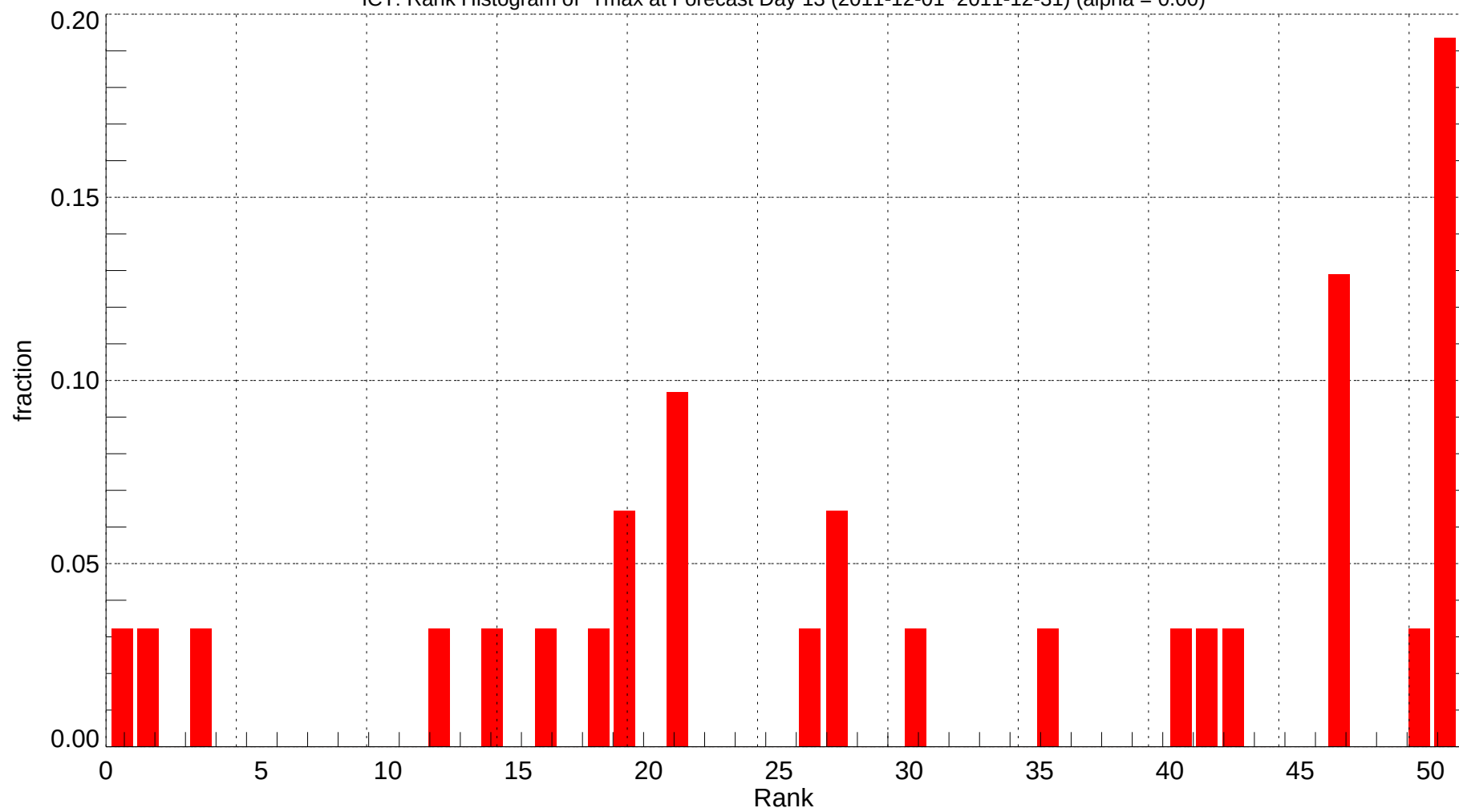
ICT: Rank Histogram of Tmax at Forecast Day 13 (2011-12-01~2011-12-31) (alpha = 0.00)
