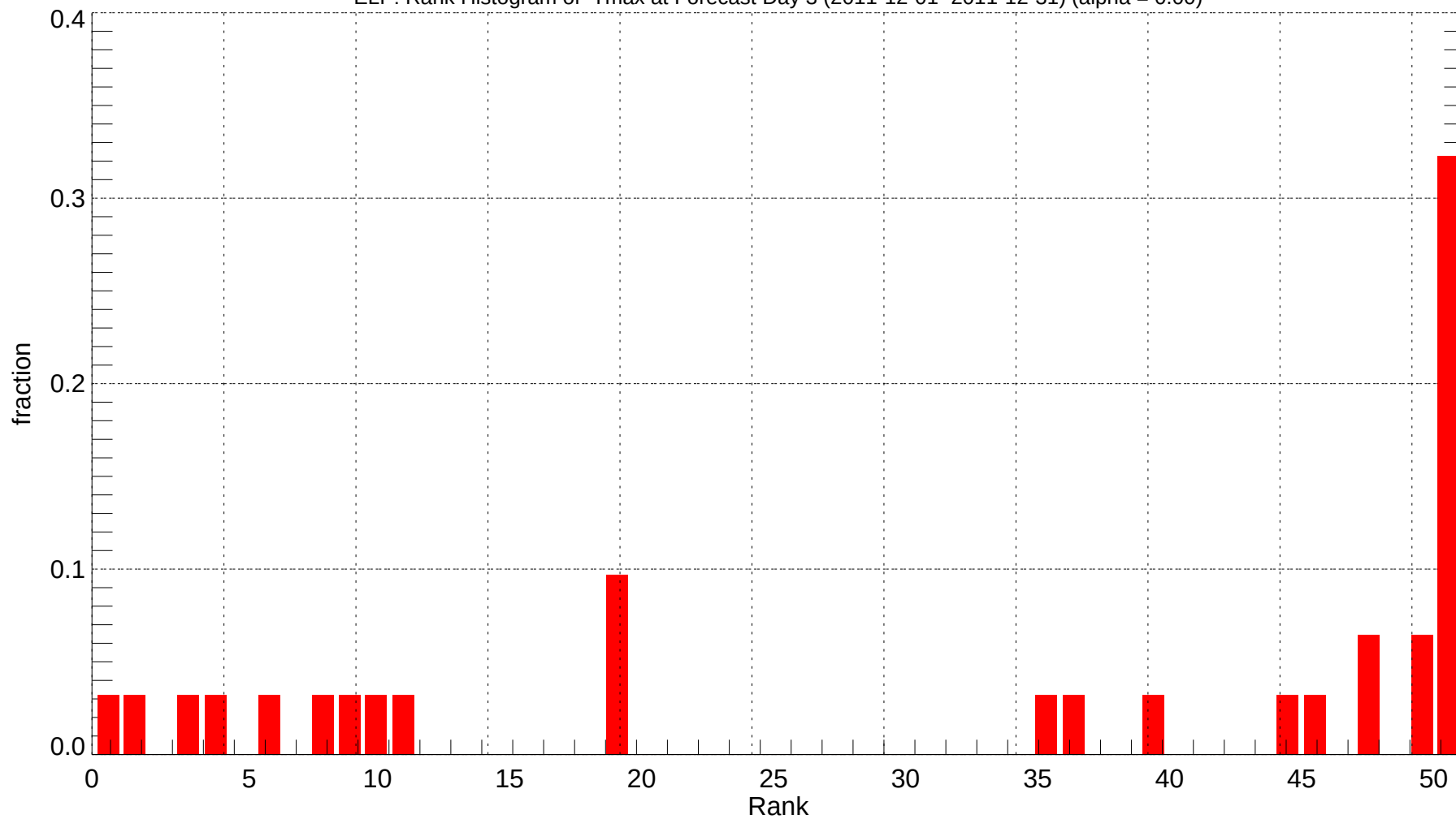
ELP: Rank Histogram of Tmax at Forecast Day 3 (2011-12-01~2011-12-31) (alpha = 0.00)
