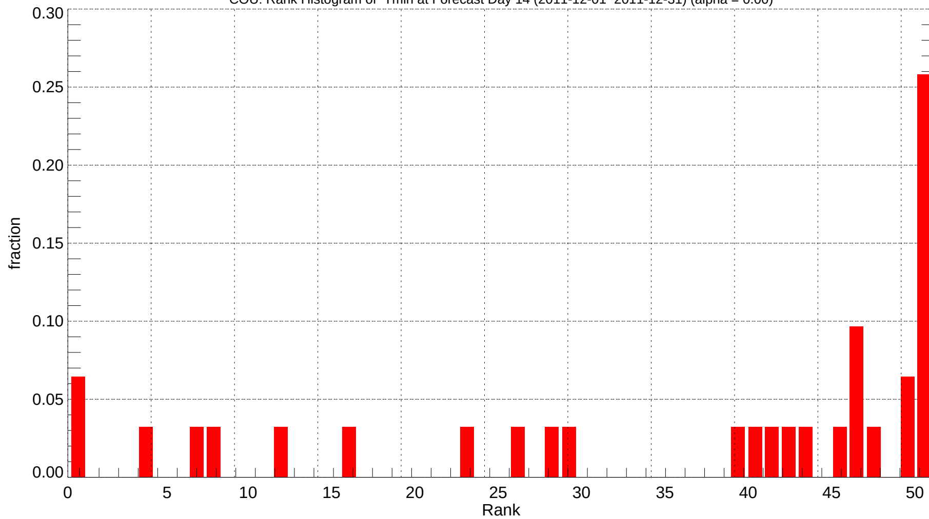
COU: Rank Histogram of Tmin at Forecast Day 14 (2011-12-01~2011-12-31) (alpha = 0.00)
