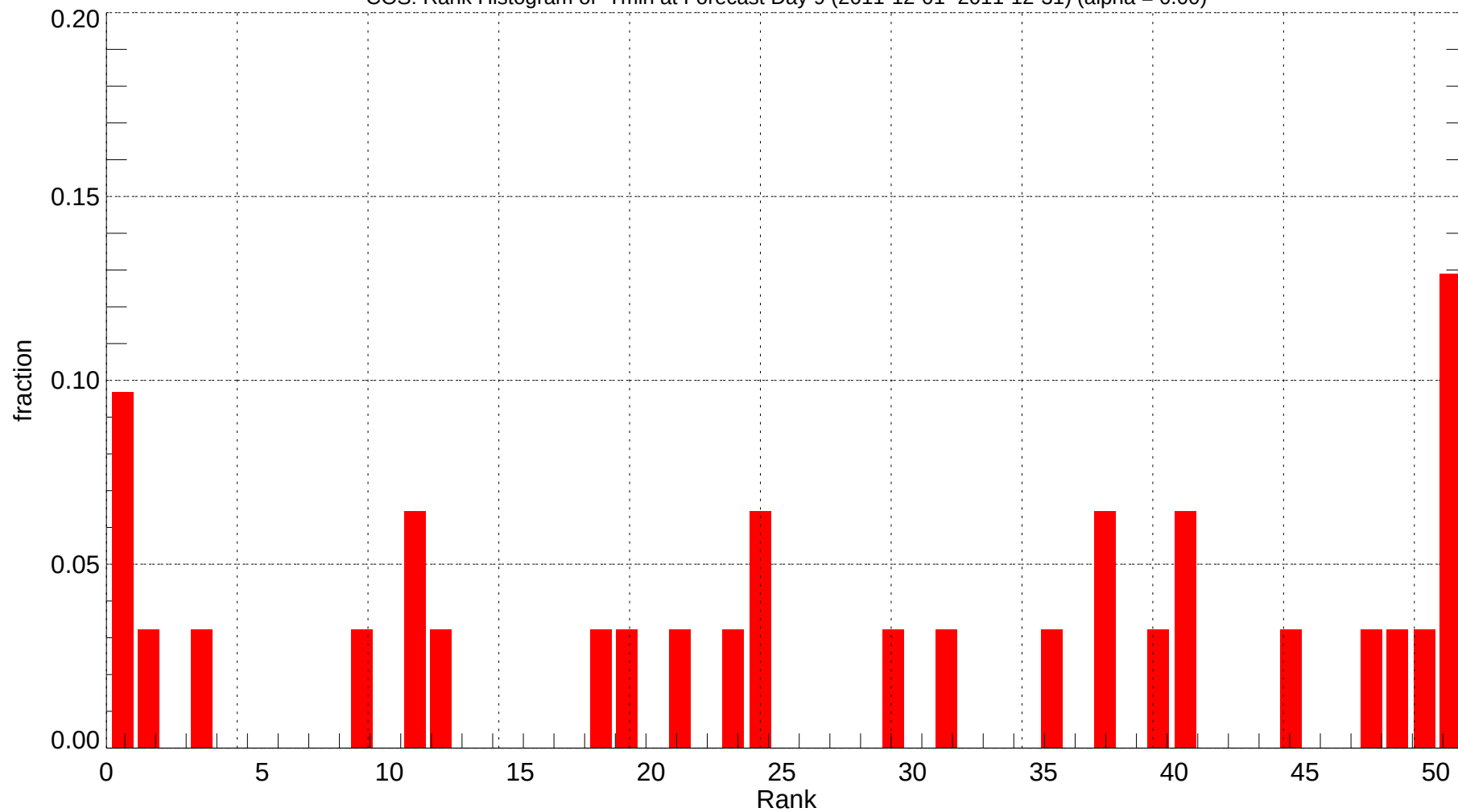
COS: Rank Histogram of Tmin at Forecast Day 9 (2011-12-01~2011-12-31) (alpha = 0.00)
