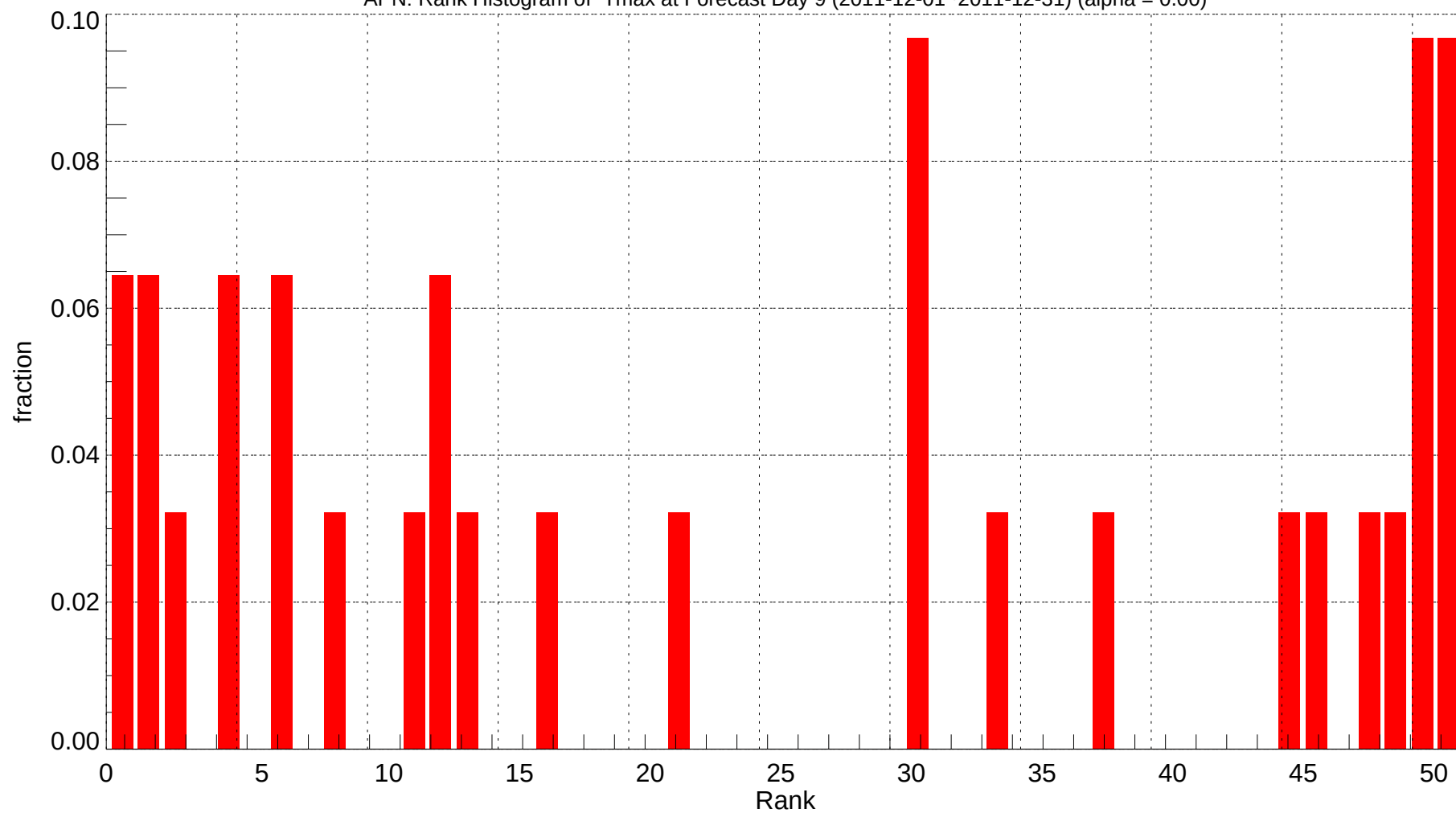
APN: Rank Histogram of Tmax at Forecast Day 9 (2011-12-01~2011-12-31) (alpha = 0.00)
