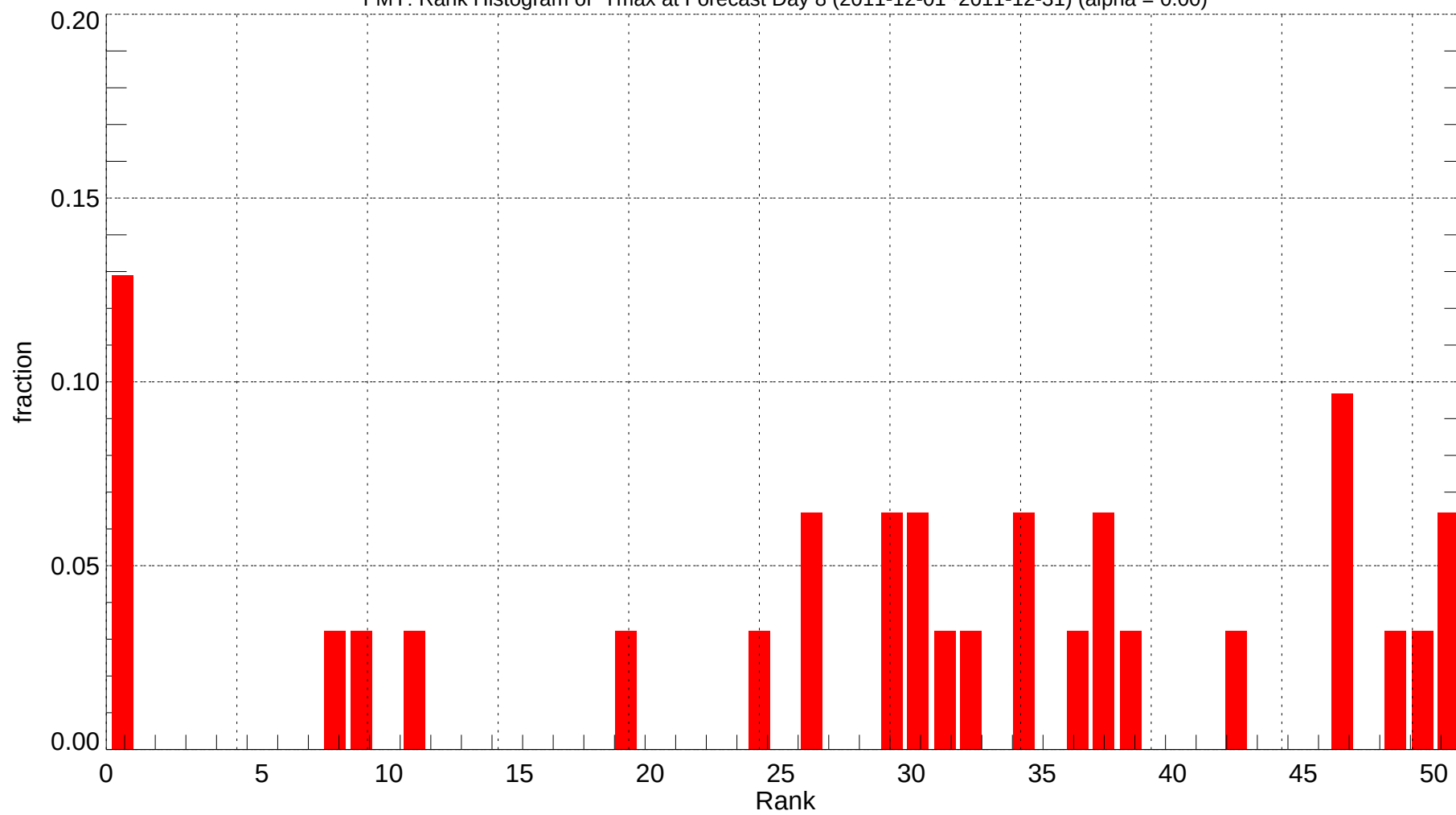
FMY: Rank Histogram of Tmax at Forecast Day 8 (2011-12-01~2011-12-31) (alpha = 0.00)
