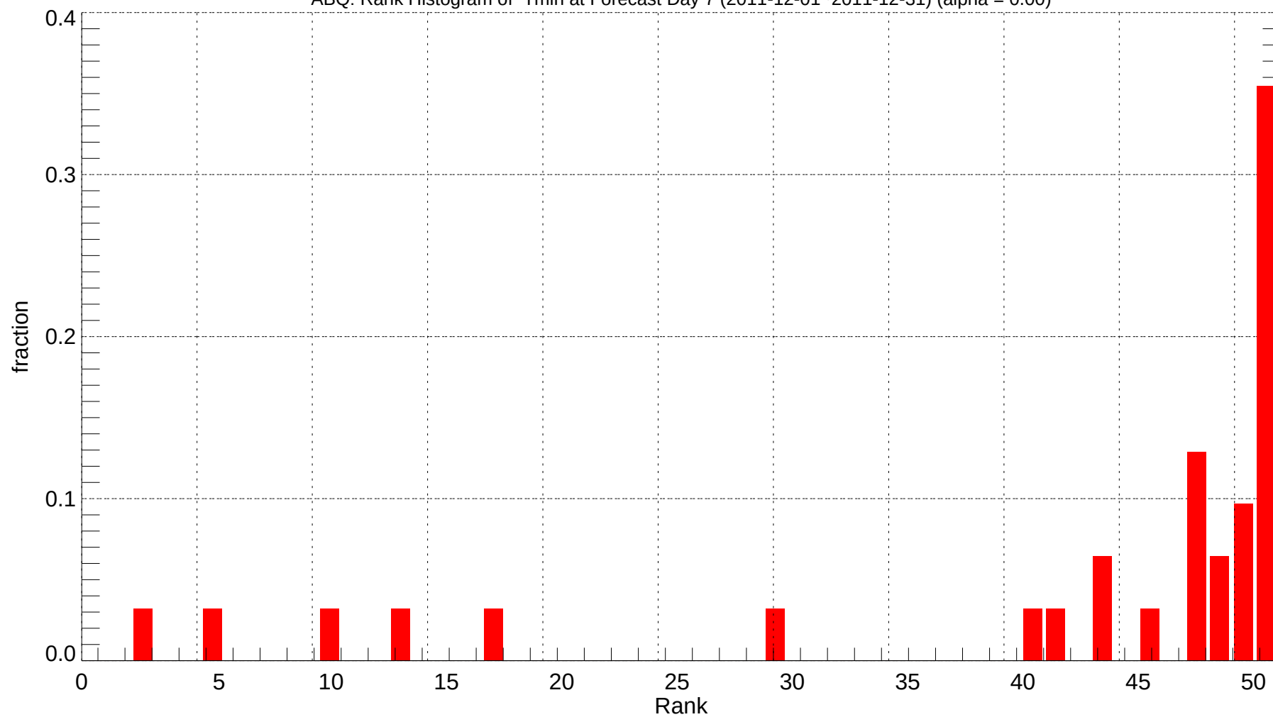
ABQ: Rank Histogram of Tmin at Forecast Day 7 (2011-12-01~2011-12-31) (alpha = 0.00)
