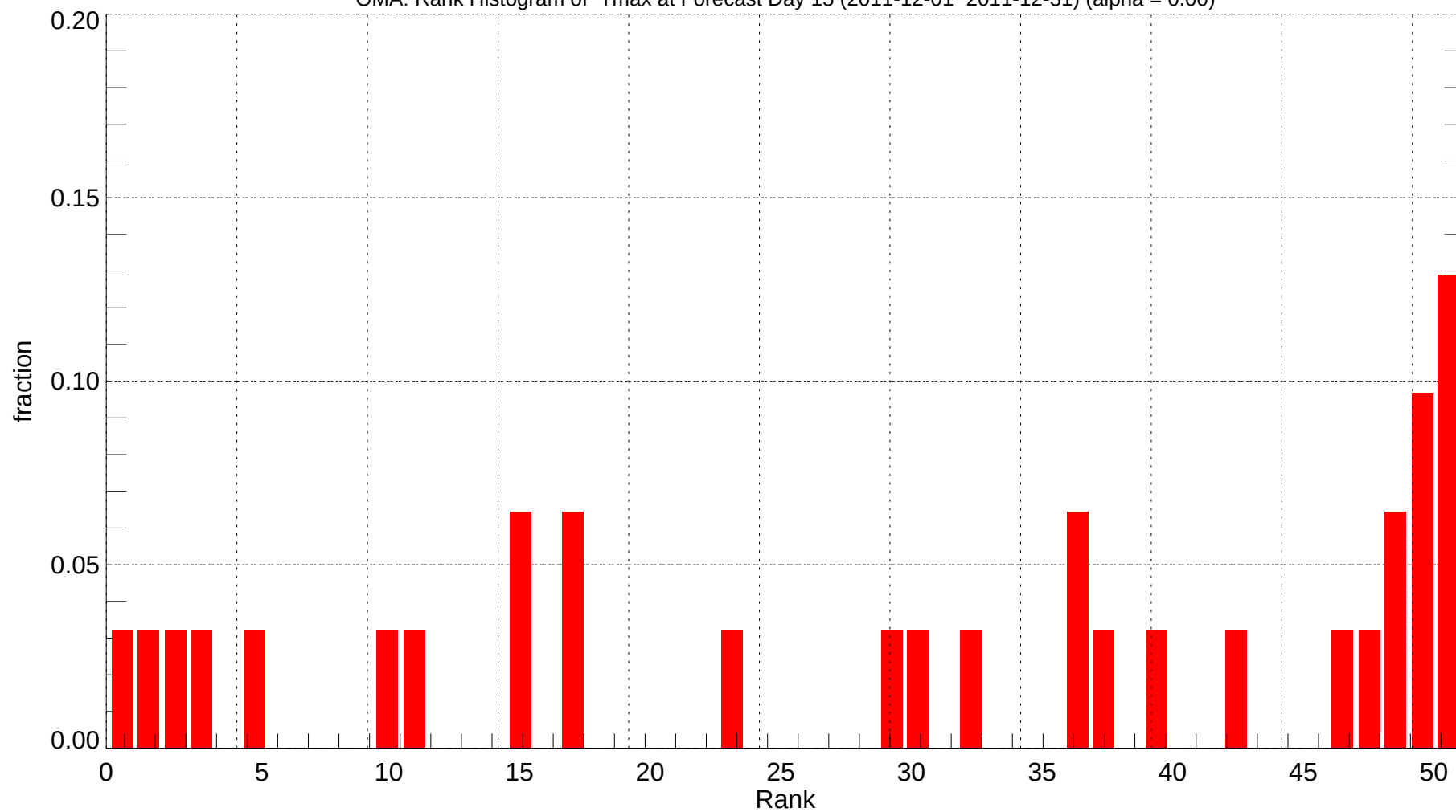
OMA: Rank Histogram of Tmax at Forecast Day 15 (2011-12-01~2011-12-31) (alpha = 0.00)
