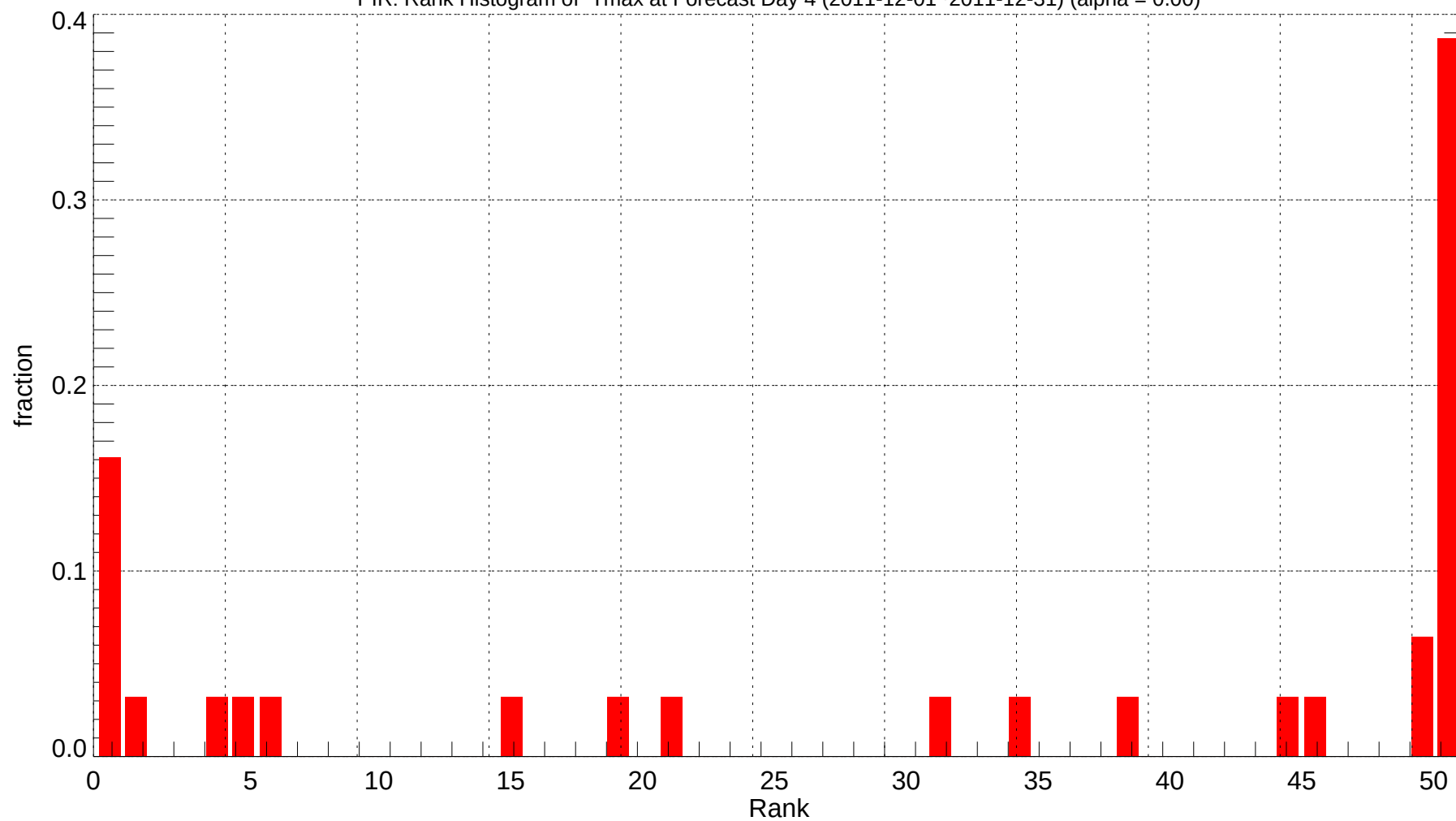
PIR: Rank Histogram of Tmax at Forecast Day 4 (2011-12-01~2011-12-31) (alpha = 0.00)
