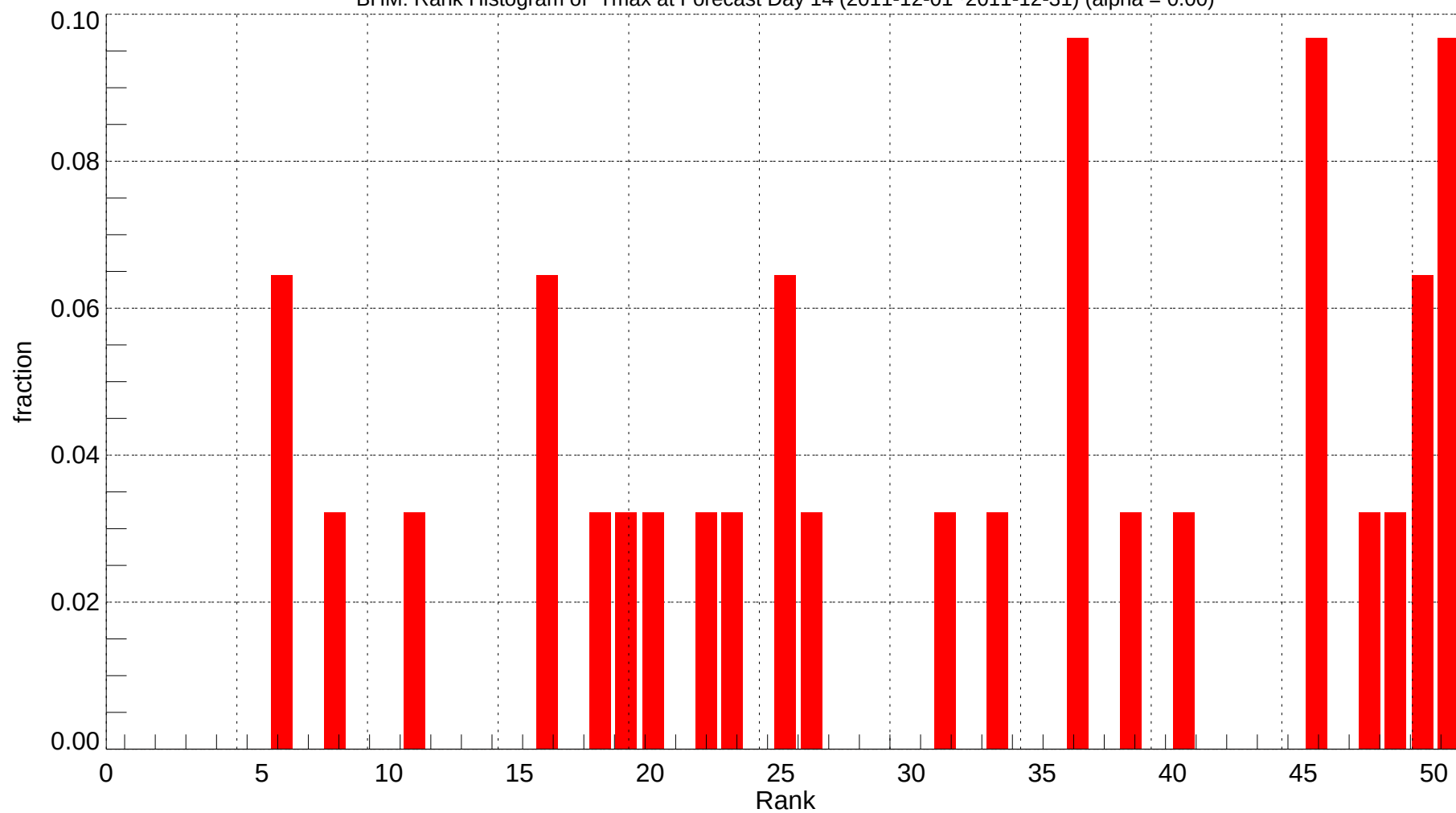
BHM: Rank Histogram of Tmax at Forecast Day 14 (2011-12-01~2011-12-31) (alpha = 0.00)
