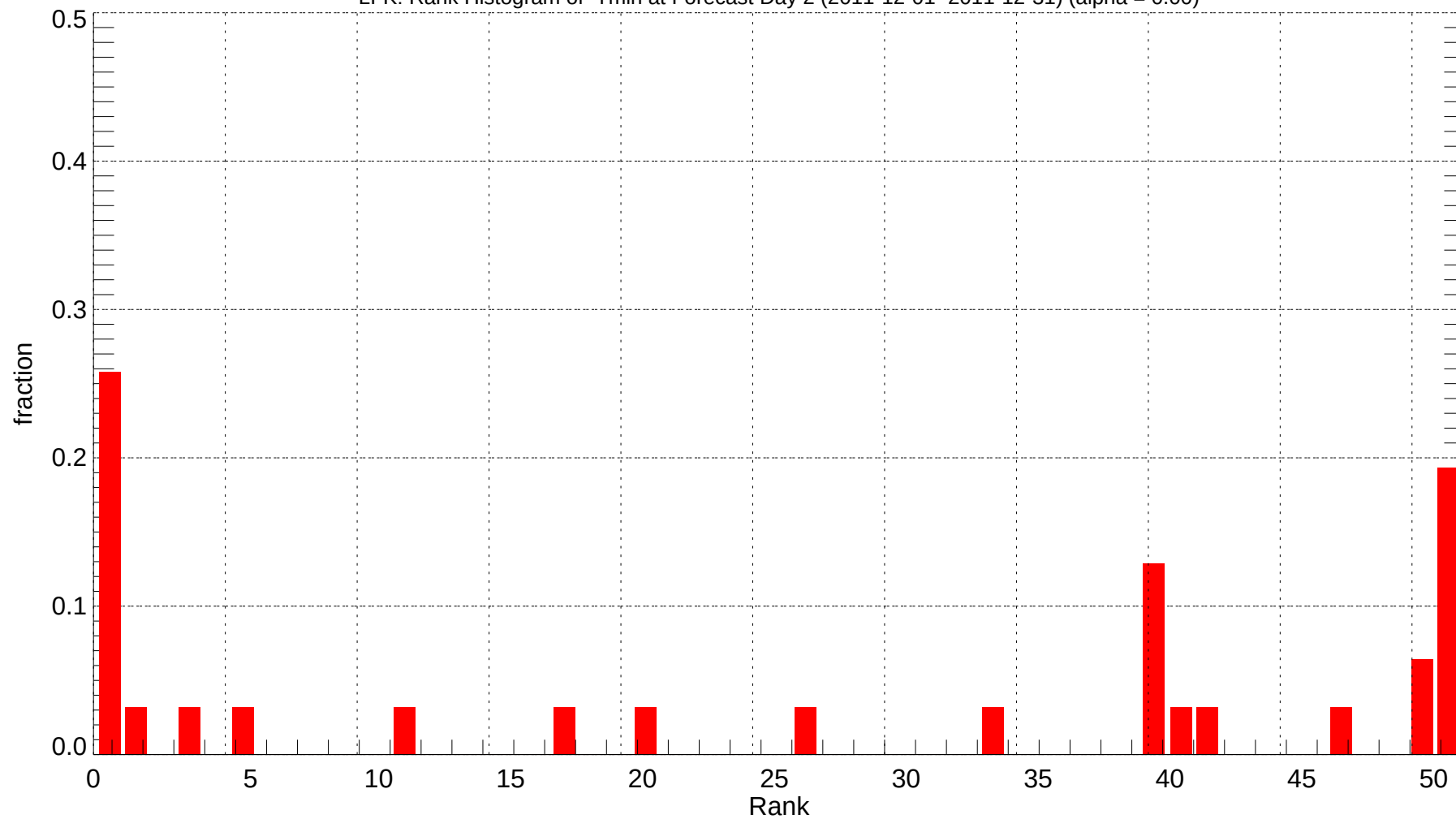
LFK: Rank Histogram of Tmin at Forecast Day 2 (2011-12-01~2011-12-31) (alpha = 0.00)
