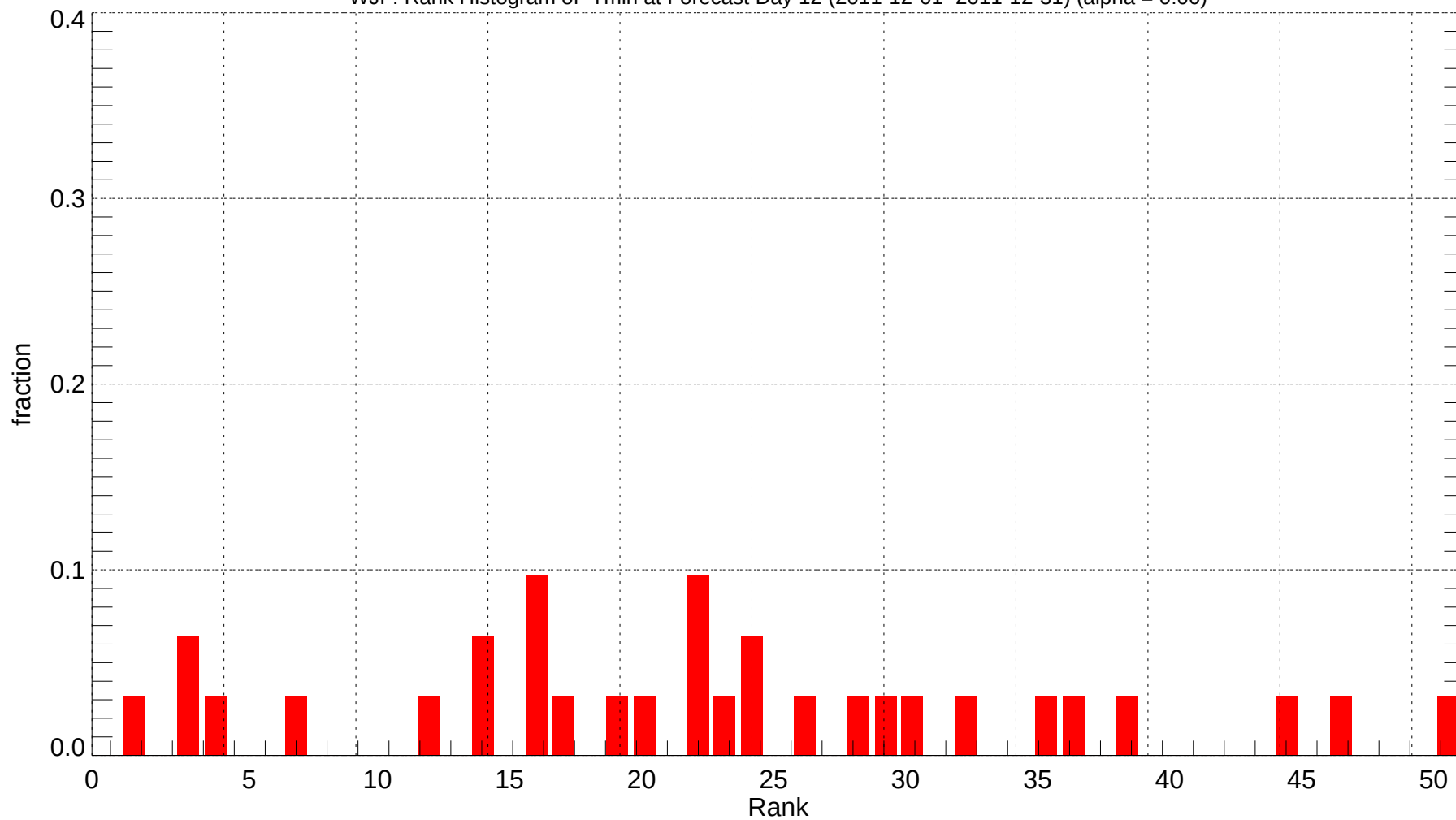
WJF: Rank Histogram of Tmin at Forecast Day 12 (2011-12-01~2011-12-31) (alpha = 0.00)
