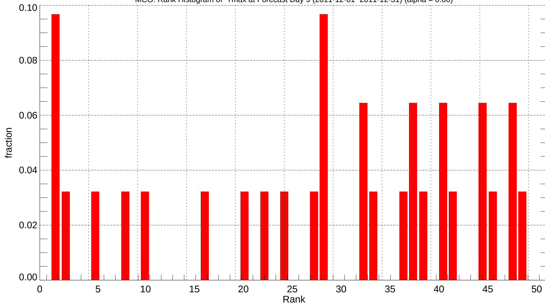
MCO: Rank Histogram of Tmax at Forecast Day 9 (2011-12-01~2011-12-31) (alpha = 0.00)
