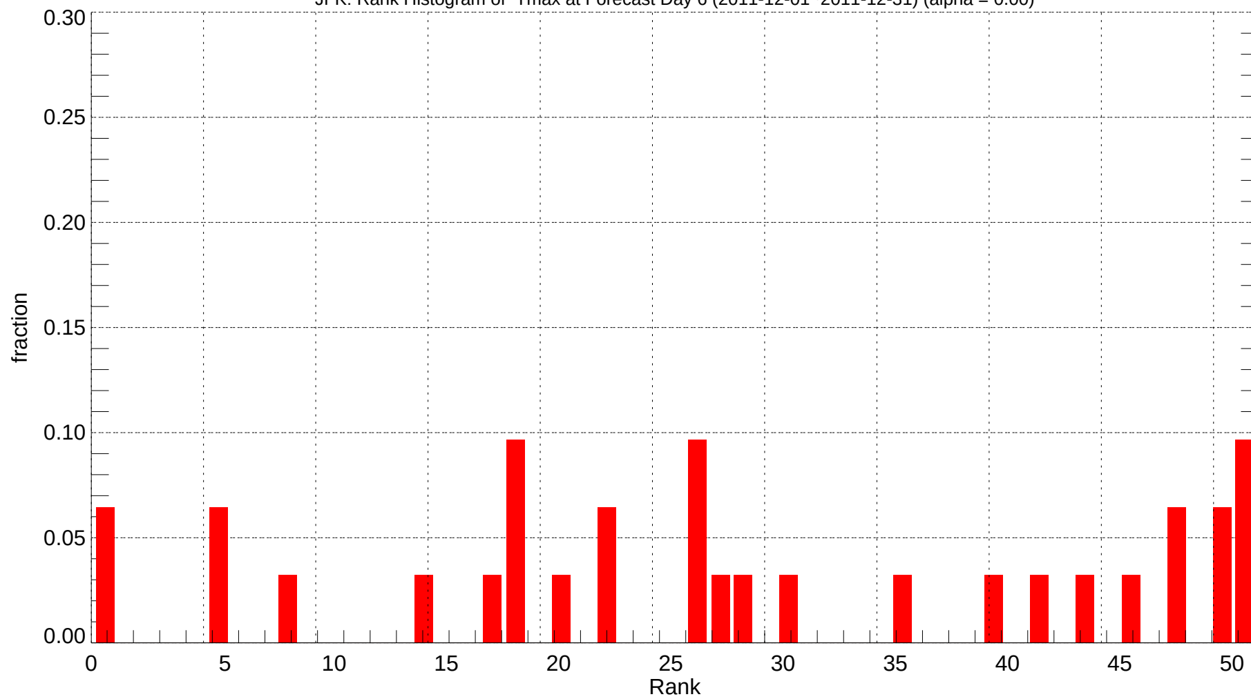
JFK: Rank Histogram of Tmax at Forecast Day 6 (2011-12-01~2011-12-31) (alpha = 0.00)
