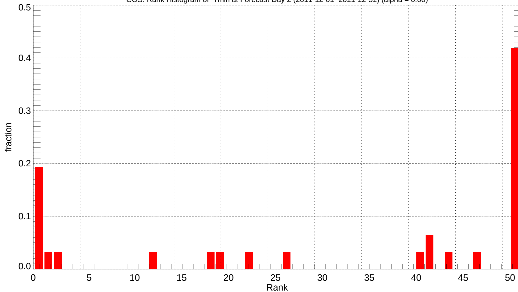
COS: Rank Histogram of Tmin at Forecast Day 2 (2011-12-01~2011-12-31) (alpha = 0.00)
