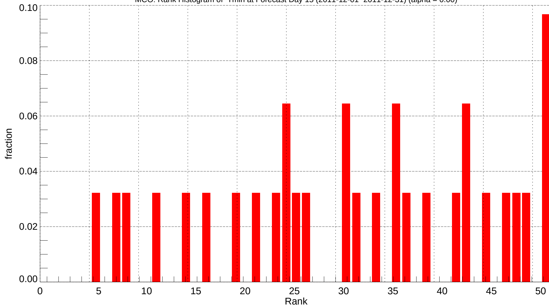
MCO: Rank Histogram of Tmin at Forecast Day 15 (2011-12-01~2011-12-31) (alpha = 0.00)
