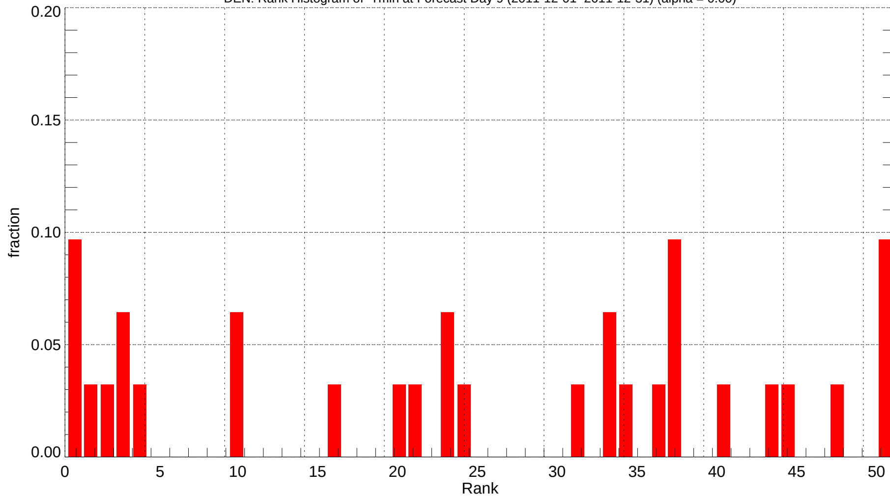
DEN: Rank Histogram of Tmin at Forecast Day 9 (2011-12-01~2011-12-31) (alpha = 0.00)
