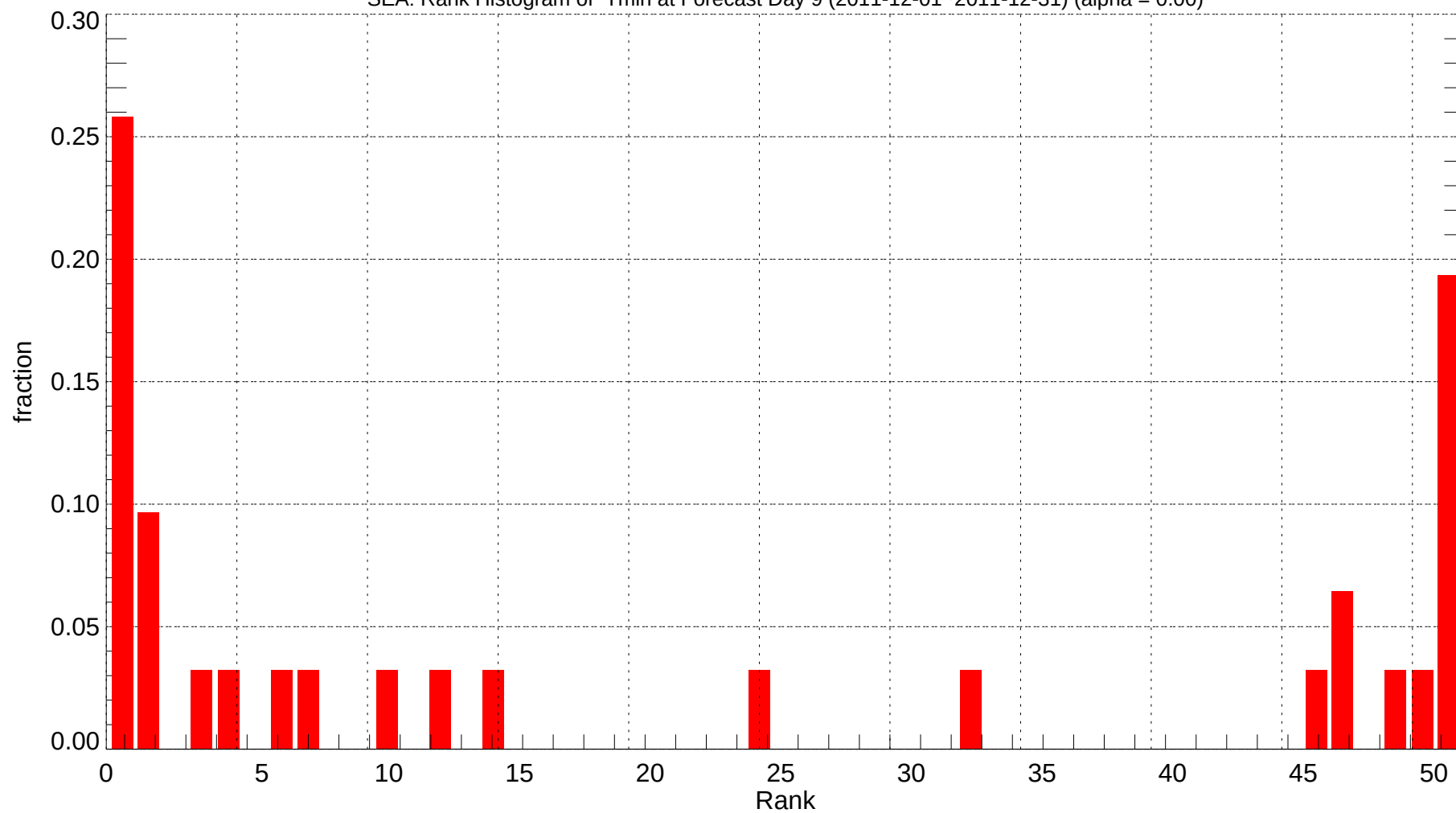
SEA: Rank Histogram of Tmin at Forecast Day 9 (2011-12-01~2011-12-31) (alpha = 0.00)
