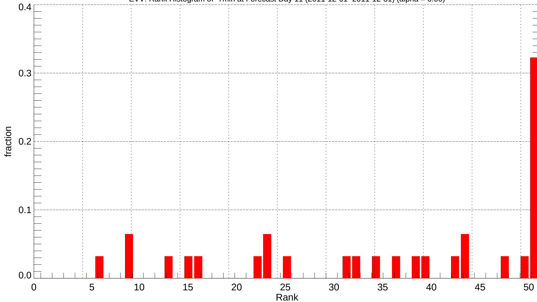
EVV: Rank Histogram of Tmin at Forecast Day 11 (2011-12-01~2011-12-31) (alpha = 0.00)
