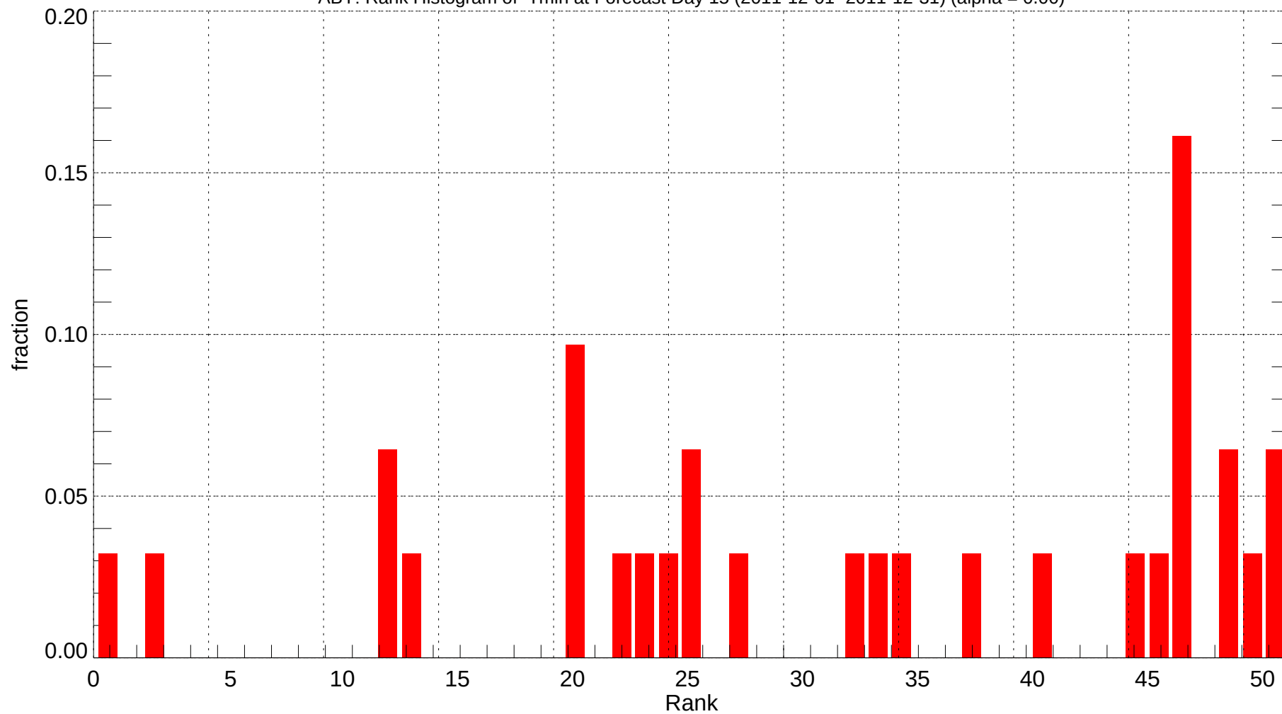
ABY: Rank Histogram of Tmin at Forecast Day 15 (2011-12-01~2011-12-31) (alpha = 0.00)
