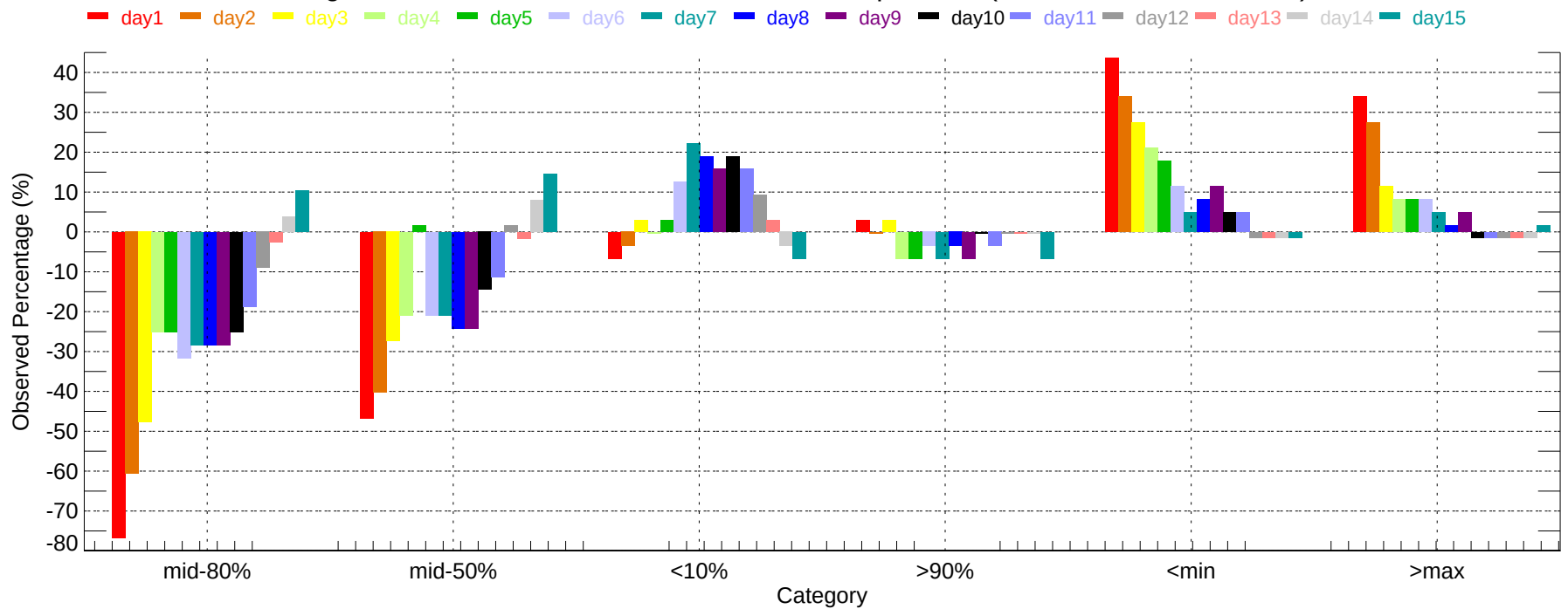
Observed Percentage Deviation of Ensembles - RNO: Max Temperature (2011-12-01~2011-12-31)
