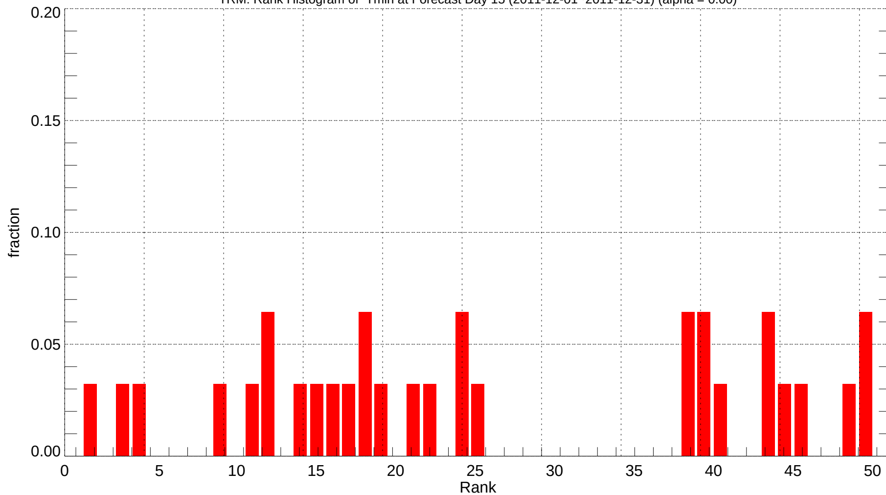
TRM: Rank Histogram of Tmin at Forecast Day 15 (2011-12-01~2011-12-31) (alpha = 0.00)
