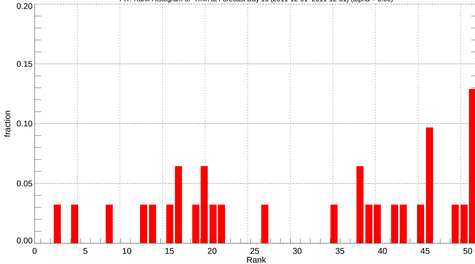
PIT: Rank Histogram of Tmin at Forecast Day 10 (2011-12-01~2011-12-31) (alpha = 0.00)
