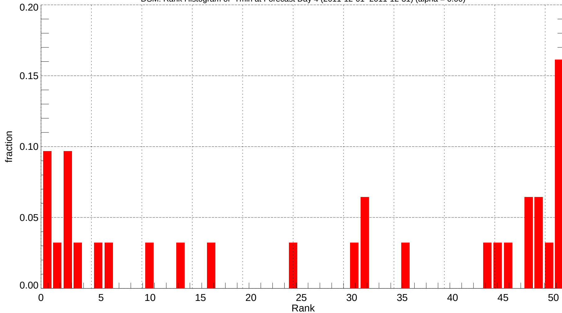
DSM: Rank Histogram of Tmin at Forecast Day 4 (2011-12-01~2011-12-31) (alpha = 0.00)
