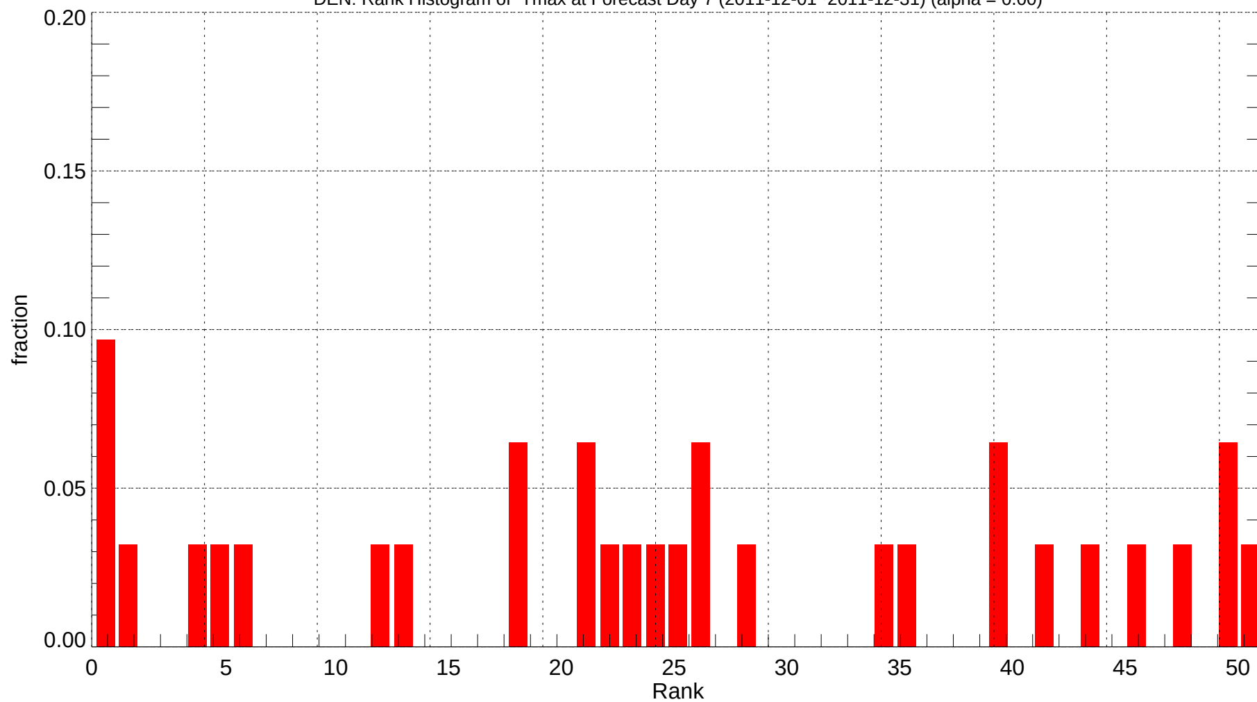
DEN: Rank Histogram of Tmax at Forecast Day 7 (2011-12-01~2011-12-31) (alpha = 0.00)
