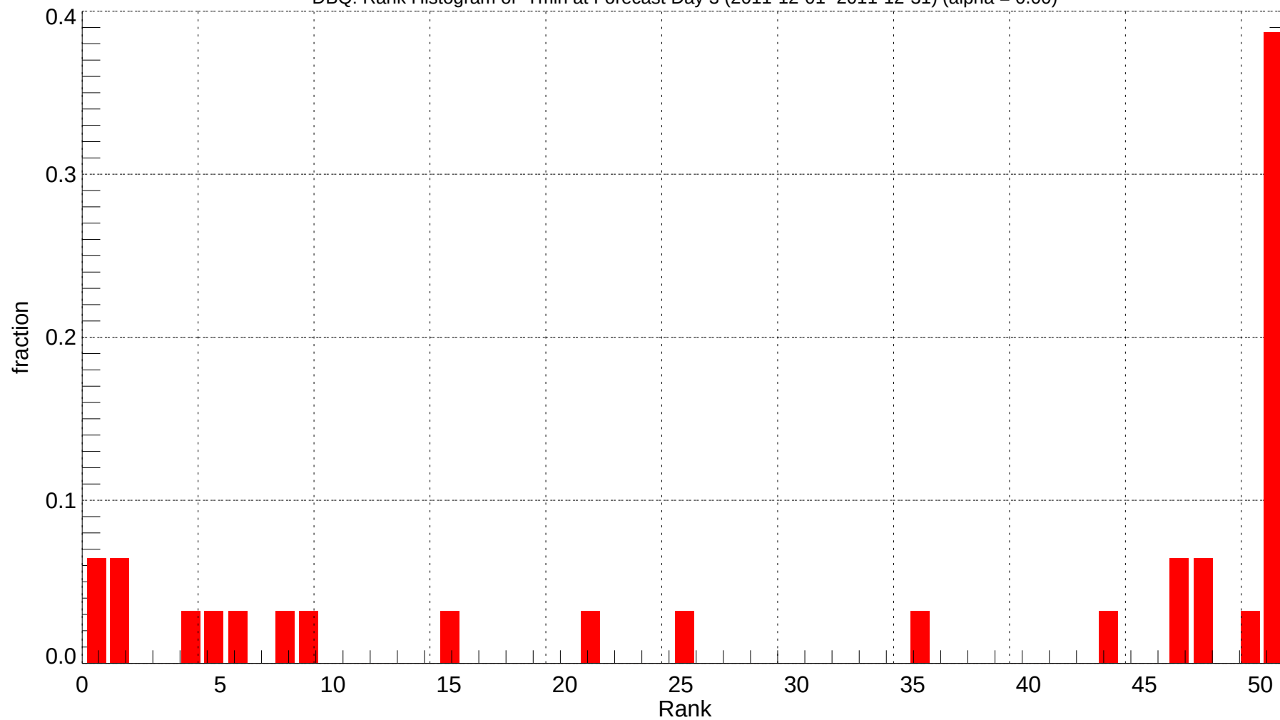
DBQ: Rank Histogram of Tmin at Forecast Day 3 (2011-12-01~2011-12-31) (alpha = 0.00)
