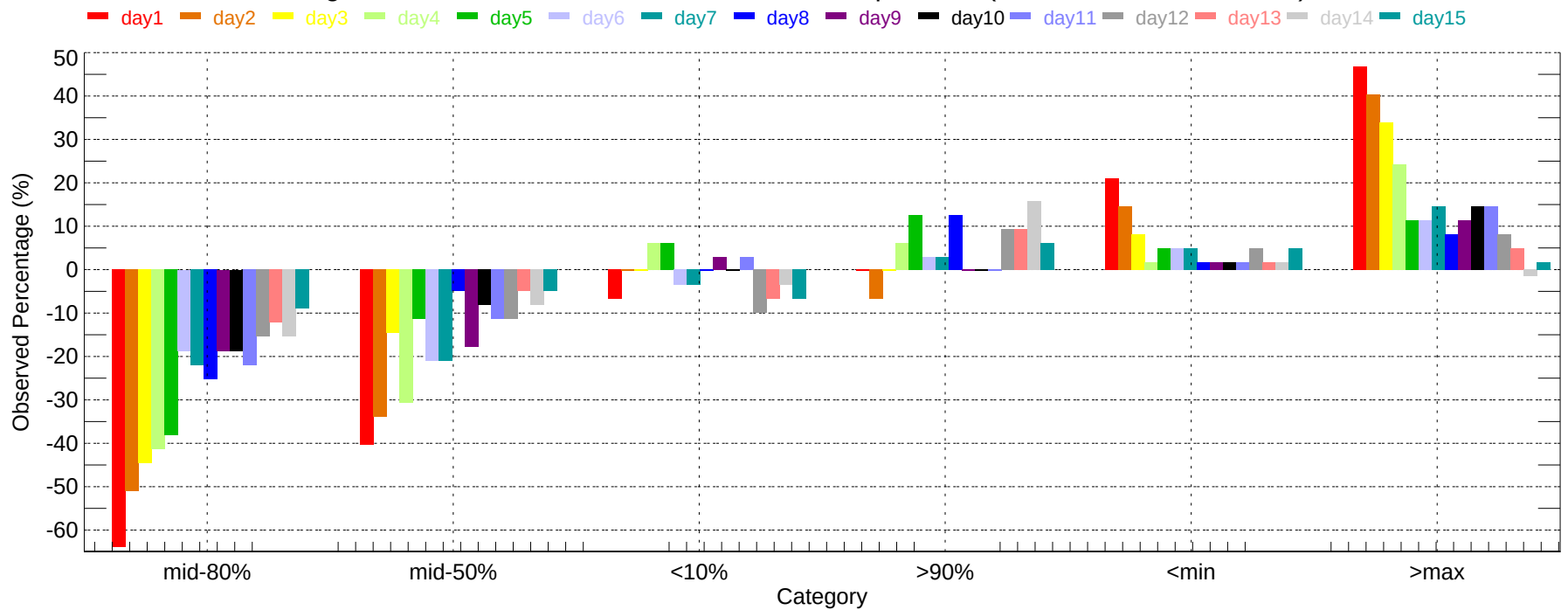
Observed Percentage Deviation of Ensembles - COS: Max Temperature (2011-12-01~2011-12-31)
