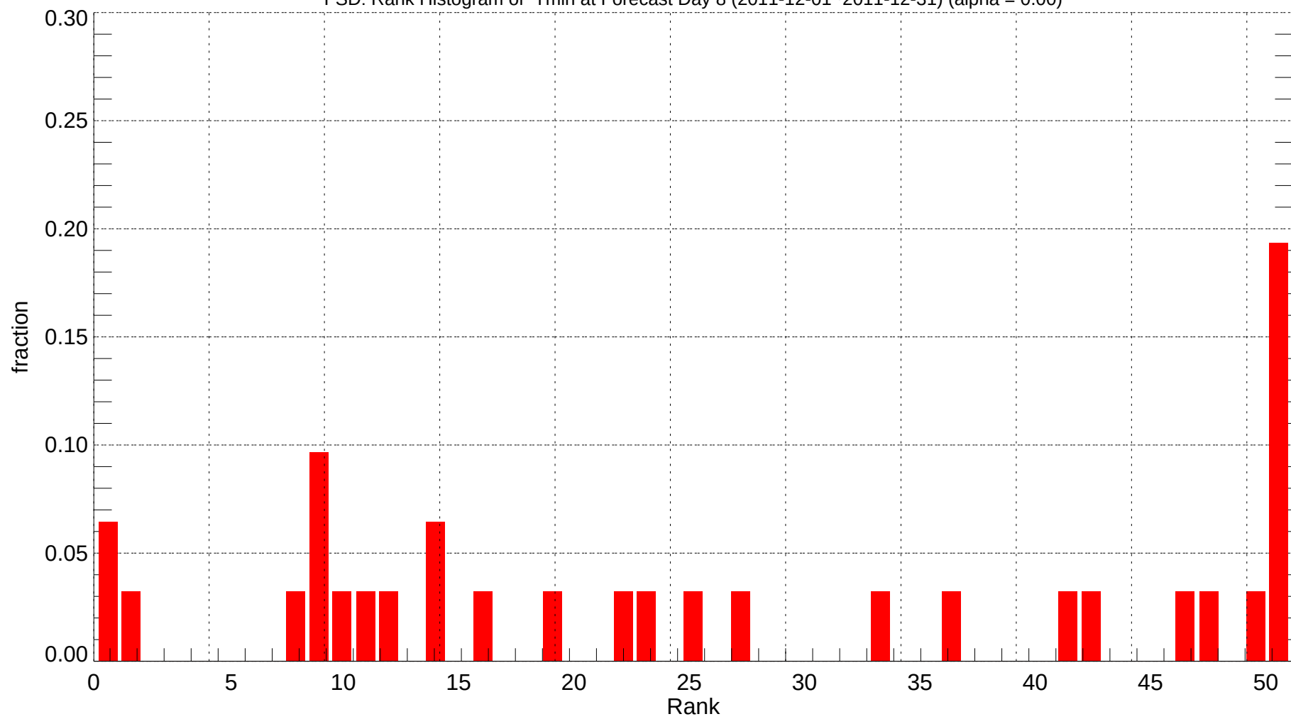
FSD: Rank Histogram of Tmin at Forecast Day 8 (2011-12-01~2011-12-31) (alpha = 0.00)
