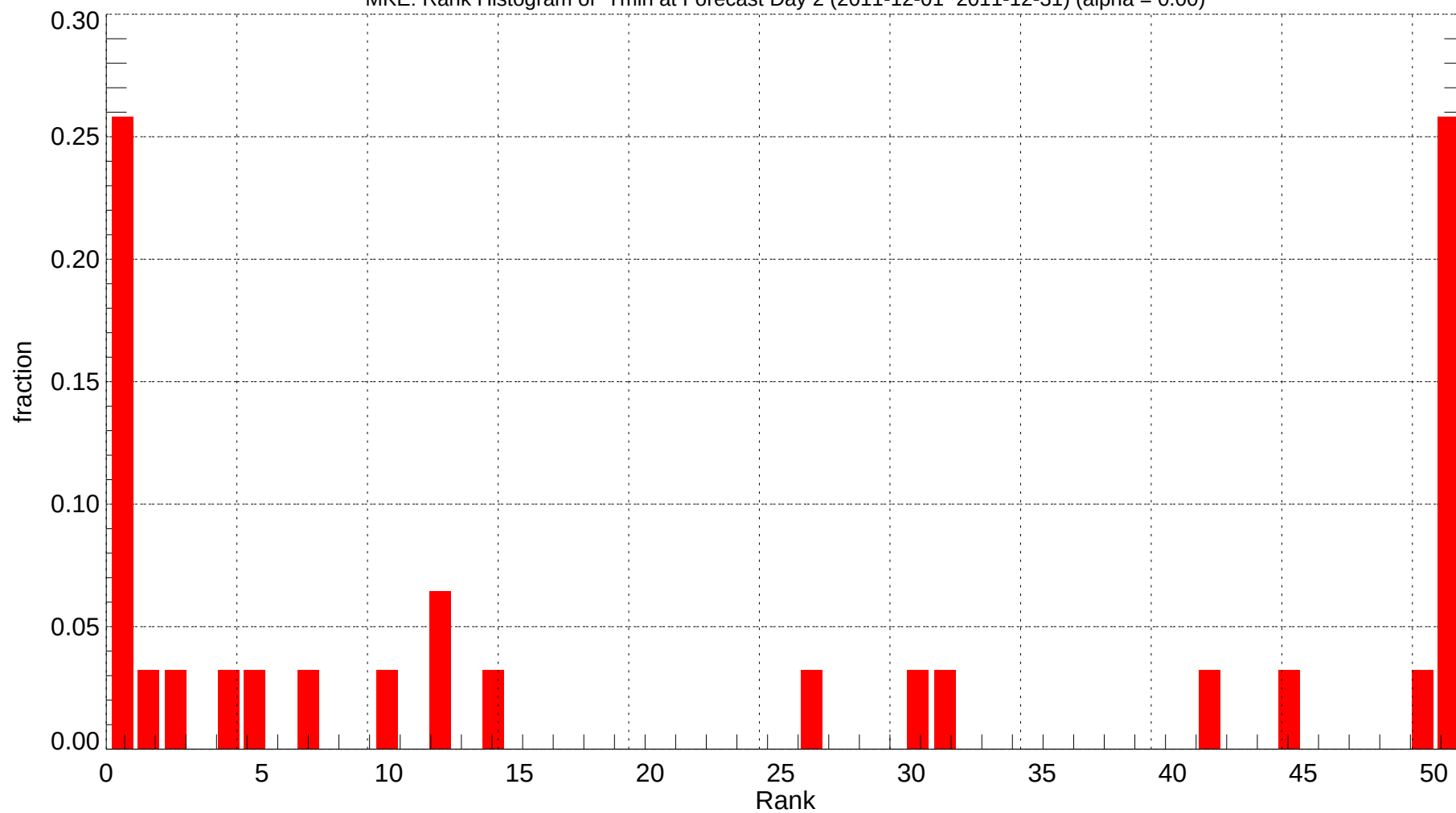
MKE: Rank Histogram of Tmin at Forecast Day 2 (2011-12-01~2011-12-31) (alpha = 0.00)
