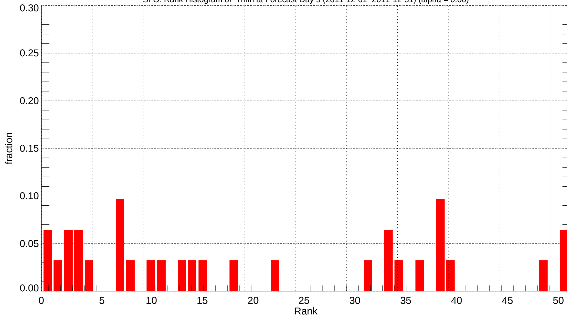
SFO: Rank Histogram of Tmin at Forecast Day 9 (2011-12-01~2011-12-31) (alpha = 0.00)
