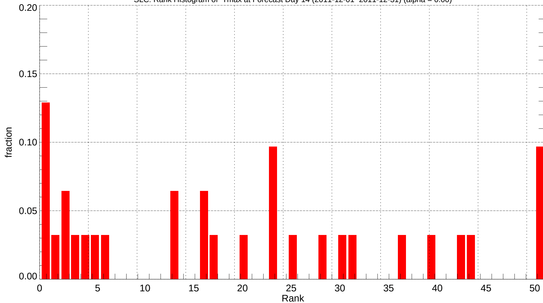
SLC: Rank Histogram of Tmax at Forecast Day 14 (2011-12-01~2011-12-31) (alpha = 0.00)
