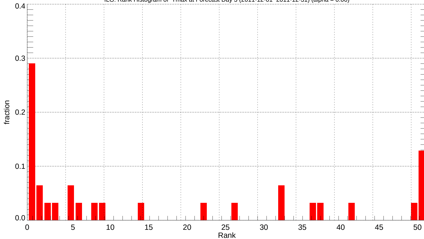
ILG: Rank Histogram of Tmax at Forecast Day 3 (2011-12-01~2011-12-31) (alpha = 0.00)
