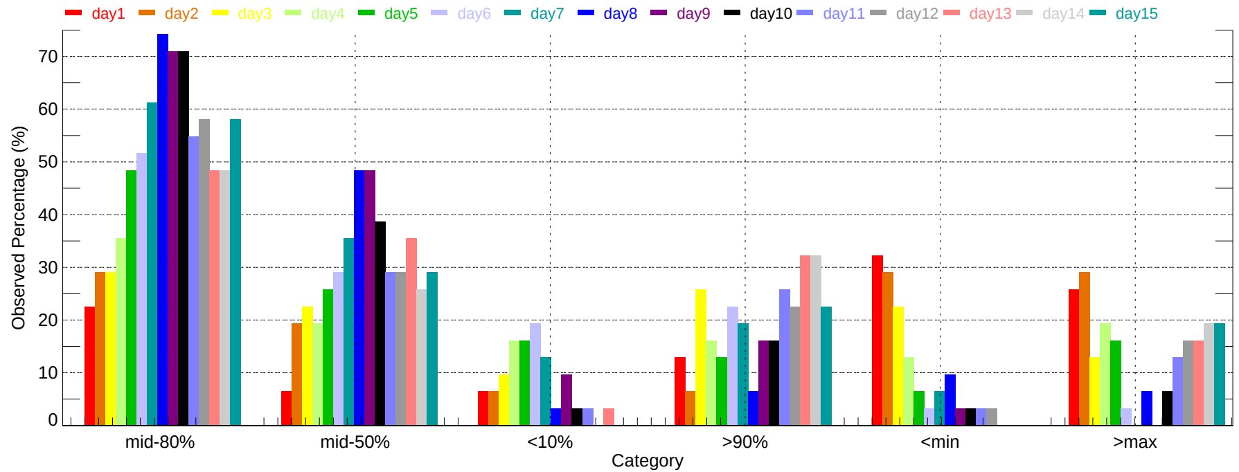
Observed Percentage of Ensembles - LGB: Max Temperature (2011-12-01~2011-12-31)
