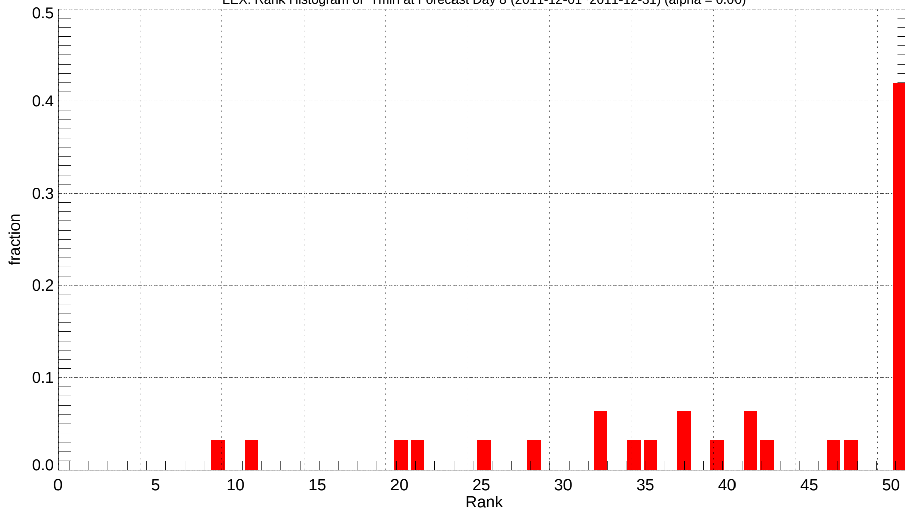
LEX: Rank Histogram of Tmin at Forecast Day 8 (2011-12-01~2011-12-31) (alpha = 0.00)
