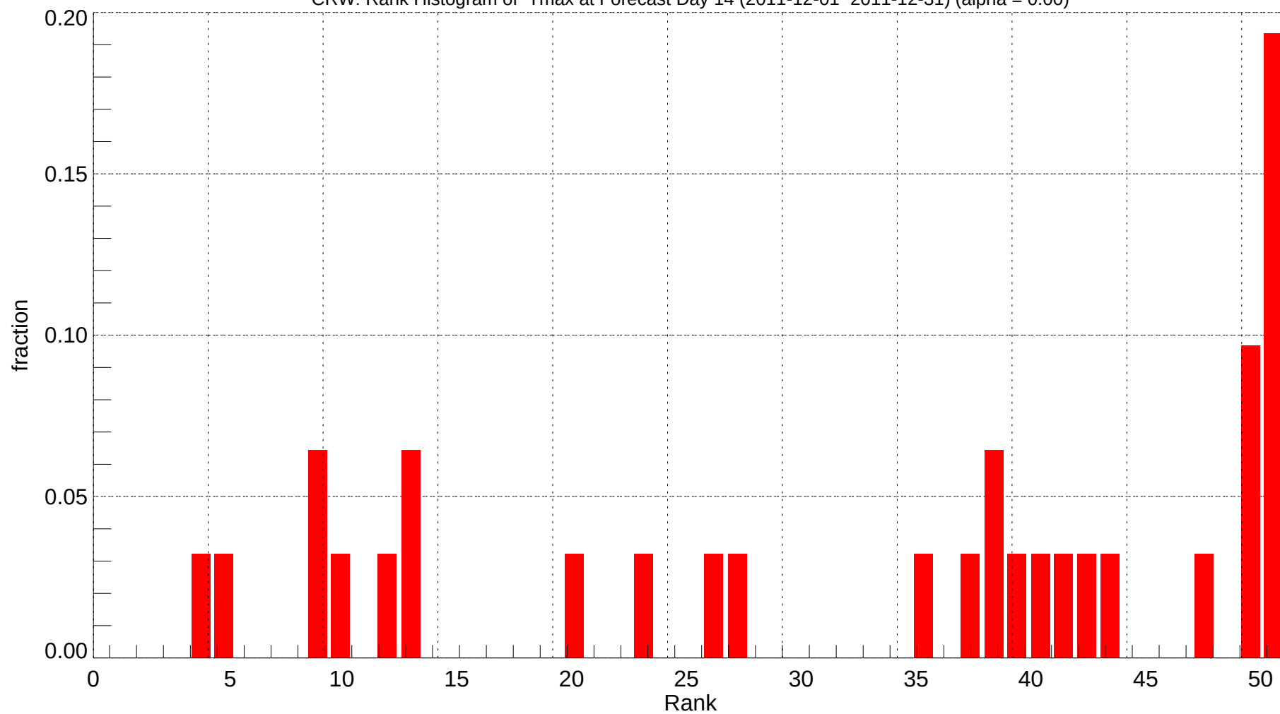
CRW: Rank Histogram of Tmax at Forecast Day 14 (2011-12-01~2011-12-31) (alpha = 0.00)
