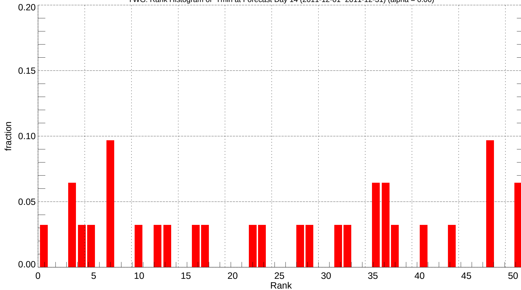
YWG: Rank Histogram of Tmin at Forecast Day 14 (2011-12-01~2011-12-31) (alpha = 0.00)
