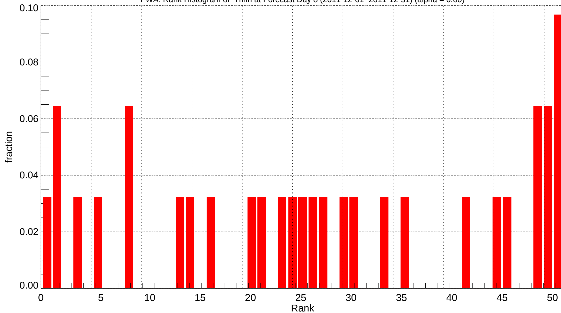
FWA: Rank Histogram of Tmin at Forecast Day 8 (2011-12-01~2011-12-31) (alpha = 0.00)
