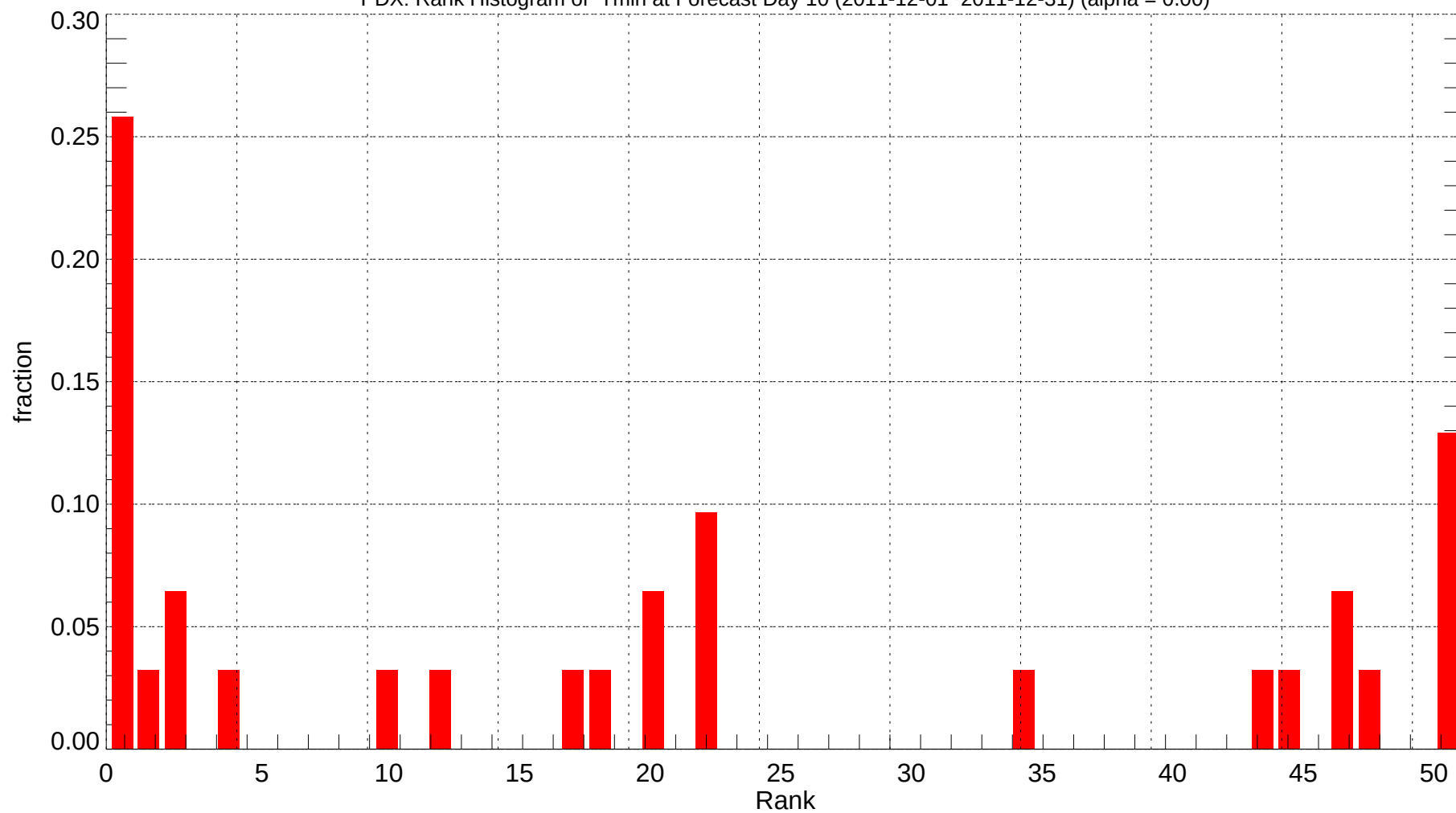
PDX: Rank Histogram of Tmin at Forecast Day 10 (2011-12-01~2011-12-31) (alpha = 0.00)
