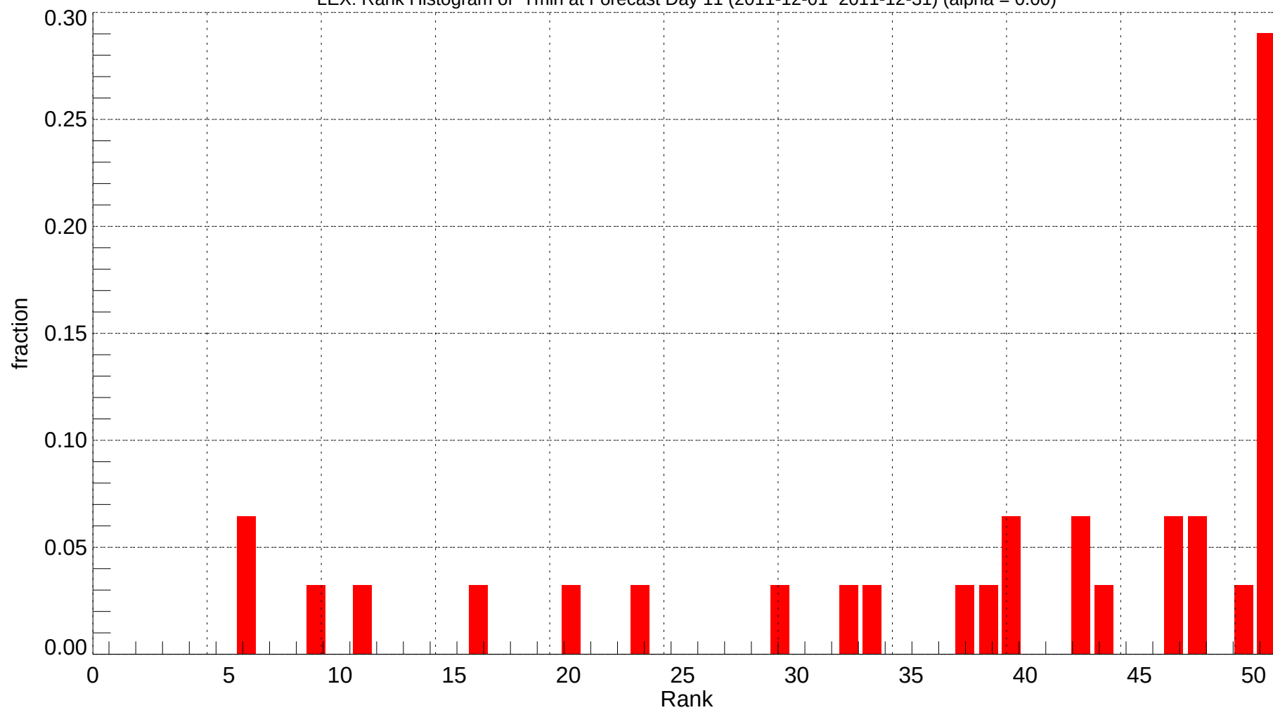
LEX: Rank Histogram of Tmin at Forecast Day 11 (2011-12-01~2011-12-31) (alpha = 0.00)
