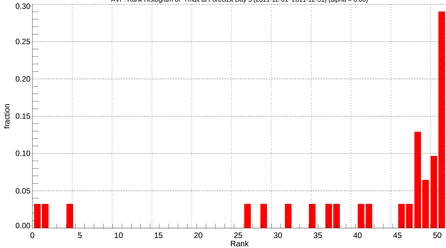
AVP: Rank Histogram of Tmax at Forecast Day 5 (2011-12-01~2011-12-31) (alpha = 0.00)
