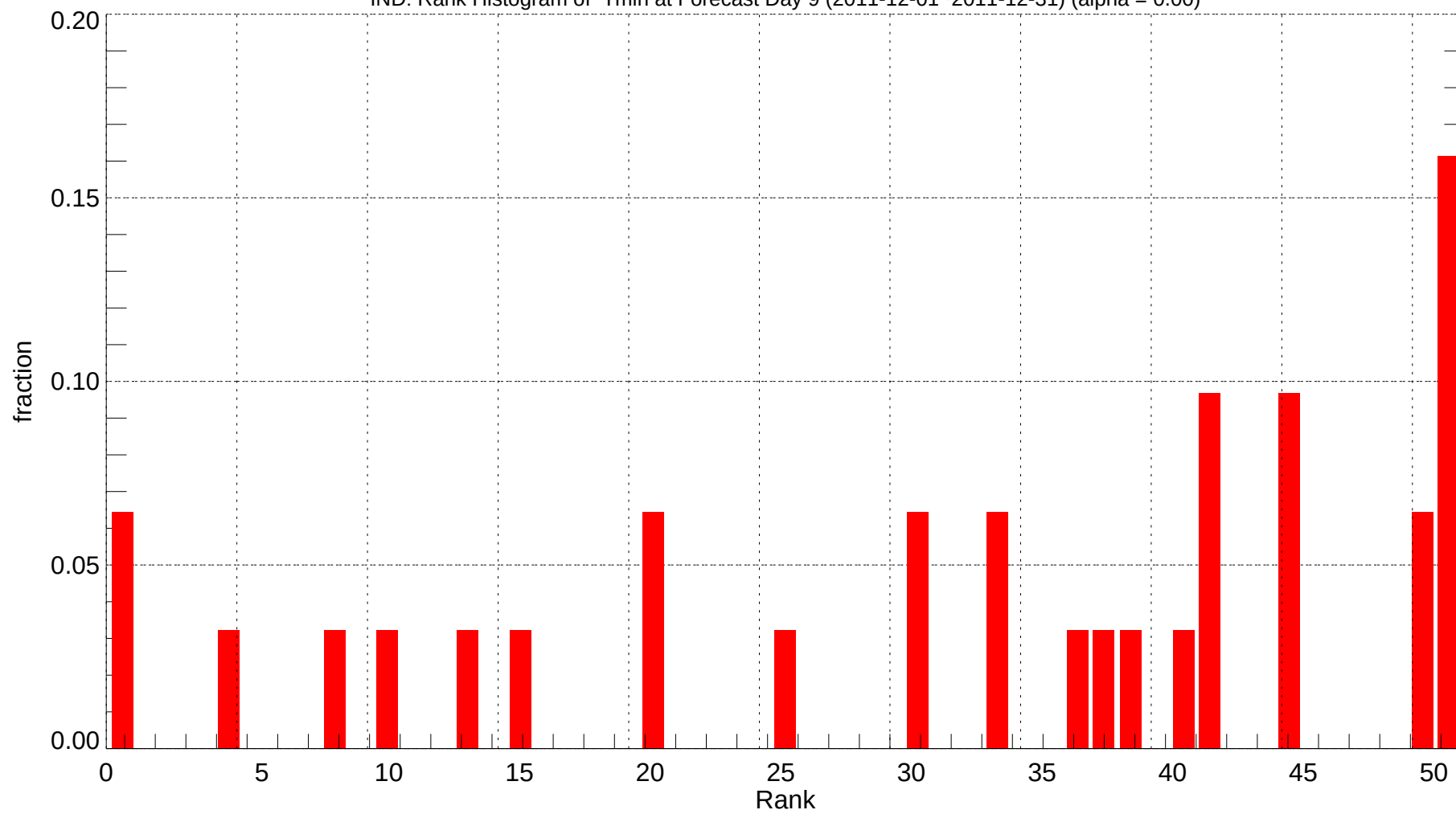
IND: Rank Histogram of Tmin at Forecast Day 9 (2011-12-01~2011-12-31) (alpha = 0.00)
