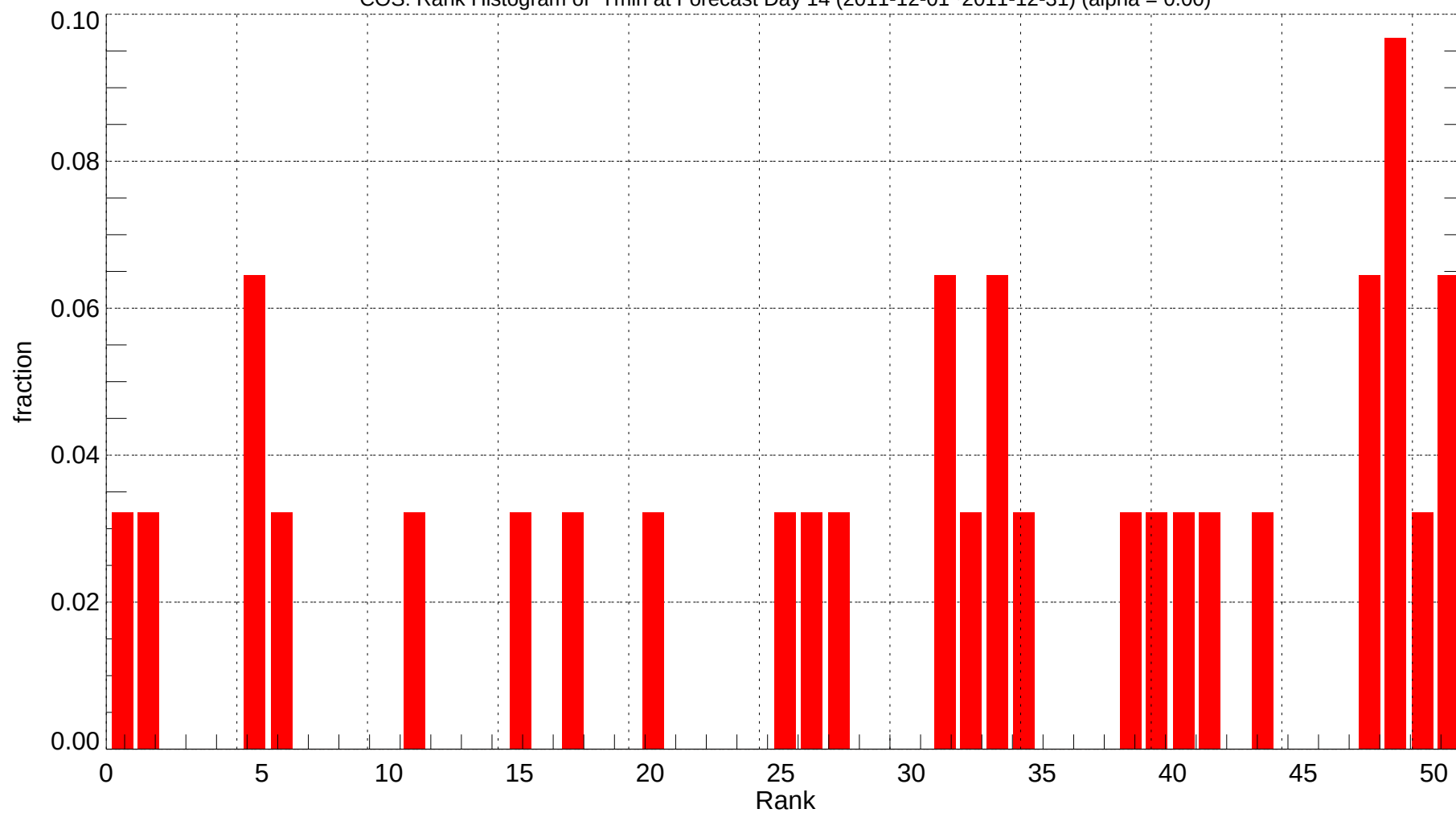
COS: Rank Histogram of Tmin at Forecast Day 14 (2011-12-01~2011-12-31) (alpha = 0.00)
