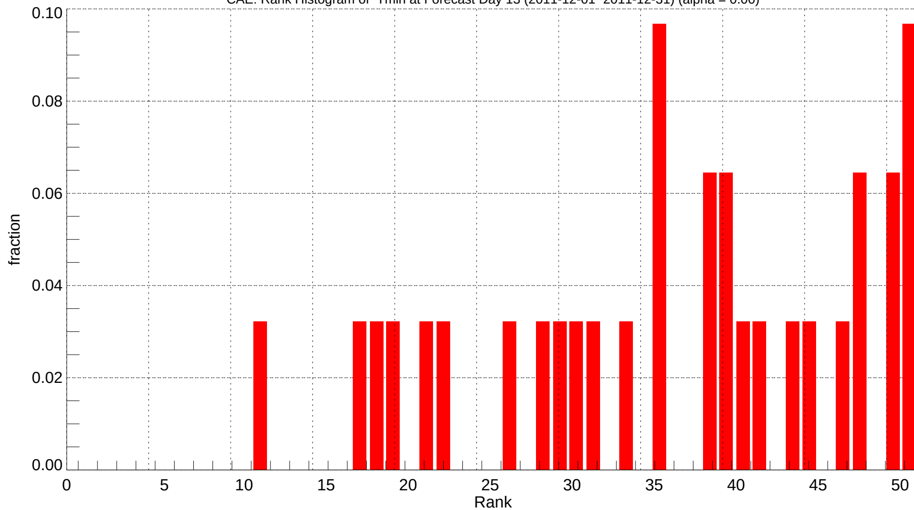
CAE: Rank Histogram of Tmin at Forecast Day 13 (2011-12-01~2011-12-31) (alpha = 0.00)
