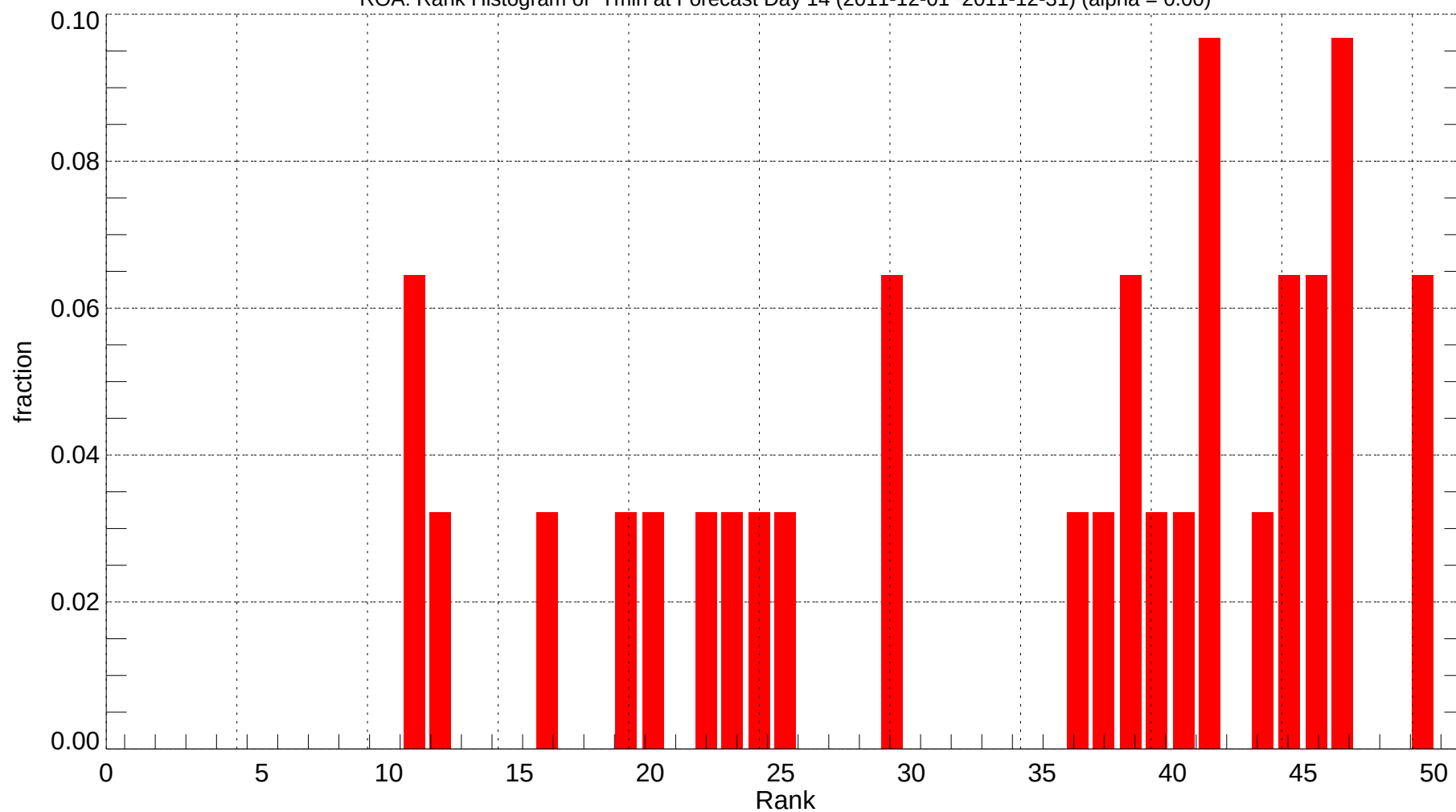
ROA: Rank Histogram of Tmin at Forecast Day 14 (2011-12-01~2011-12-31) (alpha = 0.00)
