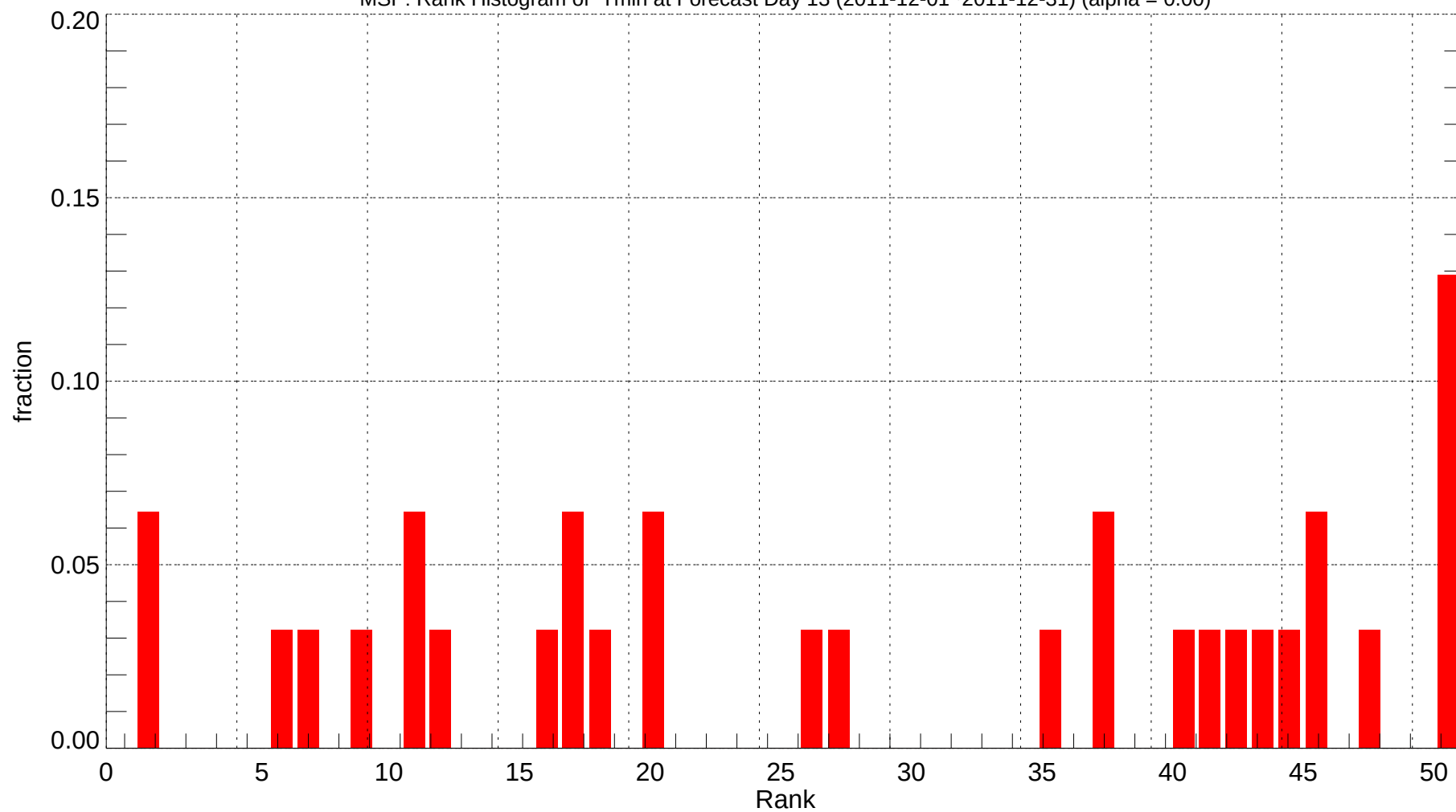
MSP: Rank Histogram of Tmin at Forecast Day 13 (2011-12-01~2011-12-31) (alpha = 0.00)
