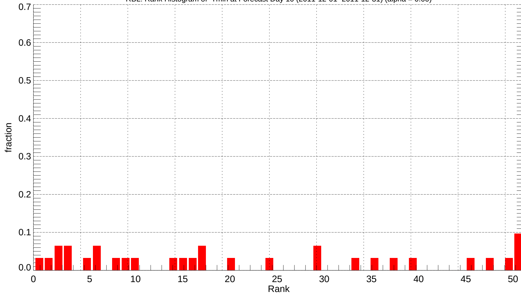
RBL: Rank Histogram of Tmin at Forecast Day 10 (2011-12-01~2011-12-31) (alpha = 0.00)
