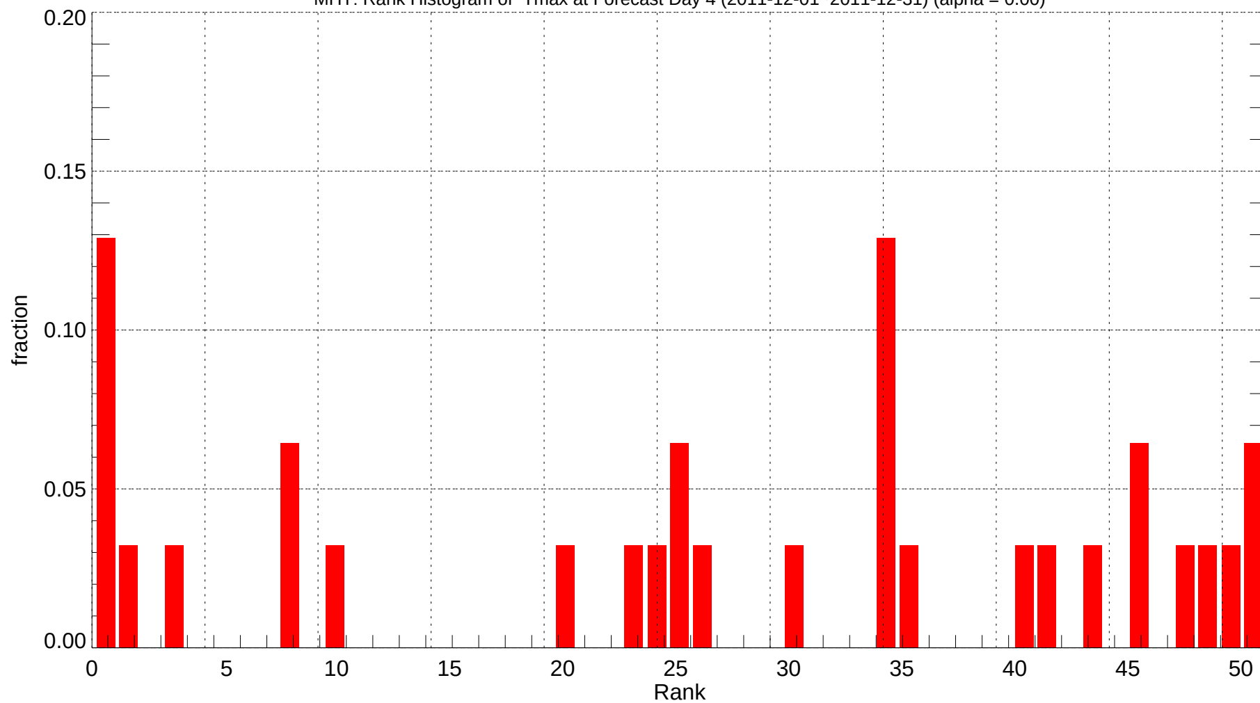
MHT: Rank Histogram of Tmax at Forecast Day 4 (2011-12-01~2011-12-31) (alpha = 0.00)
