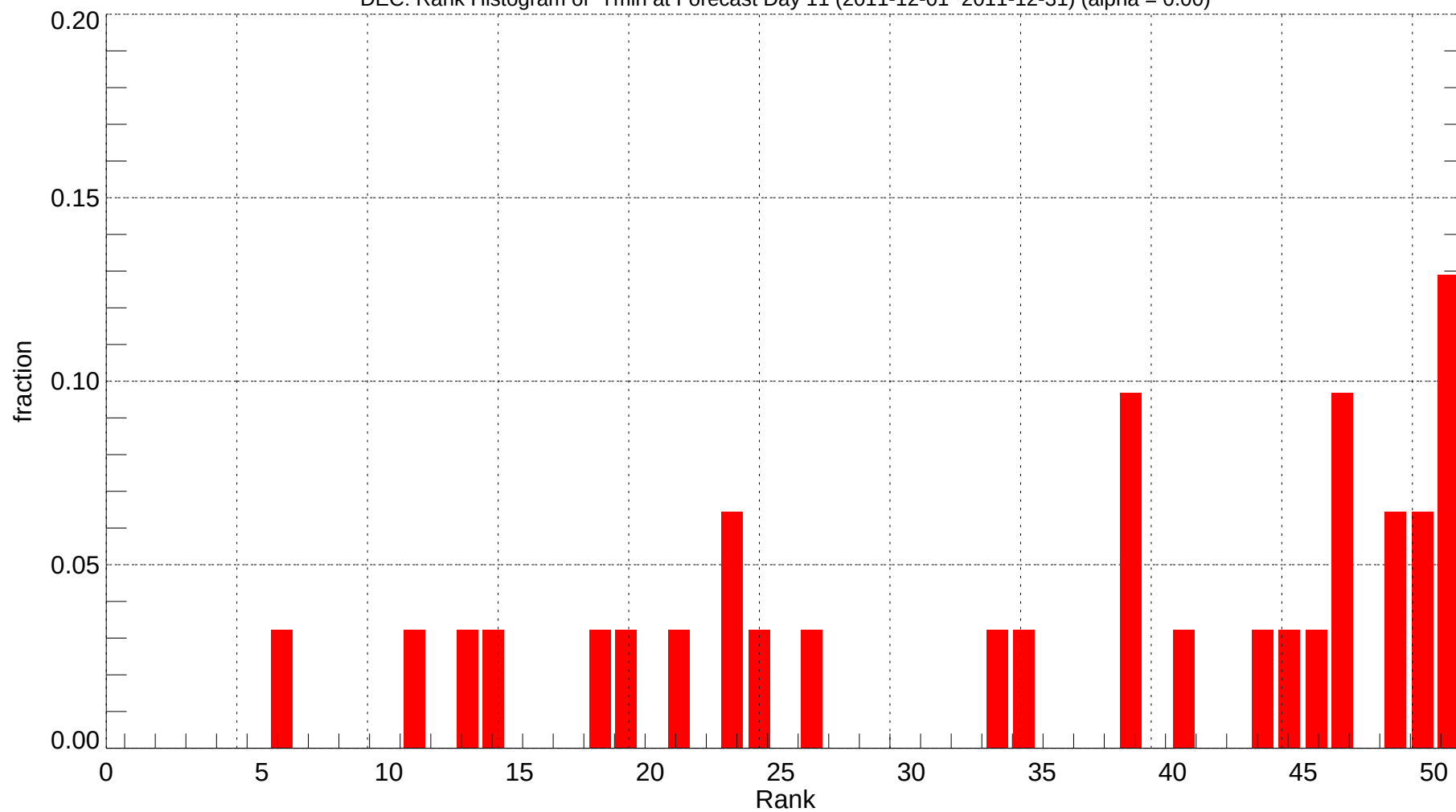
DEC: Rank Histogram of Tmin at Forecast Day 11 (2011-12-01~2011-12-31) (alpha = 0.00)
