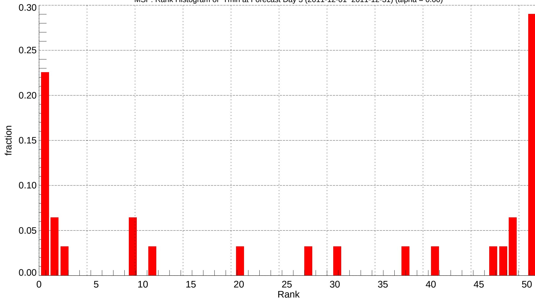
MSP: Rank Histogram of Tmin at Forecast Day 3 (2011-12-01~2011-12-31) (alpha = 0.00)
