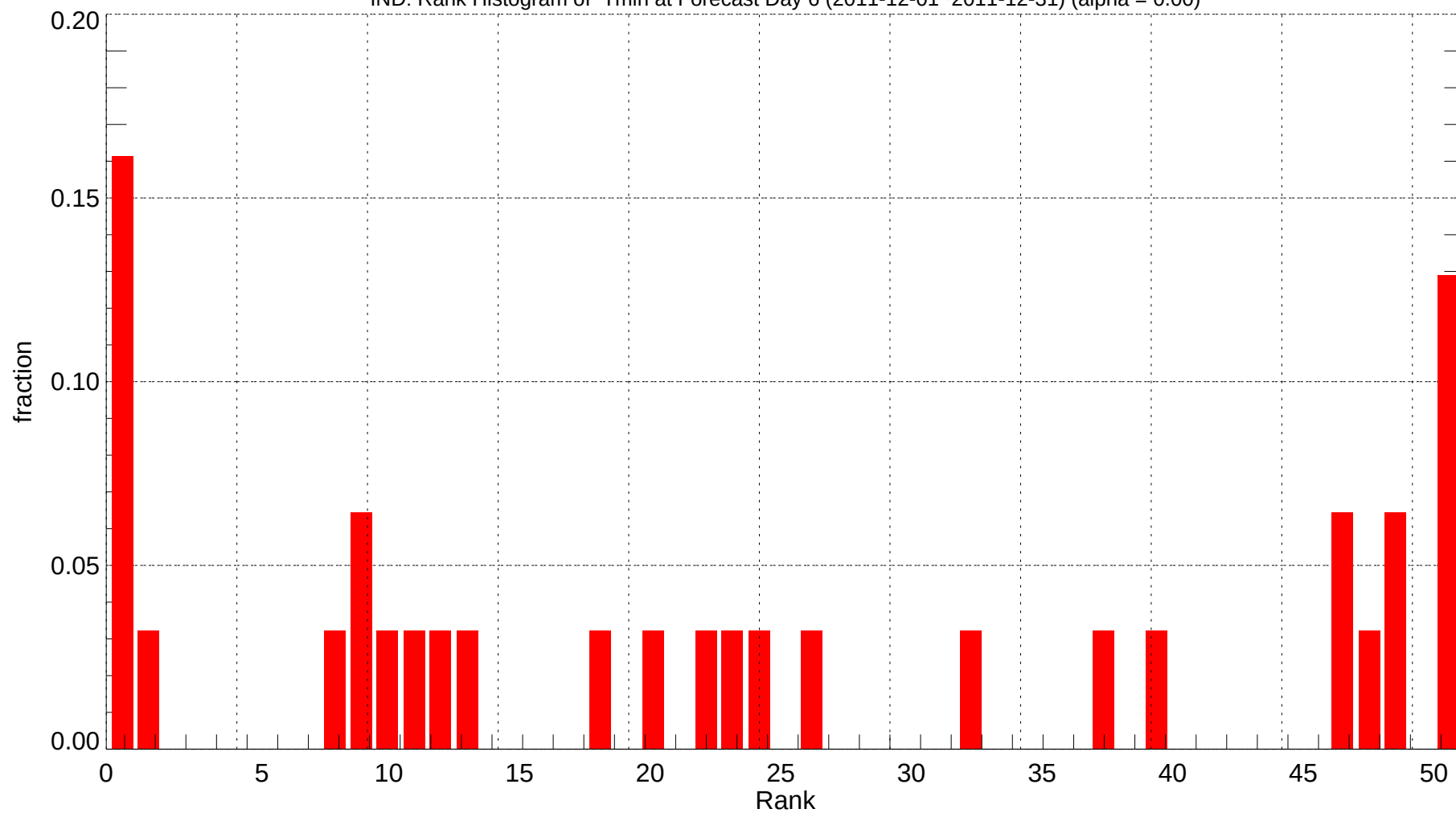
IND: Rank Histogram of Tmin at Forecast Day 6 (2011-12-01~2011-12-31) (alpha = 0.00)
