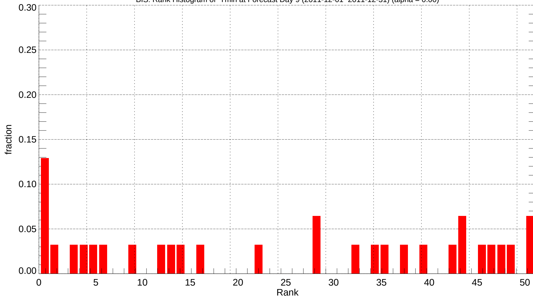
BIS: Rank Histogram of Tmin at Forecast Day 9 (2011-12-01~2011-12-31) (alpha = 0.00)
