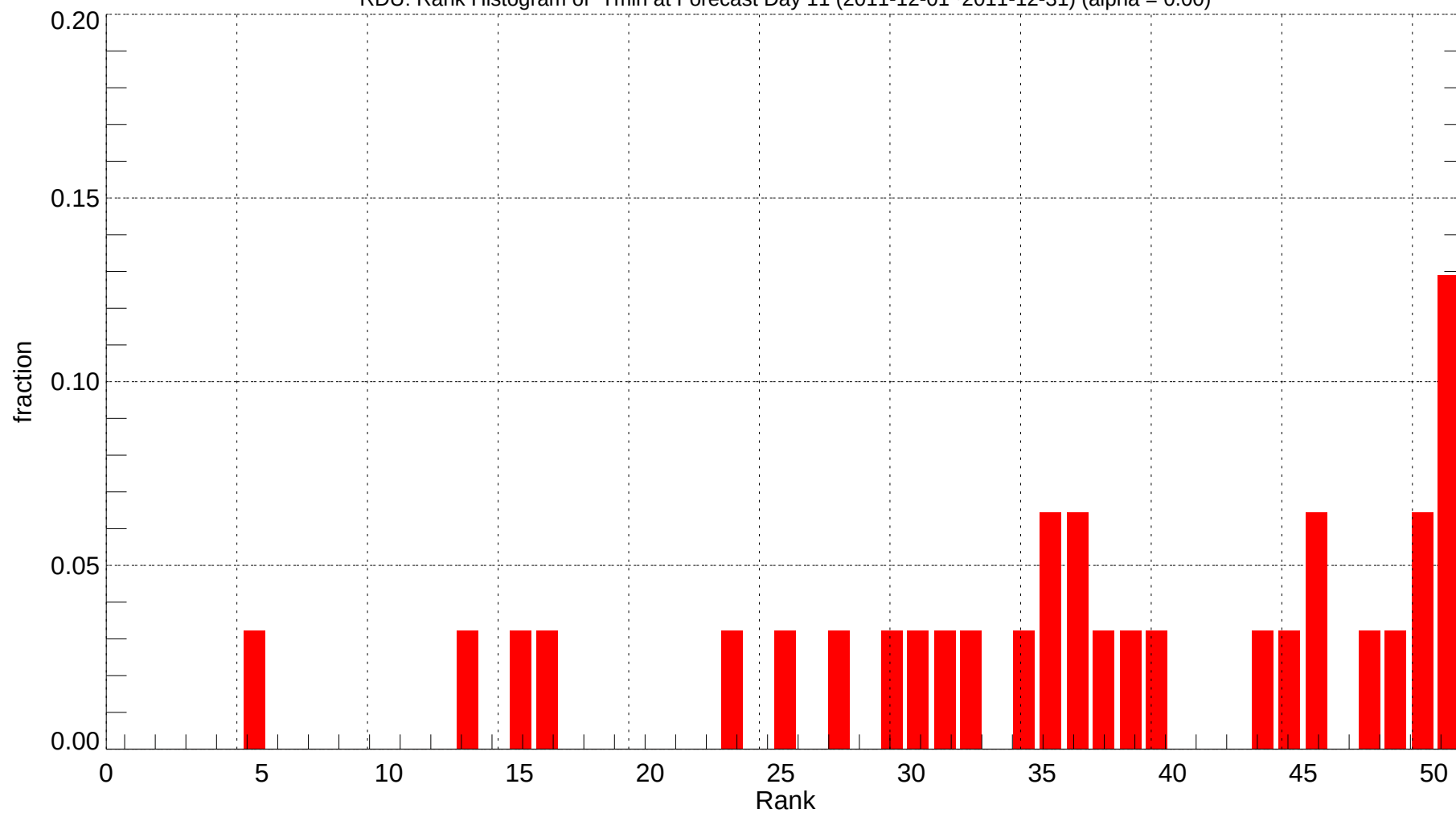
RDU: Rank Histogram of Tmin at Forecast Day 11 (2011-12-01~2011-12-31) (alpha = 0.00)
