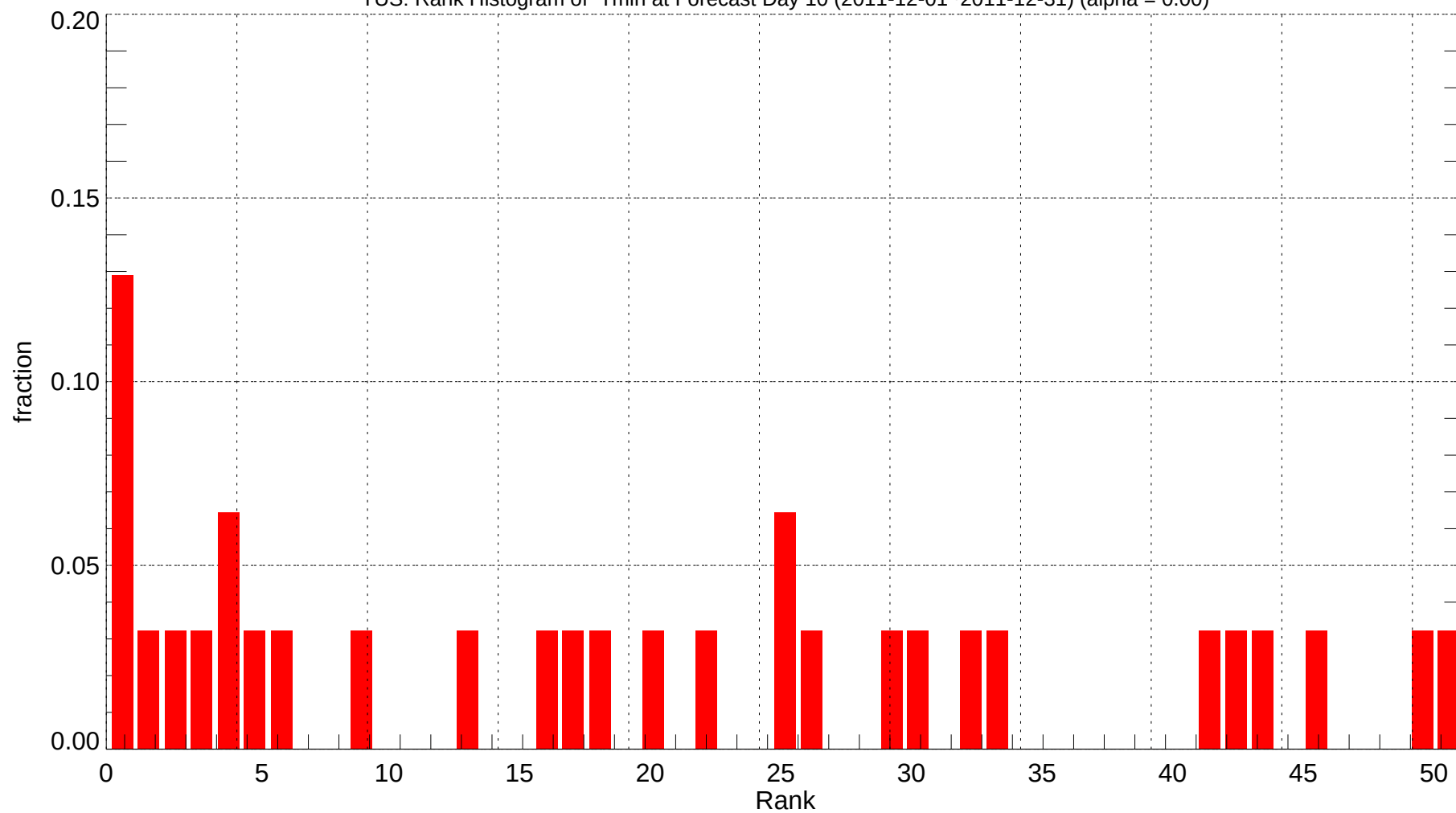
TUS: Rank Histogram of Tmin at Forecast Day 10 (2011-12-01~2011-12-31) (alpha = 0.00)
