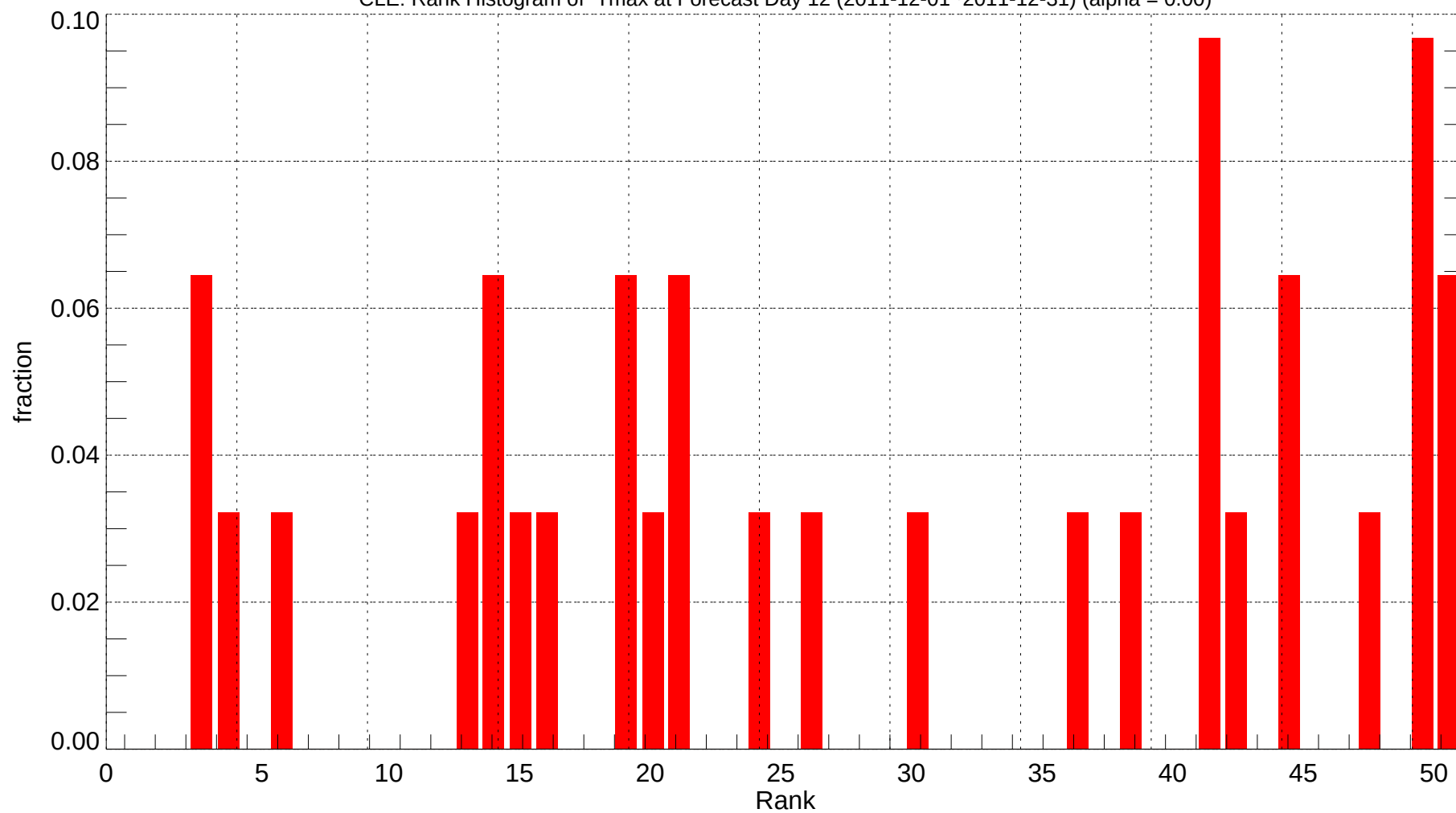
CLE: Rank Histogram of Tmax at Forecast Day 12 (2011-12-01~2011-12-31) (alpha = 0.00)
