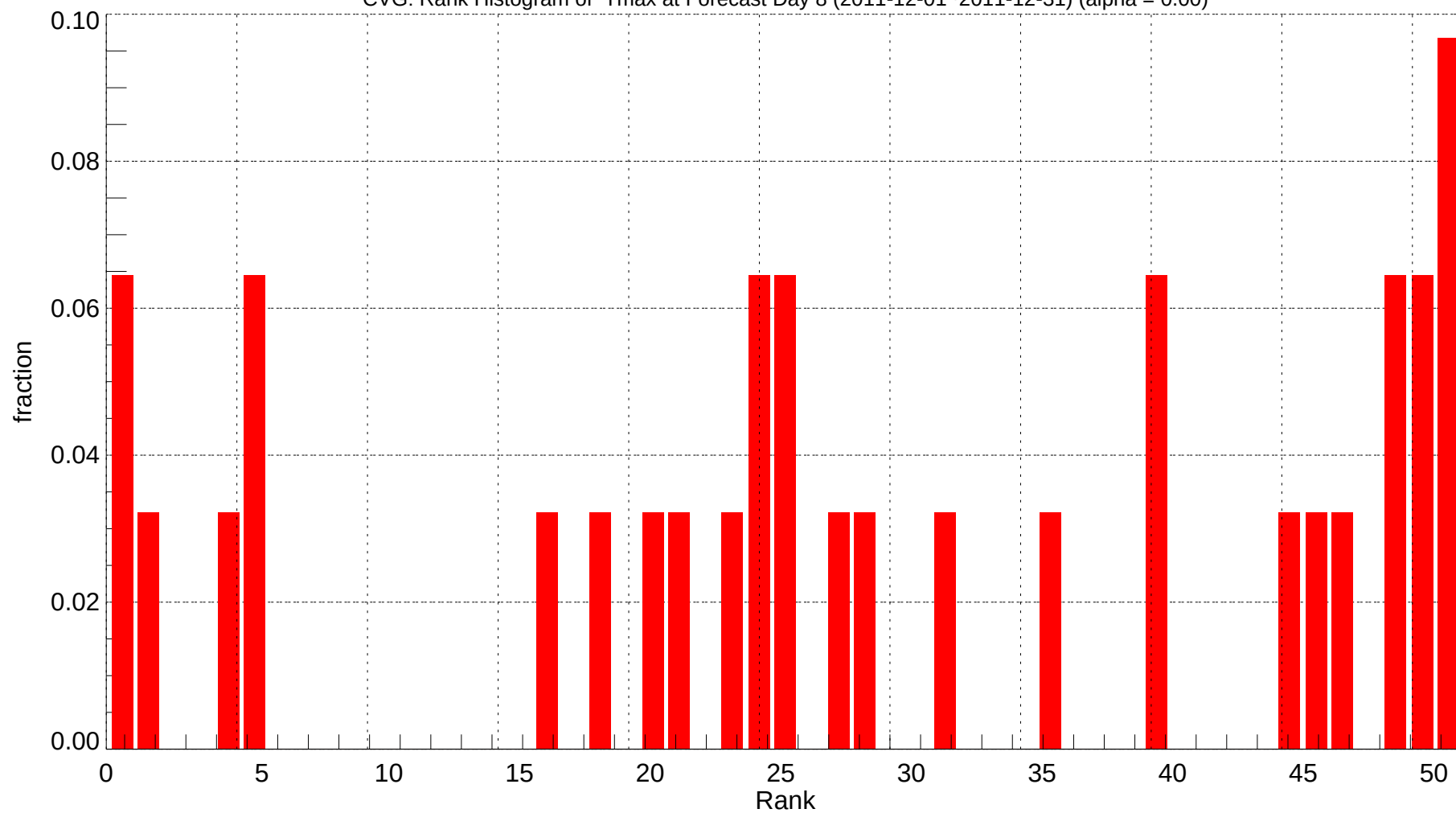
CVG: Rank Histogram of Tmax at Forecast Day 8 (2011-12-01~2011-12-31) (alpha = 0.00)
