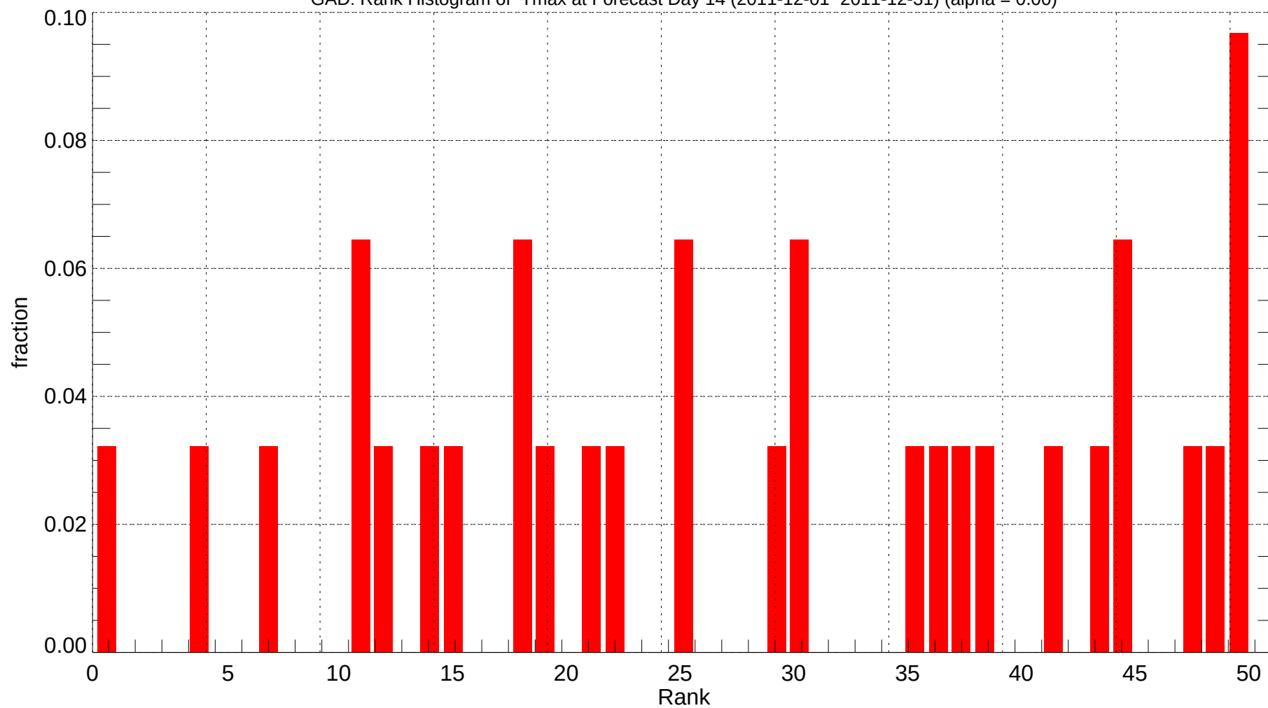
GAD: Rank Histogram of Tmax at Forecast Day 14 (2011-12-01~2011-12-31) (alpha = 0.00)
