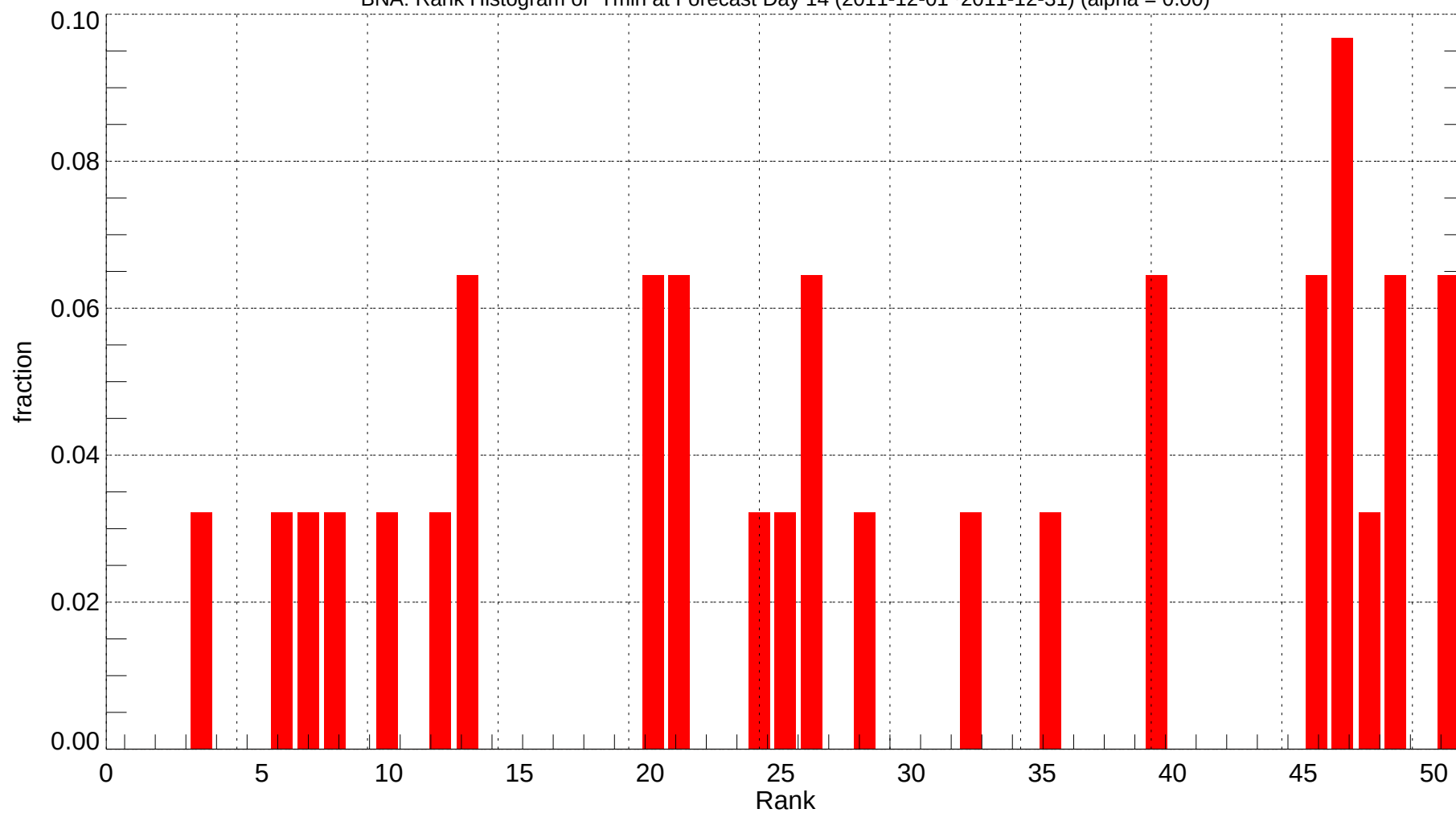
BNA: Rank Histogram of Tmin at Forecast Day 14 (2011-12-01~2011-12-31) (alpha = 0.00)
