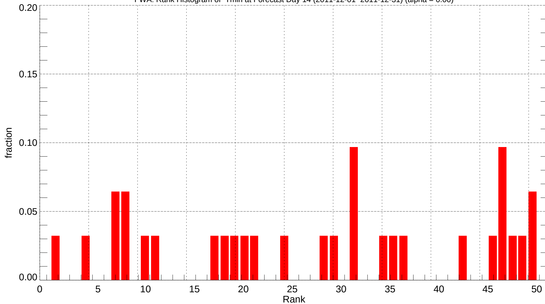
FWA: Rank Histogram of Tmin at Forecast Day 14 (2011-12-01~2011-12-31) (alpha = 0.00)
