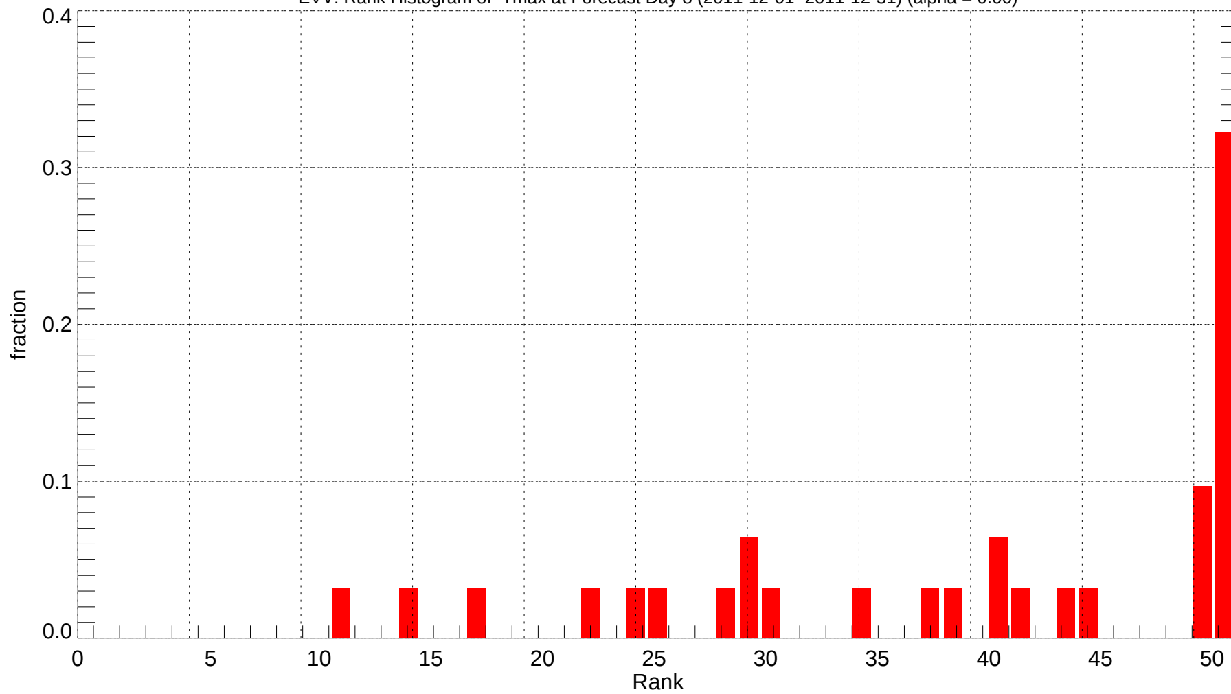
EVV: Rank Histogram of Tmax at Forecast Day 8 (2011-12-01~2011-12-31) (alpha = 0.00)
