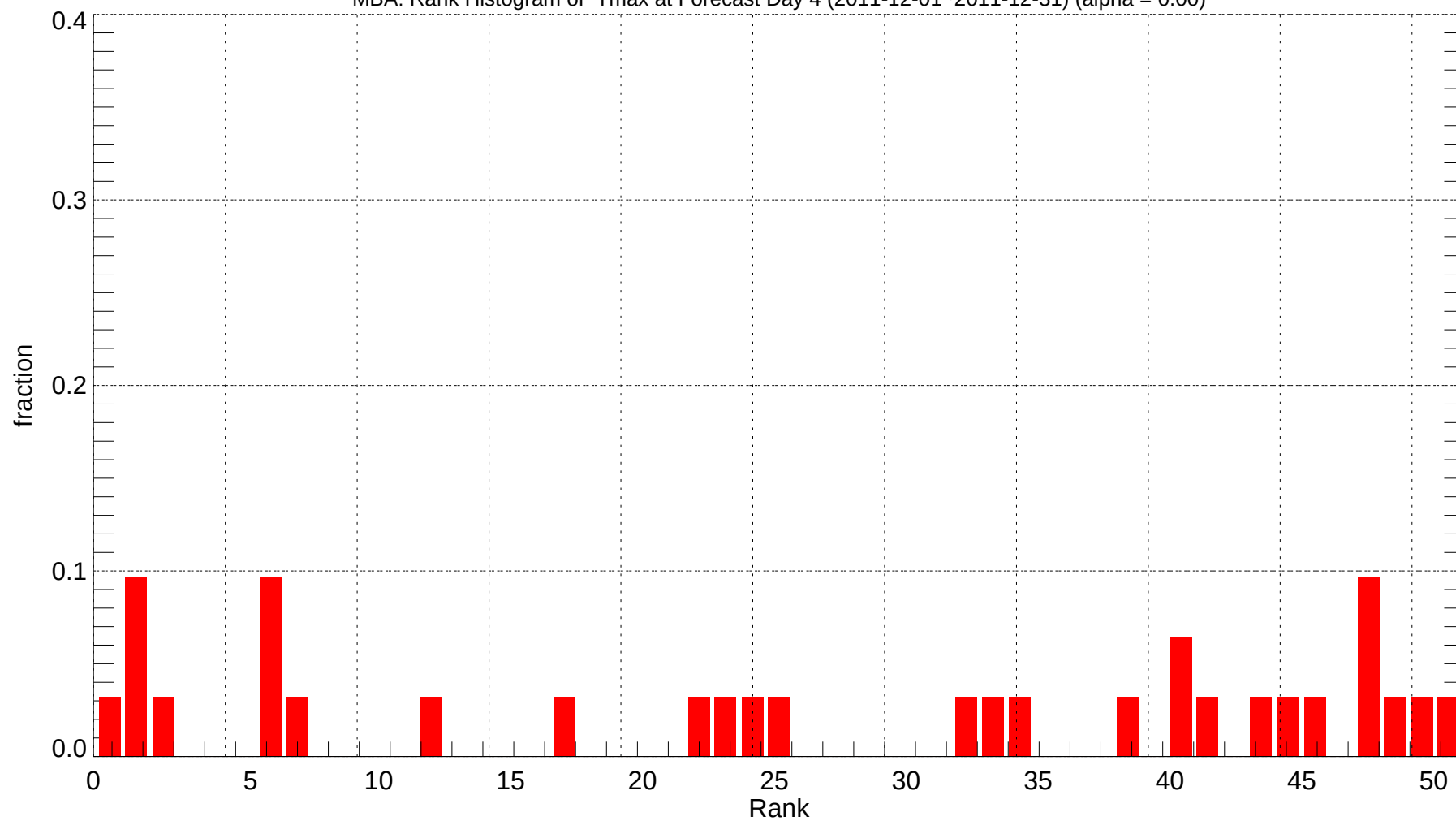
MBA: Rank Histogram of Tmax at Forecast Day 4 (2011-12-01~2011-12-31) (alpha = 0.00)
