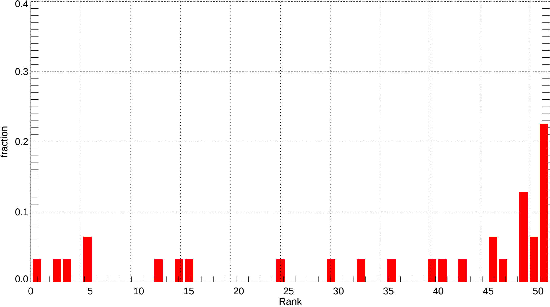
ELP: Rank Histogram of Tmin at Forecast Day 6 (2011-12-01~2011-12-31) (alpha = 0.00)
