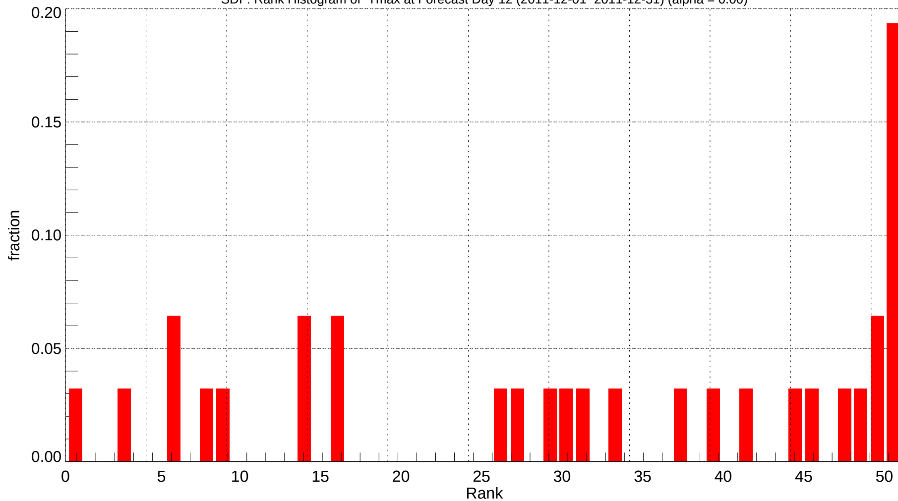
SDF: Rank Histogram of Tmax at Forecast Day 12 (2011-12-01~2011-12-31) (alpha = 0.00)
