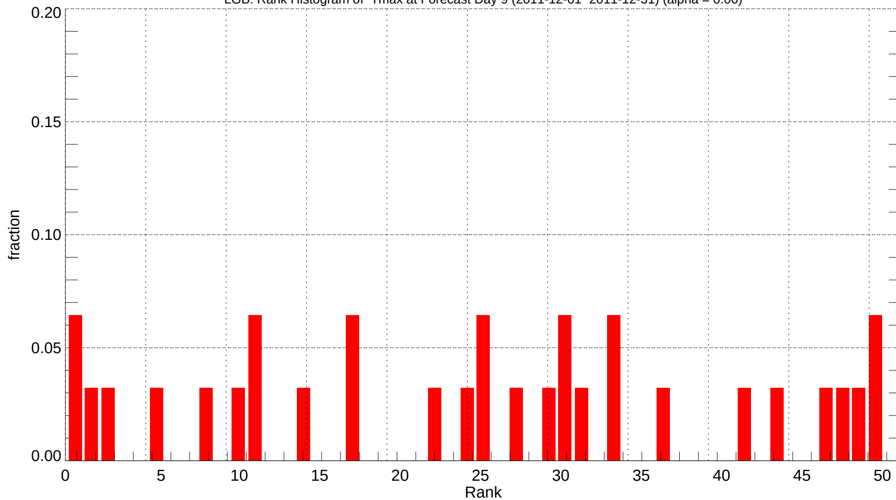
LGB: Rank Histogram of Tmax at Forecast Day 9 (2011-12-01~2011-12-31) (alpha = 0.00)
