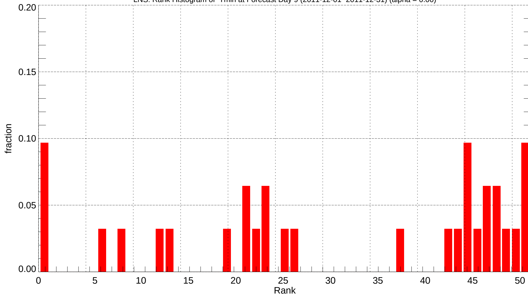
LNS: Rank Histogram of Tmin at Forecast Day 9 (2011-12-01~2011-12-31) (alpha = 0.00)
