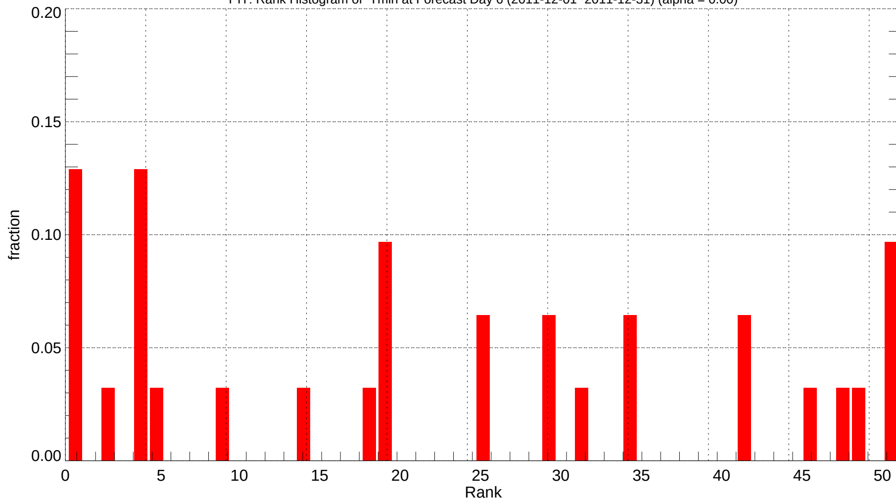
PIT: Rank Histogram of Tmin at Forecast Day 6 (2011-12-01~2011-12-31) (alpha = 0.00)
