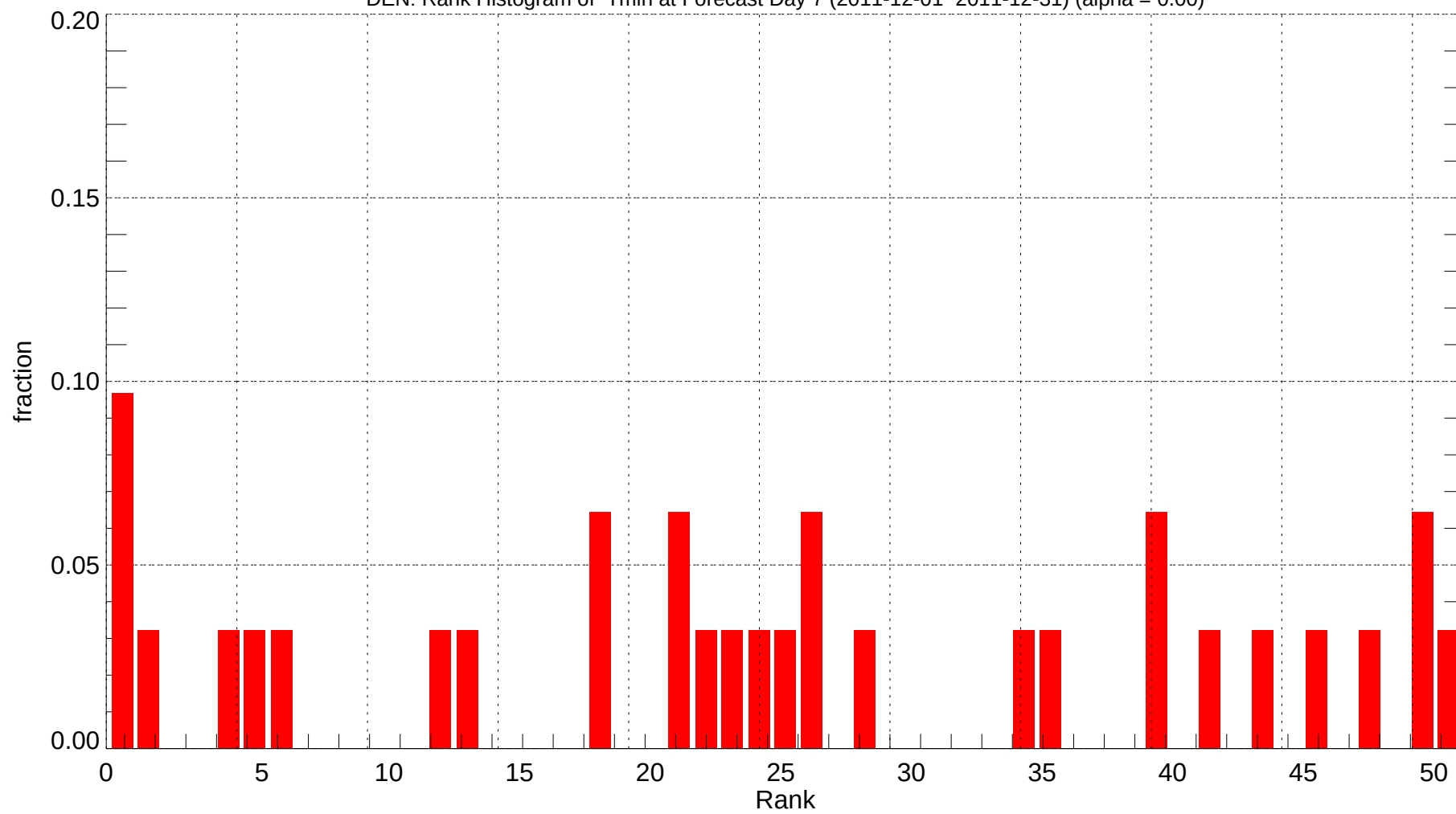
DEN: Rank Histogram of Tmin at Forecast Day 7 (2011-12-01~2011-12-31) (alpha = 0.00)
