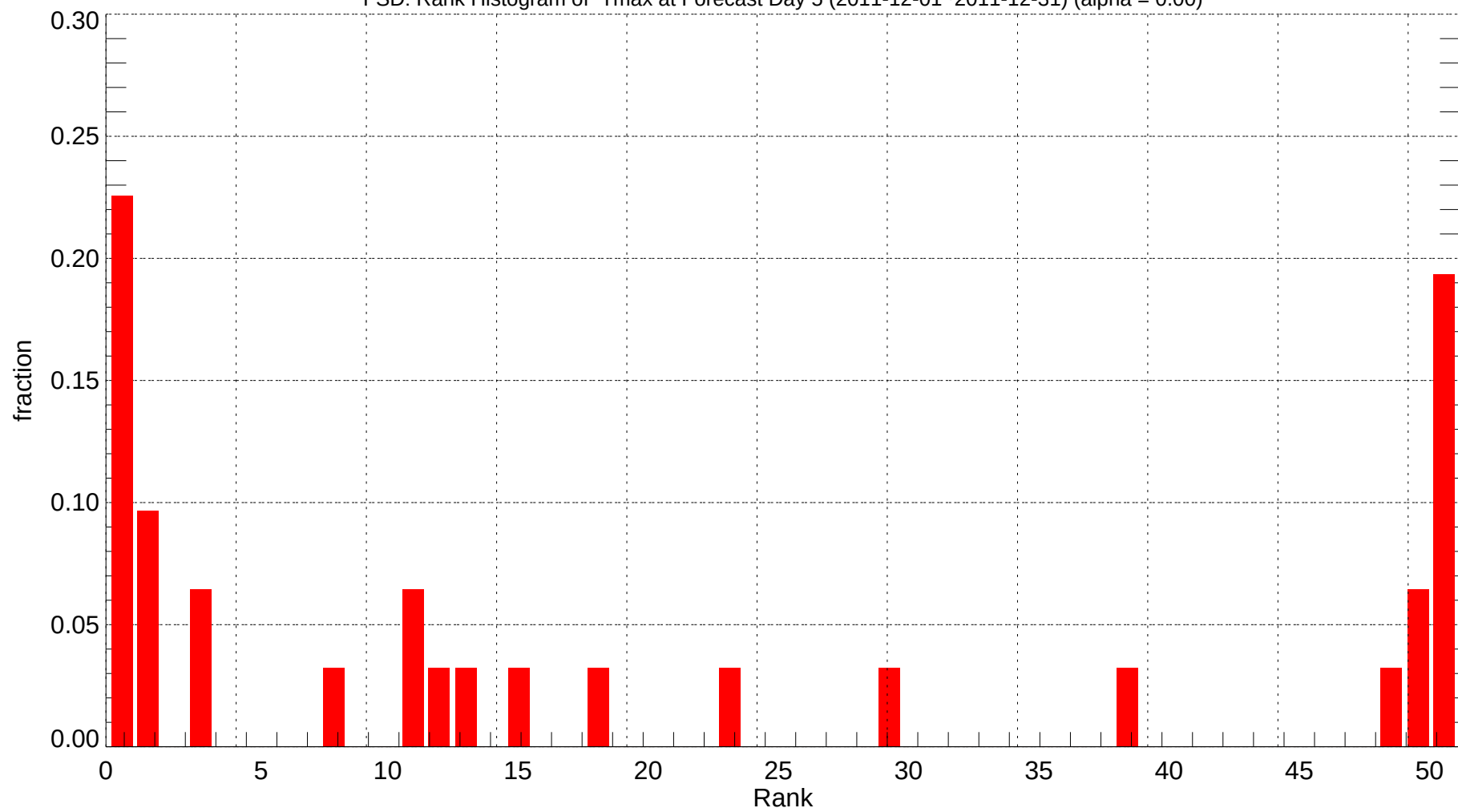
FSD: Rank Histogram of Tmax at Forecast Day 5 (2011-12-01~2011-12-31) (alpha = 0.00)
