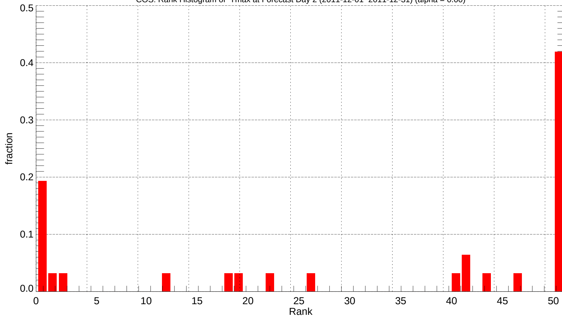
COS: Rank Histogram of Tmax at Forecast Day 2 (2011-12-01~2011-12-31) (alpha = 0.00)
