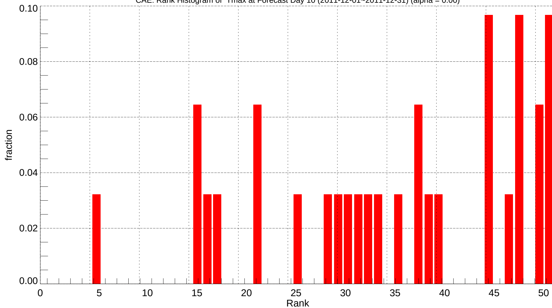
CAE: Rank Histogram of Tmax at Forecast Day 10 (2011-12-01~2011-12-31) (alpha = 0.00)
