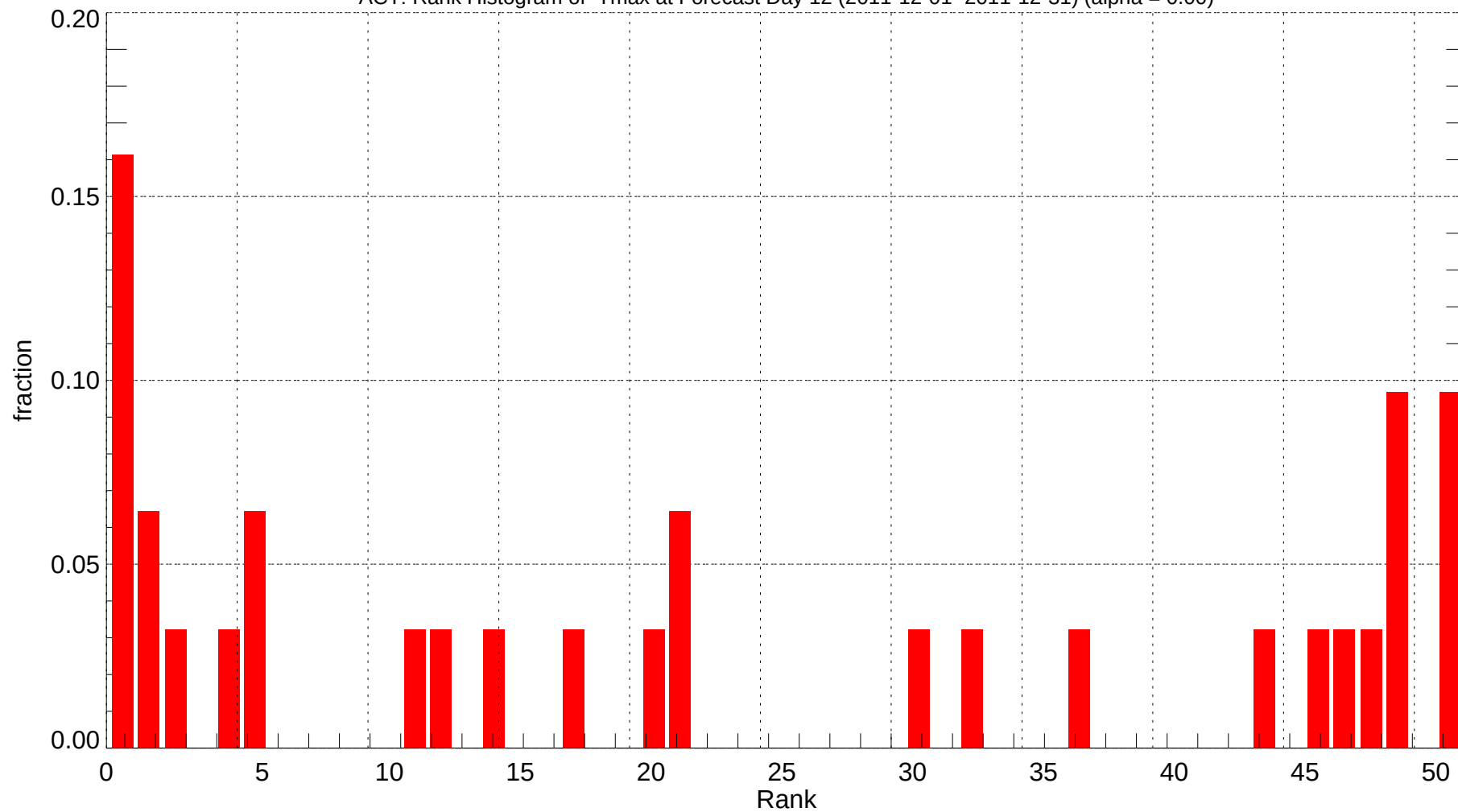
ACT: Rank Histogram of Tmax at Forecast Day 12 (2011-12-01~2011-12-31) (alpha = 0.00)
