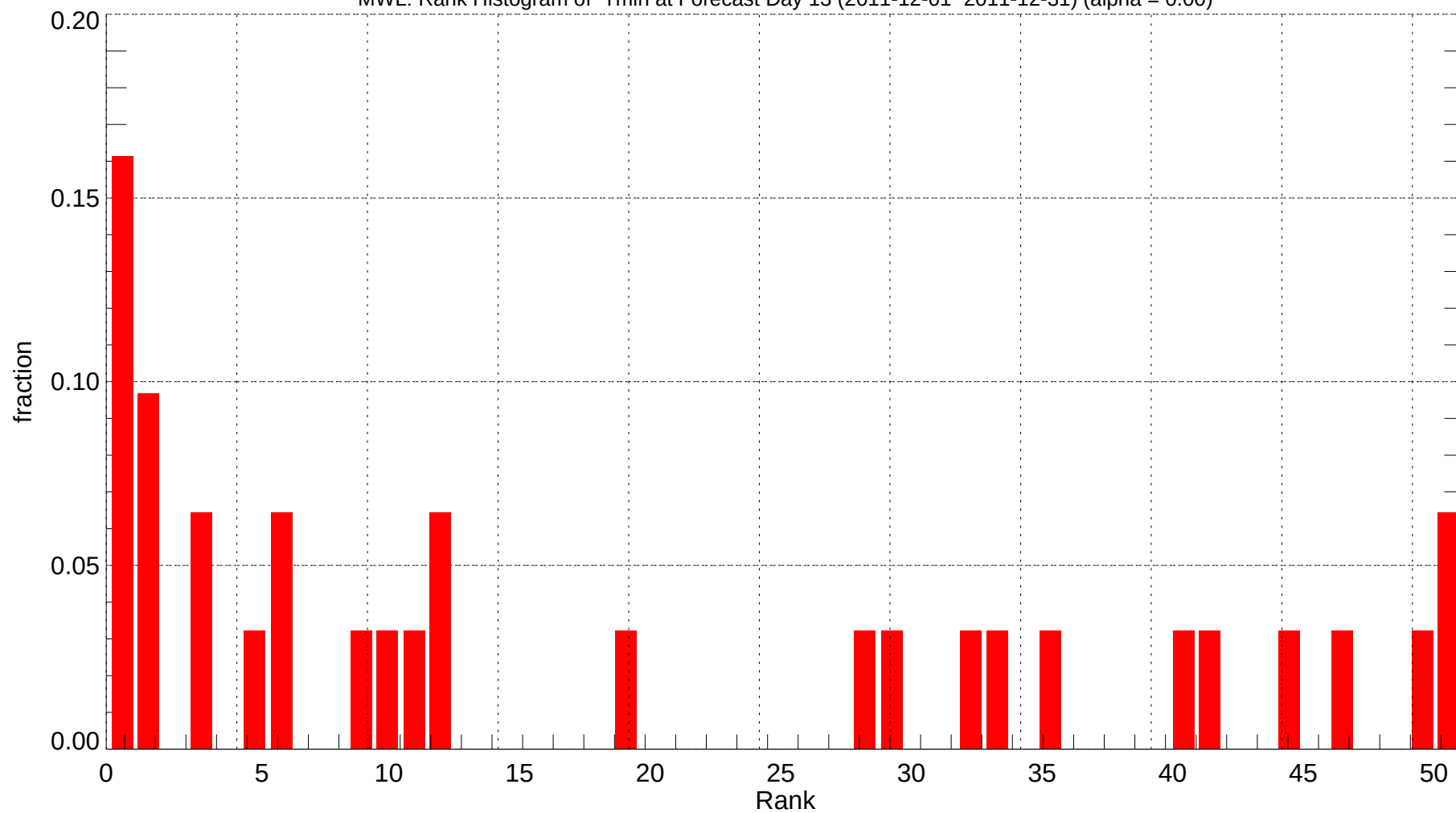
MWL: Rank Histogram of Tmin at Forecast Day 13 (2011-12-01~2011-12-31) (alpha = 0.00)
