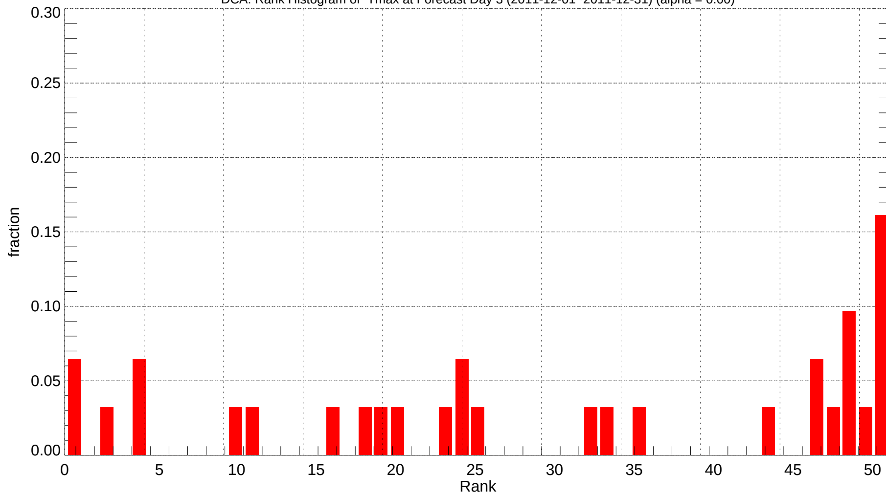
DCA: Rank Histogram of Tmax at Forecast Day 3 (2011-12-01~2011-12-31) (alpha = 0.00)
