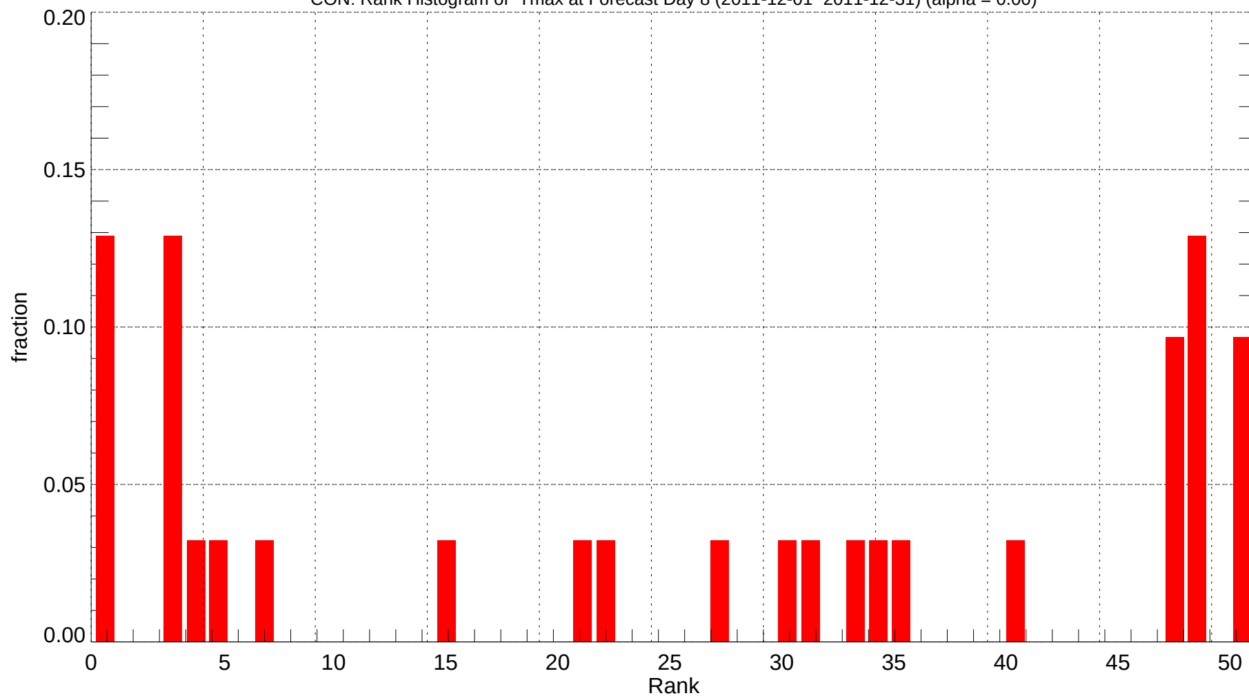
CON: Rank Histogram of Tmax at Forecast Day 8 (2011-12-01~2011-12-31) (alpha = 0.00)
