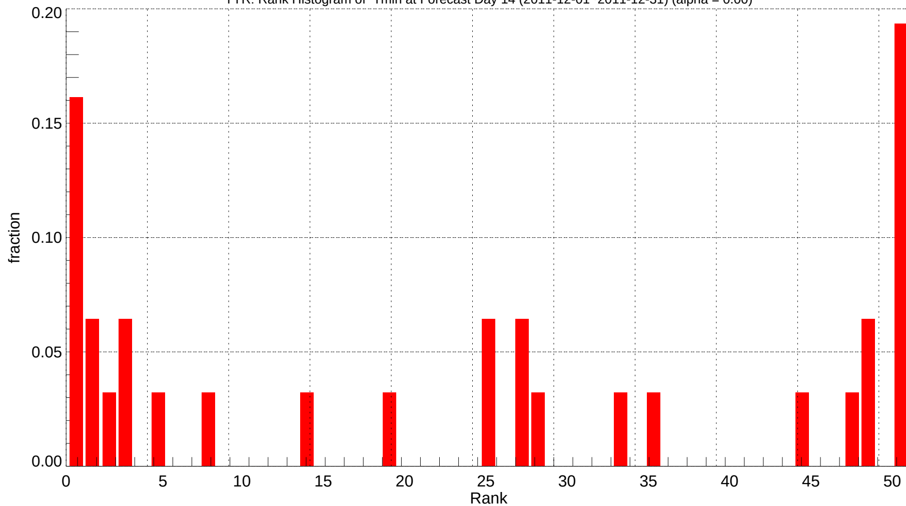
TYR: Rank Histogram of Tmin at Forecast Day 14 (2011-12-01~2011-12-31) (alpha = 0.00)
