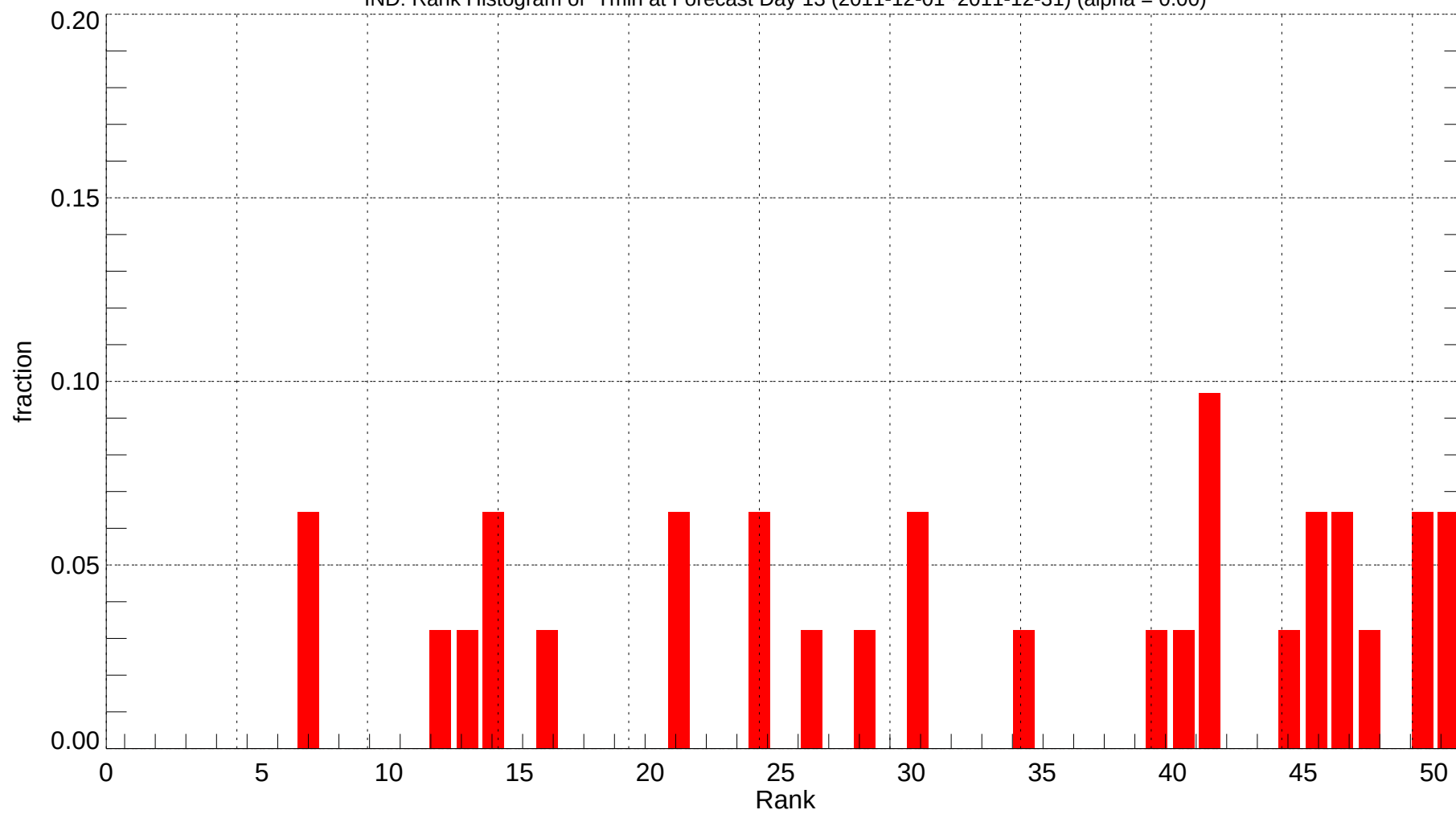
IND: Rank Histogram of Tmin at Forecast Day 13 (2011-12-01~2011-12-31) (alpha = 0.00)
