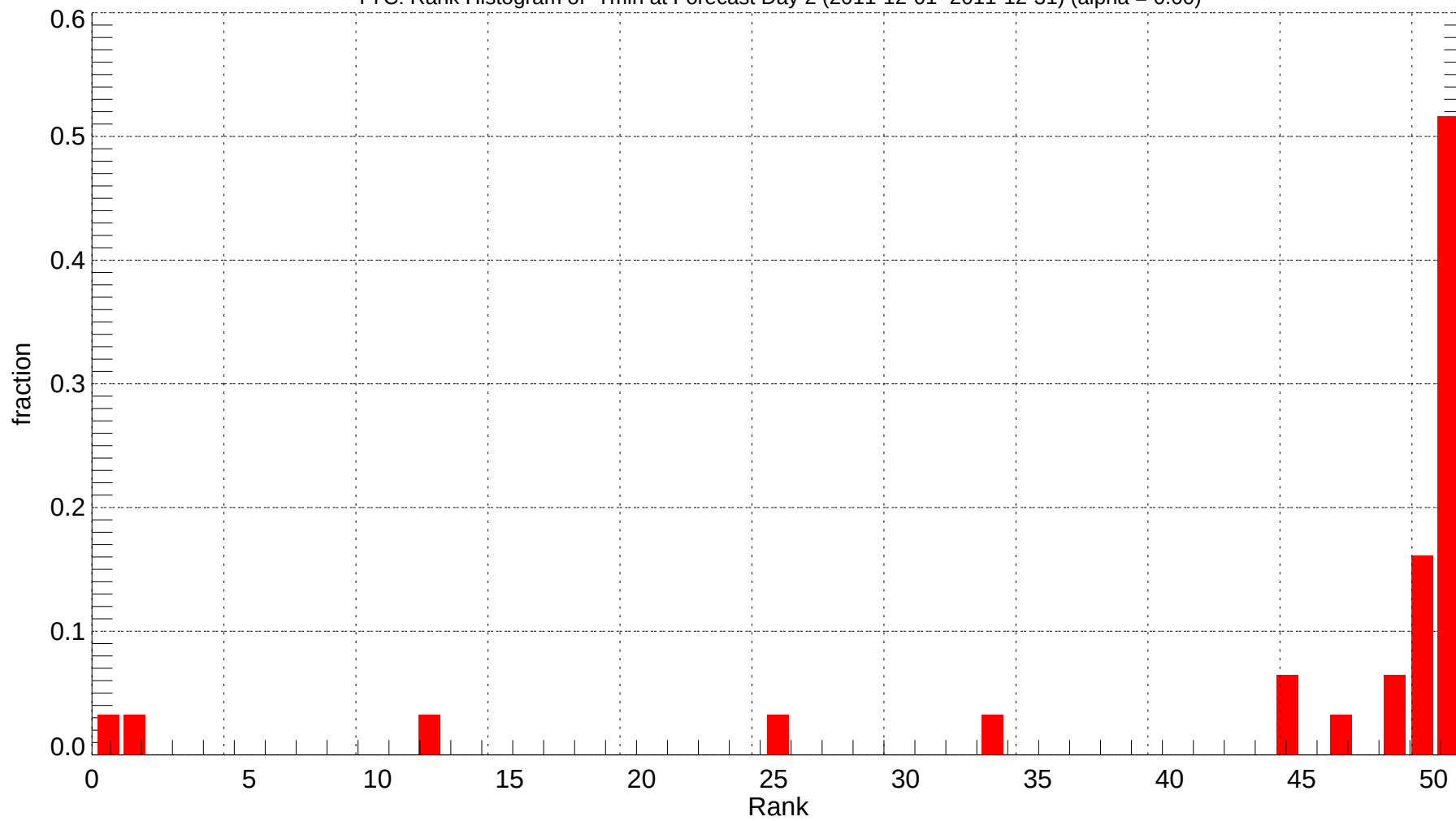
YYC: Rank Histogram of Tmin at Forecast Day 2 (2011-12-01~2011-12-31) (alpha = 0.00)
