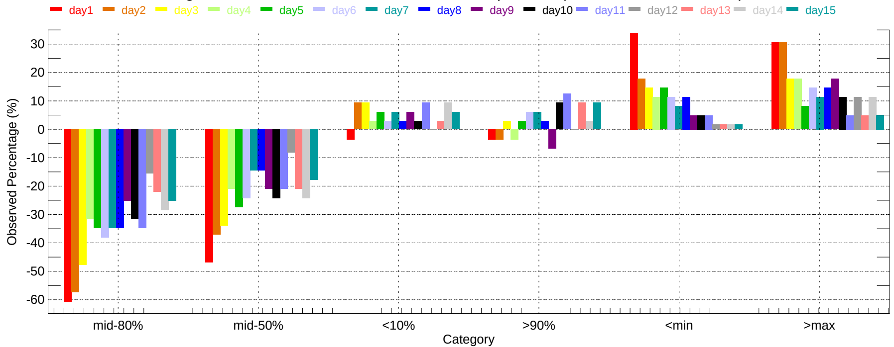
Observed Percentage Deviation of Ensembles - RAP: Max Temperature (2011-12-01~2011-12-31)
