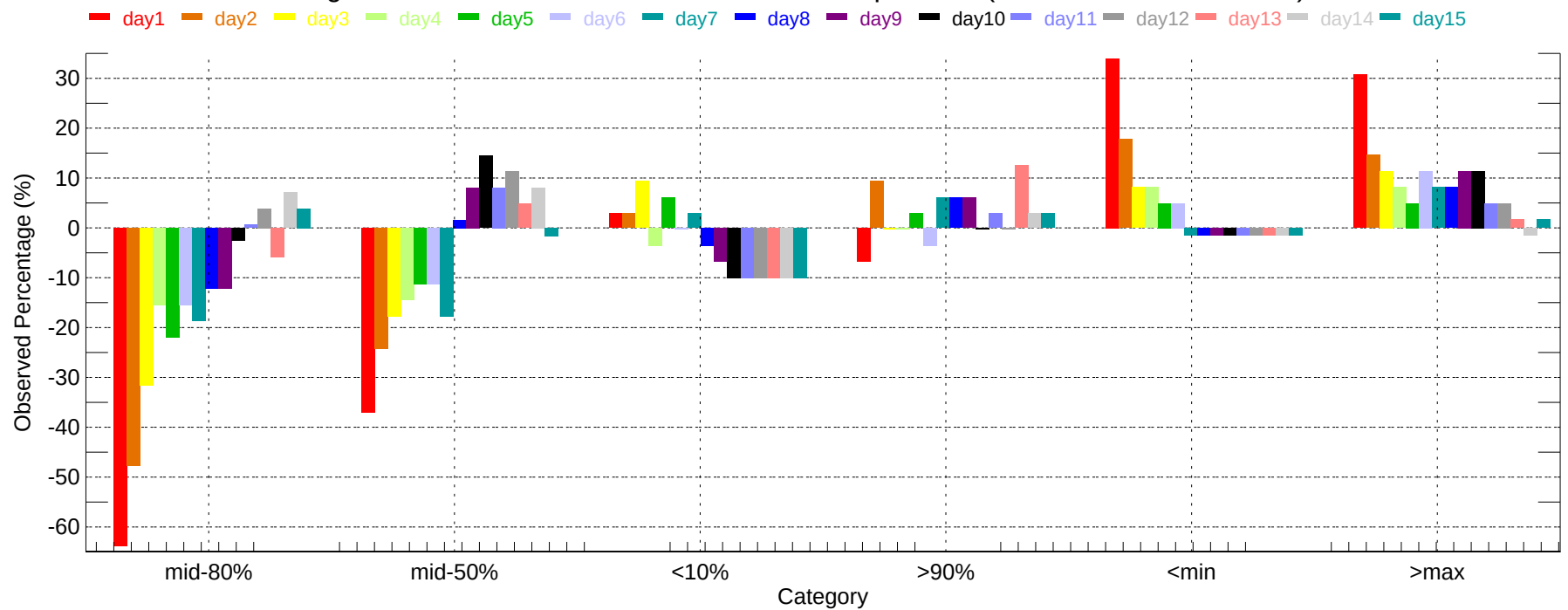
Observed Percentage Deviation of Ensembles - CHA: Max Temperature (2011-12-01~2011-12-31)
