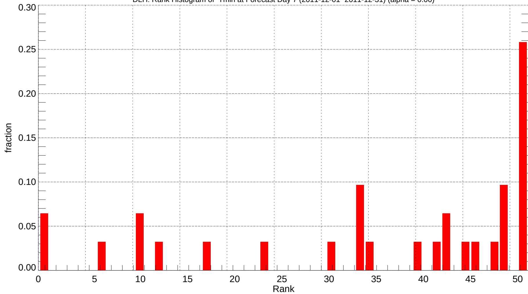
DLH: Rank Histogram of Tmin at Forecast Day 7 (2011-12-01~2011-12-31) (alpha = 0.00)
