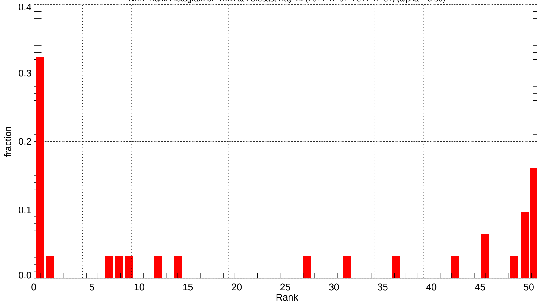
NKX: Rank Histogram of Tmin at Forecast Day 14 (2011-12-01~2011-12-31) (alpha = 0.00)
