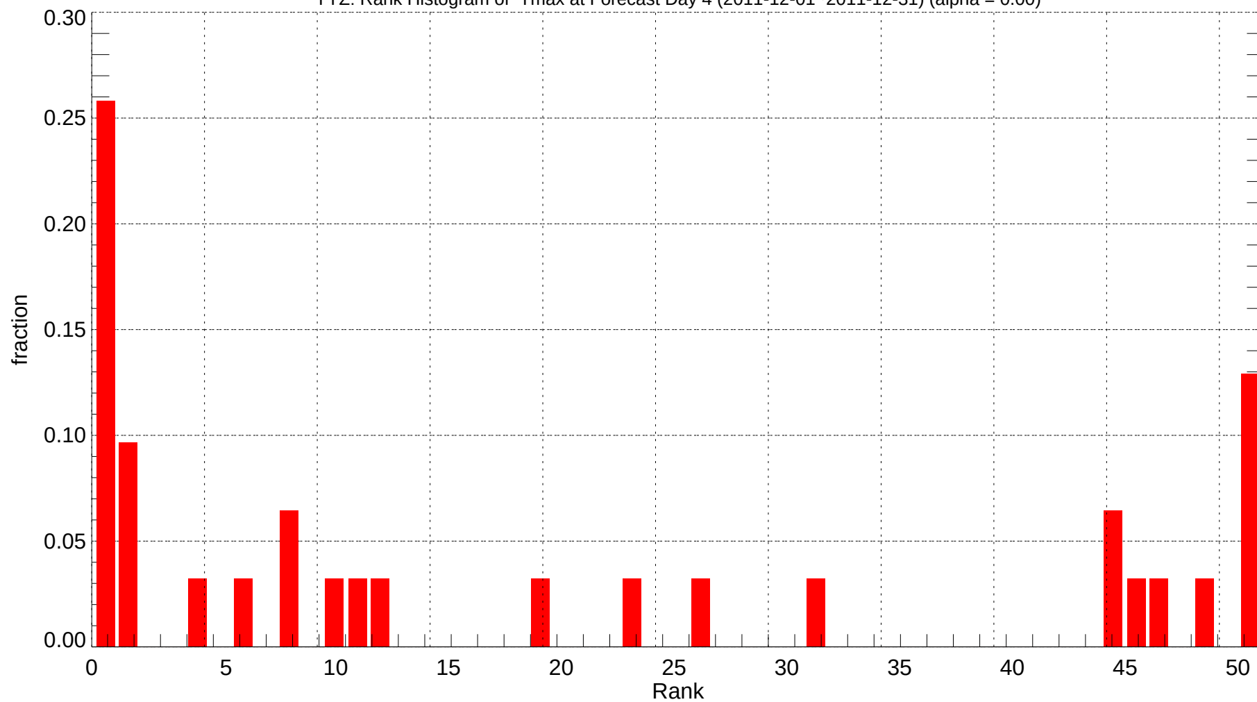
YYZ: Rank Histogram of Tmax at Forecast Day 4 (2011-12-01~2011-12-31) (alpha = 0.00)
