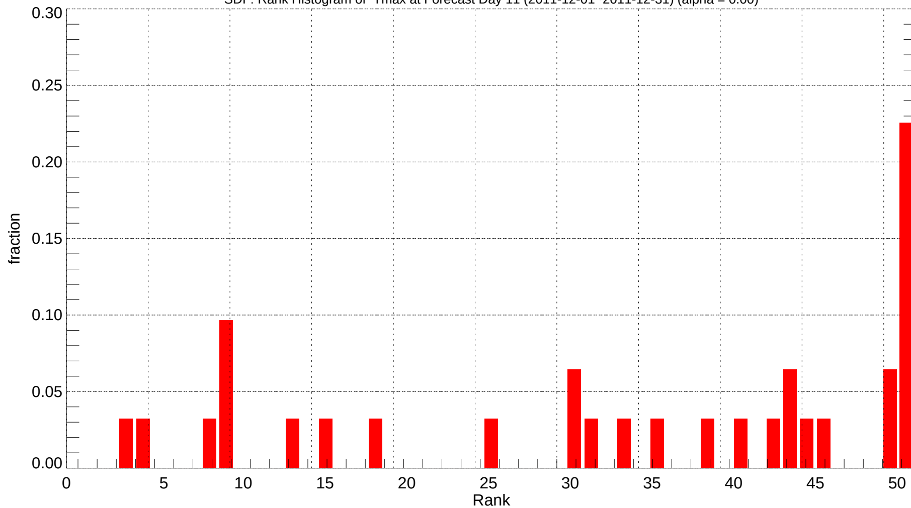
SDF: Rank Histogram of Tmax at Forecast Day 11 (2011-12-01~2011-12-31) (alpha = 0.00)
