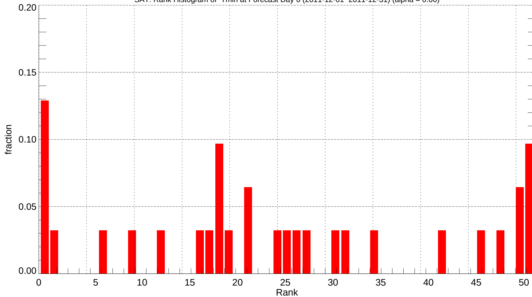
SAT: Rank Histogram of Tmin at Forecast Day 6 (2011-12-01~2011-12-31) (alpha = 0.00)
