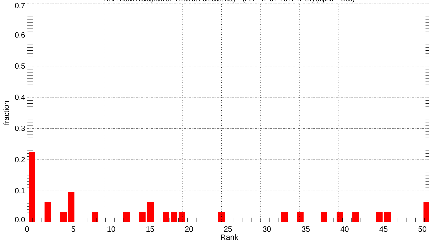
RAL: Rank Histogram of Tmax at Forecast Day 4 (2011-12-01~2011-12-31) (alpha = 0.00)
