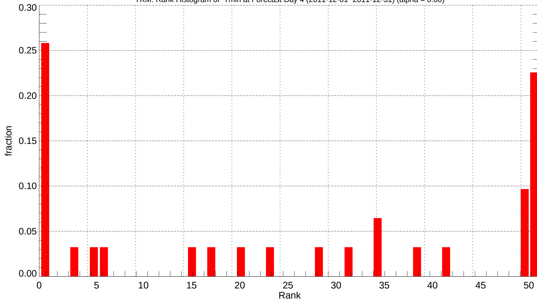
YKM: Rank Histogram of Tmin at Forecast Day 4 (2011-12-01~2011-12-31) (alpha = 0.00)
