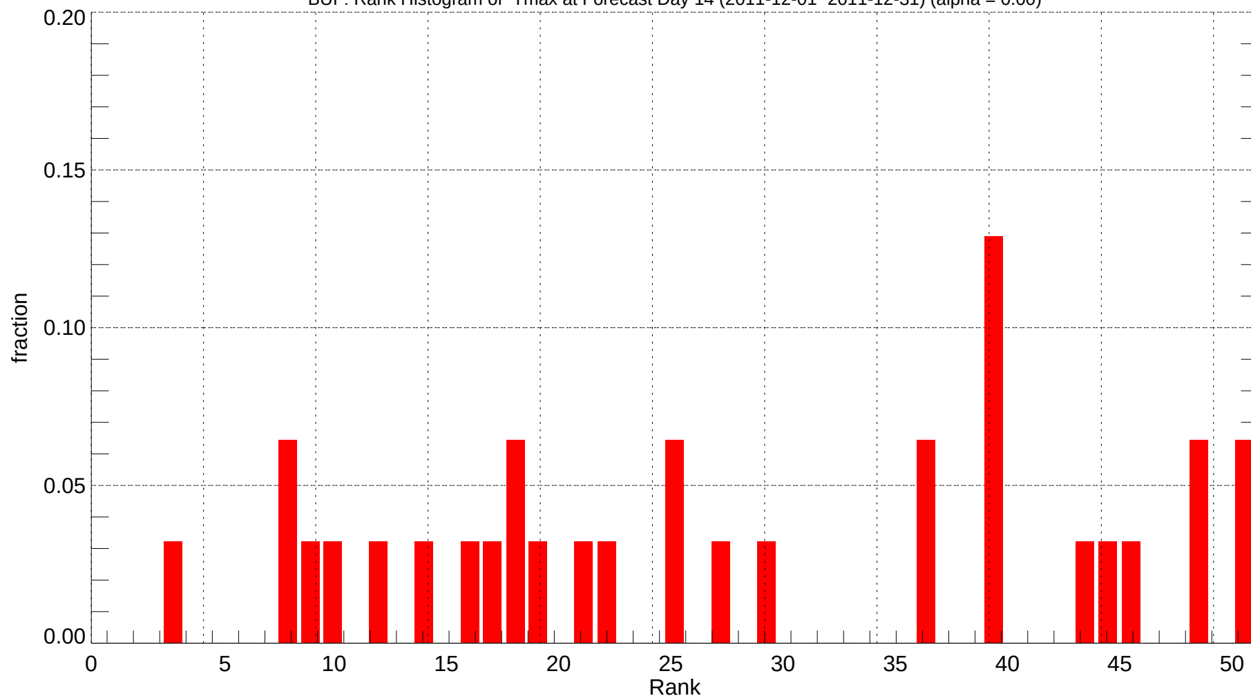
BUF: Rank Histogram of Tmax at Forecast Day 14 (2011-12-01~2011-12-31) (alpha = 0.00)
