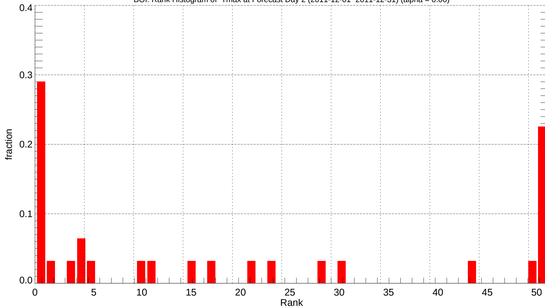
BOI: Rank Histogram of Tmax at Forecast Day 2 (2011-12-01~2011-12-31) (alpha = 0.00)
