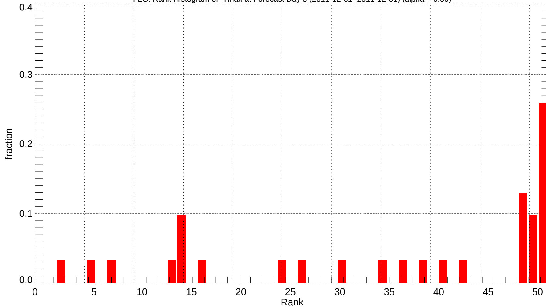
FLG: Rank Histogram of Tmax at Forecast Day 5 (2011-12-01~2011-12-31) (alpha = 0.00)
