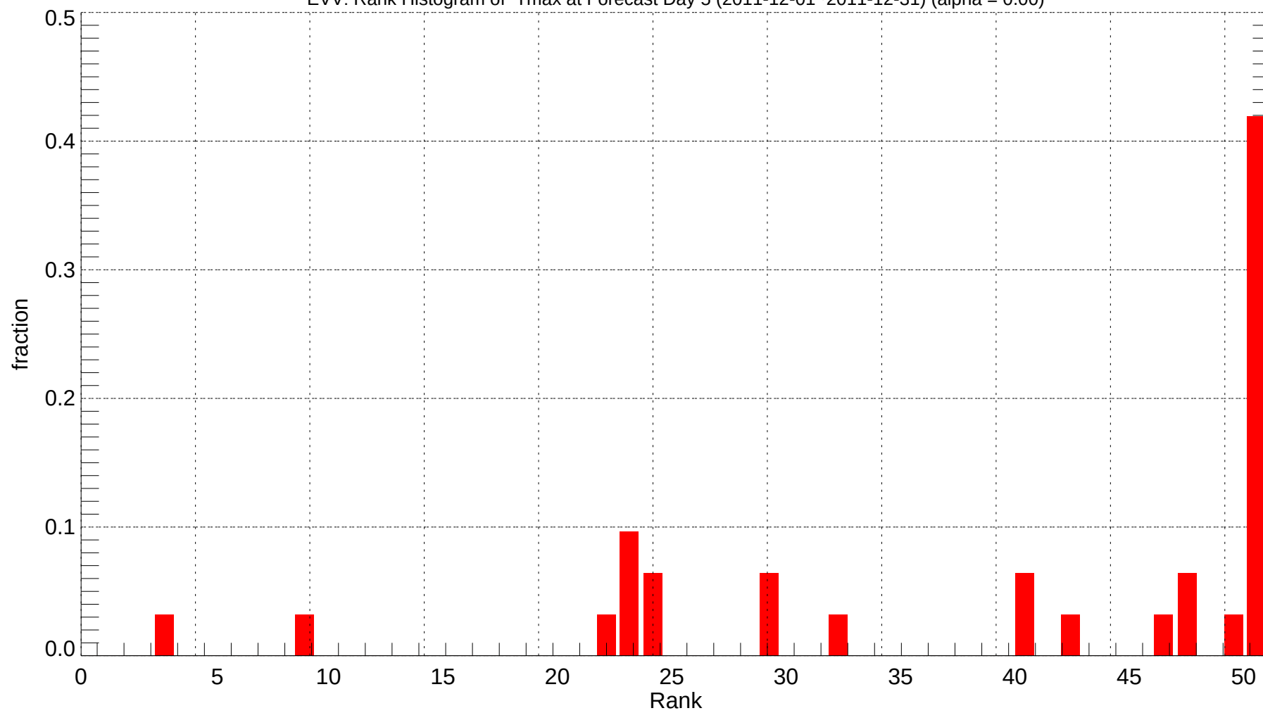
EVV: Rank Histogram of Tmax at Forecast Day 5 (2011-12-01~2011-12-31) (alpha = 0.00)
