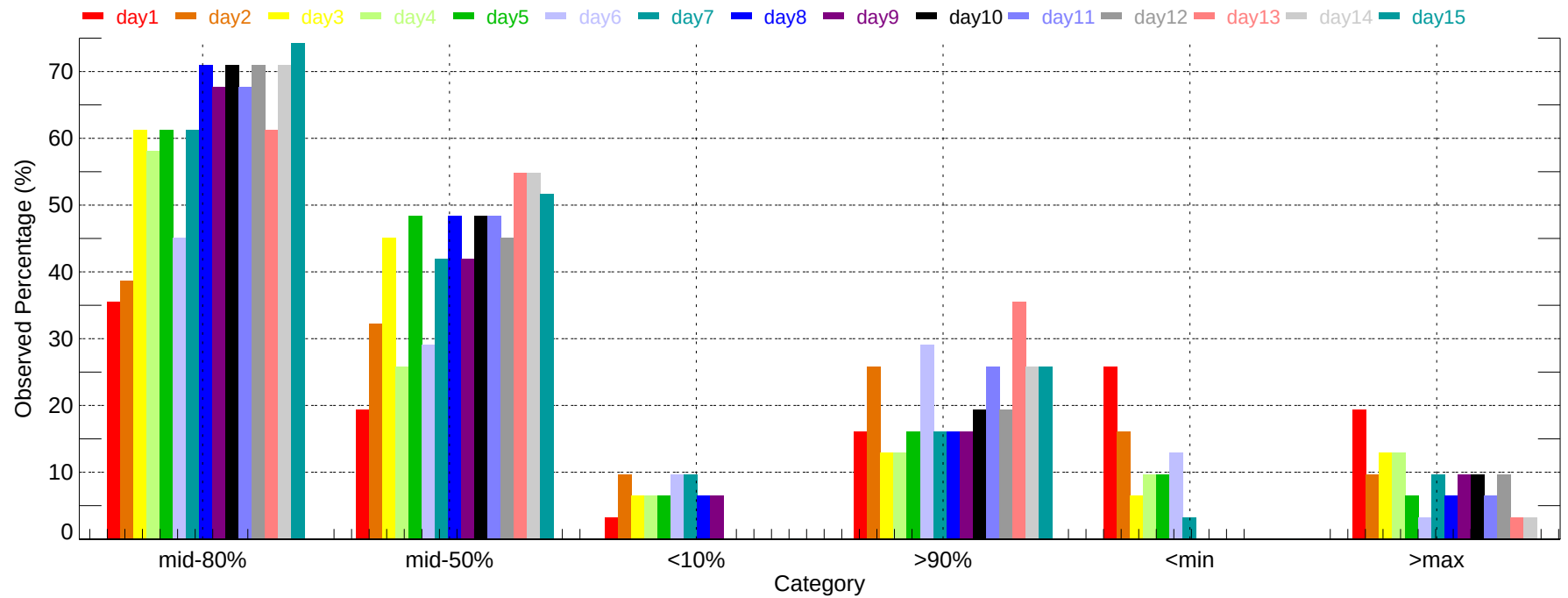
Observed Percentage of Ensembles - DEC: Min Temperature (2011-12-01~2011-12-31)
