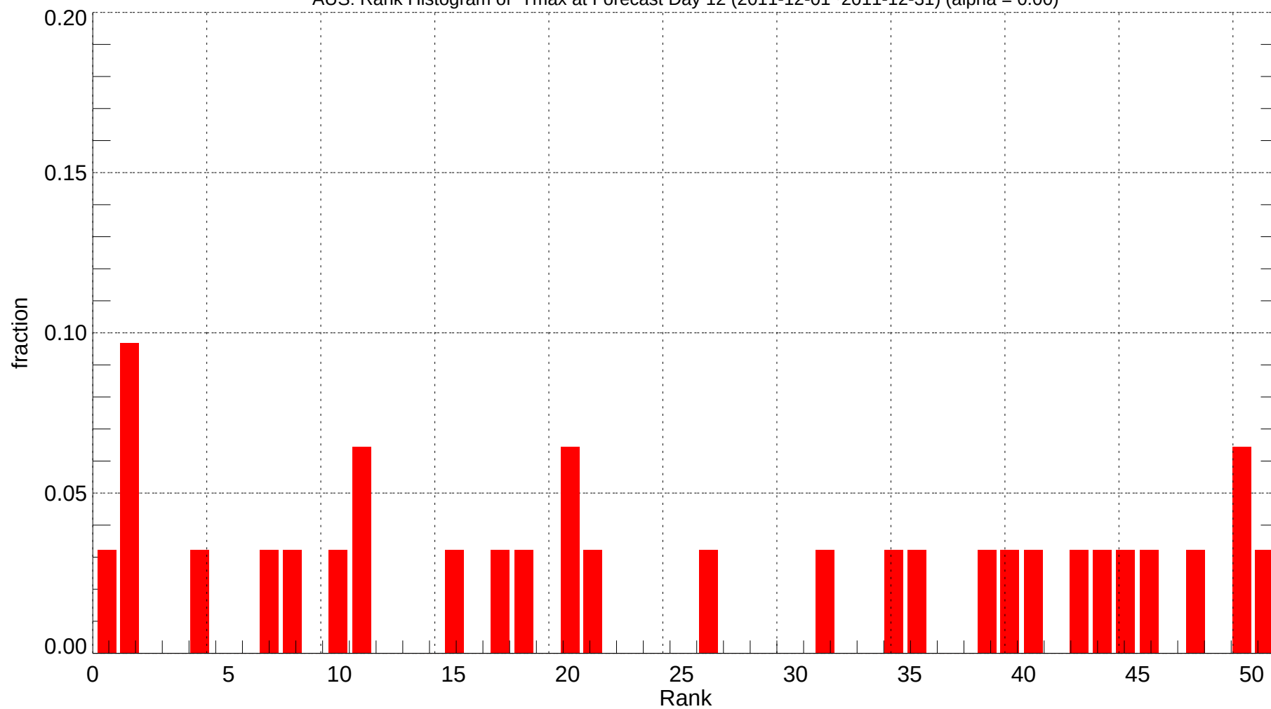
AUS: Rank Histogram of Tmax at Forecast Day 12 (2011-12-01~2011-12-31) (alpha = 0.00)
