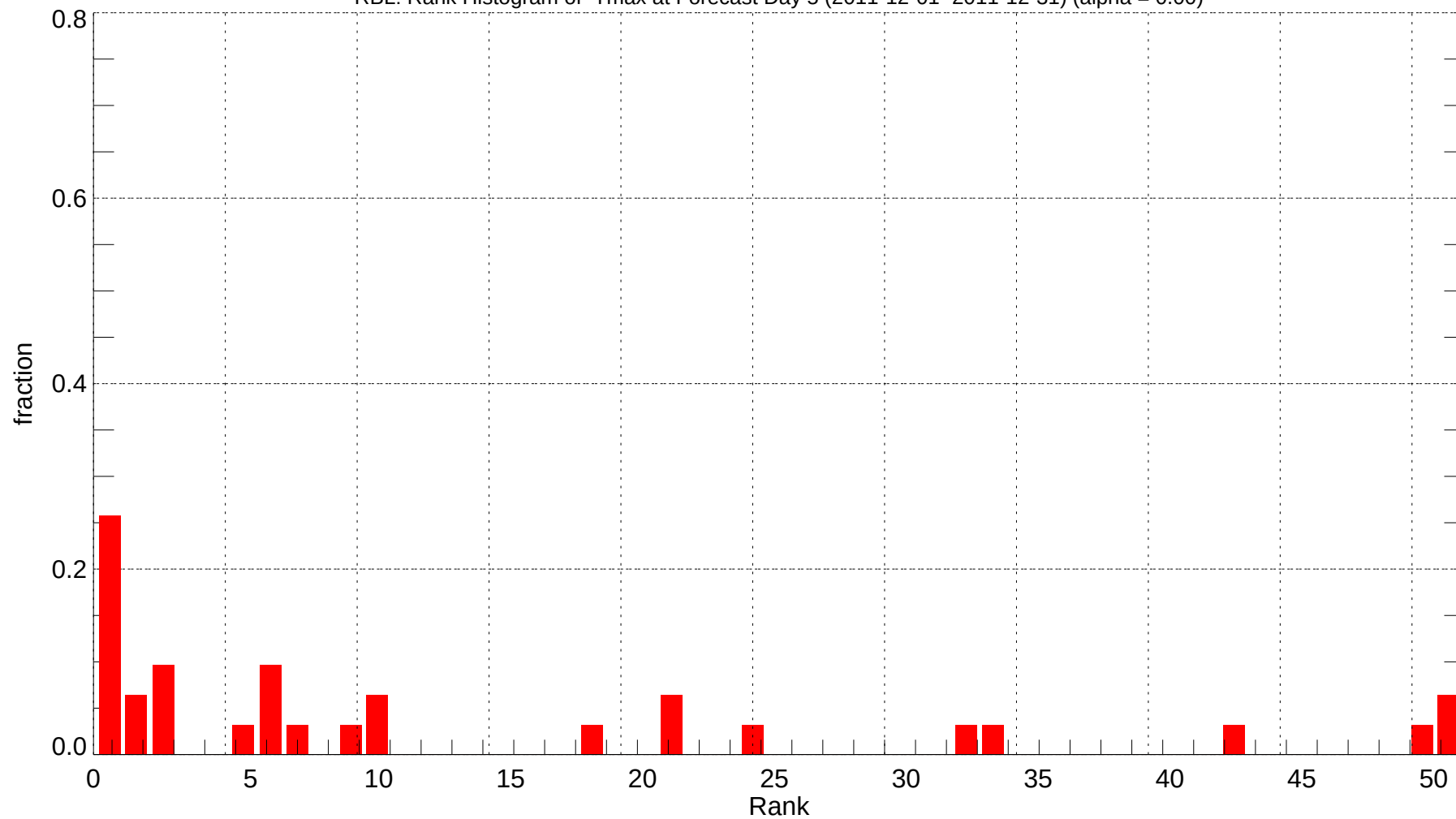
RBL: Rank Histogram of Tmax at Forecast Day 5 (2011-12-01~2011-12-31) (alpha = 0.00)
