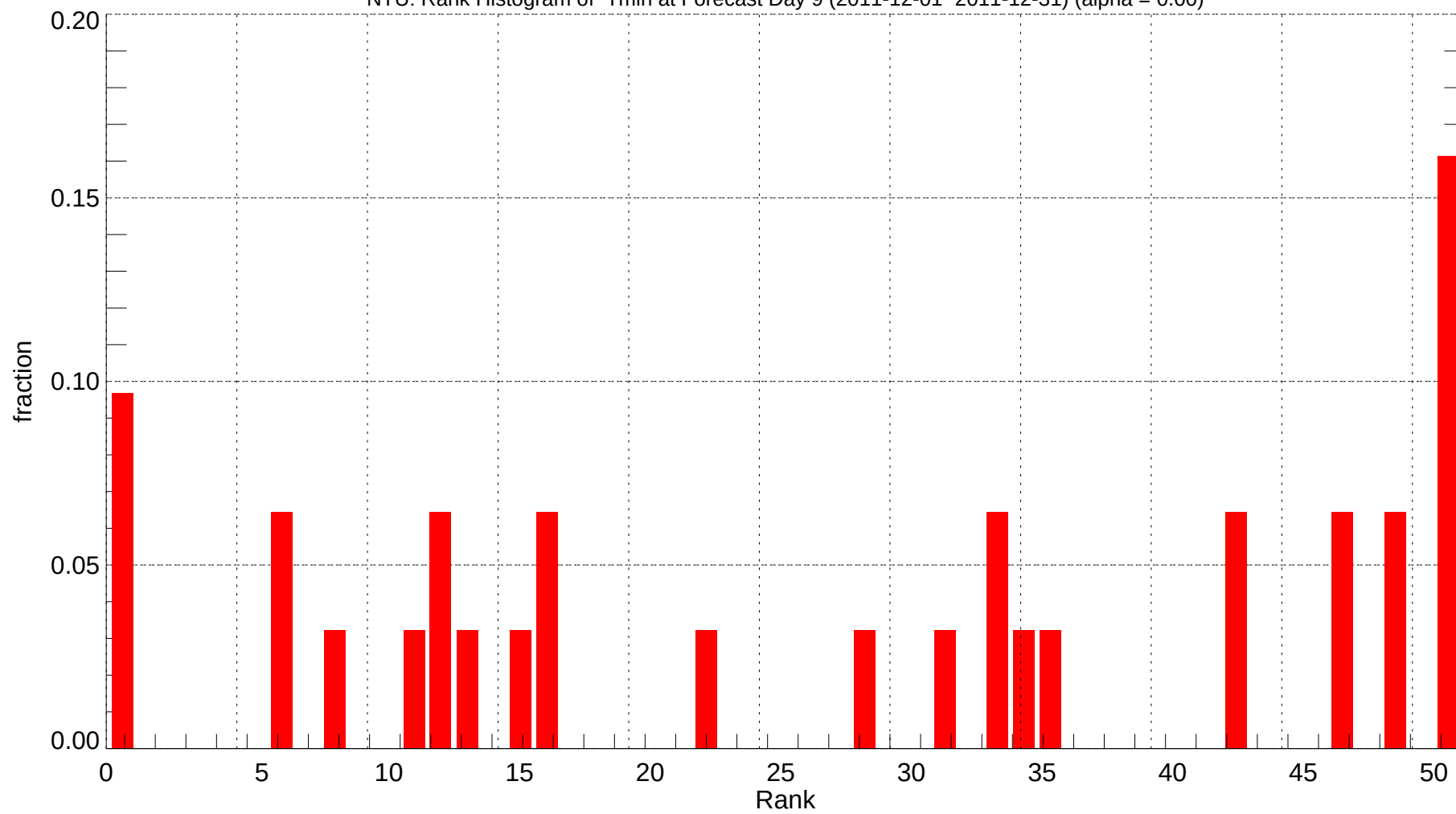
NTU: Rank Histogram of Tmin at Forecast Day 9 (2011-12-01~2011-12-31) (alpha = 0.00)
