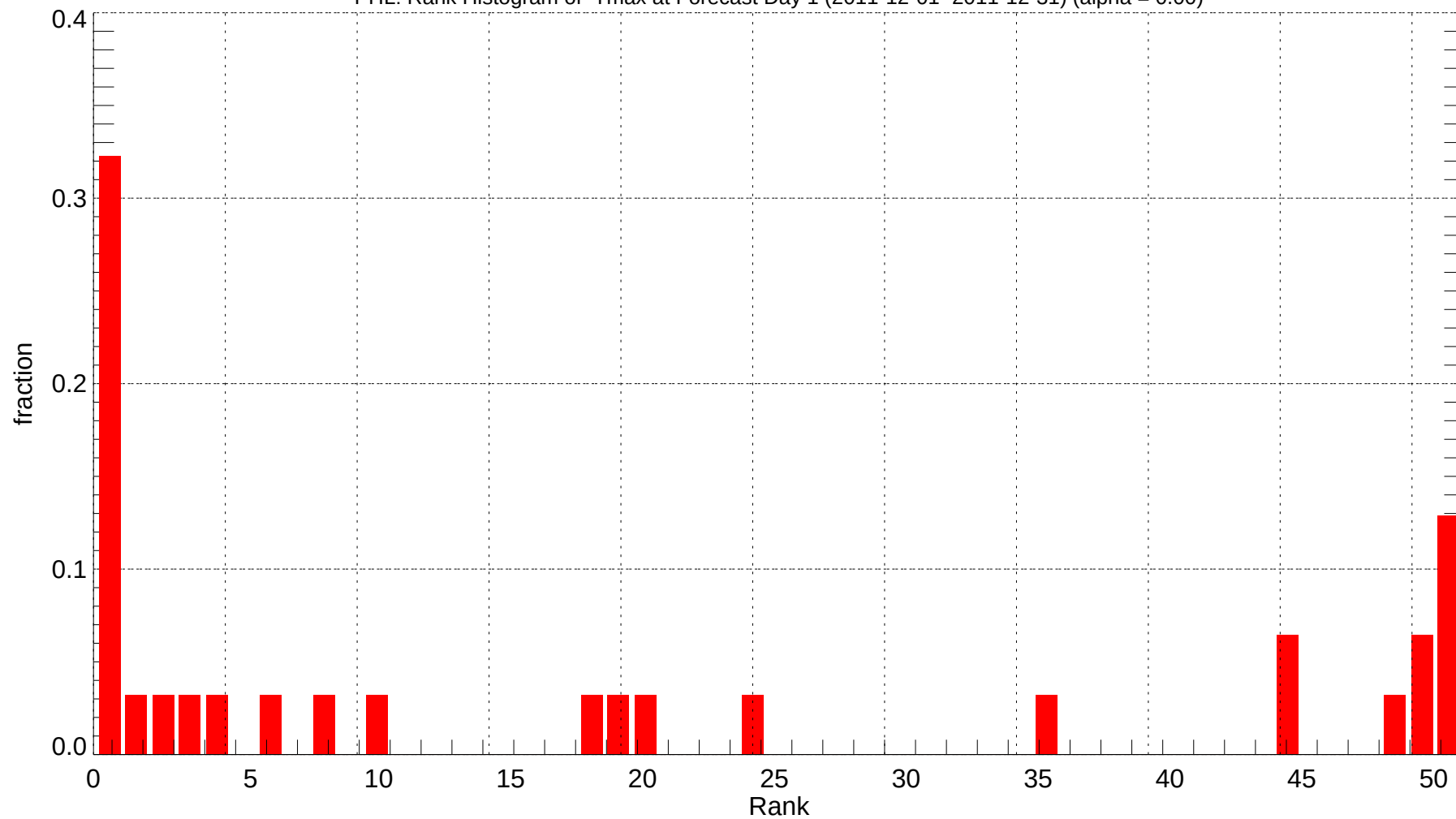
PHL: Rank Histogram of Tmax at Forecast Day 1 (2011-12-01~2011-12-31) (alpha = 0.00)
