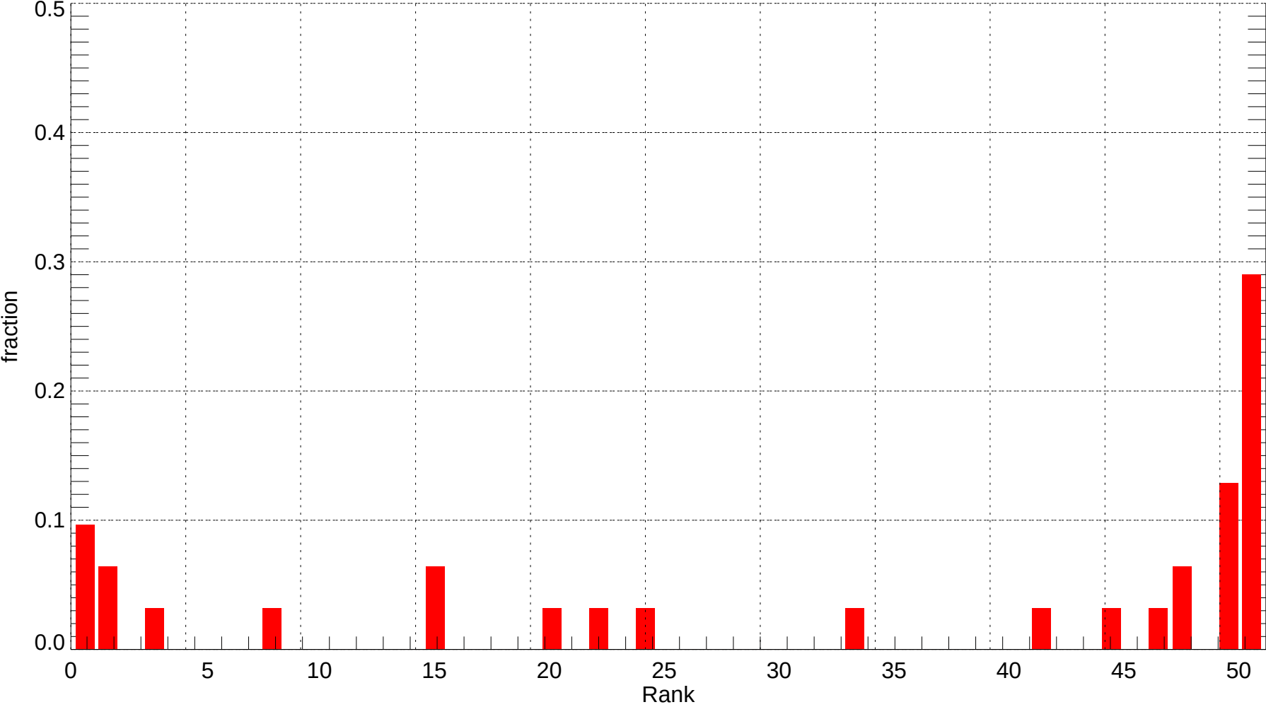
ELP: Rank Histogram of Tmin at Forecast Day 2 (2011-12-01~2011-12-31) (alpha = 0.00)
