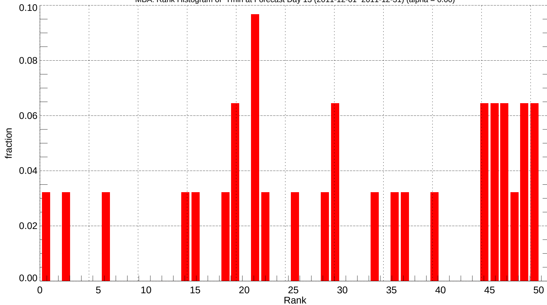
MBA: Rank Histogram of Tmin at Forecast Day 13 (2011-12-01~2011-12-31) (alpha = 0.00)
