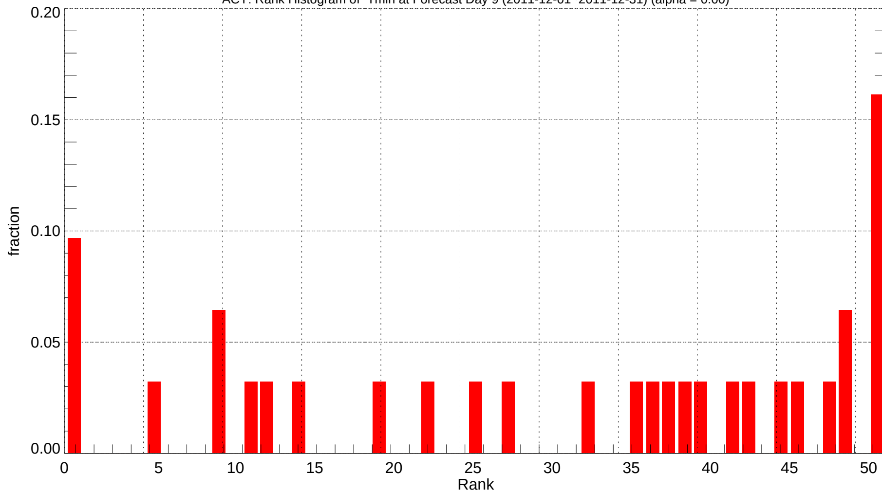
ACY: Rank Histogram of Tmin at Forecast Day 9 (2011-12-01~2011-12-31) (alpha = 0.00)
