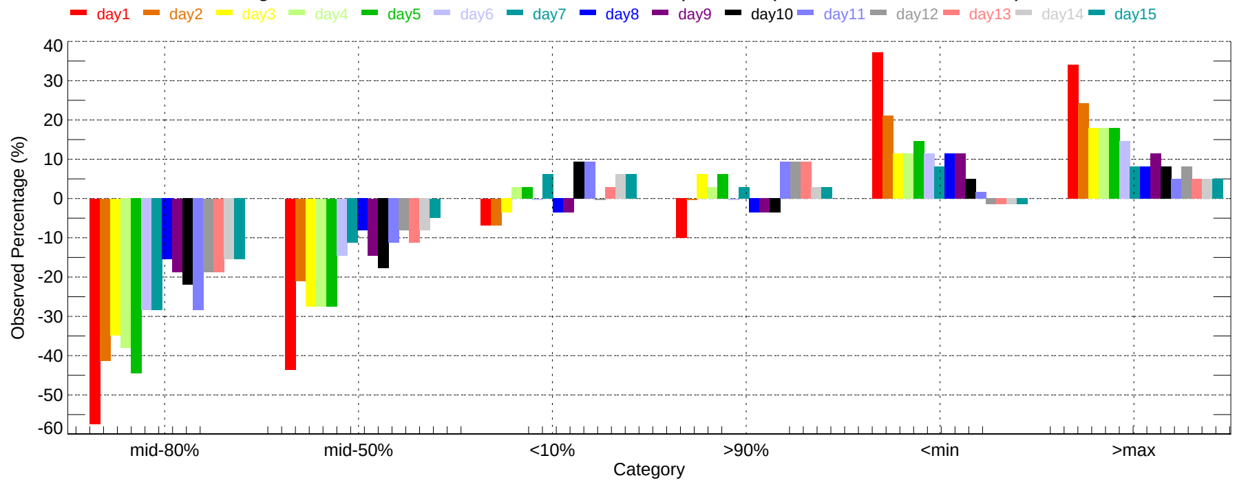
Observed Percentage Deviation of Ensembles - ABE: Min Temperature (2011-12-01~2011-12-31)
