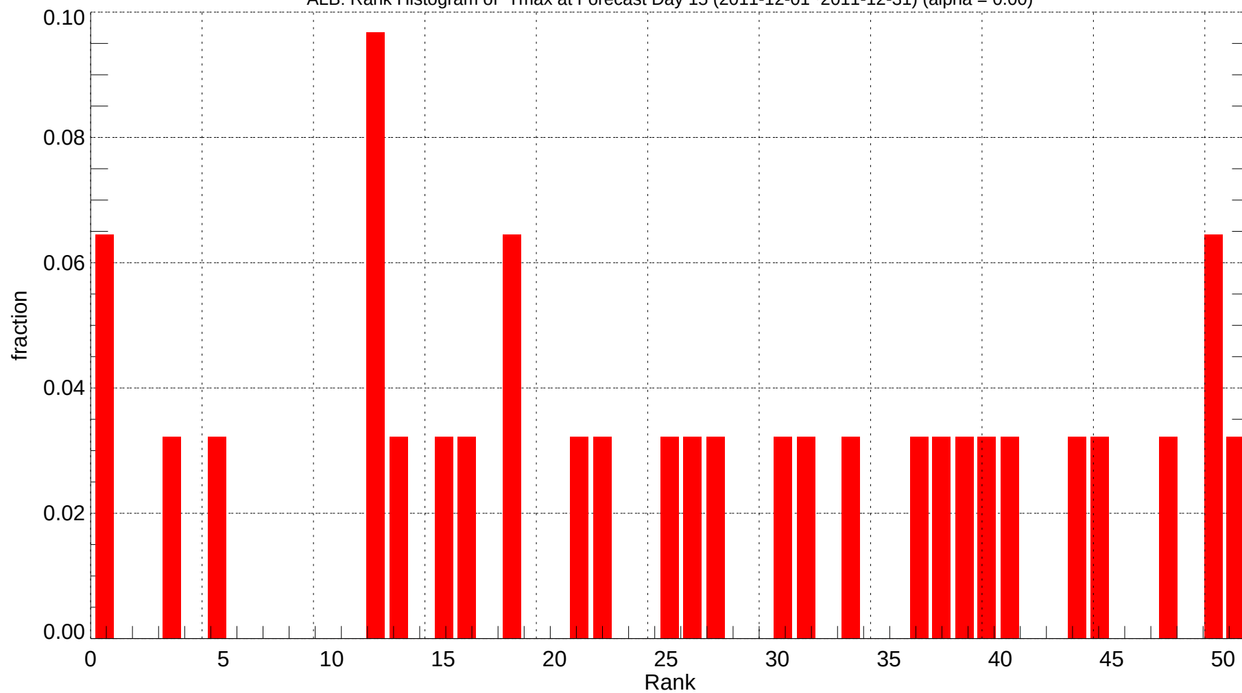
ALB: Rank Histogram of Tmax at Forecast Day 15 (2011-12-01~2011-12-31) (alpha = 0.00)
