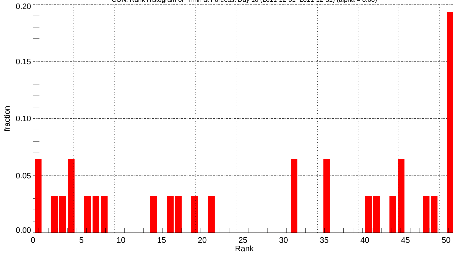
CON: Rank Histogram of Tmin at Forecast Day 10 (2011-12-01~2011-12-31) (alpha = 0.00)
