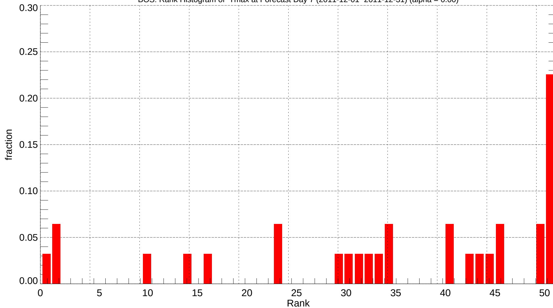
BOS: Rank Histogram of Tmax at Forecast Day 7 (2011-12-01~2011-12-31) (alpha = 0.00)
