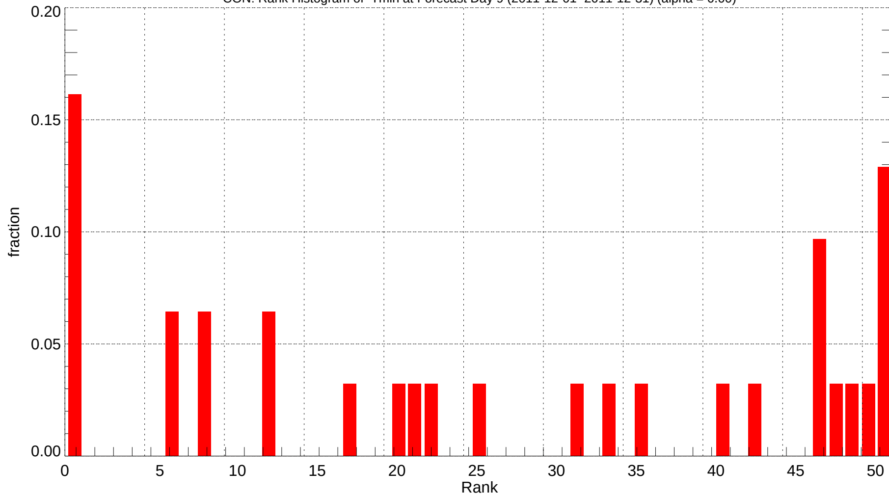
CON: Rank Histogram of Tmin at Forecast Day 9 (2011-12-01~2011-12-31) (alpha = 0.00)
