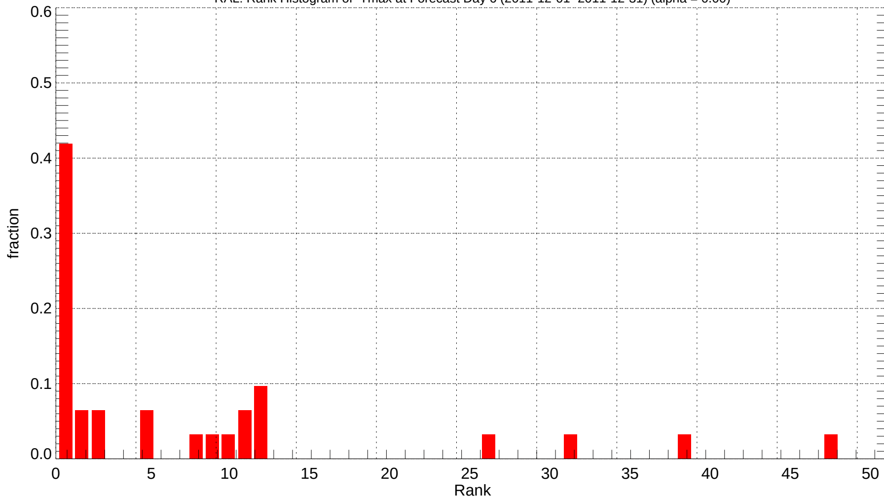
RAL: Rank Histogram of Tmax at Forecast Day 6 (2011-12-01~2011-12-31) (alpha = 0.00)
