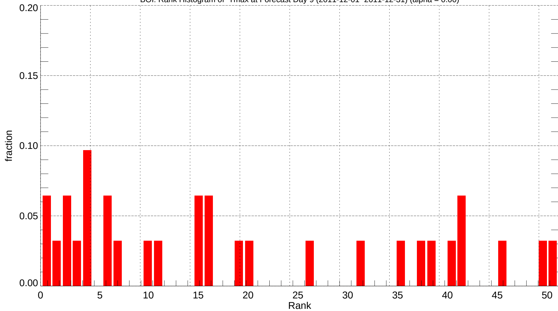
BOI: Rank Histogram of Tmax at Forecast Day 9 (2011-12-01~2011-12-31) (alpha = 0.00)
