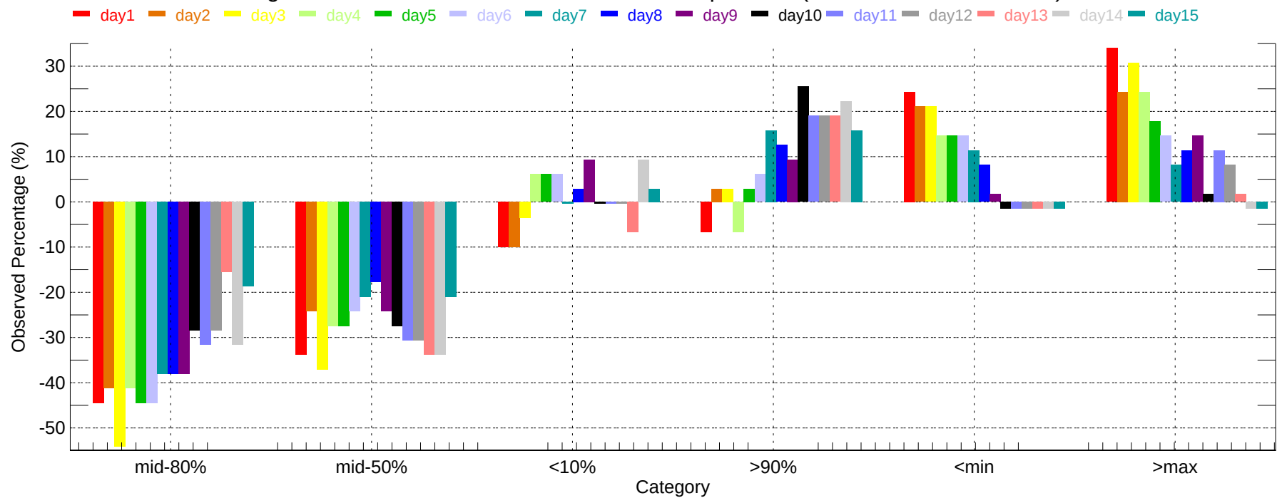
Observed Percentage Deviation of Ensembles - YNG: Min Temperature (2011-12-01~2011-12-31)
