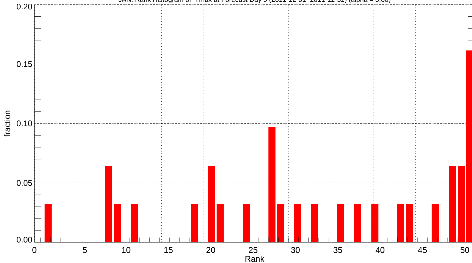
JAN: Rank Histogram of Tmax at Forecast Day 9 (2011-12-01~2011-12-31) (alpha = 0.00)
