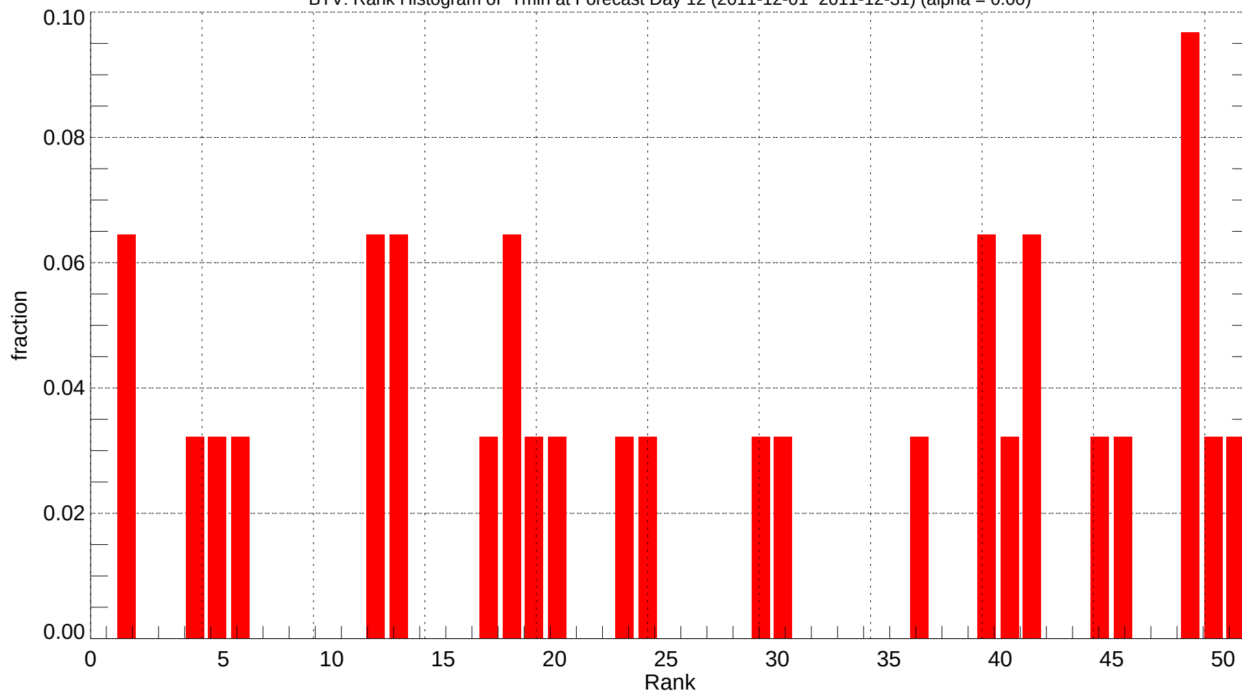
BTV: Rank Histogram of Tmin at Forecast Day 12 (2011-12-01~2011-12-31) (alpha = 0.00)
