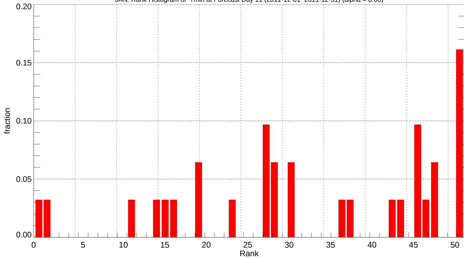
JAN: Rank Histogram of Tmin at Forecast Day 11 (2011-12-01~2011-12-31) (alpha = 0.00)
