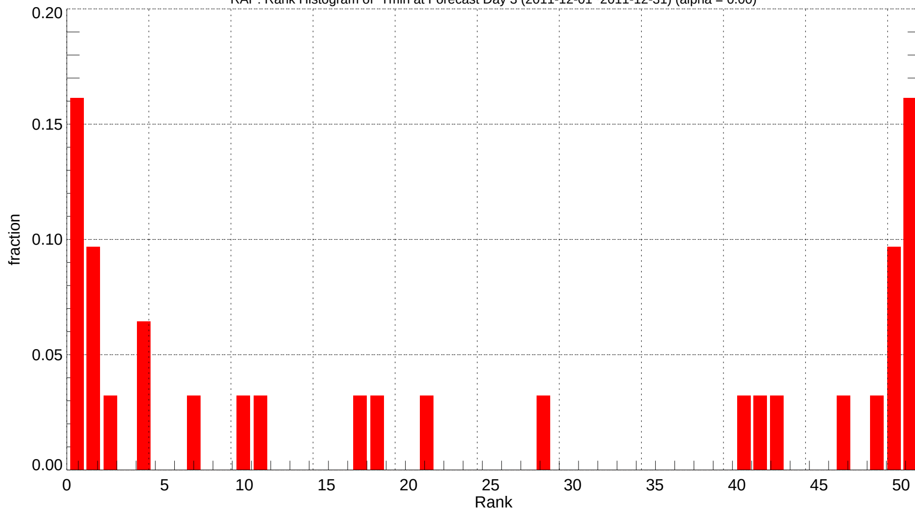
RAP: Rank Histogram of Tmin at Forecast Day 3 (2011-12-01~2011-12-31) (alpha = 0.00)
