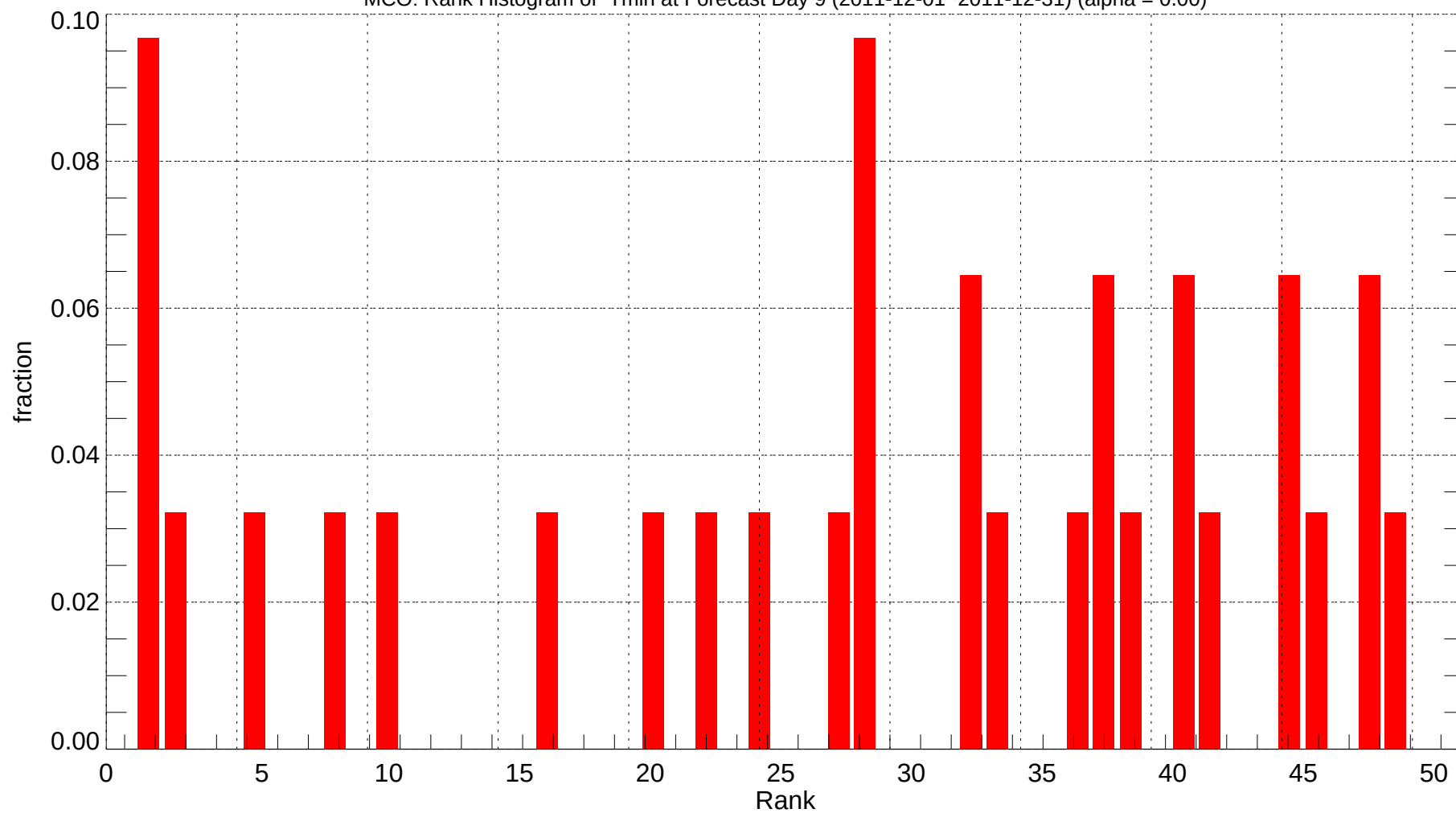
MCO: Rank Histogram of Tmin at Forecast Day 9 (2011-12-01~2011-12-31) (alpha = 0.00)
