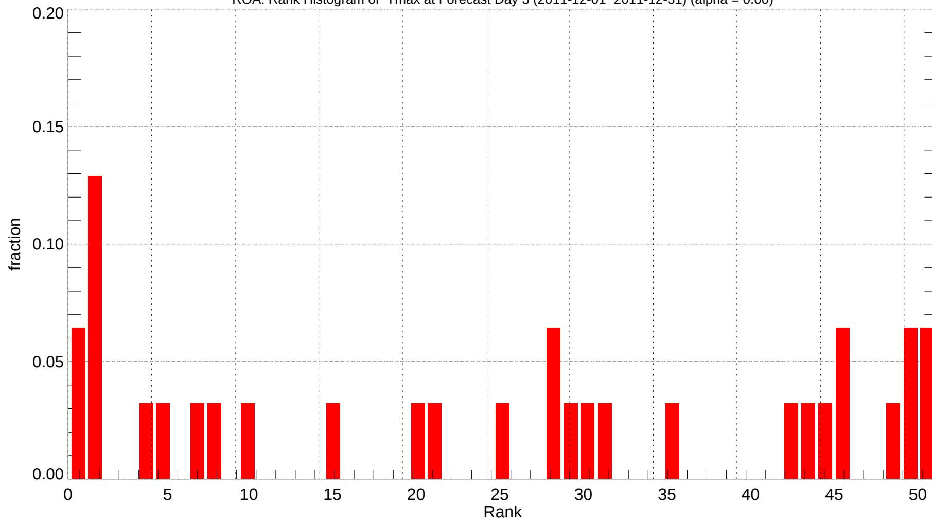
ROA: Rank Histogram of Tmax at Forecast Day 3 (2011-12-01~2011-12-31) (alpha = 0.00)
