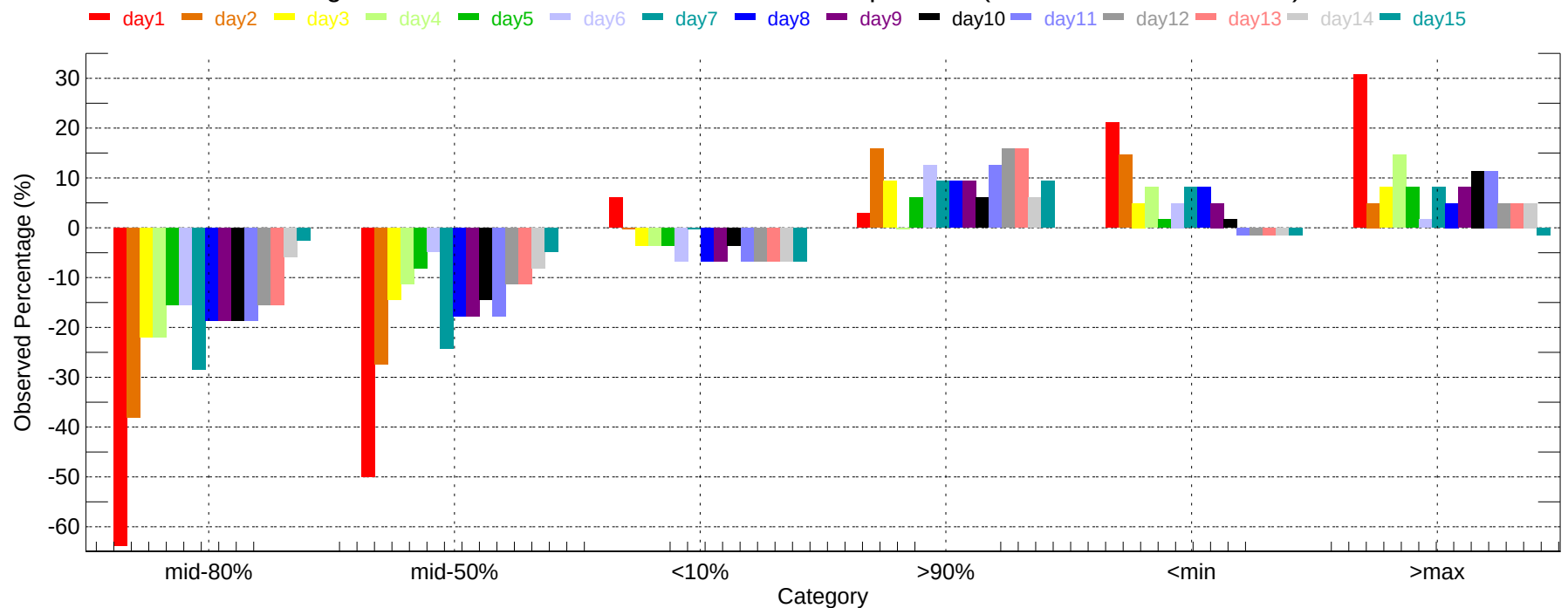
Observed Percentage Deviation of Ensembles - LNS: Max Temperature (2011-12-01~2011-12-31)
