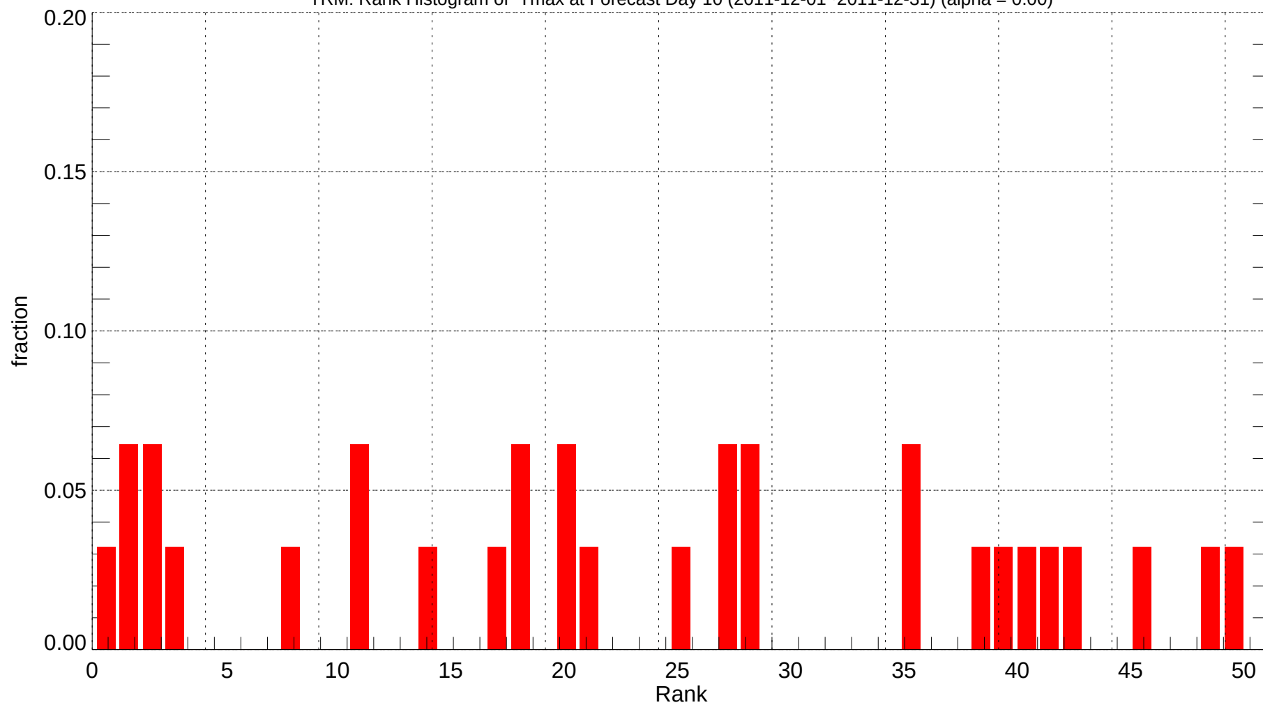
TRM: Rank Histogram of Tmax at Forecast Day 10 (2011-12-01~2011-12-31) (alpha = 0.00)
