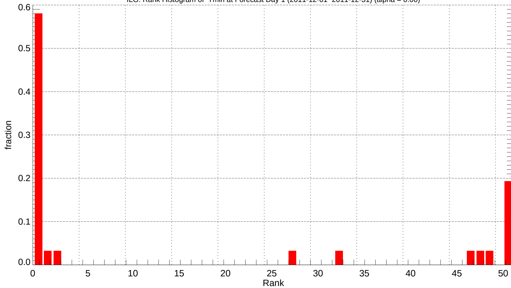
ILG: Rank Histogram of Tmin at Forecast Day 1 (2011-12-01~2011-12-31) (alpha = 0.00)
