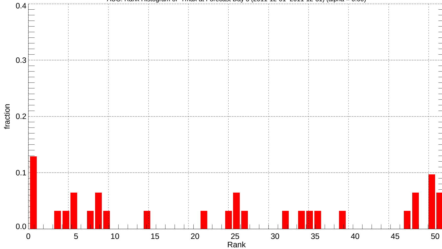
AUG: Rank Histogram of Tmax at Forecast Day 3 (2011-12-01~2011-12-31) (alpha = 0.00)
