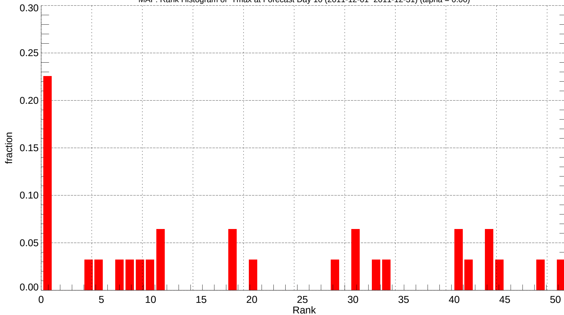
MAF: Rank Histogram of Tmax at Forecast Day 10 (2011-12-01~2011-12-31) (alpha = 0.00)
