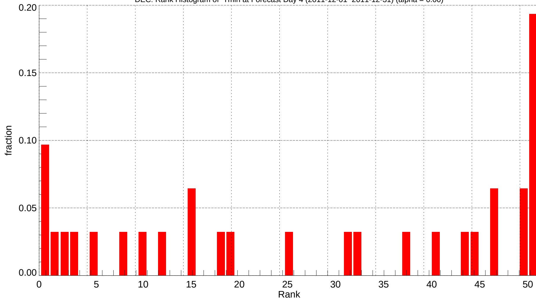
DEC: Rank Histogram of Tmin at Forecast Day 4 (2011-12-01~2011-12-31) (alpha = 0.00)
