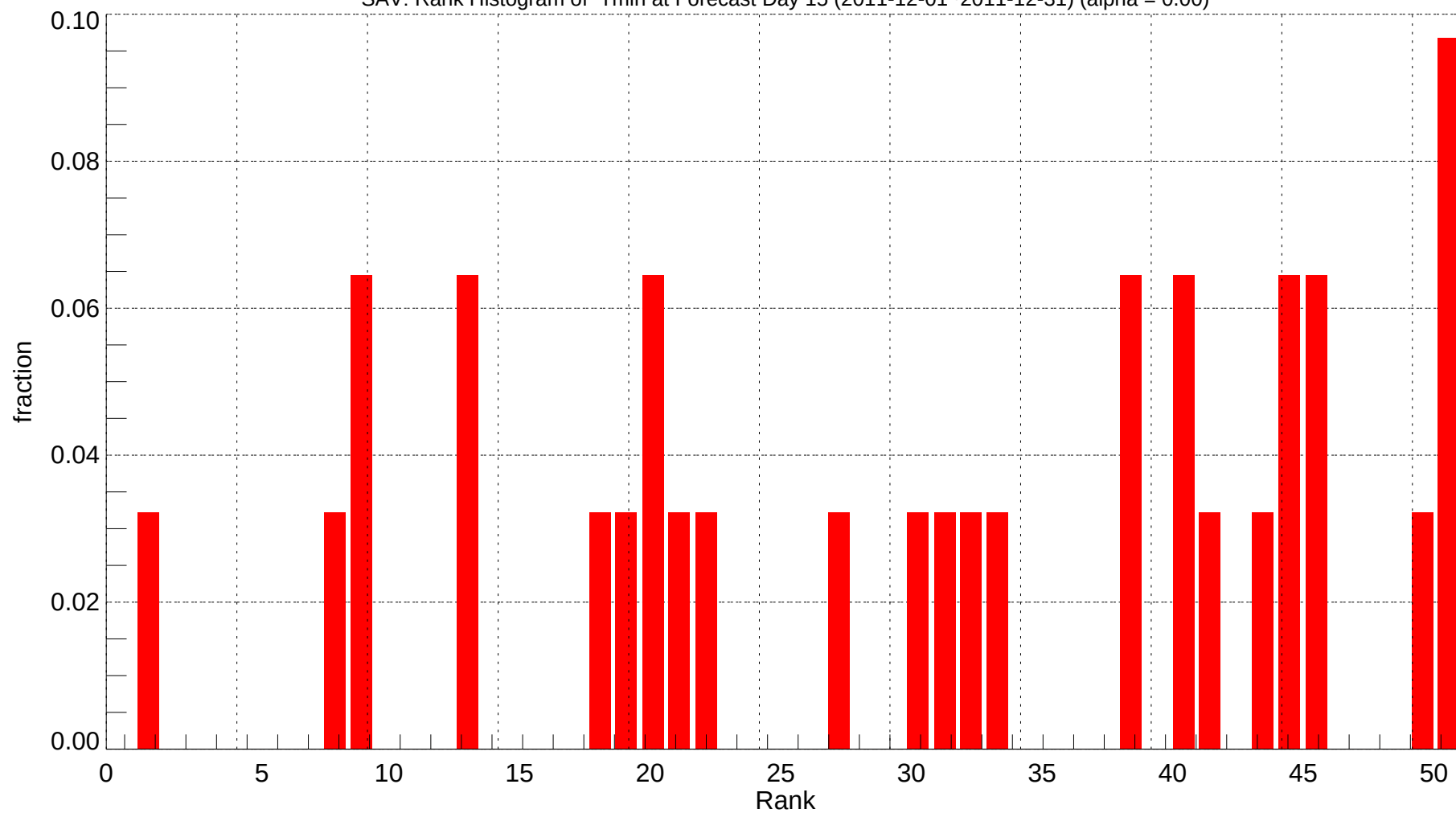
SAV: Rank Histogram of Tmin at Forecast Day 15 (2011-12-01~2011-12-31) (alpha = 0.00)
