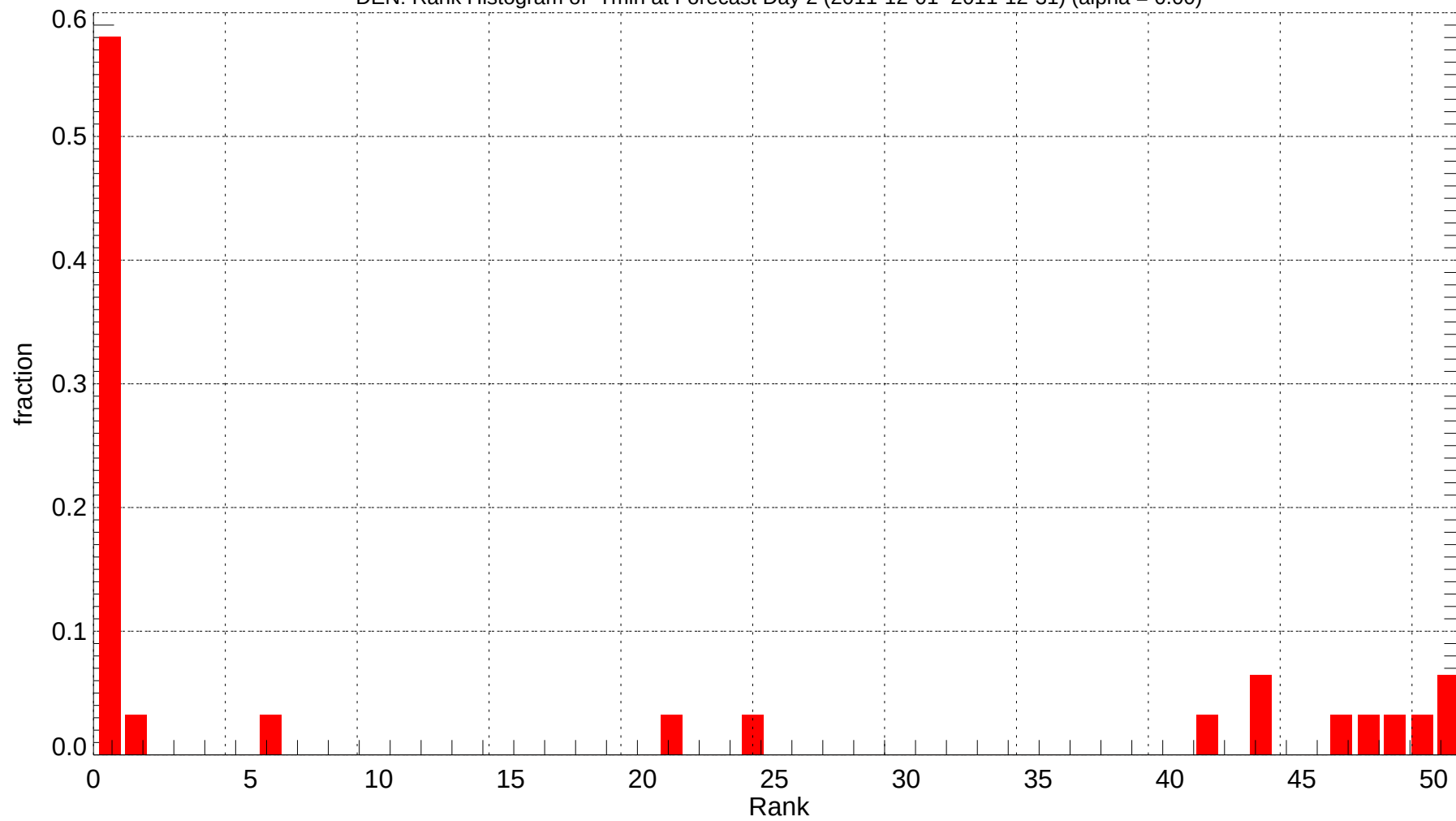
DEN: Rank Histogram of Tmin at Forecast Day 2 (2011-12-01~2011-12-31) (alpha = 0.00)
