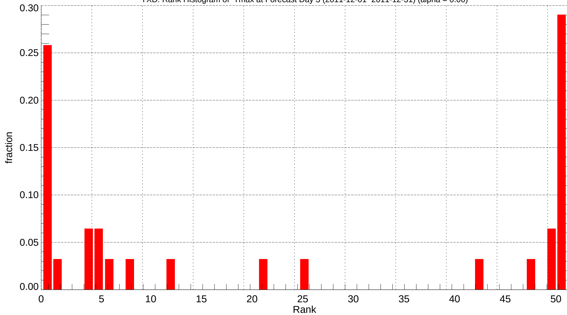
YXD: Rank Histogram of Tmax at Forecast Day 3 (2011-12-01~2011-12-31) (alpha = 0.00)
