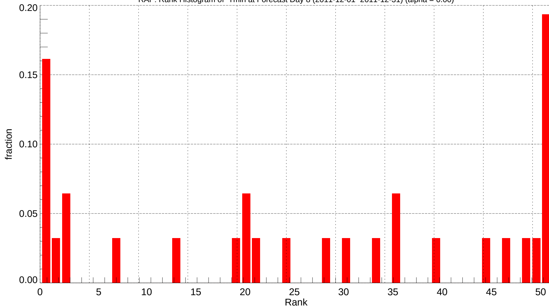
RAP: Rank Histogram of Tmin at Forecast Day 8 (2011-12-01~2011-12-31) (alpha = 0.00)
