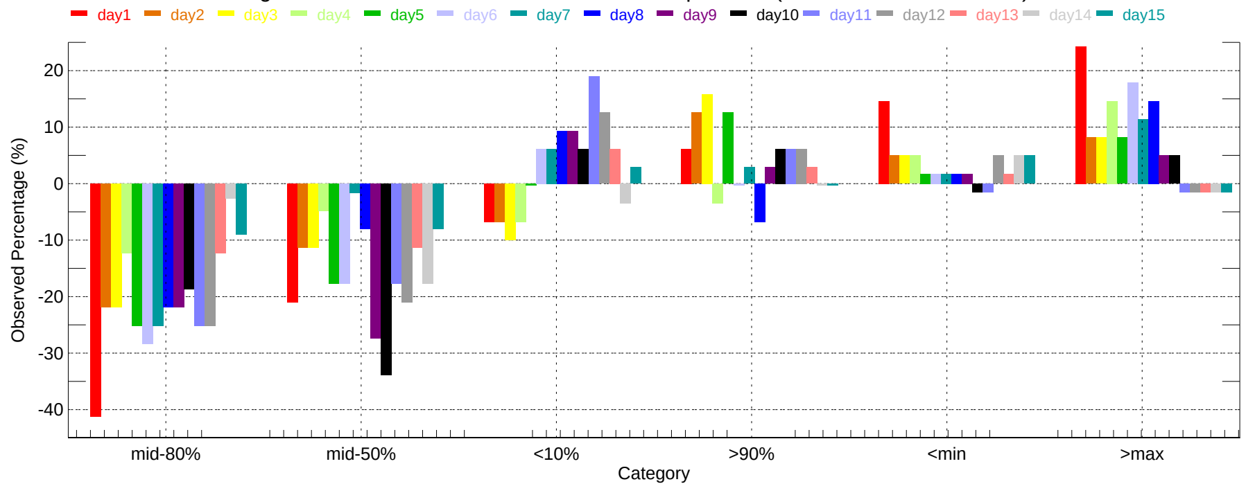
Observed Percentage Deviation of Ensembles - TUS: Min Temperature (2011-12-01~2011-12-31)
