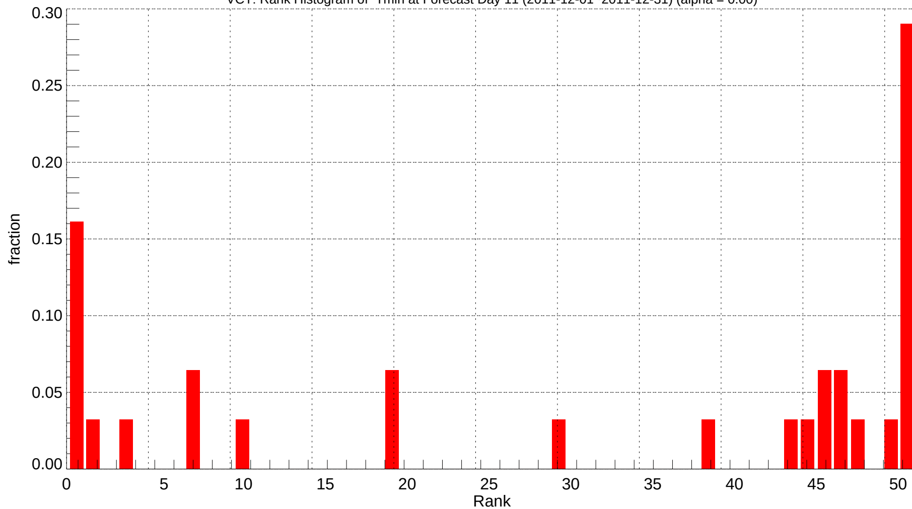
VCT: Rank Histogram of Tmin at Forecast Day 11 (2011-12-01~2011-12-31) (alpha = 0.00)
