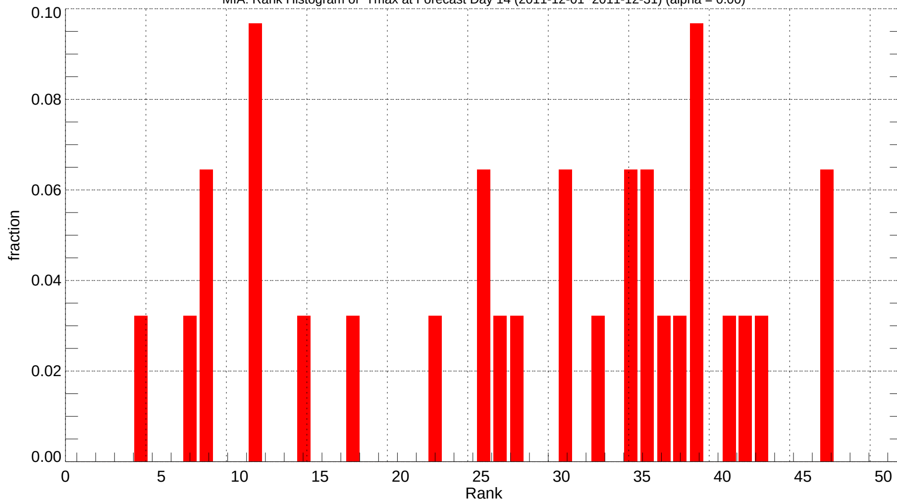
MIA: Rank Histogram of Tmax at Forecast Day 14 (2011-12-01~2011-12-31) (alpha = 0.00)
