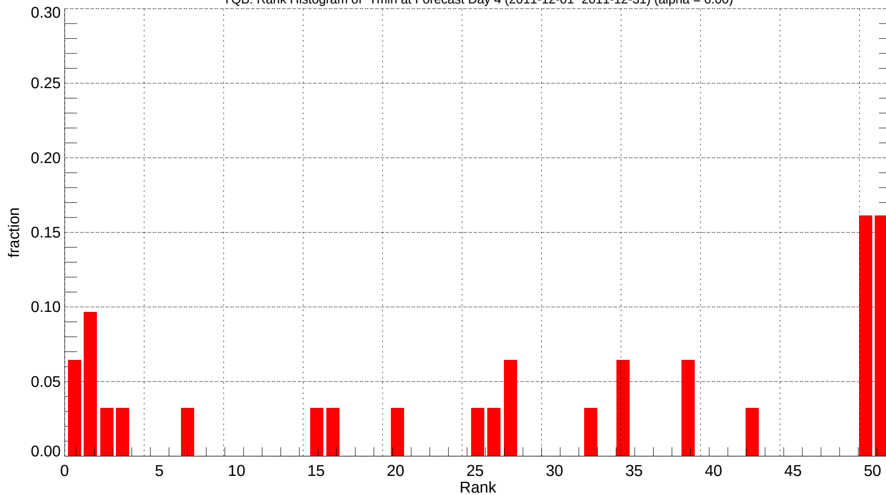
YQB: Rank Histogram of Tmin at Forecast Day 4 (2011-12-01~2011-12-31) (alpha = 0.00)
