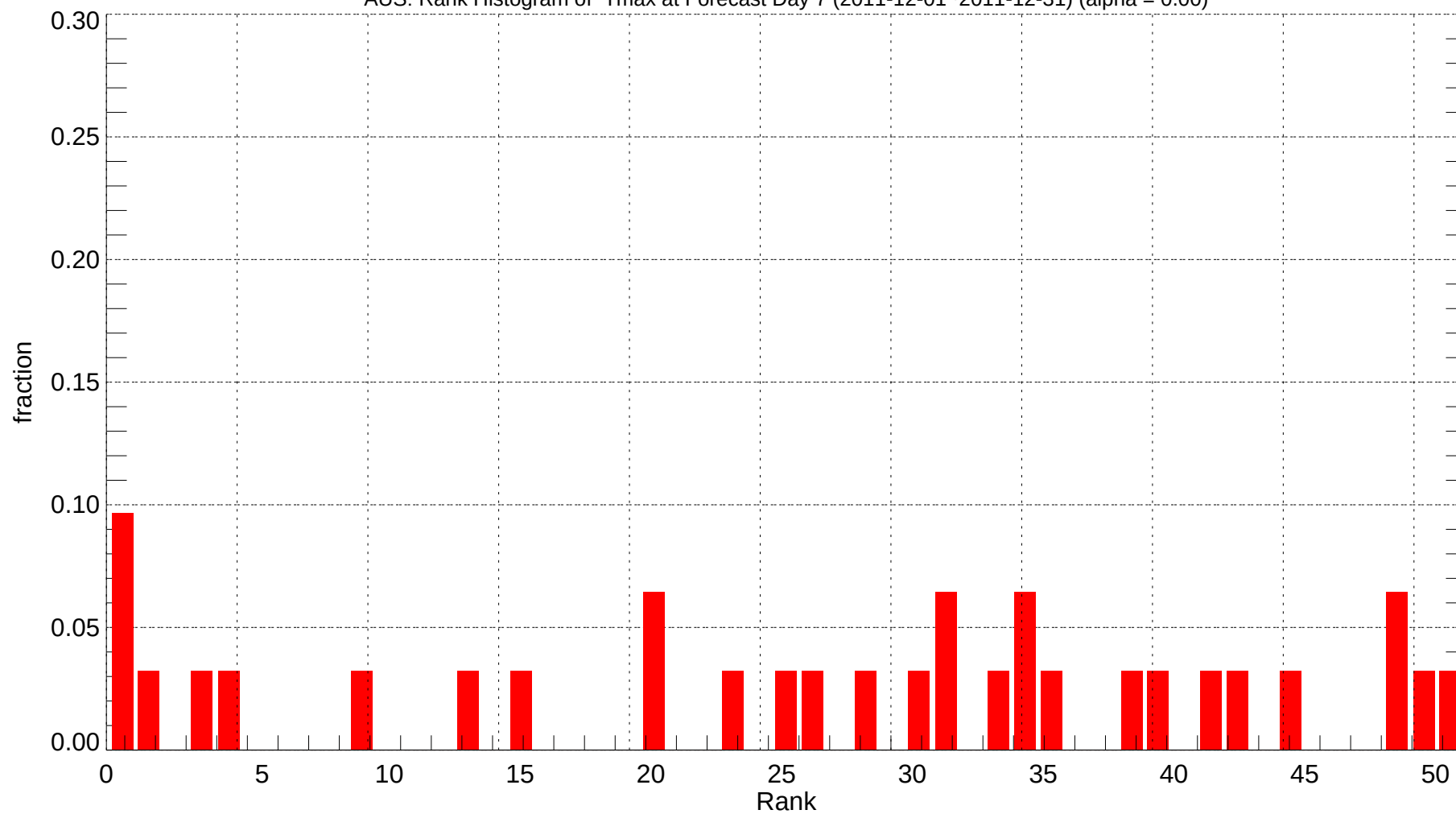
AUS: Rank Histogram of Tmax at Forecast Day 7 (2011-12-01~2011-12-31) (alpha = 0.00)
