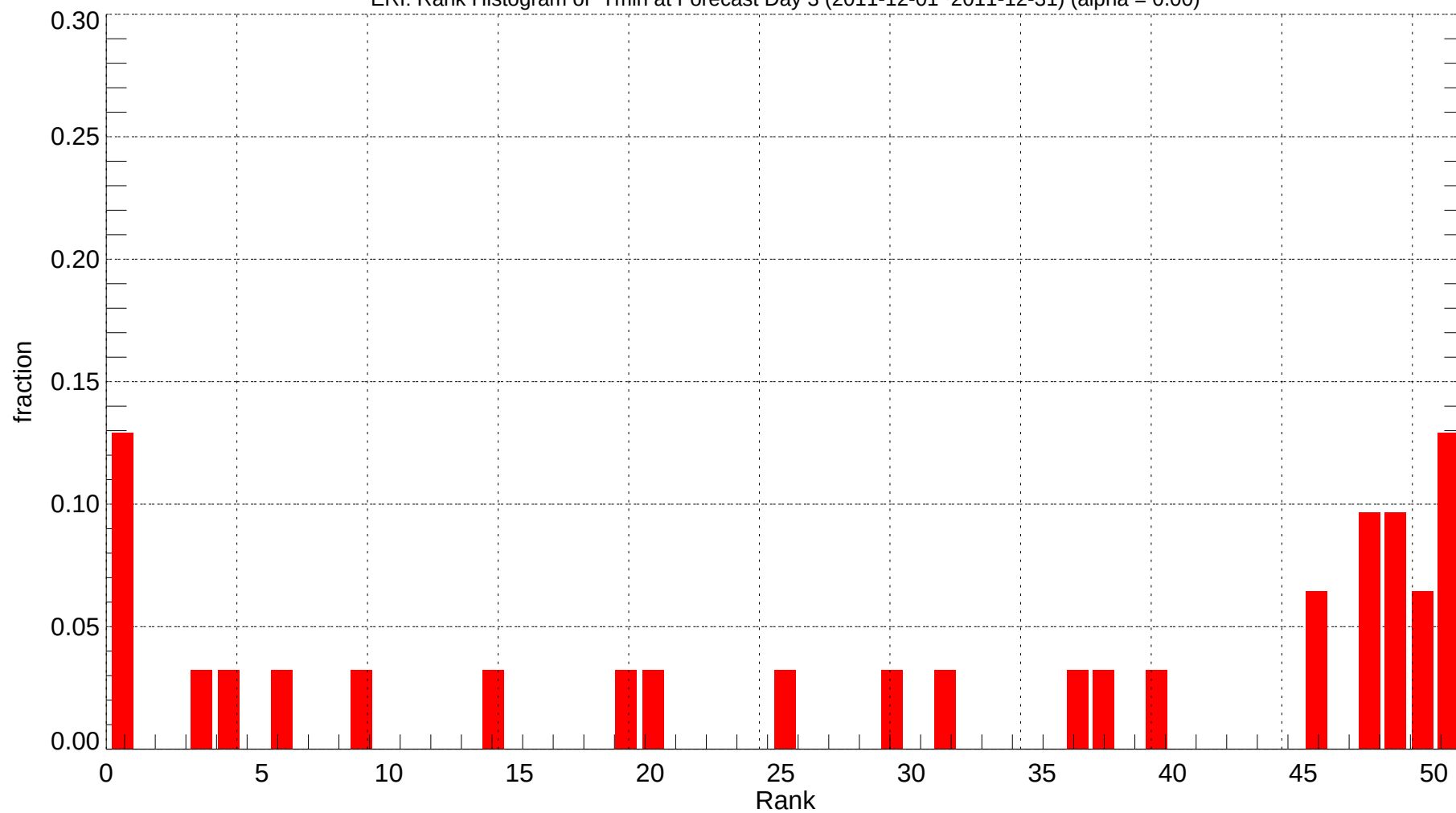
ERI: Rank Histogram of Tmin at Forecast Day 3 (2011-12-01~2011-12-31) (alpha = 0.00)
