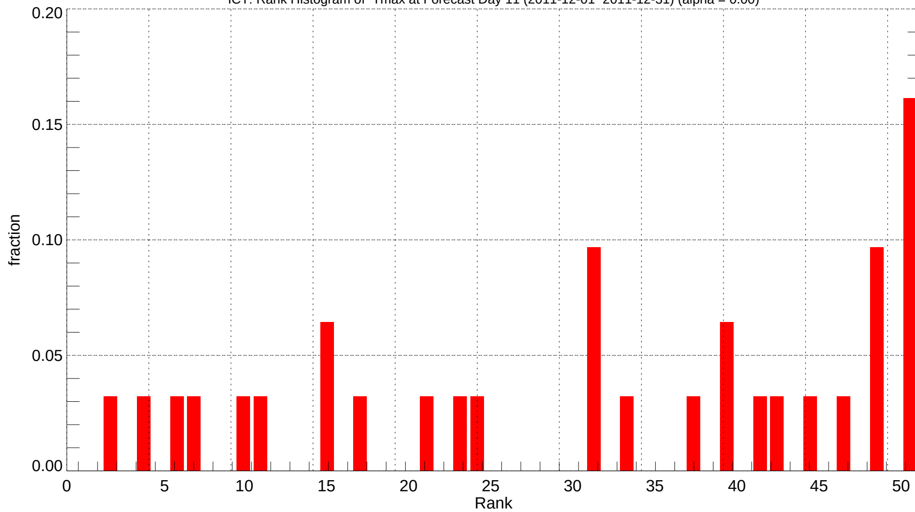
ICT: Rank Histogram of Tmax at Forecast Day 11 (2011-12-01~2011-12-31) (alpha = 0.00)
