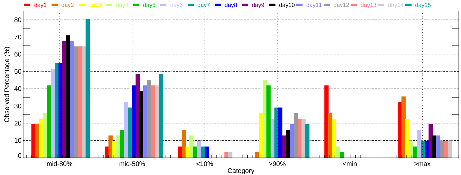
Observed Percentage of Ensembles - ICT: Min Temperature (2011-12-01~2011-12-31)
