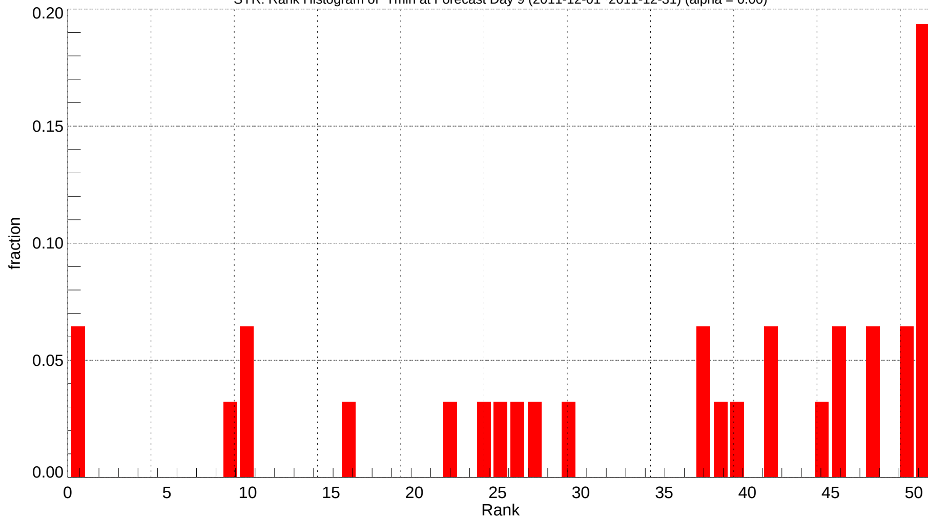
SYR: Rank Histogram of Tmin at Forecast Day 9 (2011-12-01~2011-12-31) (alpha = 0.00)
