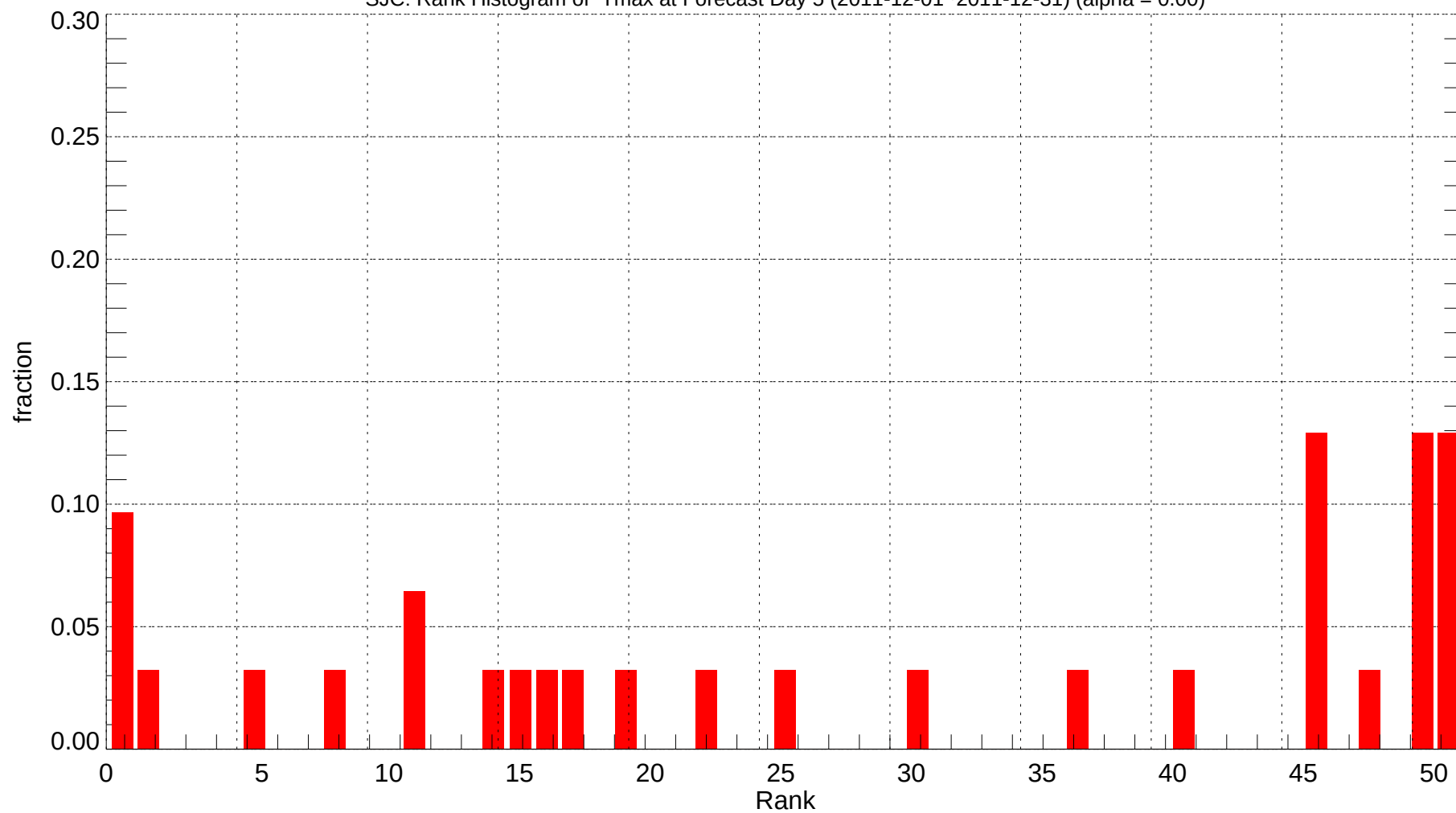
SJC: Rank Histogram of Tmax at Forecast Day 5 (2011-12-01~2011-12-31) (alpha = 0.00)
