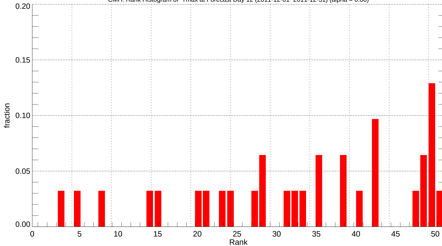
CMH: Rank Histogram of Tmax at Forecast Day 12 (2011-12-01~2011-12-31) (alpha = 0.00)
