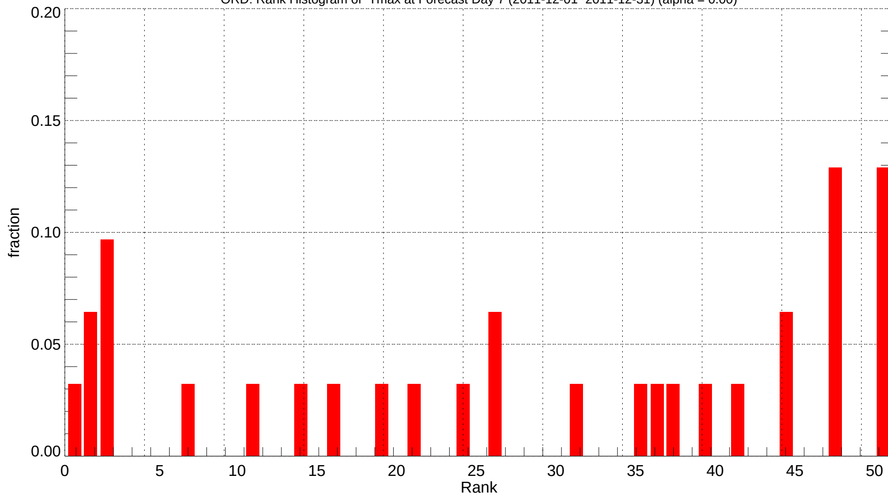
ORD: Rank Histogram of Tmax at Forecast Day 7 (2011-12-01~2011-12-31) (alpha = 0.00)
