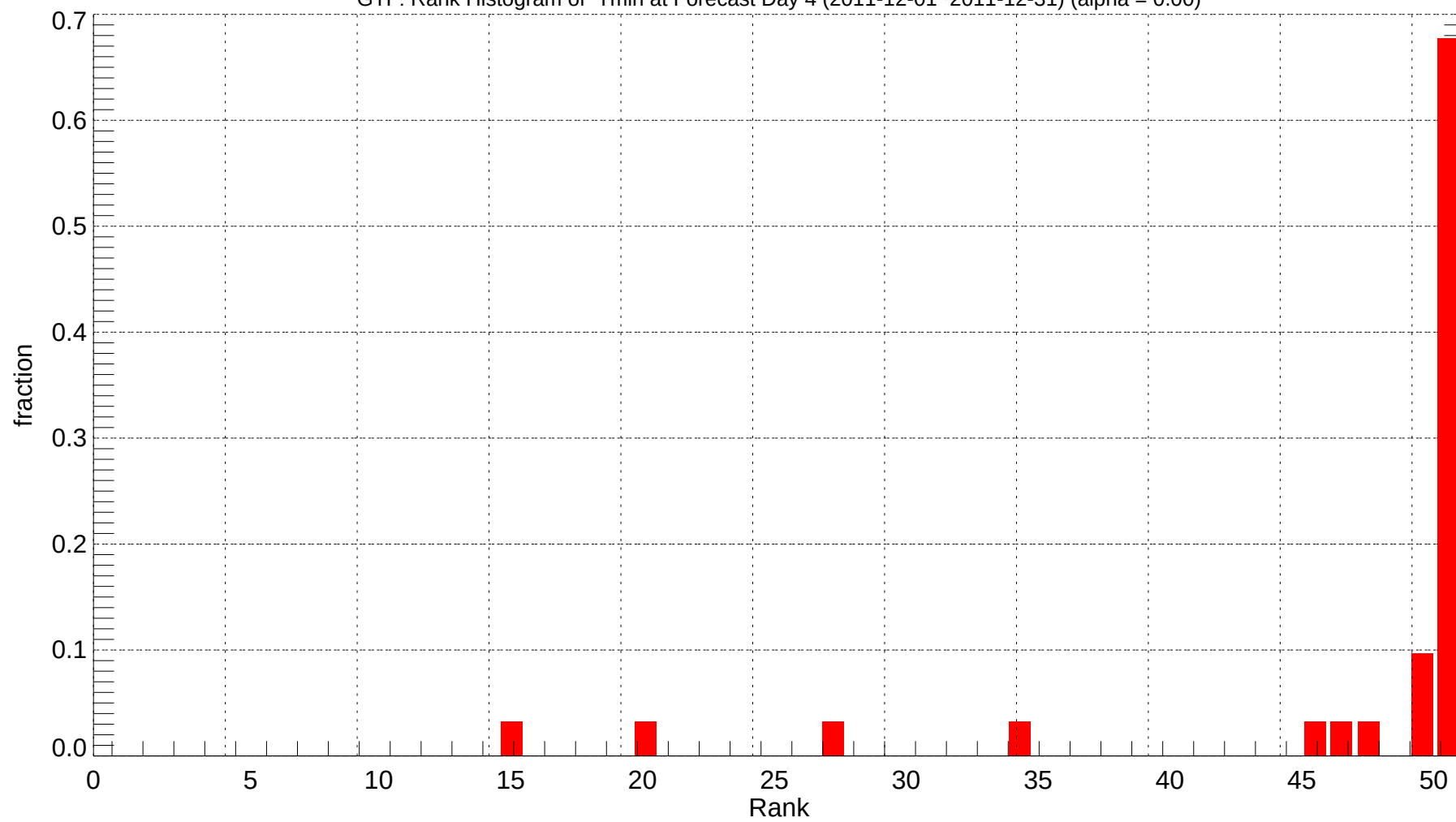
GTF: Rank Histogram of Tmin at Forecast Day 4 (2011-12-01~2011-12-31) (alpha = 0.00)
