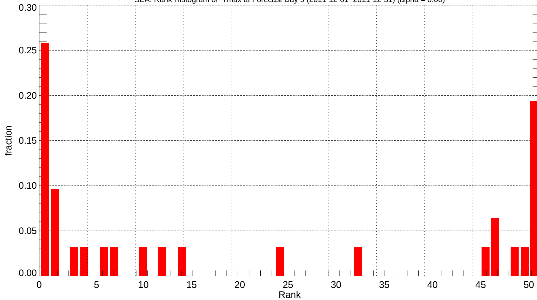
SEA: Rank Histogram of Tmax at Forecast Day 9 (2011-12-01~2011-12-31) (alpha = 0.00)
