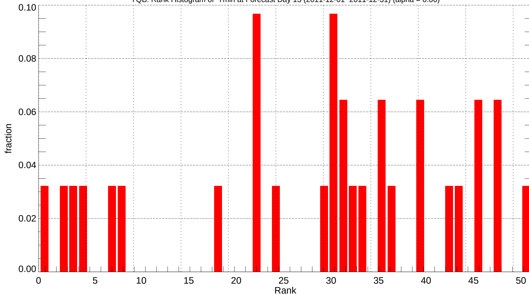
YQB: Rank Histogram of Tmin at Forecast Day 13 (2011-12-01~2011-12-31) (alpha = 0.00)
