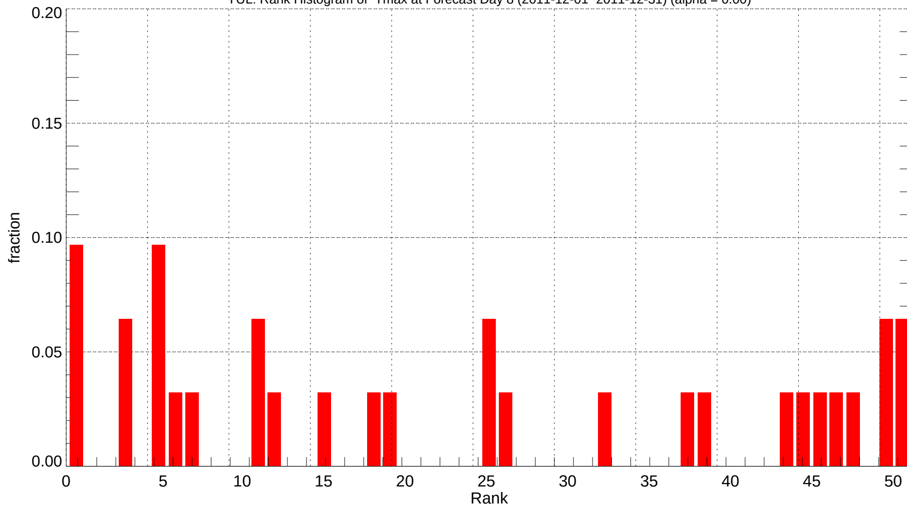
YUL: Rank Histogram of Tmax at Forecast Day 8 (2011-12-01~2011-12-31) (alpha = 0.00)
