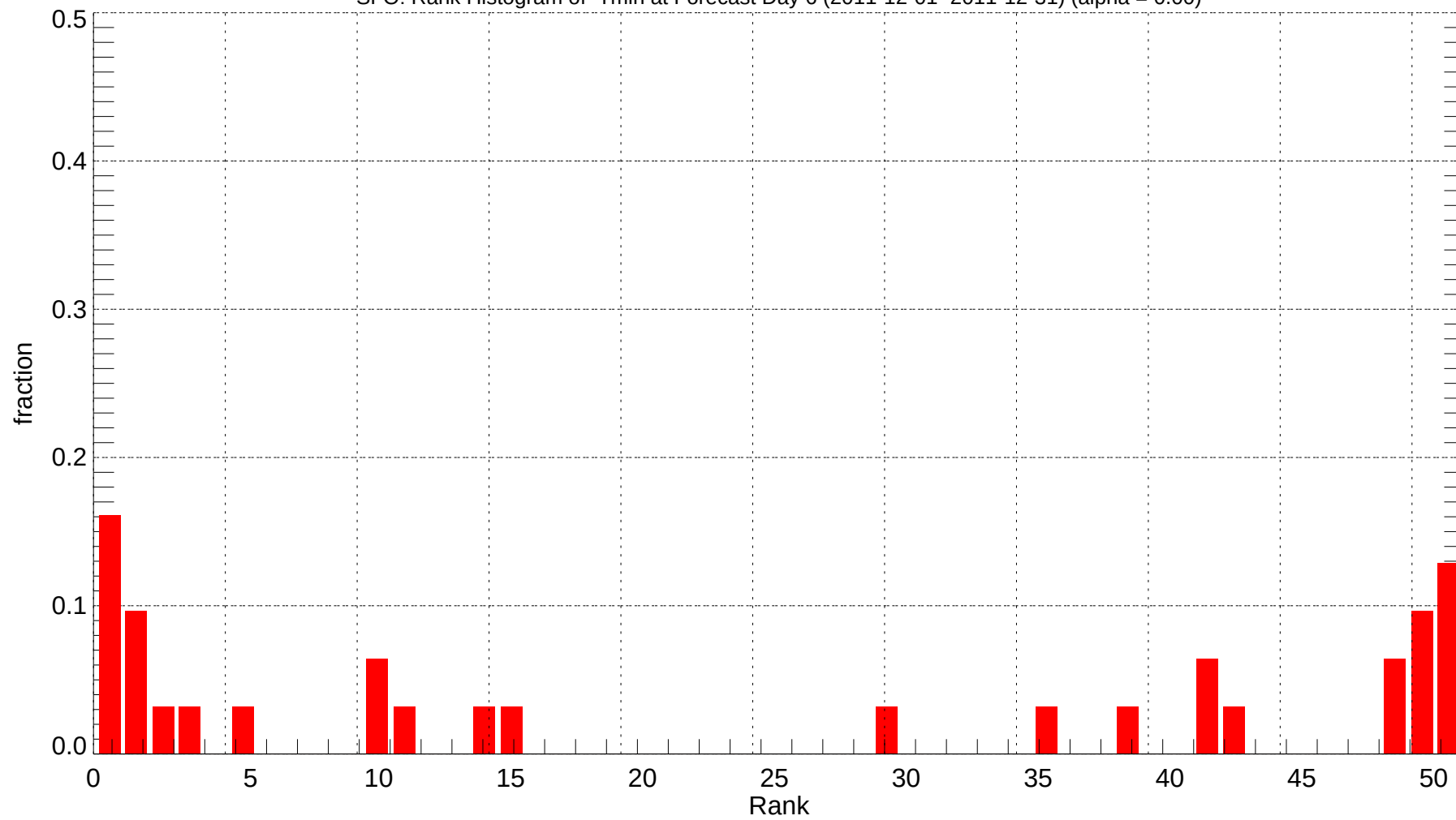
SFO: Rank Histogram of Tmin at Forecast Day 6 (2011-12-01~2011-12-31) (alpha = 0.00)
