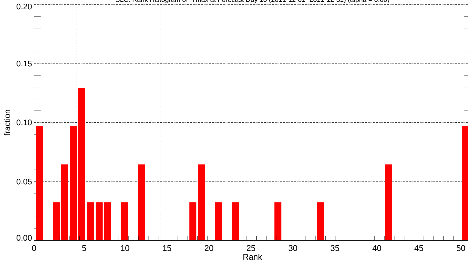
SLC: Rank Histogram of Tmax at Forecast Day 10 (2011-12-01~2011-12-31) (alpha = 0.00)
