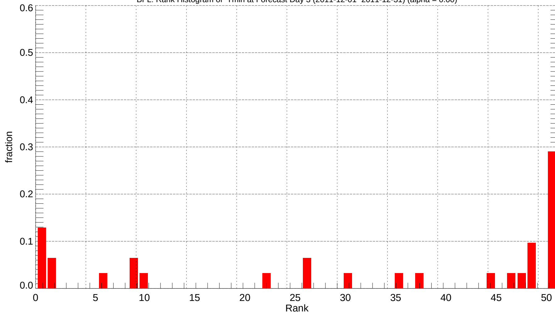
BFL: Rank Histogram of Tmin at Forecast Day 3 (2011-12-01~2011-12-31) (alpha = 0.00)
