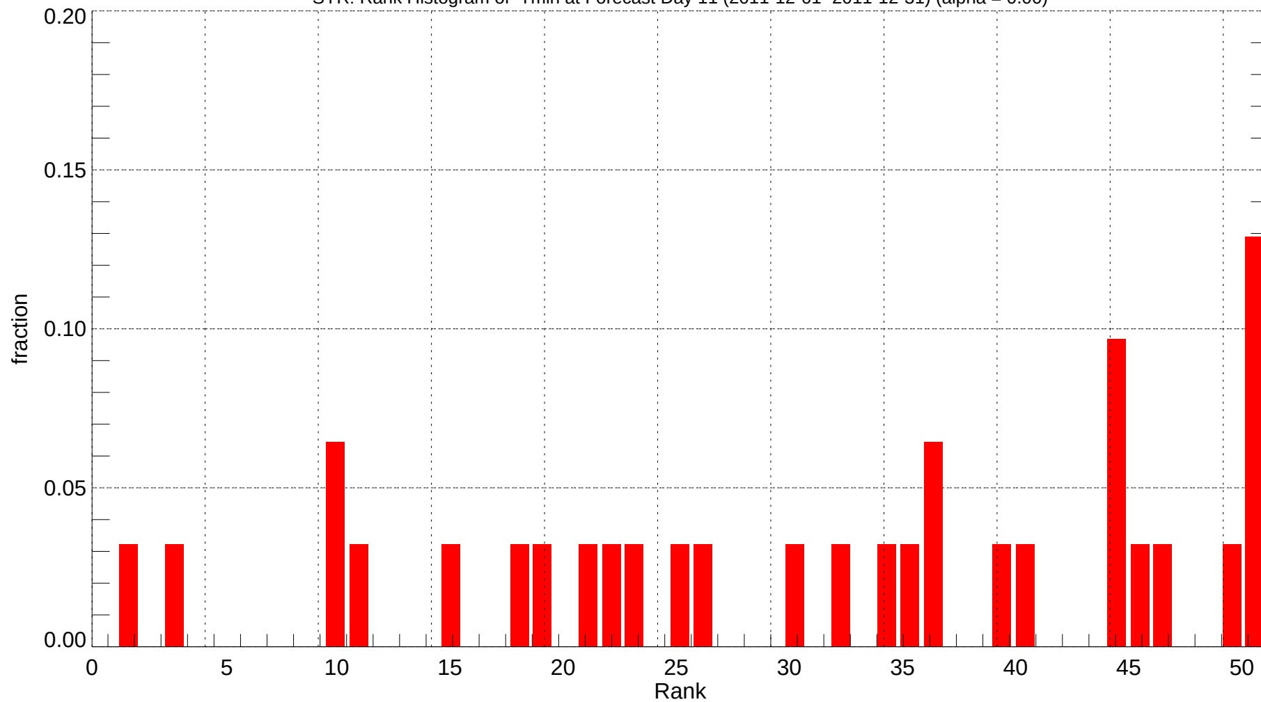
SYR: Rank Histogram of Tmin at Forecast Day 11 (2011-12-01~2011-12-31) (alpha = 0.00)
