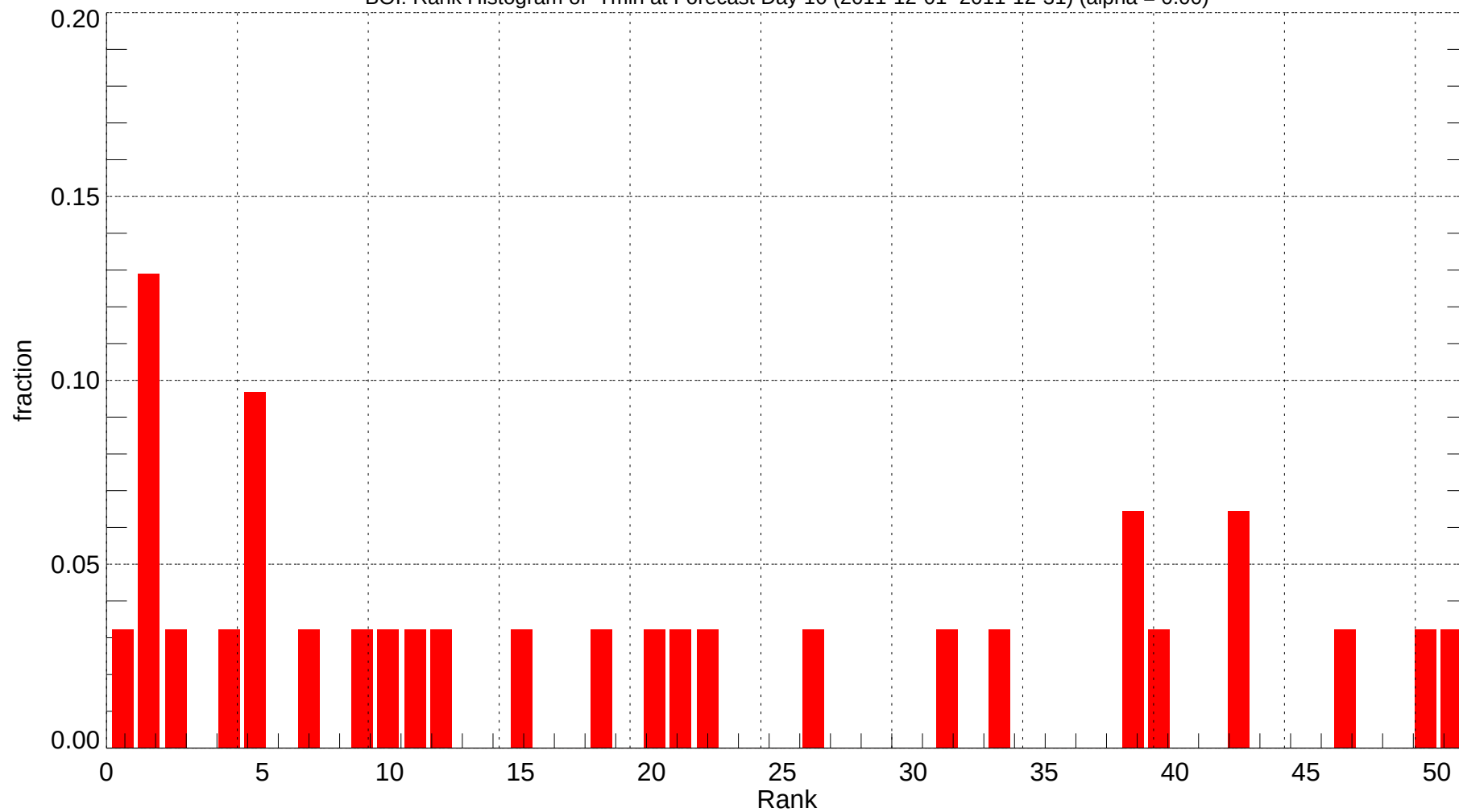
BOI: Rank Histogram of Tmin at Forecast Day 10 (2011-12-01~2011-12-31) (alpha = 0.00)
