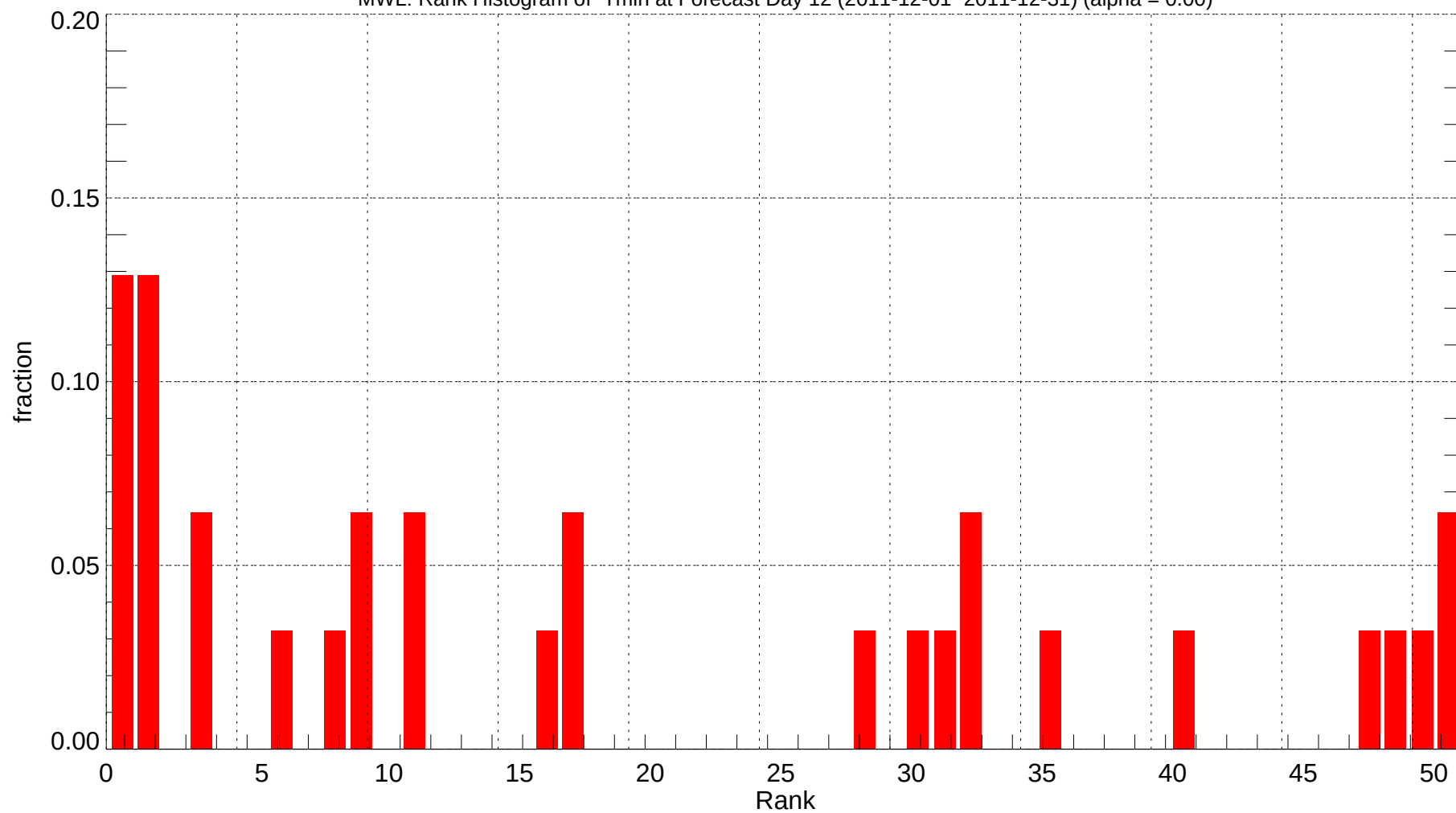
MWL: Rank Histogram of Tmin at Forecast Day 12 (2011-12-01~2011-12-31) (alpha = 0.00)
