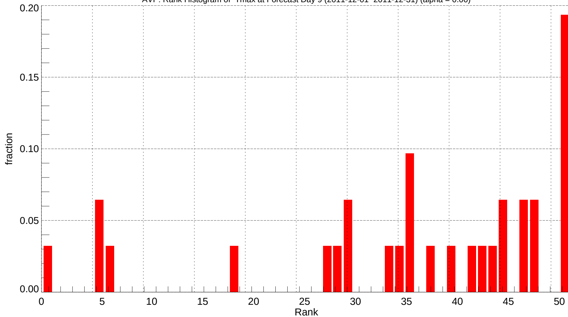
AVP: Rank Histogram of Tmax at Forecast Day 9 (2011-12-01~2011-12-31) (alpha = 0.00)
