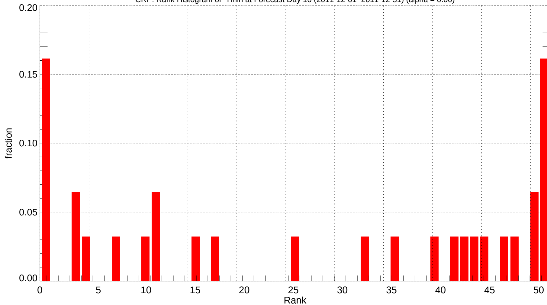
CRP: Rank Histogram of Tmin at Forecast Day 10 (2011-12-01~2011-12-31) (alpha = 0.00)
