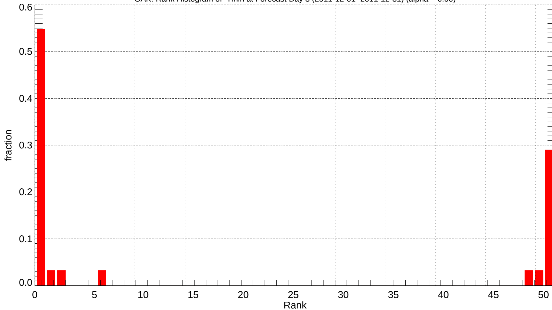
OAK: Rank Histogram of Tmin at Forecast Day 3 (2011-12-01~2011-12-31) (alpha = 0.00)
