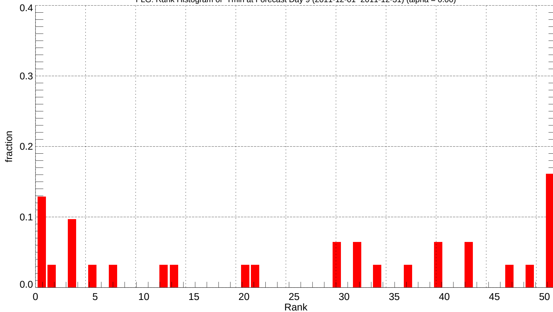
FLG: Rank Histogram of Tmin at Forecast Day 9 (2011-12-01~2011-12-31) (alpha = 0.00)
