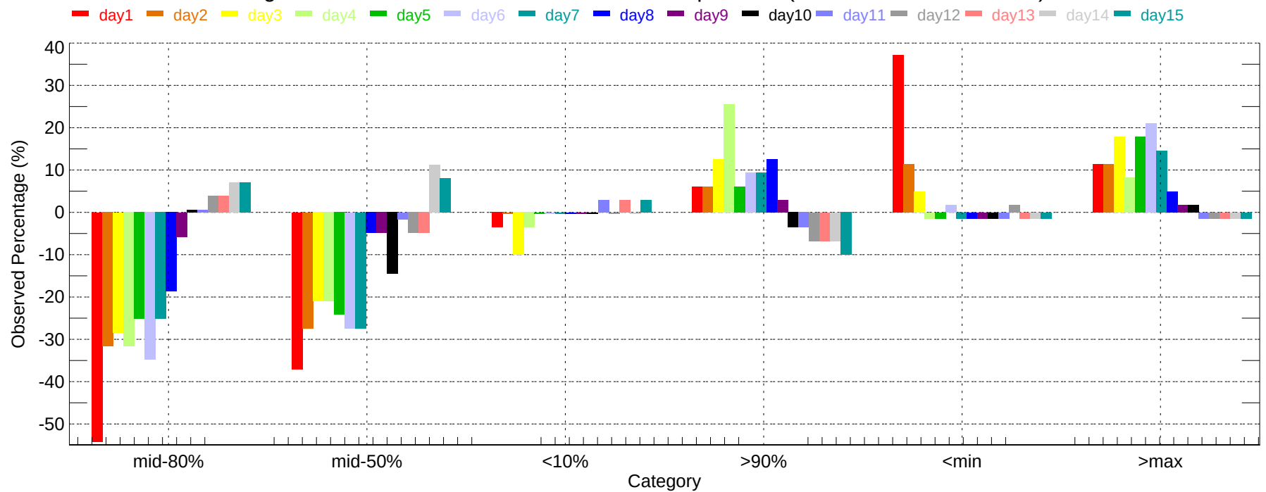
Observed Percentage Deviation of Ensembles - TYR: Min Temperature (2011-12-01~2011-12-31)
