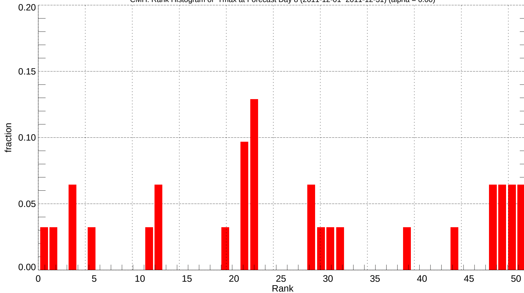
CMH: Rank Histogram of Tmax at Forecast Day 8 (2011-12-01~2011-12-31) (alpha = 0.00)
