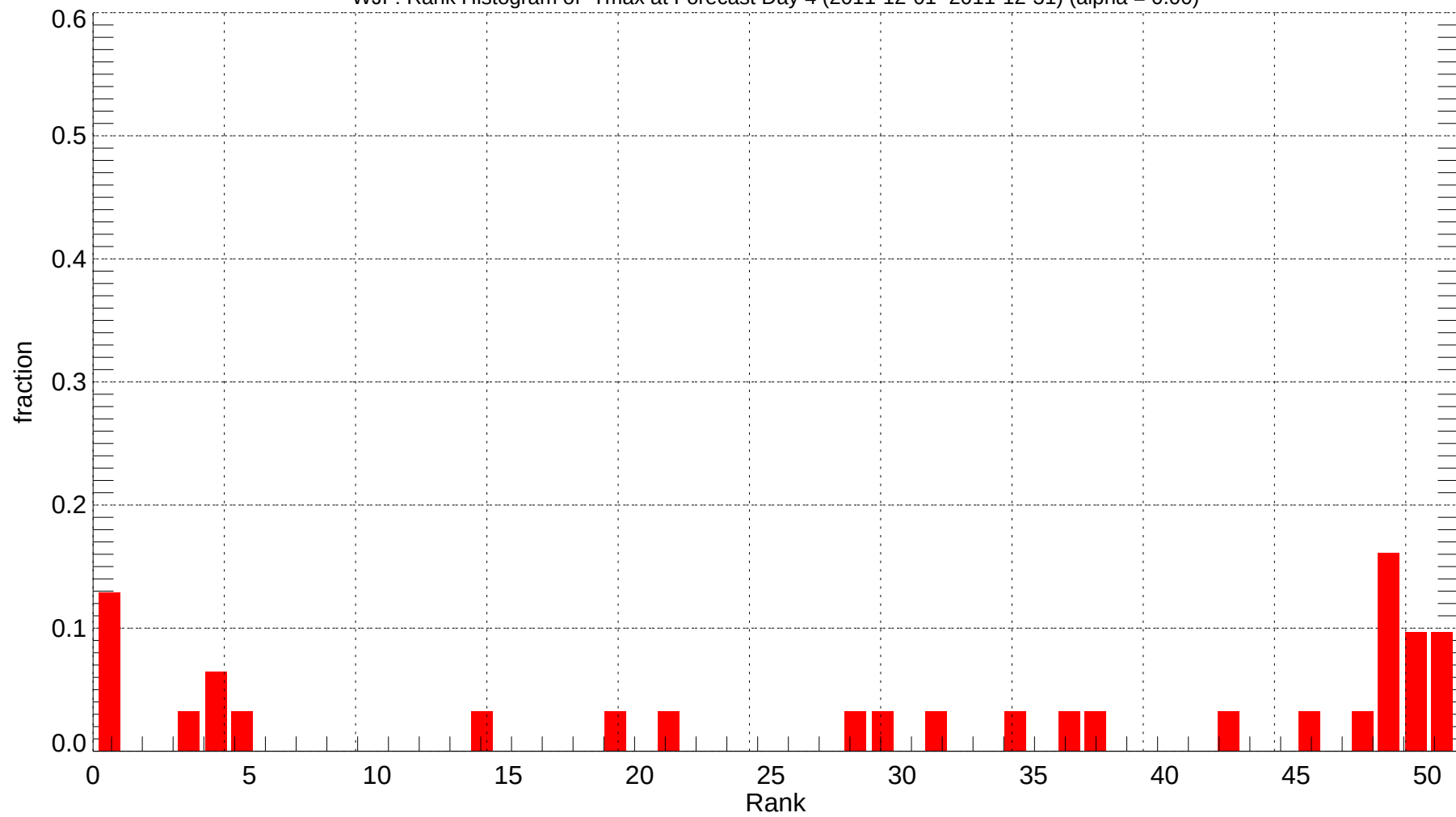
WJF: Rank Histogram of Tmax at Forecast Day 4 (2011-12-01~2011-12-31) (alpha = 0.00)
