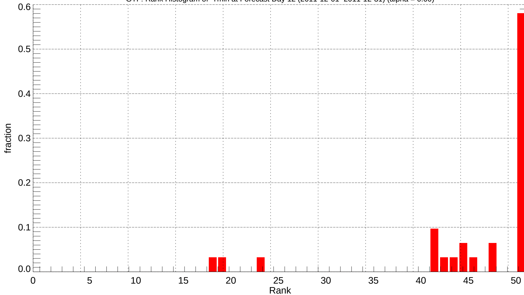
GTF: Rank Histogram of Tmin at Forecast Day 12 (2011-12-01~2011-12-31) (alpha = 0.00)
