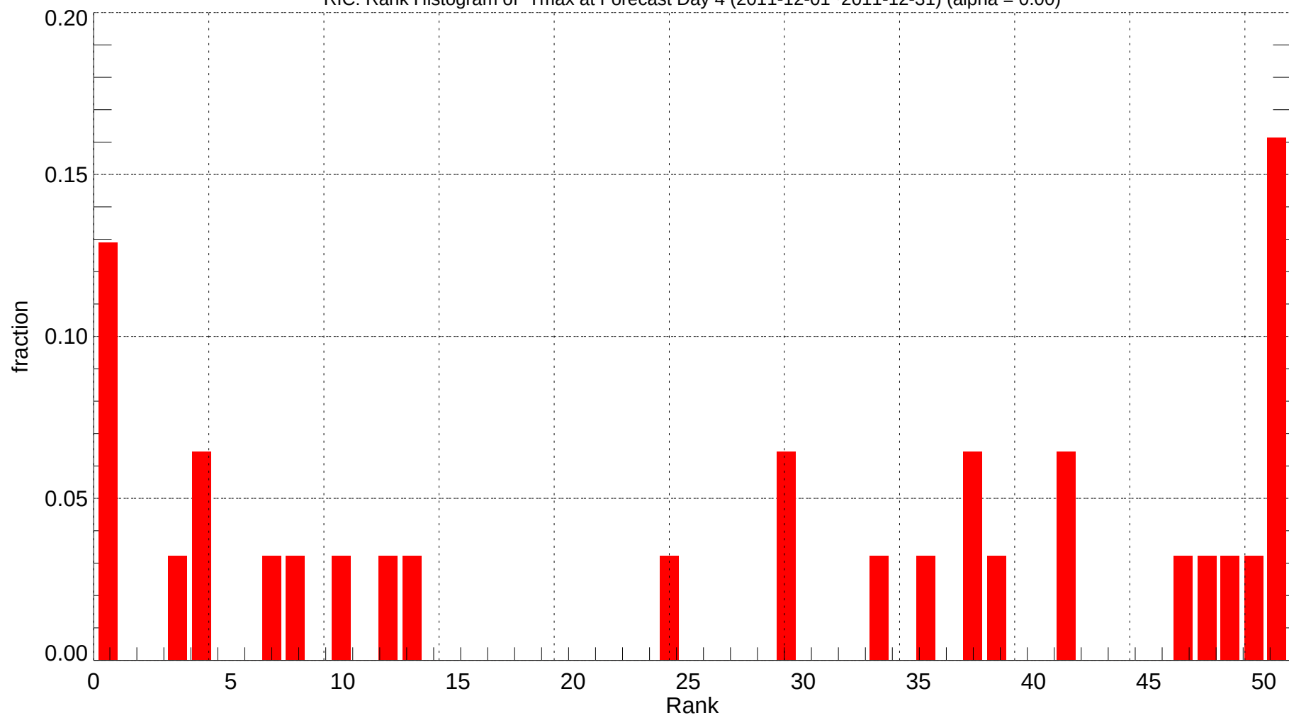
RIC: Rank Histogram of Tmax at Forecast Day 4 (2011-12-01~2011-12-31) (alpha = 0.00)
