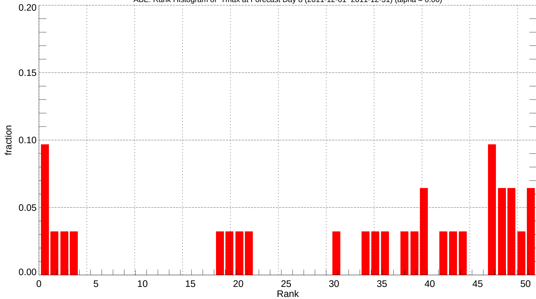
ABE: Rank Histogram of Tmax at Forecast Day 8 (2011-12-01~2011-12-31) (alpha = 0.00)
