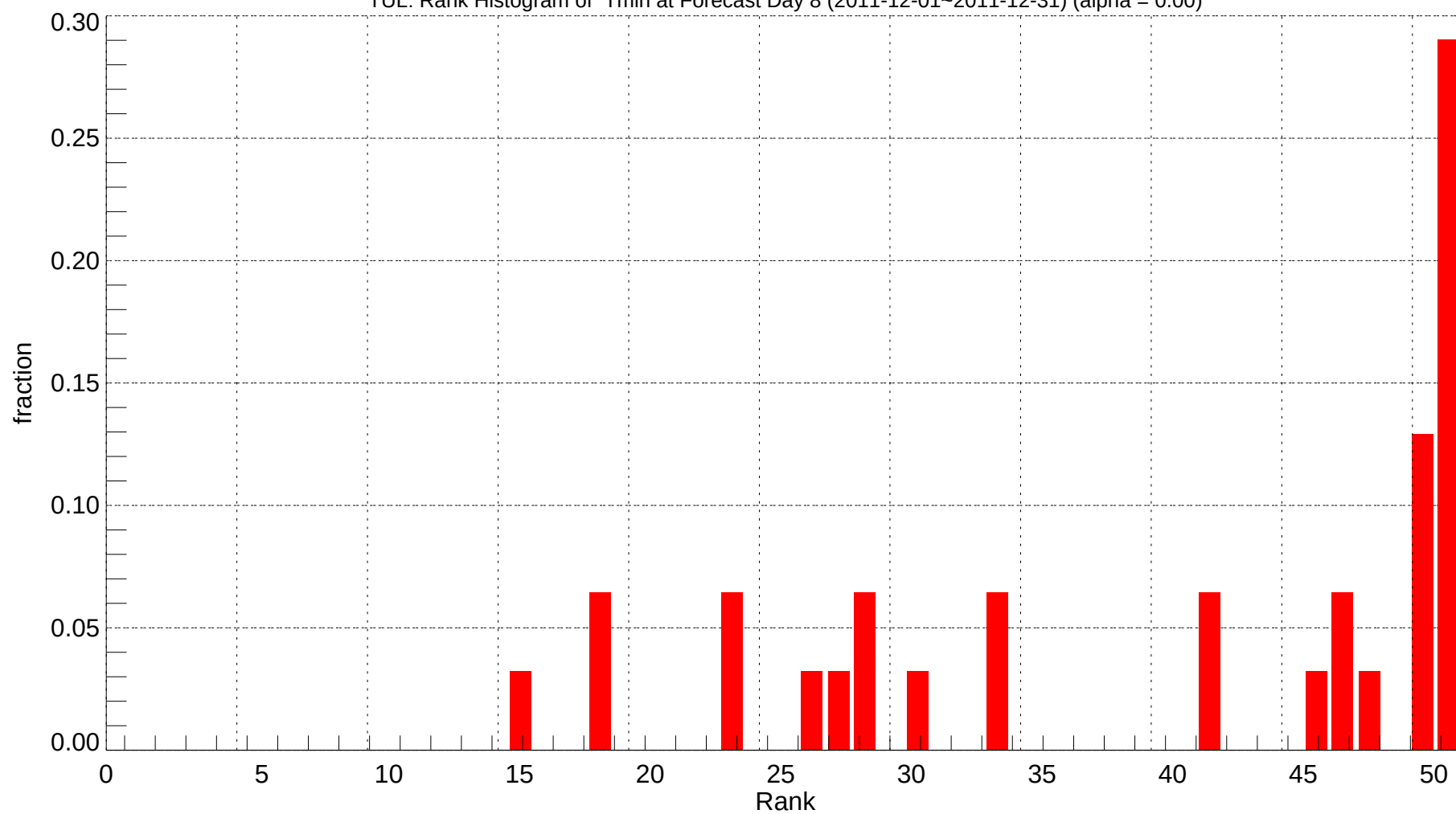
TUL: Rank Histogram of Tmin at Forecast Day 8 (2011-12-01~2011-12-31) (alpha = 0.00)
