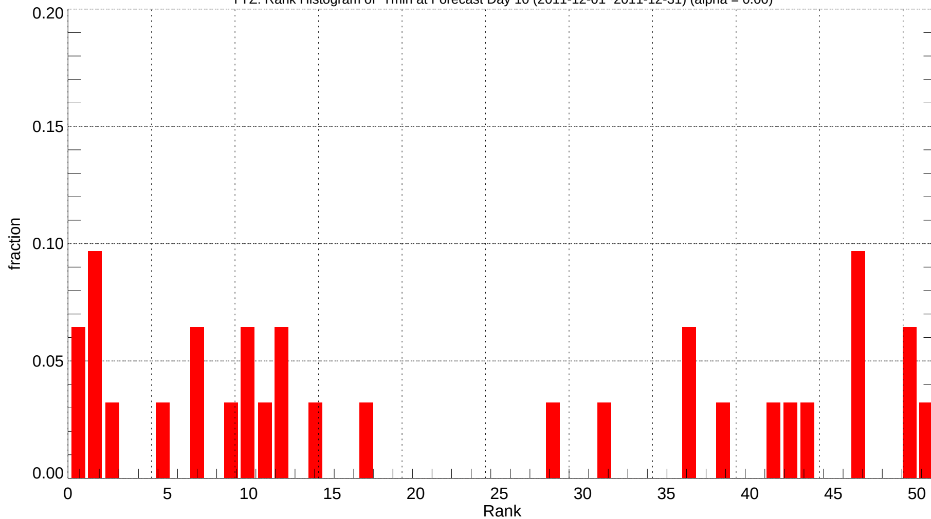
YYZ: Rank Histogram of Tmin at Forecast Day 10 (2011-12-01~2011-12-31) (alpha = 0.00)
