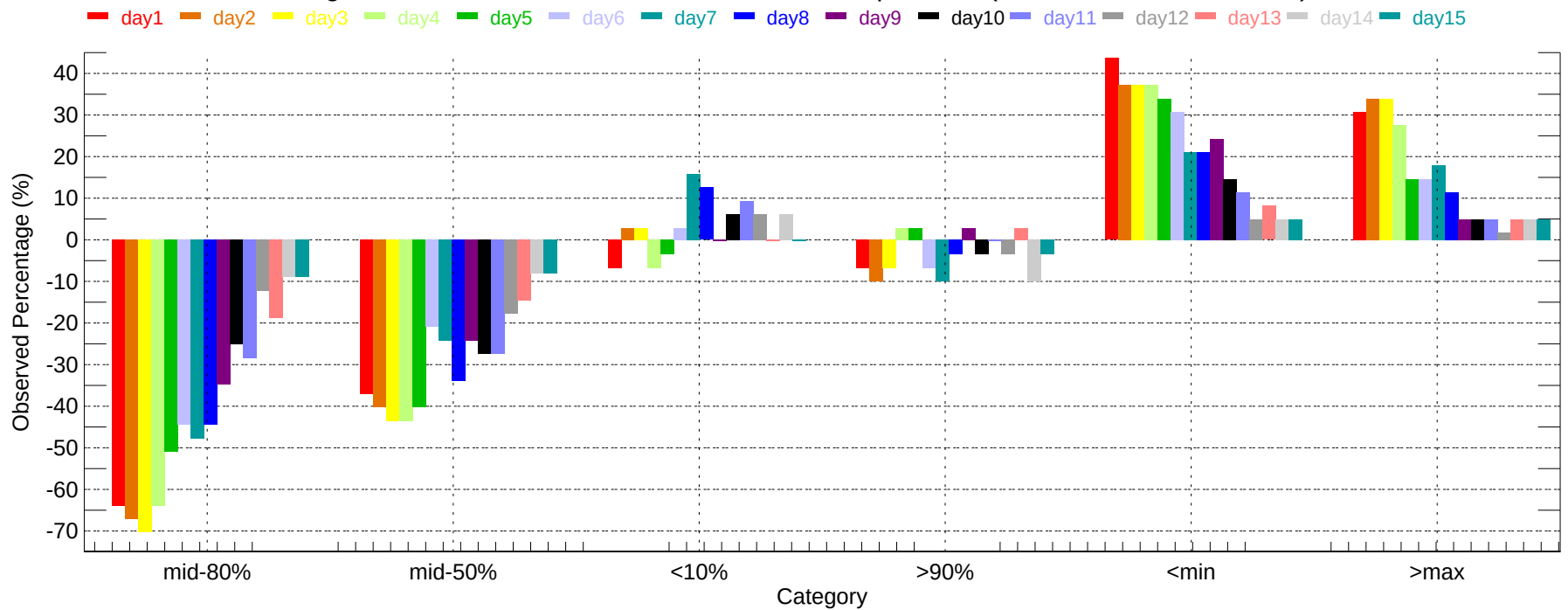
Observed Percentage Deviation of Ensembles - GEG: Max Temperature (2011-12-01~2011-12-31)
