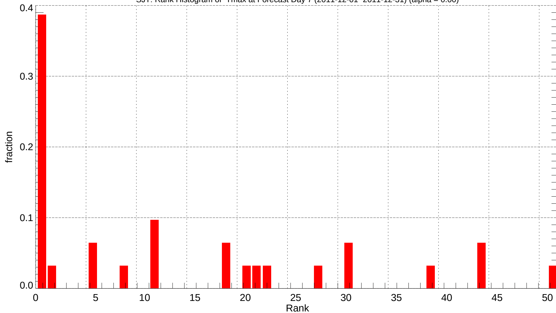
SJT: Rank Histogram of Tmax at Forecast Day 7 (2011-12-01~2011-12-31) (alpha = 0.00)
