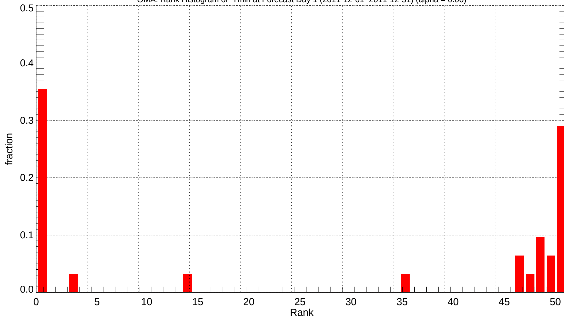
OMA: Rank Histogram of Tmin at Forecast Day 1 (2011-12-01~2011-12-31) (alpha = 0.00)
