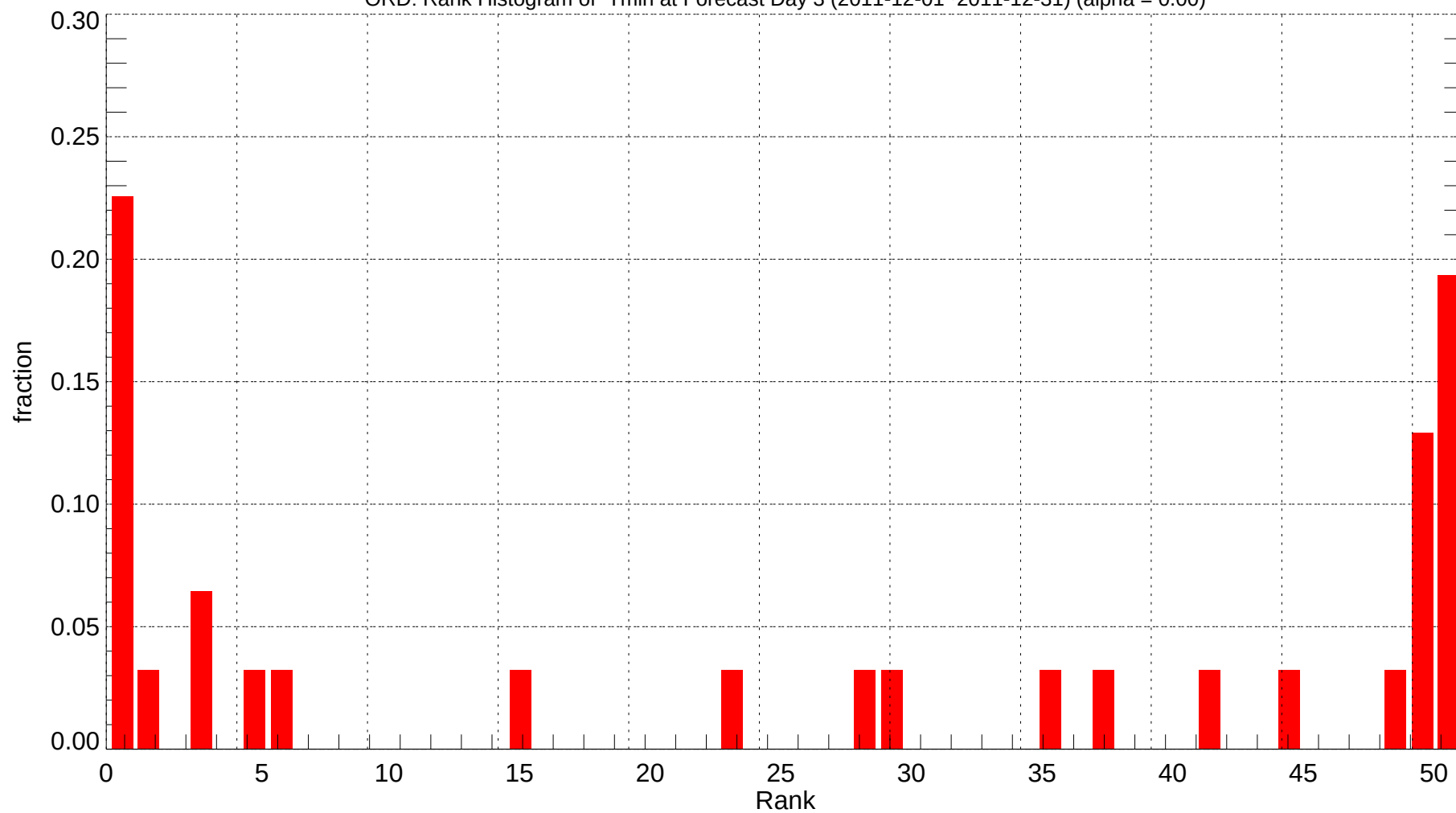
ORD: Rank Histogram of Tmin at Forecast Day 3 (2011-12-01~2011-12-31) (alpha = 0.00)
