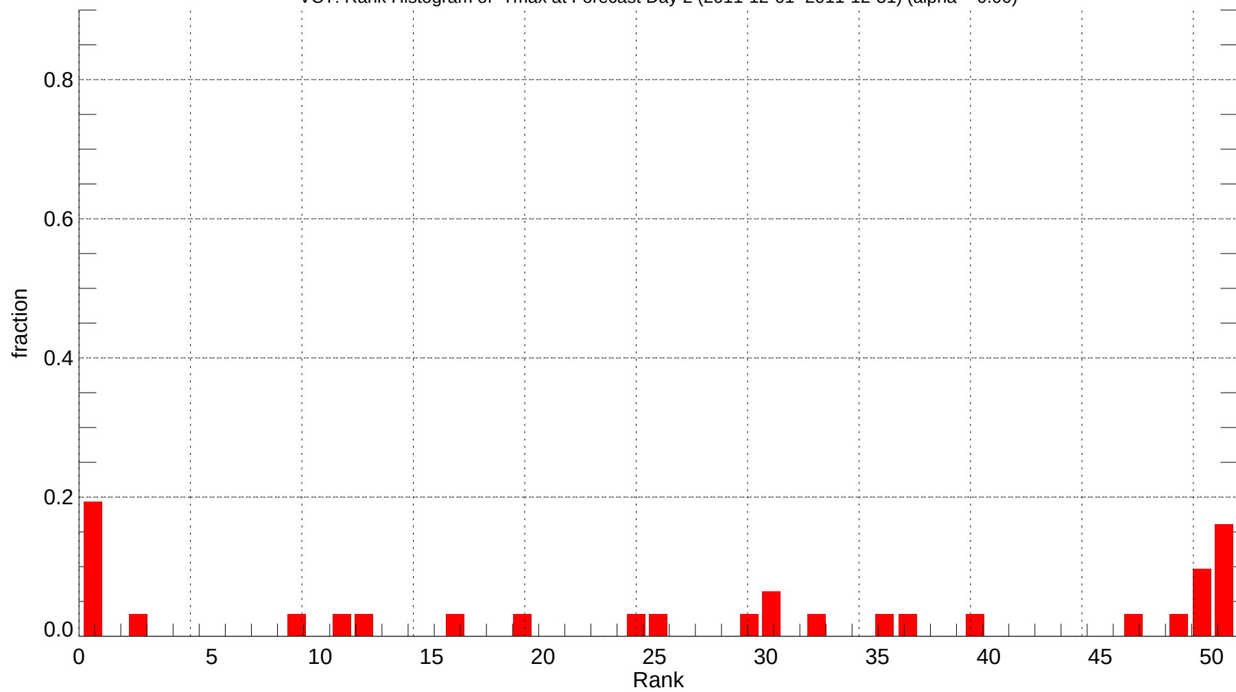
VCT: Rank Histogram of Tmax at Forecast Day 2 (2011-12-01~2011-12-31) (alpha = 0.00)
