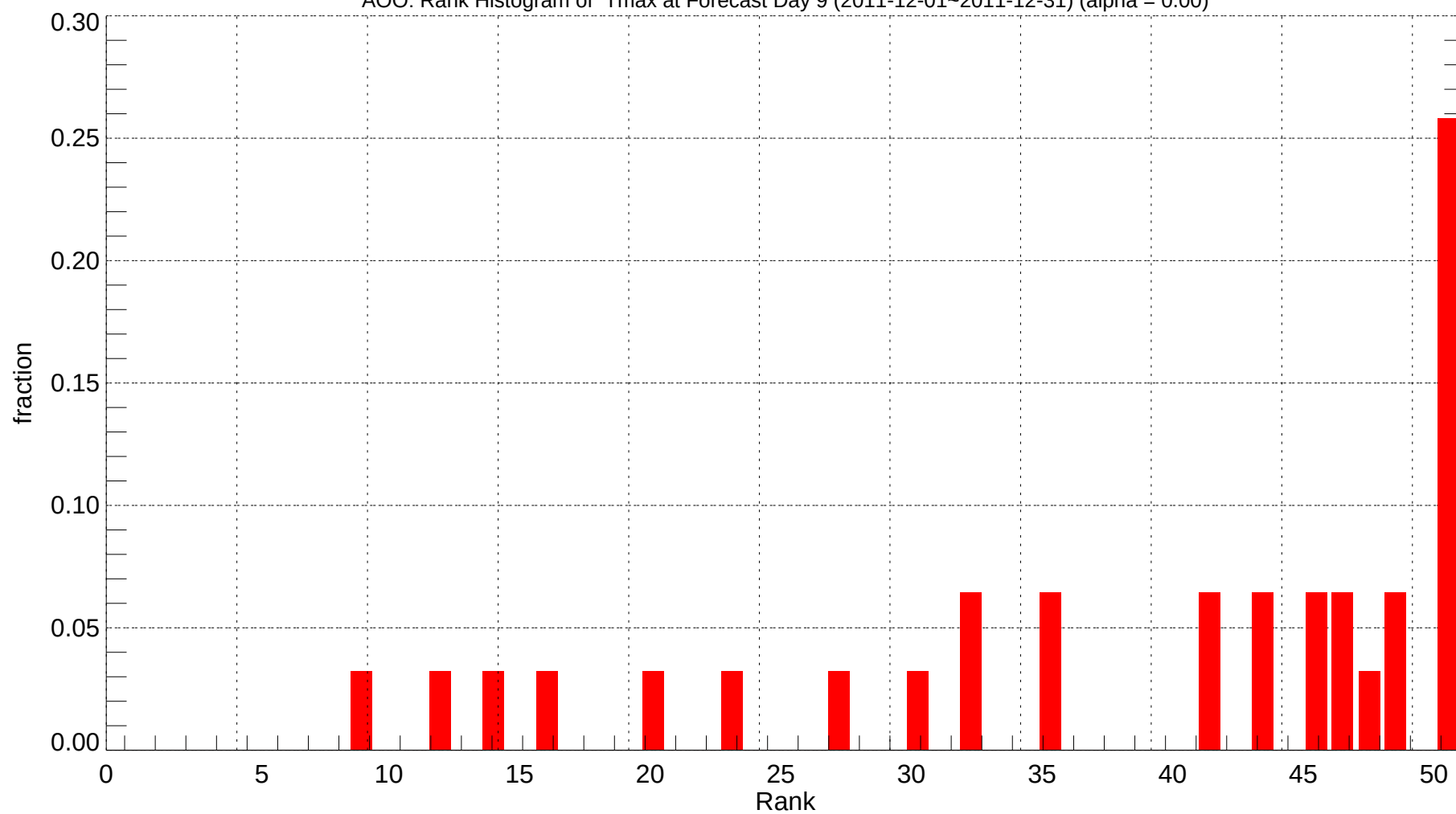
AOO: Rank Histogram of Tmax at Forecast Day 9 (2011-12-01~2011-12-31) (alpha = 0.00)
