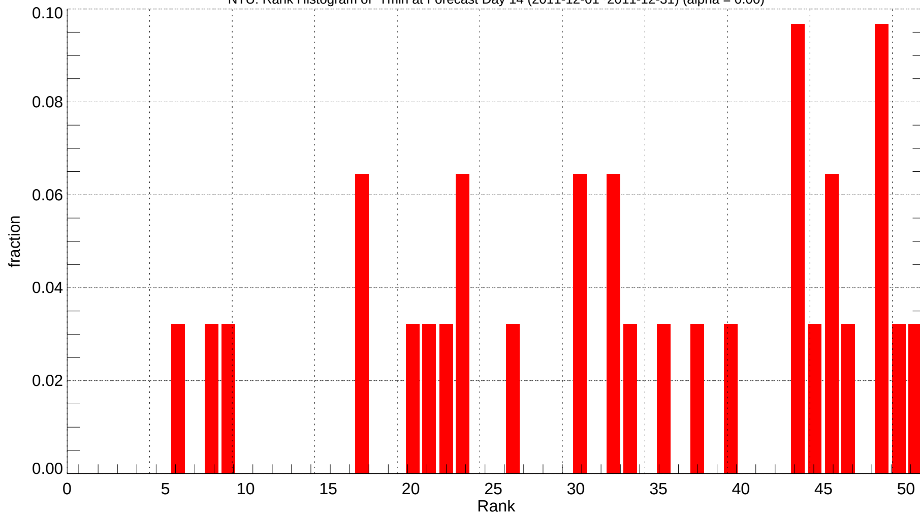
NTU: Rank Histogram of Tmin at Forecast Day 14 (2011-12-01~2011-12-31) (alpha = 0.00)
