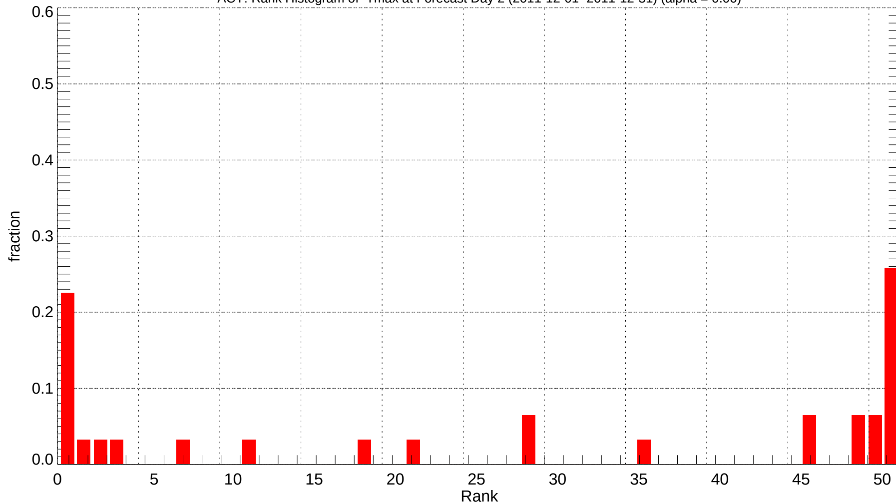
ACY: Rank Histogram of Tmax at Forecast Day 2 (2011-12-01~2011-12-31) (alpha = 0.00)
