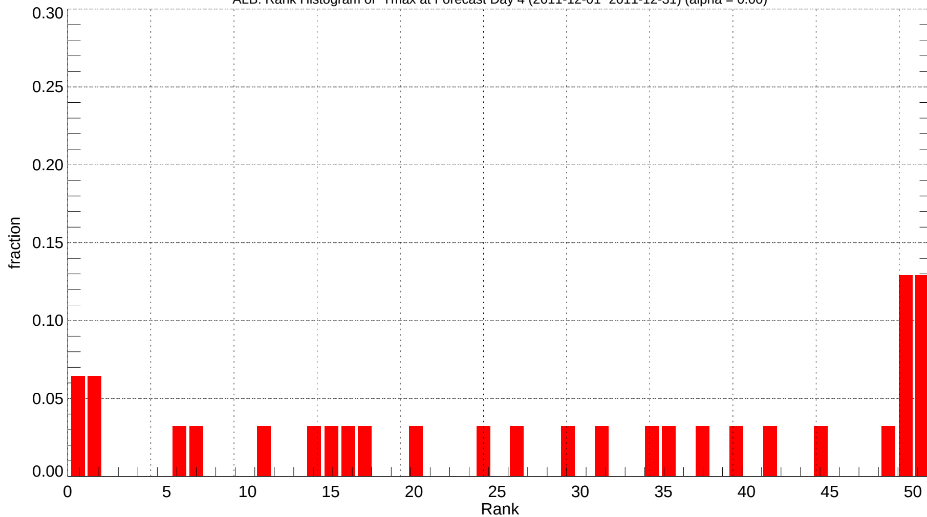
ALB: Rank Histogram of Tmax at Forecast Day 4 (2011-12-01~2011-12-31) (alpha = 0.00)
