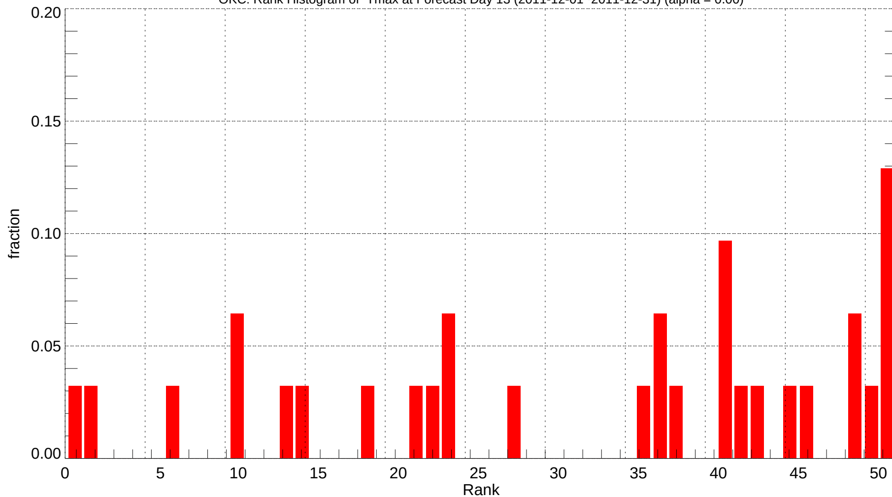
OKC: Rank Histogram of Tmax at Forecast Day 13 (2011-12-01~2011-12-31) (alpha = 0.00)
