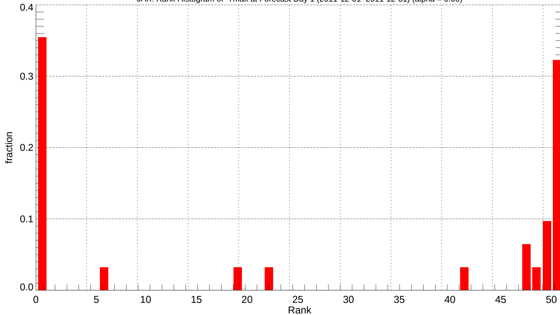
JAX: Rank Histogram of Tmax at Forecast Day 1 (2011-12-01~2011-12-31) (alpha = 0.00)
