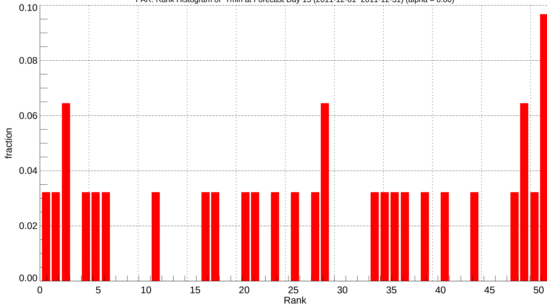
FAR: Rank Histogram of Tmin at Forecast Day 15 (2011-12-01~2011-12-31) (alpha = 0.00)
