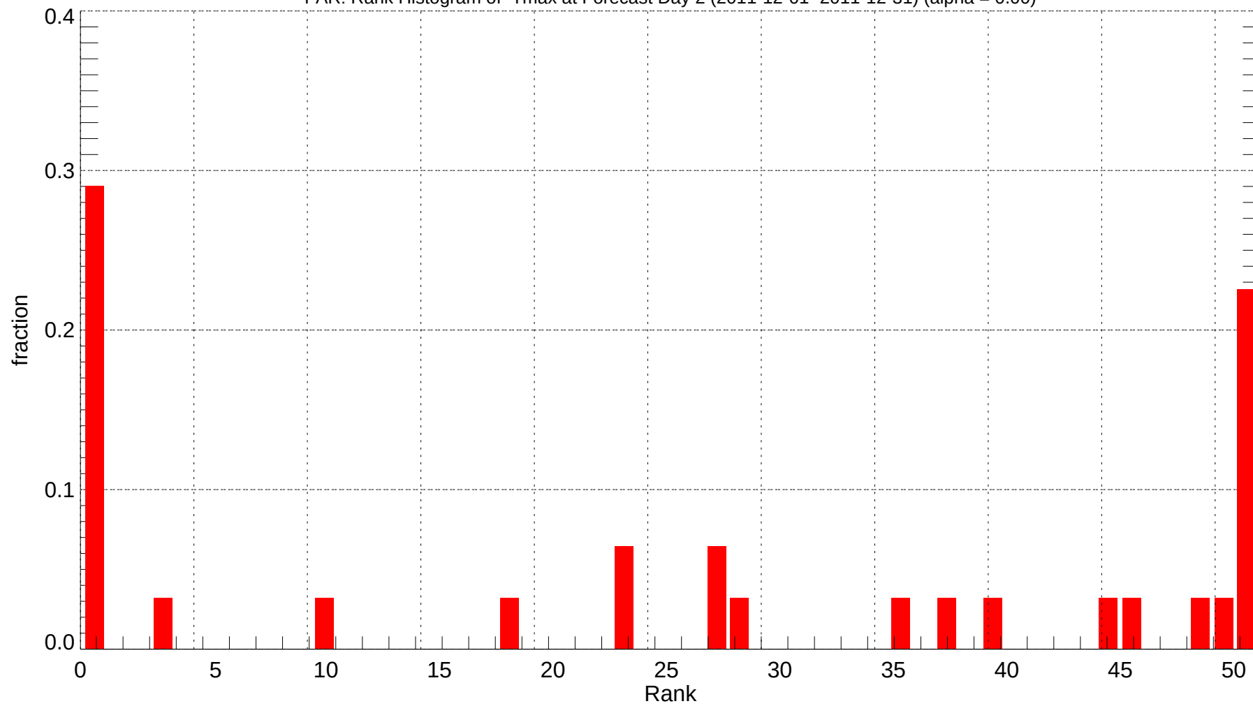
FAR: Rank Histogram of Tmax at Forecast Day 2 (2011-12-01~2011-12-31) (alpha = 0.00)
