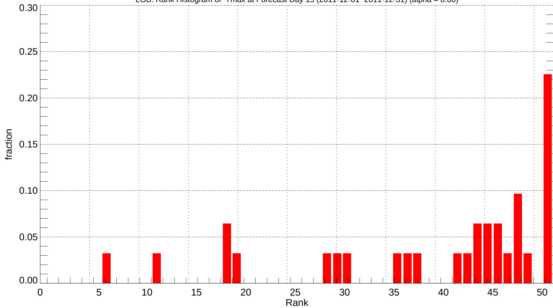
LGB: Rank Histogram of Tmax at Forecast Day 15 (2011-12-01~2011-12-31) (alpha = 0.00)
