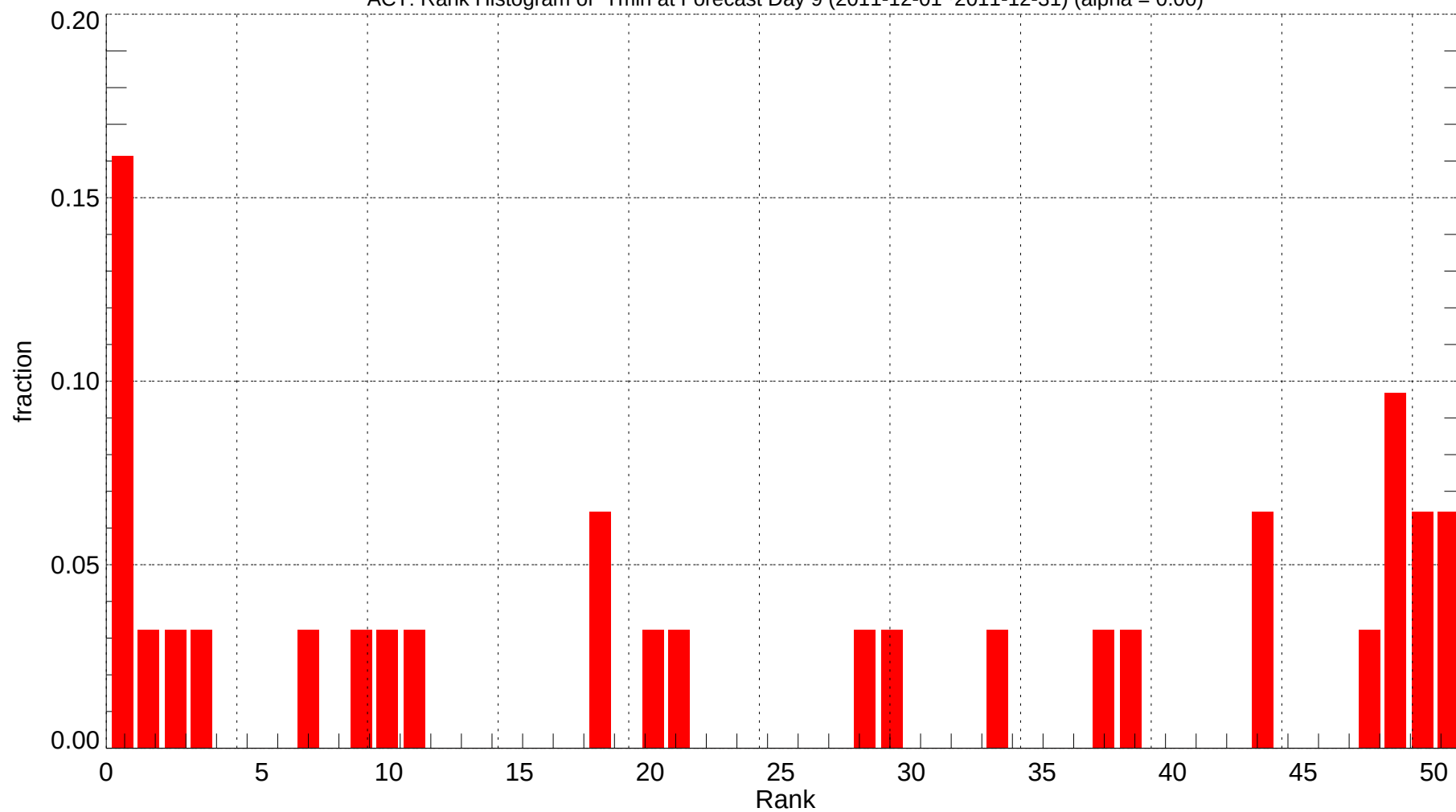
ACT: Rank Histogram of Tmin at Forecast Day 9 (2011-12-01~2011-12-31) (alpha = 0.00)
