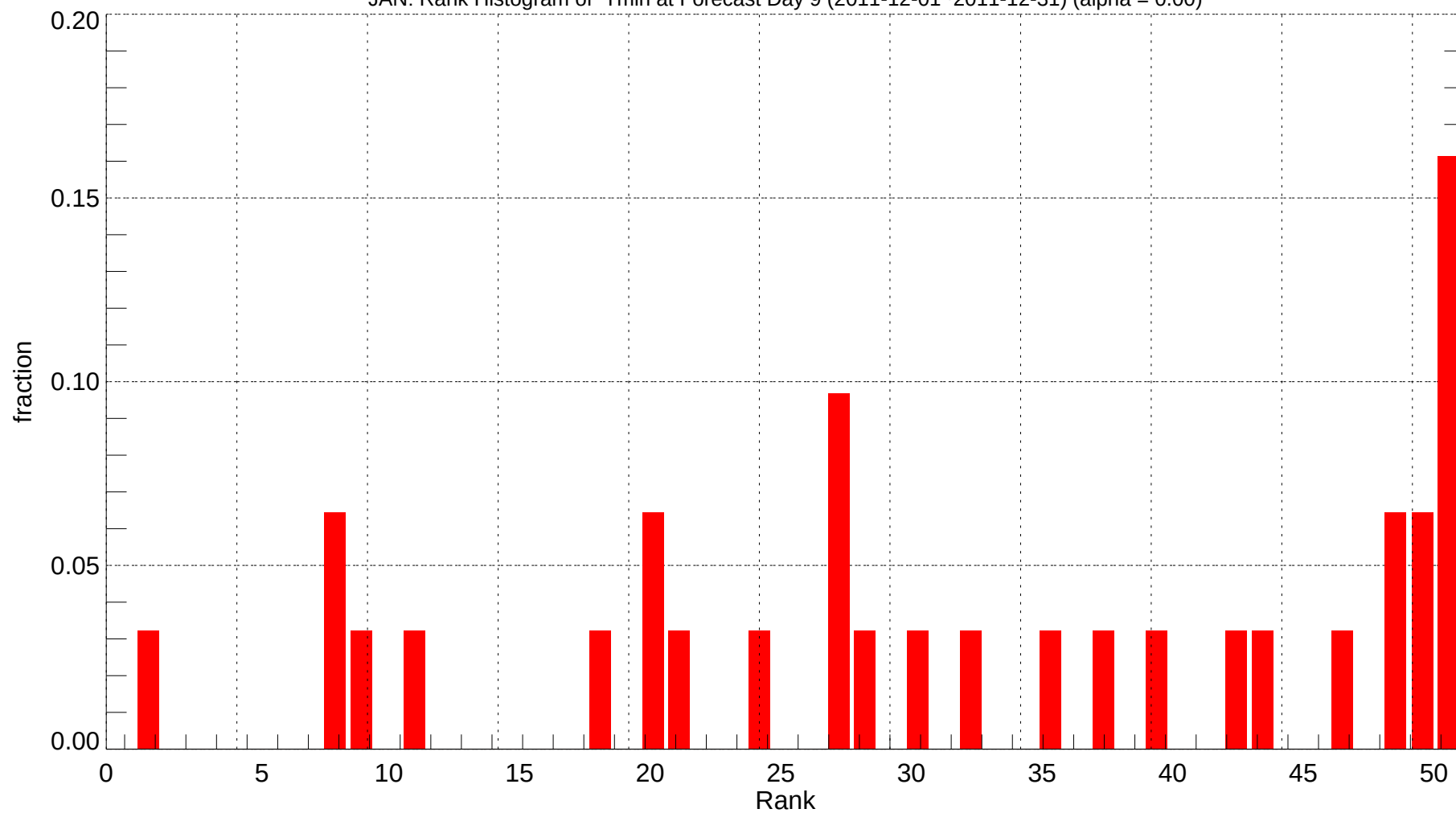
JAN: Rank Histogram of Tmin at Forecast Day 9 (2011-12-01~2011-12-31) (alpha = 0.00)
