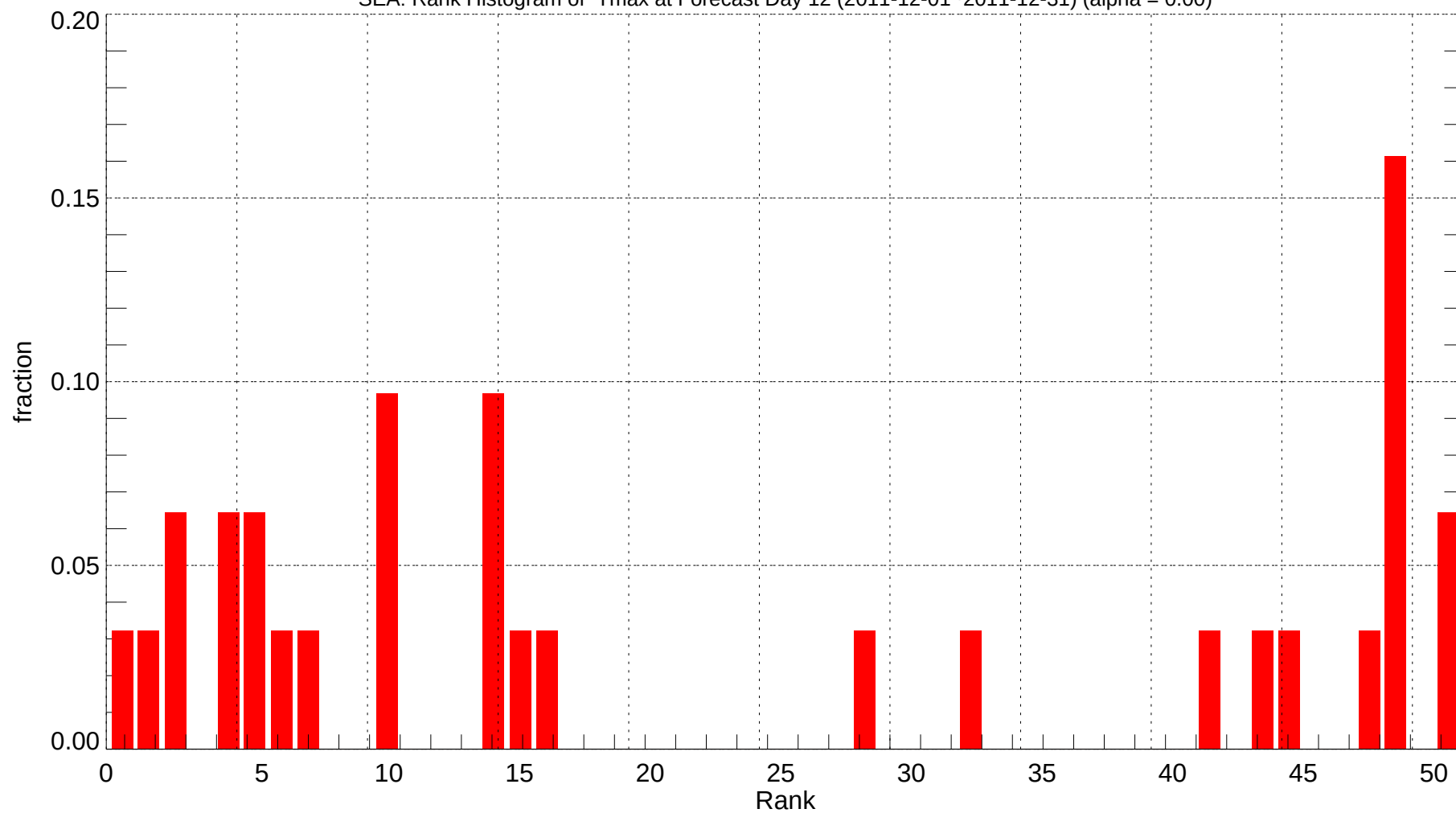
SEA: Rank Histogram of Tmax at Forecast Day 12 (2011-12-01~2011-12-31) (alpha = 0.00)
