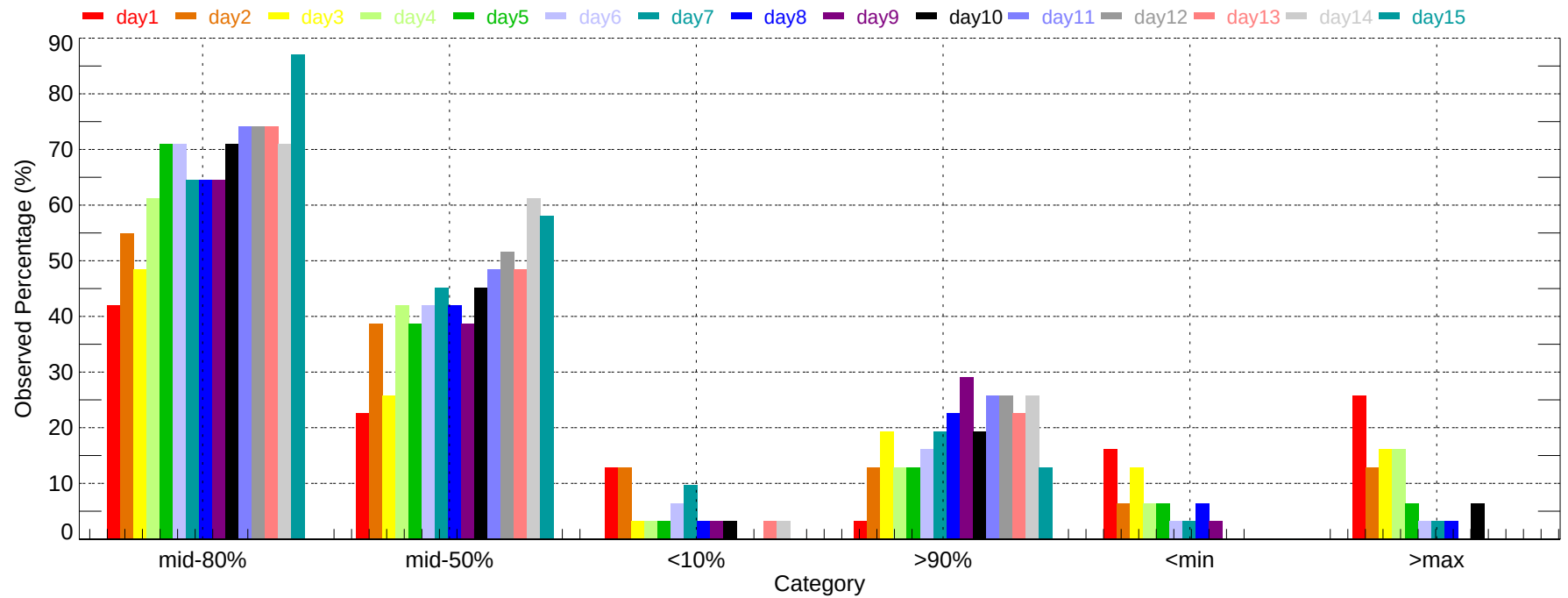
Observed Percentage of Ensembles - DTW: Min Temperature (2011-12-01~2011-12-31)
