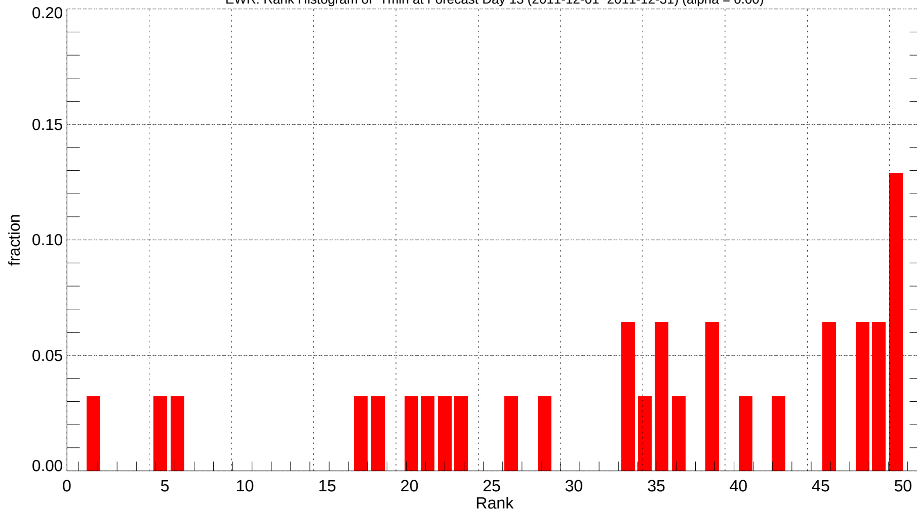
EWR: Rank Histogram of Tmin at Forecast Day 13 (2011-12-01~2011-12-31) (alpha = 0.00)
