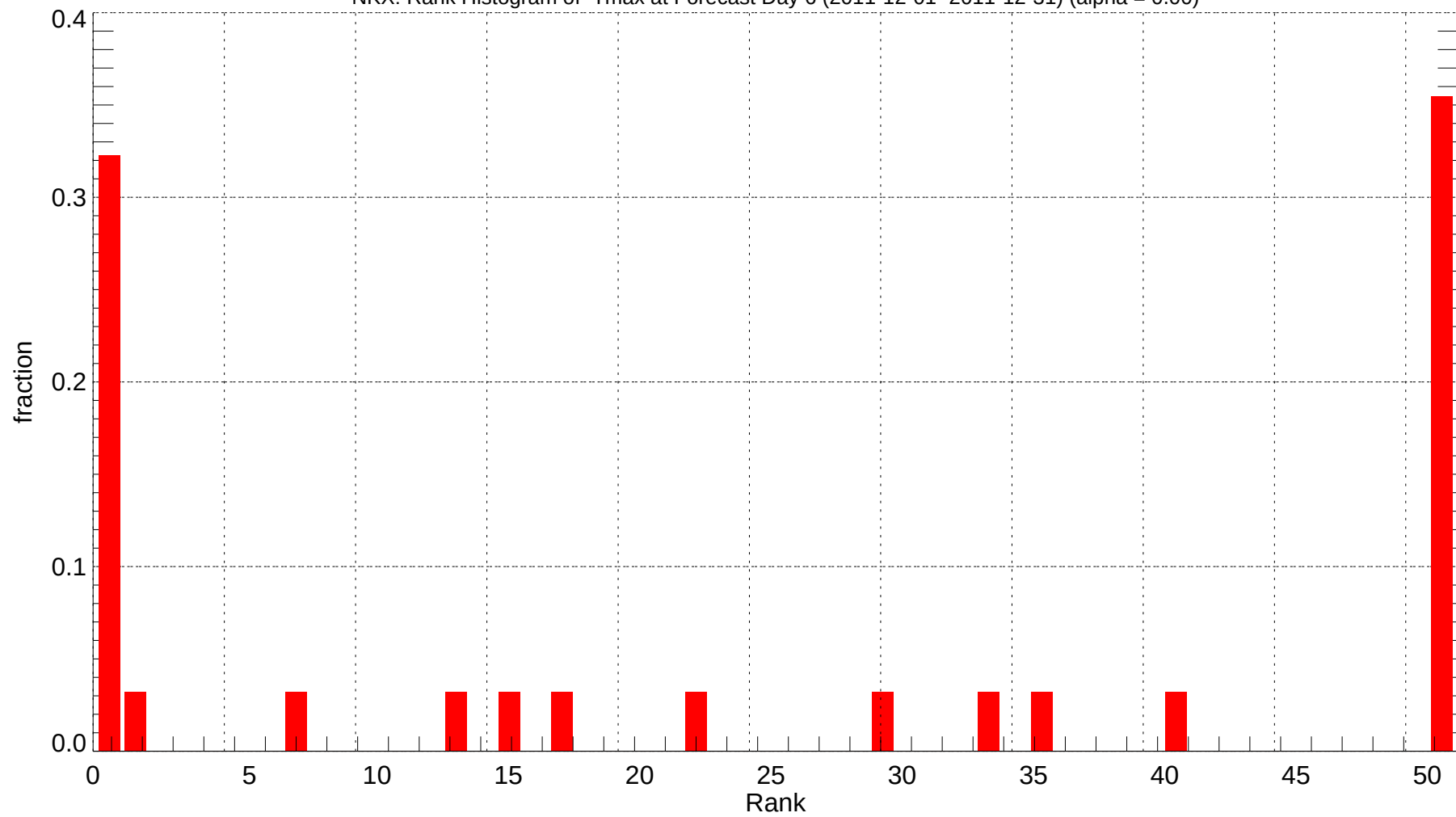
NKX: Rank Histogram of Tmax at Forecast Day 6 (2011-12-01~2011-12-31) (alpha = 0.00)
