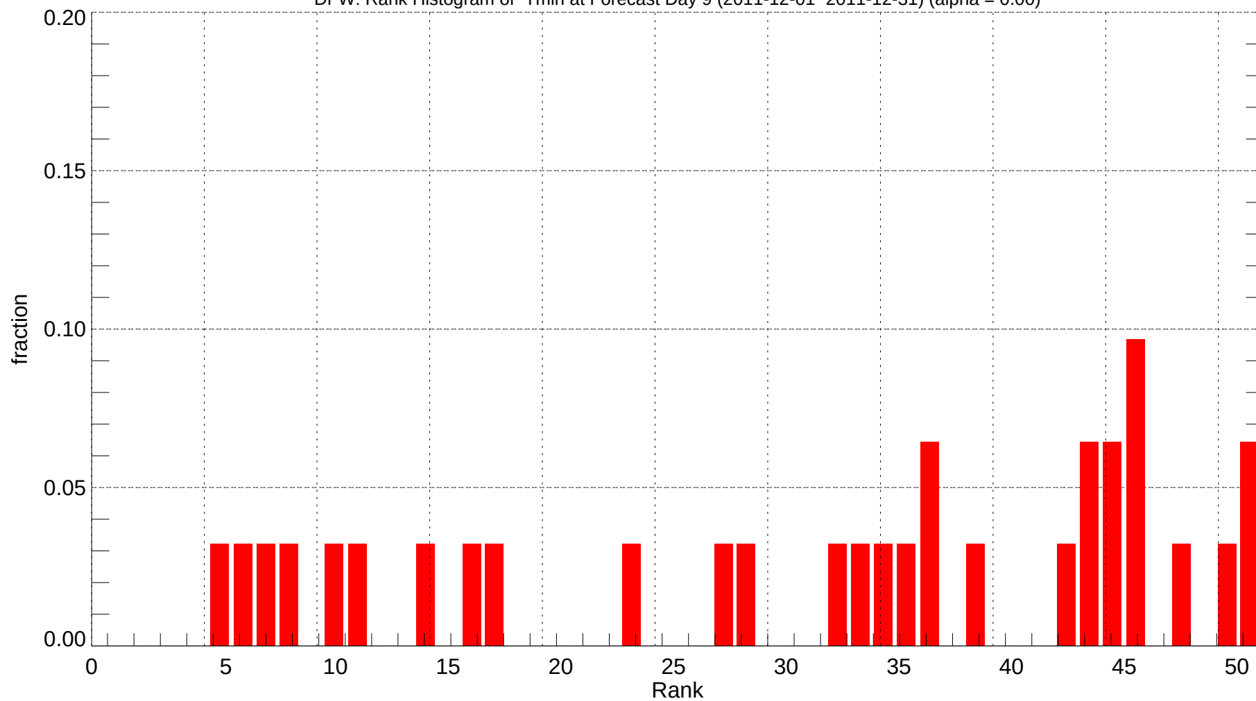
DFW: Rank Histogram of Tmin at Forecast Day 9 (2011-12-01~2011-12-31) (alpha = 0.00)
