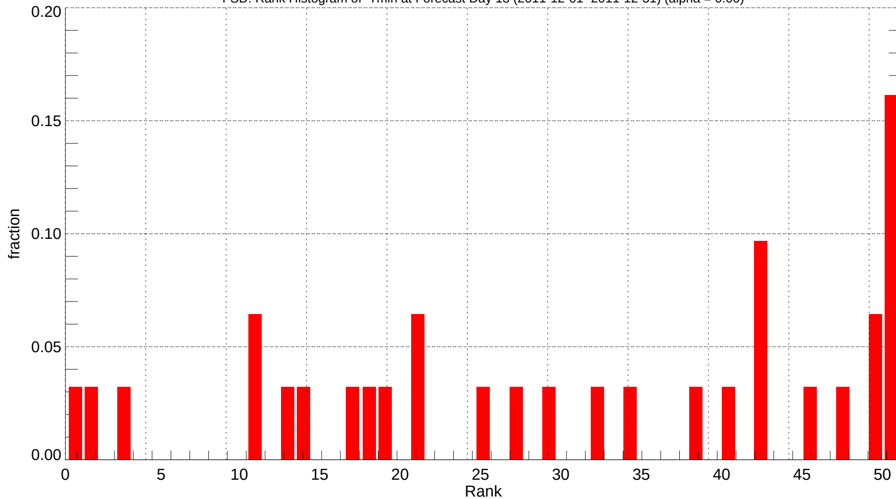
FSD: Rank Histogram of Tmin at Forecast Day 13 (2011-12-01~2011-12-31) (alpha = 0.00)
