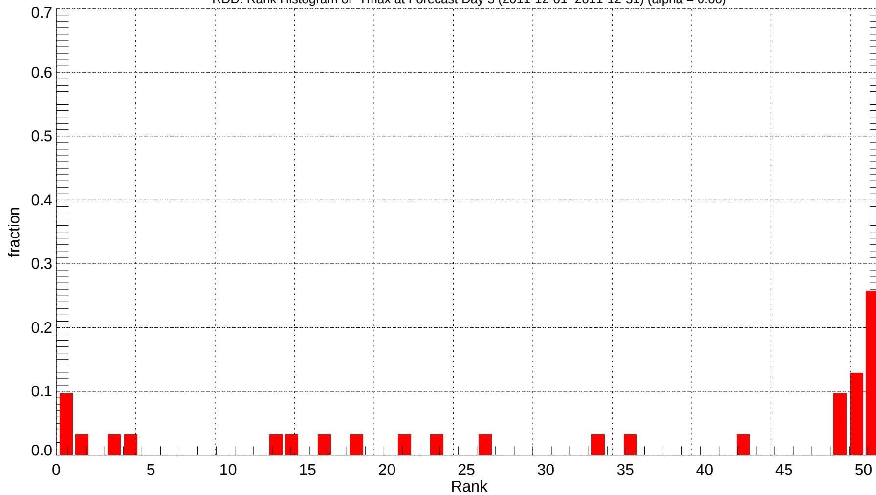
RDD: Rank Histogram of Tmax at Forecast Day 3 (2011-12-01~2011-12-31) (alpha = 0.00)
