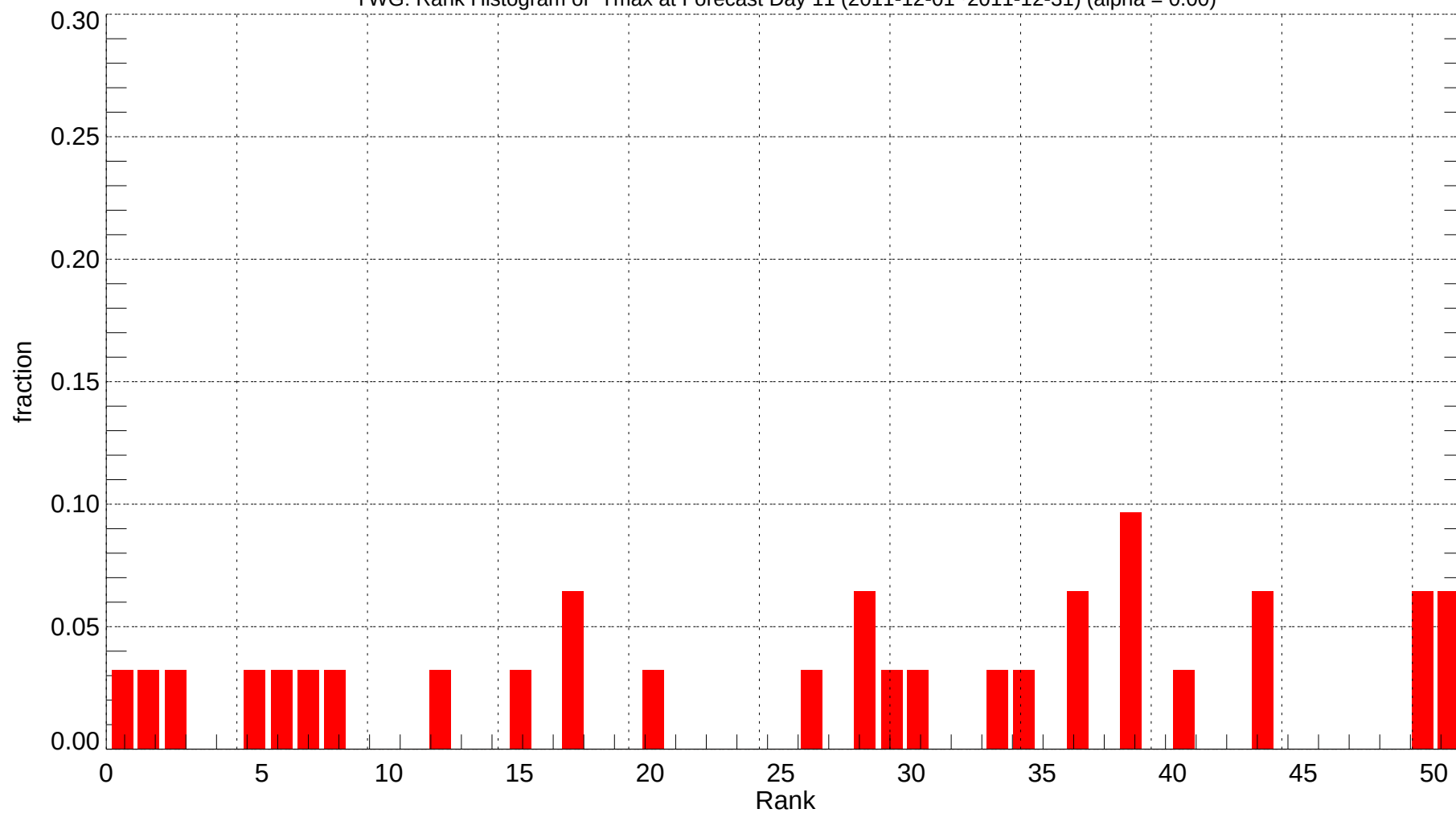
YWG: Rank Histogram of Tmax at Forecast Day 11 (2011-12-01~2011-12-31) (alpha = 0.00)
