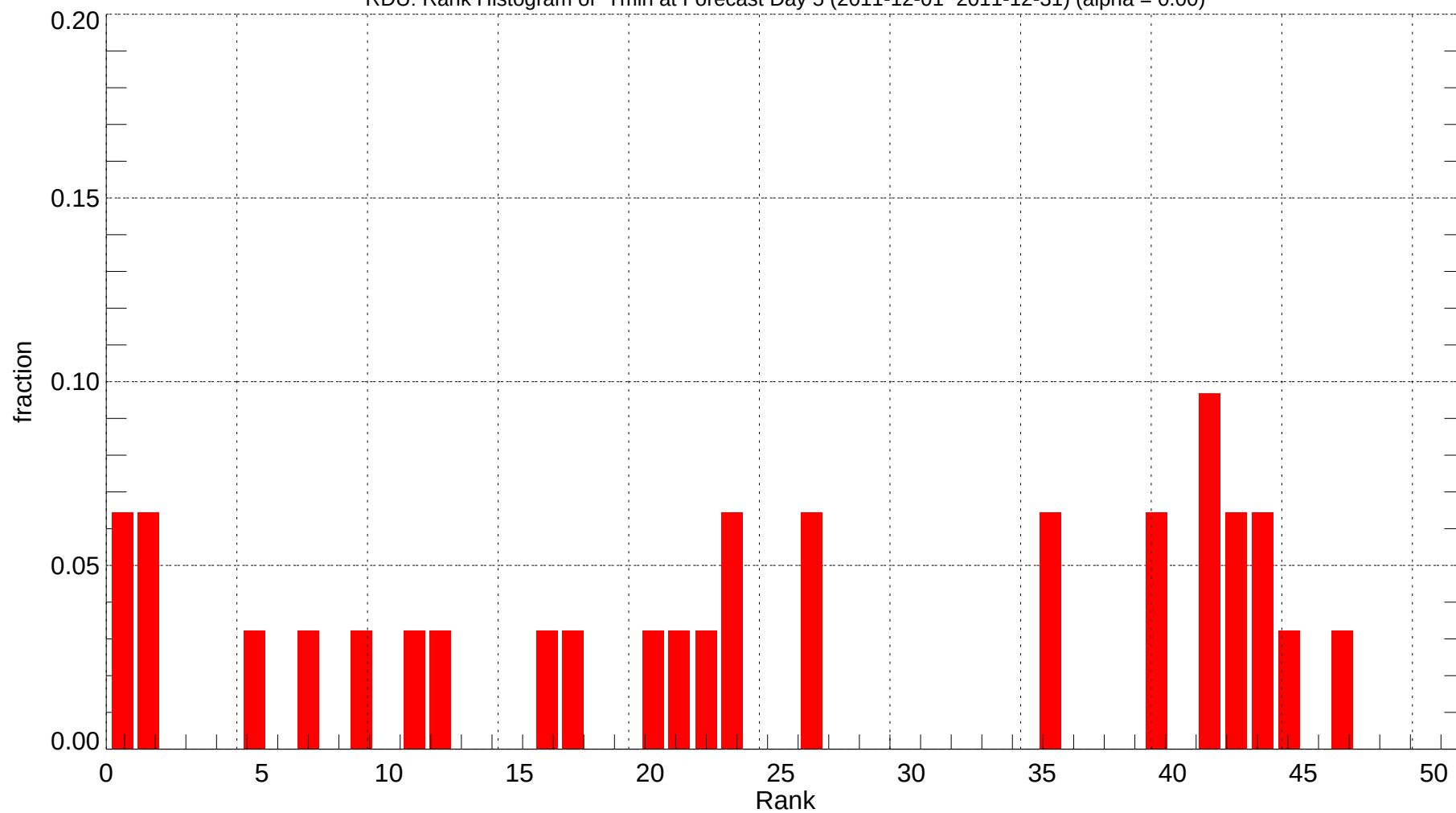
RDU: Rank Histogram of Tmin at Forecast Day 5 (2011-12-01~2011-12-31) (alpha = 0.00)
