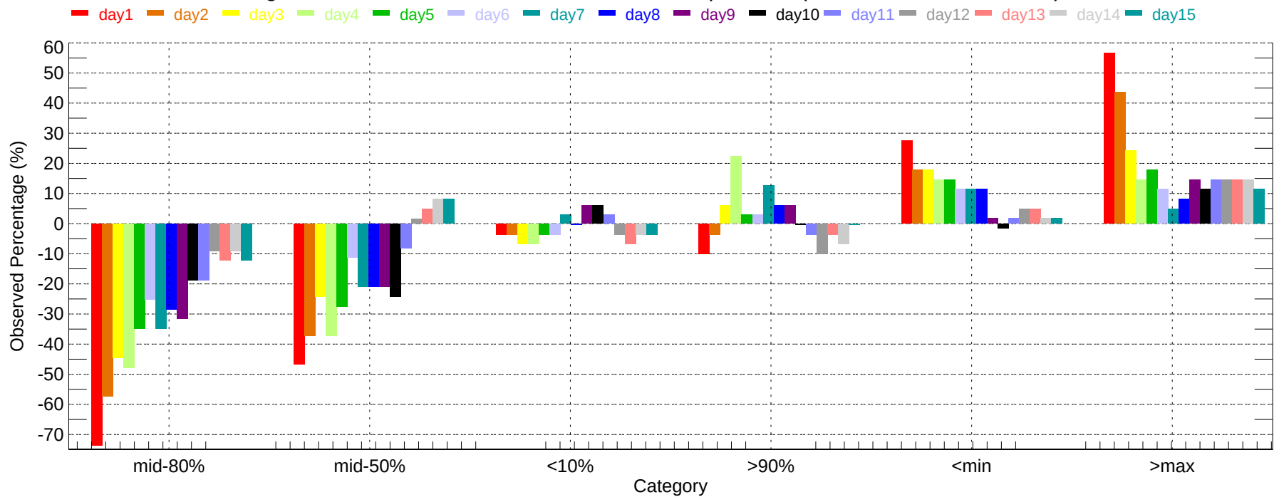
Observed Percentage Deviation of Ensembles - HOU: Min Temperature (2011-12-01~2011-12-31)
