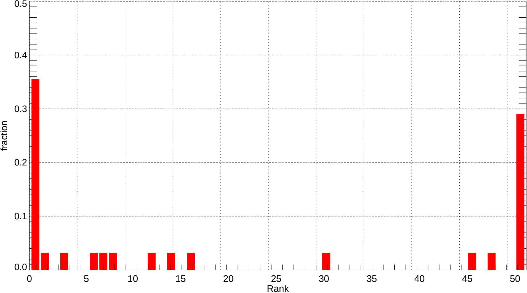
SJC: Rank Histogram of Tmin at Forecast Day 2 (2011-12-01~2011-12-31) (alpha = 0.00)
