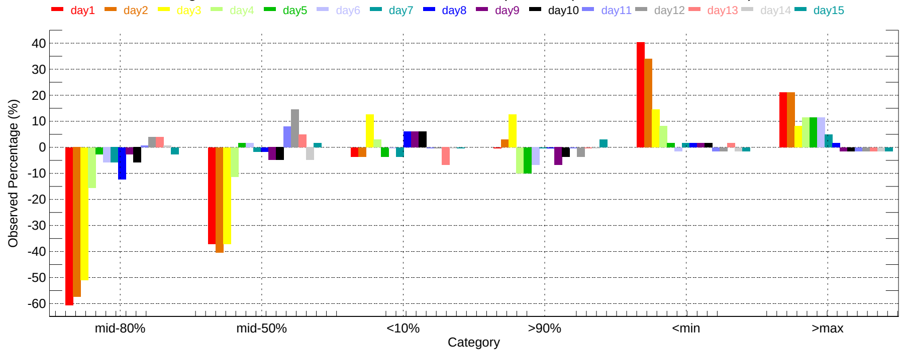
Observed Percentage Deviation of Ensembles - TRM: Max Temperature (2011-12-01~2011-12-31)
