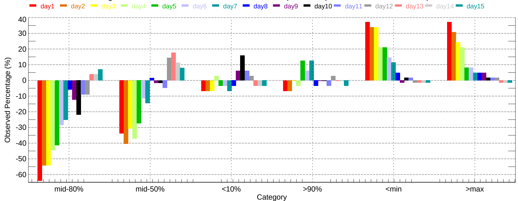
Observed Percentage Deviation of Ensembles - YKM: Min Temperature (2011-12-01~2011-12-31)
