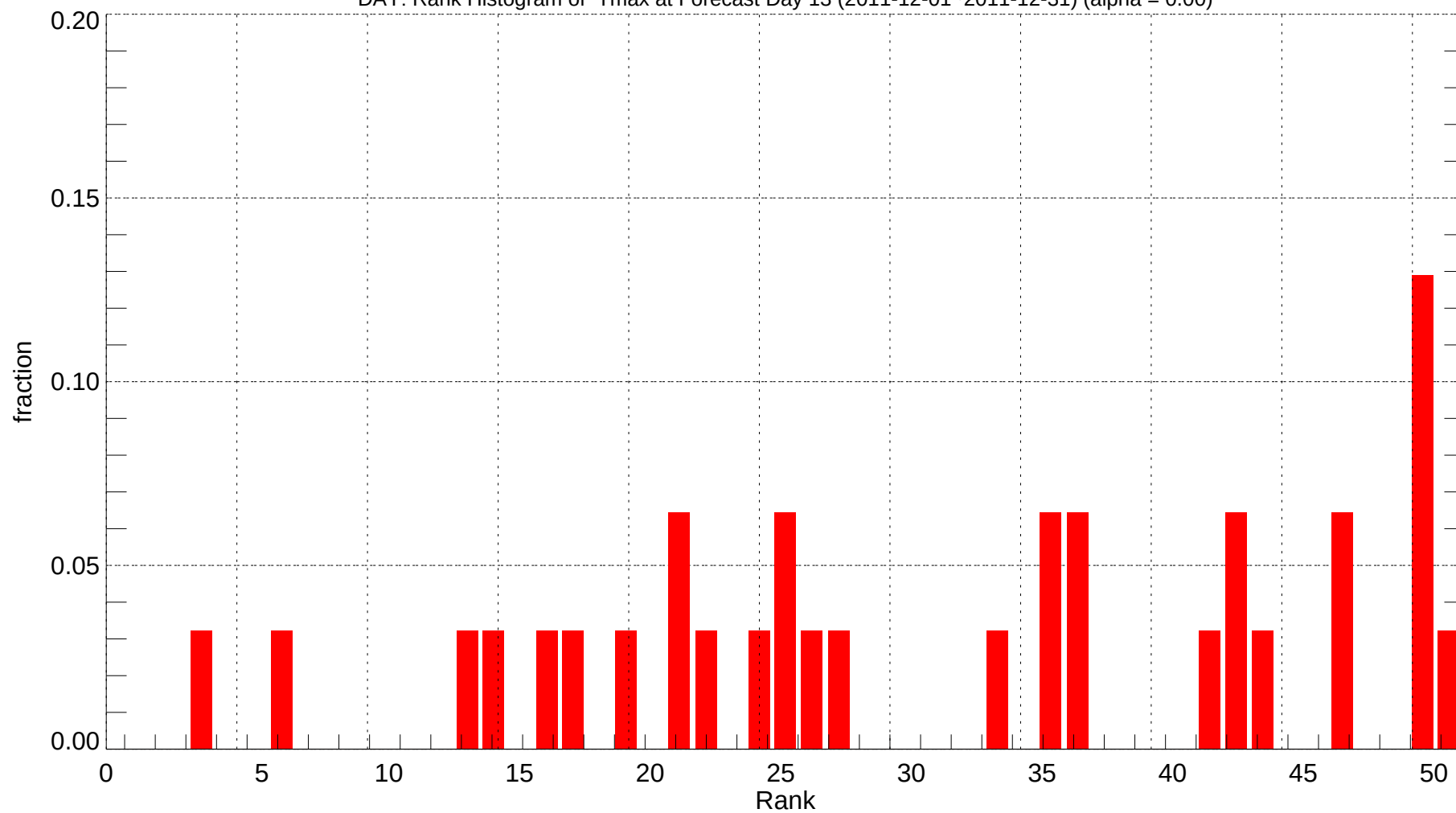
DAY: Rank Histogram of Tmax at Forecast Day 13 (2011-12-01~2011-12-31) (alpha = 0.00)
