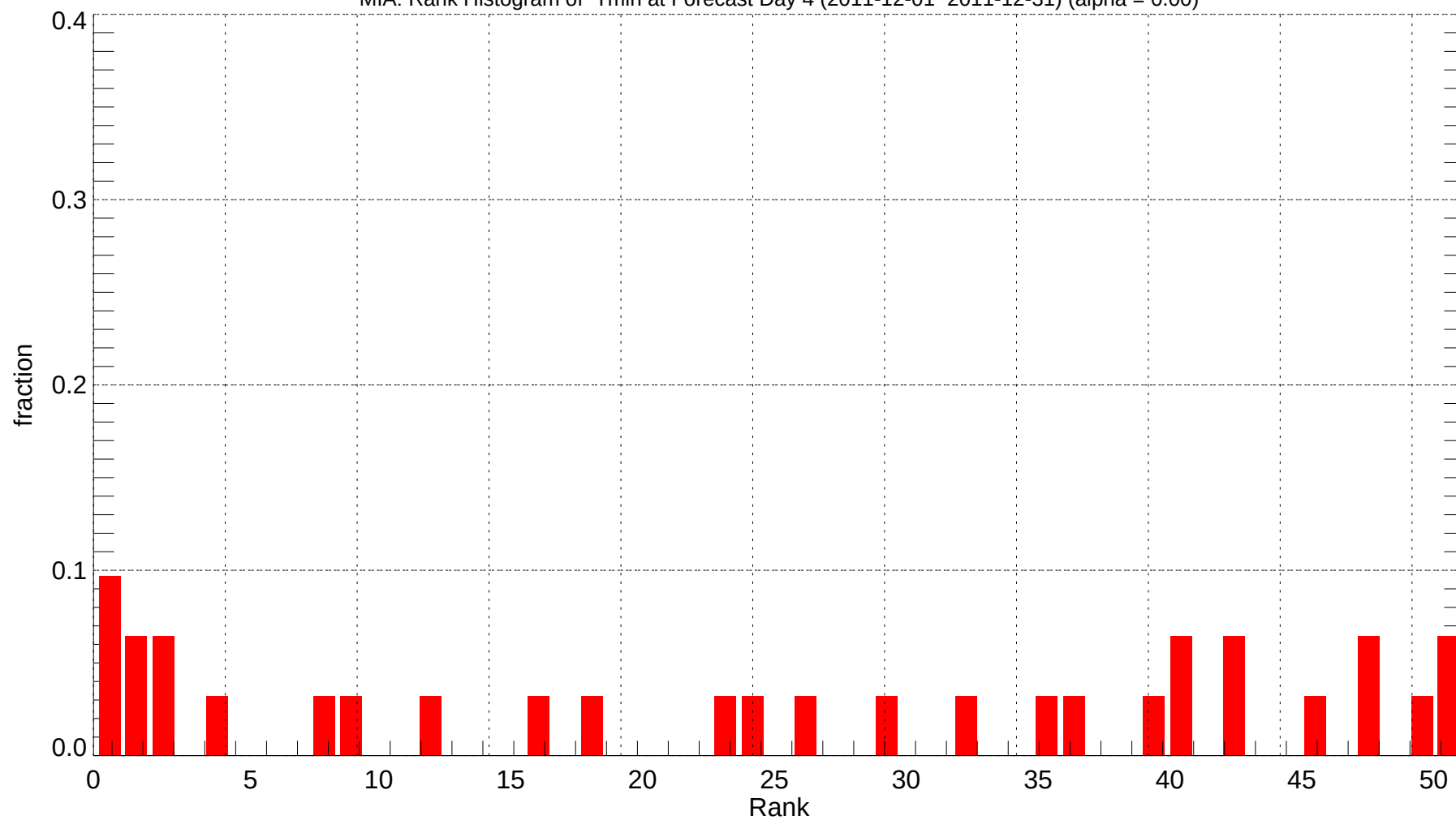
MIA: Rank Histogram of Tmin at Forecast Day 4 (2011-12-01~2011-12-31) (alpha = 0.00)
