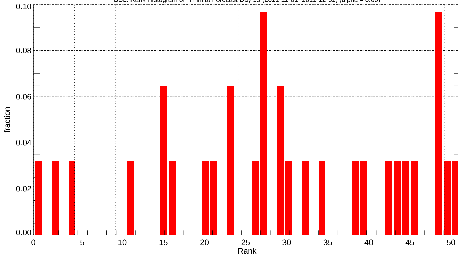
BDL: Rank Histogram of Tmin at Forecast Day 15 (2011-12-01~2011-12-31) (alpha = 0.00)
