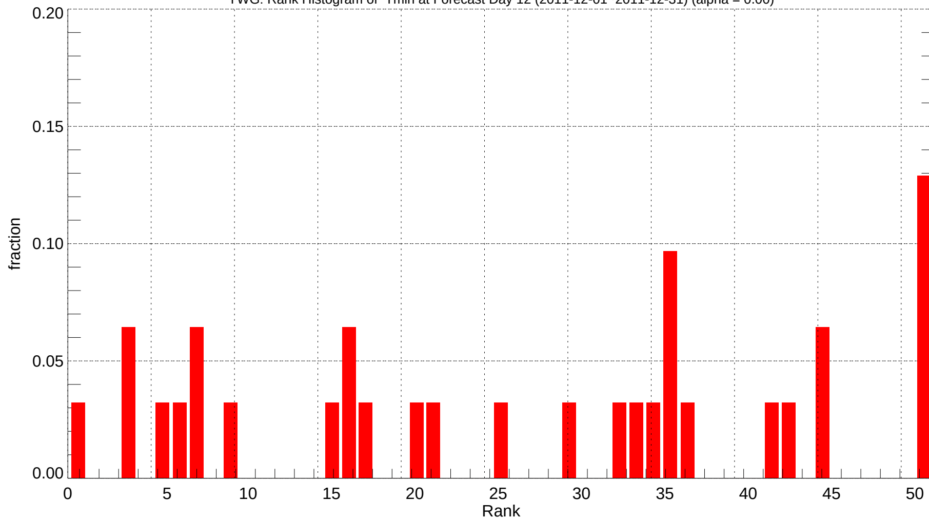
YWG: Rank Histogram of Tmin at Forecast Day 12 (2011-12-01~2011-12-31) (alpha = 0.00)
