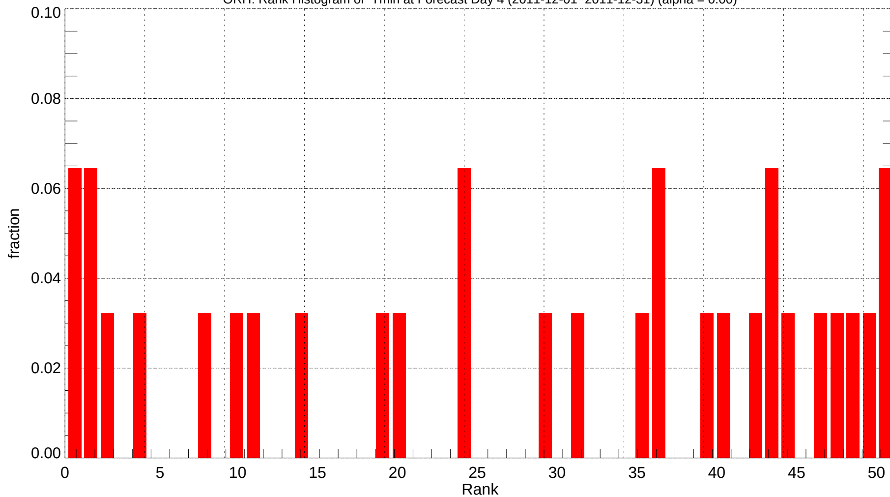
ORH: Rank Histogram of Tmin at Forecast Day 4 (2011-12-01~2011-12-31) (alpha = 0.00)
