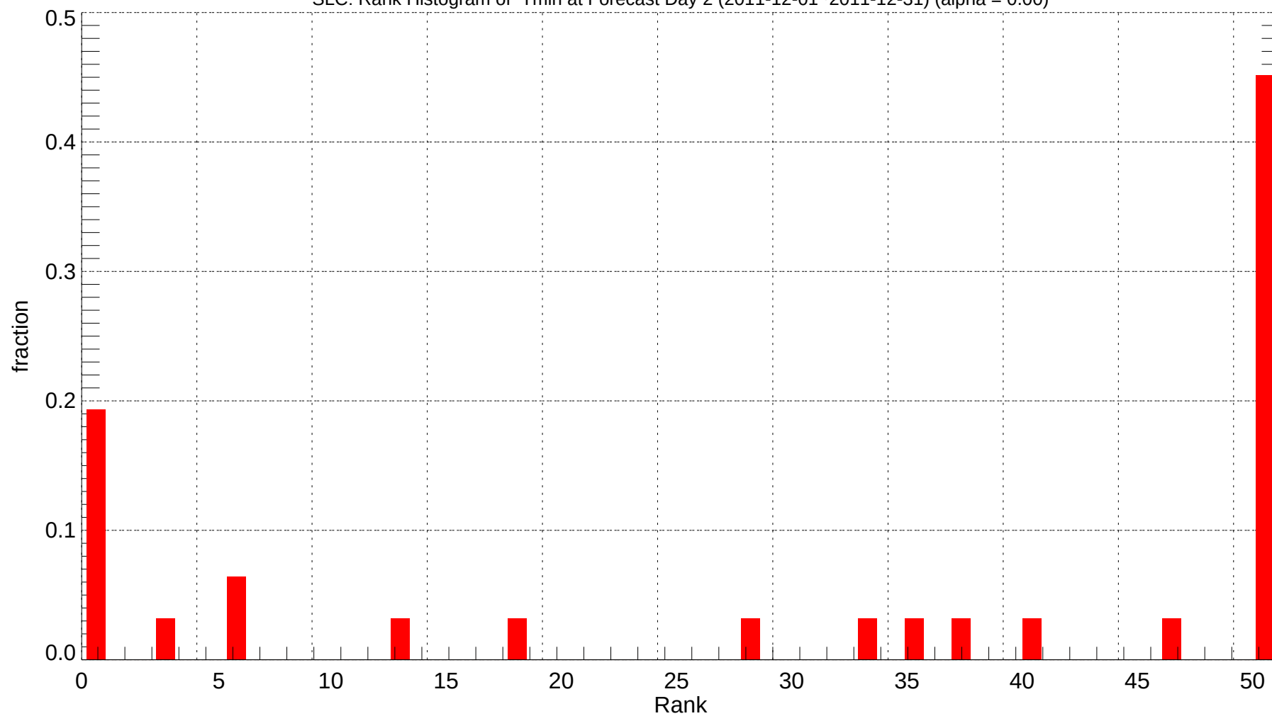
SLC: Rank Histogram of Tmin at Forecast Day 2 (2011-12-01~2011-12-31) (alpha = 0.00)
