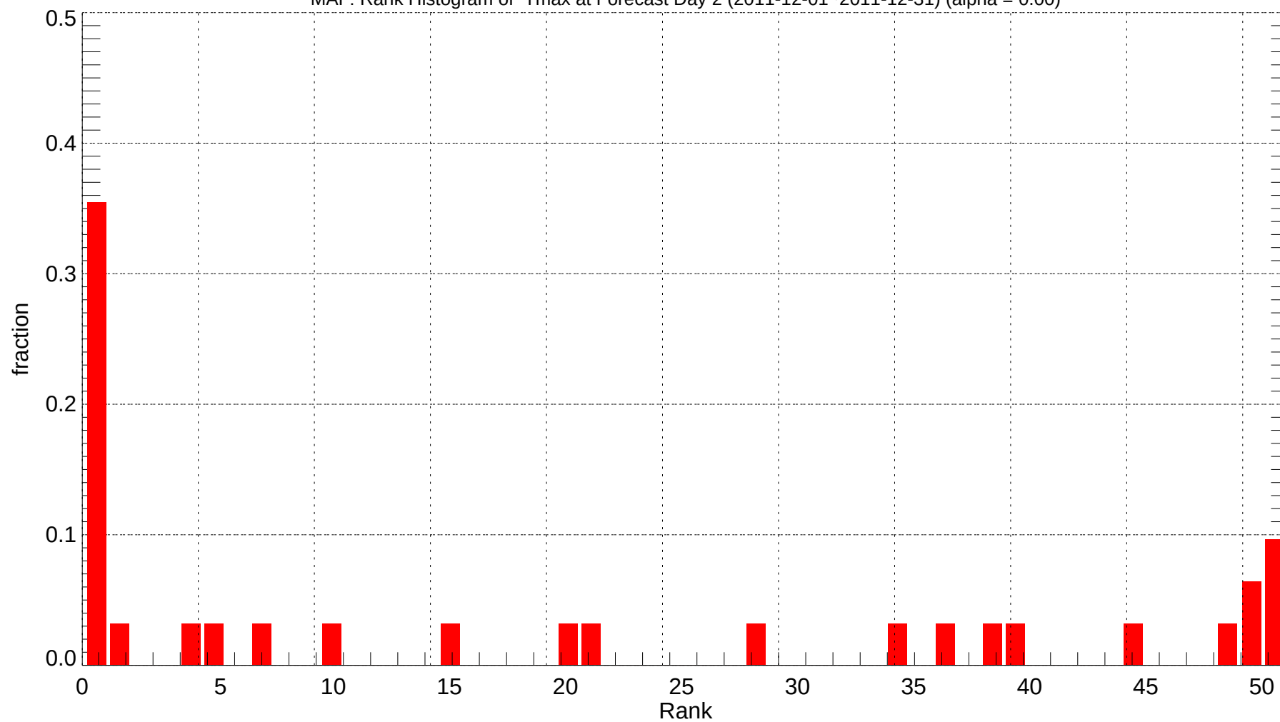
MAF: Rank Histogram of Tmax at Forecast Day 2 (2011-12-01~2011-12-31) (alpha = 0.00)
