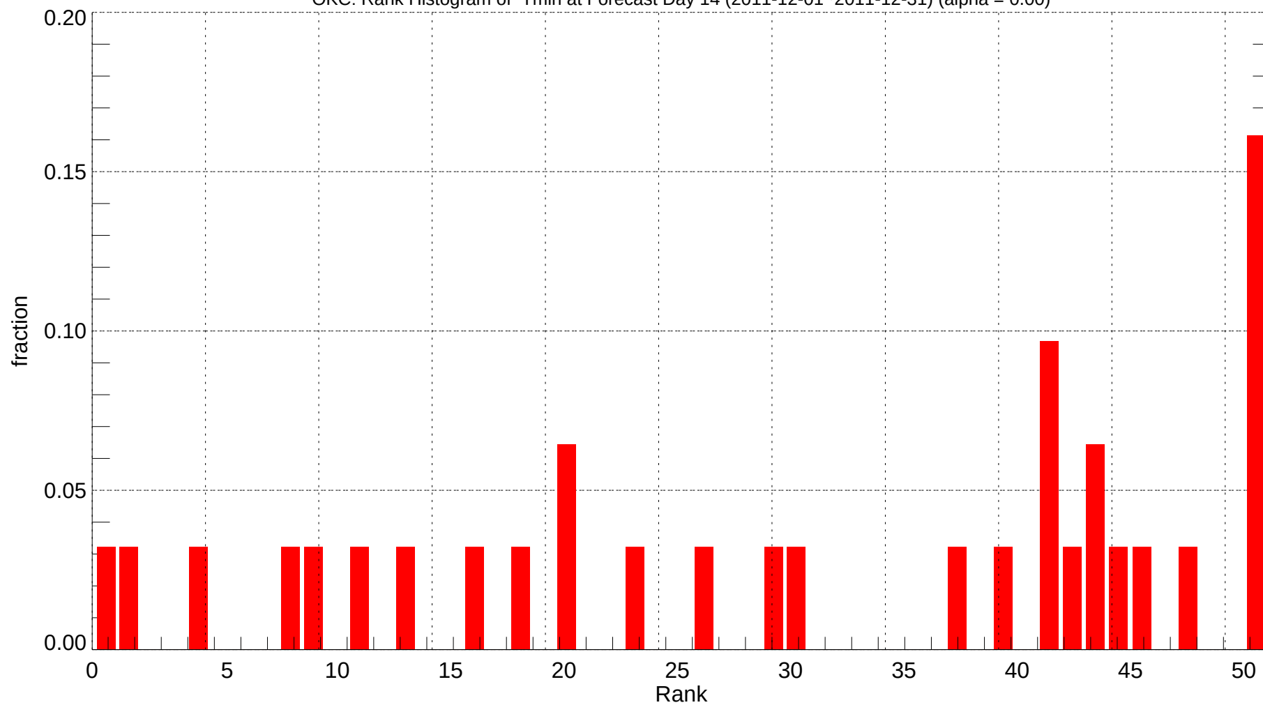
OKC: Rank Histogram of Tmin at Forecast Day 14 (2011-12-01~2011-12-31) (alpha = 0.00)
