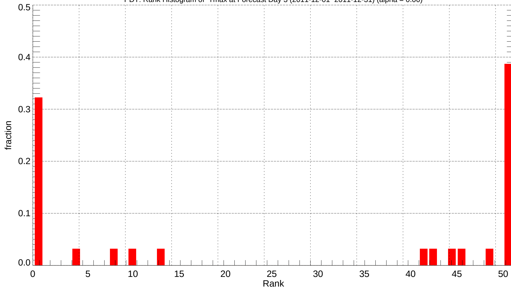
PDT: Rank Histogram of Tmax at Forecast Day 3 (2011-12-01~2011-12-31) (alpha = 0.00)
