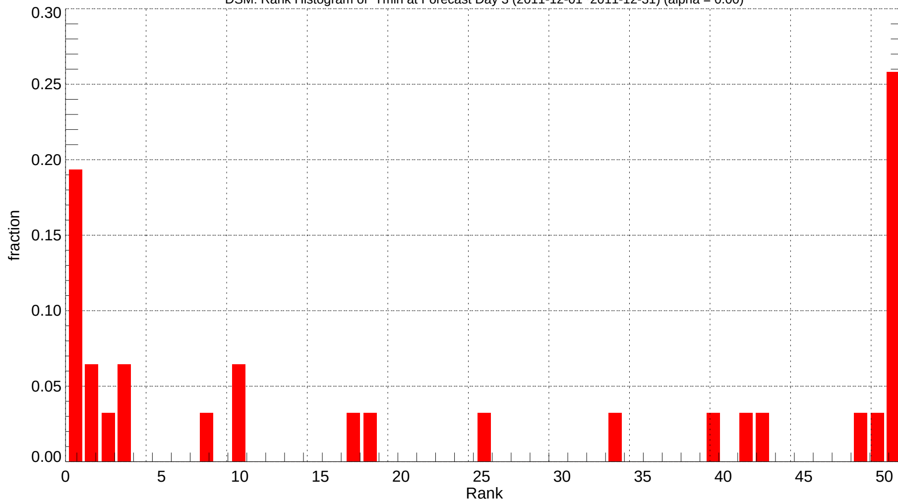
DSM: Rank Histogram of Tmin at Forecast Day 3 (2011-12-01~2011-12-31) (alpha = 0.00)
