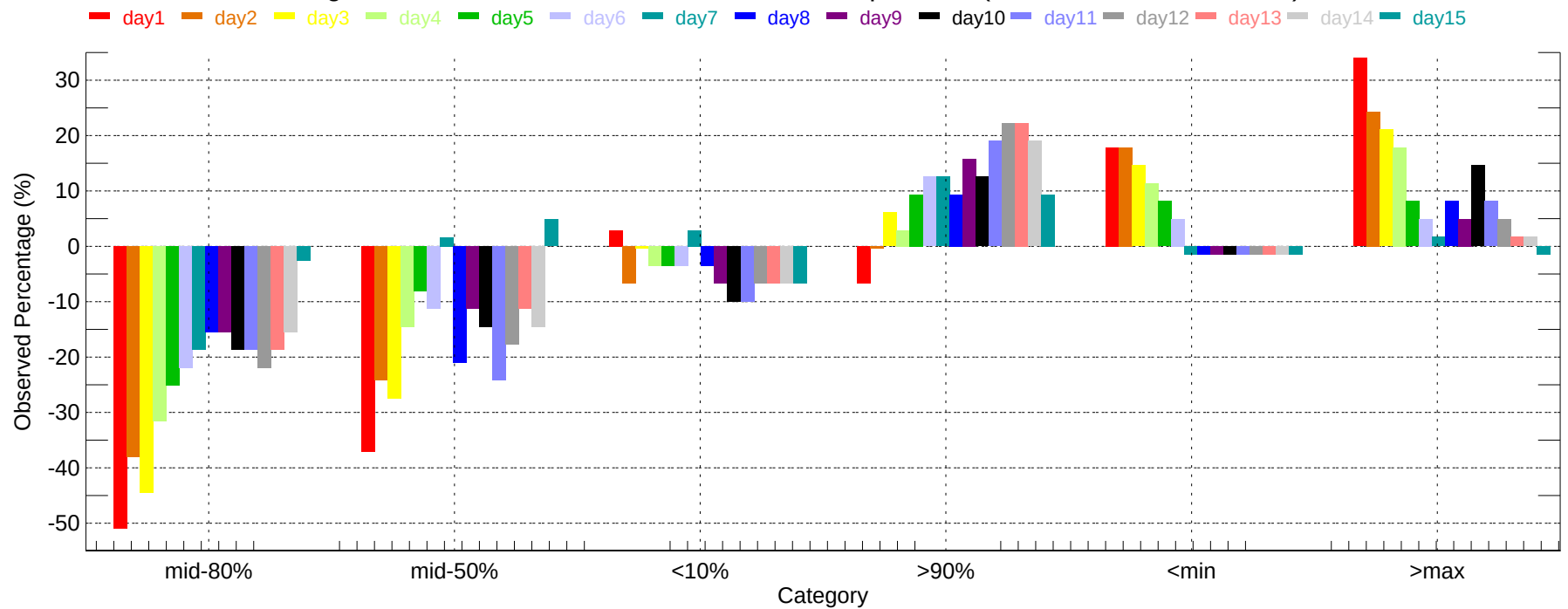
Observed Percentage Deviation of Ensembles - FWA: Min Temperature (2011-12-01~2011-12-31)
