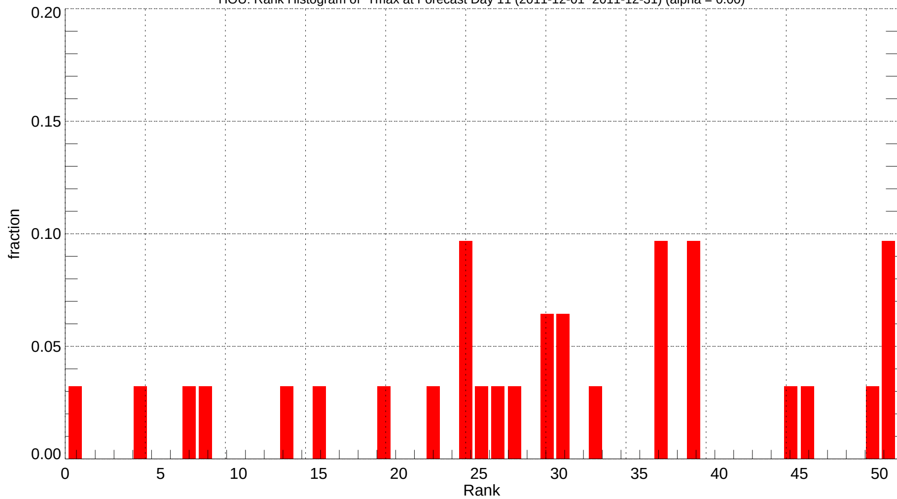
HOU: Rank Histogram of Tmax at Forecast Day 11 (2011-12-01~2011-12-31) (alpha = 0.00)
