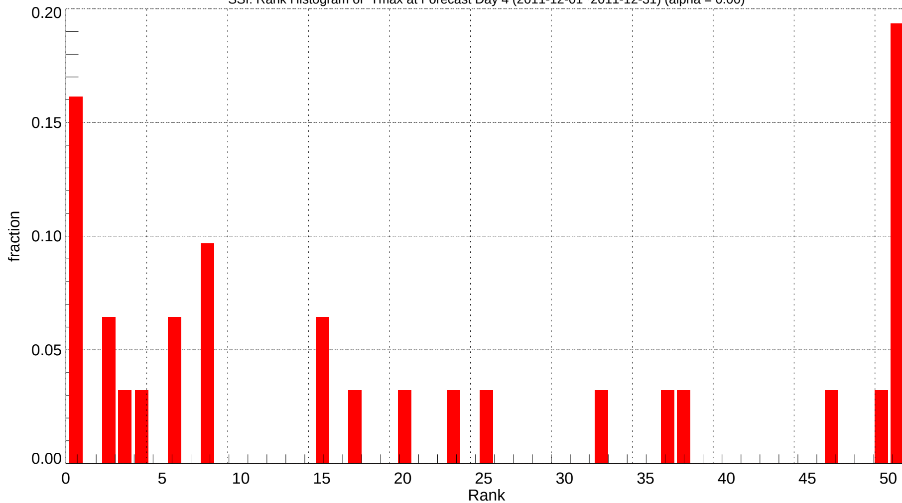
SSI: Rank Histogram of Tmax at Forecast Day 4 (2011-12-01~2011-12-31) (alpha = 0.00)
