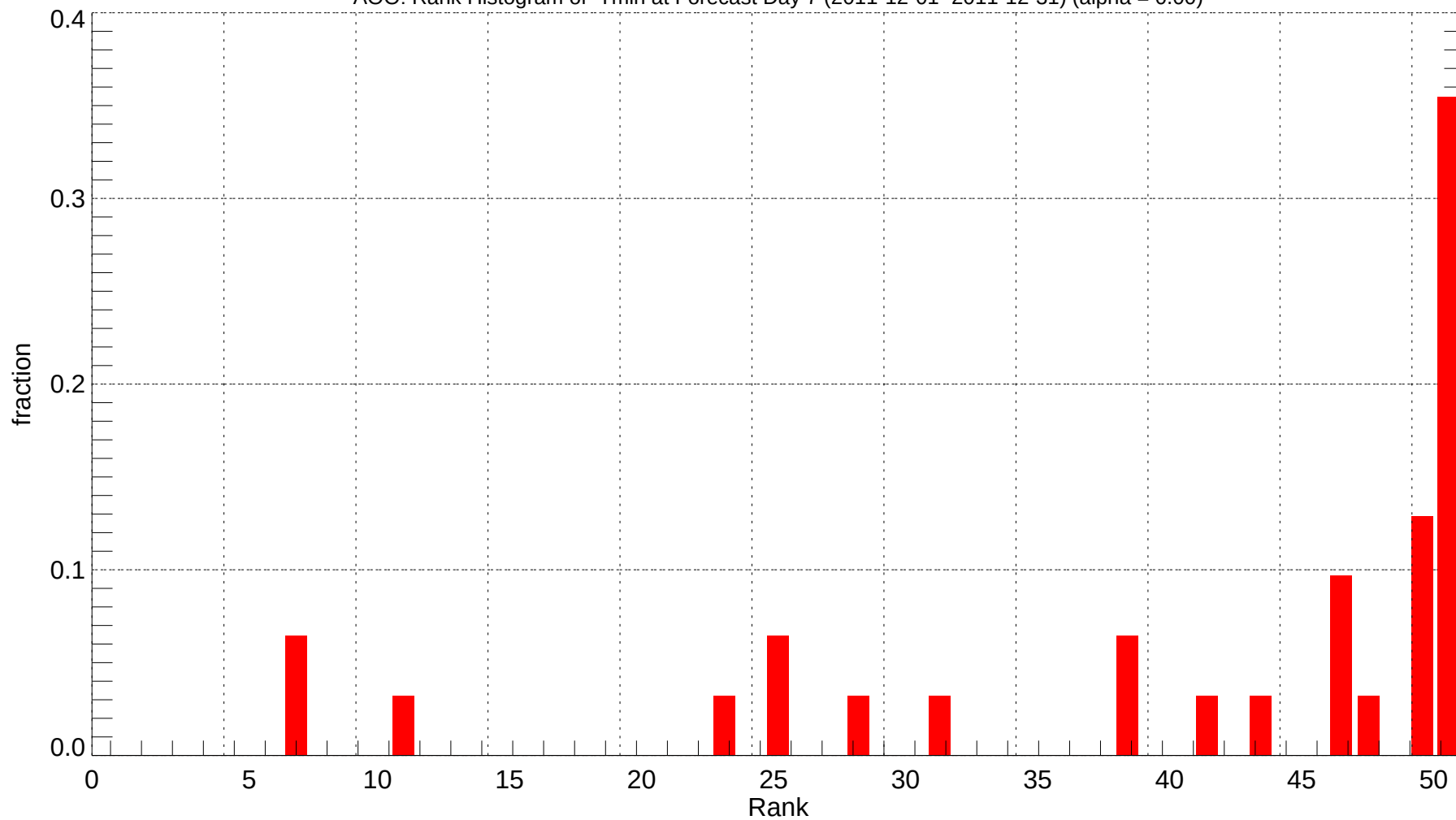
AOO: Rank Histogram of Tmin at Forecast Day 7 (2011-12-01~2011-12-31) (alpha = 0.00)
