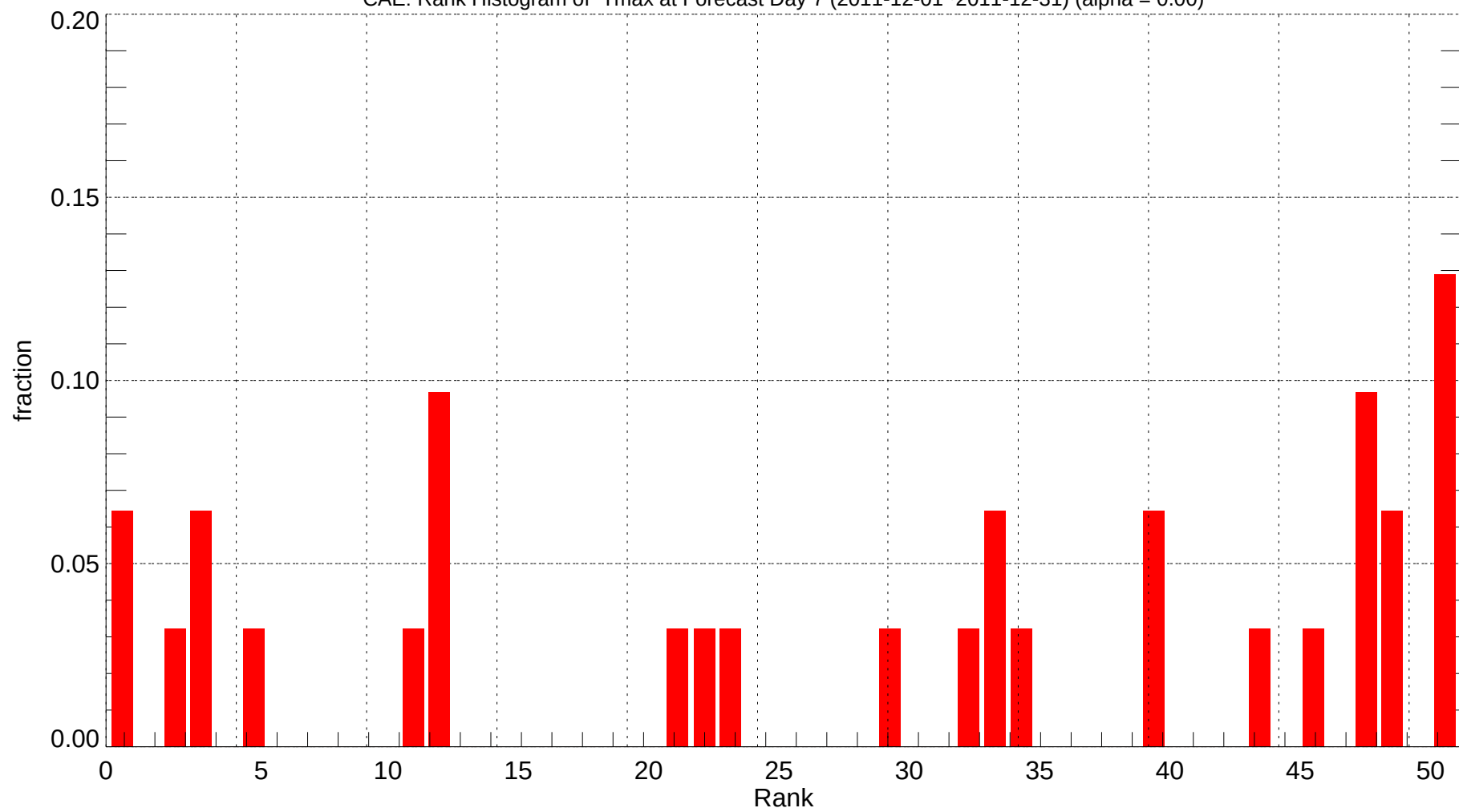
CAE: Rank Histogram of Tmax at Forecast Day 7 (2011-12-01~2011-12-31) (alpha = 0.00)
