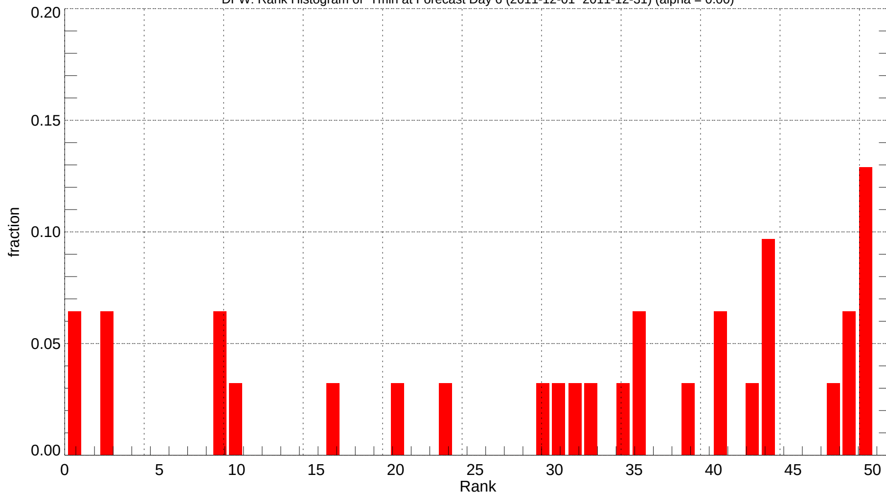
DFW: Rank Histogram of Tmin at Forecast Day 6 (2011-12-01~2011-12-31) (alpha = 0.00)
