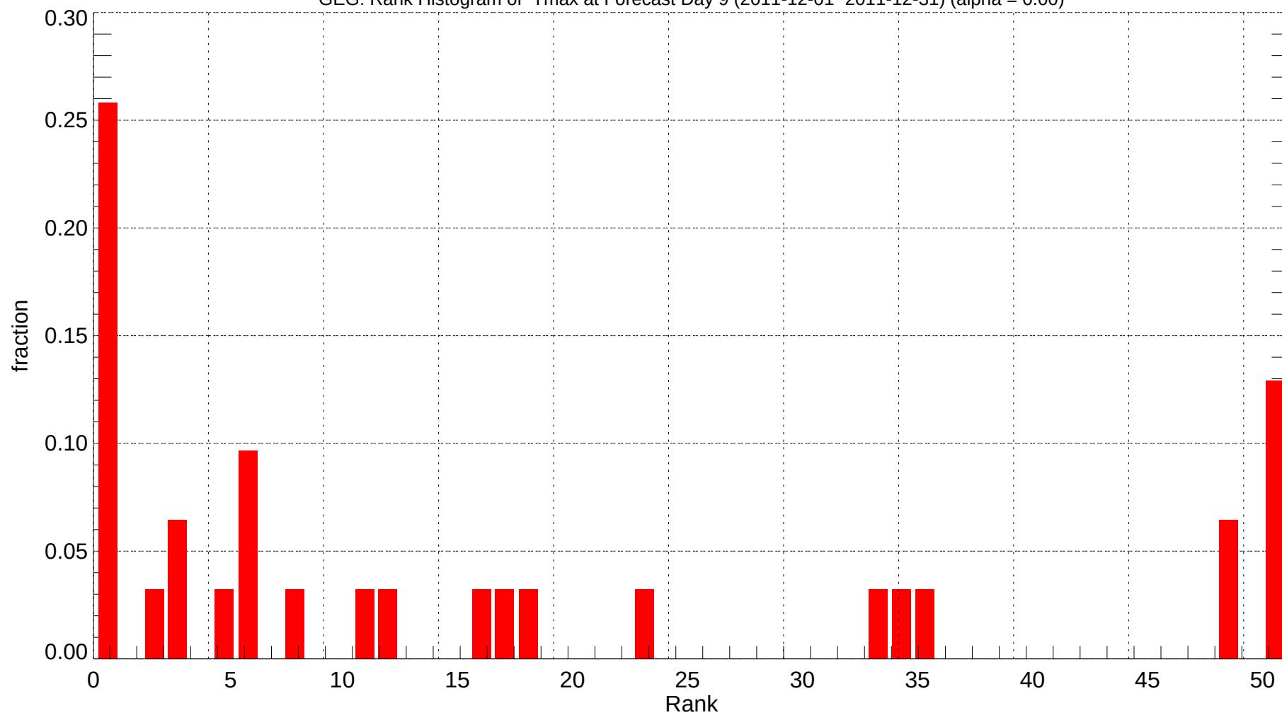
GEG: Rank Histogram of Tmax at Forecast Day 9 (2011-12-01~2011-12-31) (alpha = 0.00)
