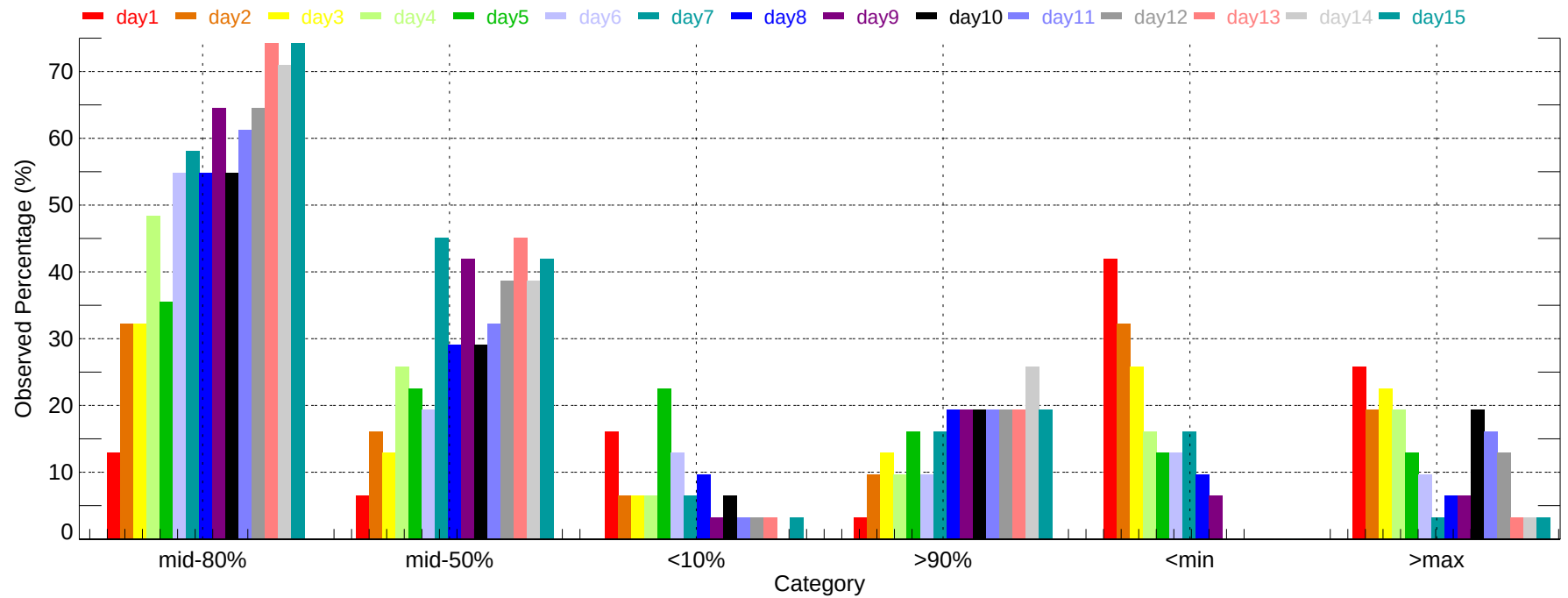
Observed Percentage of Ensembles - APN: Min Temperature (2011-12-01~2011-12-31)
