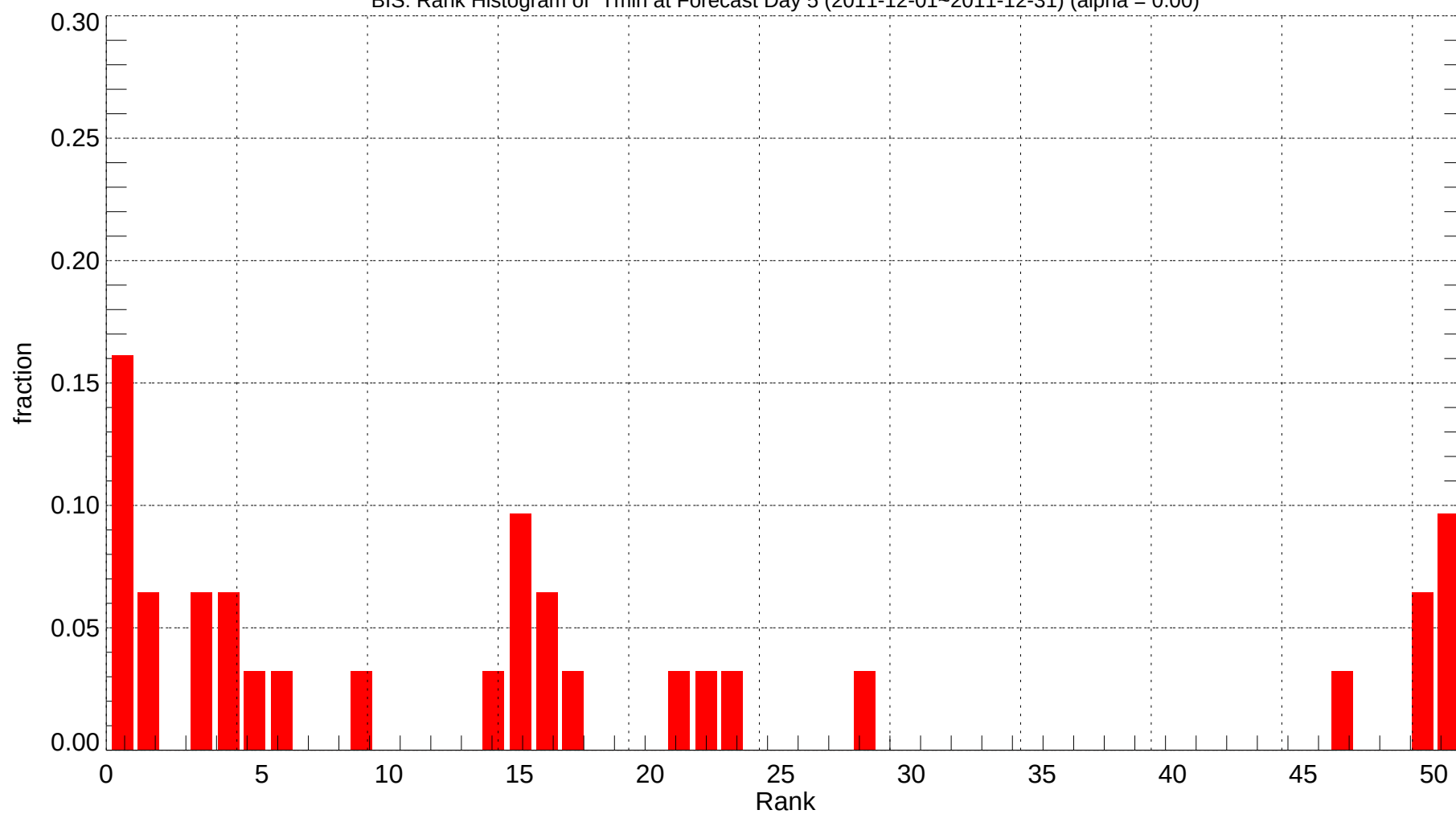
BIS: Rank Histogram of Tmin at Forecast Day 5 (2011-12-01~2011-12-31) (alpha = 0.00)
