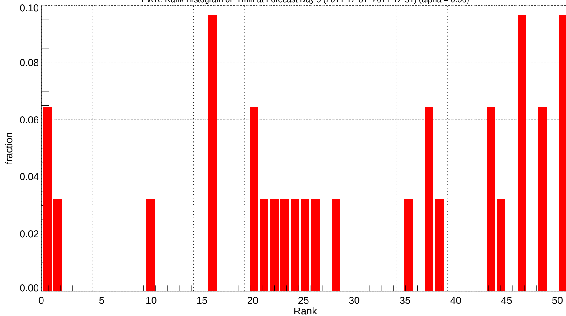
EWR: Rank Histogram of Tmin at Forecast Day 9 (2011-12-01~2011-12-31) (alpha = 0.00)
