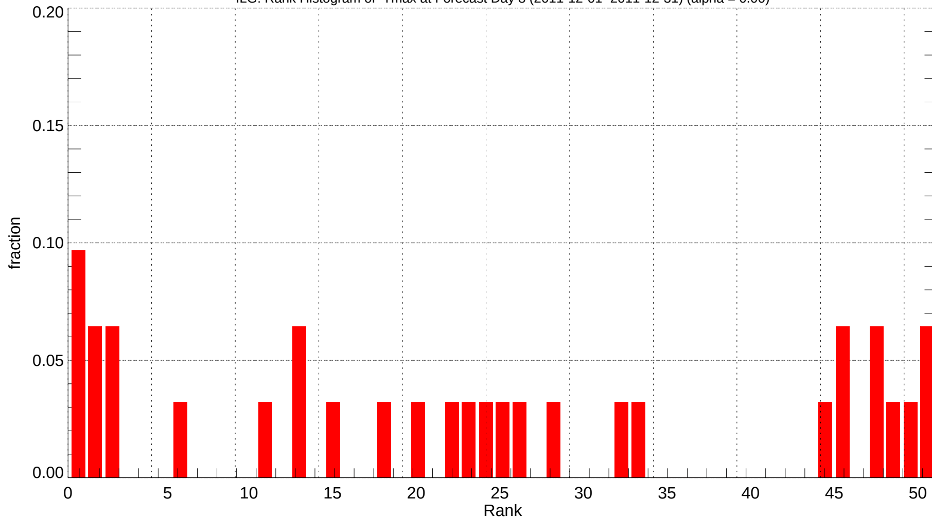
ILG: Rank Histogram of Tmax at Forecast Day 8 (2011-12-01~2011-12-31) (alpha = 0.00)
