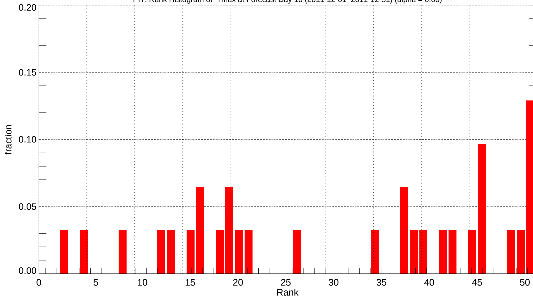
PIT: Rank Histogram of Tmax at Forecast Day 10 (2011-12-01~2011-12-31) (alpha = 0.00)
