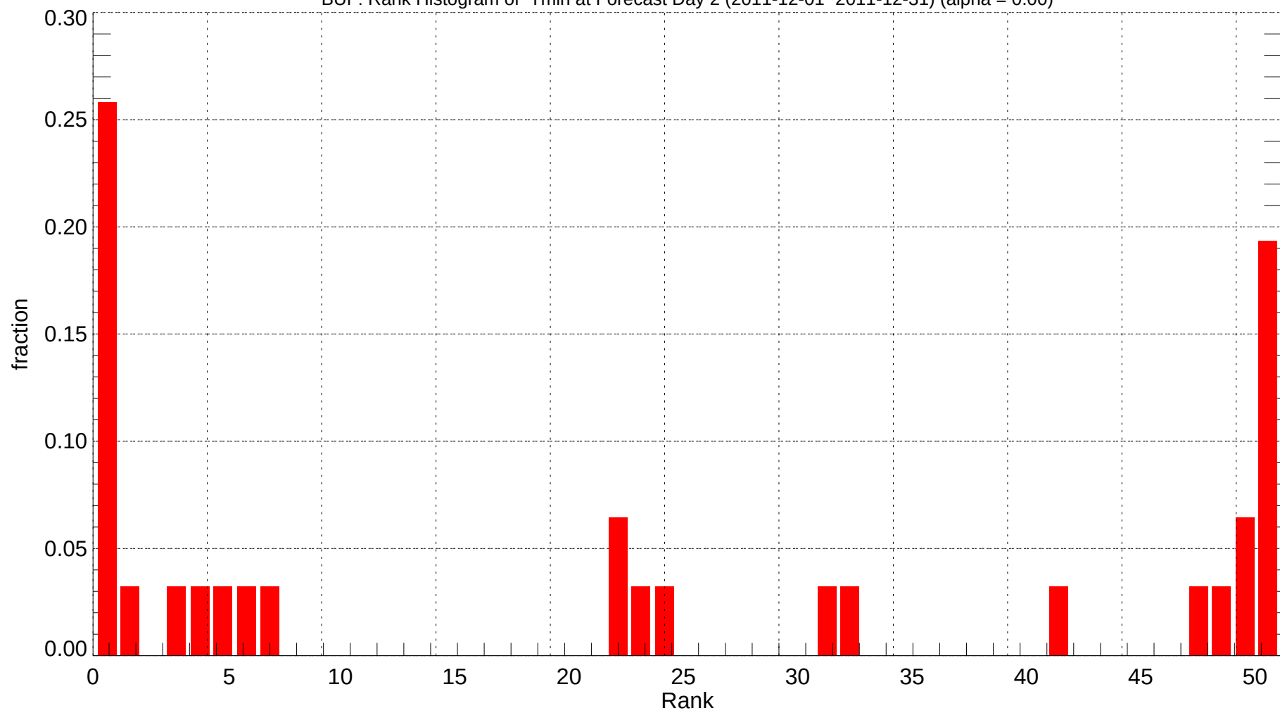
BUF: Rank Histogram of Tmin at Forecast Day 2 (2011-12-01~2011-12-31) (alpha = 0.00)
