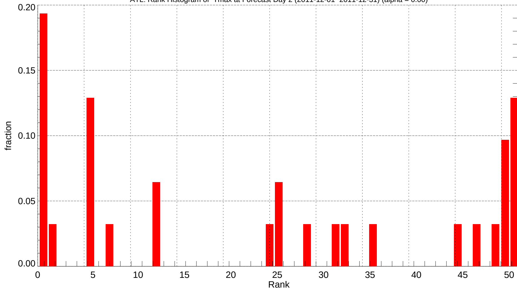
ATL: Rank Histogram of Tmax at Forecast Day 2 (2011-12-01~2011-12-31) (alpha = 0.00)
