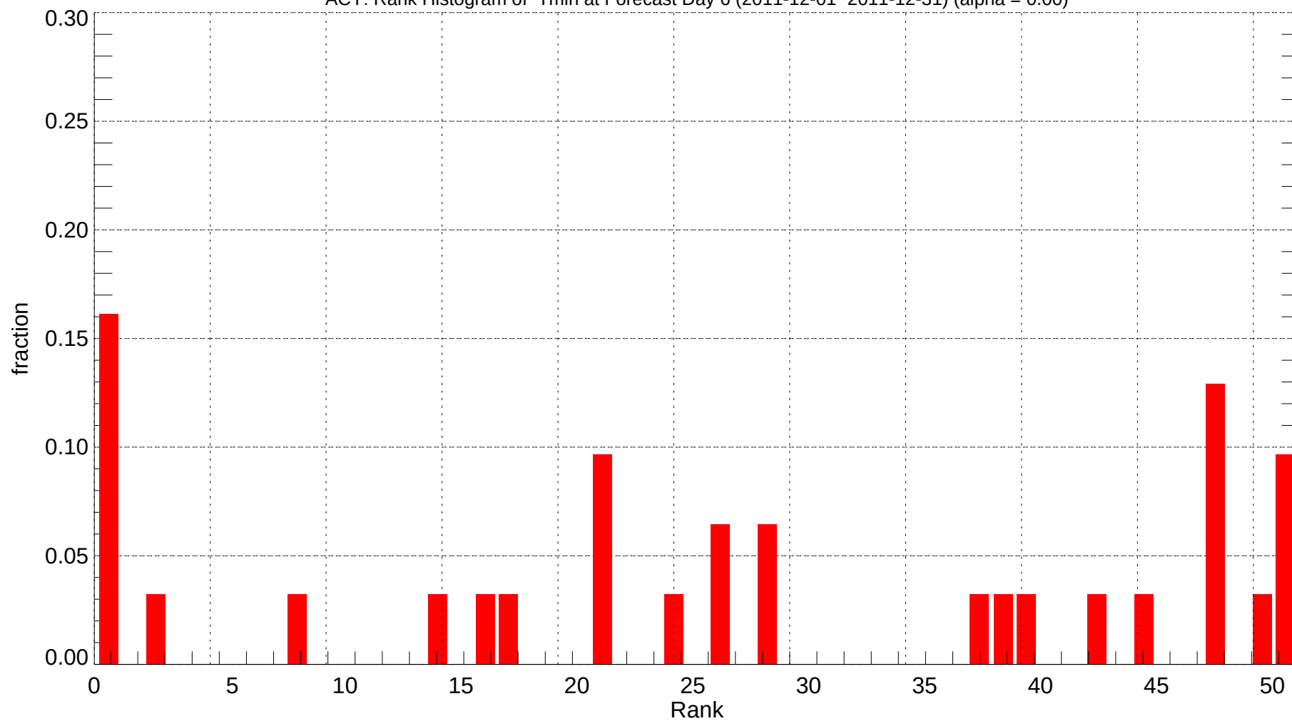
ACY: Rank Histogram of Tmin at Forecast Day 6 (2011-12-01~2011-12-31) (alpha = 0.00)
