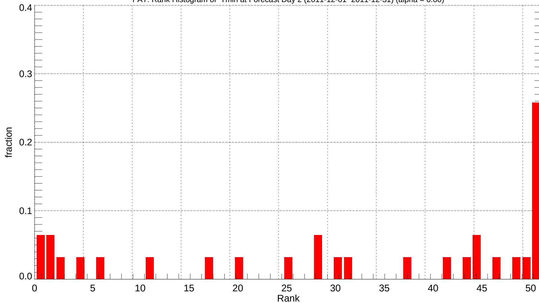
FAT: Rank Histogram of Tmin at Forecast Day 2 (2011-12-01~2011-12-31) (alpha = 0.00)
