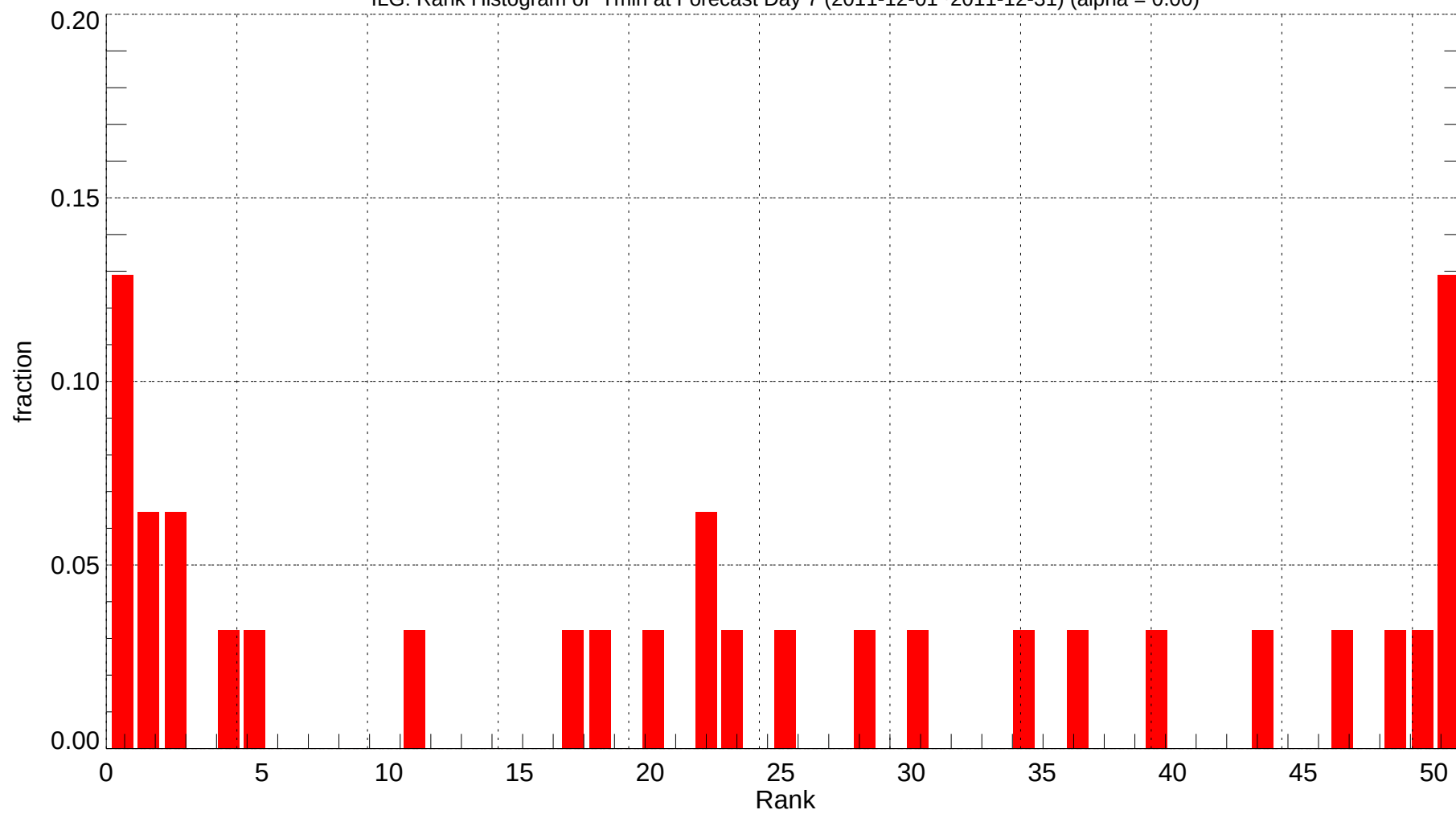
ILG: Rank Histogram of Tmin at Forecast Day 7 (2011-12-01~2011-12-31) (alpha = 0.00)
