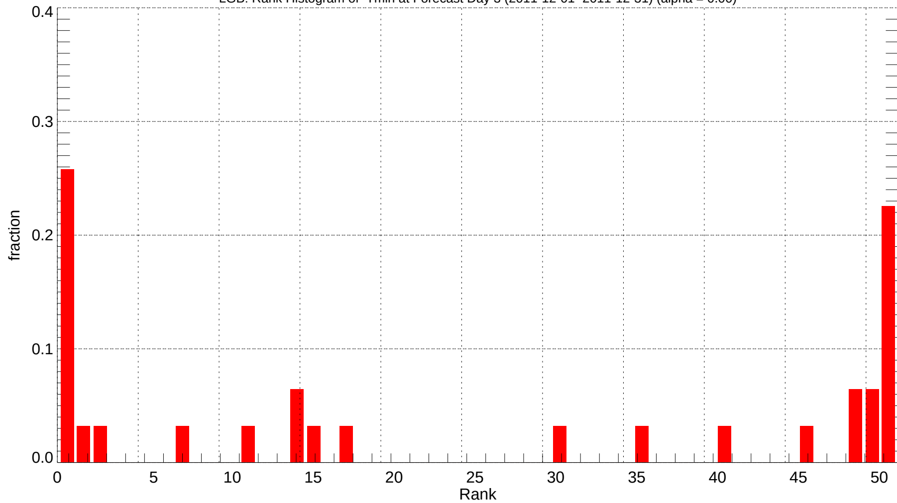
LGB: Rank Histogram of Tmin at Forecast Day 3 (2011-12-01~2011-12-31) (alpha = 0.00)
