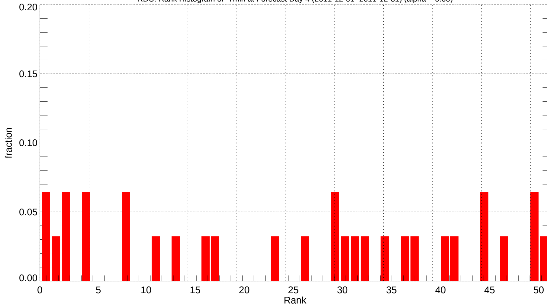
RDU: Rank Histogram of Tmin at Forecast Day 4 (2011-12-01~2011-12-31) (alpha = 0.00)
