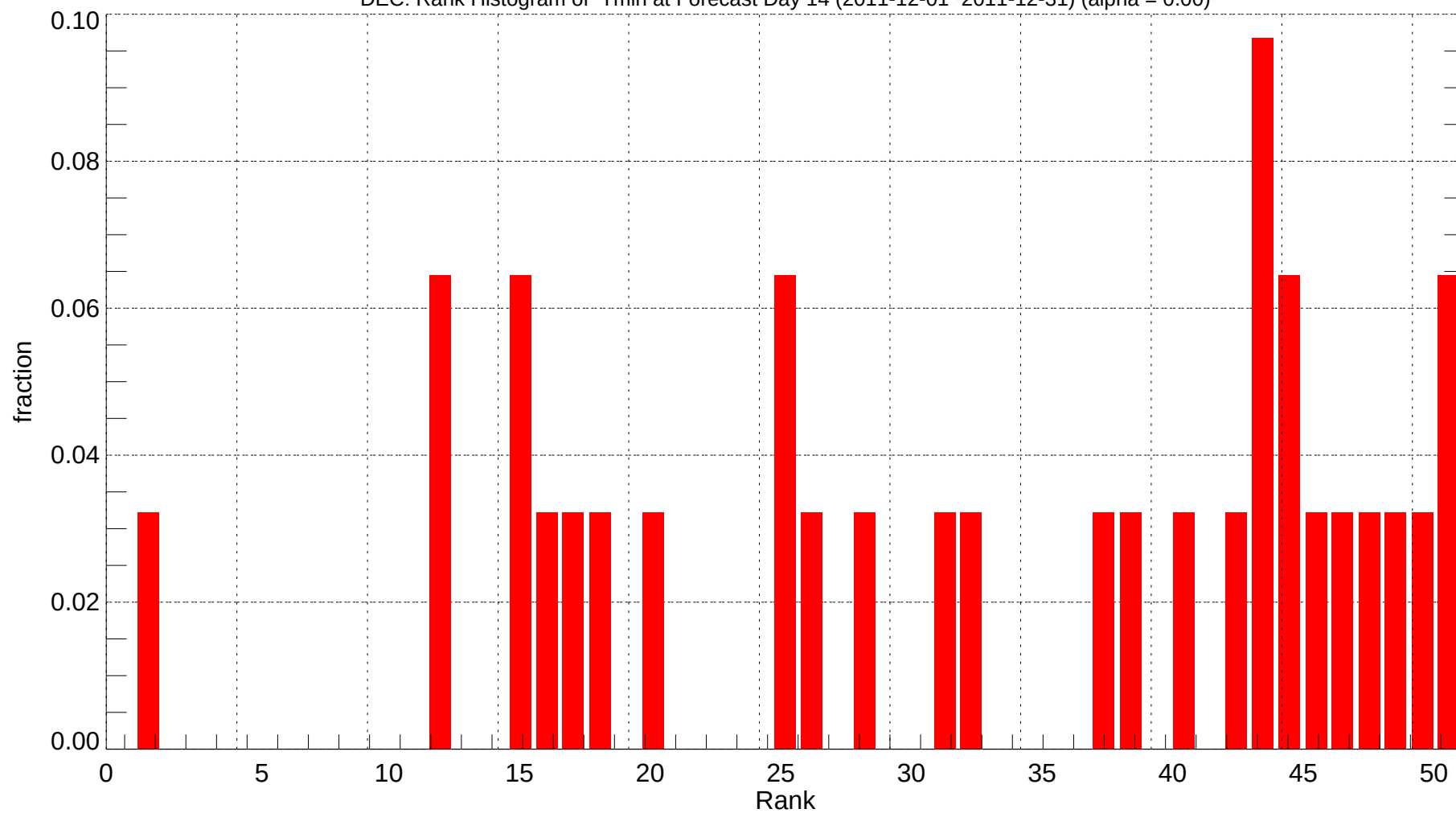
DEC: Rank Histogram of Tmin at Forecast Day 14 (2011-12-01~2011-12-31) (alpha = 0.00)
