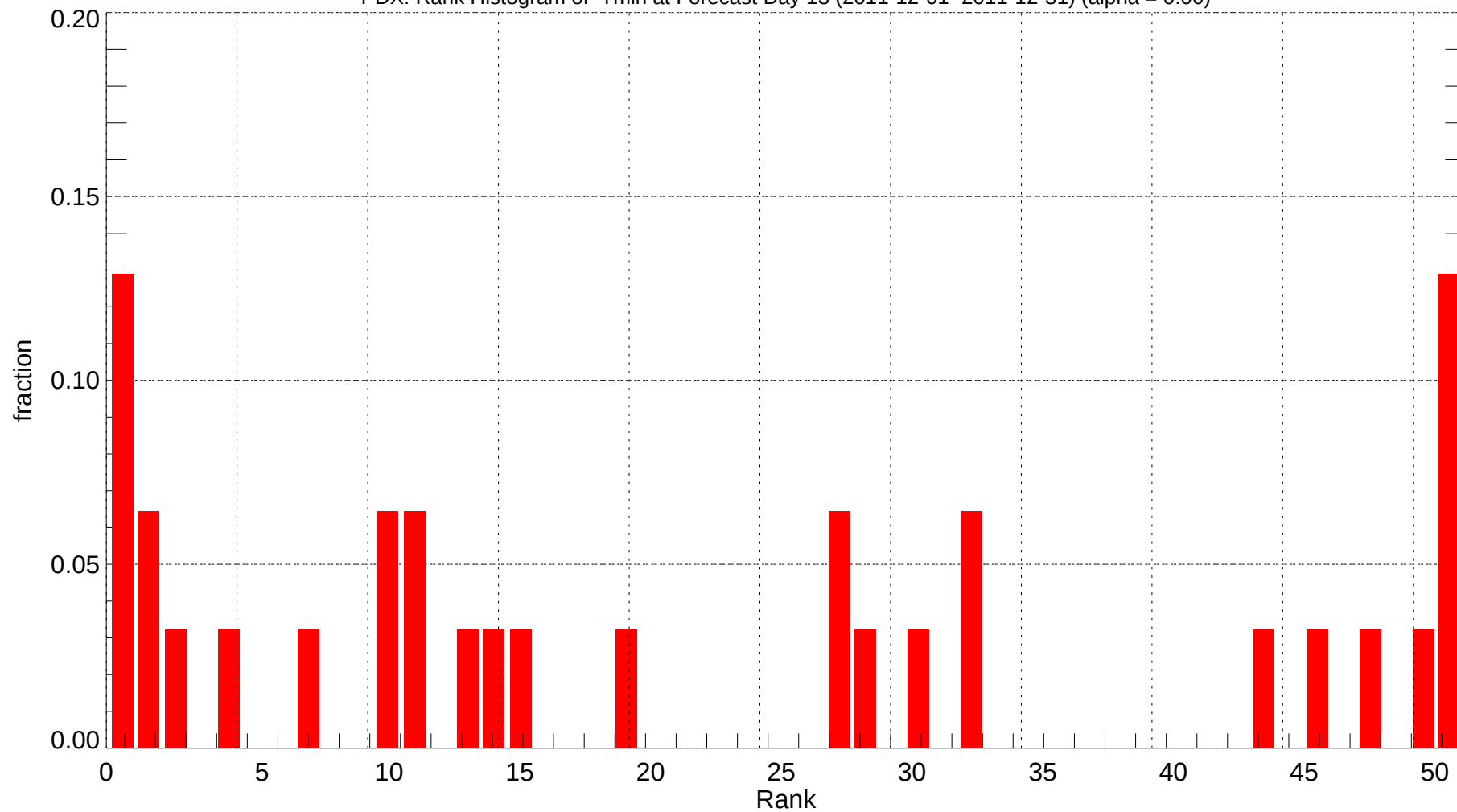
PDX: Rank Histogram of Tmin at Forecast Day 13 (2011-12-01~2011-12-31) (alpha = 0.00)
