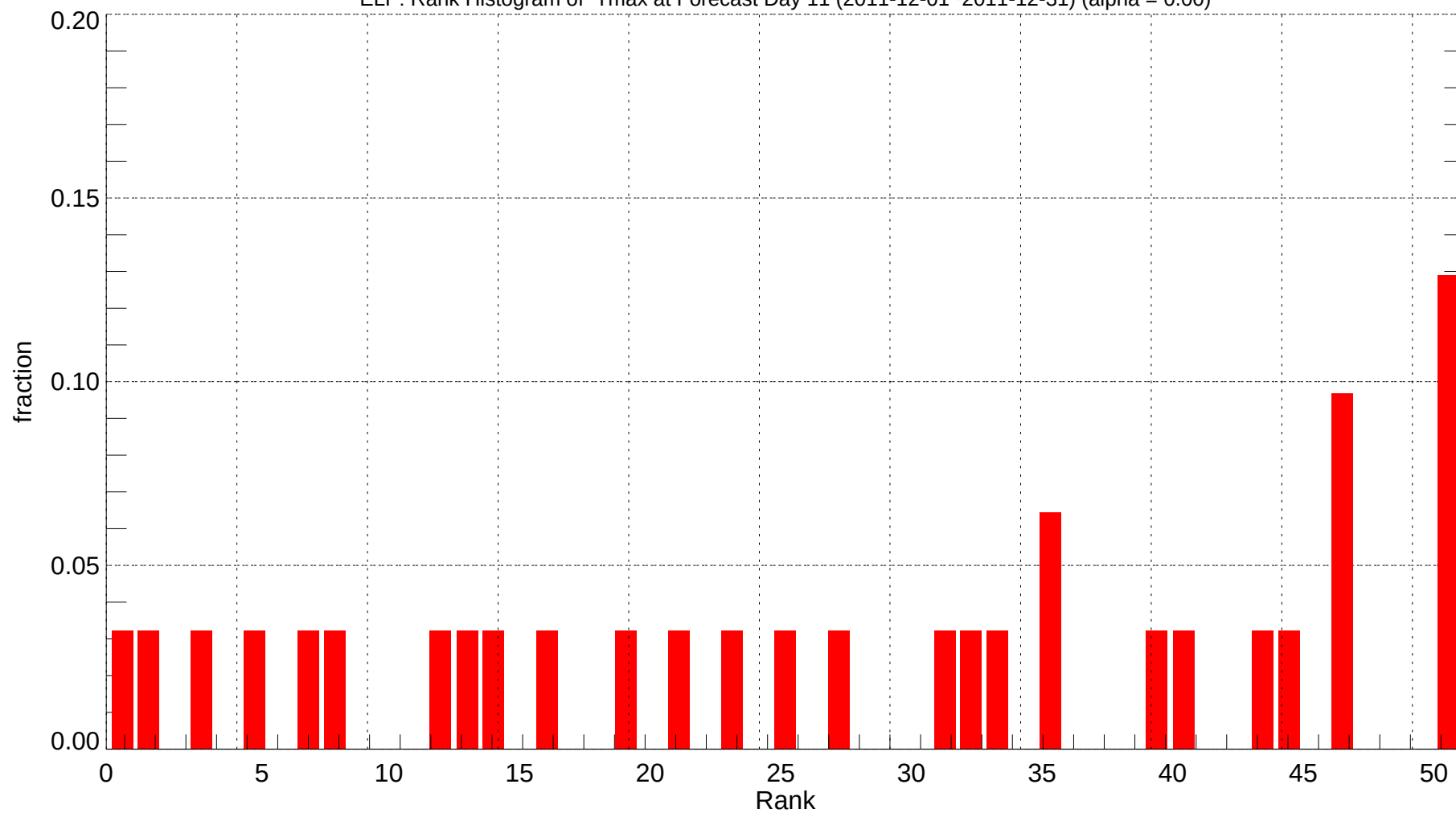
ELP: Rank Histogram of Tmax at Forecast Day 11 (2011-12-01~2011-12-31) (alpha = 0.00)
