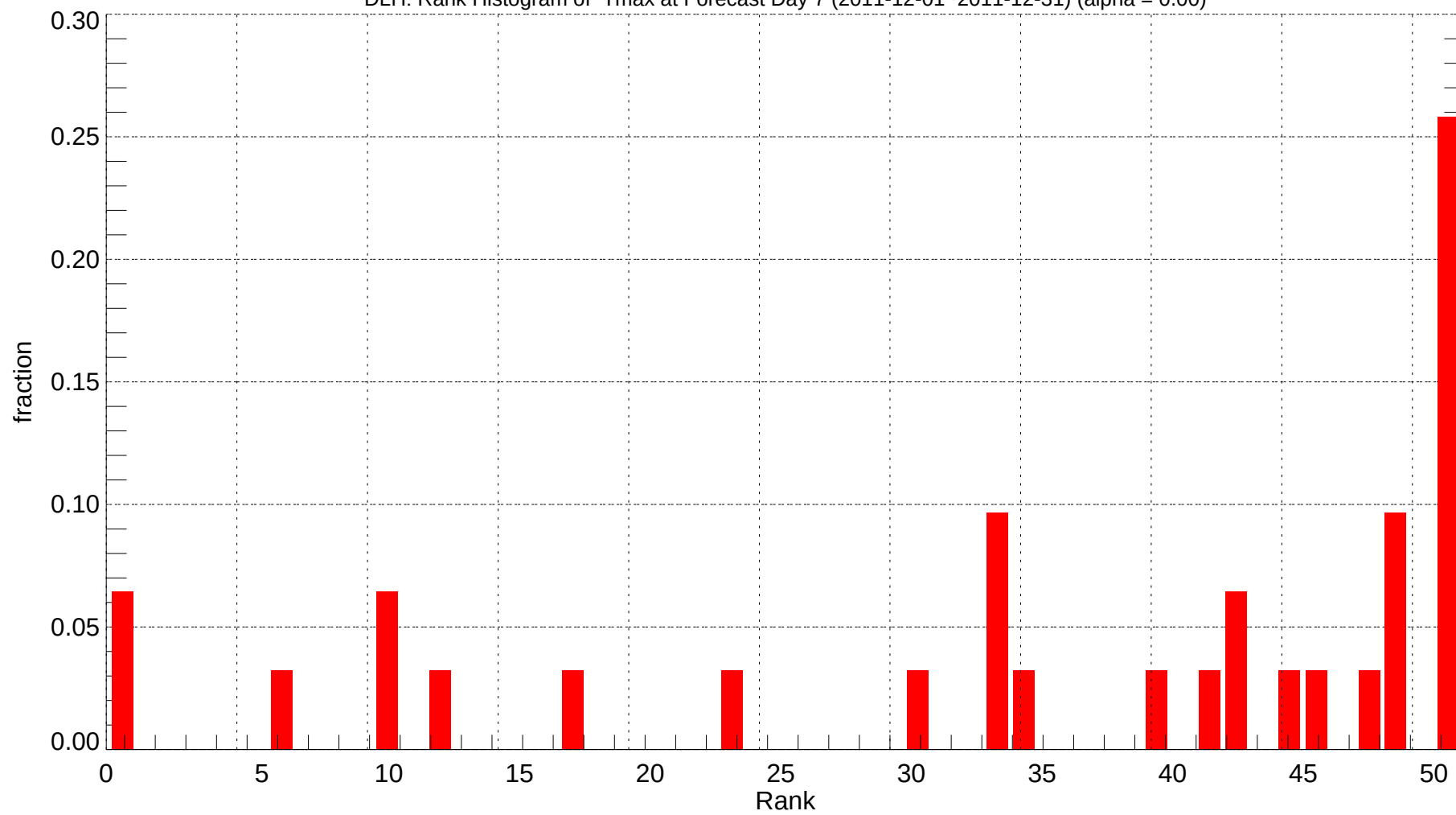
DLH: Rank Histogram of Tmax at Forecast Day 7 (2011-12-01~2011-12-31) (alpha = 0.00)
