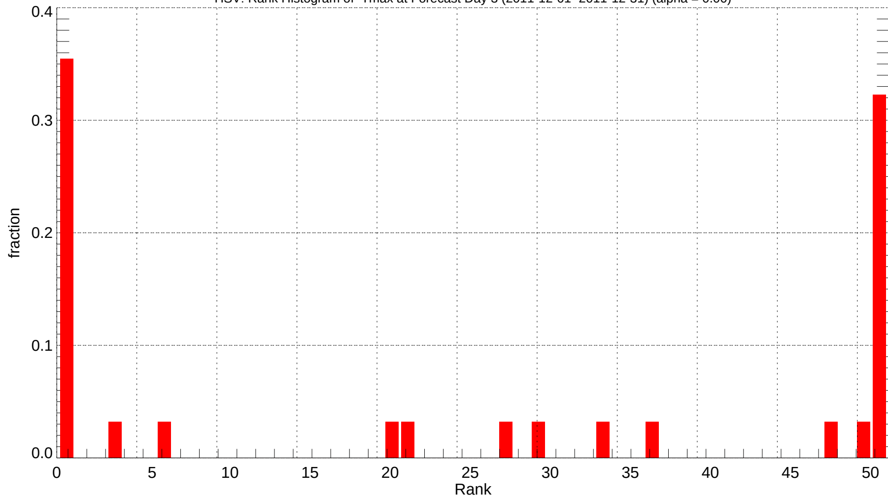
HSV: Rank Histogram of Tmax at Forecast Day 3 (2011-12-01~2011-12-31) (alpha = 0.00)
