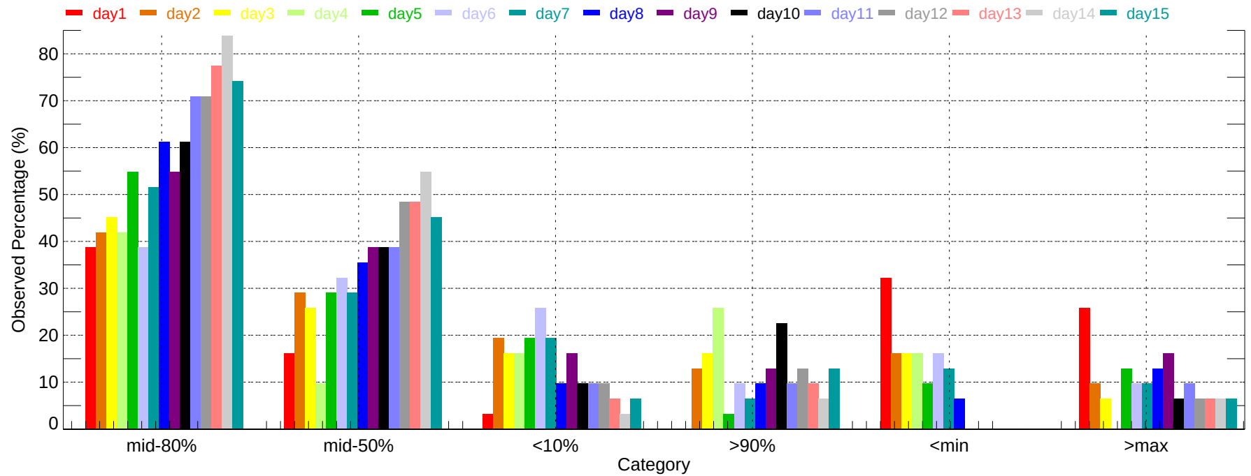
Observed Percentage of Ensembles - CLE: Max Temperature (2011-12-01~2011-12-31)
