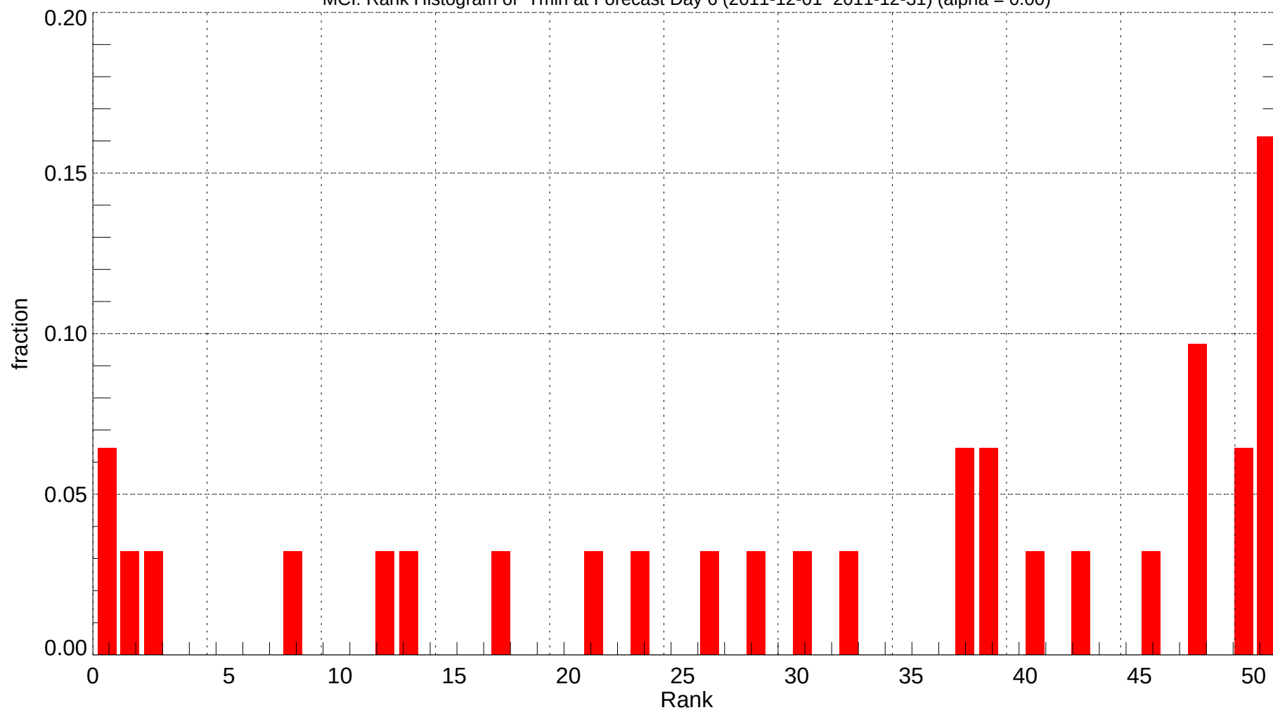
MCI: Rank Histogram of Tmin at Forecast Day 6 (2011-12-01~2011-12-31) (alpha = 0.00)
