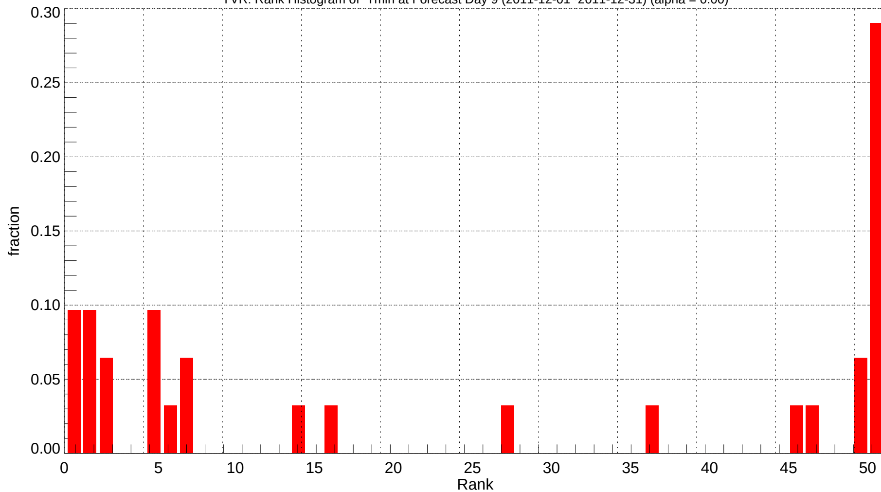
YVR: Rank Histogram of Tmin at Forecast Day 9 (2011-12-01~2011-12-31) (alpha = 0.00)
