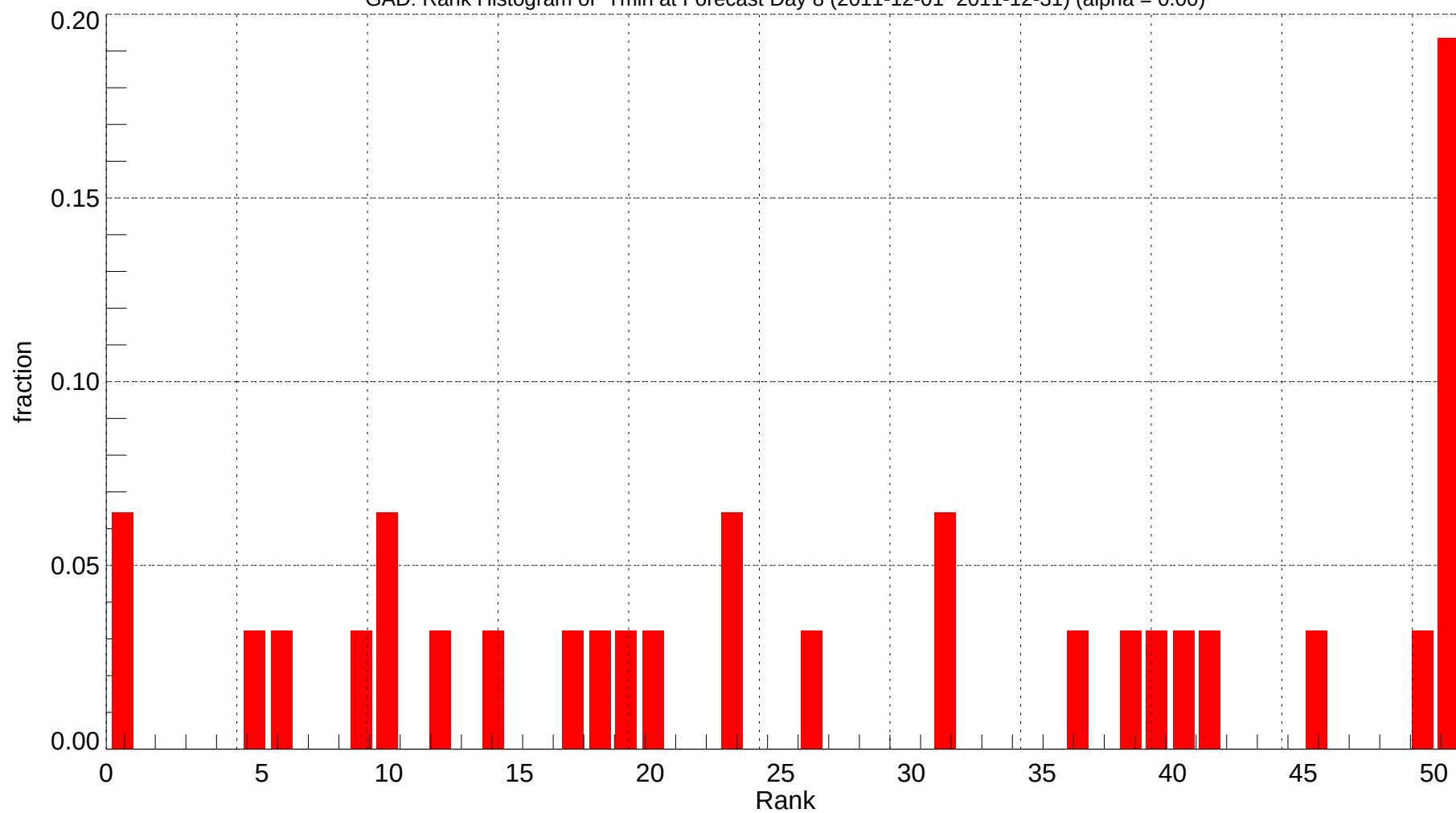
GAD: Rank Histogram of Tmin at Forecast Day 8 (2011-12-01~2011-12-31) (alpha = 0.00)
