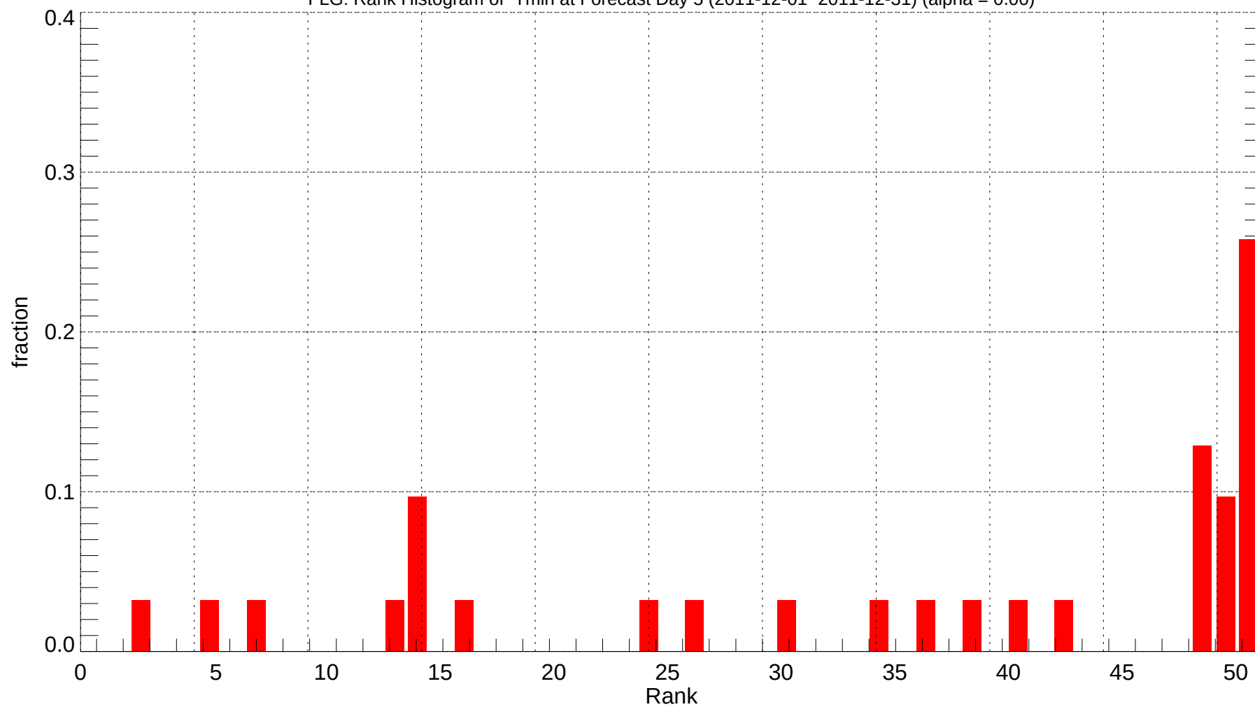
FLG: Rank Histogram of Tmin at Forecast Day 5 (2011-12-01~2011-12-31) (alpha = 0.00)
