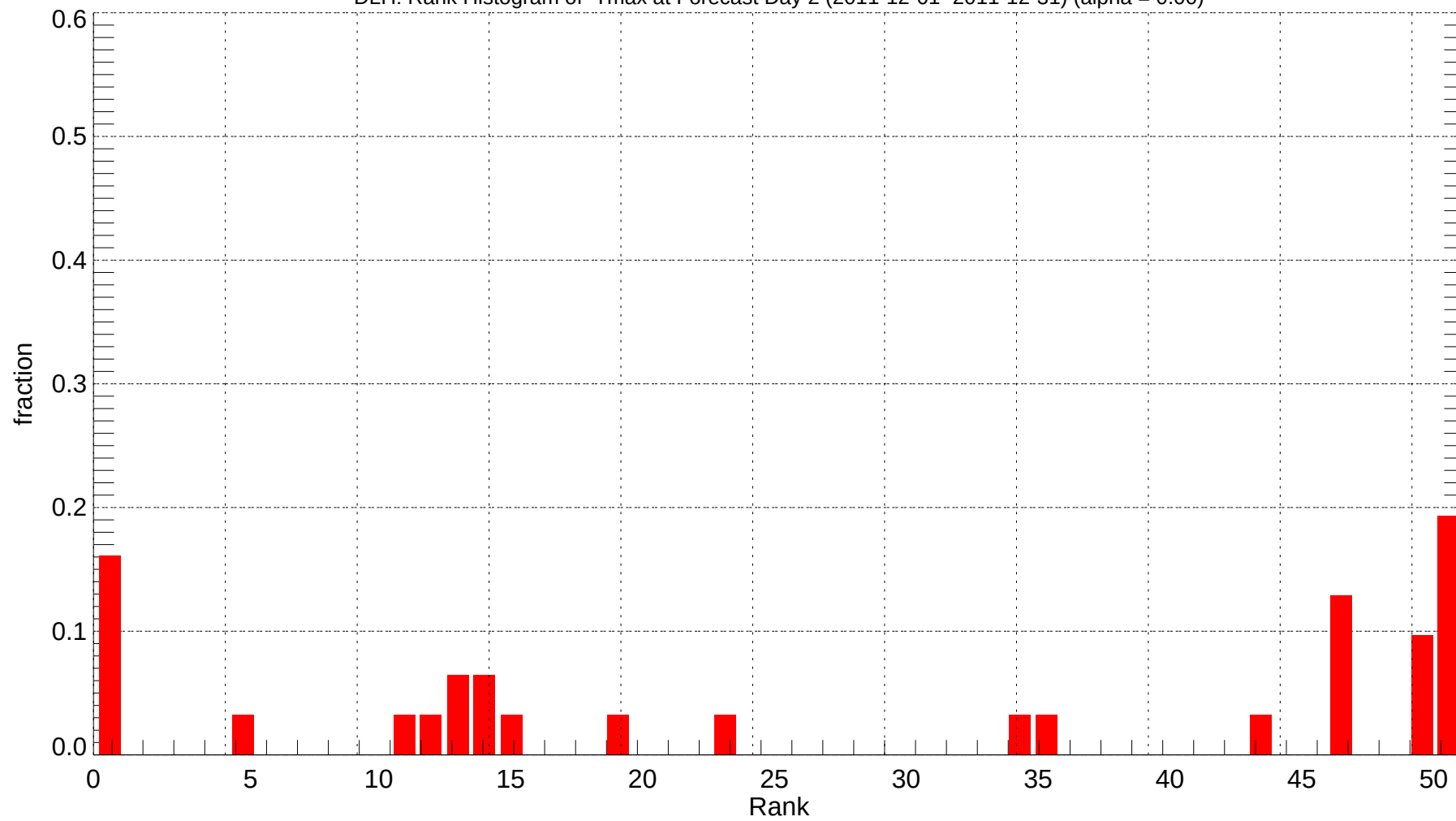
DLH: Rank Histogram of Tmax at Forecast Day 2 (2011-12-01~2011-12-31) (alpha = 0.00)
