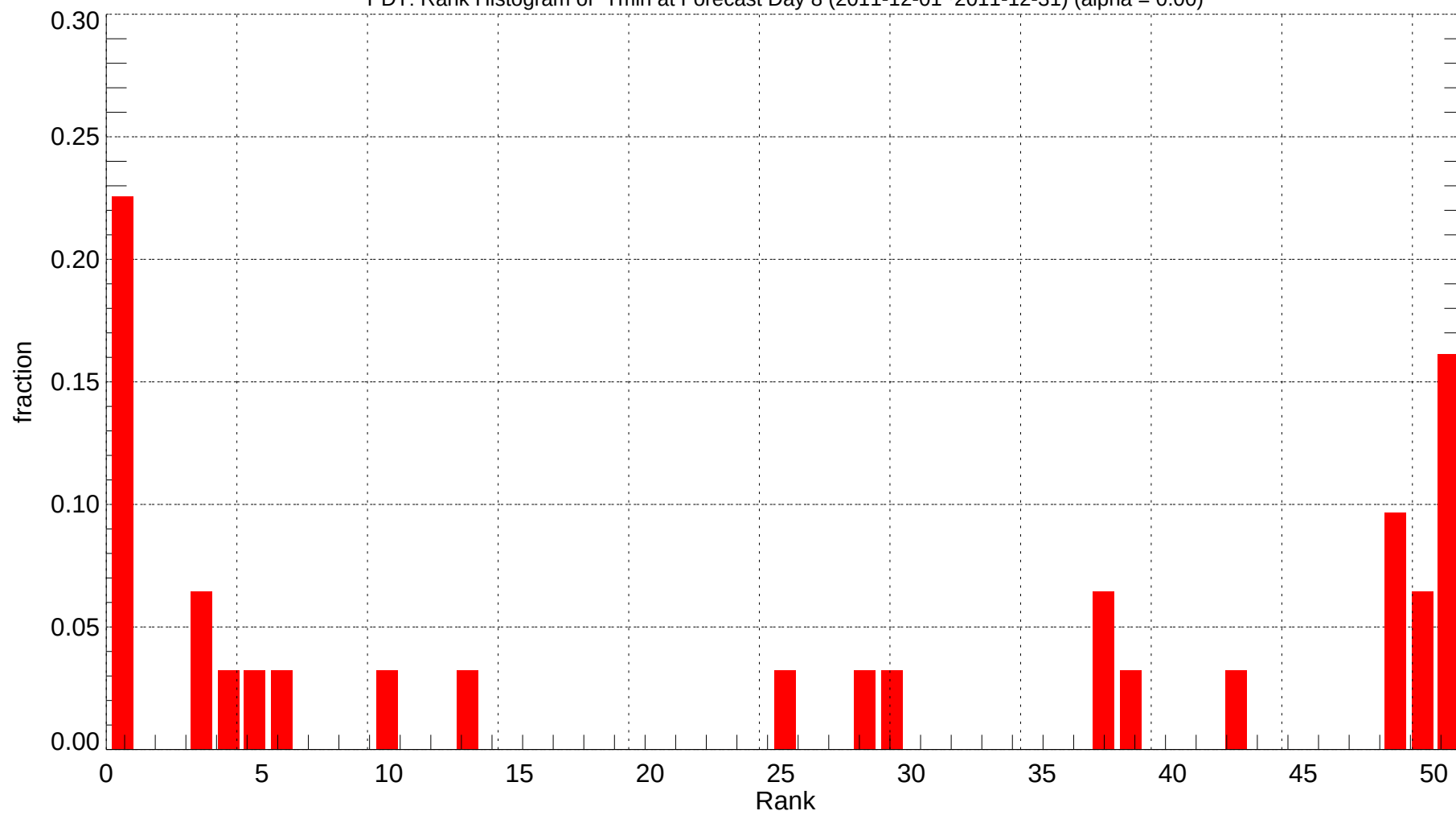
PDT: Rank Histogram of Tmin at Forecast Day 8 (2011-12-01~2011-12-31) (alpha = 0.00)
