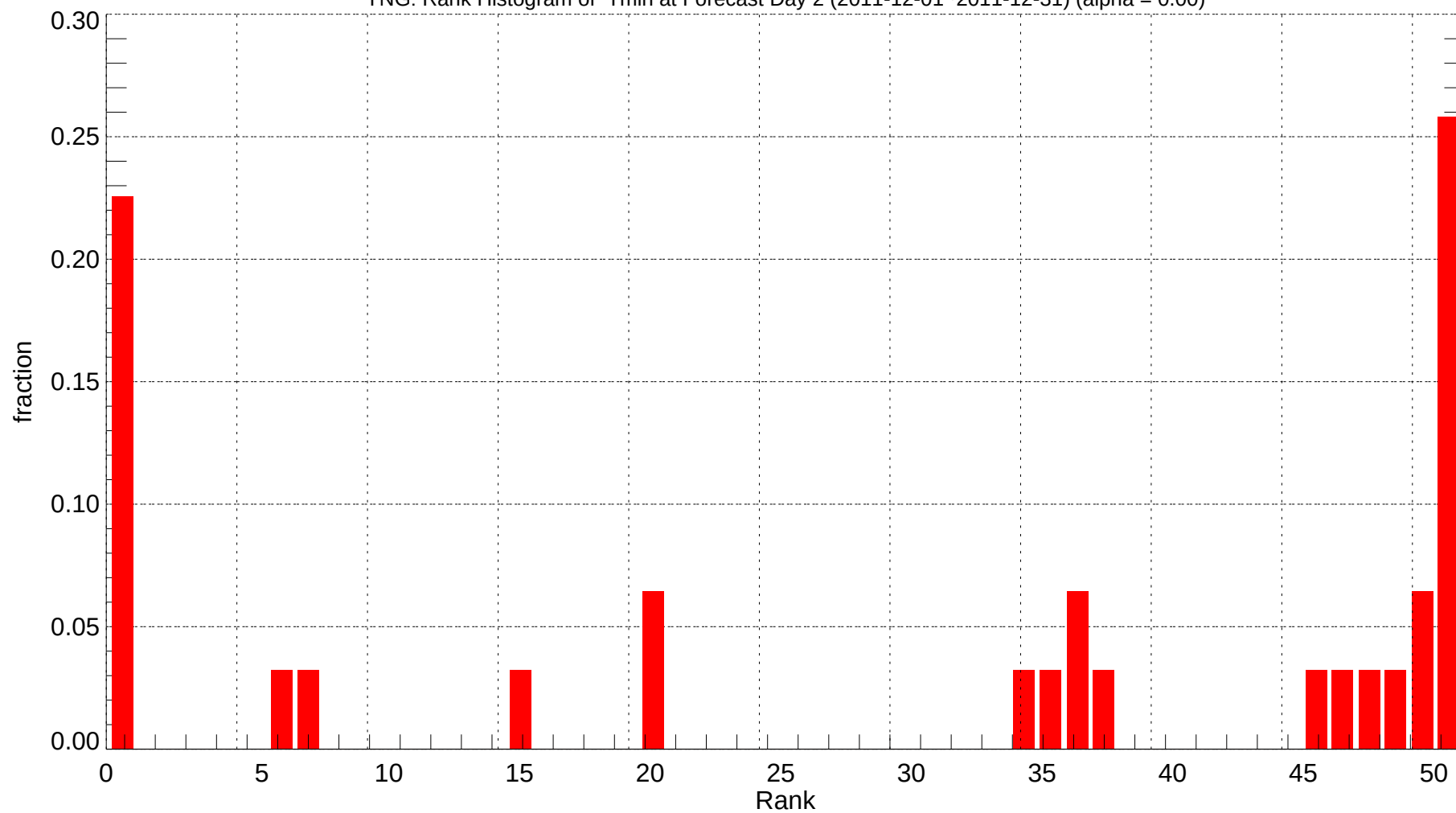
YNG: Rank Histogram of Tmin at Forecast Day 2 (2011-12-01~2011-12-31) (alpha = 0.00)
