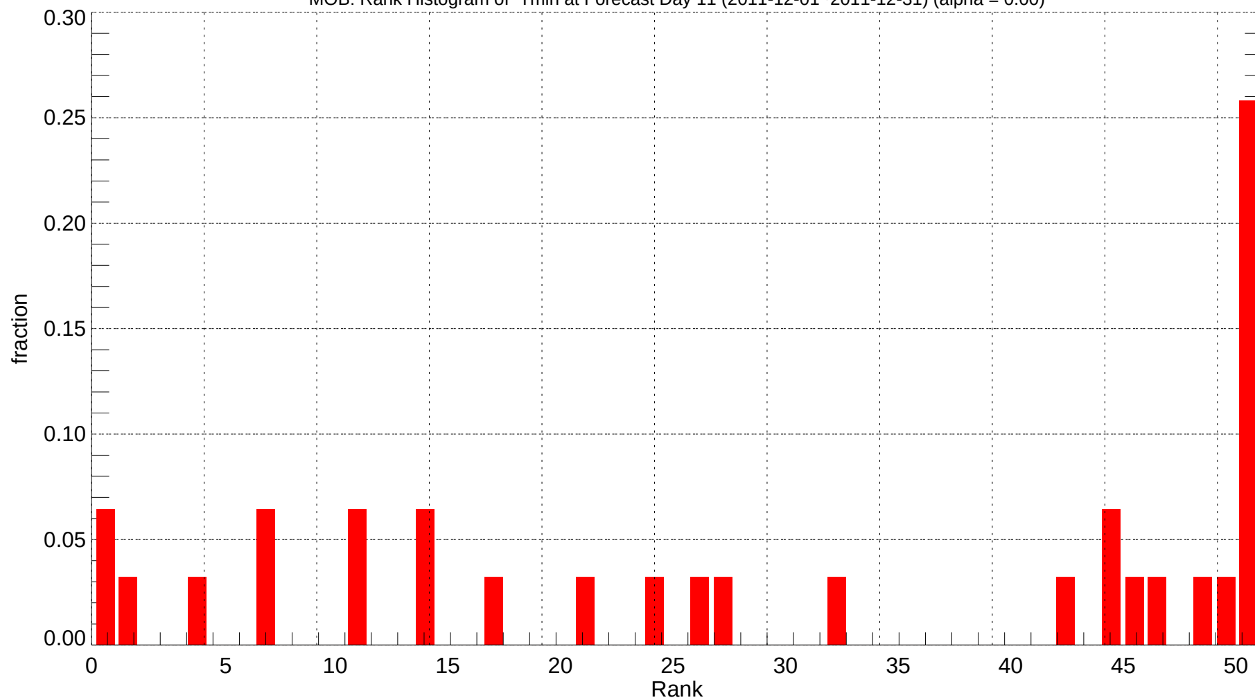
MOB: Rank Histogram of Tmin at Forecast Day 11 (2011-12-01~2011-12-31) (alpha = 0.00)
