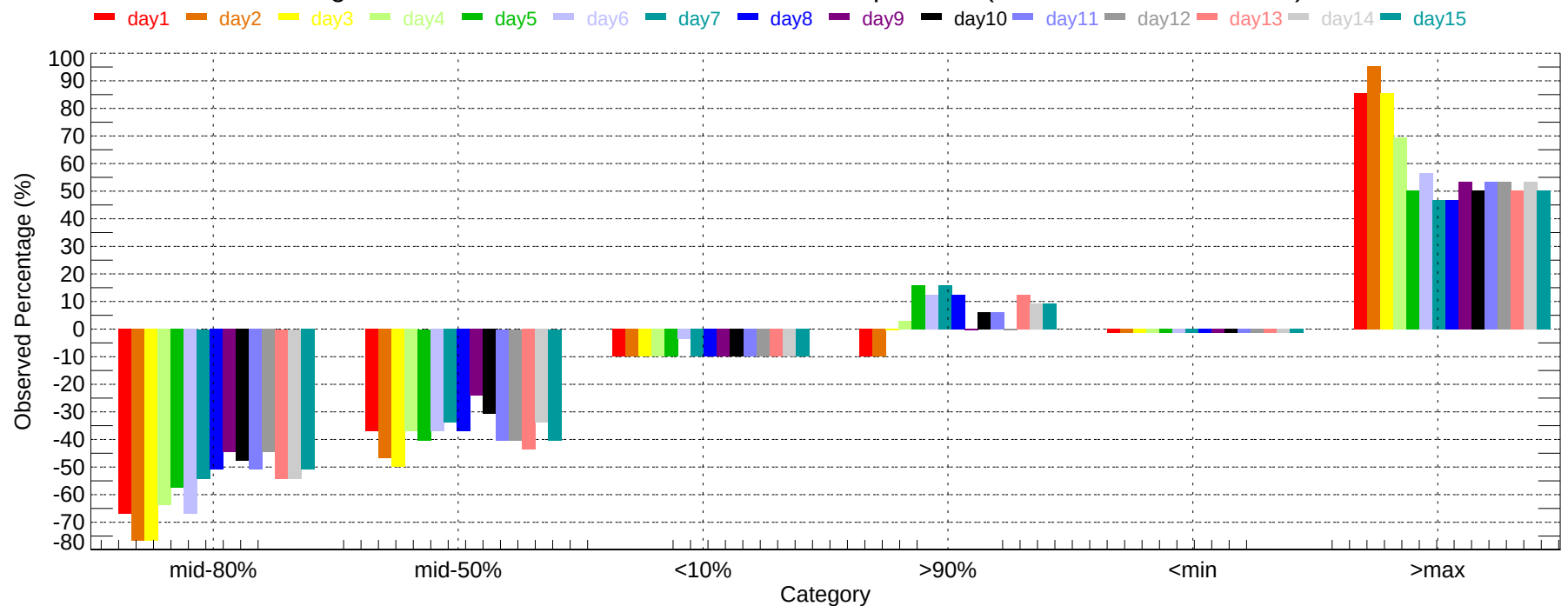
Observed Percentage Deviation of Ensembles - GTF: Max Temperature (2011-12-01~2011-12-31)
