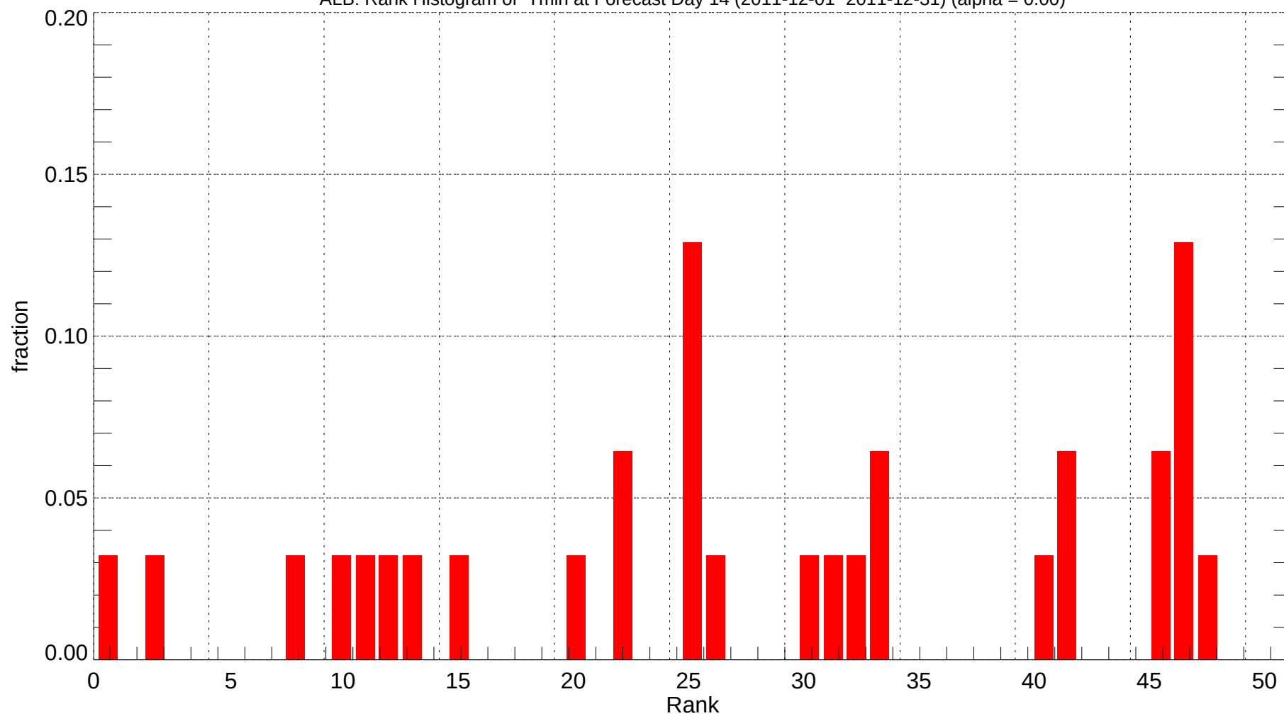
ALB: Rank Histogram of Tmin at Forecast Day 14 (2011-12-01~2011-12-31) (alpha = 0.00)
