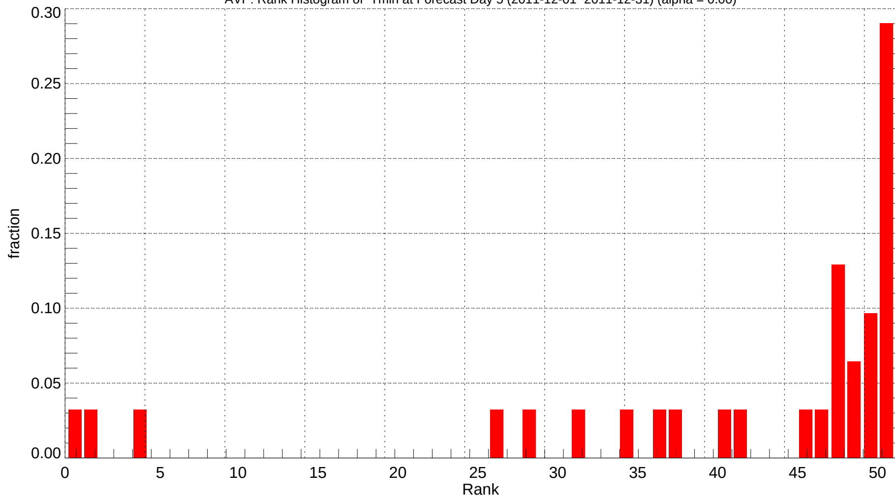
AVP: Rank Histogram of Tmin at Forecast Day 5 (2011-12-01~2011-12-31) (alpha = 0.00)
