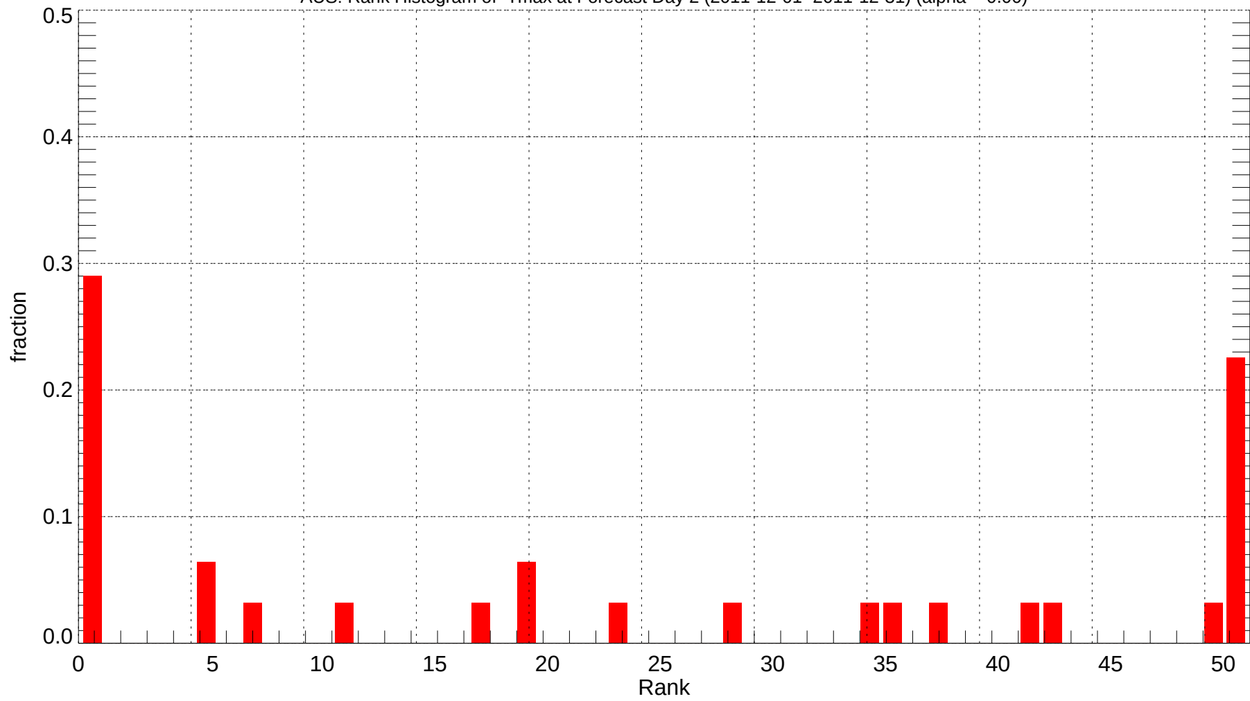
AUS: Rank Histogram of Tmax at Forecast Day 2 (2011-12-01~2011-12-31) (alpha = 0.00)
