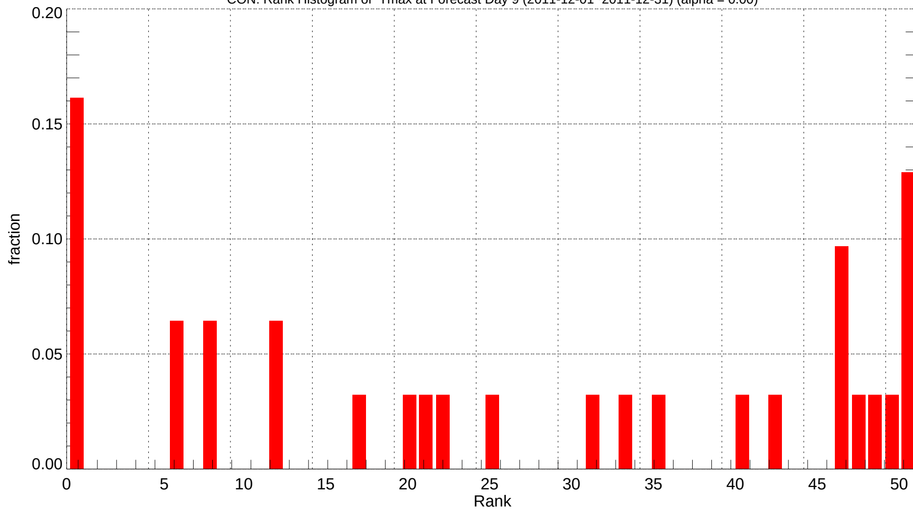
CON: Rank Histogram of Tmax at Forecast Day 9 (2011-12-01~2011-12-31) (alpha = 0.00)
