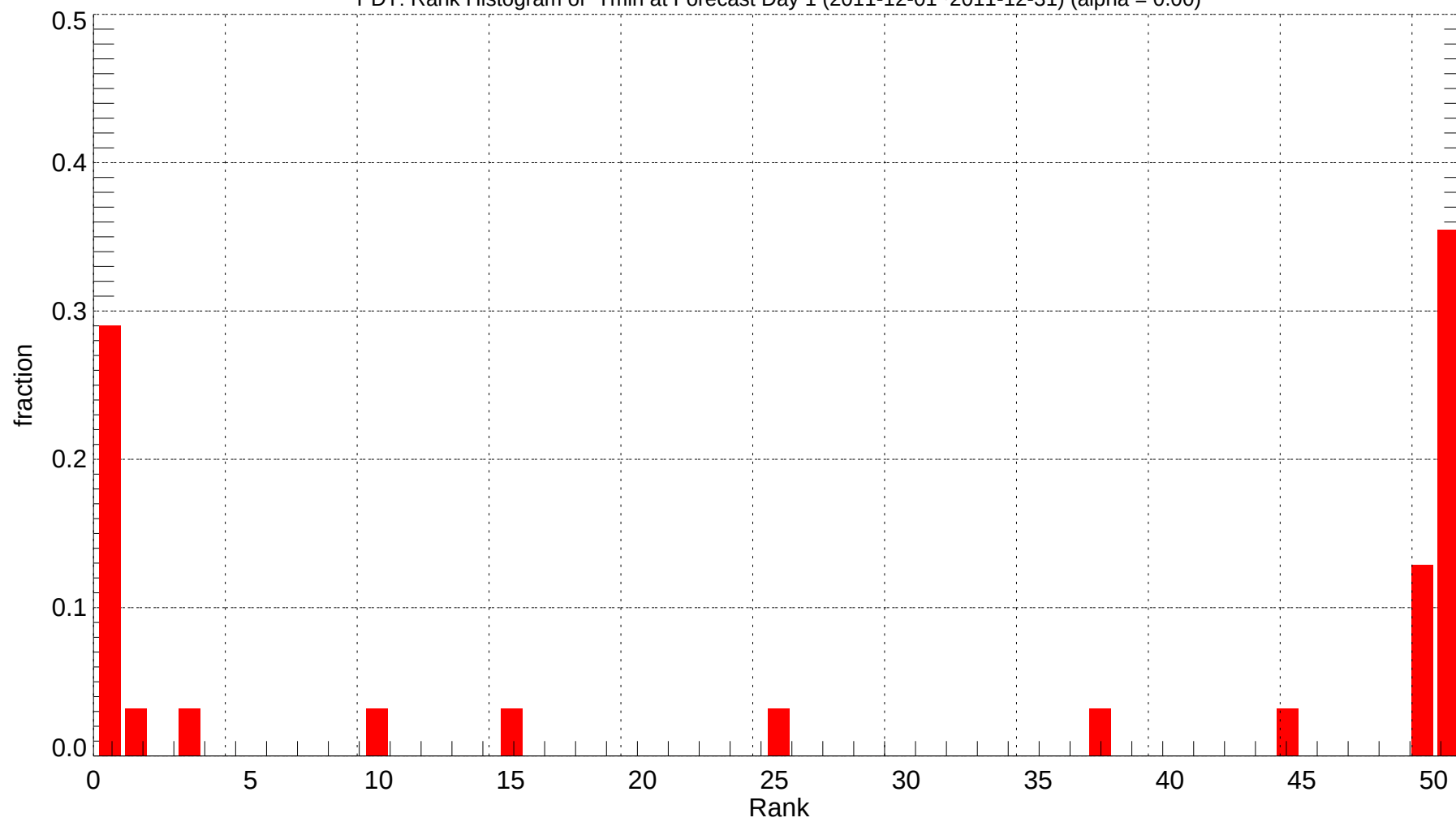
PDT: Rank Histogram of Tmin at Forecast Day 1 (2011-12-01~2011-12-31) (alpha = 0.00)
