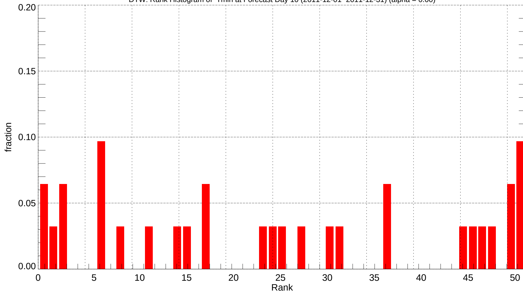
DTW: Rank Histogram of Tmin at Forecast Day 10 (2011-12-01~2011-12-31) (alpha = 0.00)
