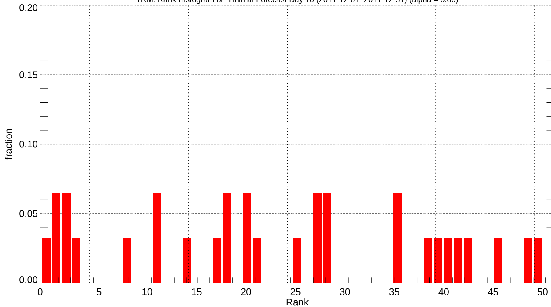
TRM: Rank Histogram of Tmin at Forecast Day 10 (2011-12-01~2011-12-31) (alpha = 0.00)
