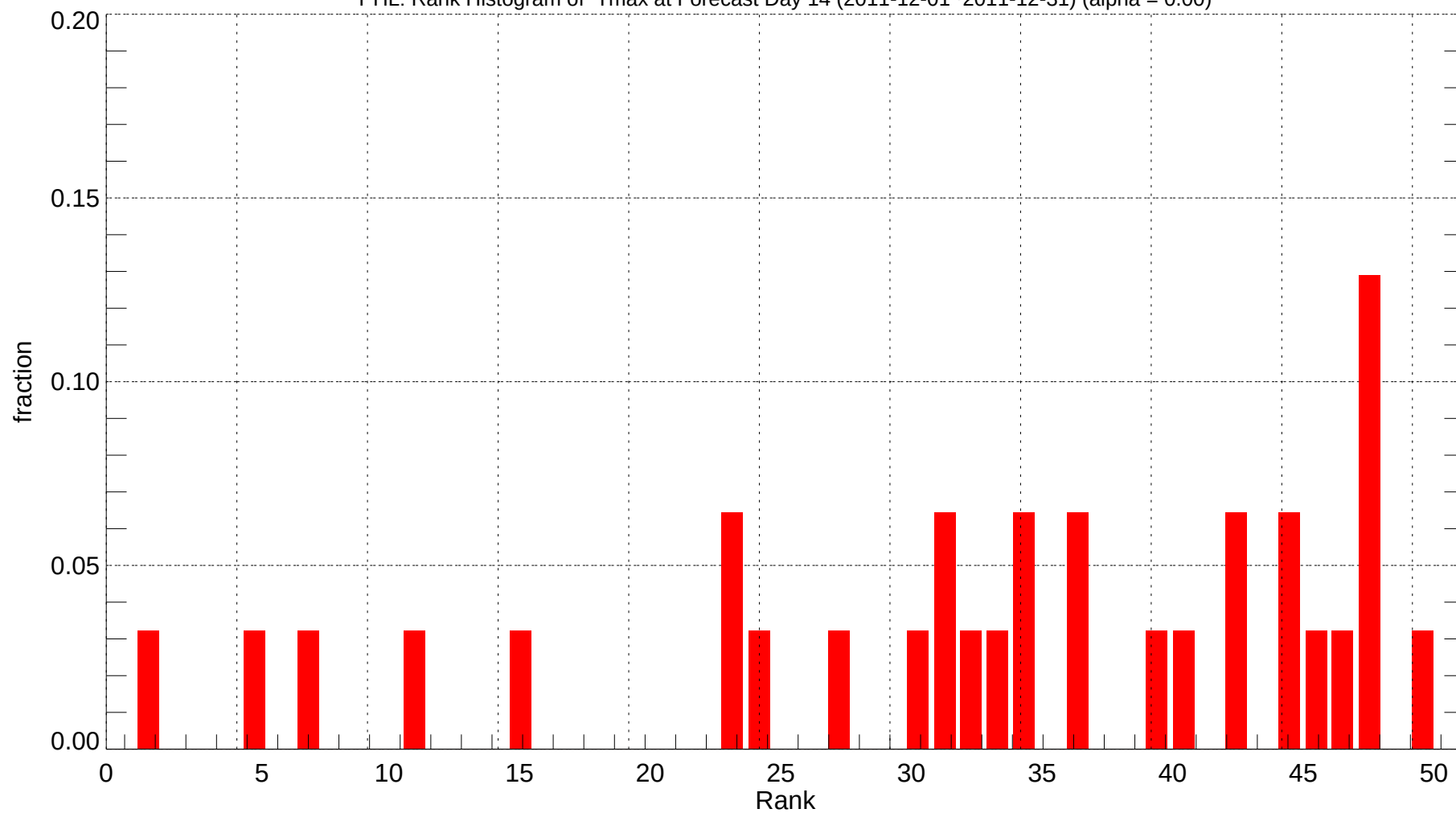
PHL: Rank Histogram of Tmax at Forecast Day 14 (2011-12-01~2011-12-31) (alpha = 0.00)
