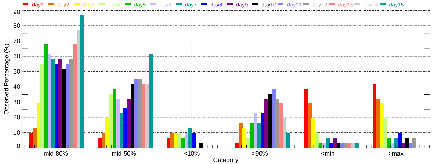
Observed Percentage of Ensembles - GAD: Min Temperature (2011-12-01~2011-12-31)
