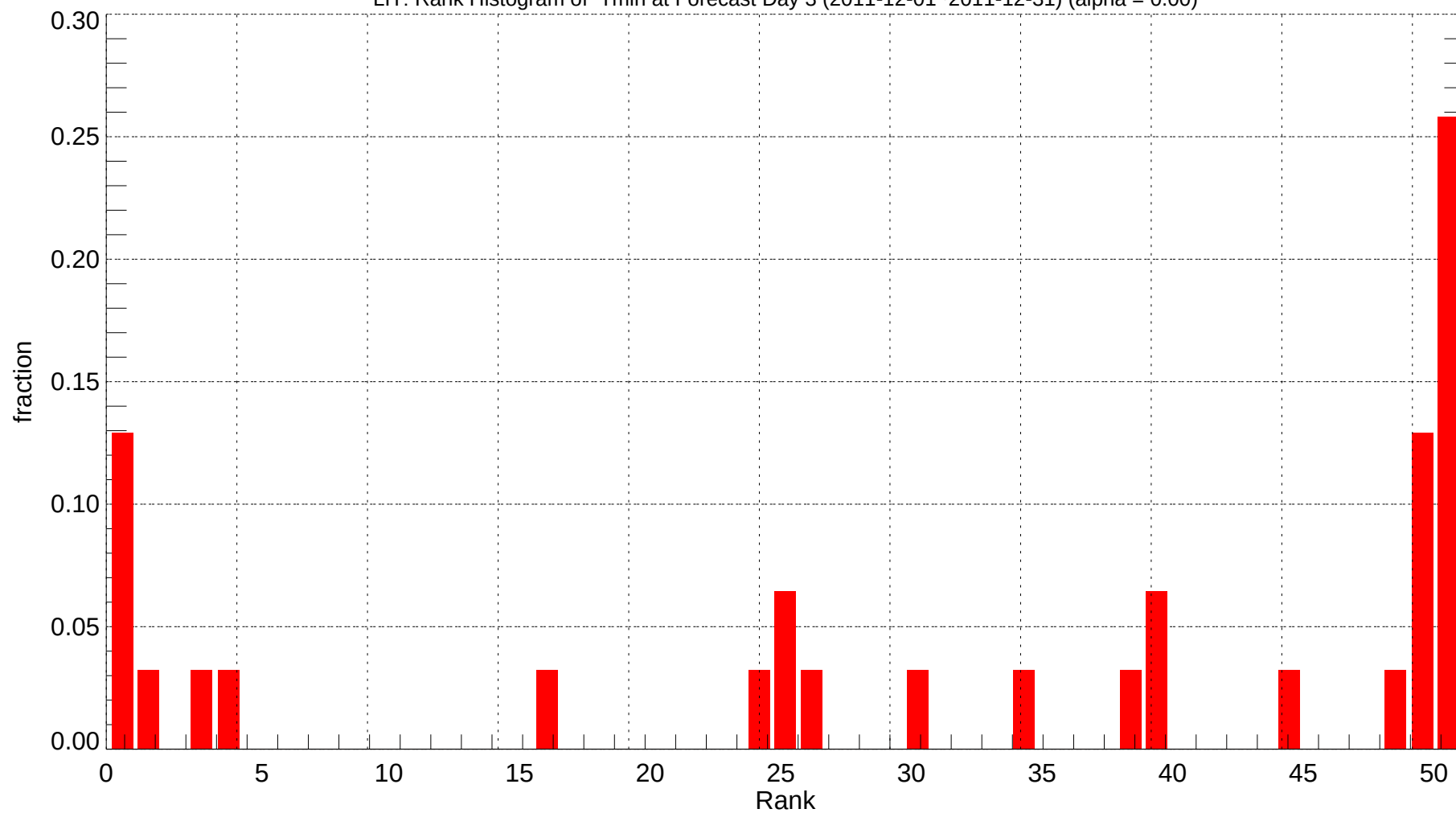
LIT: Rank Histogram of Tmin at Forecast Day 3 (2011-12-01~2011-12-31) (alpha = 0.00)
