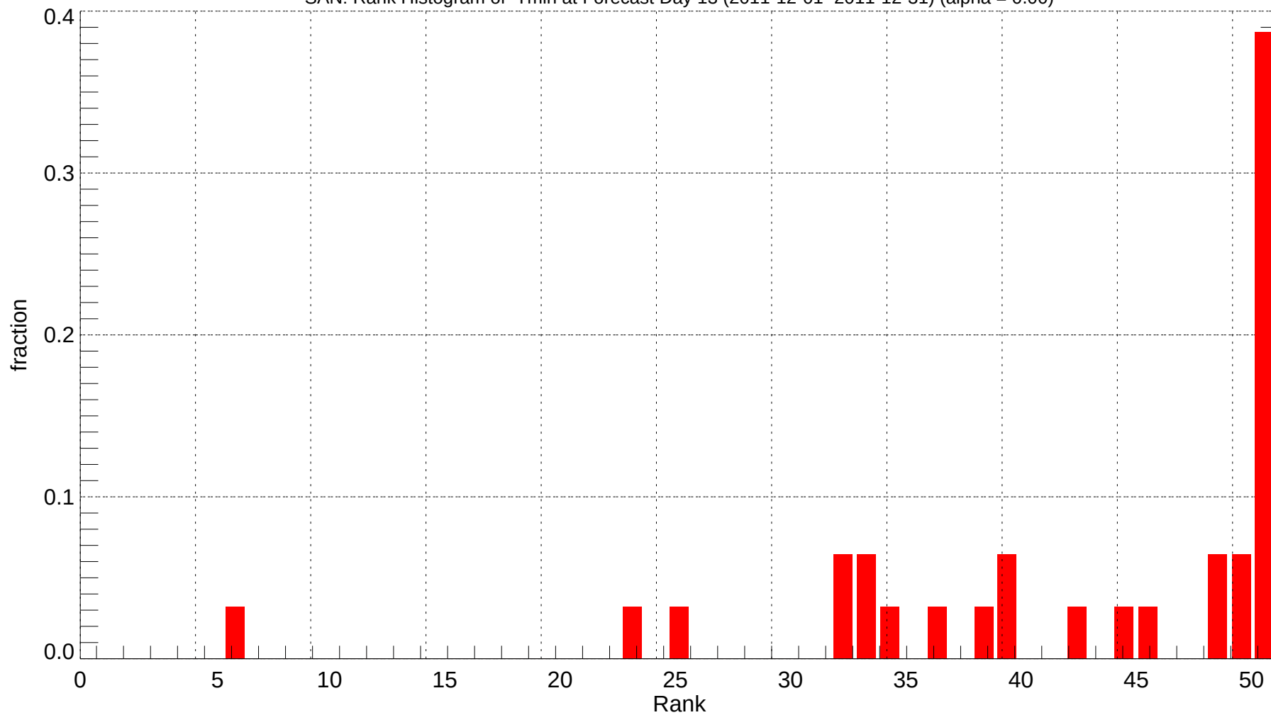
SAN: Rank Histogram of Tmin at Forecast Day 13 (2011-12-01~2011-12-31) (alpha = 0.00)
