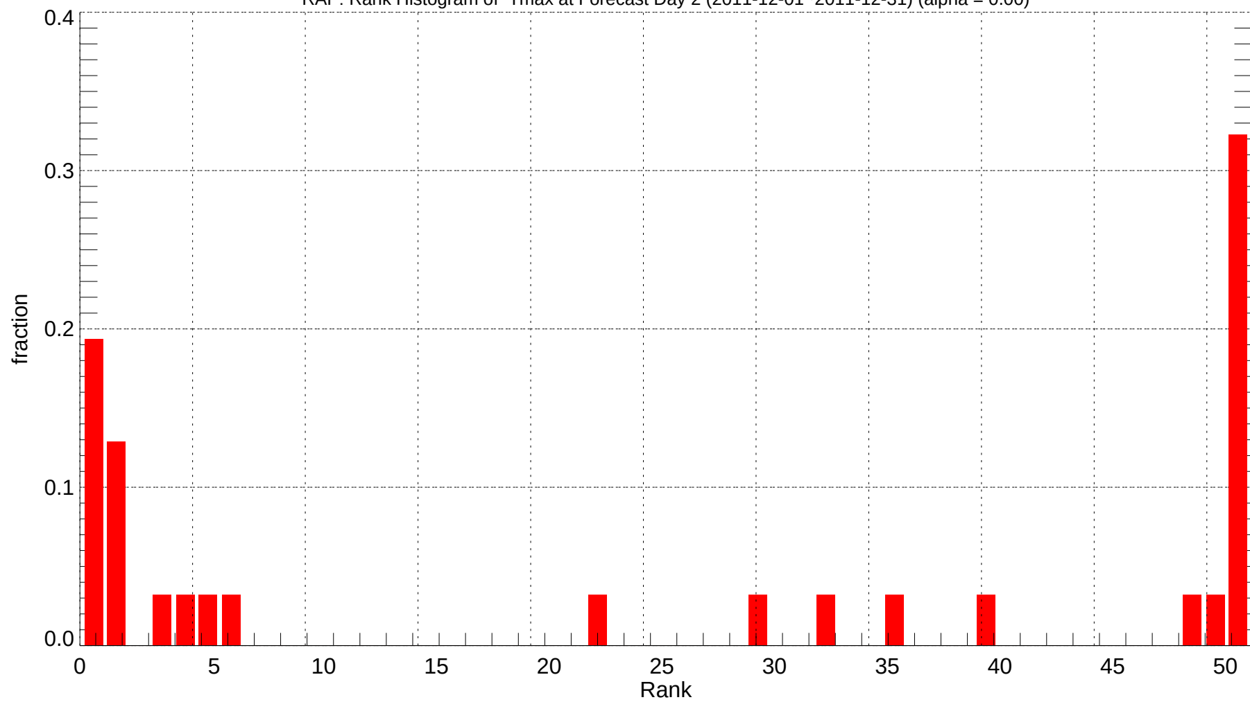
RAP: Rank Histogram of Tmax at Forecast Day 2 (2011-12-01~2011-12-31) (alpha = 0.00)
