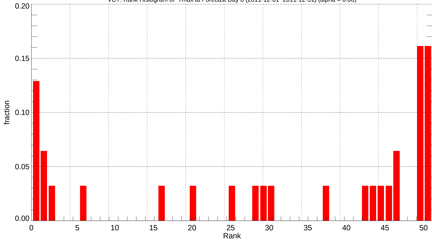
VCT: Rank Histogram of Tmax at Forecast Day 8 (2011-12-01~2011-12-31) (alpha = 0.00)
