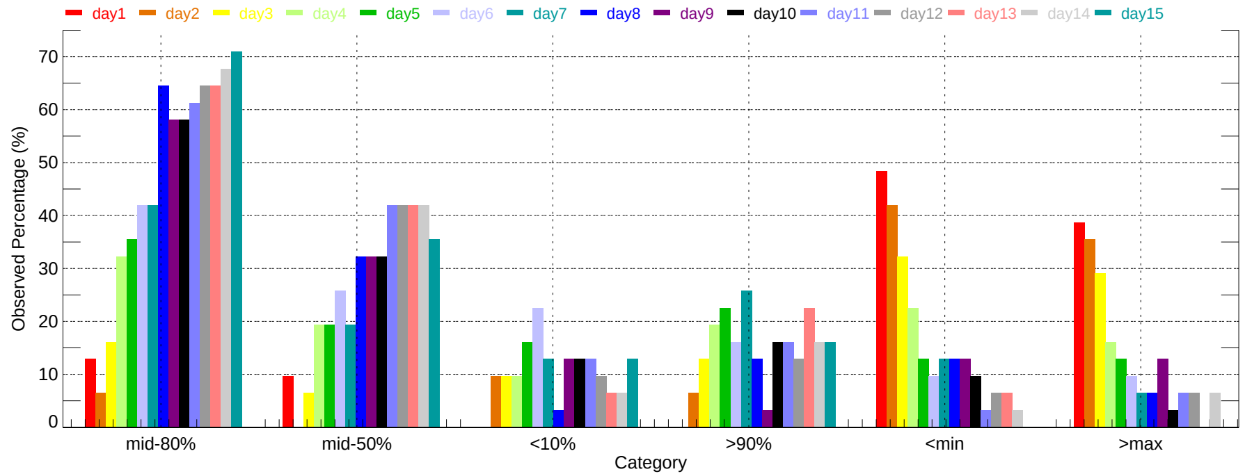
Observed Percentage of Ensembles - SJC: Min Temperature (2011-12-01~2011-12-31)
