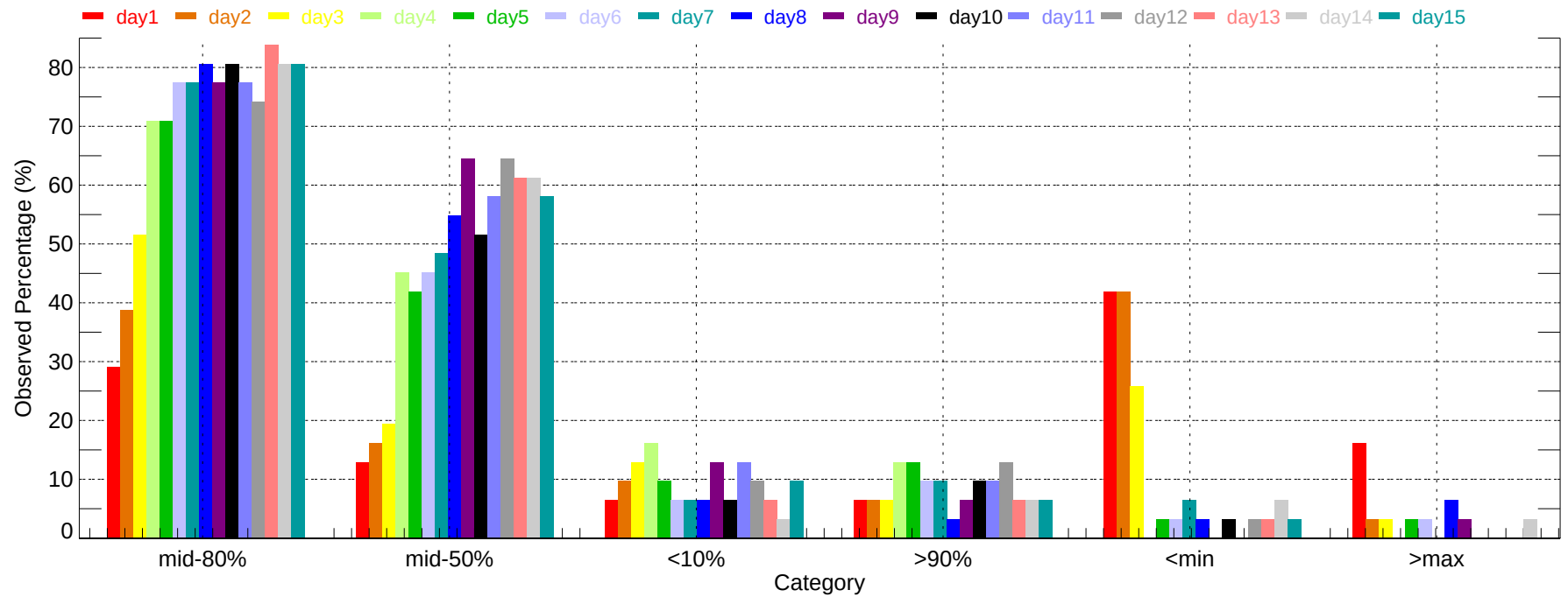
Observed Percentage of Ensembles - MAF: Min Temperature (2011-12-01~2011-12-31)
