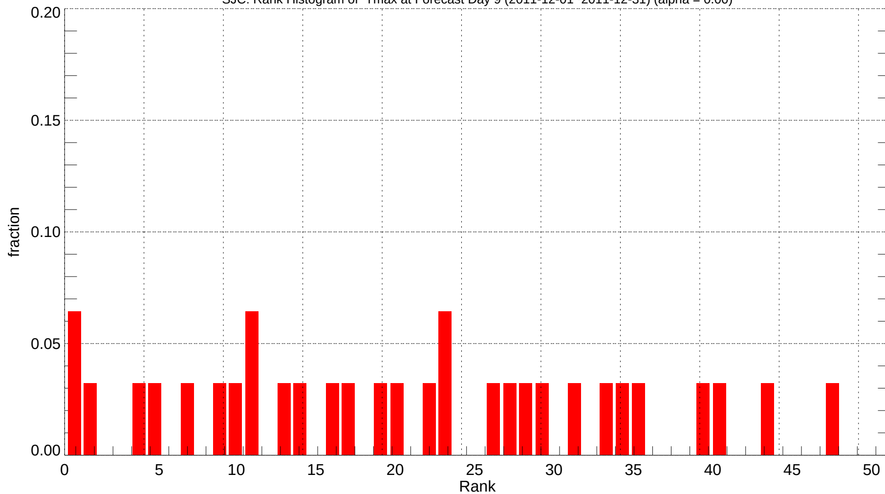
SJC: Rank Histogram of Tmax at Forecast Day 9 (2011-12-01~2011-12-31) (alpha = 0.00)
