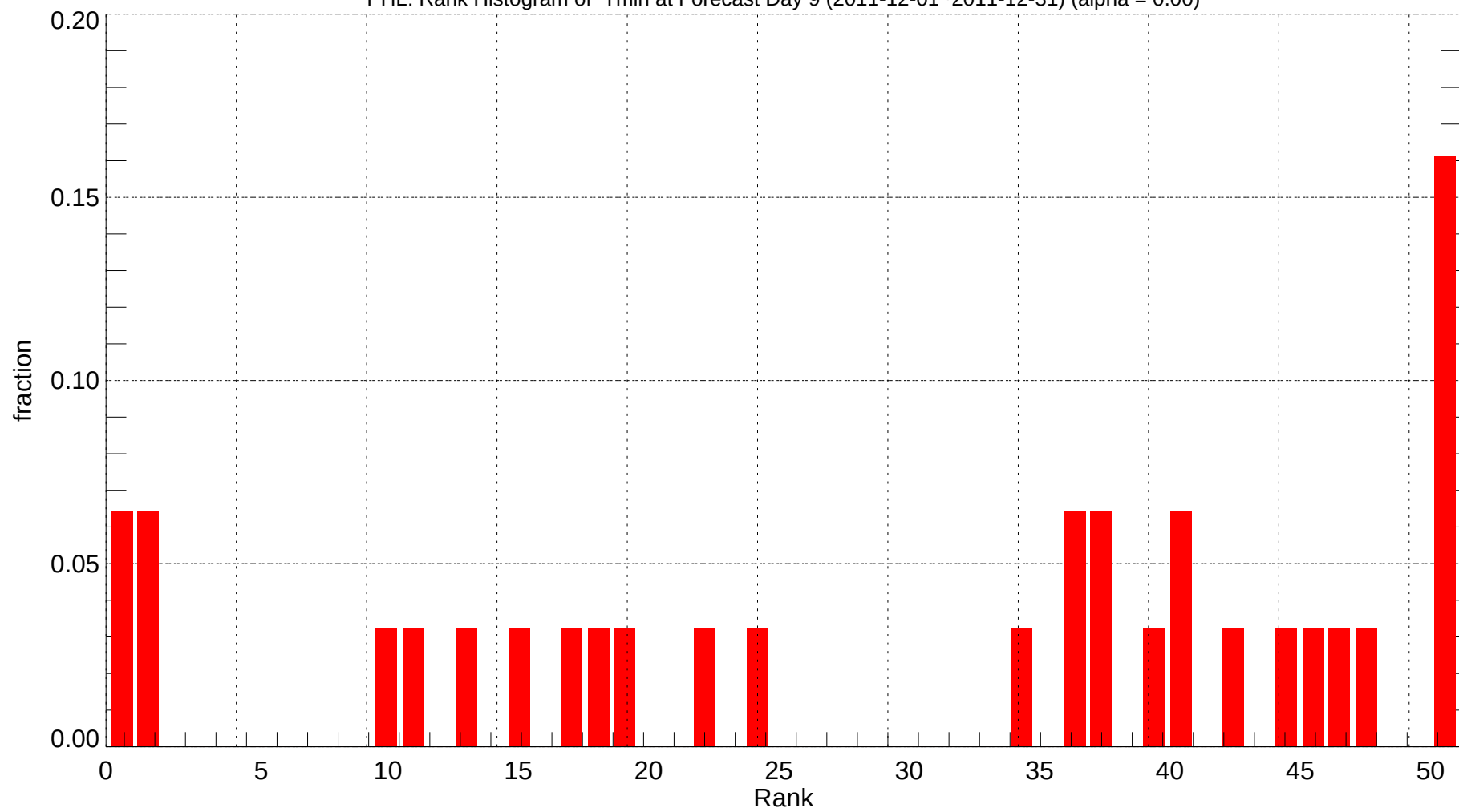
PHL: Rank Histogram of Tmin at Forecast Day 9 (2011-12-01~2011-12-31) (alpha = 0.00)
