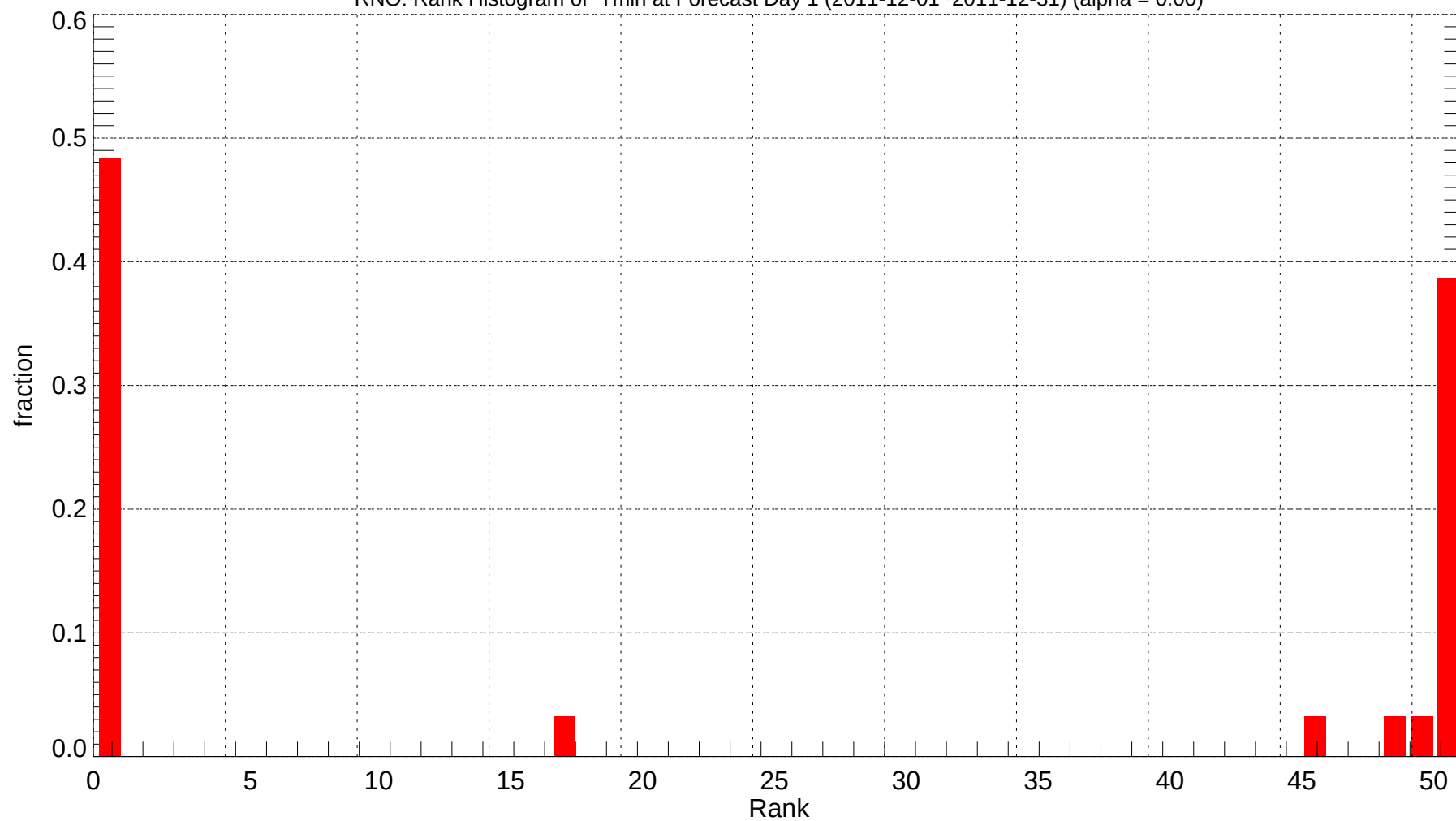
RNO: Rank Histogram of Tmin at Forecast Day 1 (2011-12-01~2011-12-31) (alpha = 0.00)
