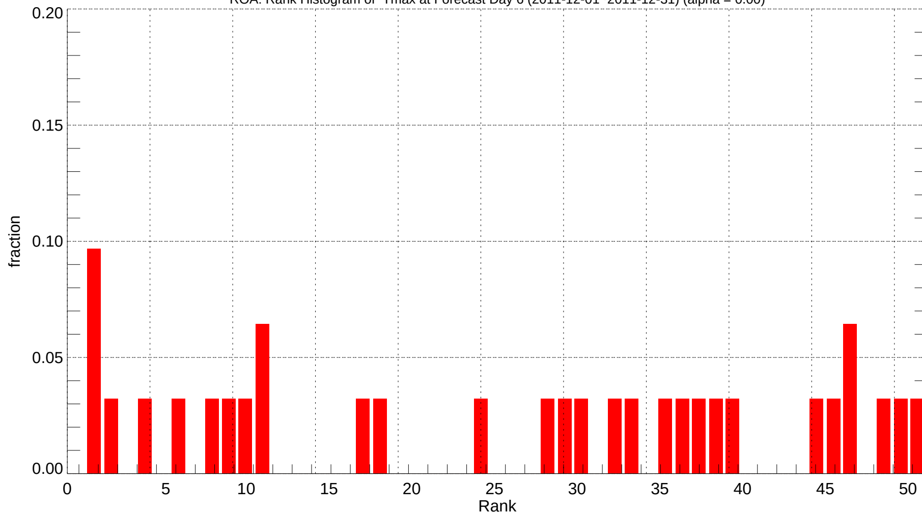
ROA: Rank Histogram of Tmax at Forecast Day 6 (2011-12-01~2011-12-31) (alpha = 0.00)
