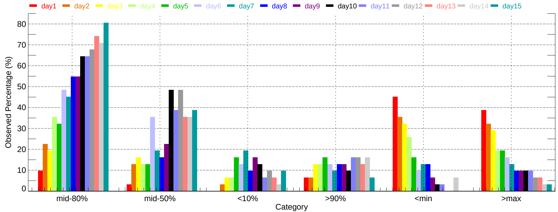
Observed Percentage of Ensembles - ILG: Min Temperature (2011-12-01~2011-12-31)
