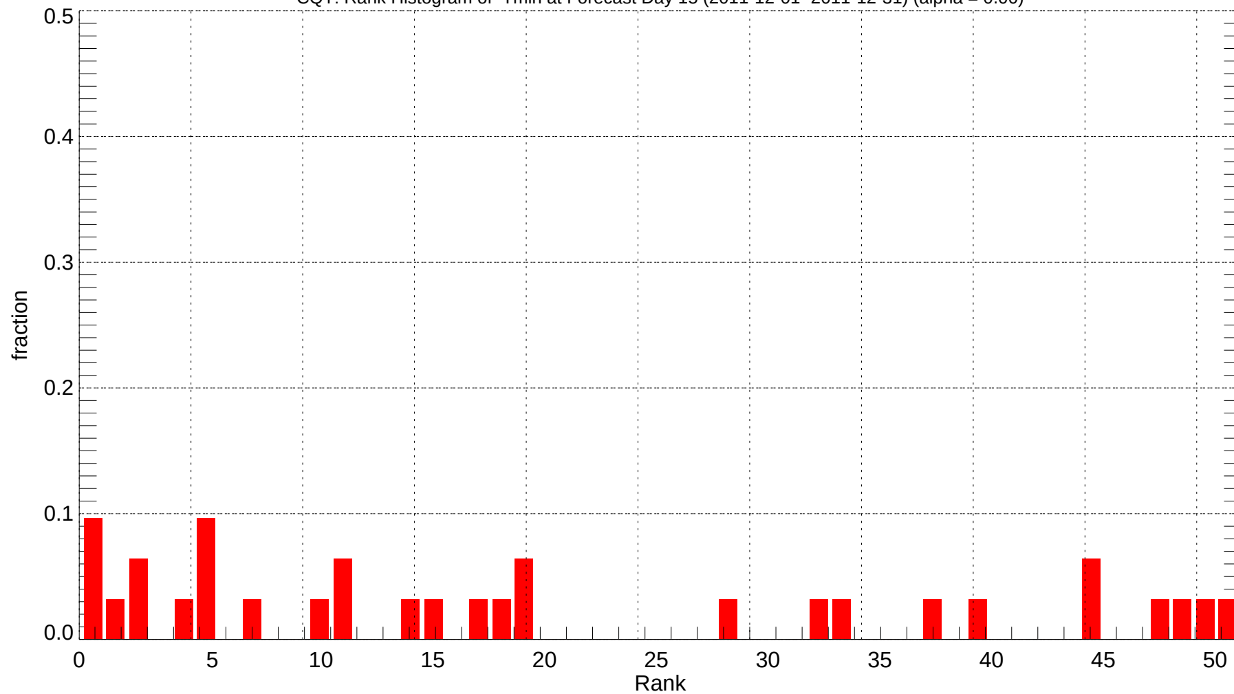
CQT: Rank Histogram of Tmin at Forecast Day 15 (2011-12-01~2011-12-31) (alpha = 0.00)
