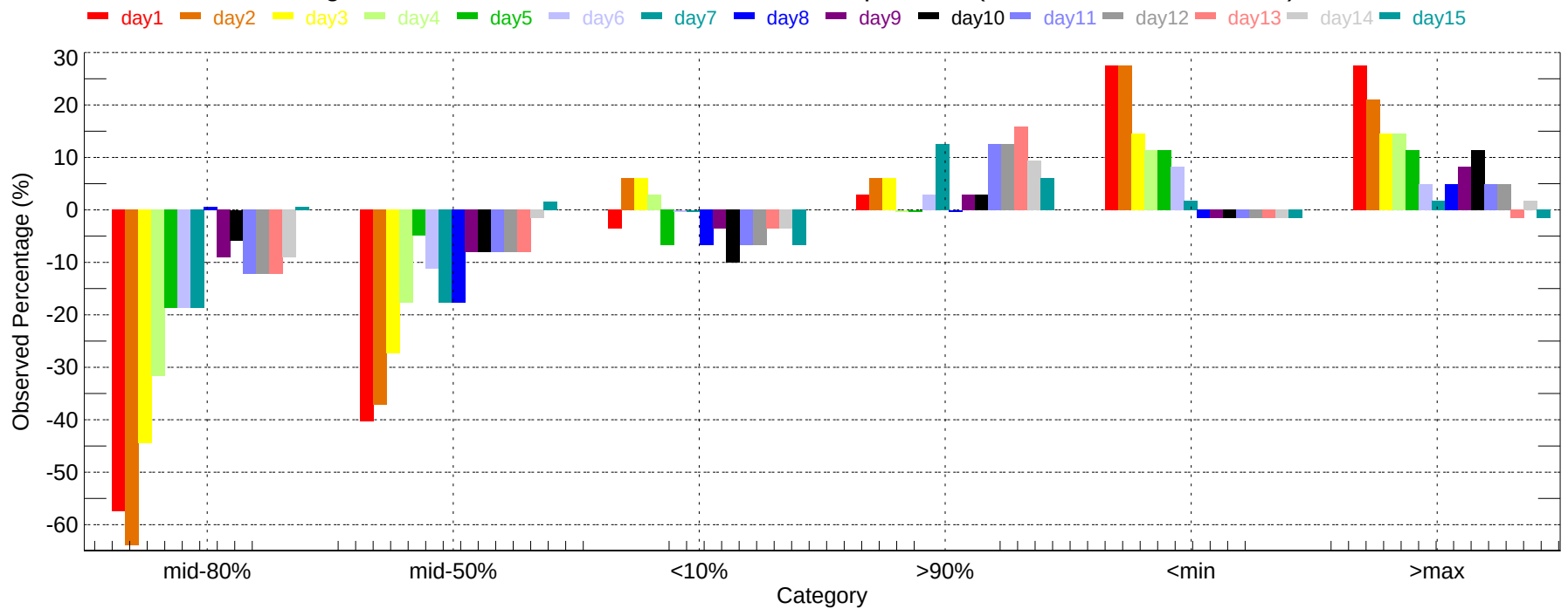
Observed Percentage Deviation of Ensembles - DAY: Min Temperature (2011-12-01~2011-12-31)
