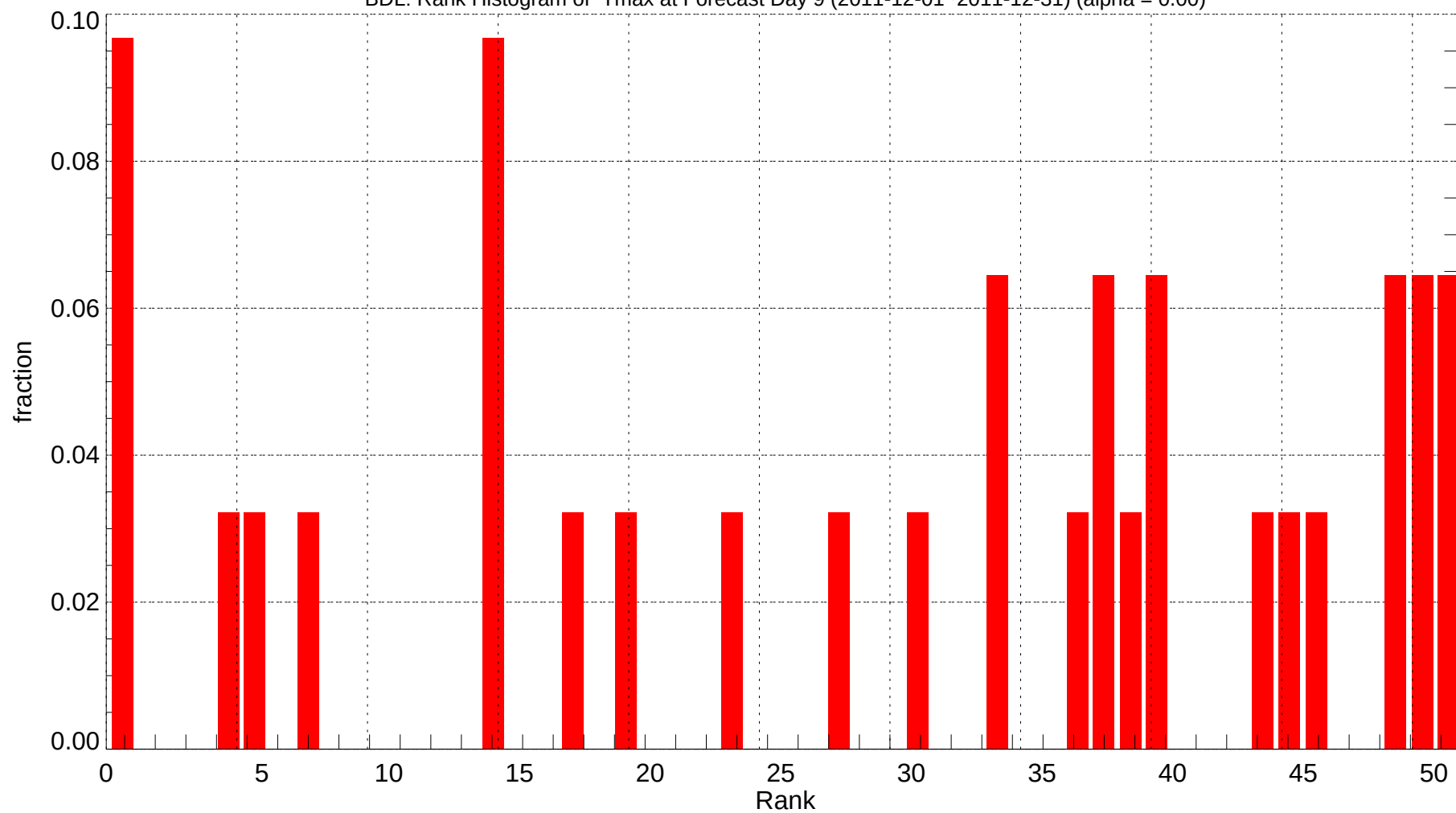
BDL: Rank Histogram of Tmax at Forecast Day 9 (2011-12-01~2011-12-31) (alpha = 0.00)
