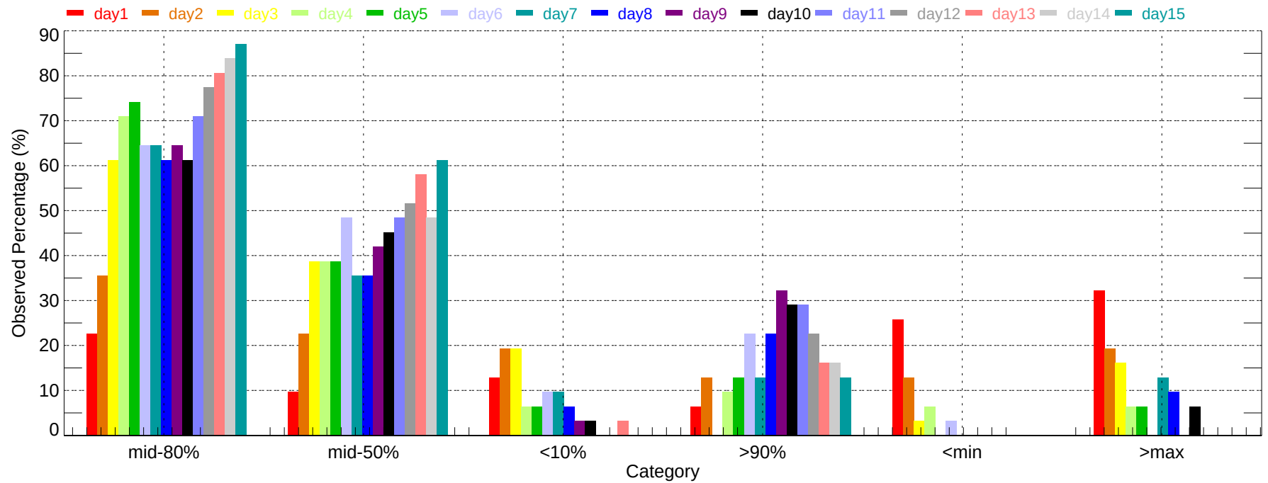
Observed Percentage of Ensembles - MEM: Min Temperature (2011-12-01~2011-12-31)
