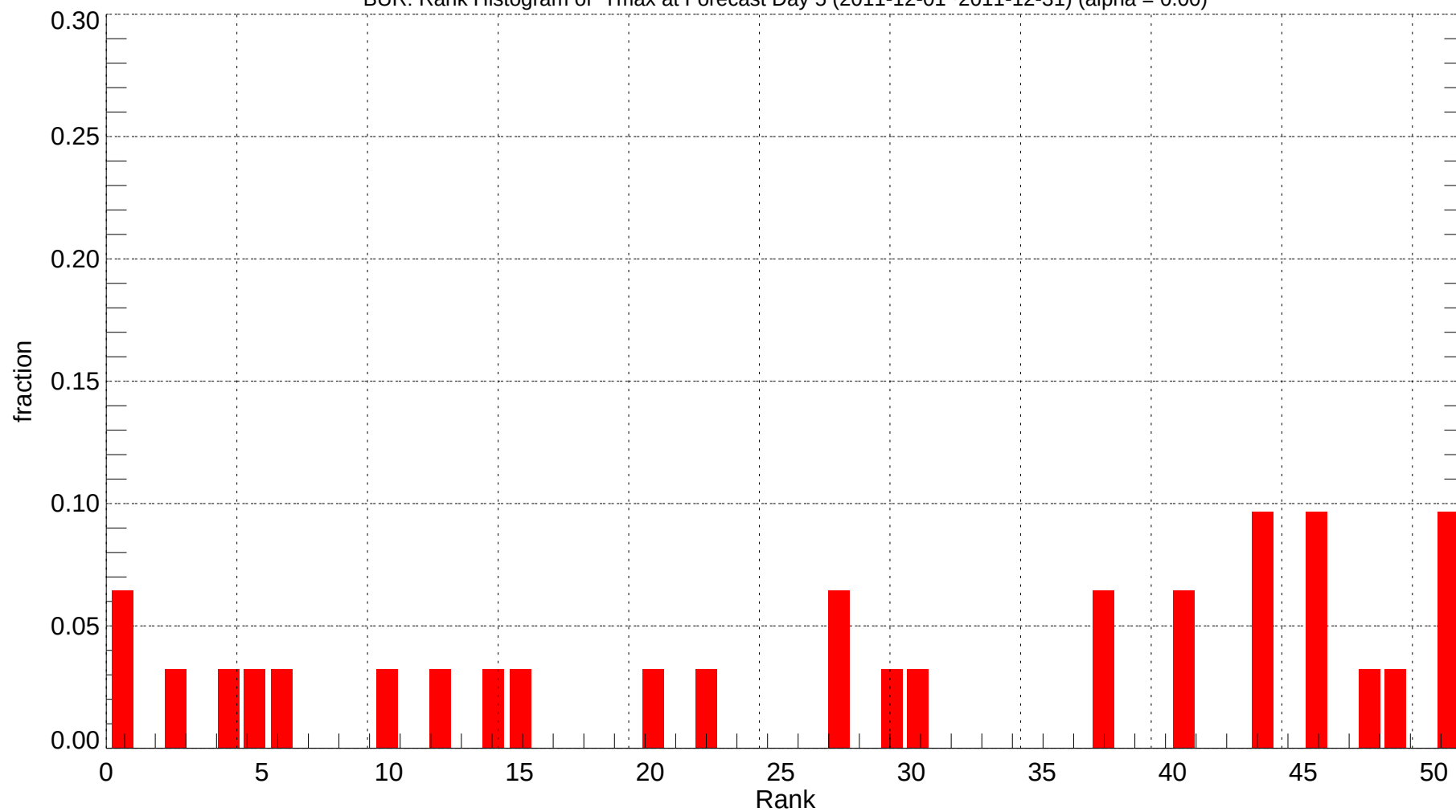
BUR: Rank Histogram of Tmax at Forecast Day 5 (2011-12-01~2011-12-31) (alpha = 0.00)
