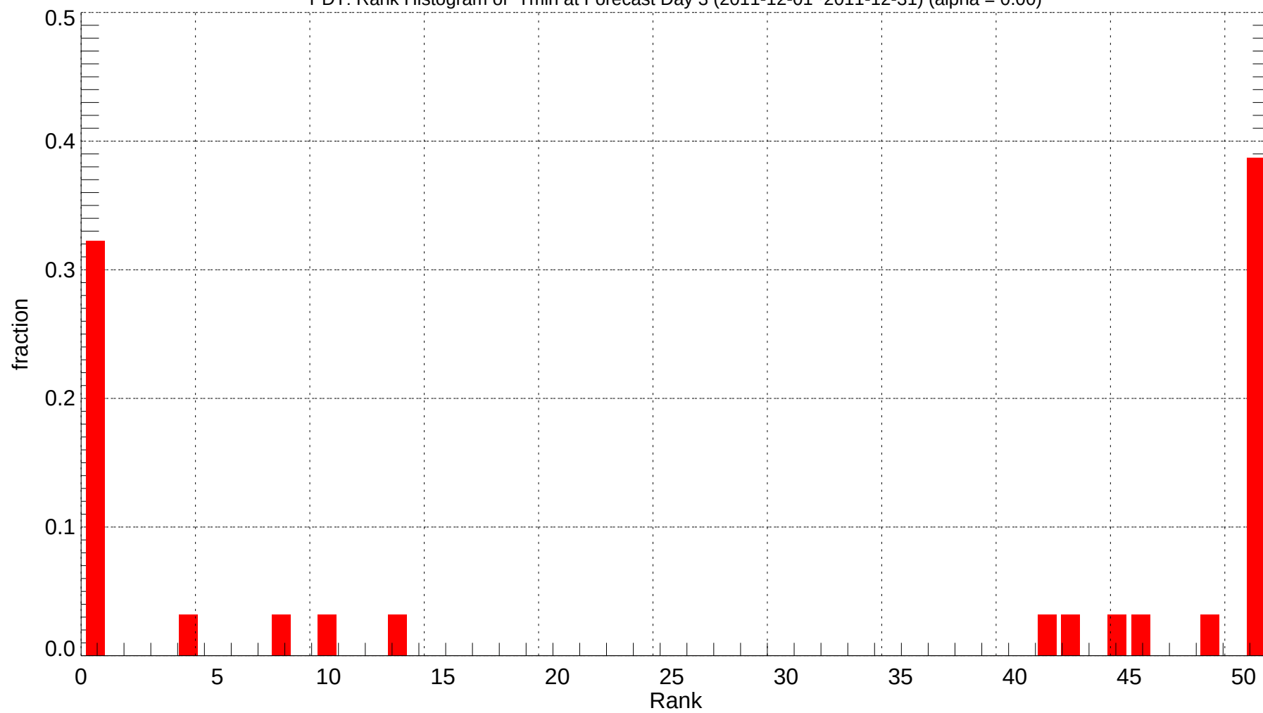
PDT: Rank Histogram of Tmin at Forecast Day 3 (2011-12-01~2011-12-31) (alpha = 0.00)
