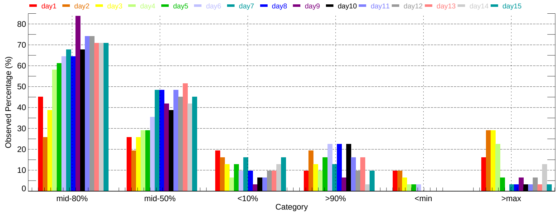
Observed Percentage of Ensembles - DFW: Max Temperature (2011-12-01~2011-12-31)
