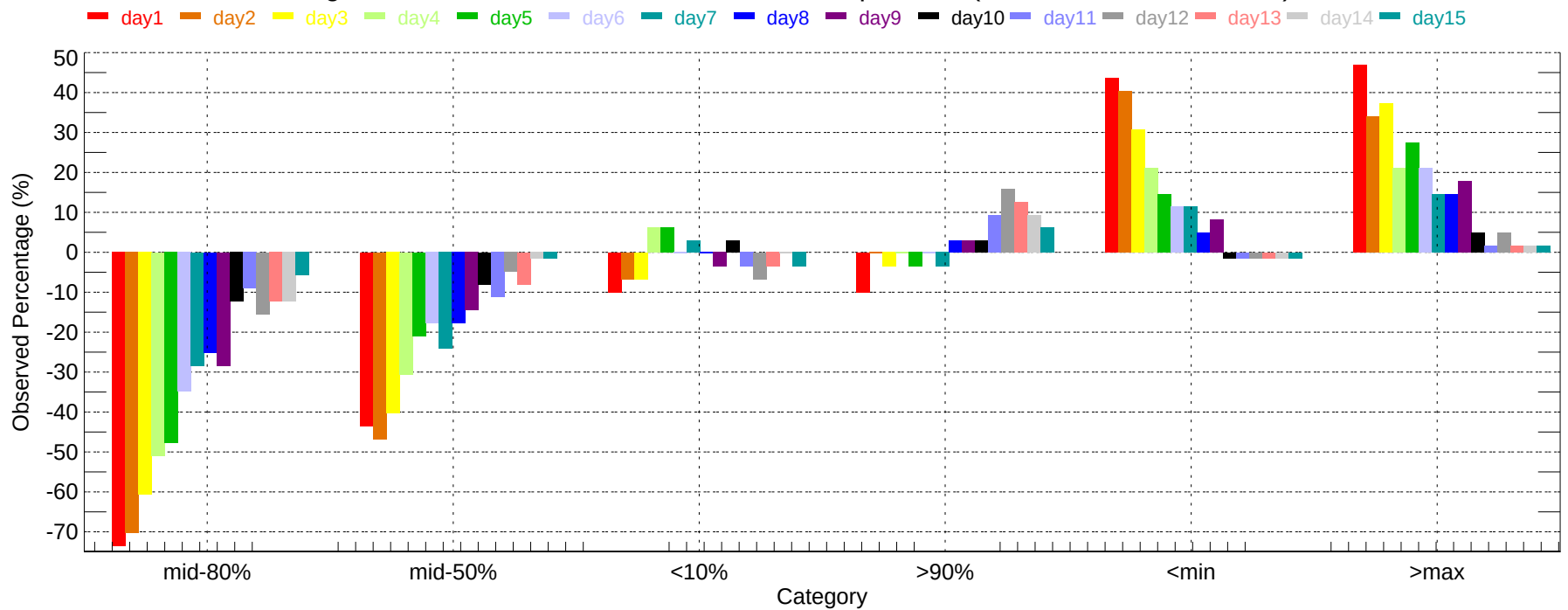
Observed Percentage Deviation of Ensembles - BWI: Min Temperature (2011-12-01~2011-12-31)
