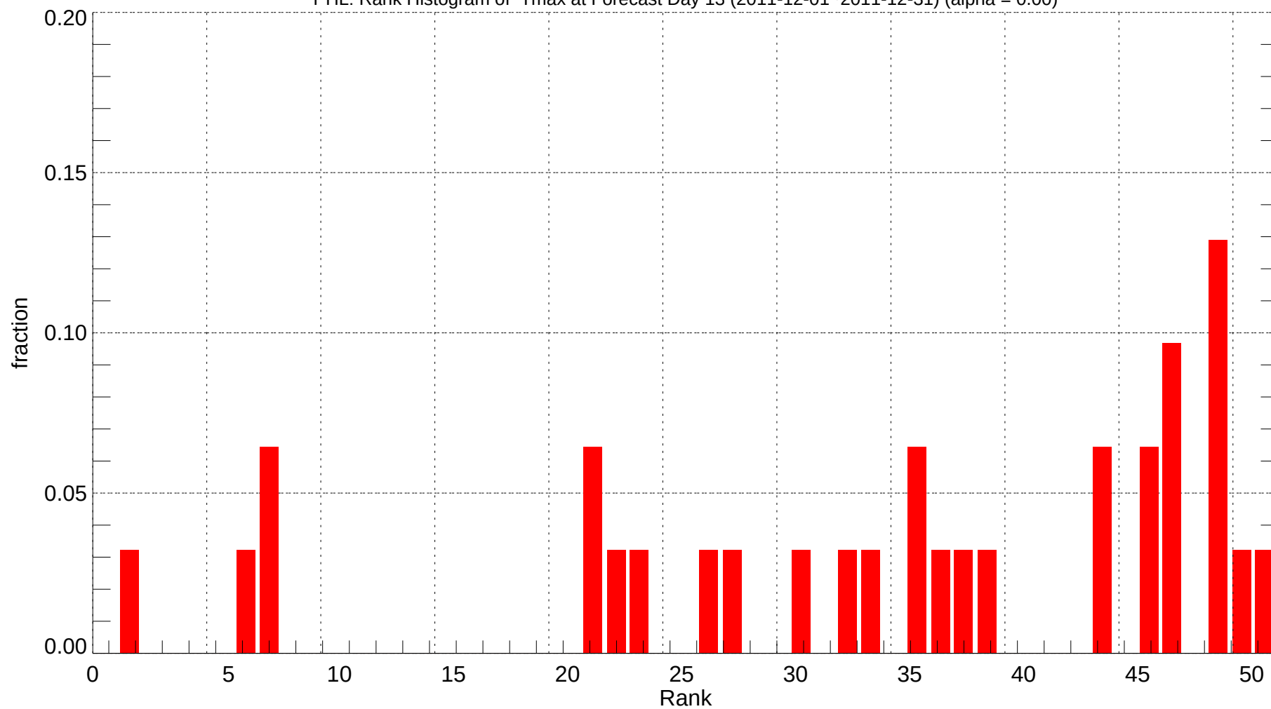
PHL: Rank Histogram of Tmax at Forecast Day 13 (2011-12-01~2011-12-31) (alpha = 0.00)
