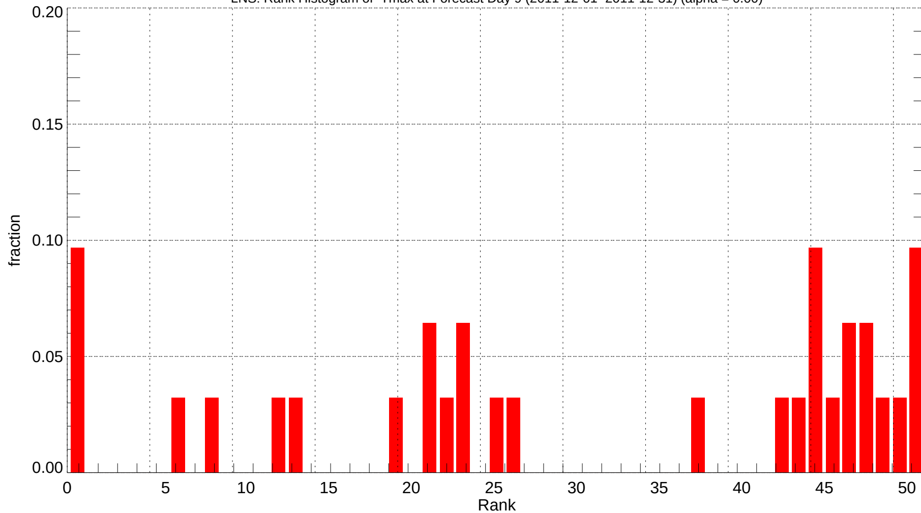
LNS: Rank Histogram of Tmax at Forecast Day 9 (2011-12-01~2011-12-31) (alpha = 0.00)
