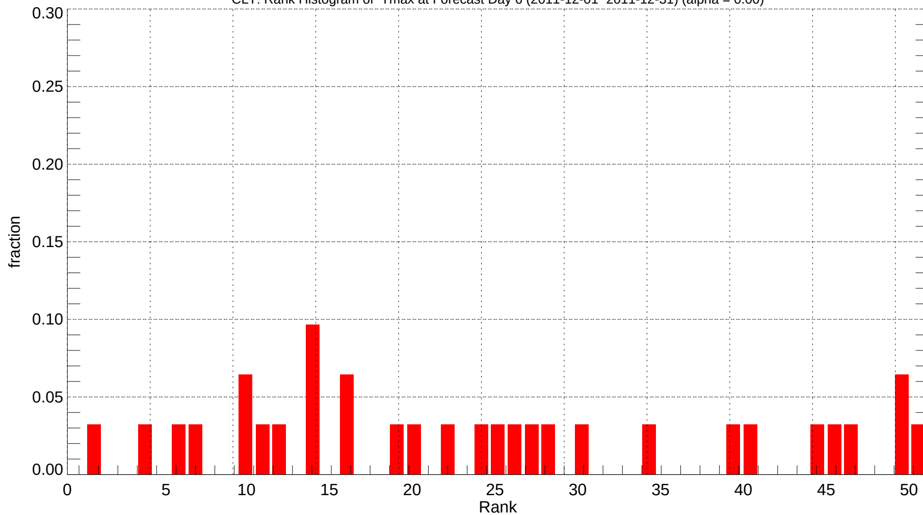
CLT: Rank Histogram of Tmax at Forecast Day 6 (2011-12-01~2011-12-31) (alpha = 0.00)
