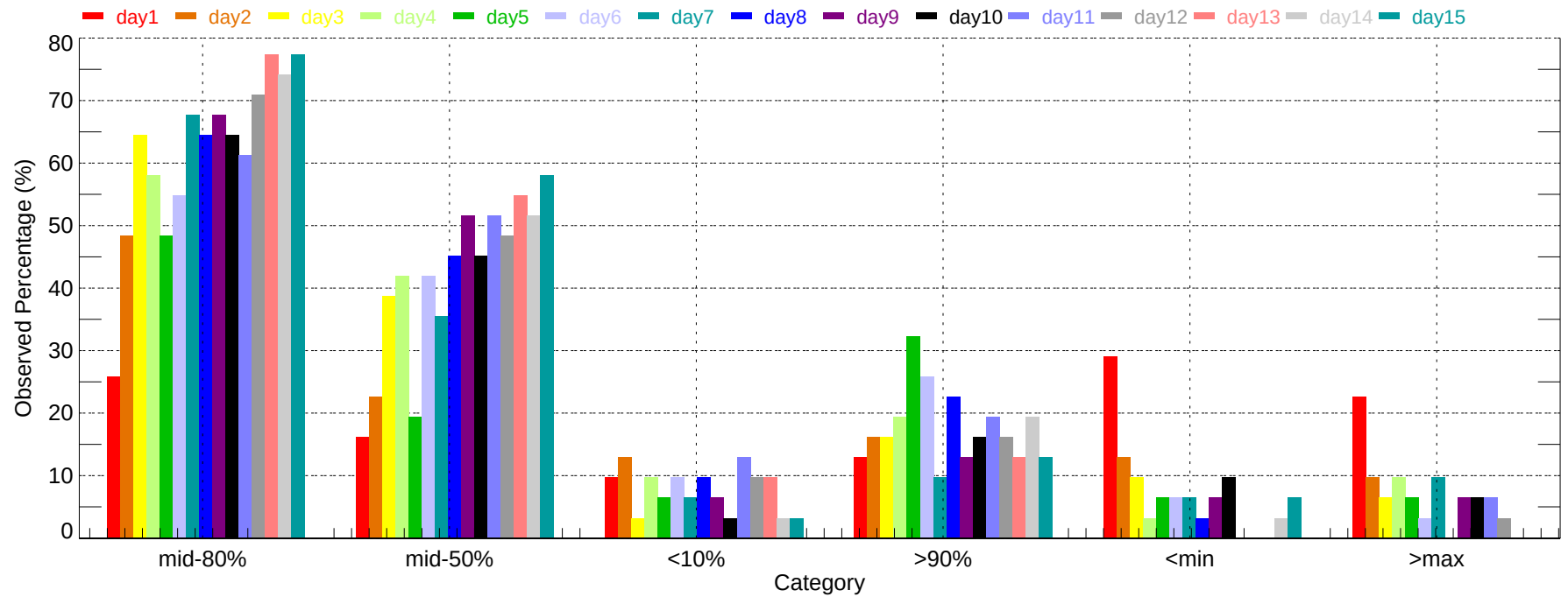
Observed Percentage of Ensembles - ALB: Max Temperature (2011-12-01~2011-12-31)
