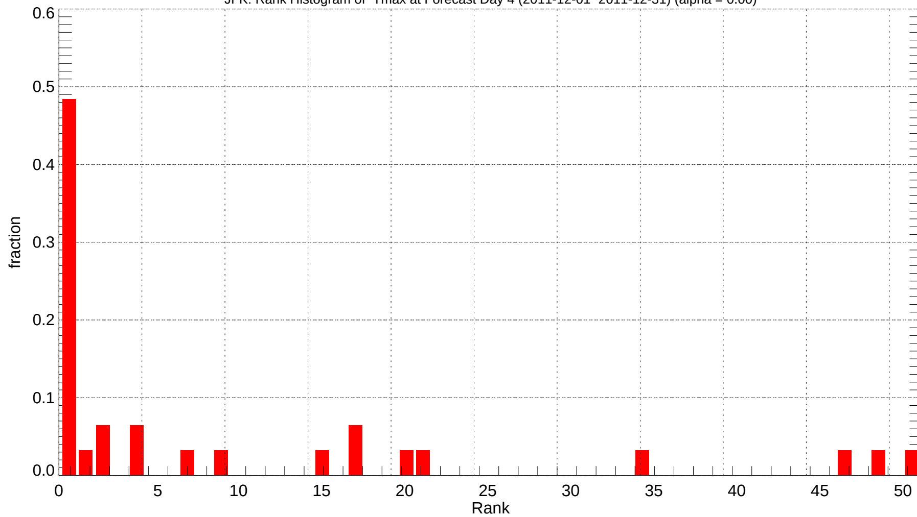
JFK: Rank Histogram of Tmax at Forecast Day 4 (2011-12-01~2011-12-31) (alpha = 0.00)
