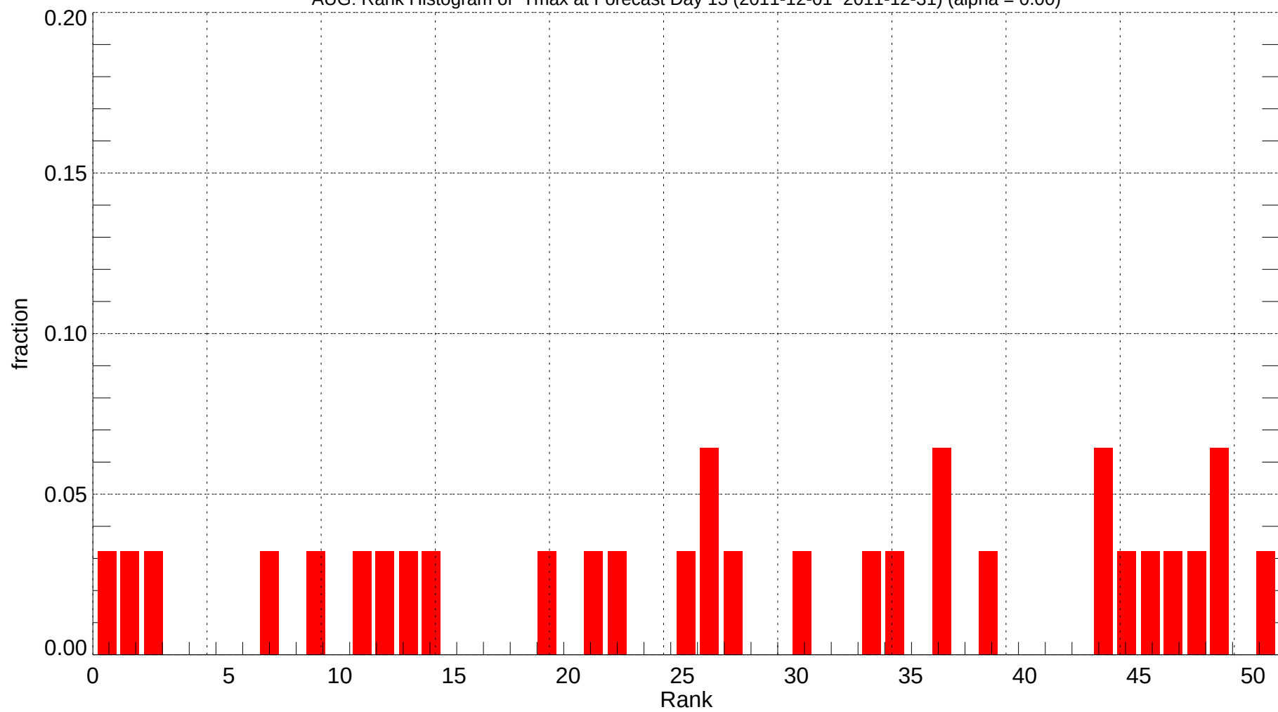
AUG: Rank Histogram of Tmax at Forecast Day 13 (2011-12-01~2011-12-31) (alpha = 0.00)
