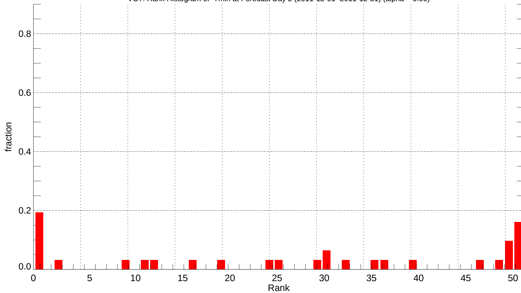
VCT: Rank Histogram of Tmin at Forecast Day 2 (2011-12-01~2011-12-31) (alpha = 0.00)
