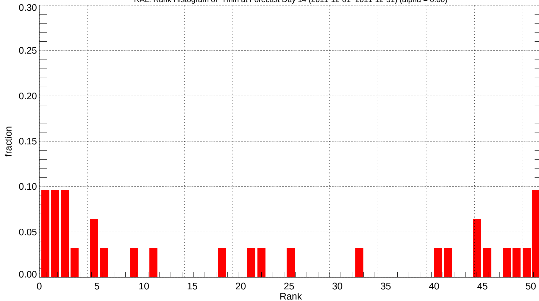
RAL: Rank Histogram of Tmin at Forecast Day 14 (2011-12-01~2011-12-31) (alpha = 0.00)
