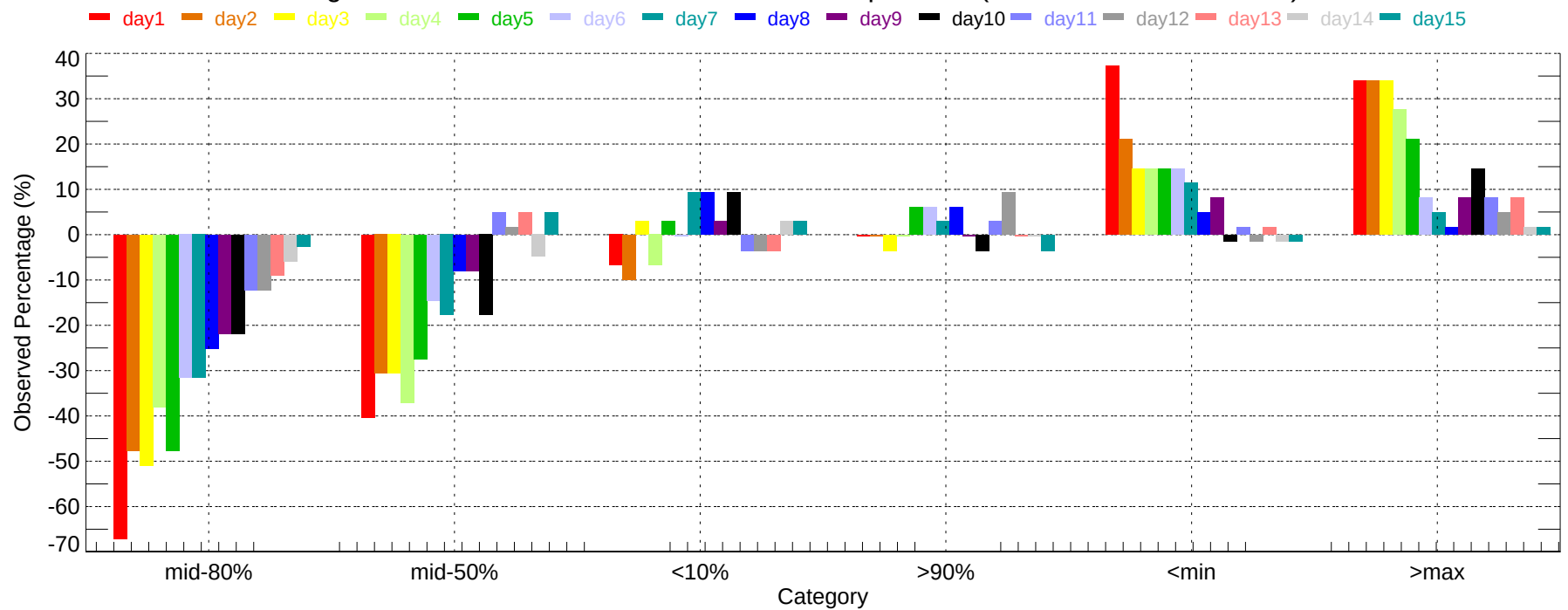
Observed Percentage Deviation of Ensembles - MBA: Min Temperature (2011-12-01~2011-12-31)
