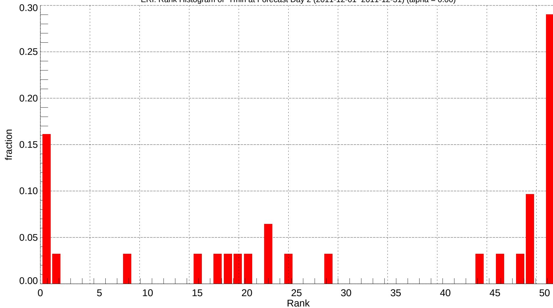
ERI: Rank Histogram of Tmin at Forecast Day 2 (2011-12-01~2011-12-31) (alpha = 0.00)
