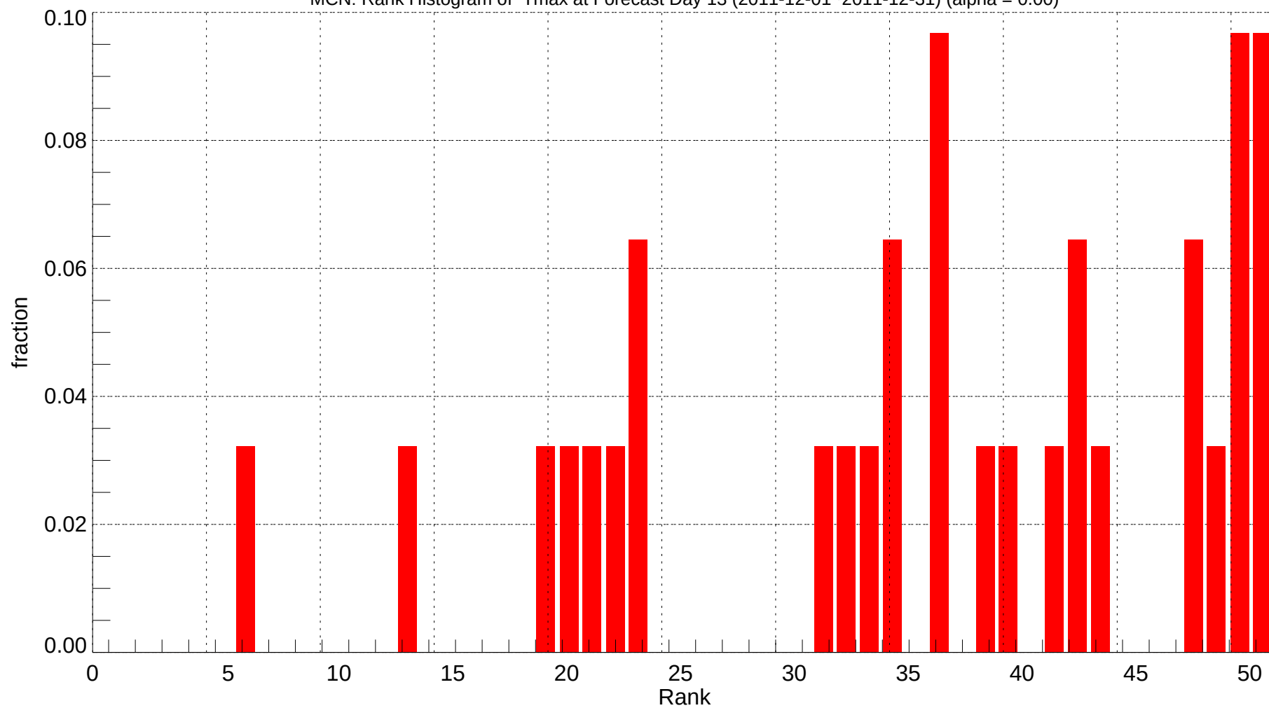
MCN: Rank Histogram of Tmax at Forecast Day 13 (2011-12-01~2011-12-31) (alpha = 0.00)
