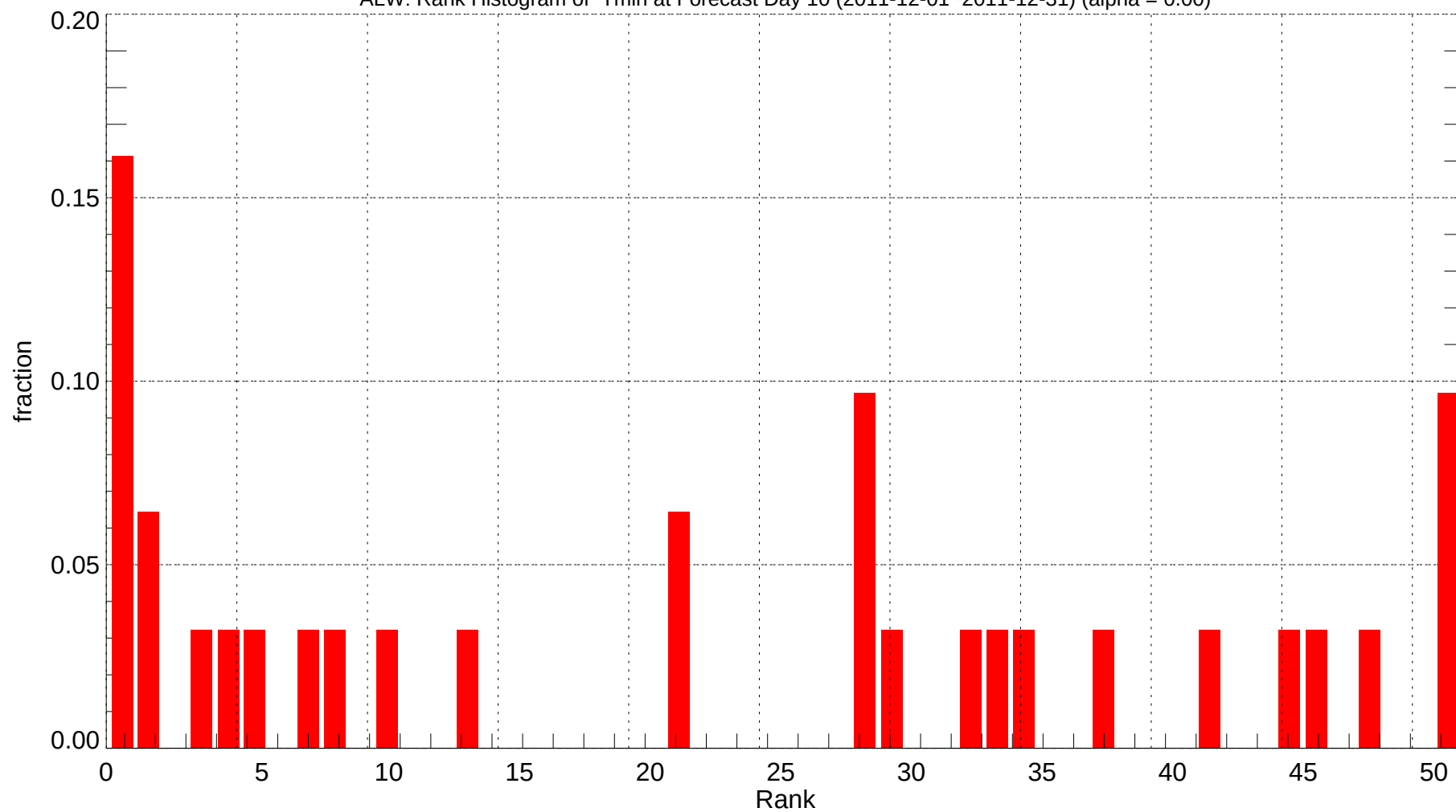
ALW: Rank Histogram of Tmin at Forecast Day 10 (2011-12-01~2011-12-31) (alpha = 0.00)
