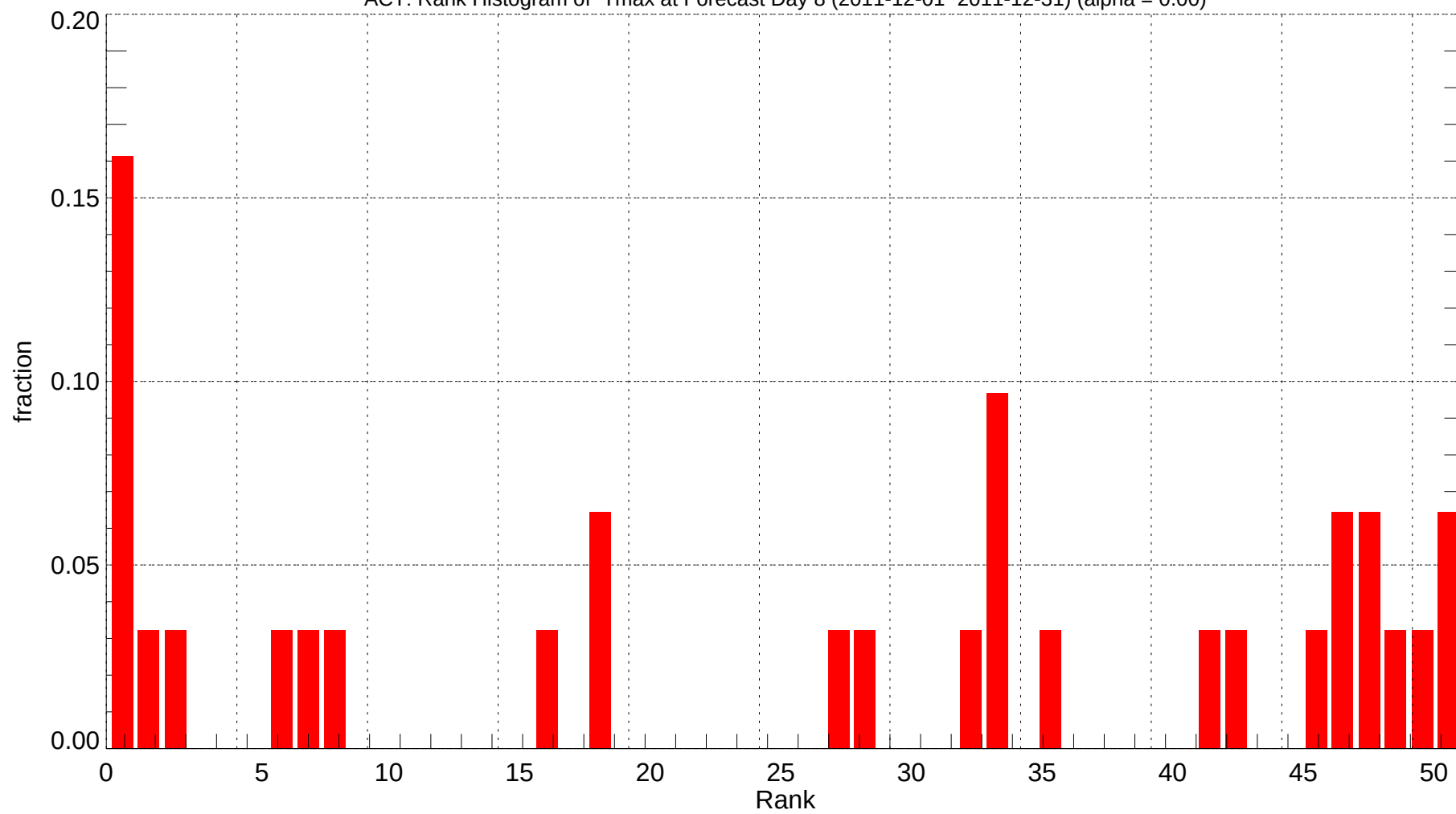
ACT: Rank Histogram of Tmax at Forecast Day 8 (2011-12-01~2011-12-31) (alpha = 0.00)
