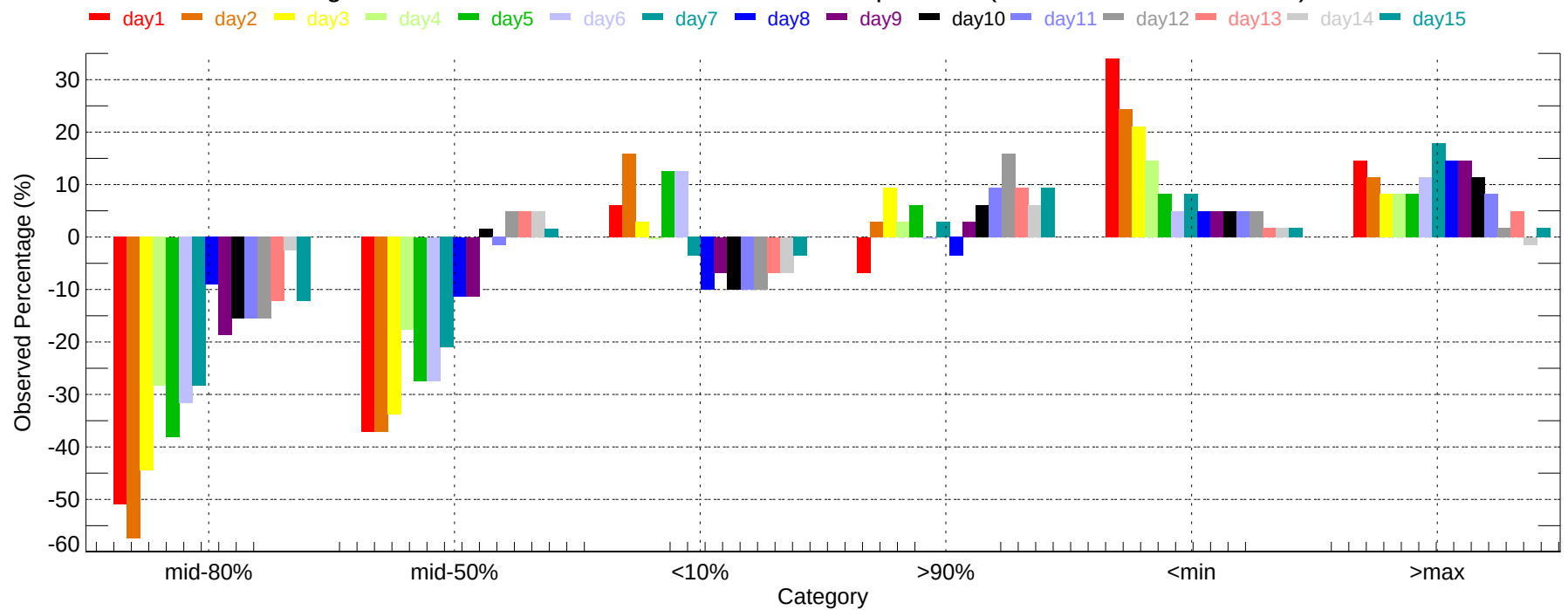
Observed Percentage Deviation of Ensembles - GAD: Max Temperature (2011-12-01~2011-12-31)
