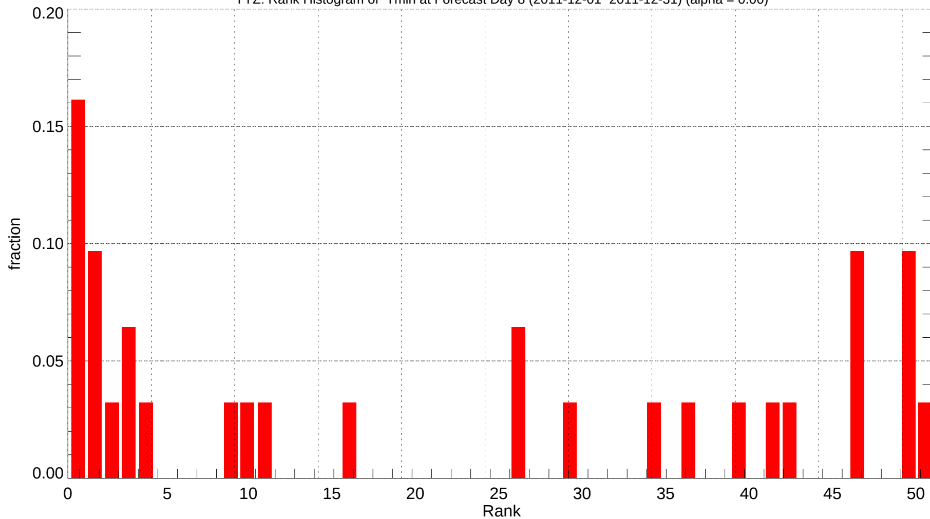
YYZ: Rank Histogram of Tmin at Forecast Day 8 (2011-12-01~2011-12-31) (alpha = 0.00)
