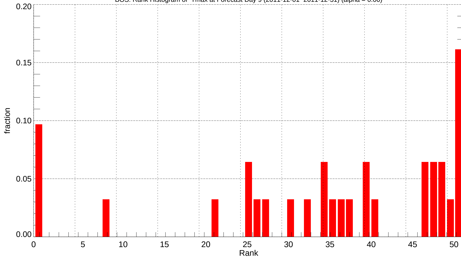
BOS: Rank Histogram of Tmax at Forecast Day 9 (2011-12-01~2011-12-31) (alpha = 0.00)
