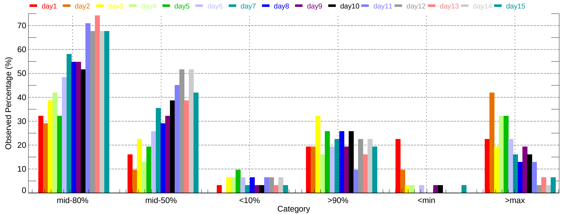
Observed Percentage of Ensembles - SYR: Max Temperature (2011-12-01~2011-12-31)
