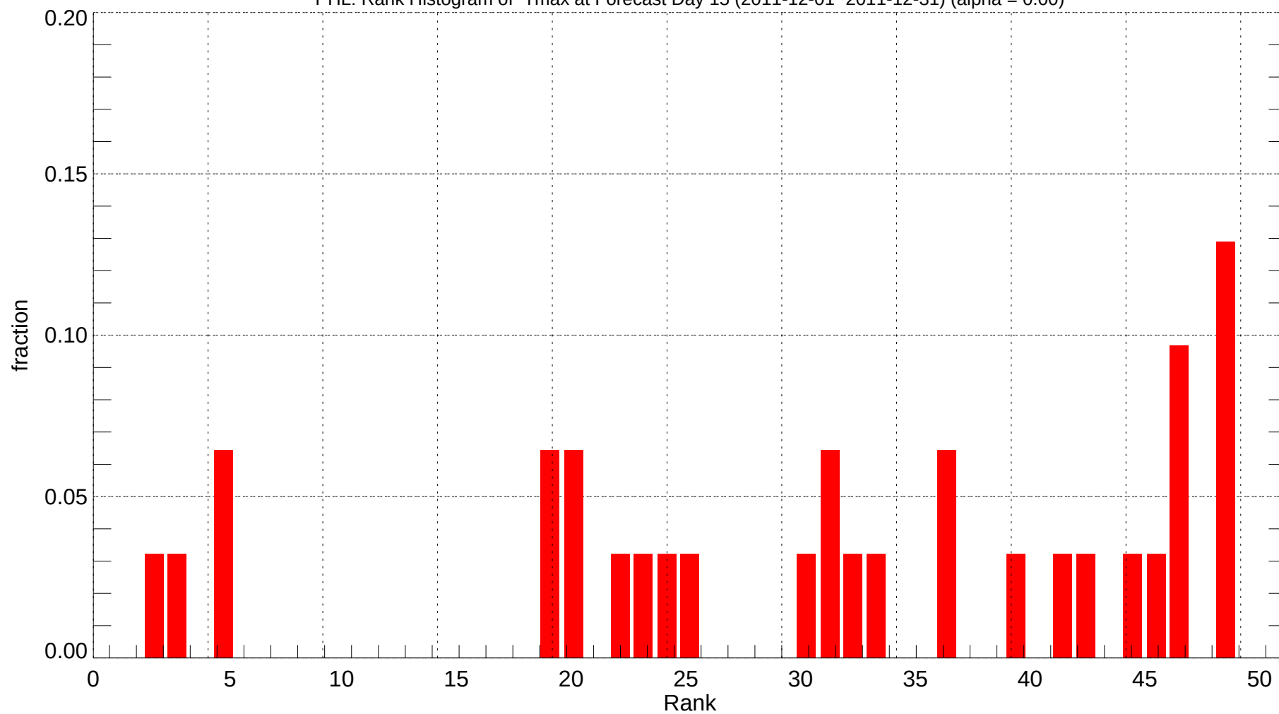
PHL: Rank Histogram of Tmax at Forecast Day 15 (2011-12-01~2011-12-31) (alpha = 0.00)
