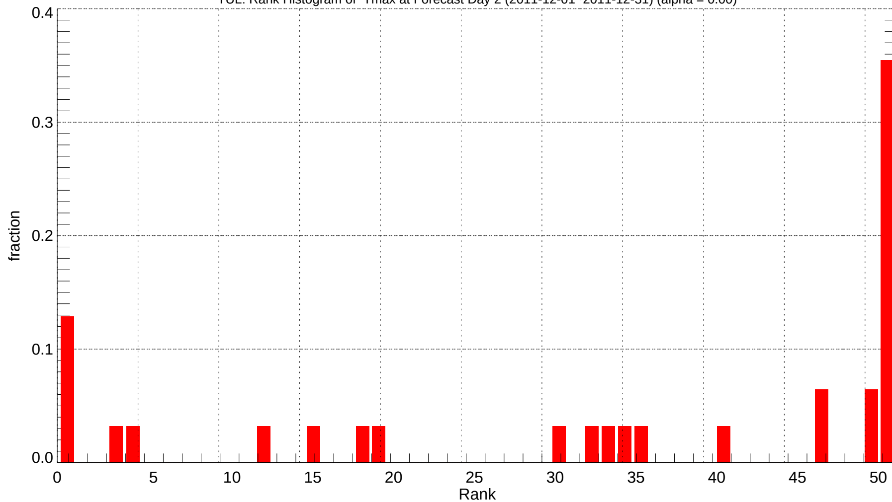
TUL: Rank Histogram of Tmax at Forecast Day 2 (2011-12-01~2011-12-31) (alpha = 0.00)
