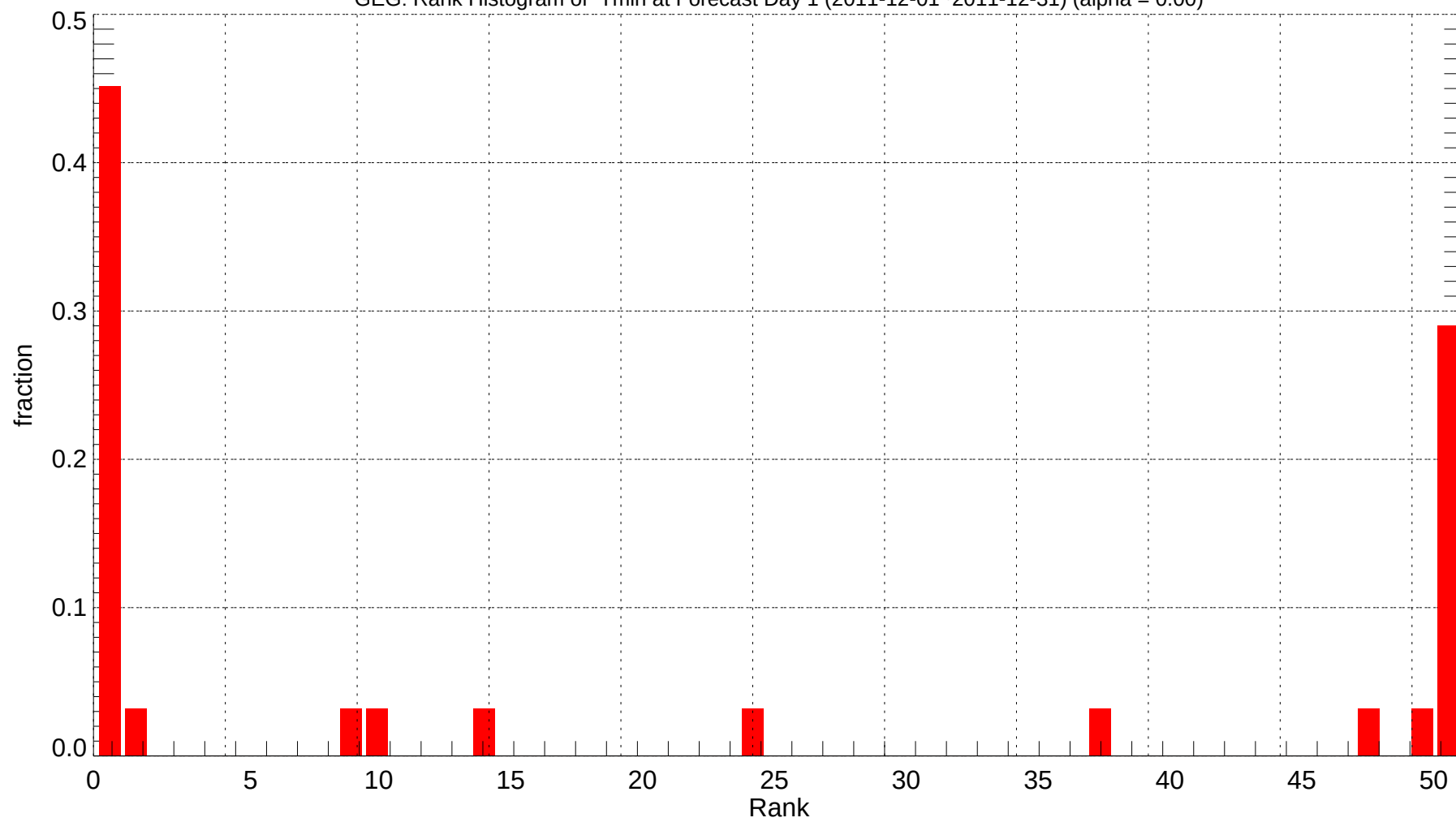
GEG: Rank Histogram of Tmin at Forecast Day 1 (2011-12-01~2011-12-31) (alpha = 0.00)
