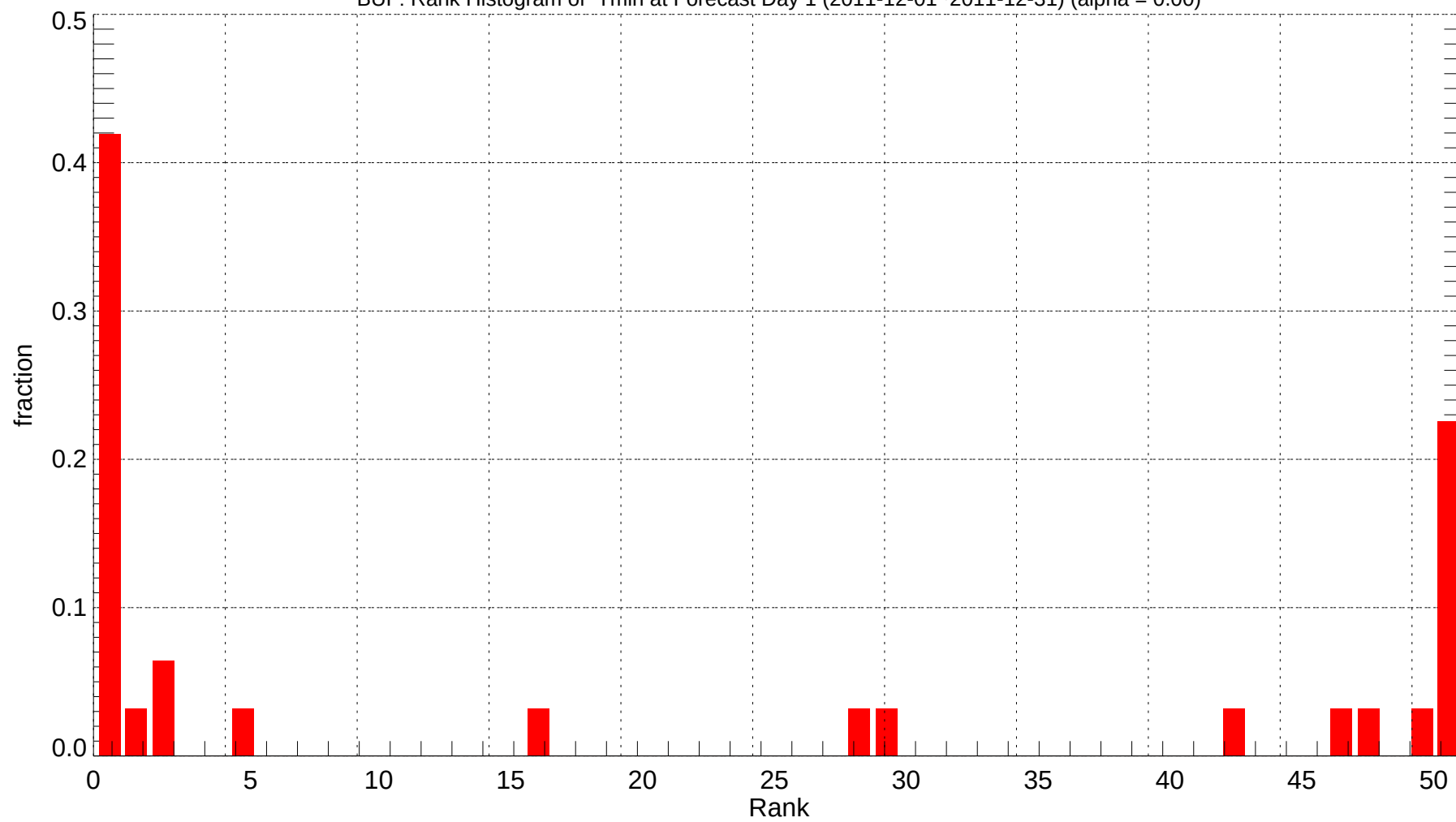
BUF: Rank Histogram of Tmin at Forecast Day 1 (2011-12-01~2011-12-31) (alpha = 0.00)
