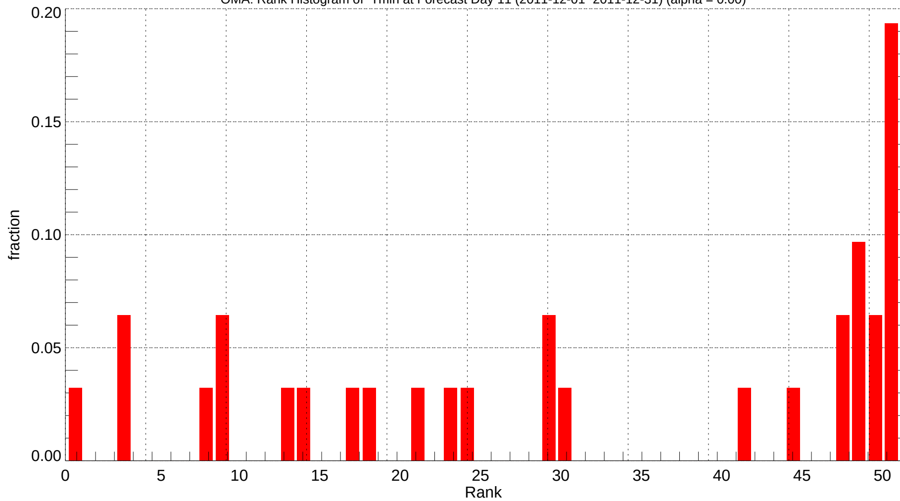
OMA: Rank Histogram of Tmin at Forecast Day 11 (2011-12-01~2011-12-31) (alpha = 0.00)
