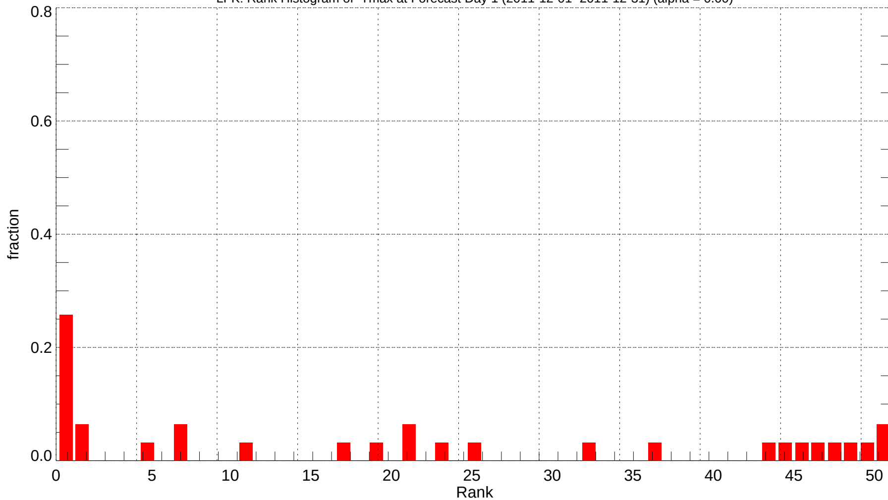
LFK: Rank Histogram of Tmax at Forecast Day 1 (2011-12-01~2011-12-31) (alpha = 0.00)
