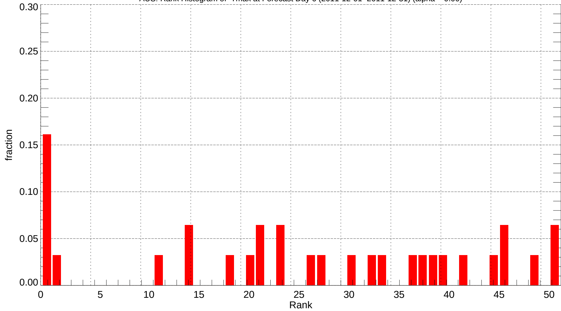
AUS: Rank Histogram of Tmax at Forecast Day 6 (2011-12-01~2011-12-31) (alpha = 0.00)
