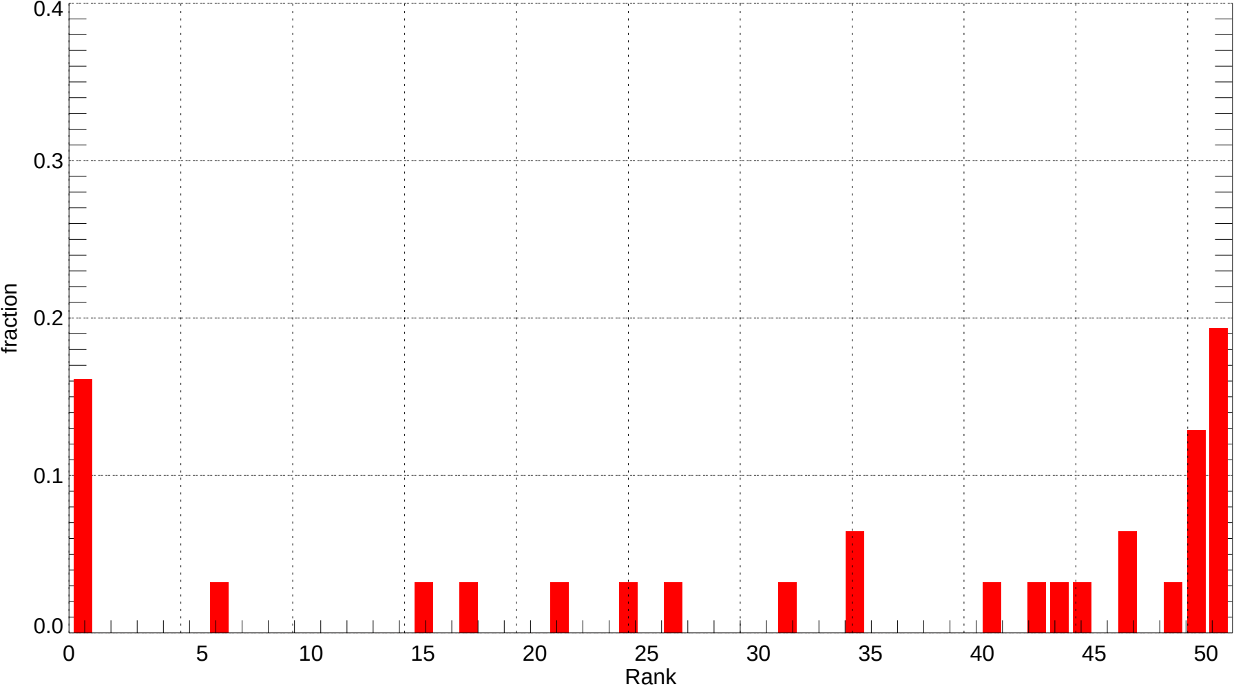
LAX: Rank Histogram of Tmin at Forecast Day 7 (2011-12-01~2011-12-31) (alpha = 0.00)
