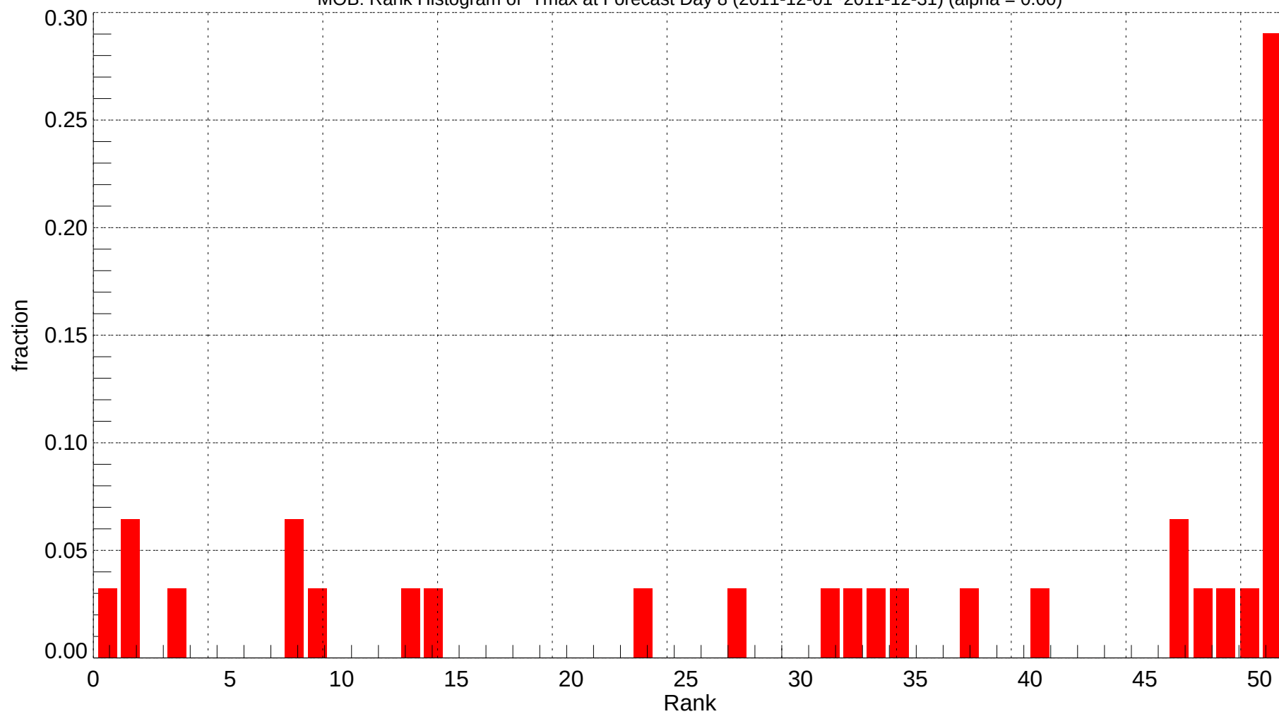
MOB: Rank Histogram of Tmax at Forecast Day 8 (2011-12-01~2011-12-31) (alpha = 0.00)
