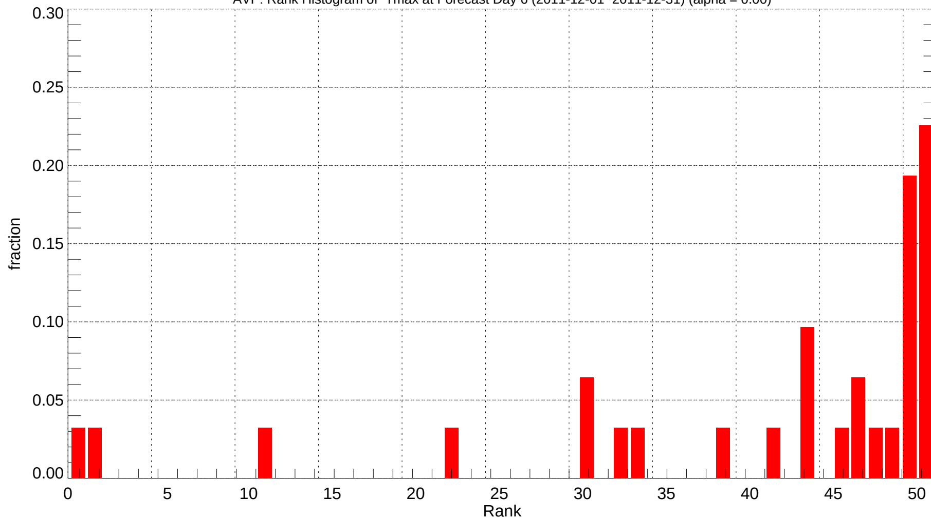
AVP: Rank Histogram of Tmax at Forecast Day 6 (2011-12-01~2011-12-31) (alpha = 0.00)
