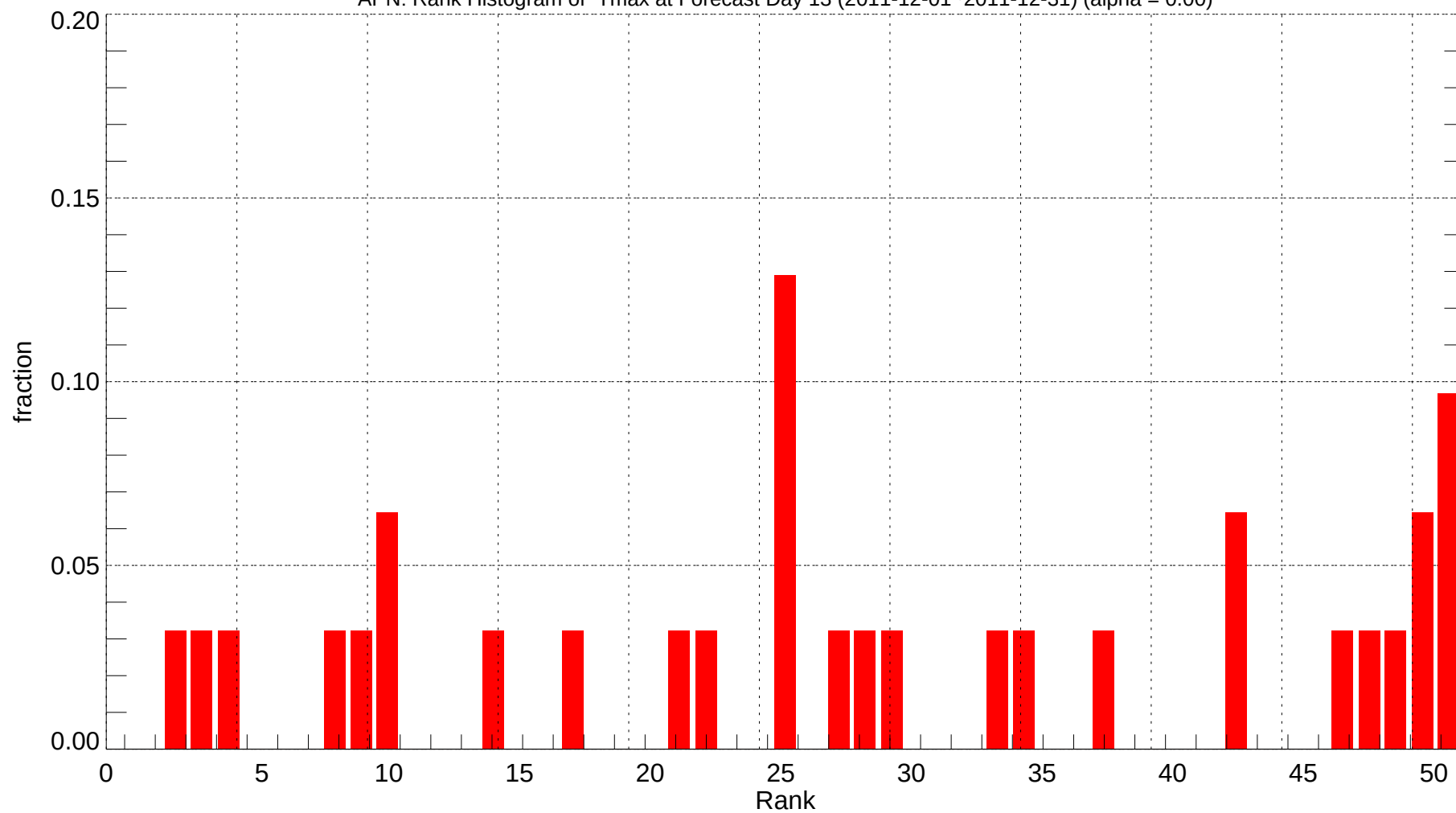
APN: Rank Histogram of Tmax at Forecast Day 13 (2011-12-01~2011-12-31) (alpha = 0.00)
