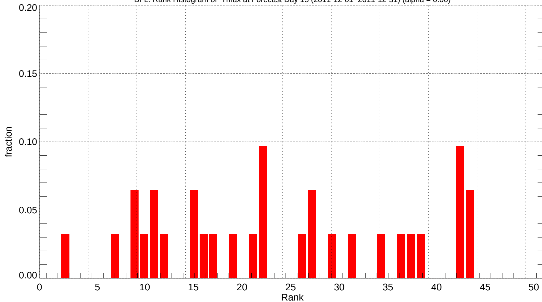
BFL: Rank Histogram of Tmax at Forecast Day 13 (2011-12-01~2011-12-31) (alpha = 0.00)
