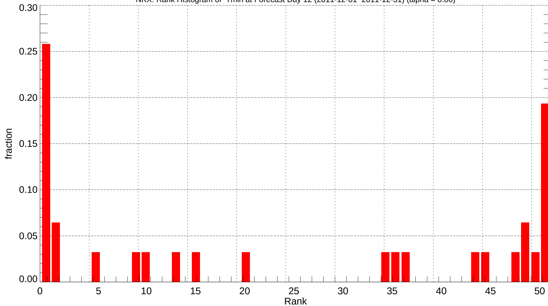
NKX: Rank Histogram of Tmin at Forecast Day 12 (2011-12-01~2011-12-31) (alpha = 0.00)
