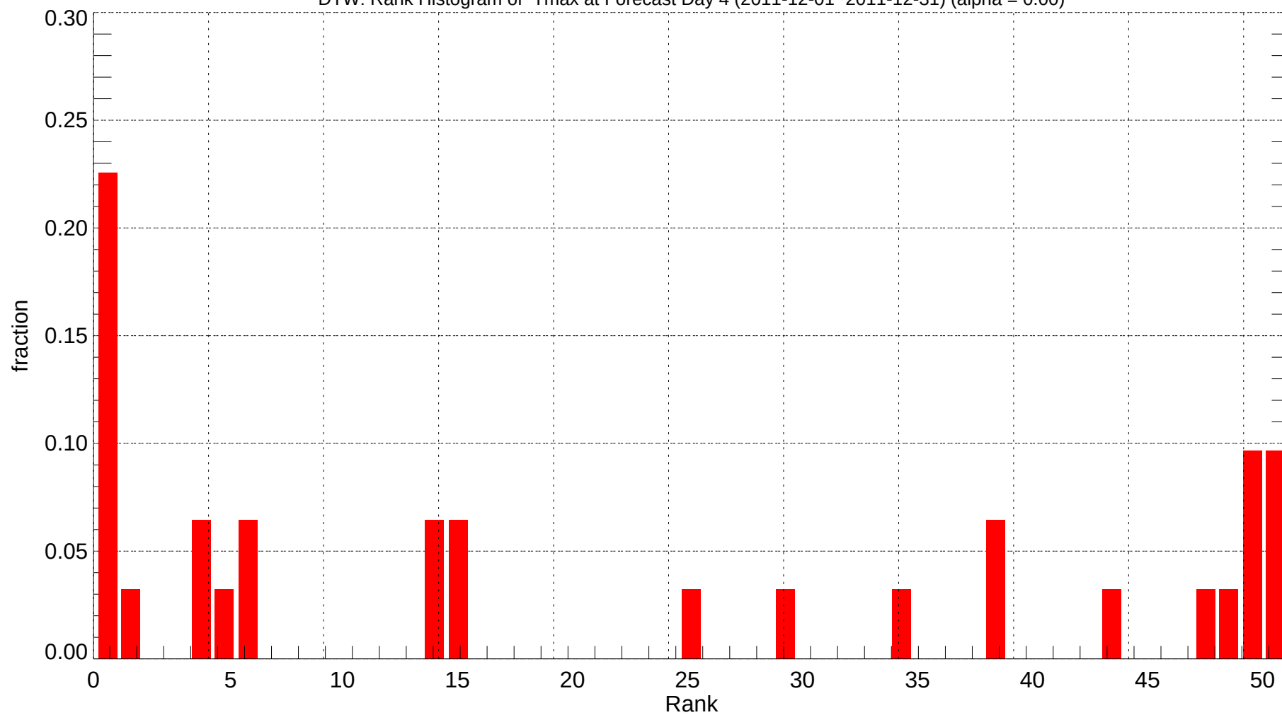
DTW: Rank Histogram of Tmax at Forecast Day 4 (2011-12-01~2011-12-31) (alpha = 0.00)
