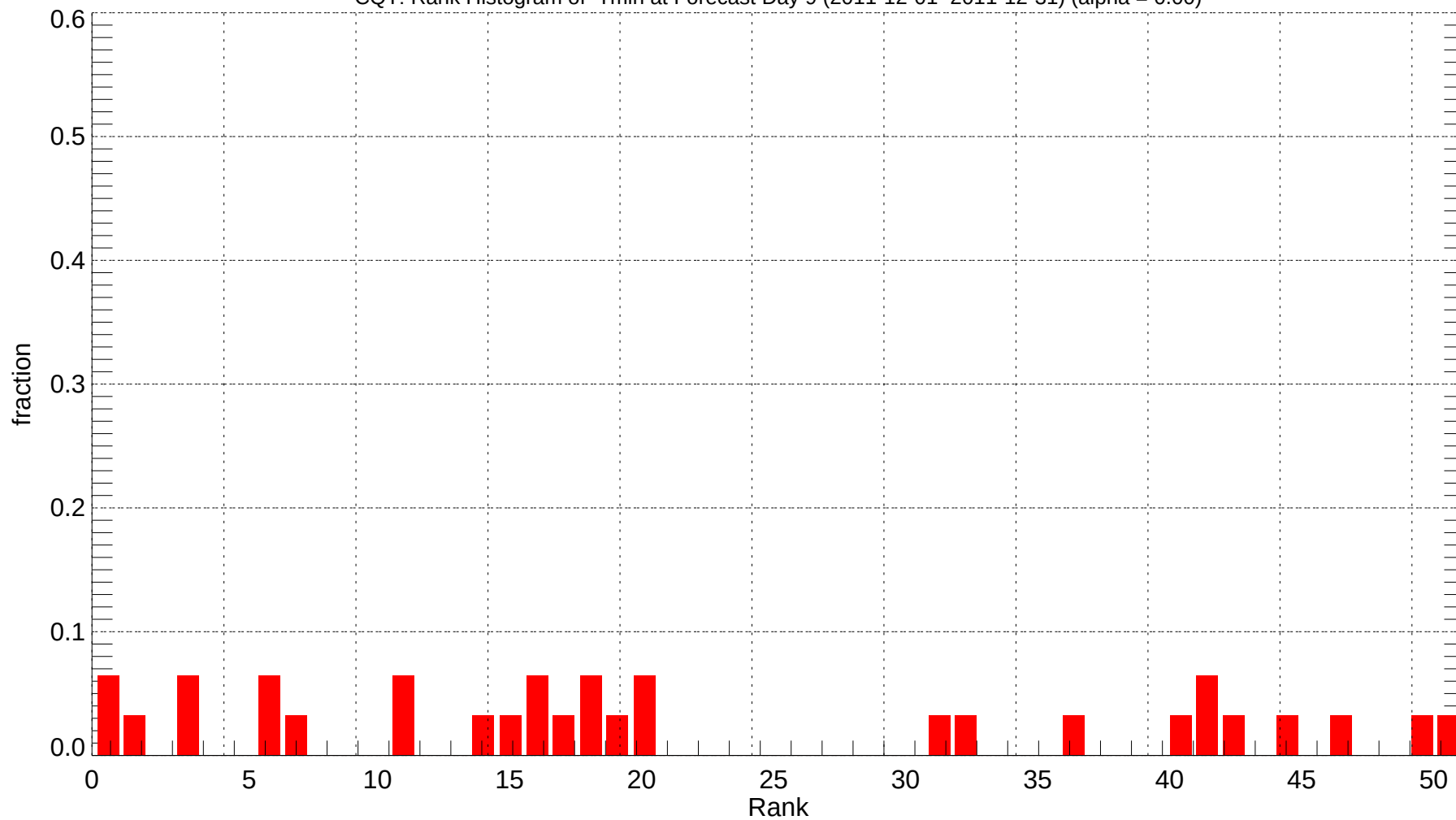
CQT: Rank Histogram of Tmin at Forecast Day 9 (2011-12-01~2011-12-31) (alpha = 0.00)
