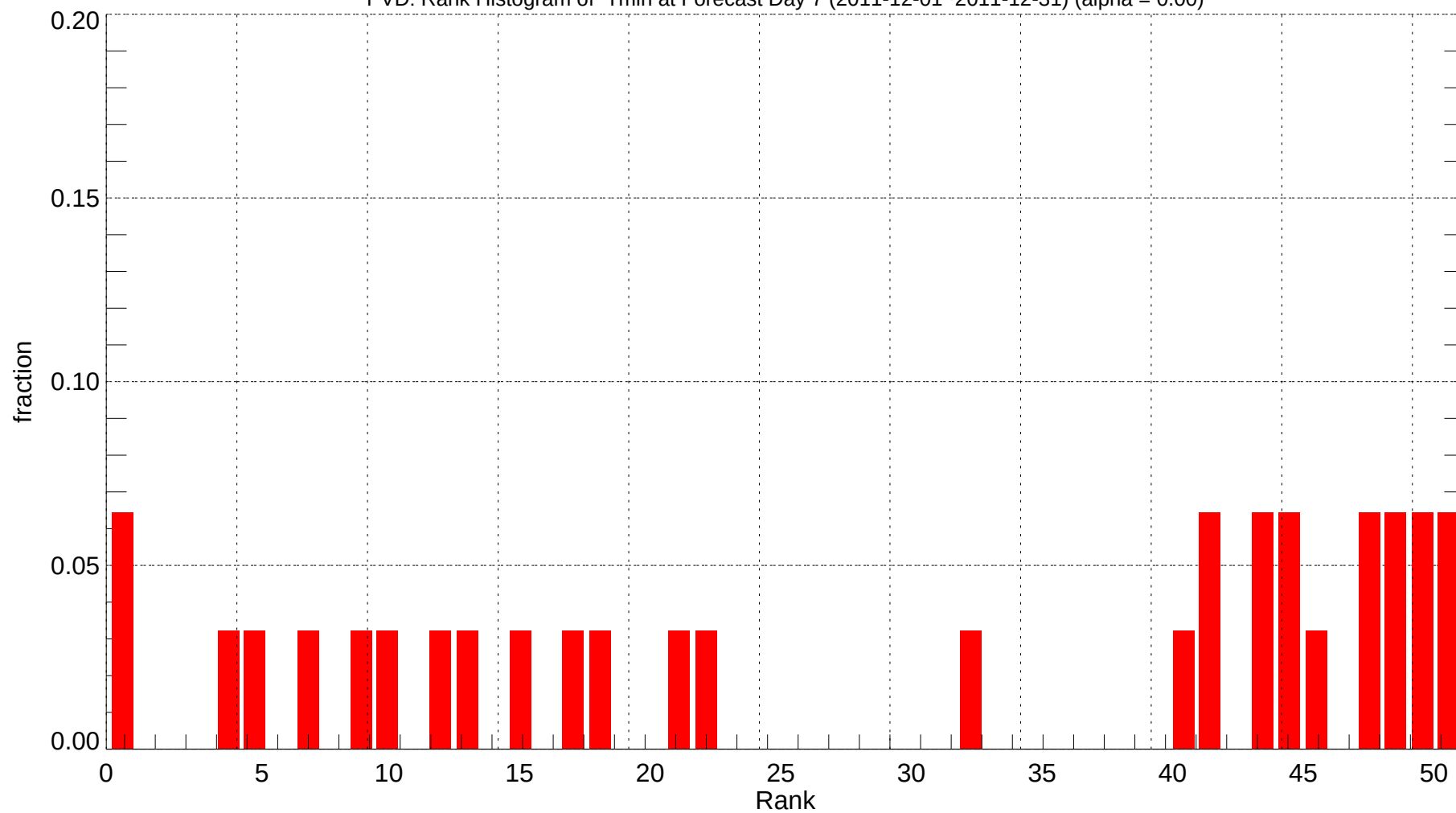
PVD: Rank Histogram of Tmin at Forecast Day 7 (2011-12-01~2011-12-31) (alpha = 0.00)
