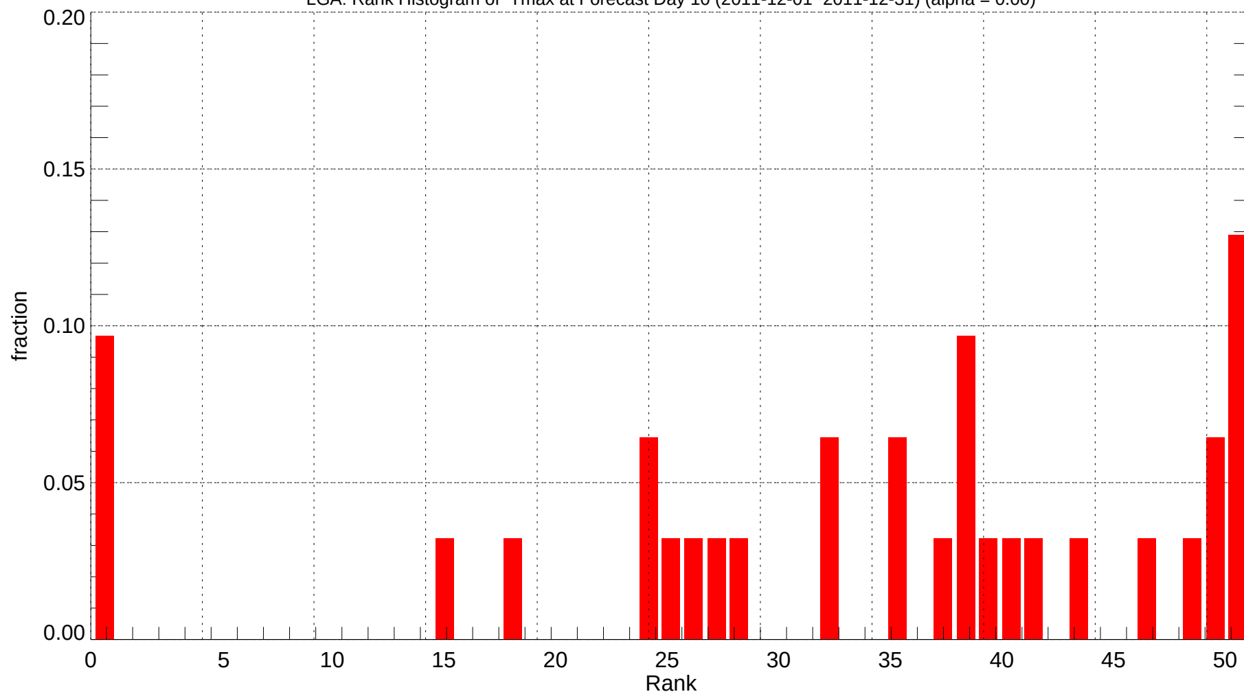
LGA: Rank Histogram of Tmax at Forecast Day 10 (2011-12-01~2011-12-31) (alpha = 0.00)
