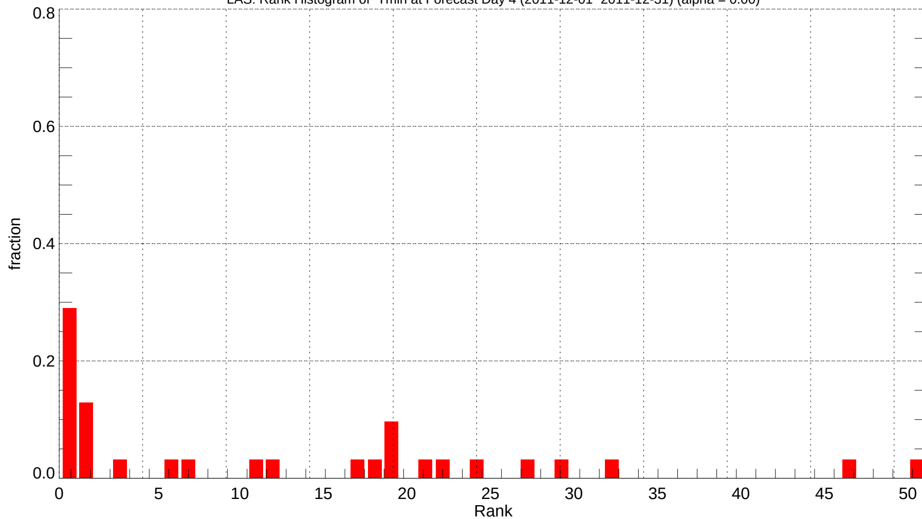
LAS: Rank Histogram of Tmin at Forecast Day 4 (2011-12-01~2011-12-31) (alpha = 0.00)
