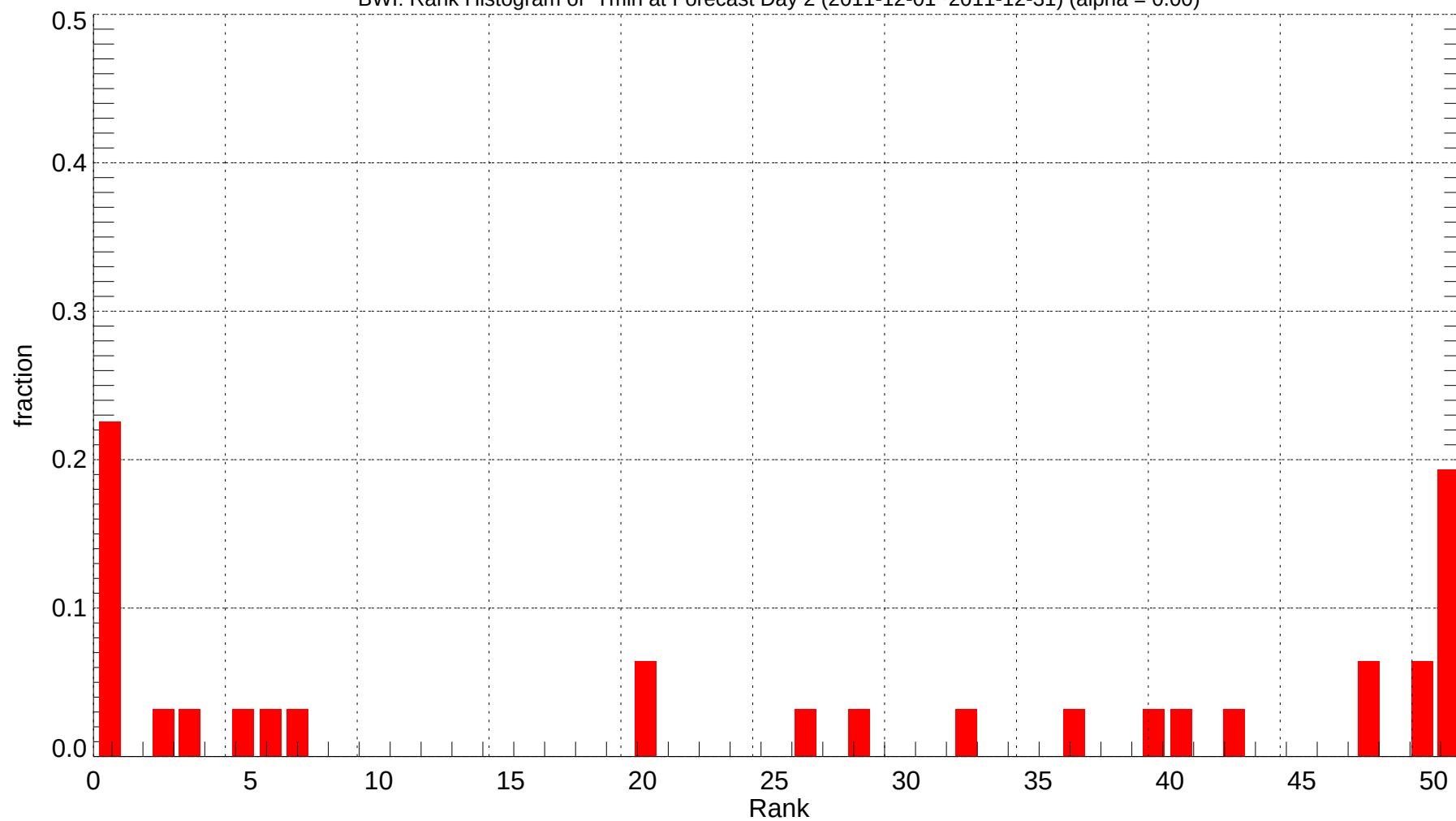
BWI: Rank Histogram of Tmin at Forecast Day 2 (2011-12-01~2011-12-31) (alpha = 0.00)
