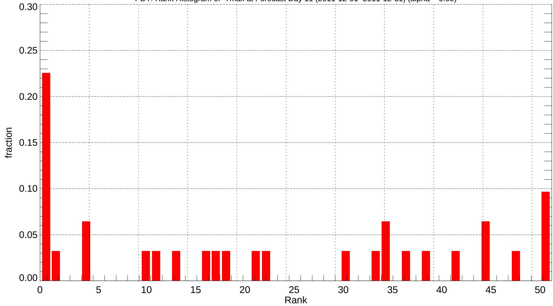
PDT: Rank Histogram of Tmax at Forecast Day 11 (2011-12-01~2011-12-31) (alpha = 0.00)
