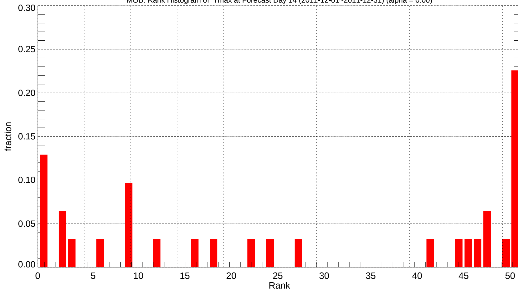
MOB: Rank Histogram of Tmax at Forecast Day 14 (2011-12-01~2011-12-31) (alpha = 0.00)
