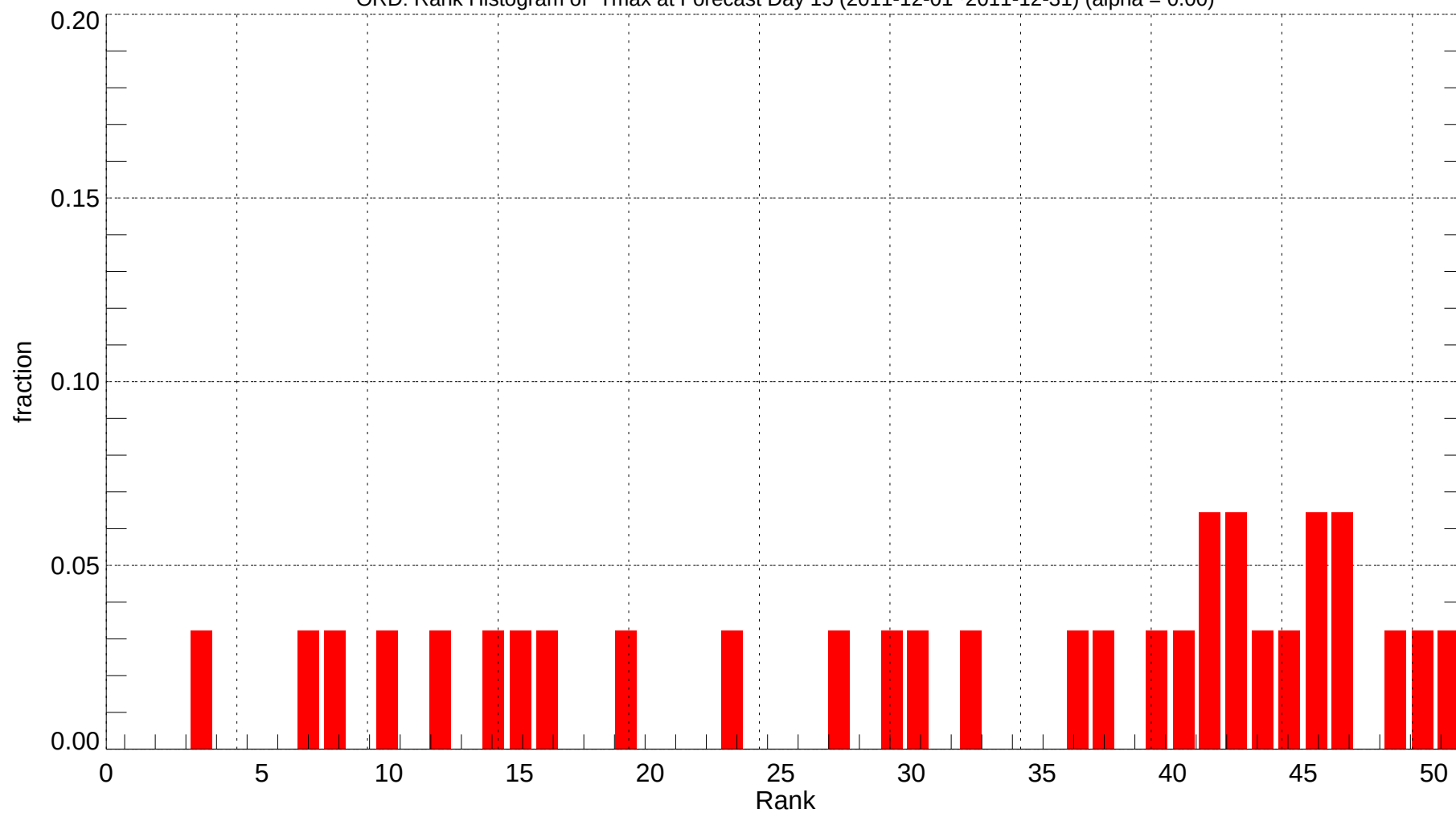
ORD: Rank Histogram of Tmax at Forecast Day 15 (2011-12-01~2011-12-31) (alpha = 0.00)
