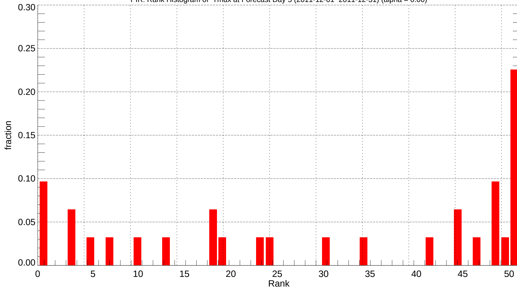
PIR: Rank Histogram of Tmax at Forecast Day 5 (2011-12-01~2011-12-31) (alpha = 0.00)
