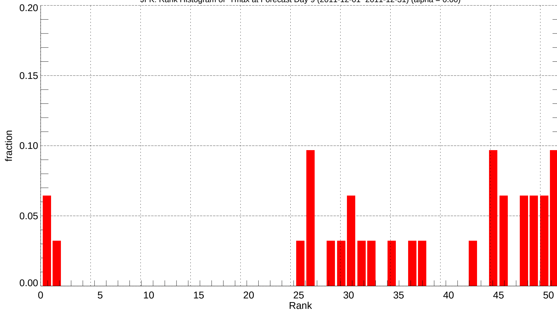
JFK: Rank Histogram of Tmax at Forecast Day 9 (2011-12-01~2011-12-31) (alpha = 0.00)
