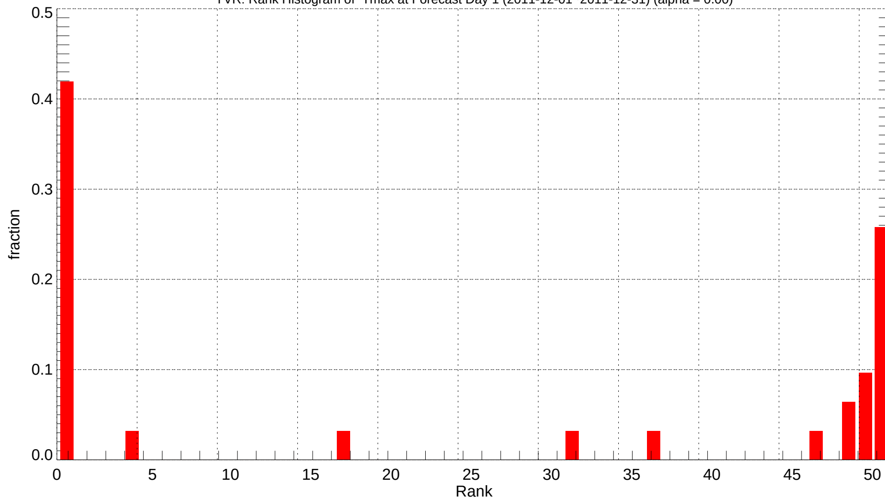
YVR: Rank Histogram of Tmax at Forecast Day 1 (2011-12-01~2011-12-31) (alpha = 0.00)
