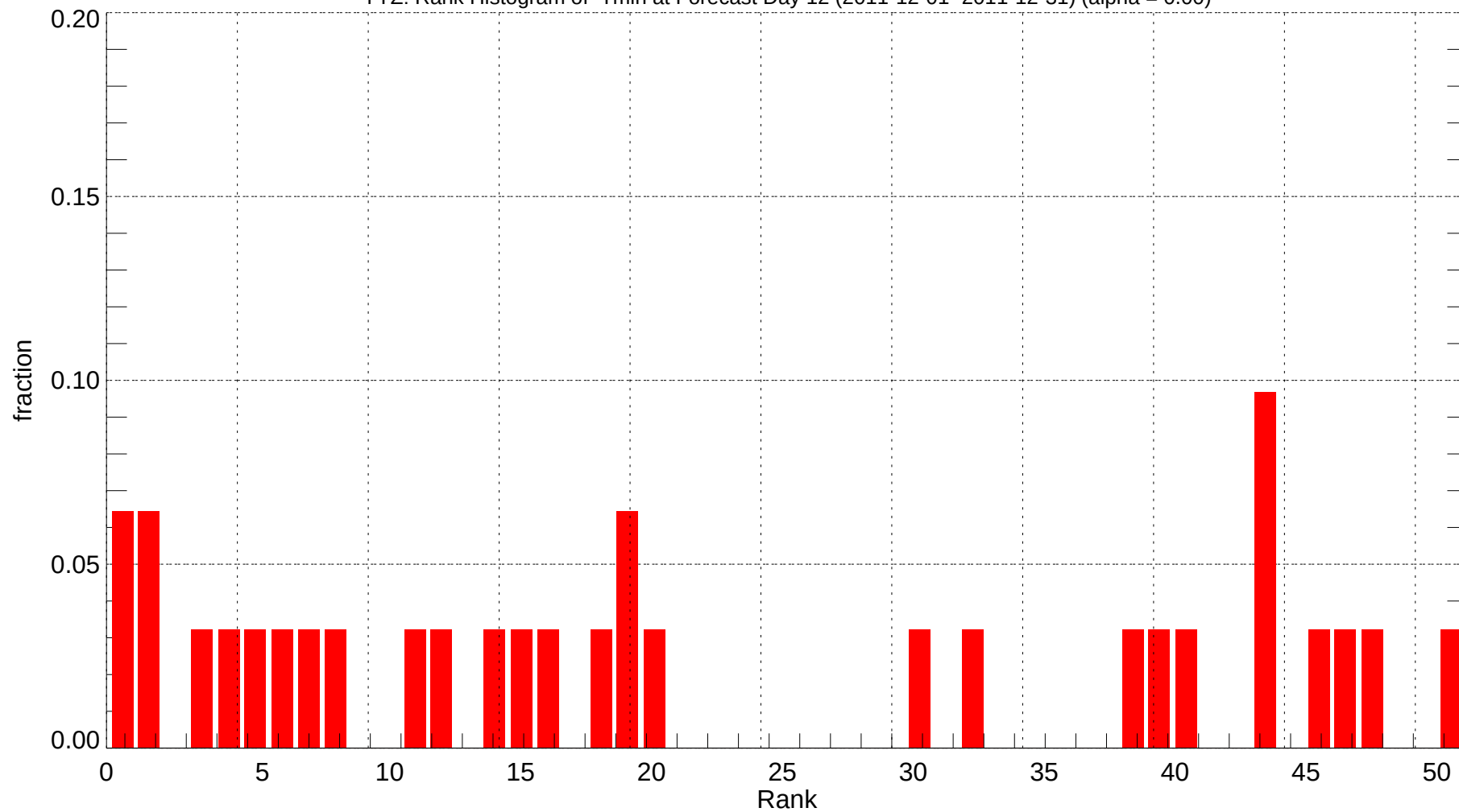
YYZ: Rank Histogram of Tmin at Forecast Day 12 (2011-12-01~2011-12-31) (alpha = 0.00)
