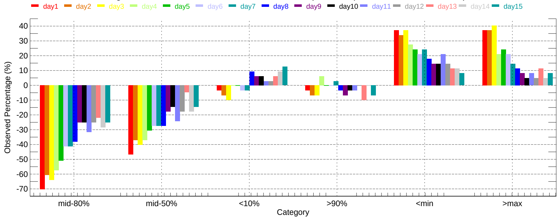
Observed Percentage Deviation of Ensembles - ALW: Max Temperature (2011-12-01~2011-12-31)
