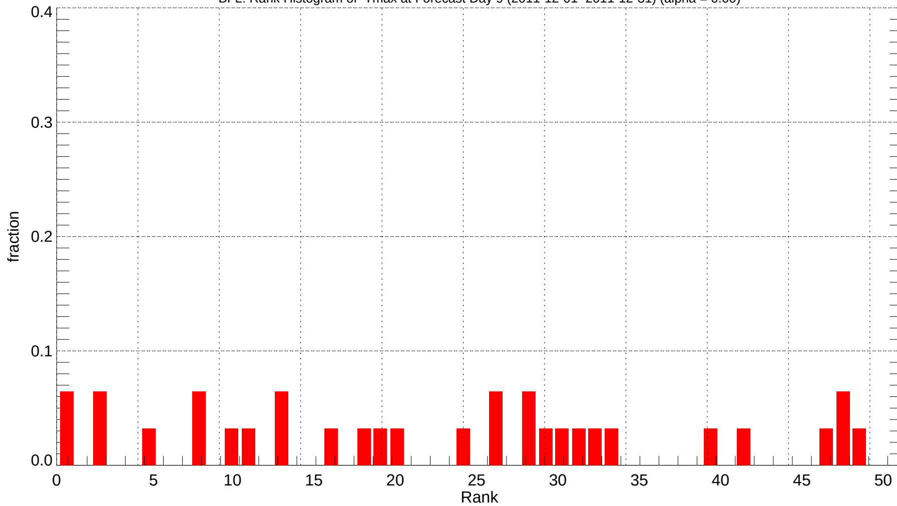
BFL: Rank Histogram of Tmax at Forecast Day 9 (2011-12-01~2011-12-31) (alpha = 0.00)
