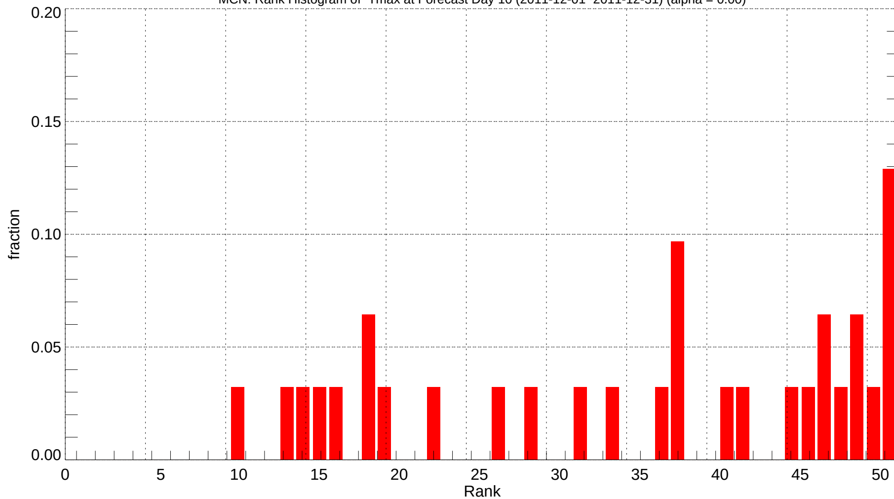
MCN: Rank Histogram of Tmax at Forecast Day 10 (2011-12-01~2011-12-31) (alpha = 0.00)
