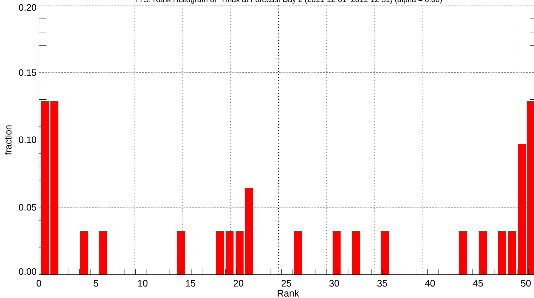
TYS: Rank Histogram of Tmax at Forecast Day 2 (2011-12-01~2011-12-31) (alpha = 0.00)
