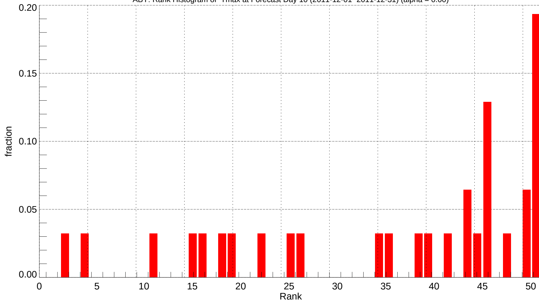
ABY: Rank Histogram of Tmax at Forecast Day 10 (2011-12-01~2011-12-31) (alpha = 0.00)
