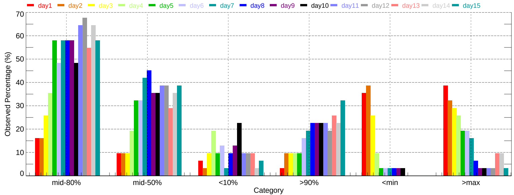
Observed Percentage of Ensembles - YXD: Max Temperature (2011-12-01~2011-12-31)
