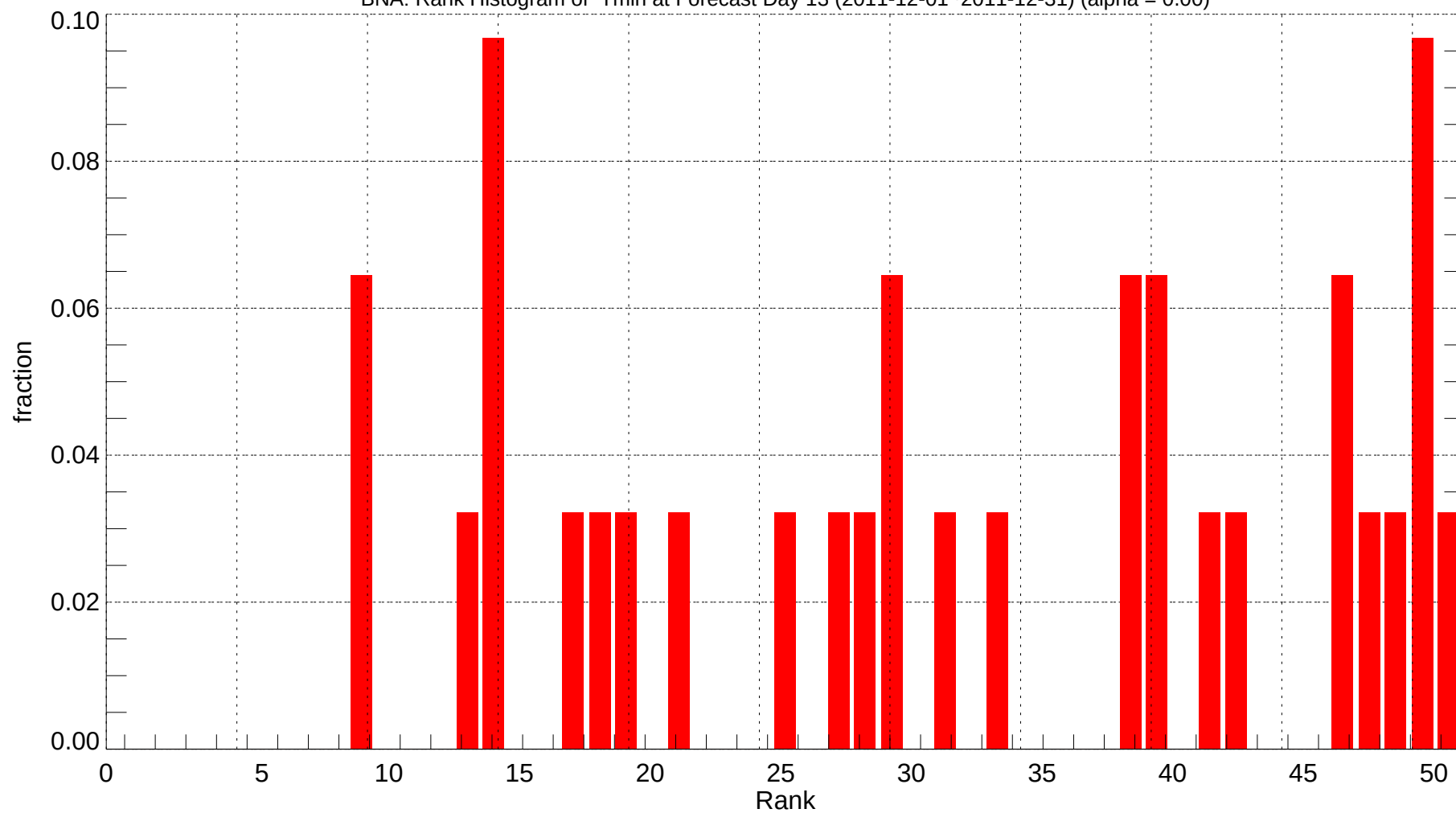
BNA: Rank Histogram of Tmin at Forecast Day 13 (2011-12-01~2011-12-31) (alpha = 0.00)
