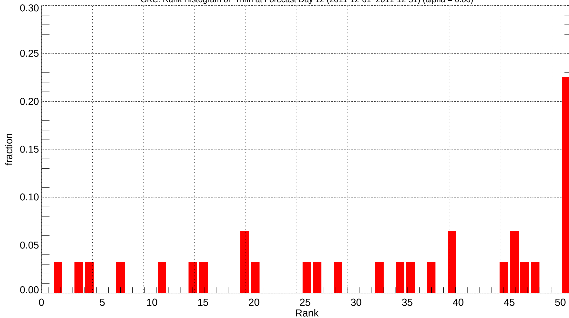
OKC: Rank Histogram of Tmin at Forecast Day 12 (2011-12-01~2011-12-31) (alpha = 0.00)
