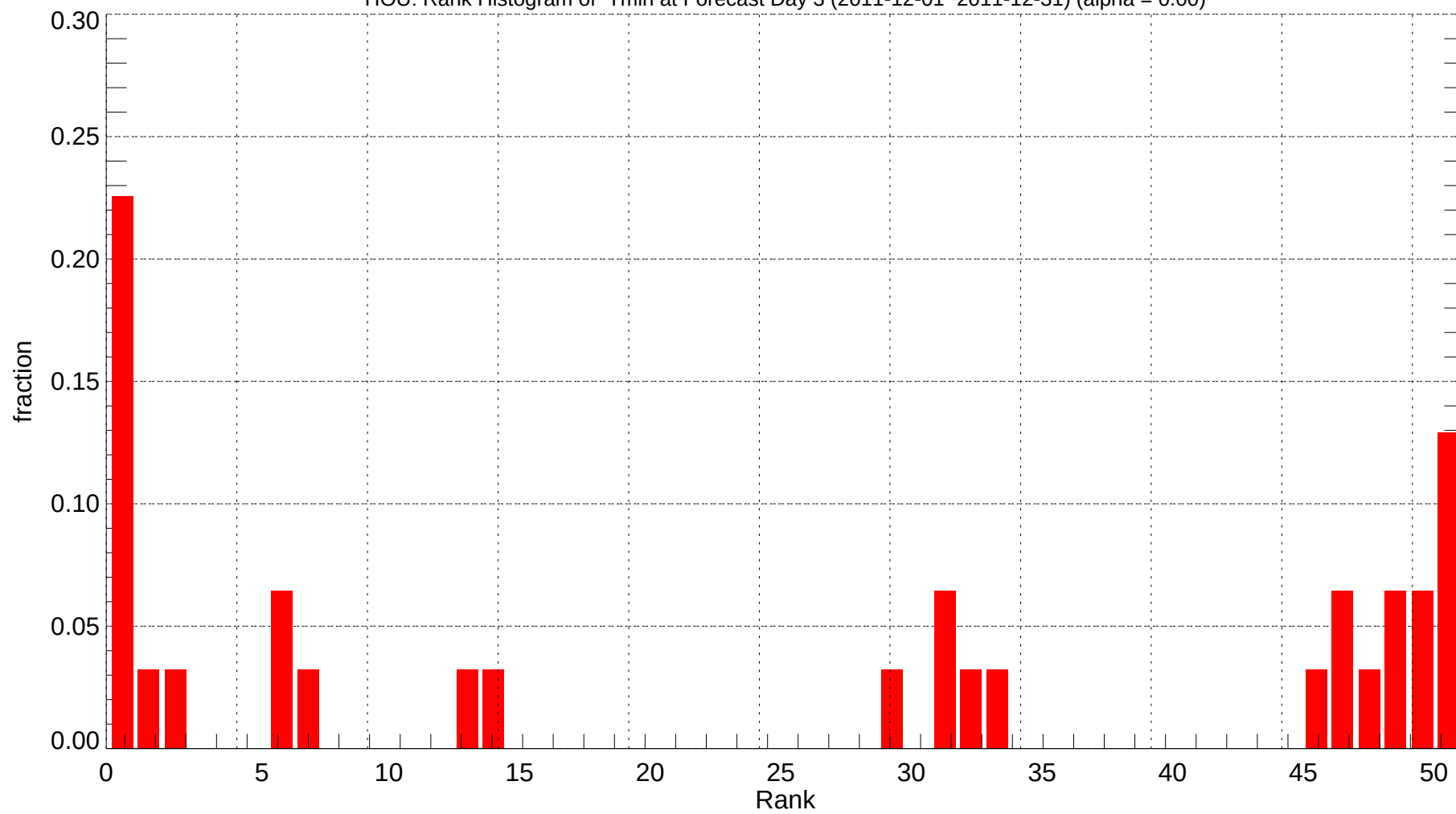
HOU: Rank Histogram of Tmin at Forecast Day 3 (2011-12-01~2011-12-31) (alpha = 0.00)
