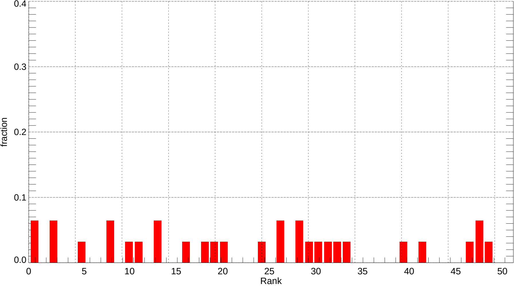
BFL: Rank Histogram of Tmin at Forecast Day 9 (2011-12-01~2011-12-31) (alpha = 0.00)
