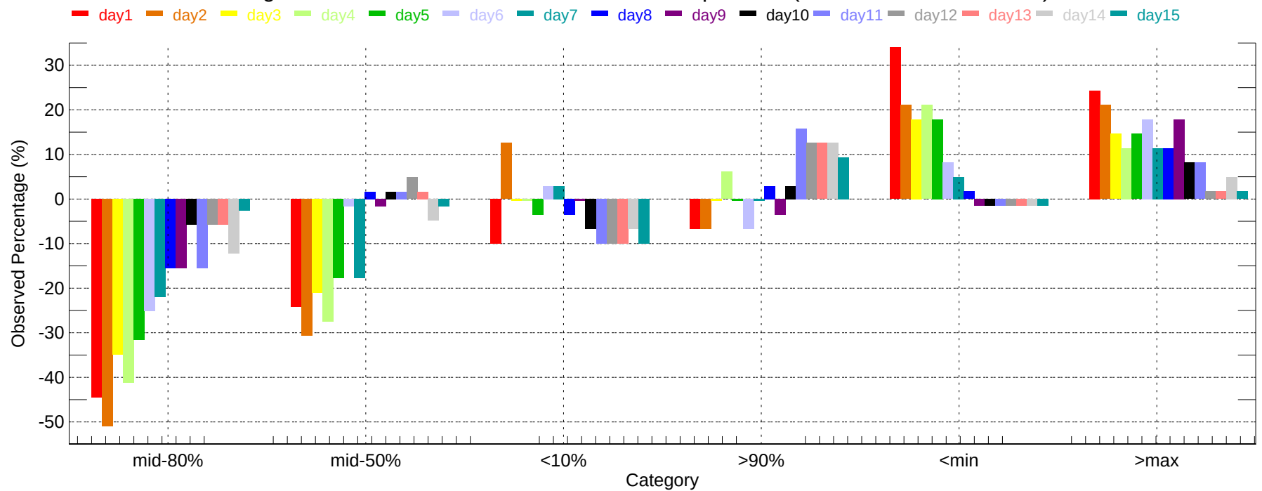
Observed Percentage Deviation of Ensembles - BNA: Max Temperature (2011-12-01~2011-12-31)
