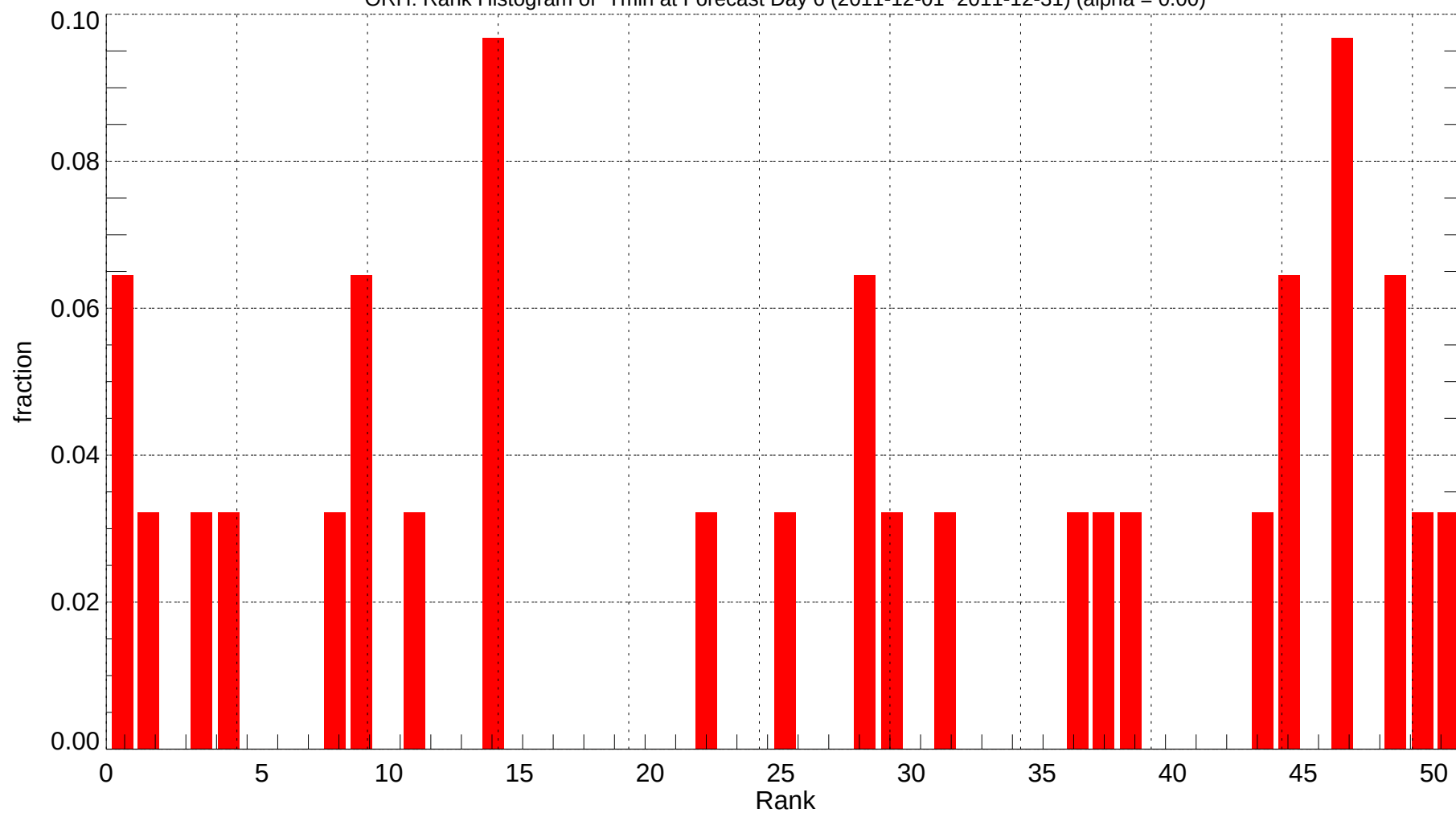
ORH: Rank Histogram of Tmin at Forecast Day 6 (2011-12-01~2011-12-31) (alpha = 0.00)
