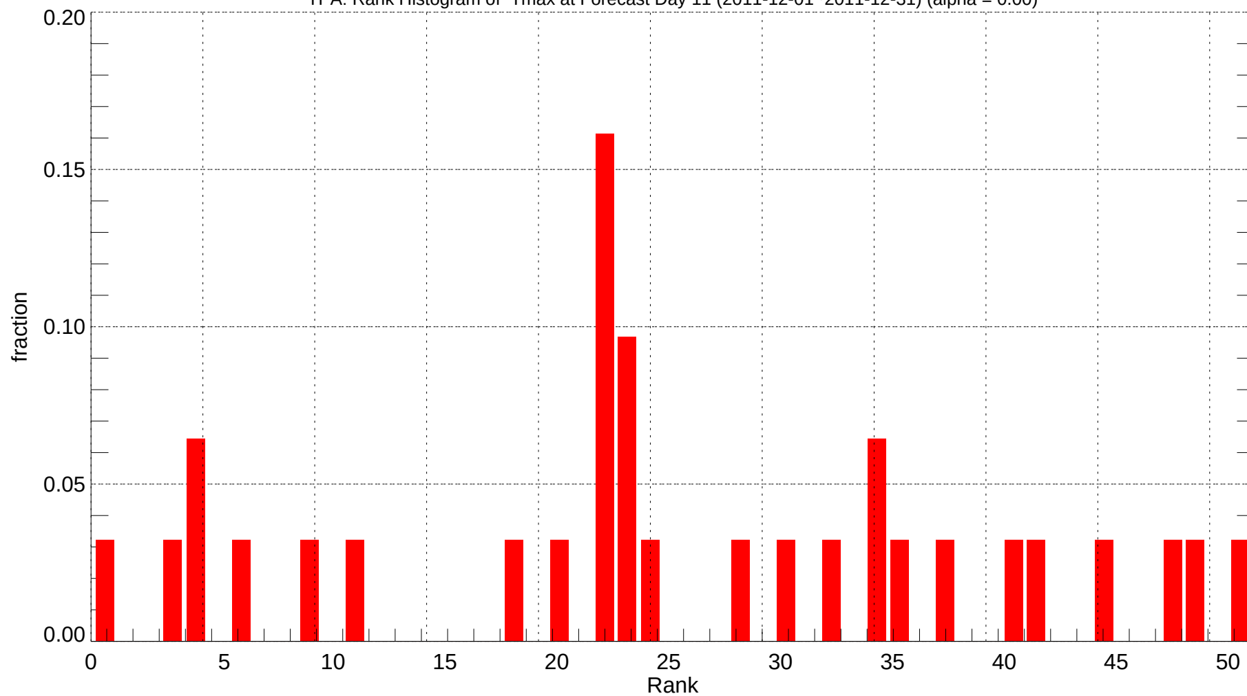
TPA: Rank Histogram of Tmax at Forecast Day 11 (2011-12-01~2011-12-31) (alpha = 0.00)
