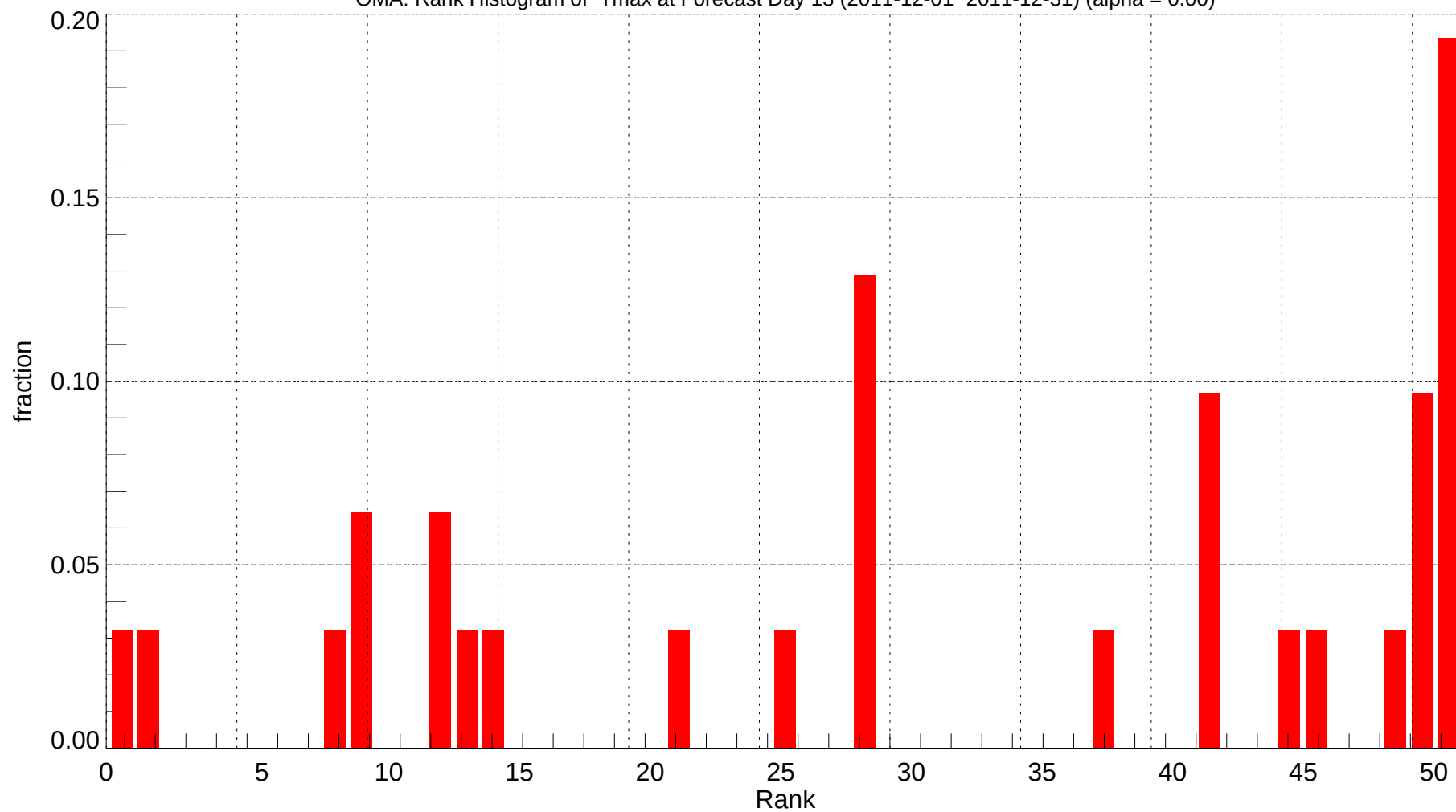
OMA: Rank Histogram of Tmax at Forecast Day 13 (2011-12-01~2011-12-31) (alpha = 0.00)
