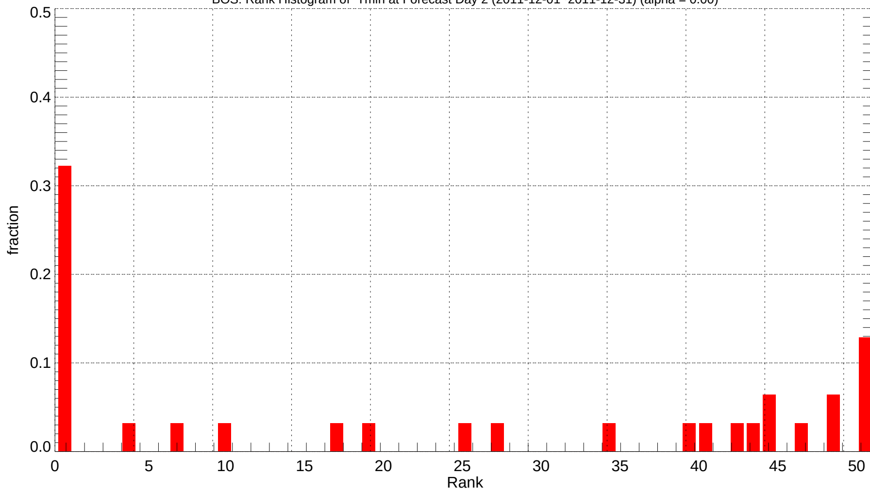
BOS: Rank Histogram of Tmin at Forecast Day 2 (2011-12-01~2011-12-31) (alpha = 0.00)
