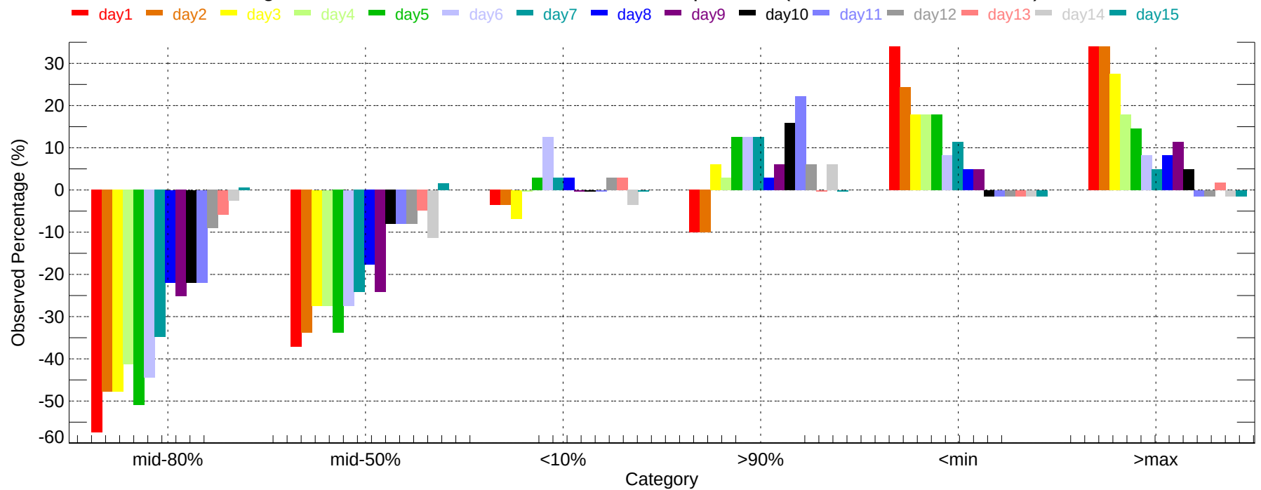
Observed Percentage Deviation of Ensembles - YYZ: Min Temperature (2011-12-01~2011-12-31)
