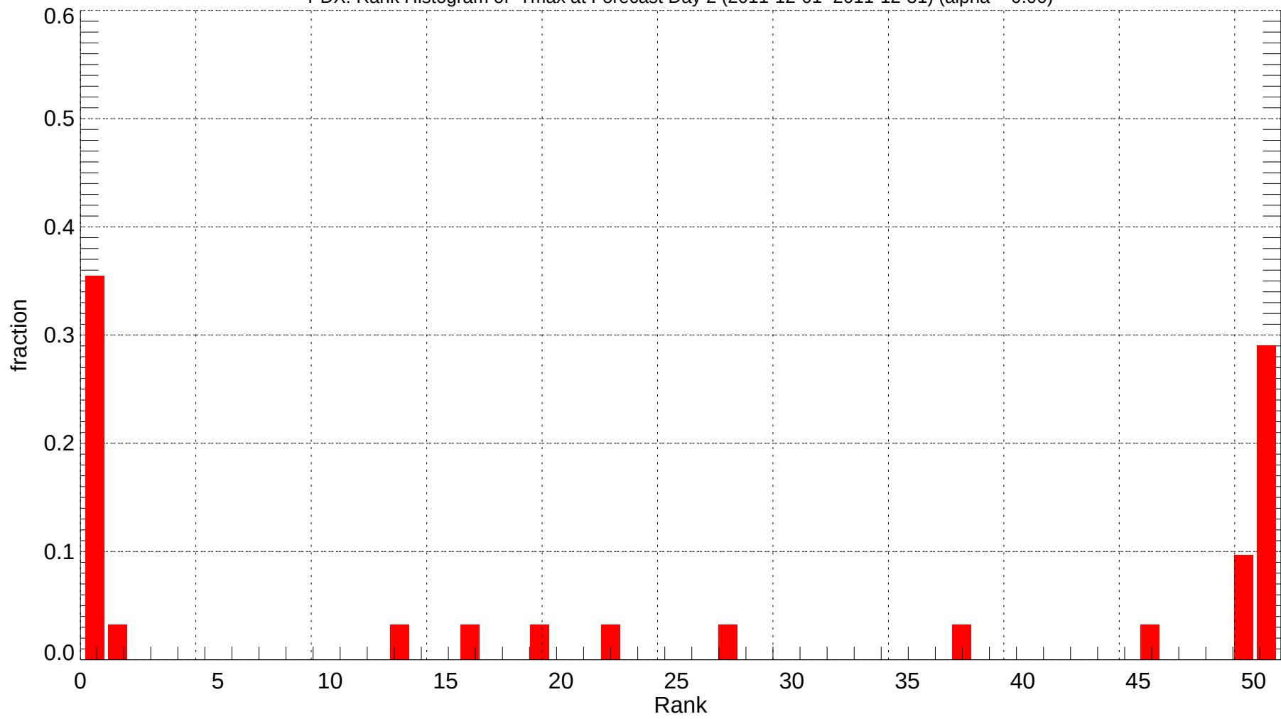
PDX: Rank Histogram of Tmax at Forecast Day 2 (2011-12-01~2011-12-31) (alpha = 0.00)
