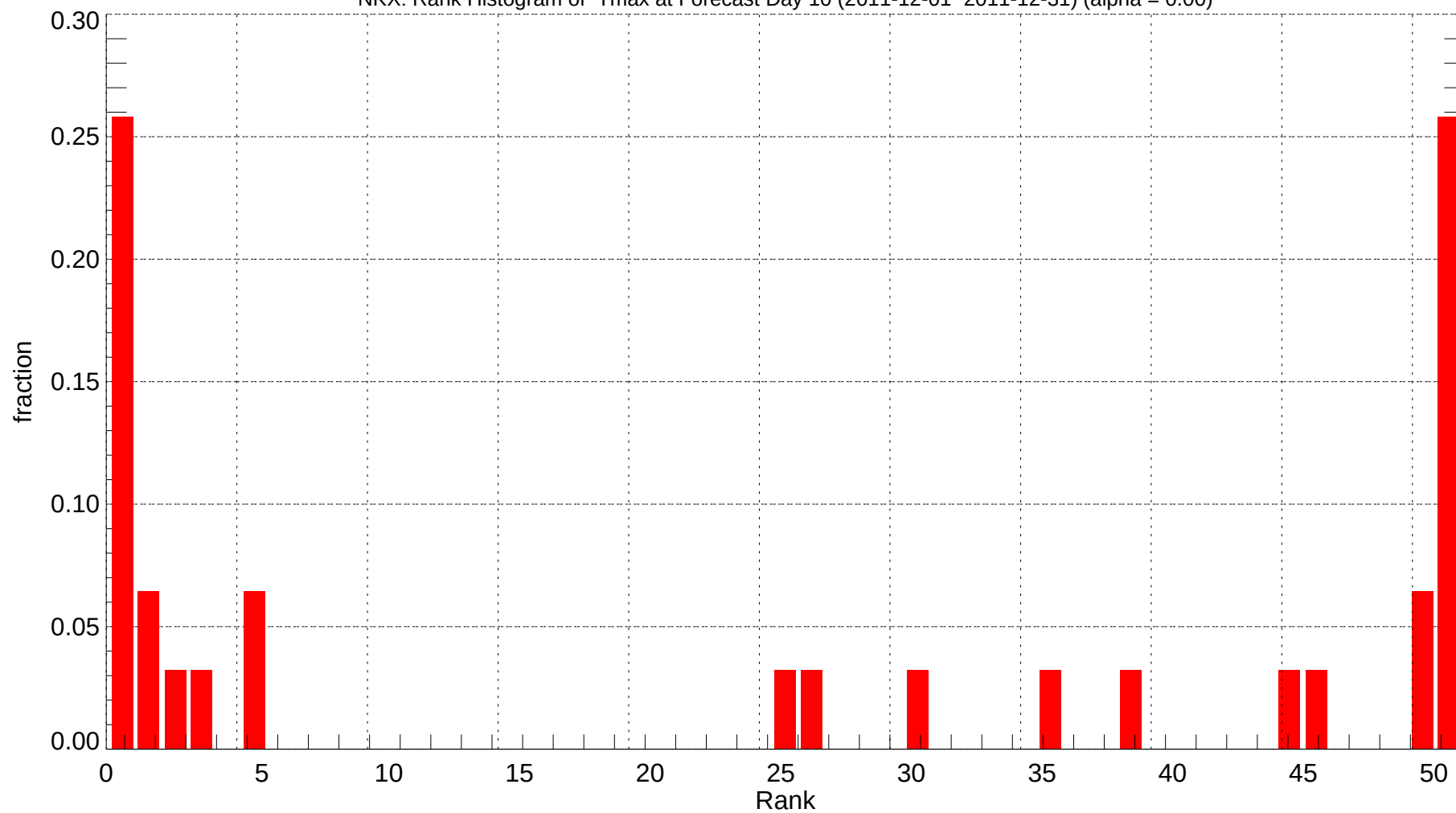
NKX: Rank Histogram of Tmax at Forecast Day 10 (2011-12-01~2011-12-31) (alpha = 0.00)
