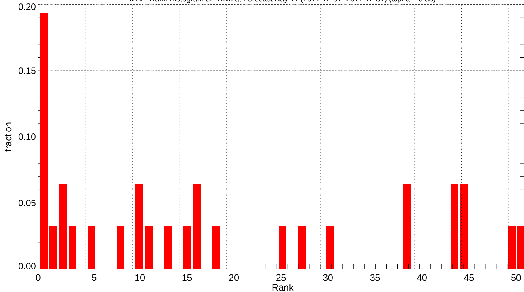
MAF: Rank Histogram of Tmin at Forecast Day 11 (2011-12-01~2011-12-31) (alpha = 0.00)
