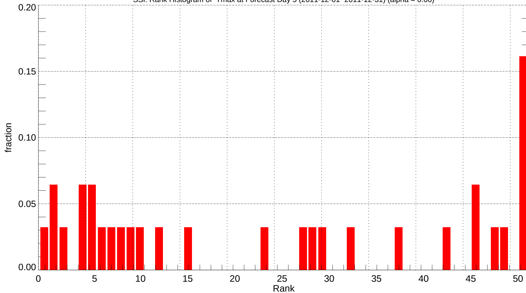
SSI: Rank Histogram of Tmax at Forecast Day 5 (2011-12-01~2011-12-31) (alpha = 0.00)
