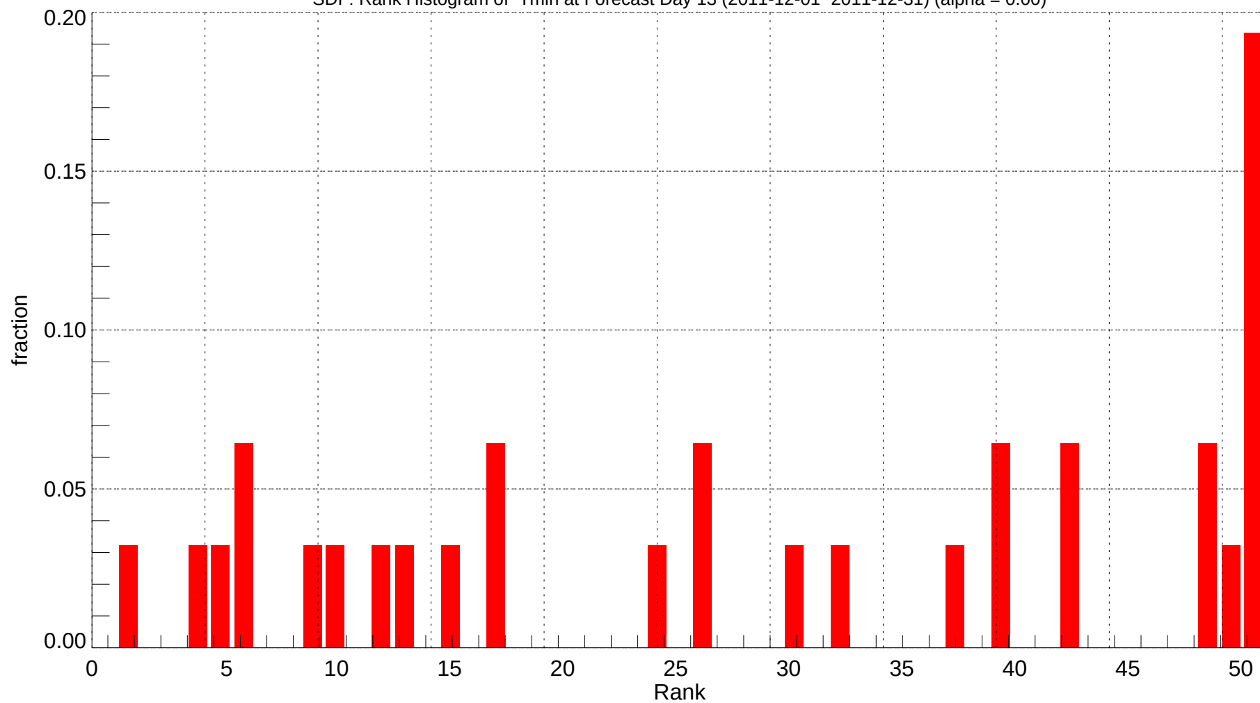
SDF: Rank Histogram of Tmin at Forecast Day 13 (2011-12-01~2011-12-31) (alpha = 0.00)
