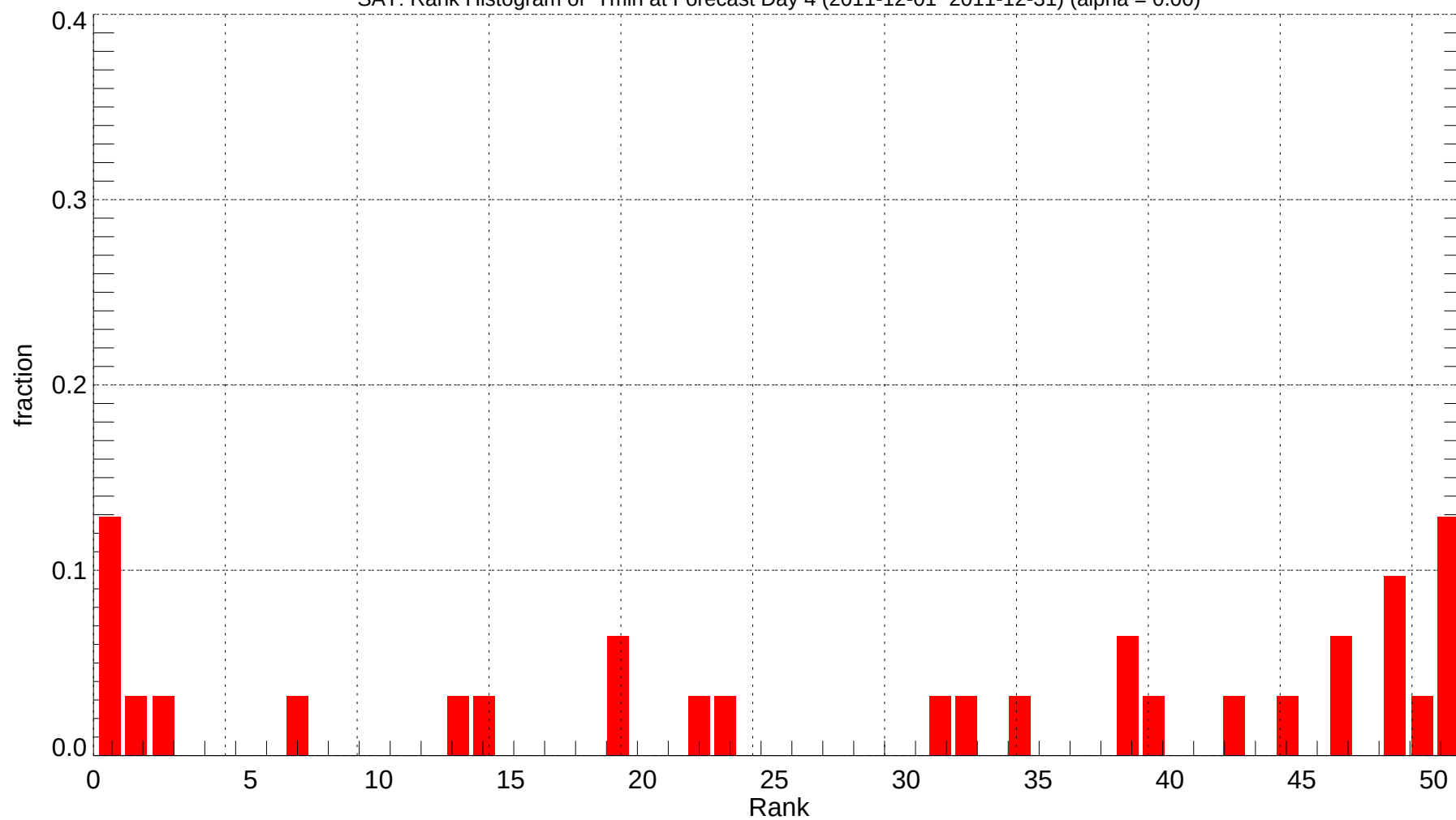
SAT: Rank Histogram of Tmin at Forecast Day 4 (2011-12-01~2011-12-31) (alpha = 0.00)
