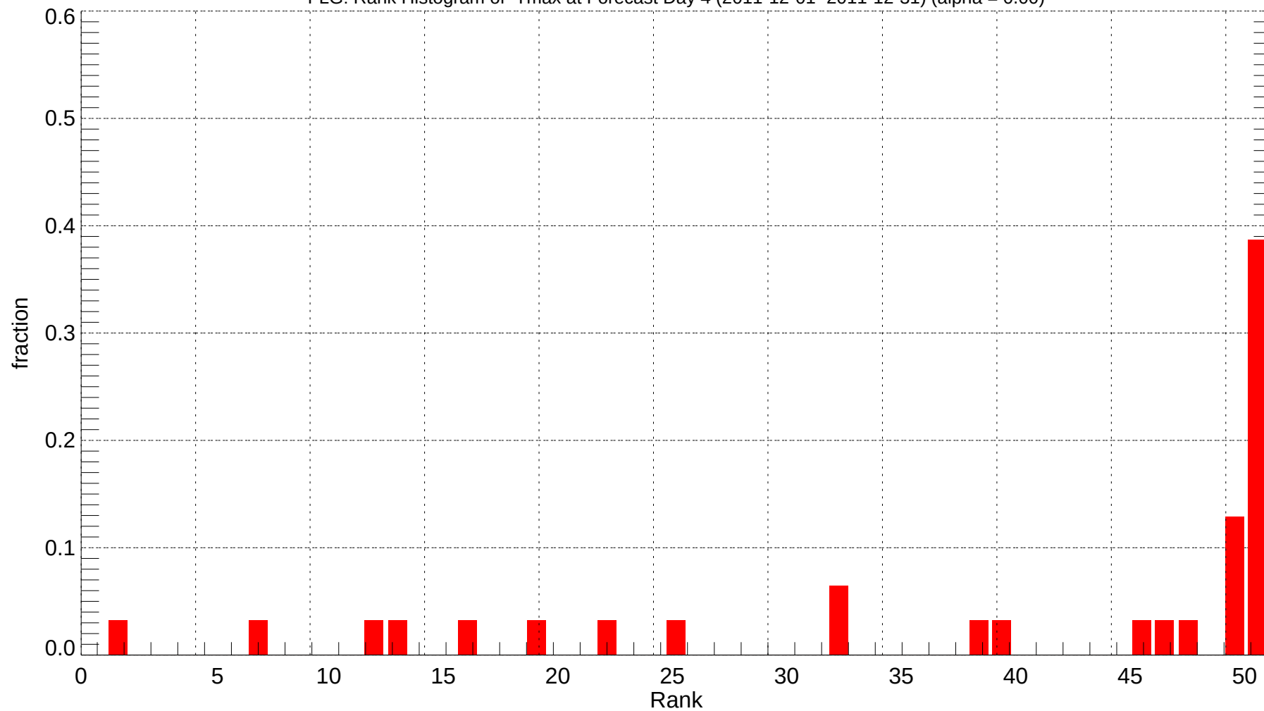
FLG: Rank Histogram of Tmax at Forecast Day 4 (2011-12-01~2011-12-31) (alpha = 0.00)
