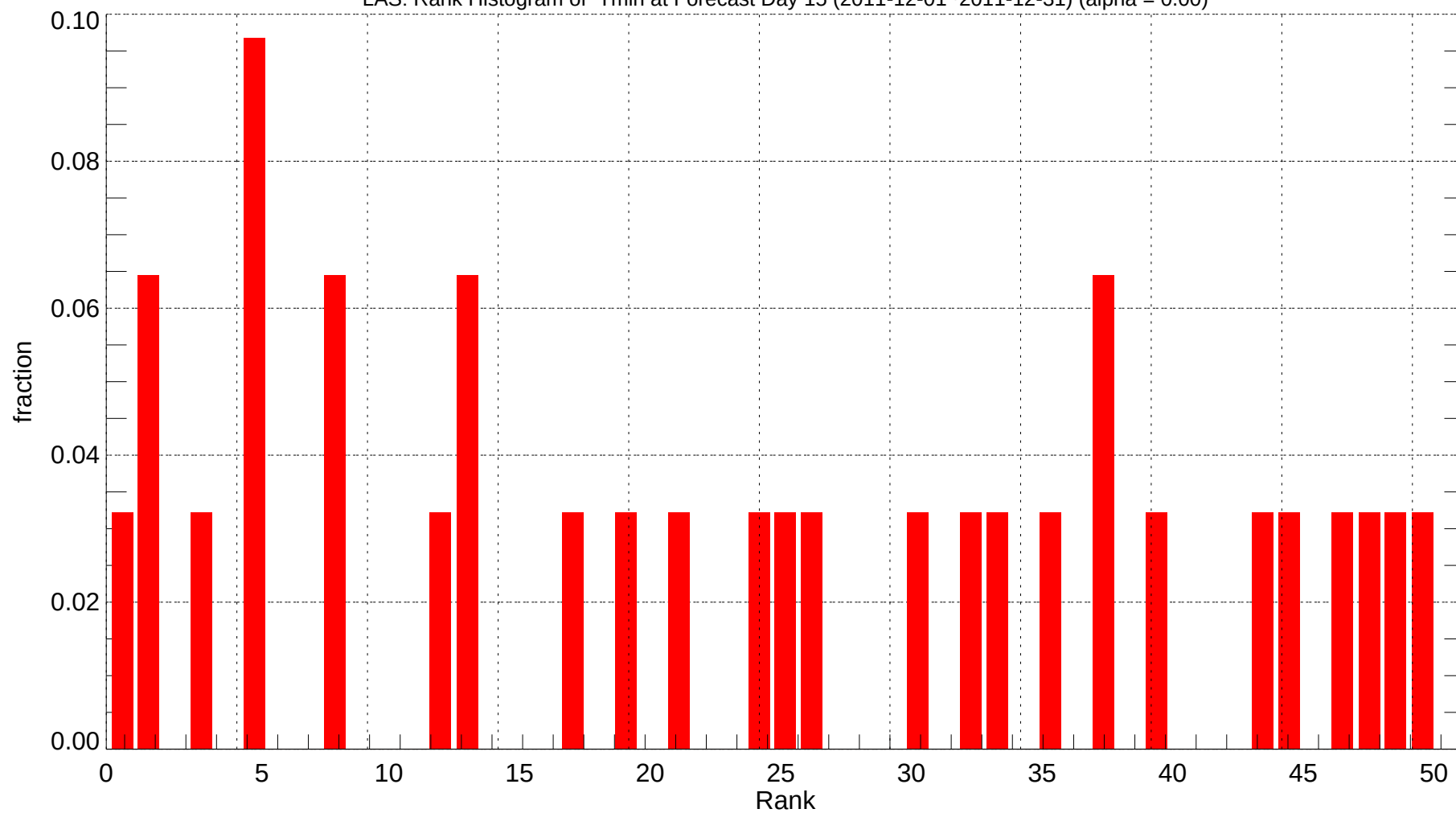
LAS: Rank Histogram of Tmin at Forecast Day 15 (2011-12-01~2011-12-31) (alpha = 0.00)
