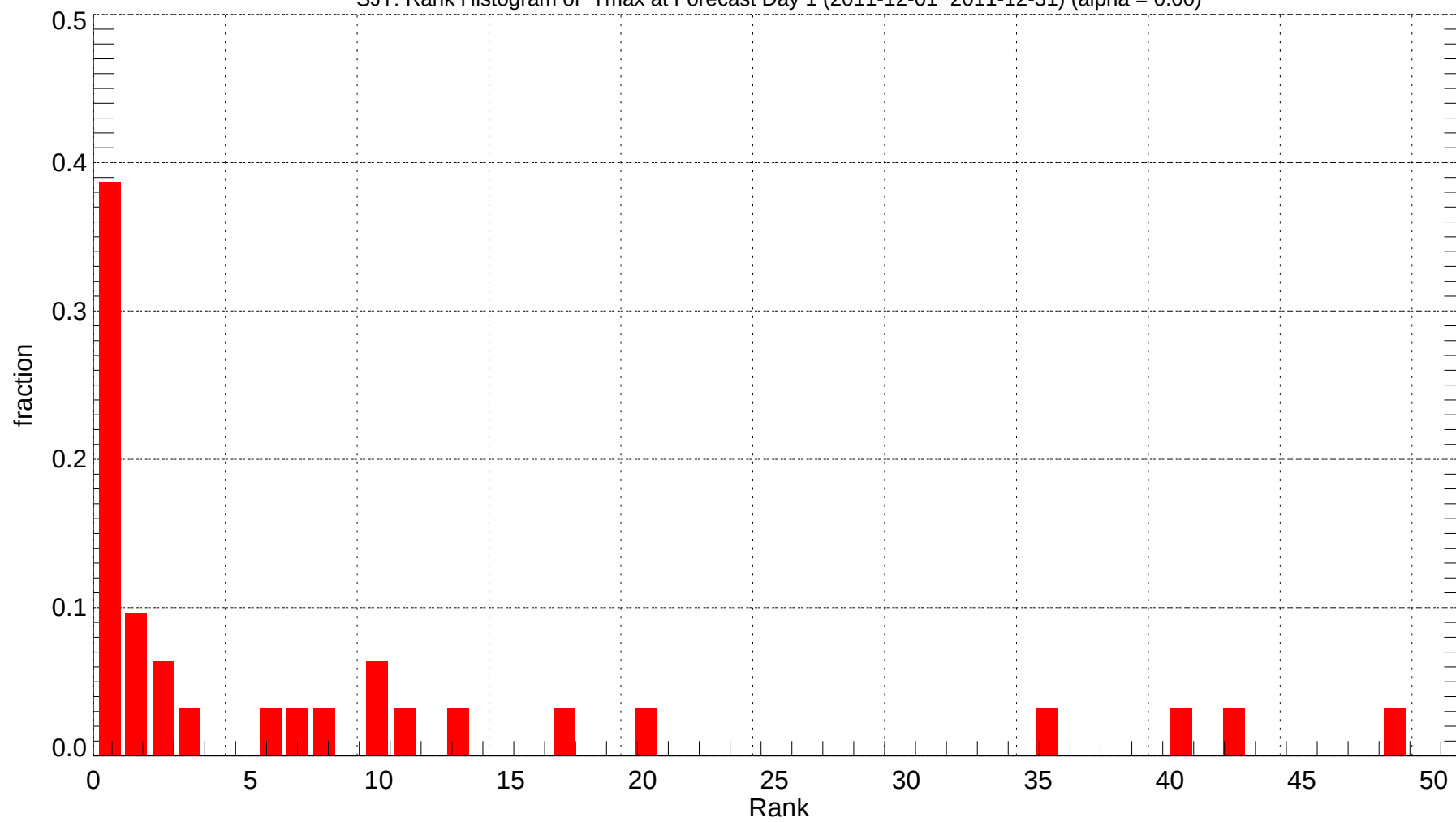
SJT: Rank Histogram of Tmax at Forecast Day 1 (2011-12-01~2011-12-31) (alpha = 0.00)
