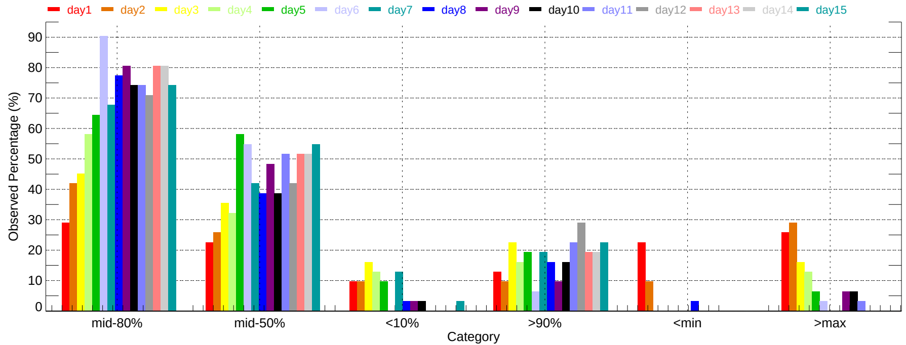
Observed Percentage of Ensembles - DCA: Max Temperature (2011-12-01~2011-12-31)
