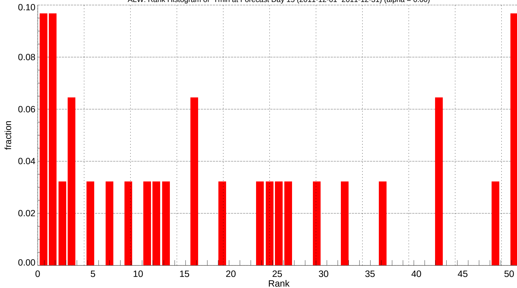
ALW: Rank Histogram of Tmin at Forecast Day 15 (2011-12-01~2011-12-31) (alpha = 0.00)
