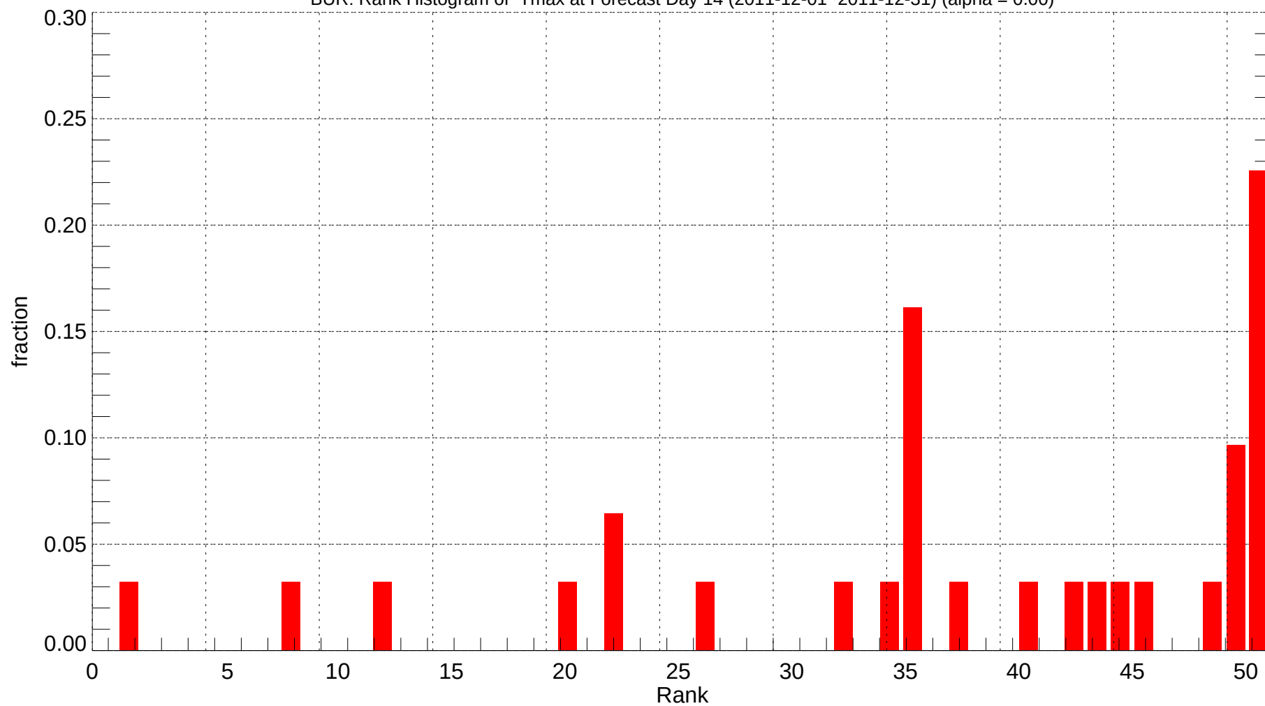
BUR: Rank Histogram of Tmax at Forecast Day 14 (2011-12-01~2011-12-31) (alpha = 0.00)
