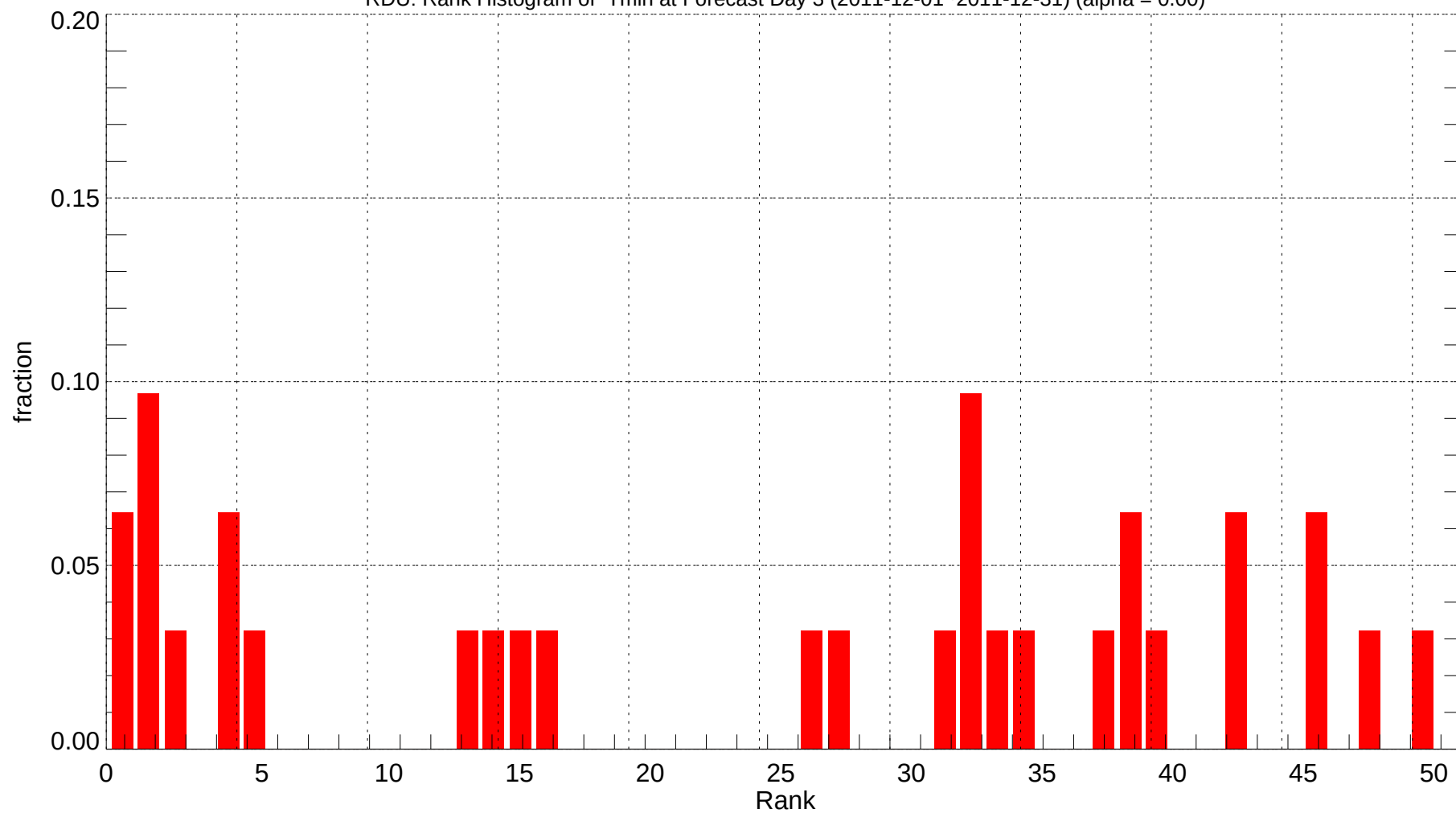
RDU: Rank Histogram of Tmin at Forecast Day 3 (2011-12-01~2011-12-31) (alpha = 0.00)
