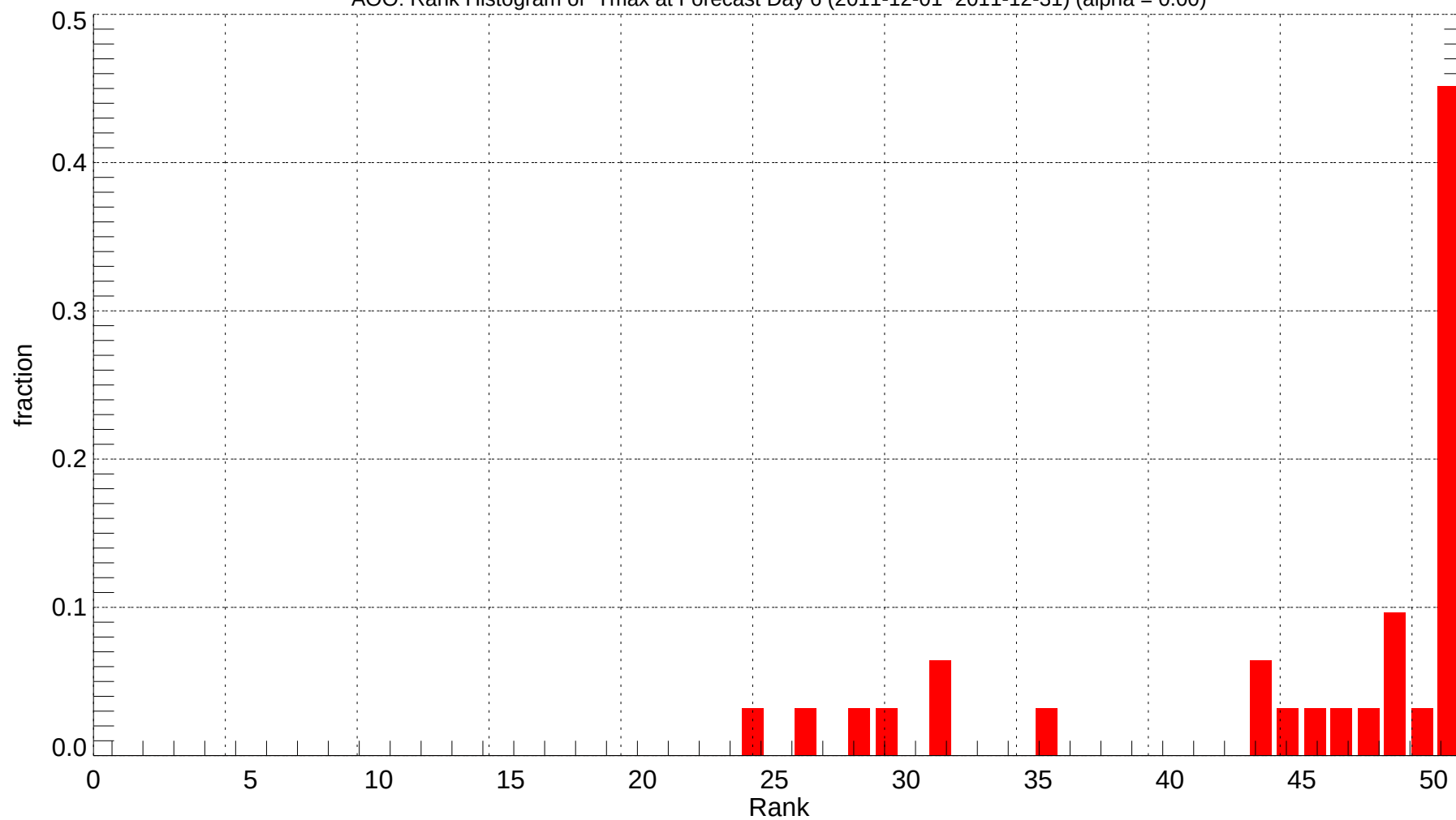
AOO: Rank Histogram of Tmax at Forecast Day 6 (2011-12-01~2011-12-31) (alpha = 0.00)
