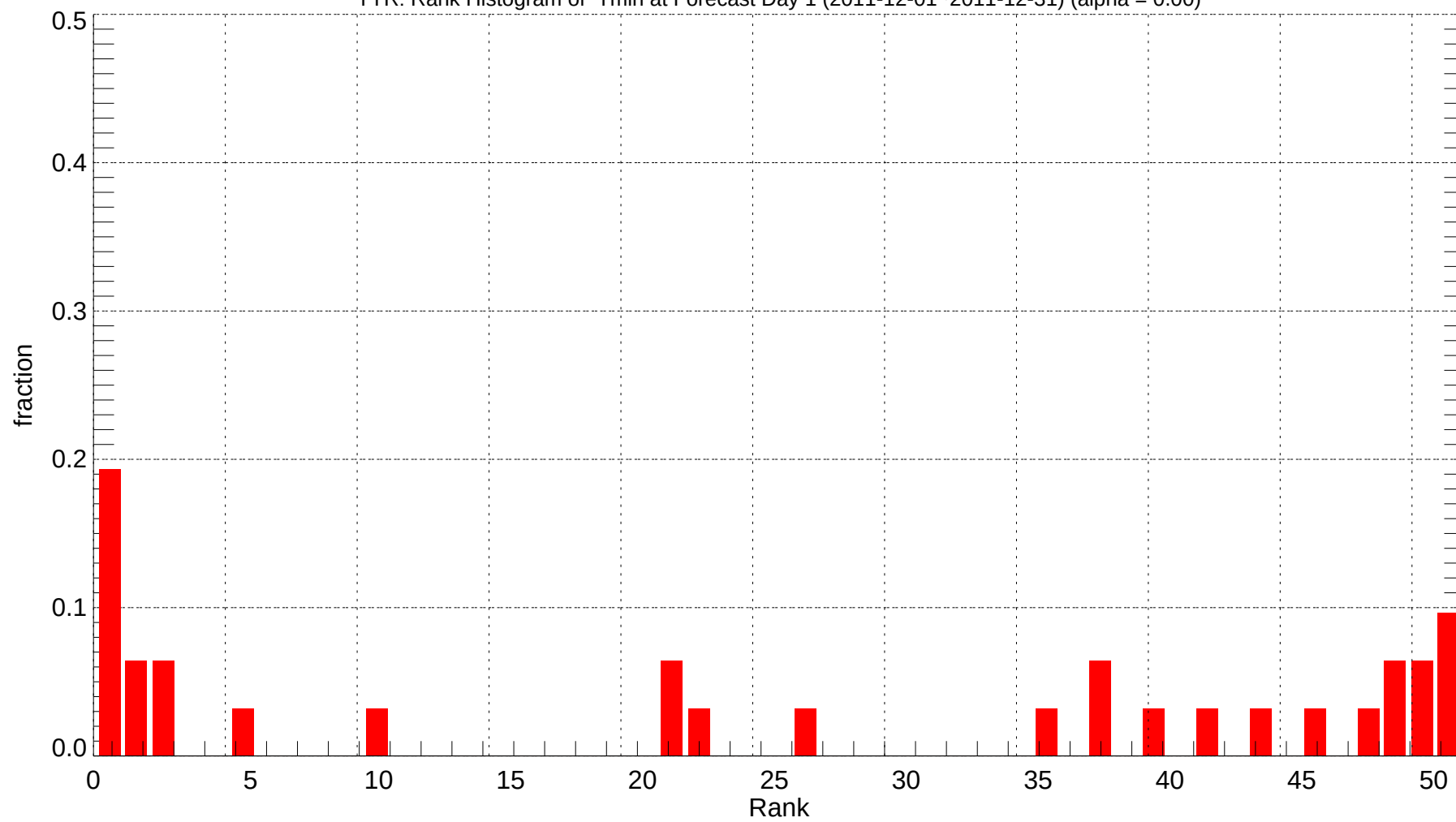
TYR: Rank Histogram of Tmin at Forecast Day 1 (2011-12-01~2011-12-31) (alpha = 0.00)
