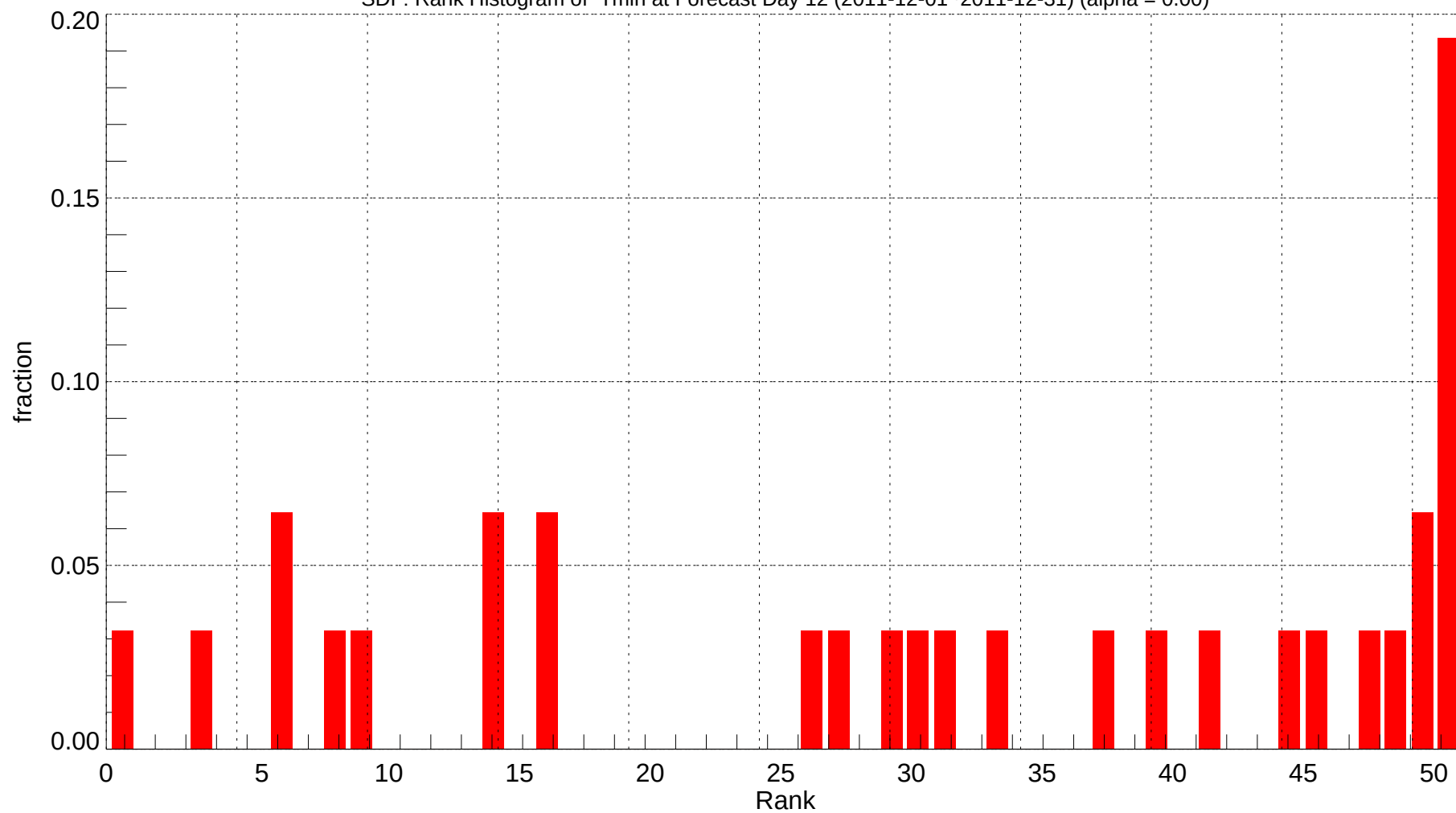
SDF: Rank Histogram of Tmin at Forecast Day 12 (2011-12-01~2011-12-31) (alpha = 0.00)
