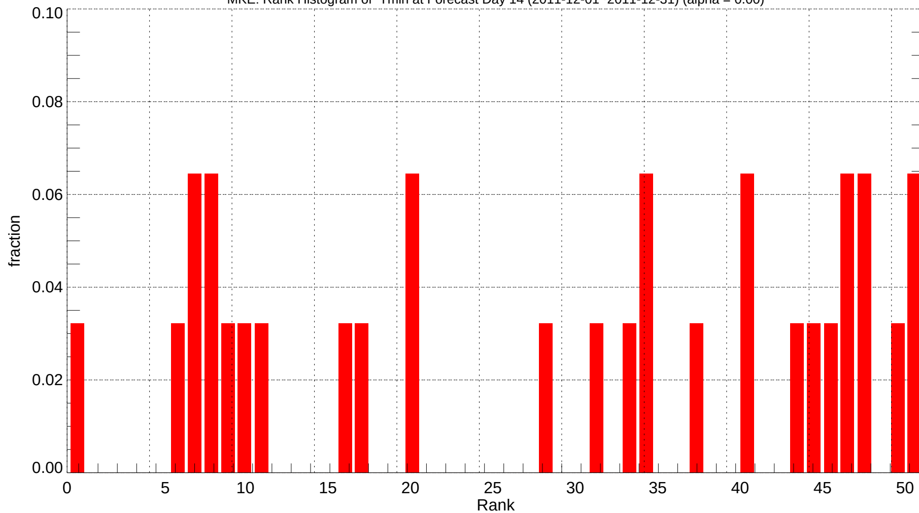
MKE: Rank Histogram of Tmin at Forecast Day 14 (2011-12-01~2011-12-31) (alpha = 0.00)
