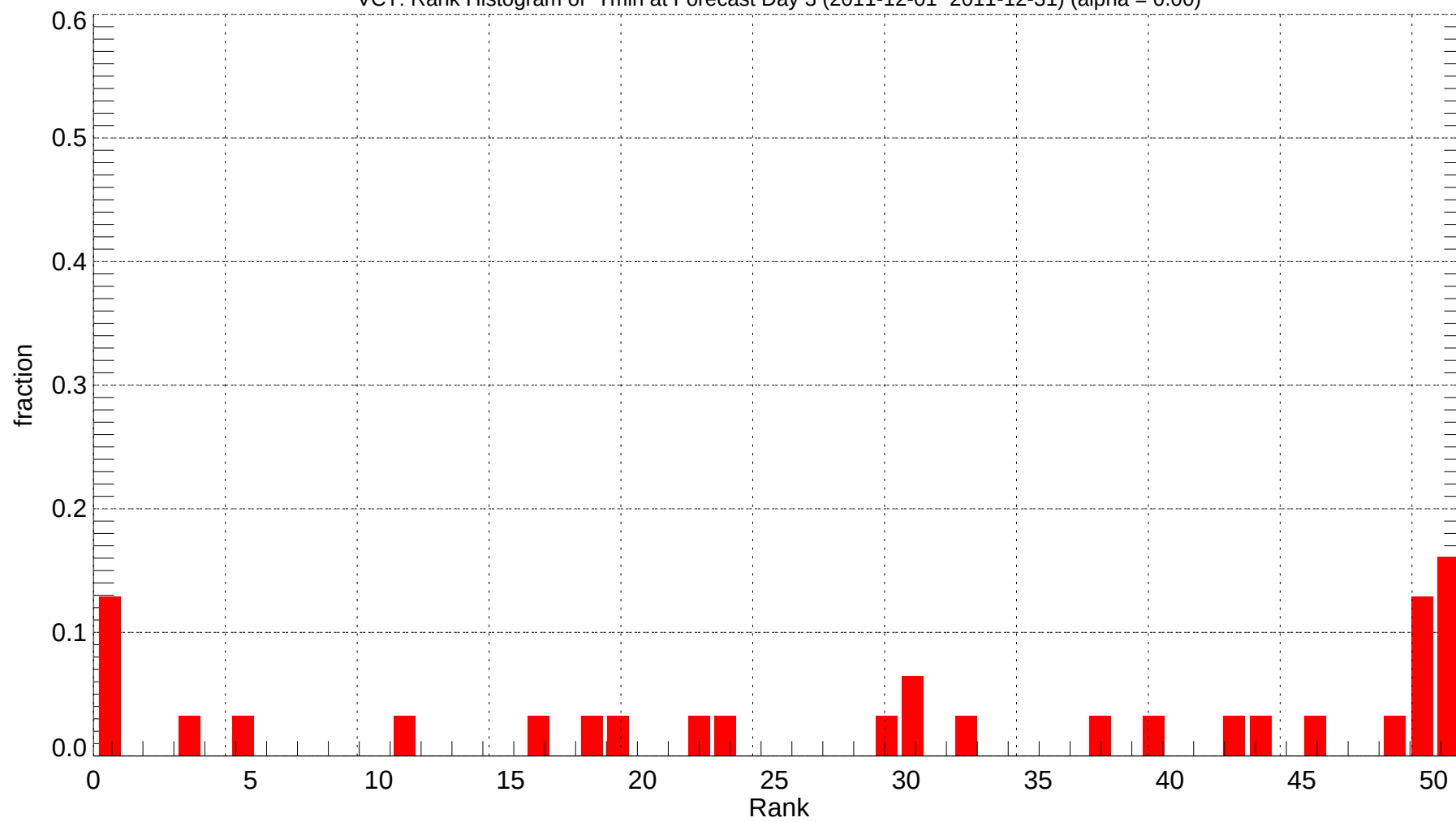
VCT: Rank Histogram of Tmin at Forecast Day 3 (2011-12-01~2011-12-31) (alpha = 0.00)
