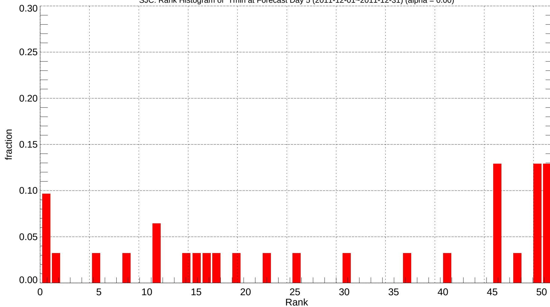
SJC: Rank Histogram of Tmin at Forecast Day 5 (2011-12-01~2011-12-31) (alpha = 0.00)
