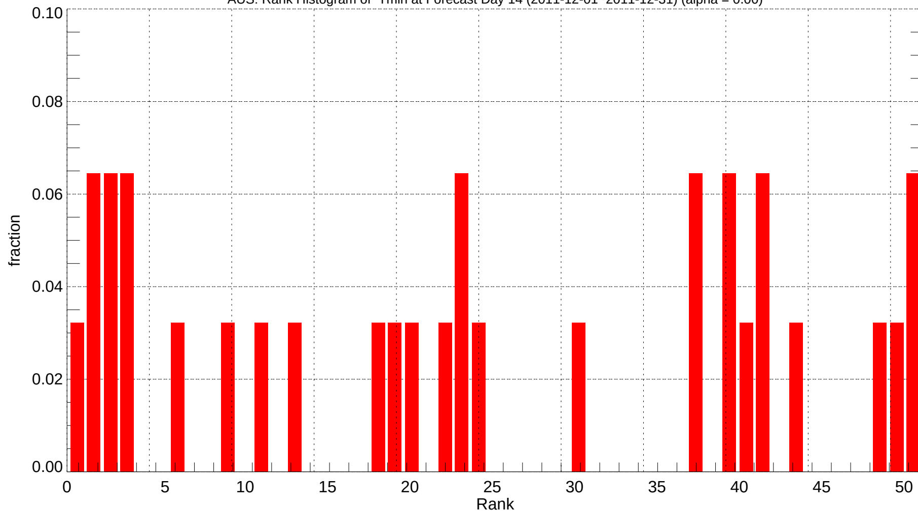
AUS: Rank Histogram of Tmin at Forecast Day 14 (2011-12-01~2011-12-31) (alpha = 0.00)
