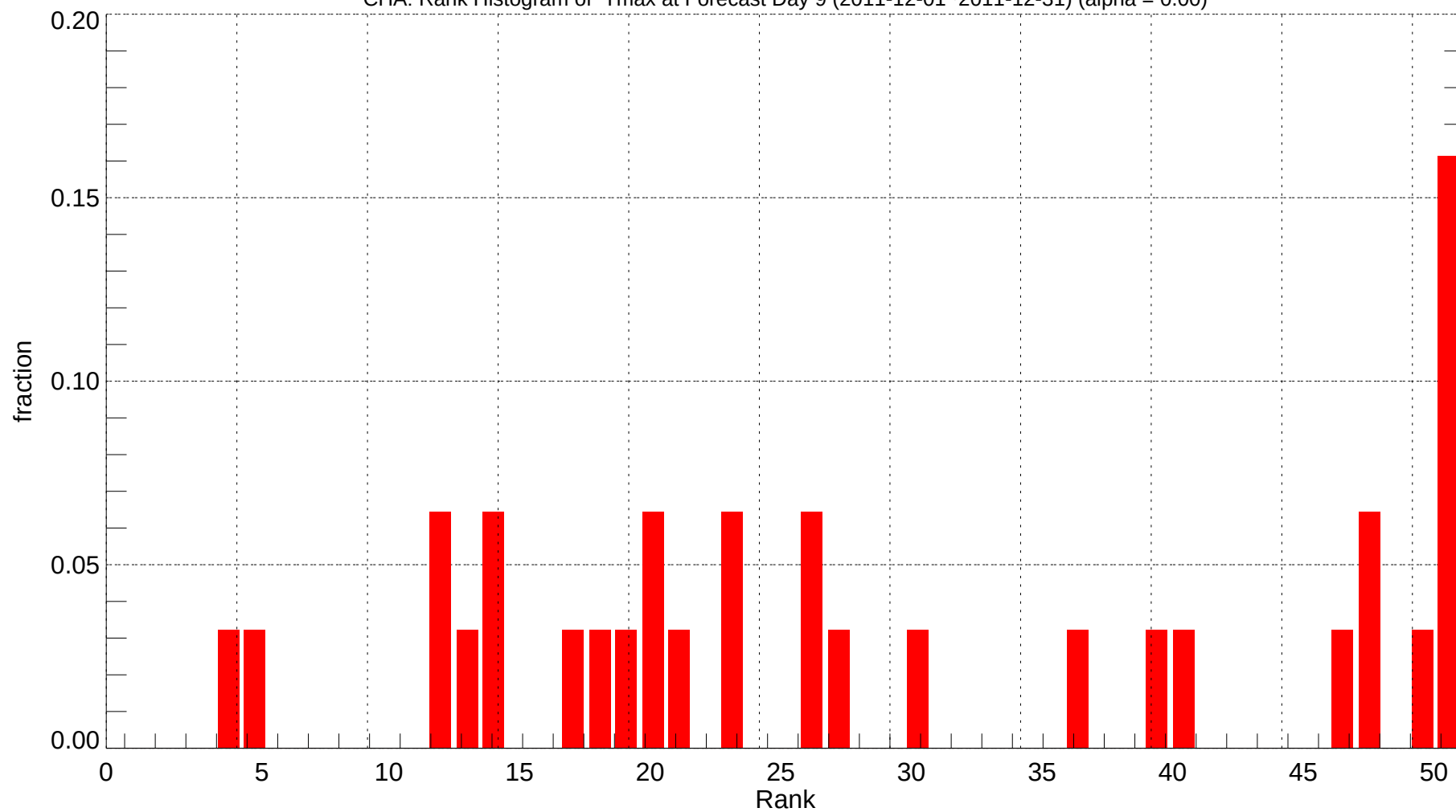
CHA: Rank Histogram of Tmax at Forecast Day 9 (2011-12-01~2011-12-31) (alpha = 0.00)
