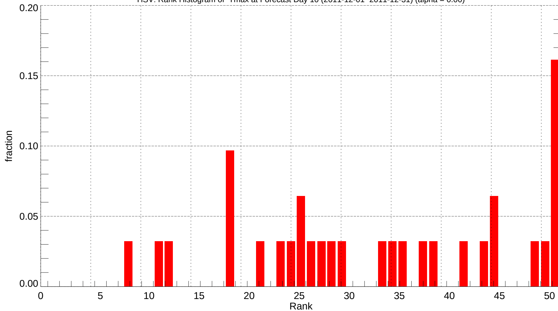
HSV: Rank Histogram of Tmax at Forecast Day 10 (2011-12-01~2011-12-31) (alpha = 0.00)
