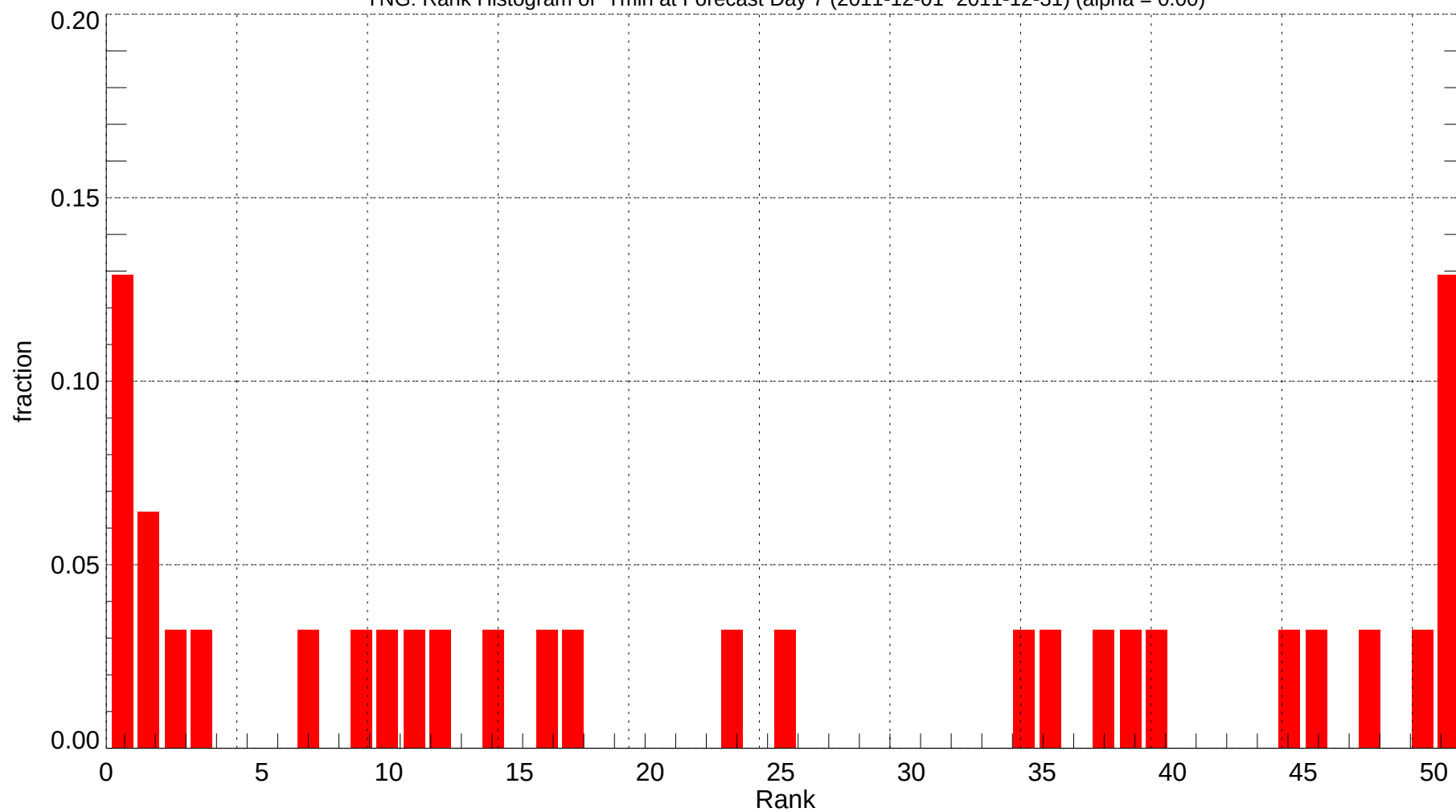
YNG: Rank Histogram of Tmin at Forecast Day 7 (2011-12-01~2011-12-31) (alpha = 0.00)
