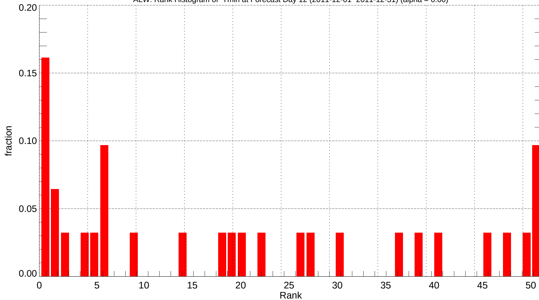
ALW: Rank Histogram of Tmin at Forecast Day 12 (2011-12-01~2011-12-31) (alpha = 0.00)
