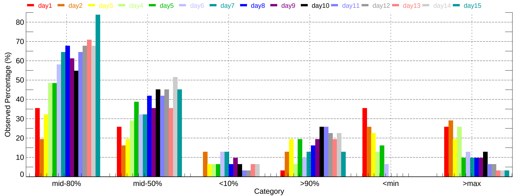
Observed Percentage of Ensembles - CVG: Min Temperature (2011-12-01~2011-12-31)
