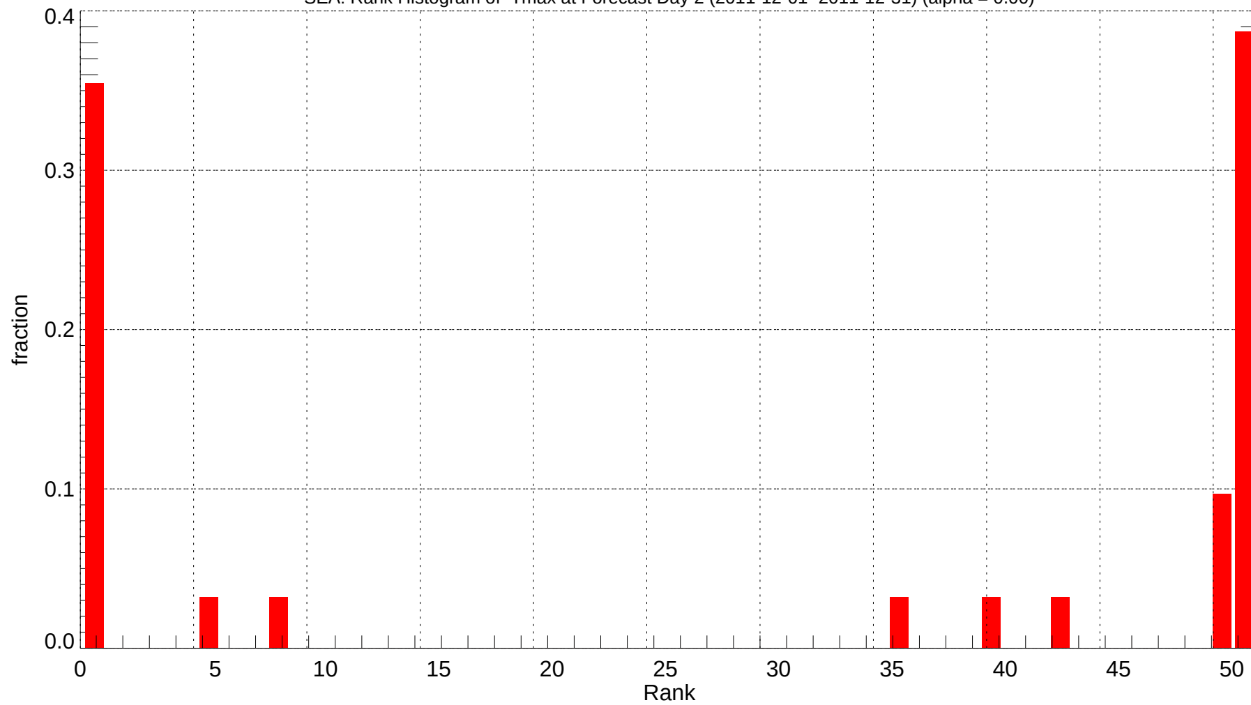
SEA: Rank Histogram of Tmax at Forecast Day 2 (2011-12-01~2011-12-31) (alpha = 0.00)
