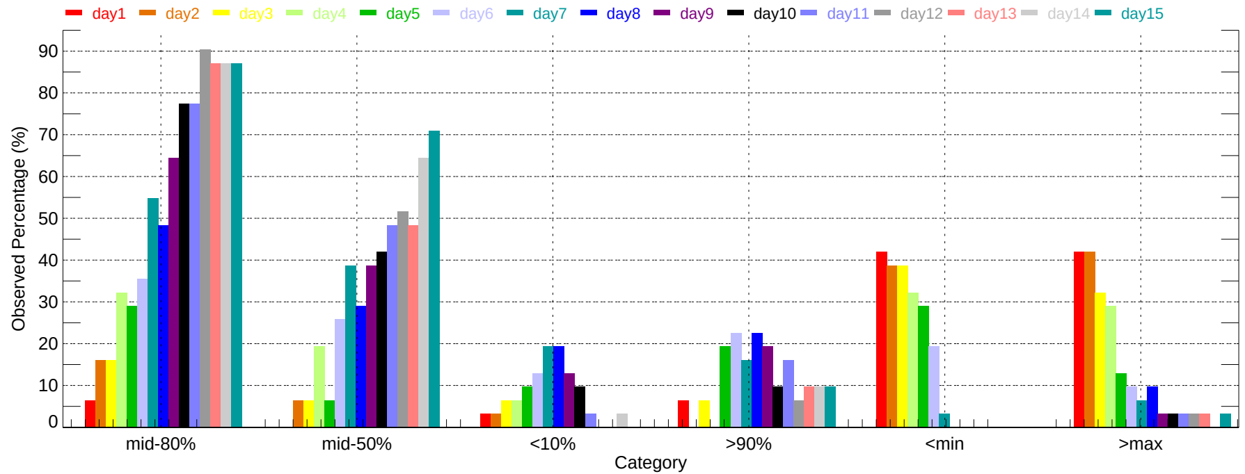
Observed Percentage of Ensembles - GEG: Min Temperature (2011-12-01~2011-12-31)
