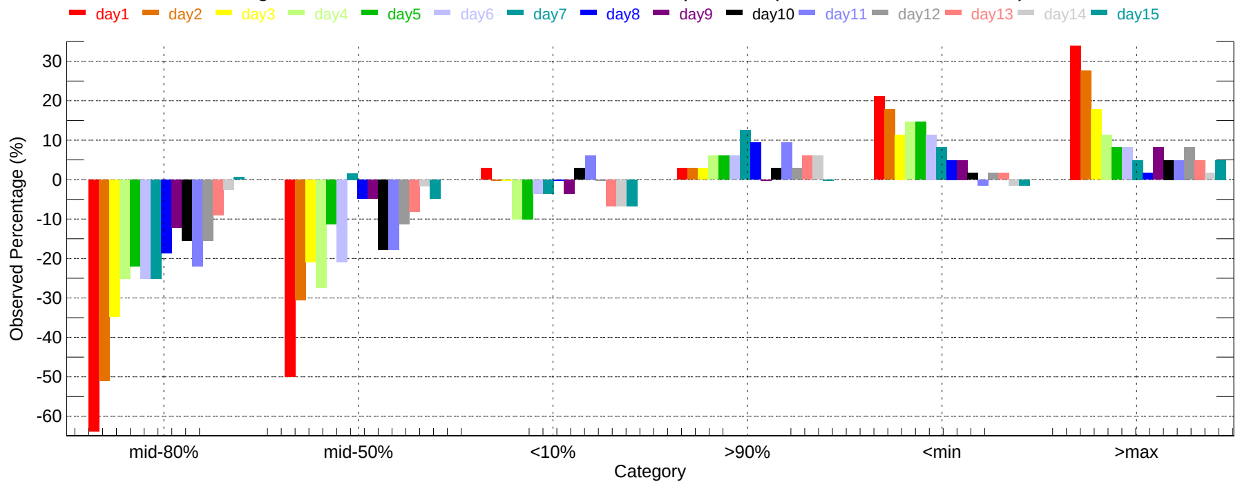
Observed Percentage Deviation of Ensembles - YVR: Min Temperature (2011-12-01~2011-12-31)
