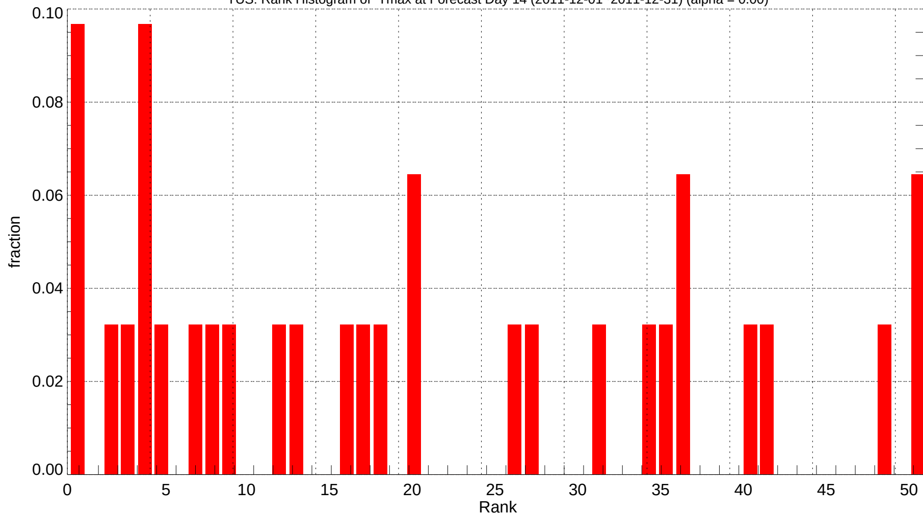
TUS: Rank Histogram of Tmax at Forecast Day 14 (2011-12-01~2011-12-31) (alpha = 0.00)
