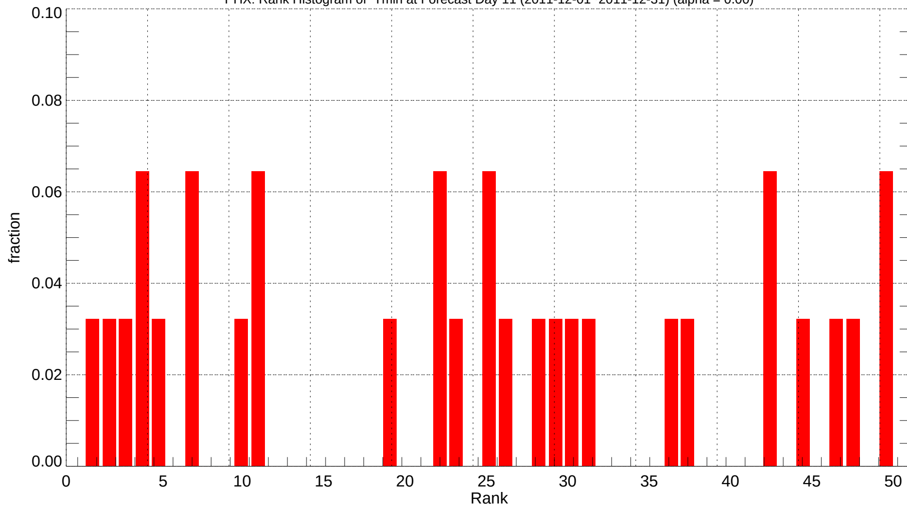
PHX: Rank Histogram of Tmin at Forecast Day 11 (2011-12-01~2011-12-31) (alpha = 0.00)
