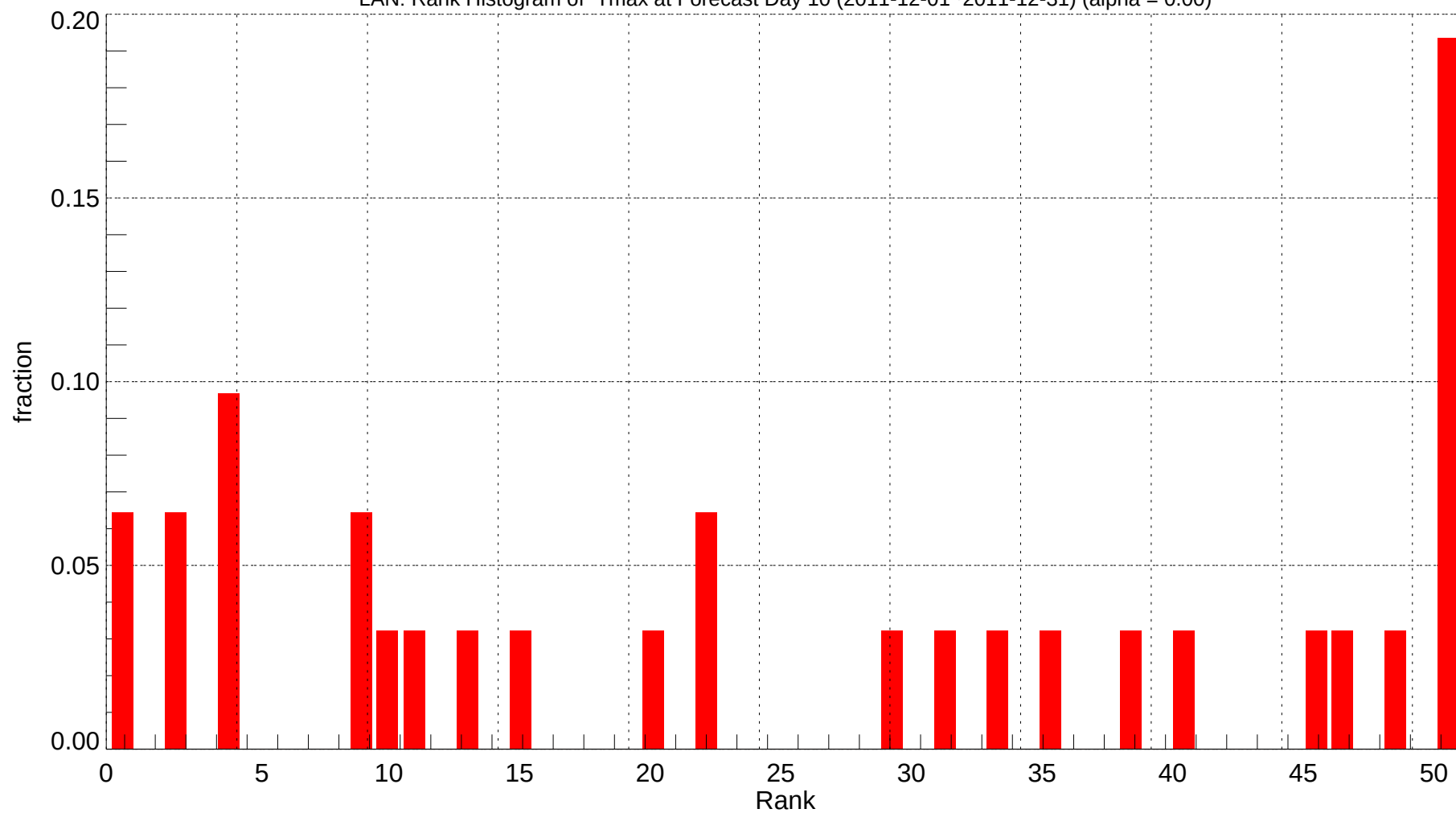
LAN: Rank Histogram of Tmax at Forecast Day 10 (2011-12-01~2011-12-31) (alpha = 0.00)
