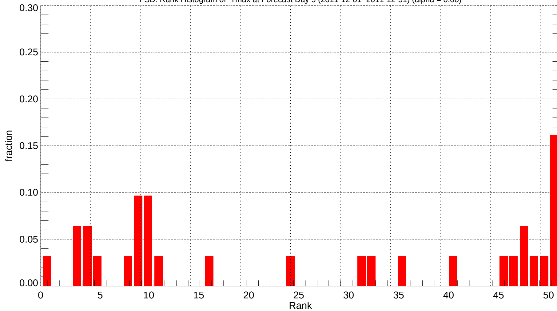
FSD: Rank Histogram of Tmax at Forecast Day 9 (2011-12-01~2011-12-31) (alpha = 0.00)
