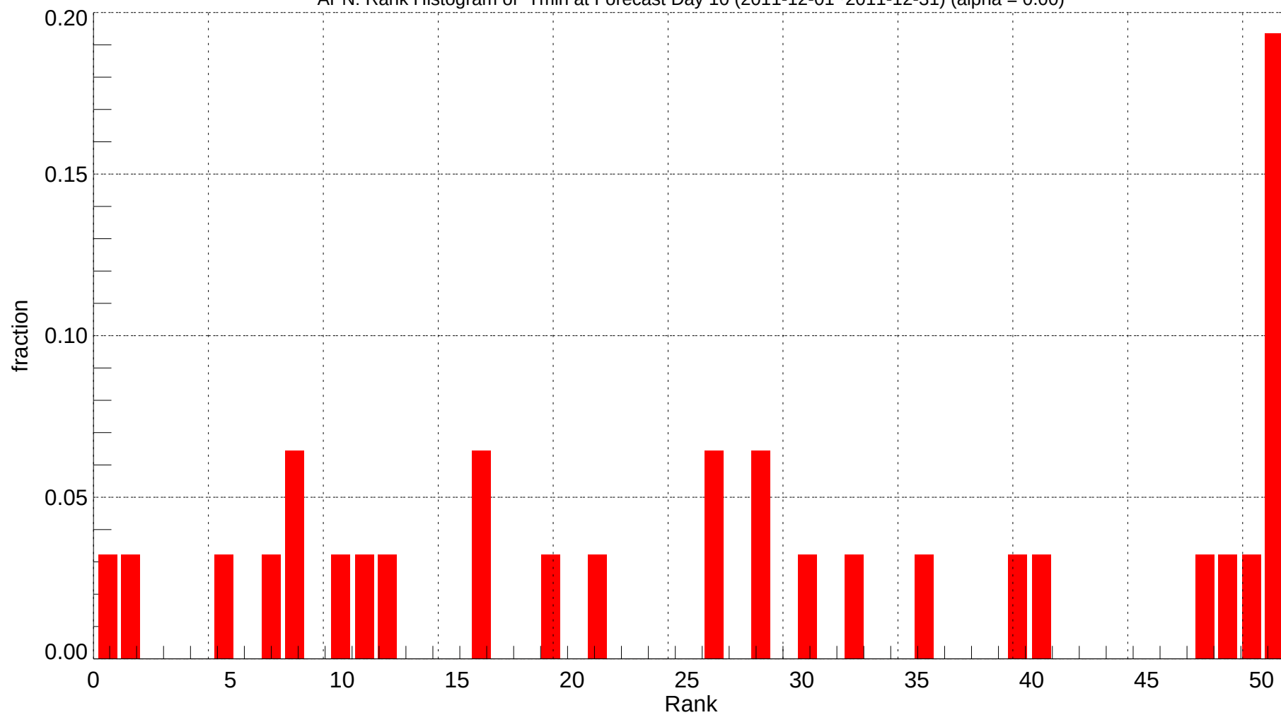
APN: Rank Histogram of Tmin at Forecast Day 10 (2011-12-01~2011-12-31) (alpha = 0.00)
