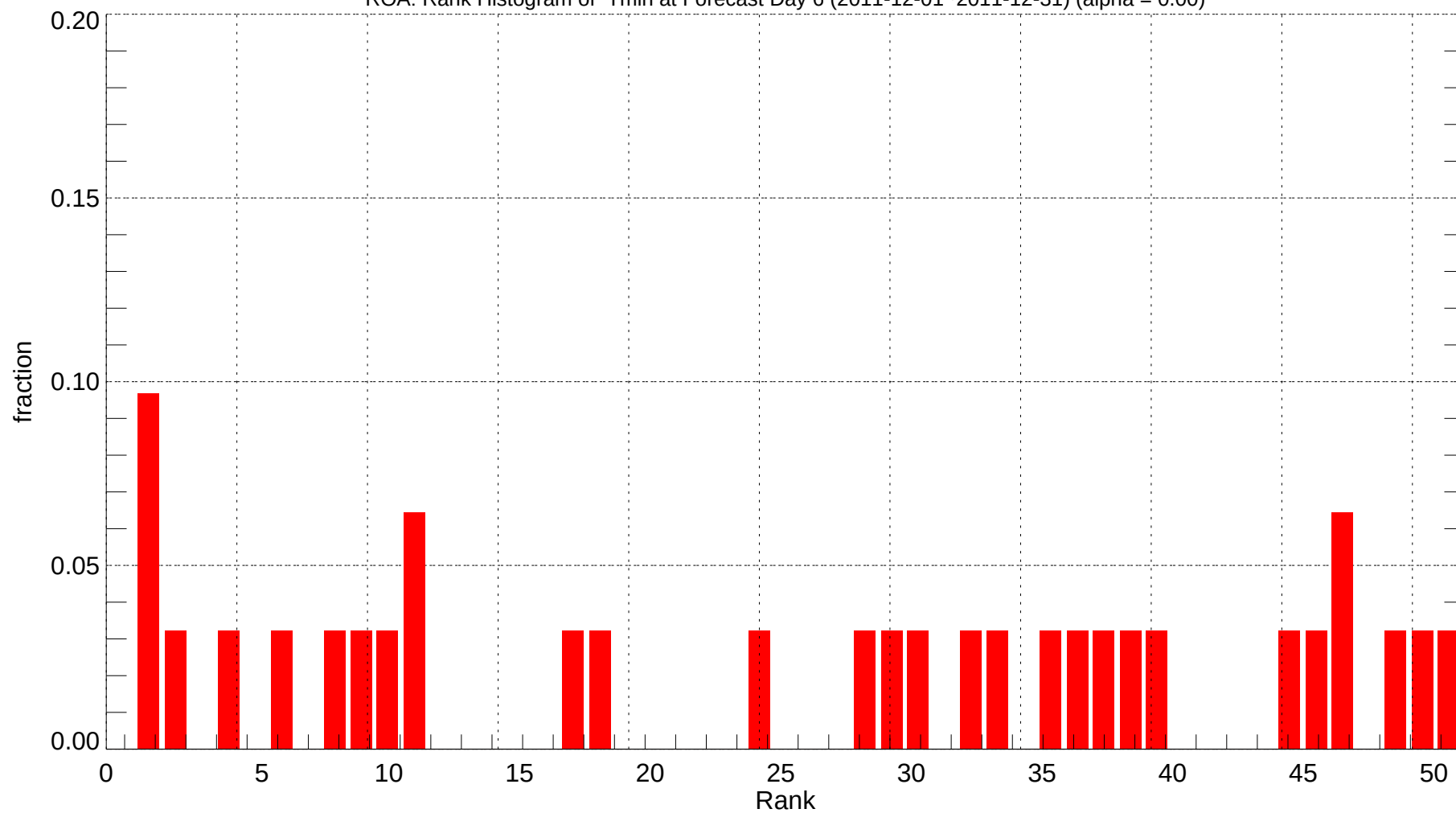
ROA: Rank Histogram of Tmin at Forecast Day 6 (2011-12-01~2011-12-31) (alpha = 0.00)
