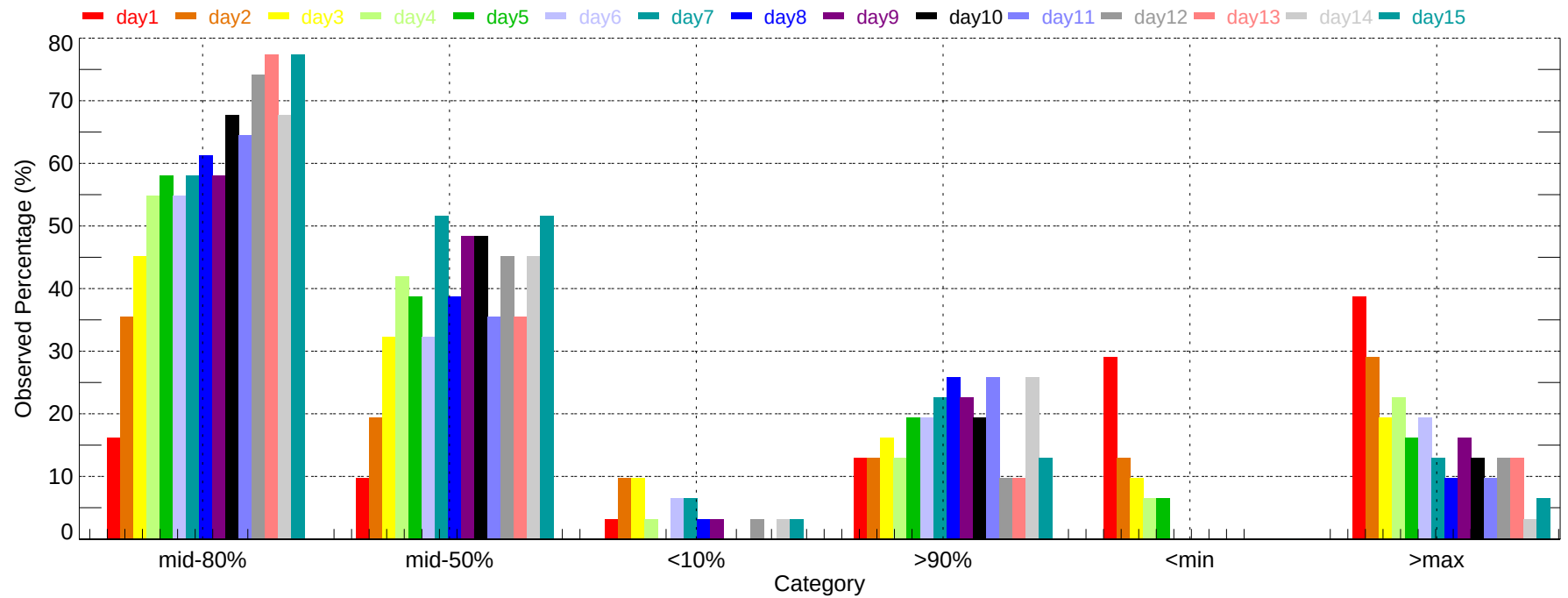
Observed Percentage of Ensembles - TUL: Min Temperature (2011-12-01~2011-12-31)
