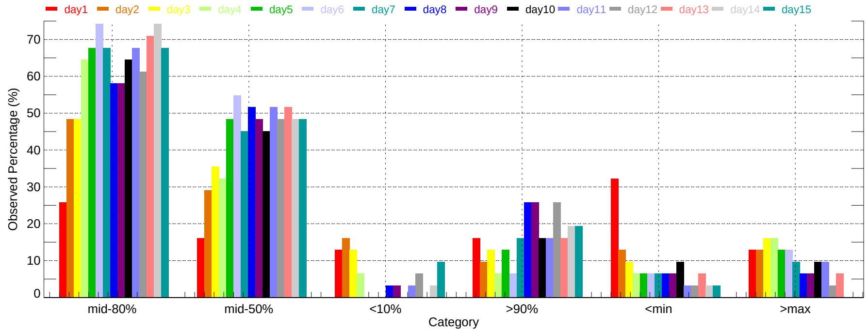
Observed Percentage of Ensembles - LGA: Max Temperature (2011-12-01~2011-12-31)
