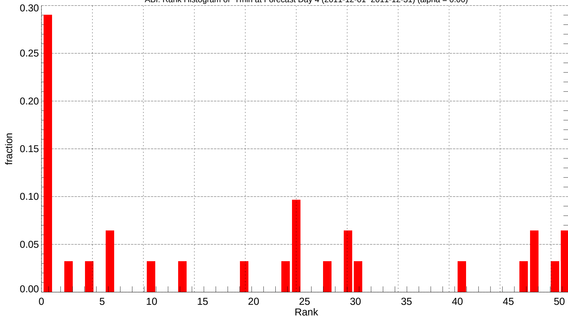
ABI: Rank Histogram of Tmin at Forecast Day 4 (2011-12-01~2011-12-31) (alpha = 0.00)
