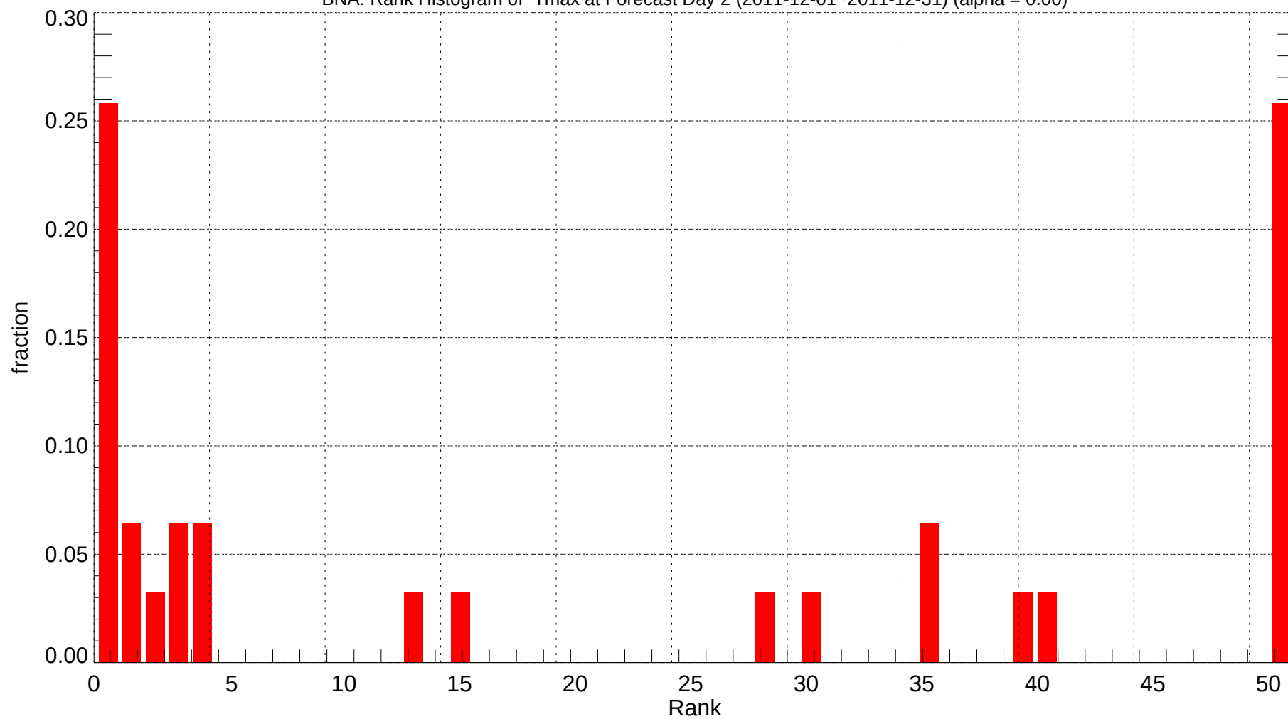
BNA: Rank Histogram of Tmax at Forecast Day 2 (2011-12-01~2011-12-31) (alpha = 0.00)
