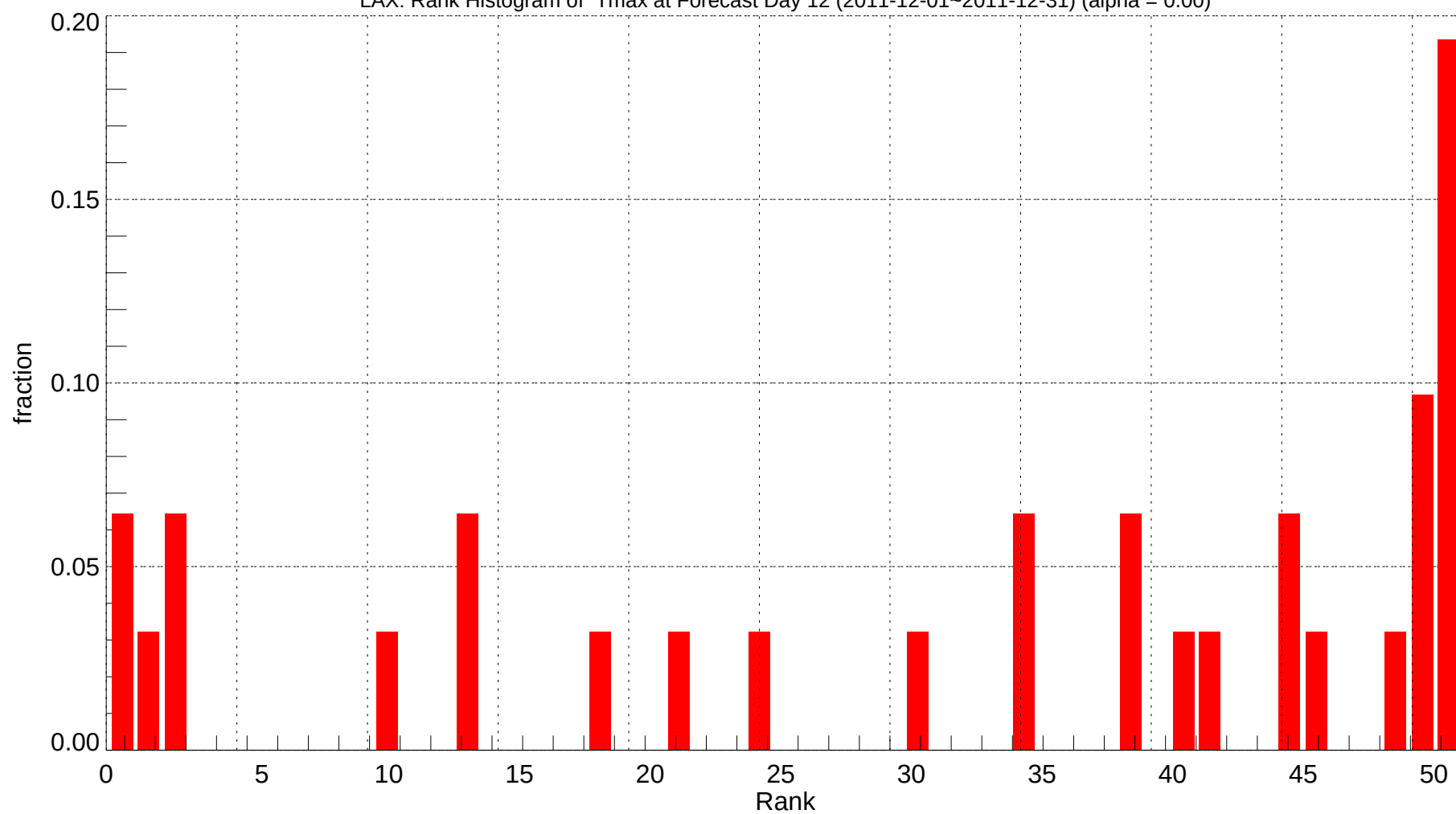
LAX: Rank Histogram of Tmax at Forecast Day 12 (2011-12-01~2011-12-31) (alpha = 0.00)
