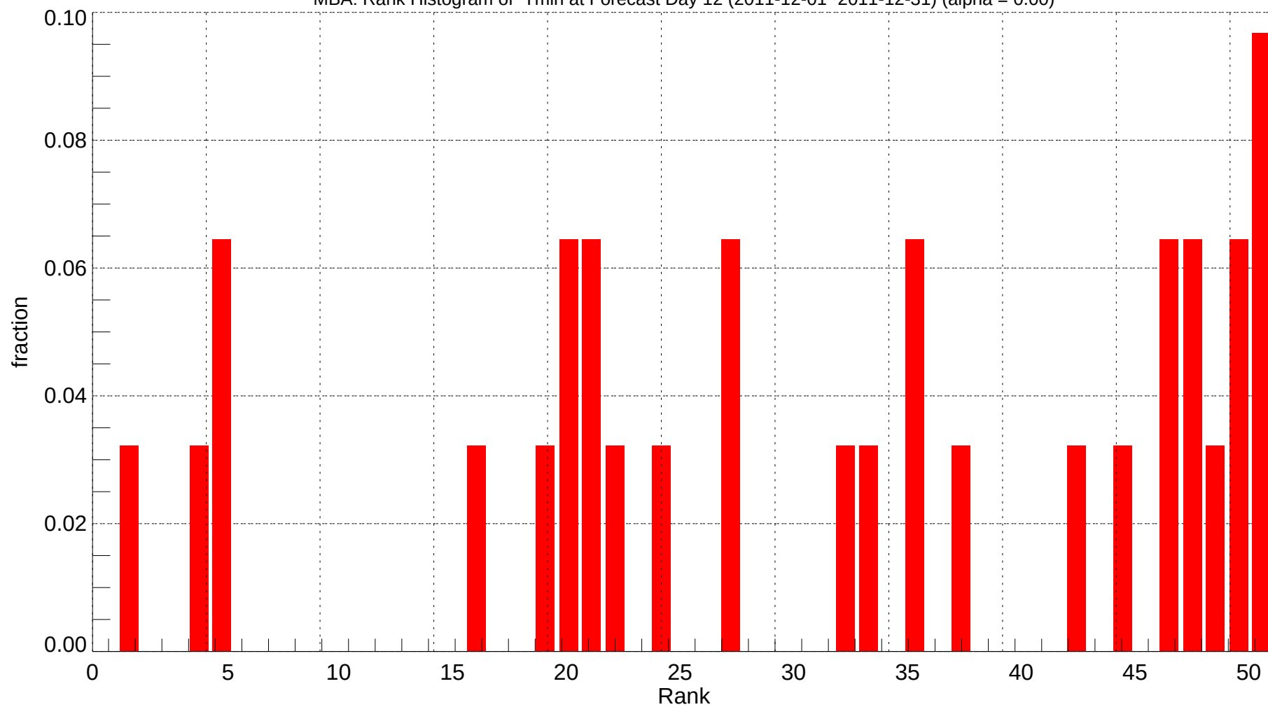
MBA: Rank Histogram of Tmin at Forecast Day 12 (2011-12-01~2011-12-31) (alpha = 0.00)
