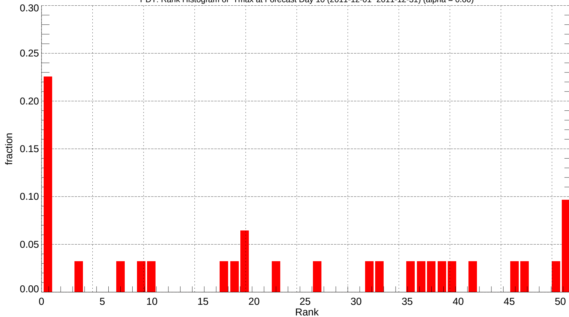
PDT: Rank Histogram of Tmax at Forecast Day 10 (2011-12-01~2011-12-31) (alpha = 0.00)
