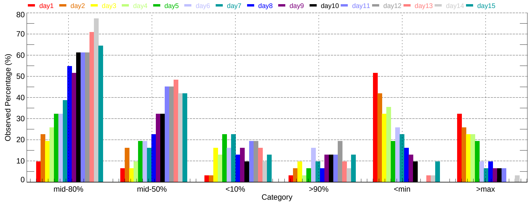
Observed Percentage of Ensembles - ROC: Max Temperature (2011-12-01~2011-12-31)
