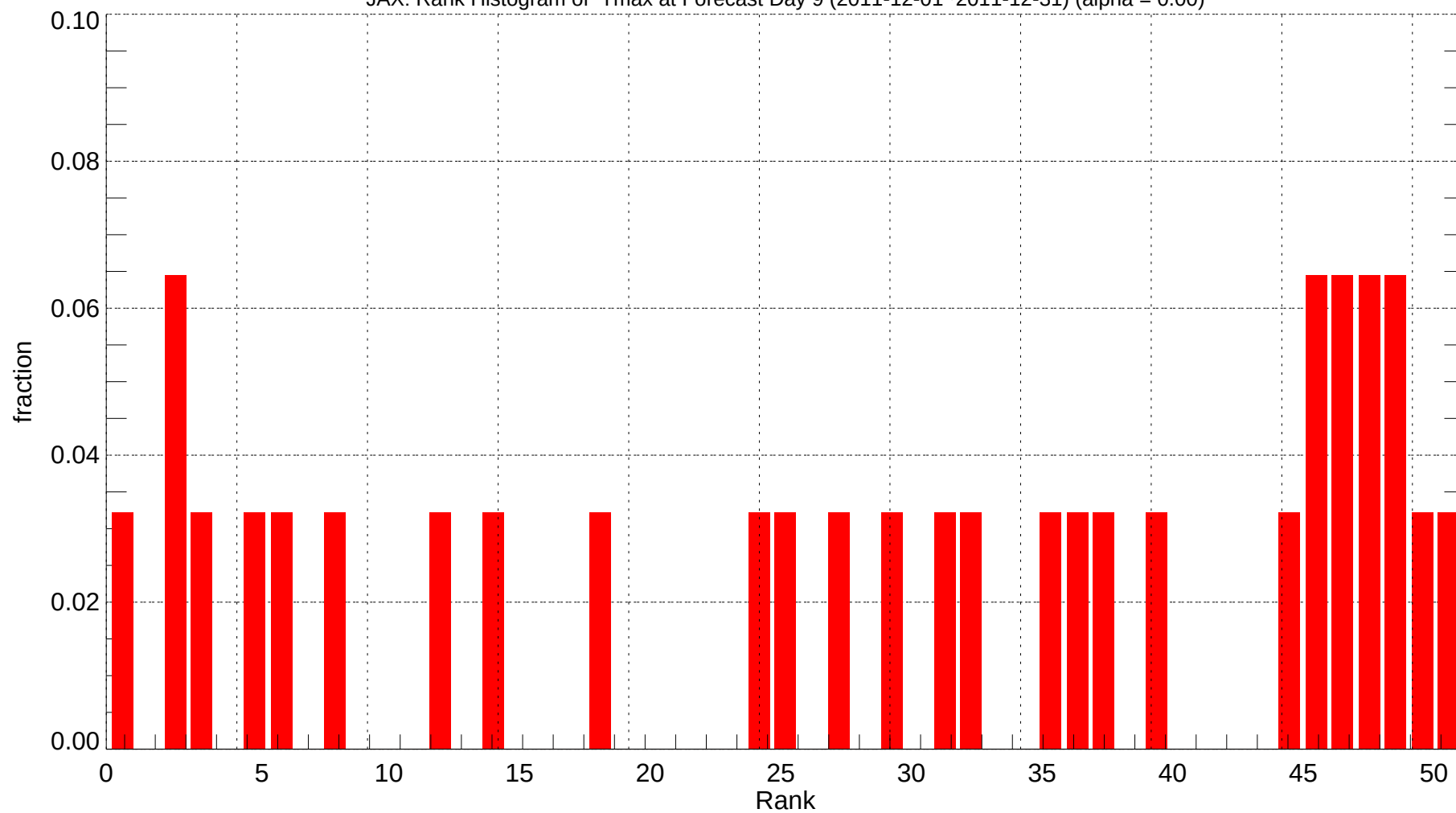
JAX: Rank Histogram of Tmax at Forecast Day 9 (2011-12-01~2011-12-31) (alpha = 0.00)
