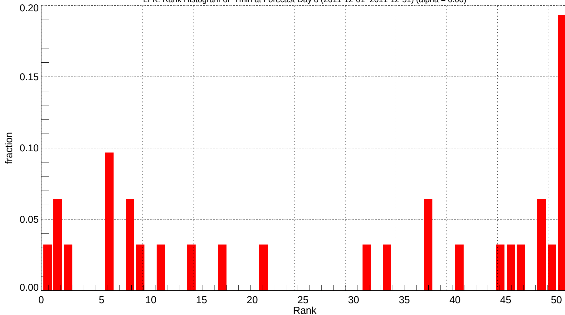
LFK: Rank Histogram of Tmin at Forecast Day 8 (2011-12-01~2011-12-31) (alpha = 0.00)
