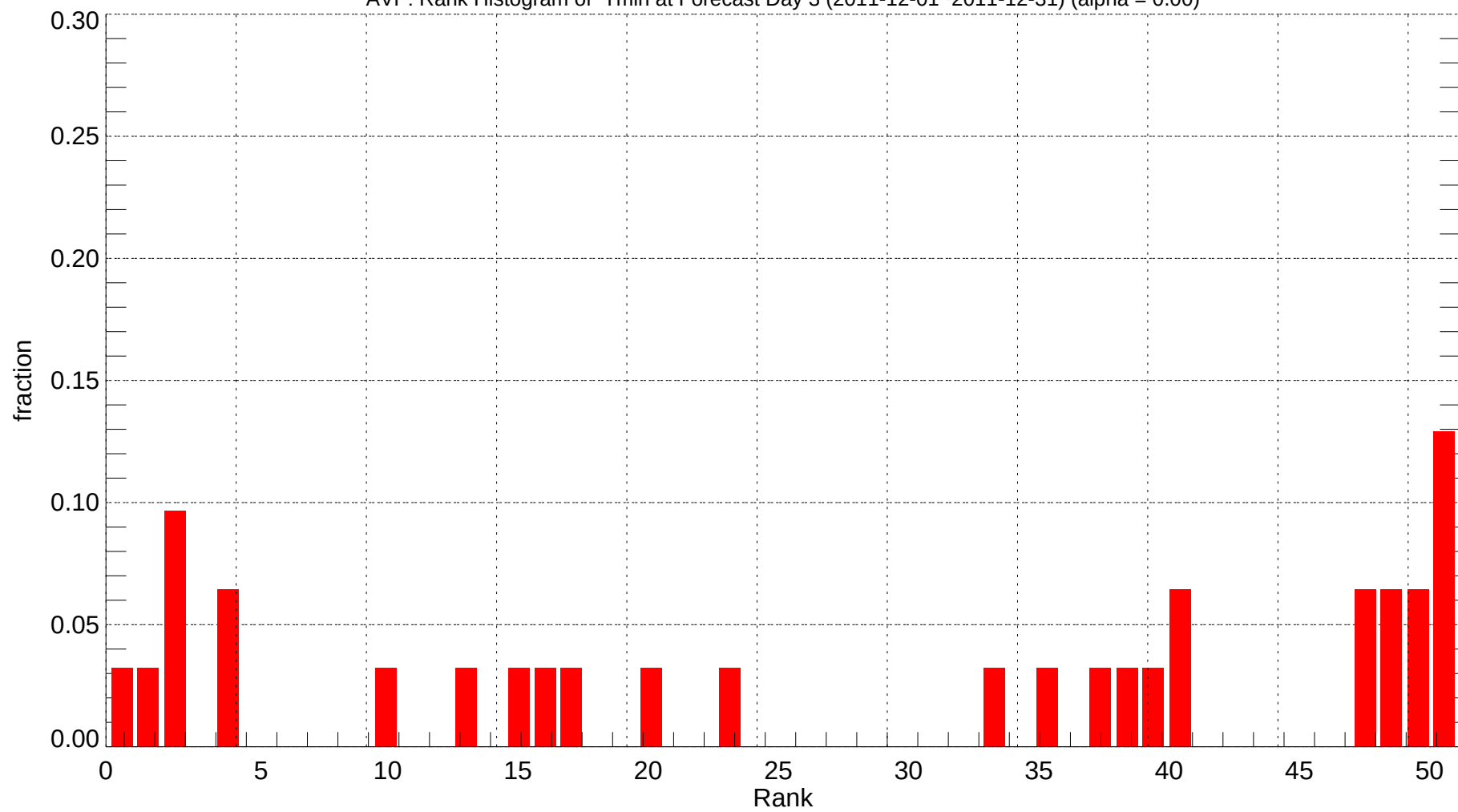
AVP: Rank Histogram of Tmin at Forecast Day 3 (2011-12-01~2011-12-31) (alpha = 0.00)
