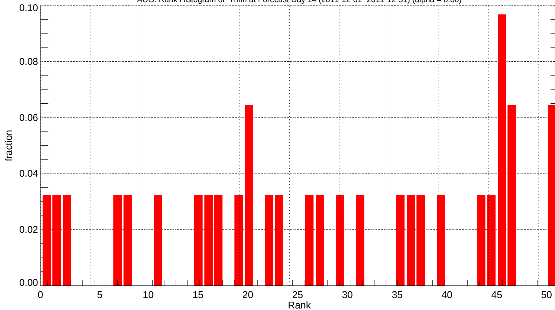
AUG: Rank Histogram of Tmin at Forecast Day 14 (2011-12-01~2011-12-31) (alpha = 0.00)
