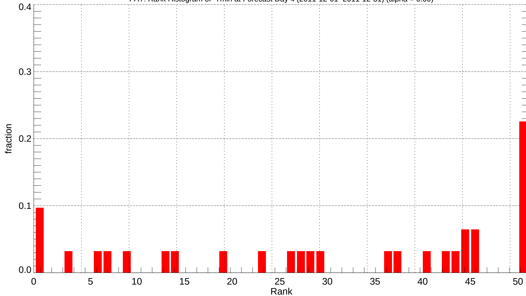
FAT: Rank Histogram of Tmin at Forecast Day 4 (2011-12-01~2011-12-31) (alpha = 0.00)
