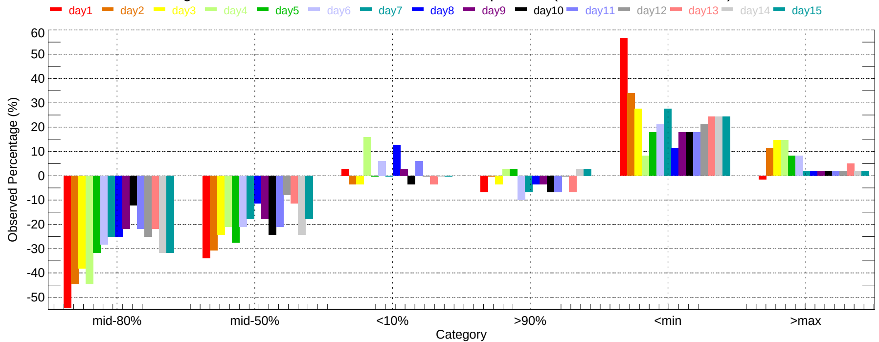
Observed Percentage Deviation of Ensembles - MAF: Max Temperature (2011-12-01~2011-12-31)
