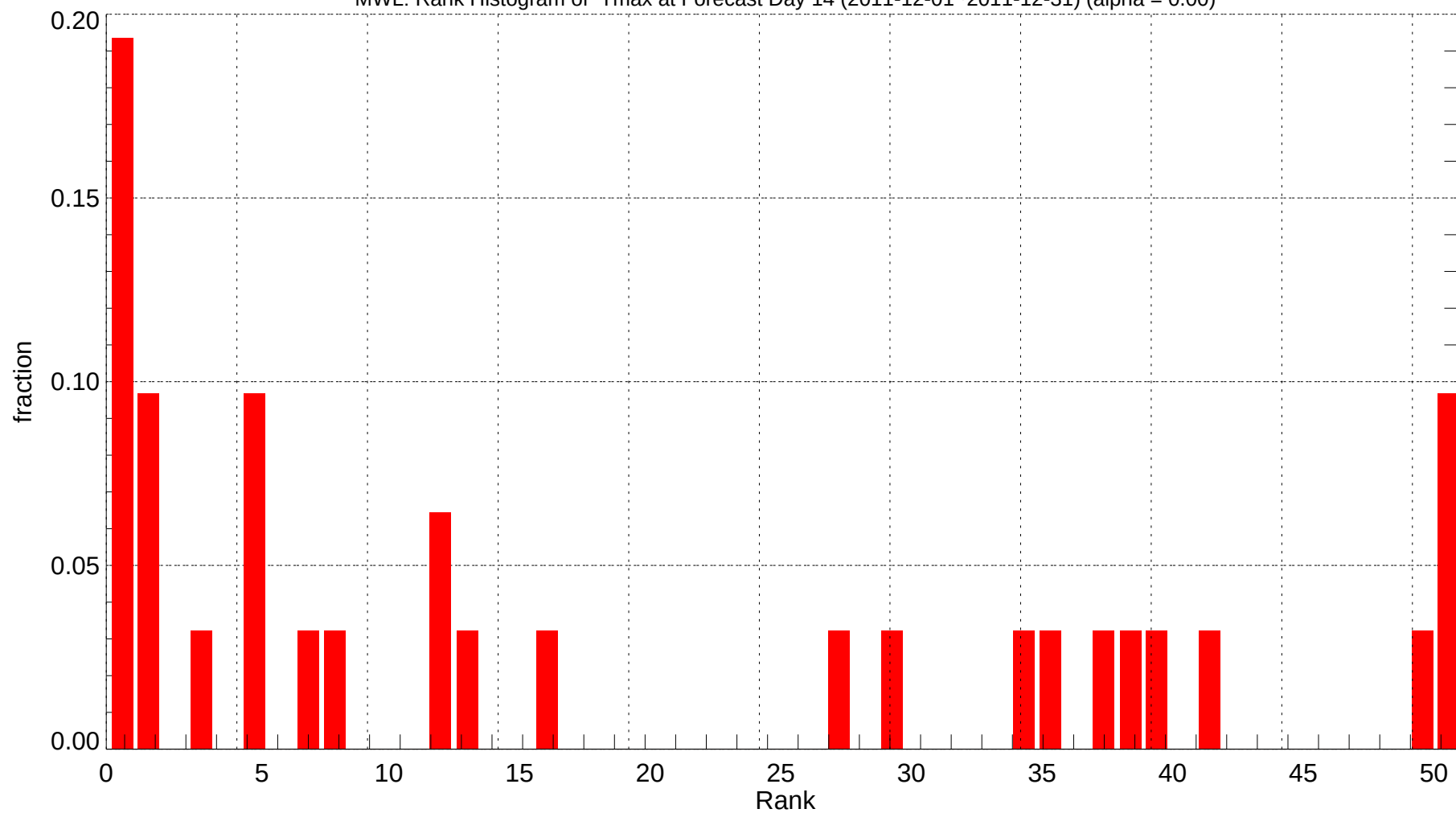
MWL: Rank Histogram of Tmax at Forecast Day 14 (2011-12-01~2011-12-31) (alpha = 0.00)
