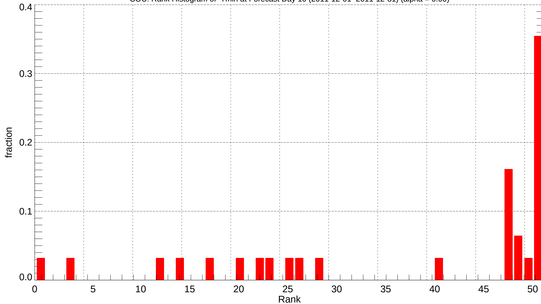
COU: Rank Histogram of Tmin at Forecast Day 10 (2011-12-01~2011-12-31) (alpha = 0.00)
