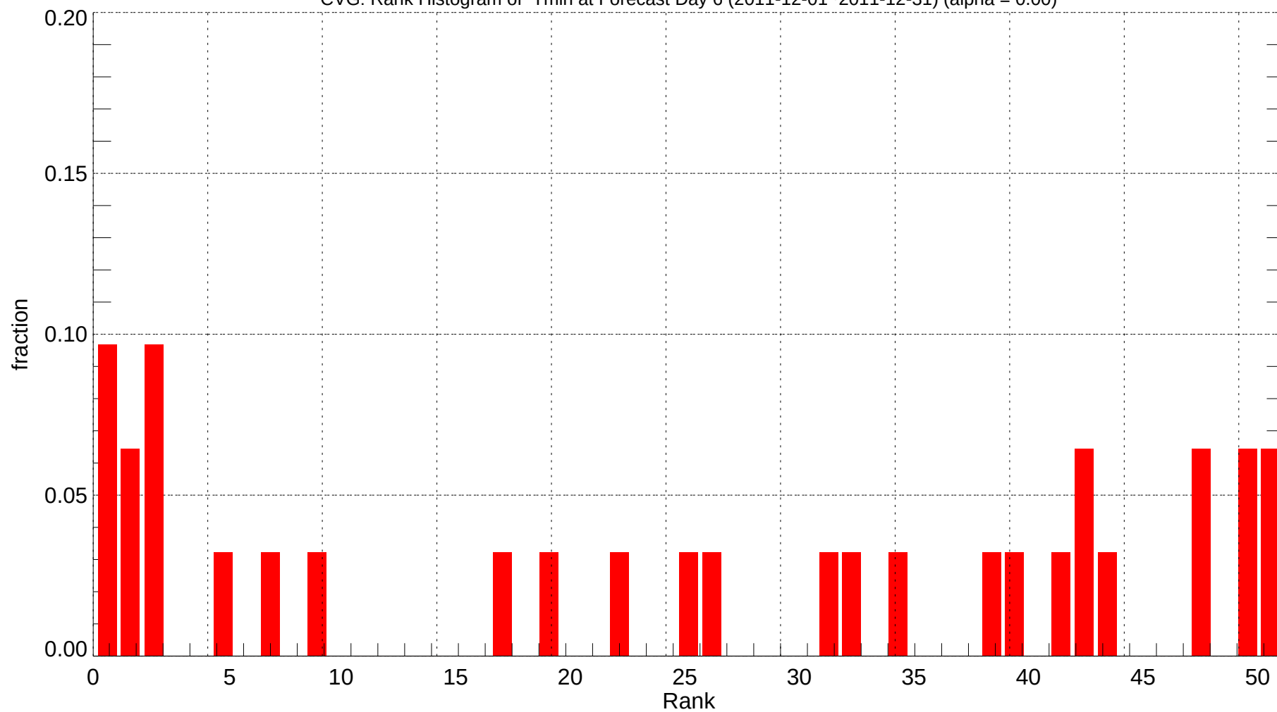
CVG: Rank Histogram of Tmin at Forecast Day 6 (2011-12-01~2011-12-31) (alpha = 0.00)
