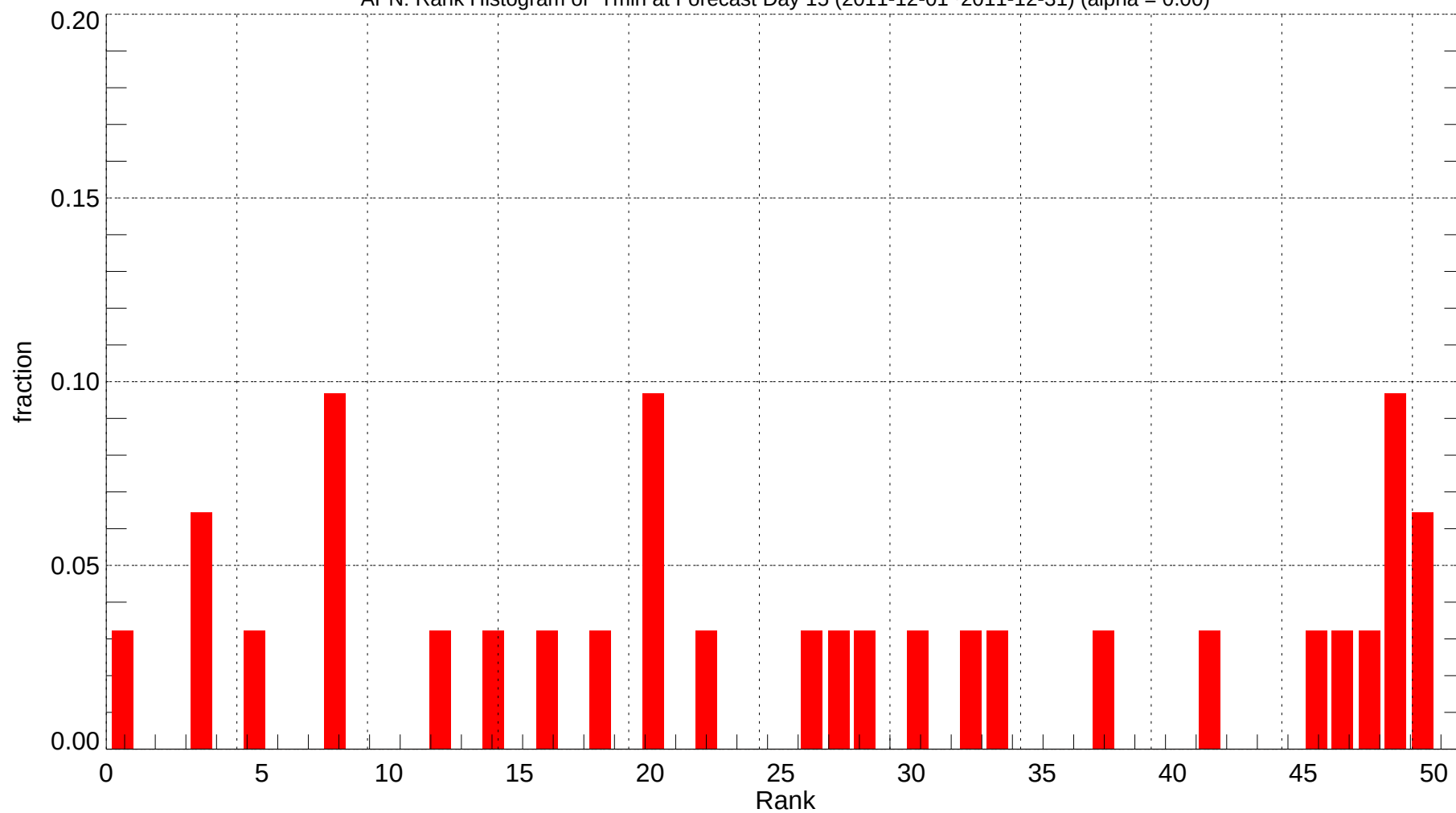
APN: Rank Histogram of Tmin at Forecast Day 15 (2011-12-01~2011-12-31) (alpha = 0.00)
