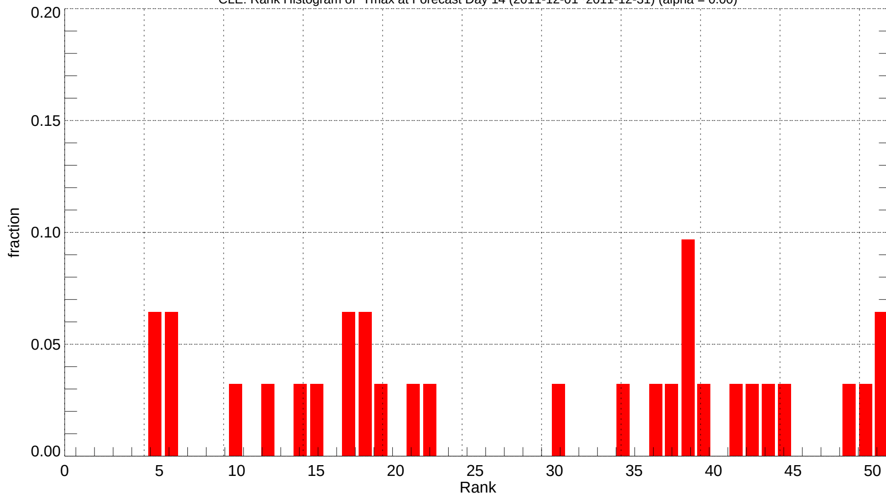
CLE: Rank Histogram of Tmax at Forecast Day 14 (2011-12-01~2011-12-31) (alpha = 0.00)
