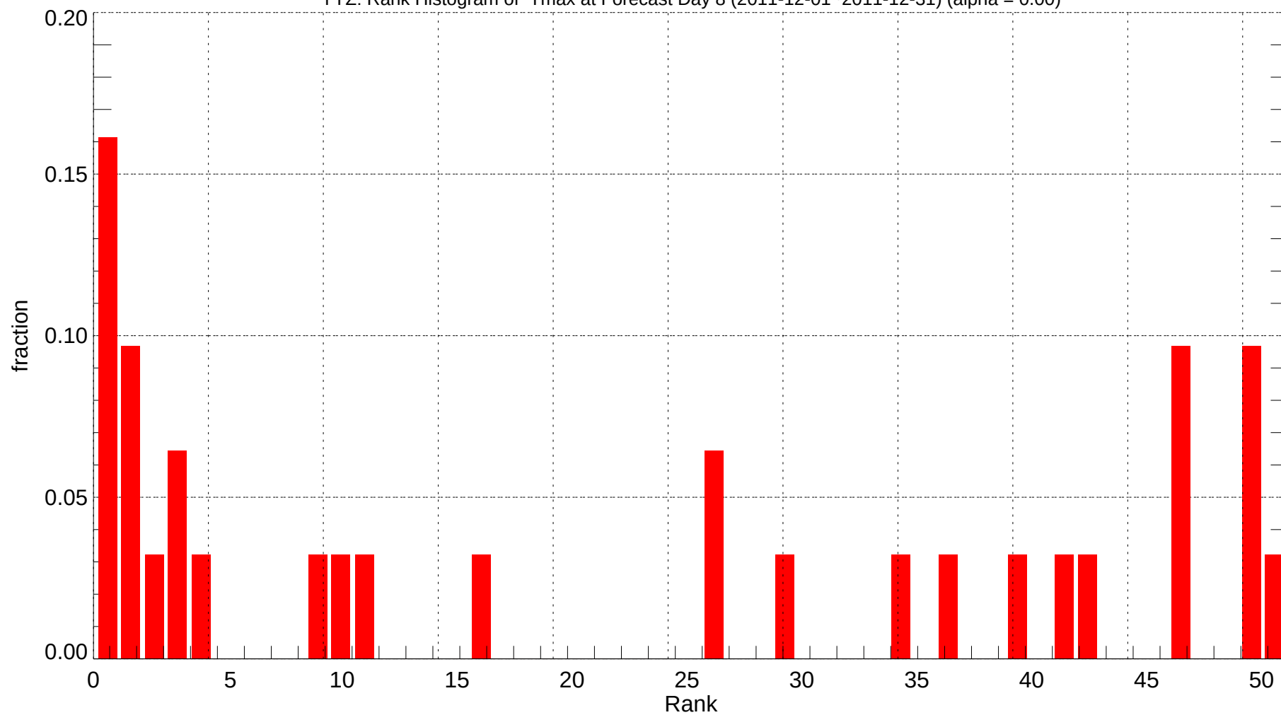
YYZ: Rank Histogram of Tmax at Forecast Day 8 (2011-12-01~2011-12-31) (alpha = 0.00)
