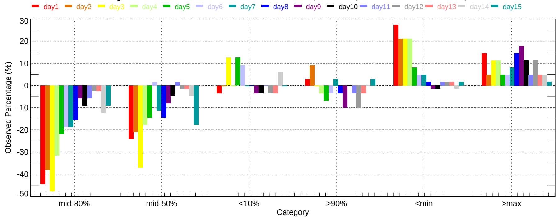
Observed Percentage Deviation of Ensembles - YWG: Max Temperature (2011-12-01~2011-12-31)
