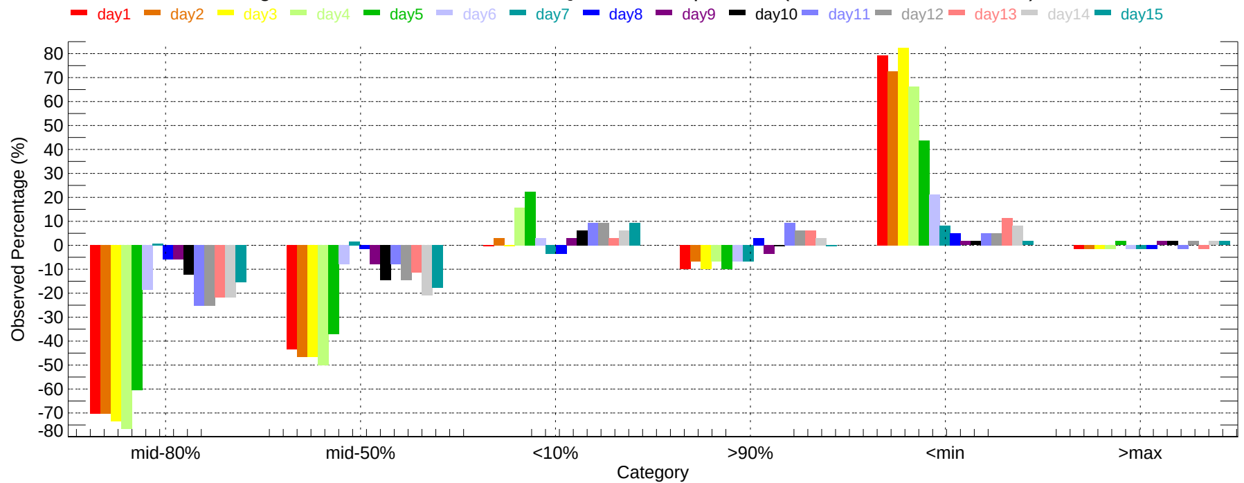
Observed Percentage Deviation of Ensembles - CQT: Max Temperature (2011-12-01~2011-12-31)
