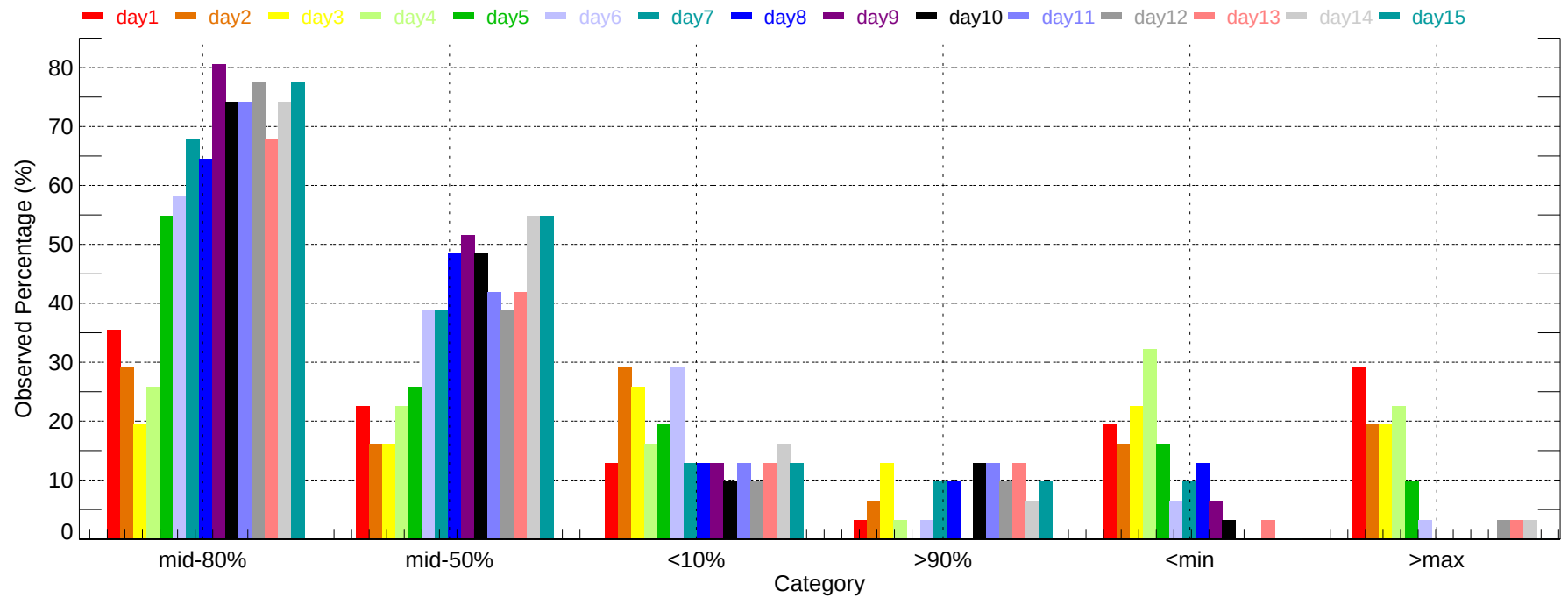
Observed Percentage of Ensembles - MIA: Min Temperature (2011-12-01~2011-12-31)
