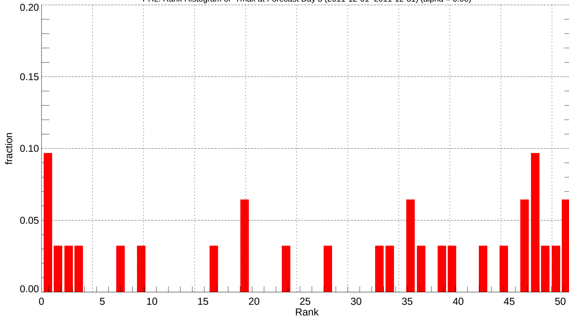
PHL: Rank Histogram of Tmax at Forecast Day 8 (2011-12-01~2011-12-31) (alpha = 0.00)
