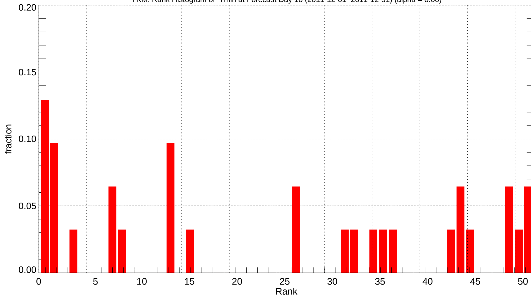
YKM: Rank Histogram of Tmin at Forecast Day 10 (2011-12-01~2011-12-31) (alpha = 0.00)
