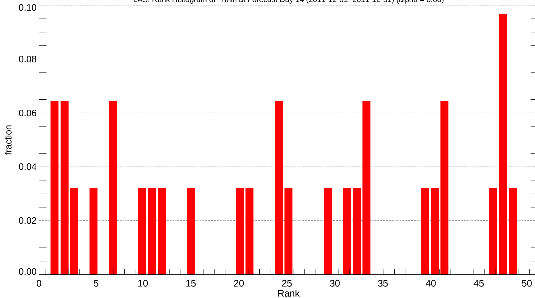
LAS: Rank Histogram of Tmin at Forecast Day 14 (2011-12-01~2011-12-31) (alpha = 0.00)
