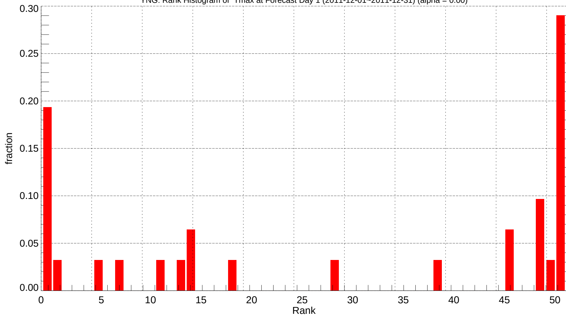
YNG: Rank Histogram of Tmax at Forecast Day 1 (2011-12-01~2011-12-31) (alpha = 0.00)
