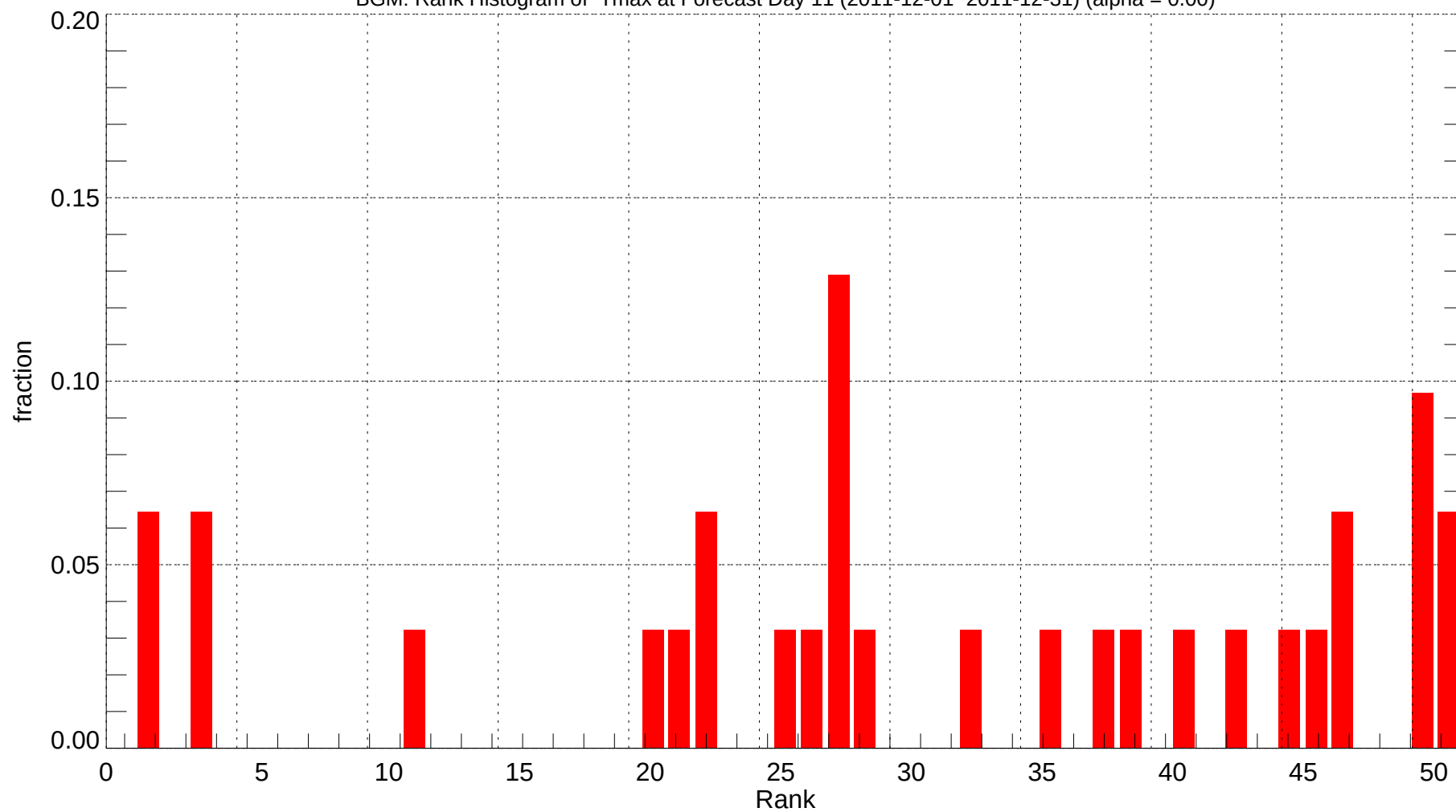
BGM: Rank Histogram of Tmax at Forecast Day 11 (2011-12-01~2011-12-31) (alpha = 0.00)
