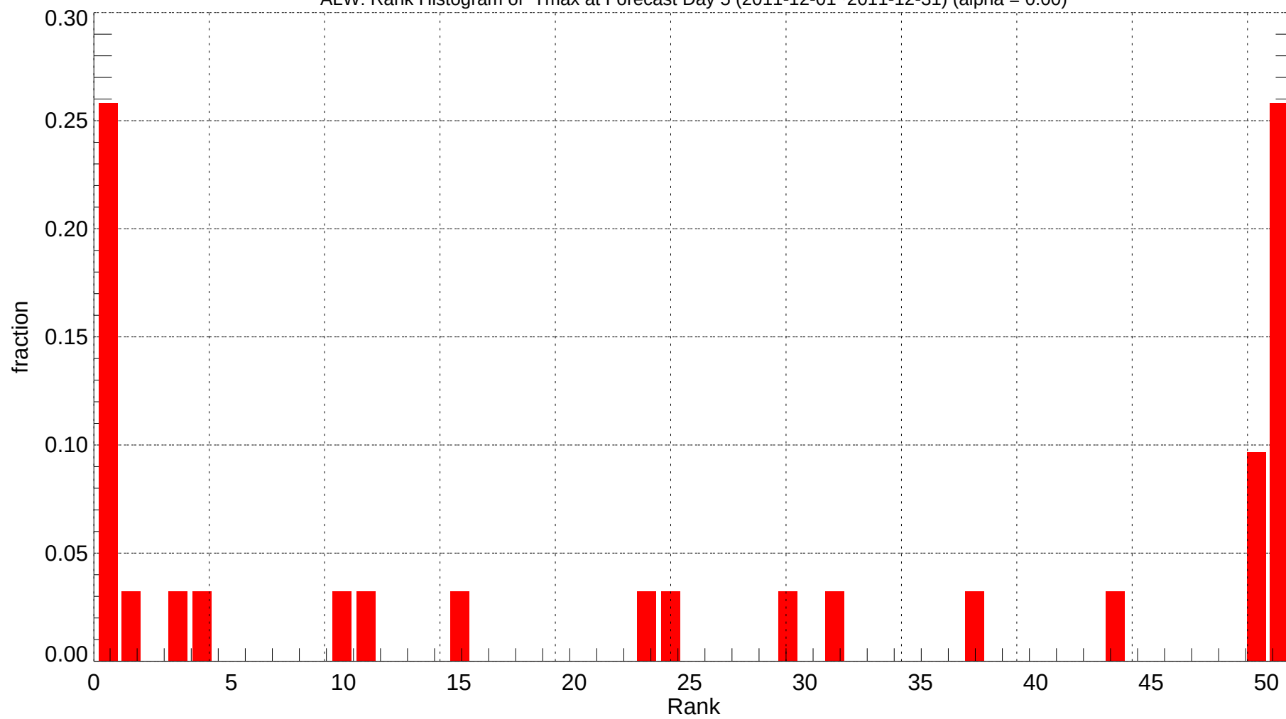
ALW: Rank Histogram of Tmax at Forecast Day 5 (2011-12-01~2011-12-31) (alpha = 0.00)
