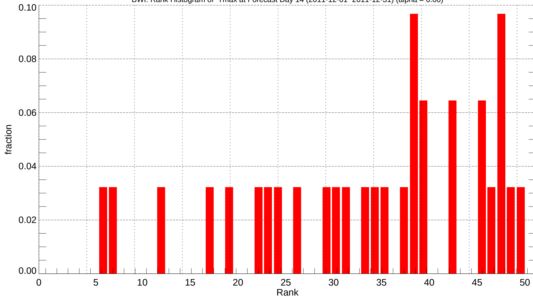
BWI: Rank Histogram of Tmax at Forecast Day 14 (2011-12-01~2011-12-31) (alpha = 0.00)
