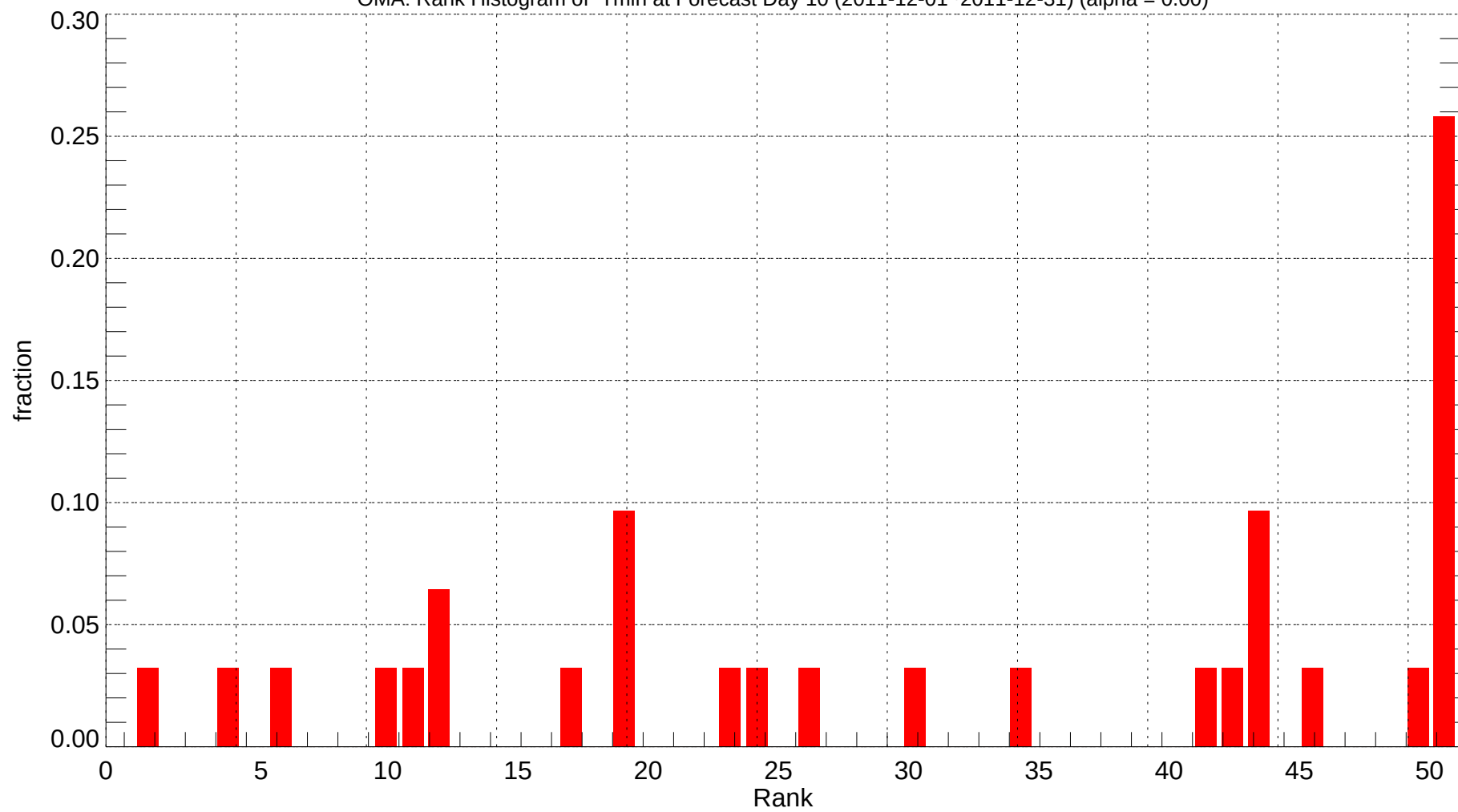
OMA: Rank Histogram of Tmin at Forecast Day 10 (2011-12-01~2011-12-31) (alpha = 0.00)
