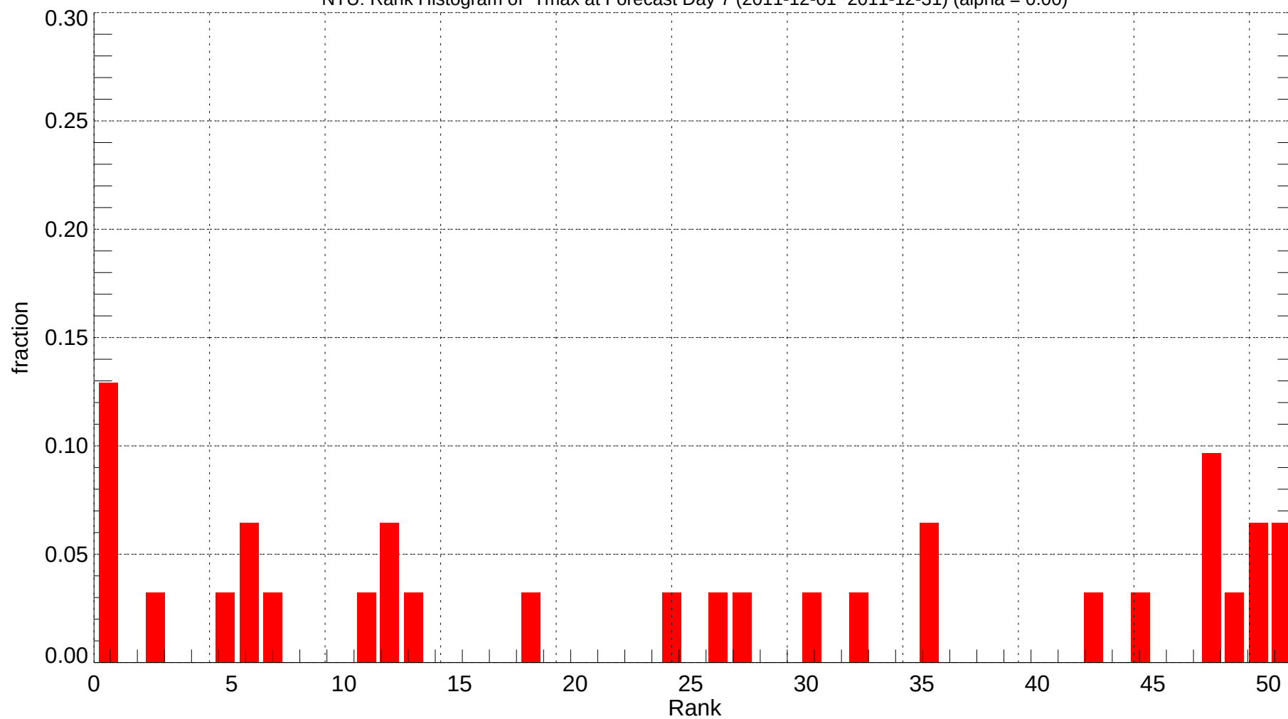
NTU: Rank Histogram of Tmax at Forecast Day 7 (2011-12-01~2011-12-31) (alpha = 0.00)
