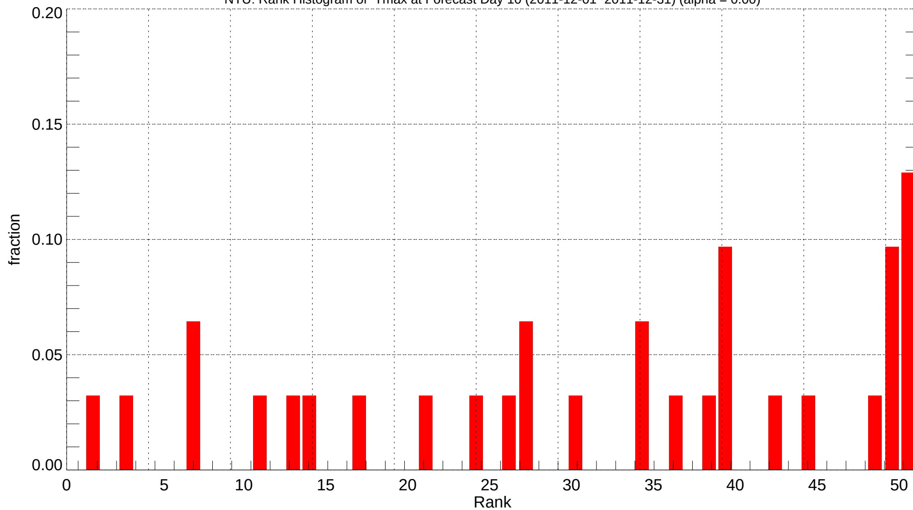
NTU: Rank Histogram of Tmax at Forecast Day 10 (2011-12-01~2011-12-31) (alpha = 0.00)
