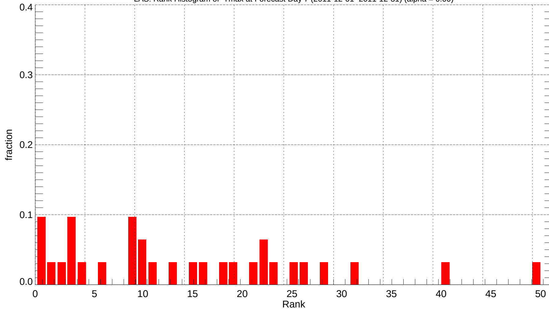
LAS: Rank Histogram of Tmax at Forecast Day 7 (2011-12-01~2011-12-31) (alpha = 0.00)
