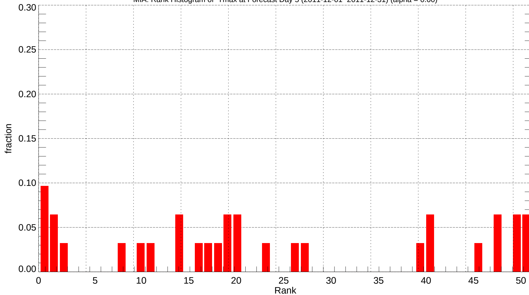
MIA: Rank Histogram of Tmax at Forecast Day 5 (2011-12-01~2011-12-31) (alpha = 0.00)
