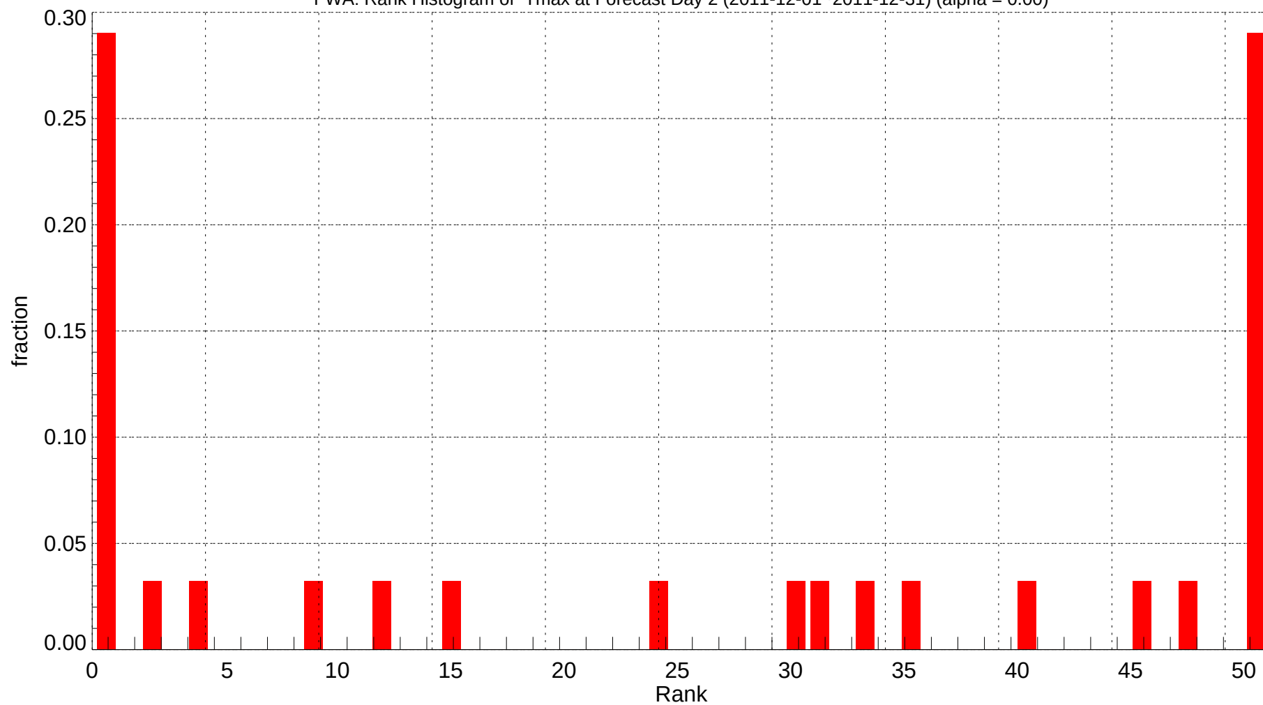
FWA: Rank Histogram of Tmax at Forecast Day 2 (2011-12-01~2011-12-31) (alpha = 0.00)
