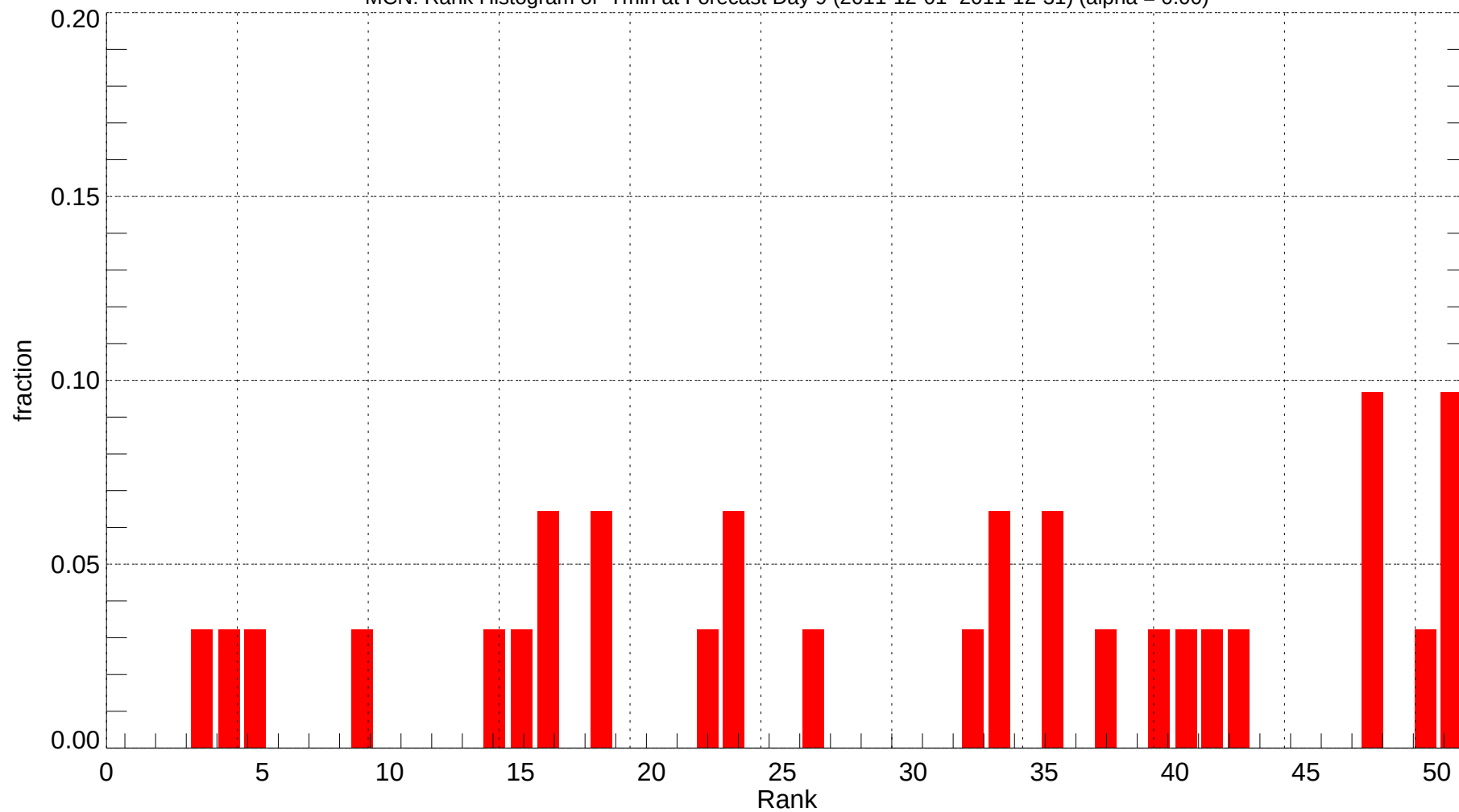
MCN: Rank Histogram of Tmin at Forecast Day 9 (2011-12-01~2011-12-31) (alpha = 0.00)
