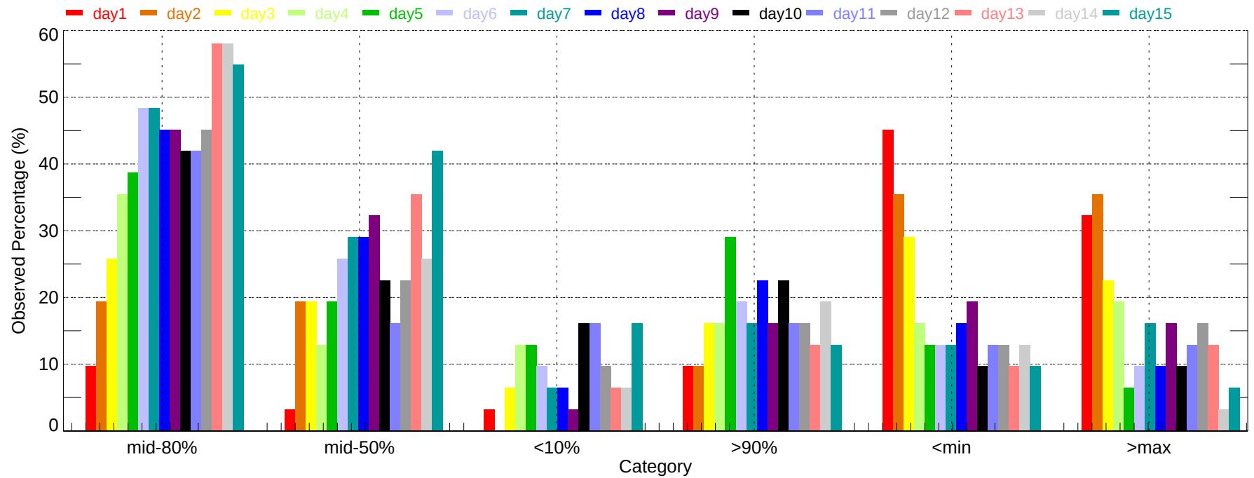
Observed Percentage of Ensembles - DEN: Min Temperature (2011-12-01~2011-12-31)
