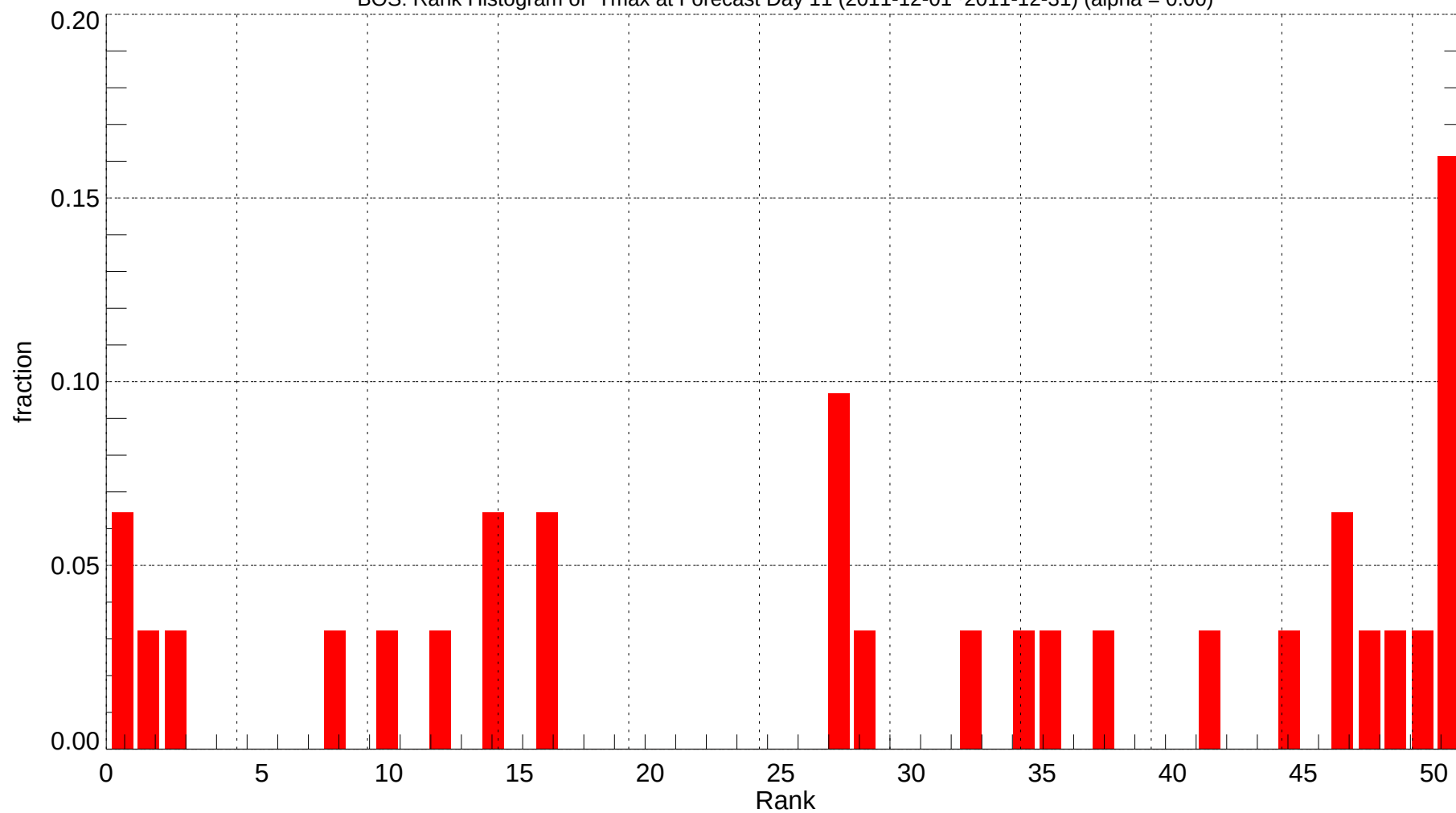
BOS: Rank Histogram of Tmax at Forecast Day 11 (2011-12-01~2011-12-31) (alpha = 0.00)
