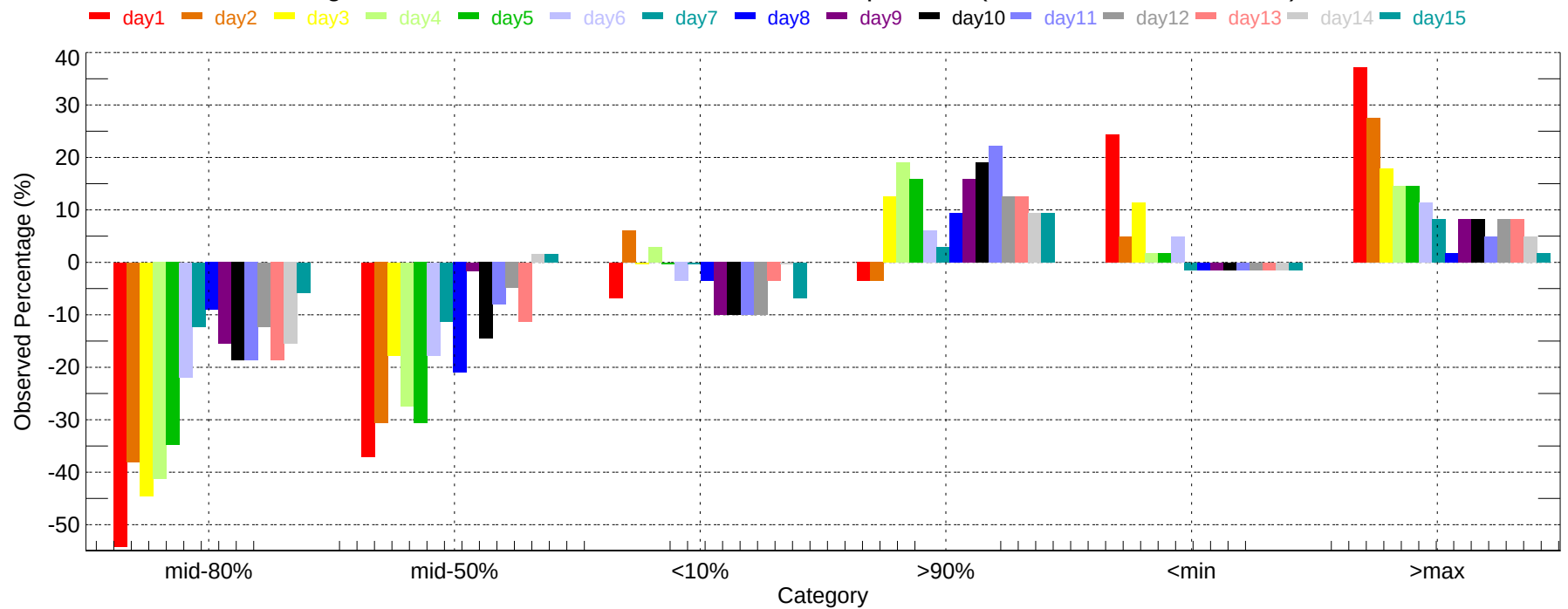
Observed Percentage Deviation of Ensembles - STL: Max Temperature (2011-12-01~2011-12-31)
