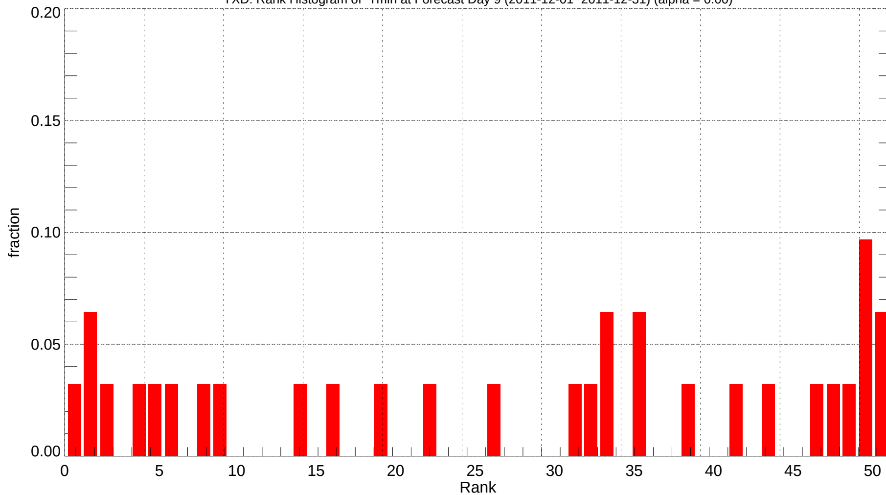
YXD: Rank Histogram of Tmin at Forecast Day 9 (2011-12-01~2011-12-31) (alpha = 0.00)
