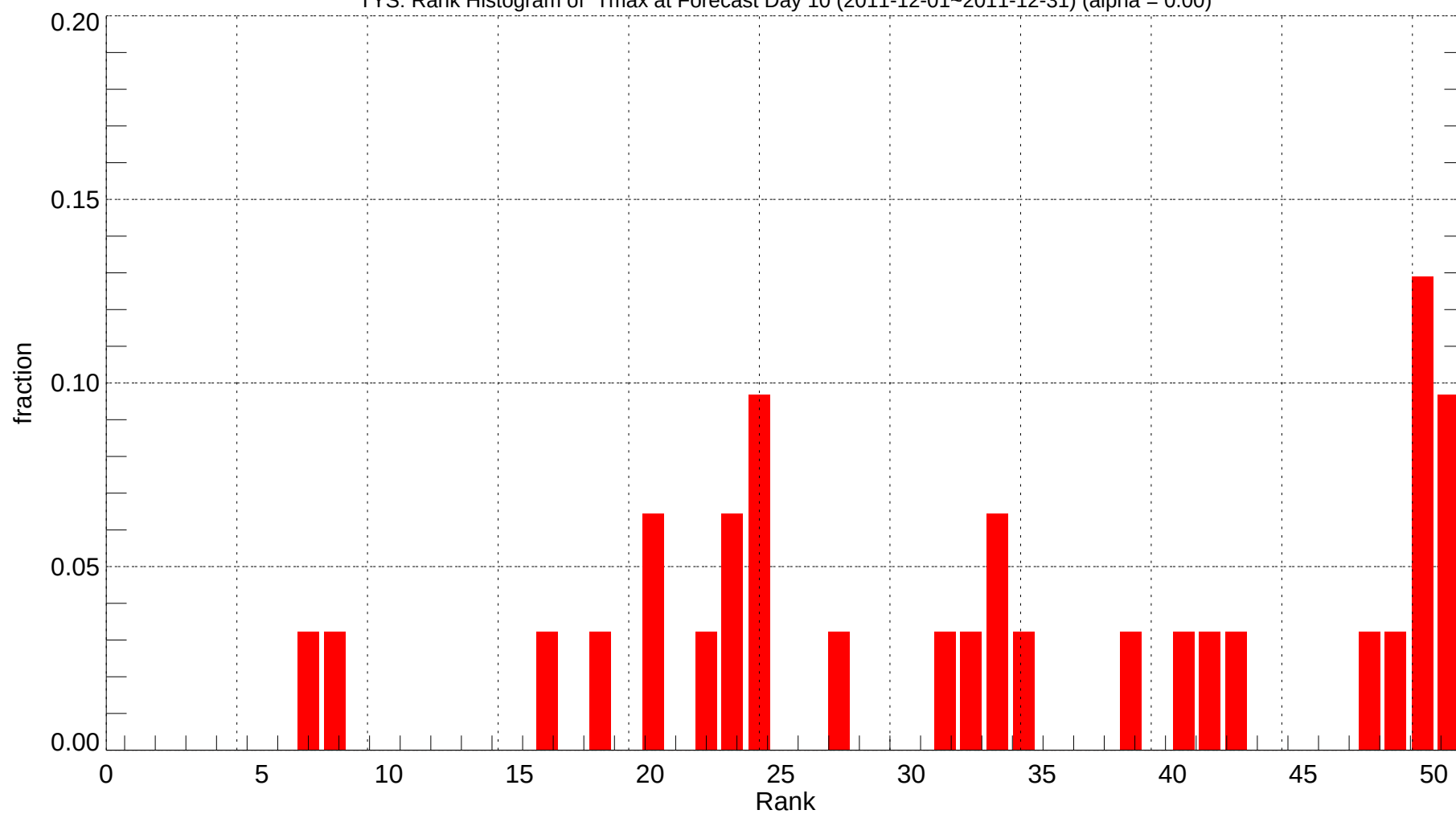
TYS: Rank Histogram of Tmax at Forecast Day 10 (2011-12-01~2011-12-31) (alpha = 0.00)
