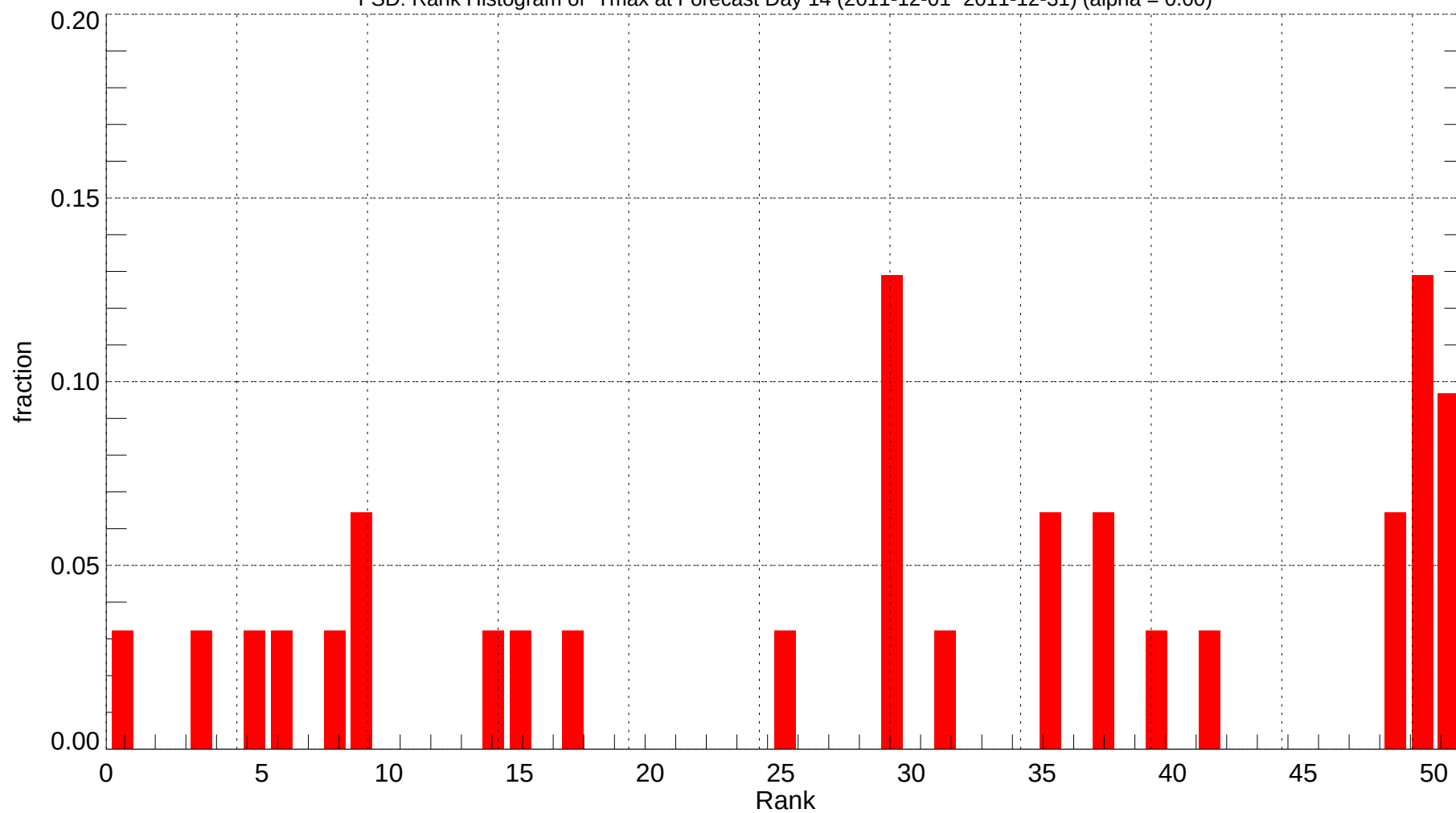
FSD: Rank Histogram of Tmax at Forecast Day 14 (2011-12-01~2011-12-31) (alpha = 0.00)
