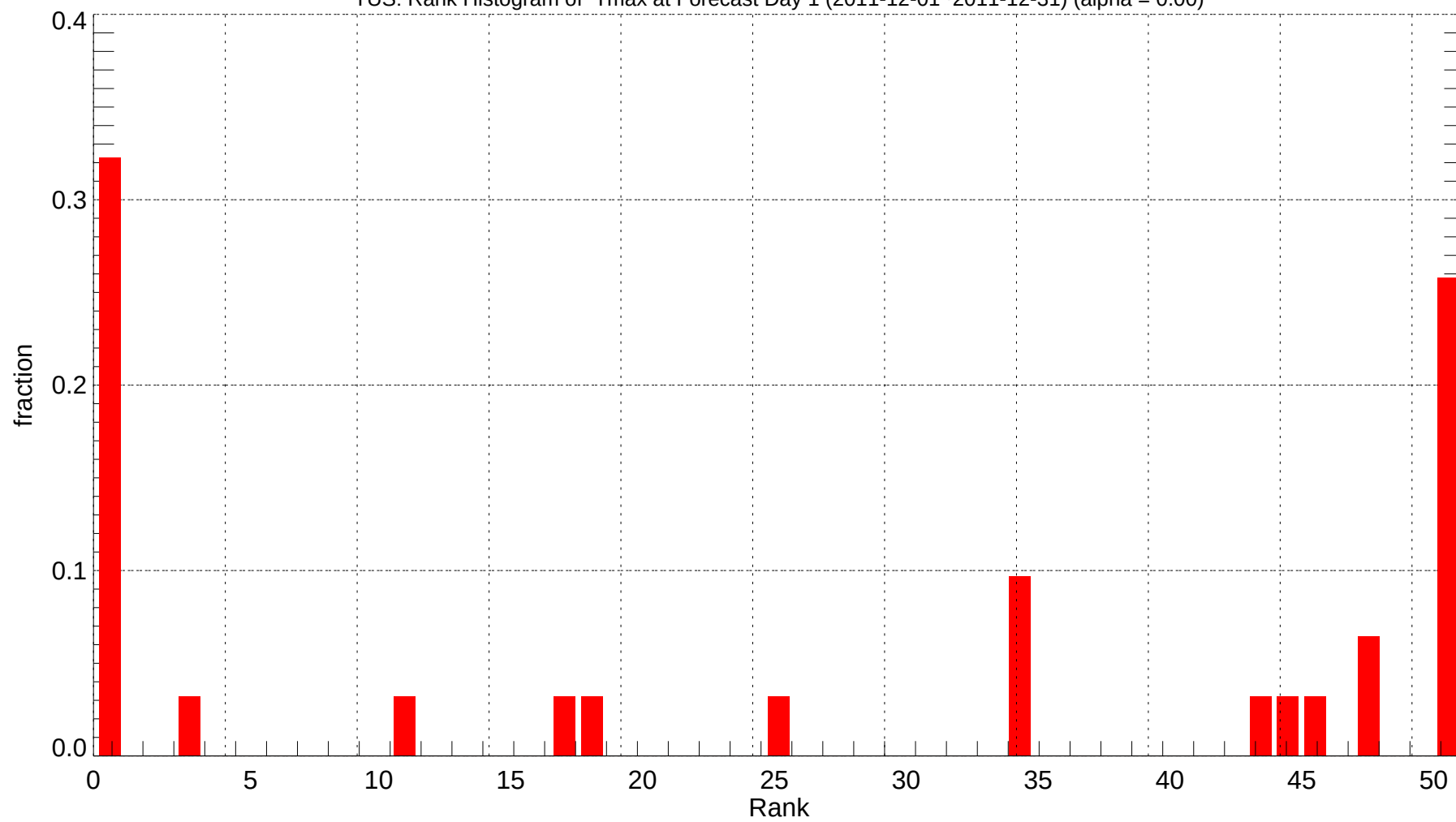
TUS: Rank Histogram of Tmax at Forecast Day 1 (2011-12-01~2011-12-31) (alpha = 0.00)
