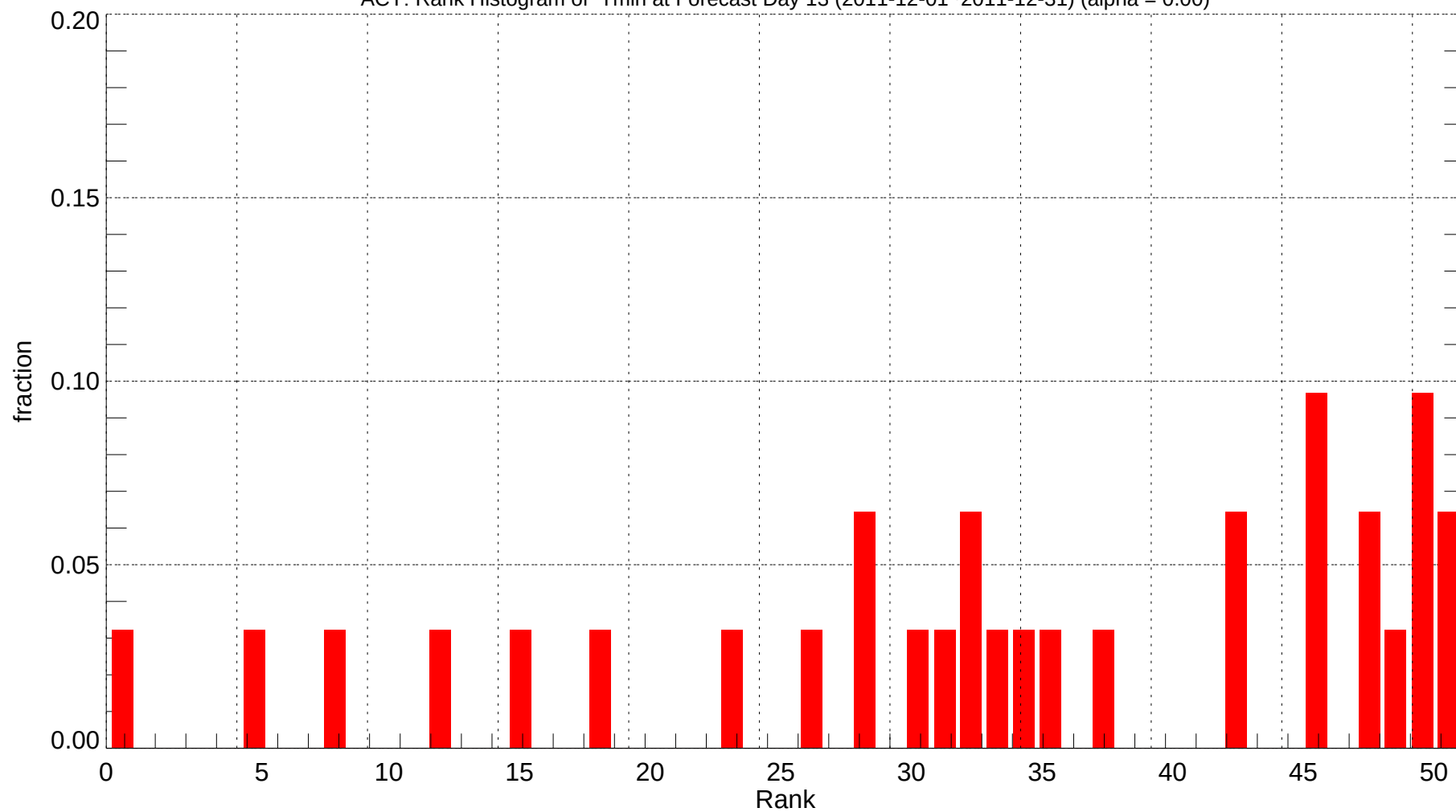
ACY: Rank Histogram of Tmin at Forecast Day 13 (2011-12-01~2011-12-31) (alpha = 0.00)
