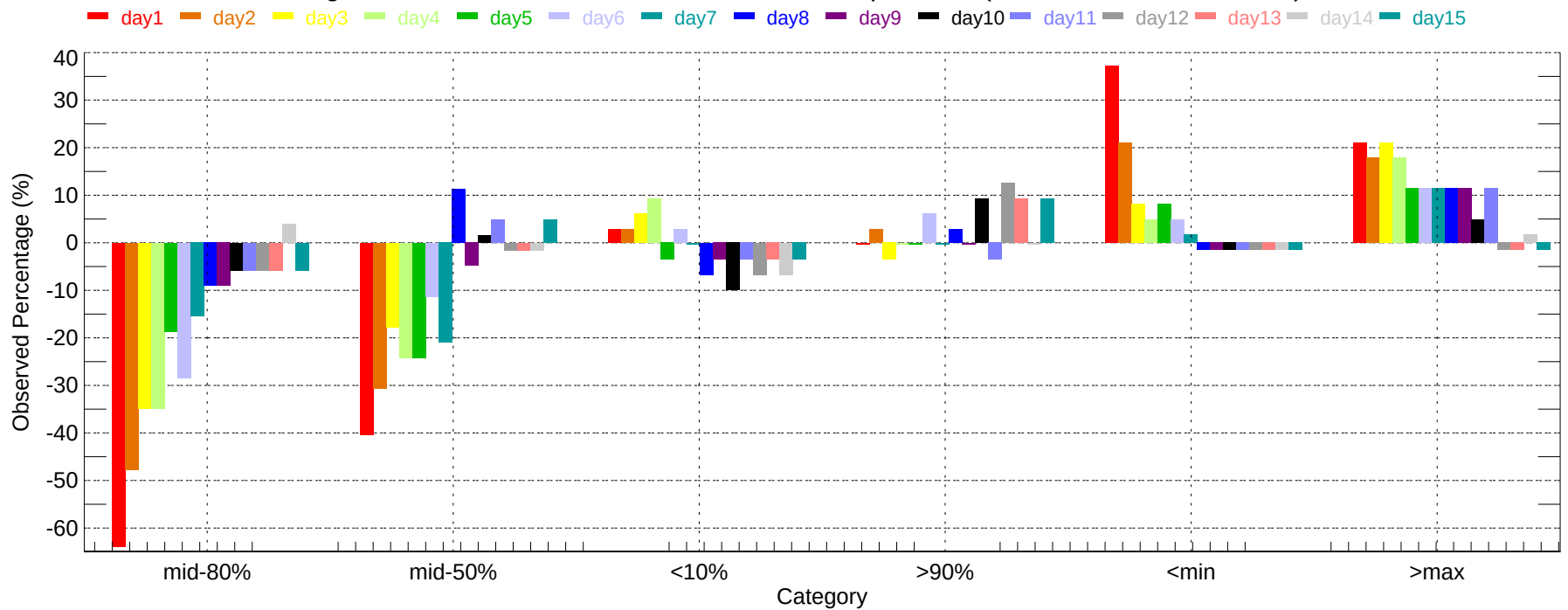
Observed Percentage Deviation of Ensembles - BUF: Max Temperature (2011-12-01~2011-12-31)
