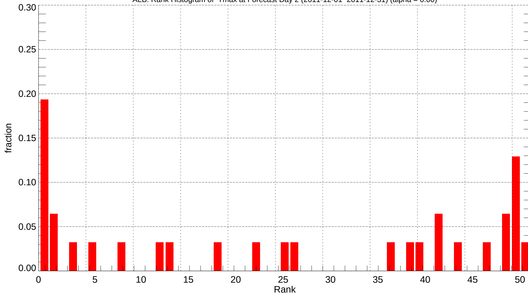
ALB: Rank Histogram of Tmax at Forecast Day 2 (2011-12-01~2011-12-31) (alpha = 0.00)
