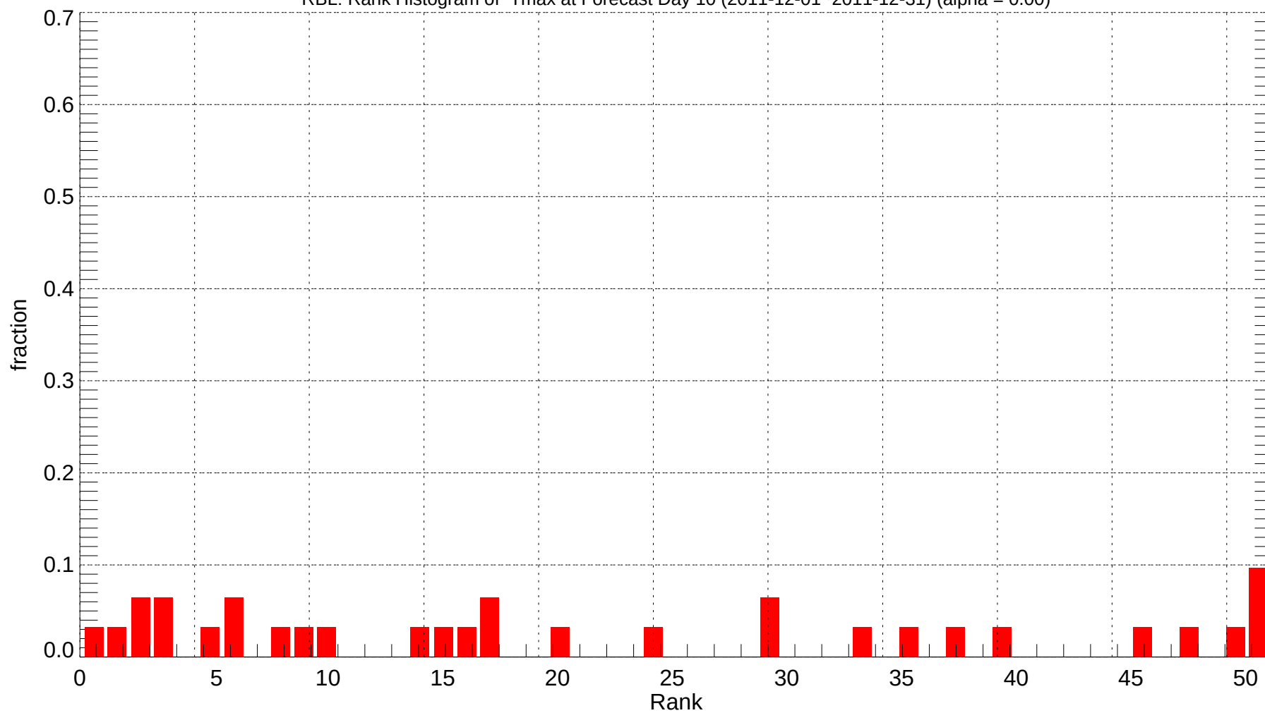
RBL: Rank Histogram of Tmax at Forecast Day 10 (2011-12-01~2011-12-31) (alpha = 0.00)
