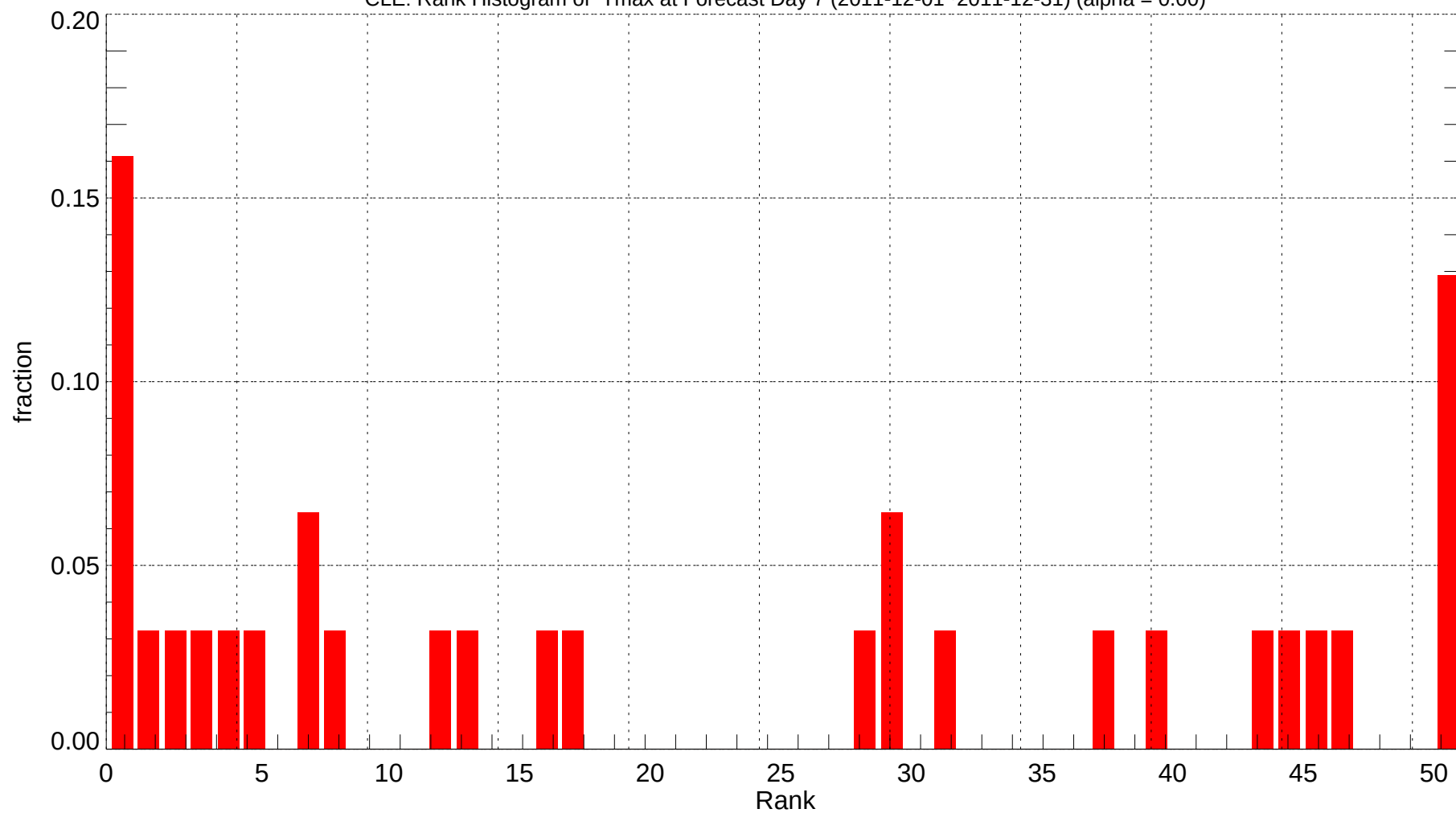
CLE: Rank Histogram of Tmax at Forecast Day 7 (2011-12-01~2011-12-31) (alpha = 0.00)
