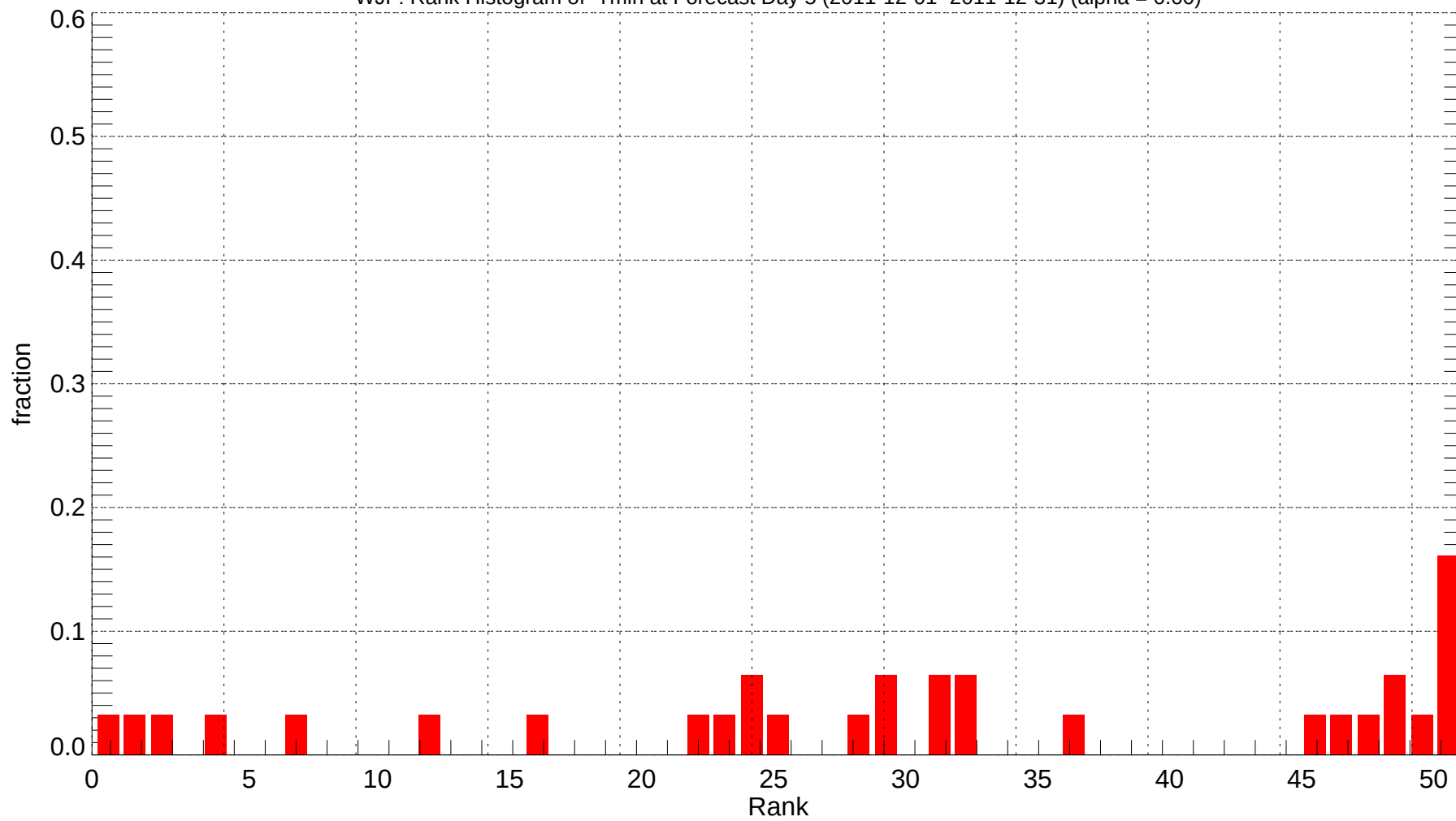
WJF: Rank Histogram of Tmin at Forecast Day 5 (2011-12-01~2011-12-31) (alpha = 0.00)
