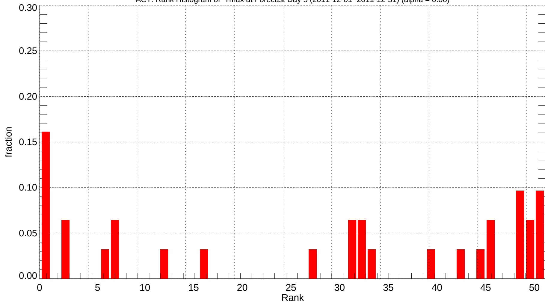
ACT: Rank Histogram of Tmax at Forecast Day 5 (2011-12-01~2011-12-31) (alpha = 0.00)
