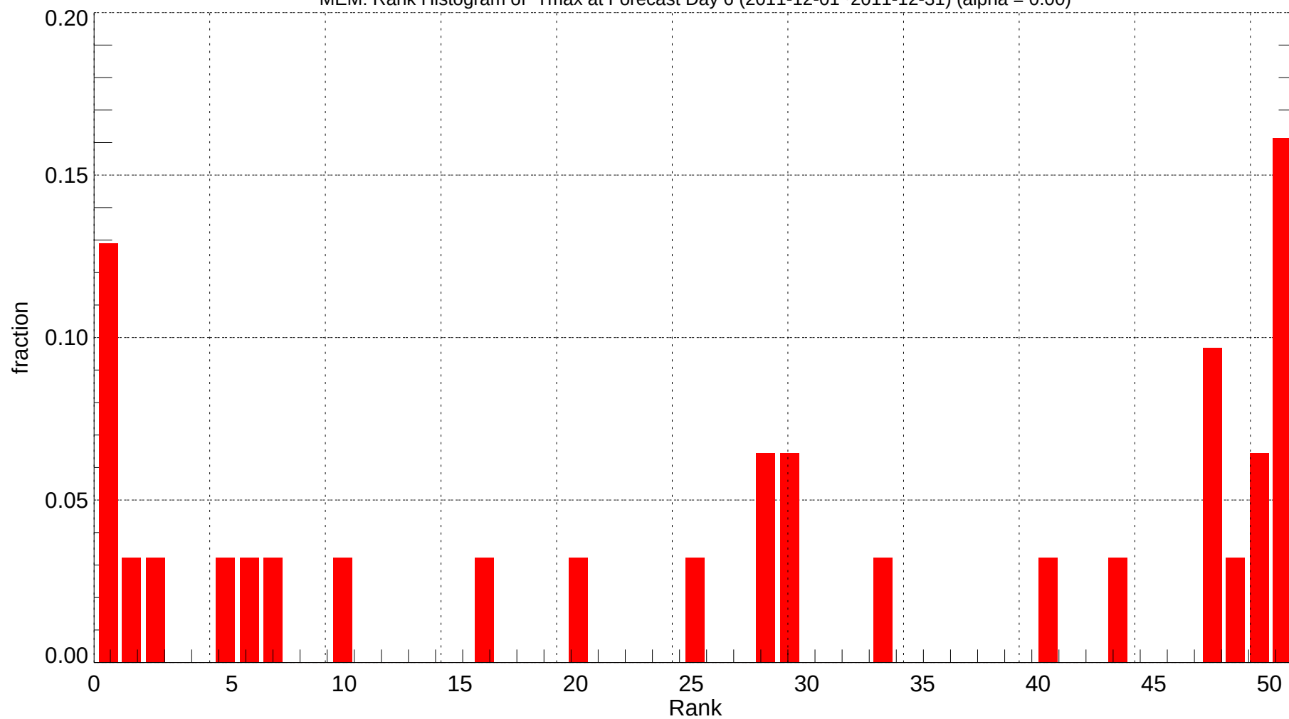
MEM: Rank Histogram of Tmax at Forecast Day 6 (2011-12-01~2011-12-31) (alpha = 0.00)
