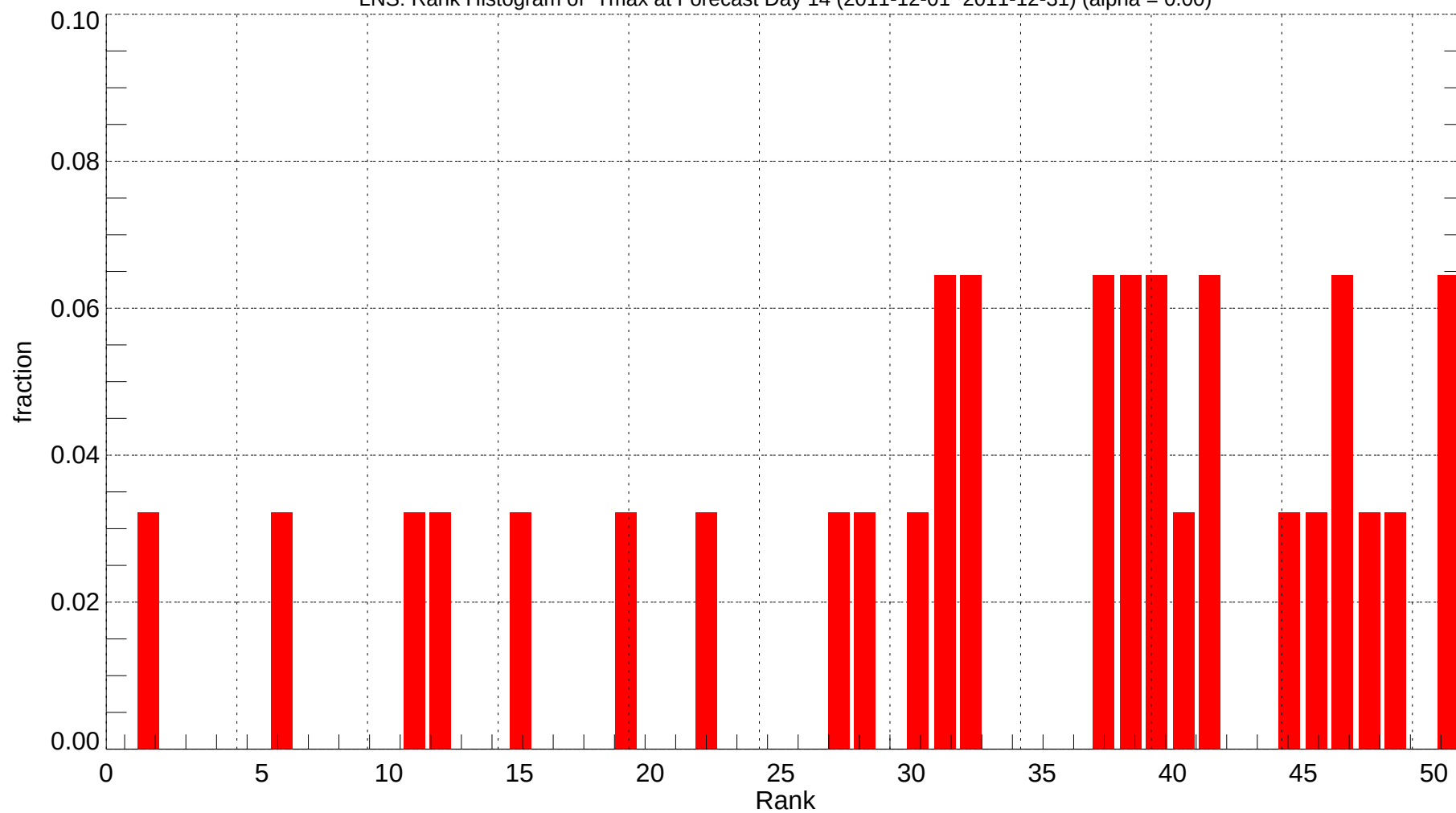
LNS: Rank Histogram of Tmax at Forecast Day 14 (2011-12-01~2011-12-31) (alpha = 0.00)
