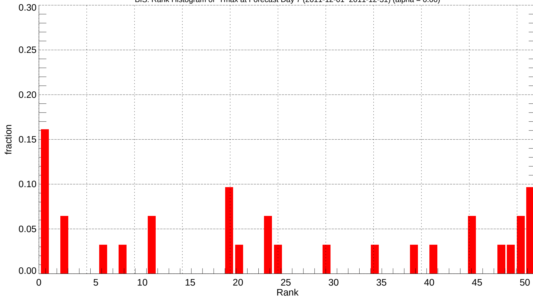
BIS: Rank Histogram of Tmax at Forecast Day 7 (2011-12-01~2011-12-31) (alpha = 0.00)
