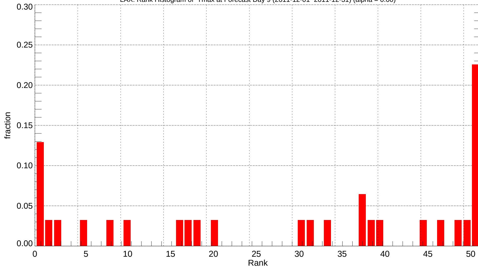
LAX: Rank Histogram of Tmax at Forecast Day 9 (2011-12-01~2011-12-31) (alpha = 0.00)
