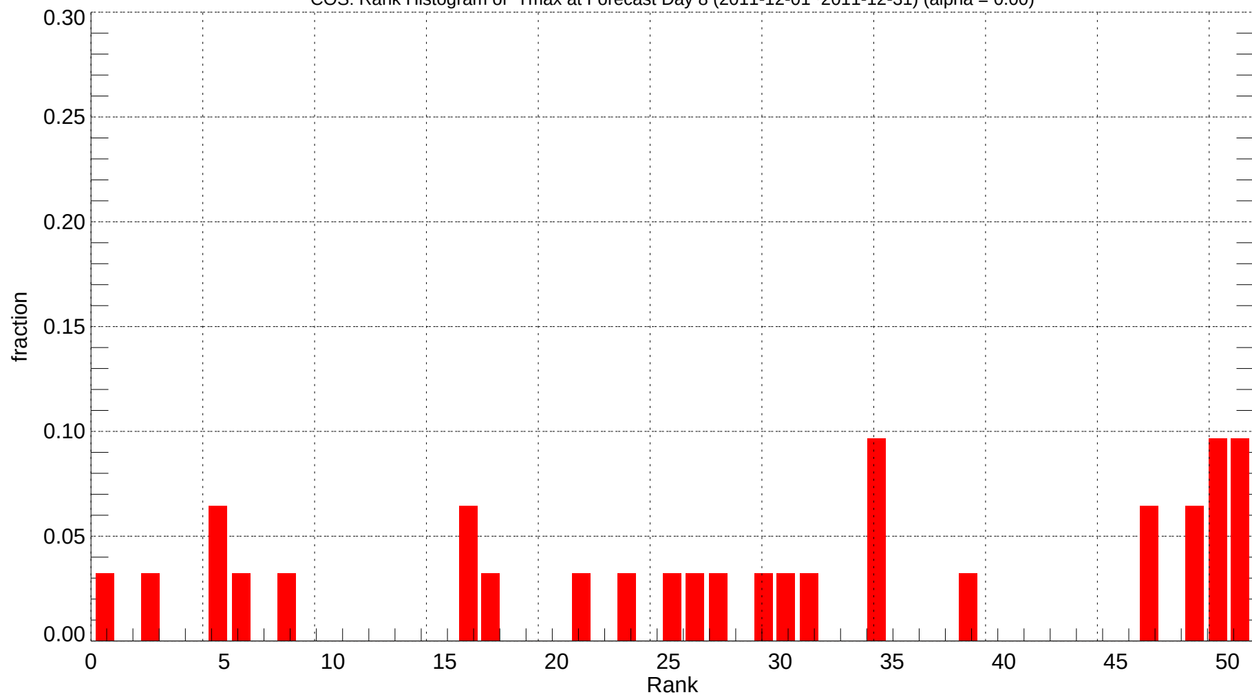
COS: Rank Histogram of Tmax at Forecast Day 8 (2011-12-01~2011-12-31) (alpha = 0.00)
