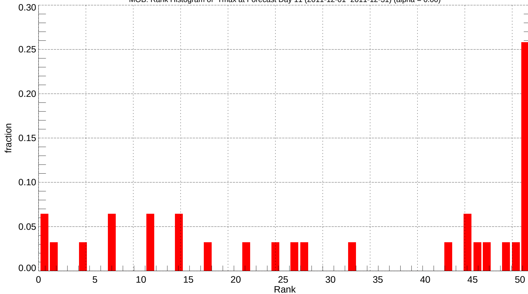
MOB: Rank Histogram of Tmax at Forecast Day 11 (2011-12-01~2011-12-31) (alpha = 0.00)
