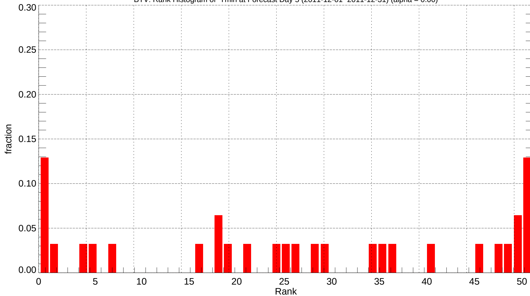
BTV: Rank Histogram of Tmin at Forecast Day 5 (2011-12-01~2011-12-31) (alpha = 0.00)
