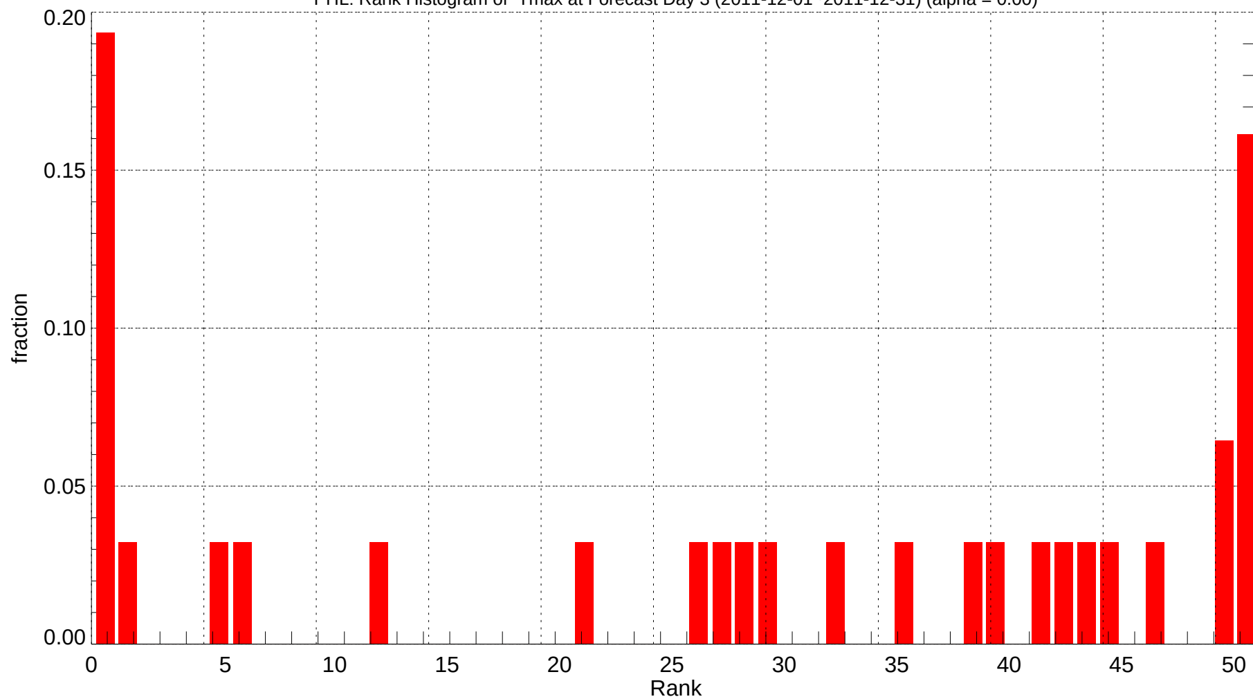
PHL: Rank Histogram of Tmax at Forecast Day 3 (2011-12-01~2011-12-31) (alpha = 0.00)
