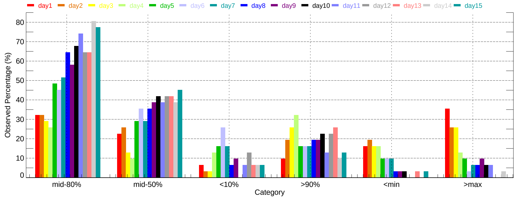
Observed Percentage of Ensembles - YNG: Max Temperature (2011-12-01~2011-12-31)
