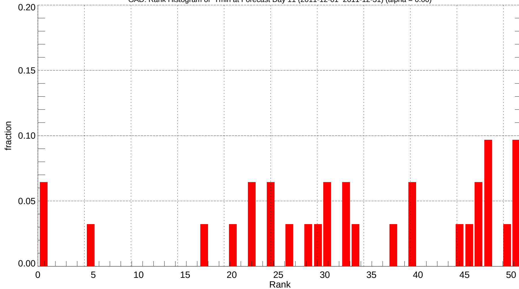
GAD: Rank Histogram of Tmin at Forecast Day 11 (2011-12-01~2011-12-31) (alpha = 0.00)
