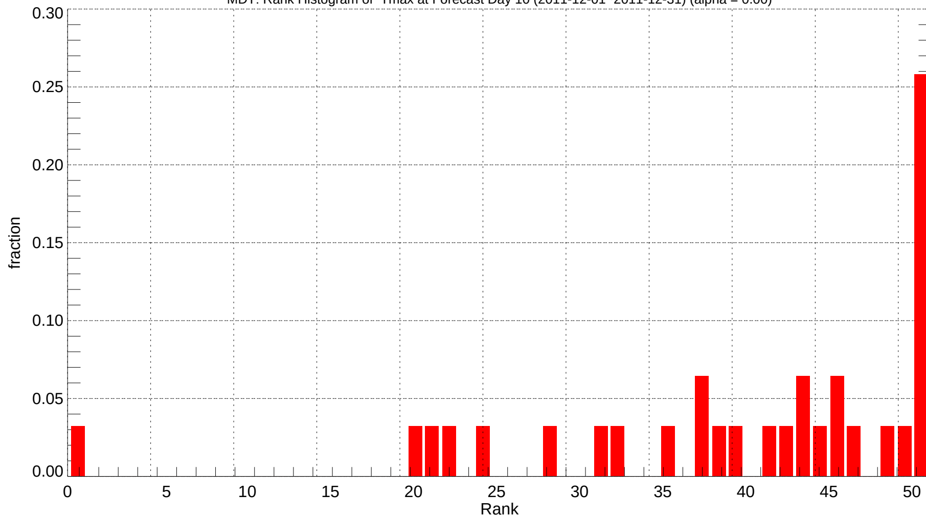
MDT: Rank Histogram of Tmax at Forecast Day 10 (2011-12-01~2011-12-31) (alpha = 0.00)
