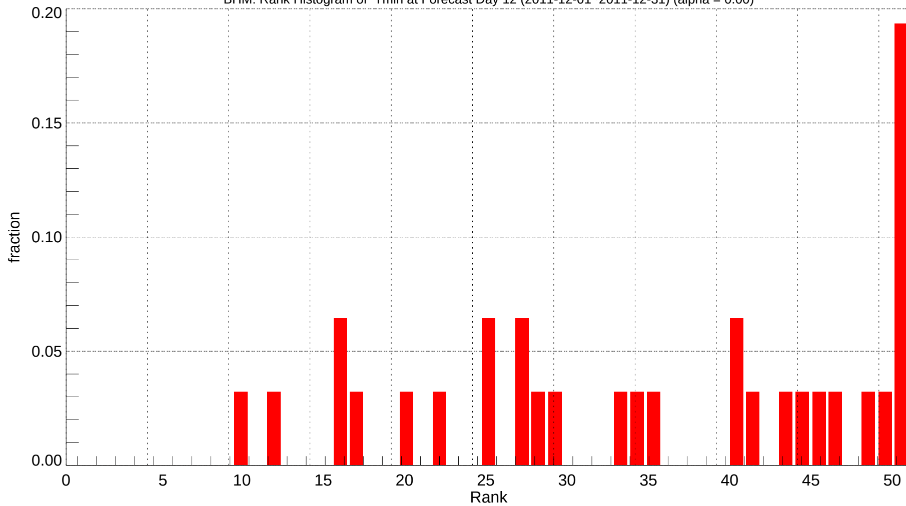
BHM: Rank Histogram of Tmin at Forecast Day 12 (2011-12-01~2011-12-31) (alpha = 0.00)
