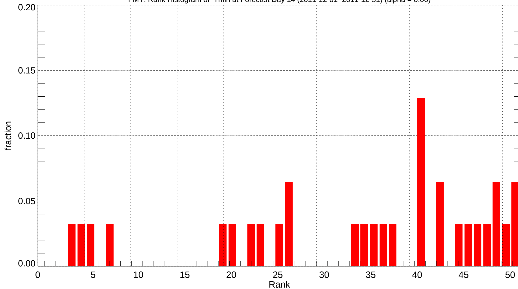
FMY: Rank Histogram of Tmin at Forecast Day 14 (2011-12-01~2011-12-31) (alpha = 0.00)
