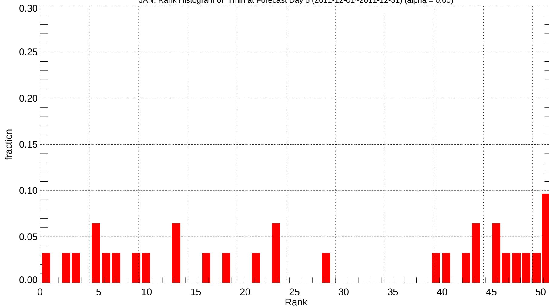
JAN: Rank Histogram of Tmin at Forecast Day 6 (2011-12-01~2011-12-31) (alpha = 0.00)
