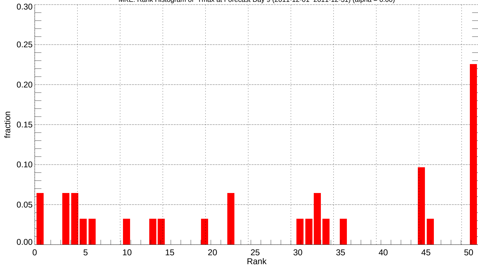
MKE: Rank Histogram of Tmax at Forecast Day 9 (2011-12-01~2011-12-31) (alpha = 0.00)
