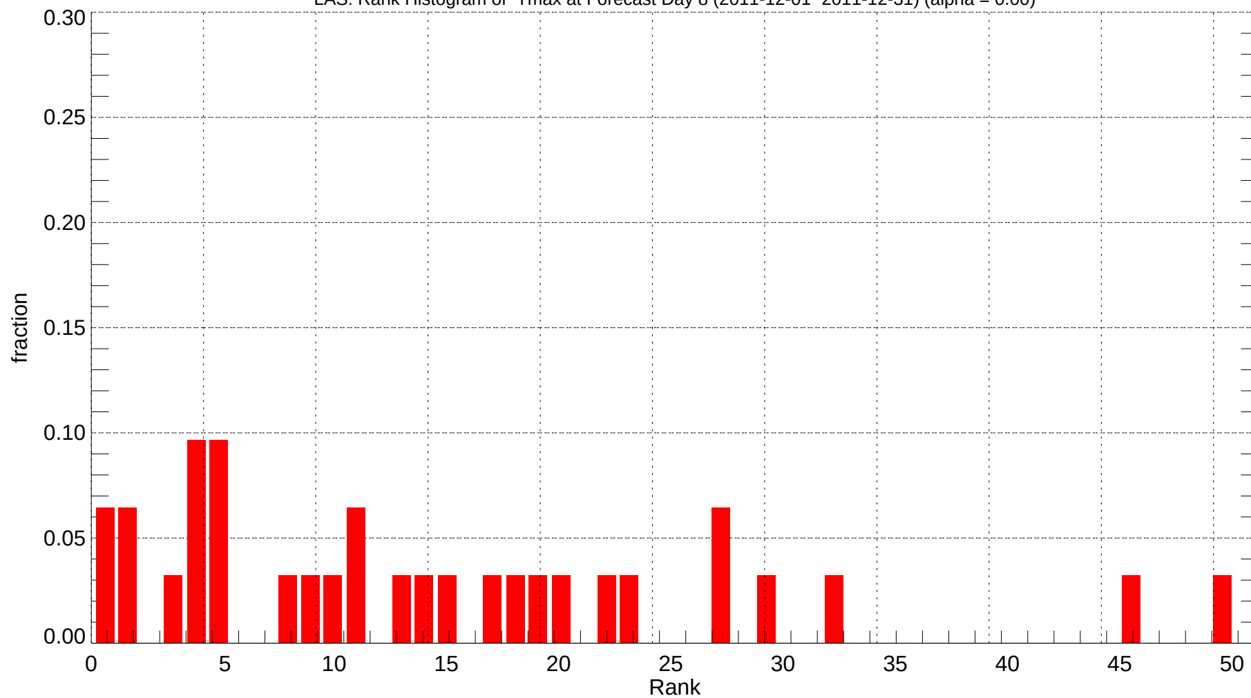
LAS: Rank Histogram of Tmax at Forecast Day 8 (2011-12-01~2011-12-31) (alpha = 0.00)
