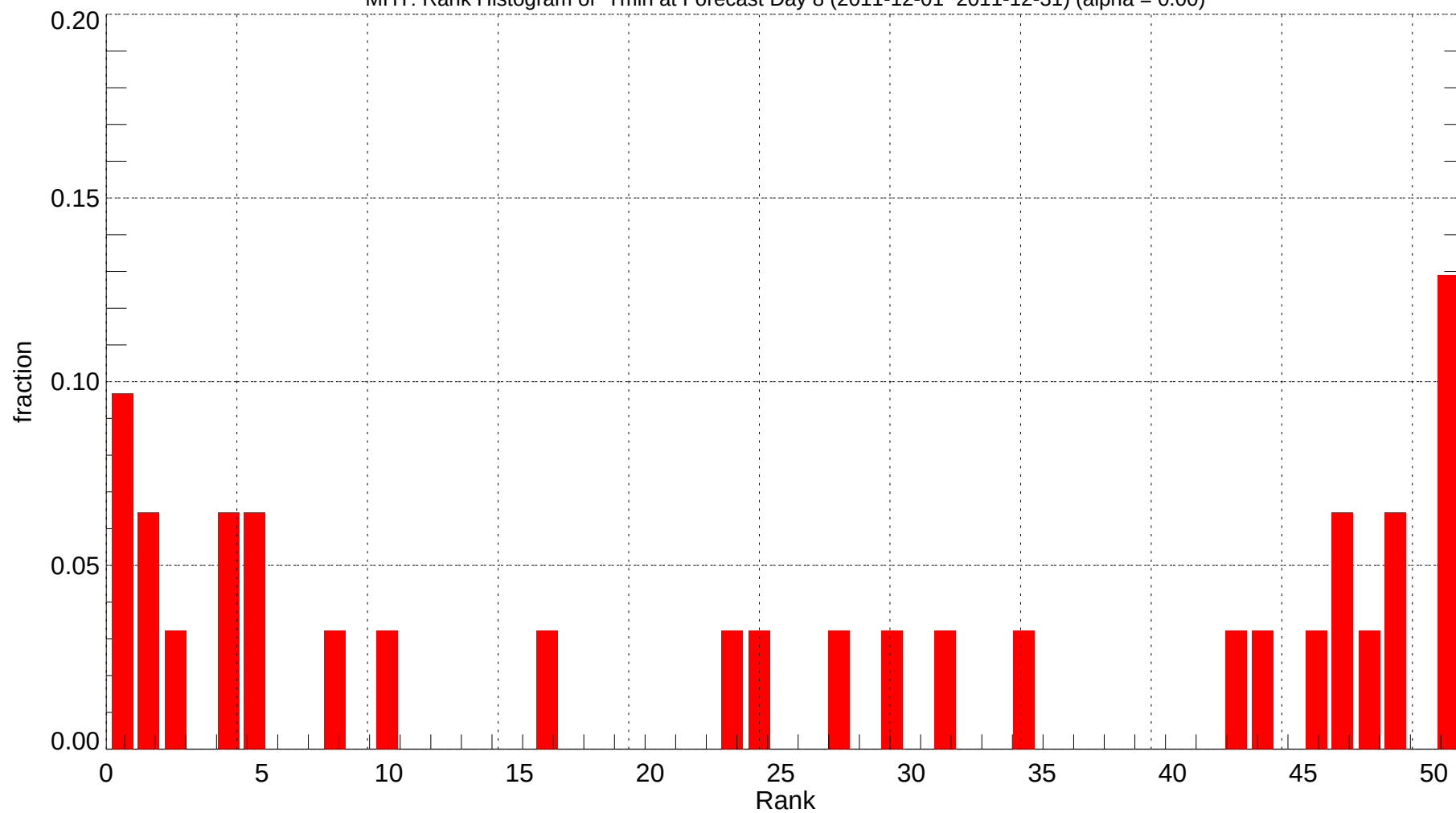
MHT: Rank Histogram of Tmin at Forecast Day 8 (2011-12-01~2011-12-31) (alpha = 0.00)
