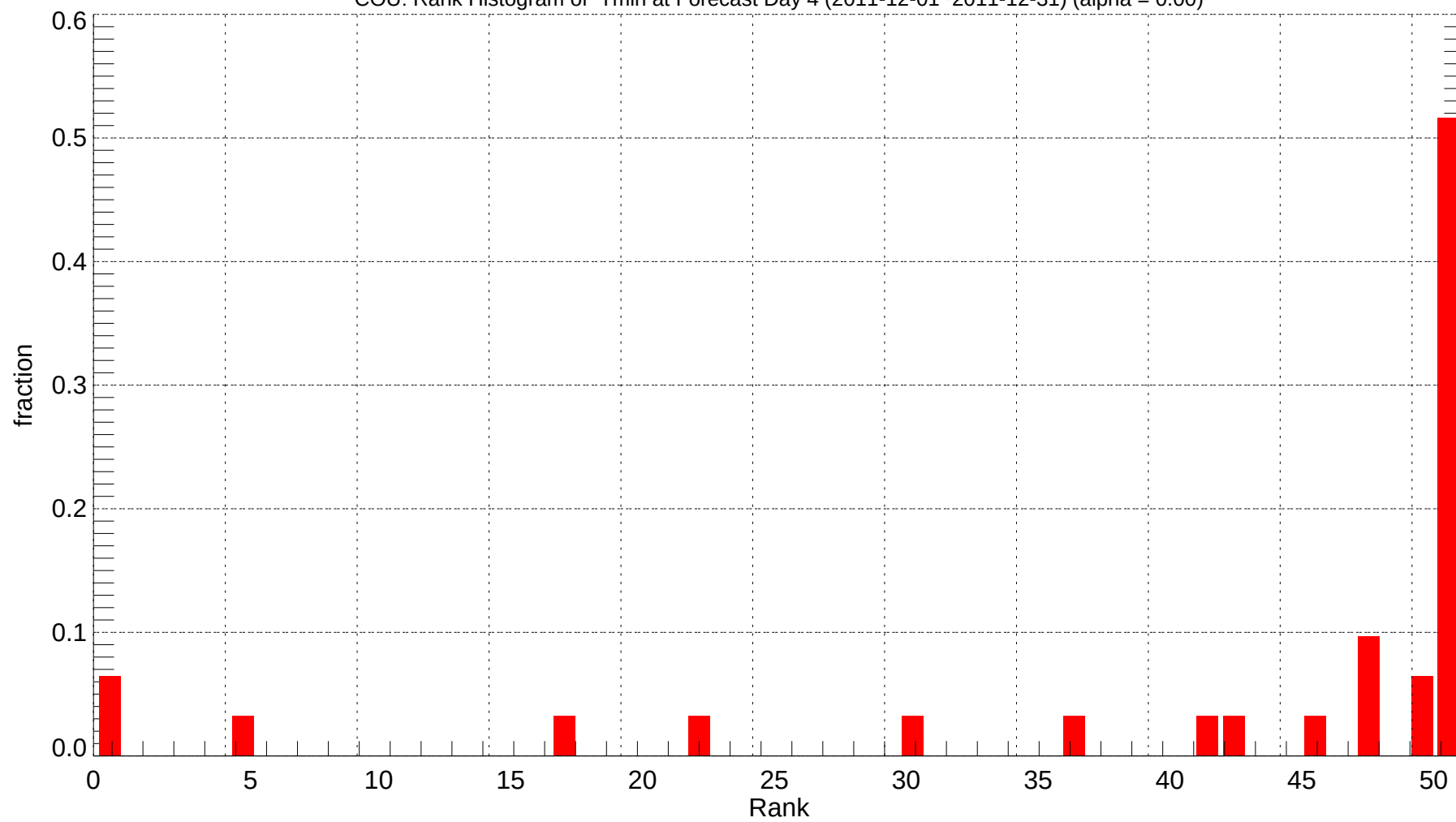
COU: Rank Histogram of Tmin at Forecast Day 4 (2011-12-01~2011-12-31) (alpha = 0.00)
