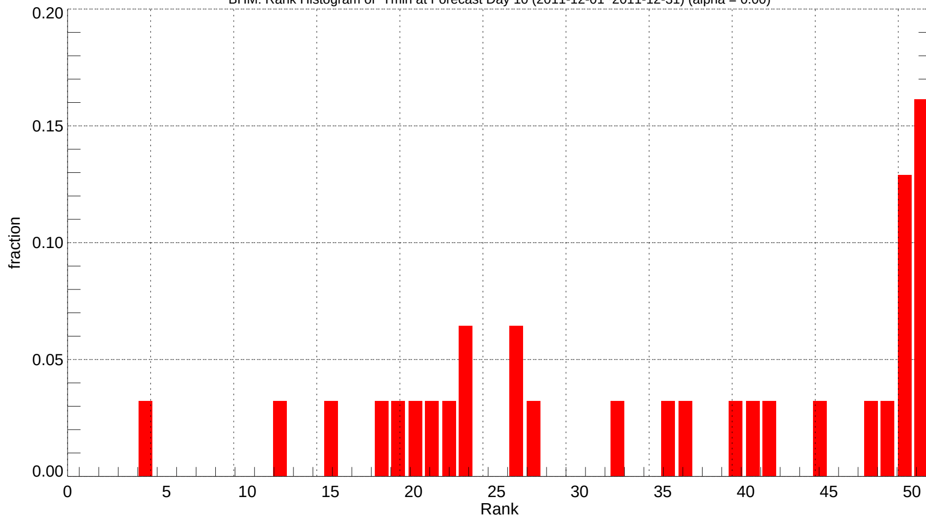
BHM: Rank Histogram of Tmin at Forecast Day 10 (2011-12-01~2011-12-31) (alpha = 0.00)
