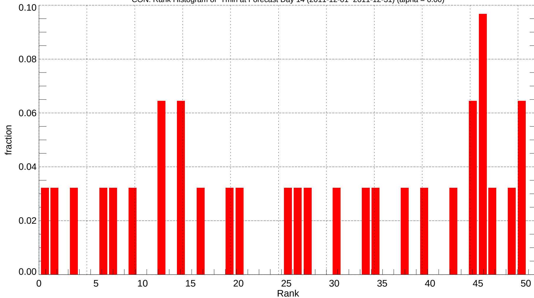
CON: Rank Histogram of Tmin at Forecast Day 14 (2011-12-01~2011-12-31) (alpha = 0.00)
