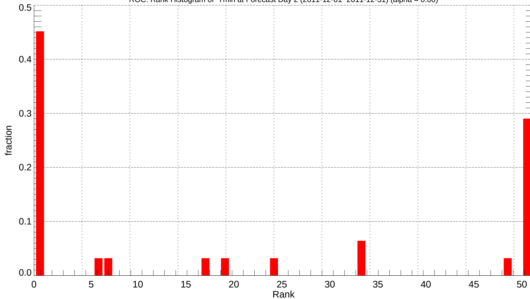
ROC: Rank Histogram of Tmin at Forecast Day 2 (2011-12-01~2011-12-31) (alpha = 0.00)
