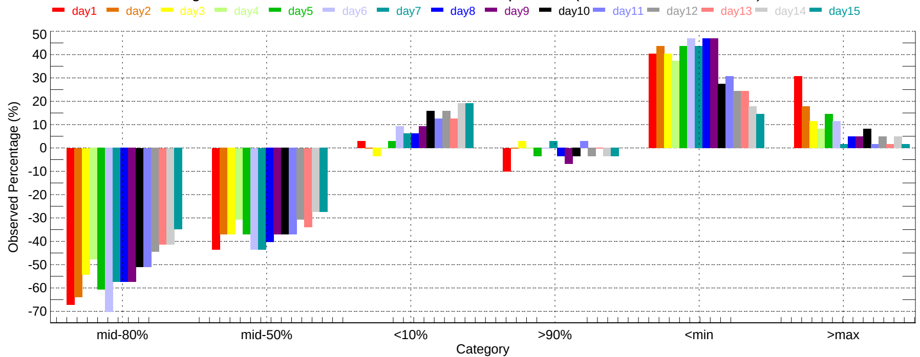
Observed Percentage Deviation of Ensembles - OAK: Min Temperature (2011-12-01~2011-12-31)
