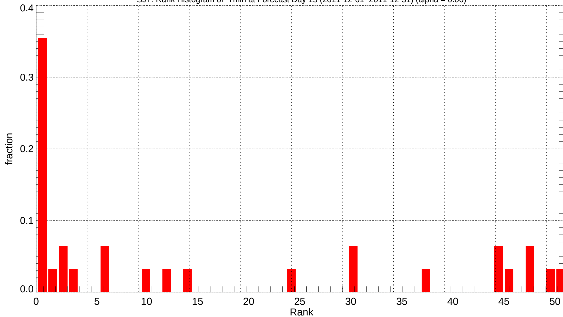
SJT: Rank Histogram of Tmin at Forecast Day 15 (2011-12-01~2011-12-31) (alpha = 0.00)
