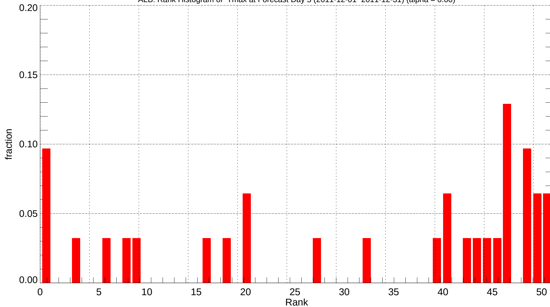
ALB: Rank Histogram of Tmax at Forecast Day 5 (2011-12-01~2011-12-31) (alpha = 0.00)
