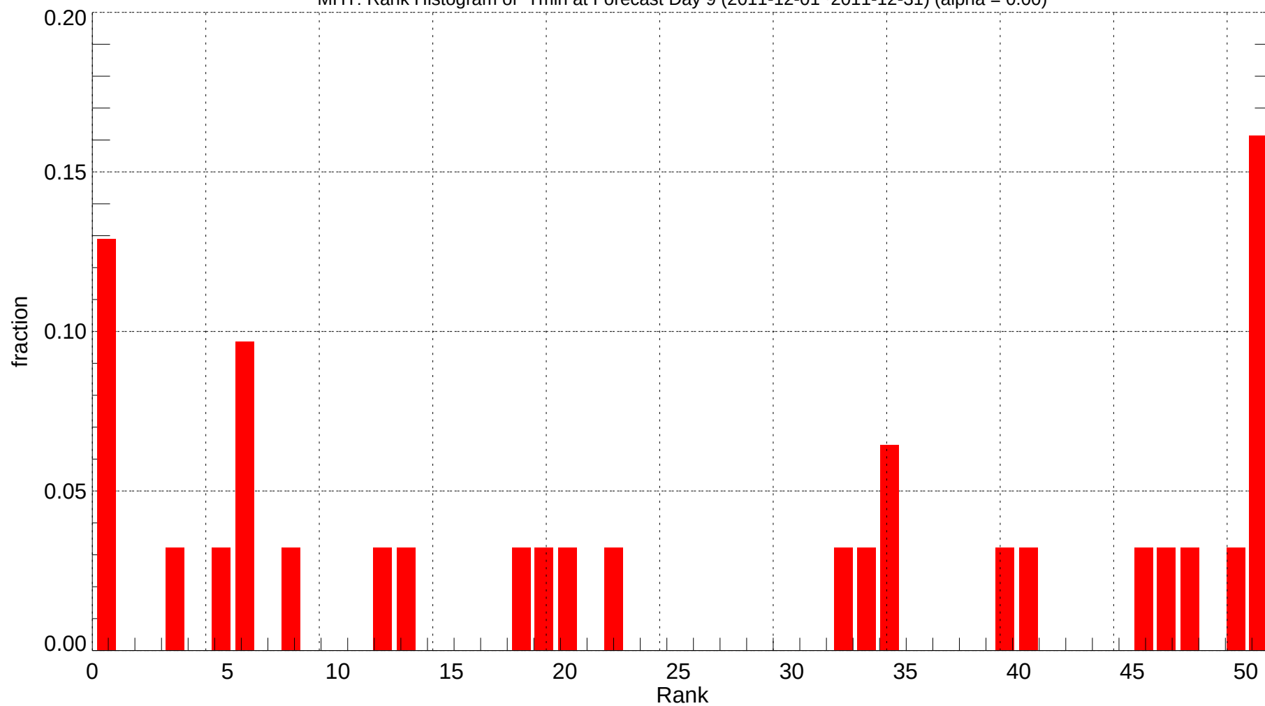
MHT: Rank Histogram of Tmin at Forecast Day 9 (2011-12-01~2011-12-31) (alpha = 0.00)
