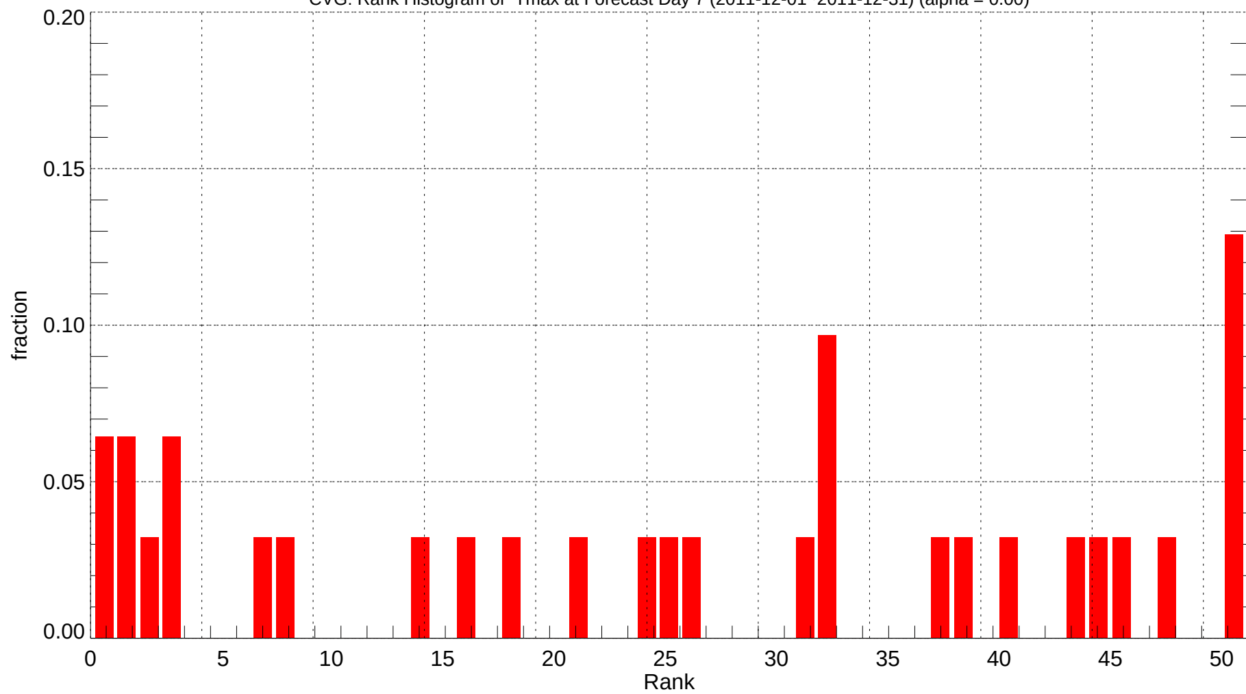
CVG: Rank Histogram of Tmax at Forecast Day 7 (2011-12-01~2011-12-31) (alpha = 0.00)
