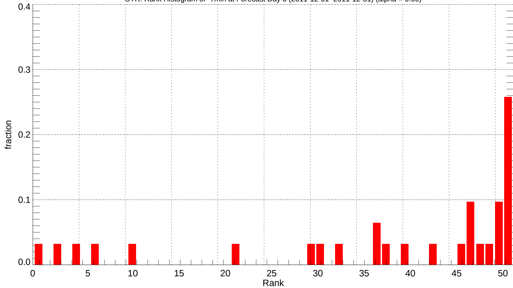
SYR: Rank Histogram of Tmin at Forecast Day 3 (2011-12-01~2011-12-31) (alpha = 0.00)
