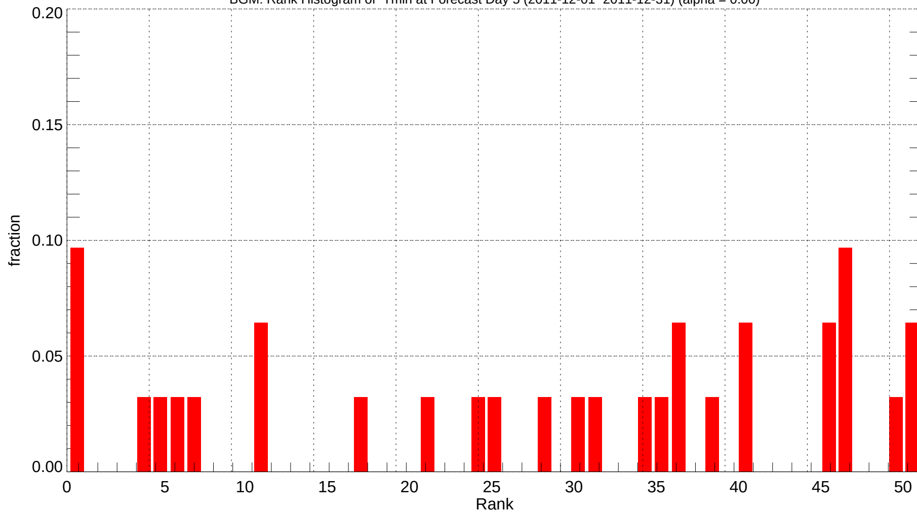
BGM: Rank Histogram of Tmin at Forecast Day 5 (2011-12-01~2011-12-31) (alpha = 0.00)
