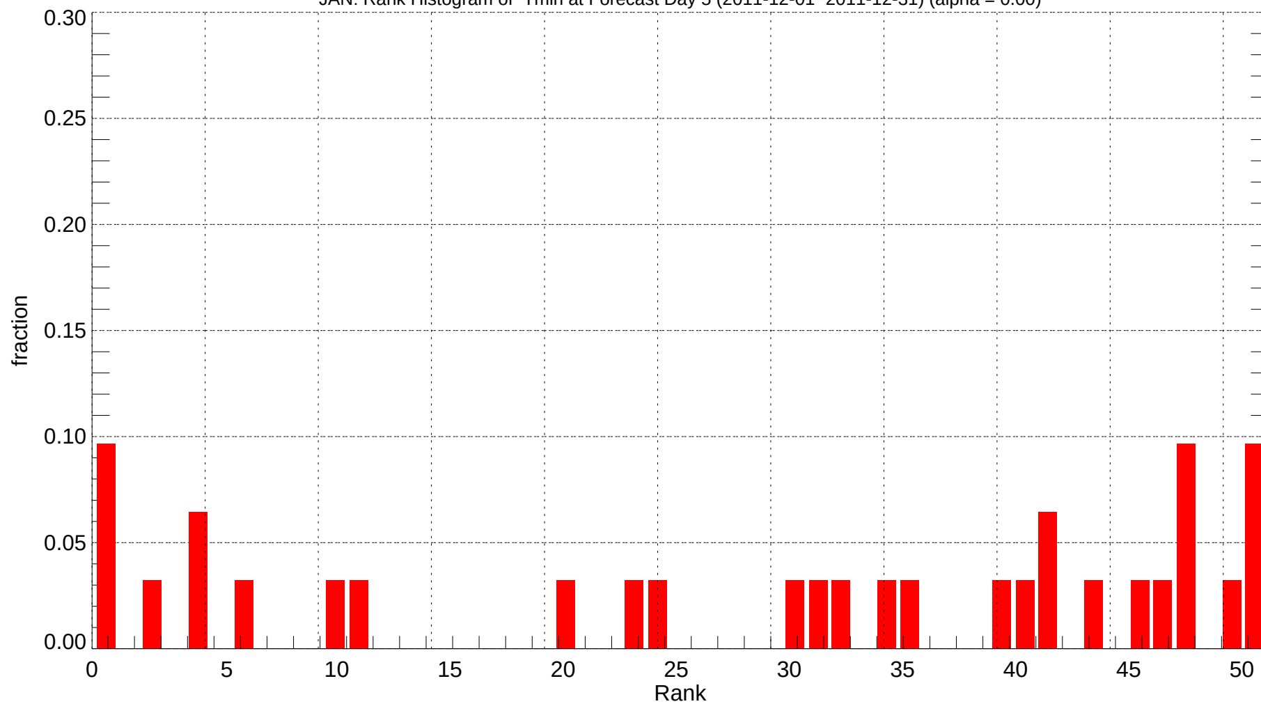
JAN: Rank Histogram of Tmin at Forecast Day 5 (2011-12-01~2011-12-31) (alpha = 0.00)
