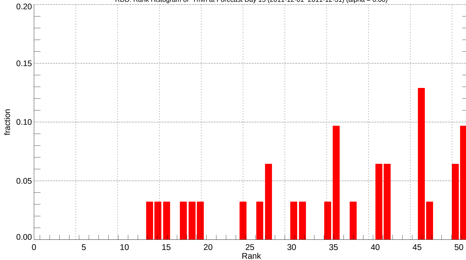
RDD: Rank Histogram of Tmin at Forecast Day 15 (2011-12-01~2011-12-31) (alpha = 0.00)
