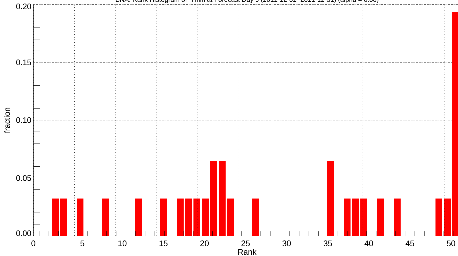
BNA: Rank Histogram of Tmin at Forecast Day 9 (2011-12-01~2011-12-31) (alpha = 0.00)
