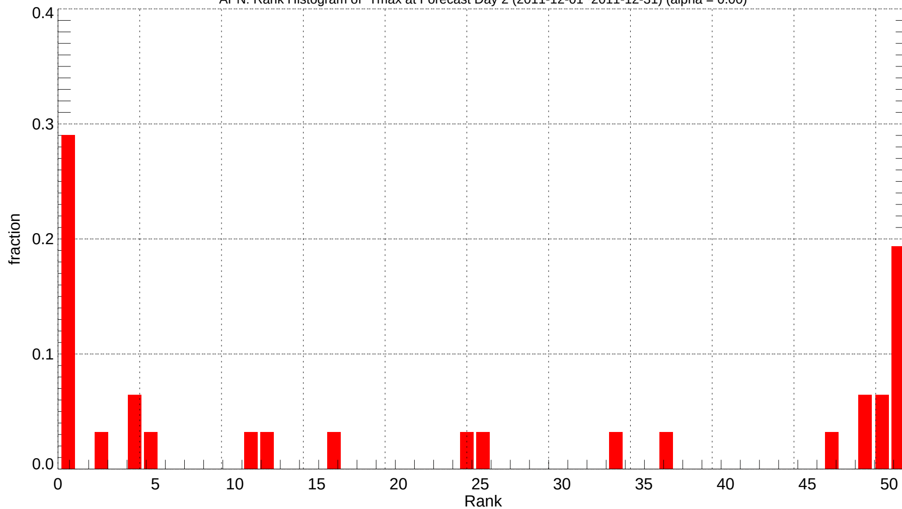
APN: Rank Histogram of Tmax at Forecast Day 2 (2011-12-01~2011-12-31) (alpha = 0.00)
