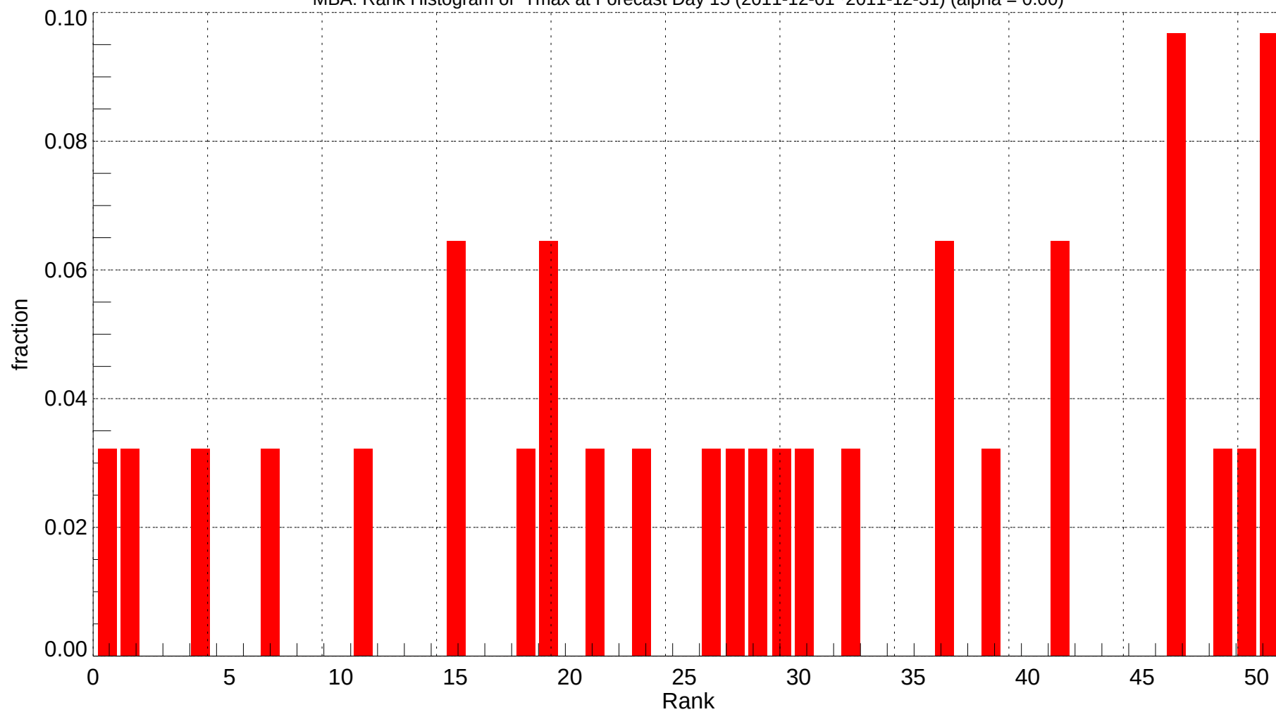
MBA: Rank Histogram of Tmax at Forecast Day 15 (2011-12-01~2011-12-31) (alpha = 0.00)
