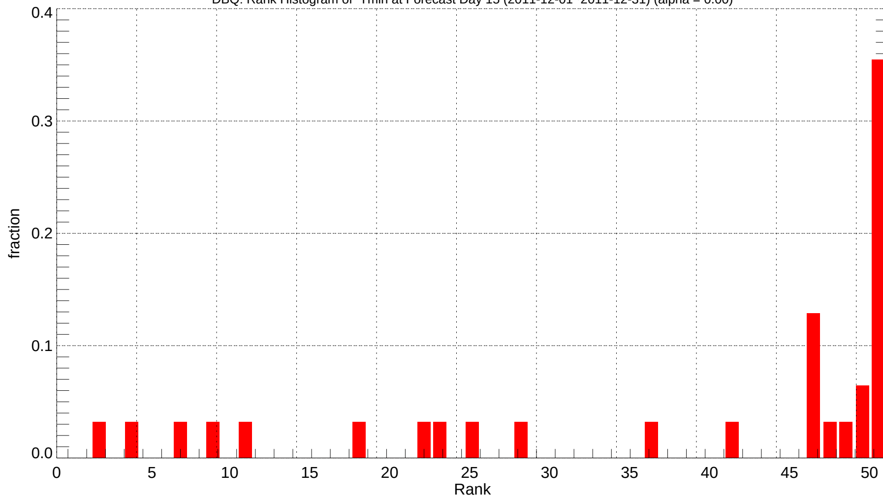
DBQ: Rank Histogram of Tmin at Forecast Day 15 (2011-12-01~2011-12-31) (alpha = 0.00)
