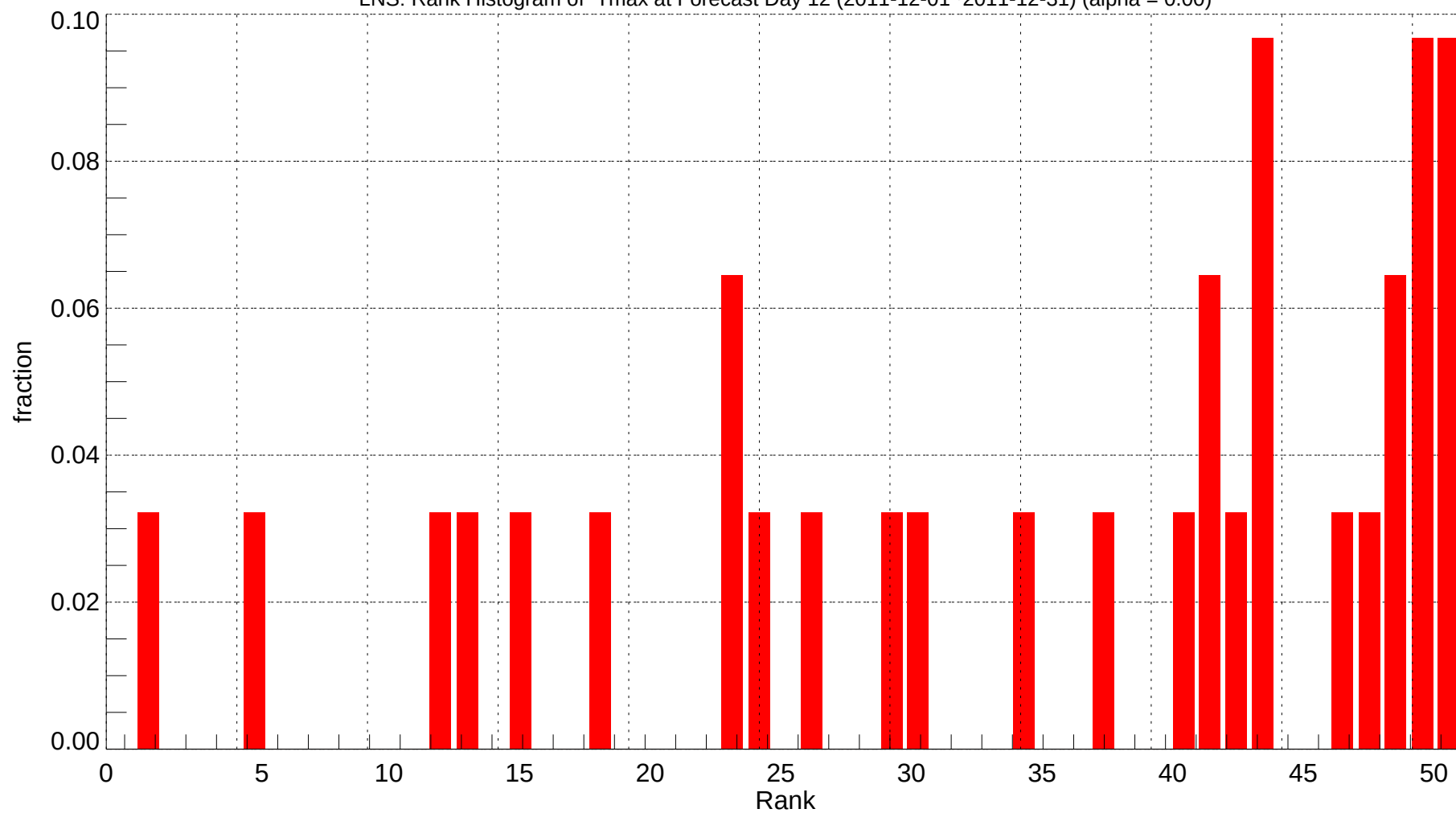
LNS: Rank Histogram of Tmax at Forecast Day 12 (2011-12-01~2011-12-31) (alpha = 0.00)
