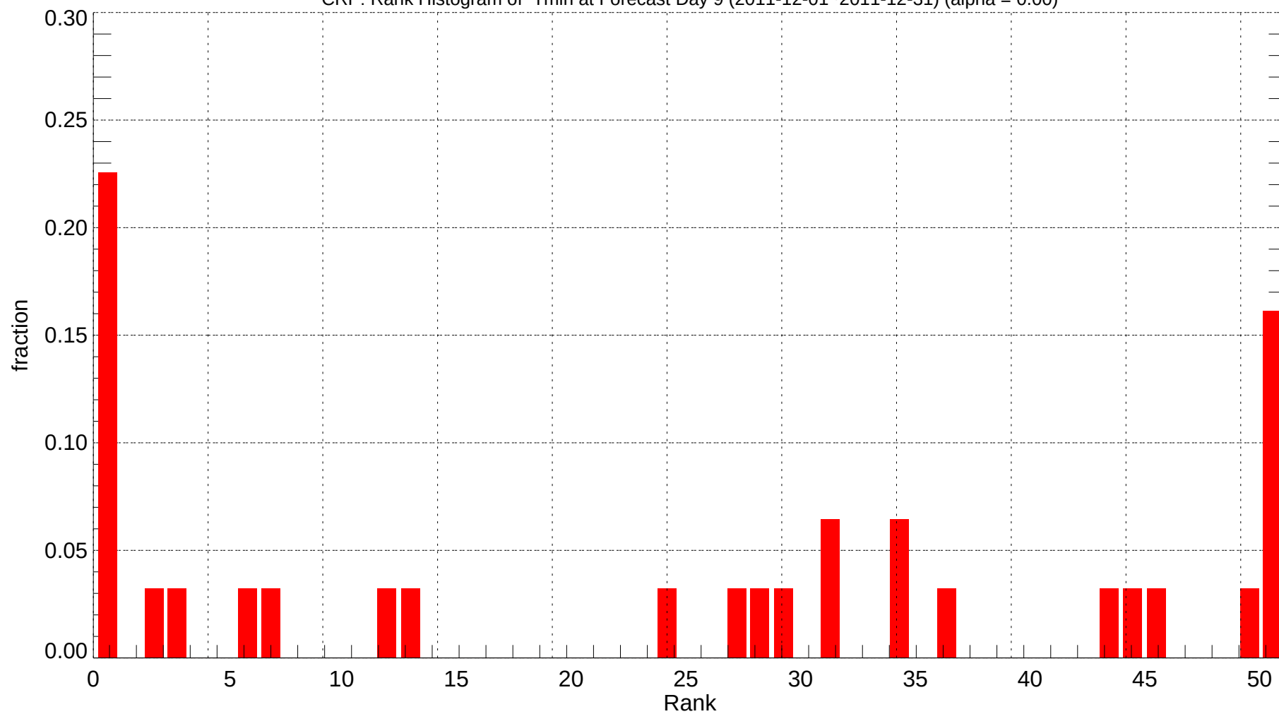
CRP: Rank Histogram of Tmin at Forecast Day 9 (2011-12-01~2011-12-31) (alpha = 0.00)
