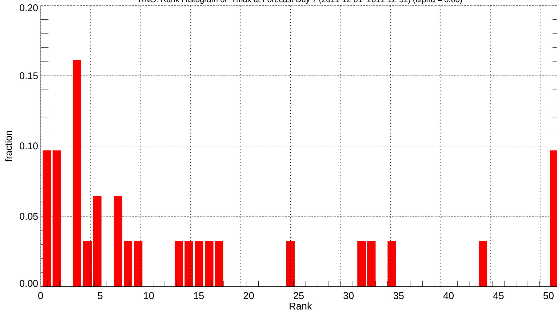
RNO: Rank Histogram of Tmax at Forecast Day 7 (2011-12-01~2011-12-31) (alpha = 0.00)
