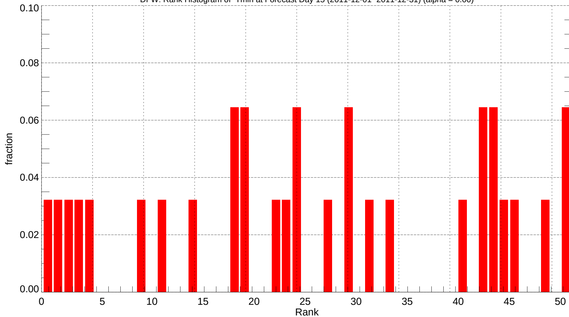
DFW: Rank Histogram of Tmin at Forecast Day 15 (2011-12-01~2011-12-31) (alpha = 0.00)
