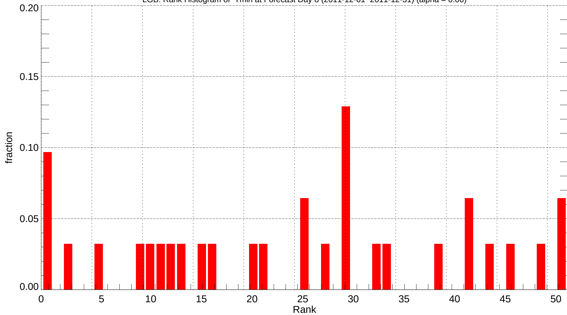
LGB: Rank Histogram of Tmin at Forecast Day 8 (2011-12-01~2011-12-31) (alpha = 0.00)
