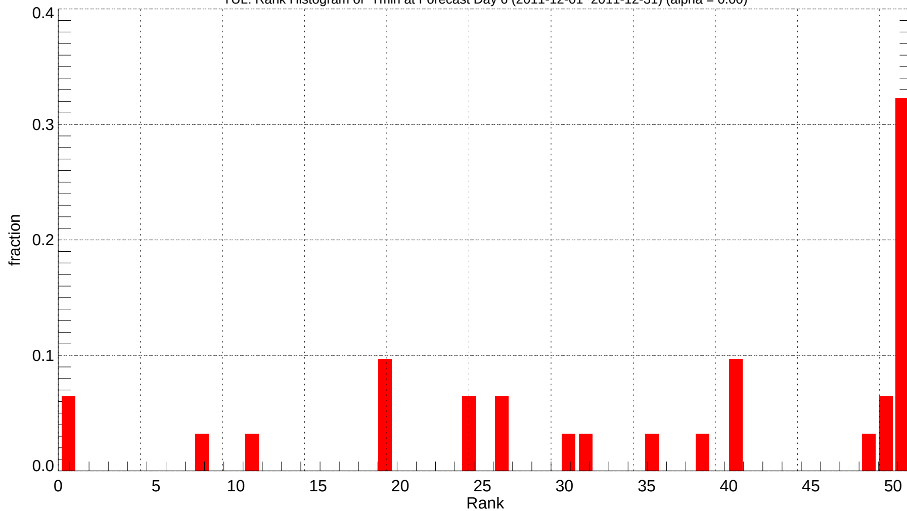
TUL: Rank Histogram of Tmin at Forecast Day 6 (2011-12-01~2011-12-31) (alpha = 0.00)
