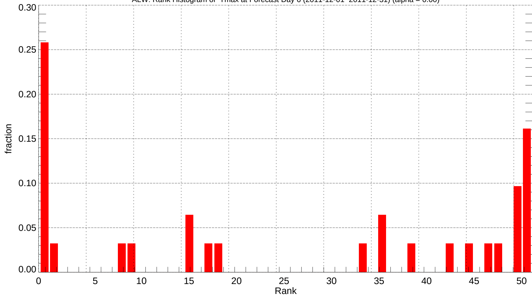
ALW: Rank Histogram of Tmax at Forecast Day 6 (2011-12-01~2011-12-31) (alpha = 0.00)
