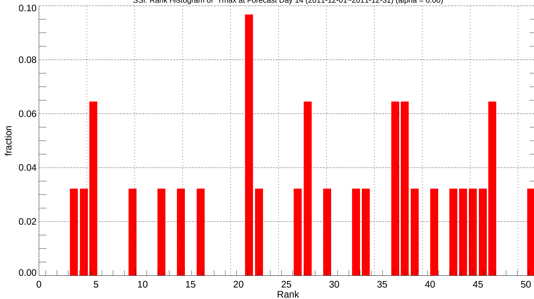
SSI: Rank Histogram of Tmax at Forecast Day 14 (2011-12-01~2011-12-31) (alpha = 0.00)
