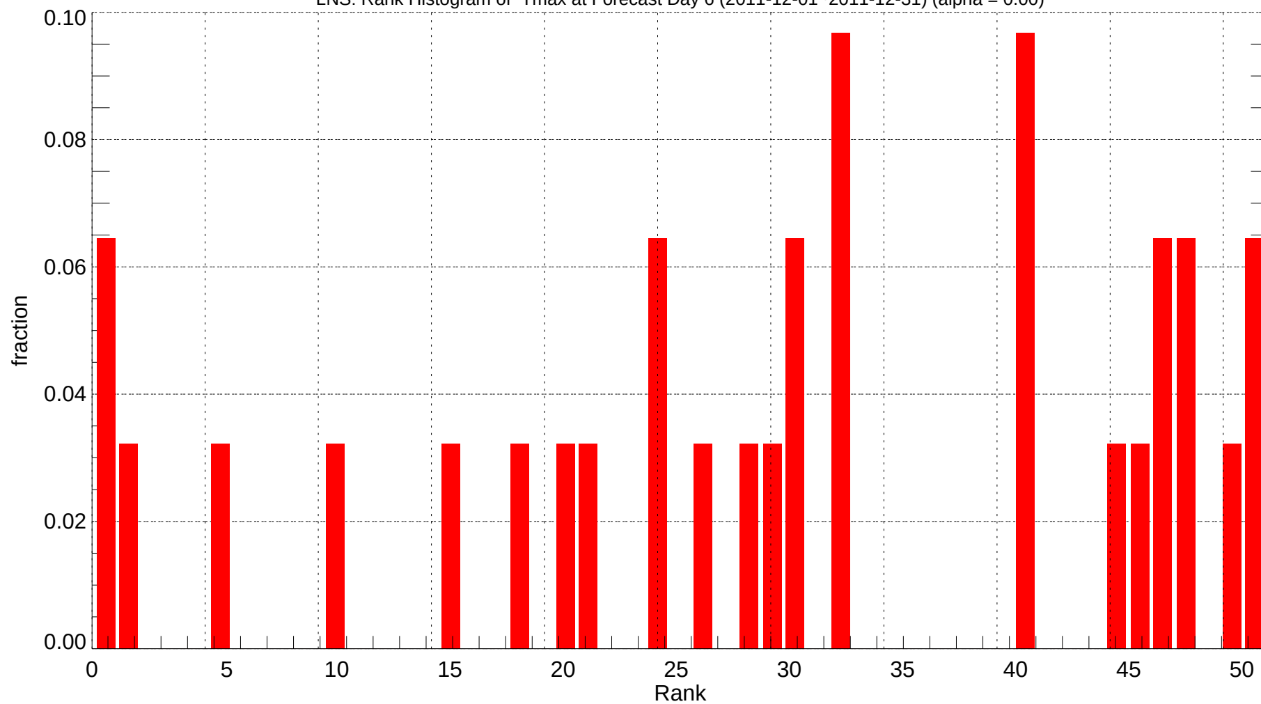
LNS: Rank Histogram of Tmax at Forecast Day 6 (2011-12-01~2011-12-31) (alpha = 0.00)
