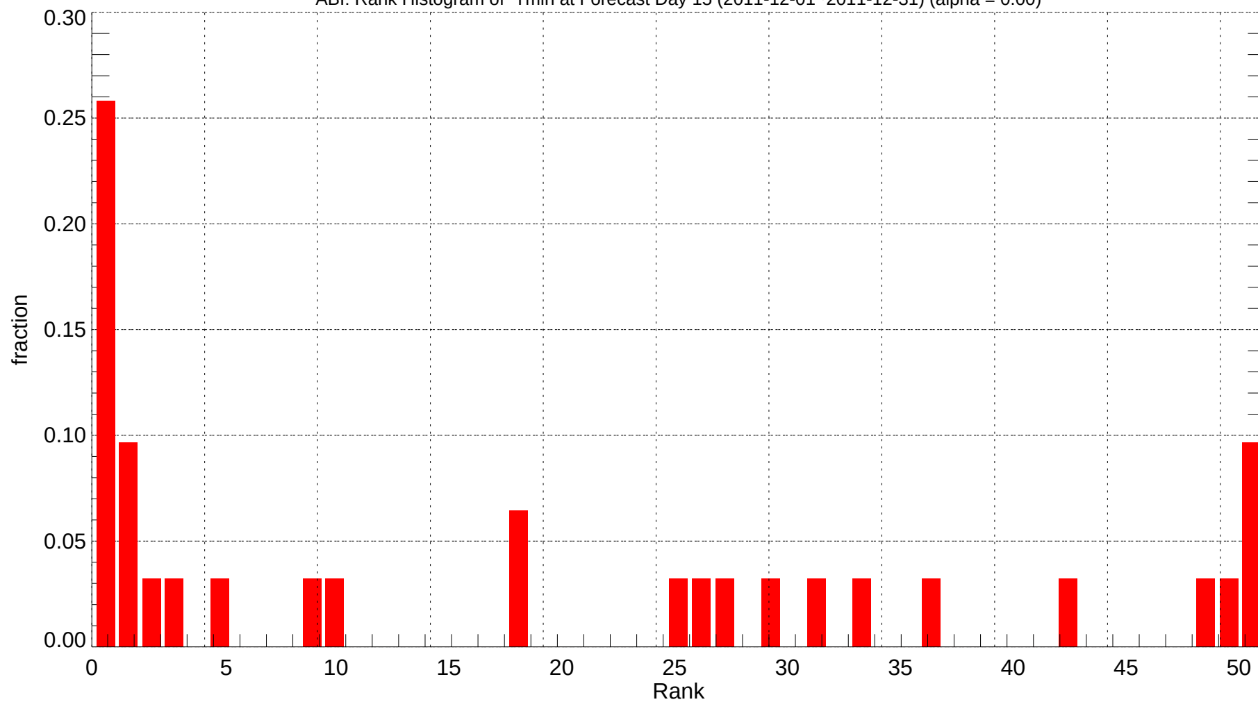
ABI: Rank Histogram of Tmin at Forecast Day 15 (2011-12-01~2011-12-31) (alpha = 0.00)
