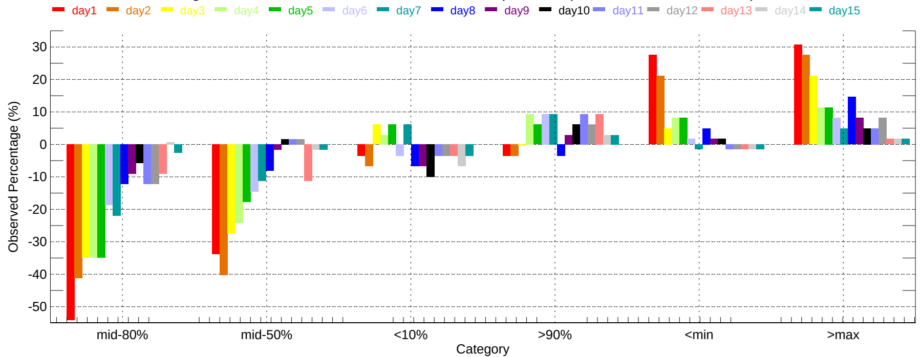
Observed Percentage Deviation of Ensembles - RIC: Min Temperature (2011-12-01~2011-12-31)
