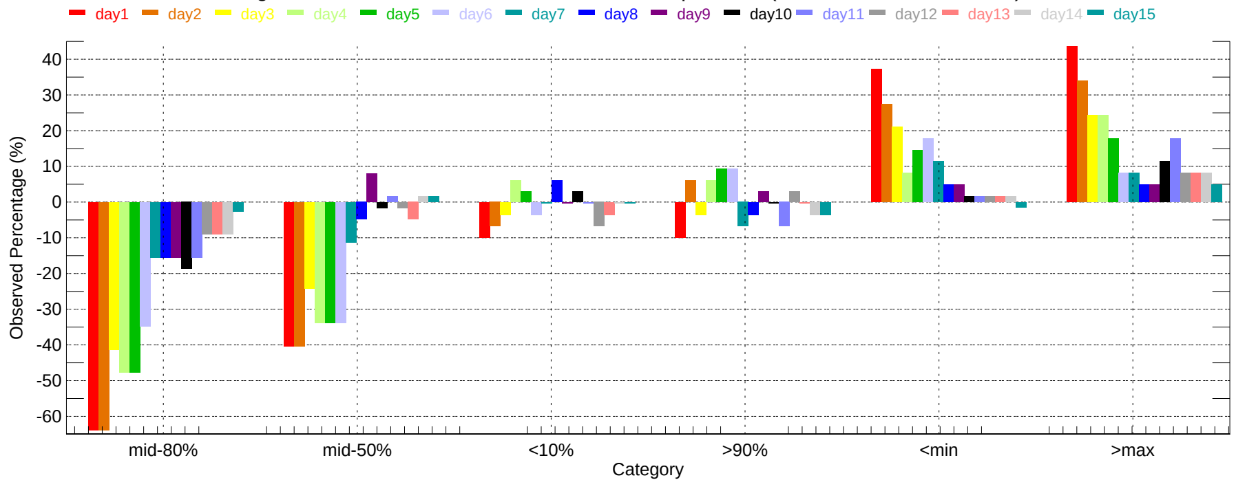
Observed Percentage Deviation of Ensembles - PVD: Min Temperature (2011-12-01~2011-12-31)
