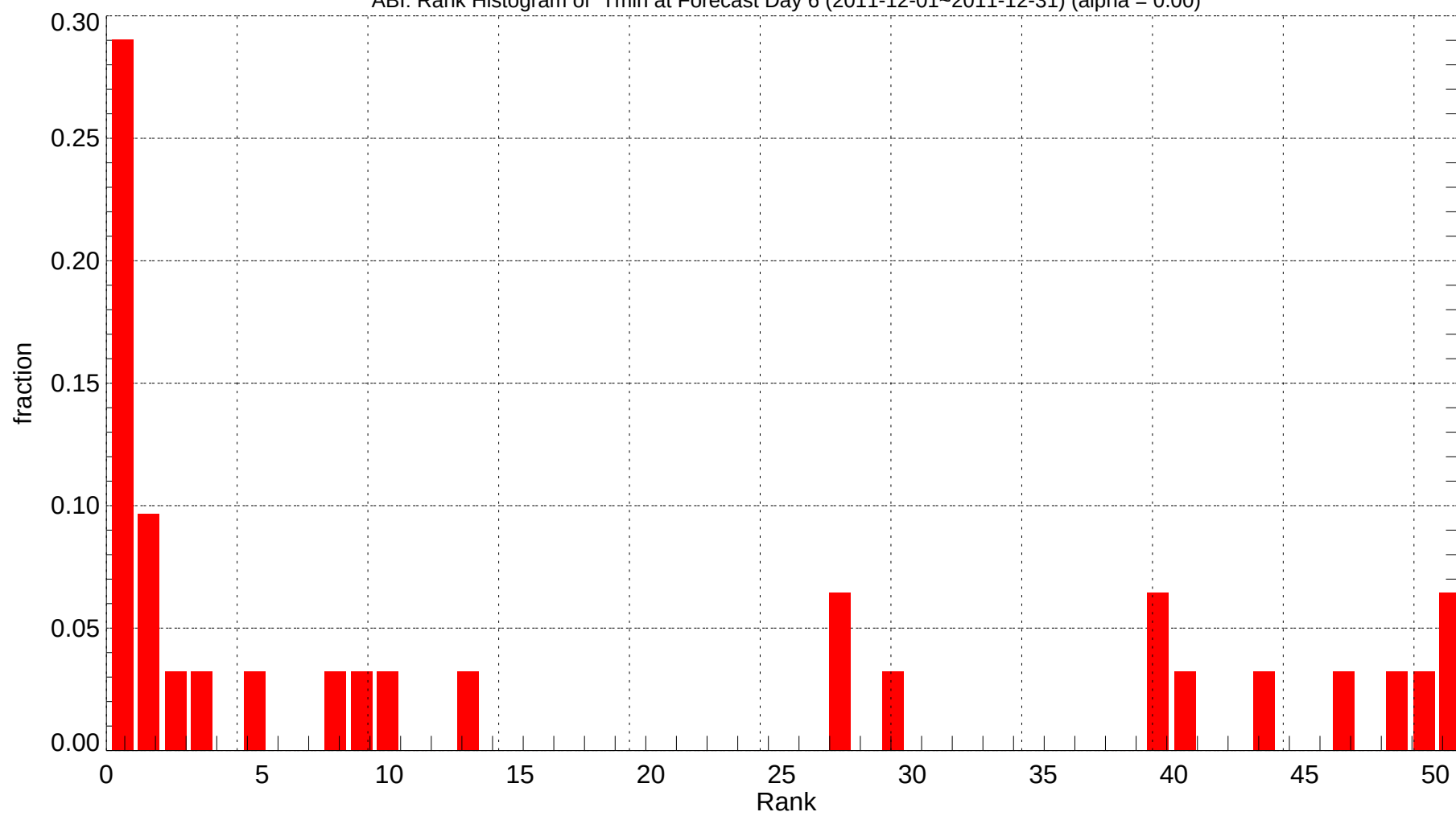
ABI: Rank Histogram of Tmin at Forecast Day 6 (2011-12-01~2011-12-31) (alpha = 0.00)
