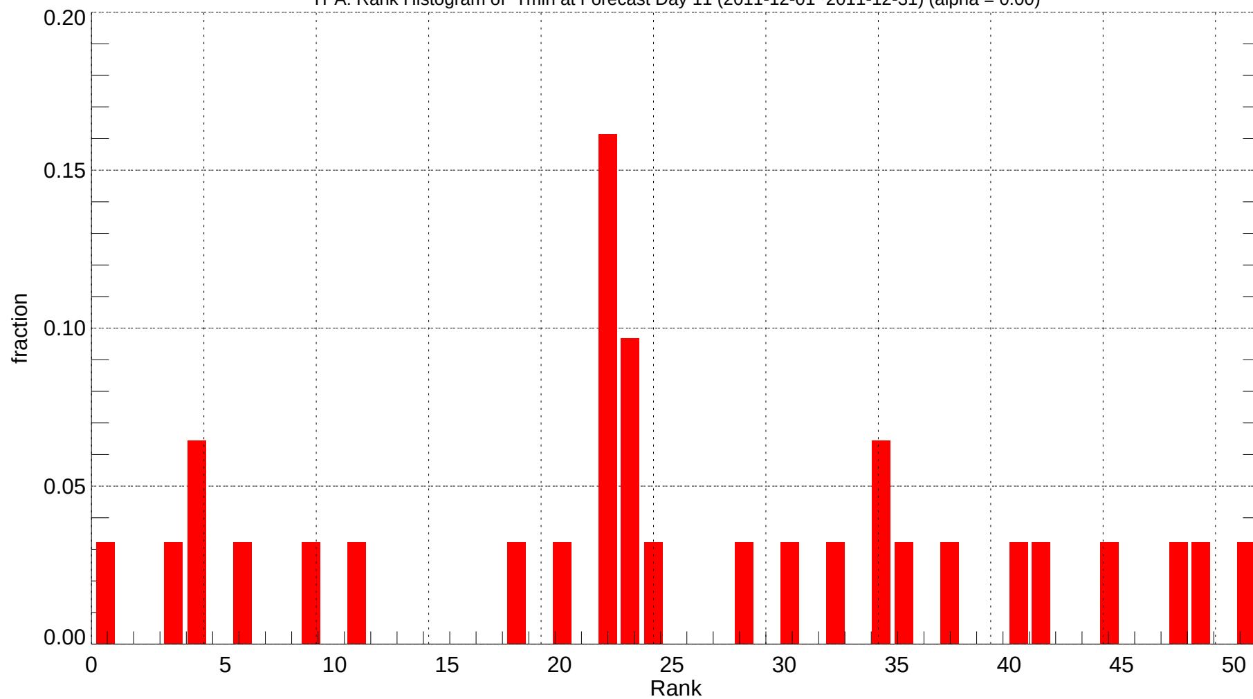
TPA: Rank Histogram of Tmin at Forecast Day 11 (2011-12-01~2011-12-31) (alpha = 0.00)
