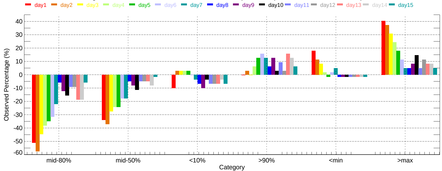
Observed Percentage Deviation of Ensembles - LIT: Max Temperature (2011-12-01~2011-12-31)
