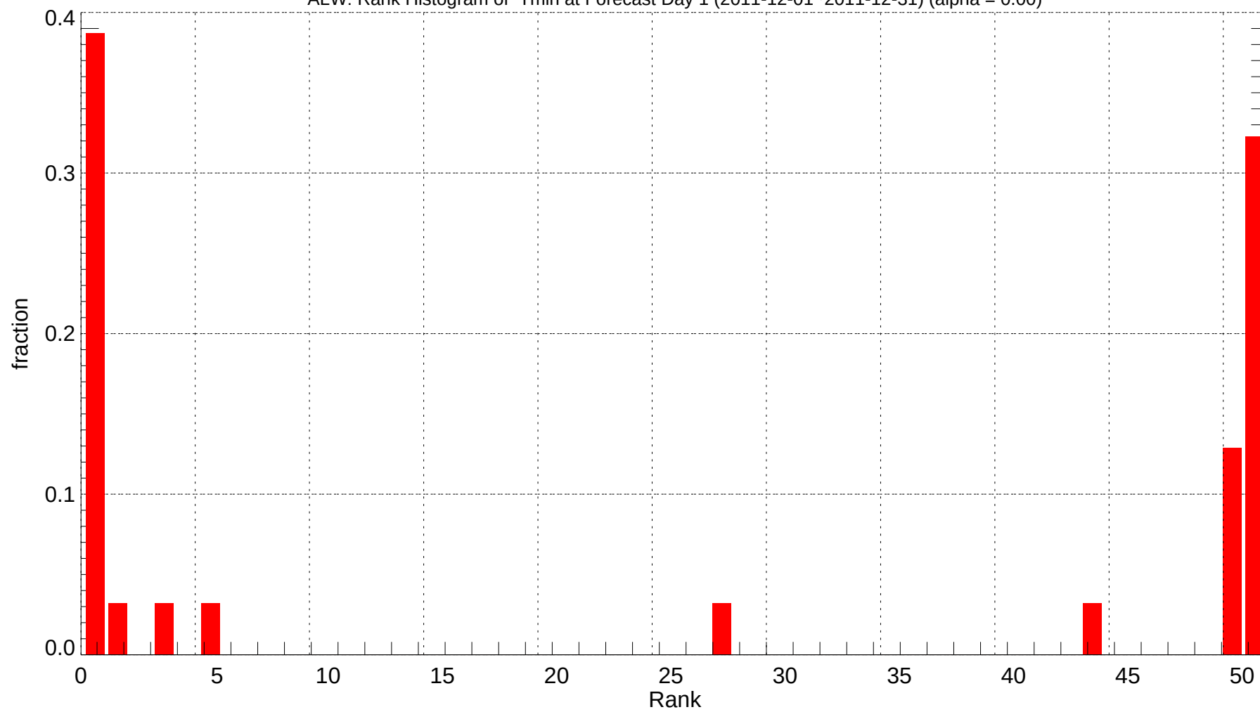
ALW: Rank Histogram of Tmin at Forecast Day 1 (2011-12-01~2011-12-31) (alpha = 0.00)
