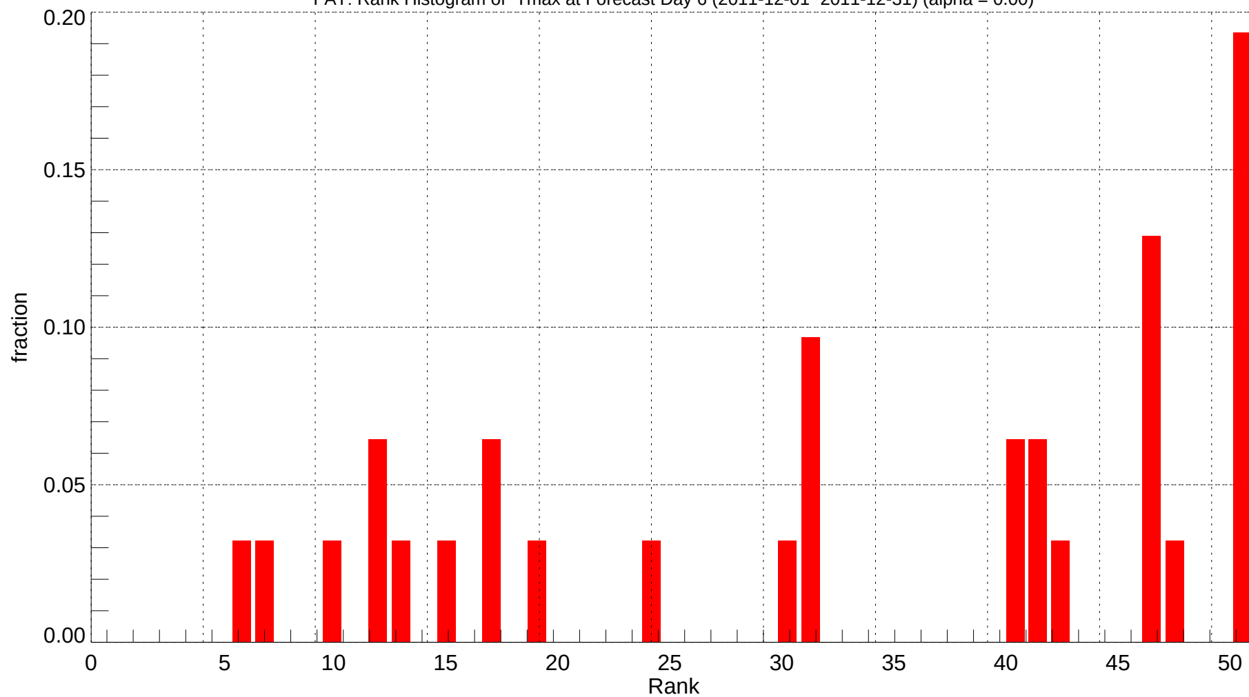
FAT: Rank Histogram of Tmax at Forecast Day 6 (2011-12-01~2011-12-31) (alpha = 0.00)
