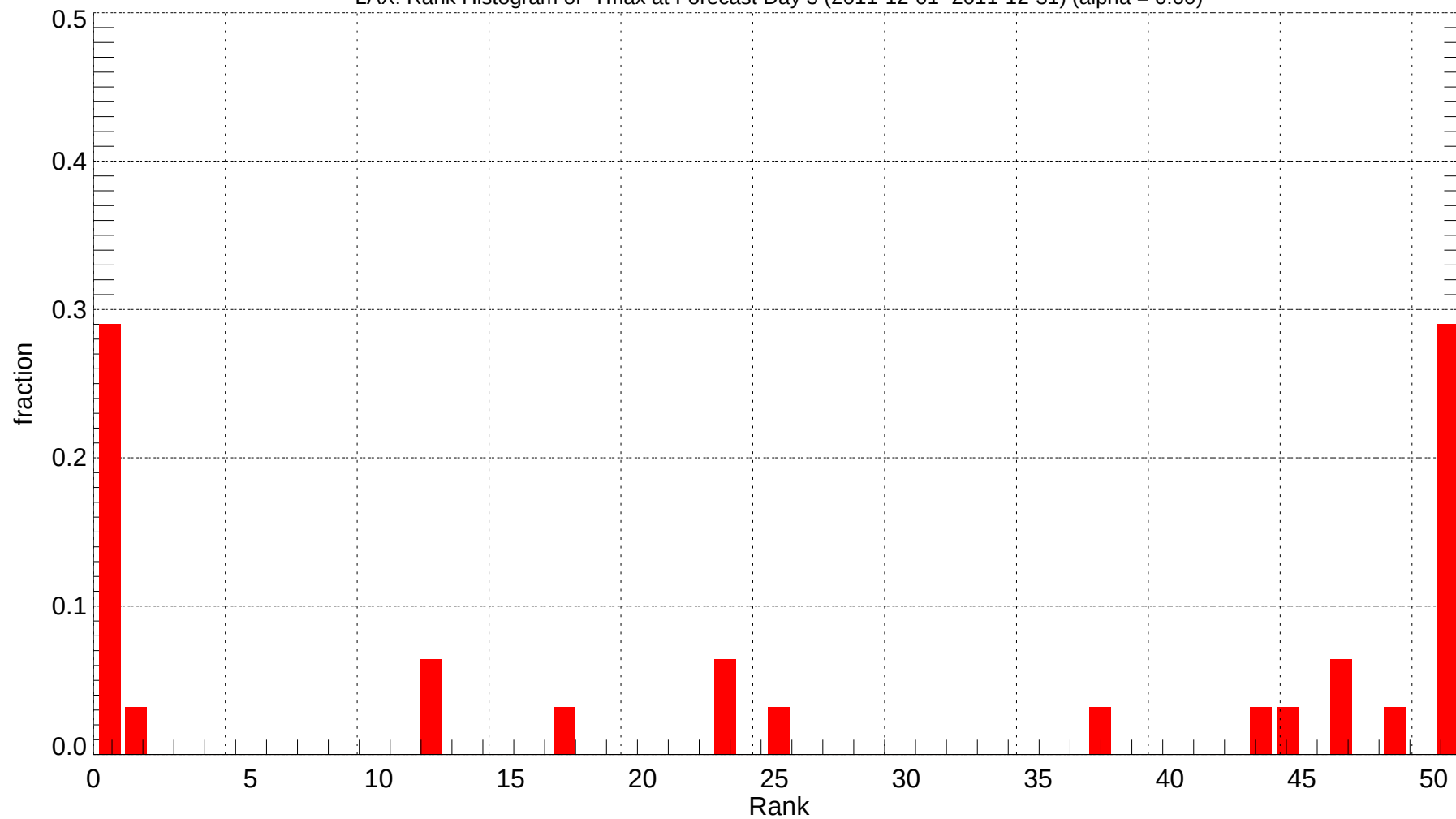
LAX: Rank Histogram of Tmax at Forecast Day 3 (2011-12-01~2011-12-31) (alpha = 0.00)
