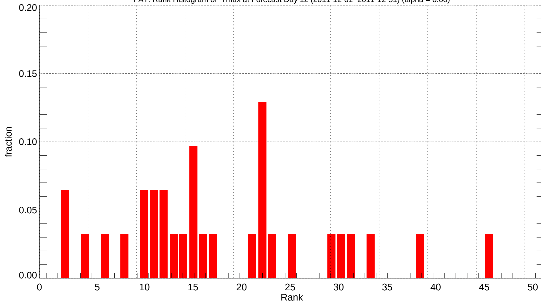
FAT: Rank Histogram of Tmax at Forecast Day 12 (2011-12-01~2011-12-31) (alpha = 0.00)
