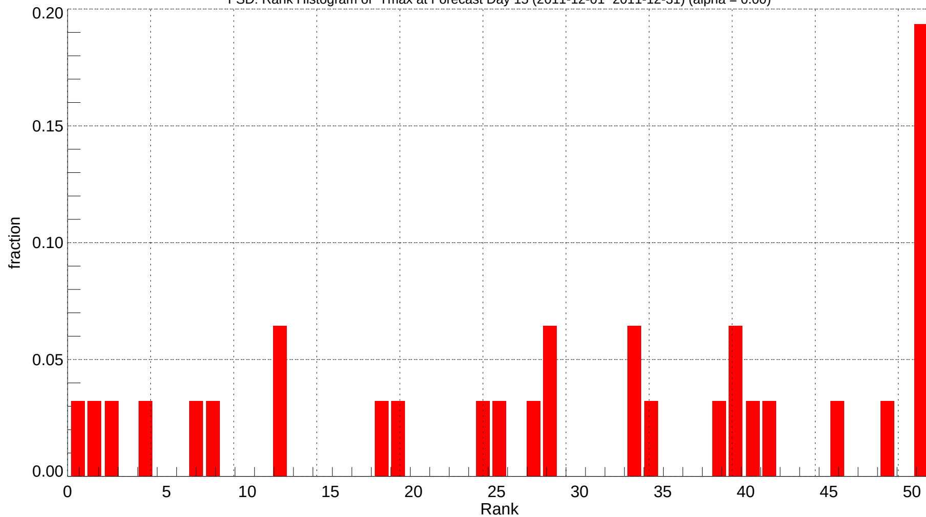
FSD: Rank Histogram of Tmax at Forecast Day 15 (2011-12-01~2011-12-31) (alpha = 0.00)
