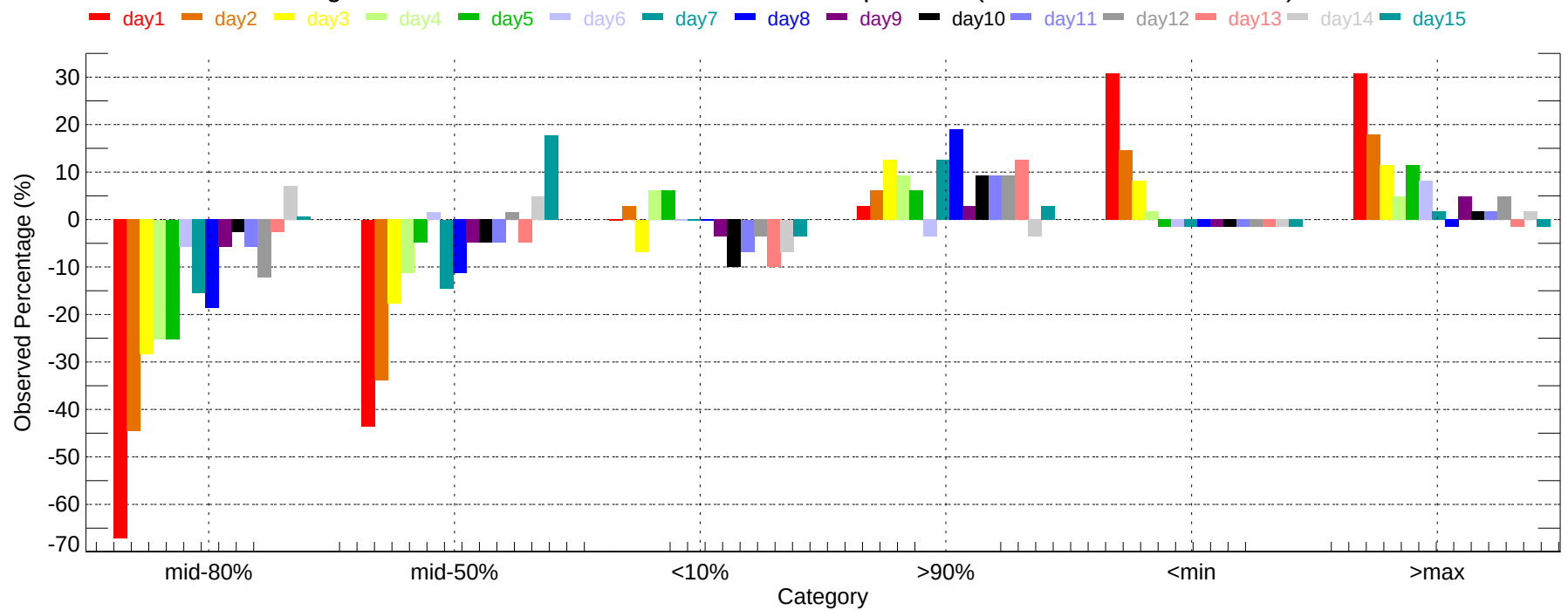
Observed Percentage Deviation of Ensembles - SAV: Min Temperature (2011-12-01~2011-12-31)
