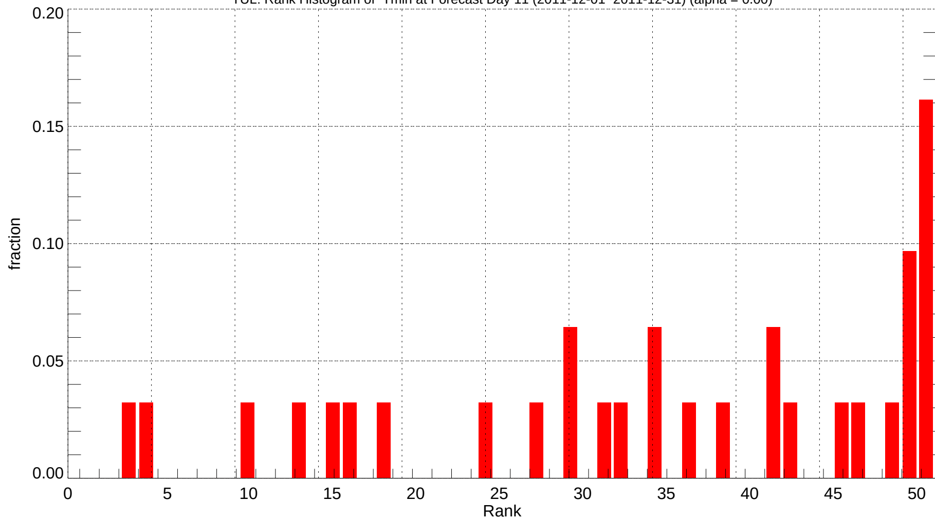
TUL: Rank Histogram of Tmin at Forecast Day 11 (2011-12-01~2011-12-31) (alpha = 0.00)
