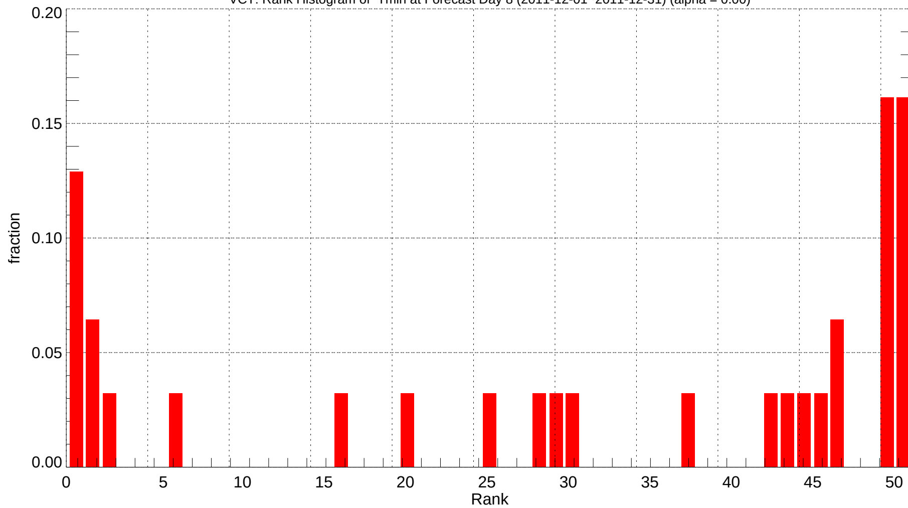
VCT: Rank Histogram of Tmin at Forecast Day 8 (2011-12-01~2011-12-31) (alpha = 0.00)
