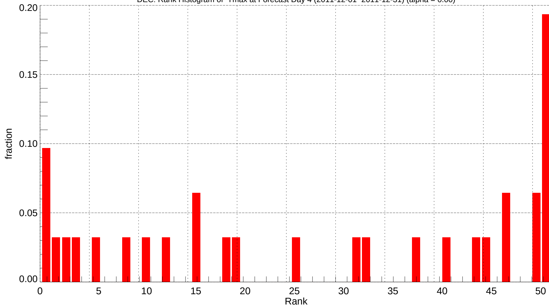
DEC: Rank Histogram of Tmax at Forecast Day 4 (2011-12-01~2011-12-31) (alpha = 0.00)
