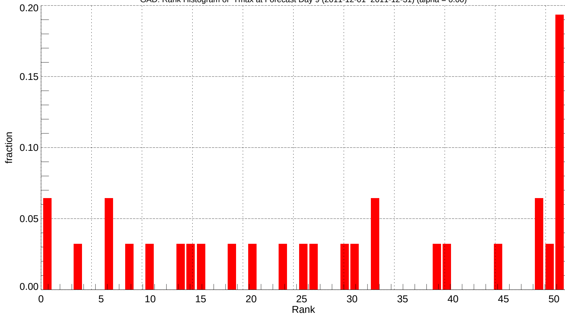
GAD: Rank Histogram of Tmax at Forecast Day 9 (2011-12-01~2011-12-31) (alpha = 0.00)
