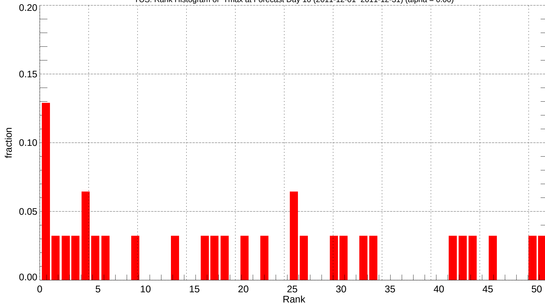
TUS: Rank Histogram of Tmax at Forecast Day 10 (2011-12-01~2011-12-31) (alpha = 0.00)
