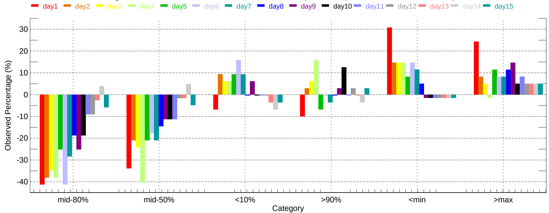
Observed Percentage Deviation of Ensembles - CLE: Max Temperature (2011-12-01~2011-12-31)
