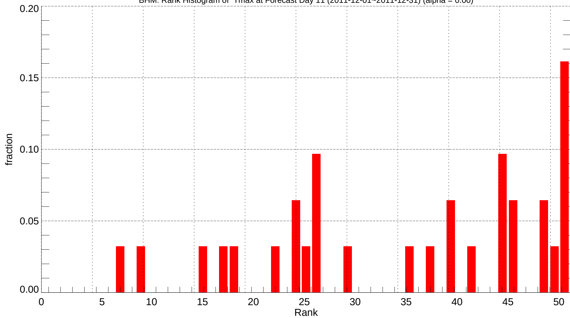
BHM: Rank Histogram of Tmax at Forecast Day 11 (2011-12-01~2011-12-31) (alpha = 0.00)
