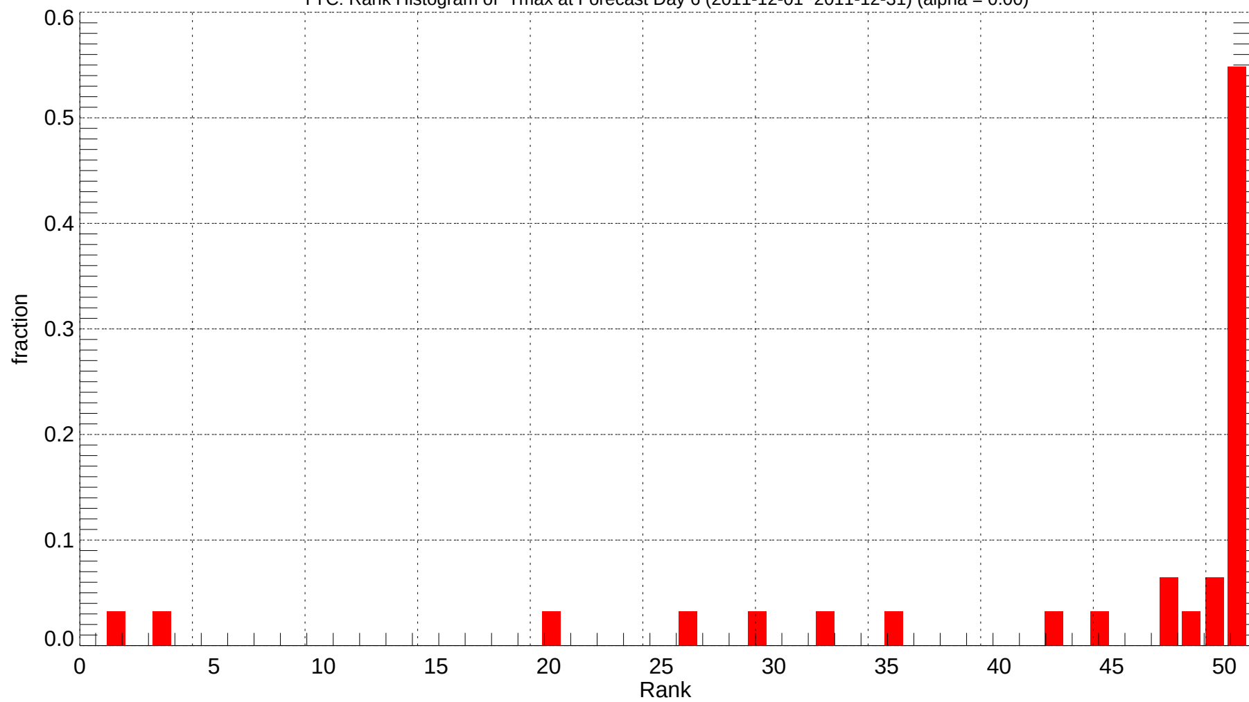
YYC: Rank Histogram of Tmax at Forecast Day 6 (2011-12-01~2011-12-31) (alpha = 0.00)
