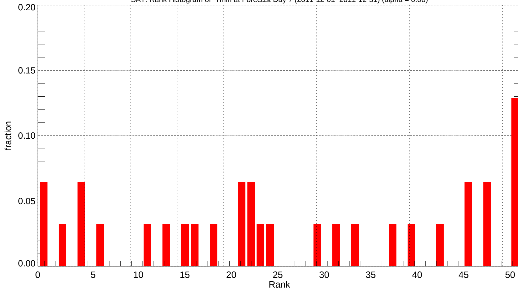
SAT: Rank Histogram of Tmin at Forecast Day 7 (2011-12-01~2011-12-31) (alpha = 0.00)
