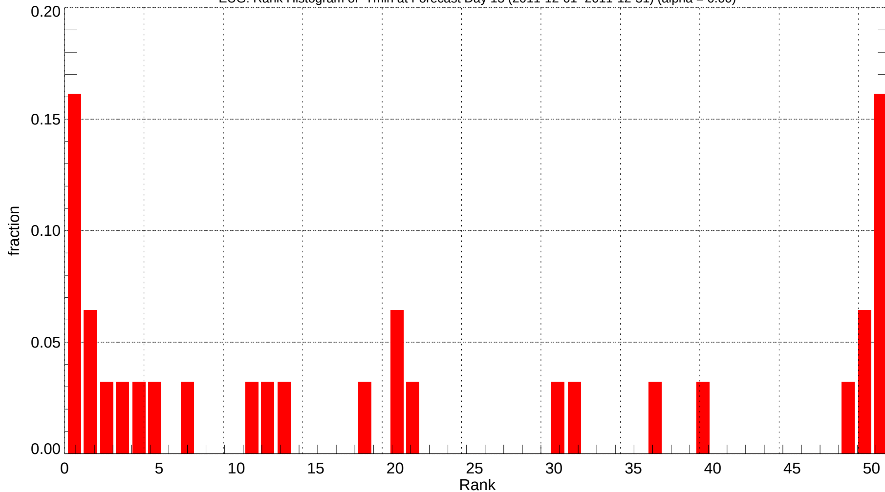
EUG: Rank Histogram of Tmin at Forecast Day 13 (2011-12-01~2011-12-31) (alpha = 0.00)
