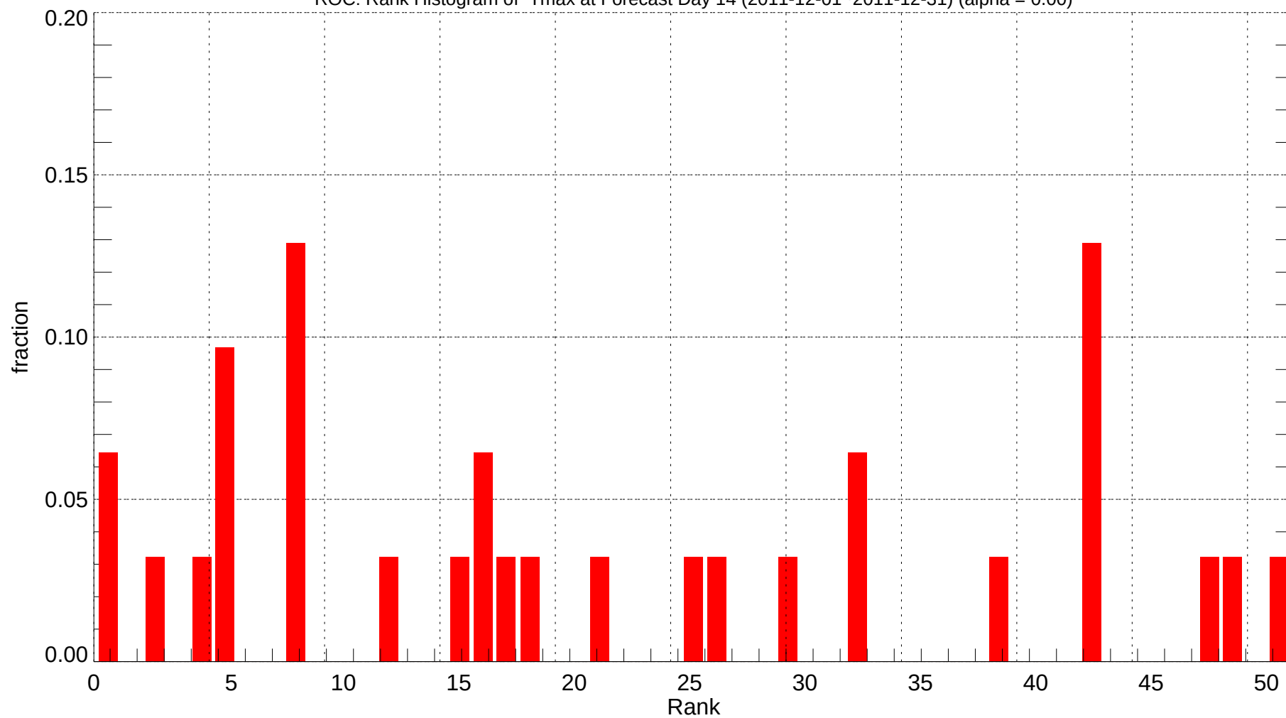
ROC: Rank Histogram of Tmax at Forecast Day 14 (2011-12-01~2011-12-31) (alpha = 0.00)
