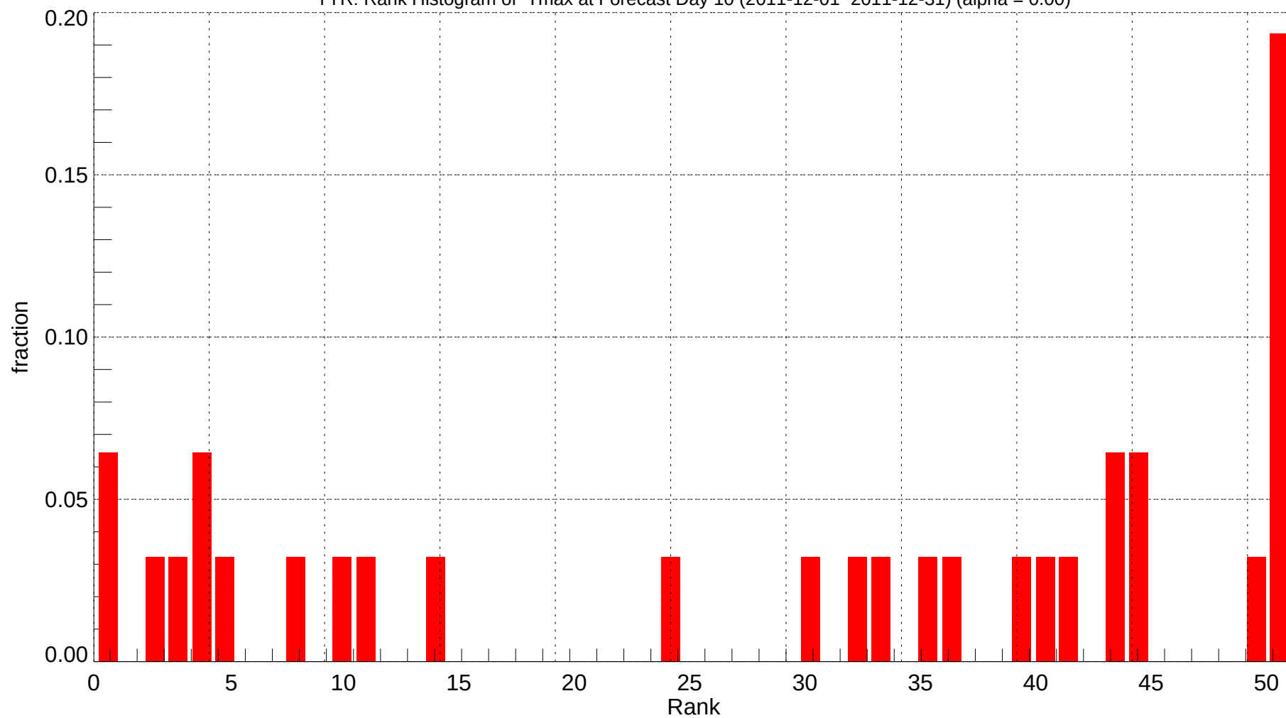
TYR: Rank Histogram of Tmax at Forecast Day 10 (2011-12-01~2011-12-31) (alpha = 0.00)
