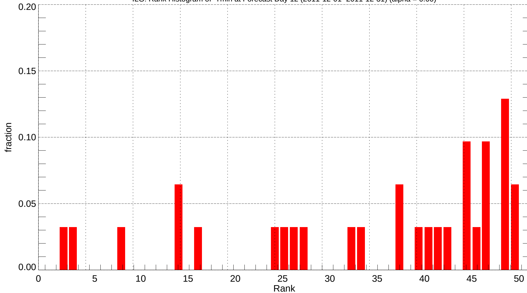
ILG: Rank Histogram of Tmin at Forecast Day 12 (2011-12-01~2011-12-31) (alpha = 0.00)
