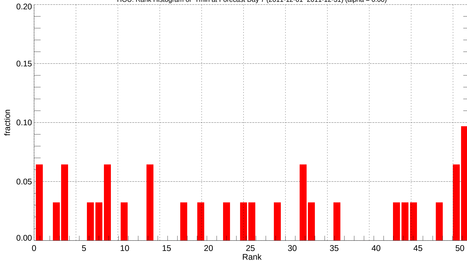
HOU: Rank Histogram of Tmin at Forecast Day 7 (2011-12-01~2011-12-31) (alpha = 0.00)
