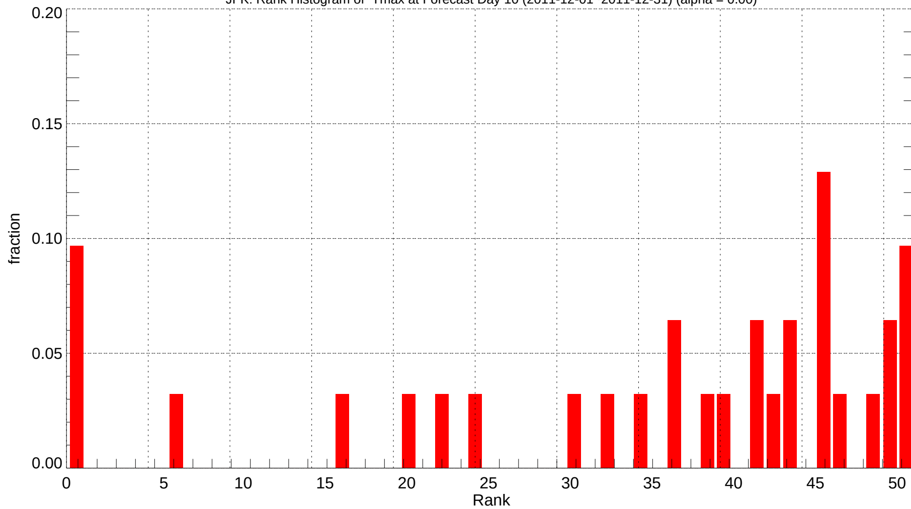
JFK: Rank Histogram of Tmax at Forecast Day 10 (2011-12-01~2011-12-31) (alpha = 0.00)
