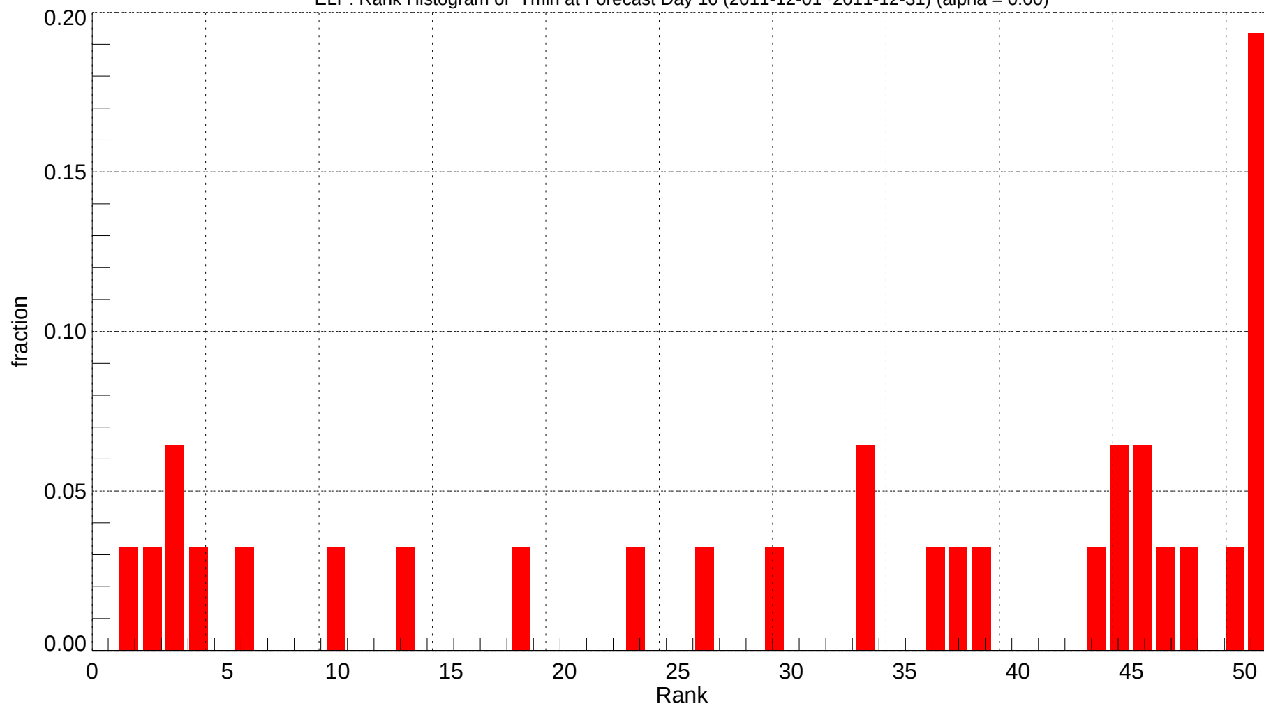
ELP: Rank Histogram of Tmin at Forecast Day 10 (2011-12-01~2011-12-31) (alpha = 0.00)
