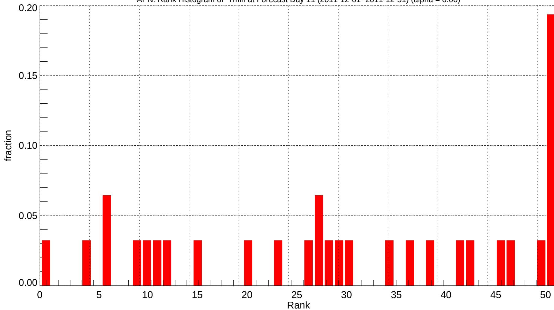
APN: Rank Histogram of Tmin at Forecast Day 11 (2011-12-01~2011-12-31) (alpha = 0.00)
