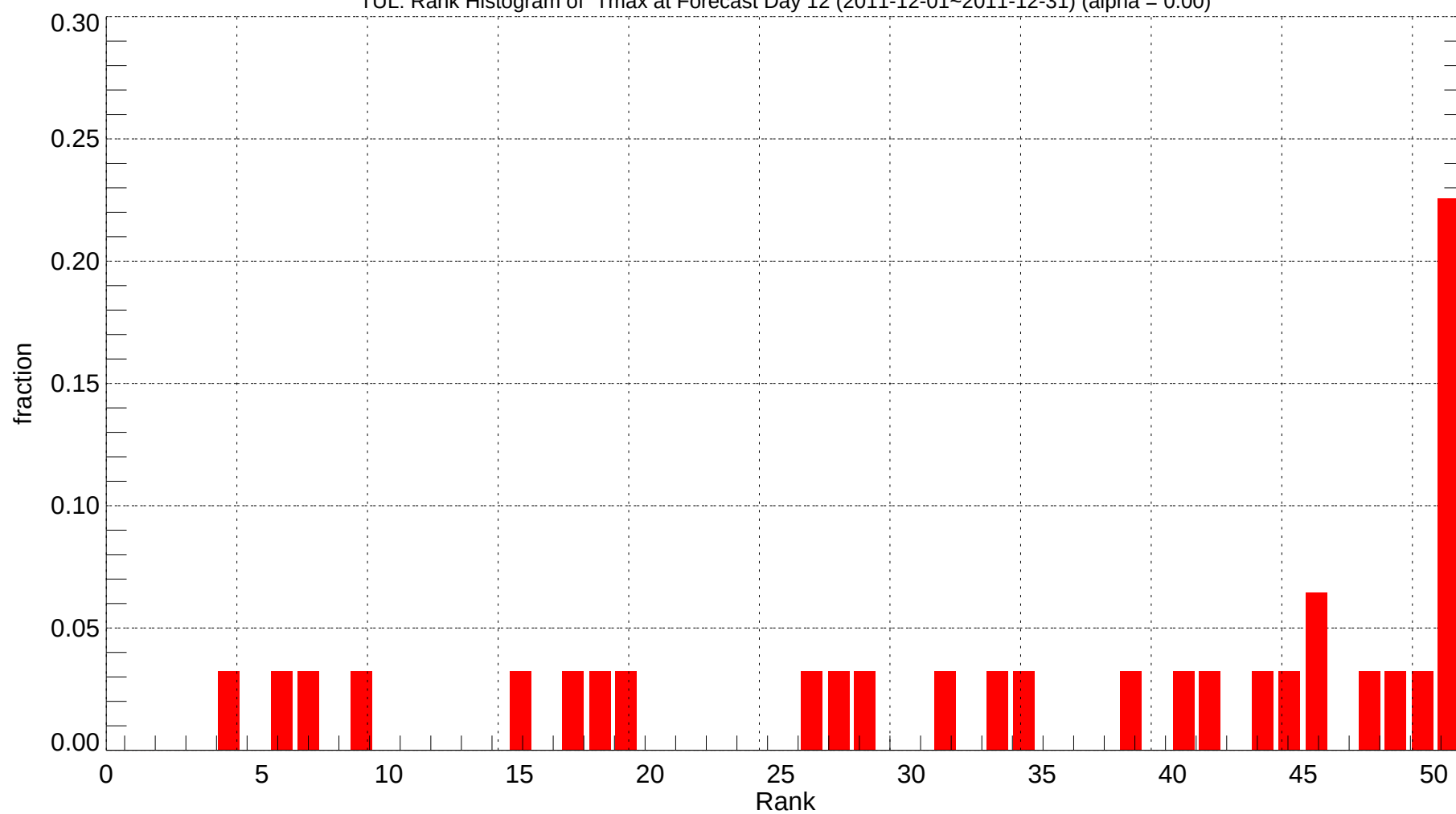
TUL: Rank Histogram of Tmax at Forecast Day 12 (2011-12-01~2011-12-31) (alpha = 0.00)
