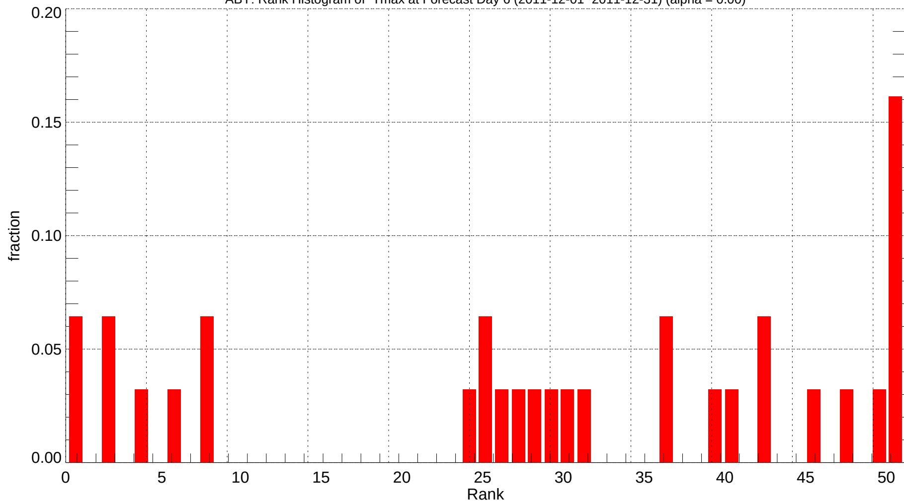
ABY: Rank Histogram of Tmax at Forecast Day 6 (2011-12-01~2011-12-31) (alpha = 0.00)
