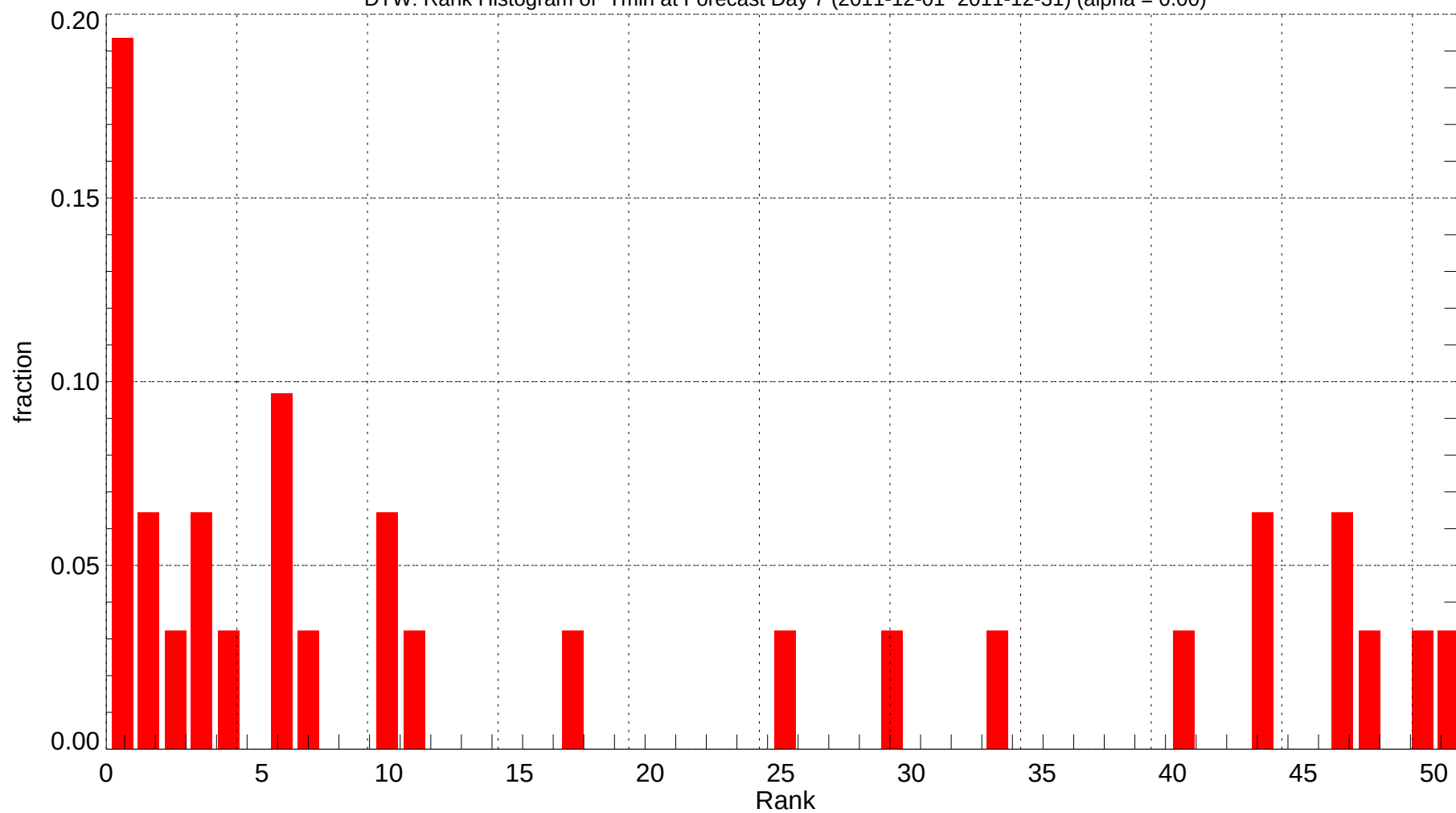
DTW: Rank Histogram of Tmin at Forecast Day 7 (2011-12-01~2011-12-31) (alpha = 0.00)
