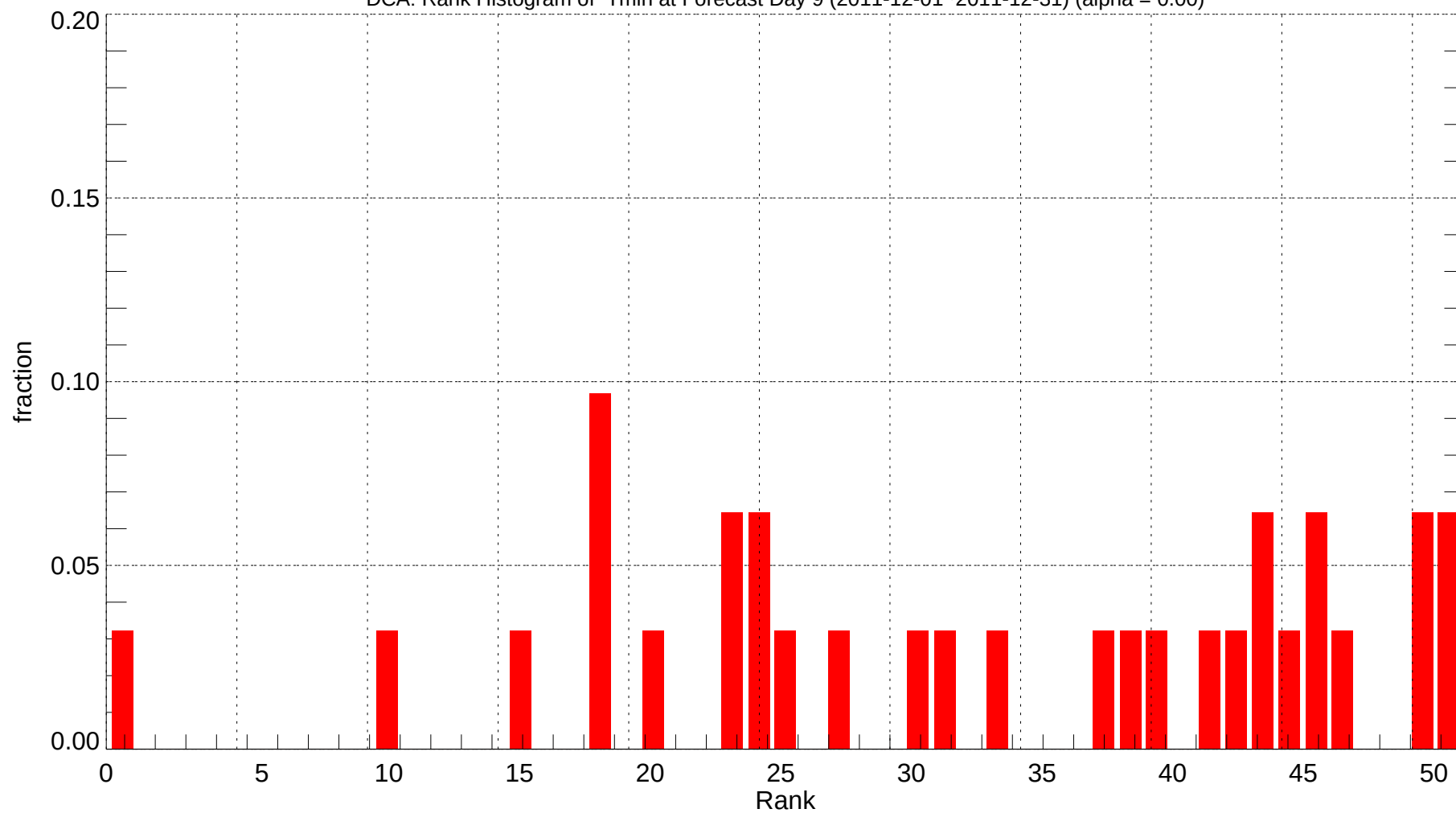
DCA: Rank Histogram of Tmin at Forecast Day 9 (2011-12-01~2011-12-31) (alpha = 0.00)
