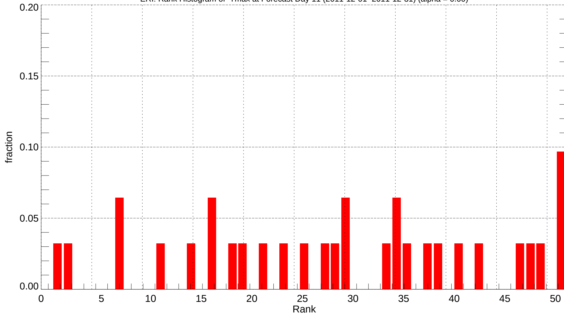
ERI: Rank Histogram of Tmax at Forecast Day 11 (2011-12-01~2011-12-31) (alpha = 0.00)
