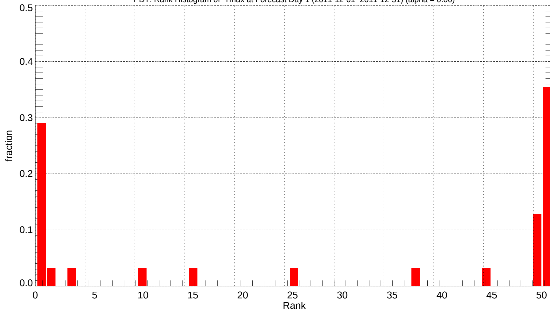
PDT: Rank Histogram of Tmax at Forecast Day 1 (2011-12-01~2011-12-31) (alpha = 0.00)
