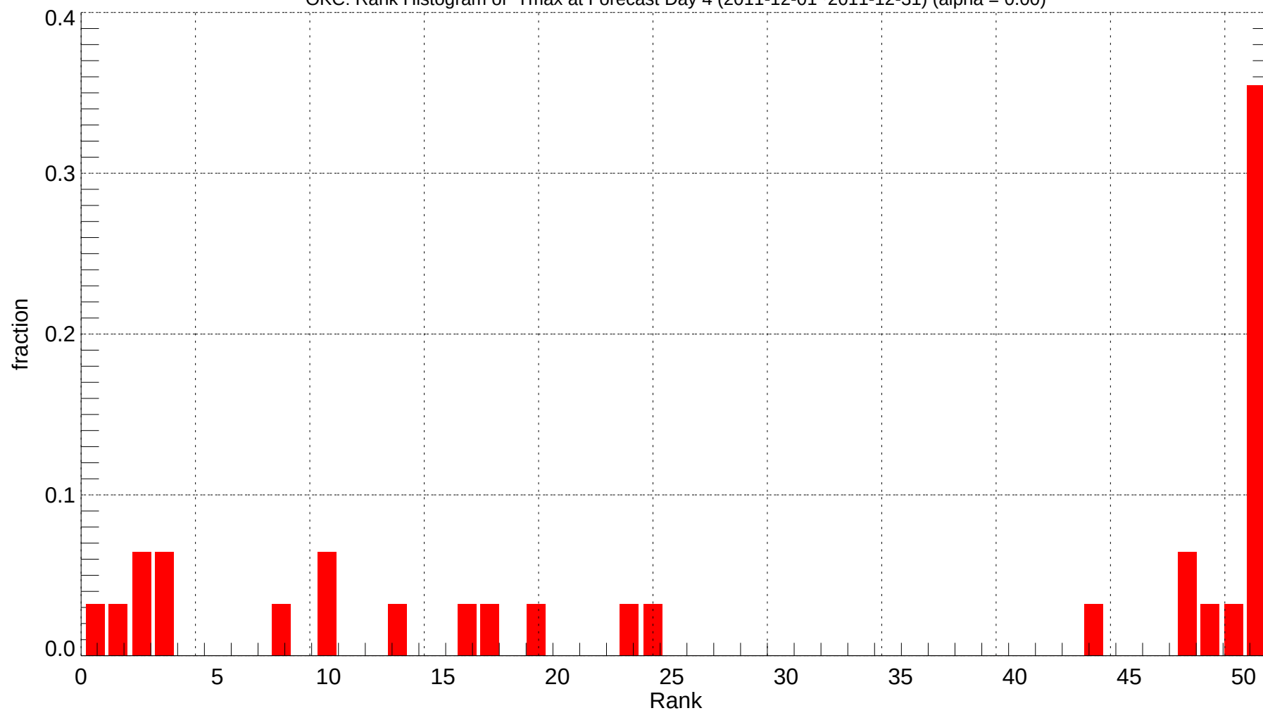
OKC: Rank Histogram of Tmax at Forecast Day 4 (2011-12-01~2011-12-31) (alpha = 0.00)
