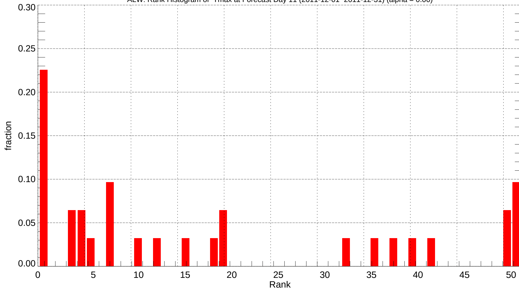
ALW: Rank Histogram of Tmax at Forecast Day 11 (2011-12-01~2011-12-31) (alpha = 0.00)
