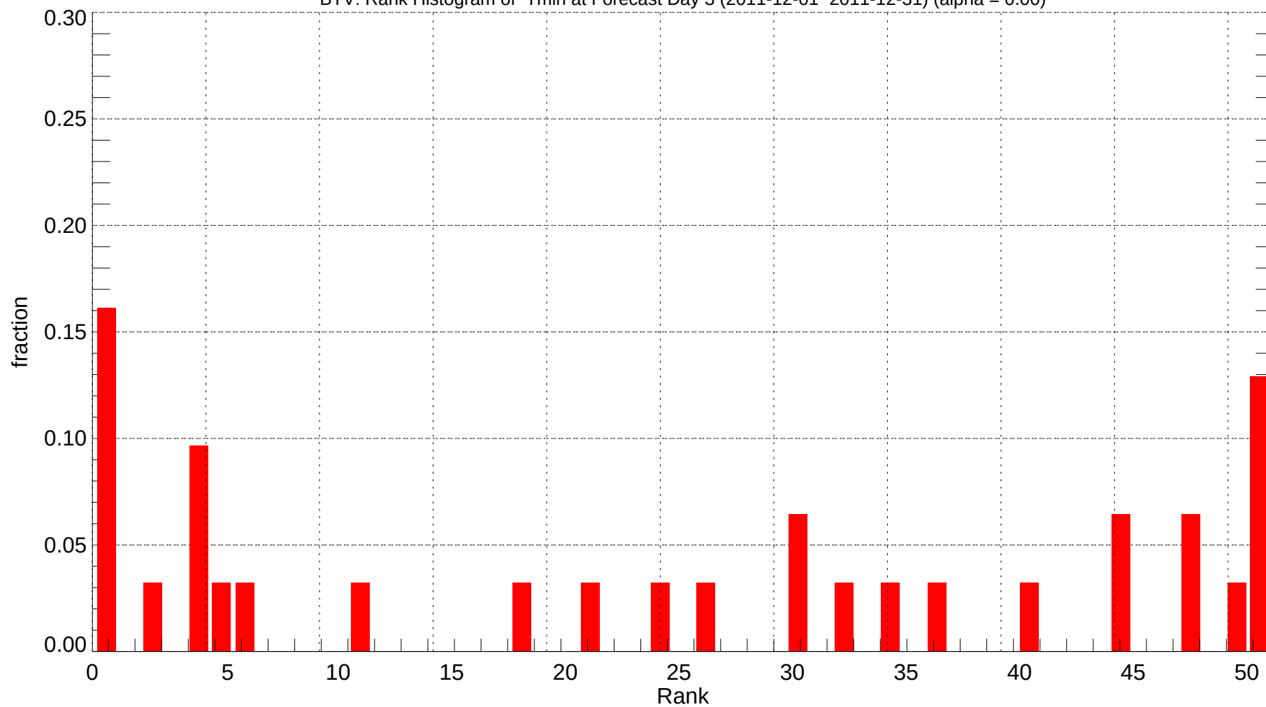
BTV: Rank Histogram of Tmin at Forecast Day 3 (2011-12-01~2011-12-31) (alpha = 0.00)
