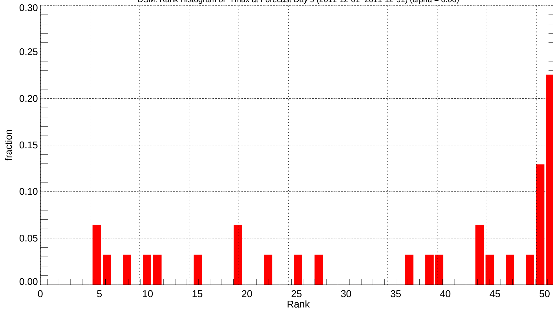
DSM: Rank Histogram of Tmax at Forecast Day 9 (2011-12-01~2011-12-31) (alpha = 0.00)
