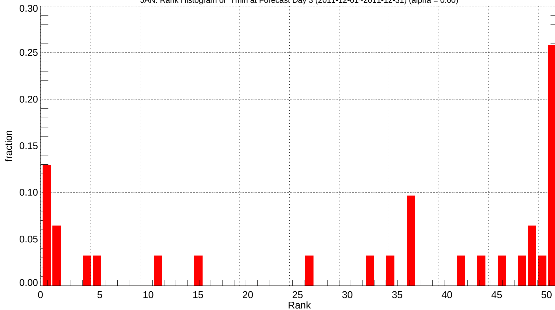
JAN: Rank Histogram of Tmin at Forecast Day 3 (2011-12-01~2011-12-31) (alpha = 0.00)
