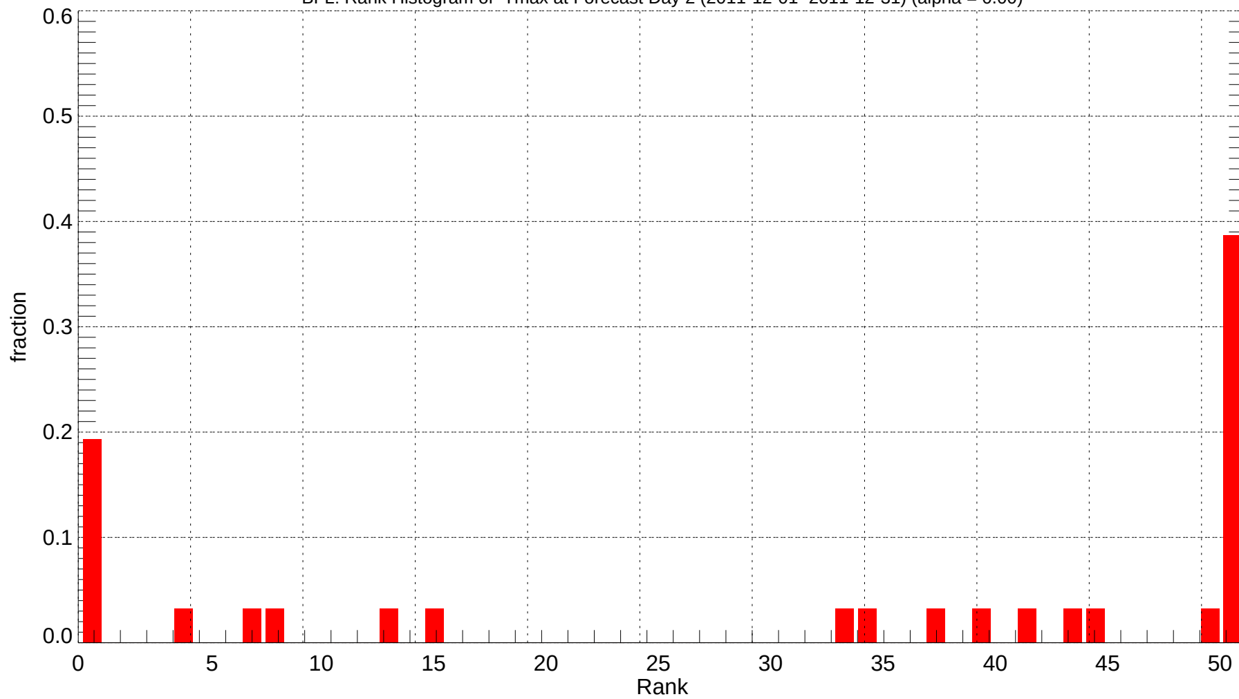
BFL: Rank Histogram of Tmax at Forecast Day 2 (2011-12-01~2011-12-31) (alpha = 0.00)
