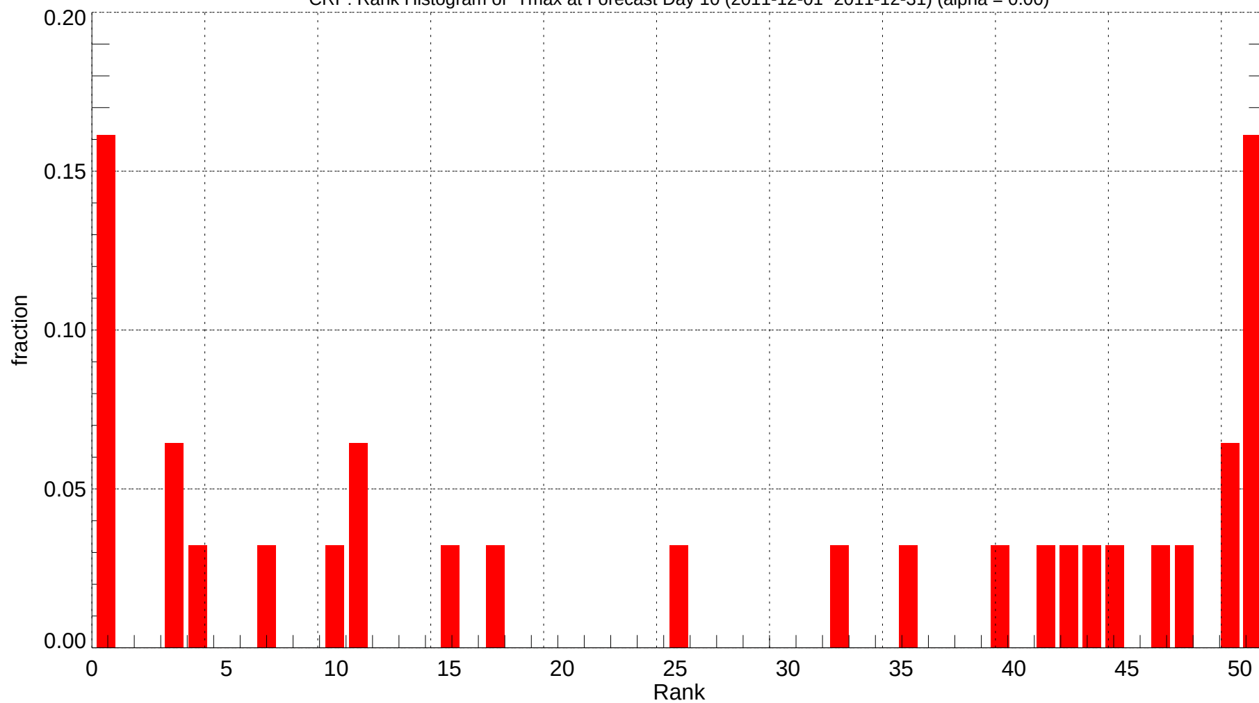
CRP: Rank Histogram of Tmax at Forecast Day 10 (2011-12-01~2011-12-31) (alpha = 0.00)
