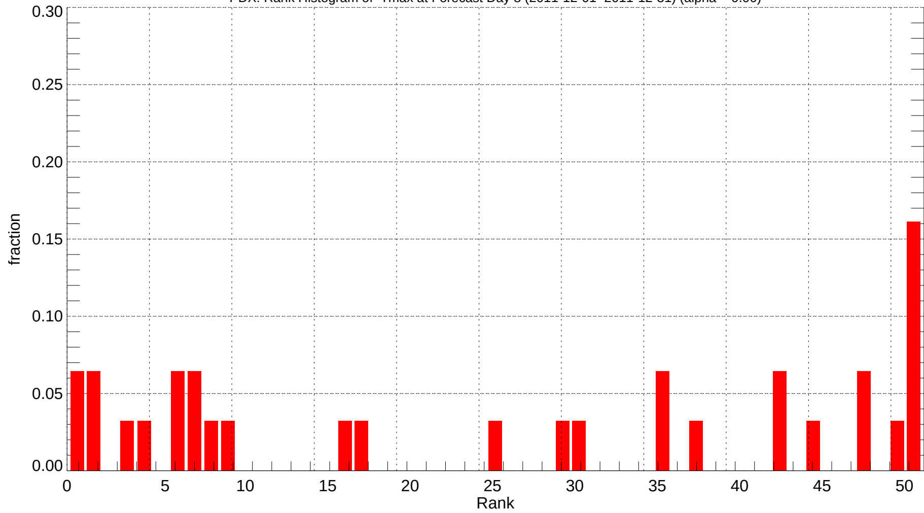
PDX: Rank Histogram of Tmax at Forecast Day 8 (2011-12-01~2011-12-31) (alpha = 0.00)
