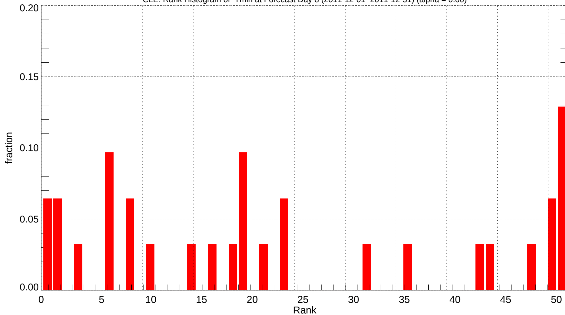
CLE: Rank Histogram of Tmin at Forecast Day 8 (2011-12-01~2011-12-31) (alpha = 0.00)
