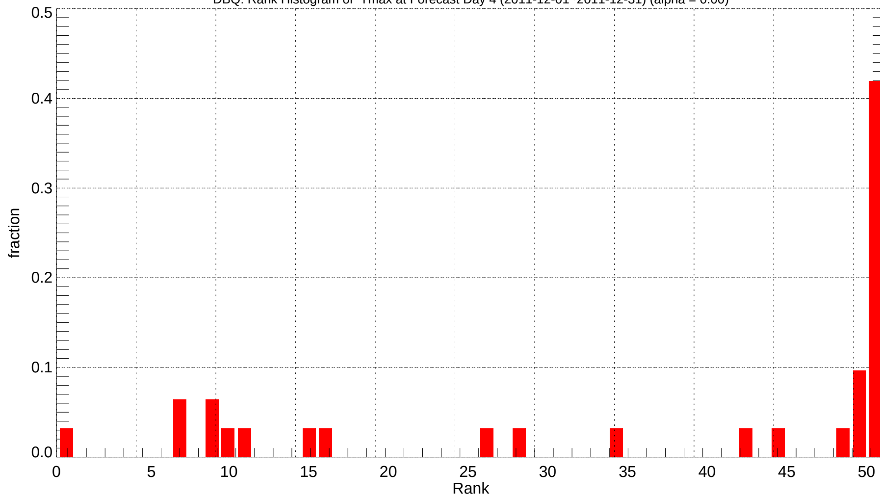
DBQ: Rank Histogram of Tmax at Forecast Day 4 (2011-12-01~2011-12-31) (alpha = 0.00)
