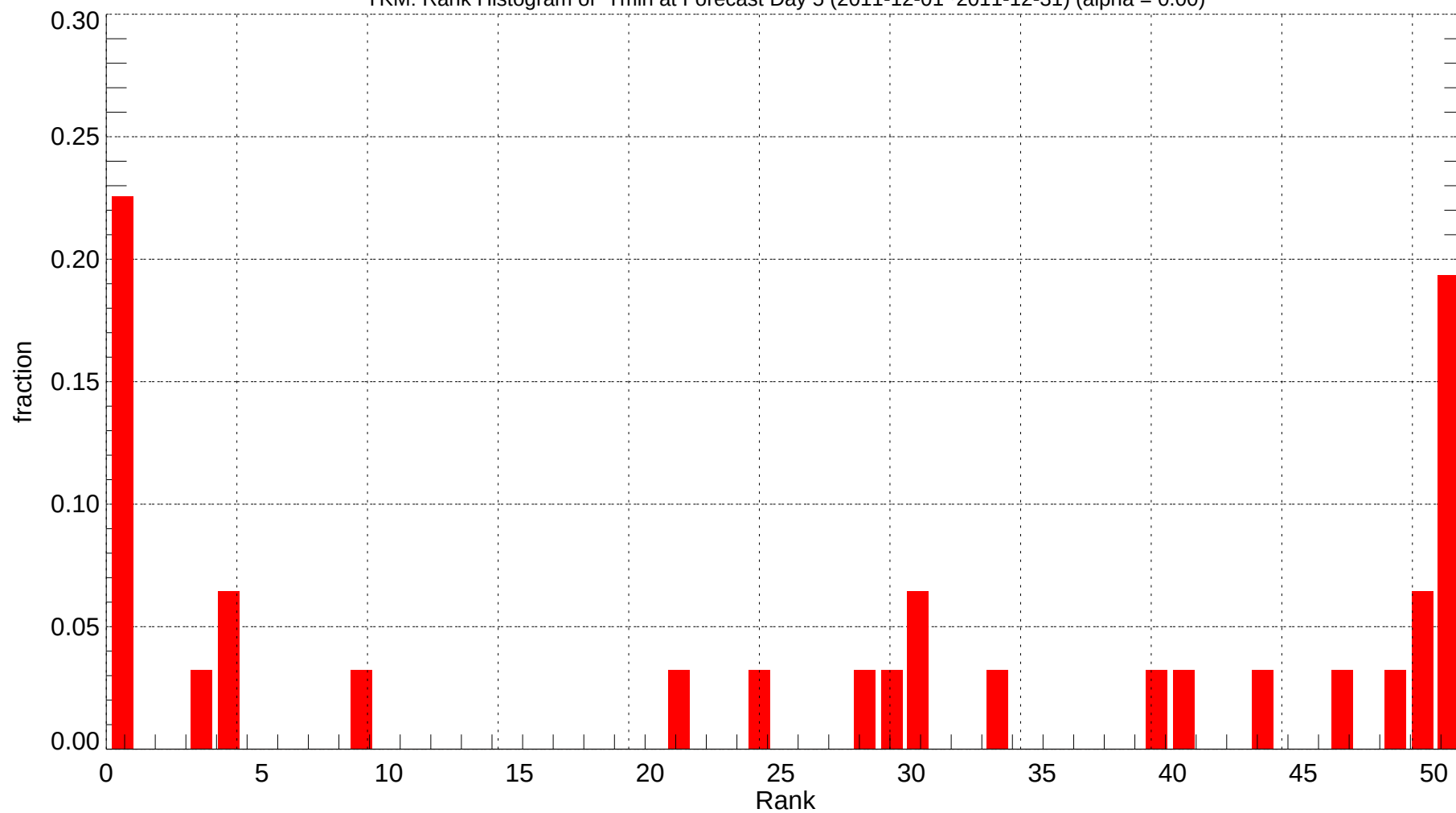
YKM: Rank Histogram of Tmin at Forecast Day 5 (2011-12-01~2011-12-31) (alpha = 0.00)
