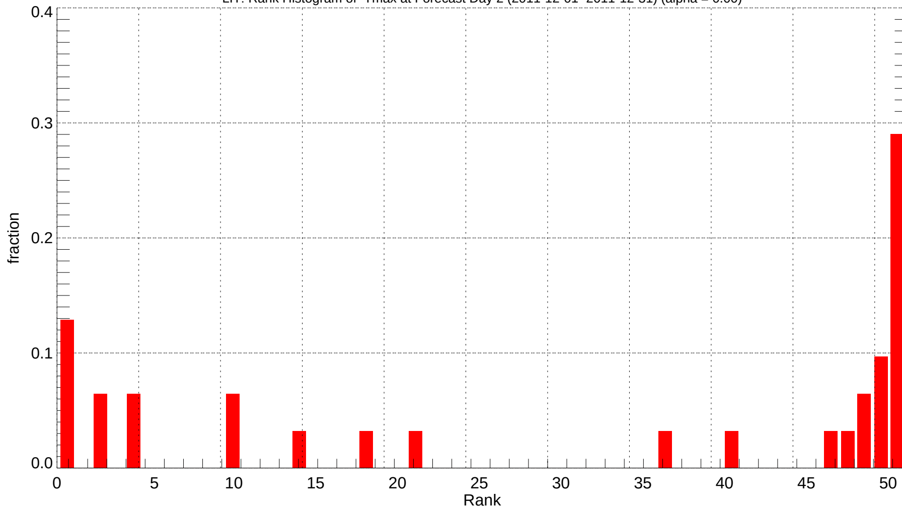
LIT: Rank Histogram of Tmax at Forecast Day 2 (2011-12-01~2011-12-31) (alpha = 0.00)
