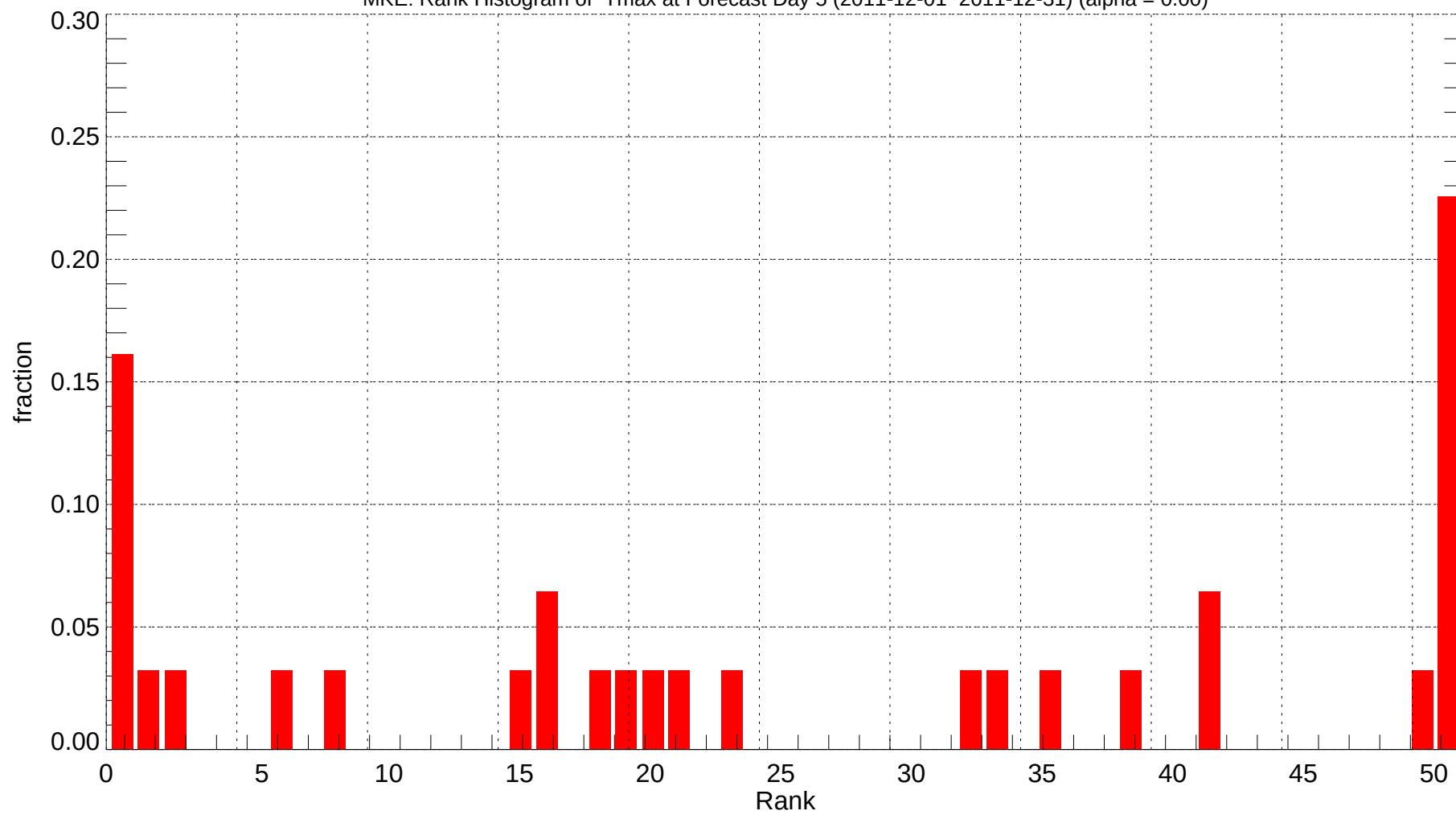
MKE: Rank Histogram of Tmax at Forecast Day 5 (2011-12-01~2011-12-31) (alpha = 0.00)
