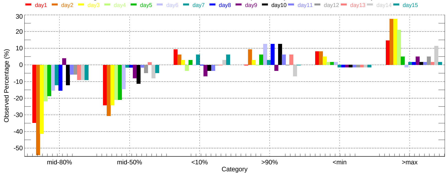
Observed Percentage Deviation of Ensembles - DFW: Max Temperature (2011-12-01~2011-12-31)
