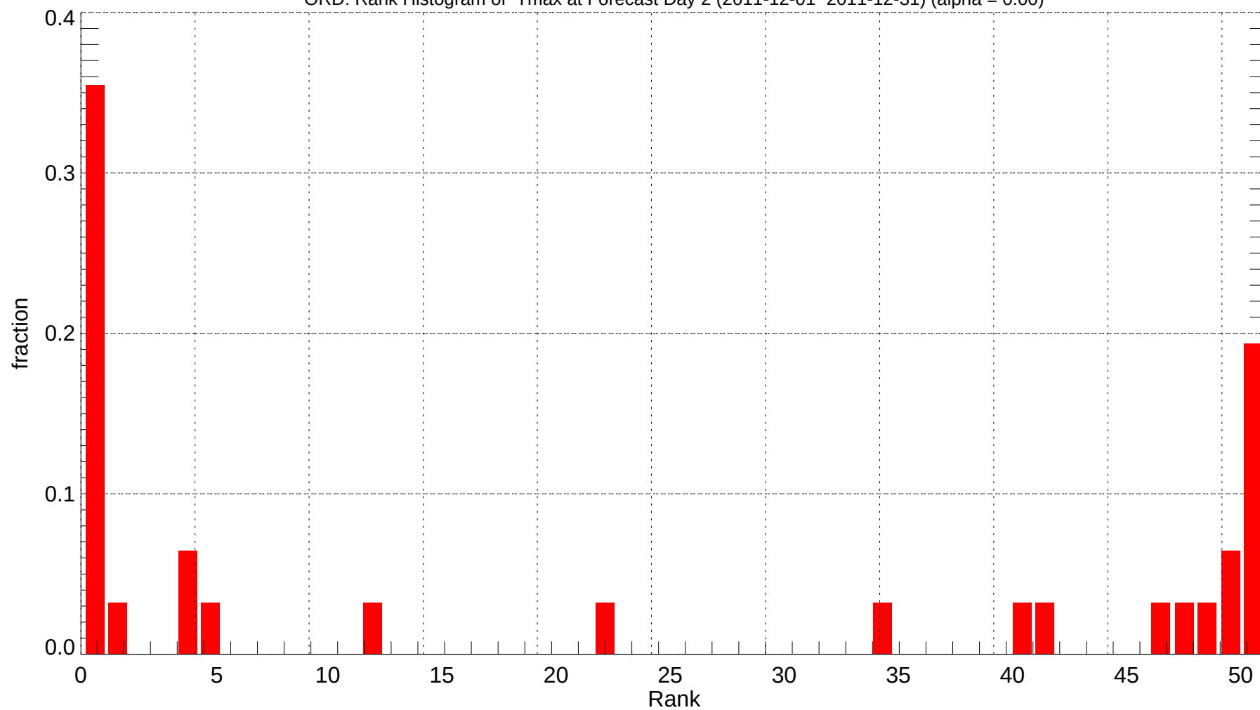
ORD: Rank Histogram of Tmax at Forecast Day 2 (2011-12-01~2011-12-31) (alpha = 0.00)
