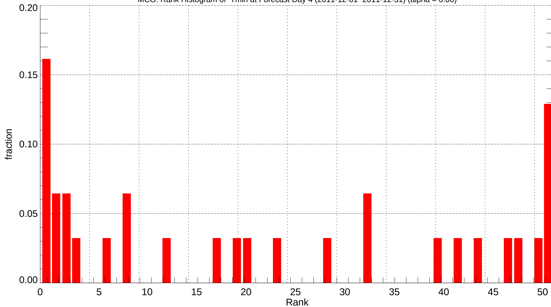
MCO: Rank Histogram of Tmin at Forecast Day 4 (2011-12-01~2011-12-31) (alpha = 0.00)
