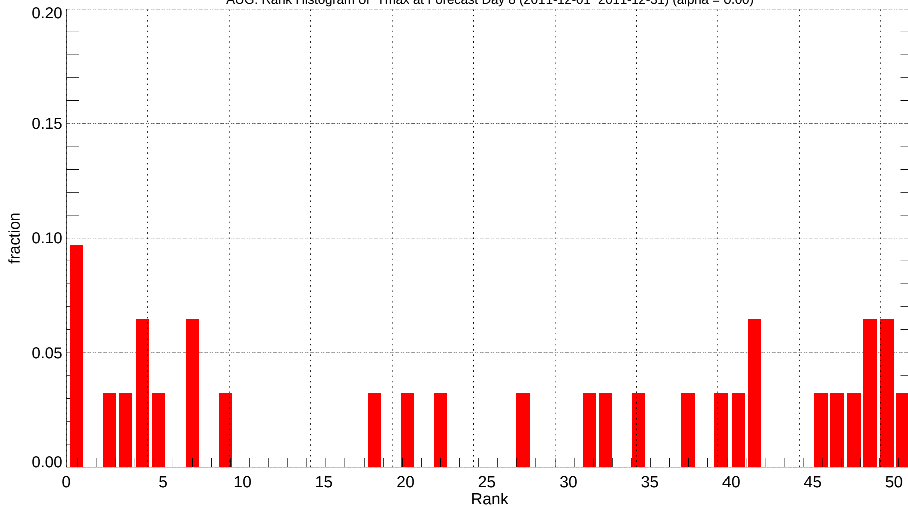
AUG: Rank Histogram of Tmax at Forecast Day 8 (2011-12-01~2011-12-31) (alpha = 0.00)
