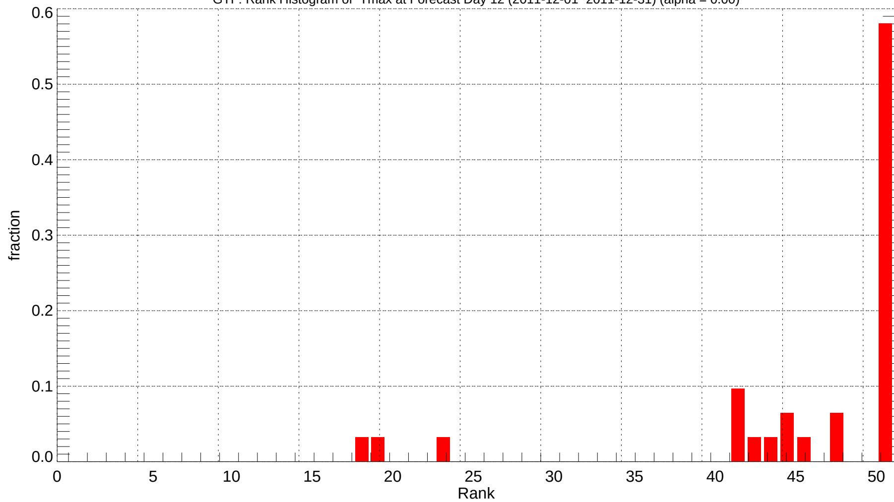
GTF: Rank Histogram of Tmax at Forecast Day 12 (2011-12-01~2011-12-31) (alpha = 0.00)
