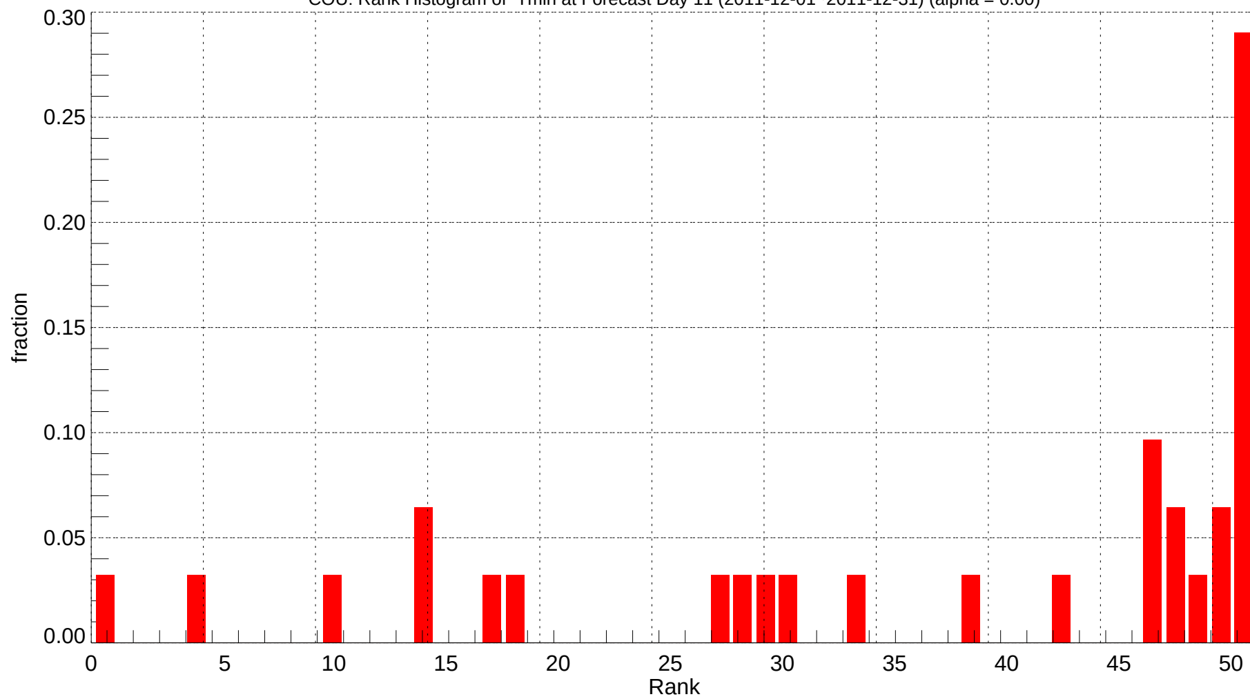
COU: Rank Histogram of Tmin at Forecast Day 11 (2011-12-01~2011-12-31) (alpha = 0.00)
