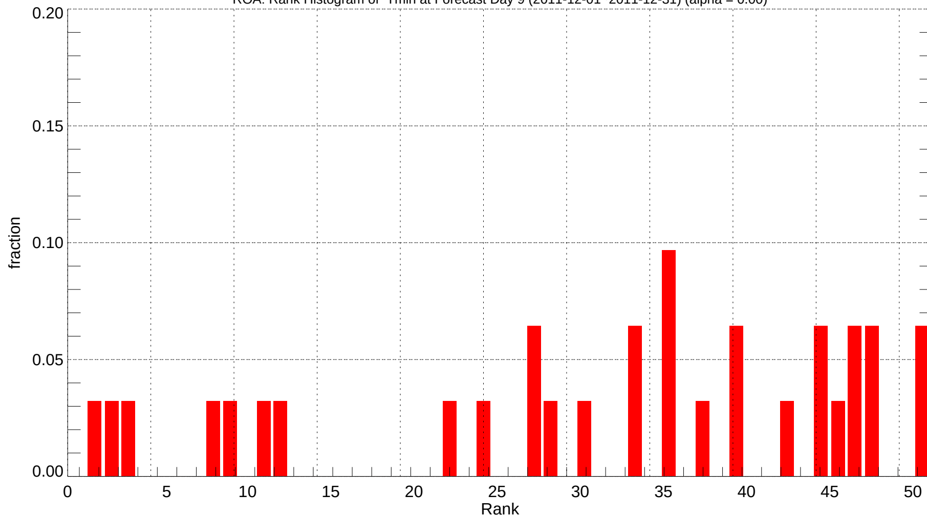
ROA: Rank Histogram of Tmin at Forecast Day 9 (2011-12-01~2011-12-31) (alpha = 0.00)
