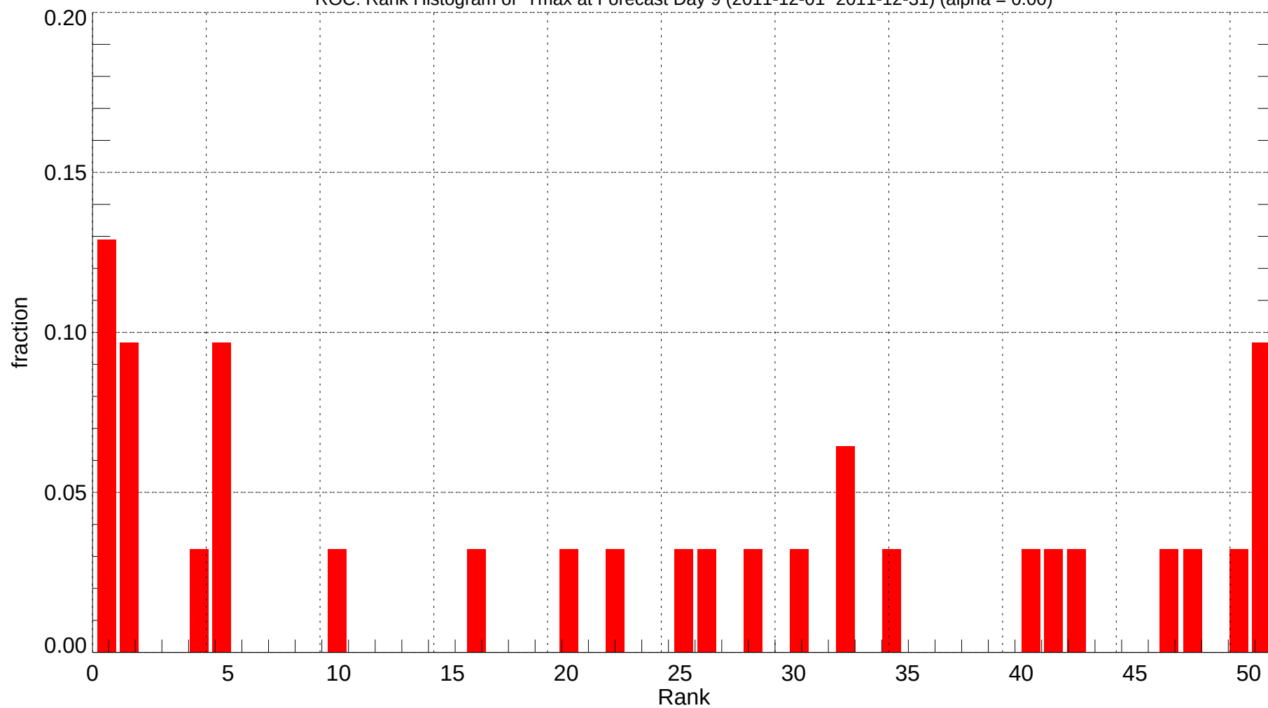
ROC: Rank Histogram of Tmax at Forecast Day 9 (2011-12-01~2011-12-31) (alpha = 0.00)
