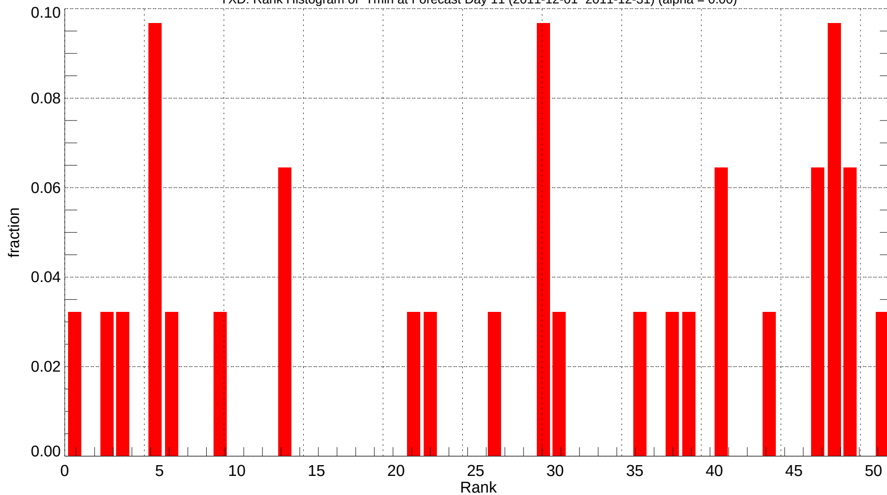
YXD: Rank Histogram of Tmin at Forecast Day 11 (2011-12-01~2011-12-31) (alpha = 0.00)
