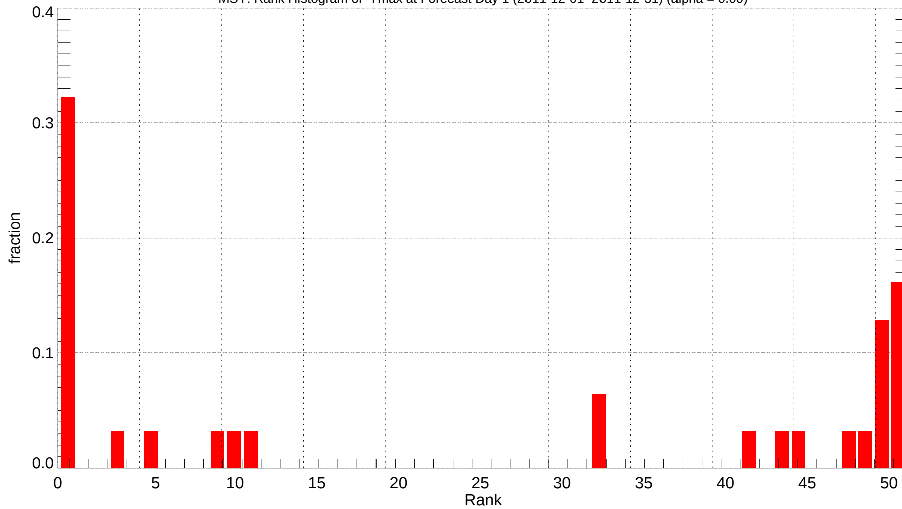
MSY: Rank Histogram of Tmax at Forecast Day 1 (2011-12-01~2011-12-31) (alpha = 0.00)
