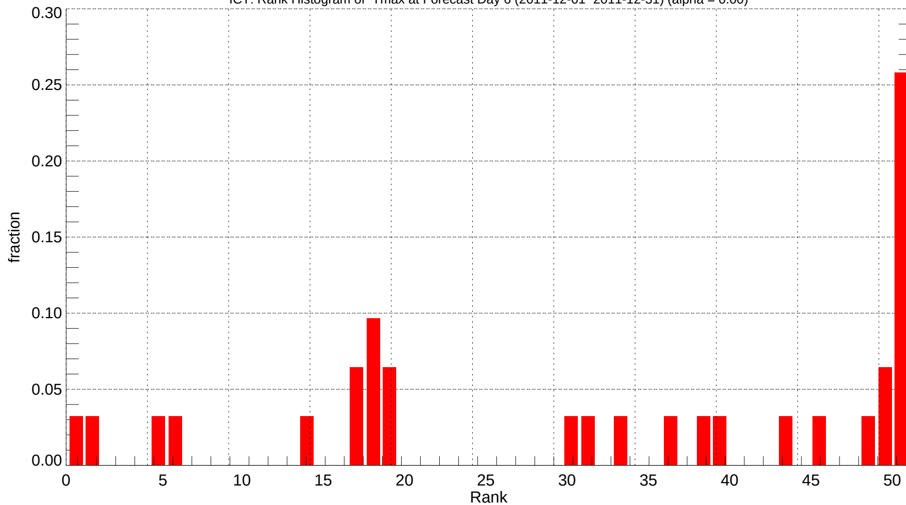
ICT: Rank Histogram of Tmax at Forecast Day 6 (2011-12-01~2011-12-31) (alpha = 0.00)
