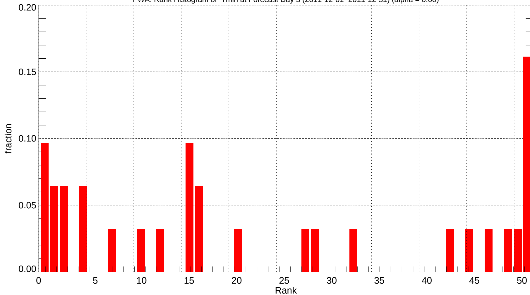
FWA: Rank Histogram of Tmin at Forecast Day 3 (2011-12-01~2011-12-31) (alpha = 0.00)
