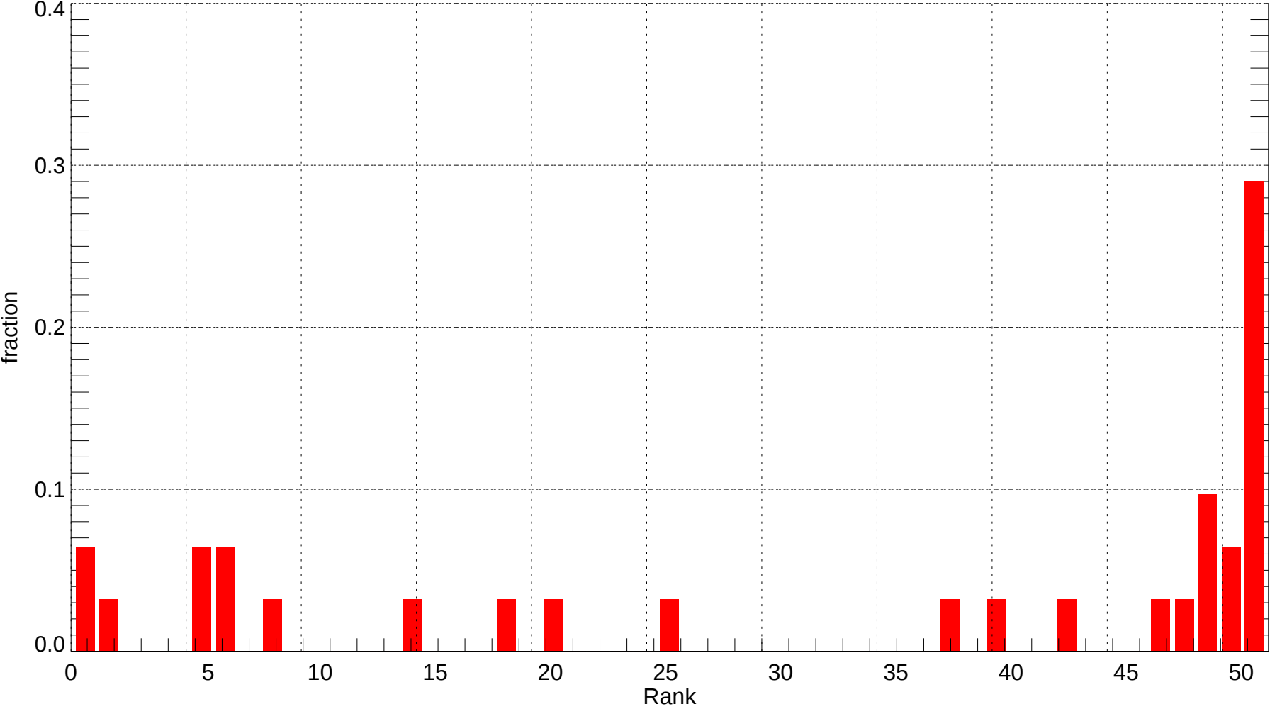
BFL: Rank Histogram of Tmin at Forecast Day 4 (2011-12-01~2011-12-31) (alpha = 0.00)
