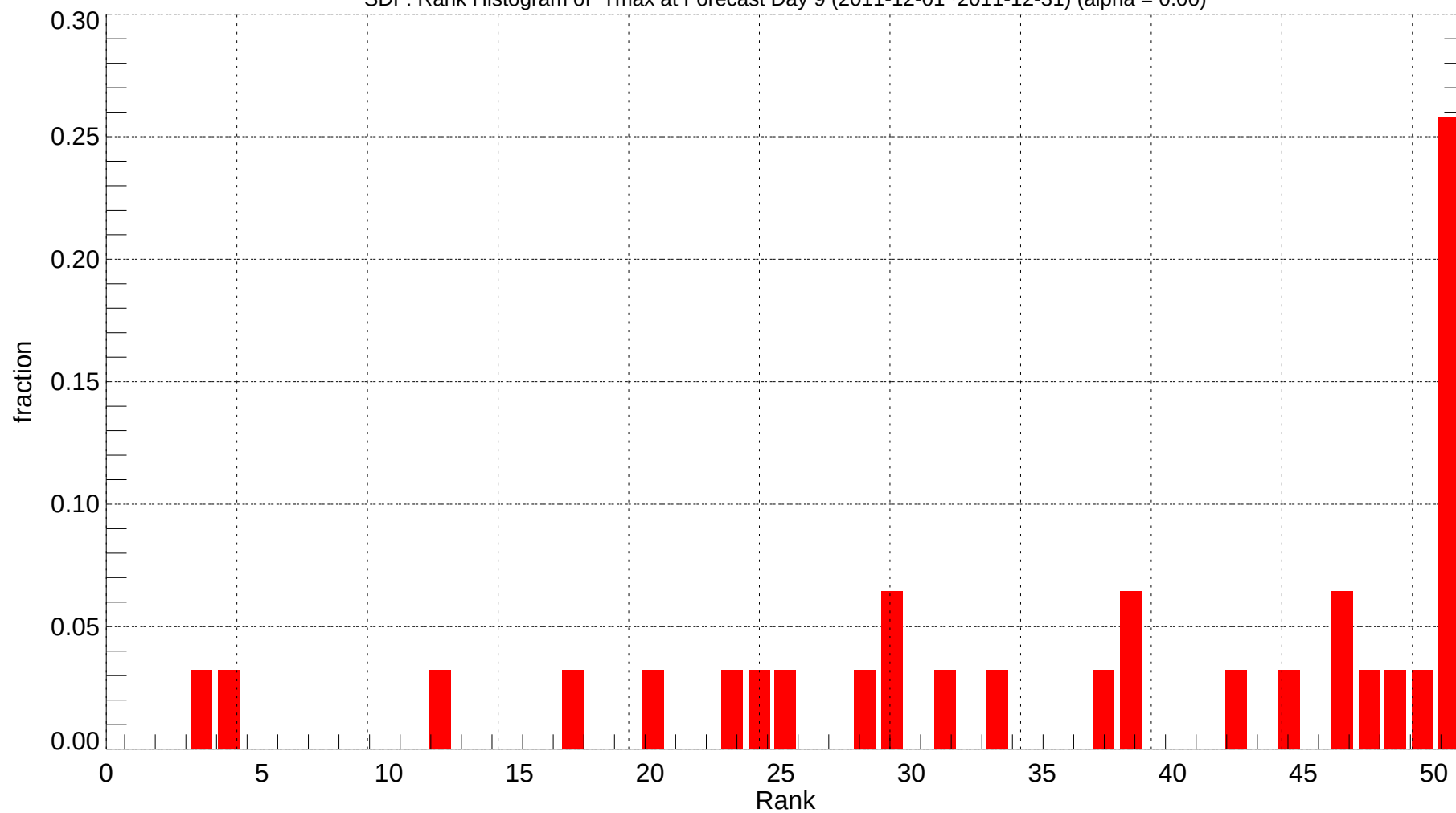
SDF: Rank Histogram of Tmax at Forecast Day 9 (2011-12-01~2011-12-31) (alpha = 0.00)
