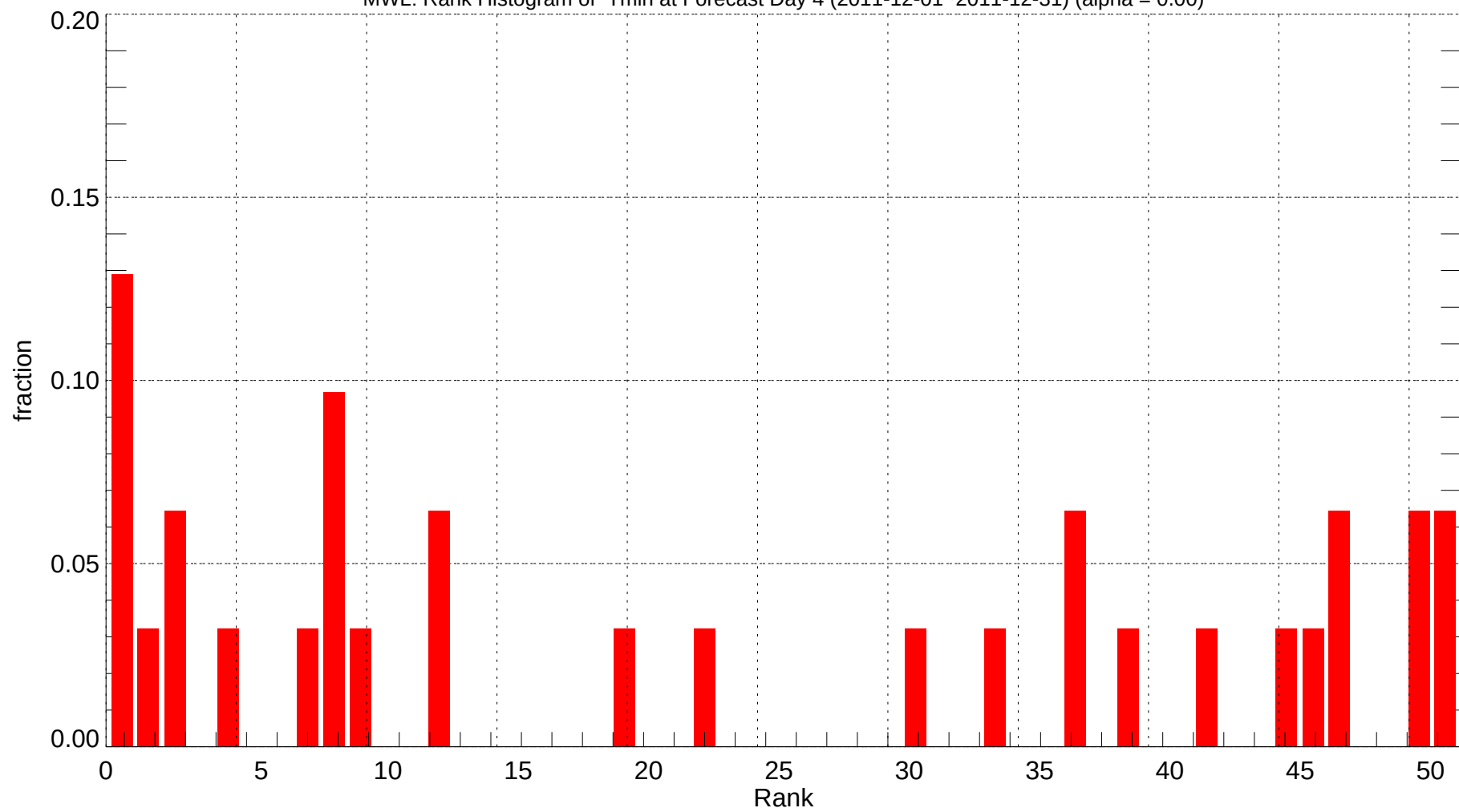
MWL: Rank Histogram of Tmin at Forecast Day 4 (2011-12-01~2011-12-31) (alpha = 0.00)
