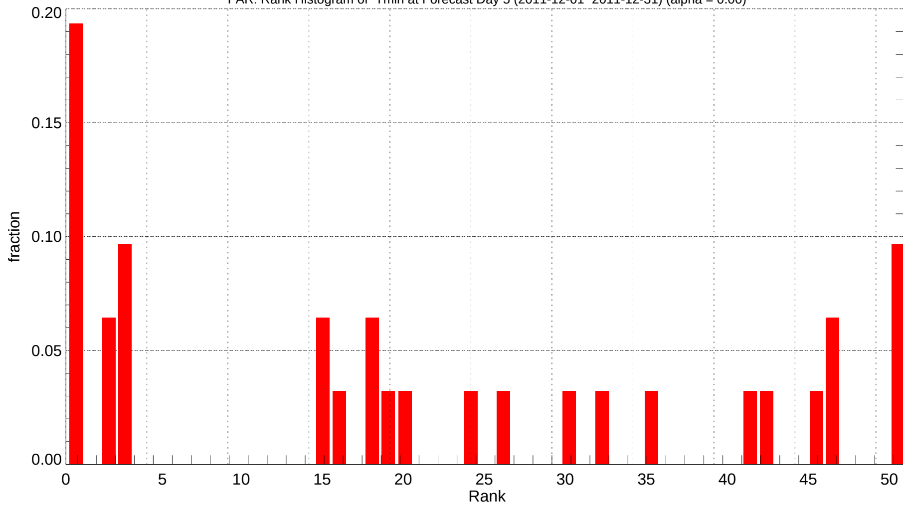
FAR: Rank Histogram of Tmin at Forecast Day 5 (2011-12-01~2011-12-31) (alpha = 0.00)
