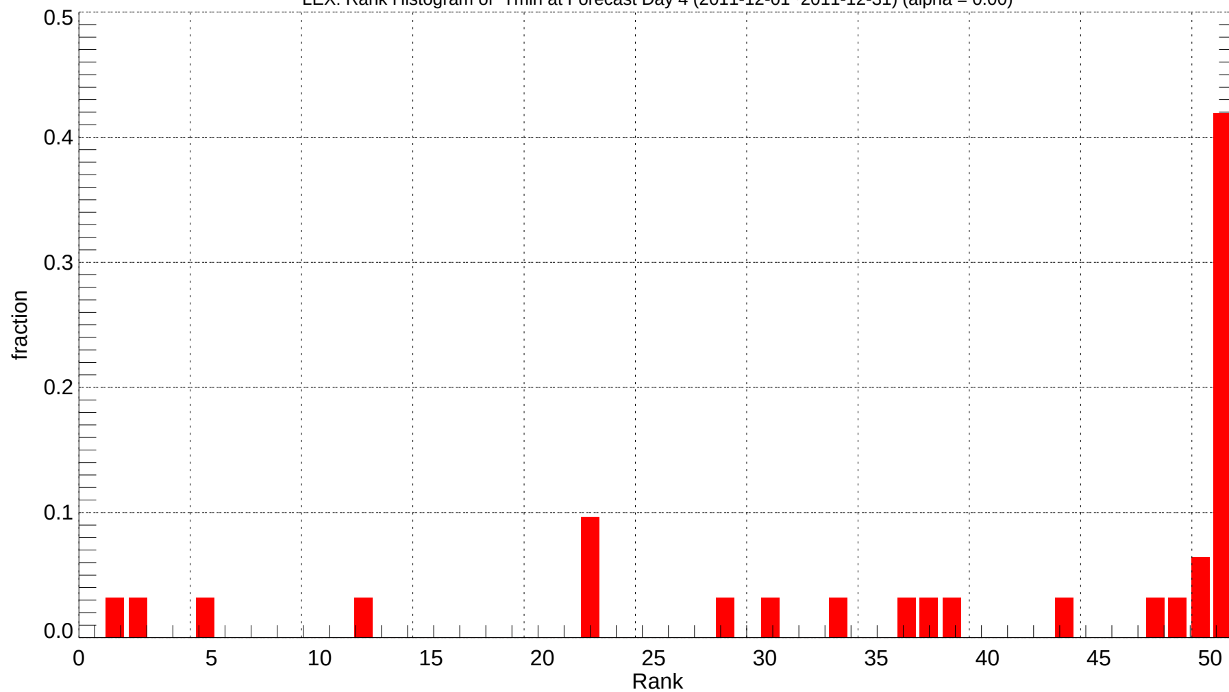
LEX: Rank Histogram of Tmin at Forecast Day 4 (2011-12-01~2011-12-31) (alpha = 0.00)
