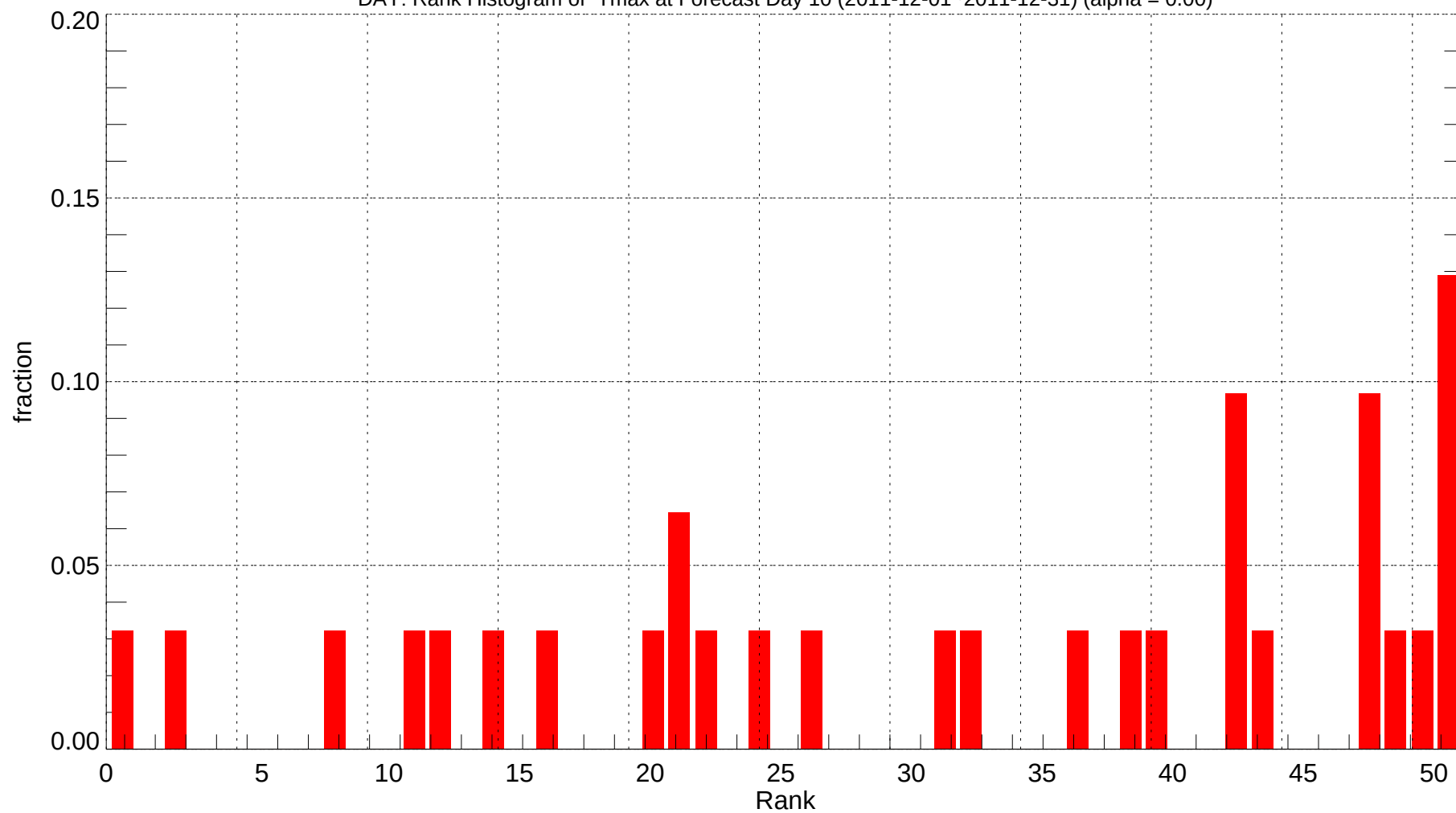
DAY: Rank Histogram of Tmax at Forecast Day 10 (2011-12-01~2011-12-31) (alpha = 0.00)
