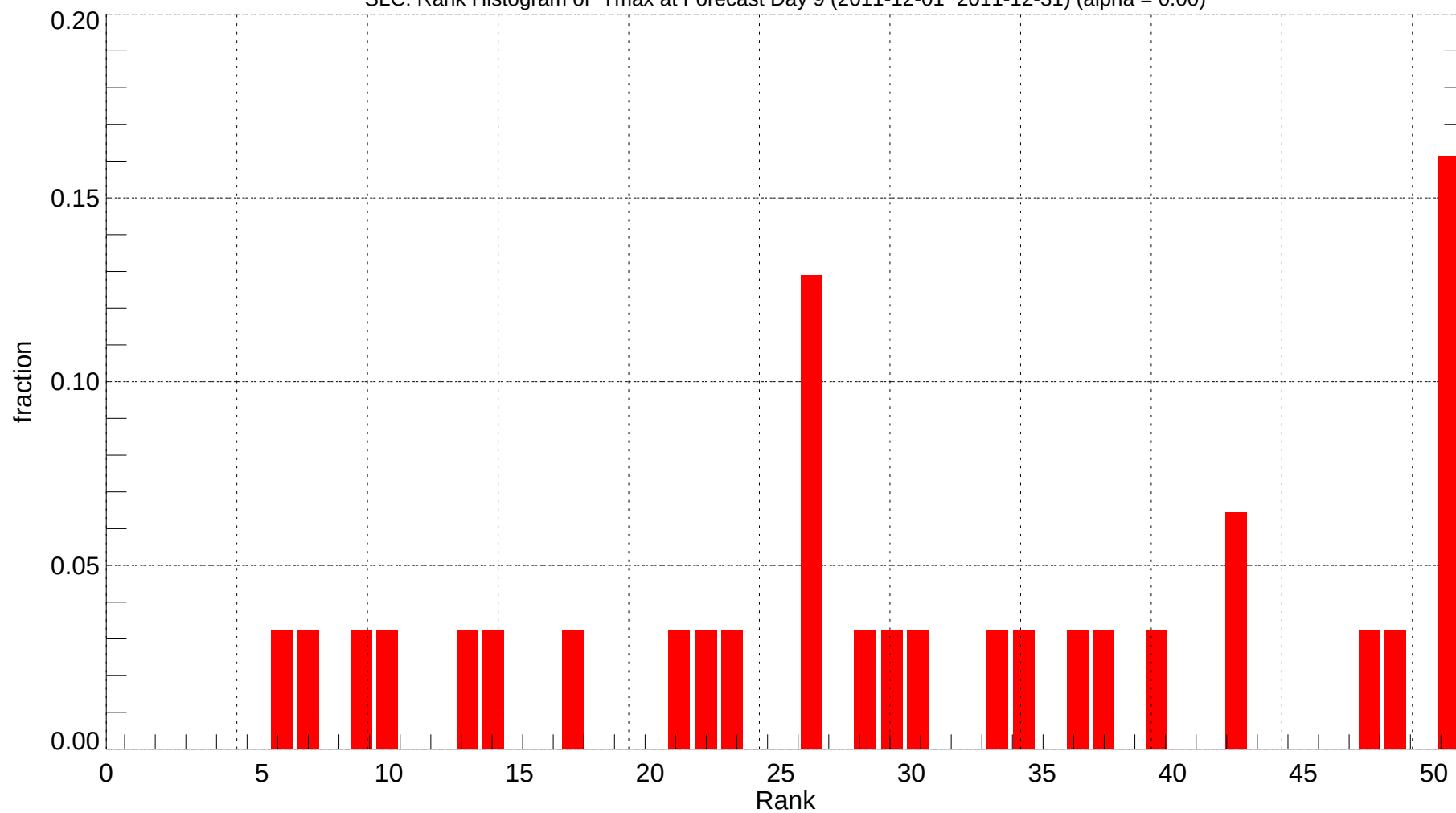
SLC: Rank Histogram of Tmax at Forecast Day 9 (2011-12-01~2011-12-31) (alpha = 0.00)
