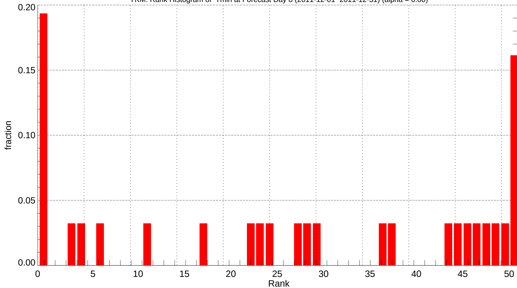
YKM: Rank Histogram of Tmin at Forecast Day 8 (2011-12-01~2011-12-31) (alpha = 0.00)
