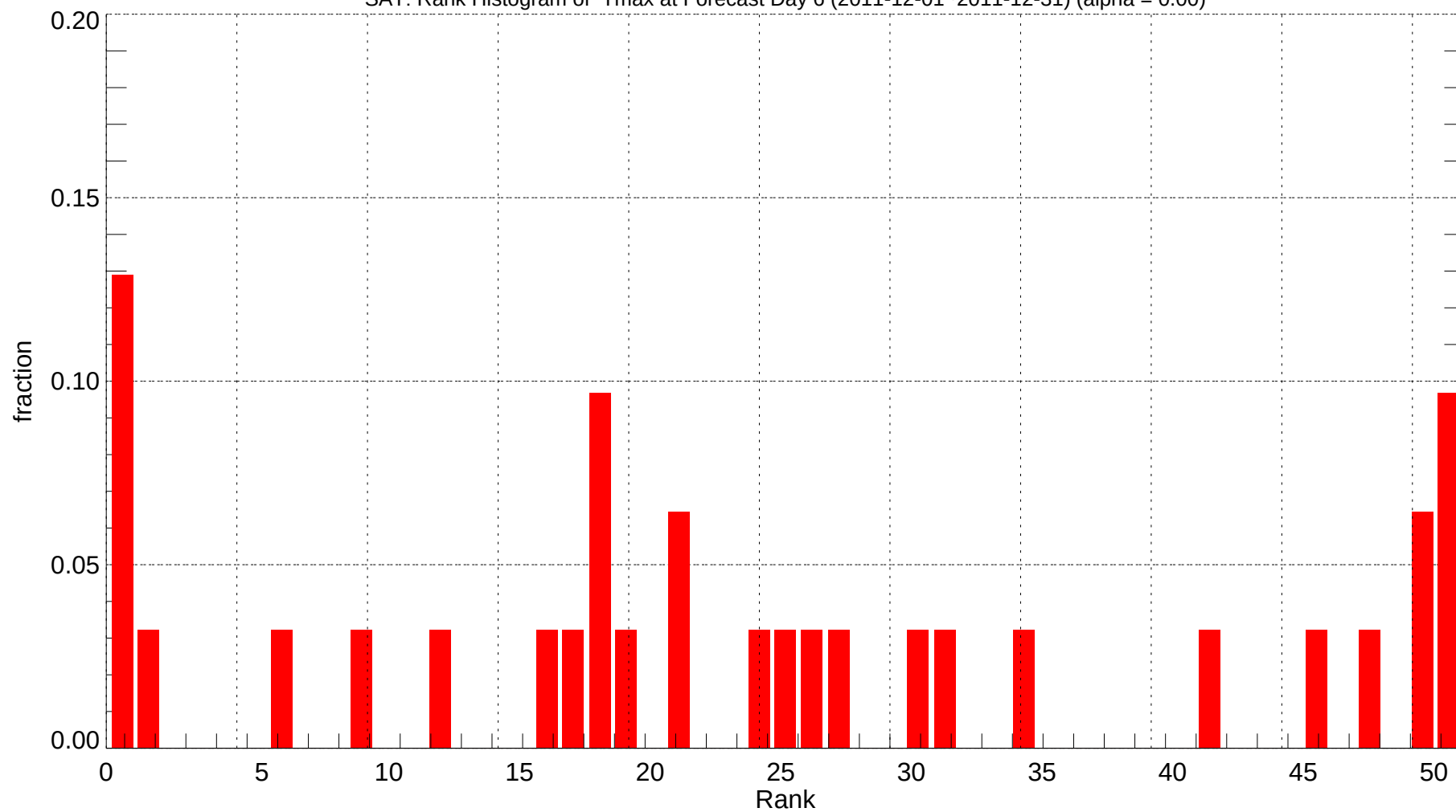
SAT: Rank Histogram of Tmax at Forecast Day 6 (2011-12-01~2011-12-31) (alpha = 0.00)
