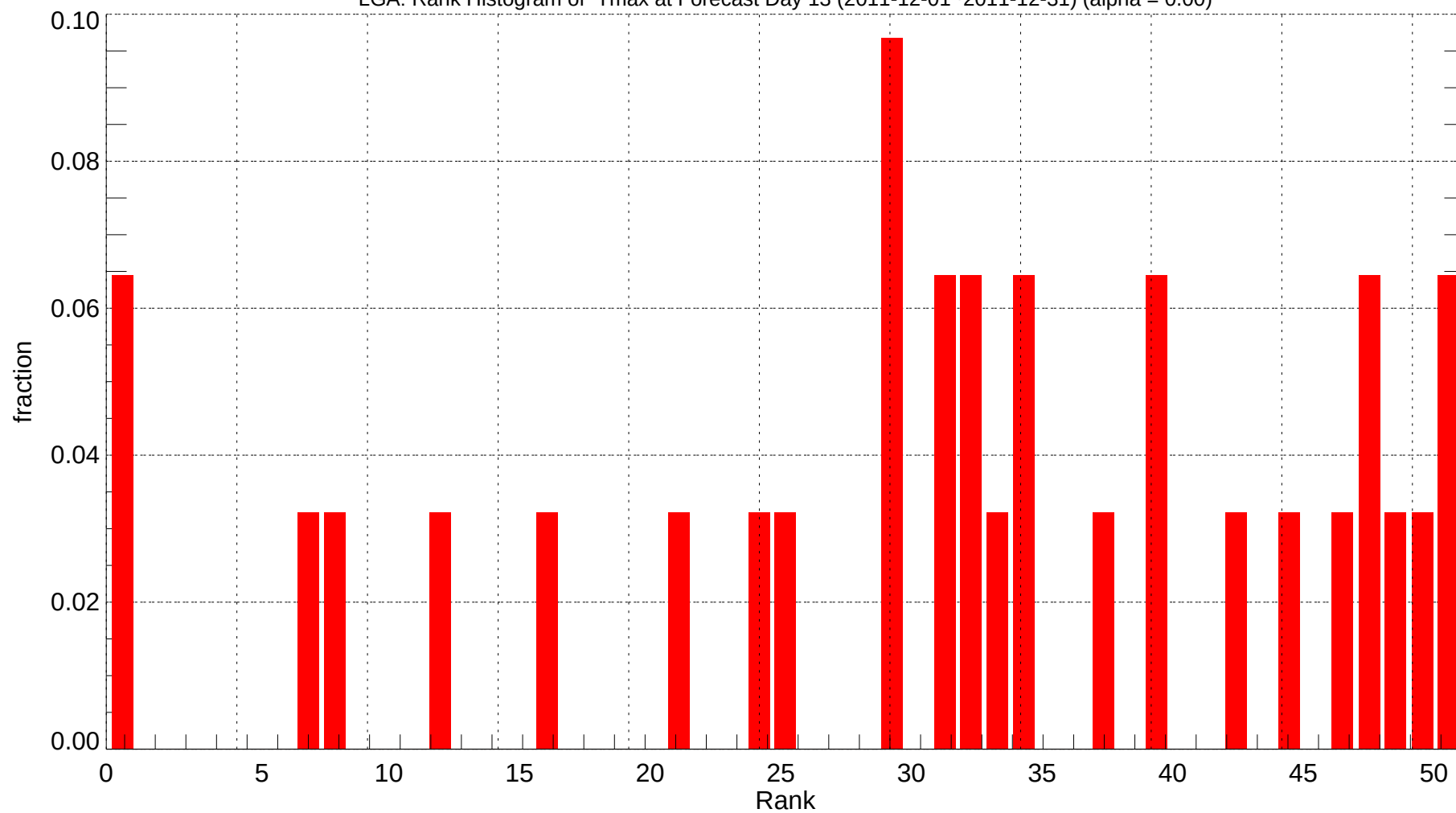
LGA: Rank Histogram of Tmax at Forecast Day 13 (2011-12-01~2011-12-31) (alpha = 0.00)
