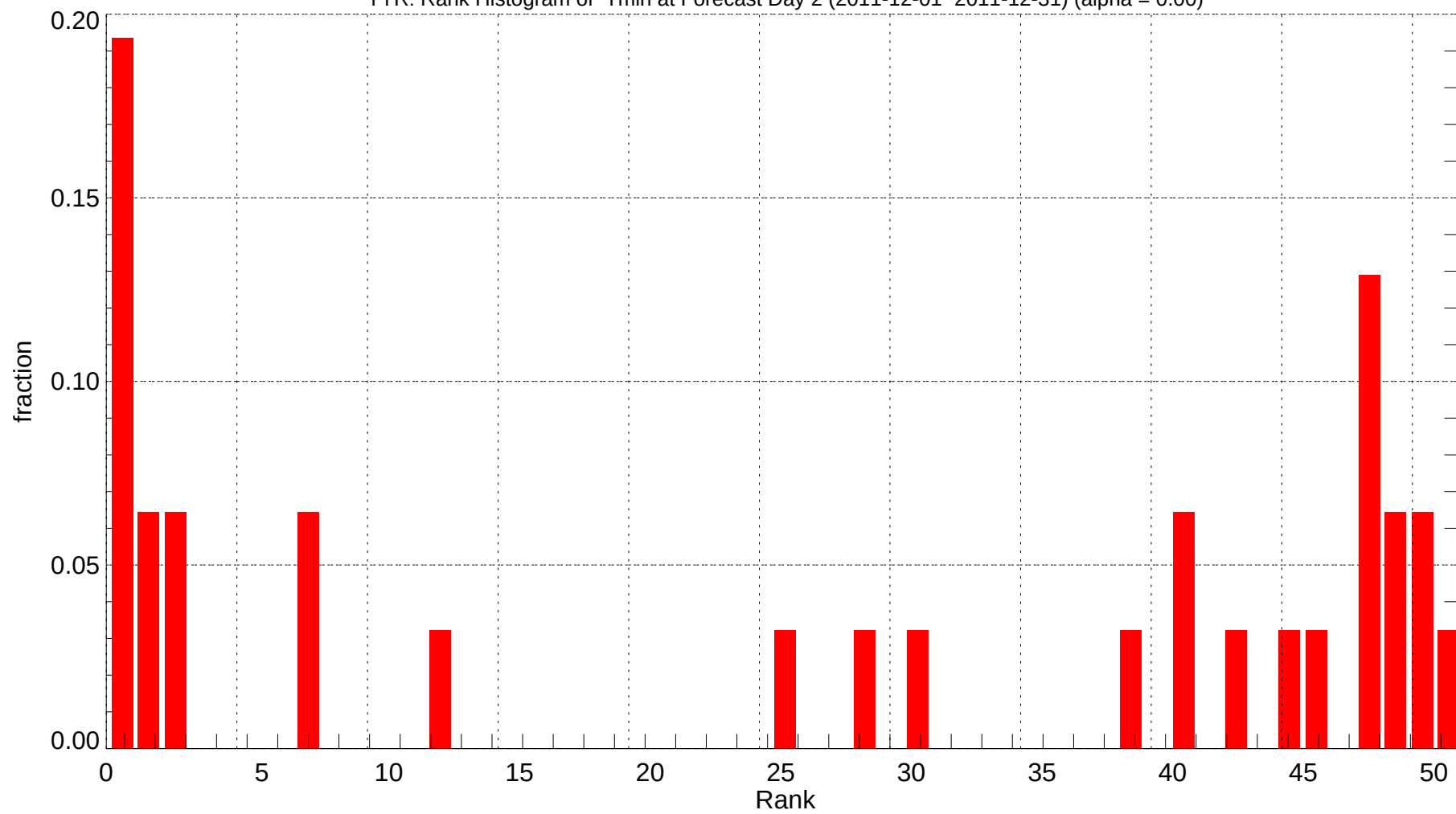
TYR: Rank Histogram of Tmin at Forecast Day 2 (2011-12-01~2011-12-31) (alpha = 0.00)
