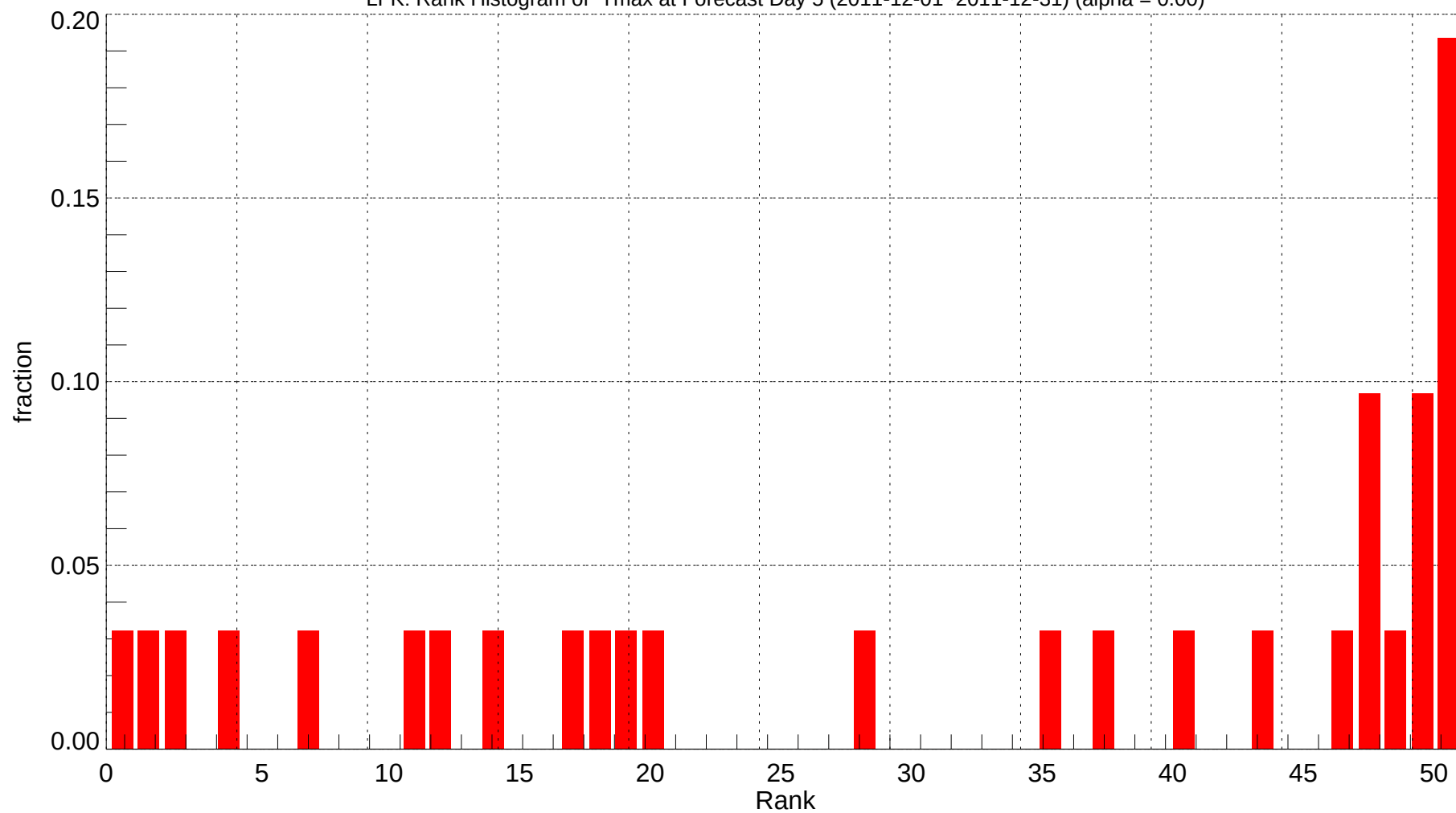
LFK: Rank Histogram of Tmax at Forecast Day 5 (2011-12-01~2011-12-31) (alpha = 0.00)
