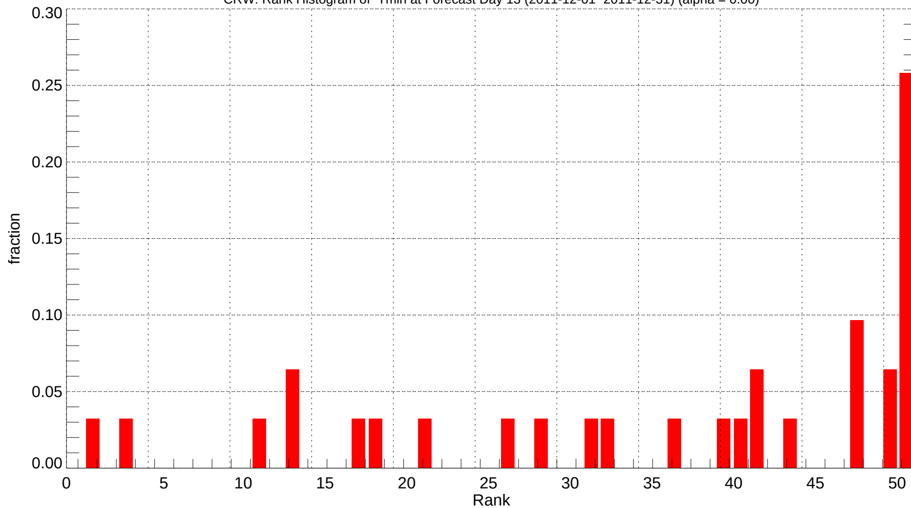
CRW: Rank Histogram of Tmin at Forecast Day 13 (2011-12-01~2011-12-31) (alpha = 0.00)
