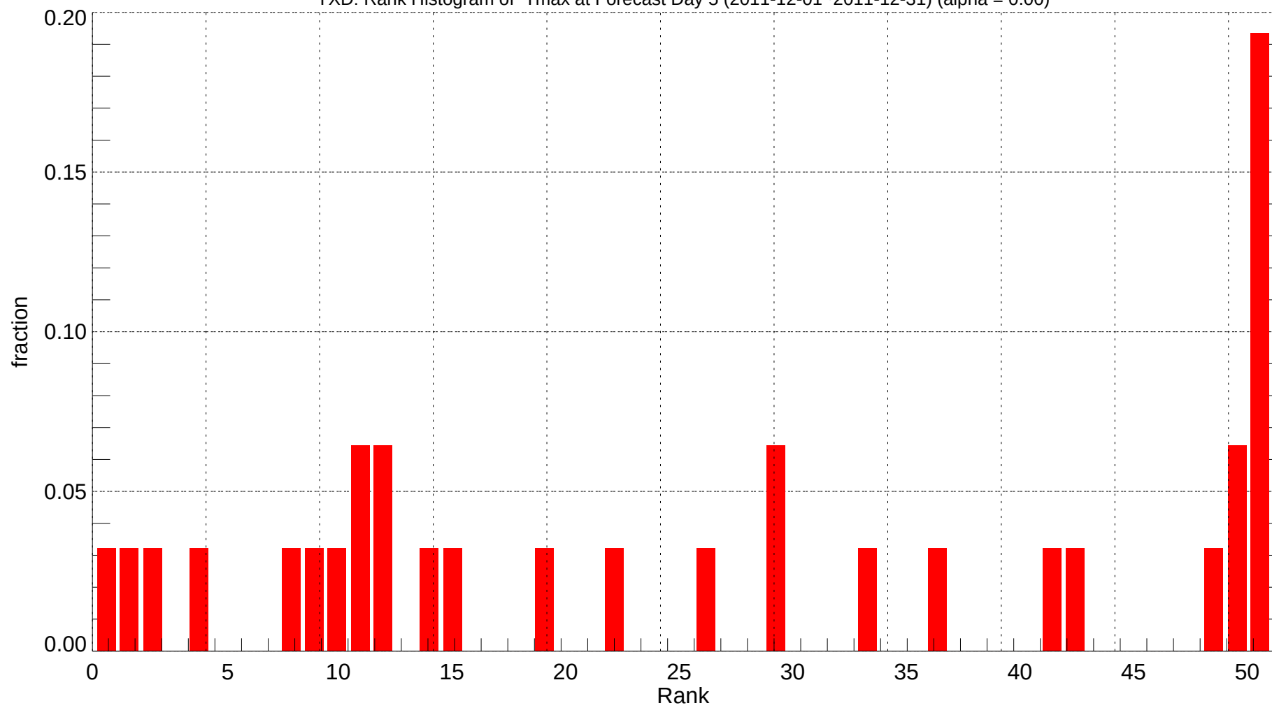
YXD: Rank Histogram of Tmax at Forecast Day 5 (2011-12-01~2011-12-31) (alpha = 0.00)
