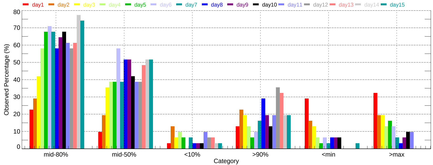
Observed Percentage of Ensembles - EWR: Max Temperature (2011-12-01~2011-12-31)
