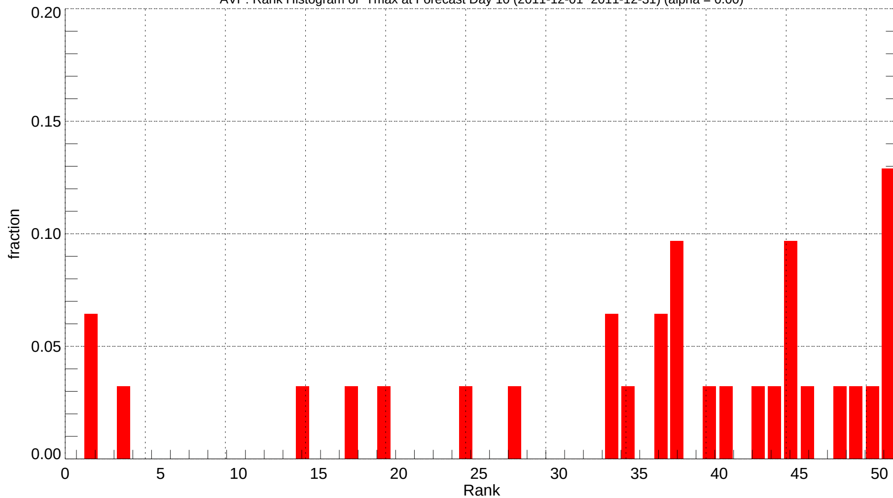
AVP: Rank Histogram of Tmax at Forecast Day 10 (2011-12-01~2011-12-31) (alpha = 0.00)
