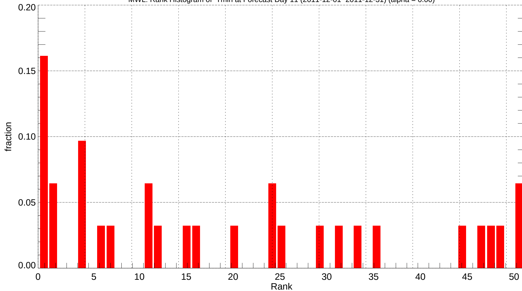
MWL: Rank Histogram of Tmin at Forecast Day 11 (2011-12-01~2011-12-31) (alpha = 0.00)
