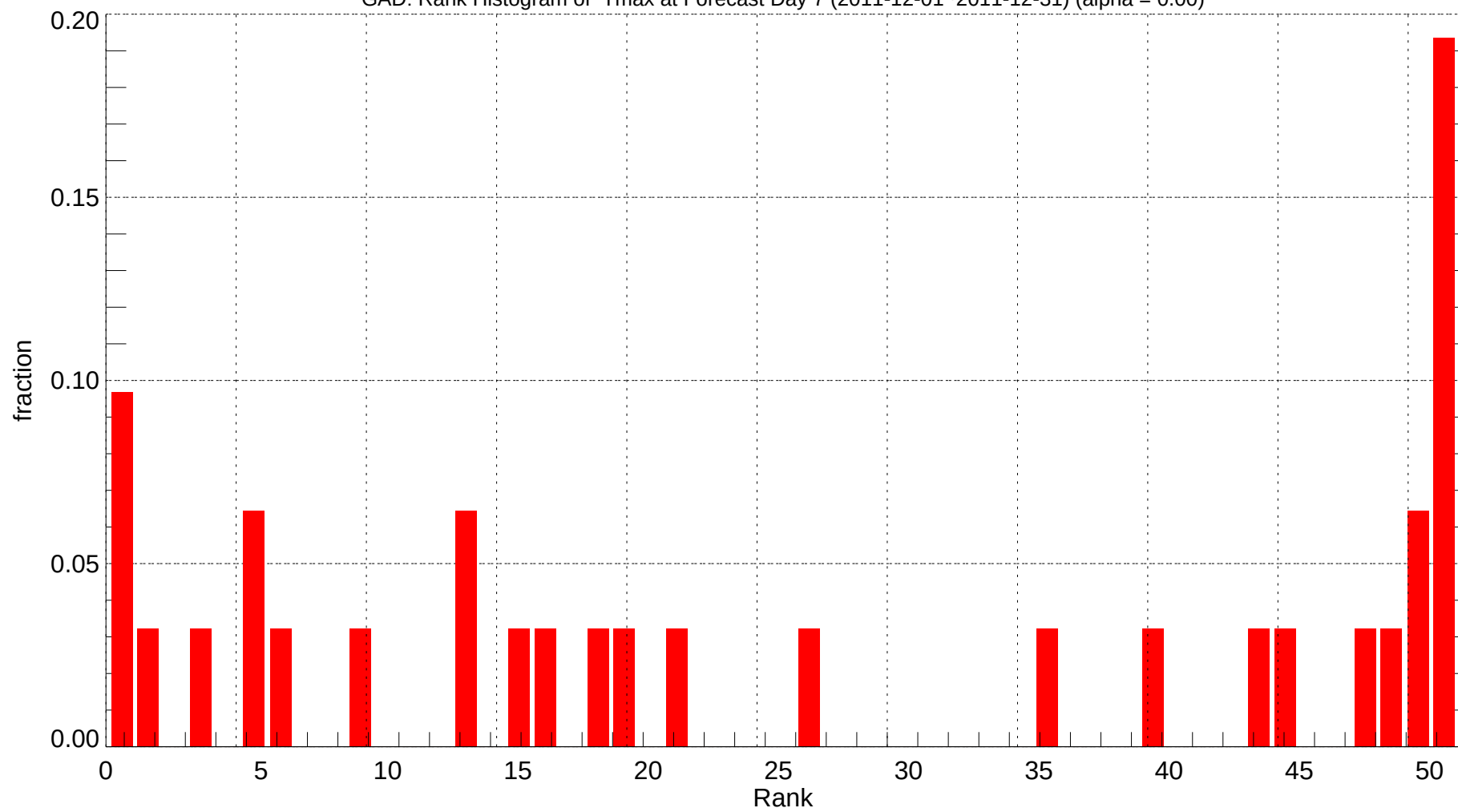
GAD: Rank Histogram of Tmax at Forecast Day 7 (2011-12-01~2011-12-31) (alpha = 0.00)
