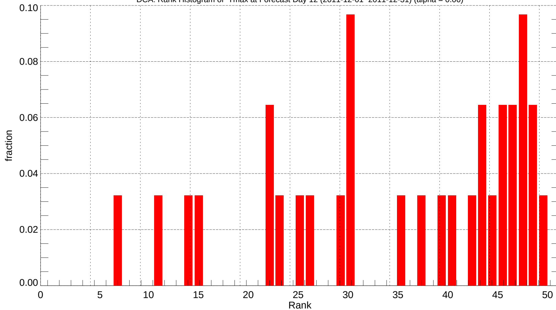
DCA: Rank Histogram of Tmax at Forecast Day 12 (2011-12-01~2011-12-31) (alpha = 0.00)
