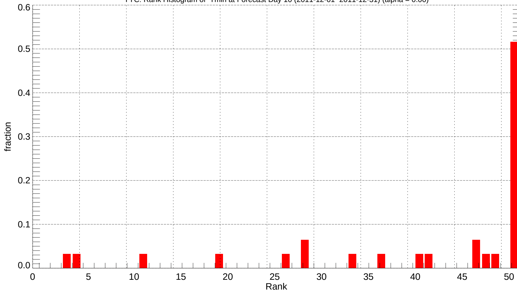
YYC: Rank Histogram of Tmin at Forecast Day 10 (2011-12-01~2011-12-31) (alpha = 0.00)
