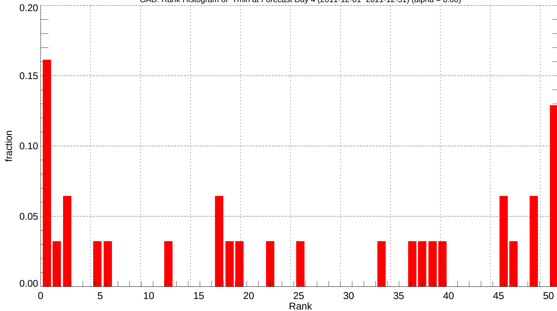
GAD: Rank Histogram of Tmin at Forecast Day 4 (2011-12-01~2011-12-31) (alpha = 0.00)
