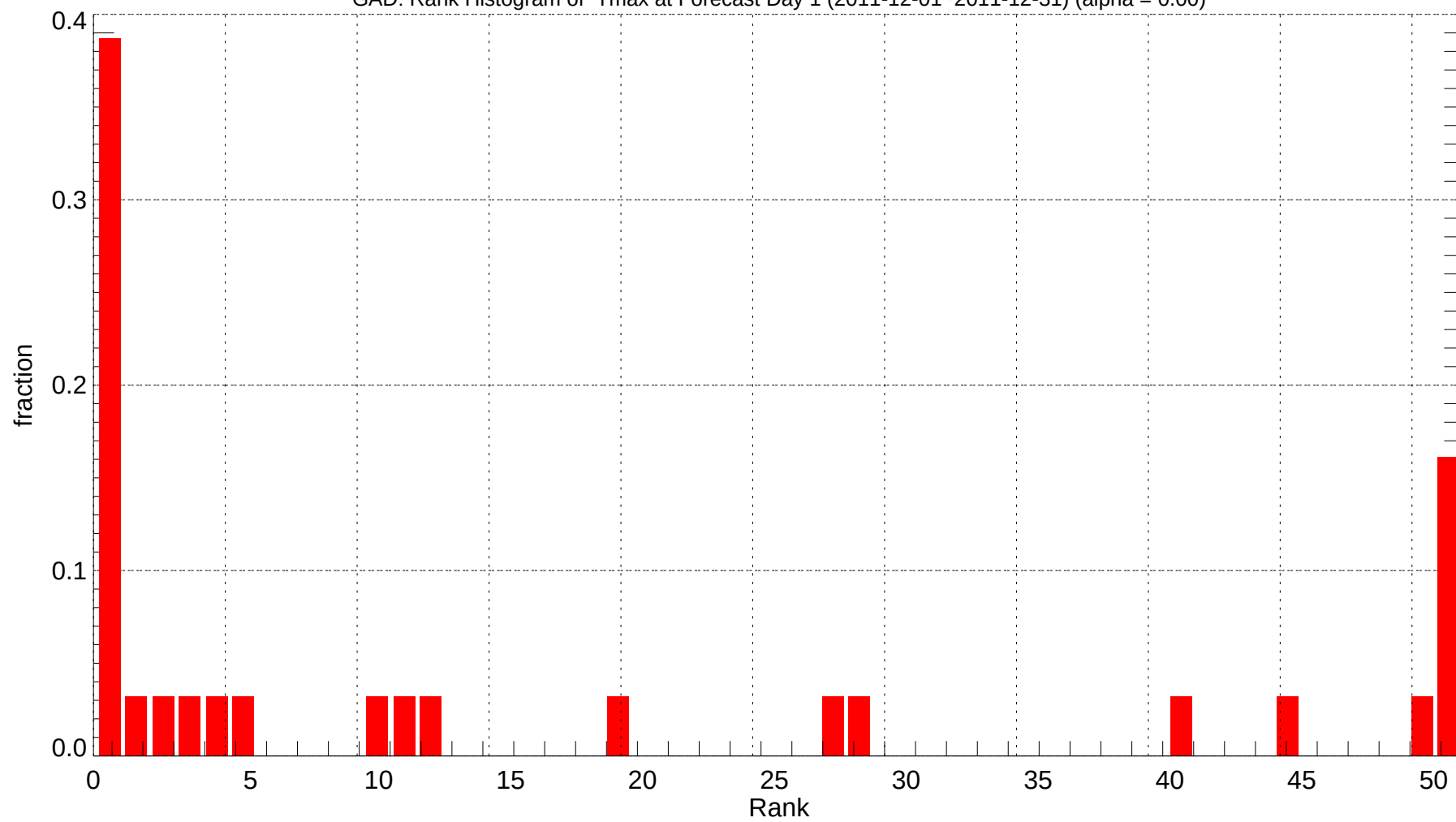
GAD: Rank Histogram of Tmax at Forecast Day 1 (2011-12-01~2011-12-31) (alpha = 0.00)
