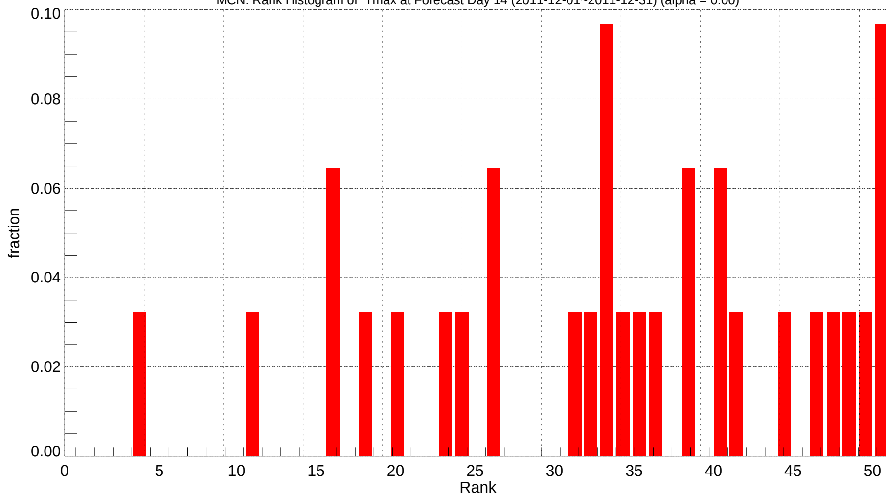
MCN: Rank Histogram of Tmax at Forecast Day 14 (2011-12-01~2011-12-31) (alpha = 0.00)
