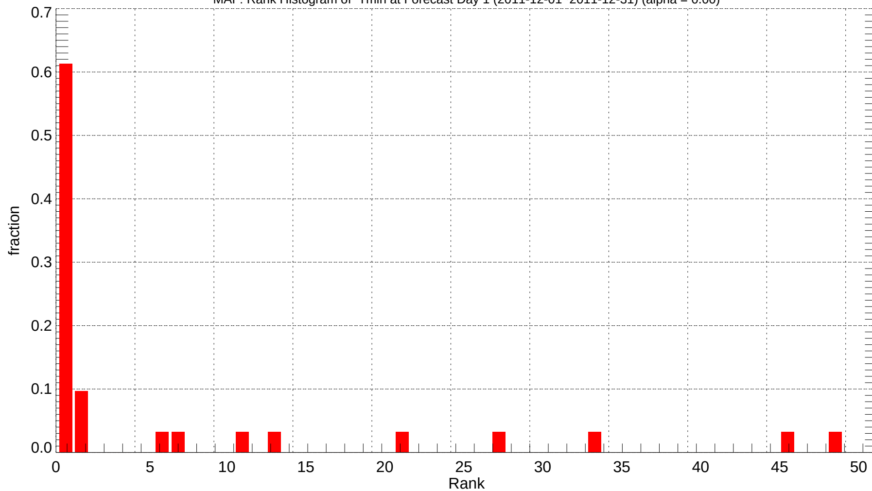
MAF: Rank Histogram of Tmin at Forecast Day 1 (2011-12-01~2011-12-31) (alpha = 0.00)
