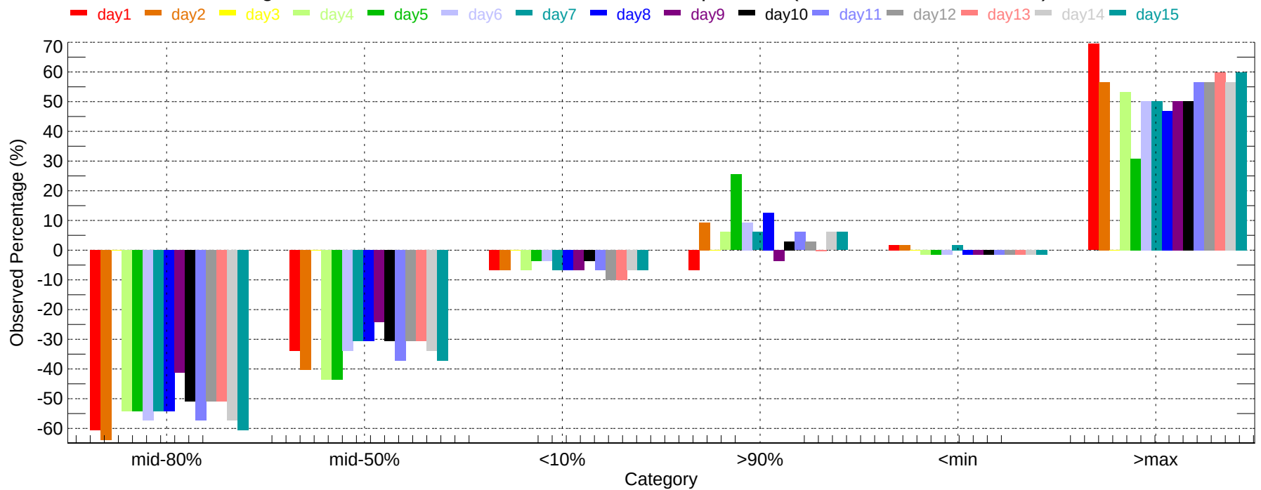
Observed Percentage Deviation of Ensembles - YYC: Max Temperature (2011-12-01~2011-12-31)
