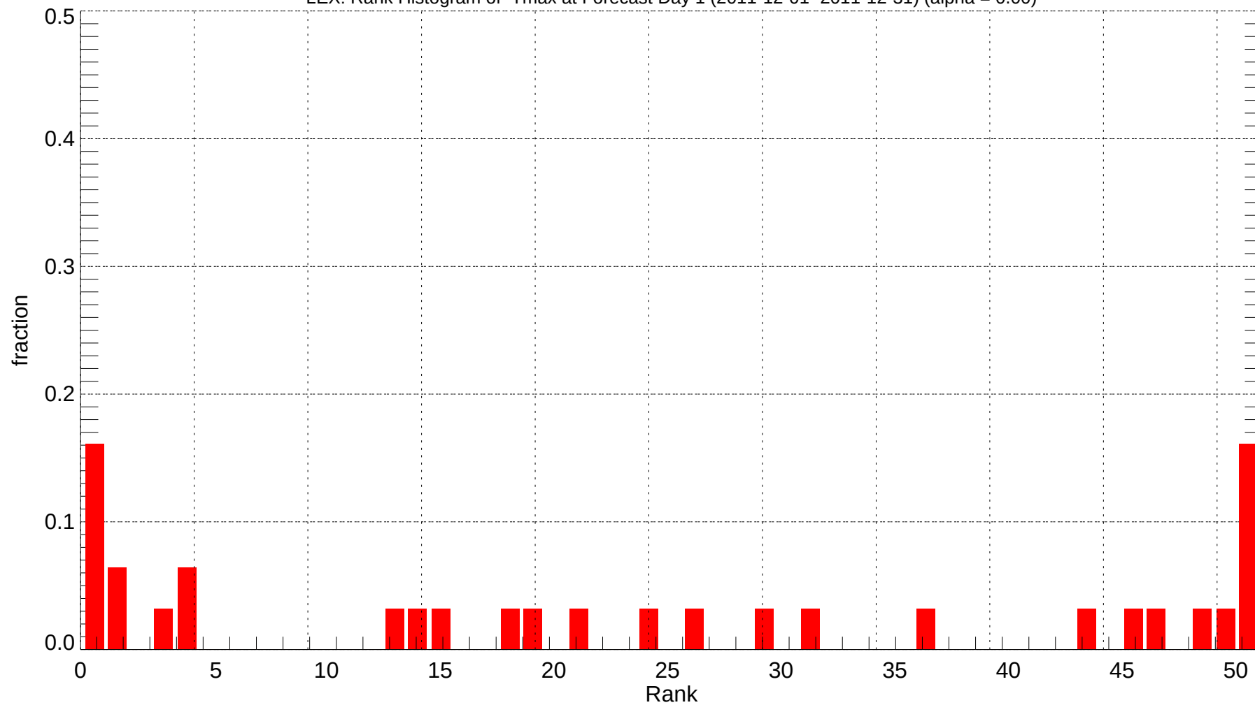
LEX: Rank Histogram of Tmax at Forecast Day 1 (2011-12-01~2011-12-31) (alpha = 0.00)
