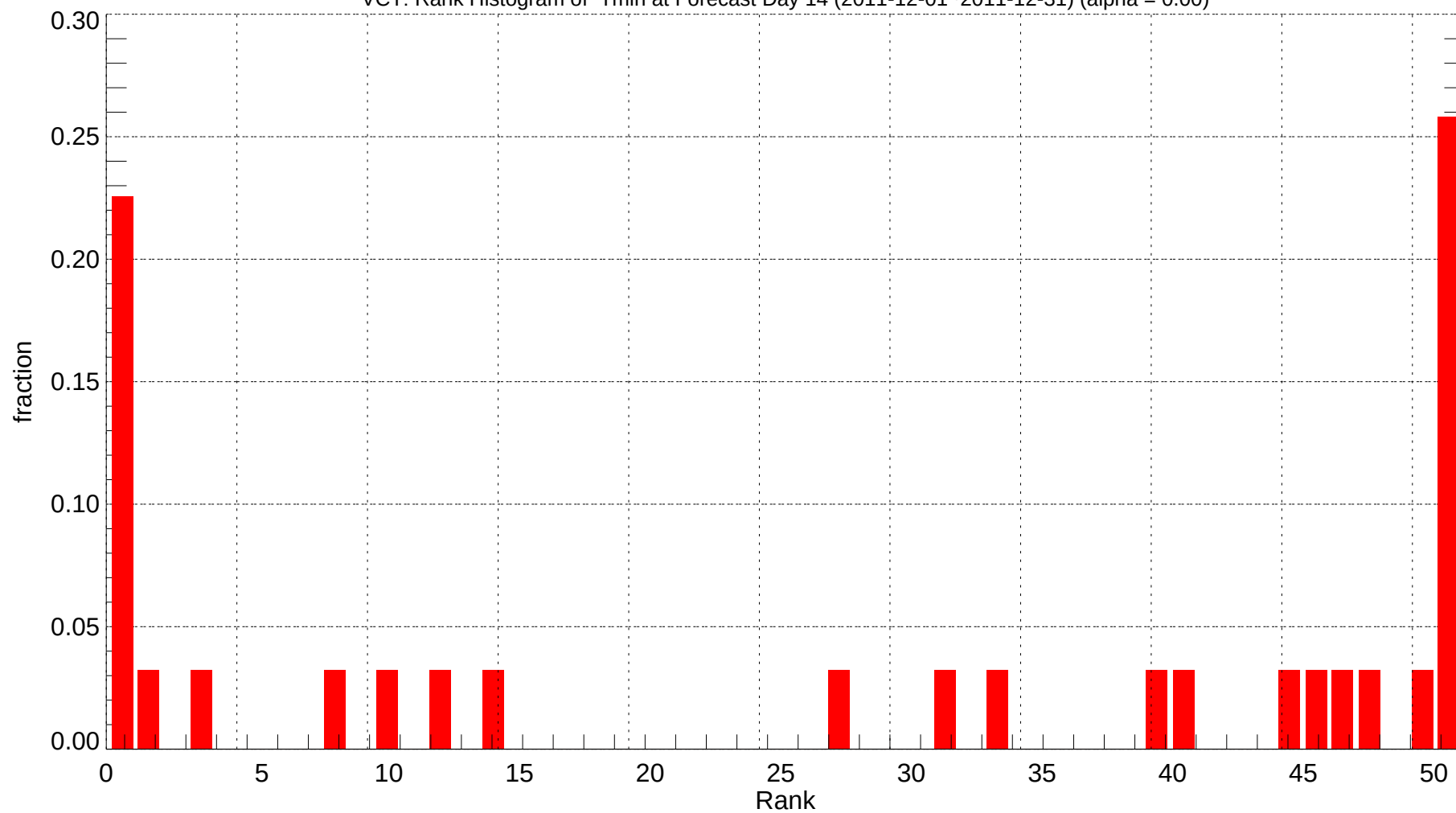
VCT: Rank Histogram of Tmin at Forecast Day 14 (2011-12-01~2011-12-31) (alpha = 0.00)
