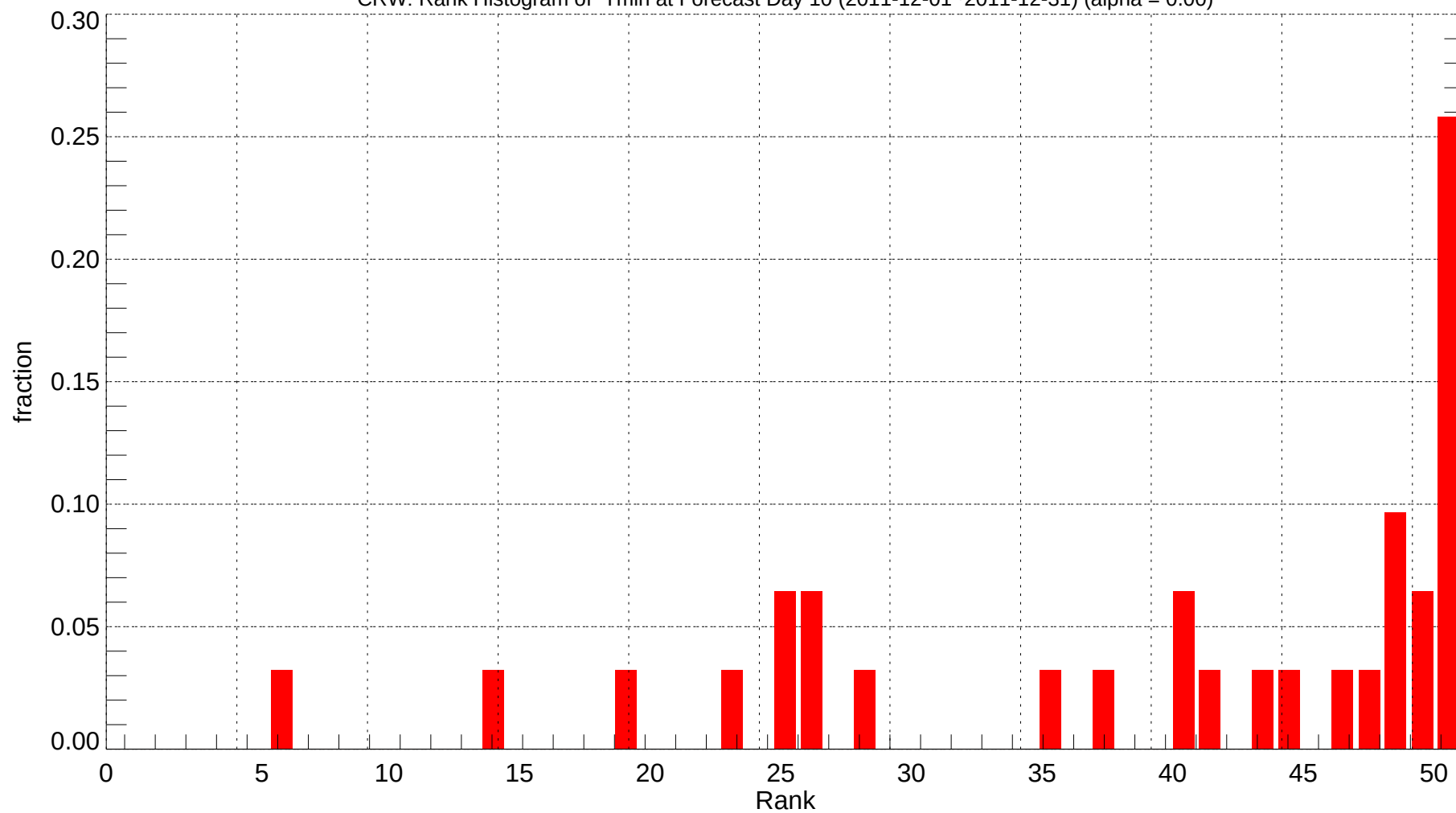
CRW: Rank Histogram of Tmin at Forecast Day 10 (2011-12-01~2011-12-31) (alpha = 0.00)
