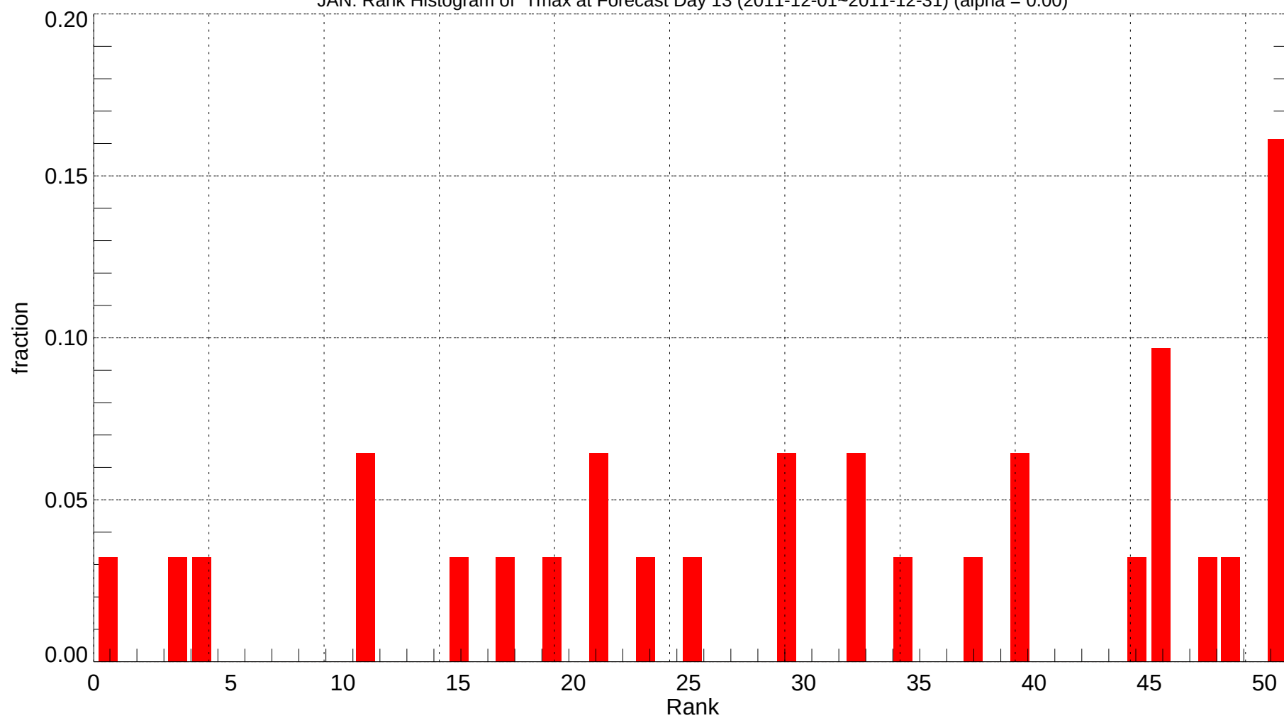
JAN: Rank Histogram of Tmax at Forecast Day 13 (2011-12-01~2011-12-31) (alpha = 0.00)
