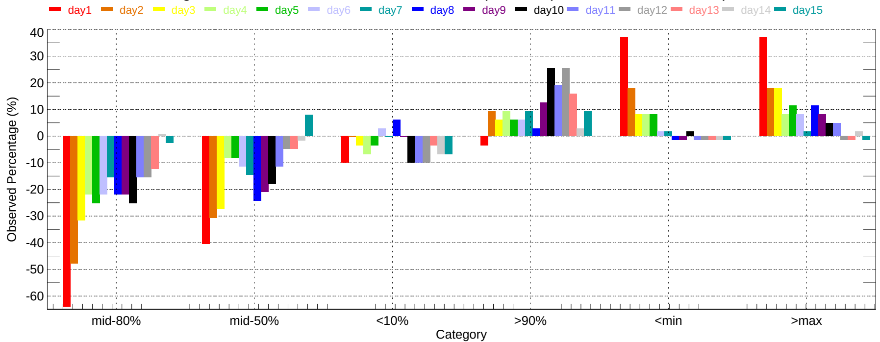
Observed Percentage Deviation of Ensembles - BNA: Min Temperature (2011-12-01~2011-12-31)
