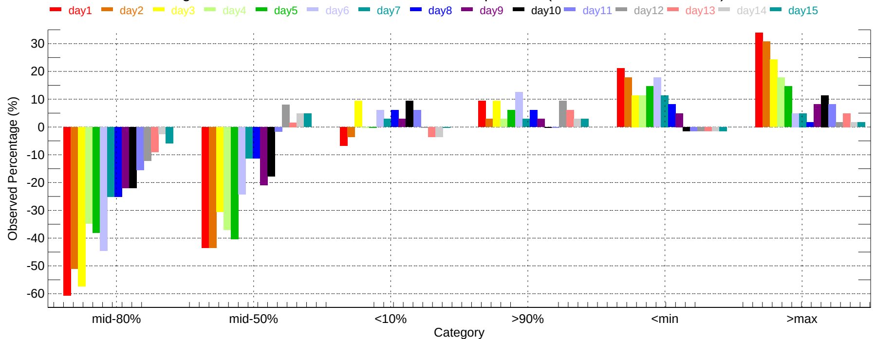
Observed Percentage Deviation of Ensembles - MHT: Min Temperature (2011-12-01~2011-12-31)
