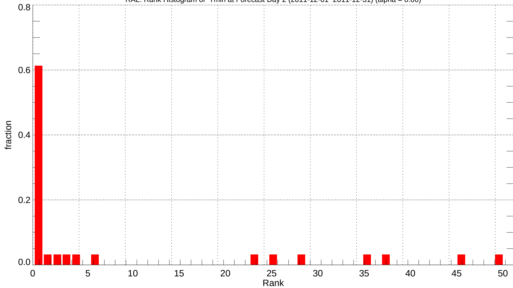
RAL: Rank Histogram of Tmin at Forecast Day 2 (2011-12-01~2011-12-31) (alpha = 0.00)
