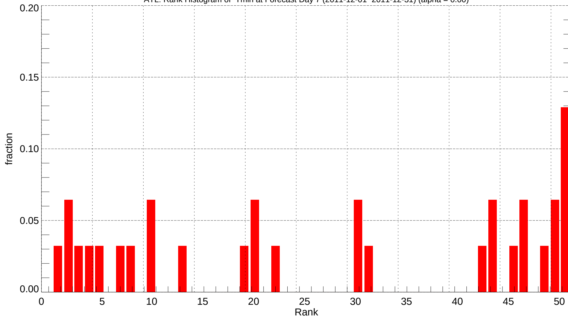
ATL: Rank Histogram of Tmin at Forecast Day 7 (2011-12-01~2011-12-31) (alpha = 0.00)
