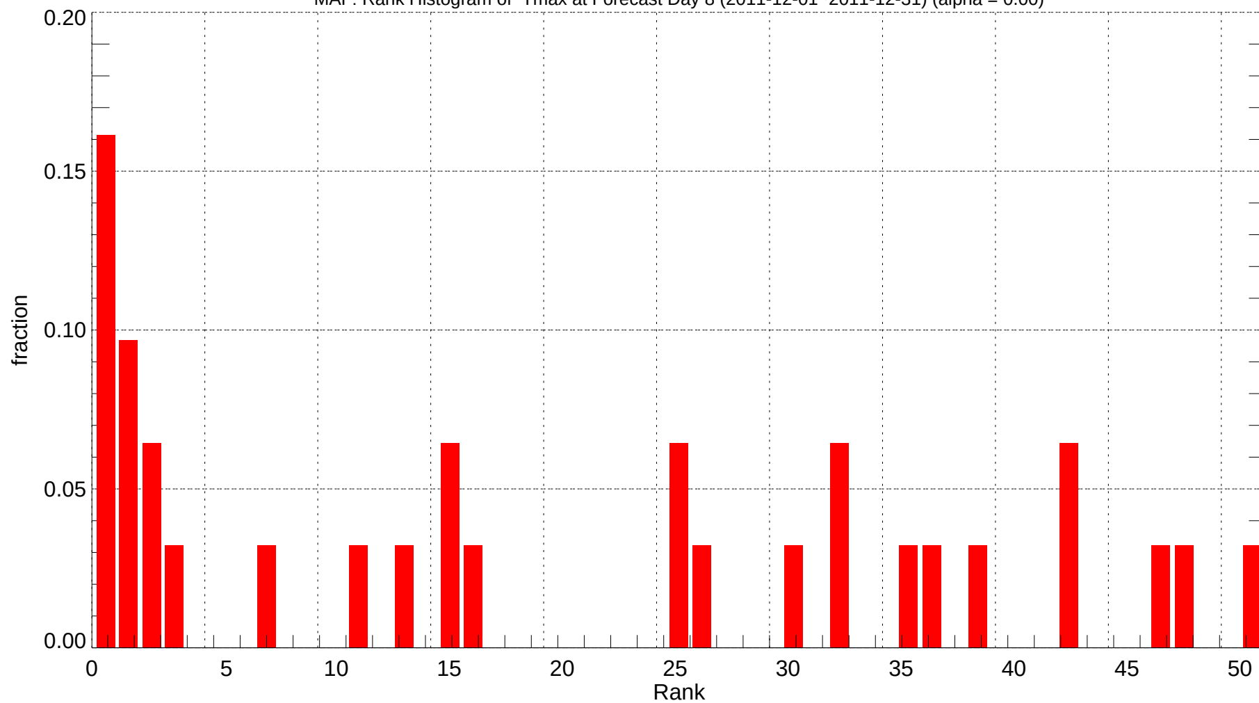
MAF: Rank Histogram of Tmax at Forecast Day 8 (2011-12-01~2011-12-31) (alpha = 0.00)
