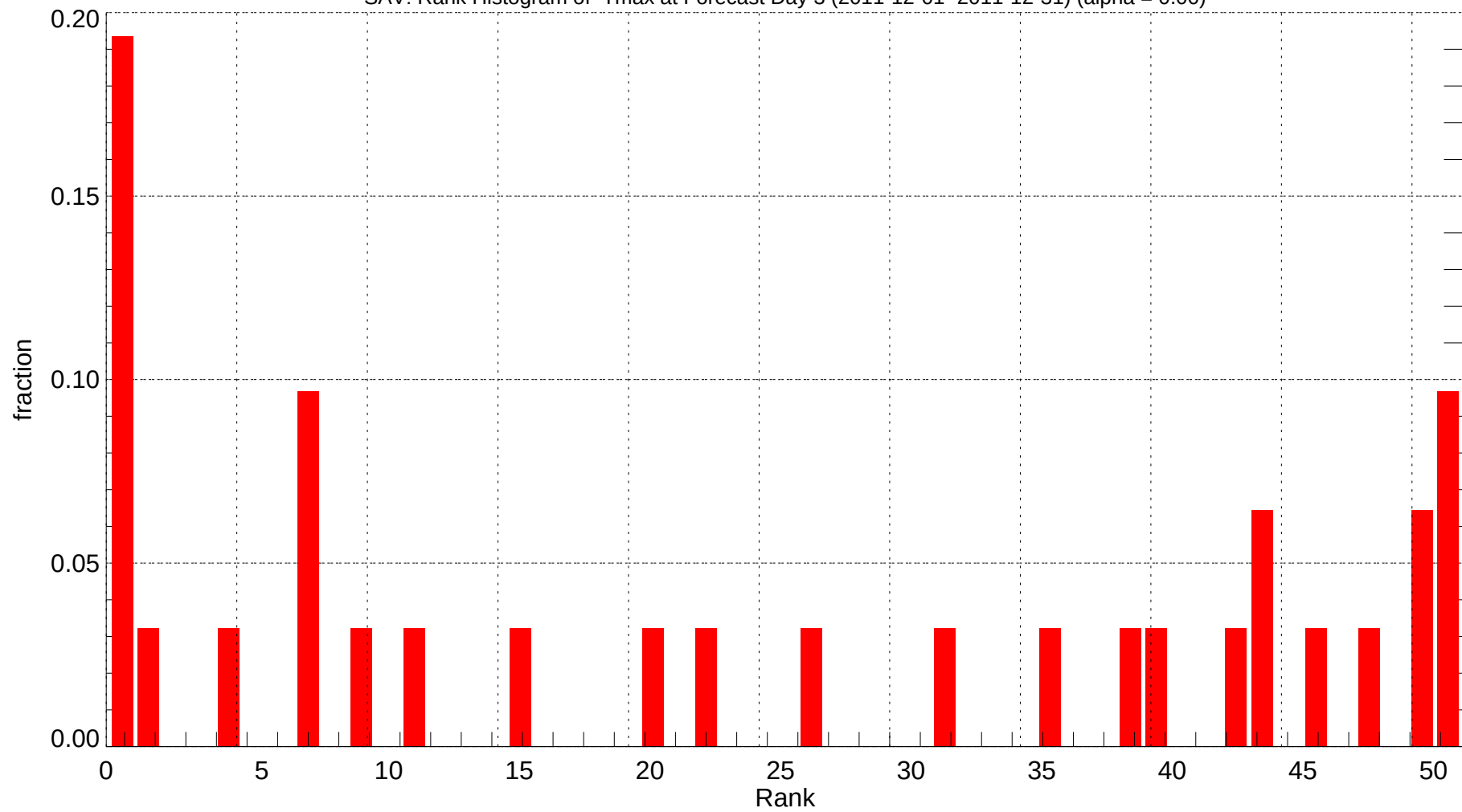
SAV: Rank Histogram of Tmax at Forecast Day 3 (2011-12-01~2011-12-31) (alpha = 0.00)
