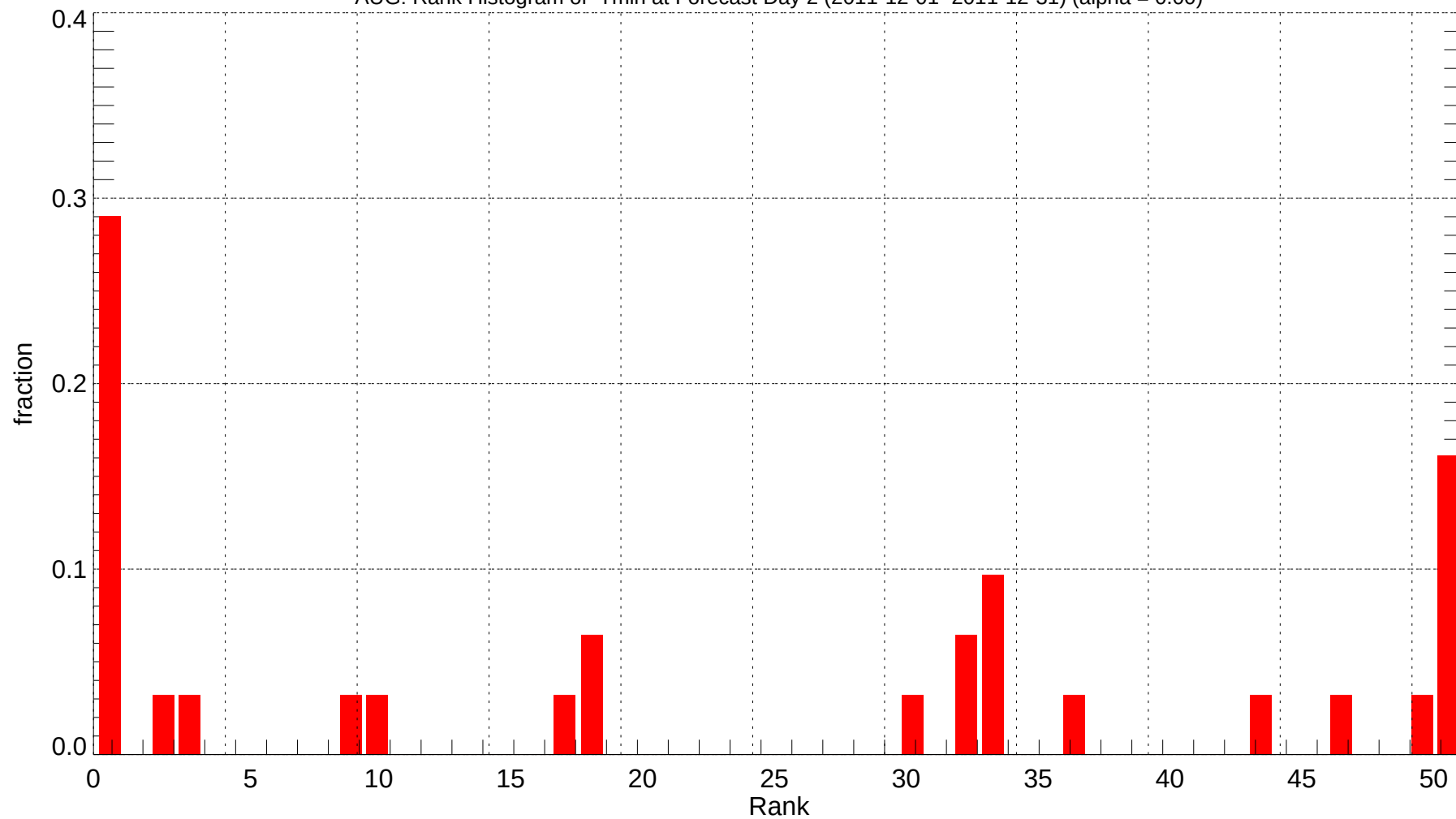
AUG: Rank Histogram of Tmin at Forecast Day 2 (2011-12-01~2011-12-31) (alpha = 0.00)
