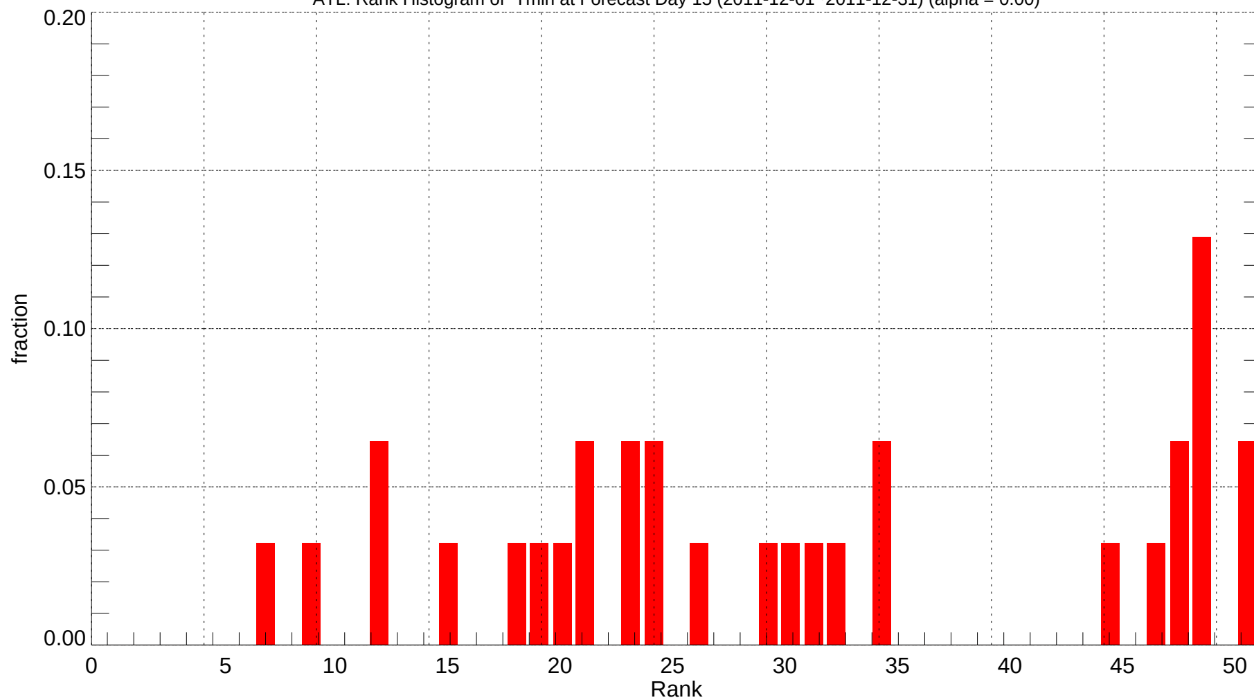
ATL: Rank Histogram of Tmin at Forecast Day 15 (2011-12-01~2011-12-31) (alpha = 0.00)
