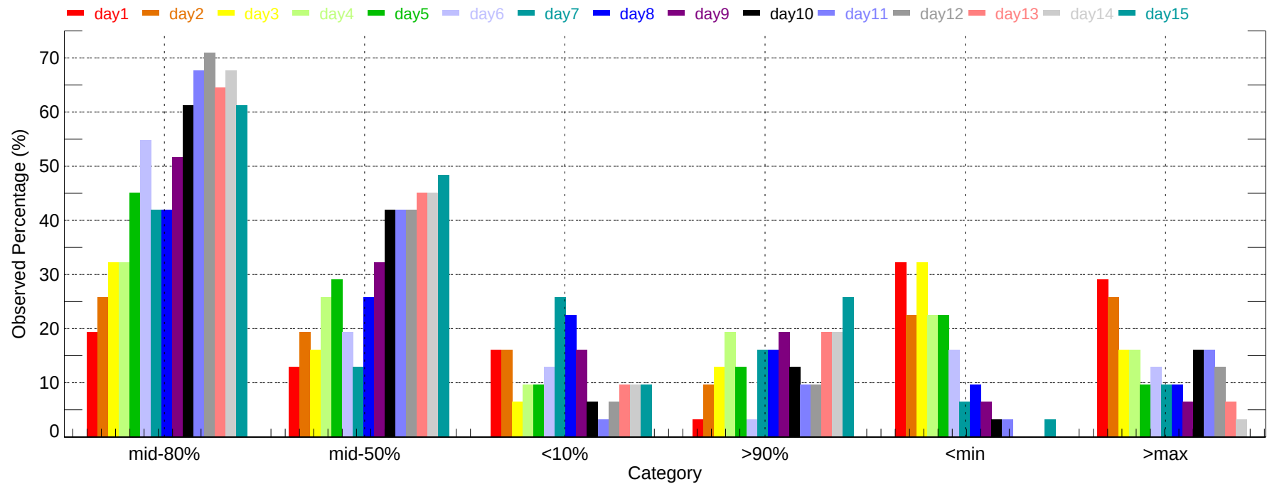
Observed Percentage of Ensembles - APN: Max Temperature (2011-12-01~2011-12-31)
