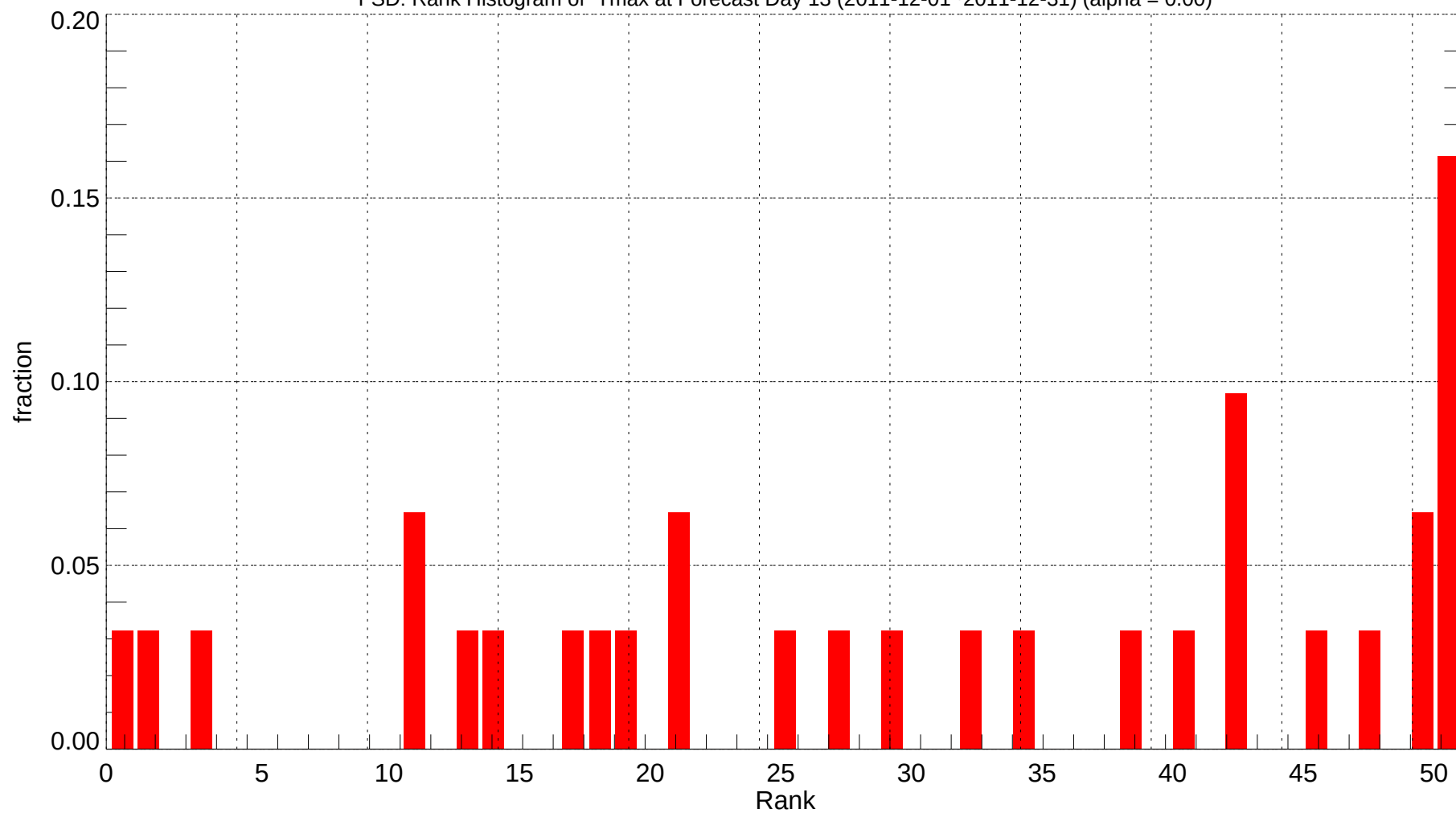
FSD: Rank Histogram of Tmax at Forecast Day 13 (2011-12-01~2011-12-31) (alpha = 0.00)
