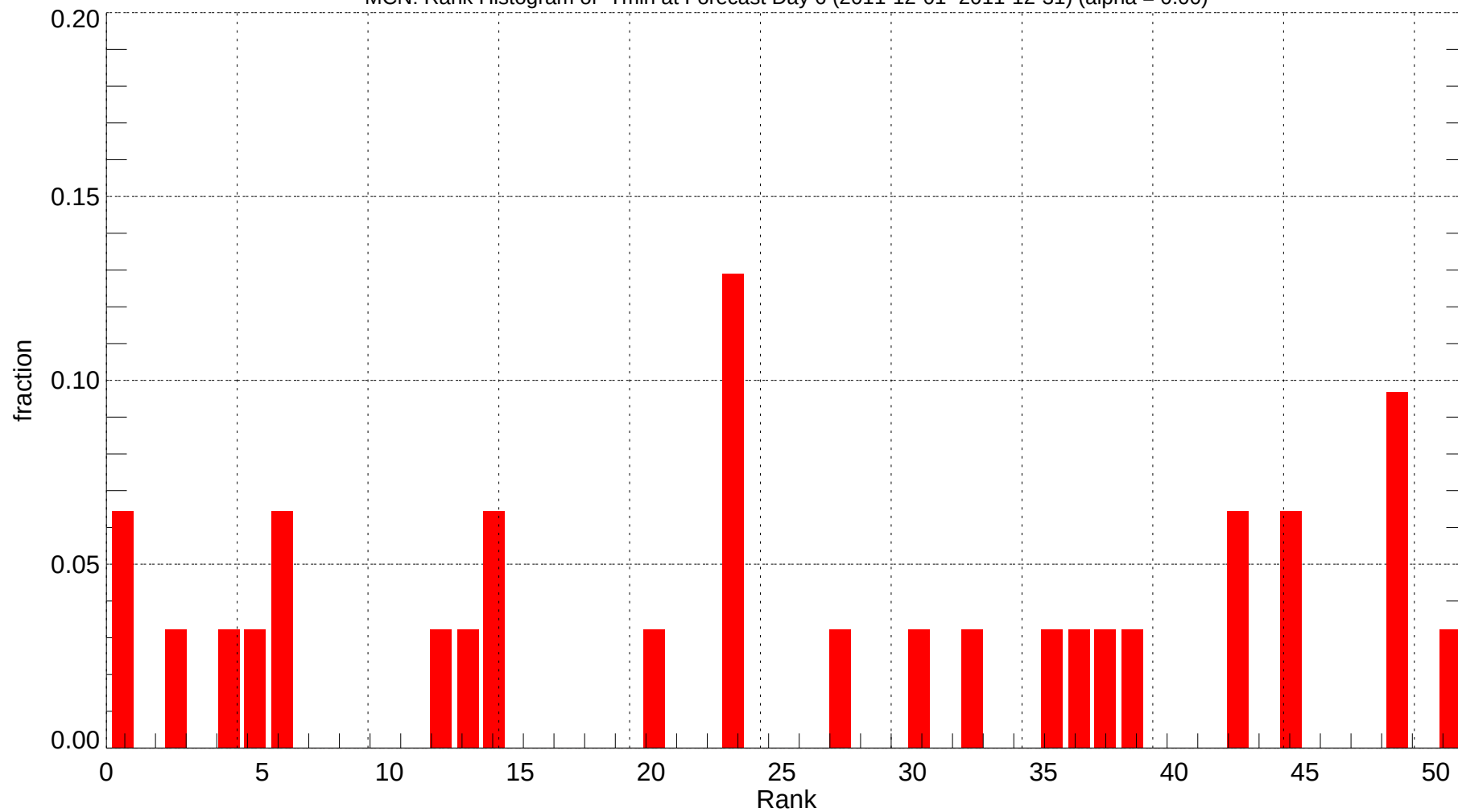
MCN: Rank Histogram of Tmin at Forecast Day 6 (2011-12-01~2011-12-31) (alpha = 0.00)
