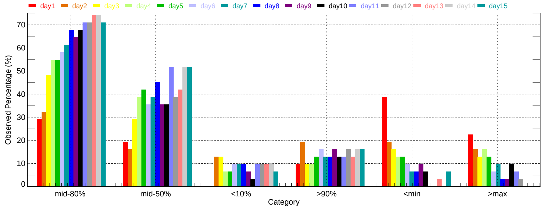
Observed Percentage of Ensembles - BTV: Max Temperature (2011-12-01~2011-12-31)
