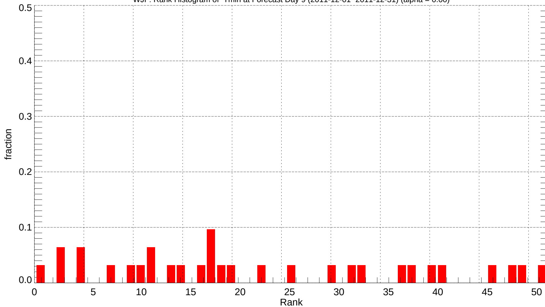
WJF: Rank Histogram of Tmin at Forecast Day 9 (2011-12-01~2011-12-31) (alpha = 0.00)
