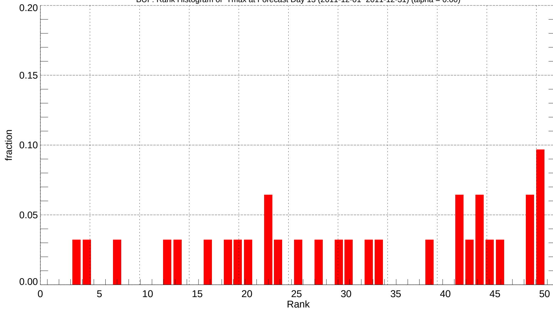
BUF: Rank Histogram of Tmax at Forecast Day 13 (2011-12-01~2011-12-31) (alpha = 0.00)
