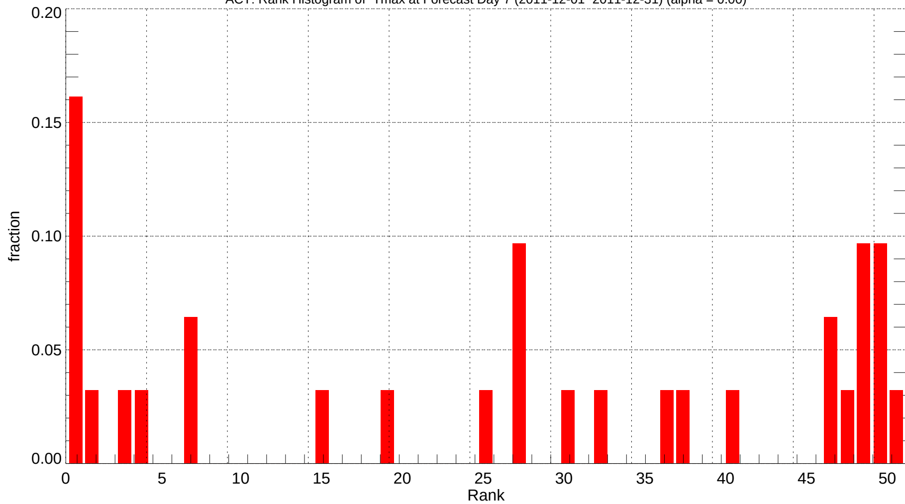
ACT: Rank Histogram of Tmax at Forecast Day 7 (2011-12-01~2011-12-31) (alpha = 0.00)
