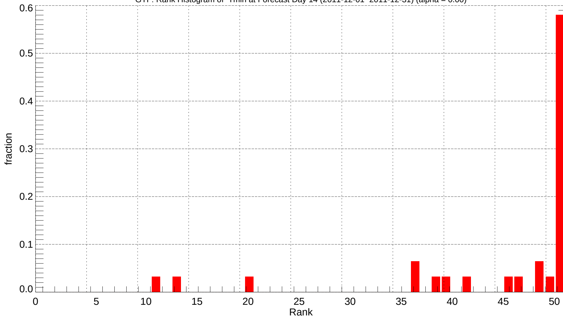
GTF: Rank Histogram of Tmin at Forecast Day 14 (2011-12-01~2011-12-31) (alpha = 0.00)
