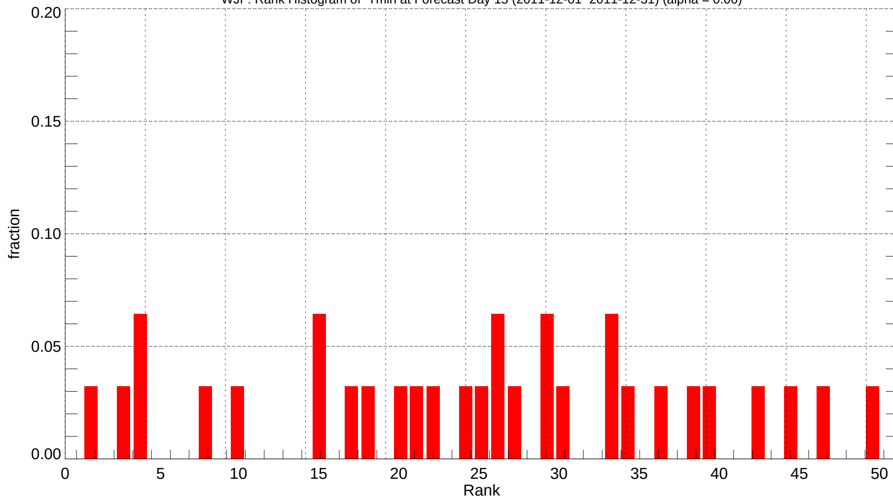
WJF: Rank Histogram of Tmin at Forecast Day 15 (2011-12-01~2011-12-31) (alpha = 0.00)
