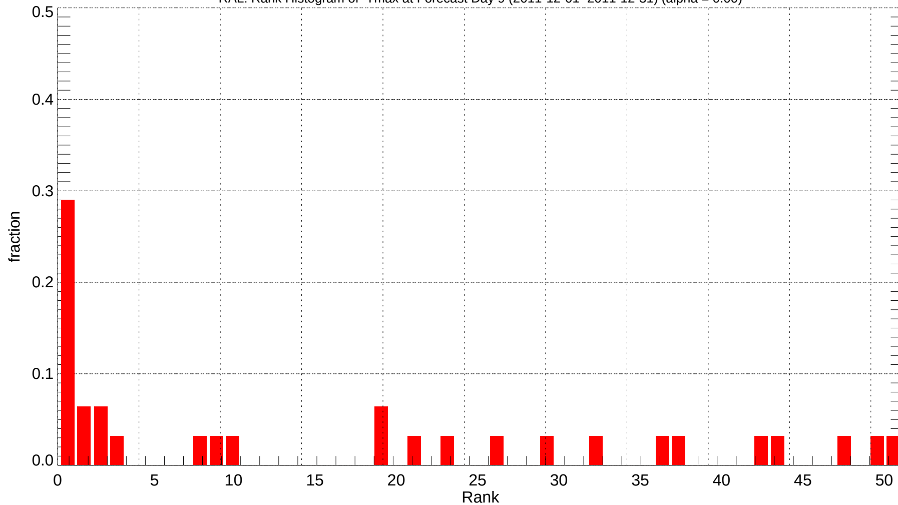
RAL: Rank Histogram of Tmax at Forecast Day 9 (2011-12-01~2011-12-31) (alpha = 0.00)
