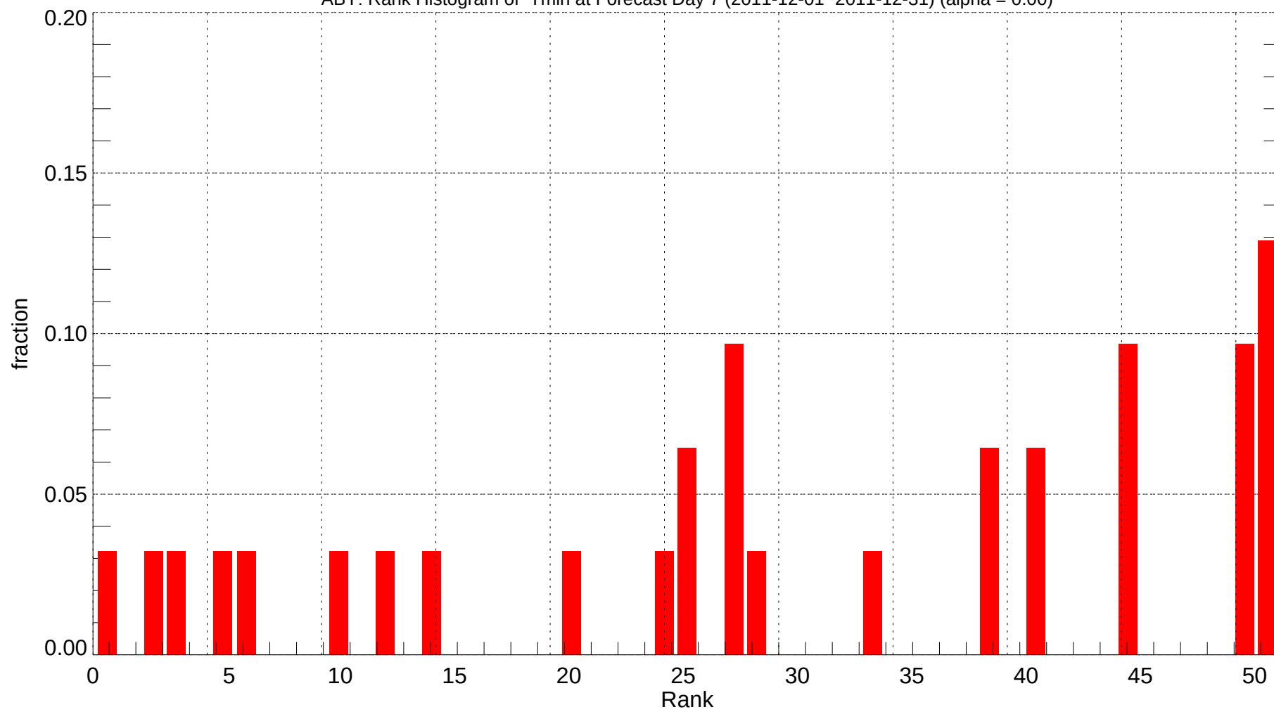
ABY: Rank Histogram of Tmin at Forecast Day 7 (2011-12-01~2011-12-31) (alpha = 0.00)
