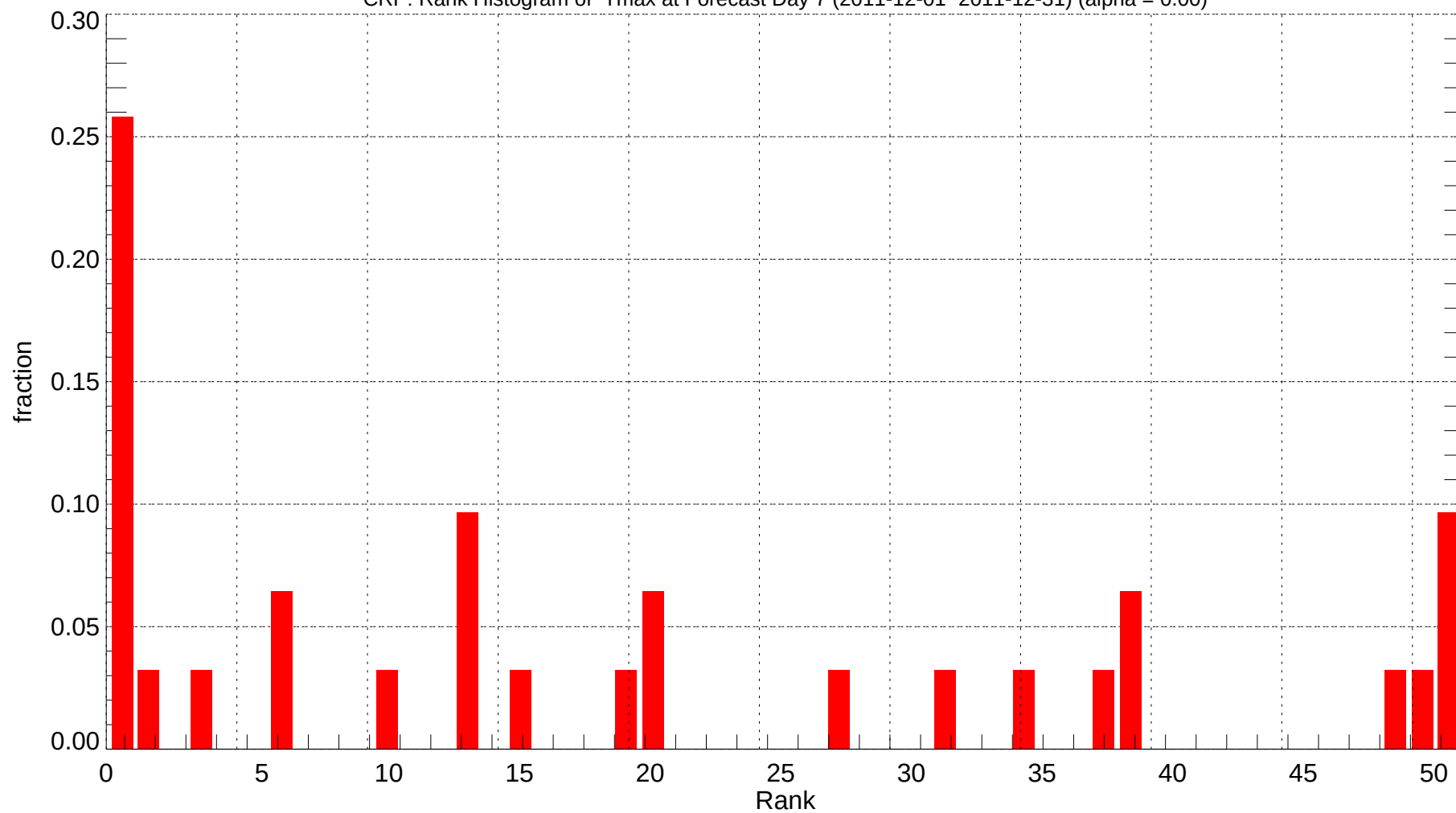
CRP: Rank Histogram of Tmax at Forecast Day 7 (2011-12-01~2011-12-31) (alpha = 0.00)
