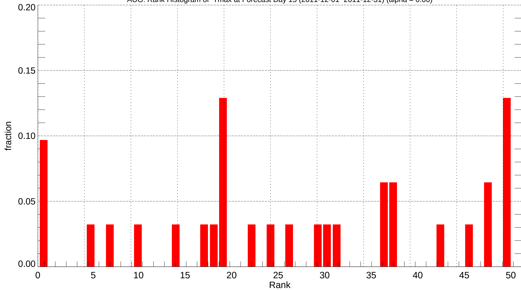
AUG: Rank Histogram of Tmax at Forecast Day 15 (2011-12-01~2011-12-31) (alpha = 0.00)
