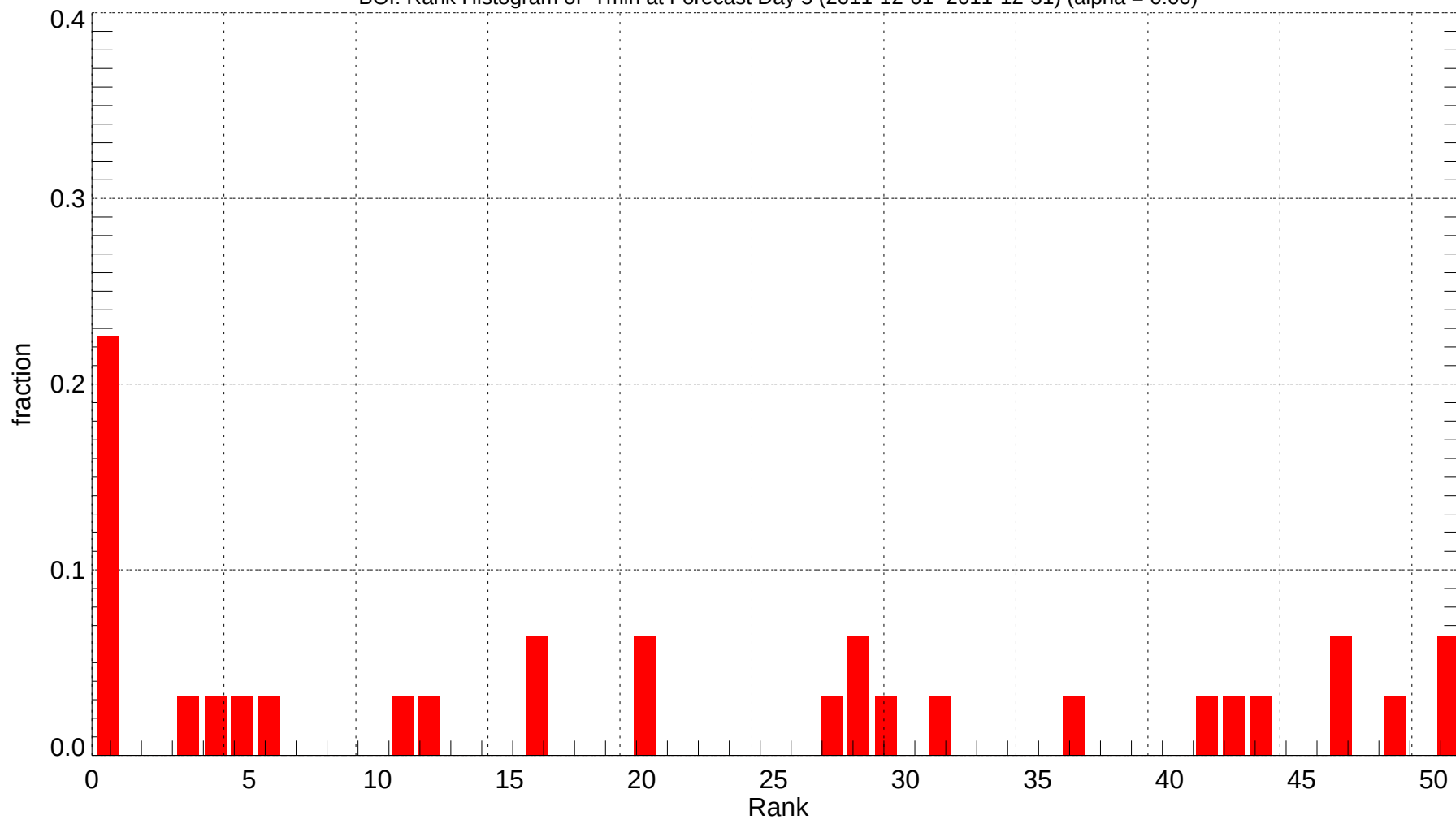
BOI: Rank Histogram of Tmin at Forecast Day 5 (2011-12-01~2011-12-31) (alpha = 0.00)
