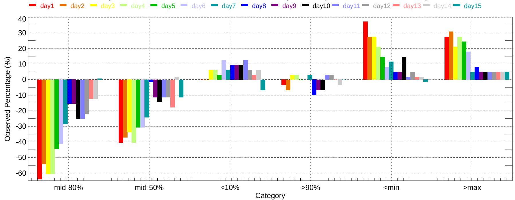
Observed Percentage Deviation of Ensembles - SFO: Max Temperature (2011-12-01~2011-12-31)
