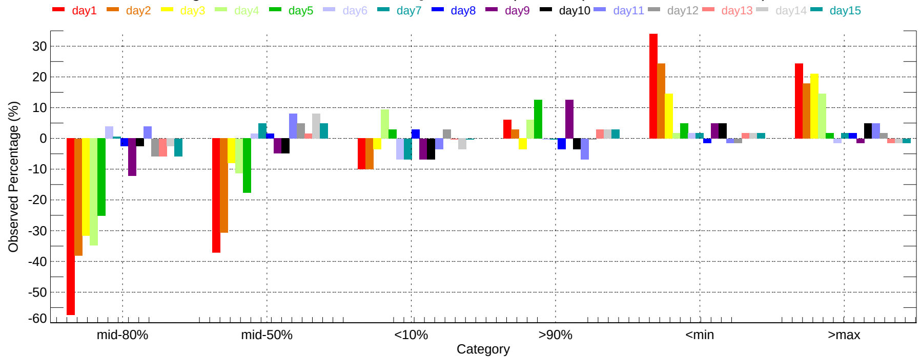
Observed Percentage Deviation of Ensembles - YQB: Max Temperature (2011-12-01~2011-12-31)
