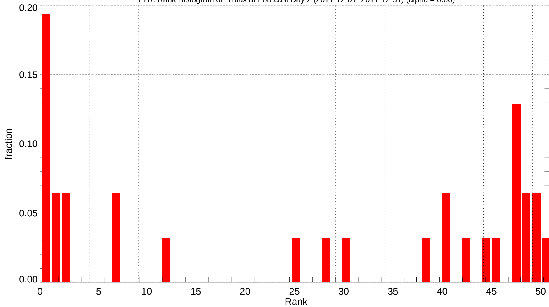
TYR: Rank Histogram of Tmax at Forecast Day 2 (2011-12-01~2011-12-31) (alpha = 0.00)
