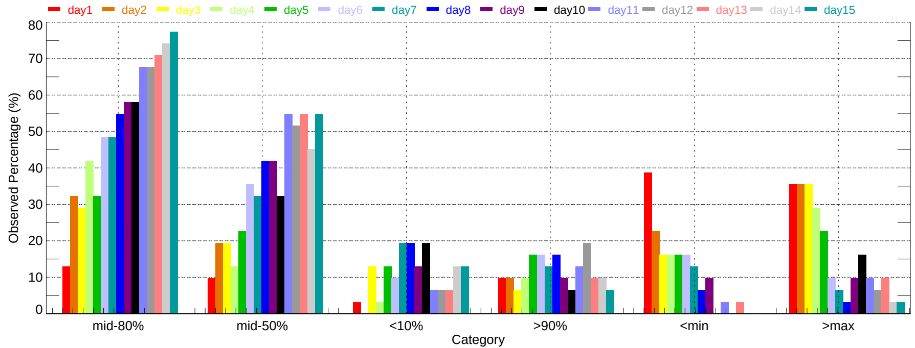
Observed Percentage of Ensembles - MBA: Min Temperature (2011-12-01~2011-12-31)
