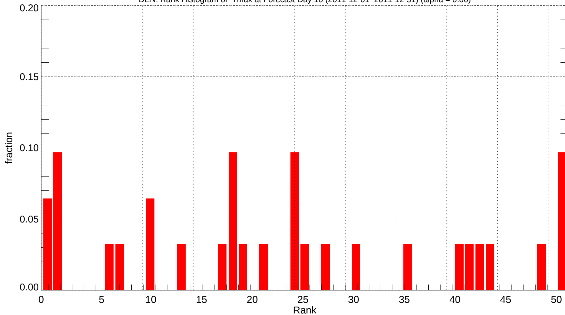
DEN: Rank Histogram of Tmax at Forecast Day 10 (2011-12-01~2011-12-31) (alpha = 0.00)
