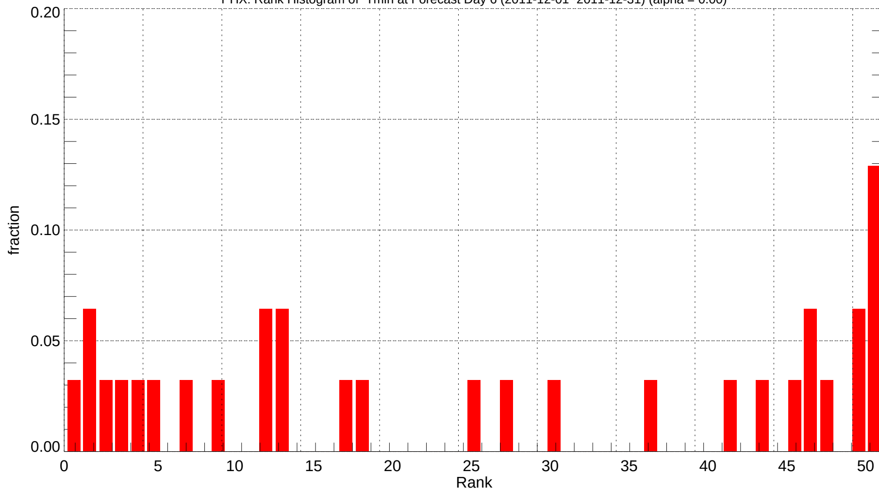
PHX: Rank Histogram of Tmin at Forecast Day 6 (2011-12-01~2011-12-31) (alpha = 0.00)
