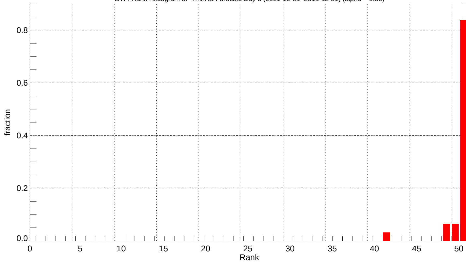
GTF: Rank Histogram of Tmin at Forecast Day 3 (2011-12-01~2011-12-31) (alpha = 0.00)
