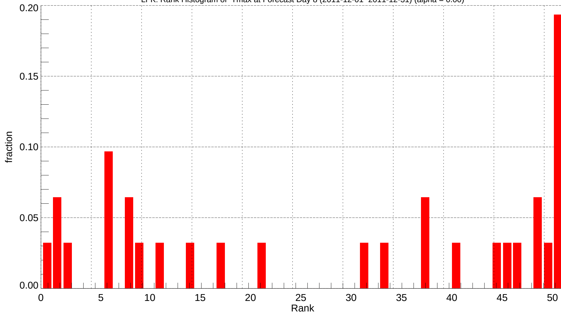
LFK: Rank Histogram of Tmax at Forecast Day 8 (2011-12-01~2011-12-31) (alpha = 0.00)
