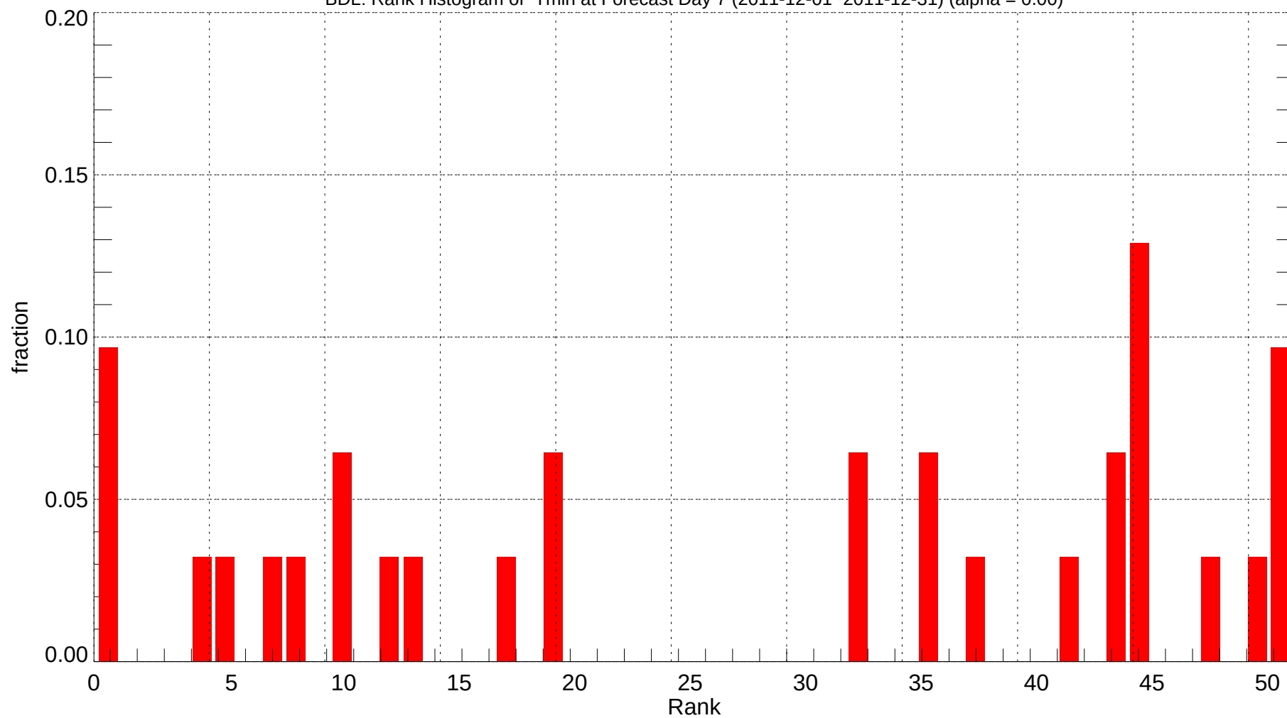
BDL: Rank Histogram of Tmin at Forecast Day 7 (2011-12-01~2011-12-31) (alpha = 0.00)
