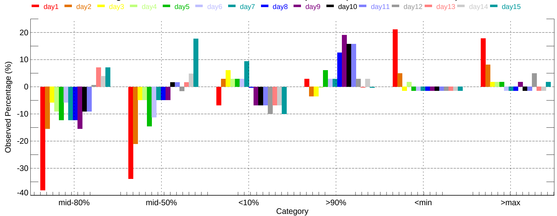
Observed Percentage Deviation of Ensembles - ATL: Min Temperature (2011-12-01~2011-12-31)
