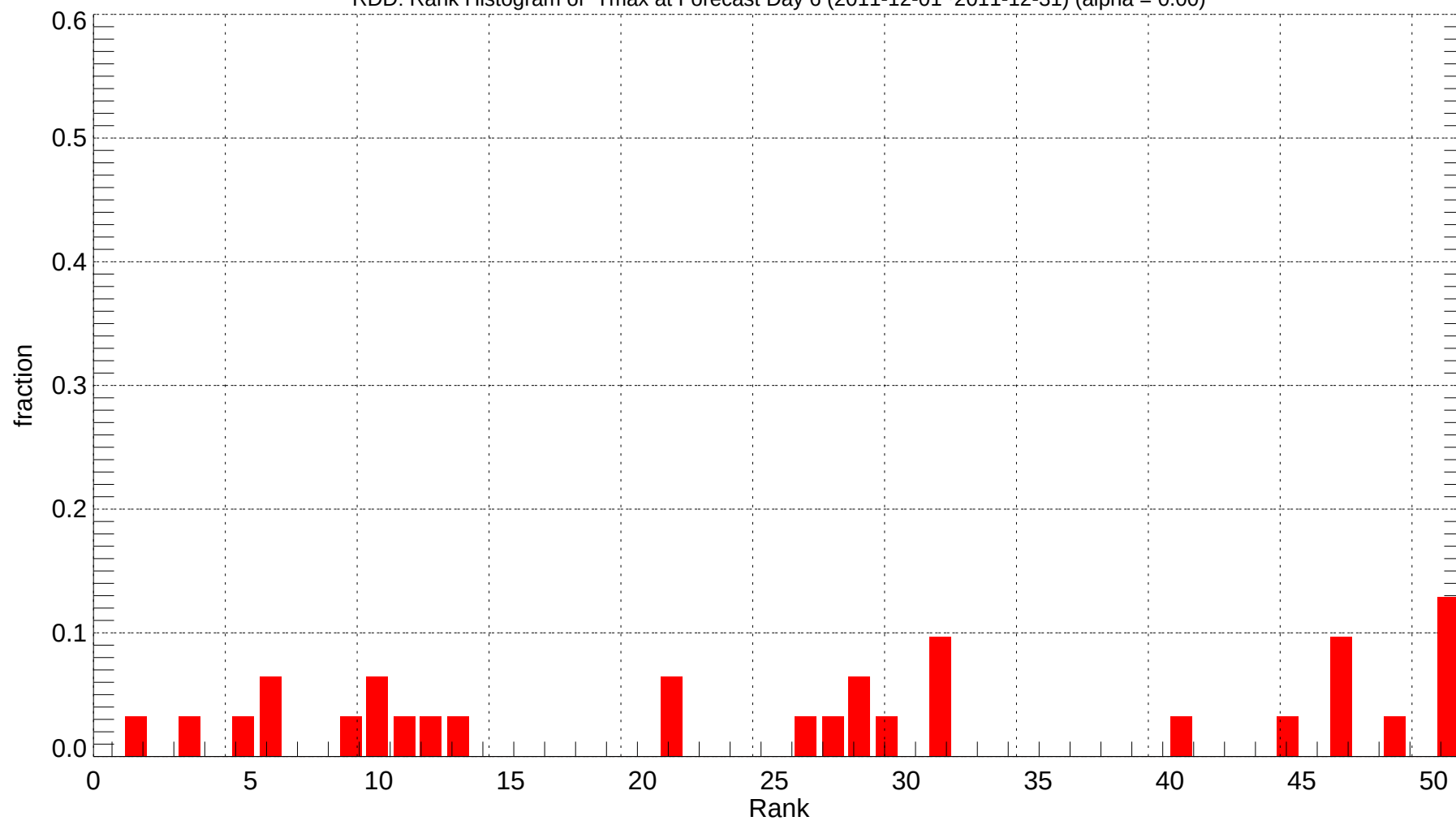
RDD: Rank Histogram of Tmax at Forecast Day 6 (2011-12-01~2011-12-31) (alpha = 0.00)
