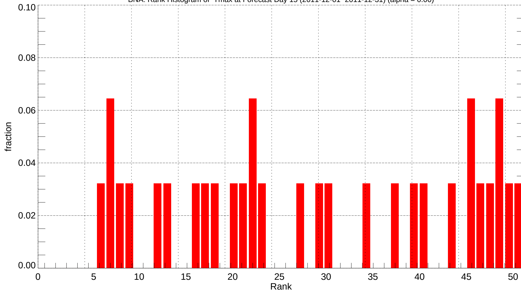
BNA: Rank Histogram of Tmax at Forecast Day 15 (2011-12-01~2011-12-31) (alpha = 0.00)
