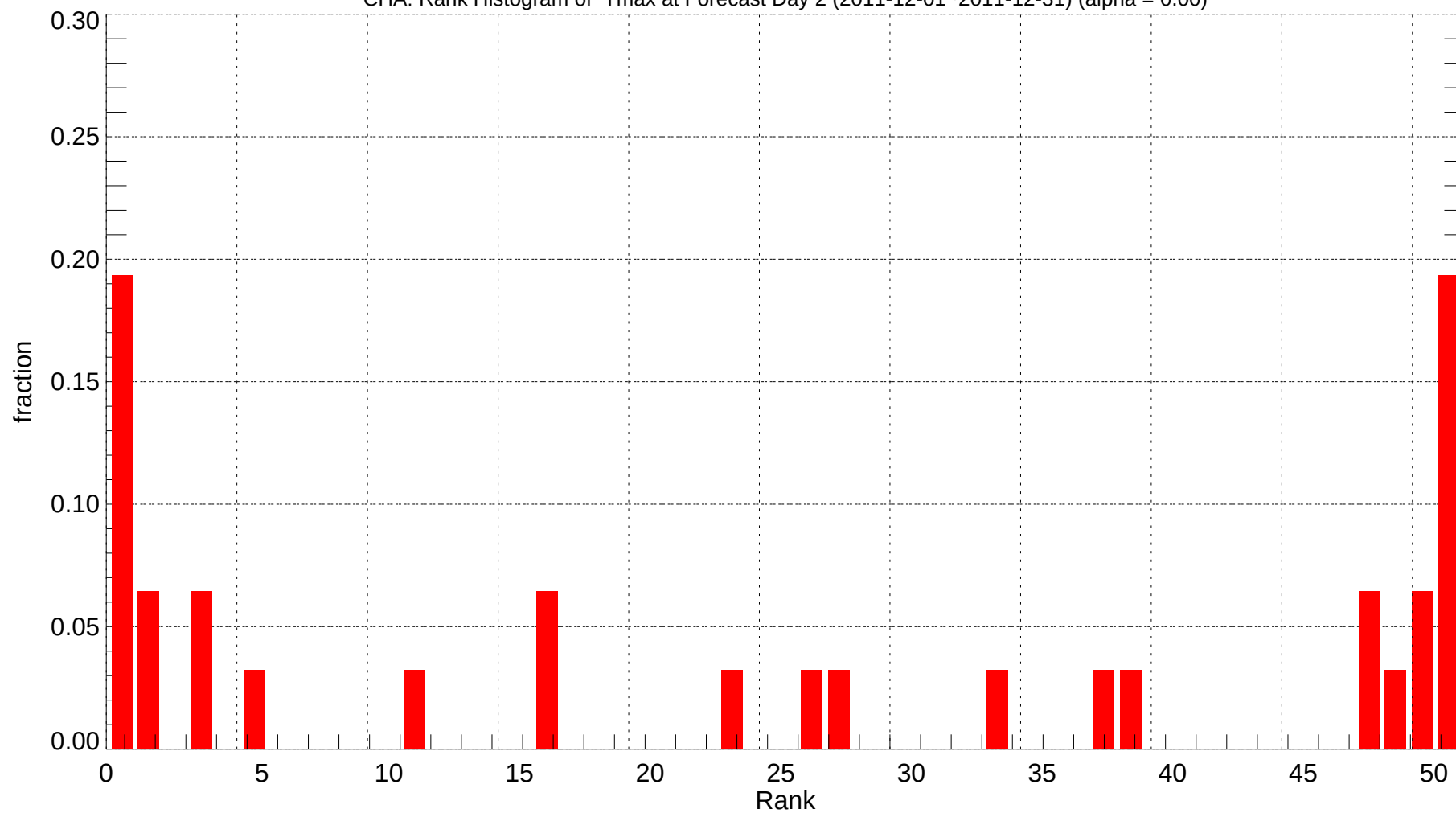
CHA: Rank Histogram of Tmax at Forecast Day 2 (2011-12-01~2011-12-31) (alpha = 0.00)
