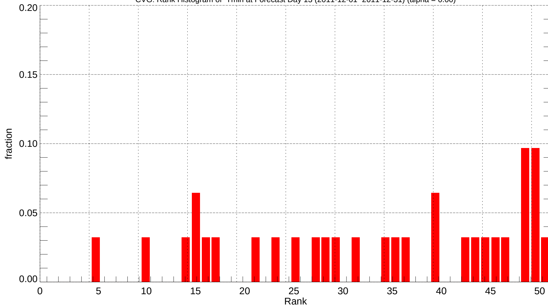
CVG: Rank Histogram of Tmin at Forecast Day 13 (2011-12-01~2011-12-31) (alpha = 0.00)
