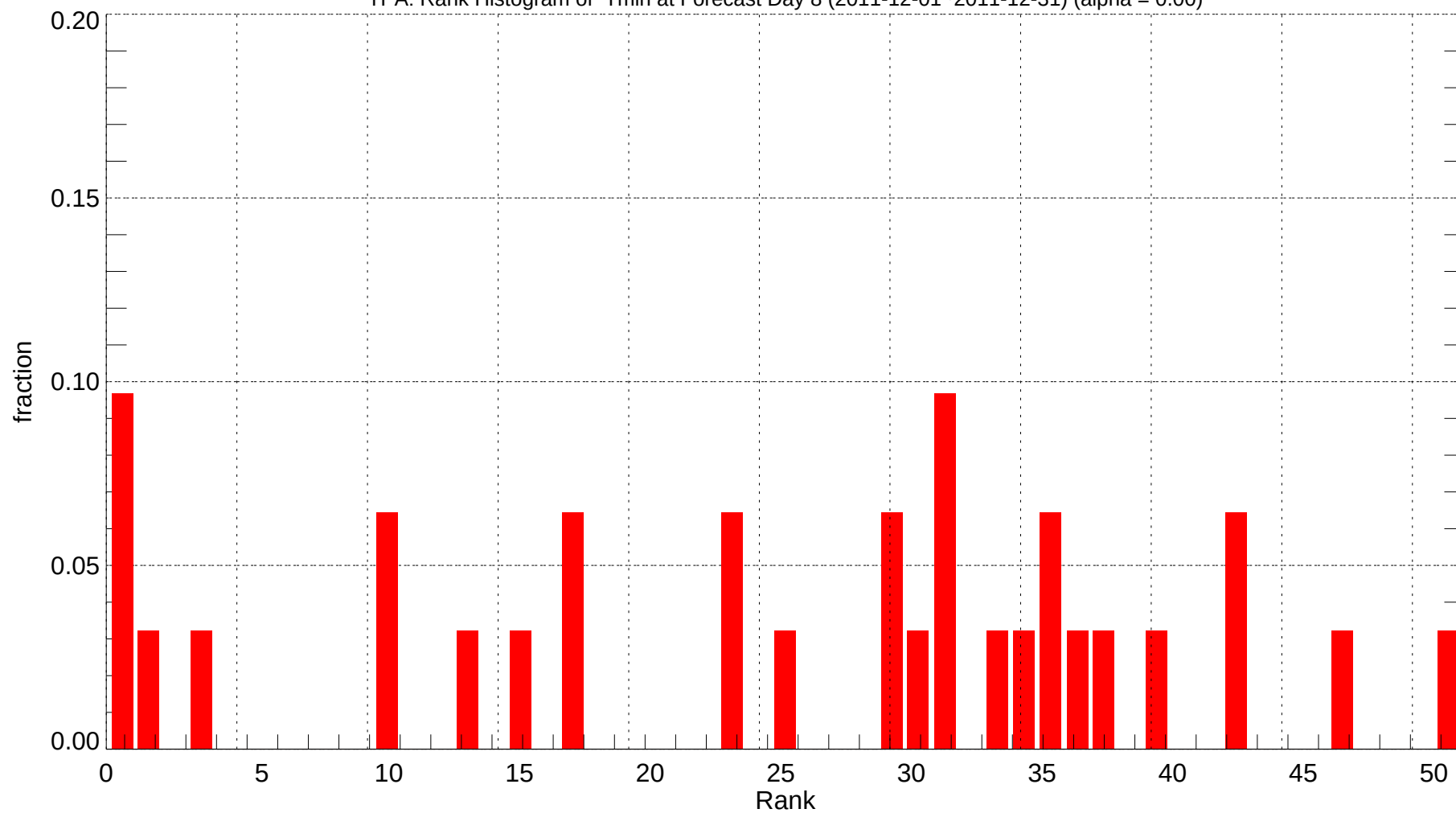
TPA: Rank Histogram of Tmin at Forecast Day 8 (2011-12-01~2011-12-31) (alpha = 0.00)
