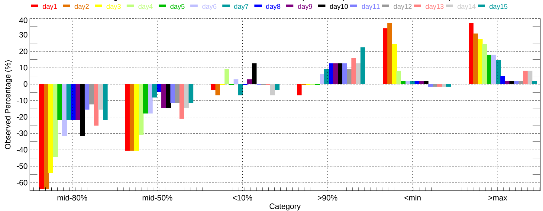
Observed Percentage Deviation of Ensembles - YXD: Max Temperature (2011-12-01~2011-12-31)
