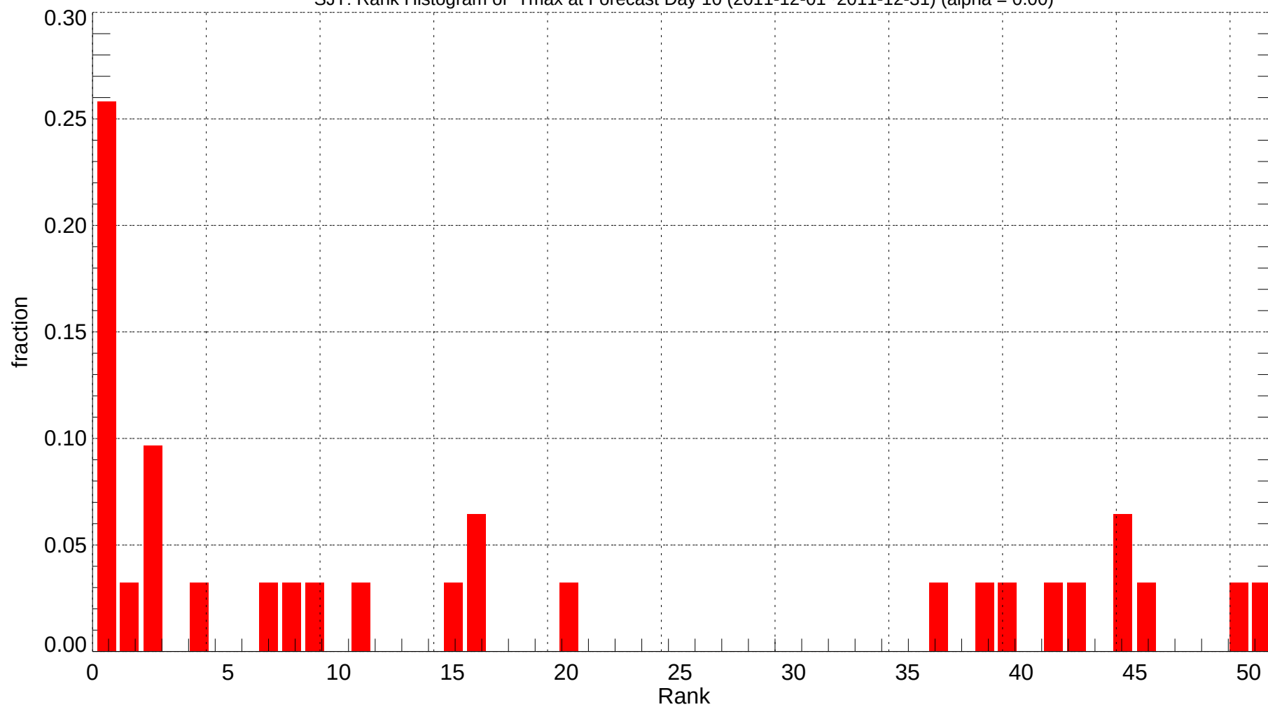
SJT: Rank Histogram of Tmax at Forecast Day 10 (2011-12-01~2011-12-31) (alpha = 0.00)
