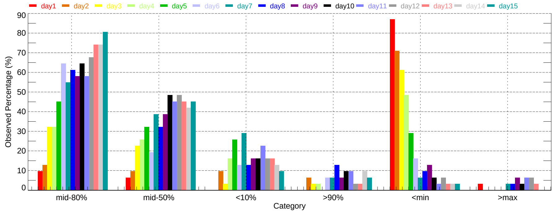
Observed Percentage of Ensembles - MDT: Min Temperature (2011-12-01~2011-12-31)
