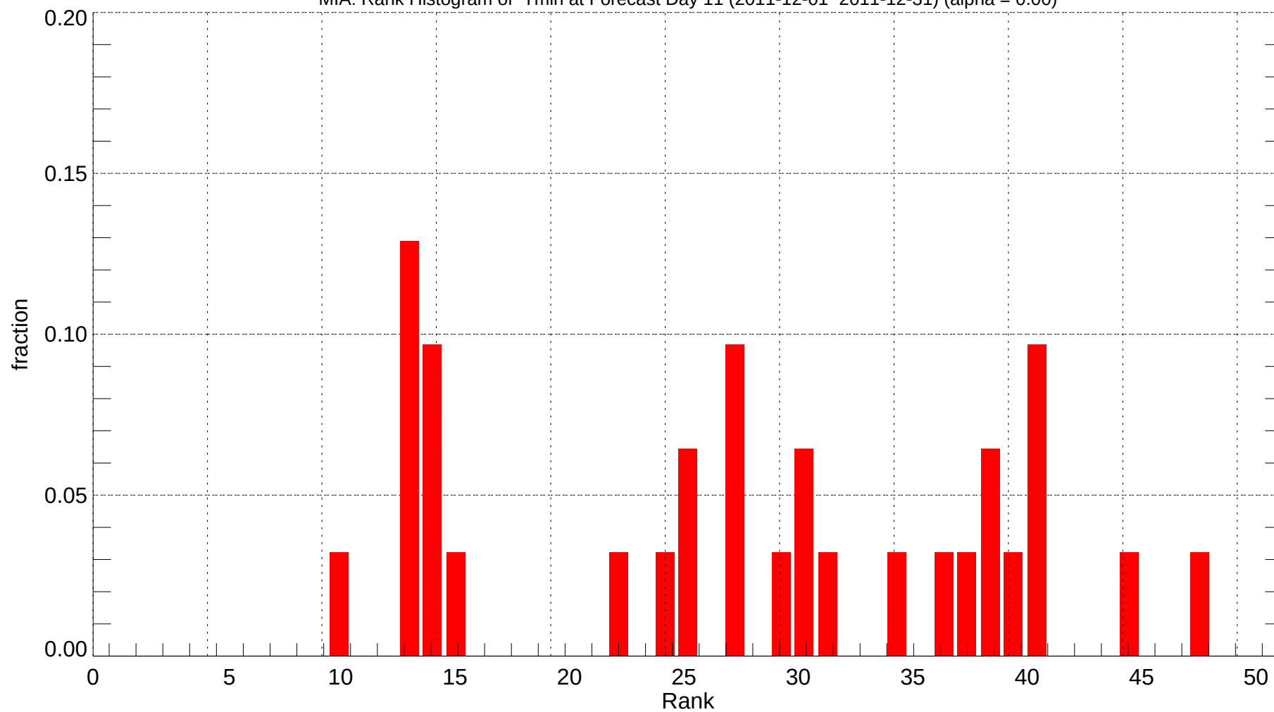
MIA: Rank Histogram of Tmin at Forecast Day 11 (2011-12-01~2011-12-31) (alpha = 0.00)
