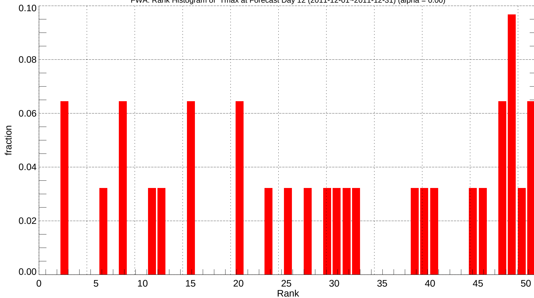
FWA: Rank Histogram of Tmax at Forecast Day 12 (2011-12-01~2011-12-31) (alpha = 0.00)
