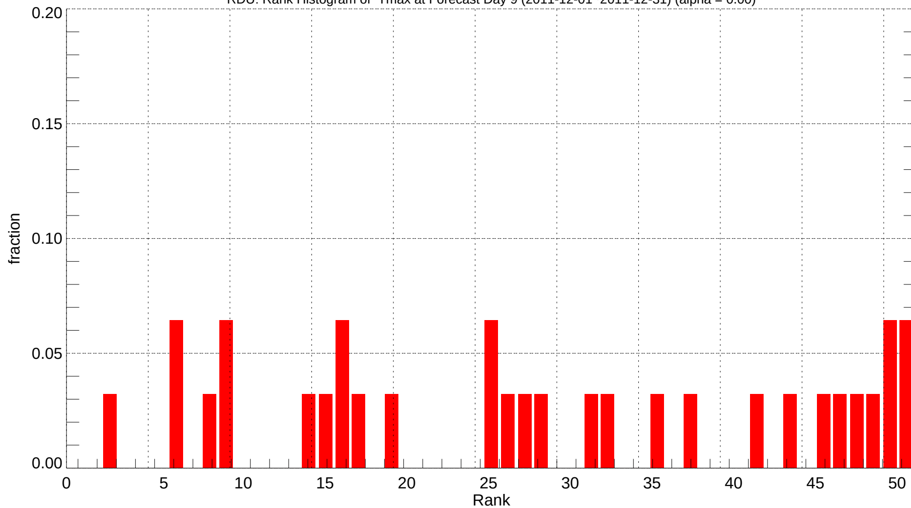
RDU: Rank Histogram of Tmax at Forecast Day 9 (2011-12-01~2011-12-31) (alpha = 0.00)
