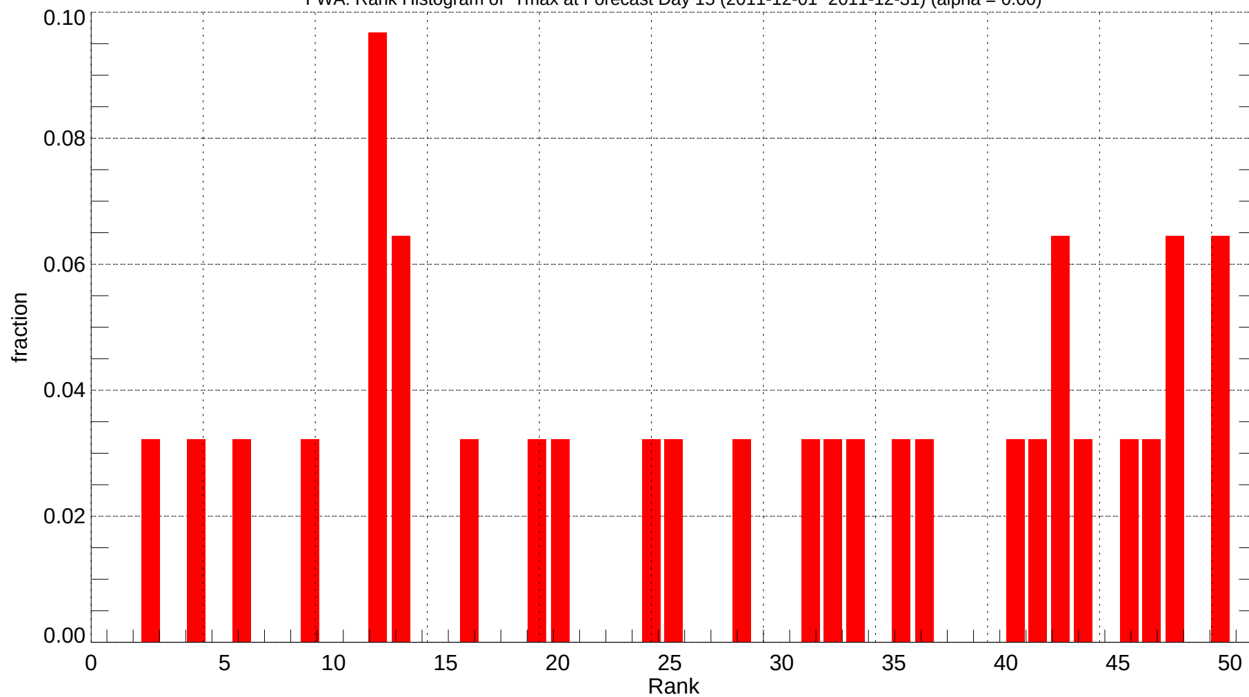
FWA: Rank Histogram of Tmax at Forecast Day 15 (2011-12-01~2011-12-31) (alpha = 0.00)
