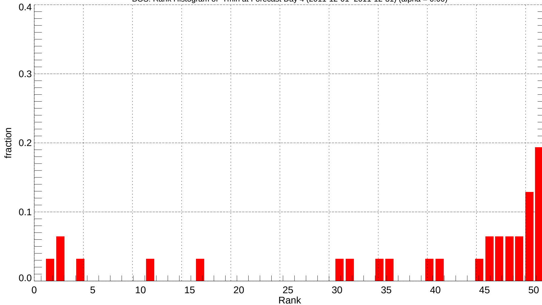
BOS: Rank Histogram of Tmin at Forecast Day 4 (2011-12-01~2011-12-31) (alpha = 0.00)
