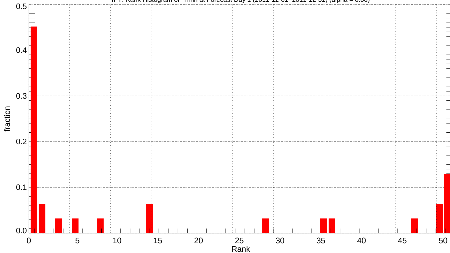
IPT: Rank Histogram of Tmin at Forecast Day 1 (2011-12-01~2011-12-31) (alpha = 0.00)
