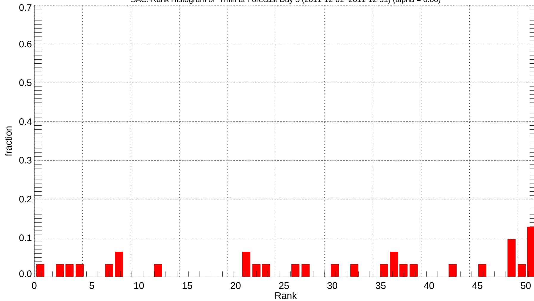
SAC: Rank Histogram of Tmin at Forecast Day 5 (2011-12-01~2011-12-31) (alpha = 0.00)
