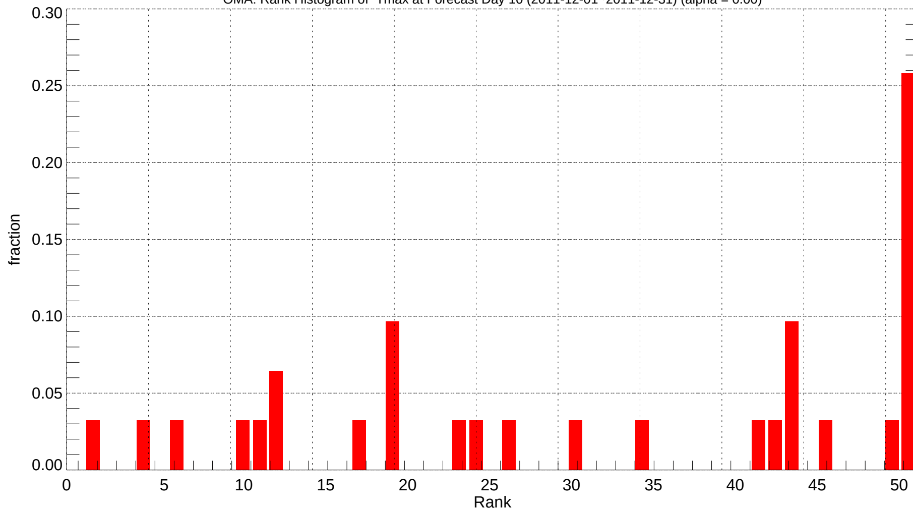
OMA: Rank Histogram of Tmax at Forecast Day 10 (2011-12-01~2011-12-31) (alpha = 0.00)
