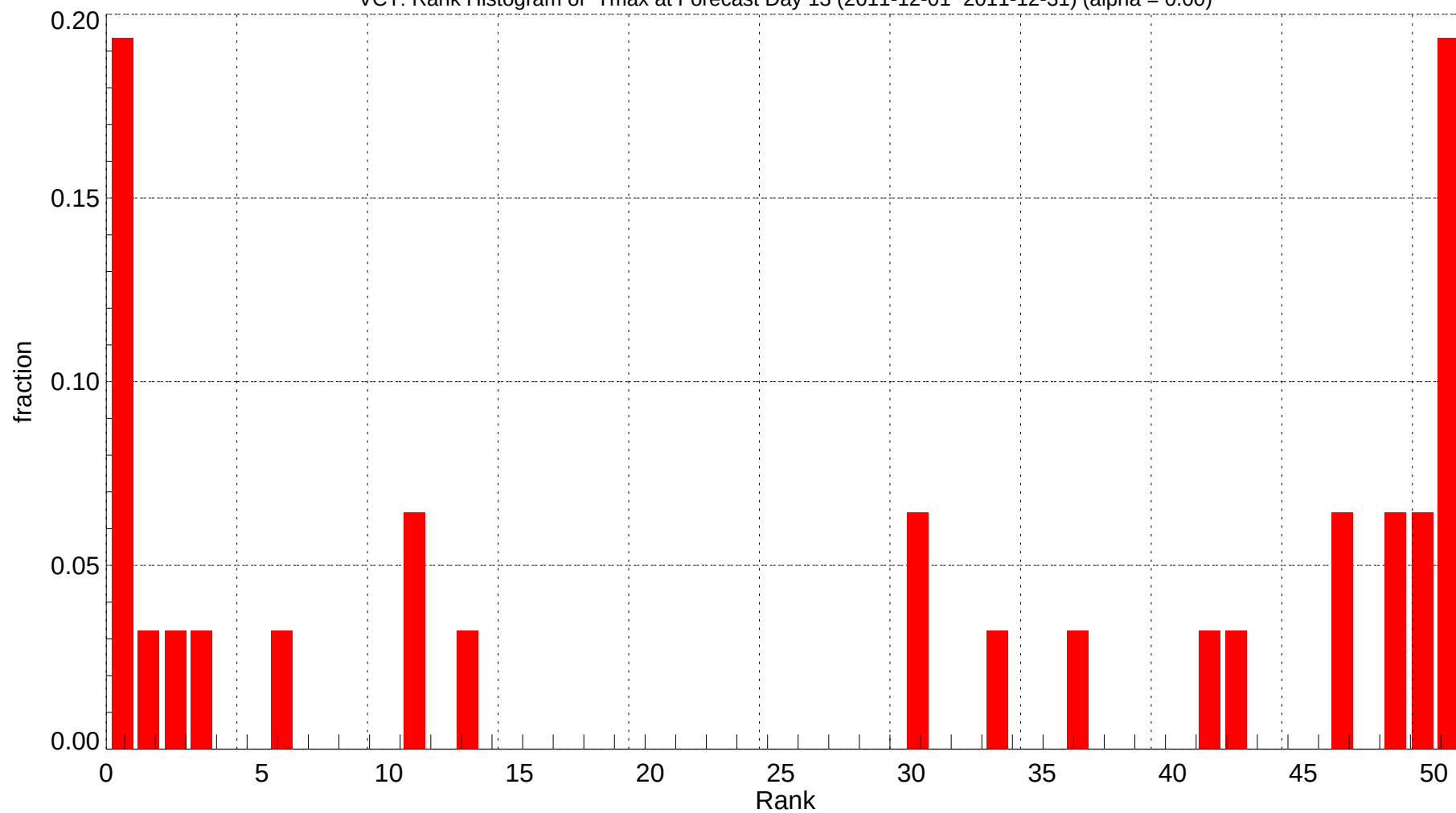
VCT: Rank Histogram of Tmax at Forecast Day 13 (2011-12-01~2011-12-31) (alpha = 0.00)
