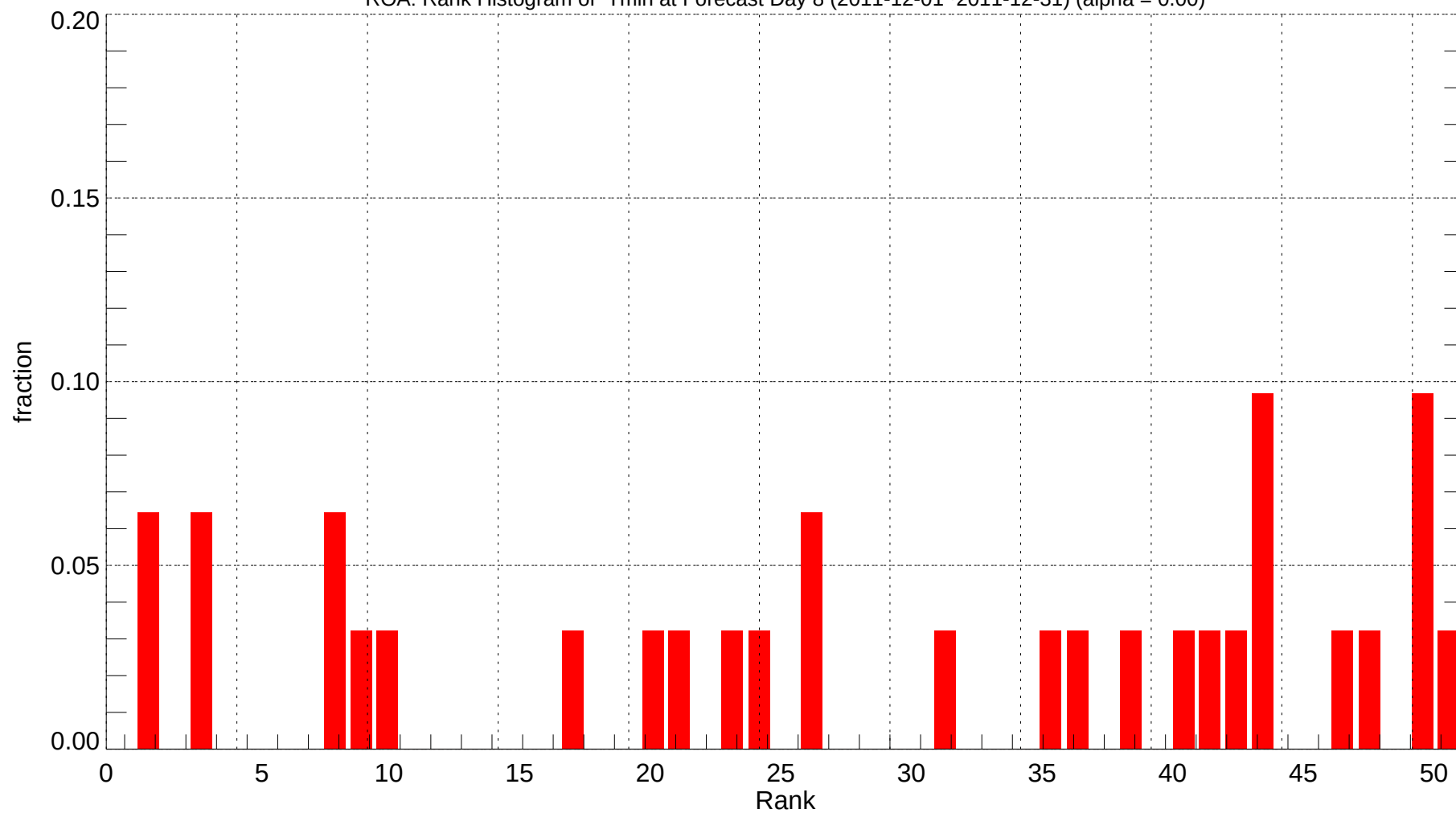
ROA: Rank Histogram of Tmin at Forecast Day 8 (2011-12-01~2011-12-31) (alpha = 0.00)
