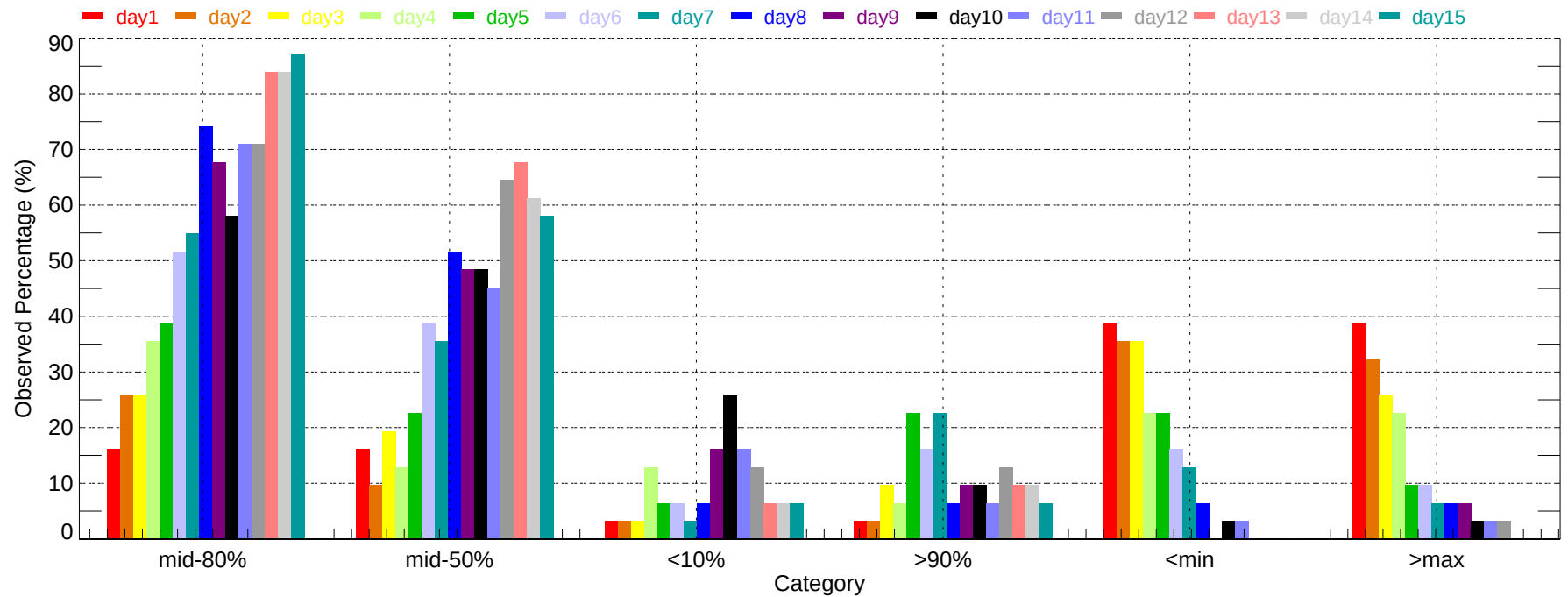
Observed Percentage of Ensembles - YKM: Min Temperature (2011-12-01~2011-12-31)
