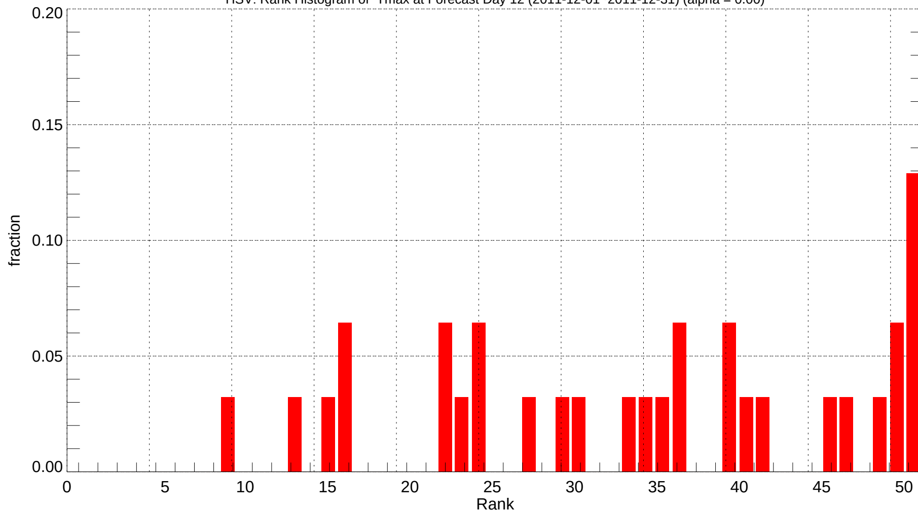
HSV: Rank Histogram of Tmax at Forecast Day 12 (2011-12-01~2011-12-31) (alpha = 0.00)
