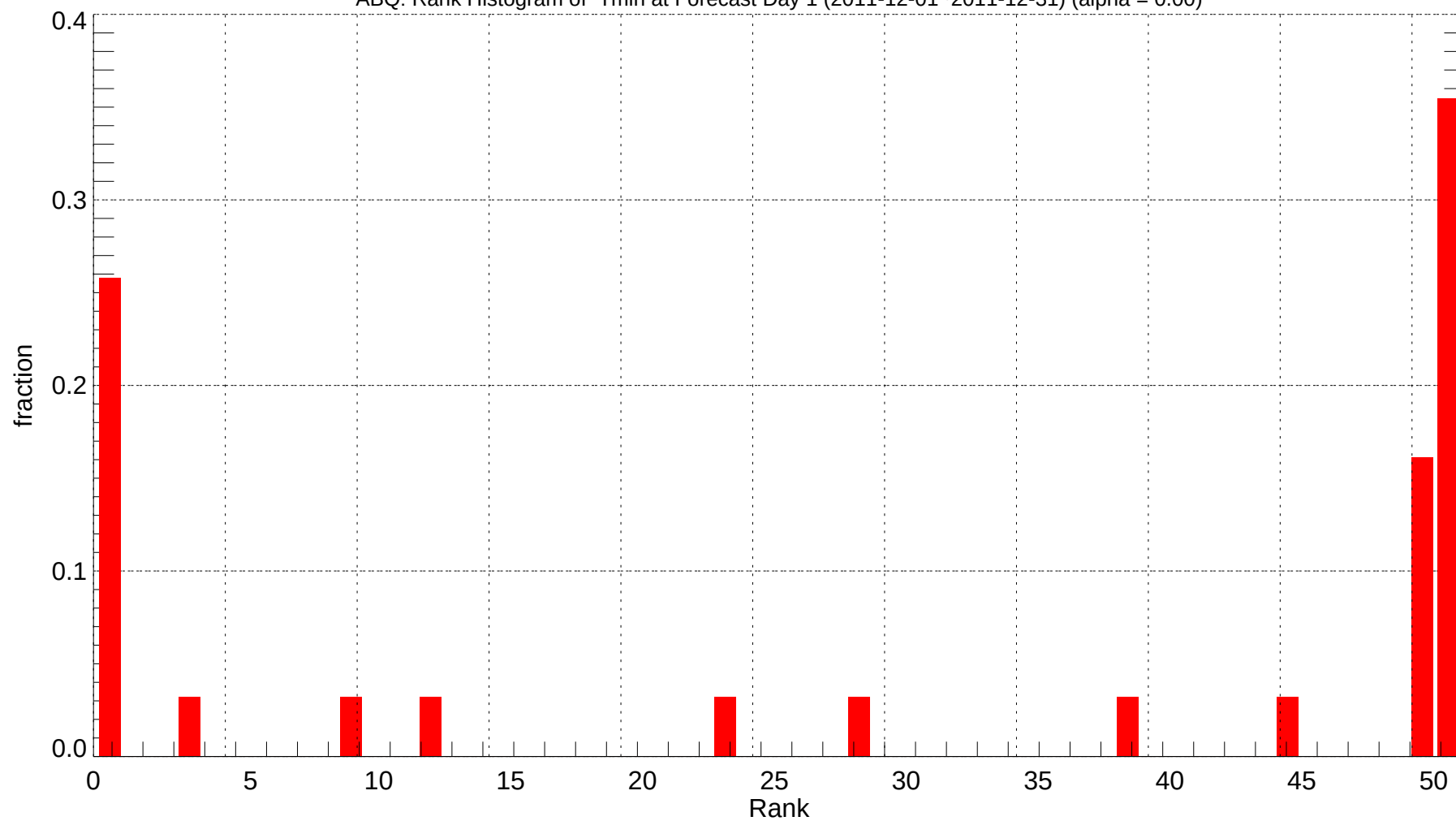
ABQ: Rank Histogram of Tmin at Forecast Day 1 (2011-12-01~2011-12-31) (alpha = 0.00)
