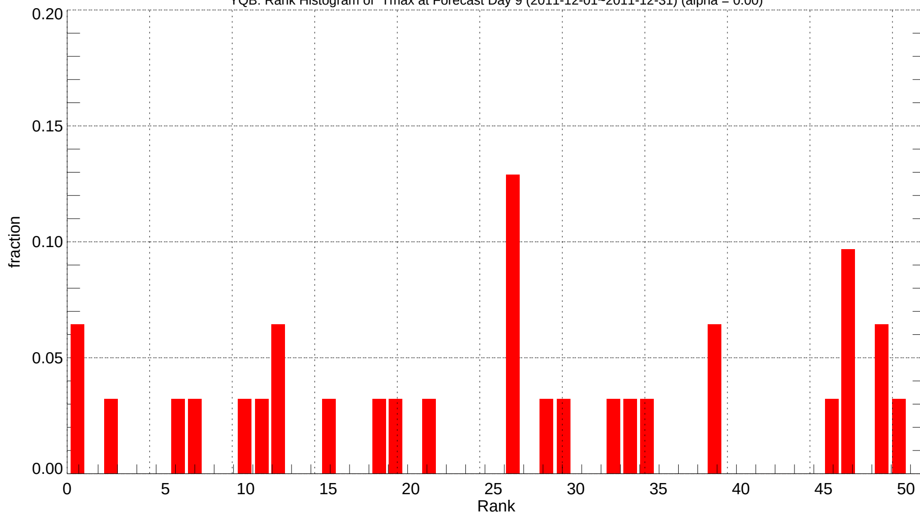
YQB: Rank Histogram of Tmax at Forecast Day 9 (2011-12-01~2011-12-31) (alpha = 0.00)
