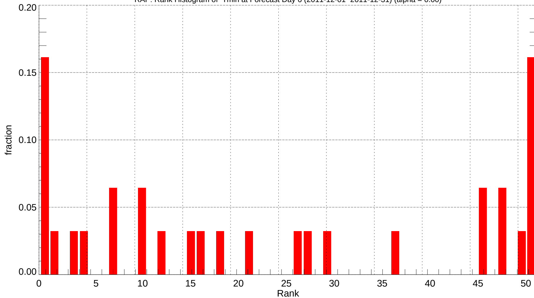
RAP: Rank Histogram of Tmin at Forecast Day 6 (2011-12-01~2011-12-31) (alpha = 0.00)
