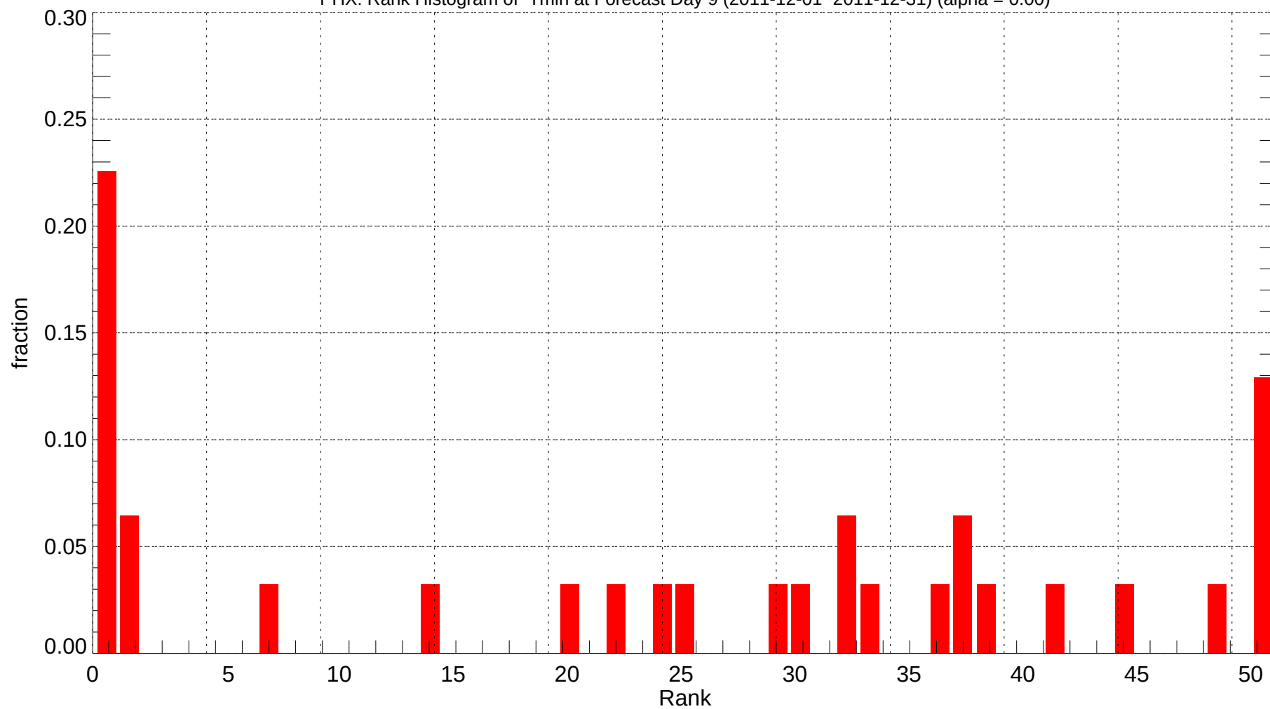
PHX: Rank Histogram of Tmin at Forecast Day 9 (2011-12-01~2011-12-31) (alpha = 0.00)
