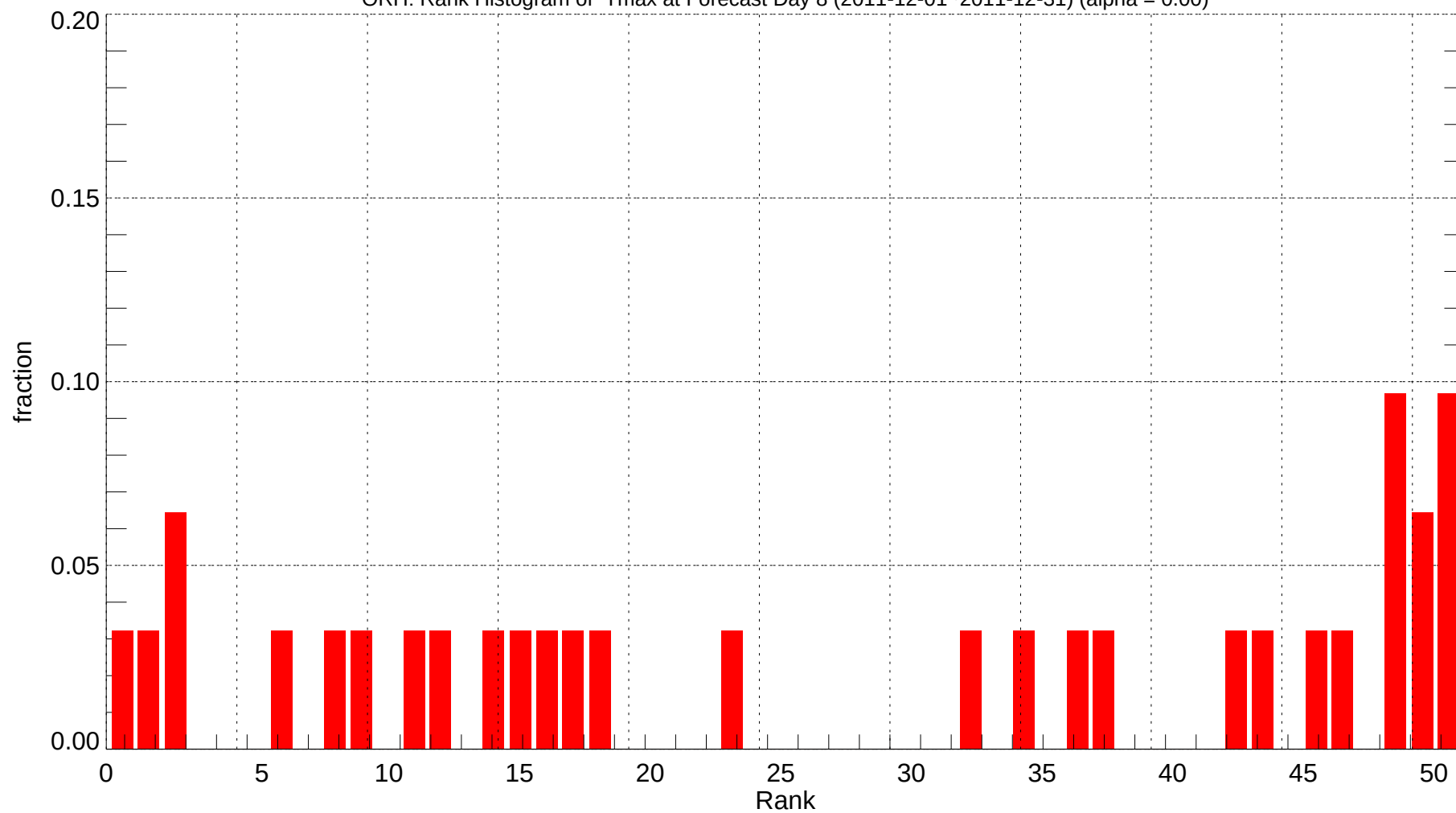
ORH: Rank Histogram of Tmax at Forecast Day 8 (2011-12-01~2011-12-31) (alpha = 0.00)
