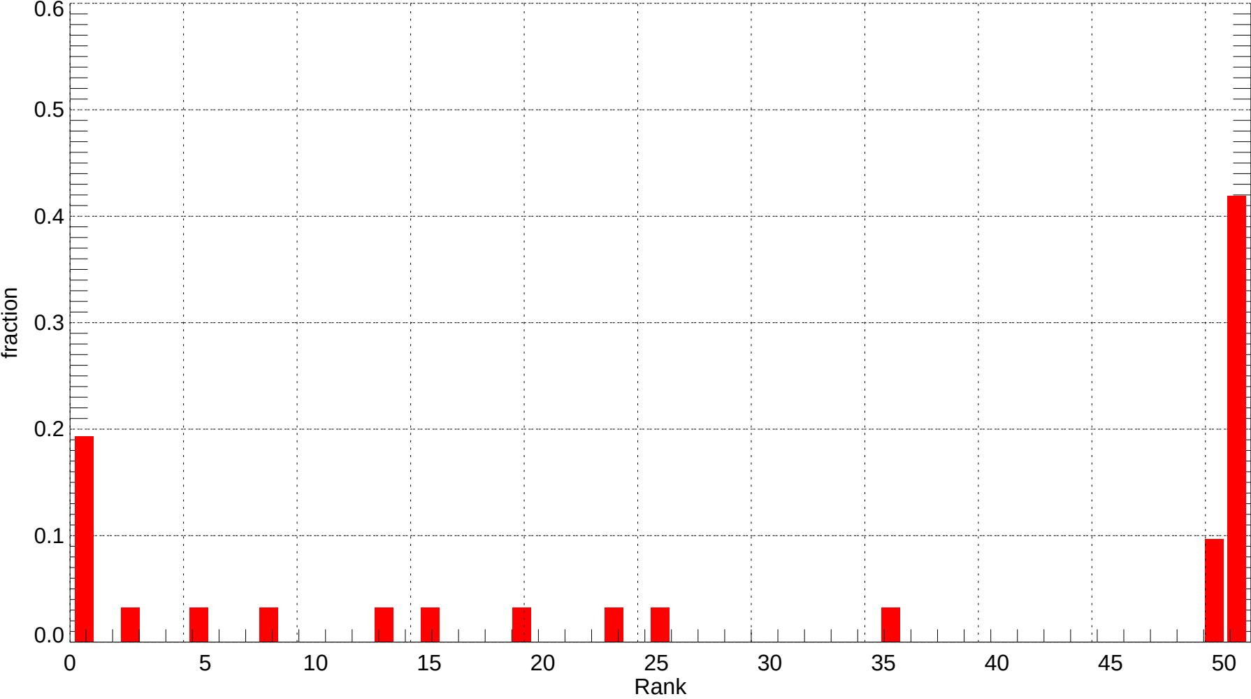
BFL: Rank Histogram of Tmin at Forecast Day 1 (2011-12-01~2011-12-31) (alpha = 0.00)
