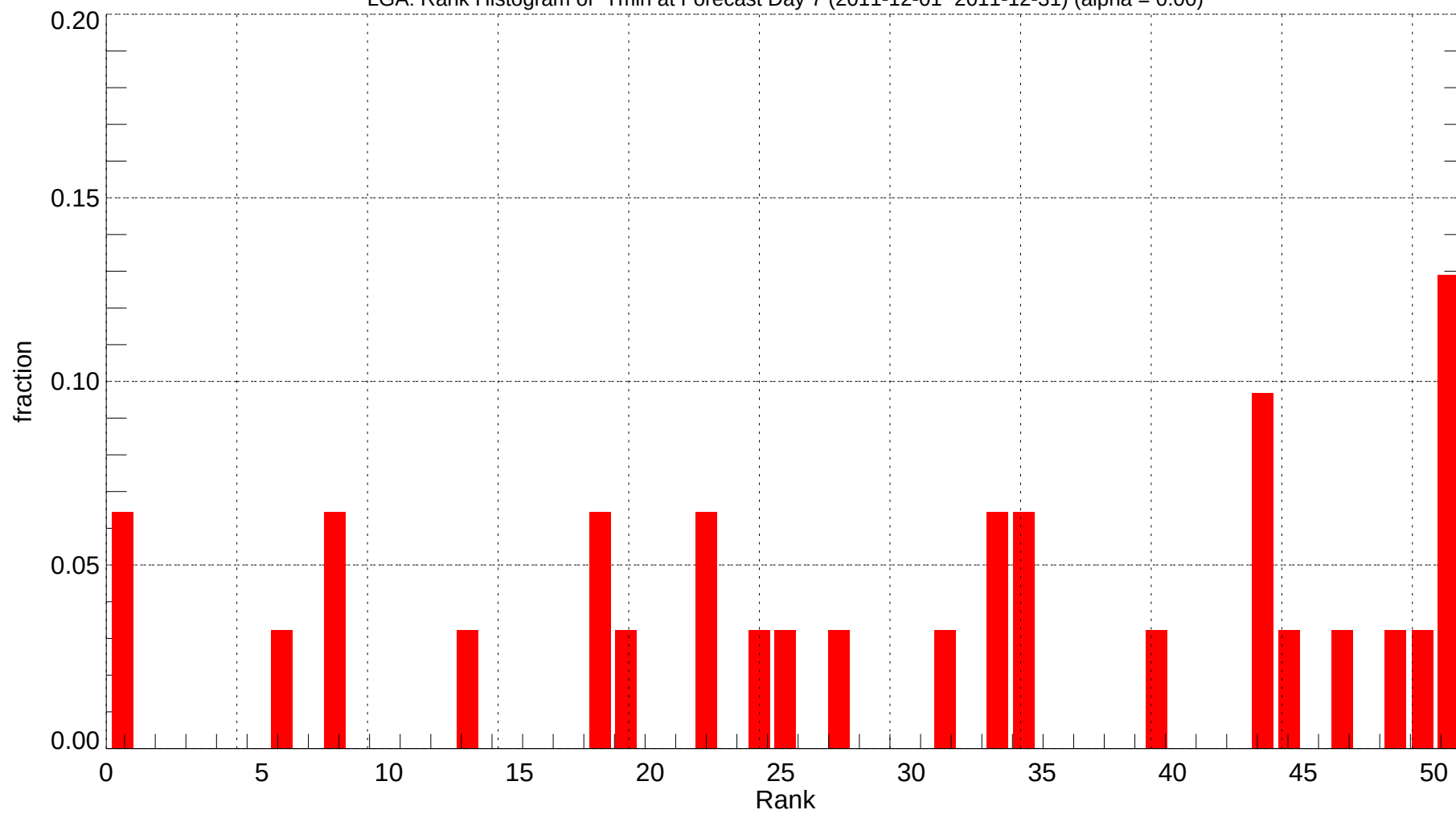
LGA: Rank Histogram of Tmin at Forecast Day 7 (2011-12-01~2011-12-31) (alpha = 0.00)
