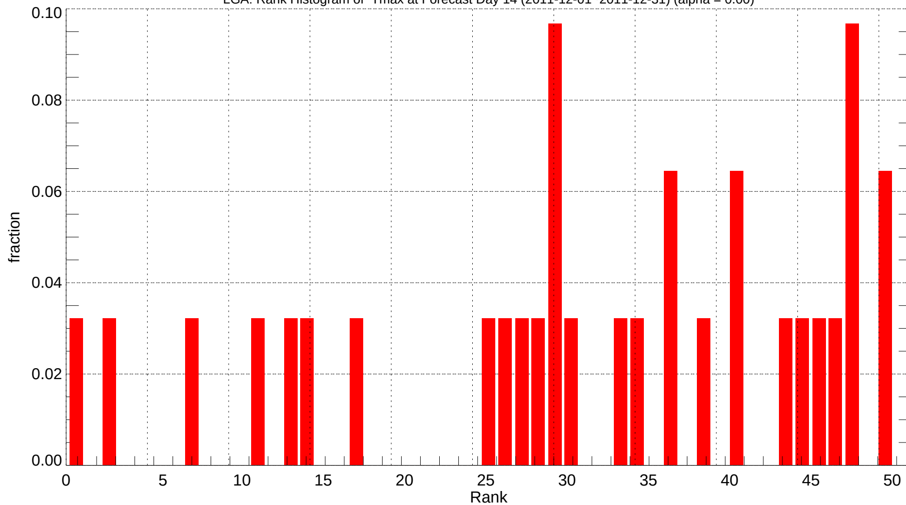
LGA: Rank Histogram of Tmax at Forecast Day 14 (2011-12-01~2011-12-31) (alpha = 0.00)
