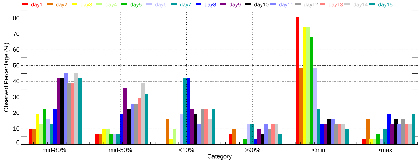
Observed Percentage of Ensembles - EUG: Max Temperature (2011-12-01~2011-12-31)
