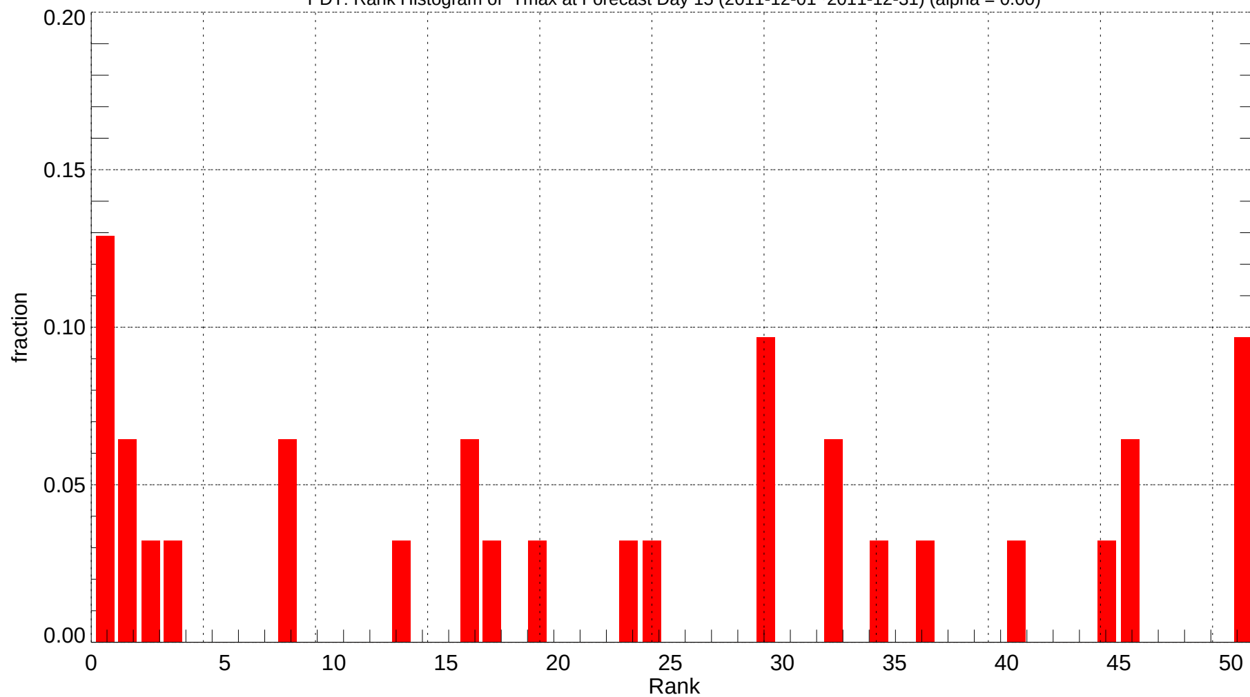
PDT: Rank Histogram of Tmax at Forecast Day 15 (2011-12-01~2011-12-31) (alpha = 0.00)
