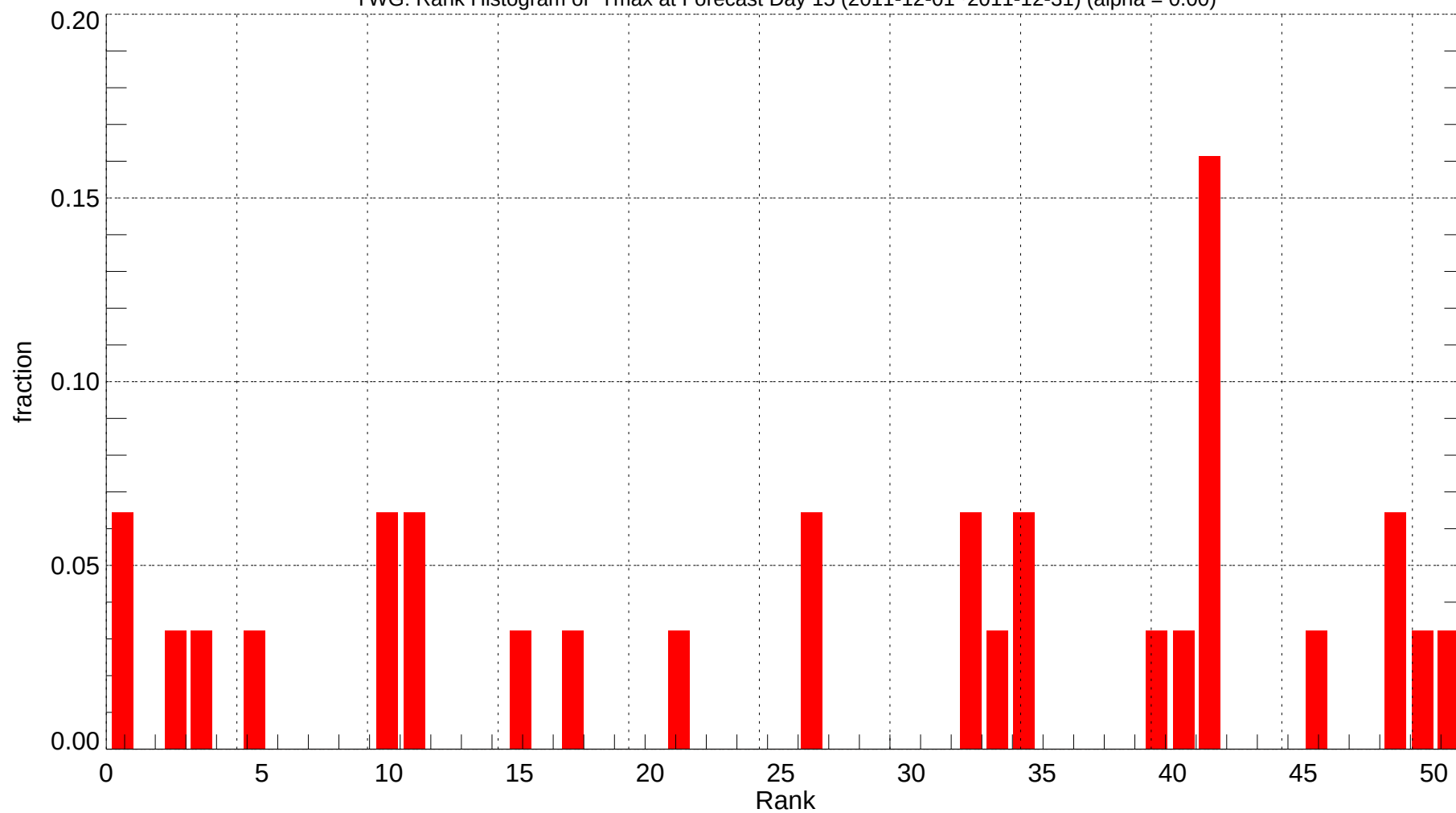
YWG: Rank Histogram of Tmax at Forecast Day 15 (2011-12-01~2011-12-31) (alpha = 0.00)
