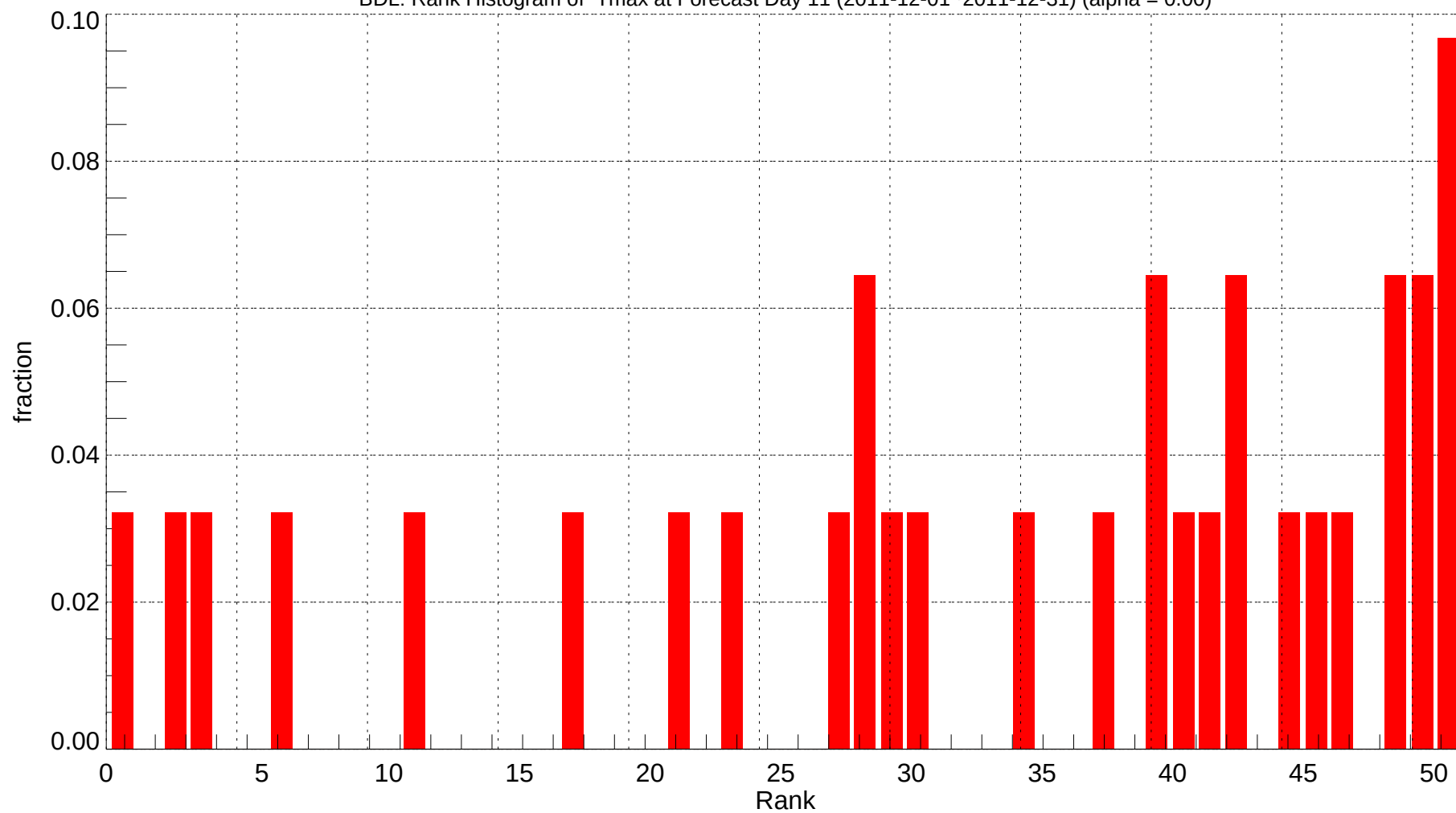
BDL: Rank Histogram of Tmax at Forecast Day 11 (2011-12-01~2011-12-31) (alpha = 0.00)
