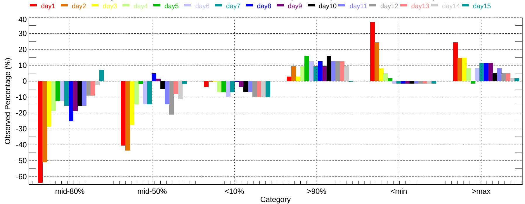
Observed Percentage Deviation of Ensembles - AOO: Min Temperature (2011-12-01~2011-12-31)
