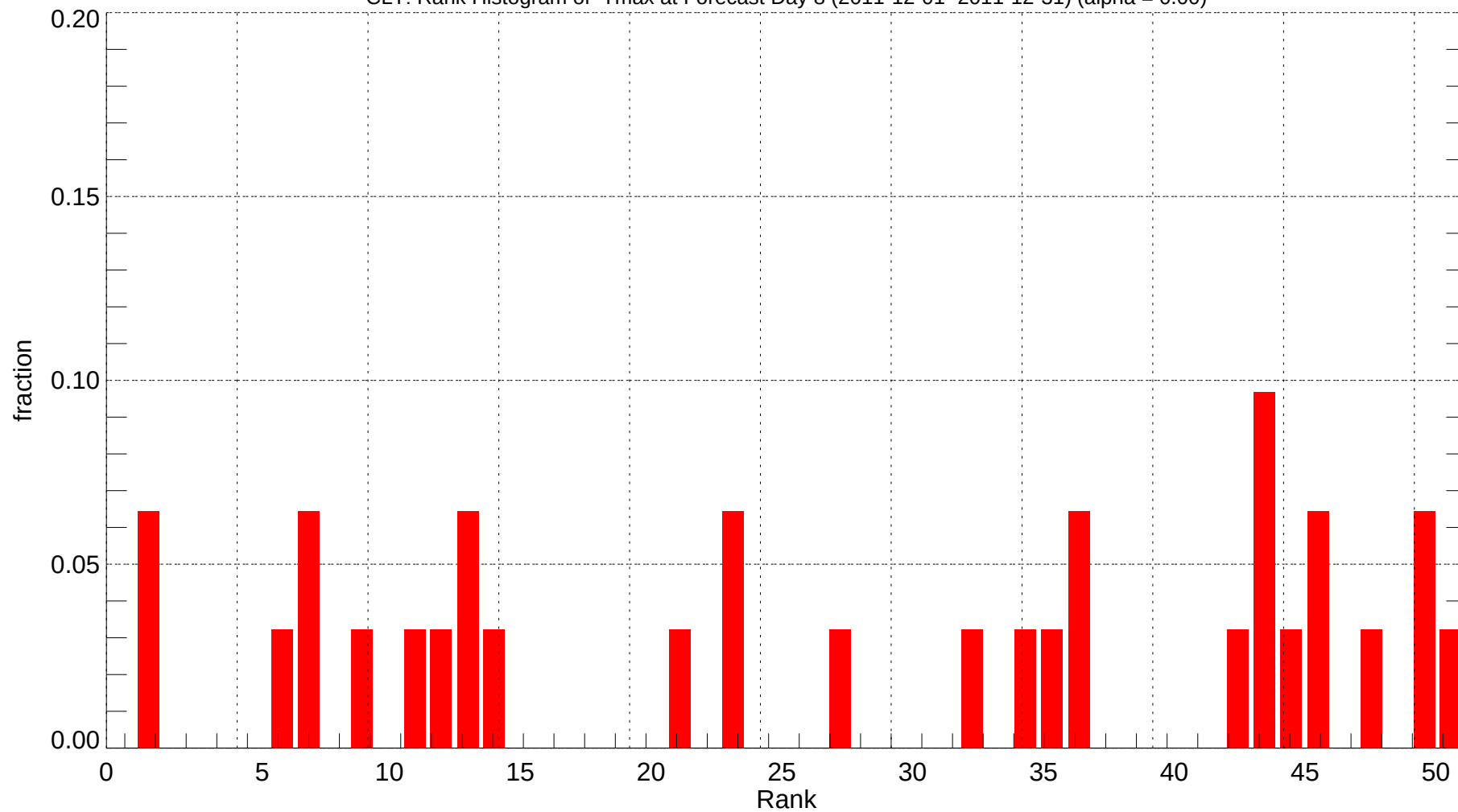
CLT: Rank Histogram of Tmax at Forecast Day 8 (2011-12-01~2011-12-31) (alpha = 0.00)
