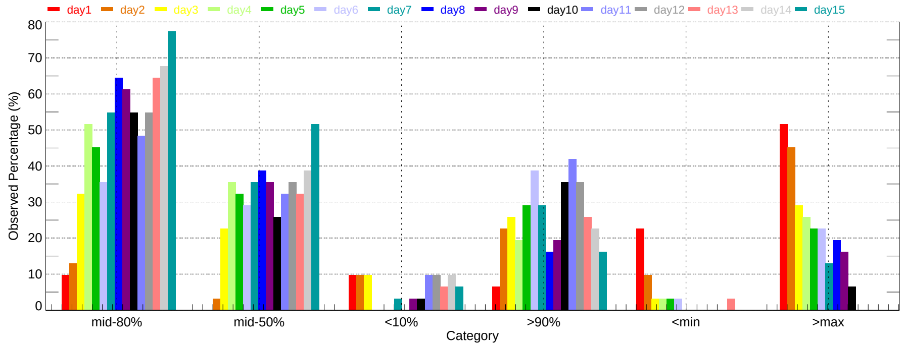
Observed Percentage of Ensembles - LEX: Min Temperature (2011-12-01~2011-12-31)
