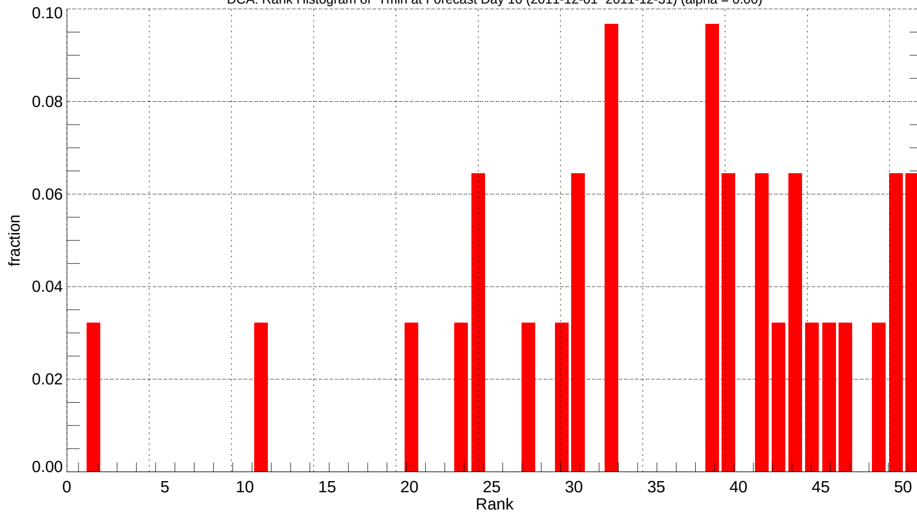
DCA: Rank Histogram of Tmin at Forecast Day 10 (2011-12-01~2011-12-31) (alpha = 0.00)
