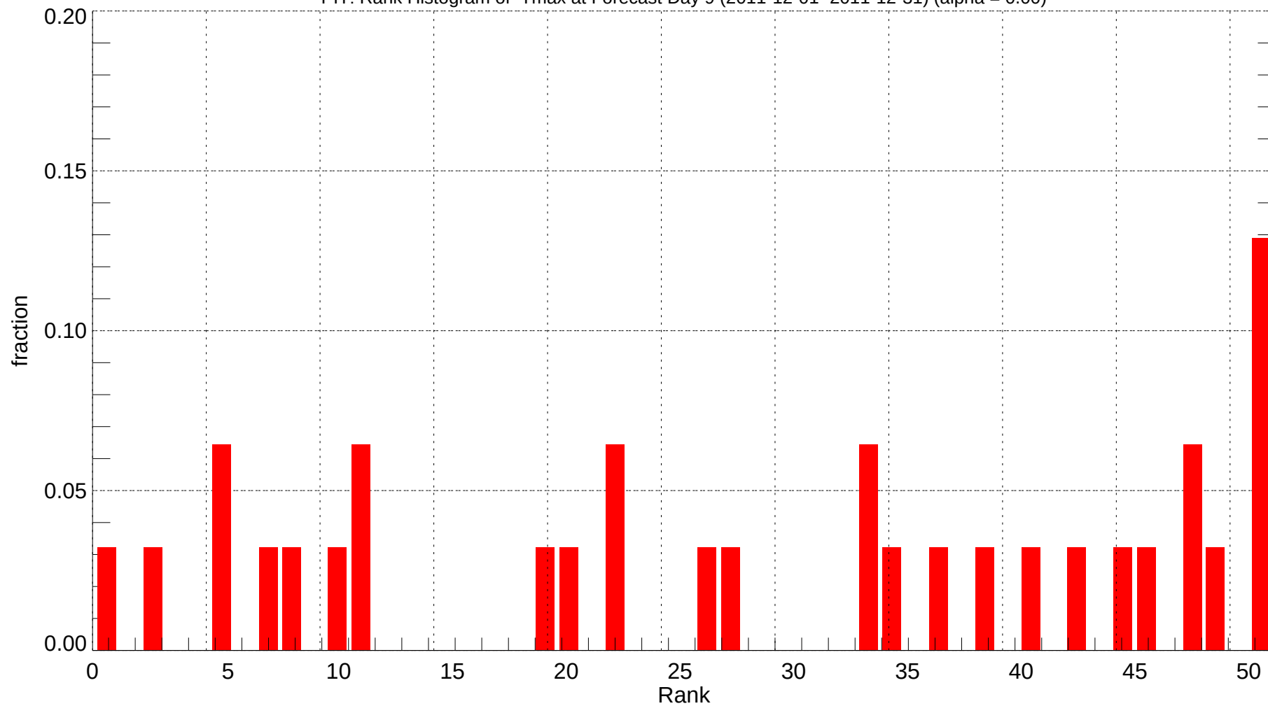
PIT: Rank Histogram of Tmax at Forecast Day 9 (2011-12-01~2011-12-31) (alpha = 0.00)
