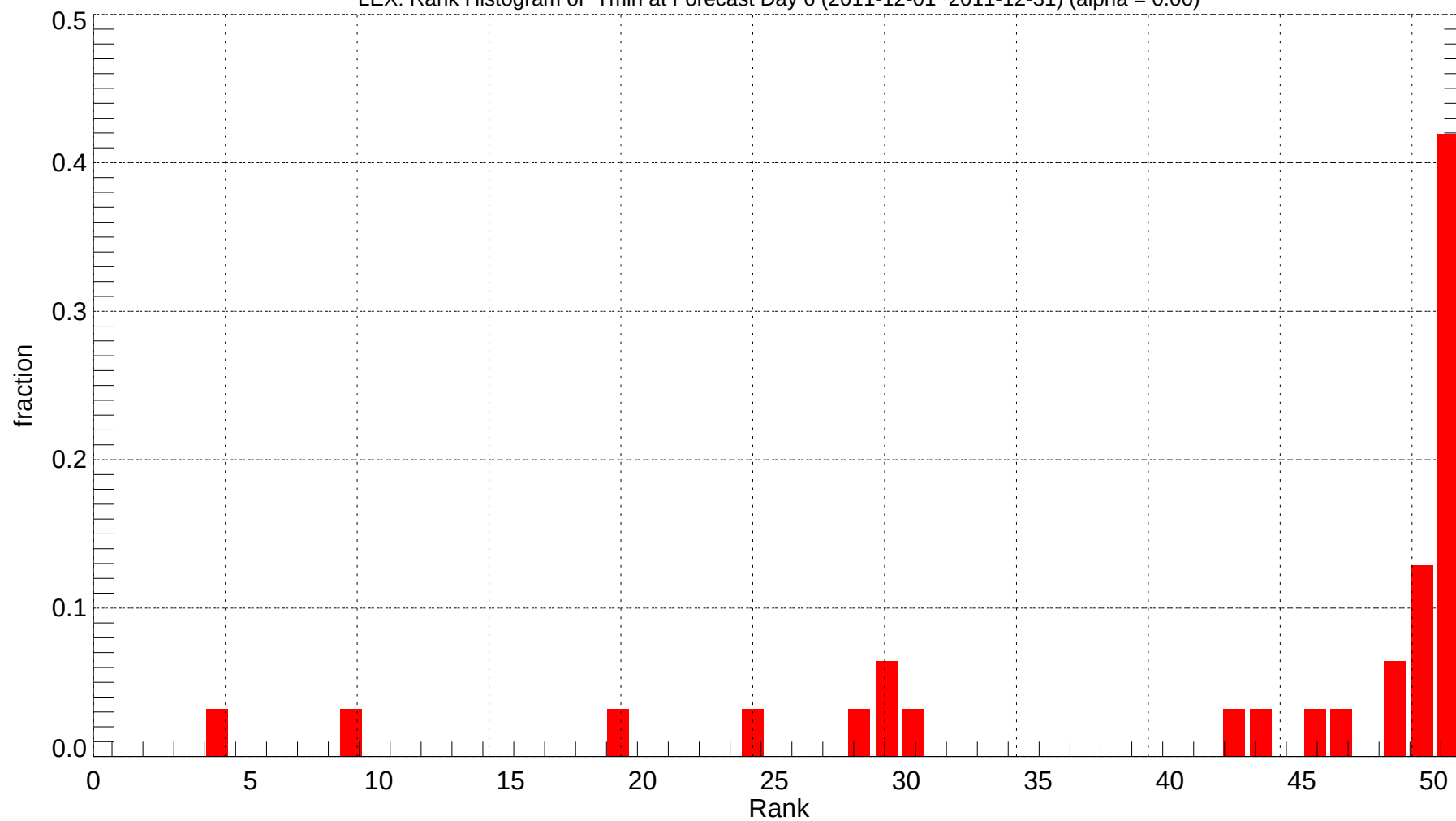
LEX: Rank Histogram of Tmin at Forecast Day 6 (2011-12-01~2011-12-31) (alpha = 0.00)
