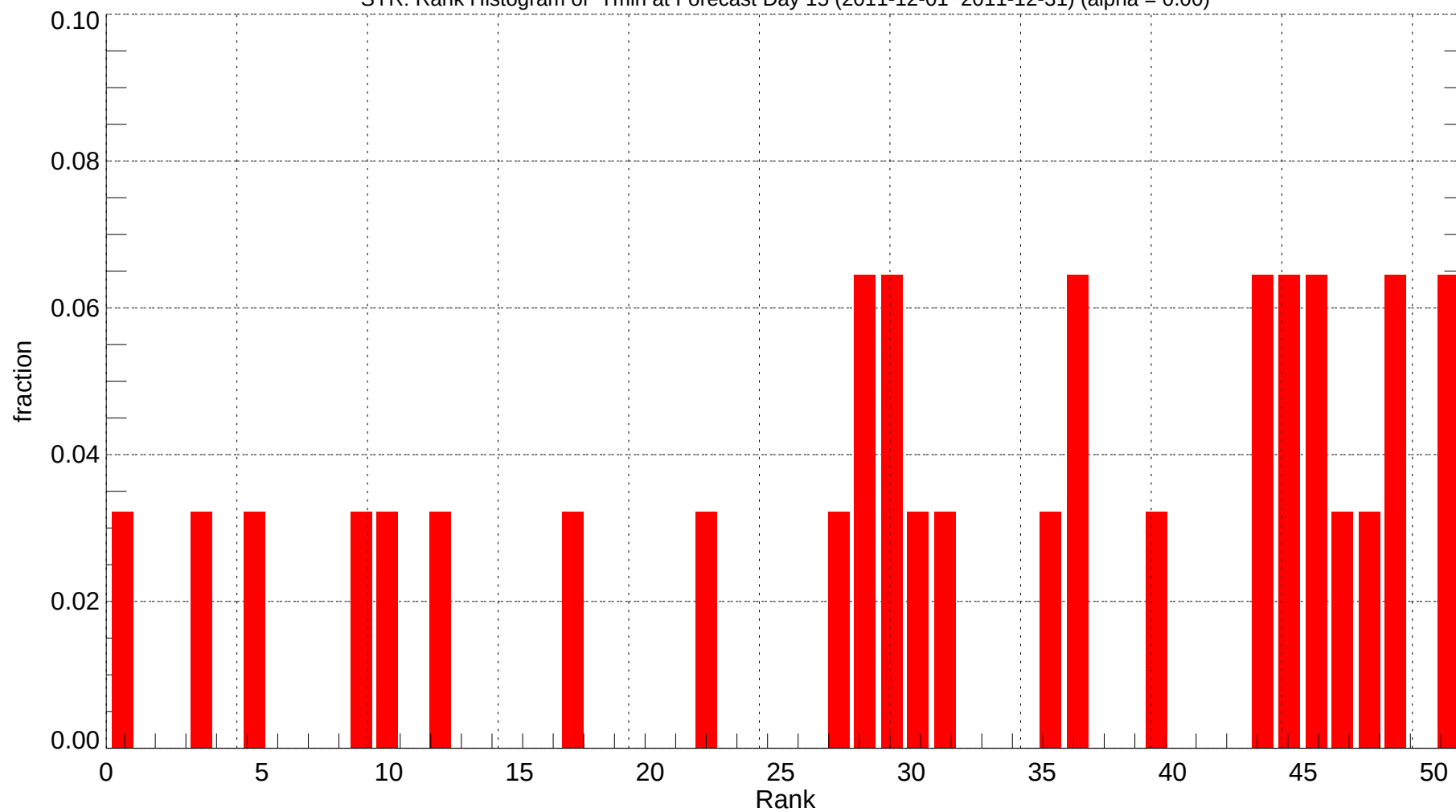
SYR: Rank Histogram of Tmin at Forecast Day 15 (2011-12-01~2011-12-31) (alpha = 0.00)
