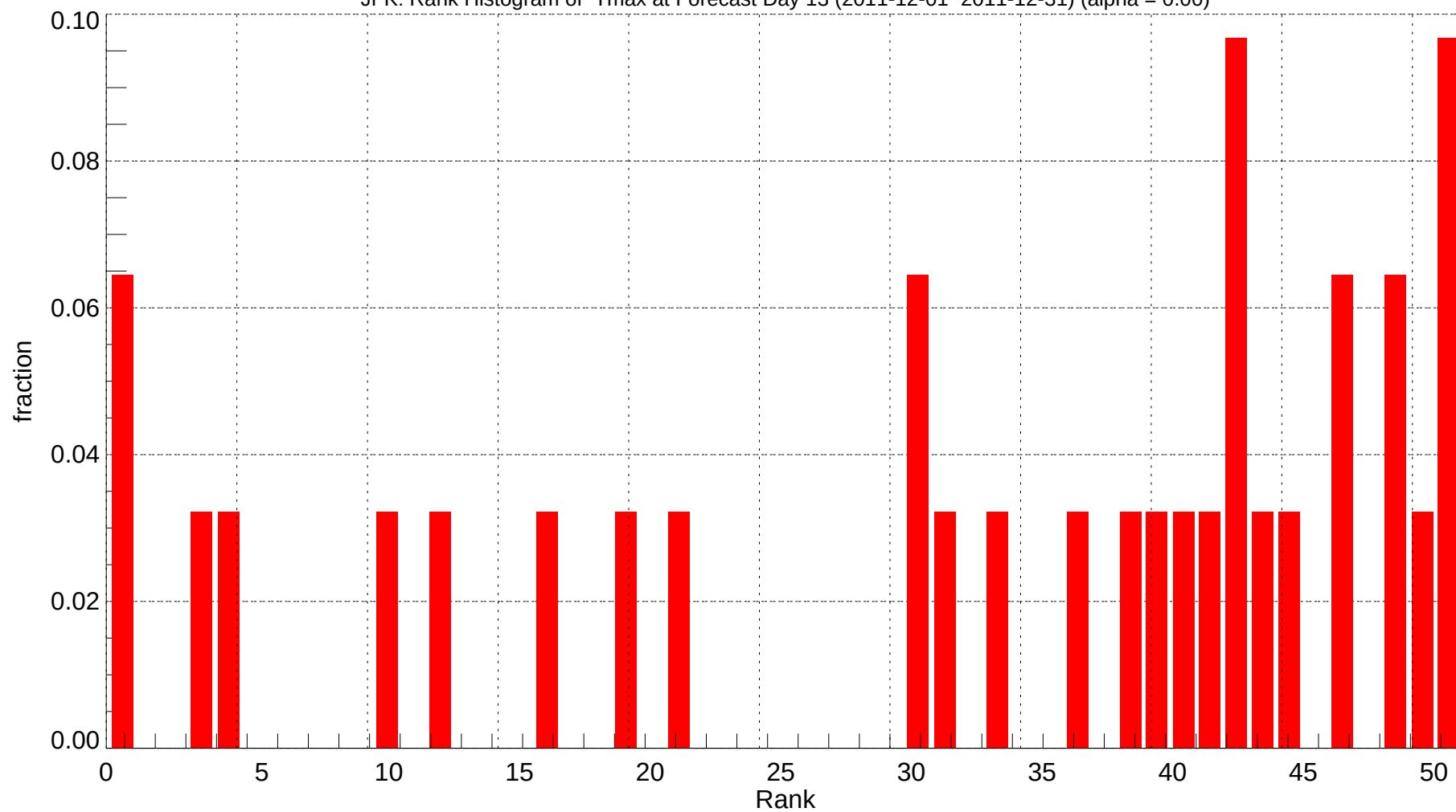
JFK: Rank Histogram of Tmax at Forecast Day 13 (2011-12-01~2011-12-31) (alpha = 0.00)
