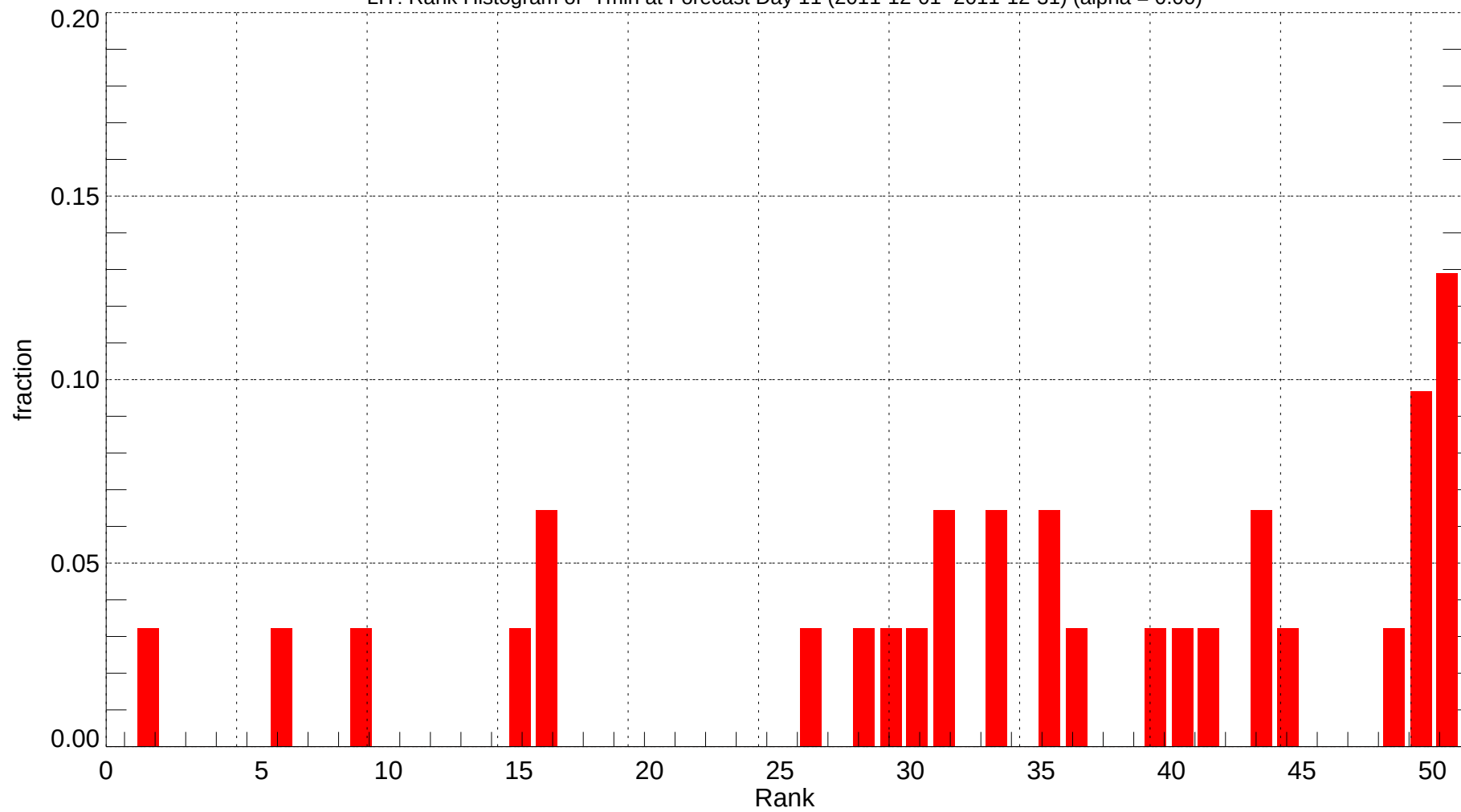
LIT: Rank Histogram of Tmin at Forecast Day 11 (2011-12-01~2011-12-31) (alpha = 0.00)
