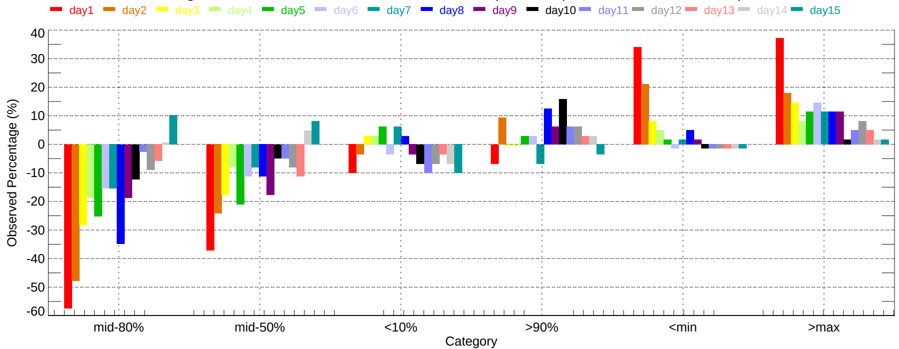
Observed Percentage Deviation of Ensembles - CAE: Min Temperature (2011-12-01~2011-12-31)
