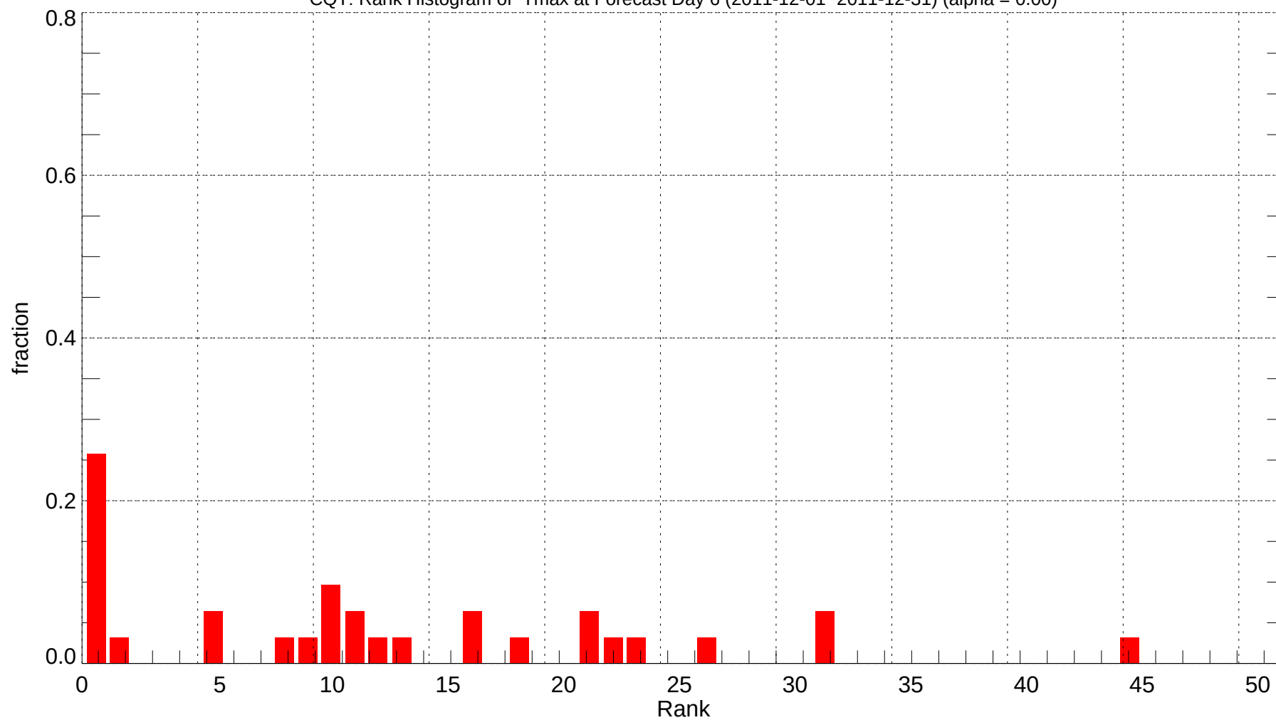
CQT: Rank Histogram of Tmax at Forecast Day 6 (2011-12-01~2011-12-31) (alpha = 0.00)
