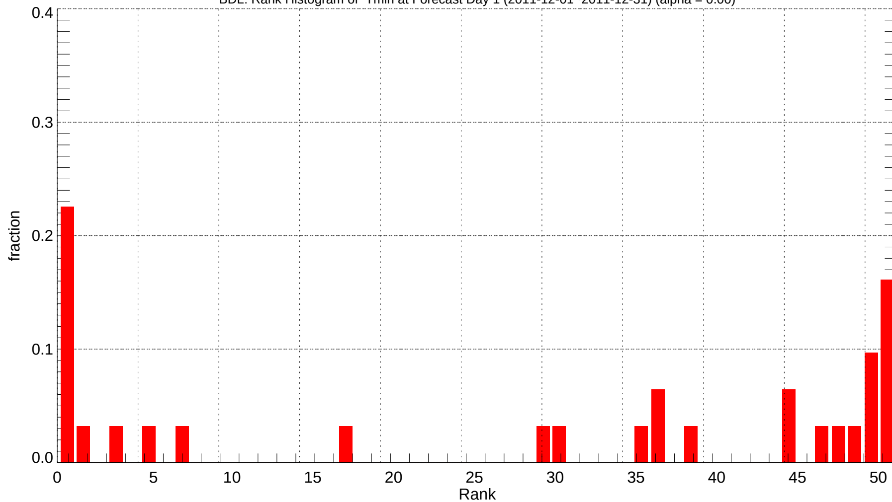
BDL: Rank Histogram of Tmin at Forecast Day 1 (2011-12-01~2011-12-31) (alpha = 0.00)
