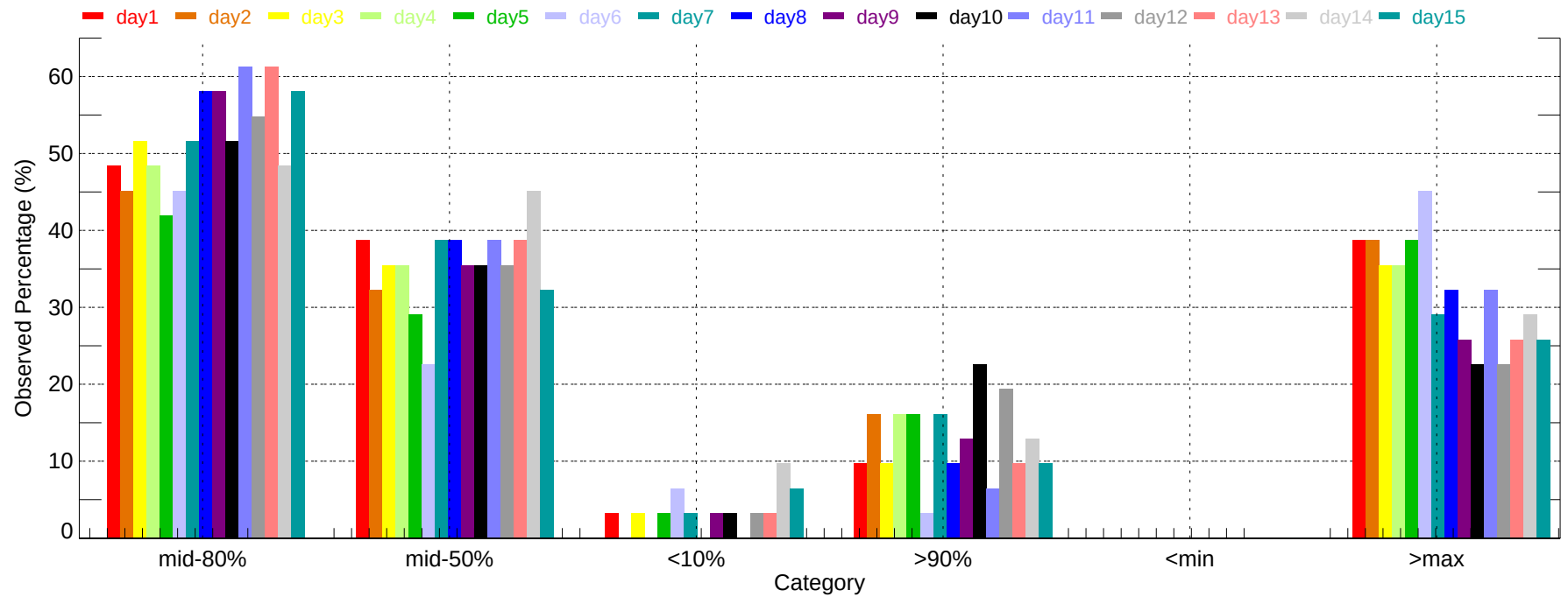
Observed Percentage of Ensembles - EVV: Max Temperature (2011-12-01~2011-12-31)
