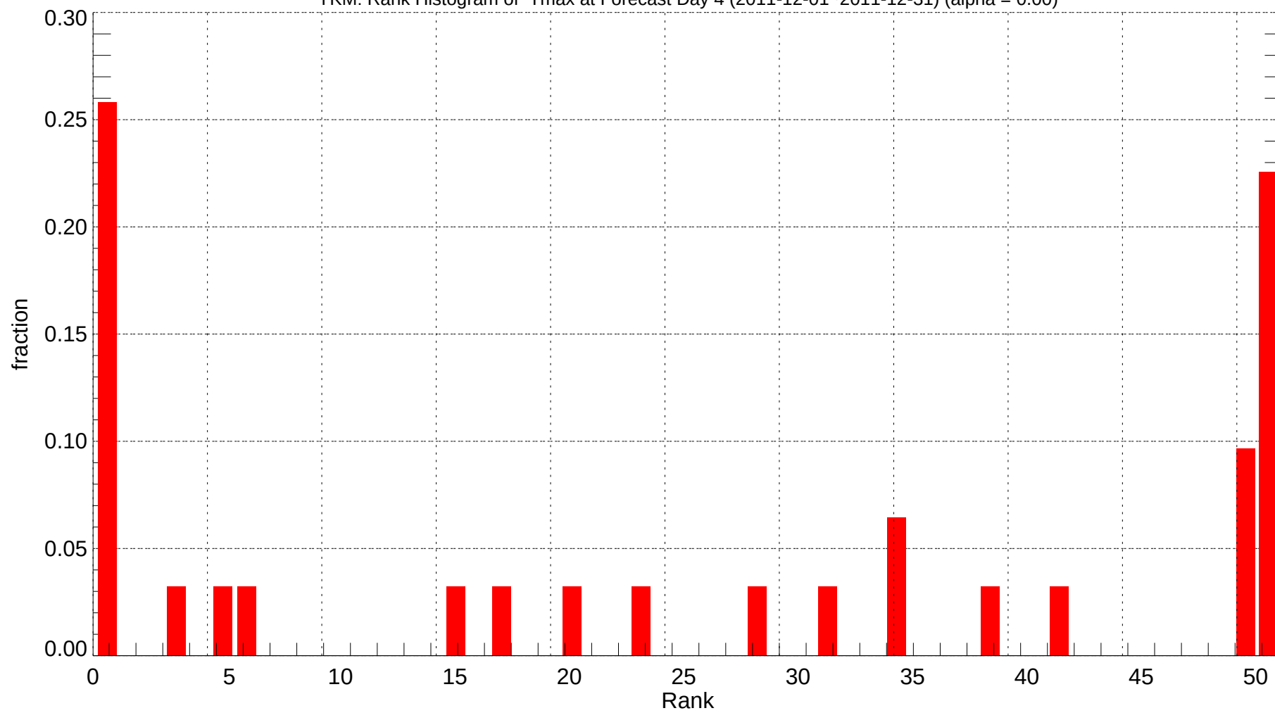
YKM: Rank Histogram of Tmax at Forecast Day 4 (2011-12-01~2011-12-31) (alpha = 0.00)
