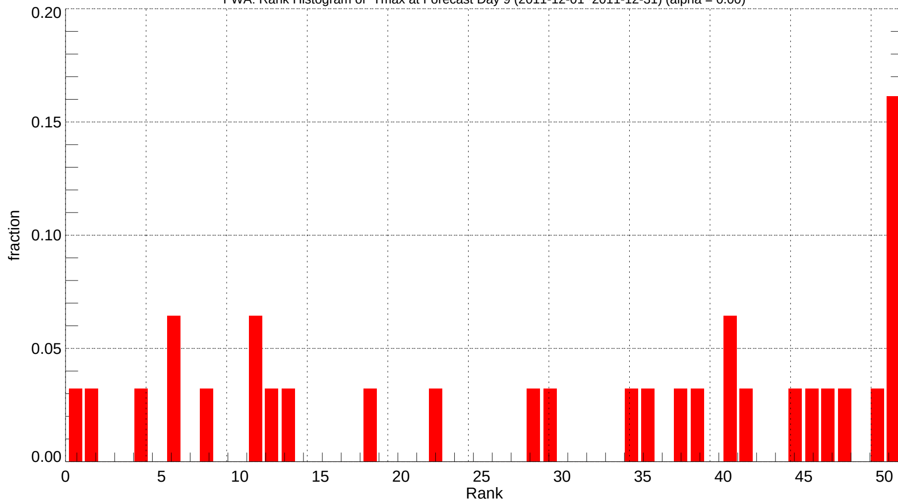
FWA: Rank Histogram of Tmax at Forecast Day 9 (2011-12-01~2011-12-31) (alpha = 0.00)
