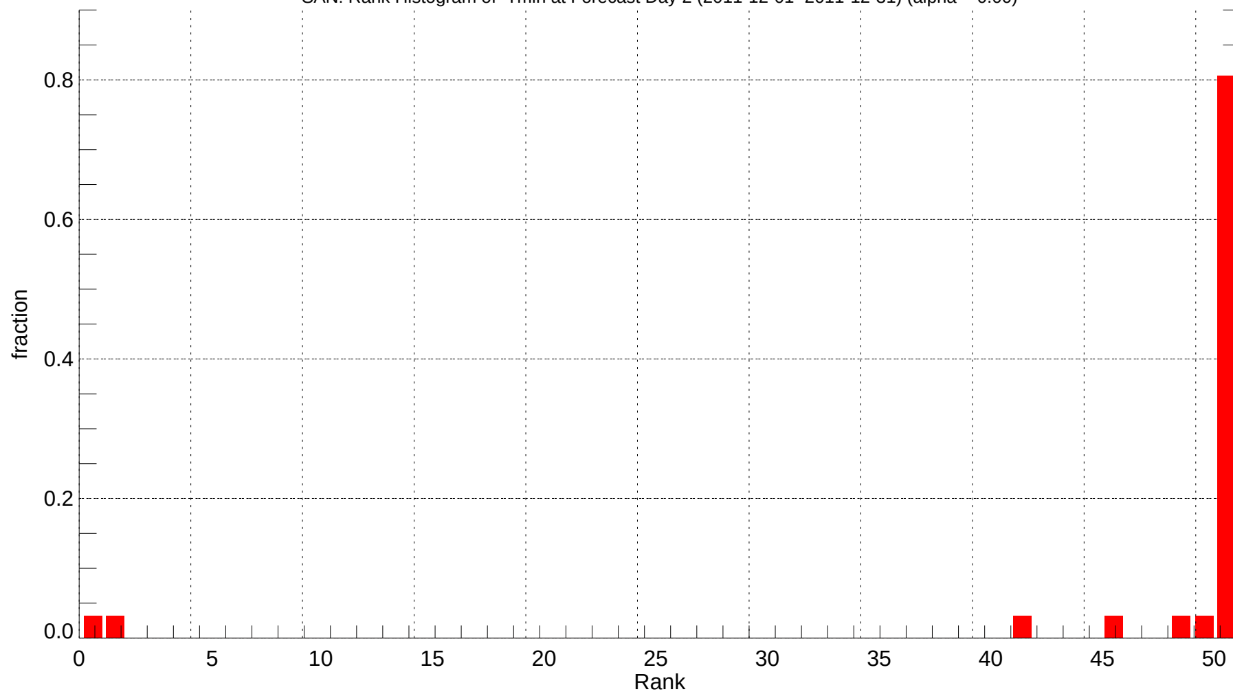
SAN: Rank Histogram of Tmin at Forecast Day 2 (2011-12-01~2011-12-31) (alpha = 0.00)
