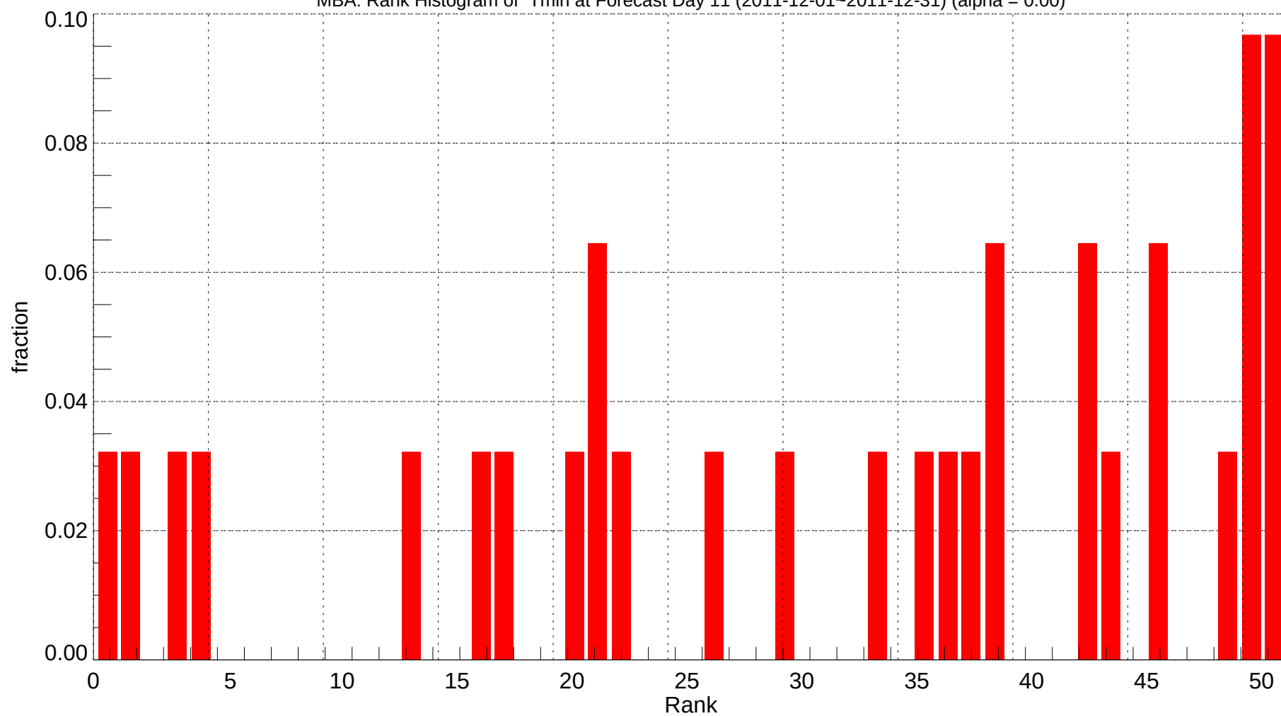
MBA: Rank Histogram of Tmin at Forecast Day 11 (2011-12-01~2011-12-31) (alpha = 0.00)
