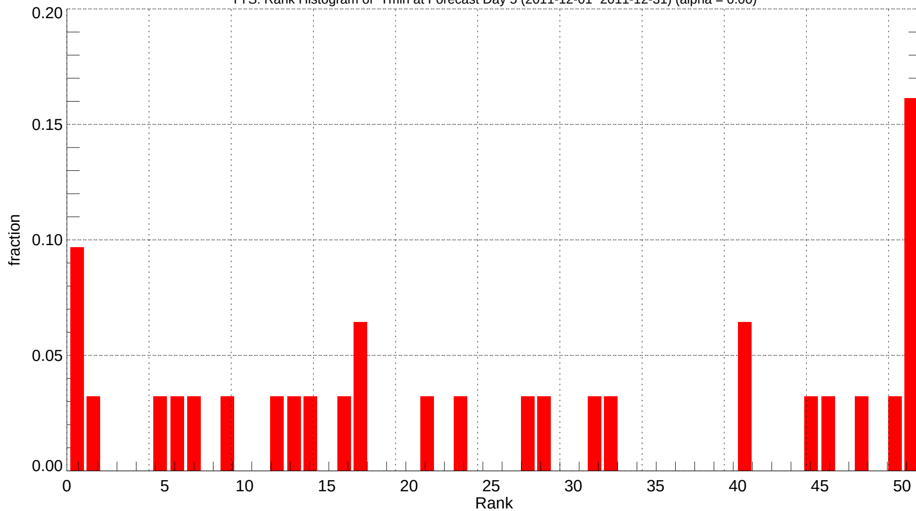
TYS: Rank Histogram of Tmin at Forecast Day 5 (2011-12-01~2011-12-31) (alpha = 0.00)
