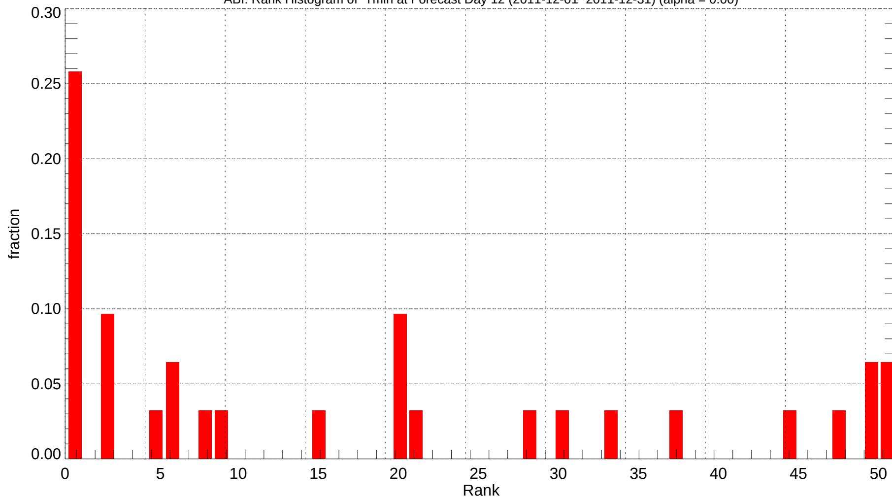
ABI: Rank Histogram of Tmin at Forecast Day 12 (2011-12-01~2011-12-31) (alpha = 0.00)
