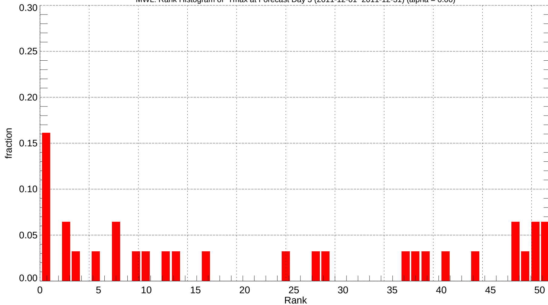
MWL: Rank Histogram of Tmax at Forecast Day 3 (2011-12-01~2011-12-31) (alpha = 0.00)
