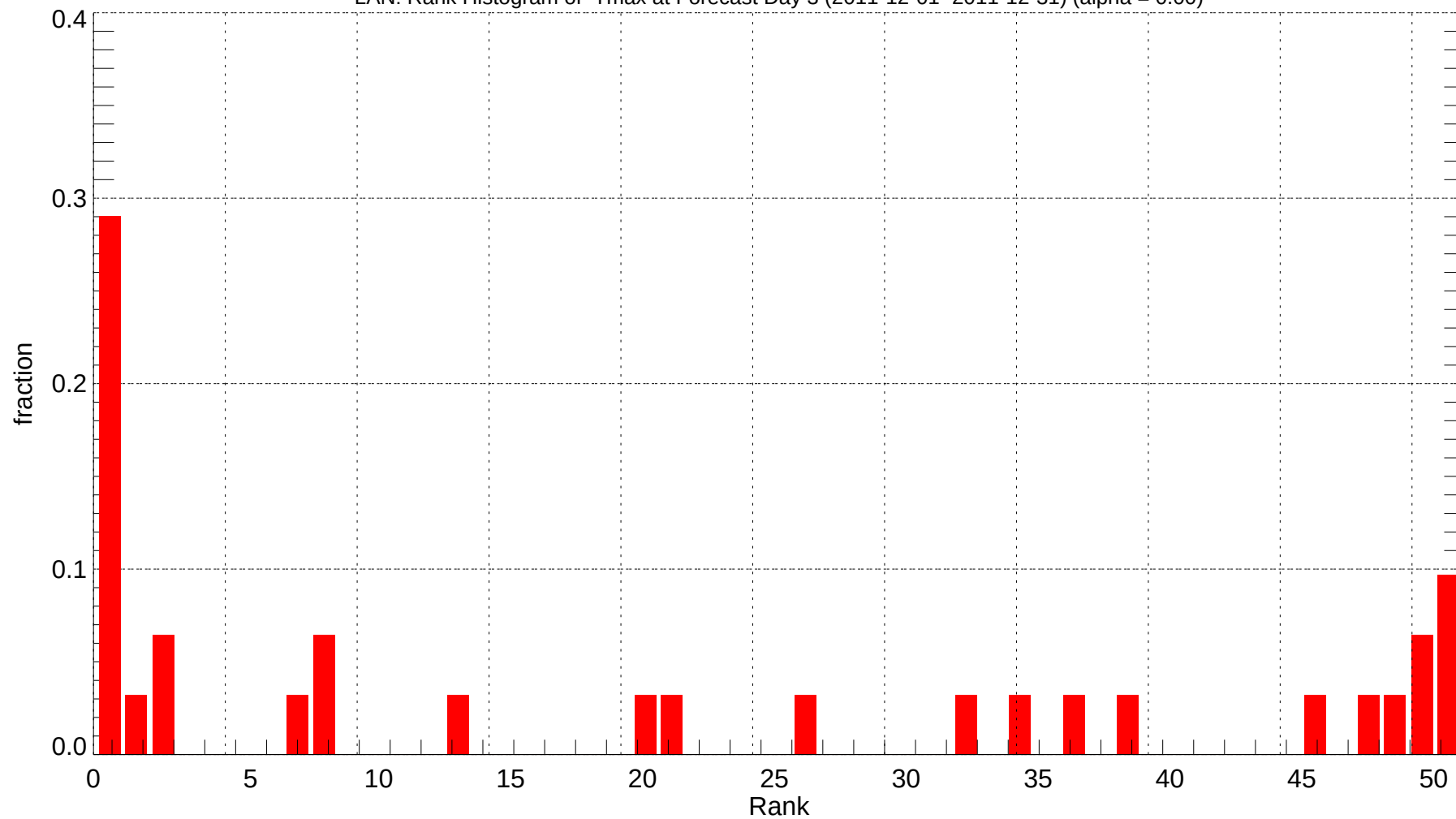
LAN: Rank Histogram of Tmax at Forecast Day 3 (2011-12-01~2011-12-31) (alpha = 0.00)
