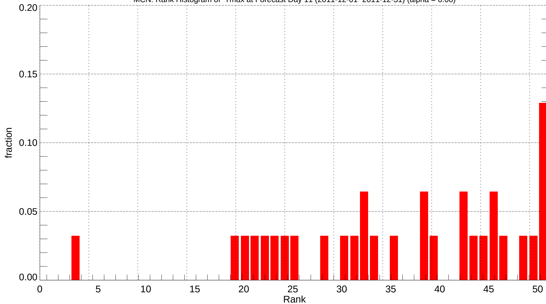
MCN: Rank Histogram of Tmax at Forecast Day 11 (2011-12-01~2011-12-31) (alpha = 0.00)
