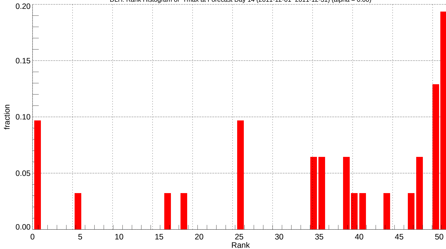
DLH: Rank Histogram of Tmax at Forecast Day 14 (2011-12-01~2011-12-31) (alpha = 0.00)
