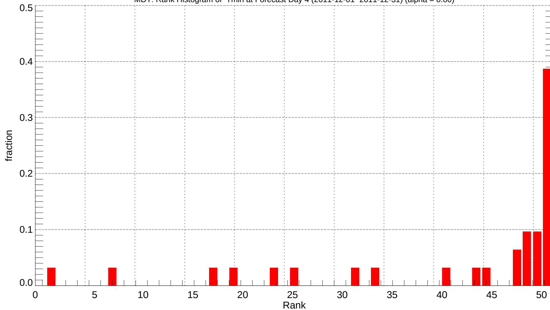
MDT: Rank Histogram of Tmin at Forecast Day 4 (2011-12-01~2011-12-31) (alpha = 0.00)
