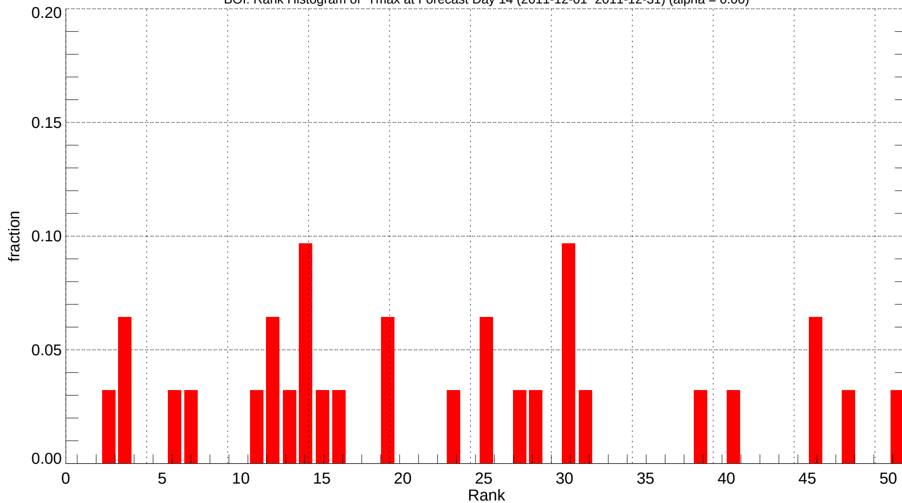
BOI: Rank Histogram of Tmax at Forecast Day 14 (2011-12-01~2011-12-31) (alpha = 0.00)
