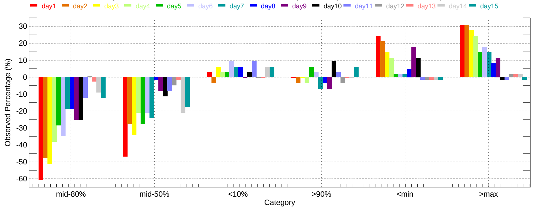
Observed Percentage Deviation of Ensembles - PHX: Max Temperature (2011-12-01~2011-12-31)
