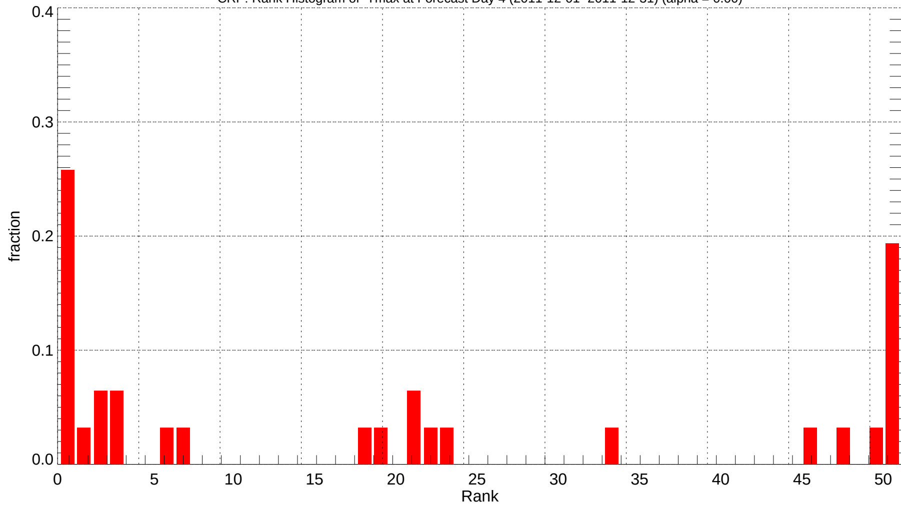
CRP: Rank Histogram of Tmax at Forecast Day 4 (2011-12-01~2011-12-31) (alpha = 0.00)
