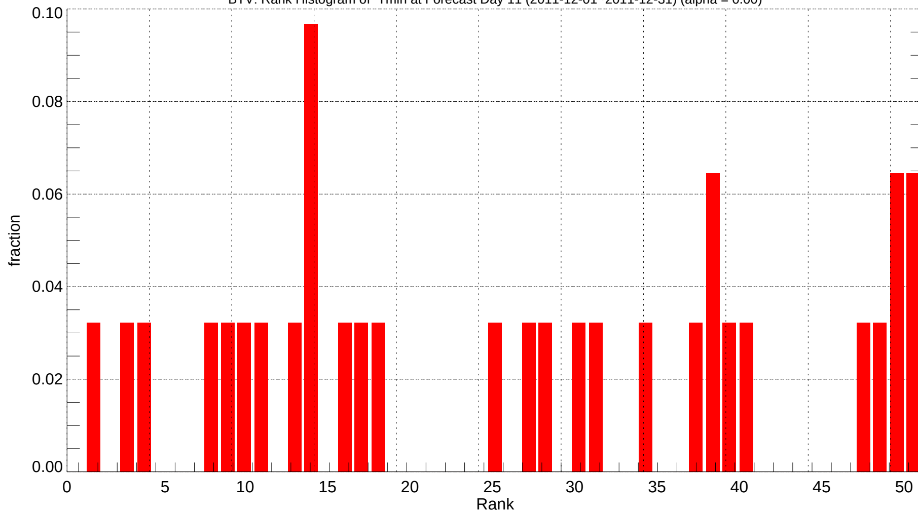
BTV: Rank Histogram of Tmin at Forecast Day 11 (2011-12-01~2011-12-31) (alpha = 0.00)
