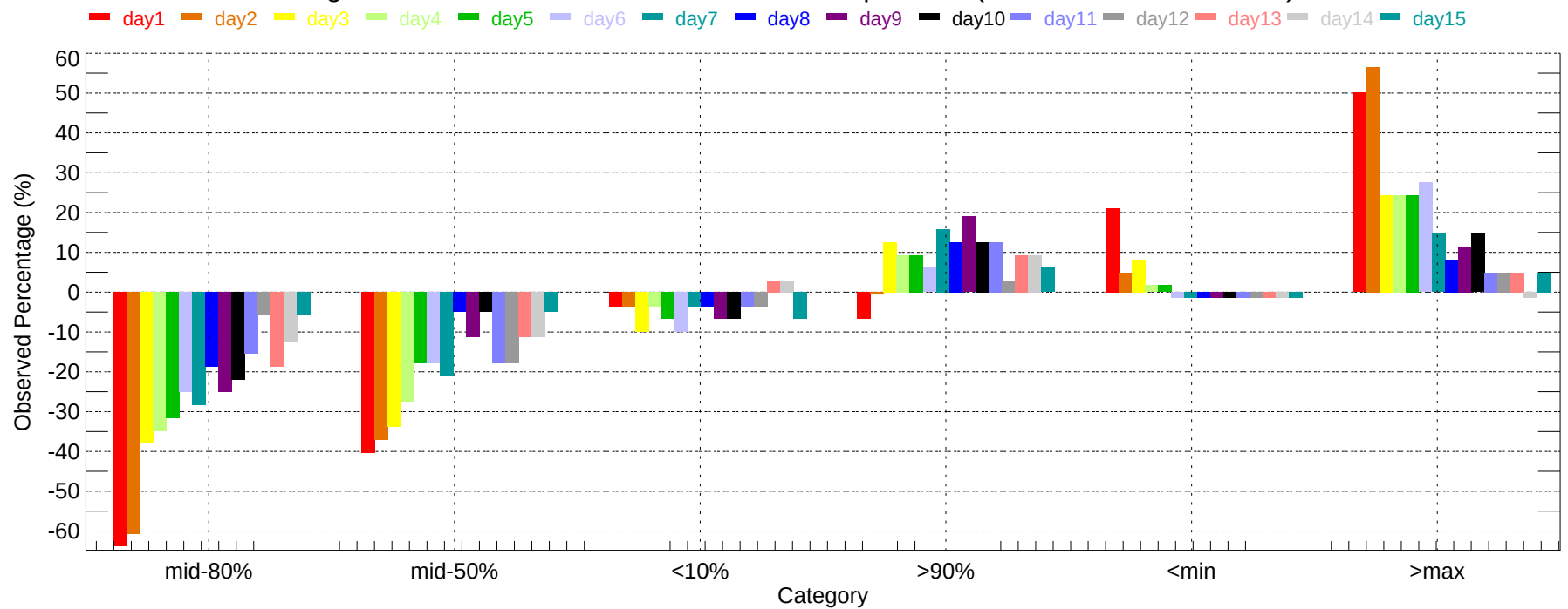
Observed Percentage Deviation of Ensembles - EVV: Min Temperature (2011-12-01~2011-12-31)
