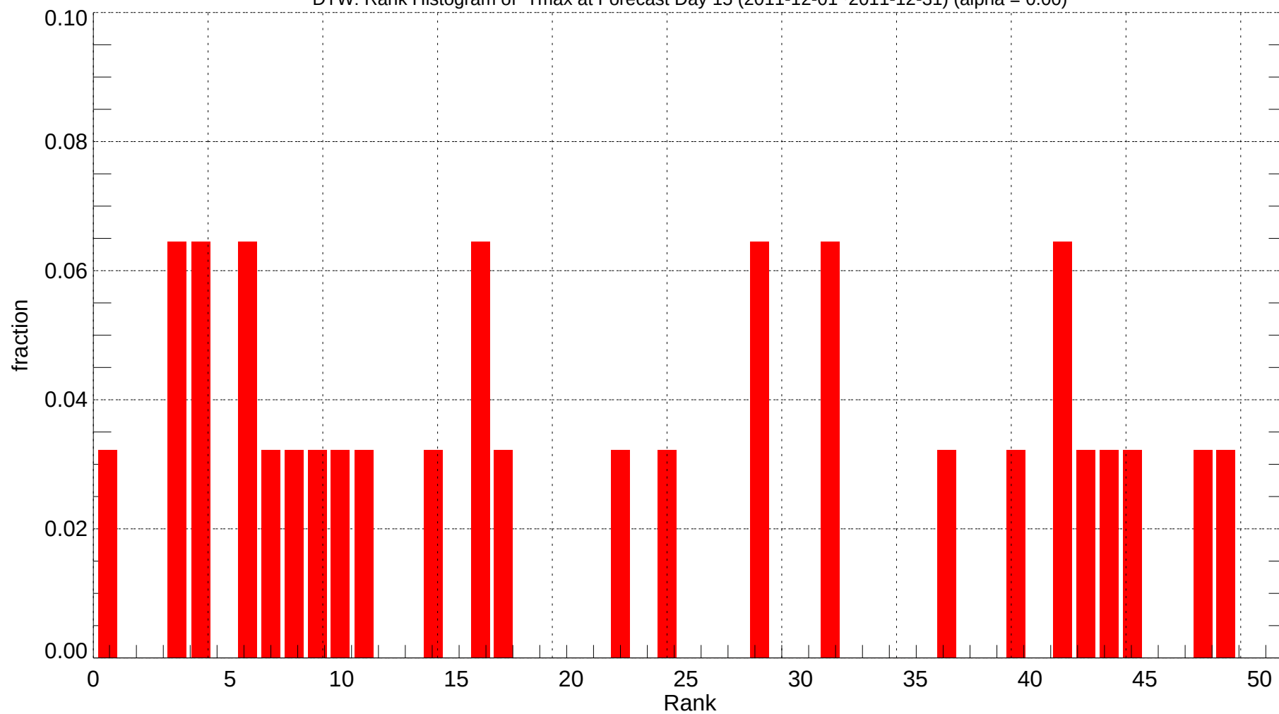
DTW: Rank Histogram of Tmax at Forecast Day 15 (2011-12-01~2011-12-31) (alpha = 0.00)
