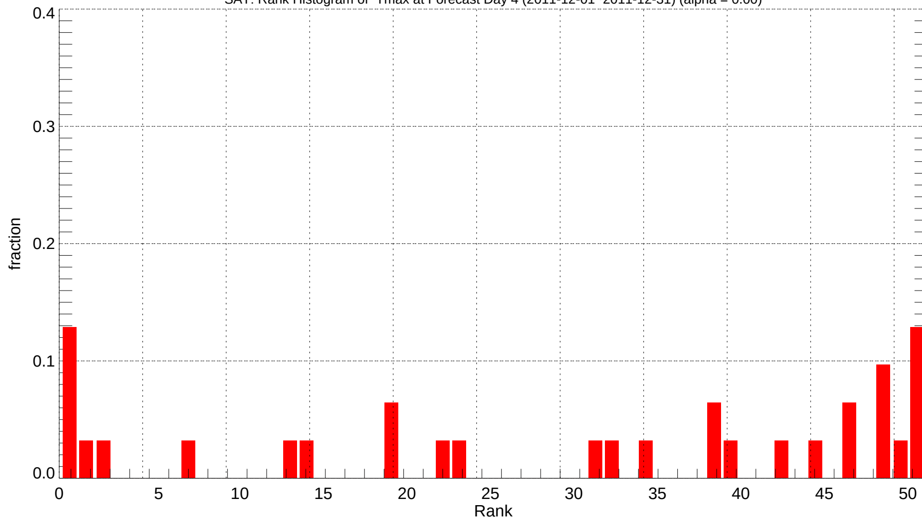
SAT: Rank Histogram of Tmax at Forecast Day 4 (2011-12-01~2011-12-31) (alpha = 0.00)
