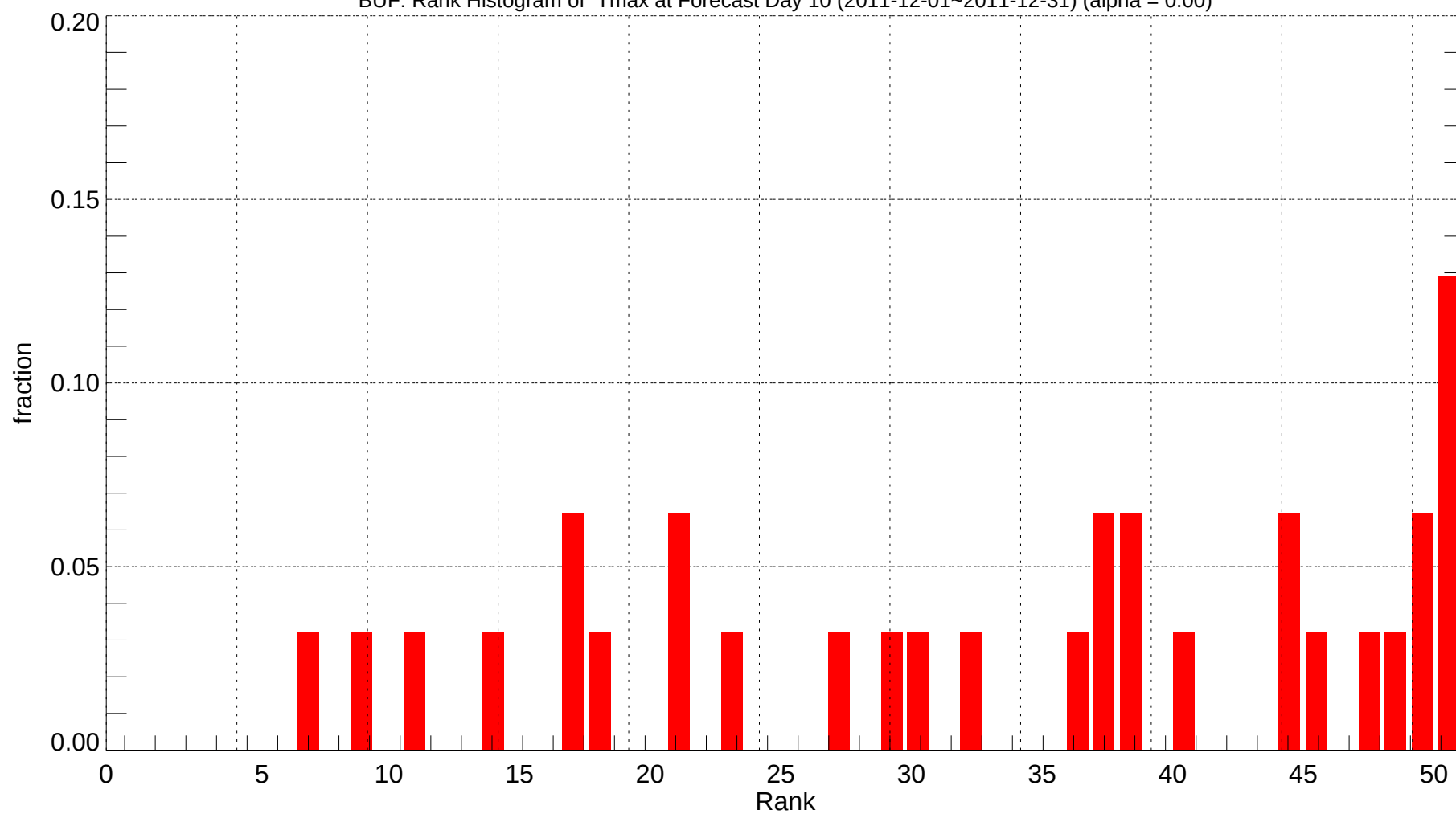
BUF: Rank Histogram of Tmax at Forecast Day 10 (2011-12-01~2011-12-31) (alpha = 0.00)
