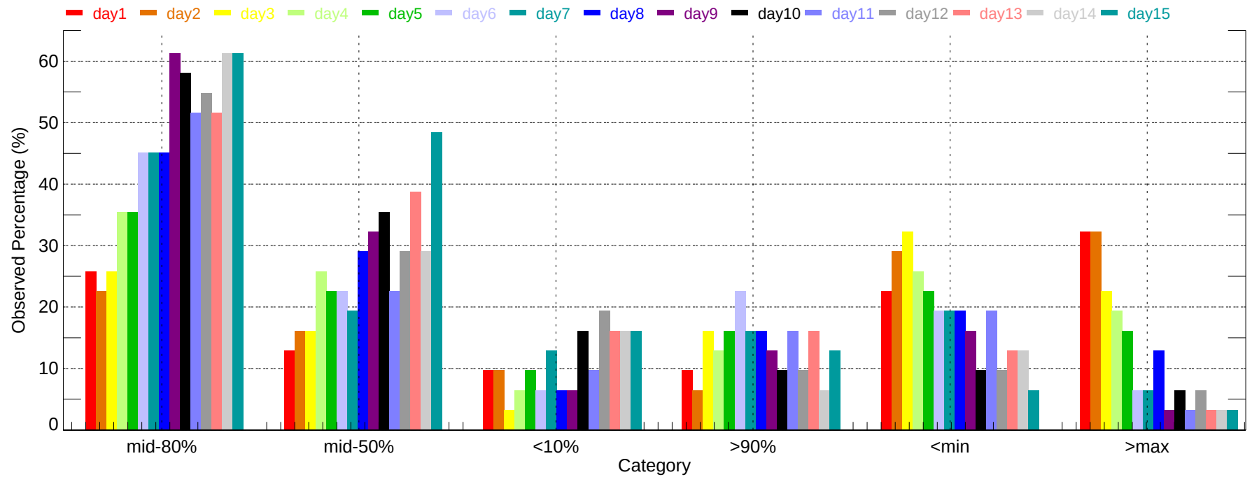
Observed Percentage of Ensembles - YKM: Max Temperature (2011-12-01~2011-12-31)
