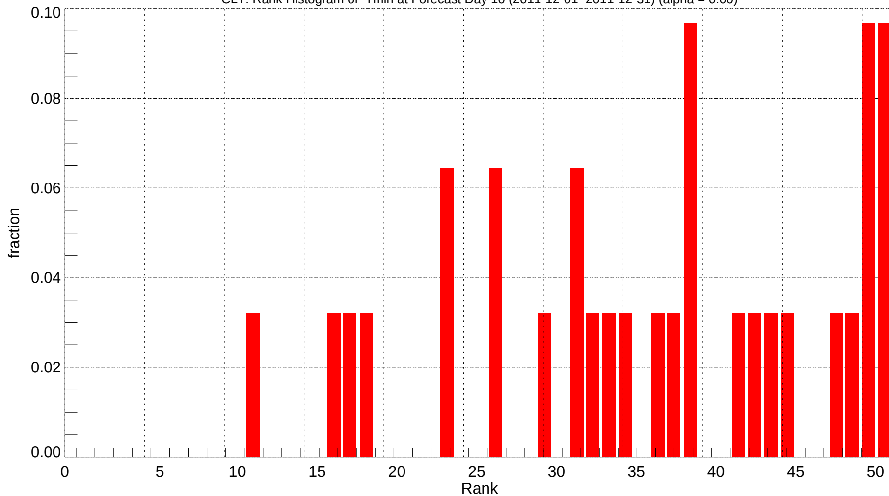
CLT: Rank Histogram of Tmin at Forecast Day 10 (2011-12-01~2011-12-31) (alpha = 0.00)
