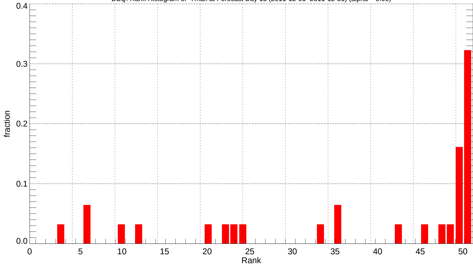
DBQ: Rank Histogram of Tmax at Forecast Day 13 (2011-12-01~2011-12-31) (alpha = 0.00)
