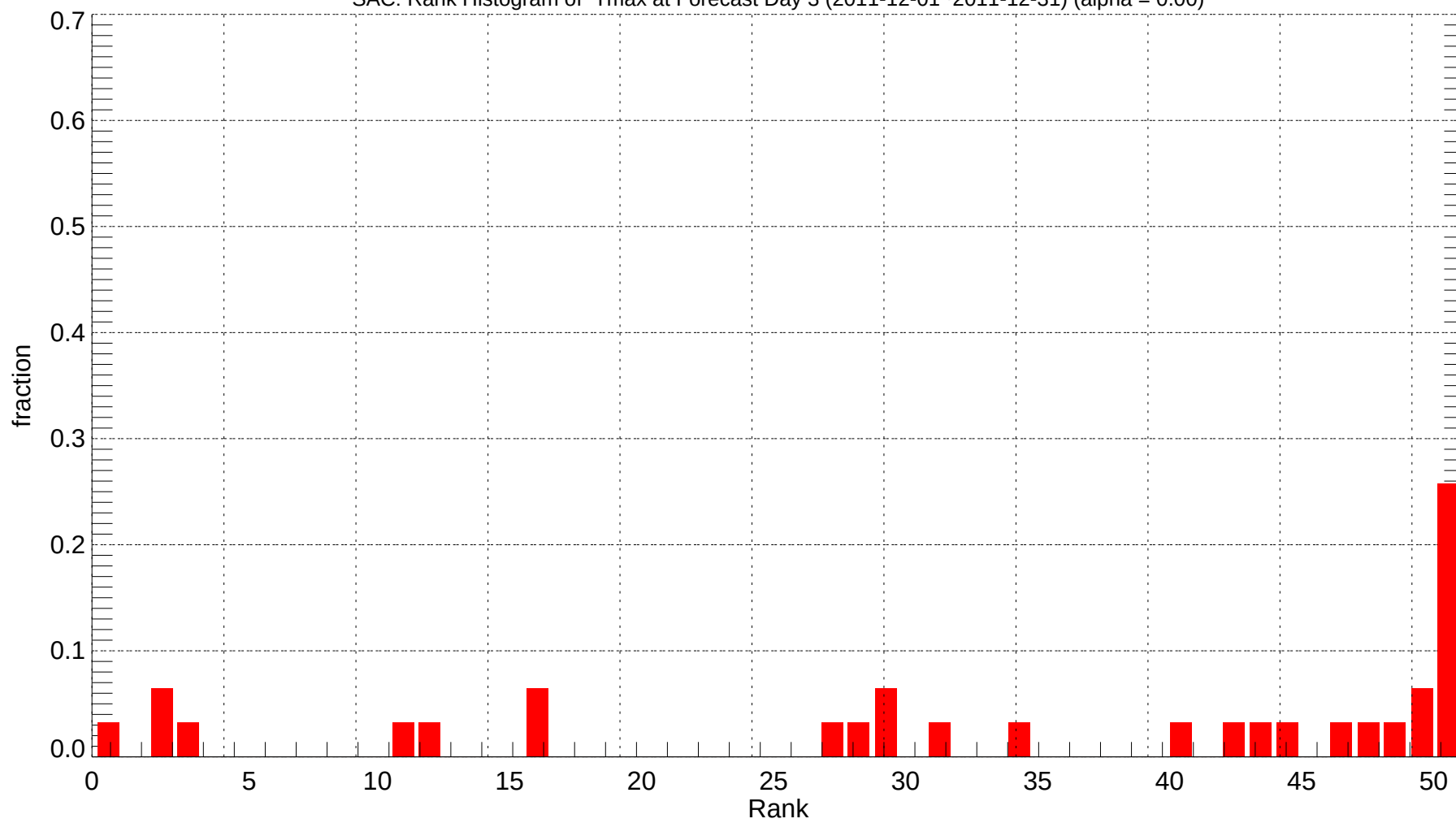
SAC: Rank Histogram of Tmax at Forecast Day 3 (2011-12-01~2011-12-31) (alpha = 0.00)
