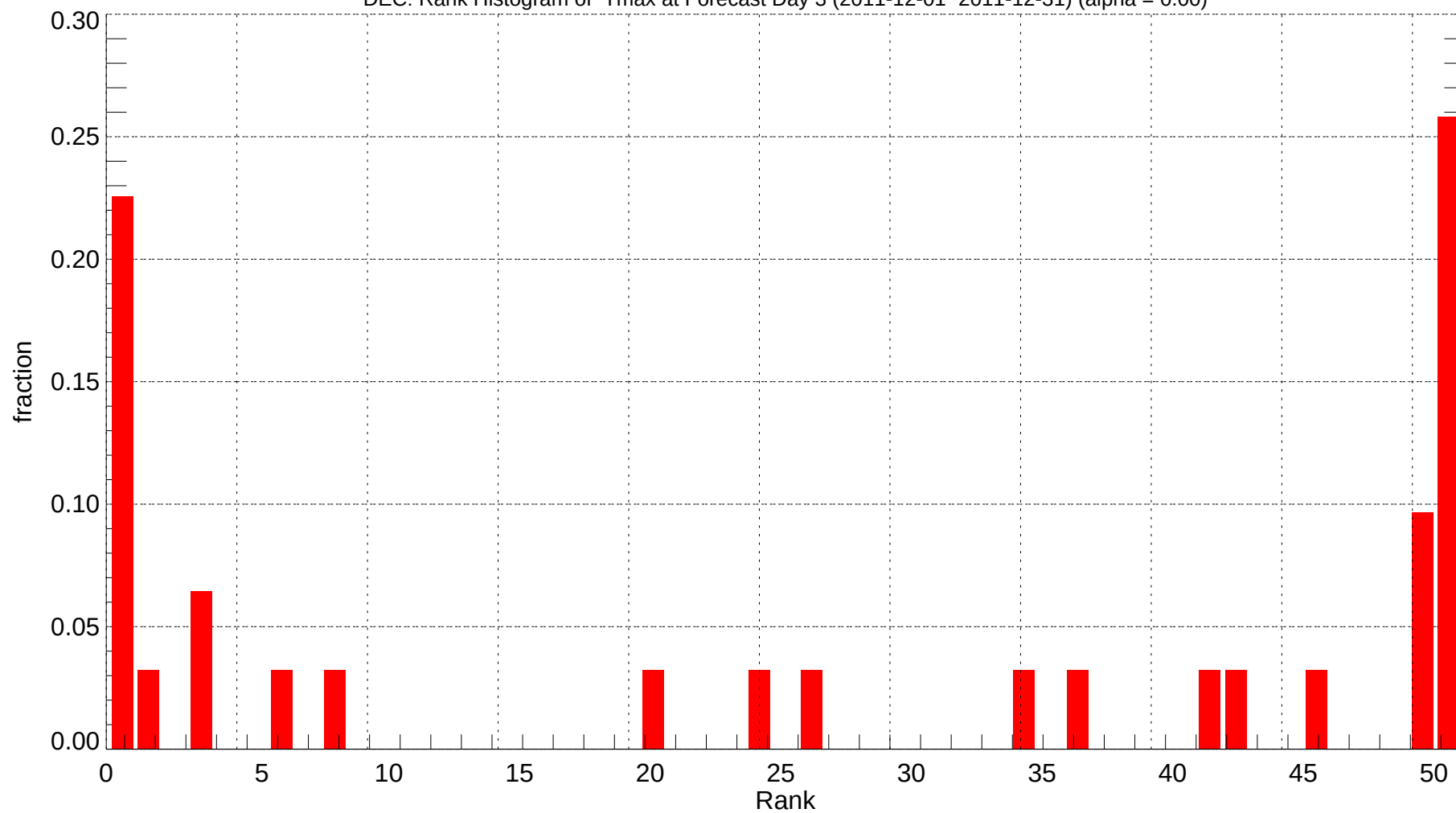
DEC: Rank Histogram of Tmax at Forecast Day 3 (2011-12-01~2011-12-31) (alpha = 0.00)
