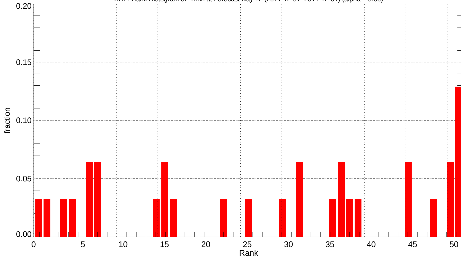
RAP: Rank Histogram of Tmin at Forecast Day 12 (2011-12-01~2011-12-31) (alpha = 0.00)
