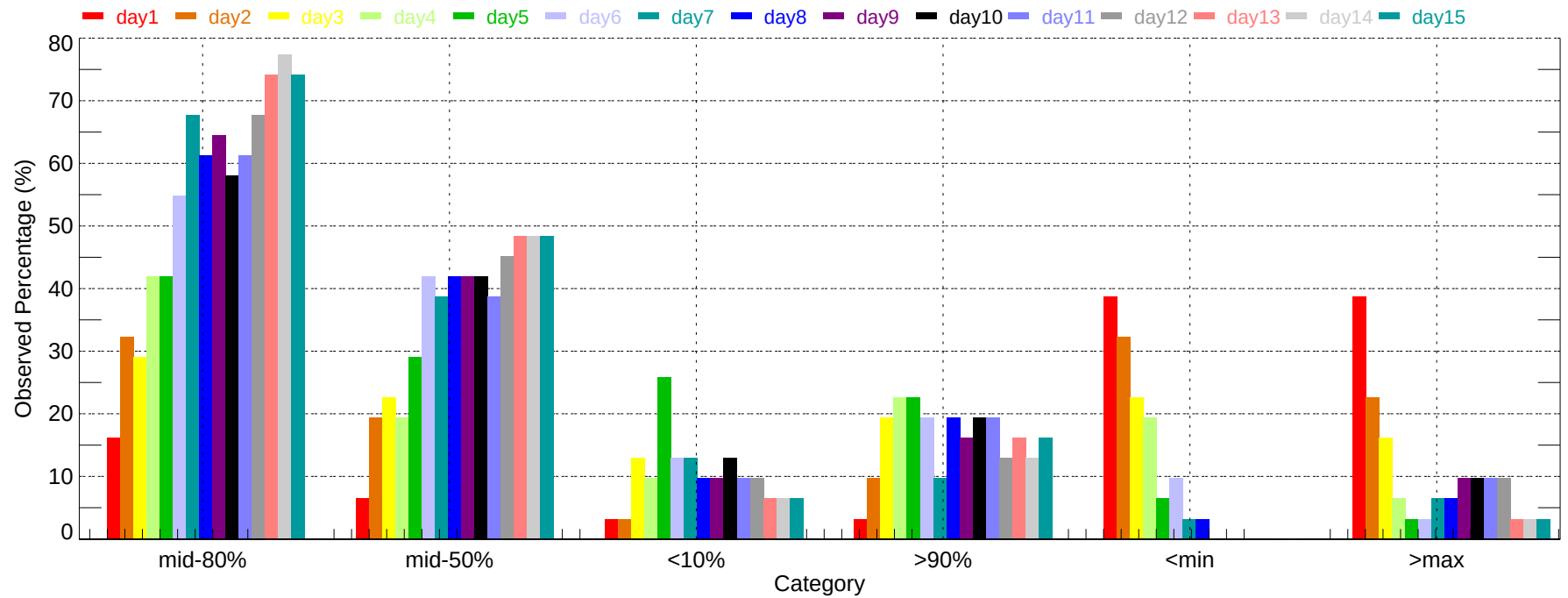
Observed Percentage of Ensembles - IPT: Min Temperature (2011-12-01~2011-12-31)
