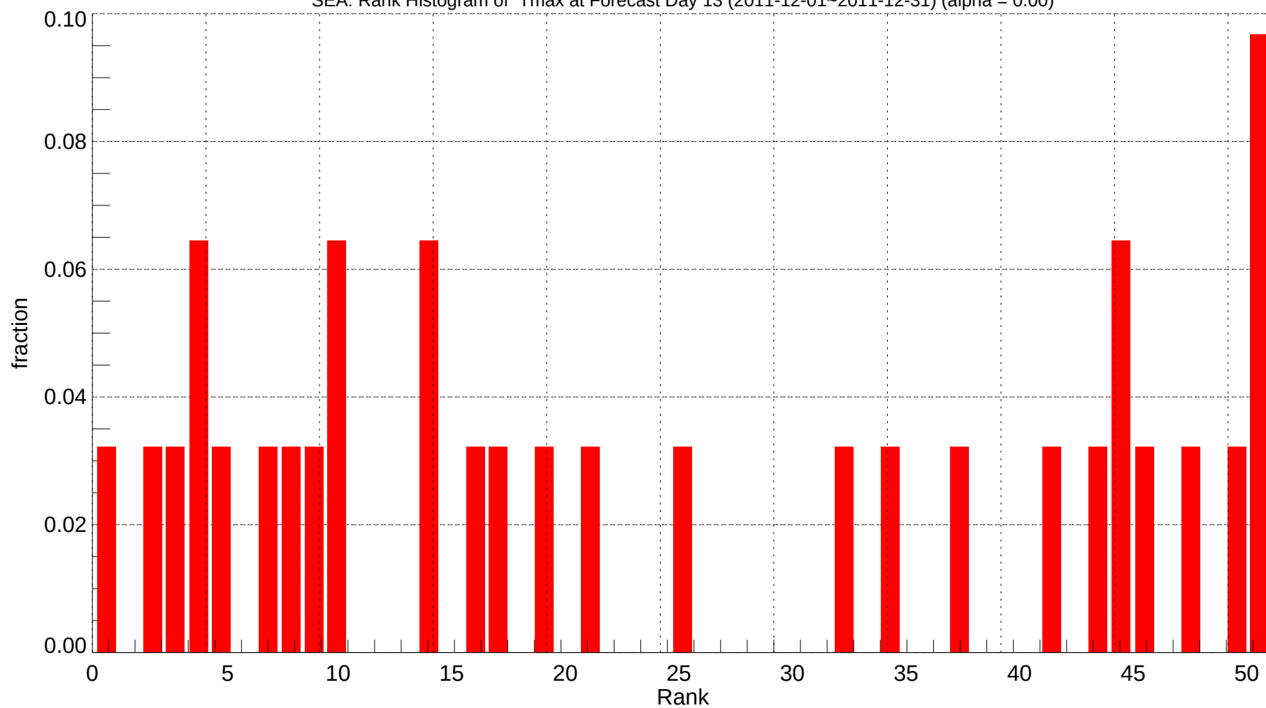
SEA: Rank Histogram of Tmax at Forecast Day 13 (2011-12-01~2011-12-31) (alpha = 0.00)
