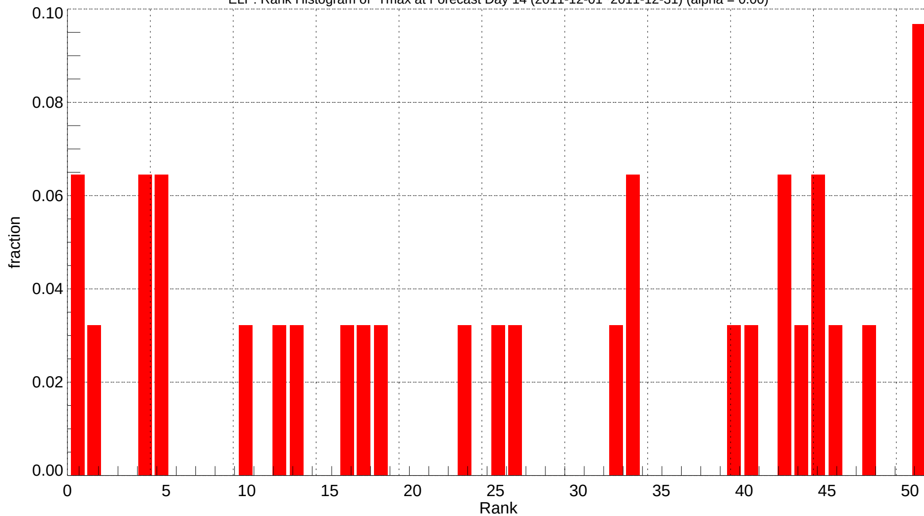
ELP: Rank Histogram of Tmax at Forecast Day 14 (2011-12-01~2011-12-31) (alpha = 0.00)
