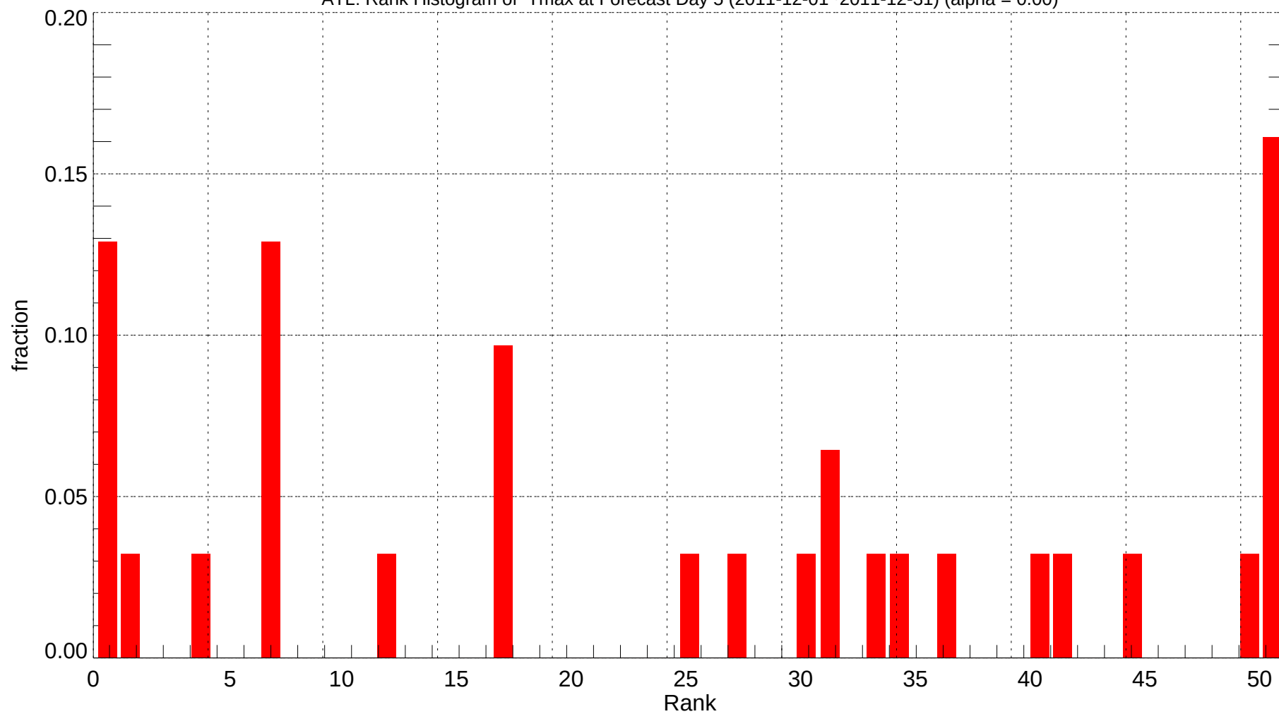
ATL: Rank Histogram of Tmax at Forecast Day 5 (2011-12-01~2011-12-31) (alpha = 0.00)
