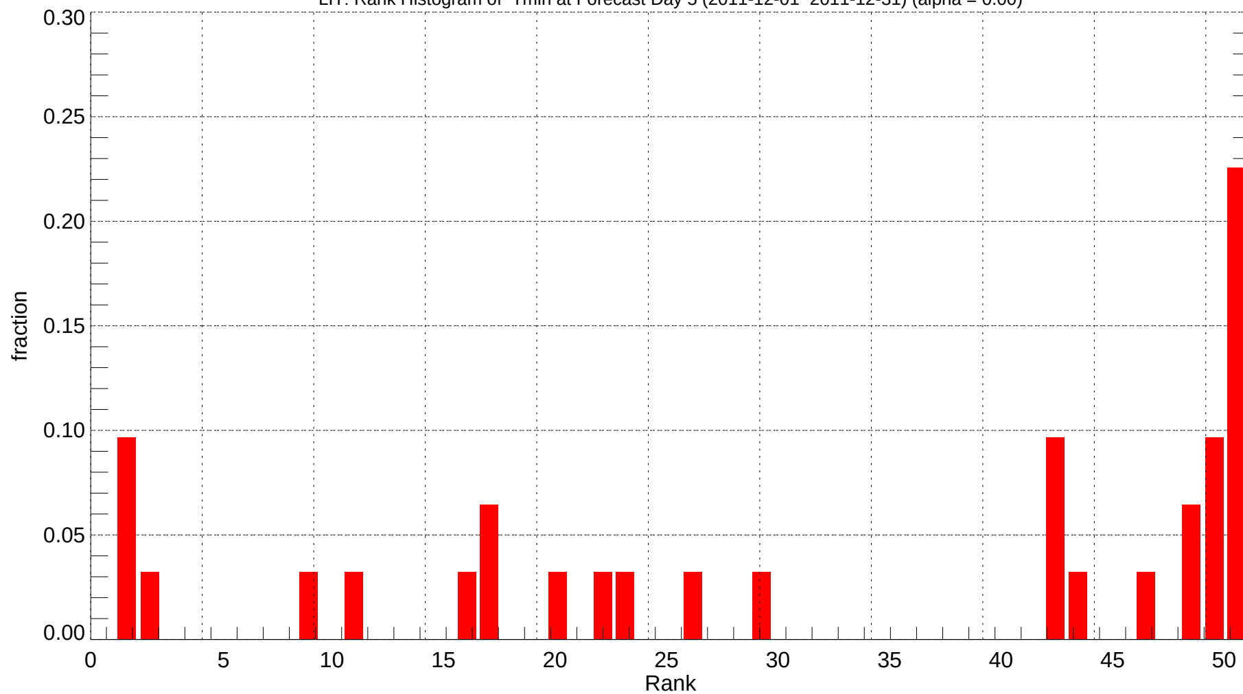
LIT: Rank Histogram of Tmin at Forecast Day 5 (2011-12-01~2011-12-31) (alpha = 0.00)
