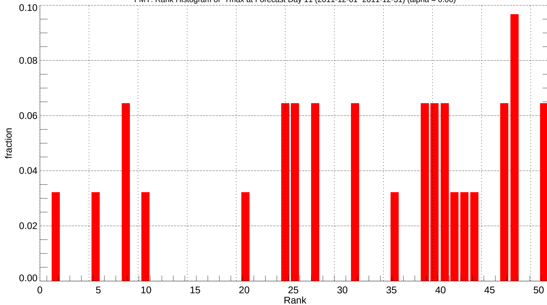
FMY: Rank Histogram of Tmax at Forecast Day 11 (2011-12-01~2011-12-31) (alpha = 0.00)
