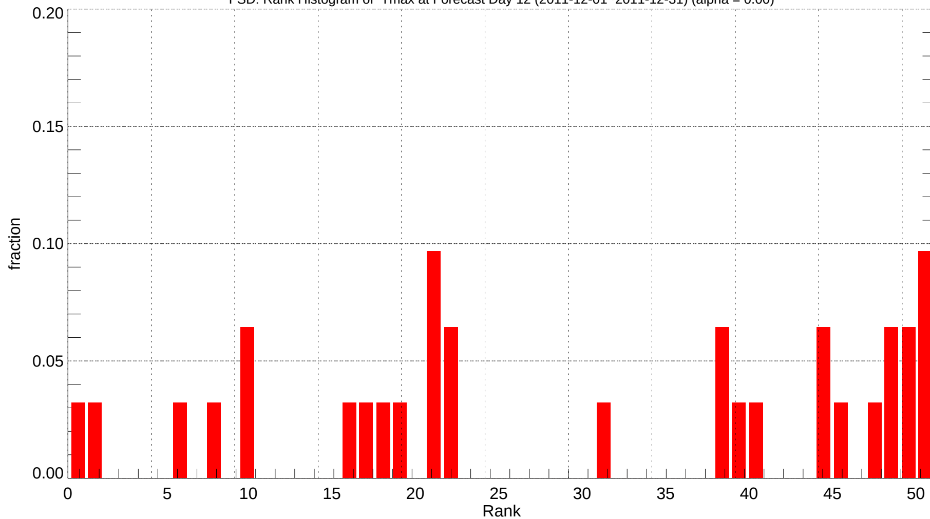
FSD: Rank Histogram of Tmax at Forecast Day 12 (2011-12-01~2011-12-31) (alpha = 0.00)
