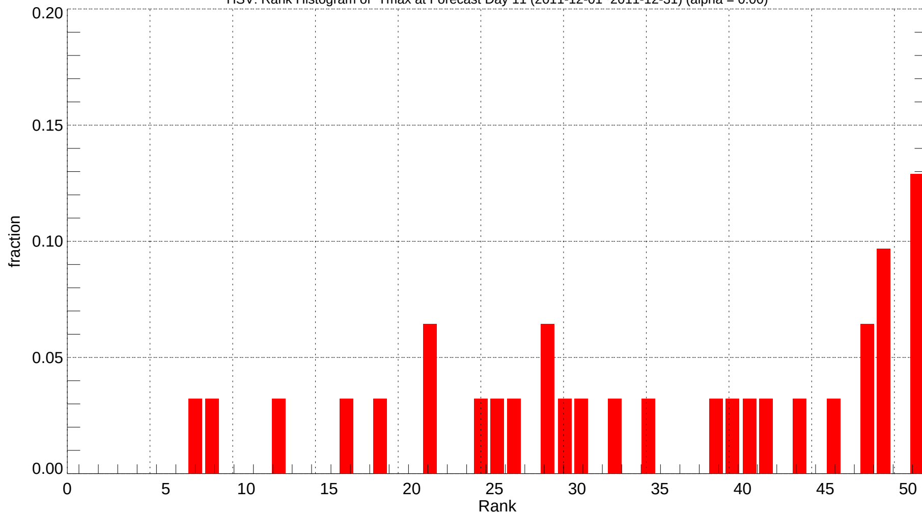
HSV: Rank Histogram of Tmax at Forecast Day 11 (2011-12-01~2011-12-31) (alpha = 0.00)
