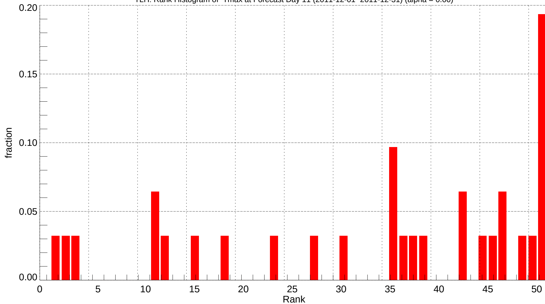
TLH: Rank Histogram of Tmax at Forecast Day 11 (2011-12-01~2011-12-31) (alpha = 0.00)
