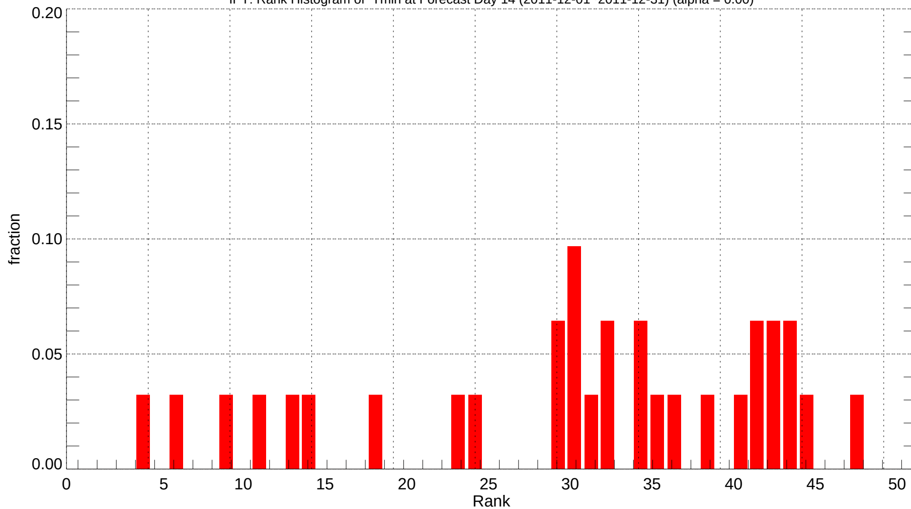
IPT: Rank Histogram of Tmin at Forecast Day 14 (2011-12-01~2011-12-31) (alpha = 0.00)
