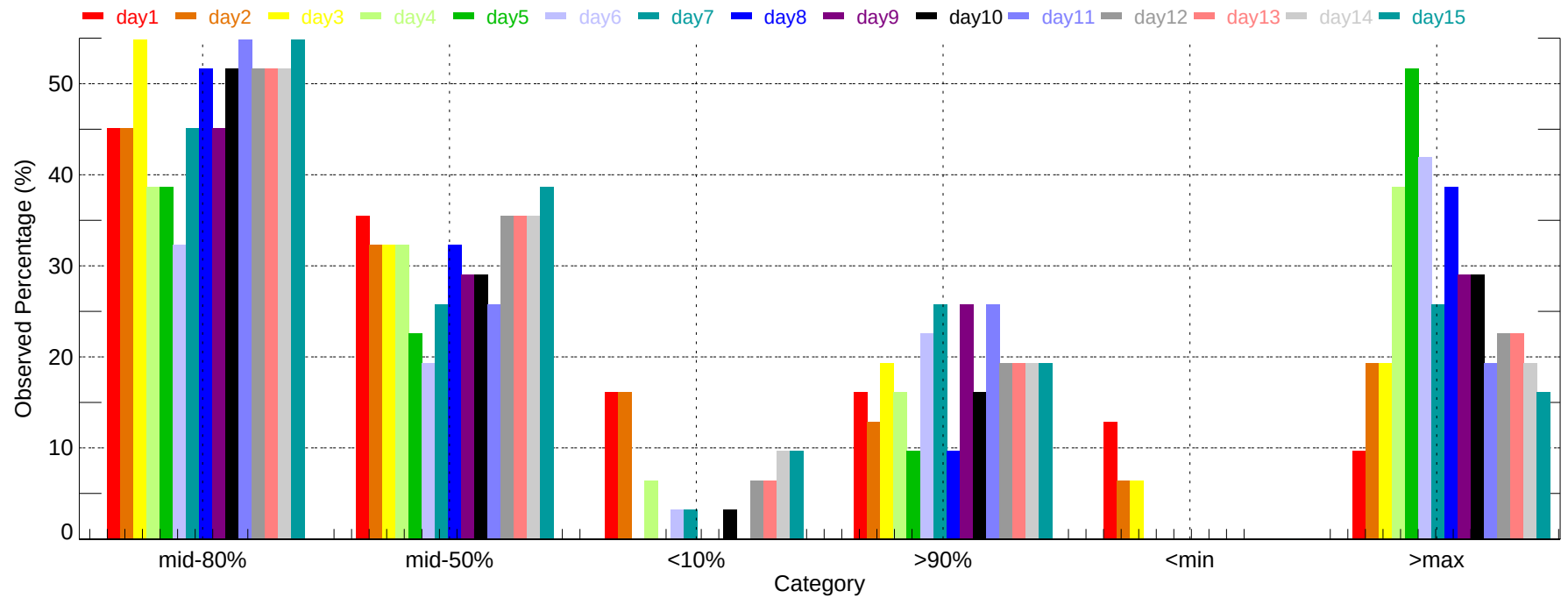
Observed Percentage of Ensembles - LEX: Max Temperature (2011-12-01~2011-12-31)
