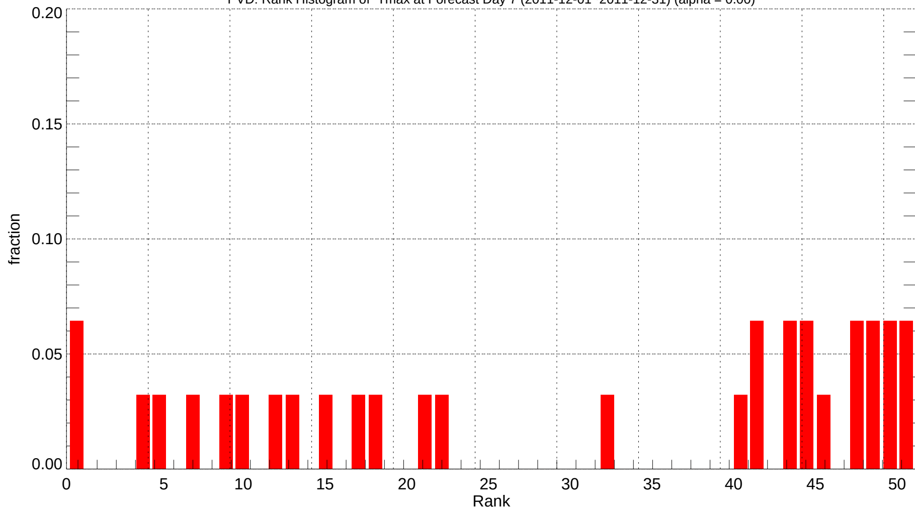
PVD: Rank Histogram of Tmax at Forecast Day 7 (2011-12-01~2011-12-31) (alpha = 0.00)
