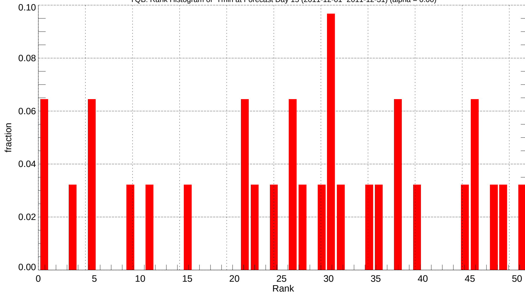
YQB: Rank Histogram of Tmin at Forecast Day 15 (2011-12-01~2011-12-31) (alpha = 0.00)
