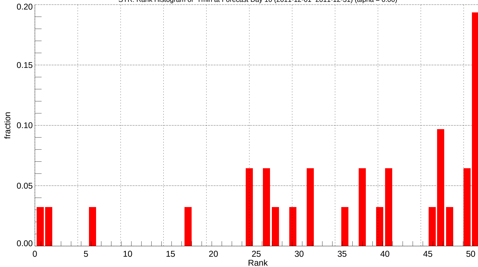
SYR: Rank Histogram of Tmin at Forecast Day 10 (2011-12-01~2011-12-31) (alpha = 0.00)
