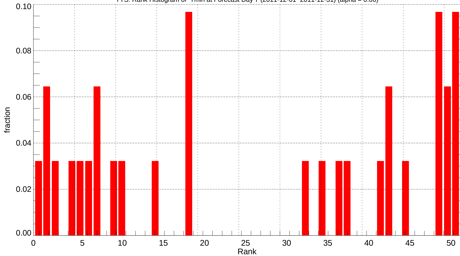
TYS: Rank Histogram of Tmin at Forecast Day 7 (2011-12-01~2011-12-31) (alpha = 0.00)
