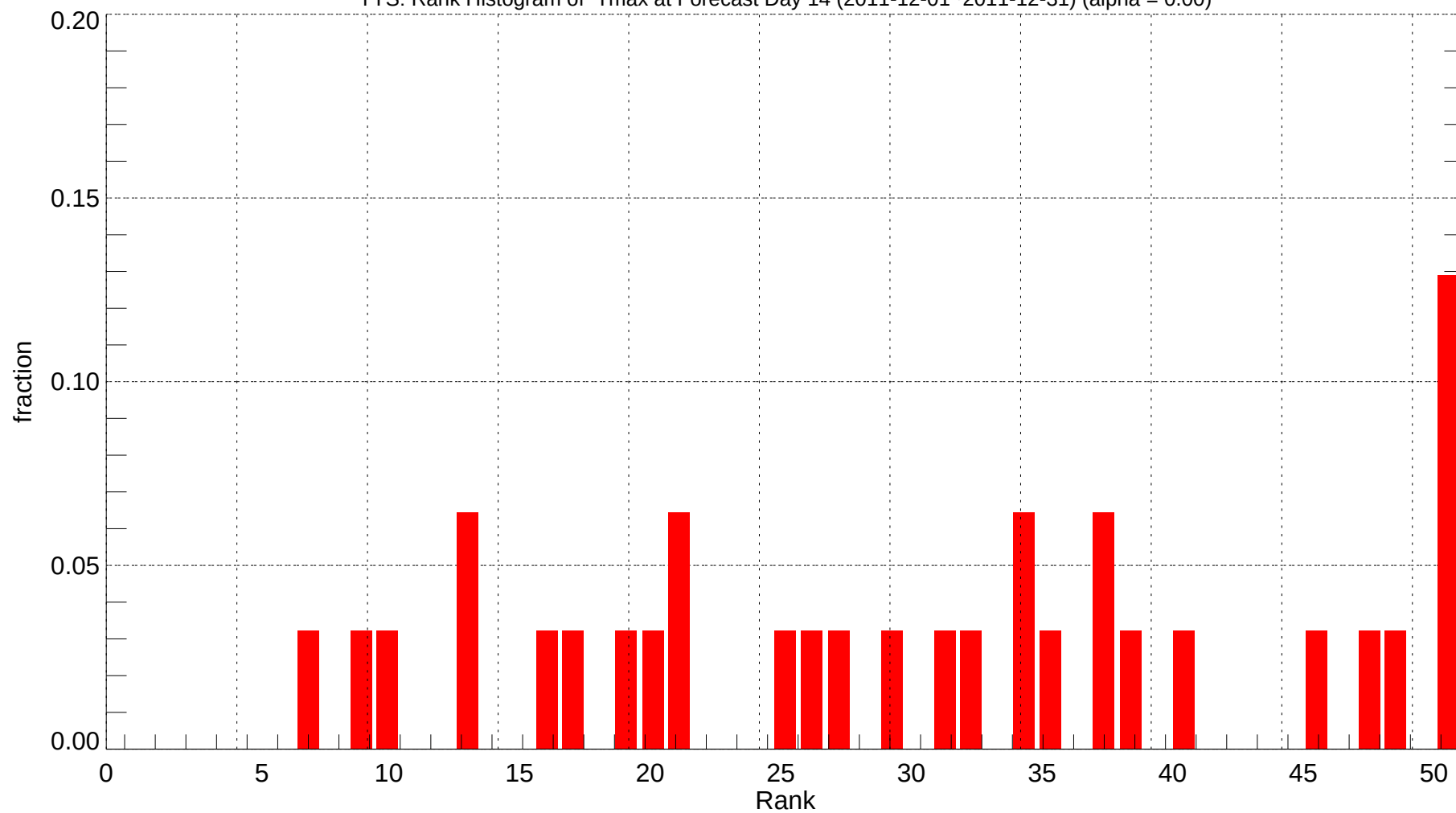
TYS: Rank Histogram of Tmax at Forecast Day 14 (2011-12-01~2011-12-31) (alpha = 0.00)
