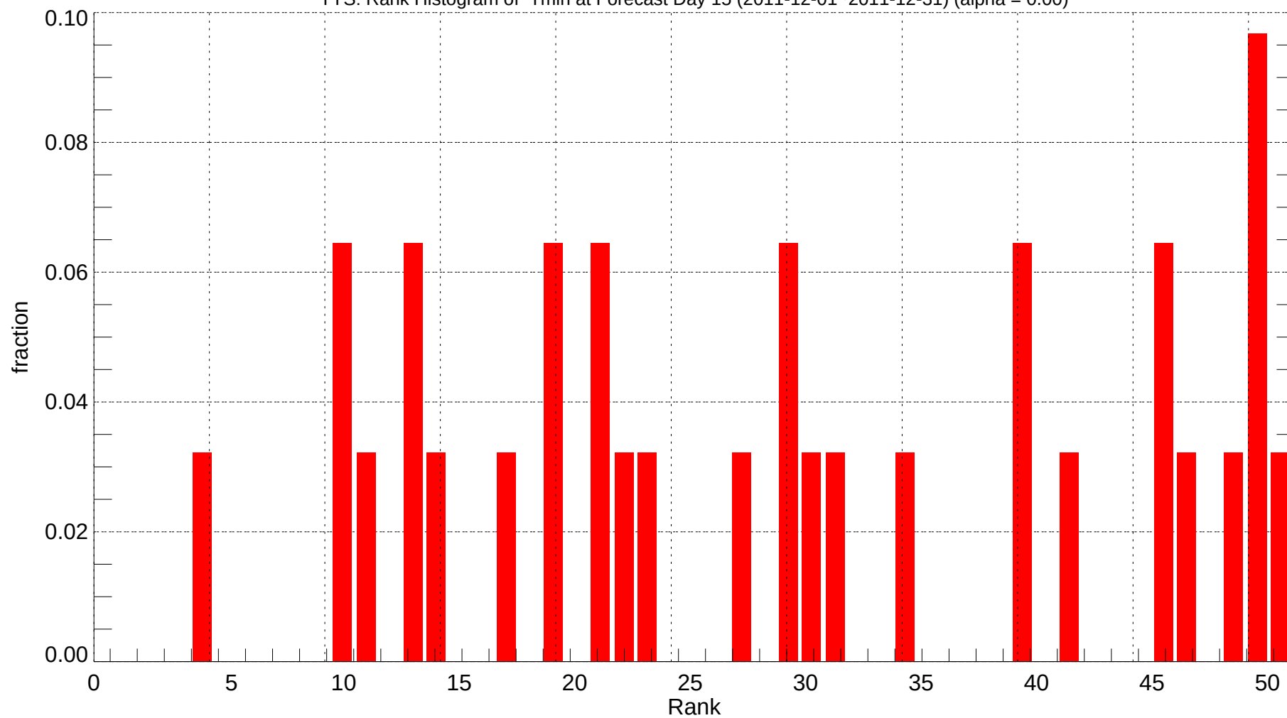
TYS: Rank Histogram of Tmin at Forecast Day 15 (2011-12-01~2011-12-31) (alpha = 0.00)
