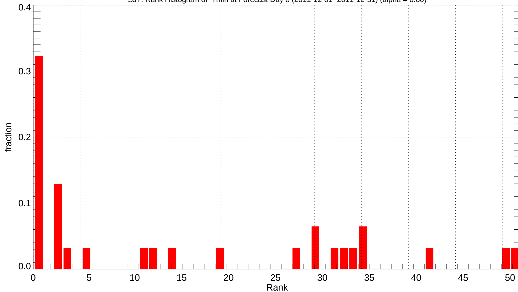
SJT: Rank Histogram of Tmin at Forecast Day 8 (2011-12-01~2011-12-31) (alpha = 0.00)
