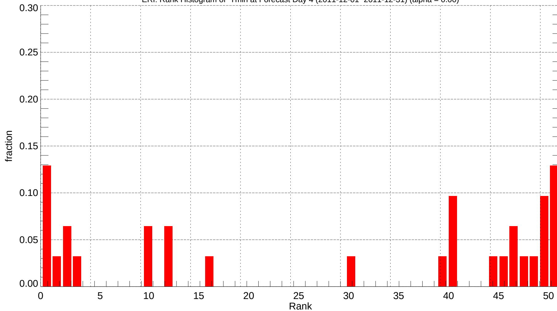
ERI: Rank Histogram of Tmin at Forecast Day 4 (2011-12-01~2011-12-31) (alpha = 0.00)
