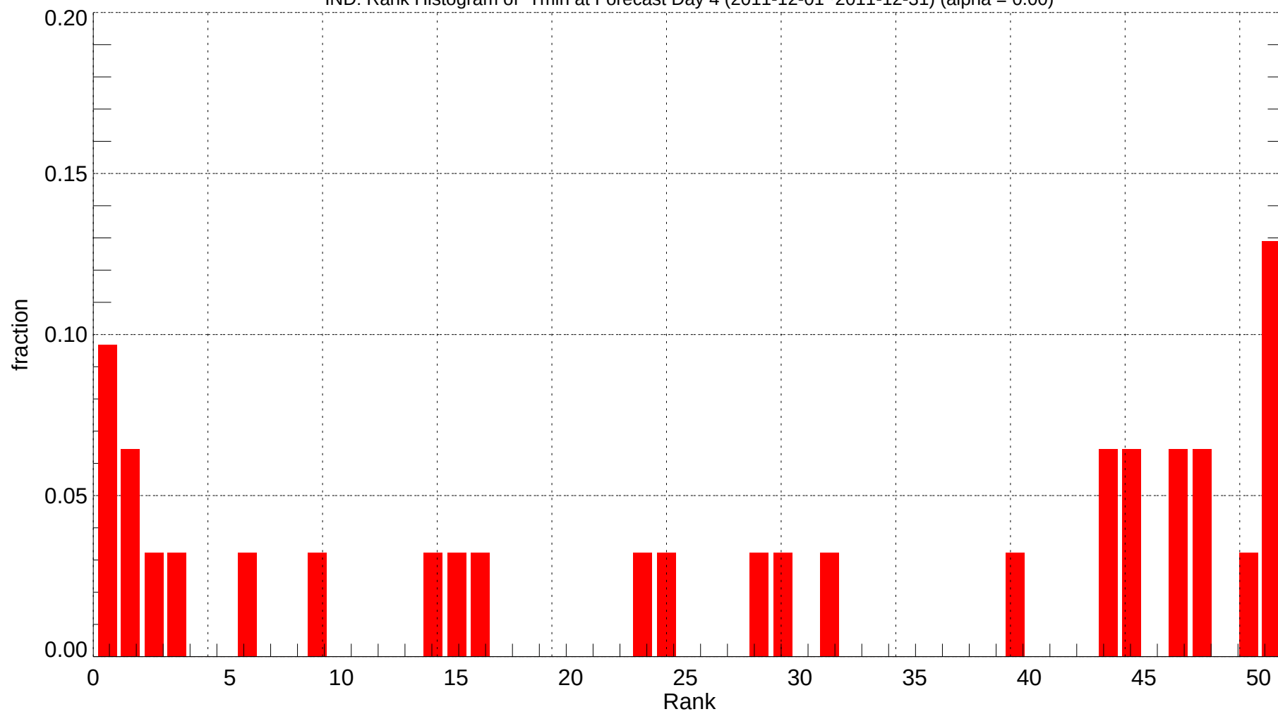
IND: Rank Histogram of Tmin at Forecast Day 4 (2011-12-01~2011-12-31) (alpha = 0.00)
