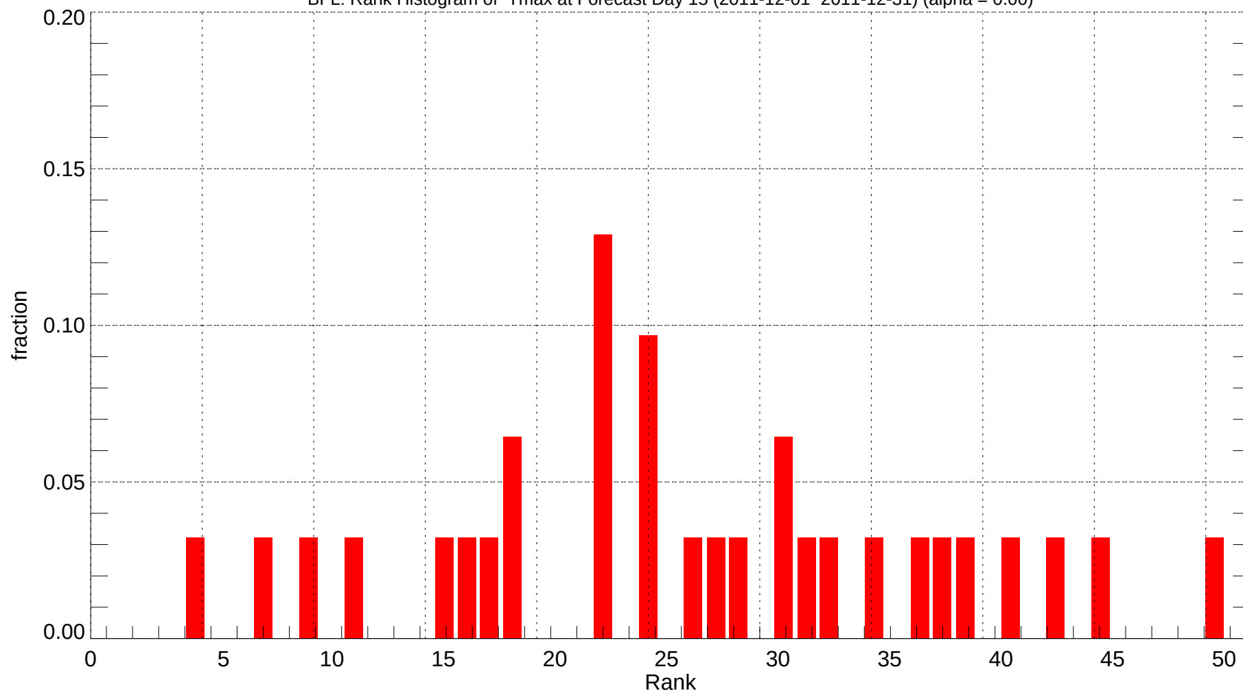
BFL: Rank Histogram of Tmax at Forecast Day 15 (2011-12-01~2011-12-31) (alpha = 0.00)
