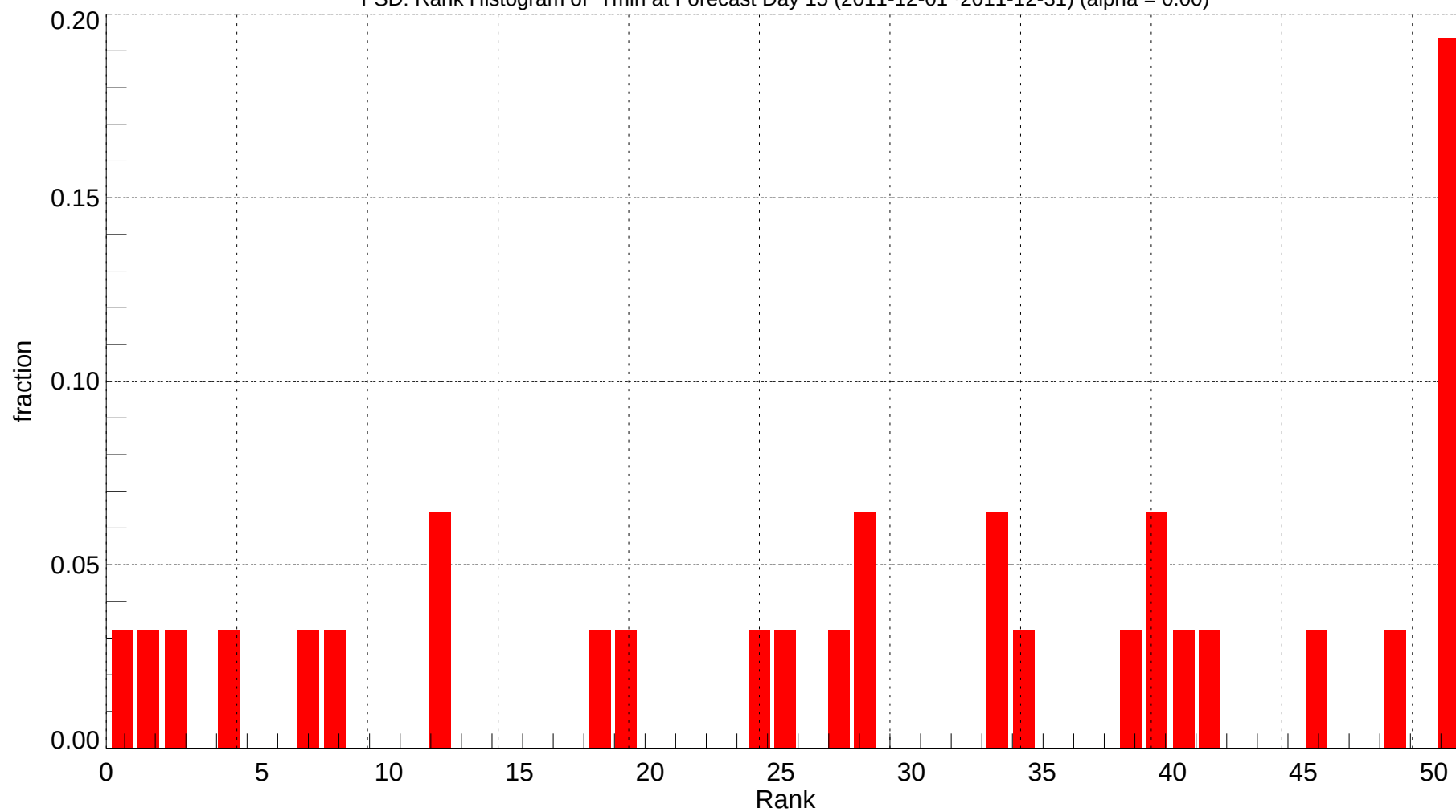
FSD: Rank Histogram of Tmin at Forecast Day 15 (2011-12-01~2011-12-31) (alpha = 0.00)
