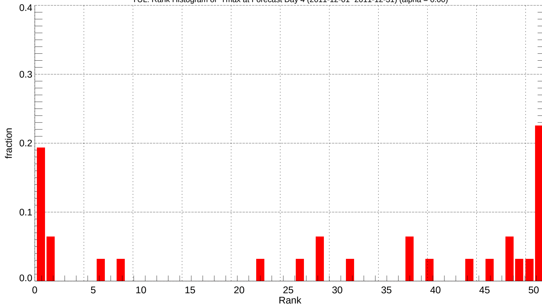
YUL: Rank Histogram of Tmax at Forecast Day 4 (2011-12-01~2011-12-31) (alpha = 0.00)
