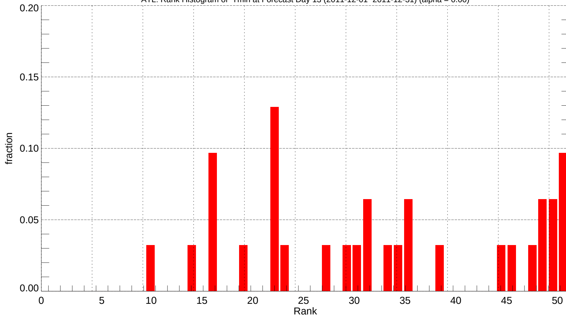
ATL: Rank Histogram of Tmin at Forecast Day 13 (2011-12-01~2011-12-31) (alpha = 0.00)
