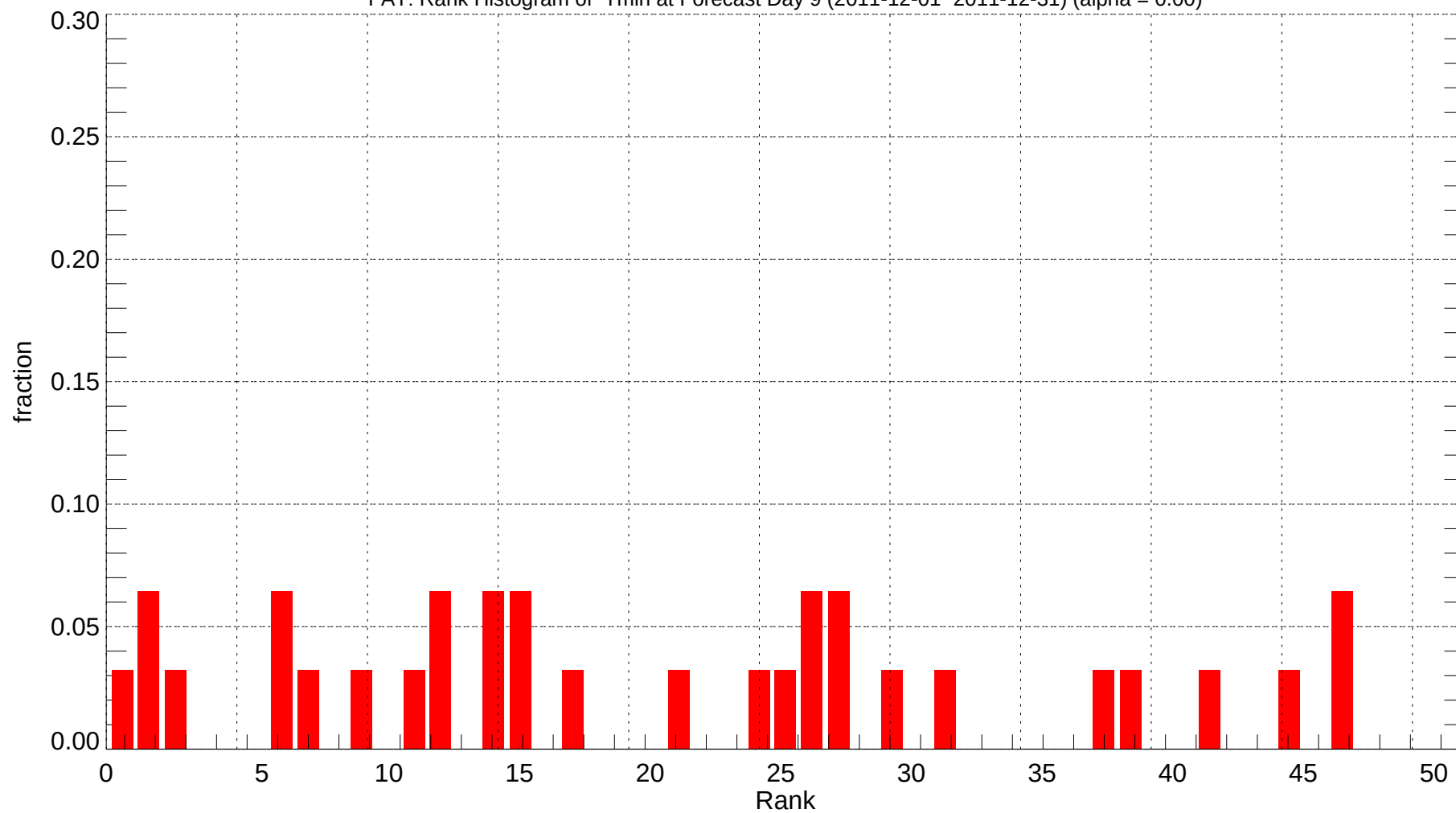
FAT: Rank Histogram of Tmin at Forecast Day 9 (2011-12-01~2011-12-31) (alpha = 0.00)
