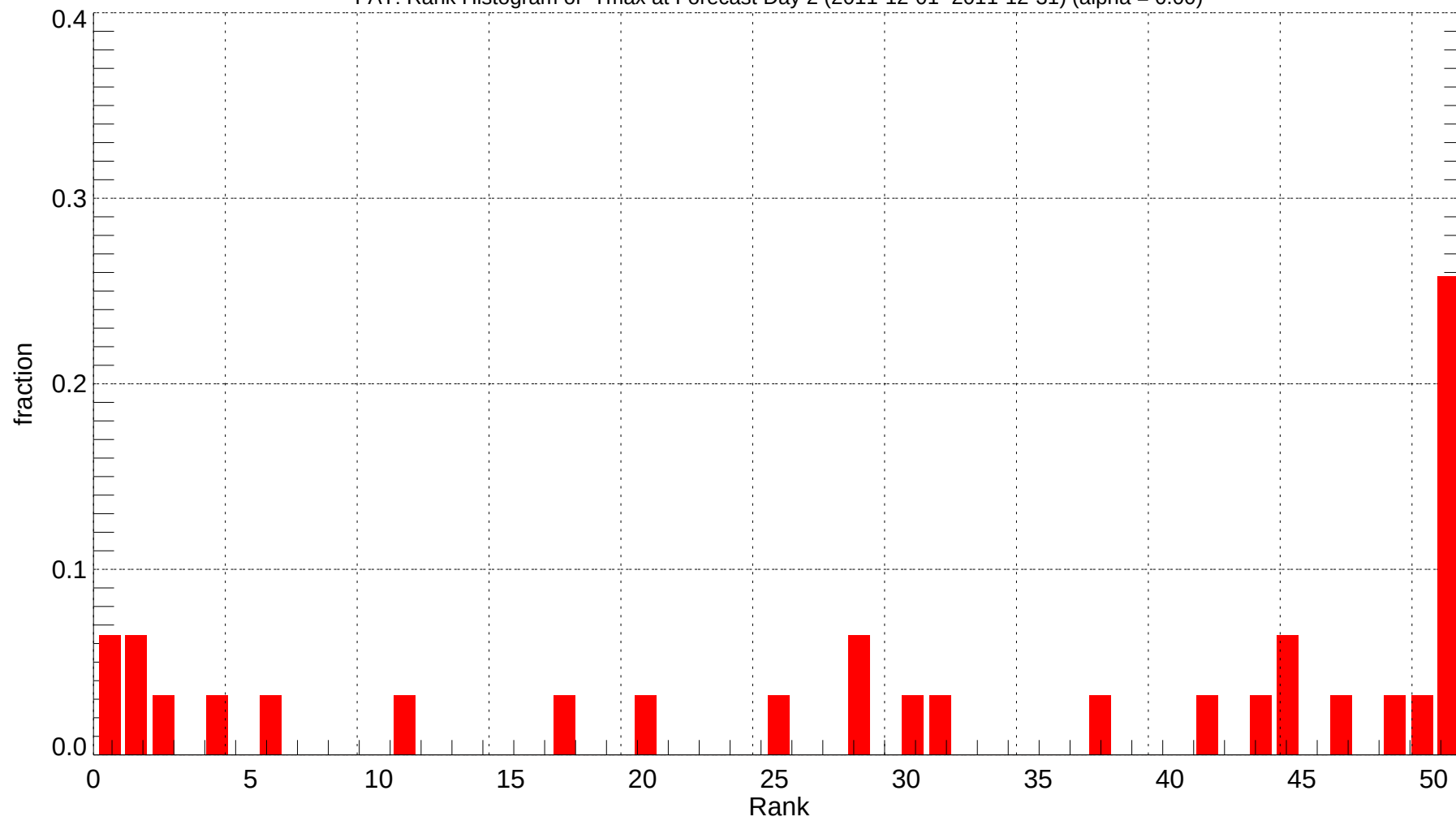
FAT: Rank Histogram of Tmax at Forecast Day 2 (2011-12-01~2011-12-31) (alpha = 0.00)
