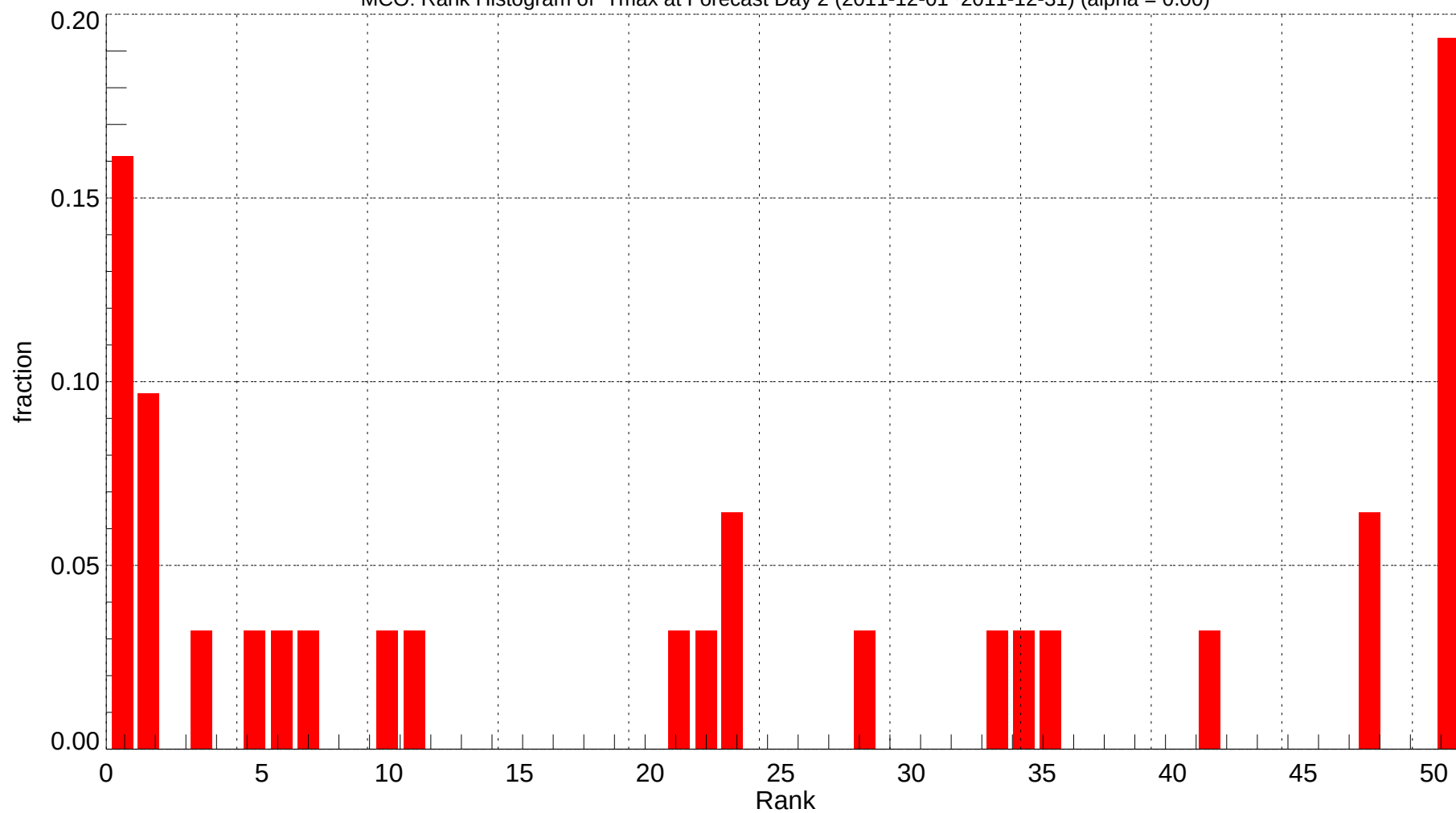
MCO: Rank Histogram of Tmax at Forecast Day 2 (2011-12-01~2011-12-31) (alpha = 0.00)
