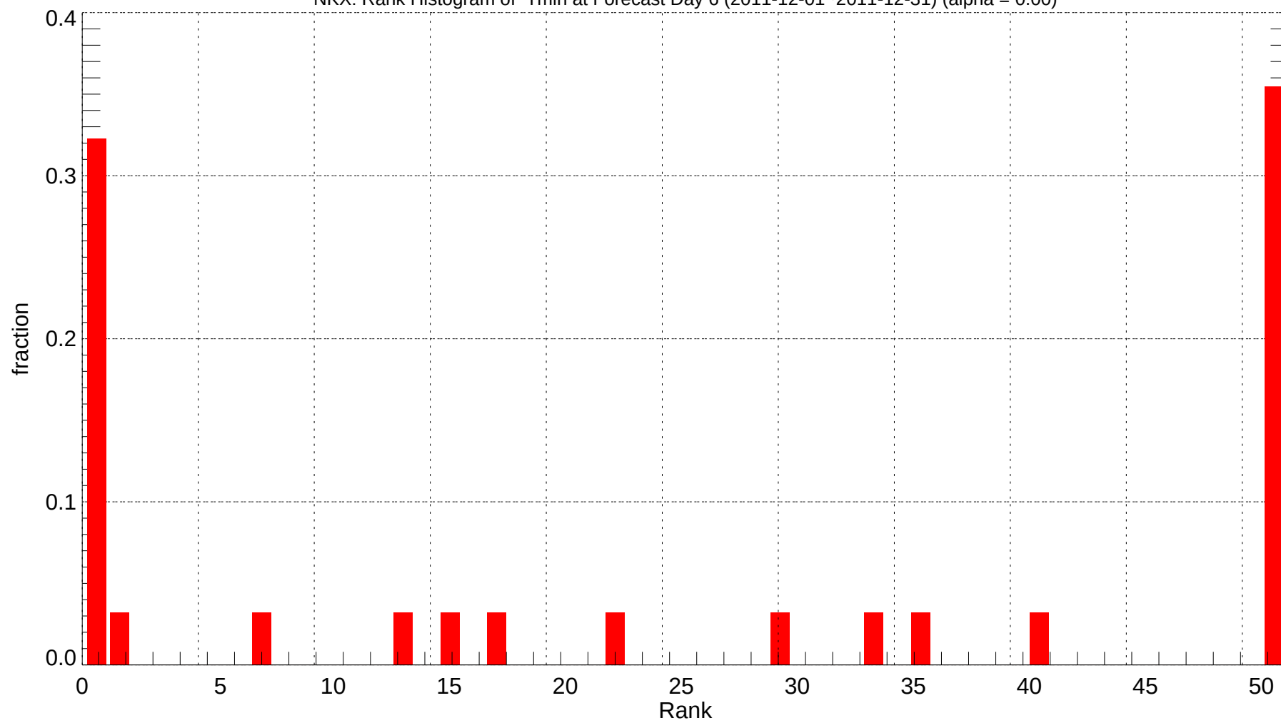
NKX: Rank Histogram of Tmin at Forecast Day 6 (2011-12-01~2011-12-31) (alpha = 0.00)
