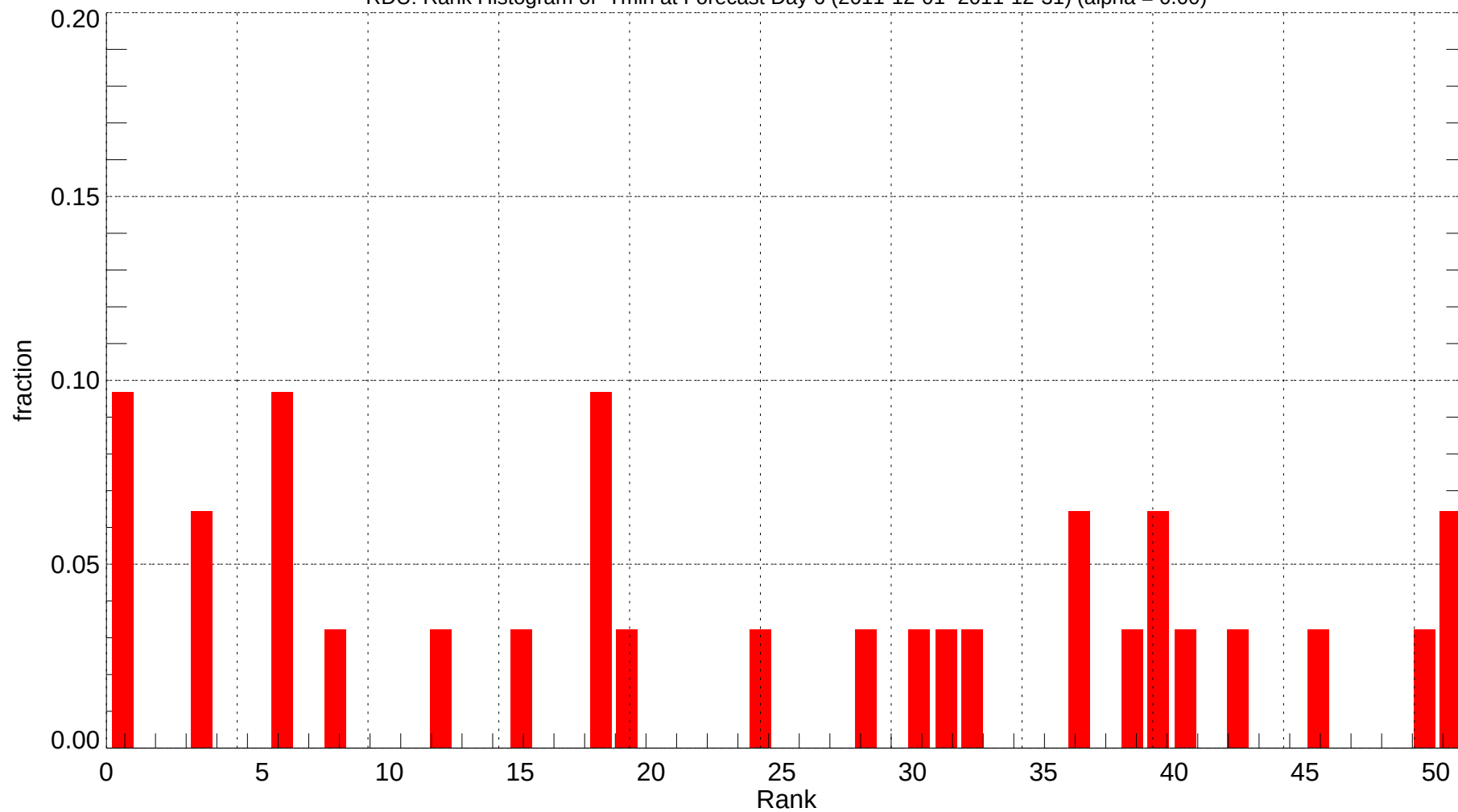
RDU: Rank Histogram of Tmin at Forecast Day 6 (2011-12-01~2011-12-31) (alpha = 0.00)
