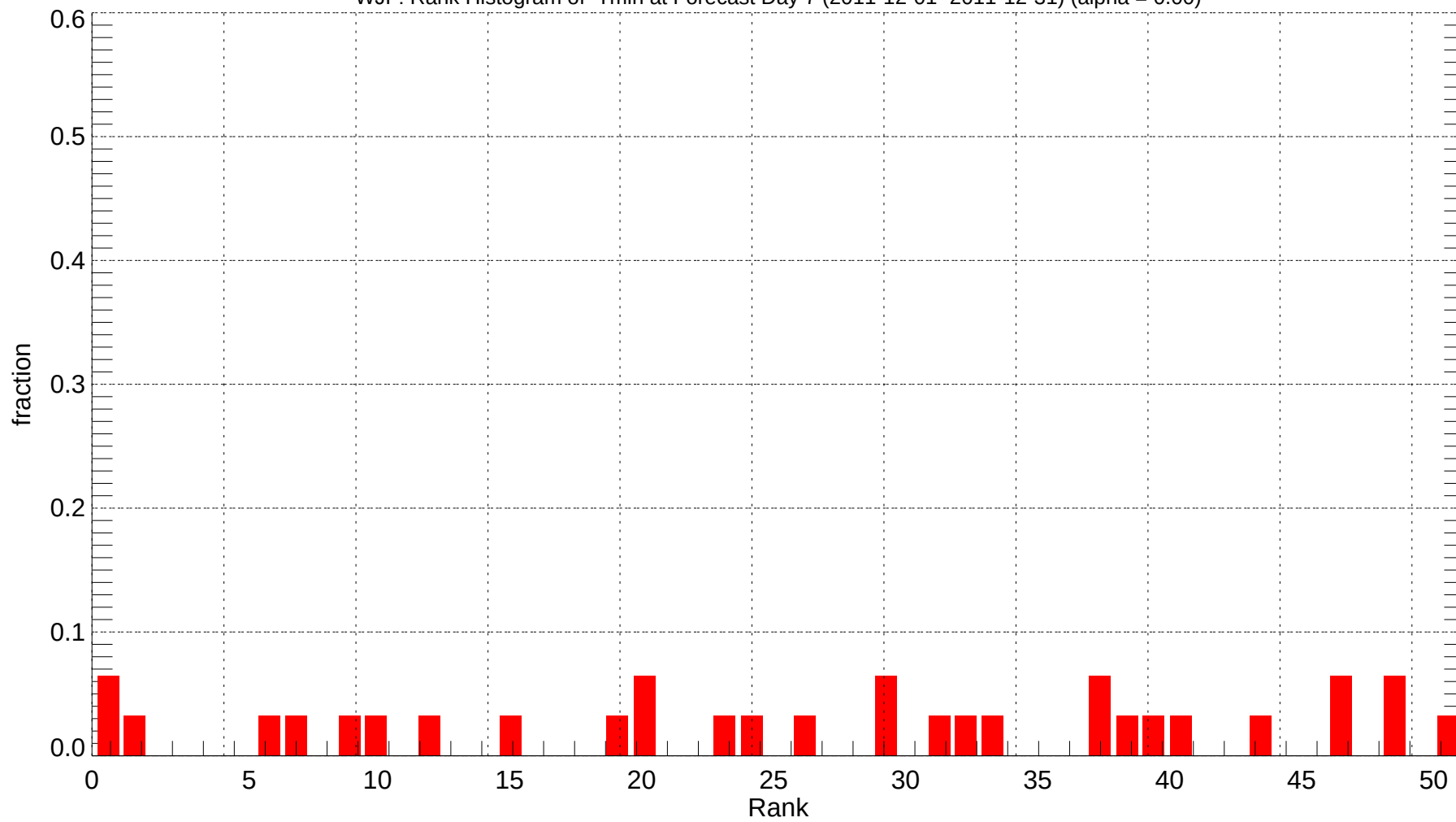
WJF: Rank Histogram of Tmin at Forecast Day 7 (2011-12-01~2011-12-31) (alpha = 0.00)
