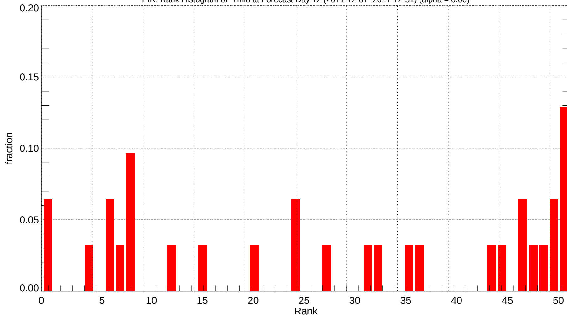
PIR: Rank Histogram of Tmin at Forecast Day 12 (2011-12-01~2011-12-31) (alpha = 0.00)
