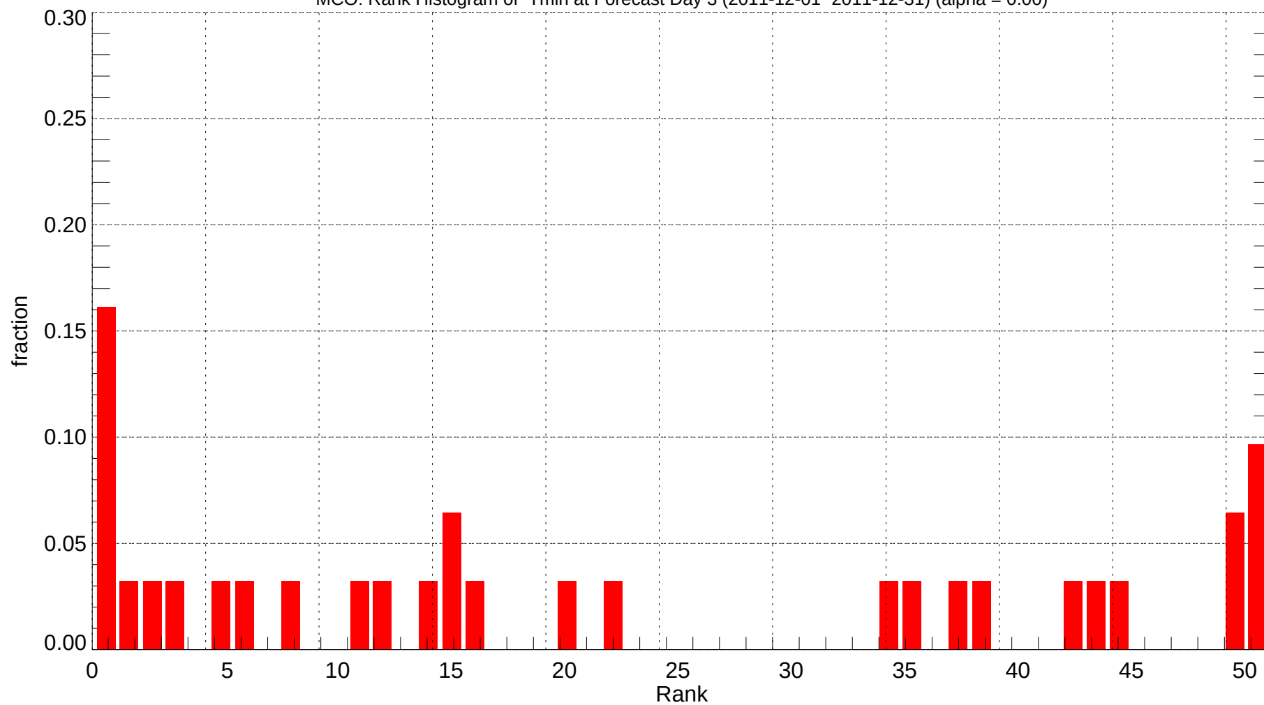
MCO: Rank Histogram of Tmin at Forecast Day 3 (2011-12-01~2011-12-31) (alpha = 0.00)
