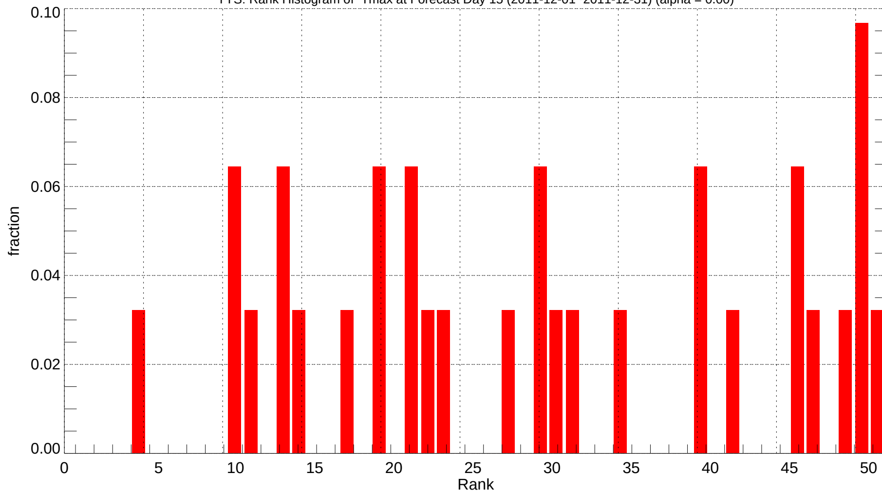
TYS: Rank Histogram of Tmax at Forecast Day 15 (2011-12-01~2011-12-31) (alpha = 0.00)
