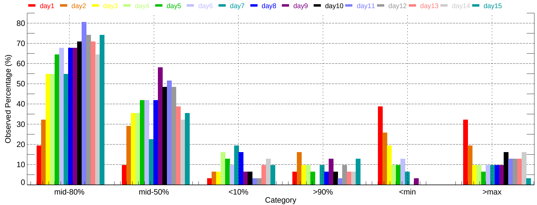
Observed Percentage of Ensembles - MSP: Min Temperature (2011-12-01~2011-12-31)
