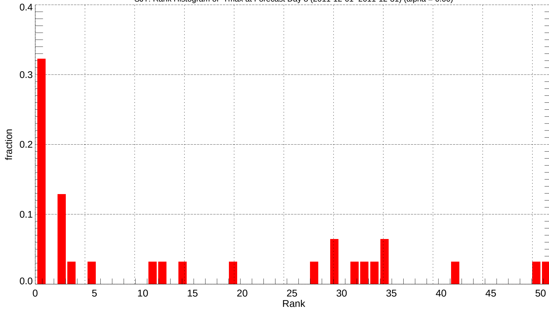
SJT: Rank Histogram of Tmax at Forecast Day 8 (2011-12-01~2011-12-31) (alpha = 0.00)
