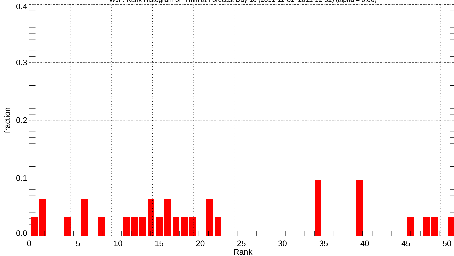
WJF: Rank Histogram of Tmin at Forecast Day 10 (2011-12-01~2011-12-31) (alpha = 0.00)
