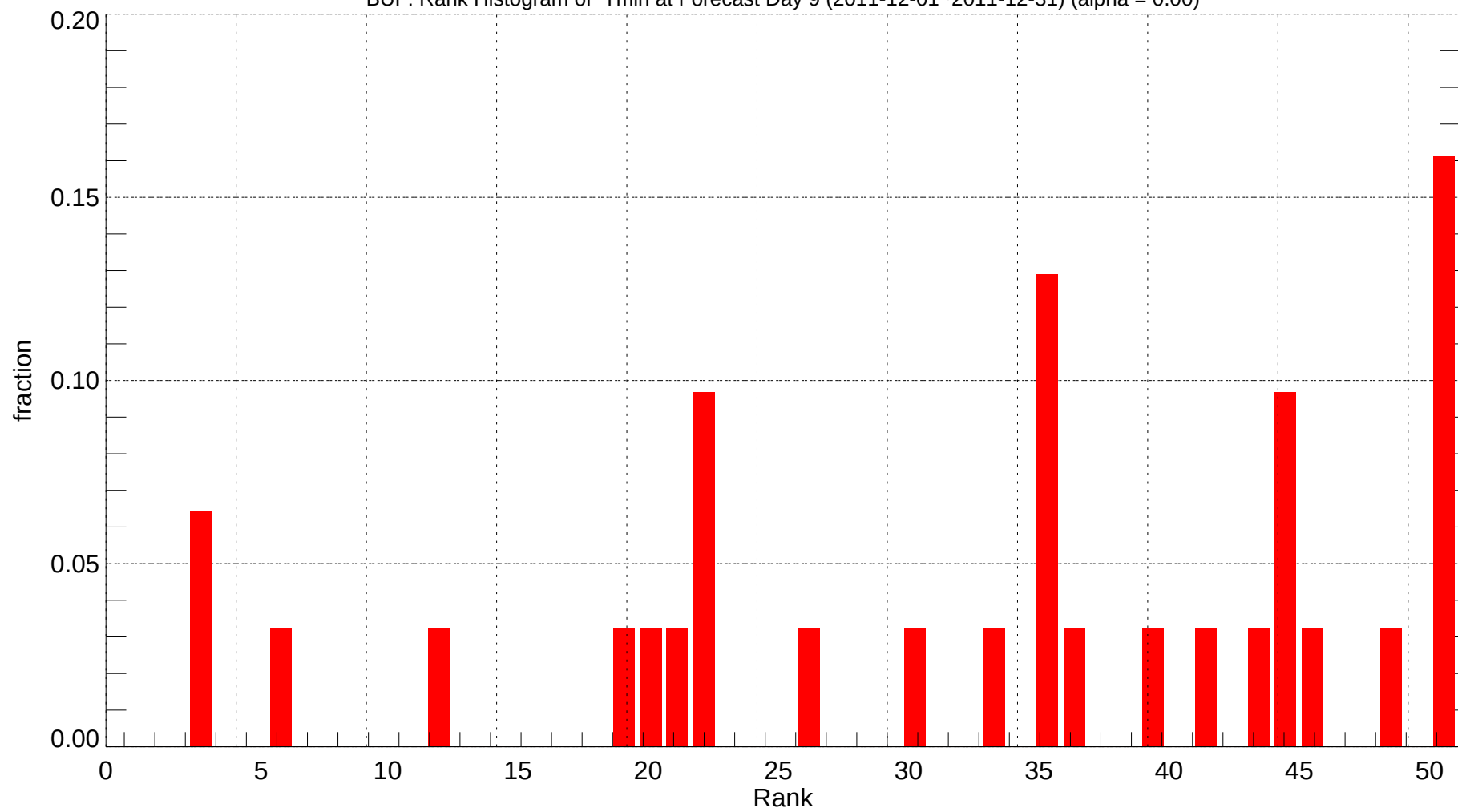
BUF: Rank Histogram of Tmin at Forecast Day 9 (2011-12-01~2011-12-31) (alpha = 0.00)
