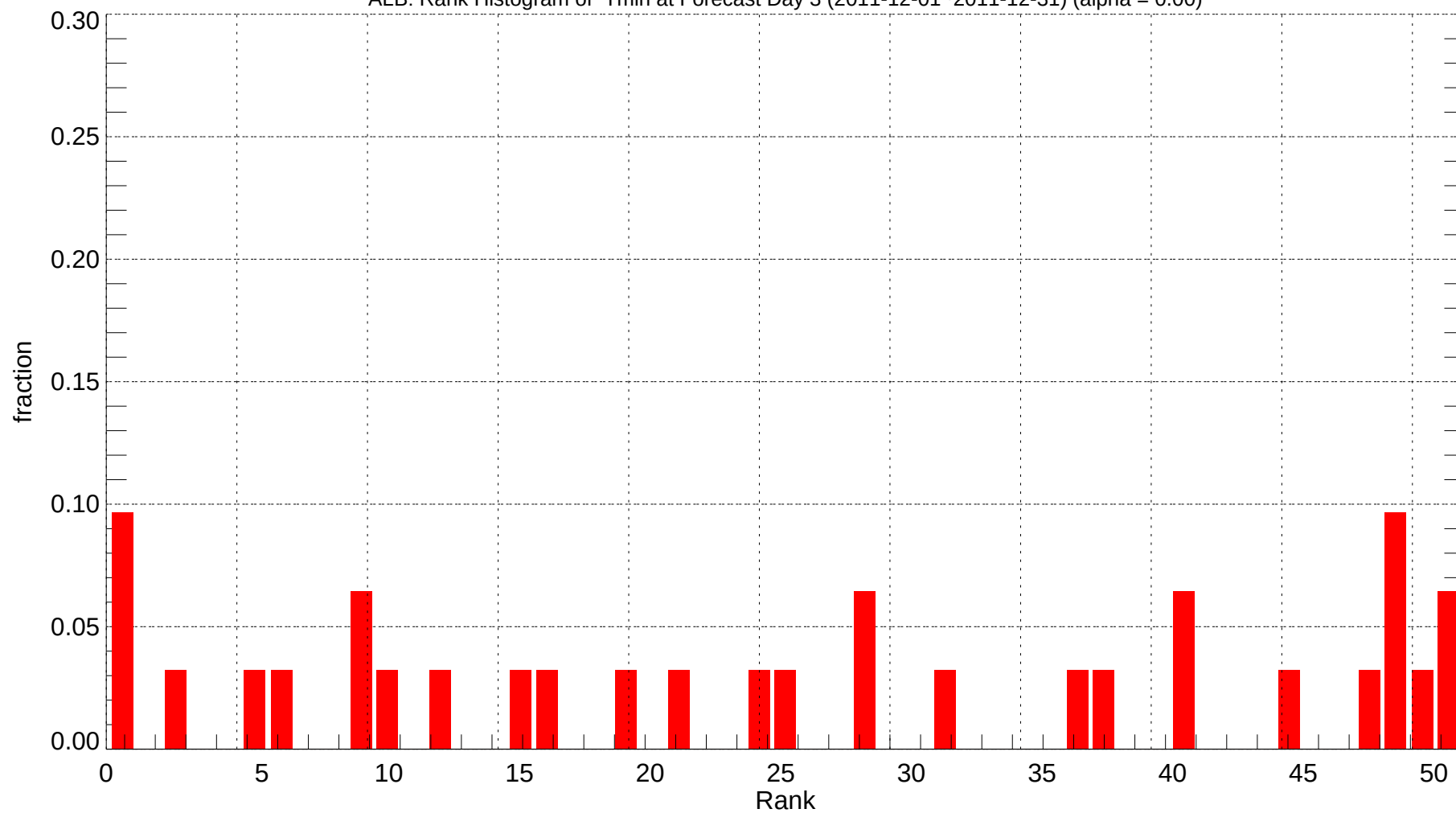
ALB: Rank Histogram of Tmin at Forecast Day 3 (2011-12-01~2011-12-31) (alpha = 0.00)
