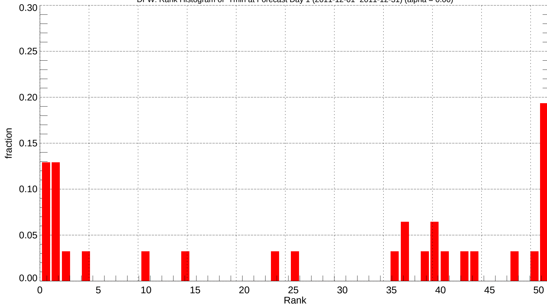
DFW: Rank Histogram of Tmin at Forecast Day 1 (2011-12-01~2011-12-31) (alpha = 0.00)
