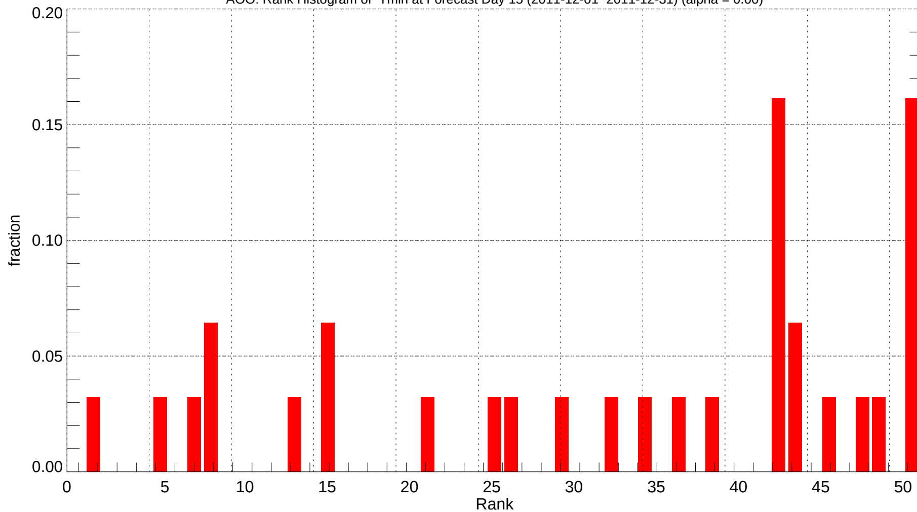
AOO: Rank Histogram of Tmin at Forecast Day 15 (2011-12-01~2011-12-31) (alpha = 0.00)
