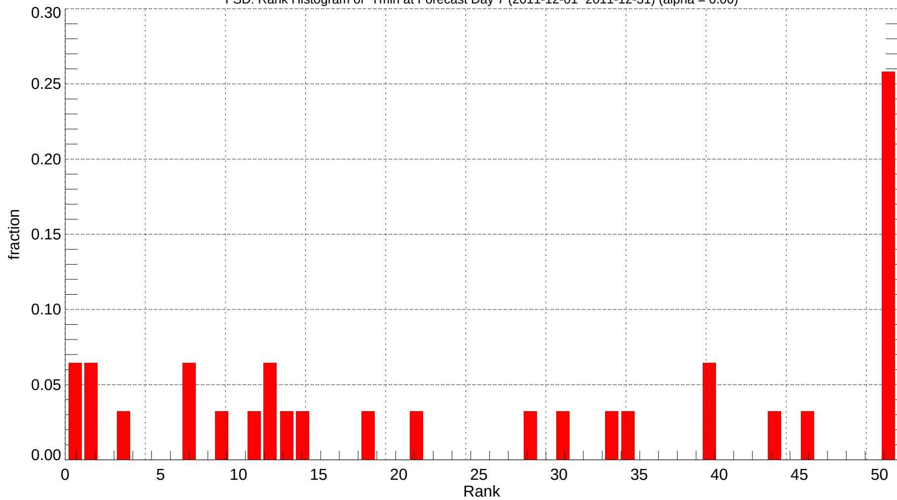
FSD: Rank Histogram of Tmin at Forecast Day 7 (2011-12-01~2011-12-31) (alpha = 0.00)
