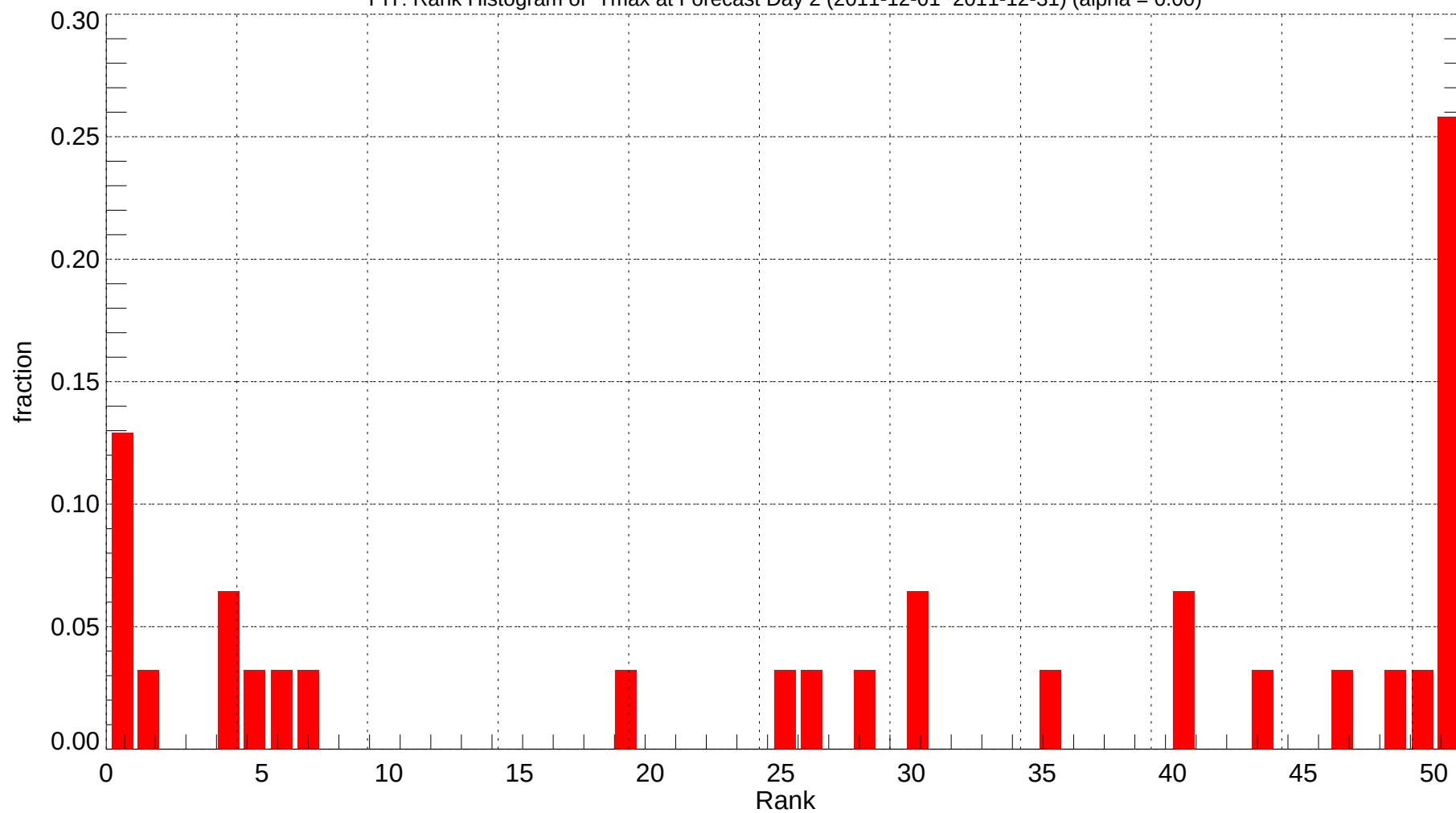
PIT: Rank Histogram of Tmax at Forecast Day 2 (2011-12-01~2011-12-31) (alpha = 0.00)
