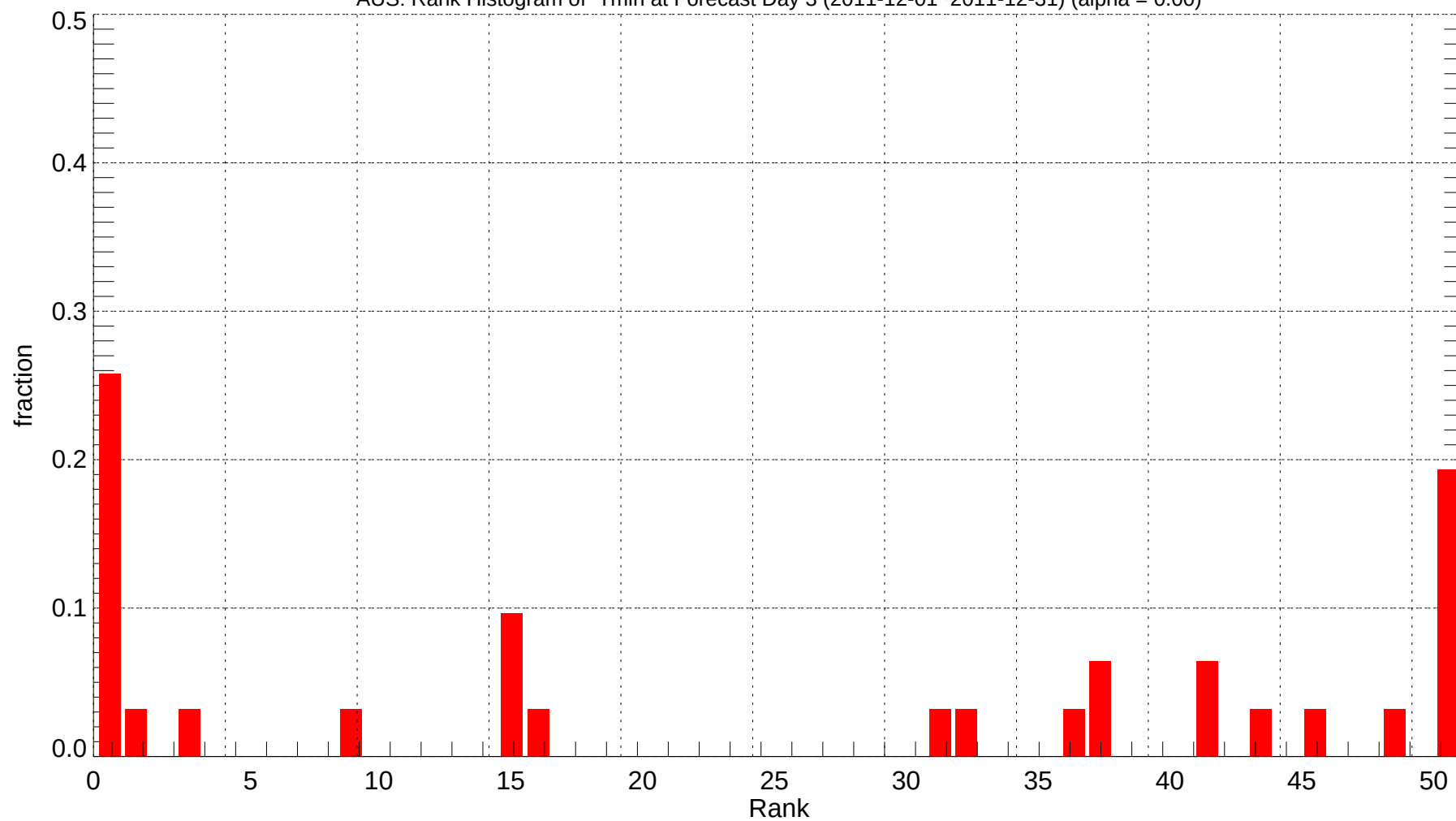
AUS: Rank Histogram of Tmin at Forecast Day 3 (2011-12-01~2011-12-31) (alpha = 0.00)
