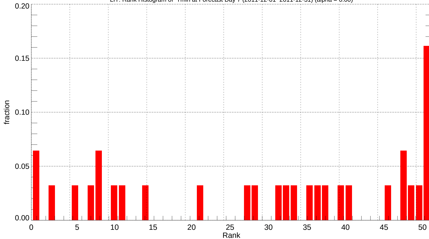
LIT: Rank Histogram of Tmin at Forecast Day 7 (2011-12-01~2011-12-31) (alpha = 0.00)
