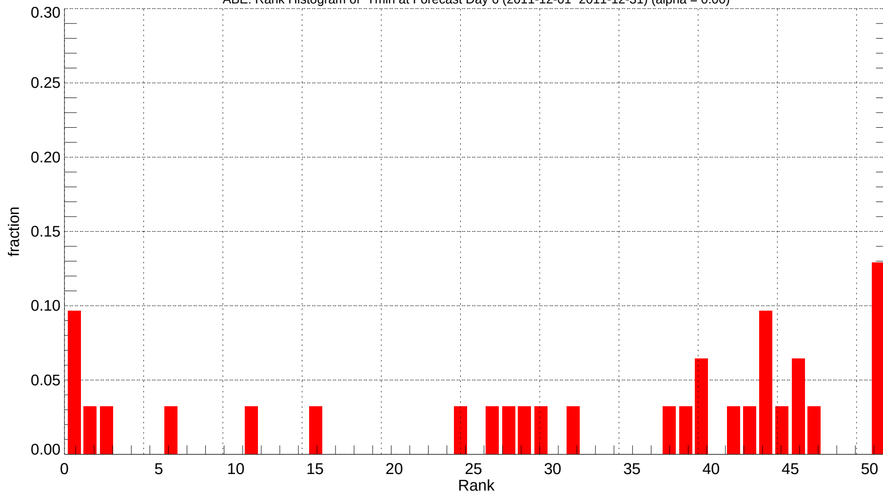
ABE: Rank Histogram of Tmin at Forecast Day 6 (2011-12-01~2011-12-31) (alpha = 0.00)
