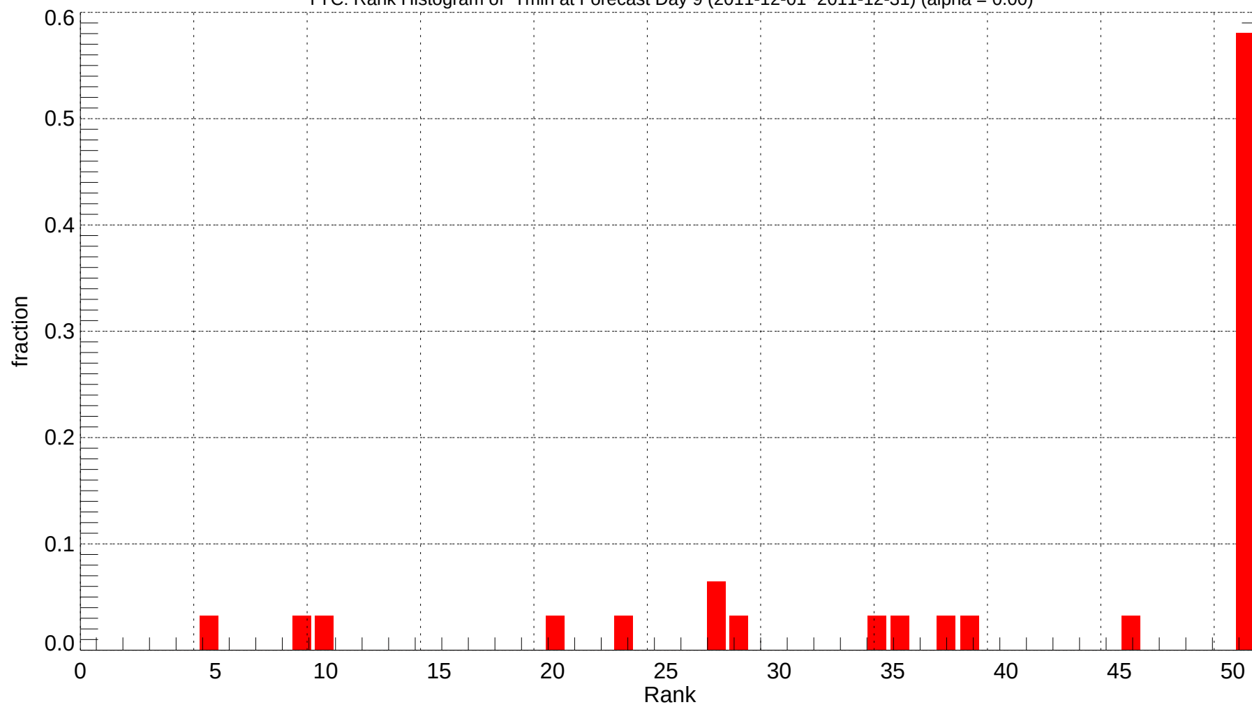
YYC: Rank Histogram of Tmin at Forecast Day 9 (2011-12-01~2011-12-31) (alpha = 0.00)
