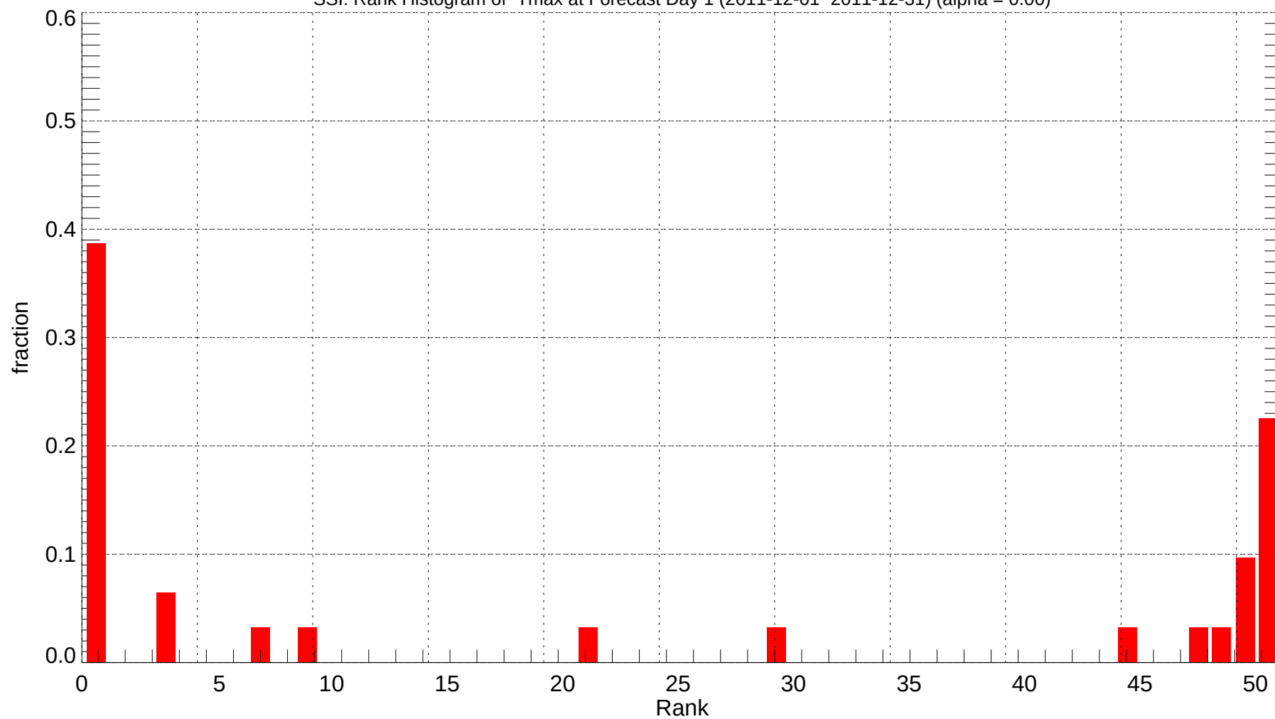
SSI: Rank Histogram of Tmax at Forecast Day 1 (2011-12-01~2011-12-31) (alpha = 0.00)
