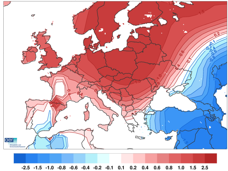
Forecasted Temperature Anomaly (C) Dec-Jan-Feb 2014
