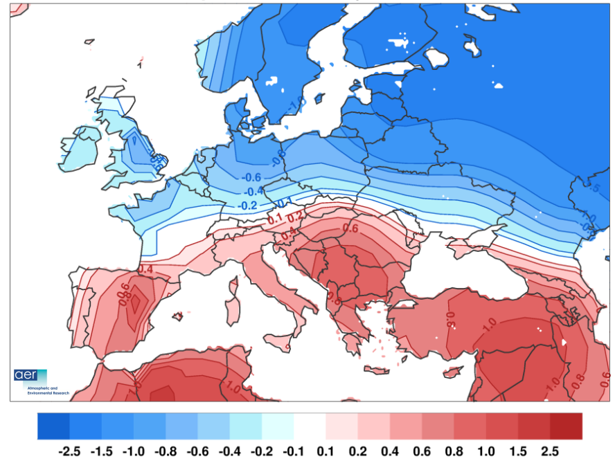
Forecasted Temperature Anomaly (C) Dec-Jan-Feb 2013
