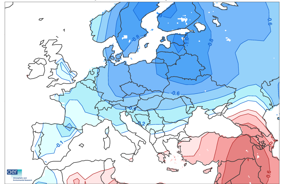
Forecast Temperature Anomaly Dec-Jan-Feb 2011
