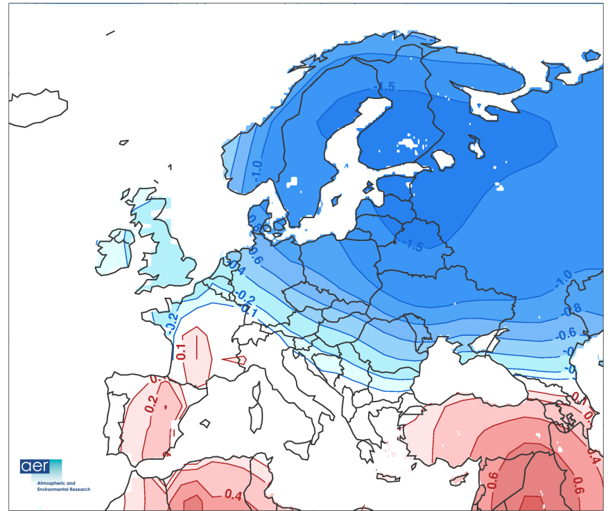
AER Forecast Temperature Anomaly Dec-Jan-Feb 2009
