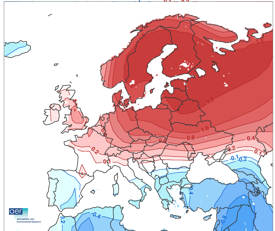
AER Forecast Temperature Anomaly Dec-Jan-Feb 2007
