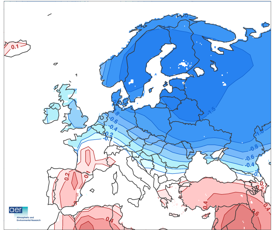
AER Forecast Temperature Anomaly Dec-Jan-Feb 2006
