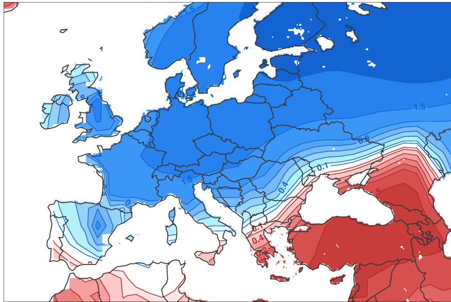
Observed Temperature Anomaly: Dec 1 - Feb 28 2011
