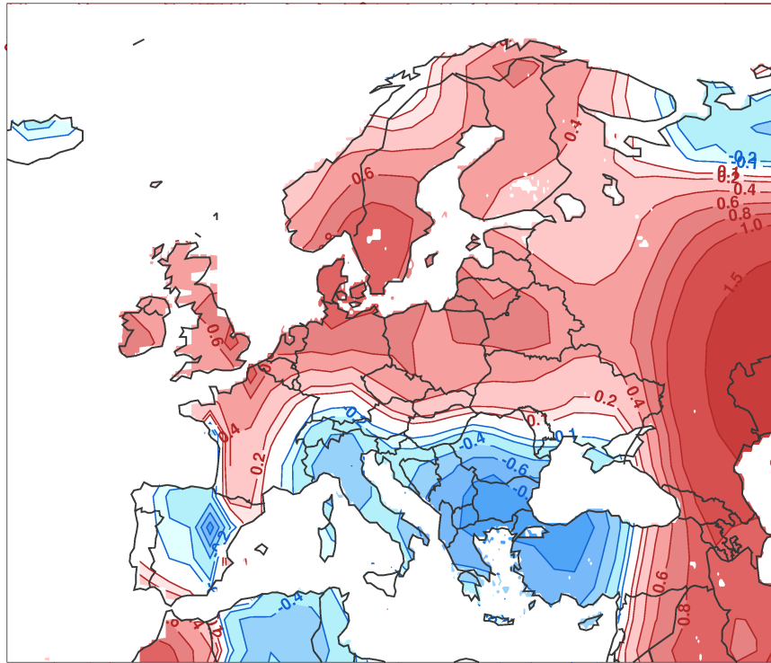
Observed Temperature Anomaly Dec-Jan-Feb 2002
