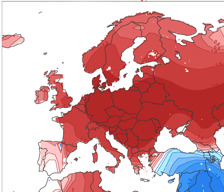
Observed Temperature Anomaly Dec-Jan-Feb 2007
