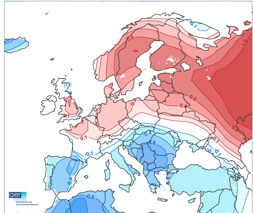
AER Forecast Temperature Anomaly Dec-Jan-Feb 2008
