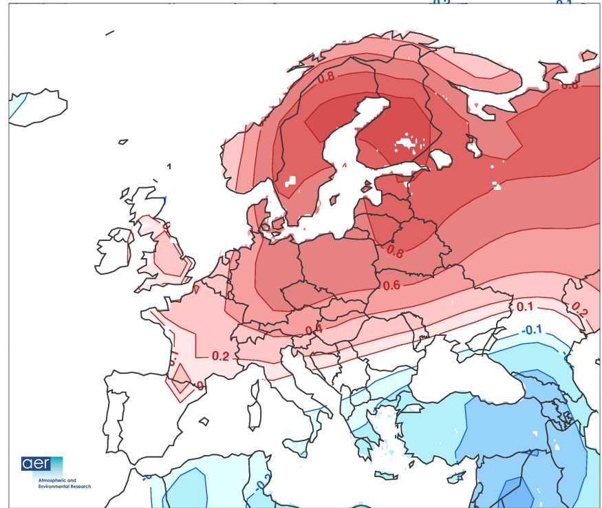
AER Forecast Temperature Anomaly Dec-Jan-Feb 2005
