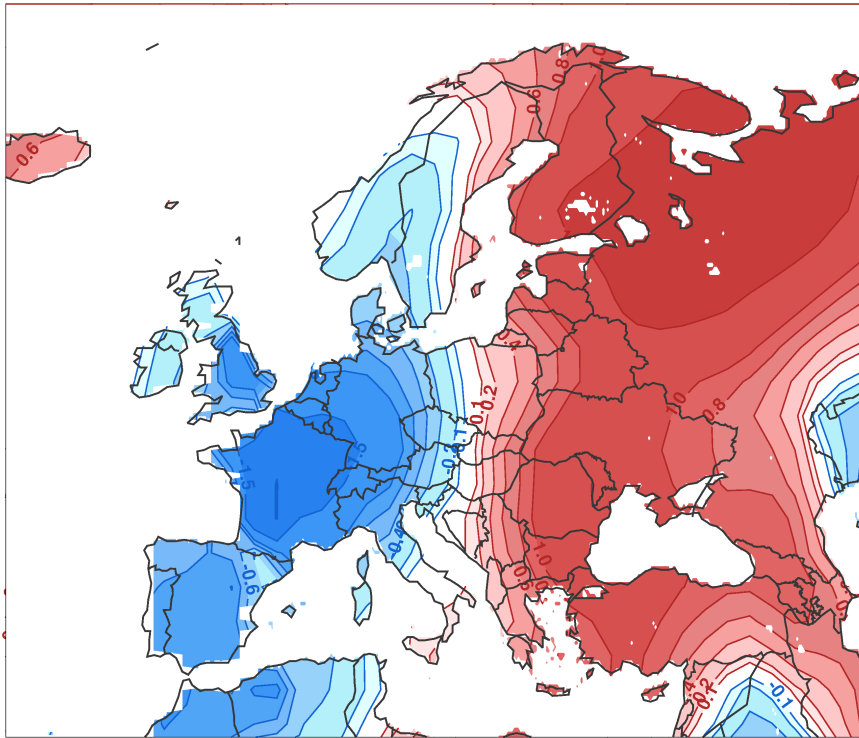
Observed Temperature Anomaly Dec-Jan-Feb 2009
