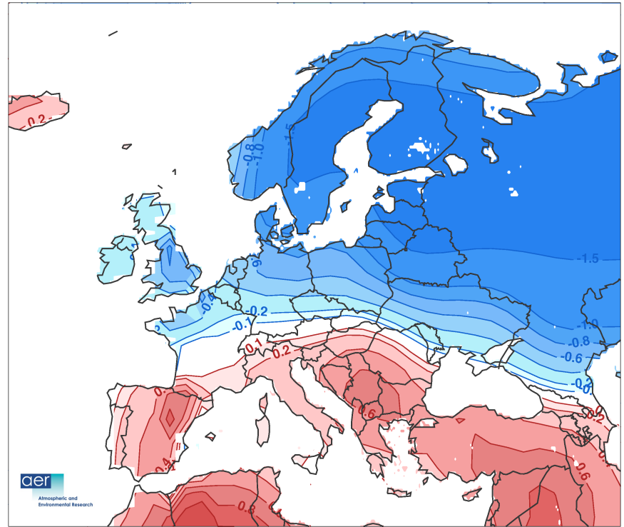
AER Forecast Temperature Anomaly Dec-Jan-Feb 2003
