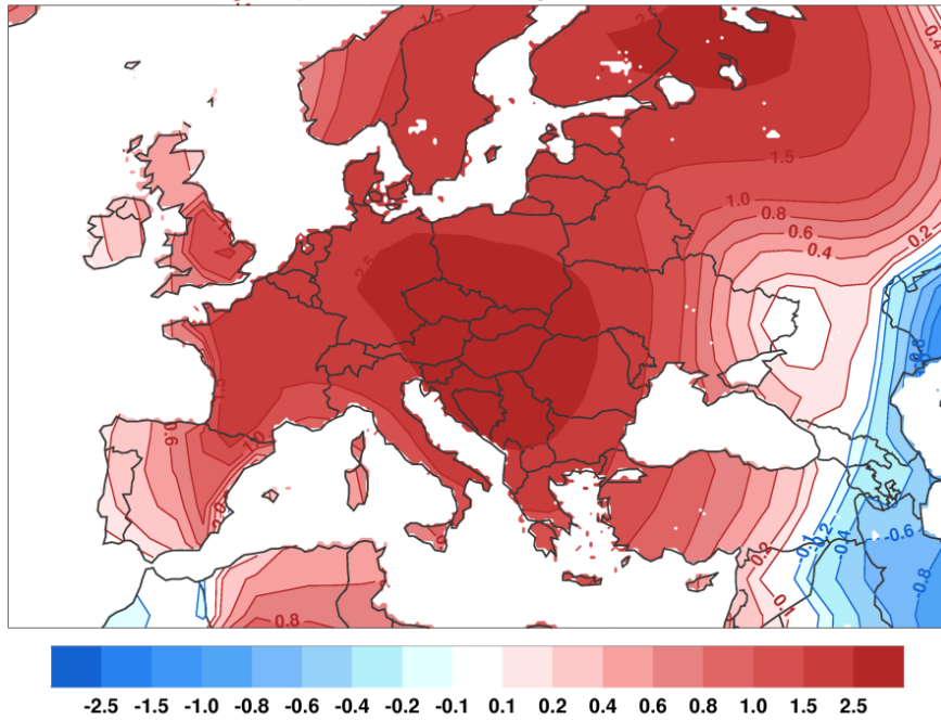
Observed Temperature Anomaly (C) Dec-Jan-Feb 2014
