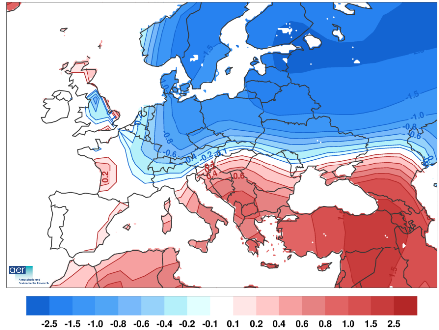
Forecasted Temperature Anomaly (C) Dec-Jan-Feb 2015
