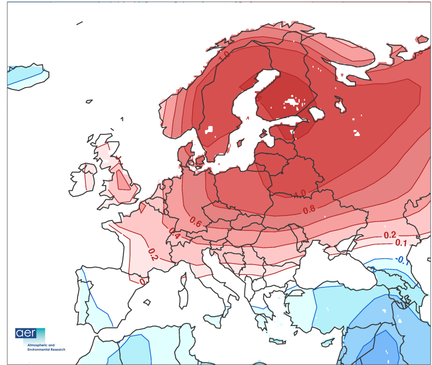
AER Forecast Temperature Anomaly Dec-Jan-Feb 2002
