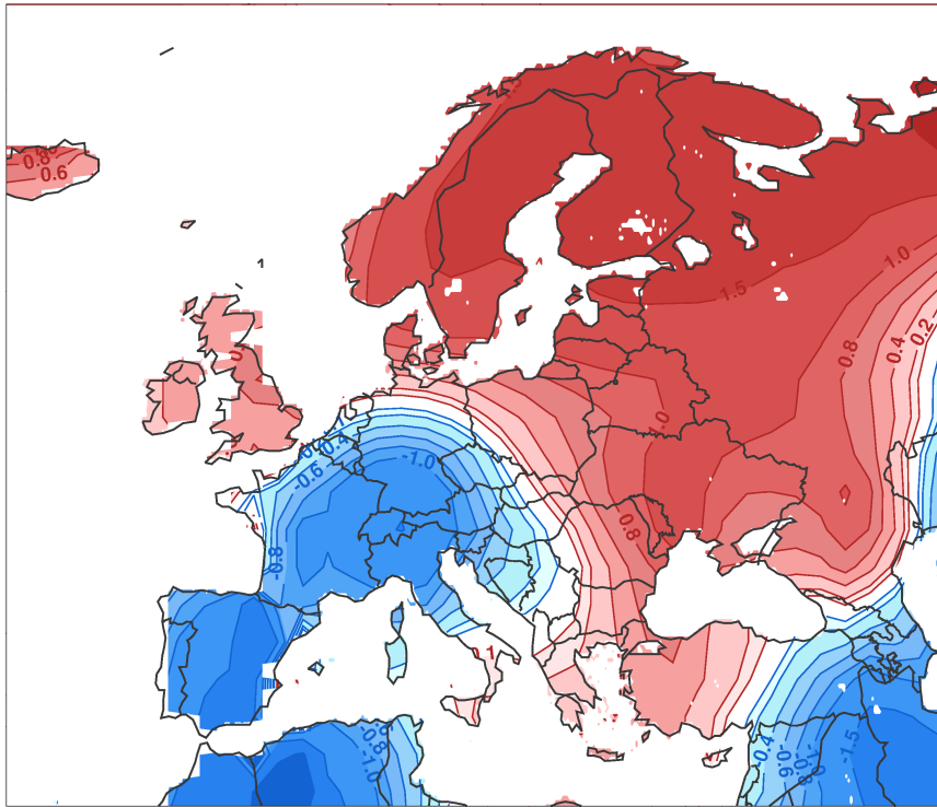
Observed Temperature Anomaly Dec-Jan-Feb 2005
