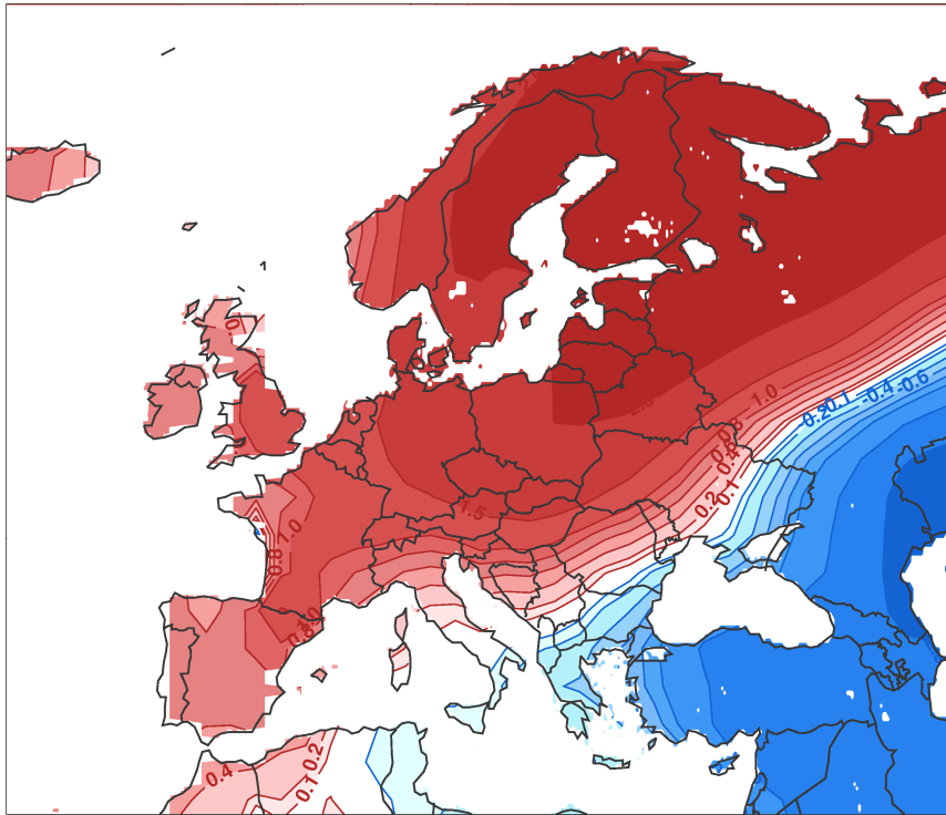
Observed Temperature Anomaly Dec-Jan-Feb 2008
