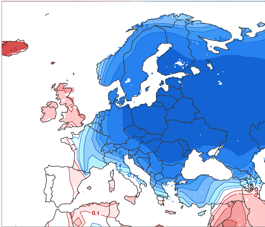
Observed Temperature Anomaly Dec-Jan-Feb 2003
