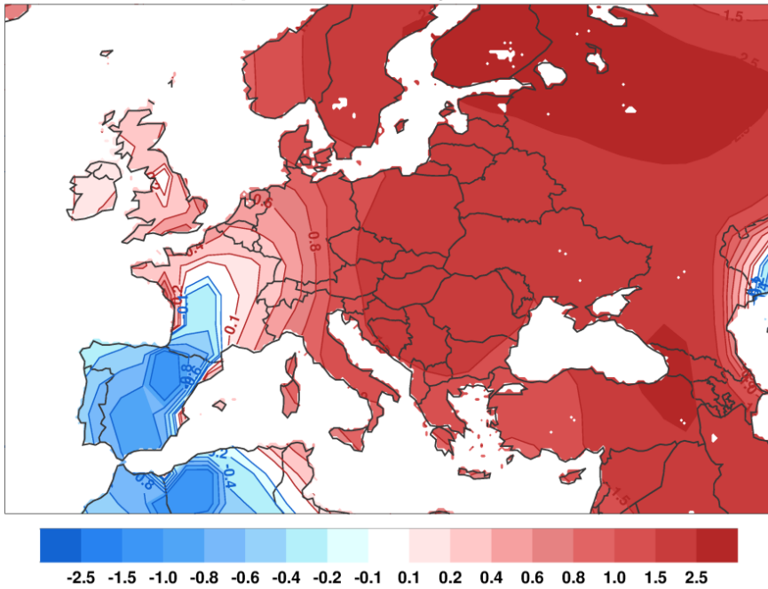
Observed Temperature Anomaly (C) Dec-Jan-Feb 2015
