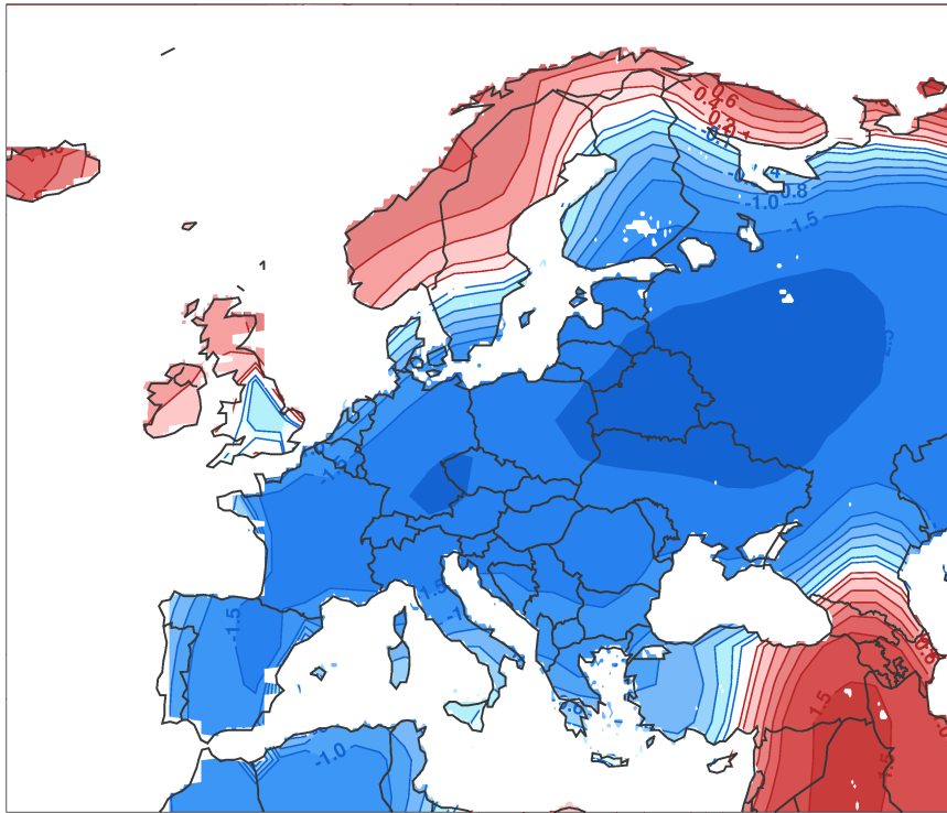
Observed Temperature Anomaly Dec-Jan-Feb 2006
