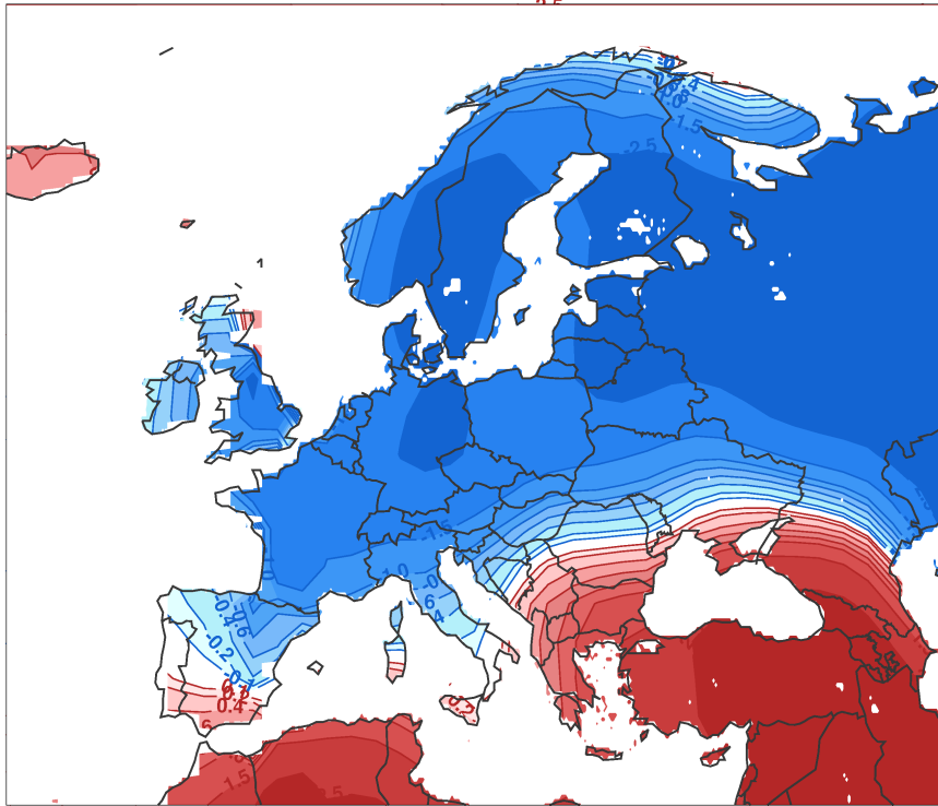
Observed Temperature Anomaly Dec-Jan-Feb 2010
