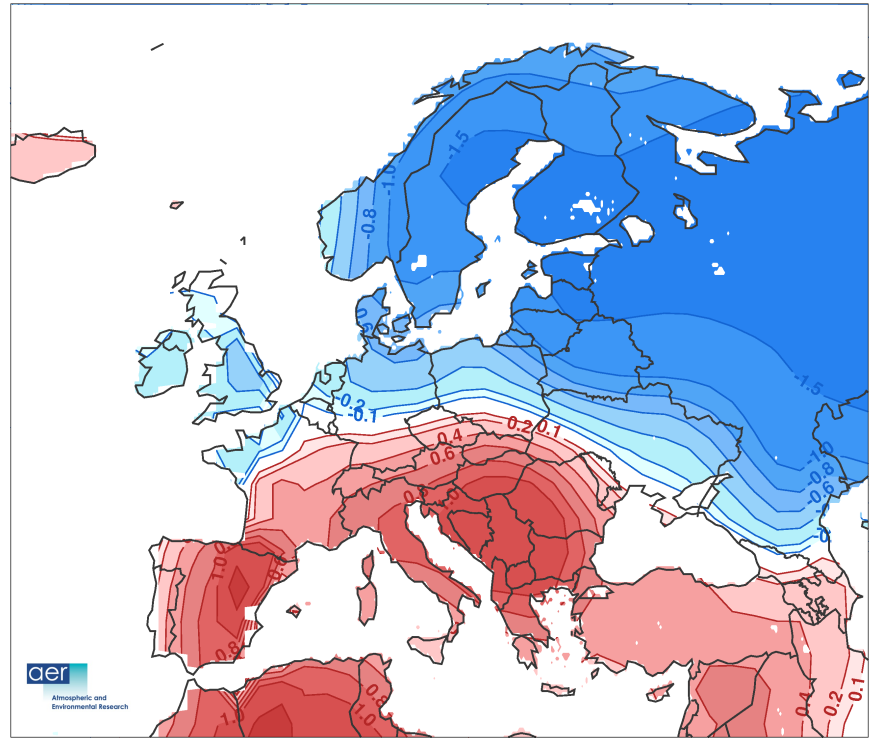
AER Forecast Temperature Anomaly Dec-Jan-Feb 2010
