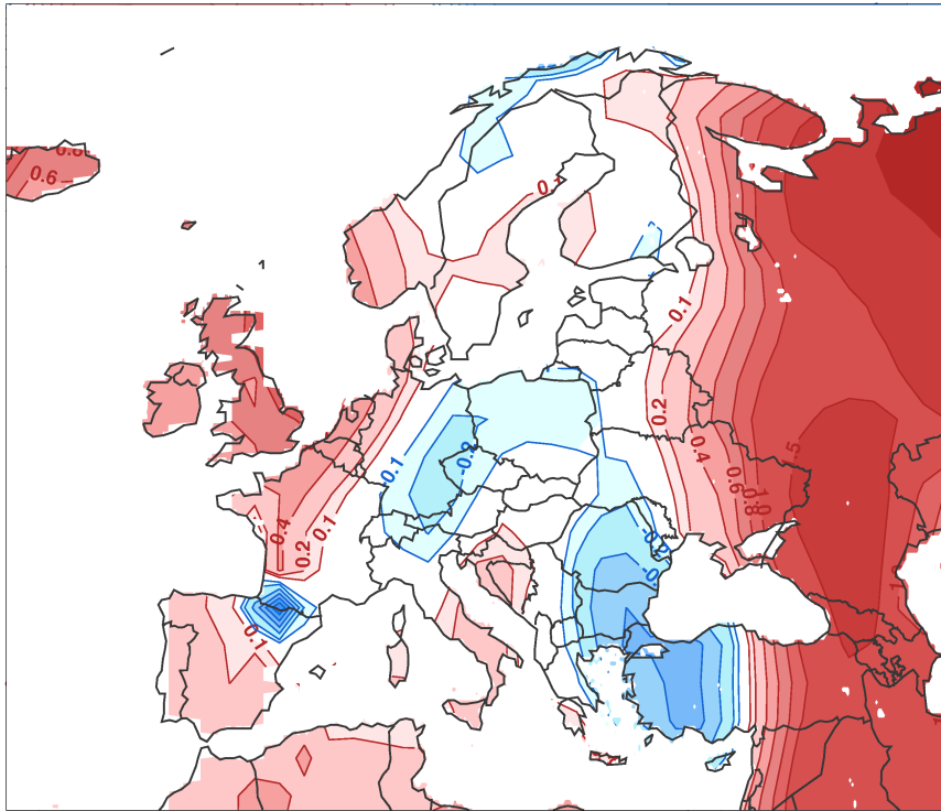
Observed Temperature Anomaly Dec-Jan-Feb 2004
