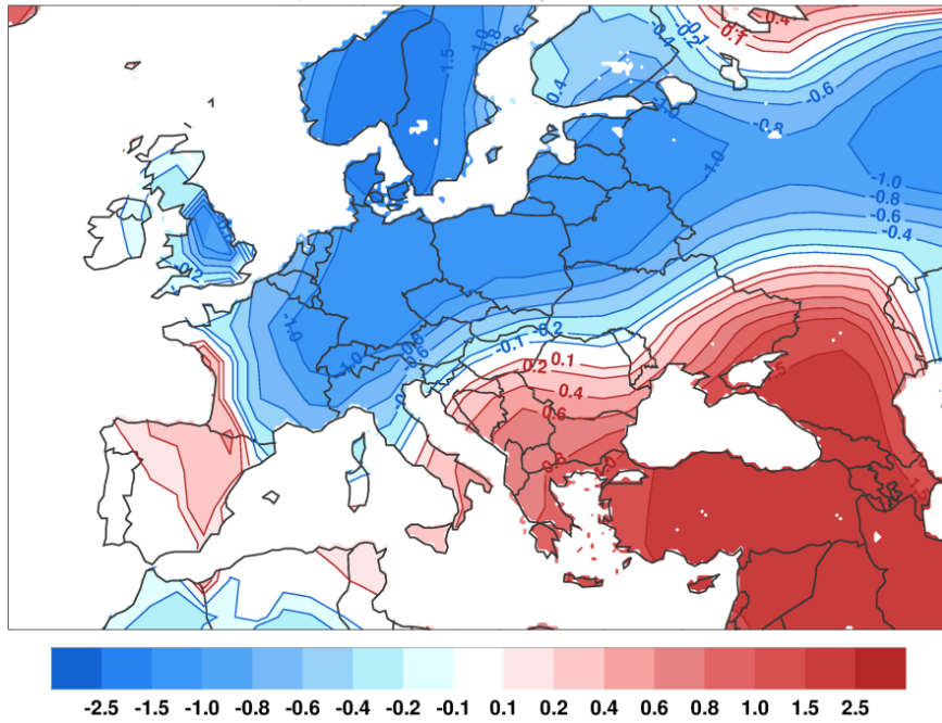
Observed Temperature Anomaly (C) Dec-Jan-Feb 2013
