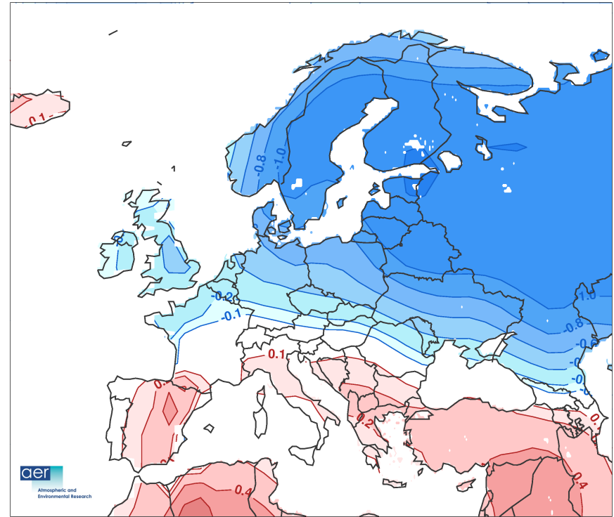
AER Forecast Temperature Anomaly Dec-Jan-Feb 2004
