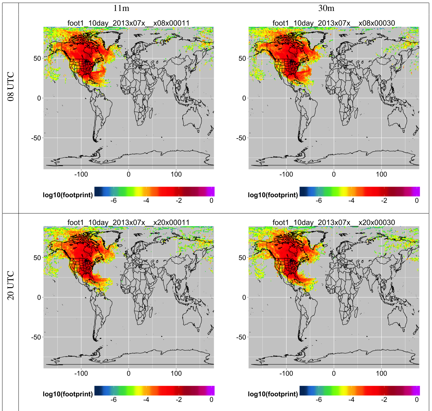
FIG. 7. Average July 10-day footprints
