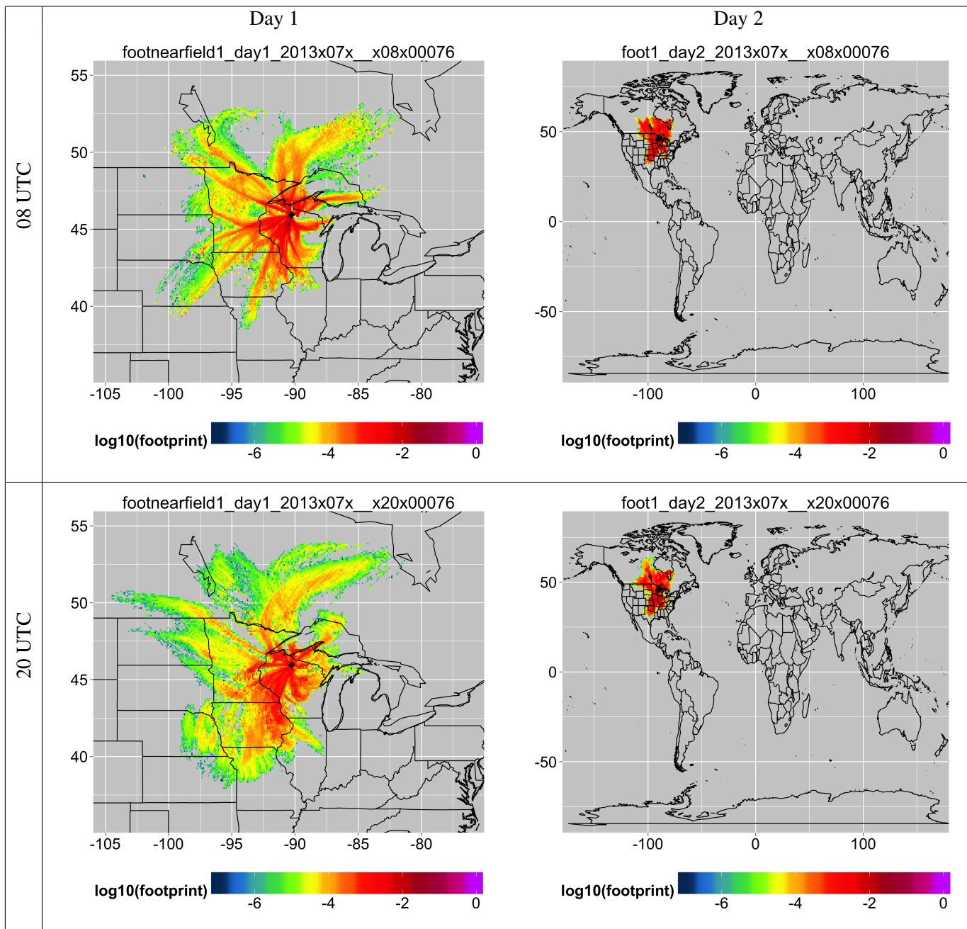
FIG. 3. Average July footprints for 76m receptor
