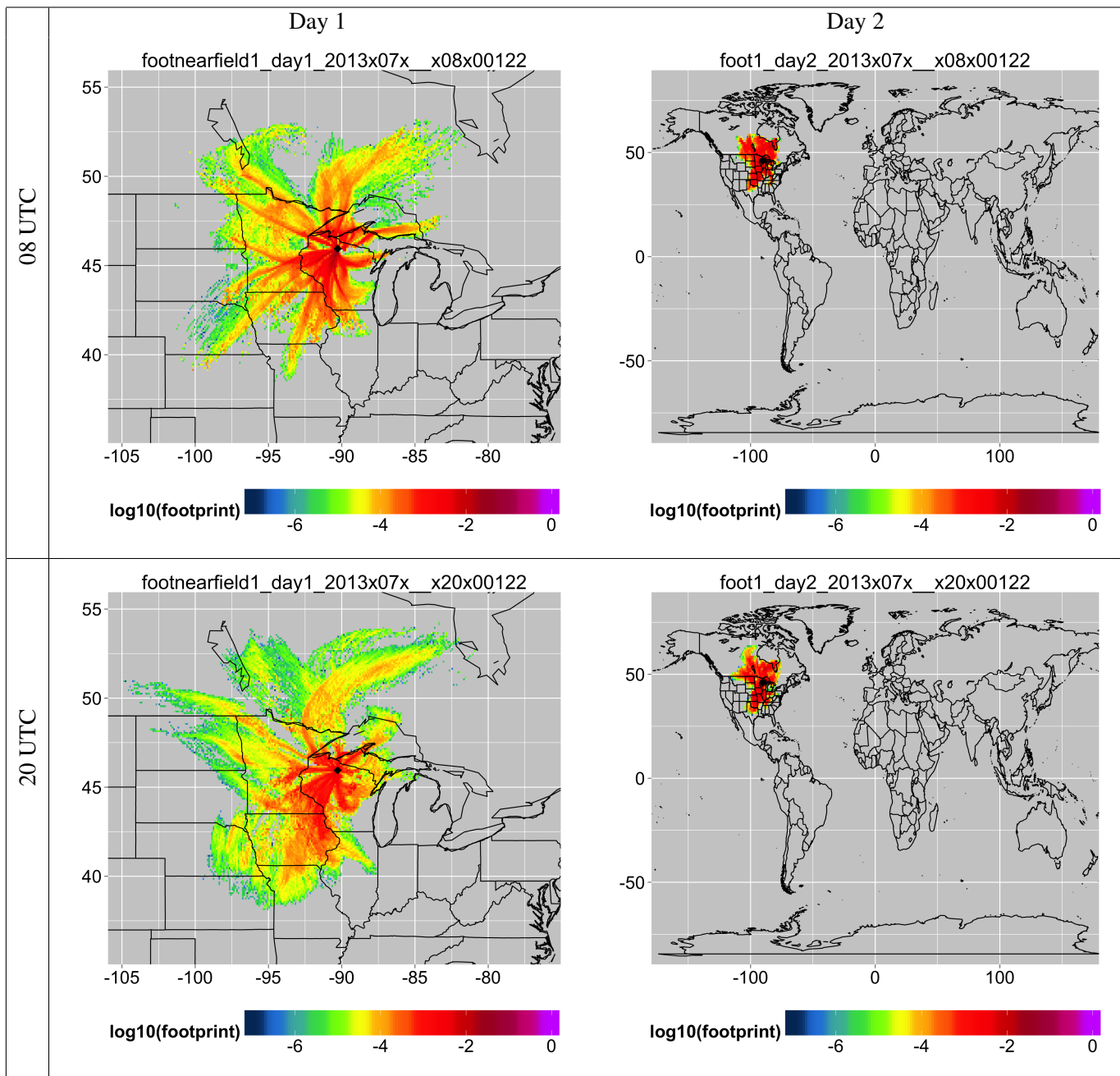
FIG. 4. Average July footprints for 122m receptor
