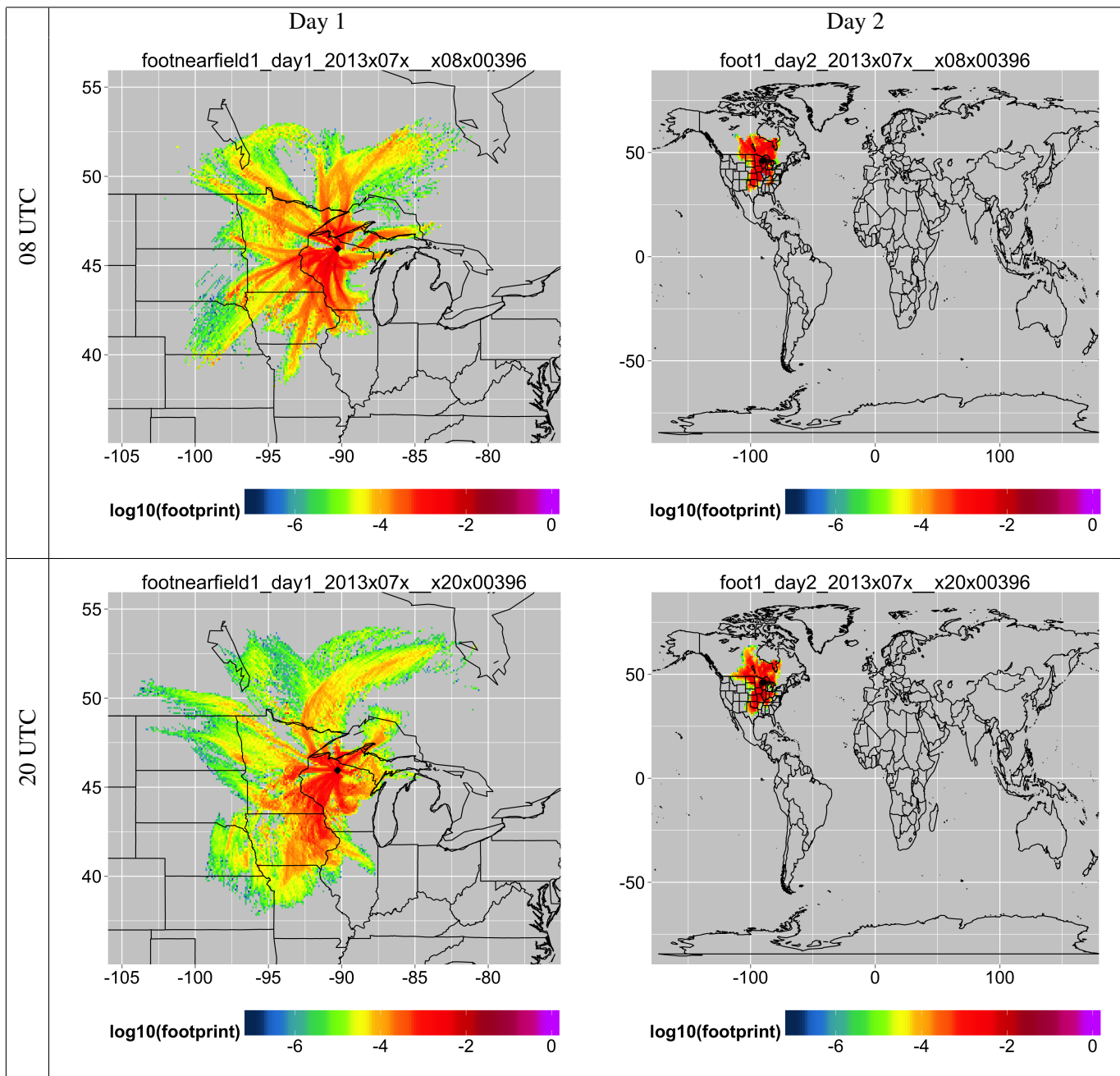
FIG. 6. Average July footprints for 396m receptor
