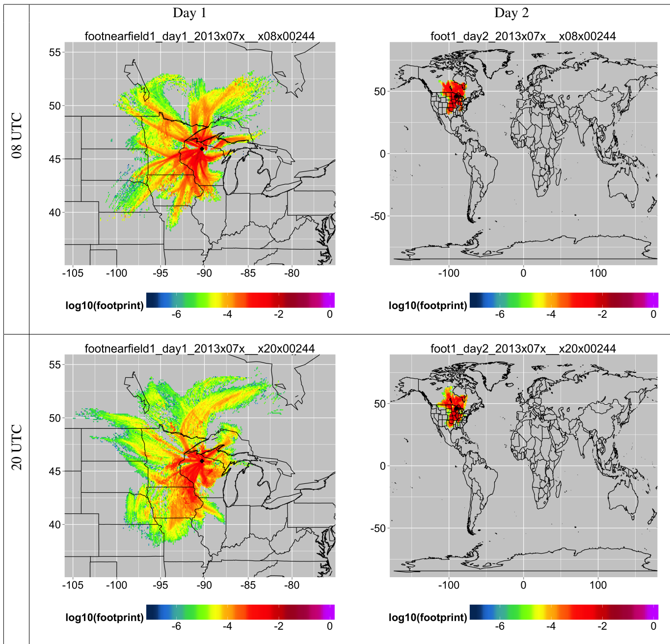
FIG. 5. Average July footprints for 244m receptor
