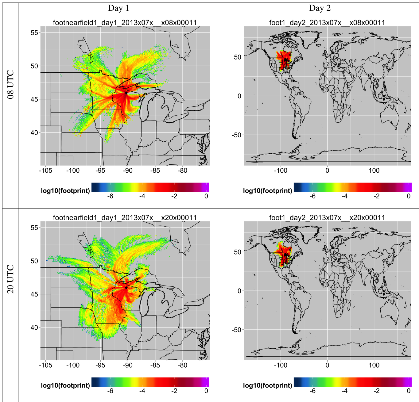
FIG. 1. Average July footprints for 11m receptor
