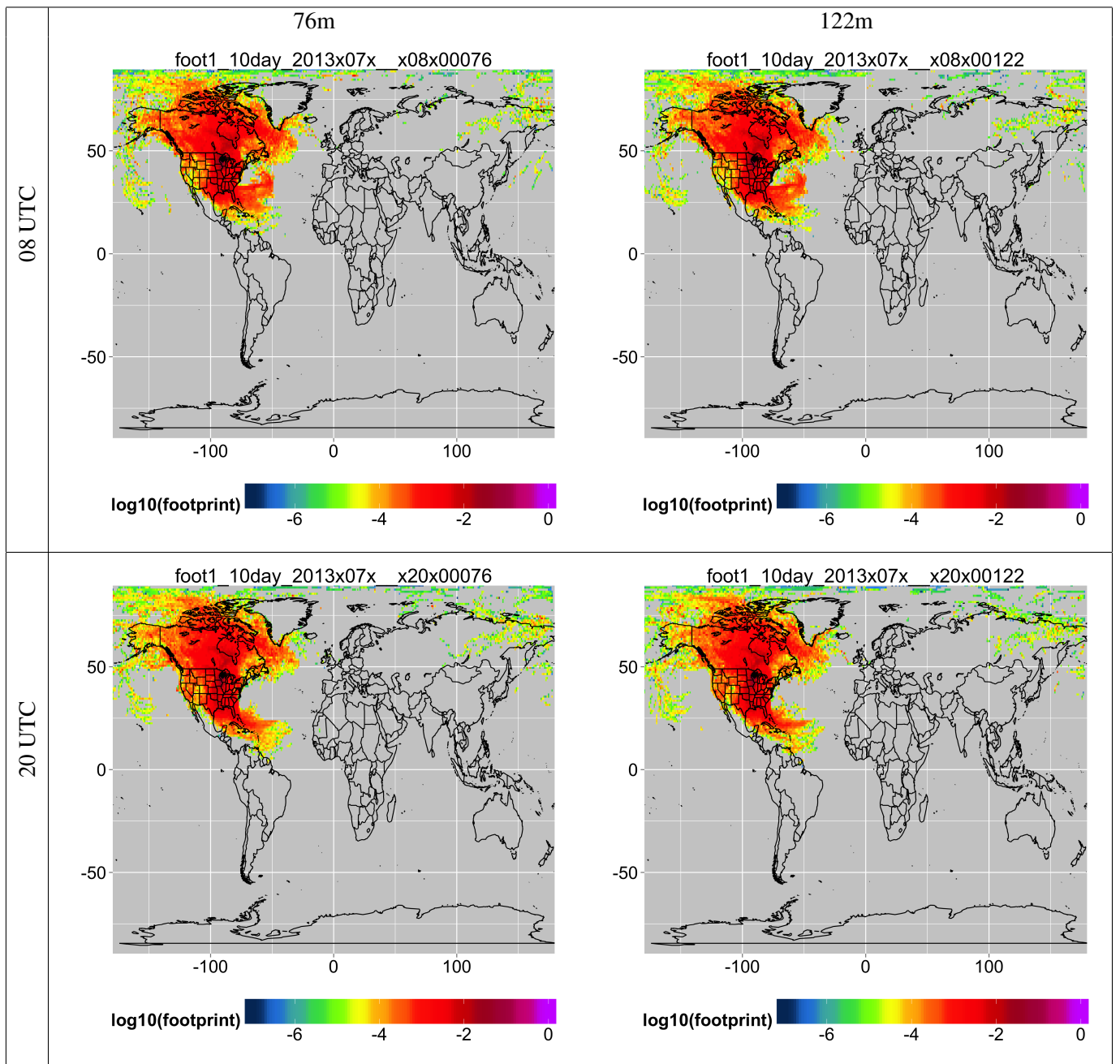
FIG. 8. Average July 10-day footprints
