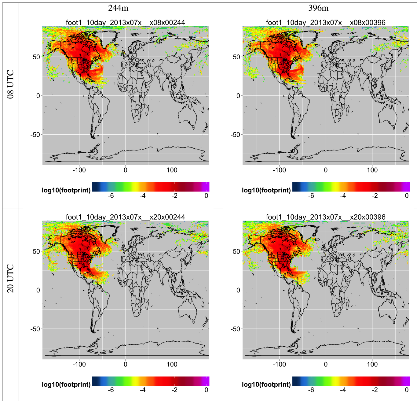
FIG. 9. Average July 10-day footprints
