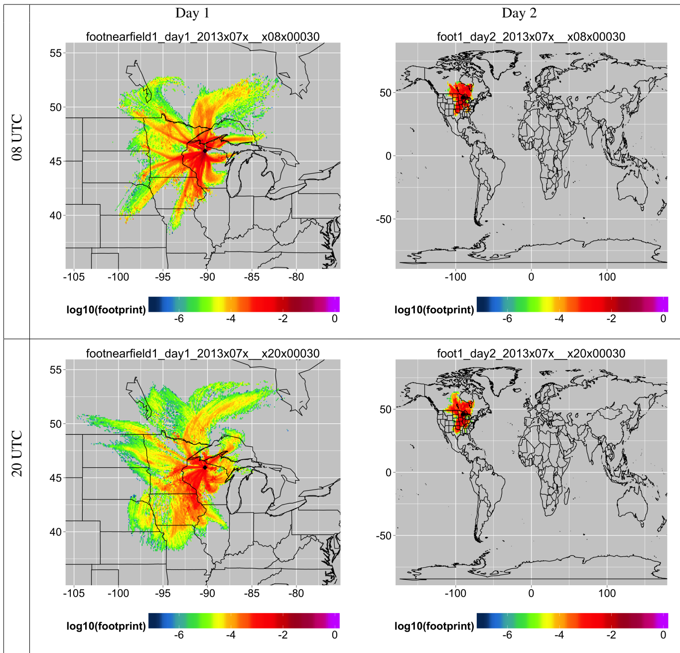
FIG. 2. Average July footprints for 30m receptor
