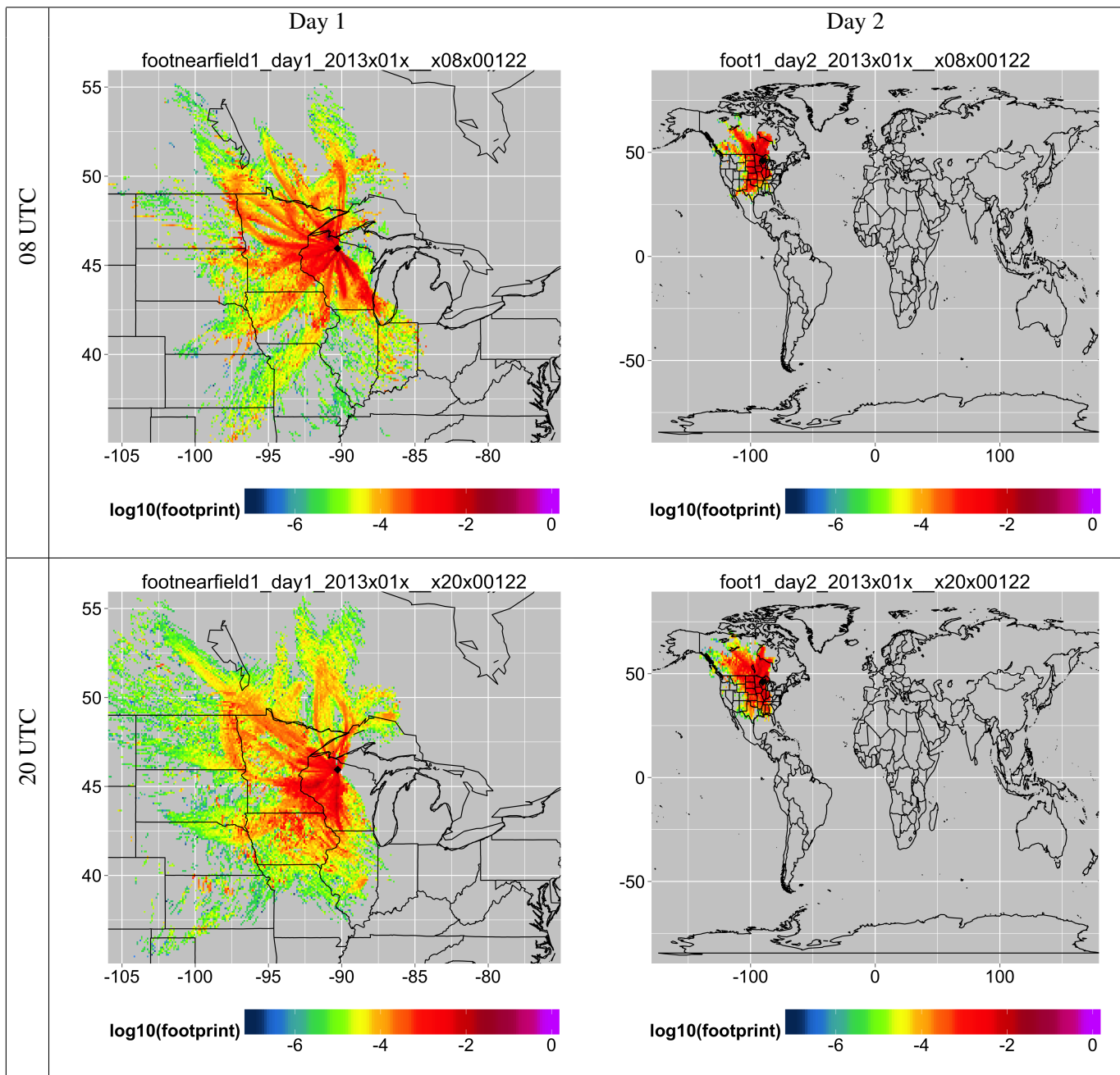
FIG. 4. Average January footprints for 122m receptor
