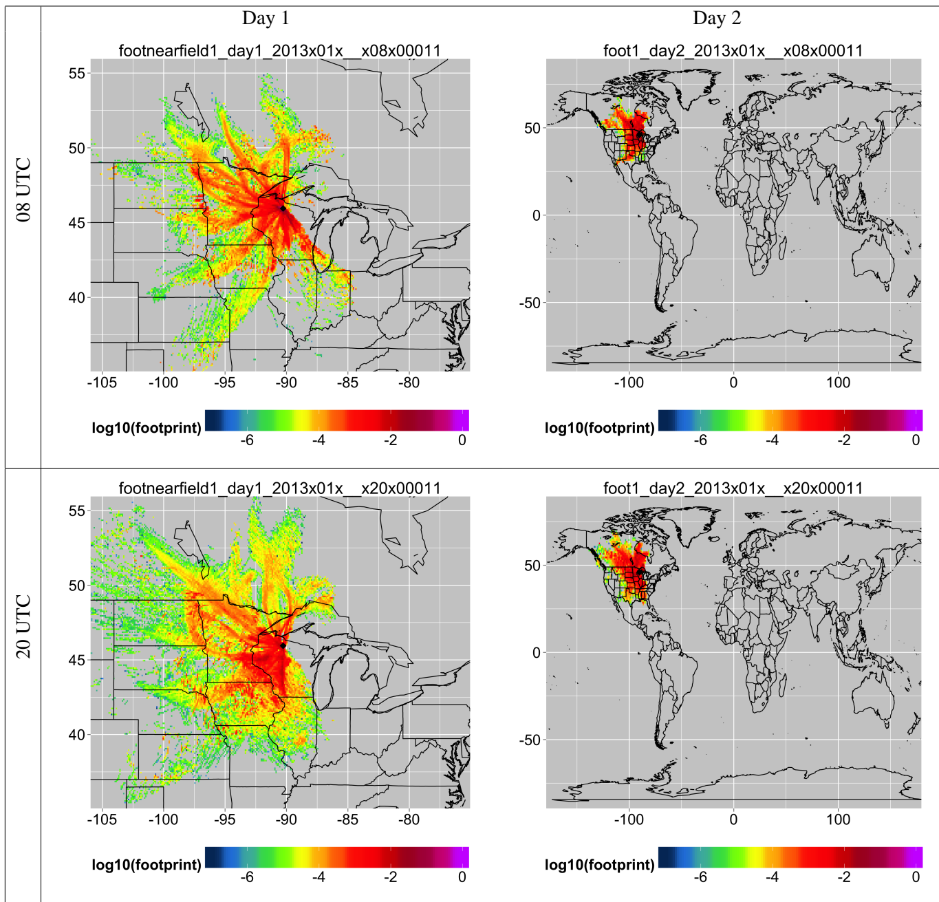
FIG. 1. Average January footprints for 11m receptor
