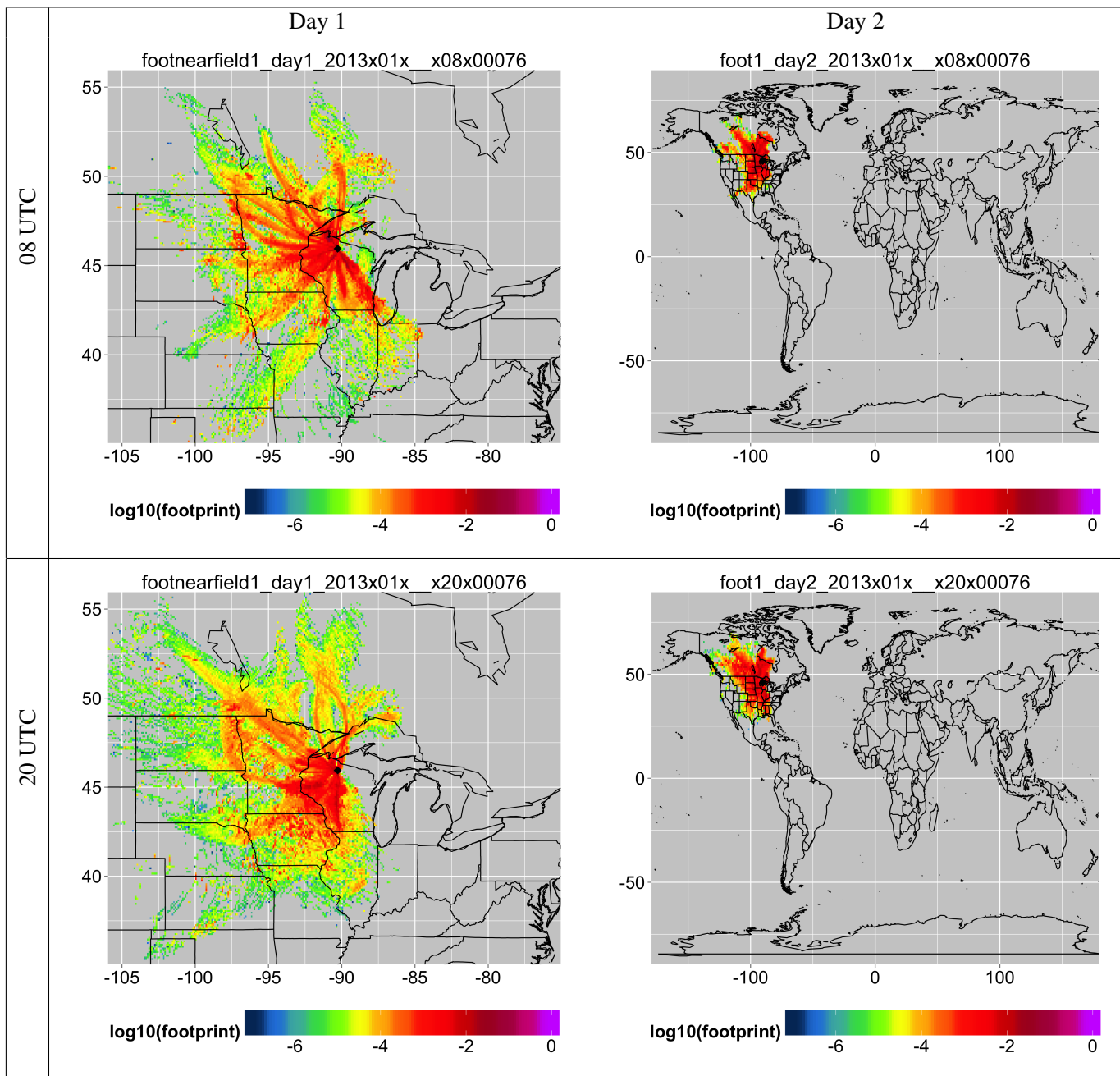
FIG. 3. Average January footprints for 76m receptor
