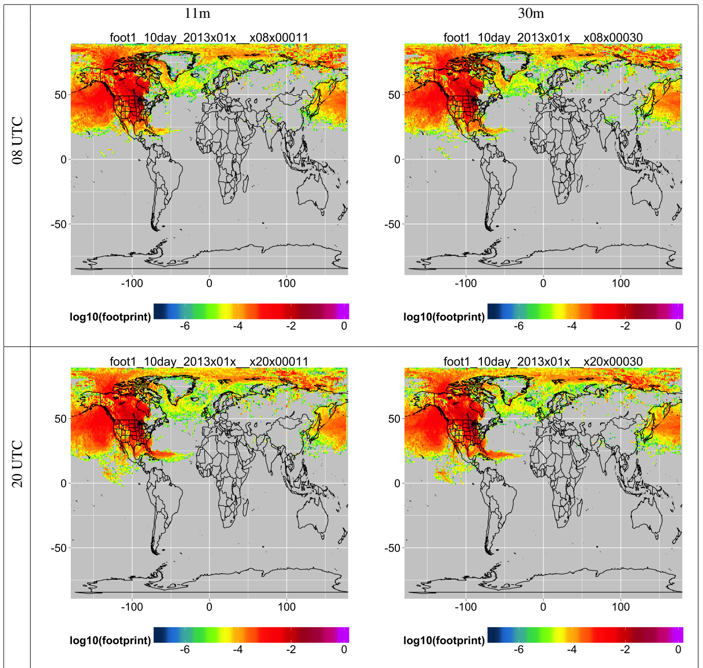
FIG. 7. Average January 10-day footprints
