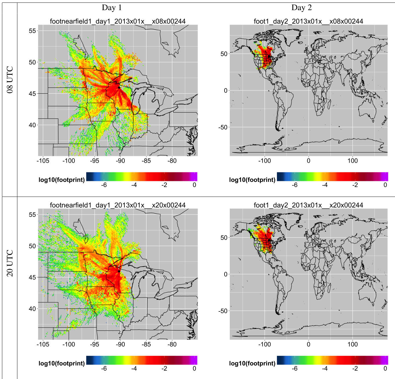
FIG. 5. Average January footprints for 244m receptor
