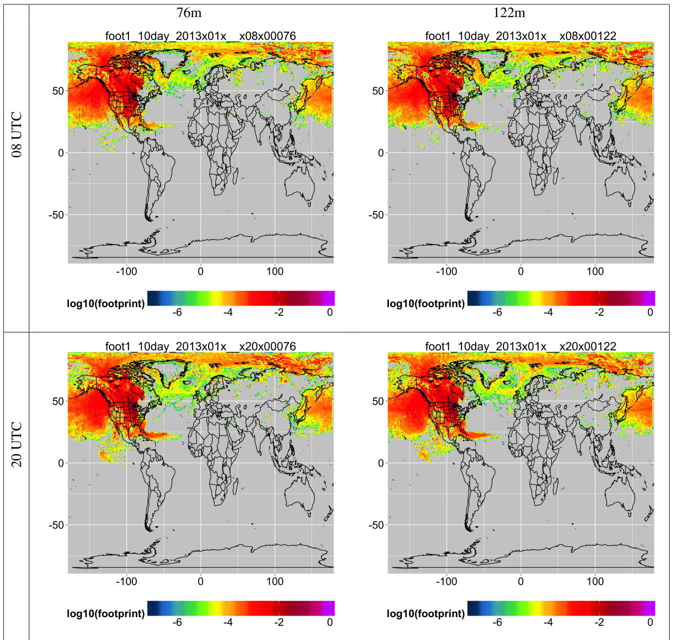
FIG. 8. Average January 10-day footprints
