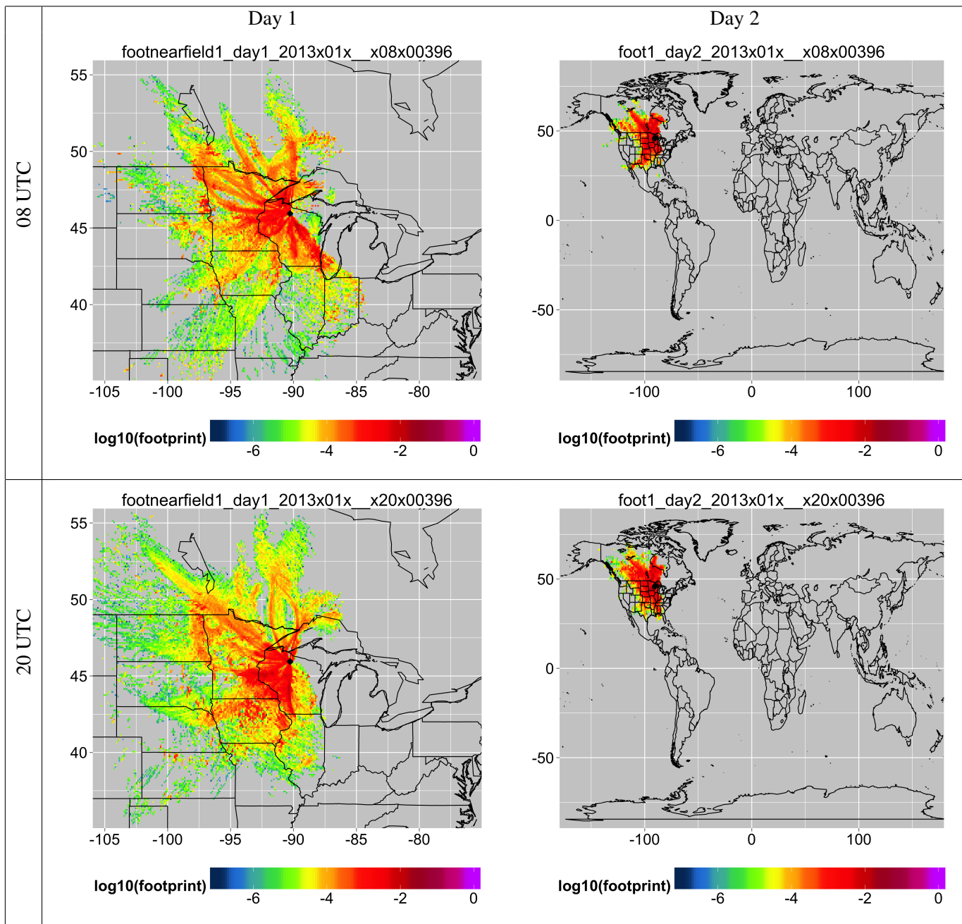
FIG. 6. Average January footprints for 396m receptor
