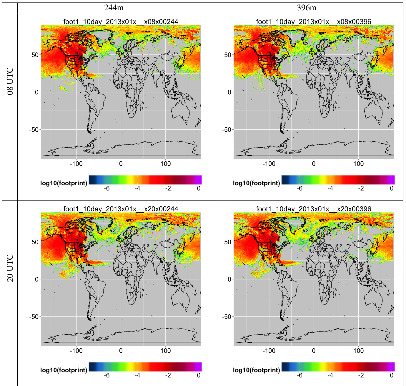
FIG. 9. Average January 10-day footprints
