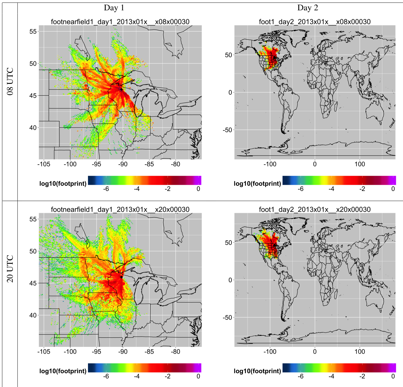
FIG. 2. Average January footprints for 30m receptor
